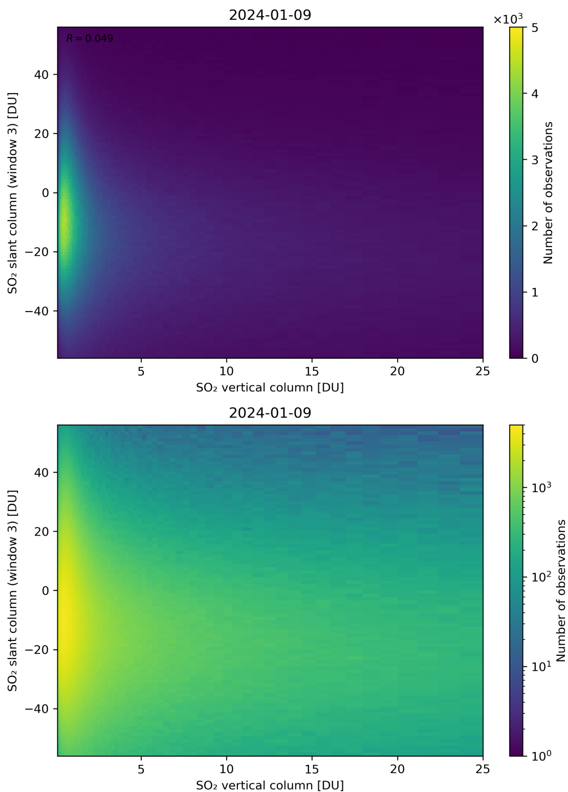
Figure 303: Scatter density plot of “SO 2 vertical column” against “SO 2 slant column (window 3)” for 2024-01-08 to 2024-01-10.
