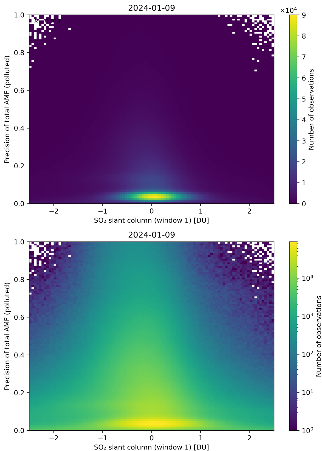
Figure 240: Scatter density plot of “SO 2 slant column (window 1)” against “Precision of total AMF (polluted)” for 2024-01-08 to 2024-01-10.
