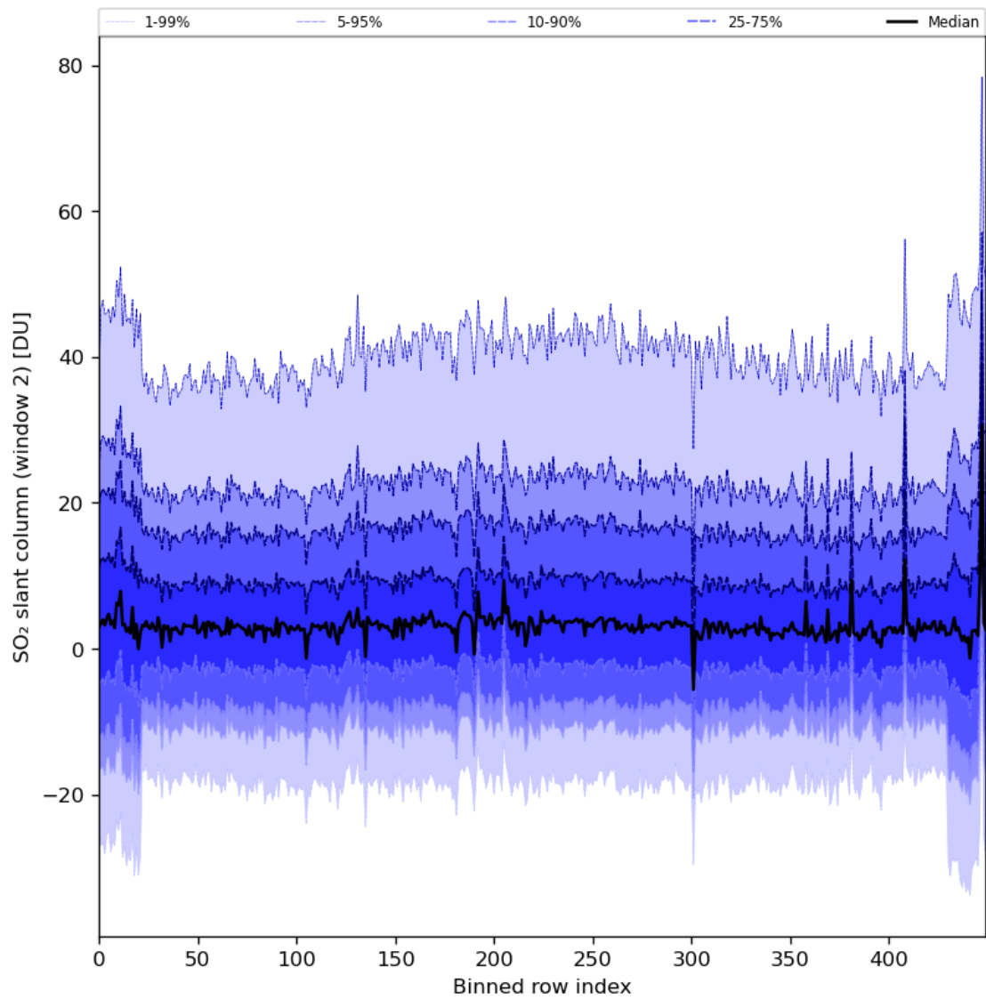
Figure 83: Along track statistics of “SO 2 slant column (window 2)” for 2024-01-08 to 2024-01-10
