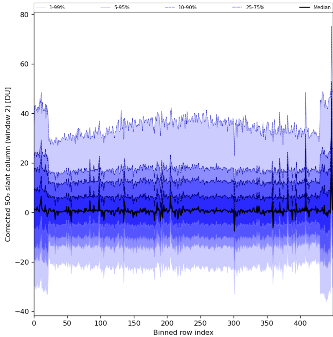
Figure 85: Along track statistics of “Corrected SO 2 slant column (window 2)” for 2024-01-08 to 2024-01-10
