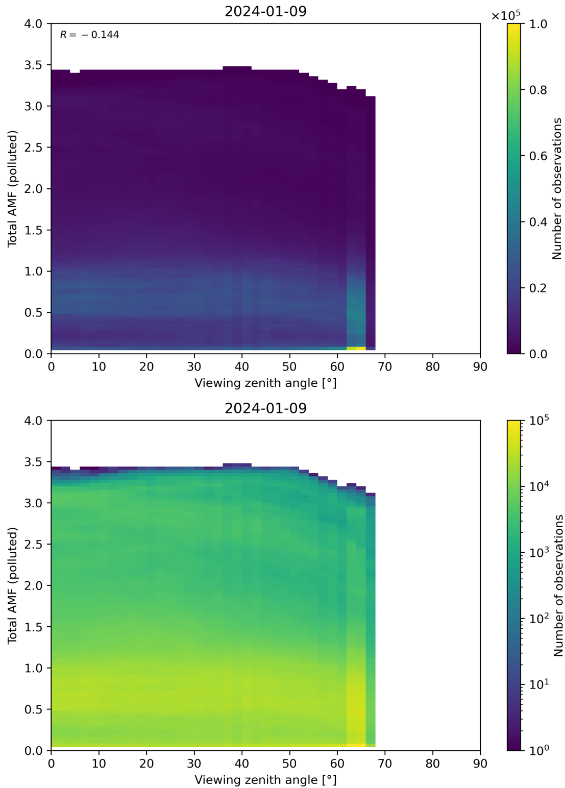
Figure 325: Scatter density plot of “Viewing zenith angle” against “Total AMF (polluted)” for 2024-01-08 to 2024-01-10.
