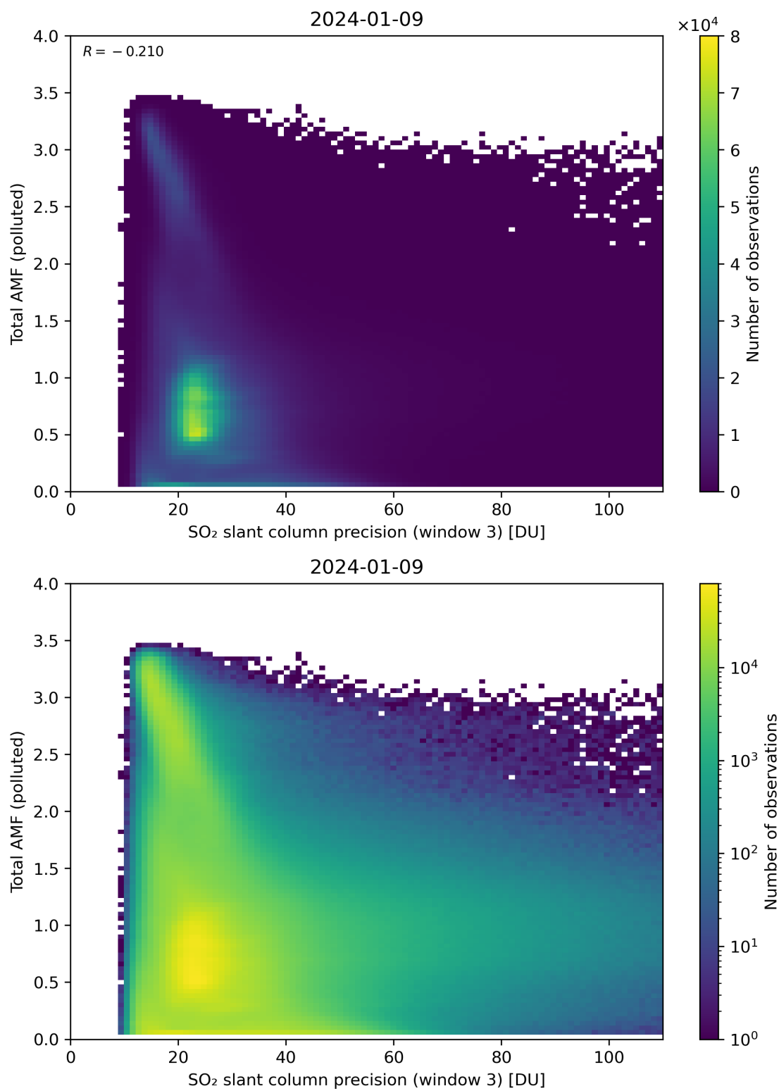
Figure 263: Scatter density plot of “SO 2 slant column precision (window 3)” against “Total AMF (polluted)” for 2024-01-08 to 2024-01-10.
