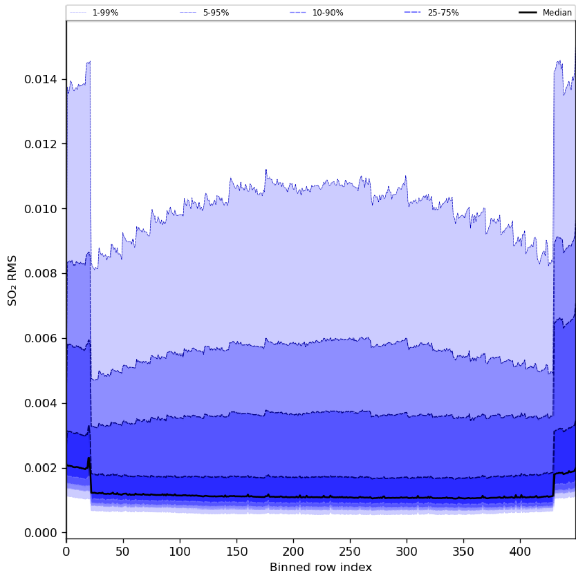
Figure 93: Along track statistics of “SO 2 RMS” for 2024-01-08 to 2024-01-10
