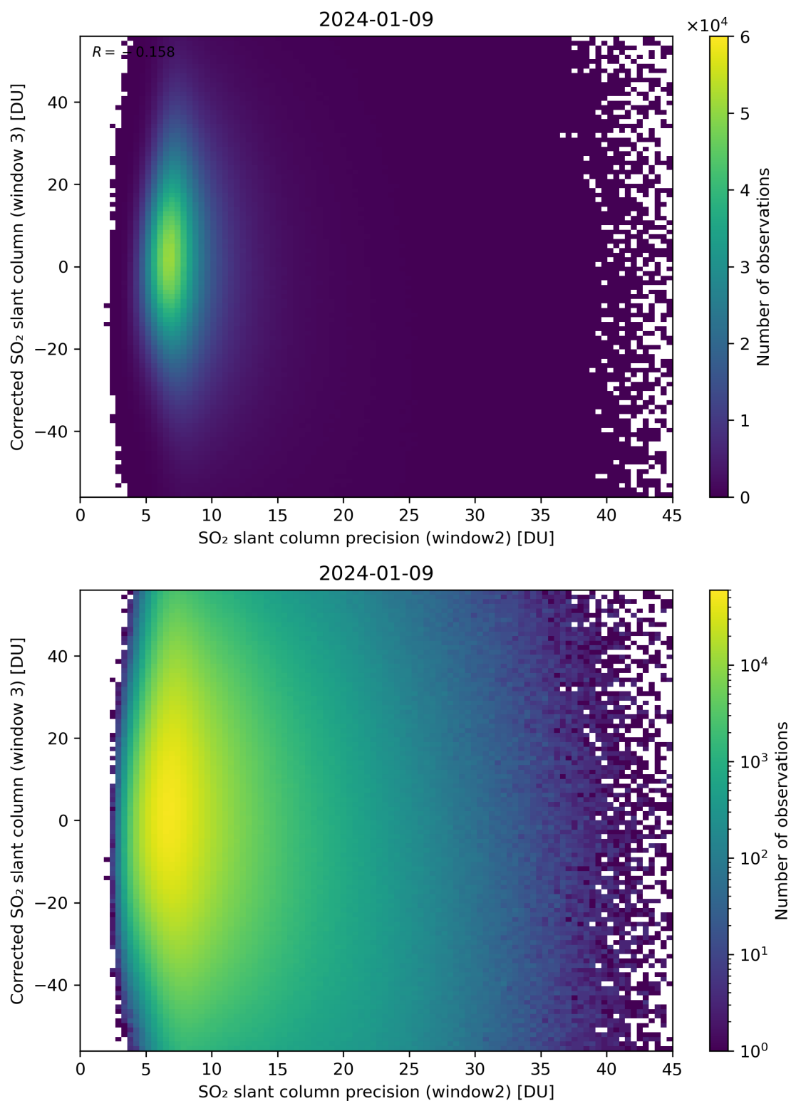
Figure 248: Scatter density plot of “SO 2 slant column precision (window2)” against “Corrected SO 2 slant column (window 3)” for 2024-01-08 to 2024-01-10.
