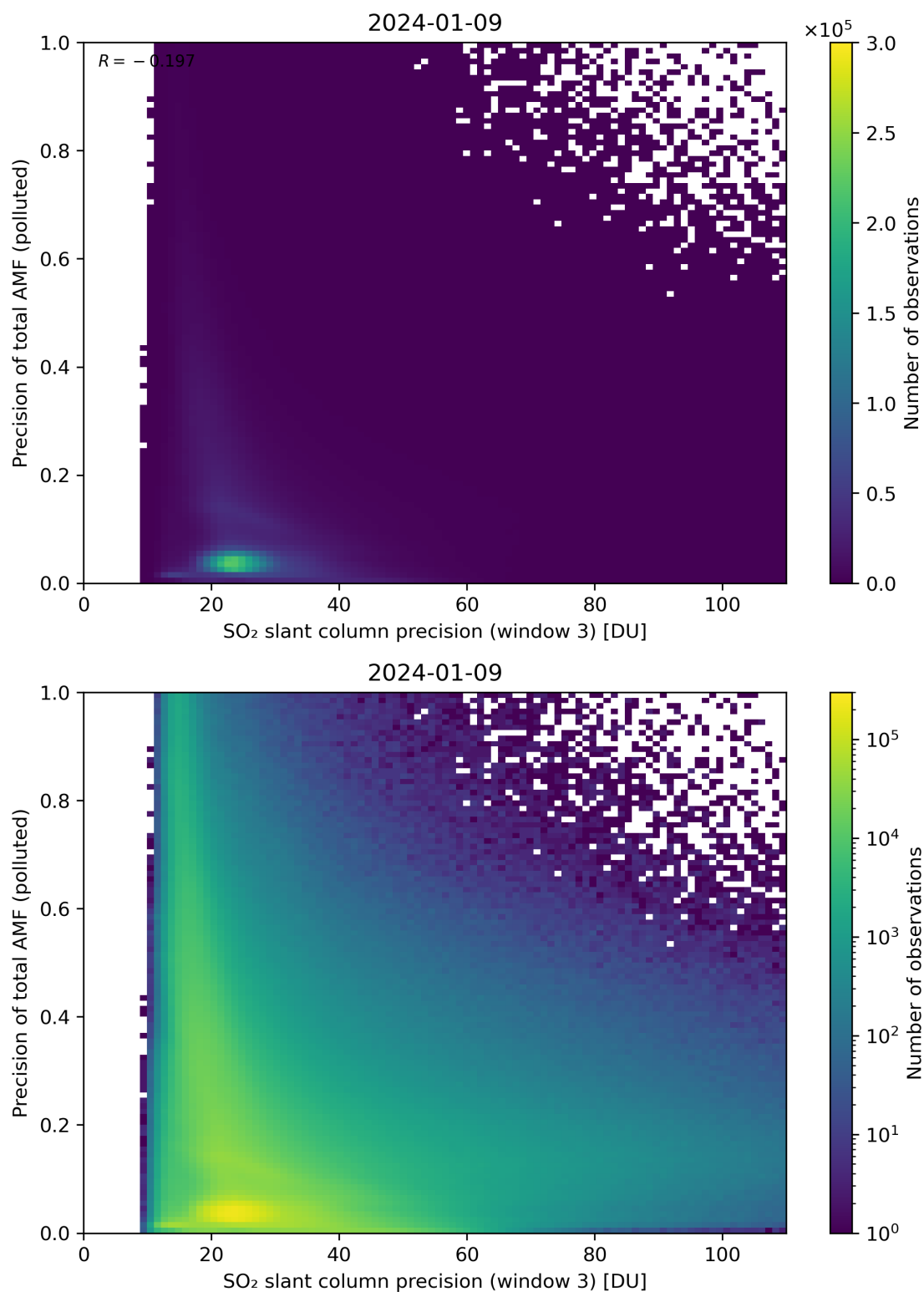
Figure 264: Scatter density plot of “SO 2 slant column precision (window 3)” against “Precision of total AMF (polluted)” for 2024-01-08 to 2024-01-10.
