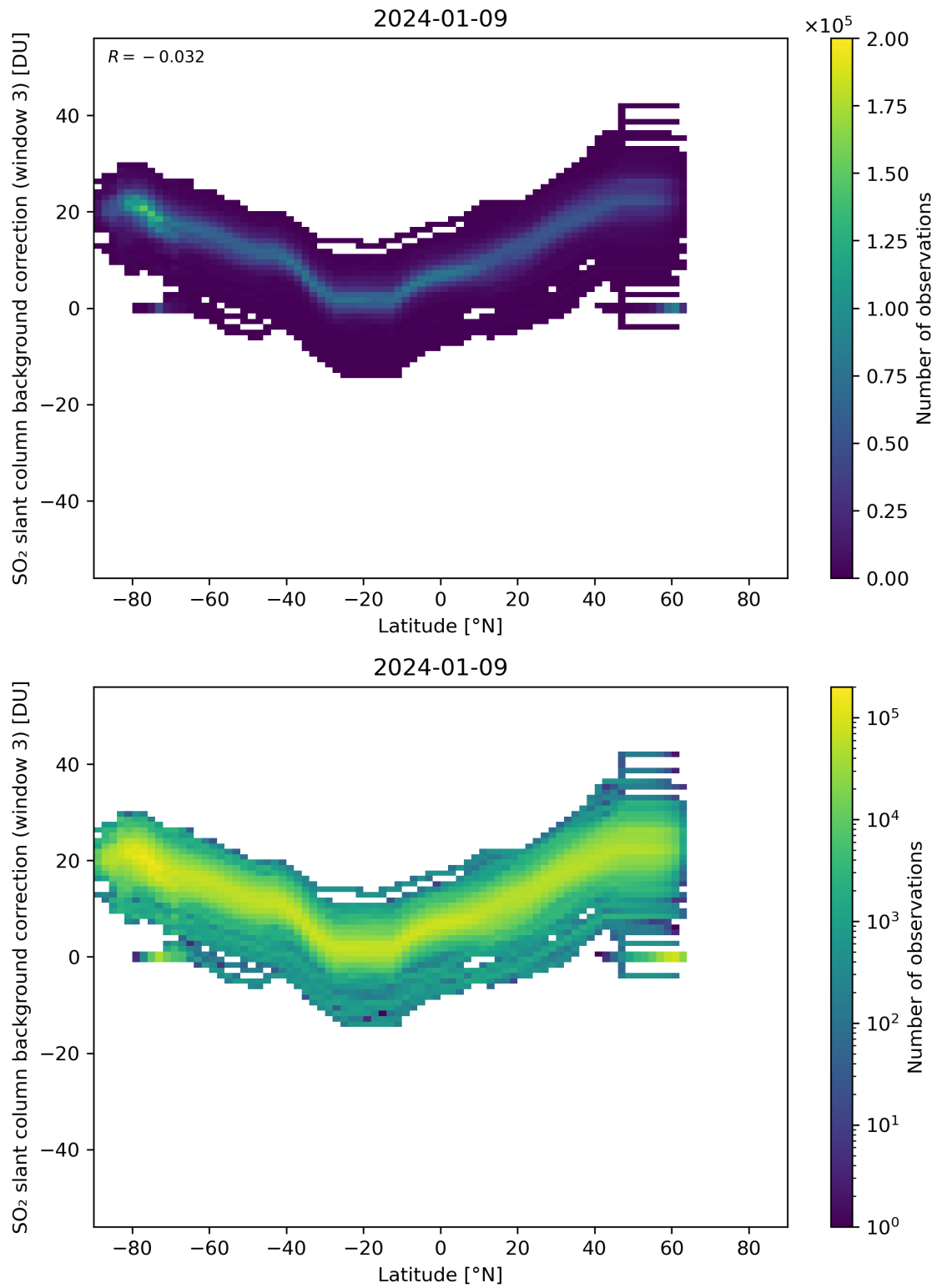
Figure 141: Scatter density plot of “Latitude” against “SO 2 slant column background correction (window 3)” for 2024-01-08 to 2024-01-10.
