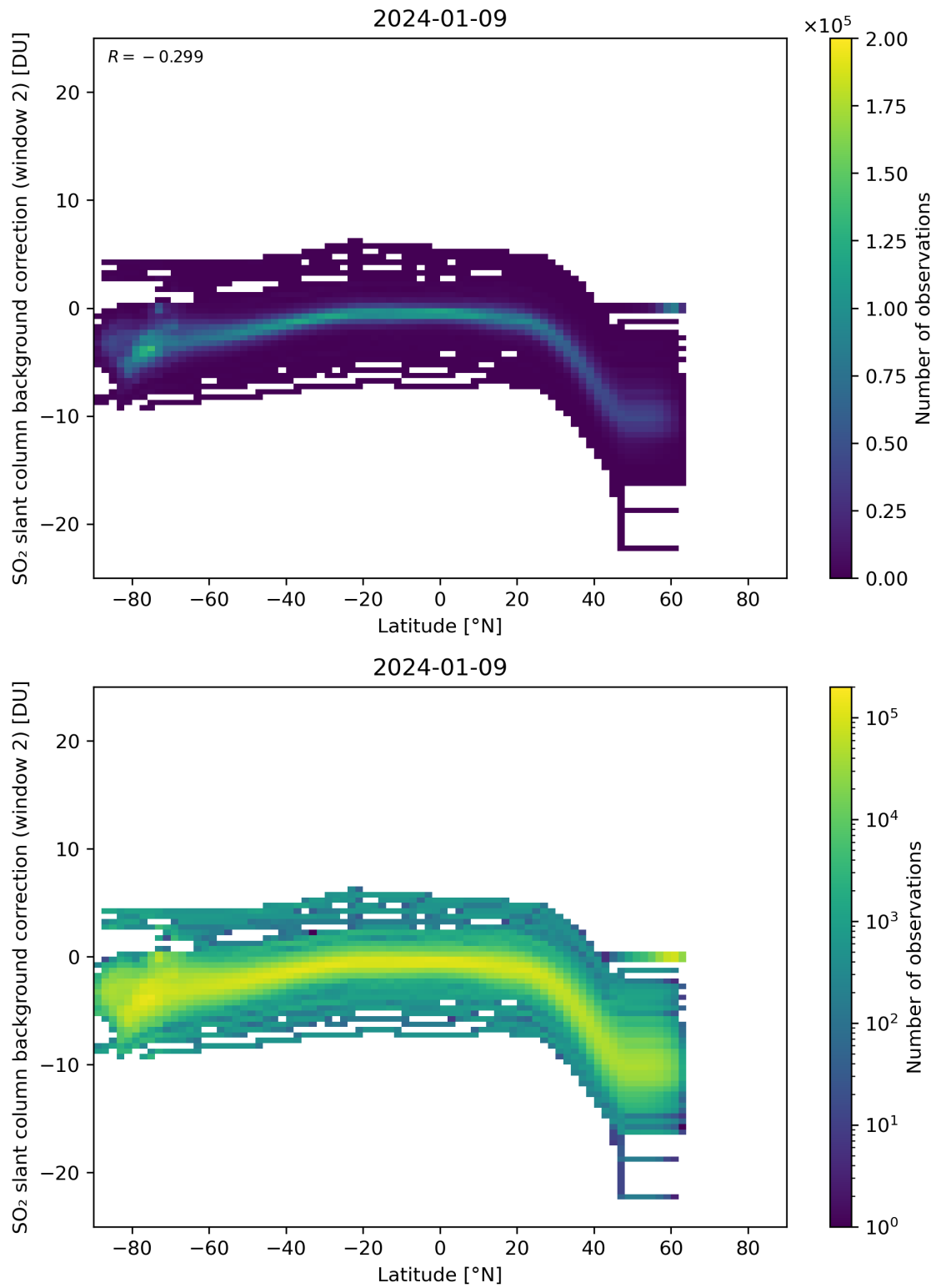
Figure 140: Scatter density plot of “Latitude” against “SO 2 slant column background correction (window 2)” for 2024-01-08 to 2024-01-10.
