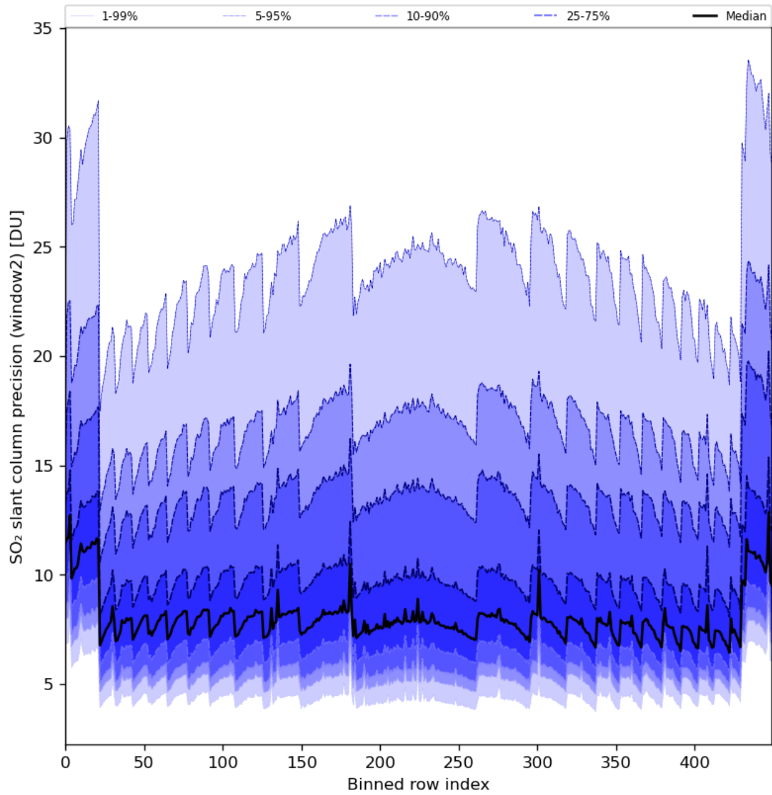
Figure 84: Along track statistics of “SO 2 slant column precision (window2)” for 2024-01-08 to 2024-01-10
