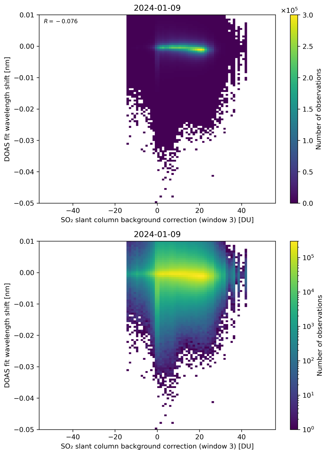
Figure 121: Scatter density plot of “SO 2 slant column background correction (window 3)” against “DOAS fit wavelength shift” for 2024-01-08 to 2024-01-10.
