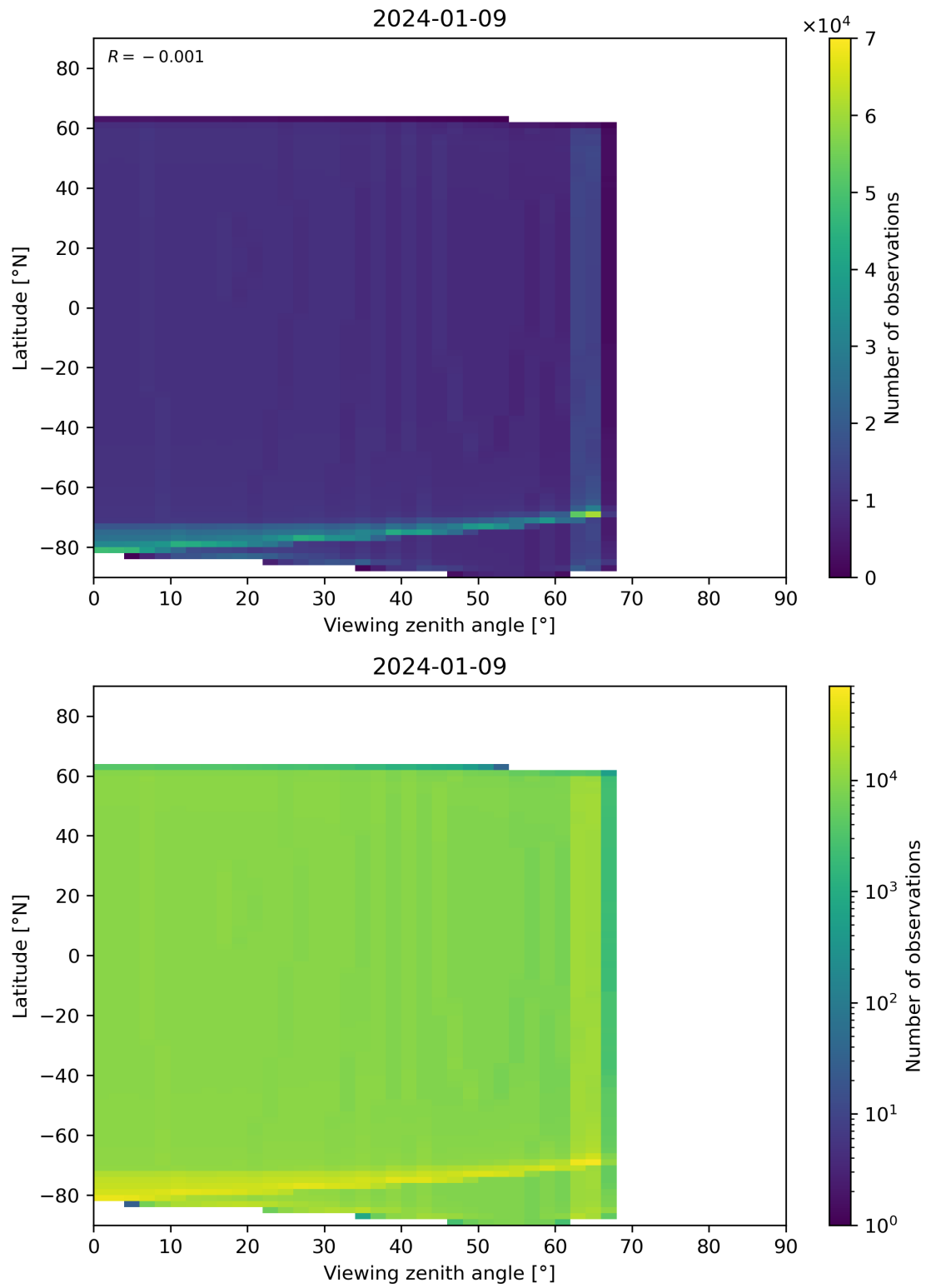
Figure 314: Scatter density plot of “Viewing zenith angle” against “Latitude” for 2024-01-08 to 2024-01-10.
