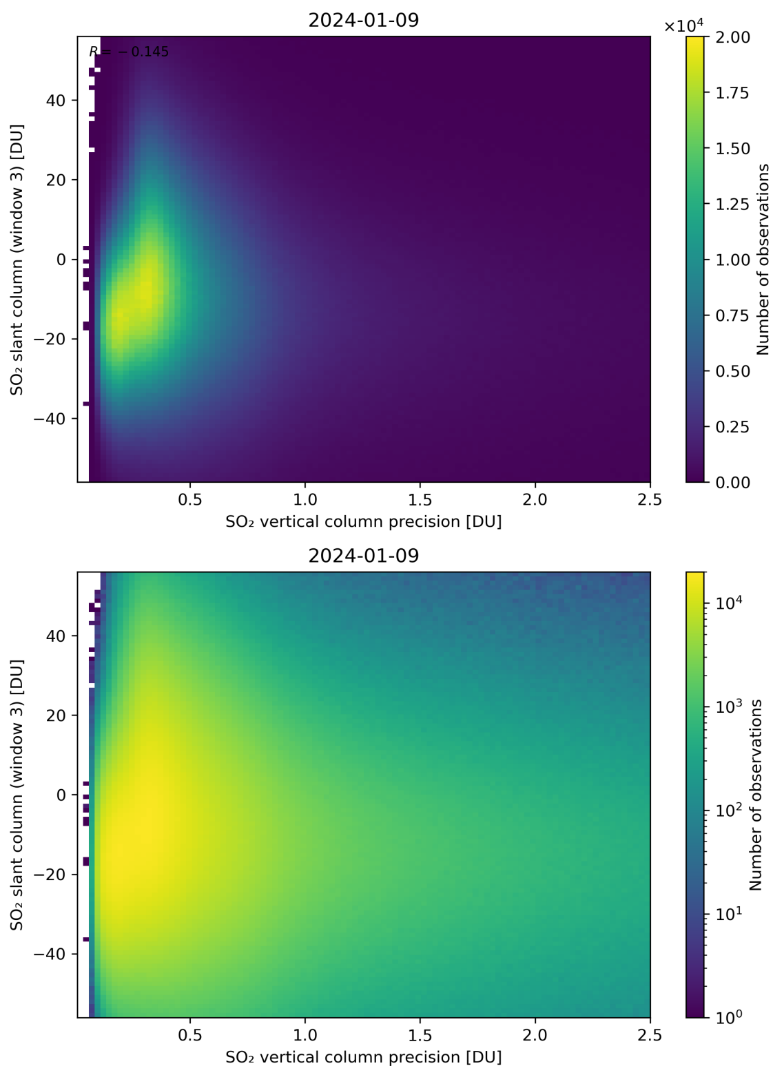
Figure 292: Scatter density plot of “SO 2 vertical column precision” against “SO 2 slant column (window 3)” for 2024-01-08 to 2024-01-10.
