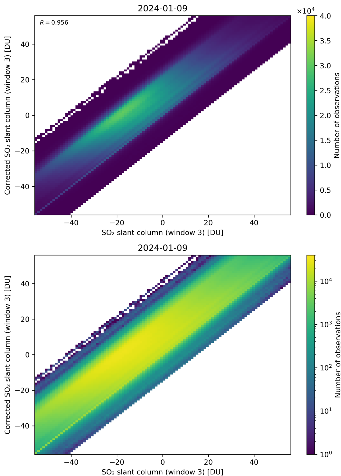
Figure 266: Scatter density plot of “SO 2 slant column (window 3)” against “Corrected SO 2 slant column (window 3)” for 2024-01-08 to 2024-01-10.
