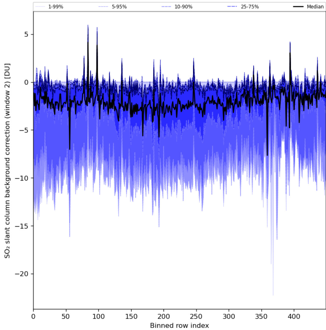
Figure 86: Along track statistics of “SO 2 slant column background correction (window 2)” for 2024-01-08 to 2024-01-10
