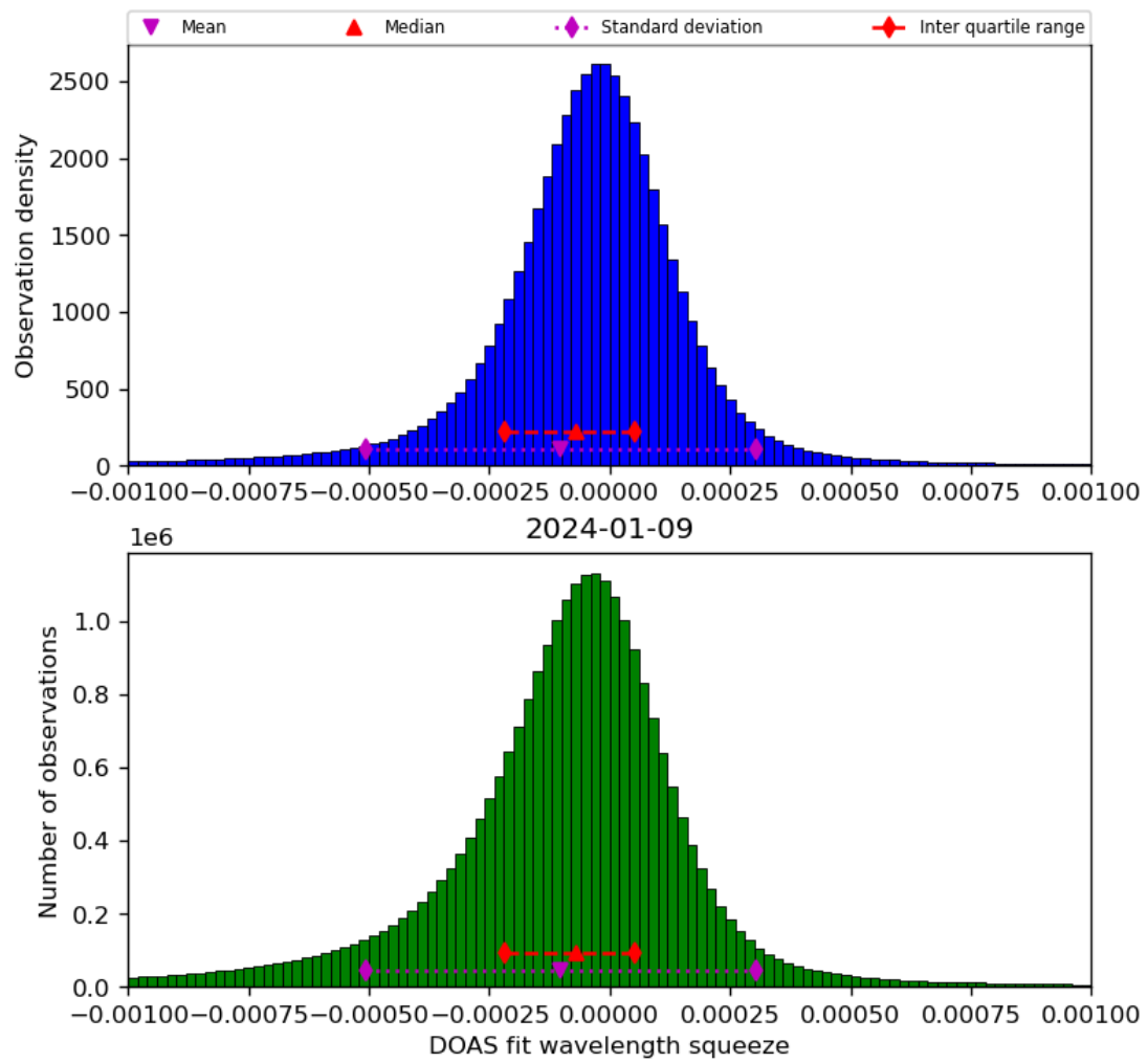
Figure 69: Histogram of “DOAS fit wavelength squeeze” for 2024-01-08 to 2024-01-10
