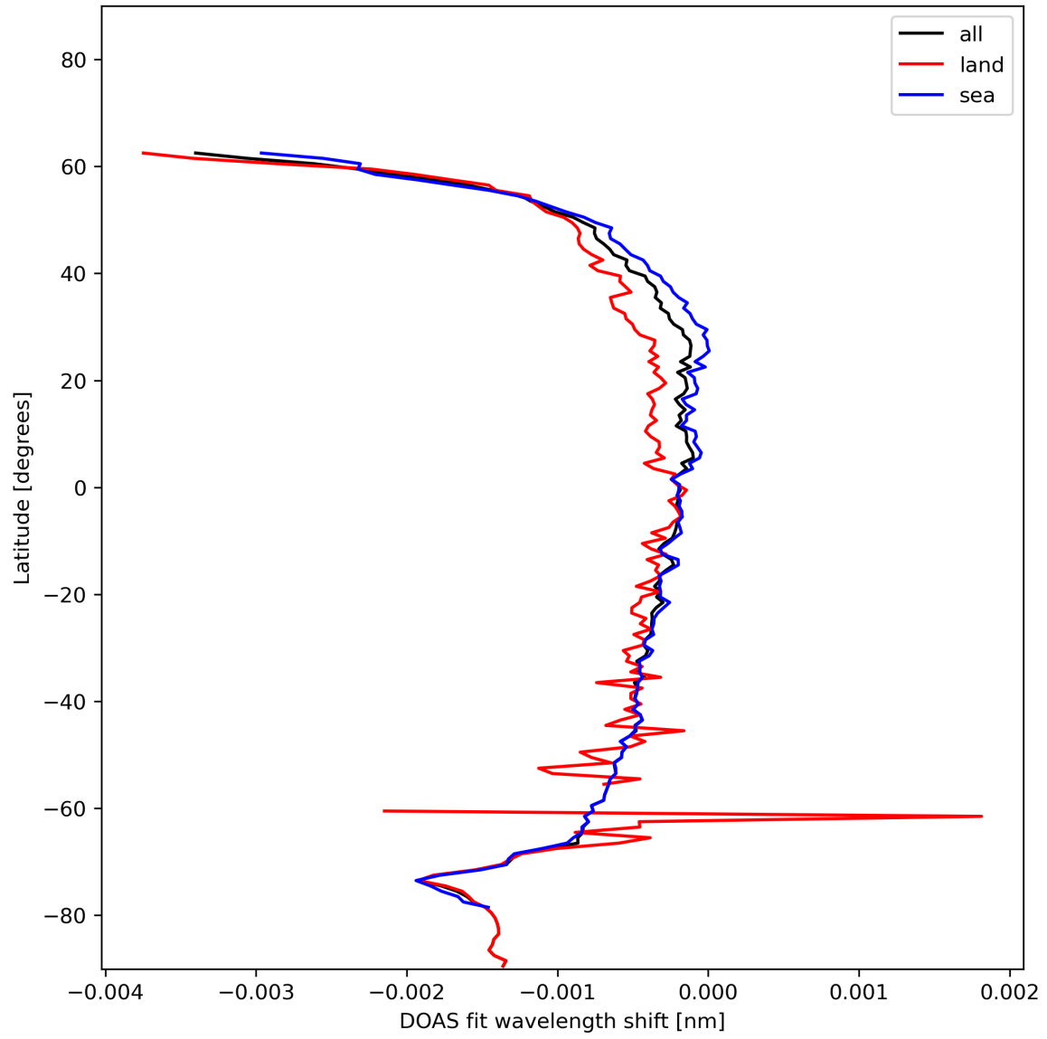
Figure 45: Zonal average of “DOAS fit wavelength shift” for 2024-01-08 to 2024-01-10.
