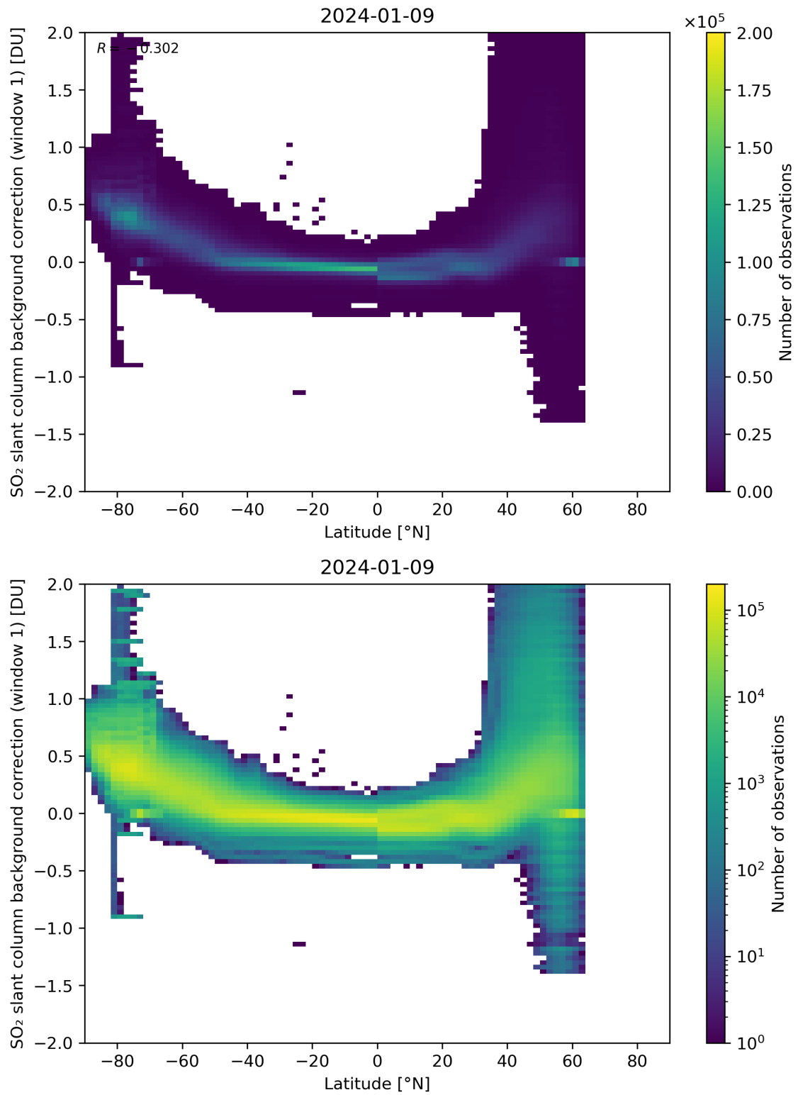
Figure 139: Scatter density plot of “Latitude” against “SO 2 slant column background correction (window 1)” for 2024-01-08 to 2024-01-10.
