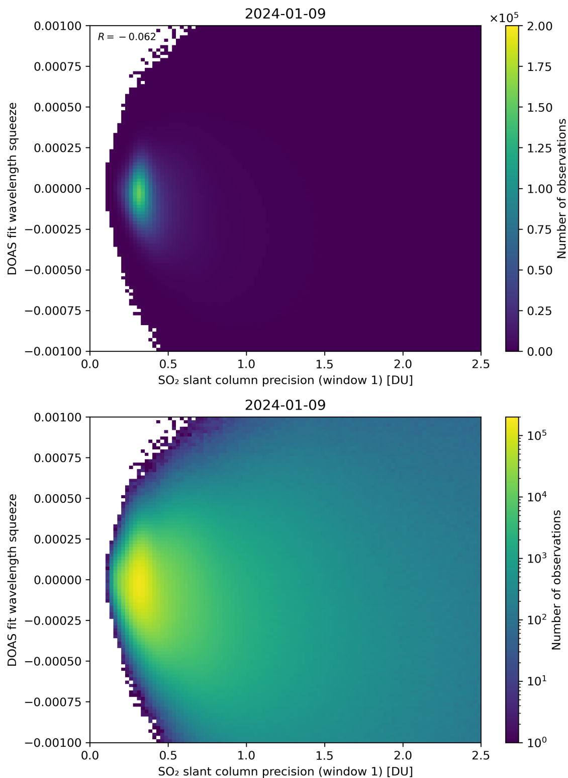
Figure 222: Scatter density plot of “SO 2 slant column precision (window 1)” against “DOAS fit wavelength squeeze” for 2024-01-08 to 2024-01-10.
