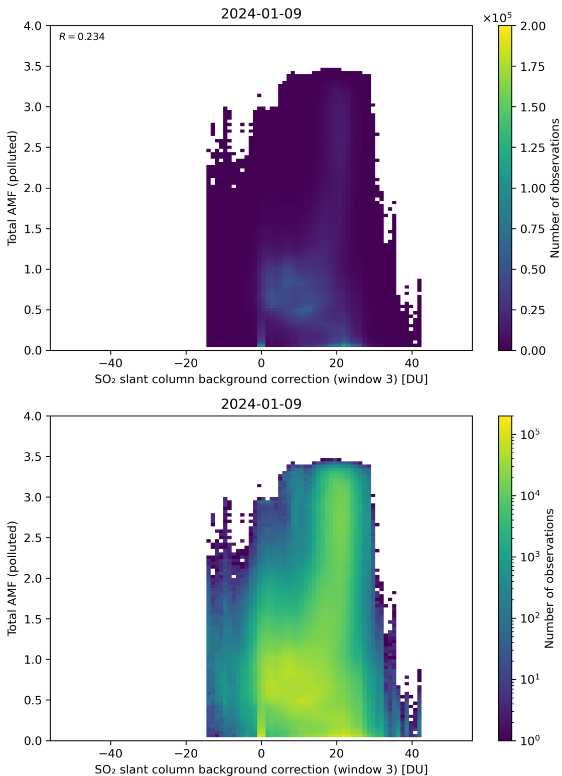
Figure 125: Scatter density plot of “SO 2 slant column background correction (window 3)” against “Total AMF (polluted)” for 2024-01-08 to 2024-01-10.
