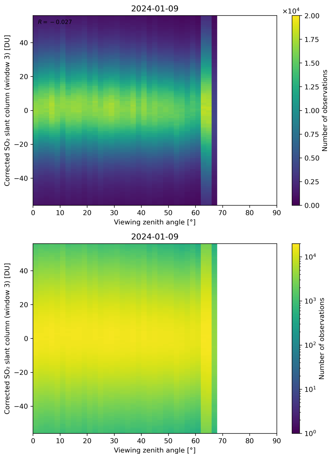
Figure 319: Scatter density plot of “Viewing zenith angle” against “Corrected SO 2 slant column (window 3)” for 2024-01-08 to 2024-01-10.
