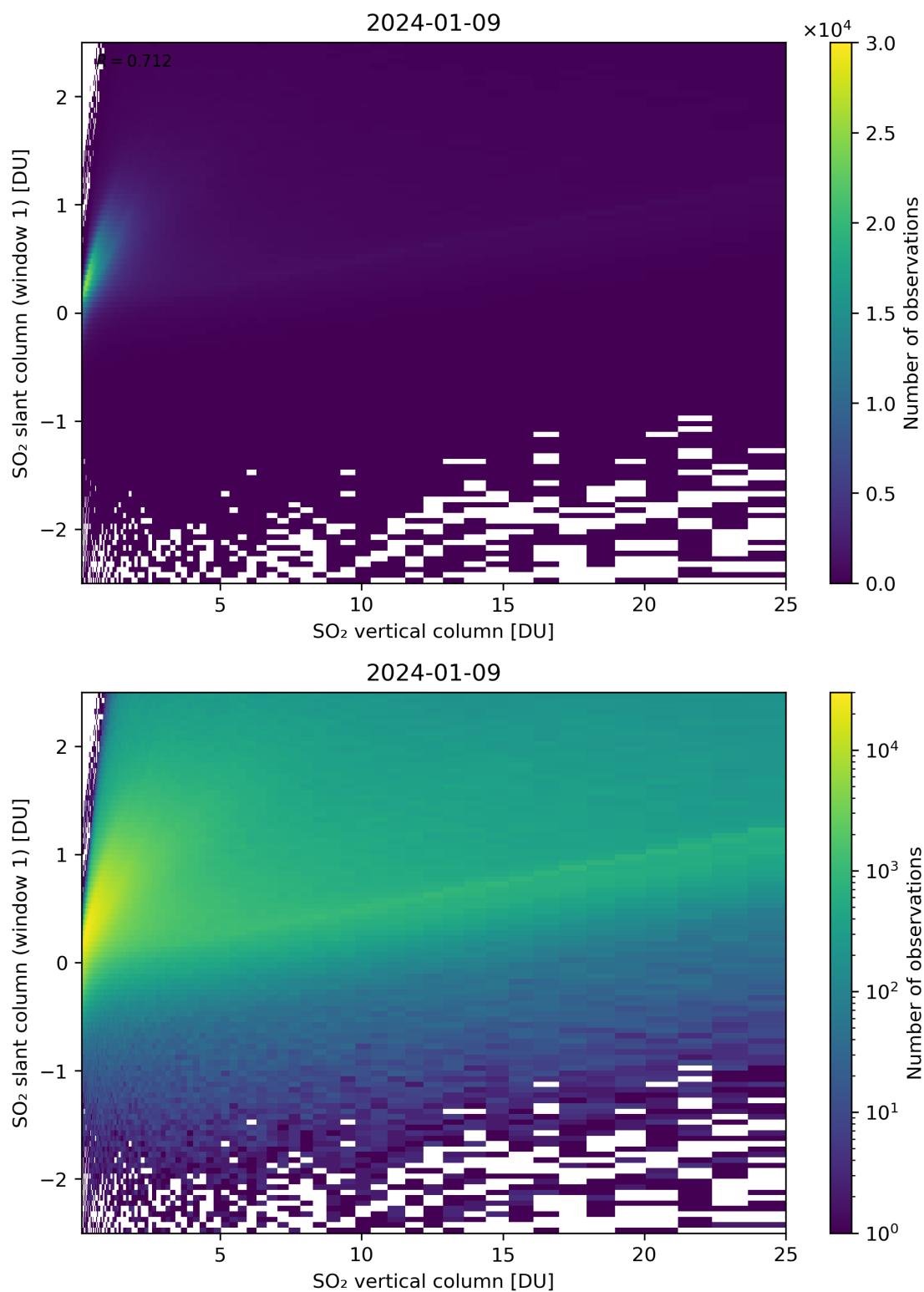
Figure 300: Scatter density plot of “SO 2 vertical column” against “SO 2 slant column (window 1)” for 2024-01-08 to 2024-01-10.
