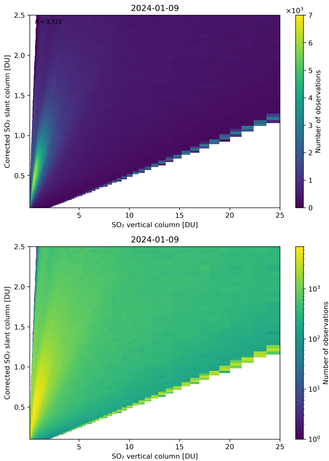
Figure 297: Scatter density plot of “SO 2 vertical column” against “Corrected SO 2 slant column” for 2024-01-08 to 2024-01-10.
