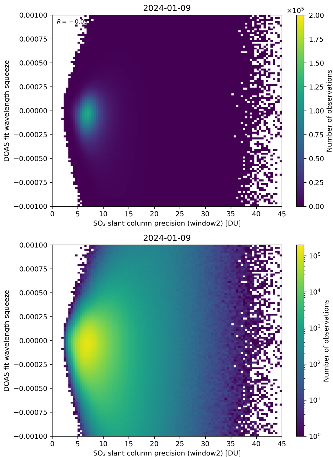
Figure 244: Scatter density plot of “SO 2 slant column precision (window2)” against “DOAS fit wavelength squeeze” for 2024-01-08 to 2024-01-10.
