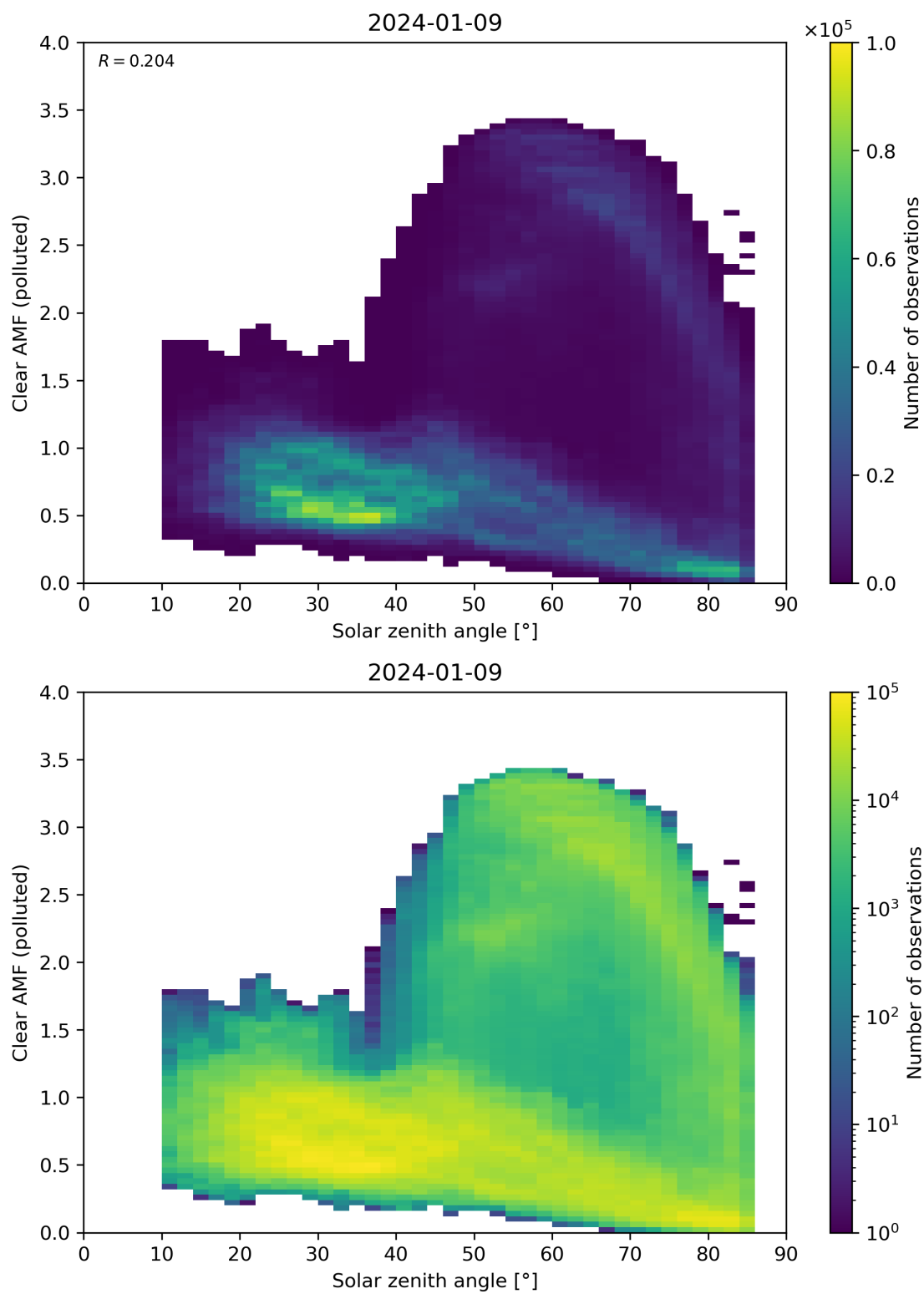
Figure 165: Scatter density plot of “Solar zenith angle” against “Clear AMF (polluted)” for 2024-01-08 to 2024-01-10.
