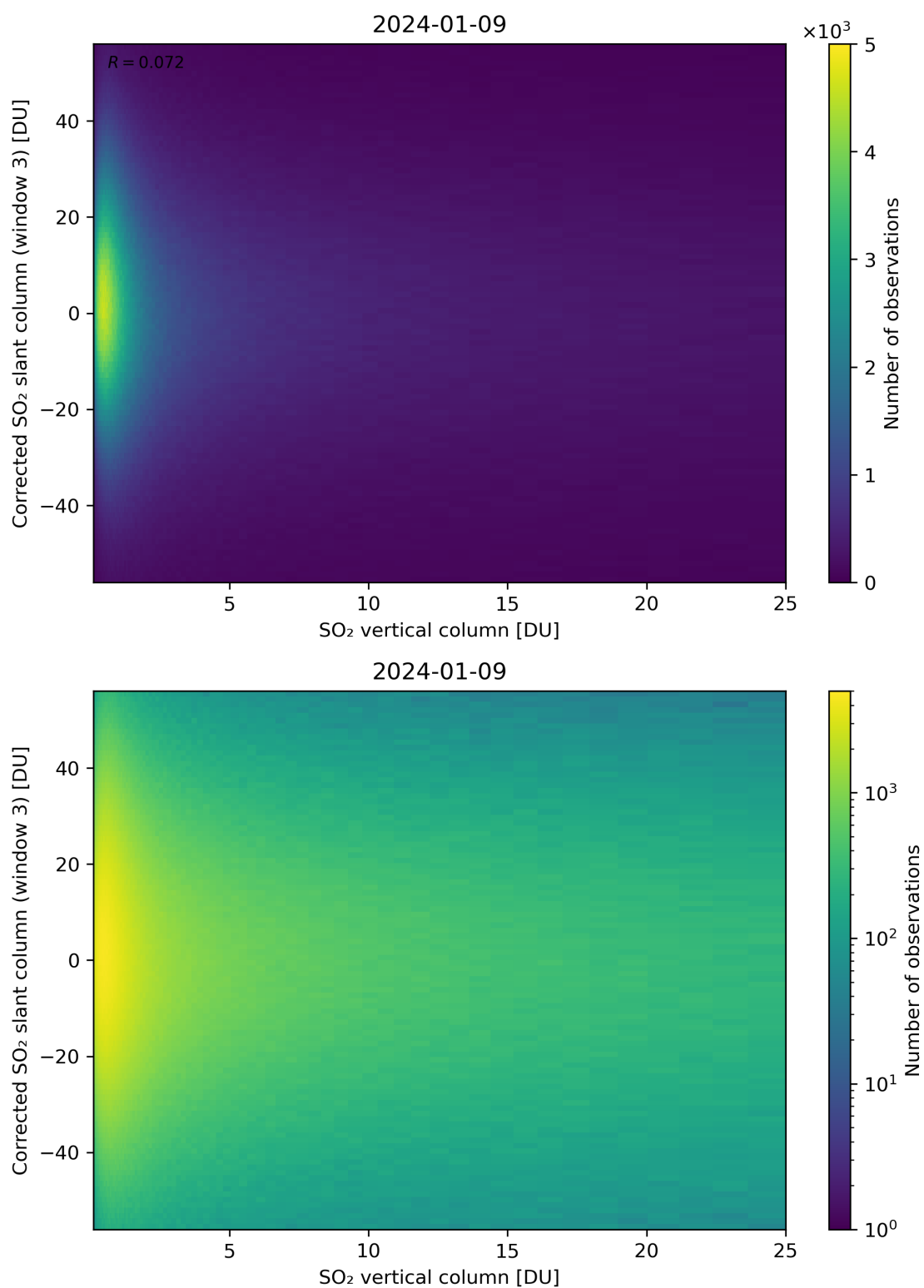
Figure 299: Scatter density plot of “SO 2 vertical column” against “Corrected SO 2 slant column (window 3)” for 2024-01-08 to 2024-01-10.
