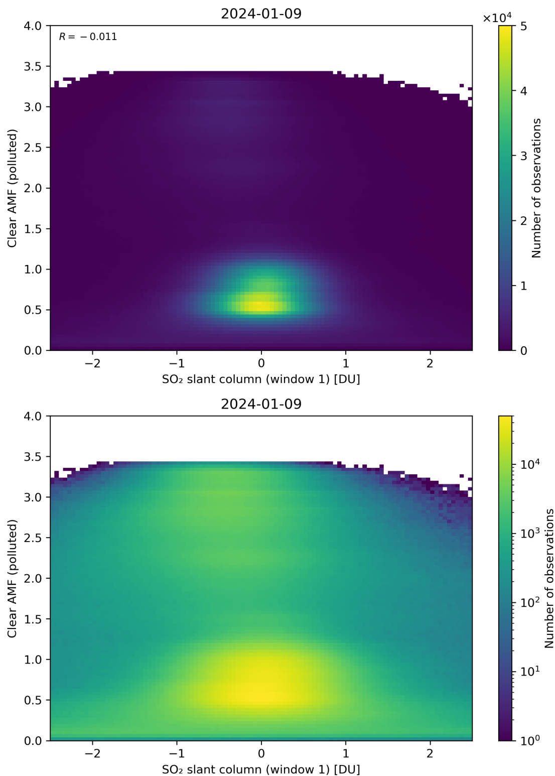
Figure 232: Scatter density plot of “SO 2 slant column (window 1)” against “Clear AMF (polluted)” for 2024-01-08 to 2024-01-10.
