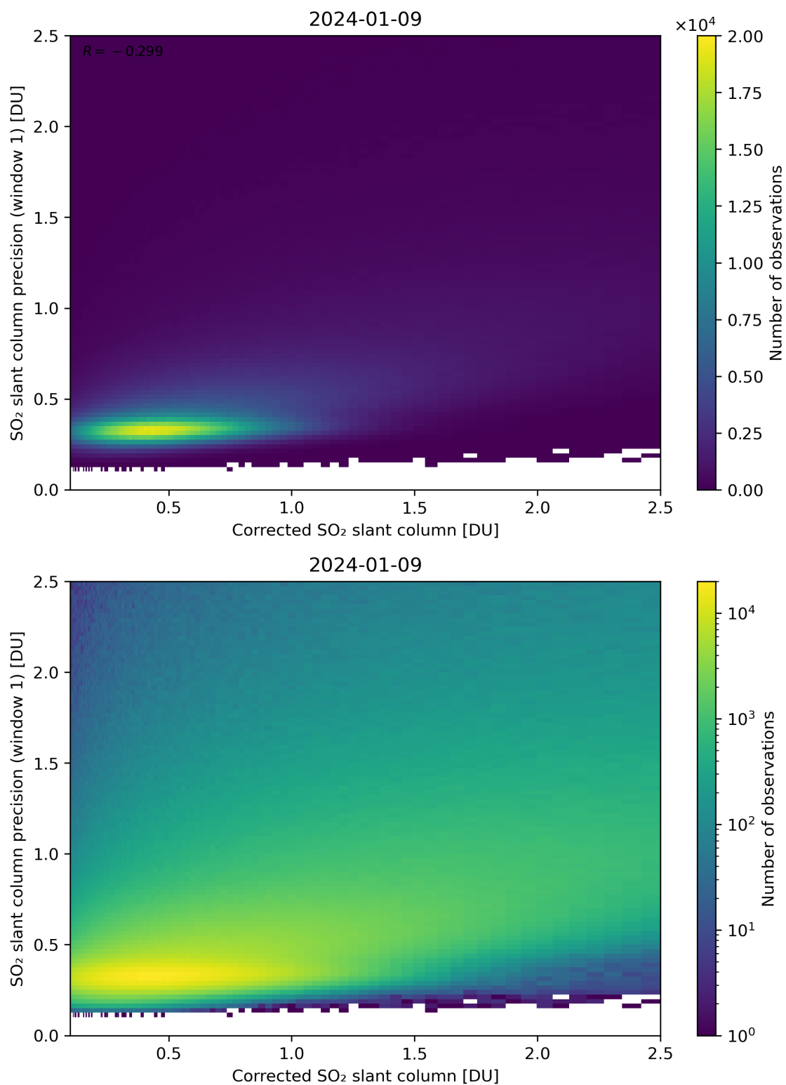
Figure 188: Scatter density plot of “Corrected SO 2 slant column” against “SO 2 slant column precision (window 1)” for 2024-01-08 to 2024-01-10.
