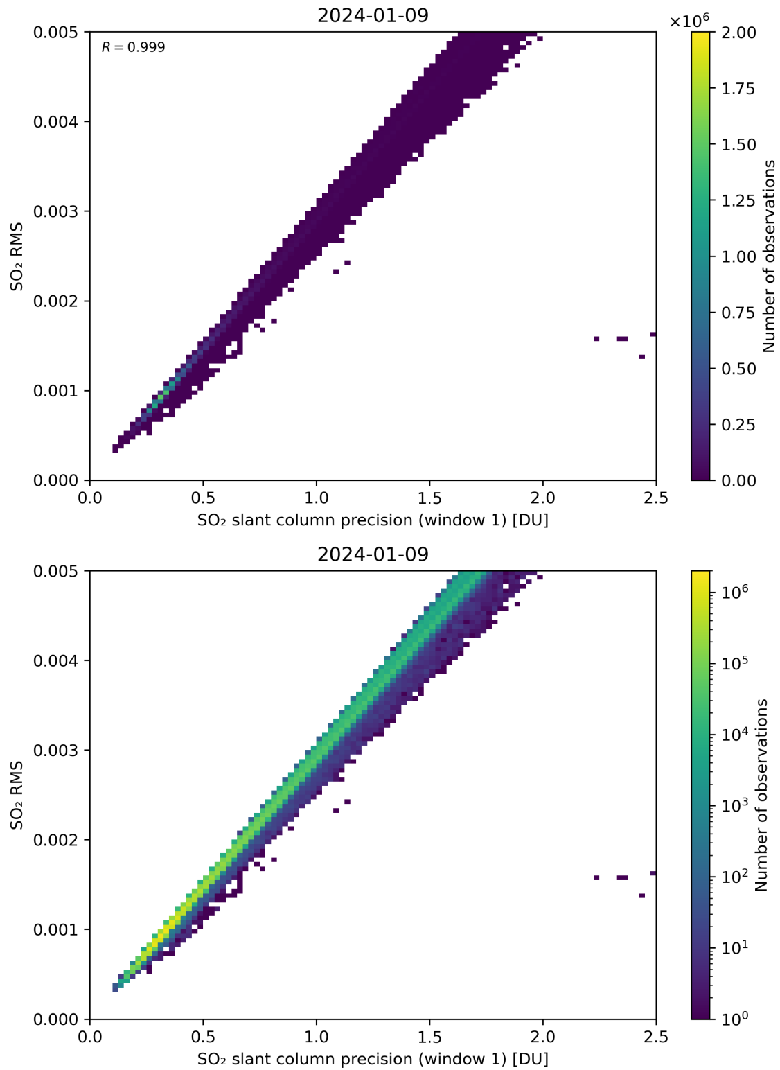
Figure 223: Scatter density plot of “SO 2 slant column precision (window 1)” against “SO 2 RMS” for 2024-01-08 to 2024-01-10.
