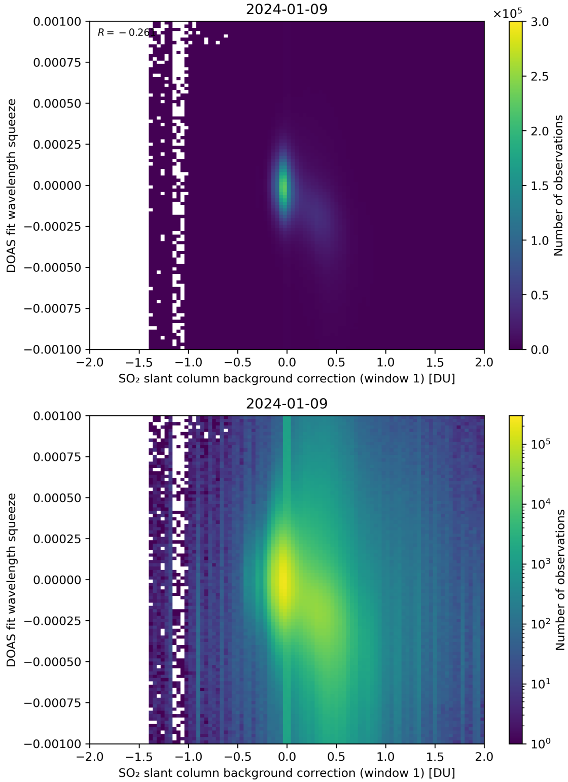
Figure 101: Scatter density plot of “SO 2 slant column background correction (window 1)” against “DOAS fit wavelength squeeze” for 2024-01-08 to 2024-01-10.
