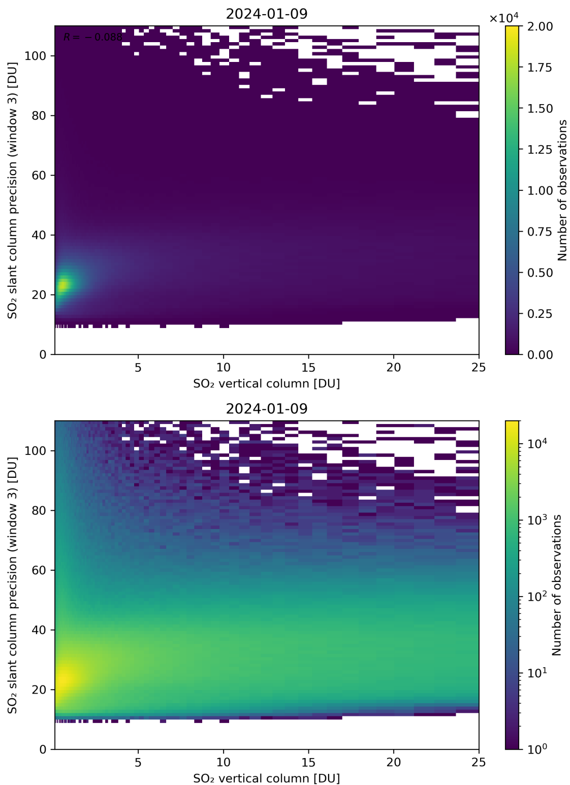
Figure 304: Scatter density plot of “SO 2 vertical column” against “SO 2 slant column precision (window 3)” for 2024-01-08 to 2024-01-10.
