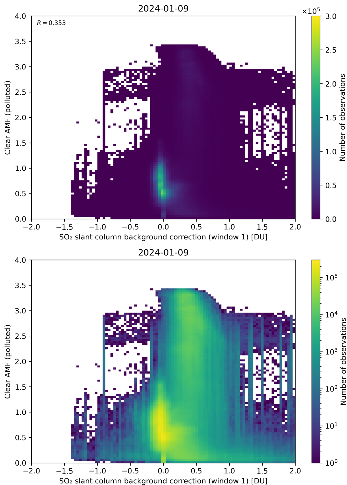
Figure 103: Scatter density plot of “SO 2 slant column background correction (window 1)” against “Clear AMF (polluted)” for 2024-01-08 to 2024-01-10.
