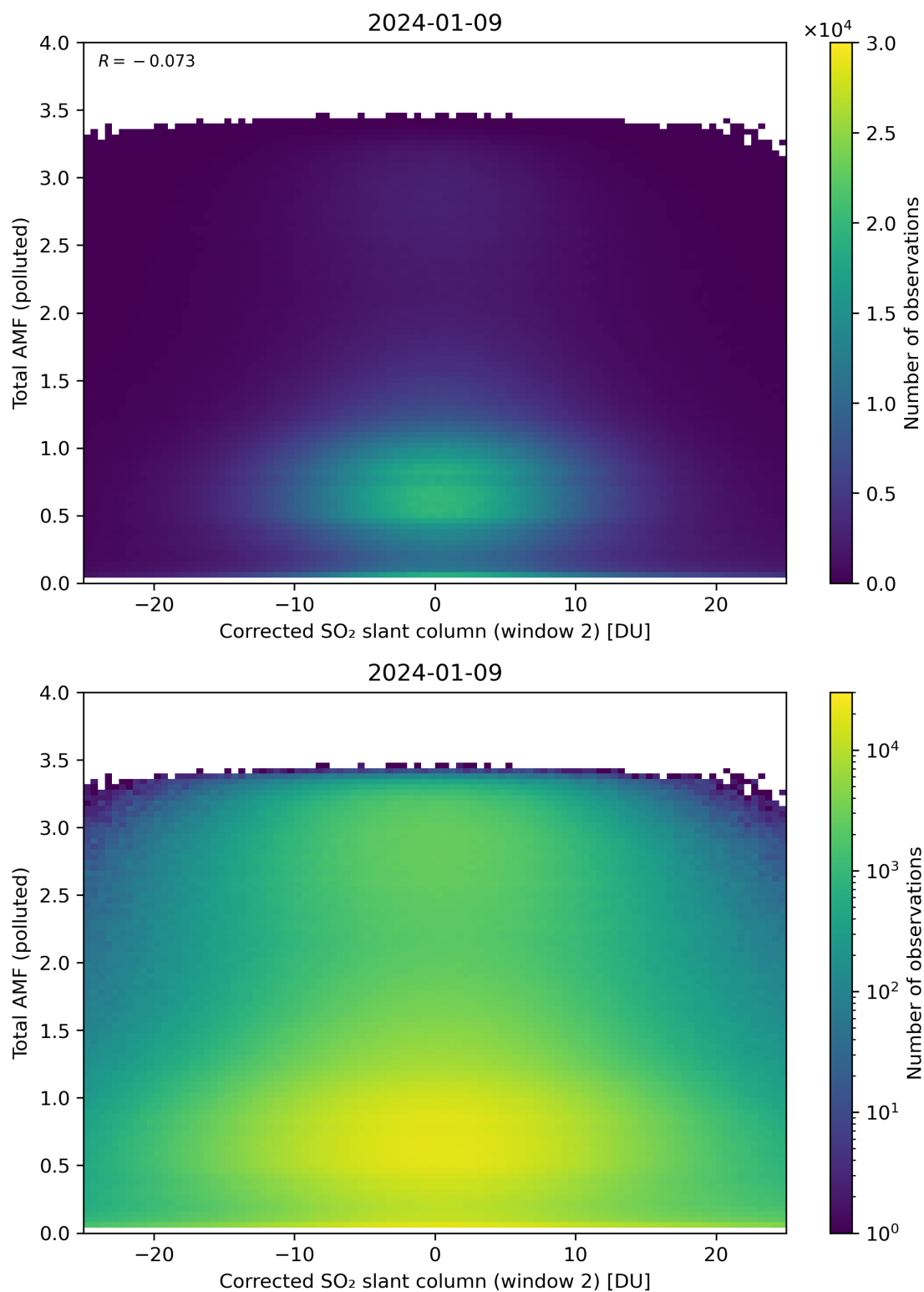
Figure 203: Scatter density plot of “Corrected SO 2 slant column (window 2)” against “Total AMF (polluted)” for 2024-01-08 to 2024-01-10.
