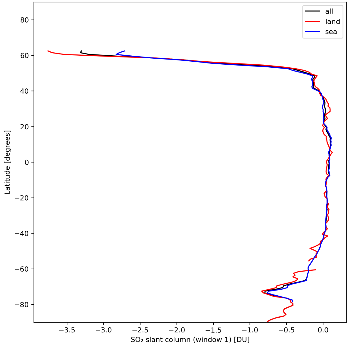
Figure 33: Zonal average of “SO 2 slant column (window 1)” for 2024-01-08 to 2024-01-10.
