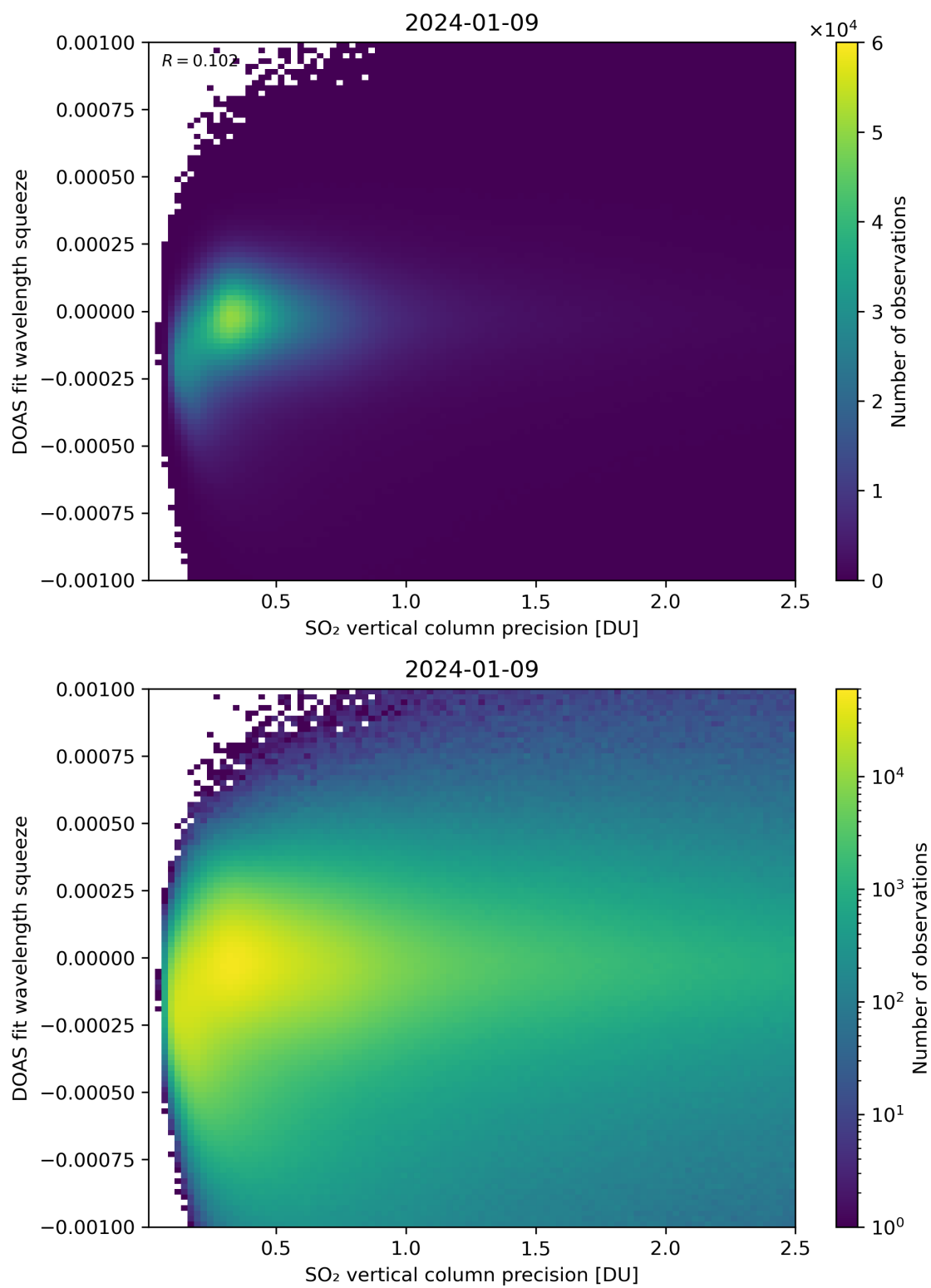
Figure 283: Scatter density plot of “SO 2 vertical column precision” against “DOAS fit wavelength squeeze” for 2024-01-08 to 2024-01-10.
