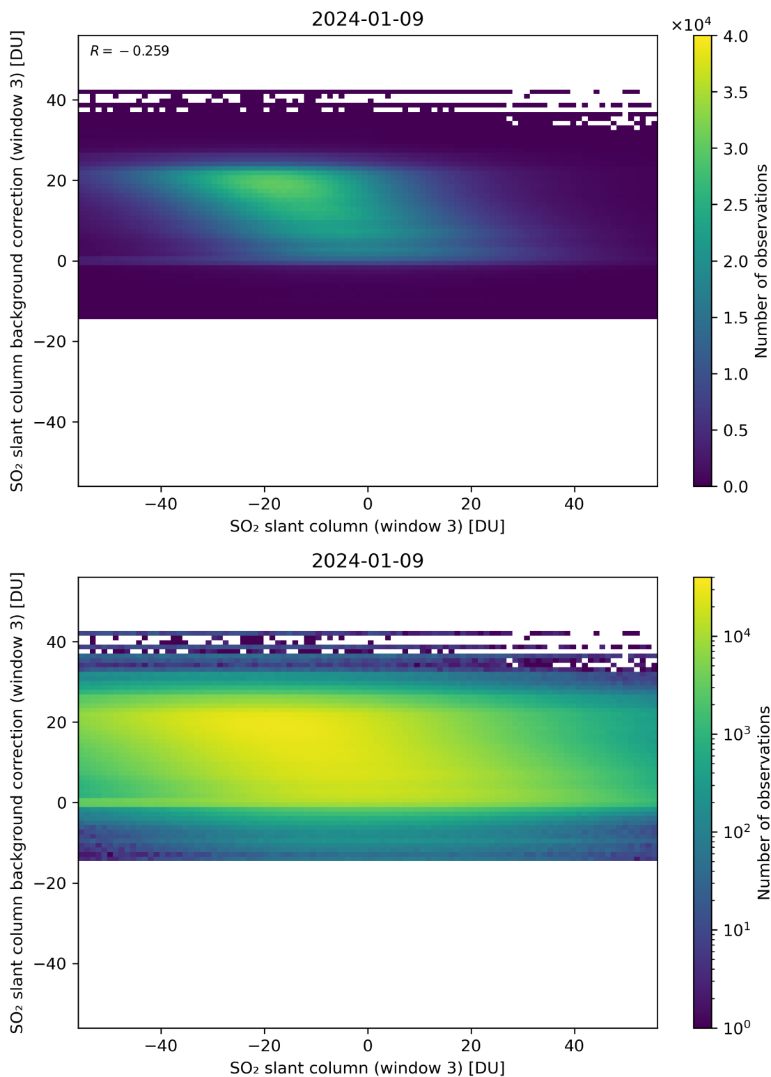
Figure 253: Scatter density plot of “SO 2 slant column (window 3)” against “SO 2 slant column background correction (window 3)” for 2024-01-08 to 2024-01-10.
