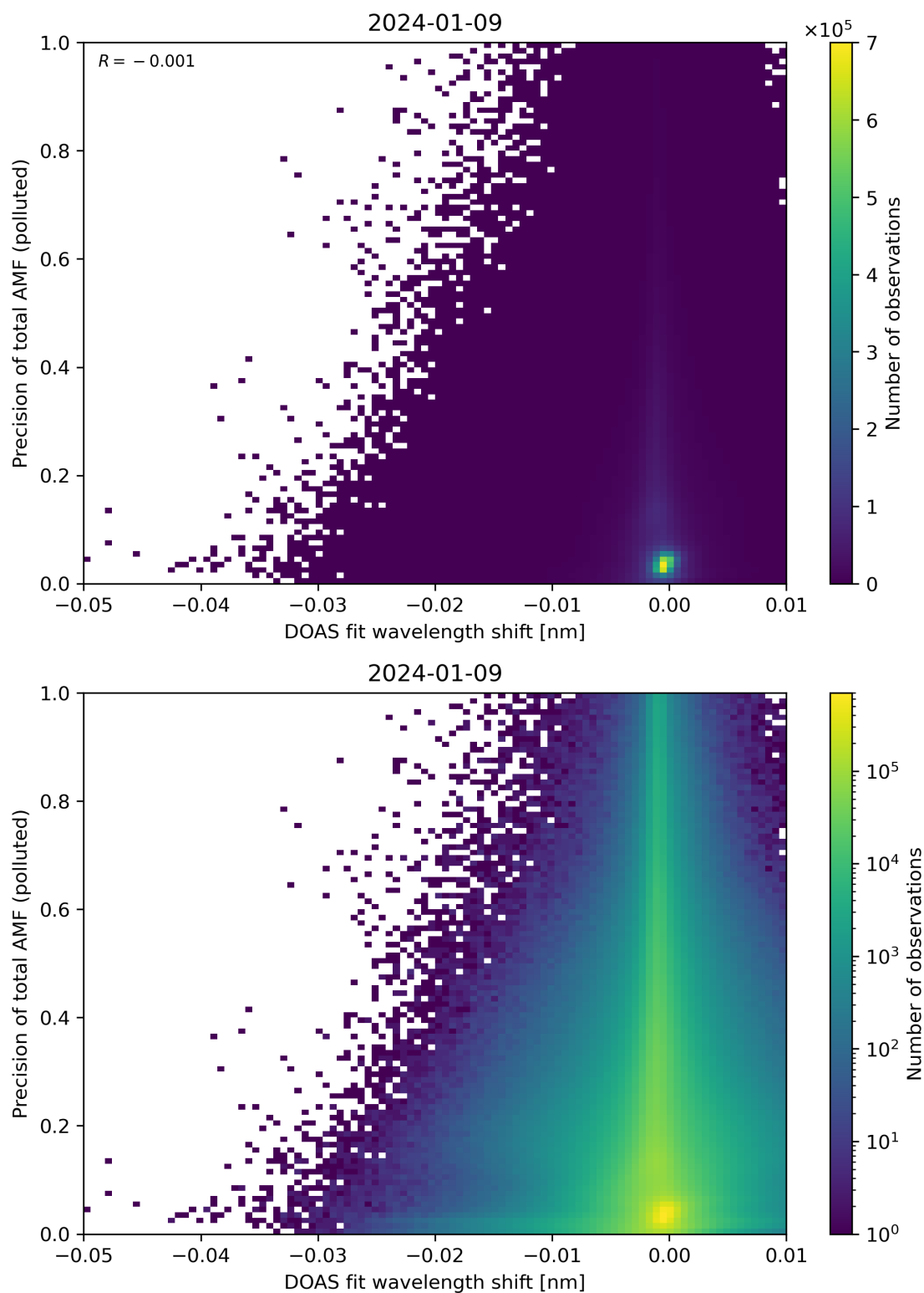
Figure 131: Scatter density plot of “DOAS fit wavelength shift” against “Precision of total AMF (polluted)” for 2024-01-08 to 2024-01-10.
