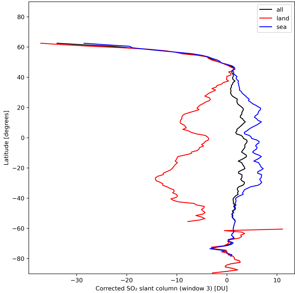
Figure 43: Zonal average of “Corrected SO 2 slant column (window 3)” for 2024-01-08 to 2024-01-10.
