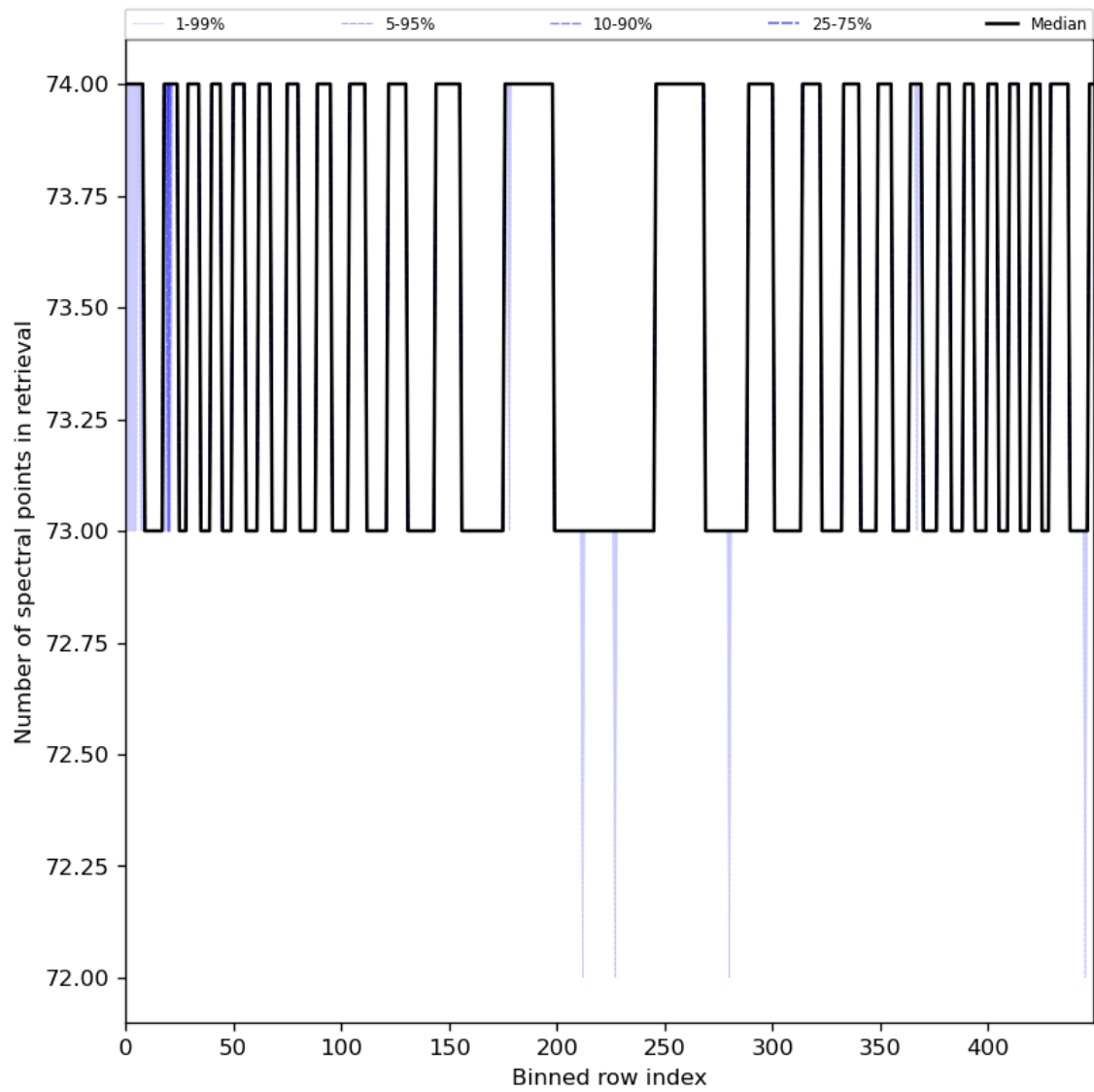
Figure 97: Along track statistics of “Number of spectral points in retrieval” for 2024-01-08 to 2024-01-10
