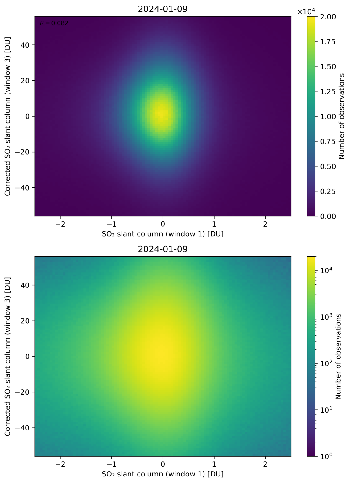
Figure 234: Scatter density plot of “SO 2 slant column (window 1)” against “Corrected SO 2 slant column (window 3)” for 2024-01-08 to 2024-01-10.
