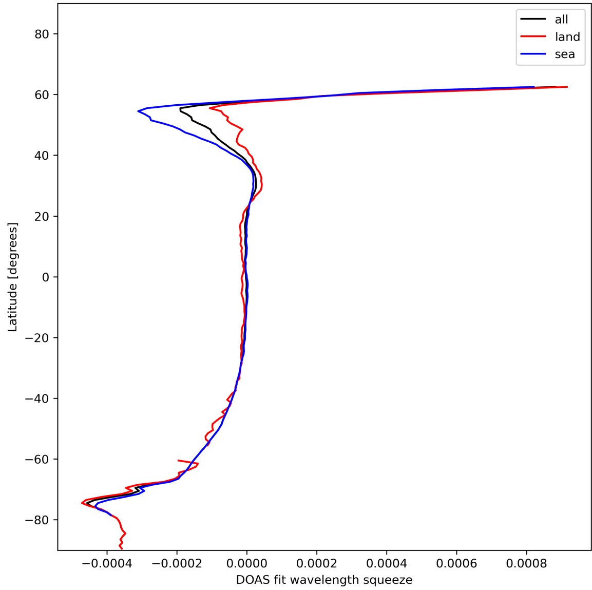
Figure 46: Zonal average of “DOAS fit wavelength squeeze” for 2024-01-08 to 2024-01-10.
