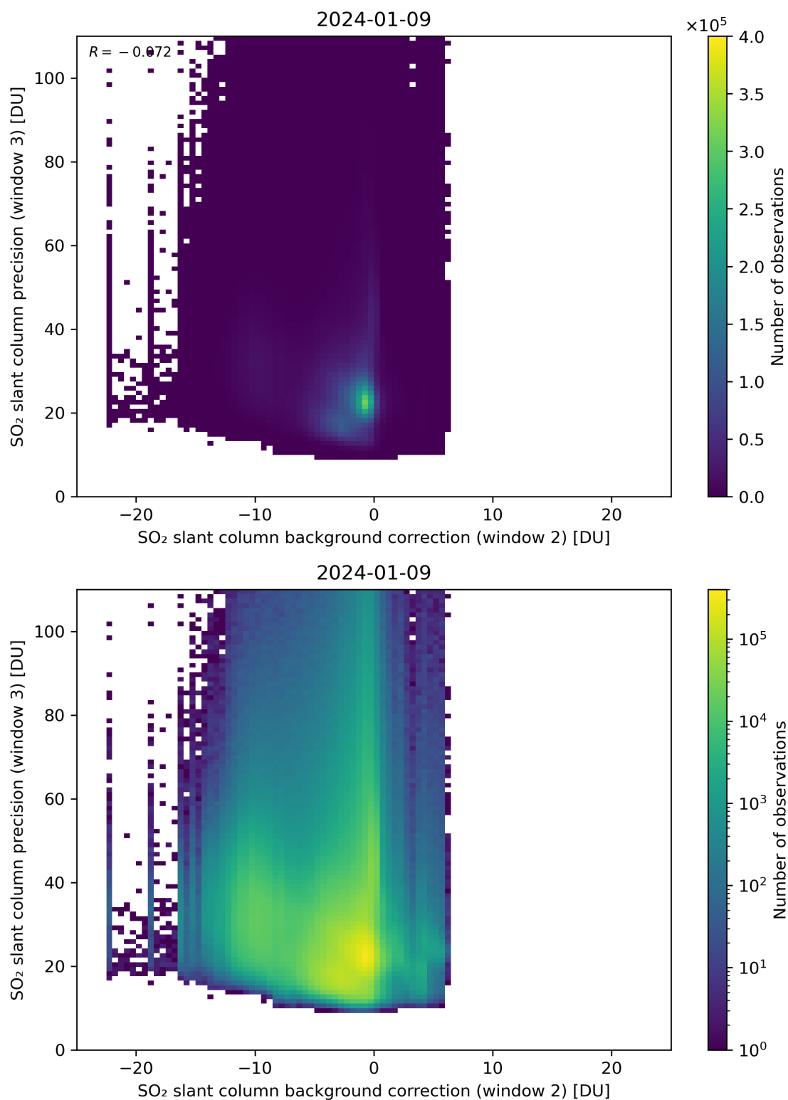
Figure 118: Scatter density plot of “SO 2 slant column background correction (window 2)” against “SO 2 slant column precision (window 3)” for 2024-01-08 to 2024-01-10.
