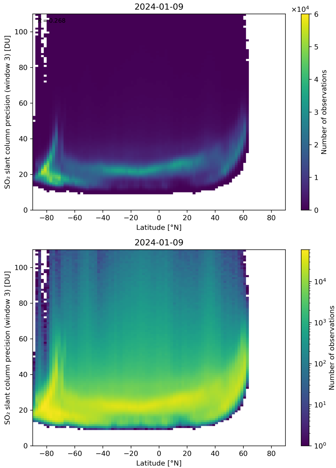
Figure 153: Scatter density plot of “Latitude” against “SO 2 slant column precision (window 3)” for 2024-01-08 to 2024-01-10.
