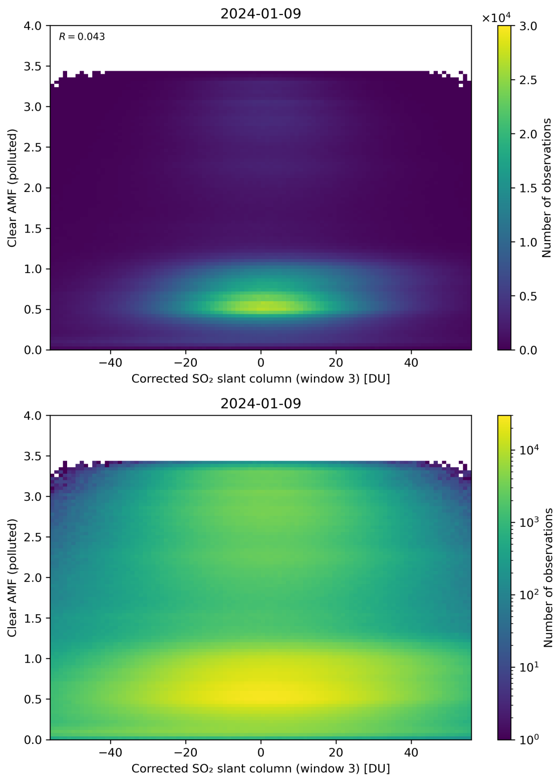
Figure 209: Scatter density plot of “Corrected SO 2 slant column (window 3)” against “Clear AMF (polluted)” for 2024-01-08 to 2024-01-10.
