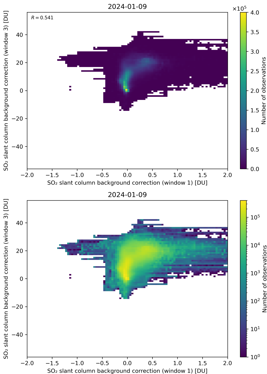
Figure 99: Scatter density plot of “SO 2 slant column background correction (window 1)” against “SO 2 slant column background correction (window 3)” for 2024-01-08 to 2024-01-10.
