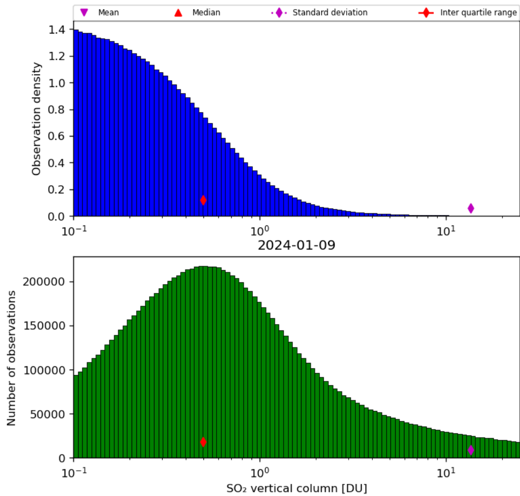
Figure 53: Histogram of “SO 2 vertical column” for 2024-01-08 to 2024-01-10
