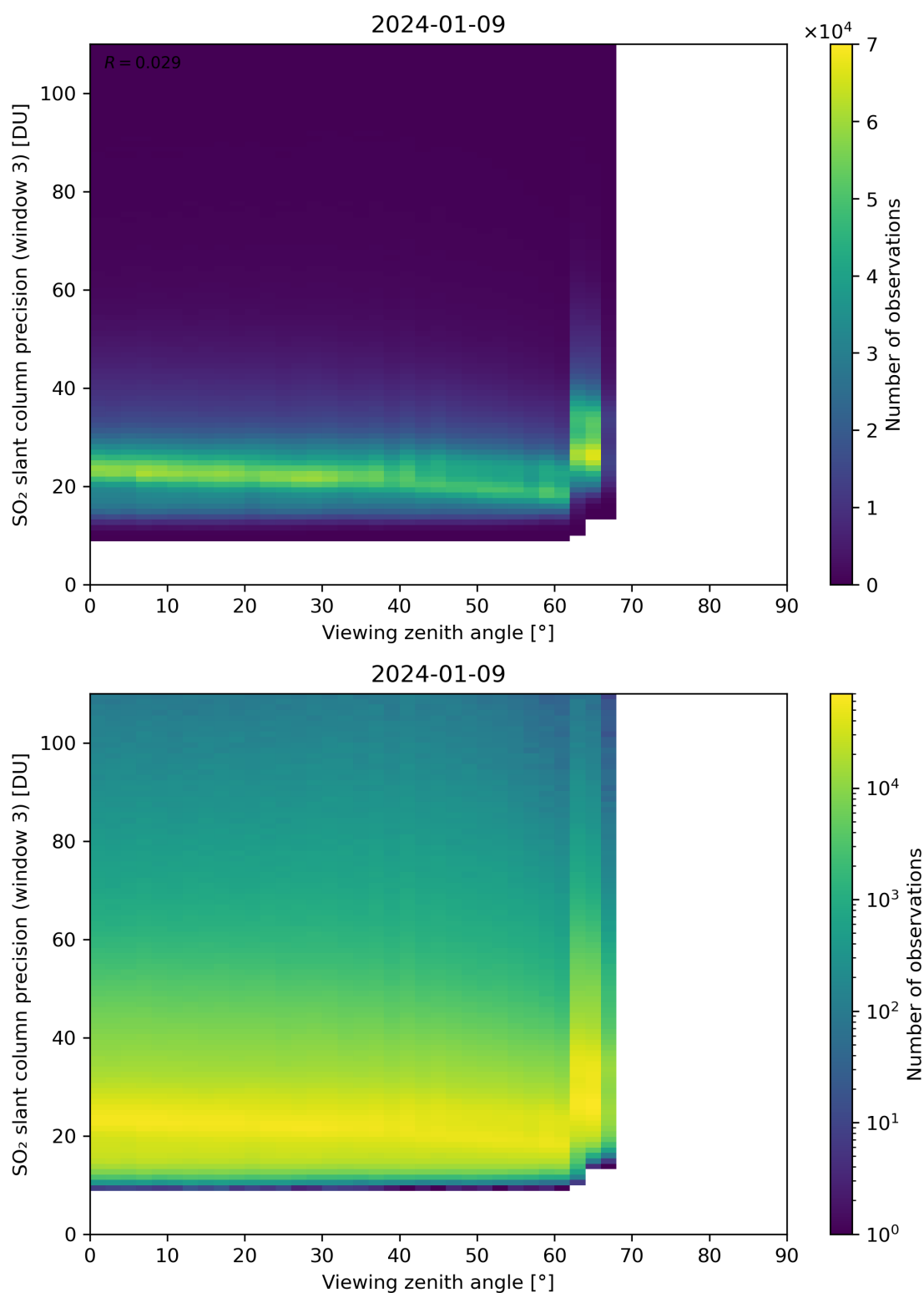
Figure 324: Scatter density plot of “Viewing zenith angle” against “SO 2 slant column precision (window 3)” for 2024-01-08 to 2024-01-10.
