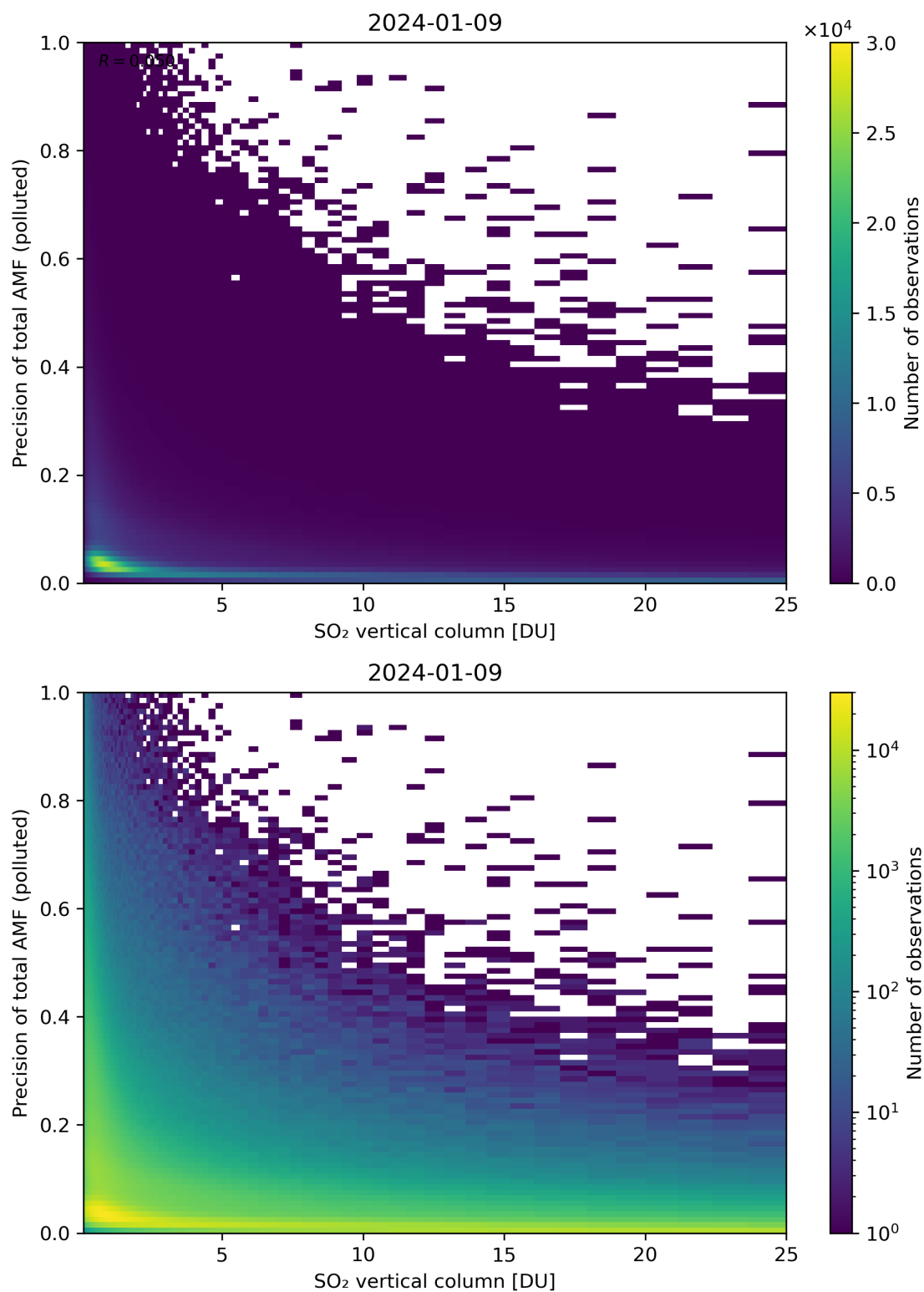
Figure 306: Scatter density plot of “SO 2 vertical column” against “Precision of total AMF (polluted)” for 2024-01-08 to 2024-01-10.
