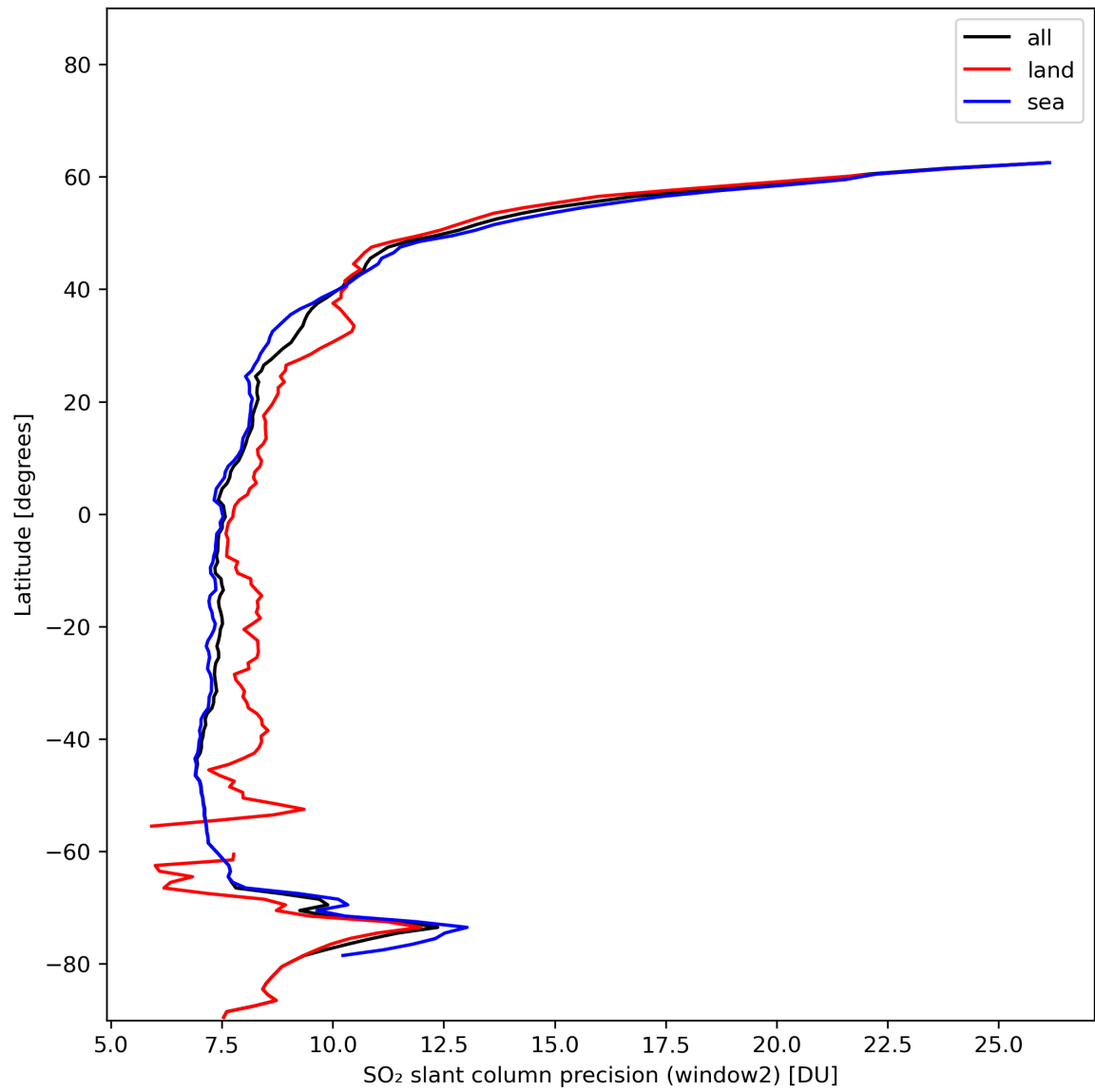
Figure 38: Zonal average of “SO 2 slant column precision (window2)” for 2024-01-08 to 2024-01-10.
