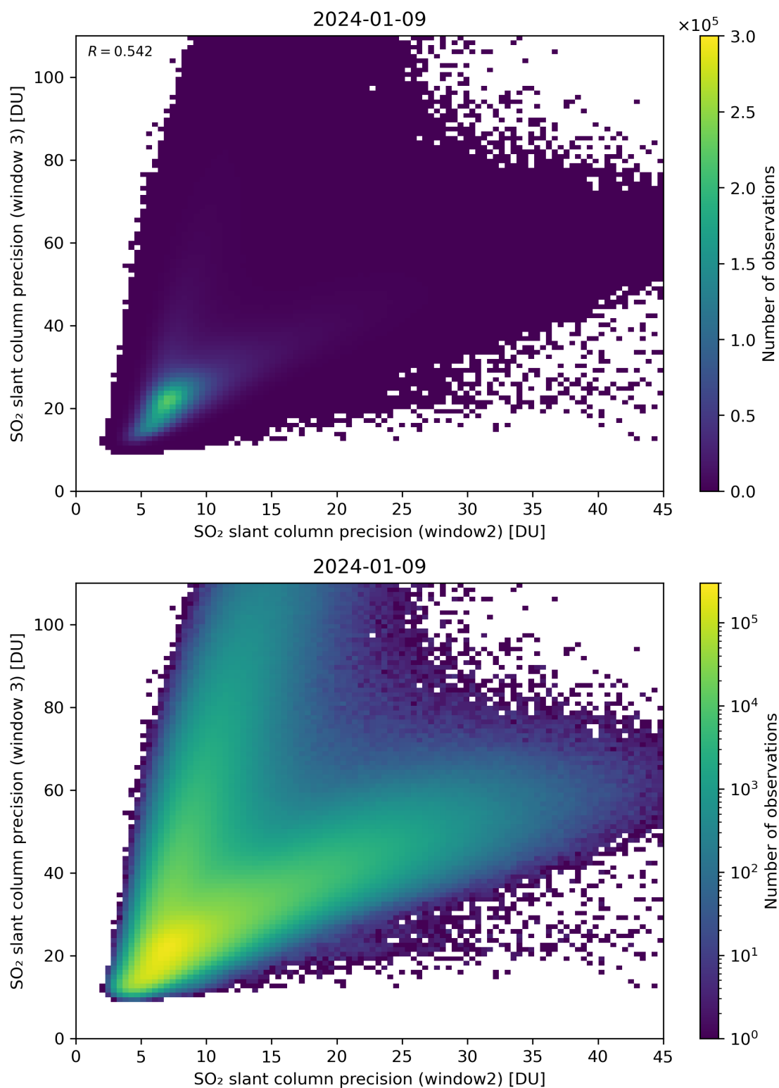
Figure 250: Scatter density plot of “SO 2 slant column precision (window2)” against “SO 2 slant column precision (window 3)” for 2024-01-08 to 2024-01-10.
