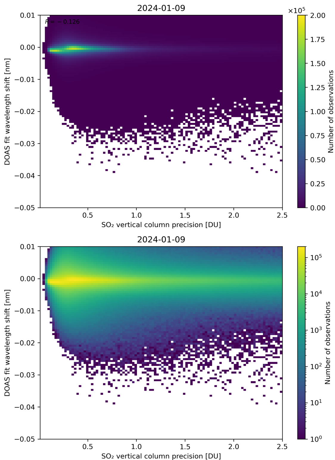
Figure 282: Scatter density plot of “SO 2 vertical column precision” against “DOAS fit wavelength shift” for 2024-01-08 to 2024-01-10.
