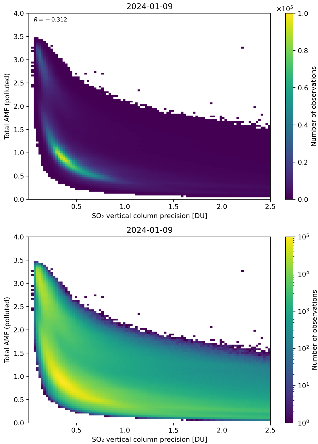
Figure 294: Scatter density plot of “SO 2 vertical column precision” against “Total AMF (polluted)” for 2024-01-08 to 2024-01-10.
