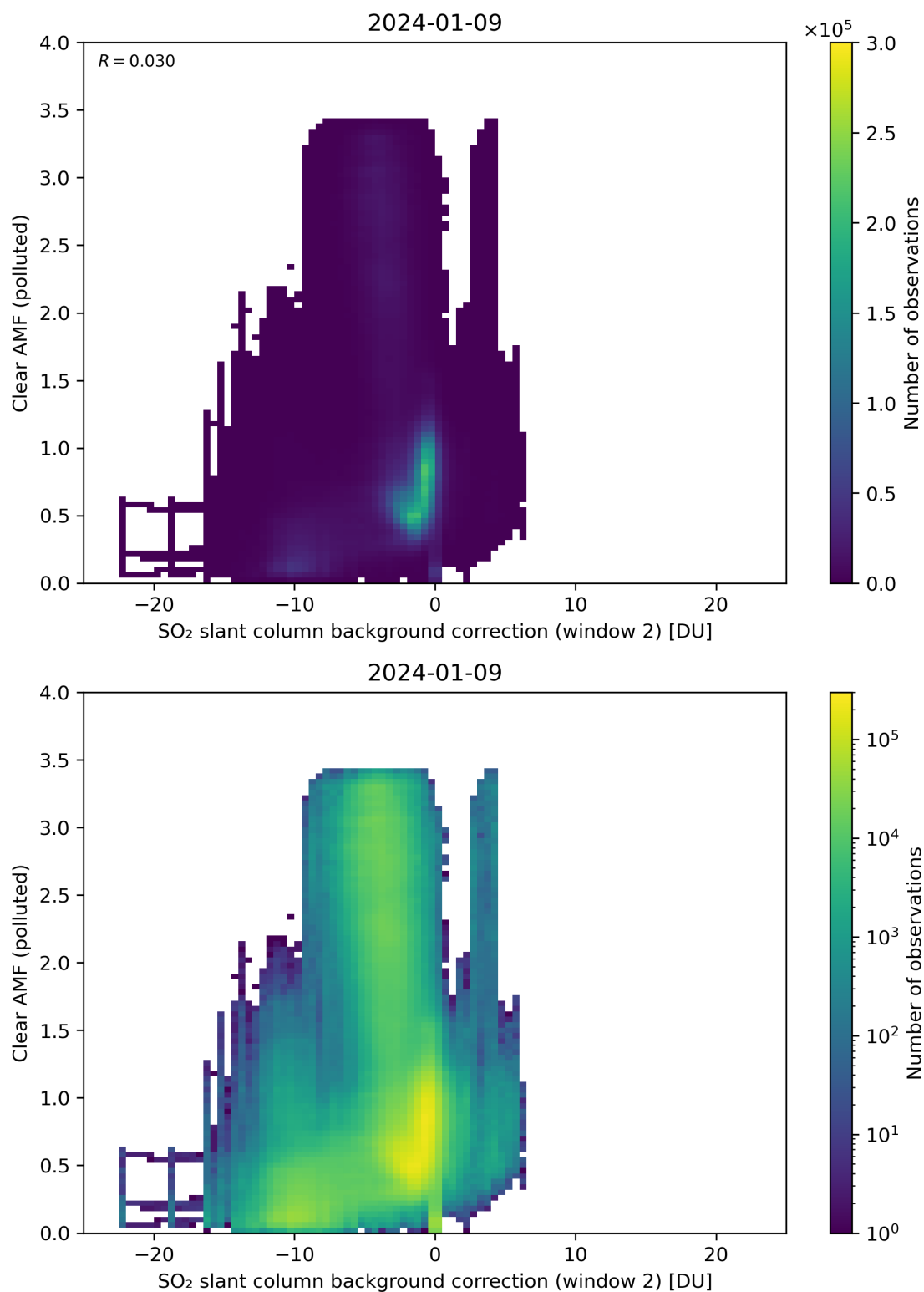
Figure 115: Scatter density plot of “SO 2 slant column background correction (window 2)” against “Clear AMF (polluted)” for 2024-01-08 to 2024-01-10.
