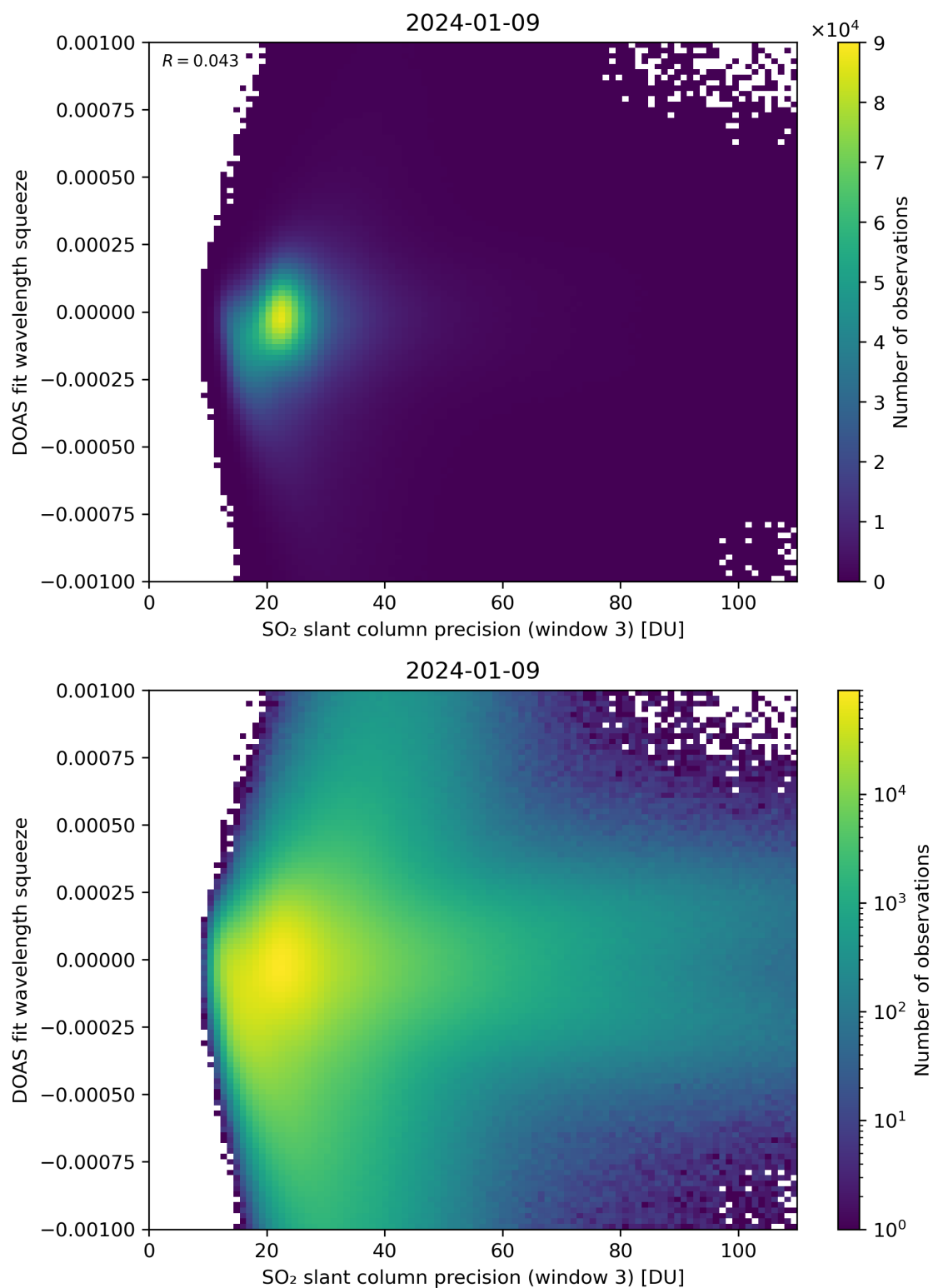
Figure 259: Scatter density plot of “SO 2 slant column precision (window 3)” against “DOAS fit wavelength squeeze” for 2024-01-08 to 2024-01-10.
