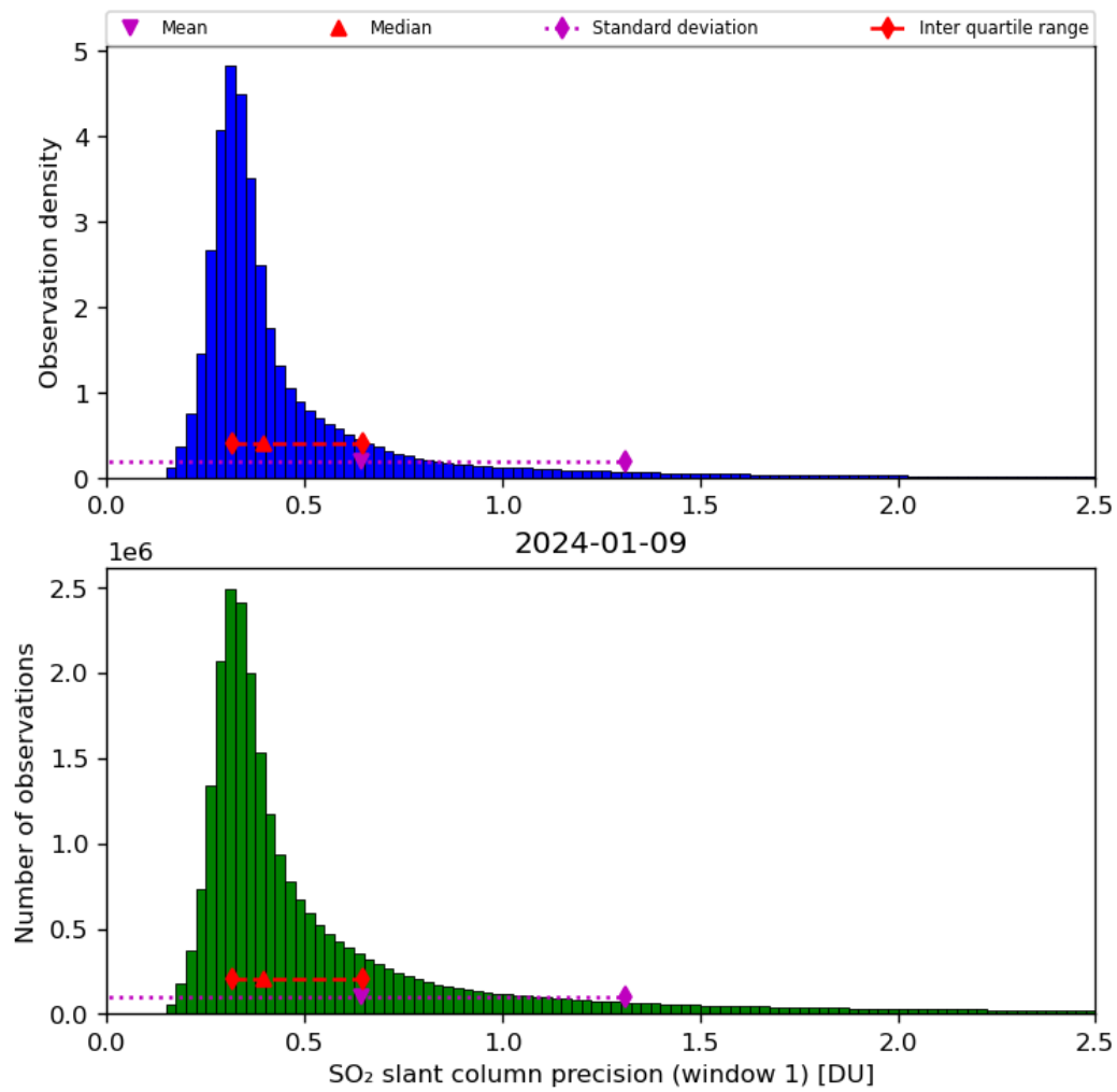
Figure 57: Histogram of “SO 2 slant column precision (window 1)” for 2024-01-08 to 2024-01-10
