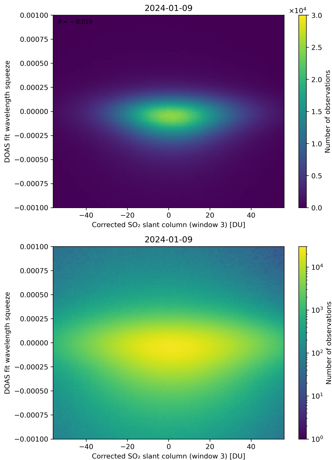
Figure 207: Scatter density plot of “Corrected SO 2 slant column (window 3)” against “DOAS fit wavelength squeeze” for 2024-01-08 to 2024-01-10.
