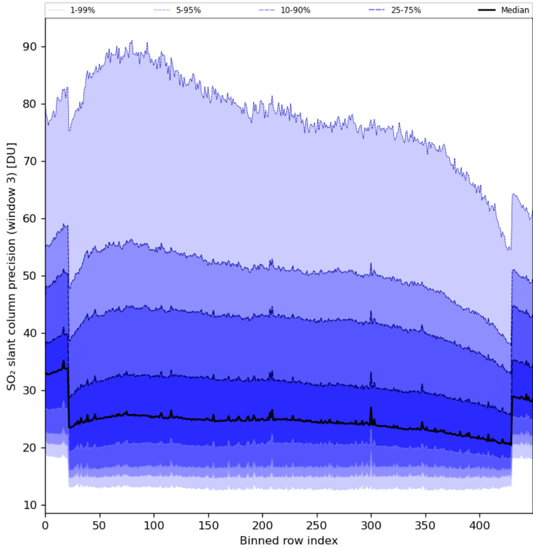
Figure 88: Along track statistics of “SO 2 slant column precision (window 3)” for 2024-01-08 to 2024-01-10
