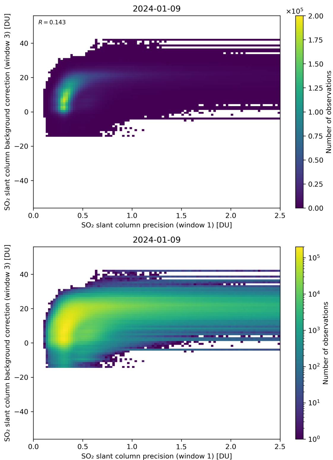
Figure 220: Scatter density plot of “SO 2 slant column precision (window 1)” against “SO 2 slant column background correction (window 3)” for 2024-01-08 to 2024-01-10.
