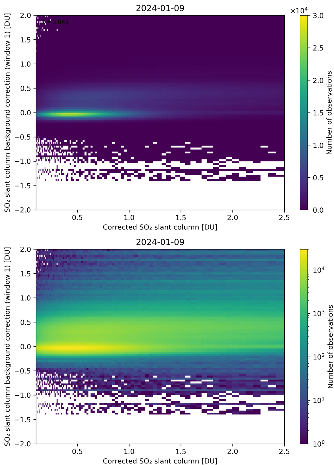
Figure 178: Scatter density plot of “Corrected SO 2 slant column” against “SO 2 slant column background correction (window 1)” for 2024-01-08 to 2024-01-10.
