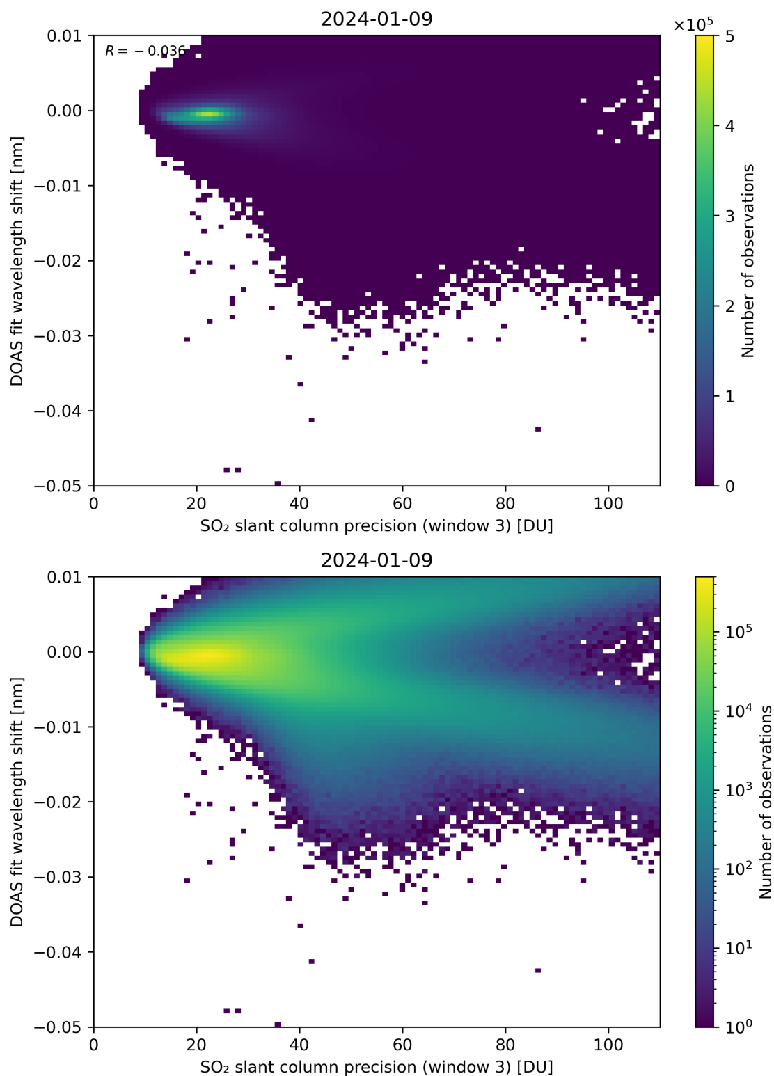
Figure 258: Scatter density plot of “SO 2 slant column precision (window 3)” against “DOAS fit wavelength shift” for 2024-01-08 to 2024-01-10.
