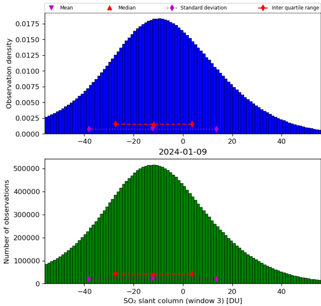
Figure 64: Histogram of “SO 2 slant column (window 3)” for 2024-01-08 to 2024-01-10
