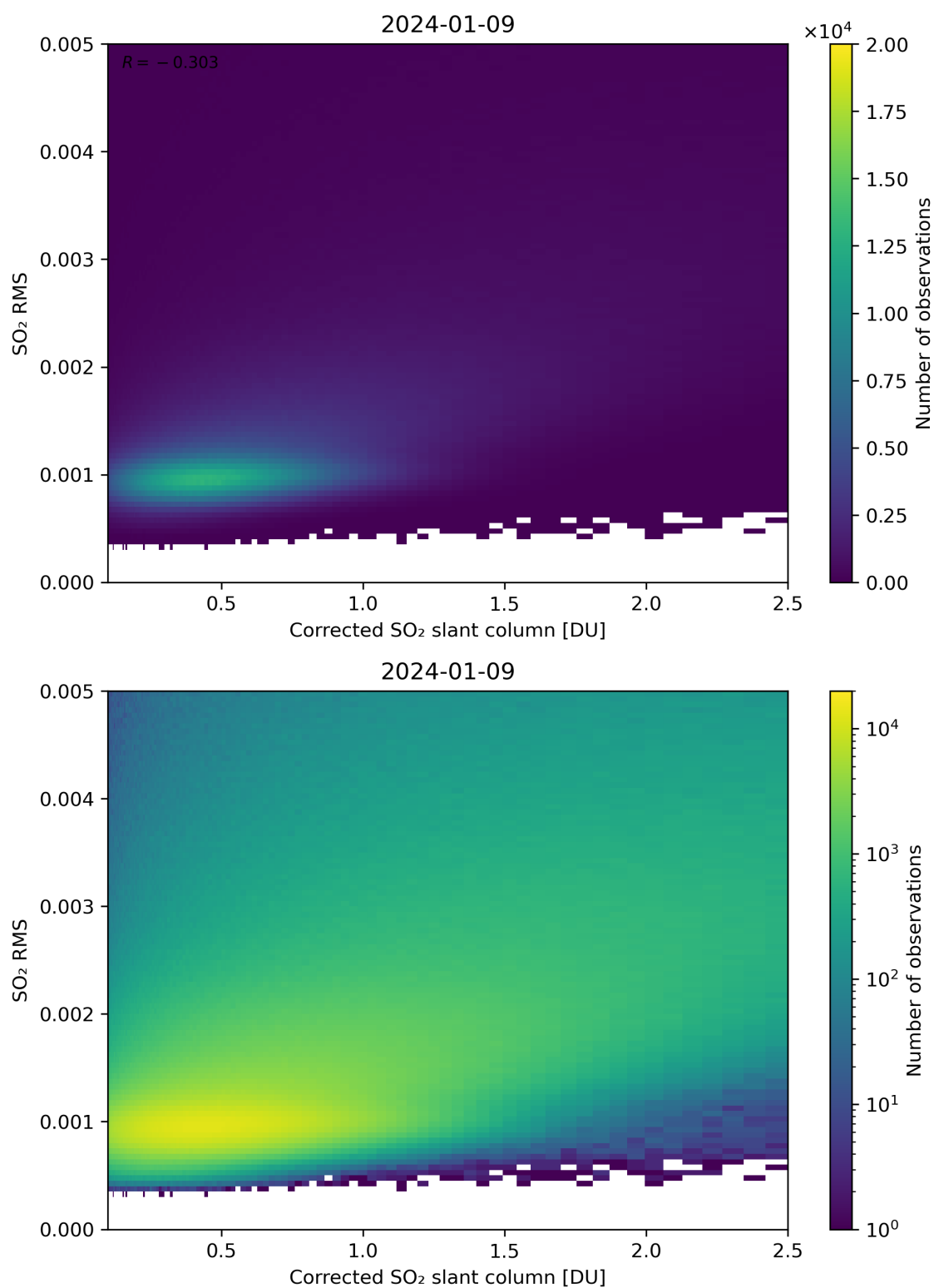
Figure 183: Scatter density plot of “Corrected SO 2 slant column” against “SO 2 RMS” for 2024-01-08 to 2024-01-10.
