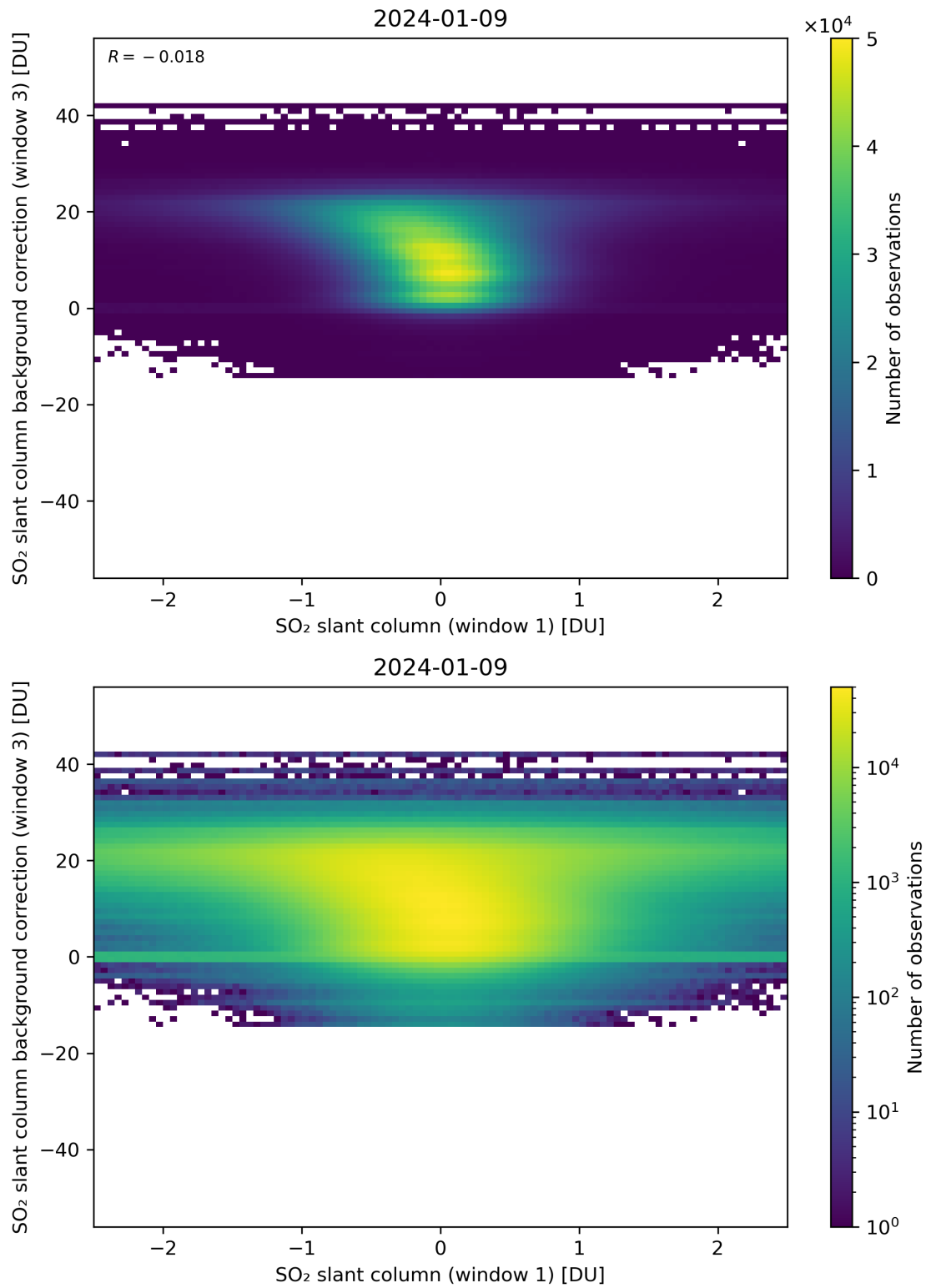
Figure 214: Scatter density plot of “SO 2 slant column (window 1)” against “SO 2 slant column background correction (window 3)” for 2024-01-08 to 2024-01-10.
