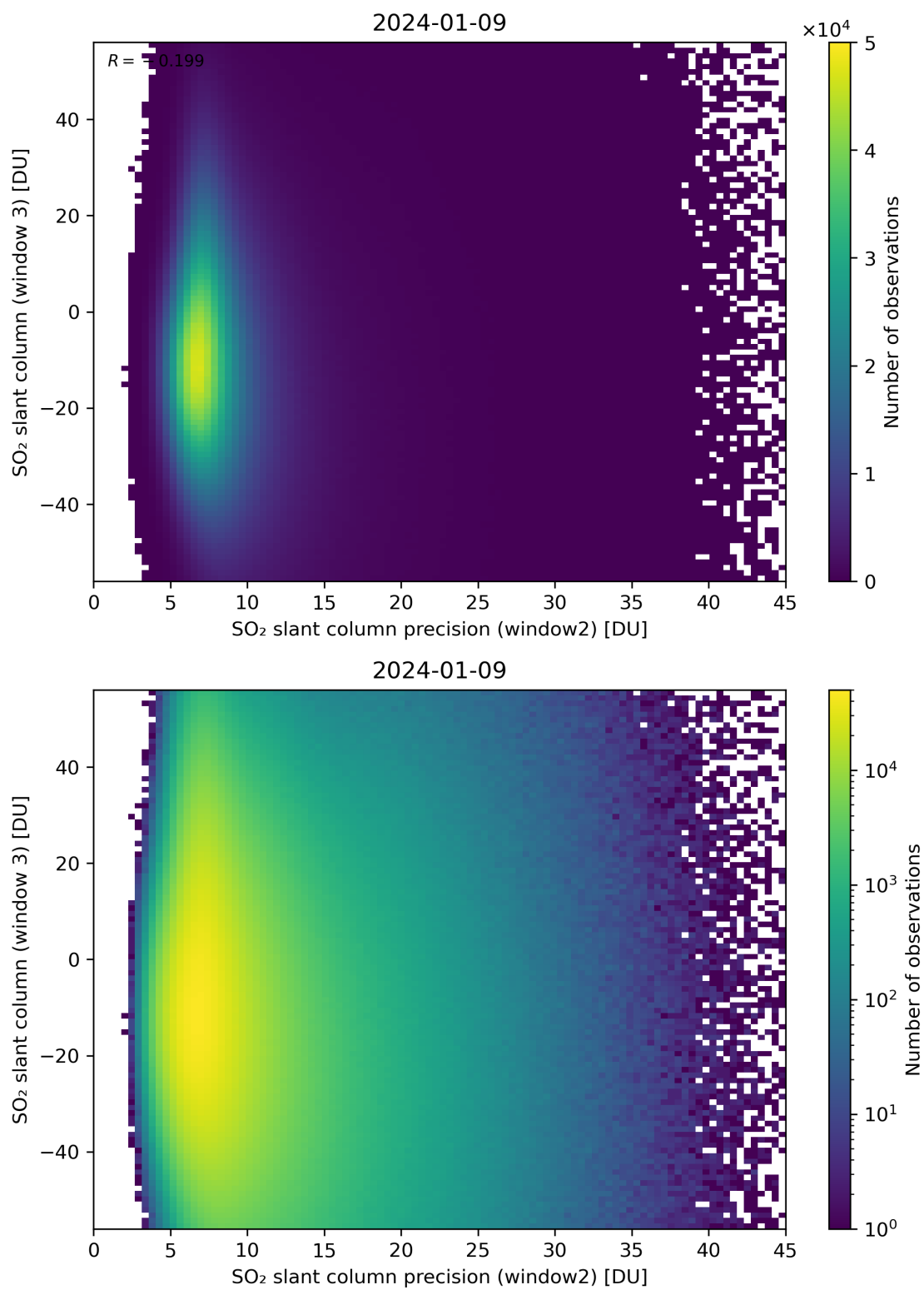
Figure 249: Scatter density plot of “SO 2 slant column precision (window2)” against “SO 2 slant column (window 3)” for 2024-01-08 to 2024-01-10.
