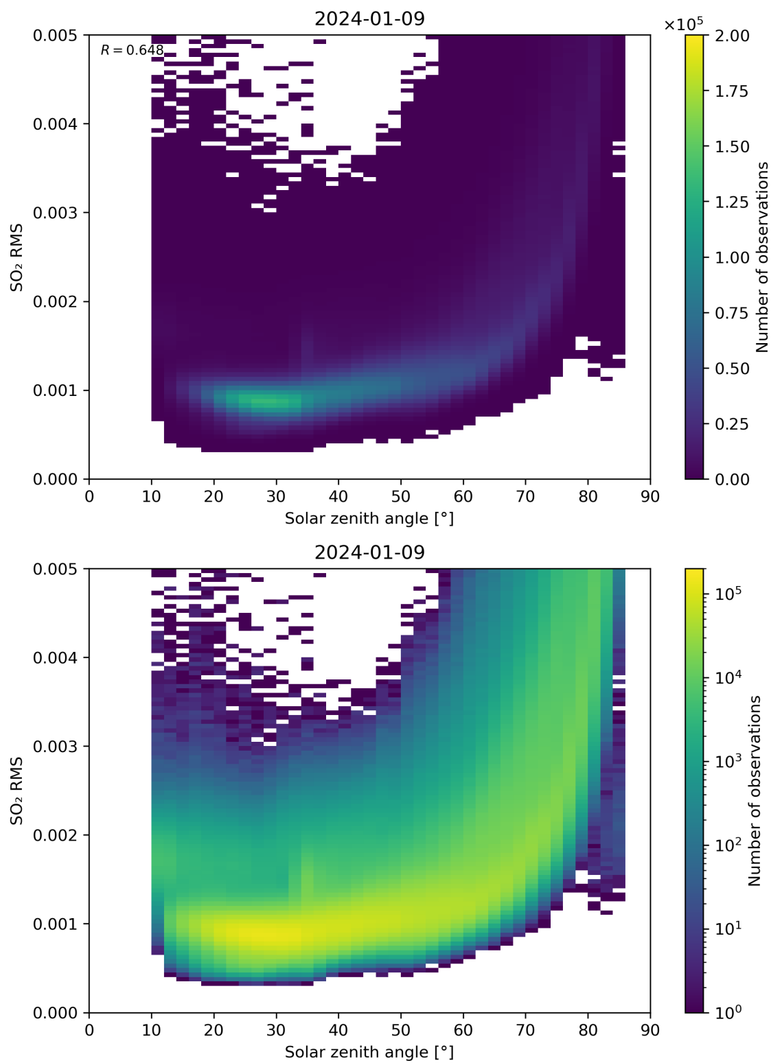
Figure 163: Scatter density plot of “Solar zenith angle” against “SO 2 RMS” for 2024-01-08 to 2024-01-10.
