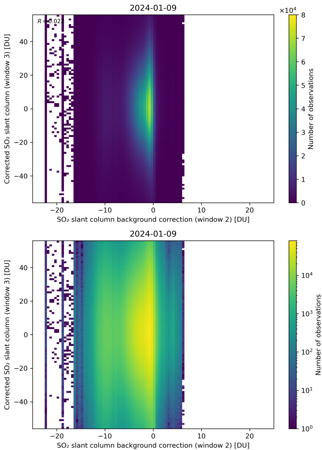
Figure 116: Scatter density plot of “SO 2 slant column background correction (window 2)” against “Corrected SO 2 slant column (window 3)” for 2024-01-08 to 2024-01-10.
