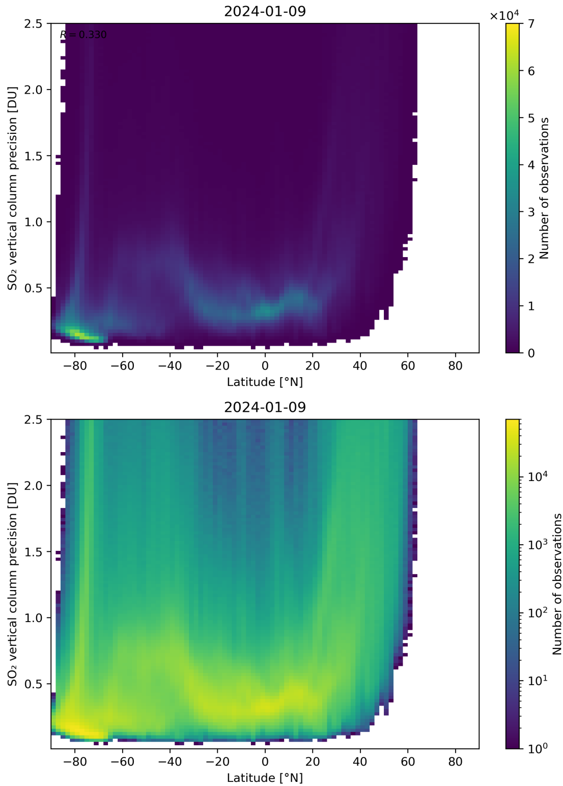
Figure 157: Scatter density plot of “Latitude” against “SO 2 vertical column precision” for 2024-01-08 to 2024-01-10.
