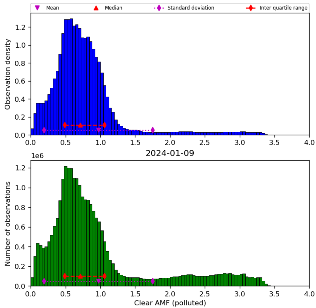
Figure 73: Histogram of “Clear AMF (polluted)” for 2024-01-08 to 2024-01-10
