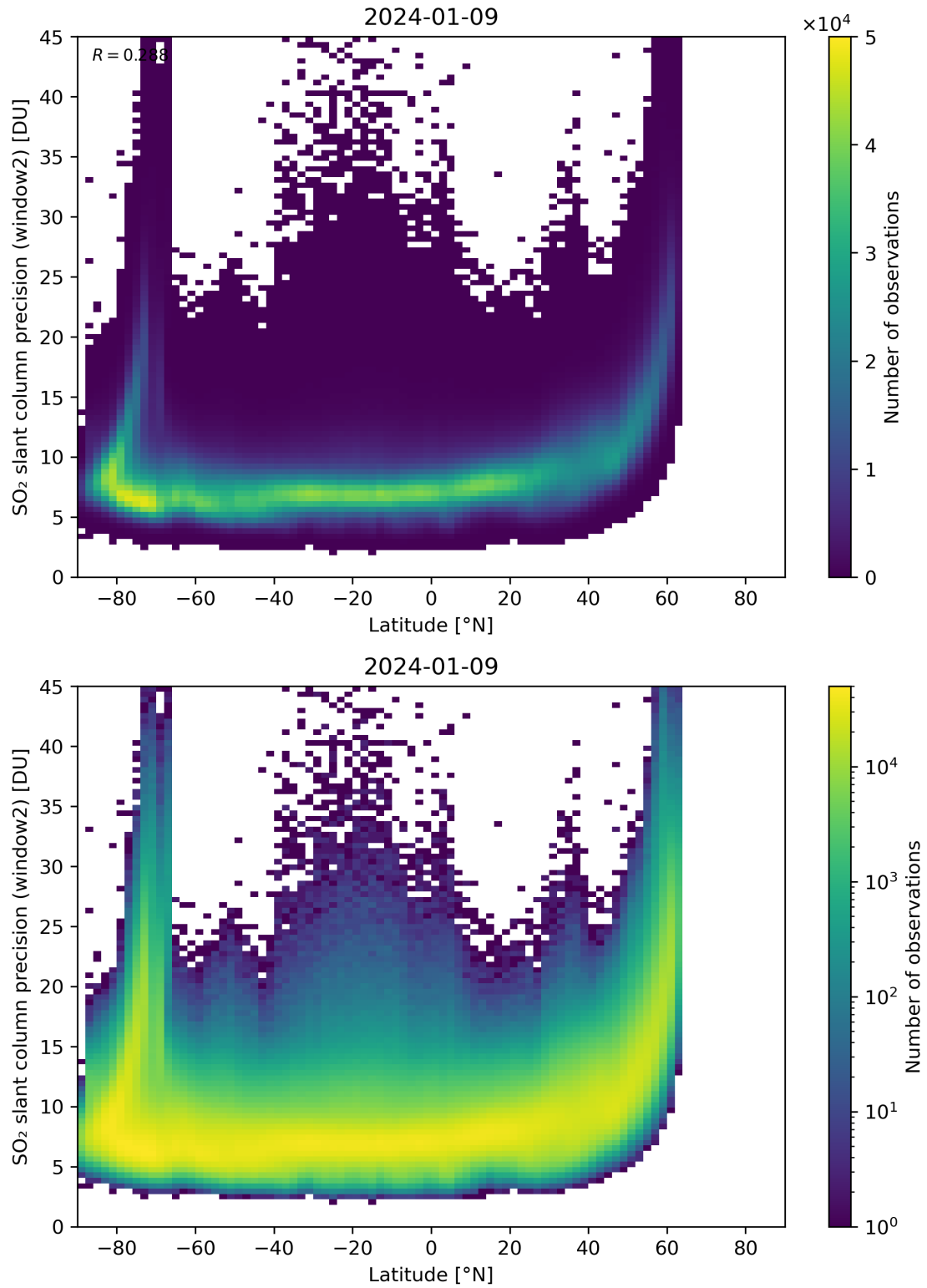
Figure 151: Scatter density plot of “Latitude” against “SO 2 slant column precision (window2)” for 2024-01-08 to 2024-01-10.
