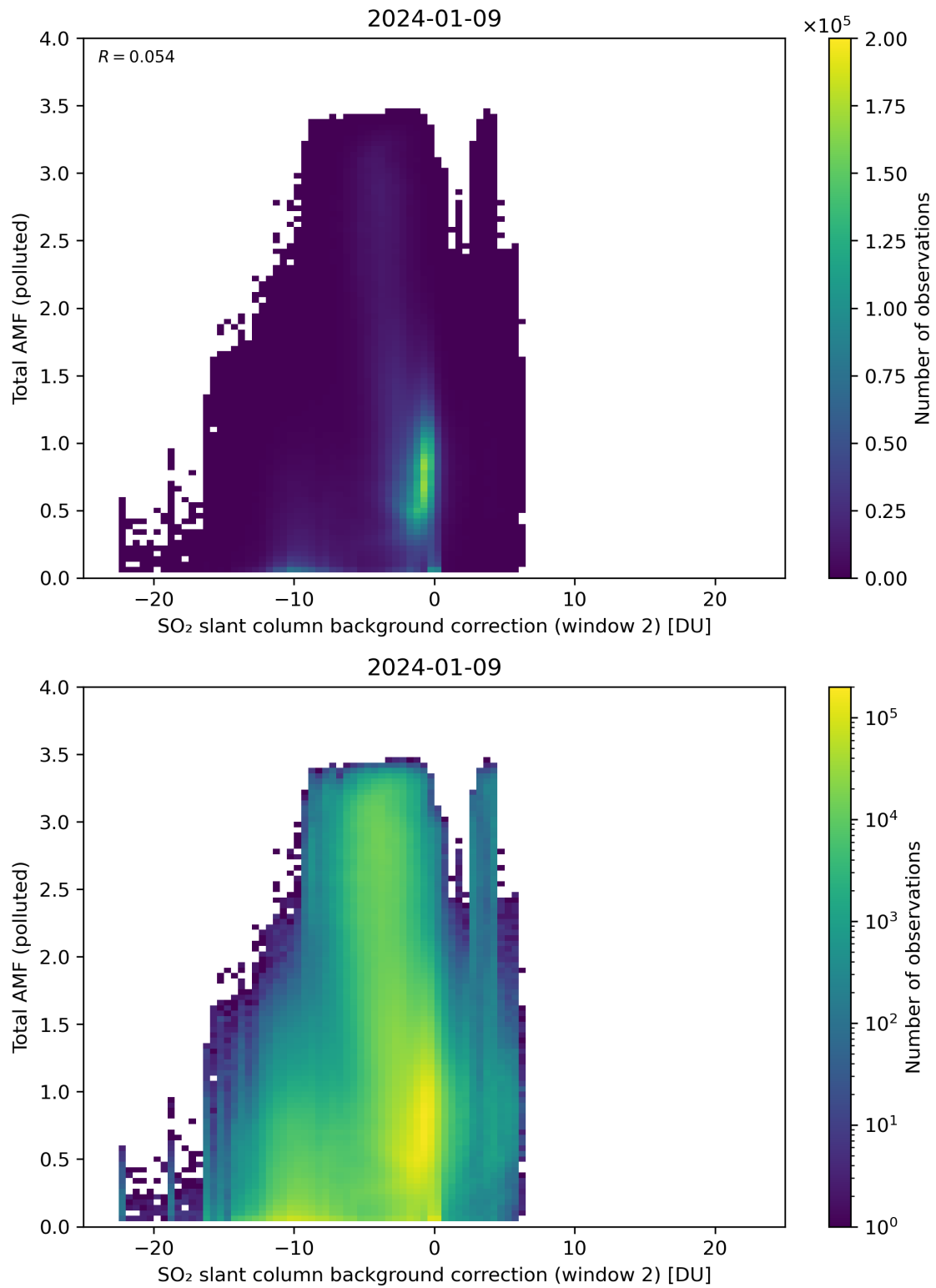
Figure 119: Scatter density plot of “SO 2 slant column background correction (window 2)” against “Total AMF (polluted)” for 2024-01-08 to 2024-01-10.
