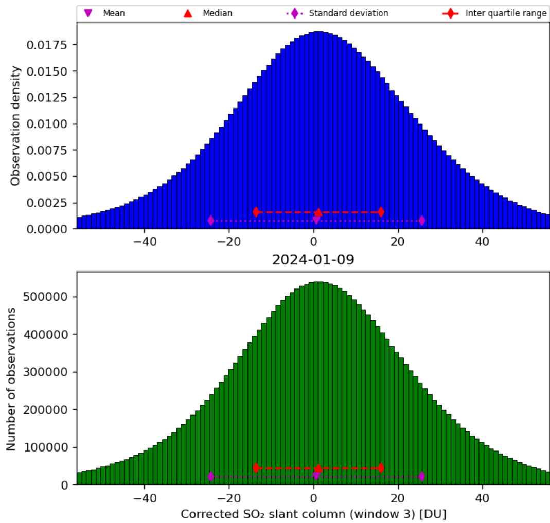
Figure 66: Histogram of “Corrected SO 2 slant column (window 3)” for 2024-01-08 to 2024-01-10
