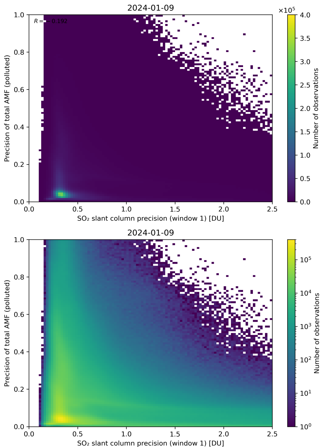
Figure 231: Scatter density plot of “SO 2 slant column precision (window 1)” against “Precision of total AMF (polluted)” for 2024-01-08 to 2024-01-10.
