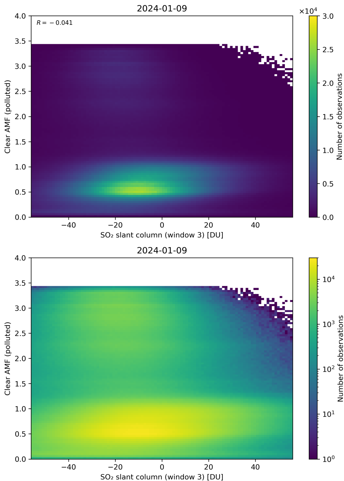
Figure 265: Scatter density plot of “SO 2 slant column (window 3)” against “Clear AMF (polluted)” for 2024-01-08 to 2024-01-10.
