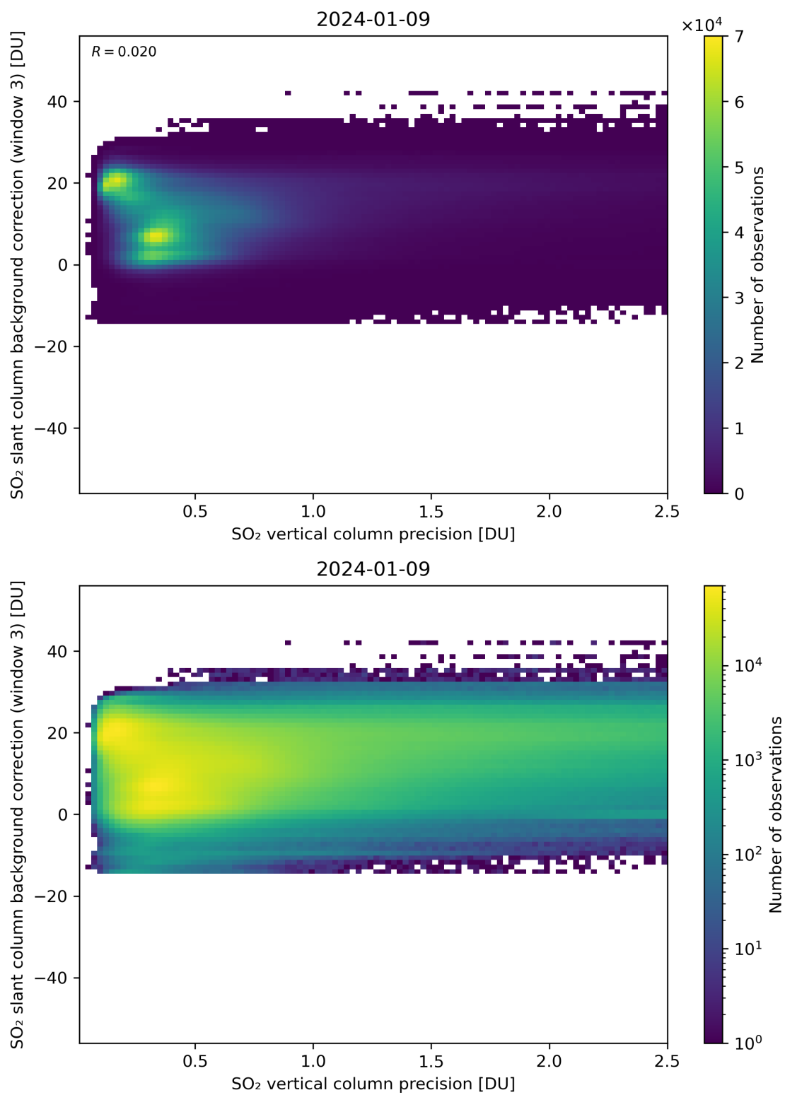
Figure 281: Scatter density plot of “SO 2 vertical column precision” against “SO 2 slant column background correction (window 3)” for 2024-01-08 to 2024-01-10.
