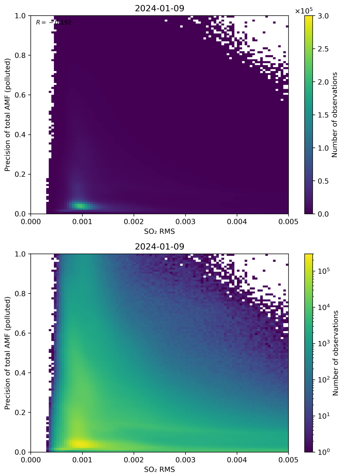
Figure 138: Scatter density plot of “SO 2 RMS” against “Precision of total AMF (polluted)” for 2024-01-08 to 2024-01-10.
