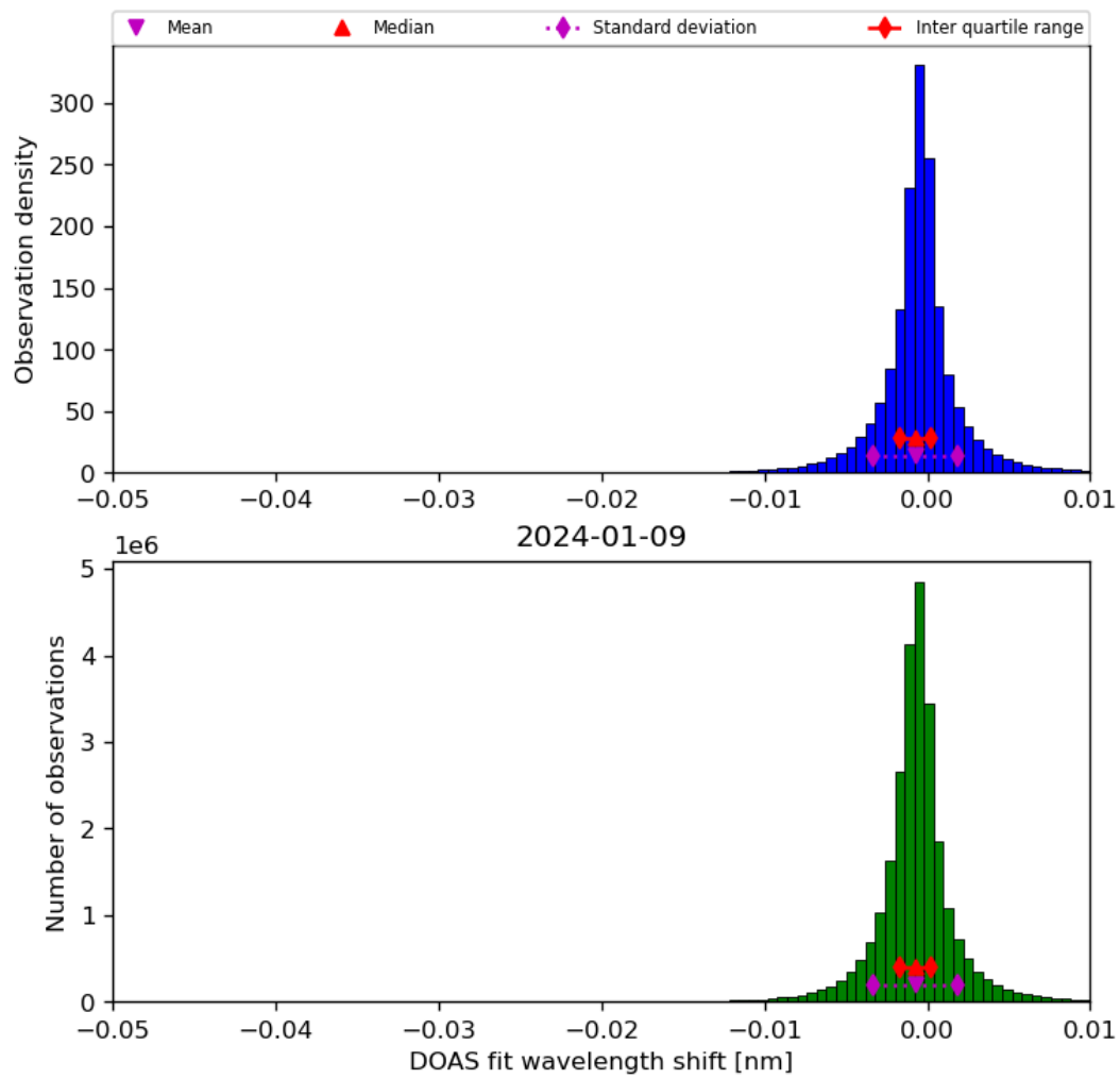
Figure 68: Histogram of “DOAS fit wavelength shift” for 2024-01-08 to 2024-01-10
