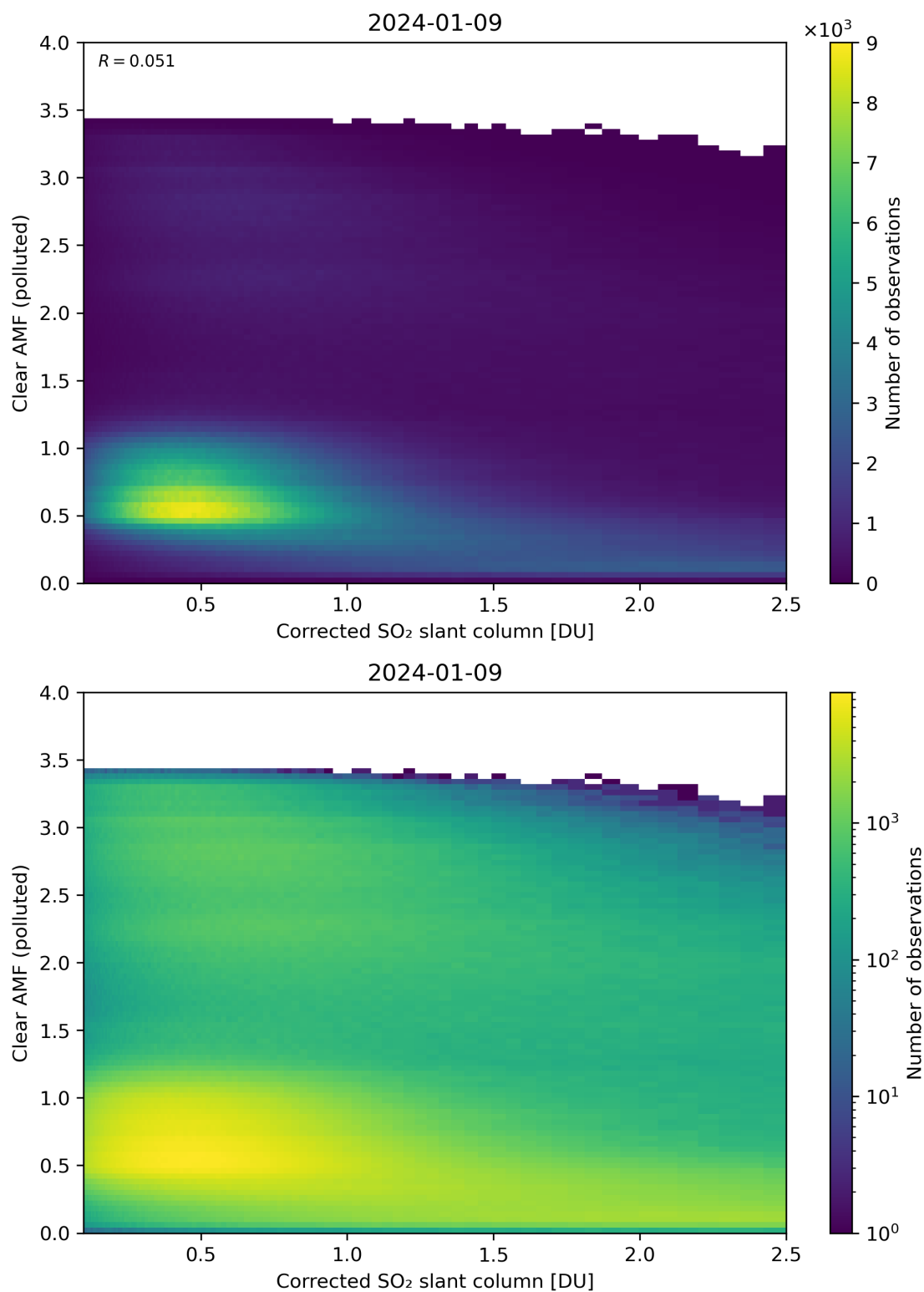
Figure 184: Scatter density plot of “Corrected SO 2 slant column” against “Clear AMF (polluted)” for 2024-01-08 to 2024-01-10.
