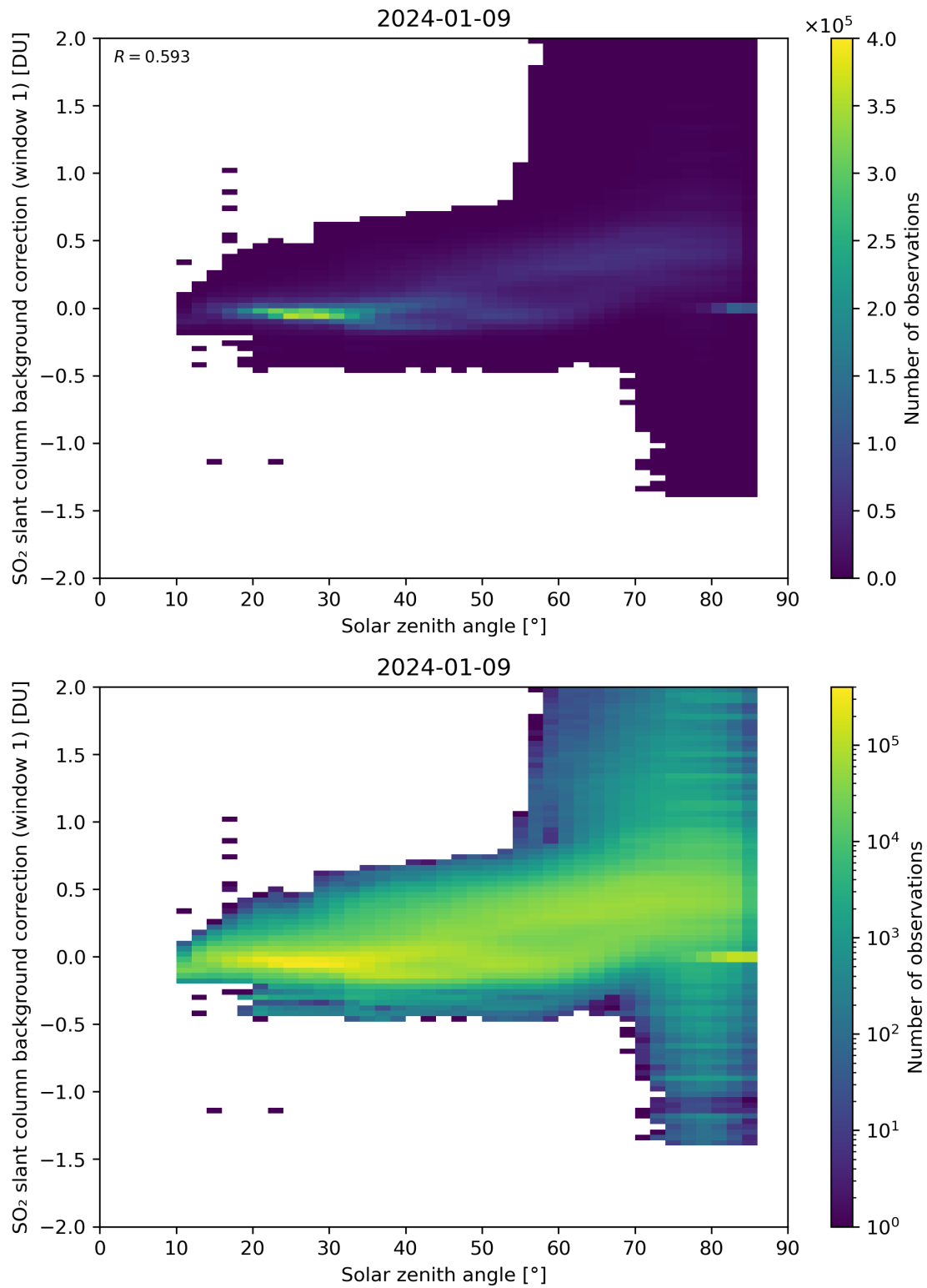
Figure 158: Scatter density plot of “Solar zenith angle” against “SO 2 slant column background correction (window 1)” for 2024-01-08 to 2024-01-10.
