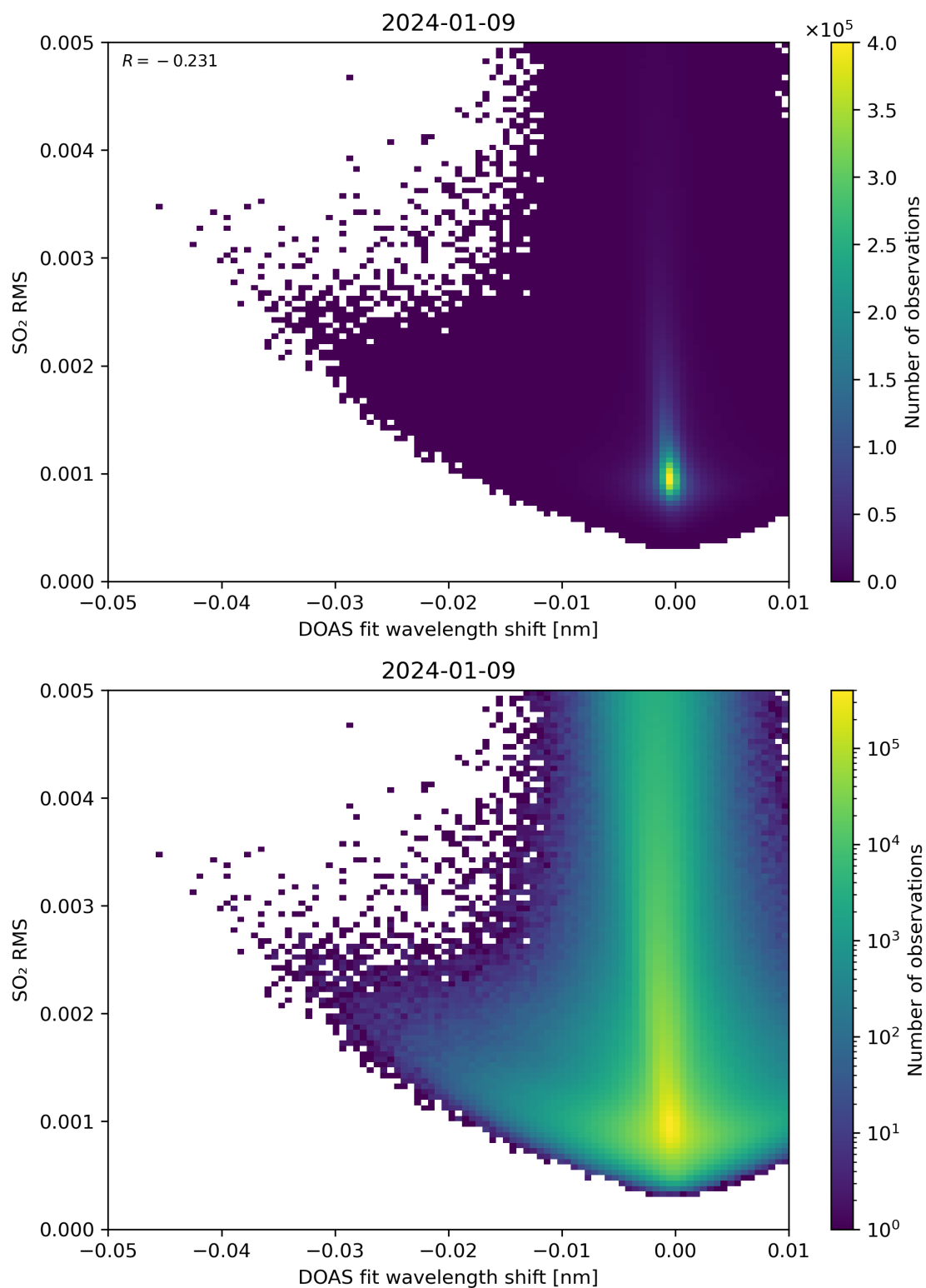
Figure 128: Scatter density plot of “DOAS fit wavelength shift” against “SO 2 RMS” for 2024-01-08 to 2024-01-10.
