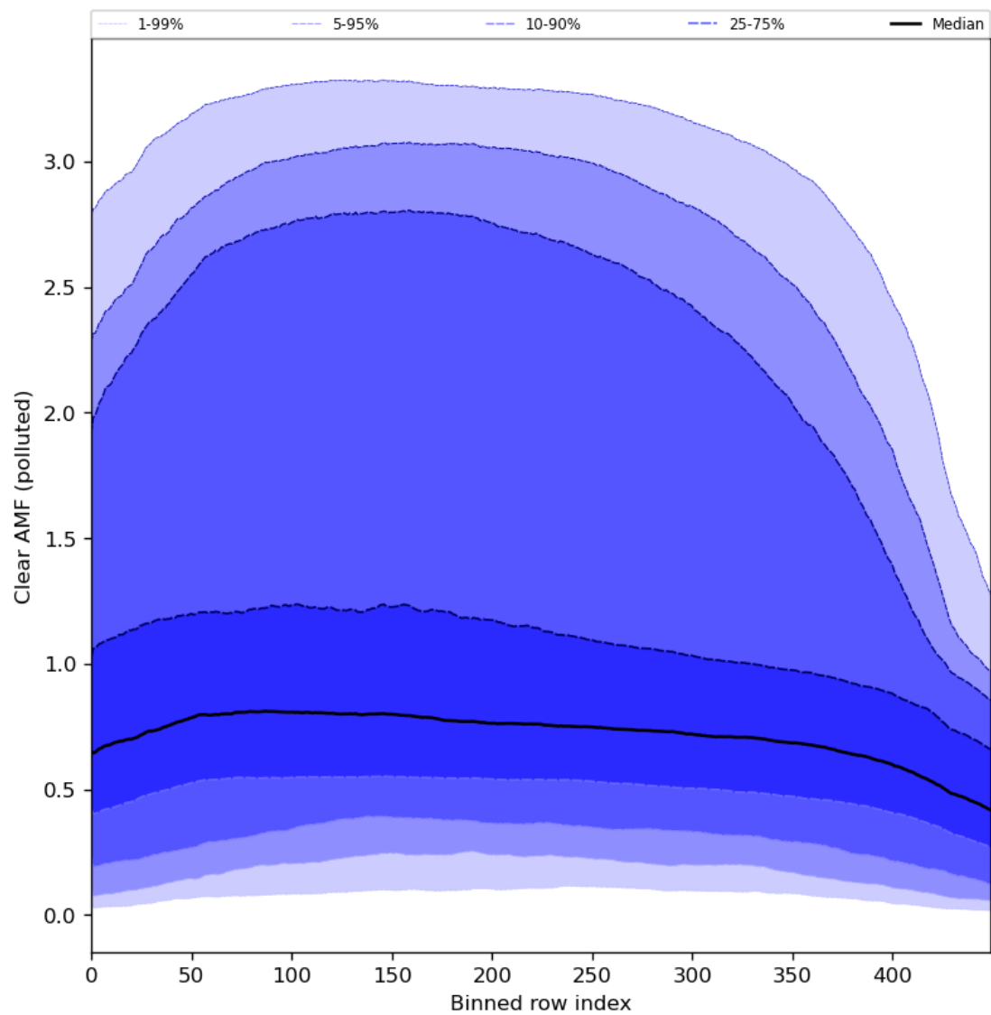
Figure 96: Along track statistics of “Clear AMF (polluted)” for 2024-01-08 to 2024-01-10
