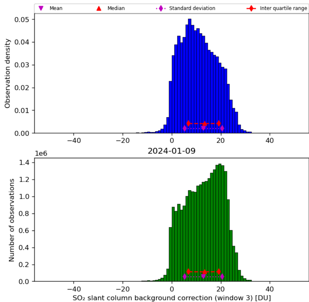
Figure 67: Histogram of “SO 2 slant column background correction (window 3)” for 2024-01-08 to 2024-01-10
