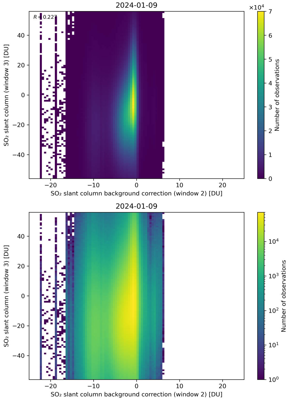
Figure 117: Scatter density plot of “SO 2 slant column background correction (window 2)” against “SO 2 slant column (window 3)” for 2024-01-08 to 2024-01-10.
