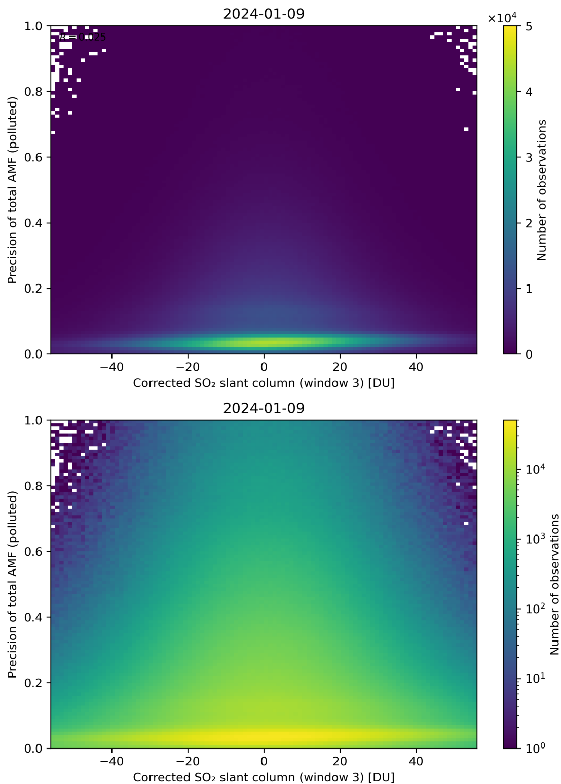
Figure 211: Scatter density plot of “Corrected SO 2 slant column (window 3)” against “Precision of total AMF (polluted)” for 2024-01-08 to 2024-01-10.
