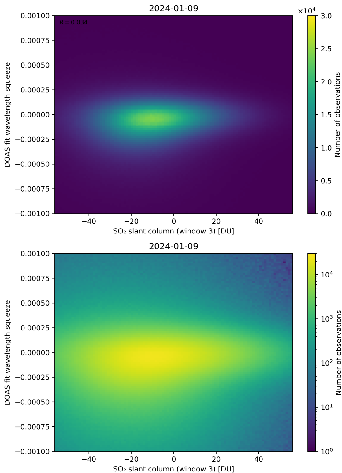
Figure 255: Scatter density plot of “SO 2 slant column (window 3)” against “DOAS fit wavelength squeeze” for 2024-01-08 to 2024-01-10.
