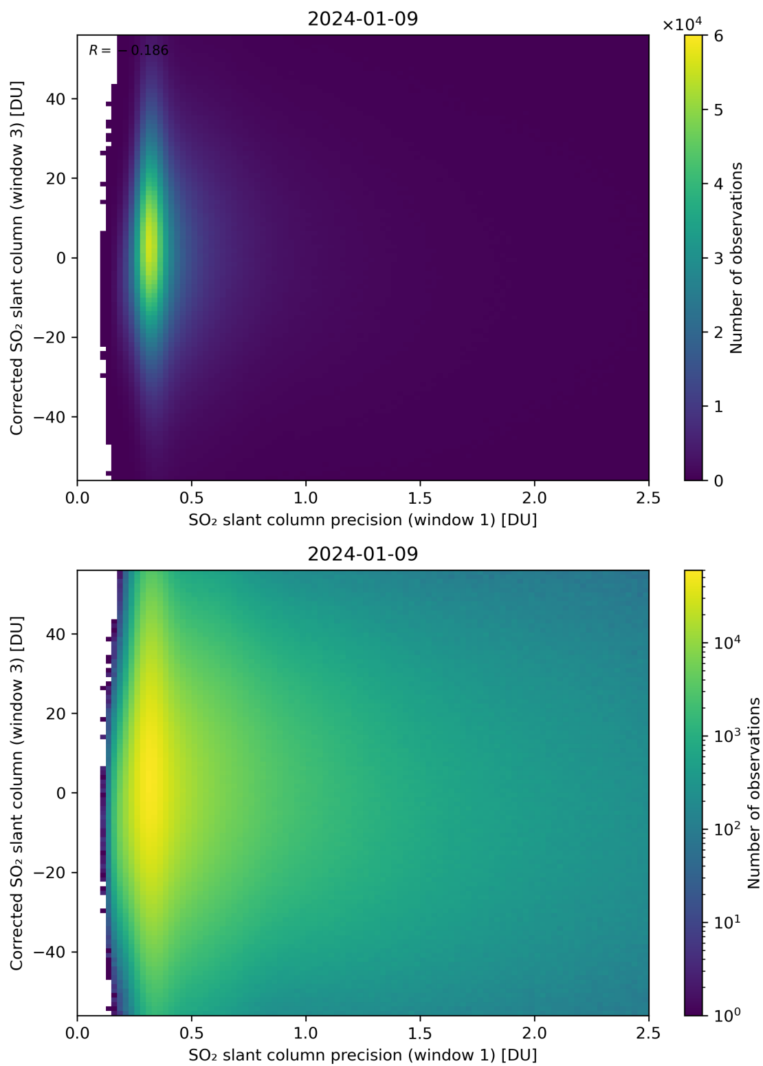
Figure 226: Scatter density plot of “SO 2 slant column precision (window 1)” against “Corrected SO 2 slant column (window 3)” for 2024-01-08 to 2024-01-10.
