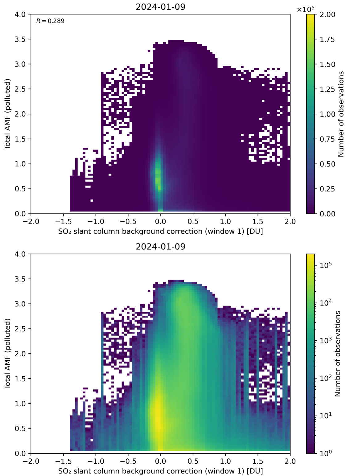
Figure 109: Scatter density plot of “SO 2 slant column background correction (window 1)” against “Total AMF (polluted)” for 2024-01-08 to 2024-01-10.
