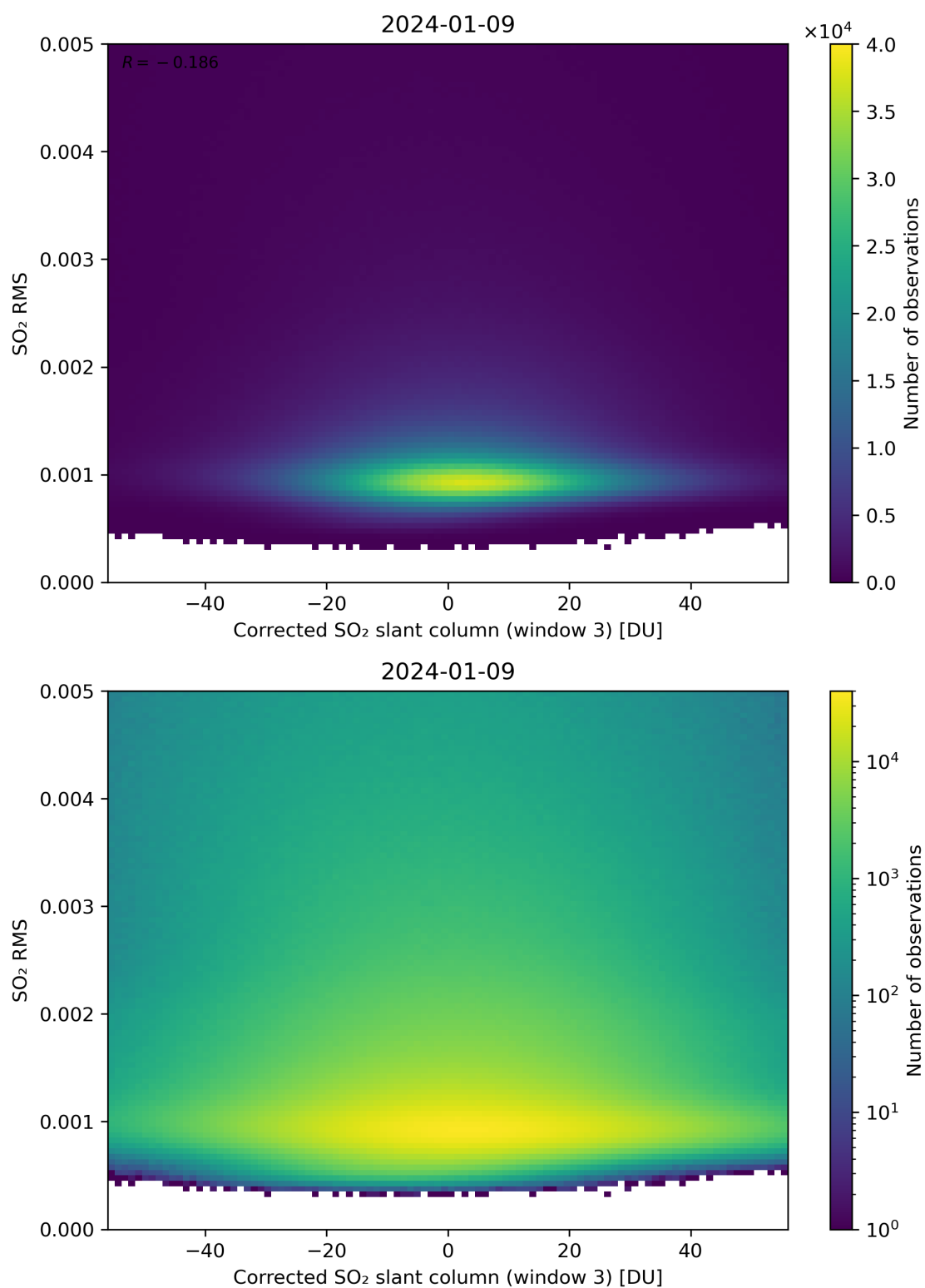
Figure 208: Scatter density plot of “Corrected SO 2 slant column (window 3)” against “SO 2 RMS” for 2024-01-08 to 2024-01-10.
