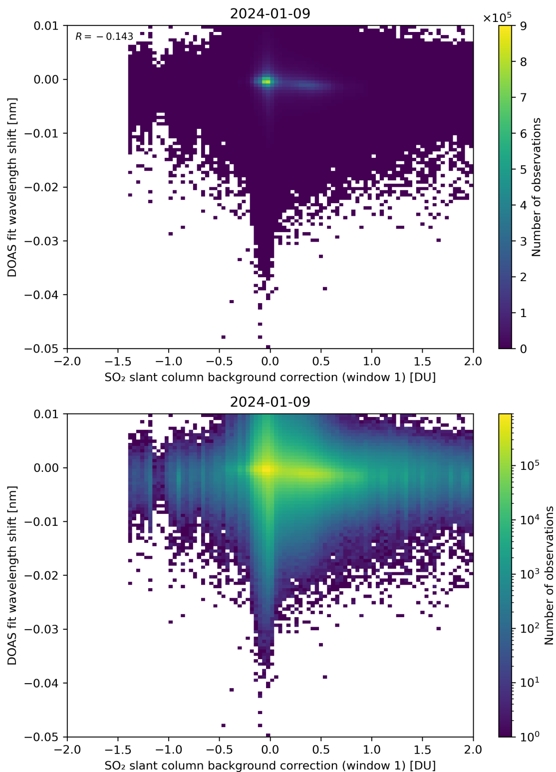
Figure 100: Scatter density plot of “SO 2 slant column background correction (window 1)” against “DOAS fit wavelength shift” for 2024-01-08 to 2024-01-10.
