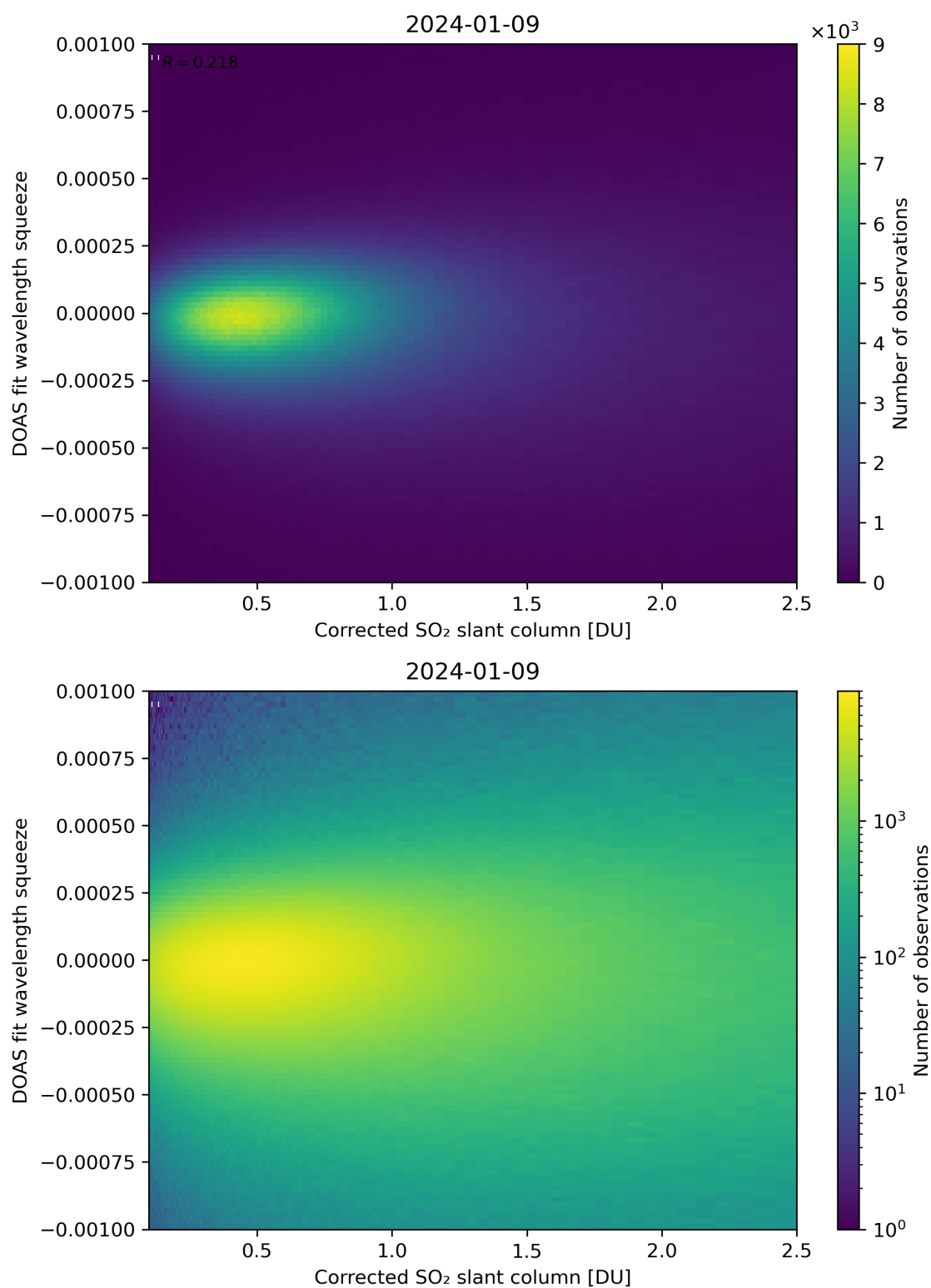
Figure 182: Scatter density plot of “Corrected SO 2 slant column” against “DOAS fit wavelength squeeze” for 2024-01-08 to 2024-01-10.
