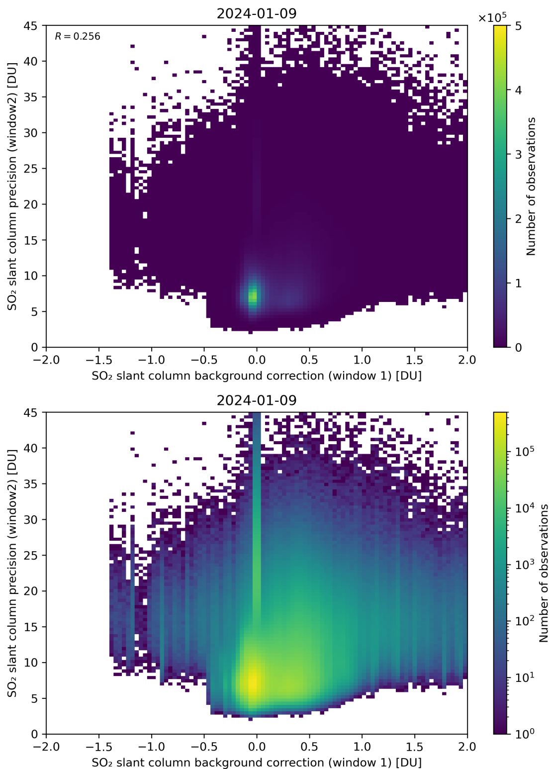
Figure 106: Scatter density plot of “SO 2 slant column background correction (window 1)” against “SO 2 slant column precision (window2)” for 2024-01-08 to 2024-01-10.
