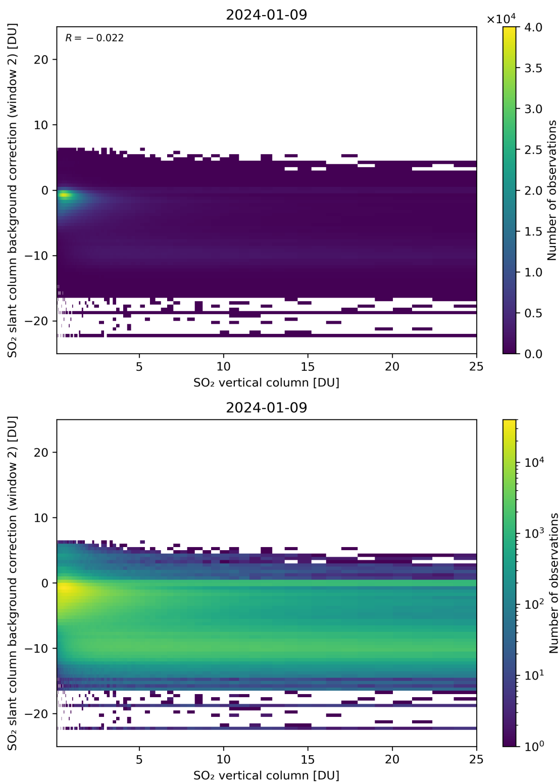
Figure 274: Scatter density plot of “SO 2 vertical column” against “SO 2 slant column background correction (window 2)” for 2024-01-08 to 2024-01-10.
