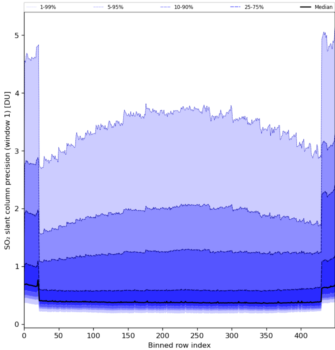
Figure 80: Along track statistics of “SO 2 slant column precision (window 1)” for 2024-01-08 to 2024-01-10
