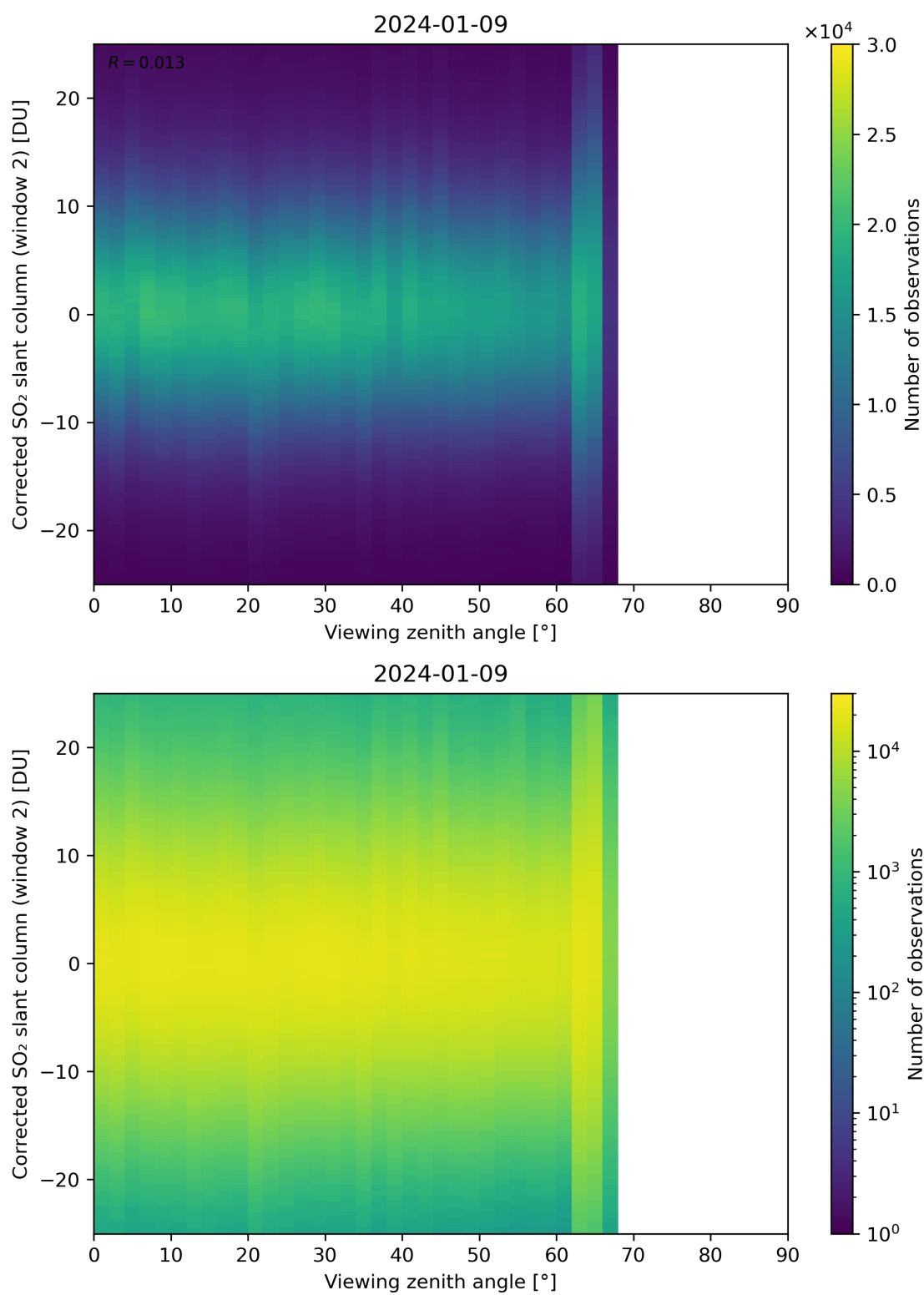
Figure 318: Scatter density plot of “Viewing zenith angle” against “Corrected SO 2 slant column (window 2)” for 2024-01-08 to 2024-01-10.
