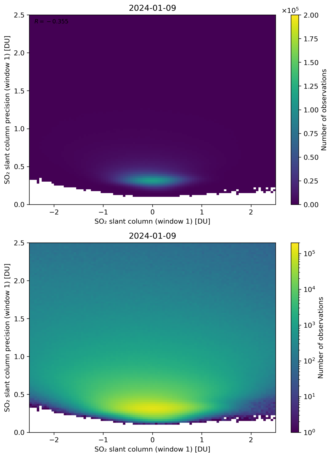
Figure 235: Scatter density plot of “SO 2 slant column (window 1)” against “SO 2 slant column precision (window 1)” for 2024-01-08 to 2024-01-10.
