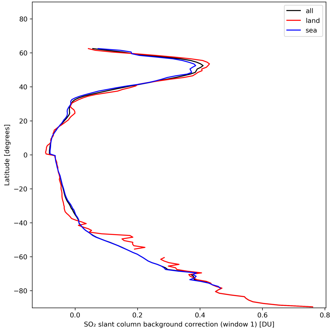
Figure 36: Zonal average of “SO 2 slant column background correction (window 1)” for 2024-01-08 to 2024-01-10.
