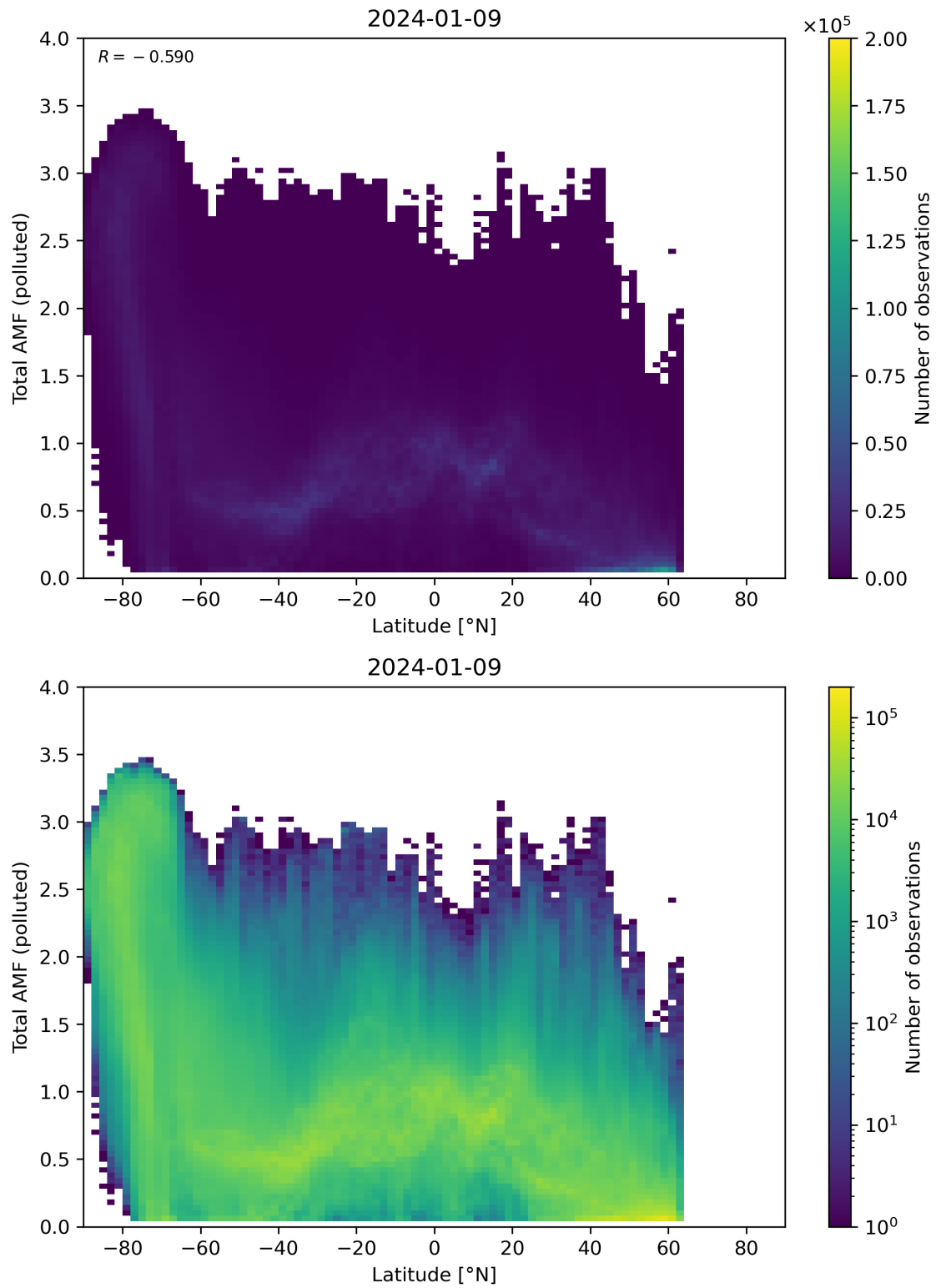
Figure 154: Scatter density plot of “Latitude” against “Total AMF (polluted)” for 2024-01-08 to 2024-01-10.
