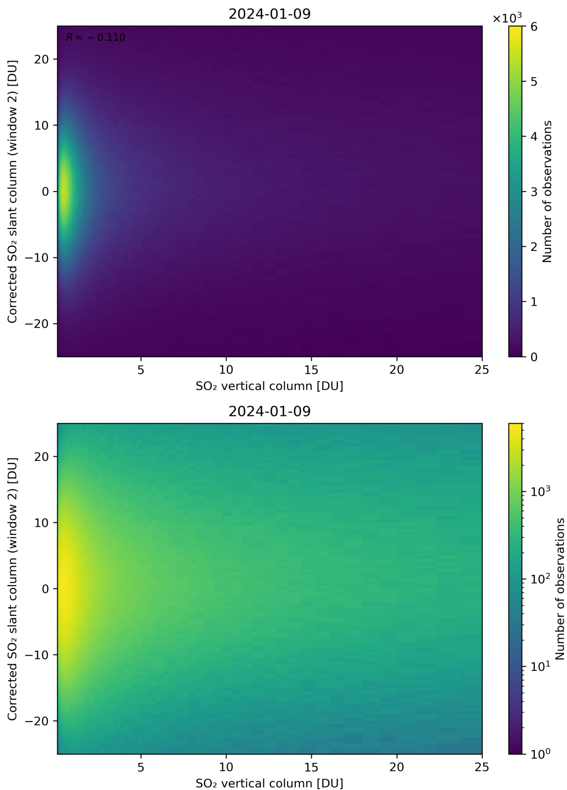
Figure 298: Scatter density plot of “SO 2 vertical column” against “Corrected SO 2 slant column (window 2)” for 2024-01-08 to 2024-01-10.
