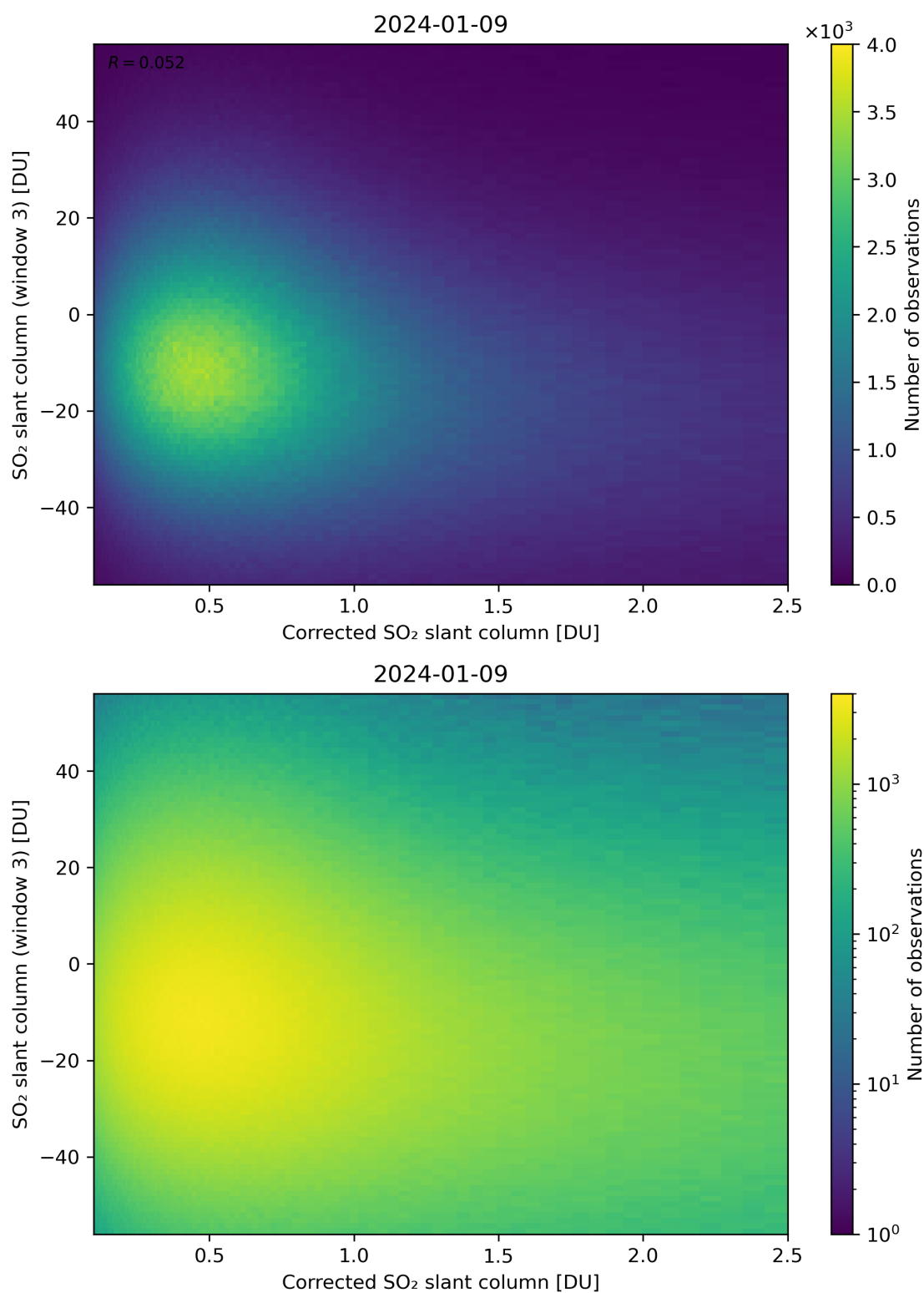
Figure 190: Scatter density plot of “Corrected SO 2 slant column” against “SO 2 slant column (window 3)” for 2024-01-08 to 2024-01-10.
