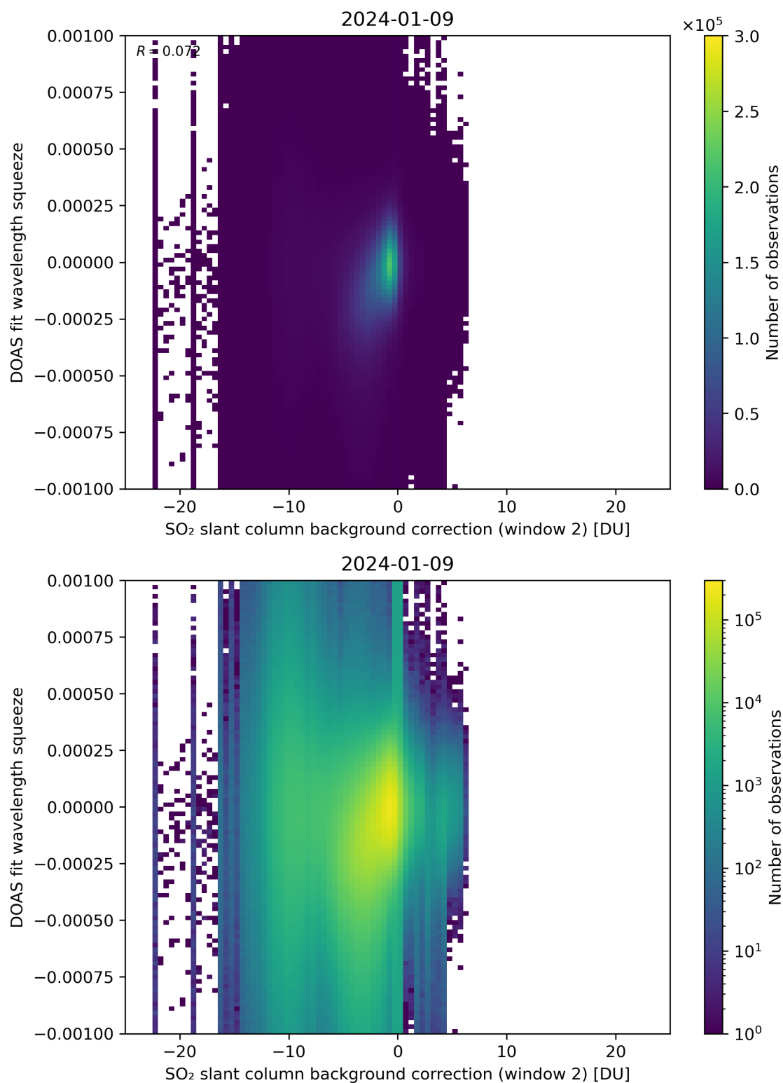
Figure 113: Scatter density plot of “SO 2 slant column background correction (window 2)” against “DOAS fit wavelength squeeze” for 2024-01-08 to 2024-01-10.
