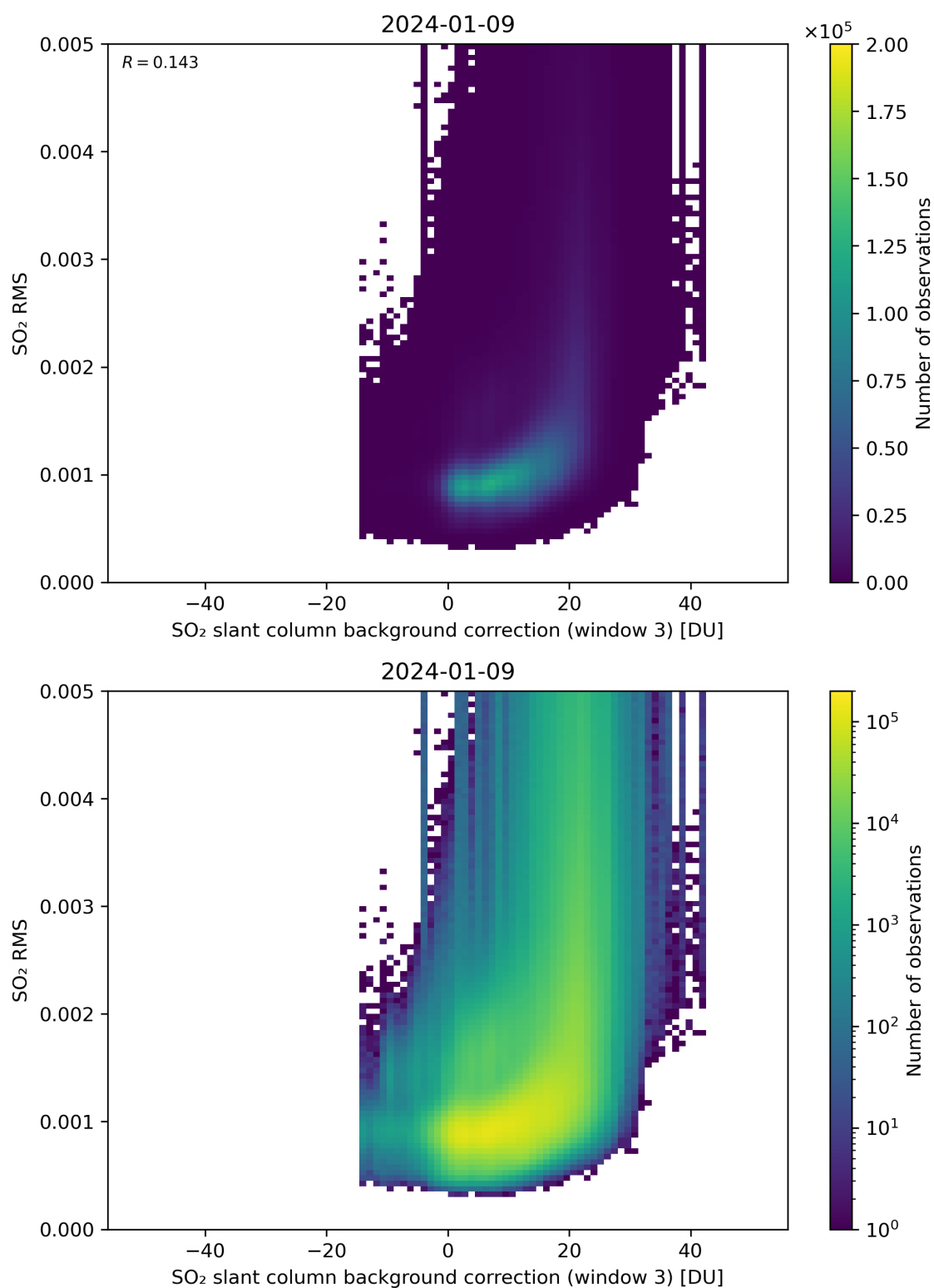
Figure 123: Scatter density plot of “SO 2 slant column background correction (window 3)” against “SO 2 RMS” for 2024-01-08 to 2024-01-10.
