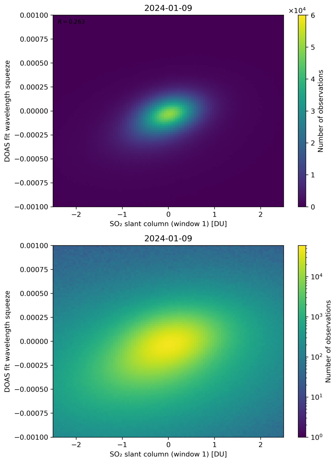
Figure 216: Scatter density plot of “SO 2 slant column (window 1)” against “DOAS fit wavelength squeeze” for 2024-01-08 to 2024-01-10.
