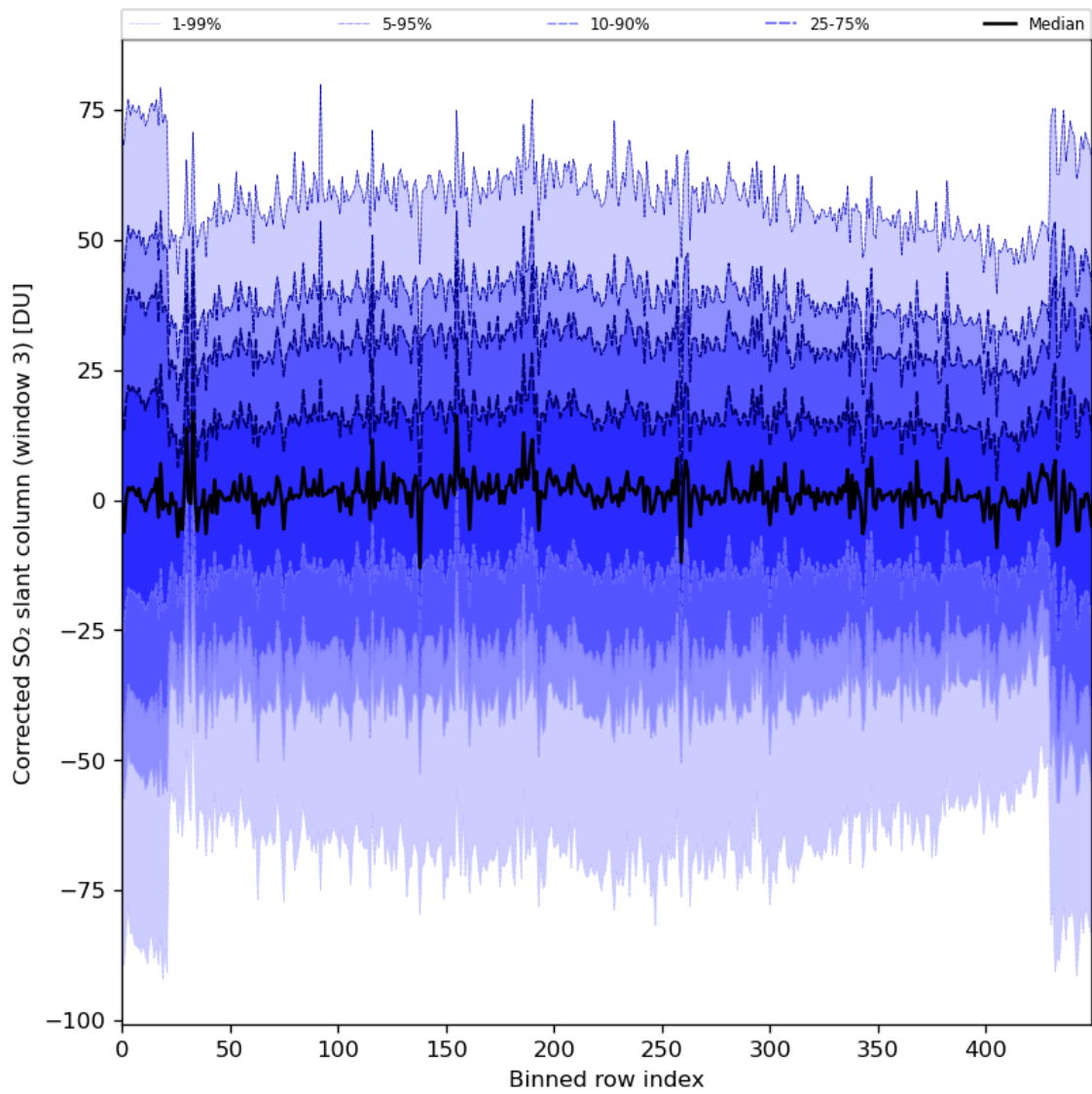
Figure 89: Along track statistics of “Corrected SO 2 slant column (window 3)” for 2024-01-08 to 2024-01-10
