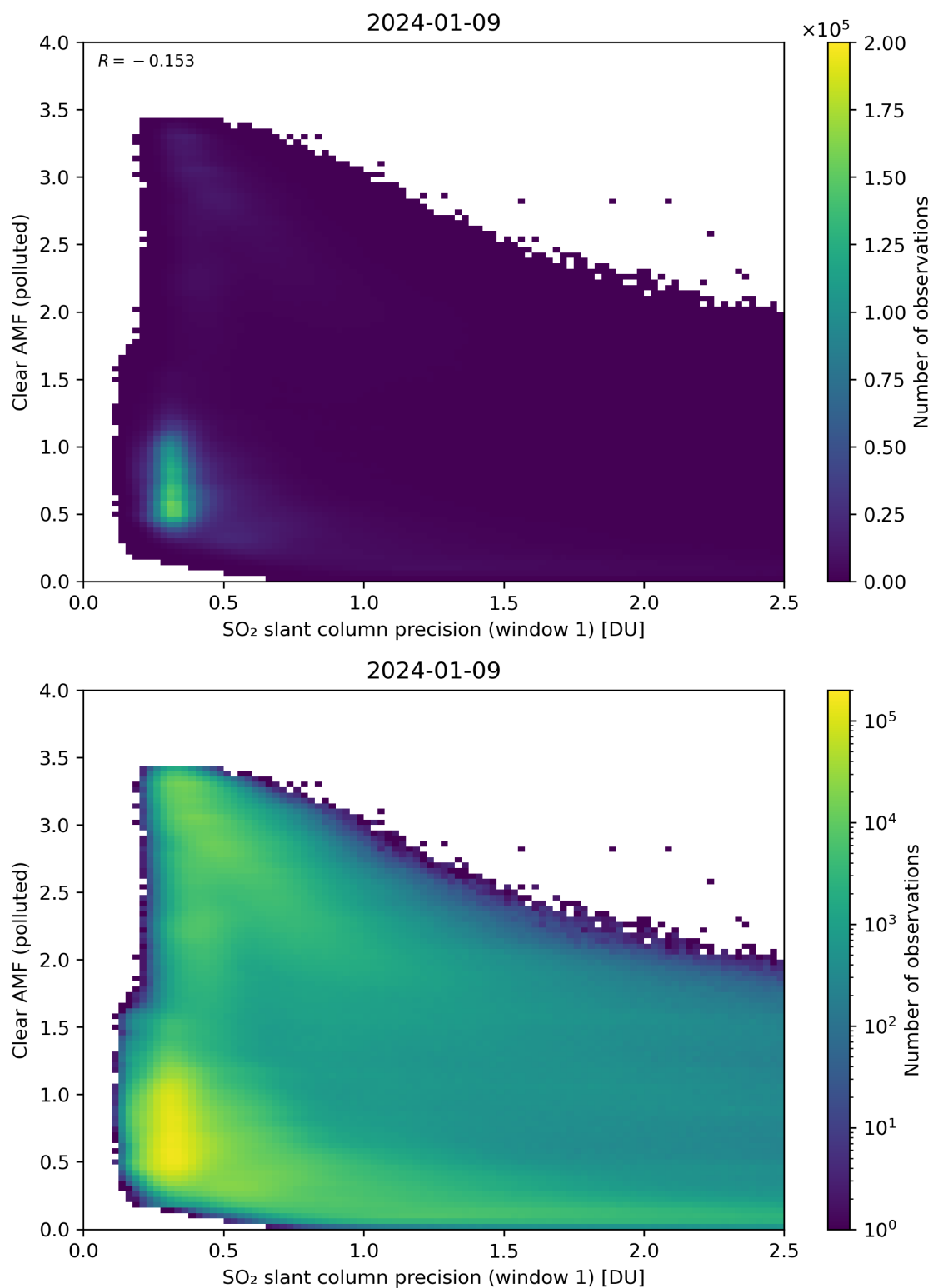
Figure 224: Scatter density plot of “SO 2 slant column precision (window 1)” against “Clear AMF (polluted)” for 2024-01-08 to 2024-01-10.
