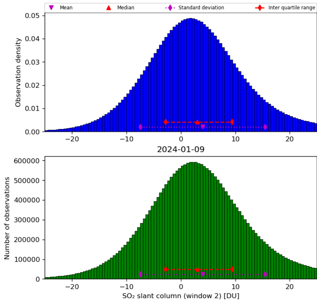
Figure 60: Histogram of “SO 2 slant column (window 2)” for 2024-01-08 to 2024-01-10
