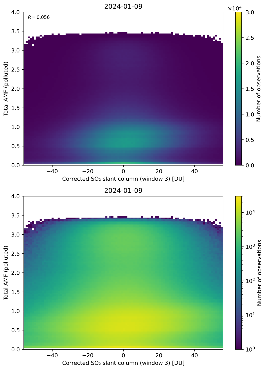
Figure 210: Scatter density plot of “Corrected SO 2 slant column (window 3)” against “Total AMF (polluted)” for 2024-01-08 to 2024-01-10.
