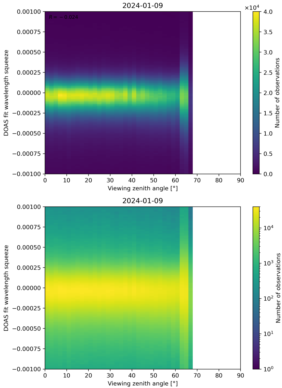
Figure 312: Scatter density plot of “Viewing zenith angle” against “DOAS fit wavelength squeeze” for 2024-01-08 to 2024-01-10.
