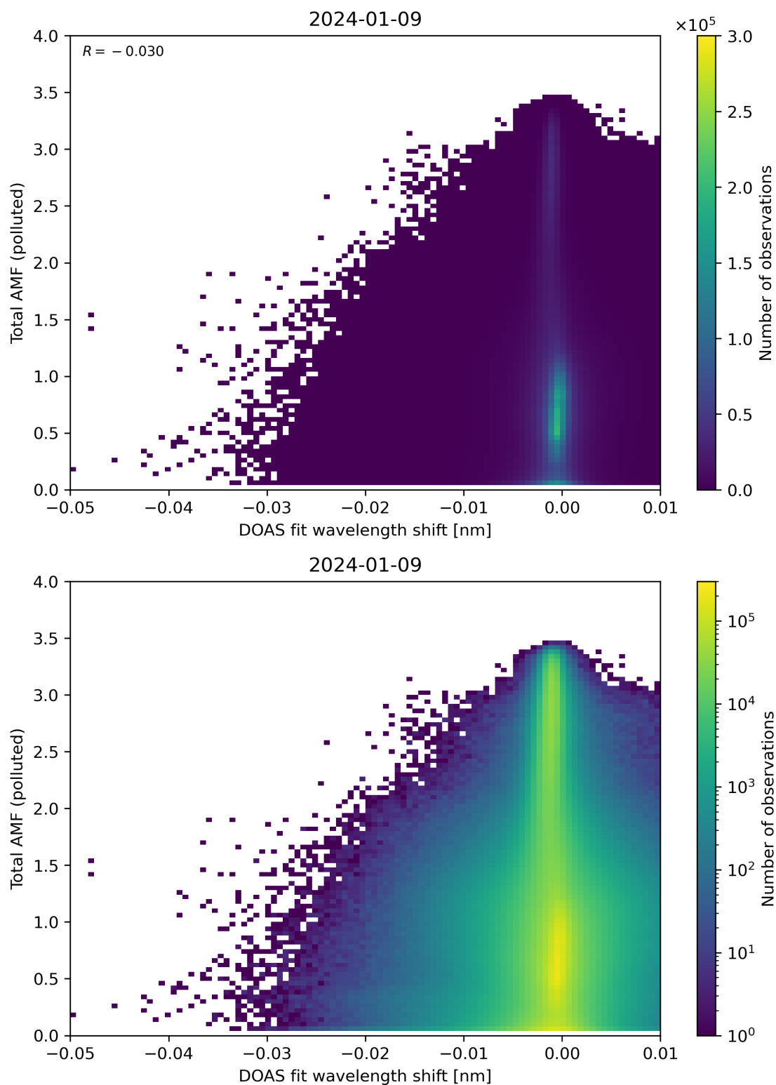
Figure 130: Scatter density plot of “DOAS fit wavelength shift” against “Total AMF (polluted)” for 2024-01-08 to 2024-01-10.
