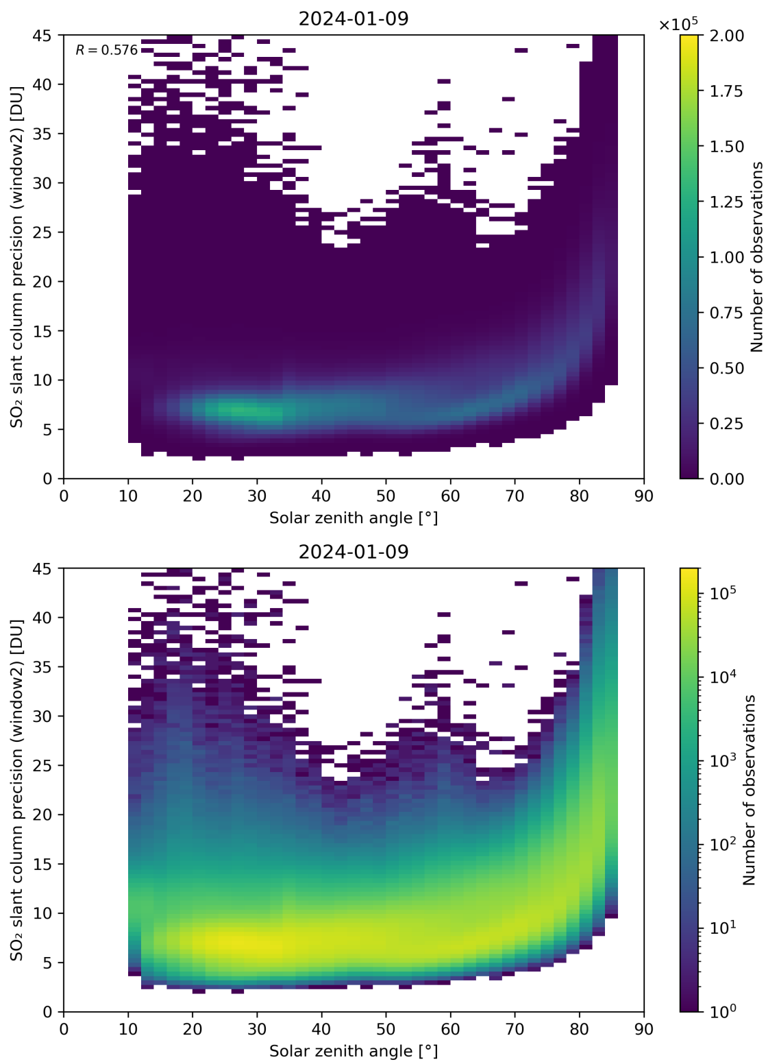
Figure 171: Scatter density plot of “Solar zenith angle” against “SO 2 slant column precision (window2)” for 2024-01-08 to 2024-01-10.
