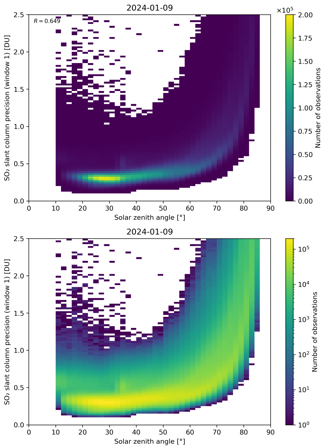
Figure 170: Scatter density plot of “Solar zenith angle” against “SO 2 slant column precision (window 1)” for 2024-01-08 to 2024-01-10.
