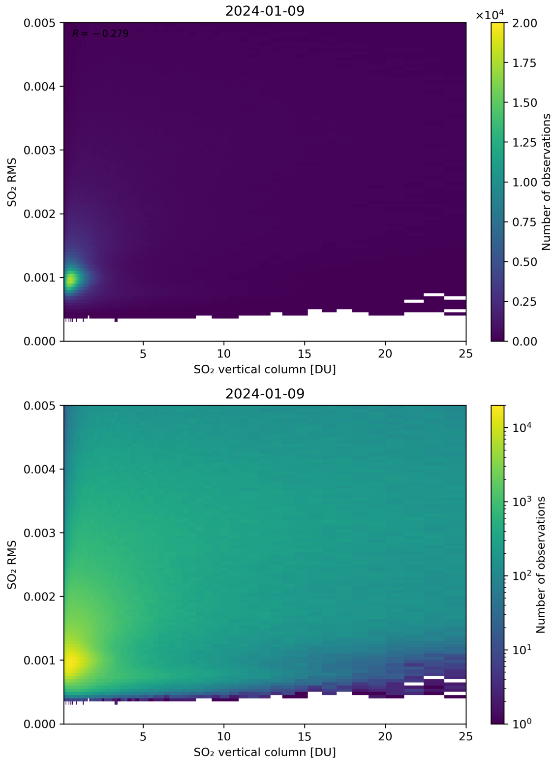
Figure 278: Scatter density plot of “SO 2 vertical column” against “SO 2 RMS” for 2024-01-08 to 2024-01-10.
