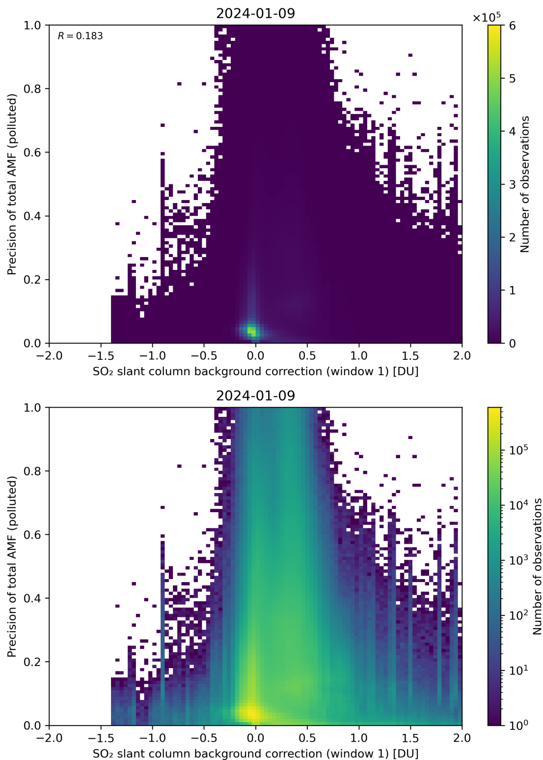
Figure 110: Scatter density plot of “SO 2 slant column background correction (window 1)” against “Precision of total AMF (polluted)” for 2024-01-08 to 2024-01-10.
