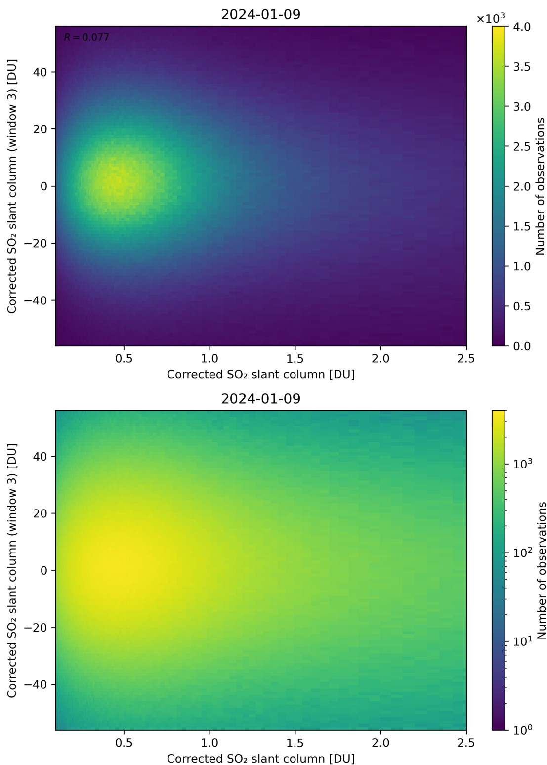
Figure 186: Scatter density plot of “Corrected SO 2 slant column” against “Corrected SO 2 slant column (window 3)” for 2024-01-08 to 2024-01-10.
