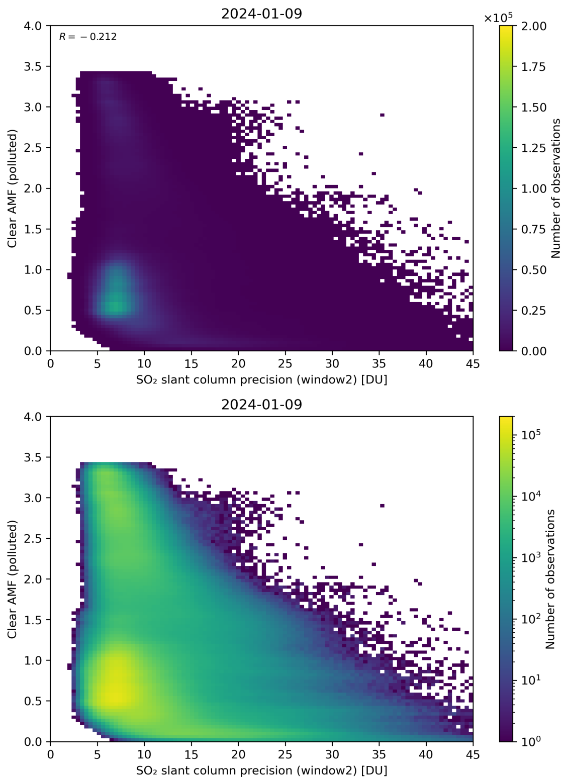
Figure 246: Scatter density plot of “SO 2 slant column precision (window2)” against “Clear AMF (polluted)” for 2024-01-08 to 2024-01-10.
