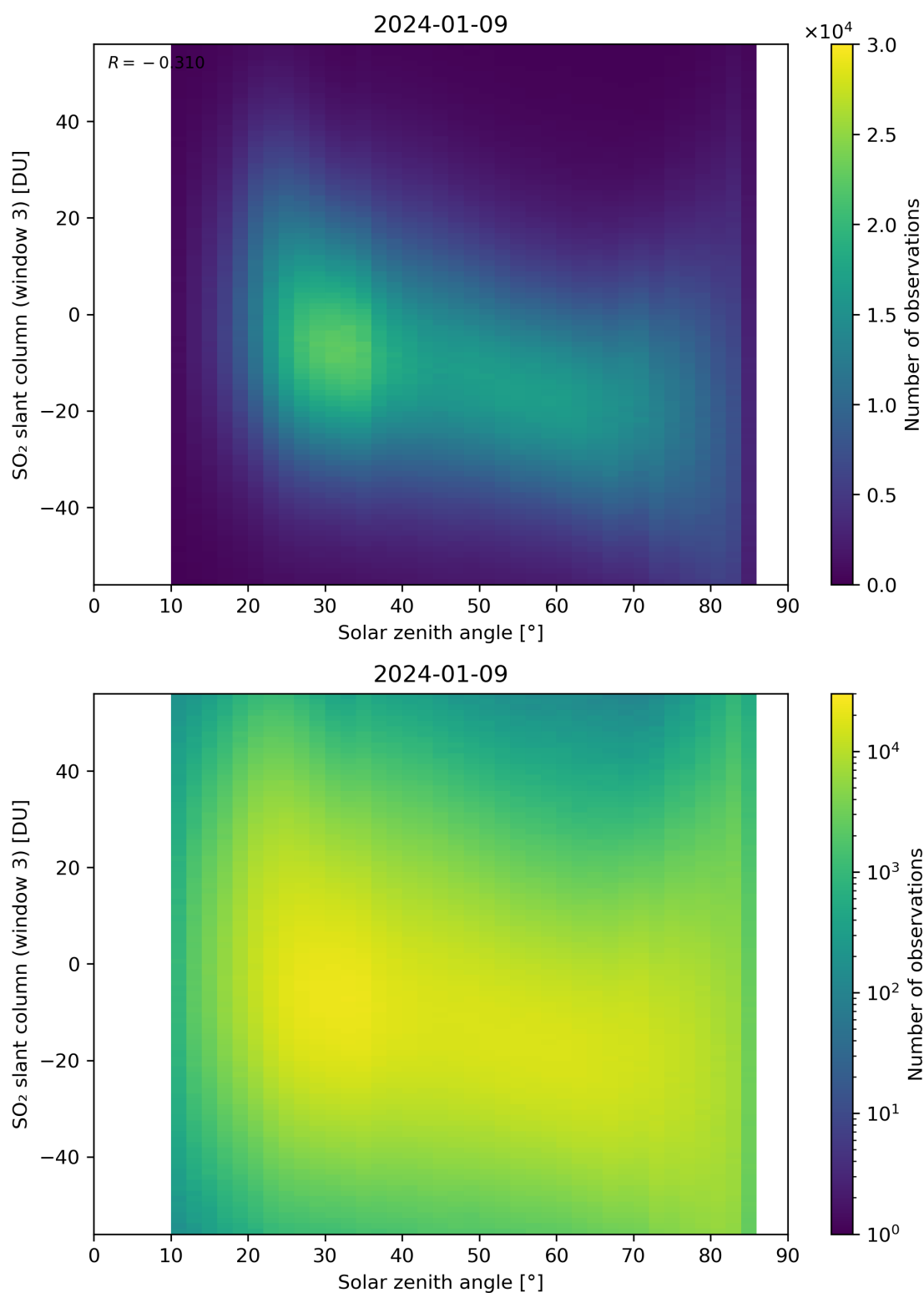
Figure 172: Scatter density plot of “Solar zenith angle” against “SO 2 slant column (window 3)” for 2024-01-08 to 2024-01-10.
