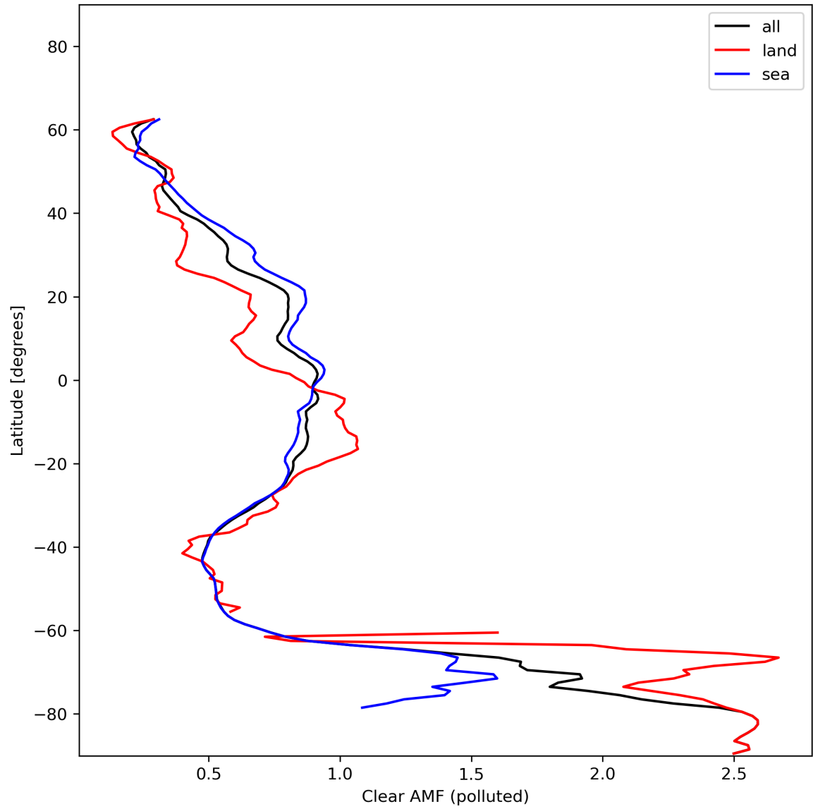
Figure 50: Zonal average of “Clear AMF (polluted)” for 2024-01-08 to 2024-01-10.
