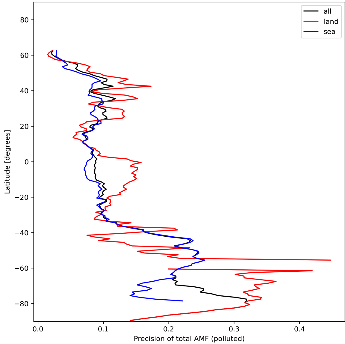
Figure 49: Zonal average of “Precision of total AMF (polluted)” for 2024-01-08 to 2024-01-10.
