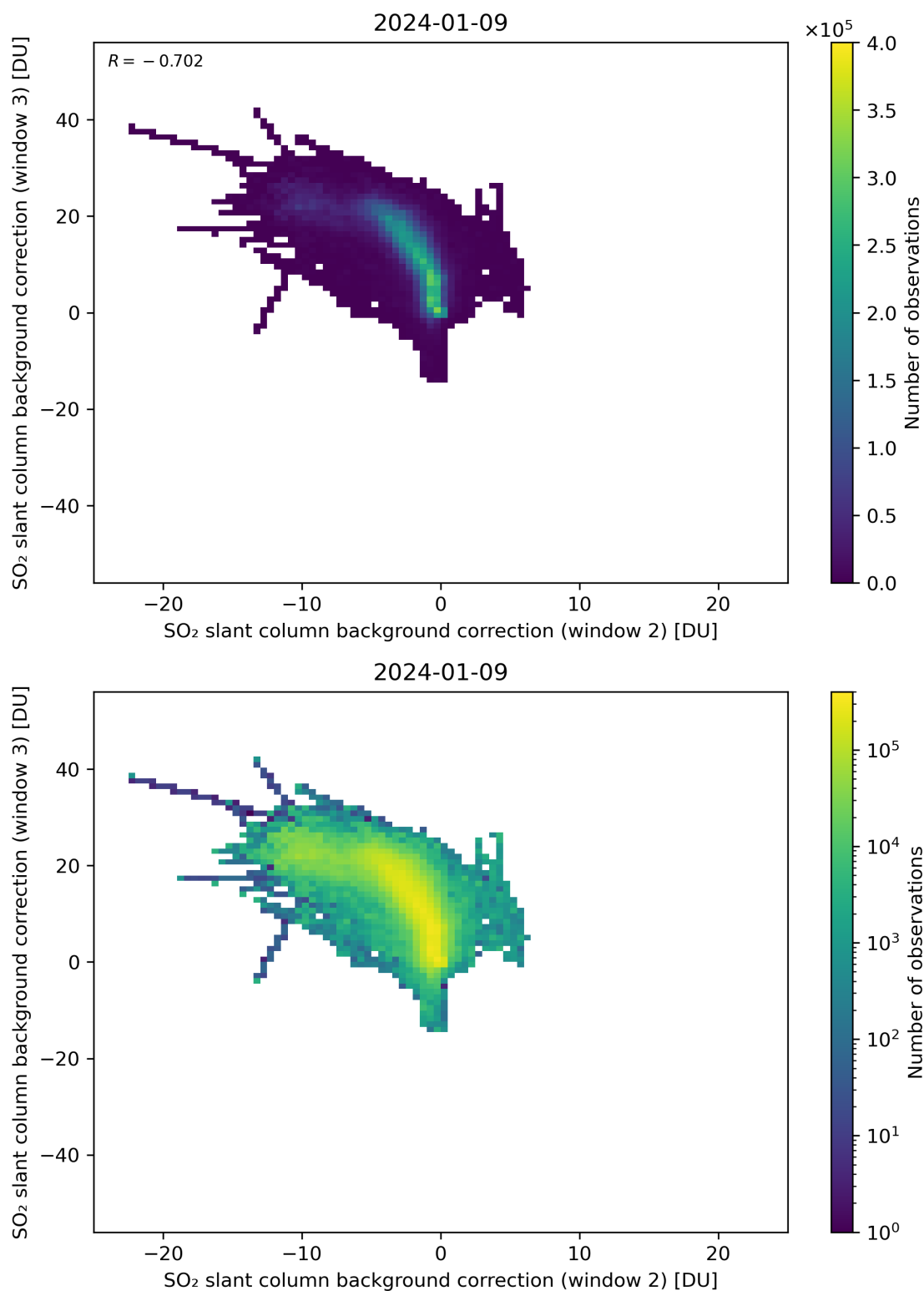
Figure 111: Scatter density plot of “SO 2 slant column background correction (window 2)” against “SO 2 slant column background correction (window 3)” for 2024-01-08 to 2024-01-10.
