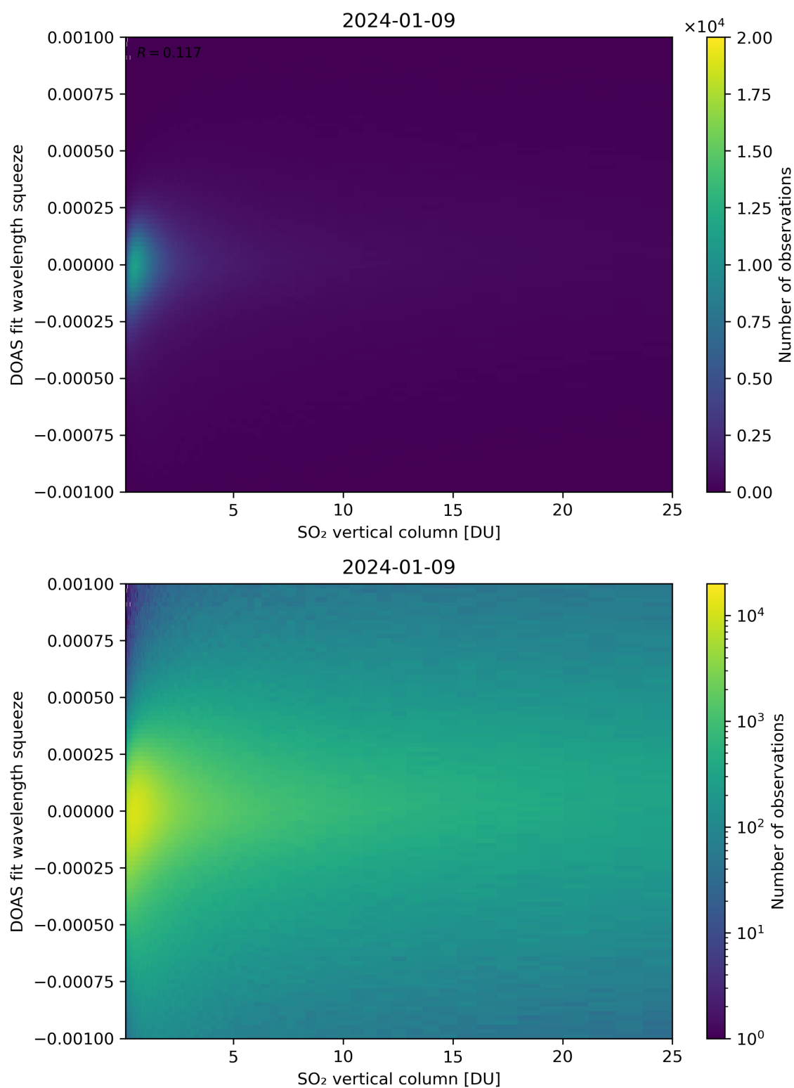
Figure 277: Scatter density plot of “SO 2 vertical column” against “DOAS fit wavelength squeeze” for 2024-01-08 to 2024-01-10.
