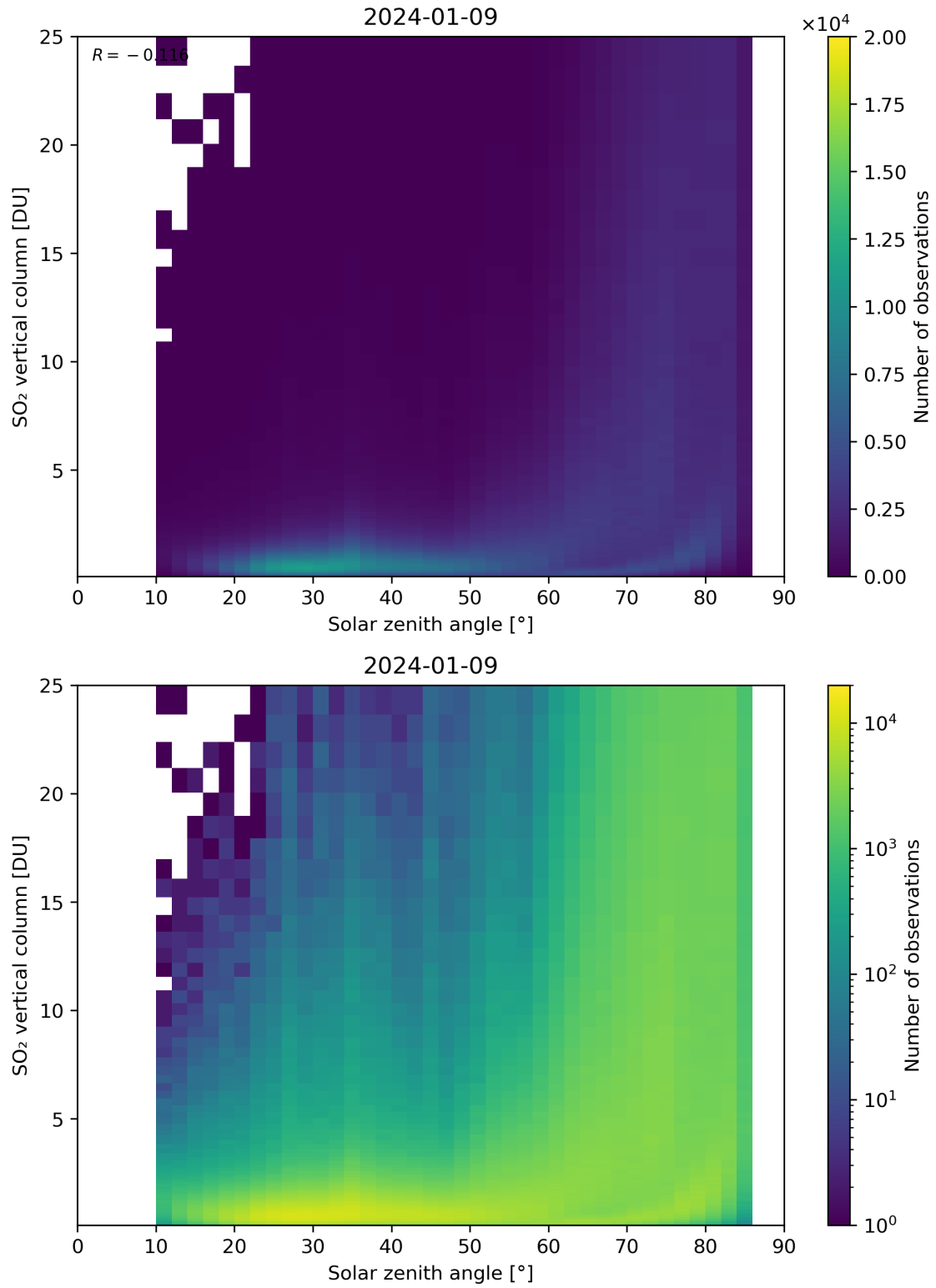
Figure 176: Scatter density plot of “Solar zenith angle” against “SO 2 vertical column” for 2024-01-08 to 2024-01-10.
