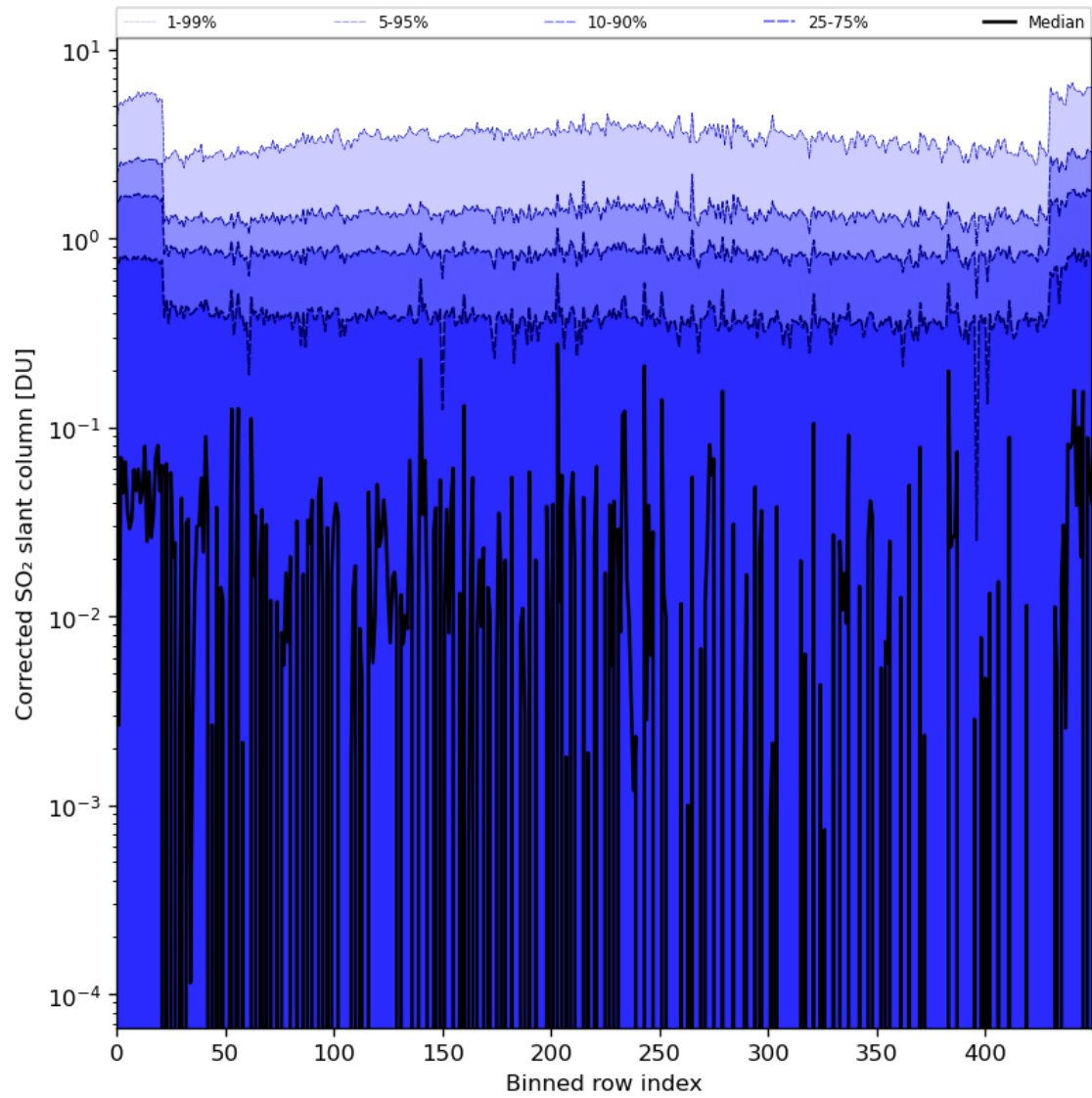
Figure 78: Along track statistics of “Corrected SO 2 slant column” for 2024-01-08 to 2024-01-10
