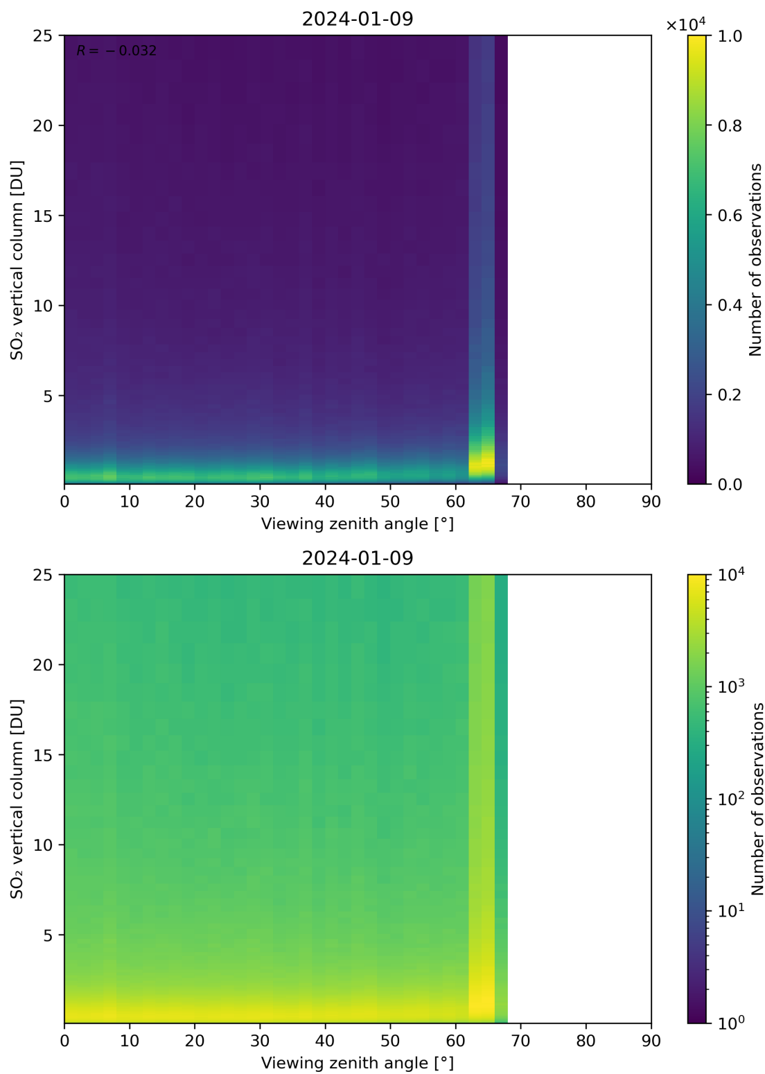
Figure 327: Scatter density plot of “Viewing zenith angle” against “SO 2 vertical column” for 2024-01-08 to 2024-01-10.
