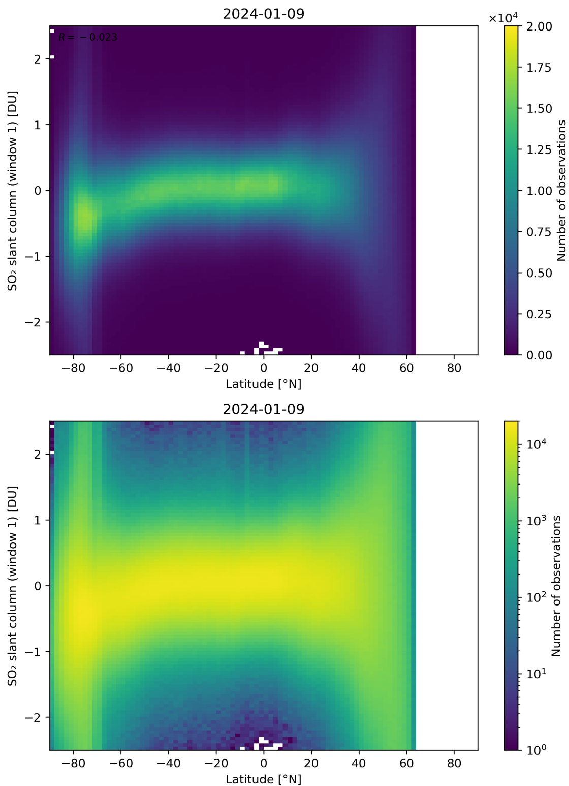
Figure 149: Scatter density plot of “Latitude” against “SO 2 slant column (window 1)” for 2024-01-08 to 2024-01-10.
