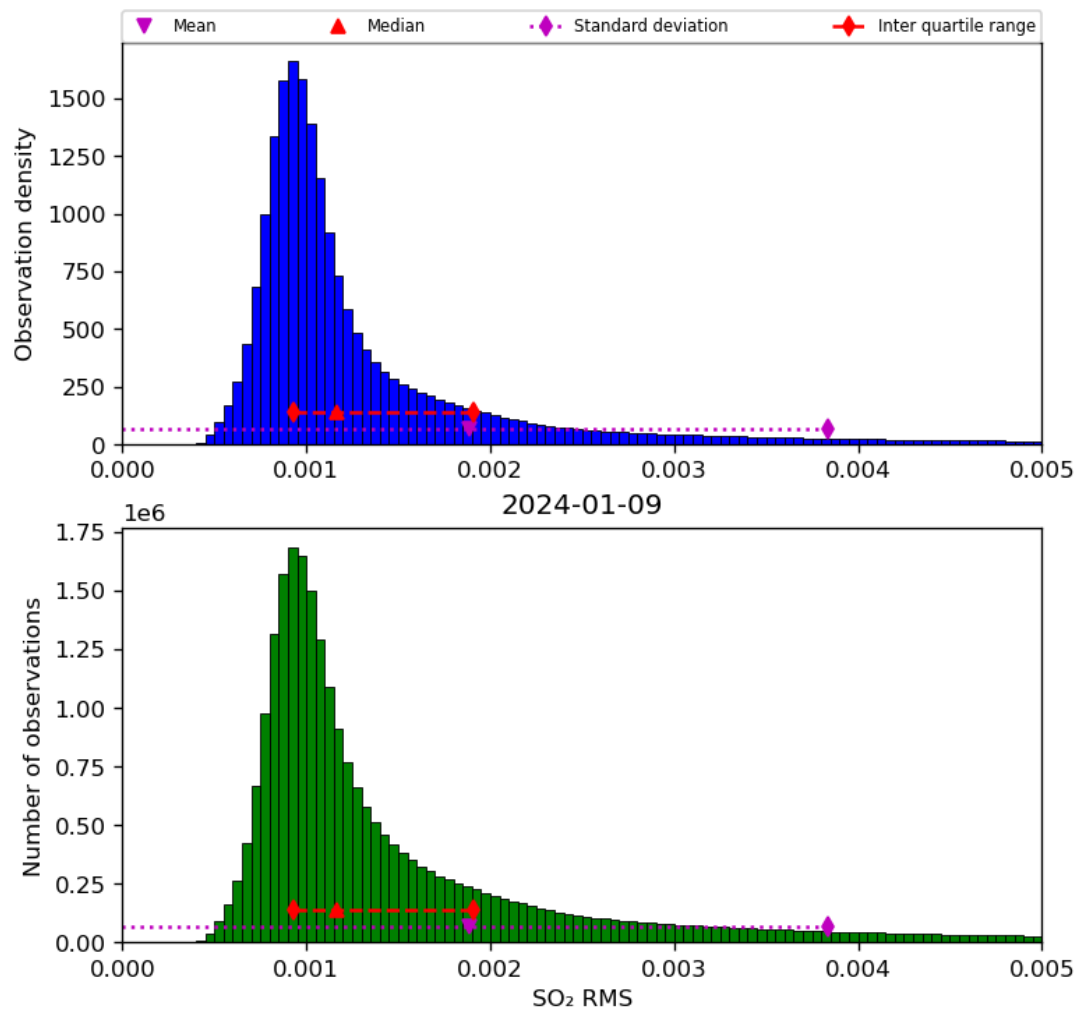
Figure 70: Histogram of “SO 2 RMS” for 2024-01-08 to 2024-01-10
