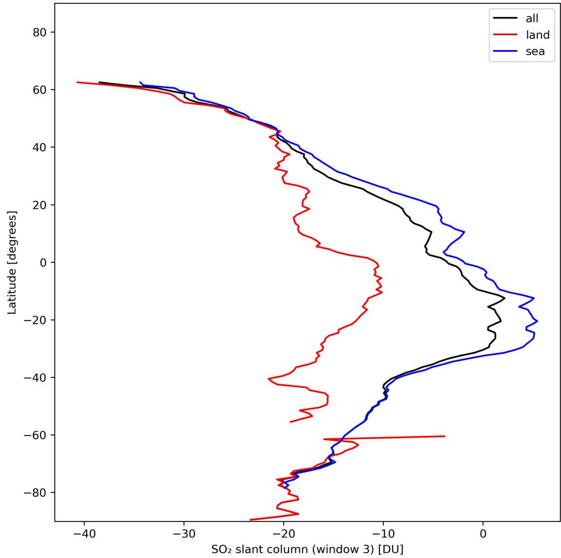
Figure 41: Zonal average of “SO 2 slant column (window 3)” for 2024-01-08 to 2024-01-10.
