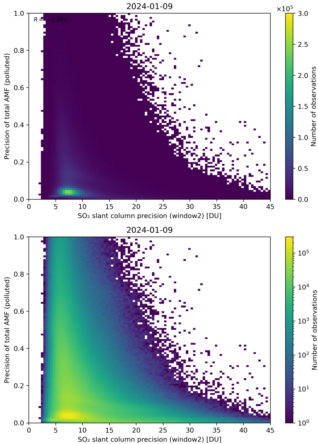
Figure 252: Scatter density plot of “SO 2 slant column precision (window2)” against “Precision of total AMF (polluted)” for 2024-01-08 to 2024-01-10.
