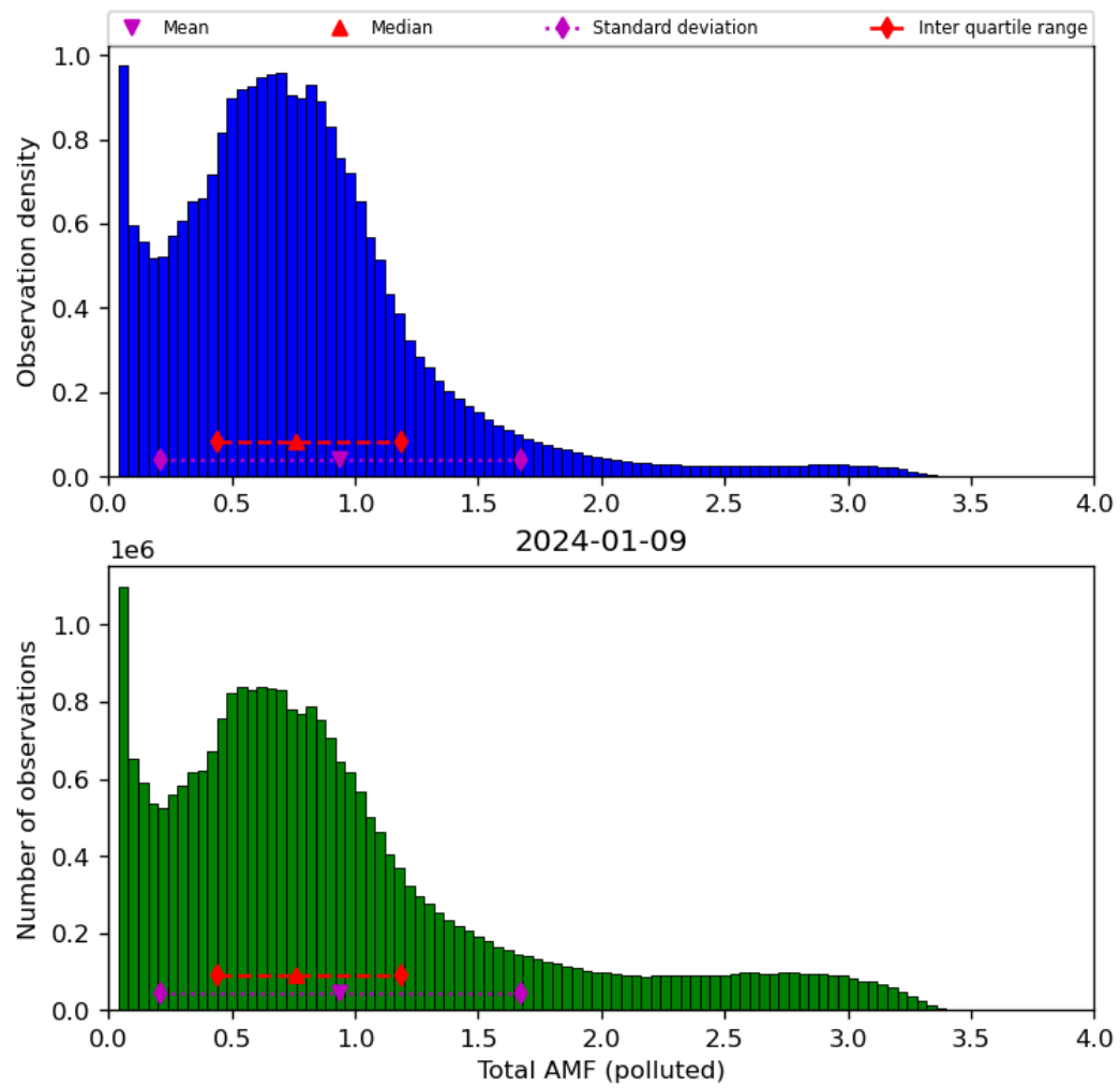
Figure 71: Histogram of “Total AMF (polluted)” for 2024-01-08 to 2024-01-10
