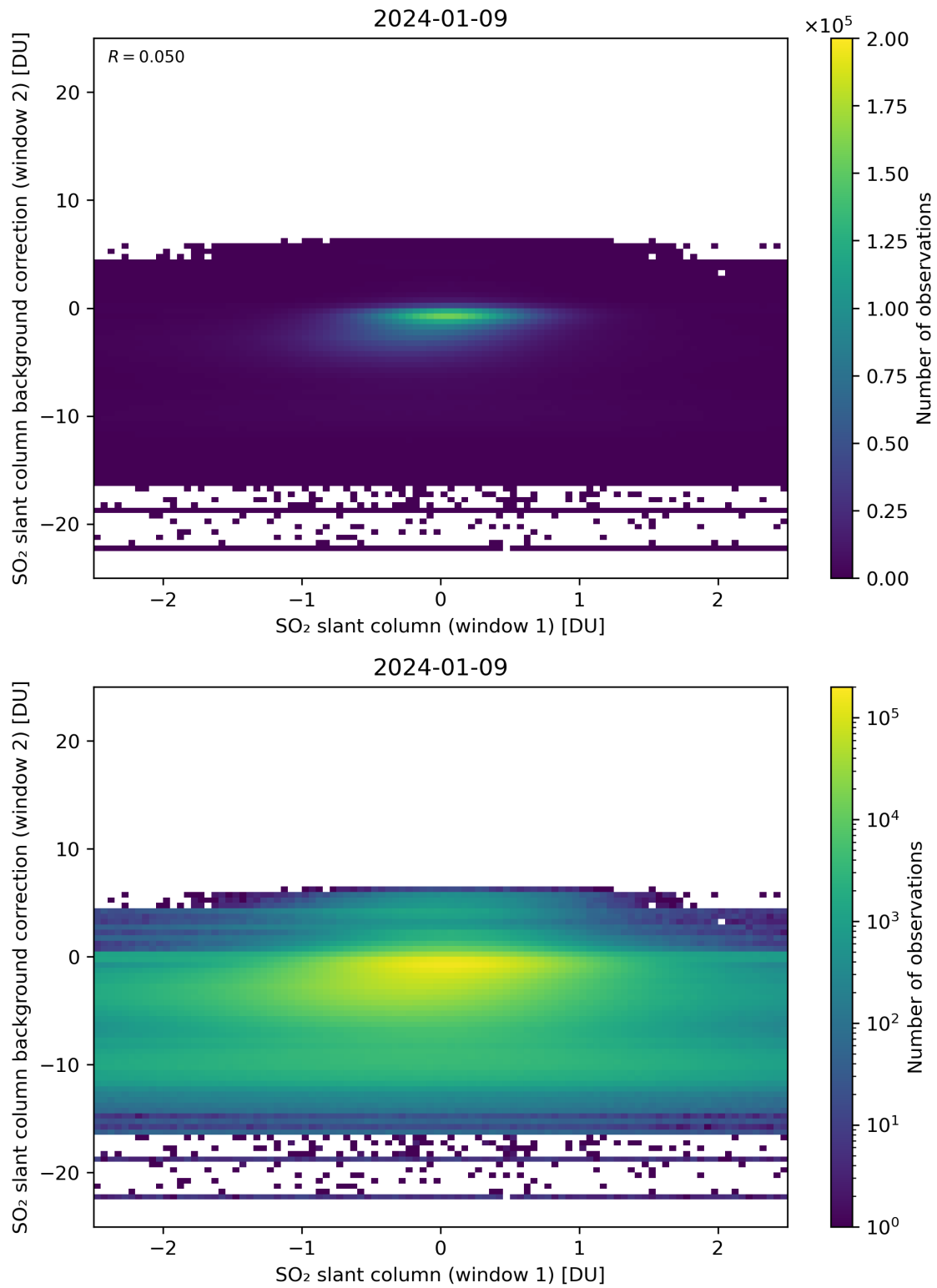
Figure 213: Scatter density plot of “SO 2 slant column (window 1)” against “SO 2 slant column background correction (window 2)” for 2024-01-08 to 2024-01-10.
