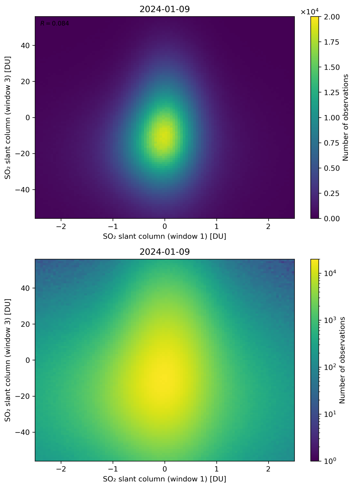
Figure 237: Scatter density plot of “SO 2 slant column (window 1)” against “SO 2 slant column (window 3)” for 2024-01-08 to 2024-01-10.
