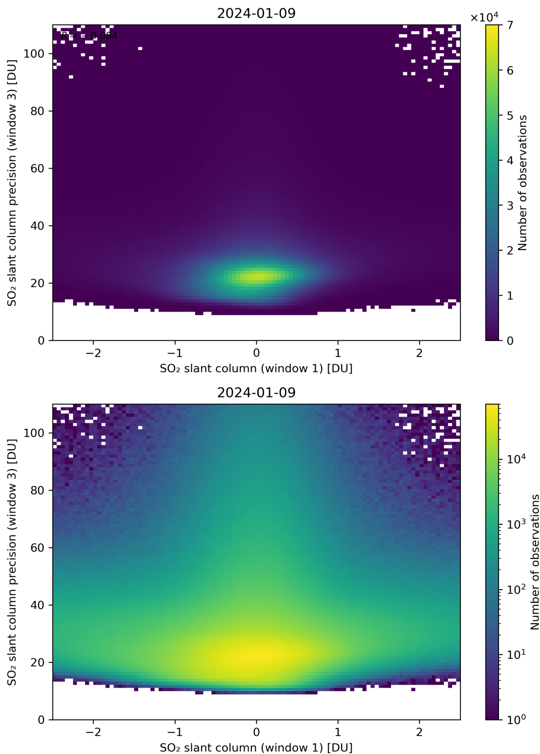
Figure 238: Scatter density plot of “SO 2 slant column (window 1)” against “SO 2 slant column precision (window 3)” for 2024-01-08 to 2024-01-10.
