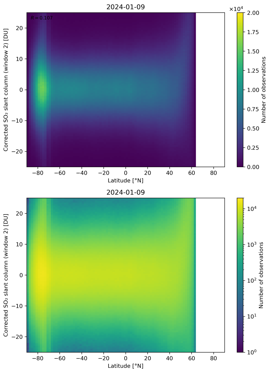
Figure 147: Scatter density plot of “Latitude” against “Corrected SO 2 slant column (window 2)” for 2024-01-08 to 2024-01-10.
