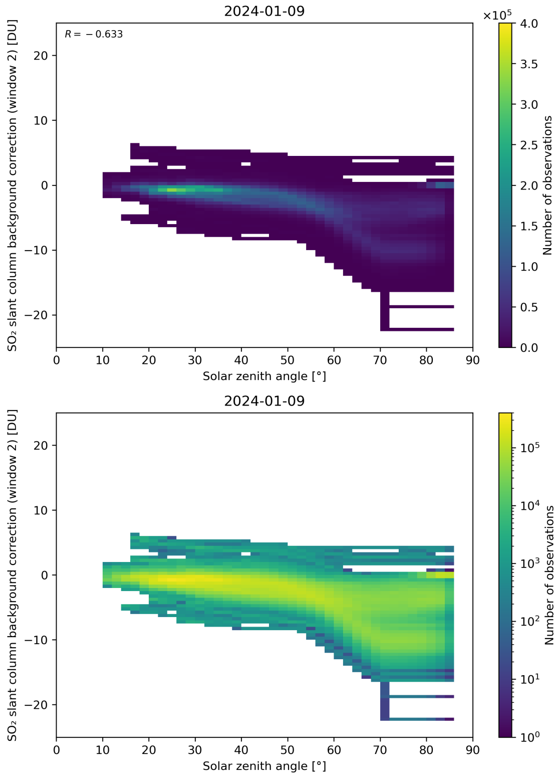
Figure 159: Scatter density plot of “Solar zenith angle” against “SO 2 slant column background correction (window 2)” for 2024-01-08 to 2024-01-10.
