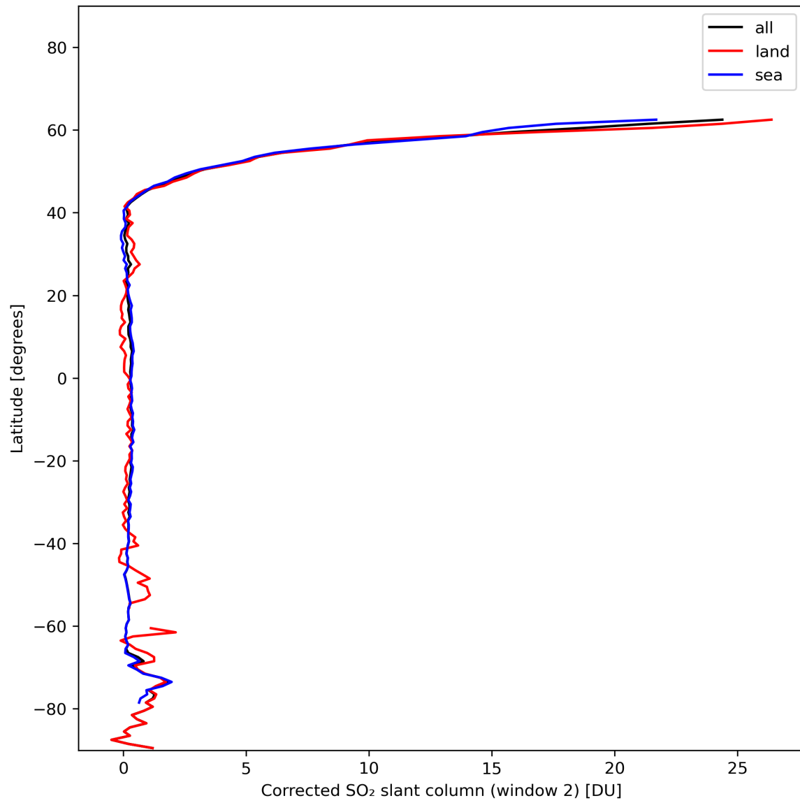
Figure 39: Zonal average of “Corrected SO 2 slant column (window 2)” for 2024-01-08 to 2024-01-10.
