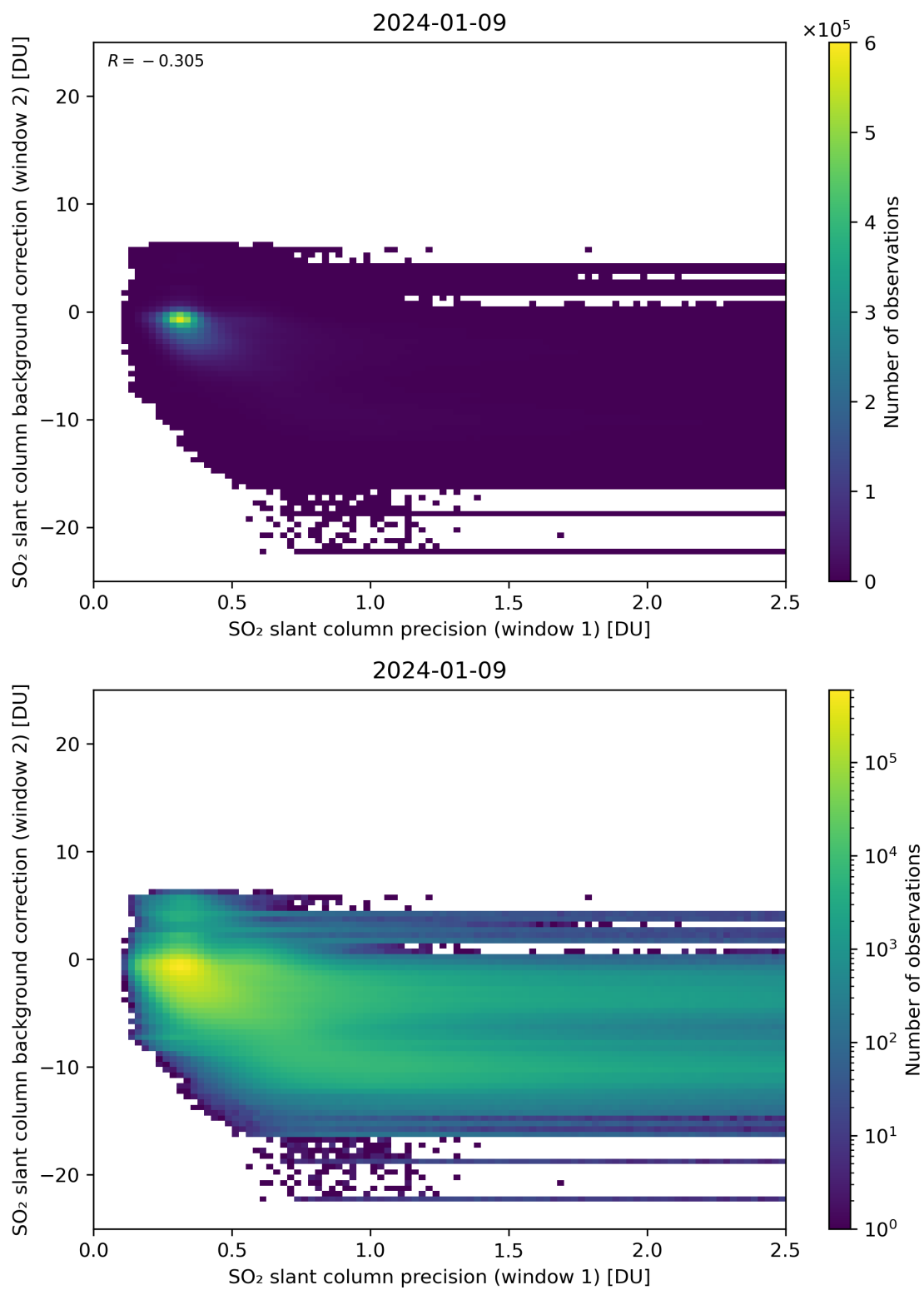
Figure 219: Scatter density plot of “SO 2 slant column precision (window 1)” against “SO 2 slant column background correction (window 2)” for 2024-01-08 to 2024-01-10.
