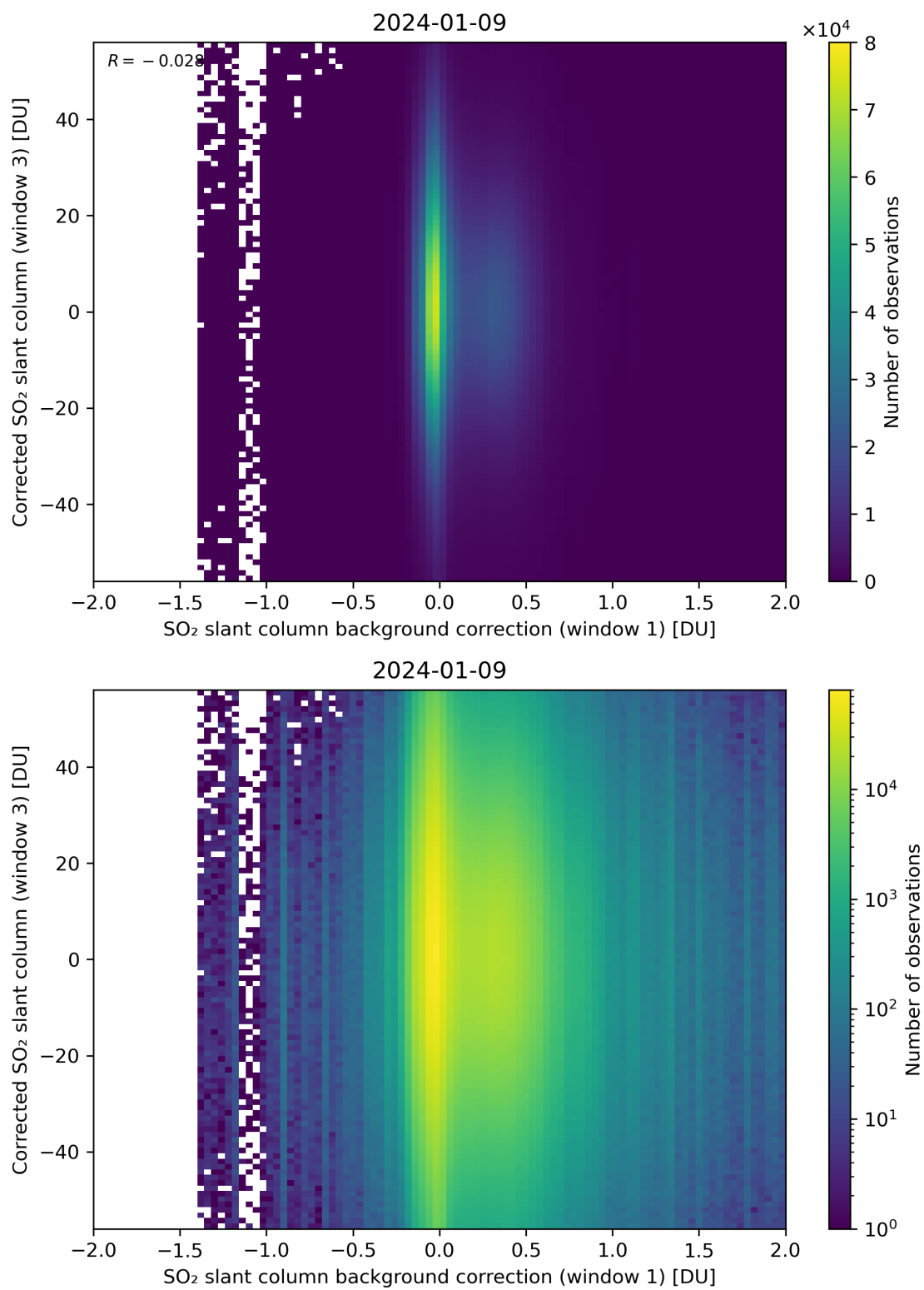
Figure 105: Scatter density plot of “SO 2 slant column background correction (window 1)” against “Corrected SO 2 slant column (window 3)” for 2024-01-08 to 2024-01-10.
