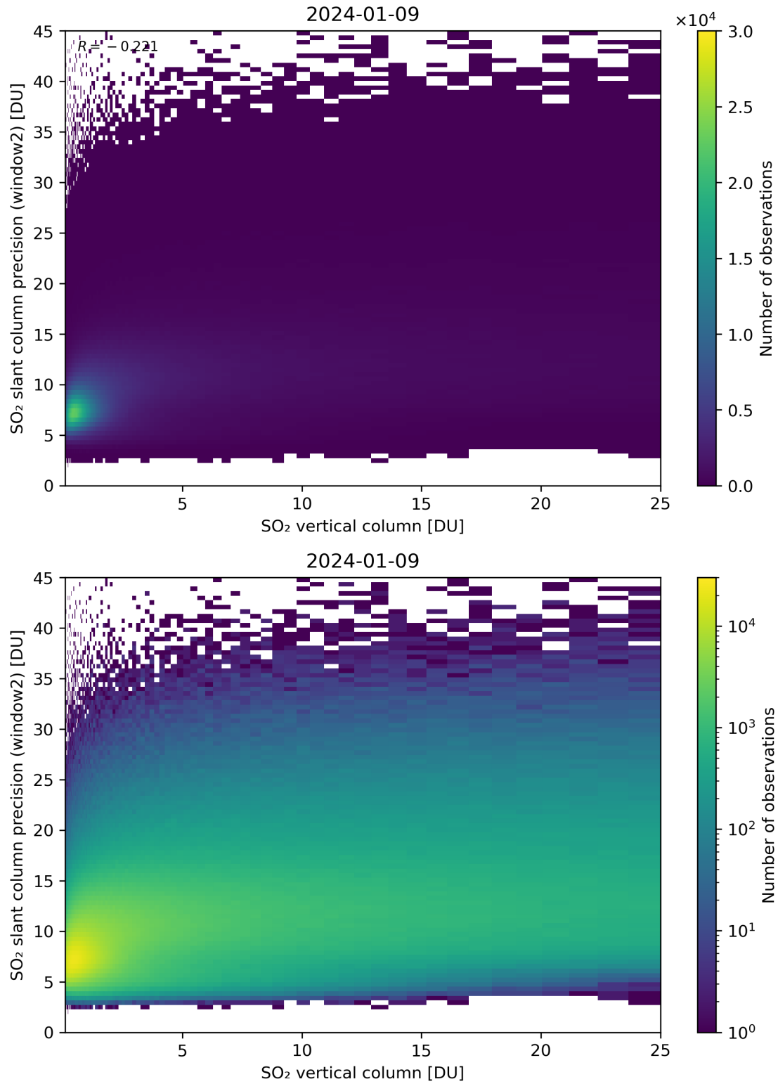
Figure 302: Scatter density plot of “SO 2 vertical column” against “SO 2 slant column precision (window2)” for 2024-01-08 to 2024-01-10.
