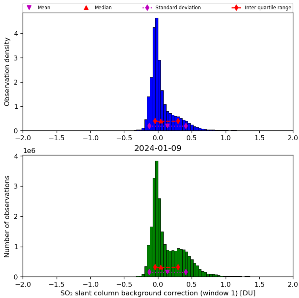
Figure 59: Histogram of “SO 2 slant column background correction (window 1)” for 2024-01-08 to 2024-01-10
