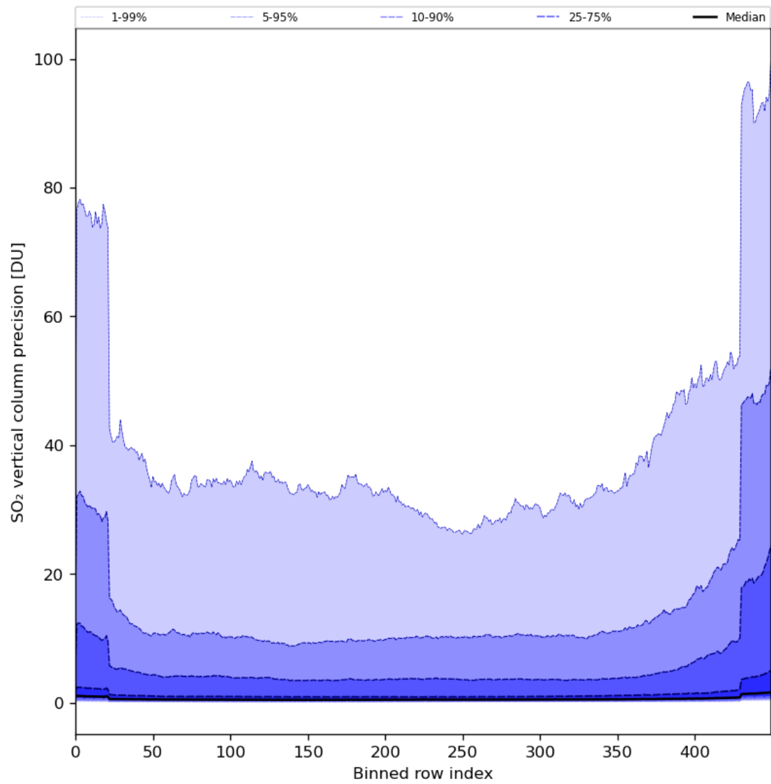
Figure 77: Along track statistics of “SO 2 vertical column precision” for 2024-01-08 to 2024-01-10
