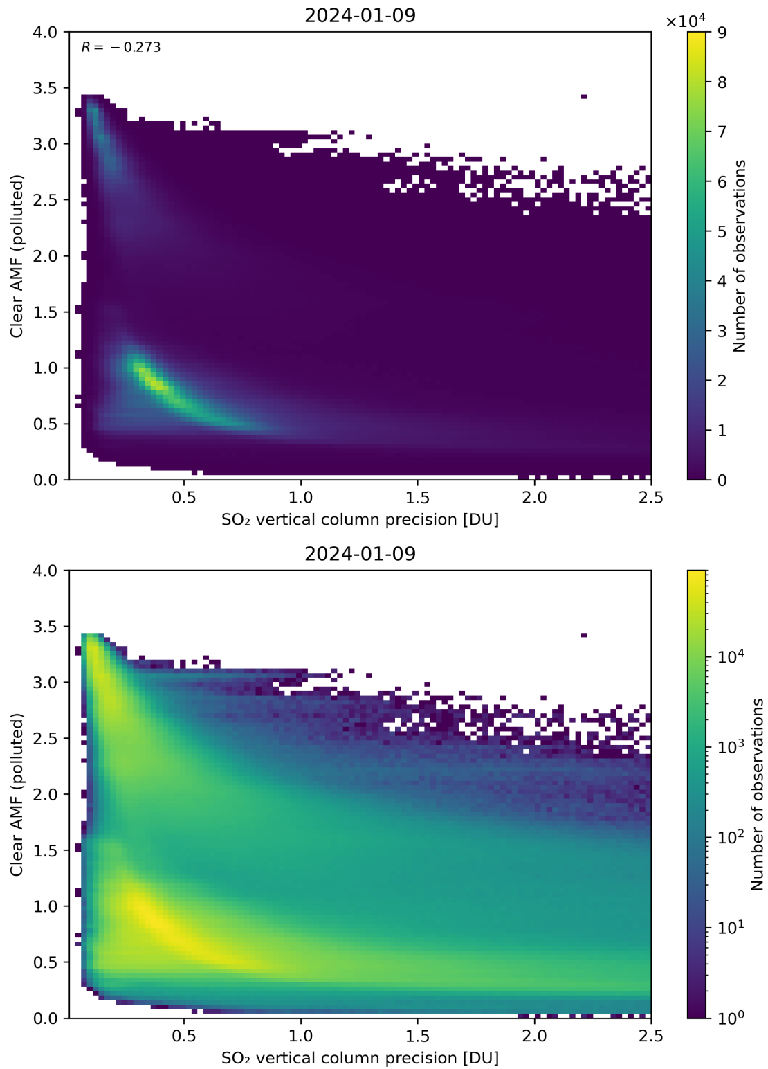
Figure 285: Scatter density plot of “SO 2 vertical column precision” against “Clear AMF (polluted)” for 2024-01-08 to 2024-01-10.
