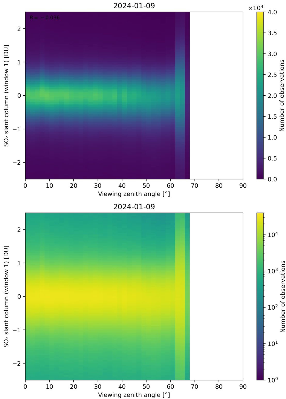
Figure 320: Scatter density plot of “Viewing zenith angle” against “SO 2 slant column (window 1)” for 2024-01-08 to 2024-01-10.
