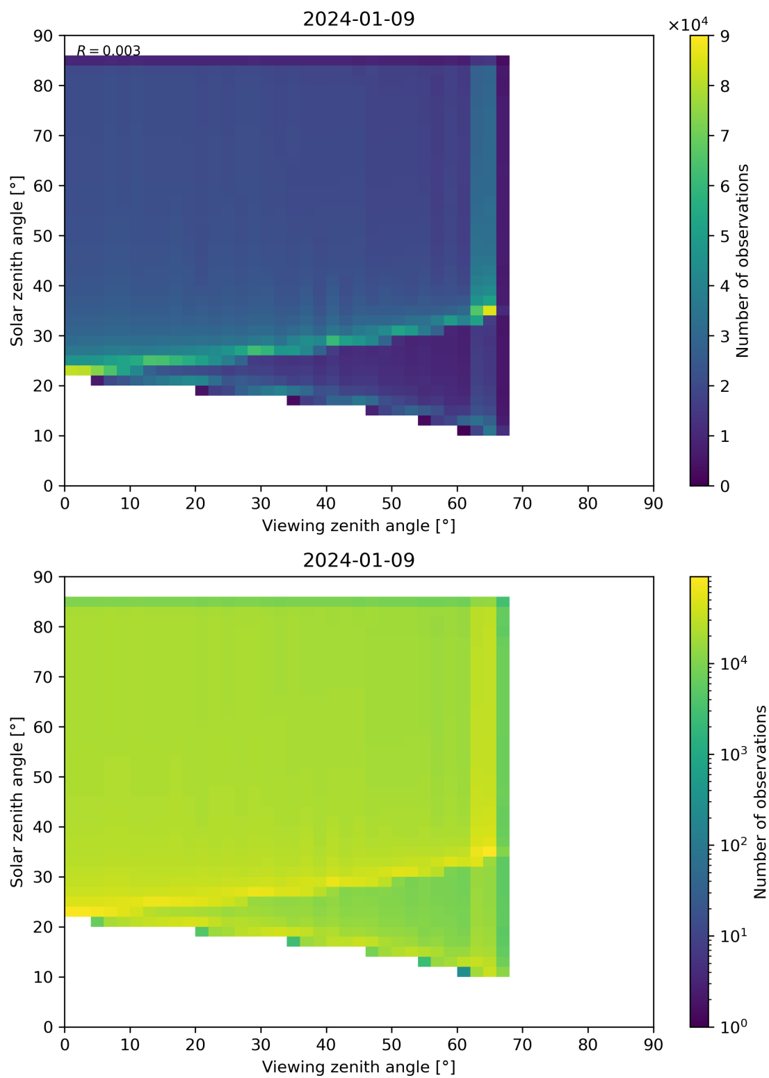
Figure 315: Scatter density plot of “Viewing zenith angle” against “Solar zenith angle” for 2024-01-08 to 2024-01-10.
