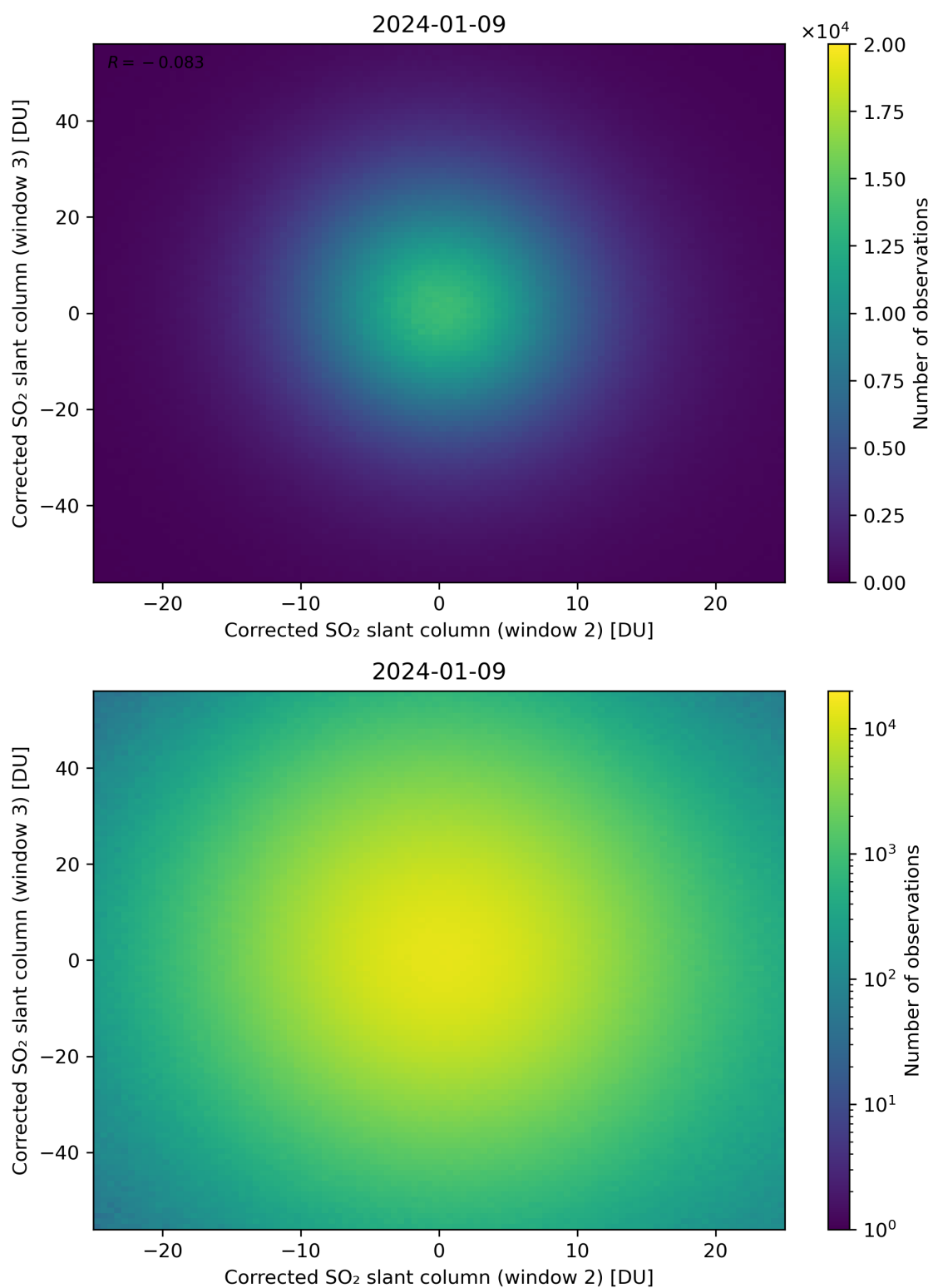
Figure 200: Scatter density plot of “Corrected SO 2 slant column (window 2)” against “Corrected SO 2 slant column (window 3)” for 2024-01-08 to 2024-01-10.
