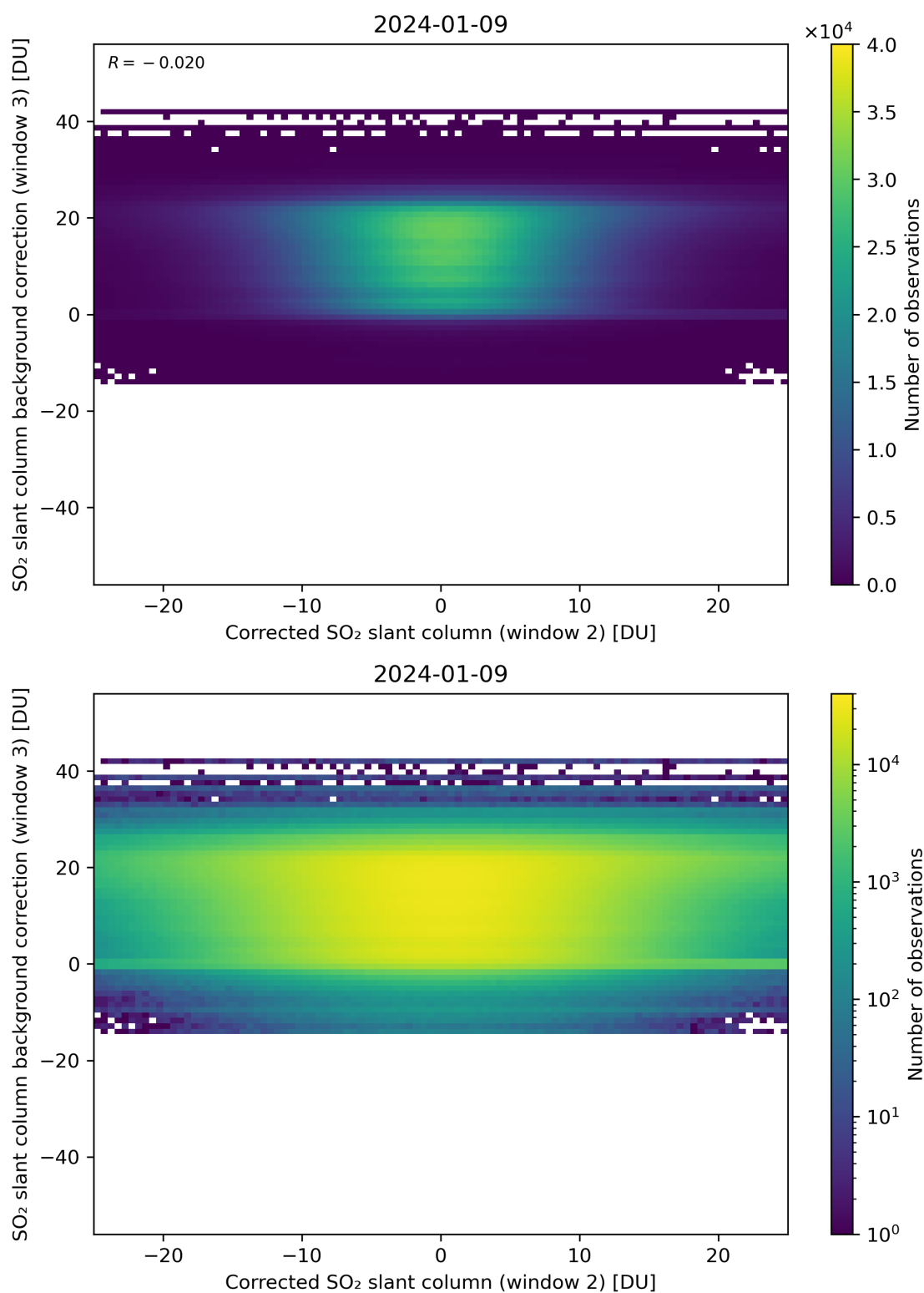
Figure 195: Scatter density plot of “Corrected SO 2 slant column (window 2)” against “SO 2 slant column background correction (window 3)” for 2024-01-08 to 2024-01-10.
