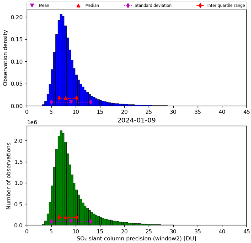
Figure 61: Histogram of “SO 2 slant column precision (window2)” for 2024-01-08 to 2024-01-10
