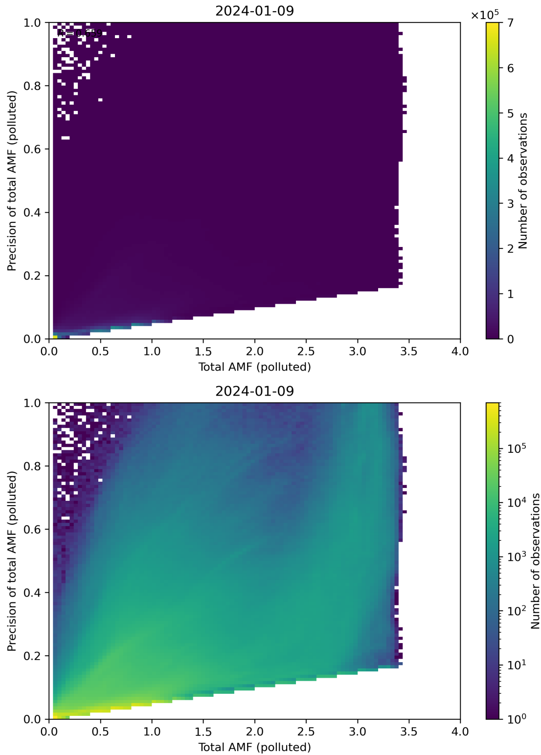
Figure 272: Scatter density plot of “Total AMF (polluted)” against “Precision of total AMF (polluted)” for 2024-01-08 to 2024-01-10.
