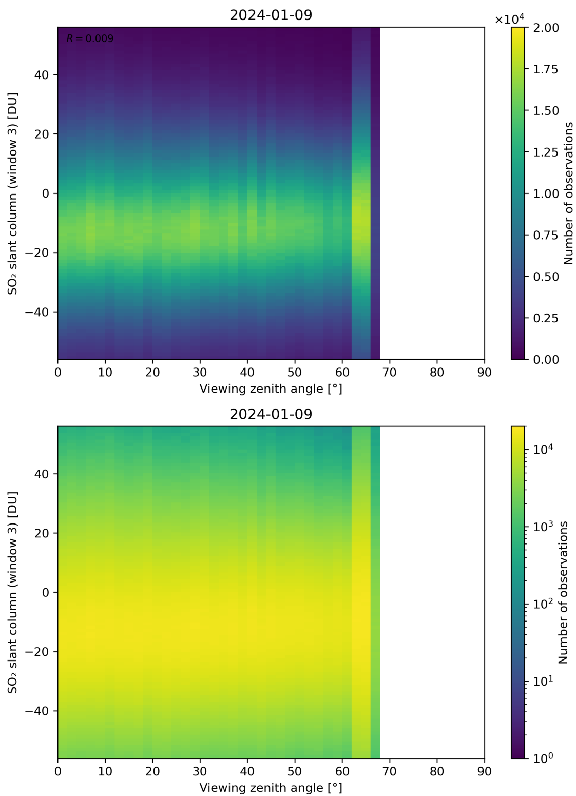
Figure 323: Scatter density plot of “Viewing zenith angle” against “SO 2 slant column (window 3)” for 2024-01-08 to 2024-01-10.
