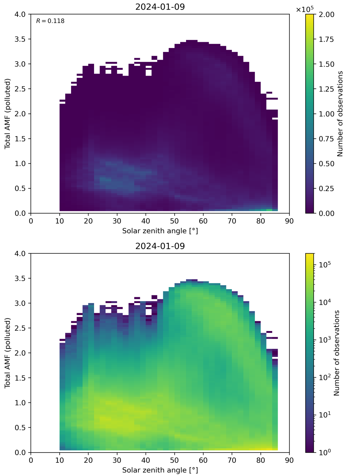
Figure 174: Scatter density plot of “Solar zenith angle” against “Total AMF (polluted)” for 2024-01-08 to 2024-01-10.
