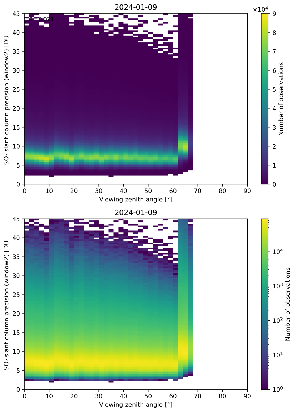
Figure 322: Scatter density plot of “Viewing zenith angle” against “SO 2 slant column precision (window2)” for 2024-01-08 to 2024-01-10.
