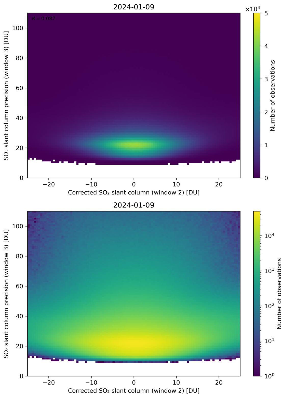
Figure 202: Scatter density plot of “Corrected SO 2 slant column (window 2)” against “SO 2 slant column precision (window 3)” for 2024-01-08 to 2024-01-10.
