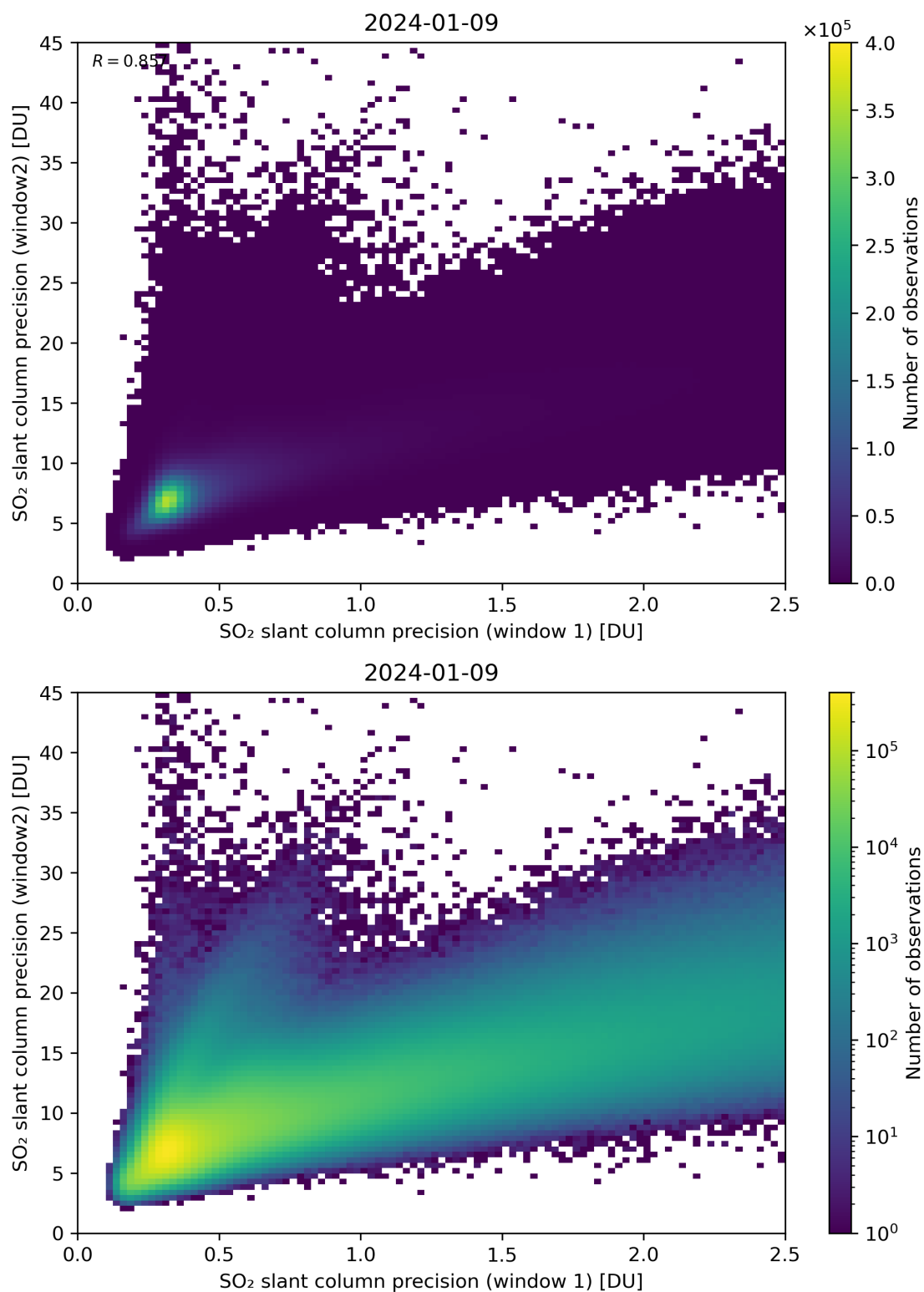
Figure 227: Scatter density plot of “SO 2 slant column precision (window 1)” against “SO 2 slant column precision (window2)” for 2024-01-08 to 2024-01-10.
