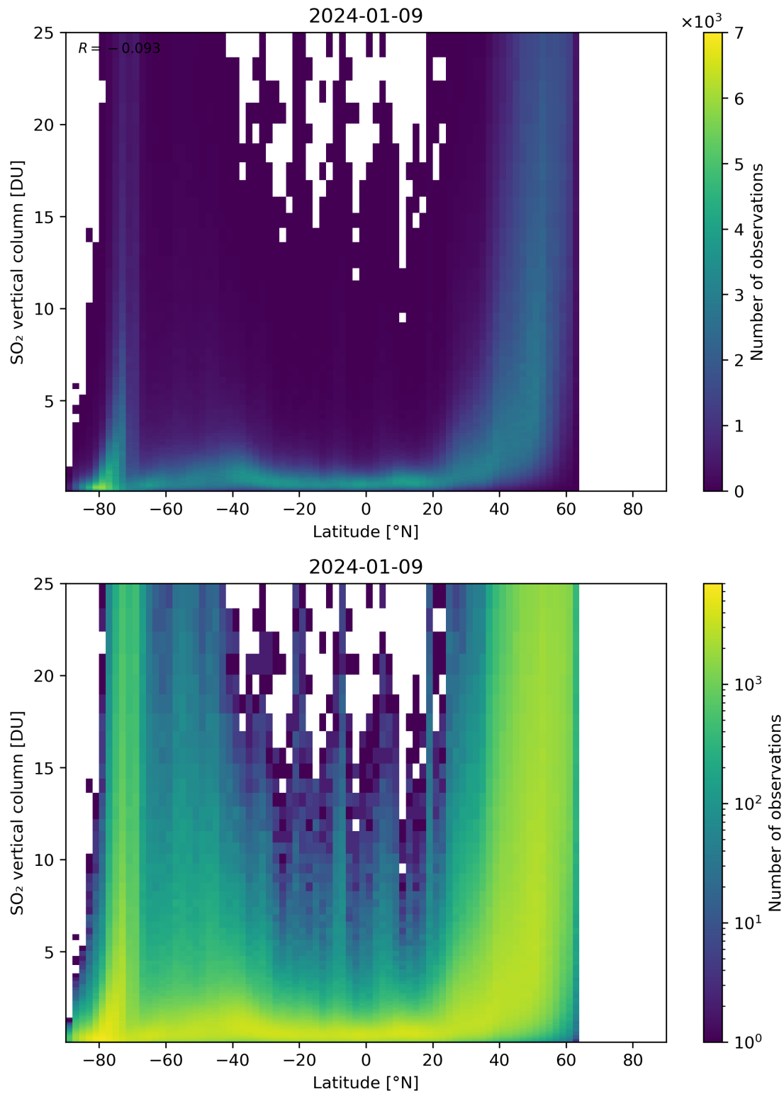
Figure 156: Scatter density plot of “Latitude” against “SO 2 vertical column” for 2024-01-08 to 2024-01-10.
