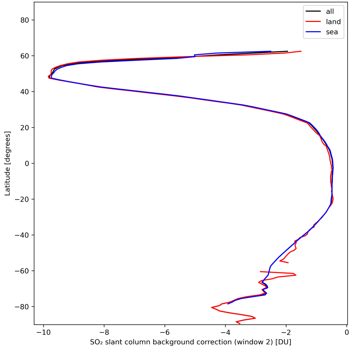
Figure 40: Zonal average of “SO 2 slant column background correction (window 2)” for 2024-01-08 to 2024-01-10.
