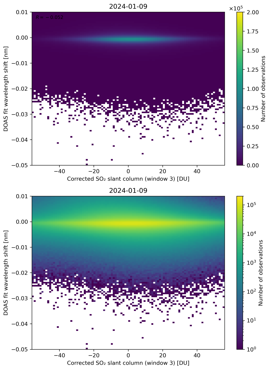
Figure 206: Scatter density plot of “Corrected SO 2 slant column (window 3)” against “DOAS fit wavelength shift” for 2024-01-08 to 2024-01-10.
