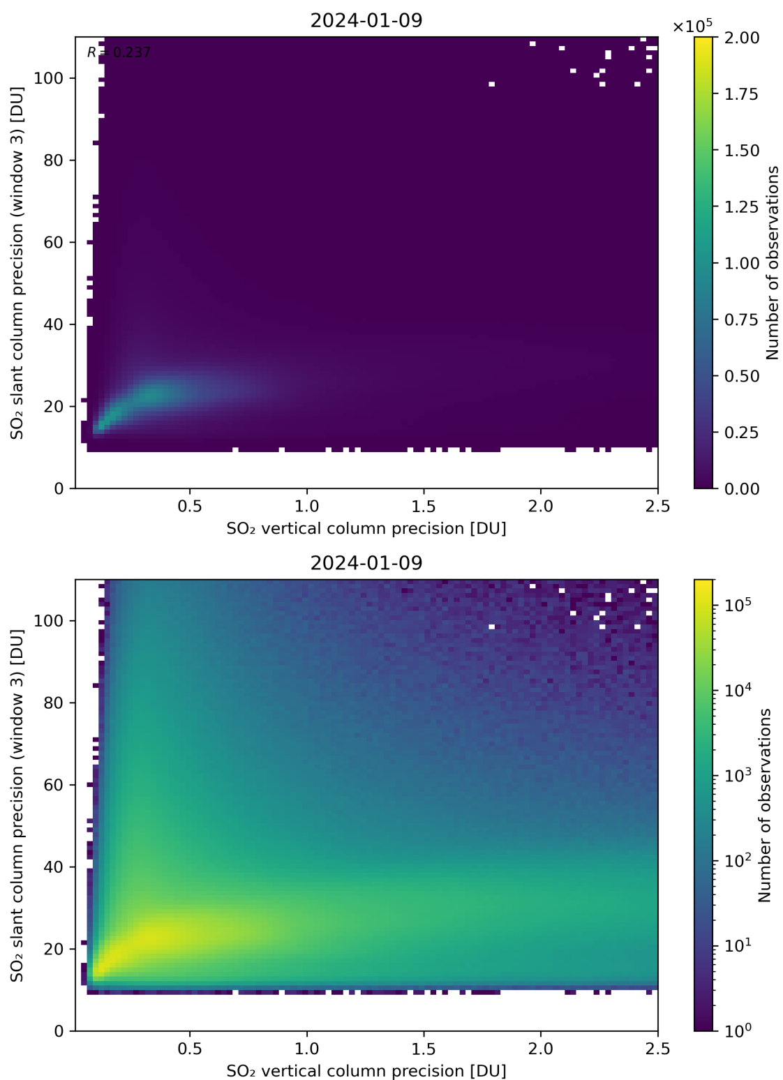
Figure 293: Scatter density plot of “SO 2 vertical column precision” against “SO 2 slant column precision (window 3)” for 2024-01-08 to 2024-01-10.
