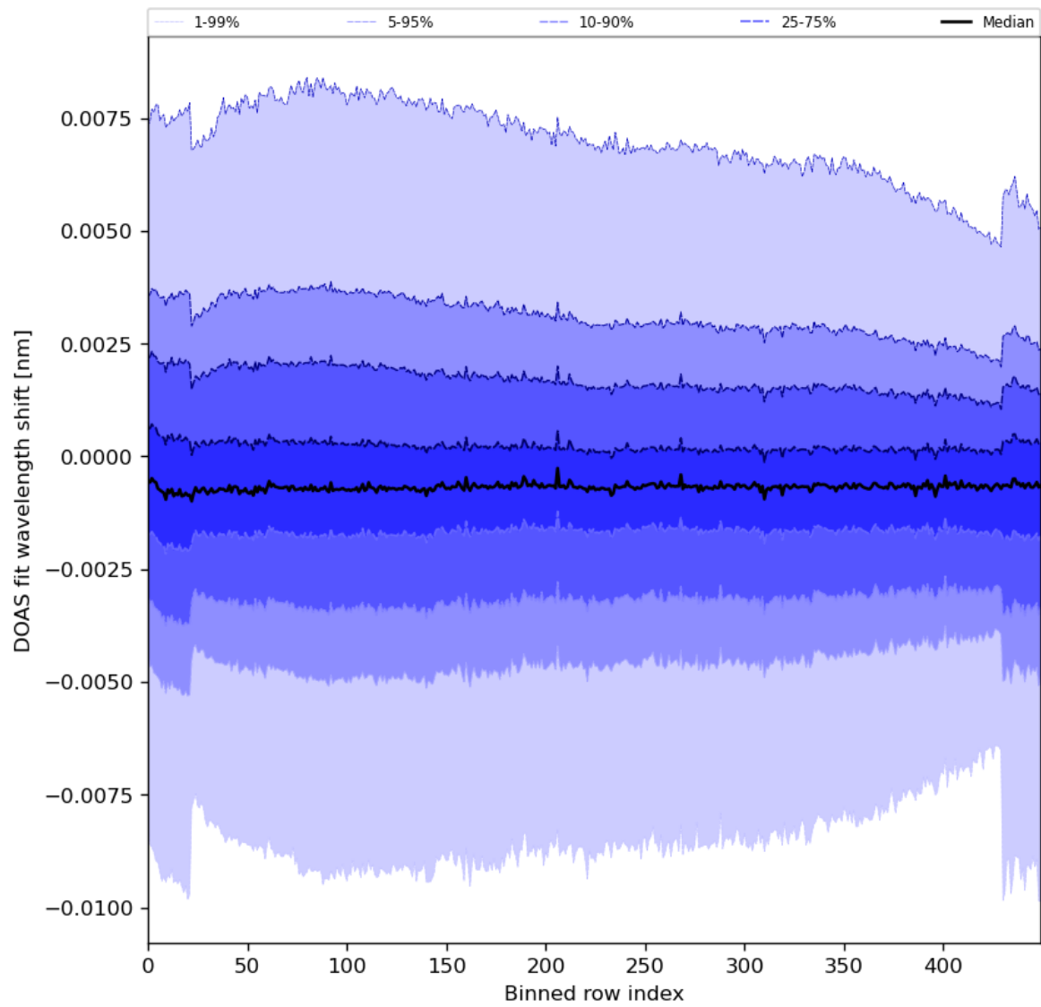
Figure 91: Along track statistics of “DOAS fit wavelength shift” for 2024-01-08 to 2024-01-10
