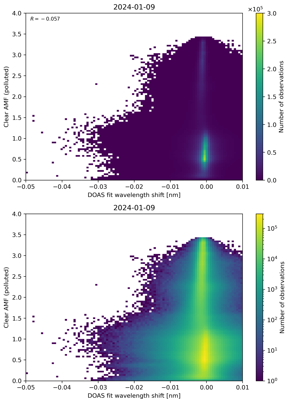
Figure 129: Scatter density plot of “DOAS fit wavelength shift” against “Clear AMF (polluted)” for 2024-01-08 to 2024-01-10.
