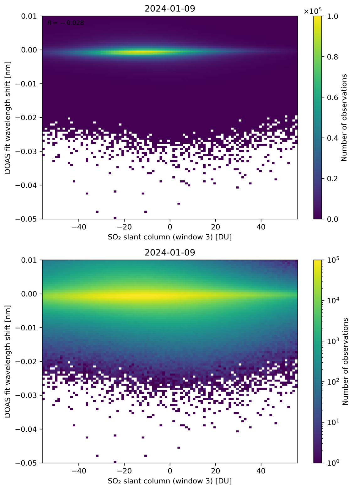
Figure 254: Scatter density plot of “SO 2 slant column (window 3)” against “DOAS fit wavelength shift” for 2024-01-08 to 2024-01-10.
