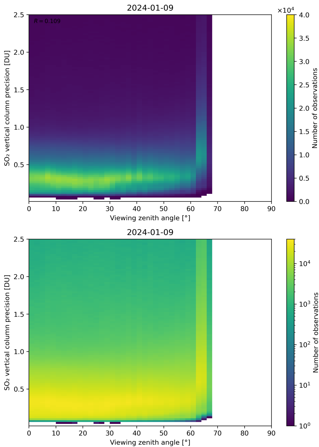
Figure 328: Scatter density plot of “Viewing zenith angle” against “SO 2 vertical column precision” for 2024-01-08 to 2024-01-10.
