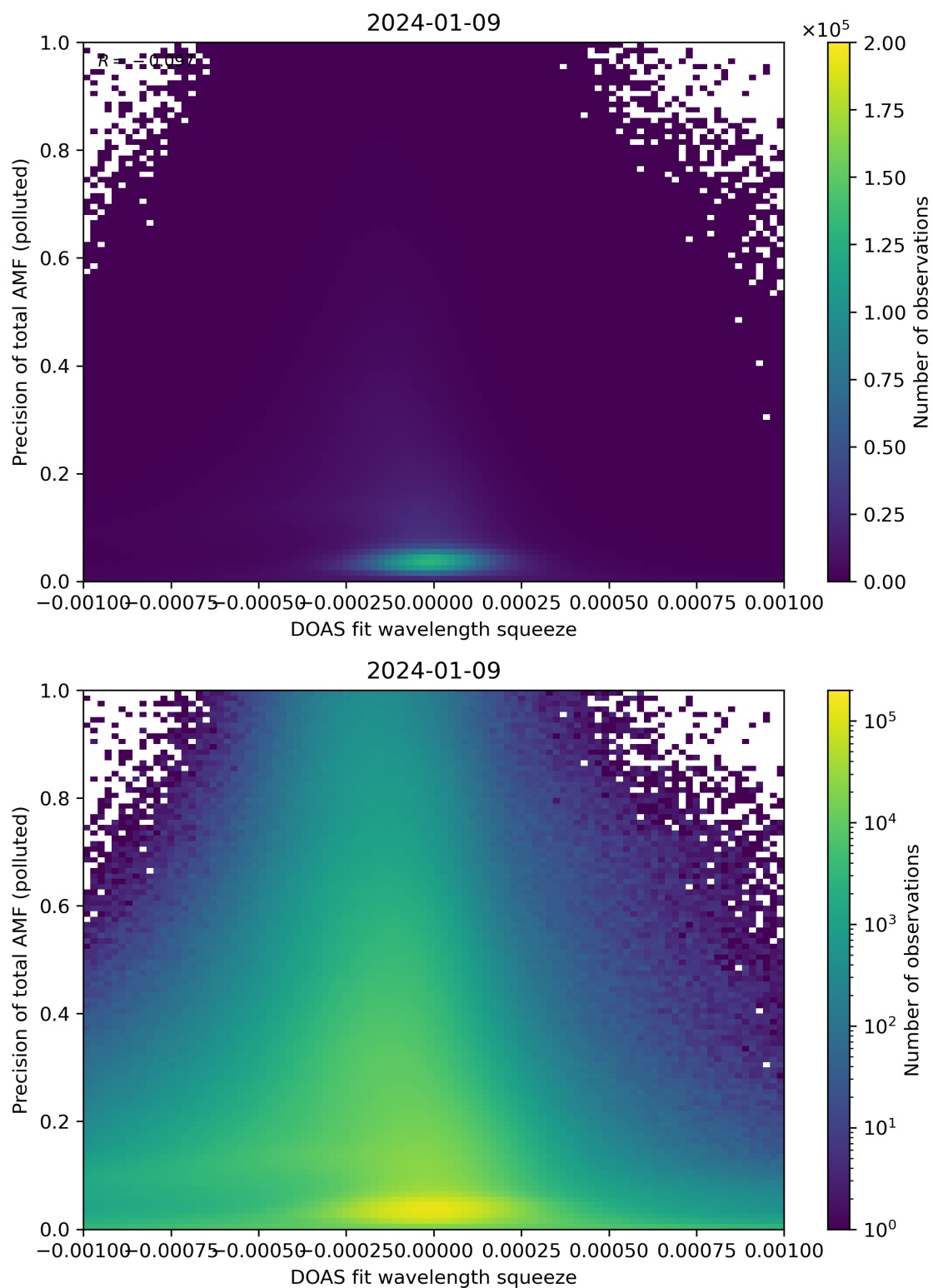
Figure 135: Scatter density plot of “DOAS fit wavelength squeeze” against “Precision of total AMF (polluted)” for 2024-01-08 to 2024-01-10.
