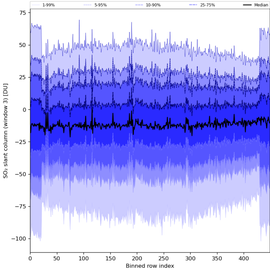
Figure 87: Along track statistics of “SO 2 slant column (window 3)” for 2024-01-08 to 2024-01-10
