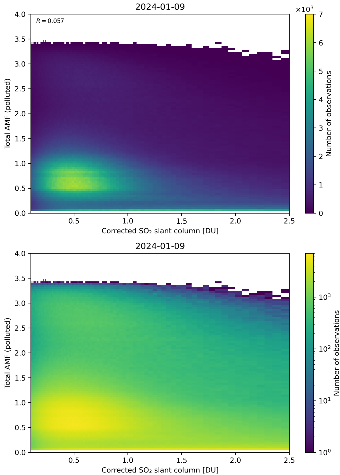
Figure 192: Scatter density plot of “Corrected SO 2 slant column” against “Total AMF (polluted)” for 2024-01-08 to 2024-01-10.
