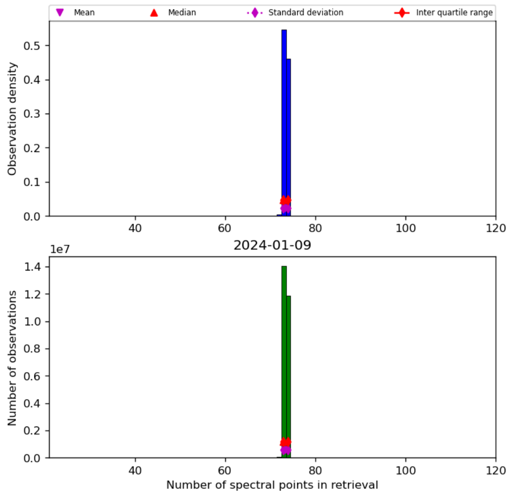
Figure 74: Histogram of “Number of spectral points in retrieval” for 2024-01-08 to 2024-01-10
