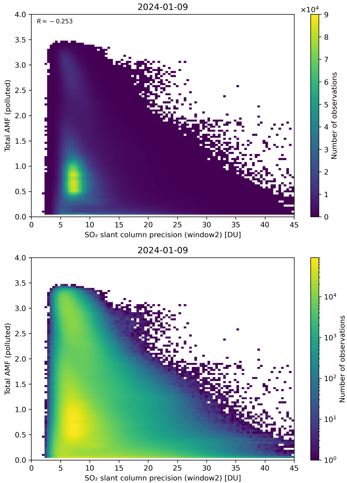
Figure 251: Scatter density plot of “SO 2 slant column precision (window2)” against “Total AMF (polluted)” for 2024-01-08 to 2024-01-10.
