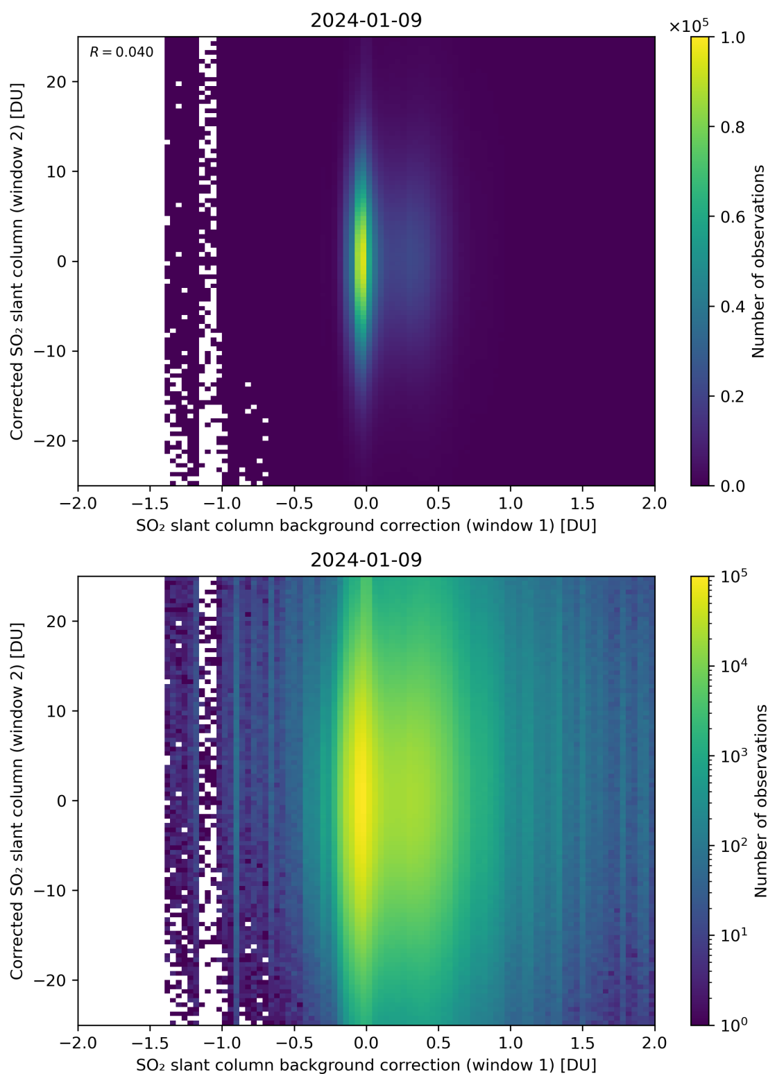
Figure 104: Scatter density plot of “SO 2 slant column background correction (window 1)” against “Corrected SO 2 slant column (window 2)” for 2024-01-08 to 2024-01-10.
