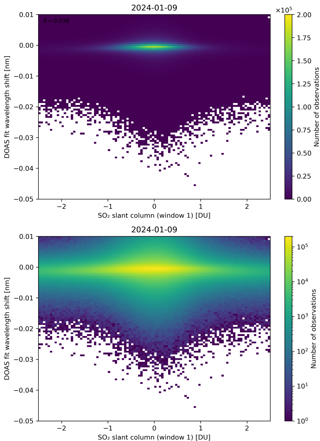
Figure 215: Scatter density plot of “SO 2 slant column (window 1)” against “DOAS fit wavelength shift” for 2024-01-08 to 2024-01-10.
