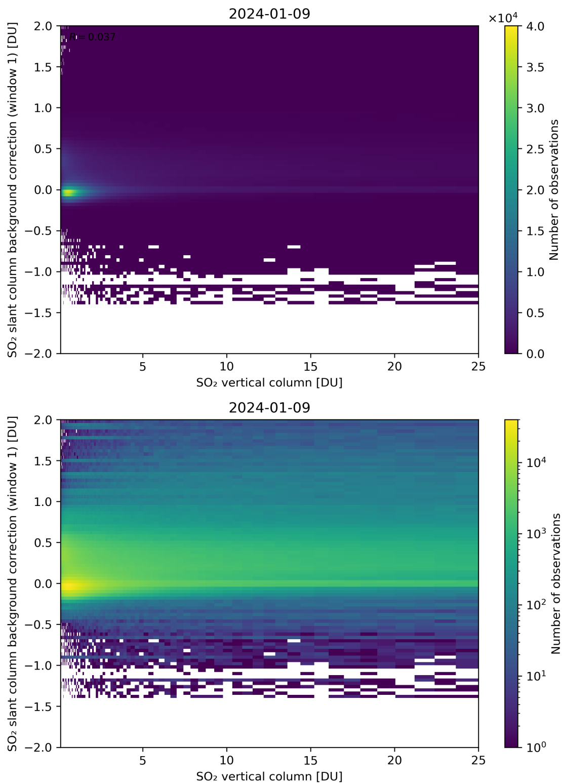
Figure 273: Scatter density plot of “SO 2 vertical column” against “SO 2 slant column background correction (window 1)” for 2024-01-08 to 2024-01-10.
