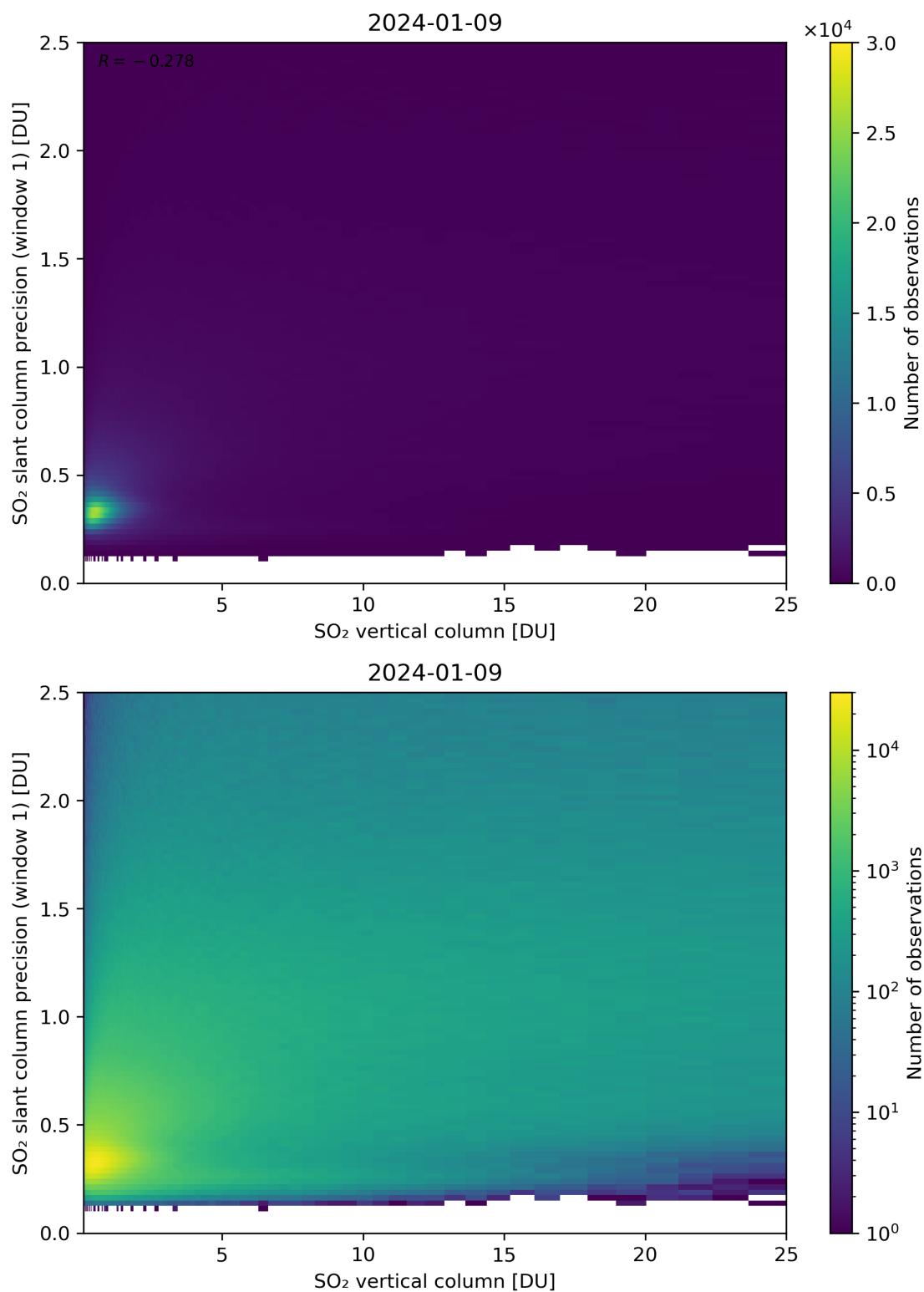
Figure 301: Scatter density plot of “SO 2 vertical column” against “SO 2 slant column precision (window 1)” for 2024-01-08 to 2024-01-10.
