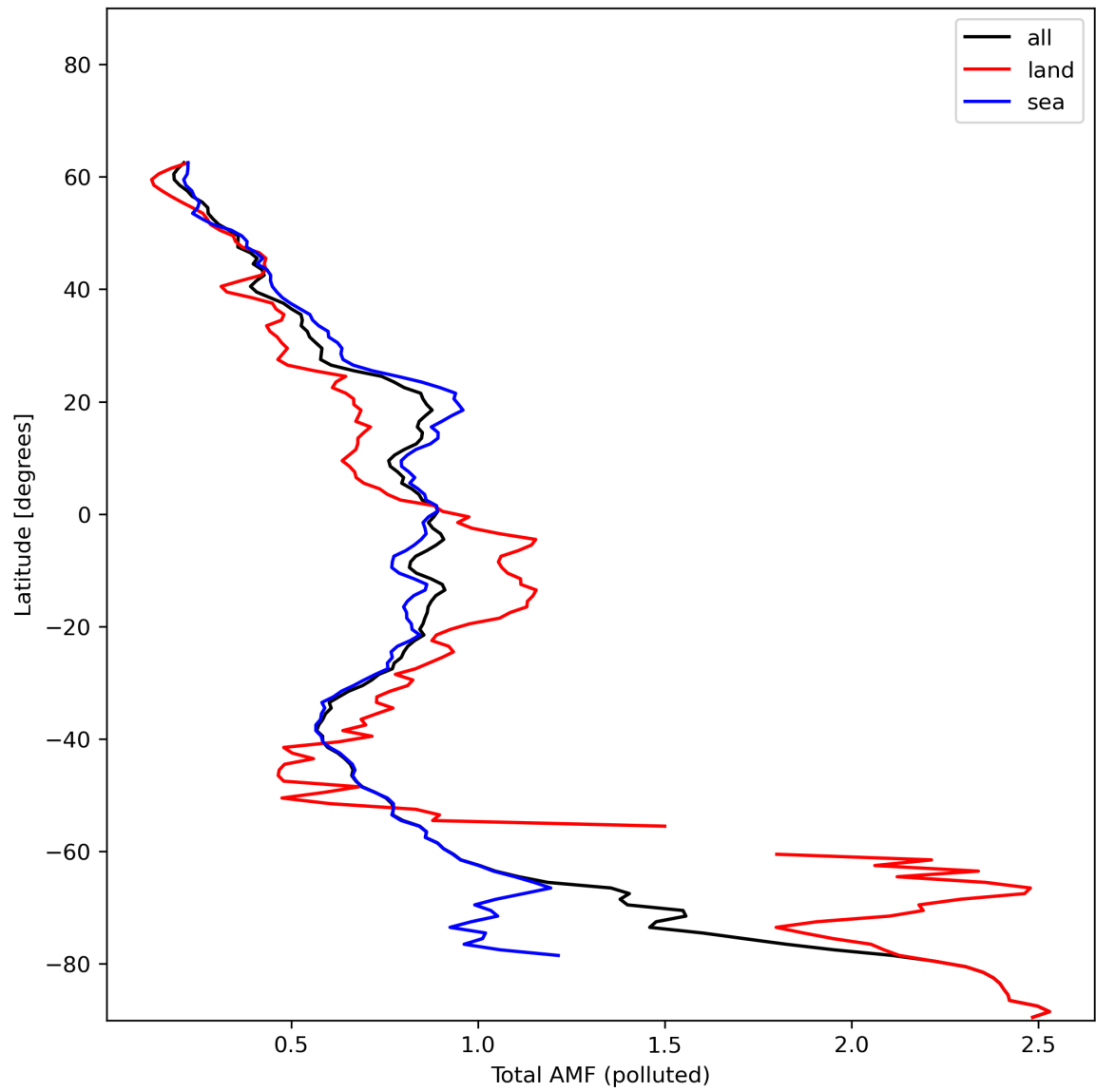
Figure 48: Zonal average of “Total AMF (polluted)” for 2024-01-08 to 2024-01-10.
