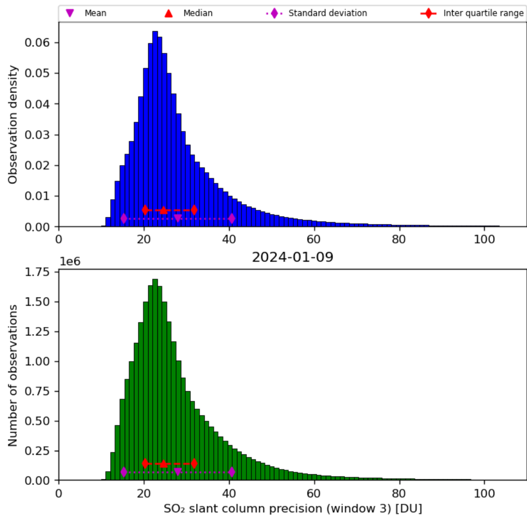
Figure 65: Histogram of “SO 2 slant column precision (window 3)” for 2024-01-08 to 2024-01-10
