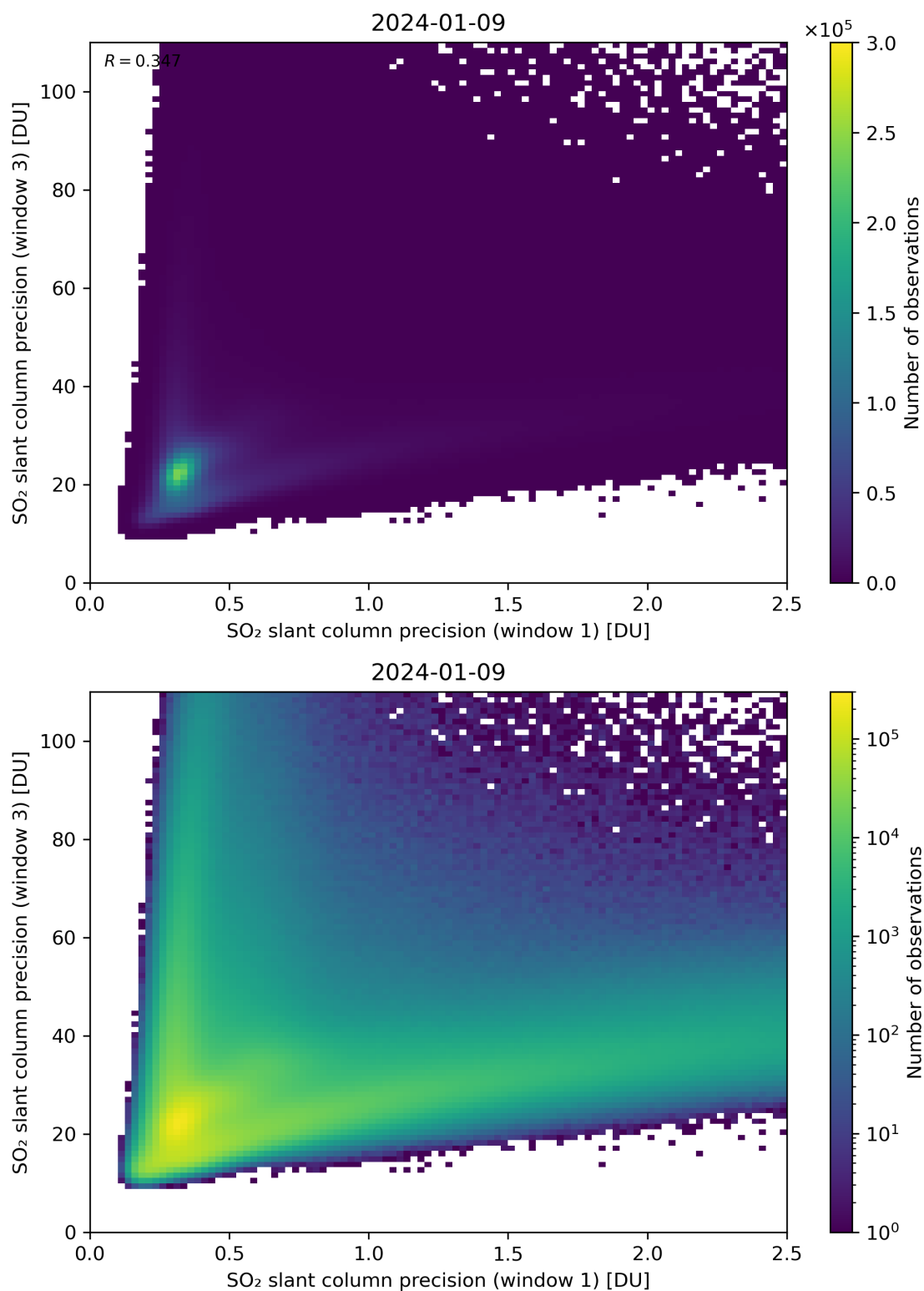
Figure 229: Scatter density plot of “SO 2 slant column precision (window 1)” against “SO 2 slant column precision (window 3)” for 2024-01-08 to 2024-01-10.
