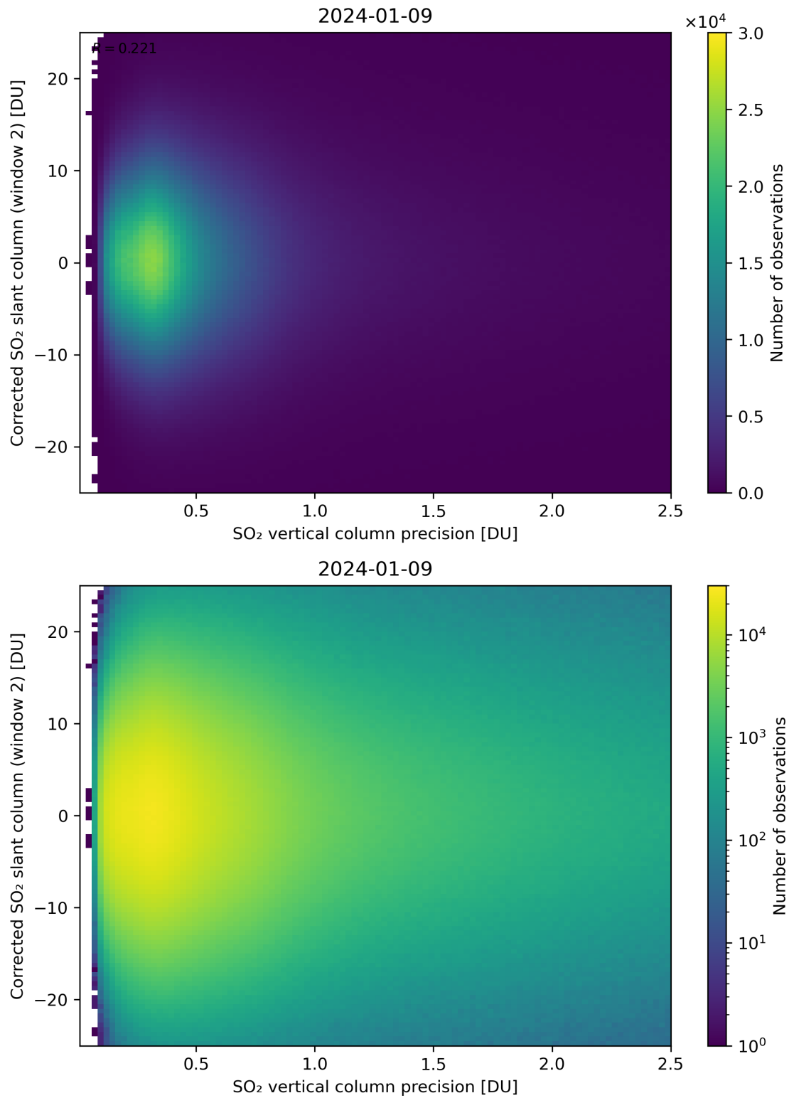
Figure 287: Scatter density plot of “SO 2 vertical column precision” against “Corrected SO 2 slant column (window 2)” for 2024-01-08 to 2024-01-10.
