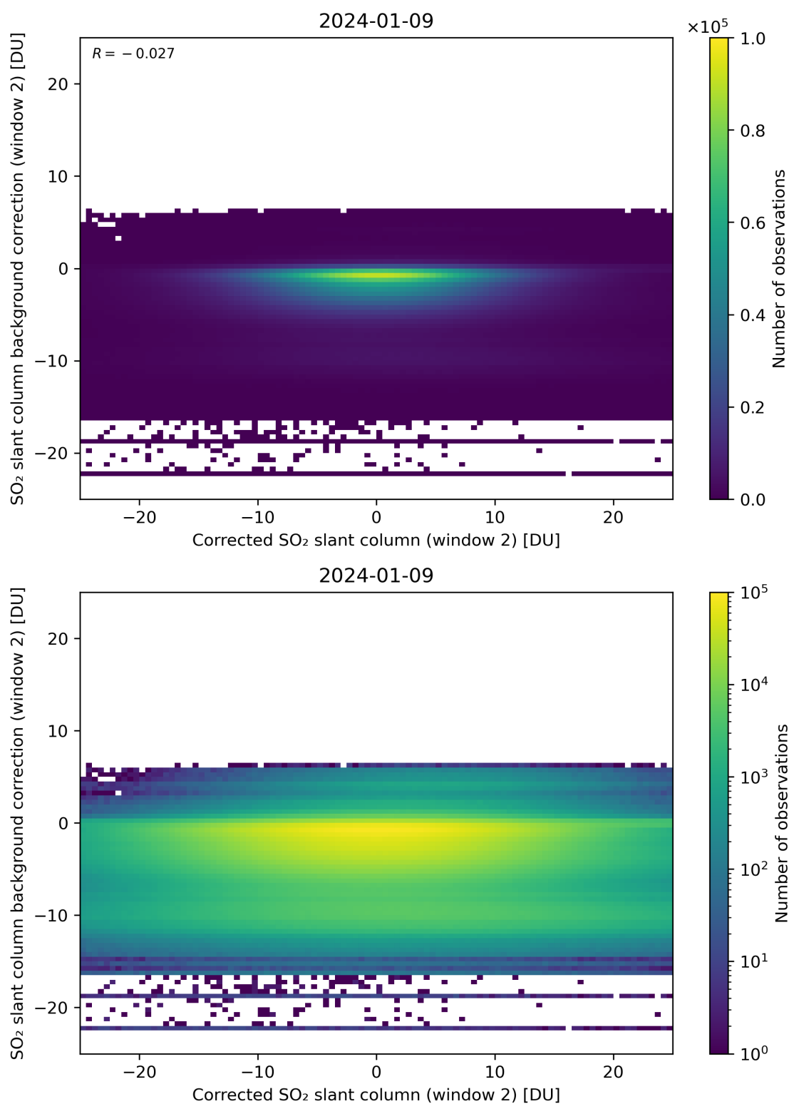
Figure 194: Scatter density plot of “Corrected SO 2 slant column (window 2)” against “SO 2 slant column background correction (window 2)” for 2024-01-08 to 2024-01-10.
