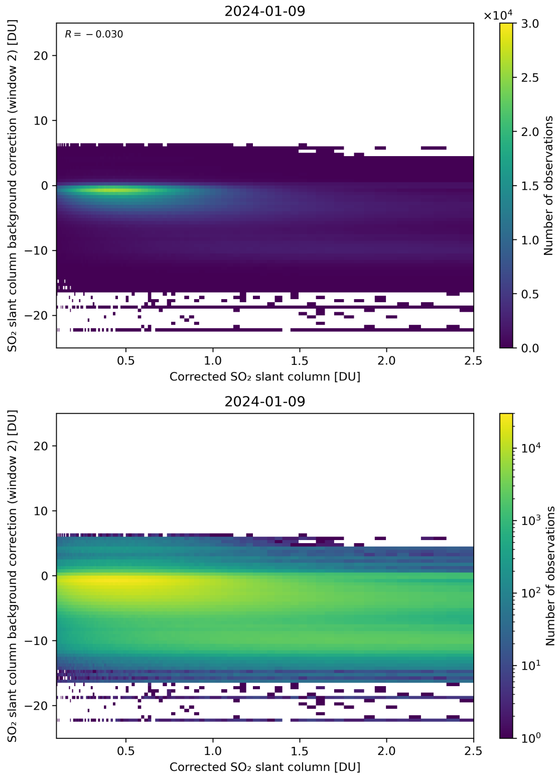
Figure 179: Scatter density plot of “Corrected SO 2 slant column” against “SO 2 slant column background correction (window 2)” for 2024-01-08 to 2024-01-10.
