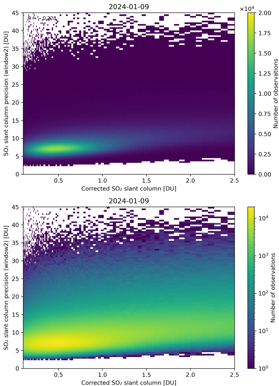
Figure 189: Scatter density plot of “Corrected SO 2 slant column” against “SO 2 slant column precision (window2)” for 2024-01-08 to 2024-01-10.
