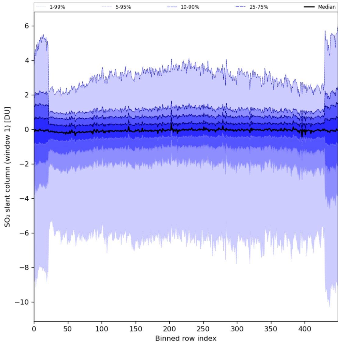
Figure 79: Along track statistics of “SO 2 slant column (window 1)” for 2024-01-08 to 2024-01-10
