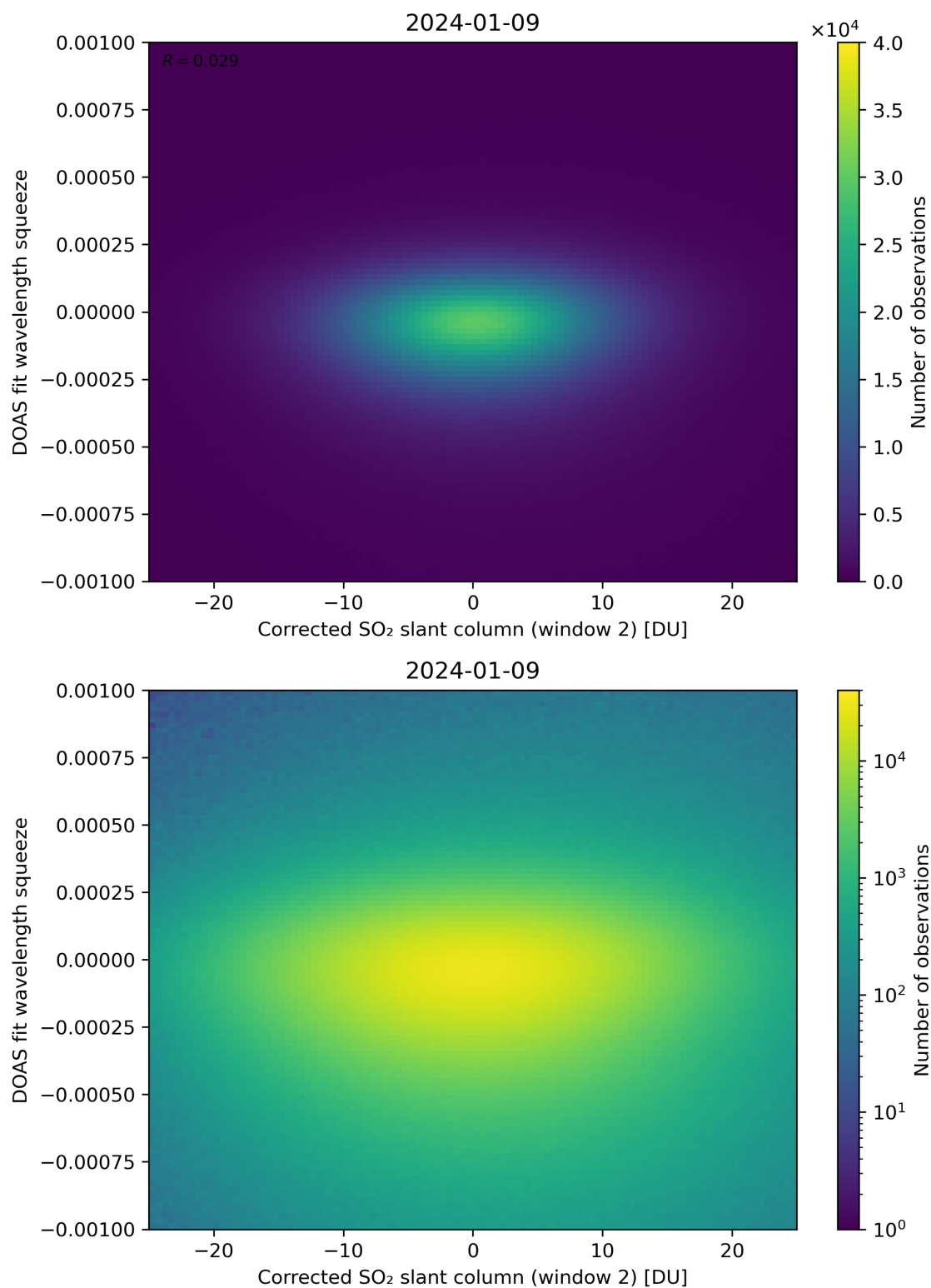
Figure 197: Scatter density plot of “Corrected SO 2 slant column (window 2)” against “DOAS fit wavelength squeeze” for 2024-01-08 to 2024-01-10.
