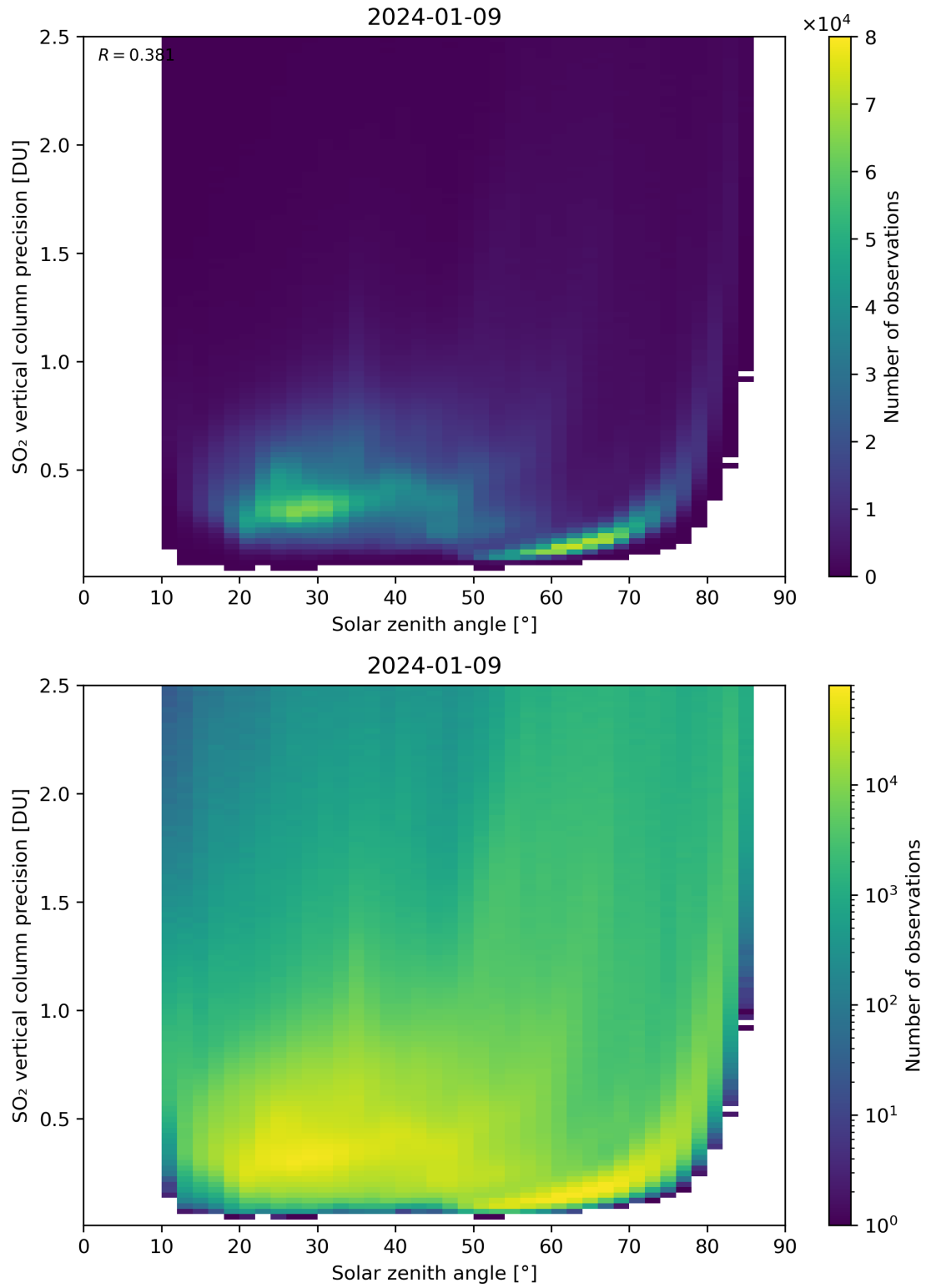
Figure 177: Scatter density plot of “Solar zenith angle” against “SO 2 vertical column precision” for 2024-01-08 to 2024-01-10.
