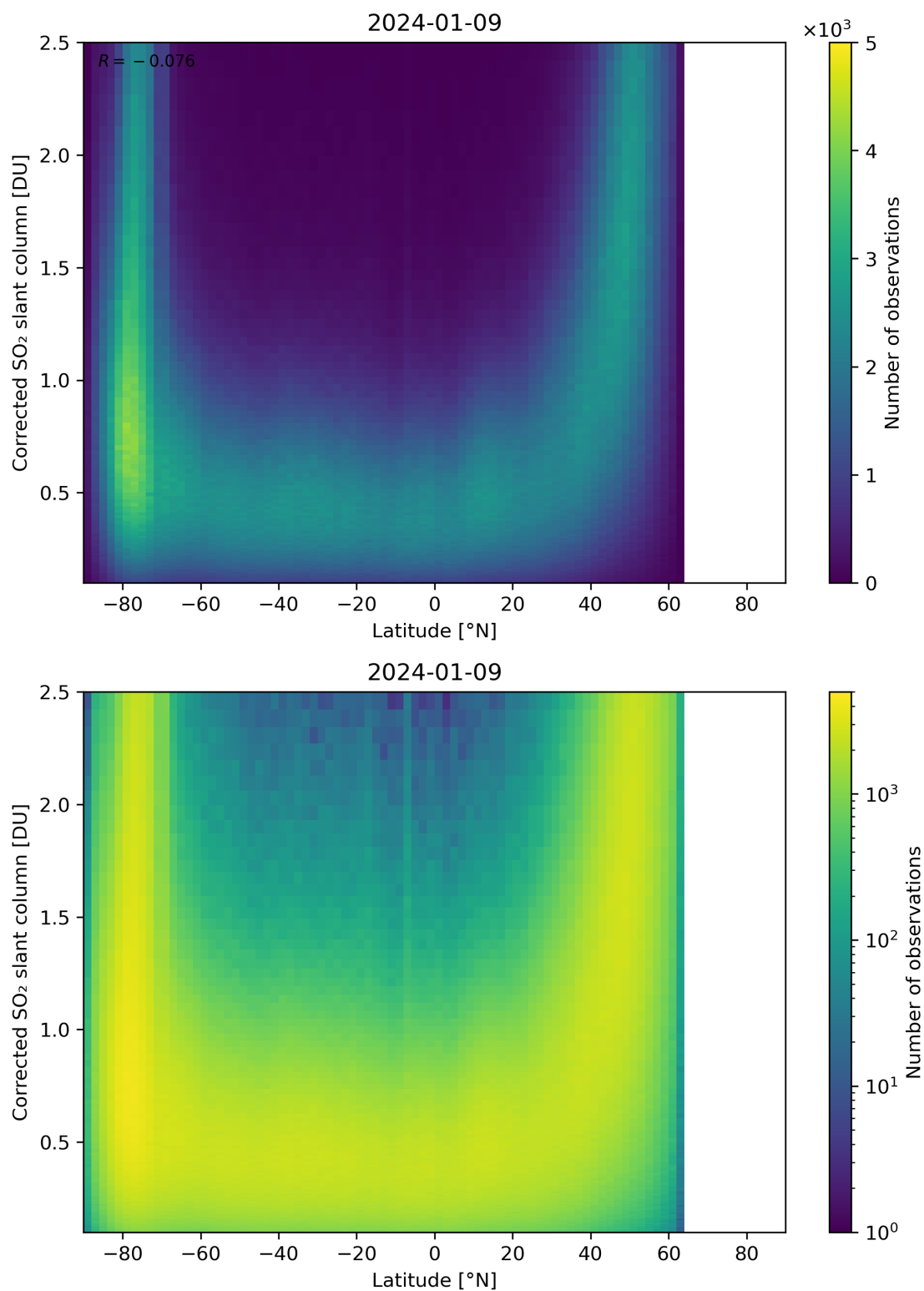
Figure 146: Scatter density plot of “Latitude” against “Corrected SO 2 slant column” for 2024-01-08 to 2024-01-10.
