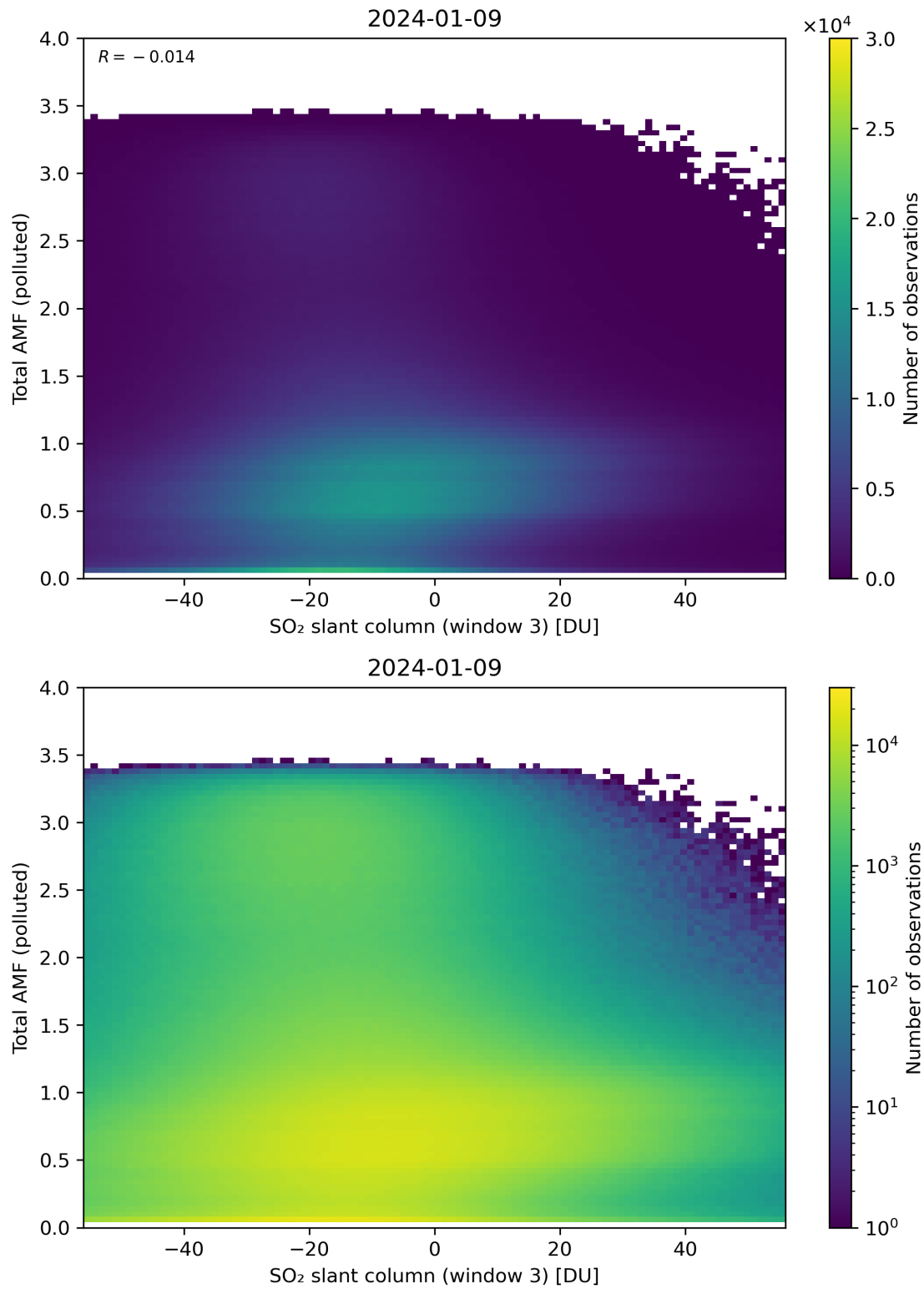
Figure 268: Scatter density plot of “SO 2 slant column (window 3)” against “Total AMF (polluted)” for 2024-01-08 to 2024-01-10.
