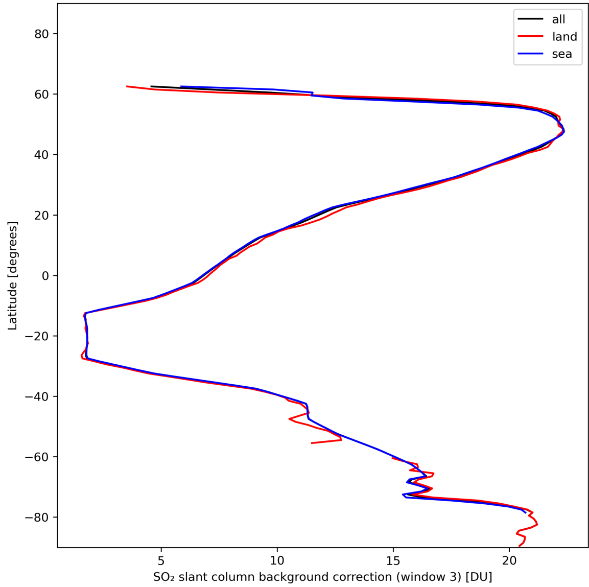
Figure 44: Zonal average of “SO 2 slant column background correction (window 3)” for 2024-01-08 to 2024-01-10.
