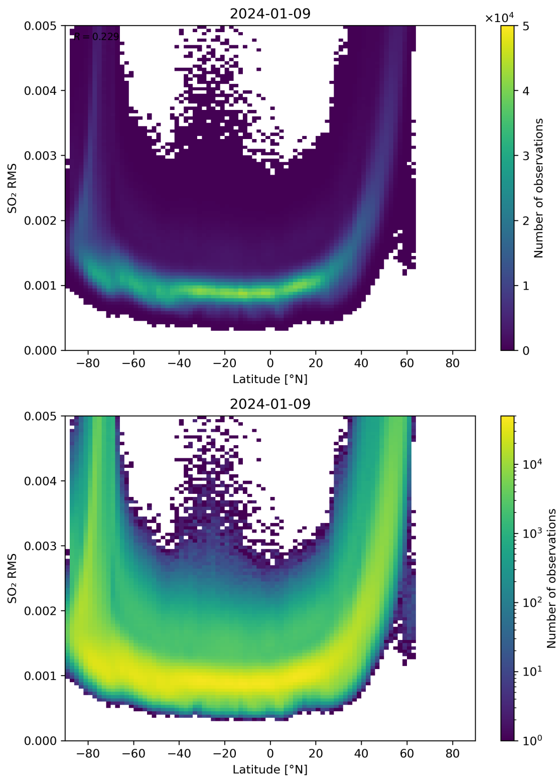
Figure 144: Scatter density plot of “Latitude” against “SO 2 RMS” for 2024-01-08 to 2024-01-10.
