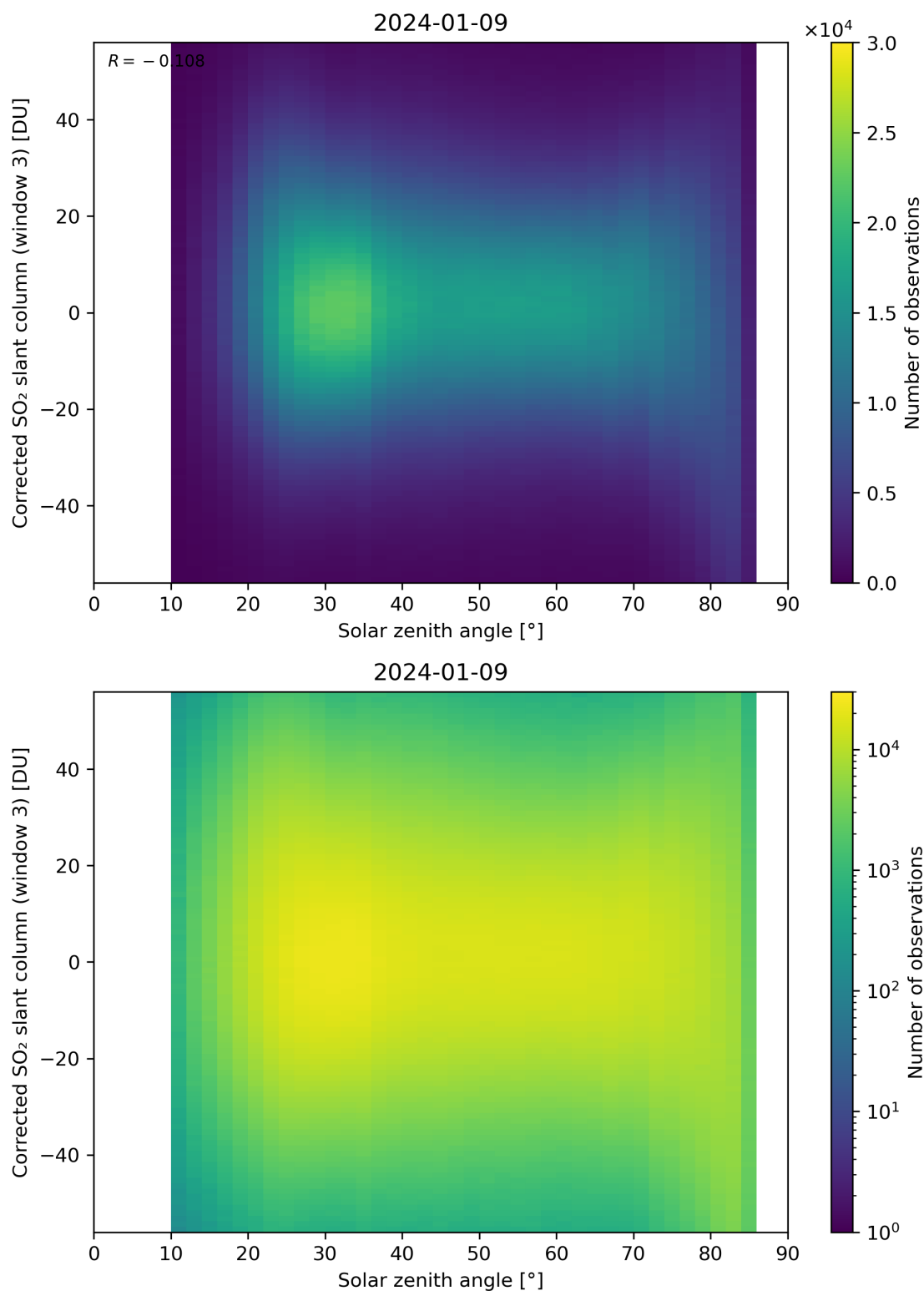
Figure 168: Scatter density plot of “Solar zenith angle” against “Corrected SO 2 slant column (window 3)” for 2024-01-08 to 2024-01-10.
