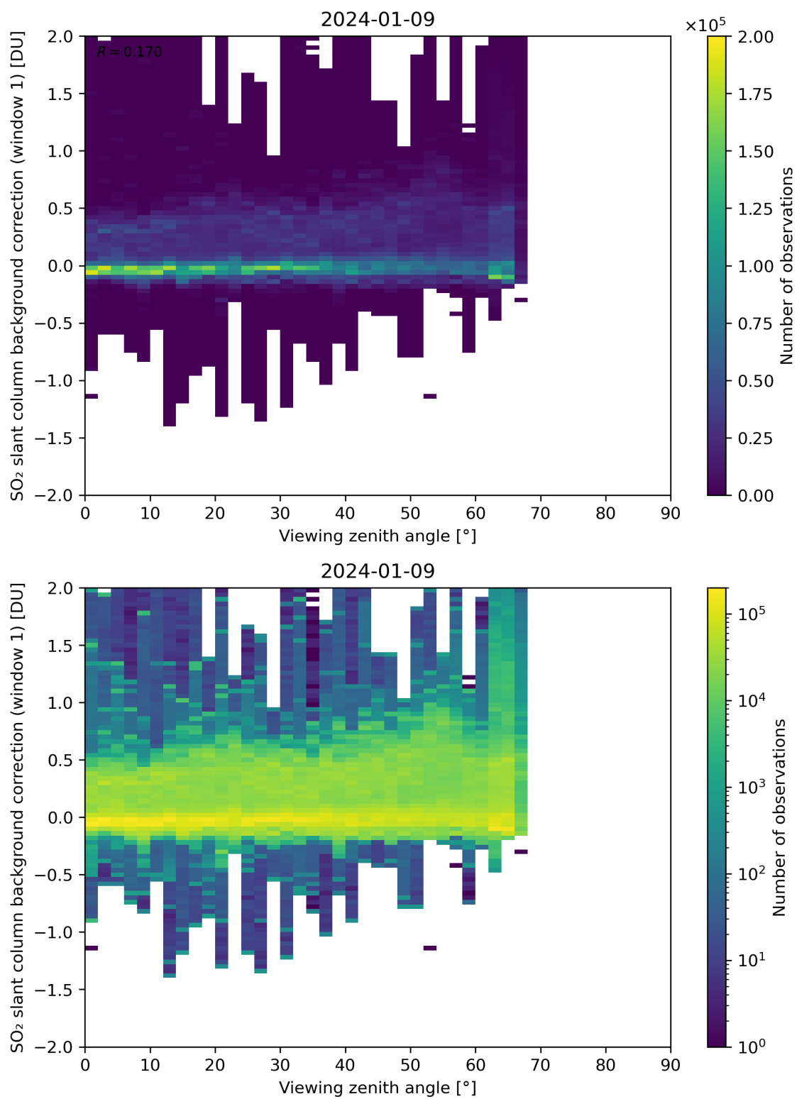
Figure 308: Scatter density plot of “Viewing zenith angle” against “SO 2 slant column background correction (window 1)” for 2024-01-08 to 2024-01-10.
