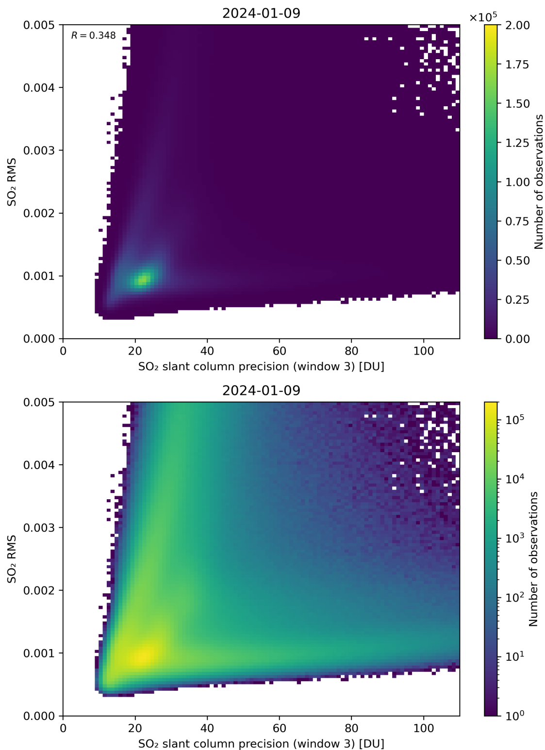
Figure 260: Scatter density plot of “SO 2 slant column precision (window 3)” against “SO 2 RMS” for 2024-01-08 to 2024-01-10.
