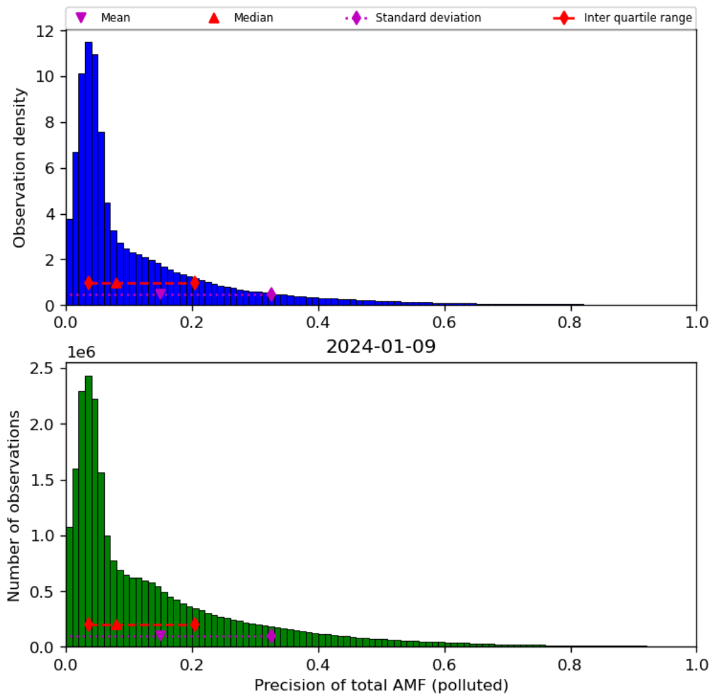
Figure 72: Histogram of “Precision of total AMF (polluted)” for 2024-01-08 to 2024-01-10
