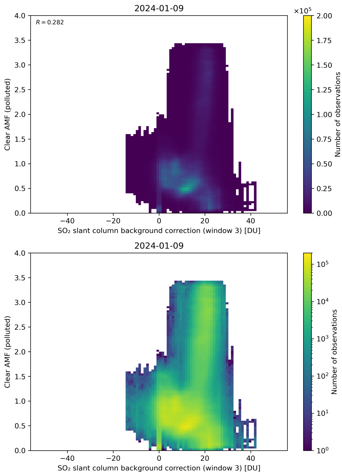
Figure 124: Scatter density plot of “SO 2 slant column background correction (window 3)” against “Clear AMF (polluted)” for 2024-01-08 to 2024-01-10.
