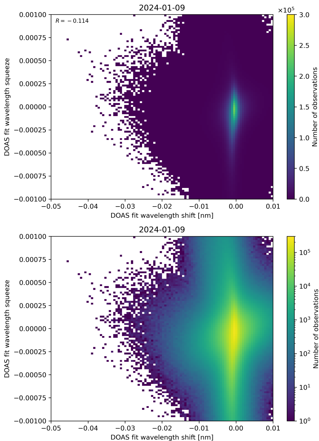
Figure 127: Scatter density plot of “DOAS fit wavelength shift” against “DOAS fit wavelength squeeze” for 2024-01-08 to 2024-01-10.
