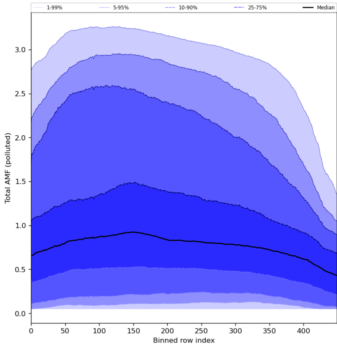
Figure 94: Along track statistics of “Total AMF (polluted)” for 2024-01-08 to 2024-01-10
