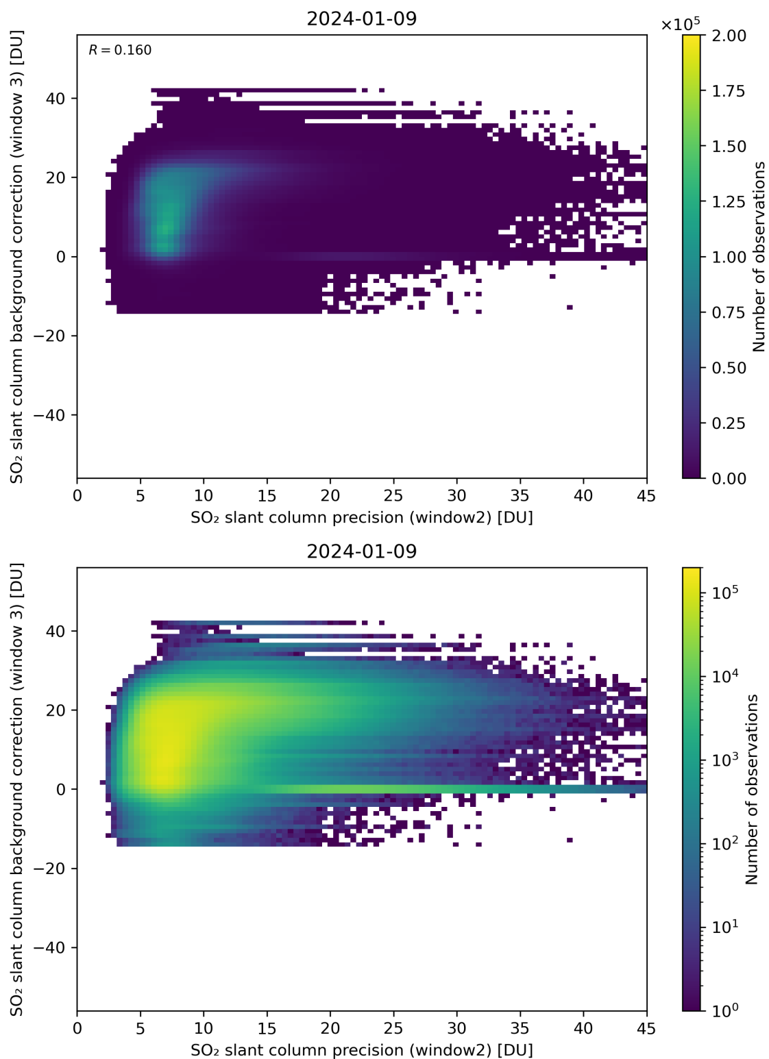
Figure 242: Scatter density plot of “SO 2 slant column precision (window2)” against “SO 2 slant column background correction (window 3)” for 2024-01-08 to 2024-01-10.
