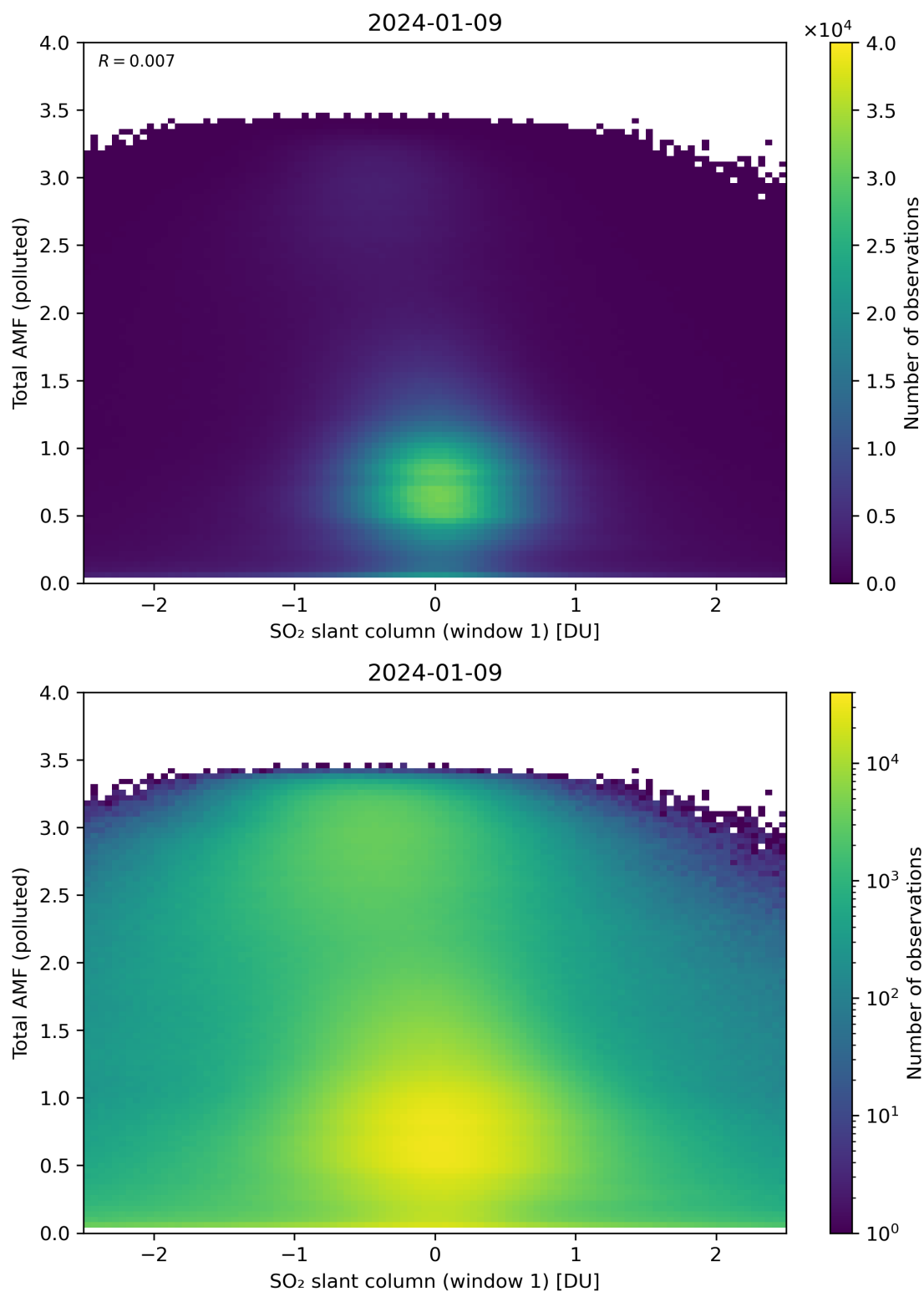
Figure 239: Scatter density plot of “SO 2 slant column (window 1)” against “Total AMF (polluted)” for 2024-01-08 to 2024-01-10.
