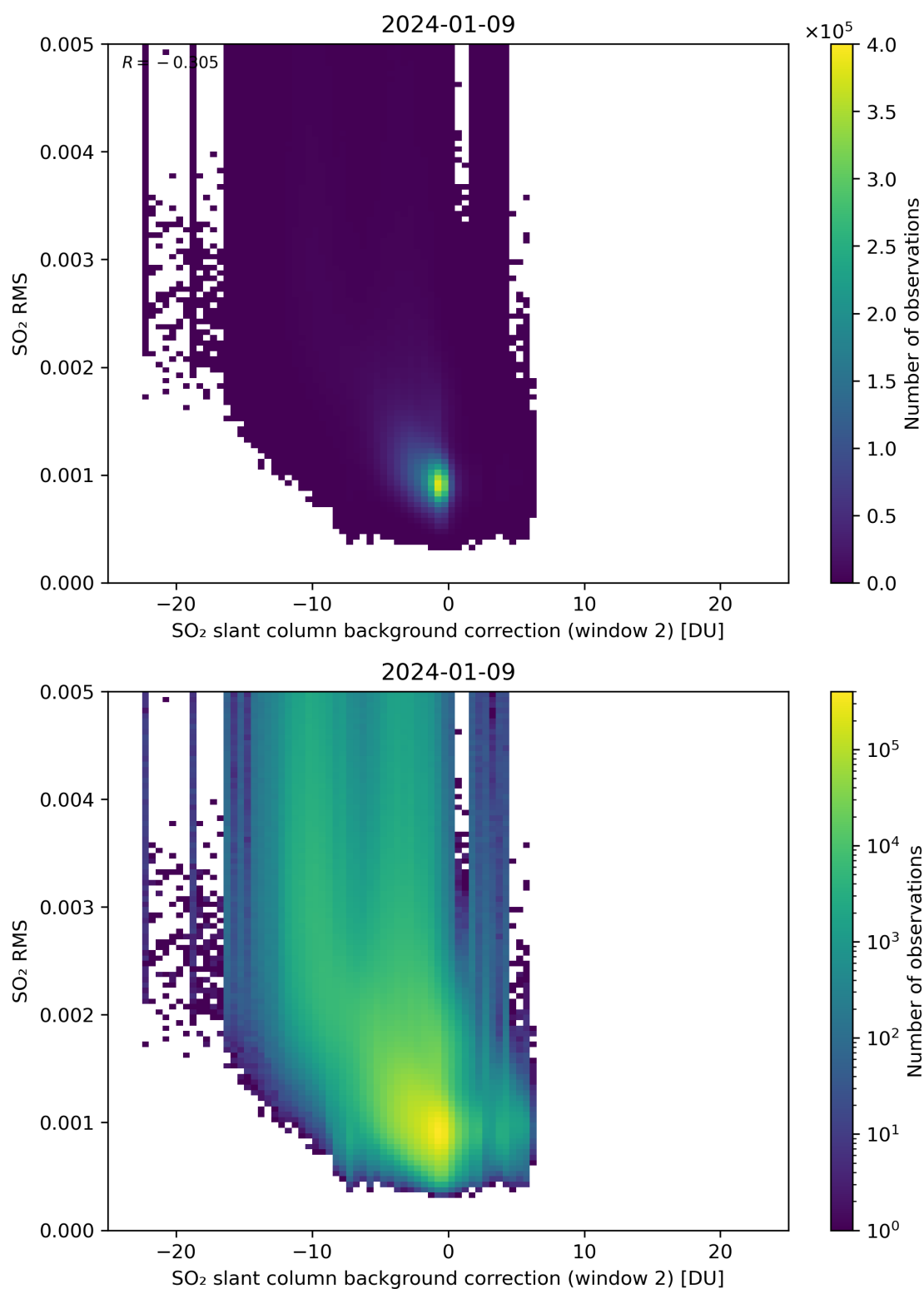
Figure 114: Scatter density plot of “SO 2 slant column background correction (window 2)” against “SO 2 RMS” for 2024-01-08 to 2024-01-10.
