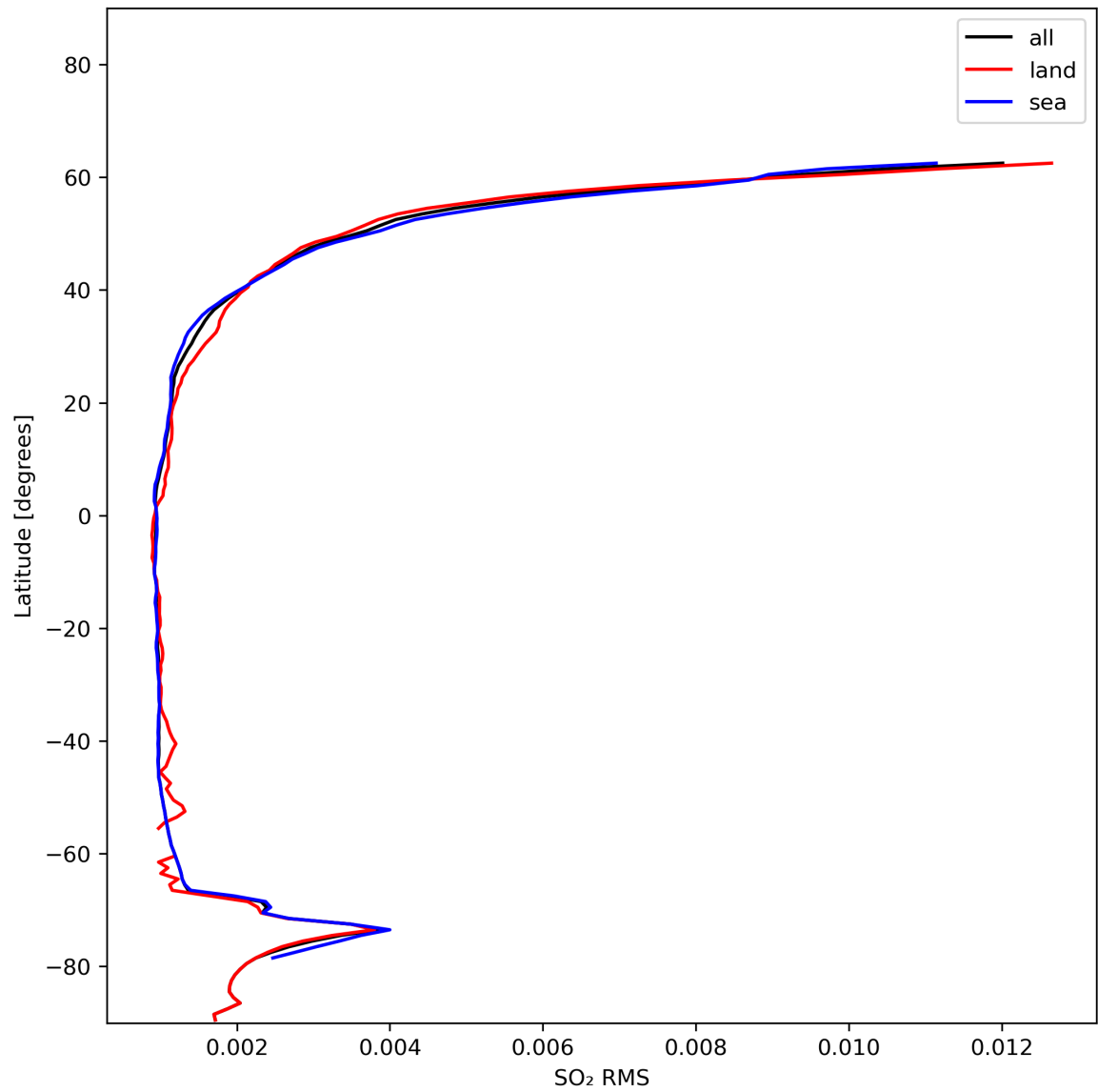
Figure 47: Zonal average of “SO 2 RMS” for 2024-01-08 to 2024-01-10.
