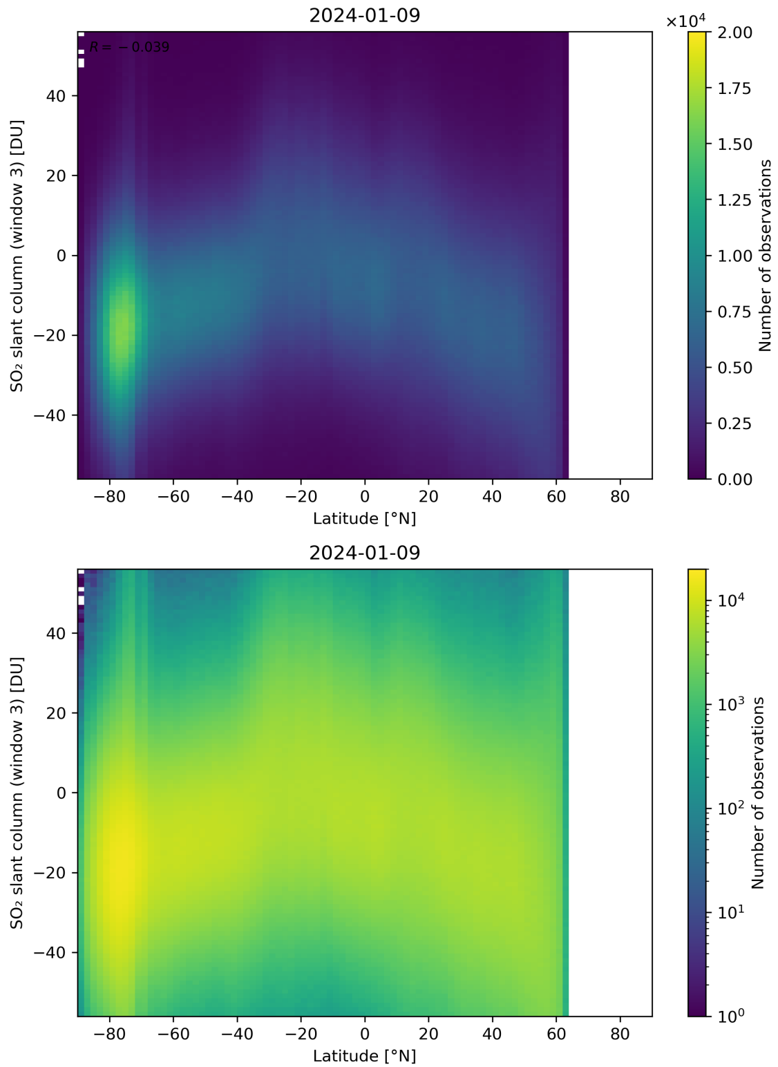
Figure 152: Scatter density plot of “Latitude” against “SO 2 slant column (window 3)” for 2024-01-08 to 2024-01-10.
