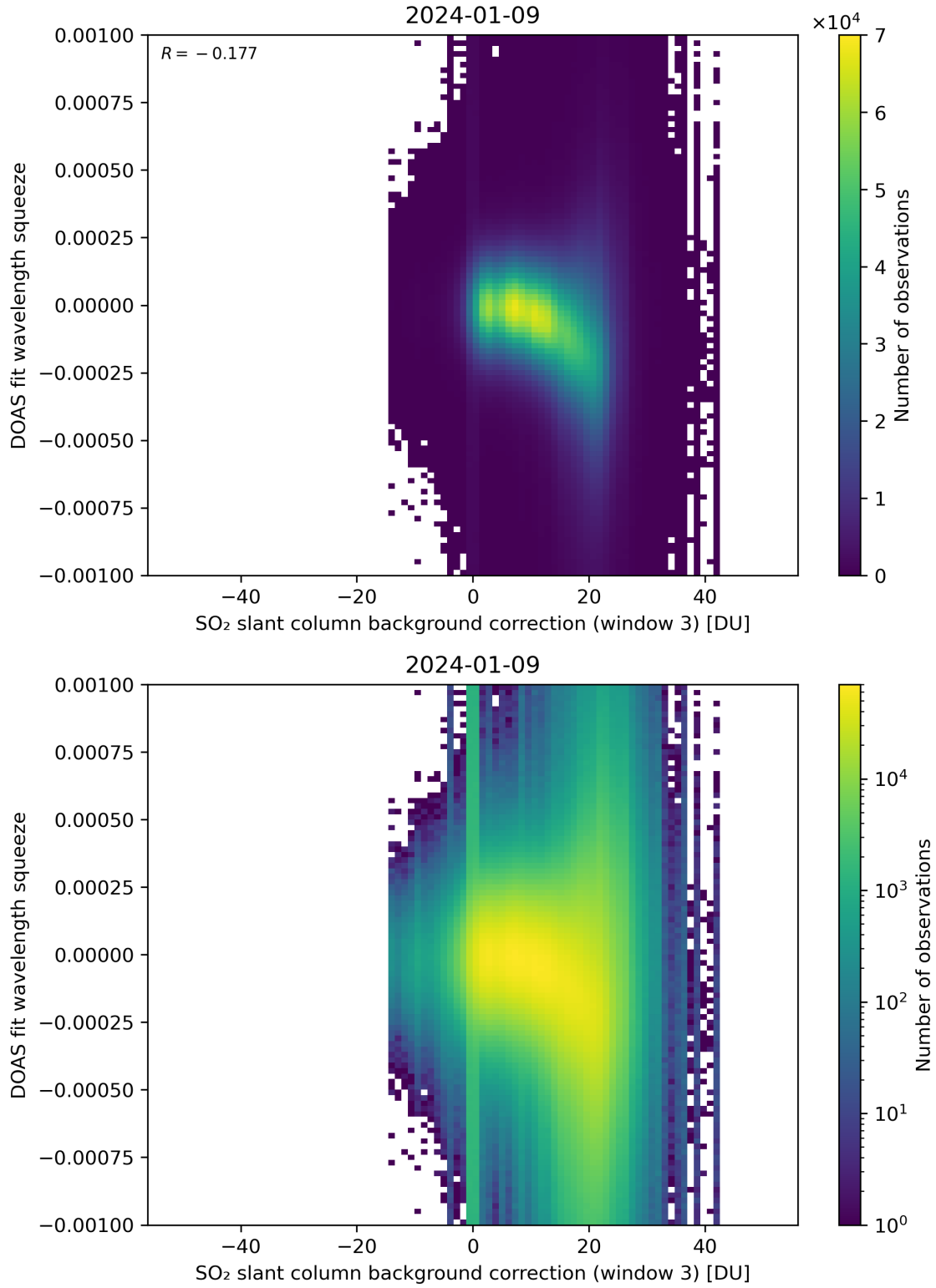
Figure 122: Scatter density plot of “SO 2 slant column background correction (window 3)” against “DOAS fit wavelength squeeze” for 2024-01-08 to 2024-01-10.
