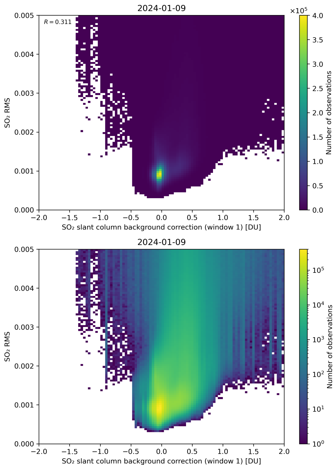
Figure 102: Scatter density plot of “SO 2 slant column background correction (window 1)” against “SO 2 RMS” for 2024-01-08 to 2024-01-10.
