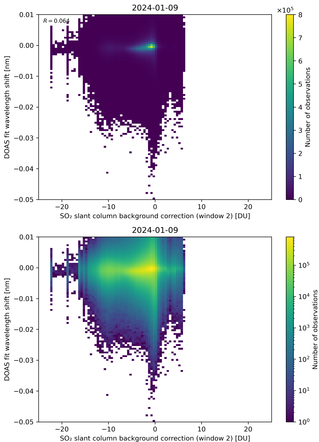
Figure 112: Scatter density plot of “SO 2 slant column background correction (window 2)” against “DOAS fit wavelength shift” for 2024-01-08 to 2024-01-10.
