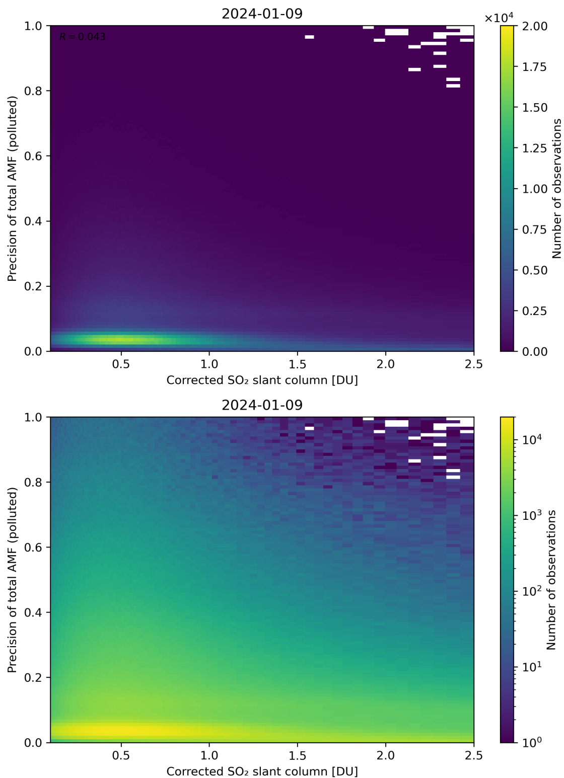
Figure 193: Scatter density plot of “Corrected SO 2 slant column” against “Precision of total AMF (polluted)” for 2024-01-08 to 2024-01-10.
