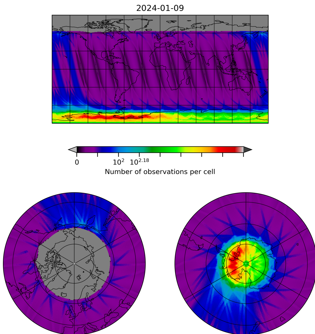
Figure 28: Map of the number of observations for 2024-01-08 to 2024-01-10
