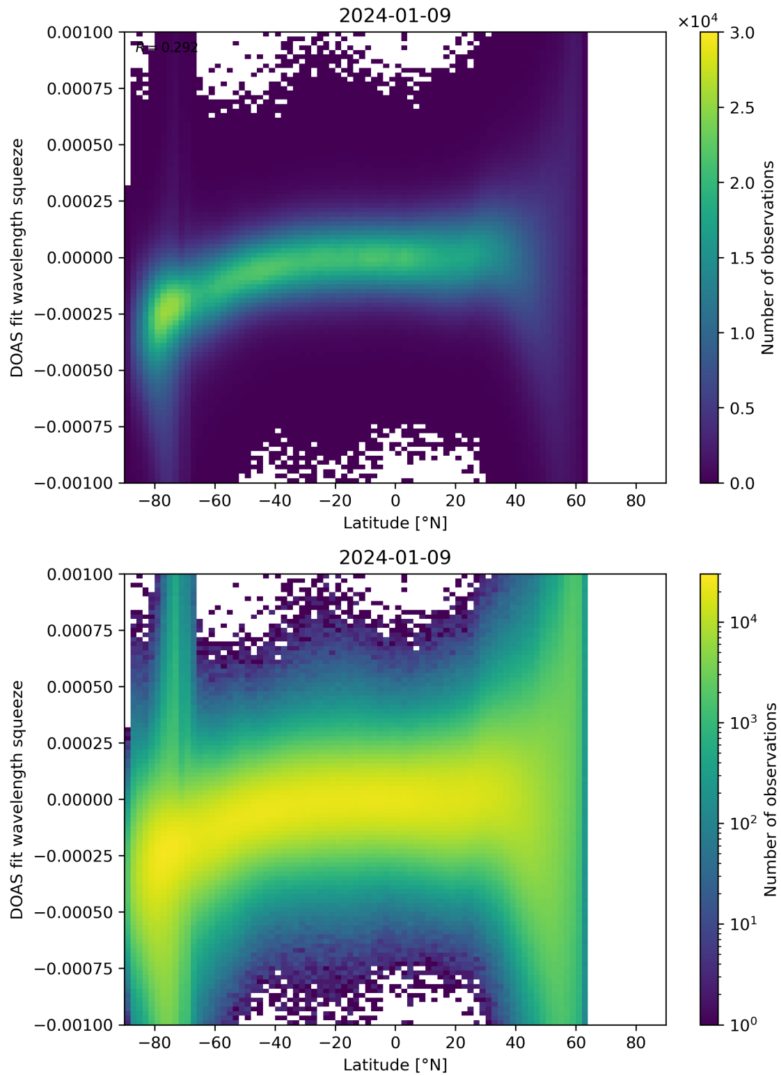
Figure 143: Scatter density plot of “Latitude” against “DOAS fit wavelength squeeze” for 2024-01-08 to 2024-01-10.
