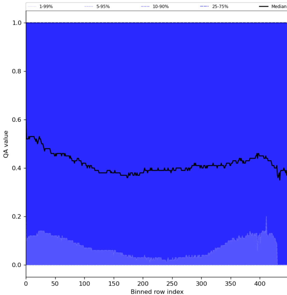
Figure 75: Along track statistics of “QA value” for 2024-01-08 to 2024-01-10
