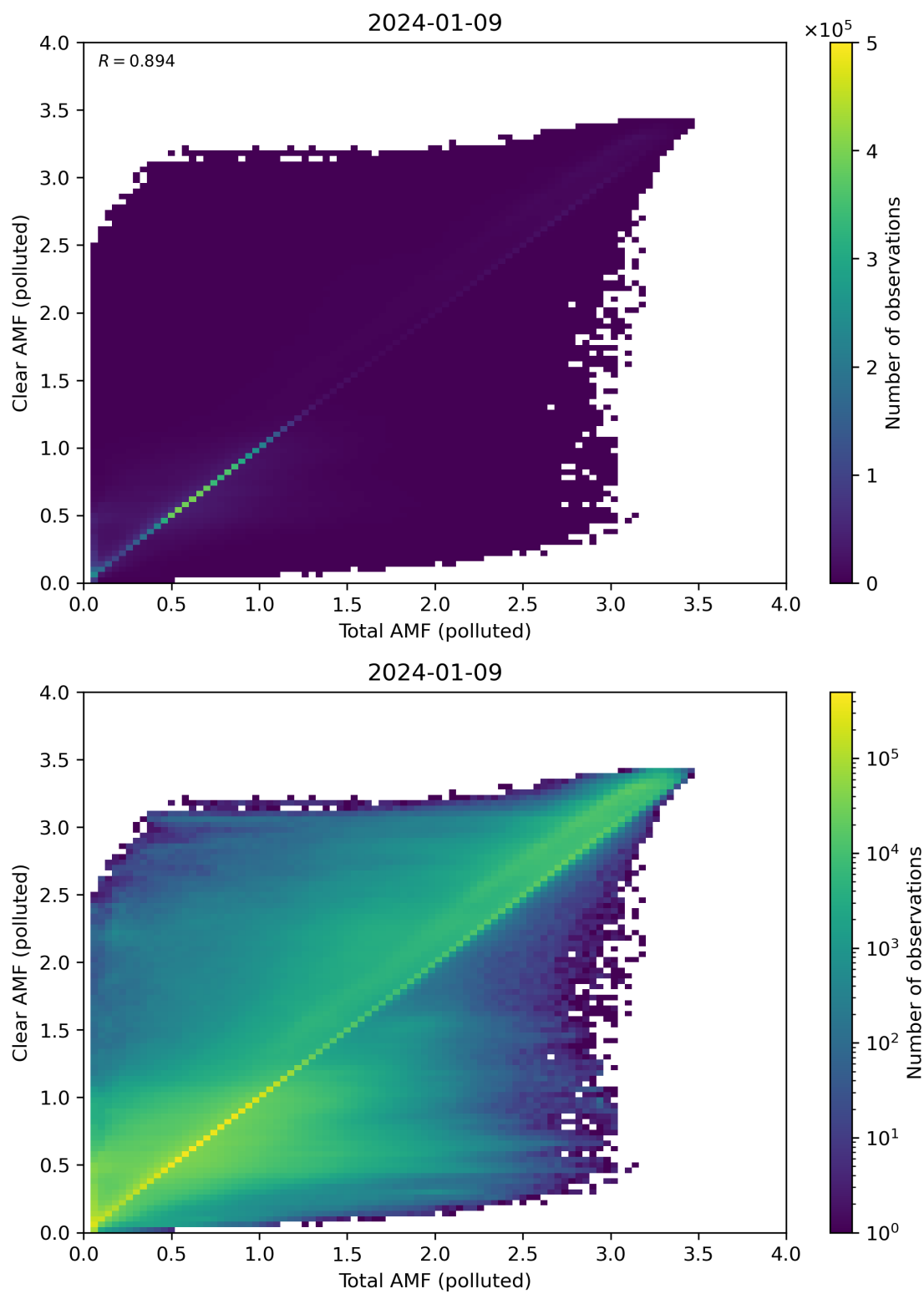
Figure 271: Scatter density plot of “Total AMF (polluted)” against “Clear AMF (polluted)” for 2024-01-08 to 2024-01-10.
