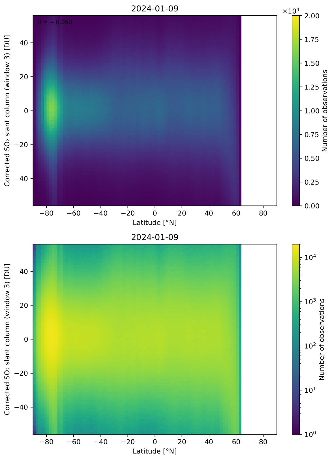
Figure 148: Scatter density plot of “Latitude” against “Corrected SO 2 slant column (window 3)” for 2024-01-08 to 2024-01-10.
