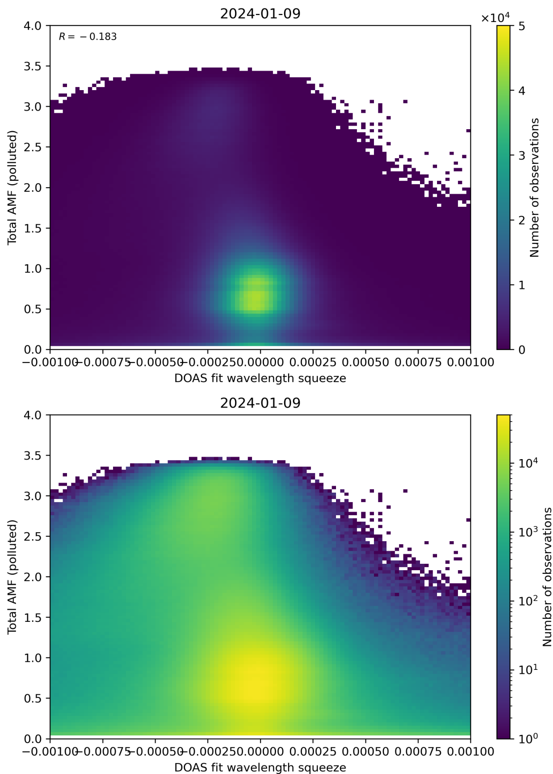
Figure 134: Scatter density plot of “DOAS fit wavelength squeeze” against “Total AMF (polluted)” for 2024-01-08 to 2024-01-10.
