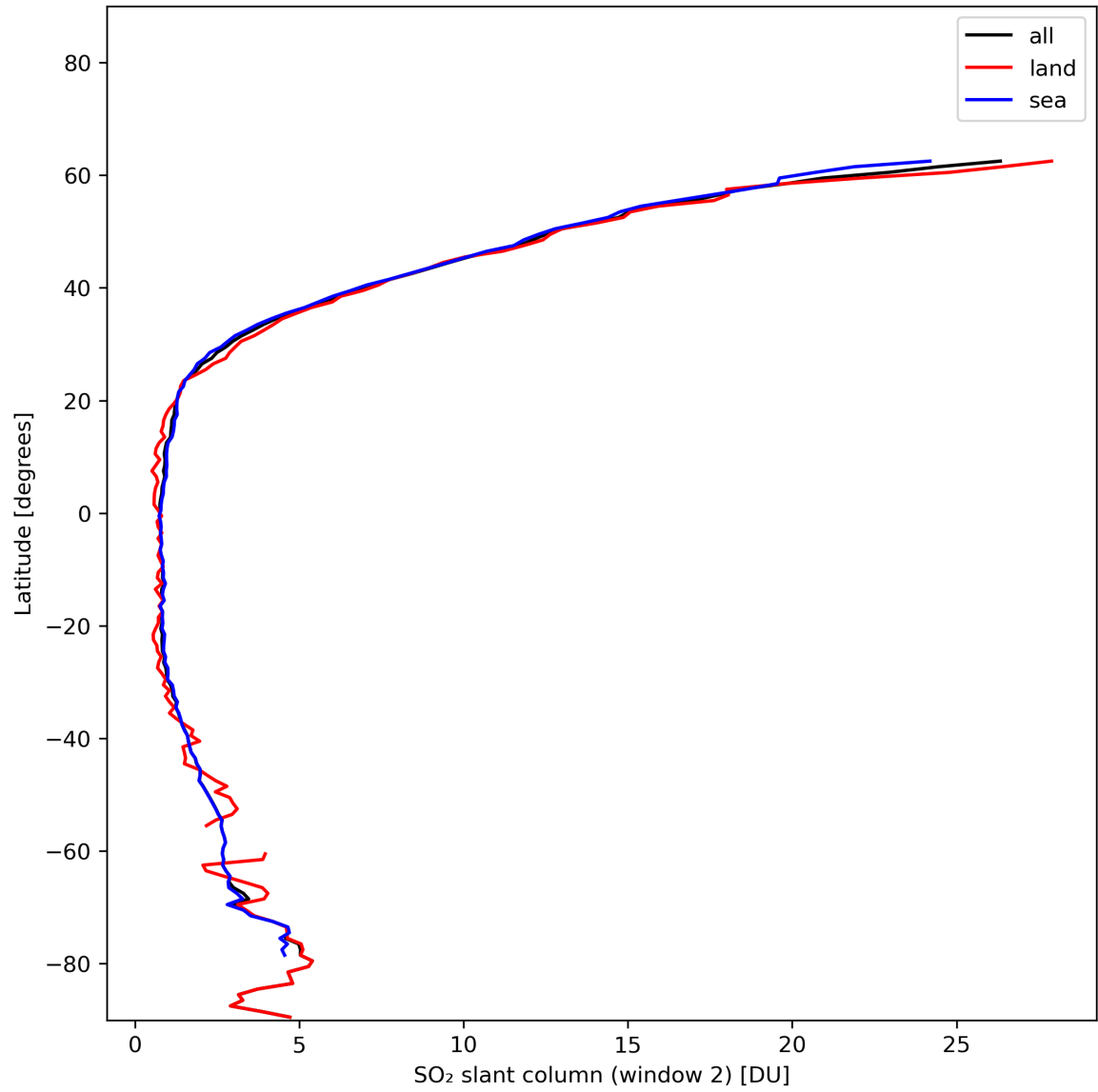
Figure 37: Zonal average of “SO 2 slant column (window 2)” for 2024-01-08 to 2024-01-10.
