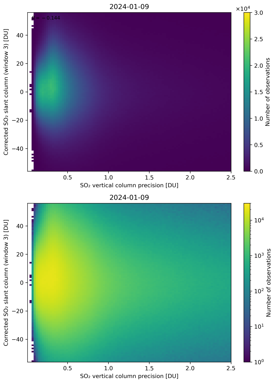
Figure 288: Scatter density plot of “SO 2 vertical column precision” against “Corrected SO 2 slant column (window 3)” for 2024-01-08 to 2024-01-10.
