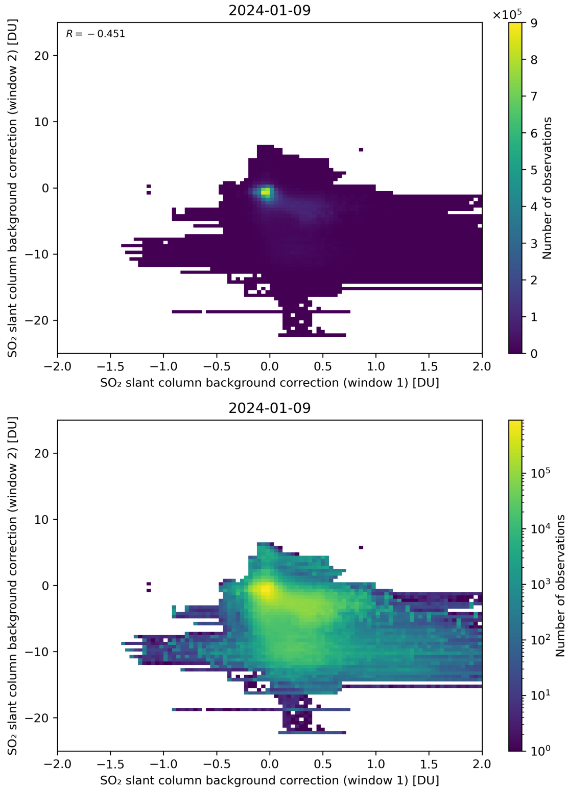
Figure 98: Scatter density plot of “SO 2 slant column background correction (window 1)” against “SO 2 slant column background correction (window 2)” for 2024-01-08 to 2024-01-10.
