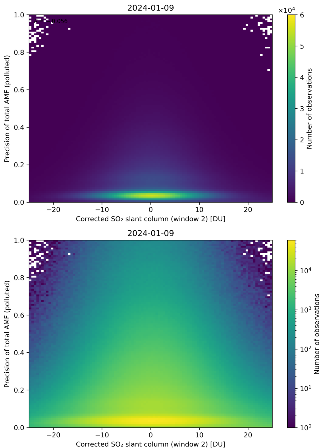
Figure 204: Scatter density plot of “Corrected SO 2 slant column (window 2)” against “Precision of total AMF (polluted)” for 2024-01-08 to 2024-01-10.
