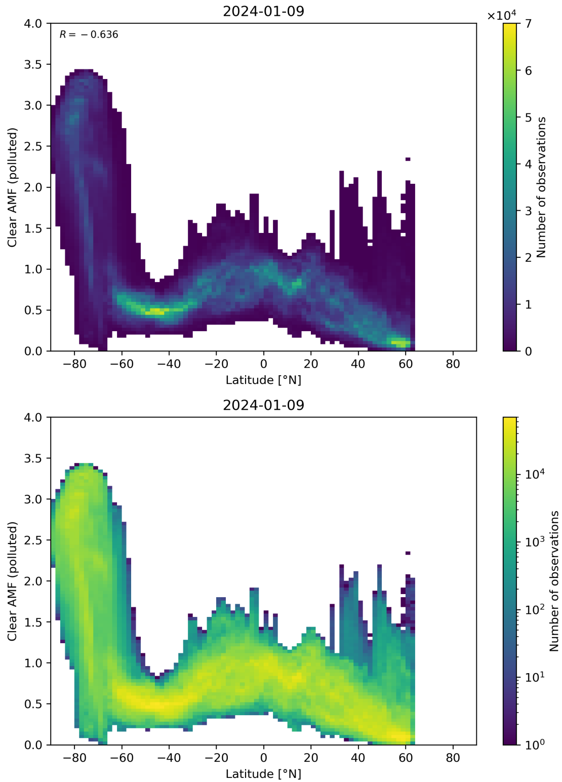
Figure 145: Scatter density plot of “Latitude” against “Clear AMF (polluted)” for 2024-01-08 to 2024-01-10.
