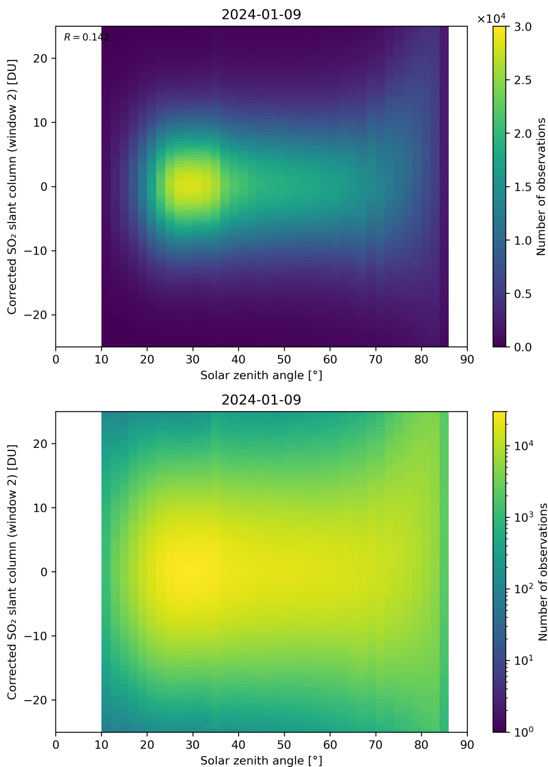
Figure 167: Scatter density plot of “Solar zenith angle” against “Corrected SO 2 slant column (window 2)” for 2024-01-08 to 2024-01-10.
