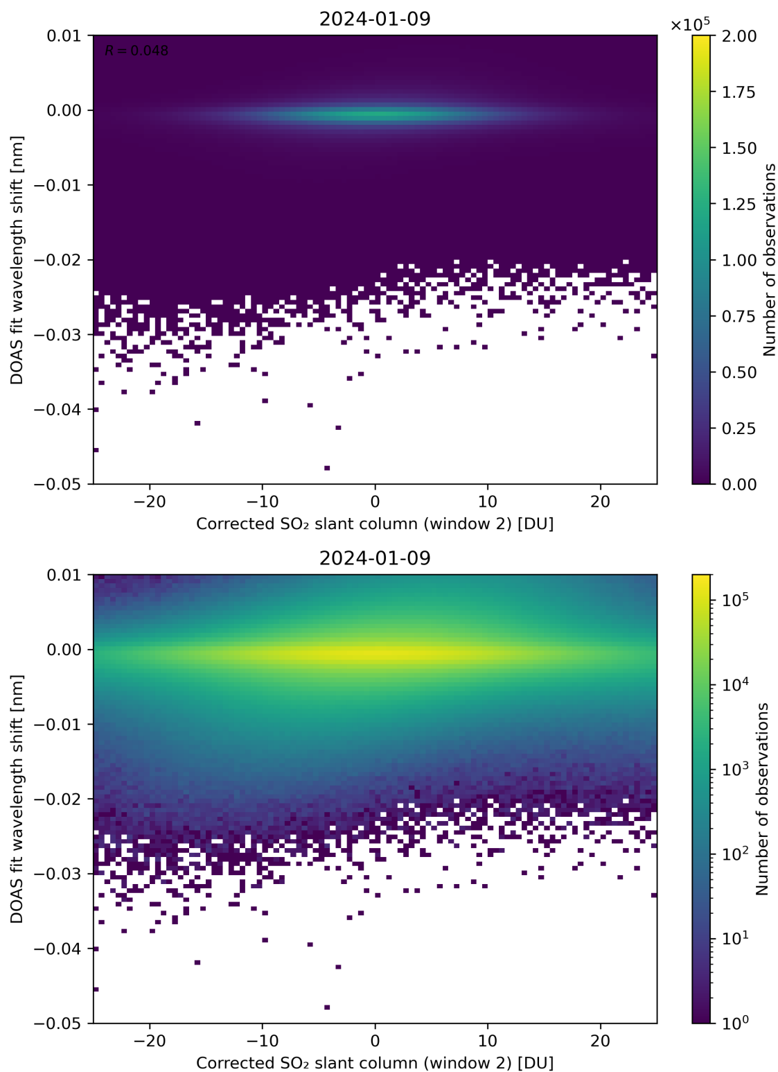
Figure 196: Scatter density plot of “Corrected SO 2 slant column (window 2)” against “DOAS fit wavelength shift” for 2024-01-08 to 2024-01-10.
