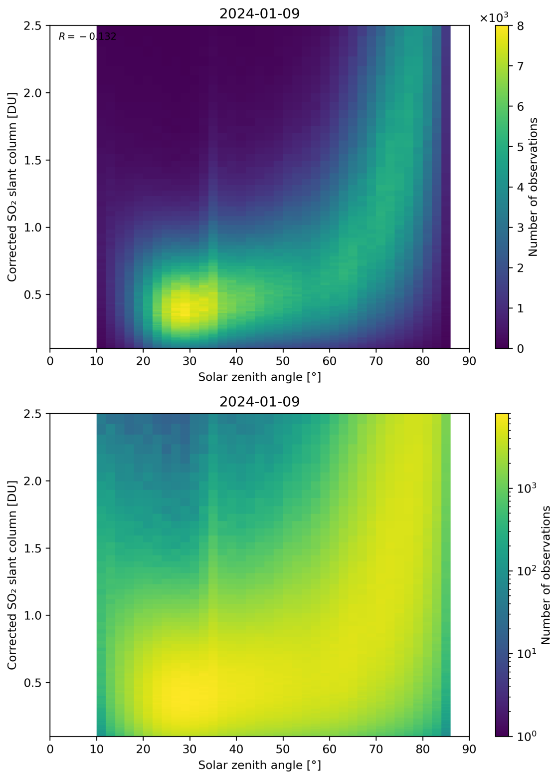
Figure 166: Scatter density plot of “Solar zenith angle” against “Corrected SO 2 slant column” for 2024-01-08 to 2024-01-10.
