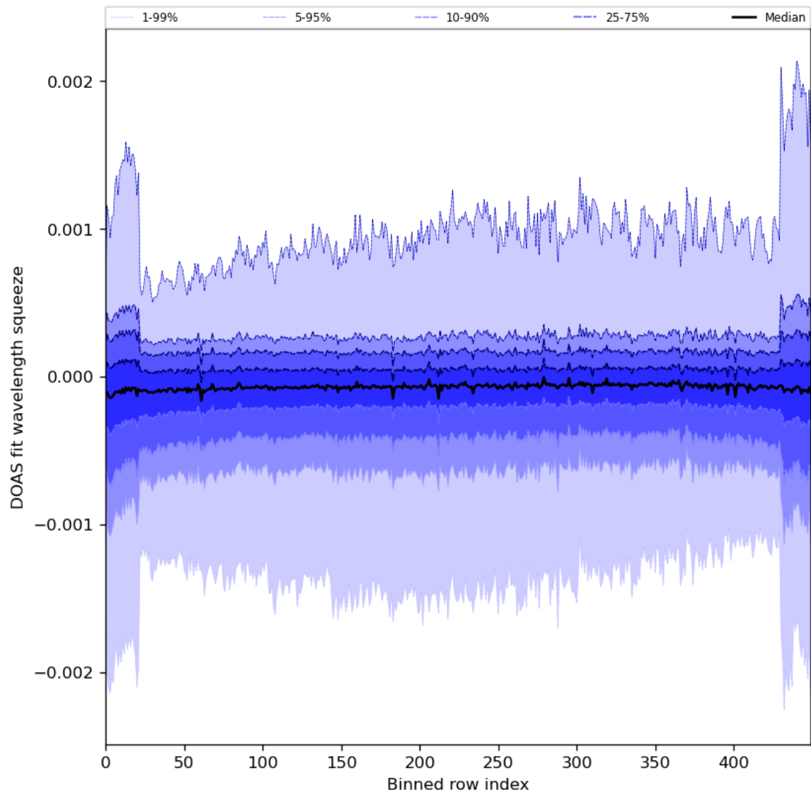
Figure 92: Along track statistics of “DOAS fit wavelength squeeze” for 2024-01-08 to 2024-01-10
