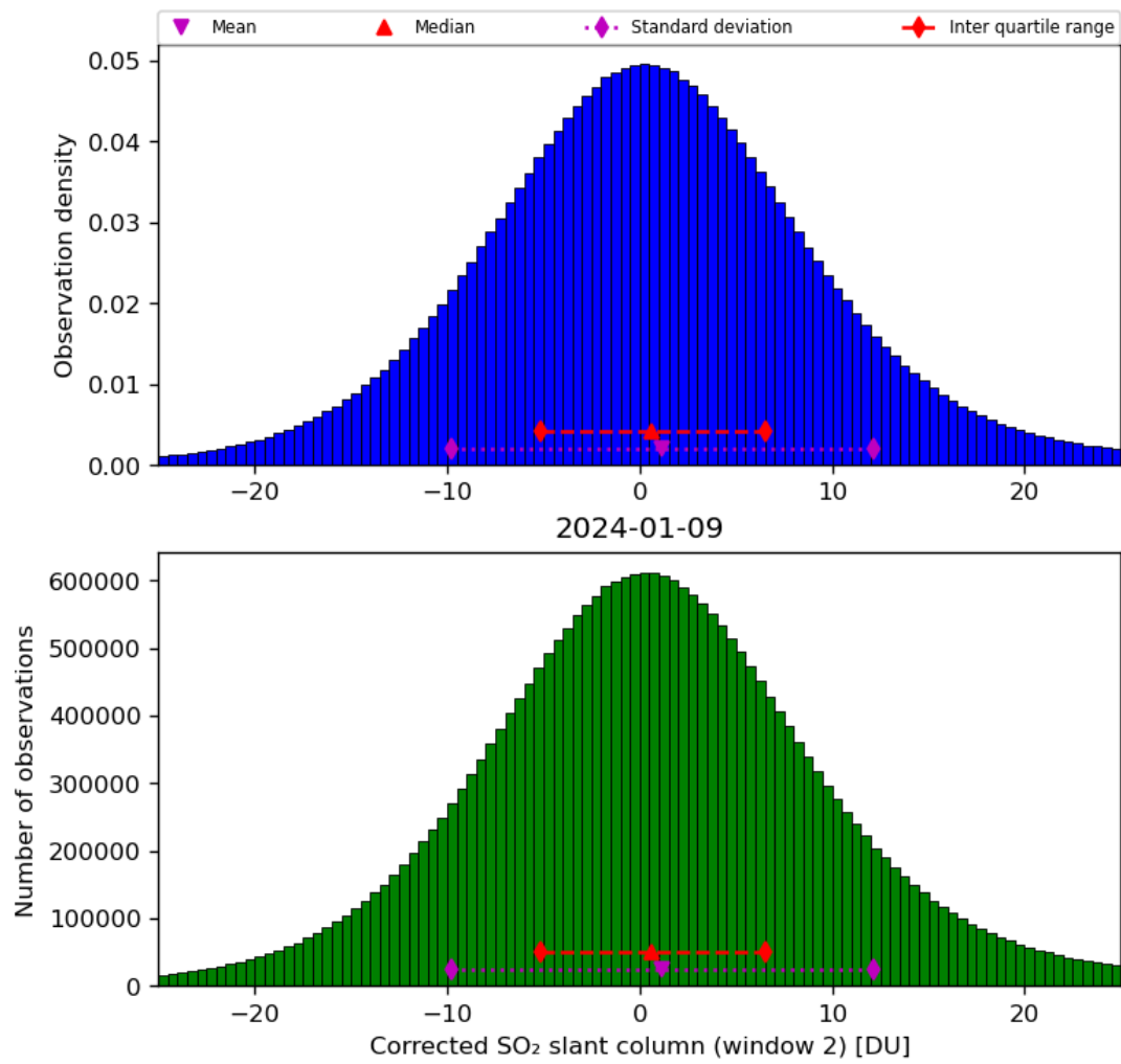
Figure 62: Histogram of “Corrected SO 2 slant column (window 2)” for 2024-01-08 to 2024-01-10
