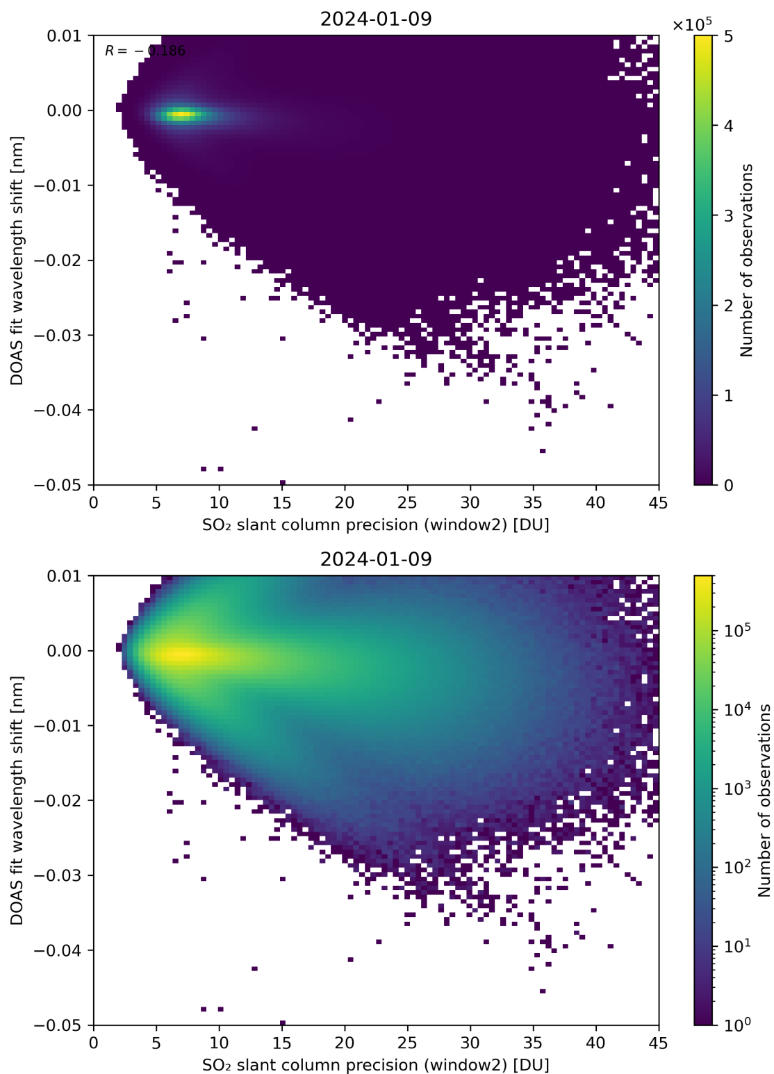
Figure 243: Scatter density plot of “SO 2 slant column precision (window2)” against “DOAS fit wavelength shift” for 2024-01-08 to 2024-01-10.
