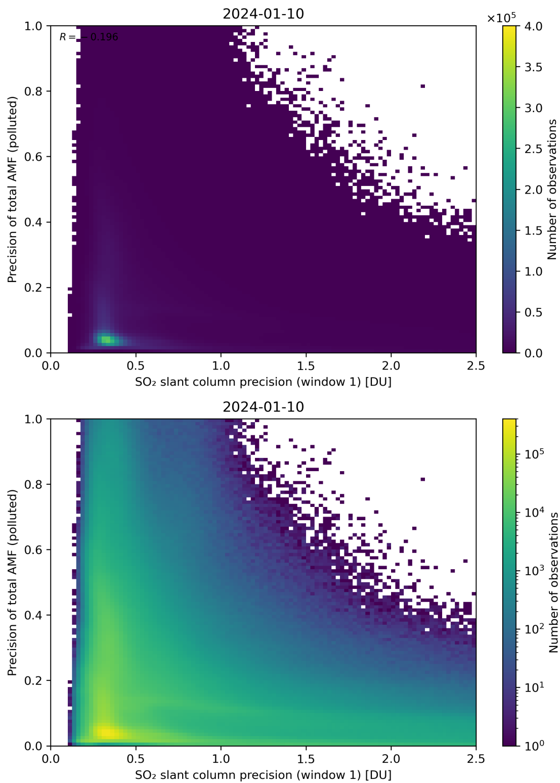
Figure 231: Scatter density plot of “SO 2 slant column precision (window 1)” against “Precision of total AMF (polluted)” for 2024-01-10 to 2024-01-11.
