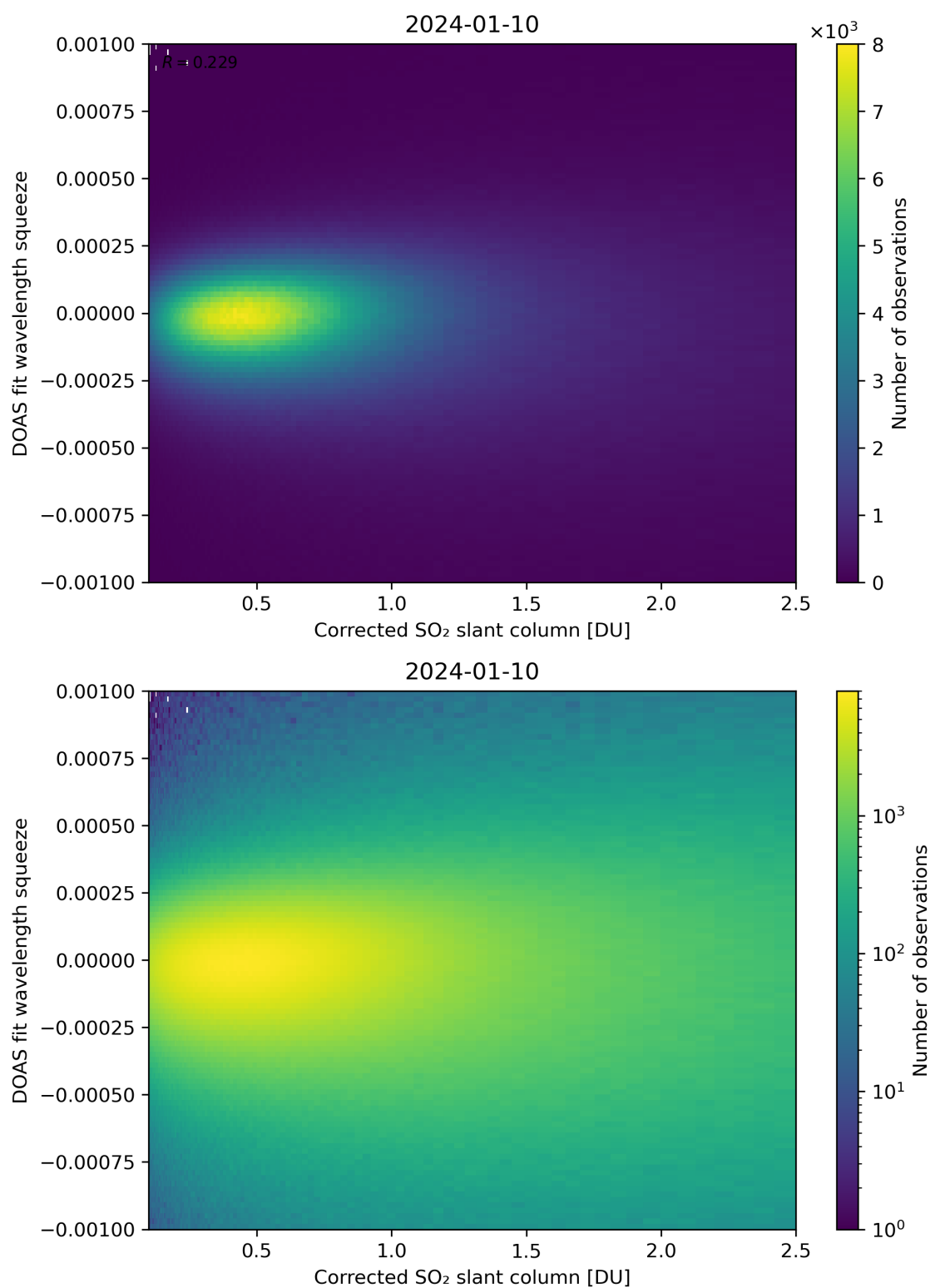
Figure 182: Scatter density plot of “Corrected SO 2 slant column” against “DOAS fit wavelength squeeze” for 2024-01-10 to 2024-01-11.
