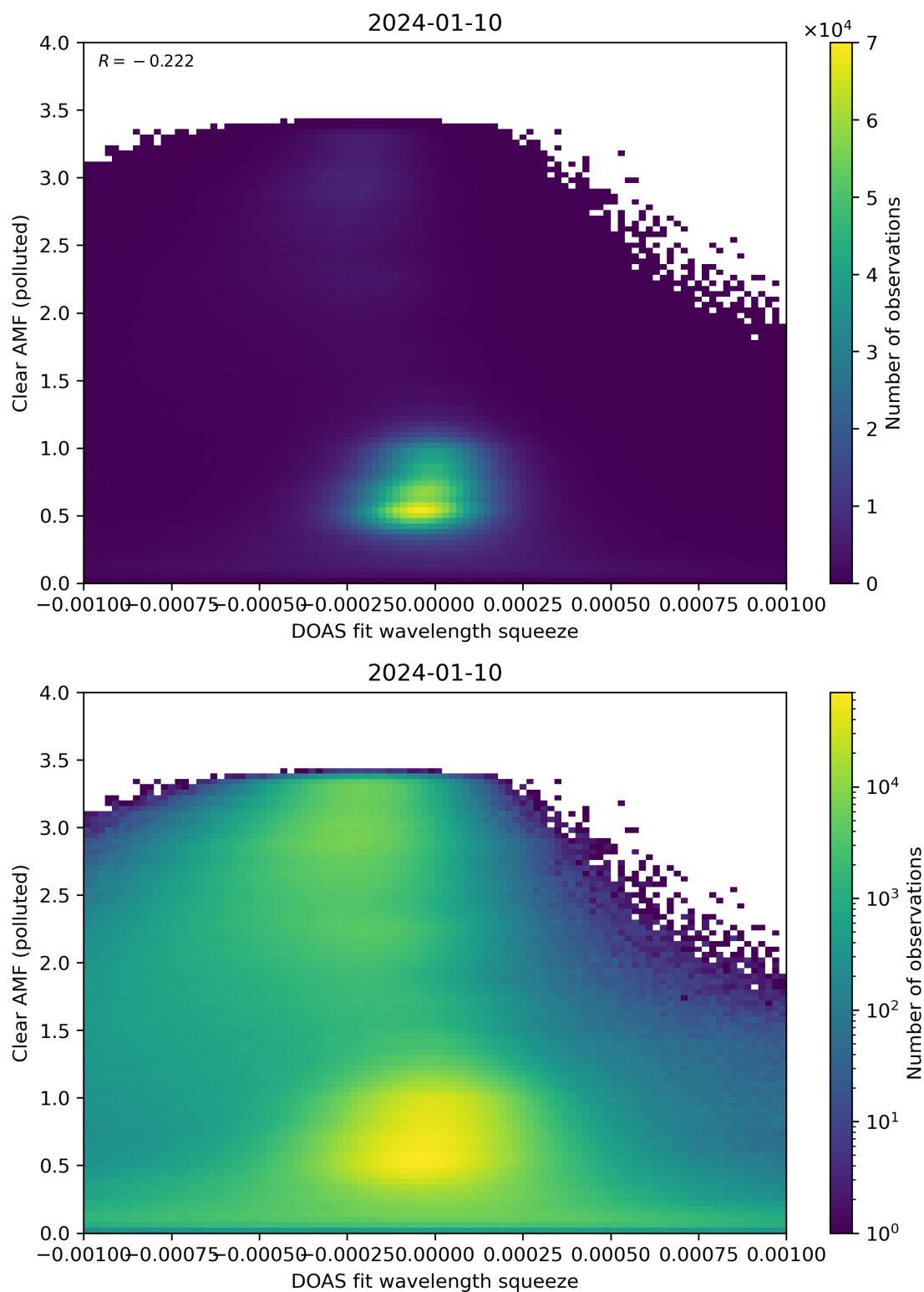
Figure 133: Scatter density plot of “DOAS fit wavelength squeeze” against “Clear AMF (polluted)” for 2024-01-10 to 2024-01-11.
