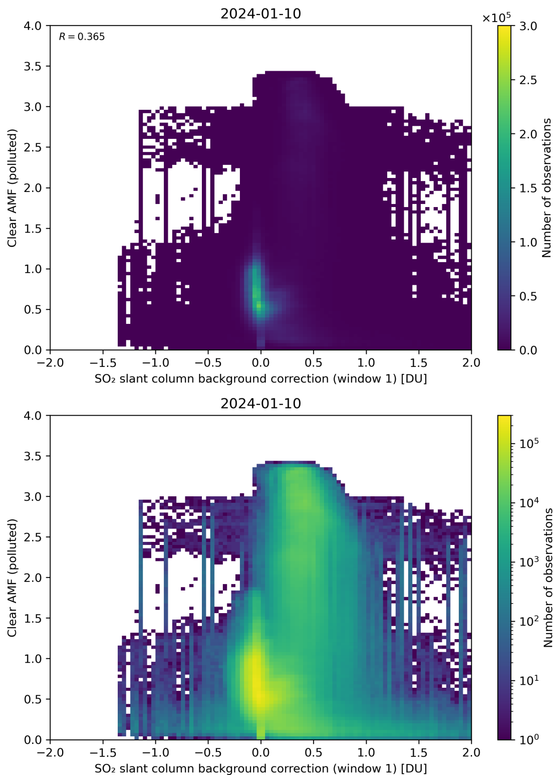
Figure 103: Scatter density plot of “SO 2 slant column background correction (window 1)” against “Clear AMF (polluted)” for 2024-01-10 to 2024-01-11.
