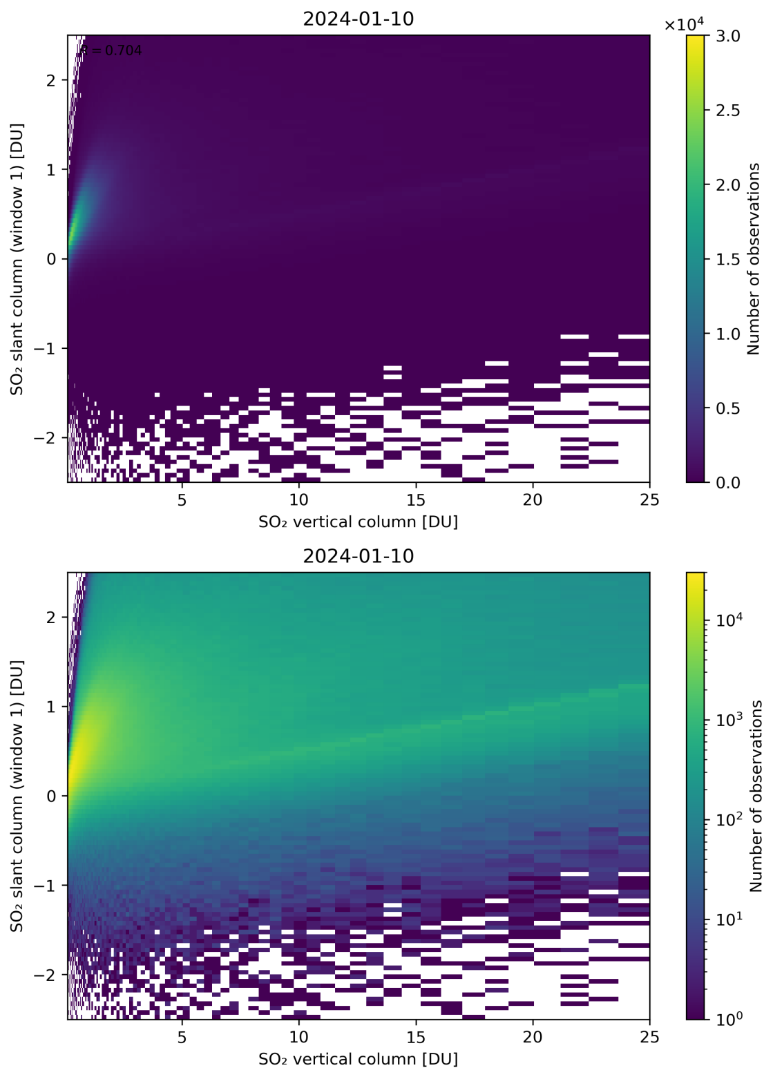
Figure 300: Scatter density plot of “SO 2 vertical column” against “SO 2 slant column (window 1)” for 2024-01-10 to 2024-01-11.
