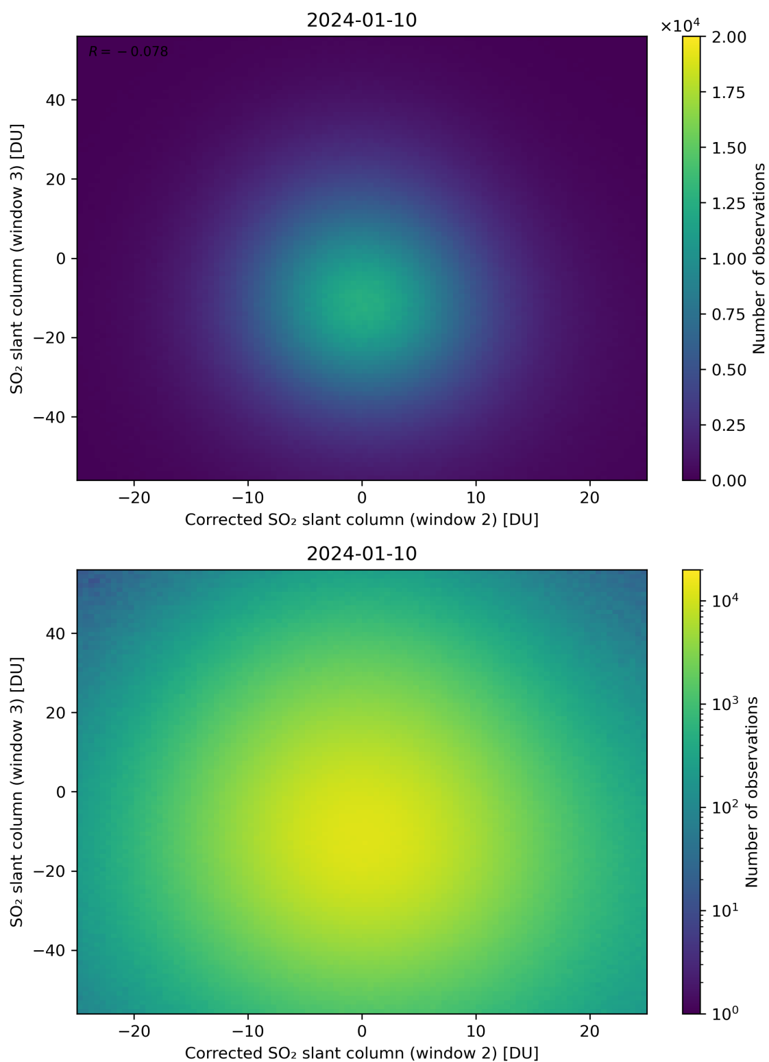
Figure 201: Scatter density plot of “Corrected SO 2 slant column (window 2)” against “SO 2 slant column (window 3)” for 2024-01-10 to 2024-01-11.
