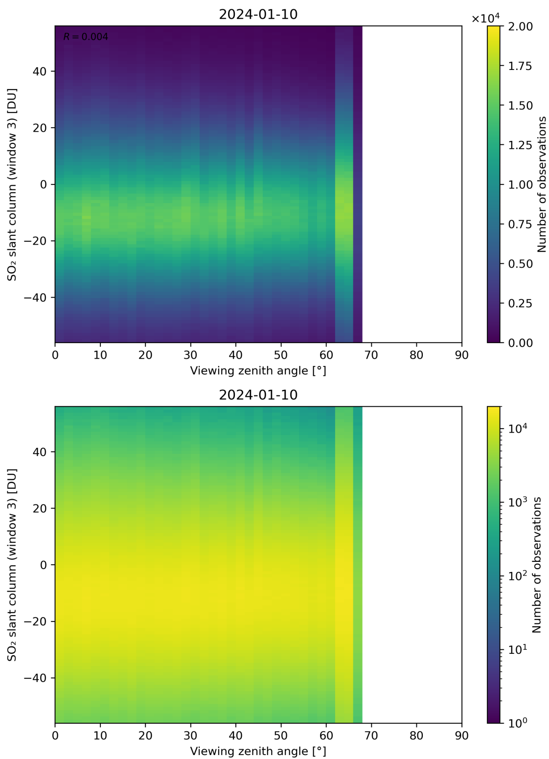
Figure 323: Scatter density plot of “Viewing zenith angle” against “SO 2 slant column (window 3)” for 2024-01-10 to 2024-01-11.
