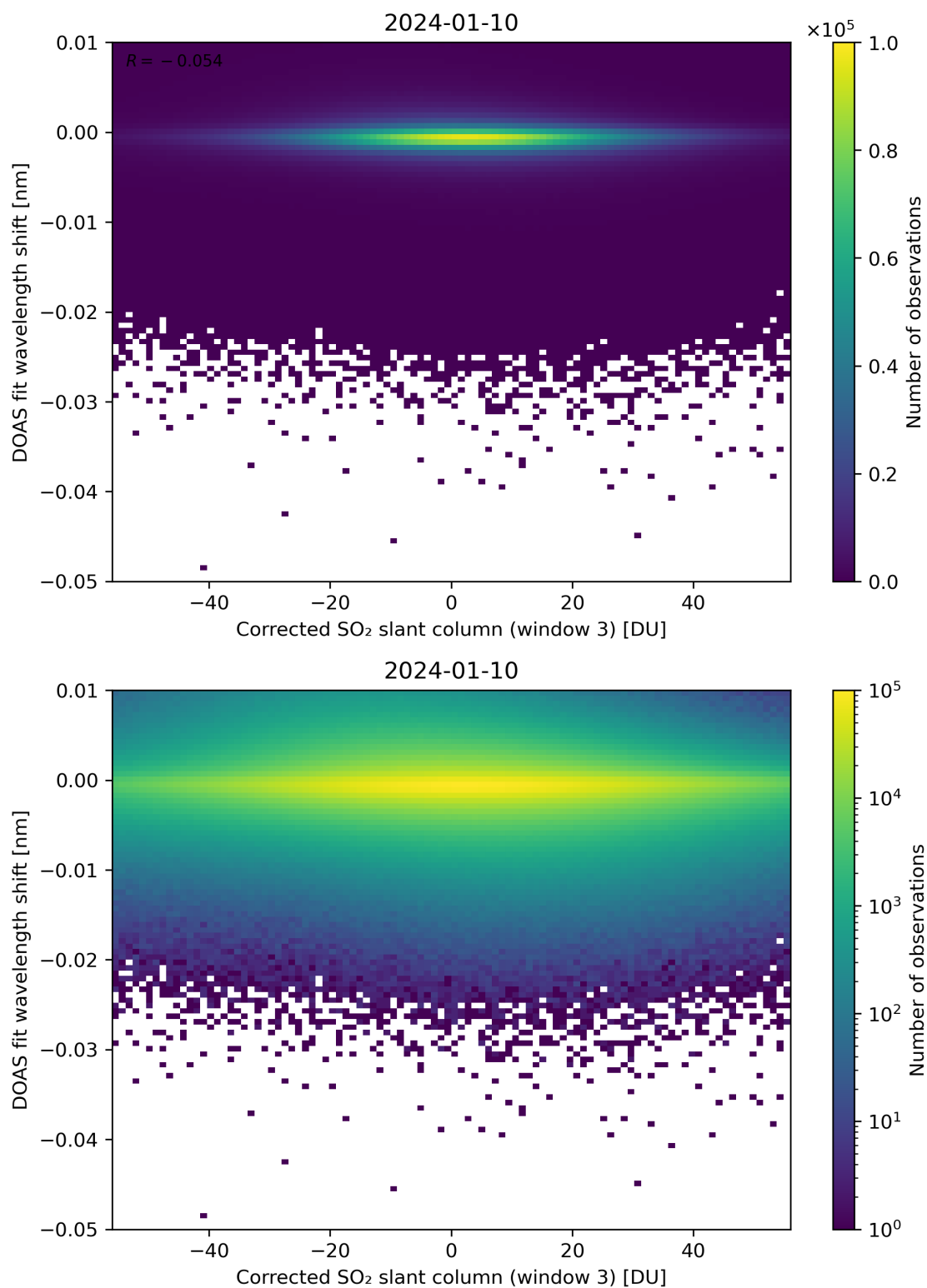
Figure 206: Scatter density plot of “Corrected SO 2 slant column (window 3)” against “DOAS fit wavelength shift” for 2024-01-10 to 2024-01-11.
