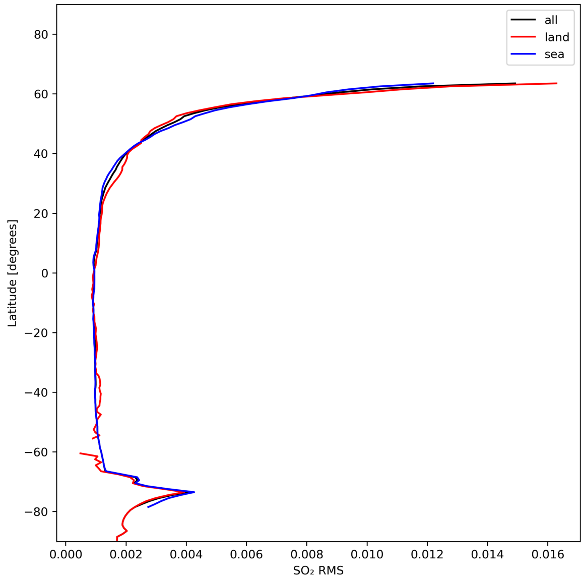
Figure 47: Zonal average of “SO 2 RMS” for 2024-01-10 to 2024-01-11.
