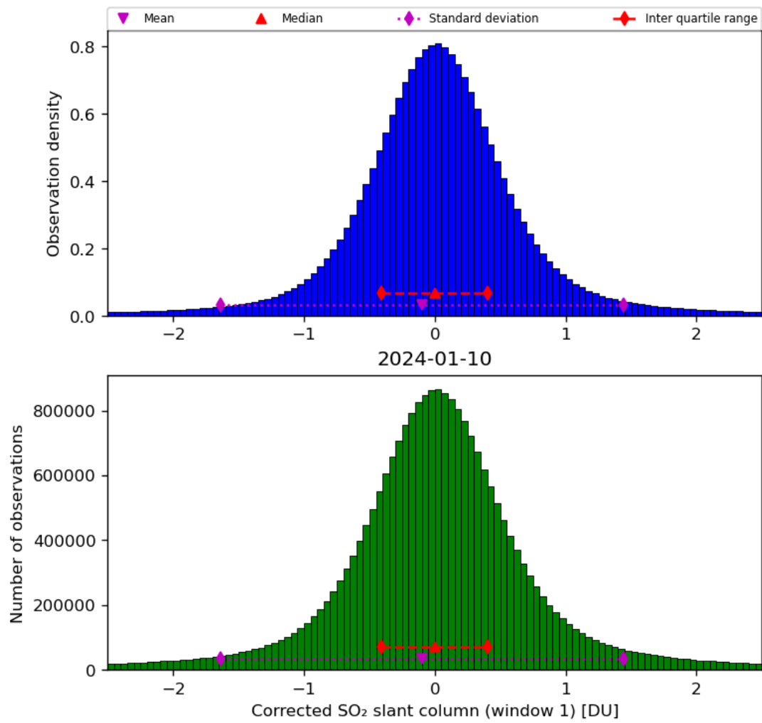
Figure 58: Histogram of “Corrected SO 2 slant column (window 1)” for 2024-01-10 to 2024-01-11
