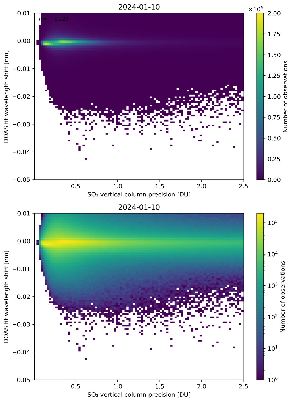
Figure 282: Scatter density plot of “SO 2 vertical column precision” against “DOAS fit wavelength shift” for 2024-01-10 to 2024-01-11.
