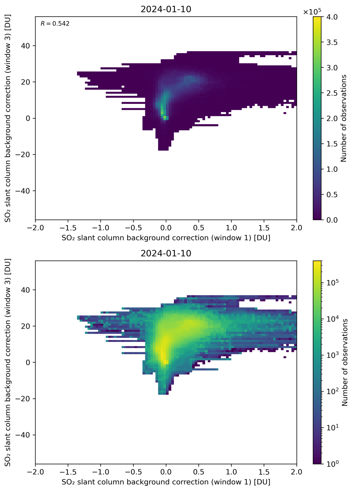
Figure 99: Scatter density plot of “SO 2 slant column background correction (window 1)” against “SO 2 slant column background correction (window 3)” for 2024-01-10 to 2024-01-11.
