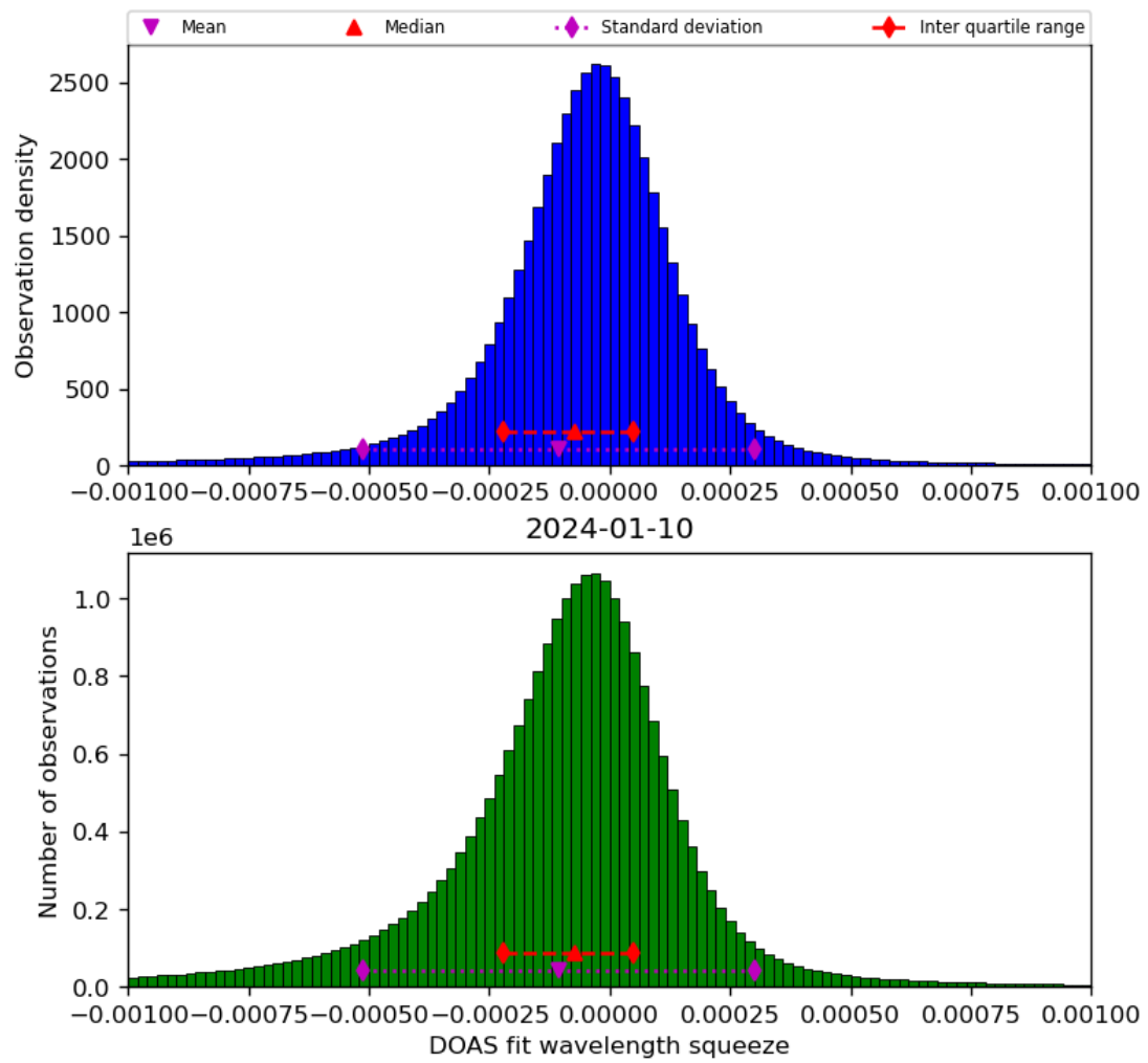
Figure 69: Histogram of “DOAS fit wavelength squeeze” for 2024-01-10 to 2024-01-11
