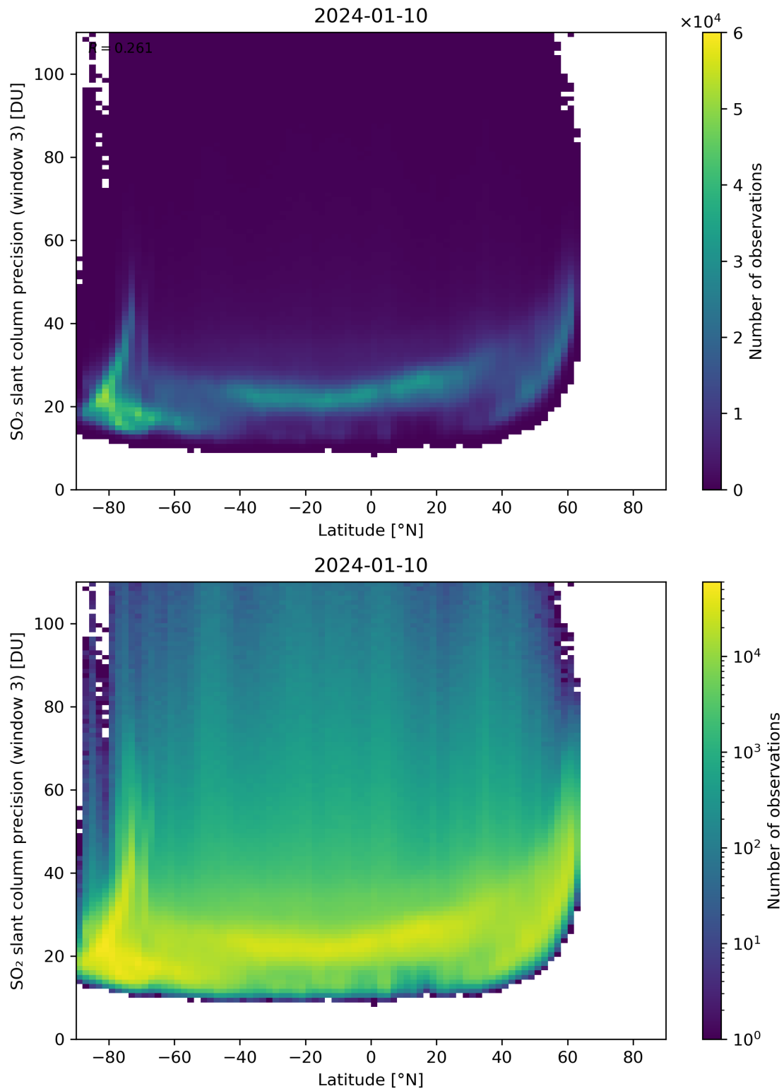
Figure 153: Scatter density plot of “Latitude” against “SO 2 slant column precision (window 3)” for 2024-01-10 to 2024-01-11.
