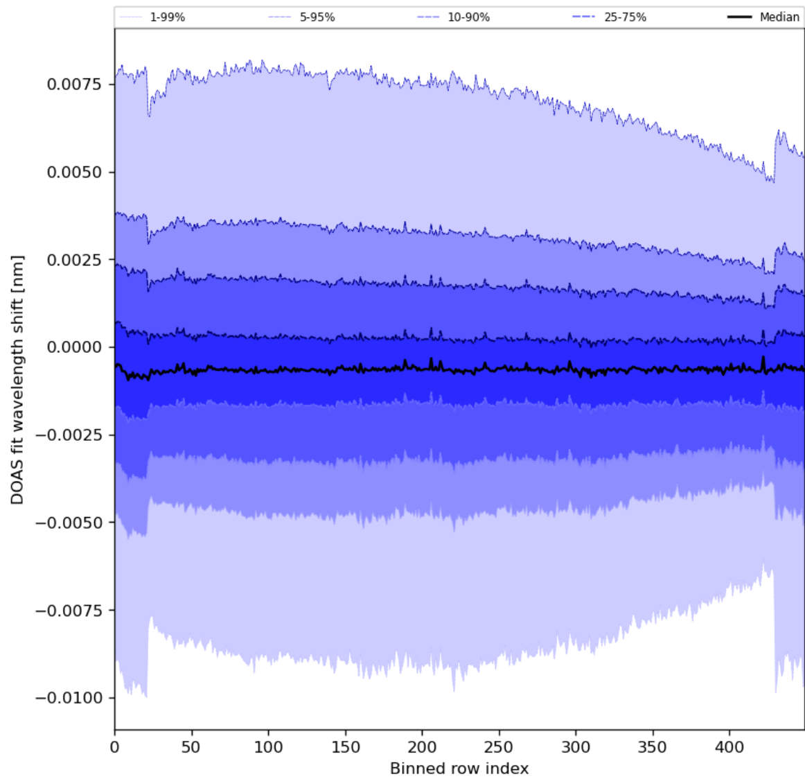
Figure 91: Along track statistics of “DOAS fit wavelength shift” for 2024-01-10 to 2024-01-11
