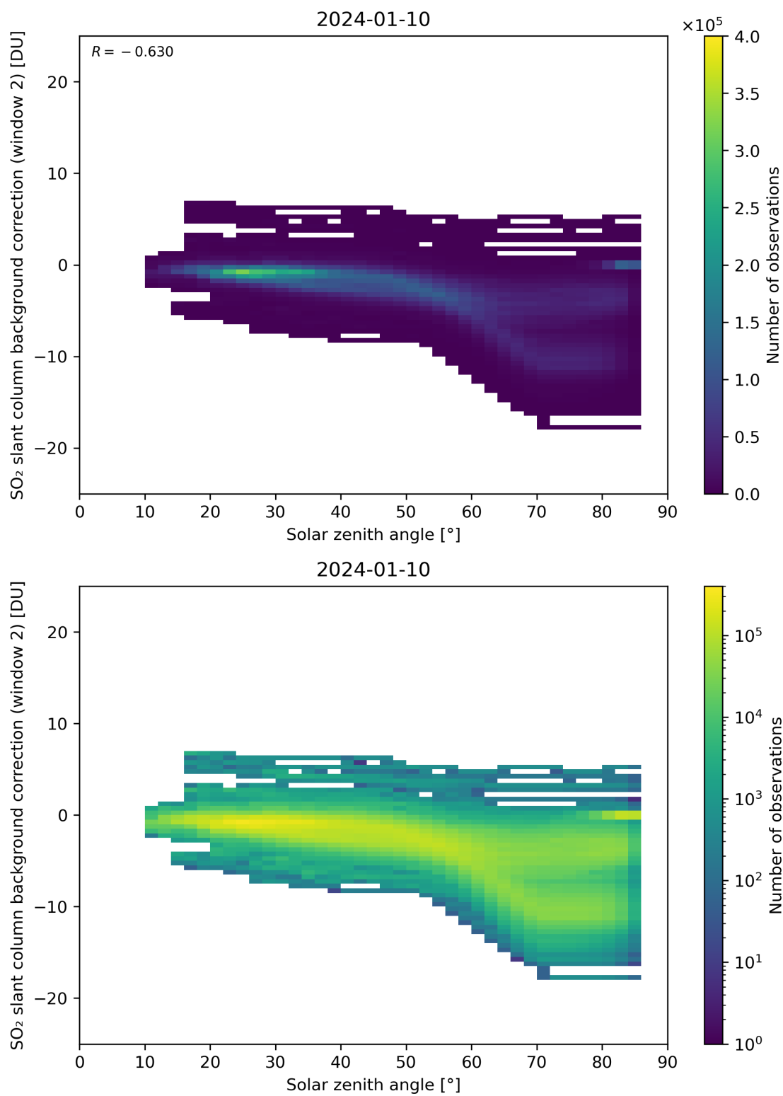
Figure 159: Scatter density plot of “Solar zenith angle” against “SO 2 slant column background correction (window 2)” for 2024-01-10 to 2024-01-11.
