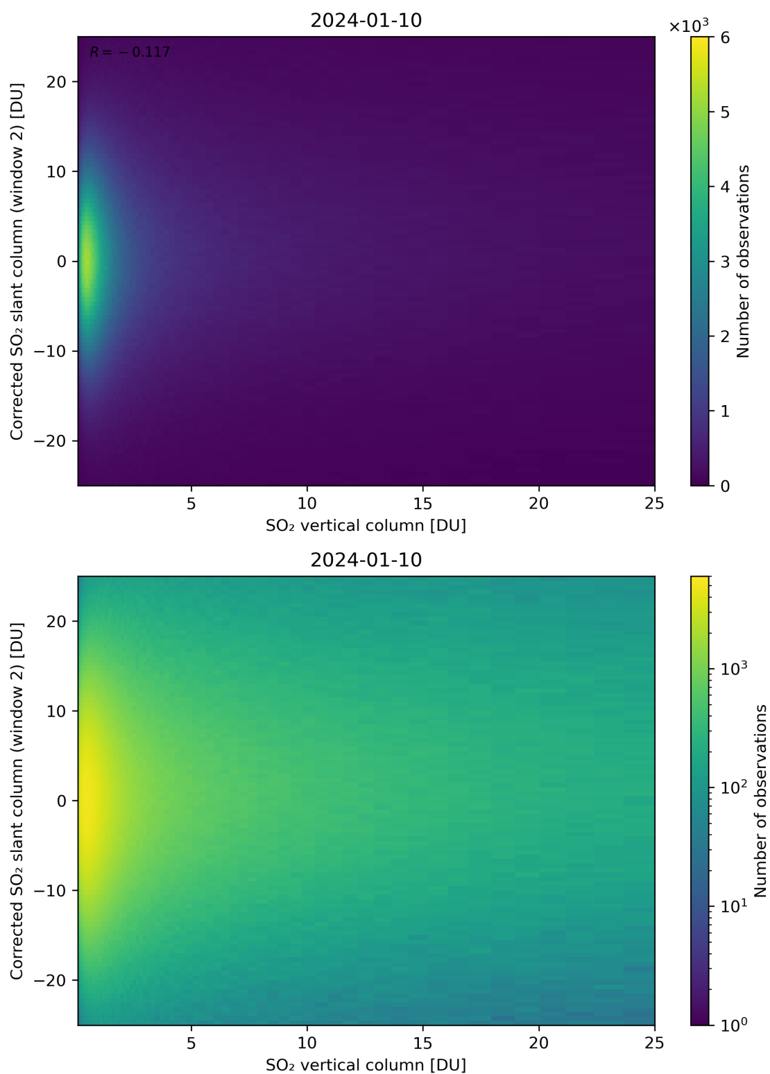
Figure 298: Scatter density plot of “SO 2 vertical column” against “Corrected SO 2 slant column (window 2)” for 2024-01-10 to 2024-01-11.
