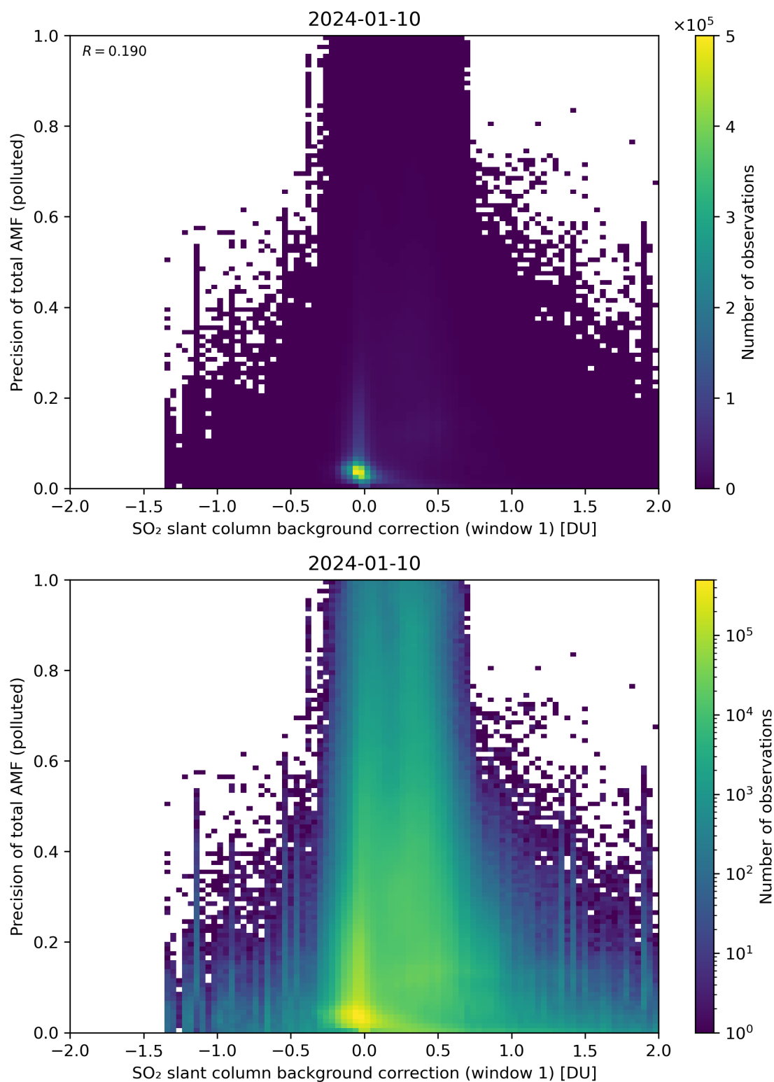
Figure 110: Scatter density plot of “SO 2 slant column background correction (window 1)” against “Precision of total AMF (polluted)” for 2024-01-10 to 2024-01-11.
