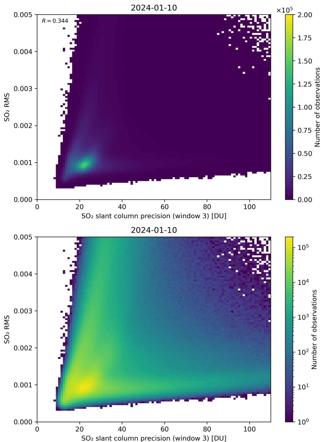
Figure 260: Scatter density plot of “SO 2 slant column precision (window 3)” against “SO 2 RMS” for 2024-01-10 to 2024-01-11.
