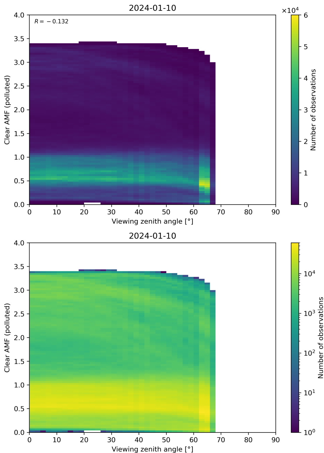
Figure 316: Scatter density plot of “Viewing zenith angle” against “Clear AMF (polluted)” for 2024-01-10 to 2024-01-11.
