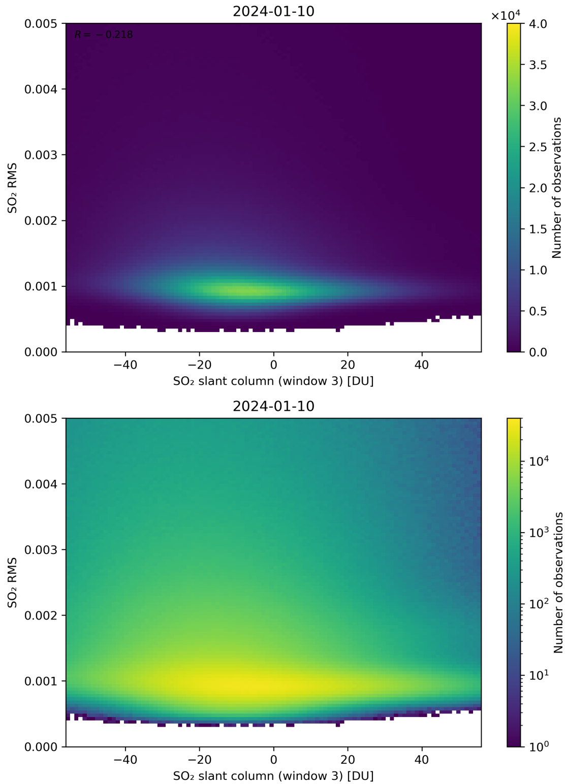
Figure 256: Scatter density plot of “SO 2 slant column (window 3)” against “SO 2 RMS” for 2024-01-10 to 2024-01-11.
