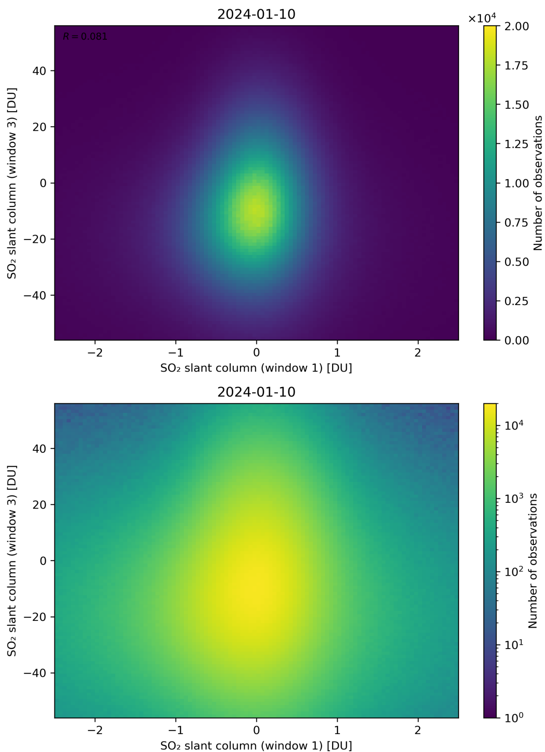
Figure 237: Scatter density plot of “SO 2 slant column (window 1)” against “SO 2 slant column (window 3)” for 2024-01-10 to 2024-01-11.
