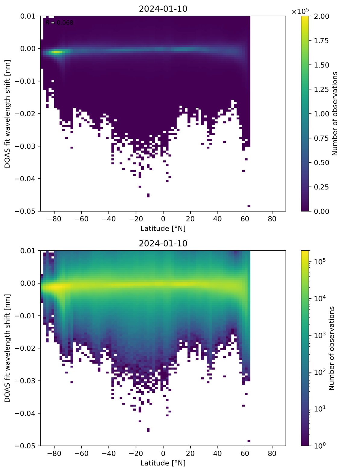
Figure 142: Scatter density plot of “Latitude” against “DOAS fit wavelength shift” for 2024-01-10 to 2024-01-11.
