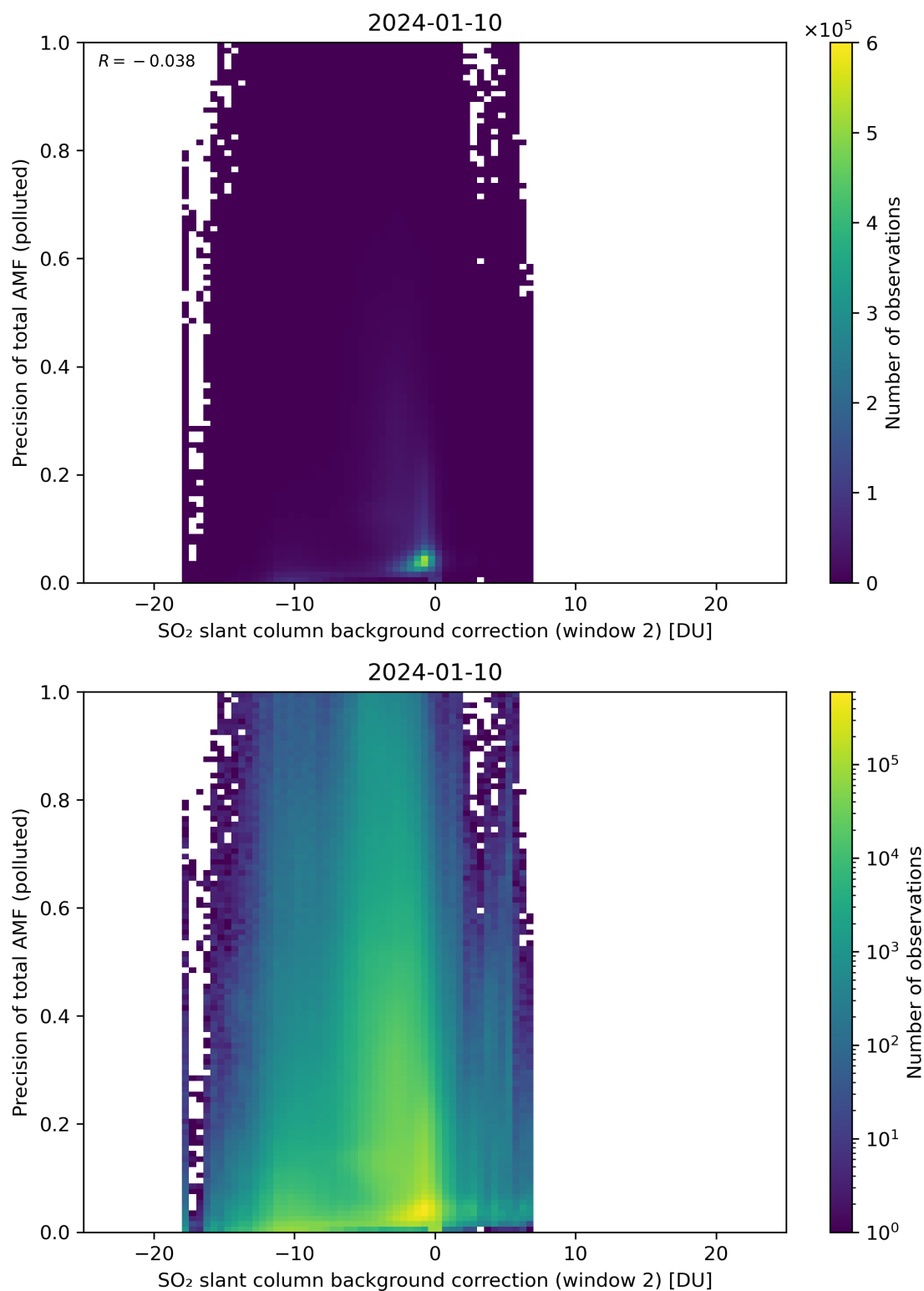
Figure 120: Scatter density plot of “SO 2 slant column background correction (window 2)” against “Precision of total AMF (polluted)” for 2024-01-10 to 2024-01-11.
