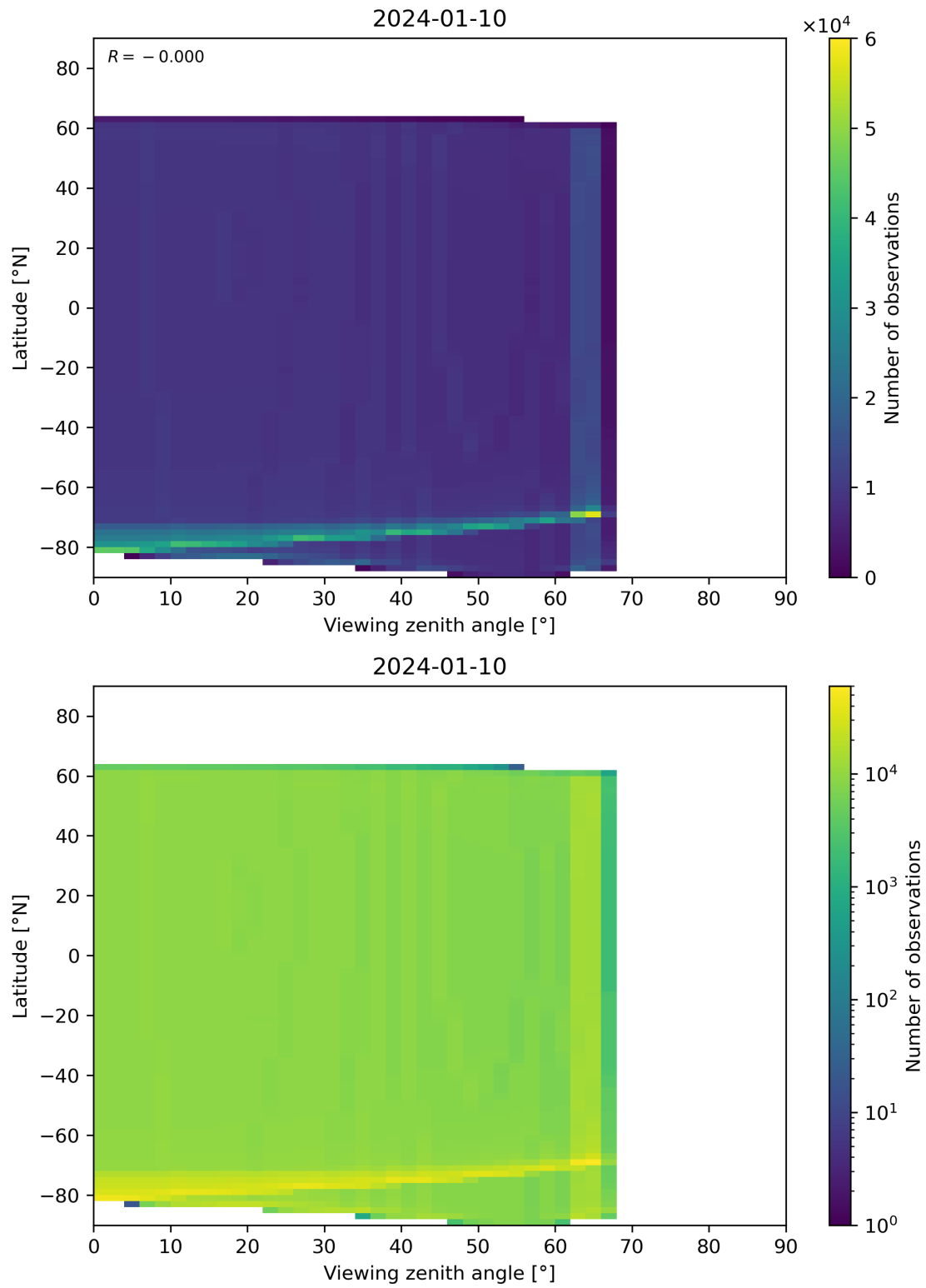
Figure 314: Scatter density plot of “Viewing zenith angle” against “Latitude” for 2024-01-10 to 2024-01-11.
