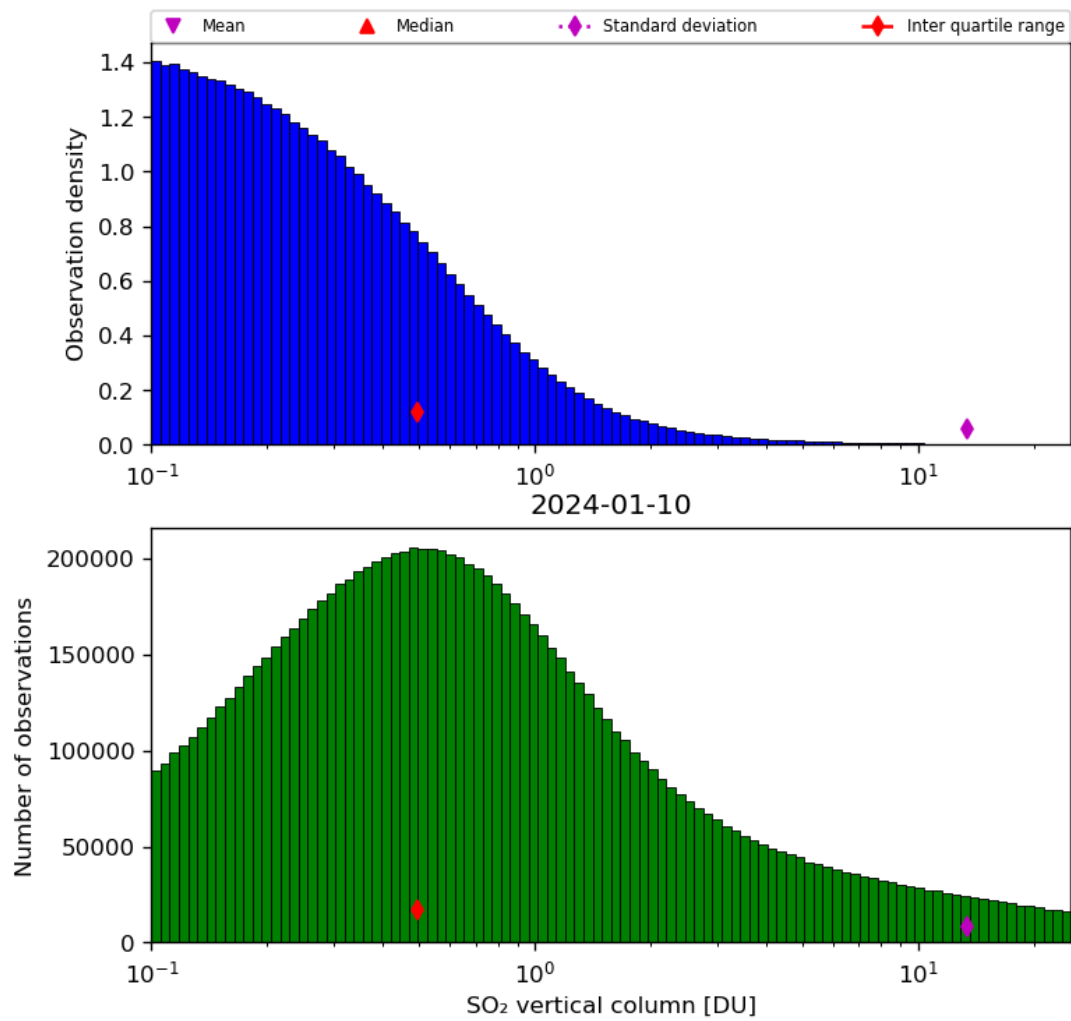
Figure 53: Histogram of “SO 2 vertical column” for 2024-01-10 to 2024-01-11
