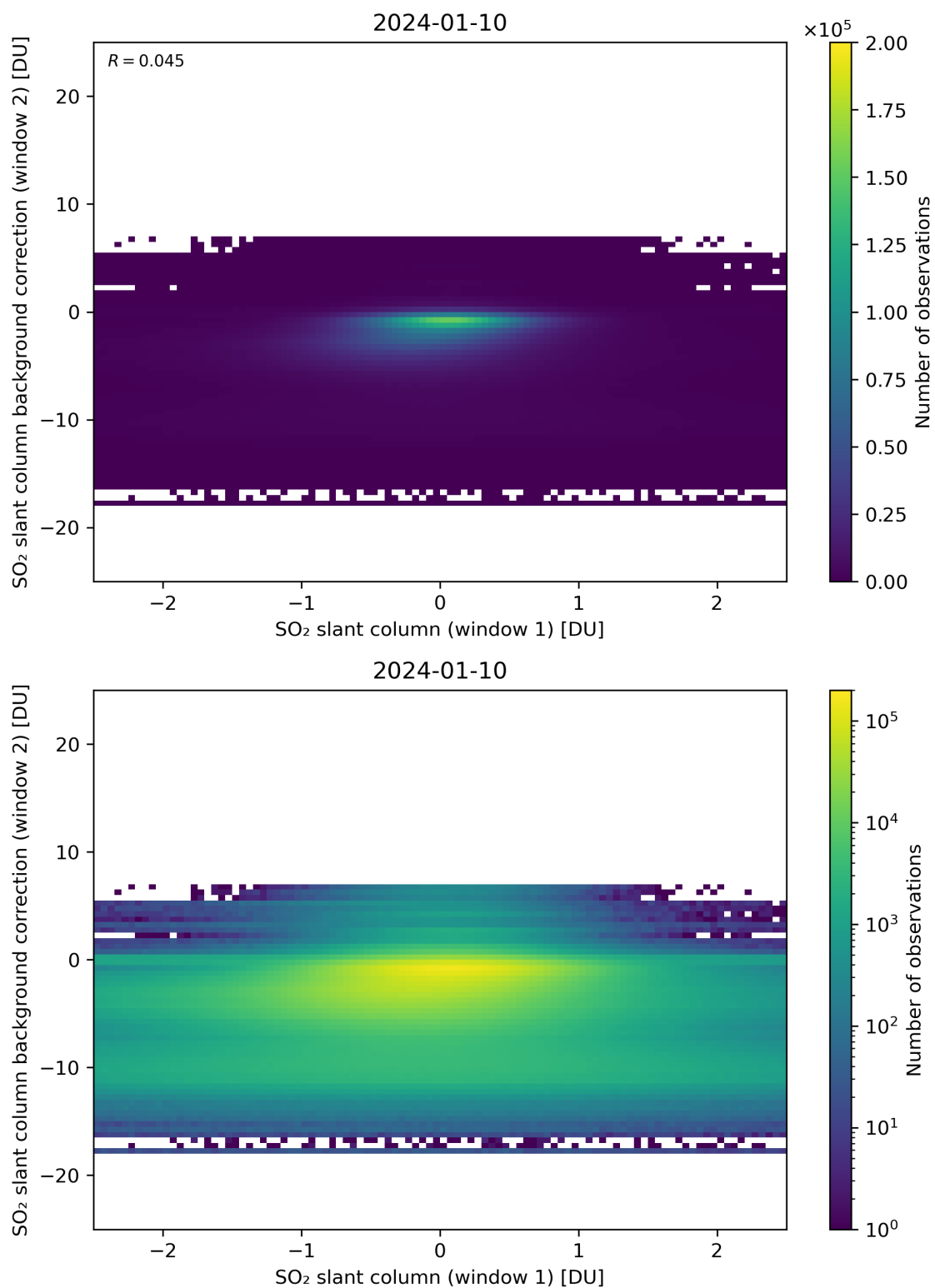
Figure 213: Scatter density plot of “SO 2 slant column (window 1)” against “SO 2 slant column background correction (window 2)” for 2024-01-10 to 2024-01-11.
