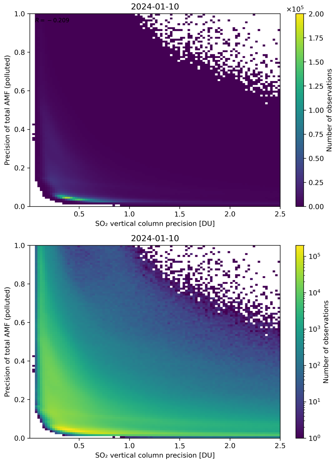
Figure 295: Scatter density plot of “SO 2 vertical column precision” against “Precision of total AMF (polluted)” for 2024-01-10 to 2024-01-11.
