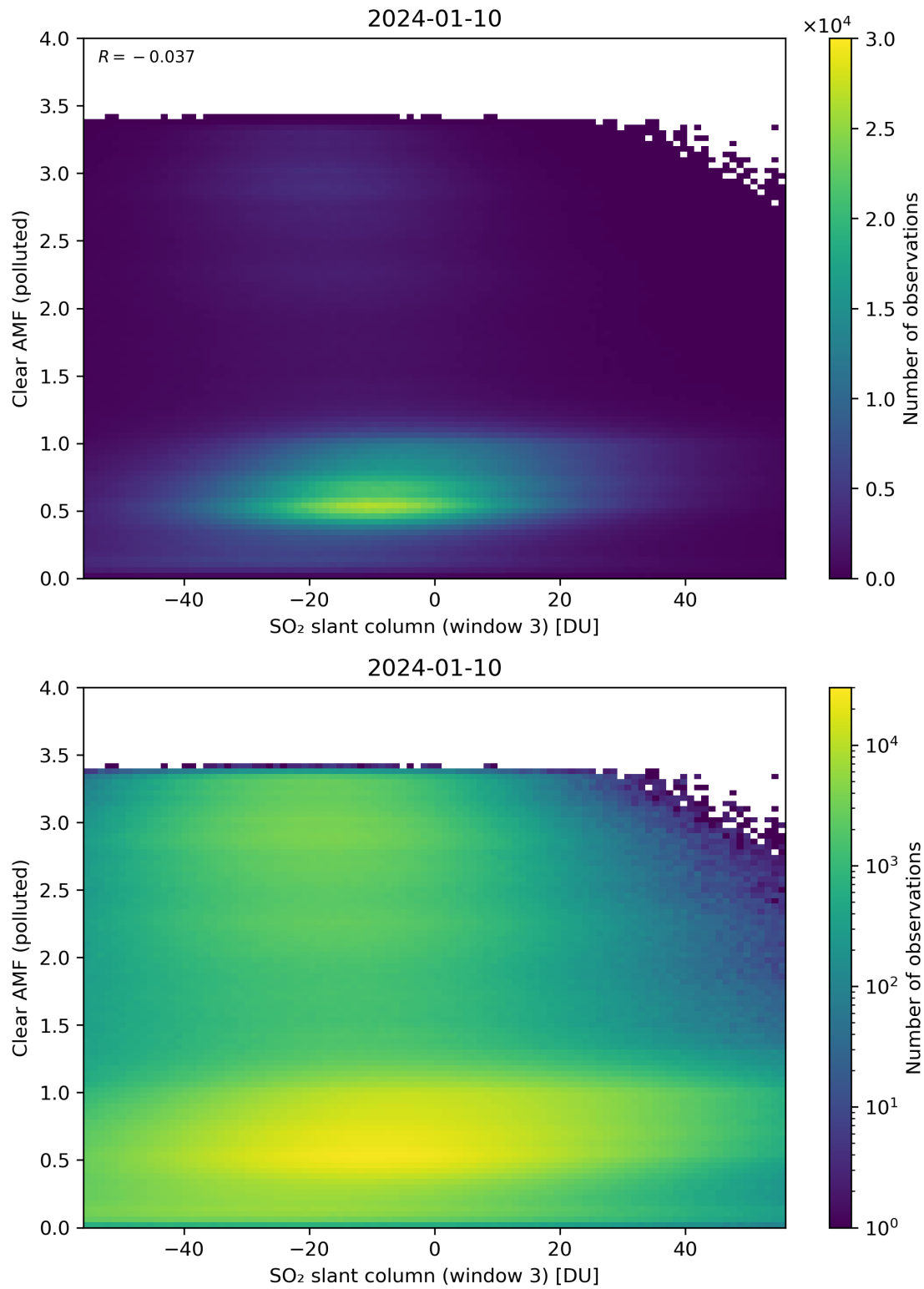
Figure 265: Scatter density plot of “SO 2 slant column (window 3)” against “Clear AMF (polluted)” for 2024-01-10 to 2024-01-11.
