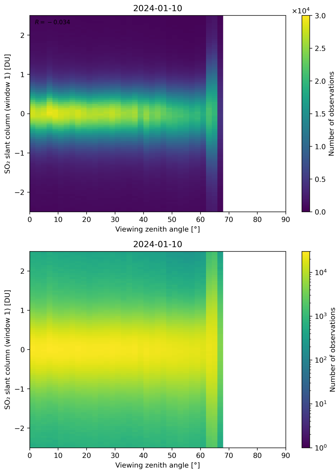
Figure 320: Scatter density plot of “Viewing zenith angle” against “SO 2 slant column (window 1)” for 2024-01-10 to 2024-01-11.
