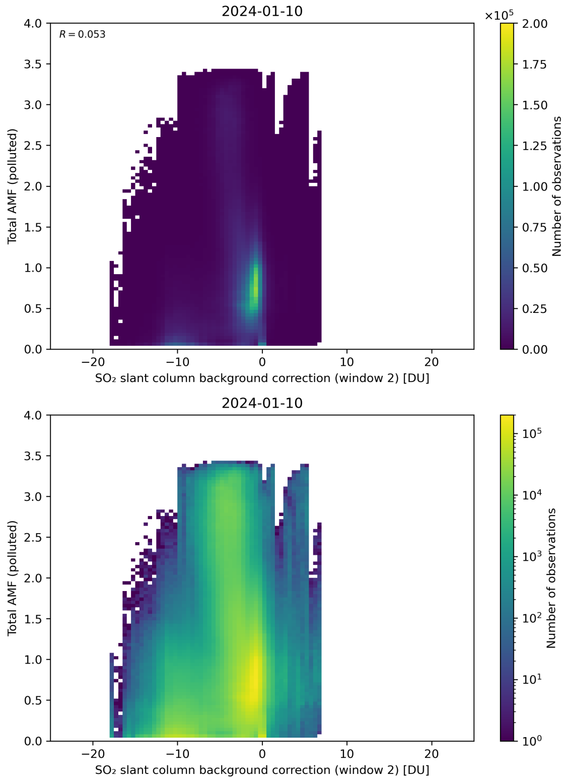
Figure 119: Scatter density plot of “SO 2 slant column background correction (window 2)” against “Total AMF (polluted)” for 2024-01-10 to 2024-01-11.
