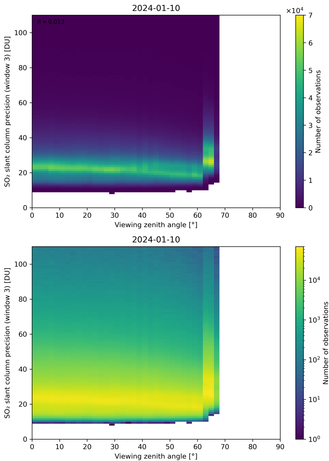
Figure 324: Scatter density plot of “Viewing zenith angle” against “SO 2 slant column precision (window 3)” for 2024-01-10 to 2024-01-11.
