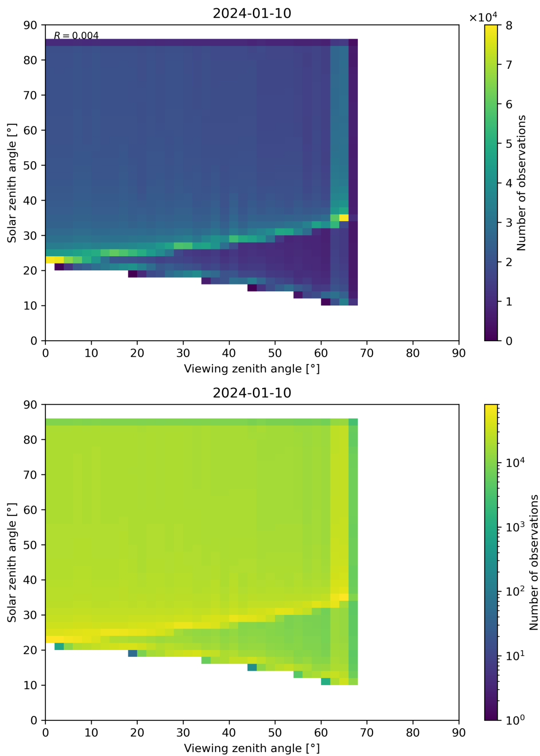
Figure 315: Scatter density plot of “Viewing zenith angle” against “Solar zenith angle” for 2024-01-10 to 2024-01-11.
