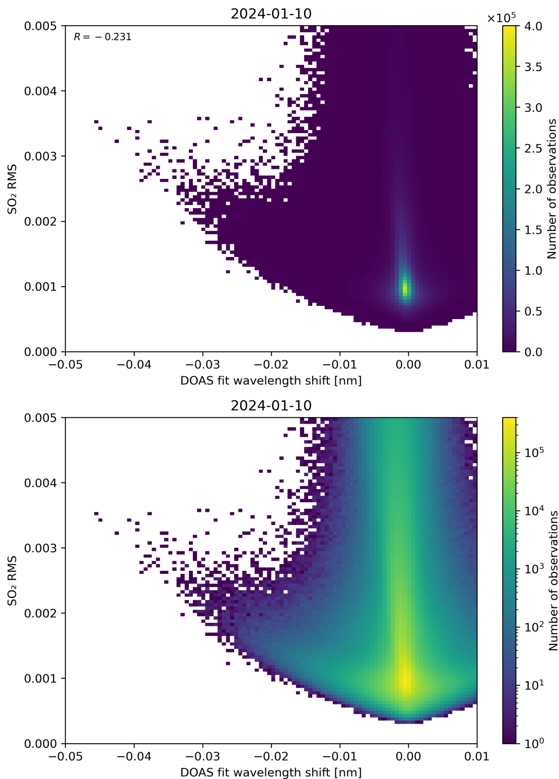
Figure 128: Scatter density plot of “DOAS fit wavelength shift” against “SO 2 RMS” for 2024-01-10 to 2024-01-11.
