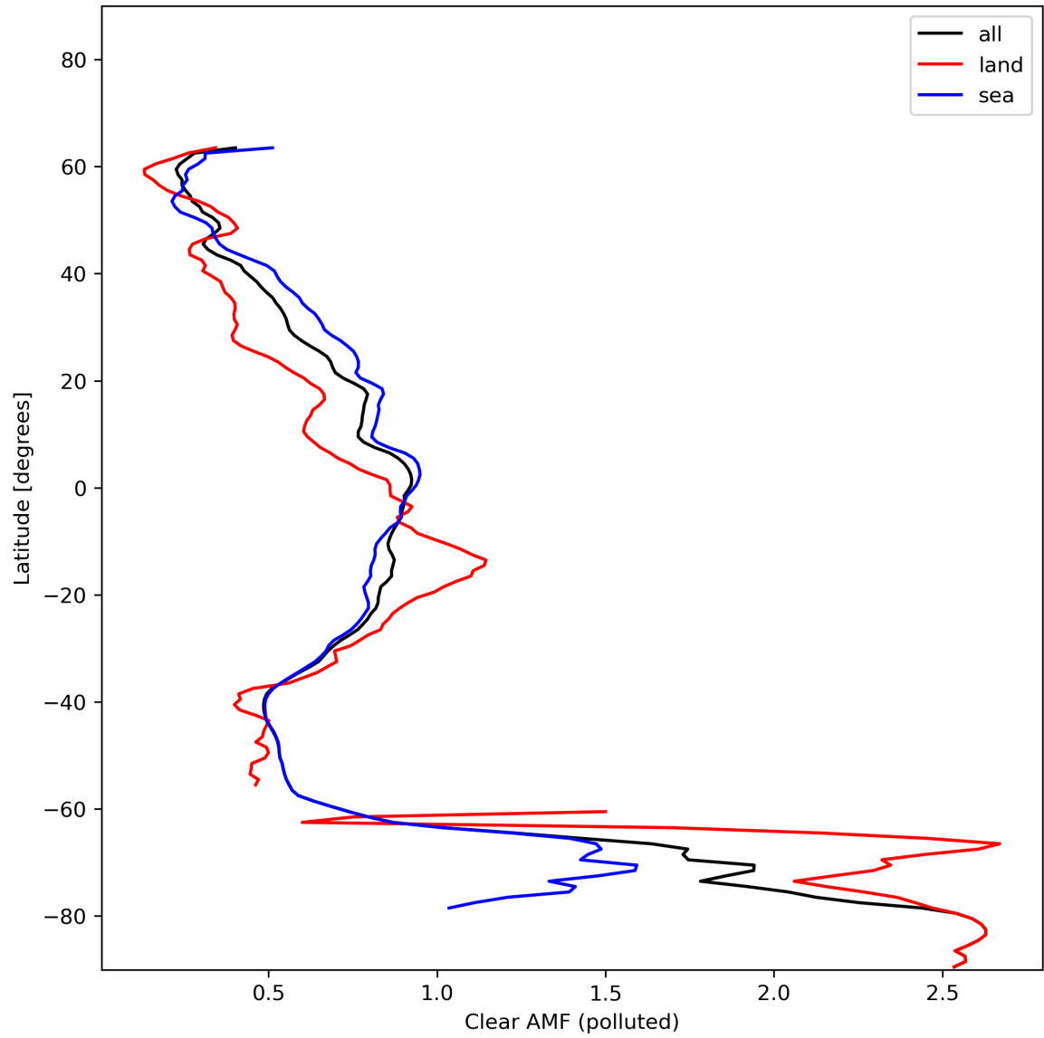
Figure 50: Zonal average of “Clear AMF (polluted)” for 2024-01-10 to 2024-01-11.
