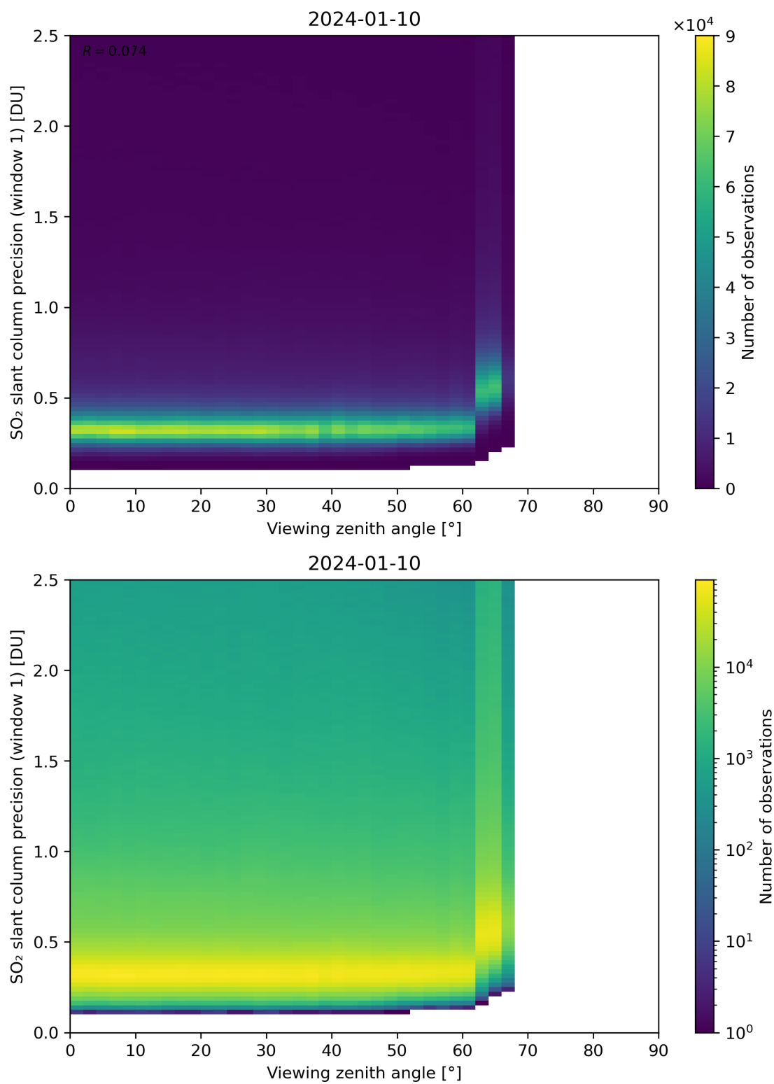
Figure 321: Scatter density plot of “Viewing zenith angle” against “SO 2 slant column precision (window 1)” for 2024-01-10 to 2024-01-11.
