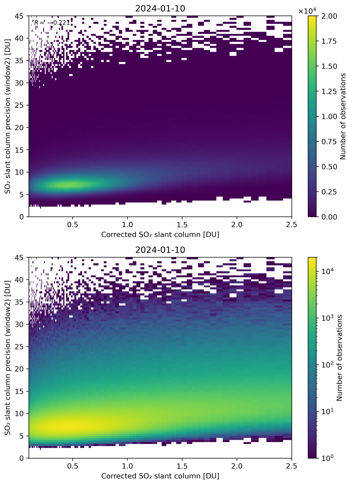
Figure 189: Scatter density plot of “Corrected SO 2 slant column” against “SO 2 slant column precision (window2)” for 2024-01-10 to 2024-01-11.
