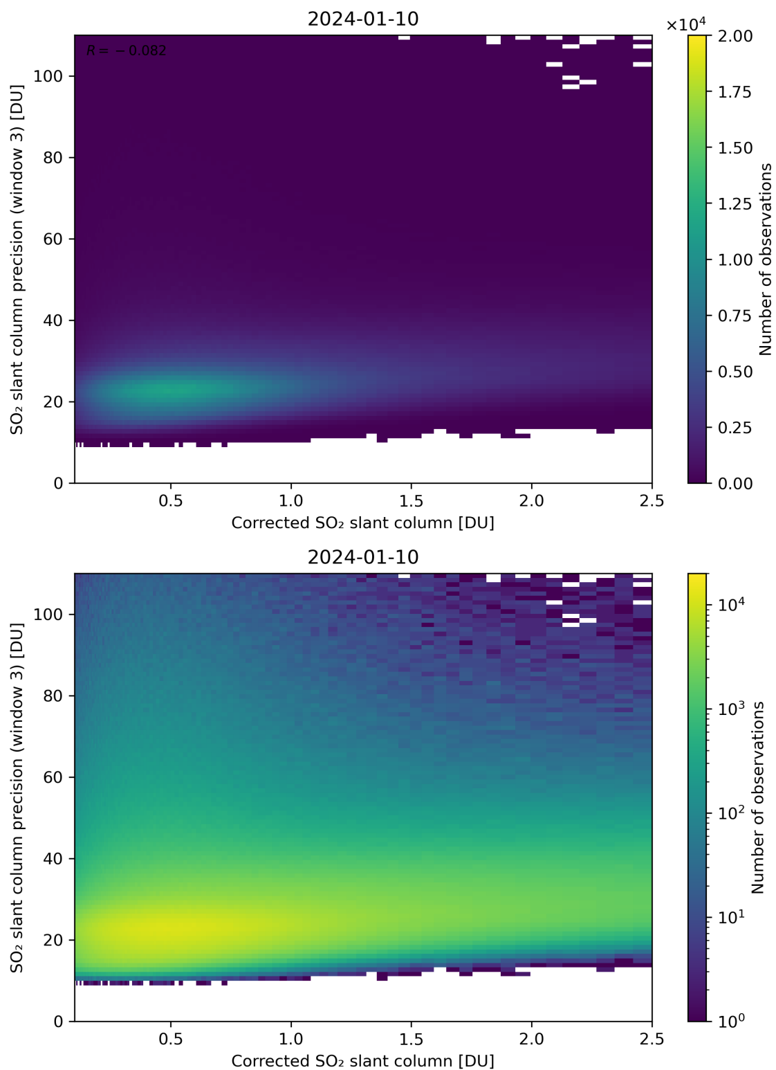
Figure 191: Scatter density plot of “Corrected SO 2 slant column” against “SO 2 slant column precision (window 3)” for 2024-01-10 to 2024-01-11.
