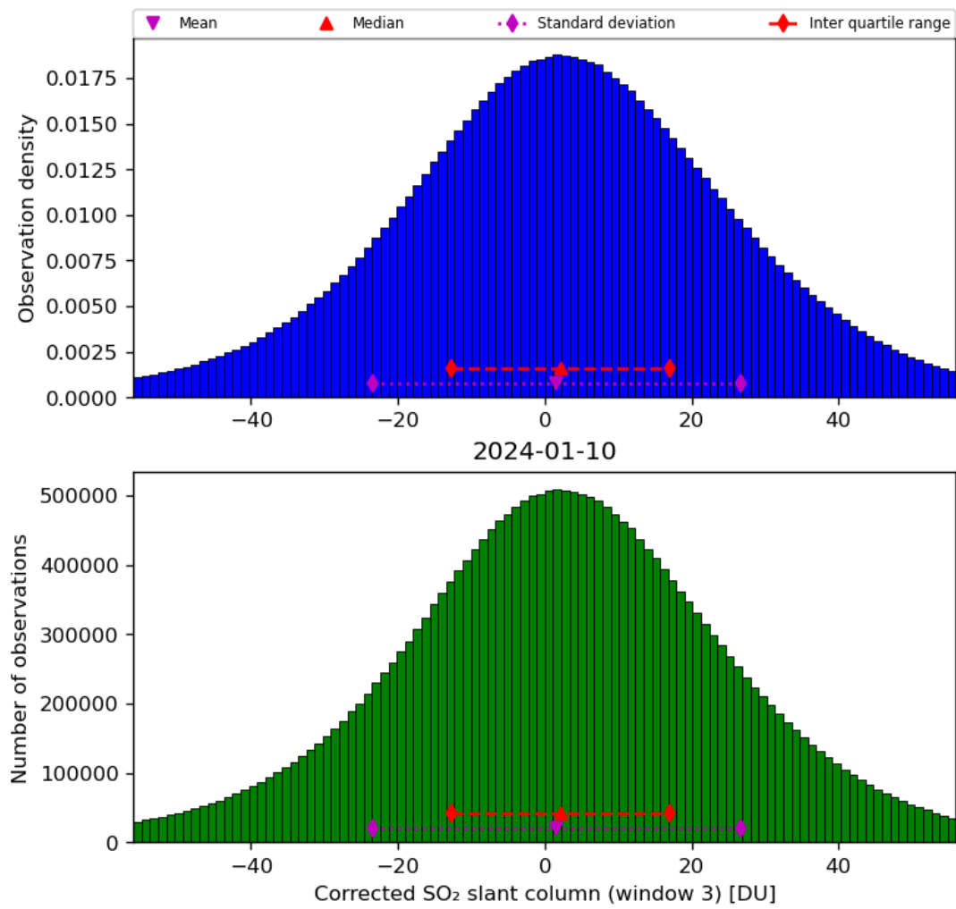
Figure 66: Histogram of “Corrected SO 2 slant column (window 3)” for 2024-01-10 to 2024-01-11
