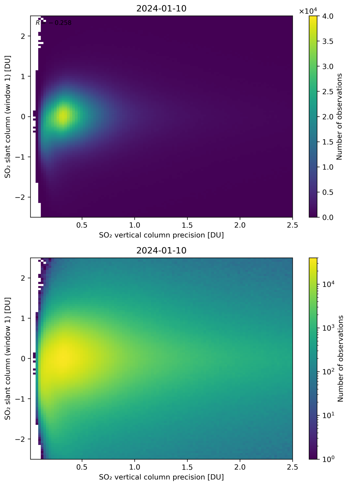
Figure 289: Scatter density plot of “SO 2 vertical column precision” against “SO 2 slant column (window 1)” for 2024-01-10 to 2024-01-11.
