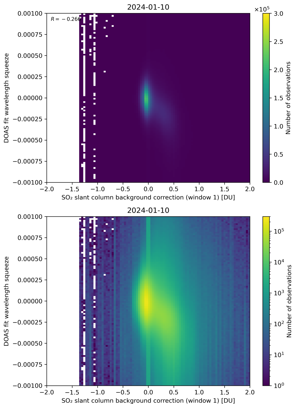
Figure 101: Scatter density plot of “SO 2 slant column background correction (window 1)” against “DOAS fit wavelength squeeze” for 2024-01-10 to 2024-01-11.
