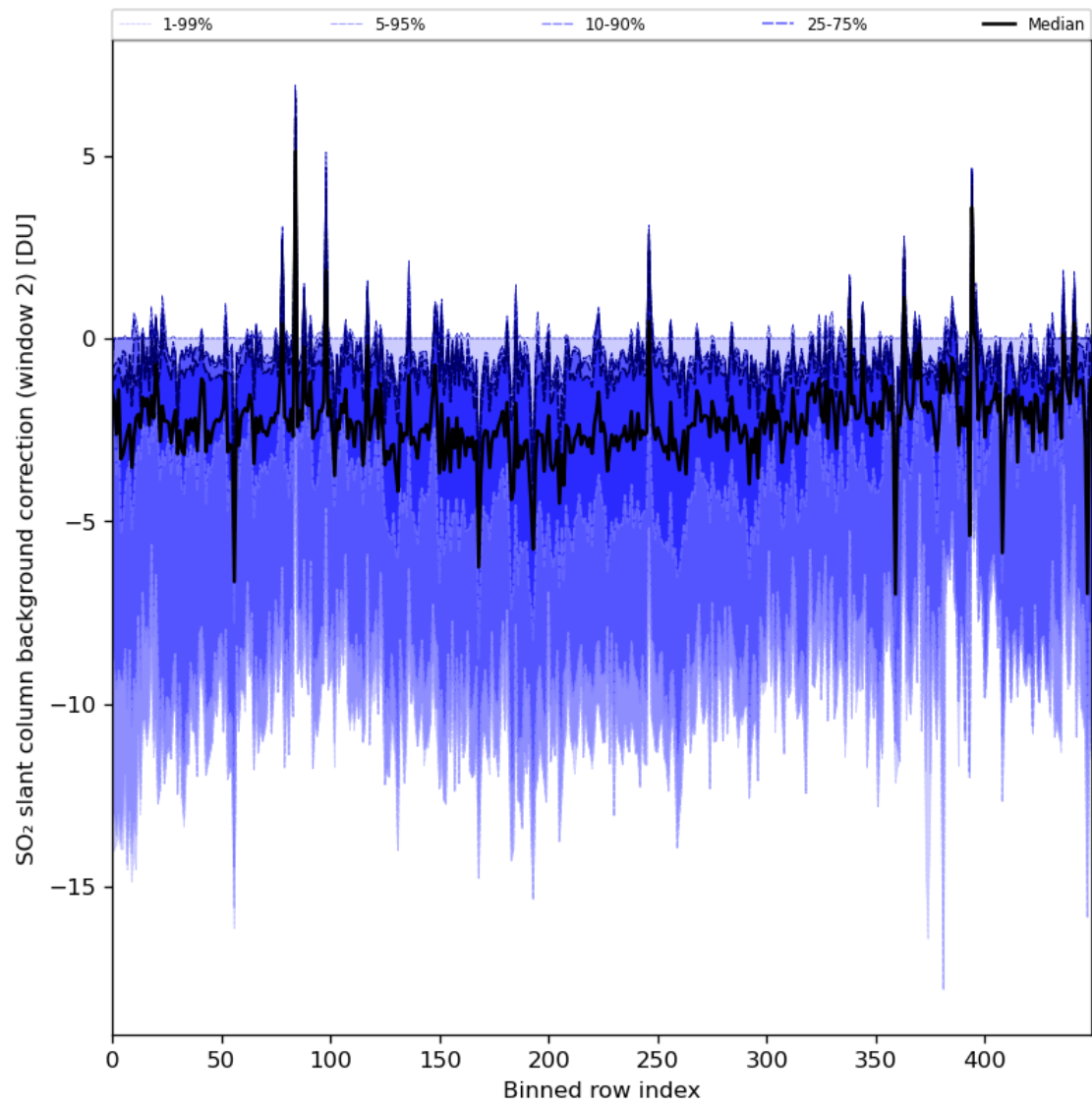
Figure 86: Along track statistics of “SO 2 slant column background correction (window 2)” for 2024-01-10 to 2024-01-11
