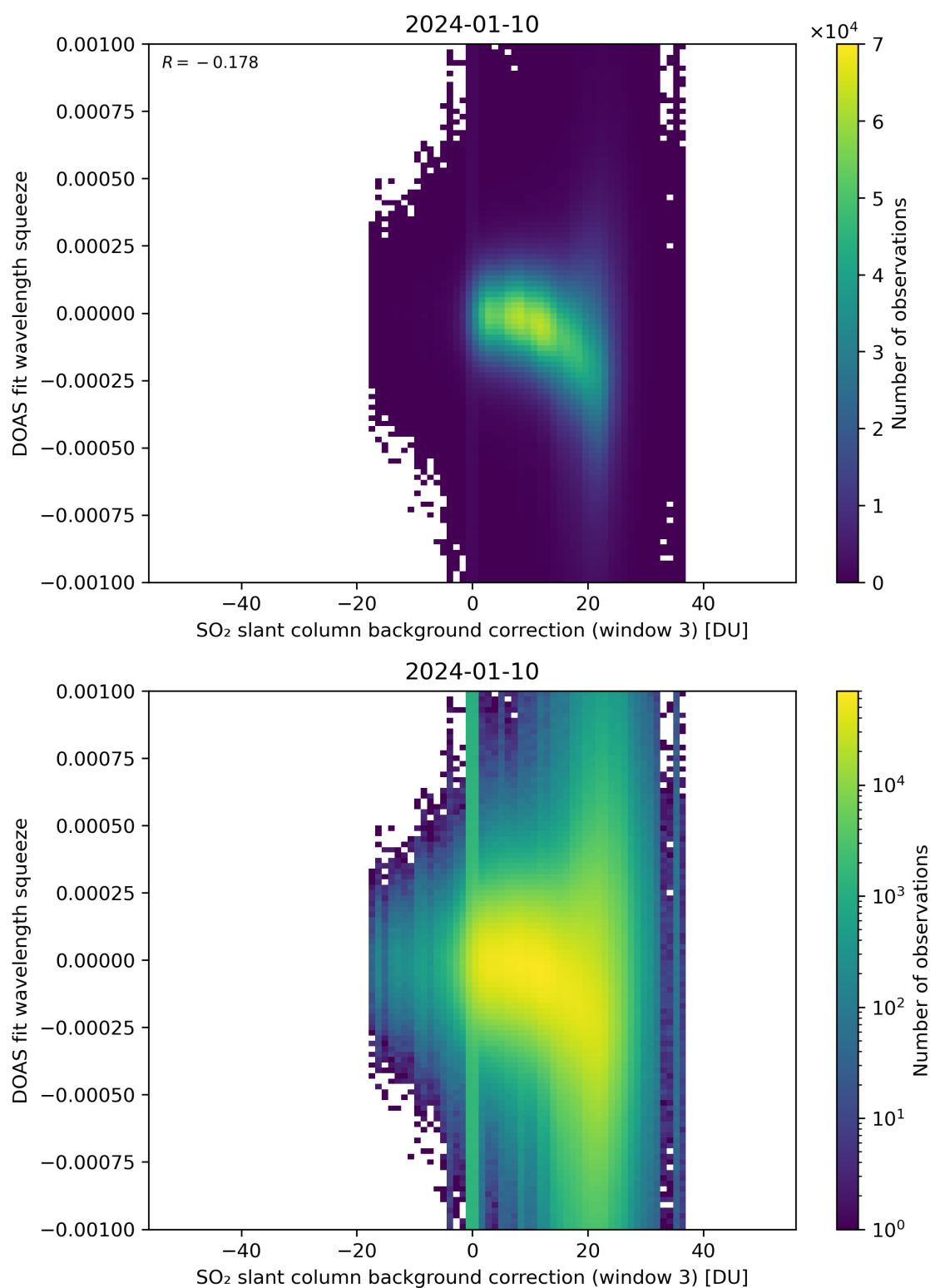
Figure 122: Scatter density plot of “SO 2 slant column background correction (window 3)” against “DOAS fit wavelength squeeze” for 2024-01-10 to 2024-01-11.
