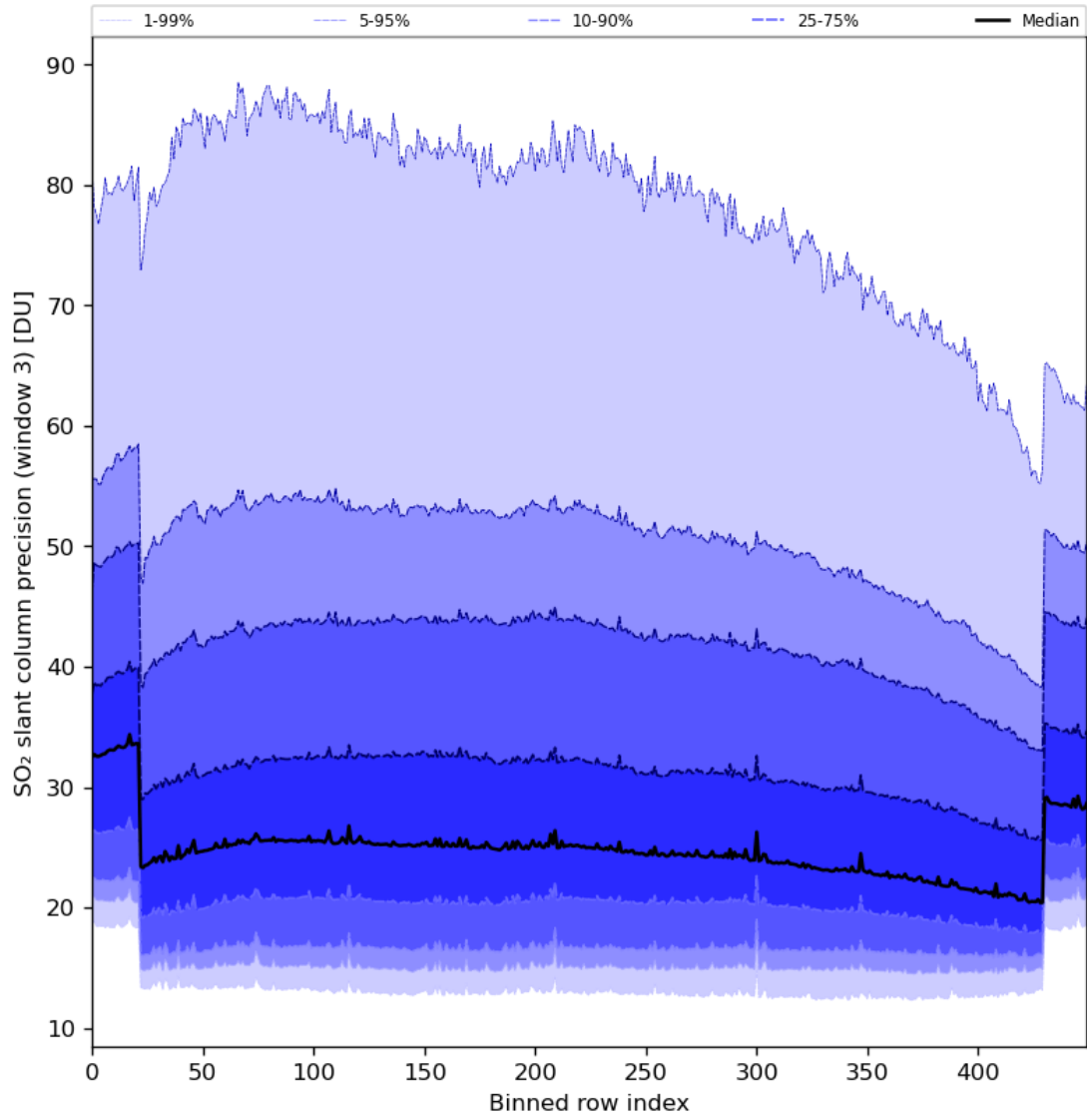
Figure 88: Along track statistics of “SO 2 slant column precision (window 3)” for 2024-01-10 to 2024-01-11
