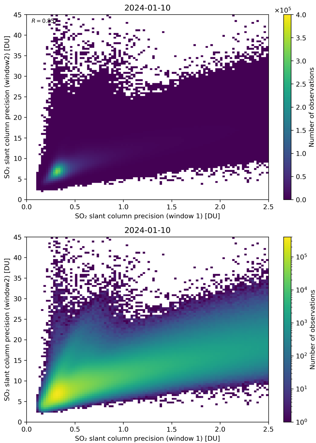
Figure 227: Scatter density plot of “SO 2 slant column precision (window 1)” against “SO 2 slant column precision (window2)” for 2024-01-10 to 2024-01-11.
