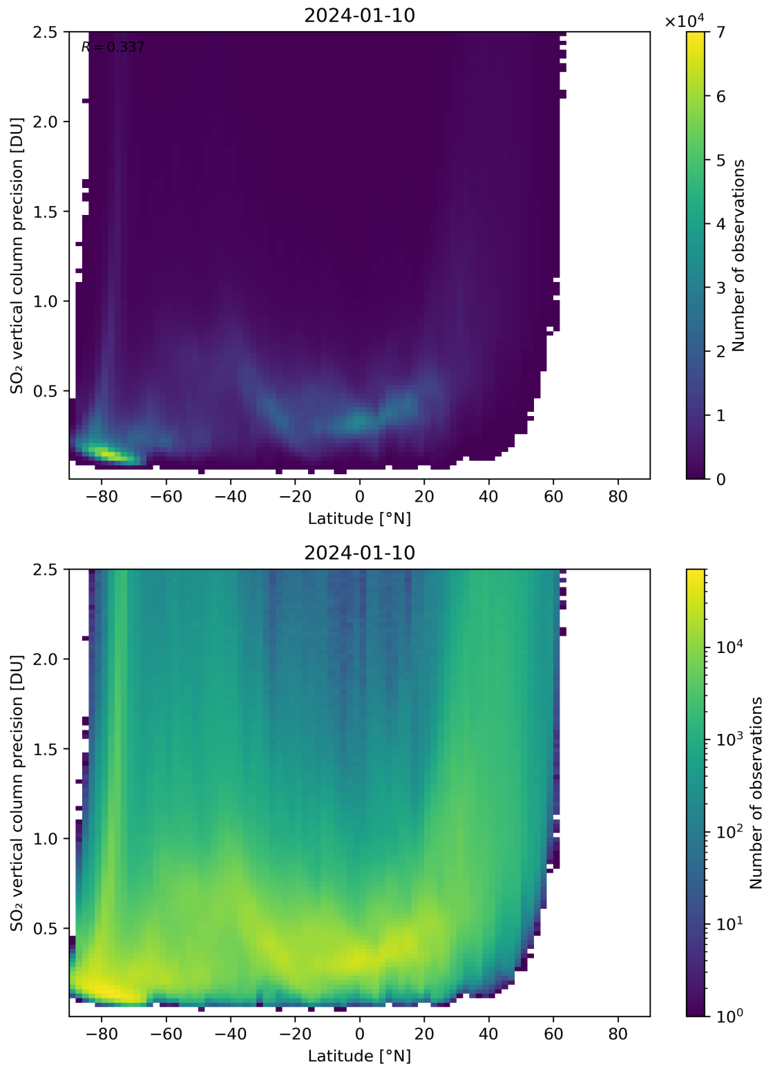
Figure 157: Scatter density plot of “Latitude” against “SO 2 vertical column precision” for 2024-01-10 to 2024-01-11.
