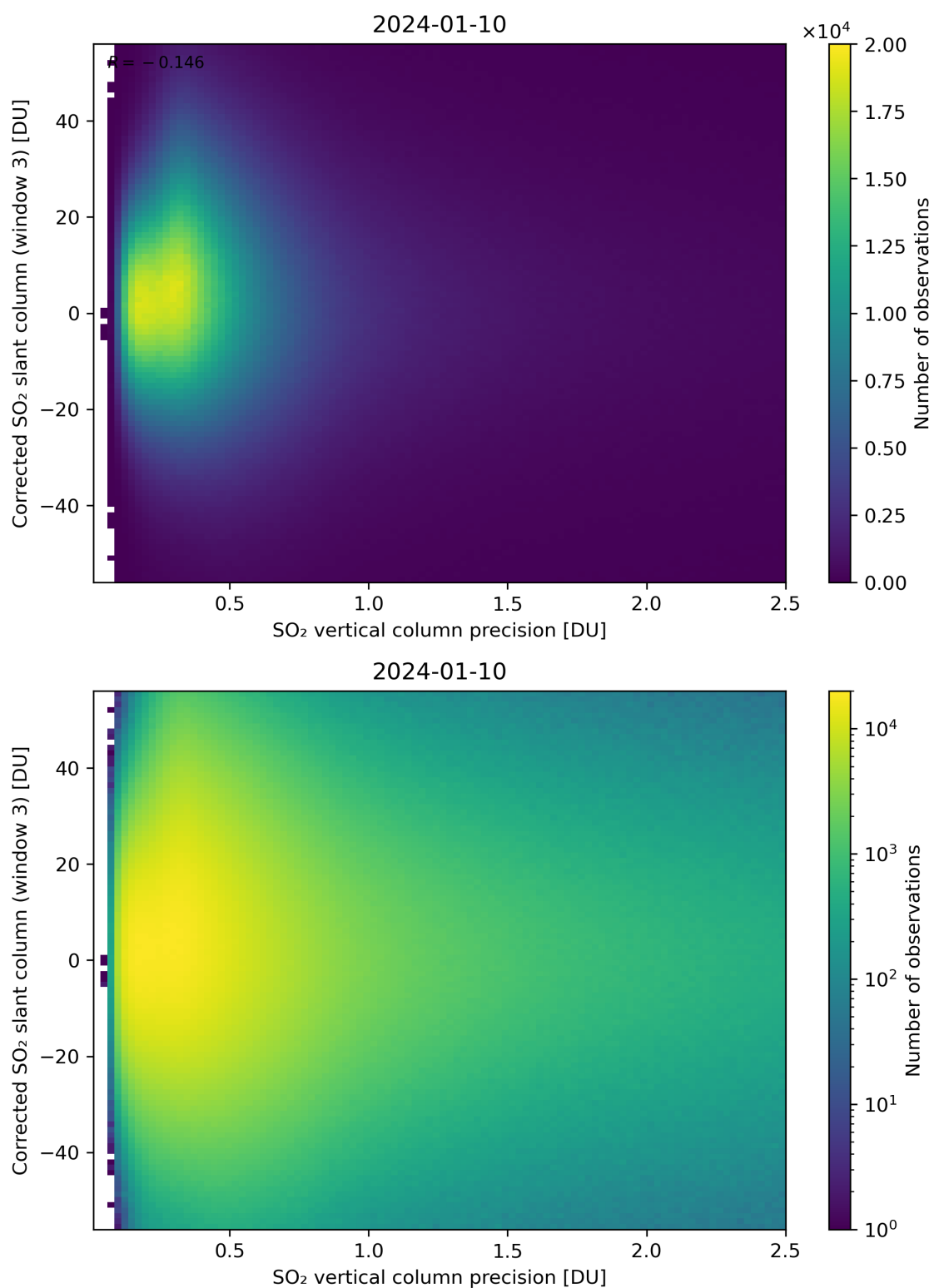
Figure 288: Scatter density plot of “SO 2 vertical column precision” against “Corrected SO 2 slant column (window 3)” for 2024-01-10 to 2024-01-11.
