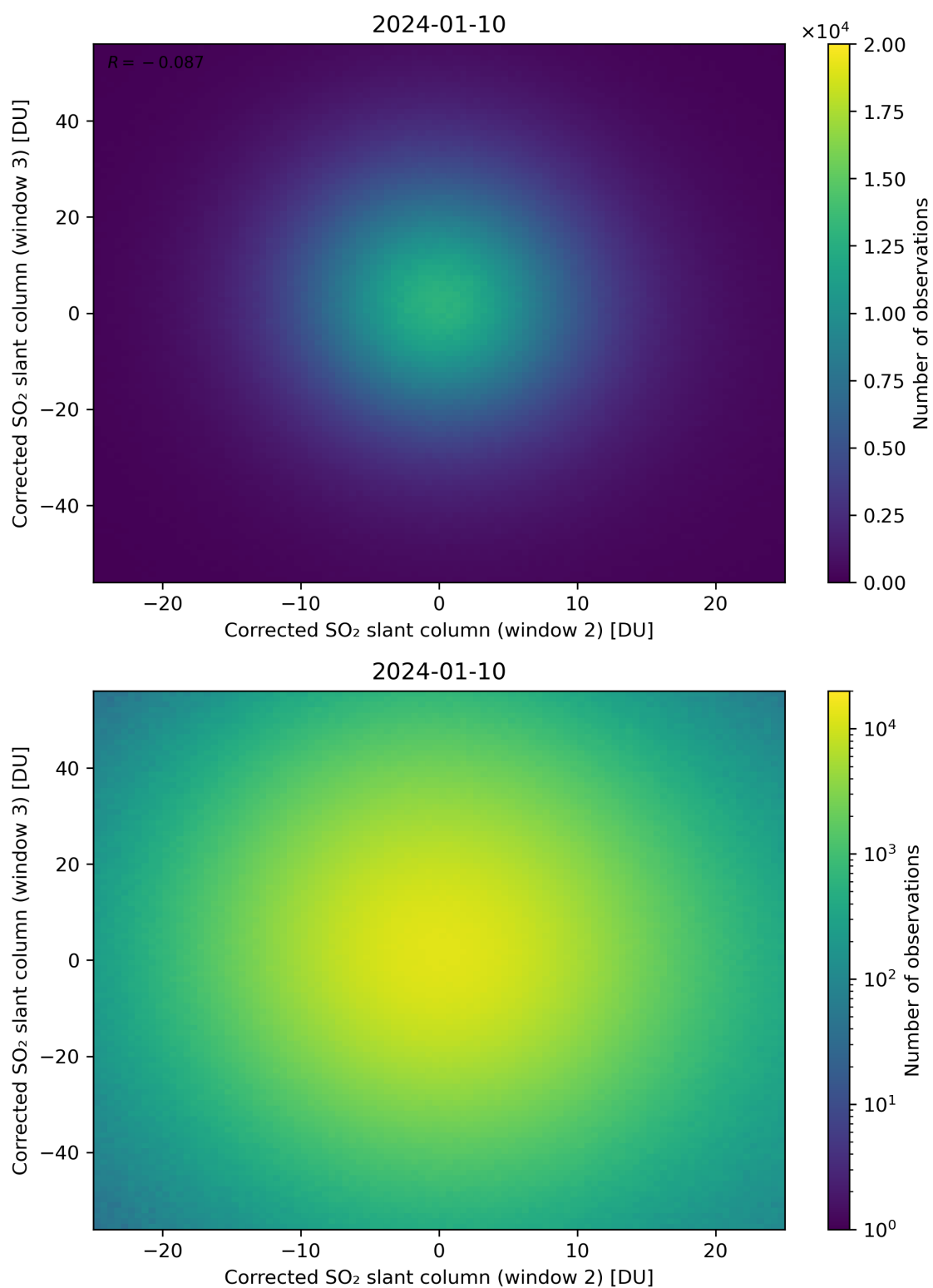
Figure 200: Scatter density plot of “Corrected SO 2 slant column (window 2)” against “Corrected SO 2 slant column (window 3)” for 2024-01-10 to 2024-01-11.
