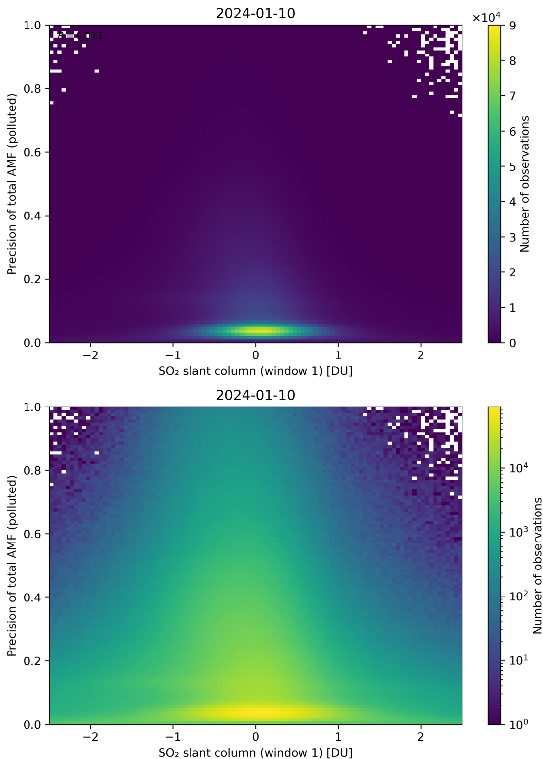
Figure 240: Scatter density plot of “SO 2 slant column (window 1)” against “Precision of total AMF (polluted)” for 2024-01-10 to 2024-01-11.
