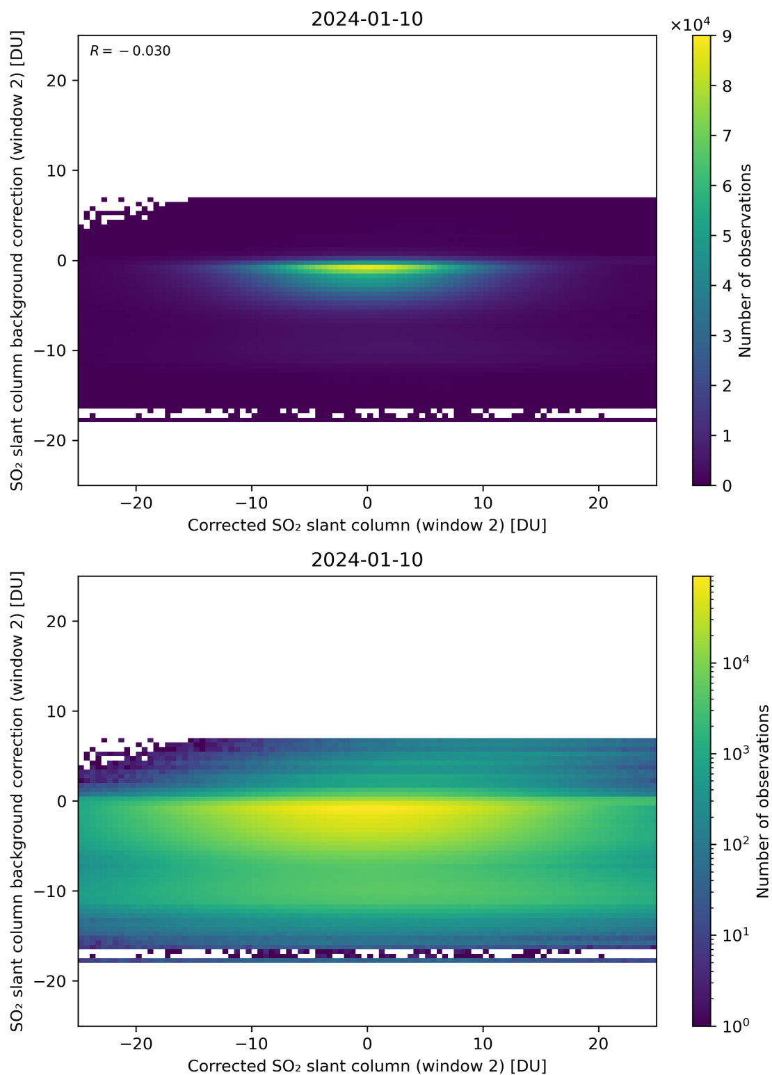
Figure 194: Scatter density plot of “Corrected SO 2 slant column (window 2)” against “SO 2 slant column background correction (window 2)” for 2024-01-10 to 2024-01-11.
