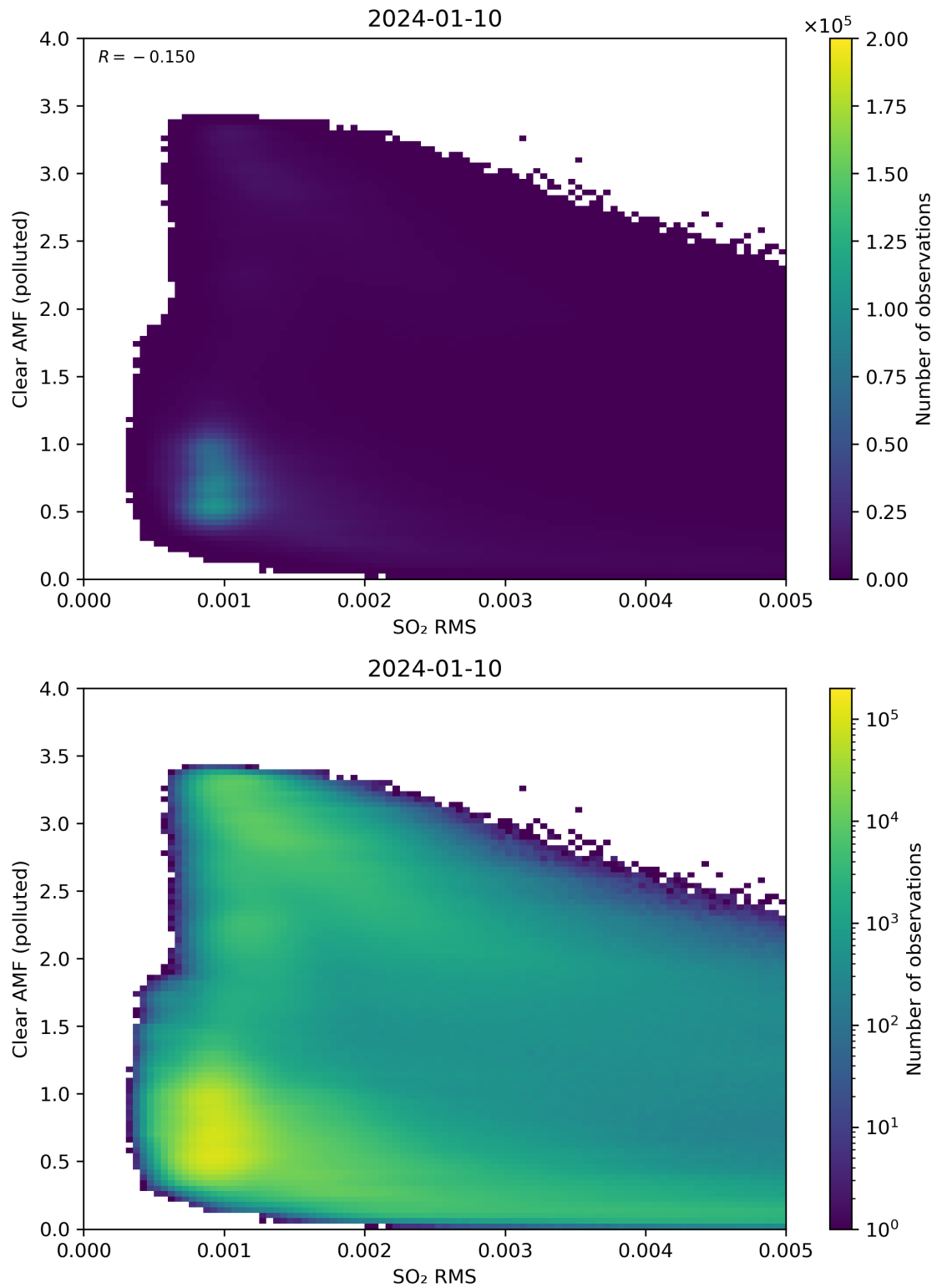
Figure 136: Scatter density plot of “SO 2 RMS” against “Clear AMF (polluted)” for 2024-01-10 to 2024-01-11.
