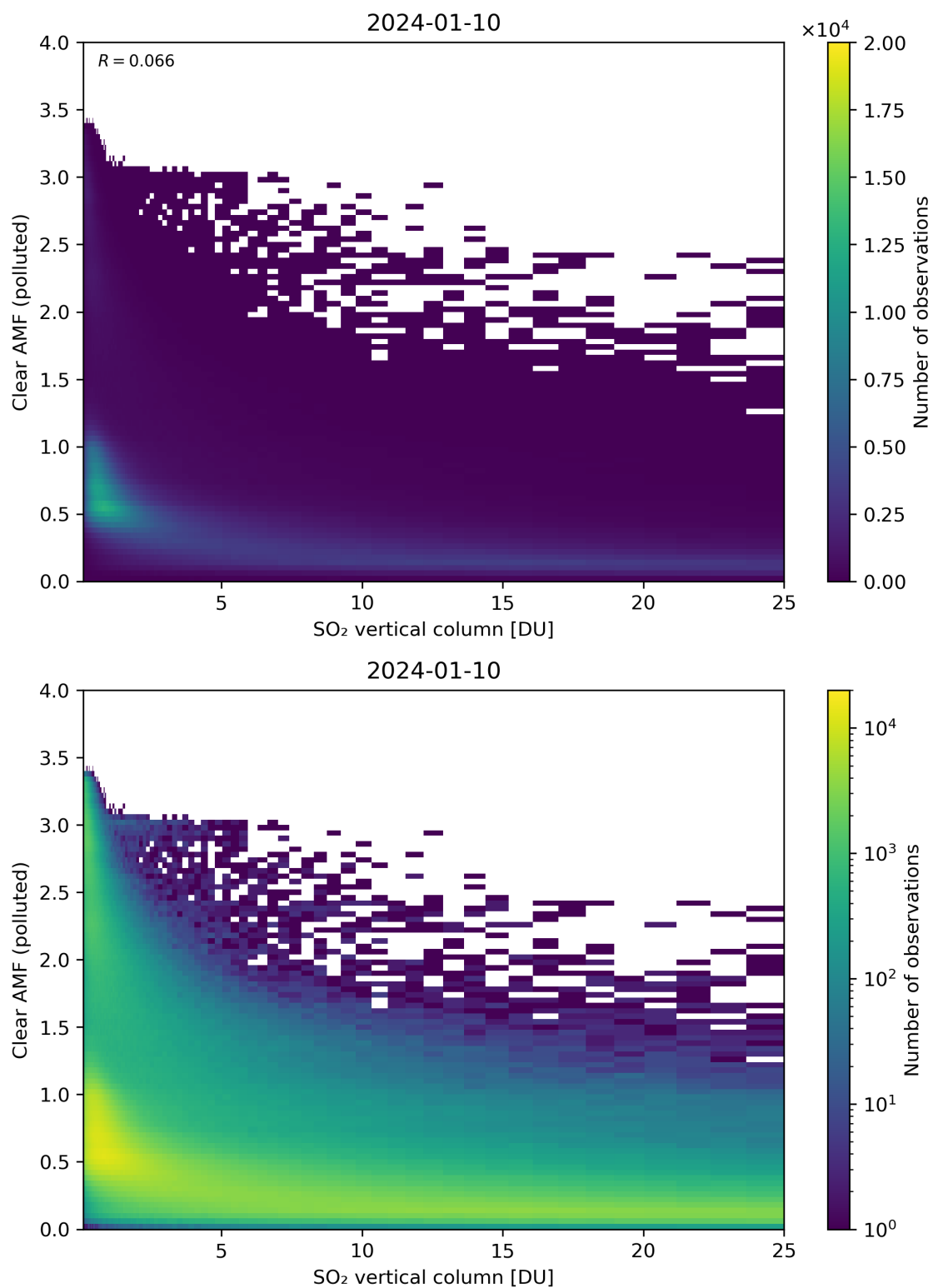
Figure 296: Scatter density plot of “SO 2 vertical column” against “Clear AMF (polluted)” for 2024-01-10 to 2024-01-11.
