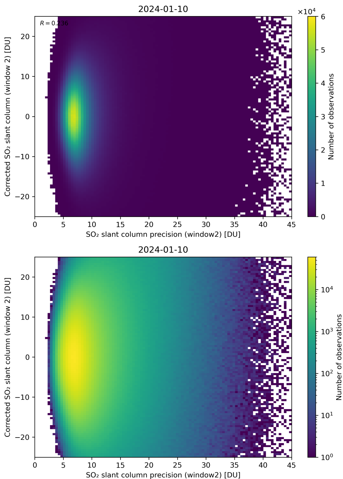
Figure 247: Scatter density plot of “SO 2 slant column precision (window2)” against “Corrected SO 2 slant column (window 2)” for 2024-01-10 to 2024-01-11.
