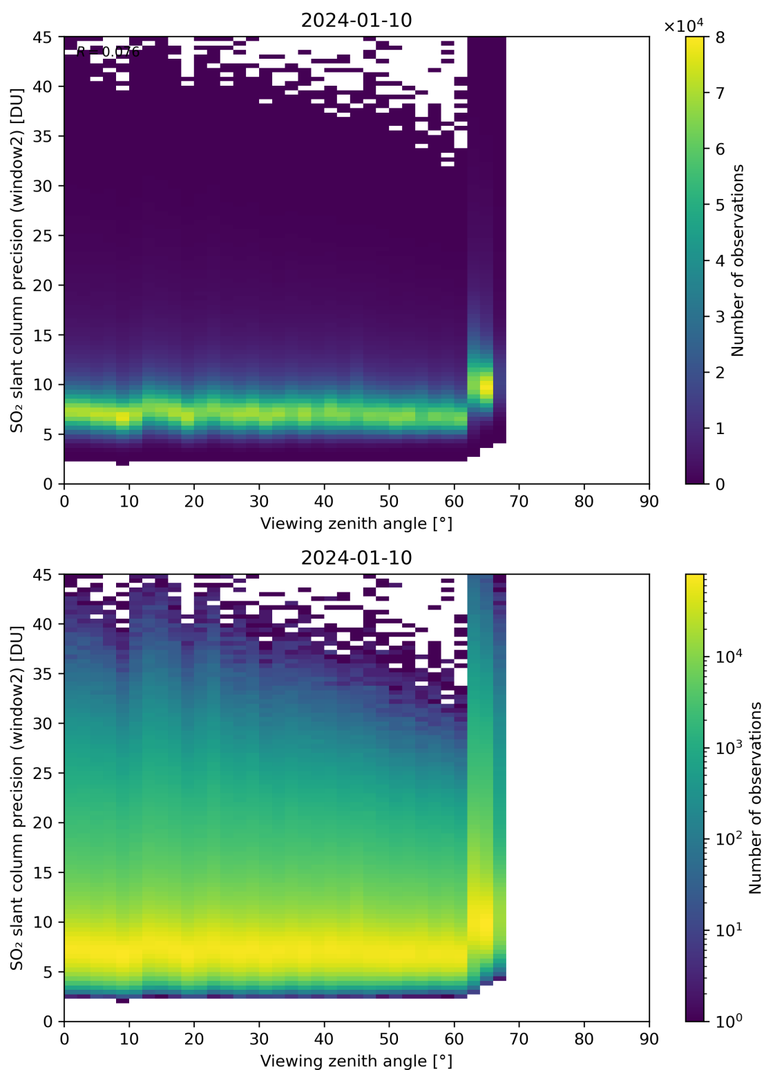
Figure 322: Scatter density plot of “Viewing zenith angle” against “SO 2 slant column precision (window2)” for 2024-01-10 to 2024-01-11.
