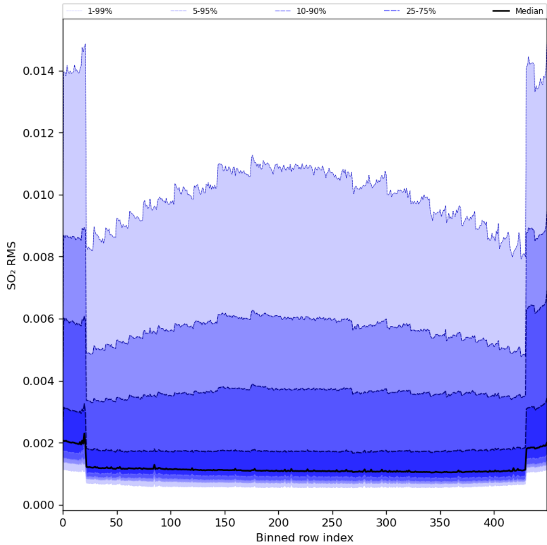
Figure 93: Along track statistics of “SO 2 RMS” for 2024-01-10 to 2024-01-11
