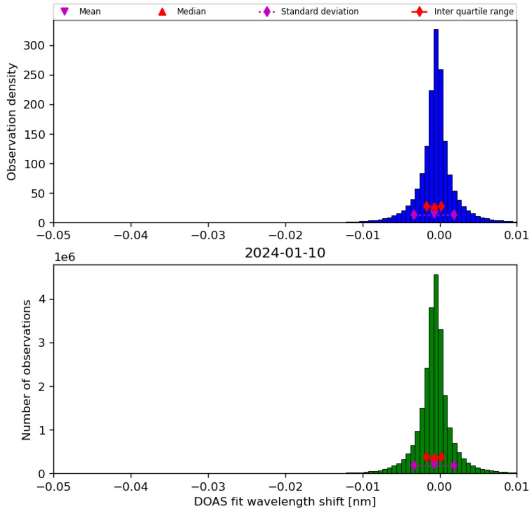
Figure 68: Histogram of “DOAS fit wavelength shift” for 2024-01-10 to 2024-01-11
