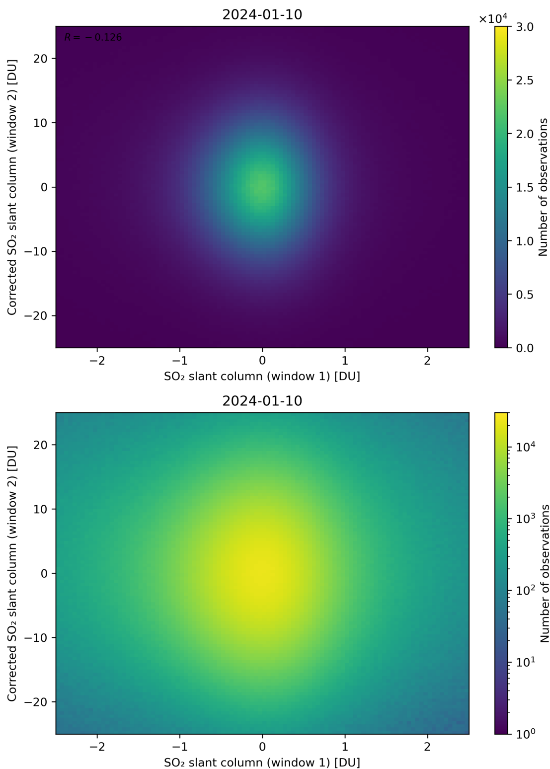
Figure 233: Scatter density plot of “SO 2 slant column (window 1)” against “Corrected SO 2 slant column (window 2)” for 2024-01-10 to 2024-01-11.
