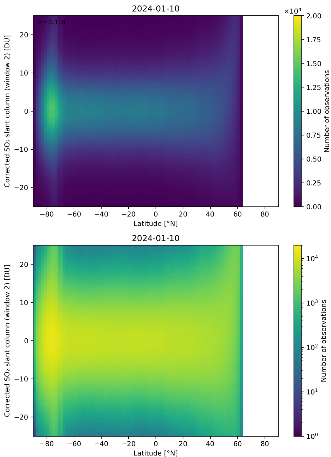
Figure 147: Scatter density plot of “Latitude” against “Corrected SO 2 slant column (window 2)” for 2024-01-10 to 2024-01-11.
