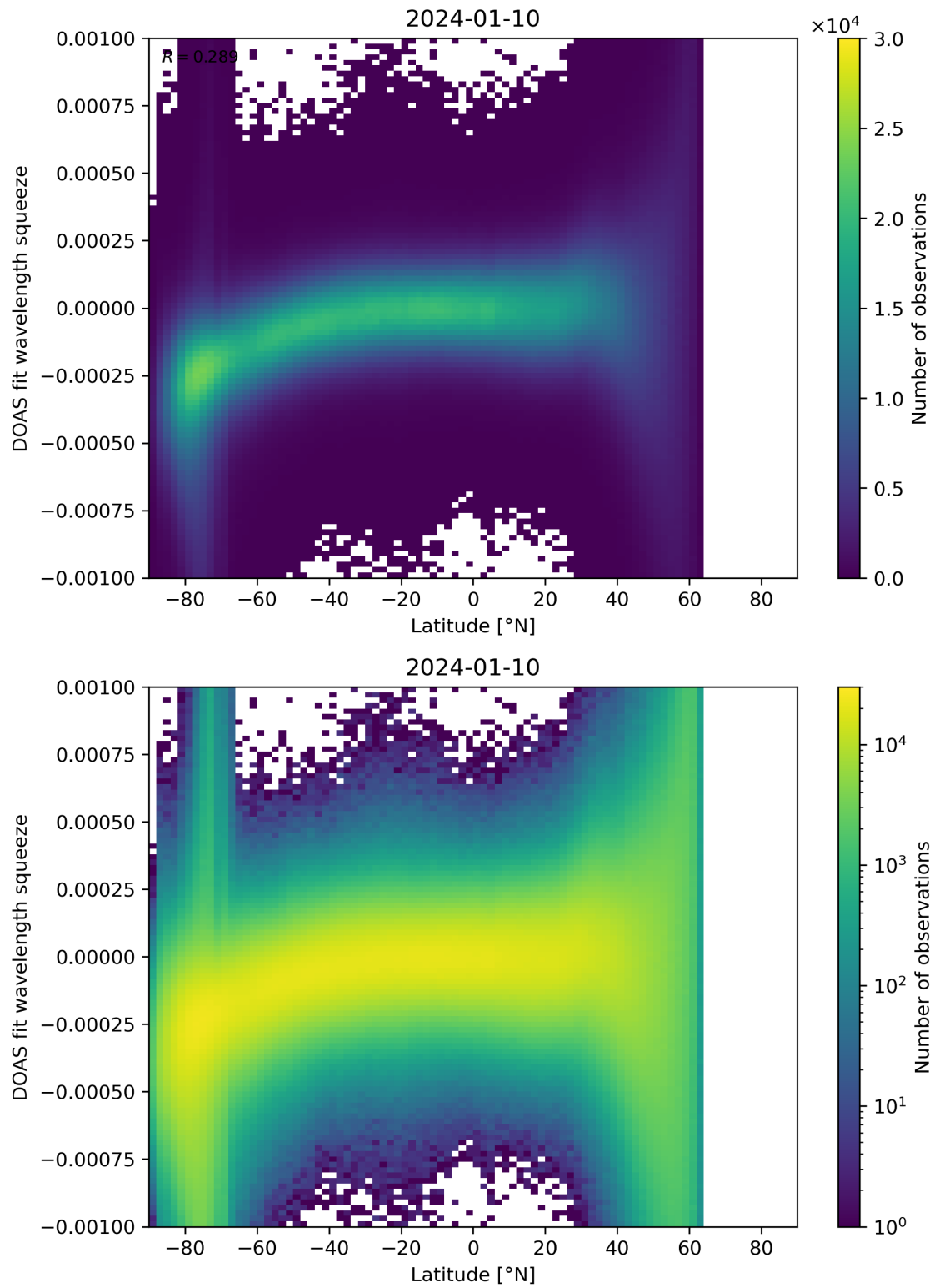
Figure 143: Scatter density plot of “Latitude” against “DOAS fit wavelength squeeze” for 2024-01-10 to 2024-01-11.
