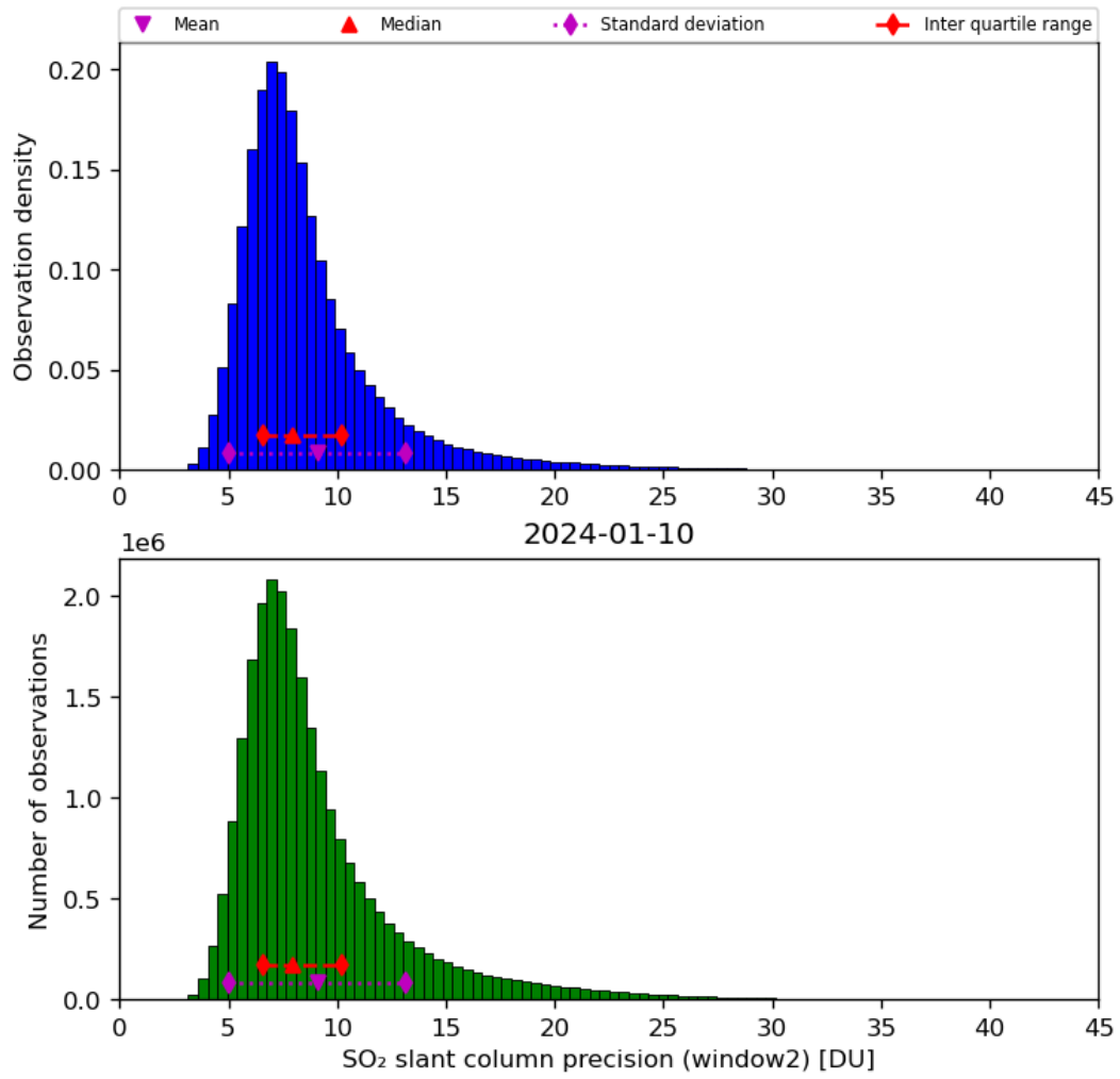
Figure 61: Histogram of “SO 2 slant column precision (window2)” for 2024-01-10 to 2024-01-11
