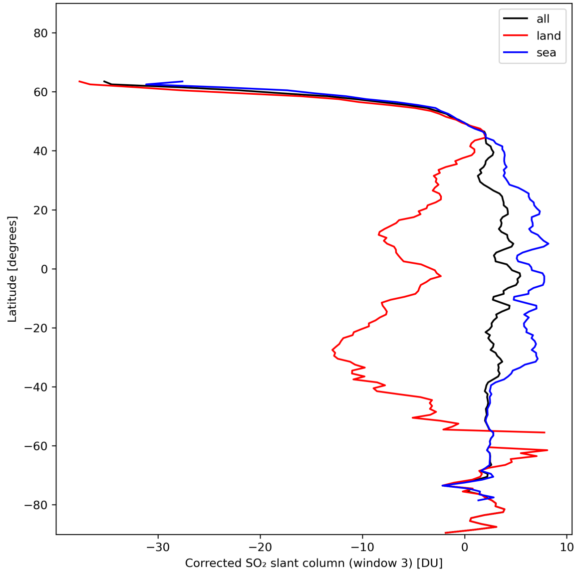
Figure 43: Zonal average of “Corrected SO 2 slant column (window 3)” for 2024-01-10 to 2024-01-11.
