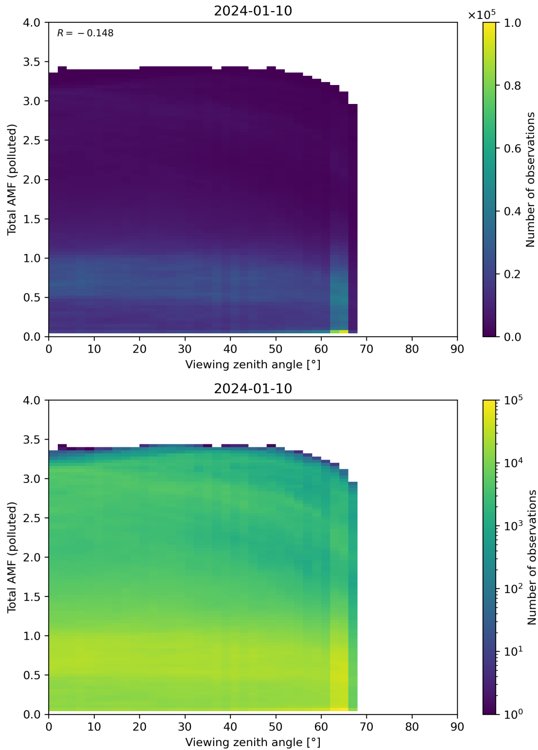
Figure 325: Scatter density plot of “Viewing zenith angle” against “Total AMF (polluted)” for 2024-01-10 to 2024-01-11.
