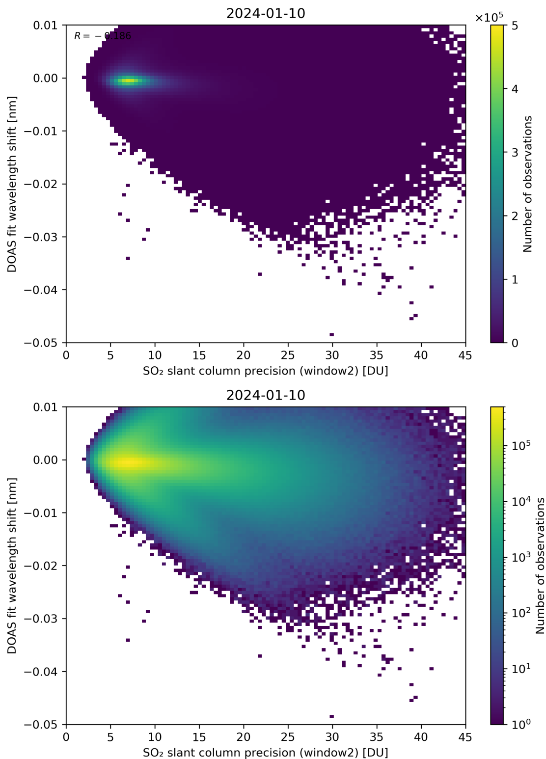
Figure 243: Scatter density plot of “SO 2 slant column precision (window2)” against “DOAS fit wavelength shift” for 2024-01-10 to 2024-01-11.
