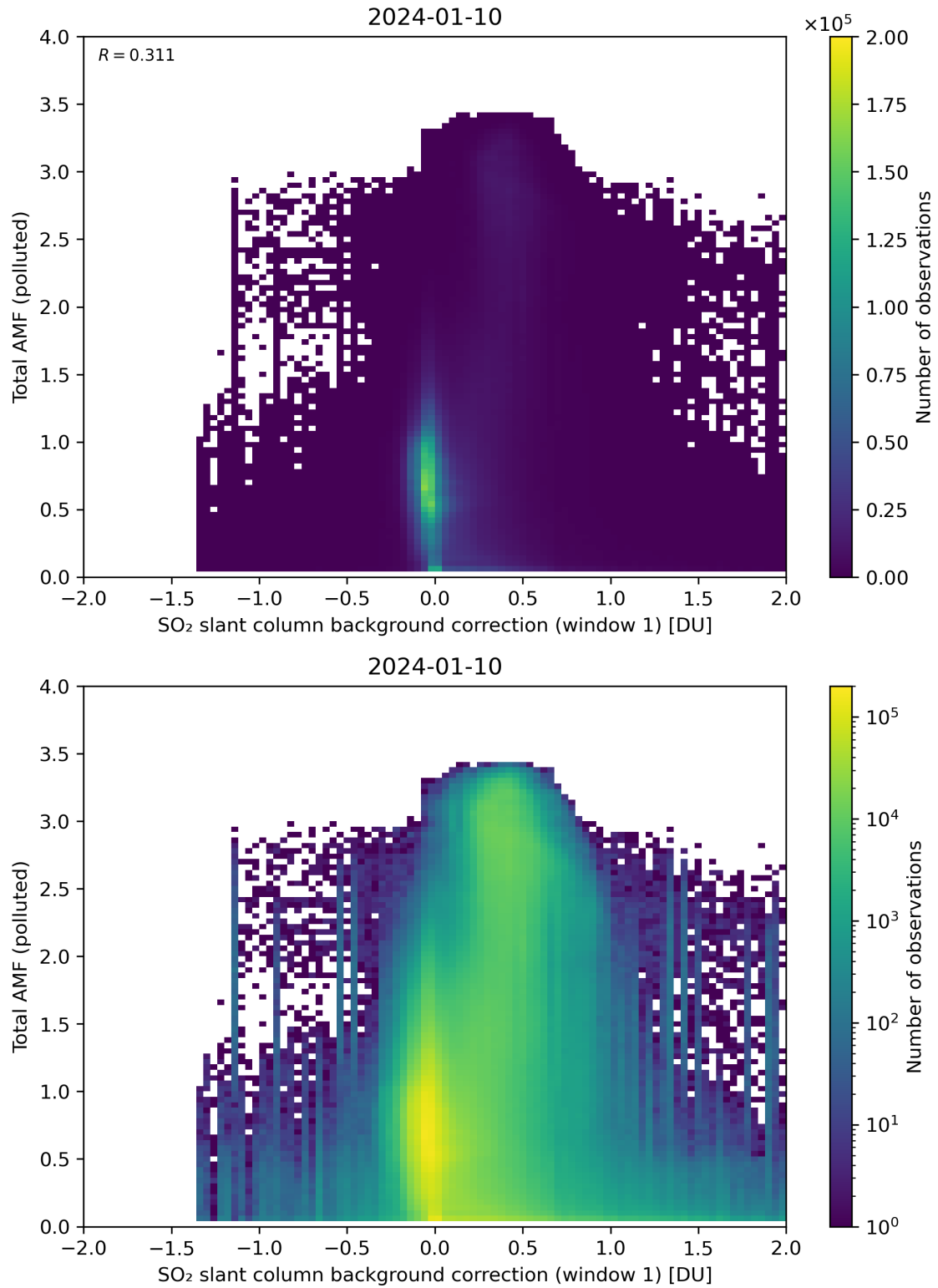
Figure 109: Scatter density plot of “SO 2 slant column background correction (window 1)” against “Total AMF (polluted)” for 2024-01-10 to 2024-01-11.
