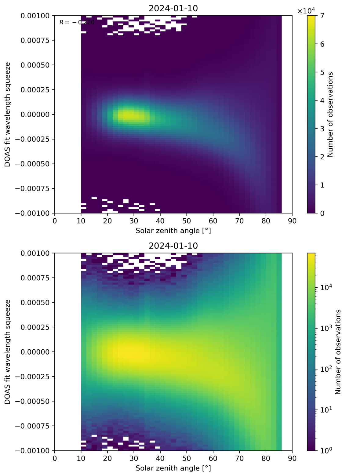
Figure 162: Scatter density plot of “Solar zenith angle” against “DOAS fit wavelength squeeze” for 2024-01-10 to 2024-01-11.
