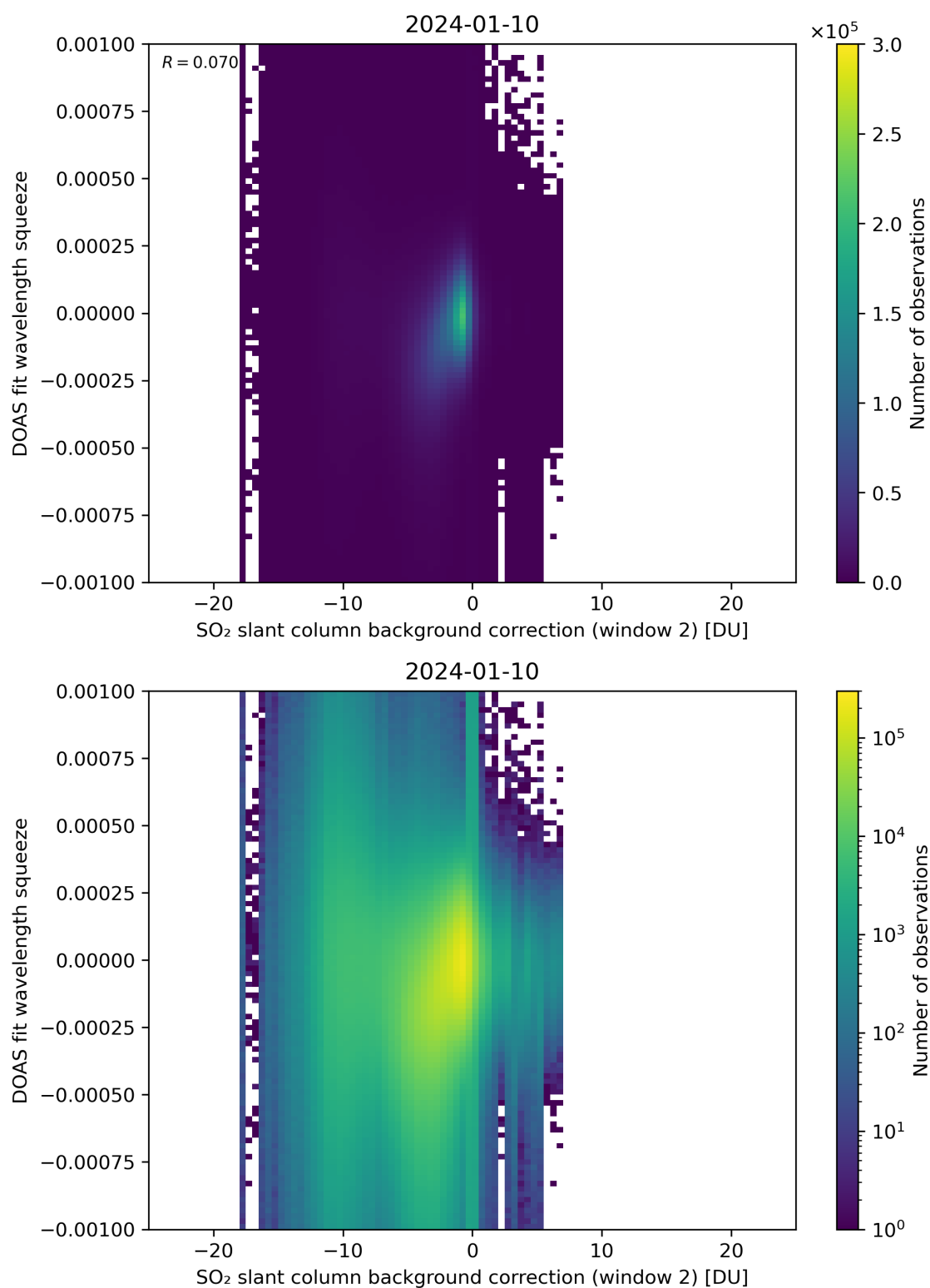
Figure 113: Scatter density plot of “SO 2 slant column background correction (window 2)” against “DOAS fit wavelength squeeze” for 2024-01-10 to 2024-01-11.
