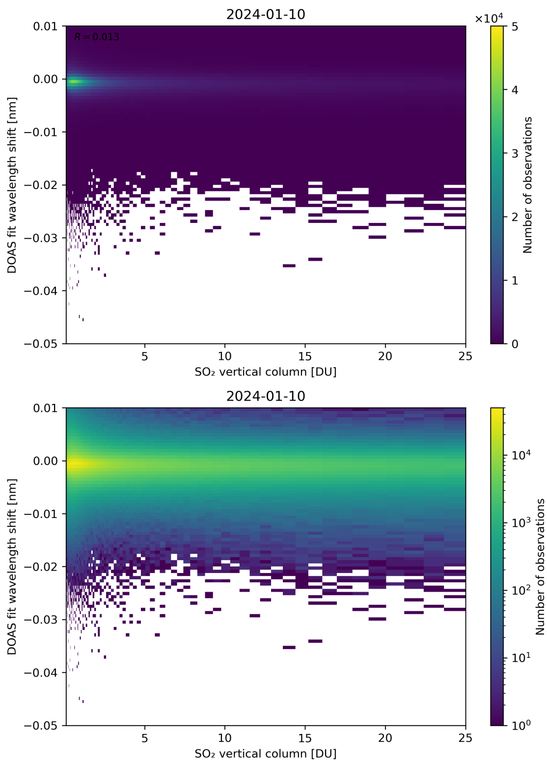
Figure 276: Scatter density plot of “SO 2 vertical column” against “DOAS fit wavelength shift” for 2024-01-10 to 2024-01-11.
