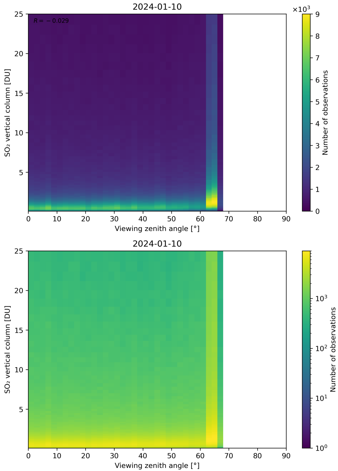
Figure 327: Scatter density plot of “Viewing zenith angle” against “SO 2 vertical column” for 2024-01-10 to 2024-01-11.
