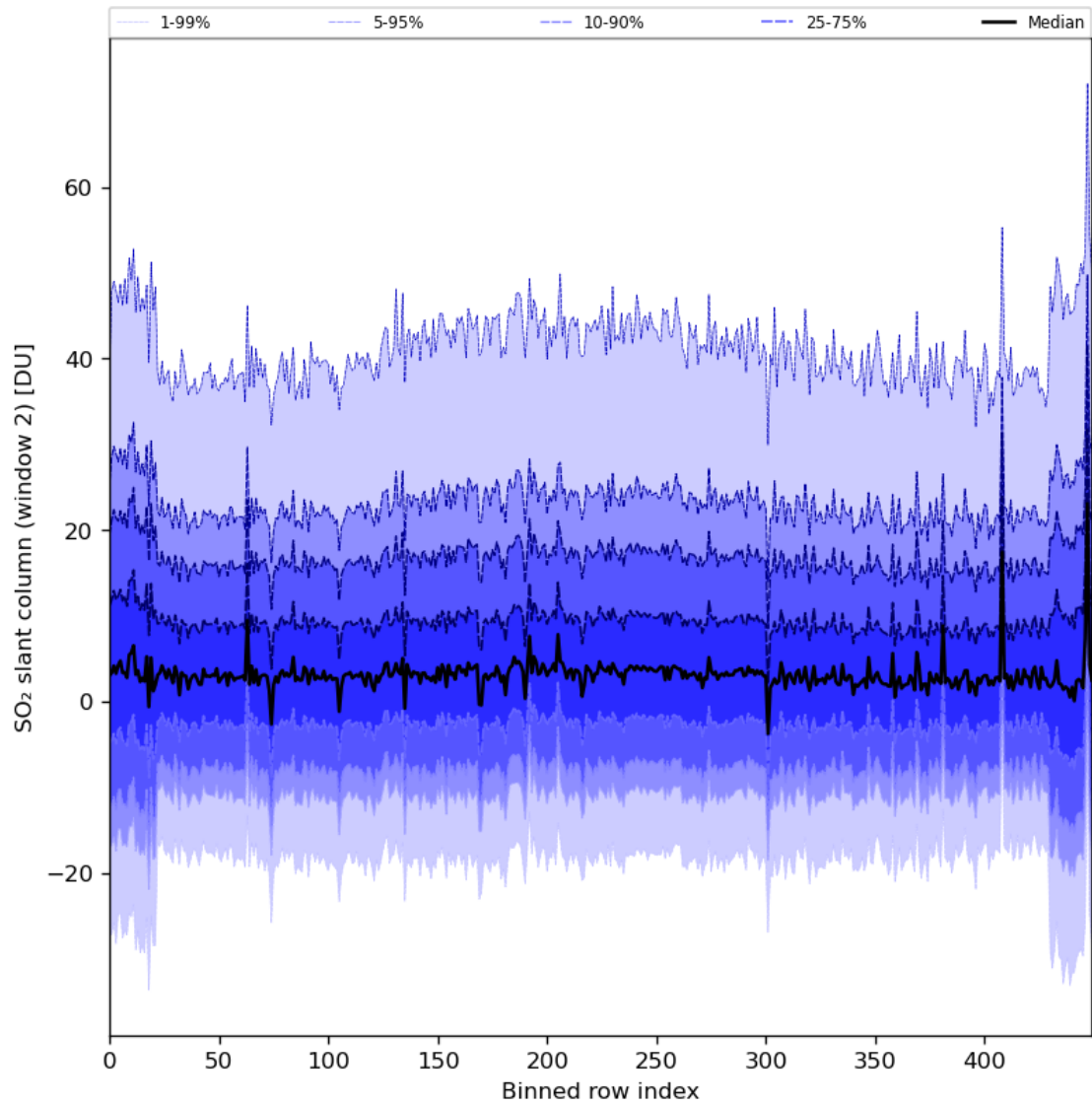
Figure 83: Along track statistics of “SO 2 slant column (window 2)” for 2024-01-10 to 2024-01-11
