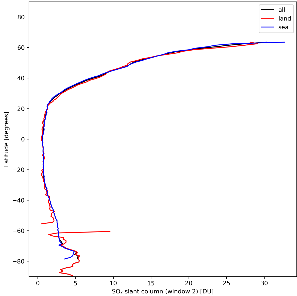
Figure 37: Zonal average of “SO 2 slant column (window 2)” for 2024-01-10 to 2024-01-11.
