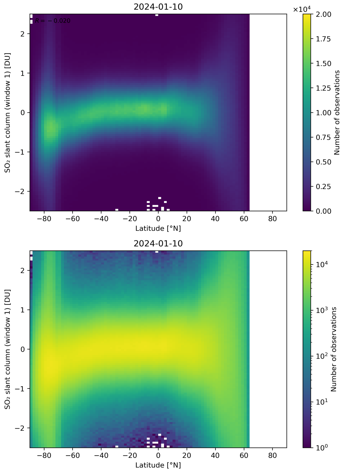
Figure 149: Scatter density plot of “Latitude” against “SO 2 slant column (window 1)” for 2024-01-10 to 2024-01-11.
