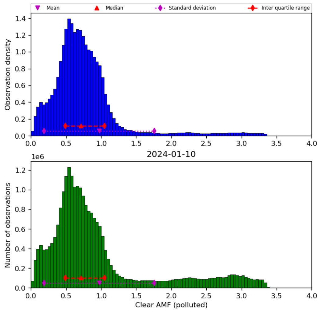
Figure 73: Histogram of “Clear AMF (polluted)” for 2024-01-10 to 2024-01-11
