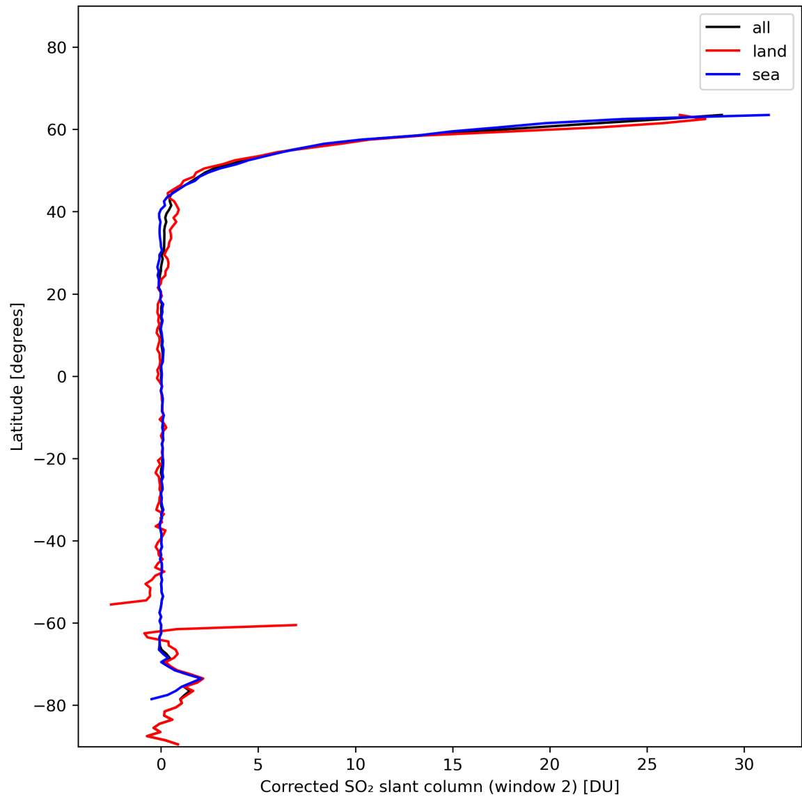
Figure 39: Zonal average of “Corrected SO 2 slant column (window 2)” for 2024-01-10 to 2024-01-11.
