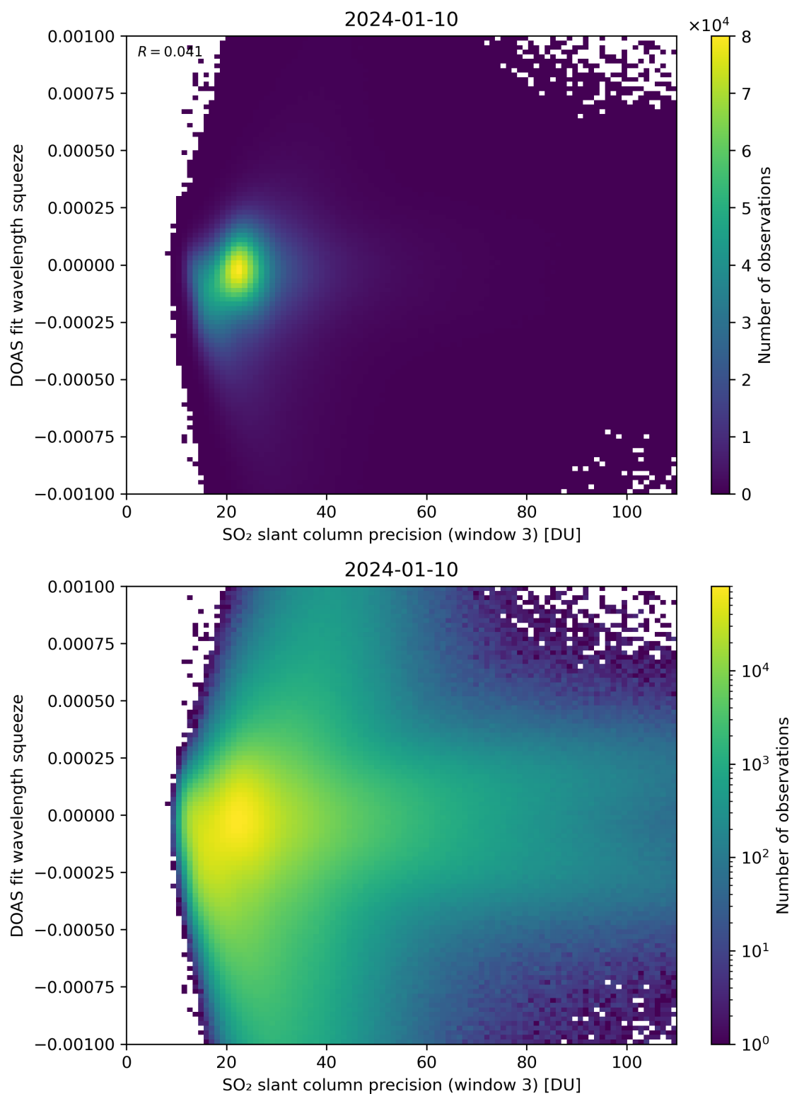
Figure 259: Scatter density plot of “SO 2 slant column precision (window 3)” against “DOAS fit wavelength squeeze” for 2024-01-10 to 2024-01-11.
