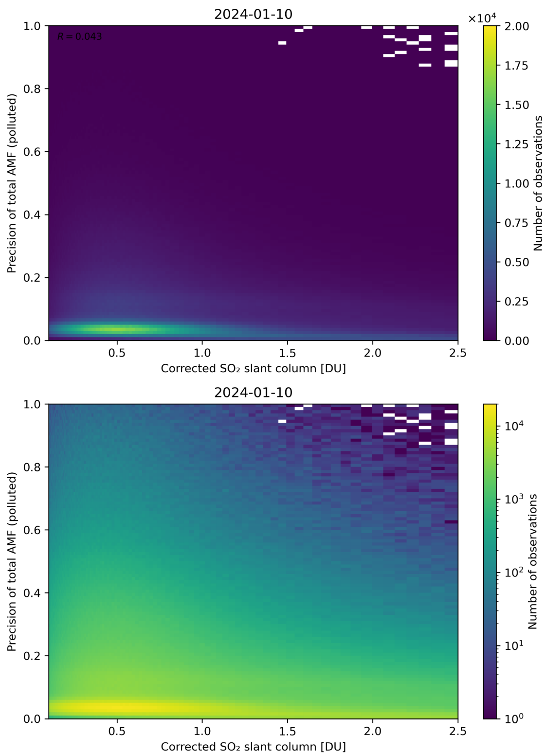
Figure 193: Scatter density plot of “Corrected SO 2 slant column” against “Precision of total AMF (polluted)” for 2024-01-10 to 2024-01-11.
