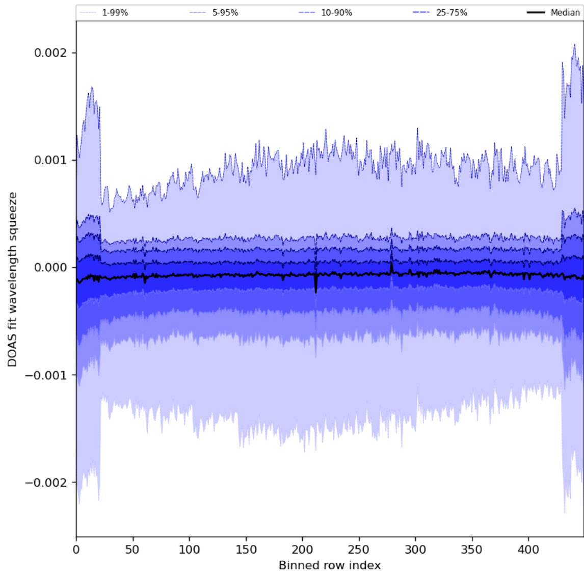
Figure 92: Along track statistics of “DOAS fit wavelength squeeze” for 2024-01-10 to 2024-01-11
