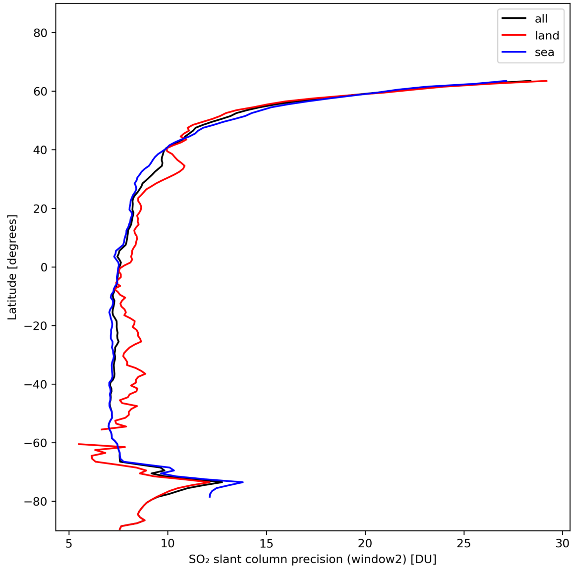
Figure 38: Zonal average of “SO 2 slant column precision (window2)” for 2024-01-10 to 2024-01-11.
