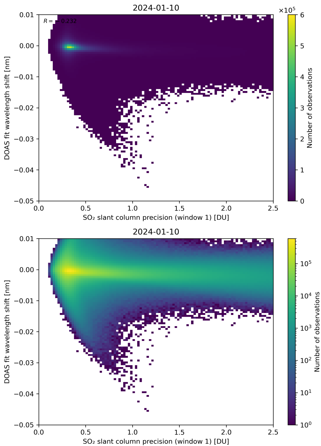
Figure 221: Scatter density plot of “SO 2 slant column precision (window 1)” against “DOAS fit wavelength shift” for 2024-01-10 to 2024-01-11.
