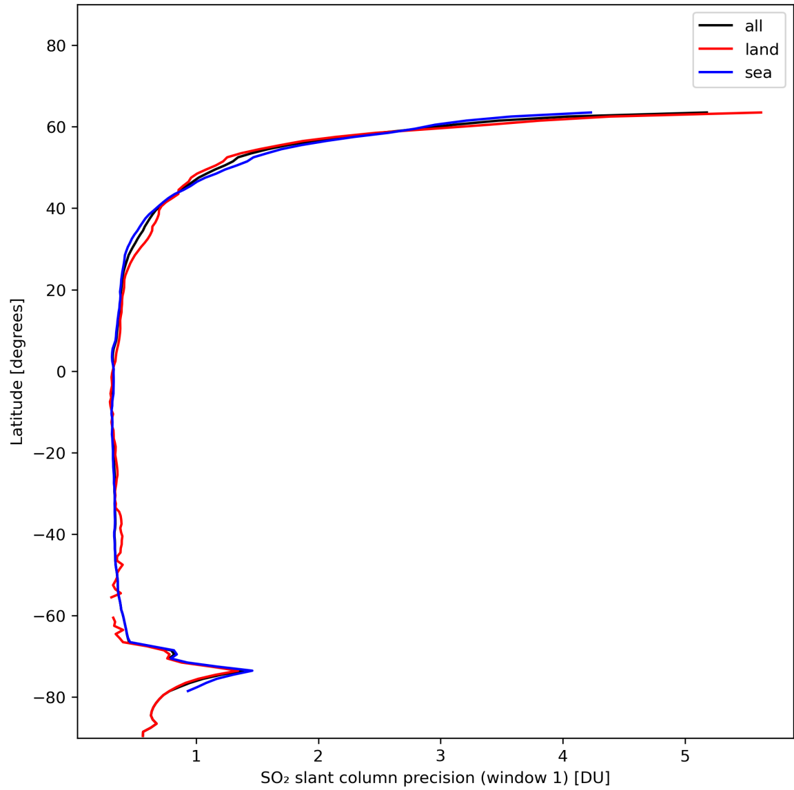
Figure 34: Zonal average of “SO 2 slant column precision (window 1)” for 2024-01-10 to 2024-01-11.
