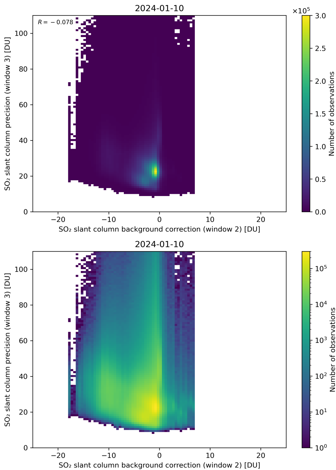
Figure 118: Scatter density plot of “SO 2 slant column background correction (window 2)” against “SO 2 slant column precision (window 3)” for 2024-01-10 to 2024-01-11.
