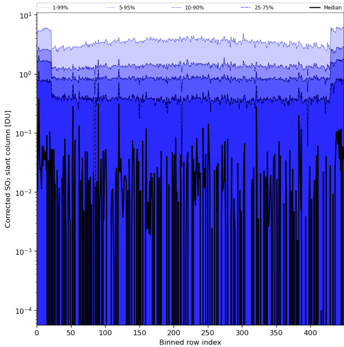
Figure 78: Along track statistics of “Corrected SO 2 slant column” for 2024-01-10 to 2024-01-11
