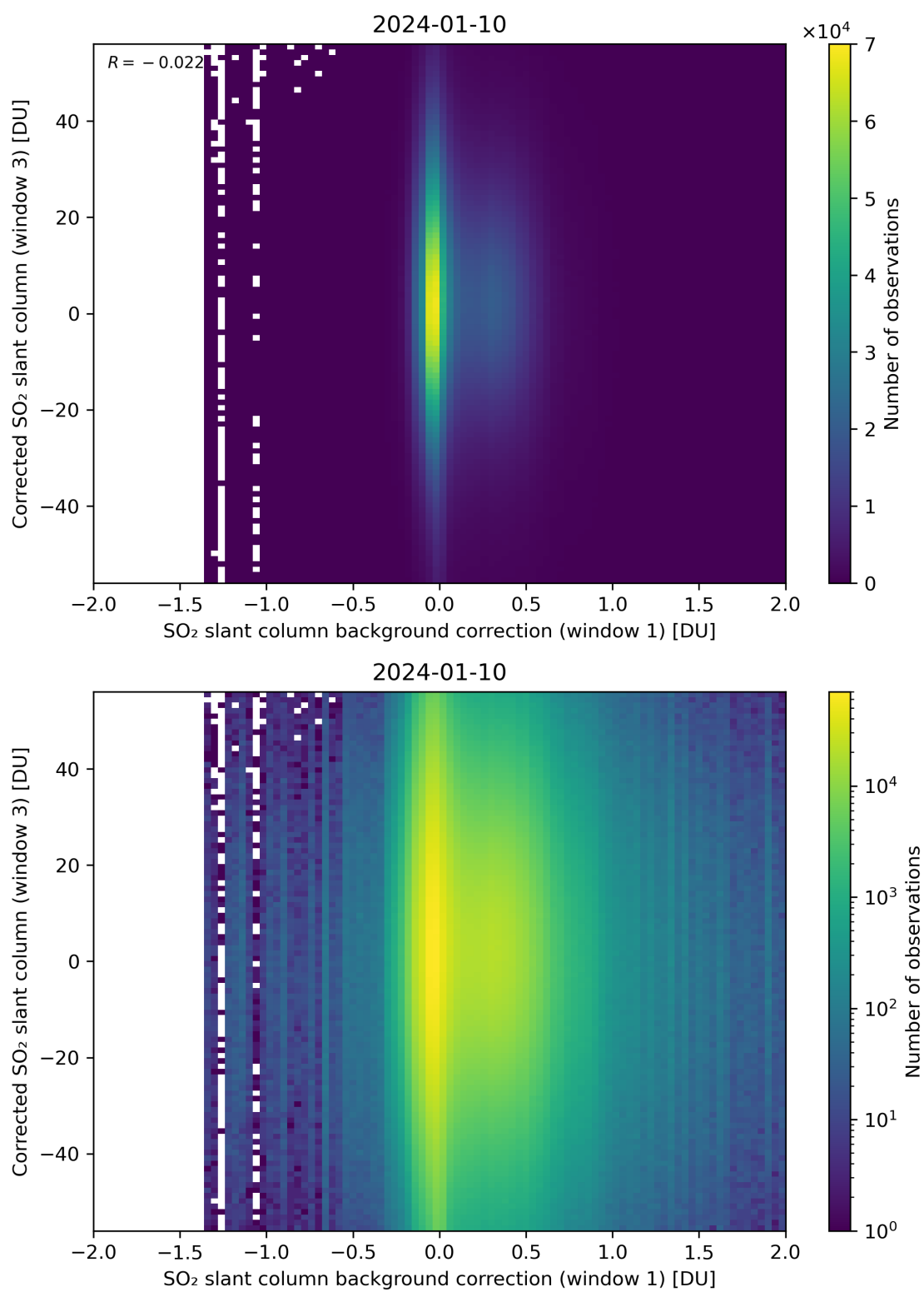
Figure 105: Scatter density plot of “SO 2 slant column background correction (window 1)” against “Corrected SO 2 slant column (window 3)” for 2024-01-10 to 2024-01-11.
