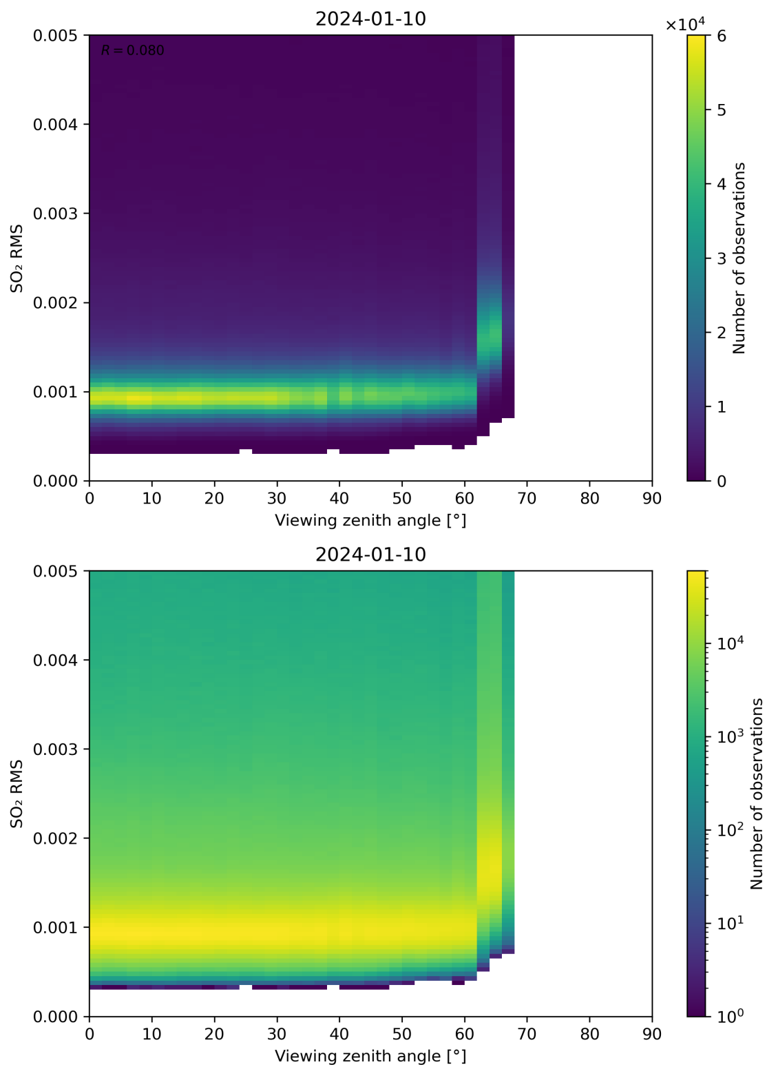
Figure 313: Scatter density plot of “Viewing zenith angle” against “SO 2 RMS” for 2024-01-10 to 2024-01-11.
