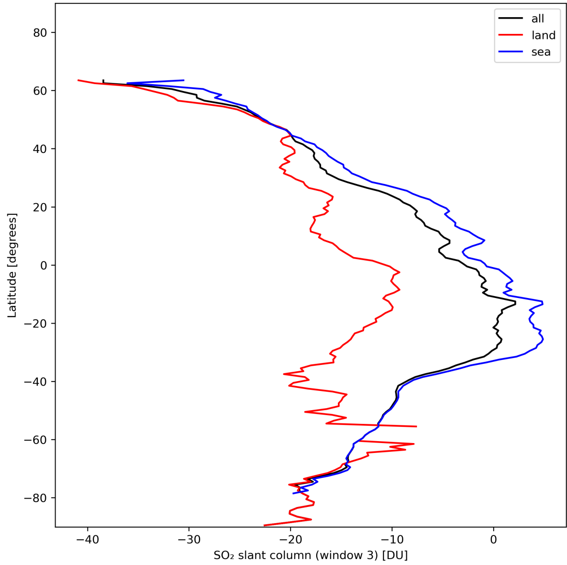
Figure 41: Zonal average of “SO 2 slant column (window 3)” for 2024-01-10 to 2024-01-11.
