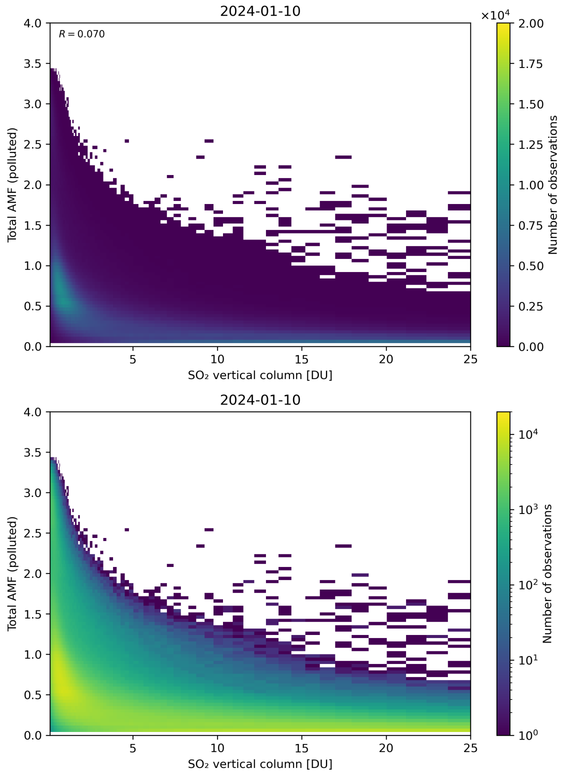
Figure 305: Scatter density plot of “SO 2 vertical column” against “Total AMF (polluted)” for 2024-01-10 to 2024-01-11.
