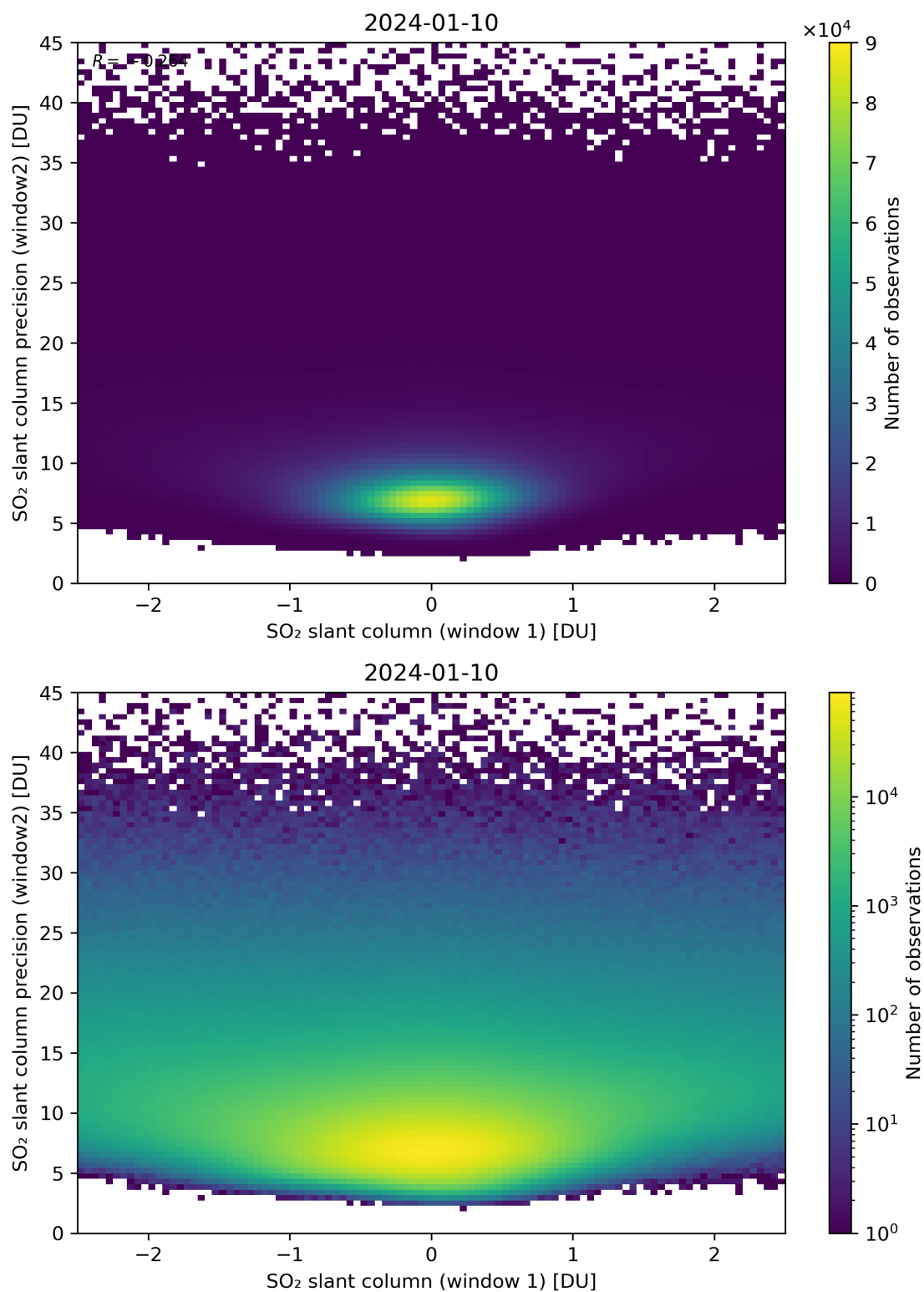
Figure 236: Scatter density plot of “SO 2 slant column (window 1)” against “SO 2 slant column precision (window2)” for 2024-01-10 to 2024-01-11.
