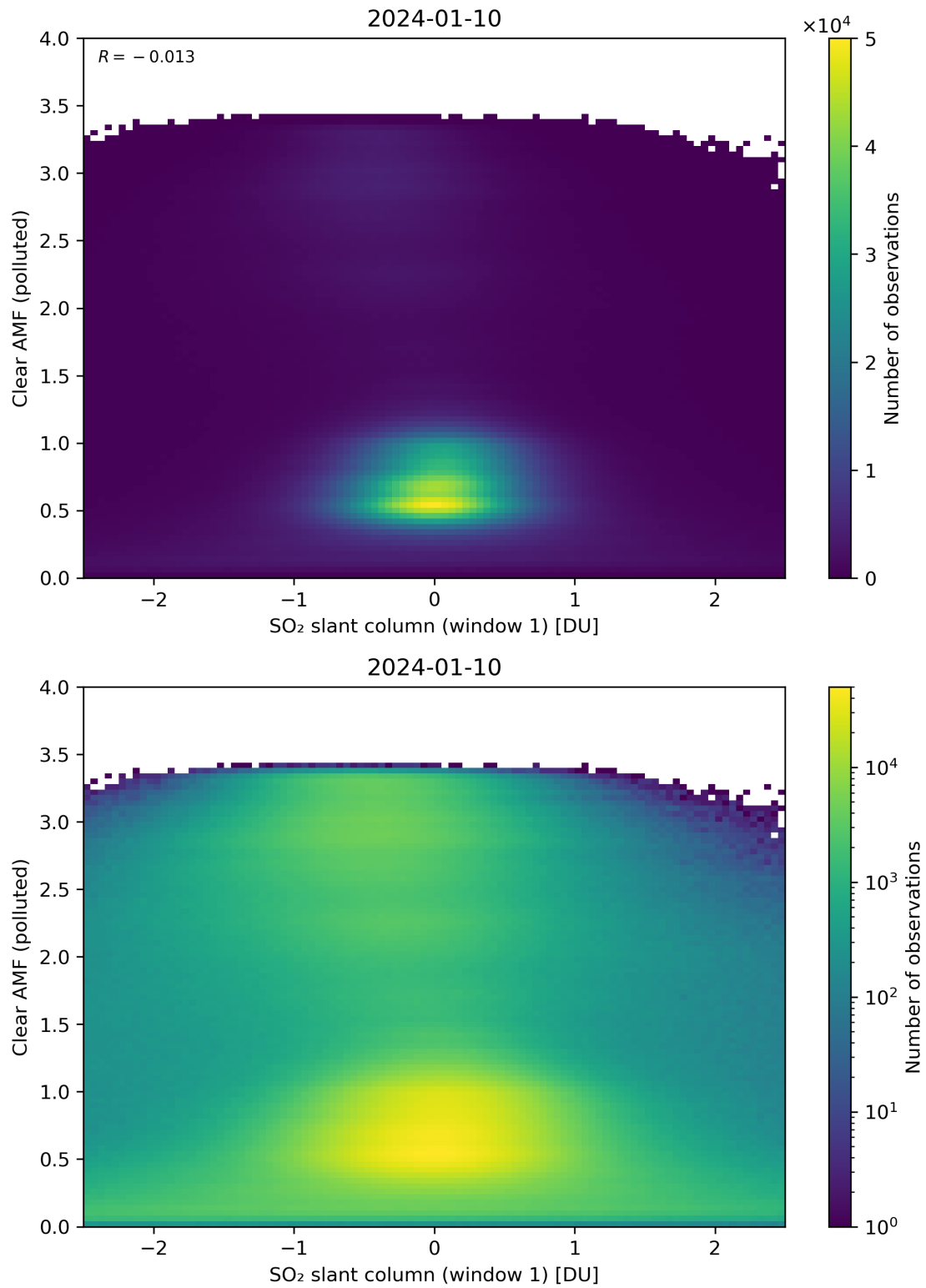
Figure 232: Scatter density plot of “SO 2 slant column (window 1)” against “Clear AMF (polluted)” for 2024-01-10 to 2024-01-11.
