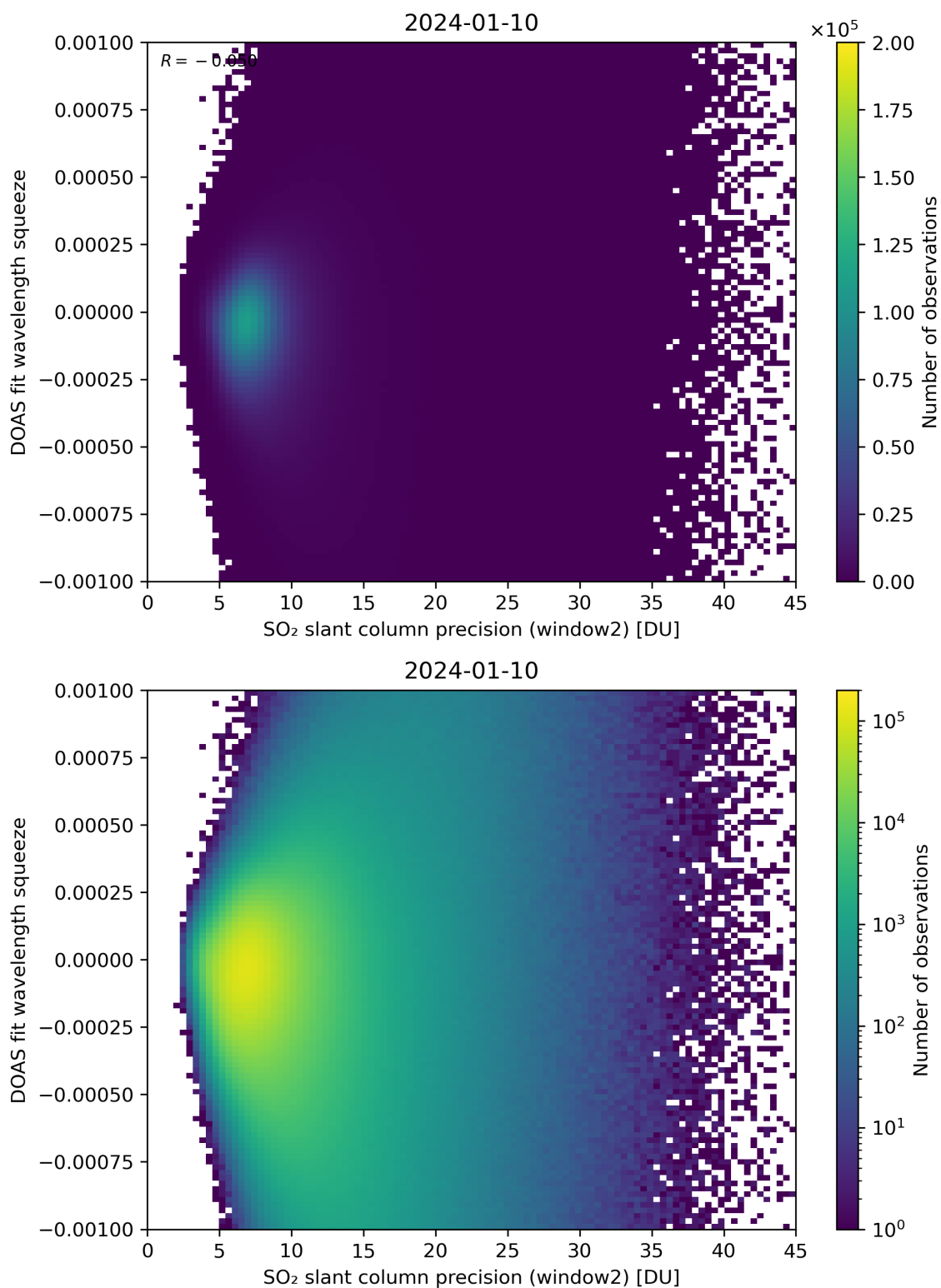
Figure 244: Scatter density plot of “SO 2 slant column precision (window2)” against “DOAS fit wavelength squeeze” for 2024-01-10 to 2024-01-11.
