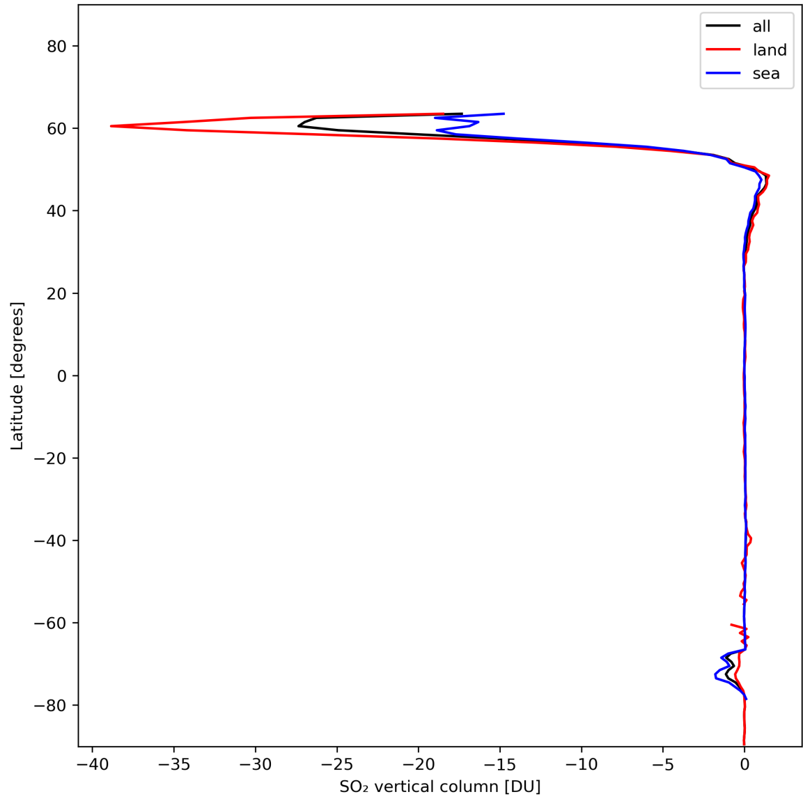
Figure 30: Zonal average of “SO 2 vertical column” for 2024-01-10 to 2024-01-11.
