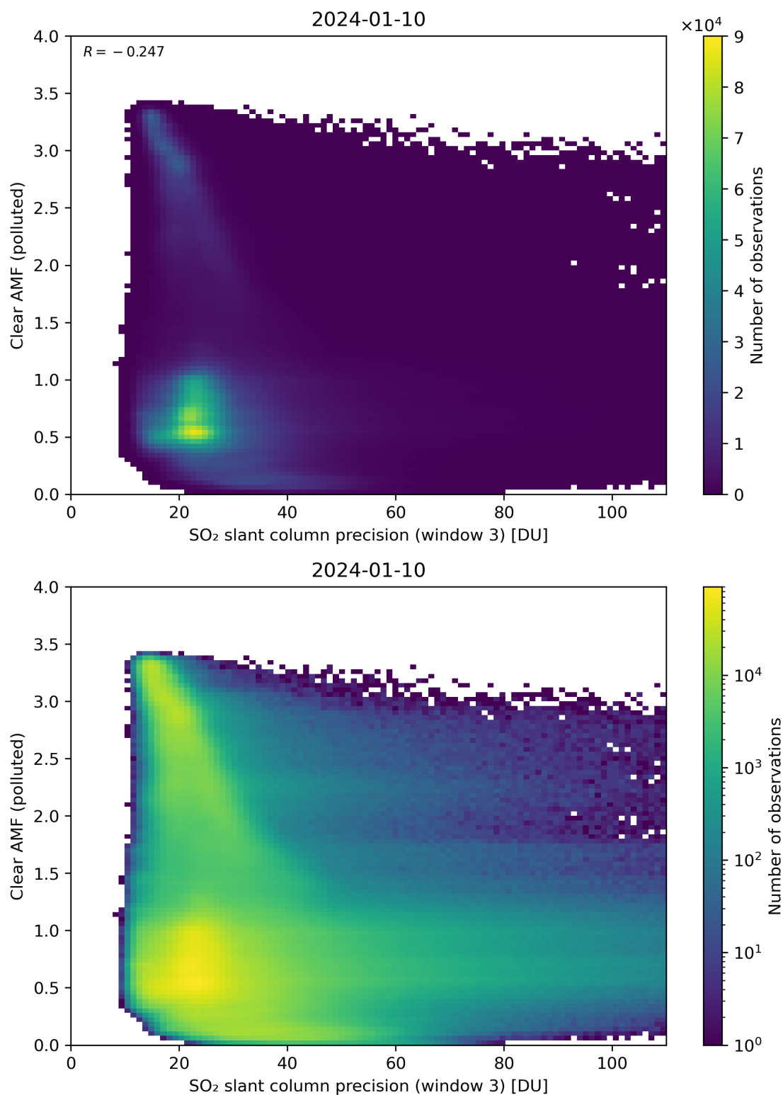
Figure 261: Scatter density plot of “SO 2 slant column precision (window 3)” against “Clear AMF (polluted)” for 2024-01-10 to 2024-01-11.
