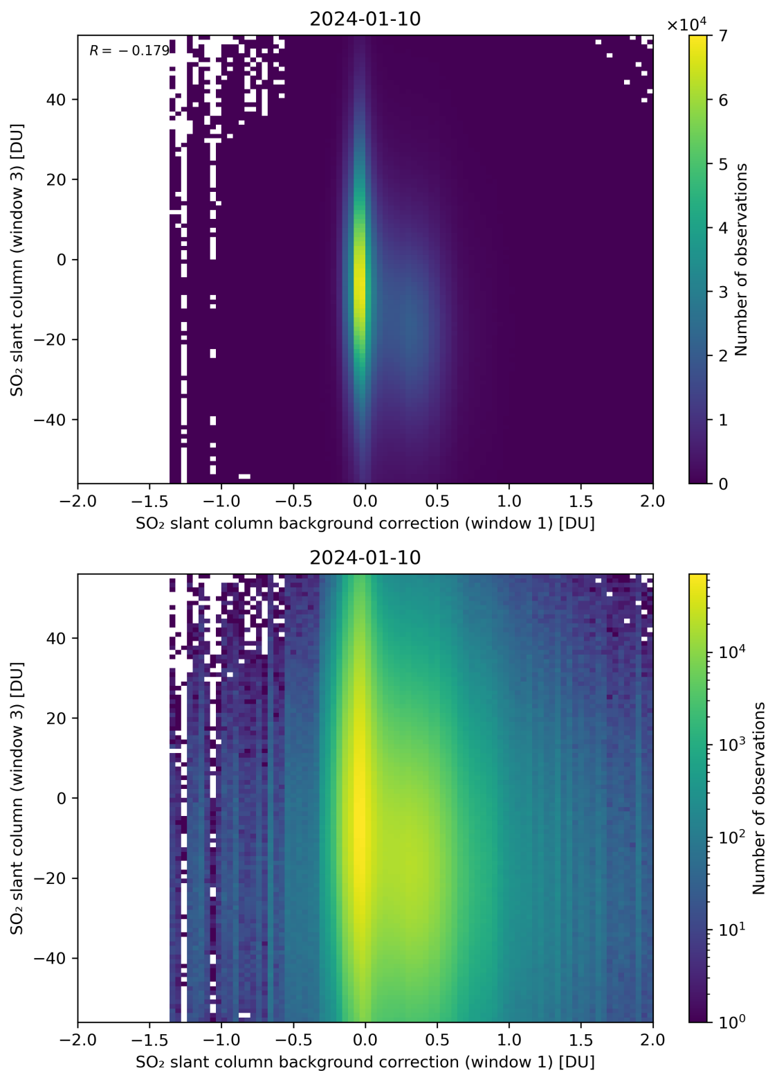
Figure 107: Scatter density plot of “SO 2 slant column background correction (window 1)” against “SO 2 slant column (window 3)” for 2024-01-10 to 2024-01-11.
