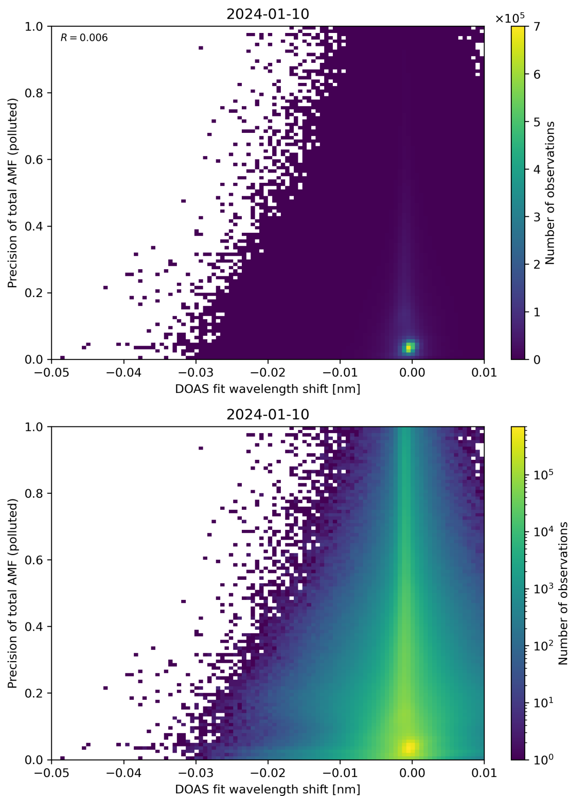
Figure 131: Scatter density plot of “DOAS fit wavelength shift” against “Precision of total AMF (polluted)” for 2024-01-10 to 2024-01-11.
