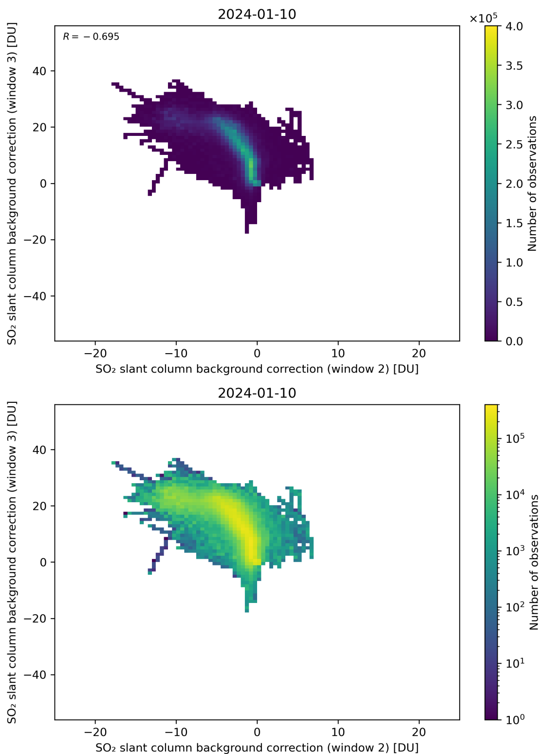
Figure 111: Scatter density plot of “SO 2 slant column background correction (window 2)” against “SO 2 slant column background correction (window 3)” for 2024-01-10 to 2024-01-11.
