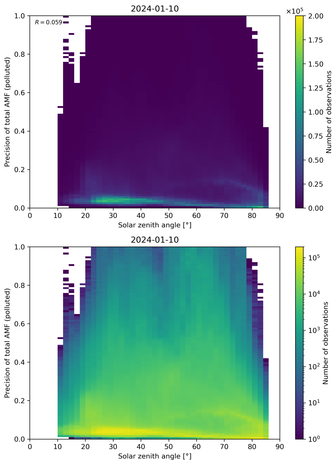
Figure 175: Scatter density plot of “Solar zenith angle” against “Precision of total AMF (polluted)” for 2024-01-10 to 2024-01-11.
