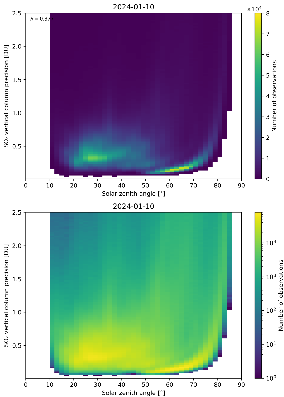
Figure 177: Scatter density plot of “Solar zenith angle” against “SO 2 vertical column precision” for 2024-01-10 to 2024-01-11.
