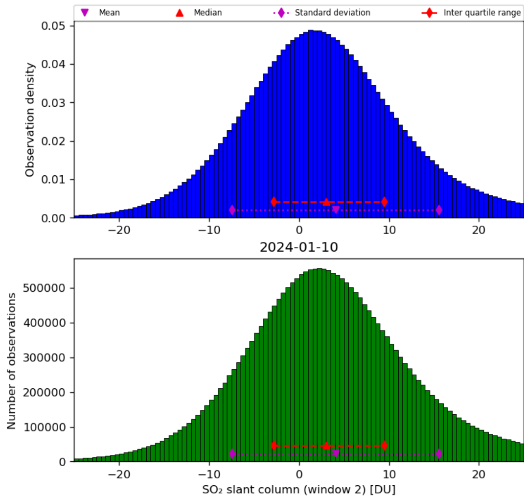
Figure 60: Histogram of “SO 2 slant column (window 2)” for 2024-01-10 to 2024-01-11
