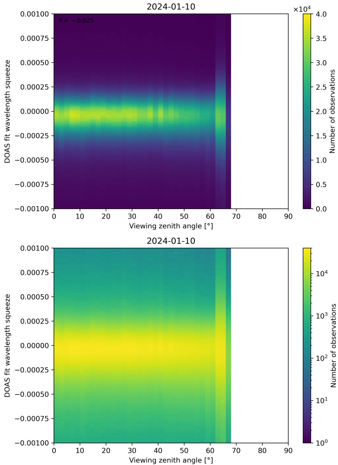
Figure 312: Scatter density plot of “Viewing zenith angle” against “DOAS fit wavelength squeeze” for 2024-01-10 to 2024-01-11.
