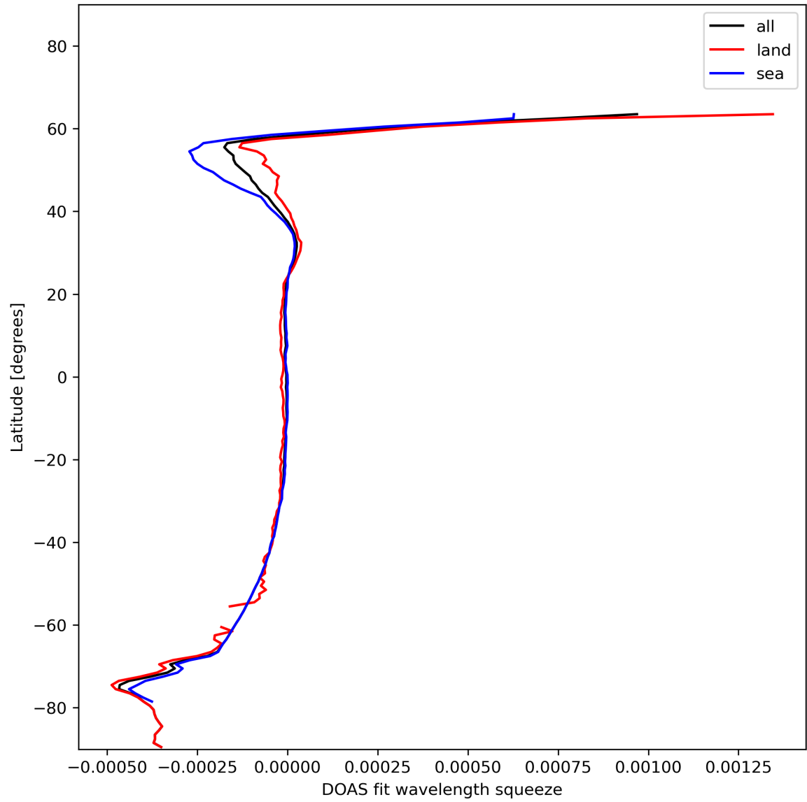
Figure 46: Zonal average of “DOAS fit wavelength squeeze” for 2024-01-10 to 2024-01-11.
