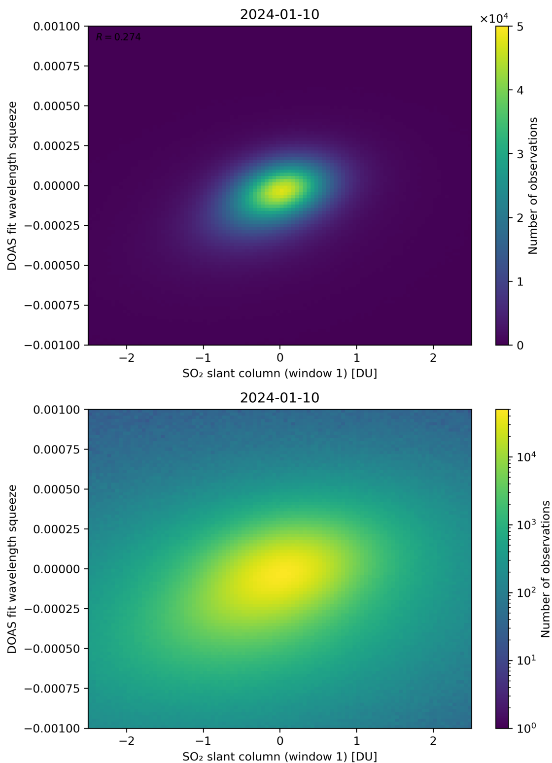
Figure 216: Scatter density plot of “SO 2 slant column (window 1)” against “DOAS fit wavelength squeeze” for 2024-01-10 to 2024-01-11.
