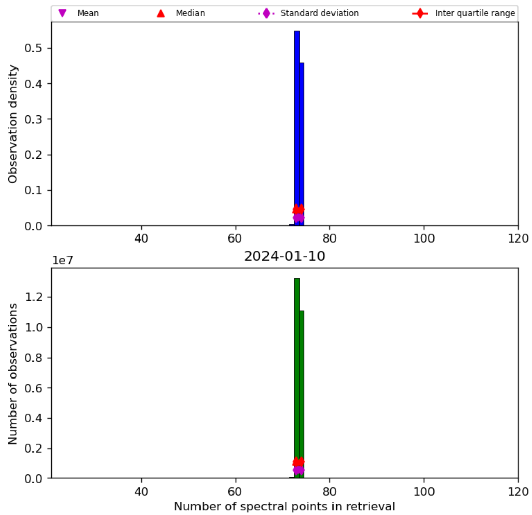
Figure 74: Histogram of “Number of spectral points in retrieval” for 2024-01-10 to 2024-01-11
