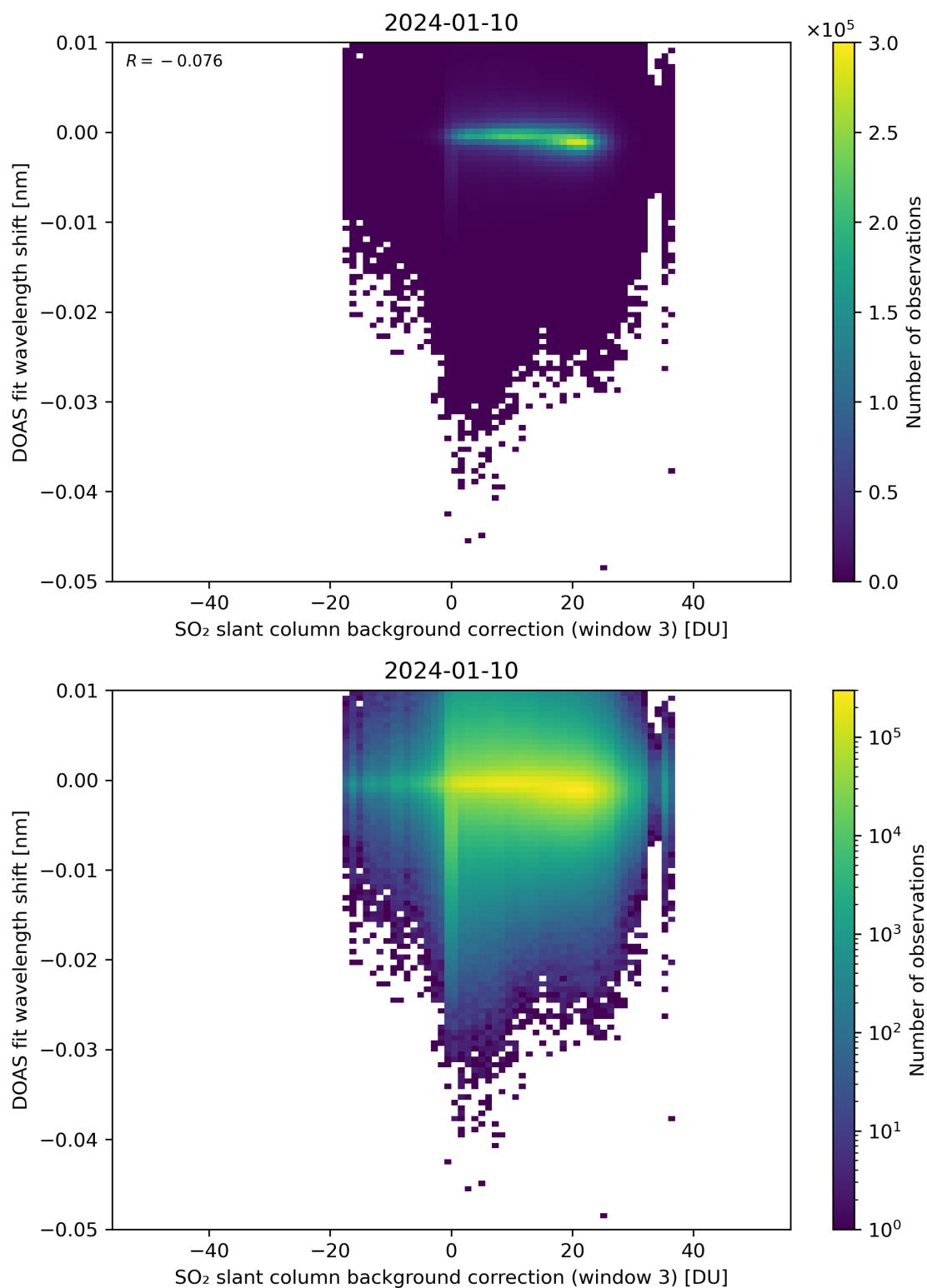
Figure 121: Scatter density plot of “SO 2 slant column background correction (window 3)” against “DOAS fit wavelength shift” for 2024-01-10 to 2024-01-11.
