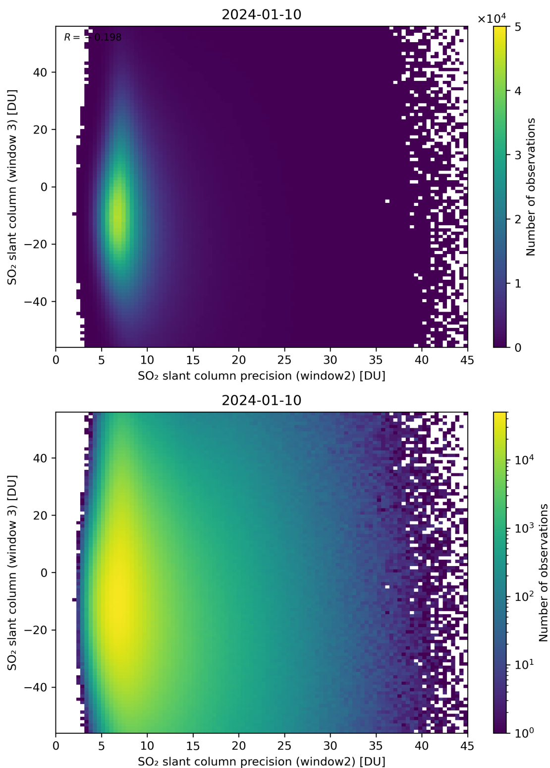
Figure 249: Scatter density plot of “SO 2 slant column precision (window2)” against “SO 2 slant column (window 3)” for 2024-01-10 to 2024-01-11.
