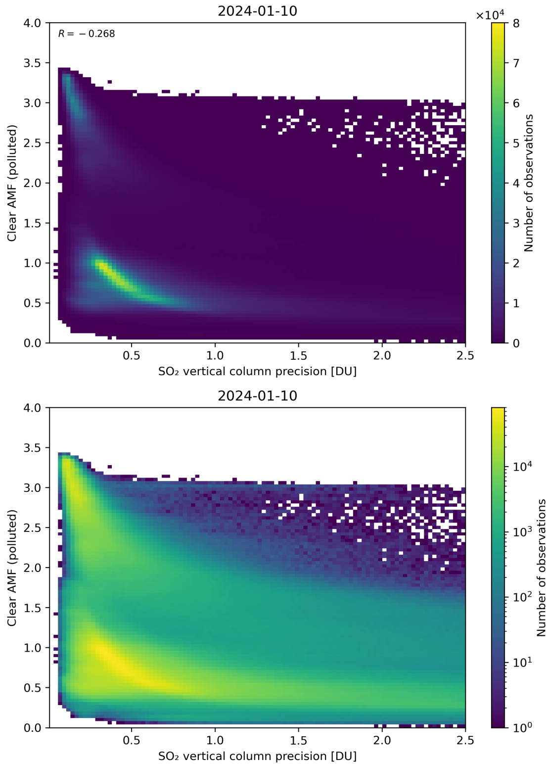
Figure 285: Scatter density plot of “SO 2 vertical column precision” against “Clear AMF (polluted)” for 2024-01-10 to 2024-01-11.
