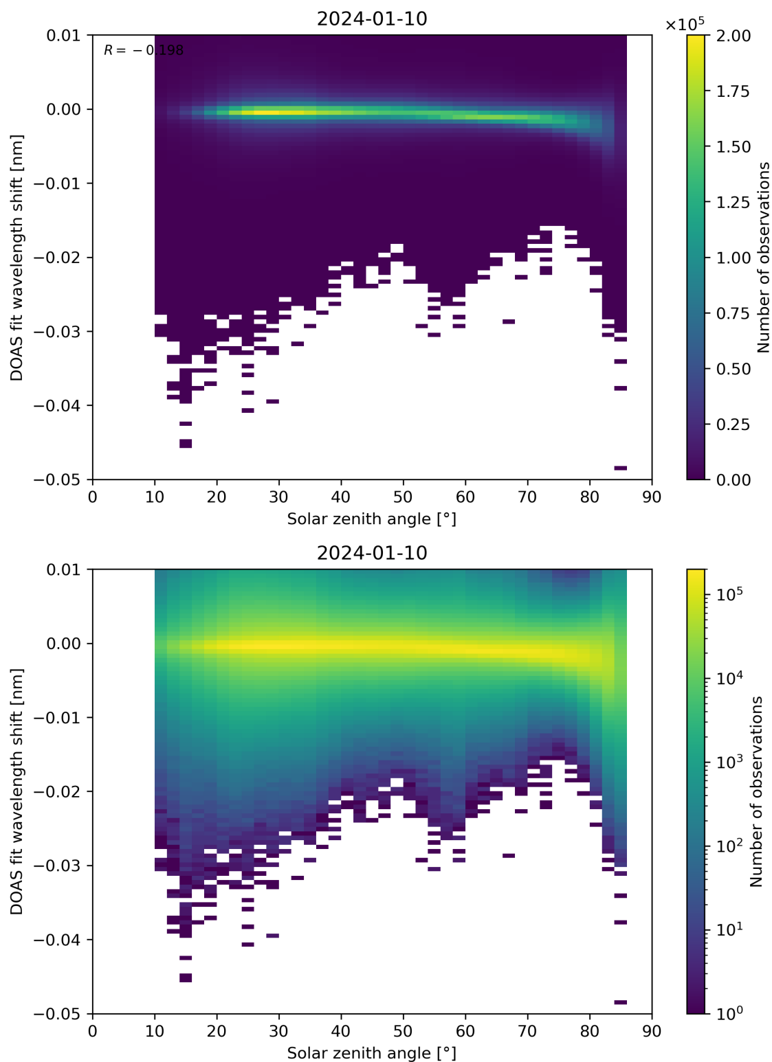
Figure 161: Scatter density plot of “Solar zenith angle” against “DOAS fit wavelength shift” for 2024-01-10 to 2024-01-11.
