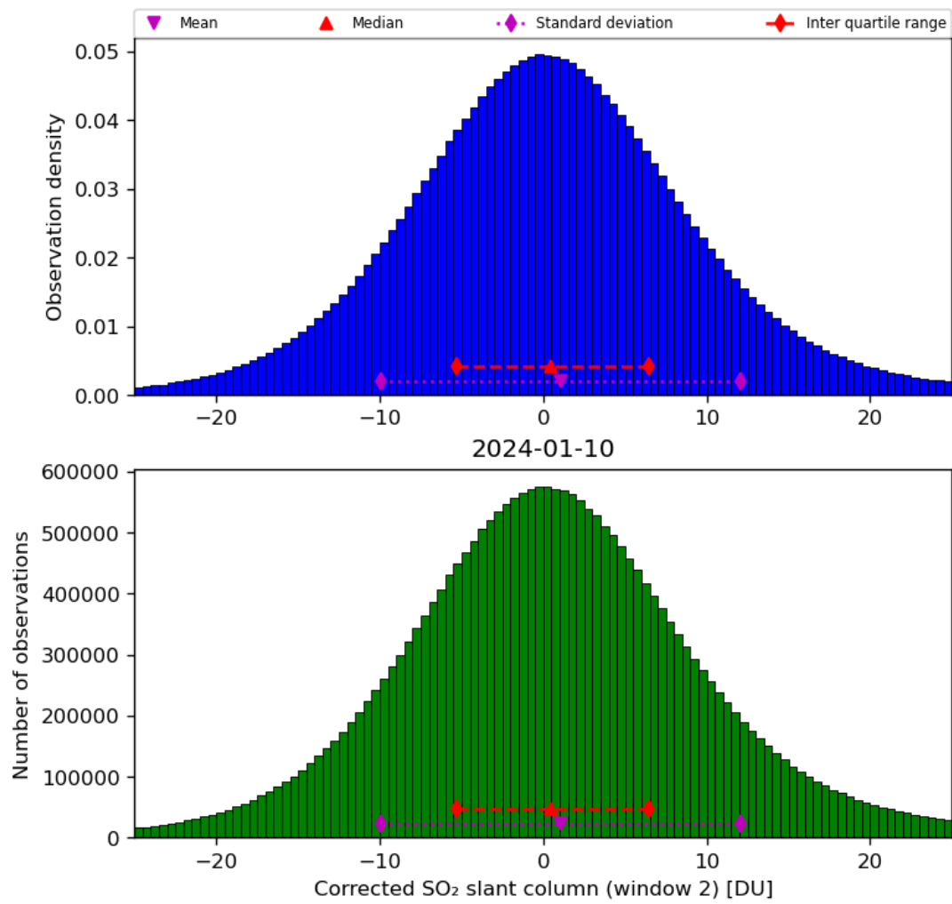
Figure 62: Histogram of “Corrected SO 2 slant column (window 2)” for 2024-01-10 to 2024-01-11
