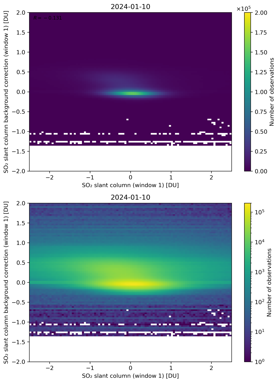
Figure 212: Scatter density plot of “SO 2 slant column (window 1)” against “SO 2 slant column background correction (window 1)” for 2024-01-10 to 2024-01-11.
