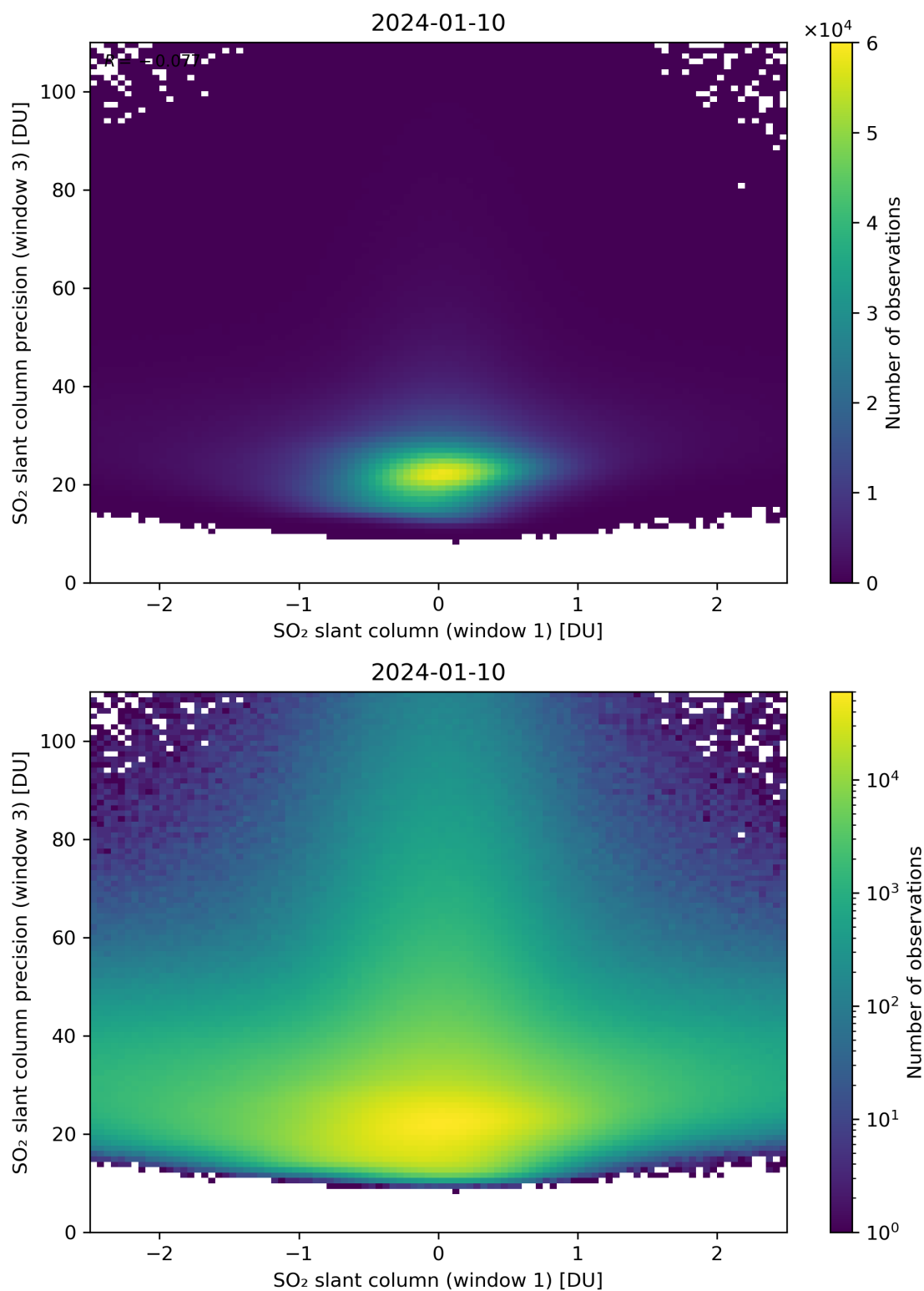
Figure 238: Scatter density plot of “SO 2 slant column (window 1)” against “SO 2 slant column precision (window 3)” for 2024-01-10 to 2024-01-11.
