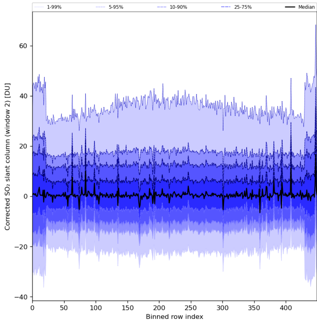
Figure 85: Along track statistics of “Corrected SO 2 slant column (window 2)” for 2024-01-10 to 2024-01-11
