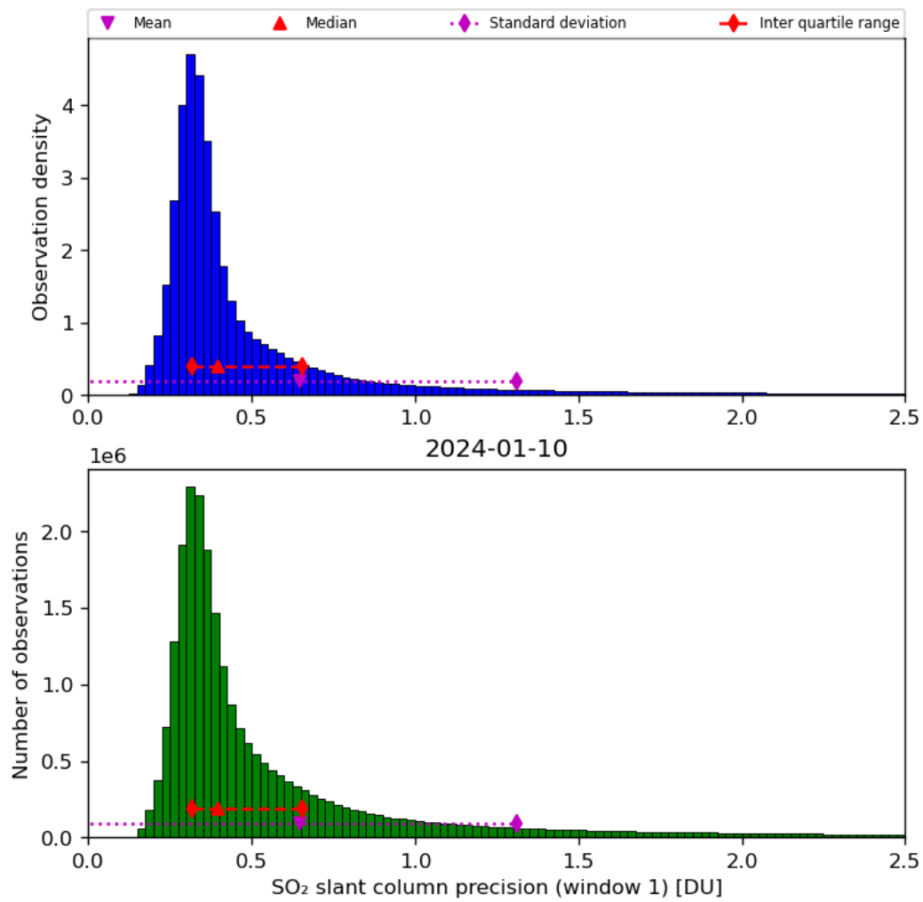
Figure 57: Histogram of “SO 2 slant column precision (window 1)” for 2024-01-10 to 2024-01-11
