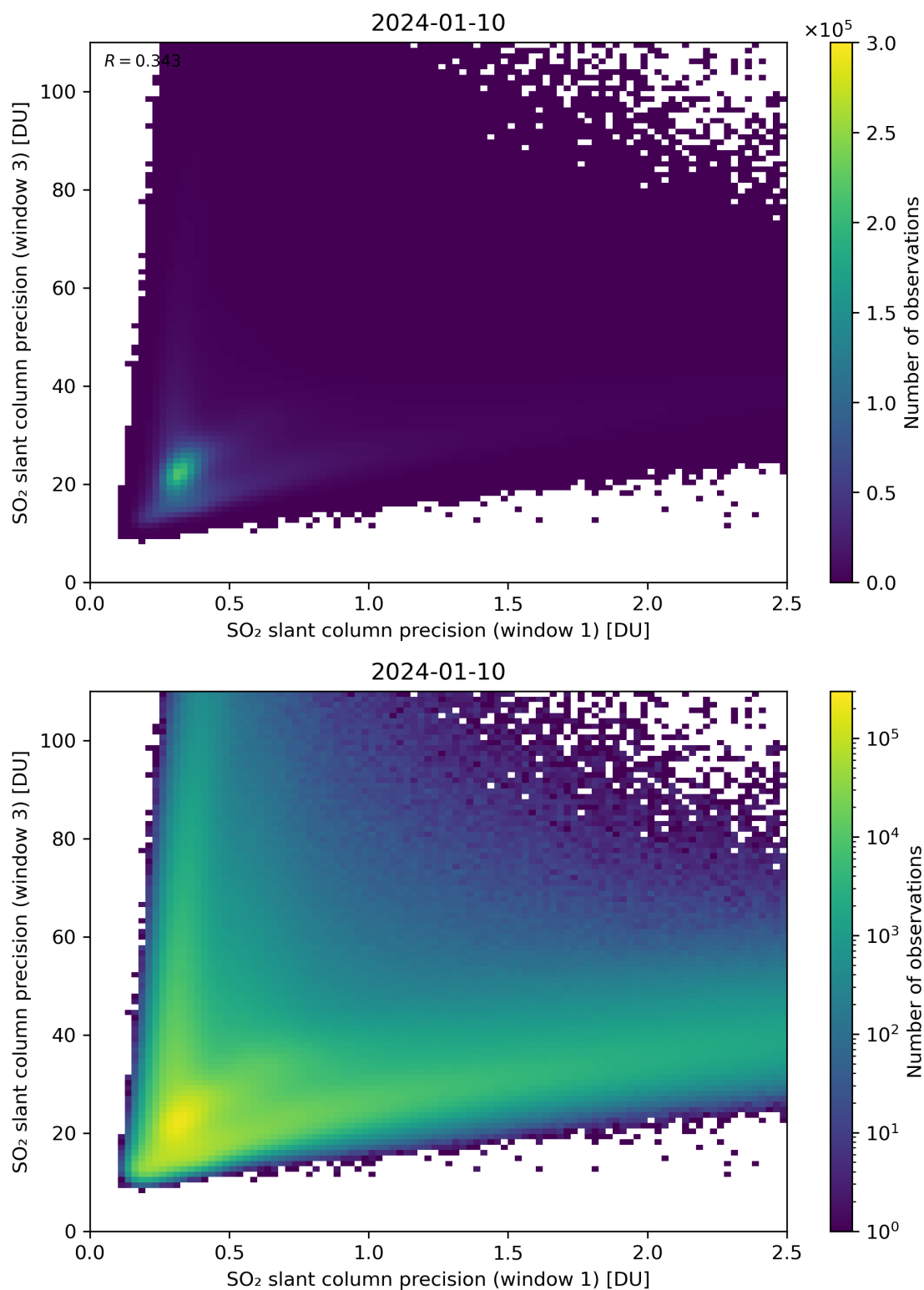
Figure 229: Scatter density plot of “SO 2 slant column precision (window 1)” against “SO 2 slant column precision (window 3)” for 2024-01-10 to 2024-01-11.
