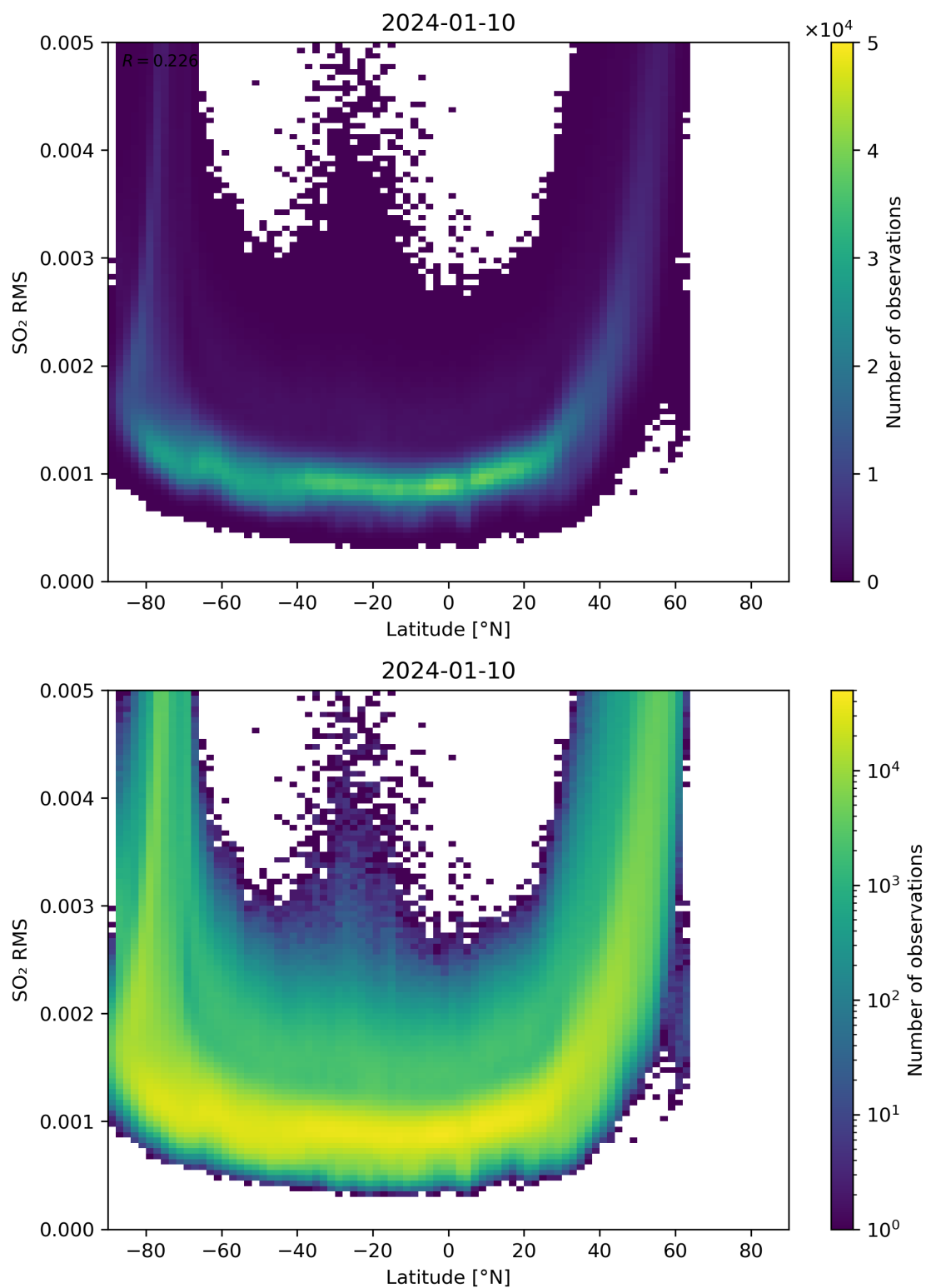
Figure 144: Scatter density plot of “Latitude” against “SO 2 RMS” for 2024-01-10 to 2024-01-11.
