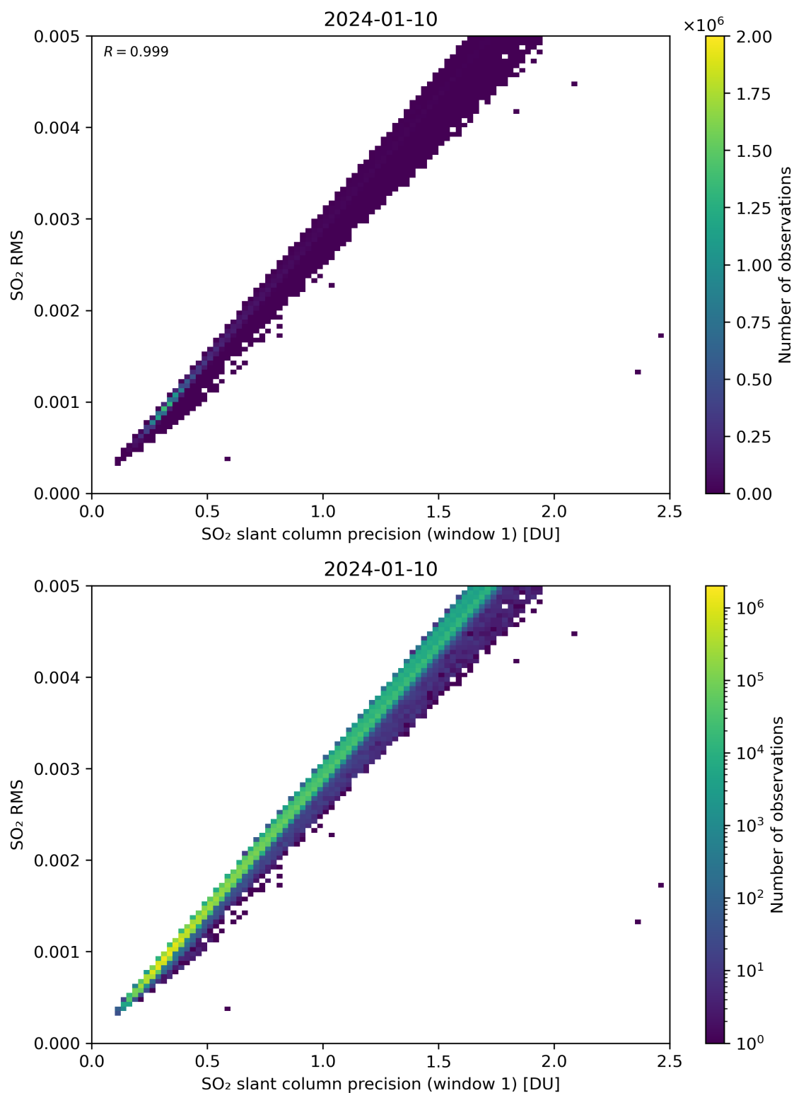
Figure 223: Scatter density plot of “SO 2 slant column precision (window 1)” against “SO 2 RMS” for 2024-01-10 to 2024-01-11.
