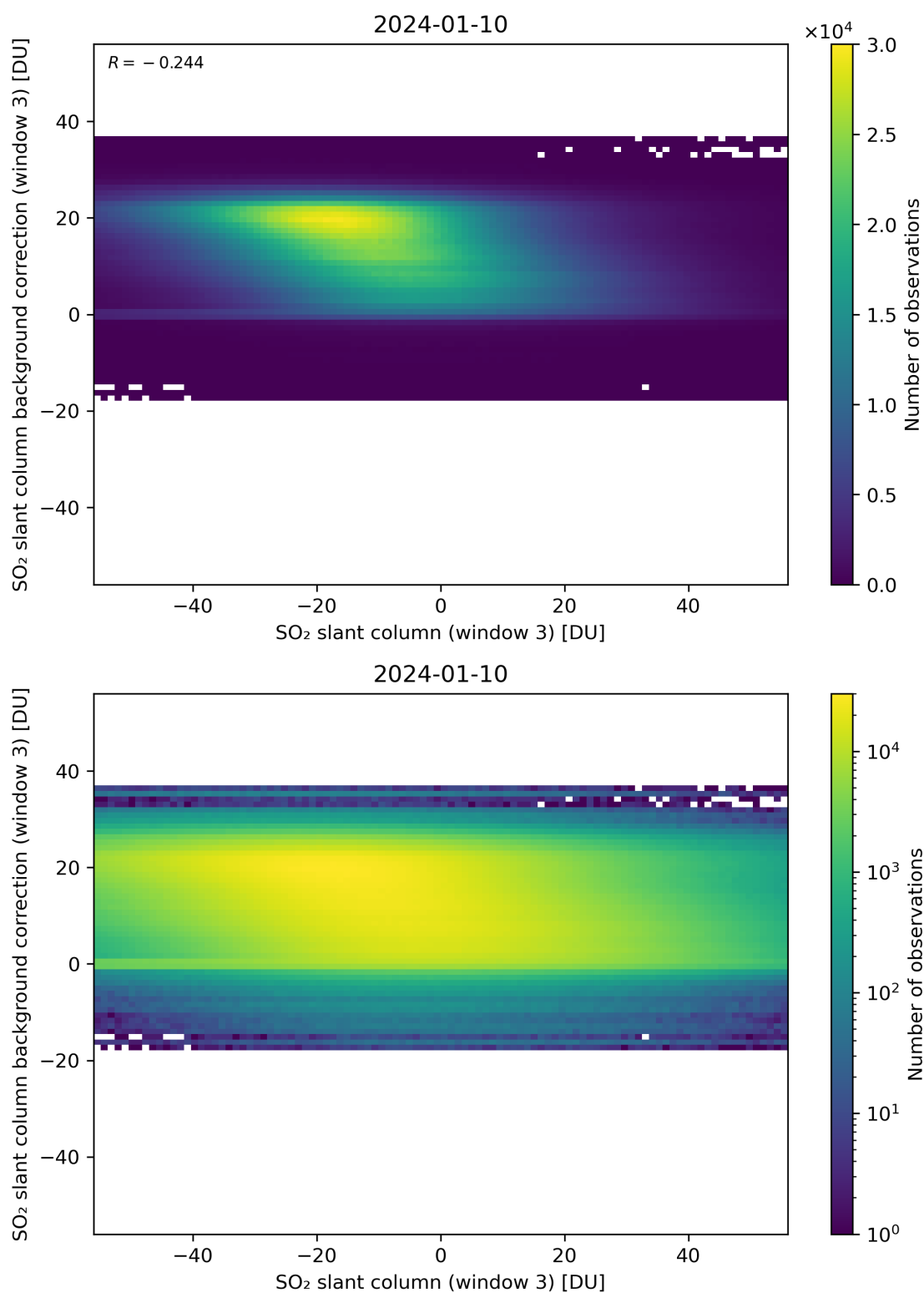
Figure 253: Scatter density plot of “SO 2 slant column (window 3)” against “SO 2 slant column background correction (window 3)” for 2024-01-10 to 2024-01-11.
