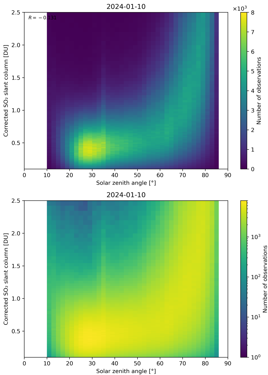
Figure 166: Scatter density plot of “Solar zenith angle” against “Corrected SO 2 slant column” for 2024-01-10 to 2024-01-11.
