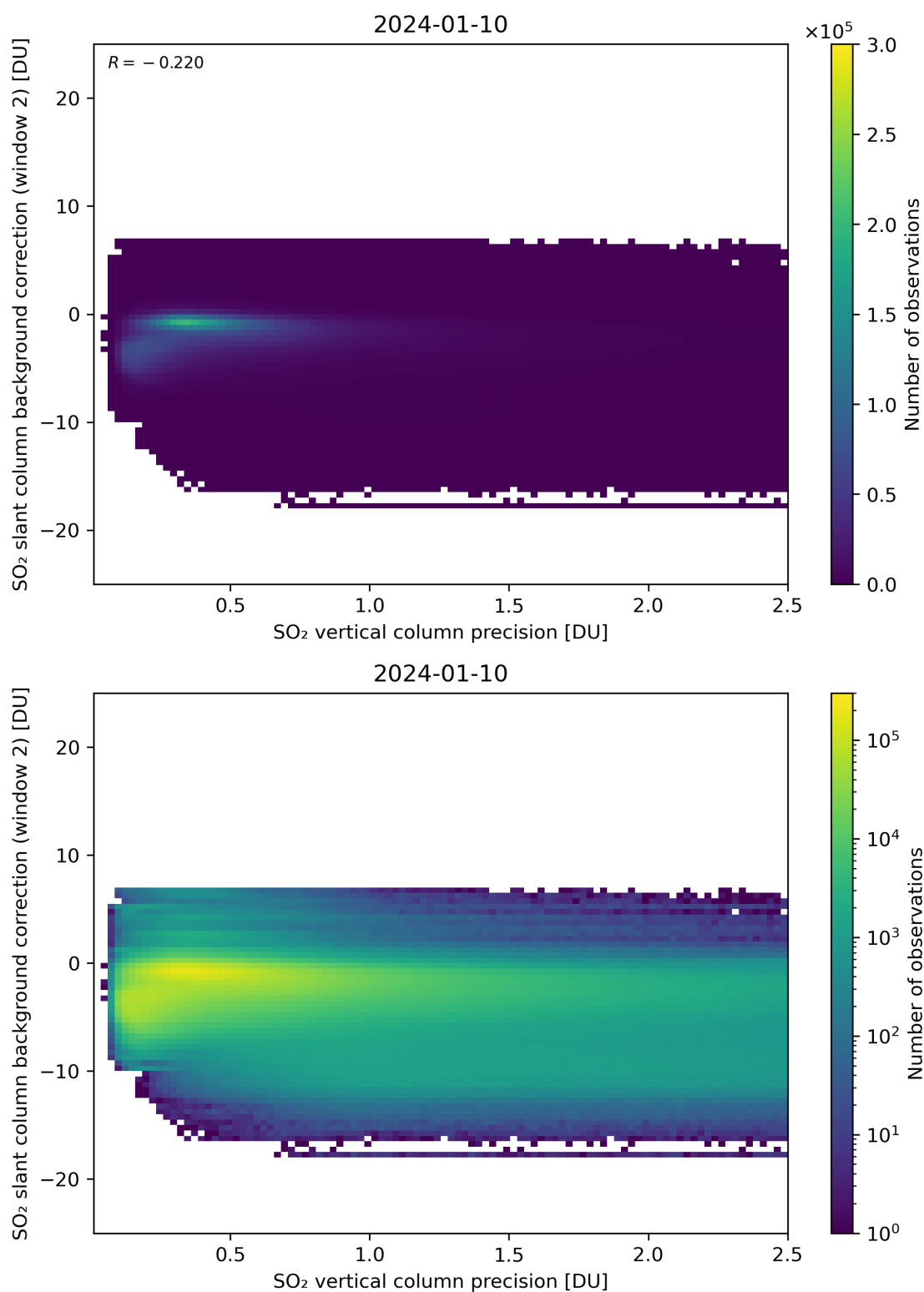
Figure 280: Scatter density plot of “SO 2 vertical column precision” against “SO 2 slant column background correction (window 2)” for 2024-01-10 to 2024-01-11.
