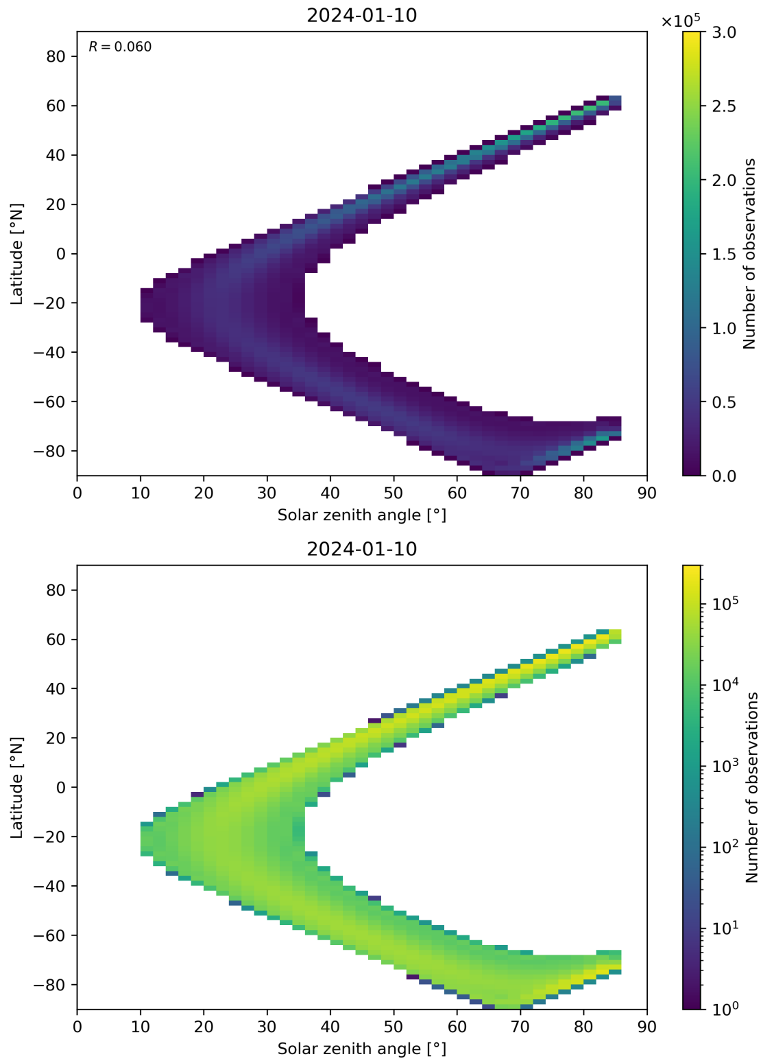
Figure 164: Scatter density plot of “Solar zenith angle” against “Latitude” for 2024-01-10 to 2024-01-11.
