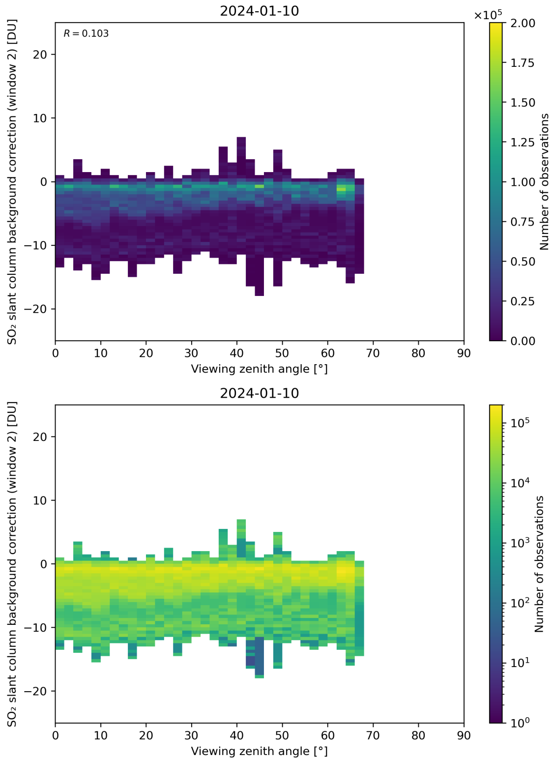
Figure 309: Scatter density plot of “Viewing zenith angle” against “SO 2 slant column background correction (window 2)” for 2024-01-10 to 2024-01-11.
