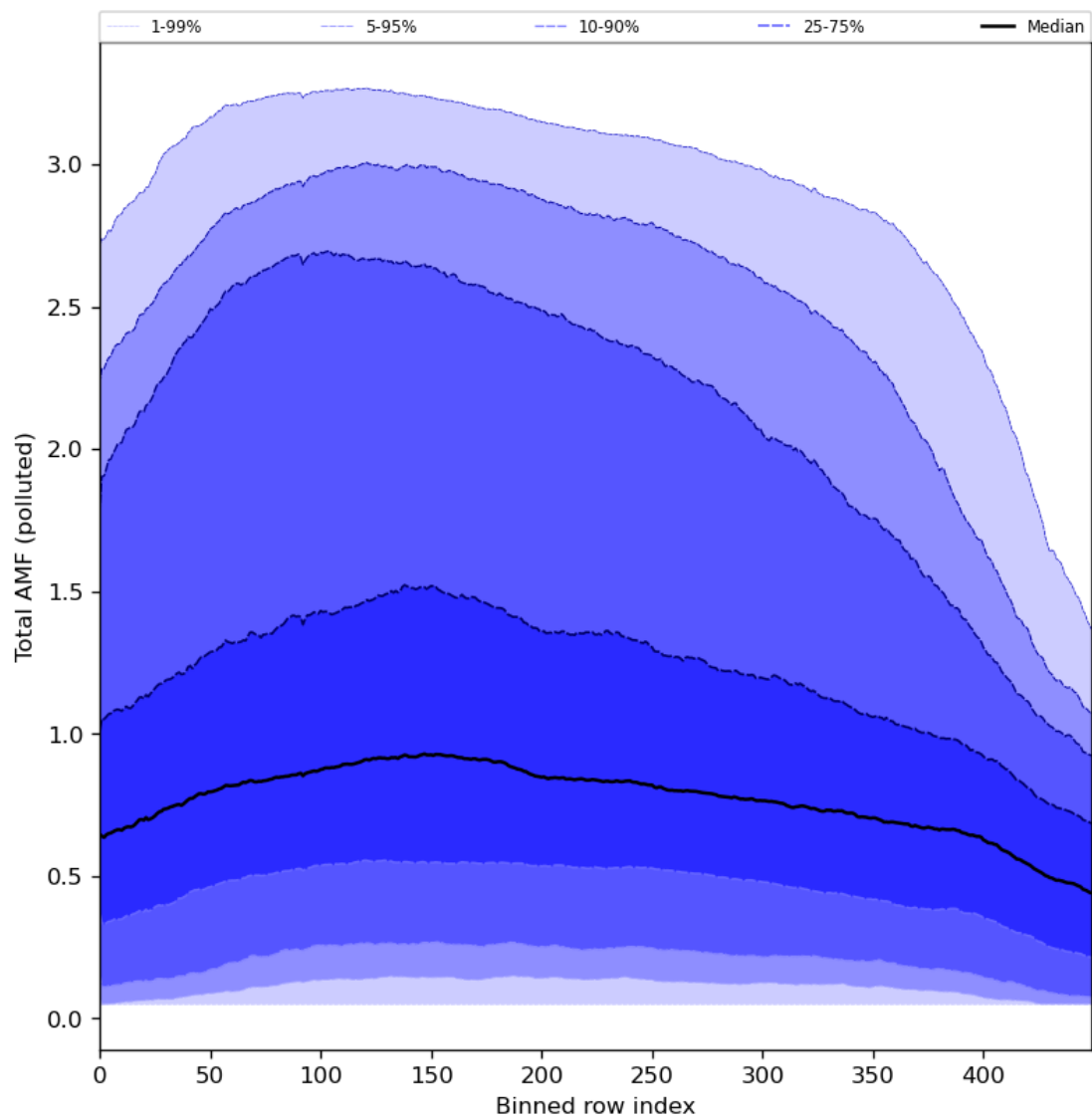
Figure 94: Along track statistics of “Total AMF (polluted)” for 2024-01-10 to 2024-01-11
