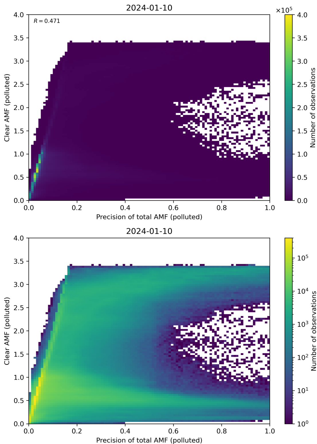
Figure 270: Scatter density plot of “Precision of total AMF (polluted)” against “Clear AMF (polluted)” for 2024-01-10 to 2024-01-11.
