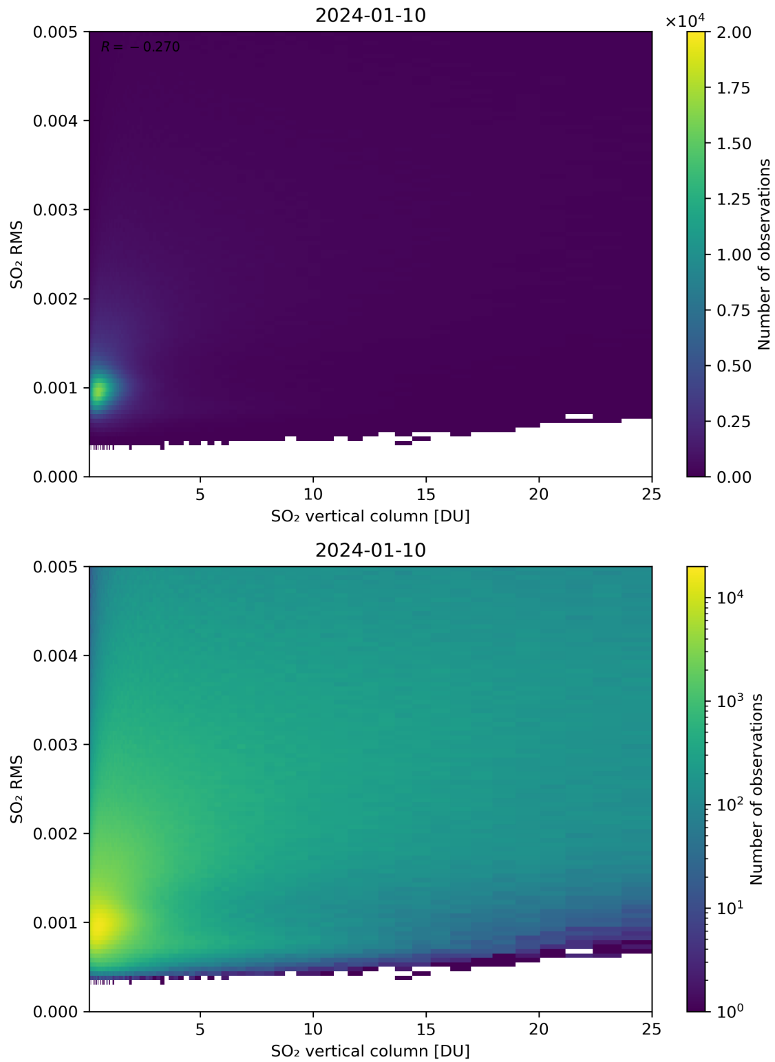
Figure 278: Scatter density plot of “SO 2 vertical column” against “SO 2 RMS” for 2024-01-10 to 2024-01-11.
