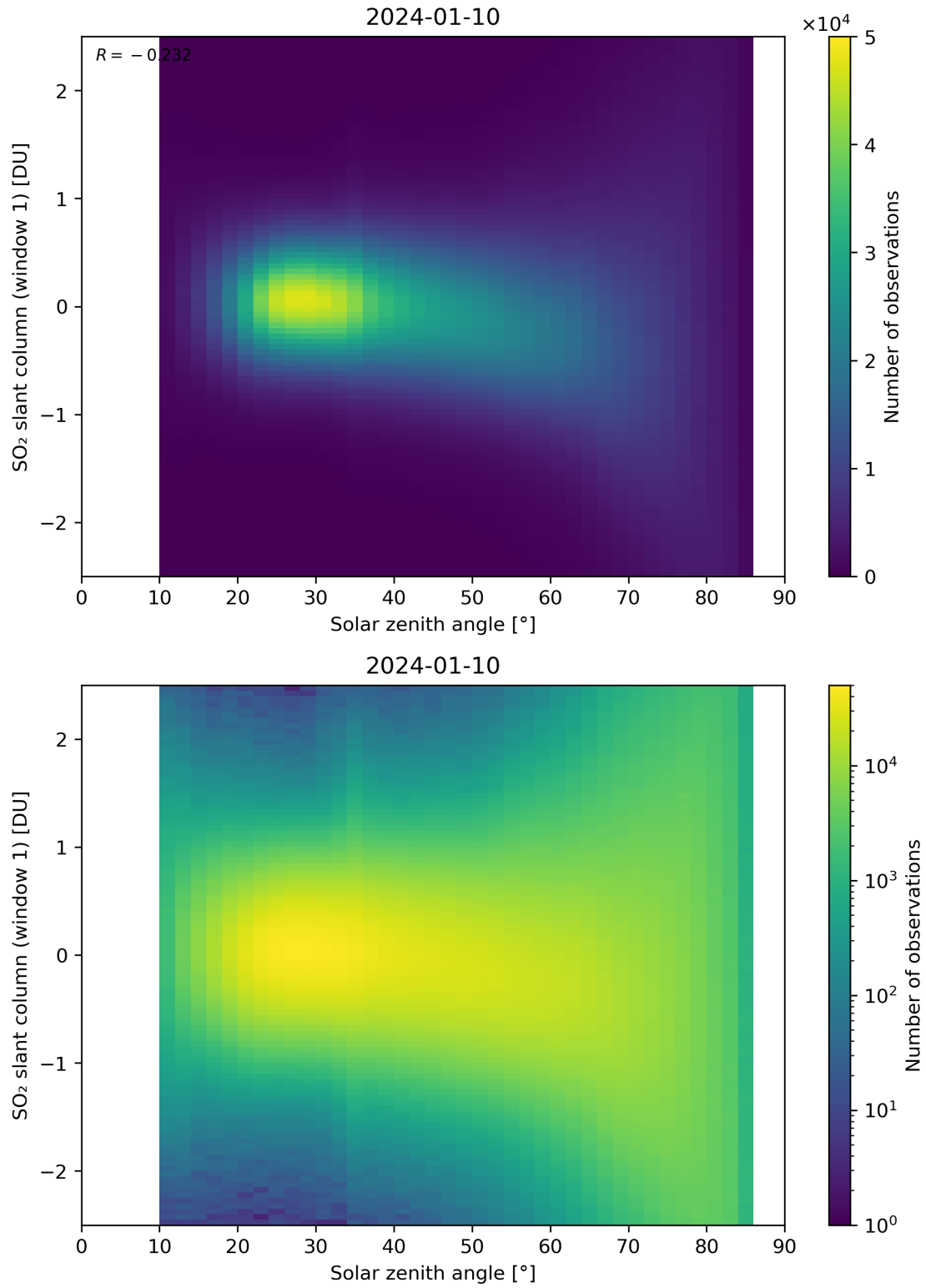
Figure 169: Scatter density plot of “Solar zenith angle” against “SO 2 slant column (window 1)” for 2024-01-10 to 2024-01-11.
