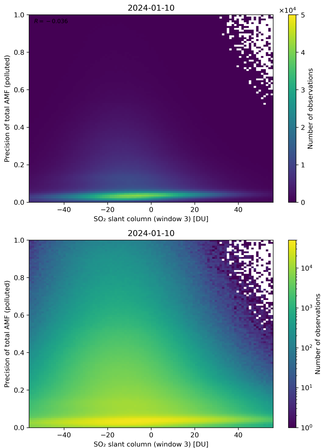
Figure 269: Scatter density plot of “SO 2 slant column (window 3)” against “Precision of total AMF (polluted)” for 2024-01-10 to 2024-01-11.
