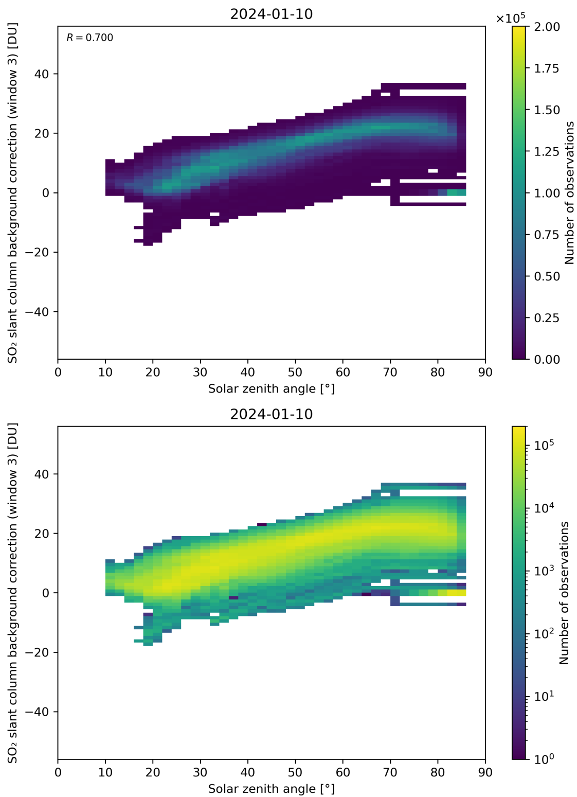
Figure 160: Scatter density plot of “Solar zenith angle” against “SO 2 slant column background correction (window 3)” for 2024-01-10 to 2024-01-11.
