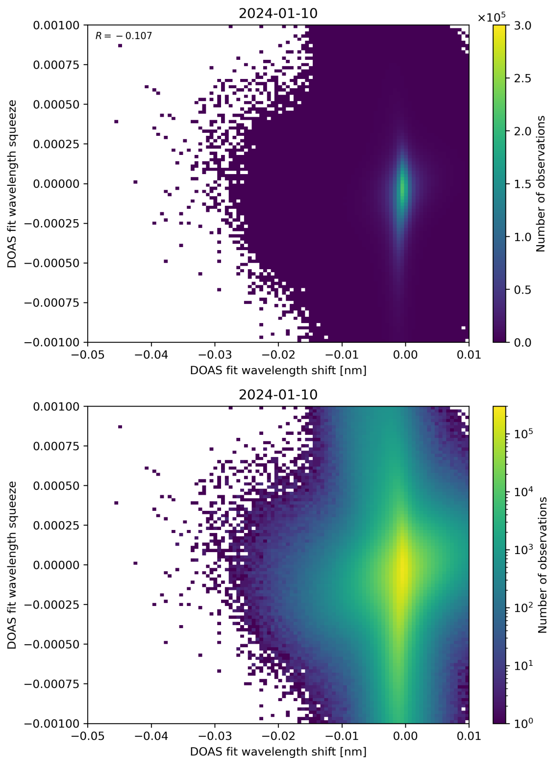
Figure 127: Scatter density plot of “DOAS fit wavelength shift” against “DOAS fit wavelength squeeze” for 2024-01-10 to 2024-01-11.
