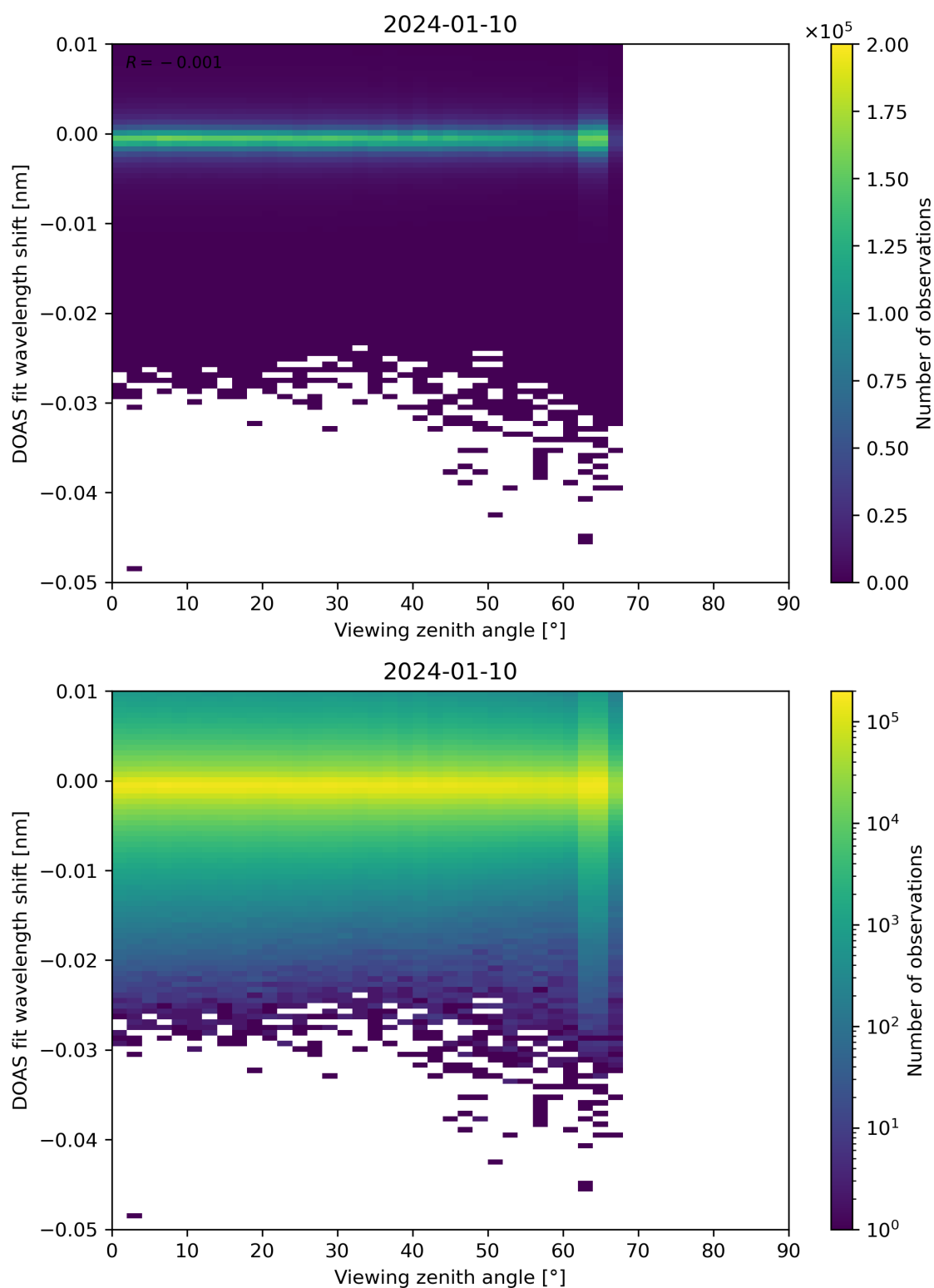
Figure 311: Scatter density plot of “Viewing zenith angle” against “DOAS fit wavelength shift” for 2024-01-10 to 2024-01-11.
