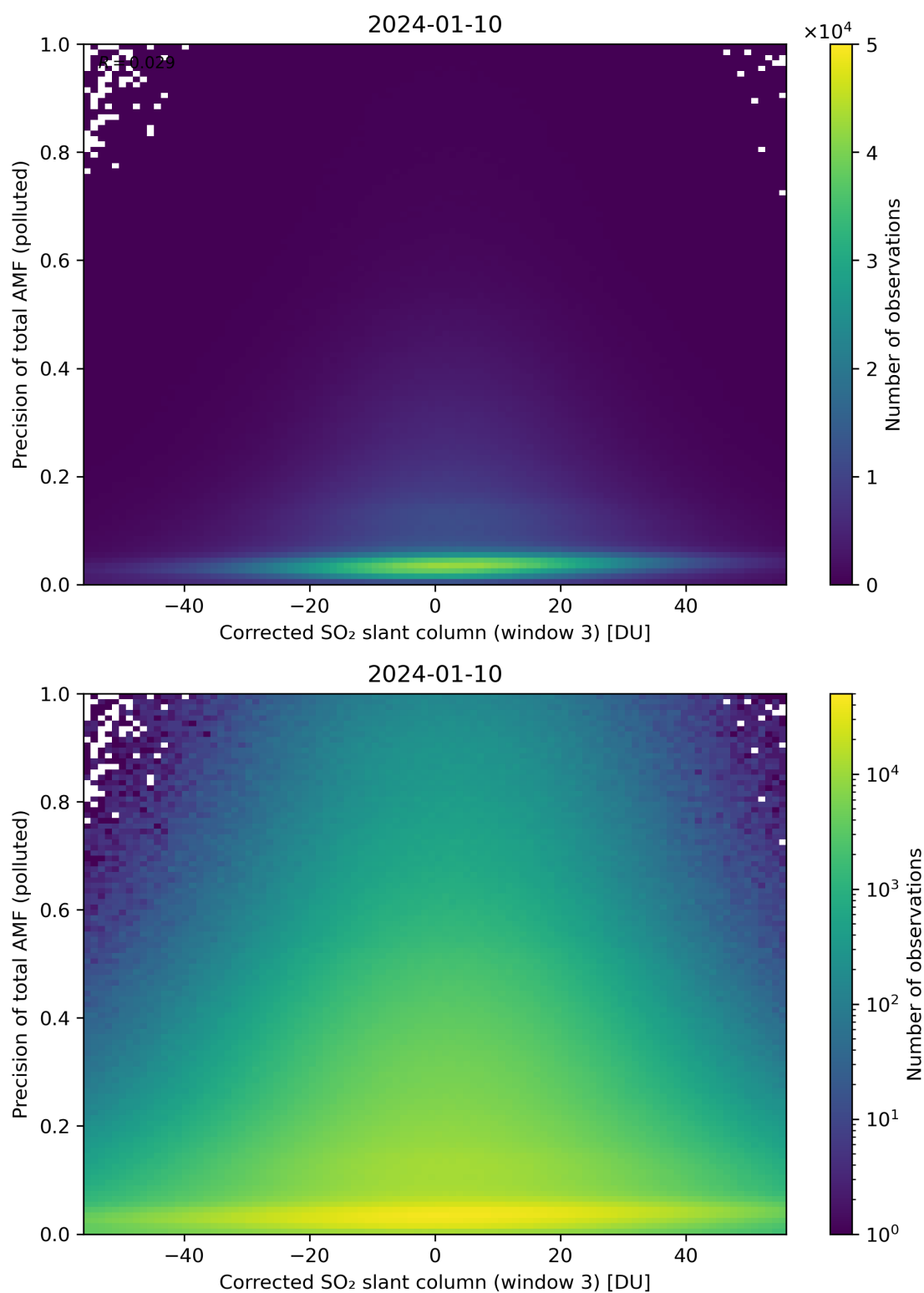
Figure 211: Scatter density plot of “Corrected SO 2 slant column (window 3)” against “Precision of total AMF (polluted)” for 2024-01-10 to 2024-01-11.
