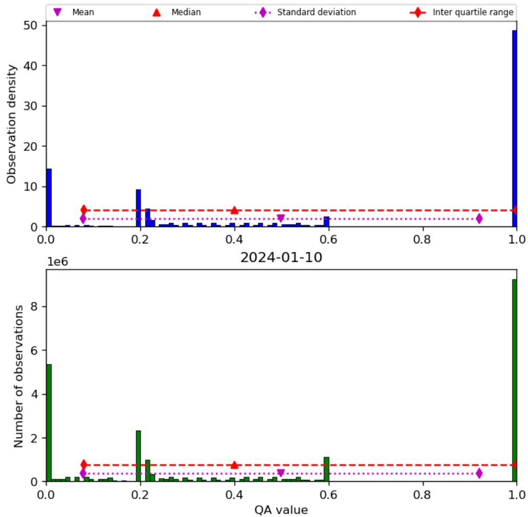
Figure 52: Histogram of “QA value” for 2024-01-10 to 2024-01-11
