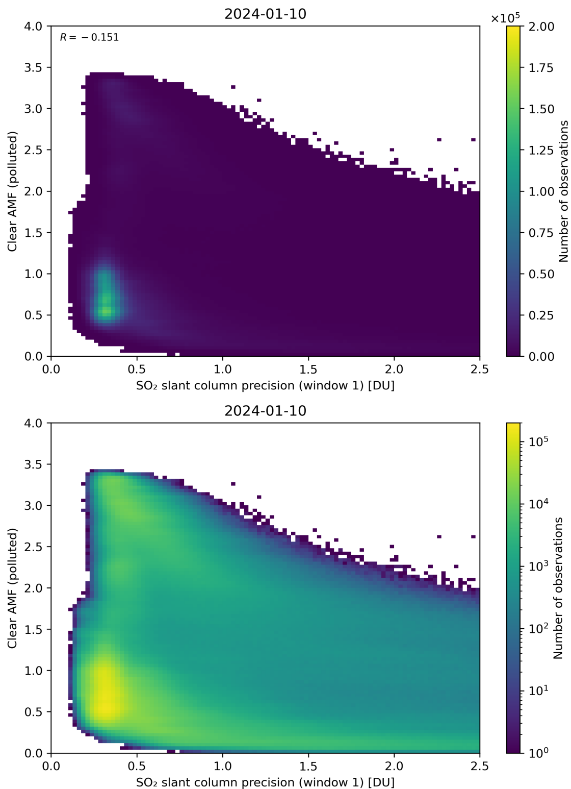
Figure 224: Scatter density plot of “SO 2 slant column precision (window 1)” against “Clear AMF (polluted)” for 2024-01-10 to 2024-01-11.
