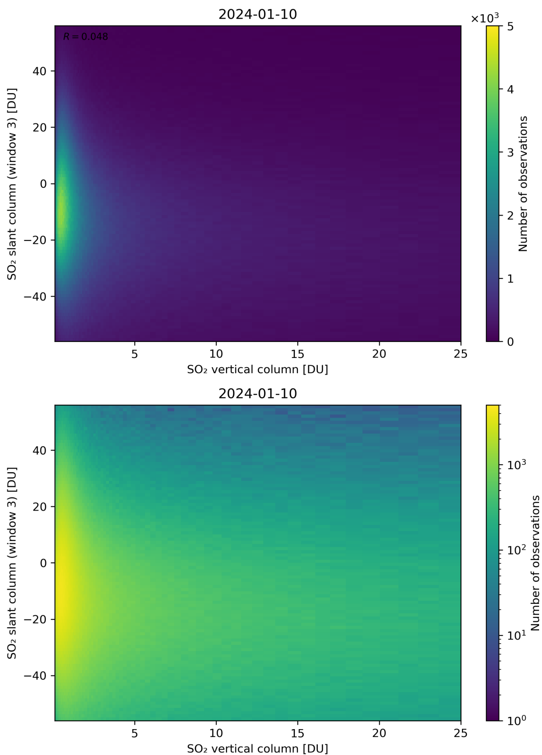
Figure 303: Scatter density plot of “SO 2 vertical column” against “SO 2 slant column (window 3)” for 2024-01-10 to 2024-01-11.
