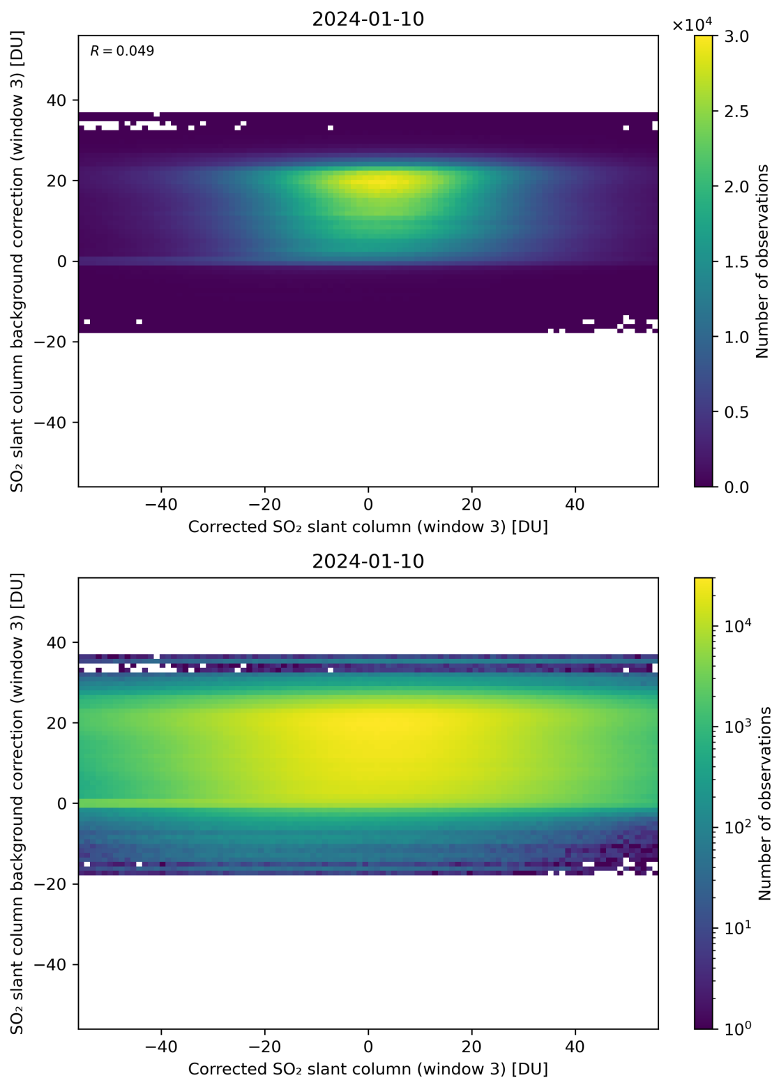
Figure 205: Scatter density plot of “Corrected SO 2 slant column (window 3)” against “SO 2 slant column background correction (window 3)” for 2024-01-10 to 2024-01-11.
