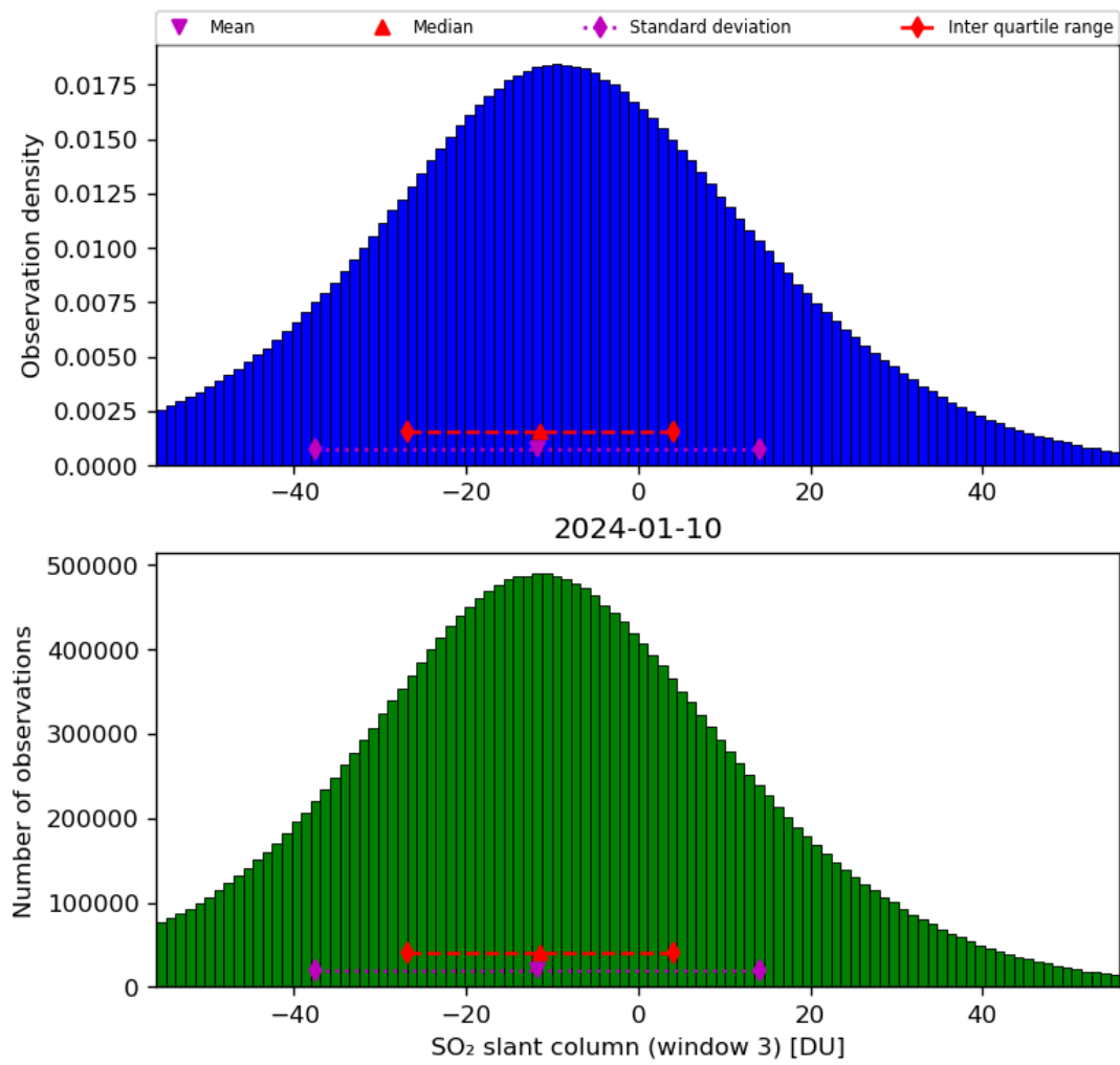
Figure 64: Histogram of “SO 2 slant column (window 3)” for 2024-01-10 to 2024-01-11
