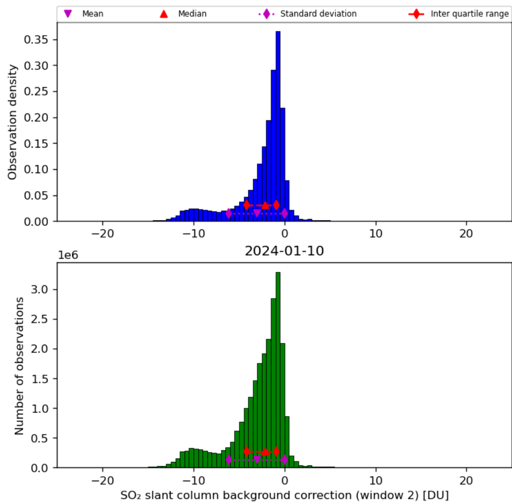
Figure 63: Histogram of “SO 2 slant column background correction (window 2)” for 2024-01-10 to 2024-01-11
