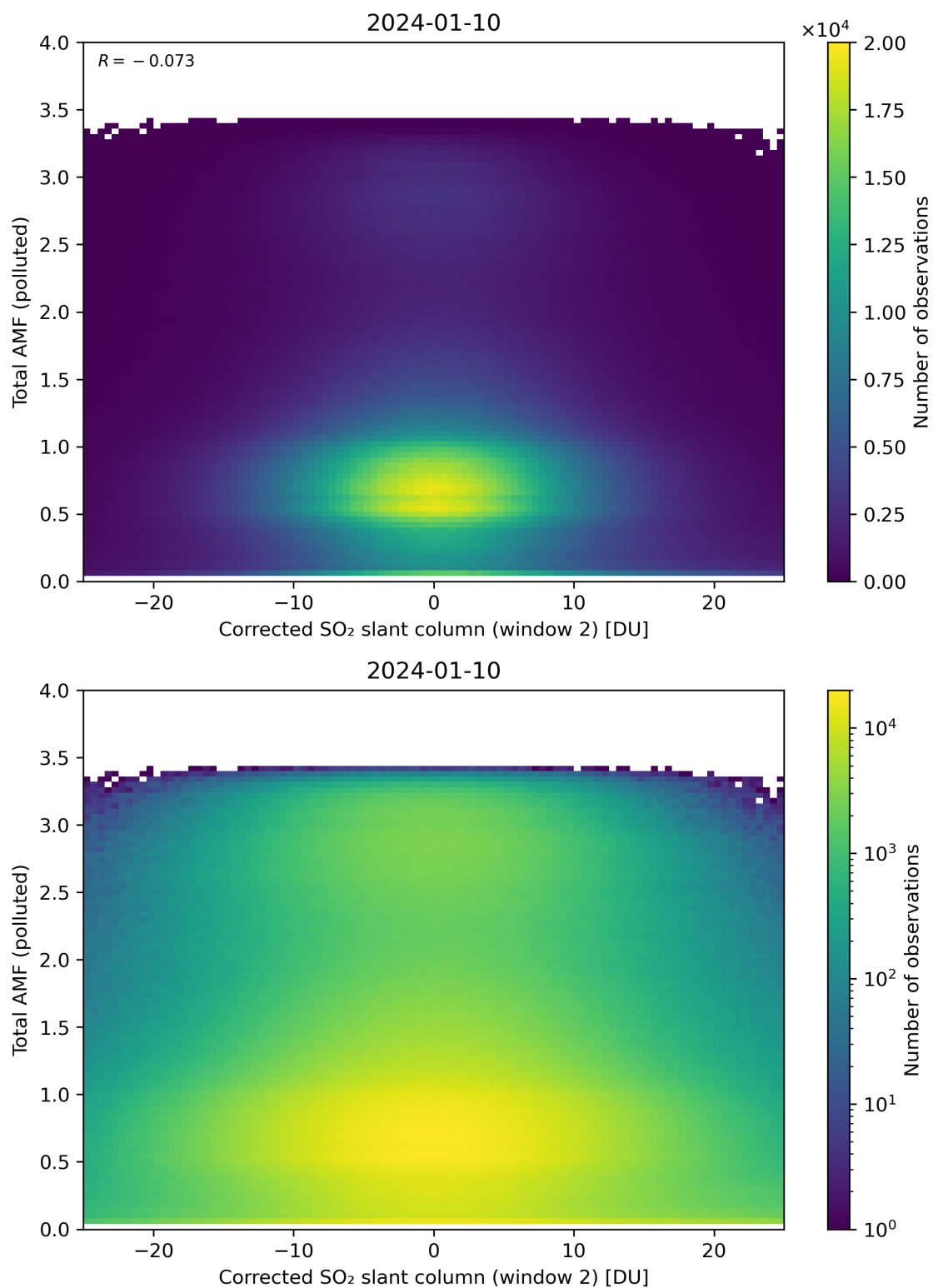
Figure 203: Scatter density plot of “Corrected SO 2 slant column (window 2)” against “Total AMF (polluted)” for 2024-01-10 to 2024-01-11.
