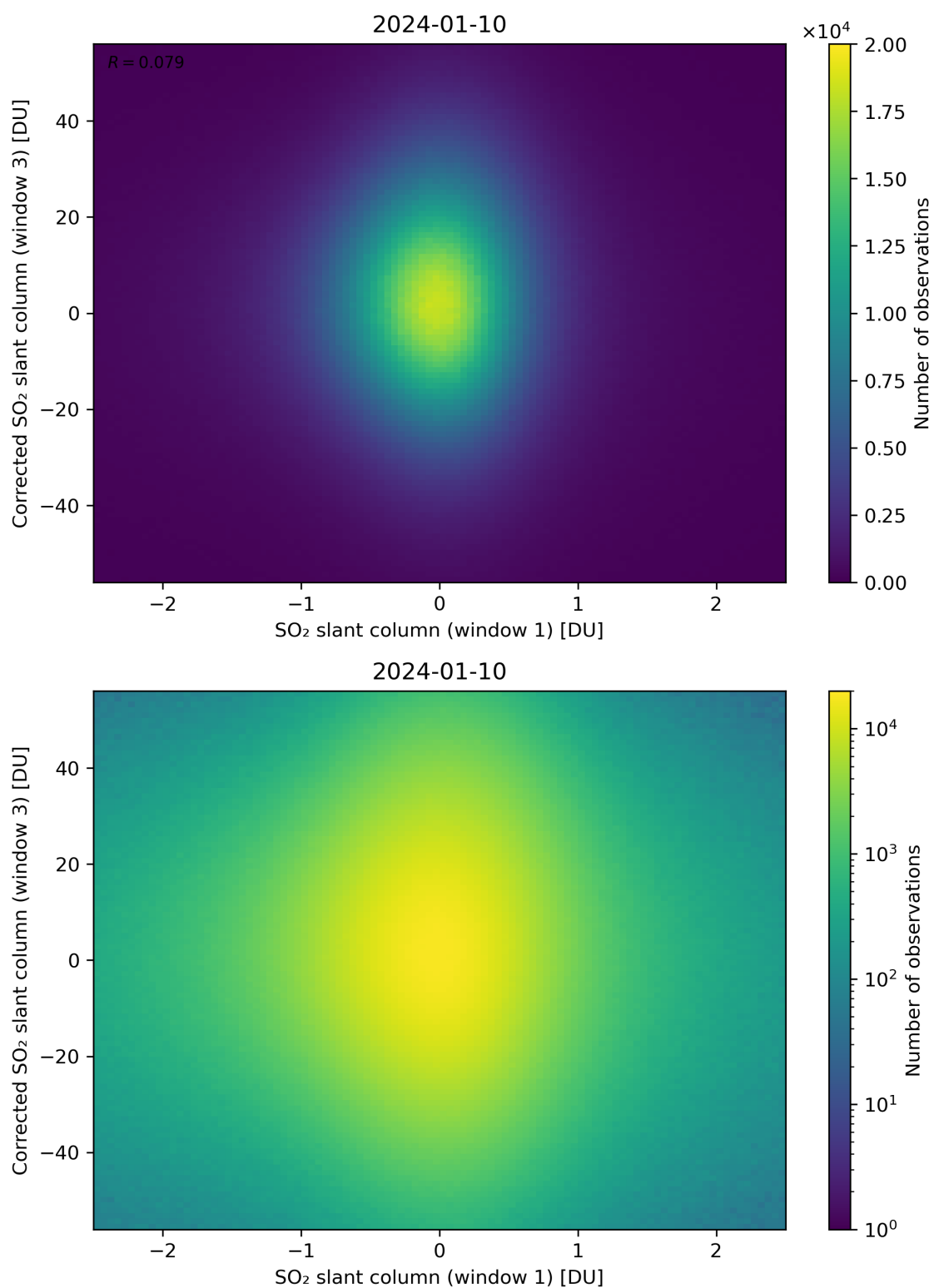
Figure 234: Scatter density plot of “SO 2 slant column (window 1)” against “Corrected SO 2 slant column (window 3)” for 2024-01-10 to 2024-01-11.
