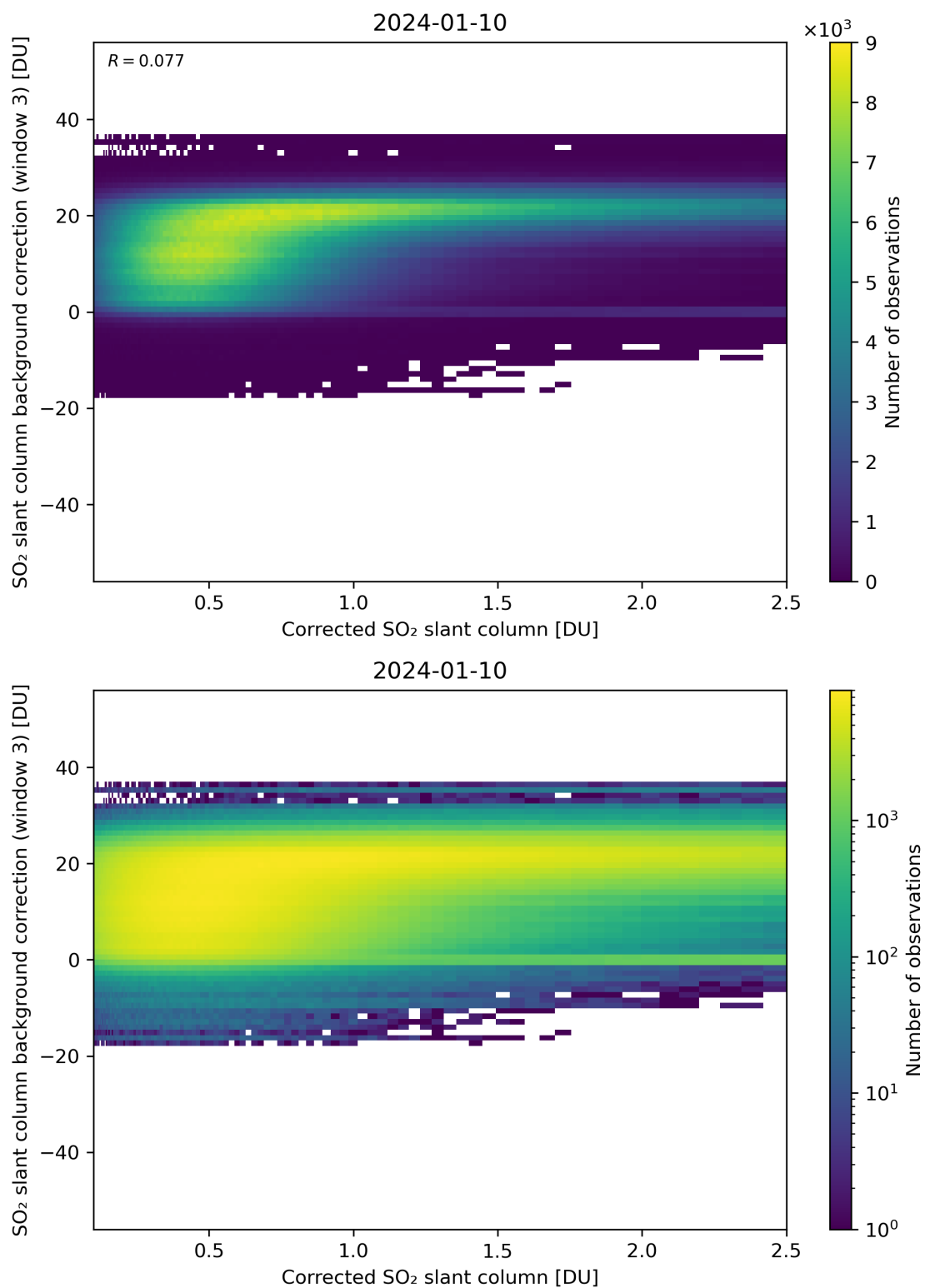
Figure 180: Scatter density plot of “Corrected SO 2 slant column” against “SO 2 slant column background correction (window 3)” for 2024-01-10 to 2024-01-11.
