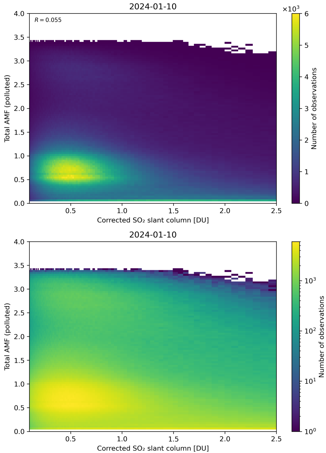
Figure 192: Scatter density plot of “Corrected SO 2 slant column” against “Total AMF (polluted)” for 2024-01-10 to 2024-01-11.
