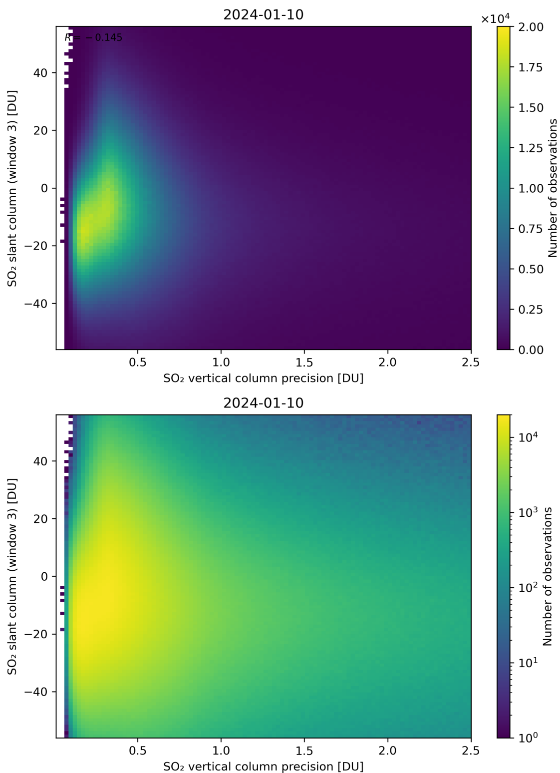
Figure 292: Scatter density plot of “SO 2 vertical column precision” against “SO 2 slant column (window 3)” for 2024-01-10 to 2024-01-11.
