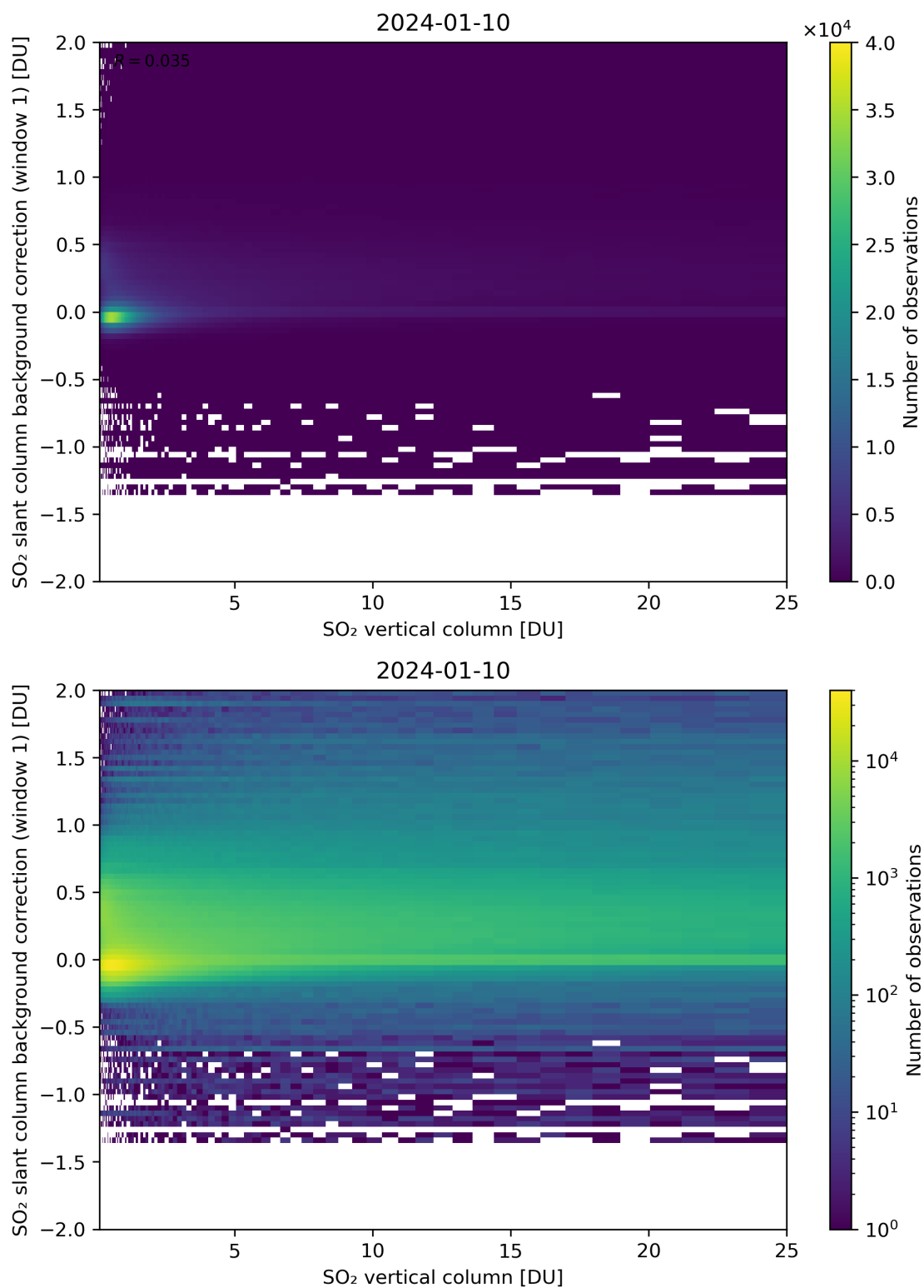
Figure 273: Scatter density plot of “SO 2 vertical column” against “SO 2 slant column background correction (window 1)” for 2024-01-10 to 2024-01-11.
