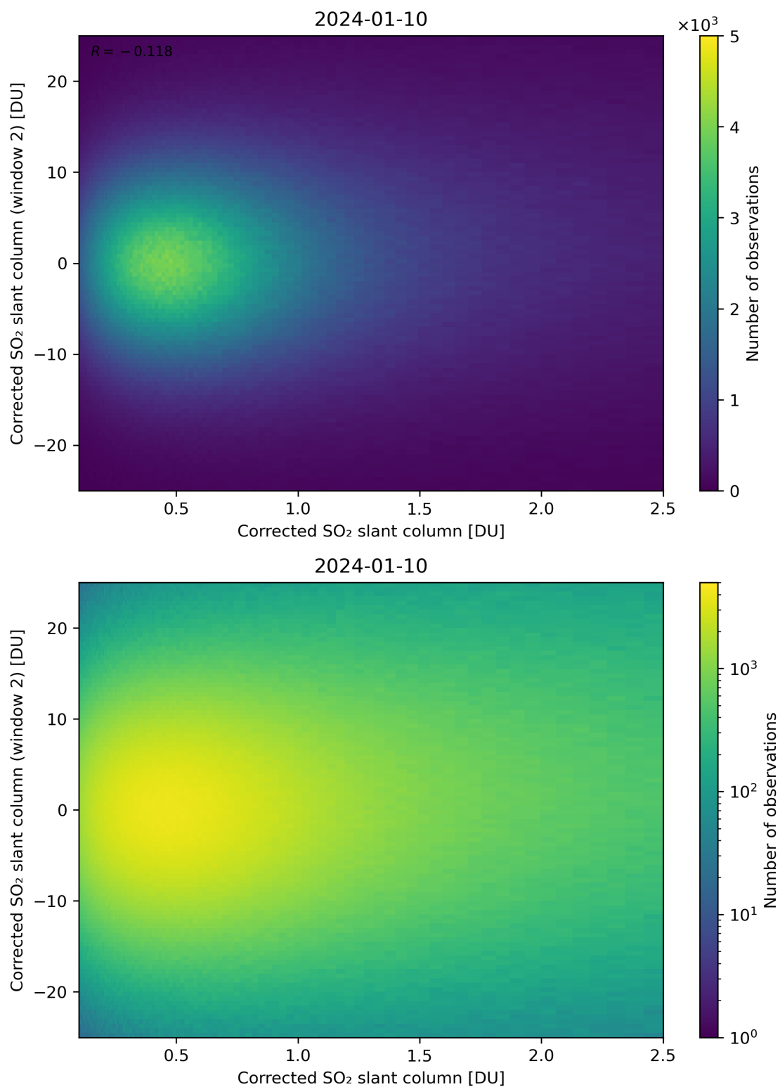
Figure 185: Scatter density plot of “Corrected SO 2 slant column” against “Corrected SO 2 slant column (window 2)” for 2024-01-10 to 2024-01-11.
