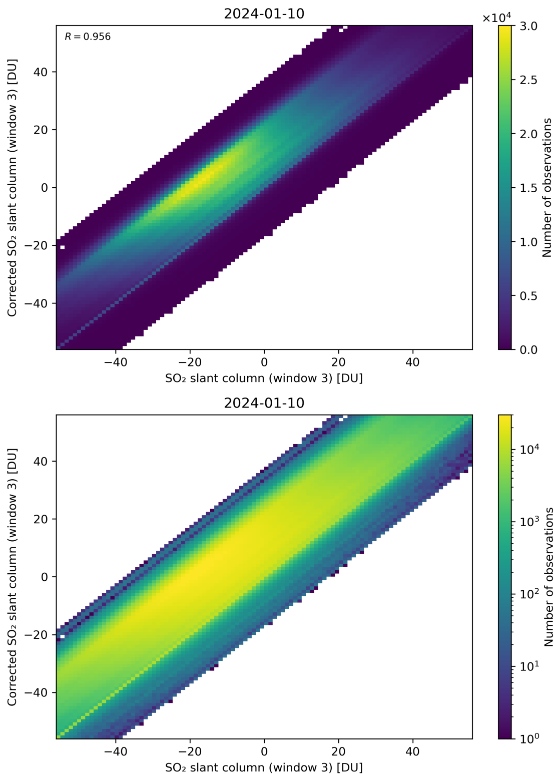
Figure 266: Scatter density plot of “SO 2 slant column (window 3)” against “Corrected SO 2 slant column (window 3)” for 2024-01-10 to 2024-01-11.
