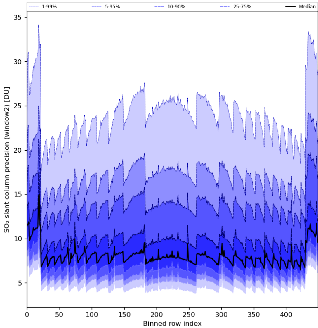
Figure 84: Along track statistics of “SO 2 slant column precision (window2)” for 2024-01-10 to 2024-01-11
