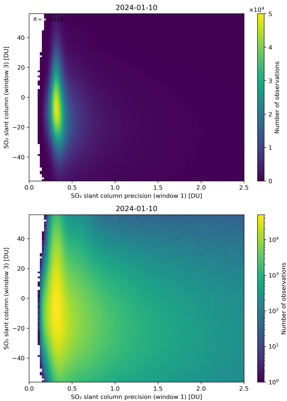
Figure 228: Scatter density plot of “SO 2 slant column precision (window 1)” against “SO 2 slant column (window 3)” for 2024-01-10 to 2024-01-11.
