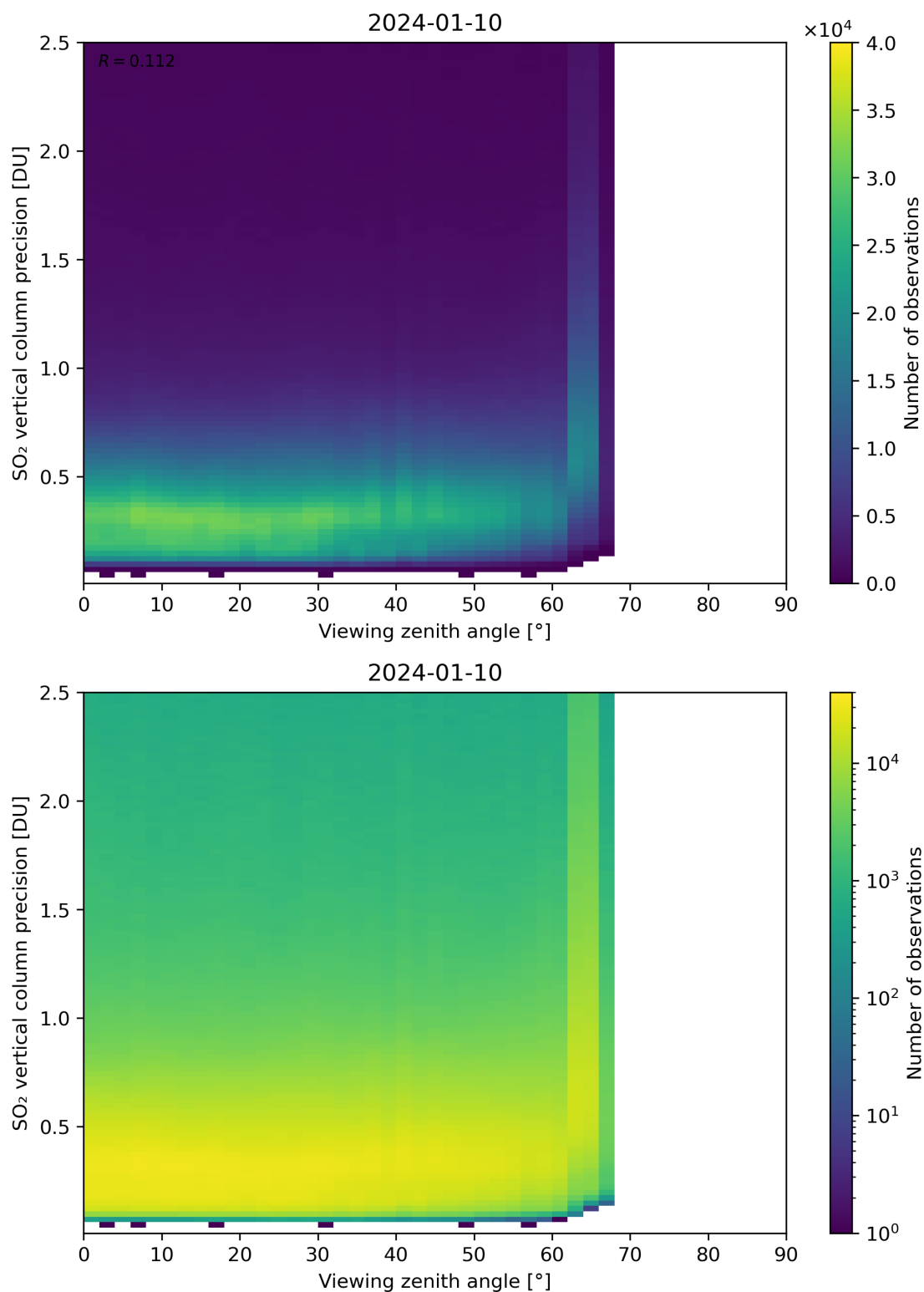
Figure 328: Scatter density plot of “Viewing zenith angle” against “SO 2 vertical column precision” for 2024-01-10 to 2024-01-11.
