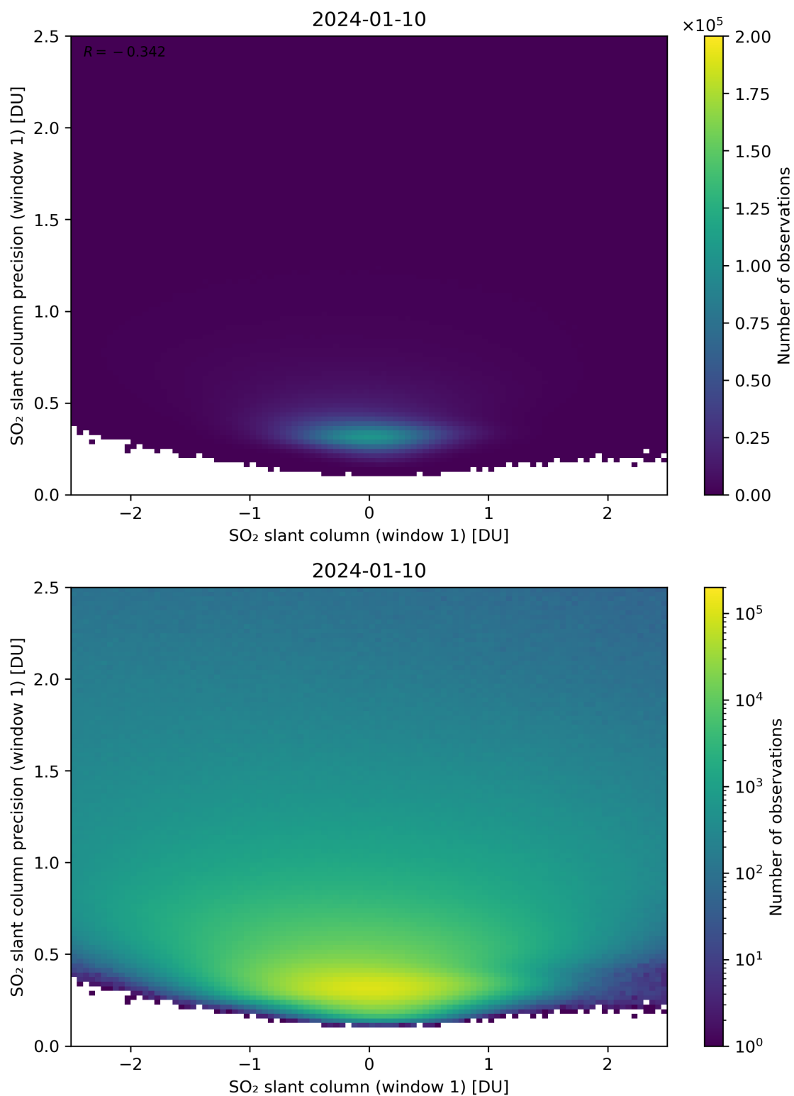
Figure 235: Scatter density plot of “SO 2 slant column (window 1)” against “SO 2 slant column precision (window 1)” for 2024-01-10 to 2024-01-11.
