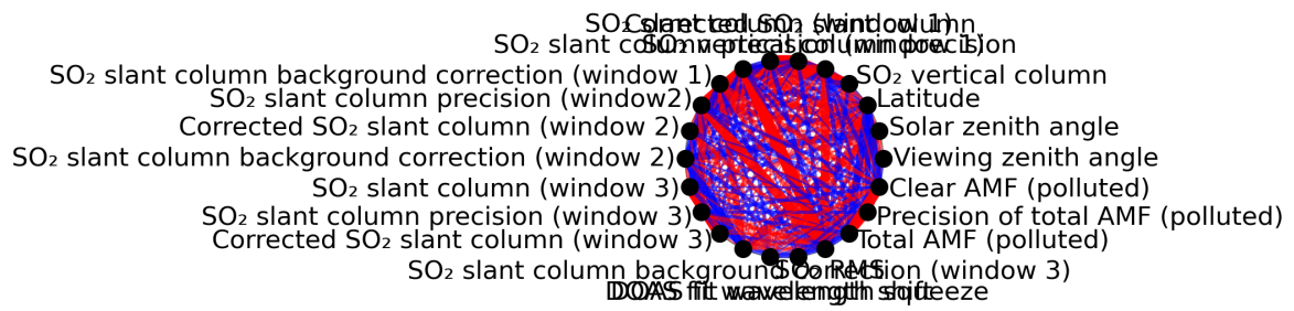
Figure 1: Map of correlation graph for 2024-01-10 to 2024-01-11.
