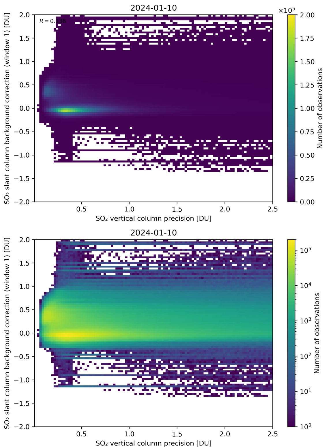
Figure 279: Scatter density plot of “SO 2 vertical column precision” against “SO 2 slant column background correction (window 1)” for 2024-01-10 to 2024-01-11.
