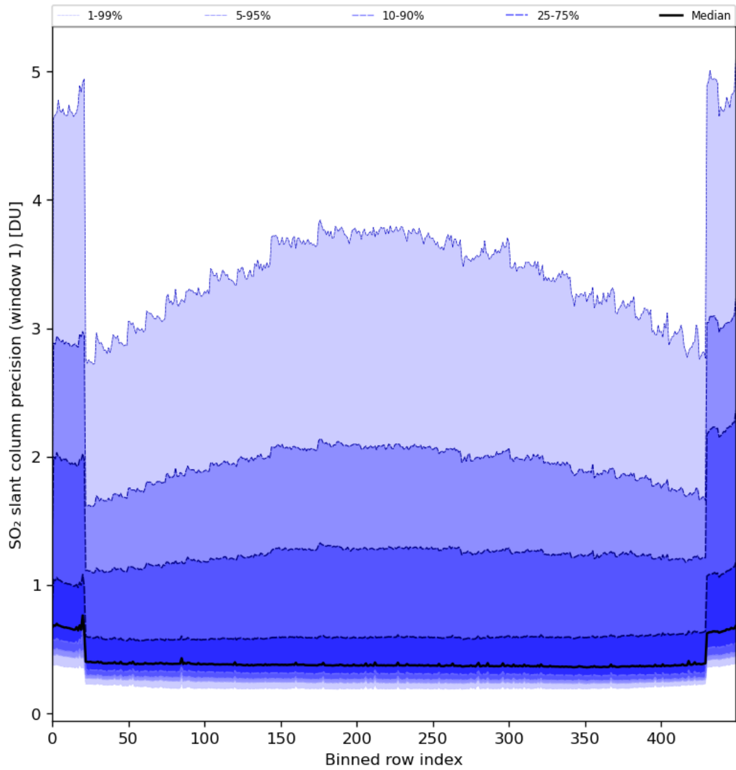
Figure 80: Along track statistics of “SO 2 slant column precision (window 1)” for 2024-01-10 to 2024-01-11
