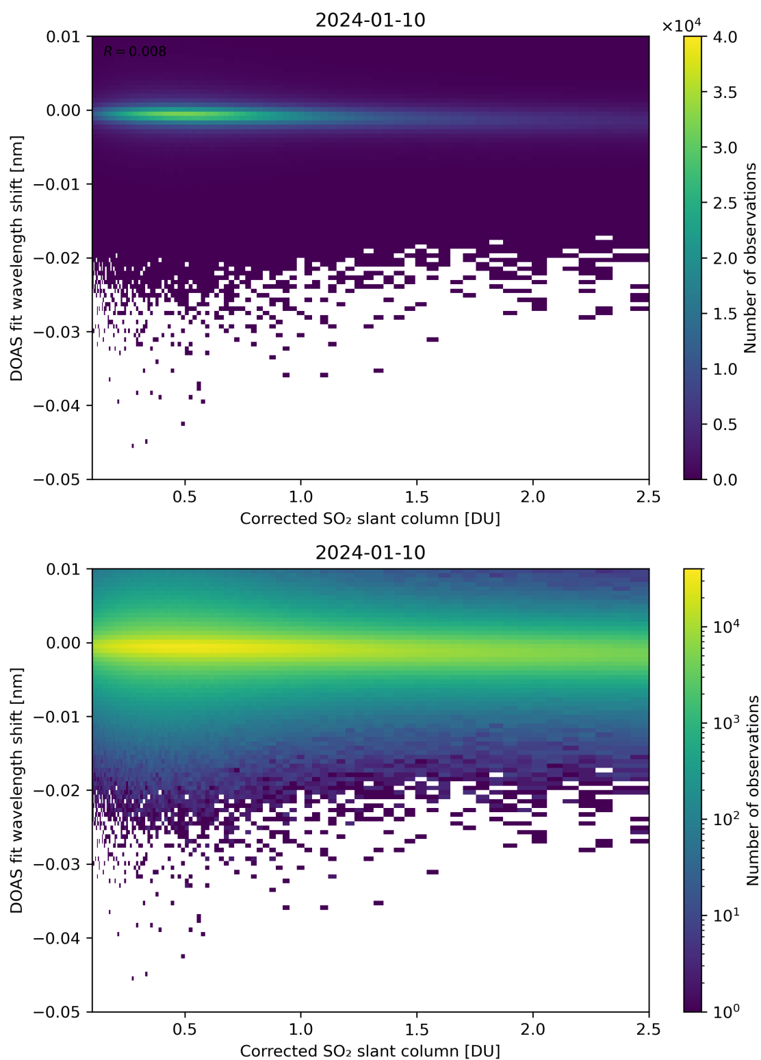
Figure 181: Scatter density plot of “Corrected SO 2 slant column” against “DOAS fit wavelength shift” for 2024-01-10 to 2024-01-11.
