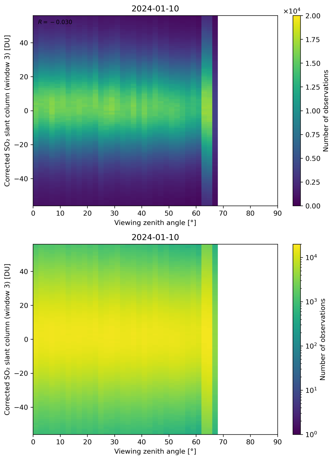
Figure 319: Scatter density plot of “Viewing zenith angle” against “Corrected SO 2 slant column (window 3)” for 2024-01-10 to 2024-01-11.
