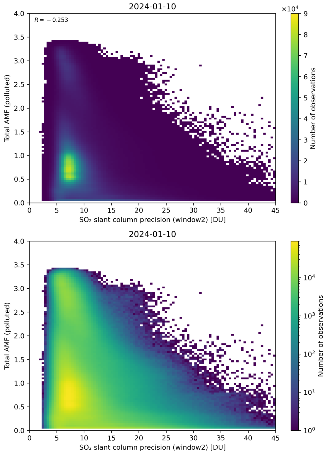
Figure 251: Scatter density plot of “SO 2 slant column precision (window2)” against “Total AMF (polluted)” for 2024-01-10 to 2024-01-11.
