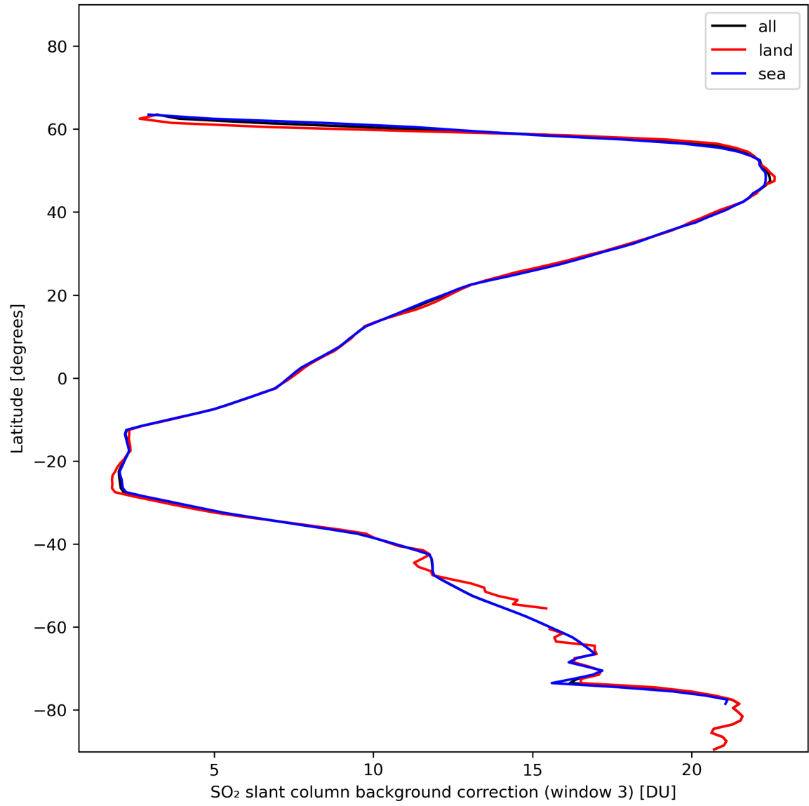
Figure 44: Zonal average of “SO 2 slant column background correction (window 3)” for 2024-01-10 to 2024-01-11.
