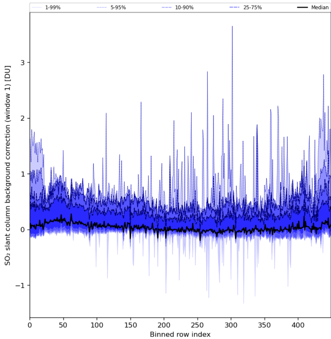
Figure 82: Along track statistics of “SO 2 slant column background correction (window 1)” for 2024-01-10 to 2024-01-11
