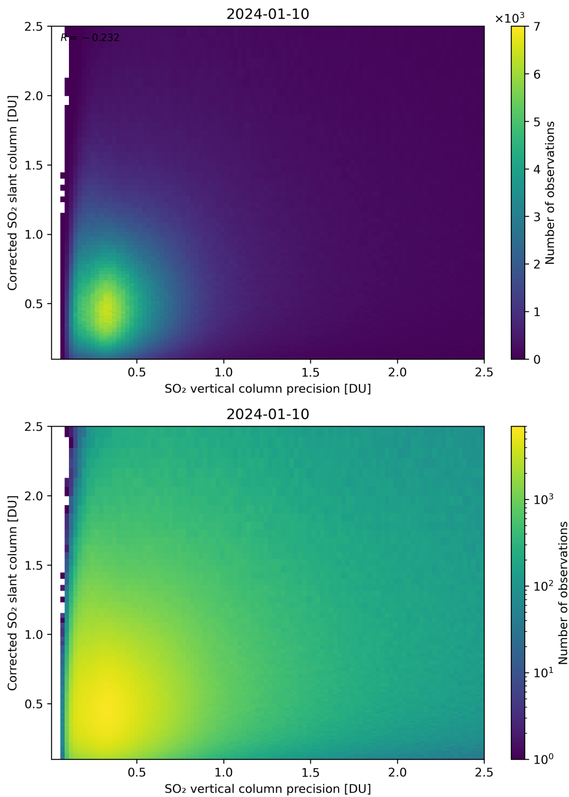
Figure 286: Scatter density plot of “SO 2 vertical column precision” against “Corrected SO 2 slant column” for 2024-01-10 to 2024-01-11.
