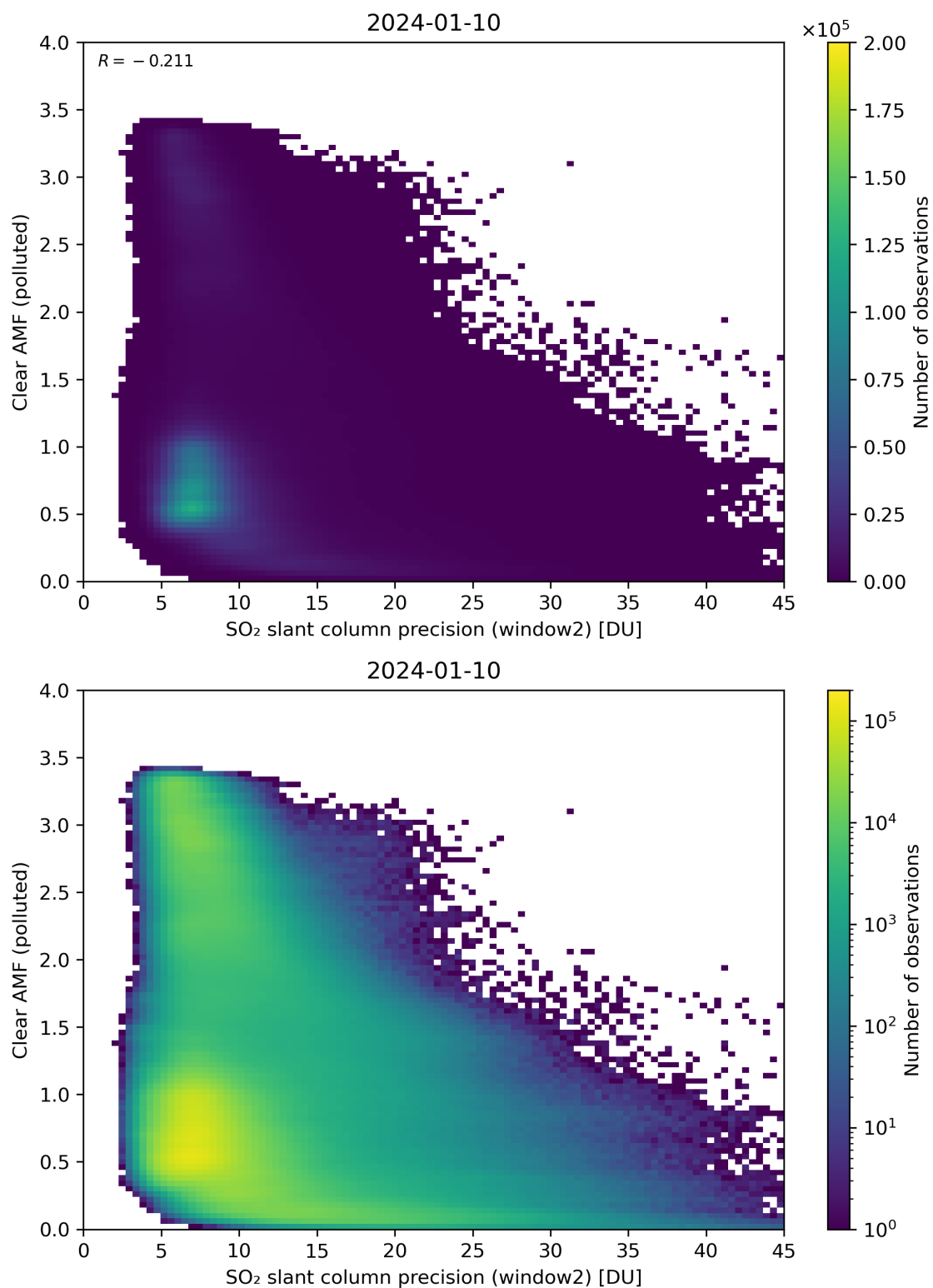
Figure 246: Scatter density plot of “SO 2 slant column precision (window2)” against “Clear AMF (polluted)” for 2024-01-10 to 2024-01-11.
