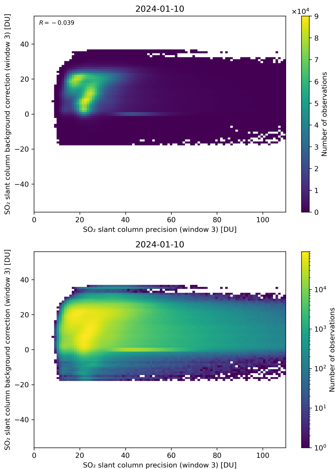
Figure 257: Scatter density plot of “SO 2 slant column precision (window 3)” against “SO 2 slant column background correction (window 3)” for 2024-01-10 to 2024-01-11.
