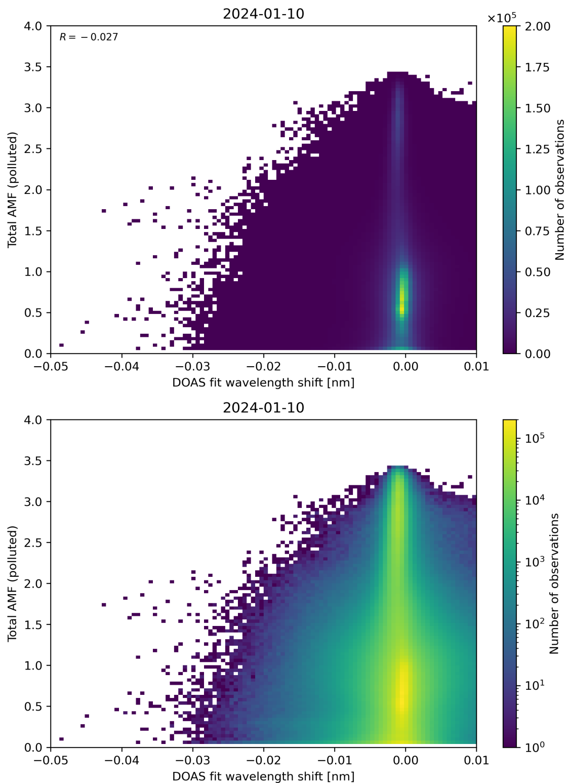
Figure 130: Scatter density plot of “DOAS fit wavelength shift” against “Total AMF (polluted)” for 2024-01-10 to 2024-01-11.
