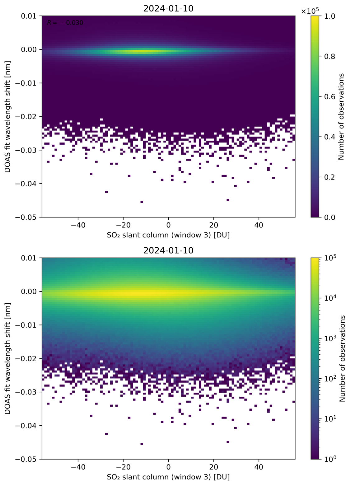
Figure 254: Scatter density plot of “SO 2 slant column (window 3)” against “DOAS fit wavelength shift” for 2024-01-10 to 2024-01-11.
