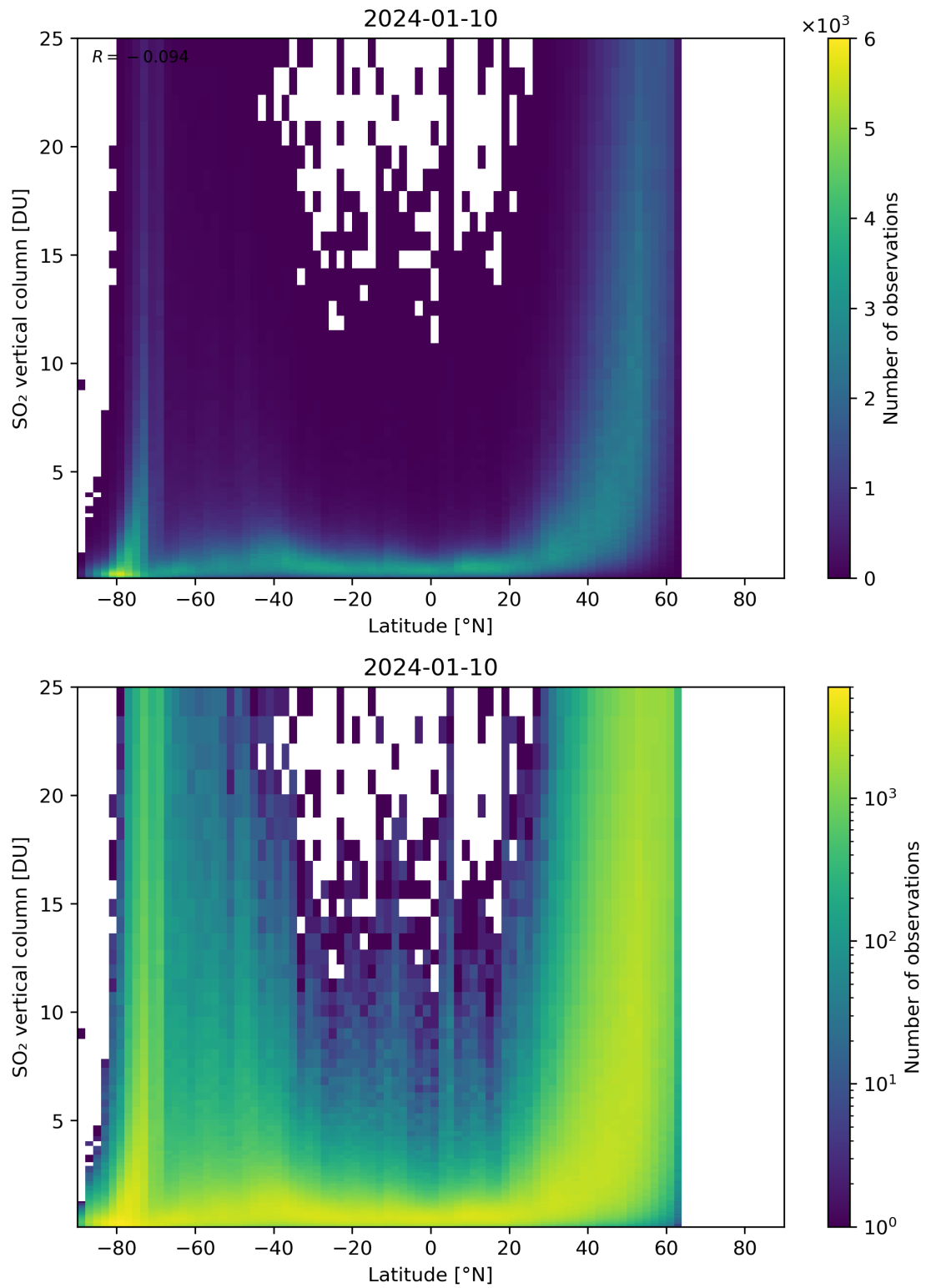
Figure 156: Scatter density plot of “Latitude” against “SO 2 vertical column” for 2024-01-10 to 2024-01-11.
