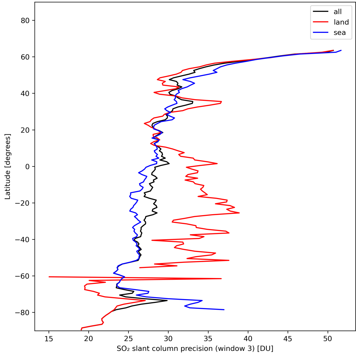
Figure 42: Zonal average of “SO 2 slant column precision (window 3)” for 2024-01-10 to 2024-01-11.
