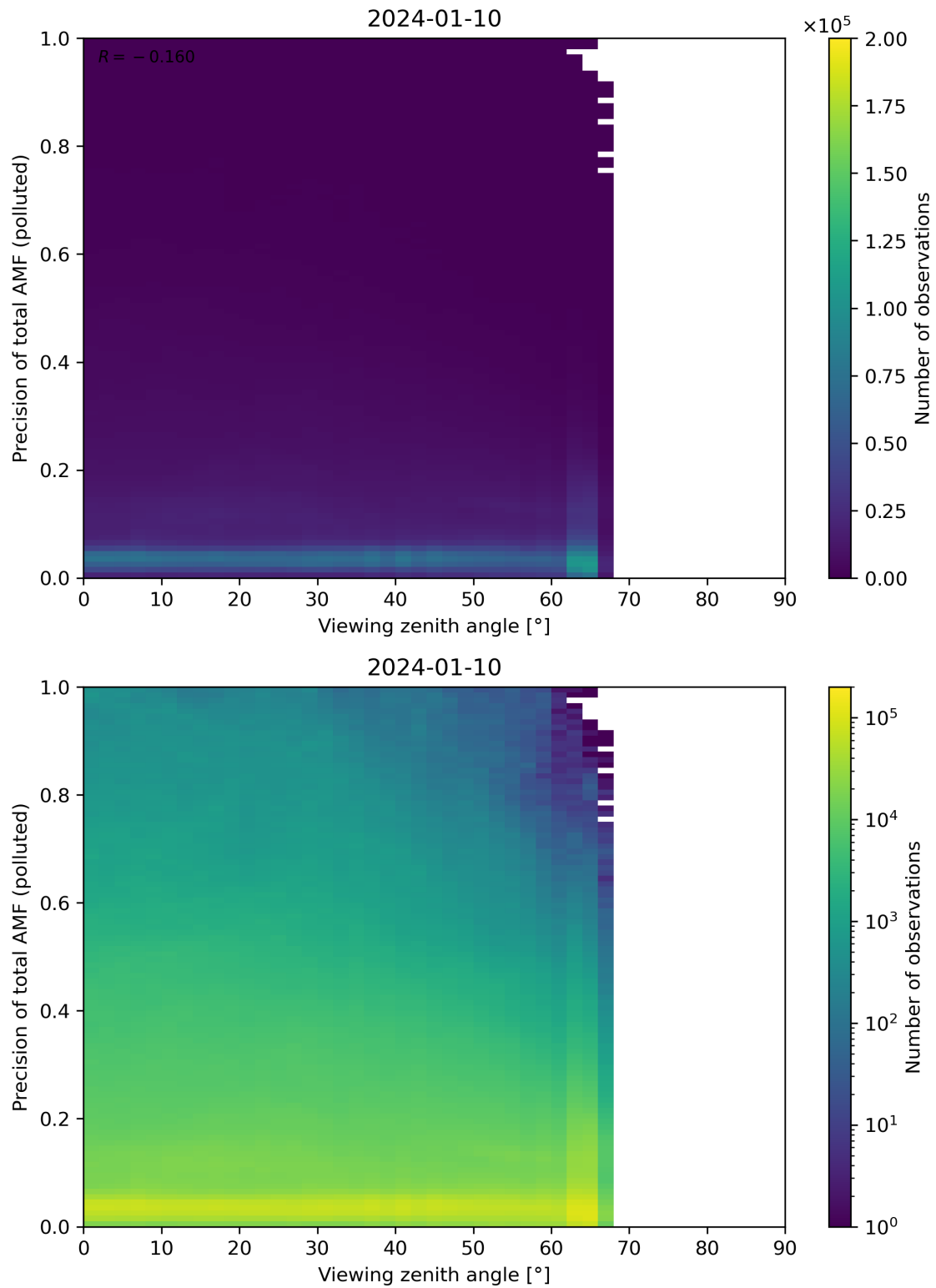
Figure 326: Scatter density plot of “Viewing zenith angle” against “Precision of total AMF (polluted)” for 2024-01-10 to 2024-01-11.
