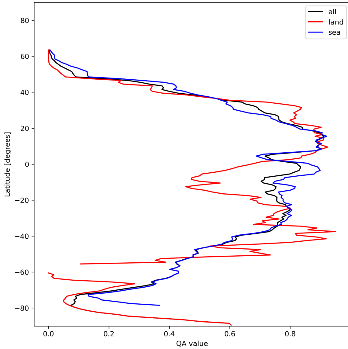
Figure 29: Zonal average of “QA value” for 2024-01-10 to 2024-01-11.
