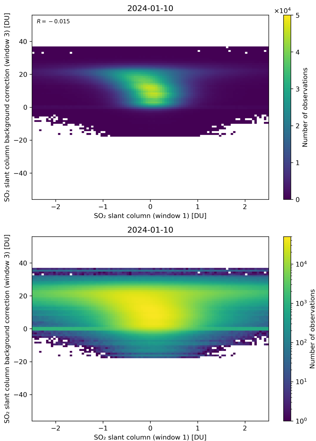
Figure 214: Scatter density plot of “SO 2 slant column (window 1)” against “SO 2 slant column background correction (window 3)” for 2024-01-10 to 2024-01-11.
