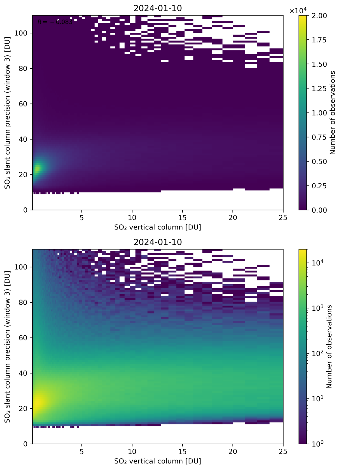
Figure 304: Scatter density plot of “SO 2 vertical column” against “SO 2 slant column precision (window 3)” for 2024-01-10 to 2024-01-11.
