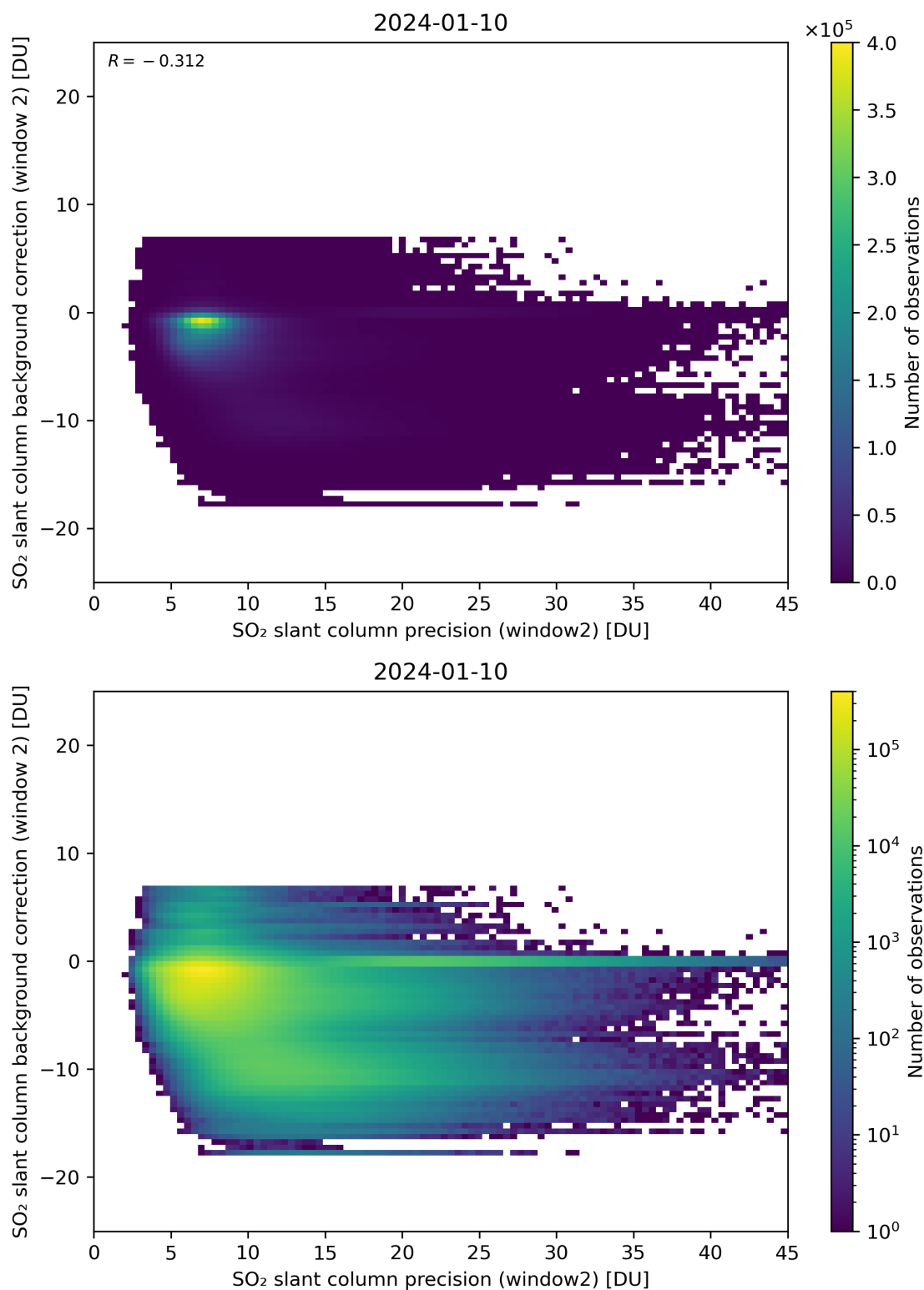
Figure 241: Scatter density plot of “SO 2 slant column precision (window2)” against “SO 2 slant column background correction (window 2)” for 2024-01-10 to 2024-01-11.
