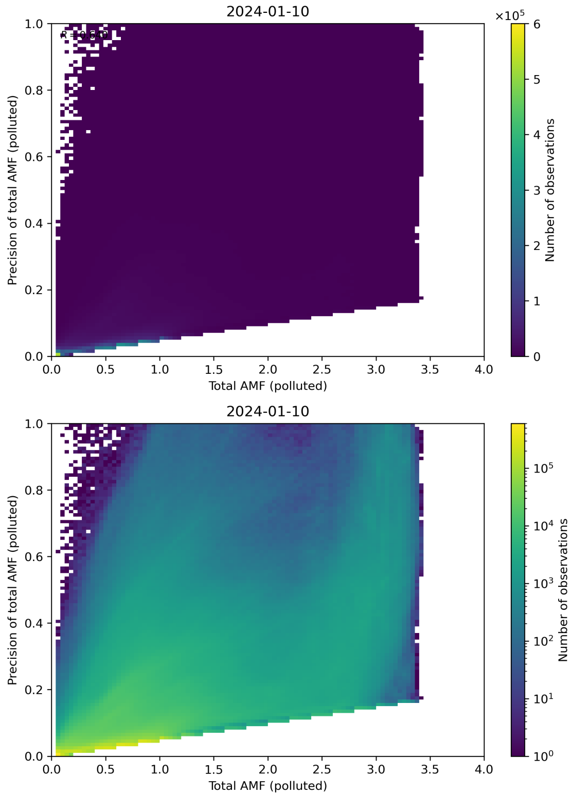
Figure 272: Scatter density plot of “Total AMF (polluted)” against “Precision of total AMF (polluted)” for 2024-01-10 to 2024-01-11.
