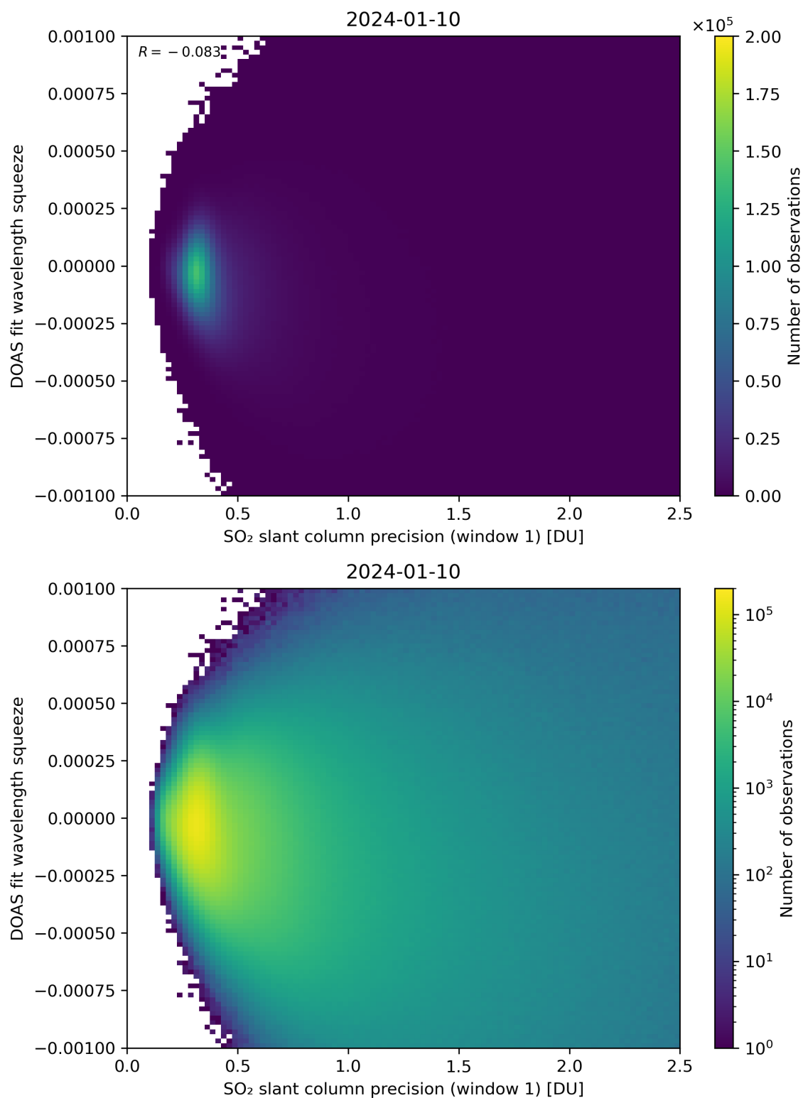
Figure 222: Scatter density plot of “SO 2 slant column precision (window 1)” against “DOAS fit wavelength squeeze” for 2024-01-10 to 2024-01-11.
