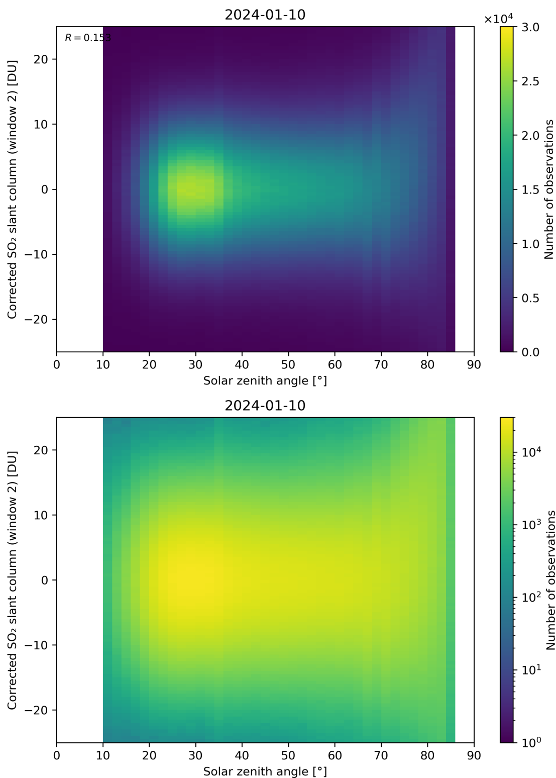
Figure 167: Scatter density plot of “Solar zenith angle” against “Corrected SO 2 slant column (window 2)” for 2024-01-10 to 2024-01-11.
