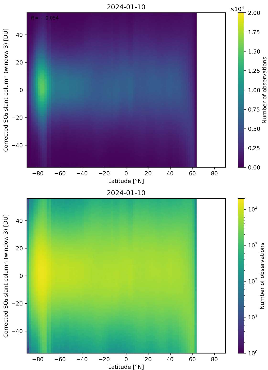
Figure 148: Scatter density plot of “Latitude” against “Corrected SO 2 slant column (window 3)” for 2024-01-10 to 2024-01-11.
