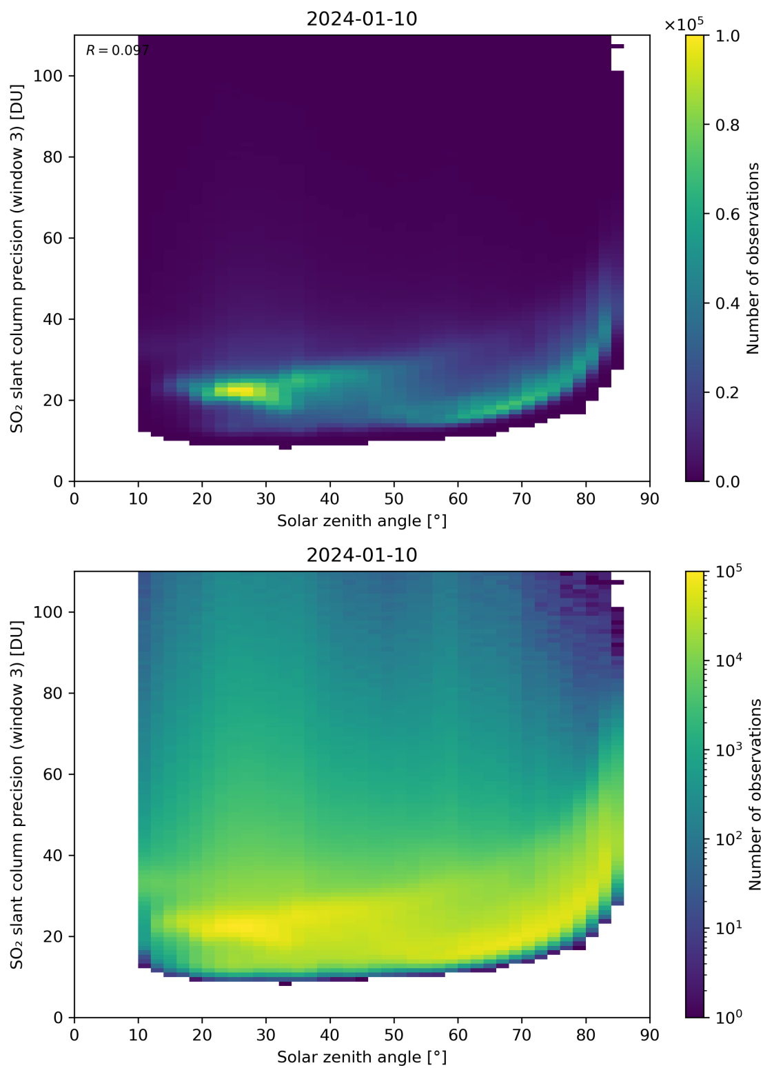
Figure 173: Scatter density plot of “Solar zenith angle” against “SO 2 slant column precision (window 3)” for 2024-01-10 to 2024-01-11.
