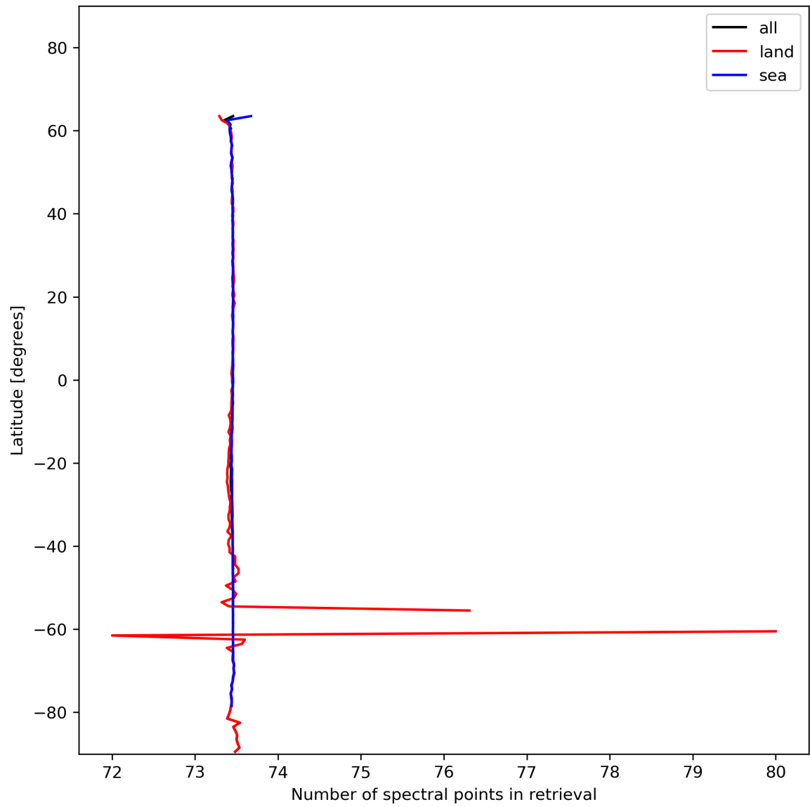
Figure 51: Zonal average of “Number of spectral points in retrieval” for 2024-01-10 to 2024-01-11.
