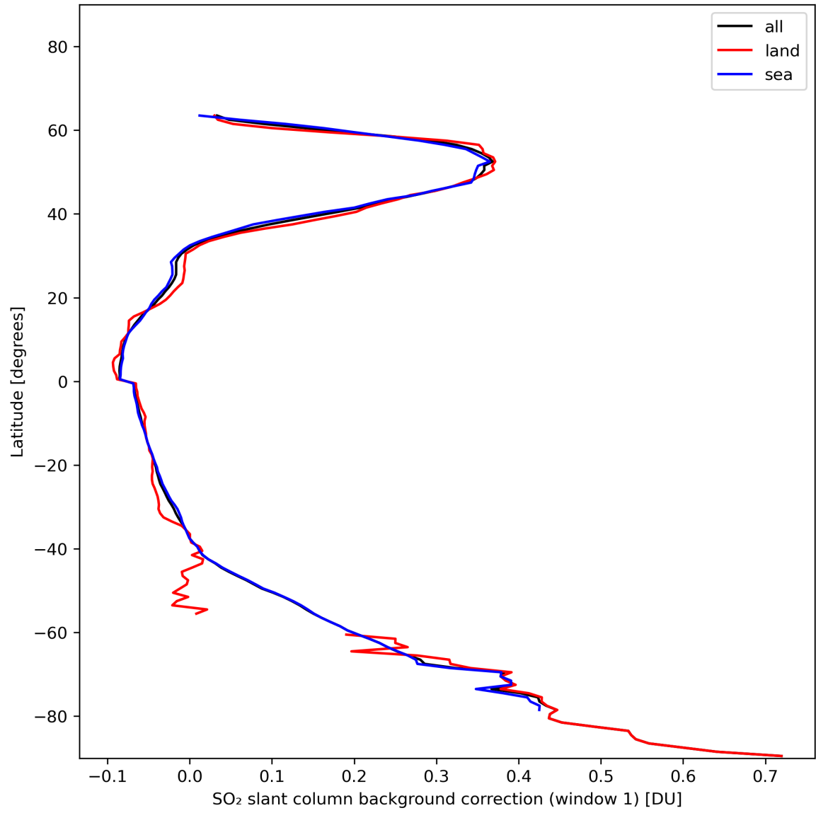
Figure 36: Zonal average of “SO 2 slant column background correction (window 1)” for 2024-01-10 to 2024-01-11.
