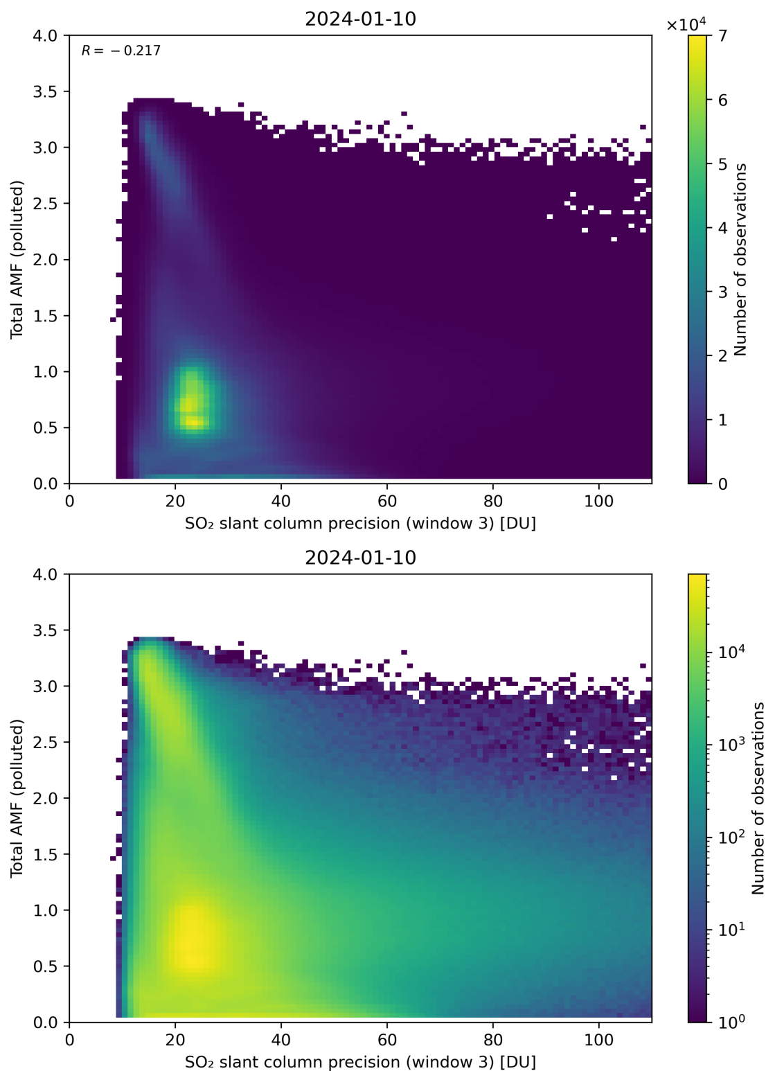
Figure 263: Scatter density plot of “SO 2 slant column precision (window 3)” against “Total AMF (polluted)” for 2024-01-10 to 2024-01-11.
