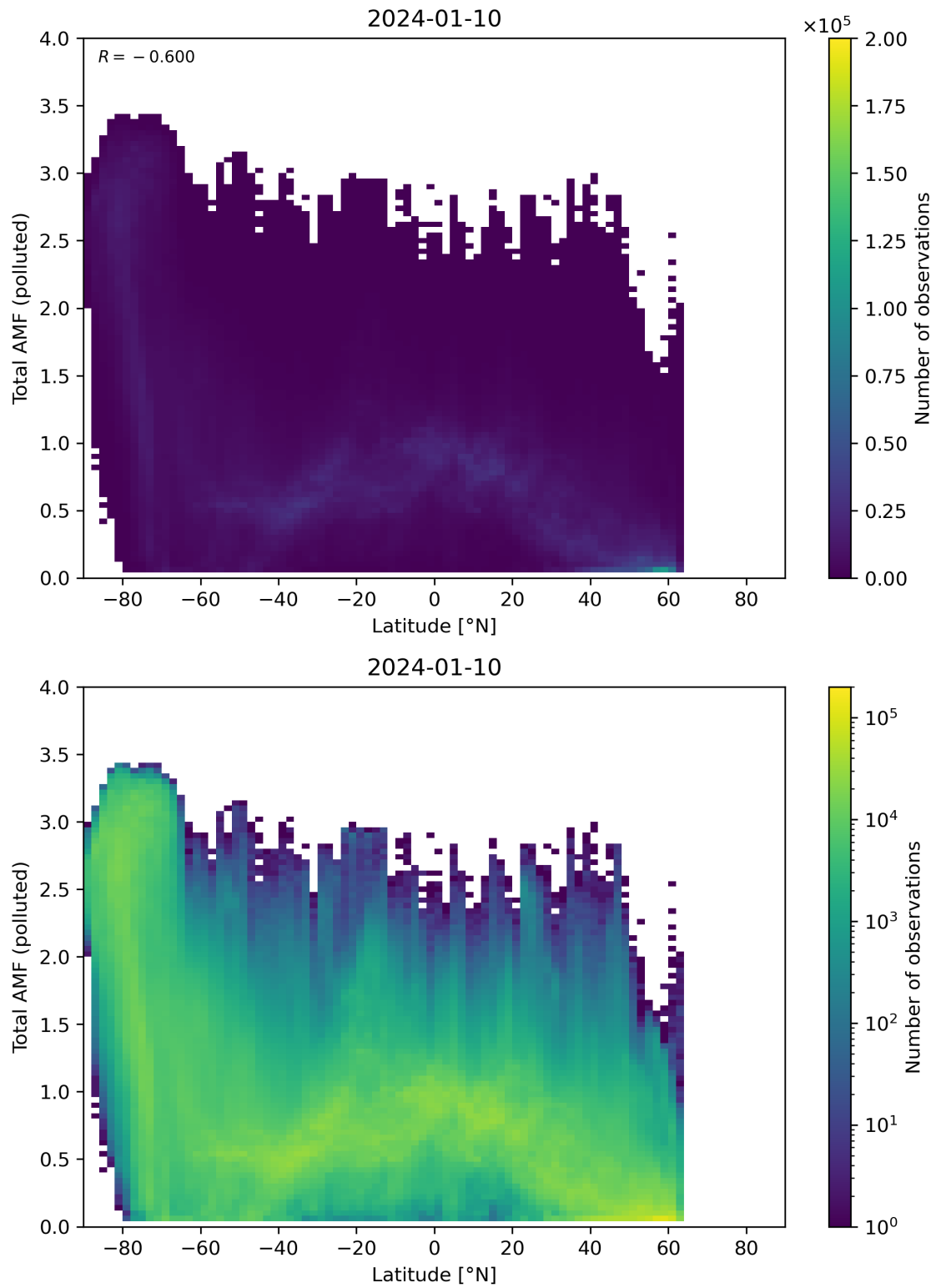
Figure 154: Scatter density plot of “Latitude” against “Total AMF (polluted)” for 2024-01-10 to 2024-01-11.
