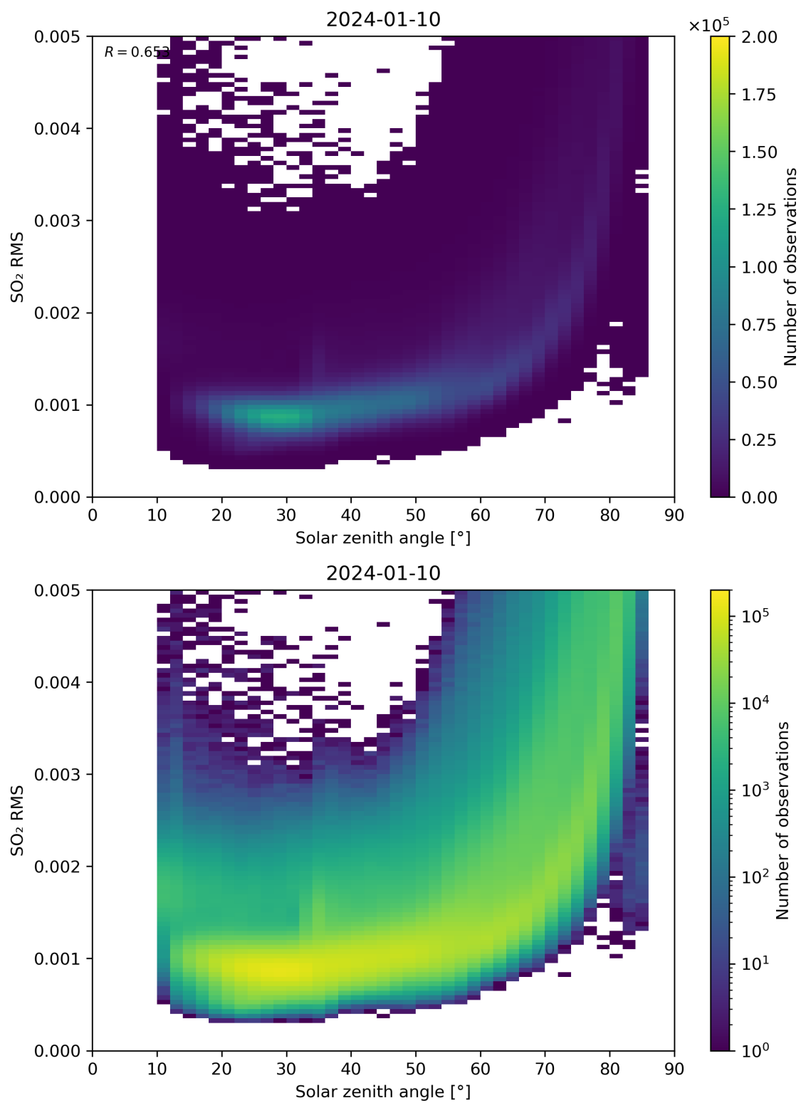
Figure 163: Scatter density plot of “Solar zenith angle” against “SO 2 RMS” for 2024-01-10 to 2024-01-11.
