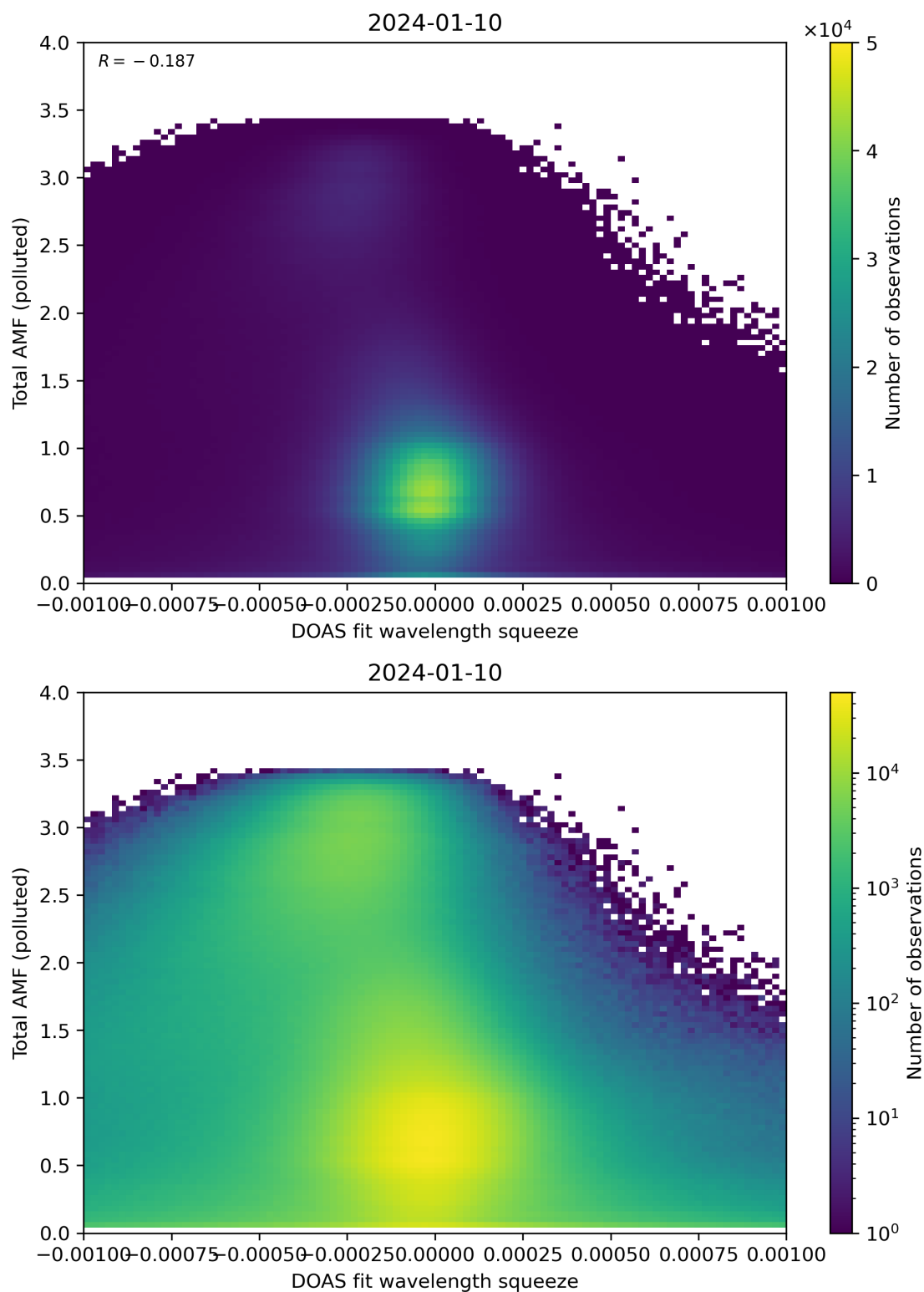
Figure 134: Scatter density plot of “DOAS fit wavelength squeeze” against “Total AMF (polluted)” for 2024-01-10 to 2024-01-11.
