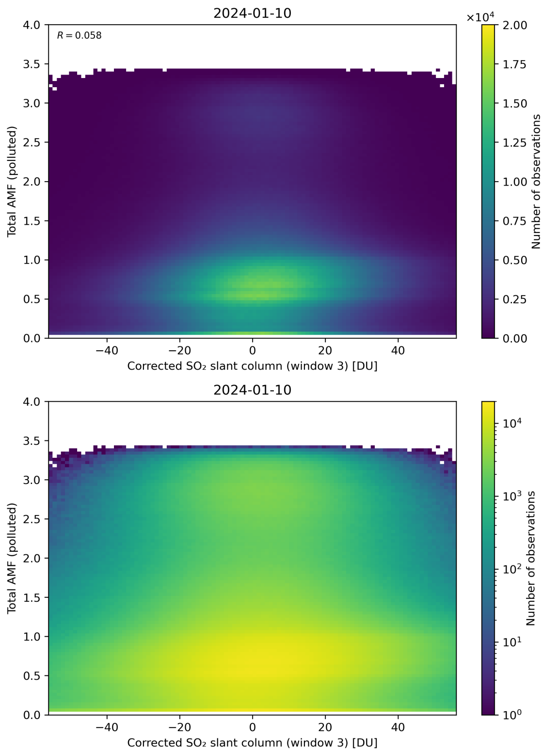
Figure 210: Scatter density plot of “Corrected SO 2 slant column (window 3)” against “Total AMF (polluted)” for 2024-01-10 to 2024-01-11.
