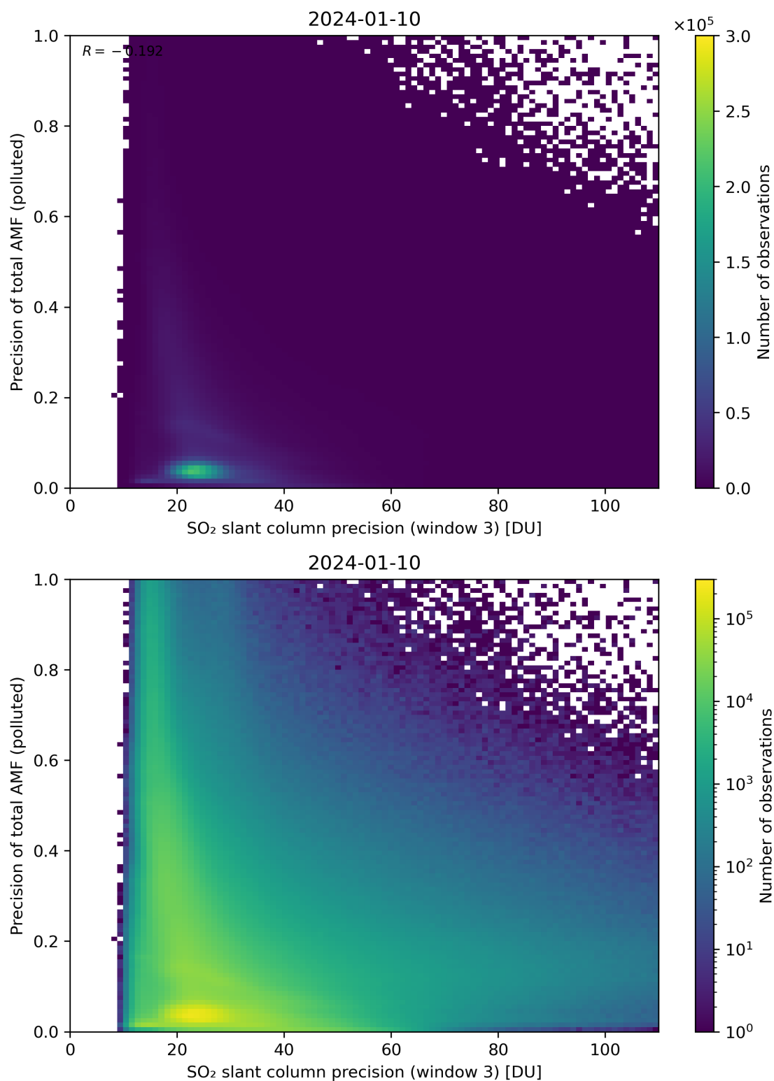
Figure 264: Scatter density plot of “SO 2 slant column precision (window 3)” against “Precision of total AMF (polluted)” for 2024-01-10 to 2024-01-11.
