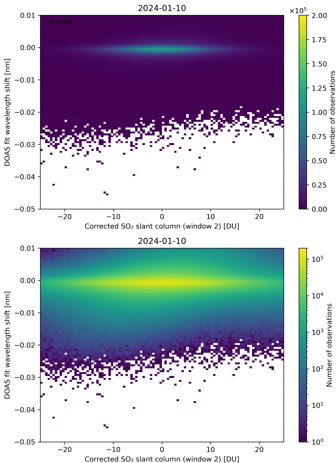
Figure 196: Scatter density plot of “Corrected SO 2 slant column (window 2)” against “DOAS fit wavelength shift” for 2024-01-10 to 2024-01-11.
