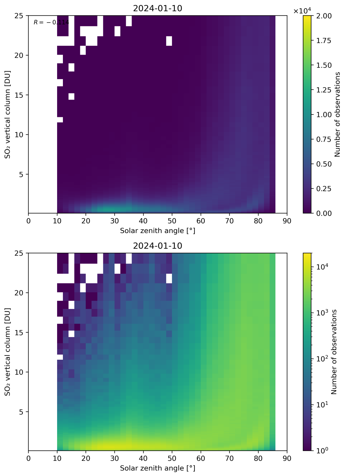
Figure 176: Scatter density plot of “Solar zenith angle” against “SO 2 vertical column” for 2024-01-10 to 2024-01-11.
