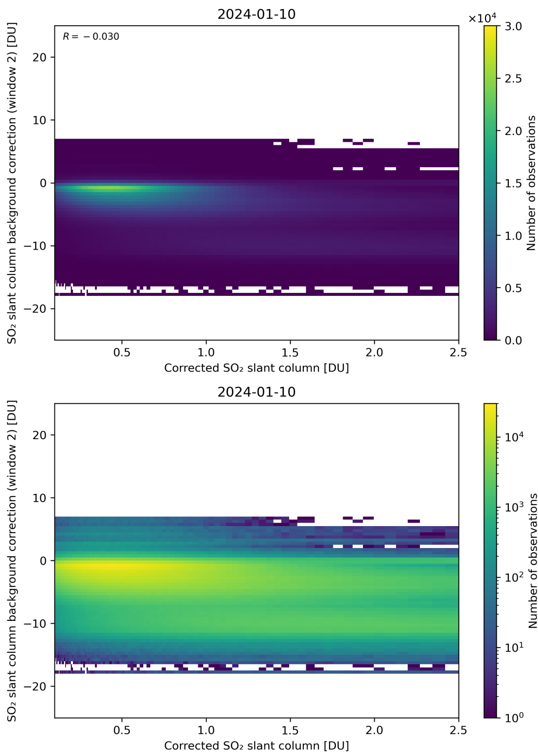
Figure 179: Scatter density plot of “Corrected SO 2 slant column” against “SO 2 slant column background correction (window 2)” for 2024-01-10 to 2024-01-11.
