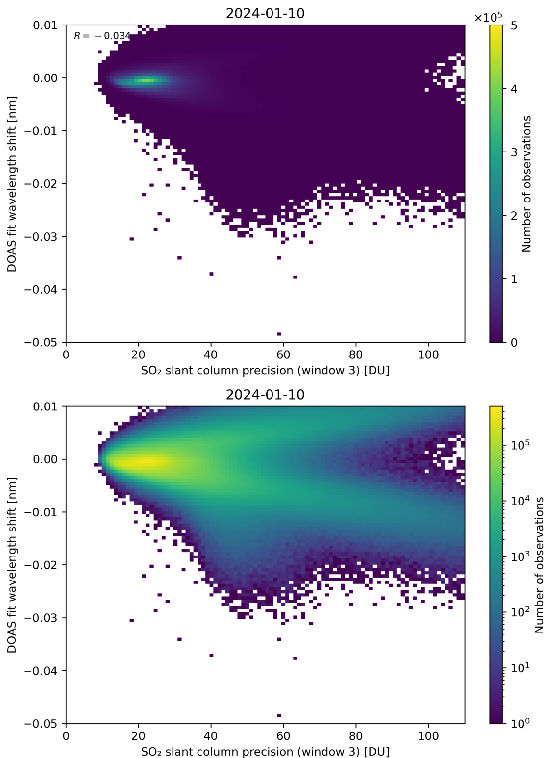
Figure 258: Scatter density plot of “SO 2 slant column precision (window 3)” against “DOAS fit wavelength shift” for 2024-01-10 to 2024-01-11.
