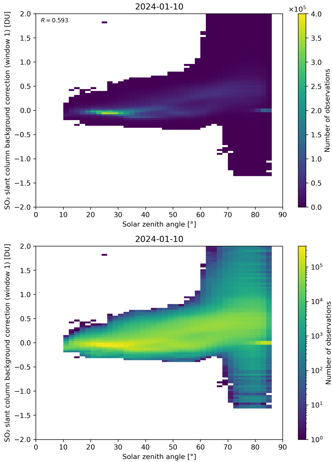
Figure 158: Scatter density plot of “Solar zenith angle” against “SO 2 slant column background correction (window 1)” for 2024-01-10 to 2024-01-11.
