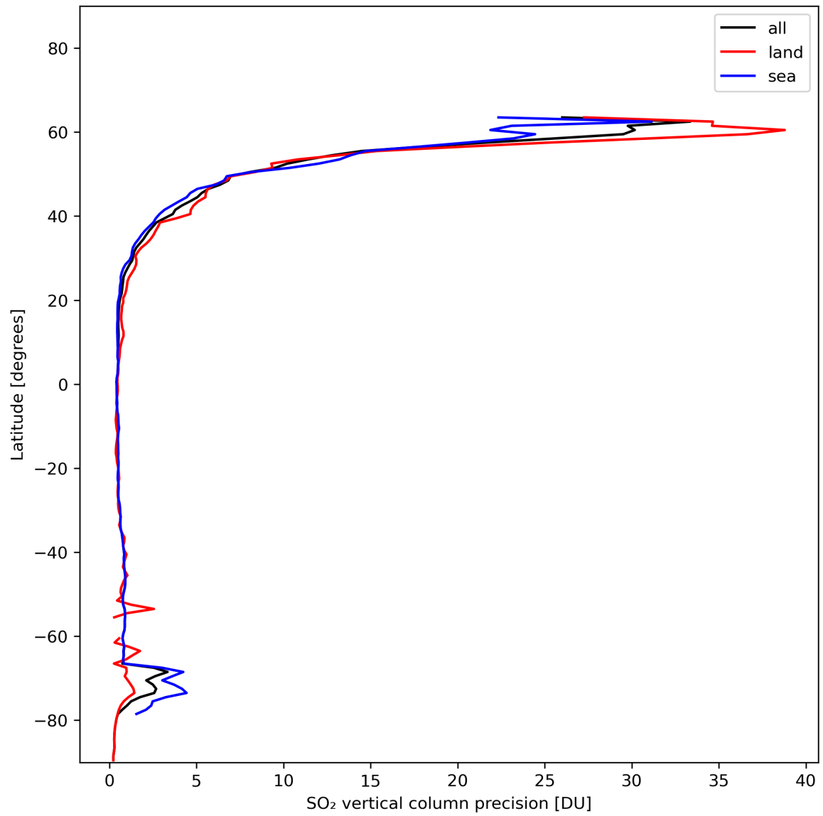
Figure 31: Zonal average of “SO 2 vertical column precision” for 2024-01-10 to 2024-01-11.
