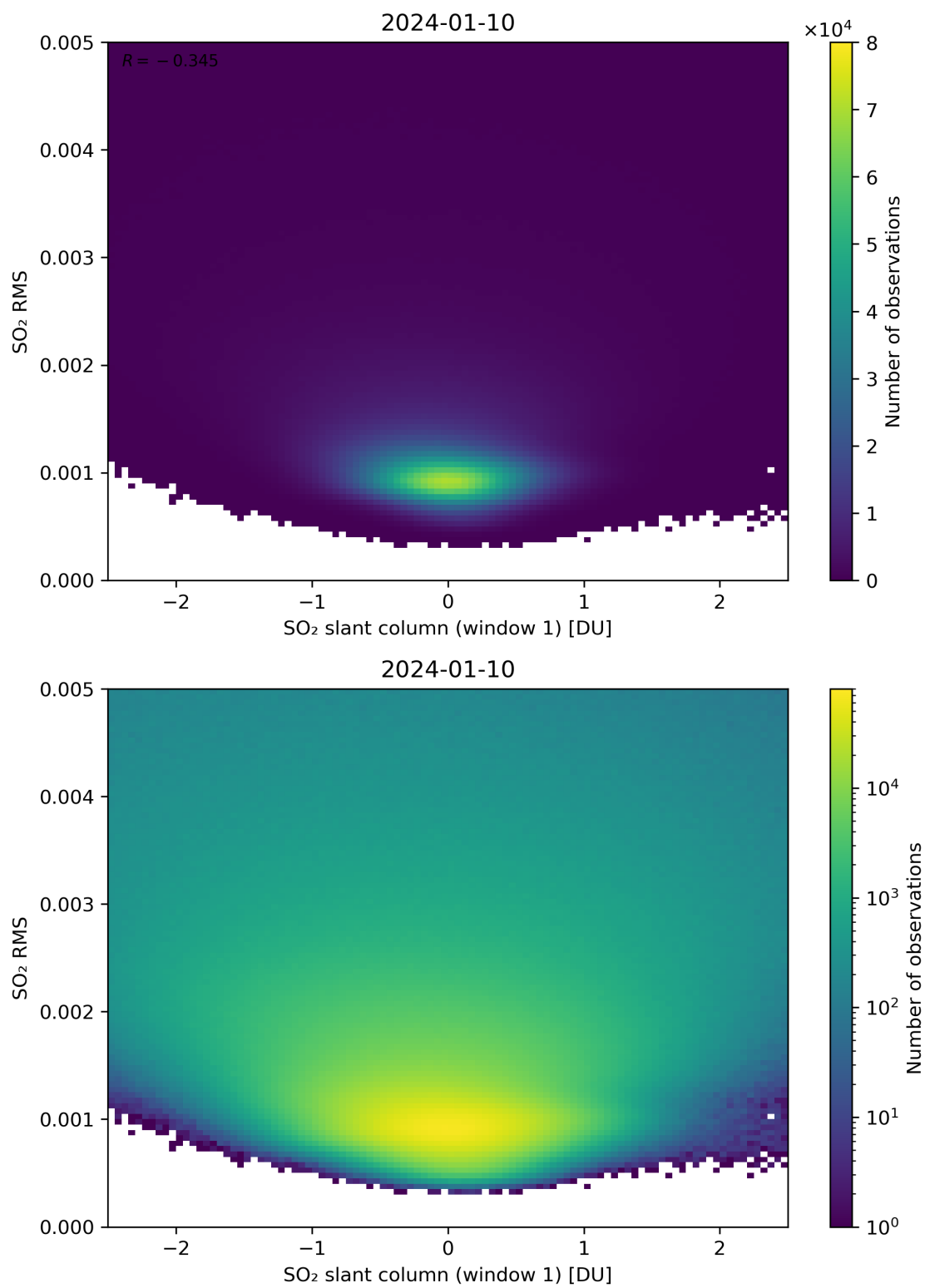
Figure 217: Scatter density plot of “SO 2 slant column (window 1)” against “SO 2 RMS” for 2024-01-10 to 2024-01-11.
