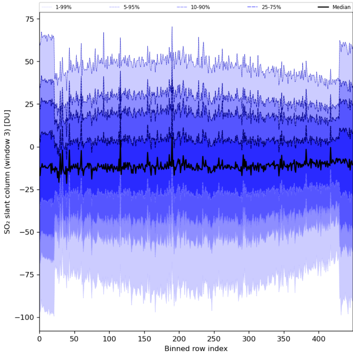
Figure 87: Along track statistics of “SO 2 slant column (window 3)” for 2024-01-10 to 2024-01-11
