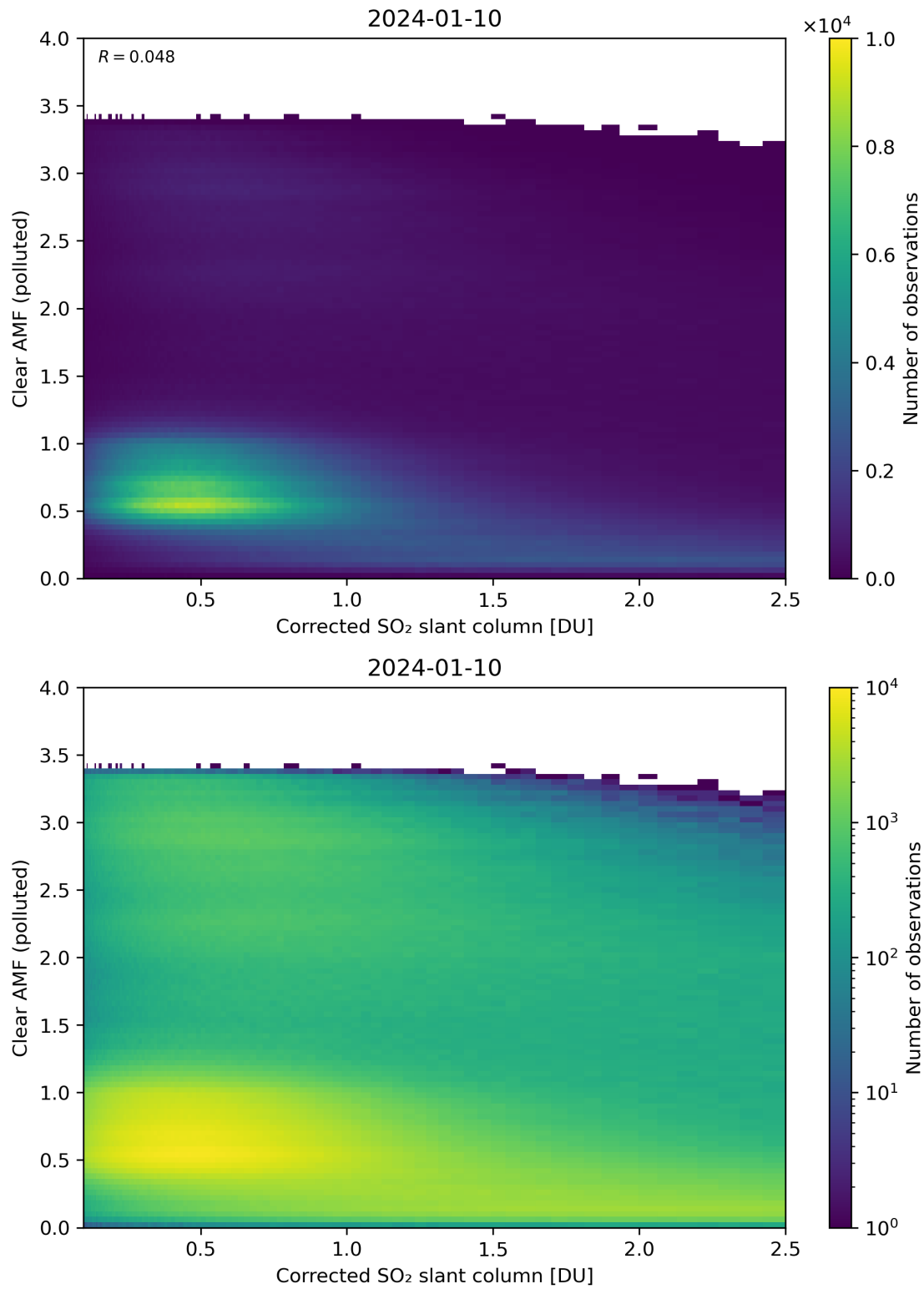
Figure 184: Scatter density plot of “Corrected SO 2 slant column” against “Clear AMF (polluted)” for 2024-01-10 to 2024-01-11.
