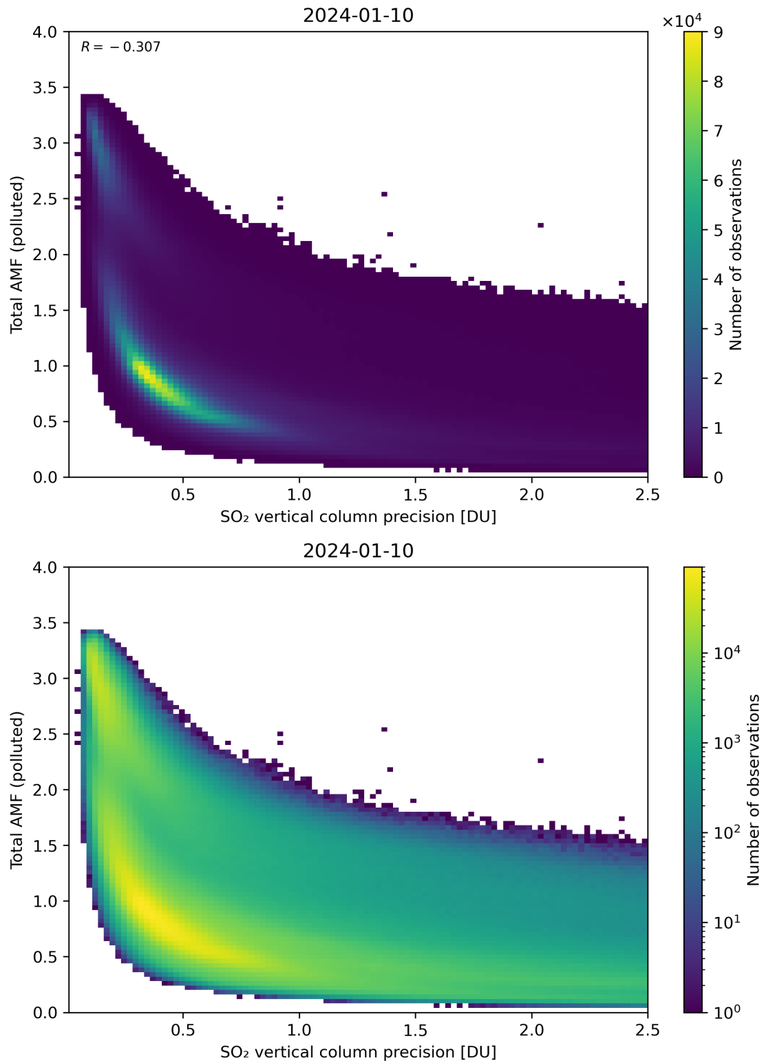
Figure 294: Scatter density plot of “SO 2 vertical column precision” against “Total AMF (polluted)” for 2024-01-10 to 2024-01-11.
