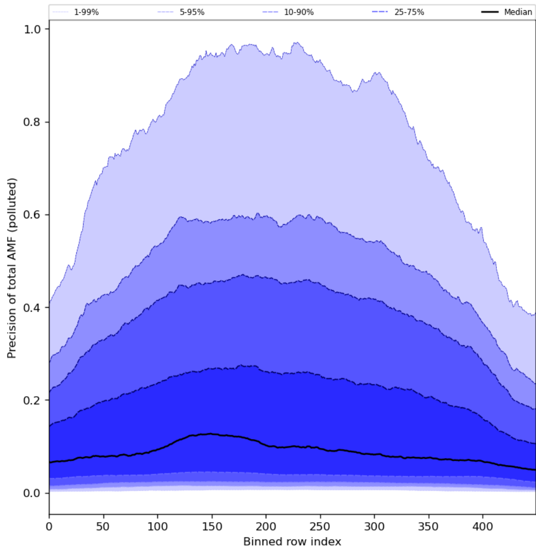
Figure 95: Along track statistics of “Precision of total AMF (polluted)” for 2024-01-10 to 2024-01-11
