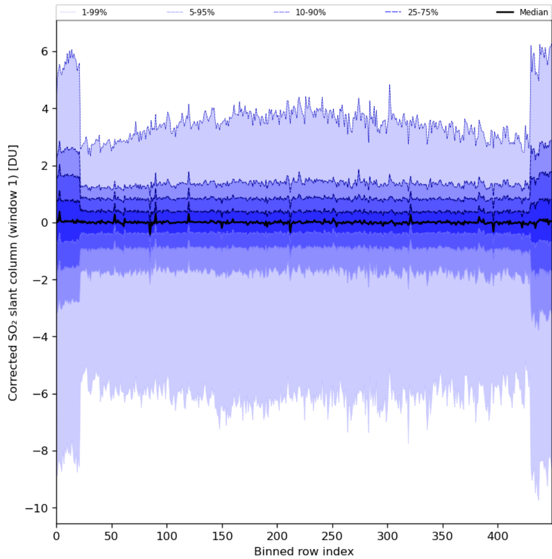
Figure 81: Along track statistics of “Corrected SO 2 slant column (window 1)” for 2024-01-10 to 2024-01-11
