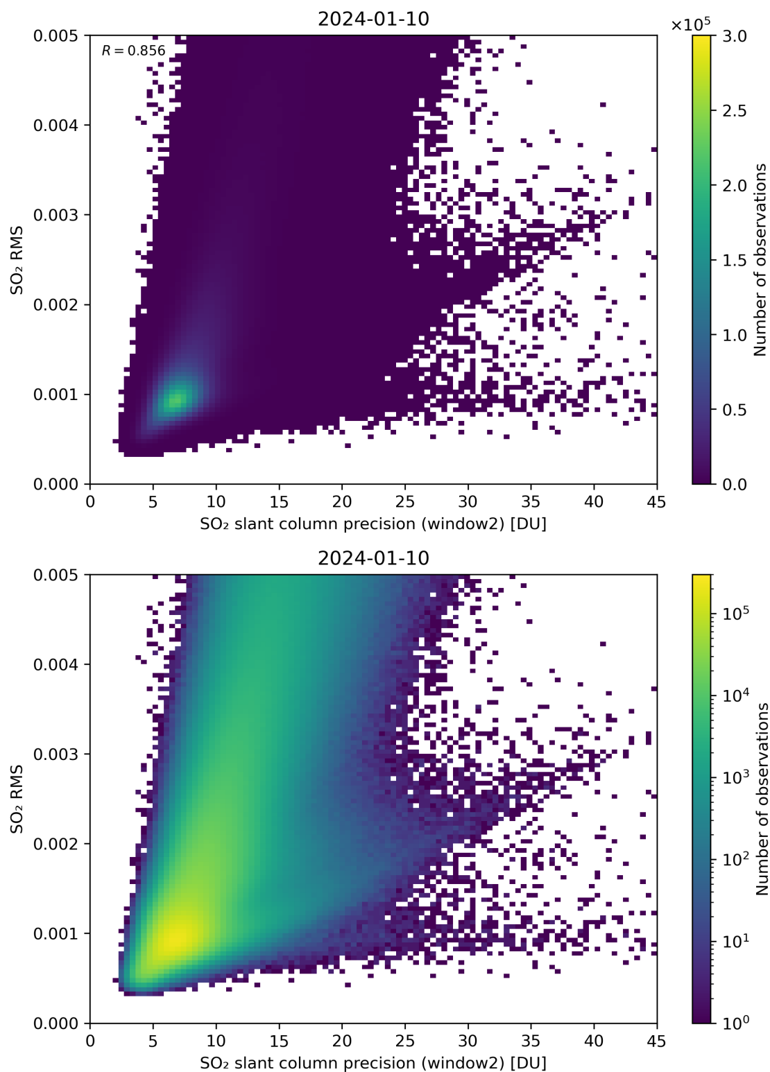
Figure 245: Scatter density plot of “SO 2 slant column precision (window2)” against “SO 2 RMS” for 2024-01-10 to 2024-01-11.
