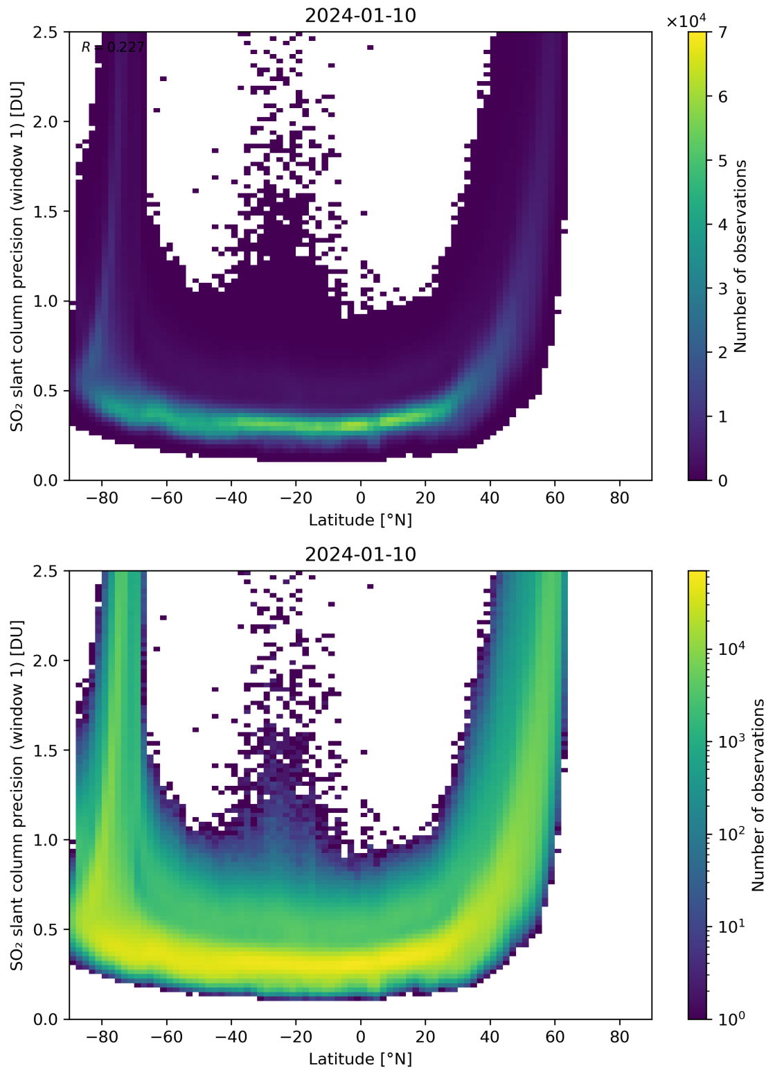
Figure 150: Scatter density plot of “Latitude” against “SO 2 slant column precision (window 1)” for 2024-01-10 to 2024-01-11.
