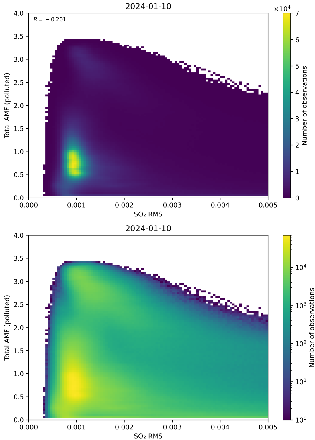
Figure 137: Scatter density plot of “SO 2 RMS” against “Total AMF (polluted)” for 2024-01-10 to 2024-01-11.
