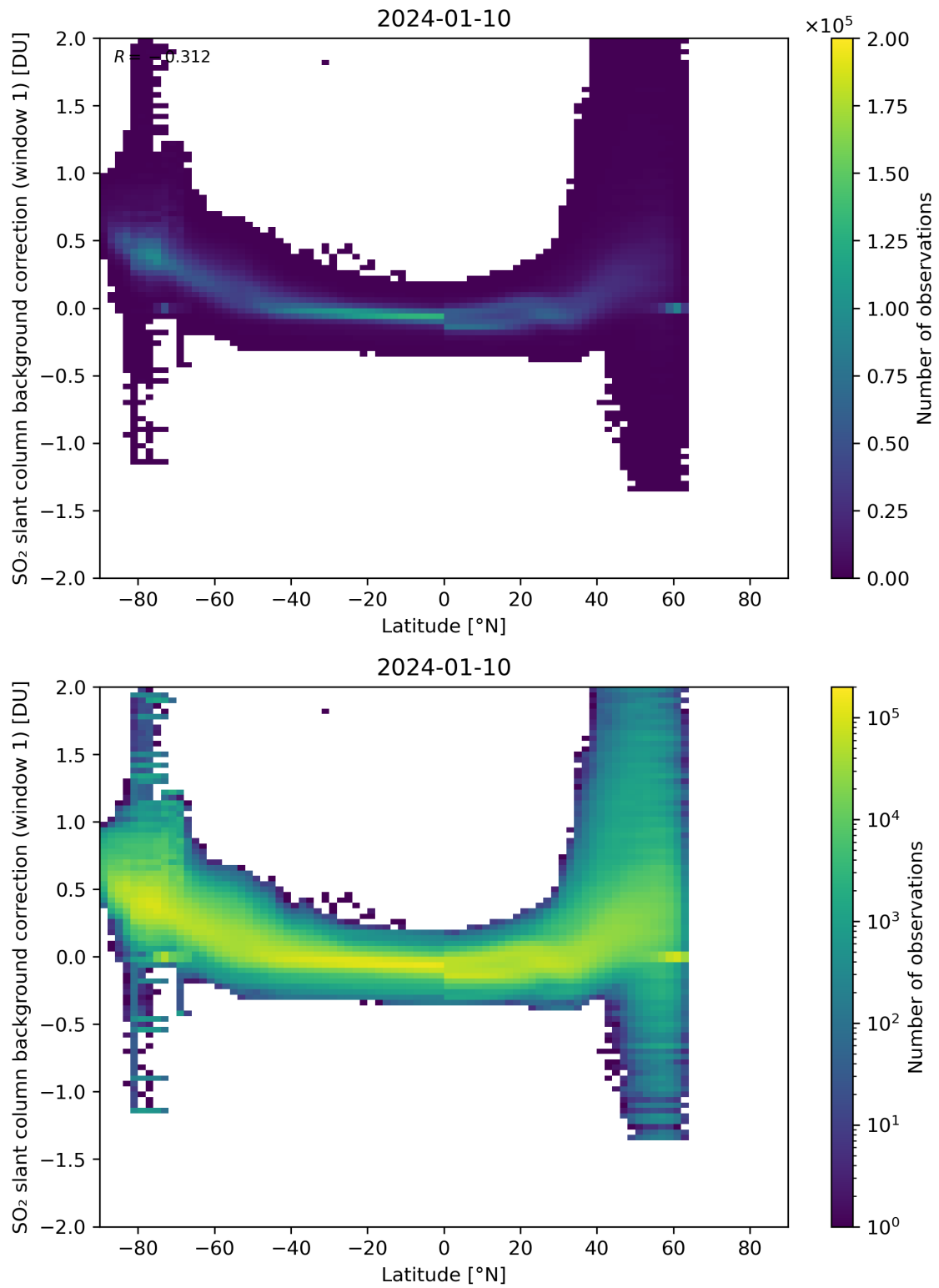
Figure 139: Scatter density plot of “Latitude” against “SO 2 slant column background correction (window 1)” for 2024-01-10 to 2024-01-11.
