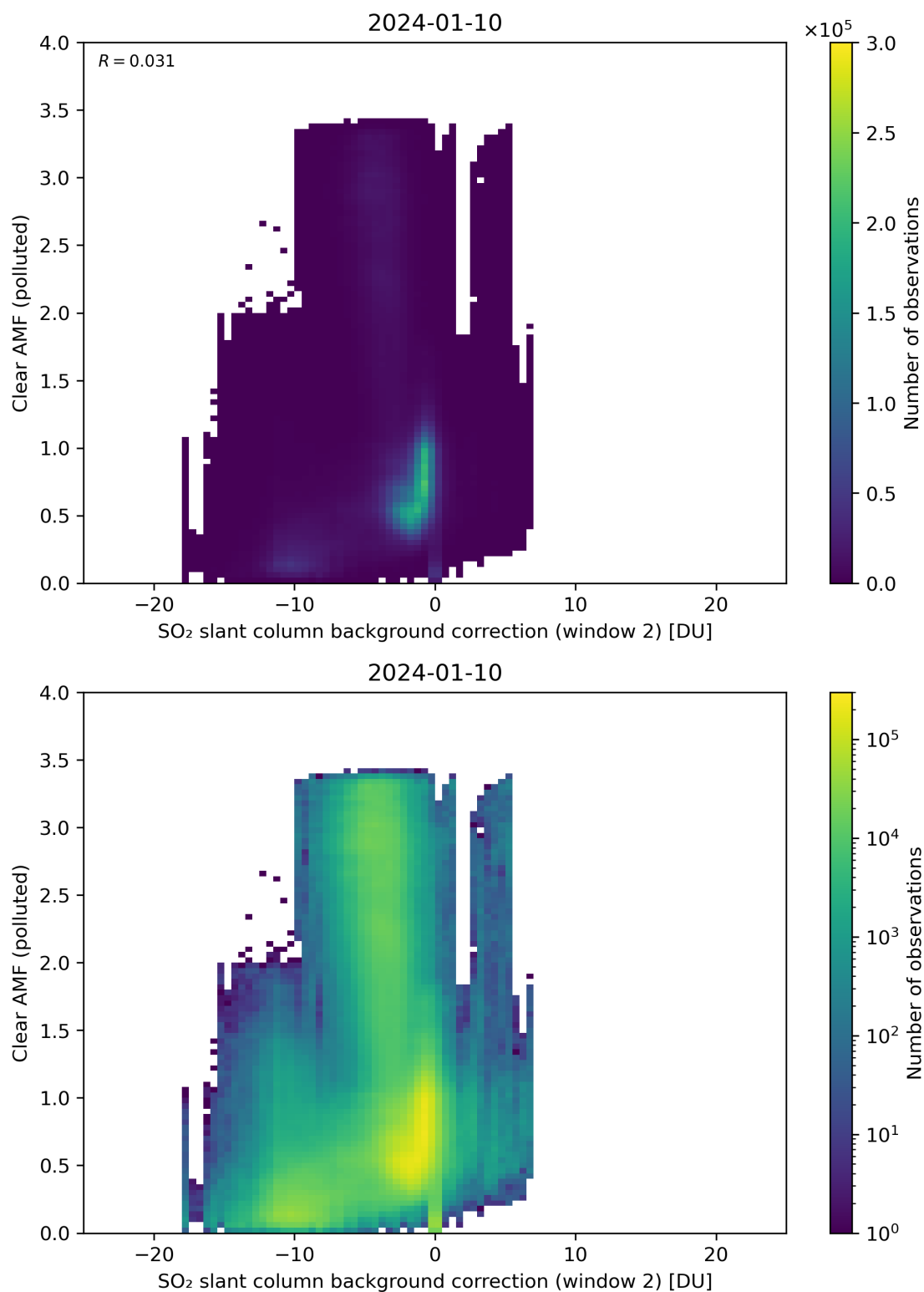
Figure 115: Scatter density plot of “SO 2 slant column background correction (window 2)” against “Clear AMF (polluted)” for 2024-01-10 to 2024-01-11.
