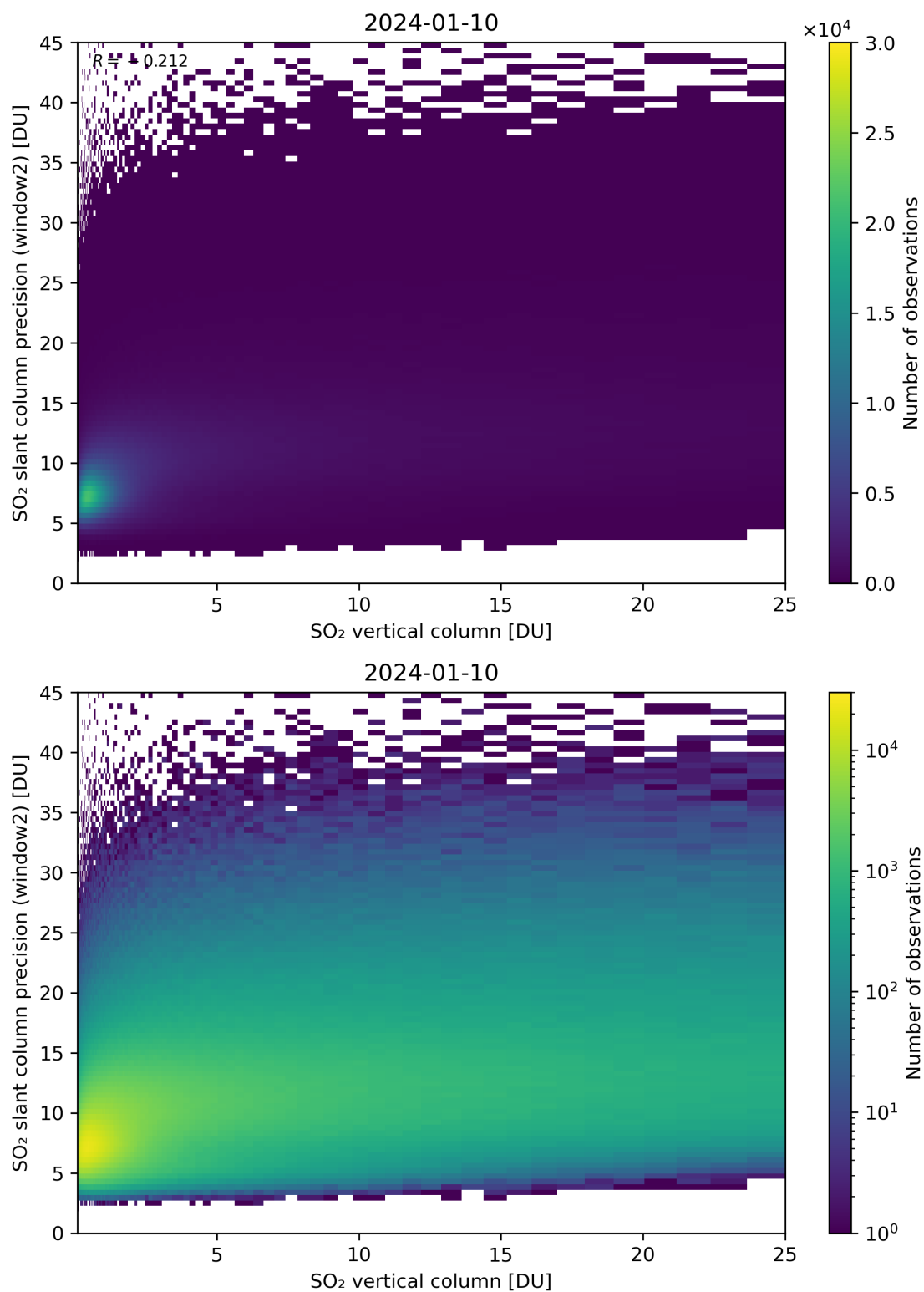
Figure 302: Scatter density plot of “SO 2 vertical column” against “SO 2 slant column precision (window2)” for 2024-01-10 to 2024-01-11.
