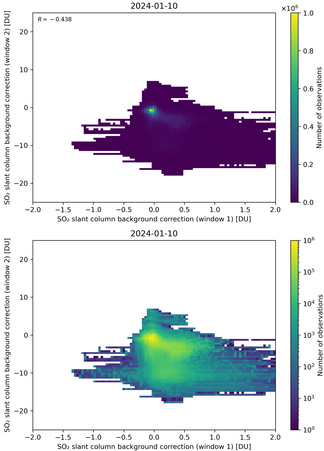
Figure 98: Scatter density plot of “SO 2 slant column background correction (window 1)” against “SO 2 slant column background correction (window 2)” for 2024-01-10 to 2024-01-11.
