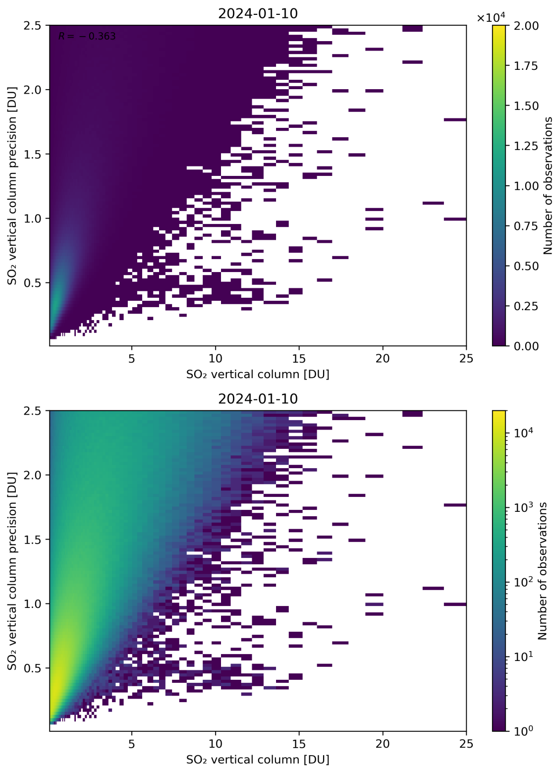
Figure 307: Scatter density plot of “SO 2 vertical column” against “SO 2 vertical column precision” for 2024-01-10 to 2024-01-11.
