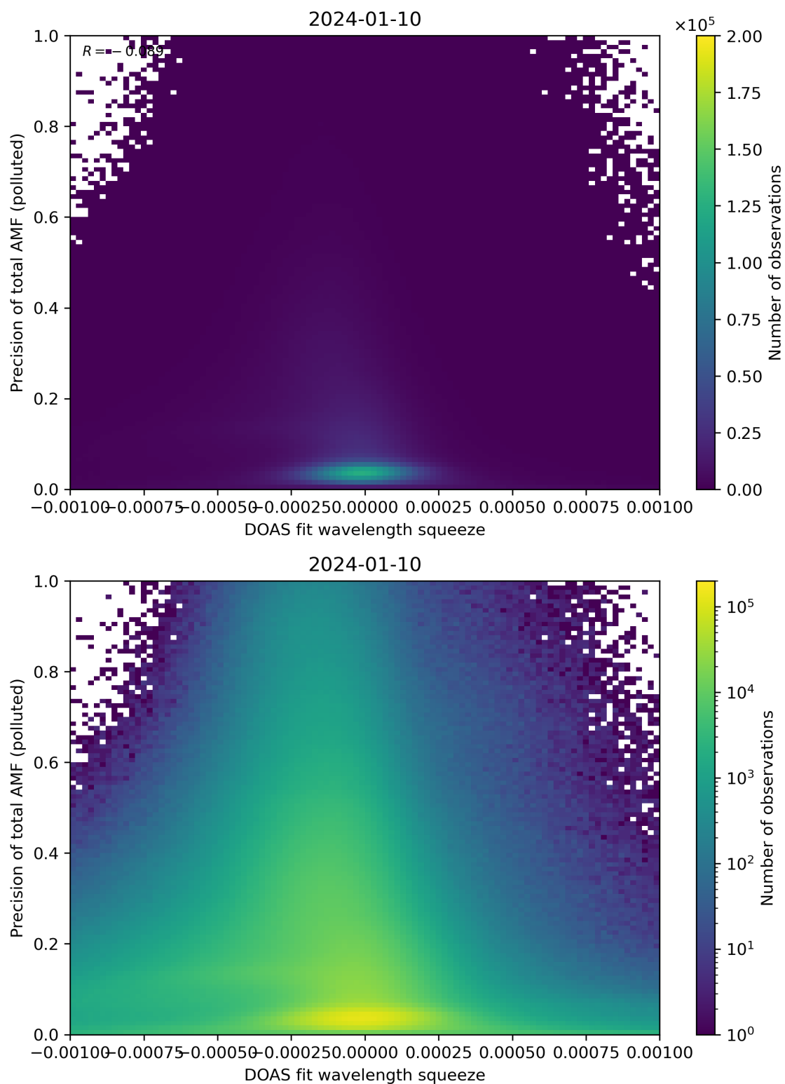
Figure 135: Scatter density plot of “DOAS fit wavelength squeeze” against “Precision of total AMF (polluted)” for 2024-01-10 to 2024-01-11.
