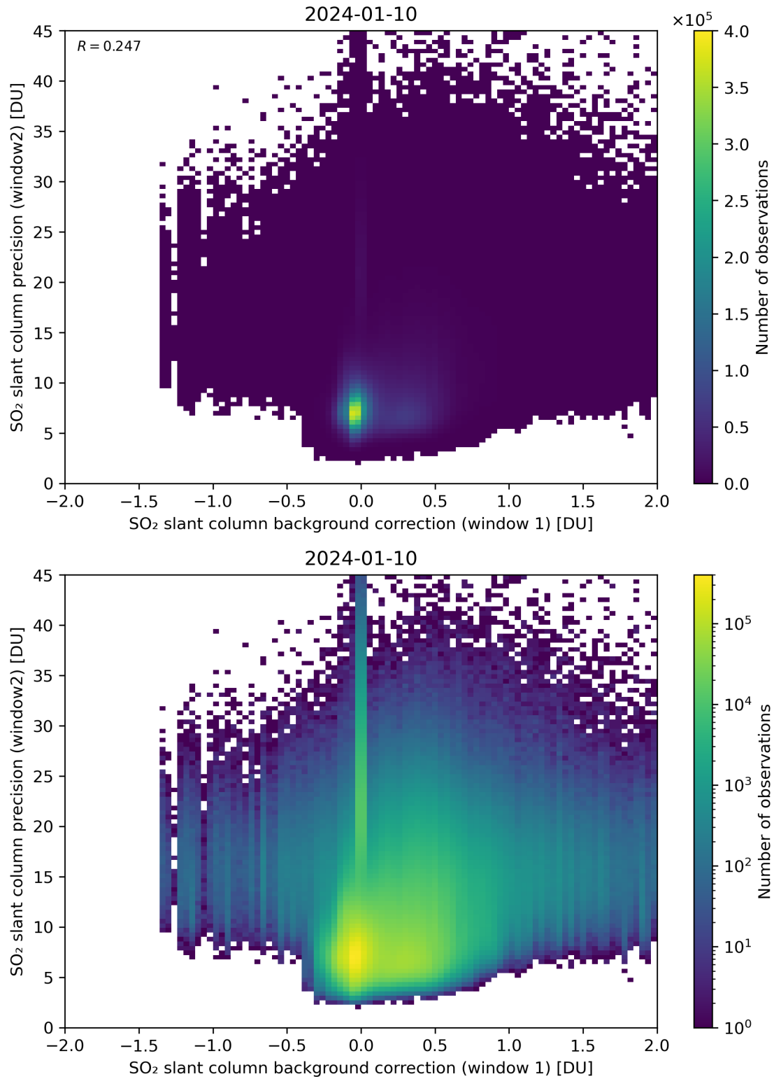
Figure 106: Scatter density plot of “SO 2 slant column background correction (window 1)” against “SO 2 slant column precision (window2)” for 2024-01-10 to 2024-01-11.
