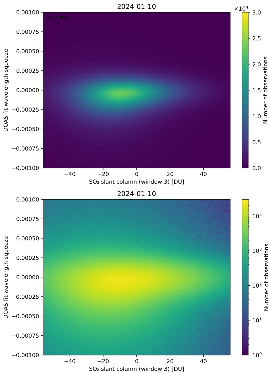
Figure 255: Scatter density plot of “SO 2 slant column (window 3)” against “DOAS fit wavelength squeeze” for 2024-01-10 to 2024-01-11.
