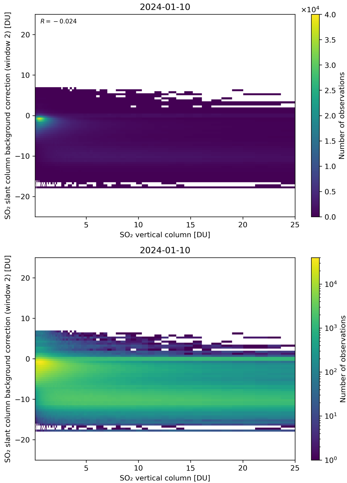
Figure 274: Scatter density plot of “SO 2 vertical column” against “SO 2 slant column background correction (window 2)” for 2024-01-10 to 2024-01-11.
