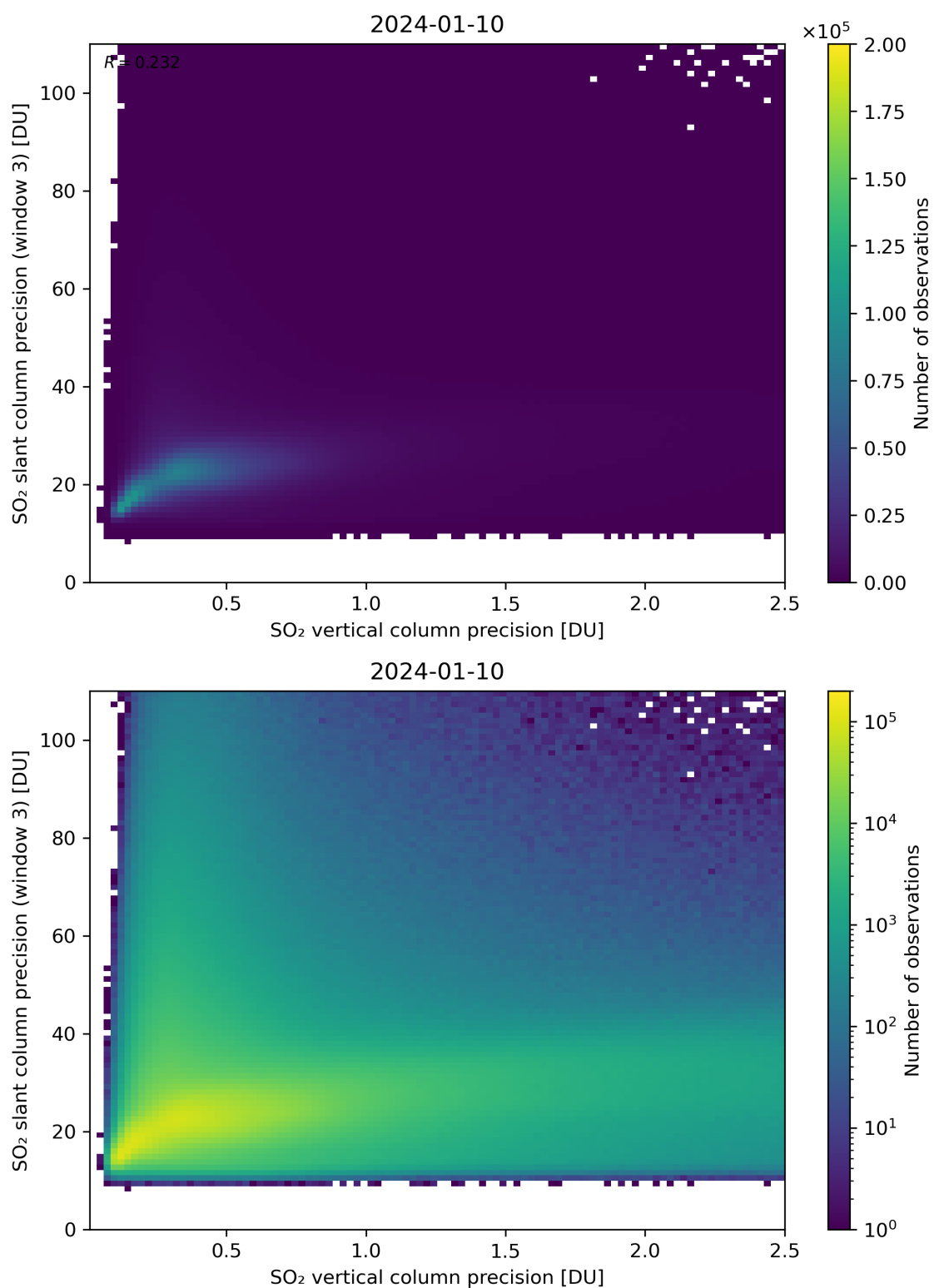
Figure 293: Scatter density plot of “SO 2 vertical column precision” against “SO 2 slant column precision (window 3)” for 2024-01-10 to 2024-01-11.
