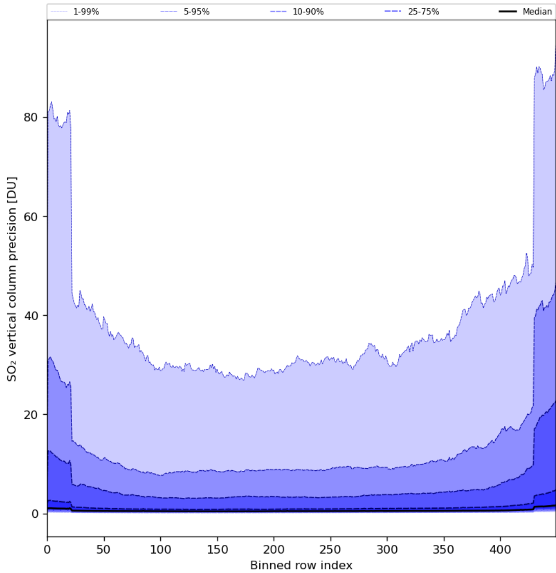
Figure 77: Along track statistics of “SO 2 vertical column precision” for 2024-01-10 to 2024-01-11
