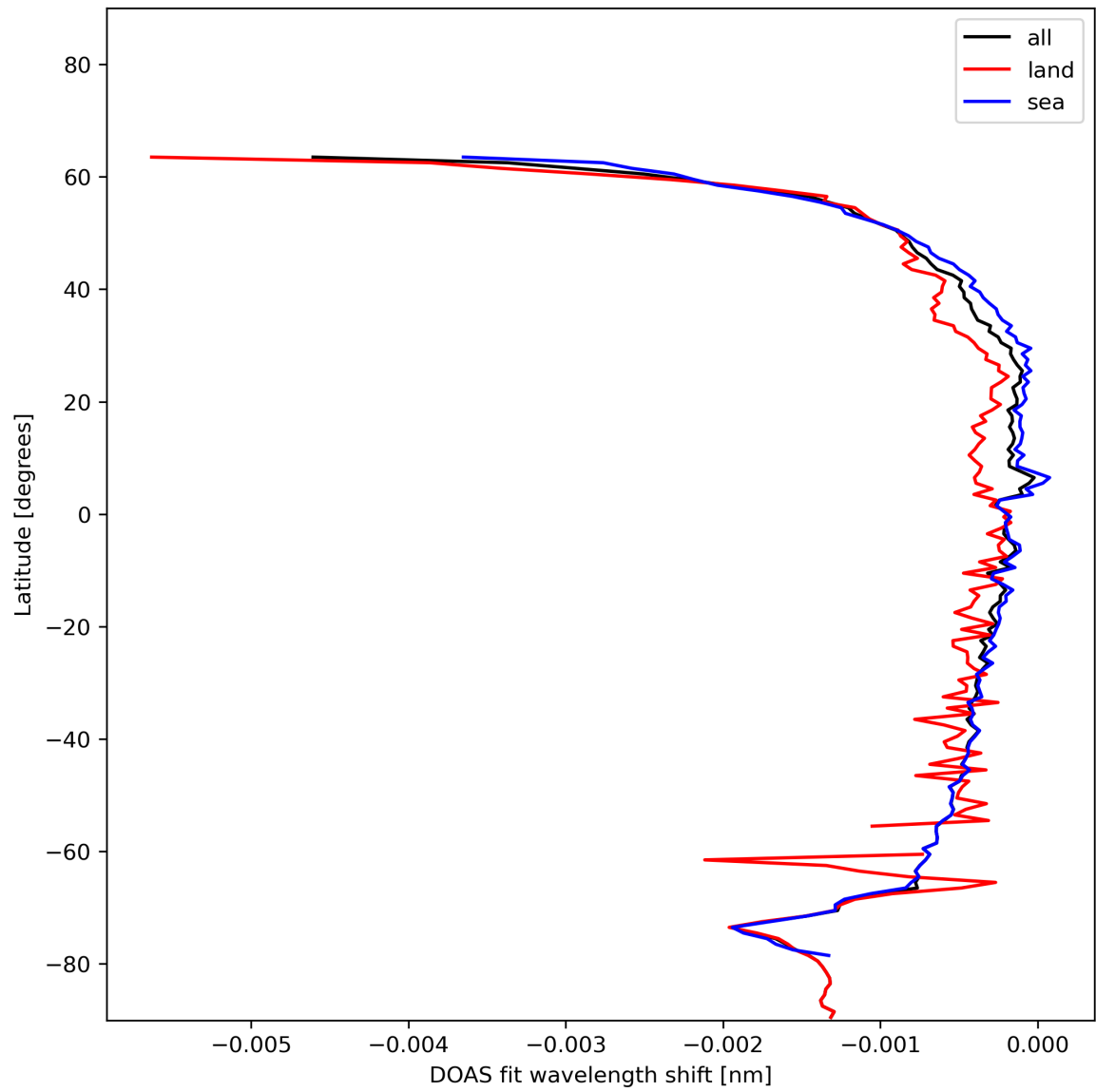
Figure 45: Zonal average of “DOAS fit wavelength shift” for 2024-01-10 to 2024-01-11.
