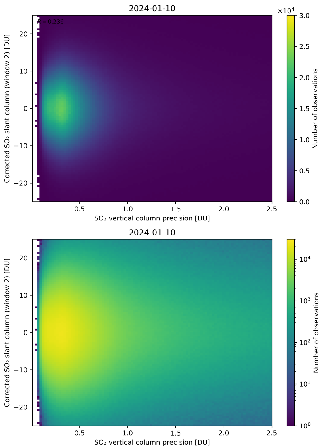
Figure 287: Scatter density plot of “SO 2 vertical column precision” against “Corrected SO 2 slant column (window 2)” for 2024-01-10 to 2024-01-11.
