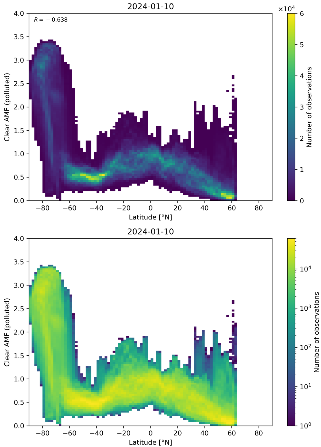
Figure 145: Scatter density plot of “Latitude” against “Clear AMF (polluted)” for 2024-01-10 to 2024-01-11.
