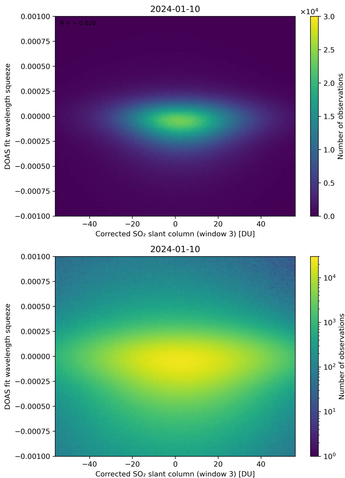
Figure 207: Scatter density plot of “Corrected SO 2 slant column (window 3)” against “DOAS fit wavelength squeeze” for 2024-01-10 to 2024-01-11.
