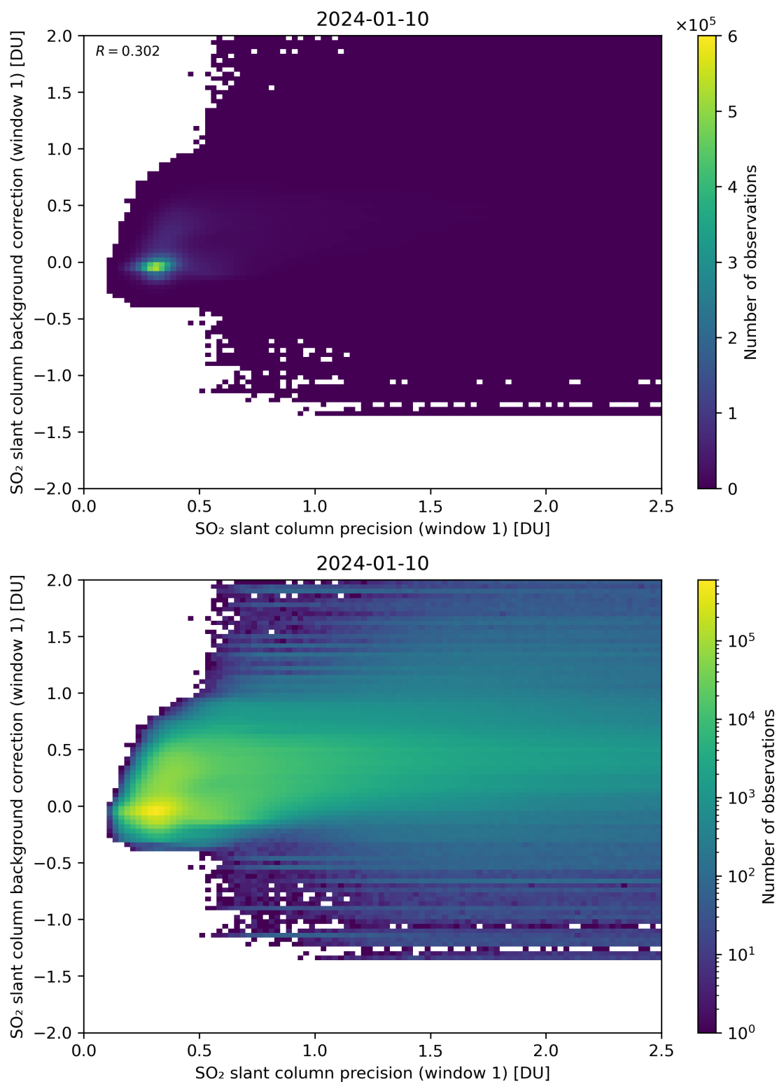
Figure 218: Scatter density plot of “SO 2 slant column precision (window 1)” against “SO 2 slant column background correction (window 1)” for 2024-01-10 to 2024-01-11.
