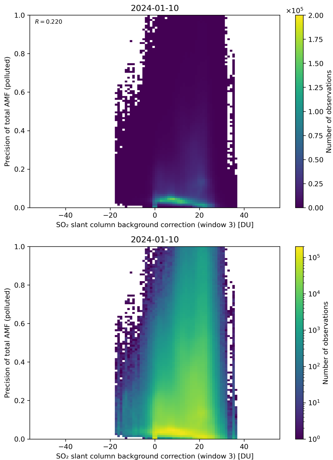
Figure 126: Scatter density plot of “SO 2 slant column background correction (window 3)” against “Precision of total AMF (polluted)” for 2024-01-10 to 2024-01-11.
