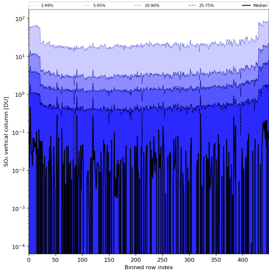
Figure 76: Along track statistics of “SO 2 vertical column” for 2024-01-10 to 2024-01-11
