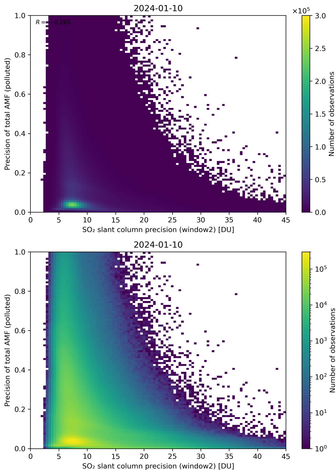
Figure 252: Scatter density plot of “SO 2 slant column precision (window2)” against “Precision of total AMF (polluted)” for 2024-01-10 to 2024-01-11.
