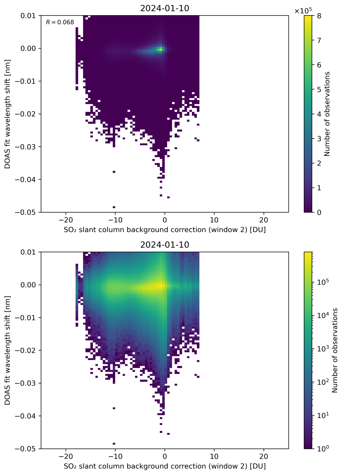
Figure 112: Scatter density plot of “SO 2 slant column background correction (window 2)” against “DOAS fit wavelength shift” for 2024-01-10 to 2024-01-11.
