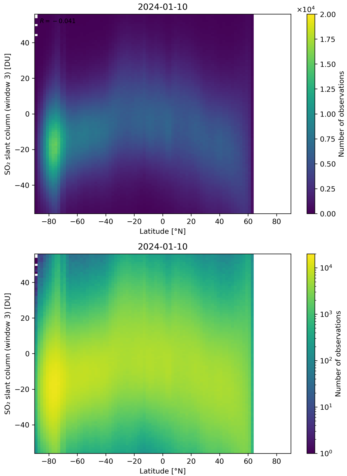
Figure 152: Scatter density plot of “Latitude” against “SO 2 slant column (window 3)” for 2024-01-10 to 2024-01-11.
