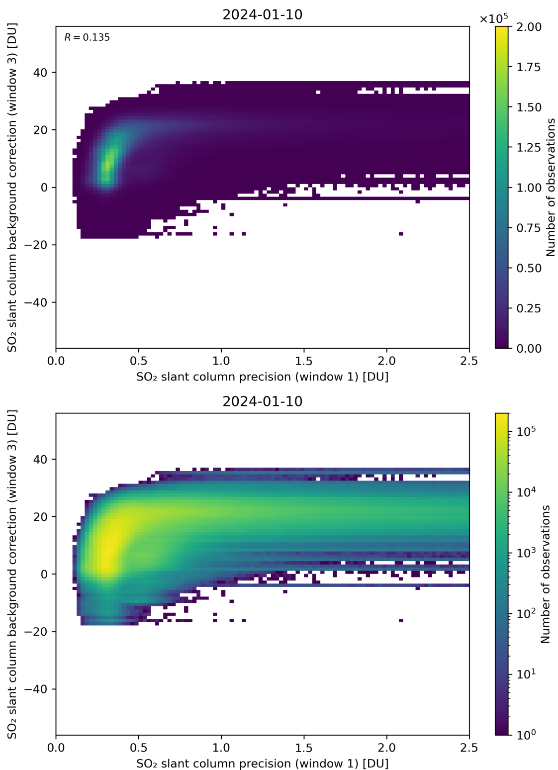
Figure 220: Scatter density plot of “SO 2 slant column precision (window 1)” against “SO 2 slant column background correction (window 3)” for 2024-01-10 to 2024-01-11.
