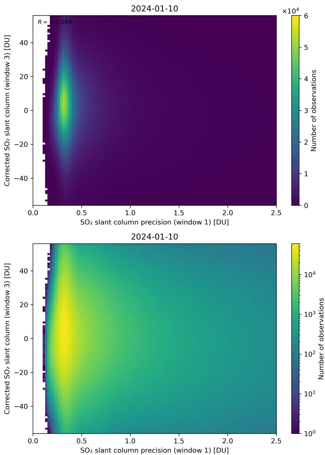
Figure 226: Scatter density plot of “SO 2 slant column precision (window 1)” against “Corrected SO 2 slant column (window 3)” for 2024-01-10 to 2024-01-11.
