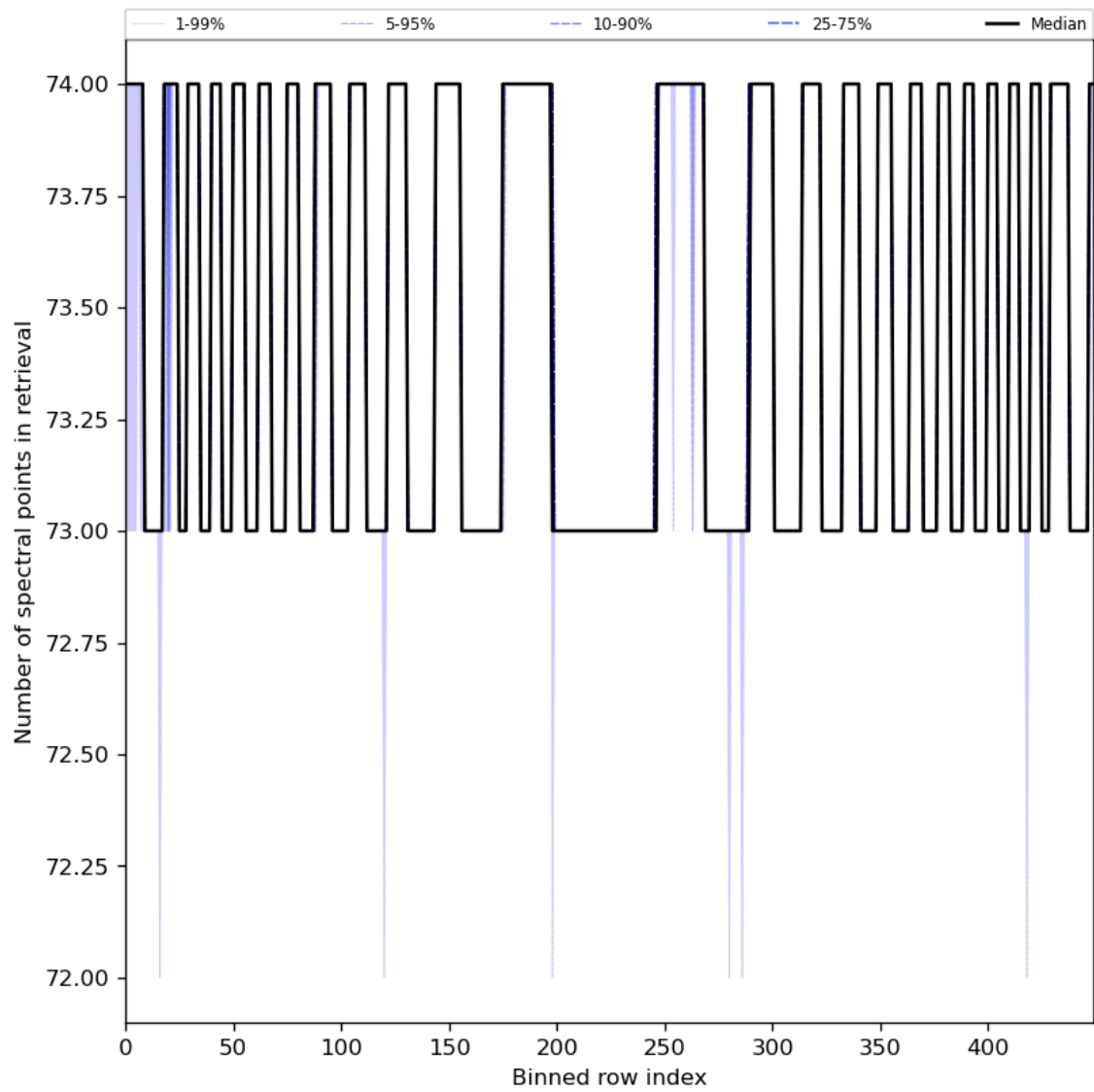
Figure 97: Along track statistics of “Number of spectral points in retrieval” for 2024-01-10 to 2024-01-11
