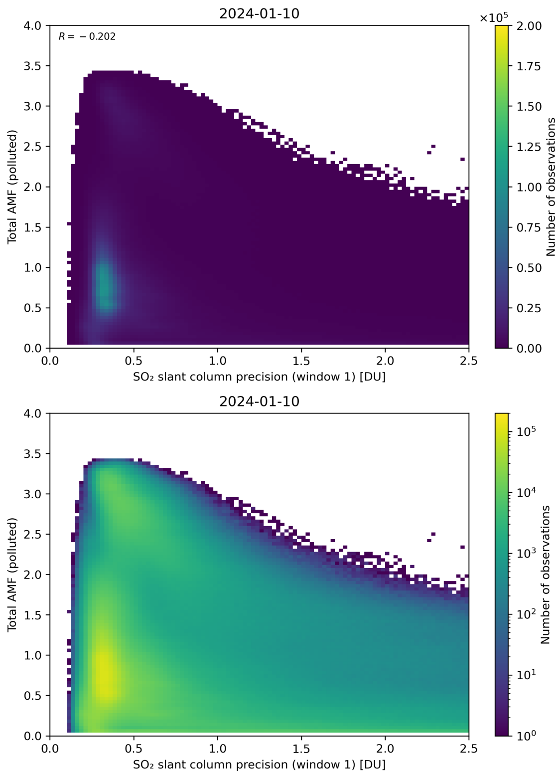
Figure 230: Scatter density plot of “SO 2 slant column precision (window 1)” against “Total AMF (polluted)” for 2024-01-10 to 2024-01-11.
