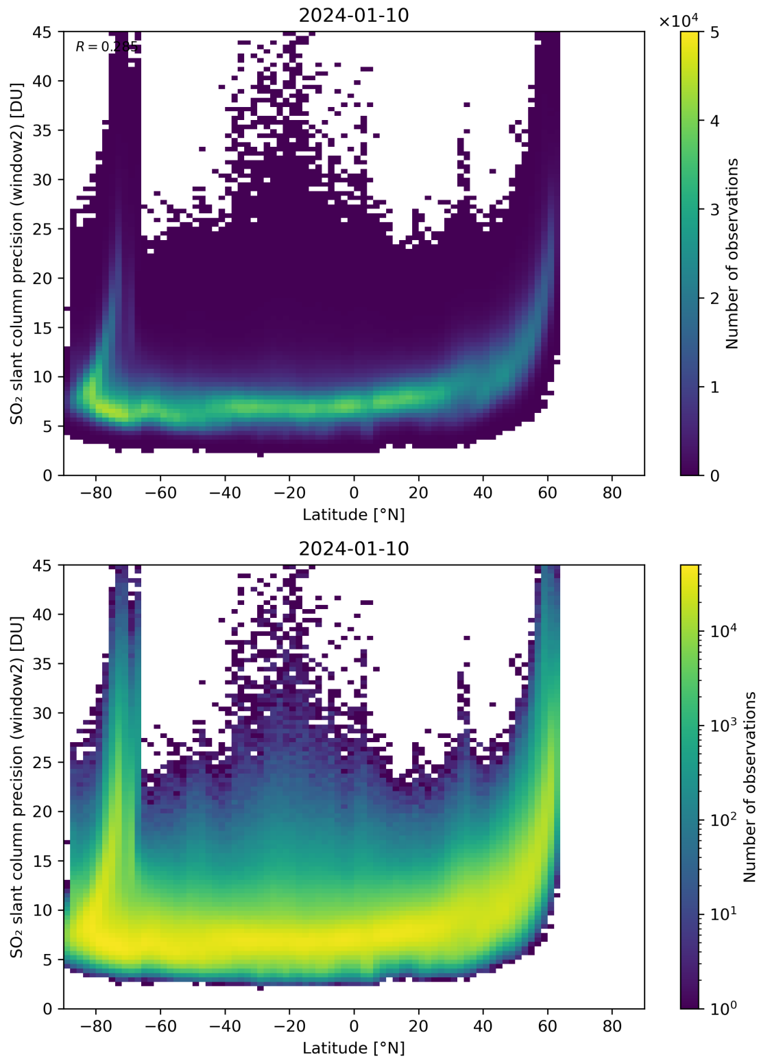
Figure 151: Scatter density plot of “Latitude” against “SO 2 slant column precision (window2)” for 2024-01-10 to 2024-01-11.
