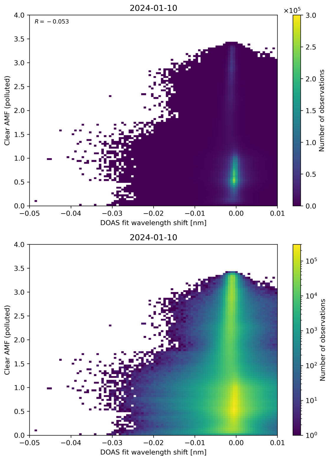
Figure 129: Scatter density plot of “DOAS fit wavelength shift” against “Clear AMF (polluted)” for 2024-01-10 to 2024-01-11.
