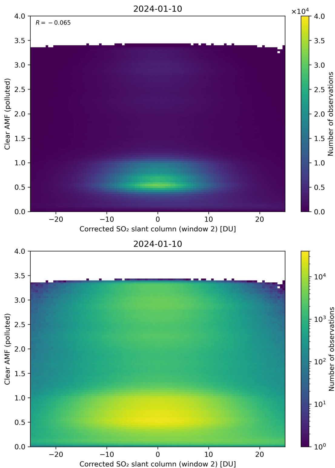
Figure 199: Scatter density plot of “Corrected SO 2 slant column (window 2)” against “Clear AMF (polluted)” for 2024-01-10 to 2024-01-11.
