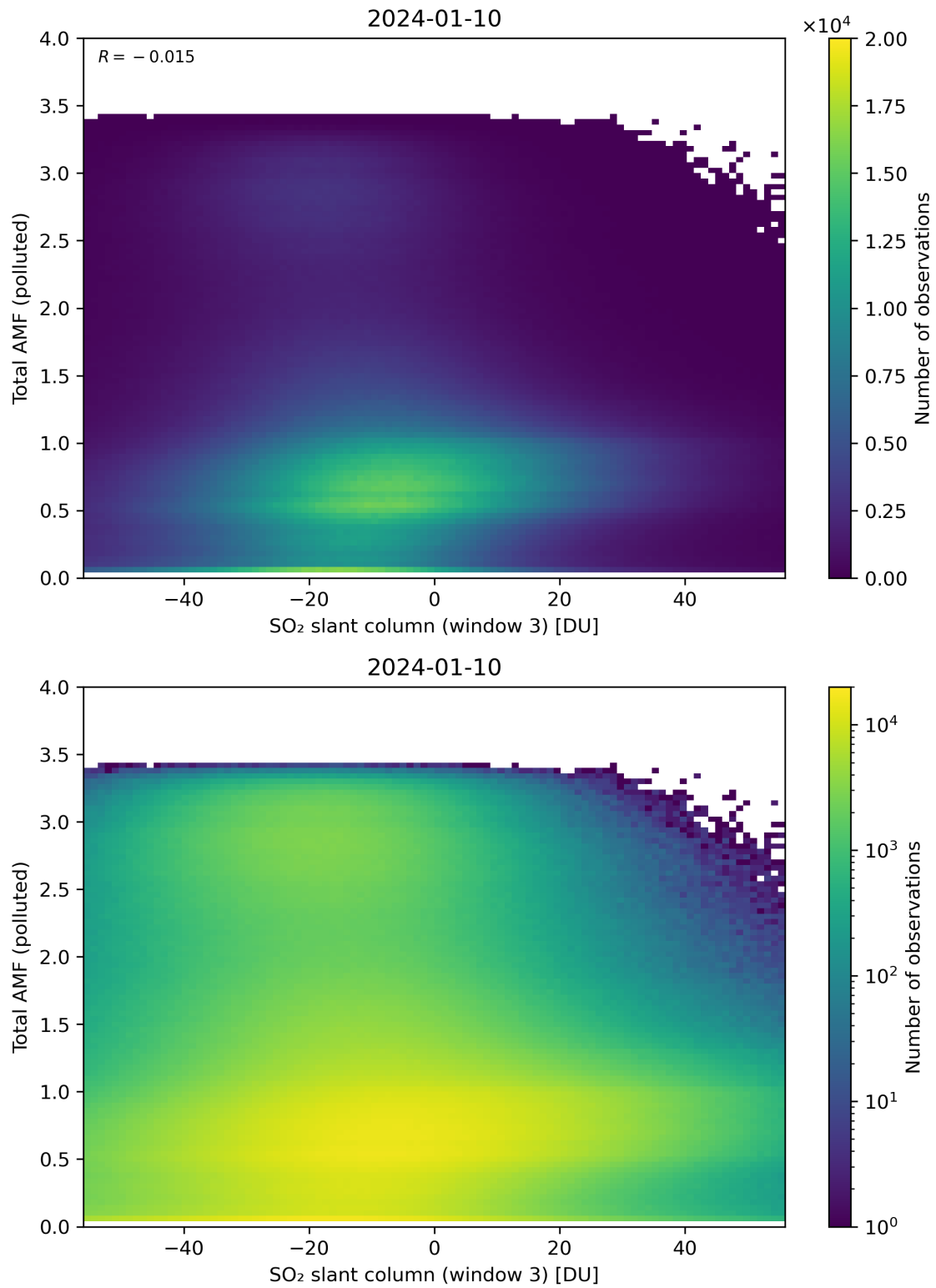
Figure 268: Scatter density plot of “SO 2 slant column (window 3)” against “Total AMF (polluted)” for 2024-01-10 to 2024-01-11.
