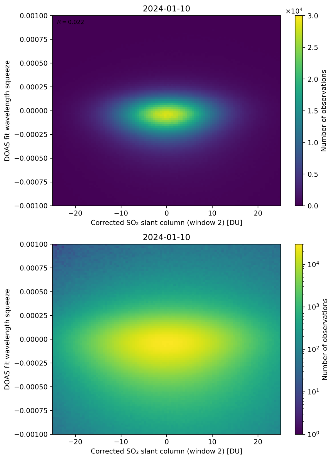
Figure 197: Scatter density plot of “Corrected SO 2 slant column (window 2)” against “DOAS fit wavelength squeeze” for 2024-01-10 to 2024-01-11.
