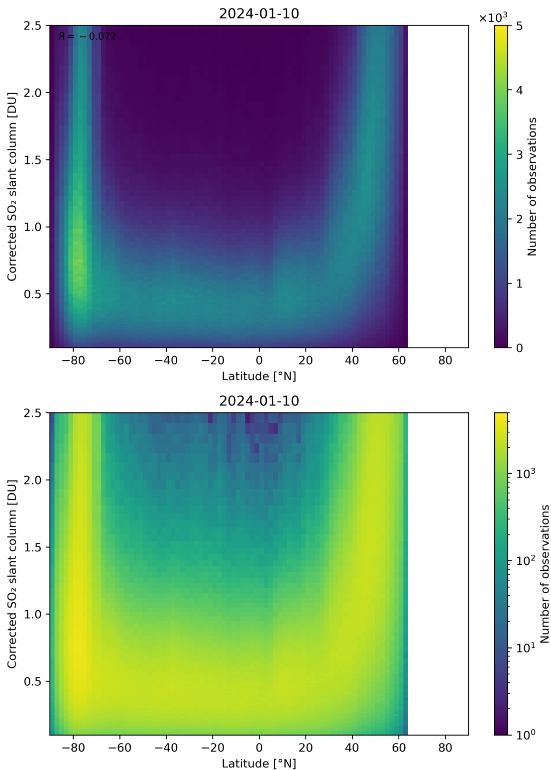
Figure 146: Scatter density plot of “Latitude” against “Corrected SO 2 slant column” for 2024-01-10 to 2024-01-11.
