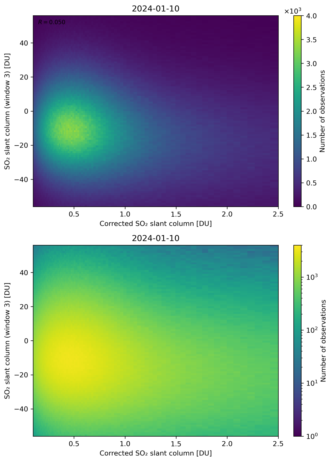
Figure 190: Scatter density plot of “Corrected SO 2 slant column” against “SO 2 slant column (window 3)” for 2024-01-10 to 2024-01-11.
