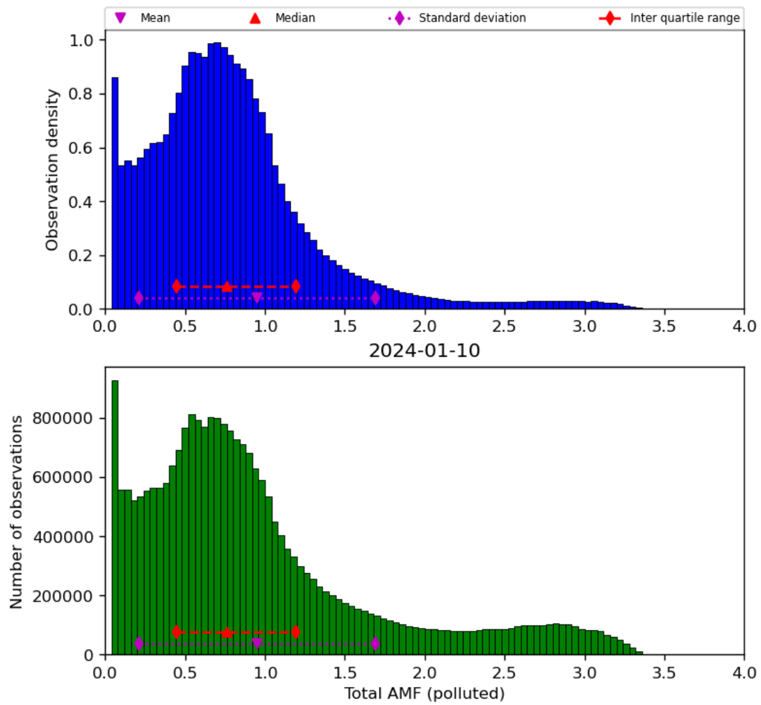
Figure 71: Histogram of “Total AMF (polluted)” for 2024-01-10 to 2024-01-11
