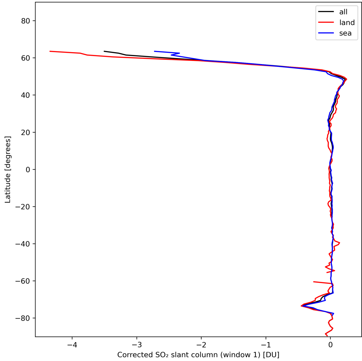
Figure 35: Zonal average of “Corrected SO 2 slant column (window 1)” for 2024-01-10 to 2024-01-11.
