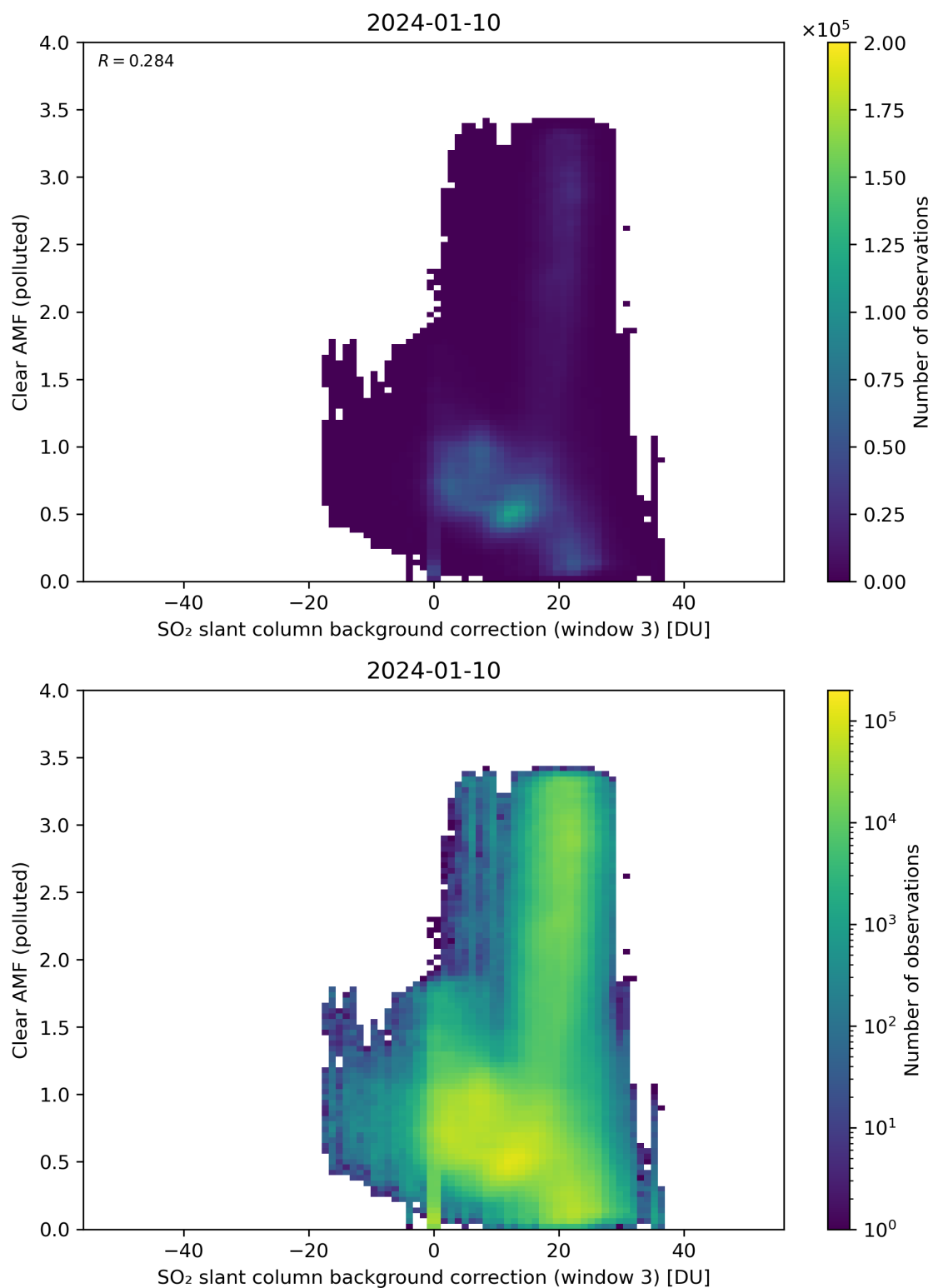
Figure 124: Scatter density plot of “SO 2 slant column background correction (window 3)” against “Clear AMF (polluted)” for 2024-01-10 to 2024-01-11.
