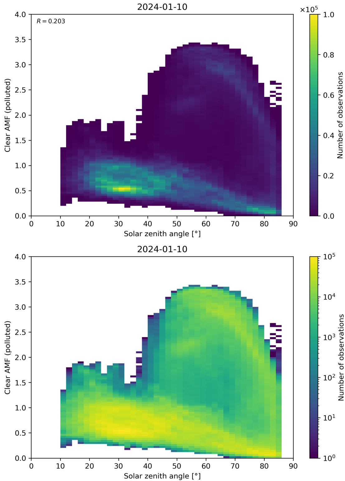
Figure 165: Scatter density plot of “Solar zenith angle” against “Clear AMF (polluted)” for 2024-01-10 to 2024-01-11.
