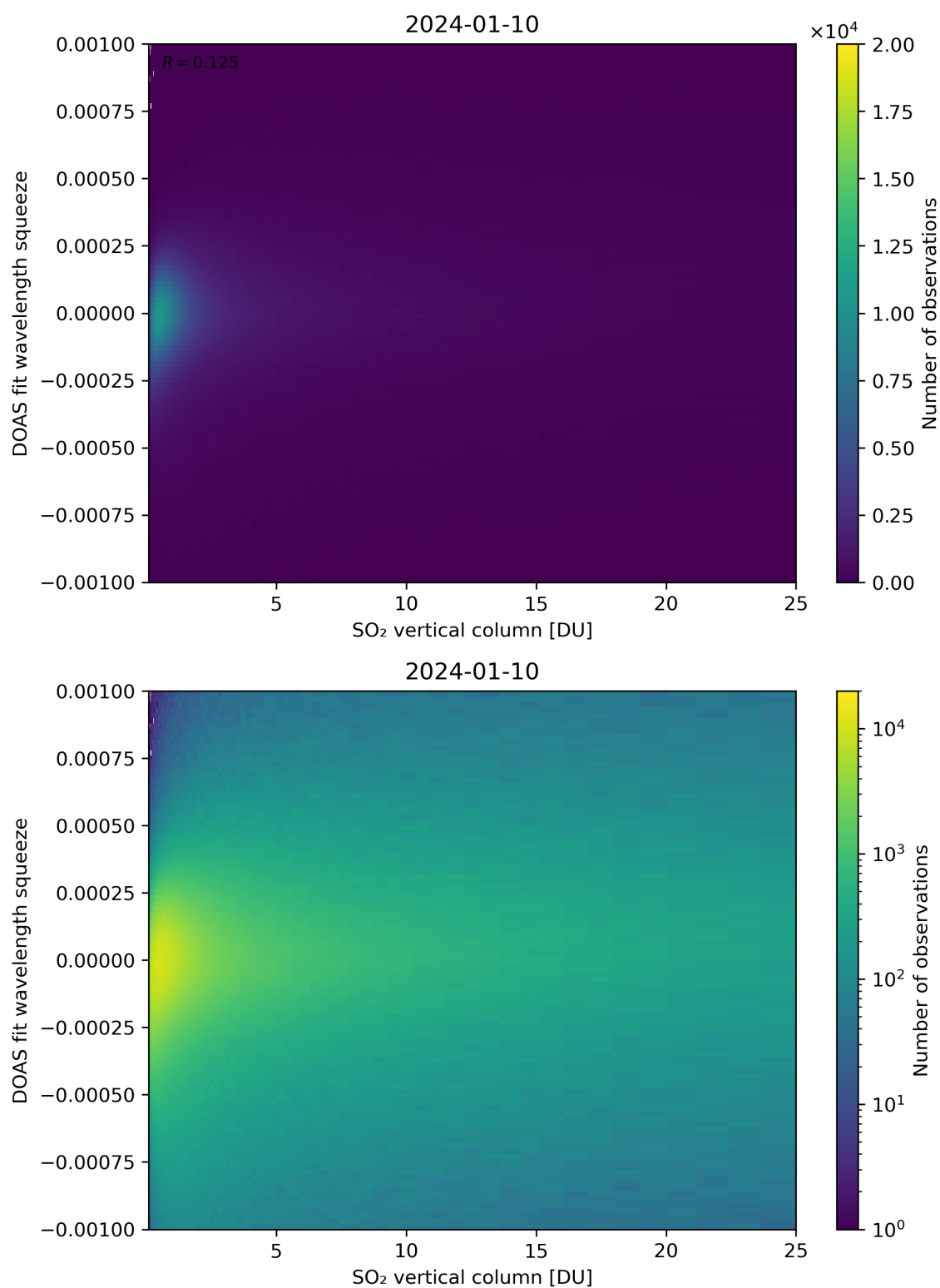
Figure 277: Scatter density plot of “SO 2 vertical column” against “DOAS fit wavelength squeeze” for 2024-01-10 to 2024-01-11.
