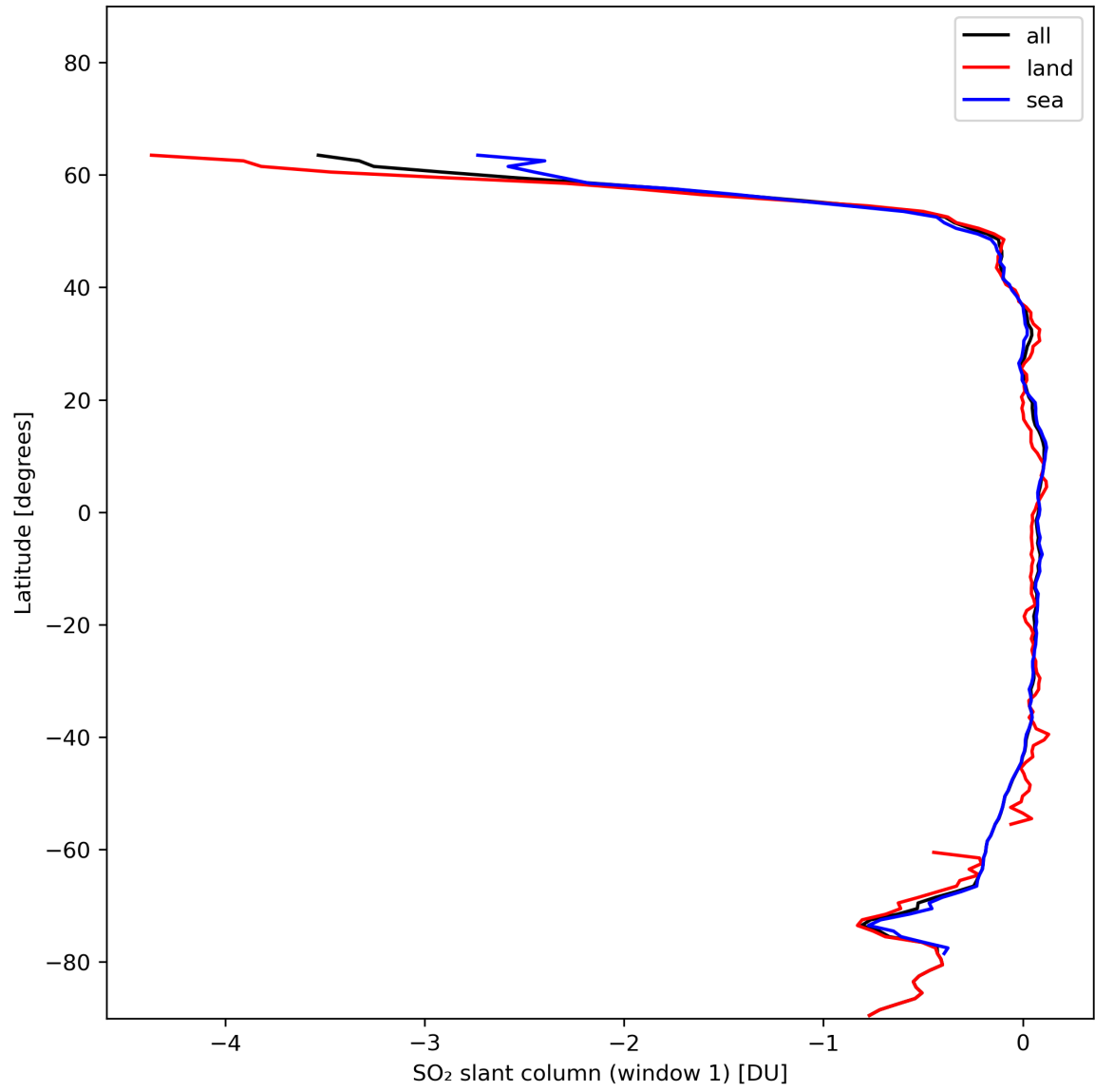
Figure 33: Zonal average of “SO 2 slant column (window 1)” for 2024-01-10 to 2024-01-11.
