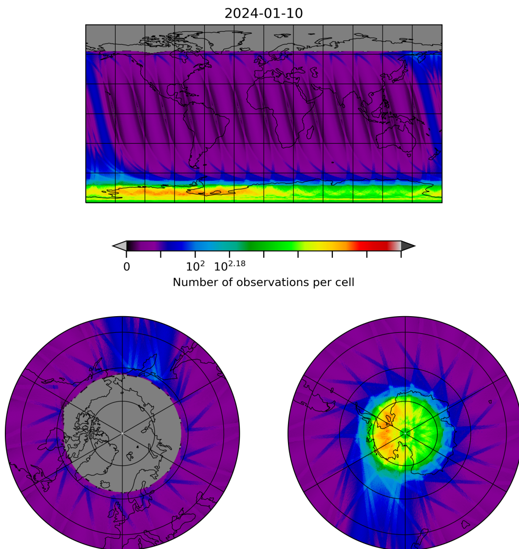
Figure 28: Map of the number of observations for 2024-01-10 to 2024-01-11
