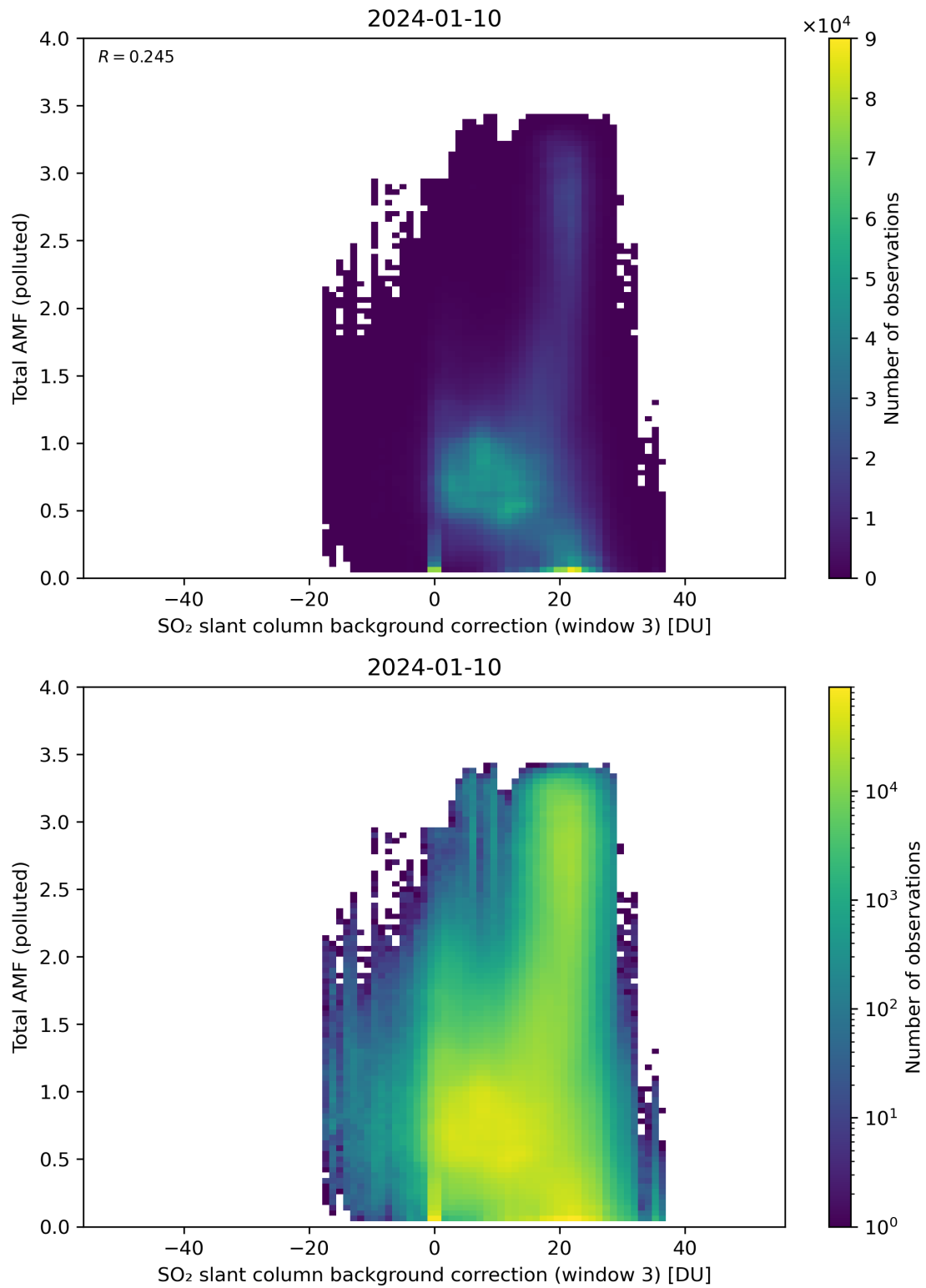
Figure 125: Scatter density plot of “SO 2 slant column background correction (window 3)” against “Total AMF (polluted)” for 2024-01-10 to 2024-01-11.
