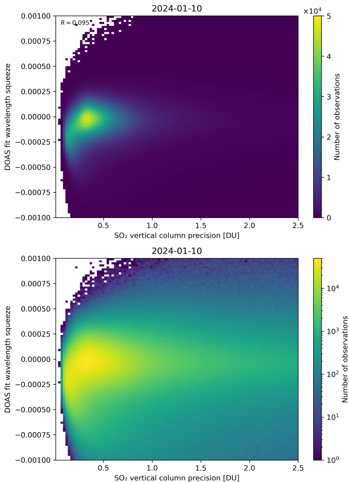
Figure 283: Scatter density plot of “SO 2 vertical column precision” against “DOAS fit wavelength squeeze” for 2024-01-10 to 2024-01-11.
