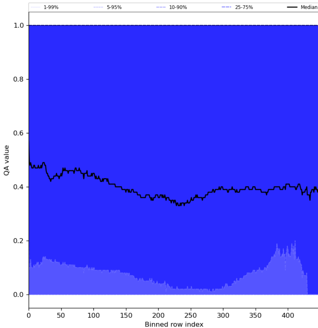
Figure 75: Along track statistics of “QA value” for 2024-01-10 to 2024-01-11
