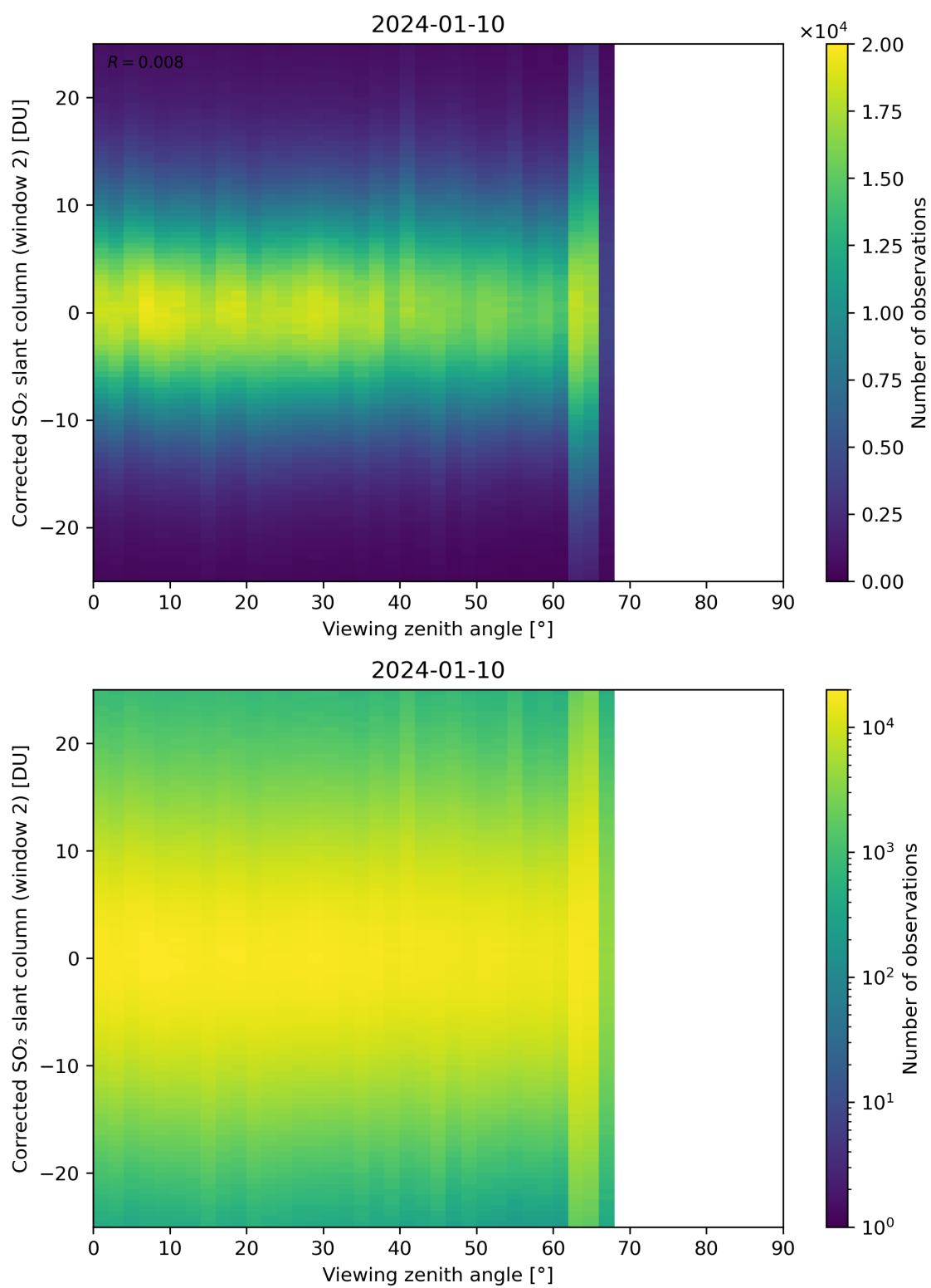
Figure 318: Scatter density plot of “Viewing zenith angle” against “Corrected SO 2 slant column (window 2)” for 2024-01-10 to 2024-01-11.
