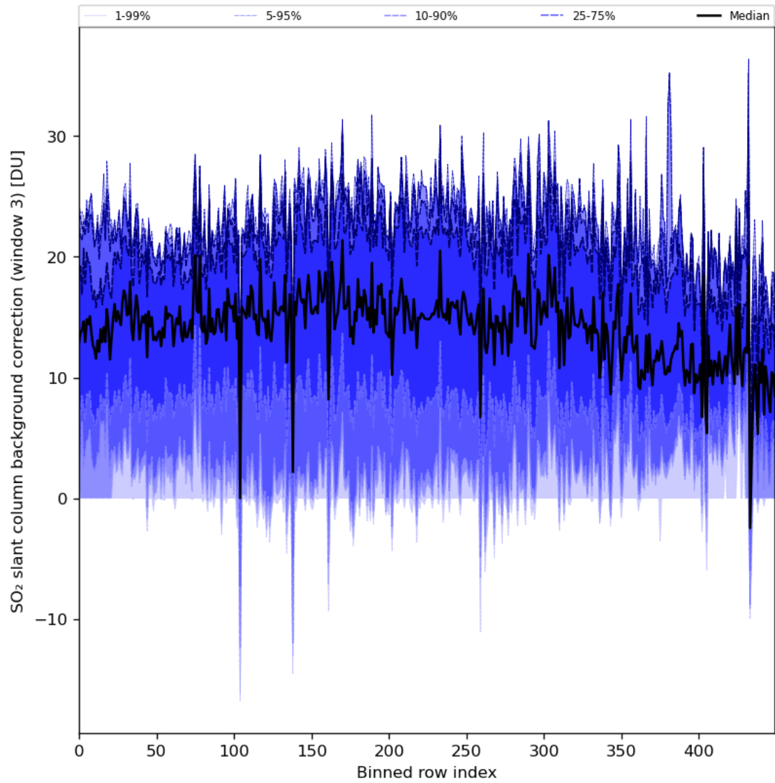
Figure 90: Along track statistics of “SO 2 slant column background correction (window 3)” for 2024-01-10 to 2024-01-11
