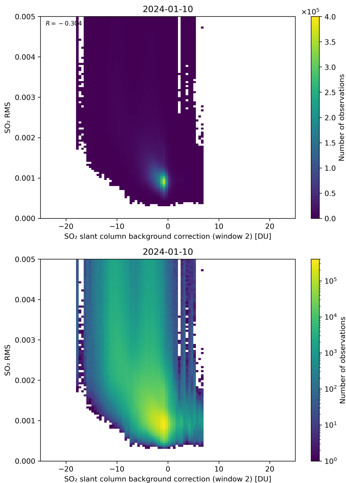
Figure 114: Scatter density plot of “SO 2 slant column background correction (window 2)” against “SO 2 RMS” for 2024-01-10 to 2024-01-11.
