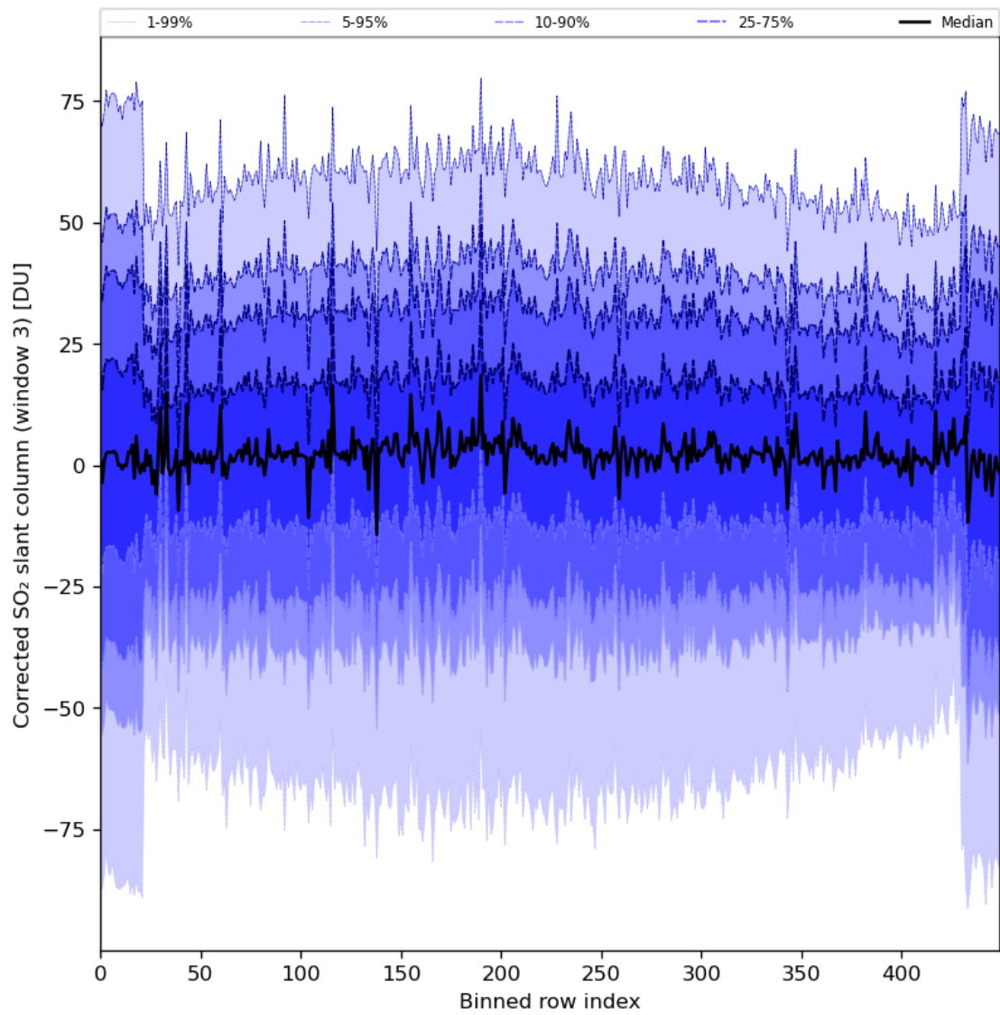
Figure 89: Along track statistics of “Corrected SO 2 slant column (window 3)” for 2024-01-10 to 2024-01-11
