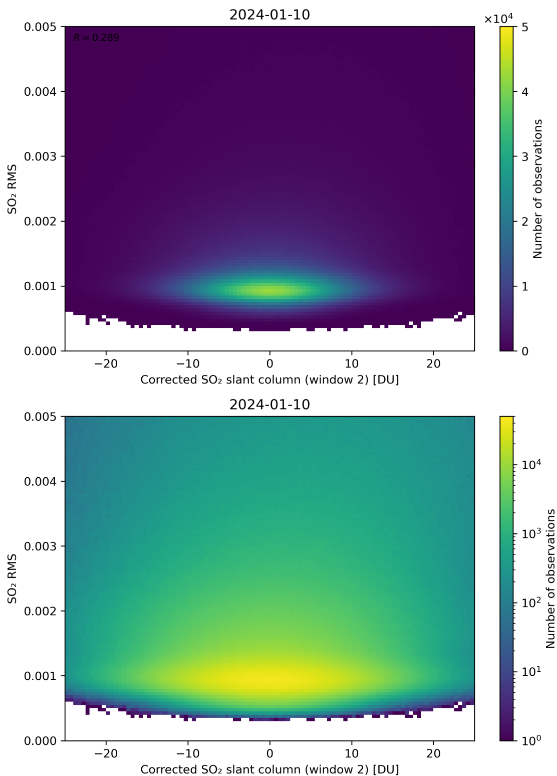
Figure 198: Scatter density plot of “Corrected SO 2 slant column (window 2)” against “SO 2 RMS” for 2024-01-10 to 2024-01-11.
