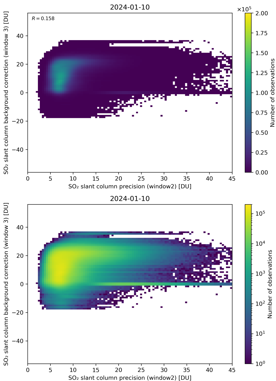
Figure 242: Scatter density plot of “SO 2 slant column precision (window2)” against “SO 2 slant column background correction (window 3)” for 2024-01-10 to 2024-01-11.
