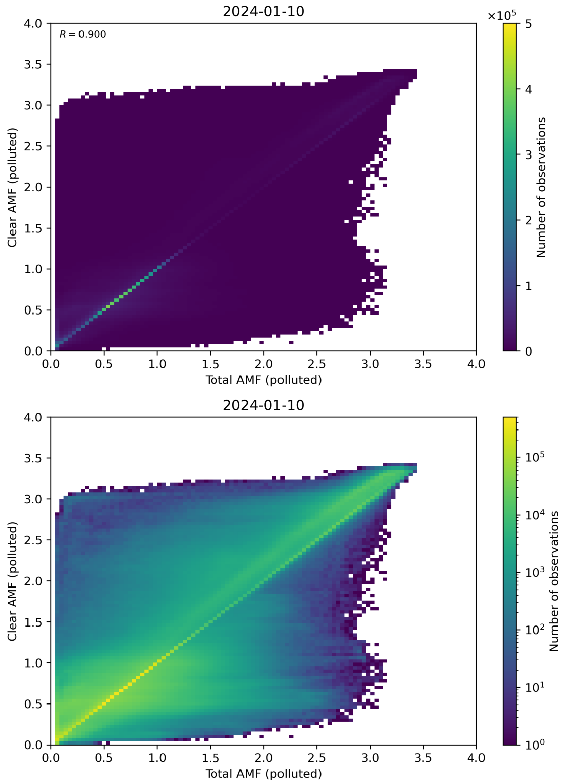
Figure 271: Scatter density plot of “Total AMF (polluted)” against “Clear AMF (polluted)” for 2024-01-10 to 2024-01-11.
