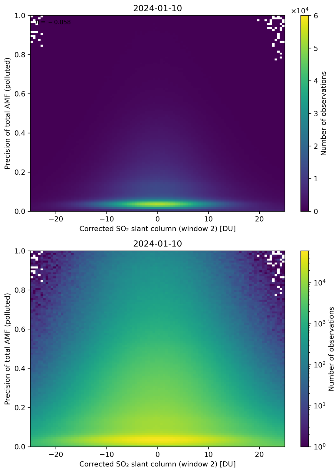
Figure 204: Scatter density plot of “Corrected SO 2 slant column (window 2)” against “Precision of total AMF (polluted)” for 2024-01-10 to 2024-01-11.
