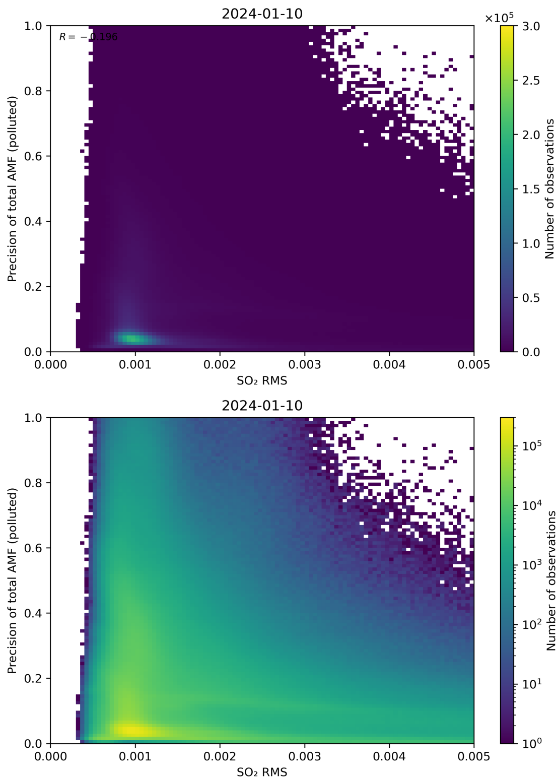
Figure 138: Scatter density plot of “SO 2 RMS” against “Precision of total AMF (polluted)” for 2024-01-10 to 2024-01-11.
