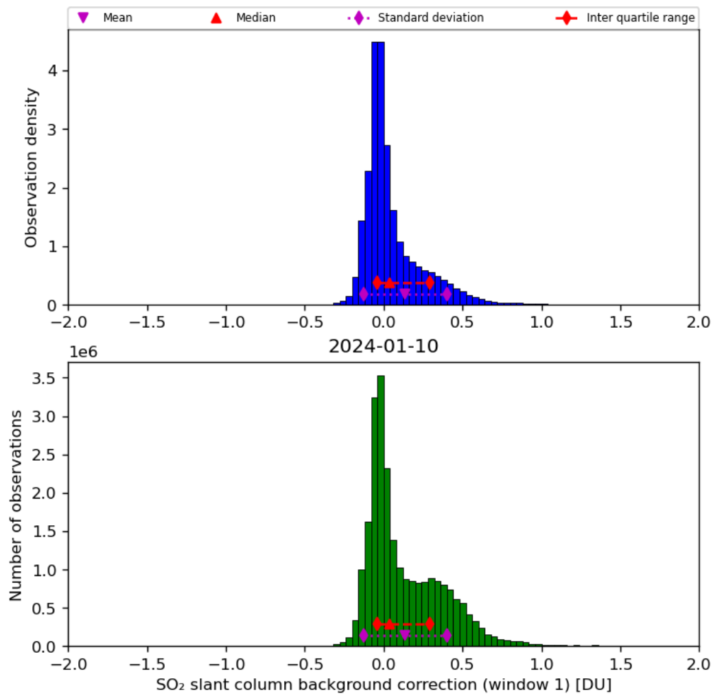
Figure 59: Histogram of “SO 2 slant column background correction (window 1)” for 2024-01-10 to 2024-01-11
