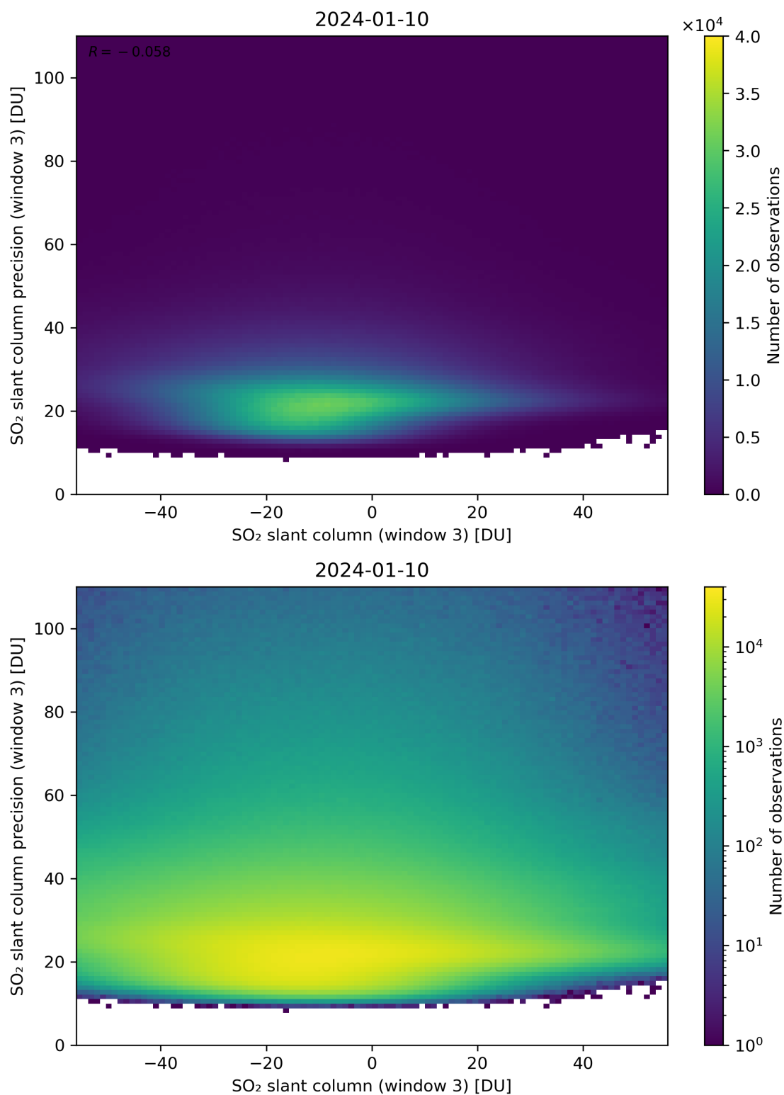
Figure 267: Scatter density plot of “SO 2 slant column (window 3)” against “SO 2 slant column precision (window 3)” for 2024-01-10 to 2024-01-11.
