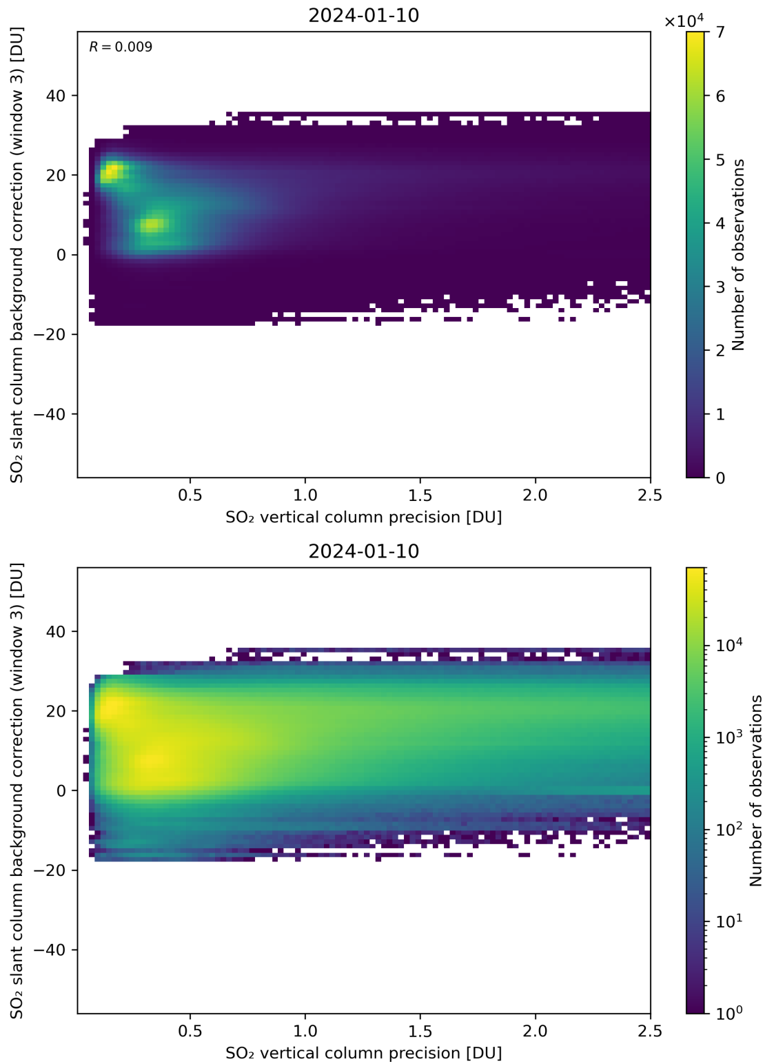
Figure 281: Scatter density plot of “SO 2 vertical column precision” against “SO 2 slant column background correction (window 3)” for 2024-01-10 to 2024-01-11.
