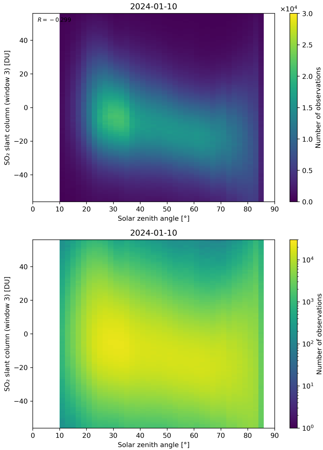
Figure 172: Scatter density plot of “Solar zenith angle” against “SO 2 slant column (window 3)” for 2024-01-10 to 2024-01-11.
