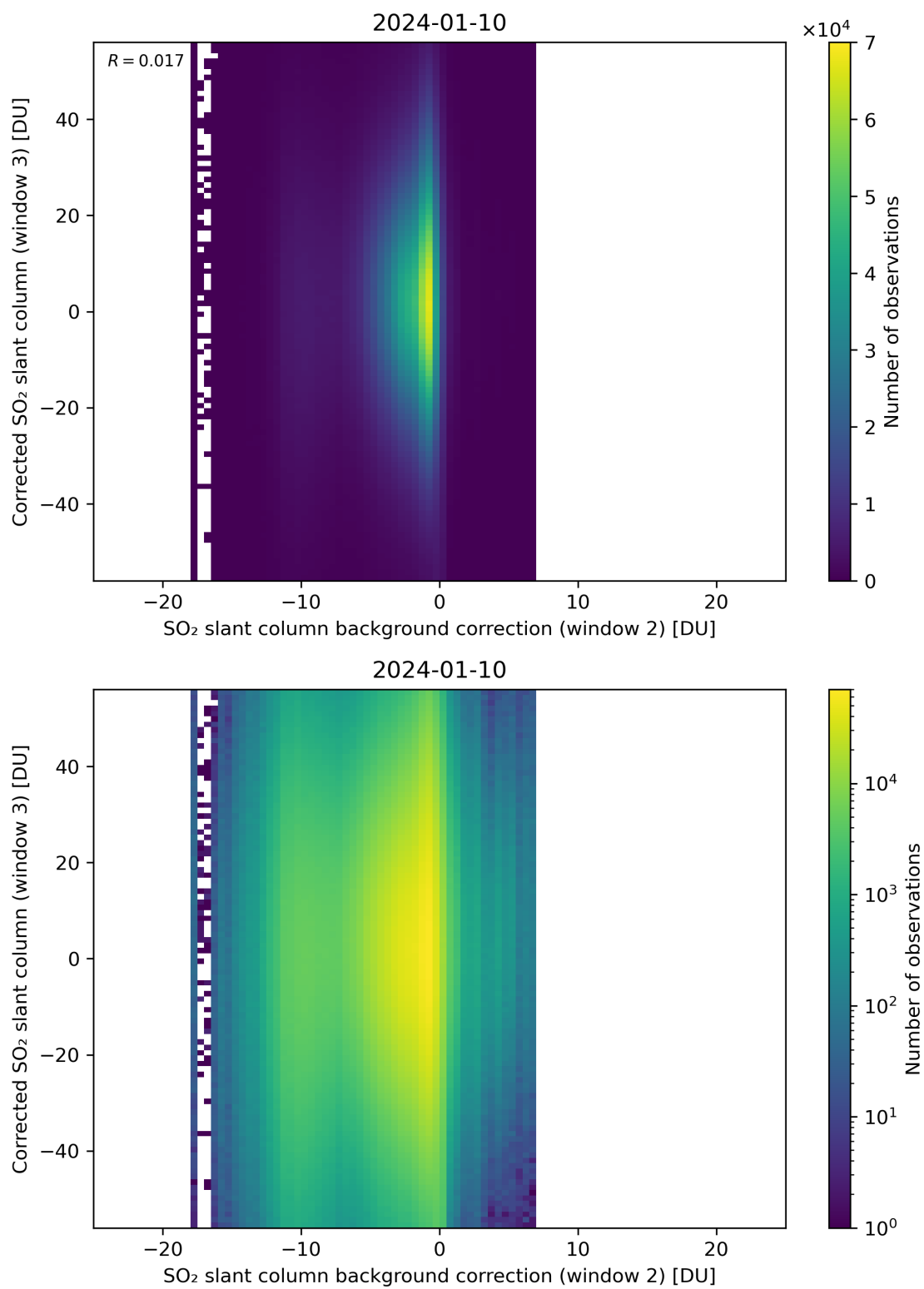
Figure 116: Scatter density plot of “SO 2 slant column background correction (window 2)” against “Corrected SO 2 slant column (window 3)” for 2024-01-10 to 2024-01-11.
