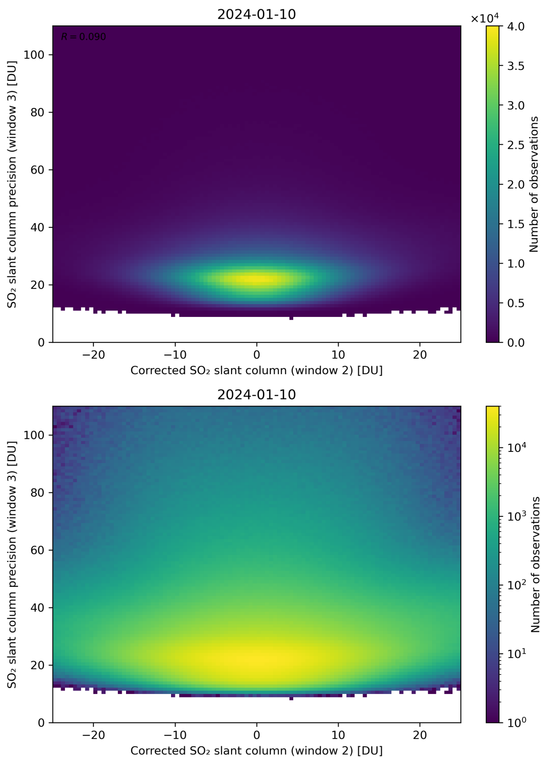
Figure 202: Scatter density plot of “Corrected SO 2 slant column (window 2)” against “SO 2 slant column precision (window 3)” for 2024-01-10 to 2024-01-11.
