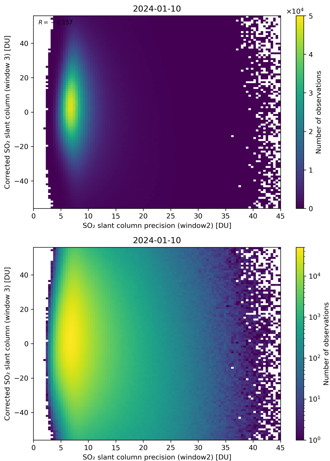
Figure 248: Scatter density plot of “SO 2 slant column precision (window2)” against “Corrected SO 2 slant column (window 3)” for 2024-01-10 to 2024-01-11.
