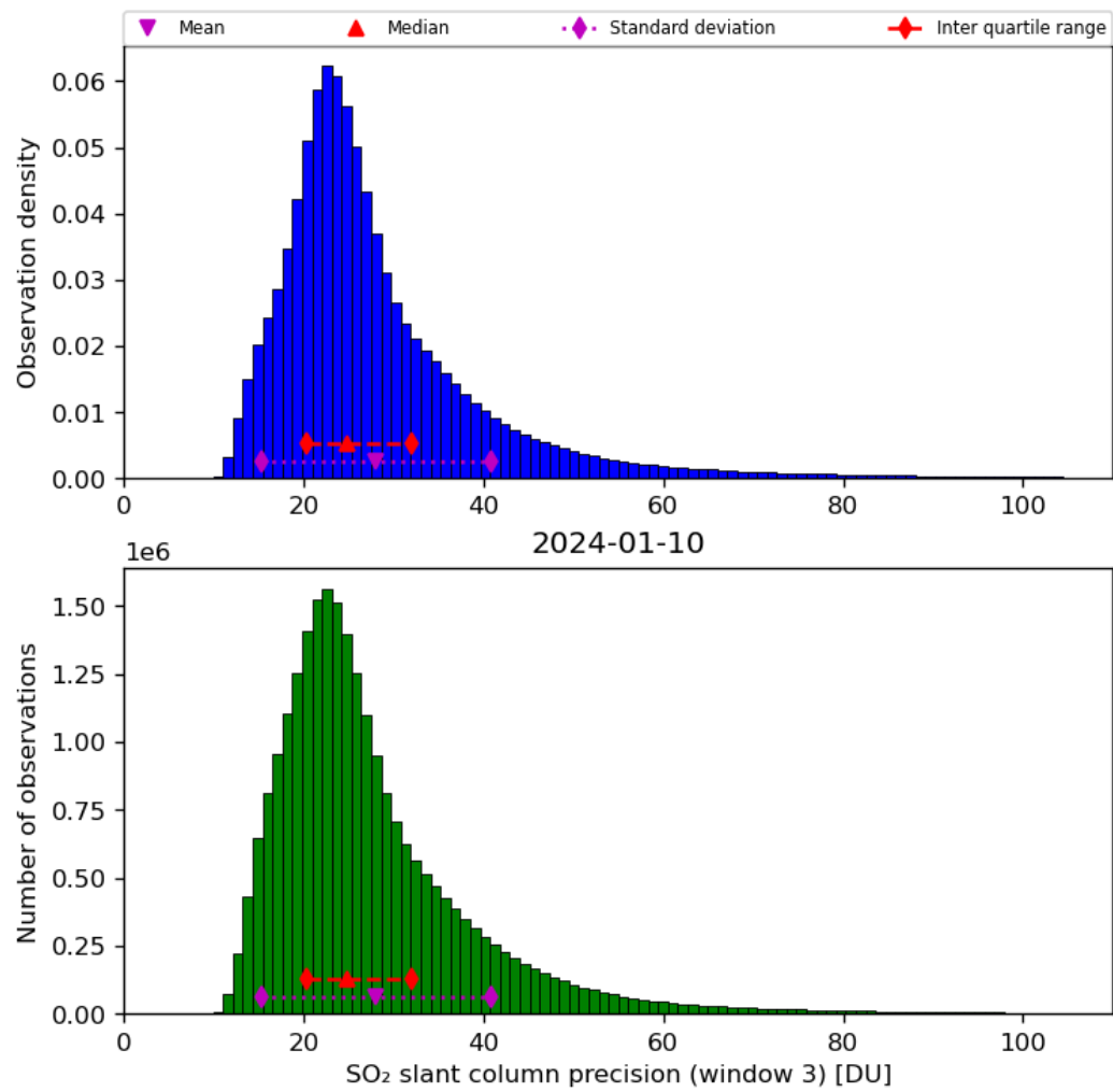
Figure 65: Histogram of “SO 2 slant column precision (window 3)” for 2024-01-10 to 2024-01-11
