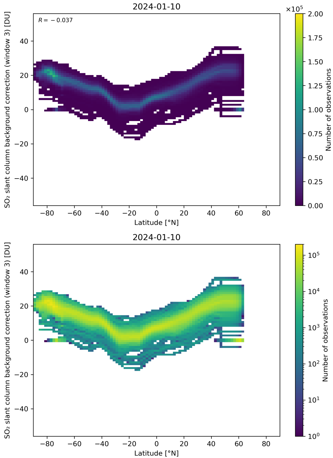
Figure 141: Scatter density plot of “Latitude” against “SO 2 slant column background correction (window 3)” for 2024-01-10 to 2024-01-11.
