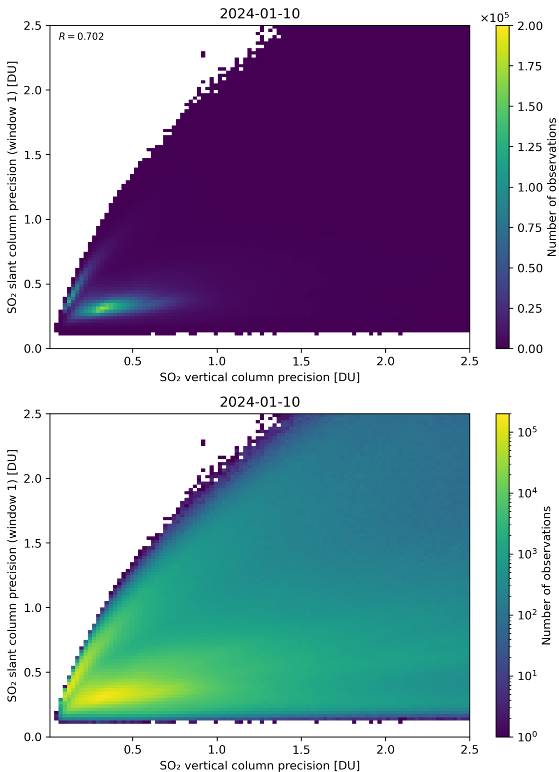
Figure 290: Scatter density plot of “SO 2 vertical column precision” against “SO 2 slant column precision (window 1)” for 2024-01-10 to 2024-01-11.
