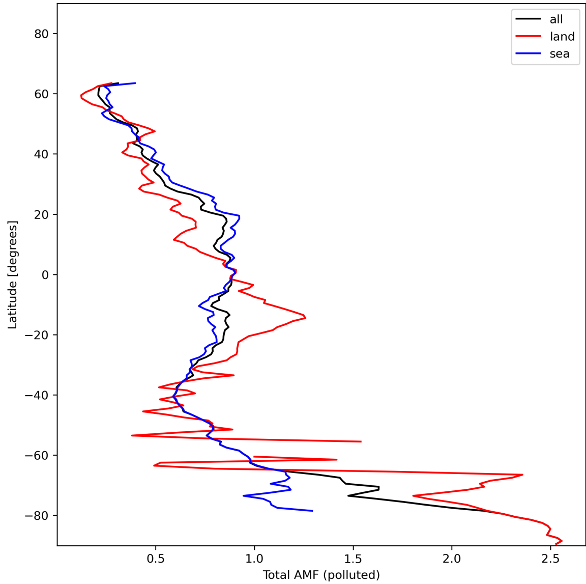
Figure 48: Zonal average of “Total AMF (polluted)” for 2024-01-10 to 2024-01-11.
