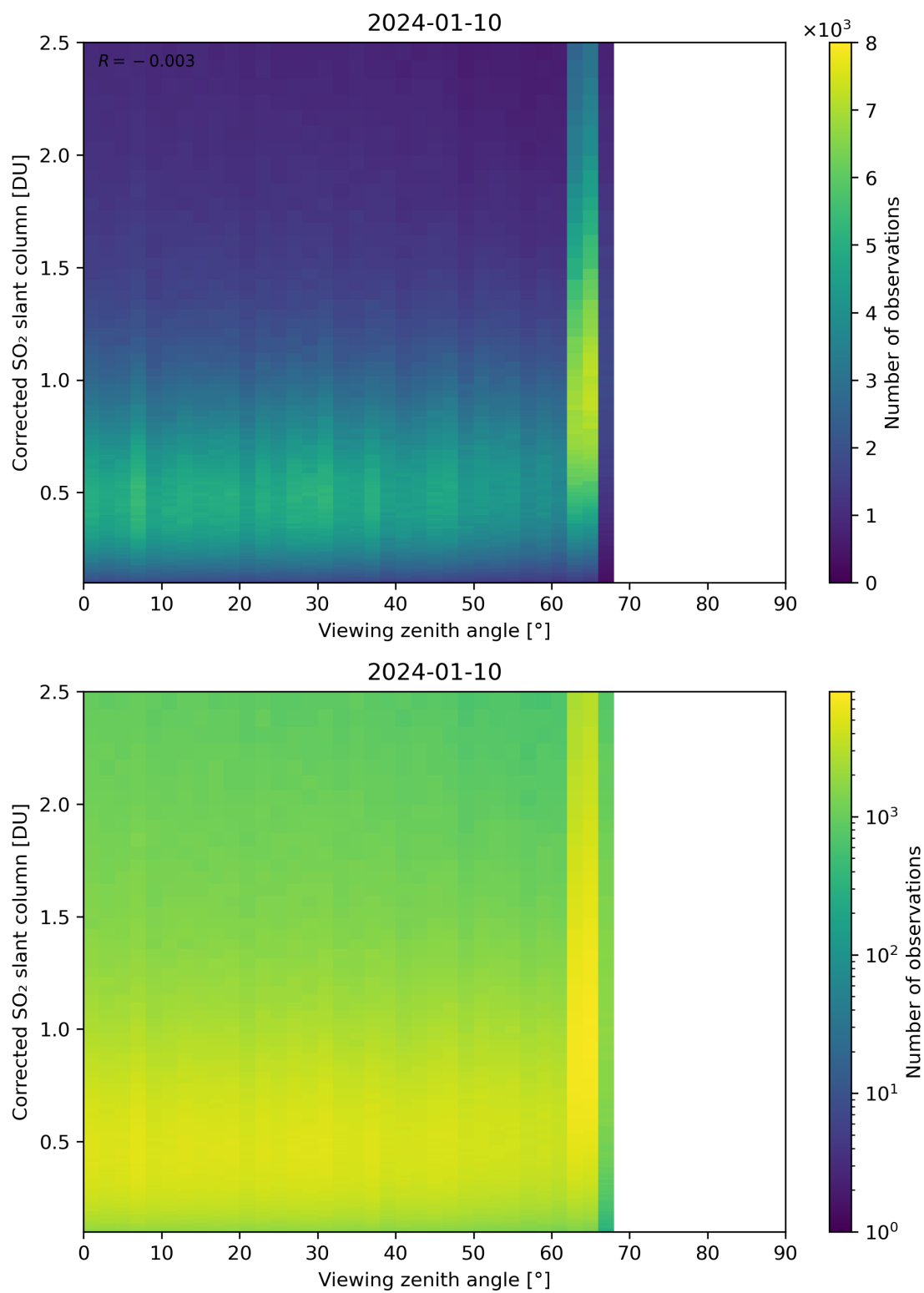
Figure 317: Scatter density plot of “Viewing zenith angle” against “Corrected SO 2 slant column” for 2024-01-10 to 2024-01-11.
