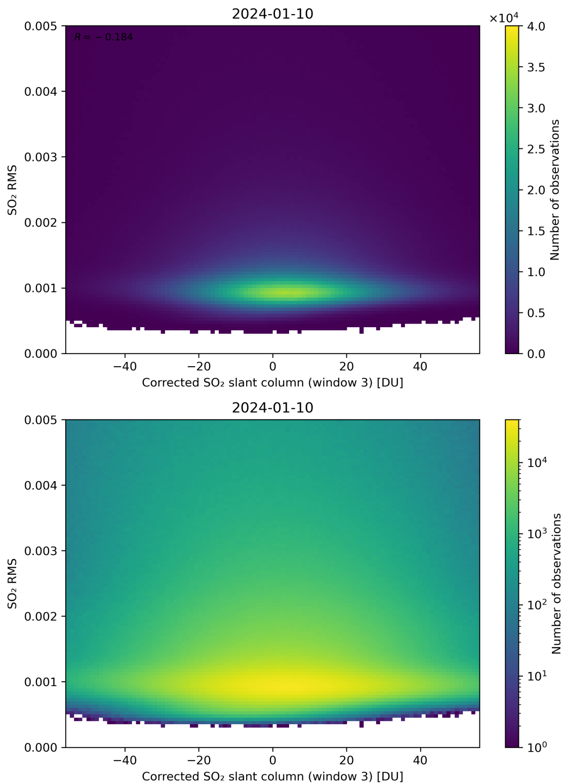
Figure 208: Scatter density plot of “Corrected SO 2 slant column (window 3)” against “SO 2 RMS” for 2024-01-10 to 2024-01-11.
