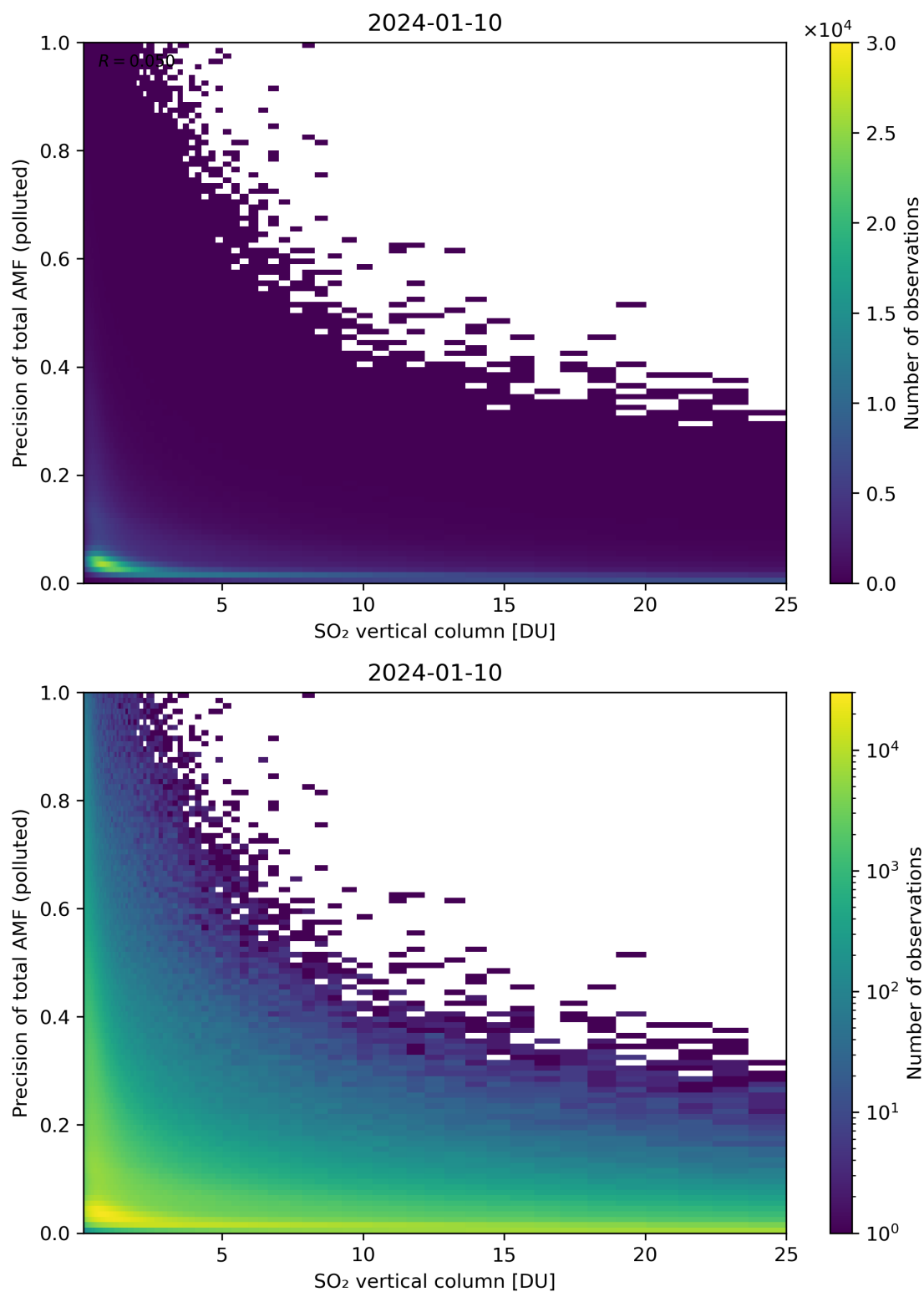
Figure 306: Scatter density plot of “SO 2 vertical column” against “Precision of total AMF (polluted)” for 2024-01-10 to 2024-01-11.
