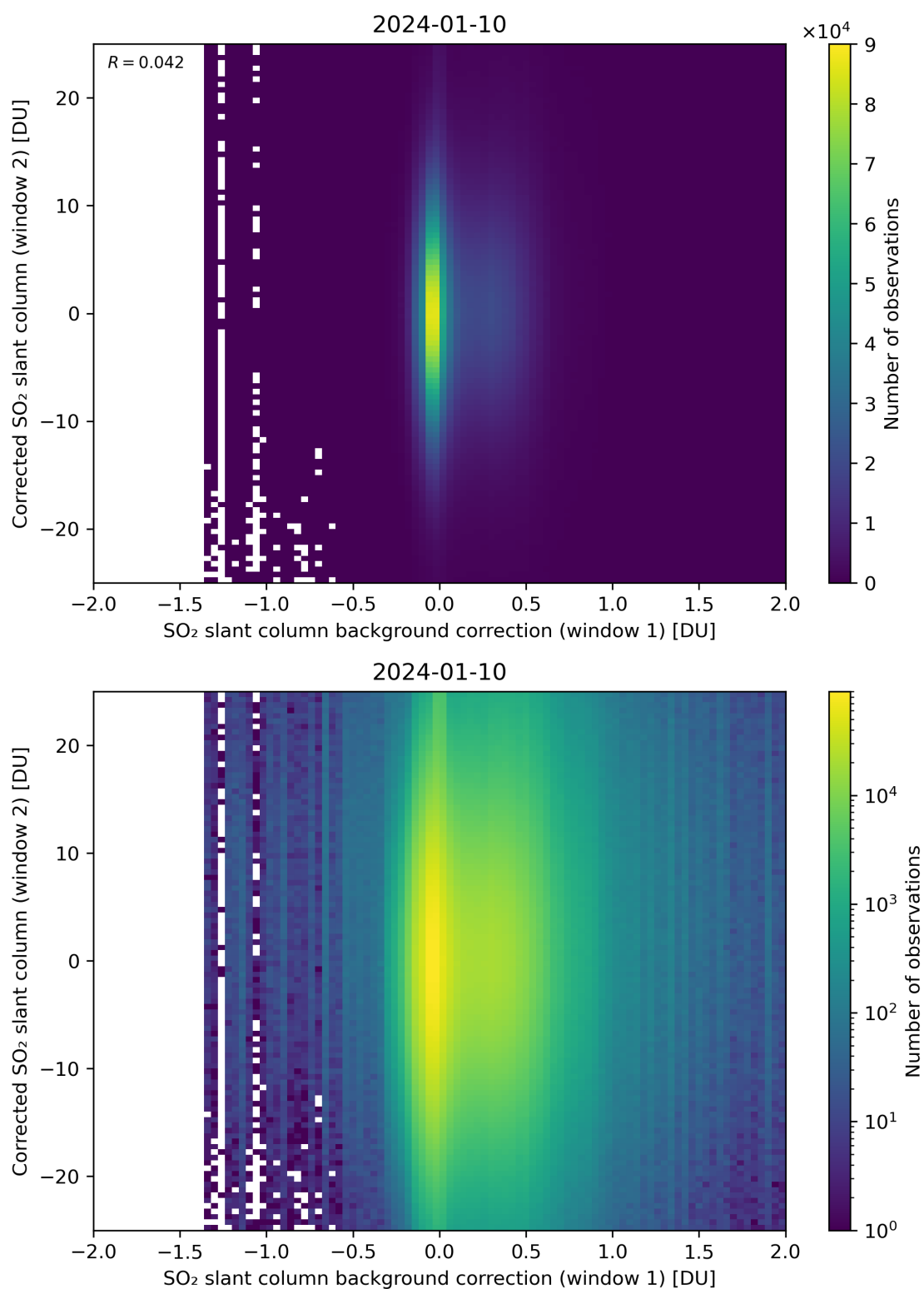
Figure 104: Scatter density plot of “SO 2 slant column background correction (window 1)” against “Corrected SO 2 slant column (window 2)” for 2024-01-10 to 2024-01-11.
