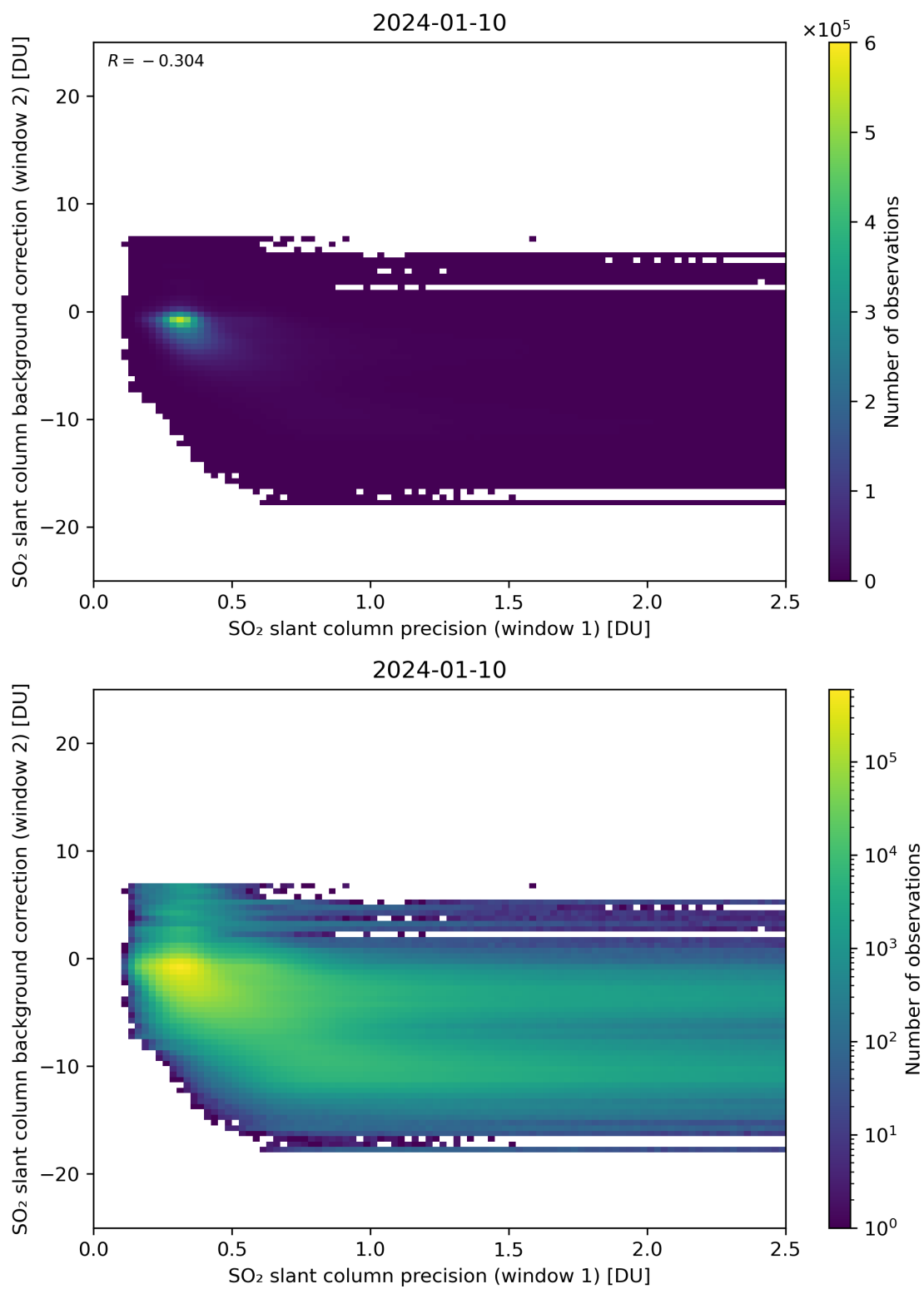
Figure 219: Scatter density plot of “SO 2 slant column precision (window 1)” against “SO 2 slant column background correction (window 2)” for 2024-01-10 to 2024-01-11.
