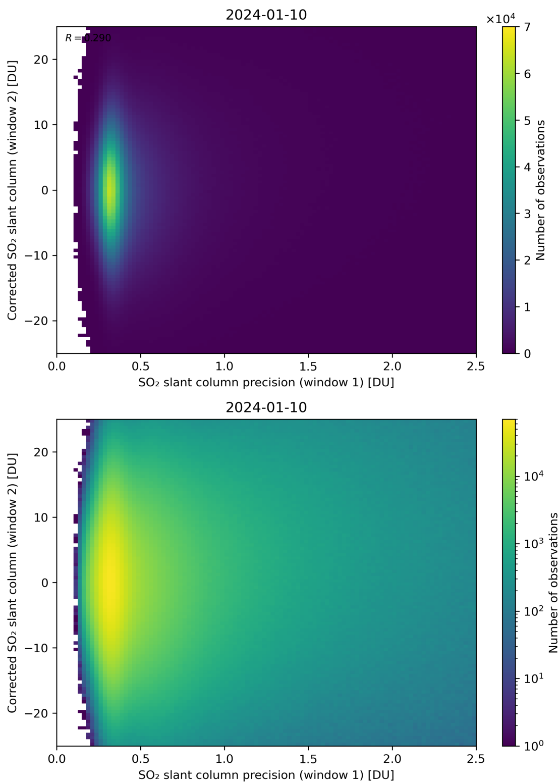
Figure 225: Scatter density plot of “SO 2 slant column precision (window 1)” against “Corrected SO 2 slant column (window 2)” for 2024-01-10 to 2024-01-11.
