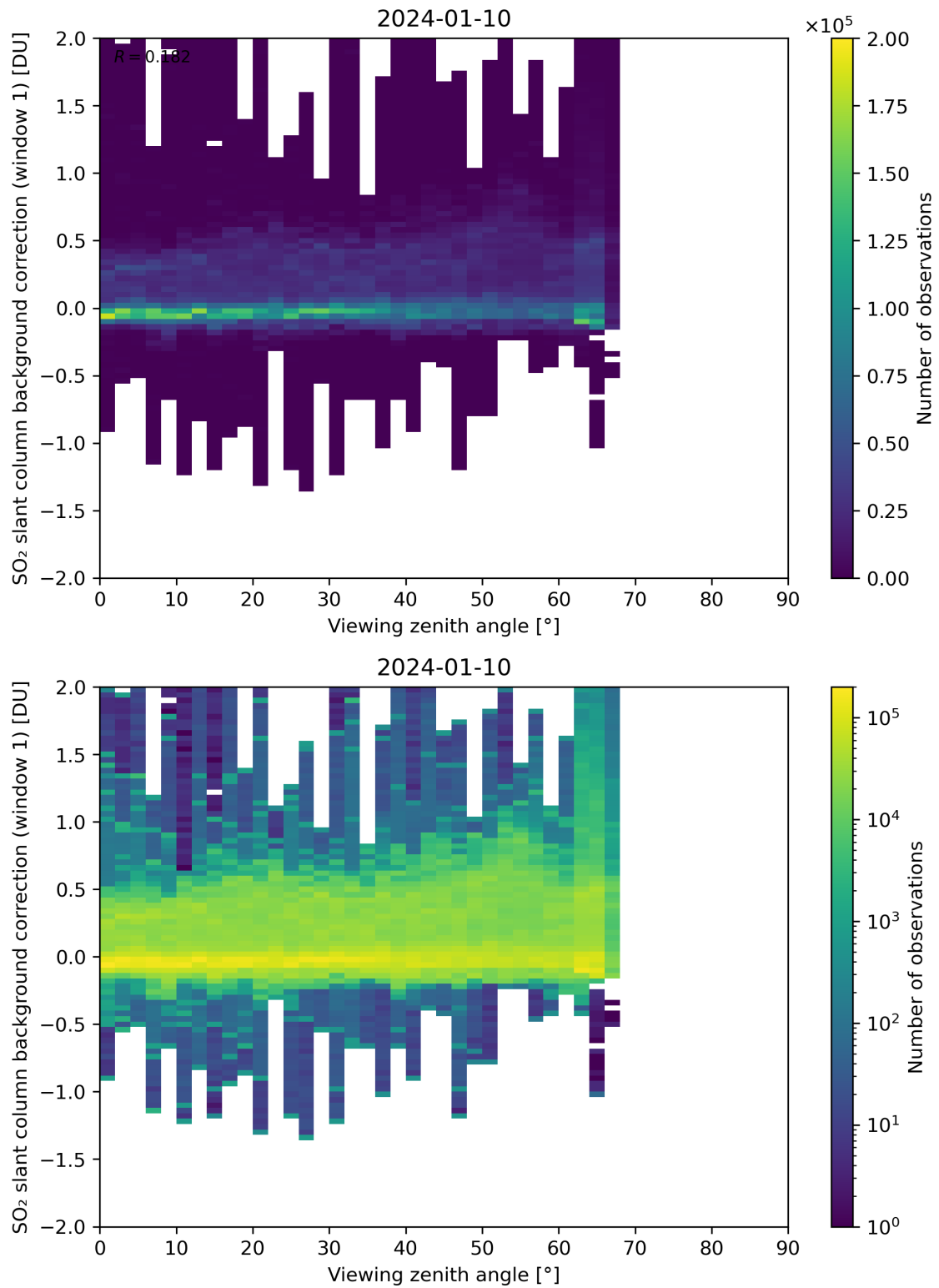
Figure 308: Scatter density plot of “Viewing zenith angle” against “SO 2 slant column background correction (window 1)” for 2024-01-10 to 2024-01-11.
