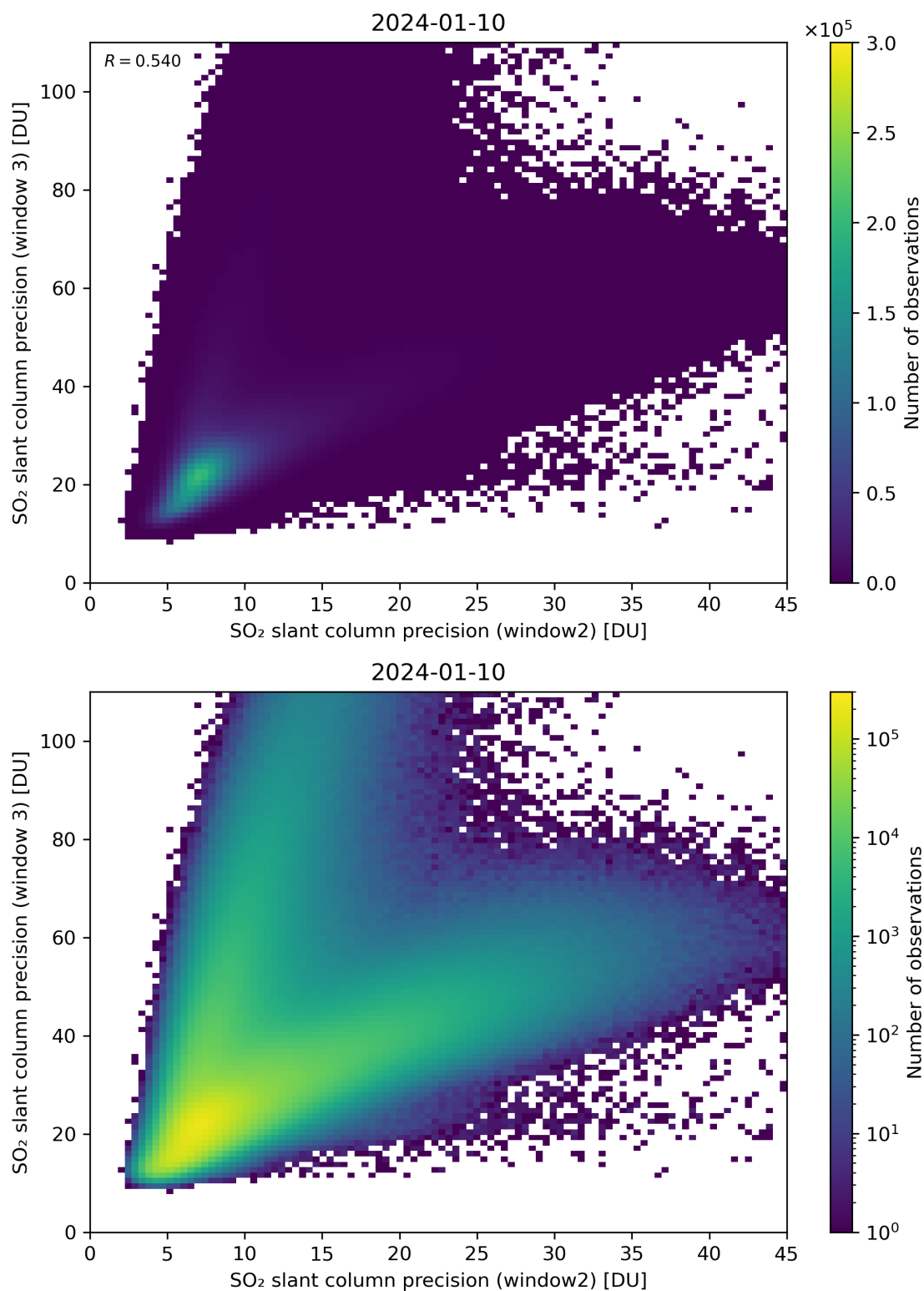
Figure 250: Scatter density plot of “SO 2 slant column precision (window2)” against “SO 2 slant column precision (window 3)” for 2024-01-10 to 2024-01-11.
