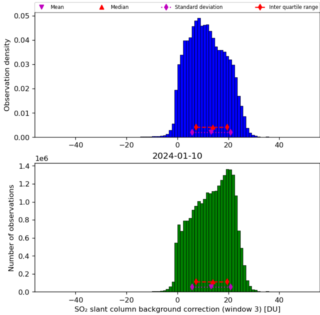
Figure 67: Histogram of “SO 2 slant column background correction (window 3)” for 2024-01-10 to 2024-01-11
