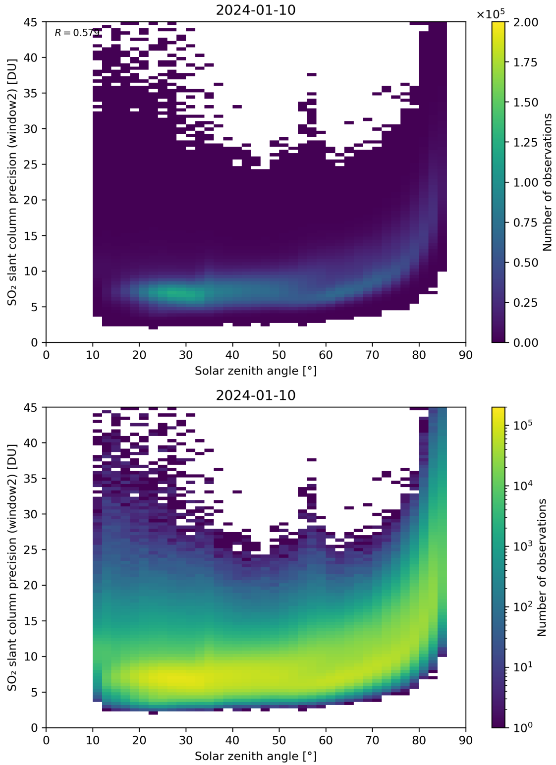
Figure 171: Scatter density plot of “Solar zenith angle” against “SO 2 slant column precision (window2)” for 2024-01-10 to 2024-01-11.
