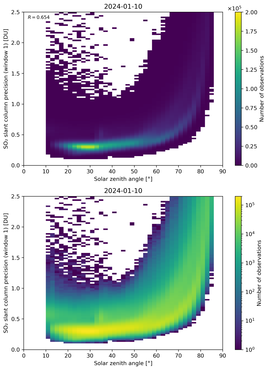
Figure 170: Scatter density plot of “Solar zenith angle” against “SO 2 slant column precision (window 1)” for 2024-01-10 to 2024-01-11.
