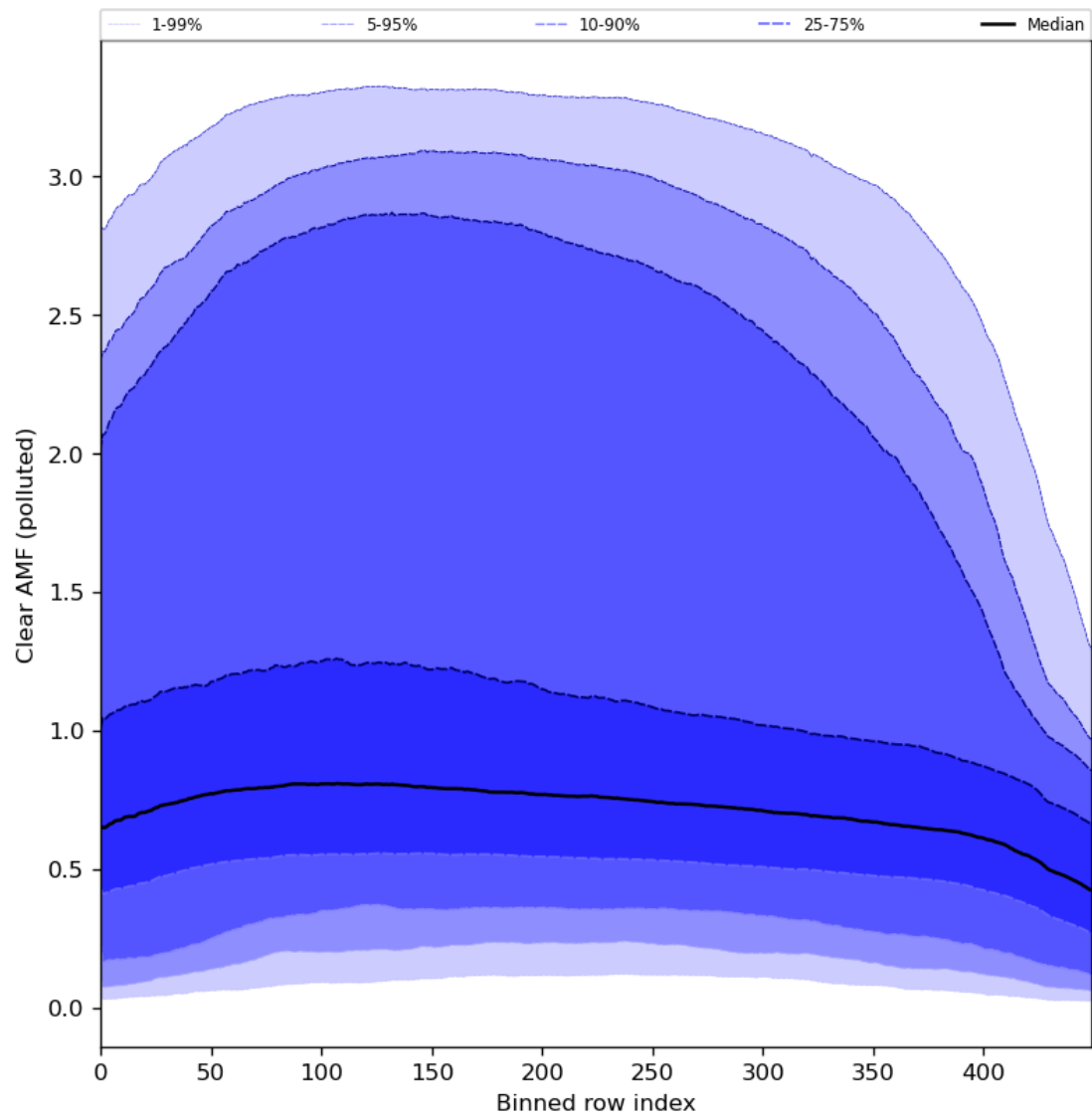
Figure 96: Along track statistics of “Clear AMF (polluted)” for 2024-01-10 to 2024-01-11
