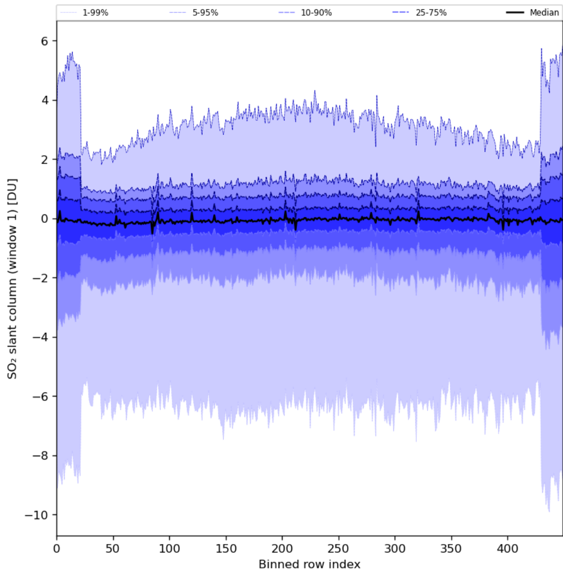
Figure 79: Along track statistics of "SO 2 slant column (window 1)" for 2024-01-10 to 2024-01-11
