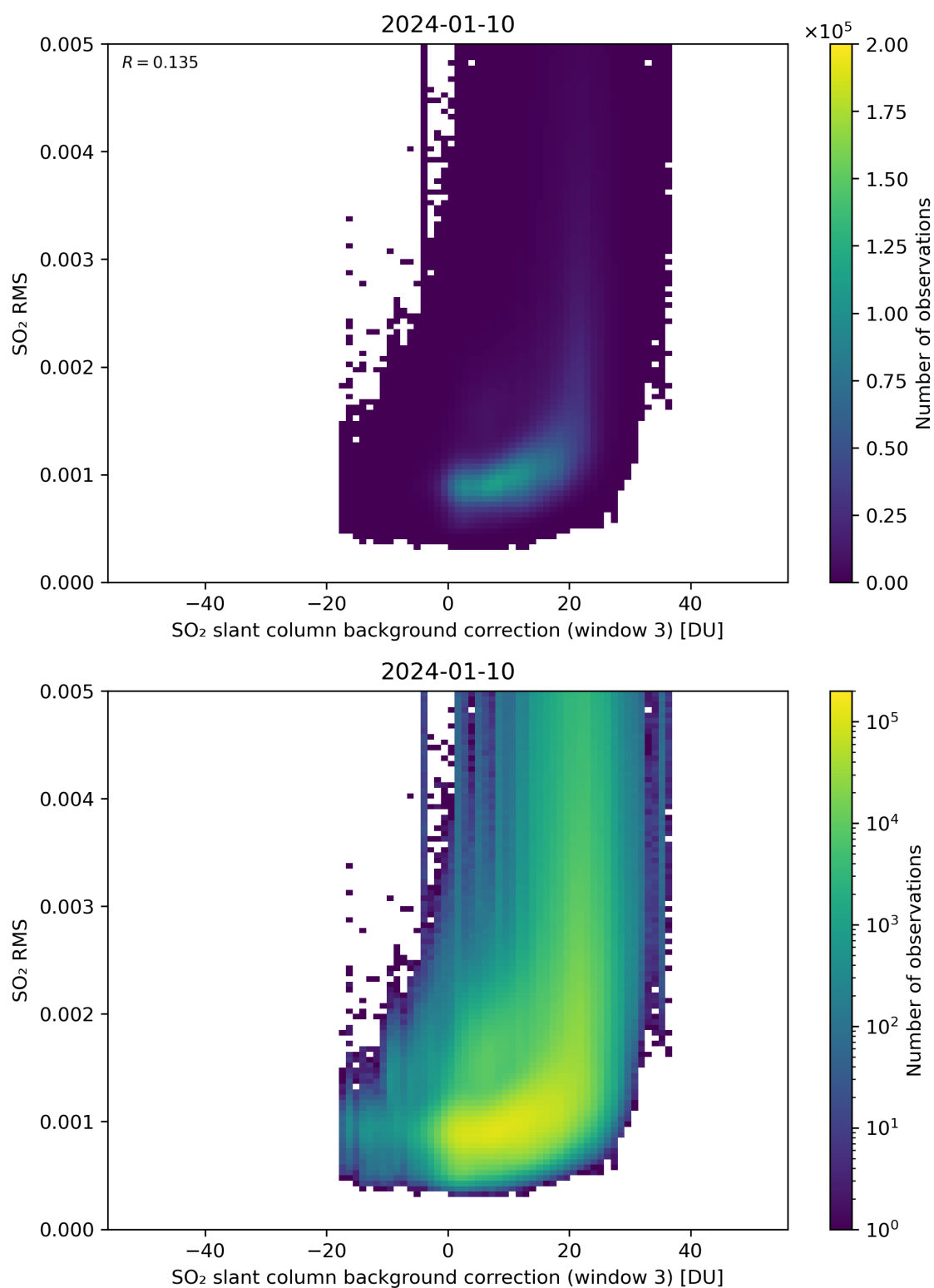
Figure 123: Scatter density plot of “SO 2 slant column background correction (window 3)” against “SO 2 RMS” for 2024-01-10 to 2024-01-11.
