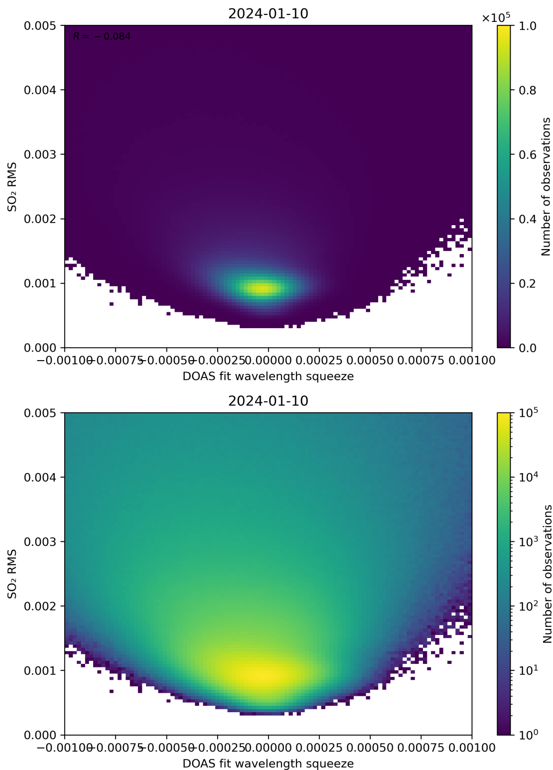
Figure 132: Scatter density plot of “DOAS fit wavelength squeeze” against “SO 2 RMS” for 2024-01-10 to 2024-01-11.
