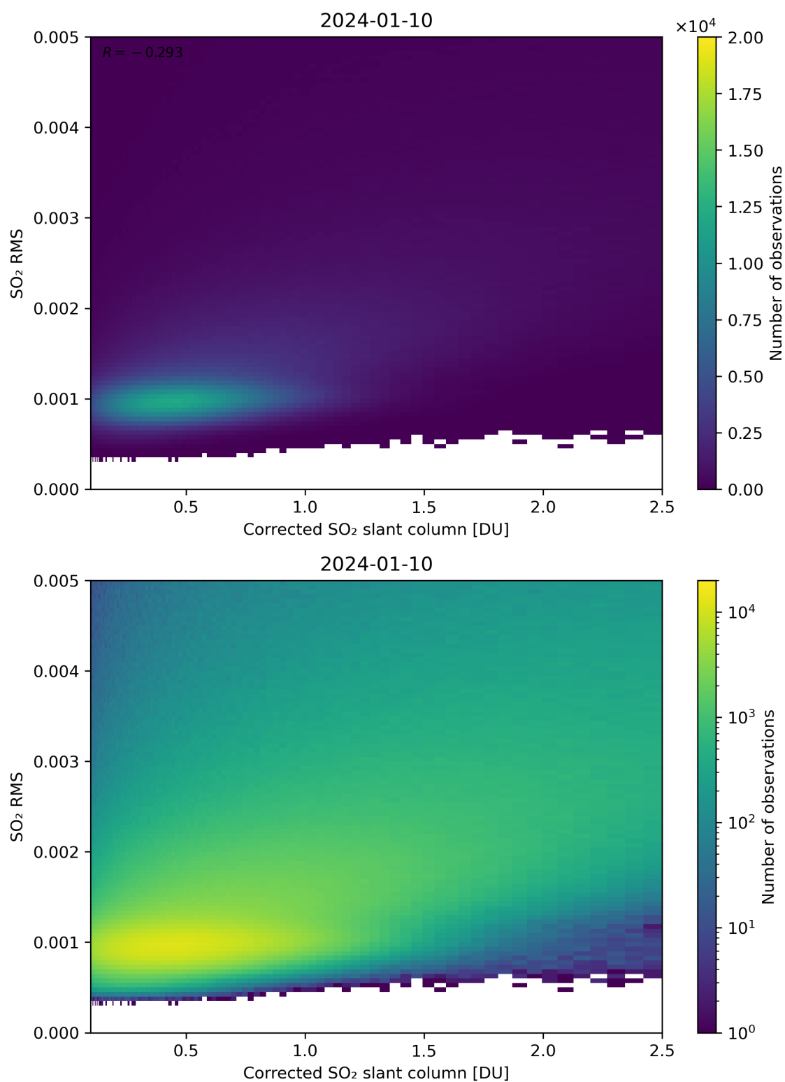
Figure 183: Scatter density plot of “Corrected SO 2 slant column” against “SO 2 RMS” for 2024-01-10 to 2024-01-11.
