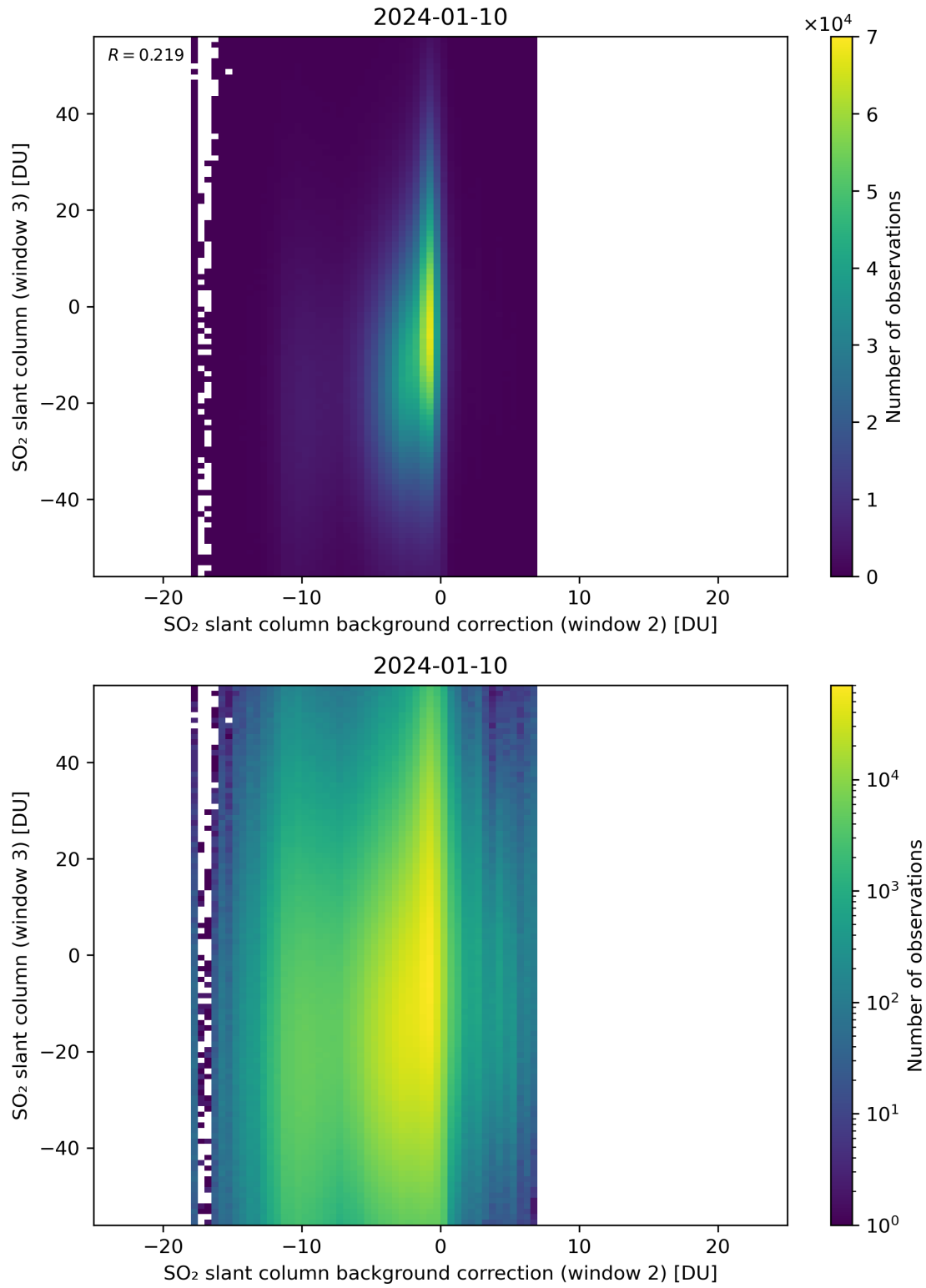
Figure 117: Scatter density plot of “SO 2 slant column background correction (window 2)” against “SO 2 slant column (window 3)” for 2024-01-10 to 2024-01-11.
