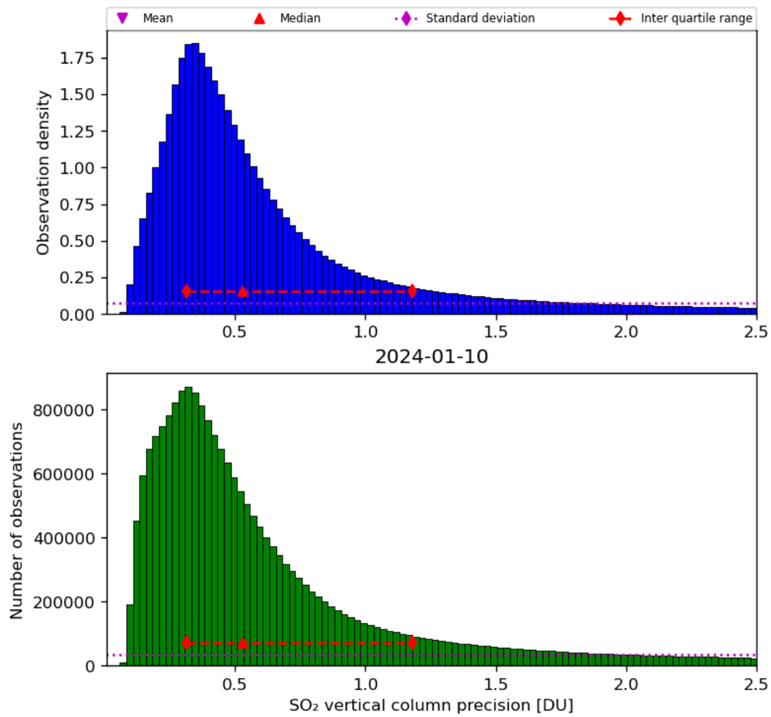
Figure 54: Histogram of “SO 2 vertical column precision” for 2024-01-10 to 2024-01-11
