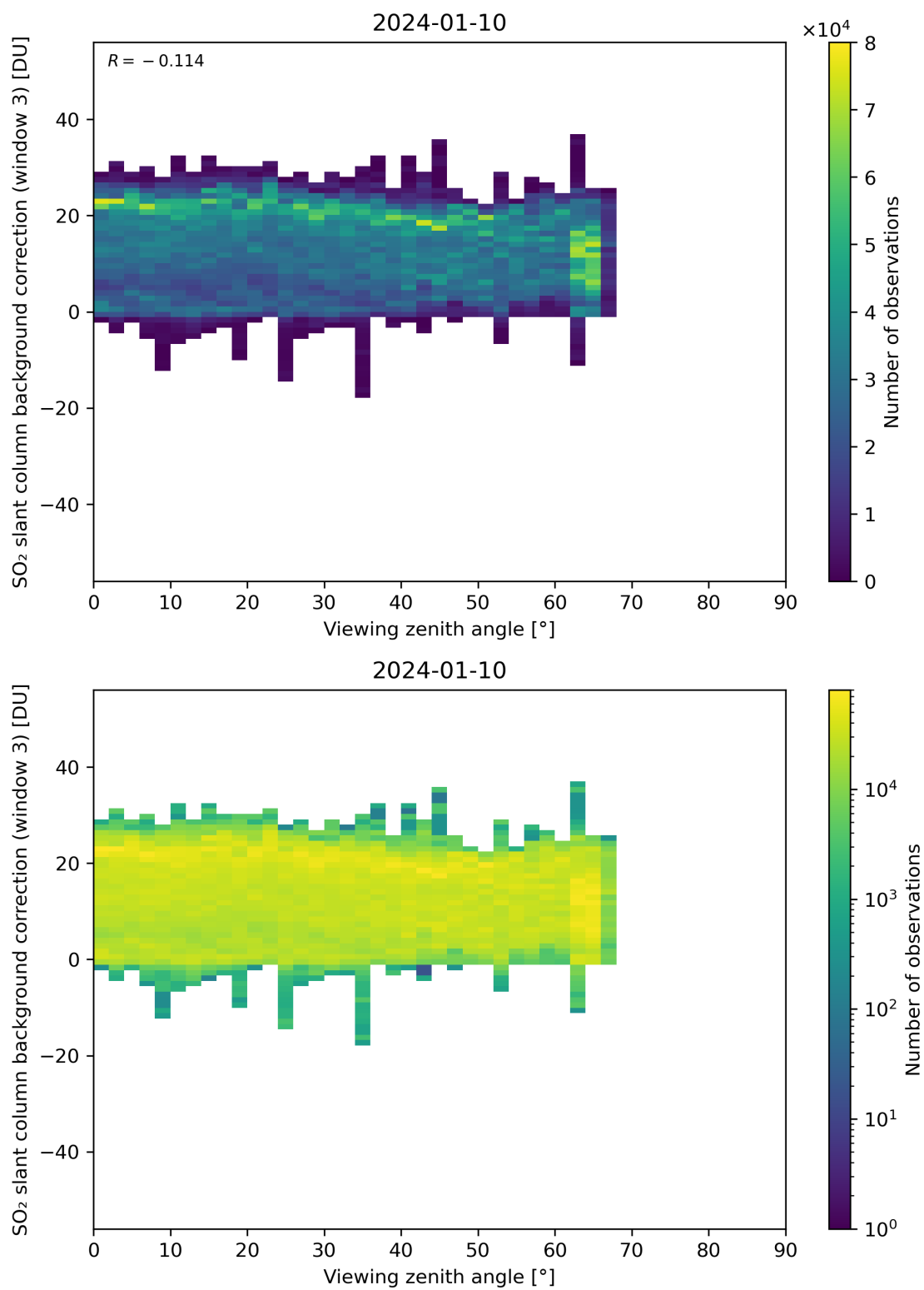
Figure 310: Scatter density plot of “Viewing zenith angle” against “SO 2 slant column background correction (window 3)” for 2024-01-10 to 2024-01-11.
