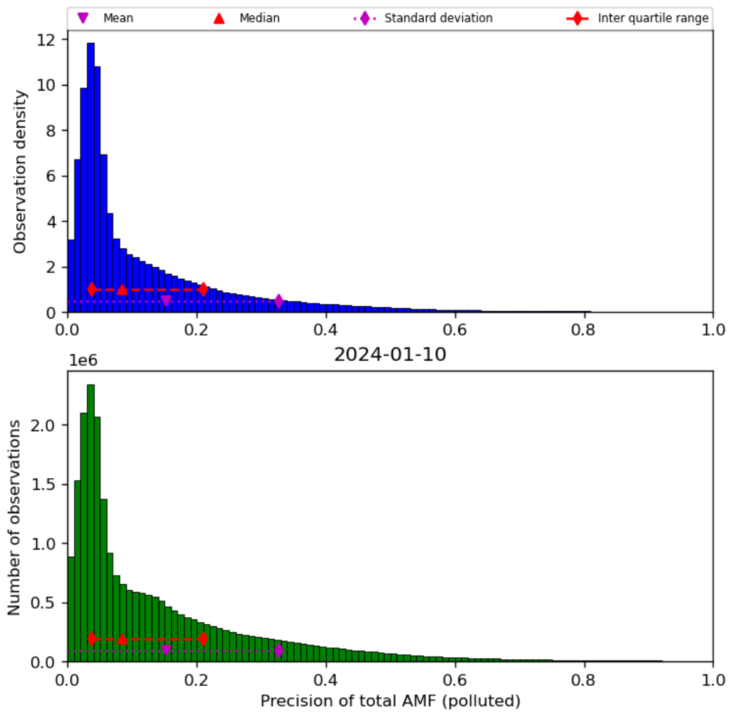
Figure 72: Histogram of “Precision of total AMF (polluted)” for 2024-01-10 to 2024-01-11
