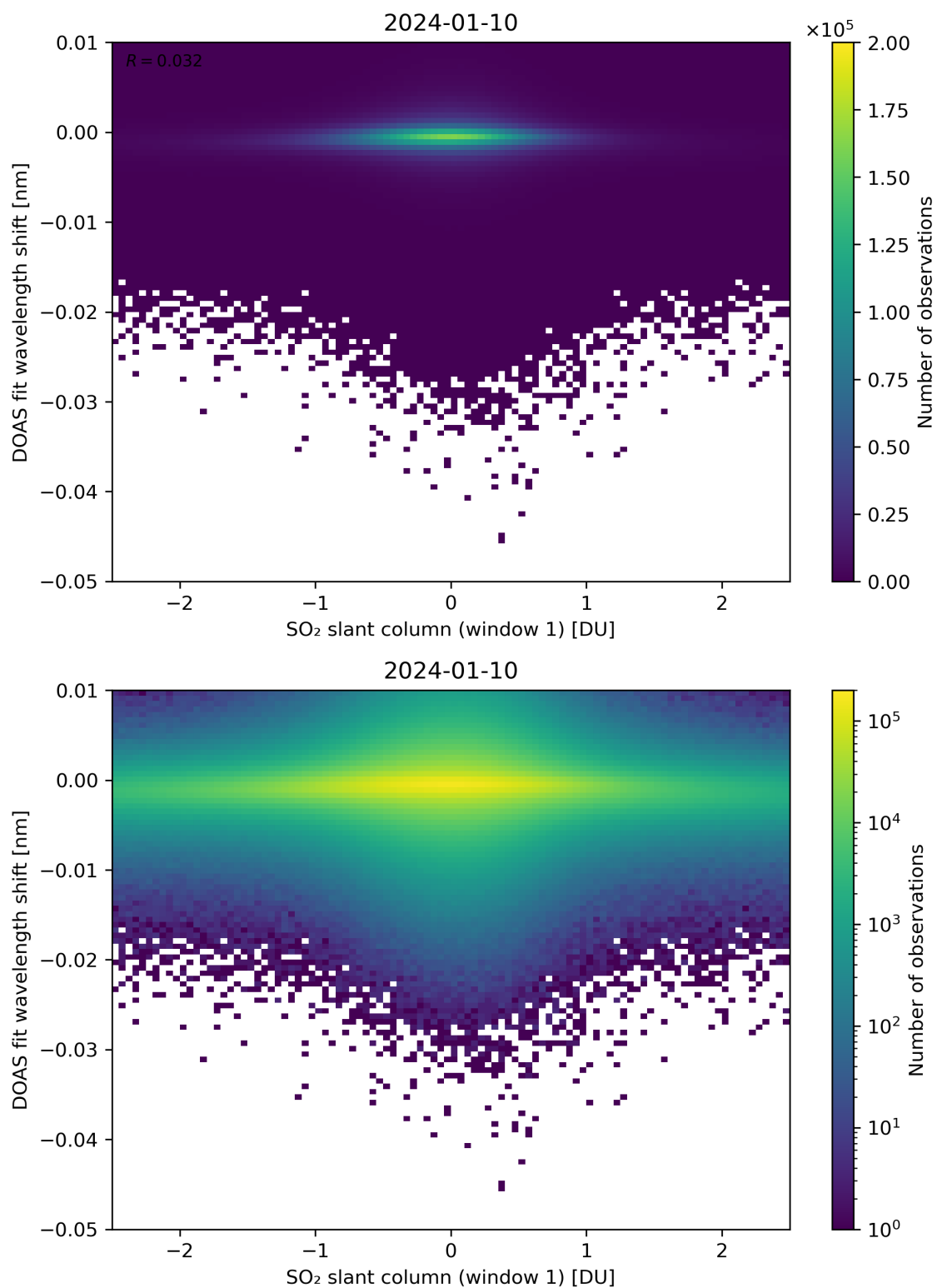
Figure 215: Scatter density plot of “SO 2 slant column (window 1)” against “DOAS fit wavelength shift” for 2024-01-10 to 2024-01-11.
