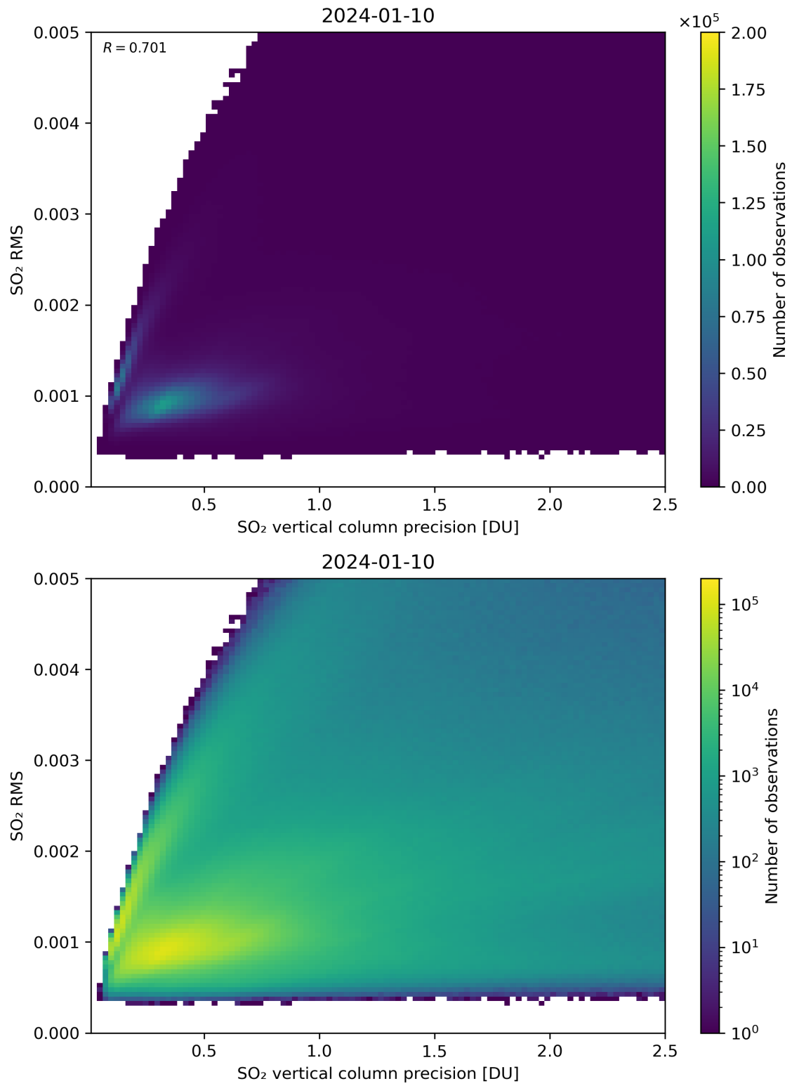
Figure 284: Scatter density plot of “SO 2 vertical column precision” against “SO 2 RMS” for 2024-01-10 to 2024-01-11.
