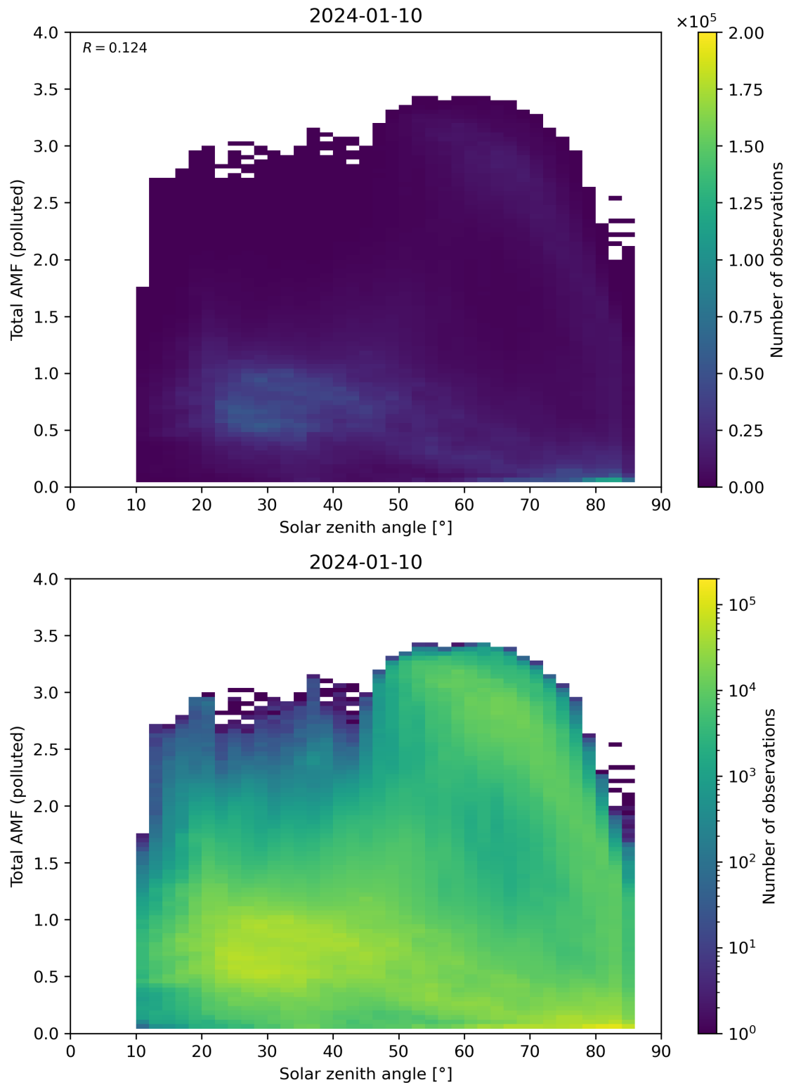
Figure 174: Scatter density plot of “Solar zenith angle” against “Total AMF (polluted)” for 2024-01-10 to 2024-01-11.
