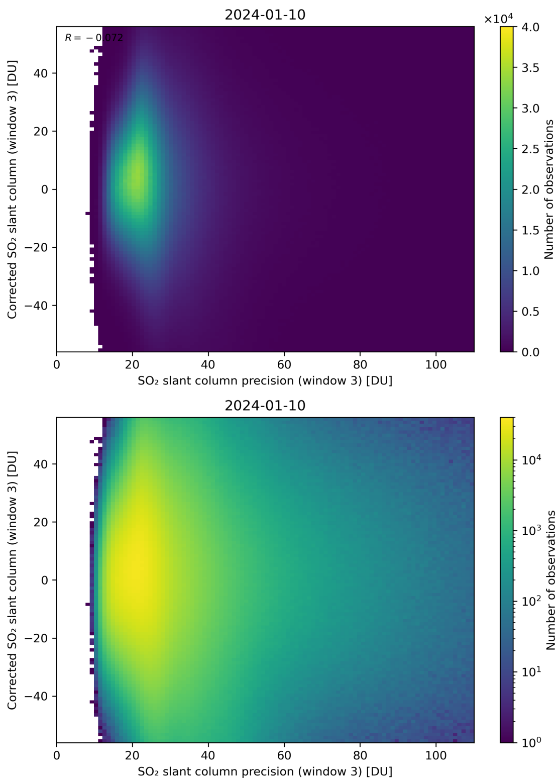
Figure 262: Scatter density plot of “SO 2 slant column precision (window 3)” against “Corrected SO 2 slant column (window 3)” for 2024-01-10 to 2024-01-11.
