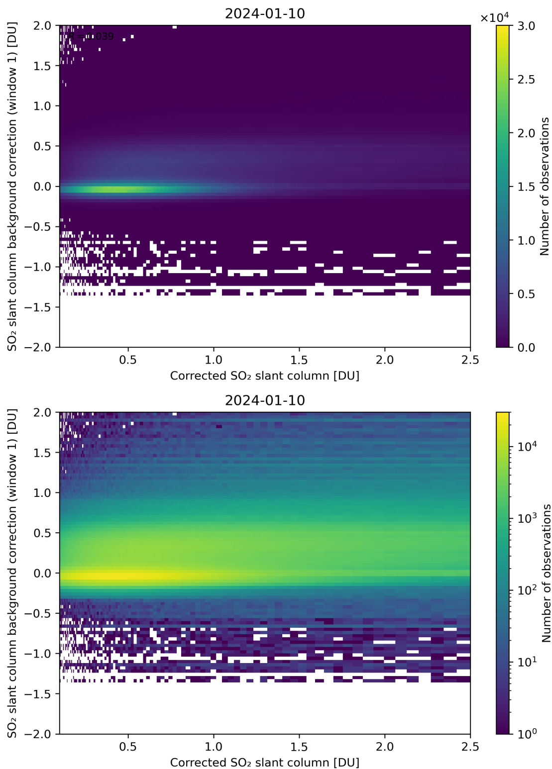
Figure 178: Scatter density plot of “Corrected SO 2 slant column” against “SO 2 slant column background correction (window 1)” for 2024-01-10 to 2024-01-11.
