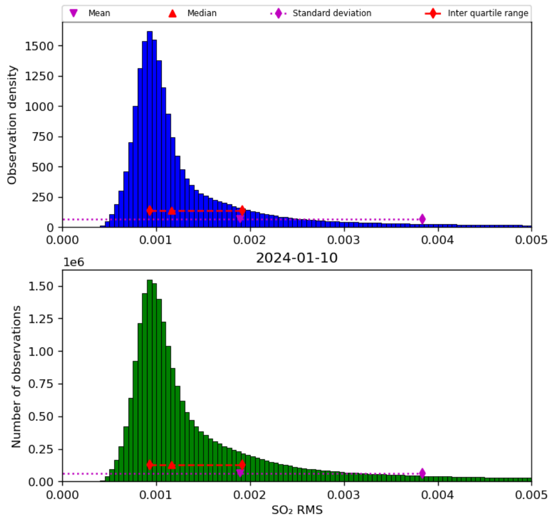
Figure 70: Histogram of “SO 2 RMS” for 2024-01-10 to 2024-01-11
