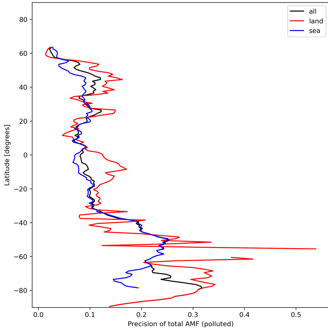
Figure 49: Zonal average of “Precision of total AMF (polluted)” for 2024-01-10 to 2024-01-11.
