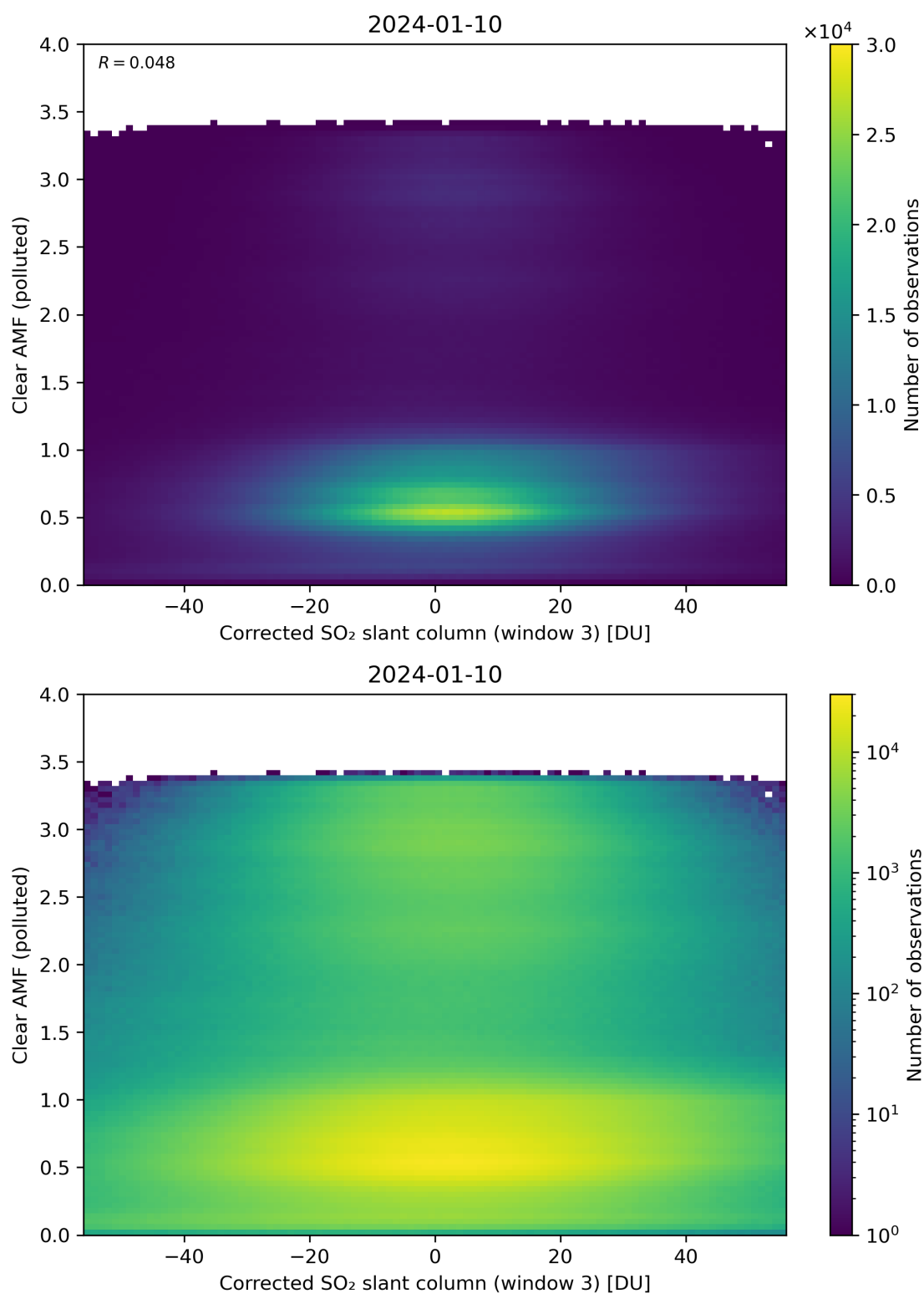
Figure 209: Scatter density plot of “Corrected SO 2 slant column (window 3)” against “Clear AMF (polluted)” for 2024-01-10 to 2024-01-11.
