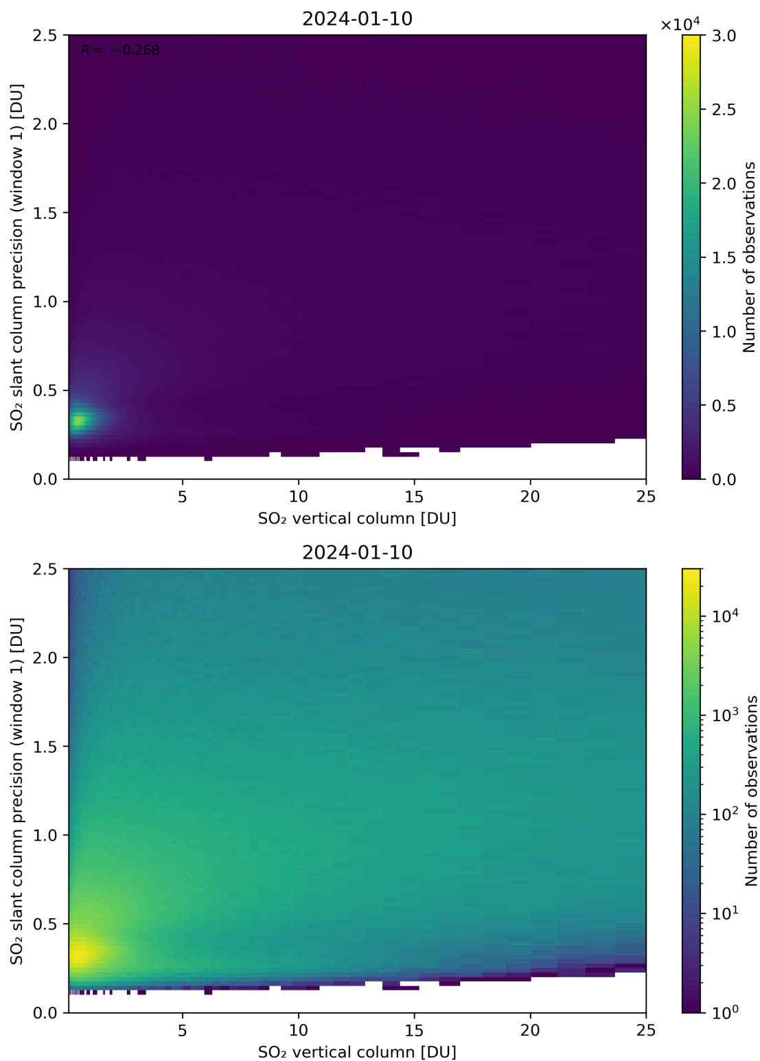
Figure 301: Scatter density plot of “SO 2 vertical column” against “SO 2 slant column precision (window 1)” for 2024-01-10 to 2024-01-11.
