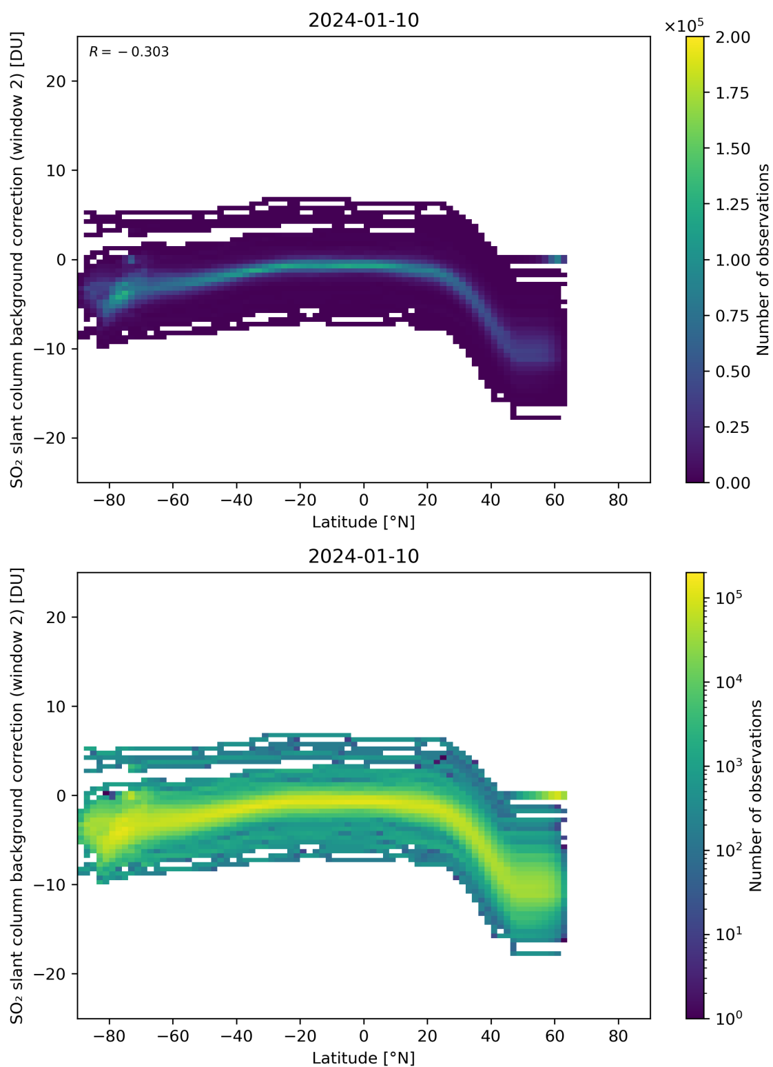
Figure 140: Scatter density plot of “Latitude” against “SO 2 slant column background correction (window 2)” for 2024-01-10 to 2024-01-11.
