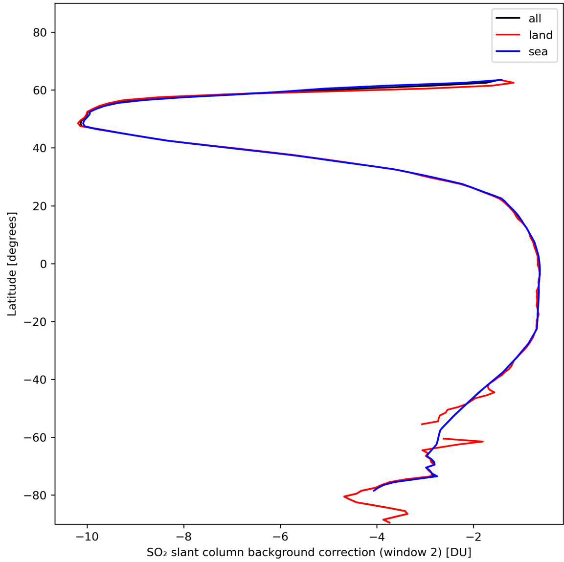
Figure 40: Zonal average of “SO 2 slant column background correction (window 2)” for 2024-01-10 to 2024-01-11.
