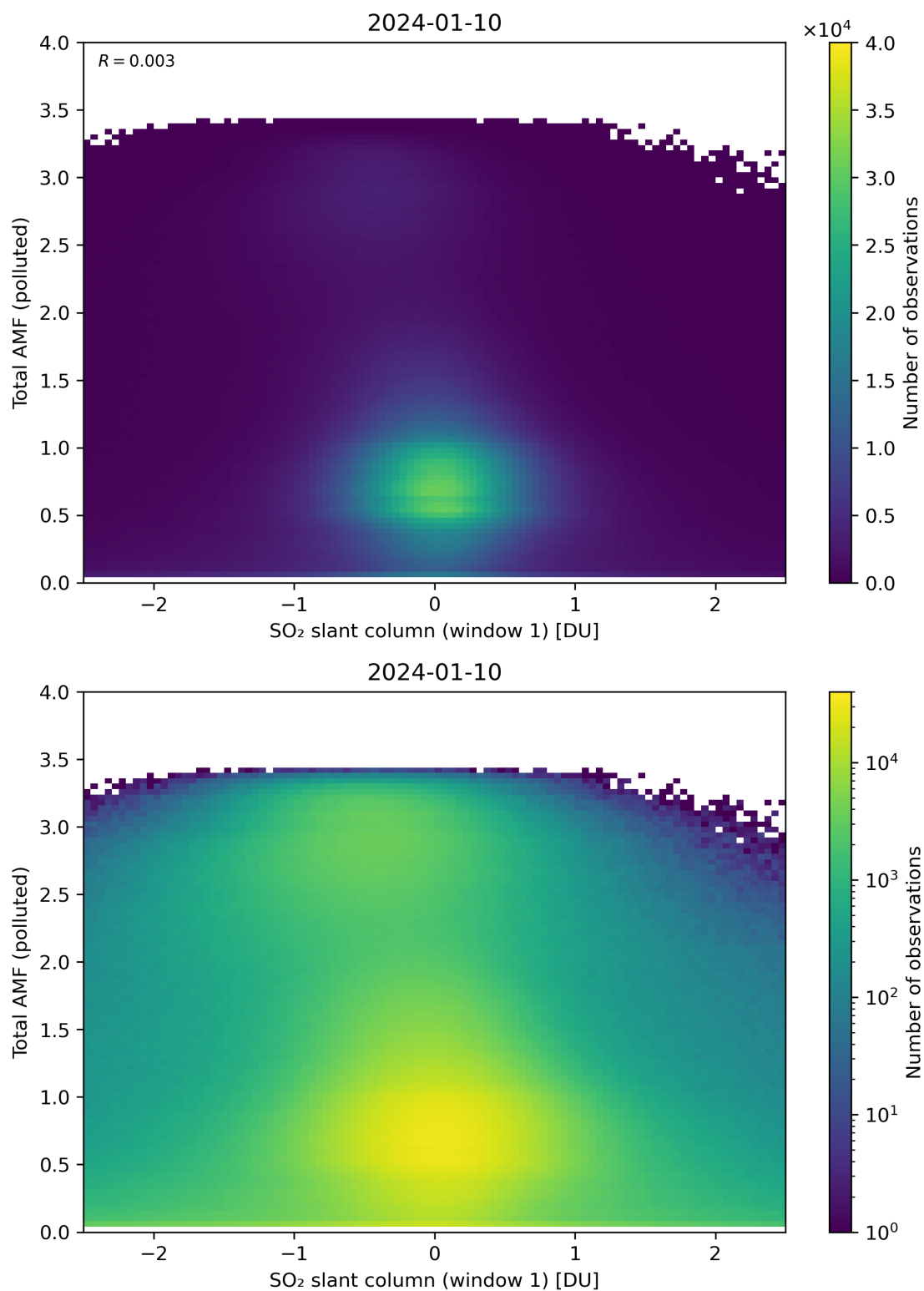
Figure 239: Scatter density plot of “SO 2 slant column (window 1)” against “Total AMF (polluted)” for 2024-01-10 to 2024-01-11.
