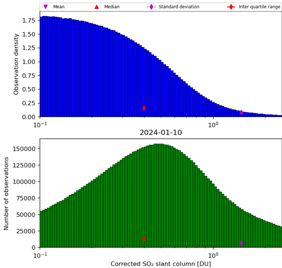
Figure 55: Histogram of “Corrected SO 2 slant column” for 2024-01-10 to 2024-01-11
