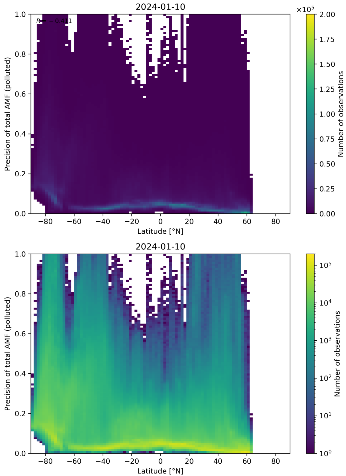
Figure 155: Scatter density plot of “Latitude” against “Precision of total AMF (polluted)” for 2024-01-10 to 2024-01-11.
