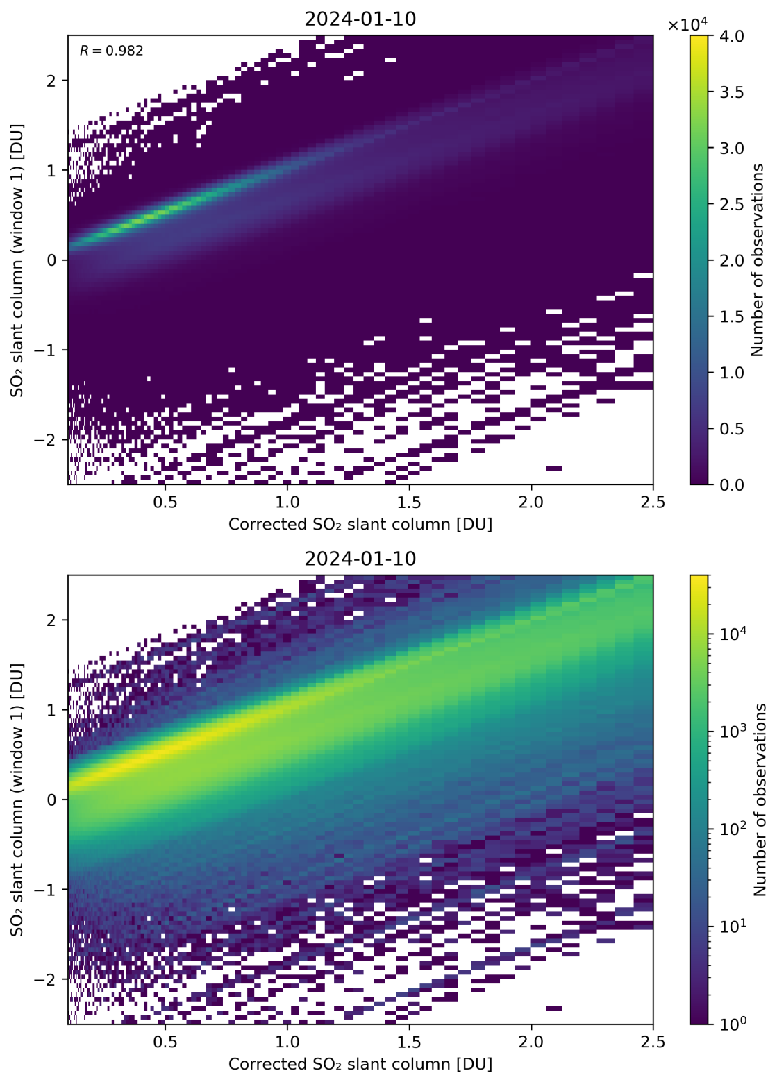
Figure 187: Scatter density plot of “Corrected SO 2 slant column” against “SO 2 slant column (window 1)” for 2024-01-10 to 2024-01-11.
