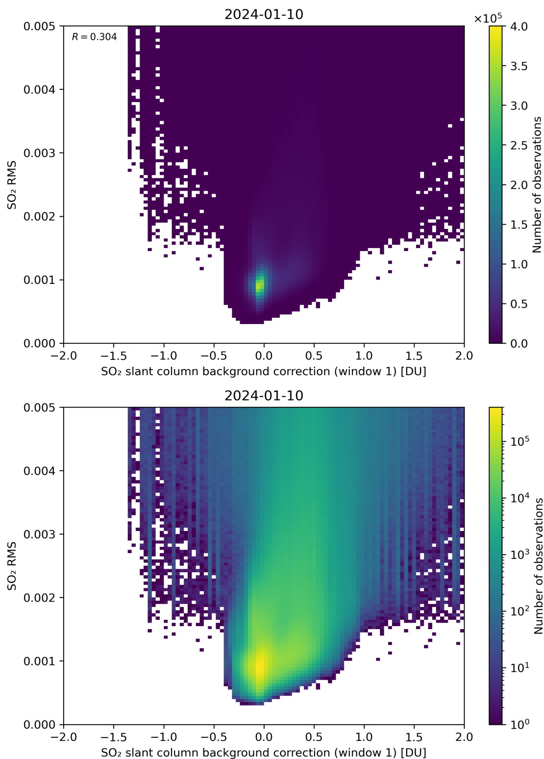
Figure 102: Scatter density plot of “SO 2 slant column background correction (window 1)” against “SO 2 RMS” for 2024-01-10 to 2024-01-11.
