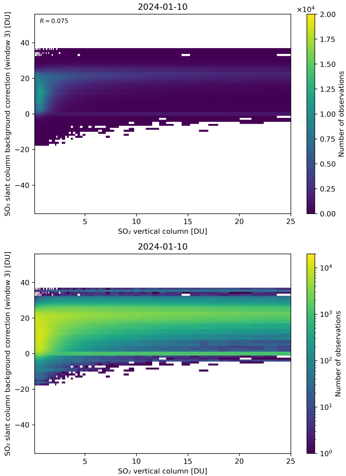
Figure 275: Scatter density plot of “SO 2 vertical column” against “SO 2 slant column background correction (window 3)” for 2024-01-10 to 2024-01-11.
