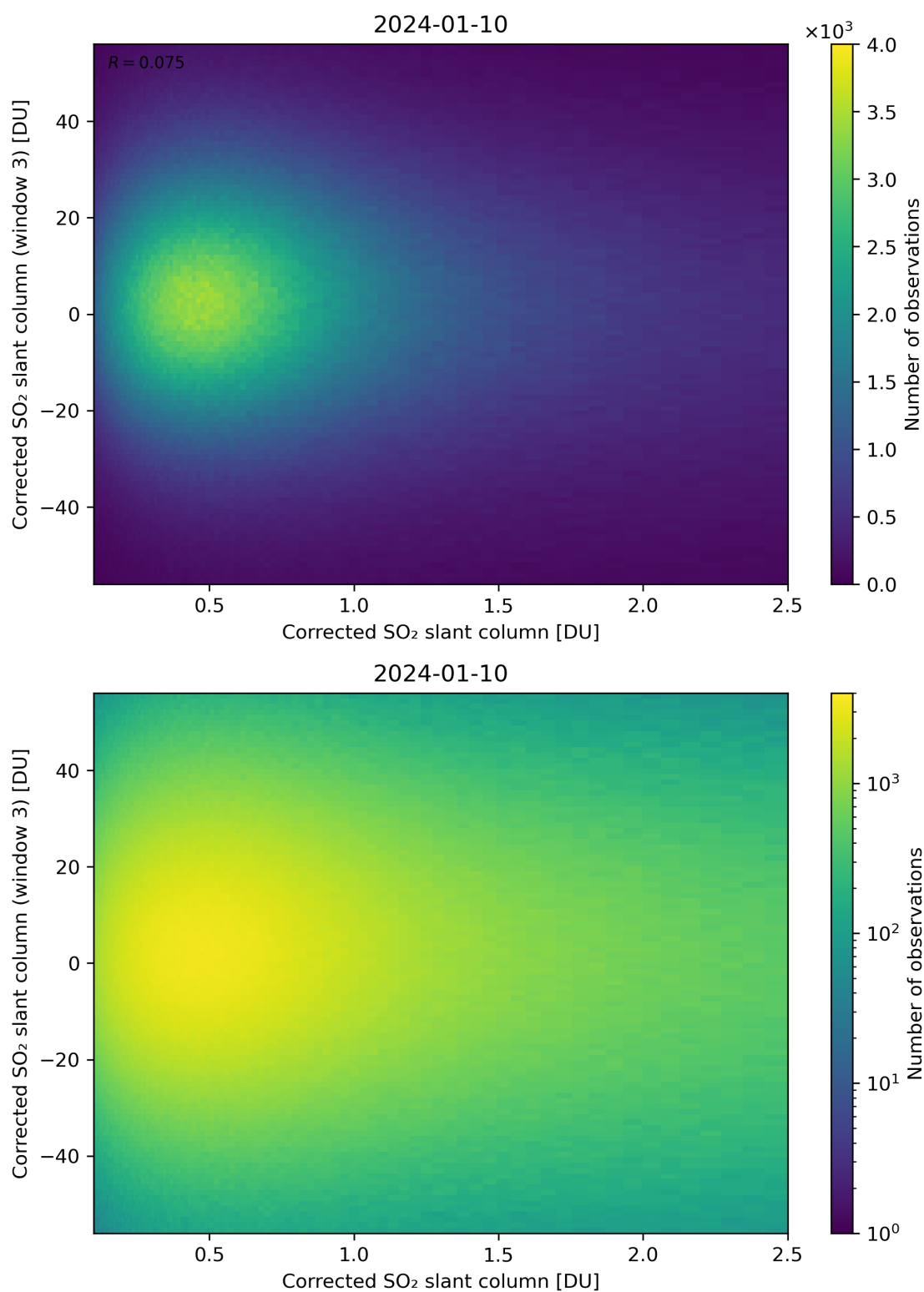
Figure 186: Scatter density plot of “Corrected SO 2 slant column” against “Corrected SO 2 slant column (window 3)” for 2024-01-10 to 2024-01-11.
