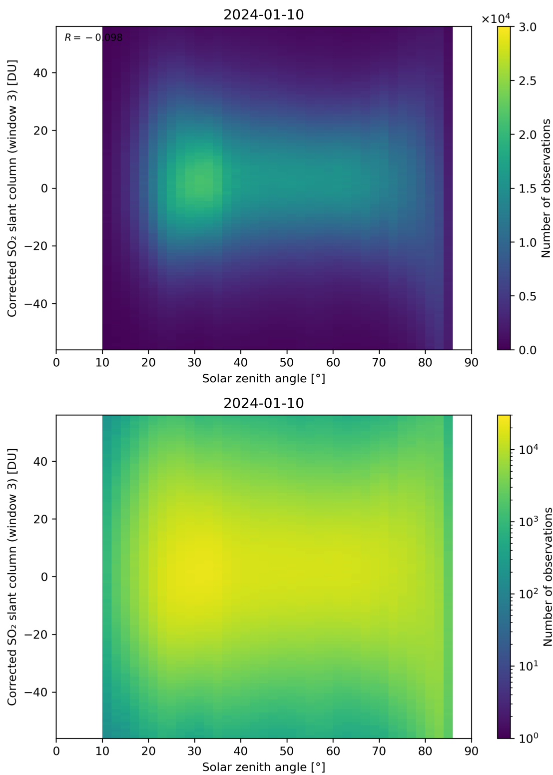
Figure 168: Scatter density plot of “Solar zenith angle” against “Corrected SO 2 slant column (window 3)” for 2024-01-10 to 2024-01-11.
