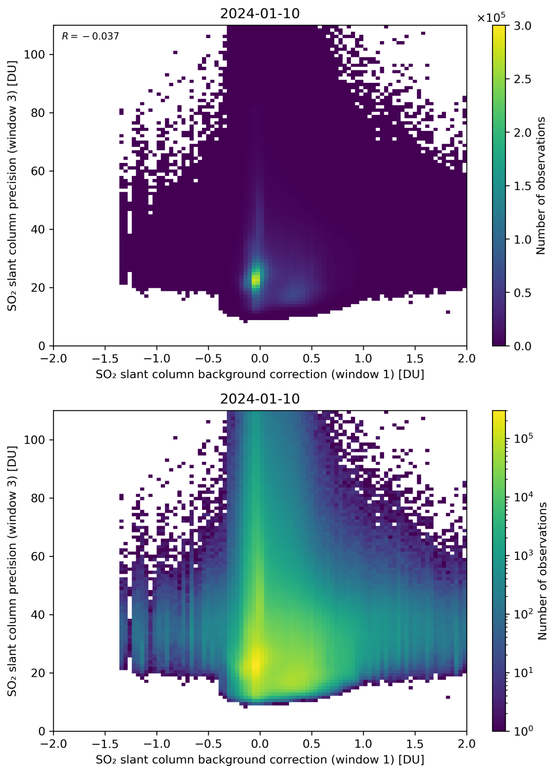
Figure 108: Scatter density plot of “SO 2 slant column background correction (window 1)” against “SO 2 slant column precision (window 3)” for 2024-01-10 to 2024-01-11.
