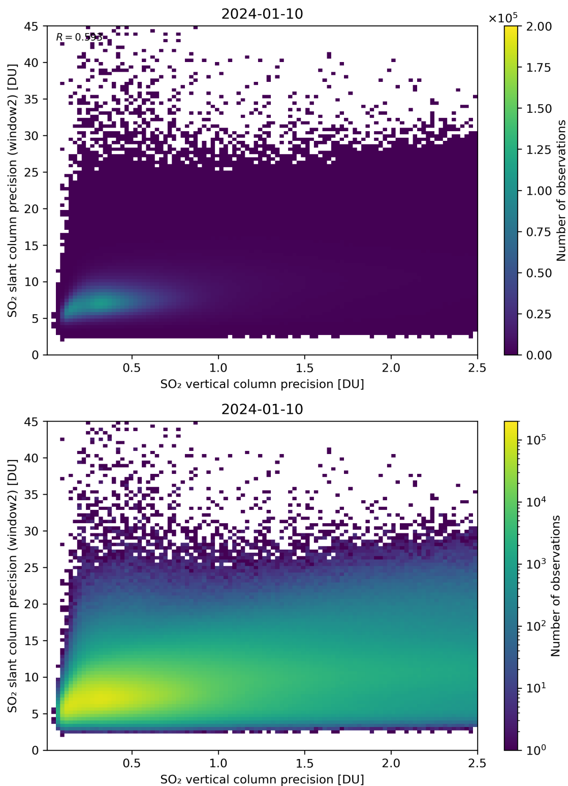
Figure 291: Scatter density plot of “SO 2 vertical column precision” against “SO 2 slant column precision (window2)” for 2024-01-10 to 2024-01-11.
