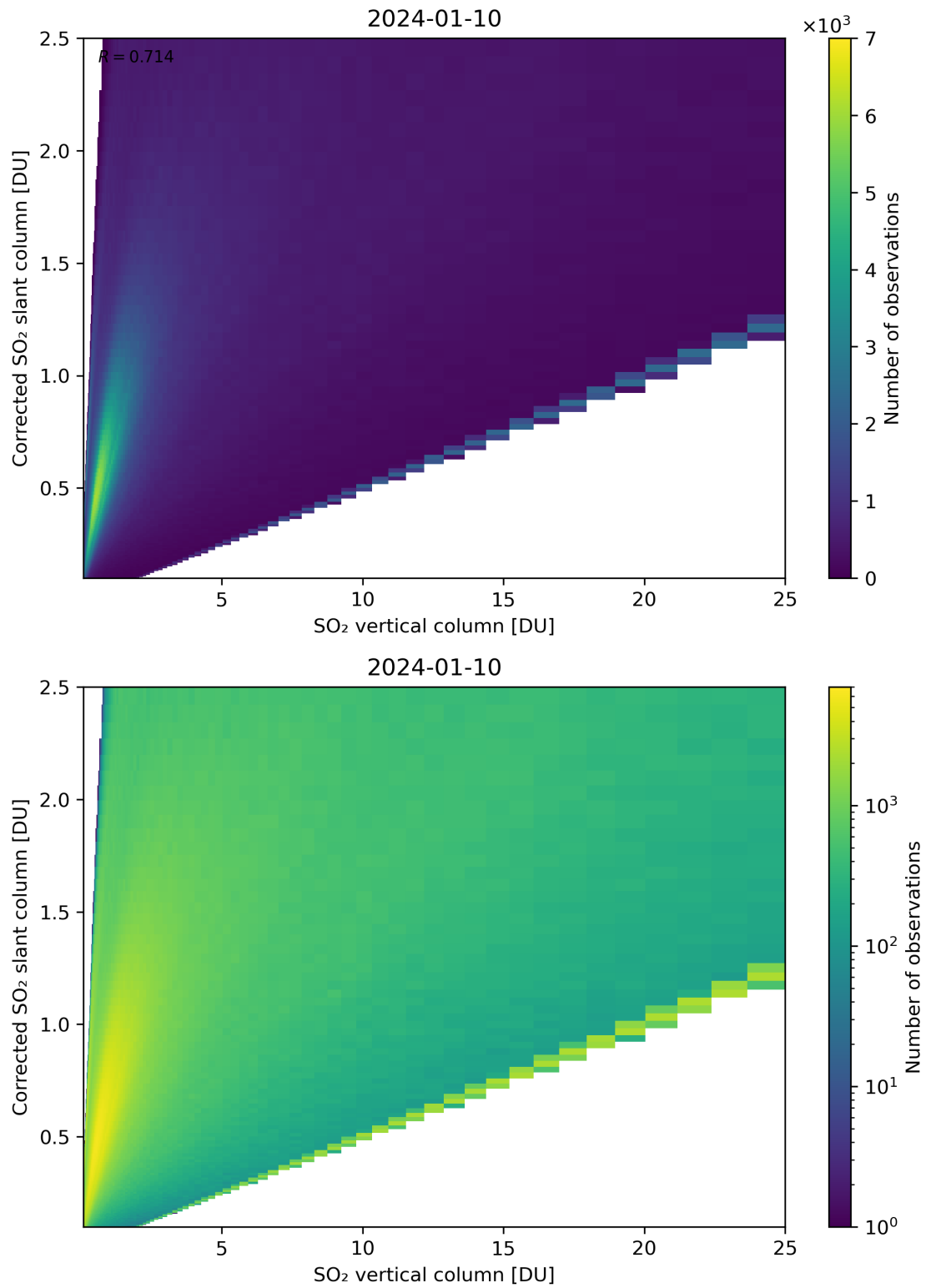
Figure 297: Scatter density plot of “SO 2 vertical column” against “Corrected SO 2 slant column” for 2024-01-10 to 2024-01-11.
