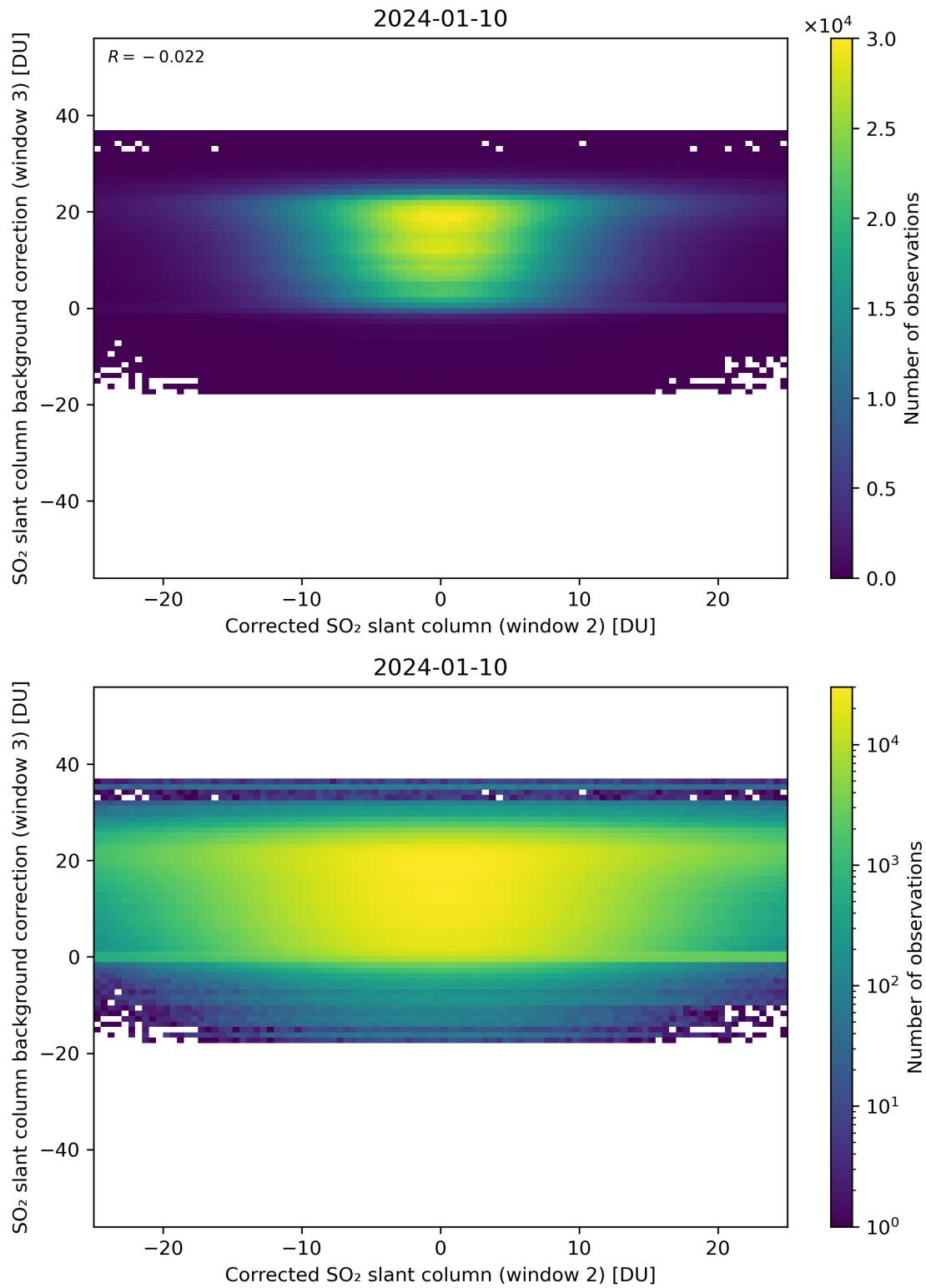
Figure 195: Scatter density plot of “Corrected SO 2 slant column (window 2)” against “SO 2 slant column background correction (window 3)” for 2024-01-10 to 2024-01-11.
