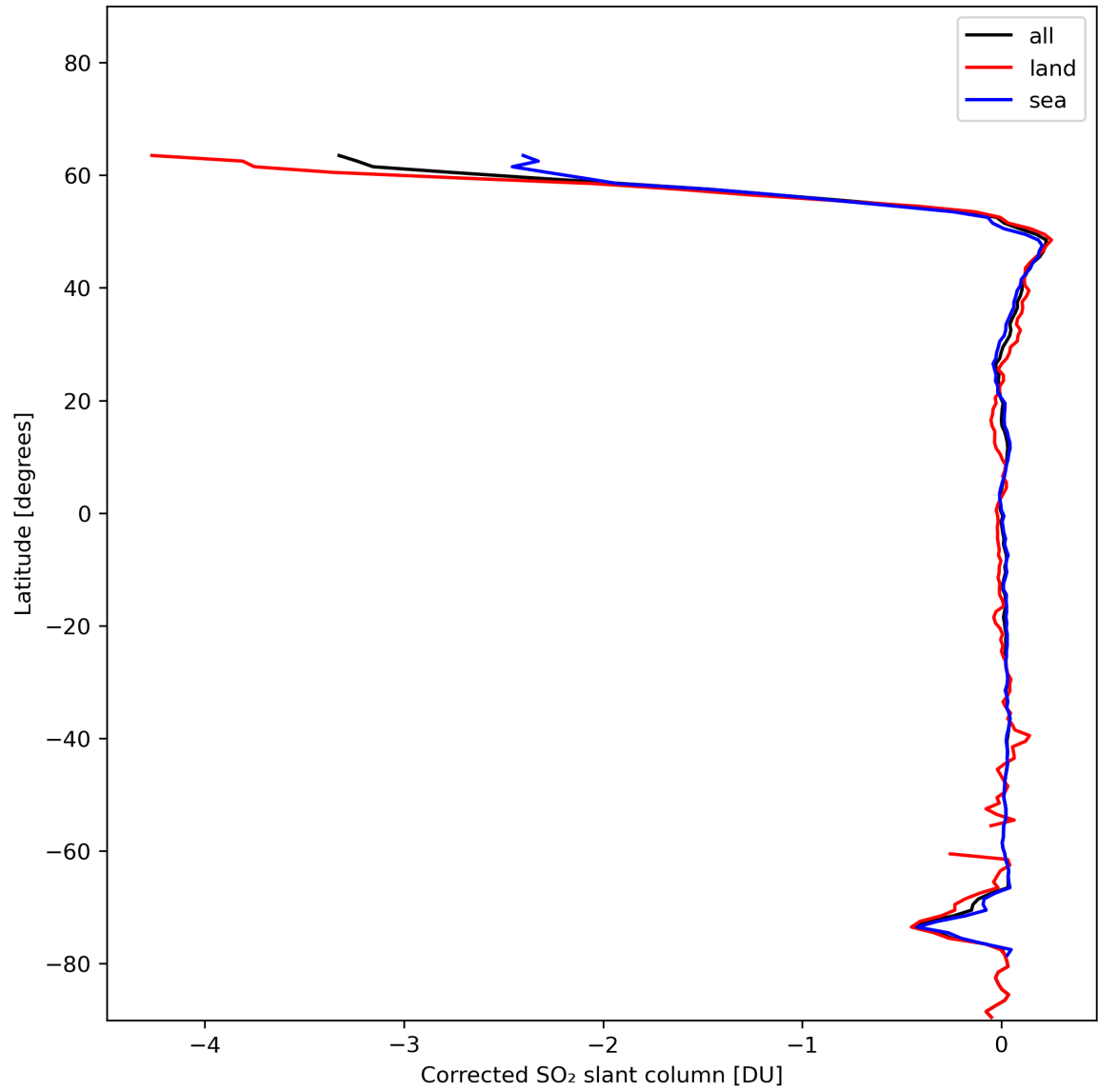
Figure 32: Zonal average of “Corrected SO 2 slant column” for 2024-01-10 to 2024-01-11.
