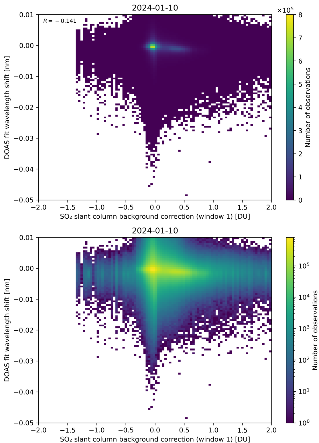
Figure 100: Scatter density plot of “SO 2 slant column background correction (window 1)” against “DOAS fit wavelength shift” for 2024-01-10 to 2024-01-11.
