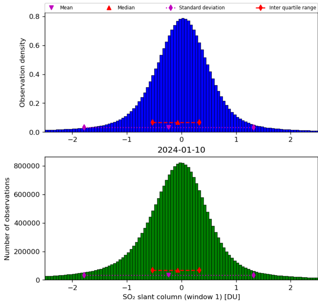
Figure 56: Histogram of “SO 2 slant column (window 1)” for 2024-01-10 to 2024-01-11
