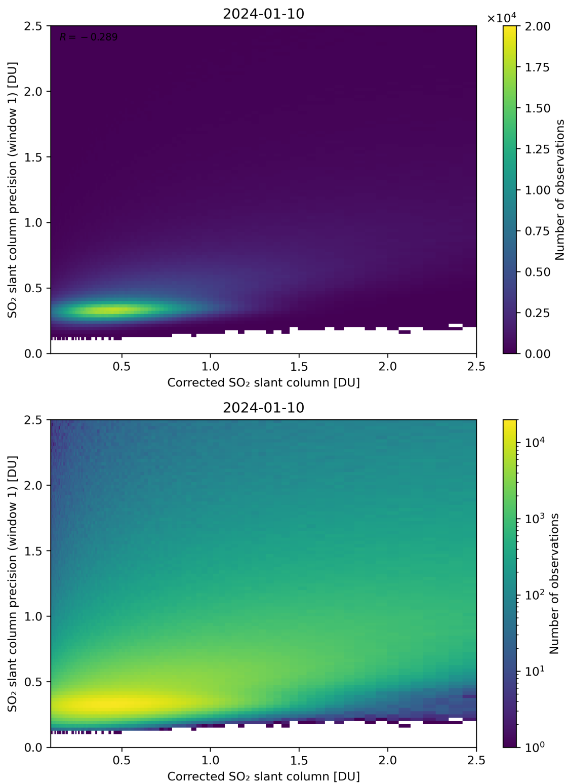
Figure 188: Scatter density plot of “Corrected SO 2 slant column” against “SO 2 slant column precision (window 1)” for 2024-01-10 to 2024-01-11.
