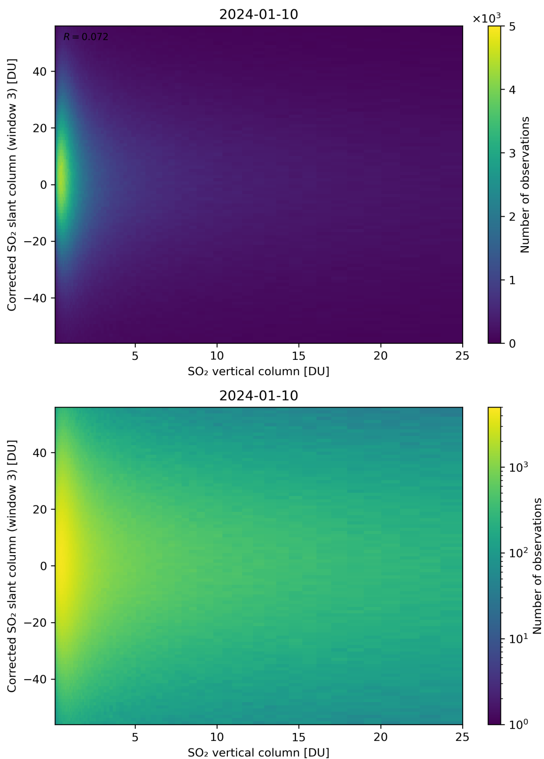
Figure 299: Scatter density plot of “SO 2 vertical column” against “Corrected SO 2 slant column (window 3)” for 2024-01-10 to 2024-01-11.
