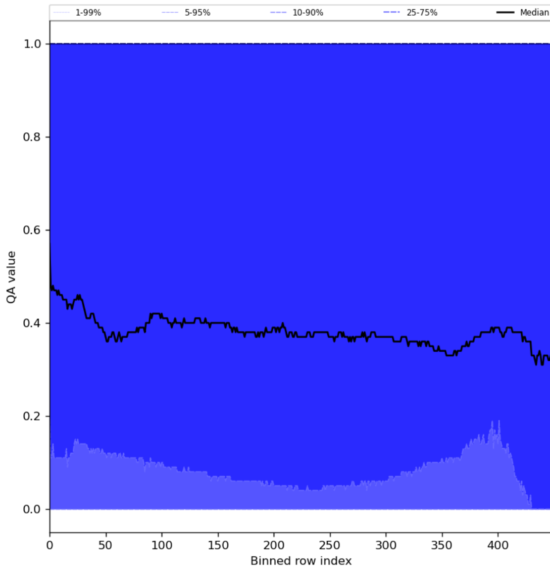
Figure 75: Along track statistics of “QA value” for 2024-01-10 to 2024-01-12
