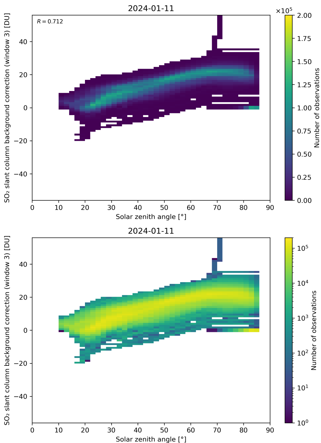
Figure 160: Scatter density plot of “Solar zenith angle” against “SO 2 slant column background correction (window 3)” for 2024-01-10 to 2024-01-12.
