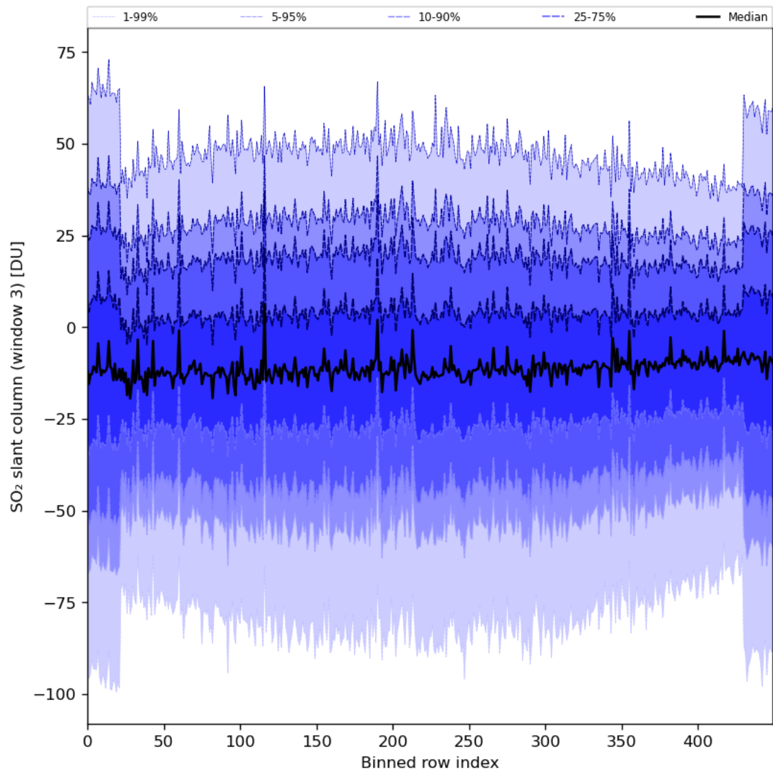
Figure 87: Along track statistics of “SO 2 slant column (window 3)” for 2024-01-10 to 2024-01-12
