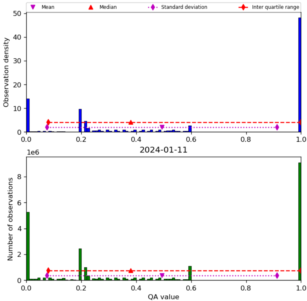
Figure 52: Histogram of “QA value” for 2024-01-10 to 2024-01-12
