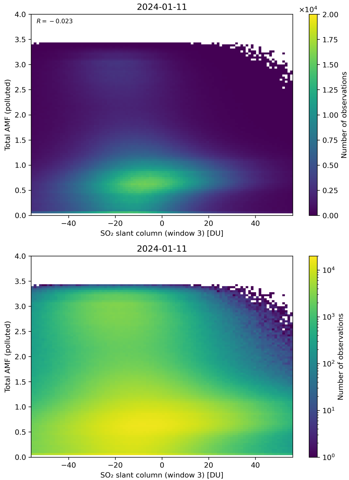
Figure 268: Scatter density plot of “SO 2 slant column (window 3)” against “Total AMF (polluted)” for 2024-01-10 to 2024-01-12.
