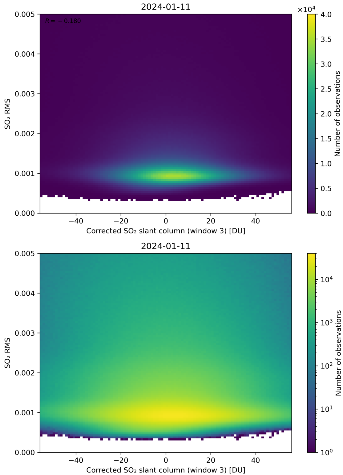
Figure 208: Scatter density plot of “Corrected SO 2 slant column (window 3)” against “SO 2 RMS” for 2024-01-10 to 2024-01-12.
