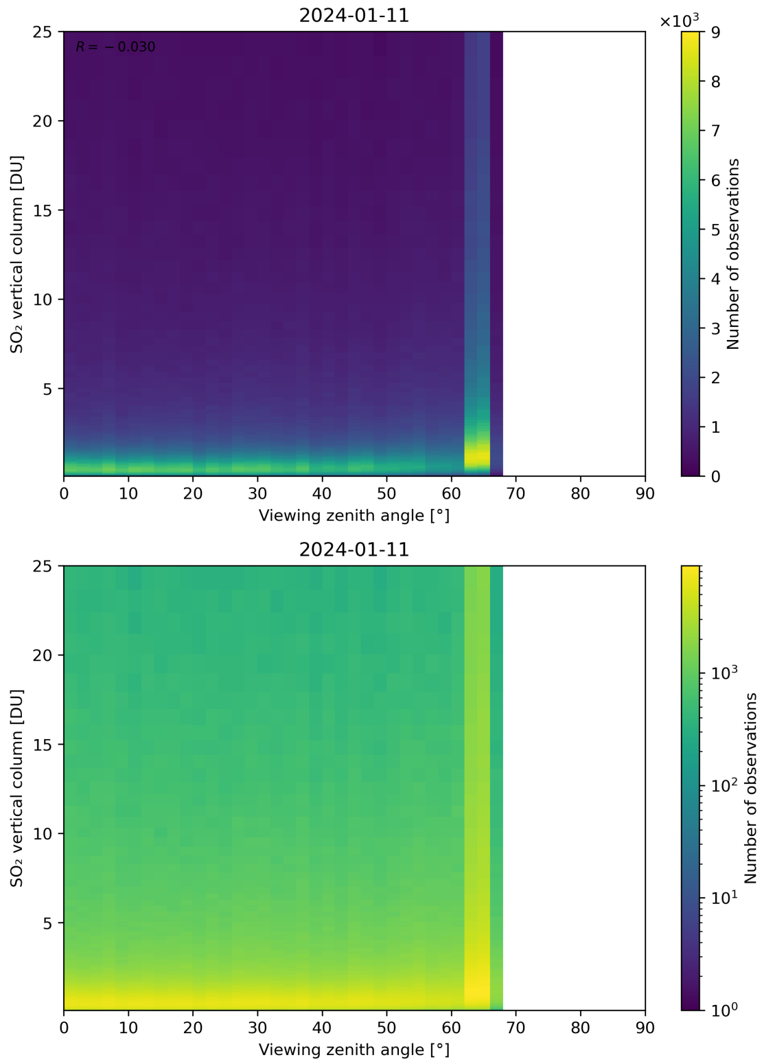
Figure 327: Scatter density plot of “Viewing zenith angle” against “SO 2 vertical column” for 2024-01-10 to 2024-01-12.
