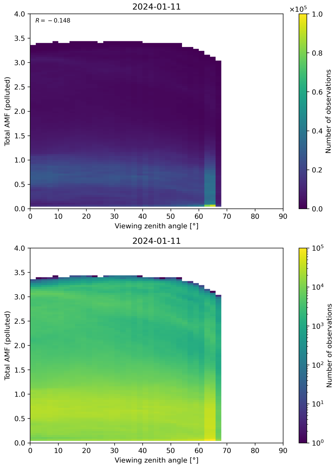
Figure 325: Scatter density plot of “Viewing zenith angle” against “Total AMF (polluted)” for 2024-01-10 to 2024-01-12.
