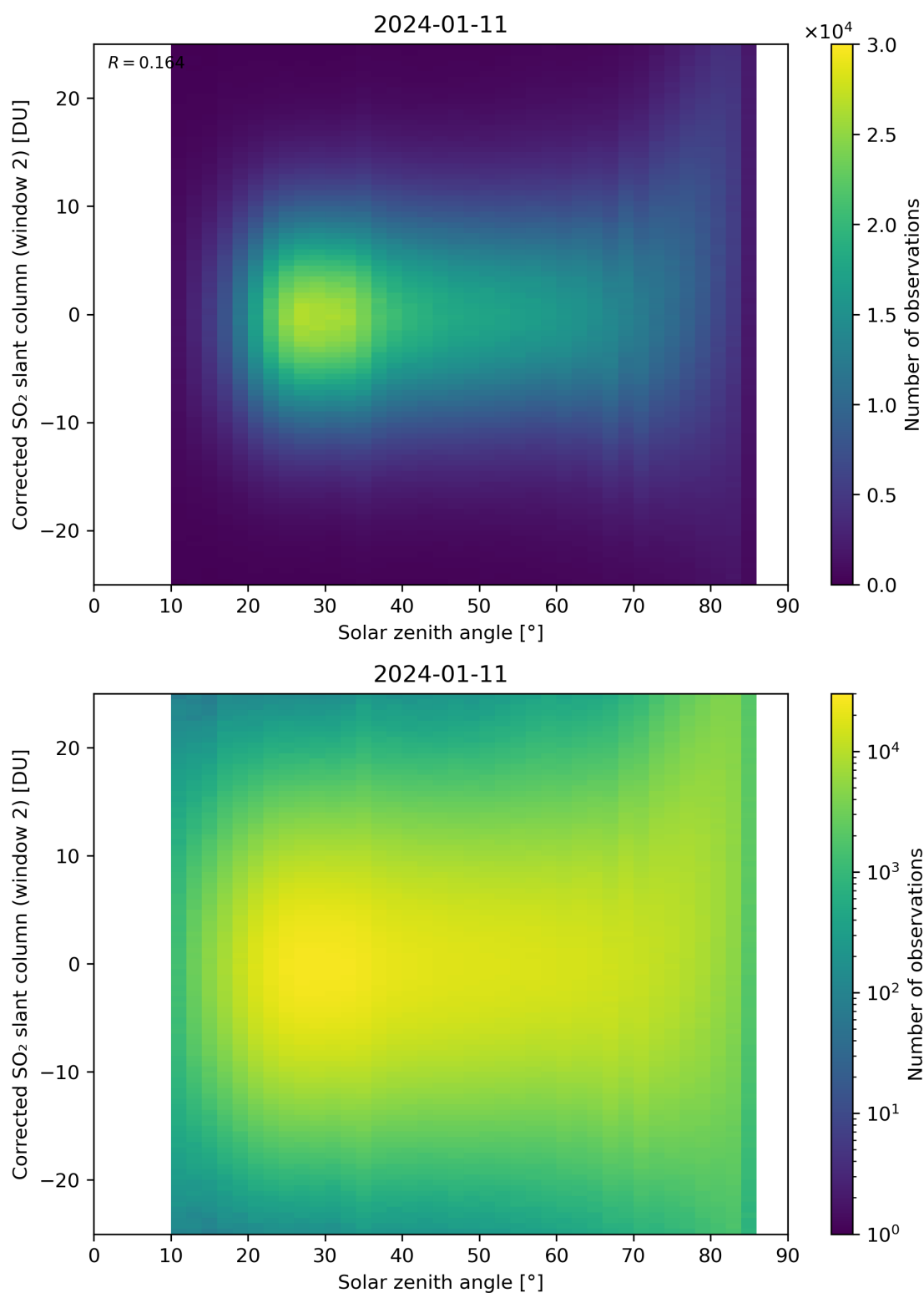
Figure 167: Scatter density plot of “Solar zenith angle” against “Corrected SO 2 slant column (window 2)” for 2024-01-10 to 2024-01-12.
