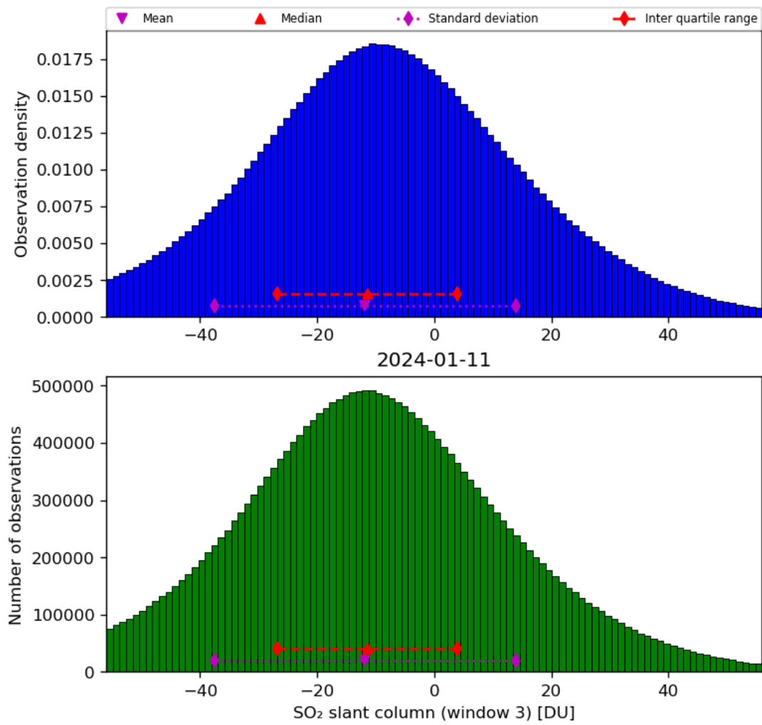
Figure 64: Histogram of “SO 2 slant column (window 3)” for 2024-01-10 to 2024-01-12
