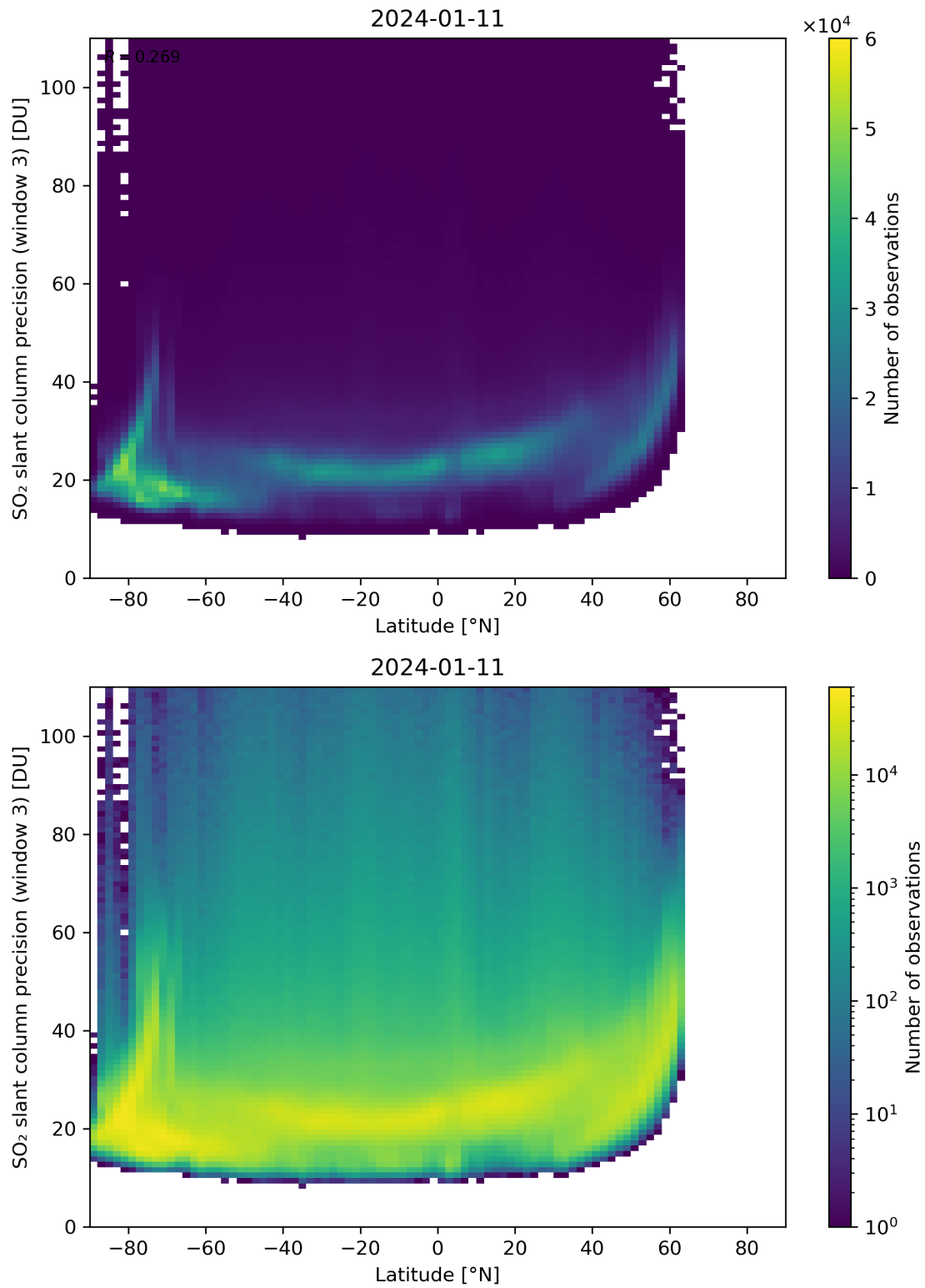
Figure 153: Scatter density plot of “Latitude” against “SO 2 slant column precision (window 3)” for 2024-01-10 to 2024-01-12.
