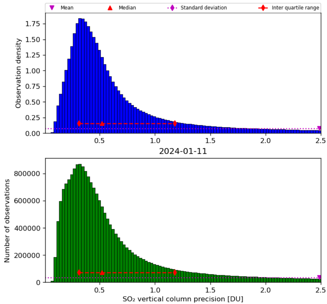
Figure 54: Histogram of “SO 2 vertical column precision” for 2024-01-10 to 2024-01-12
