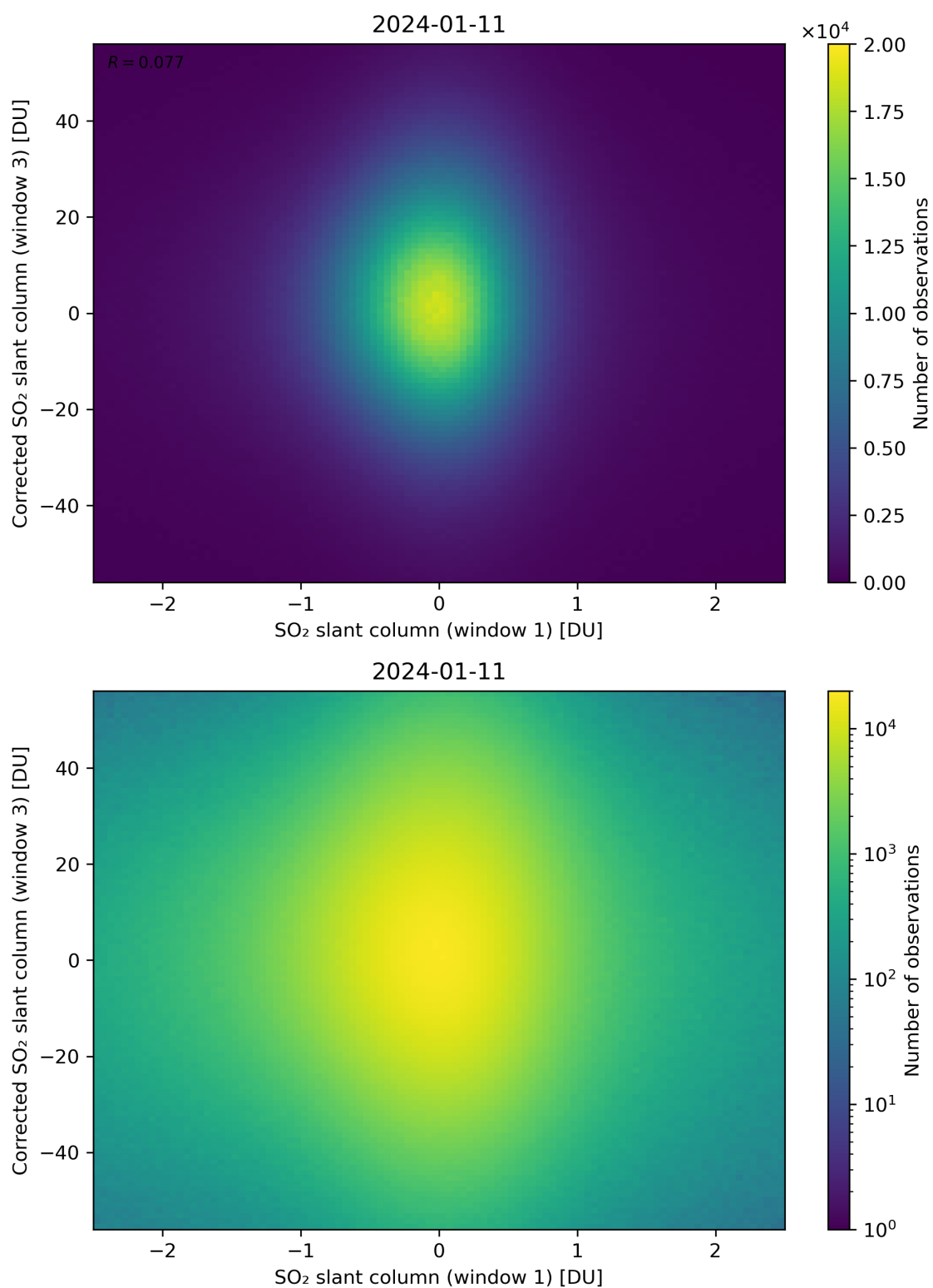
Figure 234: Scatter density plot of “SO 2 slant column (window 1)” against “Corrected SO 2 slant column (window 3)” for 2024-01-10 to 2024-01-12.
