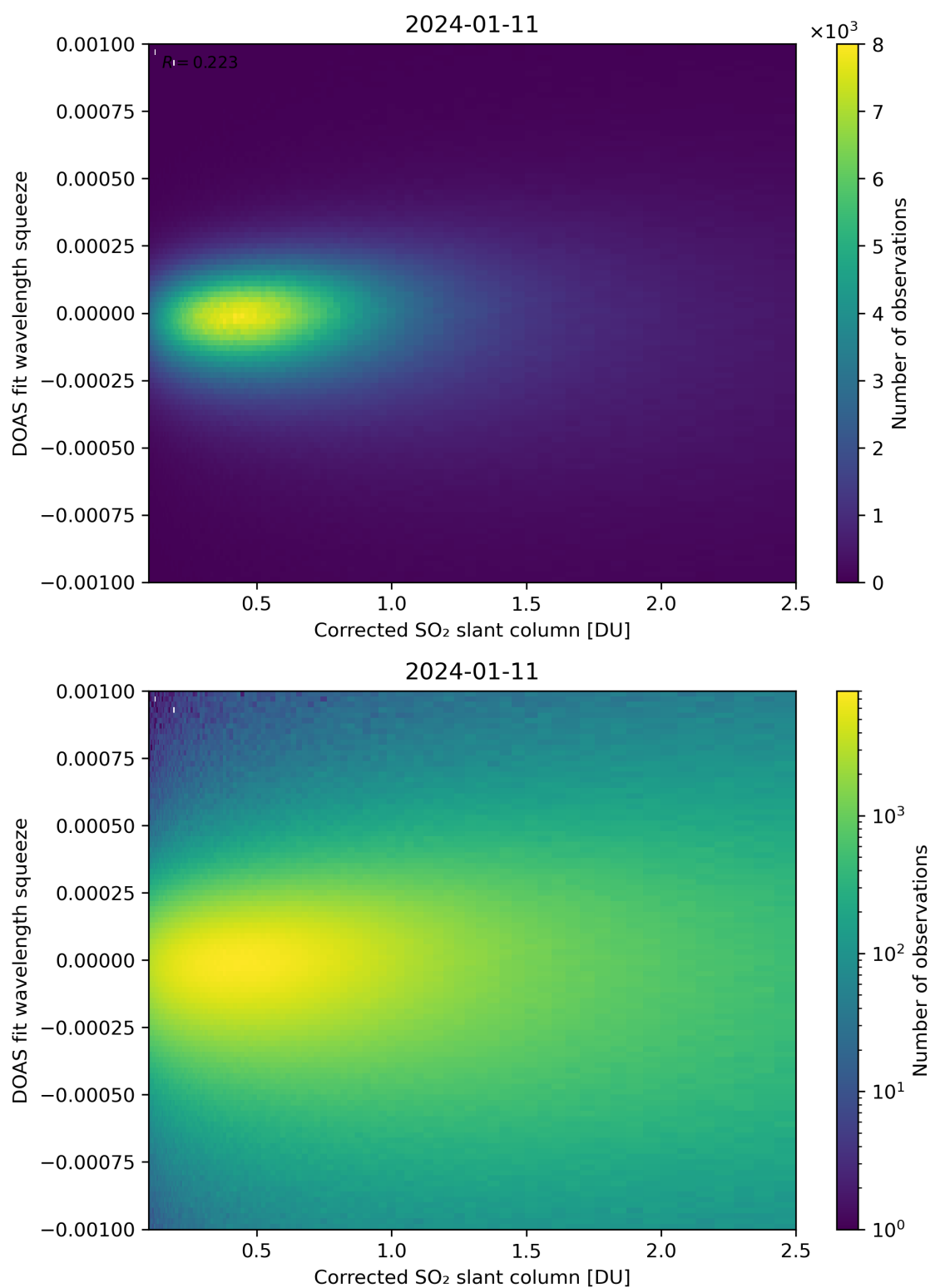
Figure 182: Scatter density plot of “Corrected SO 2 slant column” against “DOAS fit wavelength squeeze” for 2024-01-10 to 2024-01-12.
