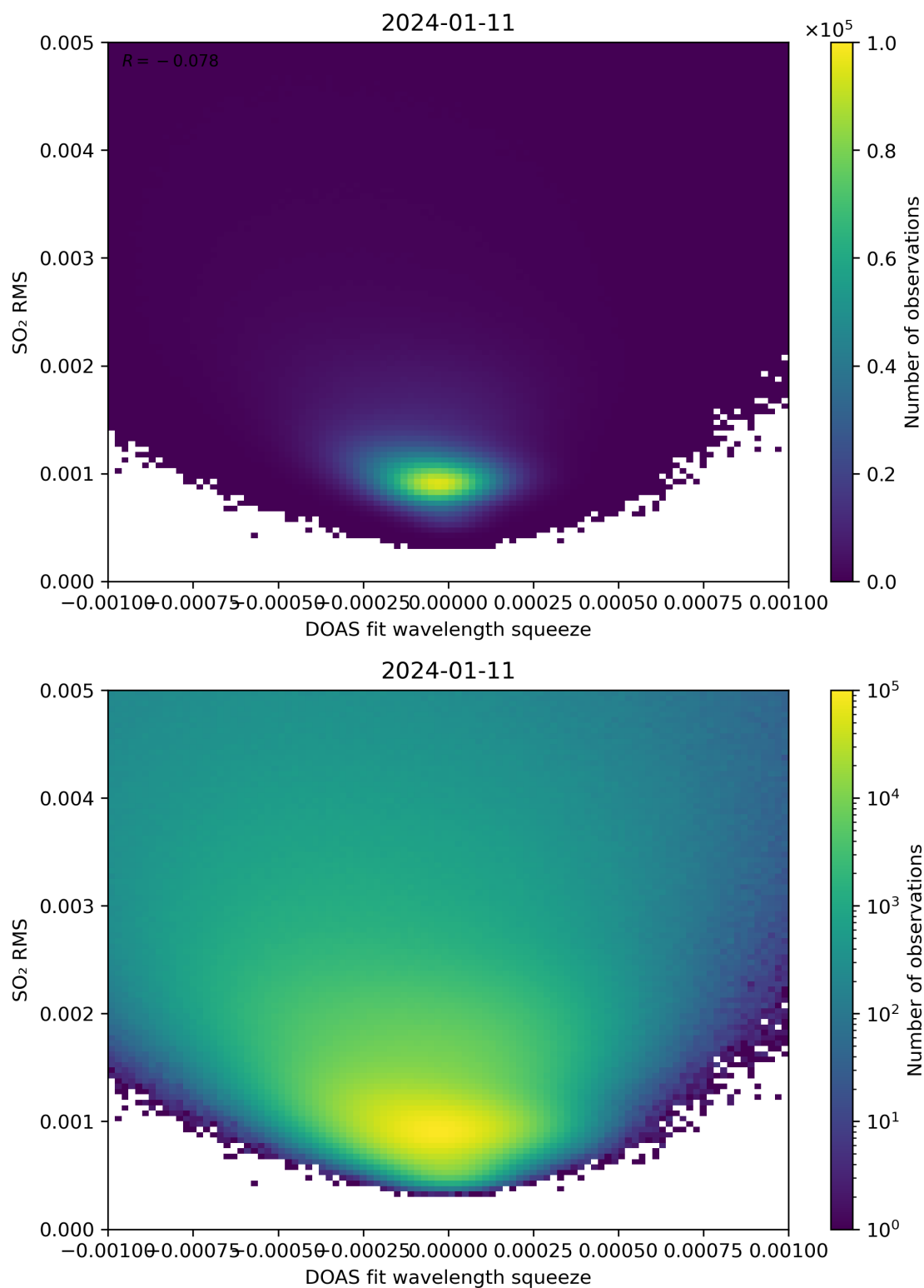
Figure 132: Scatter density plot of “DOAS fit wavelength squeeze” against “SO 2 RMS” for 2024-01-10 to 2024-01-12.
