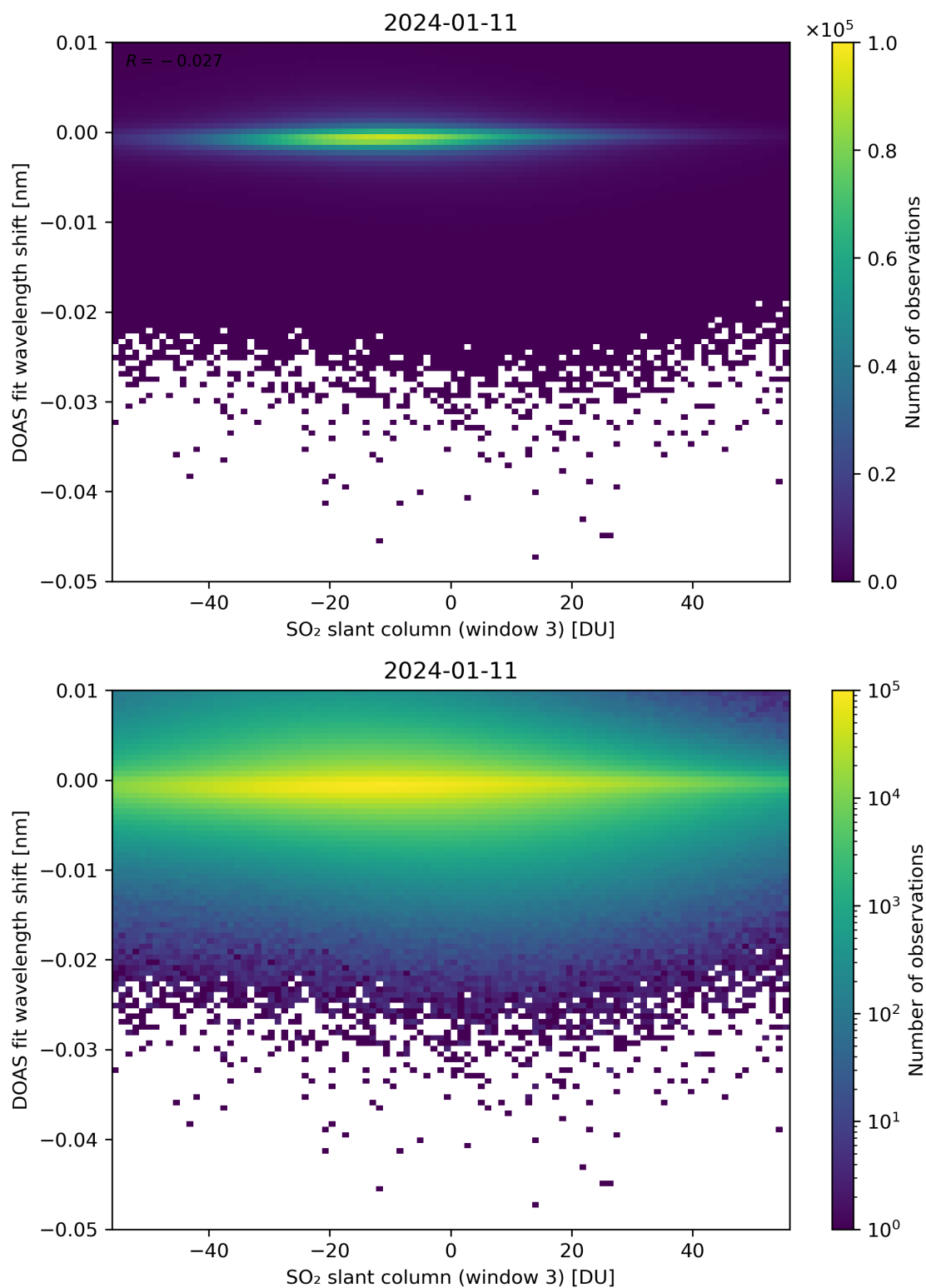
Figure 254: Scatter density plot of “SO 2 slant column (window 3)” against “DOAS fit wavelength shift” for 2024-01-10 to 2024-01-12.
