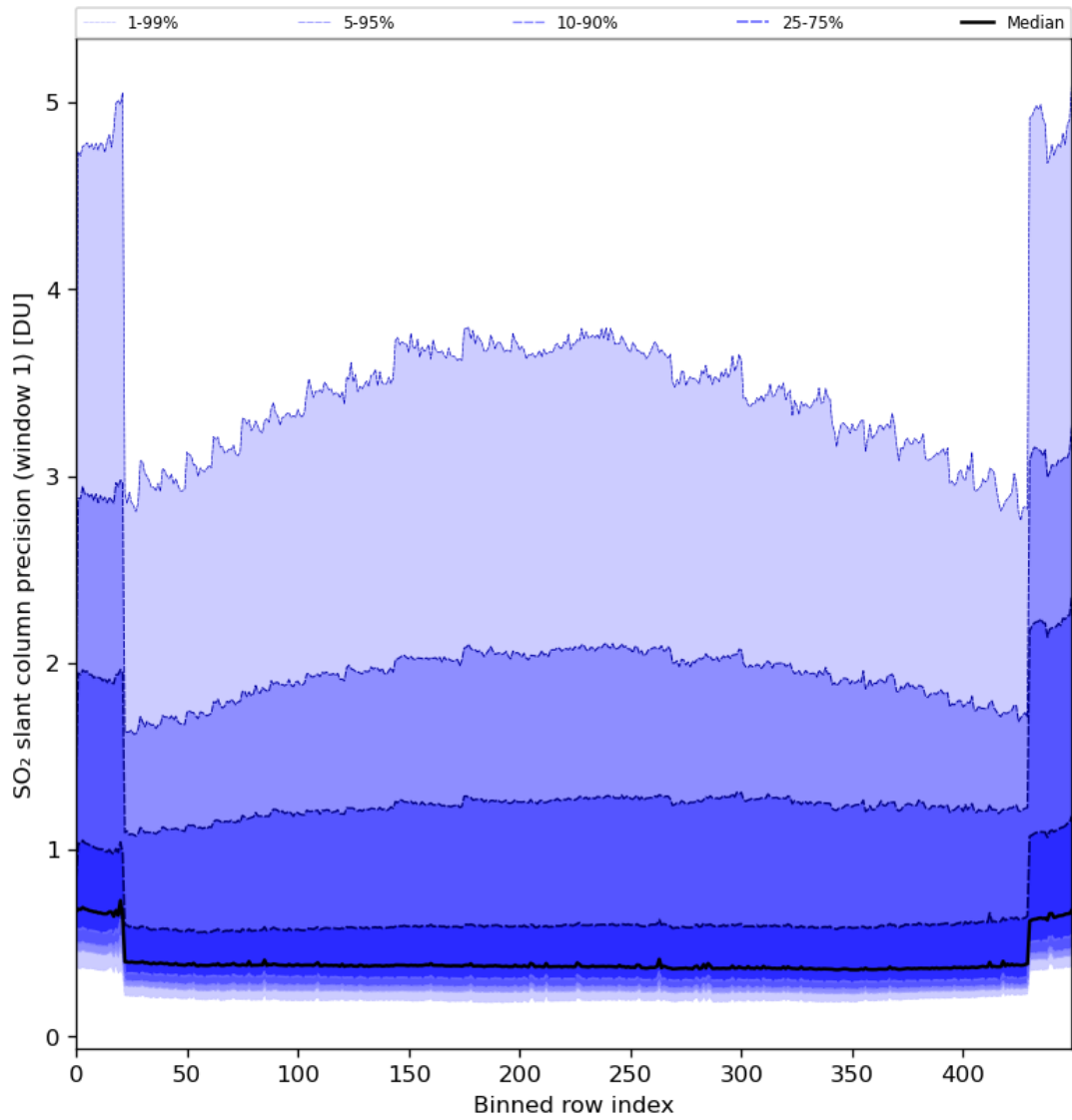
Figure 80: Along track statistics of “SO 2 slant column precision (window 1)” for 2024-01-10 to 2024-01-12
