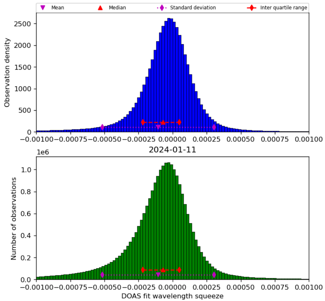
Figure 69: Histogram of “DOAS fit wavelength squeeze” for 2024-01-10 to 2024-01-12
