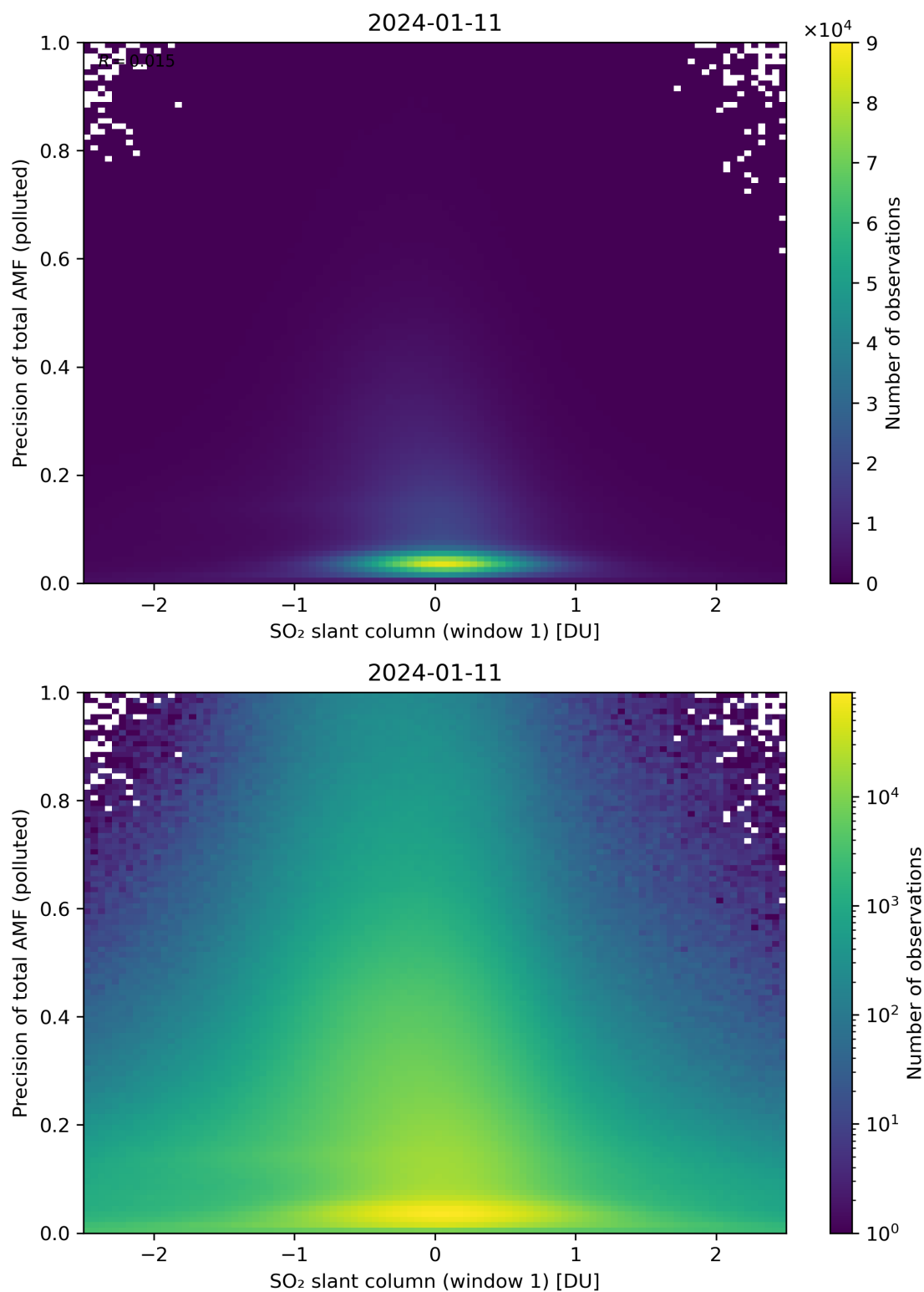
Figure 240: Scatter density plot of “SO 2 slant column (window 1)” against “Precision of total AMF (polluted)” for 2024-01-10 to 2024-01-12.
