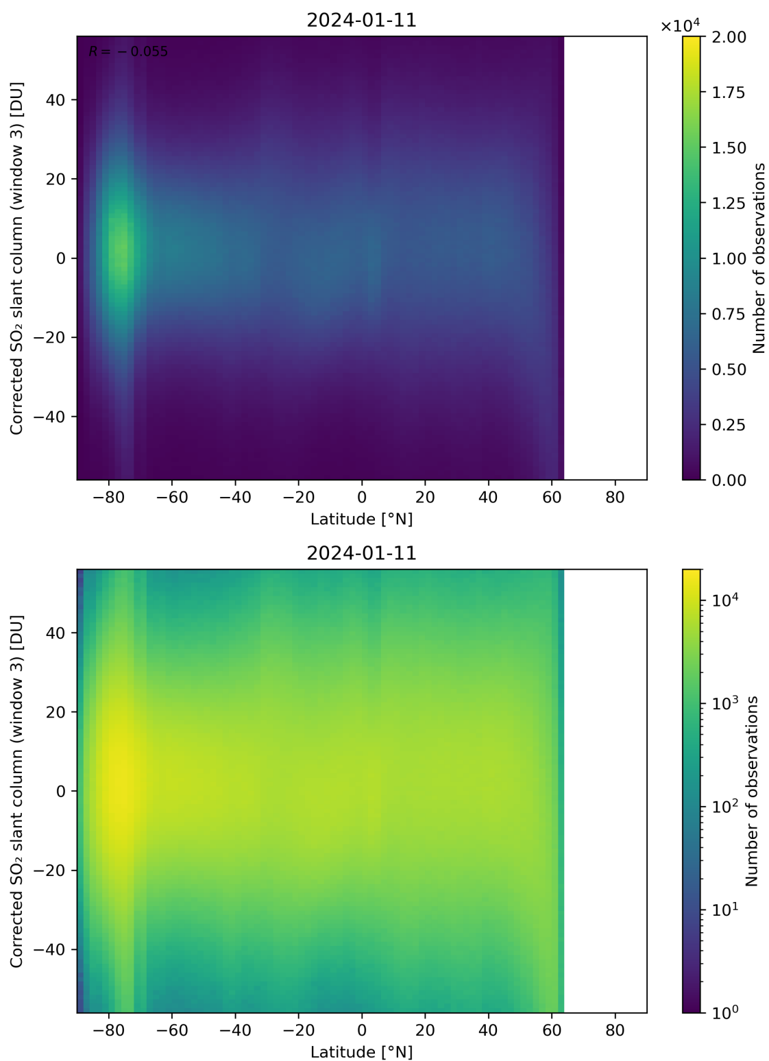
Figure 148: Scatter density plot of “Latitude” against “Corrected SO 2 slant column (window 3)” for 2024-01-10 to 2024-01-12.
