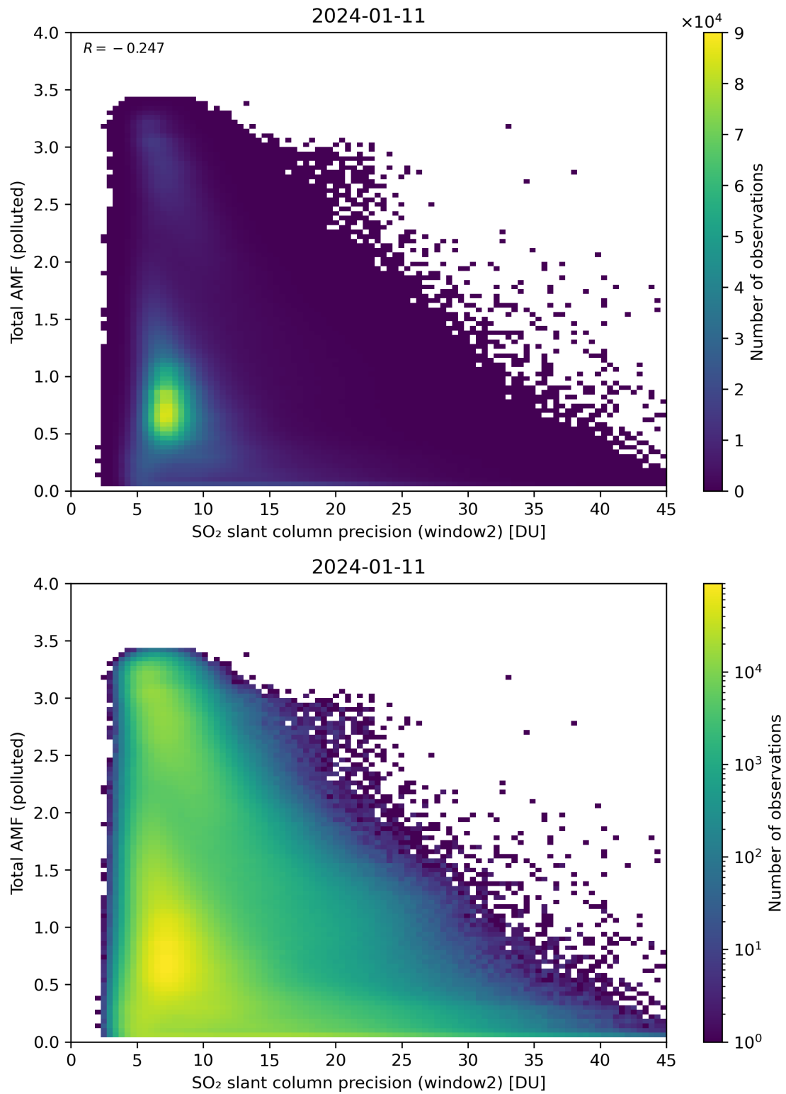
Figure 251: Scatter density plot of “SO 2 slant column precision (window2)” against “Total AMF (polluted)” for 2024-01-10 to 2024-01-12.
