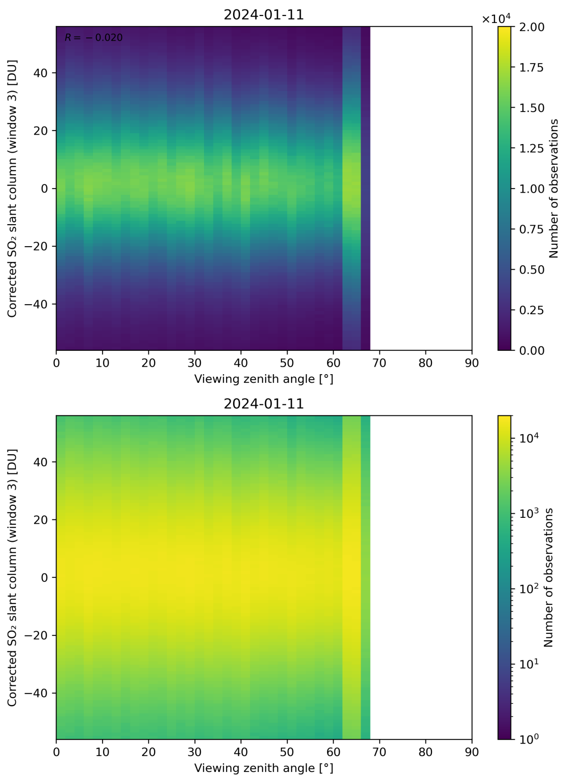
Figure 319: Scatter density plot of “Viewing zenith angle” against “Corrected SO 2 slant column (window 3)” for 2024-01-10 to 2024-01-12.
