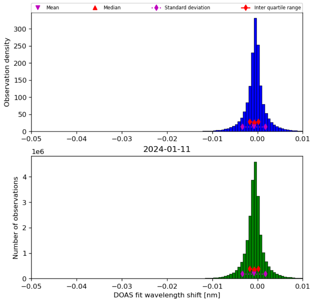
Figure 68: Histogram of “DOAS fit wavelength shift” for 2024-01-10 to 2024-01-12
