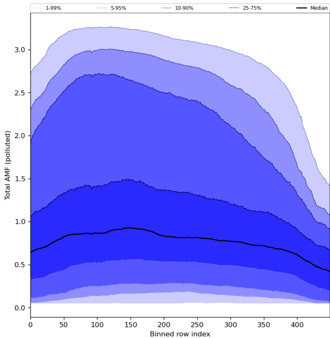
Figure 94: Along track statistics of “Total AMF (polluted)” for 2024-01-10 to 2024-01-12
