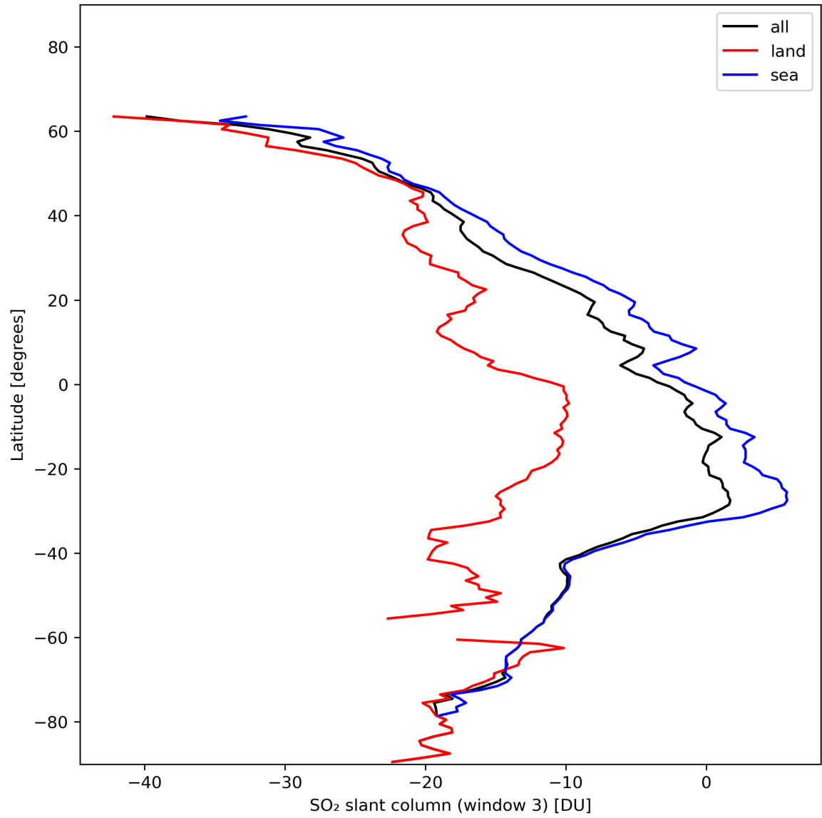
Figure 41: Zonal average of “SO 2 slant column (window 3)” for 2024-01-10 to 2024-01-12.
