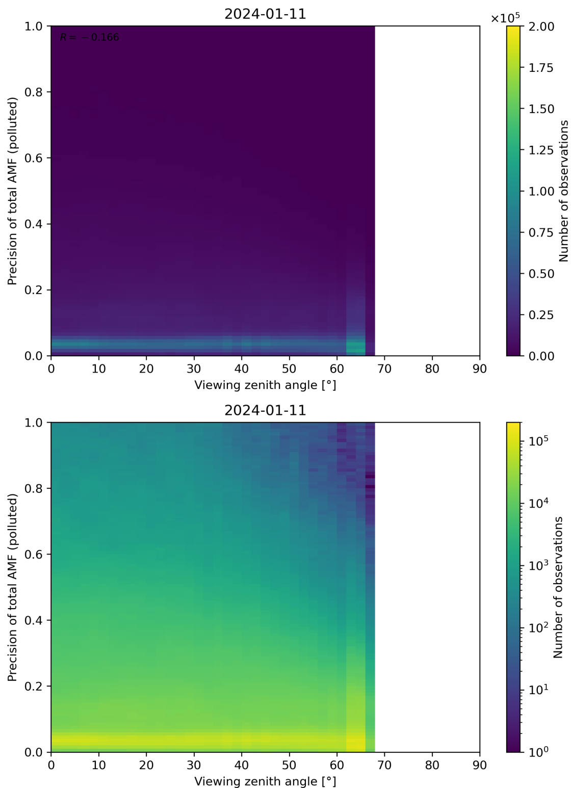
Figure 326: Scatter density plot of “Viewing zenith angle” against “Precision of total AMF (polluted)” for 2024-01-10 to 2024-01-12.
