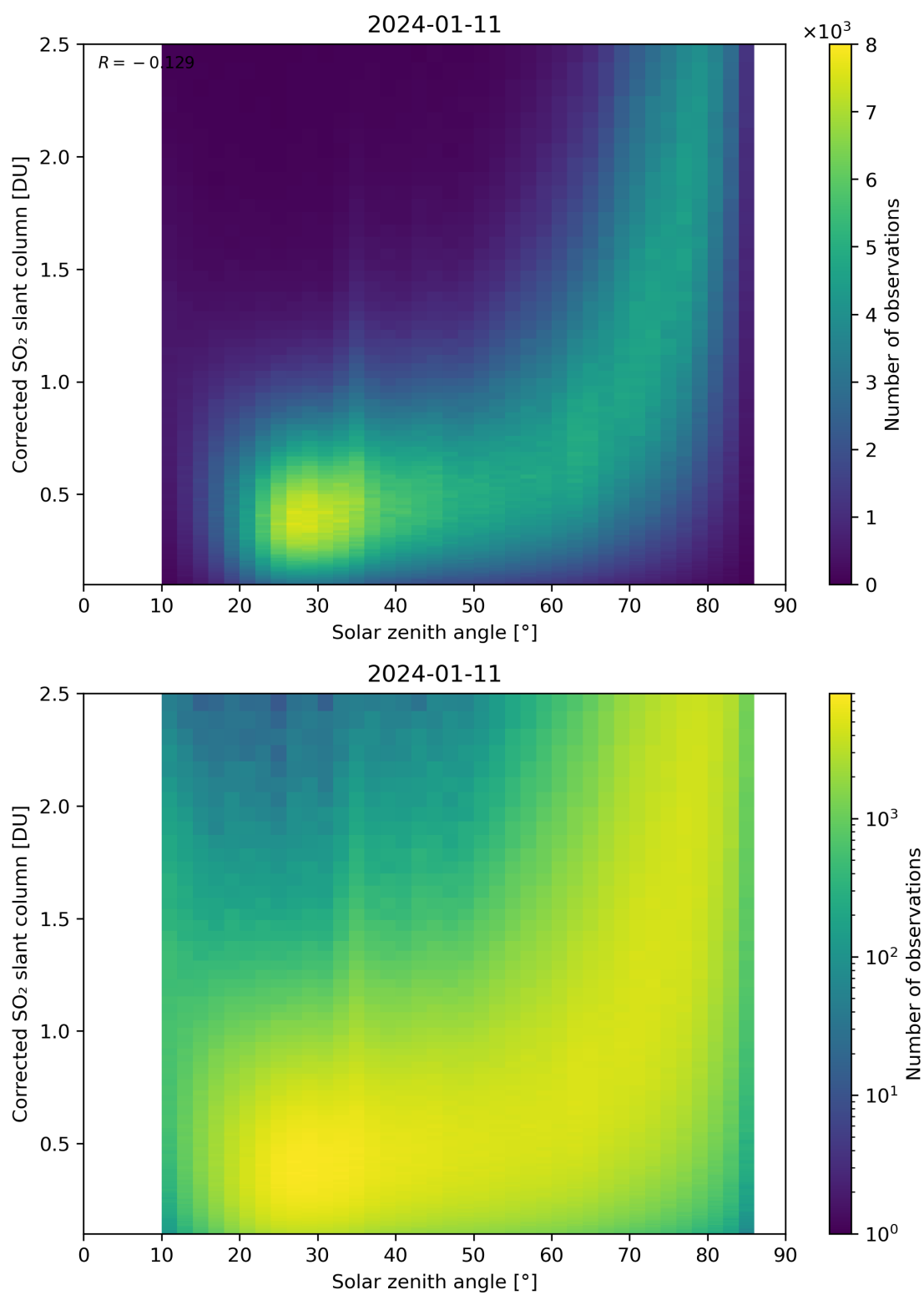
Figure 166: Scatter density plot of “Solar zenith angle” against “Corrected SO 2 slant column” for 2024-01-10 to 2024-01-12.
