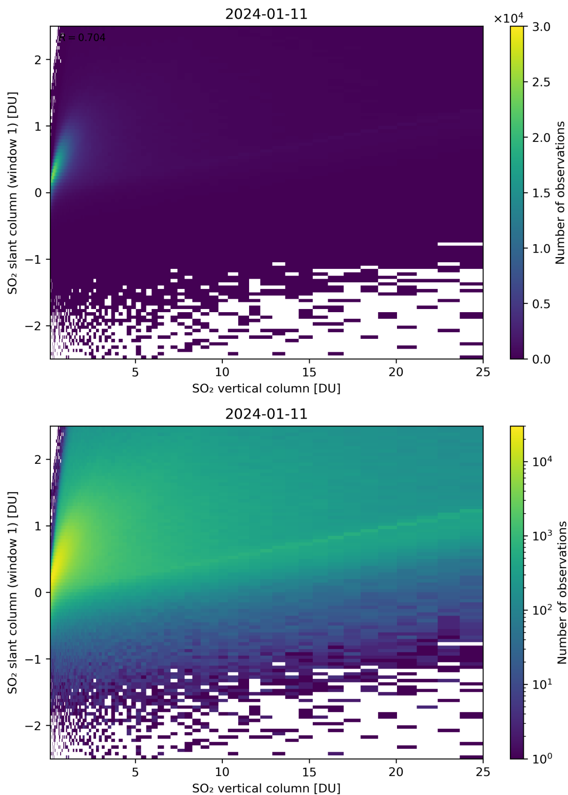
Figure 300: Scatter density plot of “SO 2 vertical column” against “SO 2 slant column (window 1)” for 2024-01-10 to 2024-01-12.
