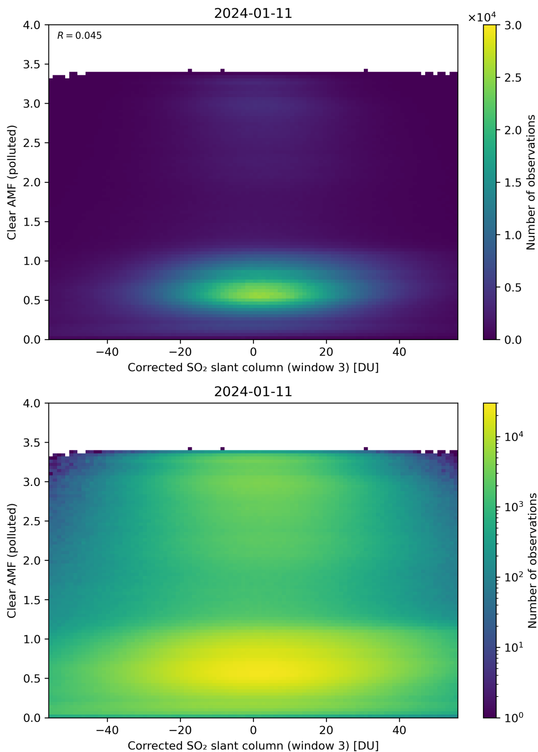
Figure 209: Scatter density plot of “Corrected SO 2 slant column (window 3)” against “Clear AMF (polluted)” for 2024-01-10 to 2024-01-12.
