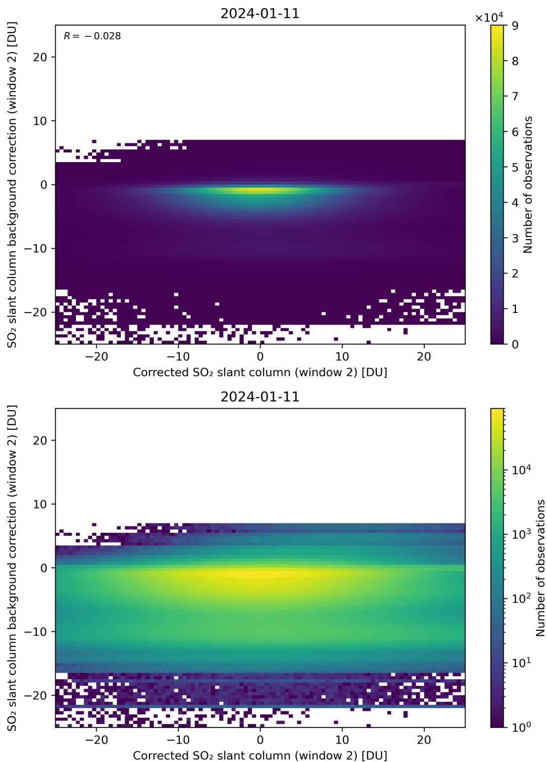
Figure 194: Scatter density plot of “Corrected SO 2 slant column (window 2)” against “SO 2 slant column background correction (window 2)” for 2024-01-10 to 2024-01-12.
