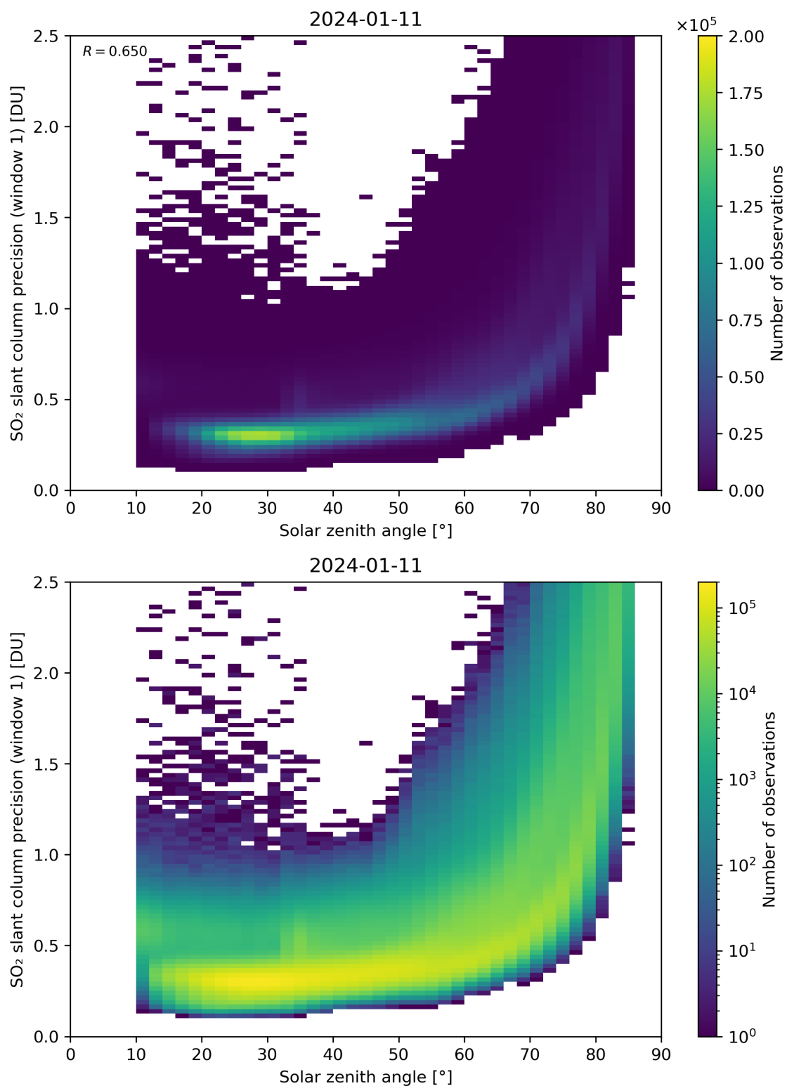
Figure 170: Scatter density plot of “Solar zenith angle” against “SO 2 slant column precision (window 1)” for 2024-01-10 to 2024-01-12.
