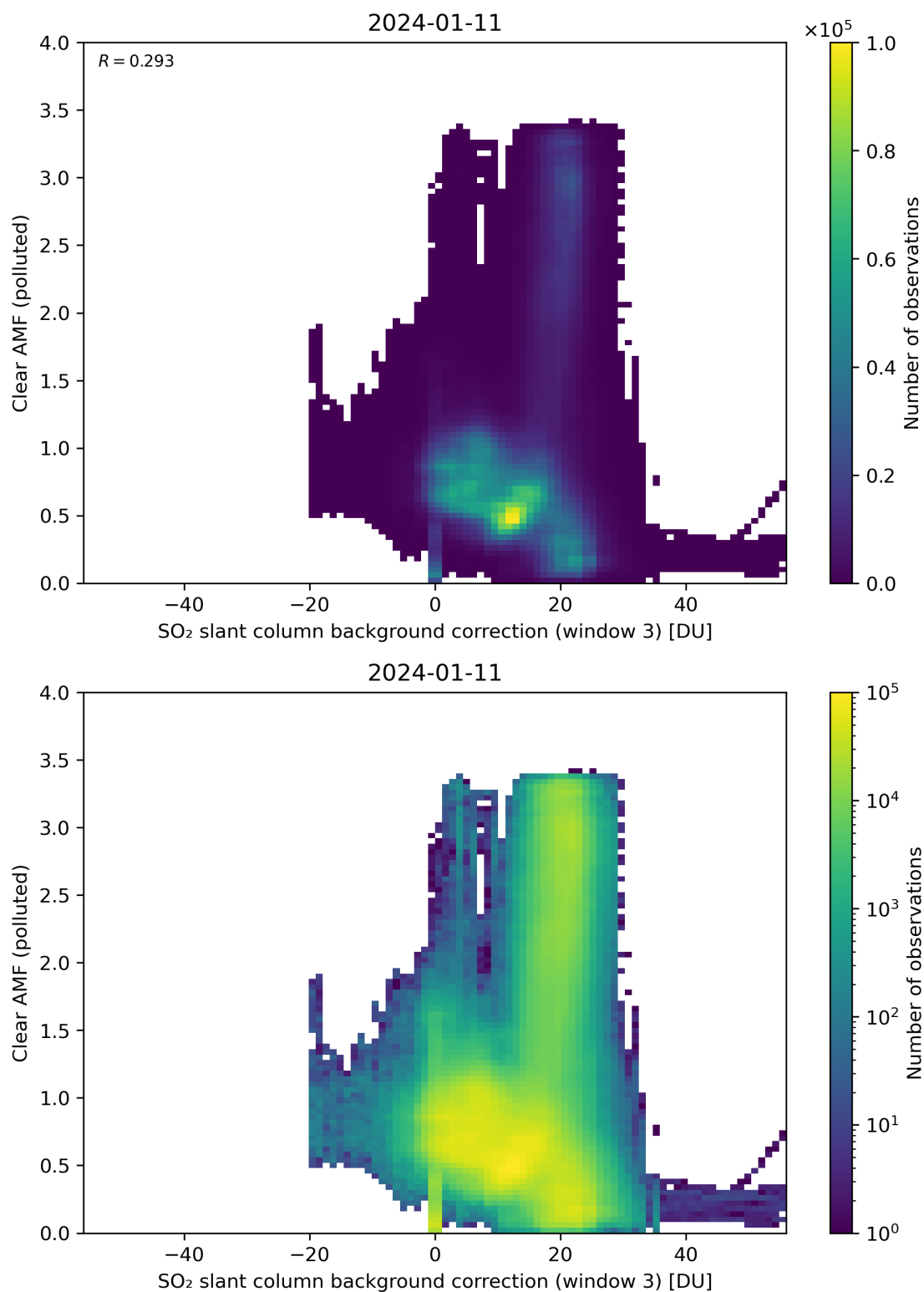
Figure 124: Scatter density plot of “SO 2 slant column background correction (window 3)” against “Clear AMF (polluted)” for 2024-01-10 to 2024-01-12.
