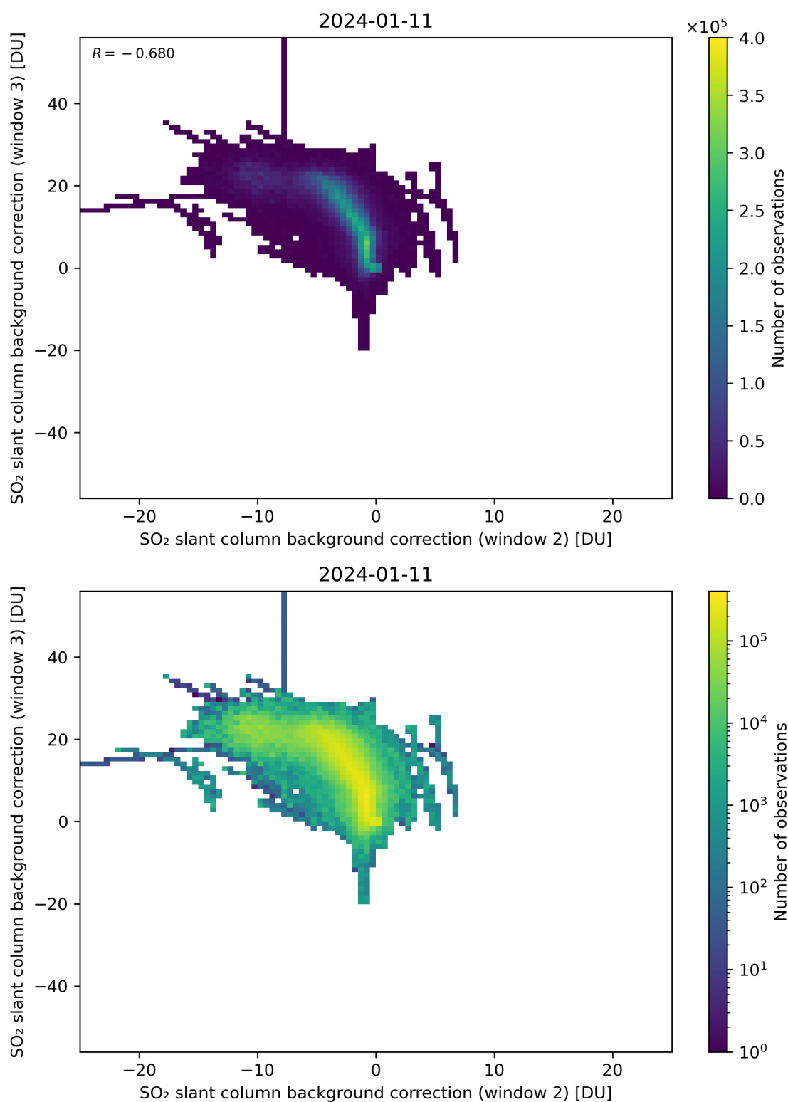
Figure 111: Scatter density plot of “SO 2 slant column background correction (window 2)” against “SO 2 slant column background correction (window 3)” for 2024-01-10 to 2024-01-12.
