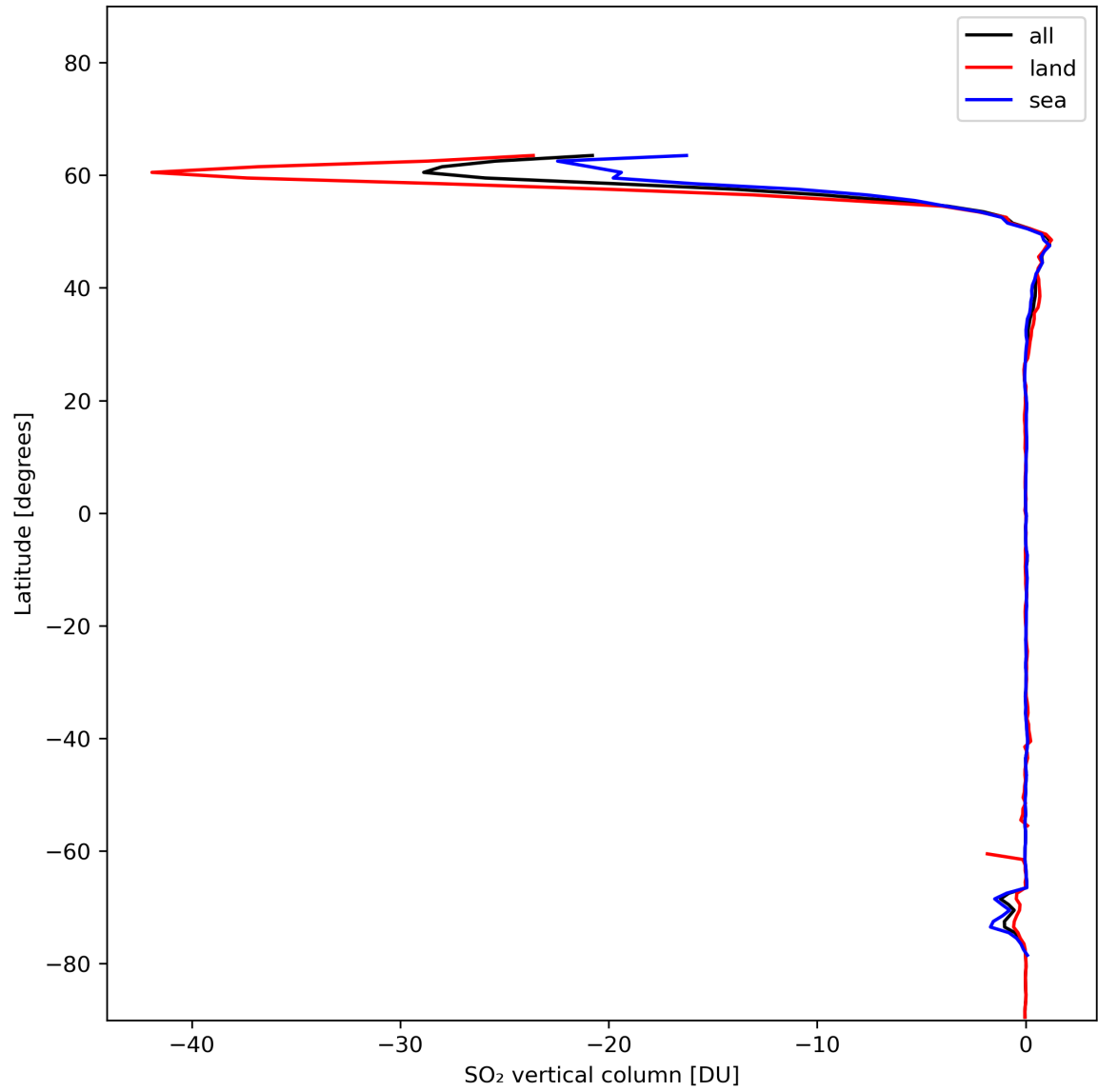
Figure 30: Zonal average of “SO 2 vertical column” for 2024-01-10 to 2024-01-12.
