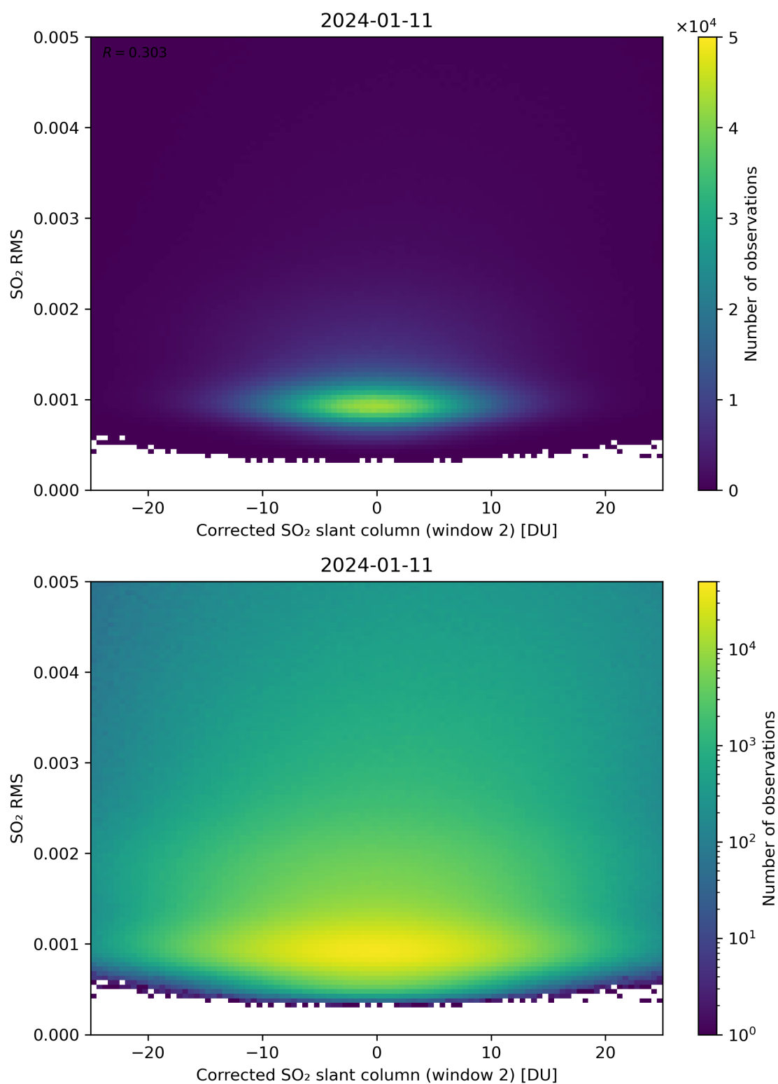
Figure 198: Scatter density plot of “Corrected SO 2 slant column (window 2)” against “SO 2 RMS” for 2024-01-10 to 2024-01-12.
