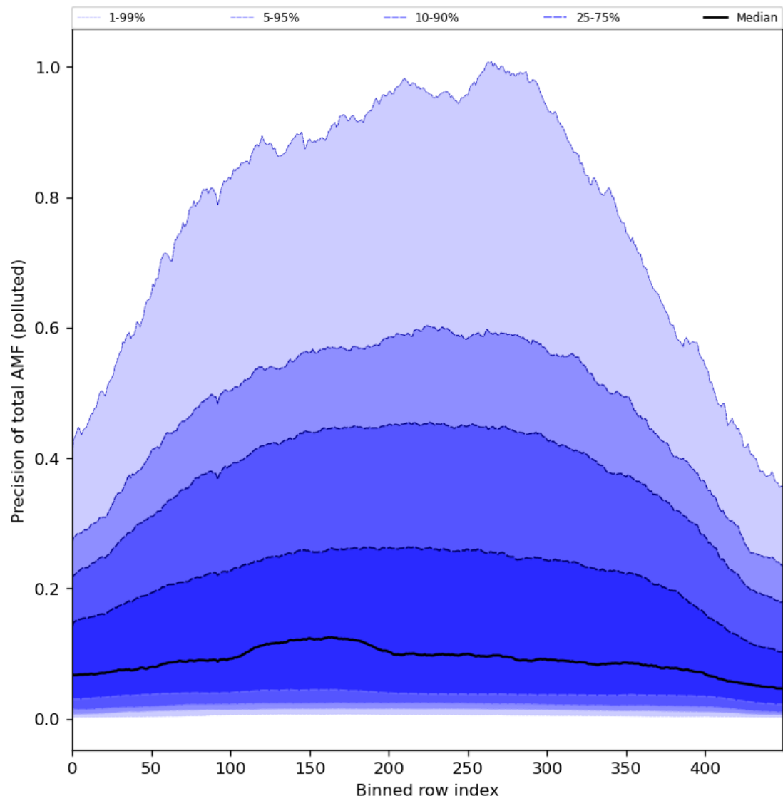
Figure 95: Along track statistics of “Precision of total AMF (polluted)” for 2024-01-10 to 2024-01-12
