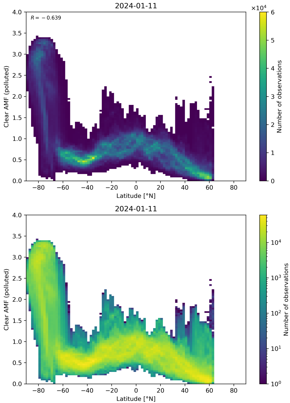
Figure 145: Scatter density plot of “Latitude” against “Clear AMF (polluted)” for 2024-01-10 to 2024-01-12.
