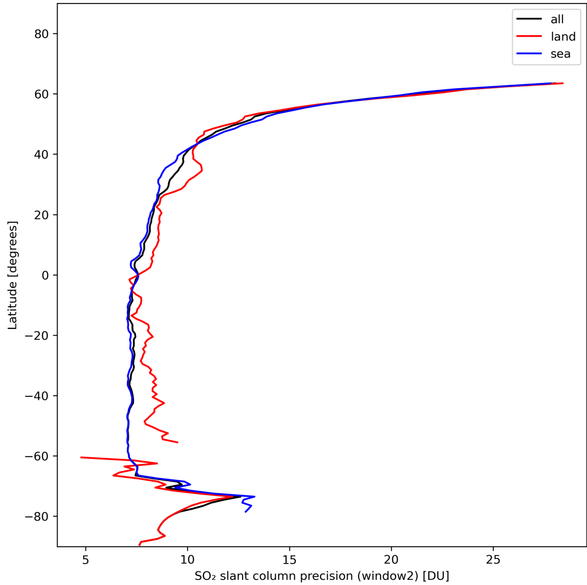
Figure 38: Zonal average of “SO 2 slant column precision (window2)” for 2024-01-10 to 2024-01-12.
