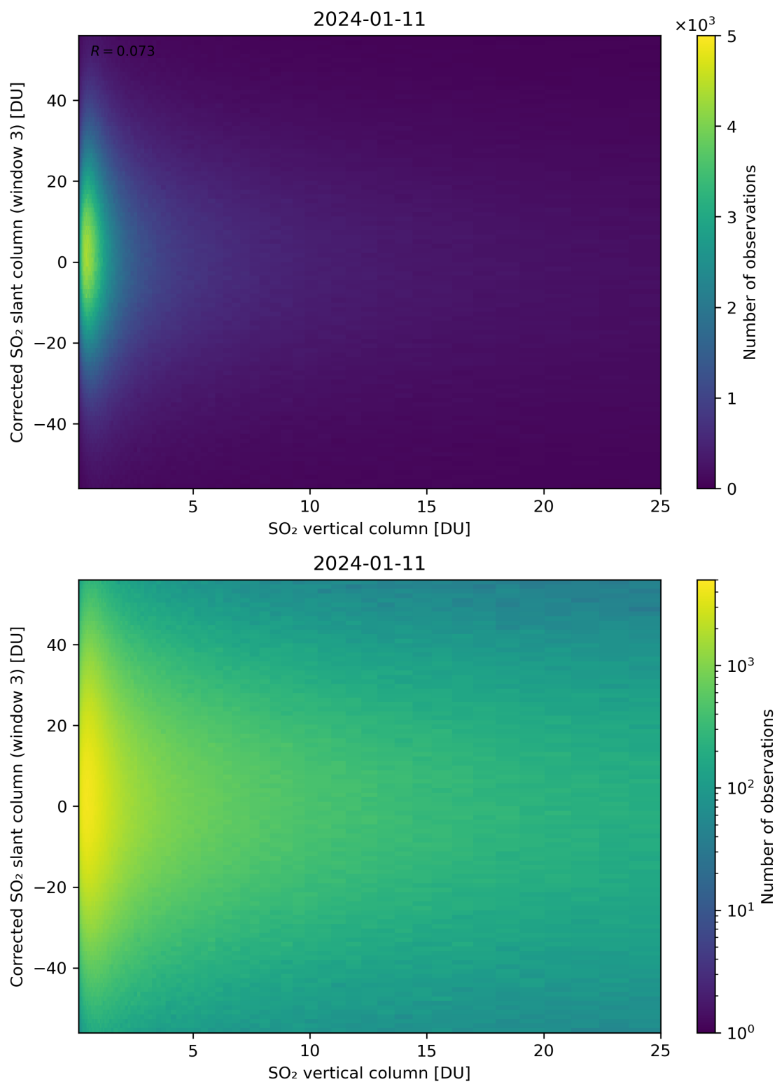
Figure 299: Scatter density plot of “SO 2 vertical column” against “Corrected SO 2 slant column (window 3)” for 2024-01-10 to 2024-01-12.
