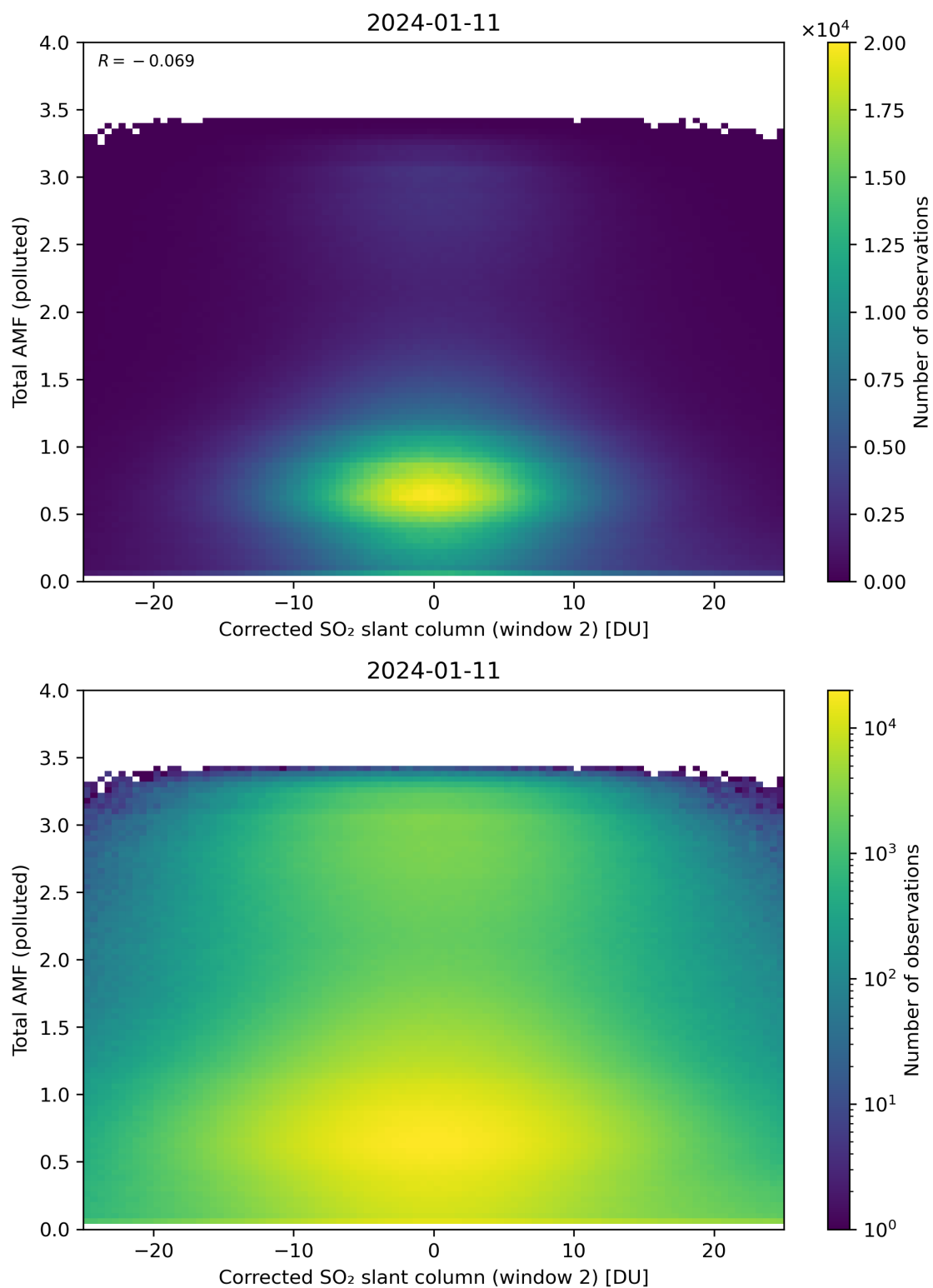
Figure 203: Scatter density plot of “Corrected SO 2 slant column (window 2)” against “Total AMF (polluted)” for 2024-01-10 to 2024-01-12.
