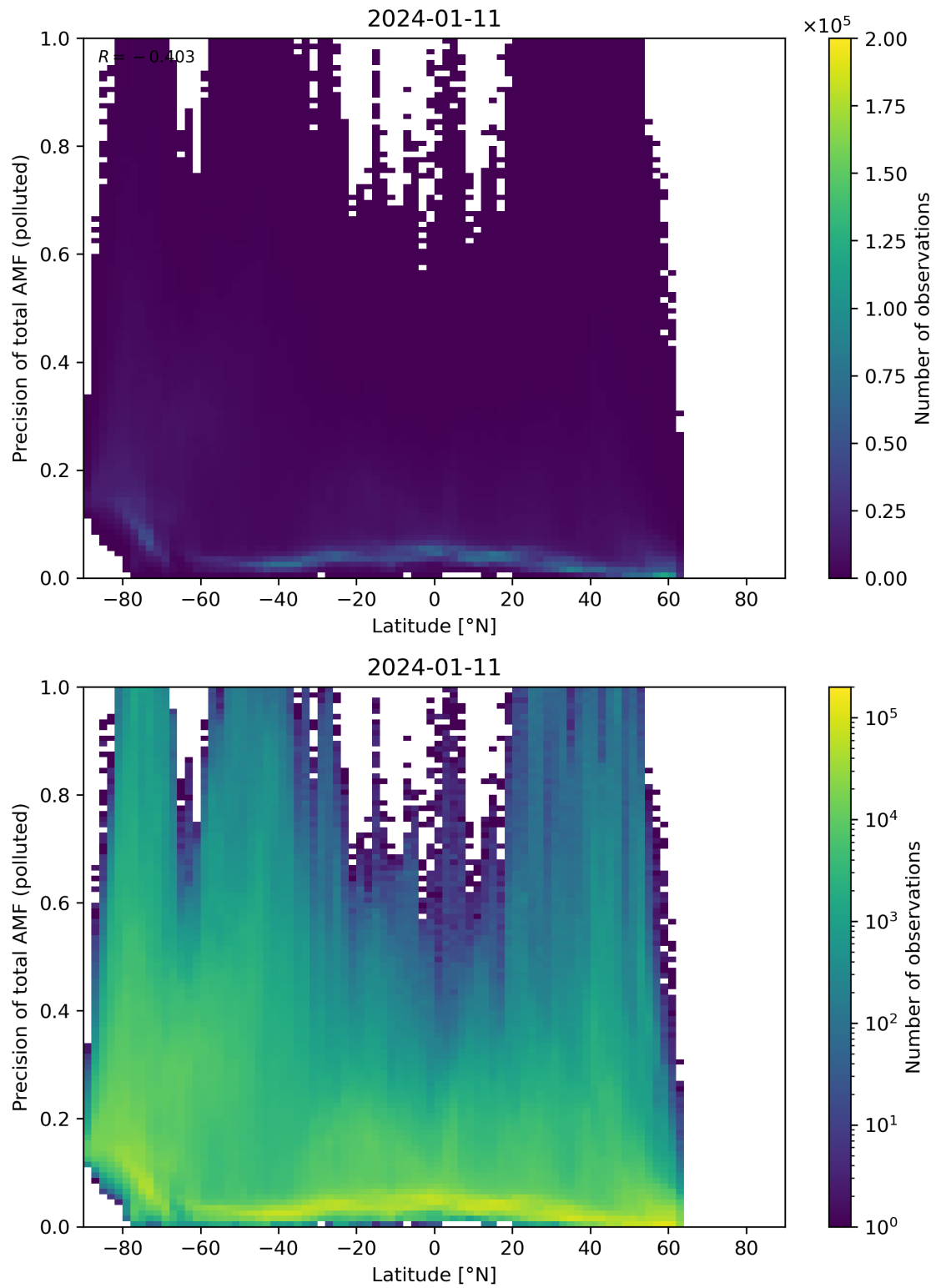
Figure 155: Scatter density plot of “Latitude” against “Precision of total AMF (polluted)” for 2024-01-10 to 2024-01-12.
