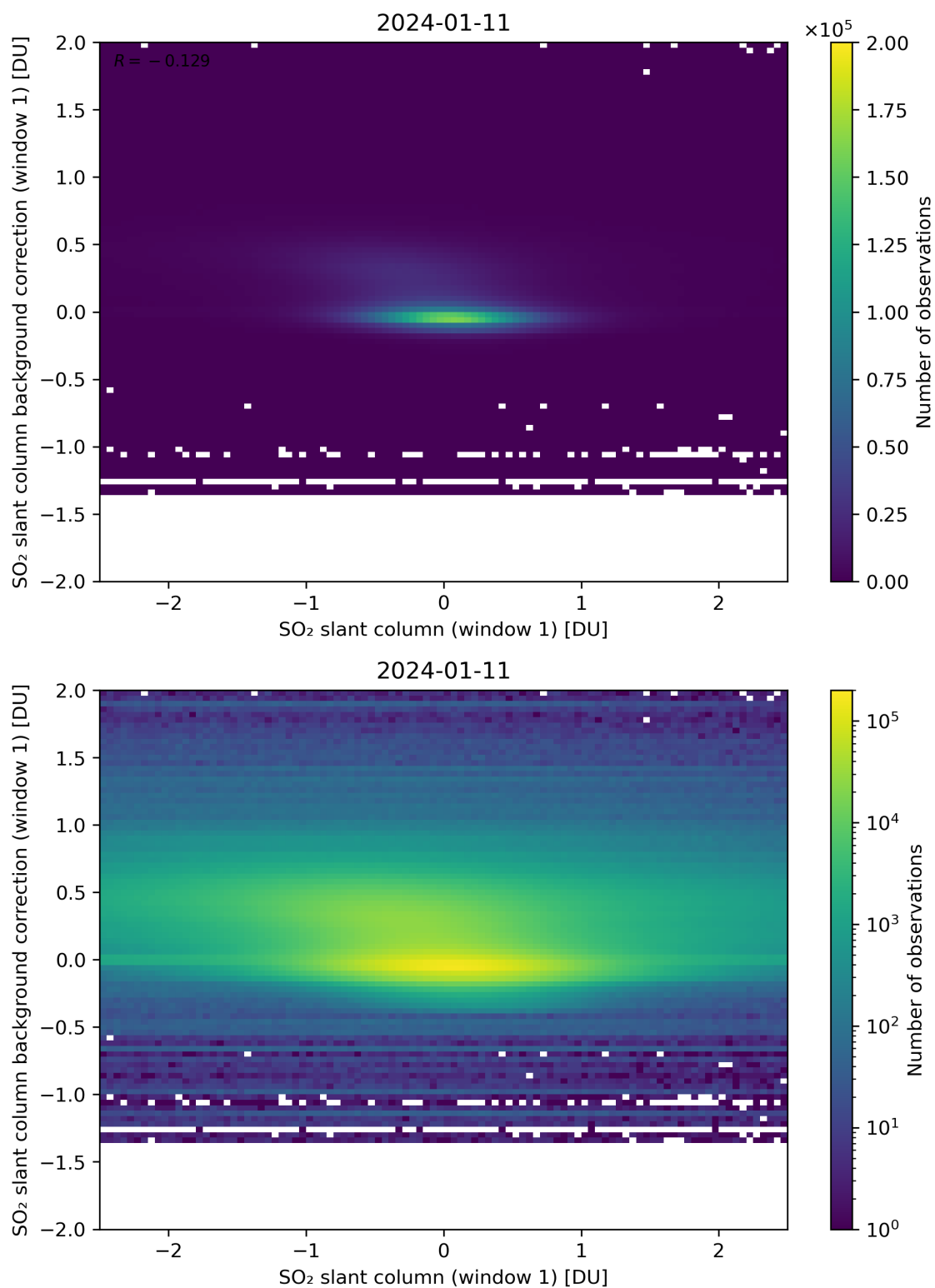
Figure 212: Scatter density plot of “SO 2 slant column (window 1)” against “SO 2 slant column background correction (window 1)” for 2024-01-10 to 2024-01-12.
