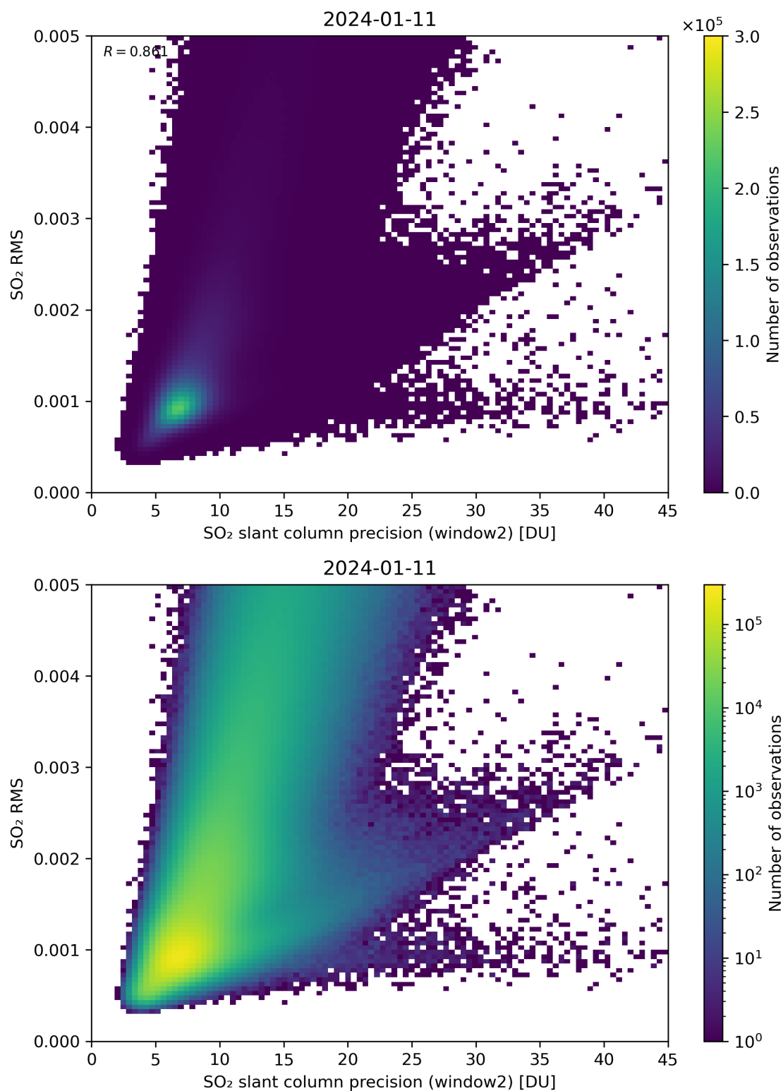
Figure 245: Scatter density plot of “SO 2 slant column precision (window2)” against “SO 2 RMS” for 2024-01-10 to 2024-01-12.
