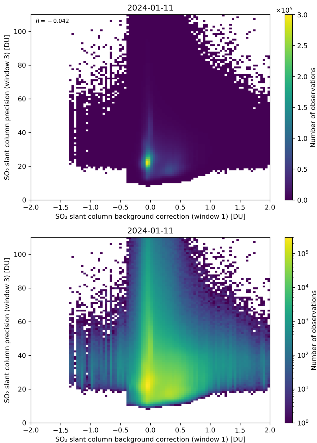
Figure 108: Scatter density plot of “SO 2 slant column background correction (window 1)” against “SO 2 slant column precision (window 3)” for 2024-01-10 to 2024-01-12.
