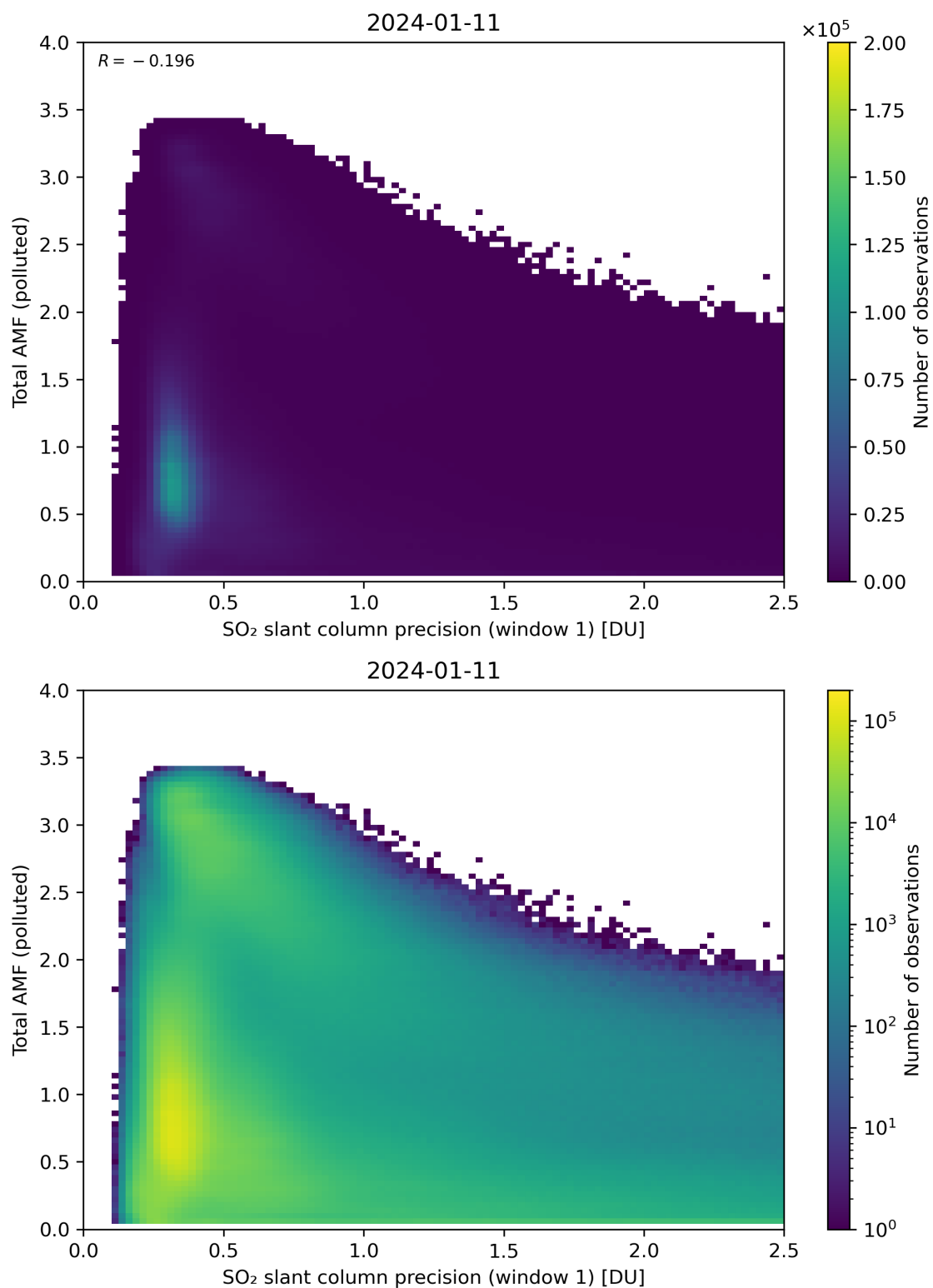
Figure 230: Scatter density plot of “SO 2 slant column precision (window 1)” against “Total AMF (polluted)” for 2024-01-10 to 2024-01-12.
