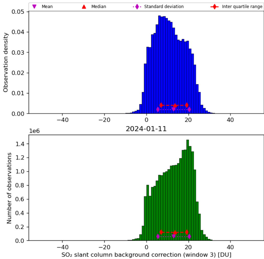
Figure 67: Histogram of “SO 2 slant column background correction (window 3)” for 2024-01-10 to 2024-01-12
