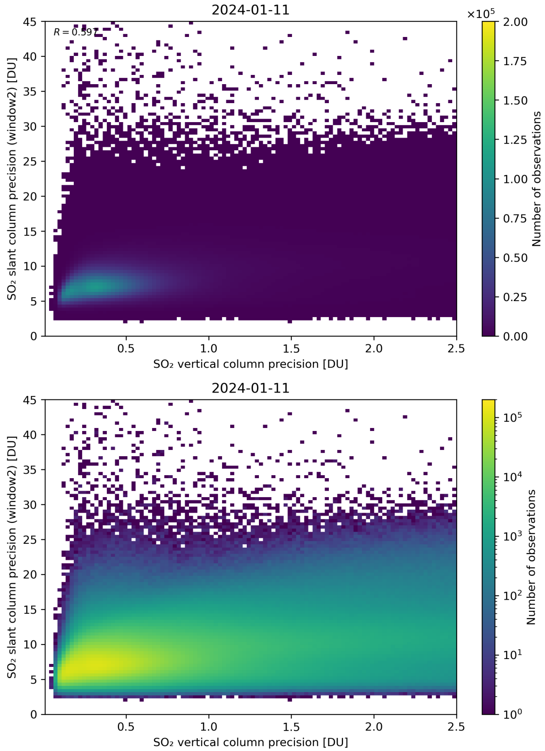
Figure 291: Scatter density plot of “SO 2 vertical column precision” against “SO 2 slant column precision (window2)” for 2024-01-10 to 2024-01-12.
