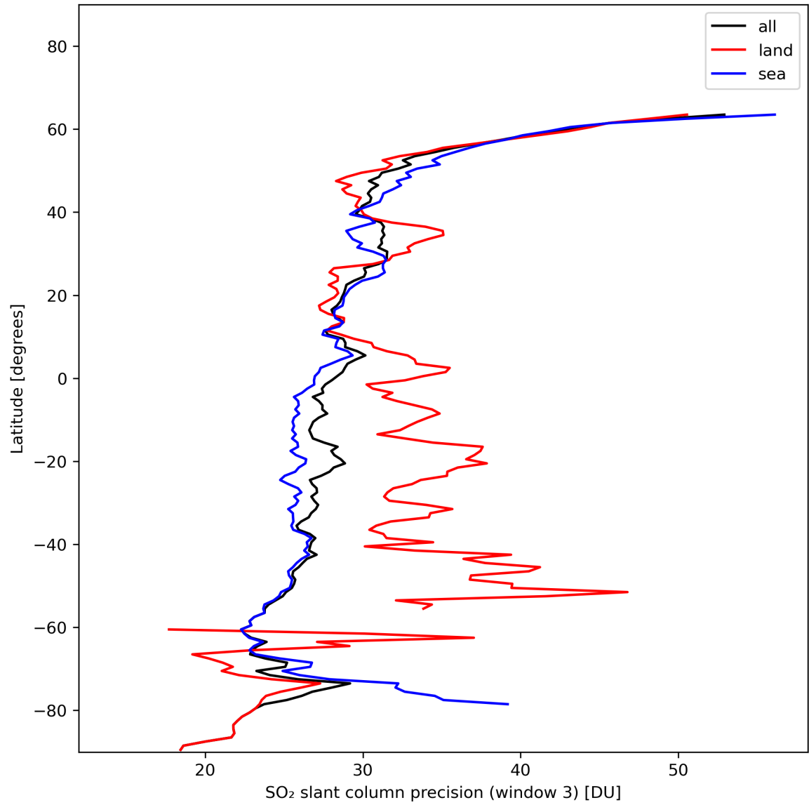
Figure 42: Zonal average of “SO 2 slant column precision (window 3)” for 2024-01-10 to 2024-01-12.
