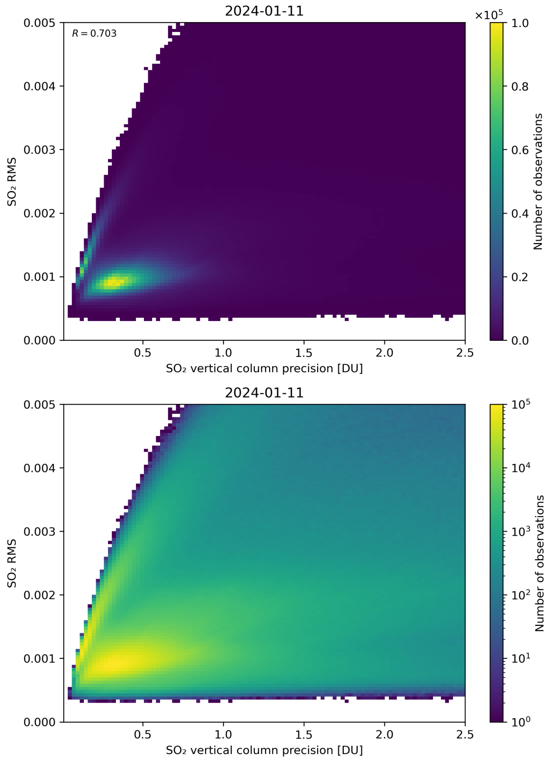
Figure 284: Scatter density plot of “SO 2 vertical column precision” against “SO 2 RMS” for 2024-01-10 to 2024-01-12.
