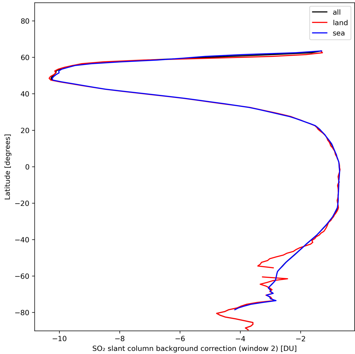
Figure 40: Zonal average of “SO 2 slant column background correction (window 2)” for 2024-01-10 to 2024-01-12.
