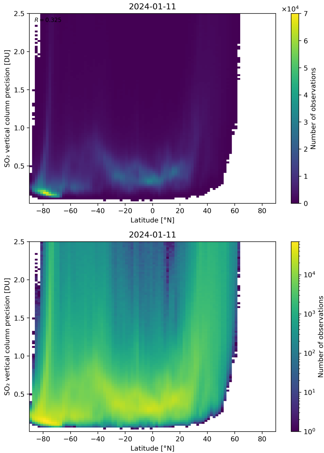
Figure 157: Scatter density plot of “Latitude” against “SO 2 vertical column precision” for 2024-01-10 to 2024-01-12.
