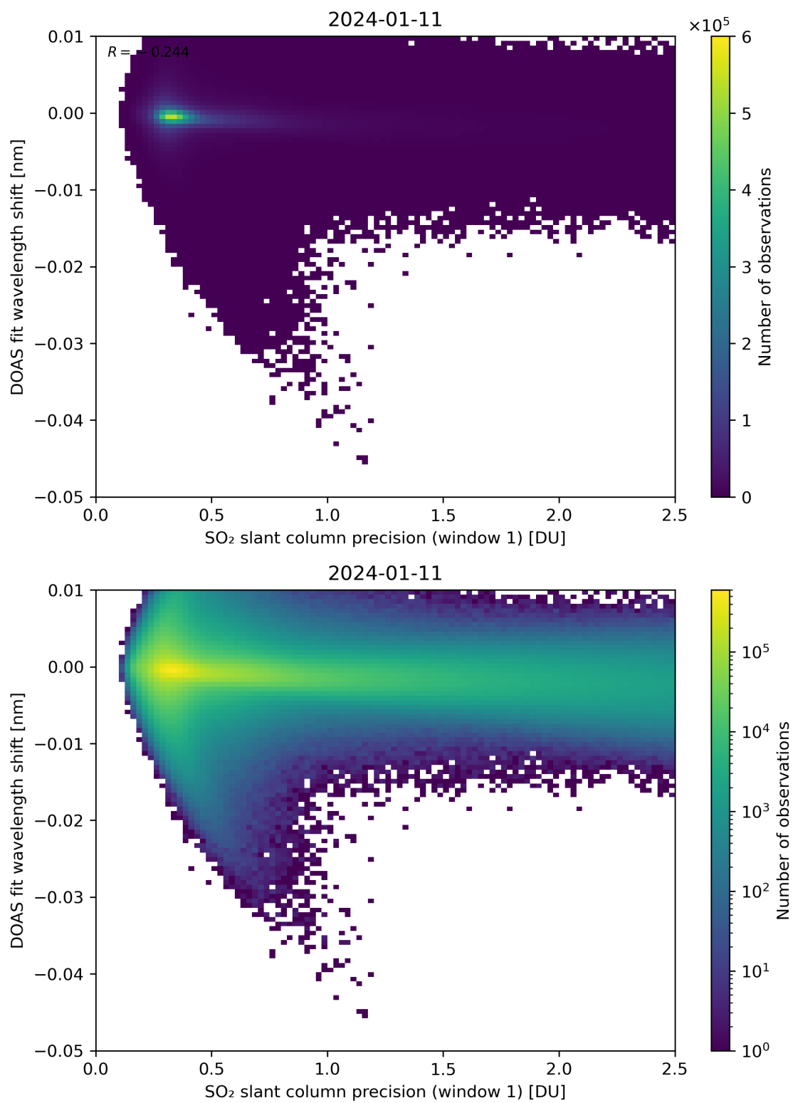
Figure 221: Scatter density plot of “SO 2 slant column precision (window 1)” against “DOAS fit wavelength shift” for 2024-01-10 to 2024-01-12.
