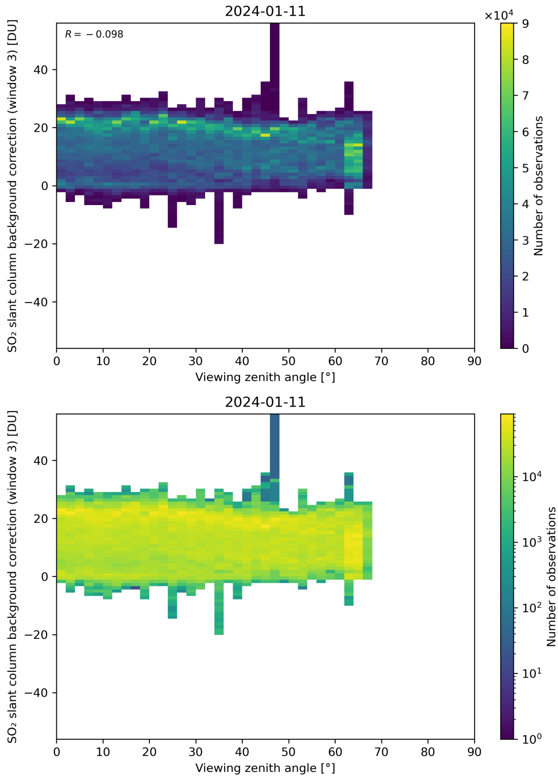
Figure 310: Scatter density plot of “Viewing zenith angle” against “SO 2 slant column background correction (window 3)” for 2024-01-10 to 2024-01-12.
