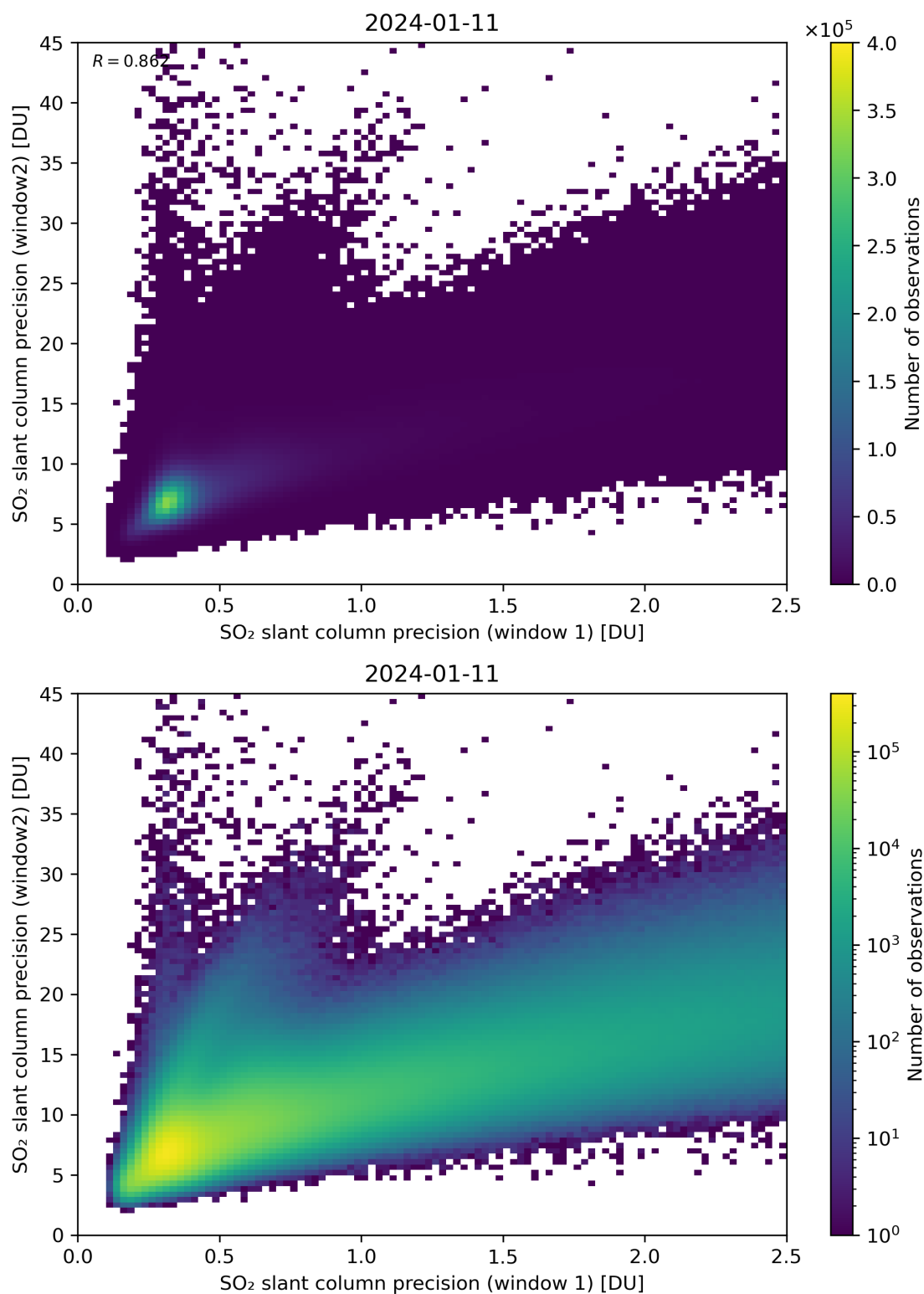
Figure 227: Scatter density plot of “SO 2 slant column precision (window 1)” against “SO 2 slant column precision (window2)” for 2024-01-10 to 2024-01-12.
