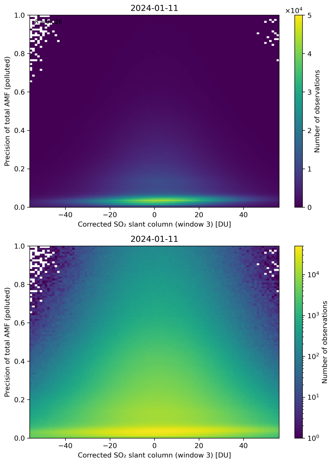
Figure 211: Scatter density plot of “Corrected SO 2 slant column (window 3)” against “Precision of total AMF (polluted)” for 2024-01-10 to 2024-01-12.
