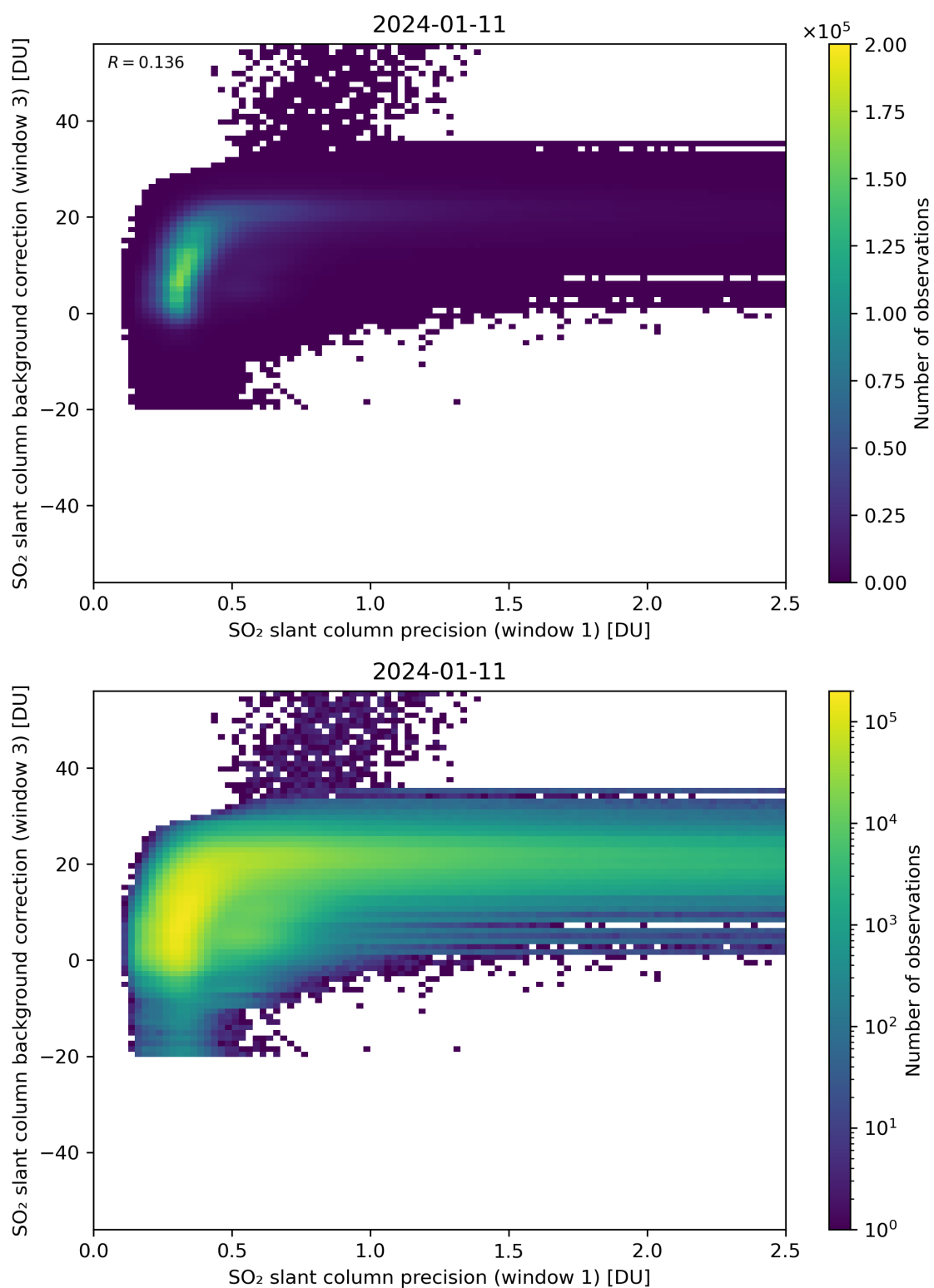
Figure 220: Scatter density plot of “SO 2 slant column precision (window 1)” against “SO 2 slant column background correction (window 3)” for 2024-01-10 to 2024-01-12.
