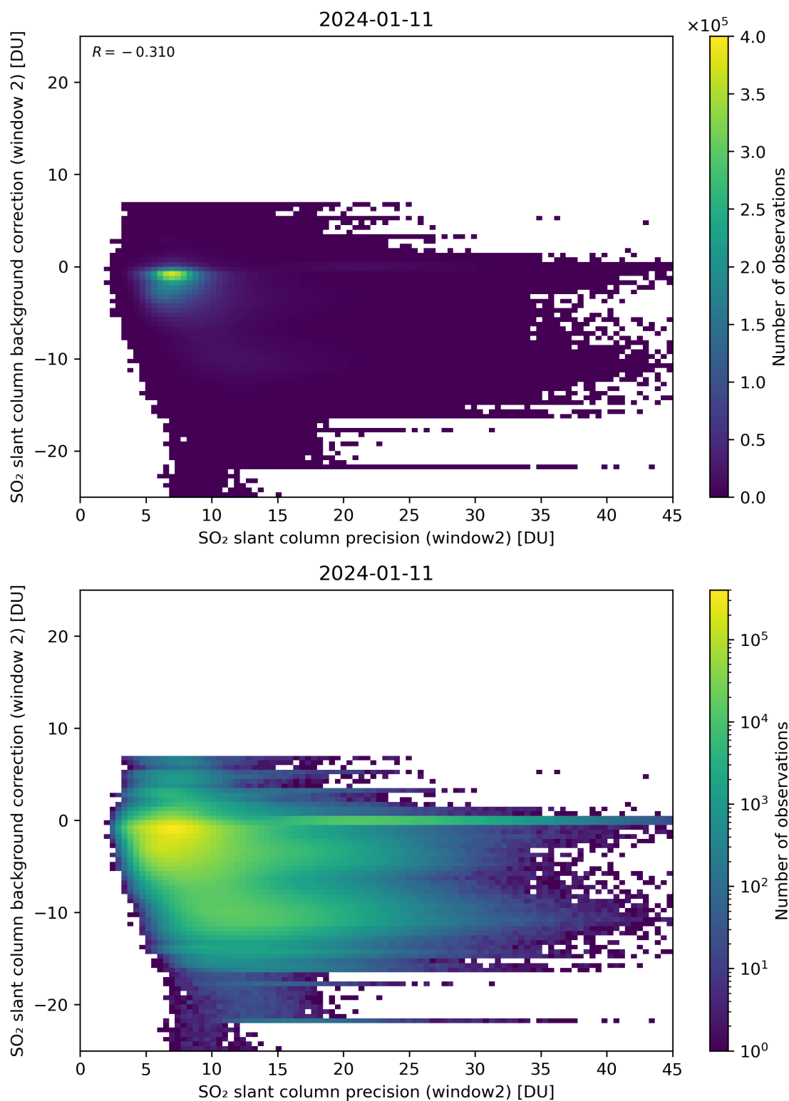
Figure 241: Scatter density plot of “SO 2 slant column precision (window2)” against “SO 2 slant column background correction (window 2)” for 2024-01-10 to 2024-01-12.
