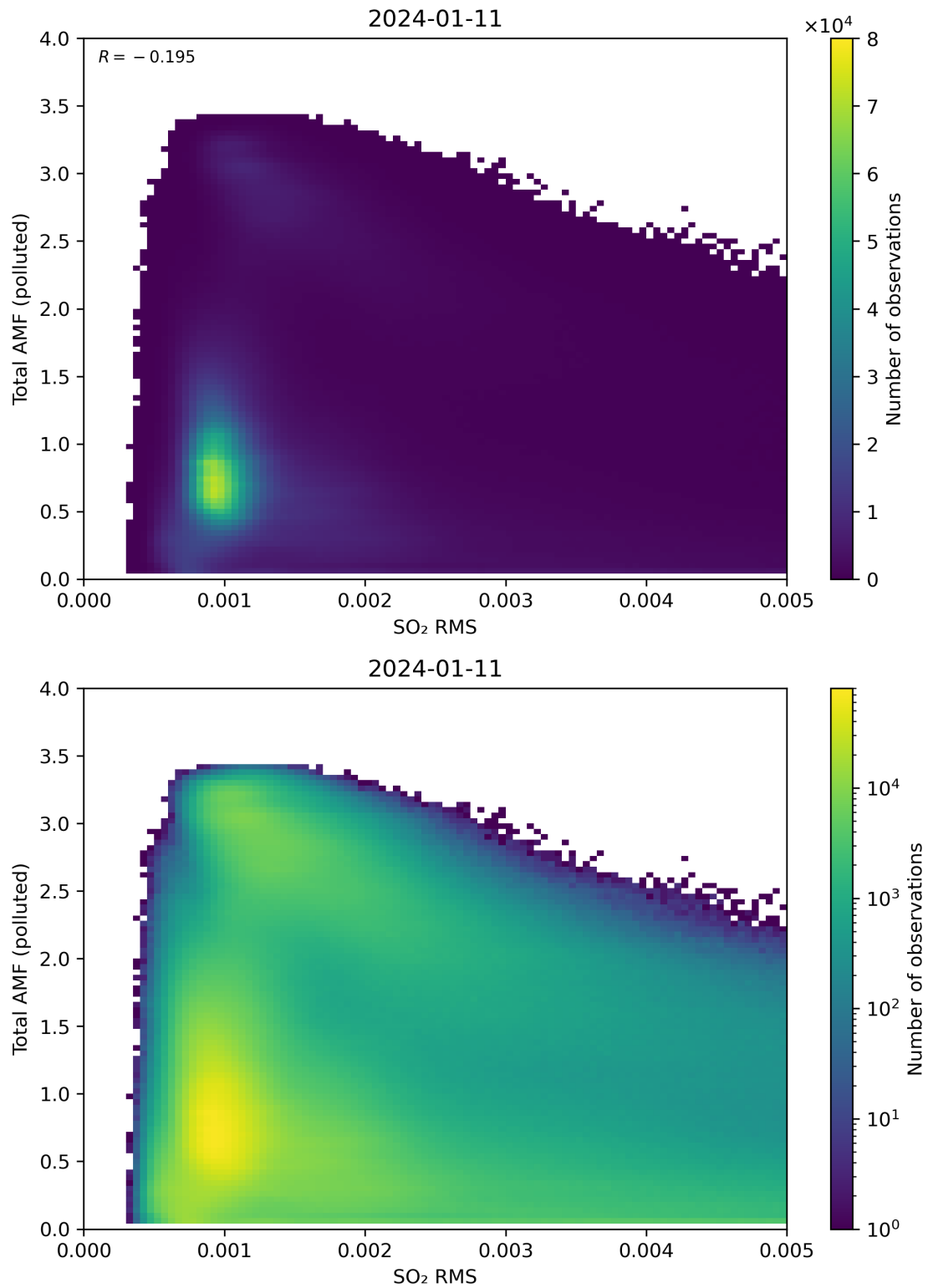
Figure 137: Scatter density plot of “SO 2 RMS” against “Total AMF (polluted)” for 2024-01-10 to 2024-01-12.
