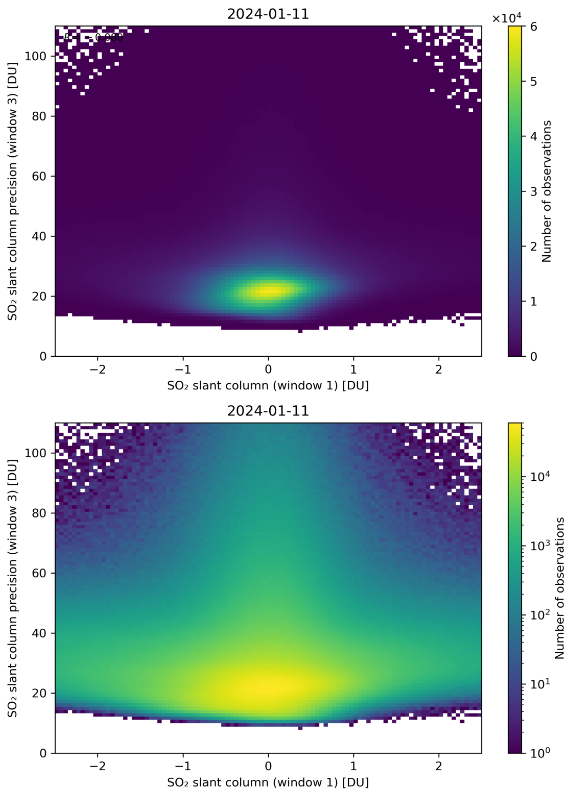
Figure 238: Scatter density plot of “SO 2 slant column (window 1)” against “SO 2 slant column precision (window 3)” for 2024-01-10 to 2024-01-12.
