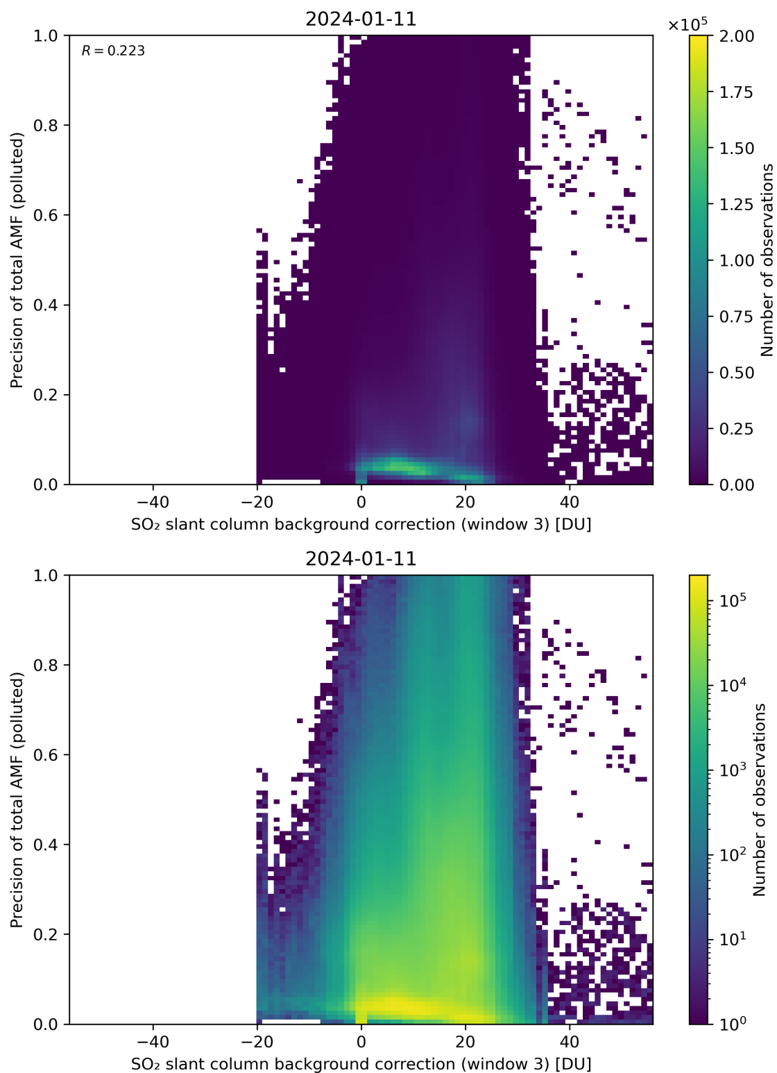
Figure 126: Scatter density plot of “SO 2 slant column background correction (window 3)” against “Precision of total AMF (polluted)” for 2024-01-10 to 2024-01-12.
