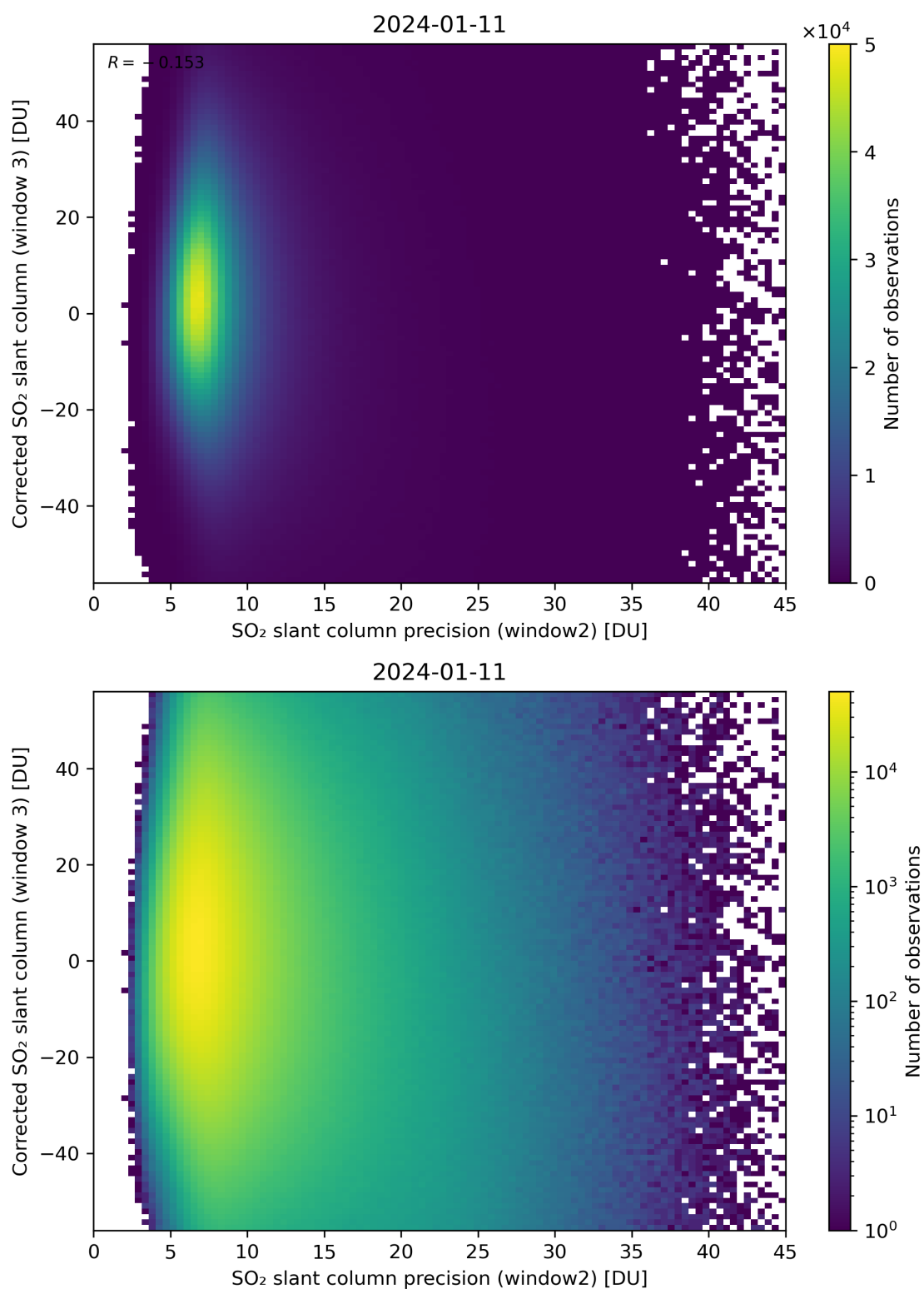
Figure 248: Scatter density plot of “SO 2 slant column precision (window2)” against “Corrected SO 2 slant column (window 3)” for 2024-01-10 to 2024-01-12.
