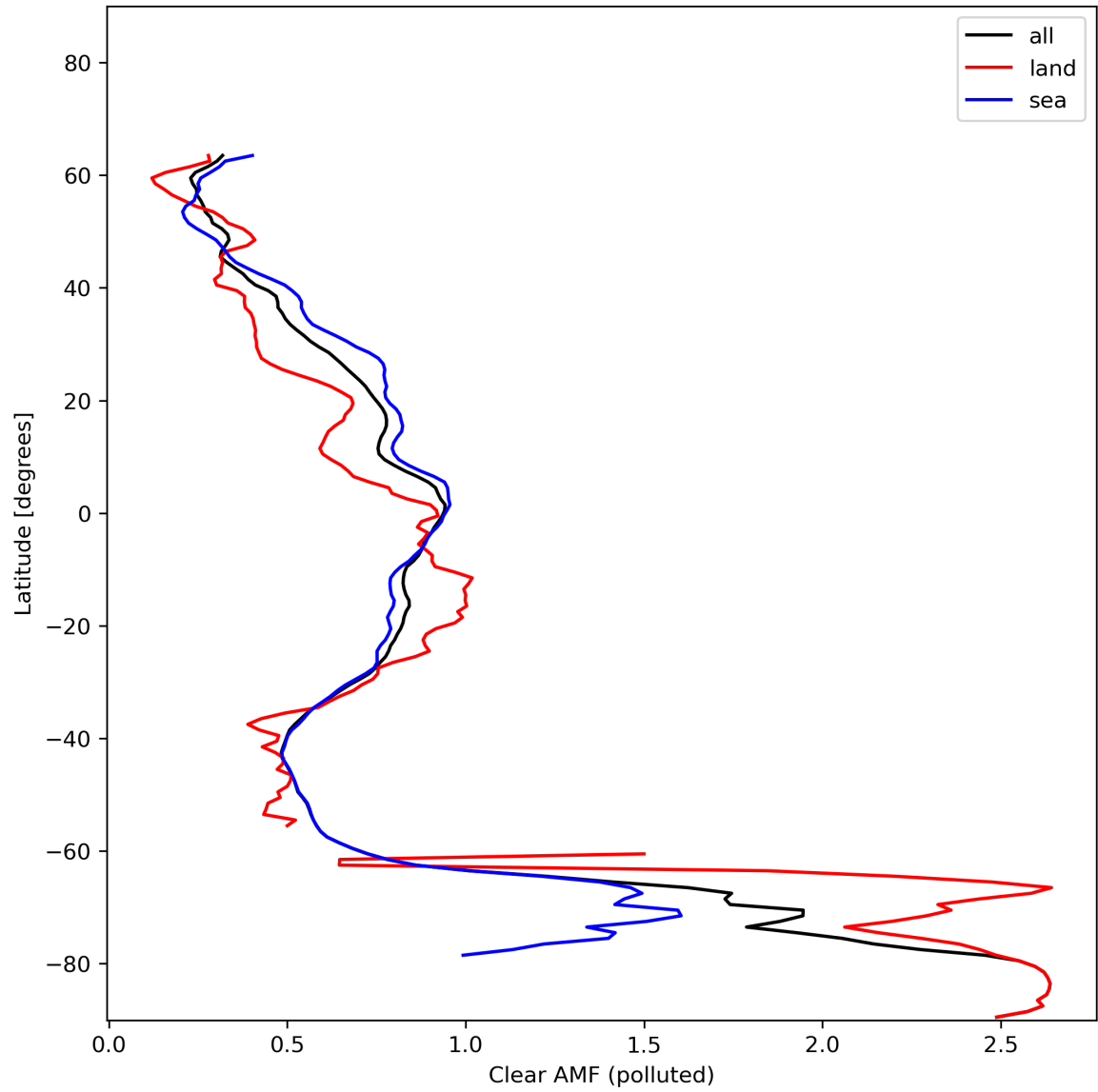
Figure 50: Zonal average of “Clear AMF (polluted)” for 2024-01-10 to 2024-01-12.
