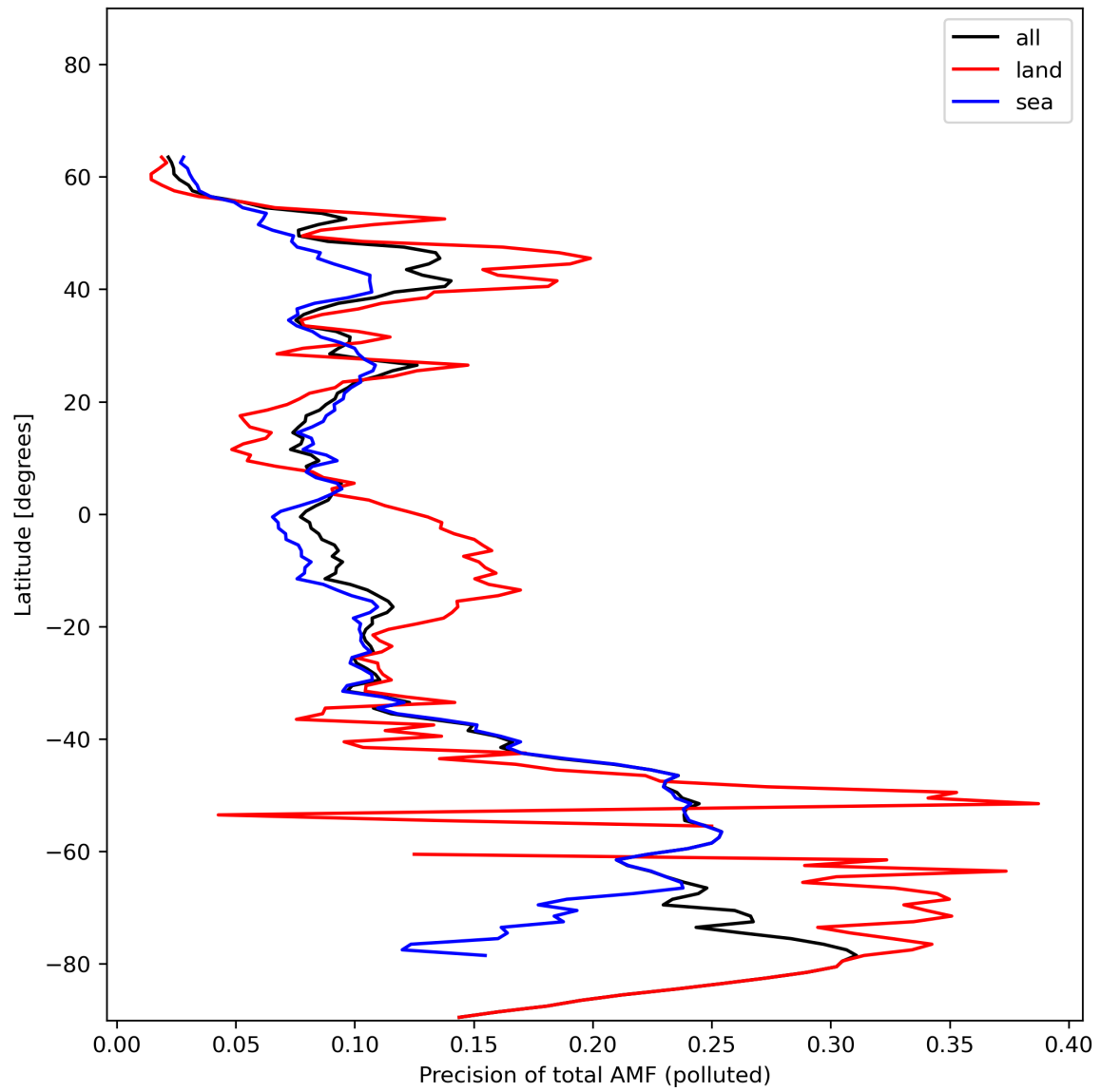
Figure 49: Zonal average of “Precision of total AMF (polluted)” for 2024-01-10 to 2024-01-12.
