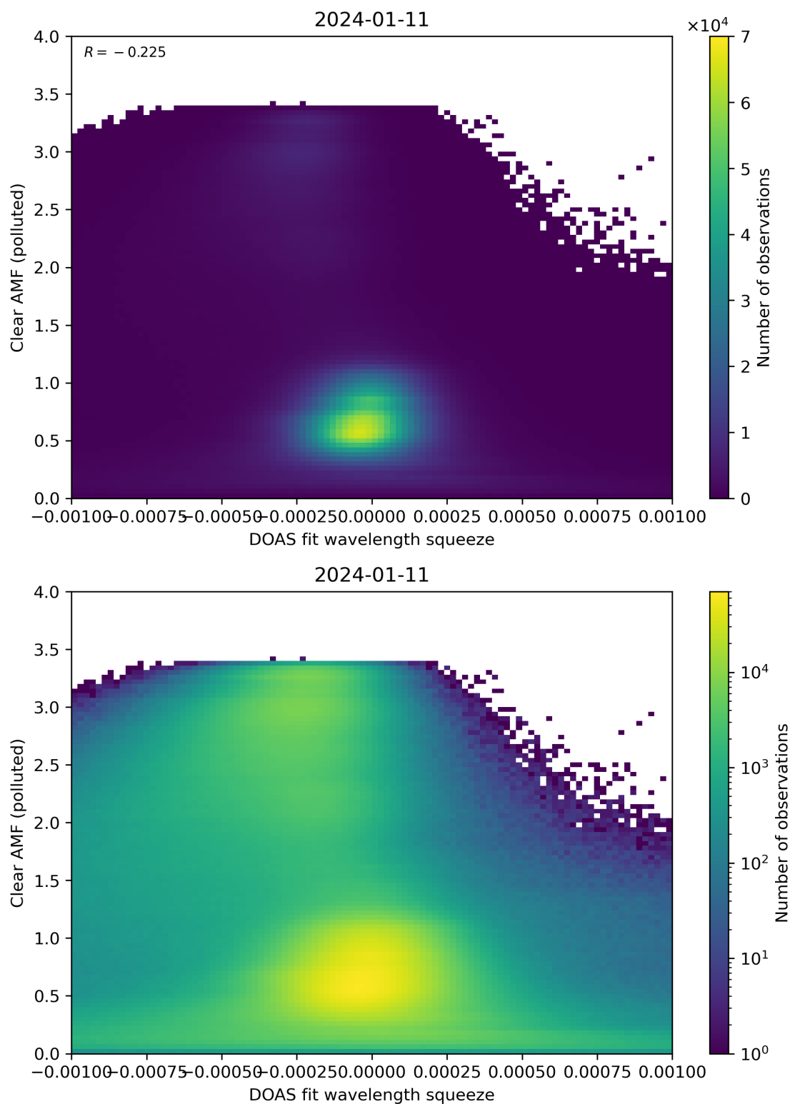
Figure 133: Scatter density plot of “DOAS fit wavelength squeeze” against “Clear AMF (polluted)” for 2024-01-10 to 2024-01-12.
