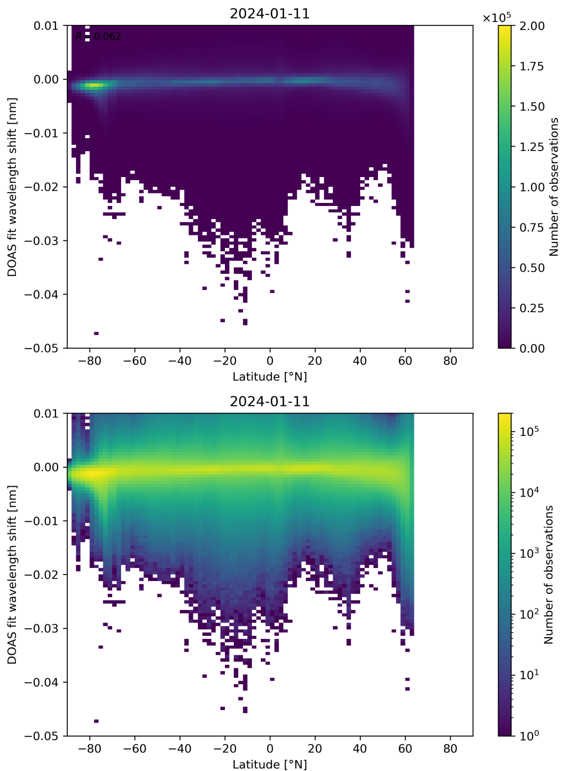
Figure 142: Scatter density plot of “Latitude” against “DOAS fit wavelength shift” for 2024-01-10 to 2024-01-12.
