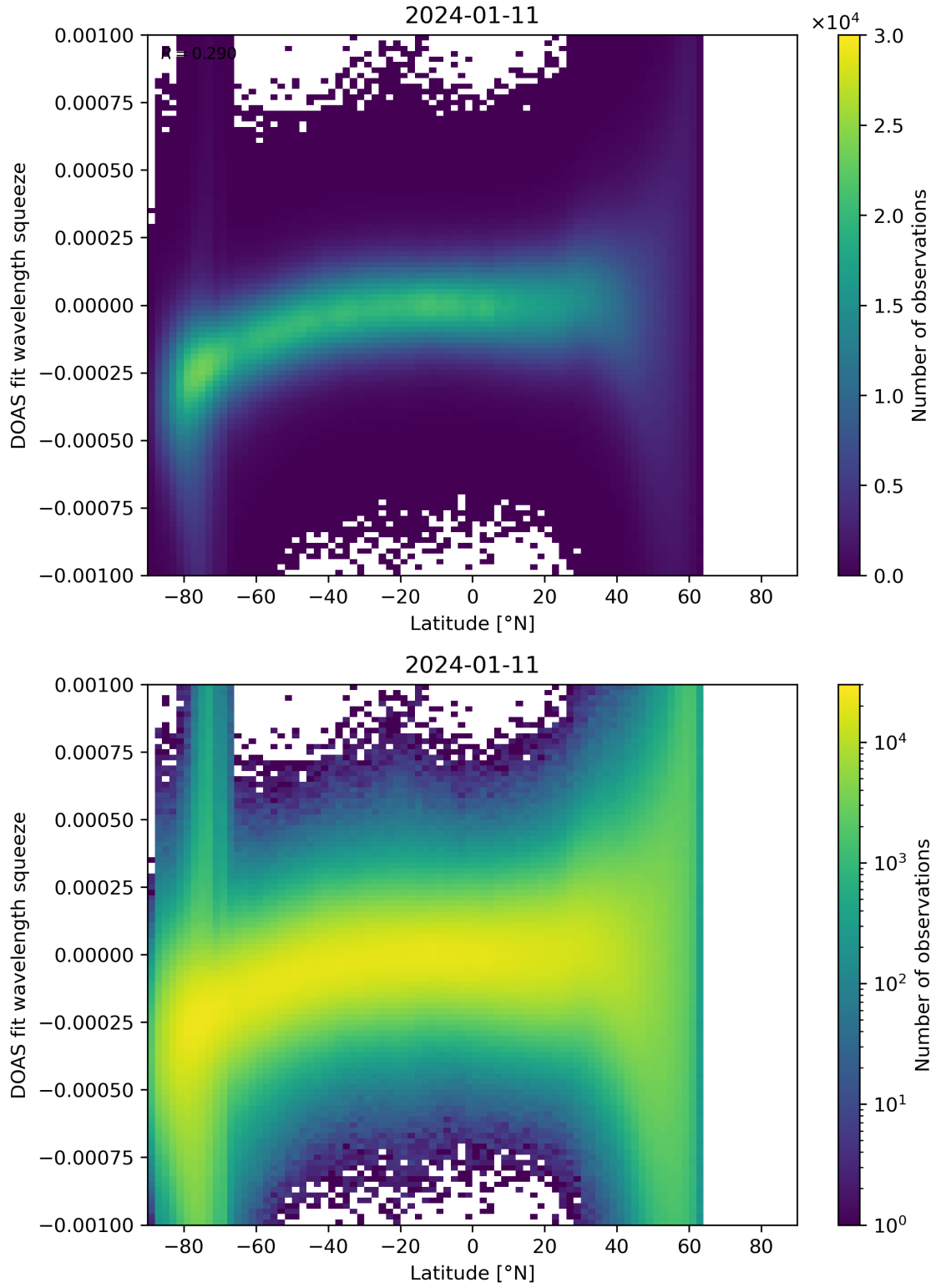
Figure 143: Scatter density plot of “Latitude” against “DOAS fit wavelength squeeze” for 2024-01-10 to 2024-01-12.
