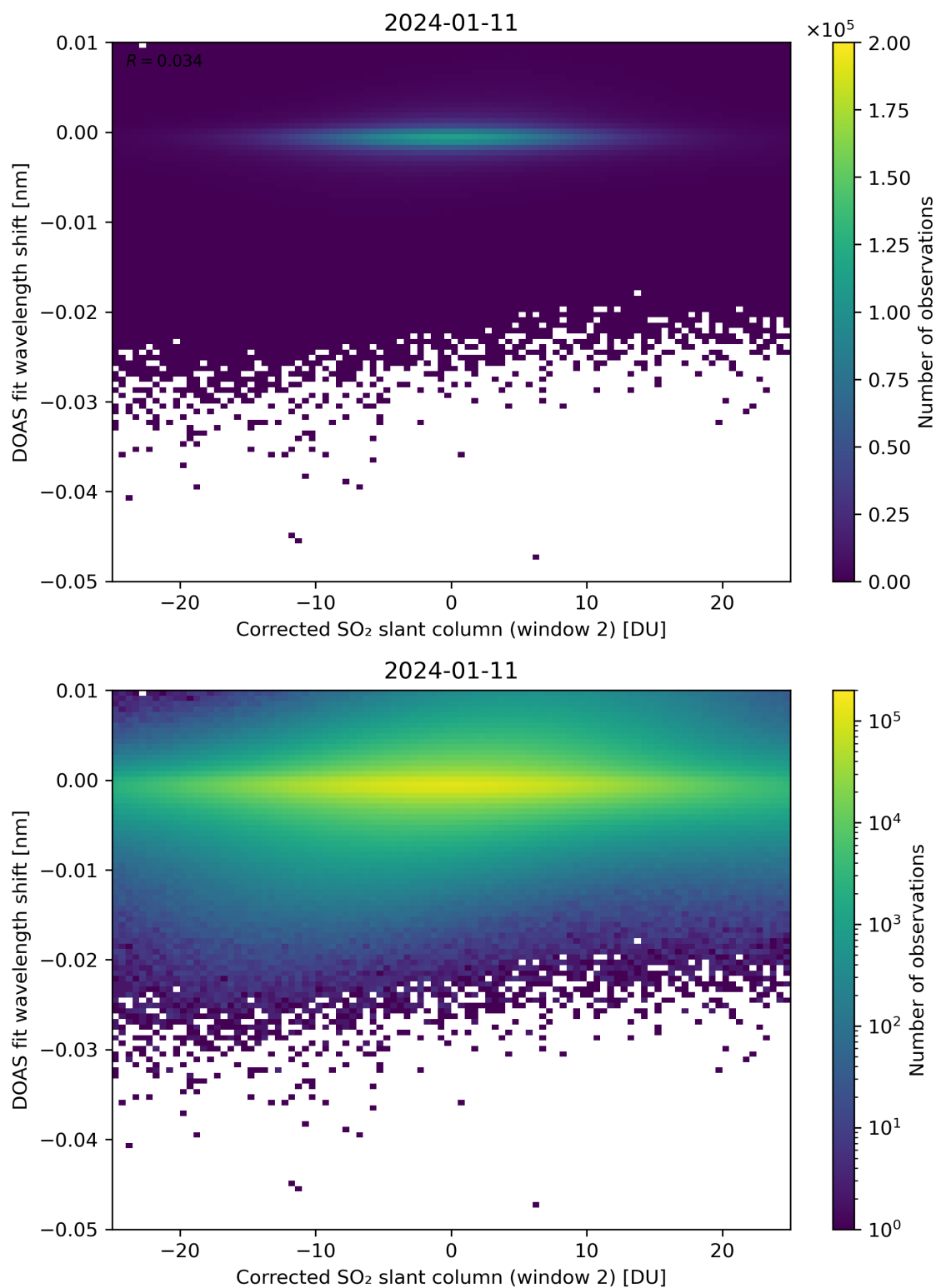
Figure 196: Scatter density plot of “Corrected SO 2 slant column (window 2)” against “DOAS fit wavelength shift” for 2024-01-10 to 2024-01-12.
