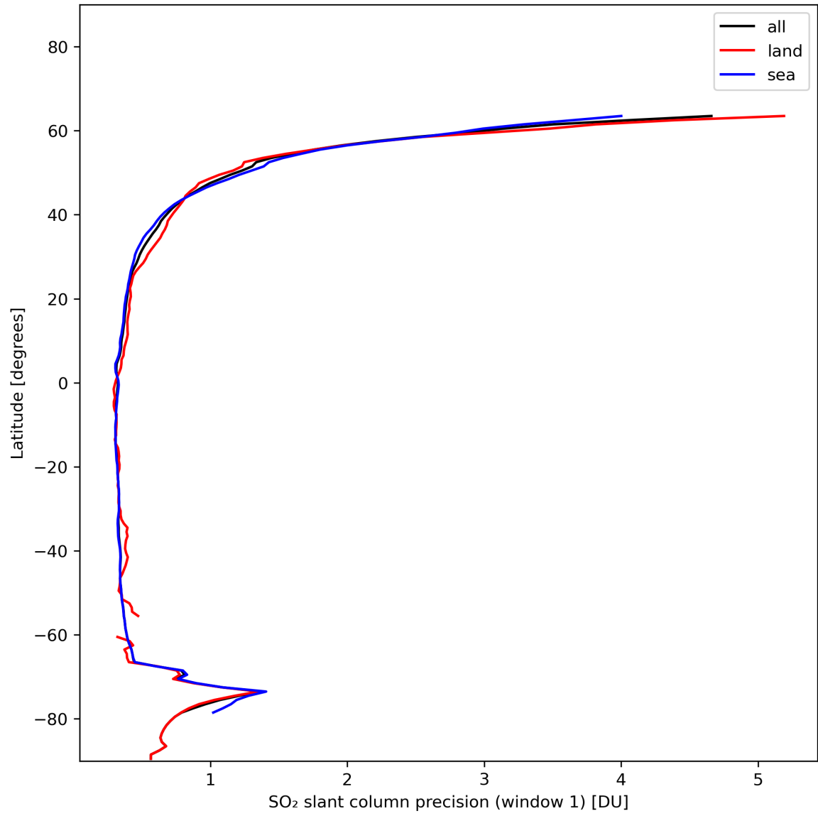
Figure 34: Zonal average of “SO 2 slant column precision (window 1)” for 2024-01-10 to 2024-01-12.
