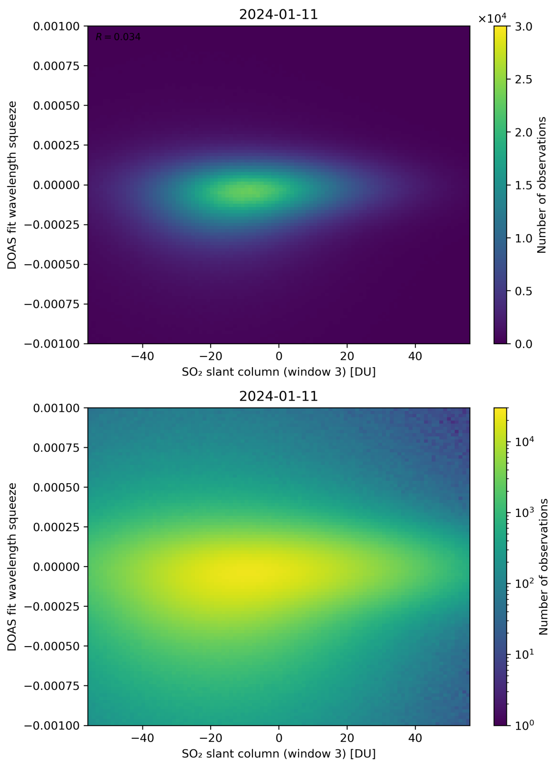
Figure 255: Scatter density plot of “SO 2 slant column (window 3)” against “DOAS fit wavelength squeeze” for 2024-01-10 to 2024-01-12.
