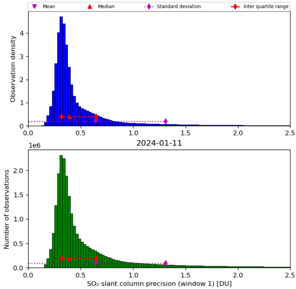
Figure 57: Histogram of “SO 2 slant column precision (window 1)” for 2024-01-10 to 2024-01-12
