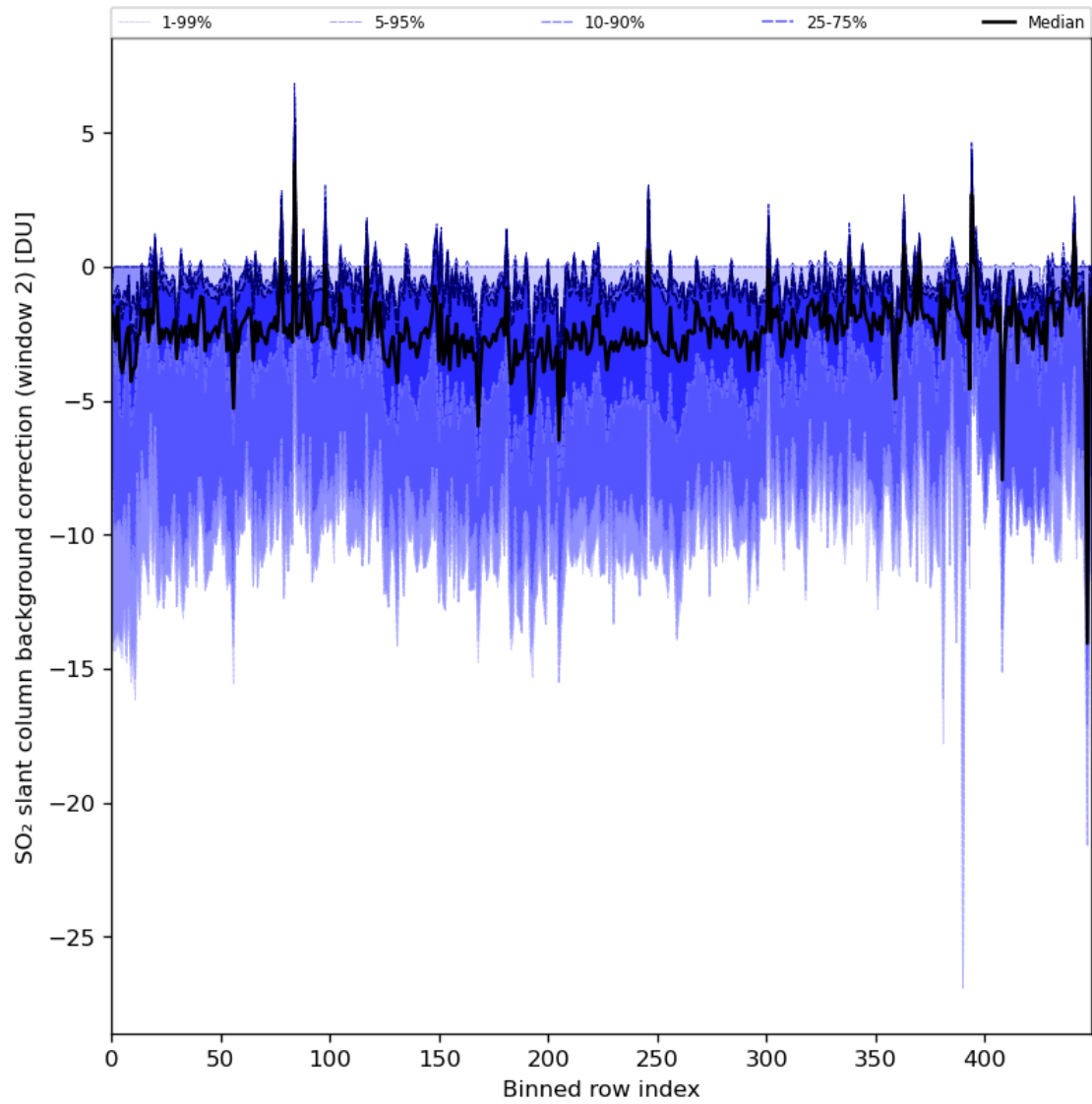
Figure 86: Along track statistics of “SO 2 slant column background correction (window 2)” for 2024-01-10 to 2024-01-12
