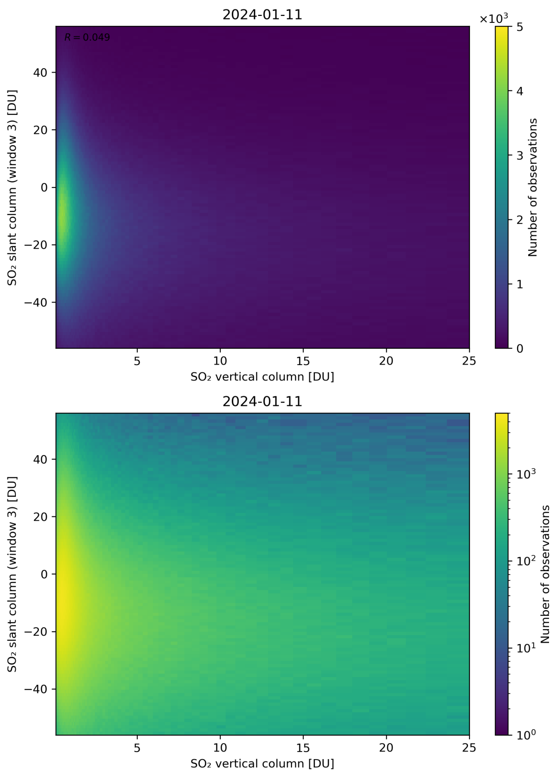
Figure 303: Scatter density plot of “SO 2 vertical column” against “SO 2 slant column (window 3)” for 2024-01-10 to 2024-01-12.
