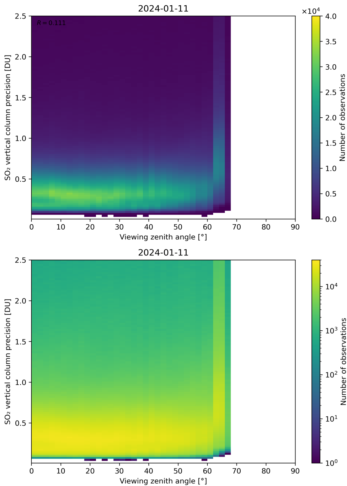
Figure 328: Scatter density plot of “Viewing zenith angle” against “SO 2 vertical column precision” for 2024-01-10 to 2024-01-12.
