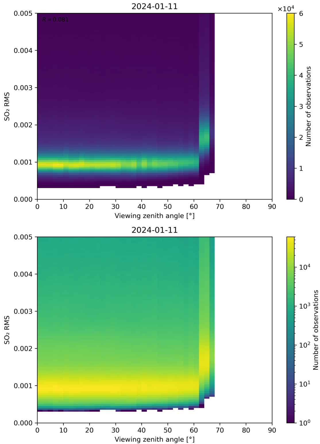
Figure 313: Scatter density plot of “Viewing zenith angle” against “SO 2 RMS” for 2024-01-10 to 2024-01-12.
