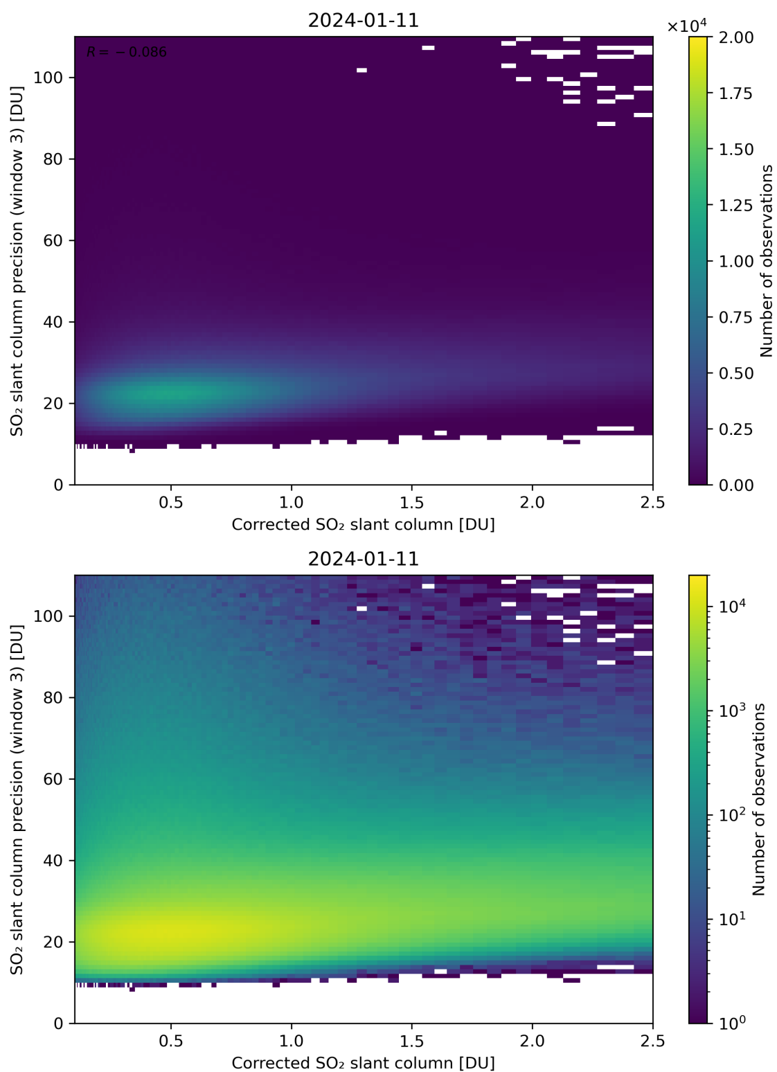
Figure 191: Scatter density plot of “Corrected SO 2 slant column” against “SO 2 slant column precision (window 3)” for 2024-01-10 to 2024-01-12.
