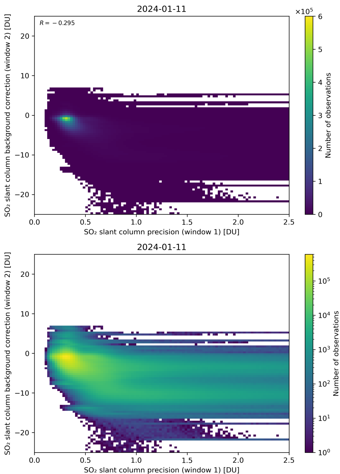
Figure 219: Scatter density plot of “SO 2 slant column precision (window 1)” against “SO 2 slant column background correction (window 2)” for 2024-01-10 to 2024-01-12.
