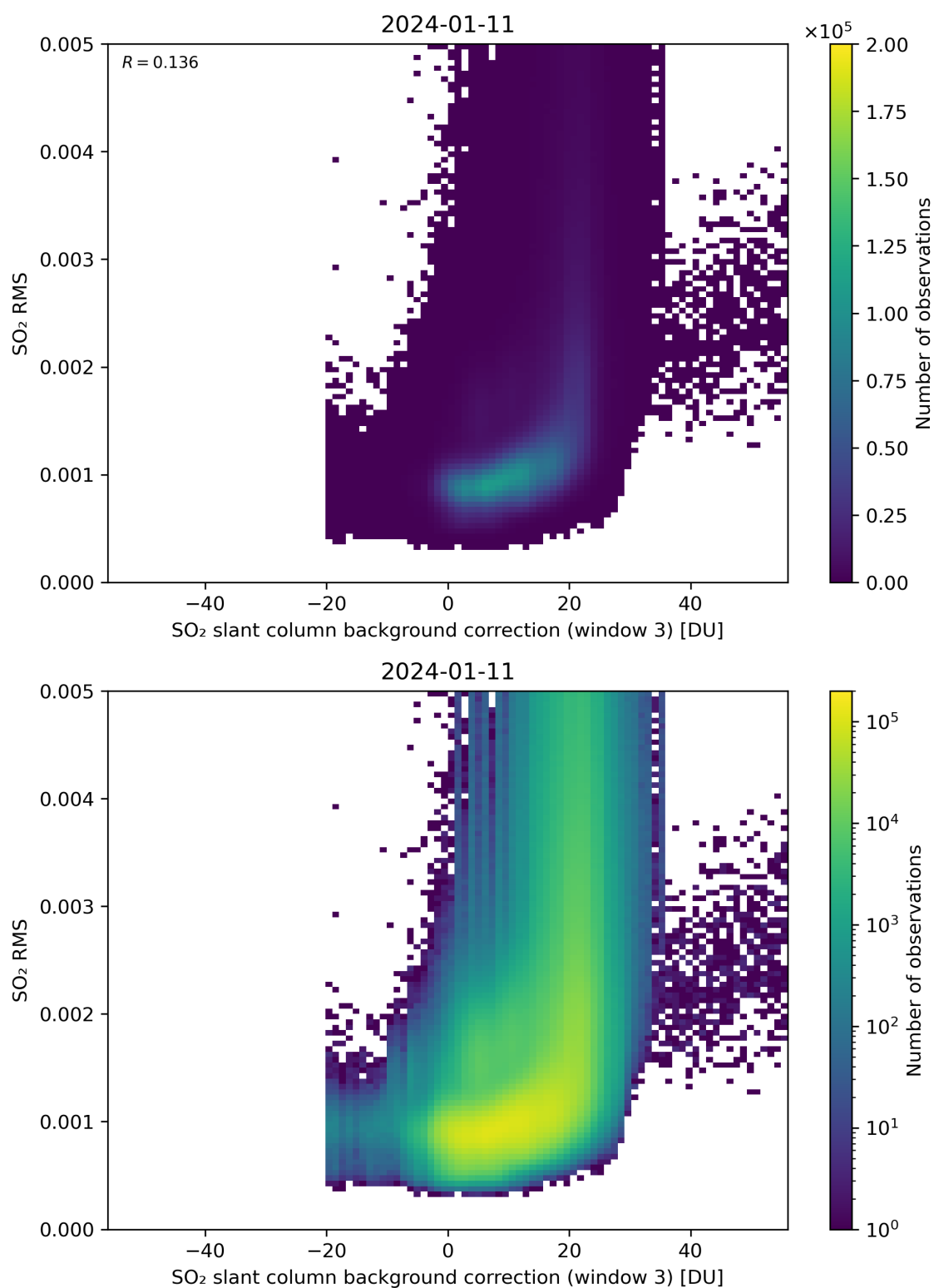
Figure 123: Scatter density plot of “SO 2 slant column background correction (window 3)” against “SO 2 RMS” for 2024-01-10 to 2024-01-12.
