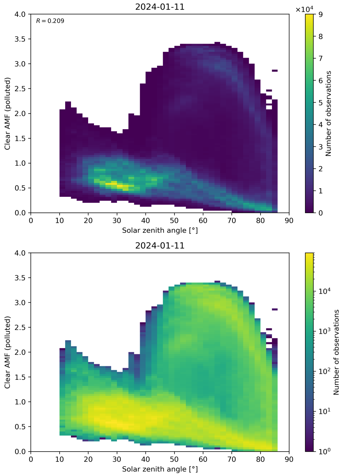
Figure 165: Scatter density plot of “Solar zenith angle” against “Clear AMF (polluted)” for 2024-01-10 to 2024-01-12.
