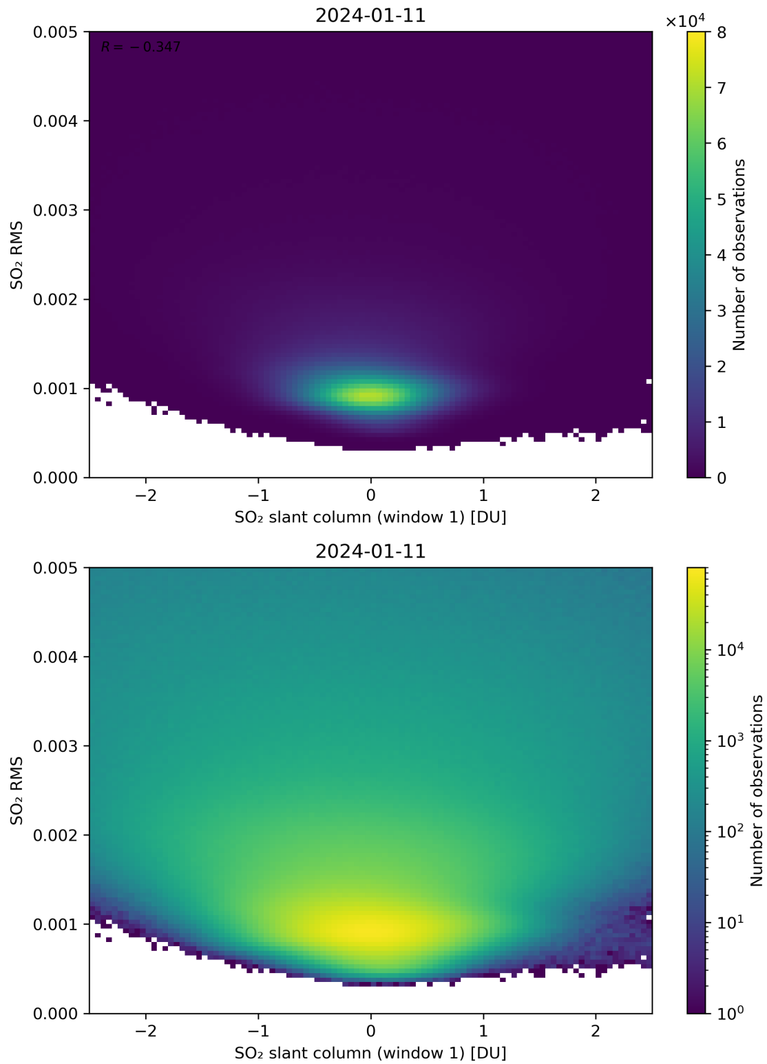
Figure 217: Scatter density plot of “SO 2 slant column (window 1)” against “SO 2 RMS” for 2024-01-10 to 2024-01-12.
