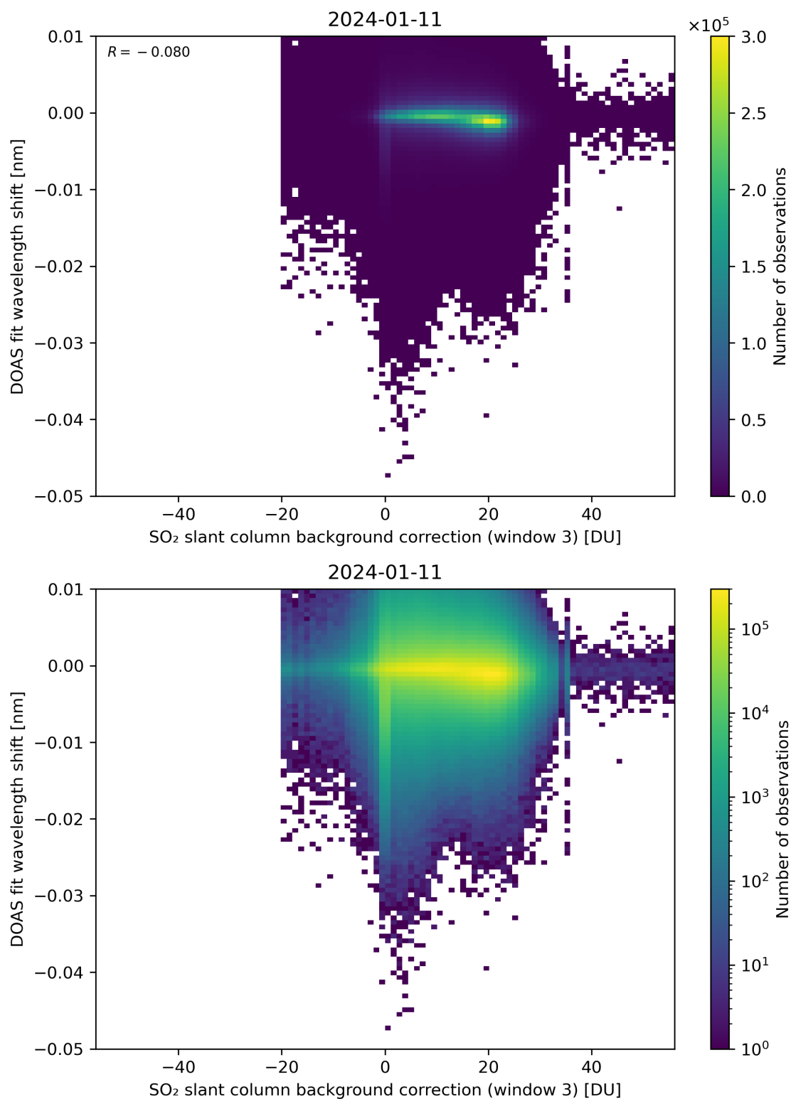
Figure 121: Scatter density plot of “SO 2 slant column background correction (window 3)” against “DOAS fit wavelength shift” for 2024-01-10 to 2024-01-12.
