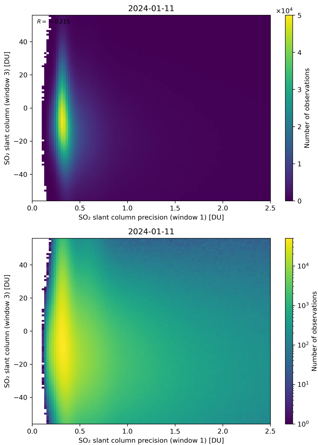
Figure 228: Scatter density plot of “SO 2 slant column precision (window 1)” against “SO 2 slant column (window 3)” for 2024-01-10 to 2024-01-12.
