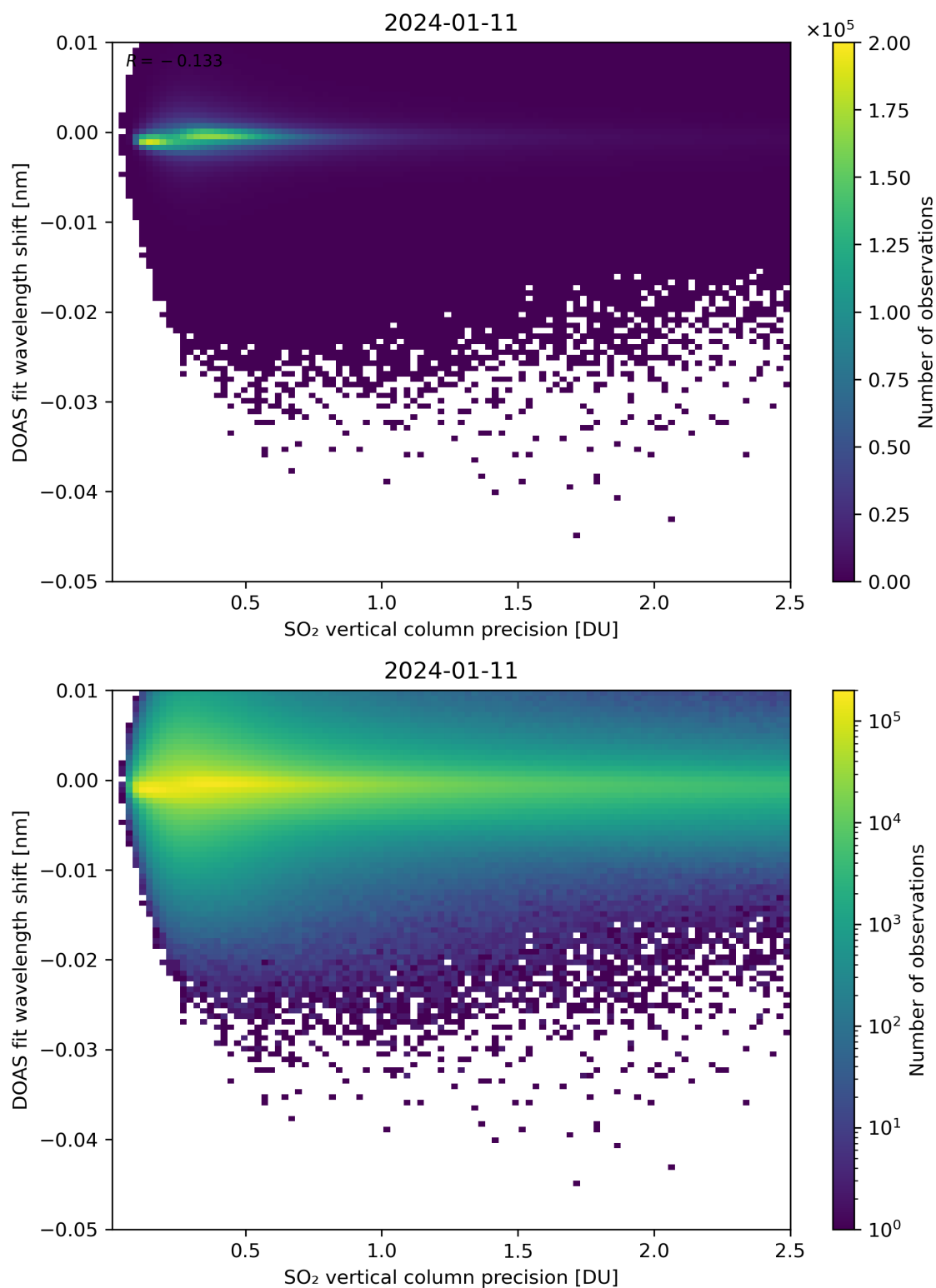
Figure 282: Scatter density plot of “SO 2 vertical column precision” against “DOAS fit wavelength shift” for 2024-01-10 to 2024-01-12.
