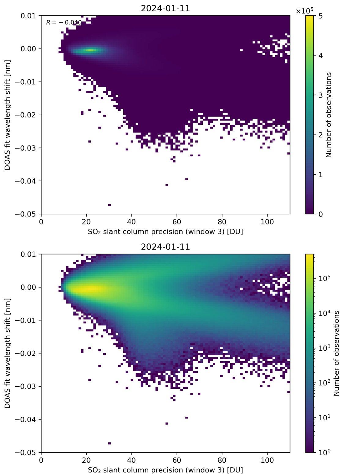
Figure 258: Scatter density plot of “SO 2 slant column precision (window 3)” against “DOAS fit wavelength shift” for 2024-01-10 to 2024-01-12.
