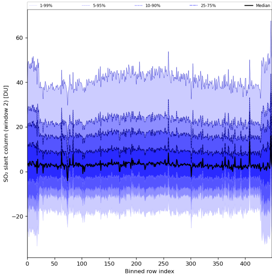
Figure 83: Along track statistics of “SO 2 slant column (window 2)” for 2024-01-10 to 2024-01-12
