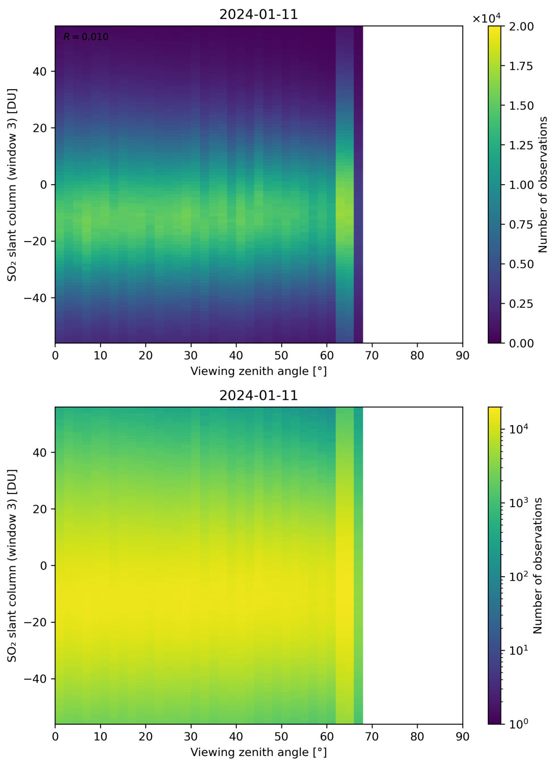
Figure 323: Scatter density plot of “Viewing zenith angle” against “SO 2 slant column (window 3)” for 2024-01-10 to 2024-01-12.
