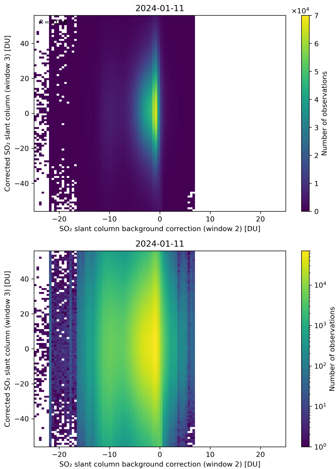
Figure 116: Scatter density plot of “SO 2 slant column background correction (window 2)” against “Corrected SO 2 slant column (window 3)” for 2024-01-10 to 2024-01-12.
