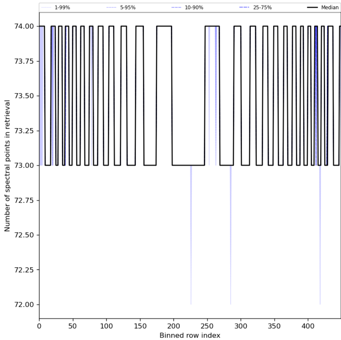
Figure 97: Along track statistics of “Number of spectral points in retrieval” for 2024-01-10 to 2024-01-12
