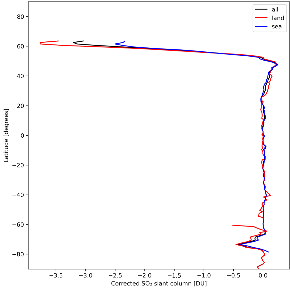
Figure 32: Zonal average of “Corrected SO 2 slant column” for 2024-01-10 to 2024-01-12.
