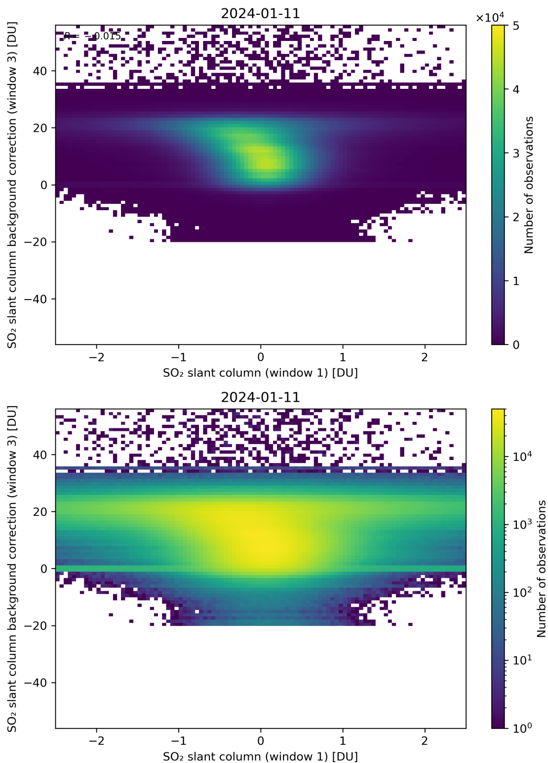
Figure 214: Scatter density plot of “SO 2 slant column (window 1)” against “SO 2 slant column background correction (window 3)” for 2024-01-10 to 2024-01-12.
