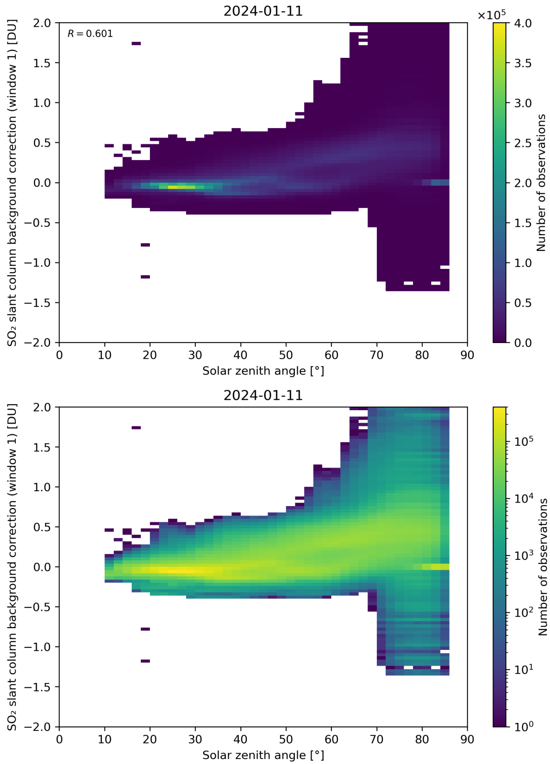
Figure 158: Scatter density plot of “Solar zenith angle” against “SO 2 slant column background correction (window 1)” for 2024-01-10 to 2024-01-12.
