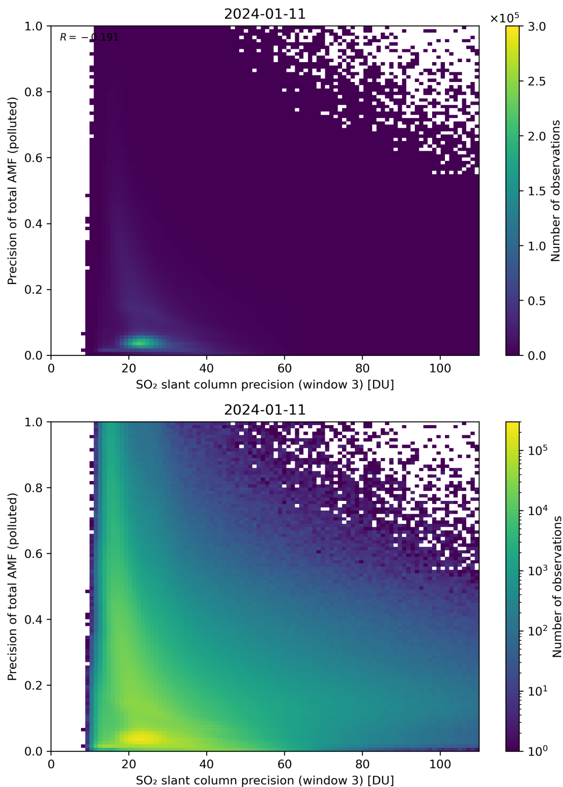
Figure 264: Scatter density plot of “SO 2 slant column precision (window 3)” against “Precision of total AMF (polluted)” for 2024-01-10 to 2024-01-12.
