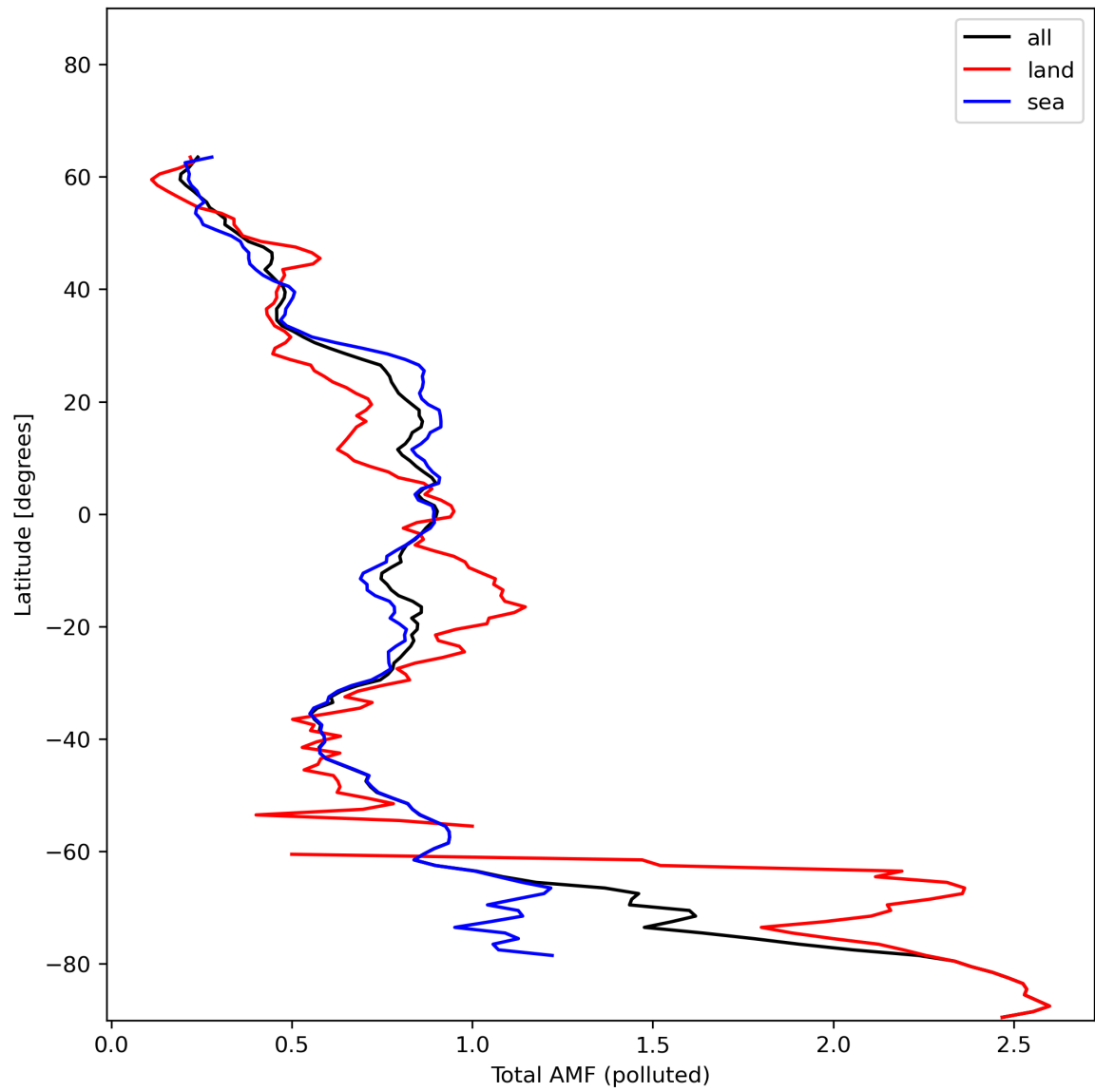
Figure 48: Zonal average of “Total AMF (polluted)” for 2024-01-10 to 2024-01-12.
