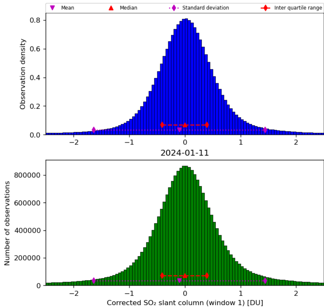
Figure 58: Histogram of “Corrected SO 2 slant column (window 1)” for 2024-01-10 to 2024-01-12
