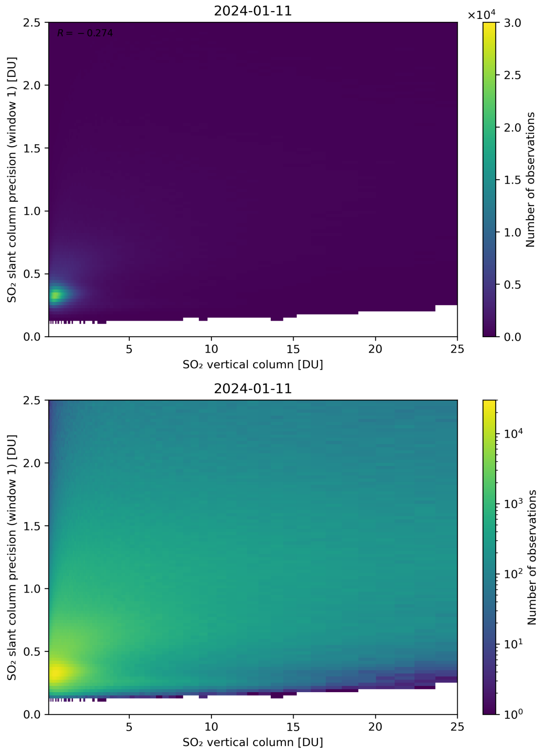
Figure 301: Scatter density plot of “SO 2 vertical column” against “SO 2 slant column precision (window 1)” for 2024-01-10 to 2024-01-12.
