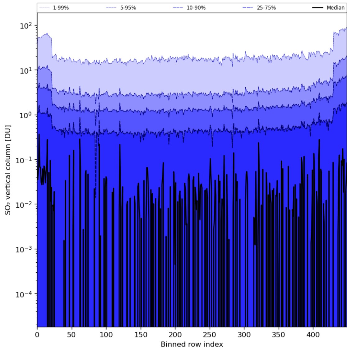
Figure 76: Along track statistics of “SO 2 vertical column” for 2024-01-10 to 2024-01-12
