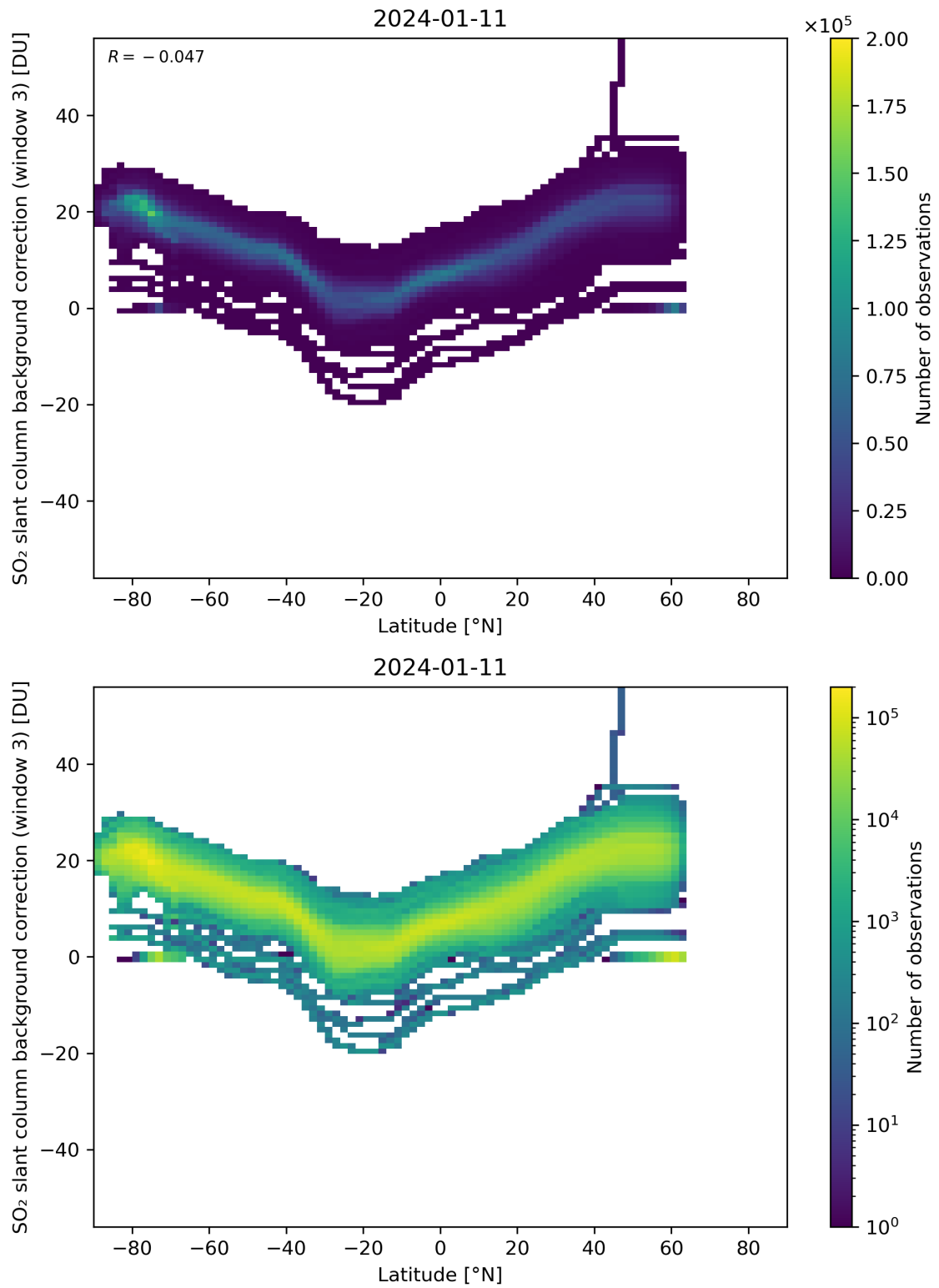
Figure 141: Scatter density plot of “Latitude” against “SO 2 slant column background correction (window 3)” for 2024-01-10 to 2024-01-12.
