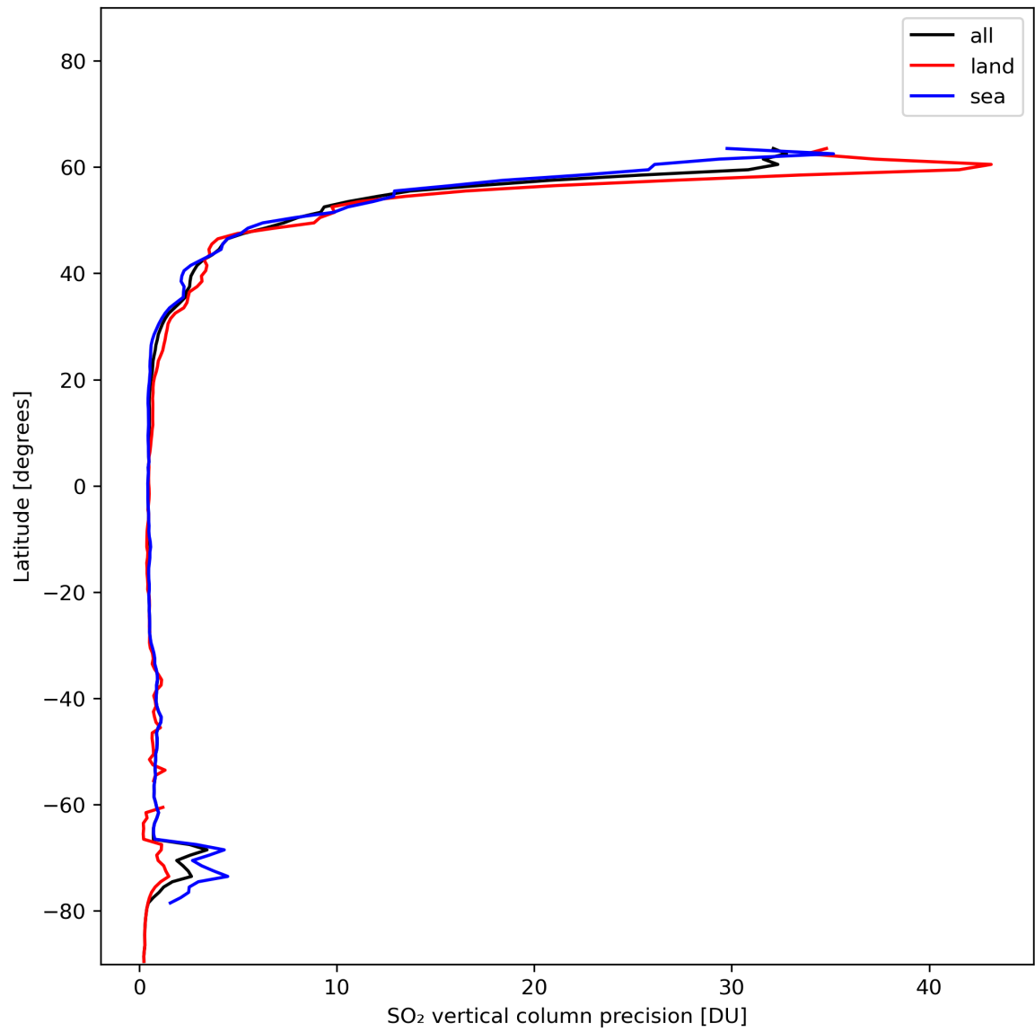
Figure 31: Zonal average of “SO 2 vertical column precision” for 2024-01-10 to 2024-01-12.
