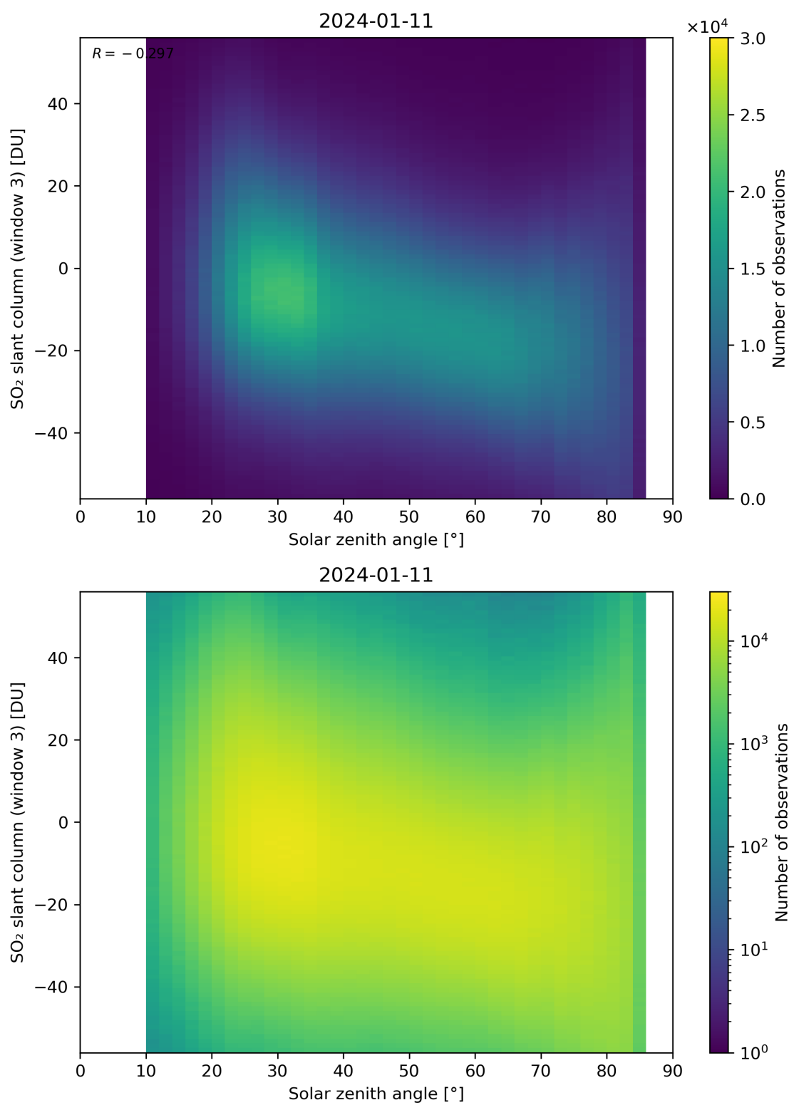
Figure 172: Scatter density plot of “Solar zenith angle” against “SO 2 slant column (window 3)” for 2024-01-10 to 2024-01-12.
