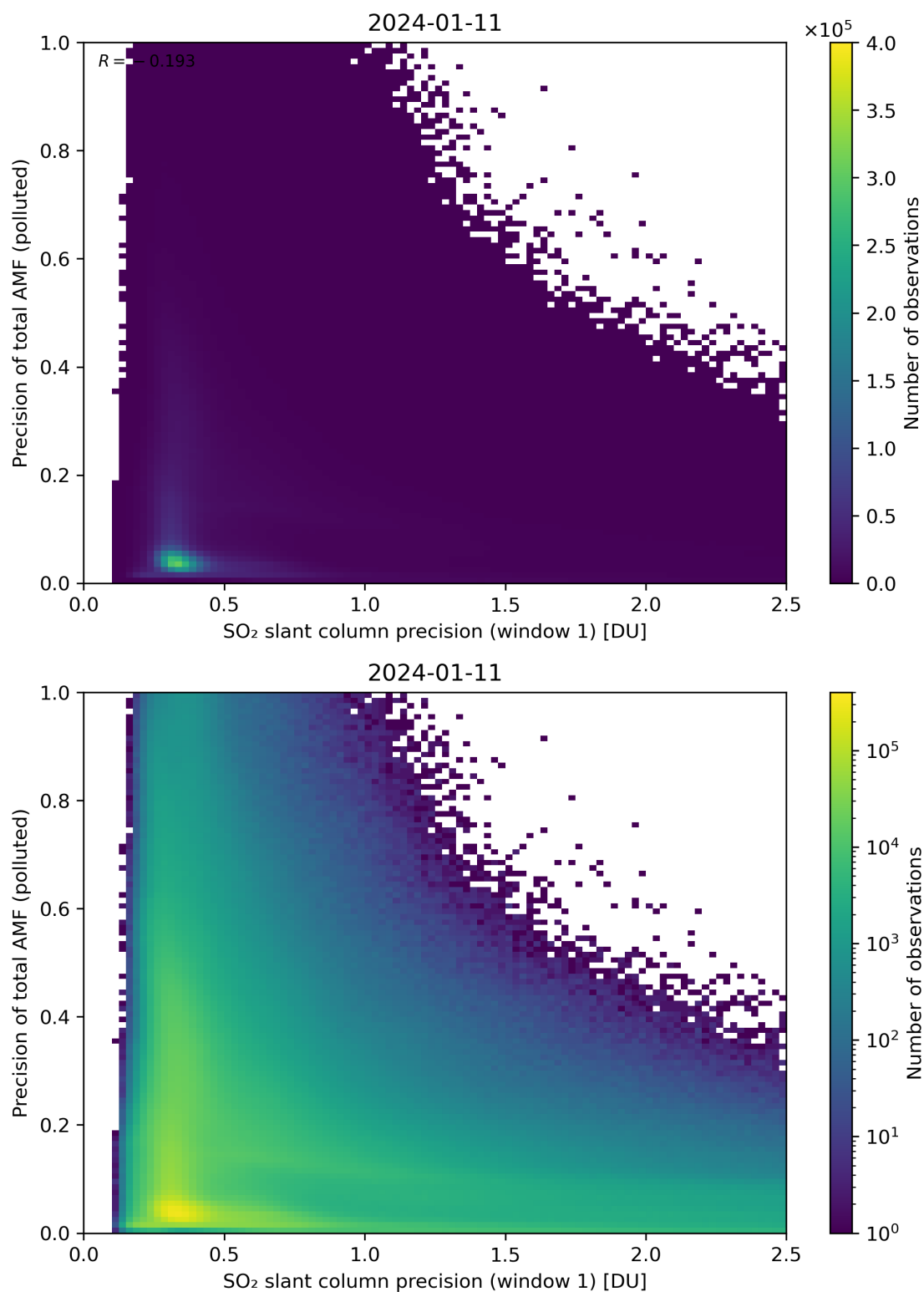
Figure 231: Scatter density plot of “SO 2 slant column precision (window 1)” against “Precision of total AMF (polluted)” for 2024-01-10 to 2024-01-12.
