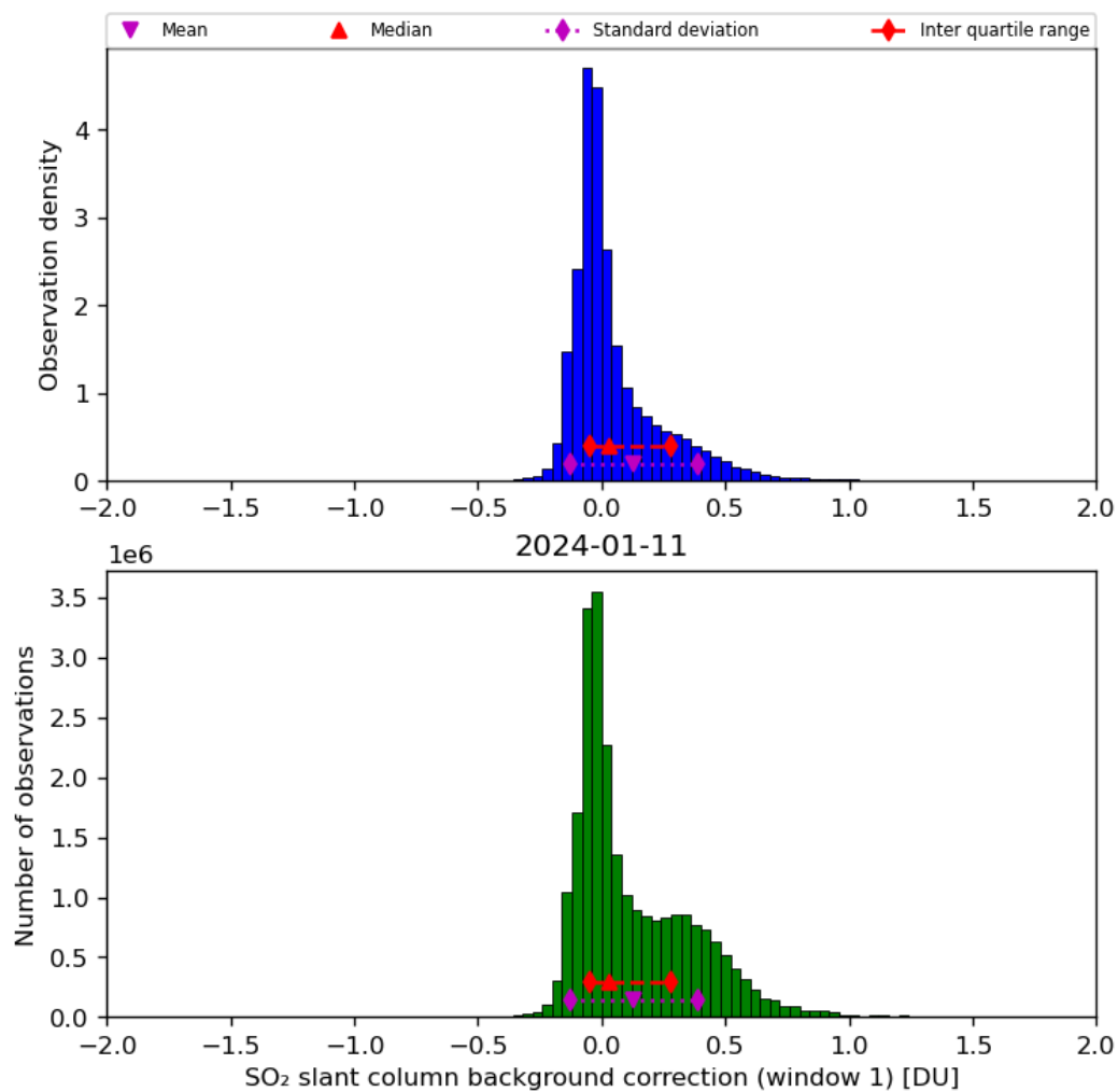
Figure 59: Histogram of “SO 2 slant column background correction (window 1)” for 2024-01-10 to 2024-01-12
