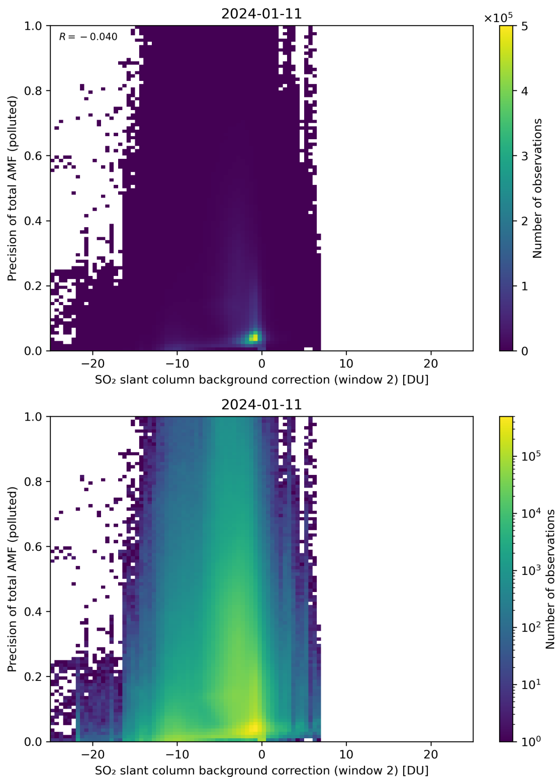
Figure 120: Scatter density plot of “SO 2 slant column background correction (window 2)” against “Precision of total AMF (polluted)” for 2024-01-10 to 2024-01-12.
