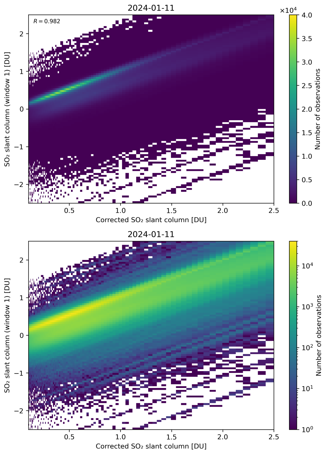
Figure 187: Scatter density plot of “Corrected SO 2 slant column” against “SO 2 slant column (window 1)” for 2024-01-10 to 2024-01-12.
