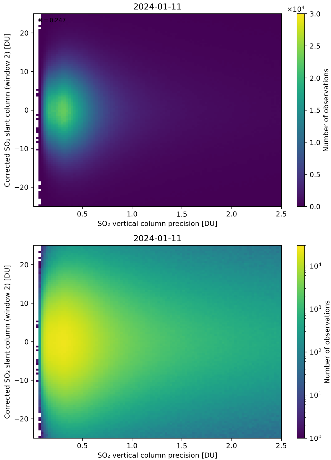
Figure 287: Scatter density plot of “SO 2 vertical column precision” against “Corrected SO 2 slant column (window 2)” for 2024-01-10 to 2024-01-12.
