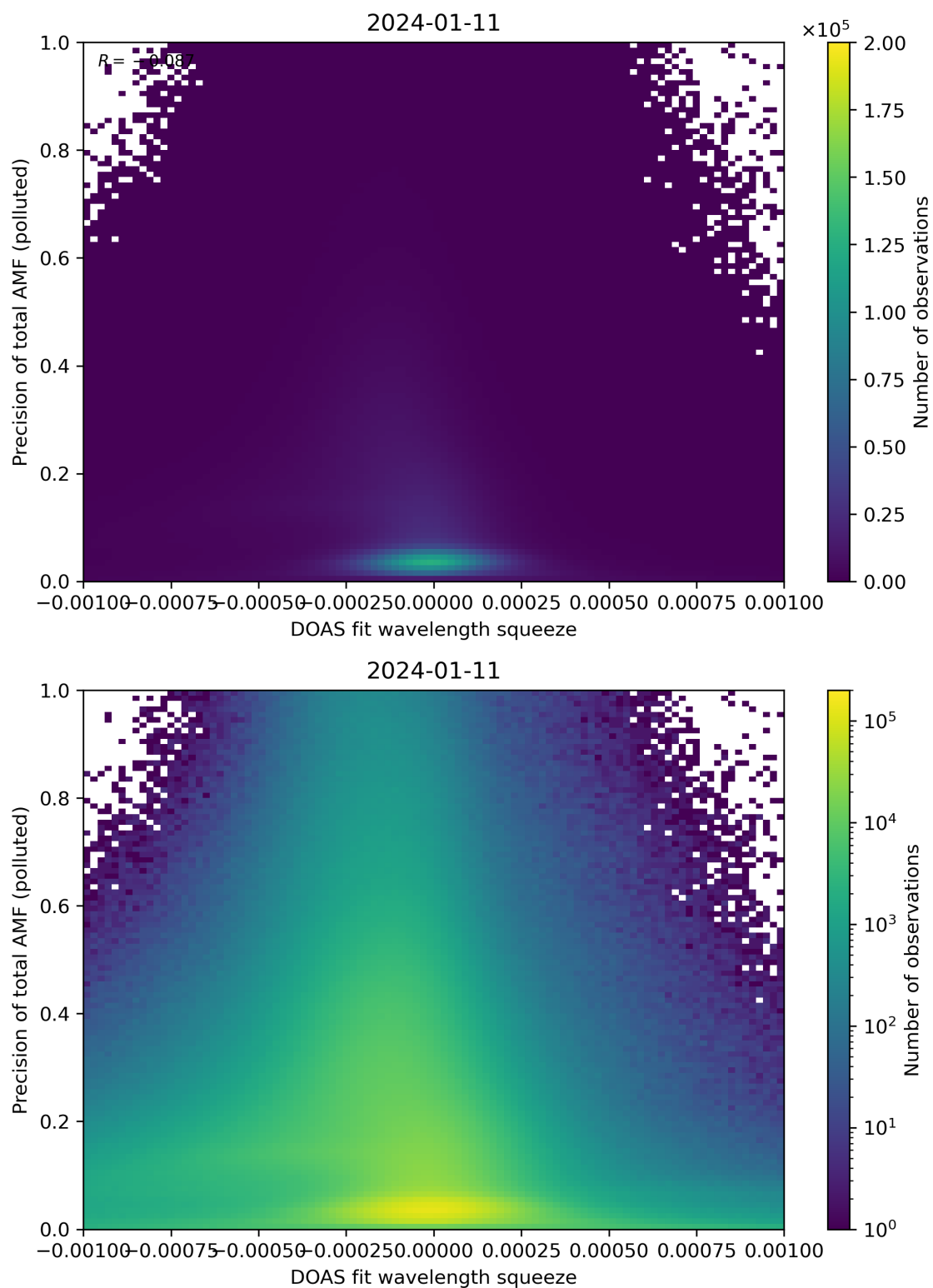
Figure 135: Scatter density plot of “DOAS fit wavelength squeeze” against “Precision of total AMF (polluted)” for 2024-01-10 to 2024-01-12.
