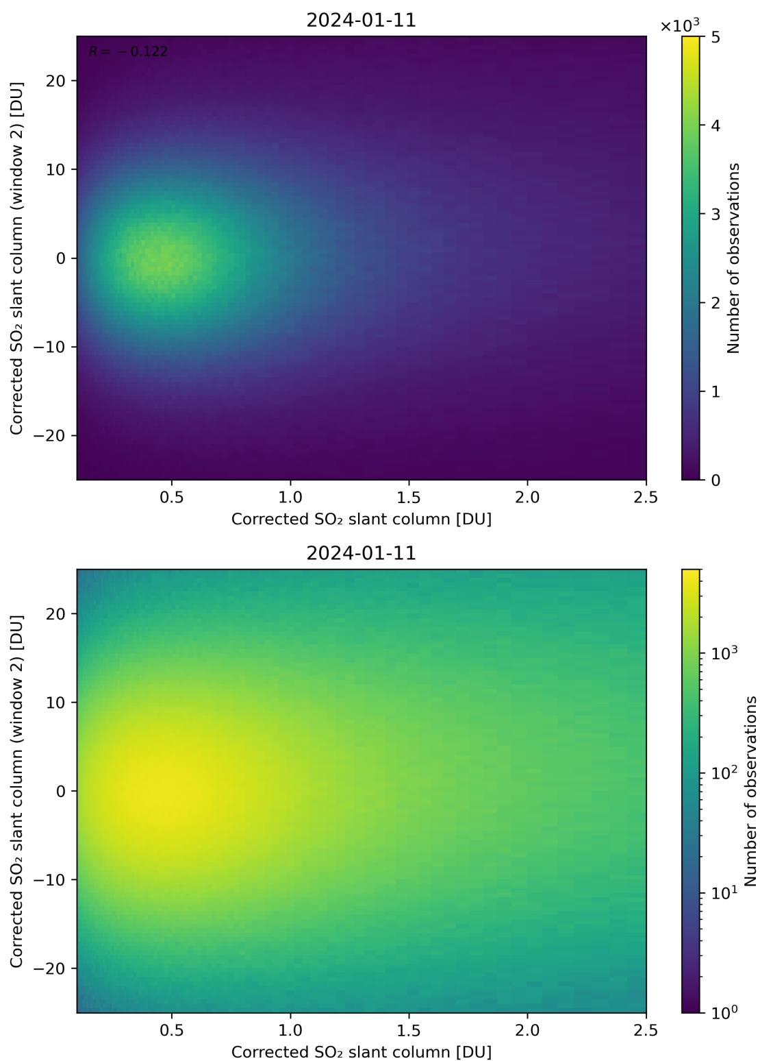
Figure 185: Scatter density plot of “Corrected SO 2 slant column” against “Corrected SO 2 slant column (window 2)” for 2024-01-10 to 2024-01-12.
