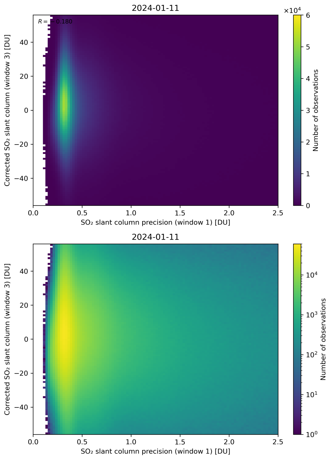
Figure 226: Scatter density plot of “SO 2 slant column precision (window 1)” against “Corrected SO 2 slant column (window 3)” for 2024-01-10 to 2024-01-12.
