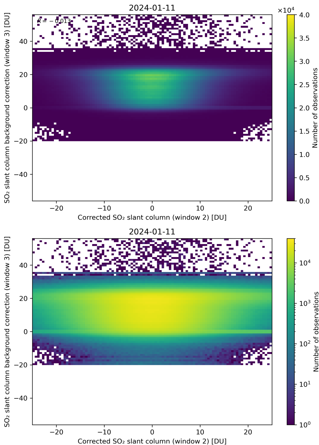
Figure 195: Scatter density plot of “Corrected SO 2 slant column (window 2)” against “SO 2 slant column background correction (window 3)” for 2024-01-10 to 2024-01-12.
