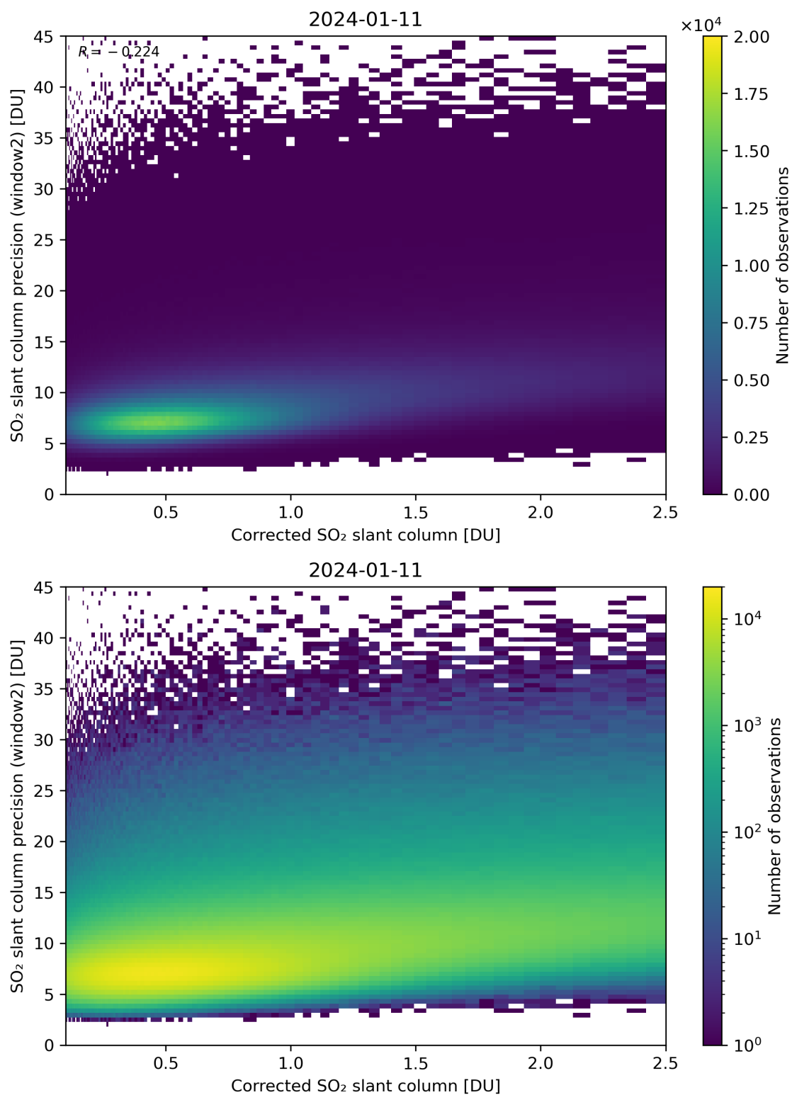
Figure 189: Scatter density plot of “Corrected SO 2 slant column” against “SO 2 slant column precision (window2)” for 2024-01-10 to 2024-01-12.
