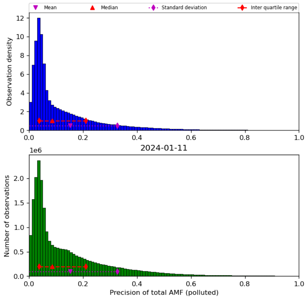
Figure 72: Histogram of “Precision of total AMF (polluted)” for 2024-01-10 to 2024-01-12
