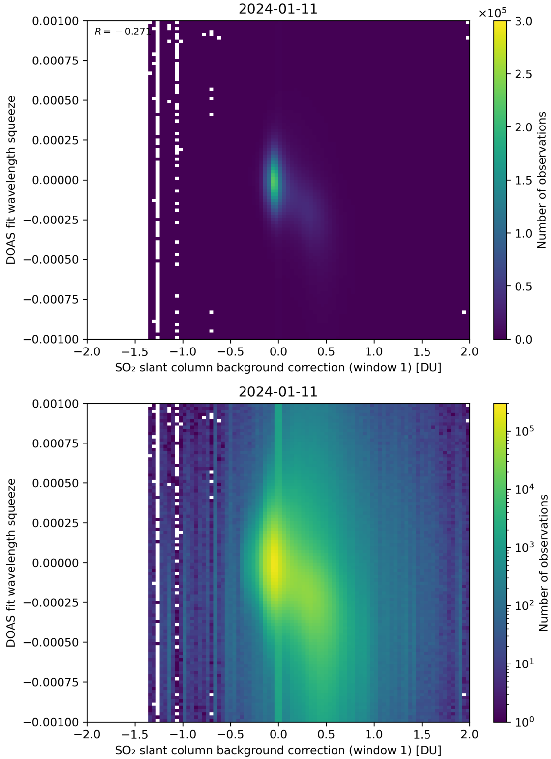
Figure 101: Scatter density plot of “SO 2 slant column background correction (window 1)” against “DOAS fit wavelength squeeze” for 2024-01-10 to 2024-01-12.
