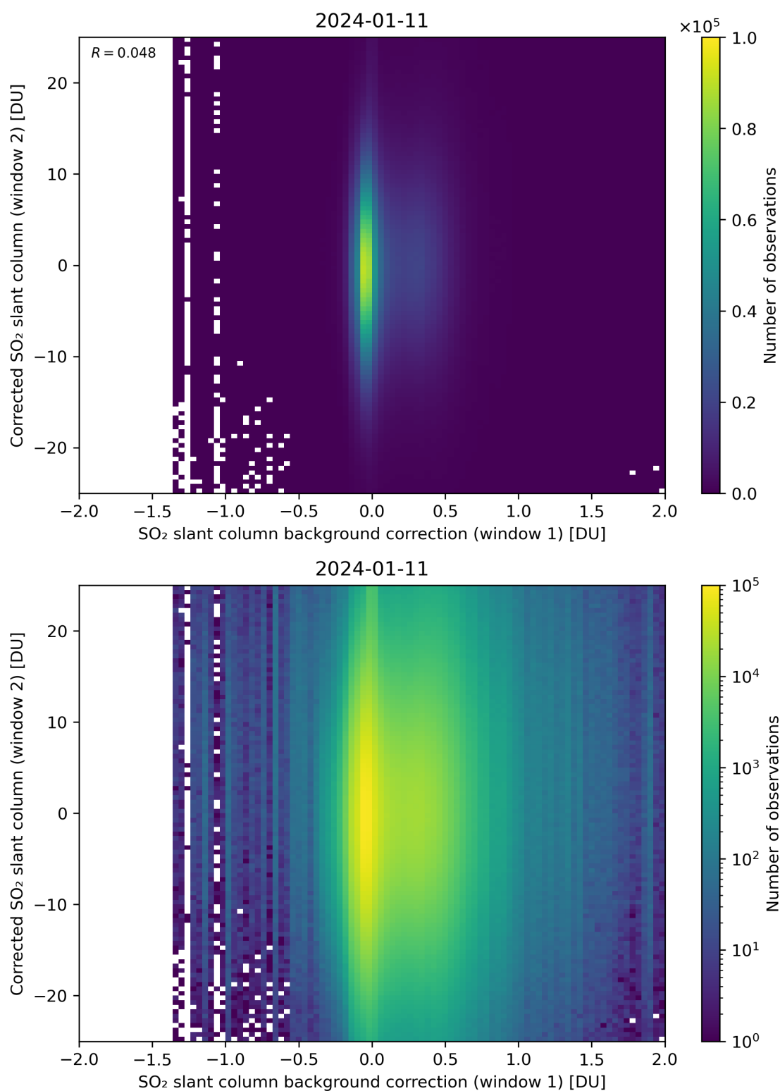
Figure 104: Scatter density plot of “SO 2 slant column background correction (window 1)” against “Corrected SO 2 slant column (window 2)” for 2024-01-10 to 2024-01-12.
