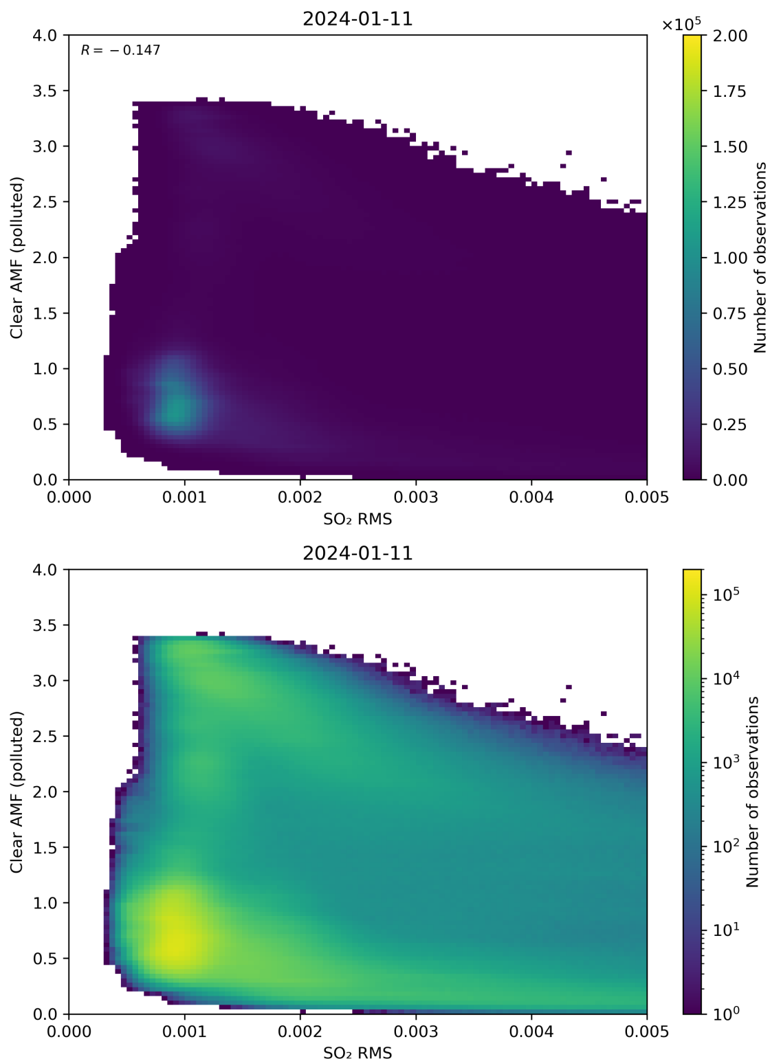
Figure 136: Scatter density plot of “SO 2 RMS” against “Clear AMF (polluted)” for 2024-01-10 to 2024-01-12.
