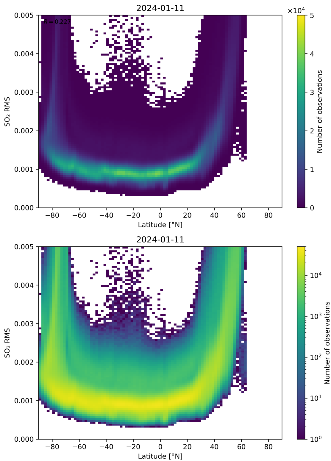
Figure 144: Scatter density plot of “Latitude” against “SO 2 RMS” for 2024-01-10 to 2024-01-12.
