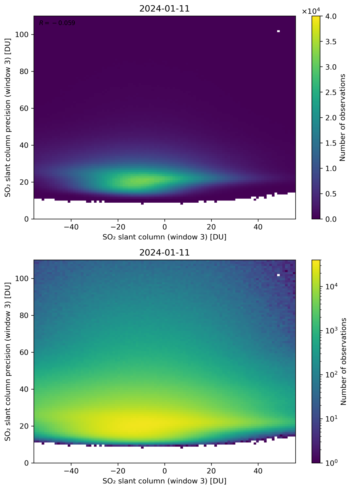
Figure 267: Scatter density plot of “SO 2 slant column (window 3)” against “SO 2 slant column precision (window 3)” for 2024-01-10 to 2024-01-12.
