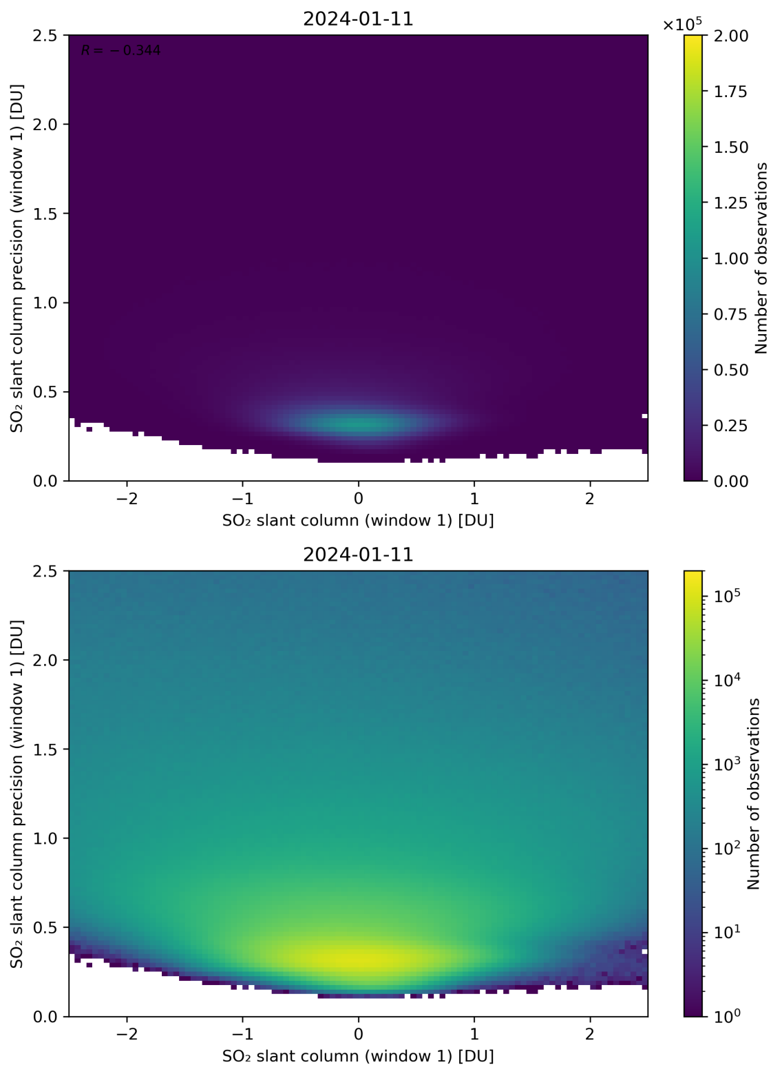
Figure 235: Scatter density plot of “SO 2 slant column (window 1)” against “SO 2 slant column precision (window 1)” for 2024-01-10 to 2024-01-12.
