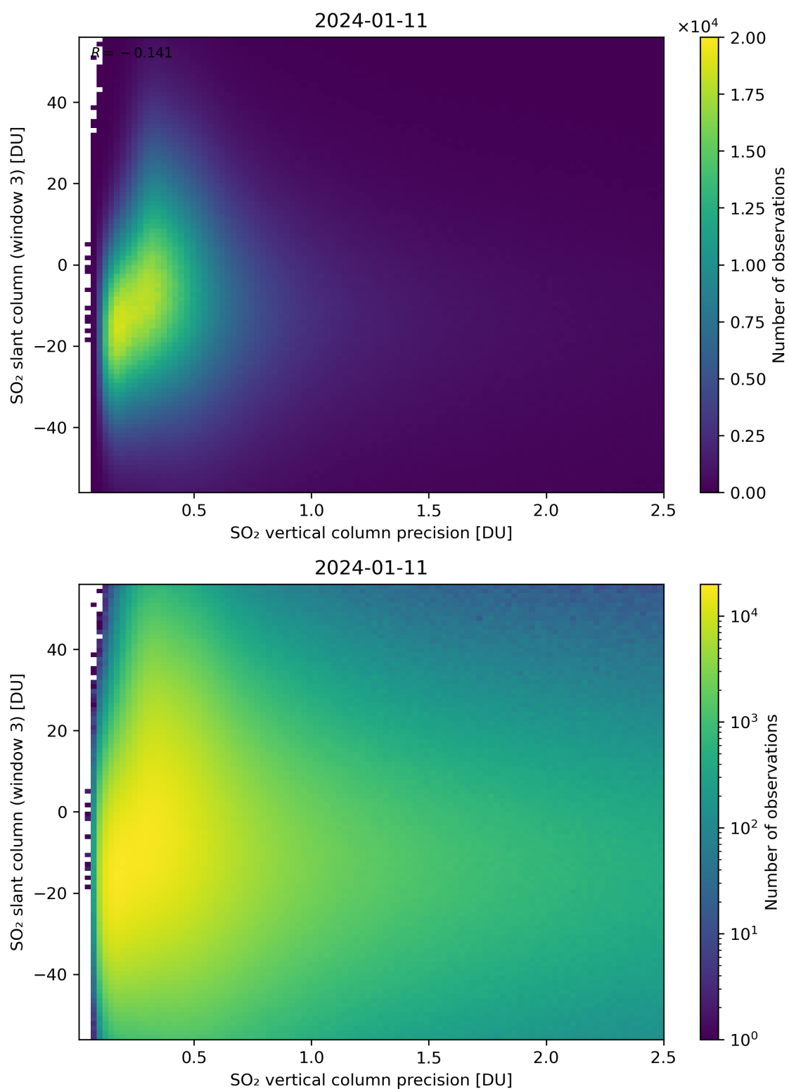
Figure 292: Scatter density plot of “SO 2 vertical column precision” against “SO 2 slant column (window 3)” for 2024-01-10 to 2024-01-12.
