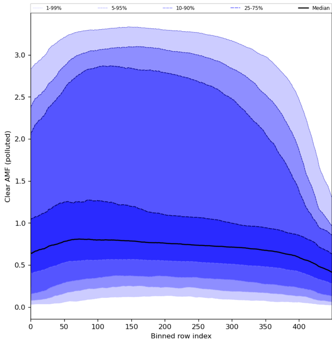
Figure 96: Along track statistics of “Clear AMF (polluted)” for 2024-01-10 to 2024-01-12
