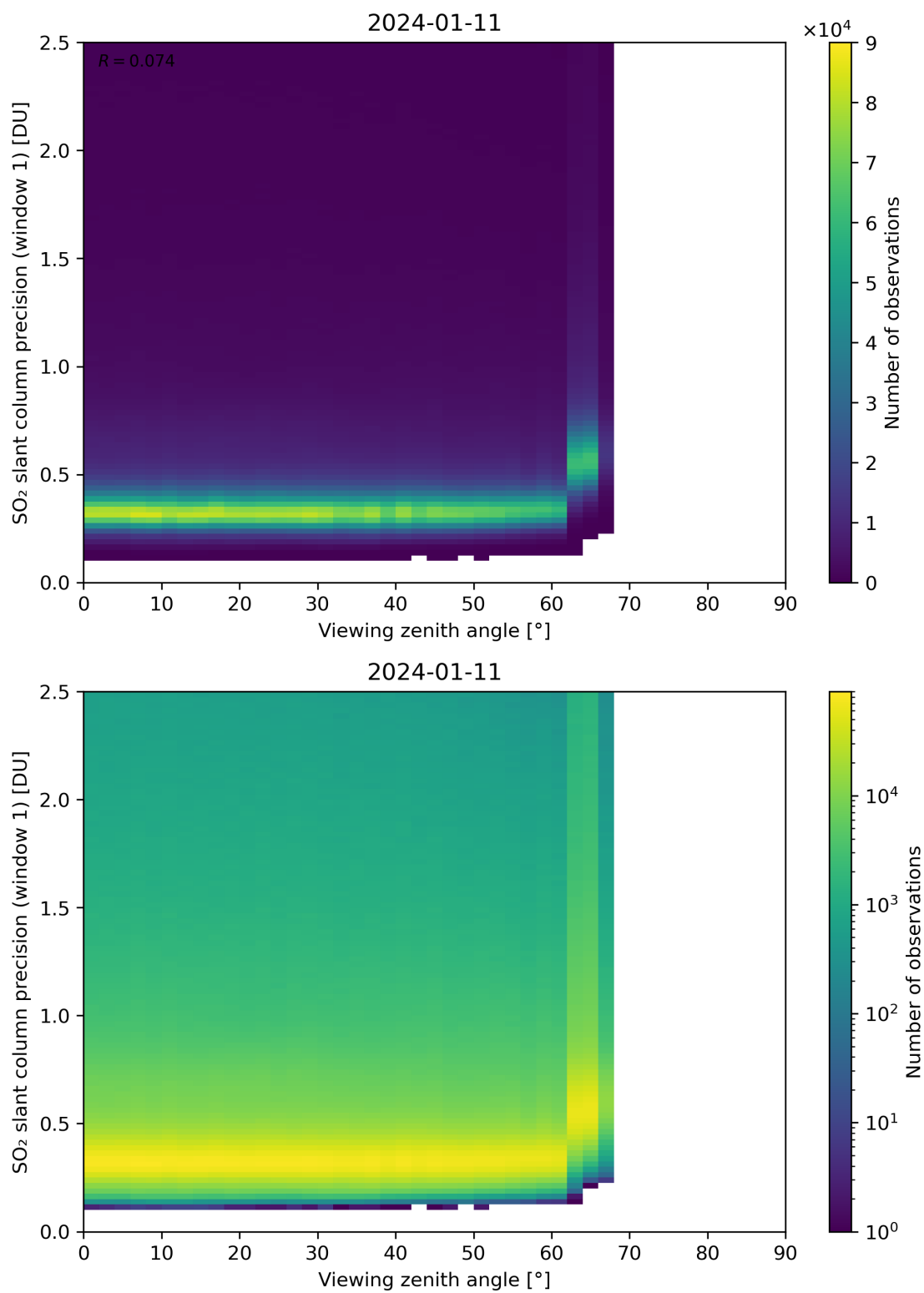
Figure 321: Scatter density plot of “Viewing zenith angle” against “SO 2 slant column precision (window 1)” for 2024-01-10 to 2024-01-12.
