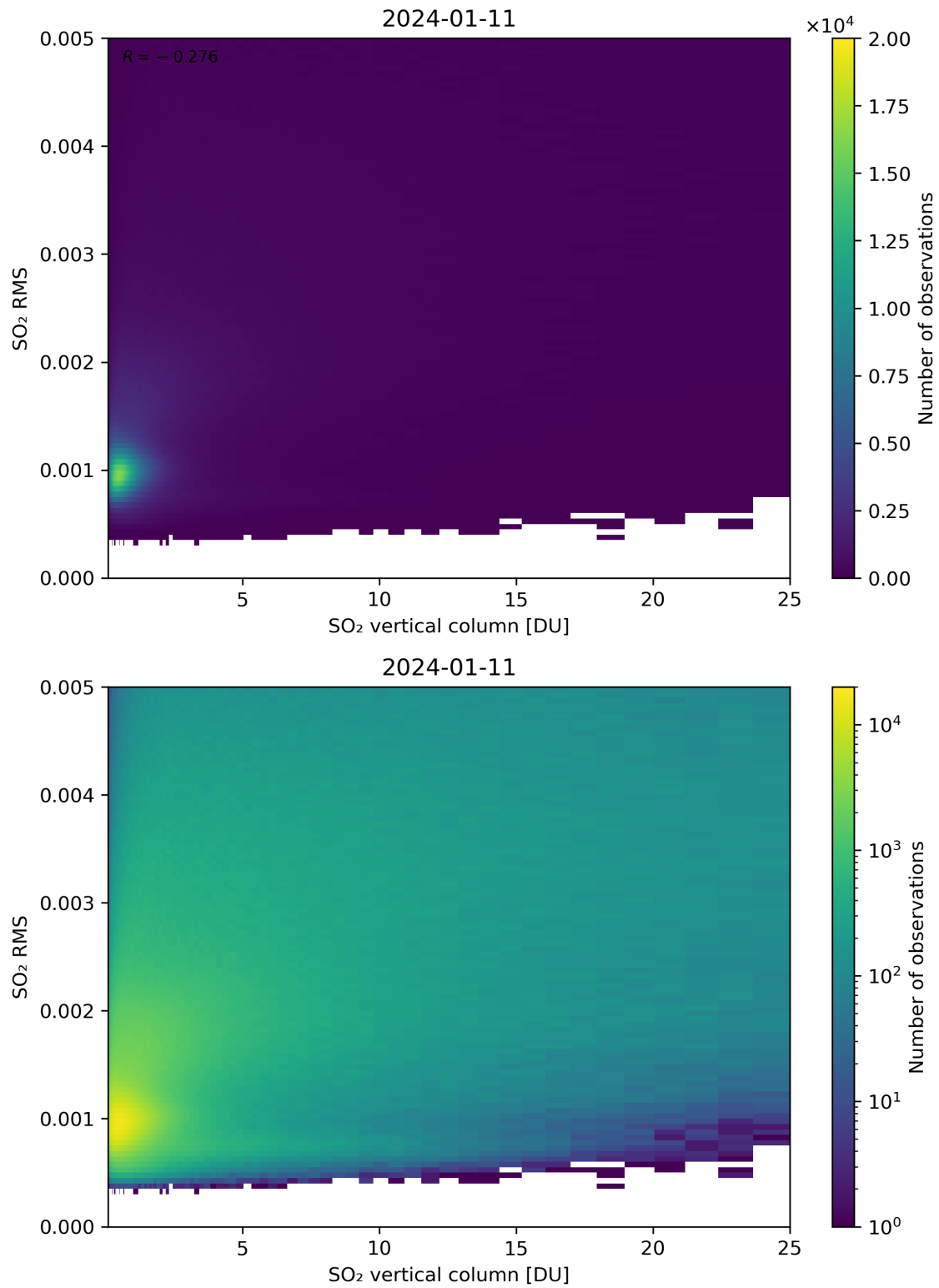
Figure 278: Scatter density plot of “SO 2 vertical column” against “SO 2 RMS” for 2024-01-10 to 2024-01-12.
