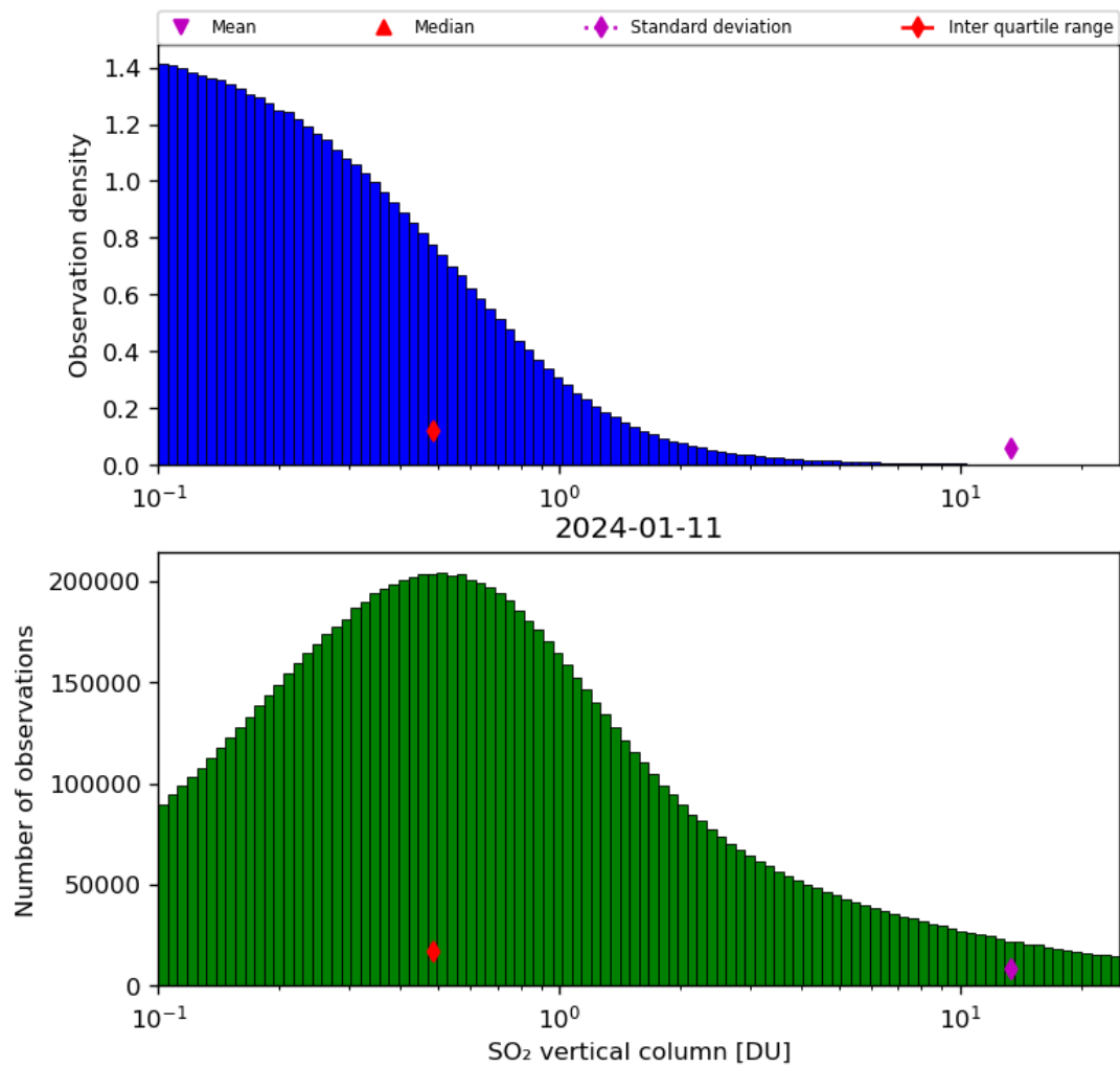
Figure 53: Histogram of “SO 2 vertical column” for 2024-01-10 to 2024-01-12
