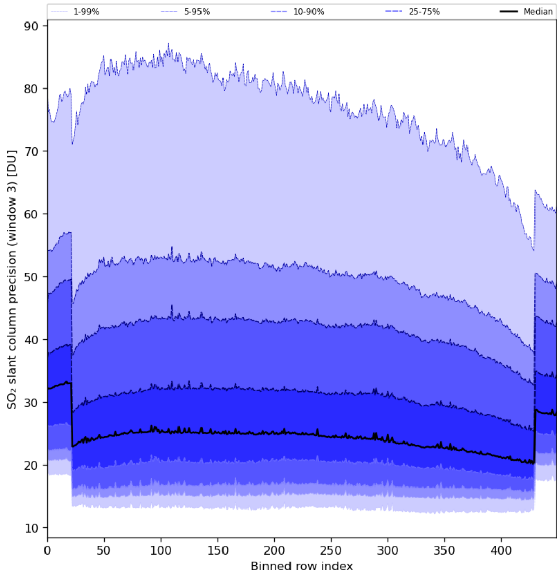
Figure 88: Along track statistics of “SO 2 slant column precision (window 3)” for 2024-01-10 to 2024-01-12
