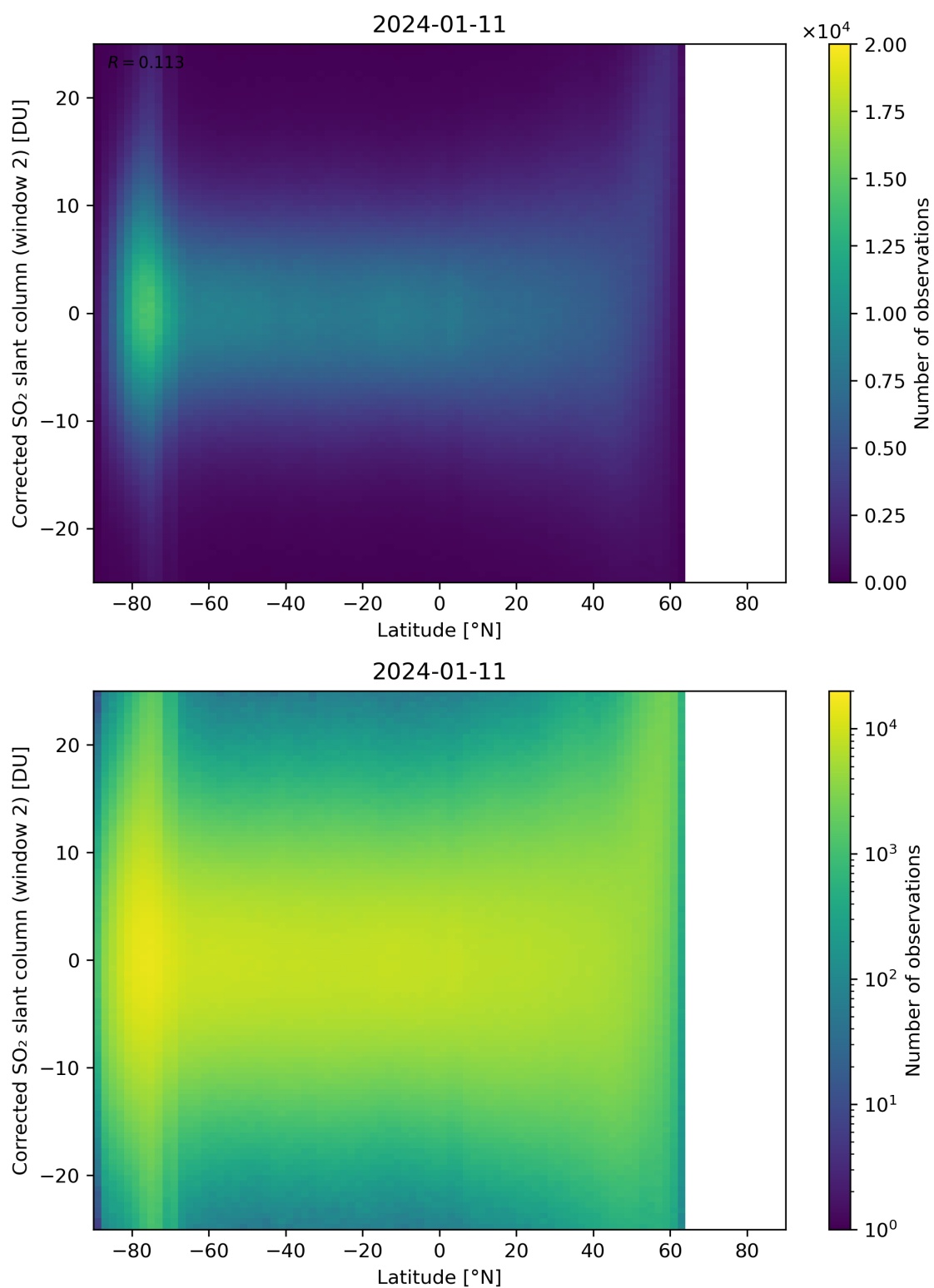
Figure 147: Scatter density plot of “Latitude” against “Corrected SO 2 slant column (window 2)” for 2024-01-10 to 2024-01-12.
