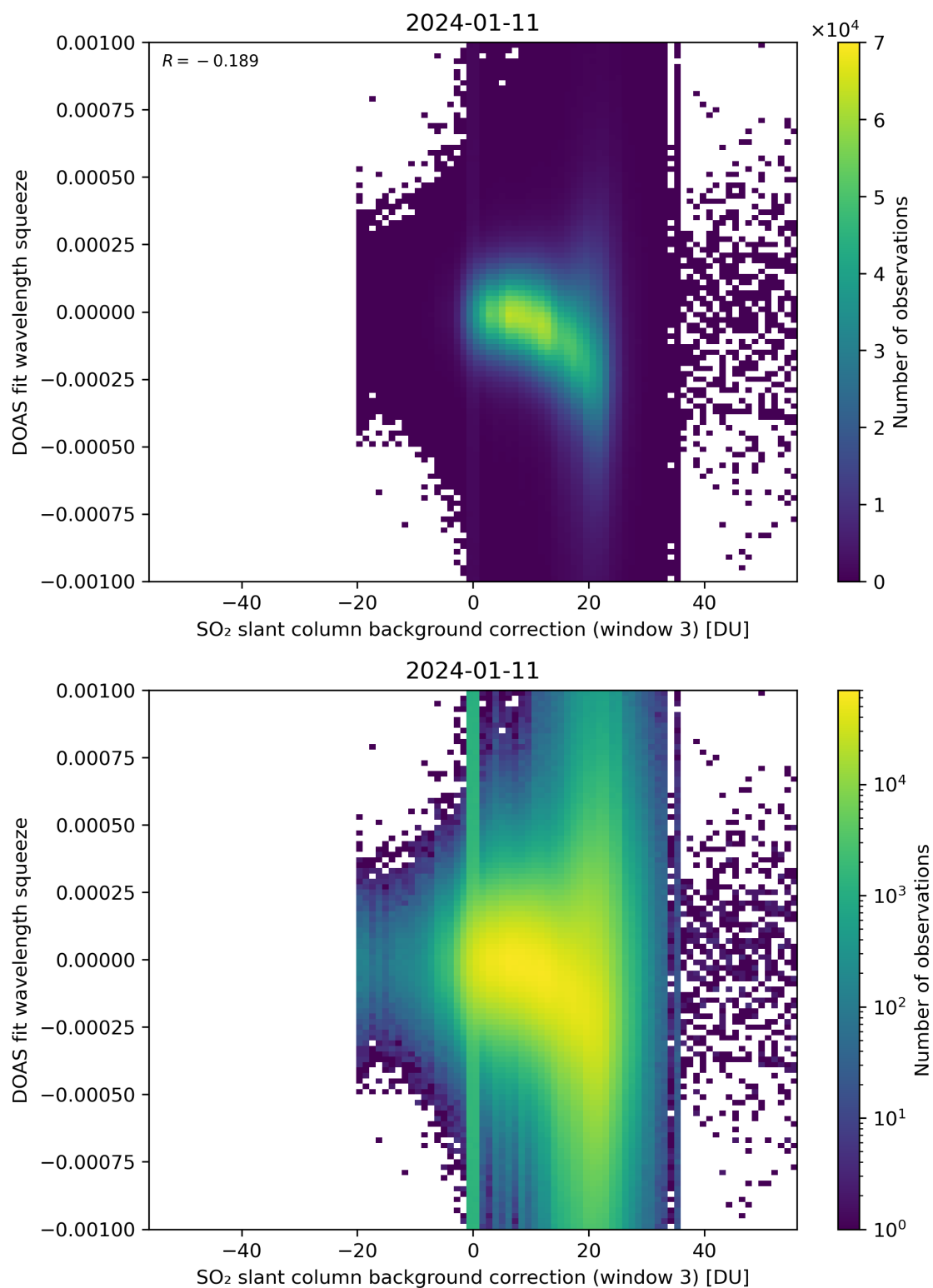
Figure 122: Scatter density plot of “SO 2 slant column background correction (window 3)” against “DOAS fit wavelength squeeze” for 2024-01-10 to 2024-01-12.
