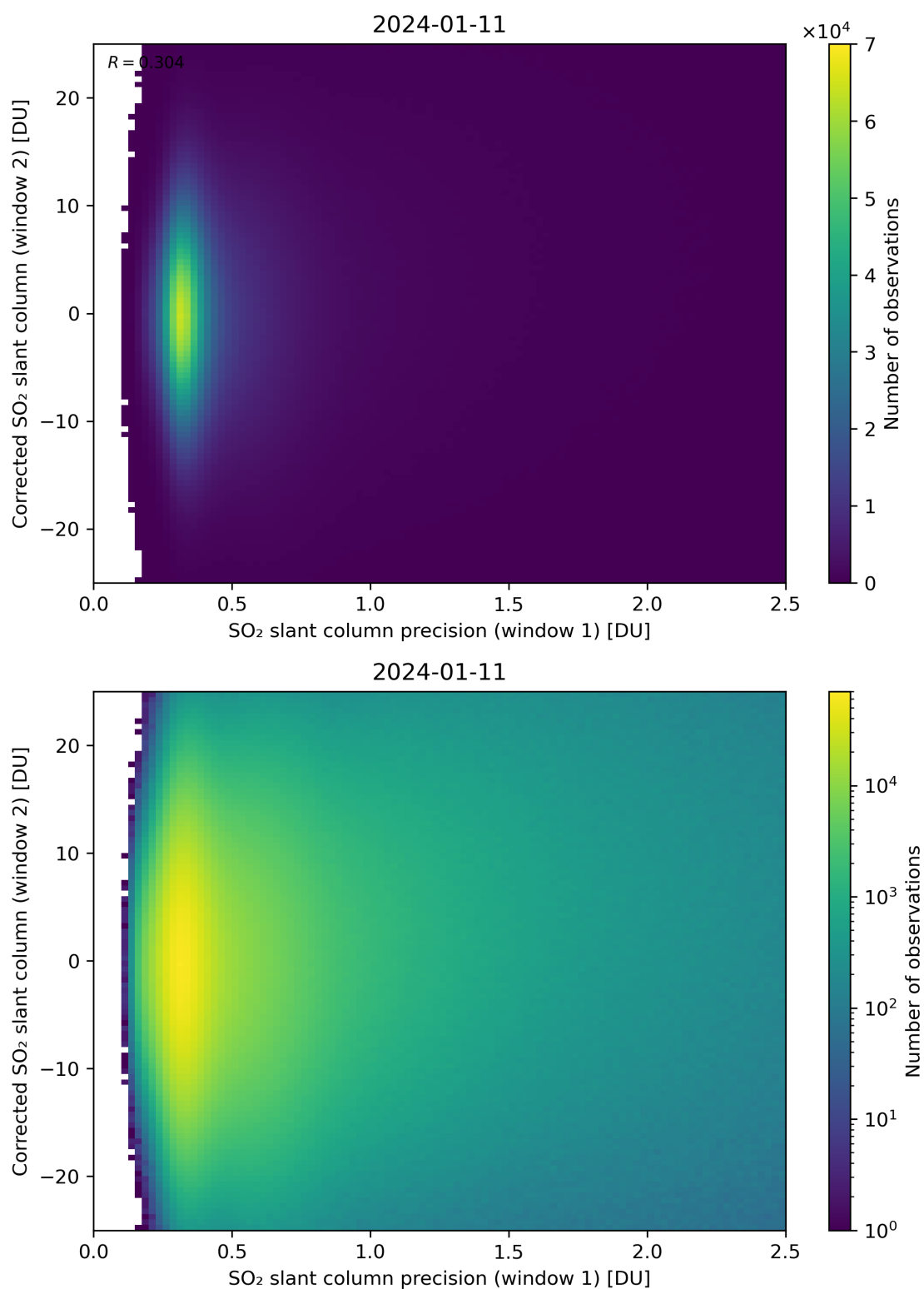
Figure 225: Scatter density plot of “SO 2 slant column precision (window 1)” against “Corrected SO 2 slant column (window 2)” for 2024-01-10 to 2024-01-12.
