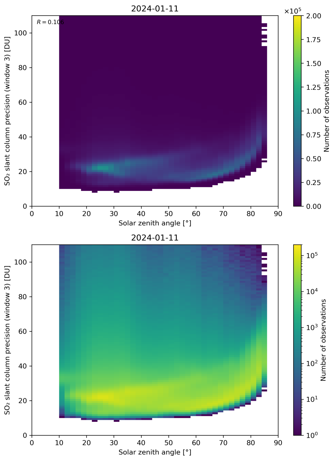
Figure 173: Scatter density plot of “Solar zenith angle” against “SO 2 slant column precision (window 3)” for 2024-01-10 to 2024-01-12.
