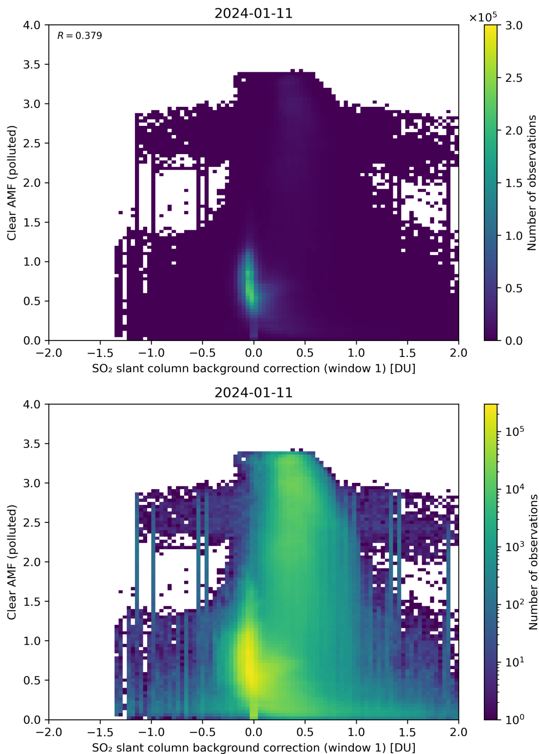
Figure 103: Scatter density plot of “SO 2 slant column background correction (window 1)” against “Clear AMF (polluted)” for 2024-01-10 to 2024-01-12.
