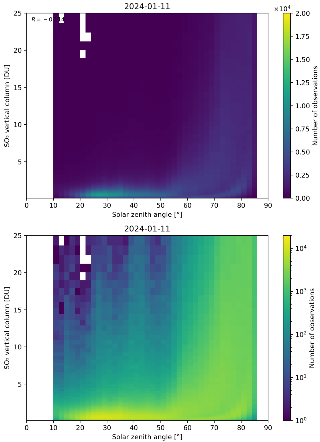
Figure 176: Scatter density plot of “Solar zenith angle” against “SO 2 vertical column” for 2024-01-10 to 2024-01-12.
