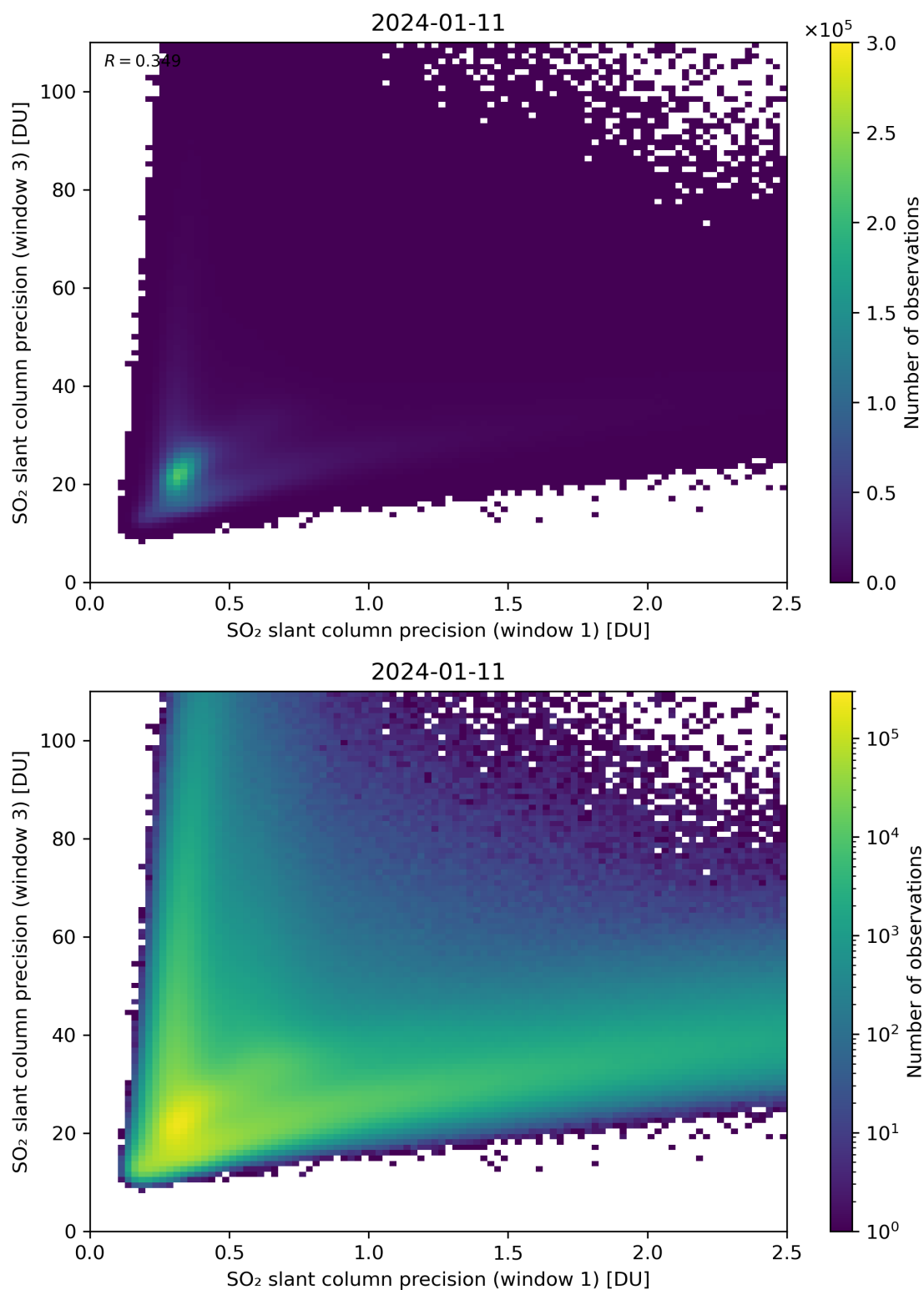
Figure 229: Scatter density plot of “SO 2 slant column precision (window 1)” against “SO 2 slant column precision (window 3)” for 2024-01-10 to 2024-01-12.
