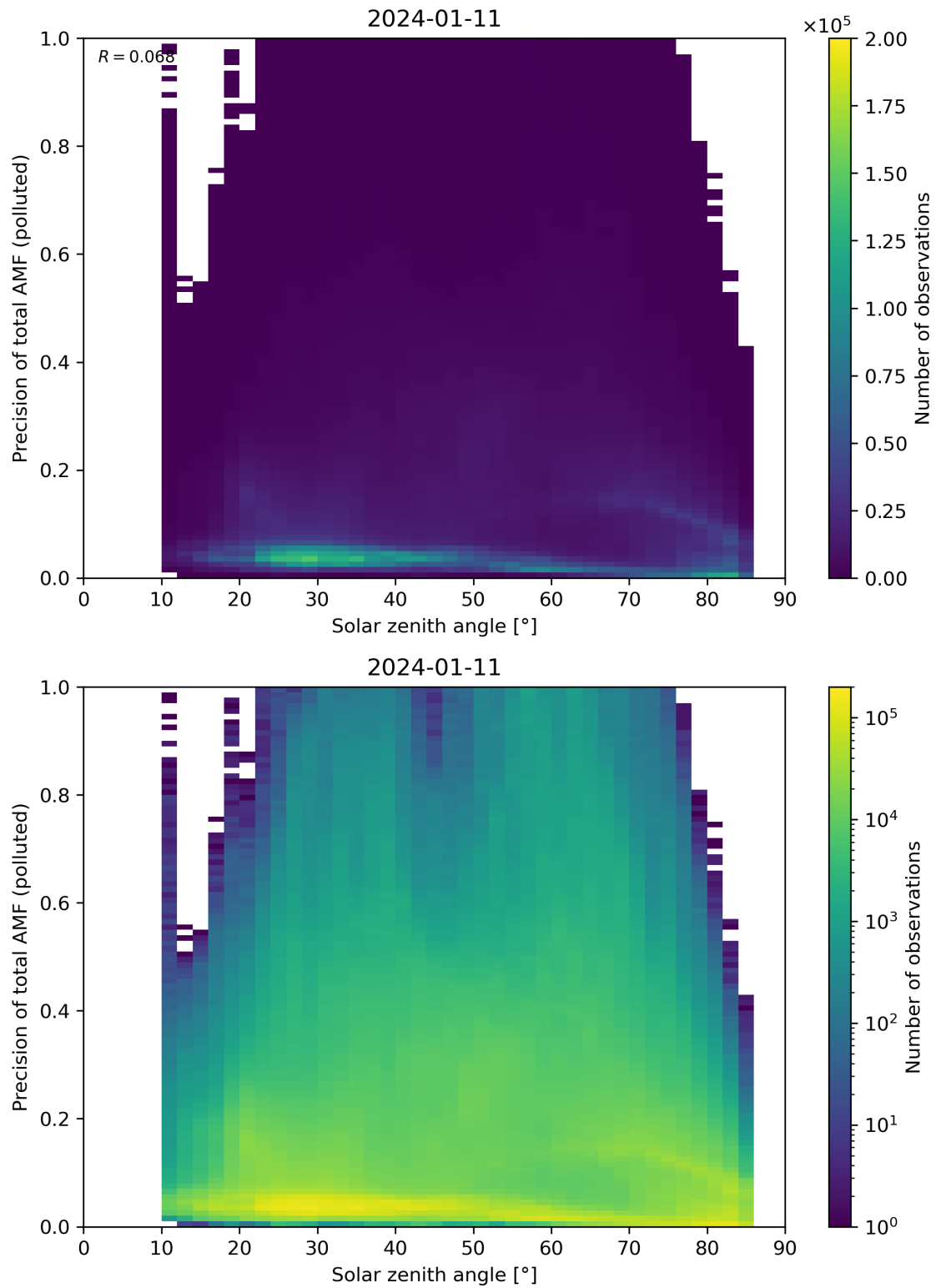
Figure 175: Scatter density plot of “Solar zenith angle” against “Precision of total AMF (polluted)” for 2024-01-10 to 2024-01-12.
