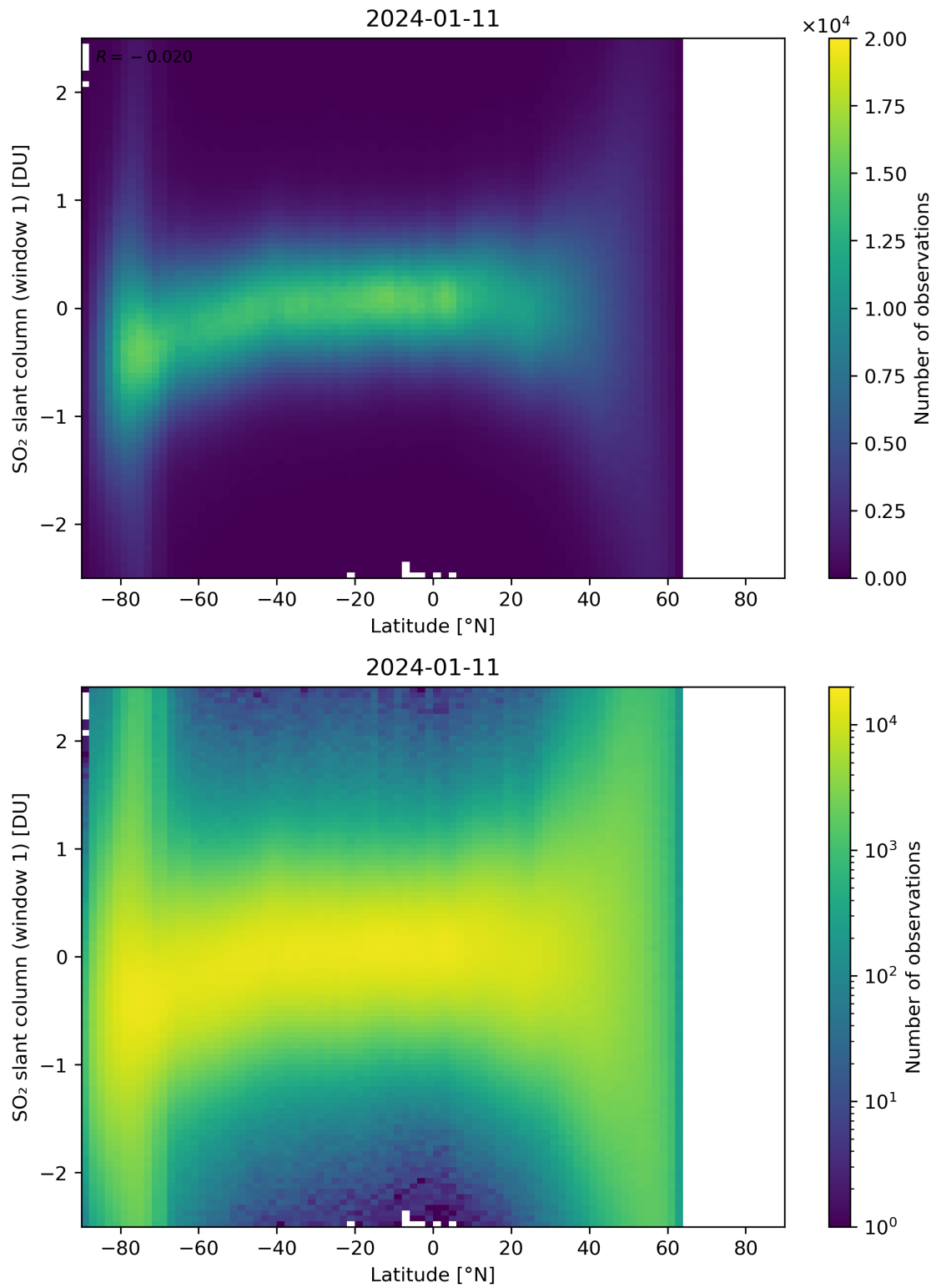
Figure 149: Scatter density plot of “Latitude” against “SO 2 slant column (window 1)” for 2024-01-10 to 2024-01-12.
