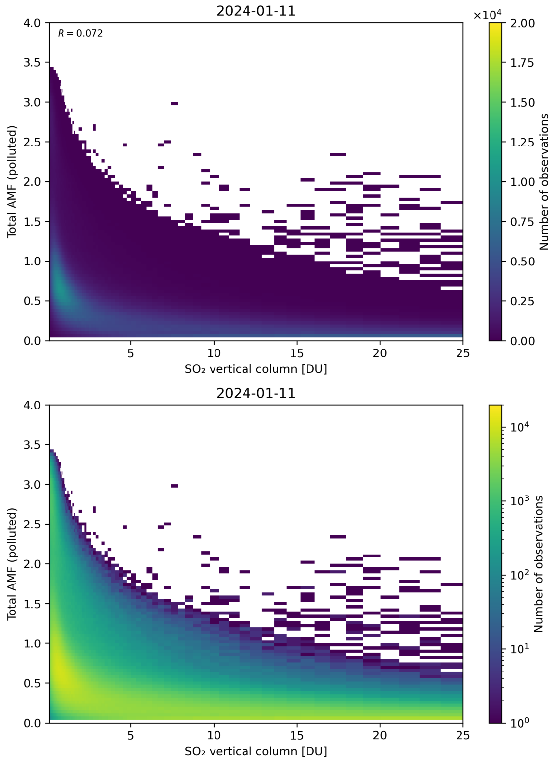
Figure 305: Scatter density plot of “SO 2 vertical column” against “Total AMF (polluted)” for 2024-01-10 to 2024-01-12.
