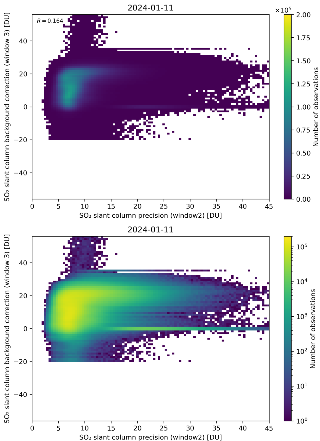
Figure 242: Scatter density plot of “SO 2 slant column precision (window2)” against “SO 2 slant column background correction (window 3)” for 2024-01-10 to 2024-01-12.
