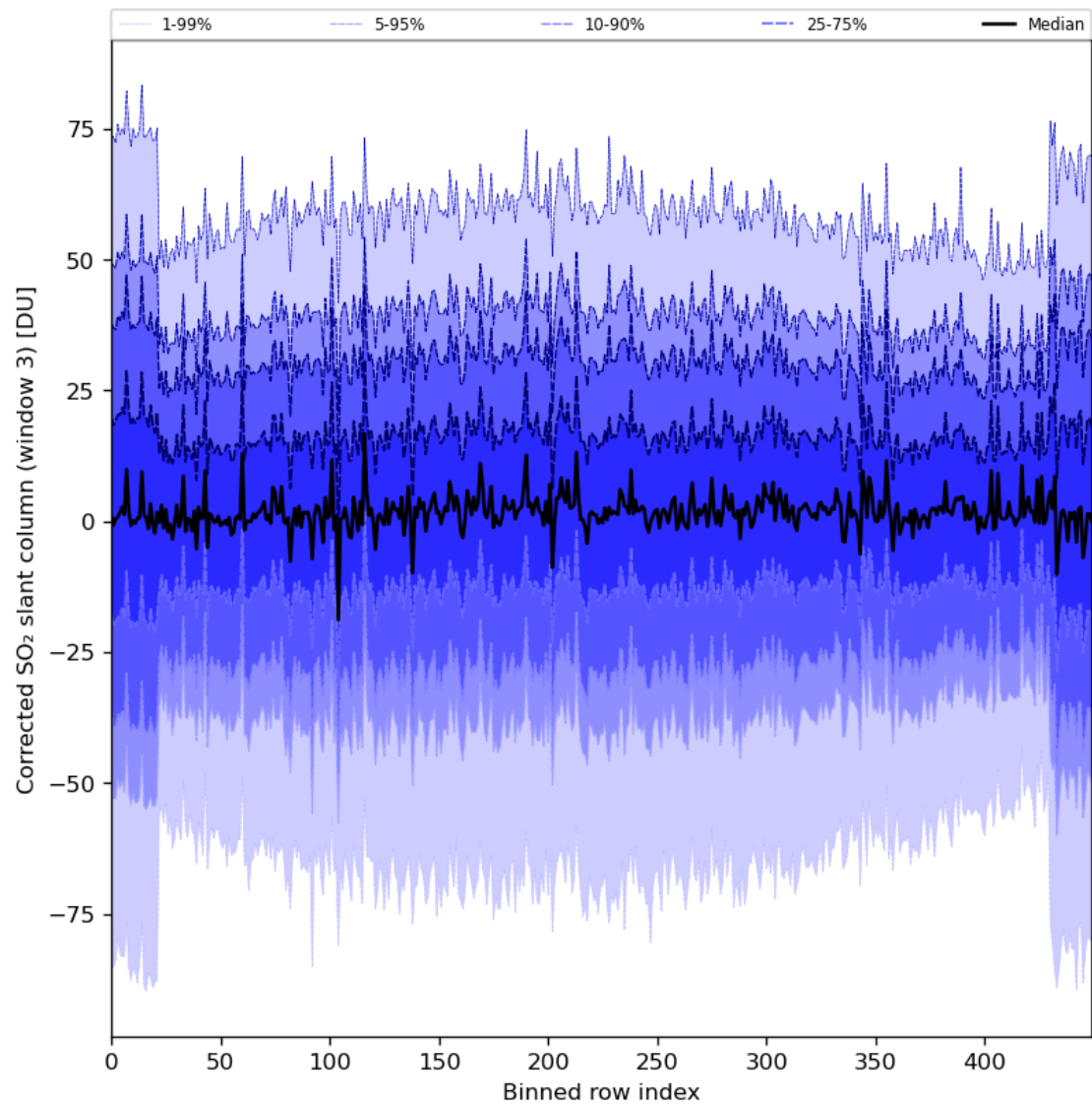
Figure 89: Along track statistics of “Corrected SO 2 slant column (window 3)” for 2024-01-10 to 2024-01-12
