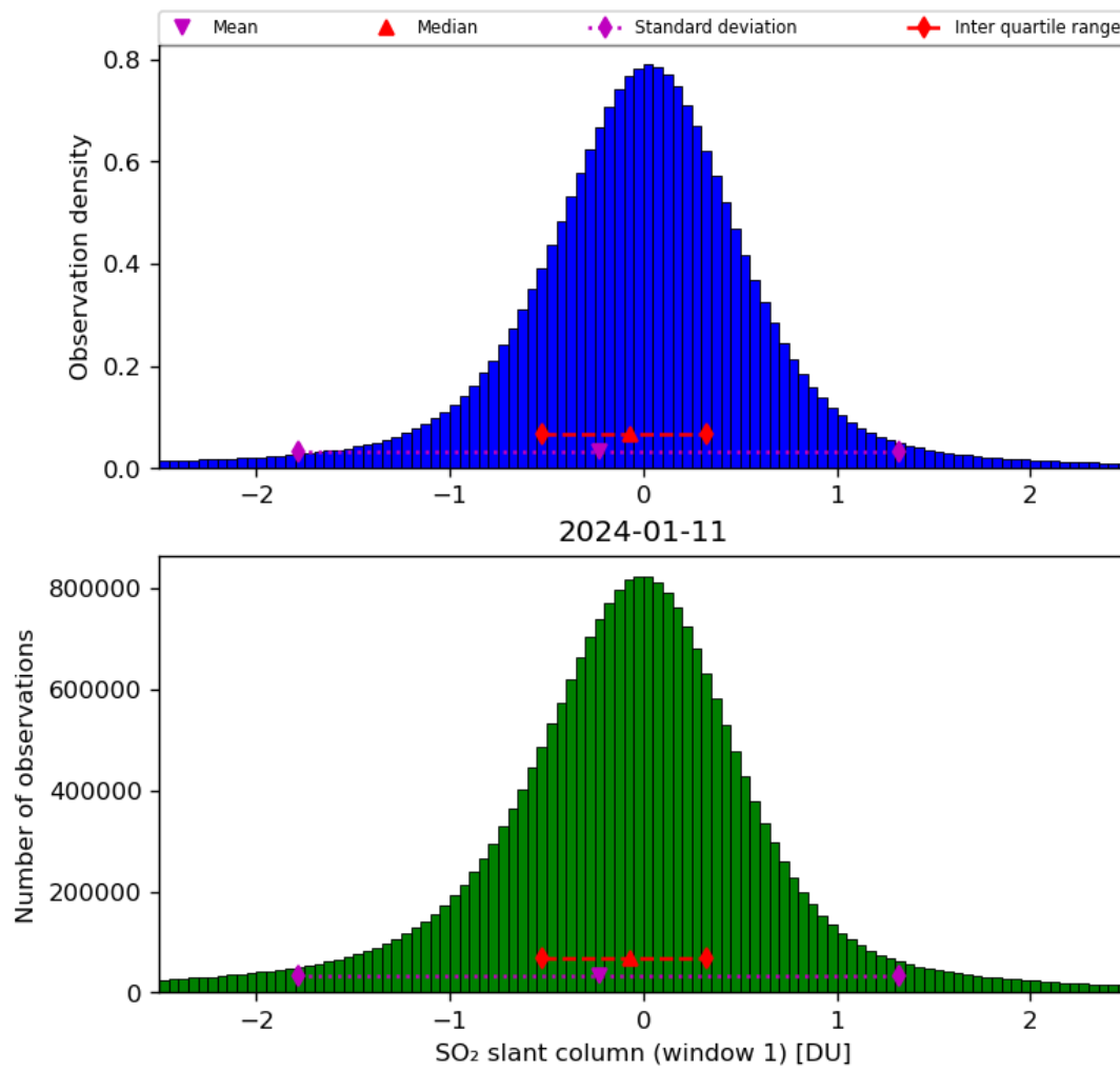
Figure 56: Histogram of “SO 2 slant column (window 1)” for 2024-01-10 to 2024-01-12
