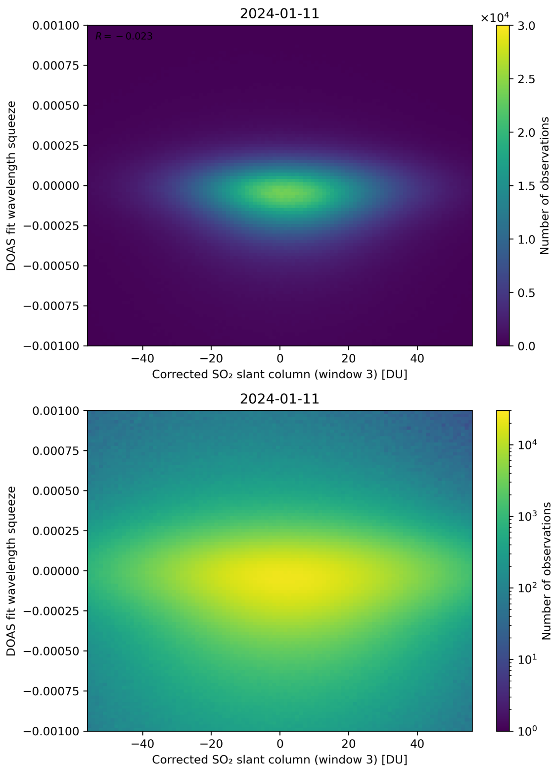
Figure 207: Scatter density plot of “Corrected SO 2 slant column (window 3)” against “DOAS fit wavelength squeeze” for 2024-01-10 to 2024-01-12.
