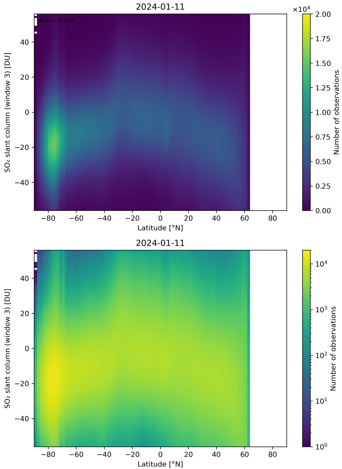
Figure 152: Scatter density plot of “Latitude” against “SO 2 slant column (window 3)” for 2024-01-10 to 2024-01-12.
