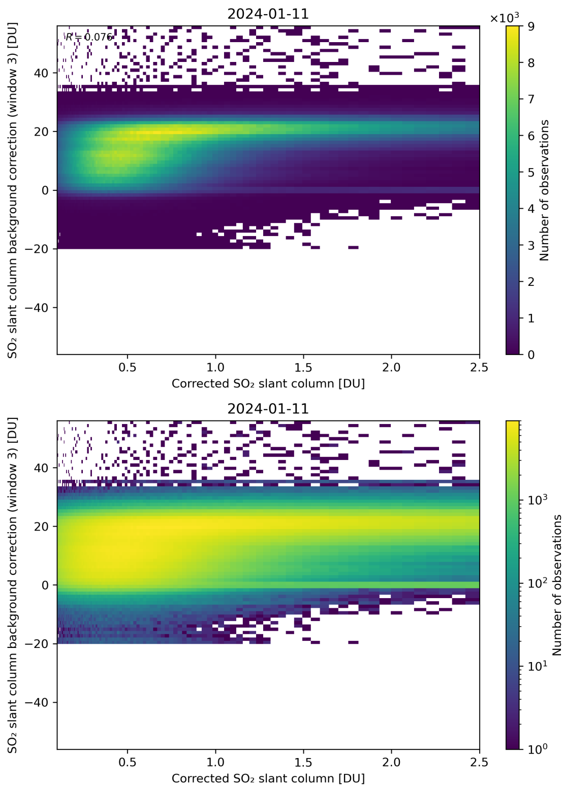
Figure 180: Scatter density plot of “Corrected SO 2 slant column” against “SO 2 slant column background correction (window 3)” for 2024-01-10 to 2024-01-12.
