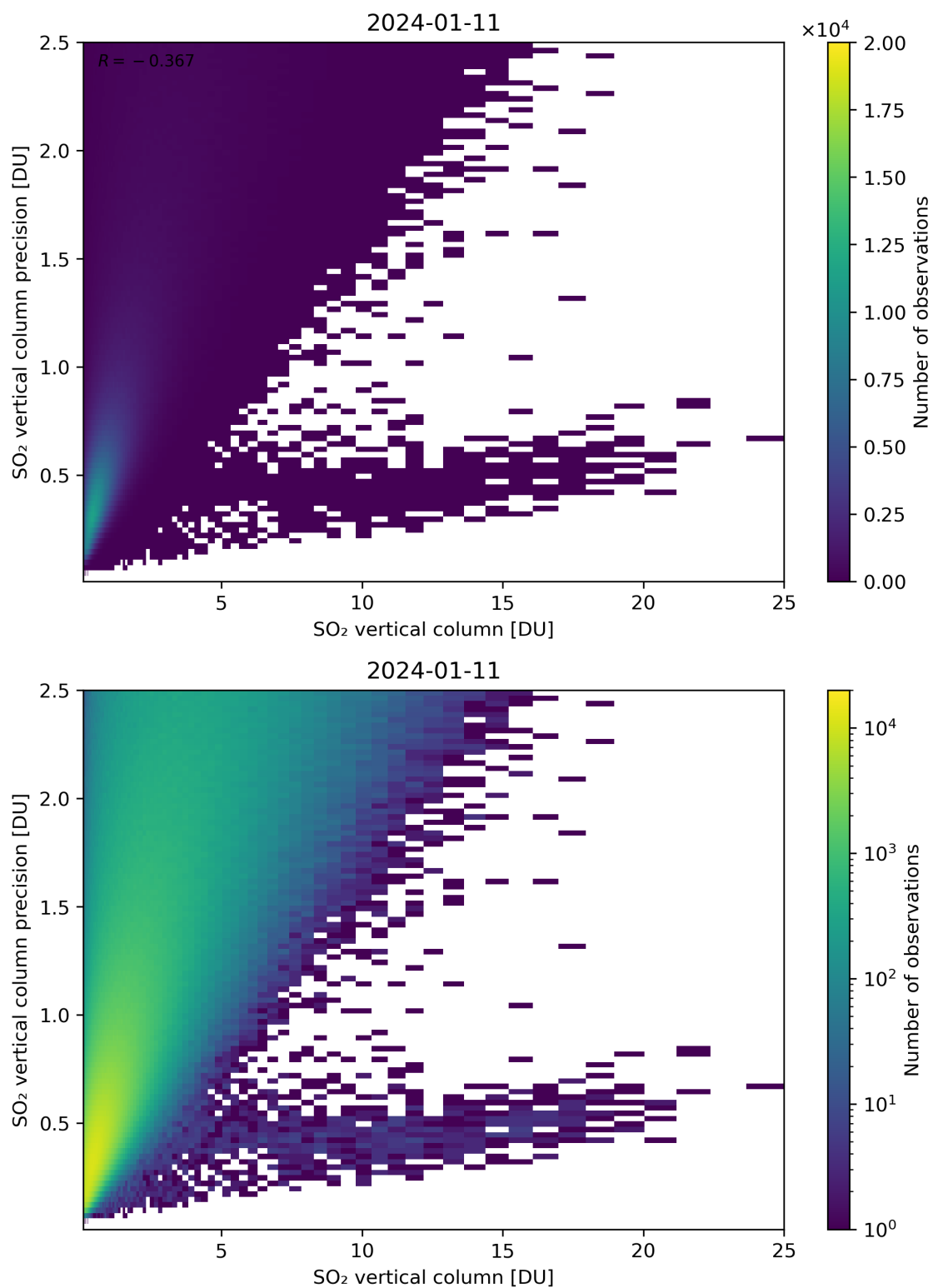
Figure 307: Scatter density plot of “SO 2 vertical column” against “SO 2 vertical column precision” for 2024-01-10 to 2024-01-12.
