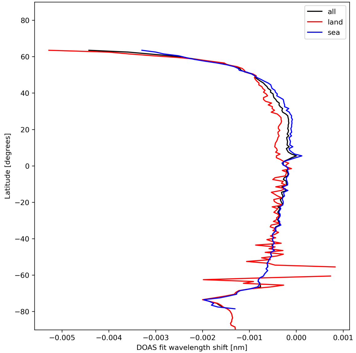
Figure 45: Zonal average of “DOAS fit wavelength shift” for 2024-01-10 to 2024-01-12.
