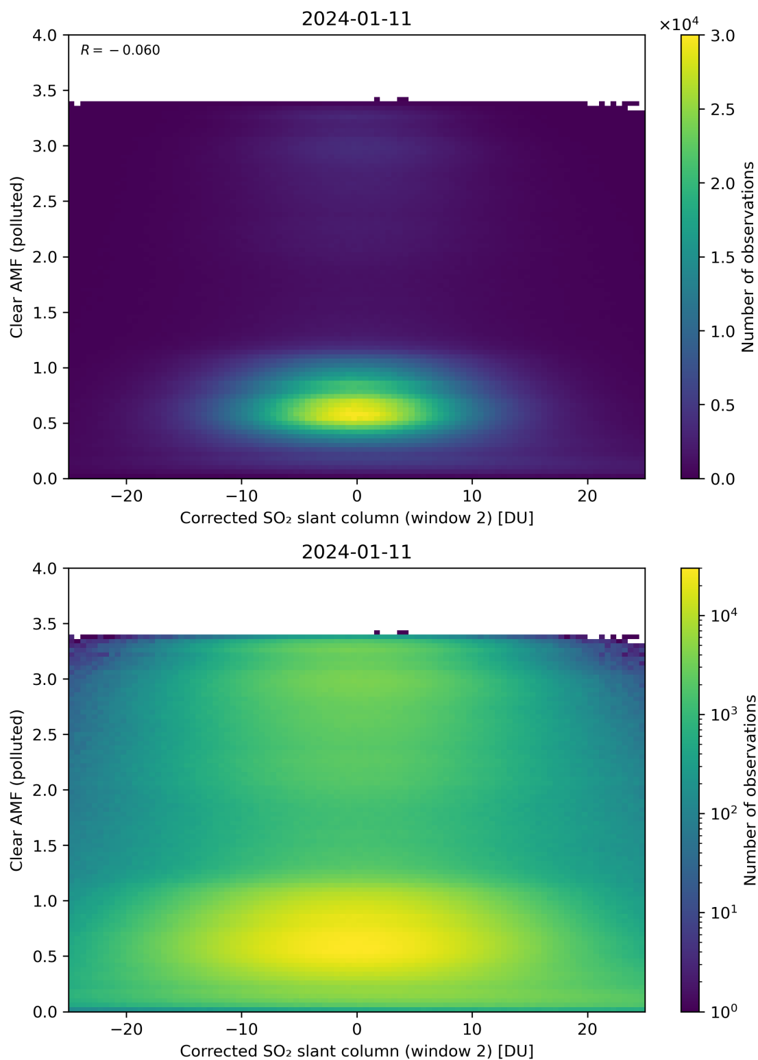
Figure 199: Scatter density plot of “Corrected SO 2 slant column (window 2)” against “Clear AMF (polluted)” for 2024-01-10 to 2024-01-12.
