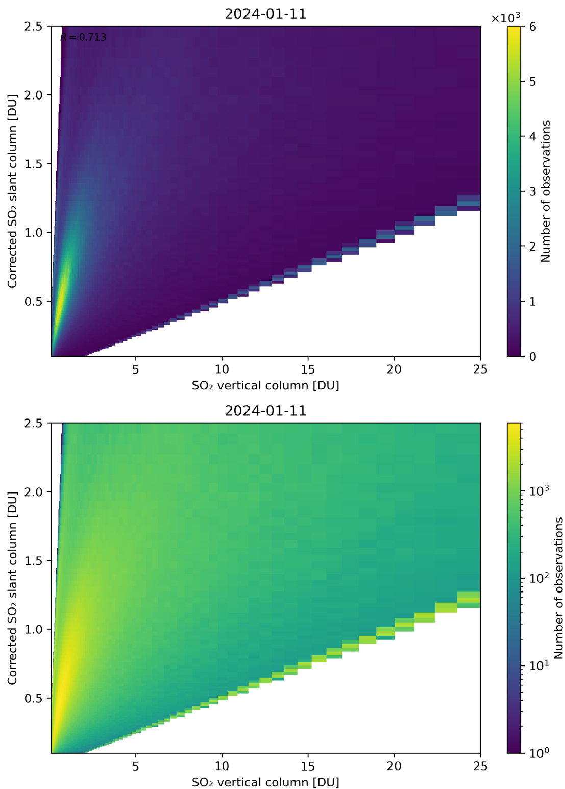
Figure 297: Scatter density plot of “SO 2 vertical column” against “Corrected SO 2 slant column” for 2024-01-10 to 2024-01-12.
