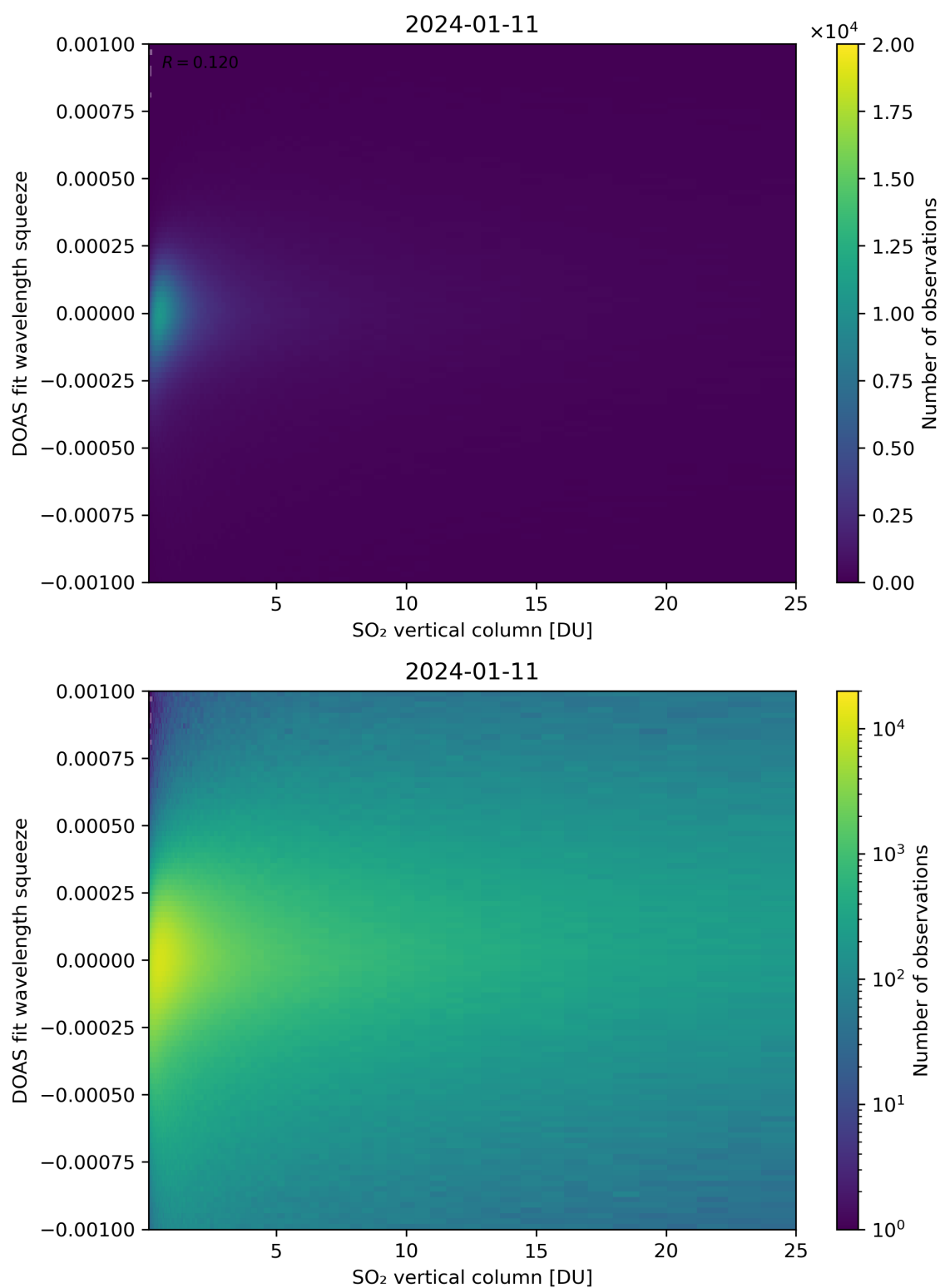
Figure 277: Scatter density plot of “SO 2 vertical column” against “DOAS fit wavelength squeeze” for 2024-01-10 to 2024-01-12.
