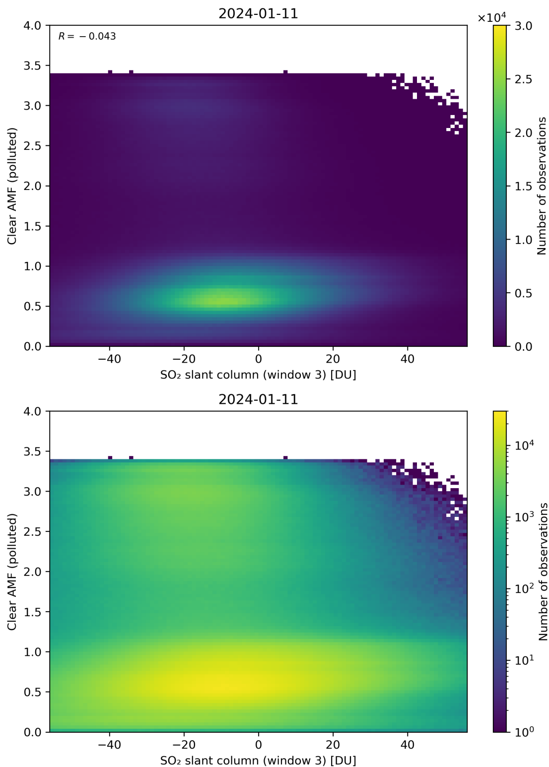
Figure 265: Scatter density plot of “SO 2 slant column (window 3)” against “Clear AMF (polluted)” for 2024-01-10 to 2024-01-12.
