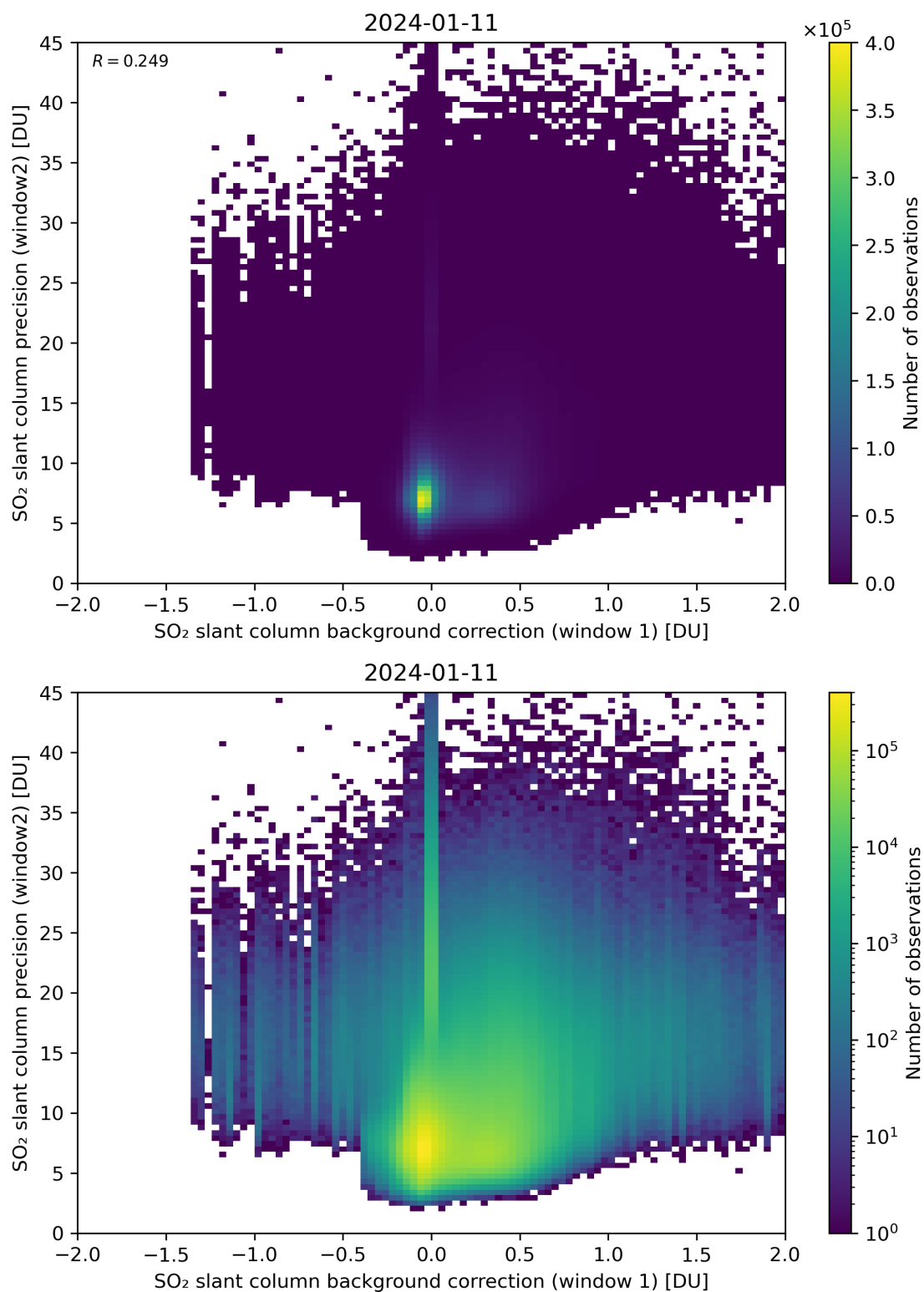
Figure 106: Scatter density plot of “SO 2 slant column background correction (window 1)” against “SO 2 slant column precision (window2)” for 2024-01-10 to 2024-01-12.
