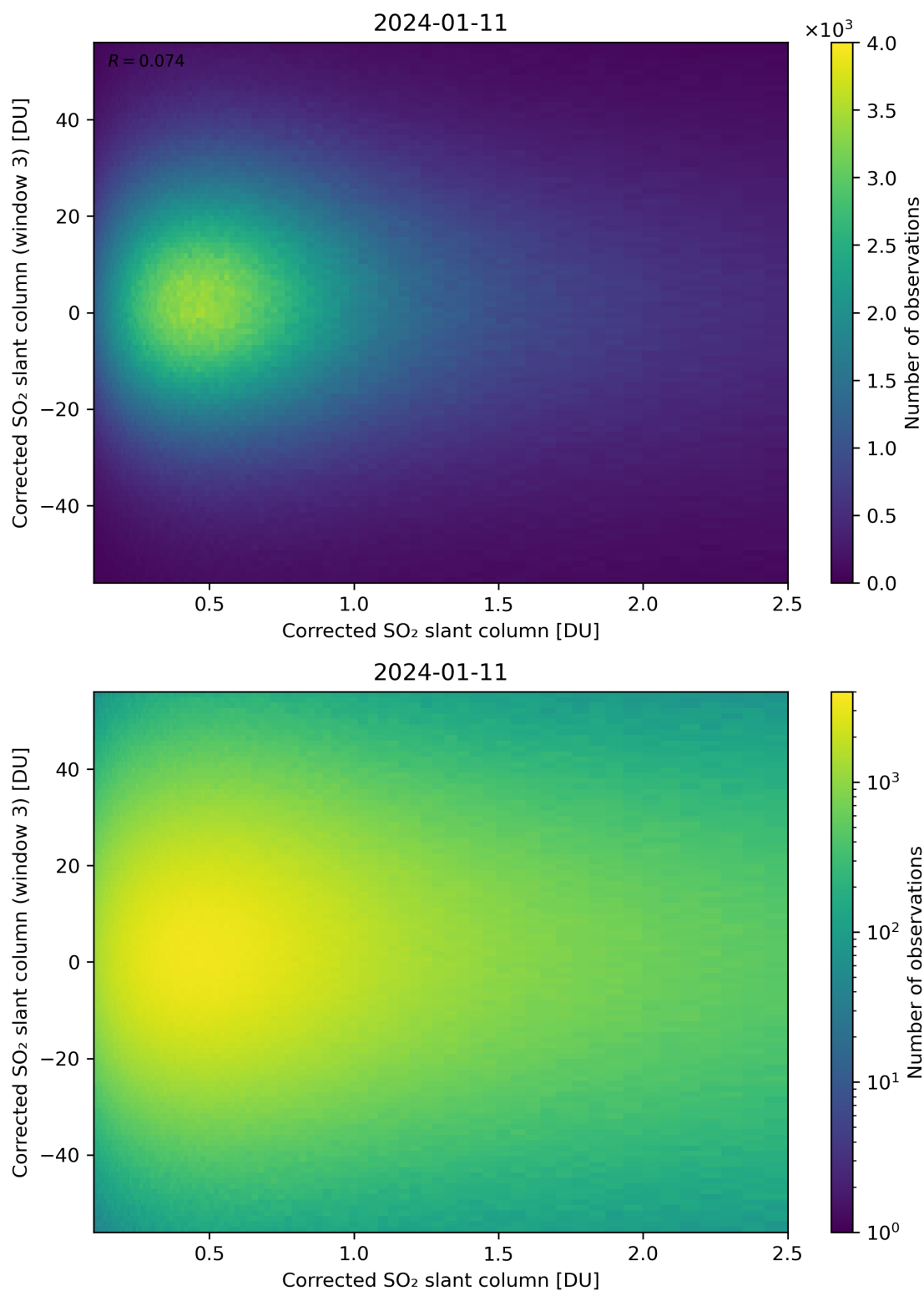
Figure 186: Scatter density plot of “Corrected SO 2 slant column” against “Corrected SO 2 slant column (window 3)” for 2024-01-10 to 2024-01-12.
