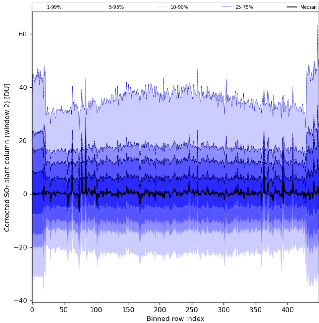
Figure 85: Along track statistics of “Corrected SO 2 slant column (window 2)” for 2024-01-10 to 2024-01-12
