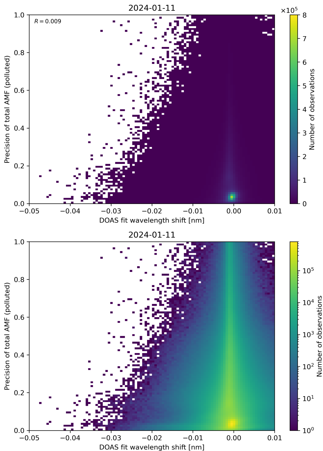
Figure 131: Scatter density plot of “DOAS fit wavelength shift” against “Precision of total AMF (polluted)” for 2024-01-10 to 2024-01-12.
