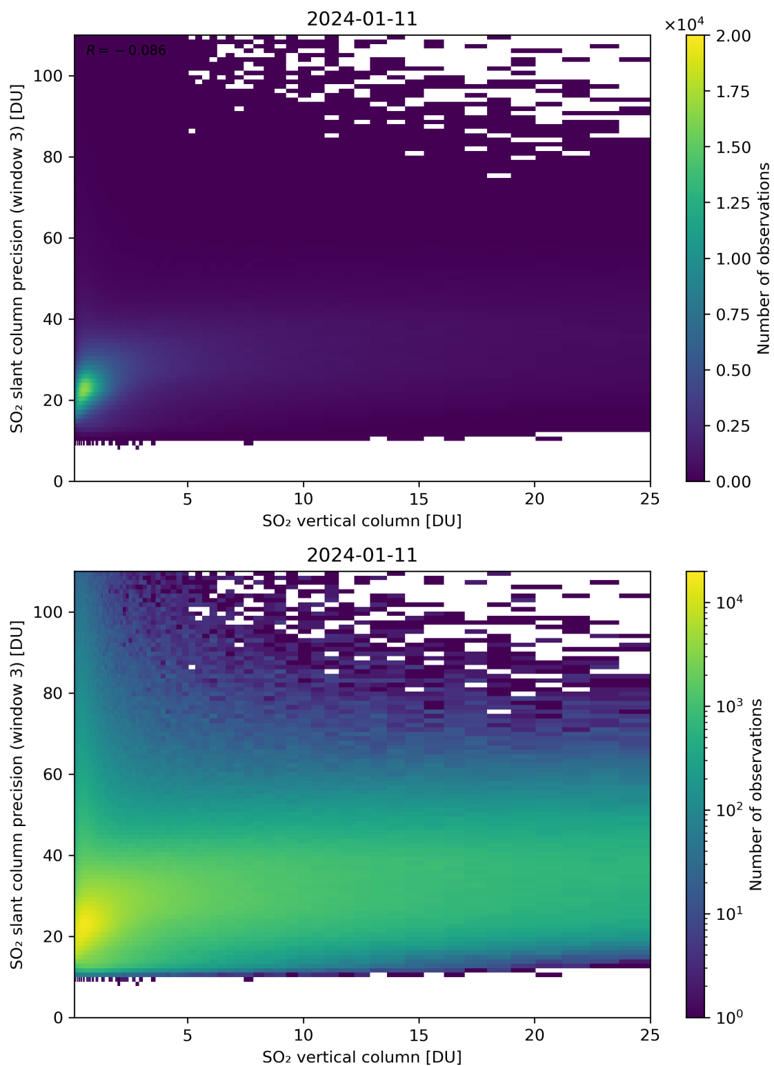
Figure 304: Scatter density plot of “SO 2 vertical column” against “SO 2 slant column precision (window 3)” for 2024-01-10 to 2024-01-12.
