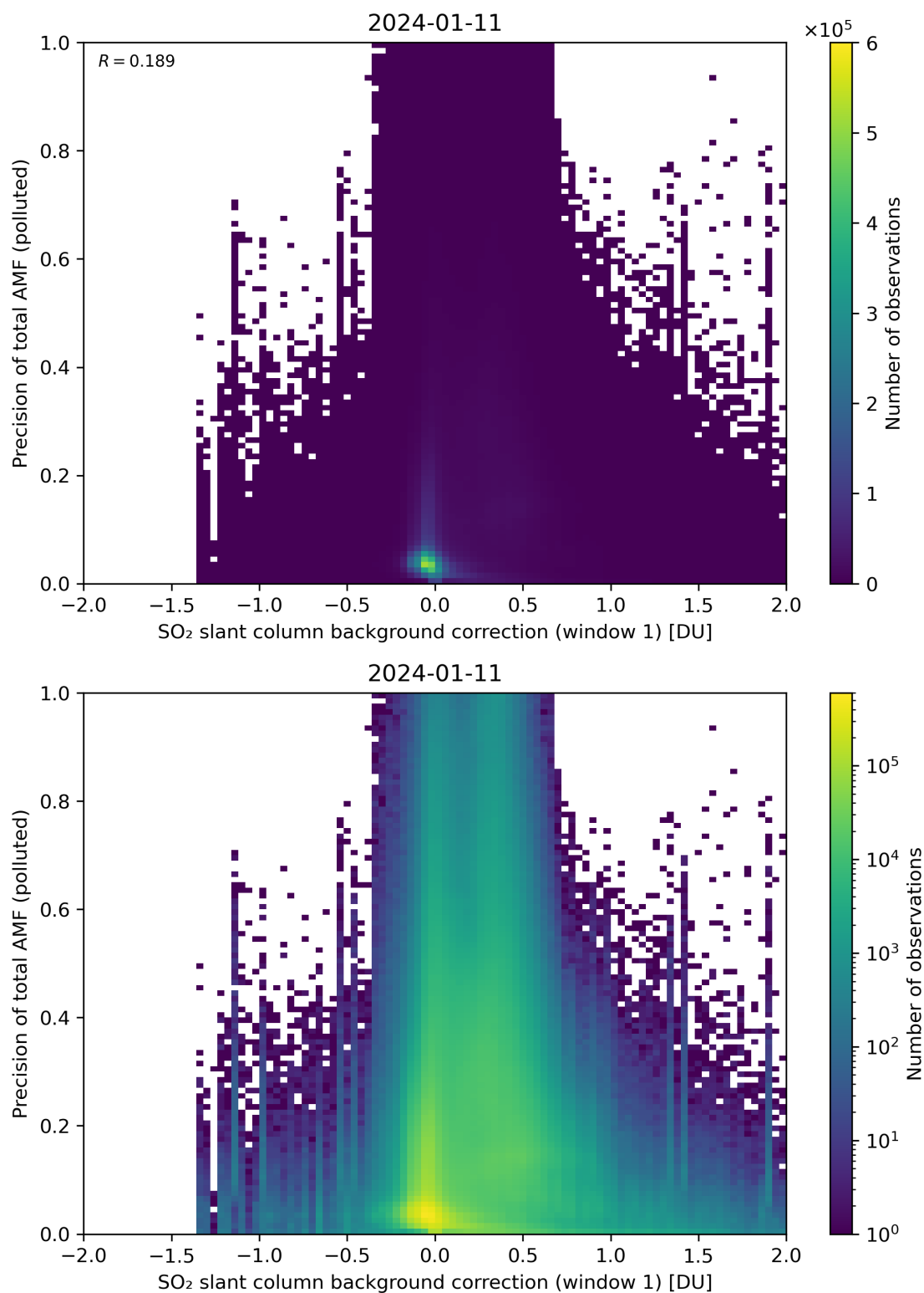
Figure 110: Scatter density plot of “SO 2 slant column background correction (window 1)” against “Precision of total AMF (polluted)” for 2024-01-10 to 2024-01-12.
