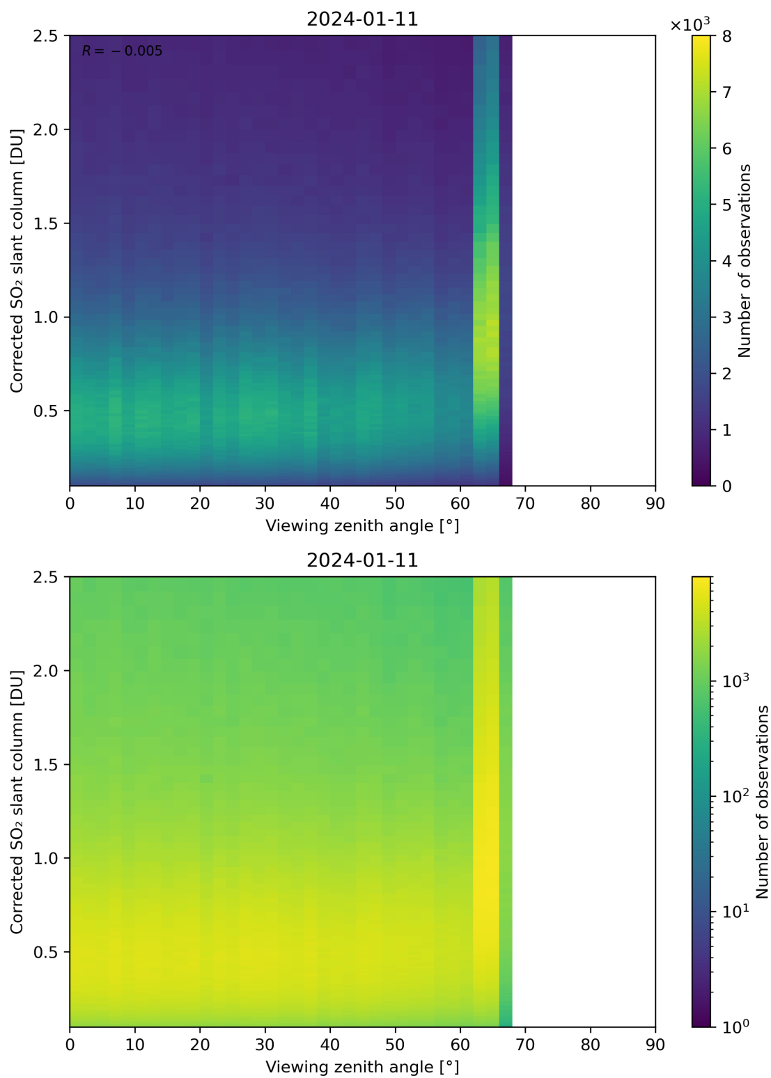
Figure 317: Scatter density plot of “Viewing zenith angle” against “Corrected SO 2 slant column” for 2024-01-10 to 2024-01-12.
