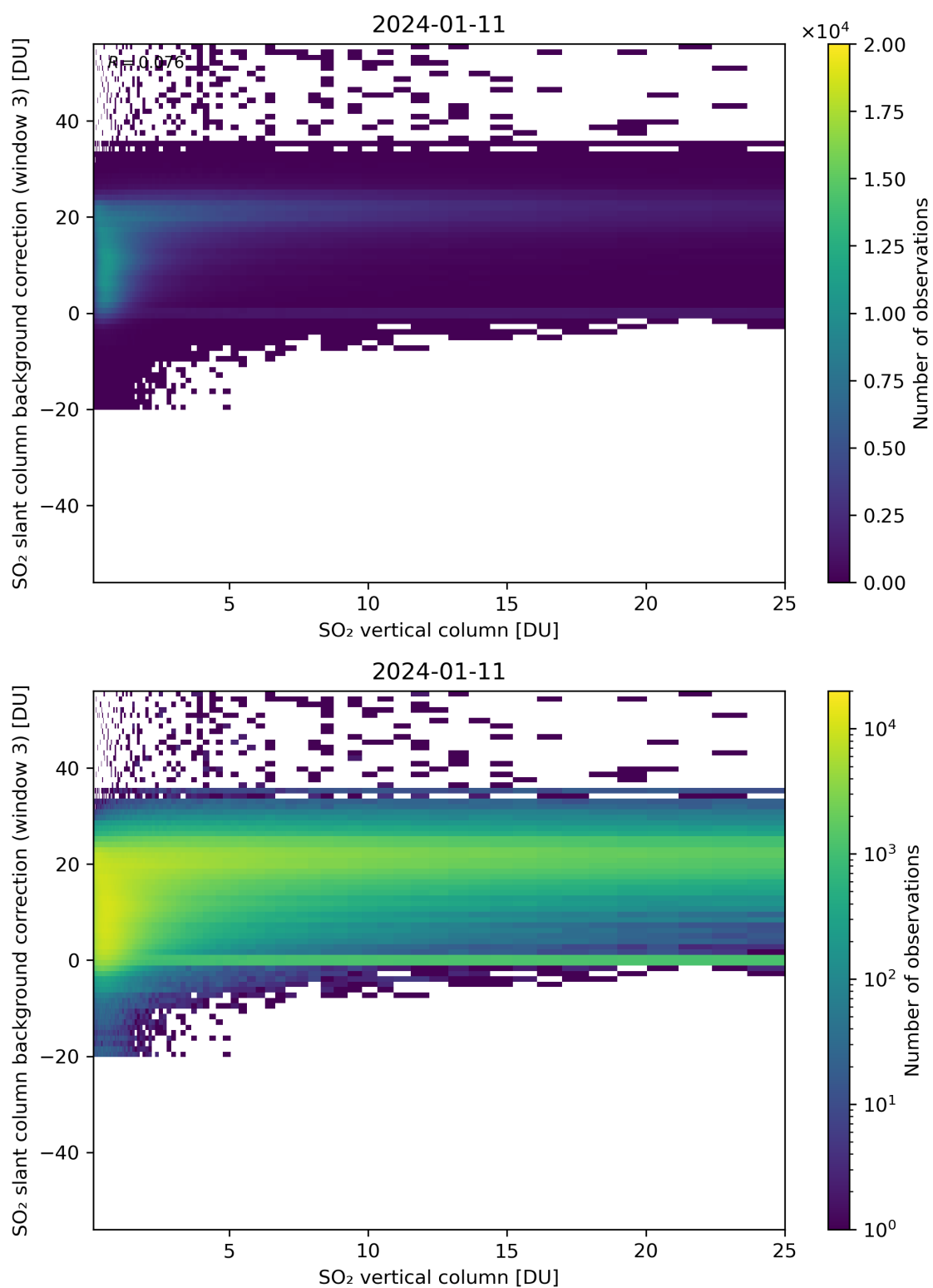
Figure 275: Scatter density plot of “SO 2 vertical column” against “SO 2 slant column background correction (window 3)” for 2024-01-10 to 2024-01-12.
