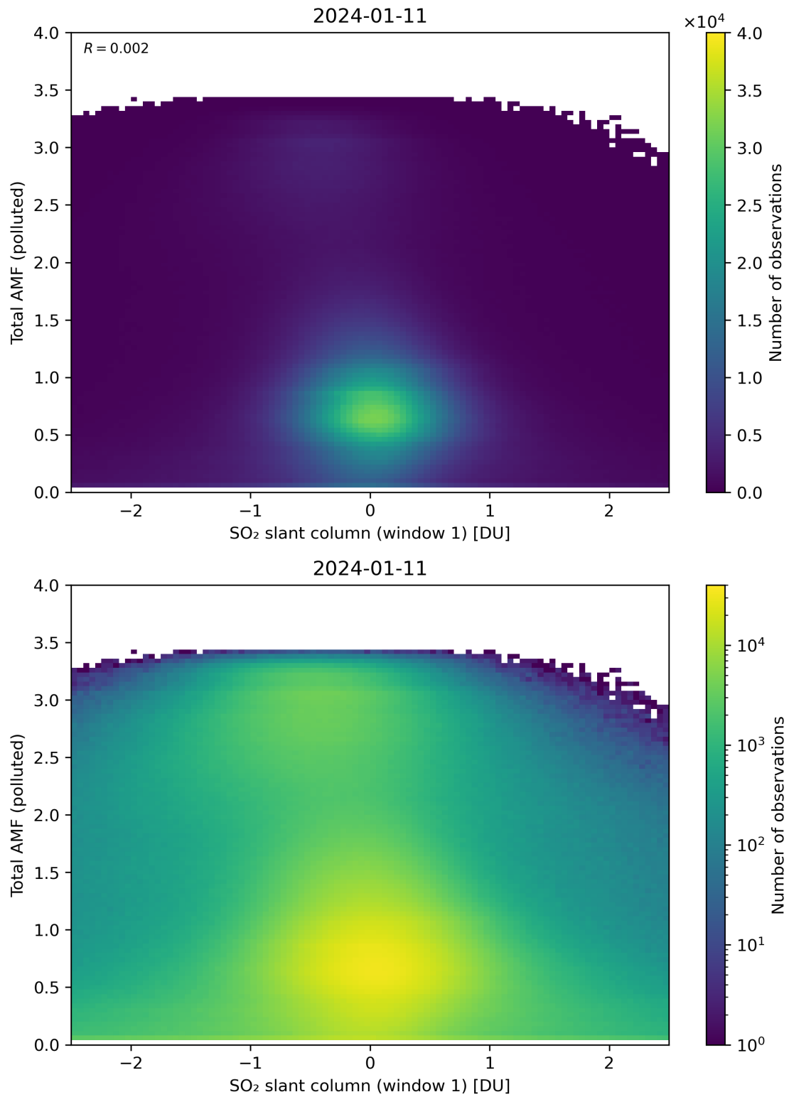
Figure 239: Scatter density plot of “SO 2 slant column (window 1)” against “Total AMF (polluted)” for 2024-01-10 to 2024-01-12.
