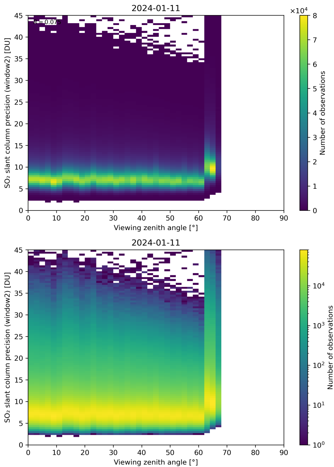
Figure 322: Scatter density plot of “Viewing zenith angle” against “SO 2 slant column precision (window2)” for 2024-01-10 to 2024-01-12.
