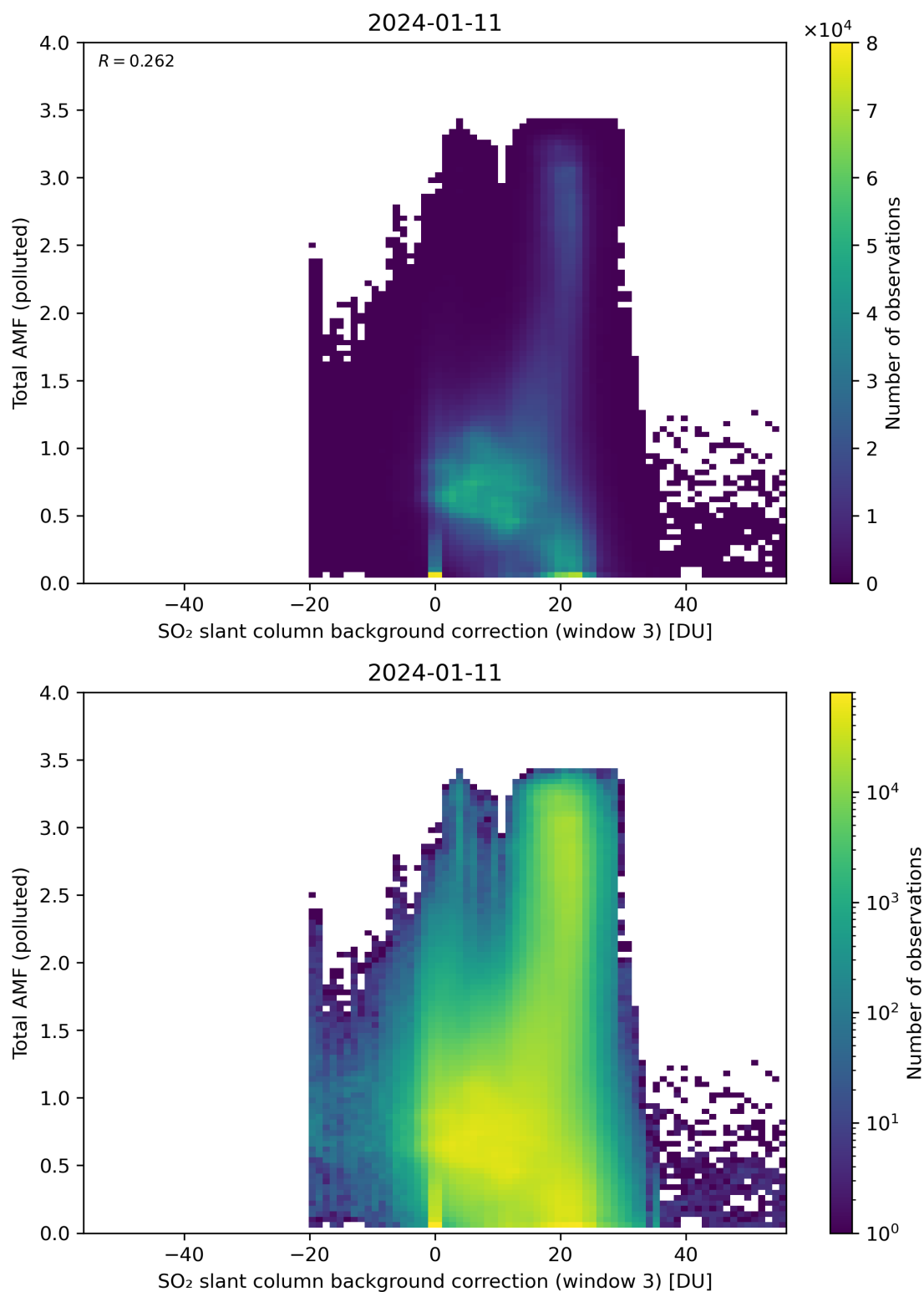
Figure 125: Scatter density plot of “SO 2 slant column background correction (window 3)” against “Total AMF (polluted)” for 2024-01-10 to 2024-01-12.
