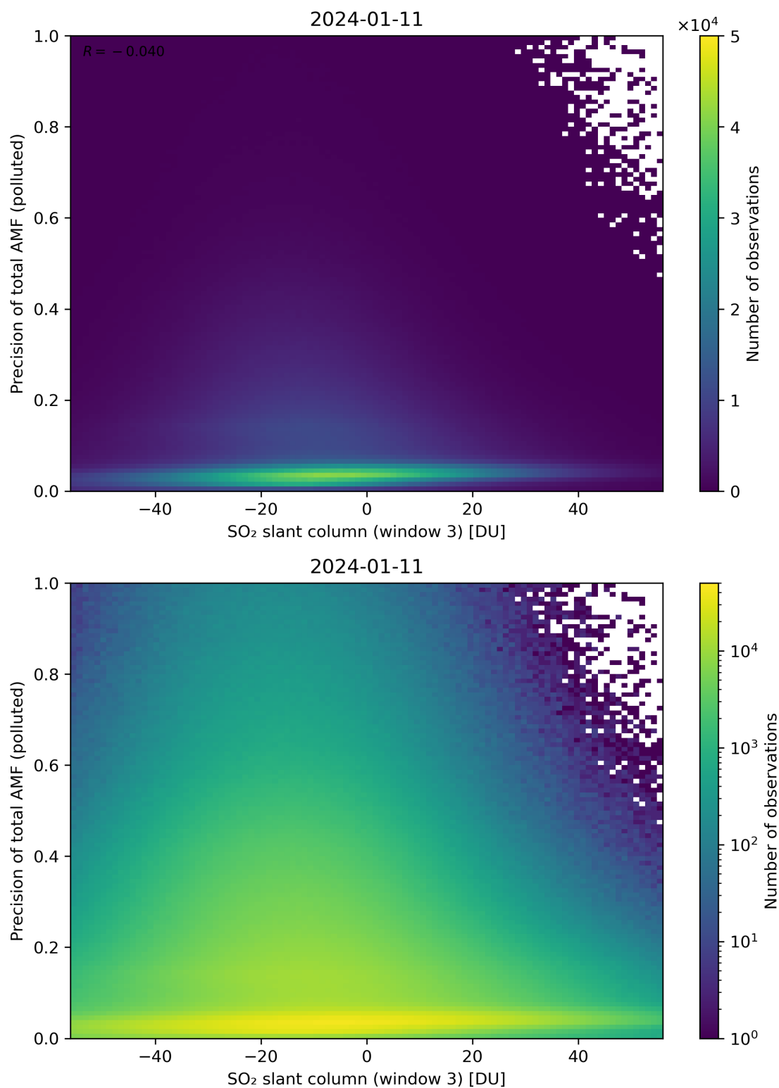
Figure 269: Scatter density plot of “SO 2 slant column (window 3)” against “Precision of total AMF (polluted)” for 2024-01-10 to 2024-01-12.
