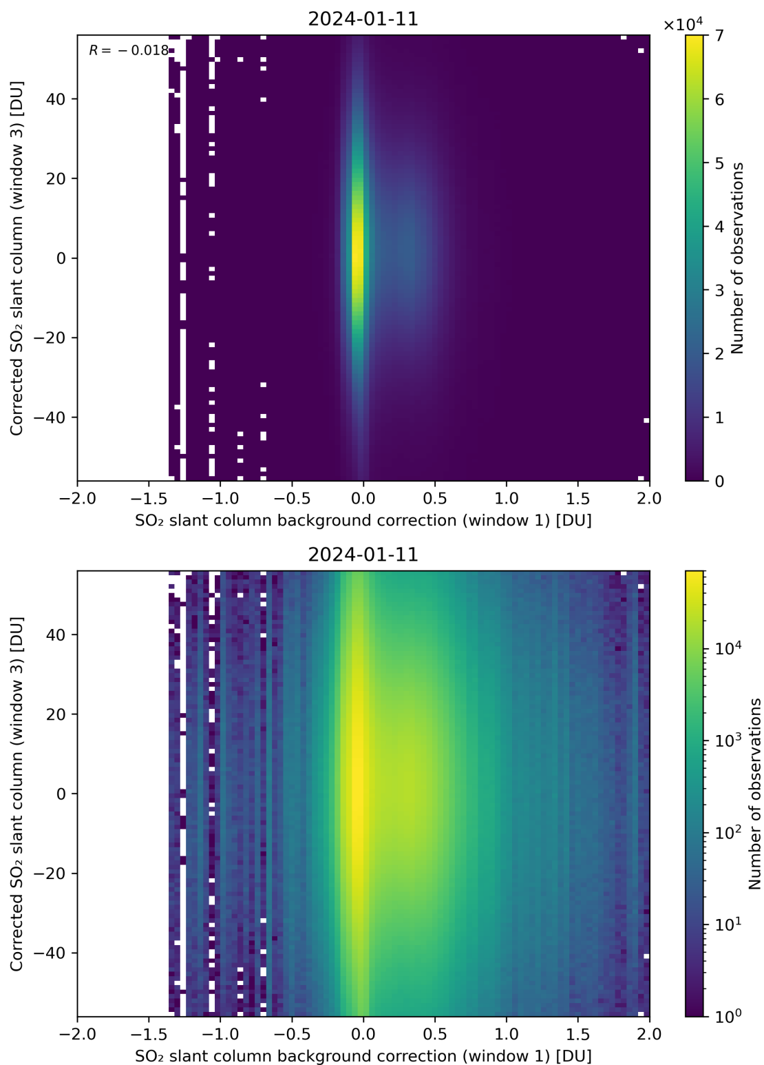
Figure 105: Scatter density plot of “SO 2 slant column background correction (window 1)” against “Corrected SO 2 slant column (window 3)” for 2024-01-10 to 2024-01-12.
