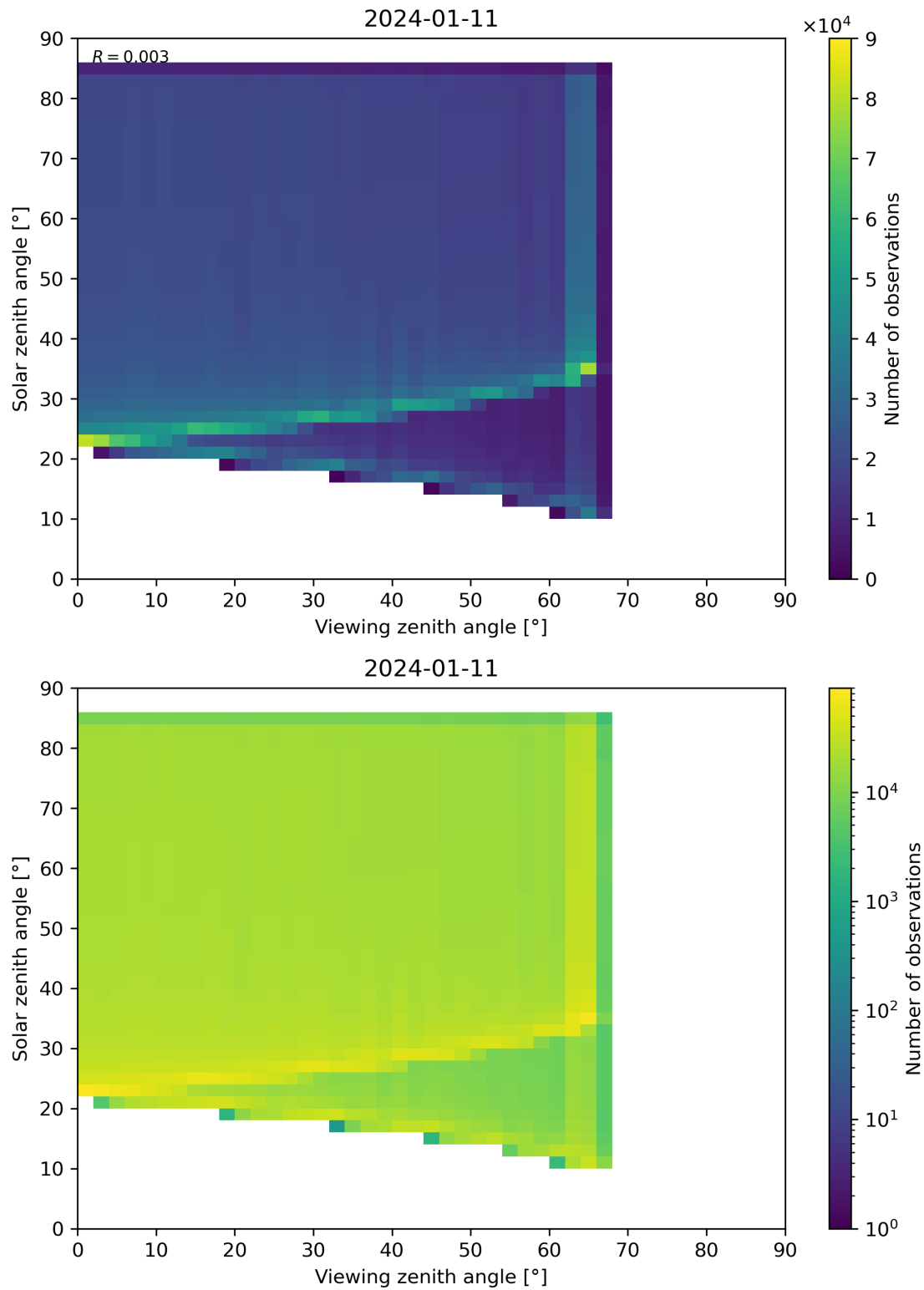
Figure 315: Scatter density plot of “Viewing zenith angle” against “Solar zenith angle” for 2024-01-10 to 2024-01-12.
