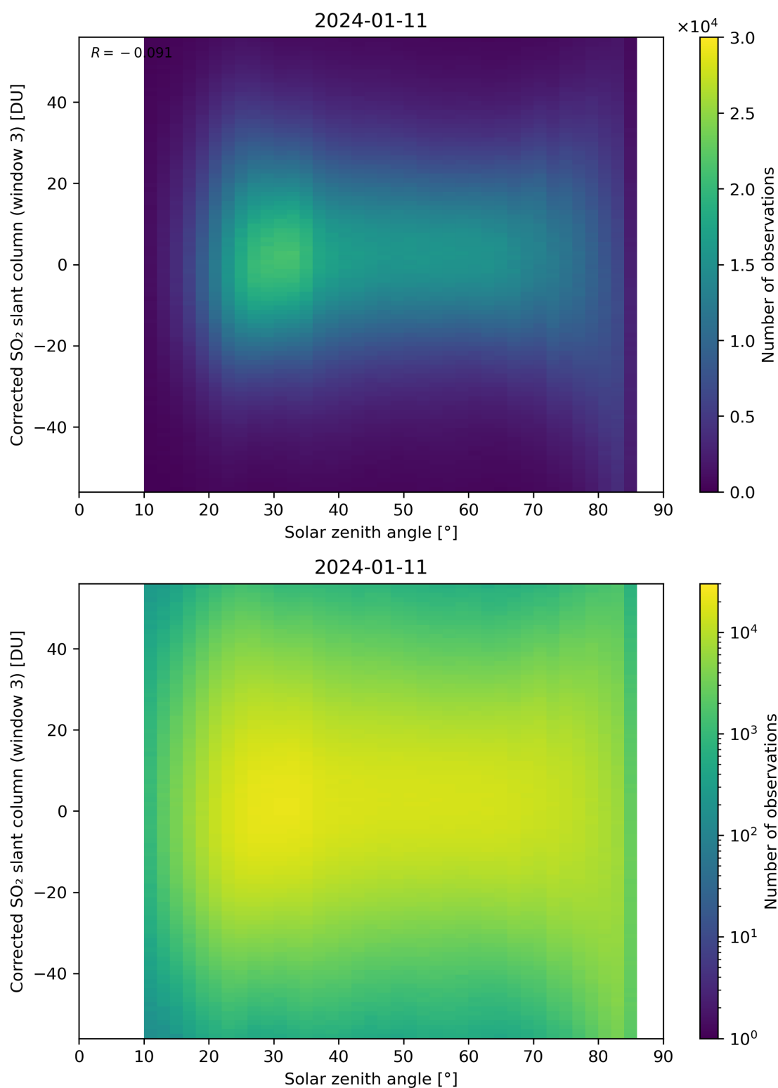
Figure 168: Scatter density plot of “Solar zenith angle” against “Corrected SO 2 slant column (window 3)” for 2024-01-10 to 2024-01-12.
