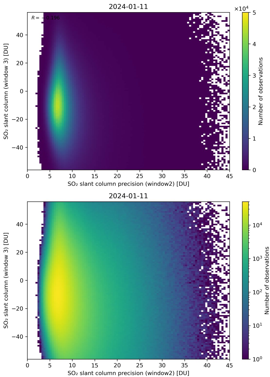
Figure 249: Scatter density plot of “SO 2 slant column precision (window2)” against “SO 2 slant column (window 3)” for 2024-01-10 to 2024-01-12.
