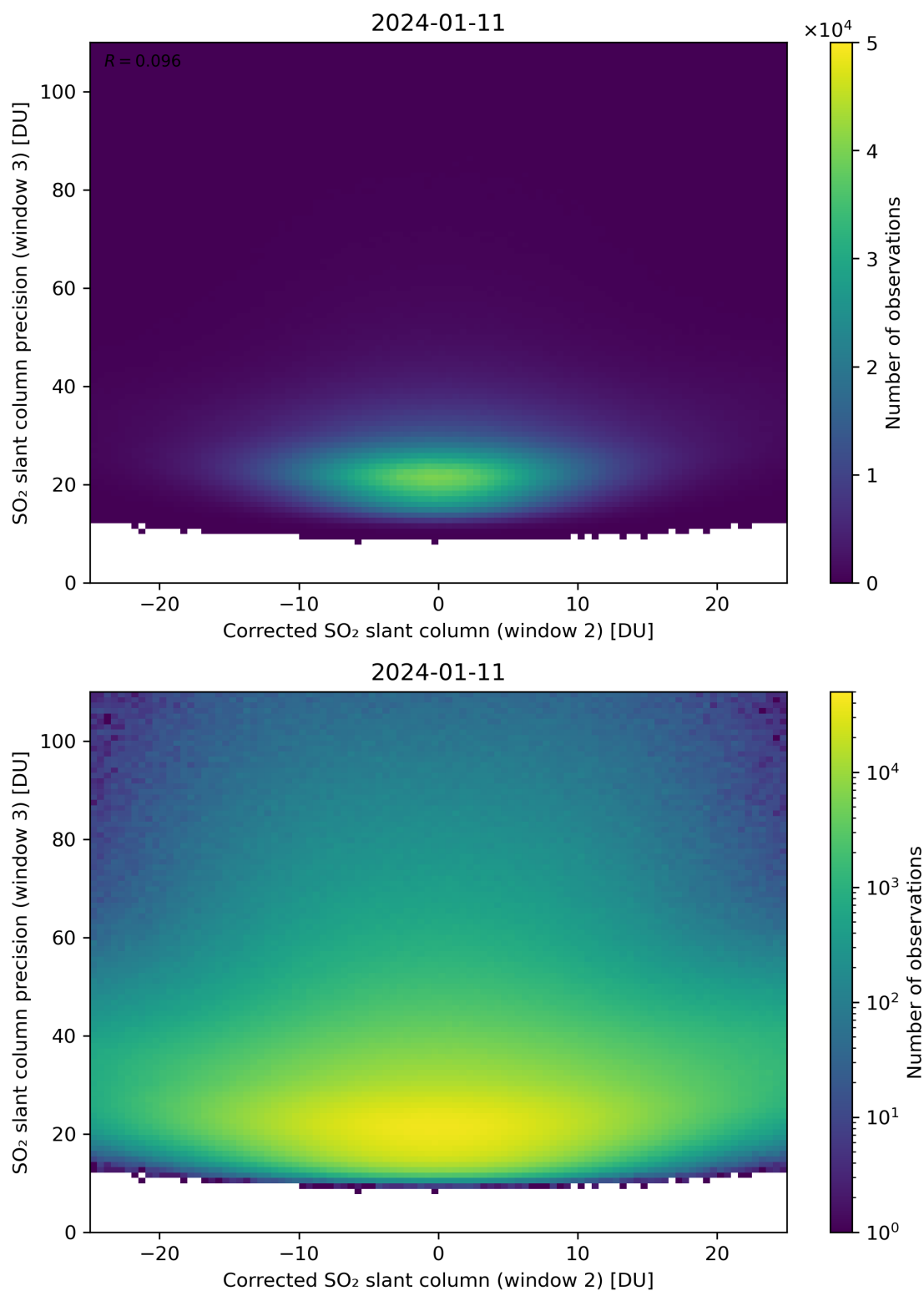
Figure 202: Scatter density plot of “Corrected SO 2 slant column (window 2)” against “SO 2 slant column precision (window 3)” for 2024-01-10 to 2024-01-12.
