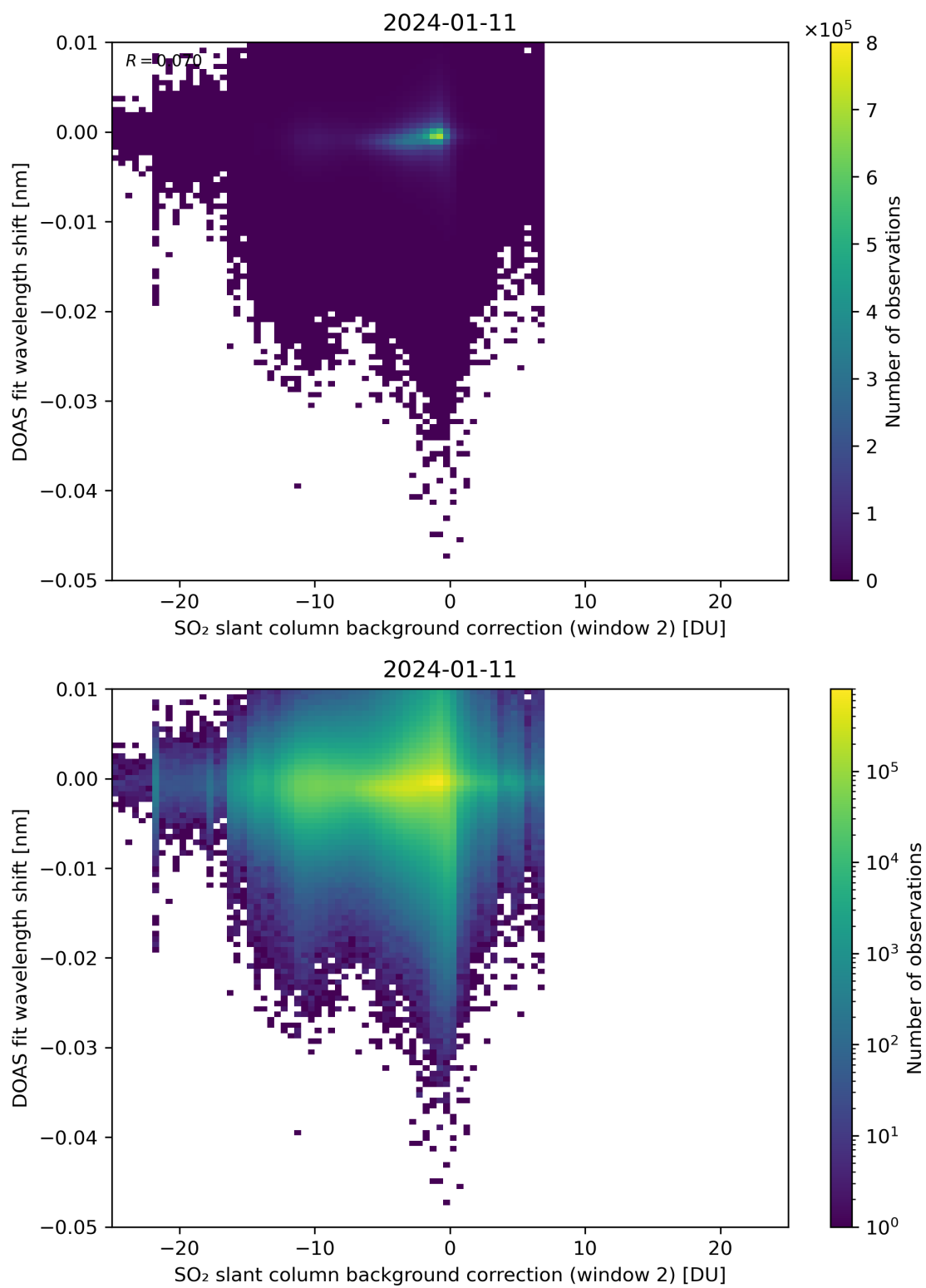
Figure 112: Scatter density plot of “SO 2 slant column background correction (window 2)” against “DOAS fit wavelength shift” for 2024-01-10 to 2024-01-12.
