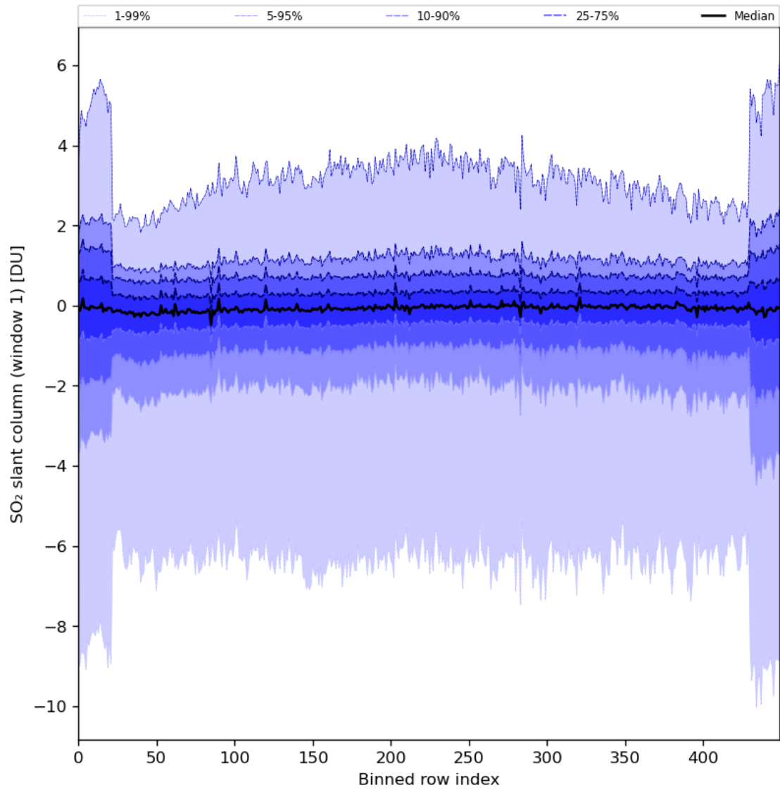
Figure 79: Along track statistics of “SO 2 slant column (window 1)” for 2024-01-10 to 2024-01-12
