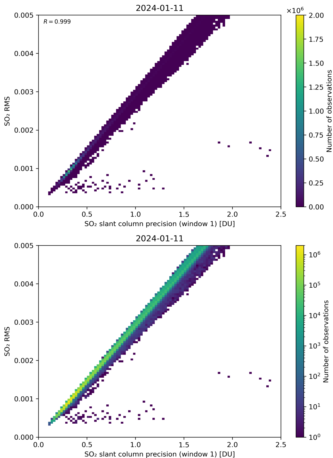
Figure 223: Scatter density plot of “SO 2 slant column precision (window 1)” against “SO 2 RMS” for 2024-01-10 to 2024-01-12.
