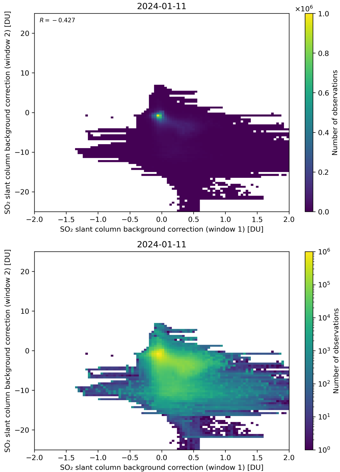
Figure 98: Scatter density plot of “SO 2 slant column background correction (window 1)” against “SO 2 slant column background correction (window 2)” for 2024-01-10 to 2024-01-12.
