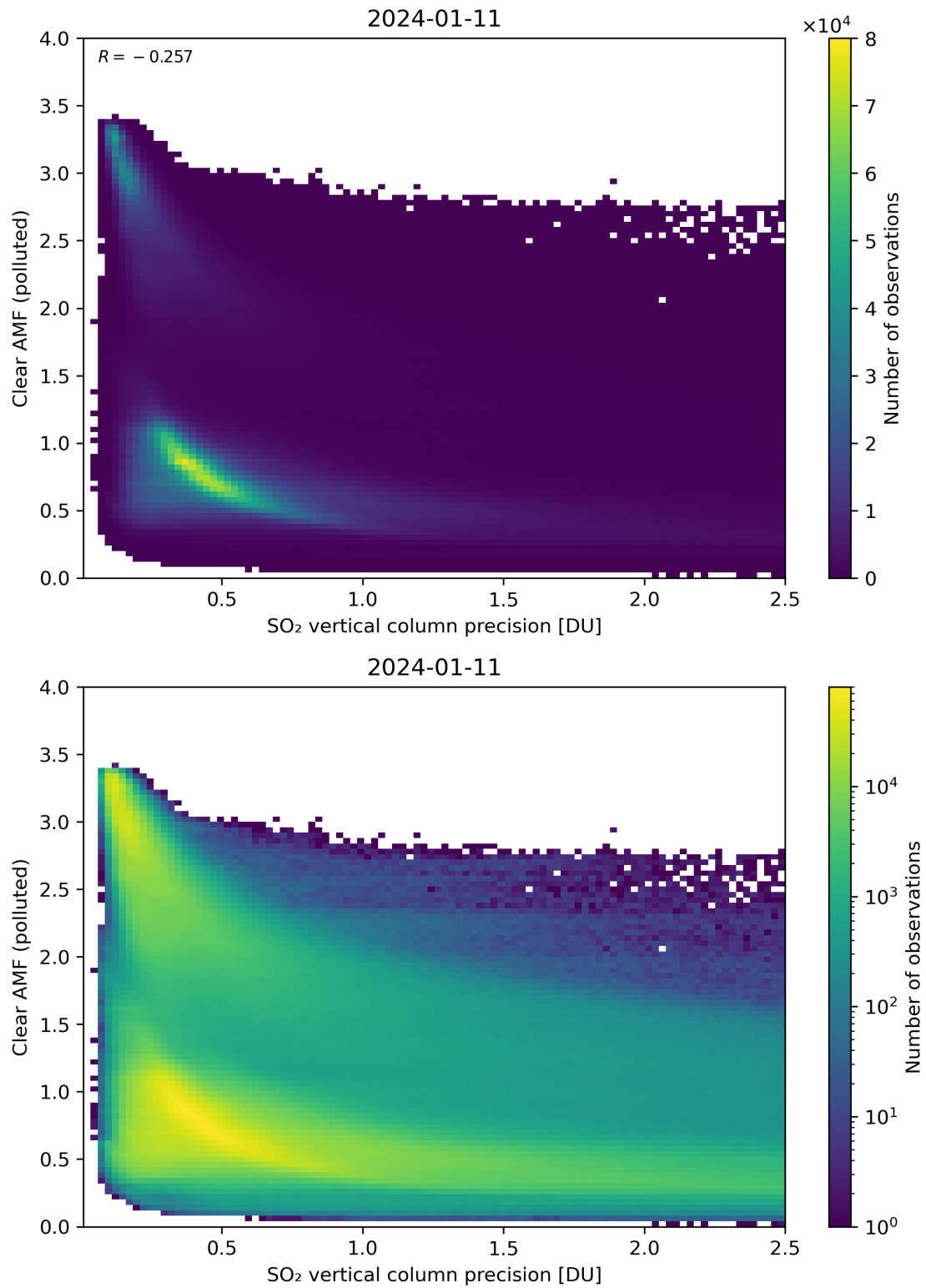
Figure 285: Scatter density plot of “SO 2 vertical column precision” against “Clear AMF (polluted)” for 2024-01-10 to 2024-01-12.
