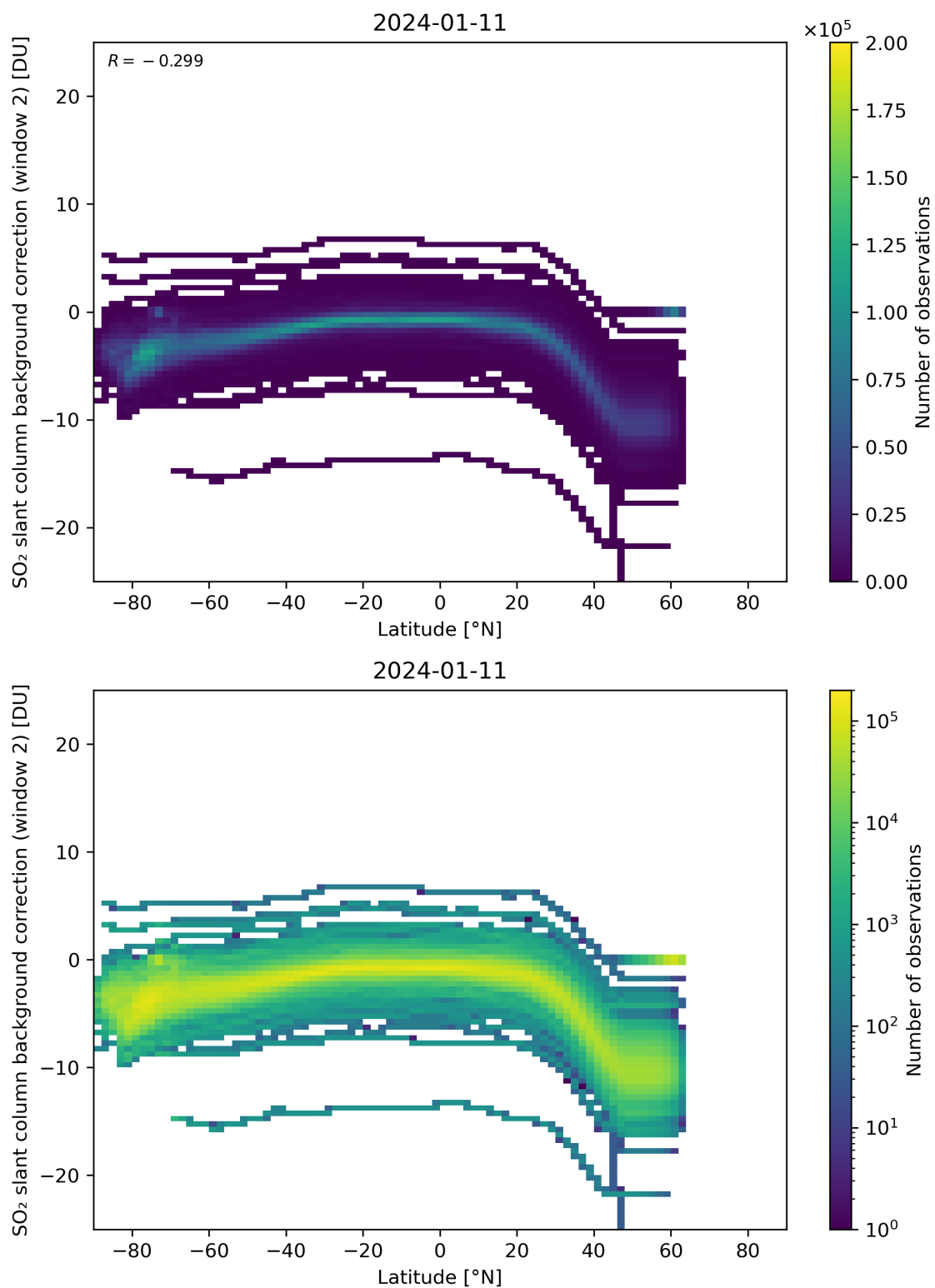
Figure 140: Scatter density plot of “Latitude” against “SO 2 slant column background correction (window 2)” for 2024-01-10 to 2024-01-12.
