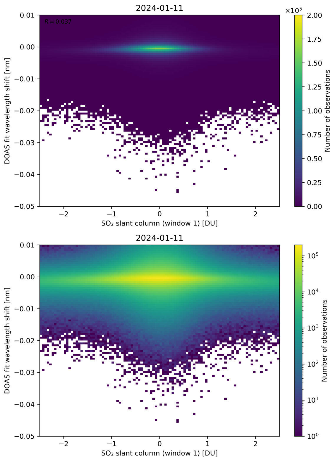
Figure 215: Scatter density plot of “SO 2 slant column (window 1)” against “DOAS fit wavelength shift” for 2024-01-10 to 2024-01-12.
