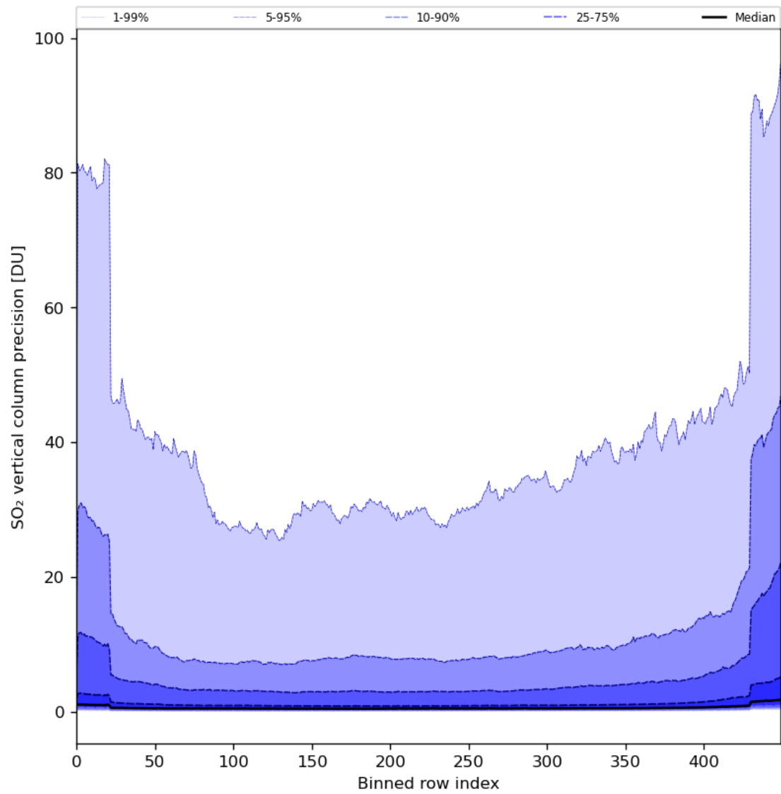
Figure 77: Along track statistics of “SO 2 vertical column precision” for 2024-01-10 to 2024-01-12
