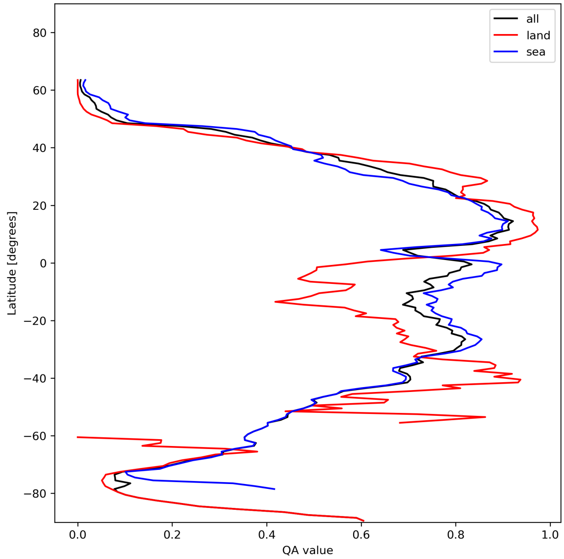
Figure 29: Zonal average of “QA value” for 2024-01-10 to 2024-01-12.
