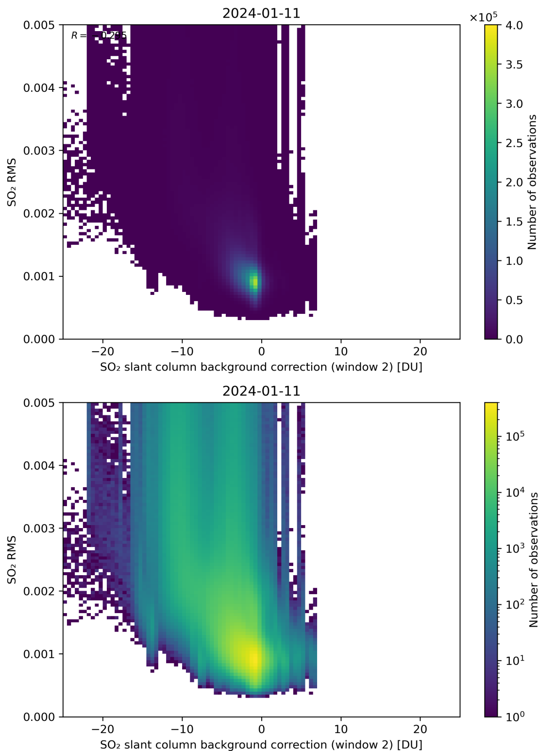
Figure 114: Scatter density plot of “SO 2 slant column background correction (window 2)” against “SO 2 RMS” for 2024-01-10 to 2024-01-12.
