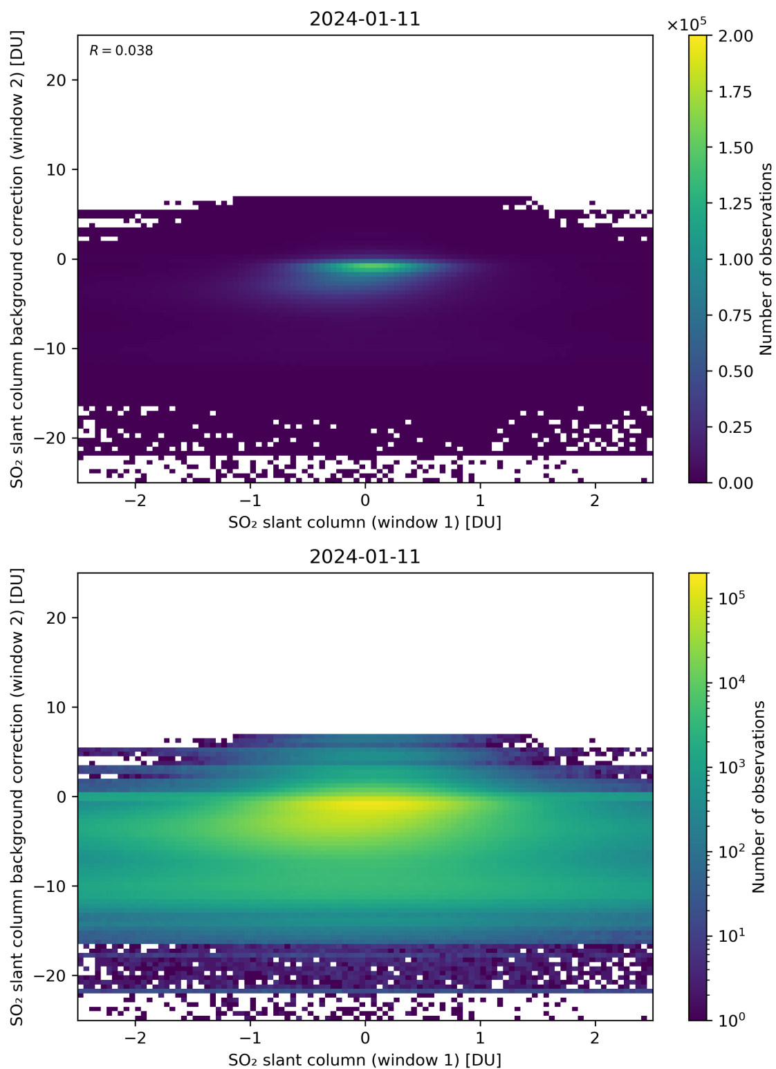
Figure 213: Scatter density plot of “SO 2 slant column (window 1)” against “SO 2 slant column background correction (window 2)” for 2024-01-10 to 2024-01-12.
