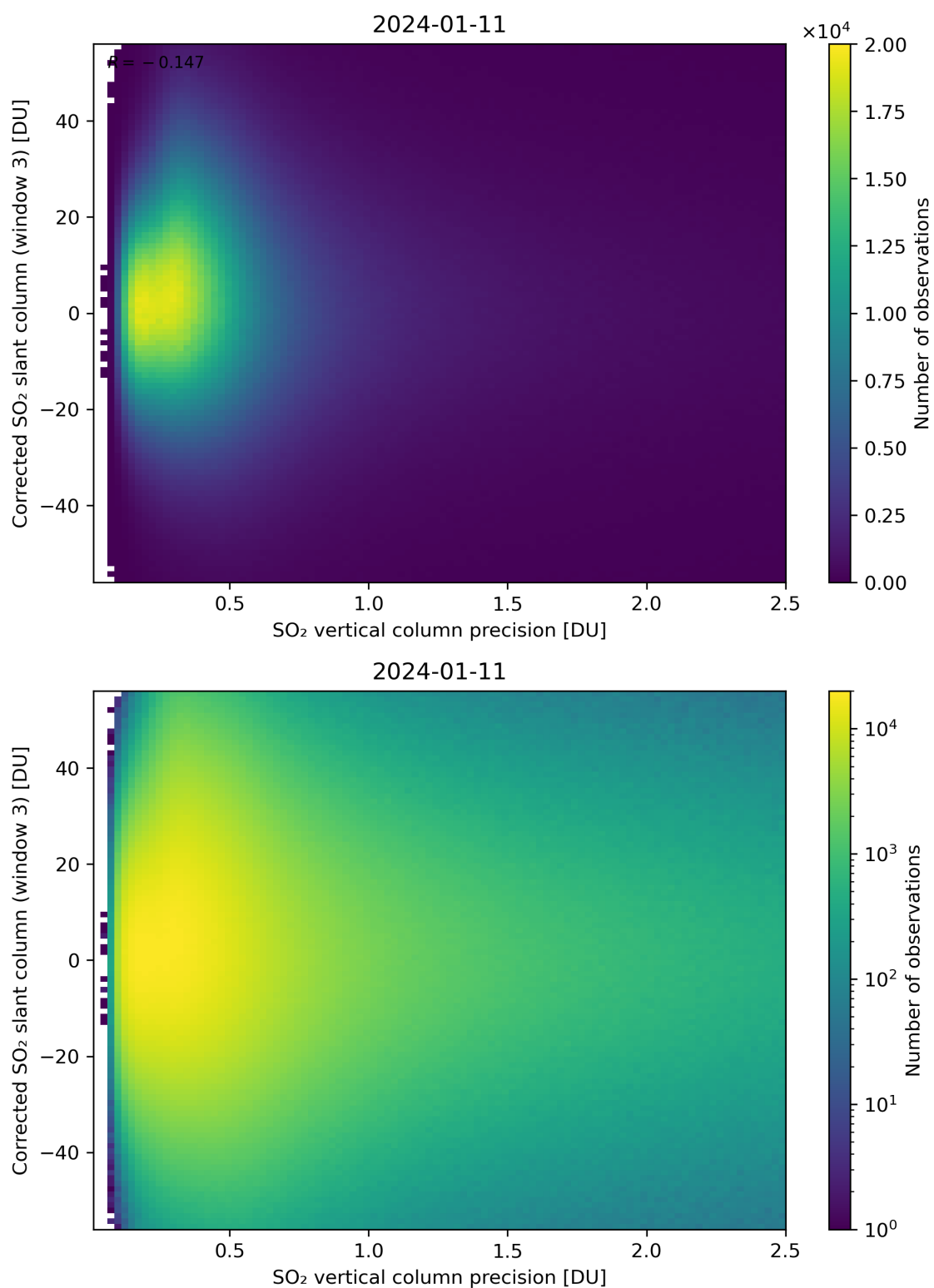
Figure 288: Scatter density plot of “SO 2 vertical column precision” against “Corrected SO 2 slant column (window 3)” for 2024-01-10 to 2024-01-12.
