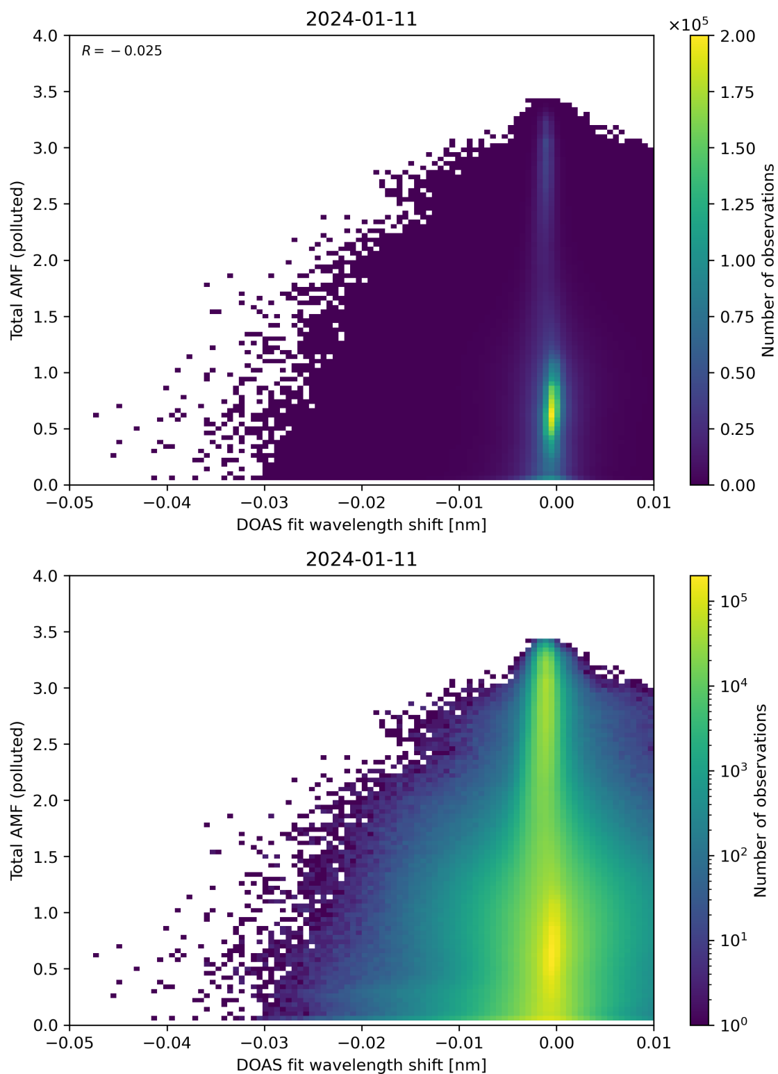
Figure 130: Scatter density plot of “DOAS fit wavelength shift” against “Total AMF (polluted)” for 2024-01-10 to 2024-01-12.
