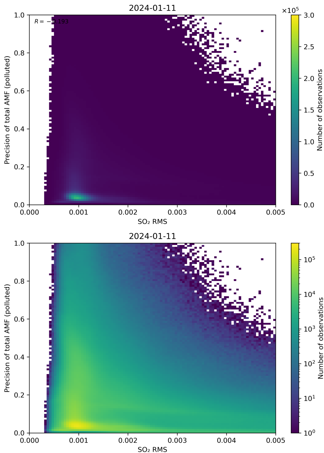
Figure 138: Scatter density plot of “SO 2 RMS” against “Precision of total AMF (polluted)” for 2024-01-10 to 2024-01-12.
