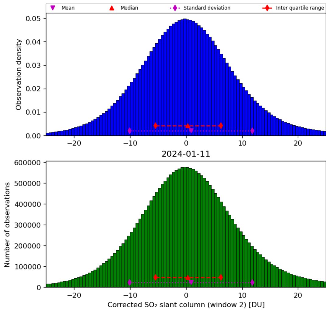
Figure 62: Histogram of “Corrected SO 2 slant column (window 2)” for 2024-01-10 to 2024-01-12
