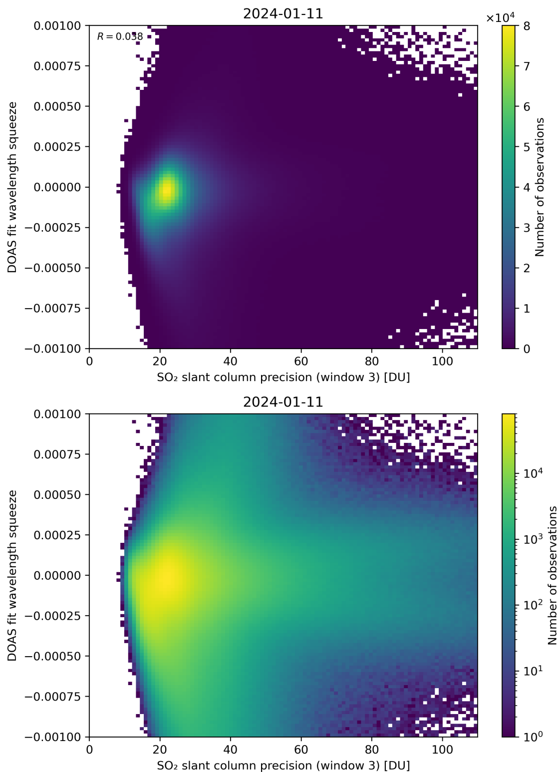
Figure 259: Scatter density plot of “SO 2 slant column precision (window 3)” against “DOAS fit wavelength squeeze” for 2024-01-10 to 2024-01-12.
