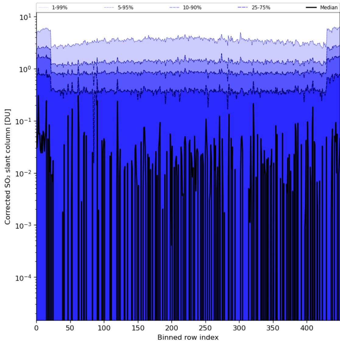
Figure 78: Along track statistics of “Corrected SO 2 slant column” for 2024-01-10 to 2024-01-12
