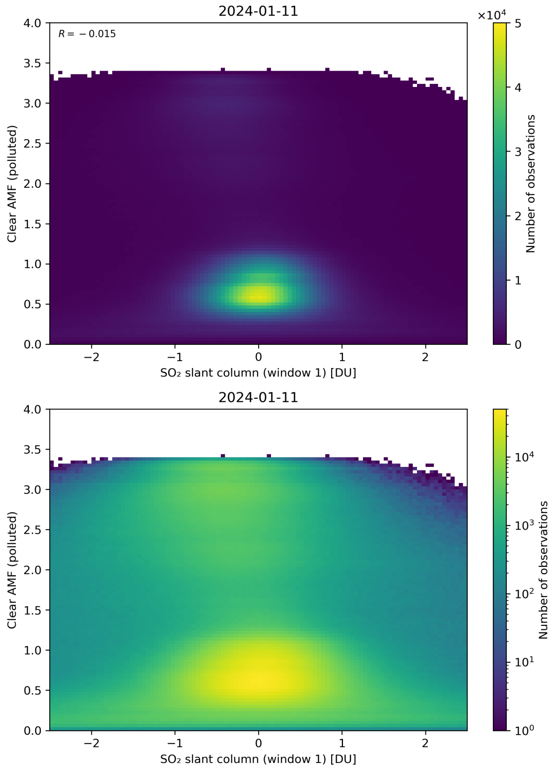
Figure 232: Scatter density plot of “SO 2 slant column (window 1)” against “Clear AMF (polluted)” for 2024-01-10 to 2024-01-12.
