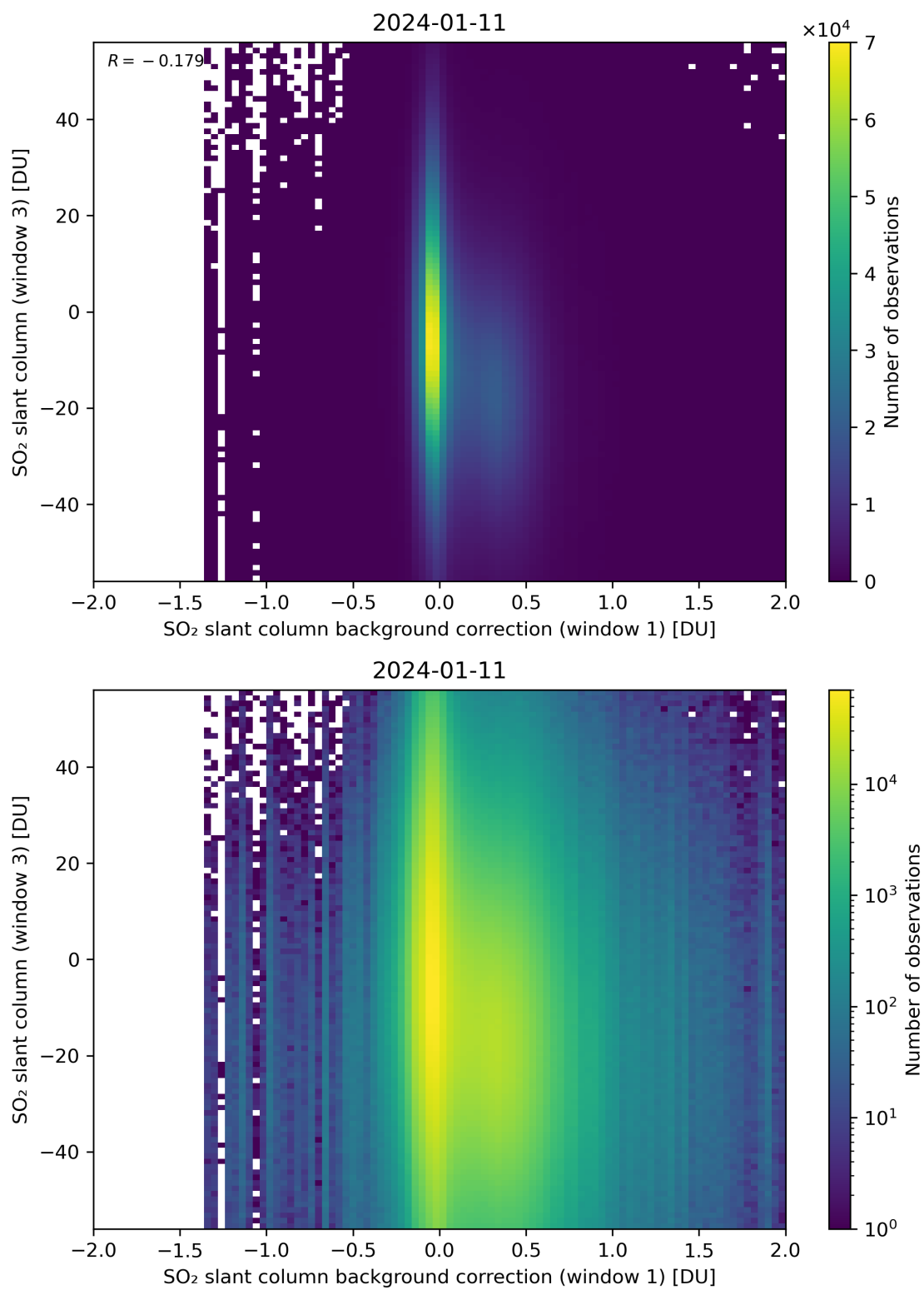
Figure 107: Scatter density plot of “SO 2 slant column background correction (window 1)” against “SO 2 slant column (window 3)” for 2024-01-10 to 2024-01-12.
