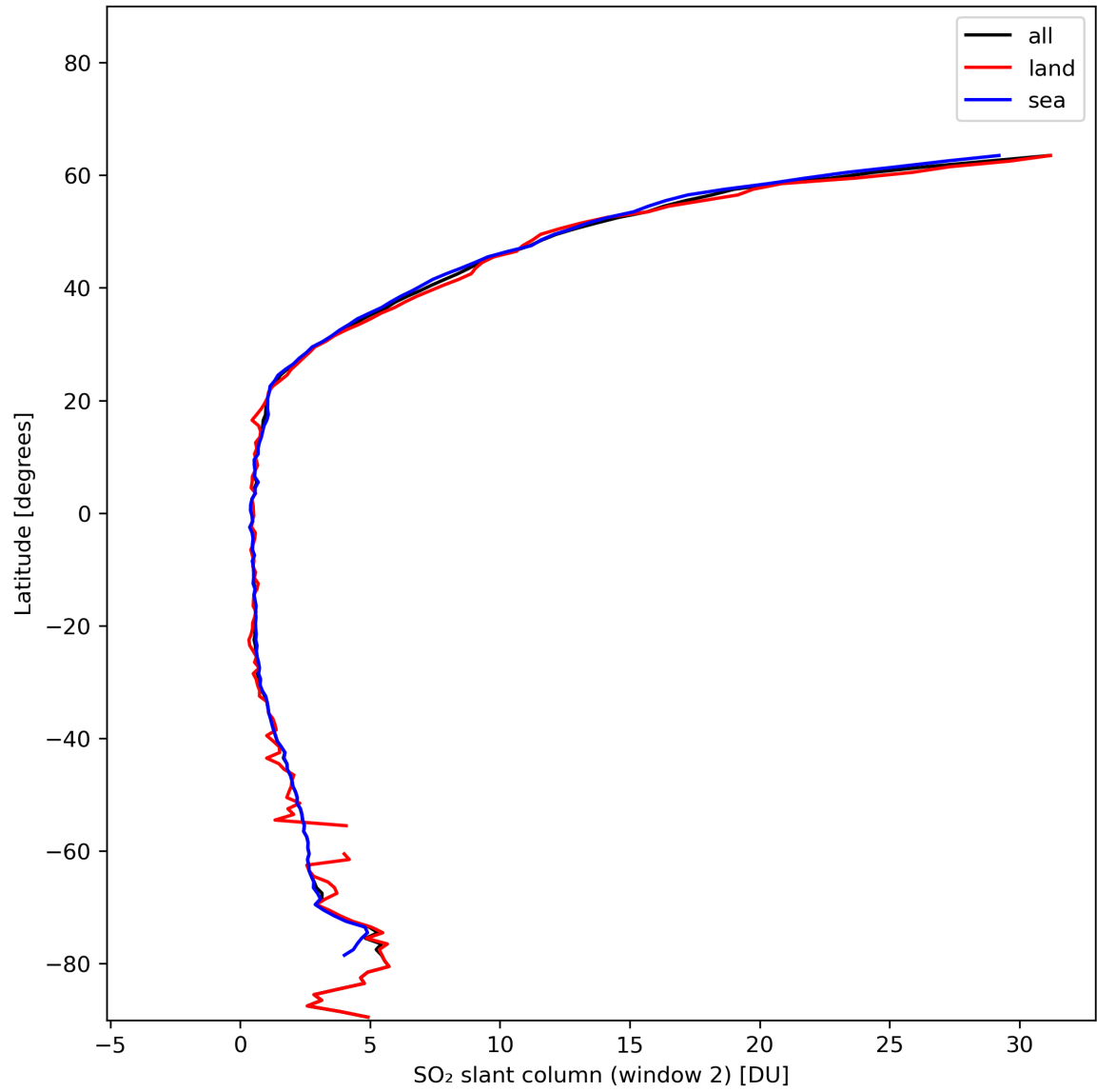
Figure 37: Zonal average of “SO 2 slant column (window 2)” for 2024-01-10 to 2024-01-12.
