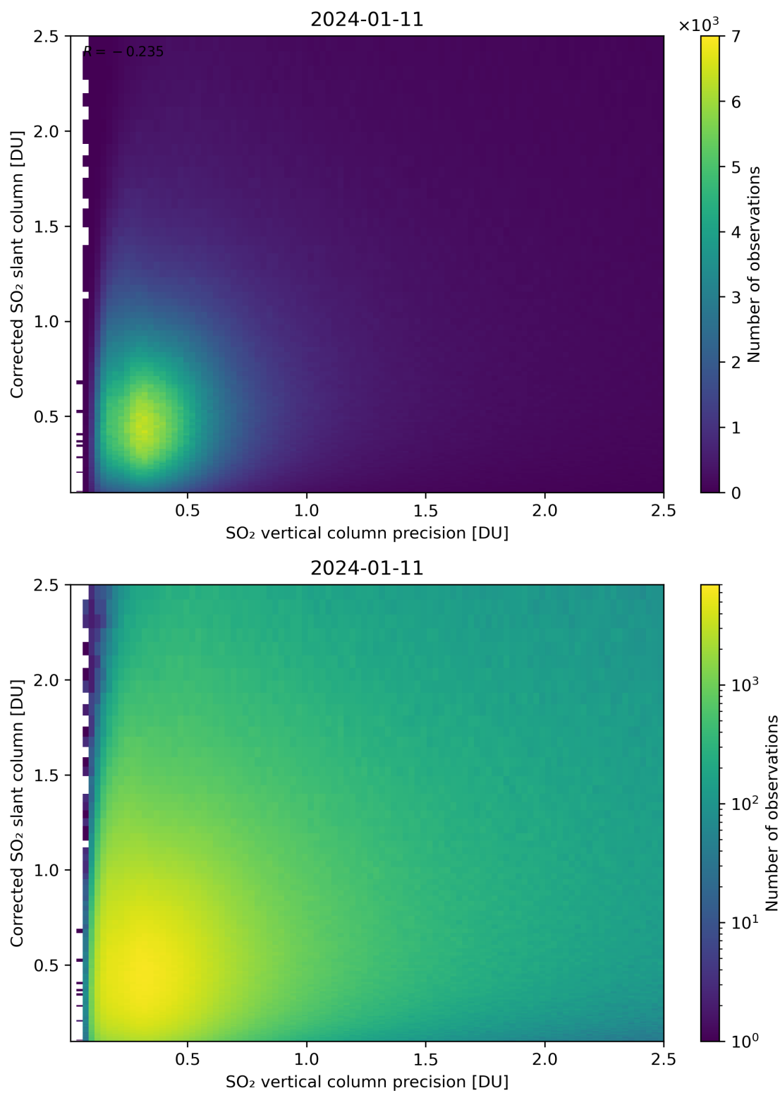
Figure 286: Scatter density plot of “SO 2 vertical column precision” against “Corrected SO 2 slant column” for 2024-01-10 to 2024-01-12.
