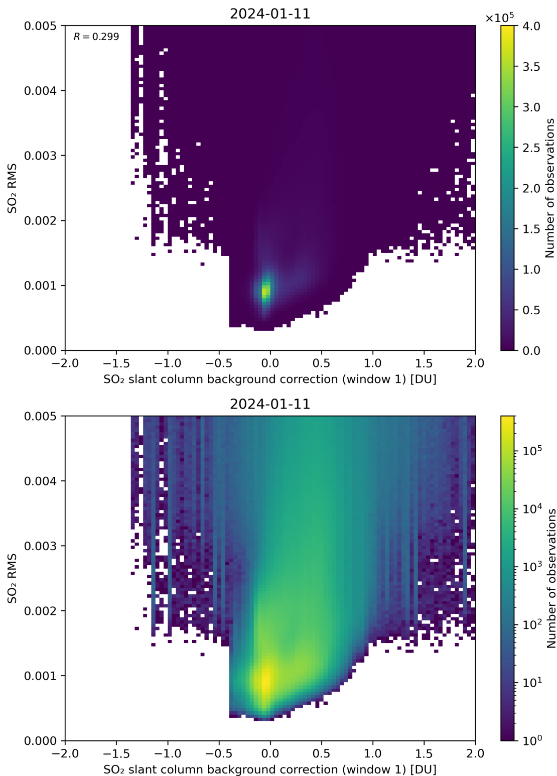
Figure 102: Scatter density plot of “SO 2 slant column background correction (window 1)” against “SO 2 RMS” for 2024-01-10 to 2024-01-12.
