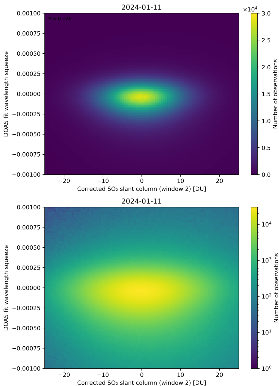
Figure 197: Scatter density plot of “Corrected SO 2 slant column (window 2)” against “DOAS fit wavelength squeeze” for 2024-01-10 to 2024-01-12.
