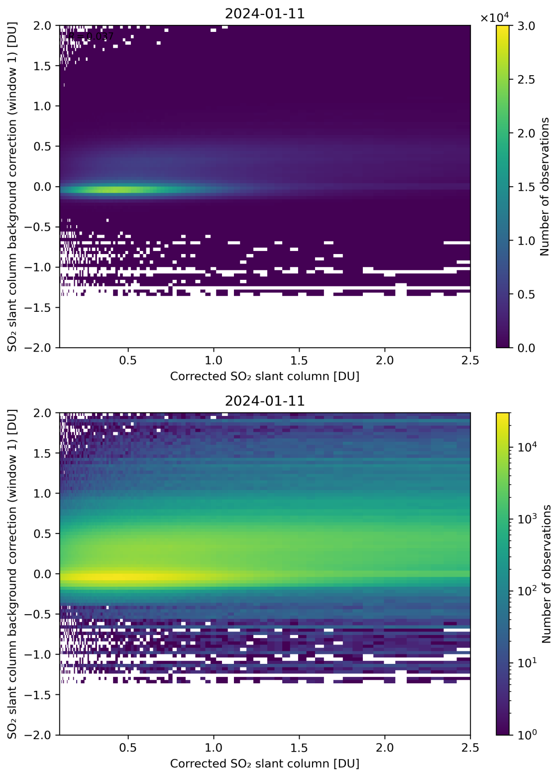
Figure 178: Scatter density plot of “Corrected SO 2 slant column” against “SO 2 slant column background correction (window 1)” for 2024-01-10 to 2024-01-12.
