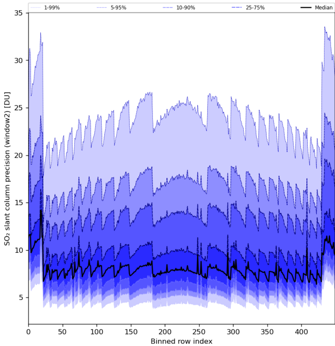
Figure 84: Along track statistics of “SO 2 slant column precision (window2)” for 2024-01-10 to 2024-01-12
