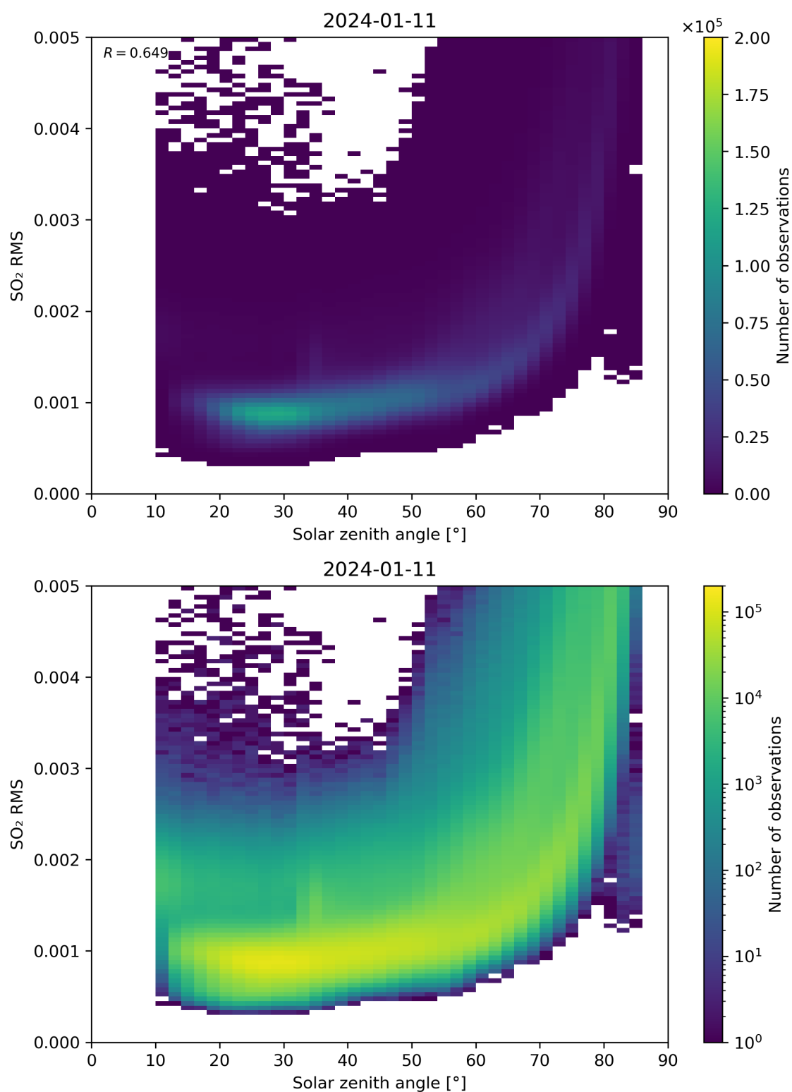
Figure 163: Scatter density plot of “Solar zenith angle” against “SO 2 RMS” for 2024-01-10 to 2024-01-12.
