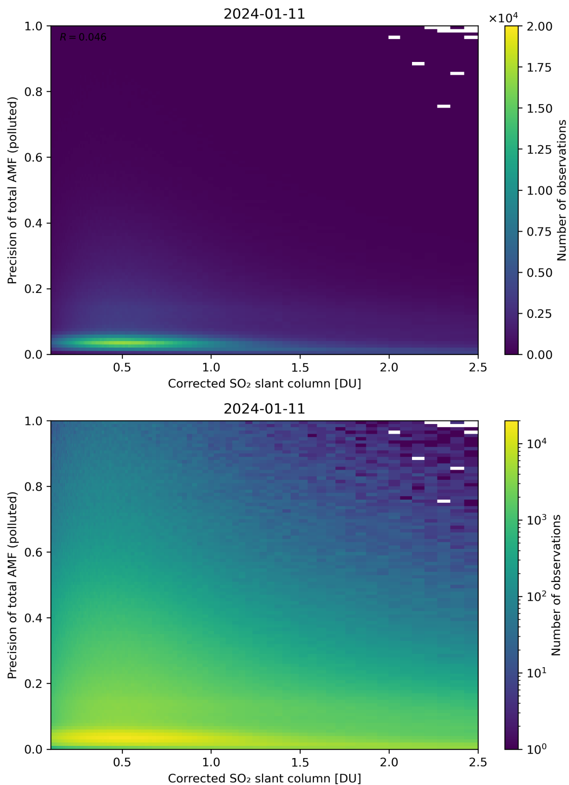
Figure 193: Scatter density plot of “Corrected SO 2 slant column” against “Precision of total AMF (polluted)” for 2024-01-10 to 2024-01-12.
