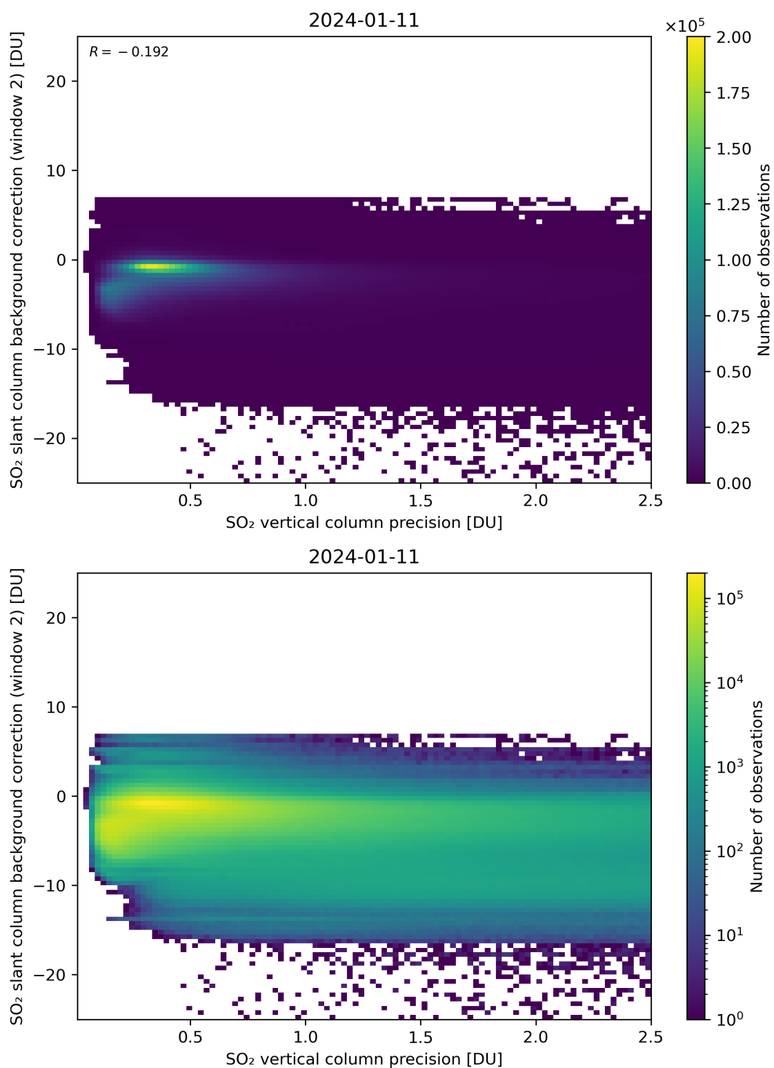
Figure 280: Scatter density plot of “SO 2 vertical column precision” against “SO 2 slant column background correction (window 2)” for 2024-01-10 to 2024-01-12.
