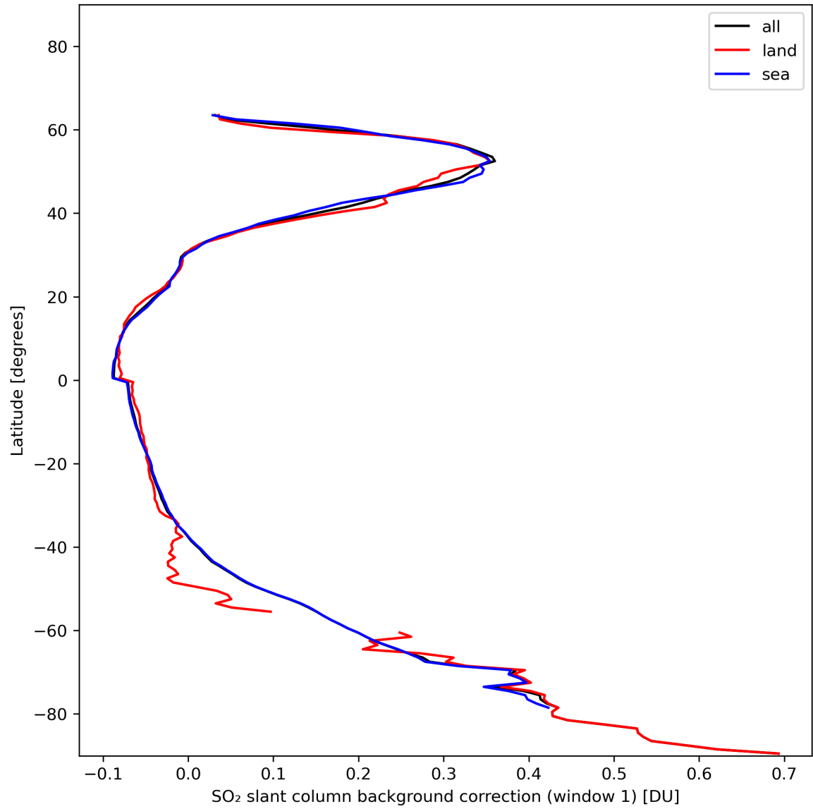
Figure 36: Zonal average of “SO 2 slant column background correction (window 1)” for 2024-01-10 to 2024-01-12.
