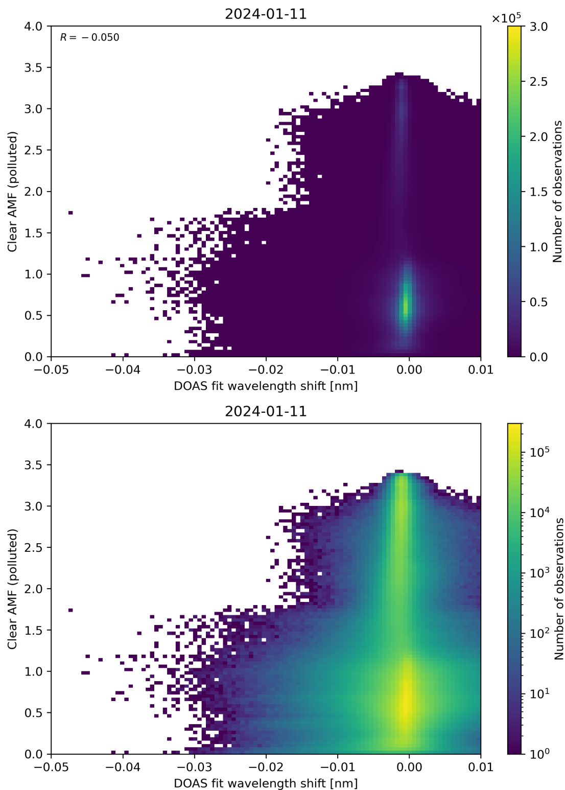
Figure 129: Scatter density plot of “DOAS fit wavelength shift” against “Clear AMF (polluted)” for 2024-01-10 to 2024-01-12.
