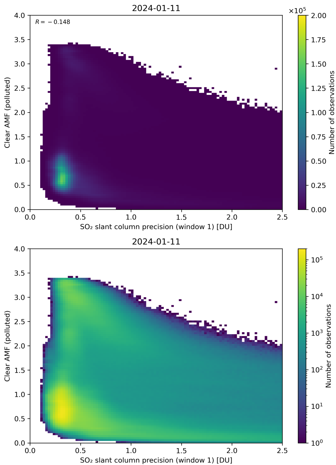
Figure 224: Scatter density plot of “SO 2 slant column precision (window 1)” against “Clear AMF (polluted)” for 2024-01-10 to 2024-01-12.
