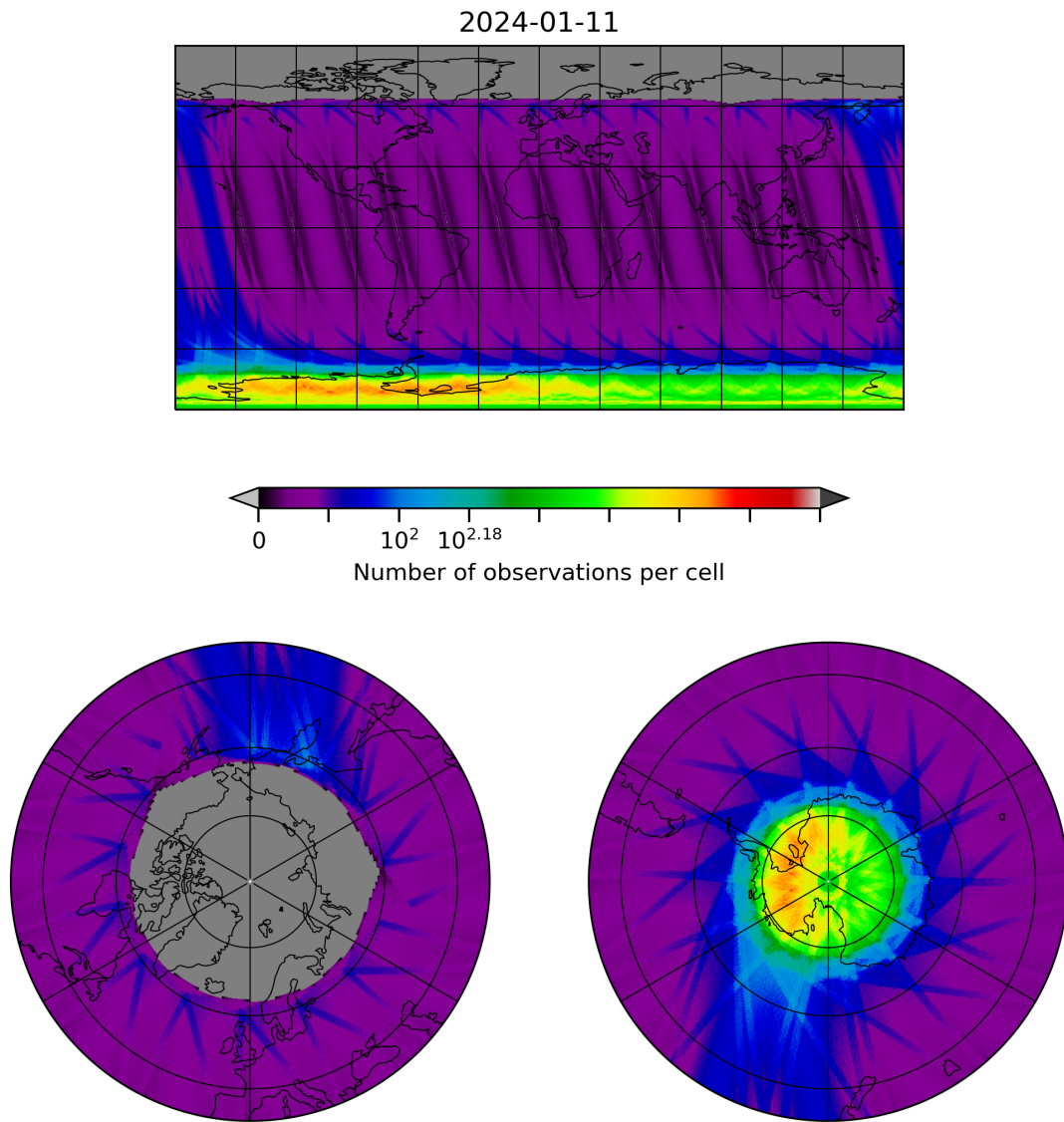
Figure 28: Map of the number of observations for 2024-01-10 to 2024-01-12
