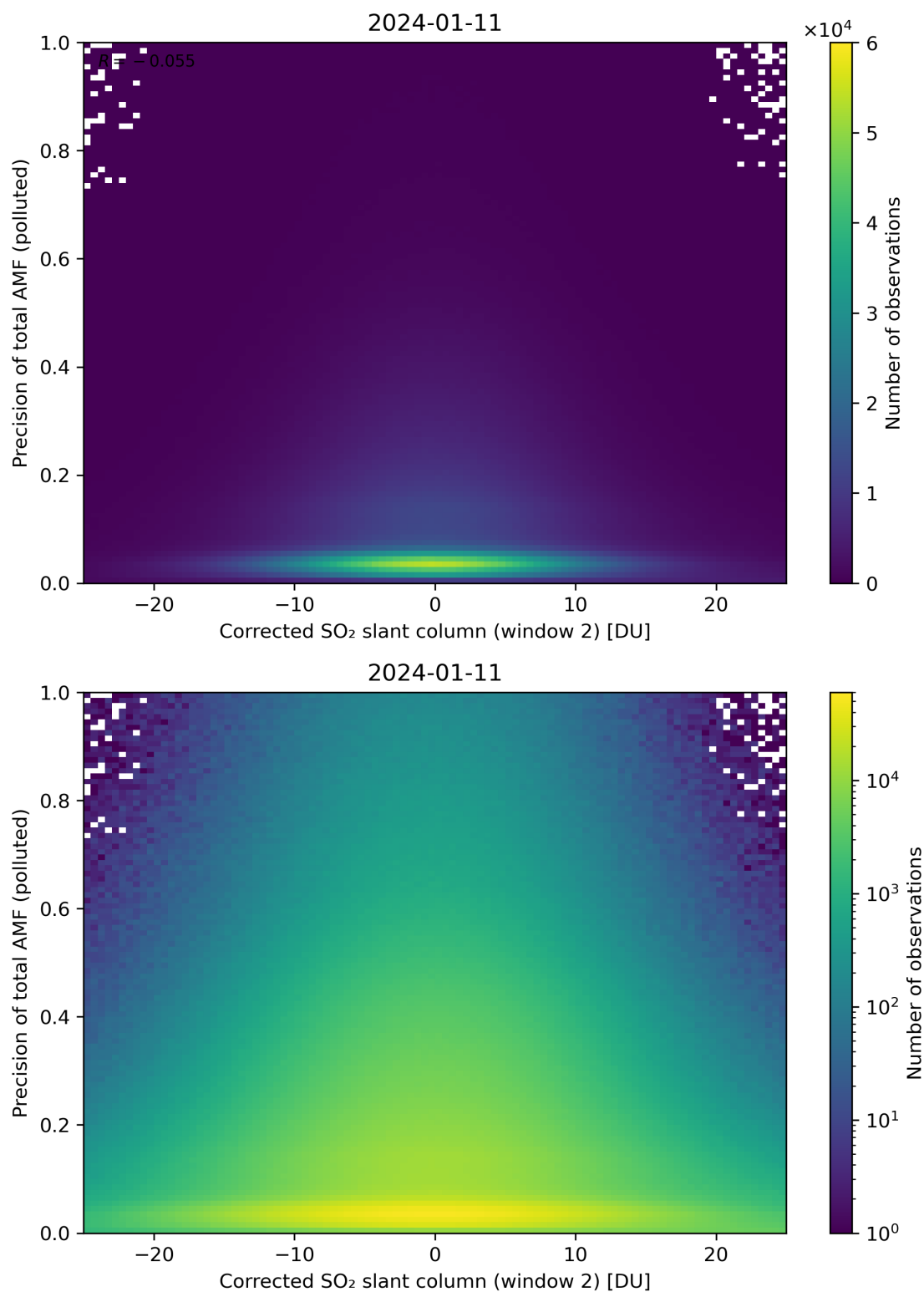
Figure 204: Scatter density plot of “Corrected SO 2 slant column (window 2)” against “Precision of total AMF (polluted)” for 2024-01-10 to 2024-01-12.
