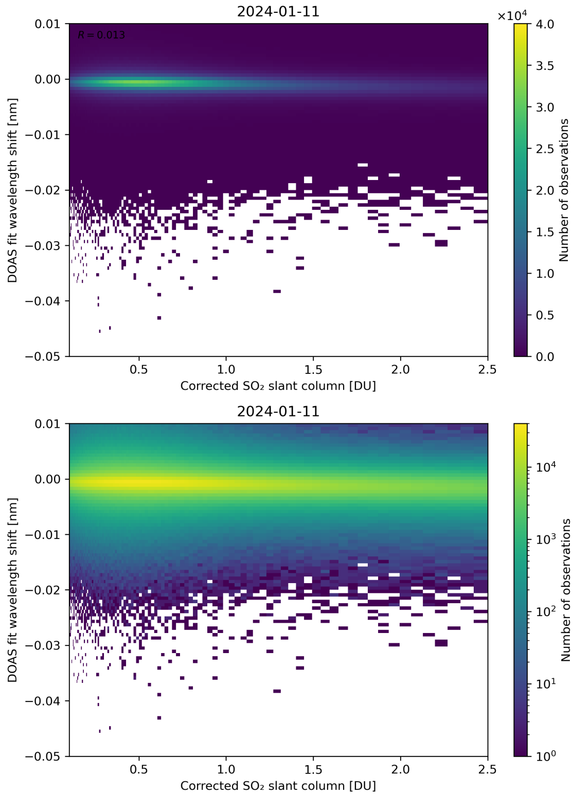
Figure 181: Scatter density plot of “Corrected SO 2 slant column” against “DOAS fit wavelength shift” for 2024-01-10 to 2024-01-12.
