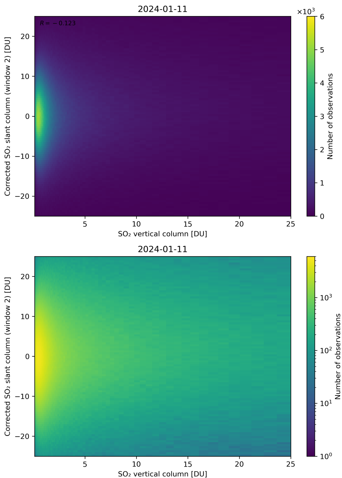
Figure 298: Scatter density plot of “SO 2 vertical column” against “Corrected SO 2 slant column (window 2)” for 2024-01-10 to 2024-01-12.
