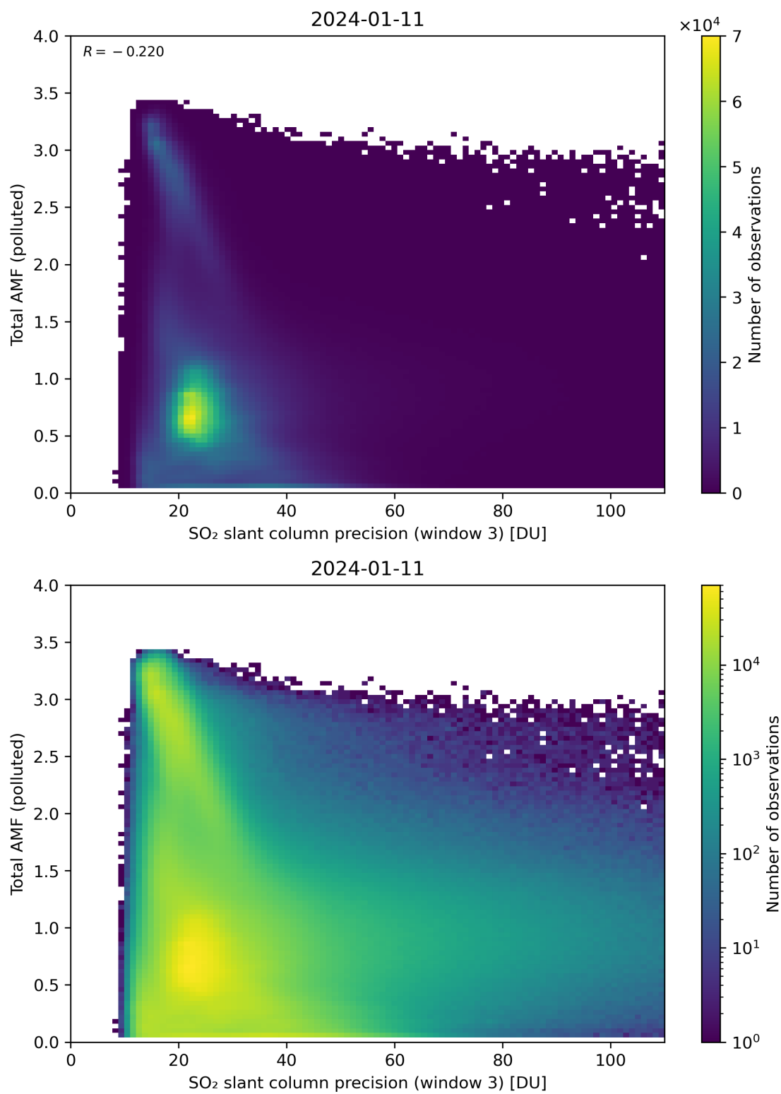
Figure 263: Scatter density plot of “SO 2 slant column precision (window 3)” against “Total AMF (polluted)” for 2024-01-10 to 2024-01-12.
