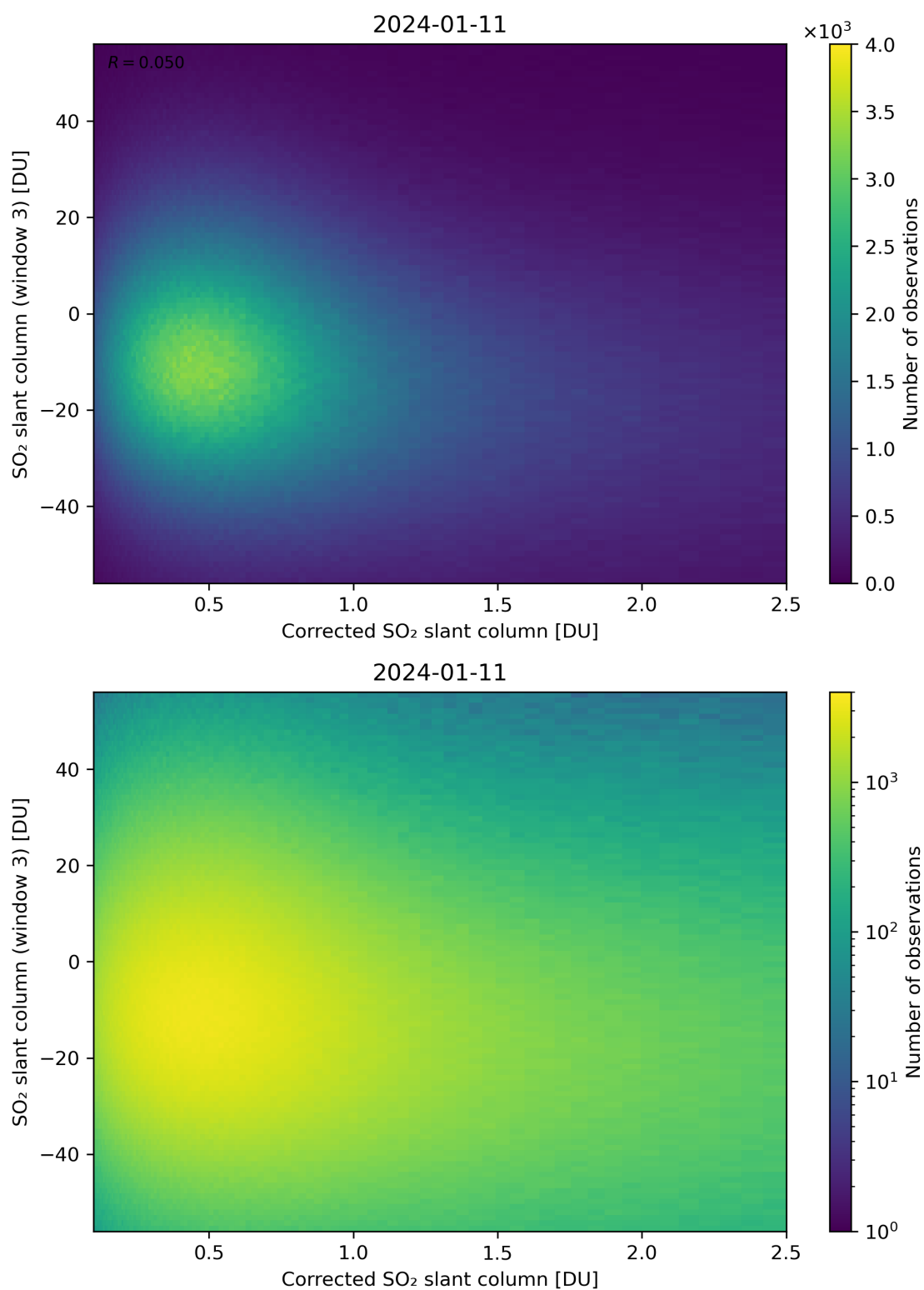
Figure 190: Scatter density plot of “Corrected SO 2 slant column” against “SO 2 slant column (window 3)” for 2024-01-10 to 2024-01-12.
