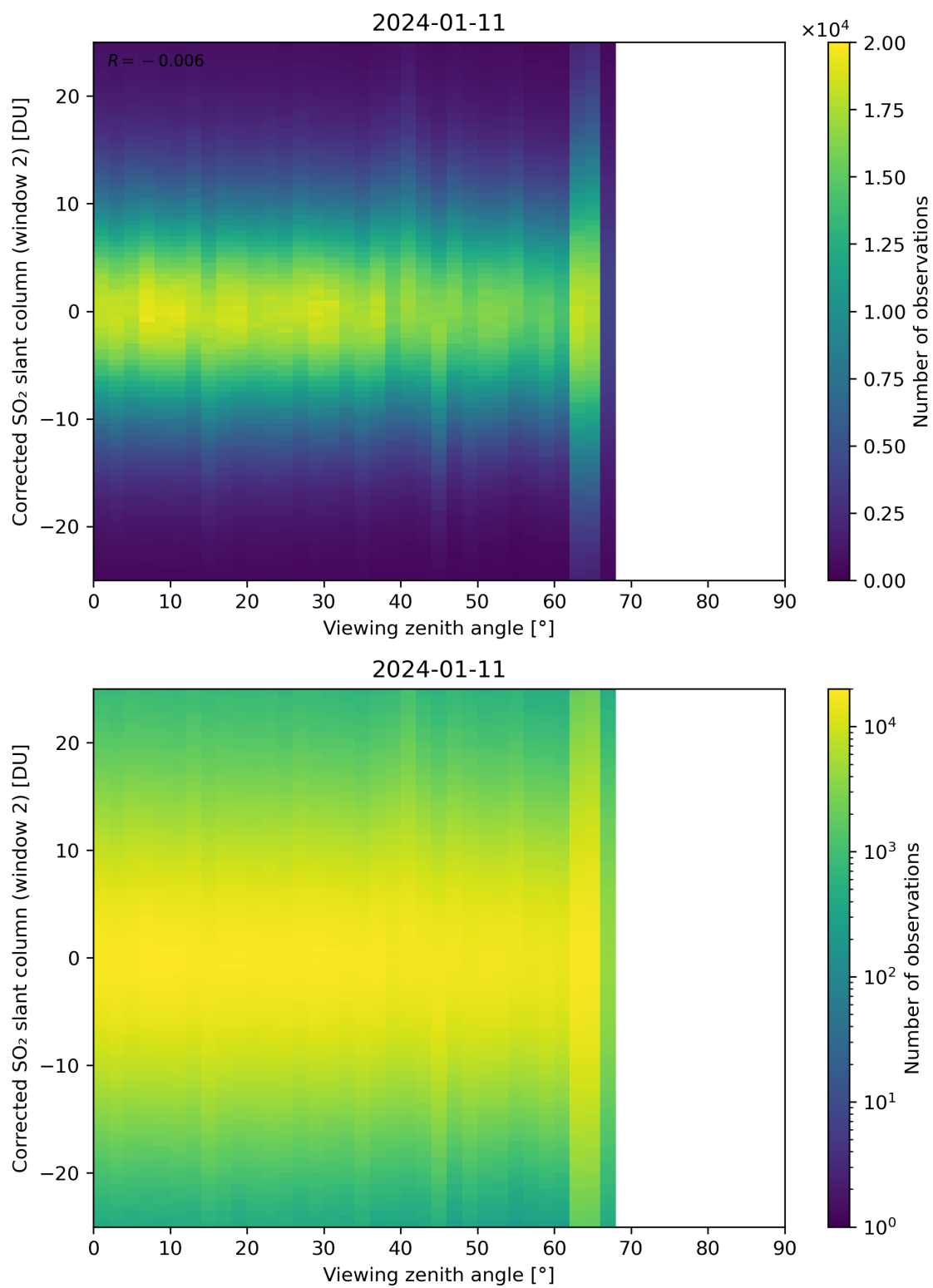
Figure 318: Scatter density plot of “Viewing zenith angle” against “Corrected SO 2 slant column (window 2)” for 2024-01-10 to 2024-01-12.
