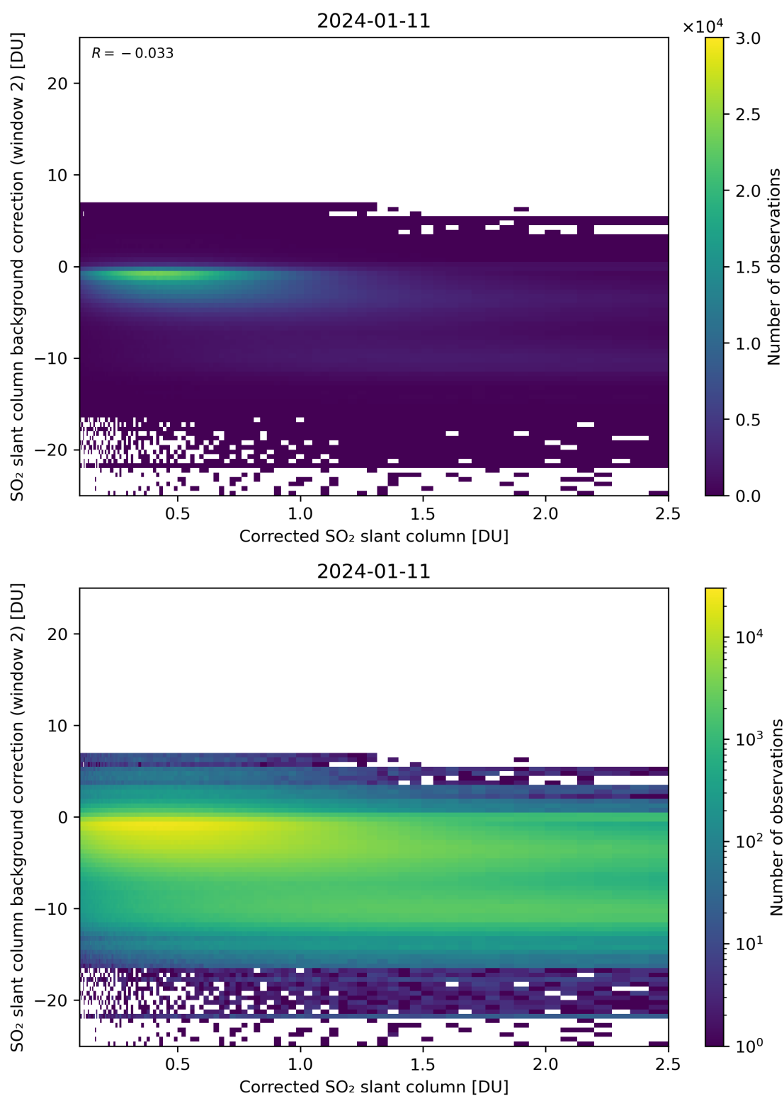
Figure 179: Scatter density plot of “Corrected SO 2 slant column” against “SO 2 slant column background correction (window 2)” for 2024-01-10 to 2024-01-12.
