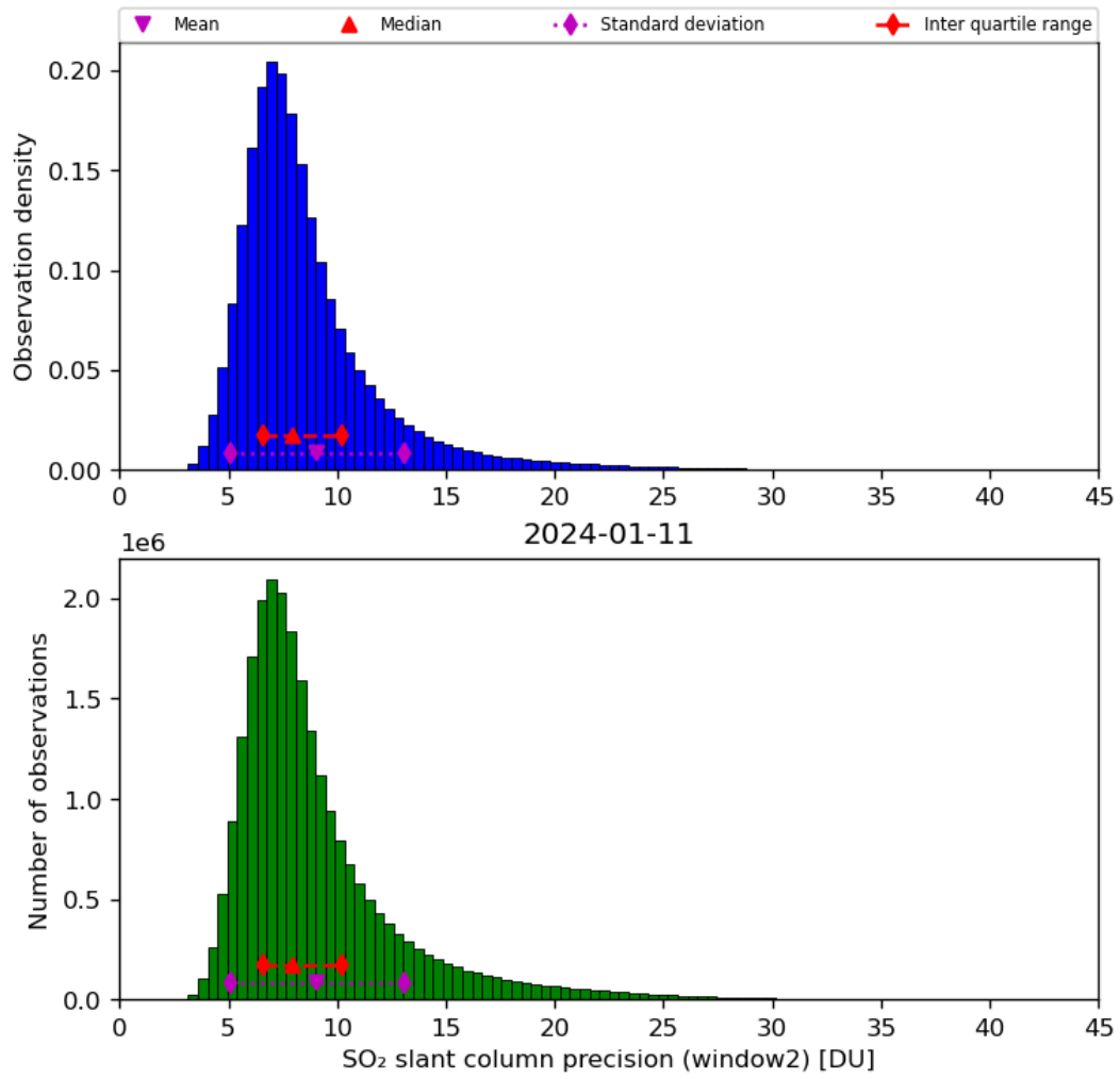
Figure 61: Histogram of “SO 2 slant column precision (window2)” for 2024-01-10 to 2024-01-12
