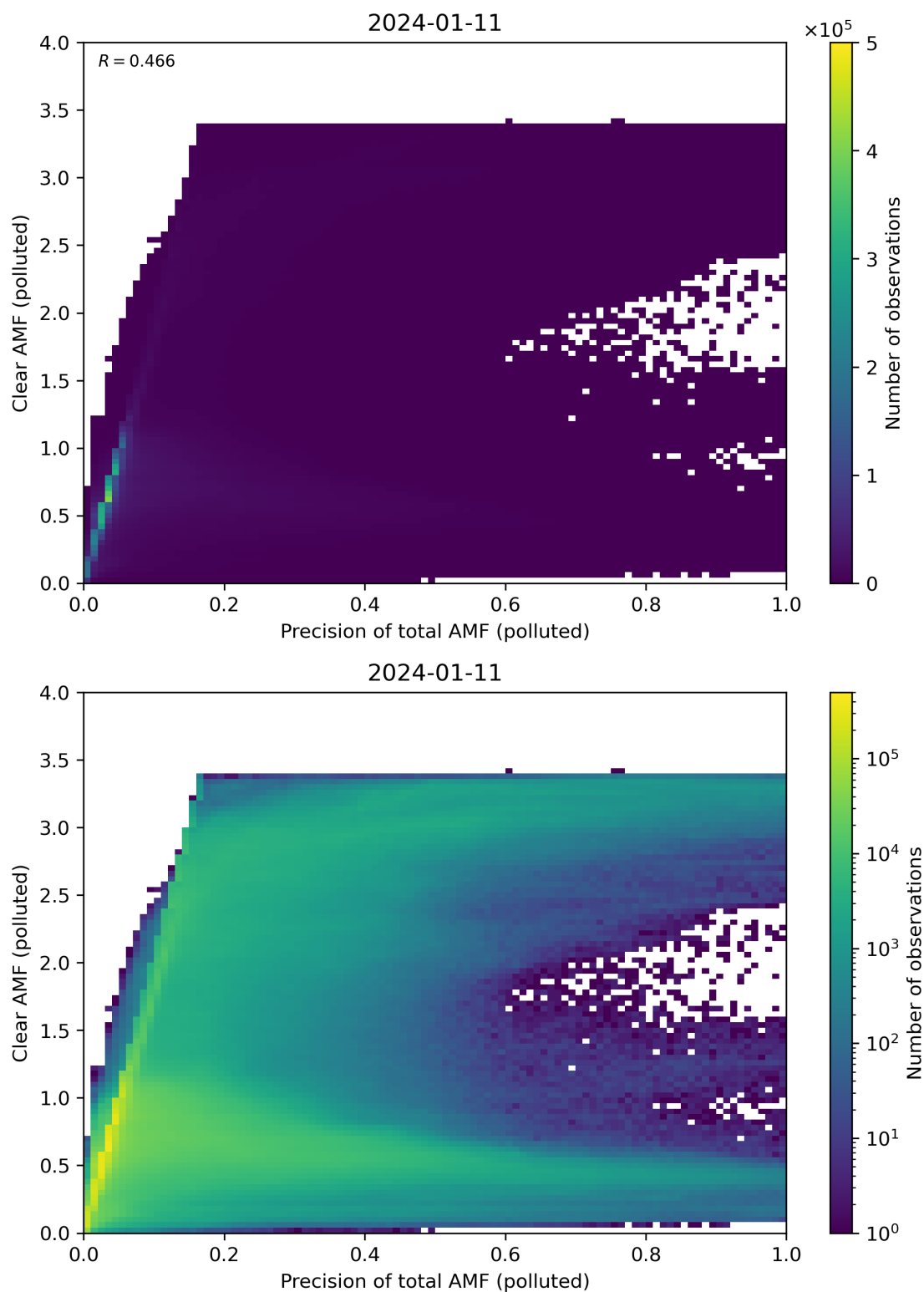
Figure 270: Scatter density plot of “Precision of total AMF (polluted)” against “Clear AMF (polluted)” for 2024-01-10 to 2024-01-12.
