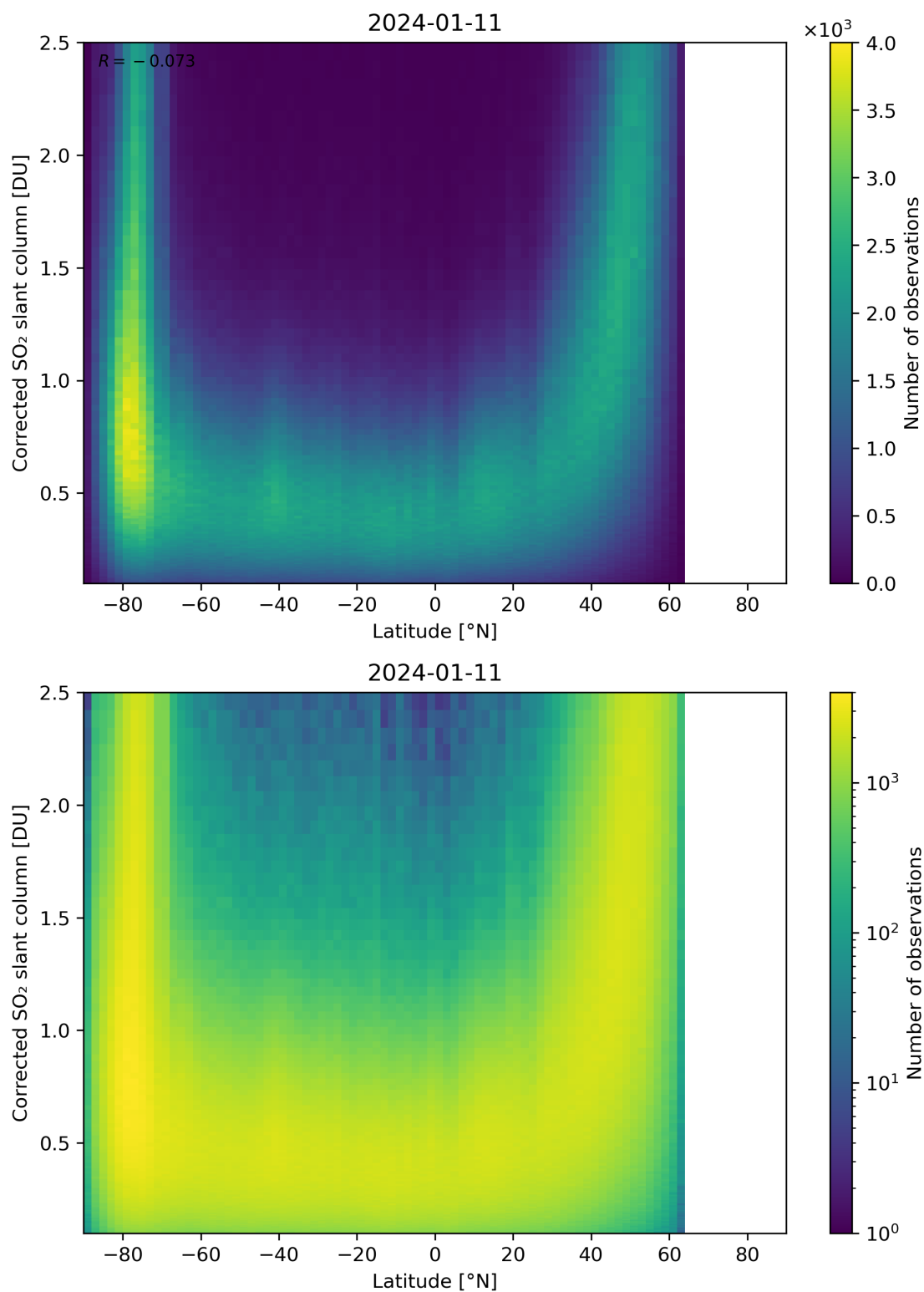
Figure 146: Scatter density plot of “Latitude” against “Corrected SO 2 slant column” for 2024-01-10 to 2024-01-12.
