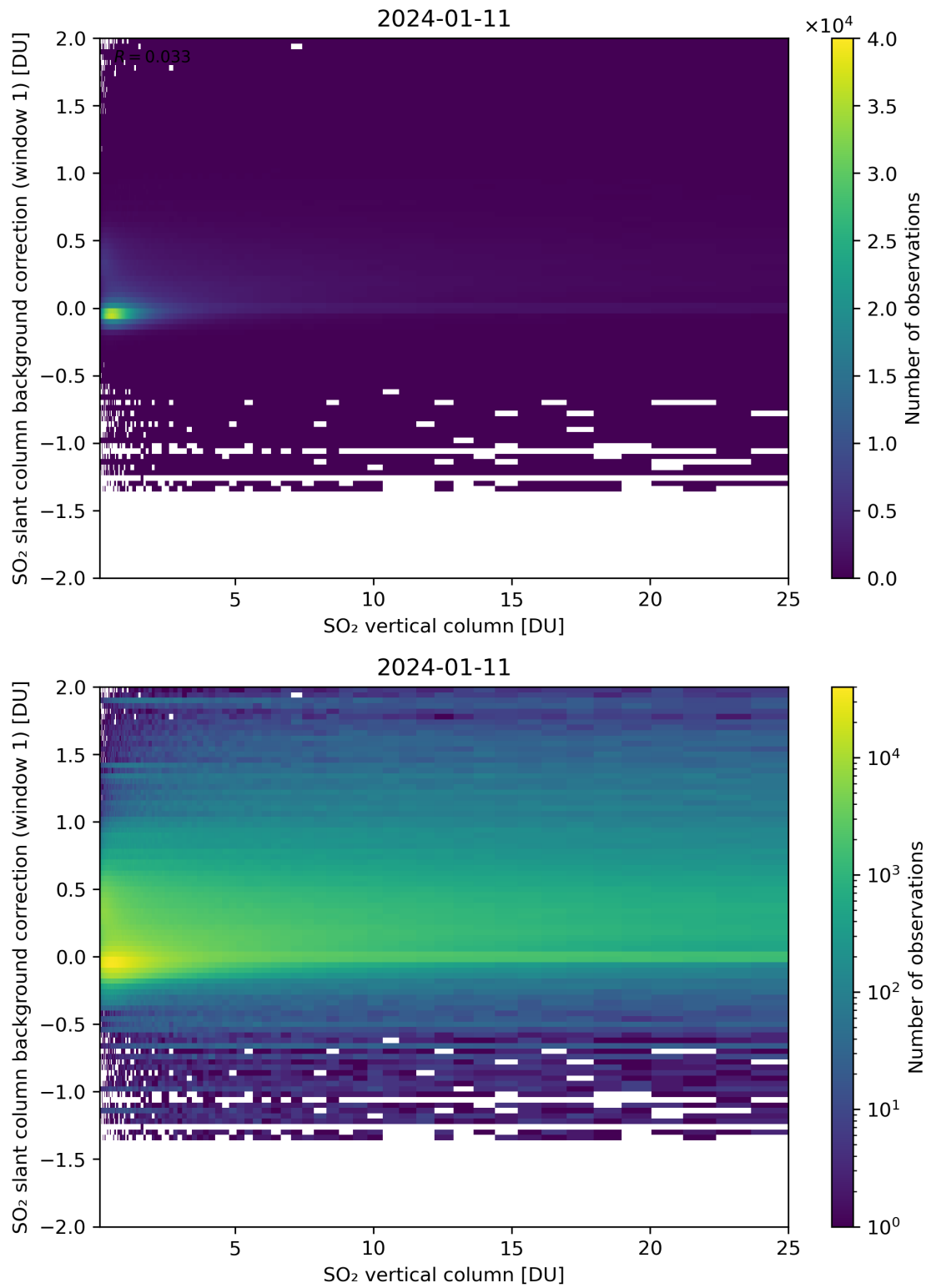
Figure 273: Scatter density plot of “SO 2 vertical column” against “SO 2 slant column background correction (window 1)” for 2024-01-10 to 2024-01-12.
