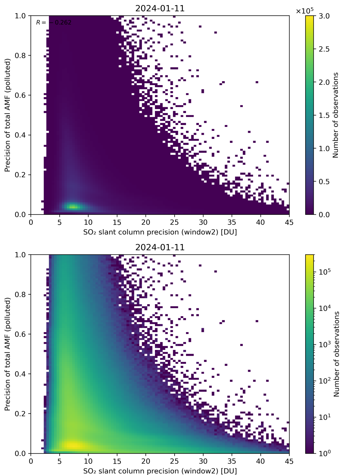
Figure 252: Scatter density plot of “SO 2 slant column precision (window2)” against “Precision of total AMF (polluted)” for 2024-01-10 to 2024-01-12.
