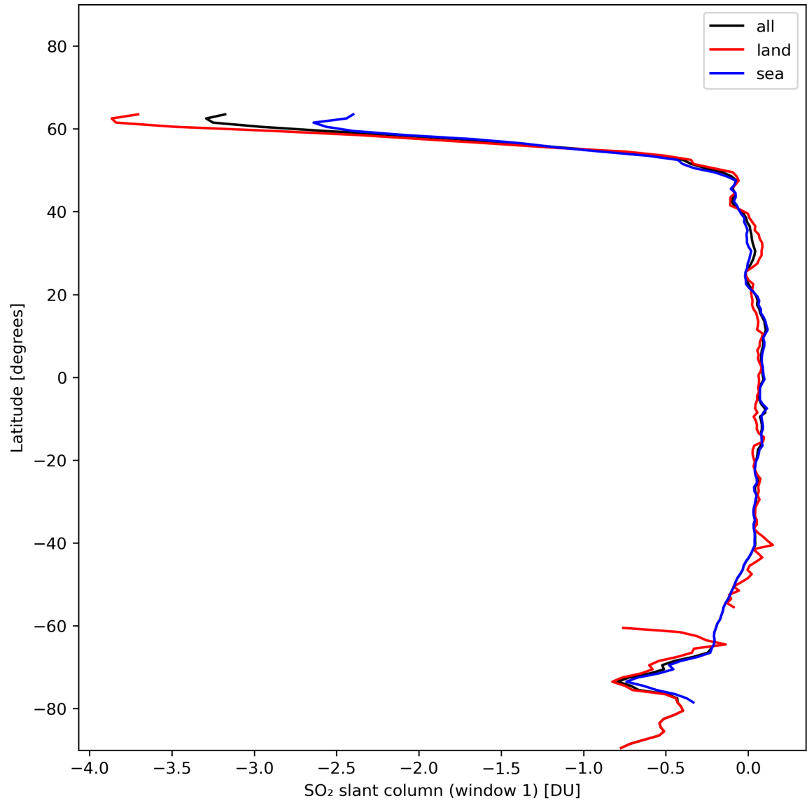
Figure 33: Zonal average of “SO 2 slant column (window 1)” for 2024-01-10 to 2024-01-12.
