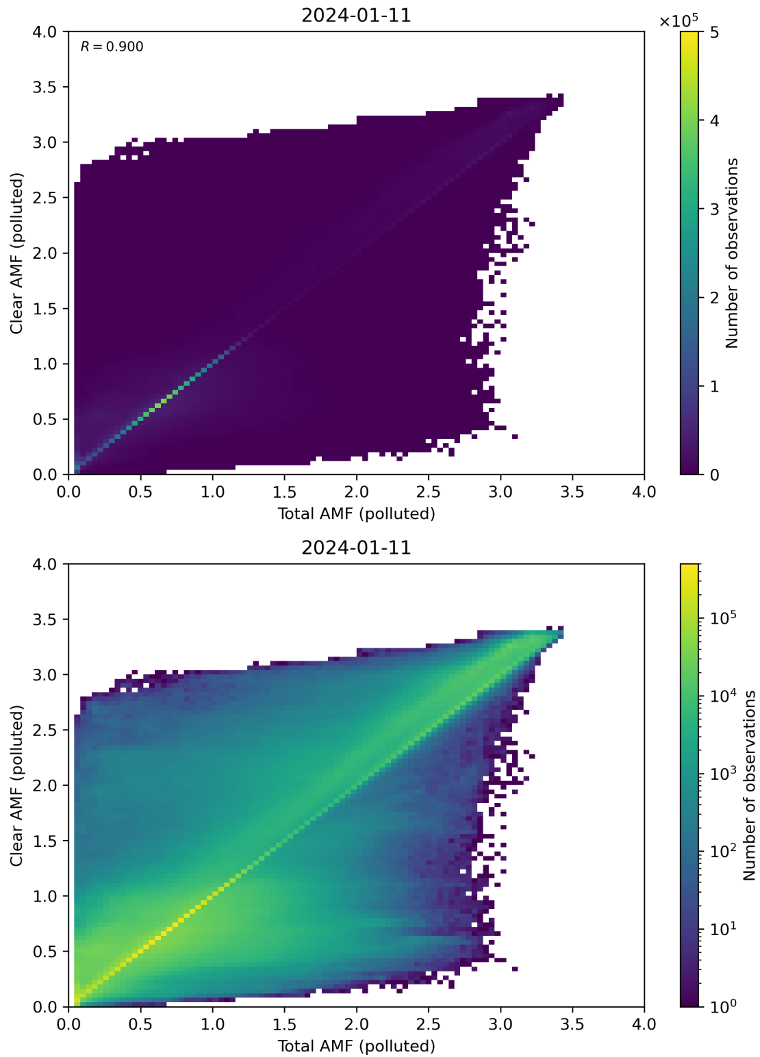
Figure 271: Scatter density plot of “Total AMF (polluted)” against “Clear AMF (polluted)” for 2024-01-10 to 2024-01-12.
