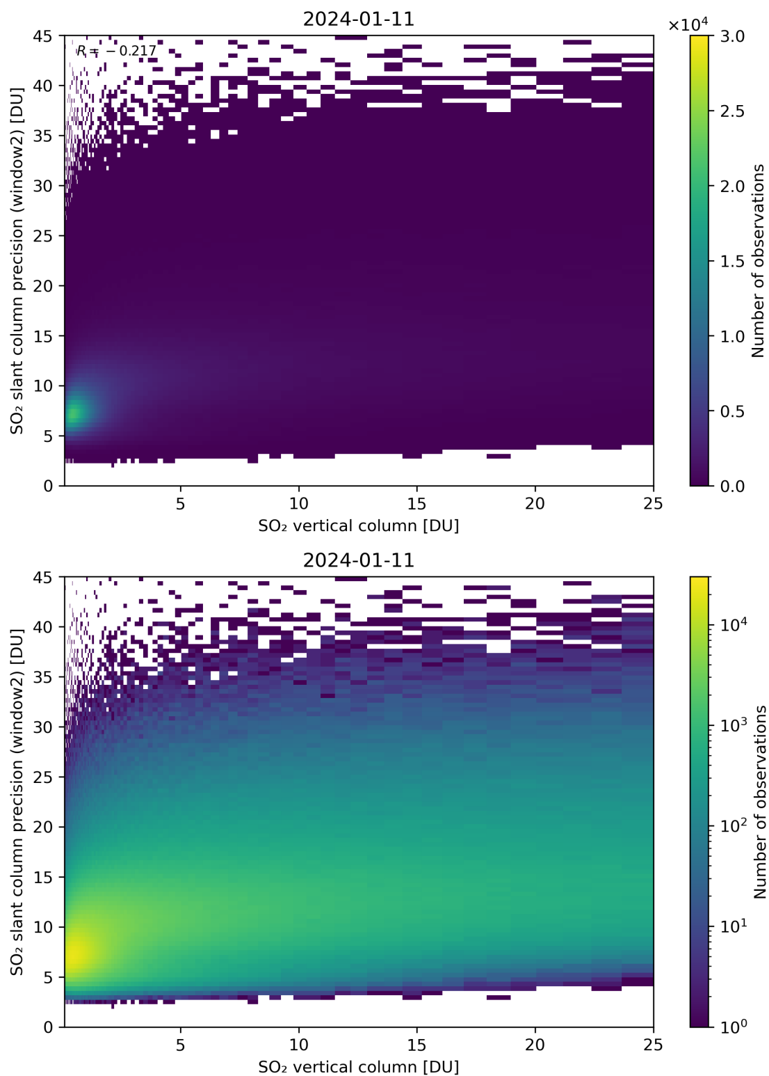
Figure 302: Scatter density plot of “SO 2 vertical column” against “SO 2 slant column precision (window2)” for 2024-01-10 to 2024-01-12.
