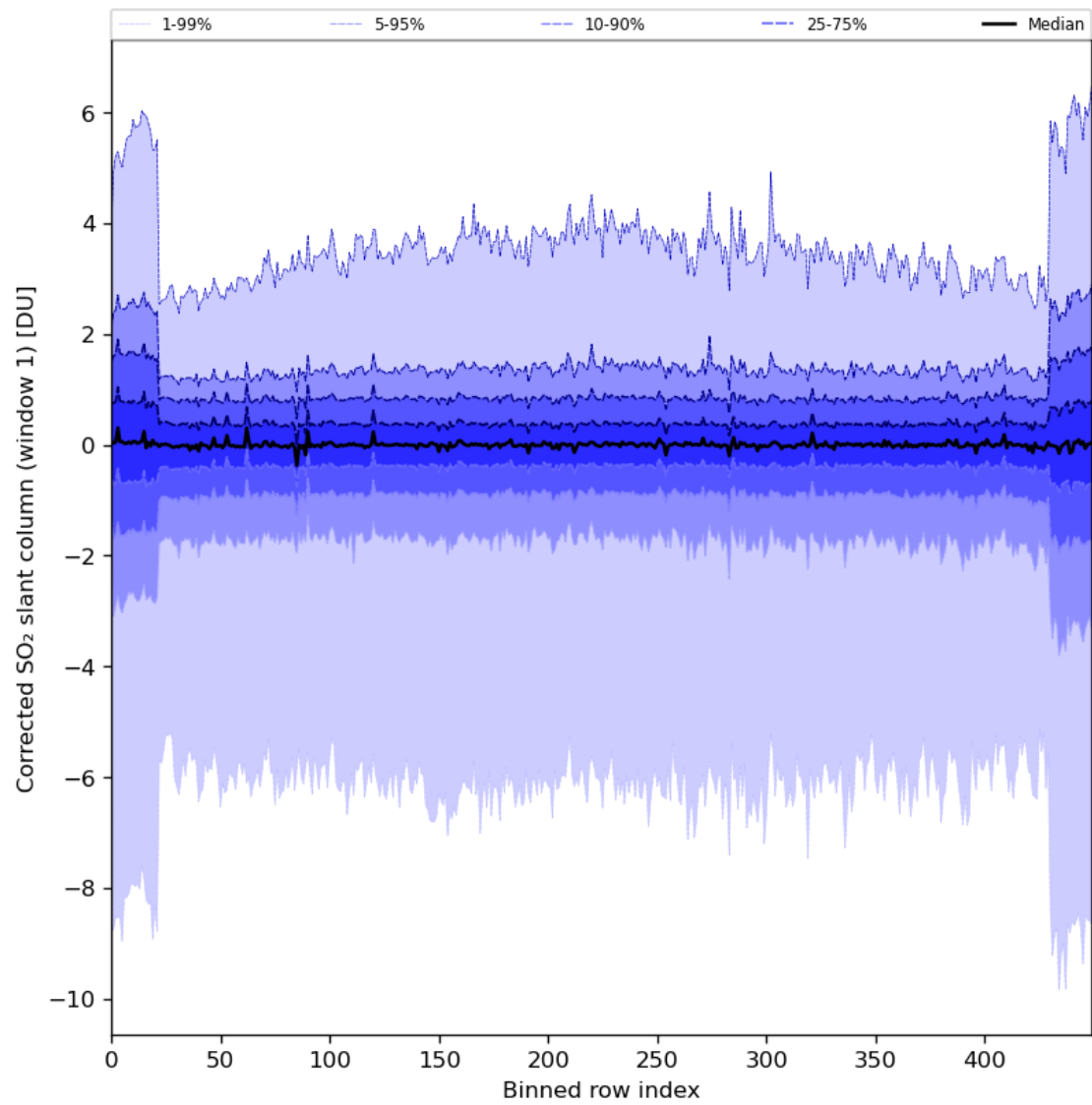
Figure 81: Along track statistics of “Corrected SO 2 slant column (window 1)” for 2024-01-10 to 2024-01-12
