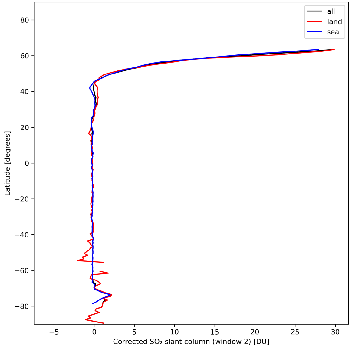
Figure 39: Zonal average of “Corrected SO 2 slant column (window 2)” for 2024-01-10 to 2024-01-12.
