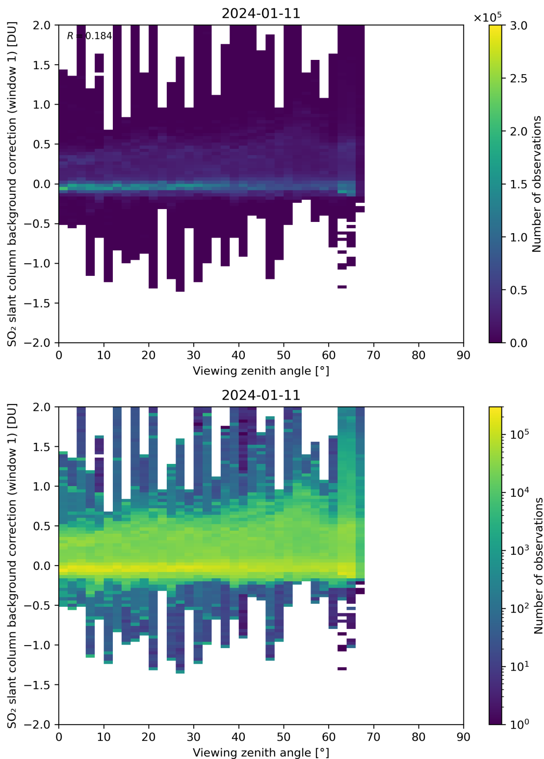
Figure 308: Scatter density plot of “Viewing zenith angle” against “SO 2 slant column background correction (window 1)” for 2024-01-10 to 2024-01-12.
