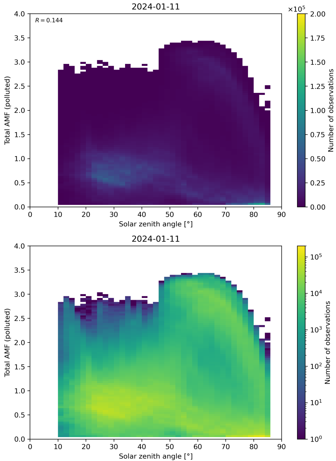
Figure 174: Scatter density plot of “Solar zenith angle” against “Total AMF (polluted)” for 2024-01-10 to 2024-01-12.
