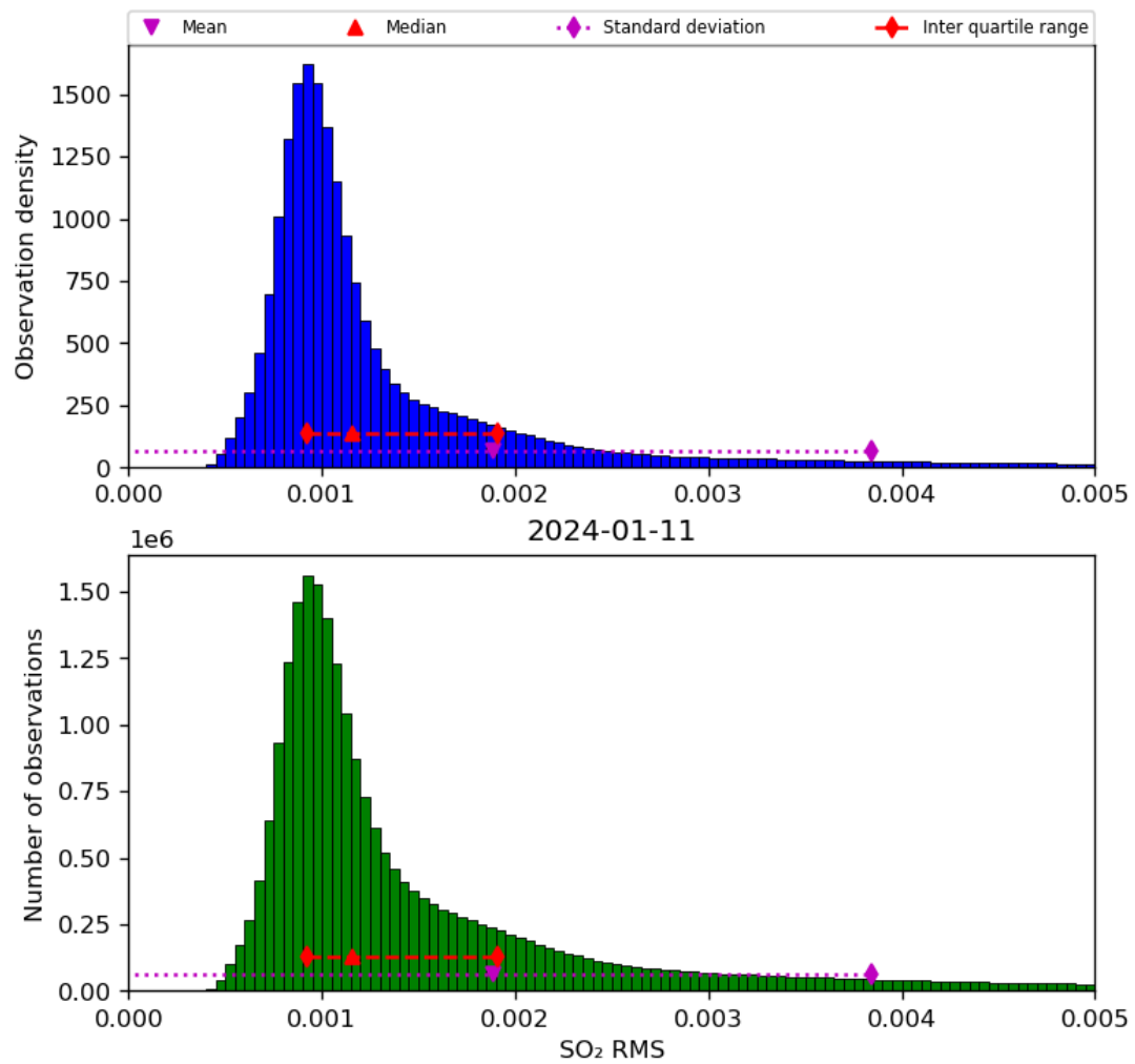
Figure 70: Histogram of “SO 2 RMS” for 2024-01-10 to 2024-01-12
