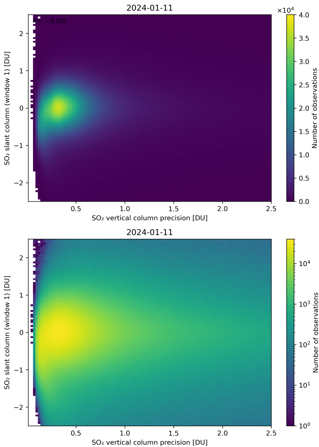
Figure 289: Scatter density plot of “SO 2 vertical column precision” against “SO 2 slant column (window 1)” for 2024-01-10 to 2024-01-12.
