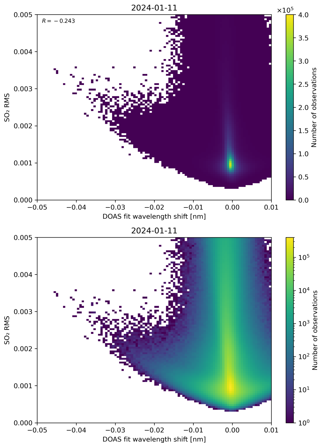
Figure 128: Scatter density plot of “DOAS fit wavelength shift” against “SO 2 RMS” for 2024-01-10 to 2024-01-12.
