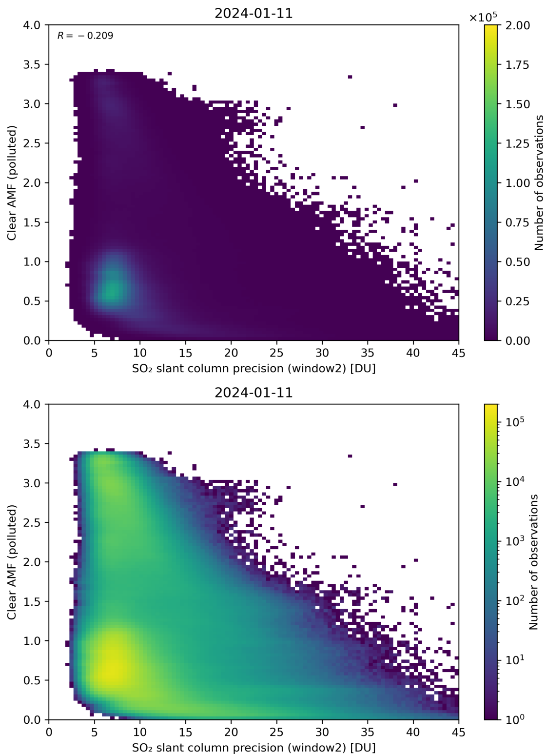
Figure 246: Scatter density plot of “SO 2 slant column precision (window2)” against “Clear AMF (polluted)” for 2024-01-10 to 2024-01-12.
