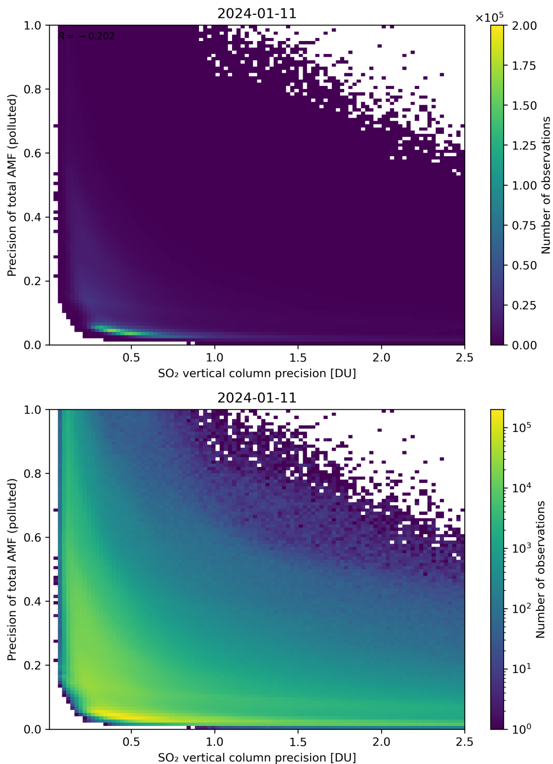
Figure 295: Scatter density plot of “SO 2 vertical column precision” against “Precision of total AMF (polluted)” for 2024-01-10 to 2024-01-12.
