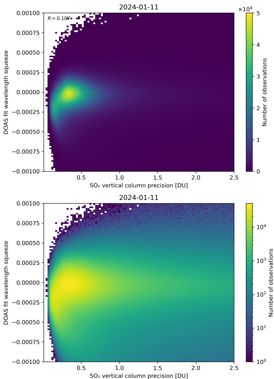
Figure 283: Scatter density plot of “SO 2 vertical column precision” against “DOAS fit wavelength squeeze” for 2024-01-10 to 2024-01-12.
