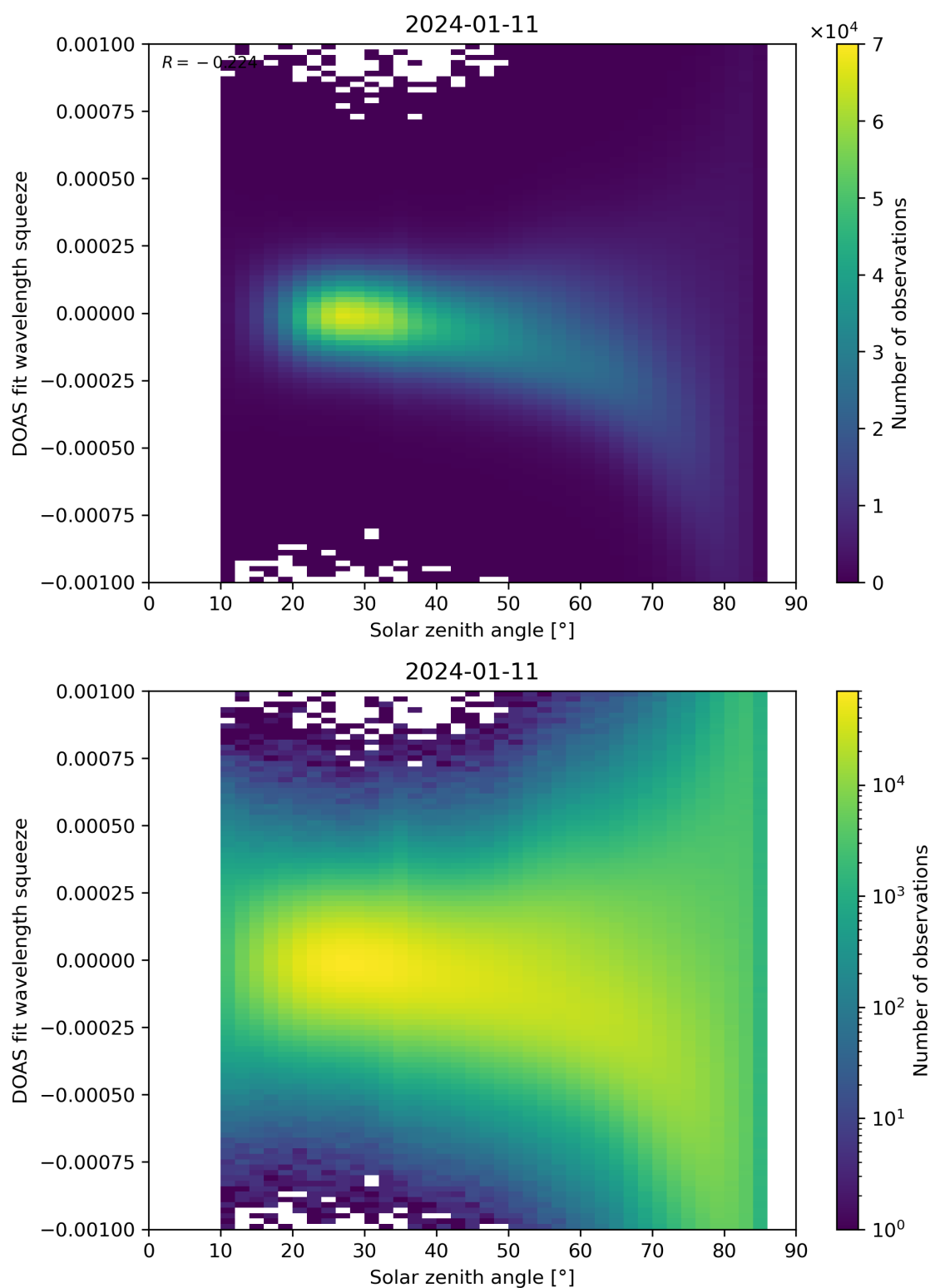
Figure 162: Scatter density plot of “Solar zenith angle” against “DOAS fit wavelength squeeze” for 2024-01-10 to 2024-01-12.
