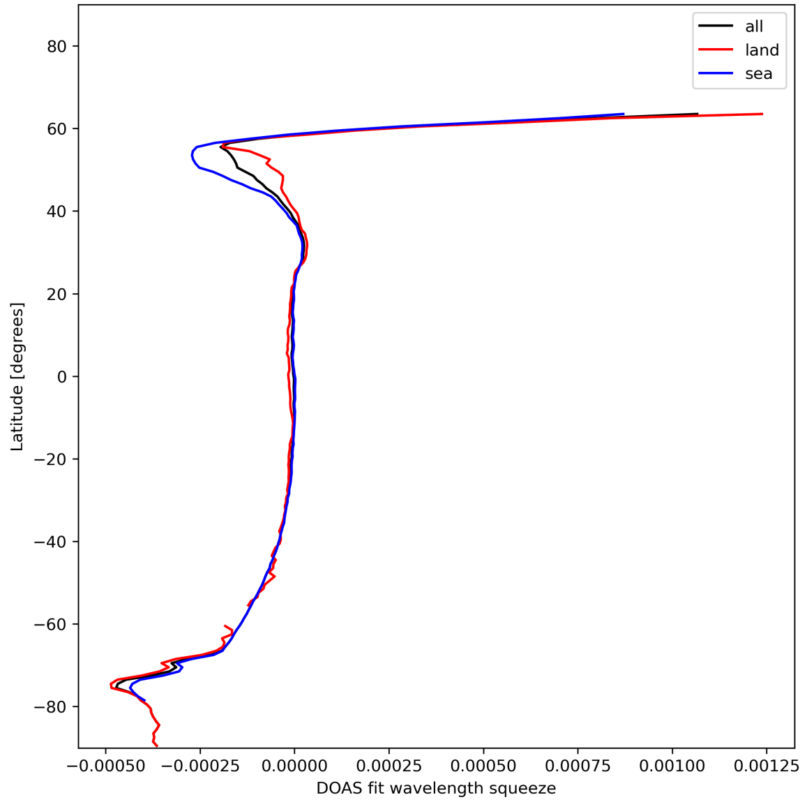
Figure 46: Zonal average of “DOAS fit wavelength squeeze” for 2024-01-10 to 2024-01-12.
