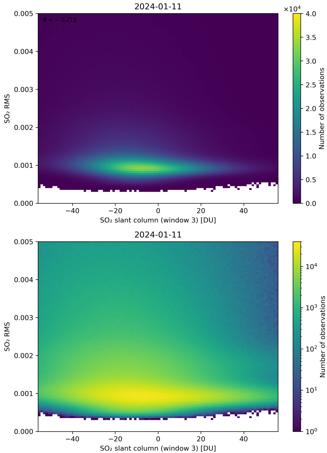
Figure 256: Scatter density plot of “SO 2 slant column (window 3)” against “SO 2 RMS” for 2024-01-10 to 2024-01-12.
