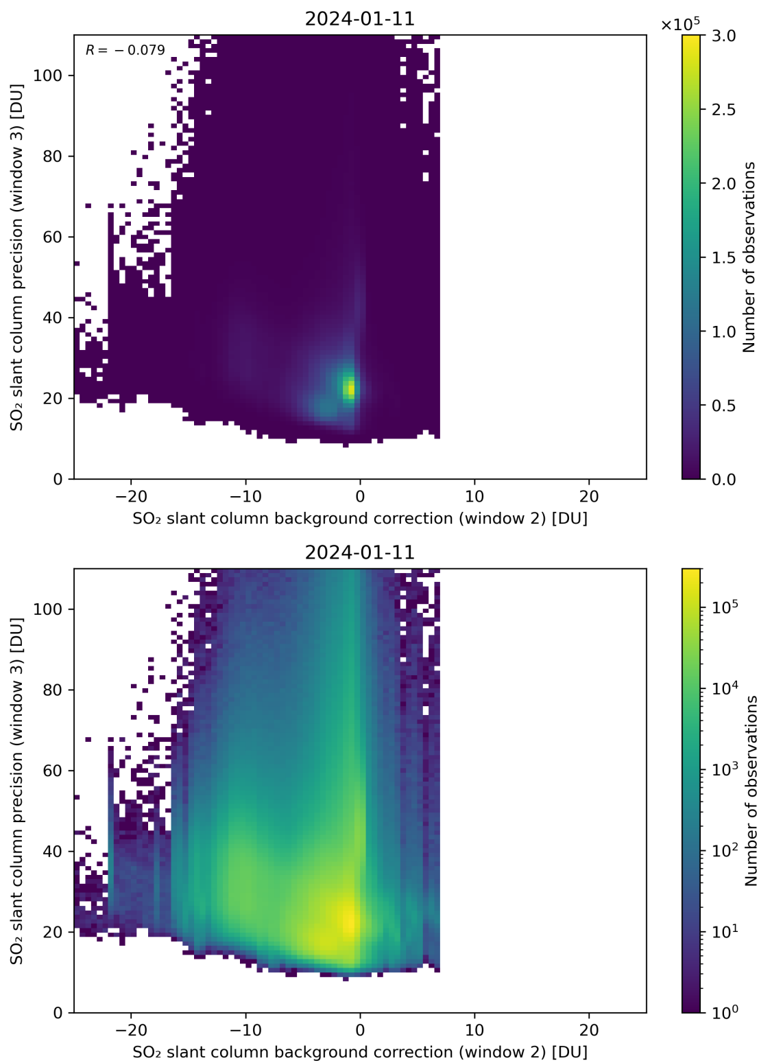
Figure 118: Scatter density plot of “SO 2 slant column background correction (window 2)” against “SO 2 slant column precision (window 3)” for 2024-01-10 to 2024-01-12.
