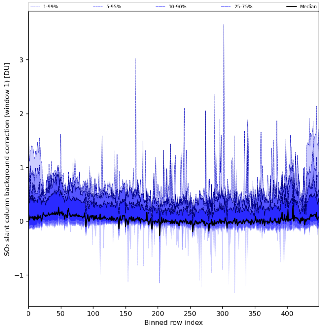
Figure 82: Along track statistics of “SO 2 slant column background correction (window 1)” for 2024-01-10 to 2024-01-12
