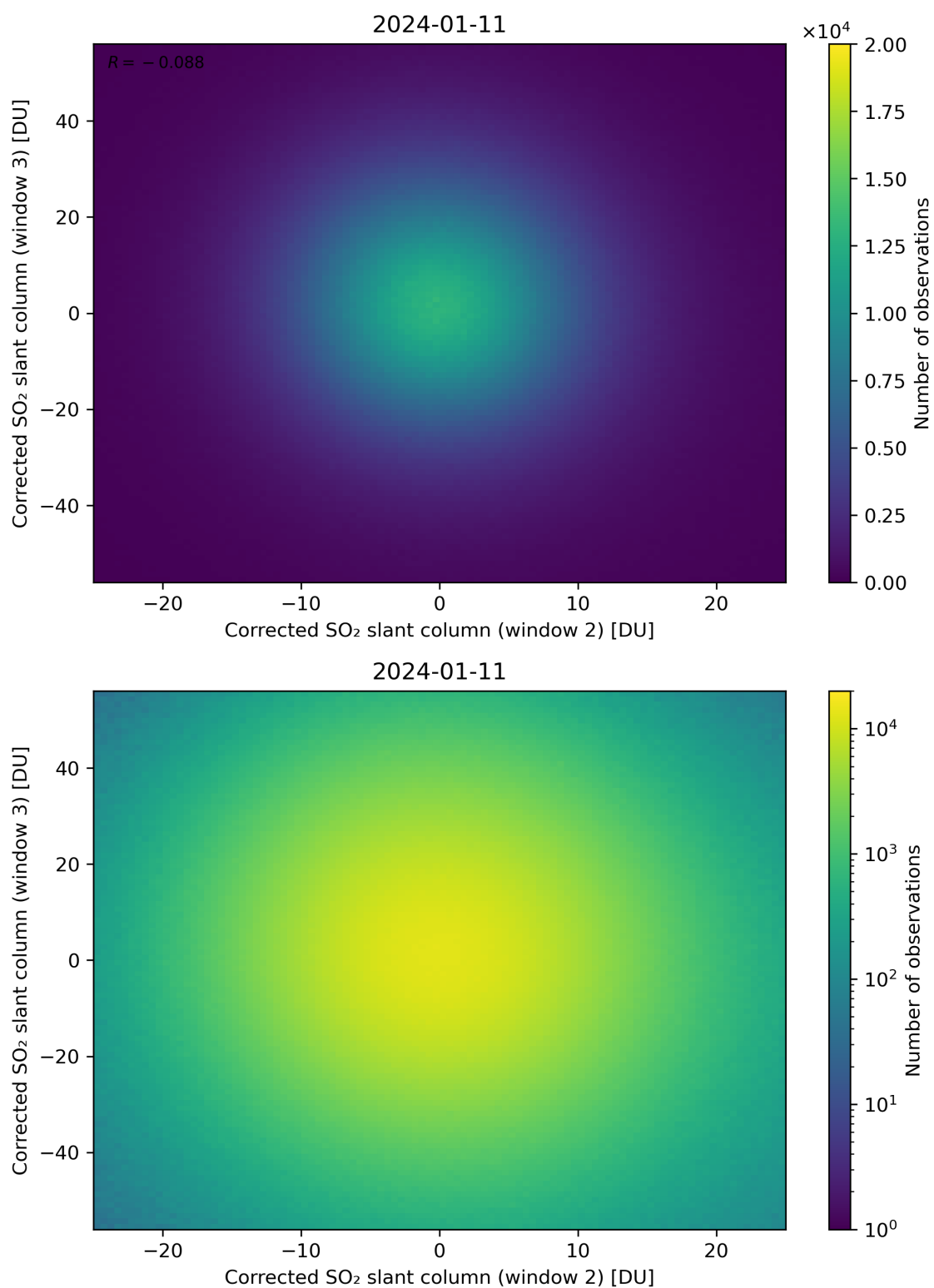
Figure 200: Scatter density plot of “Corrected SO 2 slant column (window 2)” against “Corrected SO 2 slant column (window 3)” for 2024-01-10 to 2024-01-12.
