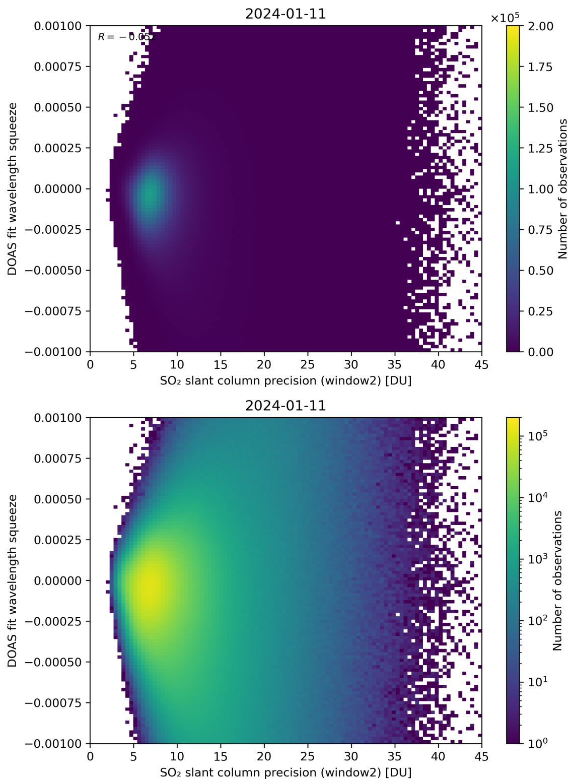
Figure 244: Scatter density plot of “SO 2 slant column precision (window2)” against “DOAS fit wavelength squeeze” for 2024-01-10 to 2024-01-12.
