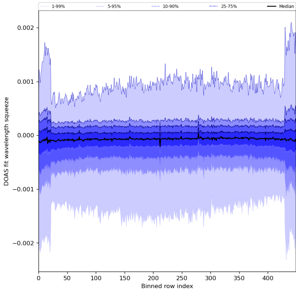
Figure 92: Along track statistics of “DOAS fit wavelength squeeze” for 2024-01-10 to 2024-01-12
