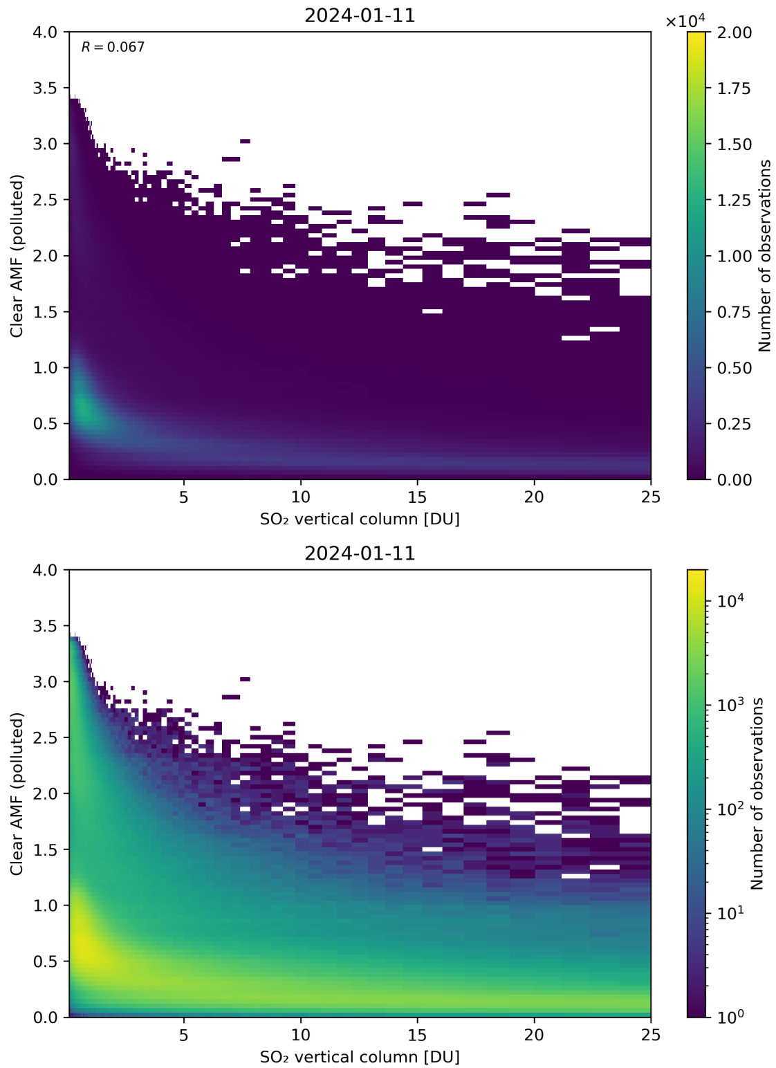
Figure 296: Scatter density plot of “SO 2 vertical column” against “Clear AMF (polluted)” for 2024-01-10 to 2024-01-12.
