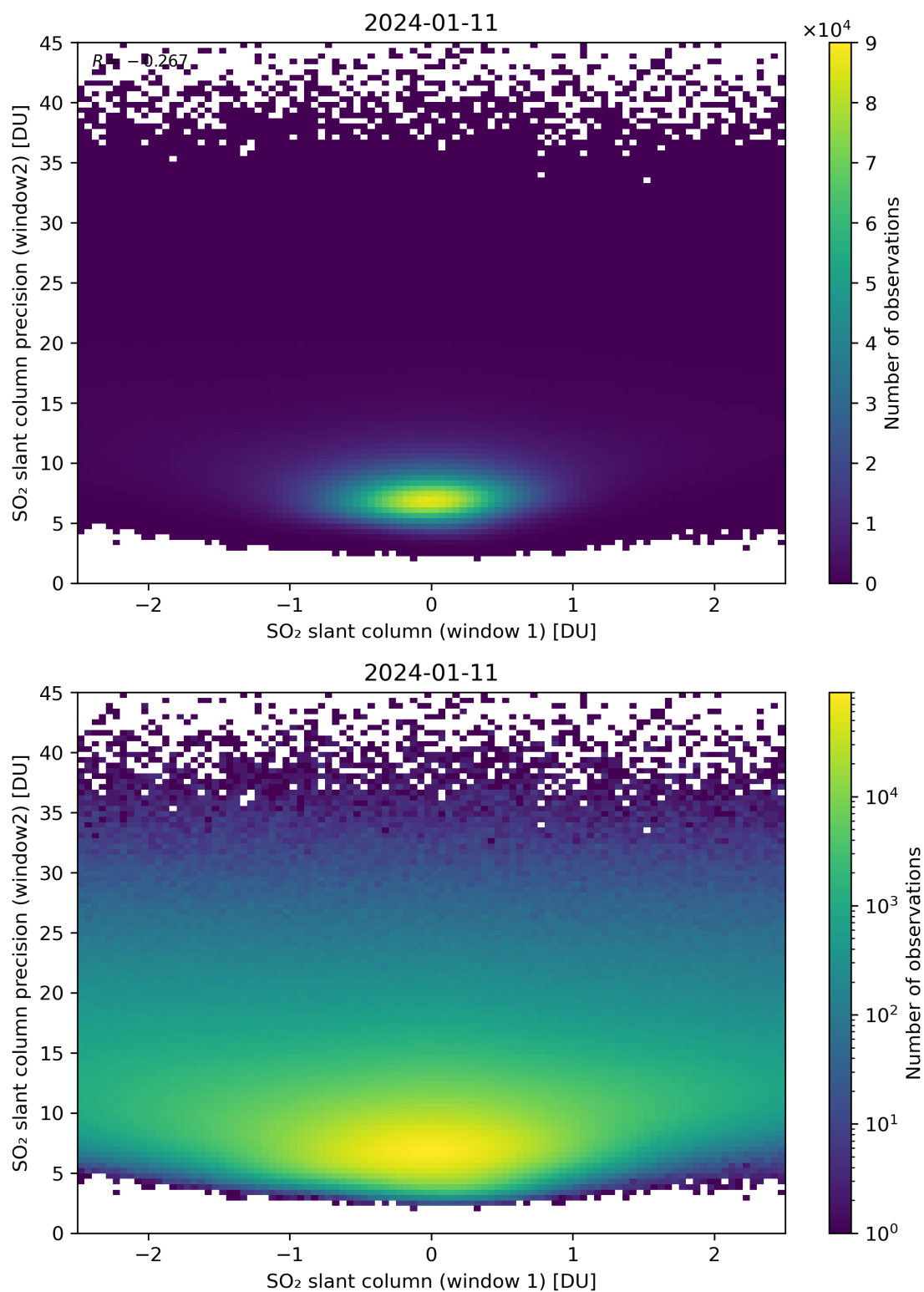
Figure 236: Scatter density plot of “SO 2 slant column (window 1)” against “SO 2 slant column precision (window2)” for 2024-01-10 to 2024-01-12.
