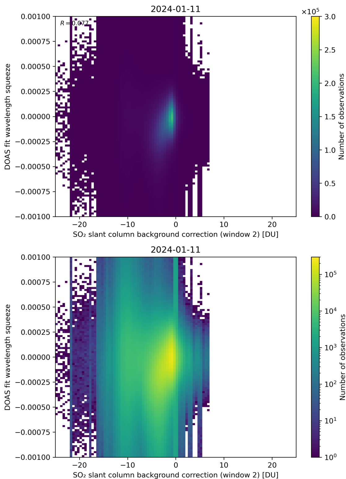
Figure 113: Scatter density plot of “SO 2 slant column background correction (window 2)” against “DOAS fit wavelength squeeze” for 2024-01-10 to 2024-01-12.
