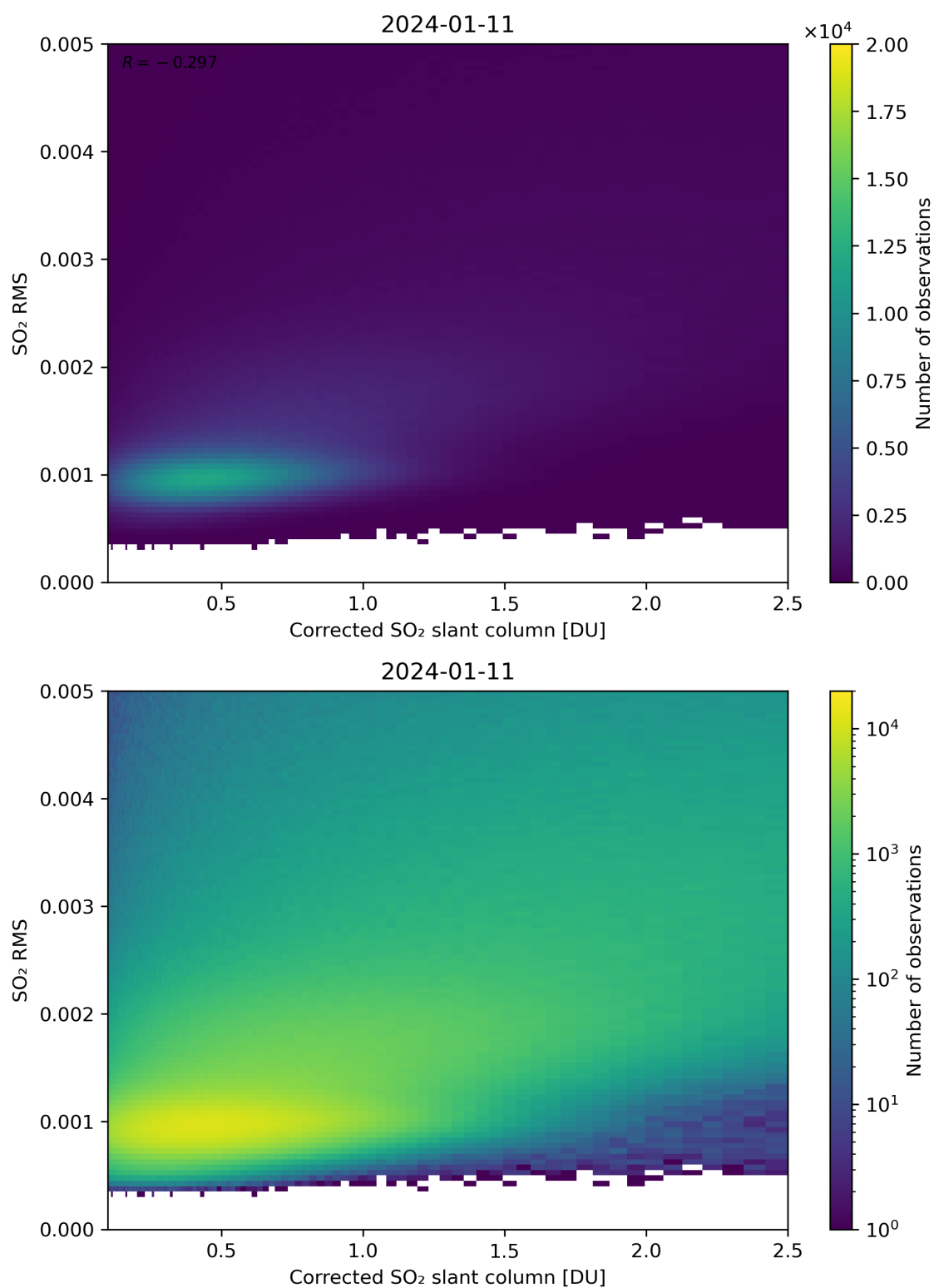
Figure 183: Scatter density plot of “Corrected SO 2 slant column” against “SO 2 RMS” for 2024-01-10 to 2024-01-12.
