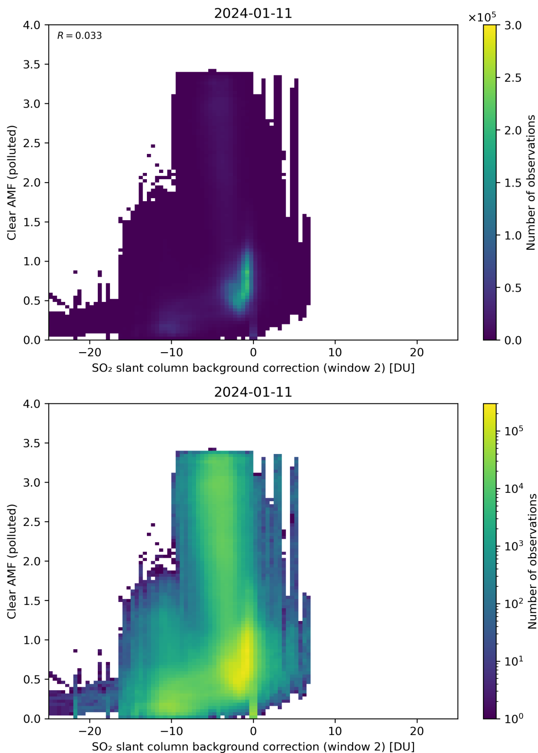
Figure 115: Scatter density plot of “SO 2 slant column background correction (window 2)” against “Clear AMF (polluted)” for 2024-01-10 to 2024-01-12.
