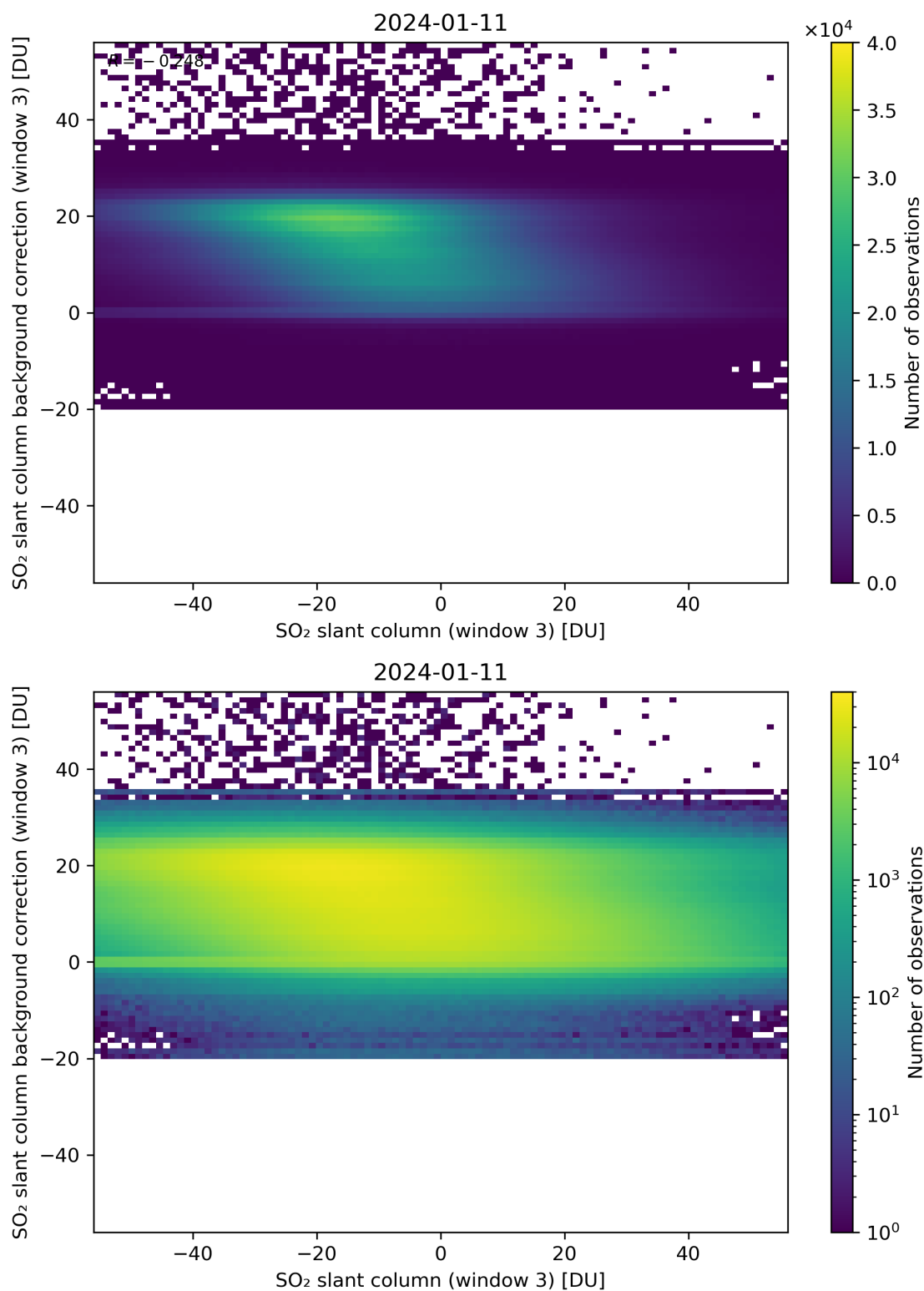
Figure 253: Scatter density plot of “SO 2 slant column (window 3)” against “SO 2 slant column background correction (window 3)” for 2024-01-10 to 2024-01-12.
