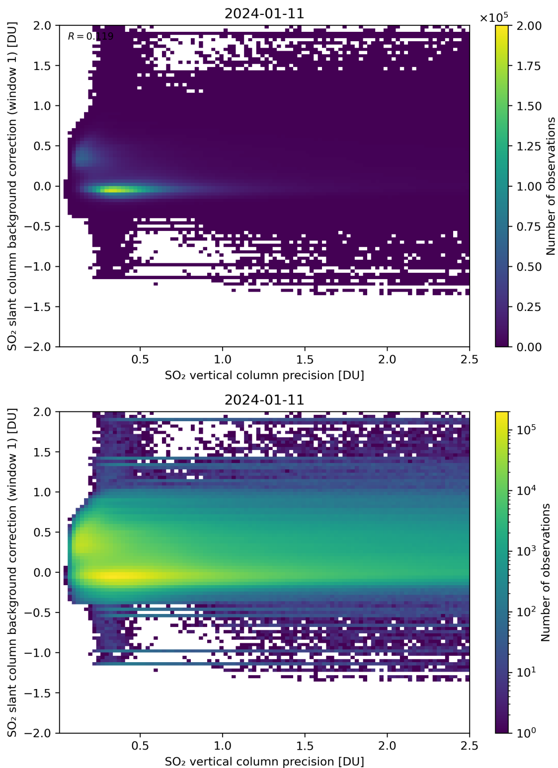
Figure 279: Scatter density plot of “SO 2 vertical column precision” against “SO 2 slant column background correction (window 1)” for 2024-01-10 to 2024-01-12.
