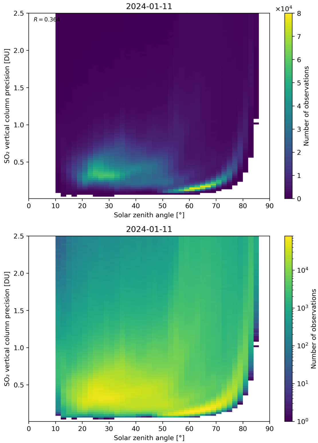
Figure 177: Scatter density plot of “Solar zenith angle” against “SO 2 vertical column precision” for 2024-01-10 to 2024-01-12.
