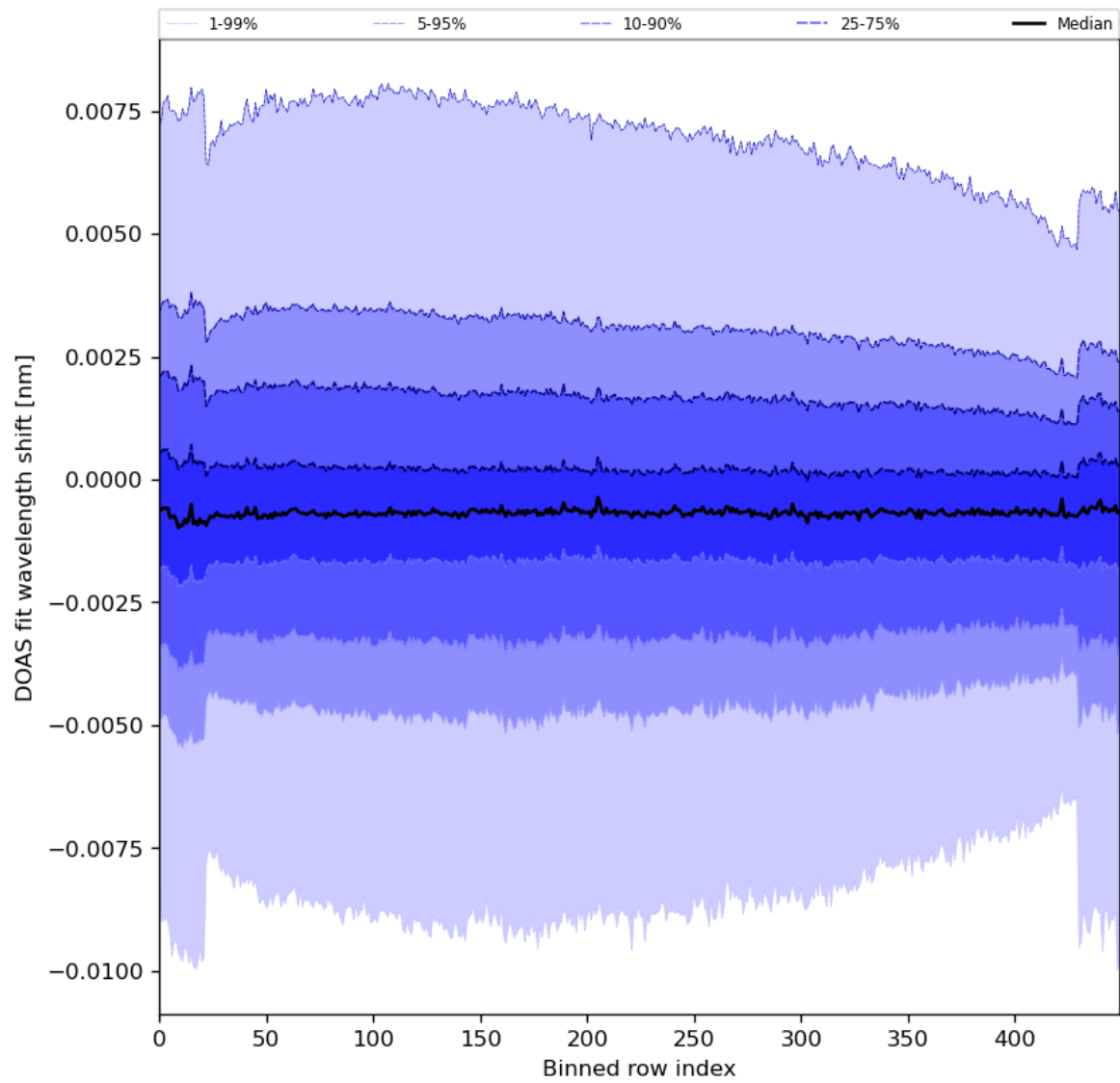
Figure 91: Along track statistics of “DOAS fit wavelength shift” for 2024-01-10 to 2024-01-12
