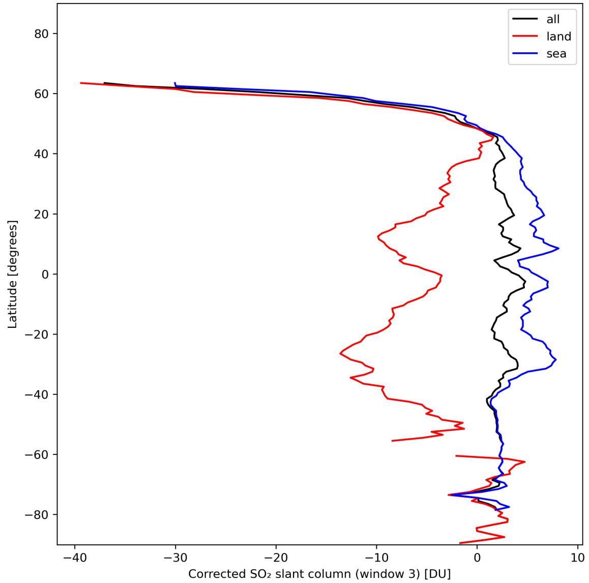
Figure 43: Zonal average of “Corrected SO 2 slant column (window 3)” for 2024-01-10 to 2024-01-12.
