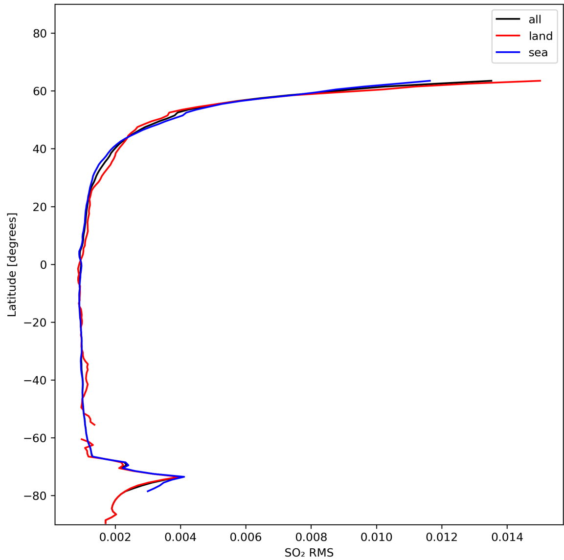
Figure 47: Zonal average of “SO 2 RMS” for 2024-01-10 to 2024-01-12.
