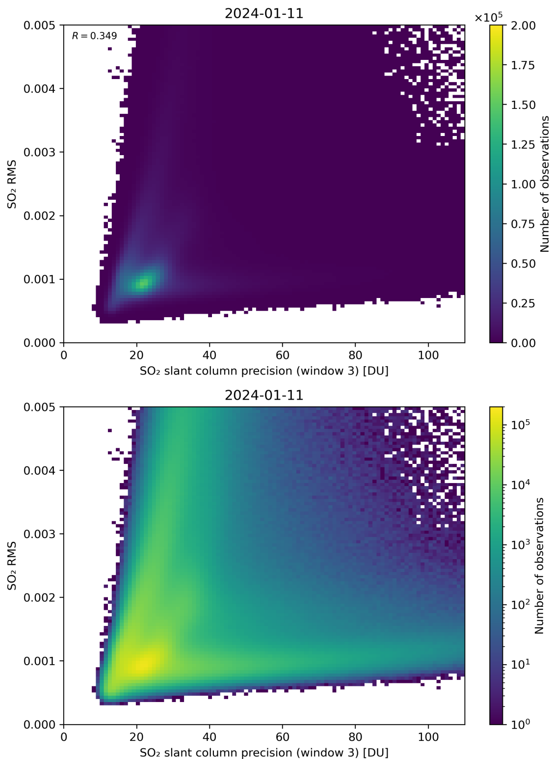
Figure 260: Scatter density plot of “SO 2 slant column precision (window 3)” against “SO 2 RMS” for 2024-01-10 to 2024-01-12.
