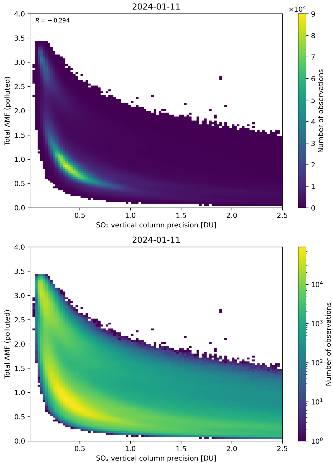
Figure 294: Scatter density plot of “SO 2 vertical column precision” against “Total AMF (polluted)” for 2024-01-10 to 2024-01-12.
