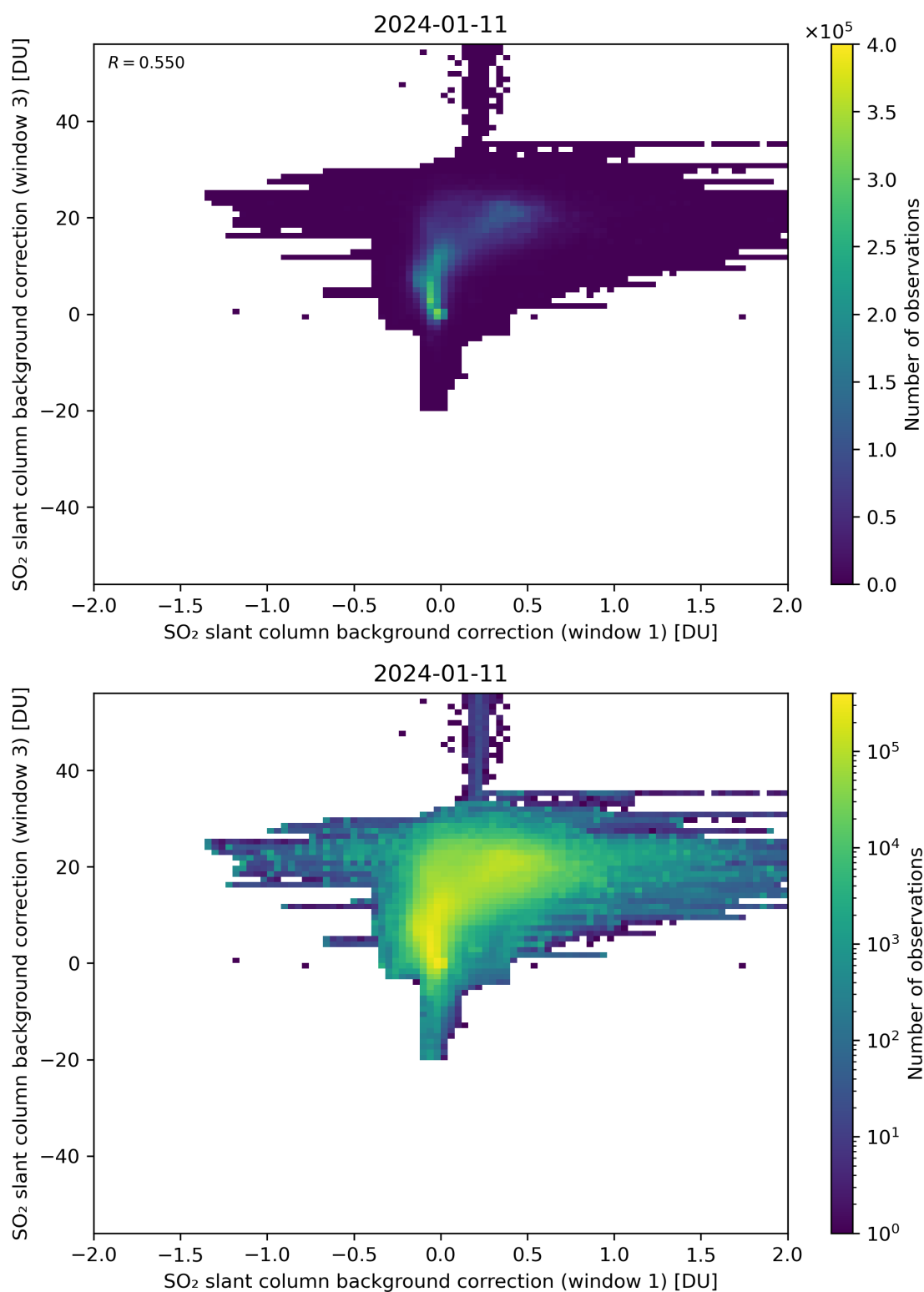
Figure 99: Scatter density plot of “SO 2 slant column background correction (window 1)” against “SO 2 slant column background correction (window 3)” for 2024-01-10 to 2024-01-12.
