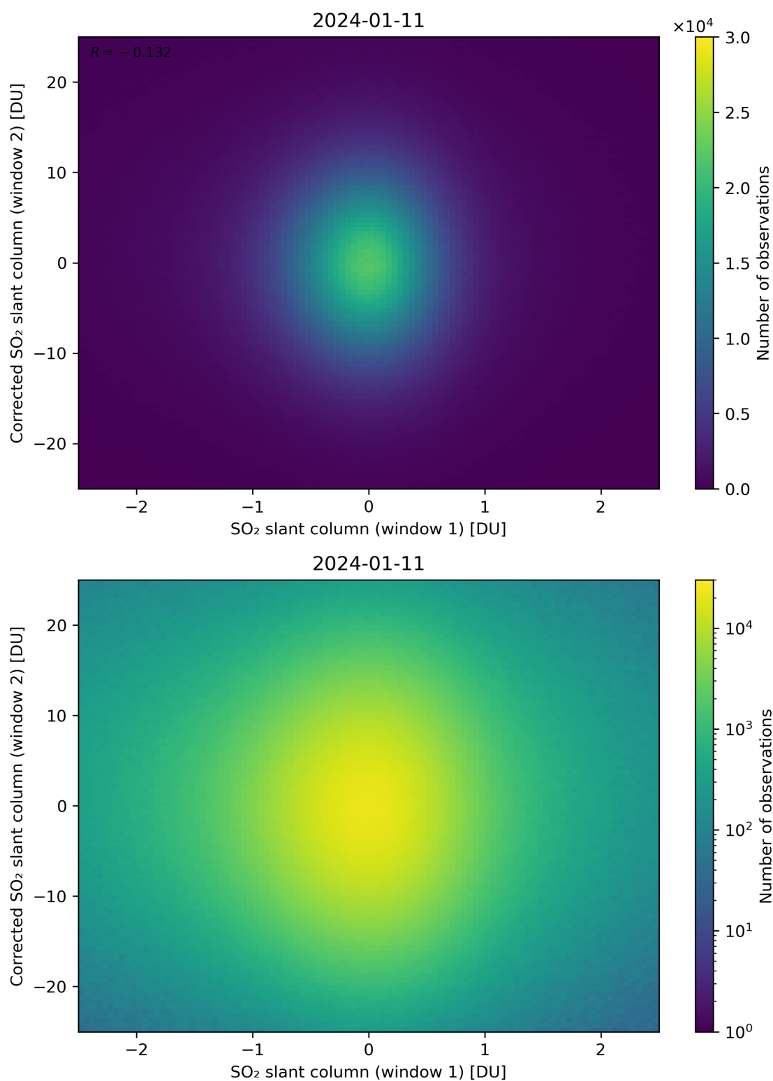
Figure 233: Scatter density plot of “SO 2 slant column (window 1)” against “Corrected SO 2 slant column (window 2)” for 2024-01-10 to 2024-01-12.
