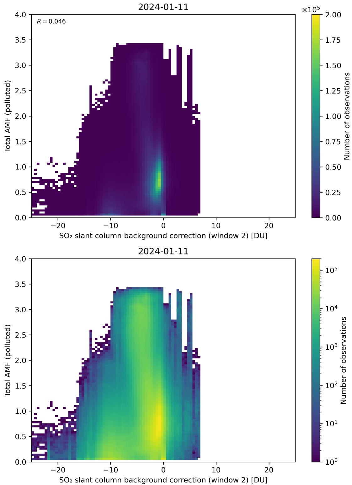
Figure 119: Scatter density plot of “SO 2 slant column background correction (window 2)” against “Total AMF (polluted)” for 2024-01-10 to 2024-01-12.
