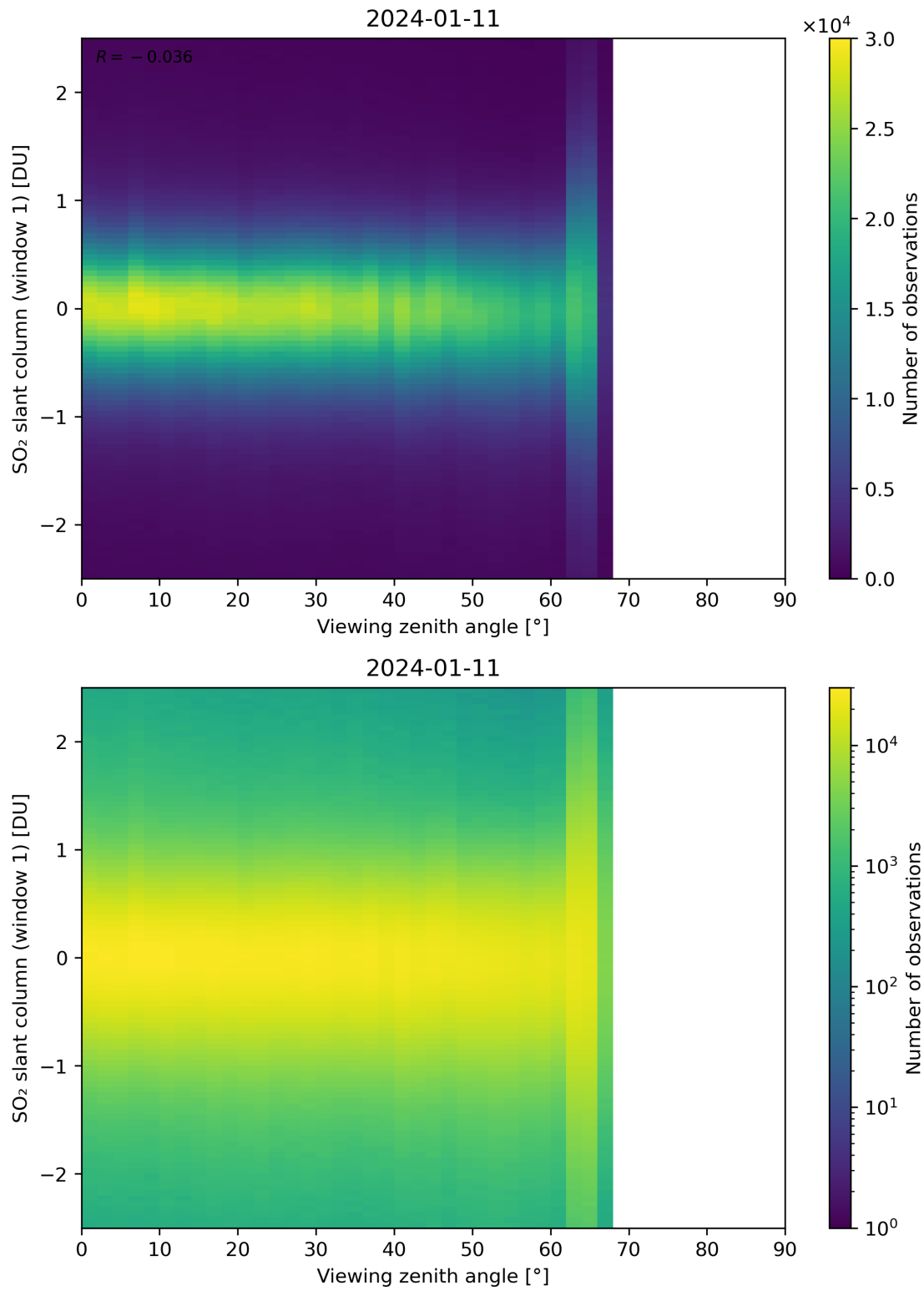
Figure 320: Scatter density plot of “Viewing zenith angle” against “SO 2 slant column (window 1)” for 2024-01-10 to 2024-01-12.
