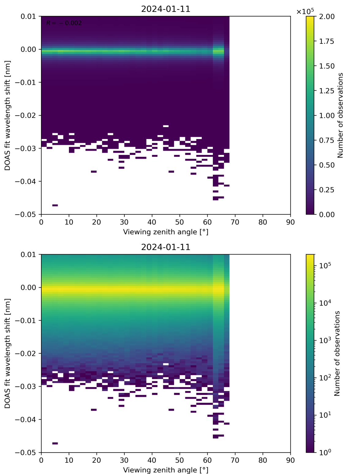
Figure 311: Scatter density plot of “Viewing zenith angle” against “DOAS fit wavelength shift” for 2024-01-10 to 2024-01-12.
