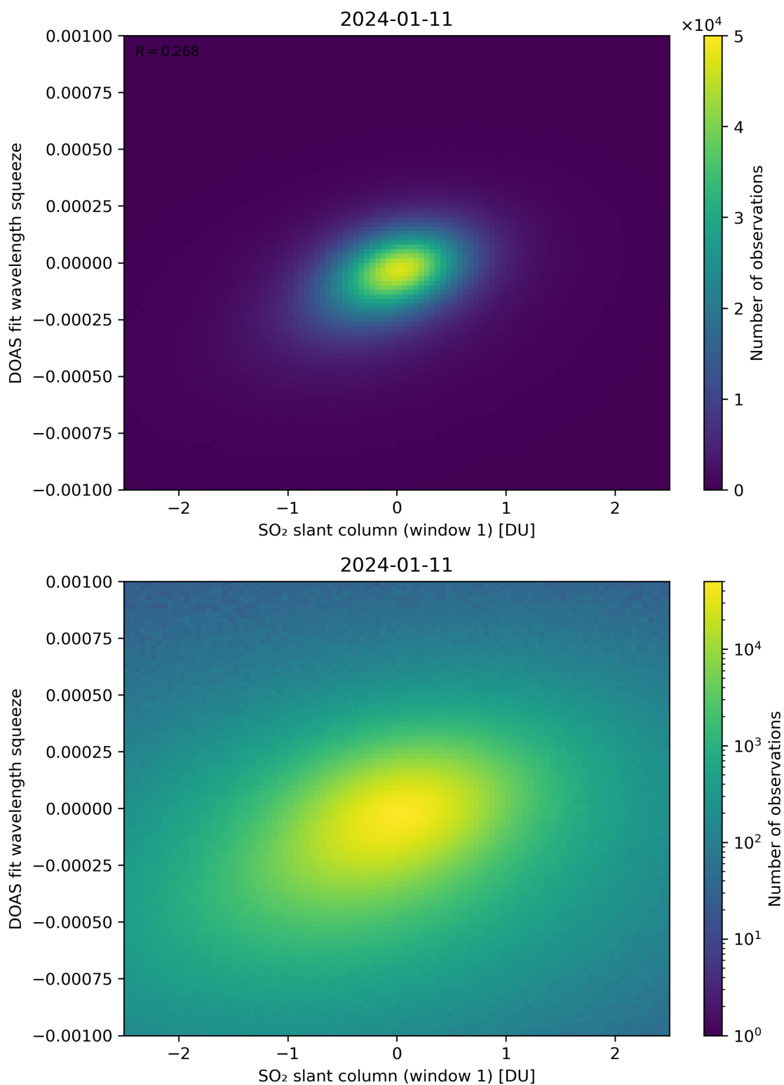
Figure 216: Scatter density plot of “SO 2 slant column (window 1)” against “DOAS fit wavelength squeeze” for 2024-01-10 to 2024-01-12.
