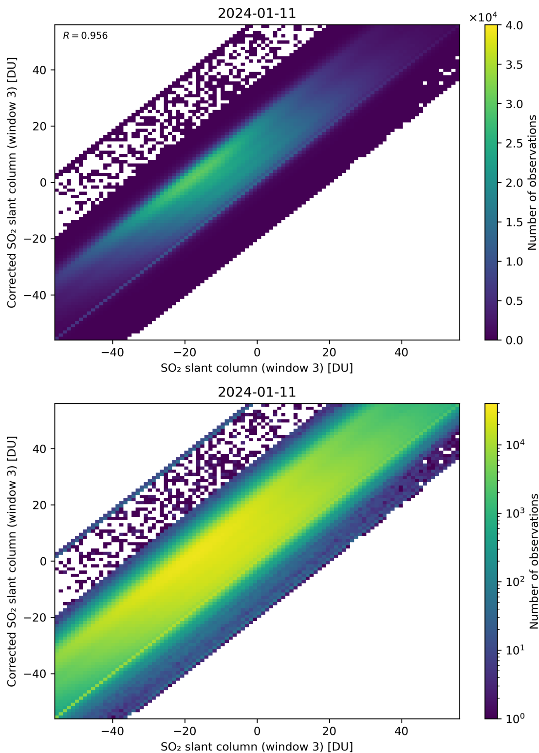
Figure 266: Scatter density plot of “SO 2 slant column (window 3)” against “Corrected SO 2 slant column (window 3)” for 2024-01-10 to 2024-01-12.
