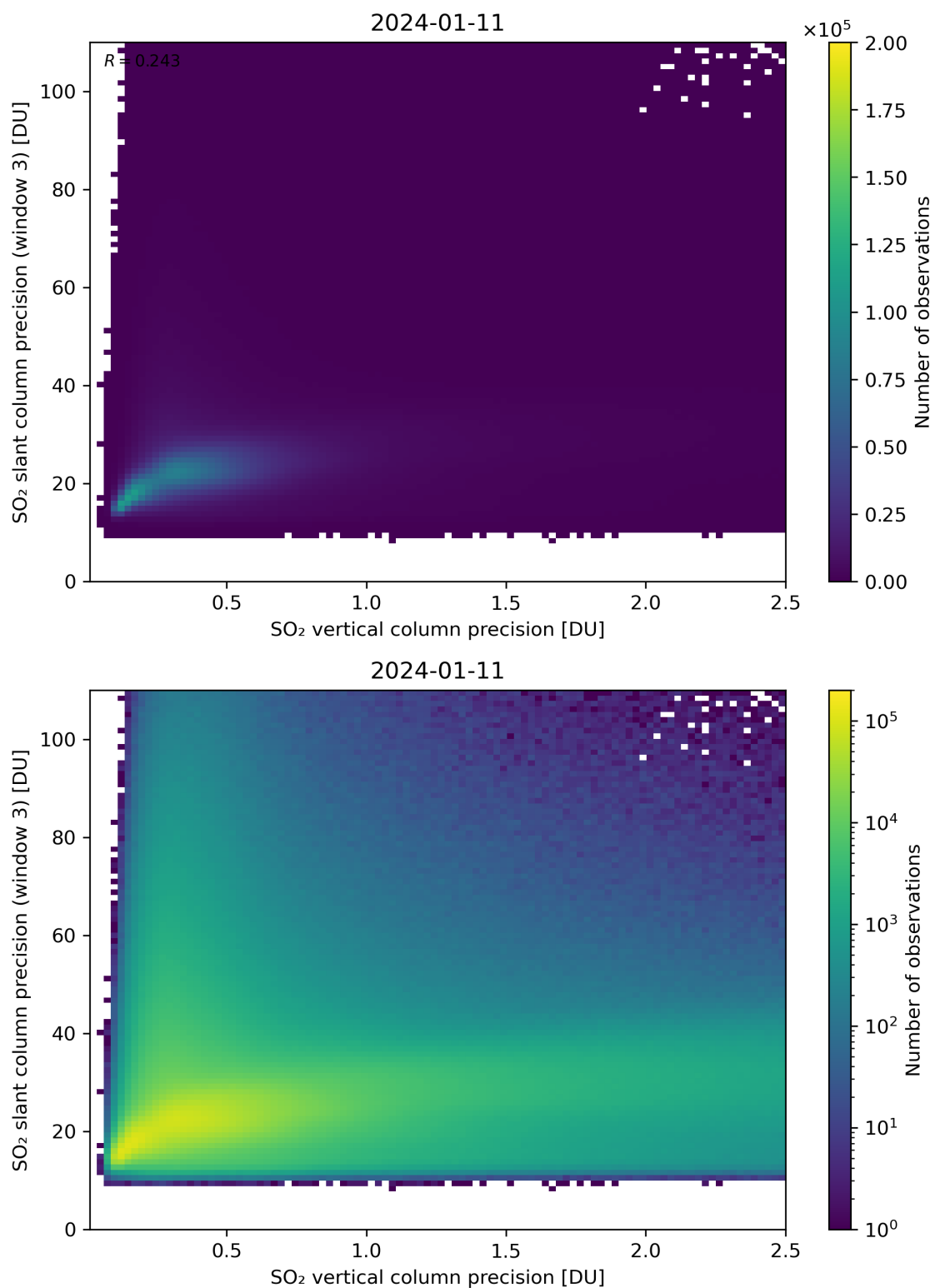
Figure 293: Scatter density plot of “SO 2 vertical column precision” against “SO 2 slant column precision (window 3)” for 2024-01-10 to 2024-01-12.
