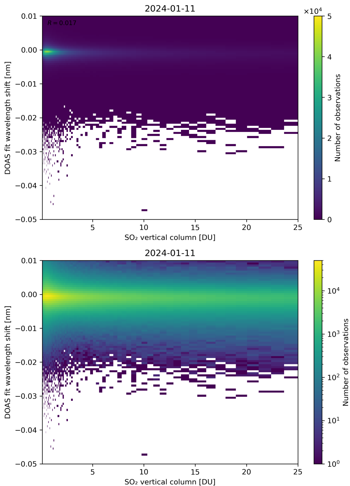
Figure 276: Scatter density plot of “SO 2 vertical column” against “DOAS fit wavelength shift” for 2024-01-10 to 2024-01-12.
