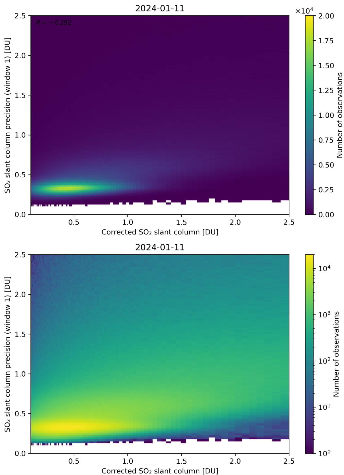
Figure 188: Scatter density plot of “Corrected SO 2 slant column” against “SO 2 slant column precision (window 1)” for 2024-01-10 to 2024-01-12.
