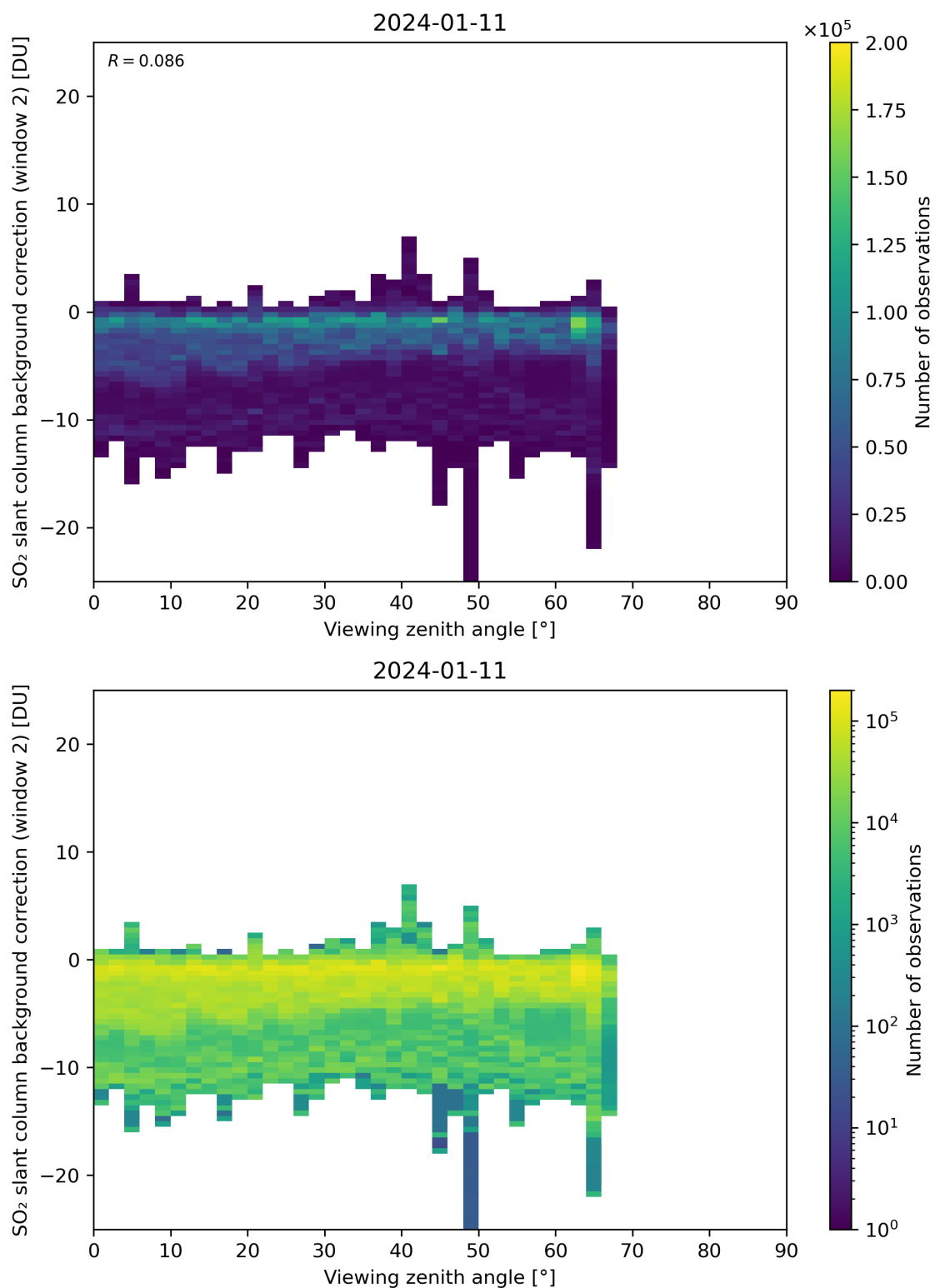
Figure 309: Scatter density plot of “Viewing zenith angle” against “SO 2 slant column background correction (window 2)” for 2024-01-10 to 2024-01-12.
