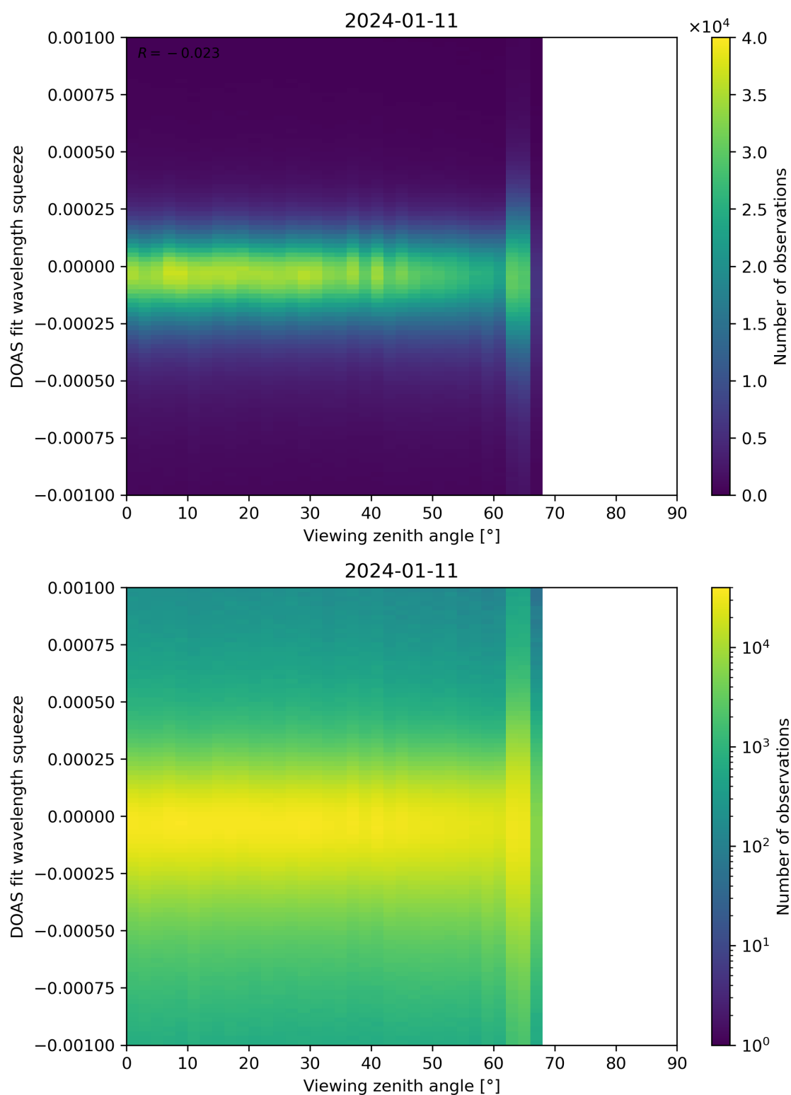
Figure 312: Scatter density plot of “Viewing zenith angle” against “DOAS fit wavelength squeeze” for 2024-01-10 to 2024-01-12.
