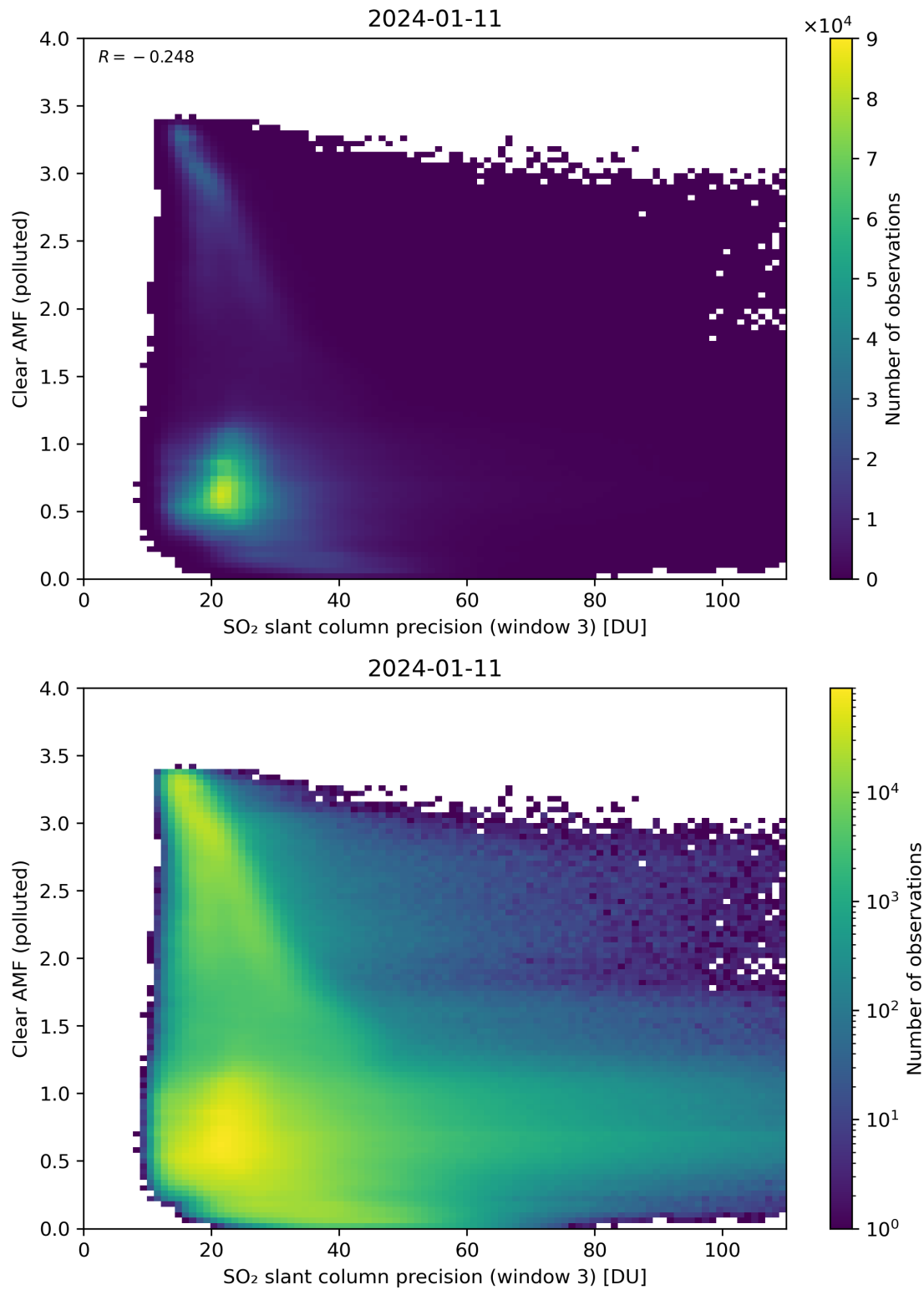
Figure 261: Scatter density plot of “SO 2 slant column precision (window 3)” against “Clear AMF (polluted)” for 2024-01-10 to 2024-01-12.
