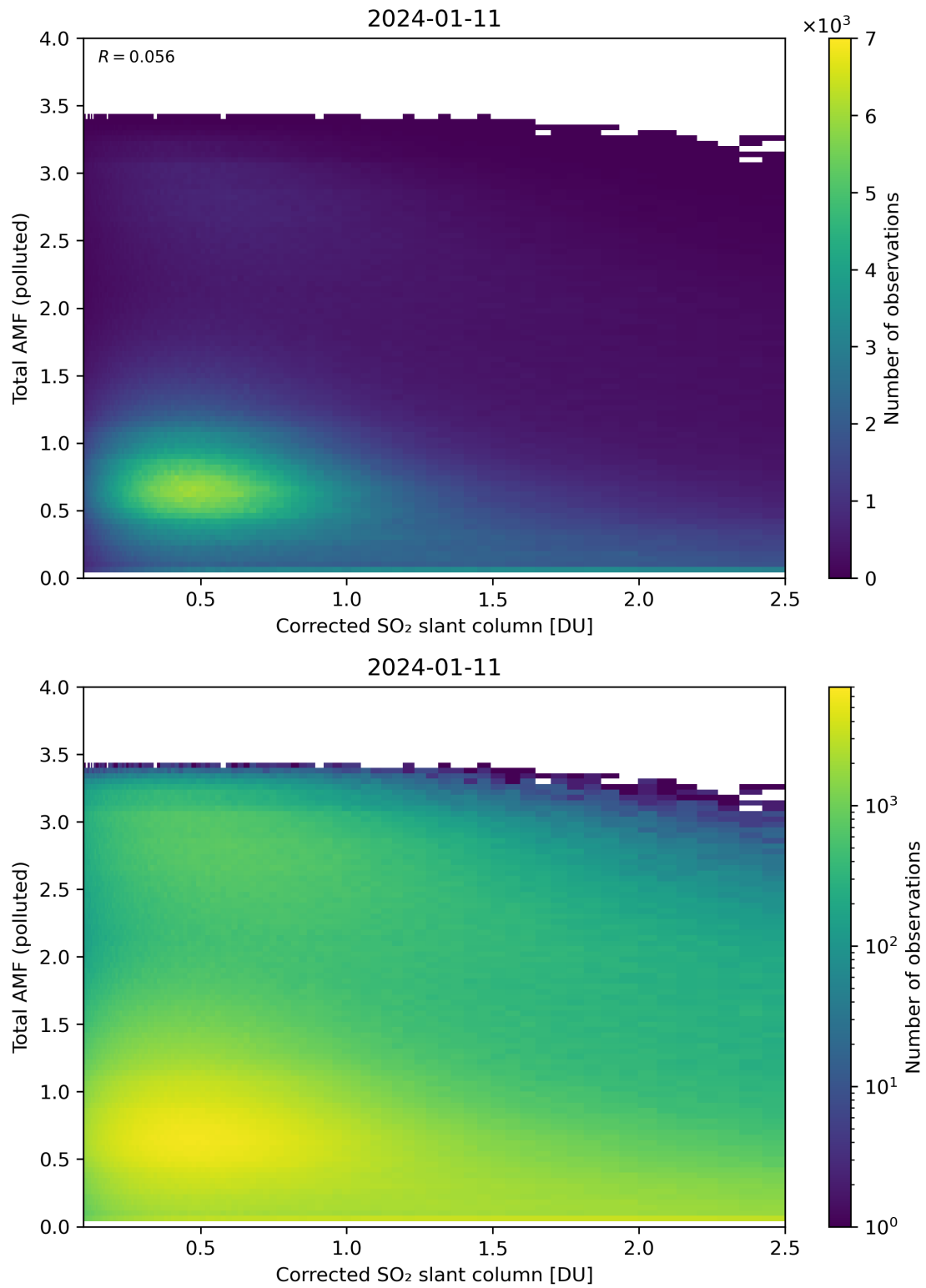
Figure 192: Scatter density plot of “Corrected SO 2 slant column” against “Total AMF (polluted)” for 2024-01-10 to 2024-01-12.
