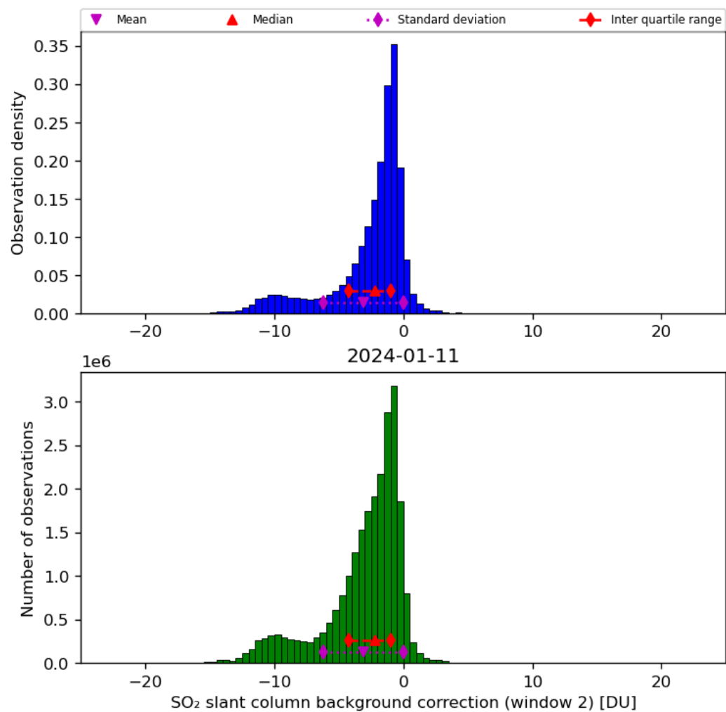
Figure 63: Histogram of “SO 2 slant column background correction (window 2)” for 2024-01-10 to 2024-01-12
