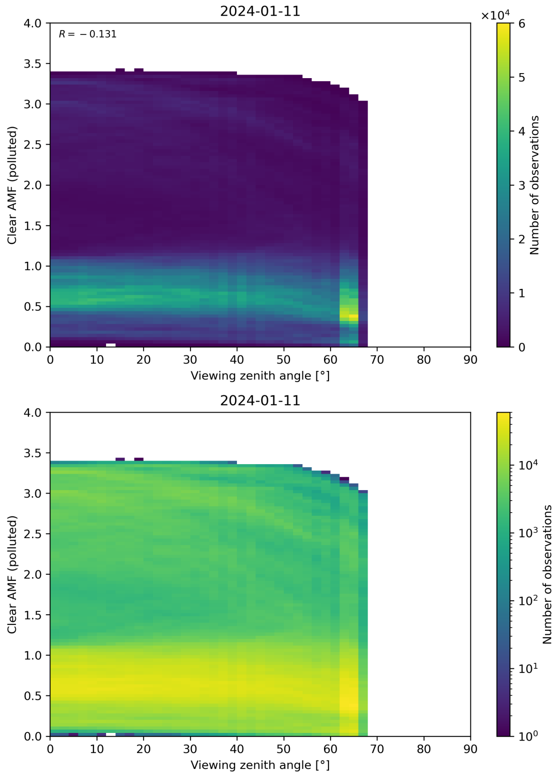
Figure 316: Scatter density plot of “Viewing zenith angle” against “Clear AMF (polluted)” for 2024-01-10 to 2024-01-12.
