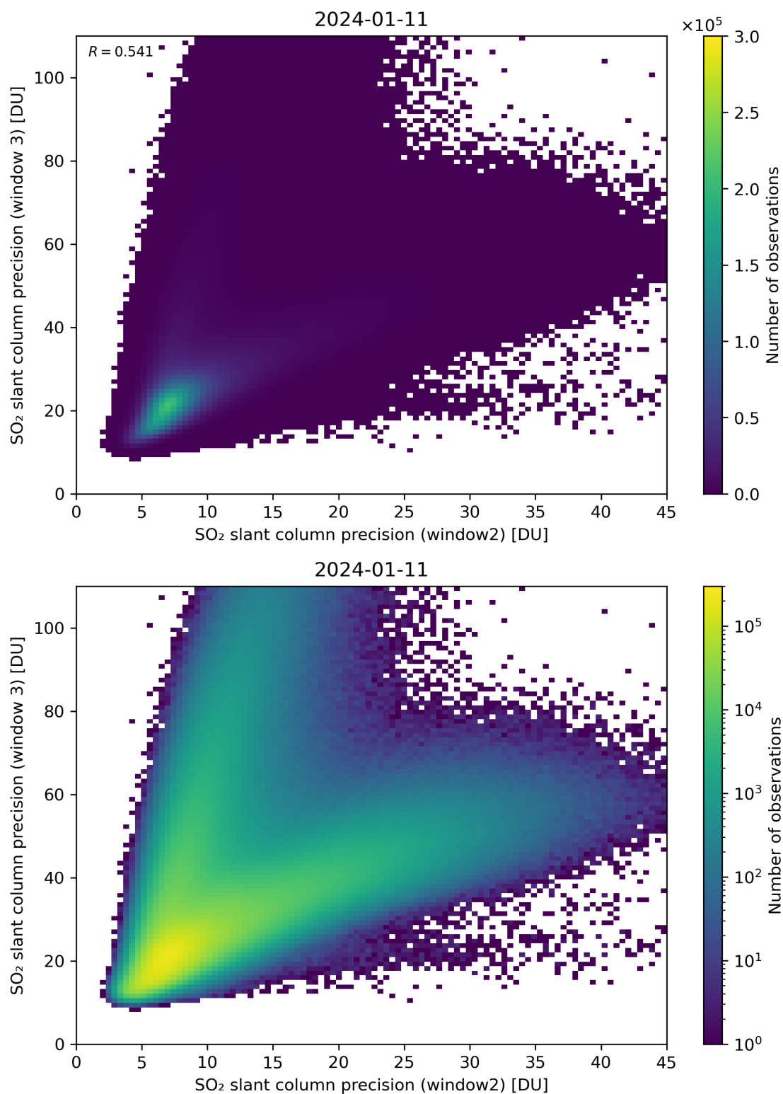
Figure 250: Scatter density plot of “SO 2 slant column precision (window2)” against “SO 2 slant column precision (window3)” for 2024-01-10 to 2024-01-12.
