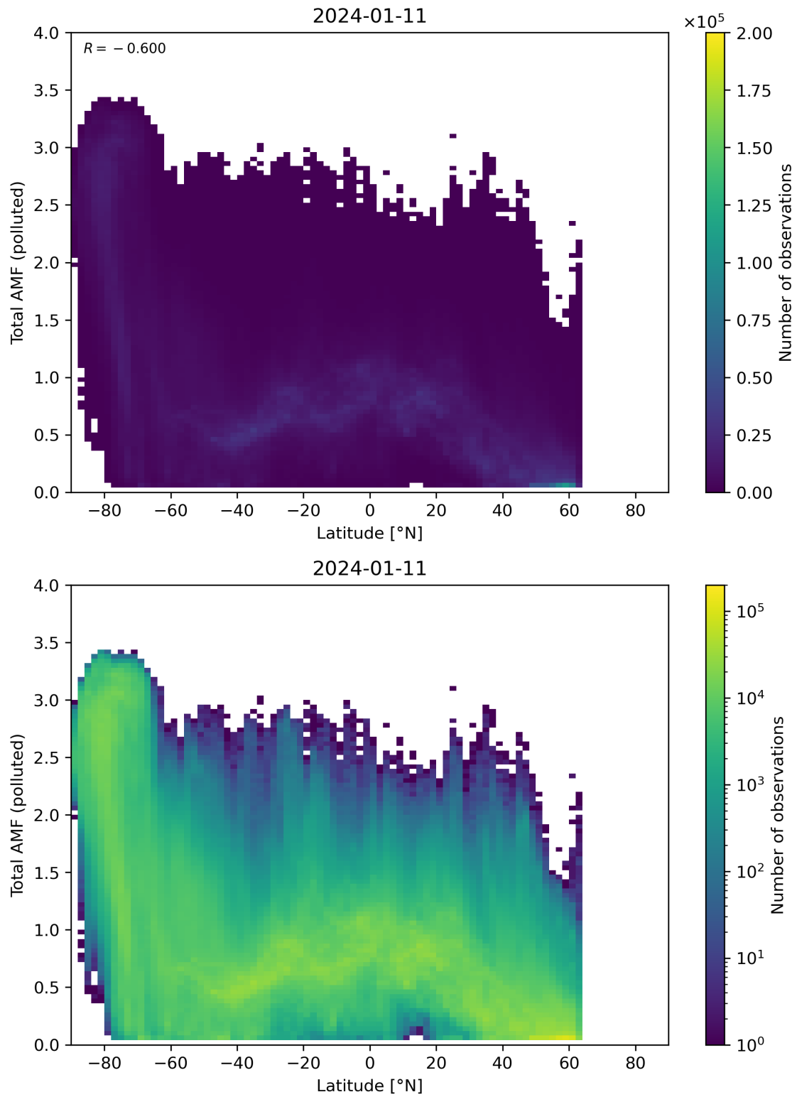
Figure 154: Scatter density plot of “Latitude” against “Total AMF (polluted)” for 2024-01-10 to 2024-01-12.
