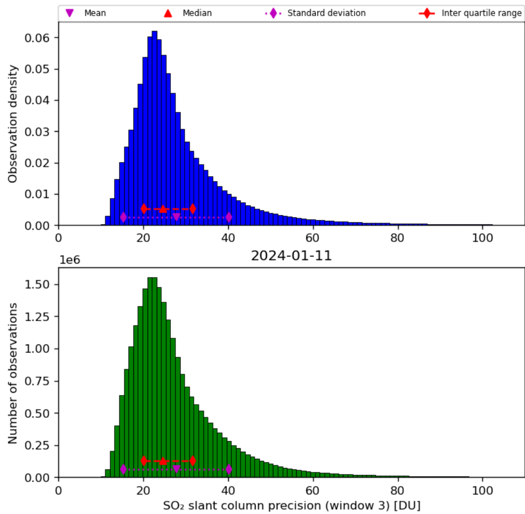
Figure 65: Histogram of “SO 2 slant column precision (window 3)” for 2024-01-10 to 2024-01-12
