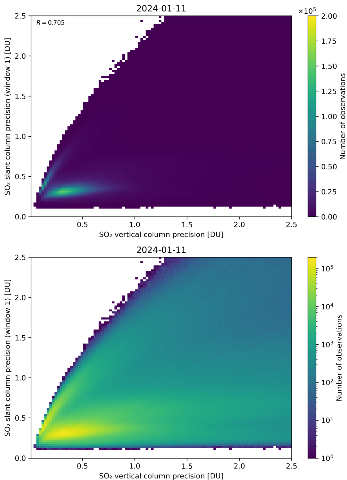
Figure 290: Scatter density plot of “SO 2 vertical column precision” against “SO 2 slant column precision (window 1)” for 2024-01-10 to 2024-01-12.
