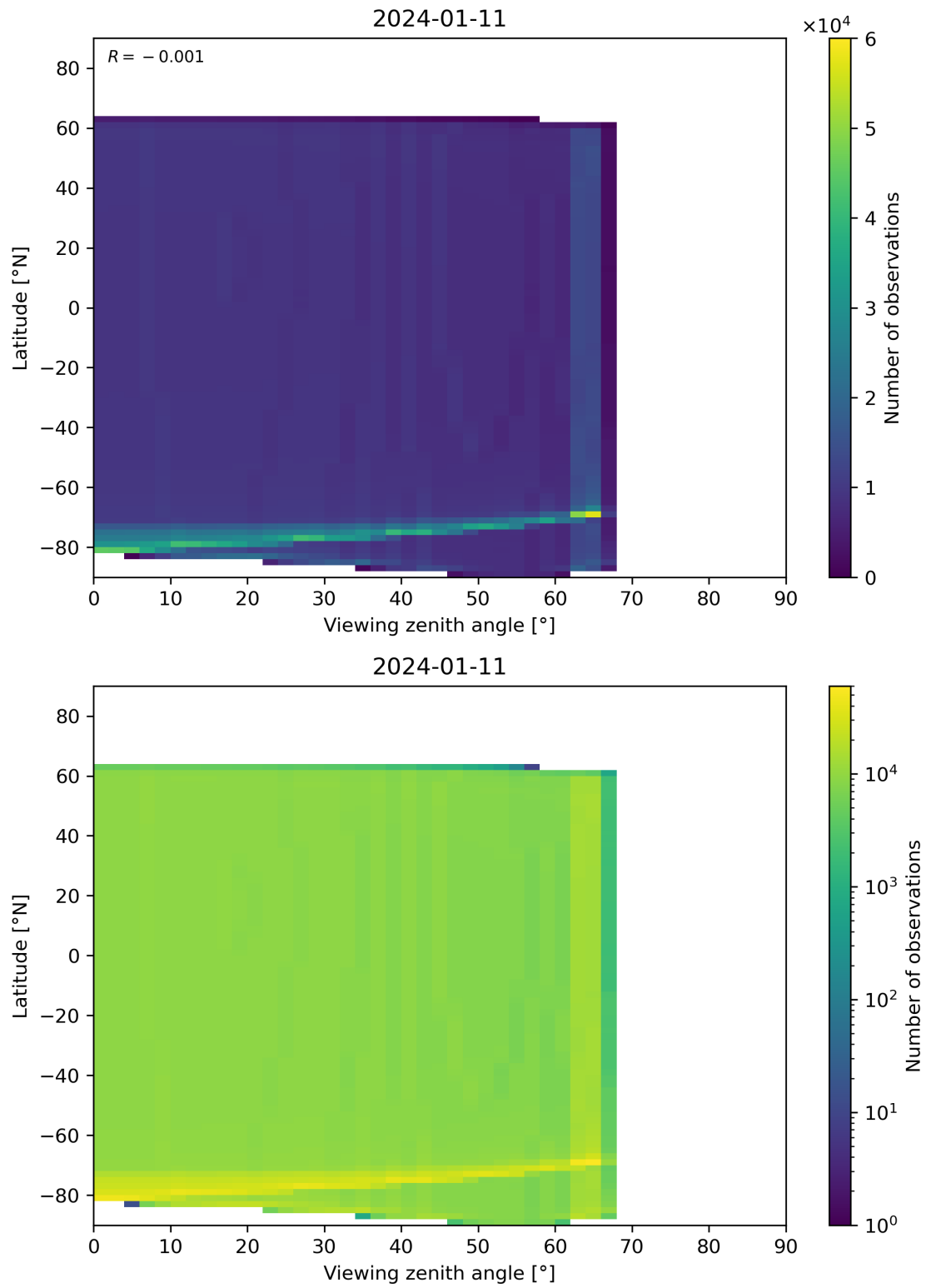
Figure 314: Scatter density plot of “Viewing zenith angle” against “Latitude” for 2024-01-10 to 2024-01-12.
