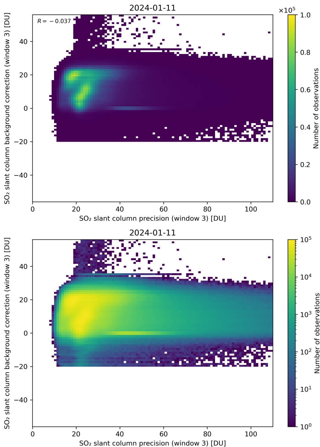
Figure 257: Scatter density plot of “SO 2 slant column precision (window 3)” against “SO 2 slant column background correction (window 3)” for 2024-01-10 to 2024-01-12.
