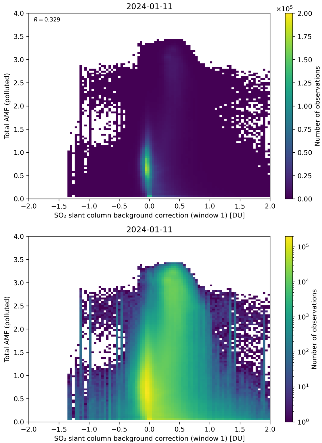
Figure 109: Scatter density plot of “SO 2 slant column background correction (window 1)” against “Total AMF (polluted)” for 2024-01-10 to 2024-01-12.
