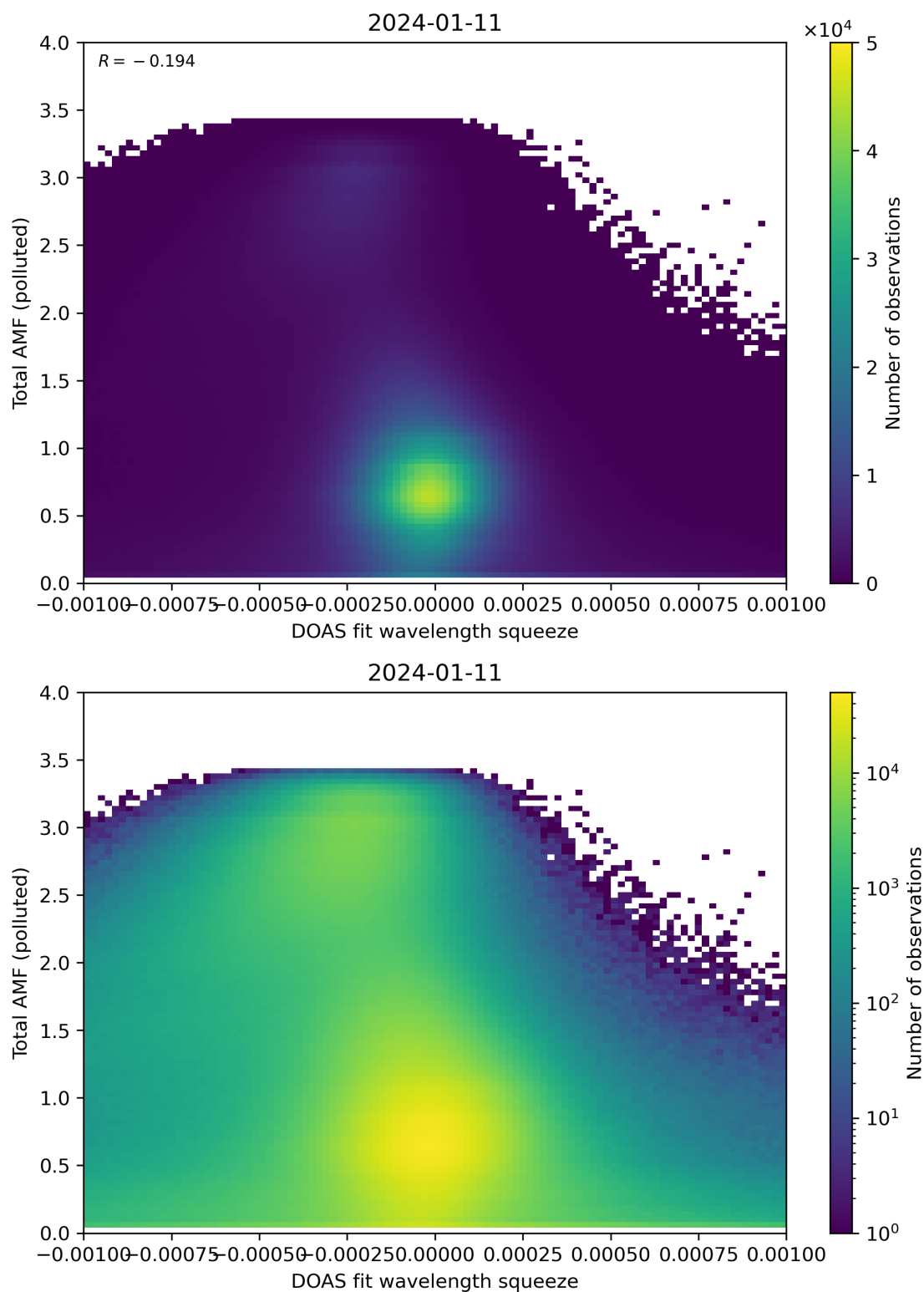
Figure 134: Scatter density plot of “DOAS fit wavelength squeeze” against “Total AMF (polluted)” for 2024-01-10 to 2024-01-12.
