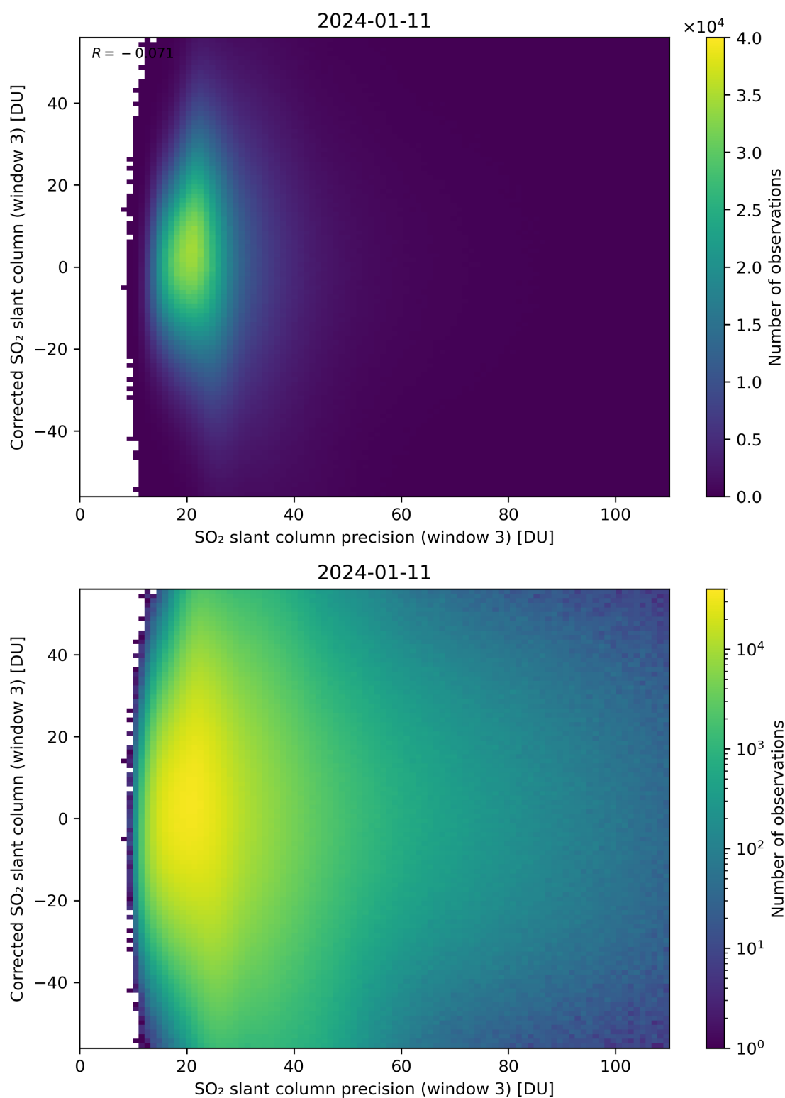
Figure 262: Scatter density plot of “SO 2 slant column precision (window 3)” against “Corrected SO 2 slant column (window 3)” for 2024-01-10 to 2024-01-12.
