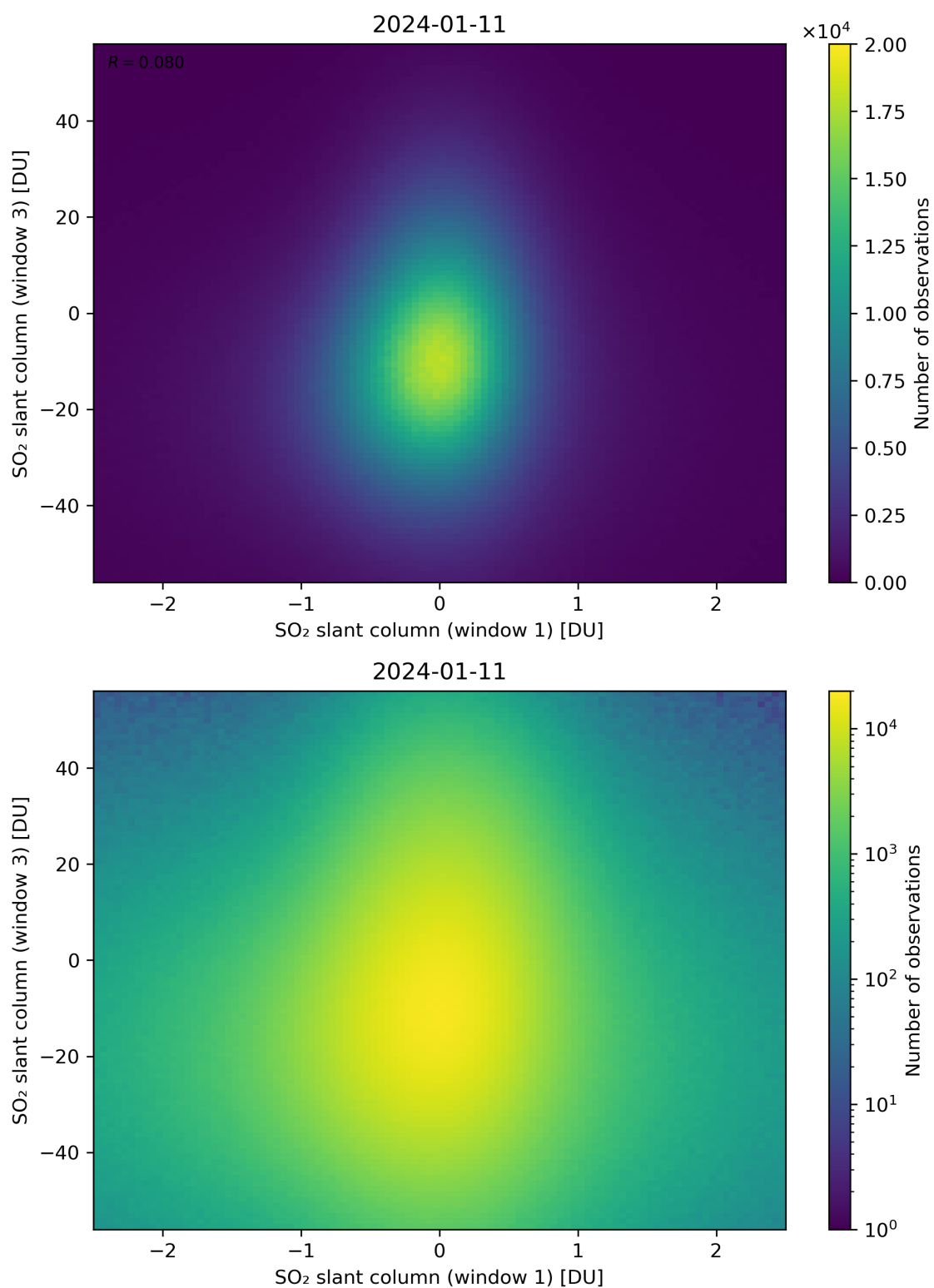
Figure 237: Scatter density plot of “SO 2 slant column (window 1)” against “SO 2 slant column (window 3)” for 2024-01-10 to 2024-01-12.
