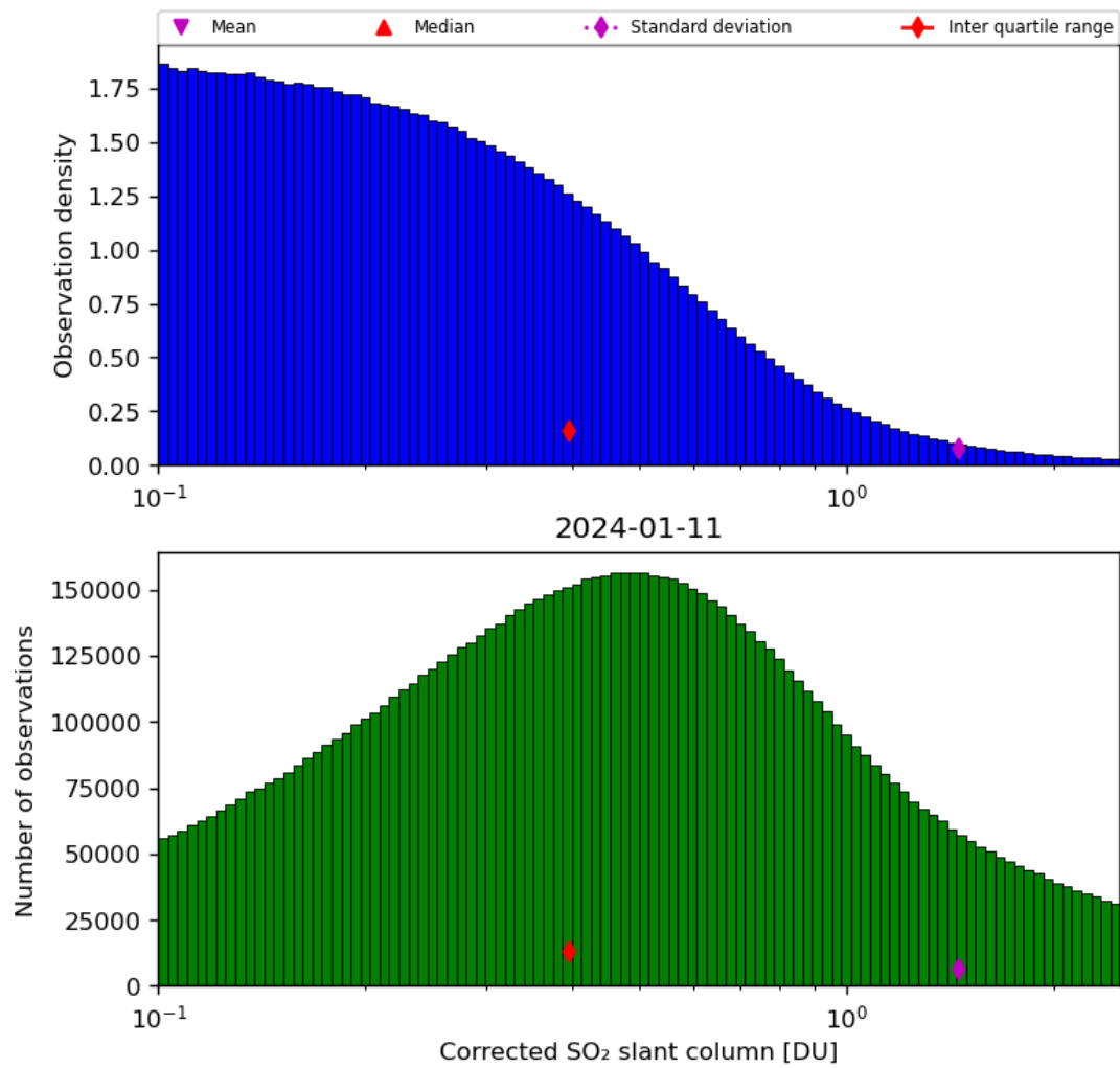
Figure 55: Histogram of “Corrected SO 2 slant column” for 2024-01-10 to 2024-01-12
