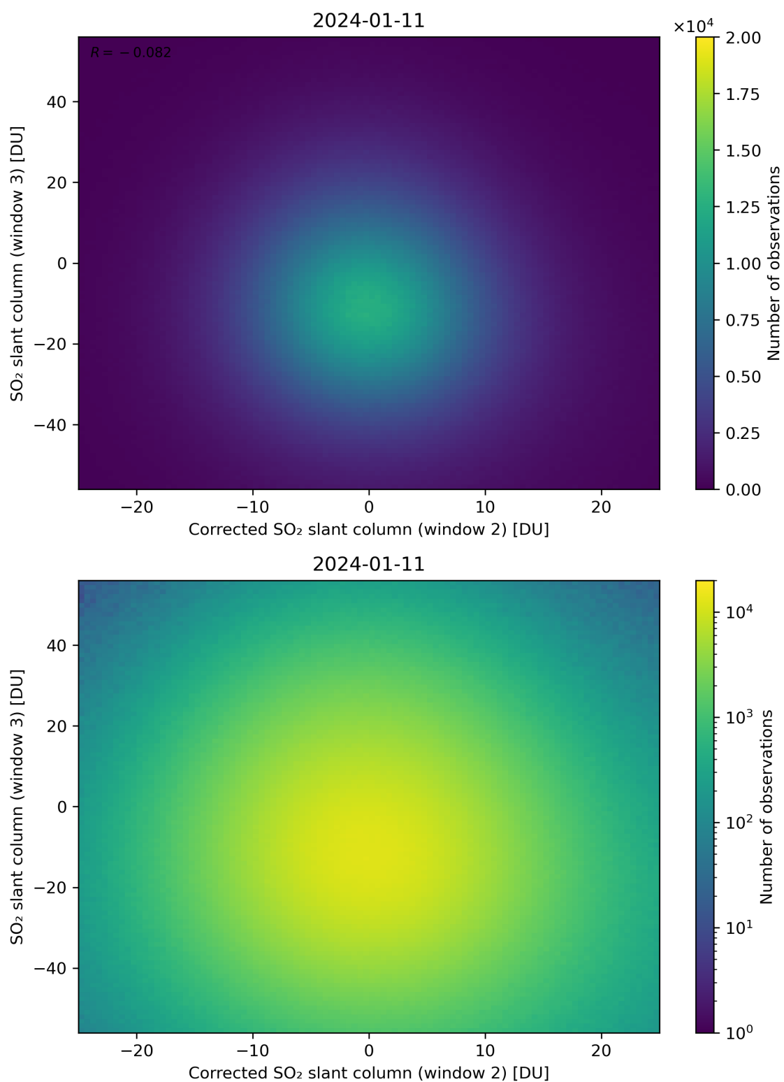
Figure 201: Scatter density plot of “Corrected SO 2 slant column (window 2)” against “SO 2 slant column (window 3)” for 2024-01-10 to 2024-01-12.
