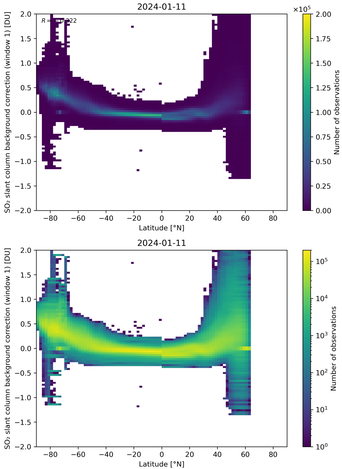
Figure 139: Scatter density plot of “Latitude” against “SO 2 slant column background correction (window 1)” for 2024-01-10 to 2024-01-12.
