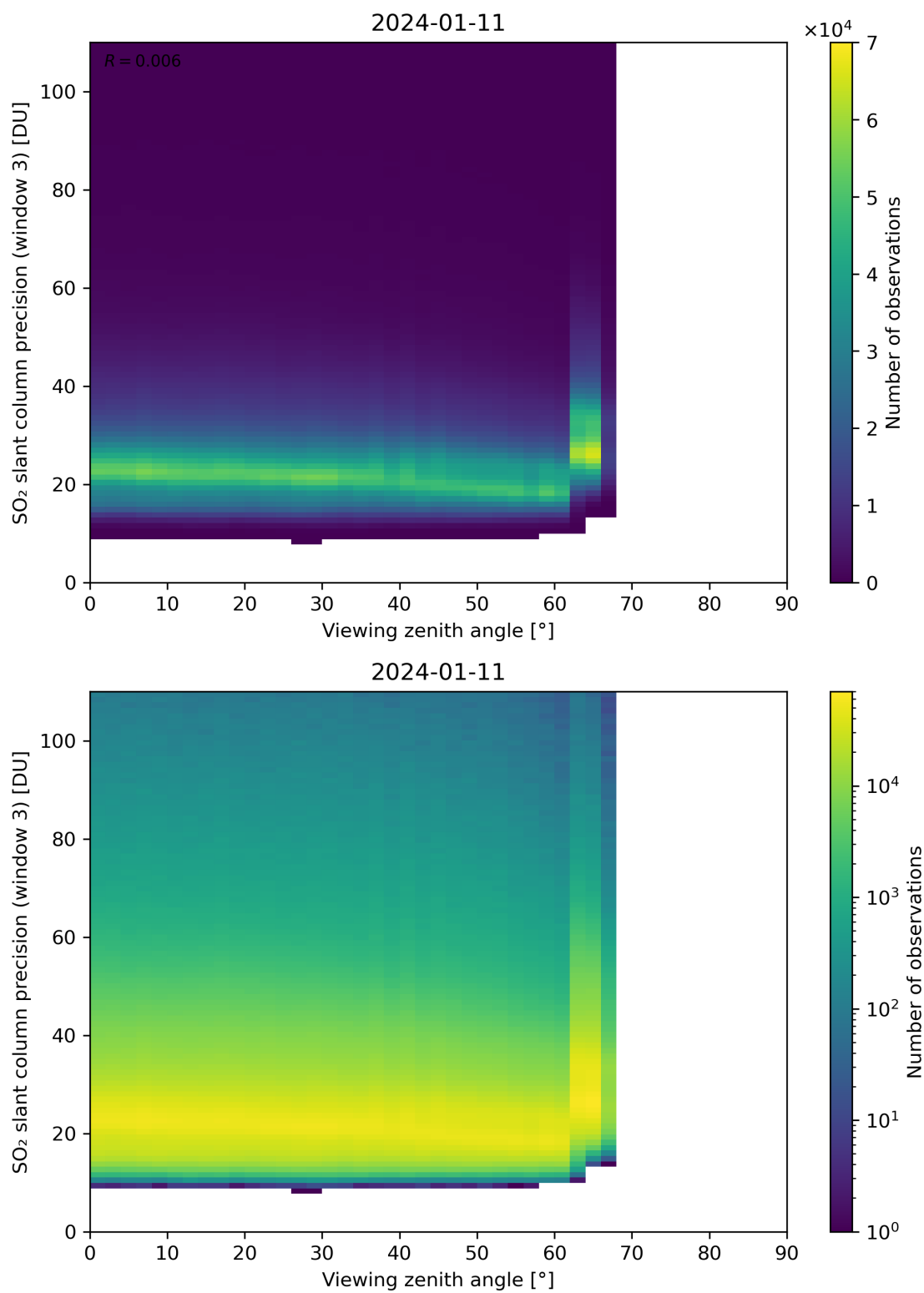
Figure 324: Scatter density plot of “Viewing zenith angle” against “SO 2 slant column precision (window 3)” for 2024-01-10 to 2024-01-12.
