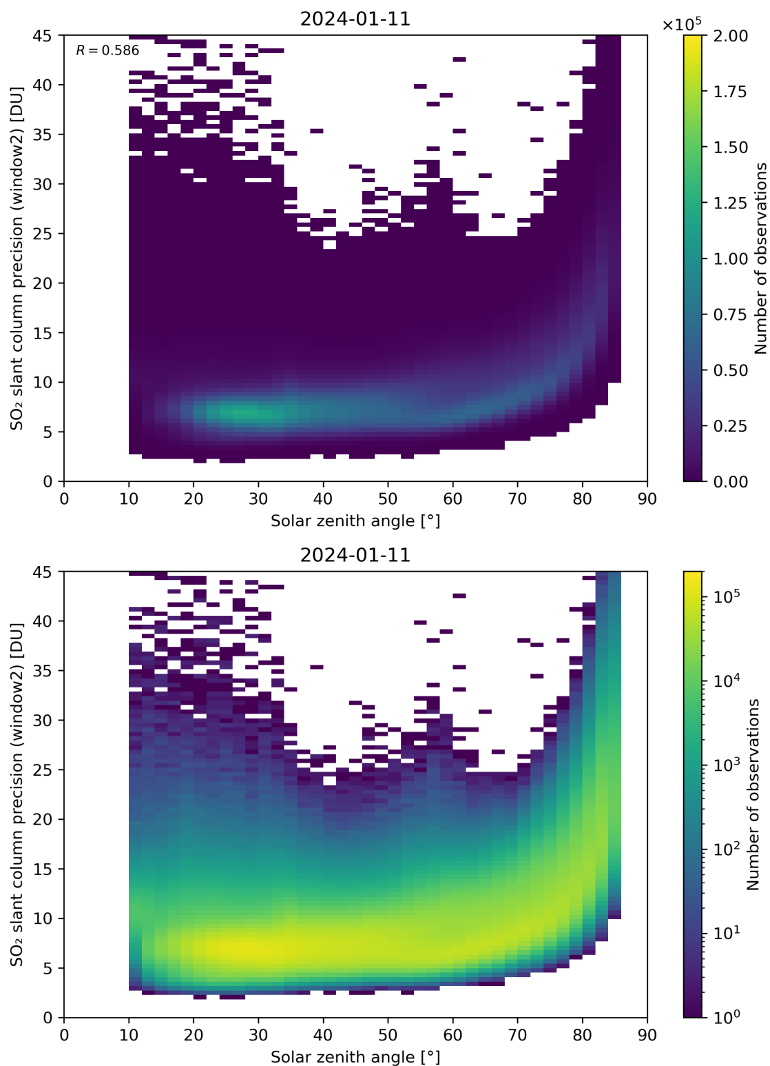
Figure 171: Scatter density plot of “Solar zenith angle” against “SO 2 slant column precision (window2)” for 2024-01-10 to 2024-01-12.
