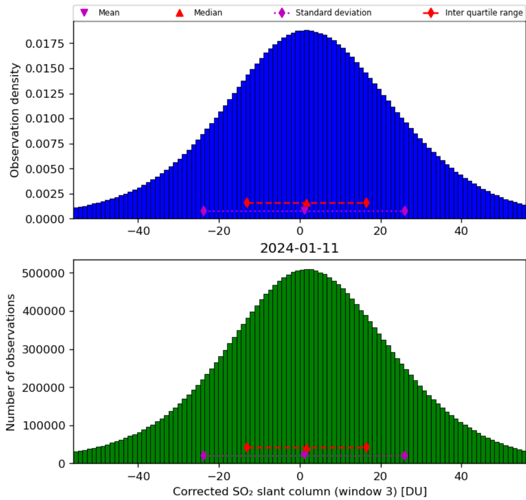
Figure 66: Histogram of “Corrected SO 2 slant column (window 3)” for 2024-01-10 to 2024-01-12
