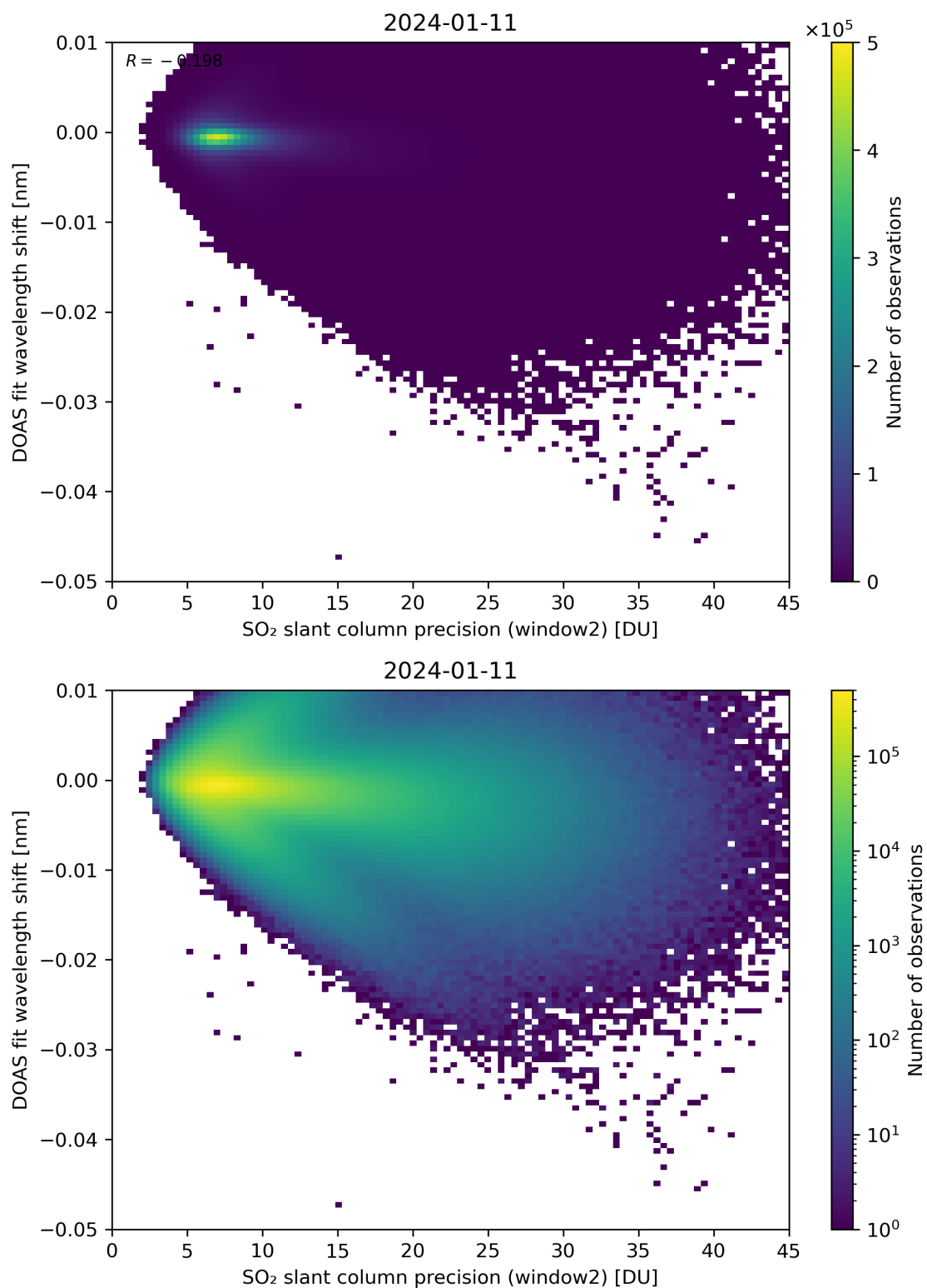
Figure 243: Scatter density plot of “SO 2 slant column precision (window2)” against “DOAS fit wavelength shift” for 2024-01-10 to 2024-01-12.
