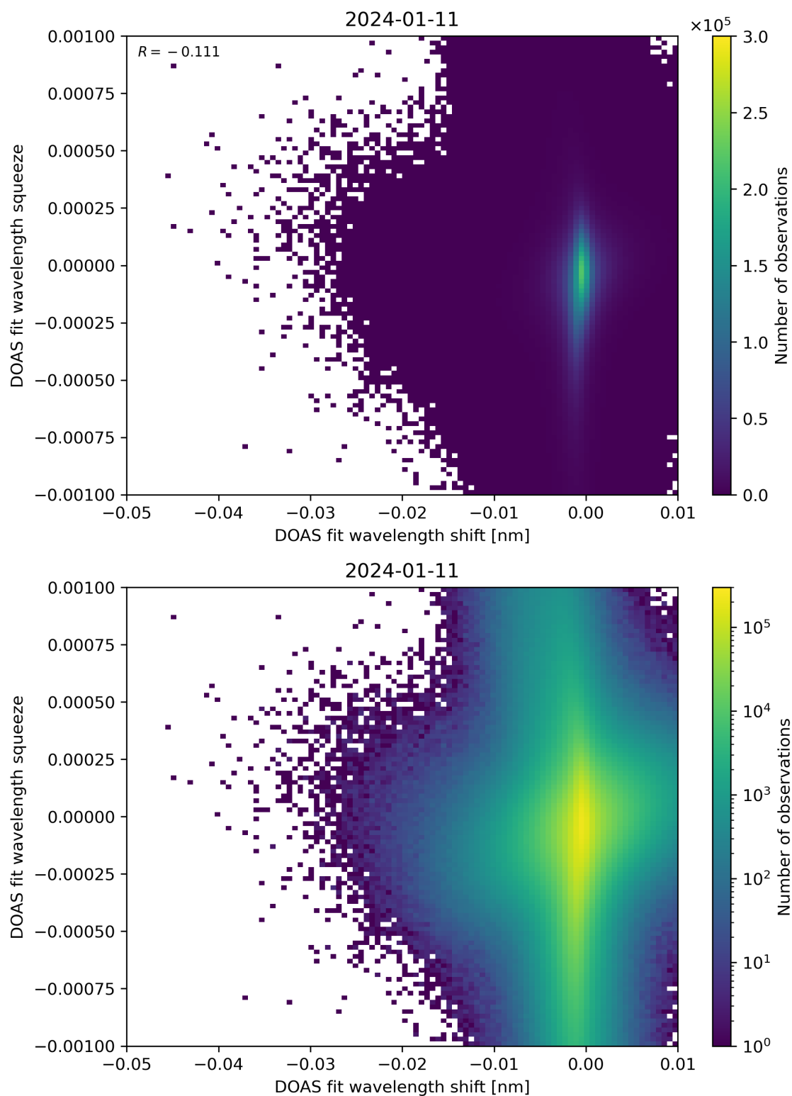
Figure 127: Scatter density plot of “DOAS fit wavelength shift” against “DOAS fit wavelength squeeze” for 2024-01-10 to 2024-01-12.
