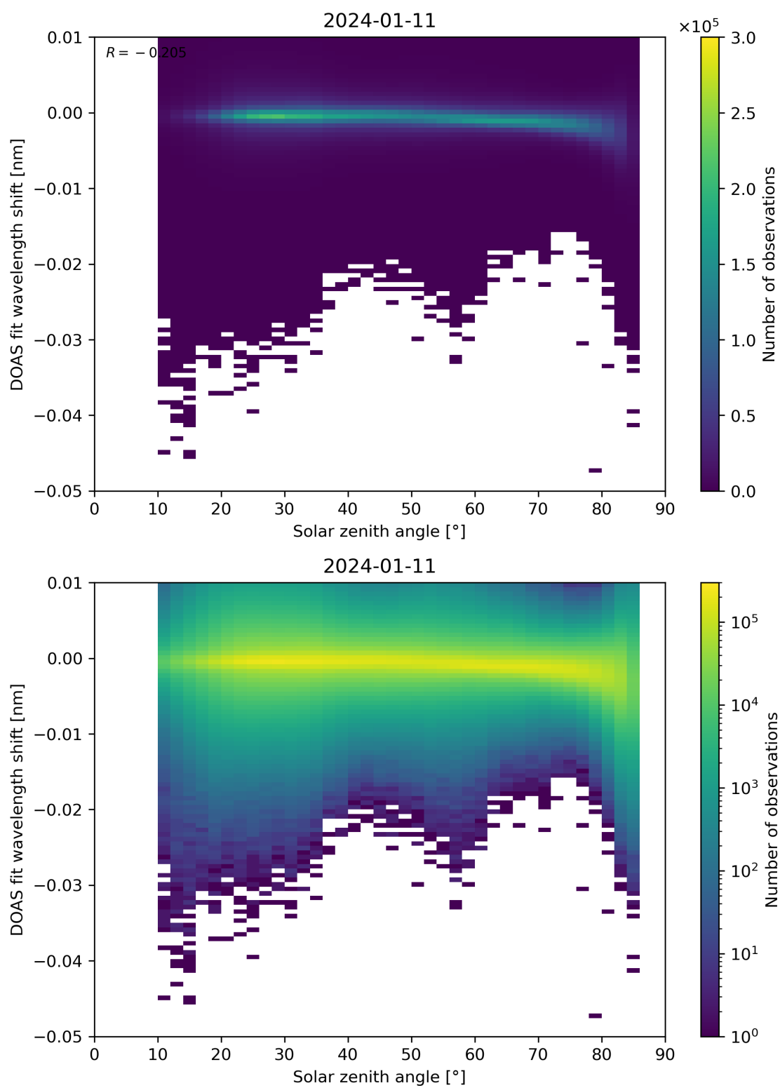
Figure 161: Scatter density plot of “Solar zenith angle” against “DOAS fit wavelength shift” for 2024-01-10 to 2024-01-12.
