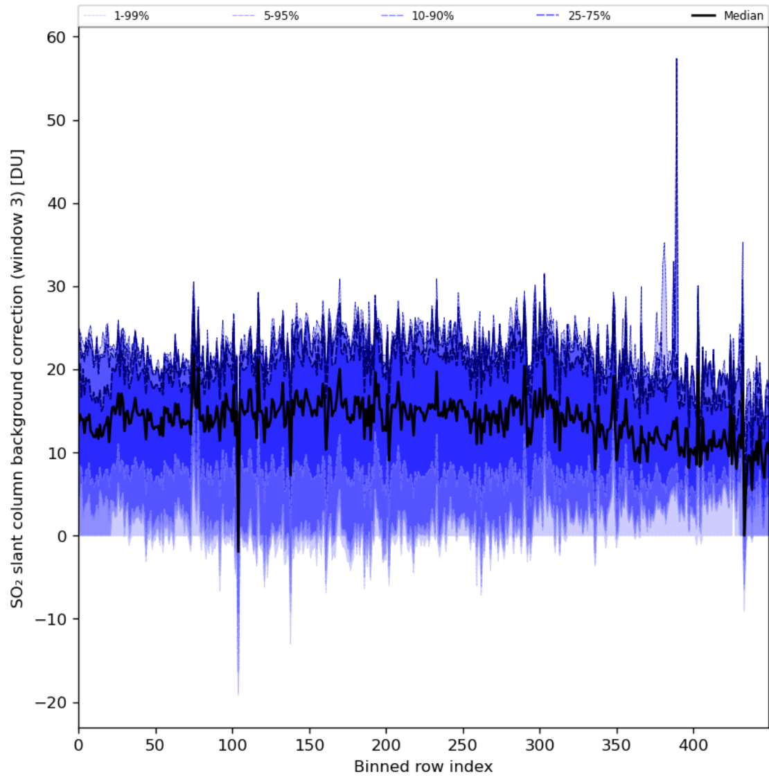
Figure 90: Along track statistics of “SO 2 slant column background correction (window 3)” for 2024-01-10 to 2024-01-12
