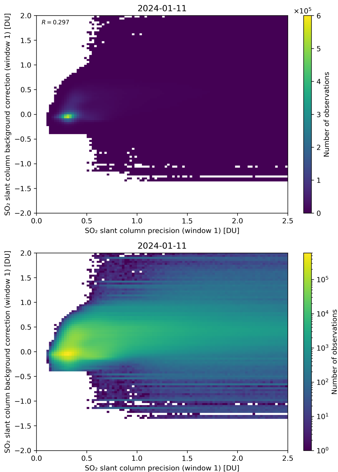
Figure 218: Scatter density plot of “SO 2 slant column precision (window 1)” against “SO 2 slant column background correction (window 1)” for 2024-01-10 to 2024-01-12.
