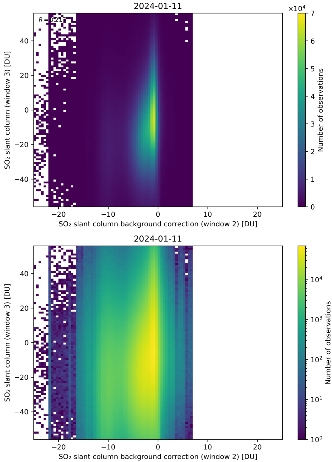
Figure 117: Scatter density plot of “SO 2 slant column background correction (window 2)” against “SO 2 slant column (window 3)” for 2024-01-10 to 2024-01-12.
