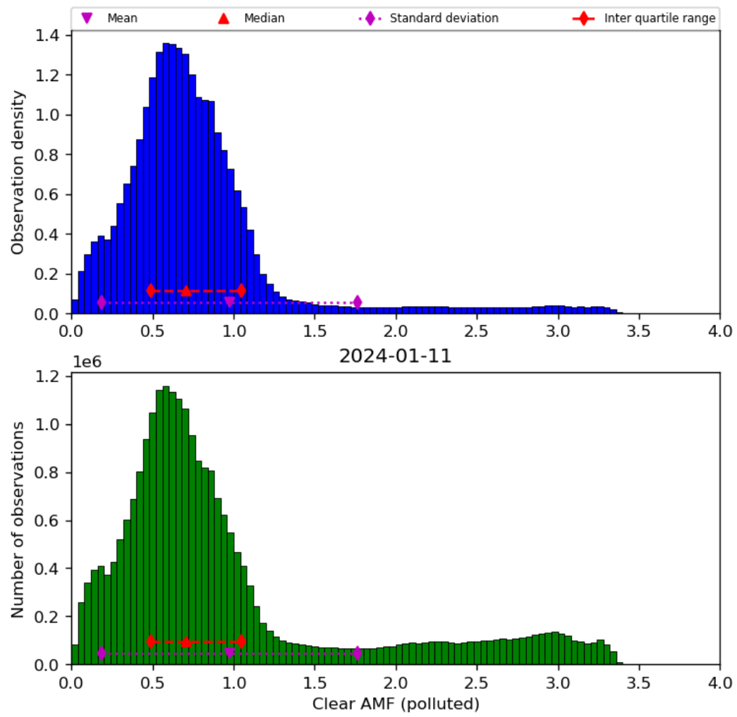
Figure 73: Histogram of “Clear AMF (polluted)” for 2024-01-10 to 2024-01-12
