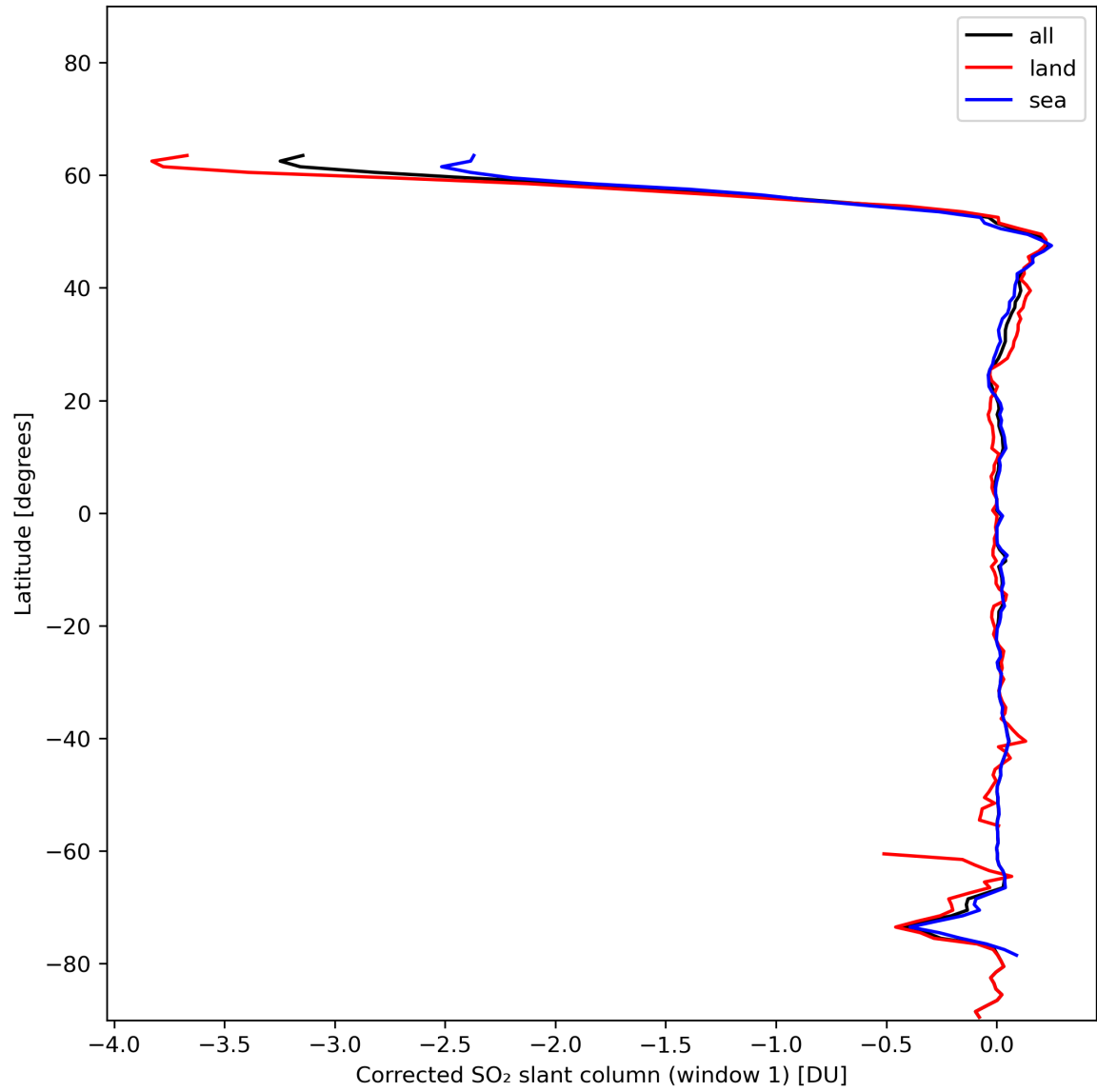
Figure 35: Zonal average of “Corrected SO 2 slant column (window 1)” for 2024-01-10 to 2024-01-12.
