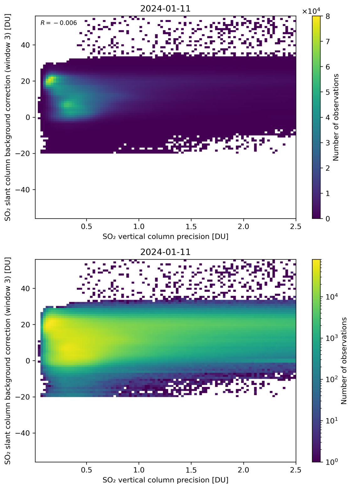
Figure 281: Scatter density plot of “SO 2 vertical column precision” against “SO 2 slant column background correction (window 3)” for 2024-01-10 to 2024-01-12.
