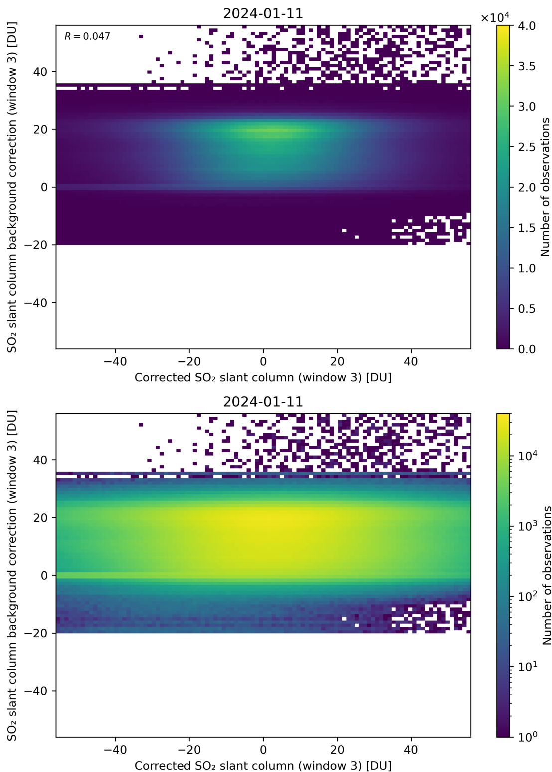
Figure 205: Scatter density plot of “Corrected SO 2 slant column (window 3)” against “SO 2 slant column background correction (window 3)” for 2024-01-10 to 2024-01-12.
