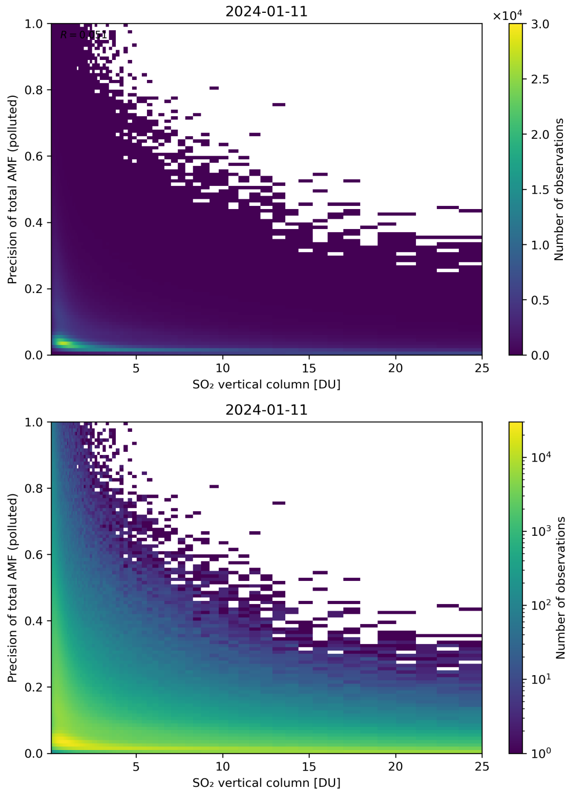
Figure 306: Scatter density plot of “SO 2 vertical column” against “Precision of total AMF (polluted)” for 2024-01-10 to 2024-01-12.
