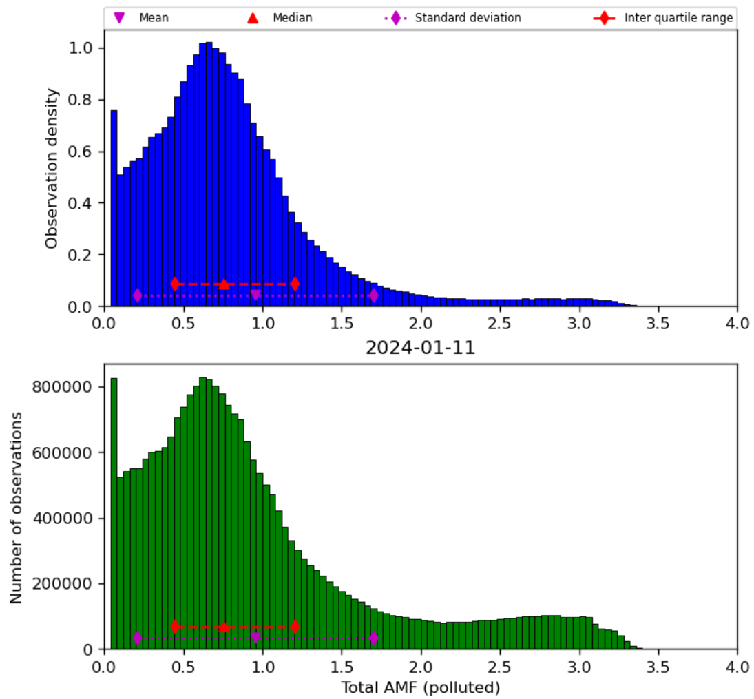
Figure 71: Histogram of “Total AMF (polluted)” for 2024-01-10 to 2024-01-12
