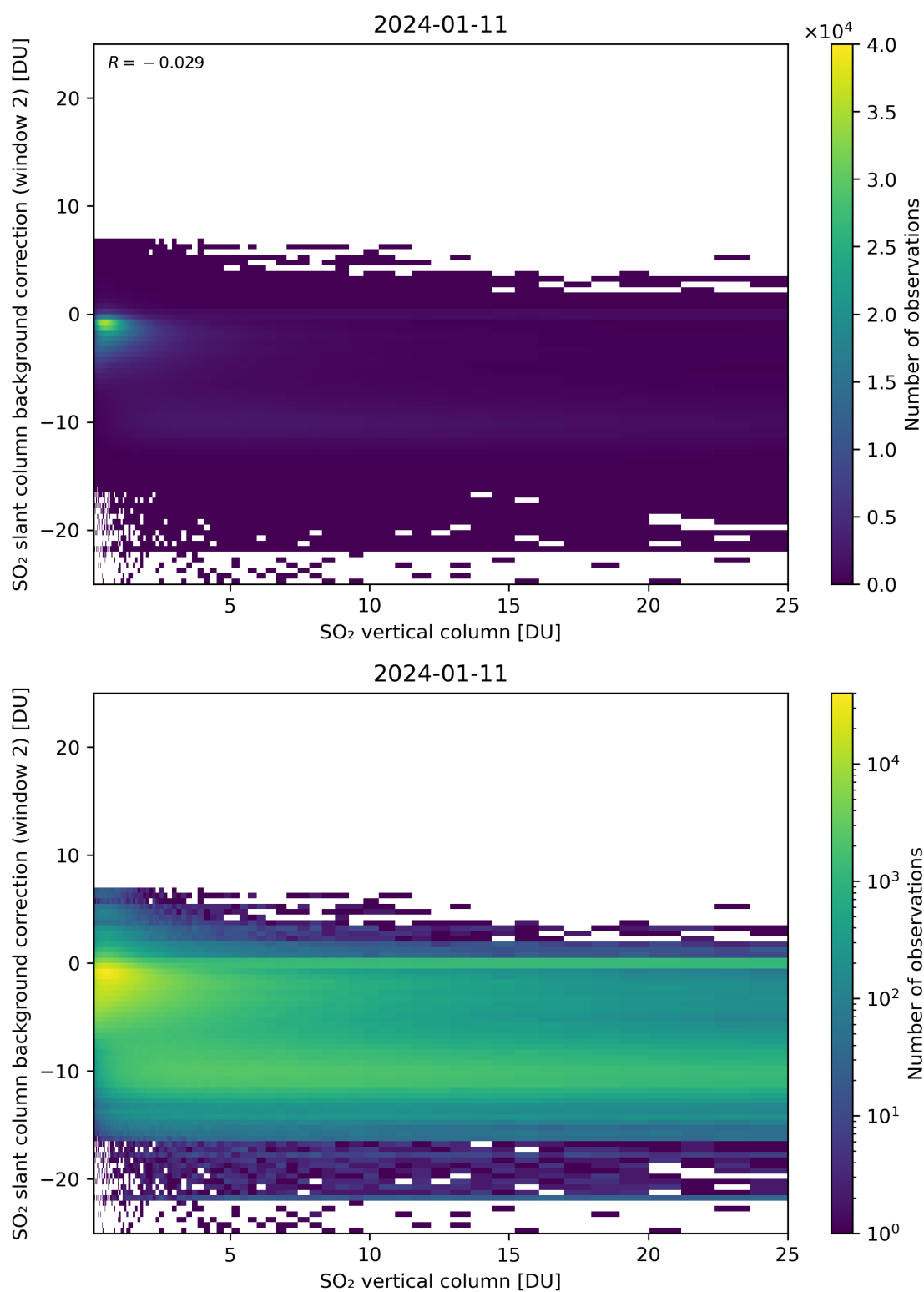
Figure 274: Scatter density plot of “SO 2 vertical column” against “SO 2 slant column background correction (window 2)” for 2024-01-10 to 2024-01-12.
