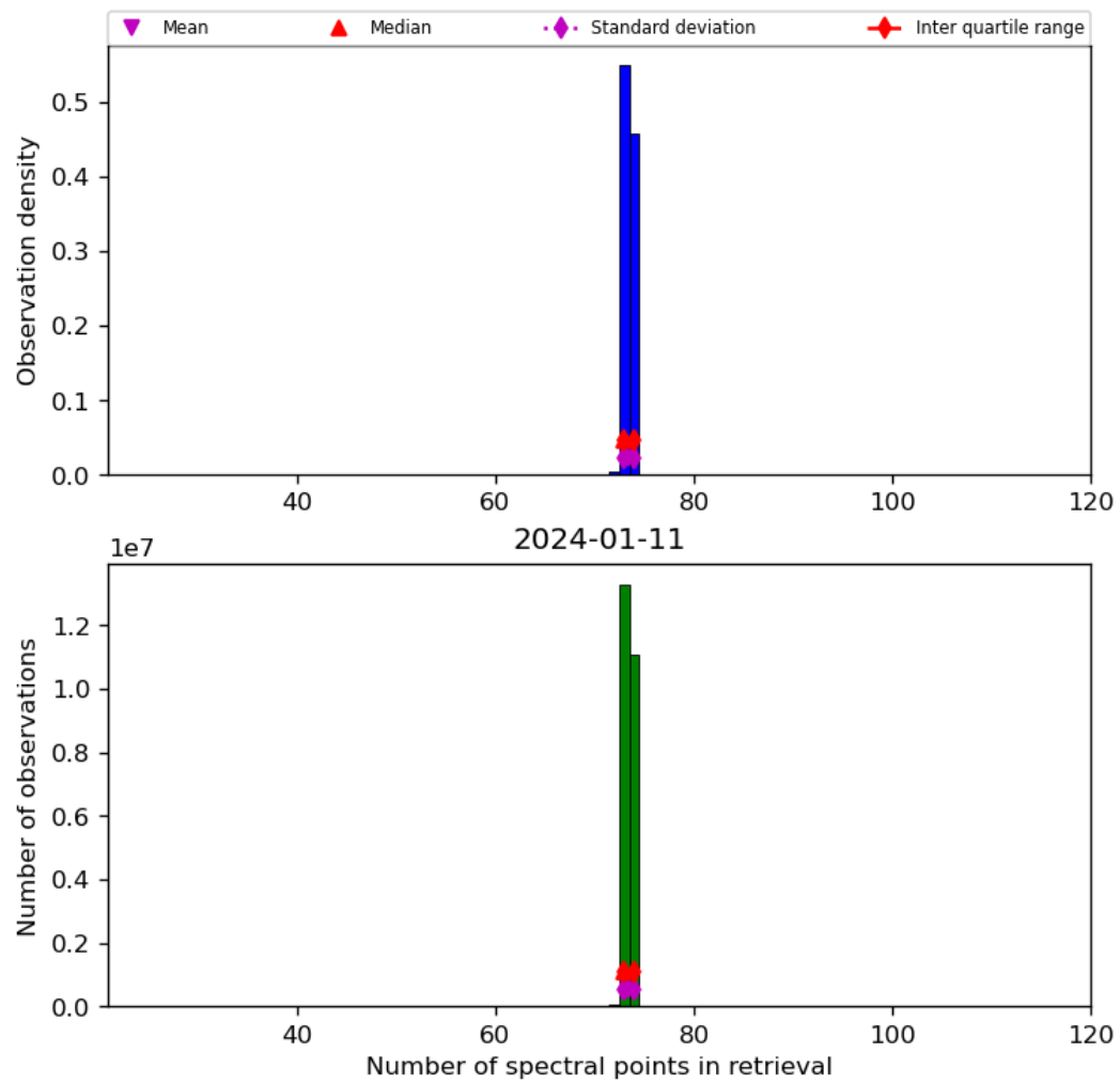
Figure 74: Histogram of “Number of spectral points in retrieval” for 2024-01-10 to 2024-01-12
