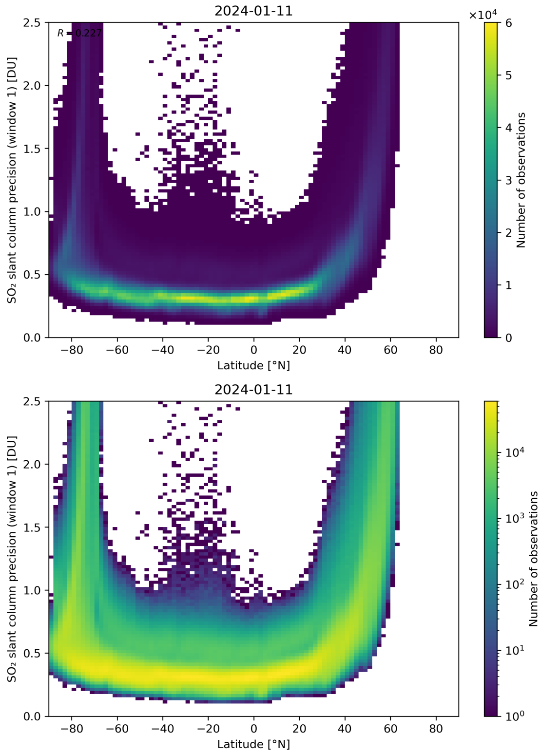
Figure 150: Scatter density plot of “Latitude” against “SO 2 slant column precision (window 1)” for 2024-01-10 to 2024-01-12.
