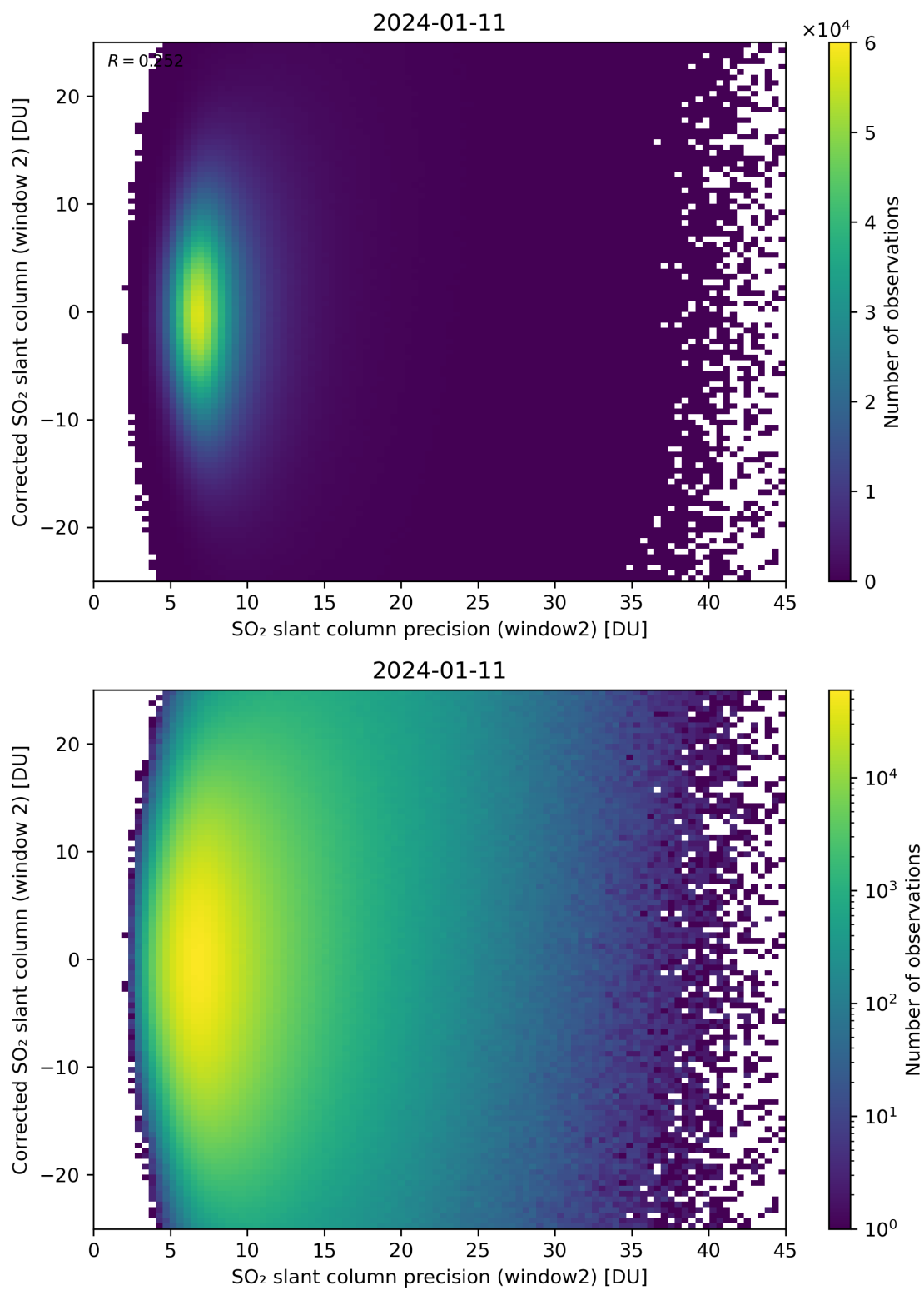
Figure 247: Scatter density plot of “SO 2 slant column precision (window2)” against “Corrected SO 2 slant column (window 2)” for 2024-01-10 to 2024-01-12.
