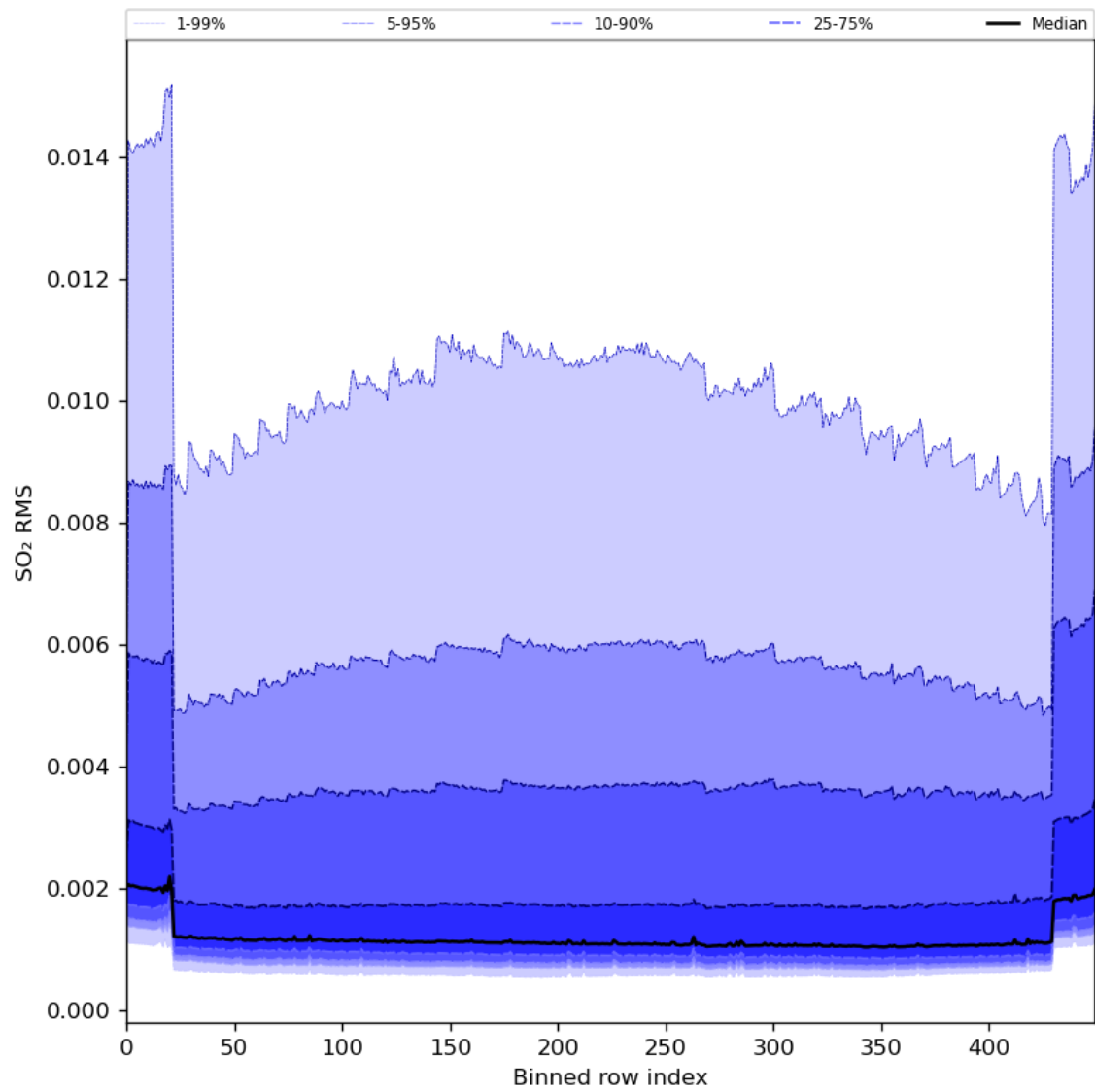
Figure 93: Along track statistics of “SO 2 RMS” for 2024-01-10 to 2024-01-12
