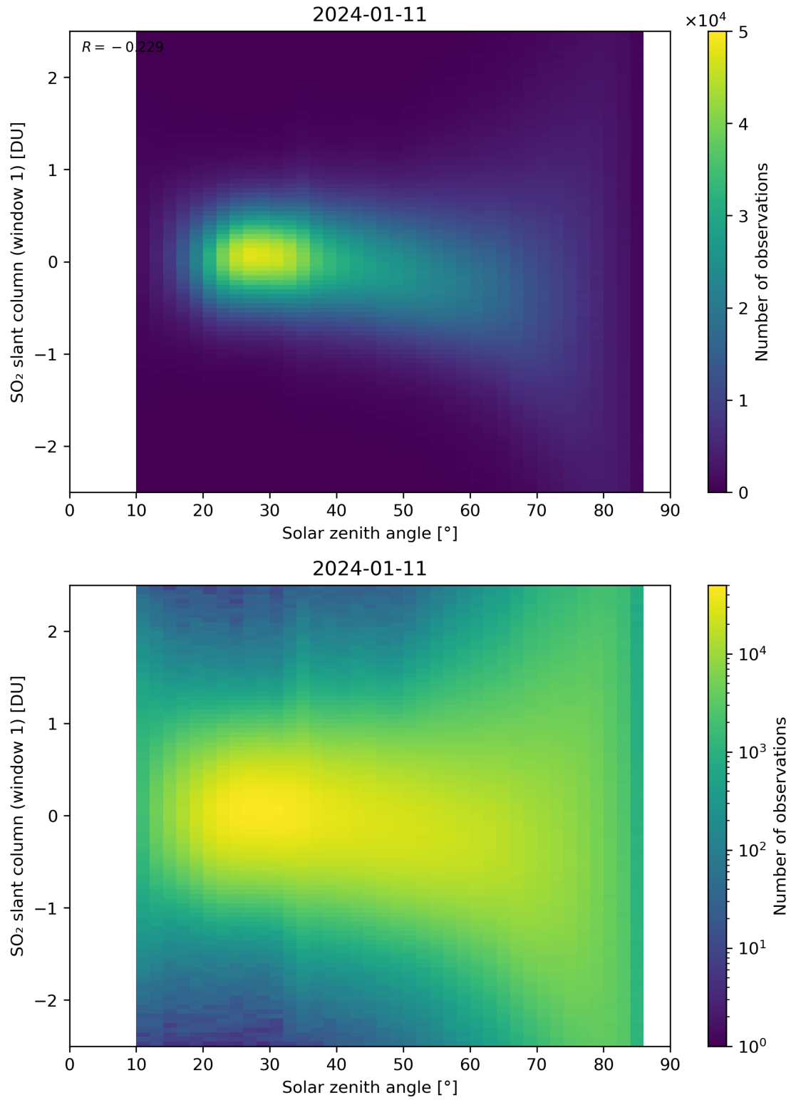
Figure 169: Scatter density plot of “Solar zenith angle” against “SO 2 slant column (window 1)” for 2024-01-10 to 2024-01-12.
