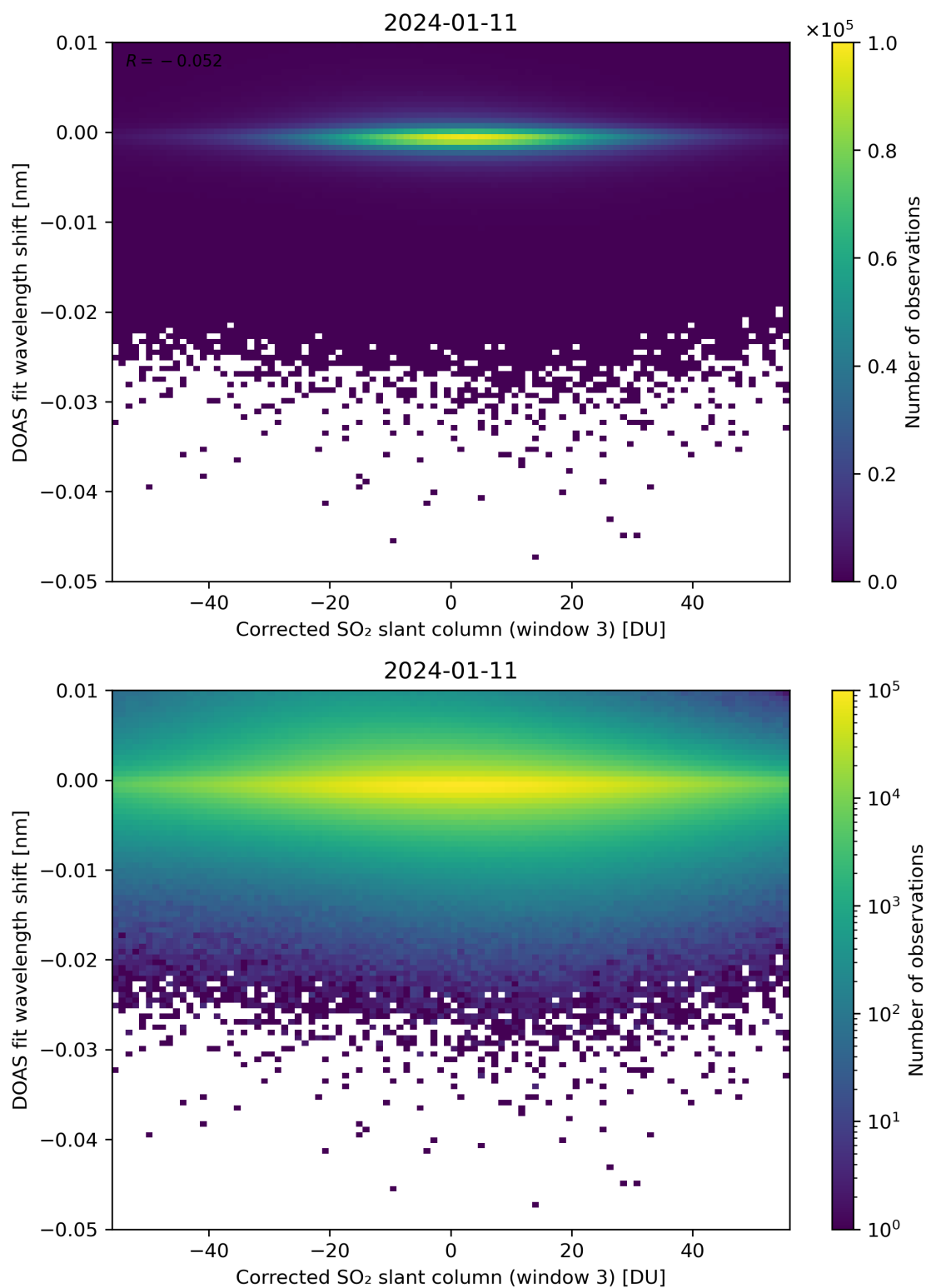
Figure 206: Scatter density plot of “Corrected SO 2 slant column (window 3)” against “DOAS fit wavelength shift” for 2024-01-10 to 2024-01-12.
