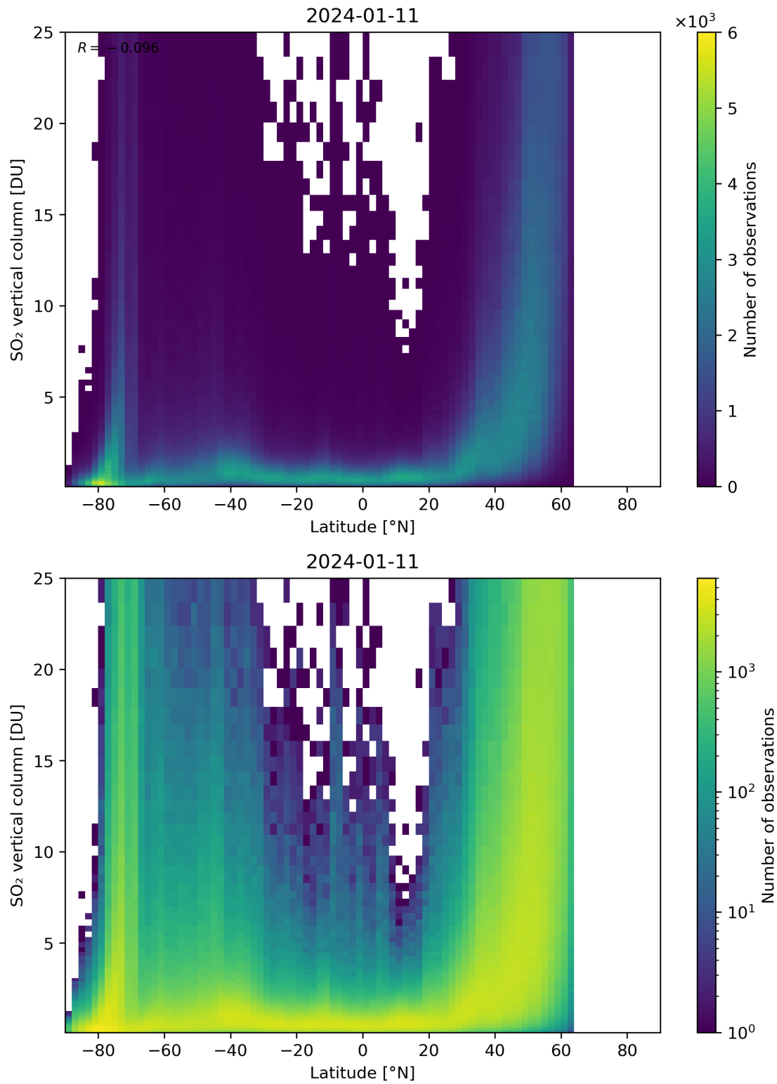
Figure 156: Scatter density plot of “Latitude” against “SO 2 vertical column” for 2024-01-10 to 2024-01-12.
