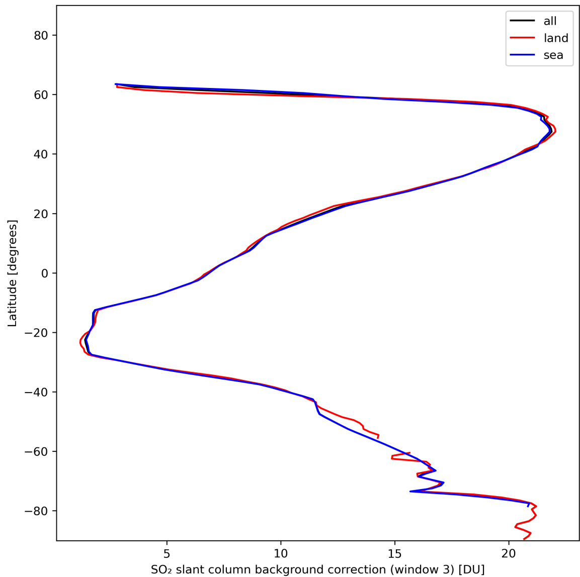
Figure 44: Zonal average of “SO 2 slant column background correction (window 3)” for 2024-01-10 to 2024-01-12.
