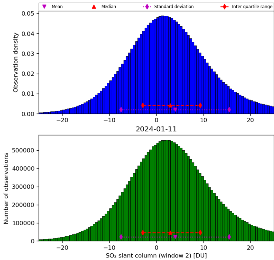
Figure 60: Histogram of “SO 2 slant column (window 2)” for 2024-01-10 to 2024-01-12
