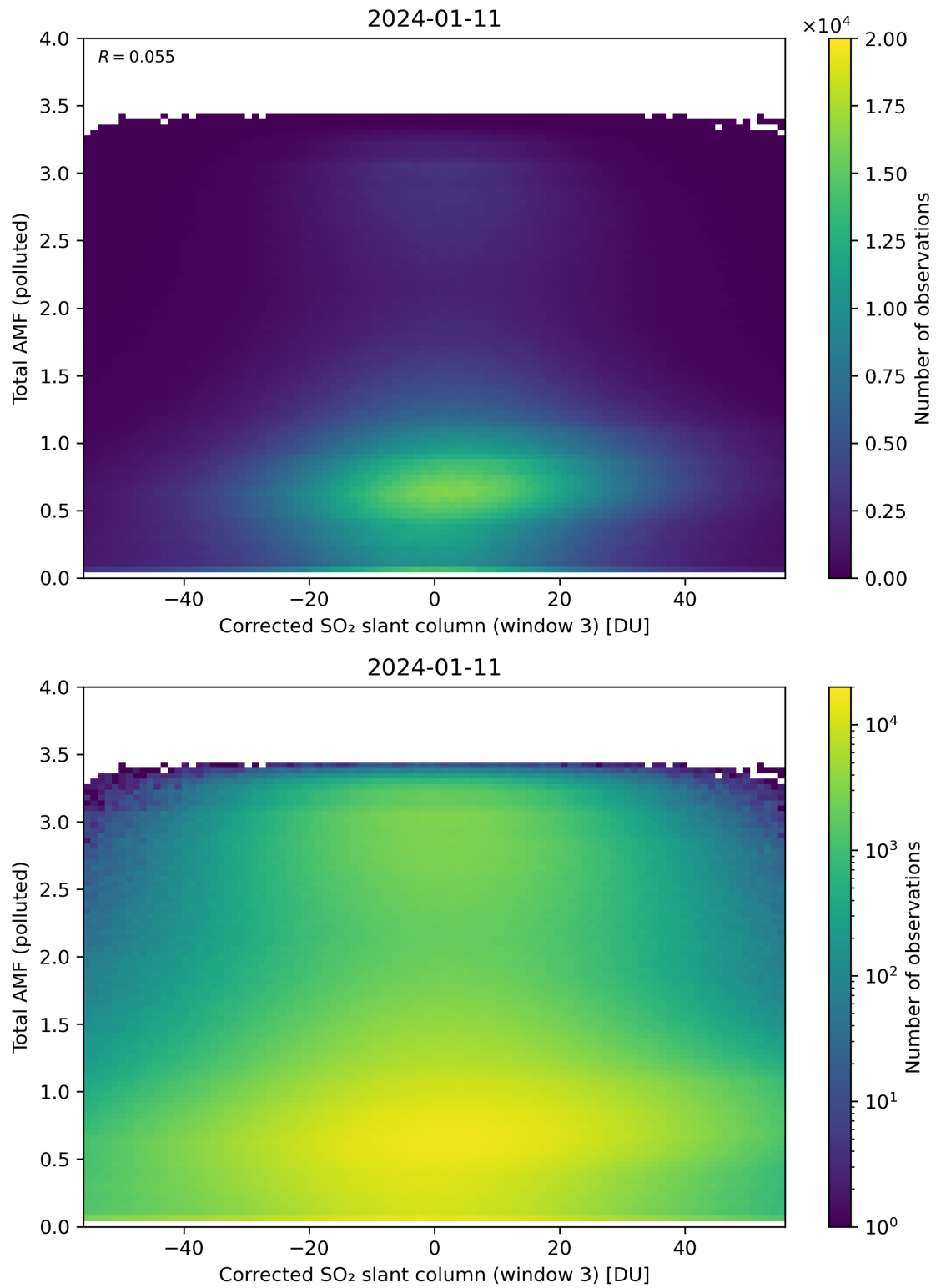
Figure 210: Scatter density plot of “Corrected SO 2 slant column (window 3)” against “Total AMF (polluted)” for 2024-01-10 to 2024-01-12.
