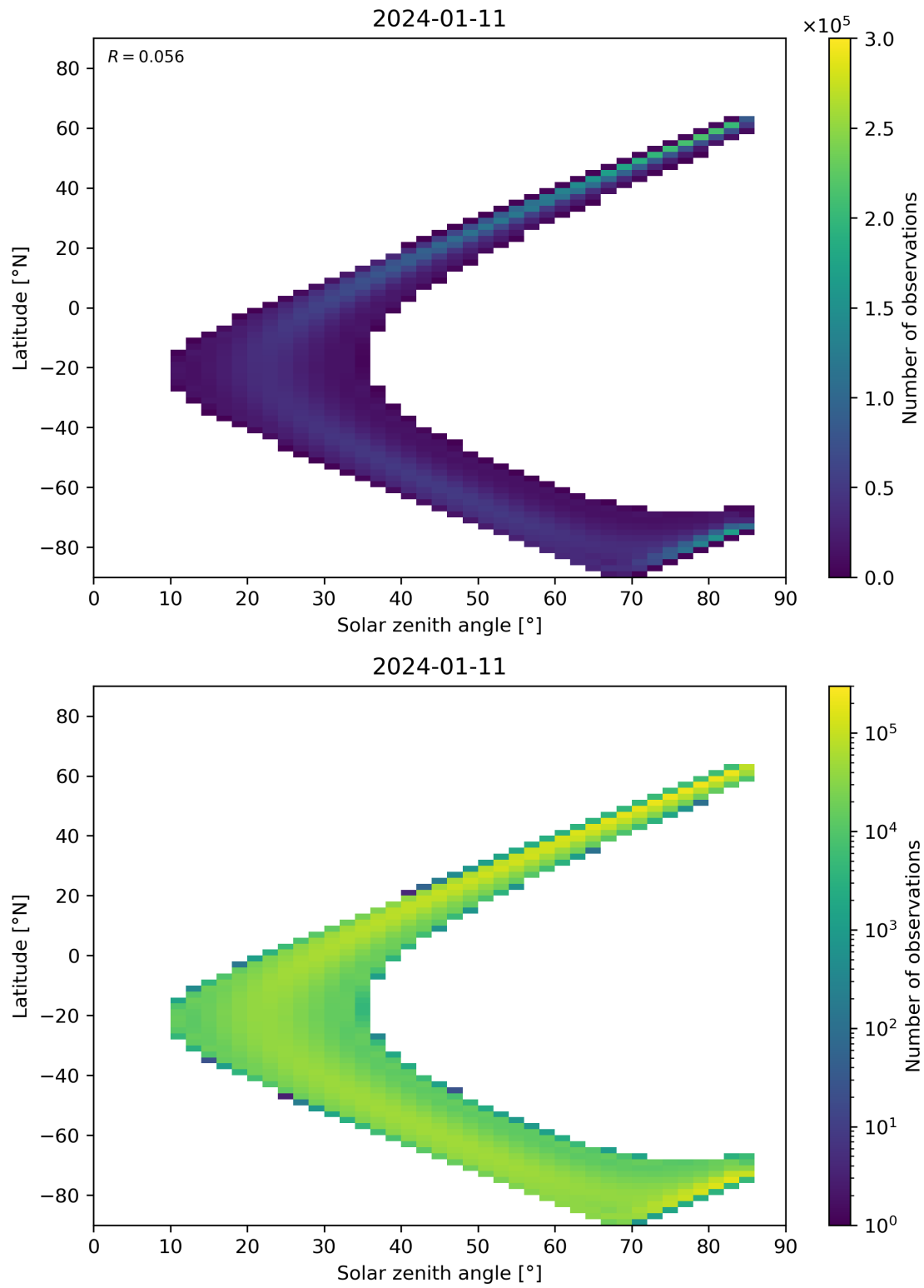
Figure 164: Scatter density plot of “Solar zenith angle” against “Latitude” for 2024-01-10 to 2024-01-12.
