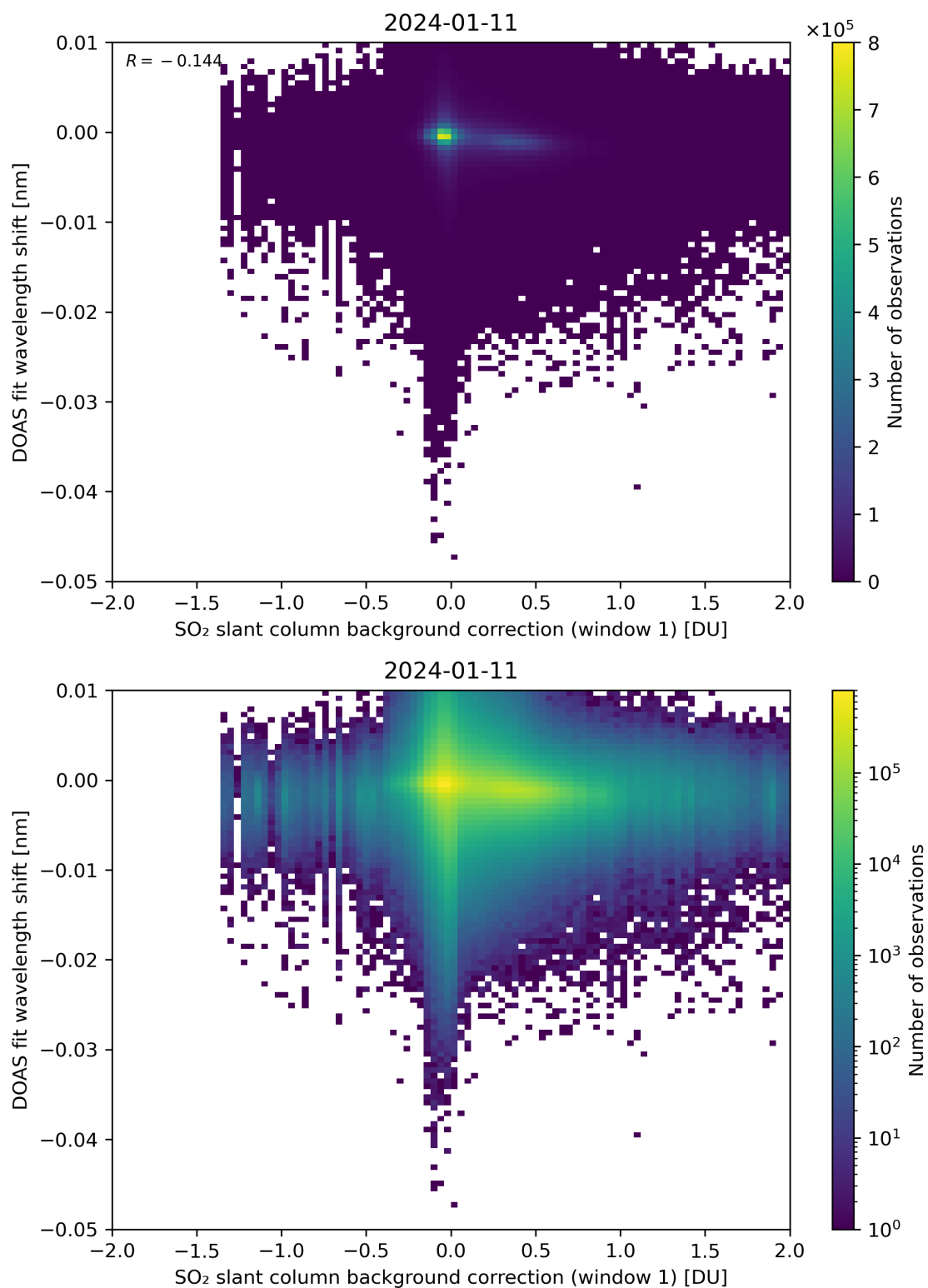
Figure 100: Scatter density plot of “SO 2 slant column background correction (window 1)” against “DOAS fit wavelength shift” for 2024-01-10 to 2024-01-12.
