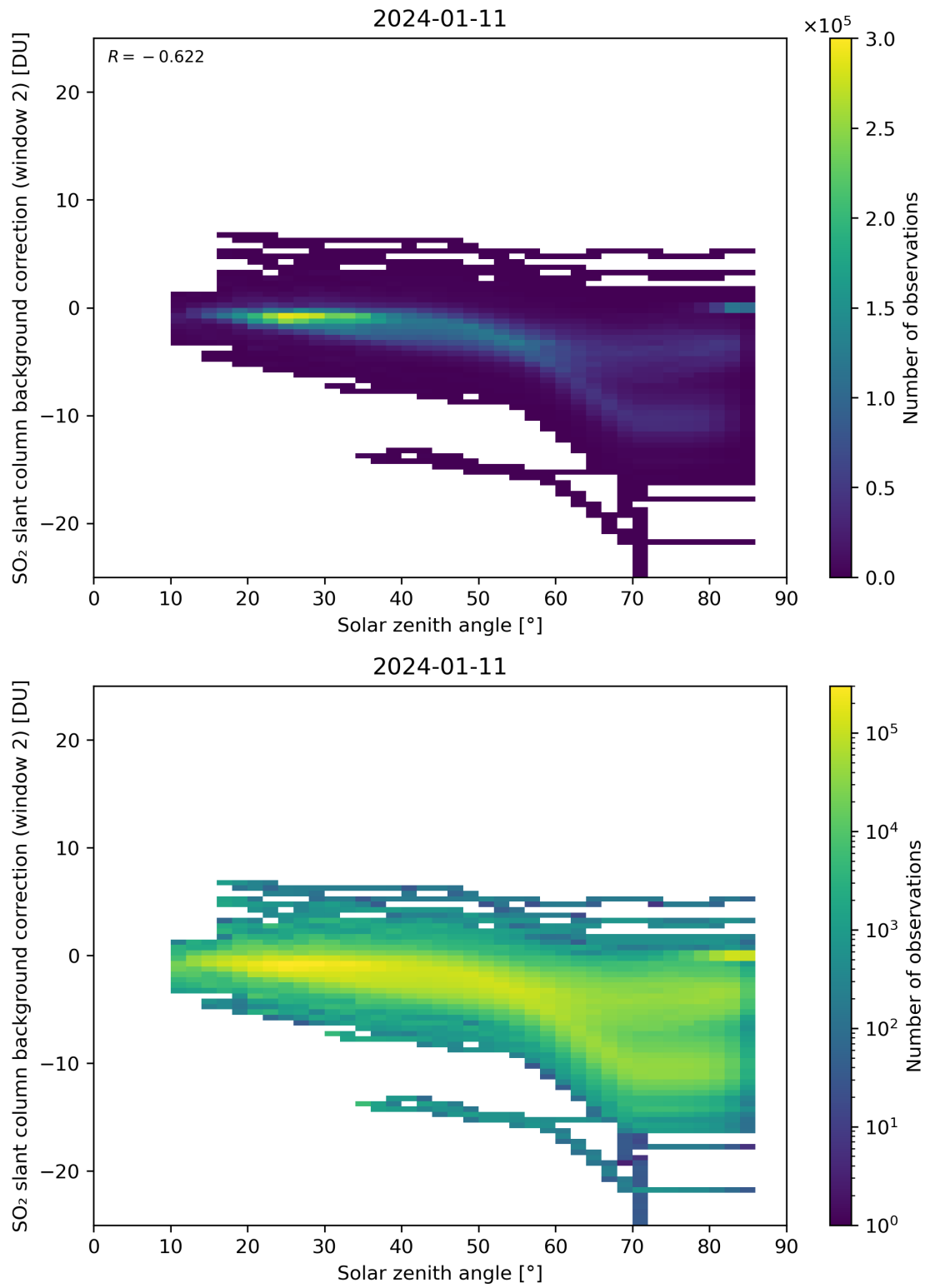
Figure 159: Scatter density plot of “Solar zenith angle” against “SO 2 slant column background correction (window 2)” for 2024-01-10 to 2024-01-12.
