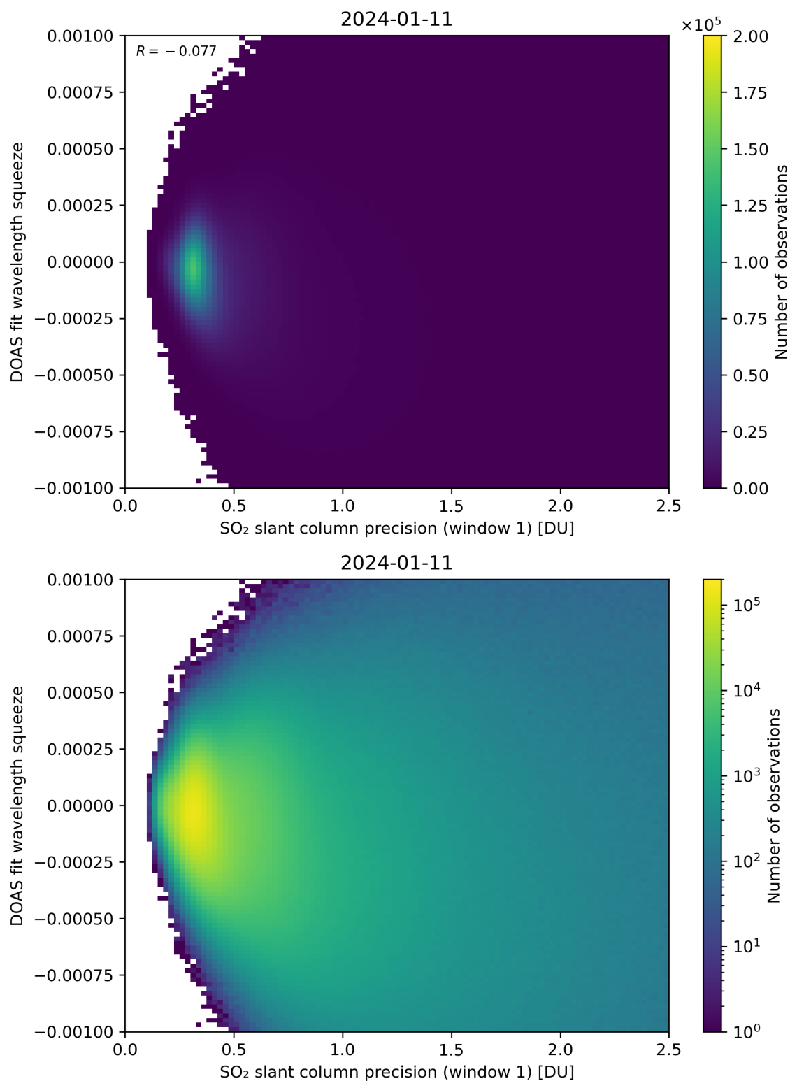
Figure 222: Scatter density plot of “SO 2 slant column precision (window 1)” against “DOAS fit wavelength squeeze” for 2024-01-10 to 2024-01-12.
