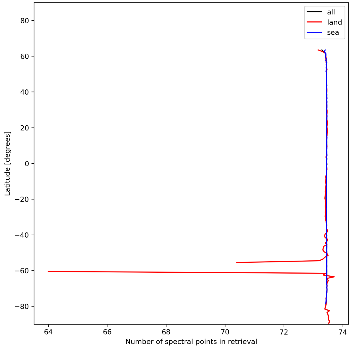
Figure 51: Zonal average of “Number of spectral points in retrieval” for 2024-01-10 to 2024-01-12.
