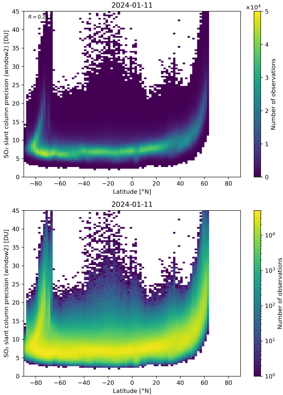
Figure 151: Scatter density plot of “Latitude” against “SO 2 slant column precision (window2)” for 2024-01-10 to 2024-01-12.
