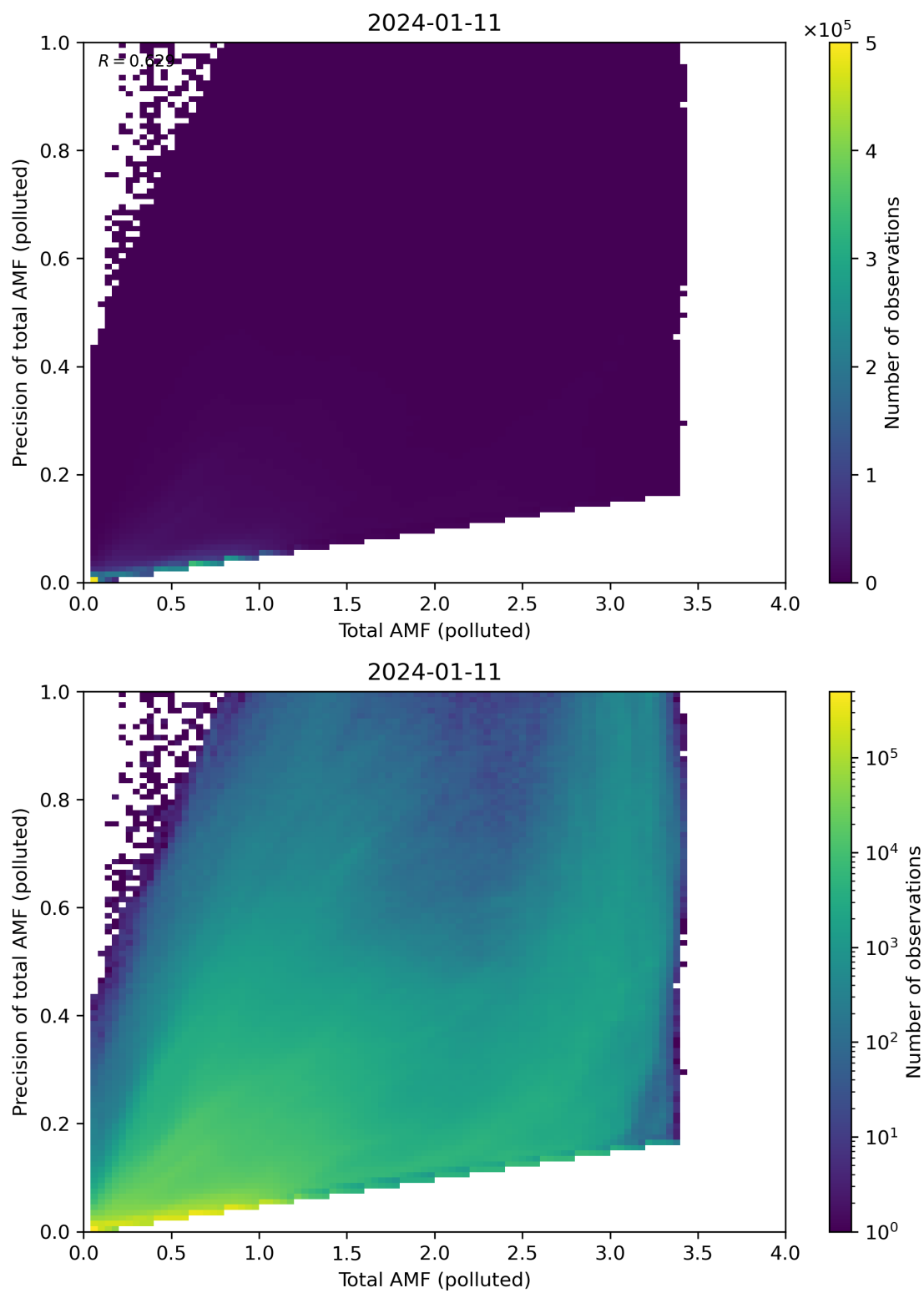
Figure 272: Scatter density plot of “Total AMF (polluted)” against “Precision of total AMF (polluted)” for 2024-01-10 to 2024-01-12.
