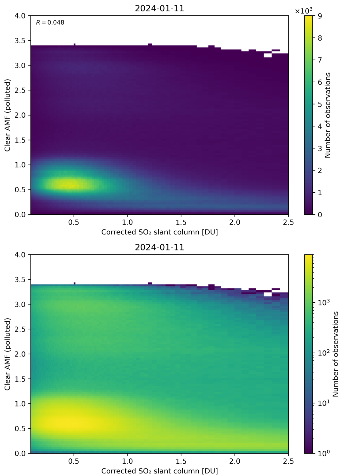
Figure 184: Scatter density plot of “Corrected SO 2 slant column” against “Clear AMF (polluted)” for 2024-01-10 to 2024-01-12.
