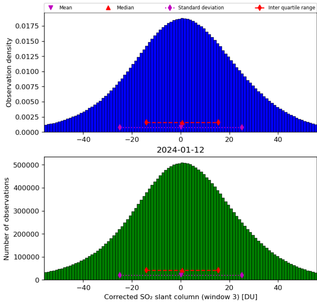
Figure 66: Histogram of “Corrected SO 2 slant column (window 3)” for 2024-01-11 to 2024-01-13
