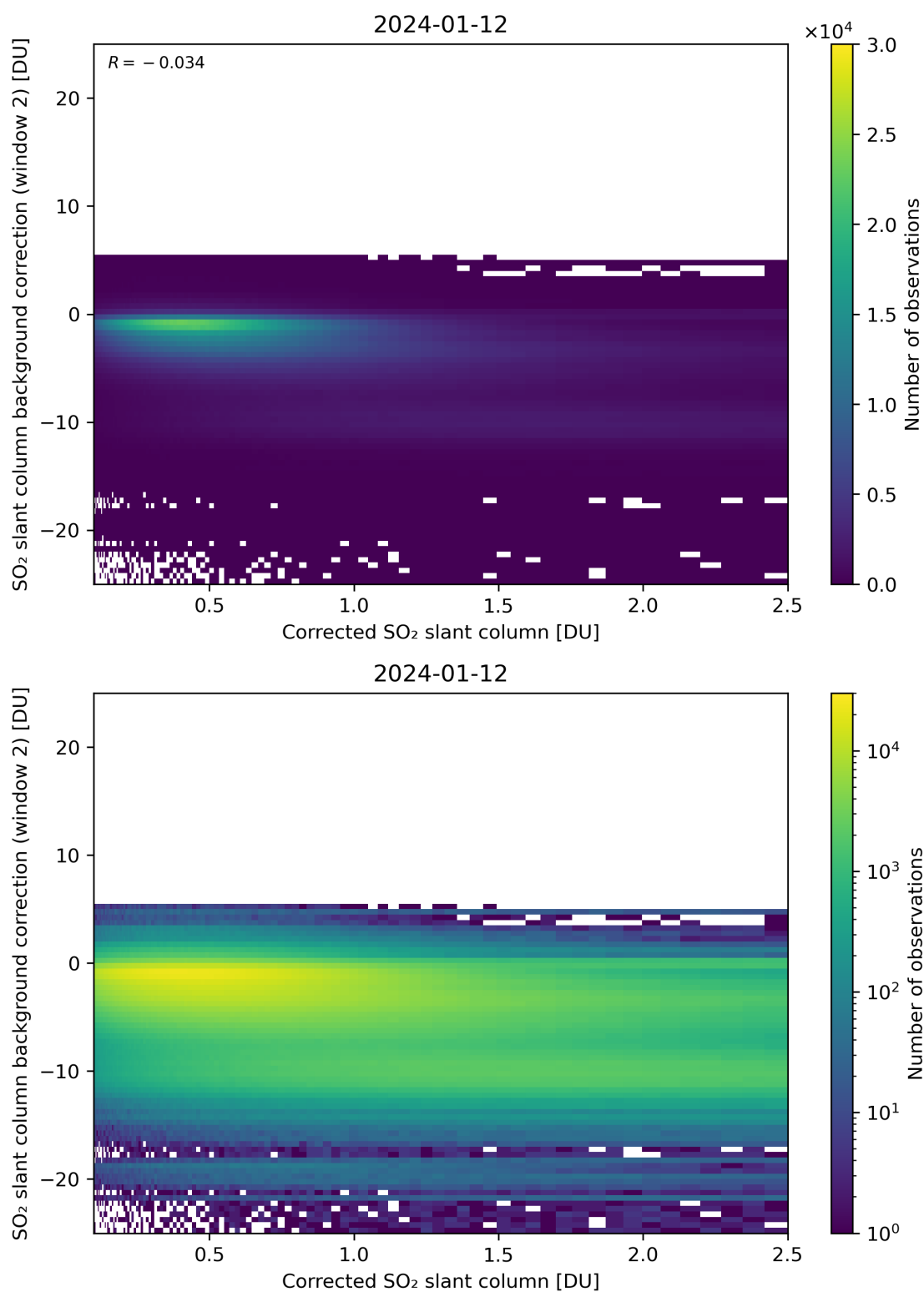
Figure 179: Scatter density plot of “Corrected SO 2 slant column” against “SO 2 slant column background correction (window 2)” for 2024-01-11 to 2024-01-13.
