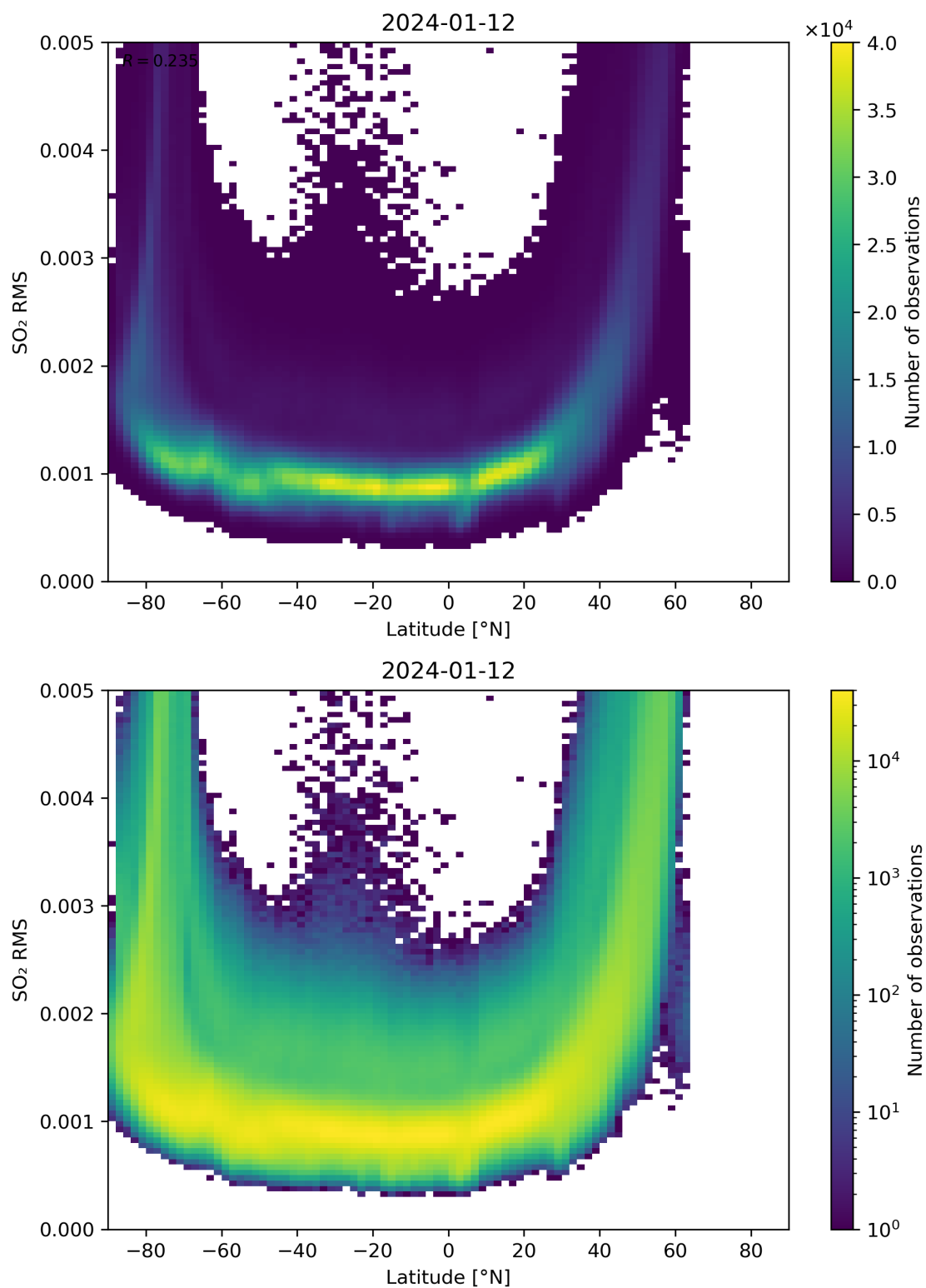
Figure 144: Scatter density plot of “Latitude” against “SO 2 RMS” for 2024-01-11 to 2024-01-13.
