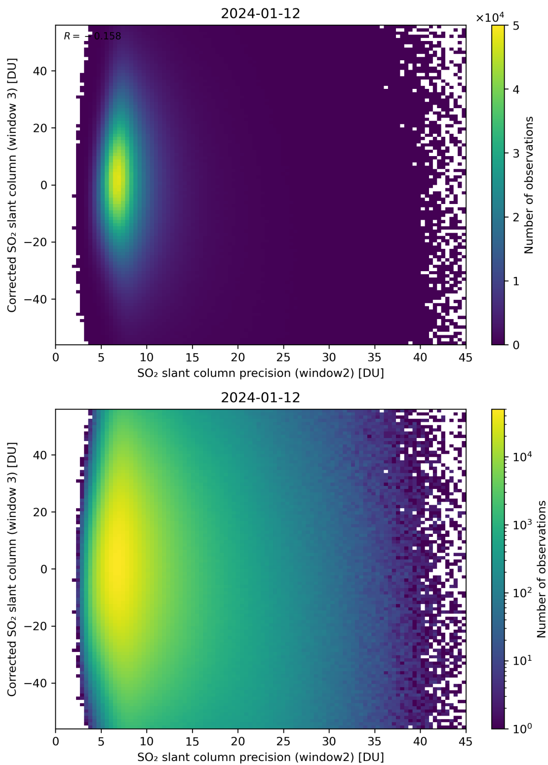
Figure 248: Scatter density plot of “SO 2 slant column precision (window2)” against “Corrected SO 2 slant column (window 3)” for 2024-01-11 to 2024-01-13.
