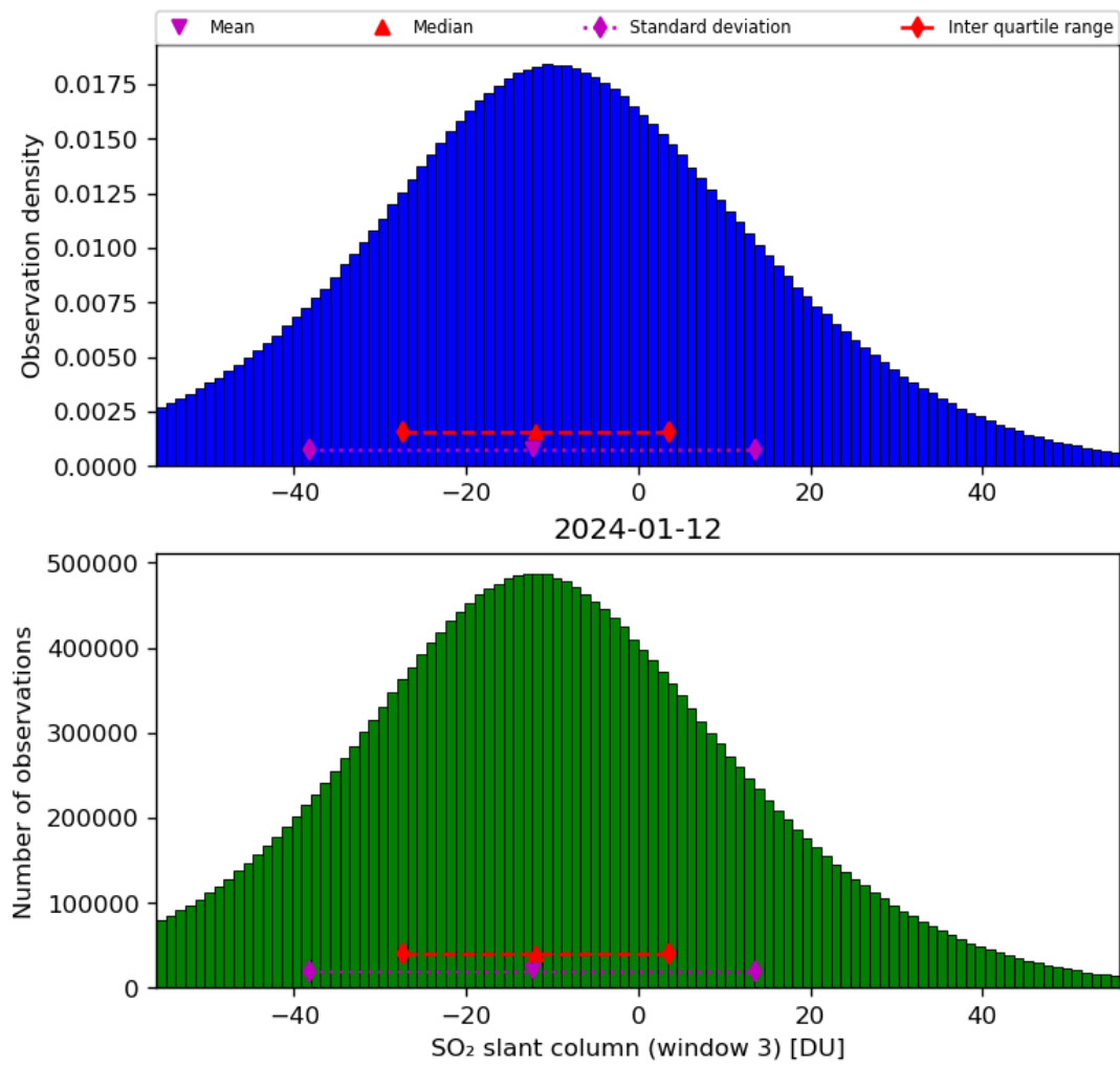
Figure 64: Histogram of “SO 2 slant column (window 3)” for 2024-01-11 to 2024-01-13
