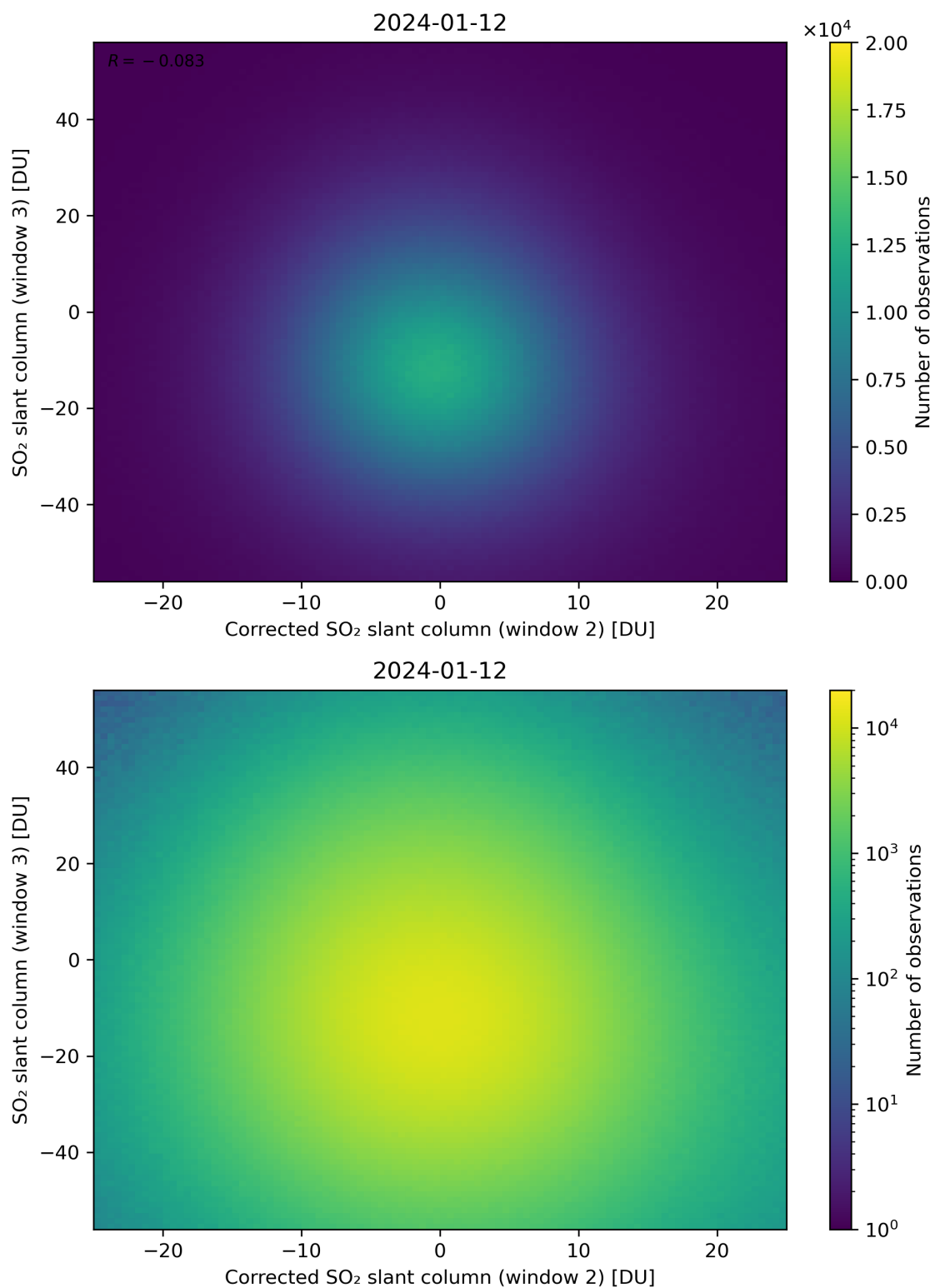
Figure 201: Scatter density plot of “Corrected SO 2 slant column (window 2)” against “SO 2 slant column (window 3)” for 2024-01-11 to 2024-01-13.
