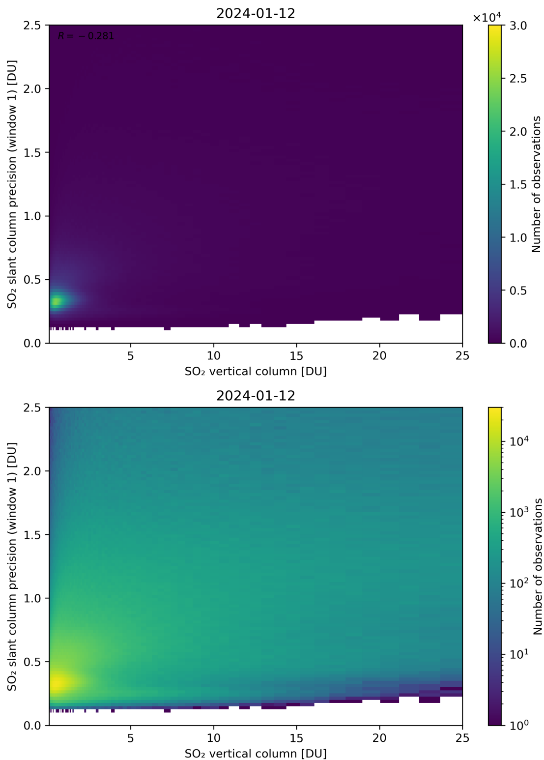
Figure 301: Scatter density plot of “SO 2 vertical column” against “SO 2 slant column precision (window 1)” for 2024-01-11 to 2024-01-13.
