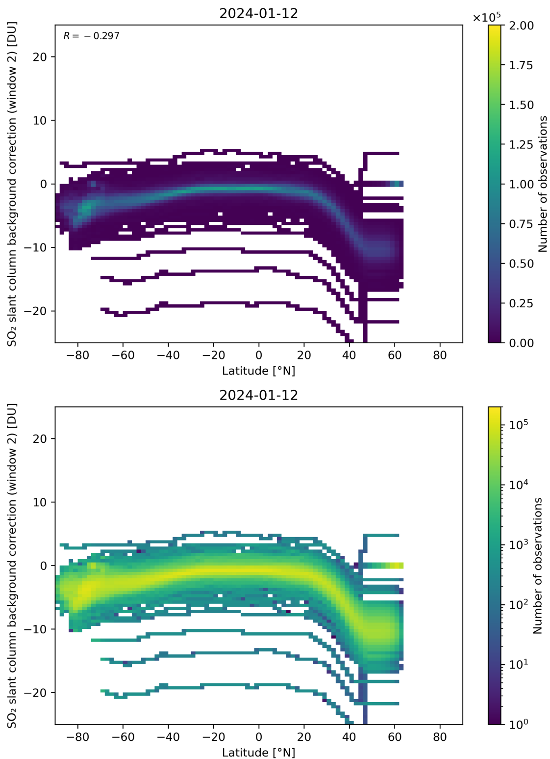
Figure 140: Scatter density plot of “Latitude” against “SO 2 slant column background correction (window 2)” for 2024-01-11 to 2024-01-13.
