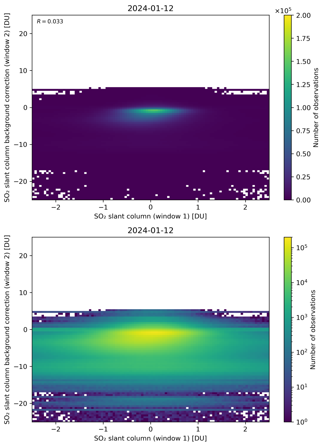
Figure 213: Scatter density plot of “SO 2 slant column (window 1)” against “SO 2 slant column background correction (window 2)” for 2024-01-11 to 2024-01-13.
