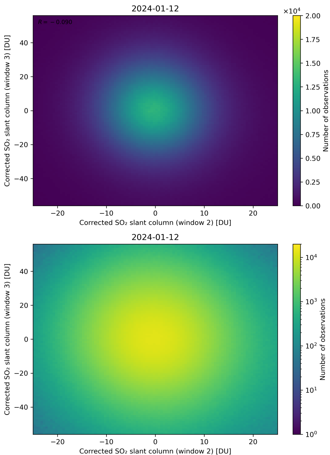
Figure 200: Scatter density plot of “Corrected SO 2 slant column (window 2)” against “Corrected SO 2 slant column (window 3)” for 2024-01-11 to 2024-01-13.
