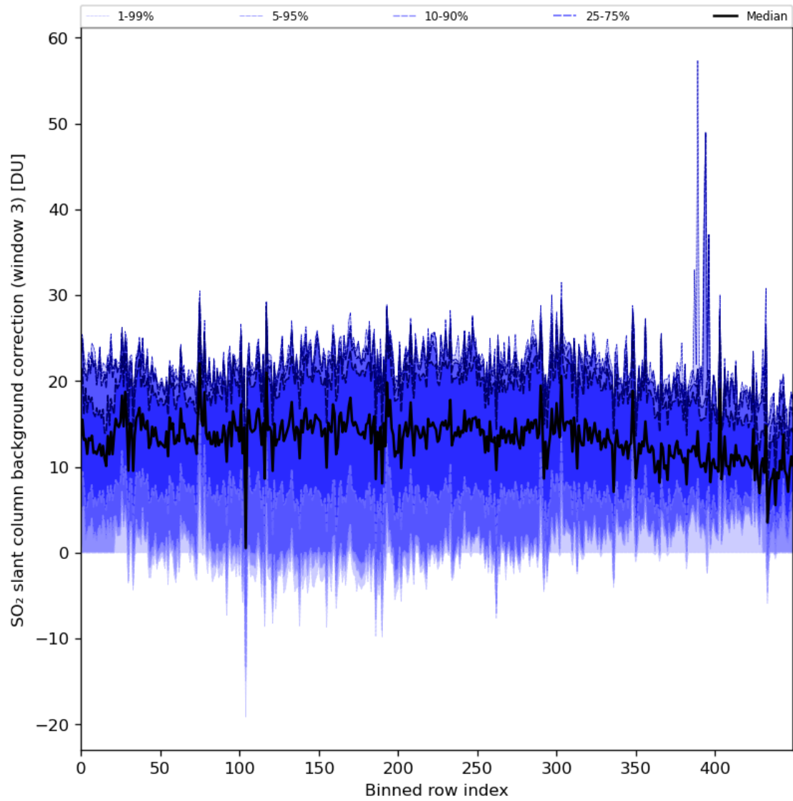
Figure 90: Along track statistics of “SO 2 slant column background correction (window 3)” for 2024-01-11 to 2024-01-13
