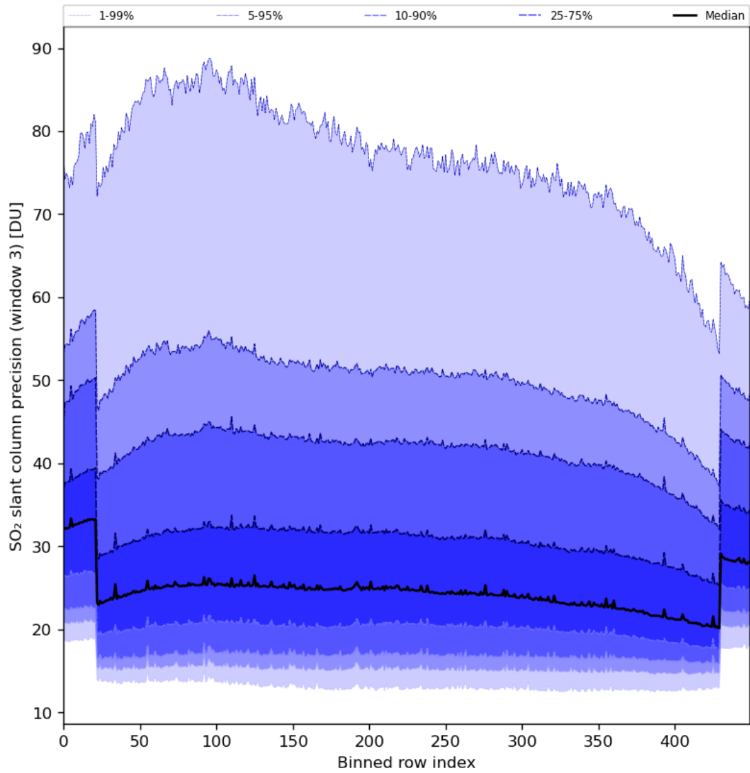
Figure 88: Along track statistics of “SO 2 slant column precision (window 3)” for 2024-01-11 to 2024-01-13
