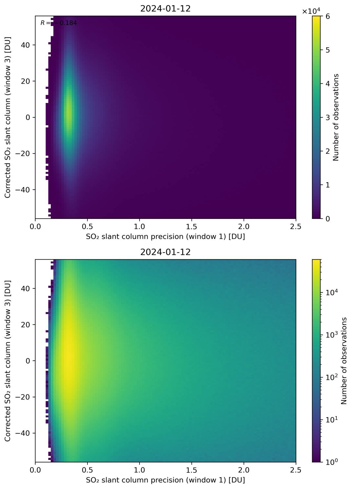
Figure 226: Scatter density plot of “SO 2 slant column precision (window 1)” against “Corrected SO 2 slant column (window 3)” for 2024-01-11 to 2024-01-13.
