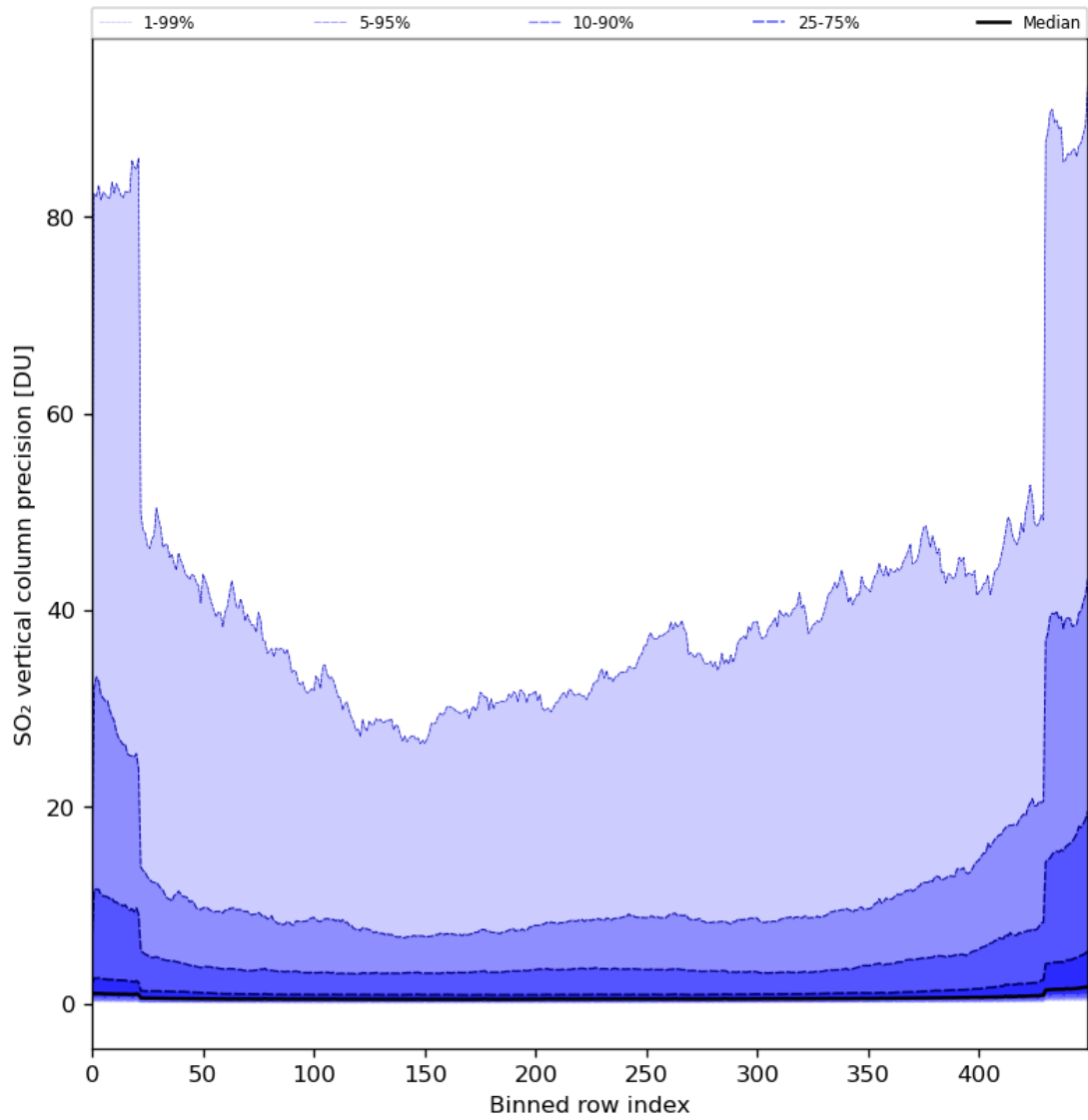
Figure 77: Along track statistics of “SO 2 vertical column precision” for 2024-01-11 to 2024-01-13
