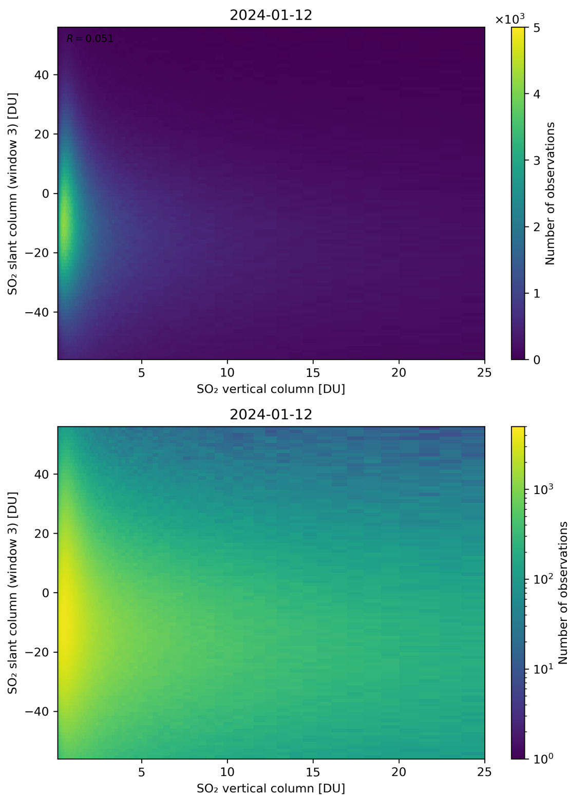
Figure 303: Scatter density plot of “SO 2 vertical column” against “SO 2 slant column (window 3)” for 2024-01-11 to 2024-01-13.
