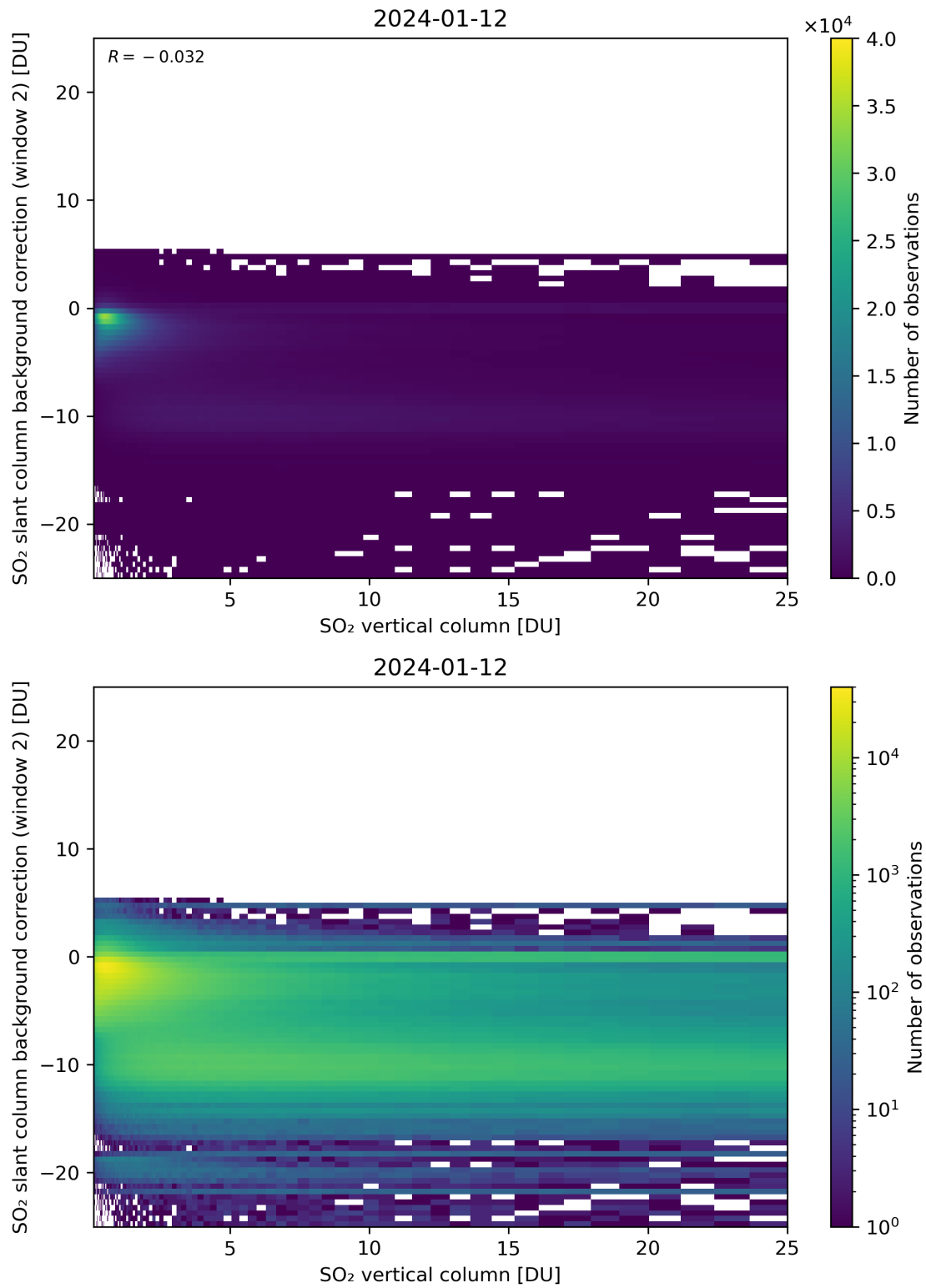
Figure 274: Scatter density plot of “SO 2 vertical column” against “SO 2 slant column background correction (window 2)” for 2024-01-11 to 2024-01-13.
