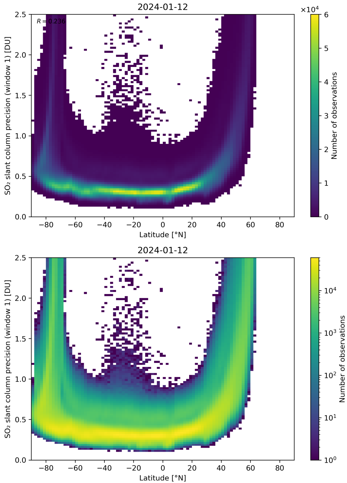
Figure 150: Scatter density plot of “Latitude” against “SO 2 slant column precision (window 1)” for 2024-01-11 to 2024-01-13.
