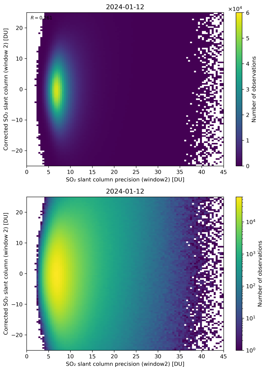
Figure 247: Scatter density plot of “SO 2 slant column precision (window2)” against “Corrected SO 2 slant column (window 2)” for 2024-01-11 to 2024-01-13.
