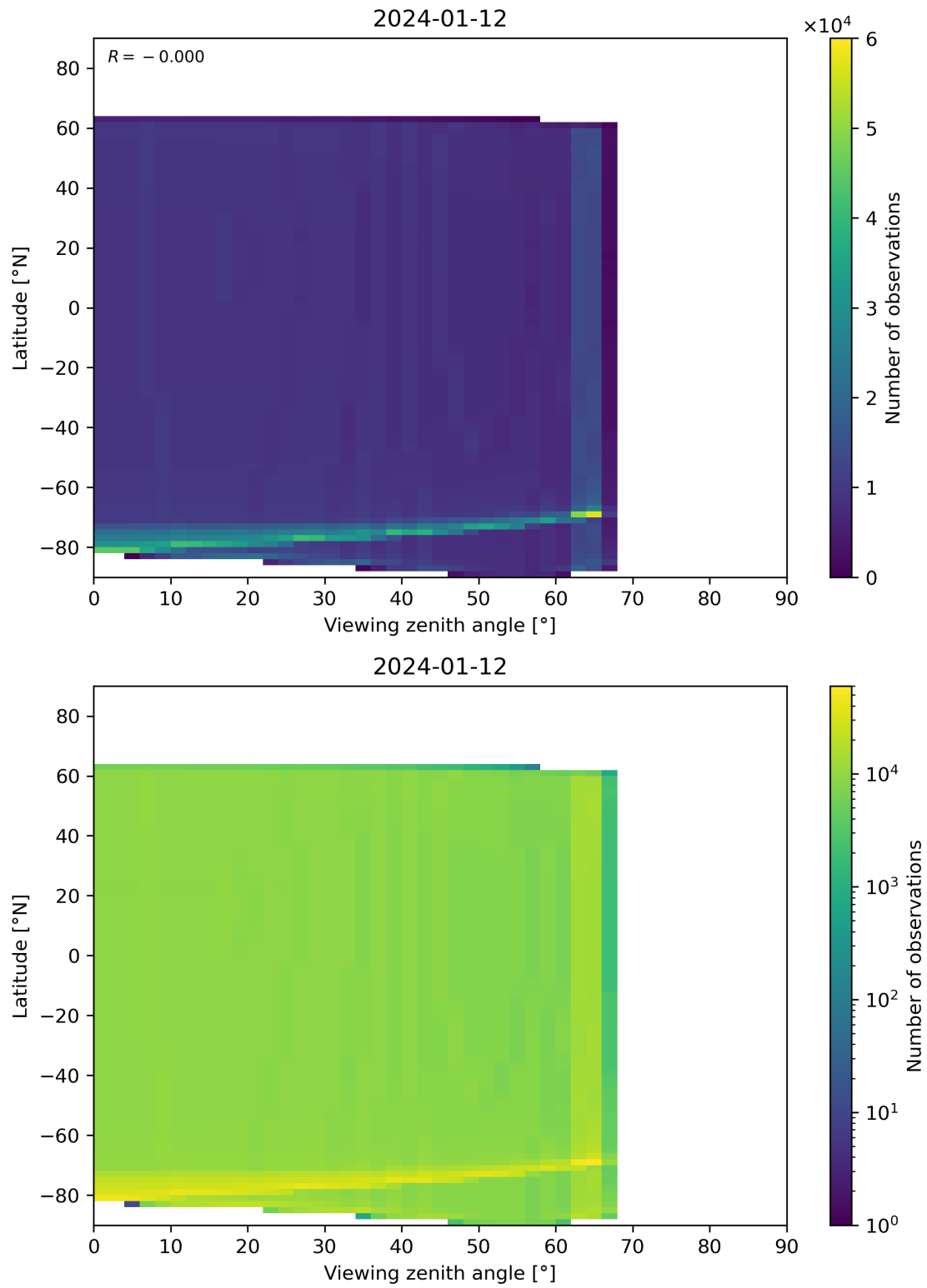
Figure 314: Scatter density plot of “Viewing zenith angle” against “Latitude” for 2024-01-11 to 2024-01-13.
