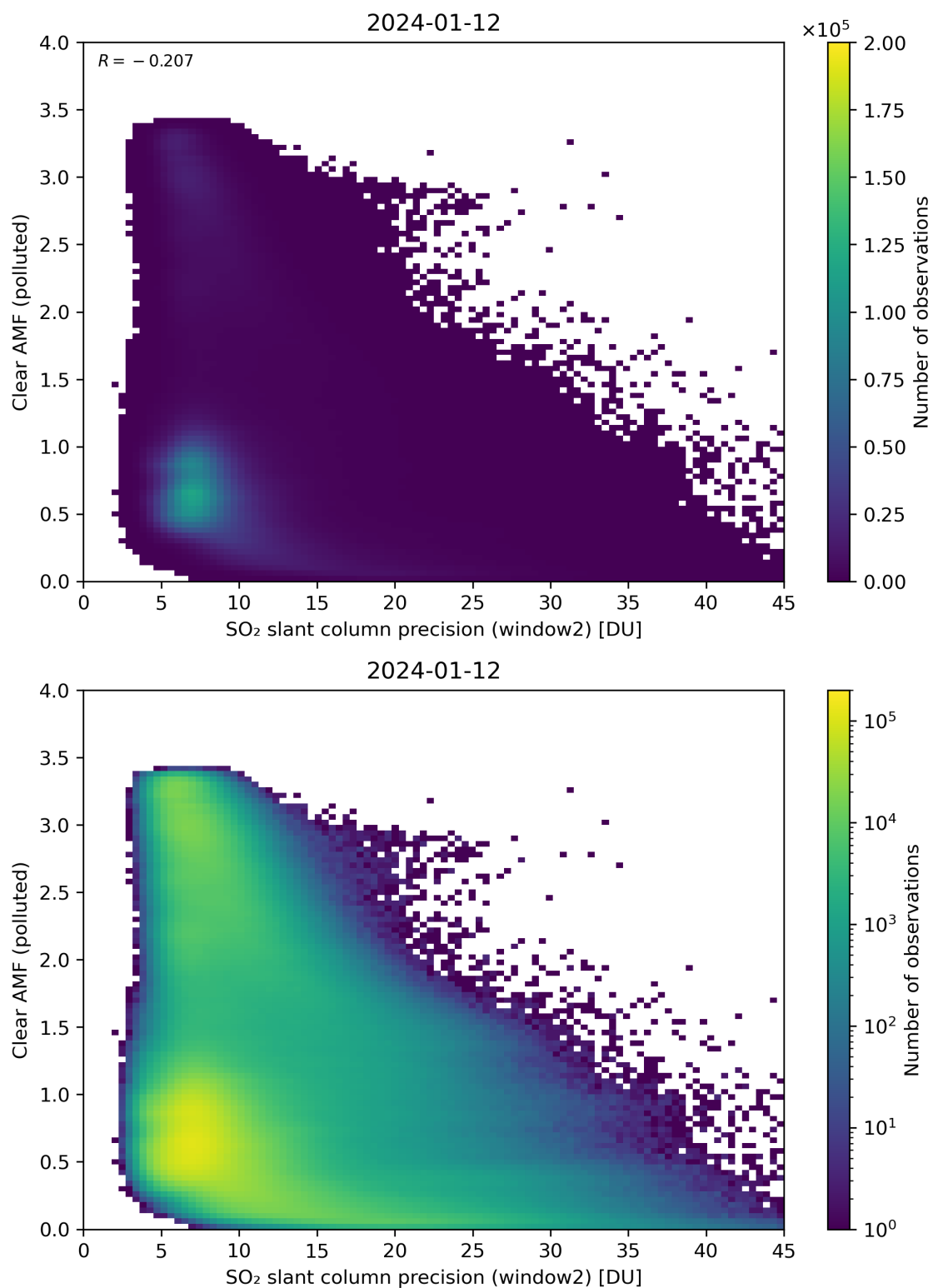
Figure 246: Scatter density plot of “SO 2 slant column precision (window2)” against “Clear AMF (polluted)” for 2024-01-11 to 2024-01-13.
