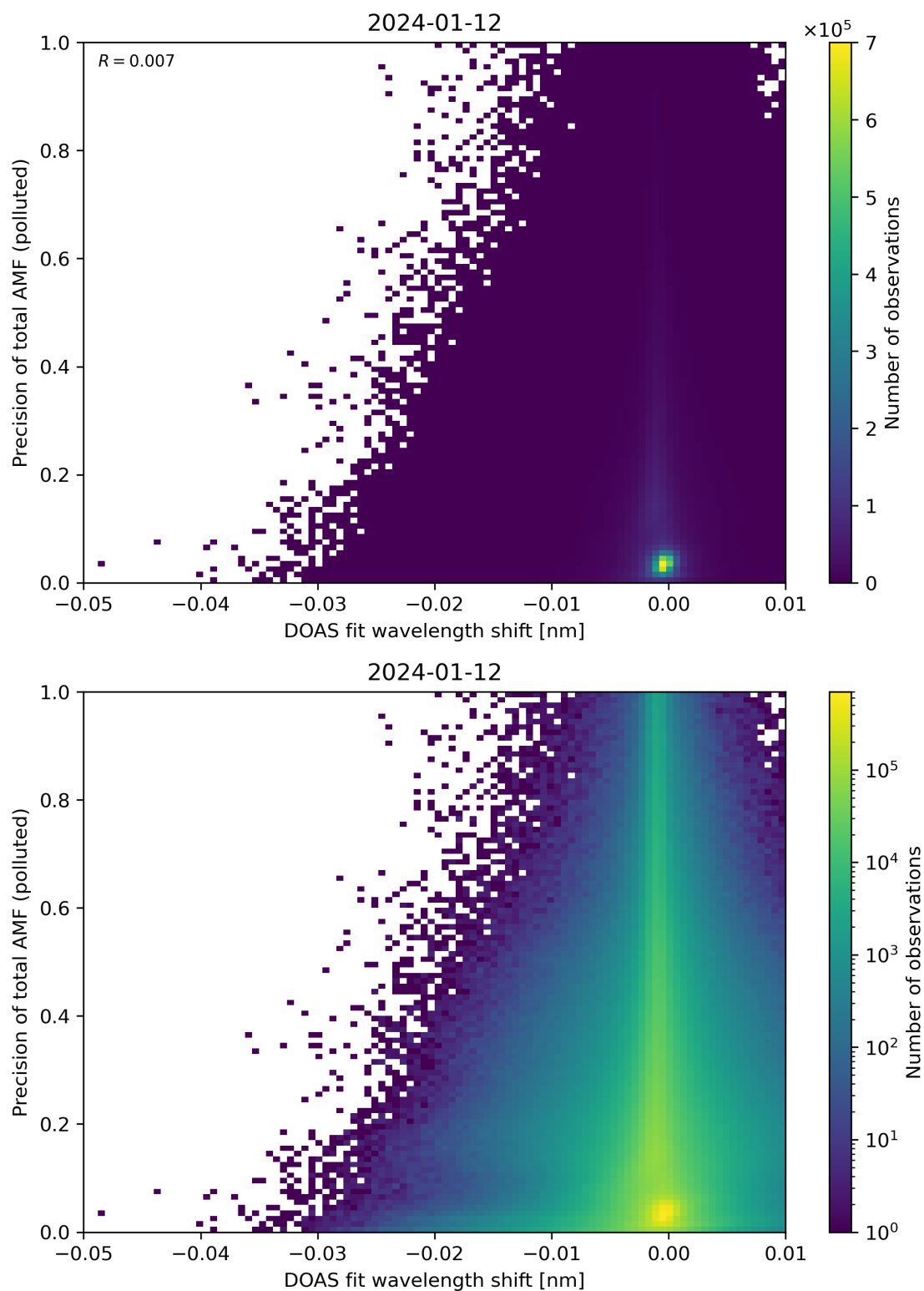
Figure 131: Scatter density plot of “DOAS fit wavelength shift” against “Precision of total AMF (polluted)” for 2024-01-11 to 2024-01-13.
