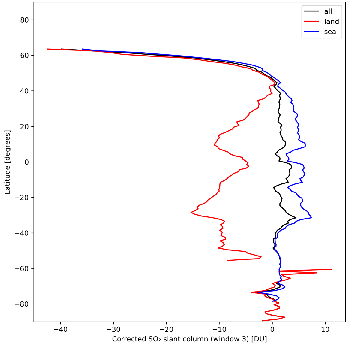
Figure 43: Zonal average of “Corrected SO 2 slant column (window 3)” for 2024-01-11 to 2024-01-13.
