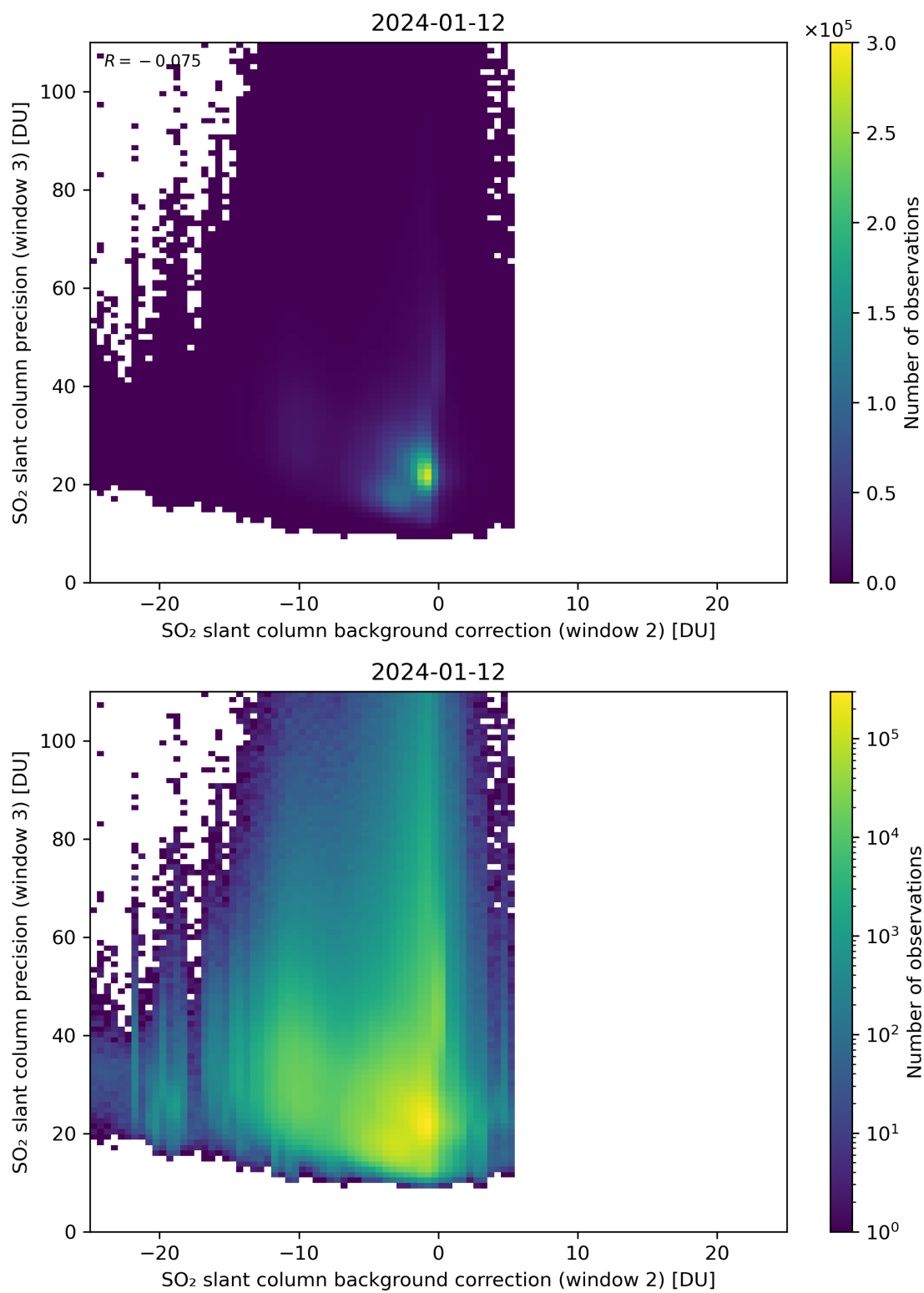
Figure 118: Scatter density plot of “SO 2 slant column background correction (window 2)” against “SO 2 slant column precision (window 3)” for 2024-01-11 to 2024-01-13.
