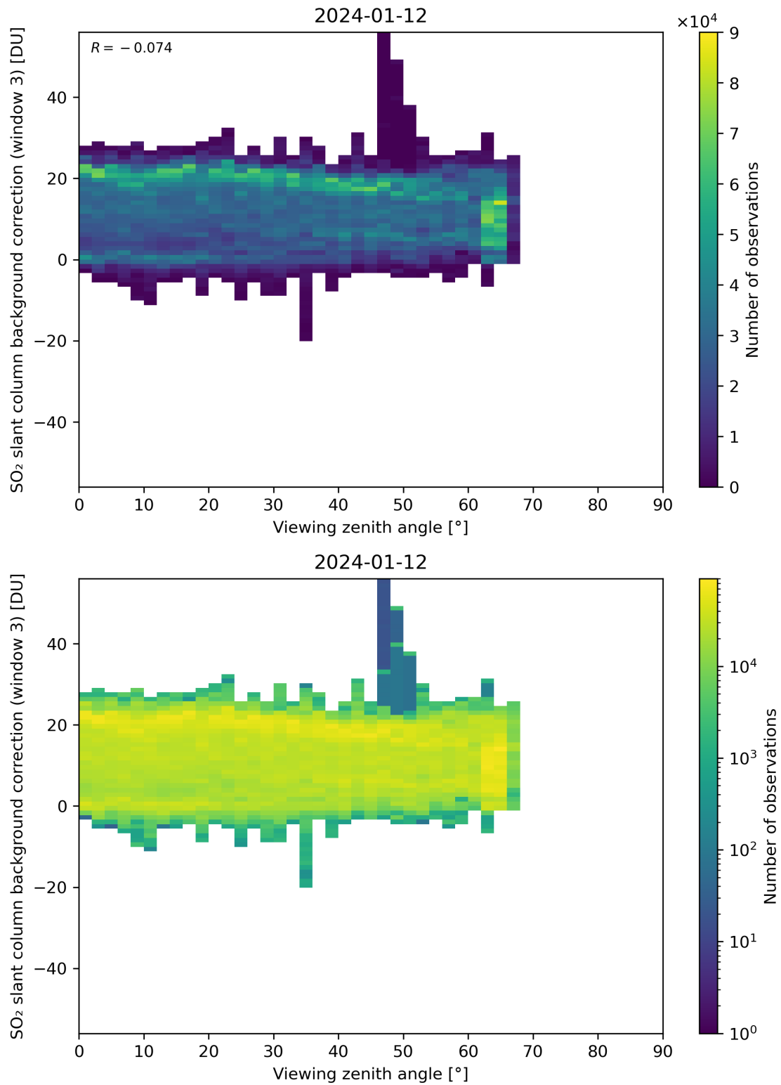
Figure 310: Scatter density plot of “Viewing zenith angle” against “SO 2 slant column background correction (window 3)” for 2024-01-11 to 2024-01-13.
