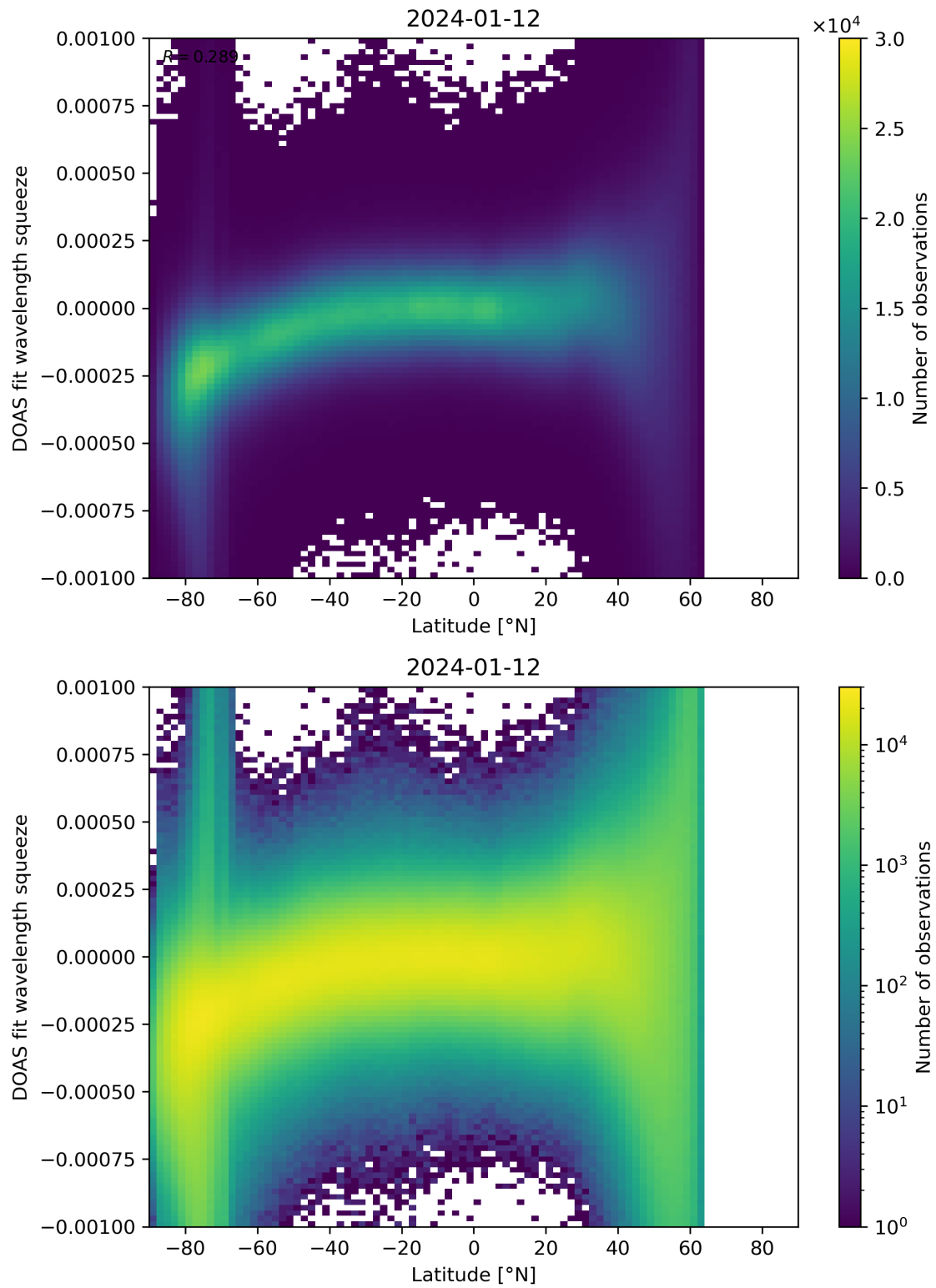
Figure 143: Scatter density plot of “Latitude” against “DOAS fit wavelength squeeze” for 2024-01-11 to 2024-01-13.
