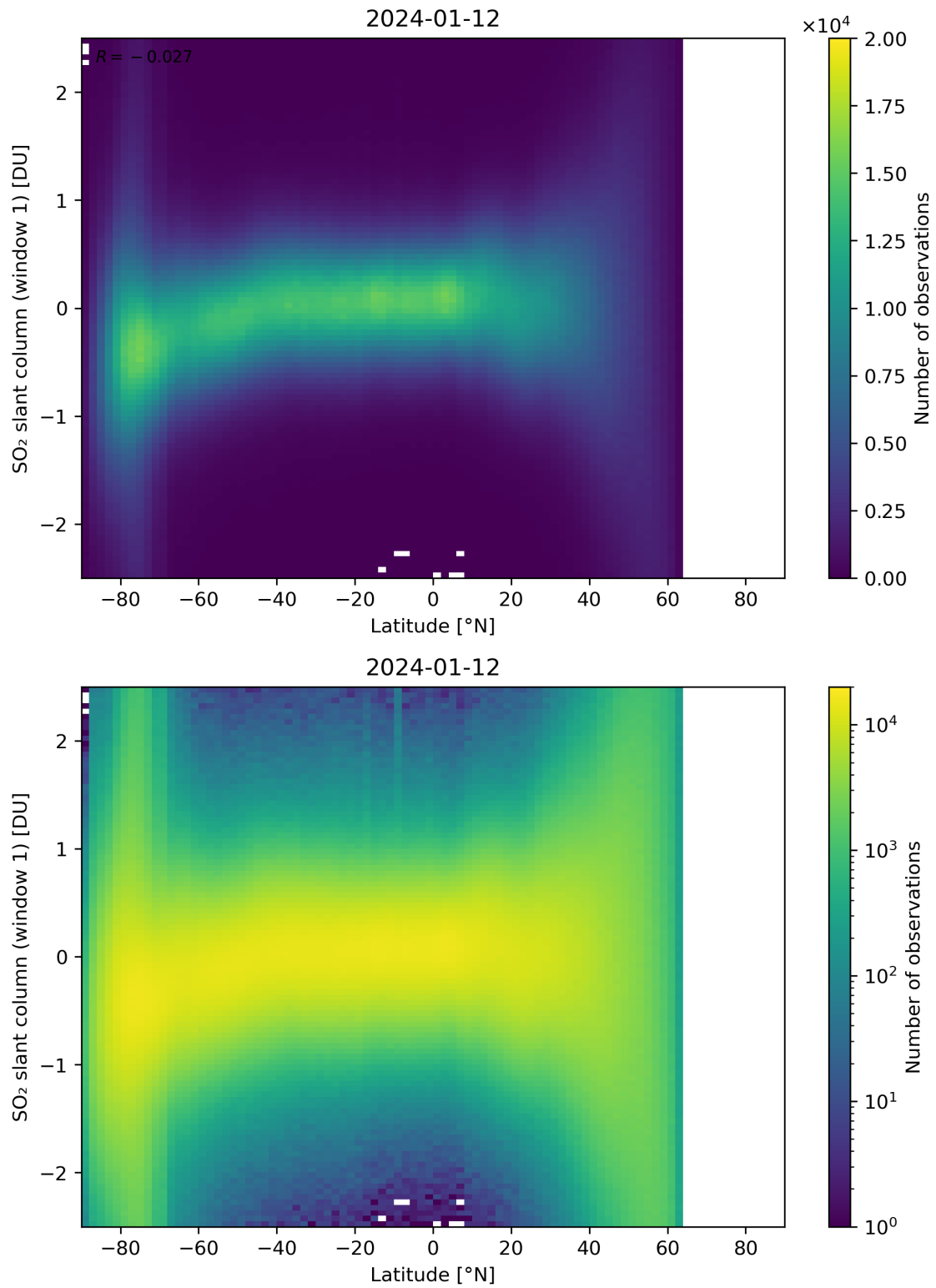
Figure 149: Scatter density plot of “Latitude” against “SO 2 slant column (window 1)” for 2024-01-11 to 2024-01-13.
