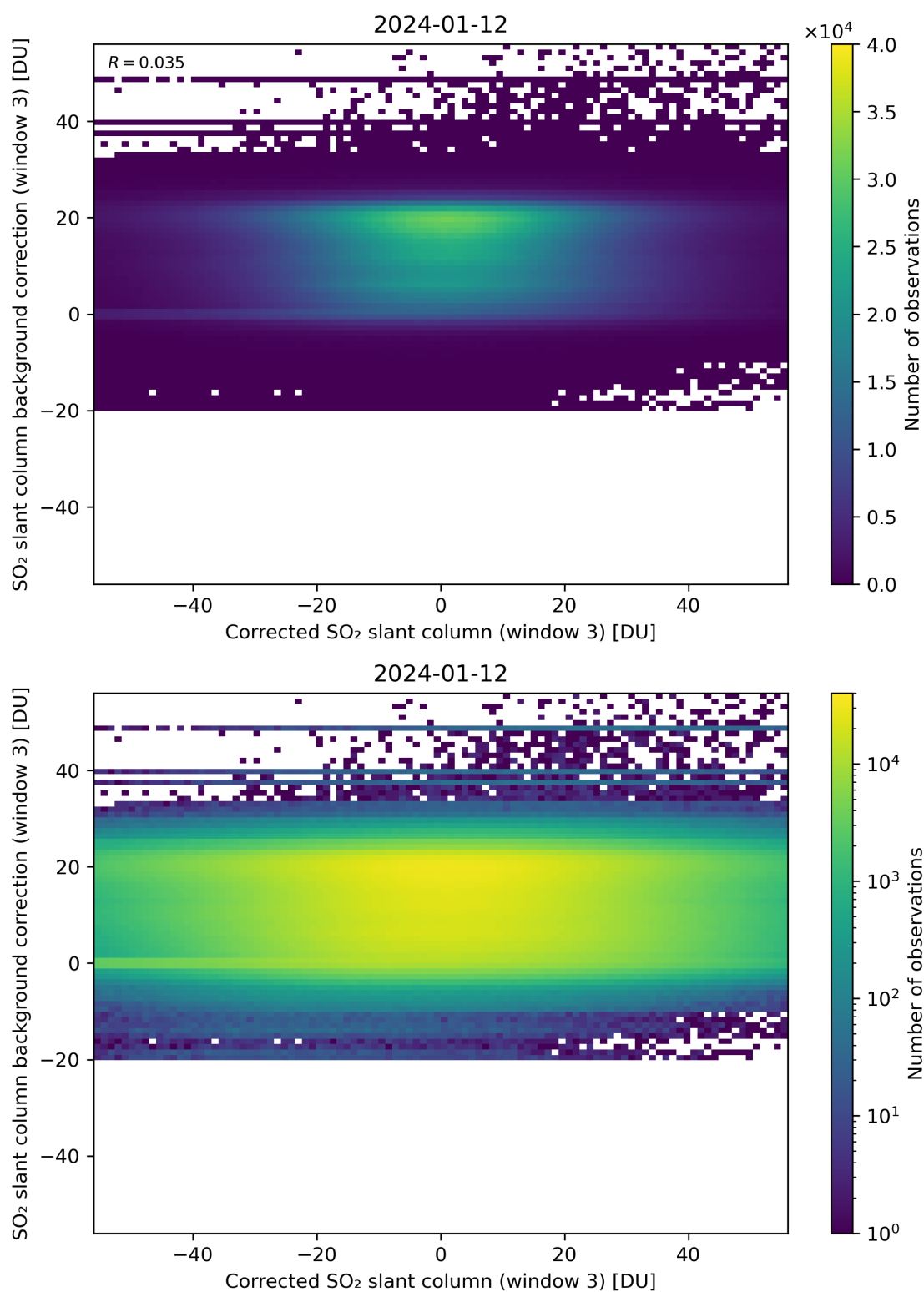
Figure 205: Scatter density plot of “Corrected SO 2 slant column (window 3)” against “SO 2 slant column background correction (window 3)” for 2024-01-11 to 2024-01-13.
