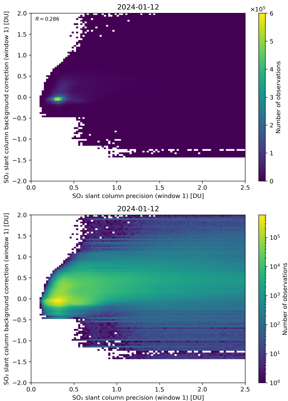
Figure 218: Scatter density plot of “SO 2 slant column precision (window 1)” against “SO 2 slant column background correction (window 1)” for 2024-01-11 to 2024-01-13.
