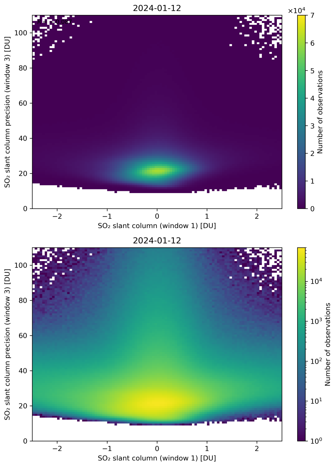
Figure 238: Scatter density plot of “SO 2 slant column (window 1)” against “SO 2 slant column precision (window 3)” for 2024-01-11 to 2024-01-13.
