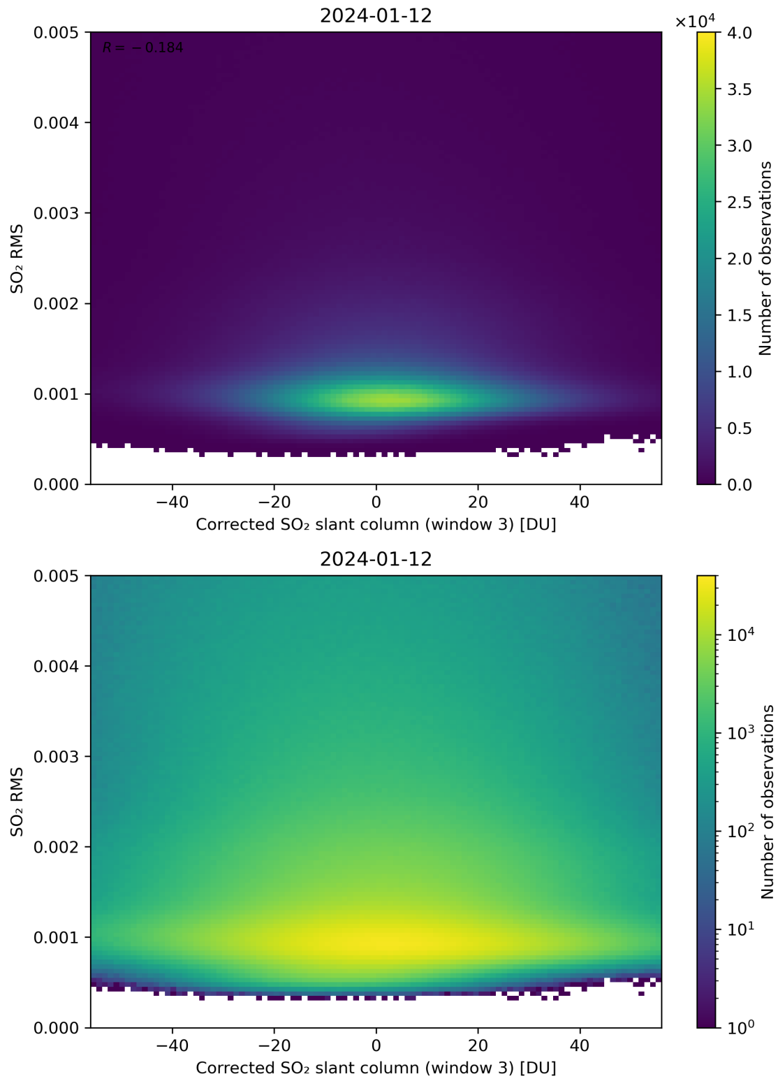
Figure 208: Scatter density plot of “Corrected SO 2 slant column (window 3)” against “SO 2 RMS” for 2024-01-11 to 2024-01-13.
