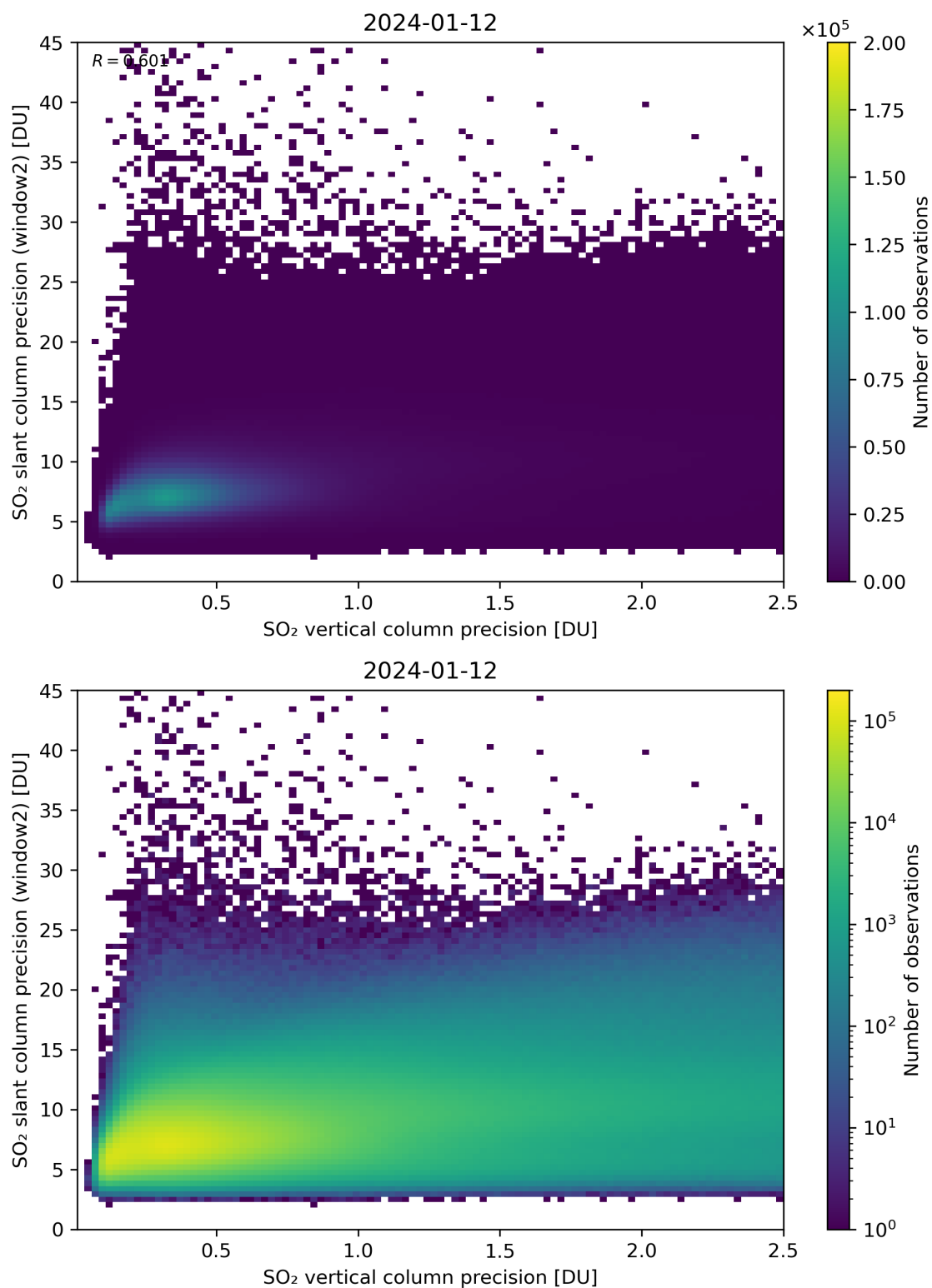
Figure 291: Scatter density plot of “SO 2 vertical column precision” against “SO 2 slant column precision (window2)” for 2024-01-11 to 2024-01-13.
