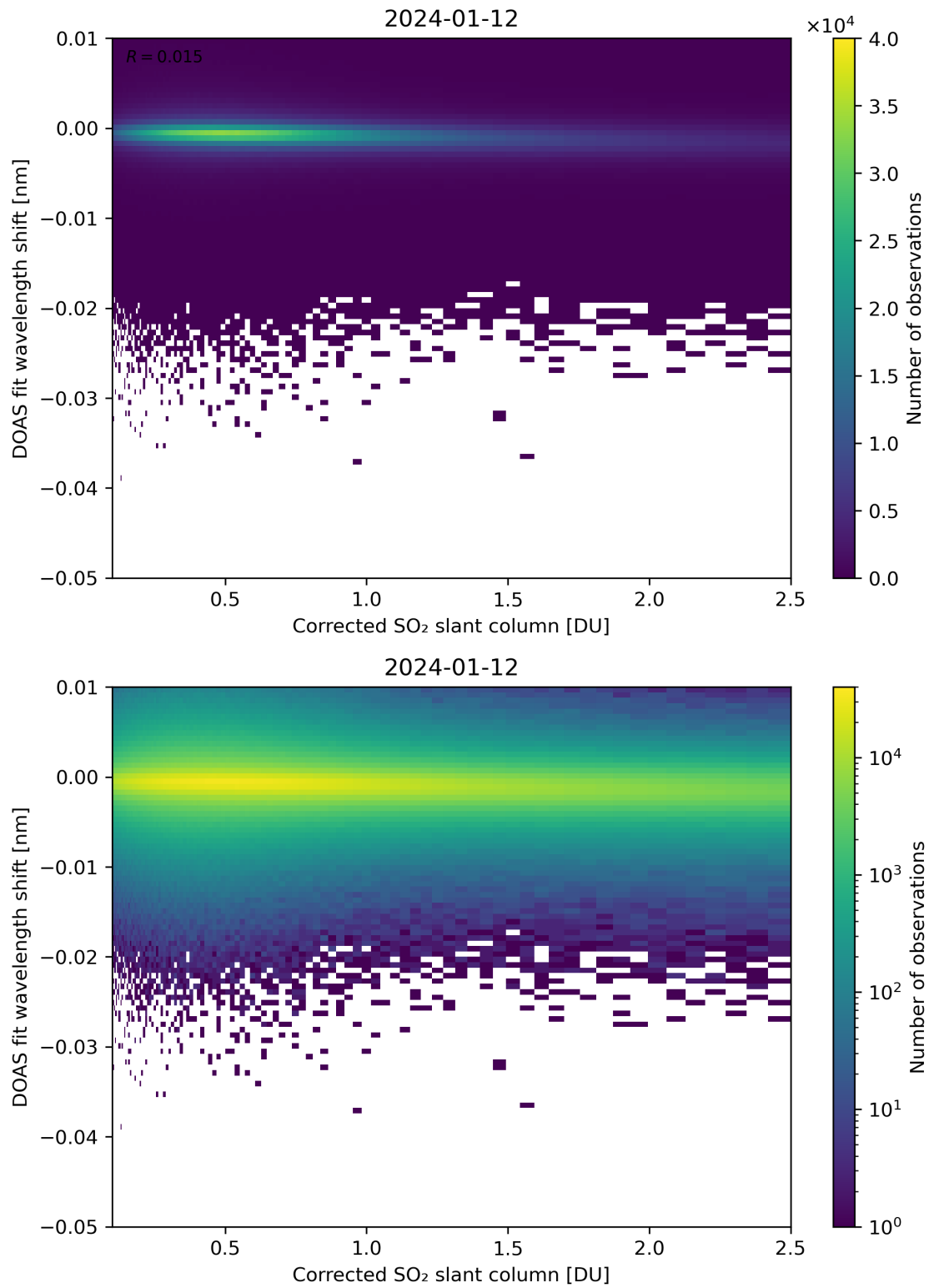
Figure 181: Scatter density plot of “Corrected SO 2 slant column” against “DOAS fit wavelength shift” for 2024-01-11 to 2024-01-13.
