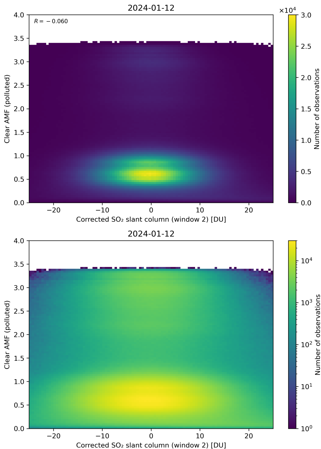
Figure 199: Scatter density plot of “Corrected SO 2 slant column (window 2)” against “Clear AMF (polluted)” for 2024-01-11 to 2024-01-13.
