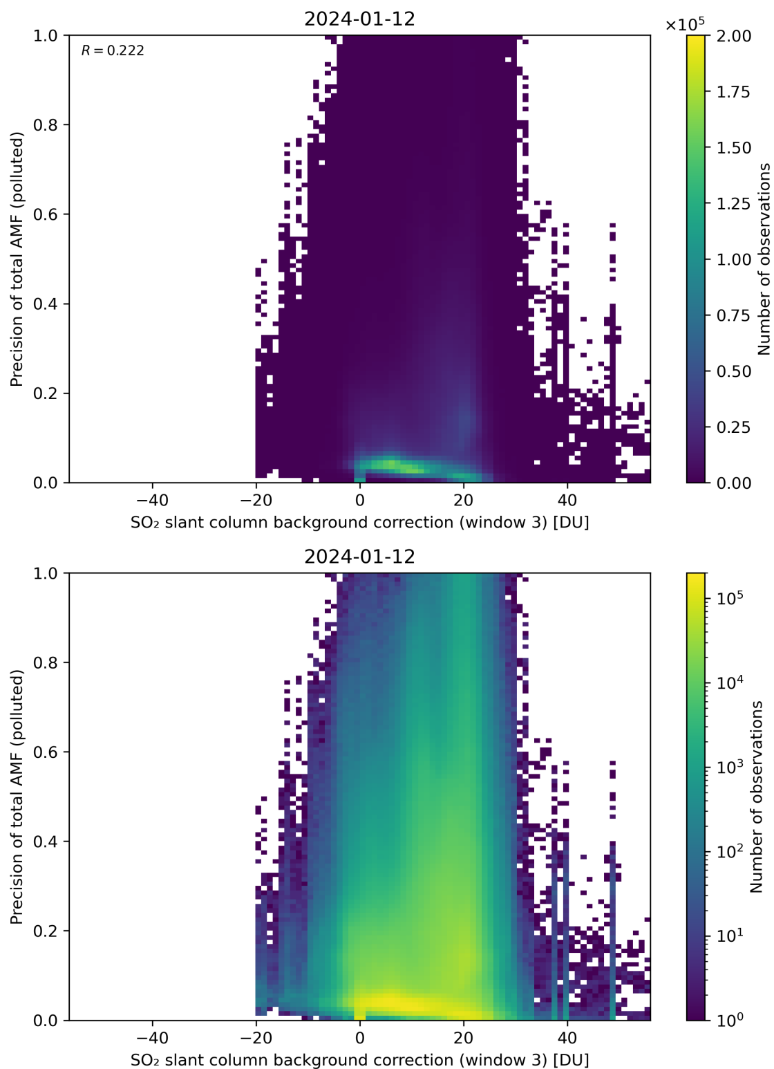
Figure 126: Scatter density plot of “SO 2 slant column background correction (window 3)” against “Precision of total AMF (polluted)” for 2024-01-11 to 2024-01-13.
