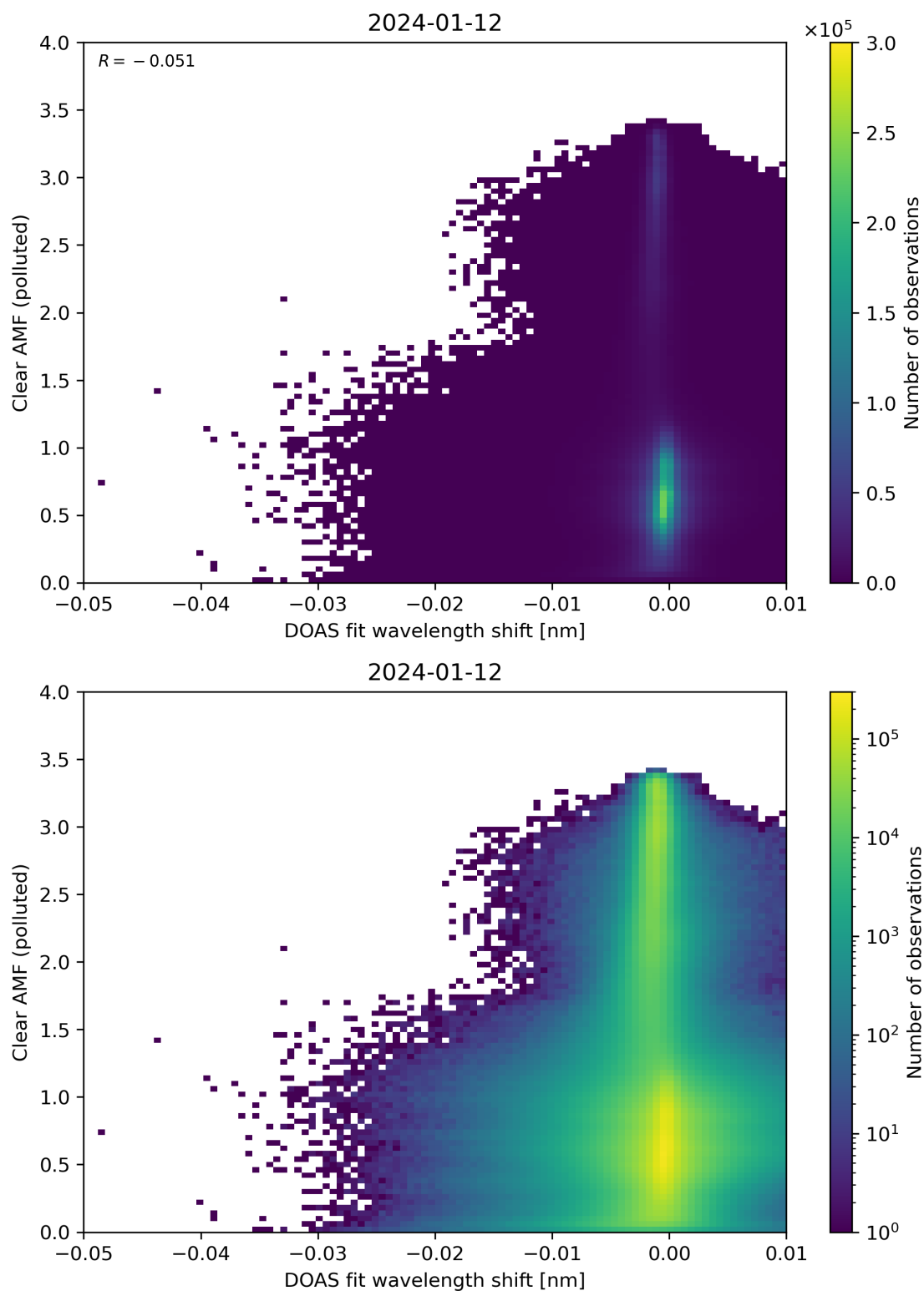
Figure 129: Scatter density plot of “DOAS fit wavelength shift” against “Clear AMF (polluted)” for 2024-01-11 to 2024-01-13.
