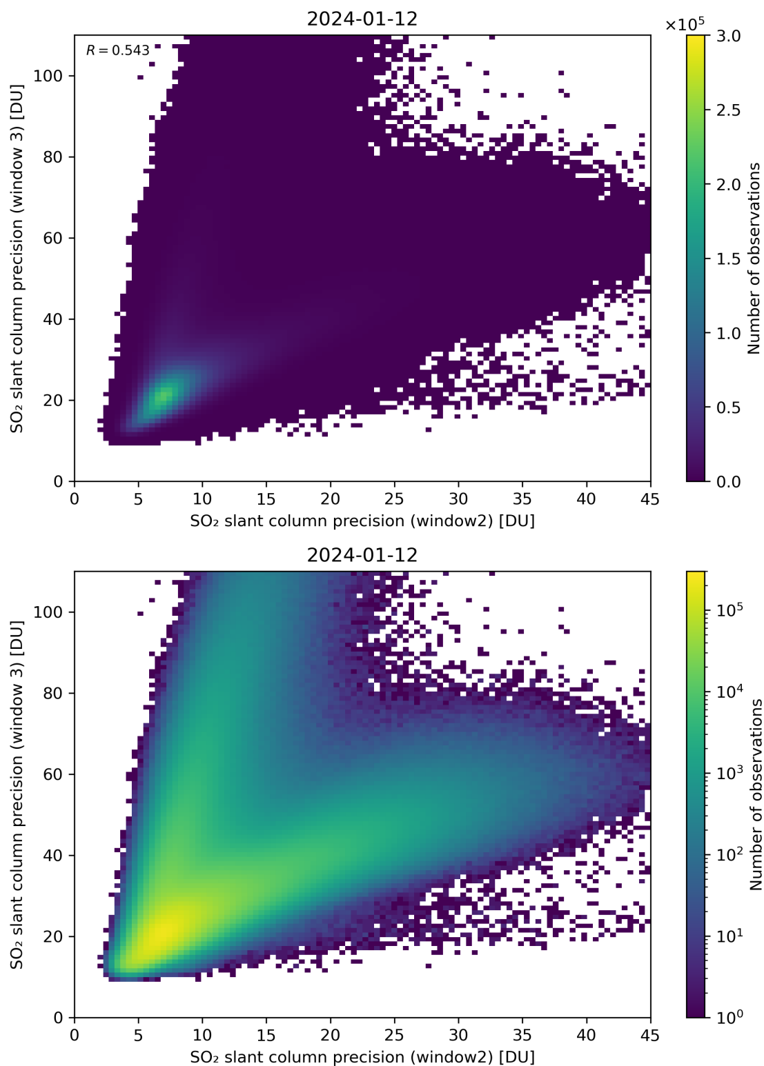
Figure 250: Scatter density plot of “SO 2 slant column precision (window2)” against “SO 2 slant column precision (window 3)” for 2024-01-11 to 2024-01-13.
