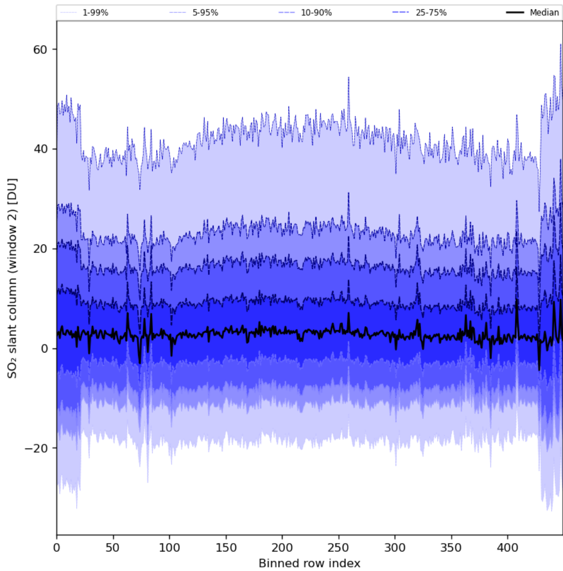
Figure 83: Along track statistics of “SO 2 slant column (window 2)” for 2024-01-11 to 2024-01-13
