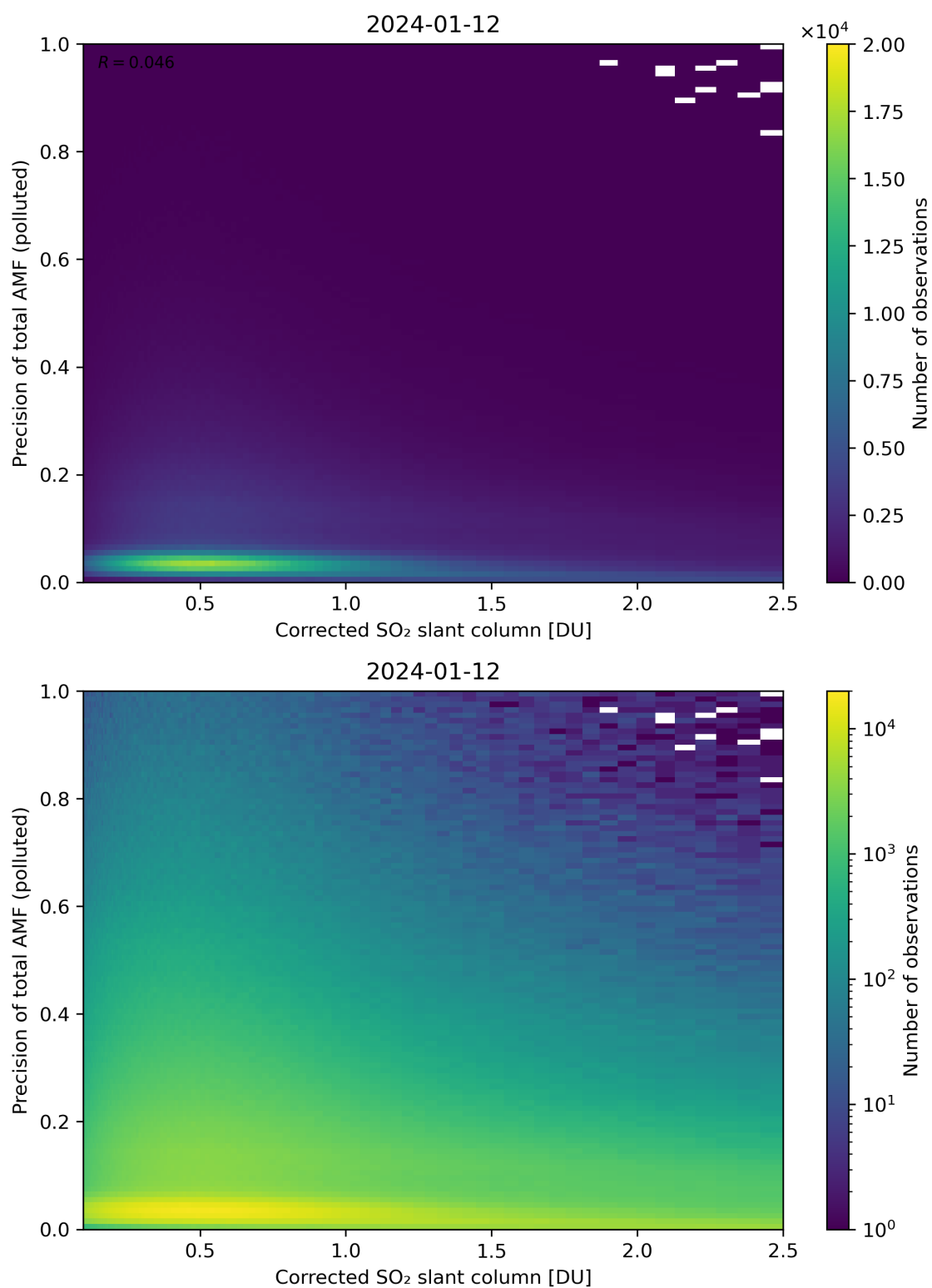
Figure 193: Scatter density plot of “Corrected SO 2 slant column” against “Precision of total AMF (polluted)” for 2024-01-11 to 2024-01-13.
