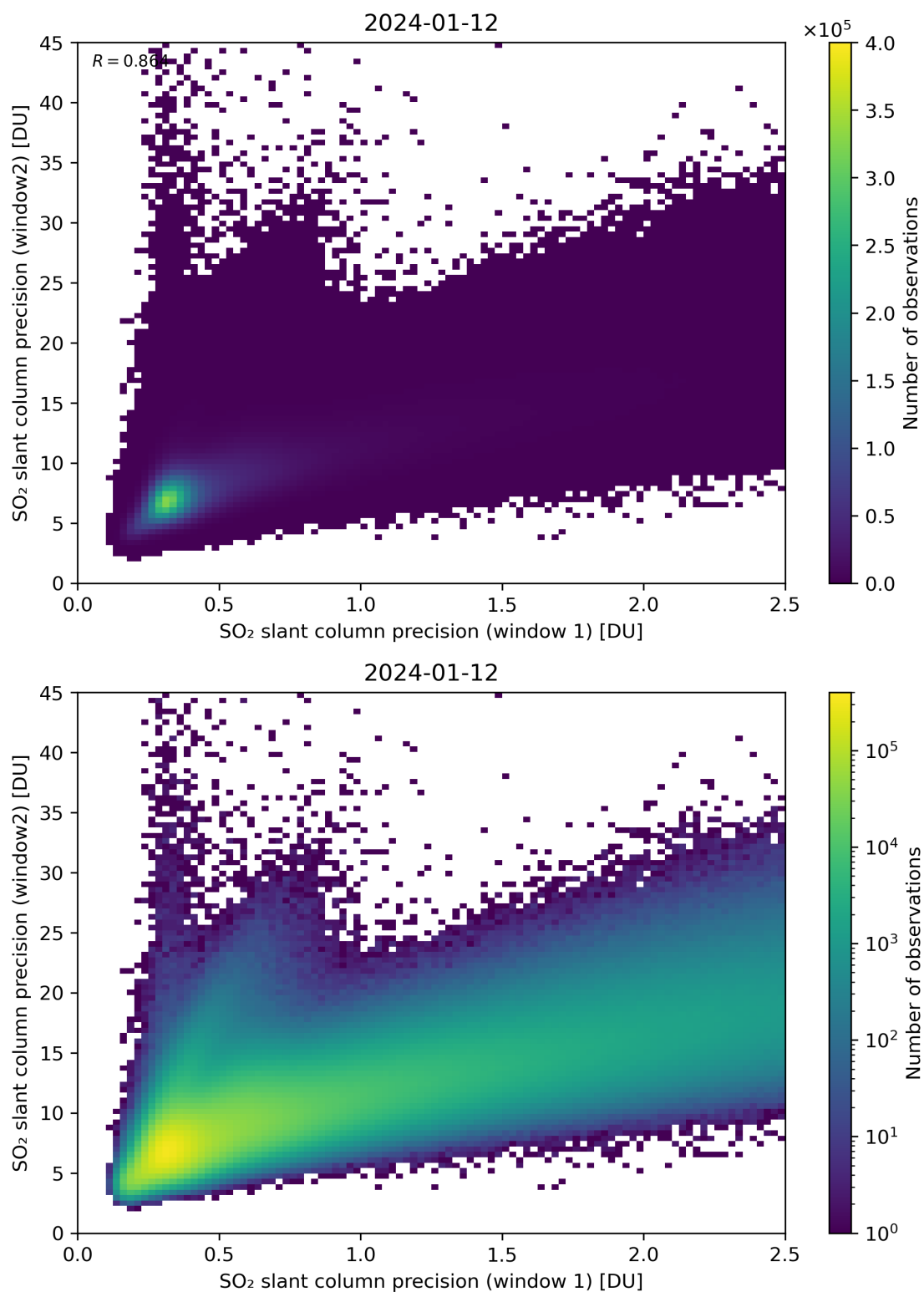
Figure 227: Scatter density plot of “SO 2 slant column precision (window 1)” against “SO 2 slant column precision (window2)” for 2024-01-11 to 2024-01-13.
