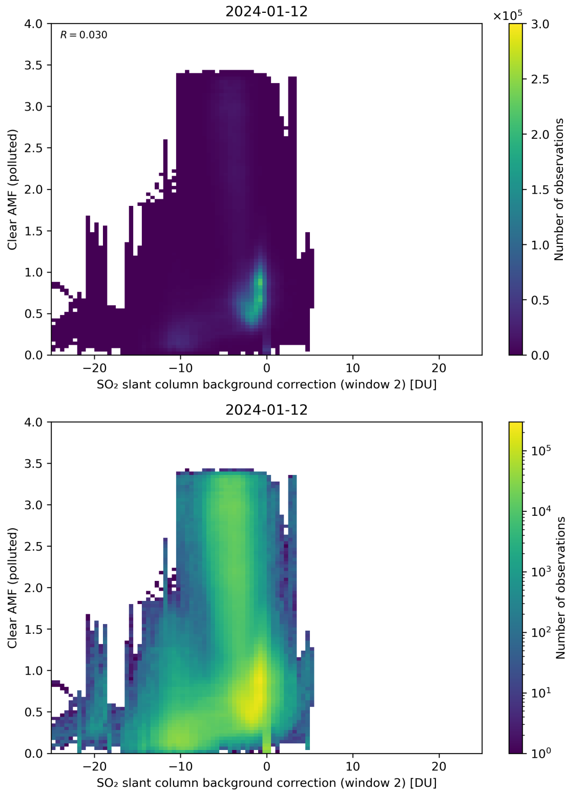
Figure 115: Scatter density plot of “SO 2 slant column background correction (window 2)” against “Clear AMF (polluted)” for 2024-01-11 to 2024-01-13.
