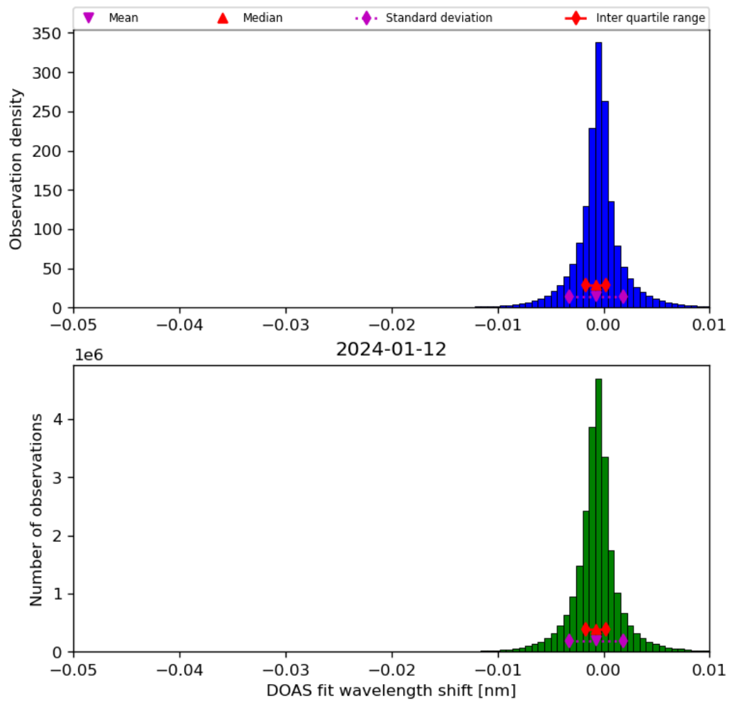
Figure 68: Histogram of “DOAS fit wavelength shift” for 2024-01-11 to 2024-01-13
