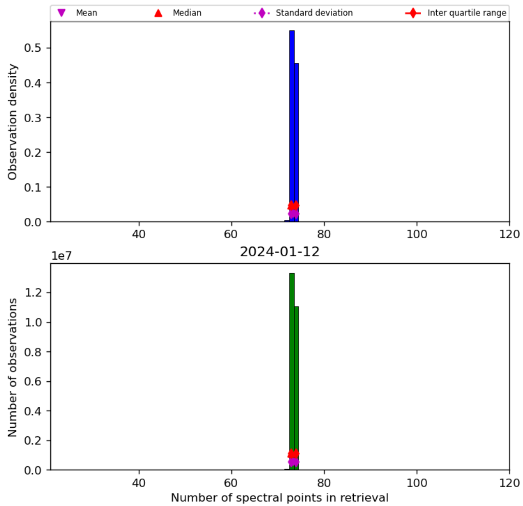
Figure 74: Histogram of “Number of spectral points in retrieval” for 2024-01-11 to 2024-01-13
