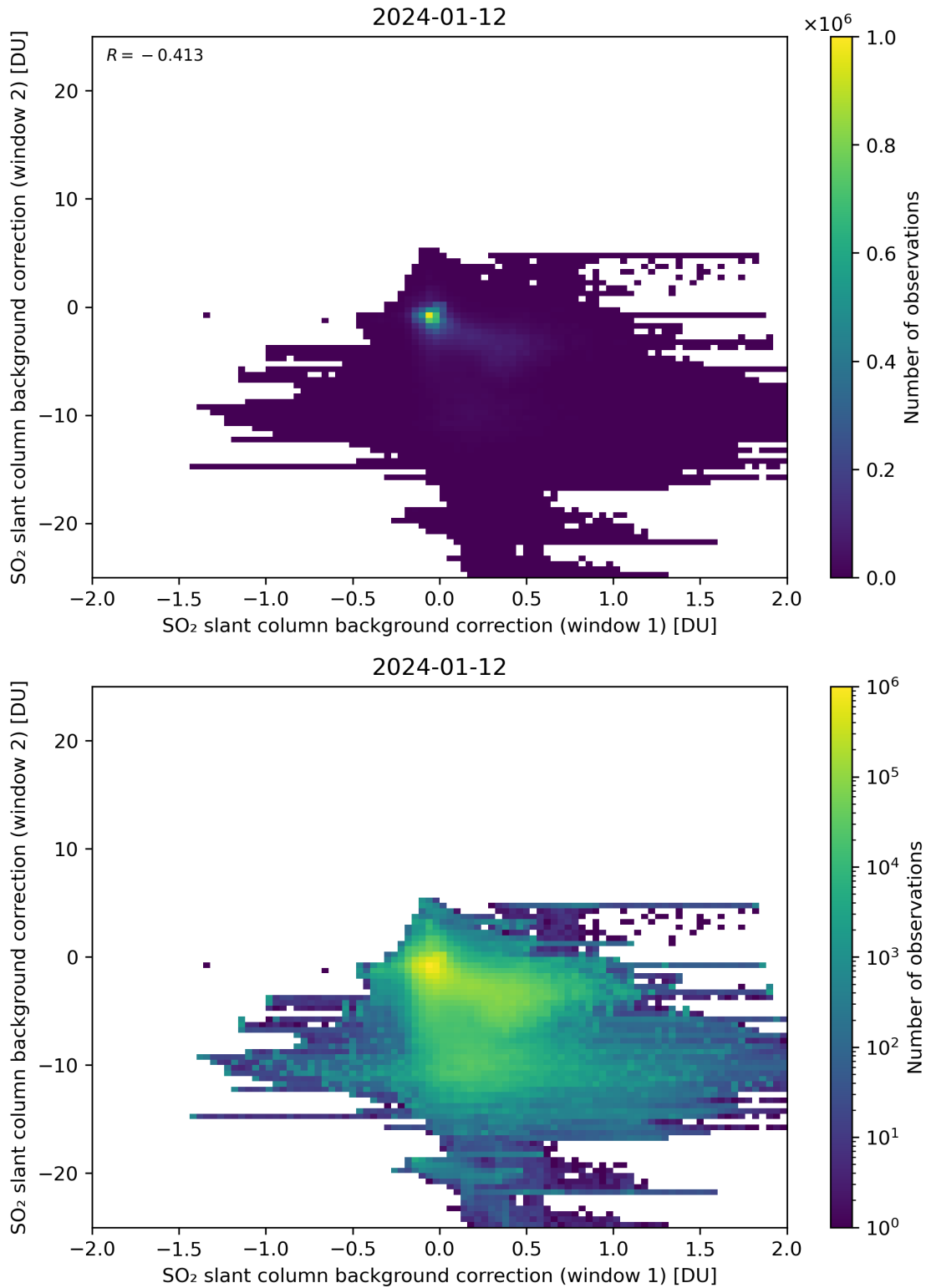
Figure 98: Scatter density plot of “SO 2 slant column background correction (window 1)” against “SO 2 slant column background correction (window 2)” for 2024-01-11 to 2024-01-13.
