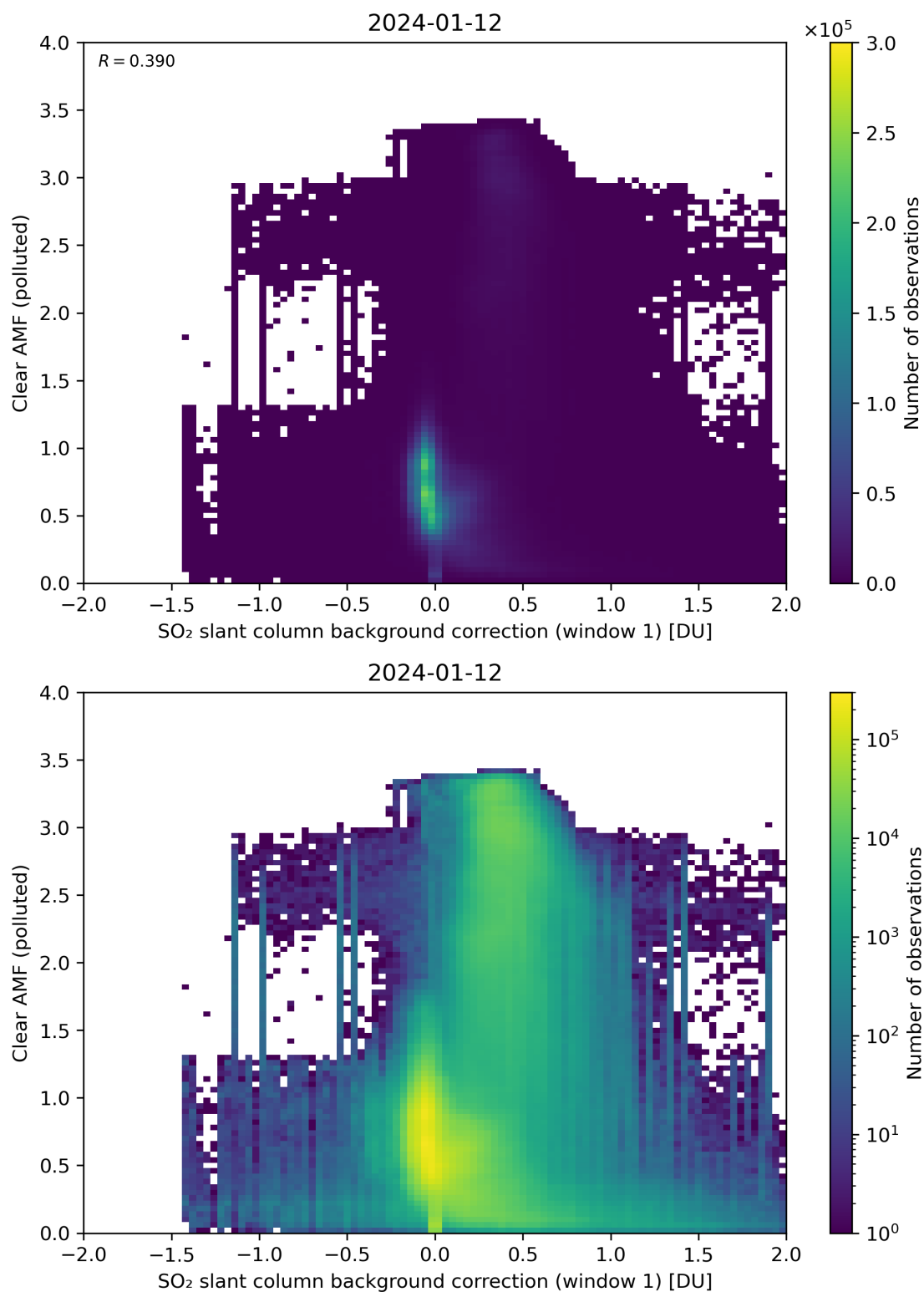
Figure 103: Scatter density plot of “SO 2 slant column background correction (window 1)” against “Clear AMF (polluted)” for 2024-01-11 to 2024-01-13.
