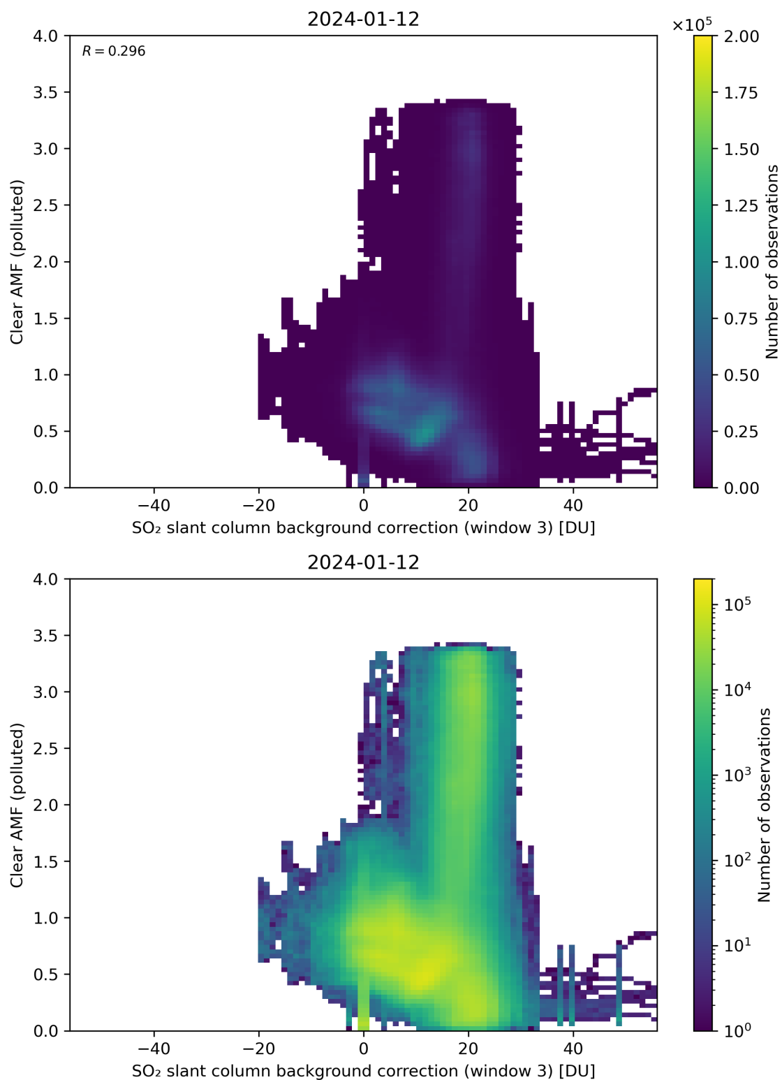
Figure 124: Scatter density plot of “SO 2 slant column background correction (window 3)” against “Clear AMF (polluted)” for 2024-01-11 to 2024-01-13.
