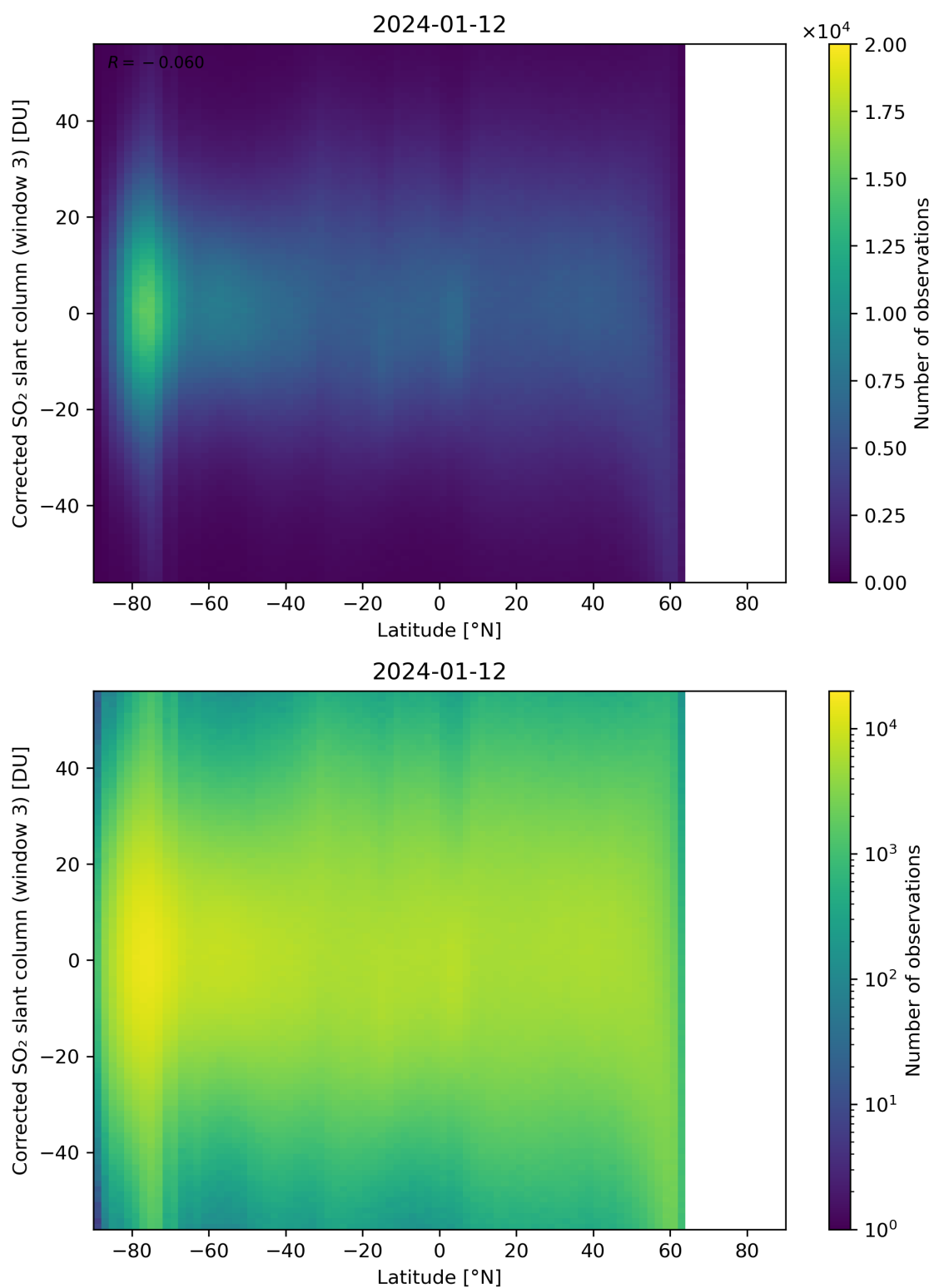
Figure 148: Scatter density plot of “Latitude” against “Corrected SO 2 slant column (window 3)” for 2024-01-11 to 2024-01-13.
