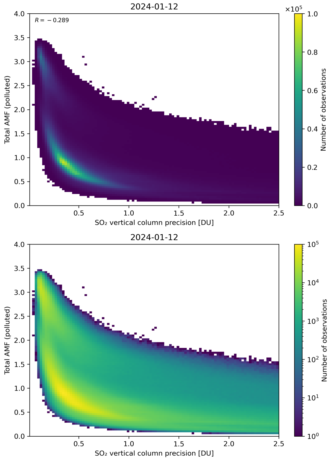
Figure 294: Scatter density plot of “SO 2 vertical column precision” against “Total AMF (polluted)” for 2024-01-11 to 2024-01-13.
