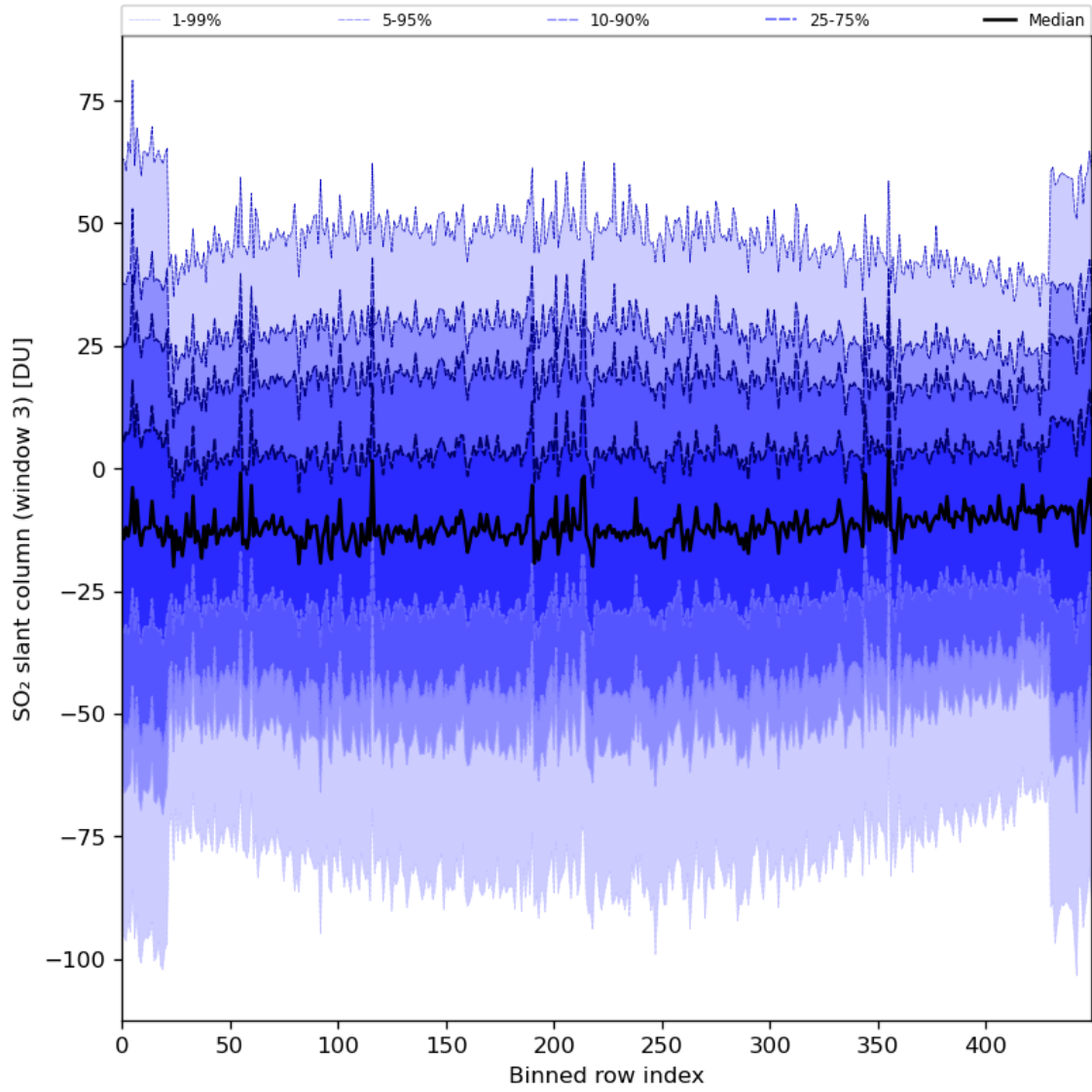
Figure 87: Along track statistics of “SO 2 slant column (window 3)” for 2024-01-11 to 2024-01-13
