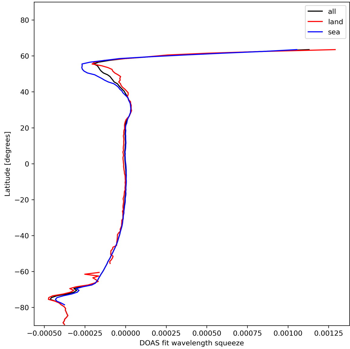
Figure 46: Zonal average of “DOAS fit wavelength squeeze” for 2024-01-11 to 2024-01-13.
