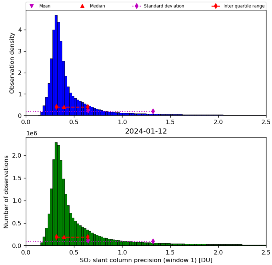
Figure 57: Histogram of “SO 2 slant column precision (window 1)” for 2024-01-11 to 2024-01-13
