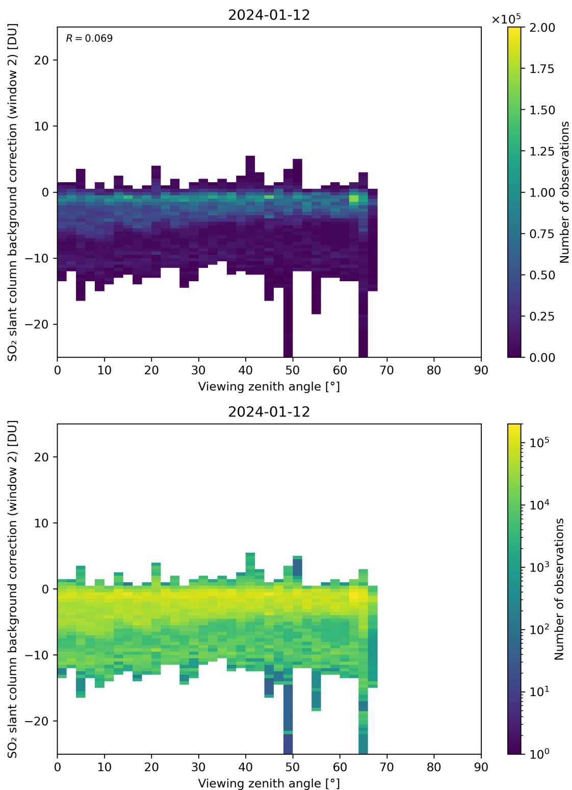
Figure 309: Scatter density plot of “Viewing zenith angle” against “SO 2 slant column background correction (window 2)” for 2024-01-11 to 2024-01-13.
