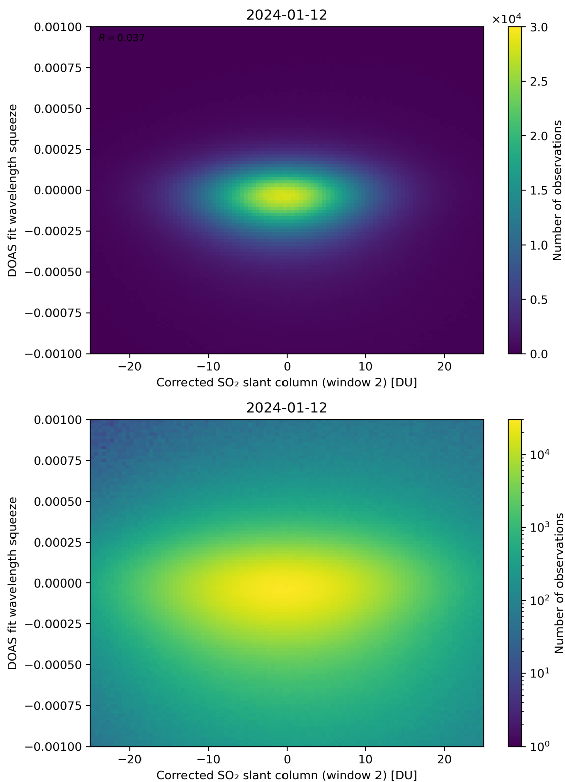
Figure 197: Scatter density plot of “Corrected SO 2 slant column (window 2)” against “DOAS fit wavelength squeeze” for 2024-01-11 to 2024-01-13.
