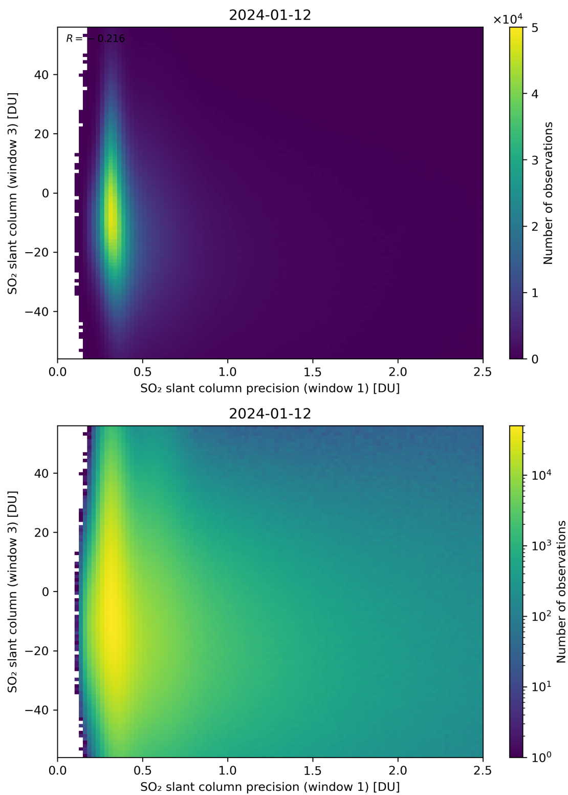
Figure 228: Scatter density plot of “SO 2 slant column precision (window 1)” against “SO 2 slant column (window 3)” for 2024-01-11 to 2024-01-13.
