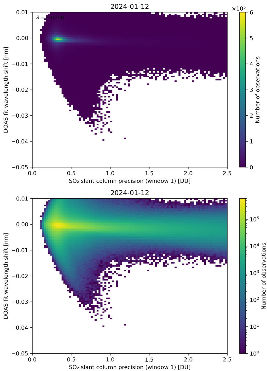
Figure 221: Scatter density plot of “SO 2 slant column precision (window 1)” against “DOAS fit wavelength shift” for 2024-01-11 to 2024-01-13.
