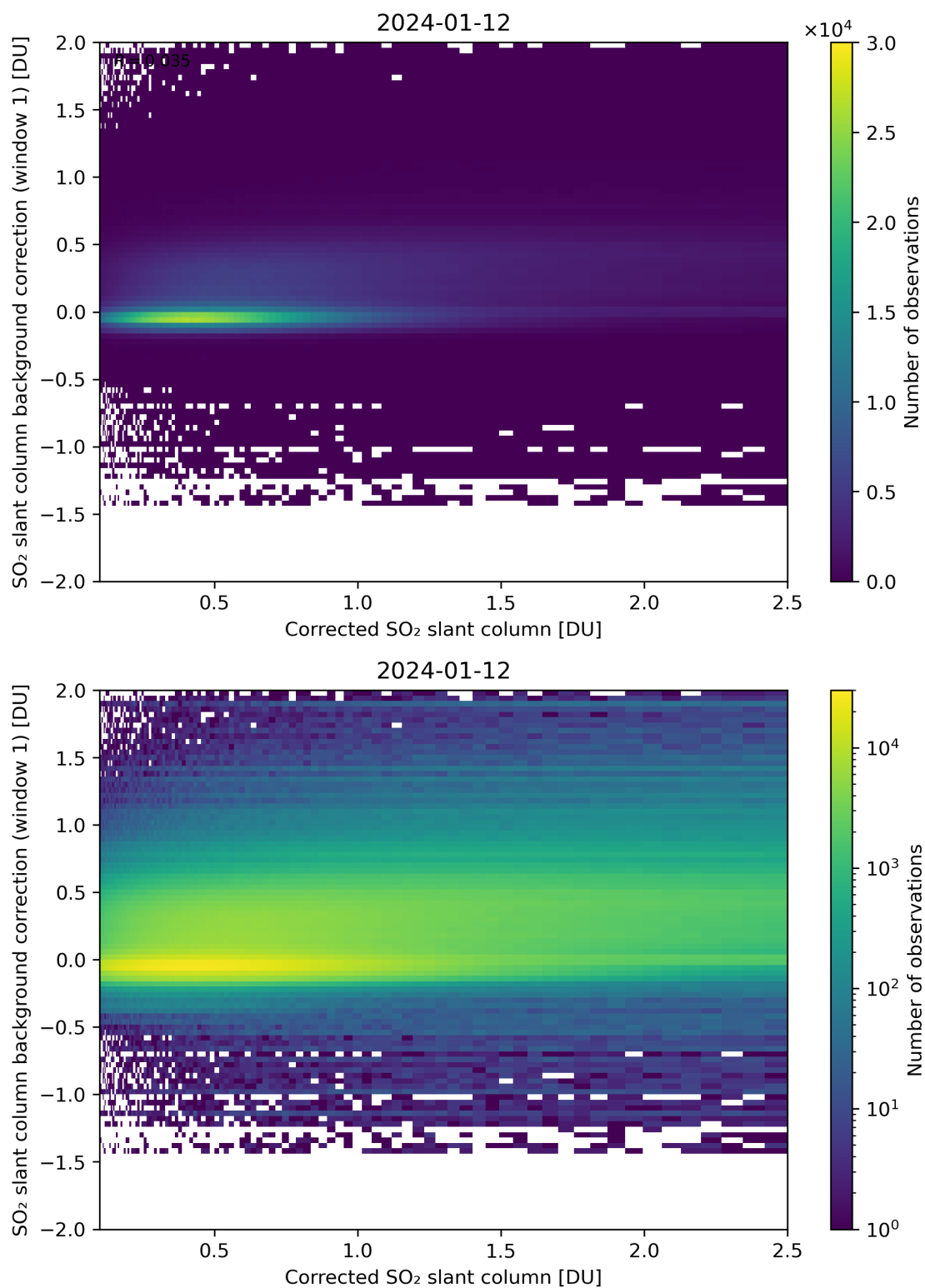
Figure 178: Scatter density plot of “Corrected SO 2 slant column” against “SO 2 slant column background correction (window 1)” for 2024-01-11 to 2024-01-13.
