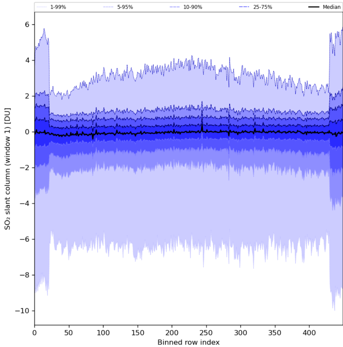
Figure 79: Along track statistics of “SO 2 slant column (window 1)” for 2024-01-11 to 2024-01-13
