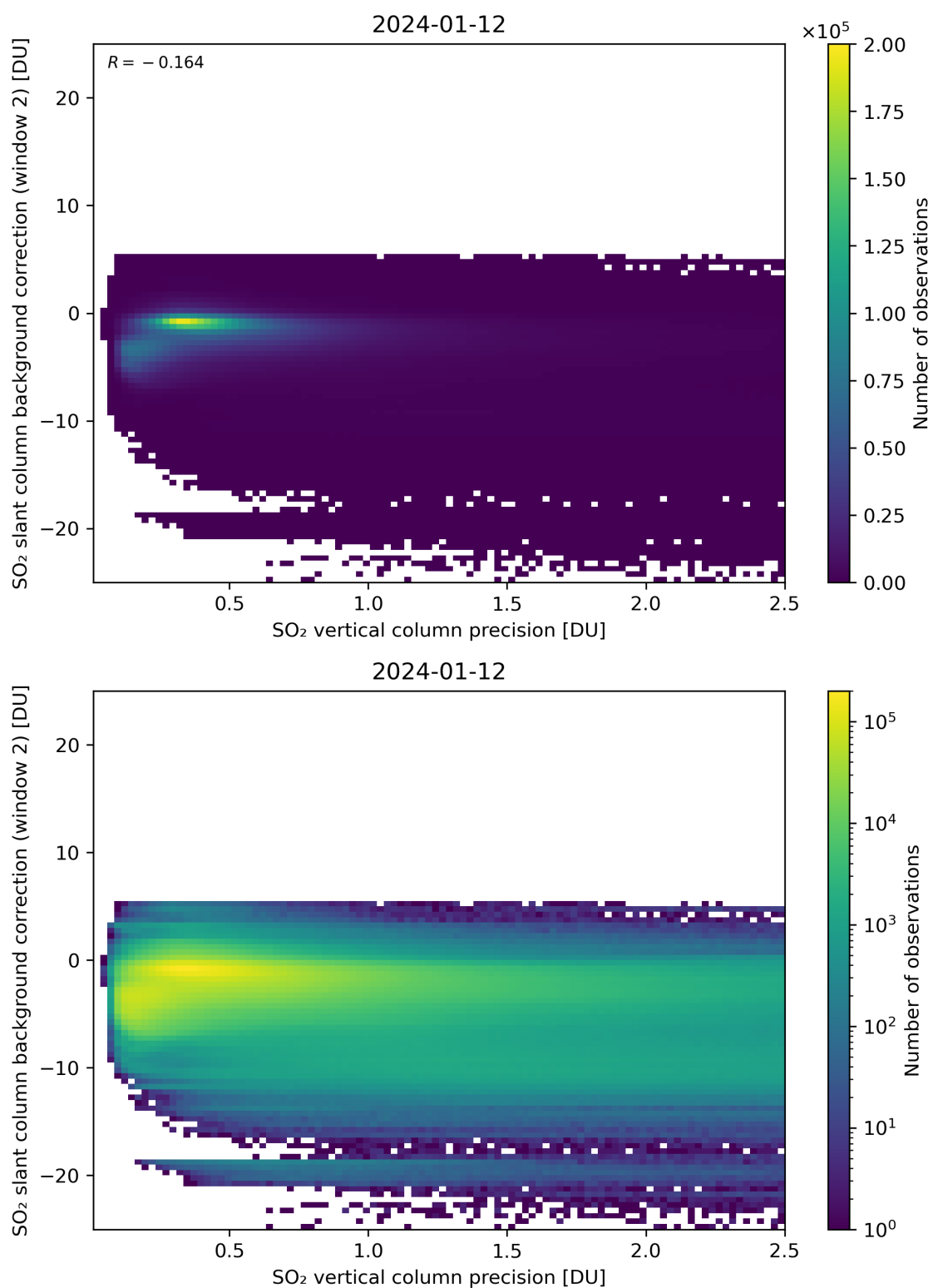
Figure 280: Scatter density plot of “SO 2 vertical column precision” against “SO 2 slant column background correction (window 2)” for 2024-01-11 to 2024-01-13.
