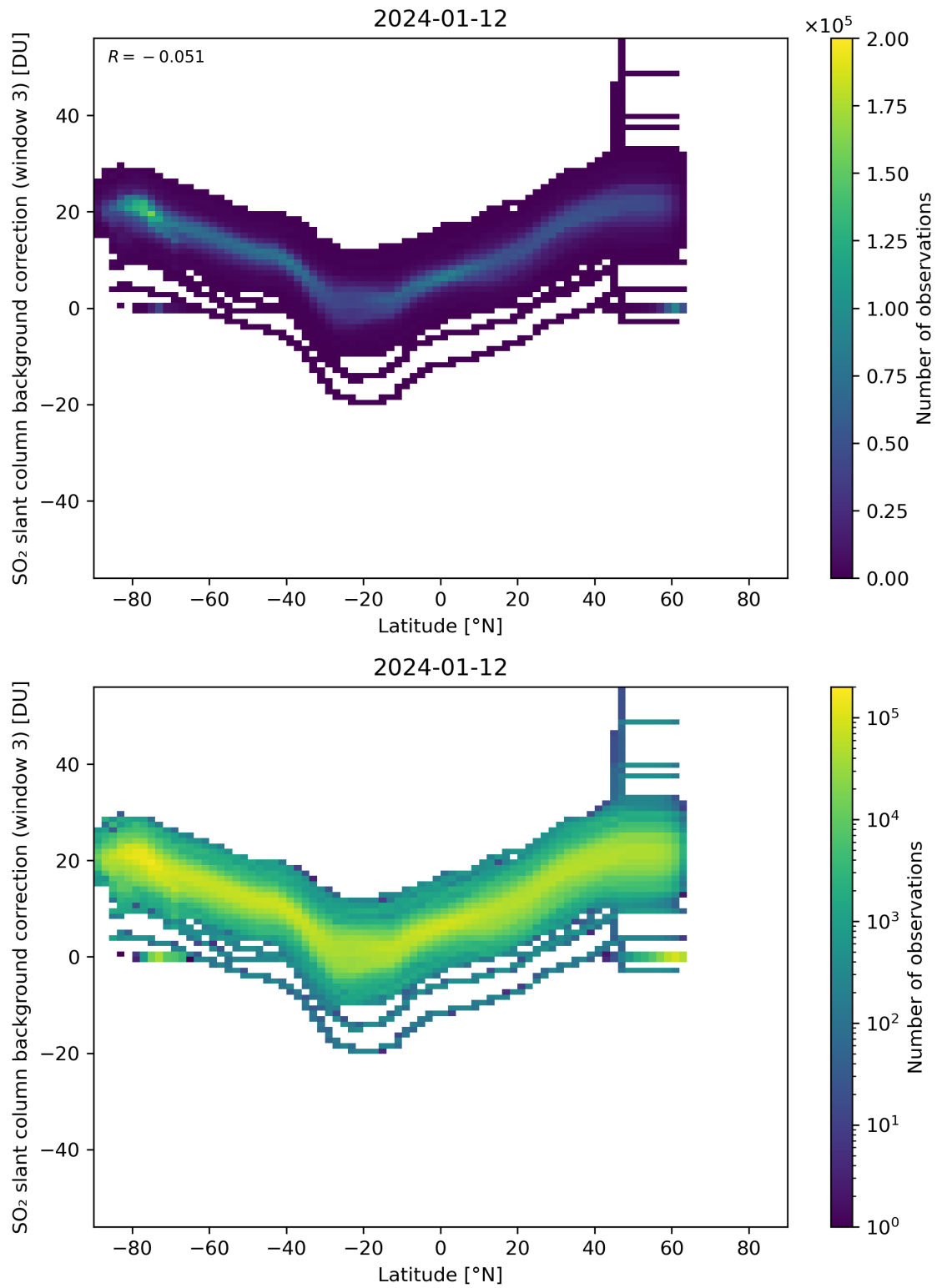
Figure 141: Scatter density plot of “Latitude” against “SO 2 slant column background correction (window 3)” for 2024-01-11 to 2024-01-13.
