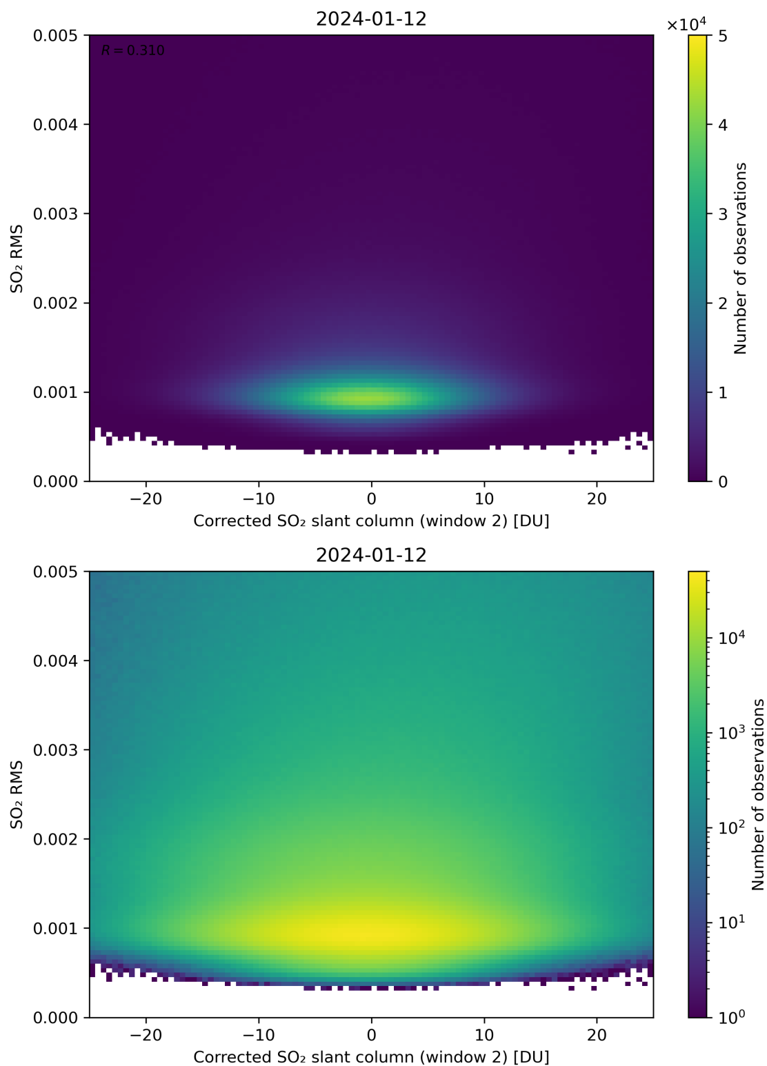
Figure 198: Scatter density plot of “Corrected SO 2 slant column (window 2)” against “SO 2 RMS” for 2024-01-11 to 2024-01-13.
