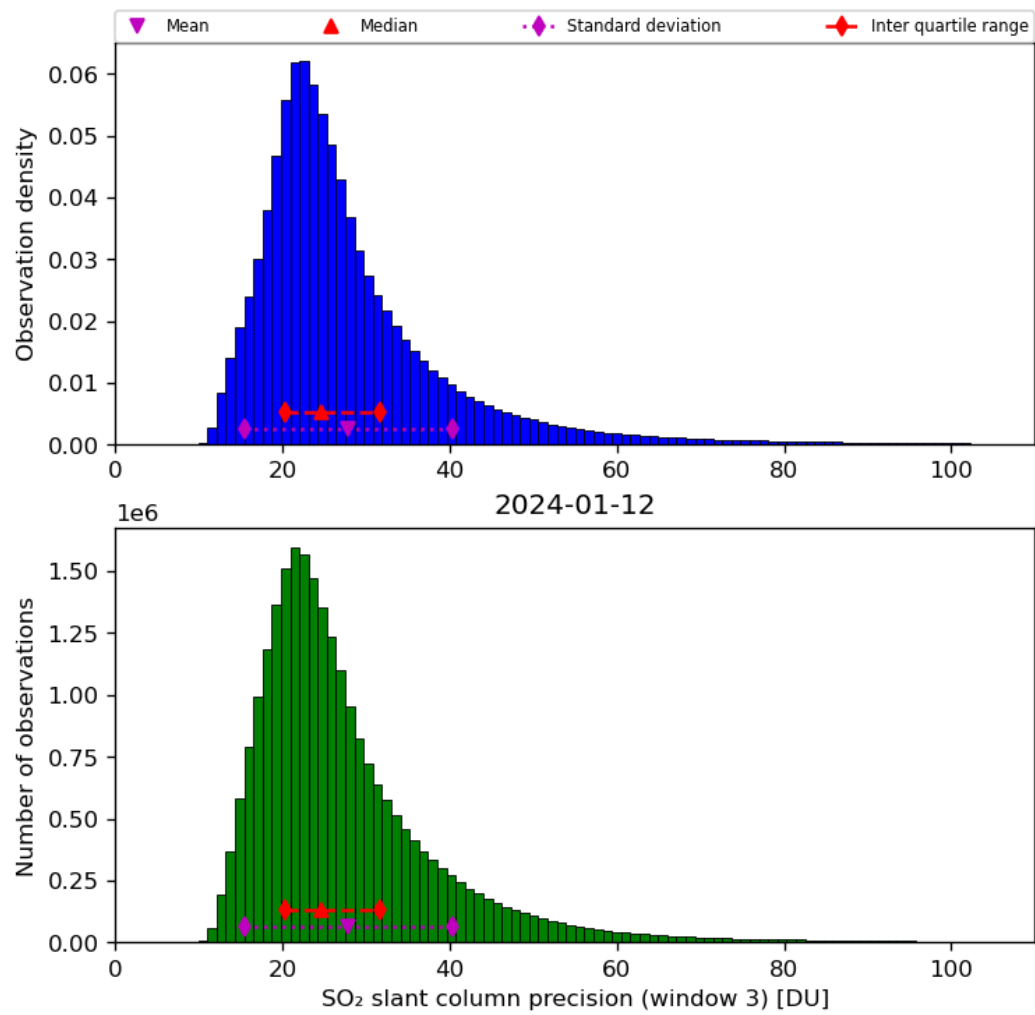
Figure 65: Histogram of “SO 2 slant column precision (window 3)” for 2024-01-11 to 2024-01-13
