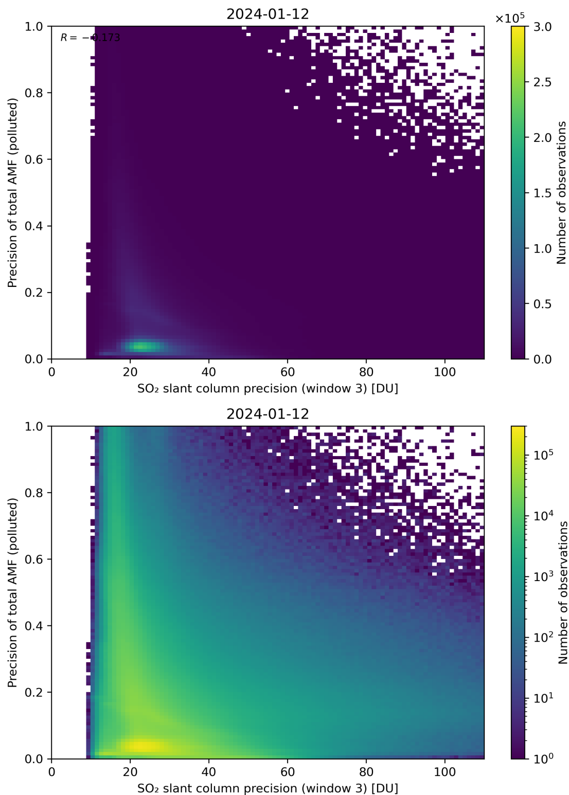
Figure 264: Scatter density plot of “SO 2 slant column precision (window 3)” against “Precision of total AMF (polluted)” for 2024-01-11 to 2024-01-13.
