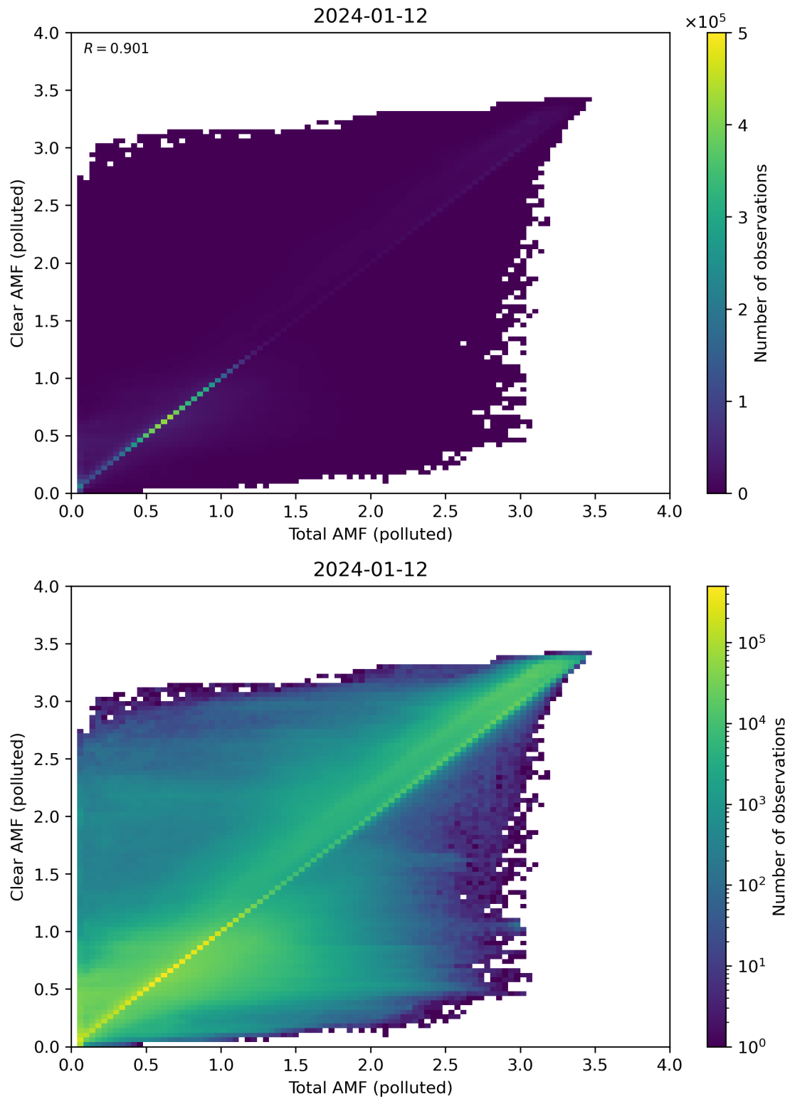
Figure 271: Scatter density plot of “Total AMF (polluted)” against “Clear AMF (polluted)” for 2024-01-11 to 2024-01-13.
