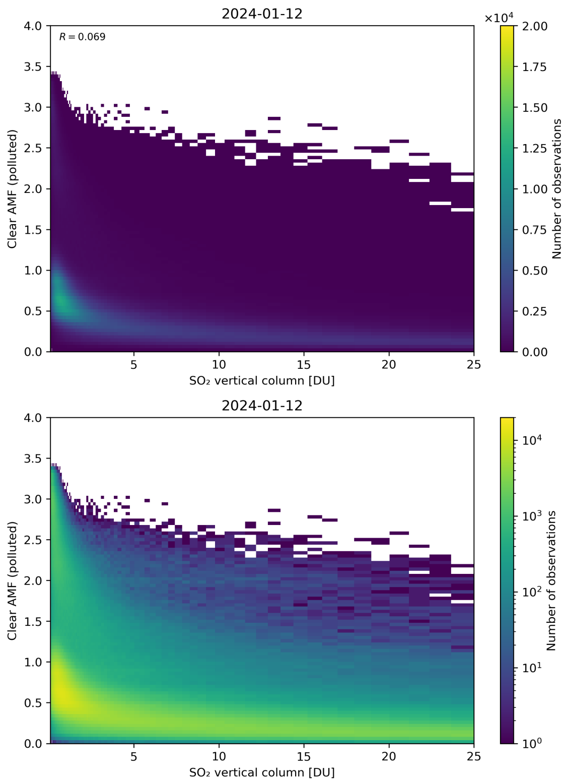
Figure 296: Scatter density plot of “SO 2 vertical column” against “Clear AMF (polluted)” for 2024-01-11 to 2024-01-13.
