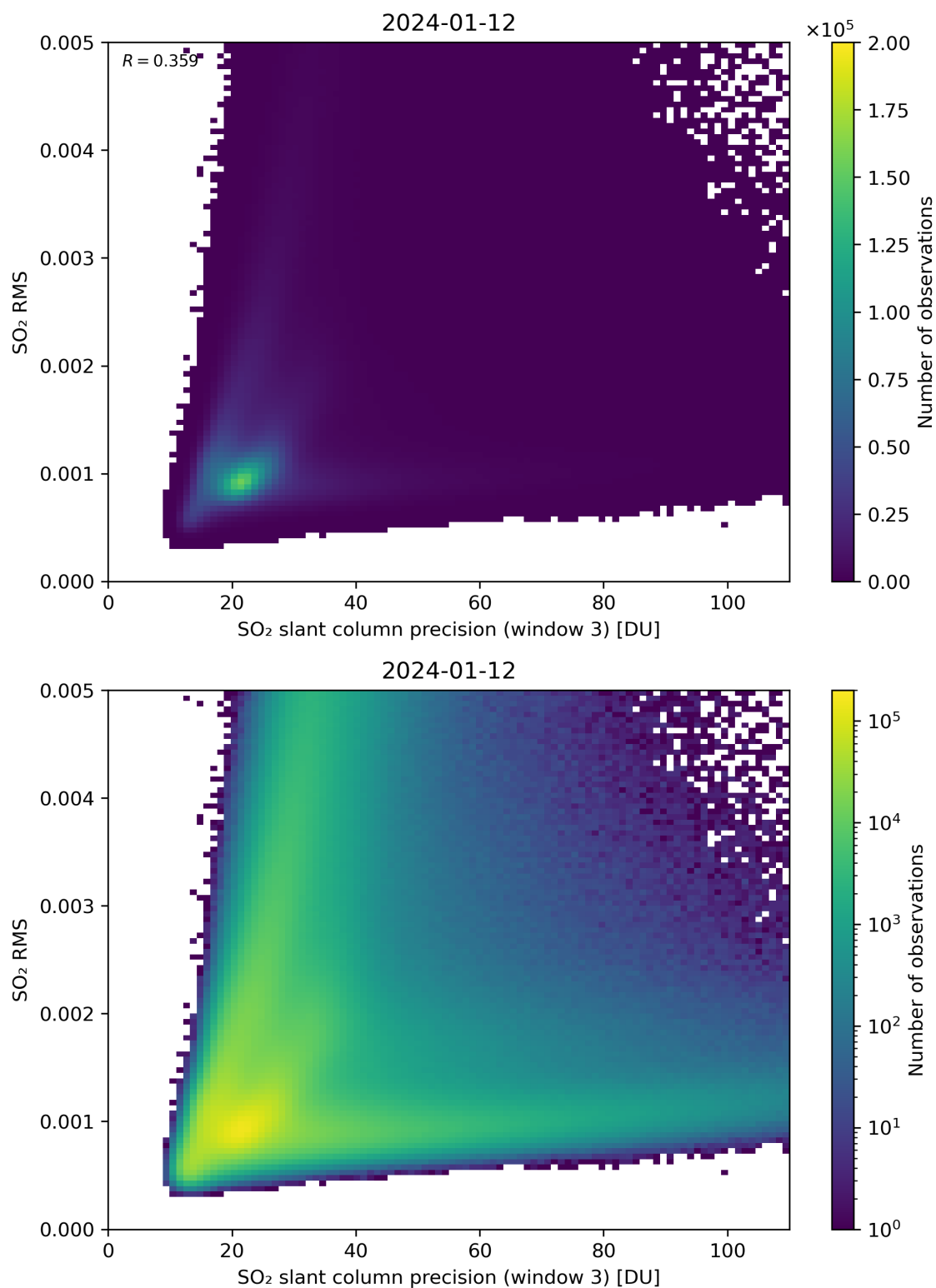
Figure 260: Scatter density plot of “SO 2 slant column precision (window 3)” against “SO 2 RMS” for 2024-01-11 to 2024-01-13.
