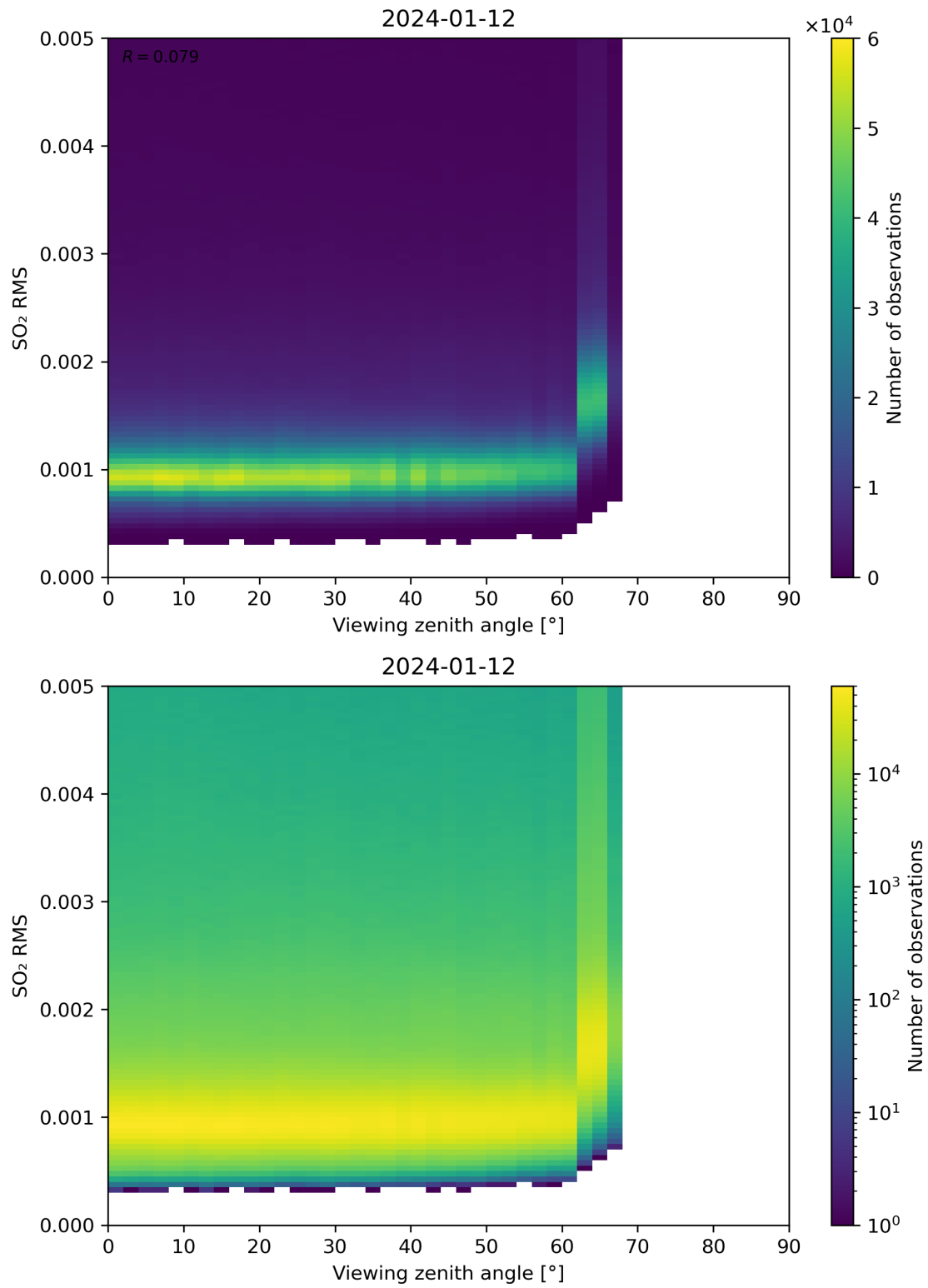
Figure 313: Scatter density plot of “Viewing zenith angle” against “SO 2 RMS” for 2024-01-11 to 2024-01-13.
