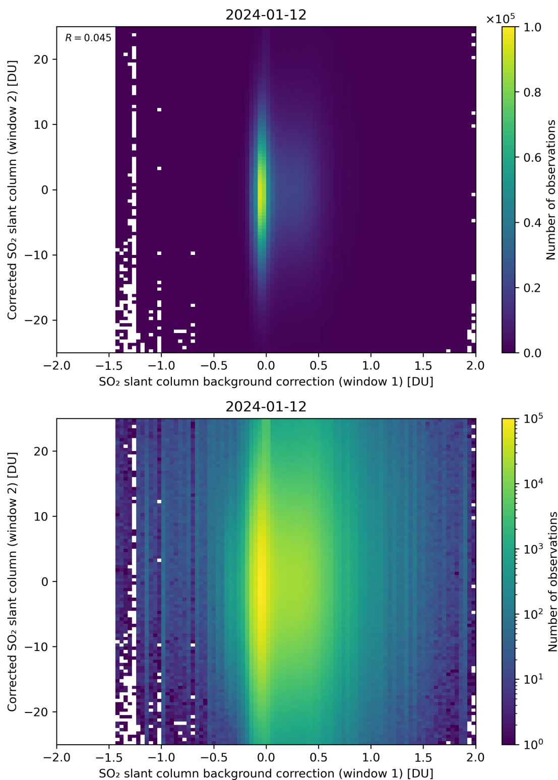
Figure 104: Scatter density plot of “SO 2 slant column background correction (window 1)” against “Corrected SO 2 slant column (window 2)” for 2024-01-11 to 2024-01-13.
