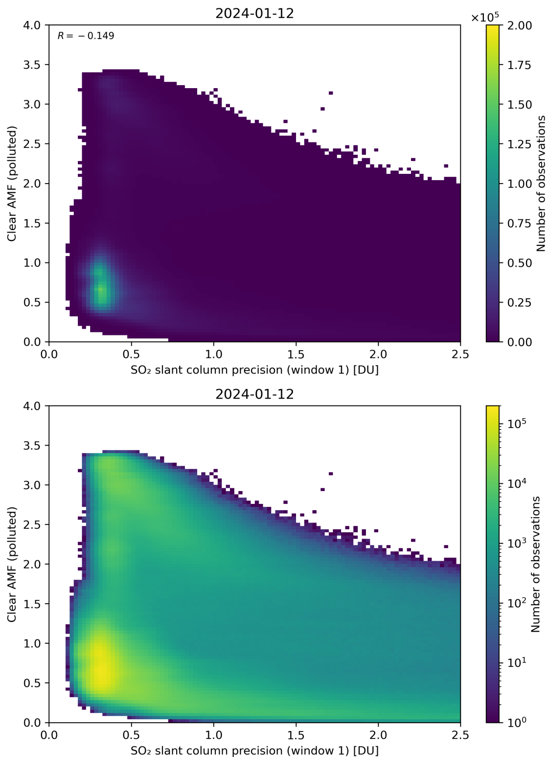
Figure 224: Scatter density plot of “SO 2 slant column precision (window 1)” against “Clear AMF (polluted)” for 2024-01-11 to 2024-01-13.
