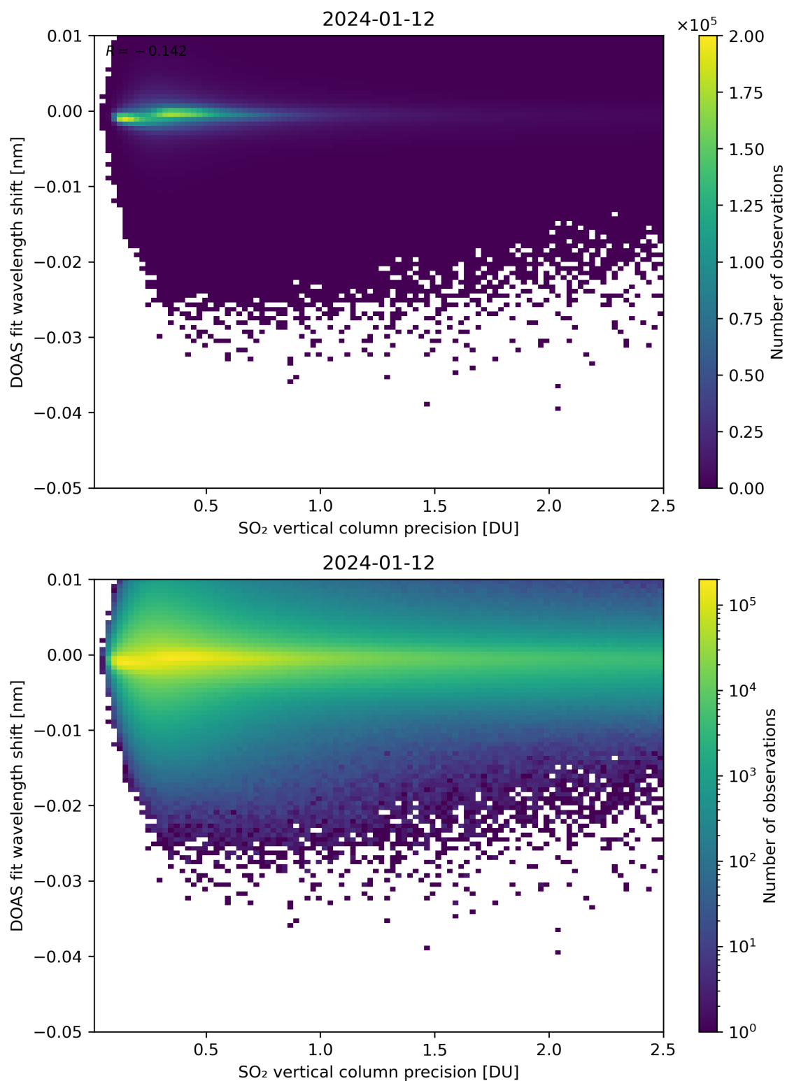
Figure 282: Scatter density plot of “SO 2 vertical column precision” against “DOAS fit wavelength shift” for 2024-01-11 to 2024-01-13.
