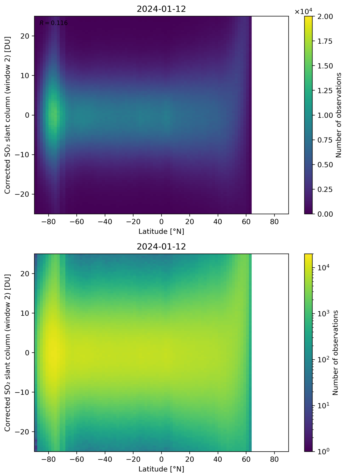
Figure 147: Scatter density plot of “Latitude” against “Corrected SO 2 slant column (window 2)” for 2024-01-11 to 2024-01-13.
