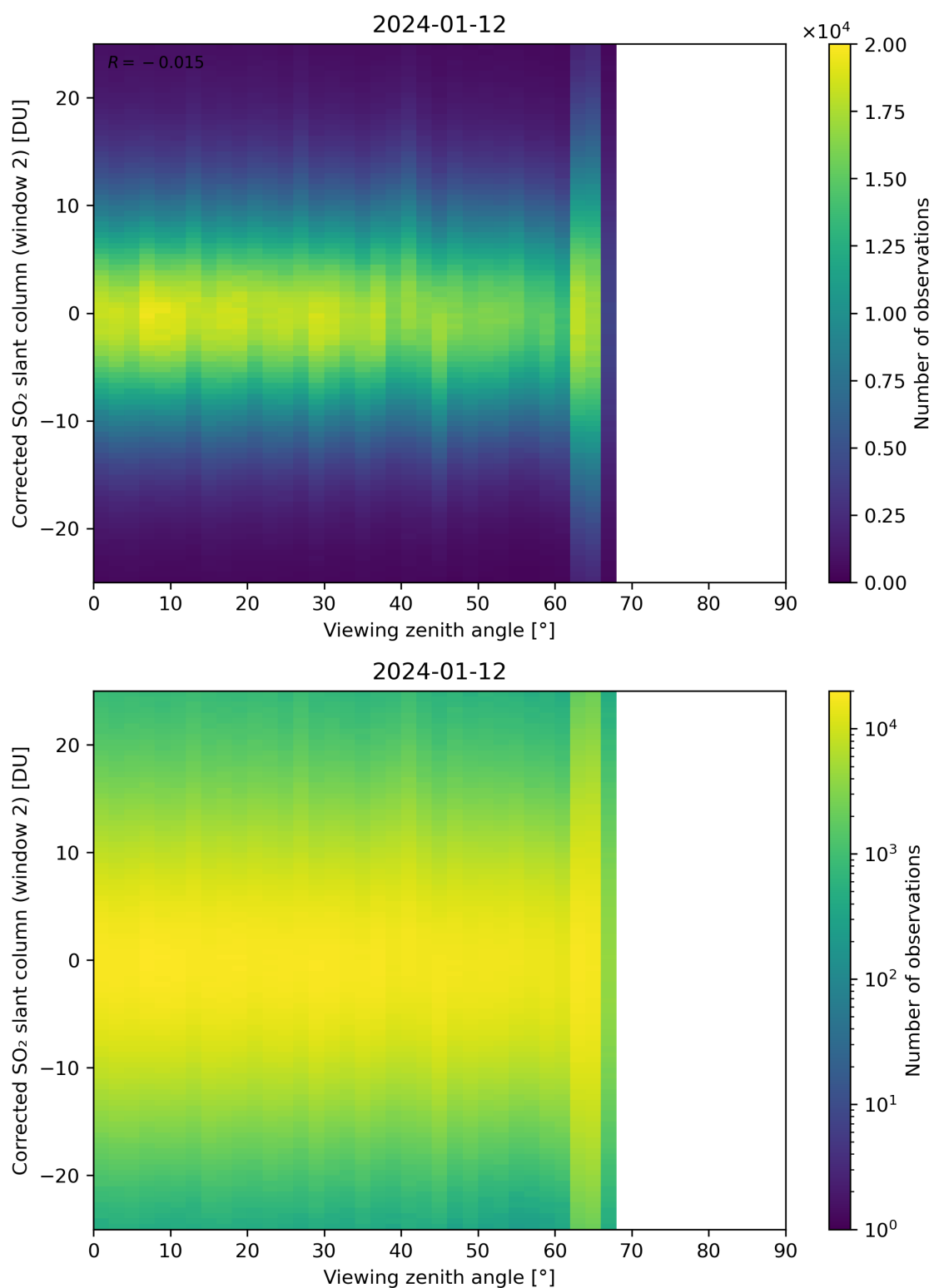
Figure 318: Scatter density plot of “Viewing zenith angle” against “Corrected SO 2 slant column (window 2)” for 2024-01-11 to 2024-01-13.
