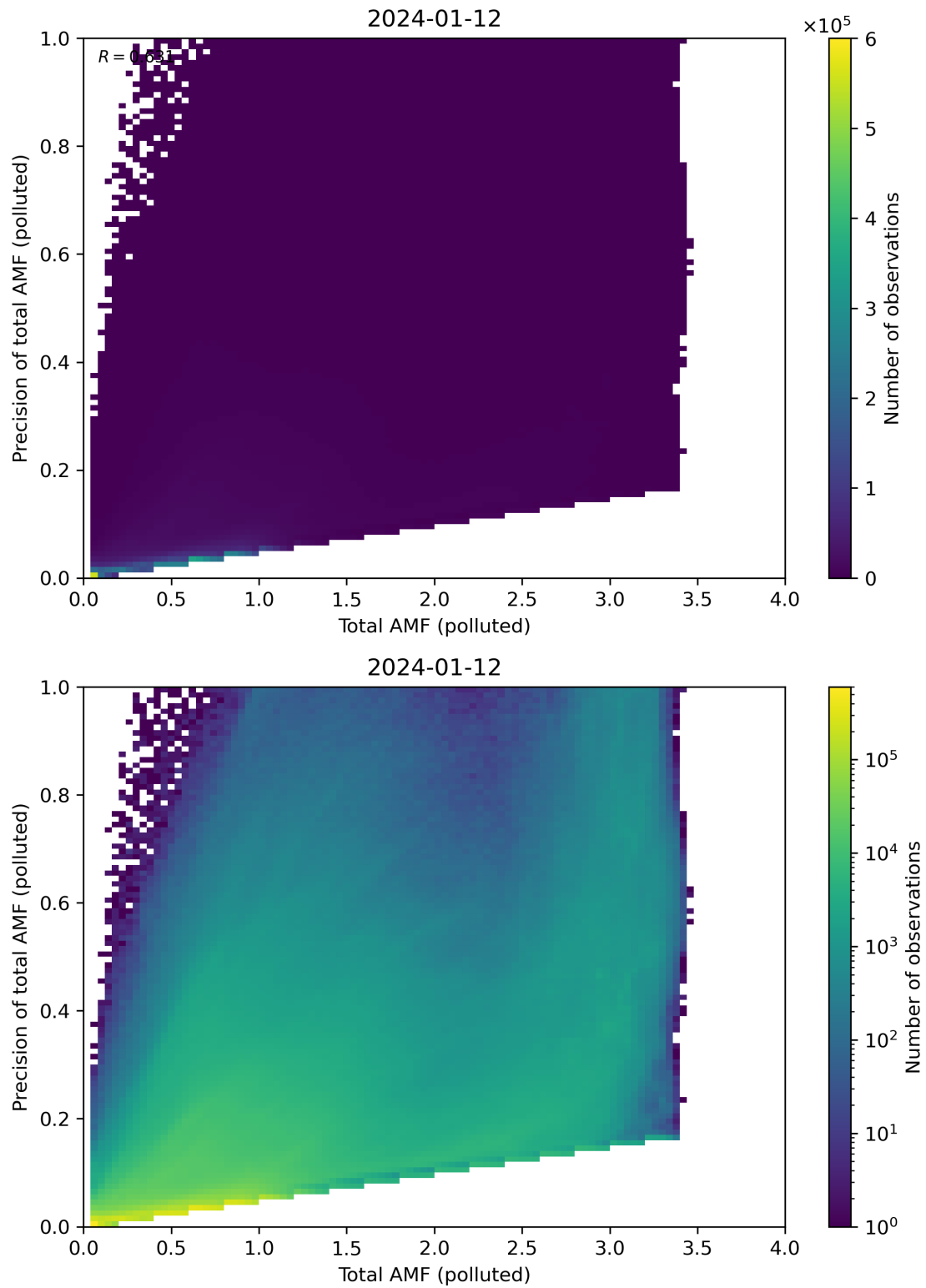
Figure 272: Scatter density plot of “Total AMF (polluted)” against “Precision of total AMF (polluted)” for 2024-01-11 to 2024-01-13.
