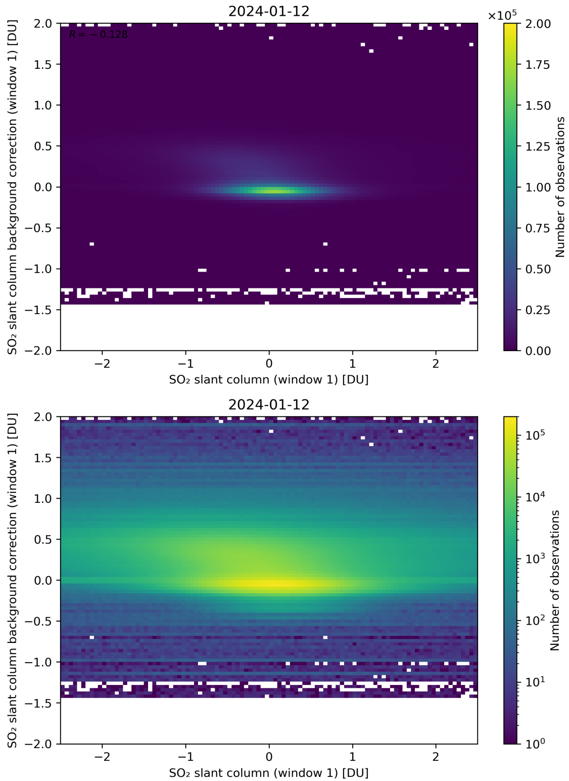
Figure 212: Scatter density plot of “SO 2 slant column (window 1)” against “SO 2 slant column background correction (window 1)” for 2024-01-11 to 2024-01-13.
