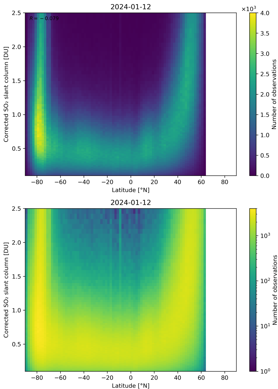
Figure 146: Scatter density plot of “Latitude” against “Corrected SO 2 slant column” for 2024-01-11 to 2024-01-13.
