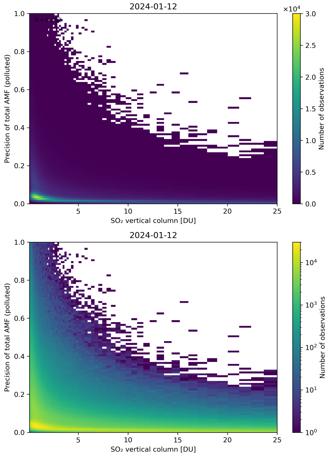
Figure 306: Scatter density plot of “SO 2 vertical column” against “Precision of total AMF (polluted)” for 2024-01-11 to 2024-01-13.
