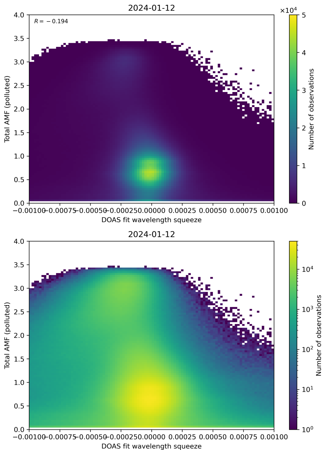
Figure 134: Scatter density plot of “DOAS fit wavelength squeeze” against “Total AMF (polluted)” for 2024-01-11 to 2024-01-13.
