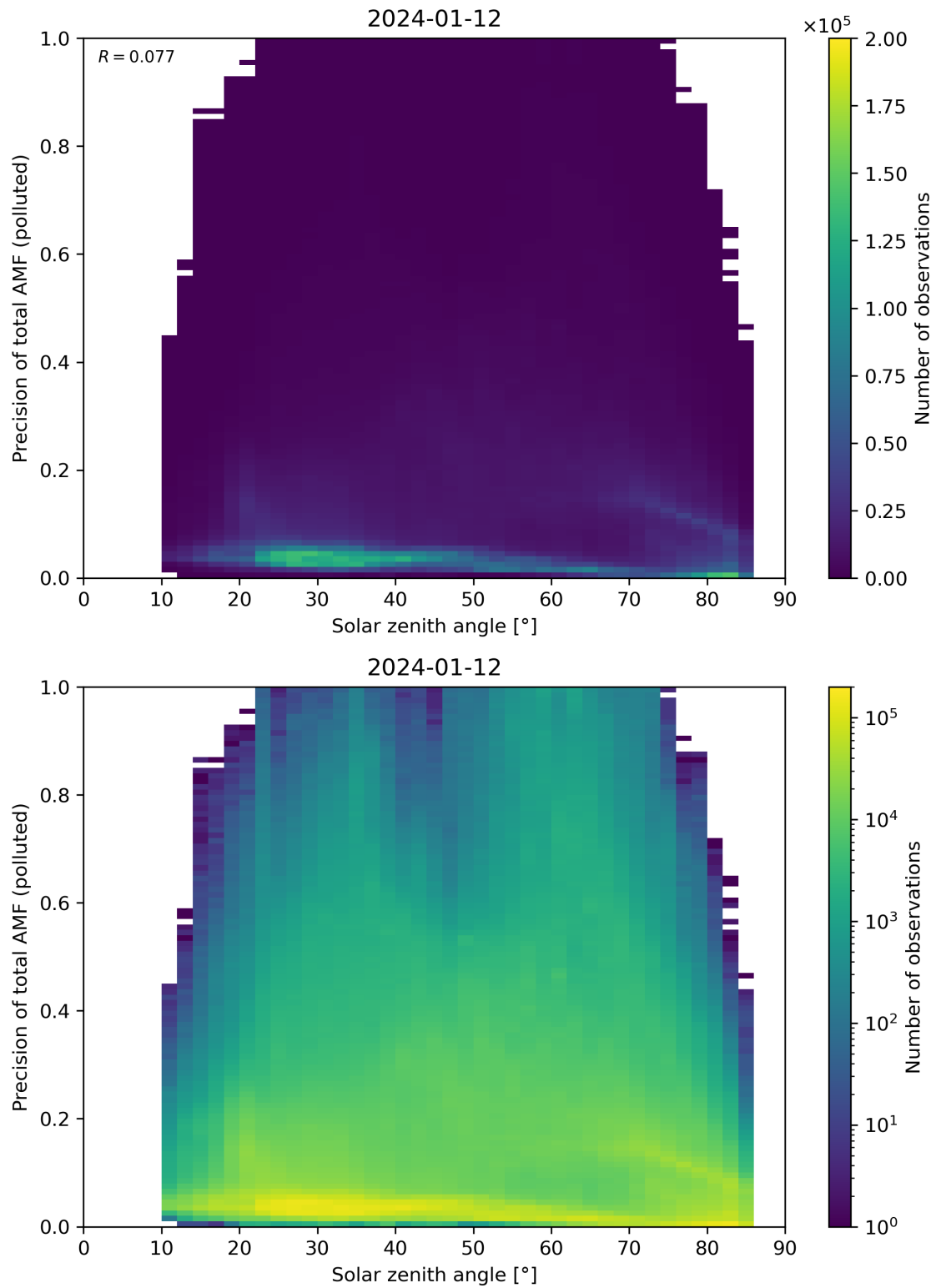
Figure 175: Scatter density plot of “Solar zenith angle” against “Precision of total AMF (polluted)” for 2024-01-11 to 2024-01-13.
