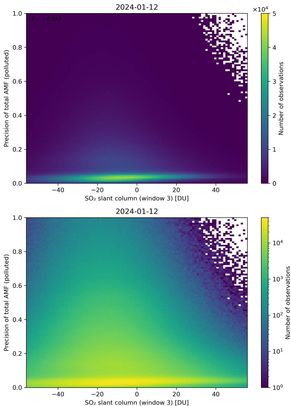
Figure 269: Scatter density plot of “SO 2 slant column (window 3)” against “Precision of total AMF (polluted)” for 2024-01-11 to 2024-01-13.
