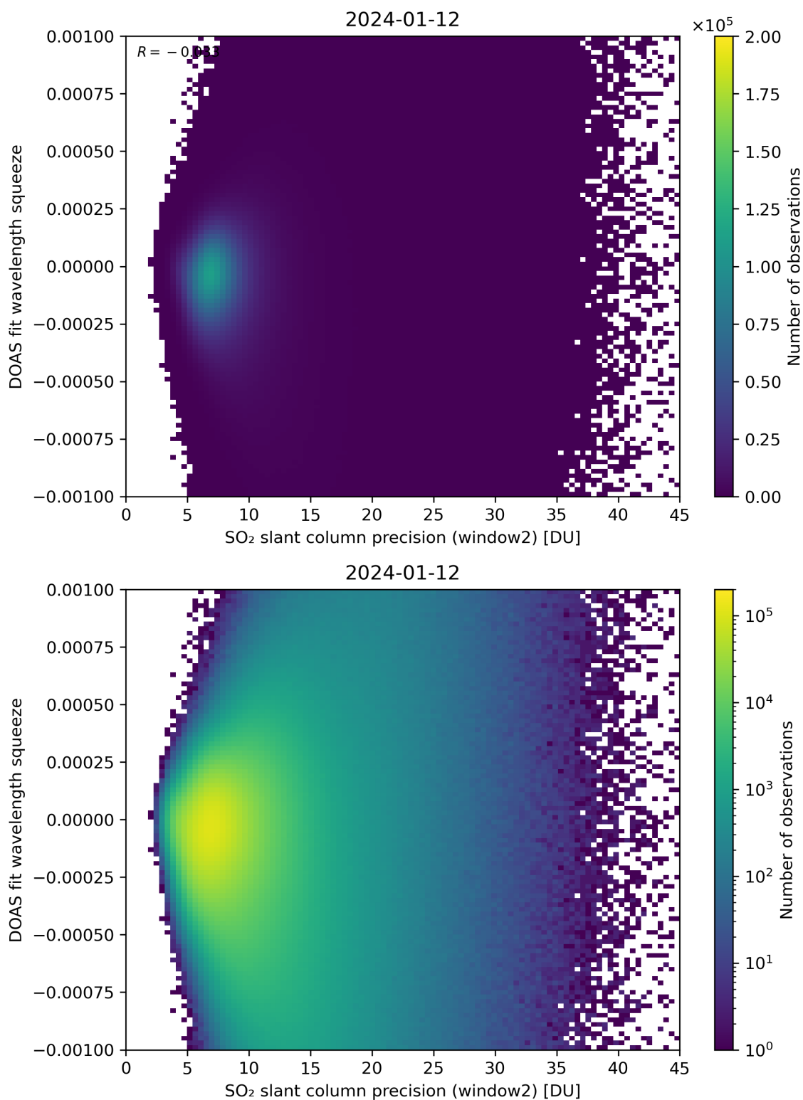
Figure 244: Scatter density plot of “SO 2 slant column precision (window2)” against “DOAS fit wavelength squeeze” for 2024-01-11 to 2024-01-13.
