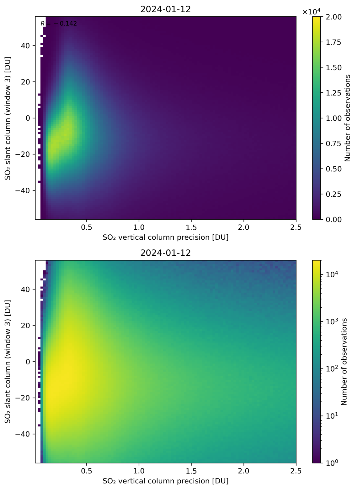
Figure 292: Scatter density plot of “SO 2 vertical column precision” against “SO 2 slant column (window 3)” for 2024-01-11 to 2024-01-13.
