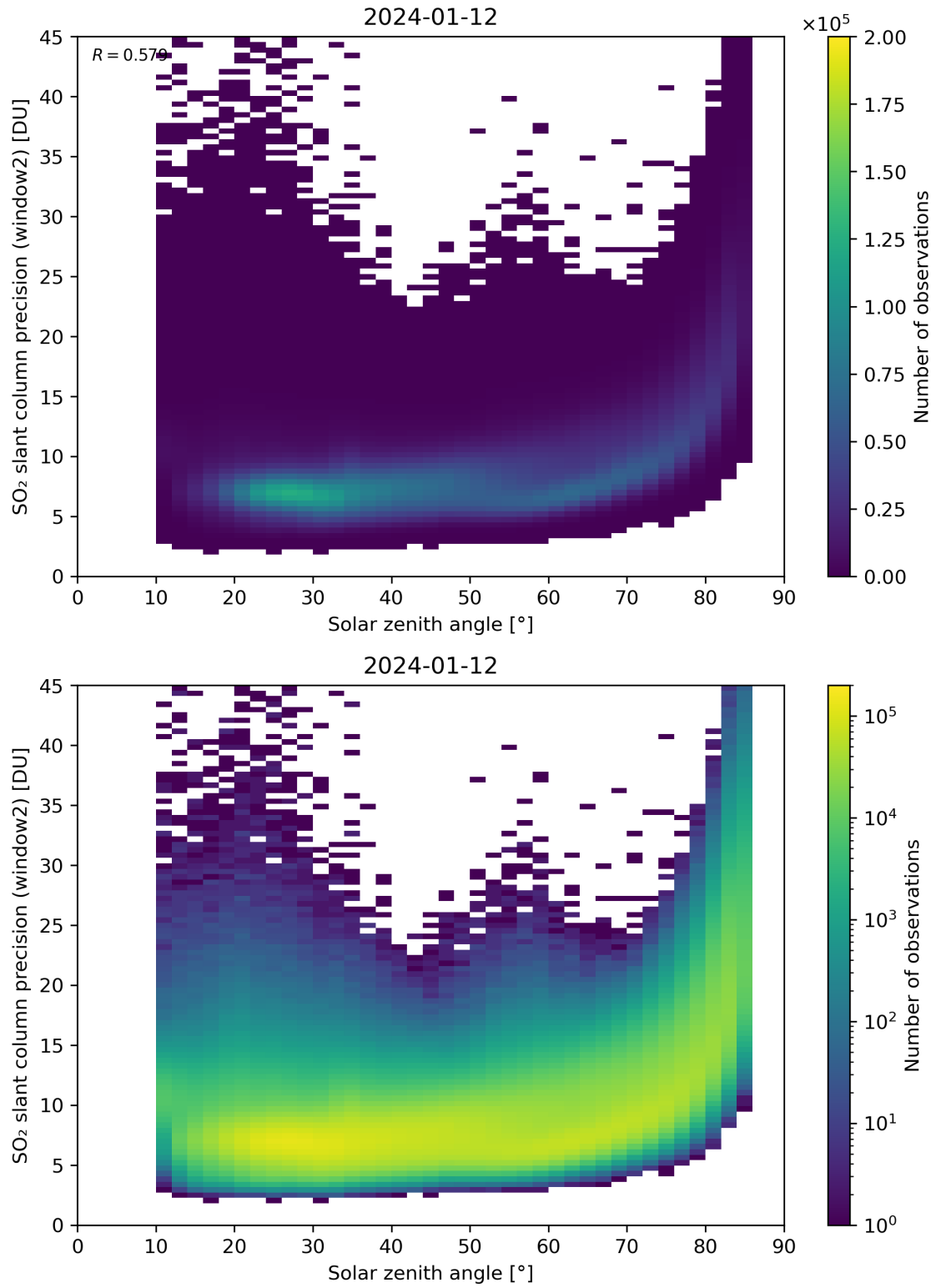
Figure 171: Scatter density plot of “Solar zenith angle” against “SO 2 slant column precision (window2)” for 2024-01-11 to 2024-01-13.
