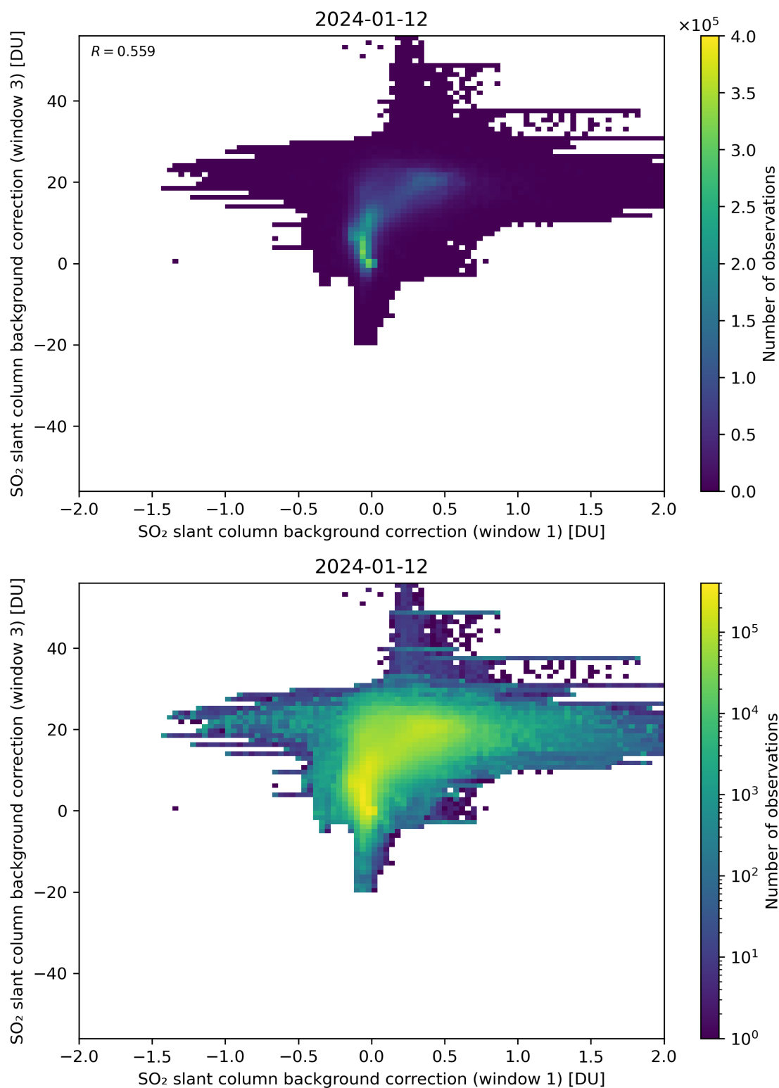
Figure 99: Scatter density plot of “SO 2 slant column background correction (window 1)” against “SO 2 slant column background correction (window 3)” for 2024-01-11 to 2024-01-13.
