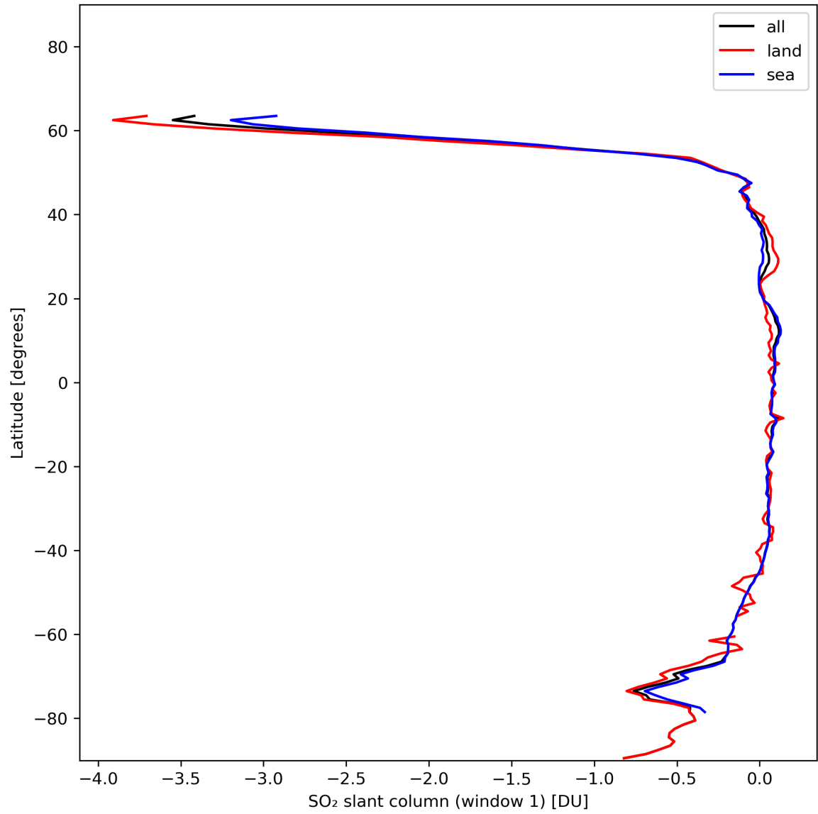
Figure 33: Zonal average of “SO 2 slant column (window 1)” for 2024-01-11 to 2024-01-13.
