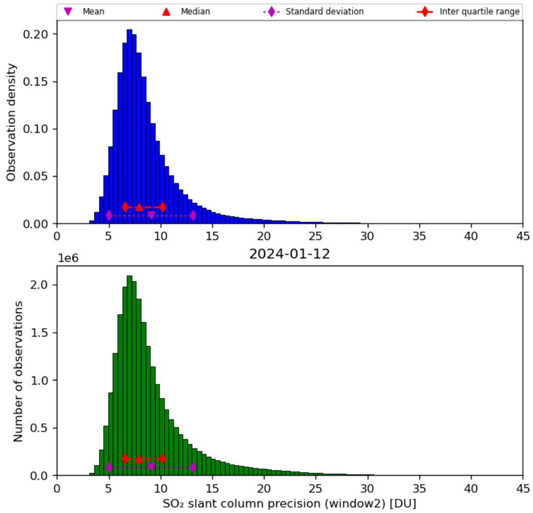
Figure 61: Histogram of “SO 2 slant column precision (window2)” for 2024-01-11 to 2024-01-13
