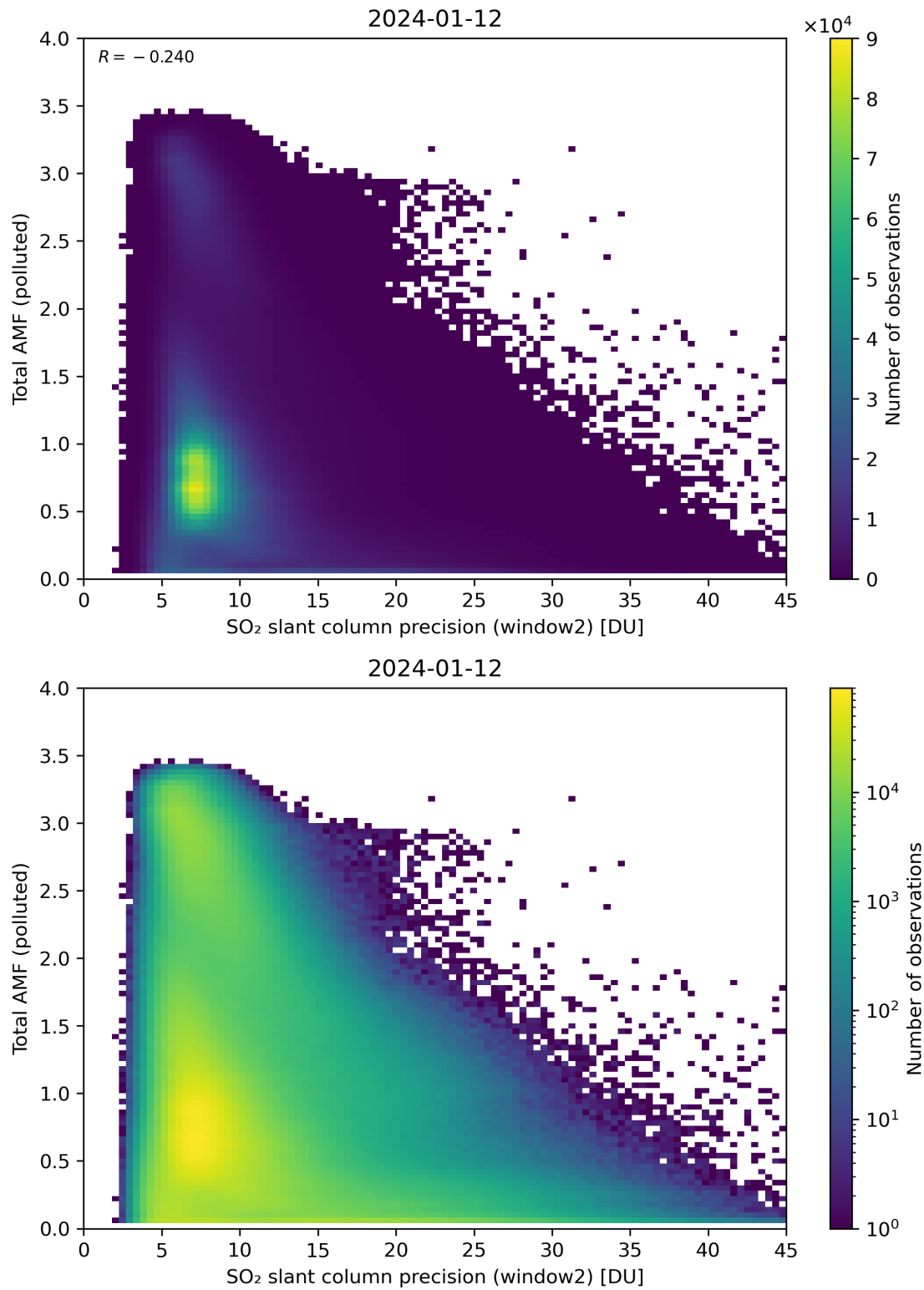
Figure 251: Scatter density plot of “SO 2 slant column precision (window2)” against “Total AMF (polluted)” for 2024-01-11 to 2024-01-13.
