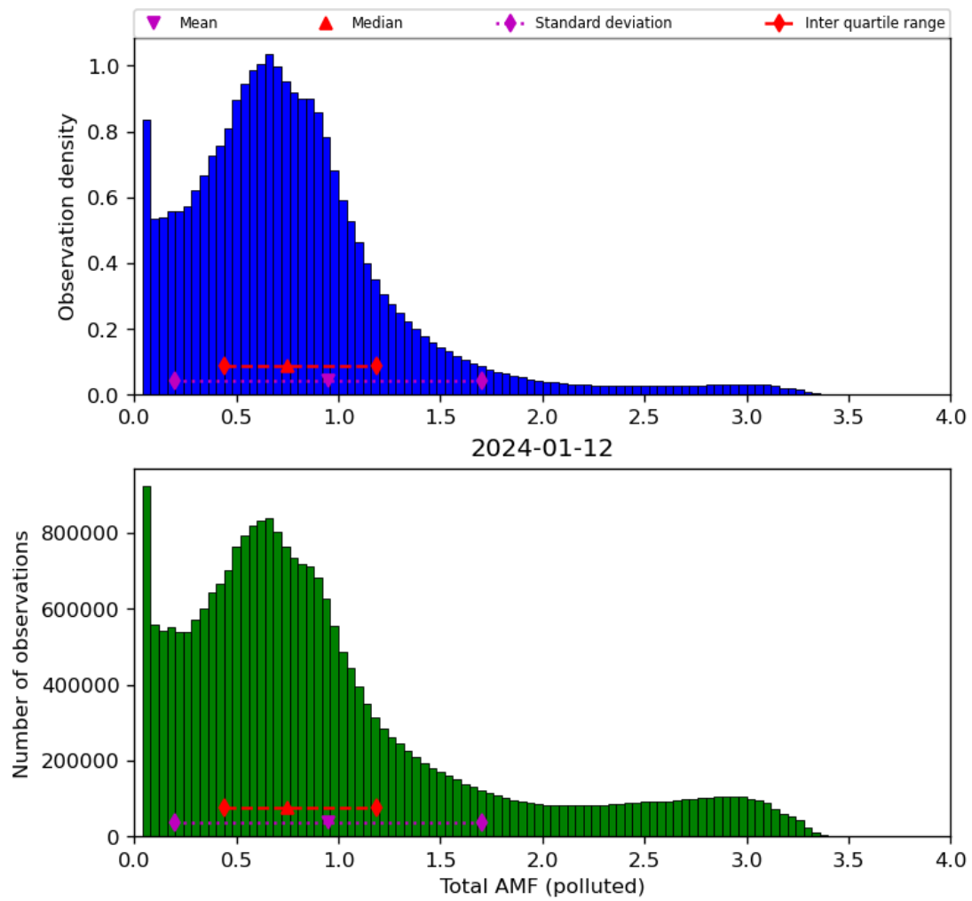
Figure 71: Histogram of “Total AMF (polluted)” for 2024-01-11 to 2024-01-13
