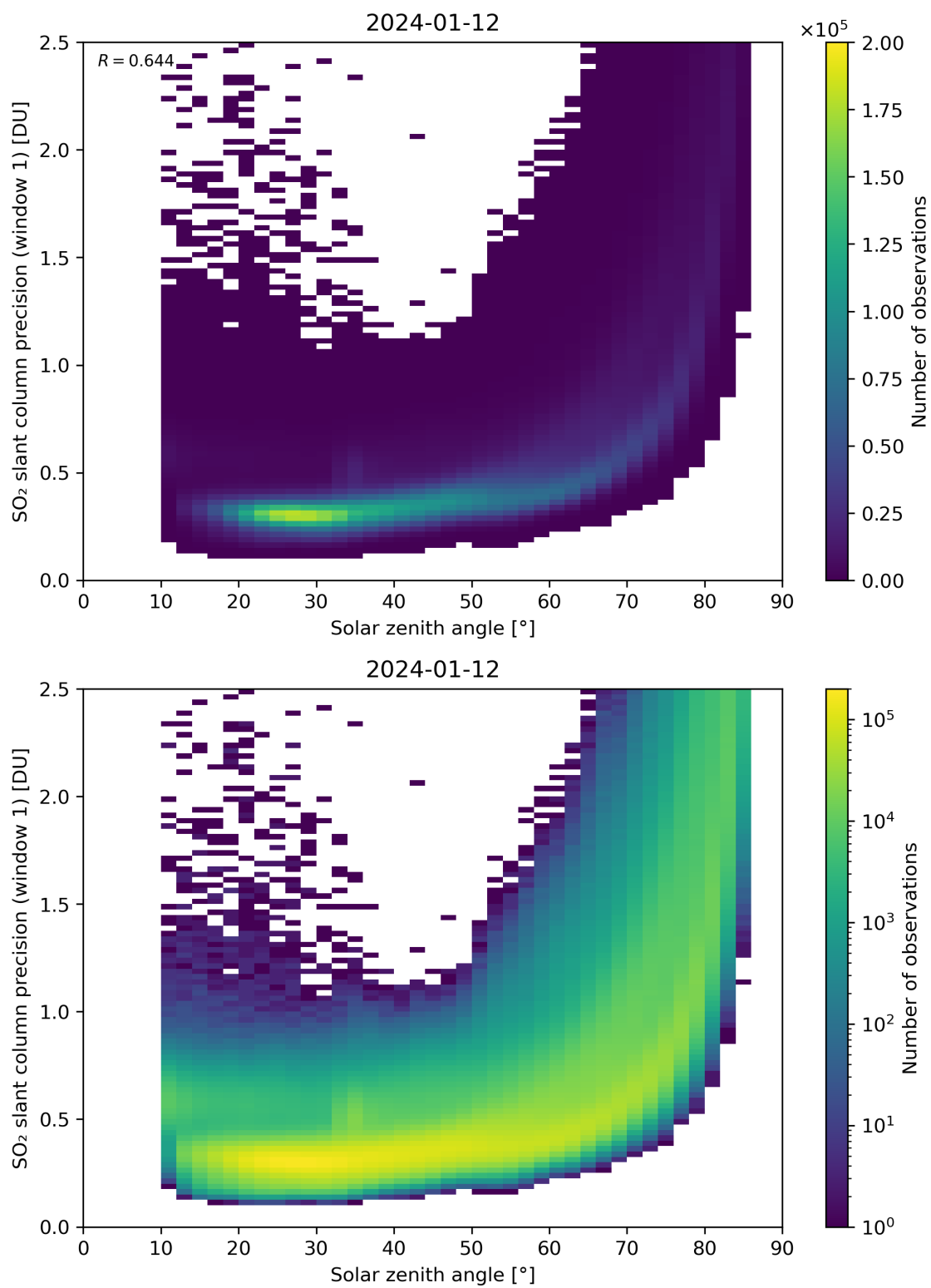
Figure 170: Scatter density plot of “Solar zenith angle” against “SO 2 slant column precision (window 1)” for 2024-01-11 to 2024-01-13.
