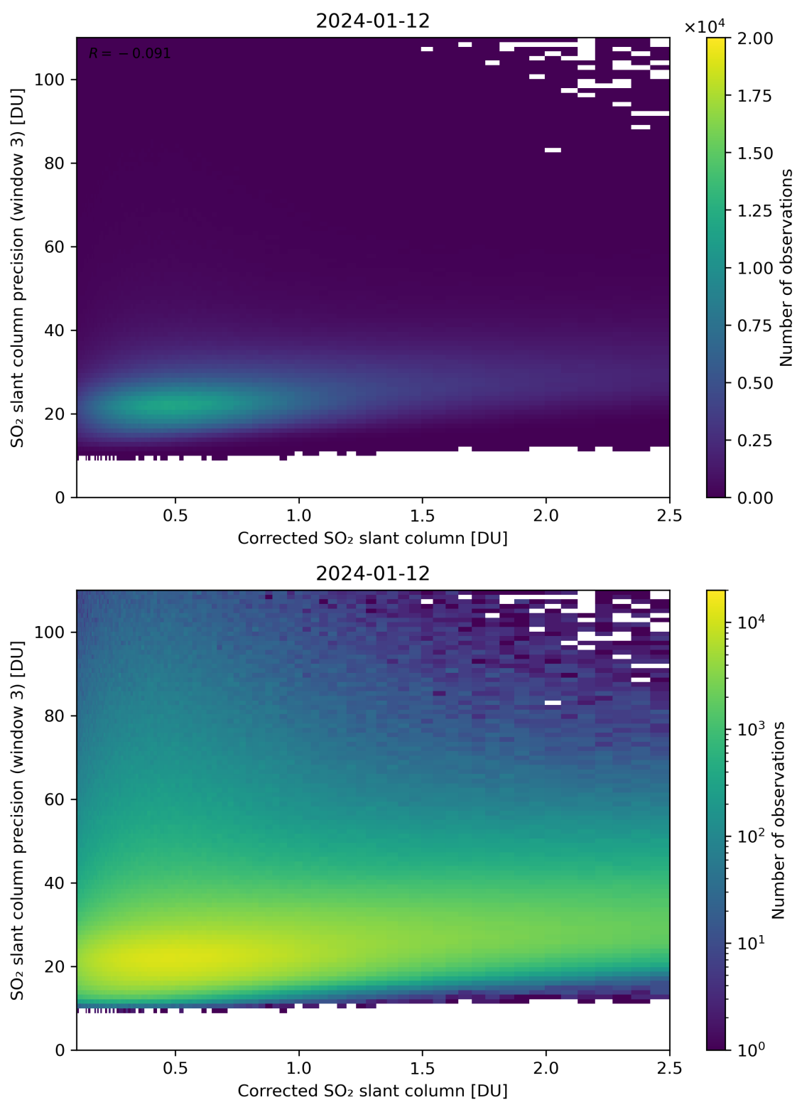
Figure 191: Scatter density plot of “Corrected SO 2 slant column” against “SO 2 slant column precision (window 3)” for 2024-01-11 to 2024-01-13.
