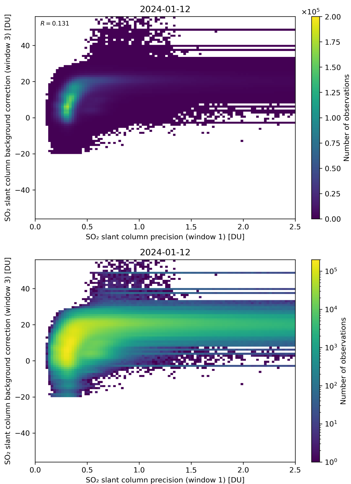
Figure 220: Scatter density plot of “SO 2 slant column precision (window 1)” against “SO 2 slant column background correction (window 3)” for 2024-01-11 to 2024-01-13.
