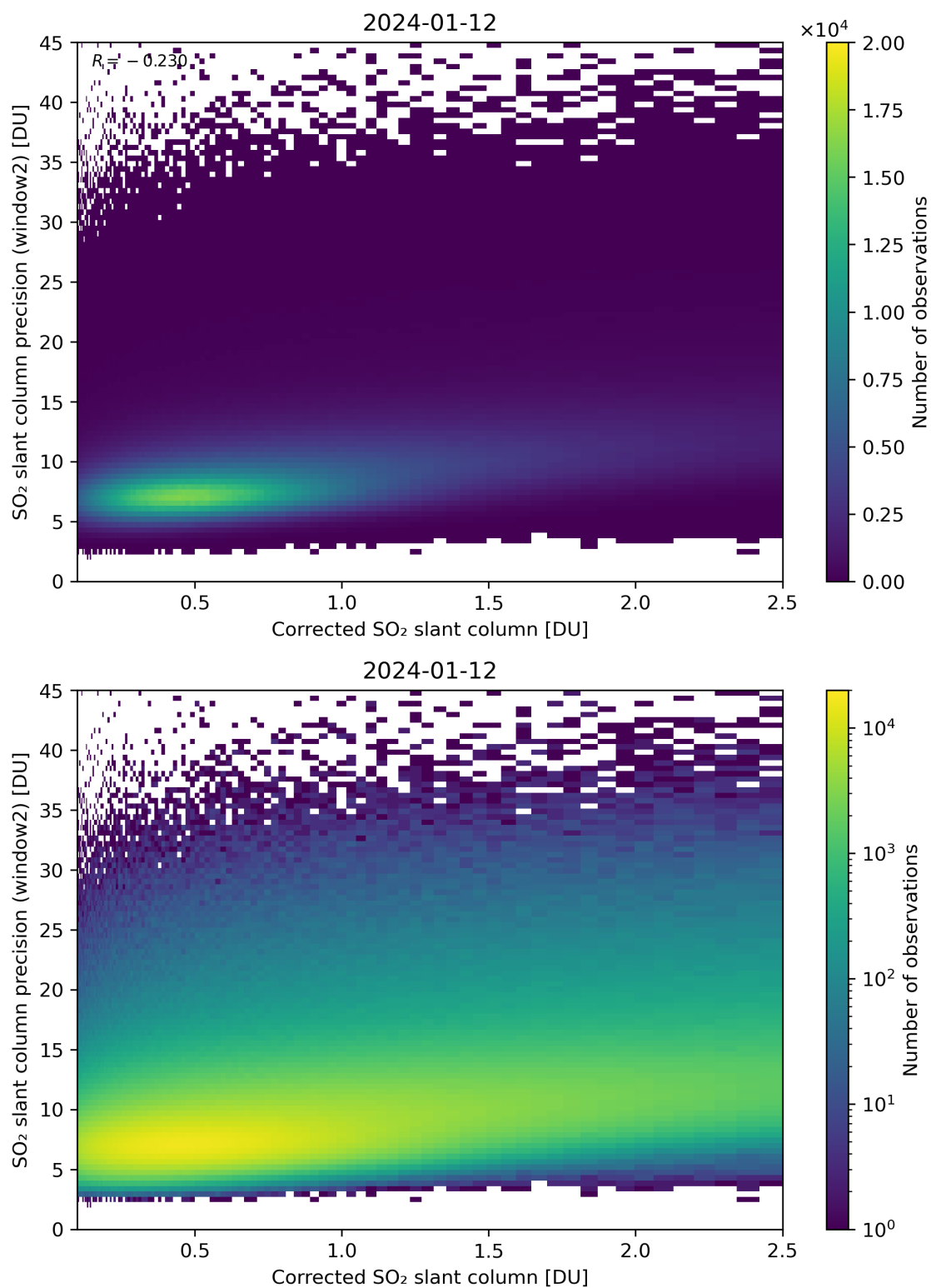
Figure 189: Scatter density plot of “Corrected SO 2 slant column” against “SO 2 slant column precision (window2)” for 2024-01-11 to 2024-01-13.
