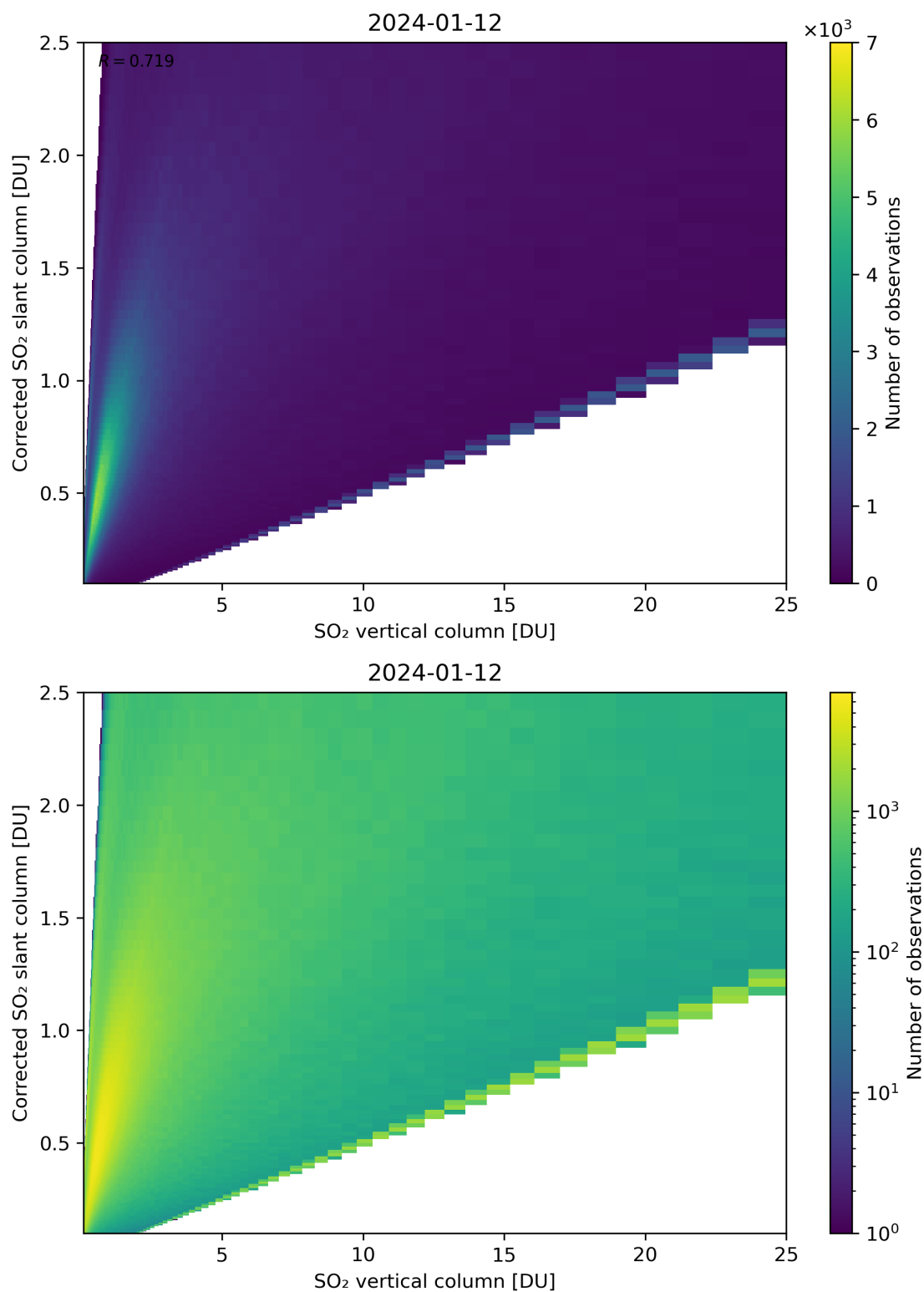
Figure 297: Scatter density plot of “SO 2 vertical column” against “Corrected SO 2 slant column” for 2024-01-11 to 2024-01-13.
