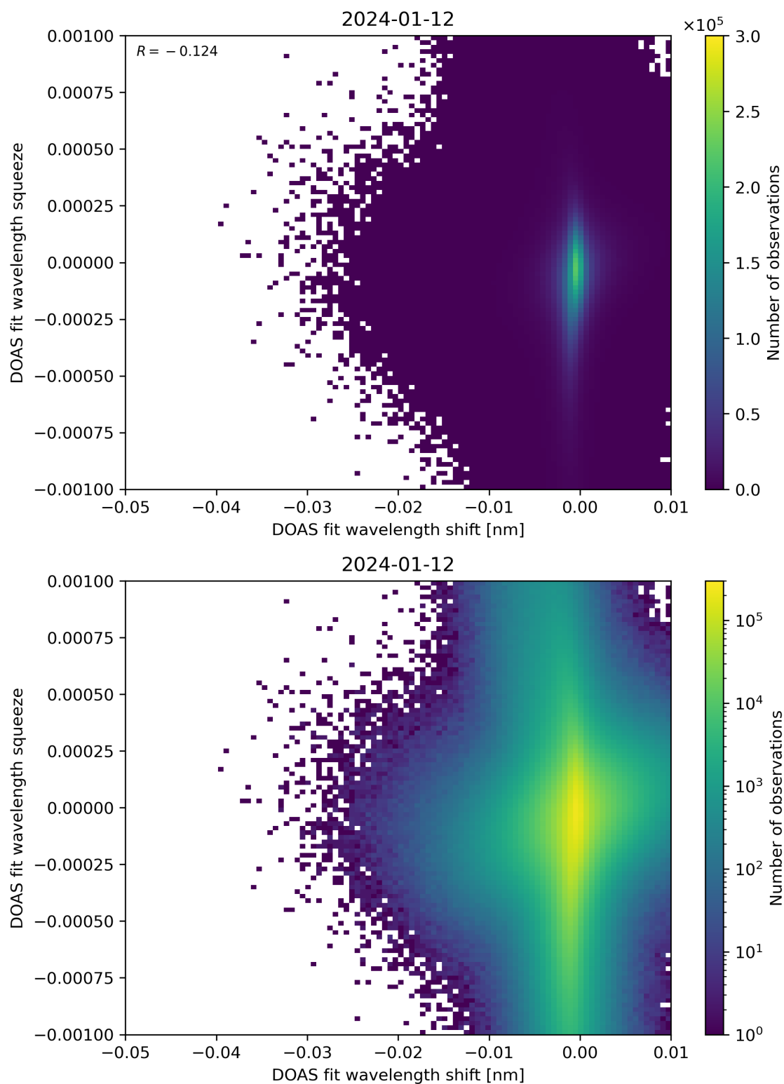
Figure 127: Scatter density plot of “DOAS fit wavelength shift” against “DOAS fit wavelength squeeze” for 2024-01-11 to 2024-01-13.
