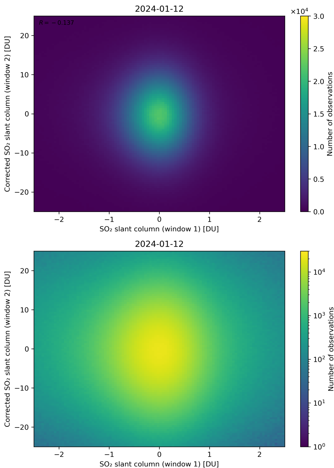
Figure 233: Scatter density plot of “SO 2 slant column (window 1)” against “Corrected SO 2 slant column (window 2)” for 2024-01-11 to 2024-01-13.
