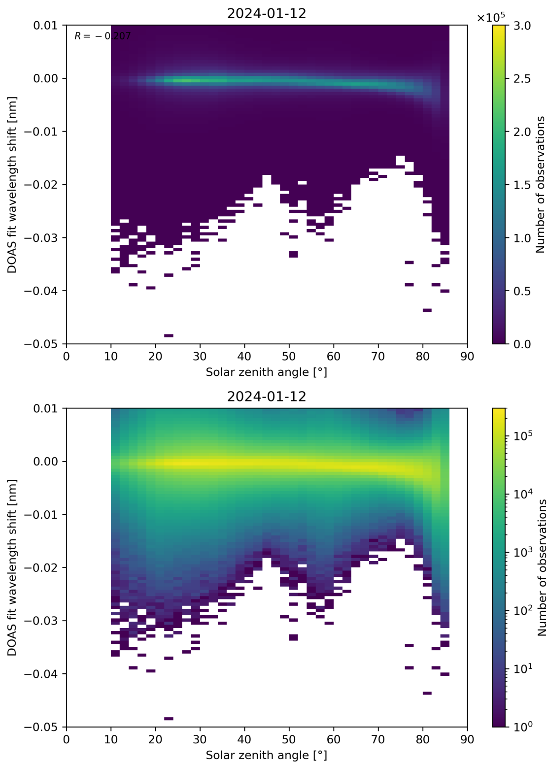
Figure 161: Scatter density plot of “Solar zenith angle” against “DOAS fit wavelength shift” for 2024-01-11 to 2024-01-13.
