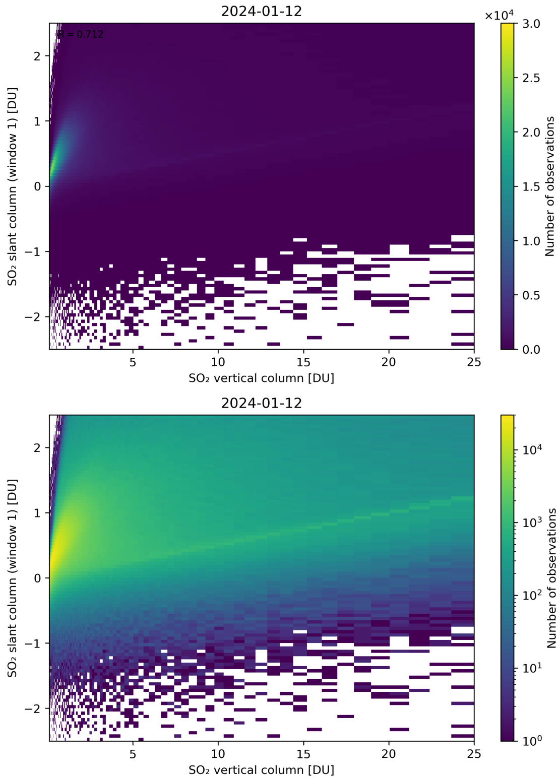
Figure 300: Scatter density plot of “SO 2 vertical column” against “SO 2 slant column (window 1)” for 2024-01-11 to 2024-01-13.
