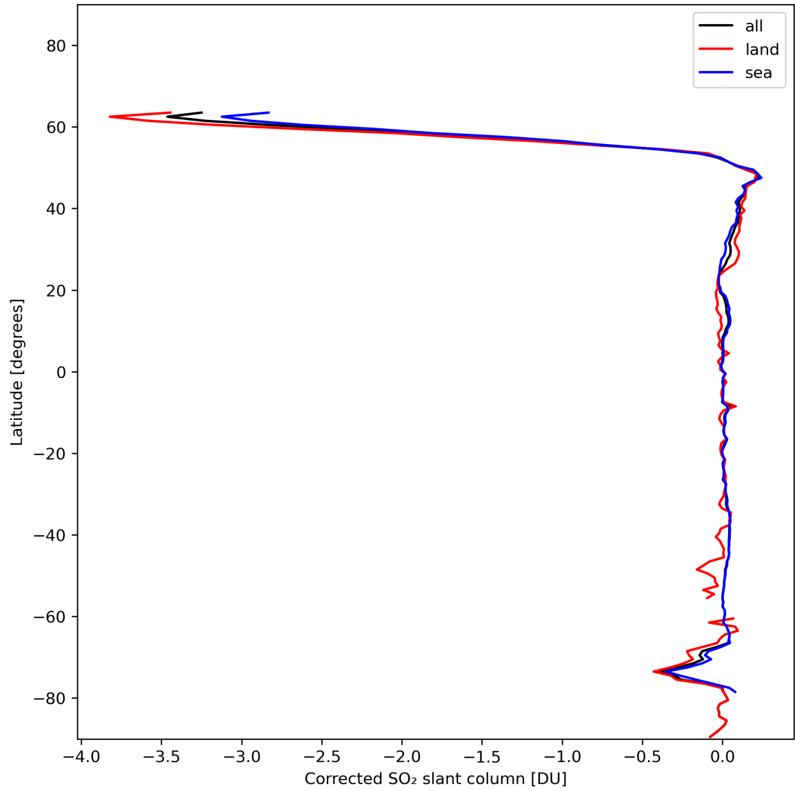
Figure 32: Zonal average of "Corrected SO 2 slant column" for 2024-01-11 to 2024-01-13.
