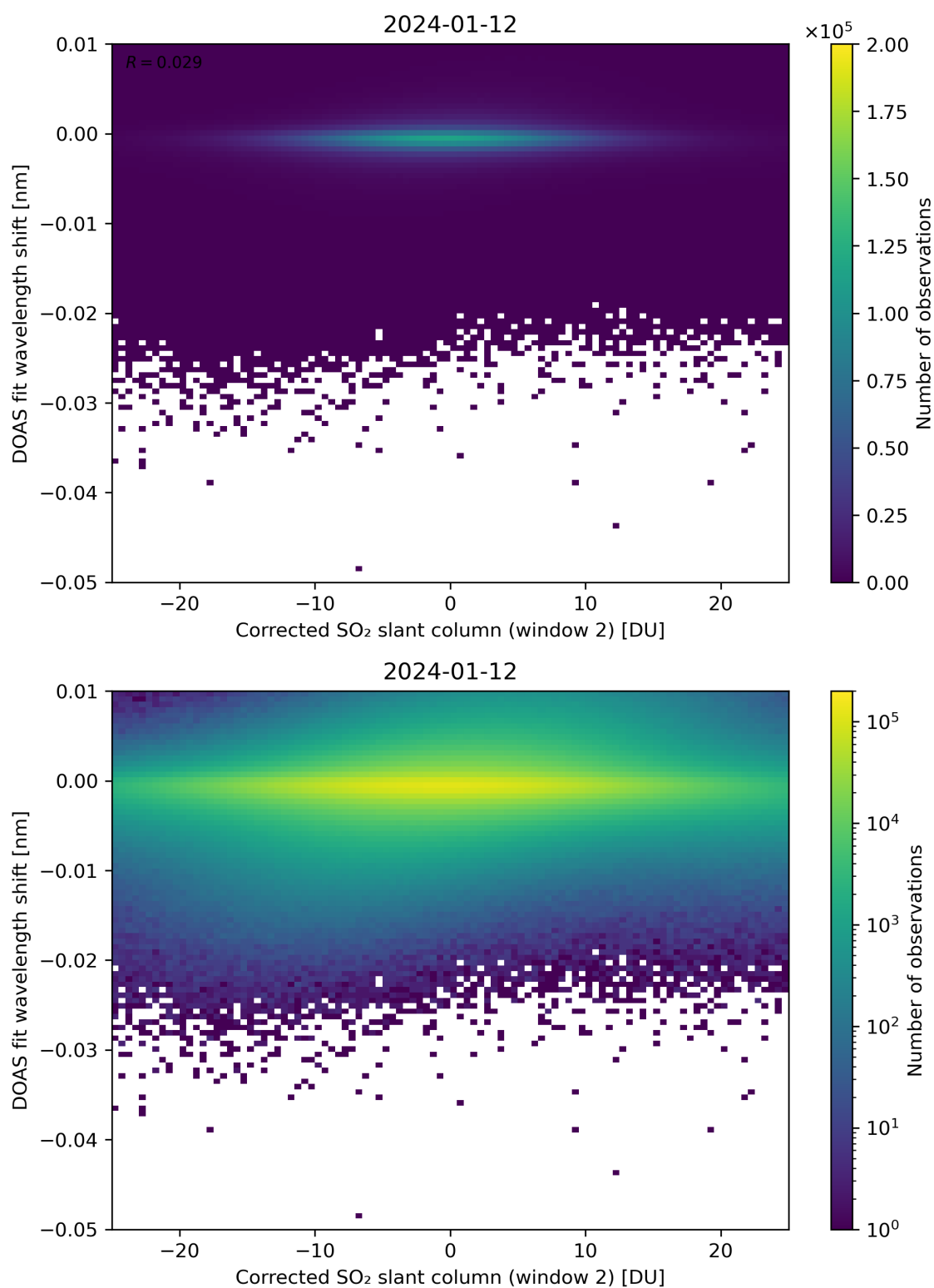
Figure 196: Scatter density plot of “Corrected SO 2 slant column (window 2)” against “DOAS fit wavelength shift” for 2024-01-11 to 2024-01-13.
