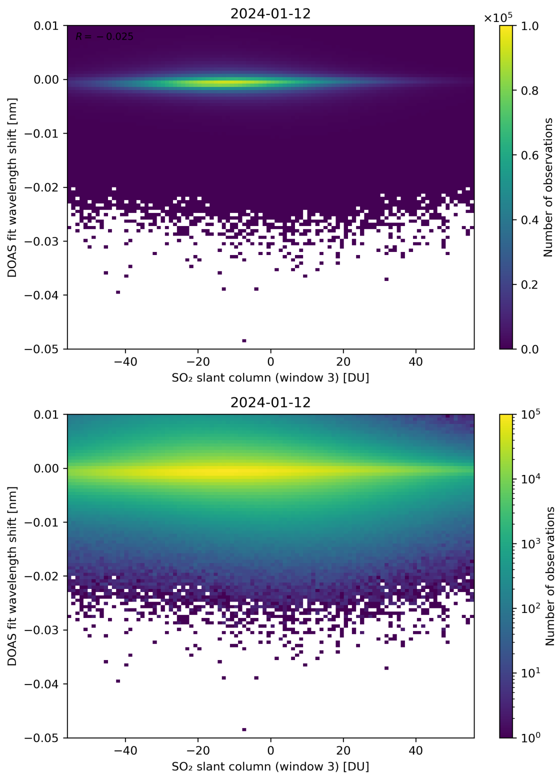
Figure 254: Scatter density plot of “SO 2 slant column (window 3)” against “DOAS fit wavelength shift” for 2024-01-11 to 2024-01-13.
