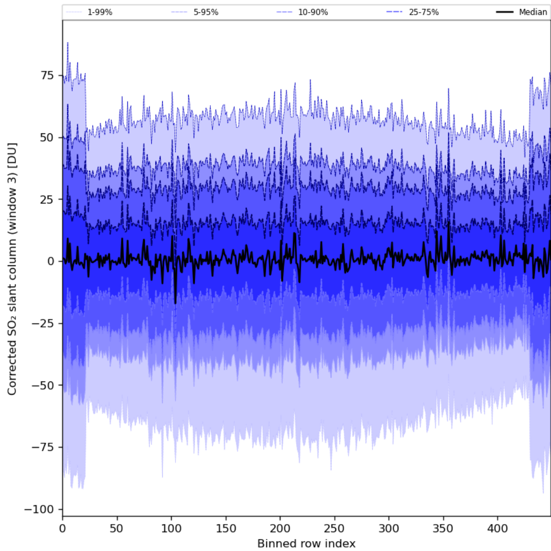
Figure 89: Along track statistics of “Corrected SO 2 slant column (window 3)” for 2024-01-11 to 2024-01-13
