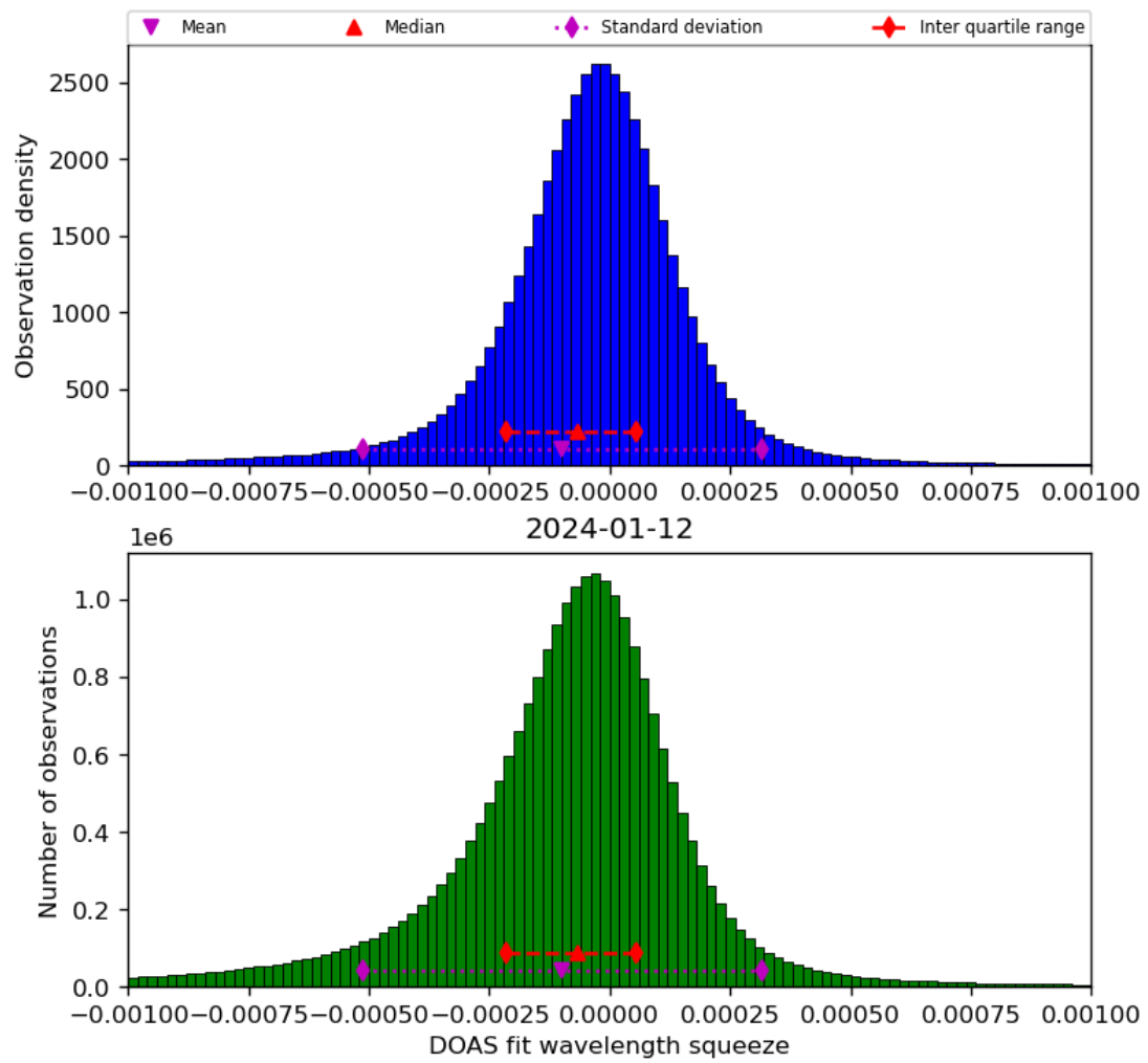
Figure 69: Histogram of “DOAS fit wavelength squeeze” for 2024-01-11 to 2024-01-13
