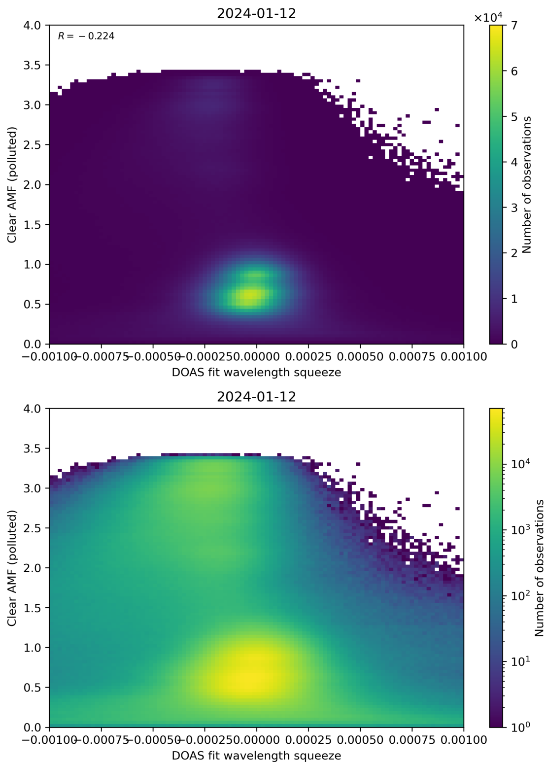
Figure 133: Scatter density plot of “DOAS fit wavelength squeeze” against “Clear AMF (polluted)” for 2024-01-11 to 2024-01-13.
