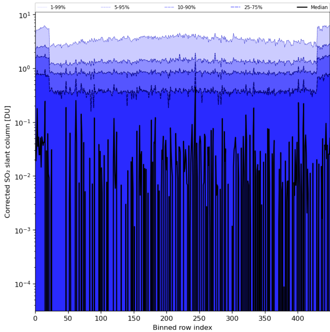
Figure 78: Along track statistics of “Corrected SO 2 slant column” for 2024-01-11 to 2024-01-13
