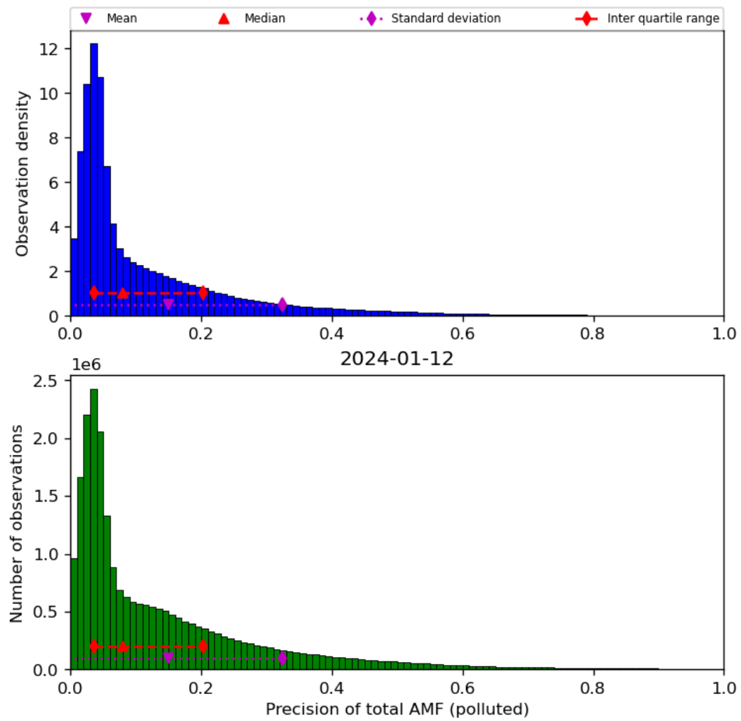
Figure 72: Histogram of “Precision of total AMF (polluted)” for 2024-01-11 to 2024-01-13
