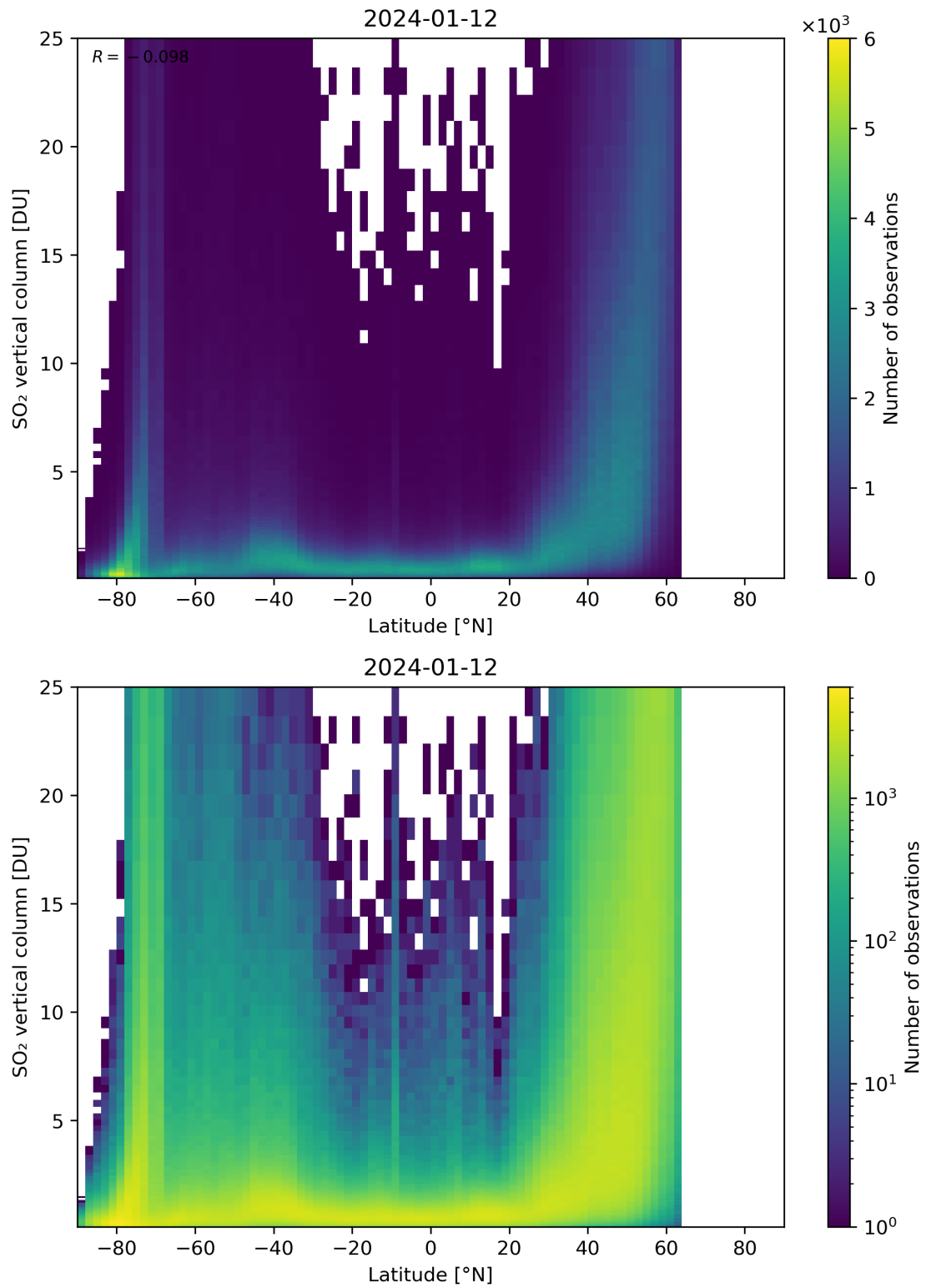
Figure 156: Scatter density plot of “Latitude” against “SO 2 vertical column” for 2024-01-11 to 2024-01-13.
