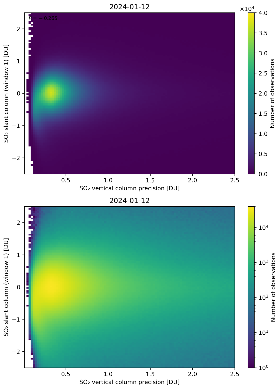
Figure 289: Scatter density plot of “SO 2 vertical column precision” against “SO 2 slant column (window 1)” for 2024-01-11 to 2024-01-13.
