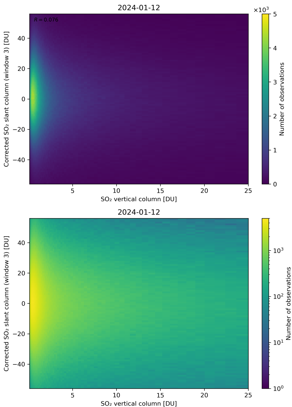
Figure 299: Scatter density plot of “SO 2 vertical column” against “Corrected SO 2 slant column (window 3)” for 2024-01-11 to 2024-01-13.
