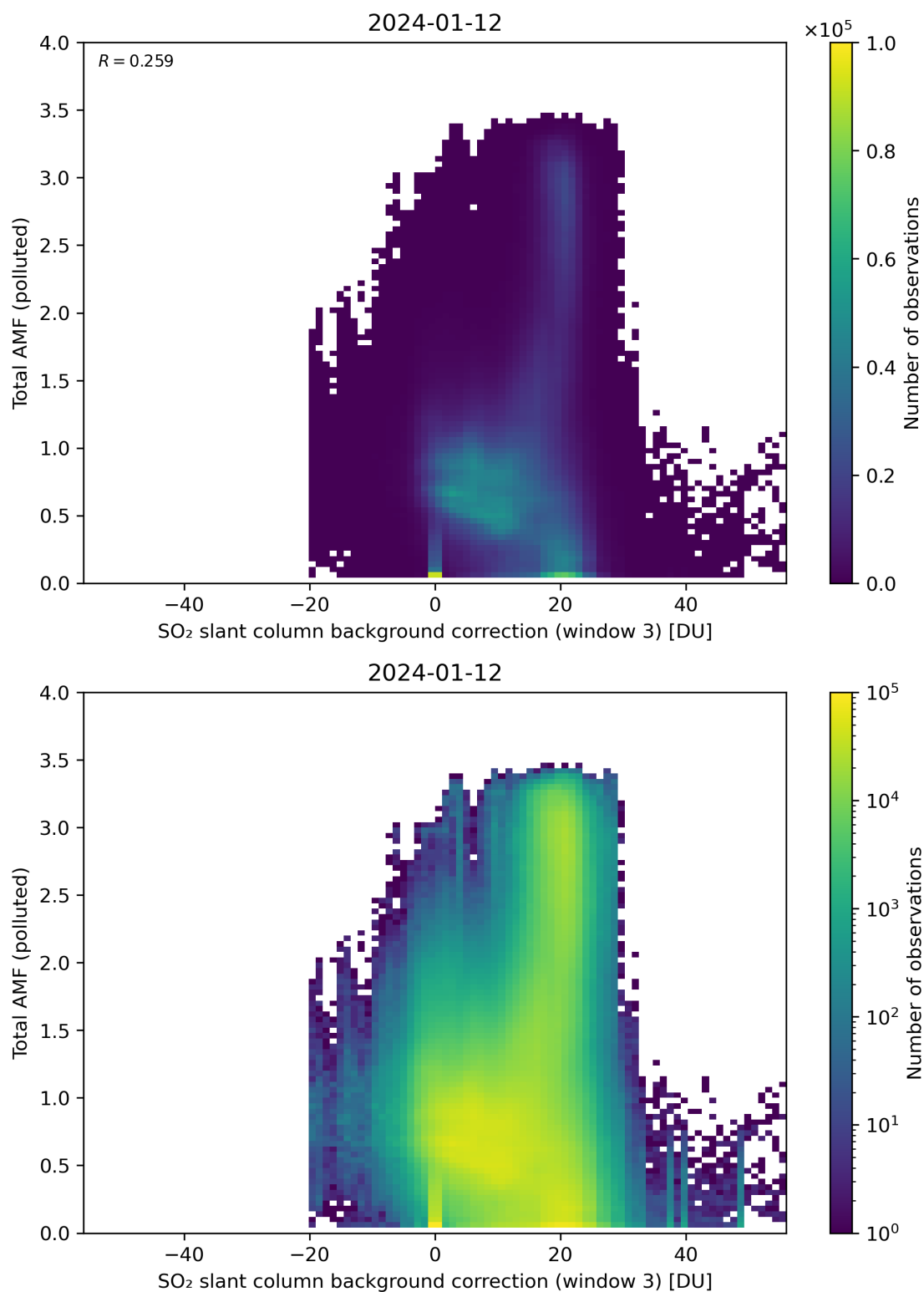
Figure 125: Scatter density plot of “SO 2 slant column background correction (window 3)” against “Total AMF (polluted)” for 2024-01-11 to 2024-01-13.
