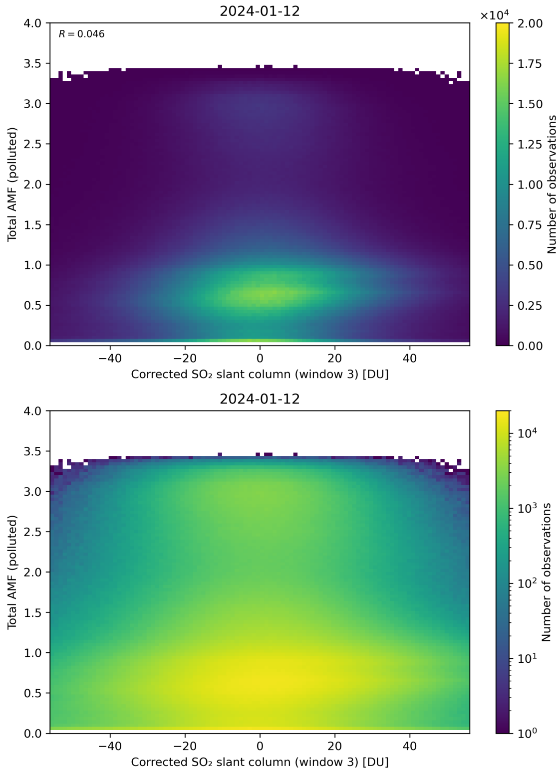
Figure 210: Scatter density plot of “Corrected SO 2 slant column (window 3)” against “Total AMF (polluted)” for 2024-01-11 to 2024-01-13.
