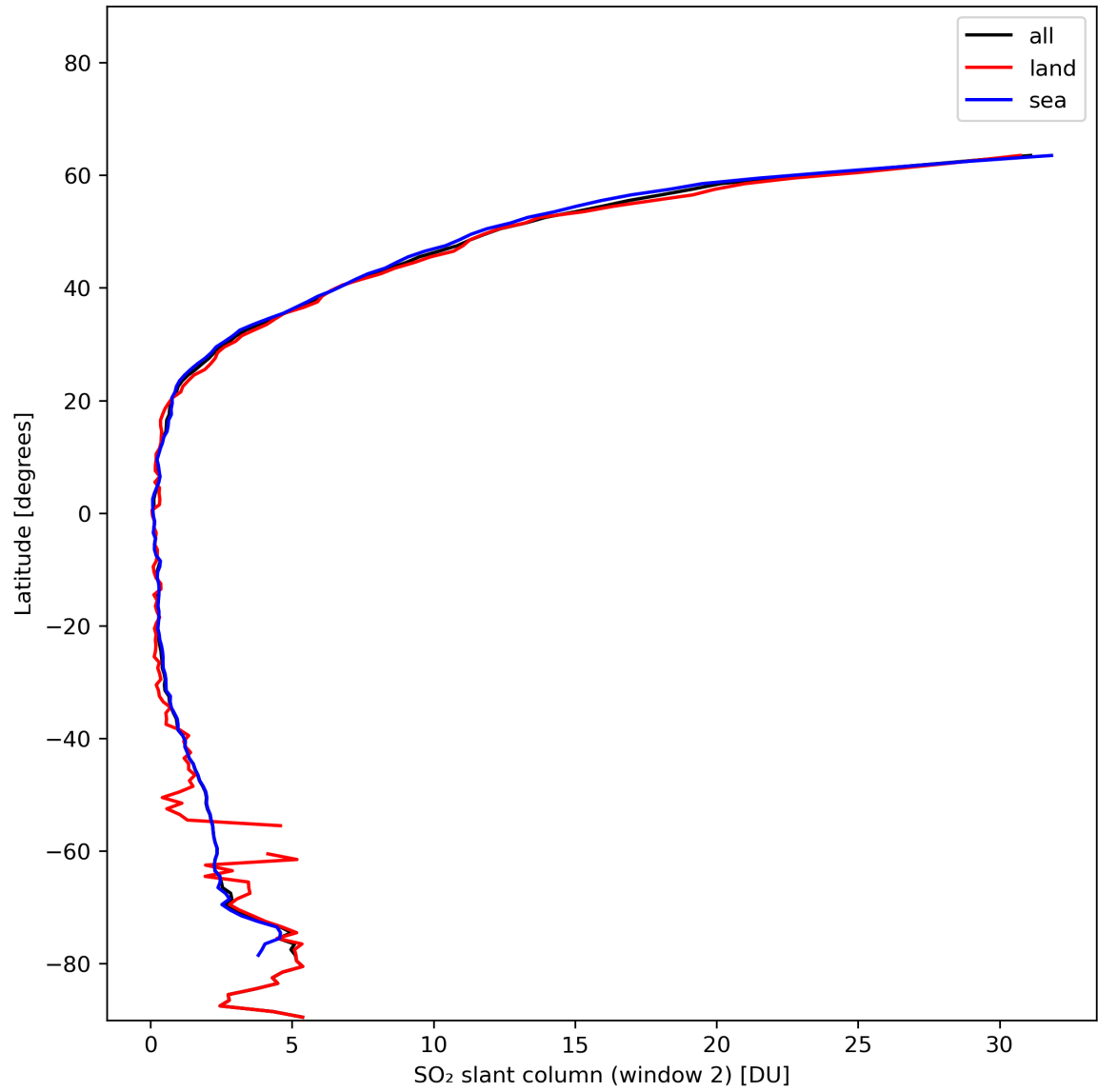
Figure 37: Zonal average of “SO 2 slant column (window 2)” for 2024-01-11 to 2024-01-13.
