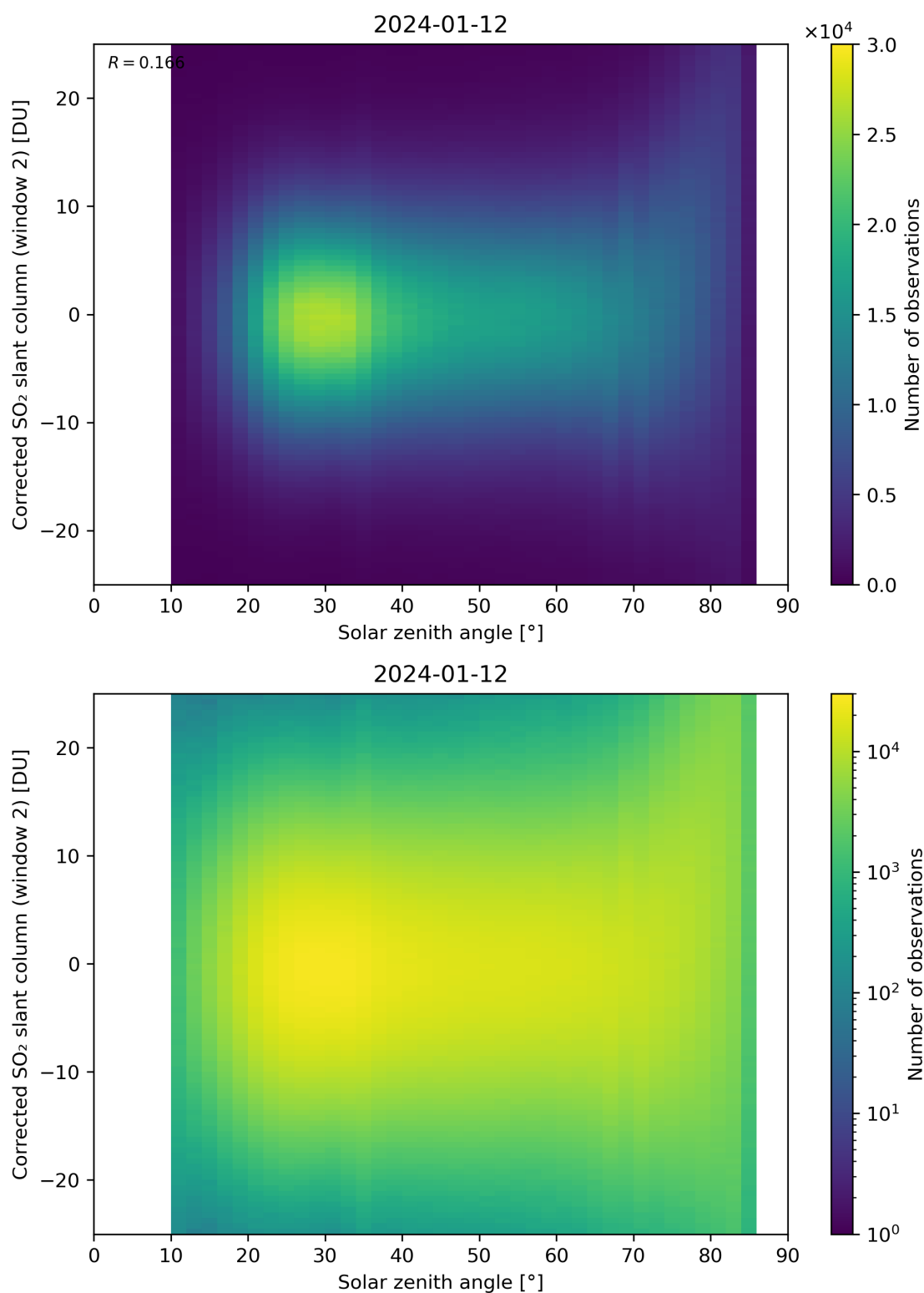
Figure 167: Scatter density plot of “Solar zenith angle” against “Corrected SO 2 slant column (window 2)” for 2024-01-11 to 2024-01-13.
