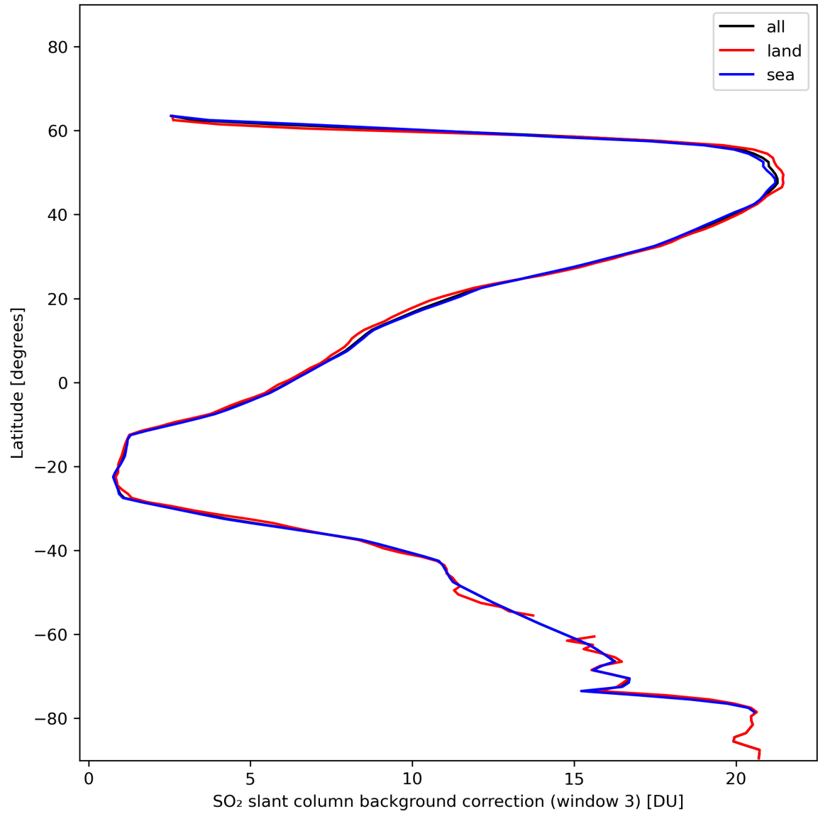
Figure 44: Zonal average of “SO 2 slant column background correction (window 3)” for 2024-01-11 to 2024-01-13.
