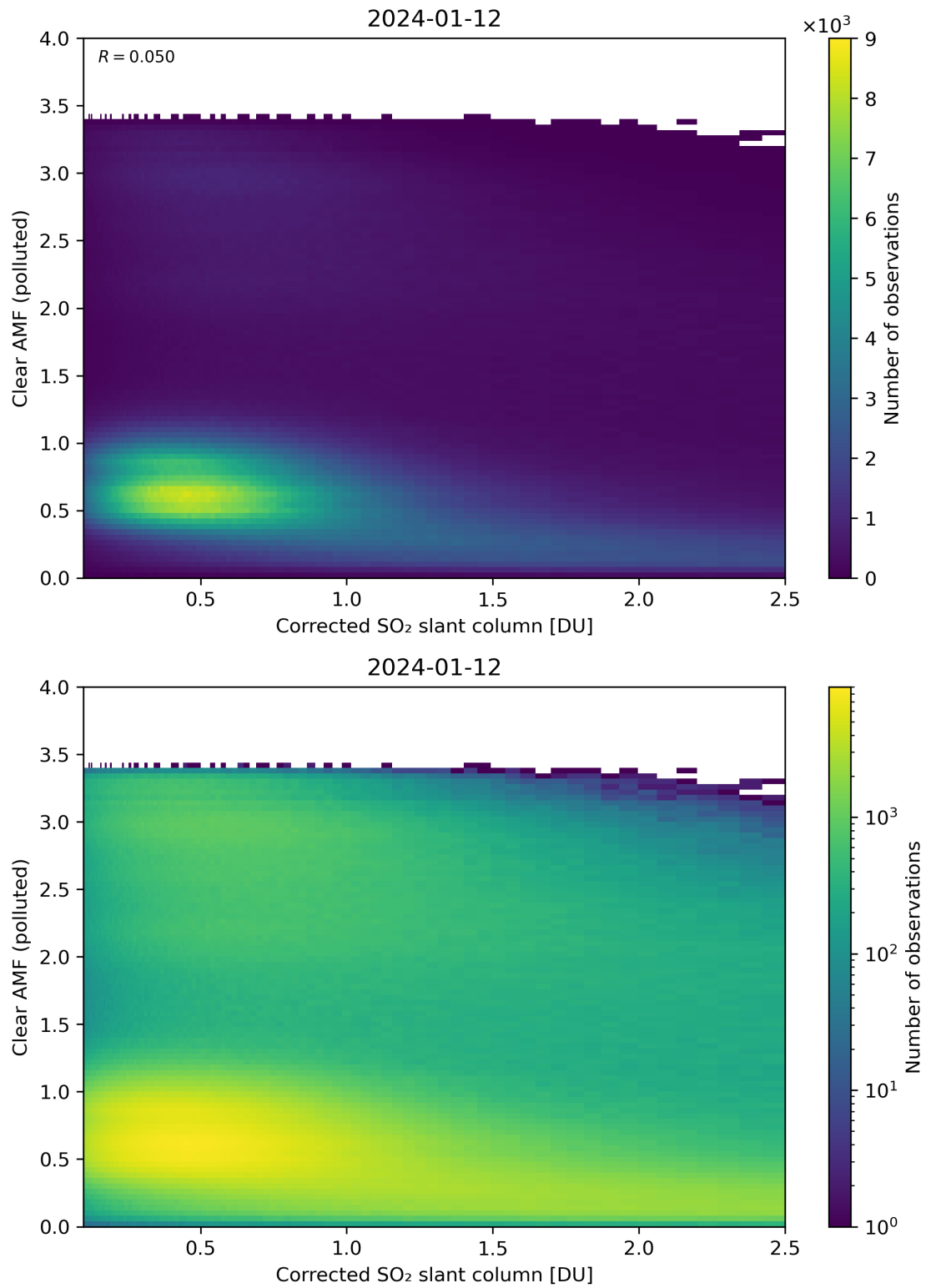
Figure 184: Scatter density plot of “Corrected SO 2 slant column” against “Clear AMF (polluted)” for 2024-01-11 to 2024-01-13.
