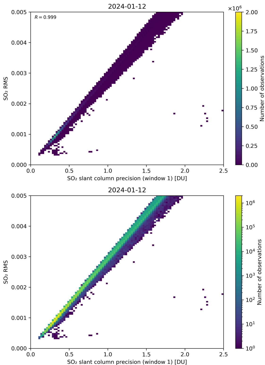
Figure 223: Scatter density plot of “SO 2 slant column precision (window 1)” against “SO 2 RMS” for 2024-01-11 to 2024-01-13.
