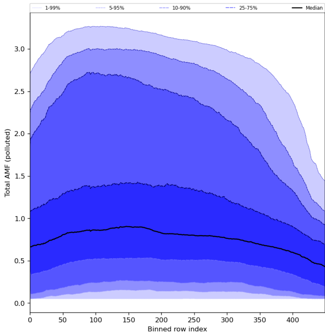
Figure 94: Along track statistics of “Total AMF (polluted)” for 2024-01-11 to 2024-01-13
