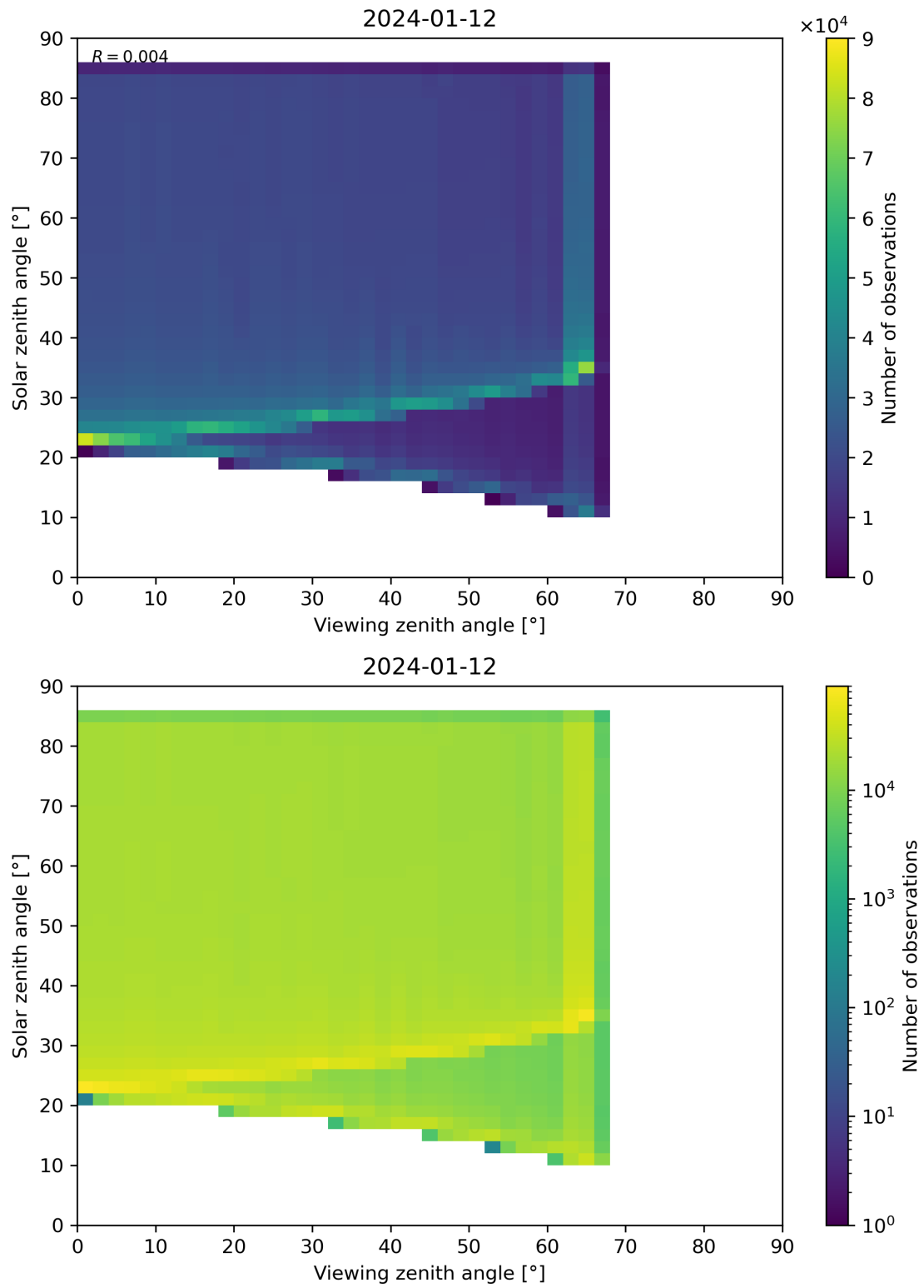
Figure 315: Scatter density plot of “Viewing zenith angle” against “Solar zenith angle” for 2024-01-11 to 2024-01-13.
