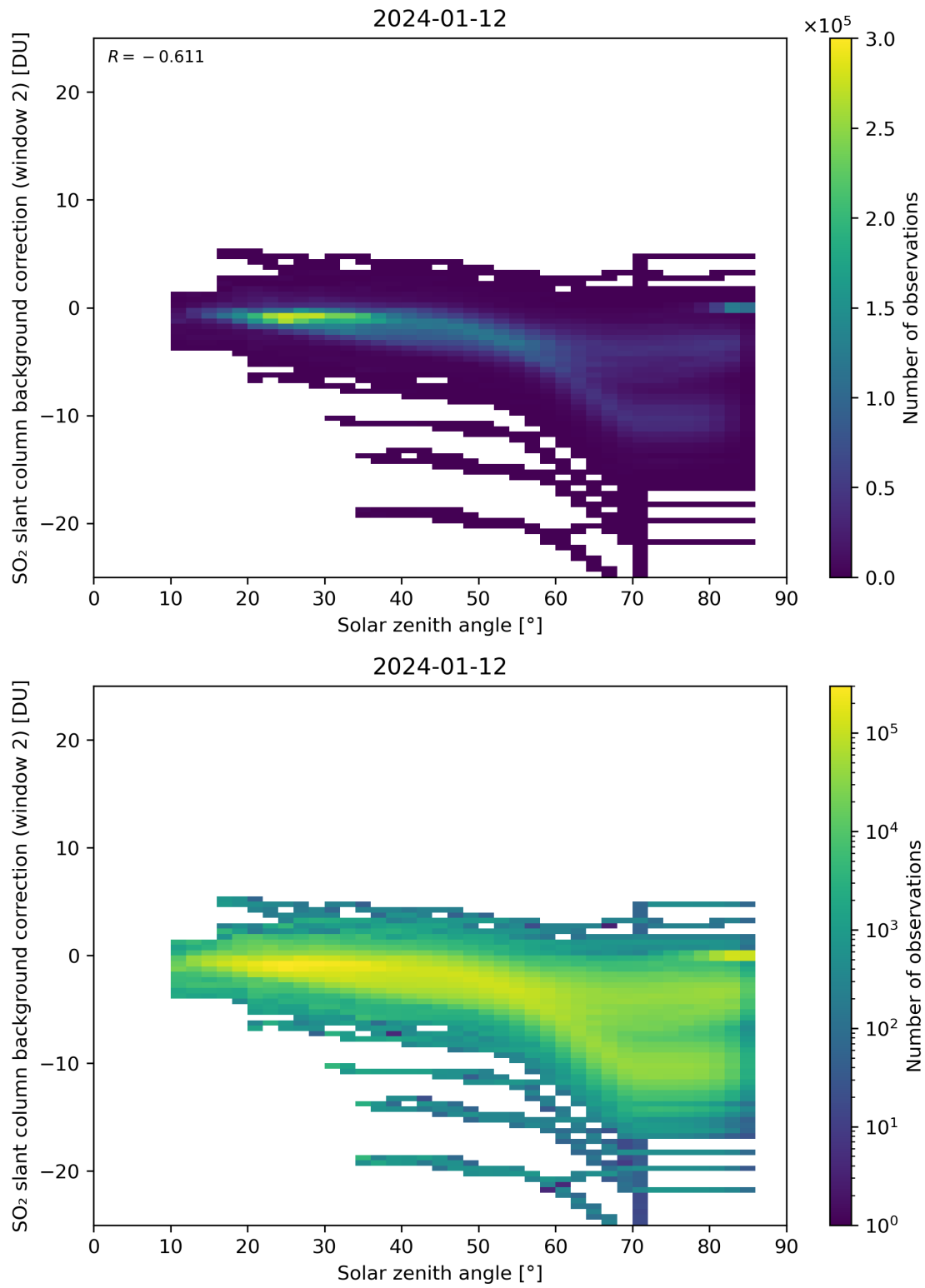
Figure 159: Scatter density plot of “Solar zenith angle” against “SO 2 slant column background correction (window 2)” for 2024-01-11 to 2024-01-13.
