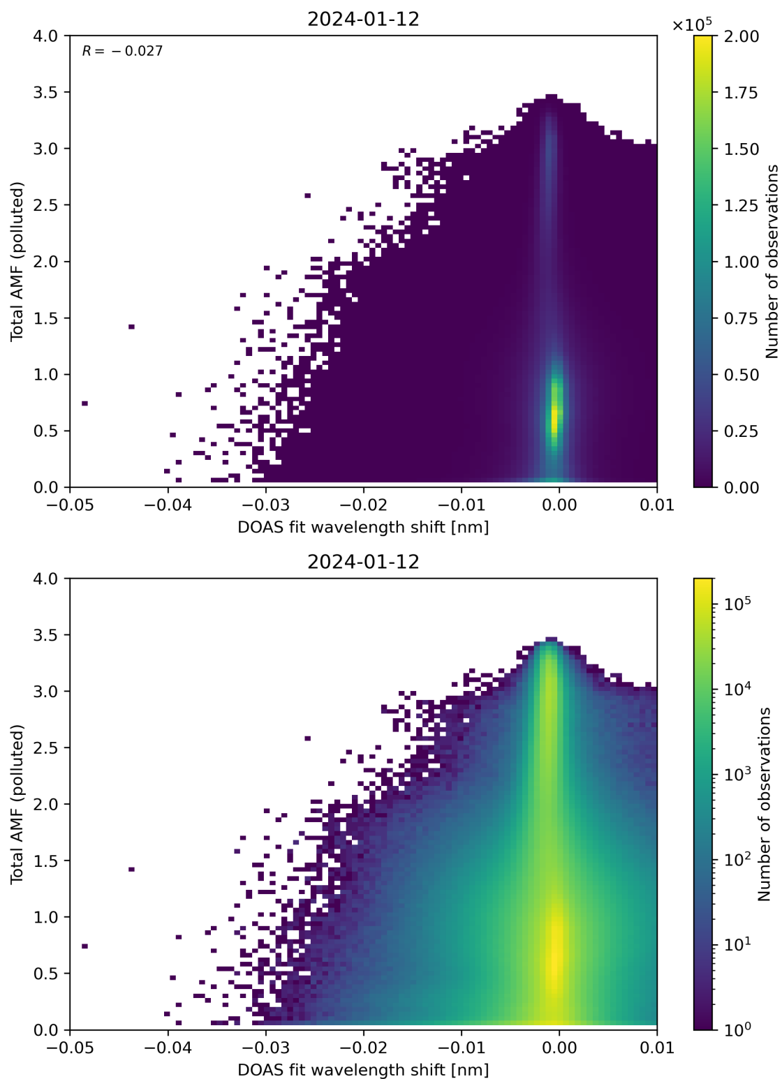
Figure 130: Scatter density plot of “DOAS fit wavelength shift” against “Total AMF (polluted)” for 2024-01-11 to 2024-01-13.
