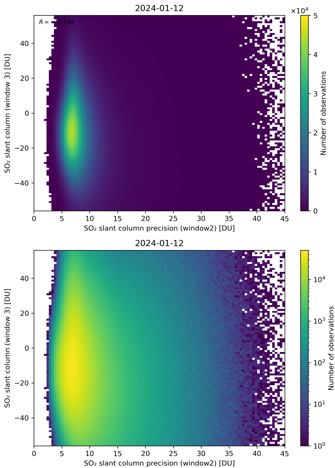
Figure 249: Scatter density plot of “SO 2 slant column precision (window2)” against “SO 2 slant column (window 3)” for 2024-01-11 to 2024-01-13.
