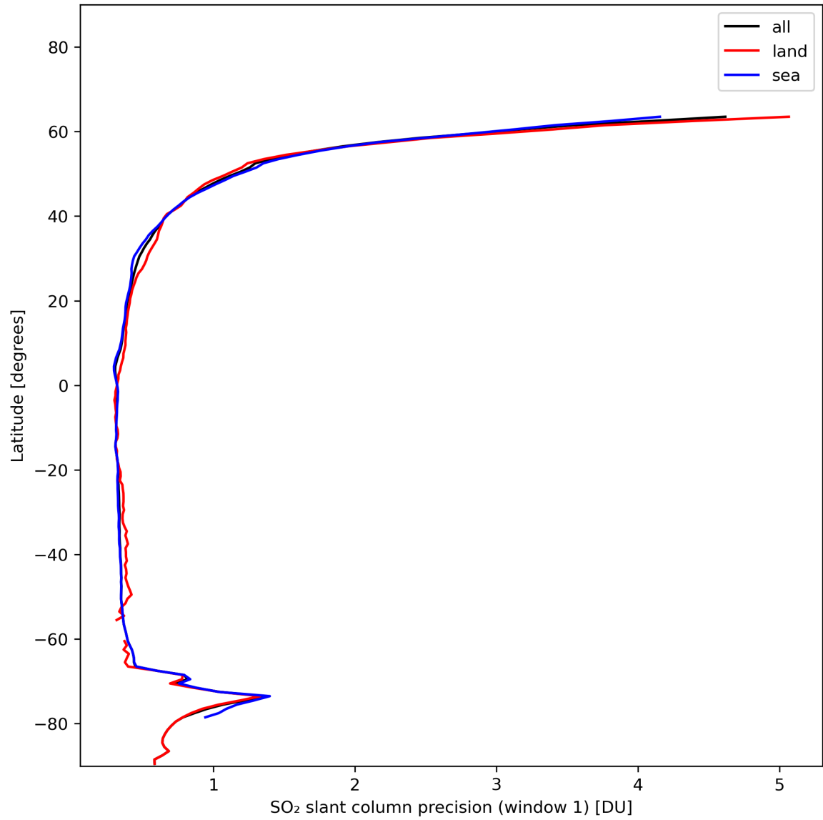
Figure 34: Zonal average of “SO 2 slant column precision (window 1)” for 2024-01-11 to 2024-01-13.
