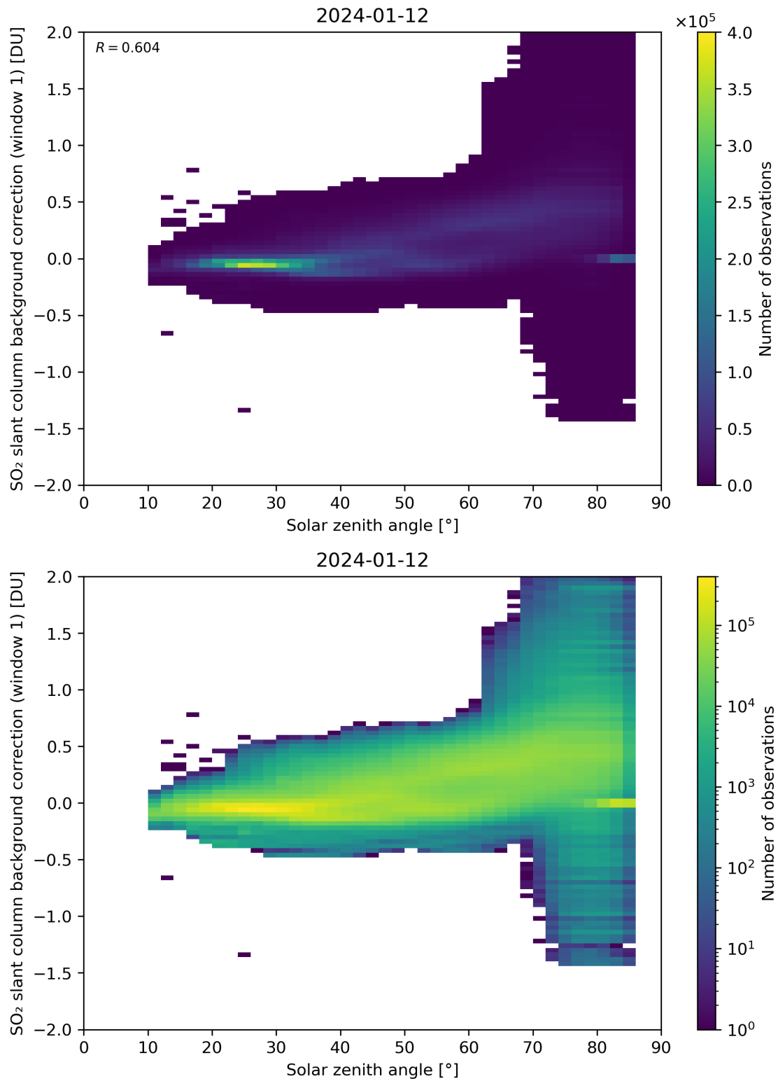
Figure 158: Scatter density plot of “Solar zenith angle” against “SO 2 slant column background correction (window 1)” for 2024-01-11 to 2024-01-13.
