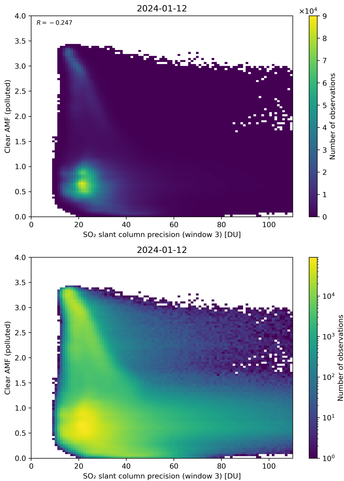
Figure 261: Scatter density plot of “SO 2 slant column precision (window 3)” against “Clear AMF (polluted)” for 2024-01-11 to 2024-01-13.
