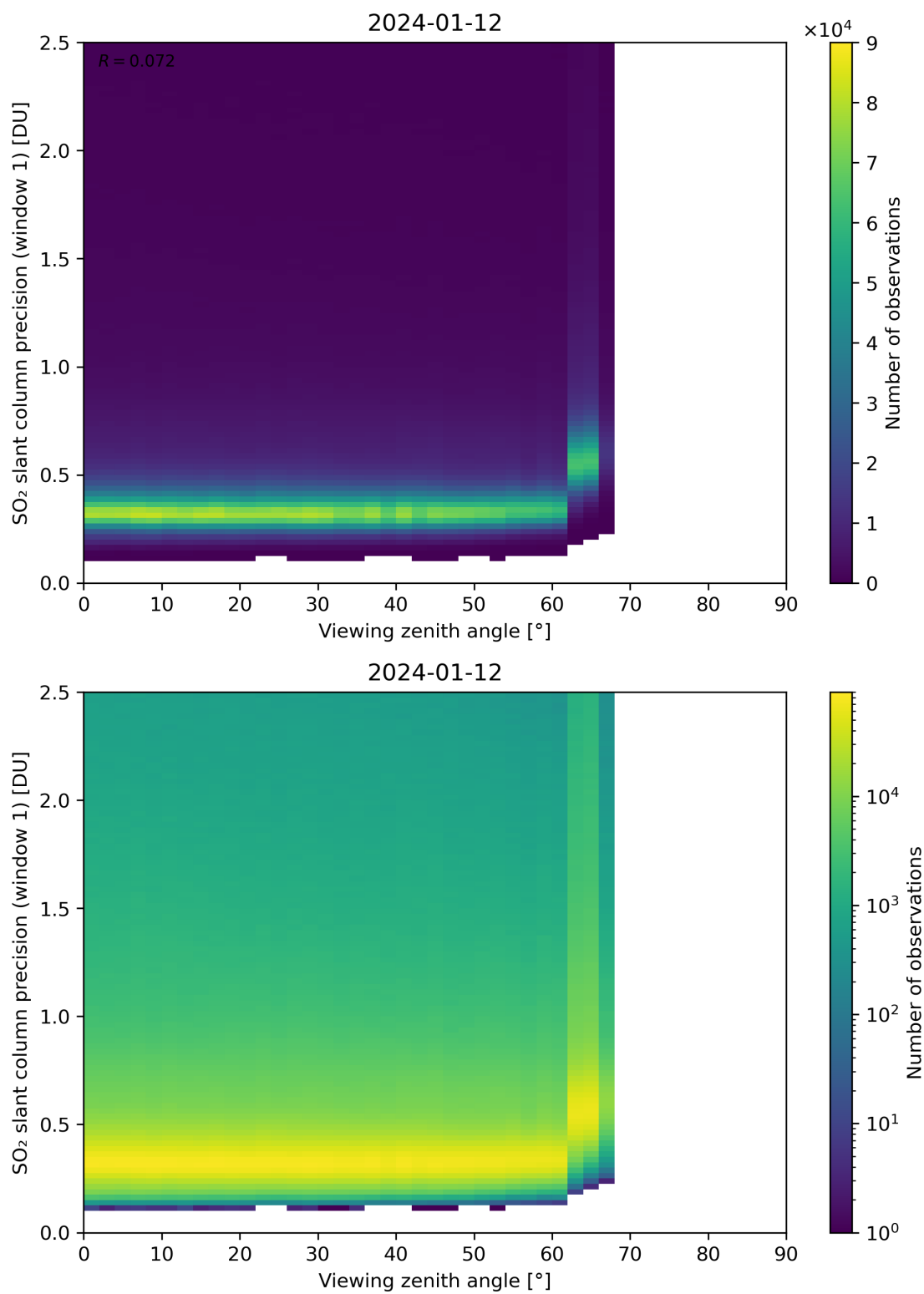
Figure 321: Scatter density plot of “Viewing zenith angle” against “SO 2 slant column precision (window 1)” for 2024-01-11 to 2024-01-13.
