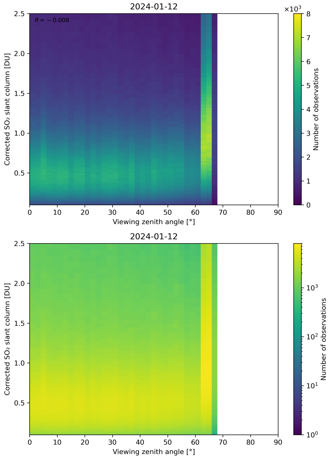
Figure 317: Scatter density plot of “Viewing zenith angle” against “Corrected SO 2 slant column” for 2024-01-11 to 2024-01-13.
