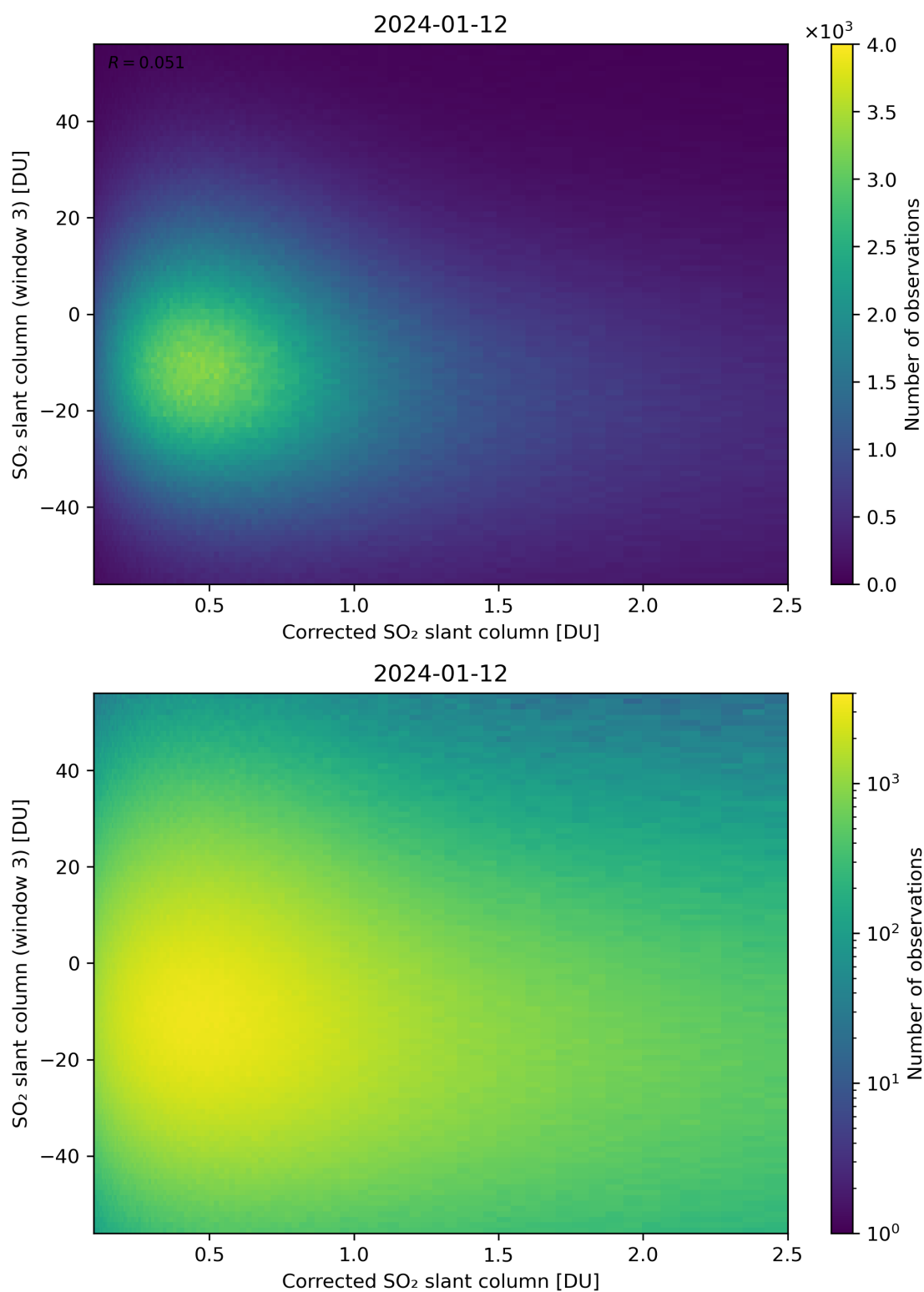
Figure 190: Scatter density plot of “Corrected SO 2 slant column” against “SO 2 slant column (window 3)” for 2024-01-11 to 2024-01-13.
