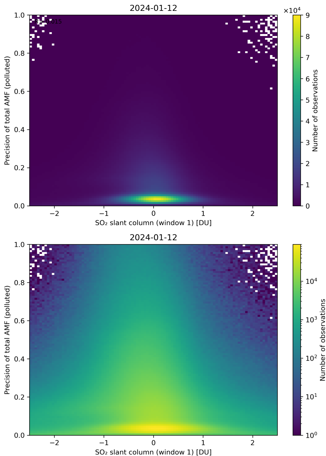
Figure 240: Scatter density plot of “SO 2 slant column (window 1)” against “Precision of total AMF (polluted)” for 2024-01-11 to 2024-01-13.
