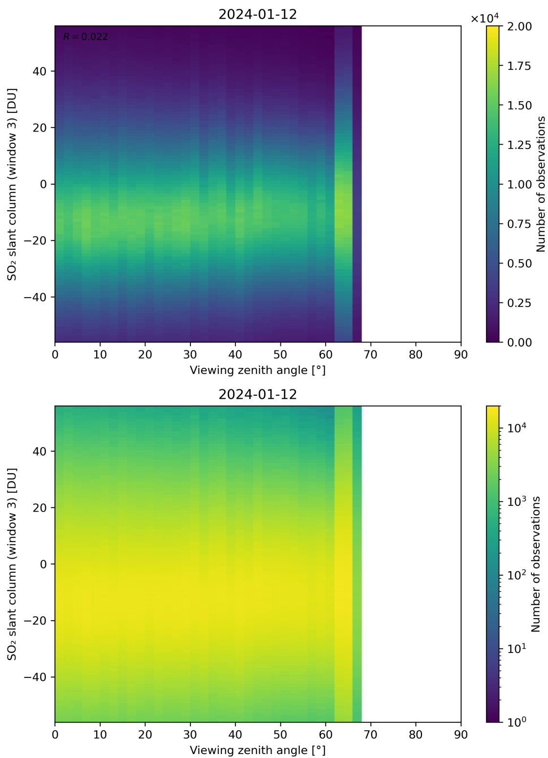
Figure 323: Scatter density plot of “Viewing zenith angle” against “SO 2 slant column (window 3)” for 2024-01-11 to 2024-01-13.
