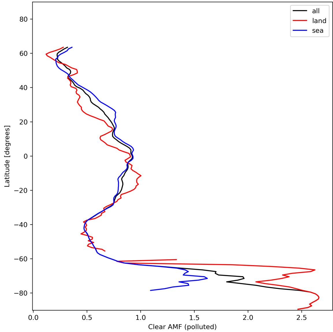
Figure 50: Zonal average of “Clear AMF (polluted)” for 2024-01-11 to 2024-01-13.
