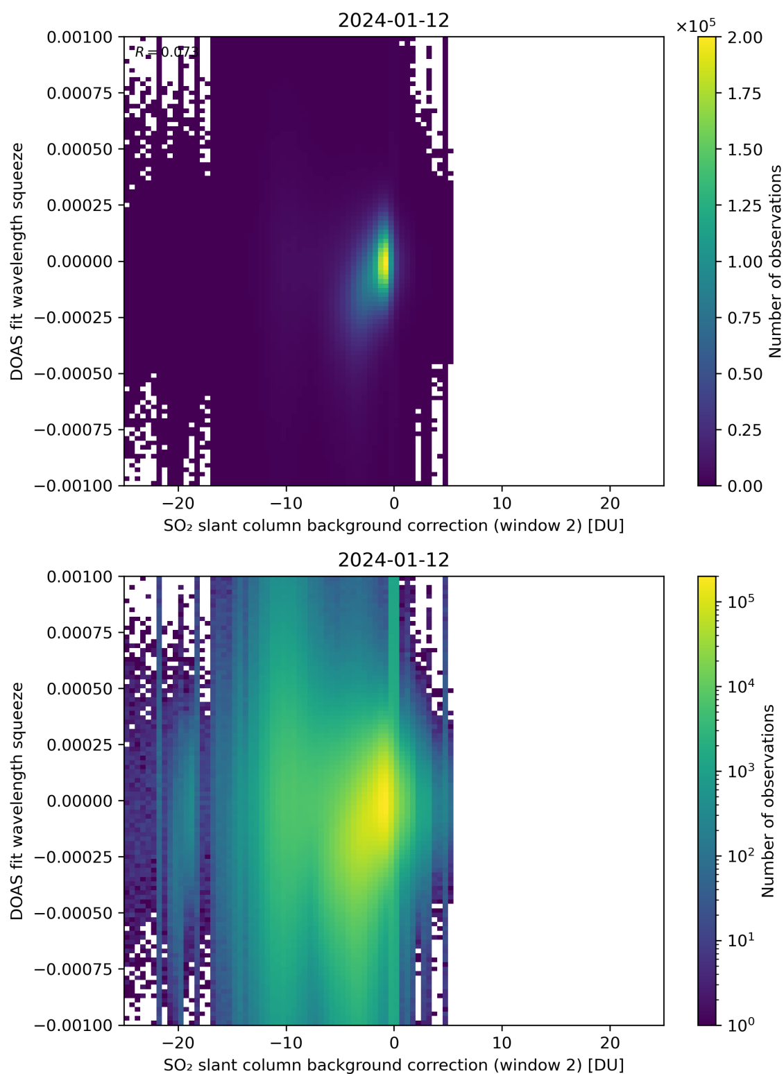
Figure 113: Scatter density plot of “SO 2 slant column background correction (window 2)” against “DOAS fit wavelength squeeze” for 2024-01-11 to 2024-01-13.
