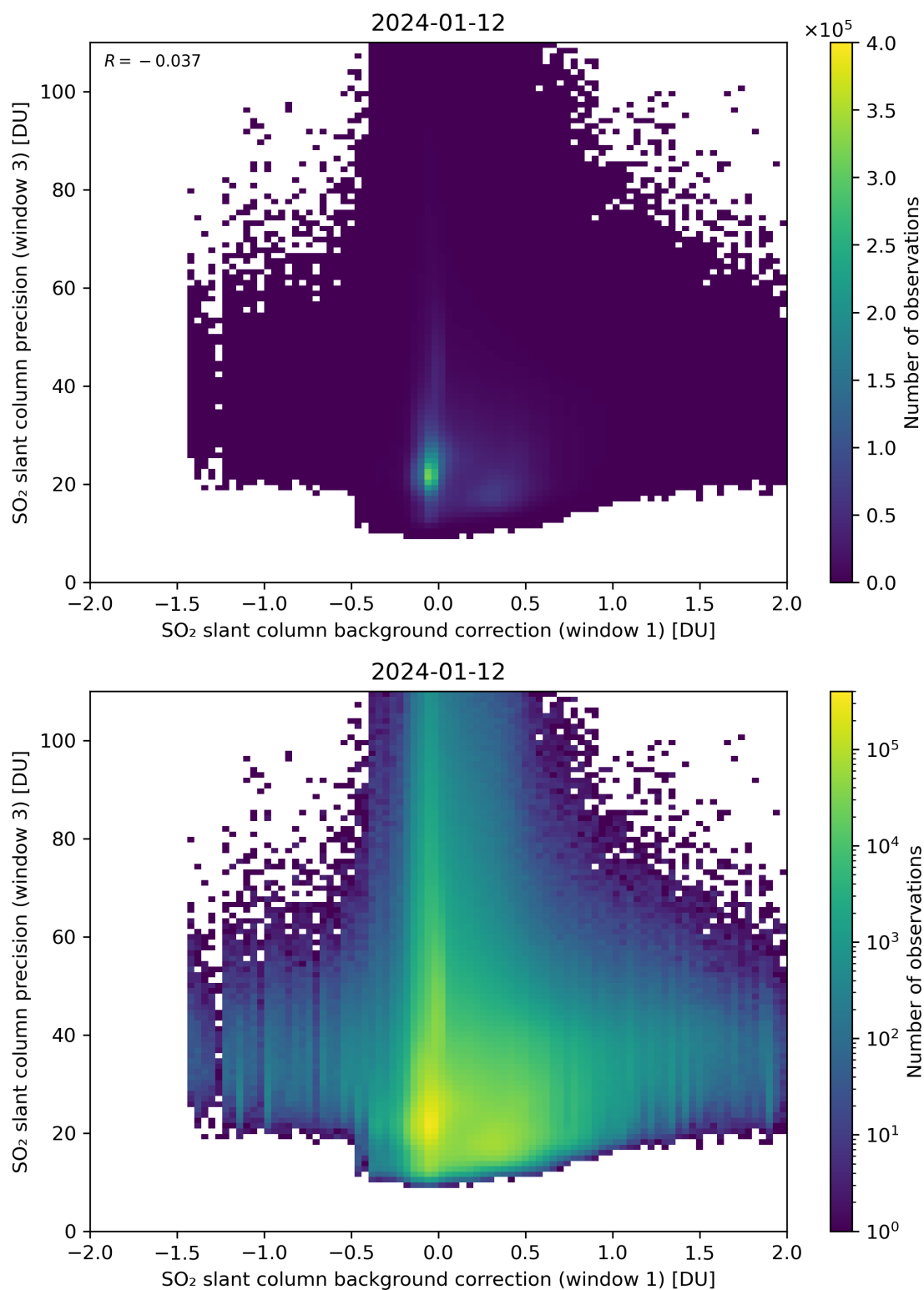
Figure 108: Scatter density plot of “SO 2 slant column background correction (window 1)” against “SO 2 slant column precision (window 3)” for 2024-01-11 to 2024-01-13.
