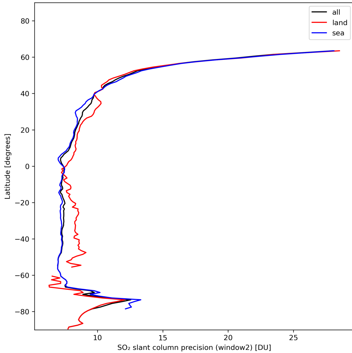
Figure 38: Zonal average of “SO 2 slant column precision (window2)” for 2024-01-11 to 2024-01-13.
