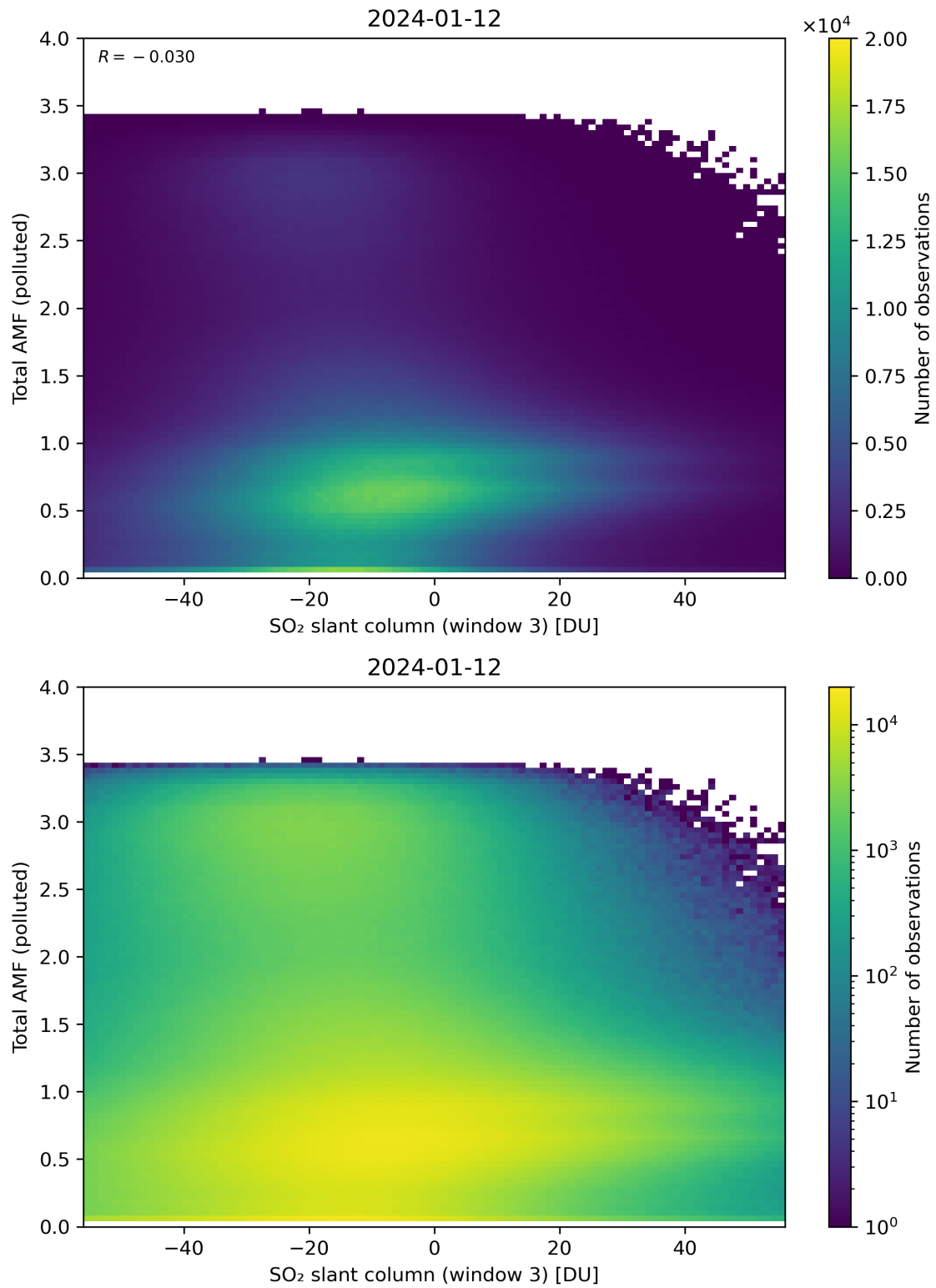
Figure 268: Scatter density plot of “SO 2 slant column (window 3)” against “Total AMF (polluted)” for 2024-01-11 to 2024-01-13.
