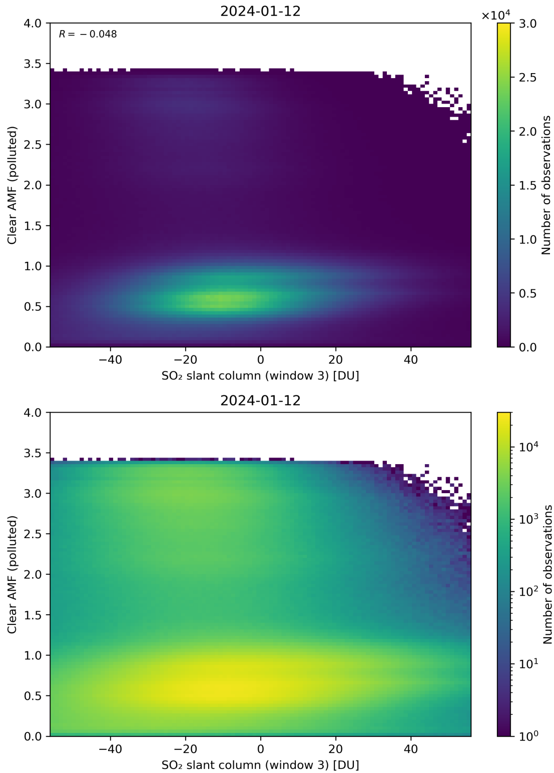
Figure 265: Scatter density plot of “SO 2 slant column (window 3)” against “Clear AMF (polluted)” for 2024-01-11 to 2024-01-13.
