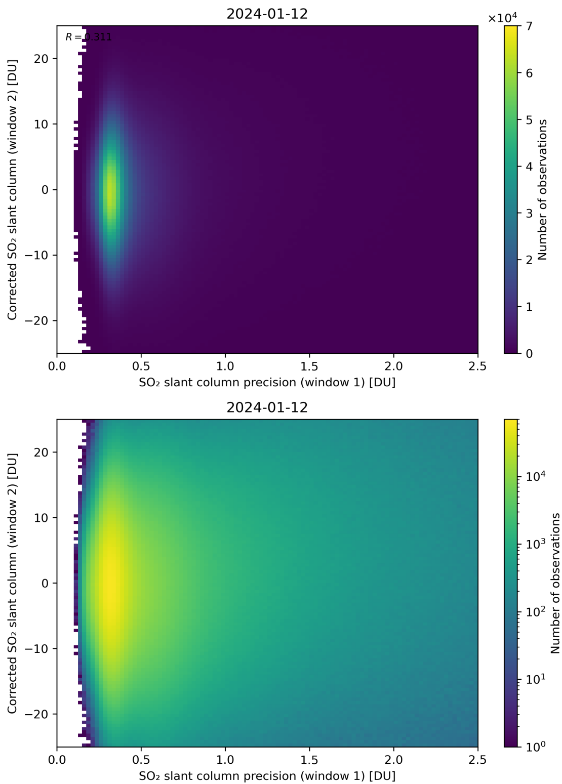
Figure 225: Scatter density plot of “SO 2 slant column precision (window 1)” against “Corrected SO 2 slant column (window 2)” for 2024-01-11 to 2024-01-13.
