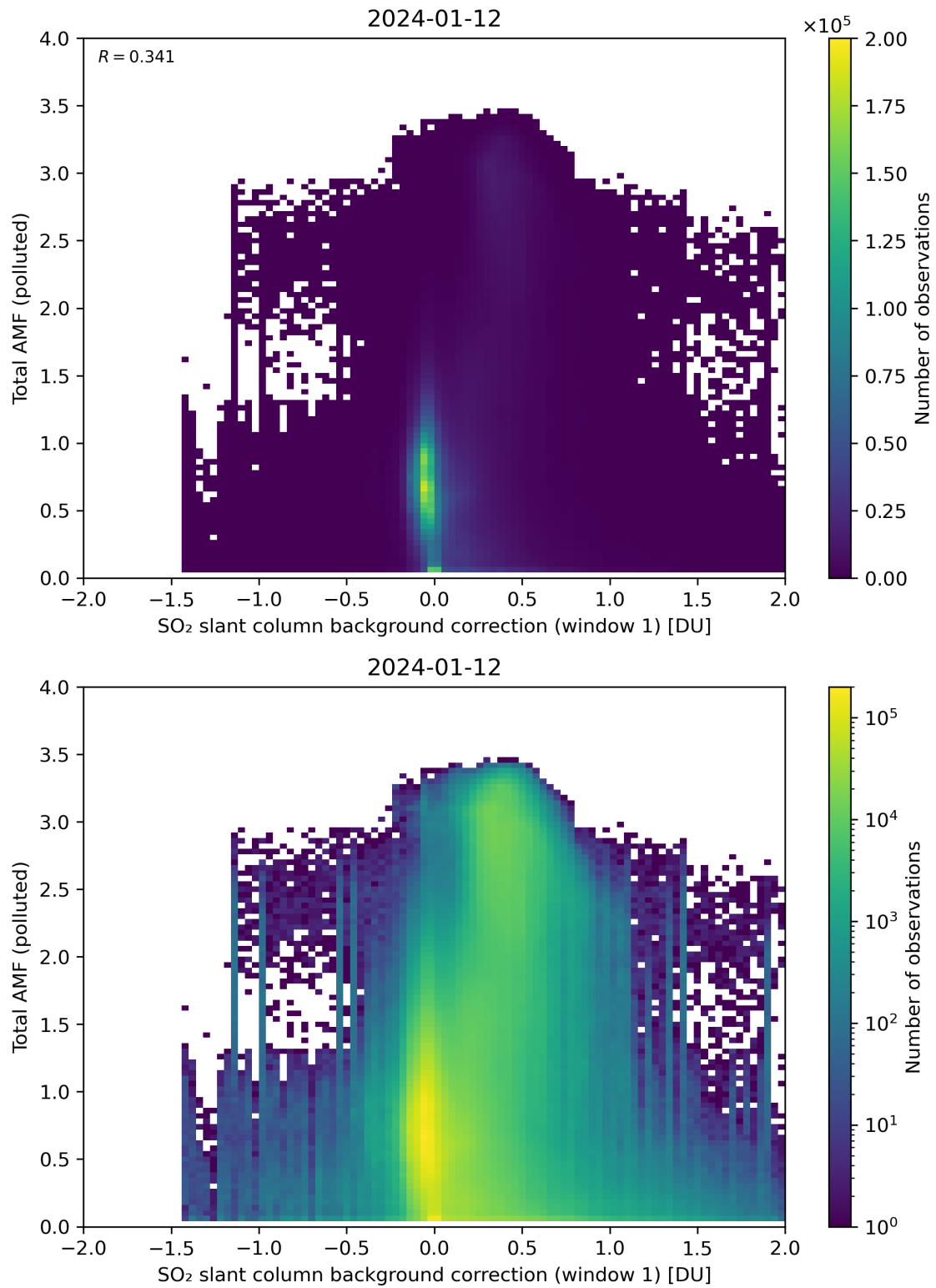
Figure 109: Scatter density plot of “SO 2 slant column background correction (window 1)” against “Total AMF (polluted)” for 2024-01-11 to 2024-01-13.
