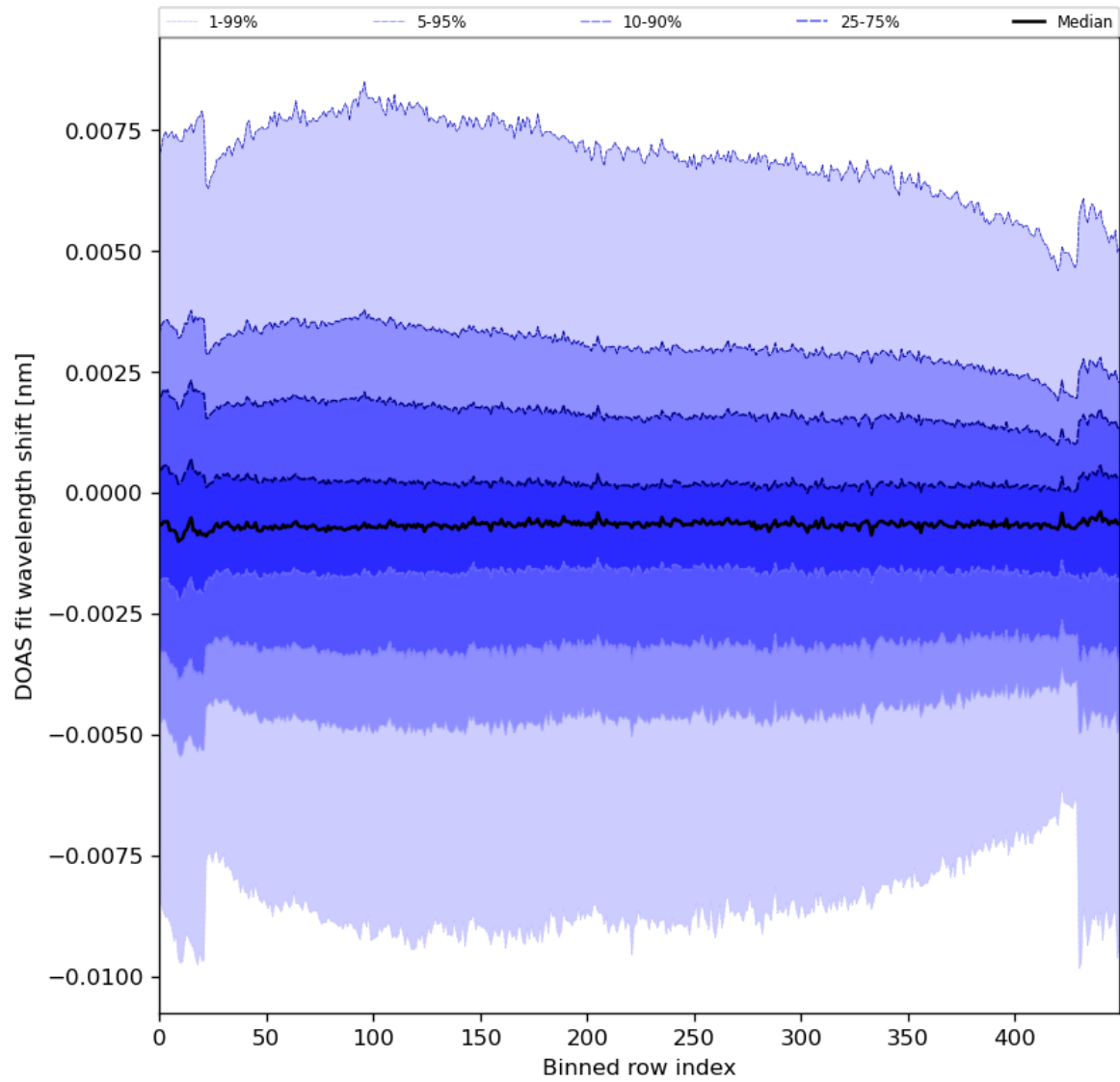
Figure 91: Along track statistics of “DOAS fit wavelength shift” for 2024-01-11 to 2024-01-13
