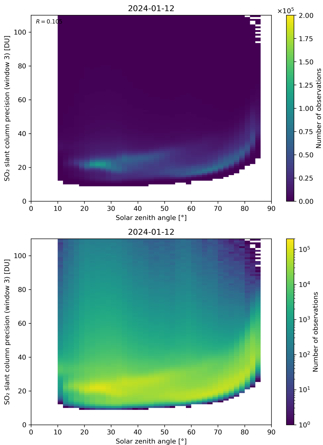
Figure 173: Scatter density plot of “Solar zenith angle” against “SO 2 slant column precision (window 3)” for 2024-01-11 to 2024-01-13.
