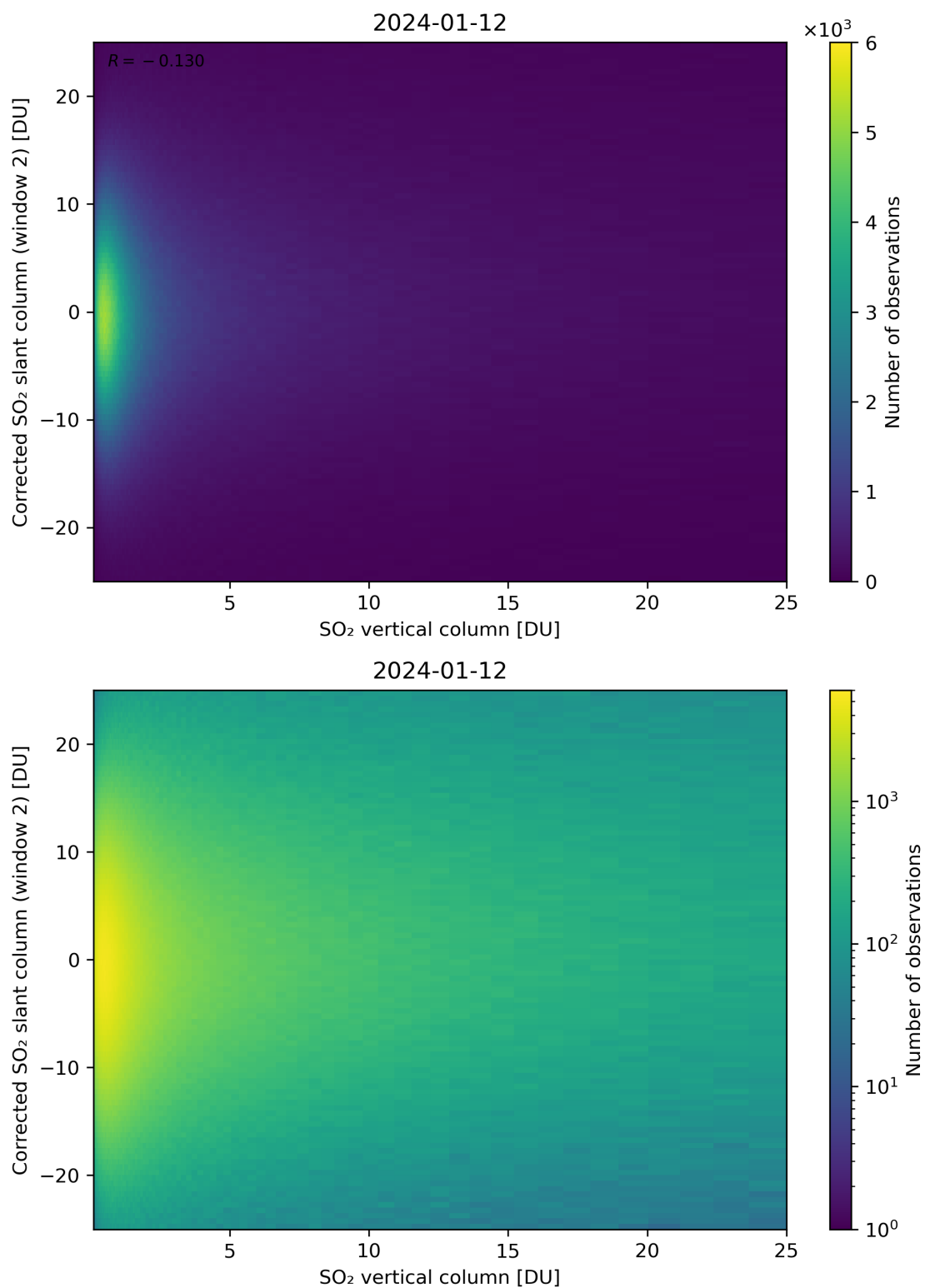
Figure 298: Scatter density plot of “SO 2 vertical column” against “Corrected SO 2 slant column (window 2)” for 2024-01-11 to 2024-01-13.
