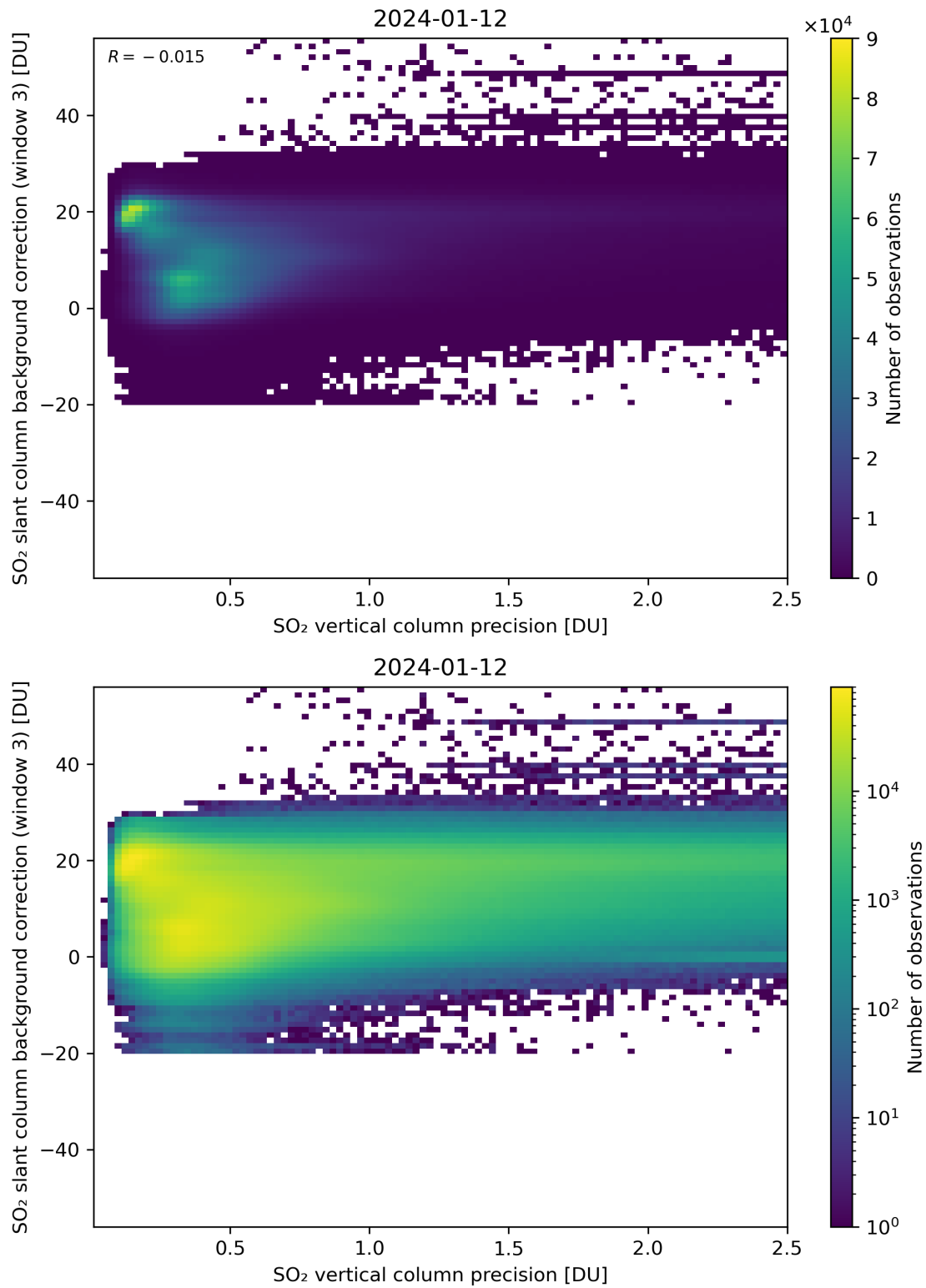
Figure 281: Scatter density plot of “SO 2 vertical column precision” against “SO 2 slant column background correction (window 3)” for 2024-01-11 to 2024-01-13.
