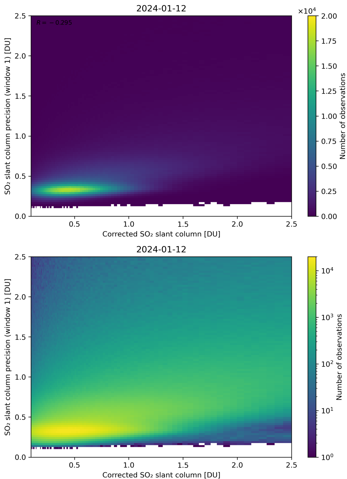
Figure 188: Scatter density plot of “Corrected SO 2 slant column” against “SO 2 slant column precision (window 1)” for 2024-01-11 to 2024-01-13.
