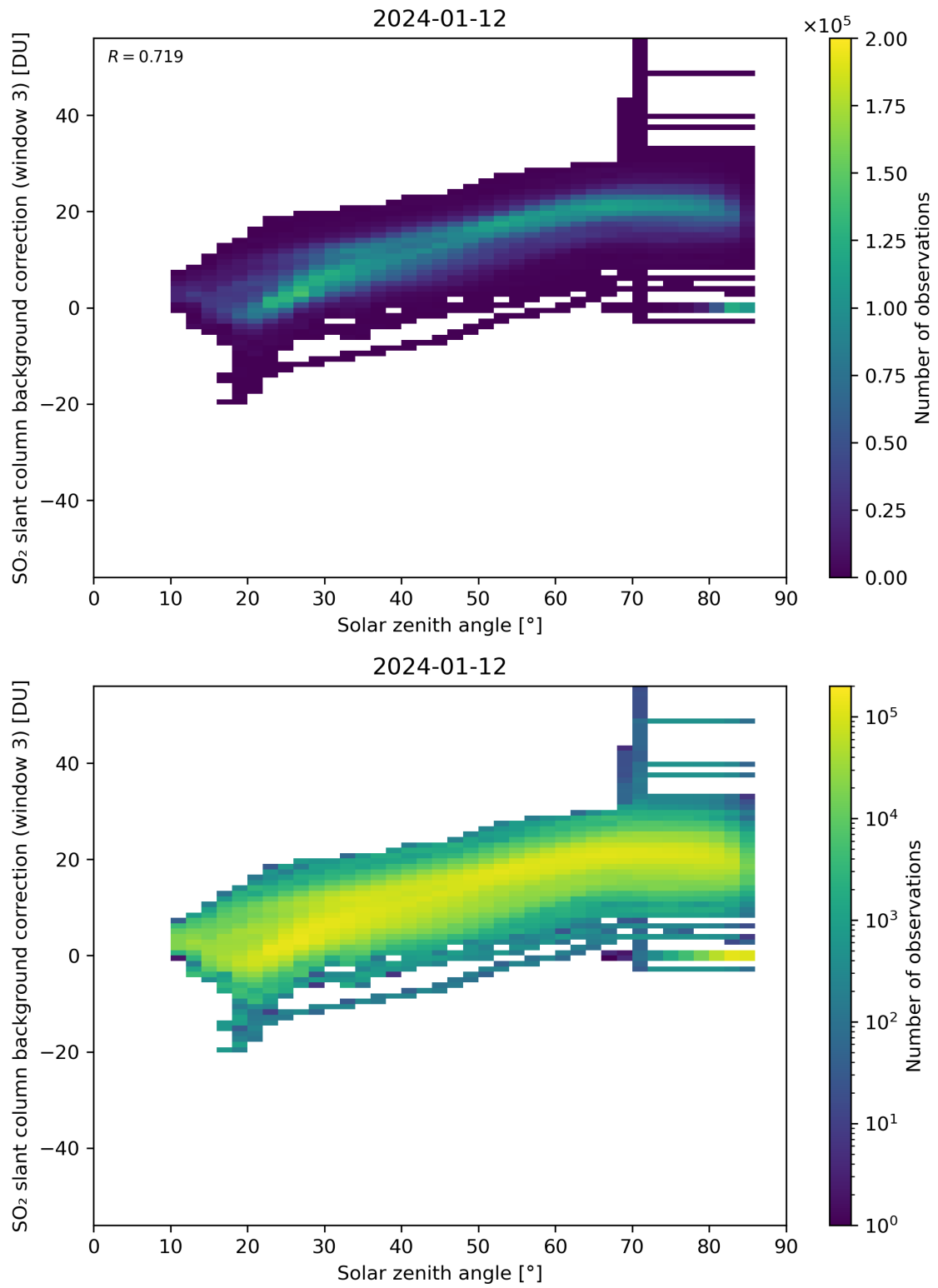
Figure 160: Scatter density plot of “Solar zenith angle” against “SO 2 slant column background correction (window 3)” for 2024-01-11 to 2024-01-13.
