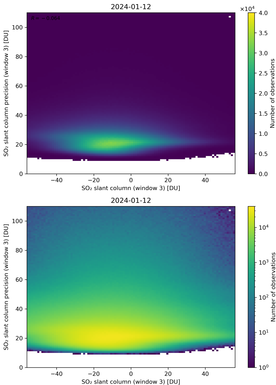
Figure 267: Scatter density plot of “SO 2 slant column (window 3)” against “SO 2 slant column precision (window 3)” for 2024-01-11 to 2024-01-13.
