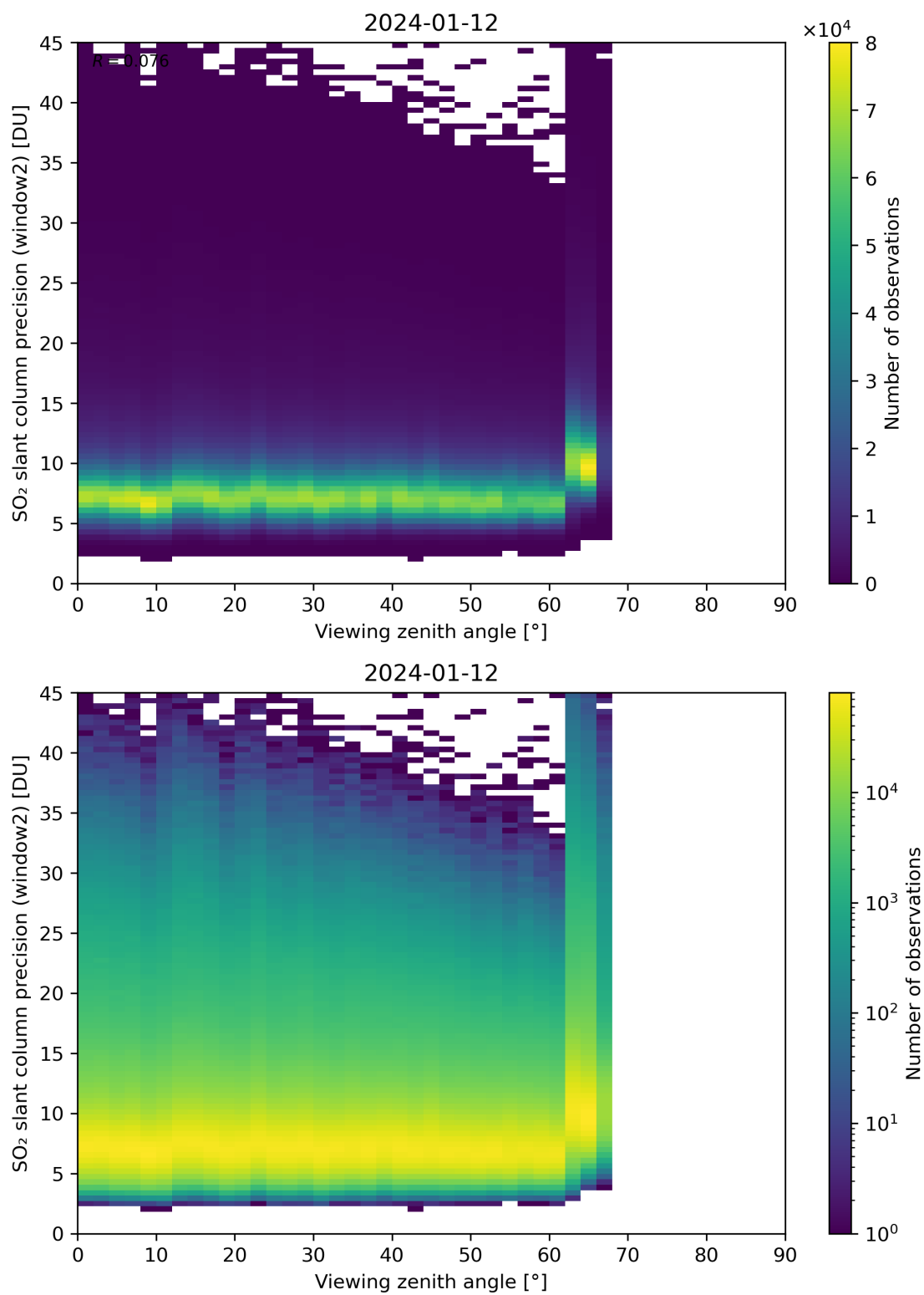
Figure 322: Scatter density plot of “Viewing zenith angle” against “SO 2 slant column precision (window2)” for 2024-01-11 to 2024-01-13.
