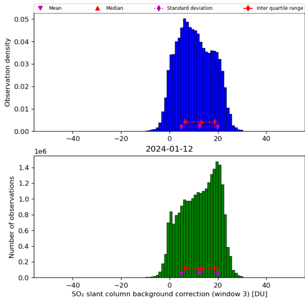
Figure 67: Histogram of “SO 2 slant column background correction (window 3)” for 2024-01-11 to 2024-01-13
