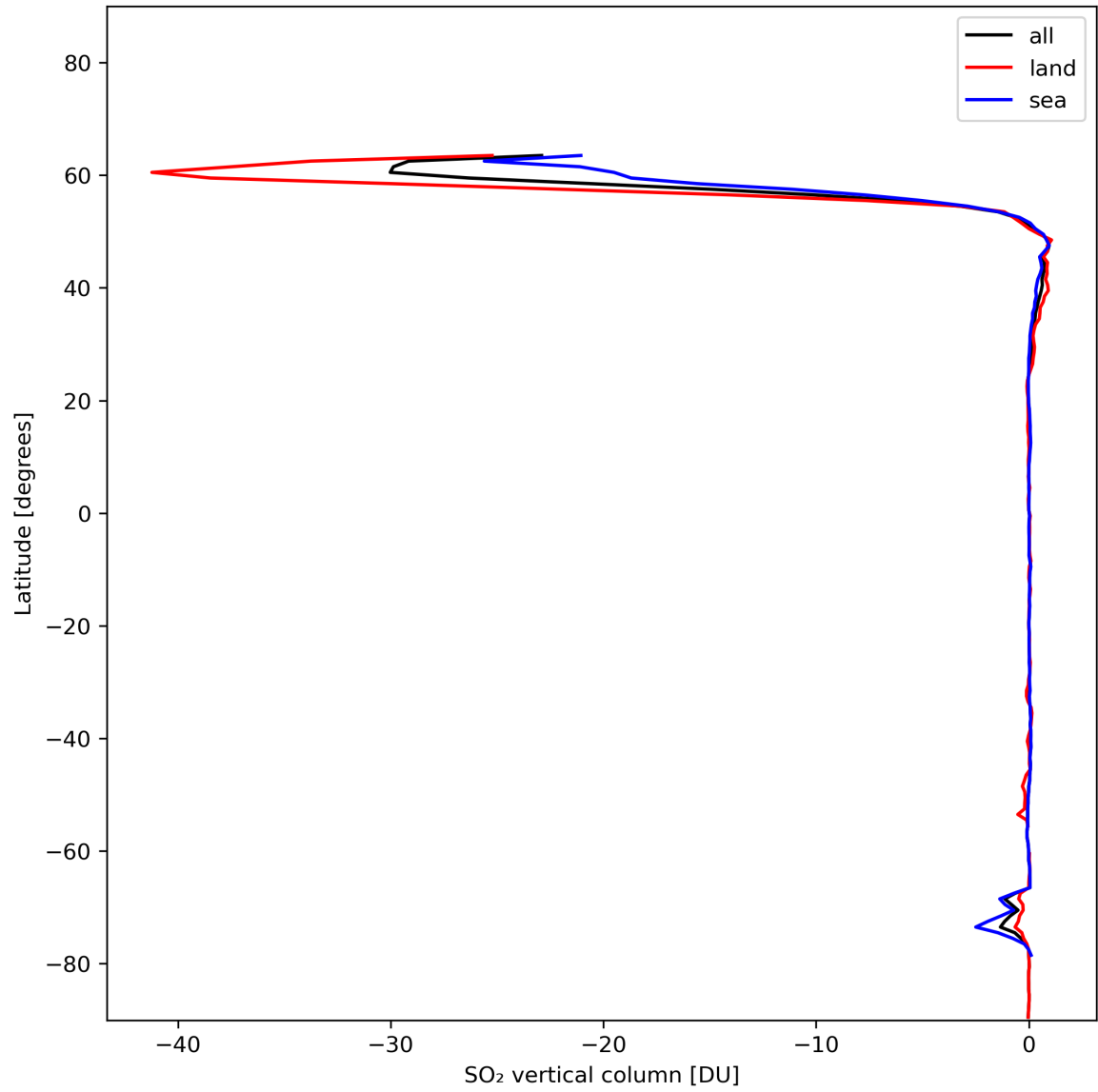
Figure 30: Zonal average of “SO 2 vertical column” for 2024-01-11 to 2024-01-13.
