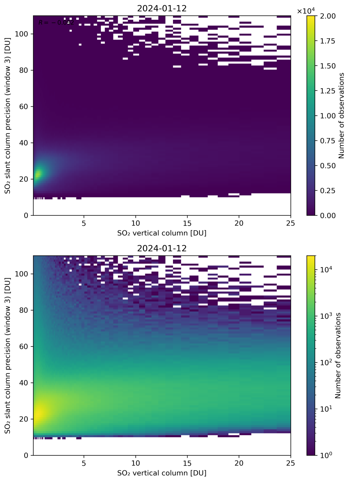
Figure 304: Scatter density plot of “SO 2 vertical column” against “SO 2 slant column precision (window 3)” for 2024-01-11 to 2024-01-13.
