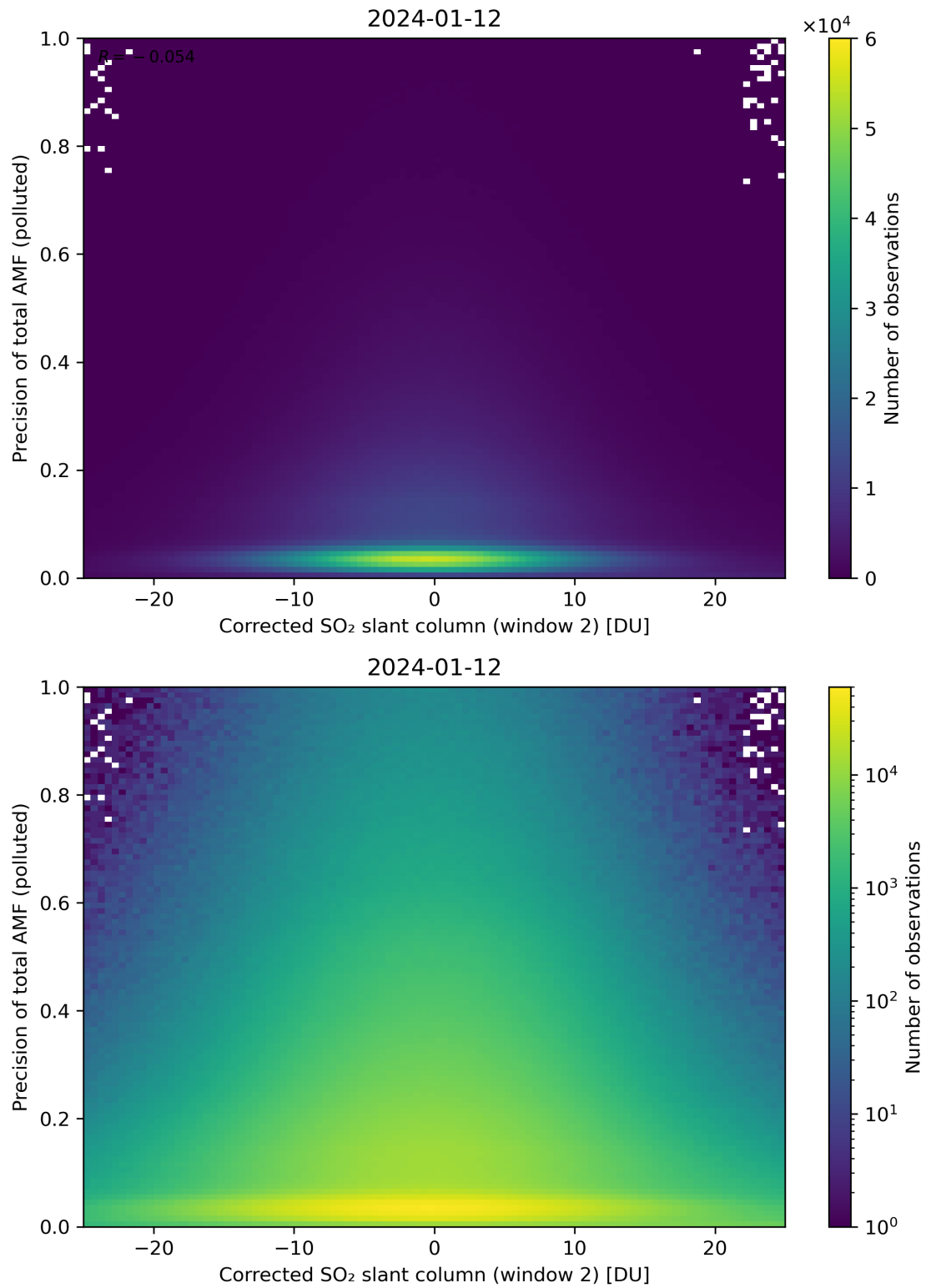
Figure 204: Scatter density plot of “Corrected SO 2 slant column (window 2)” against “Precision of total AMF (polluted)” for 2024-01-11 to 2024-01-13.
