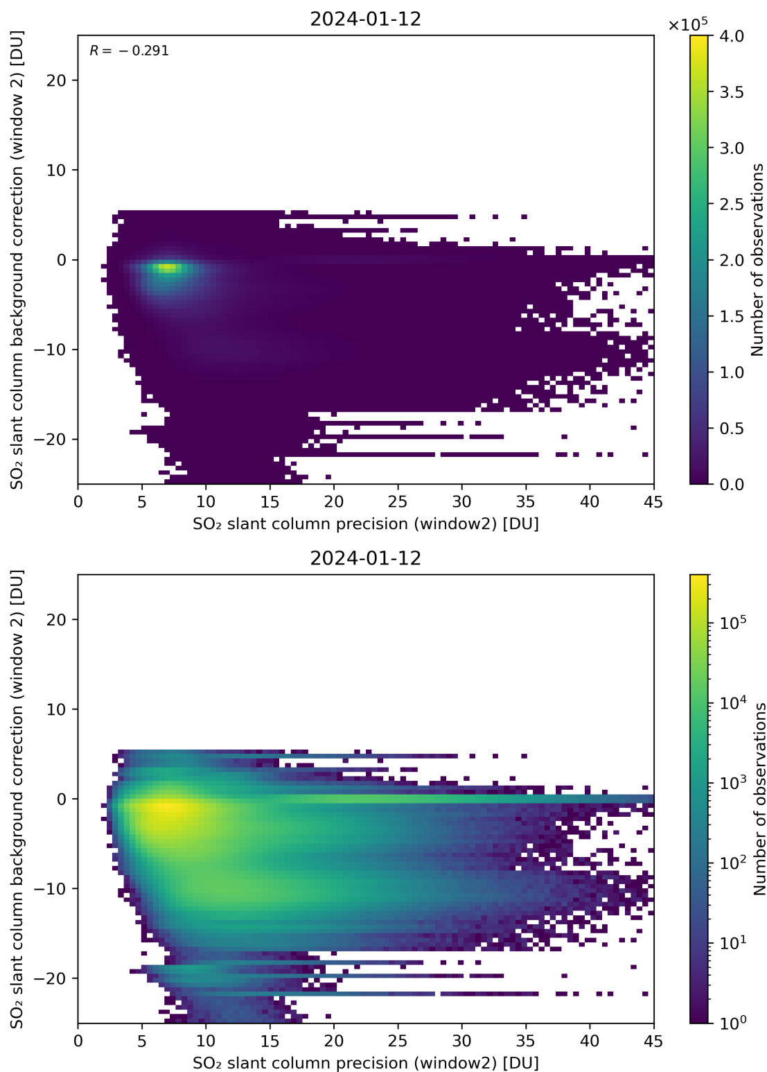
Figure 241: Scatter density plot of “SO 2 slant column precision (window2)” against “SO 2 slant column background correction (window 2)” for 2024-01-11 to 2024-01-13.
