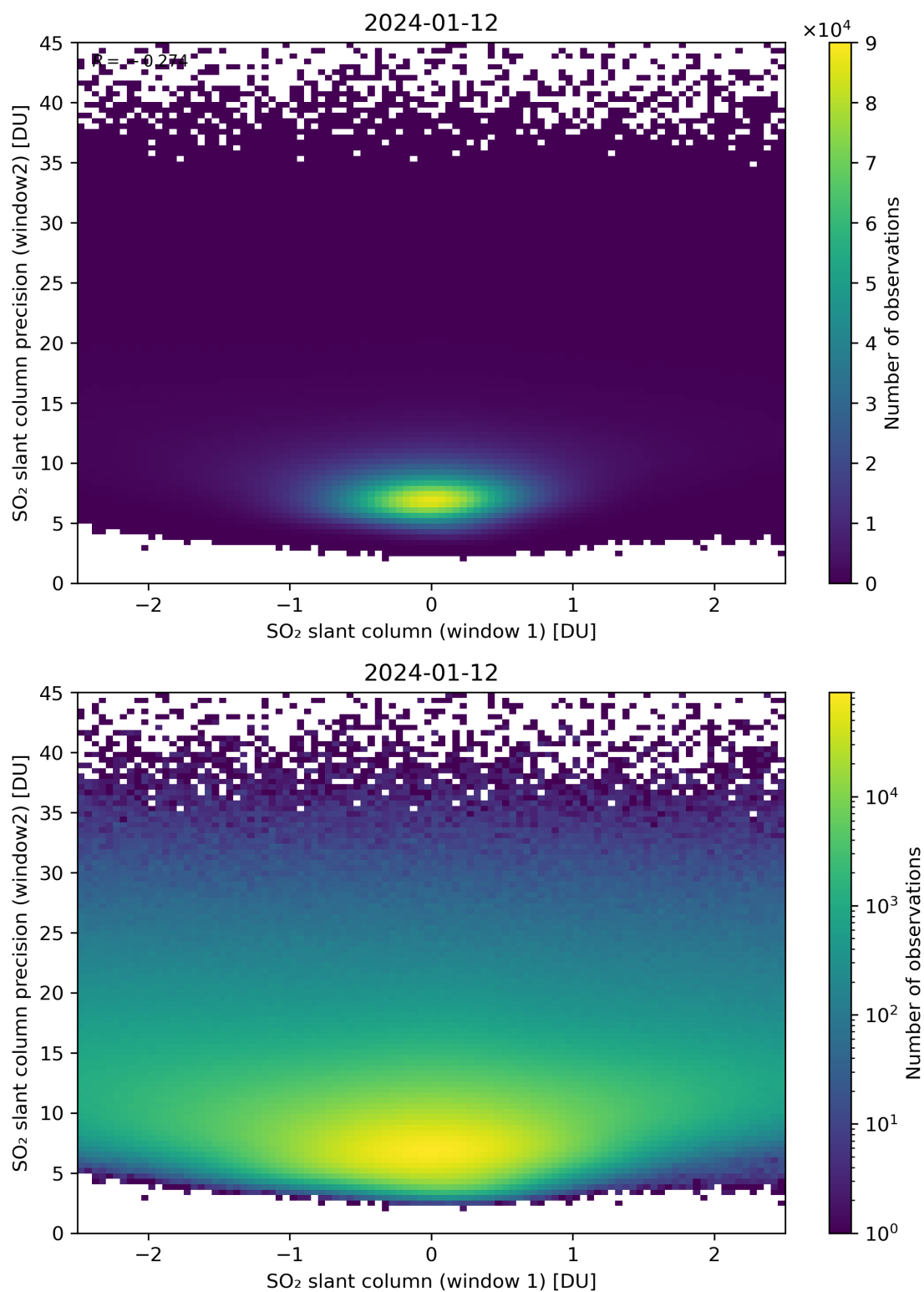
Figure 236: Scatter density plot of “SO 2 slant column (window 1)” against “SO 2 slant column precision (window2)” for 2024-01-11 to 2024-01-13.
