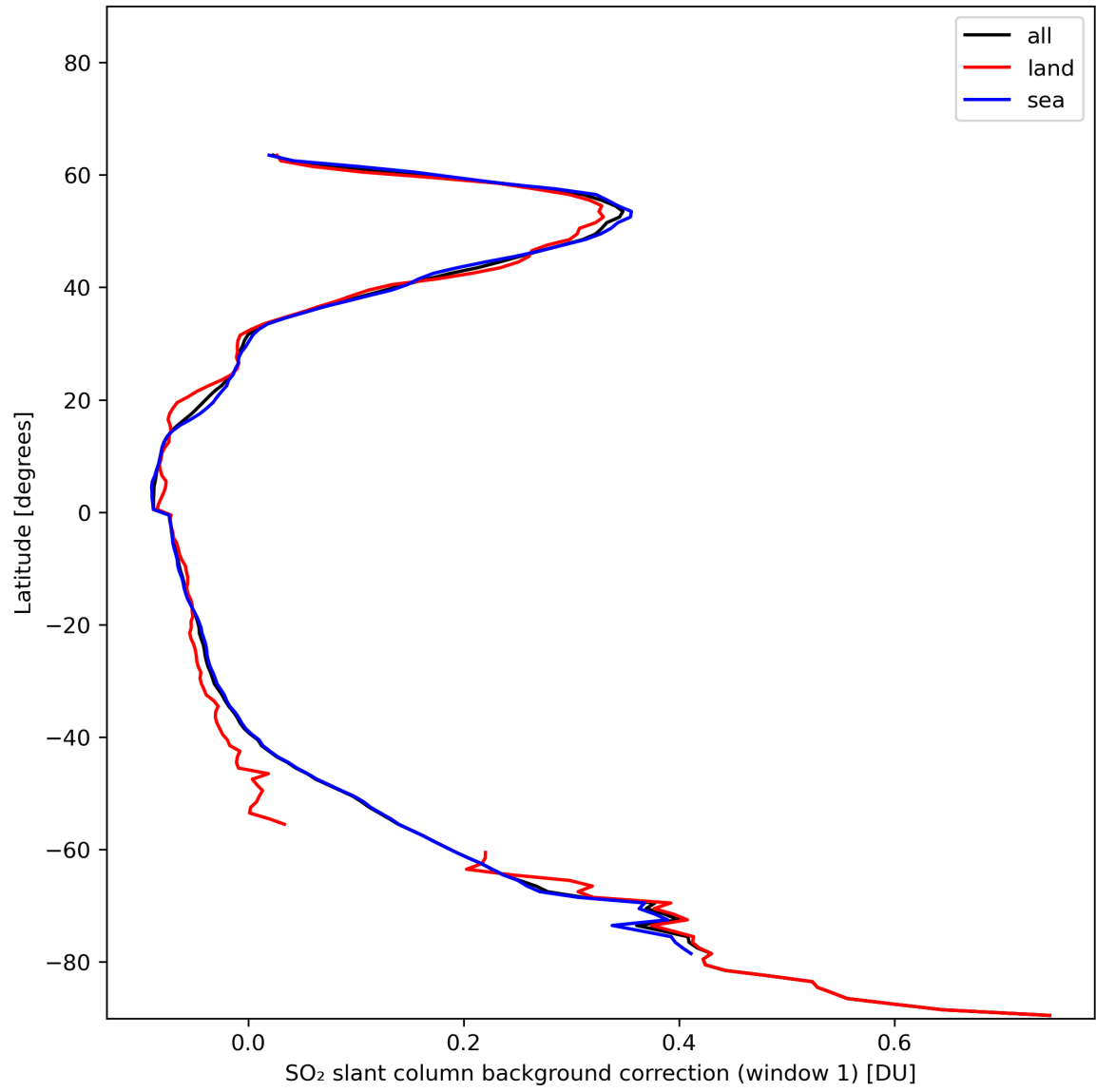
Figure 36: Zonal average of “SO 2 slant column background correction (window 1)” for 2024-01-11 to 2024-01-13.
