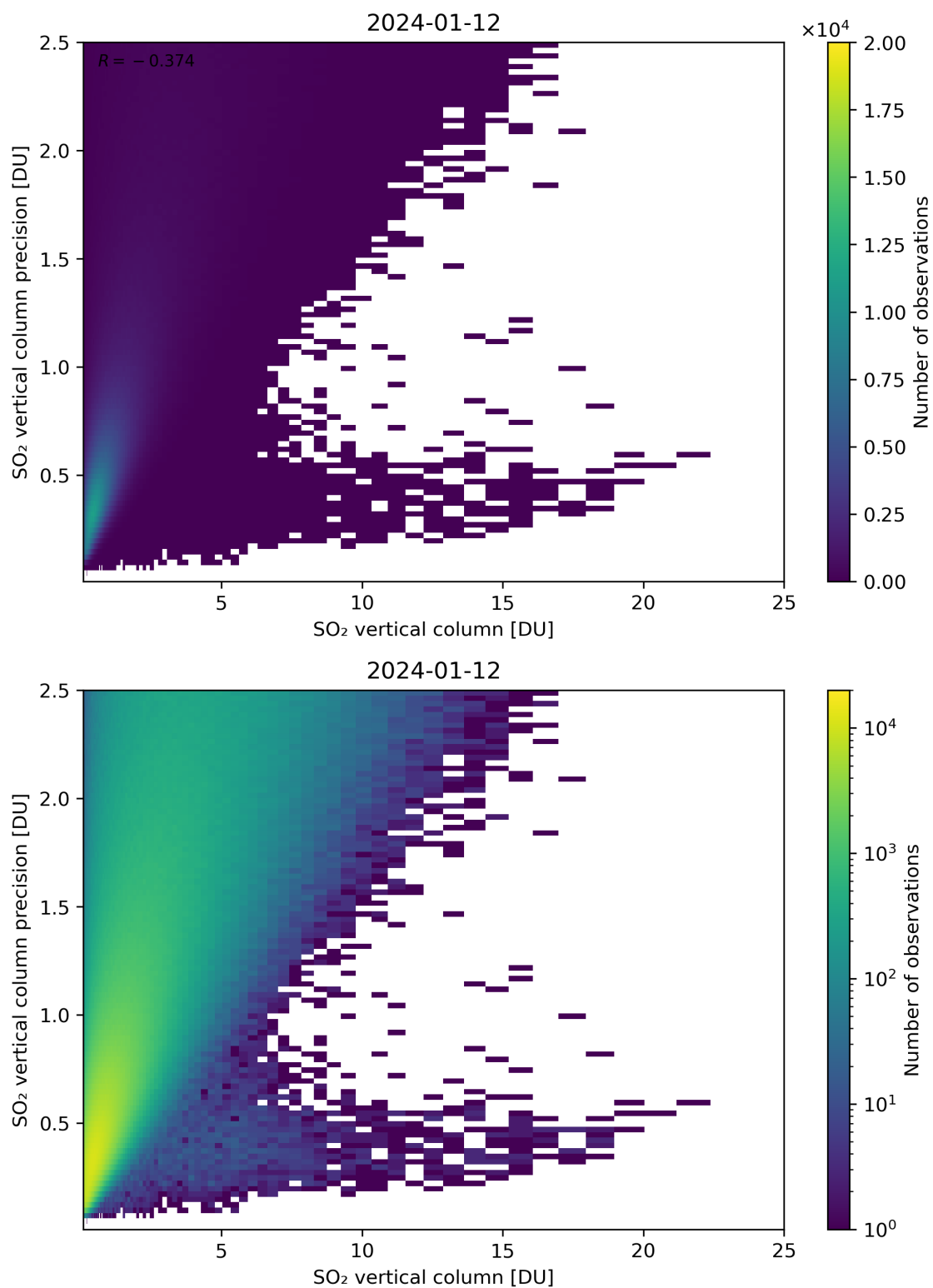
Figure 307: Scatter density plot of “SO 2 vertical column” against “SO 2 vertical column precision” for 2024-01-11 to 2024-01-13.
