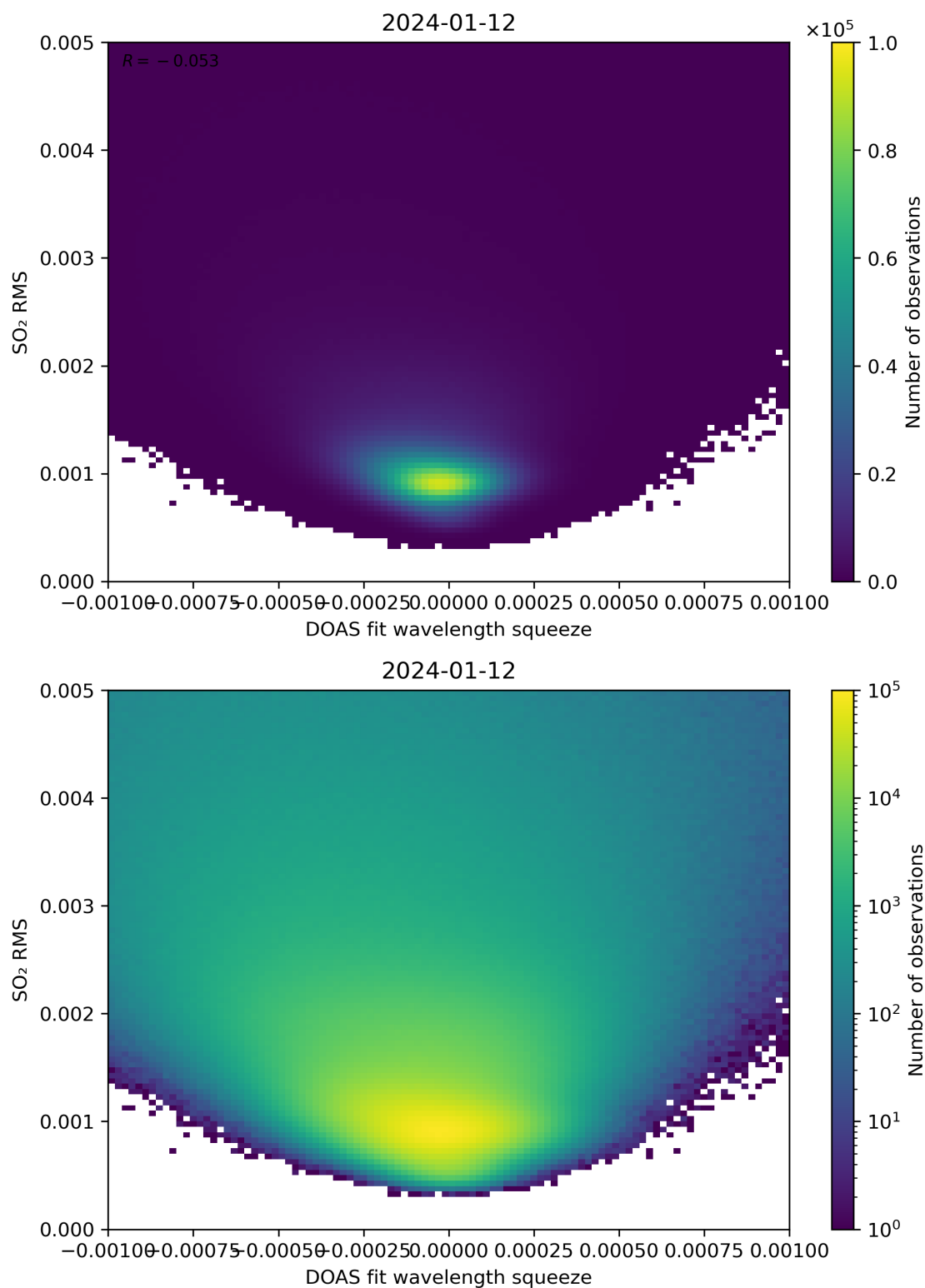
Figure 132: Scatter density plot of “DOAS fit wavelength squeeze” against “SO 2 RMS” for 2024-01-11 to 2024-01-13.
