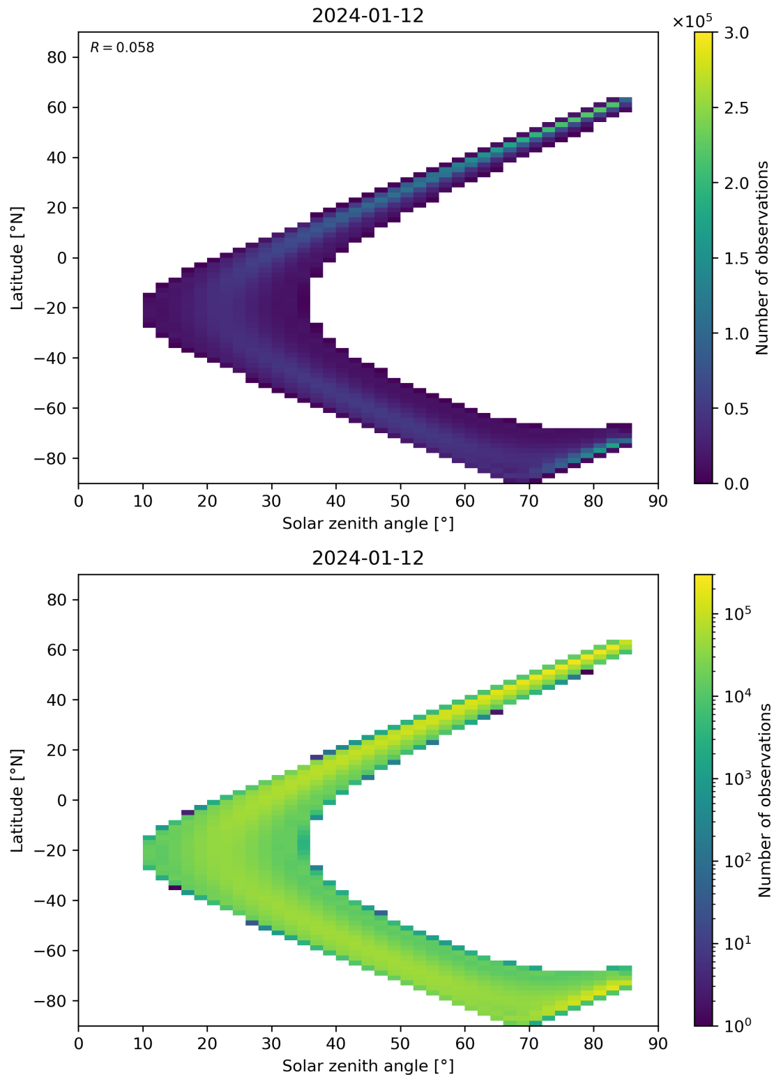
Figure 164: Scatter density plot of “Solar zenith angle” against “Latitude” for 2024-01-11 to 2024-01-13.
