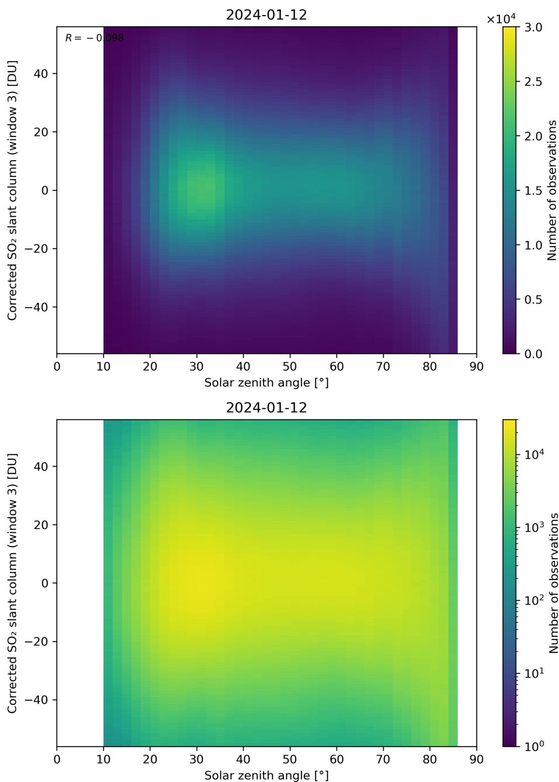
Figure 168: Scatter density plot of “Solar zenith angle” against “Corrected SO 2 slant column (window 3)” for 2024-01-11 to 2024-01-13.
