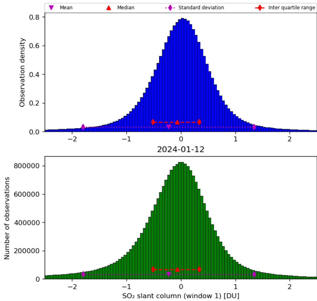
Figure 56: Histogram of “SO 2 slant column (window 1)” for 2024-01-11 to 2024-01-13
