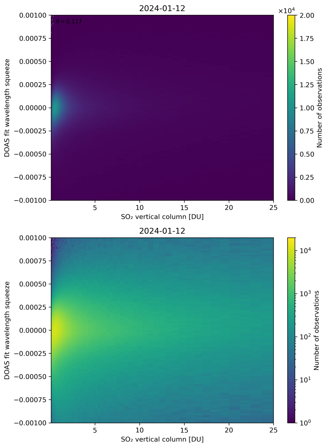
Figure 277: Scatter density plot of “SO 2 vertical column” against “DOAS fit wavelength squeeze” for 2024-01-11 to 2024-01-13.
