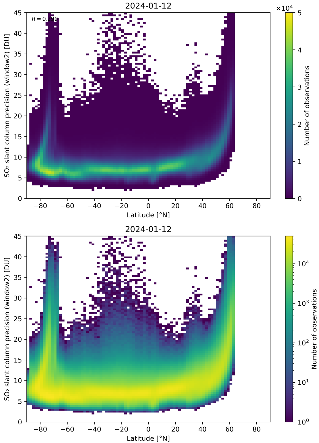
Figure 151: Scatter density plot of “Latitude” against “SO 2 slant column precision (window2)” for 2024-01-11 to 2024-01-13.
