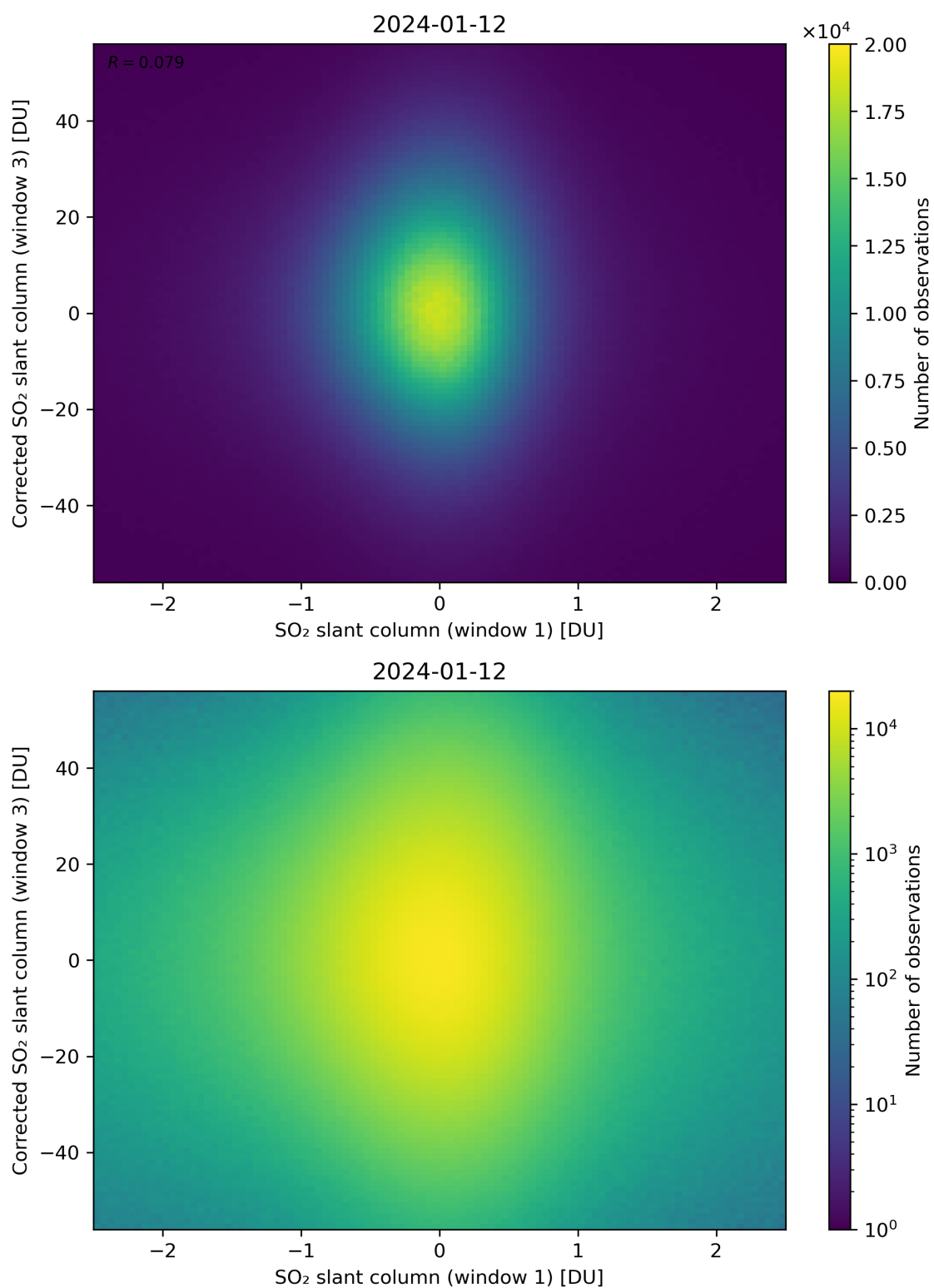
Figure 234: Scatter density plot of “SO 2 slant column (window 1)” against “Corrected SO 2 slant column (window 3)” for 2024-01-11 to 2024-01-13.
