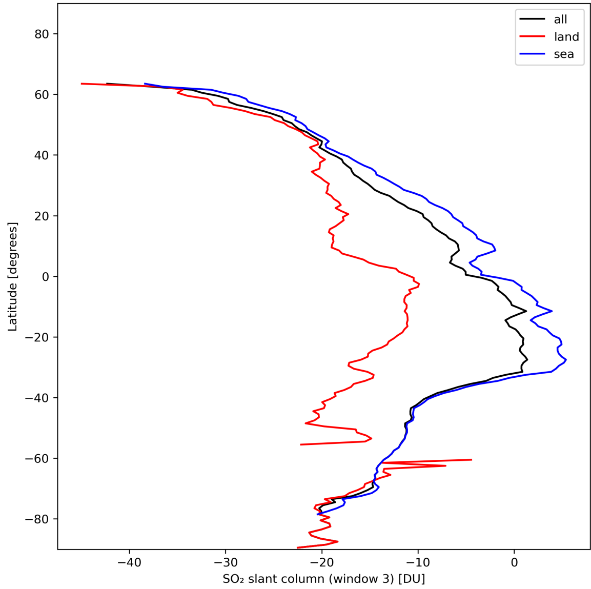
Figure 41: Zonal average of “SO 2 slant column (window 3)” for 2024-01-11 to 2024-01-13.
