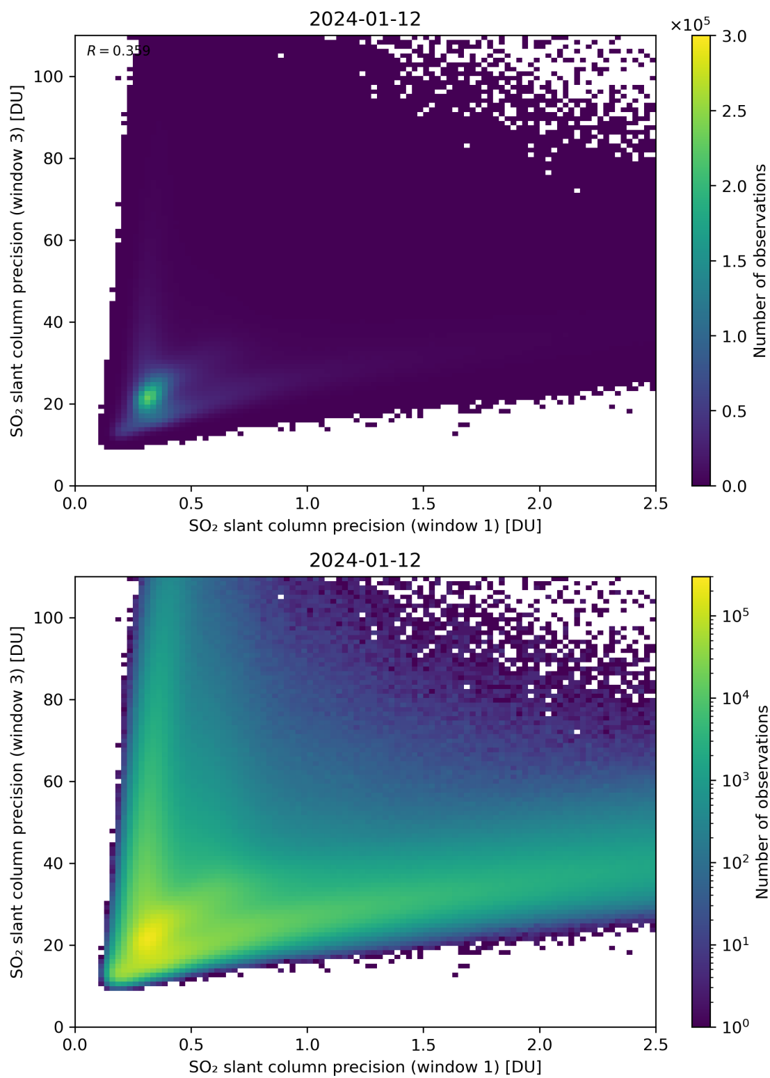
Figure 229: Scatter density plot of “SO 2 slant column precision (window 1)” against “SO 2 slant column precision (window 3)” for 2024-01-11 to 2024-01-13.
