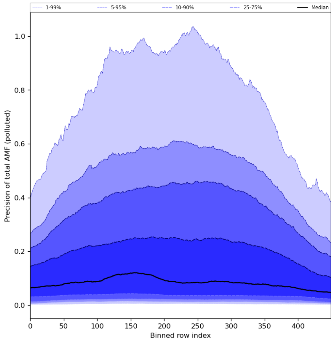
Figure 95: Along track statistics of “Precision of total AMF (polluted)” for 2024-01-11 to 2024-01-13
