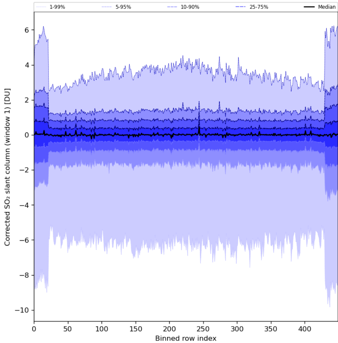
Figure 81: Along track statistics of “Corrected SO 2 slant column (window 1)” for 2024-01-11 to 2024-01-13
