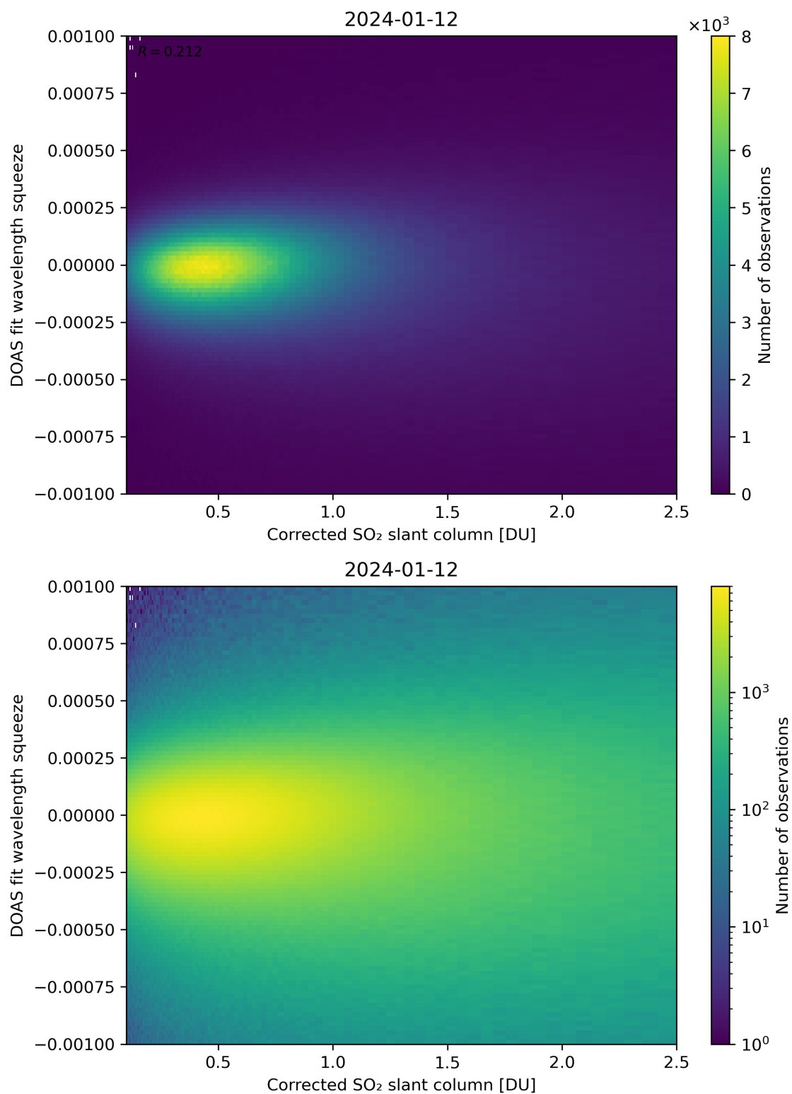
Figure 182: Scatter density plot of “Corrected SO 2 slant column” against “DOAS fit wavelength squeeze” for 2024-01-11 to 2024-01-13.
