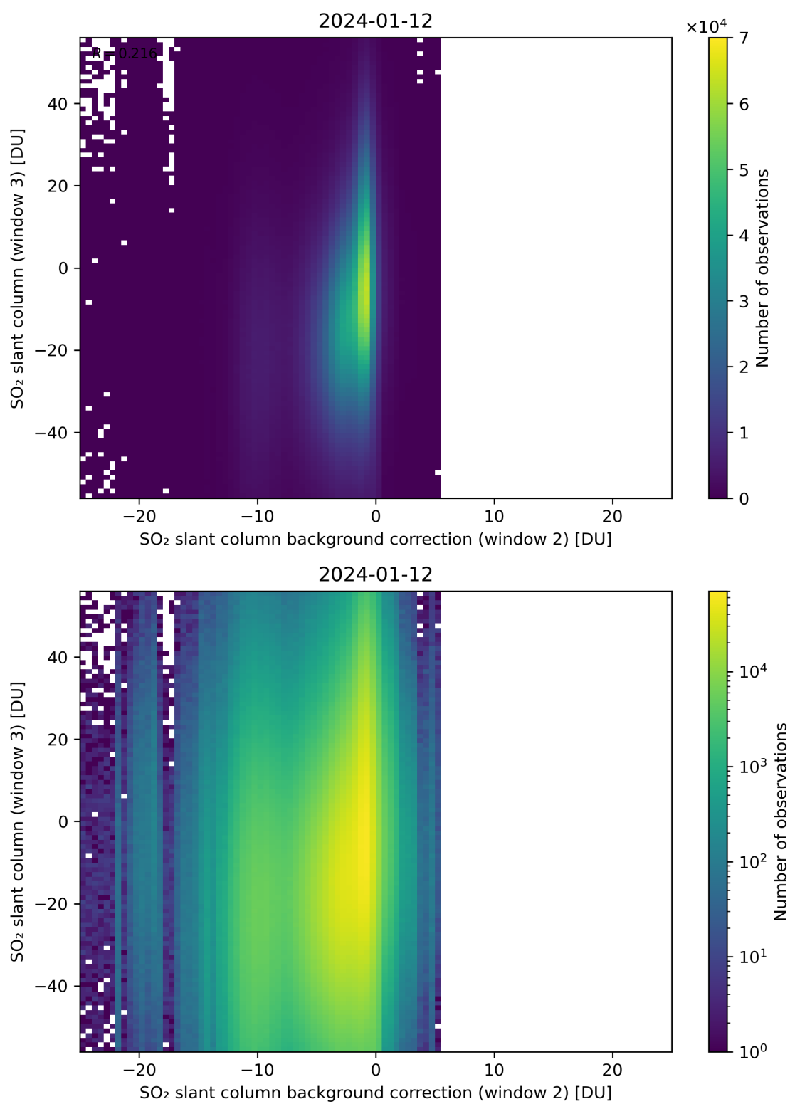
Figure 117: Scatter density plot of “SO 2 slant column background correction (window 2)” against “SO 2 slant column (window 3)” for 2024-01-11 to 2024-01-13.
