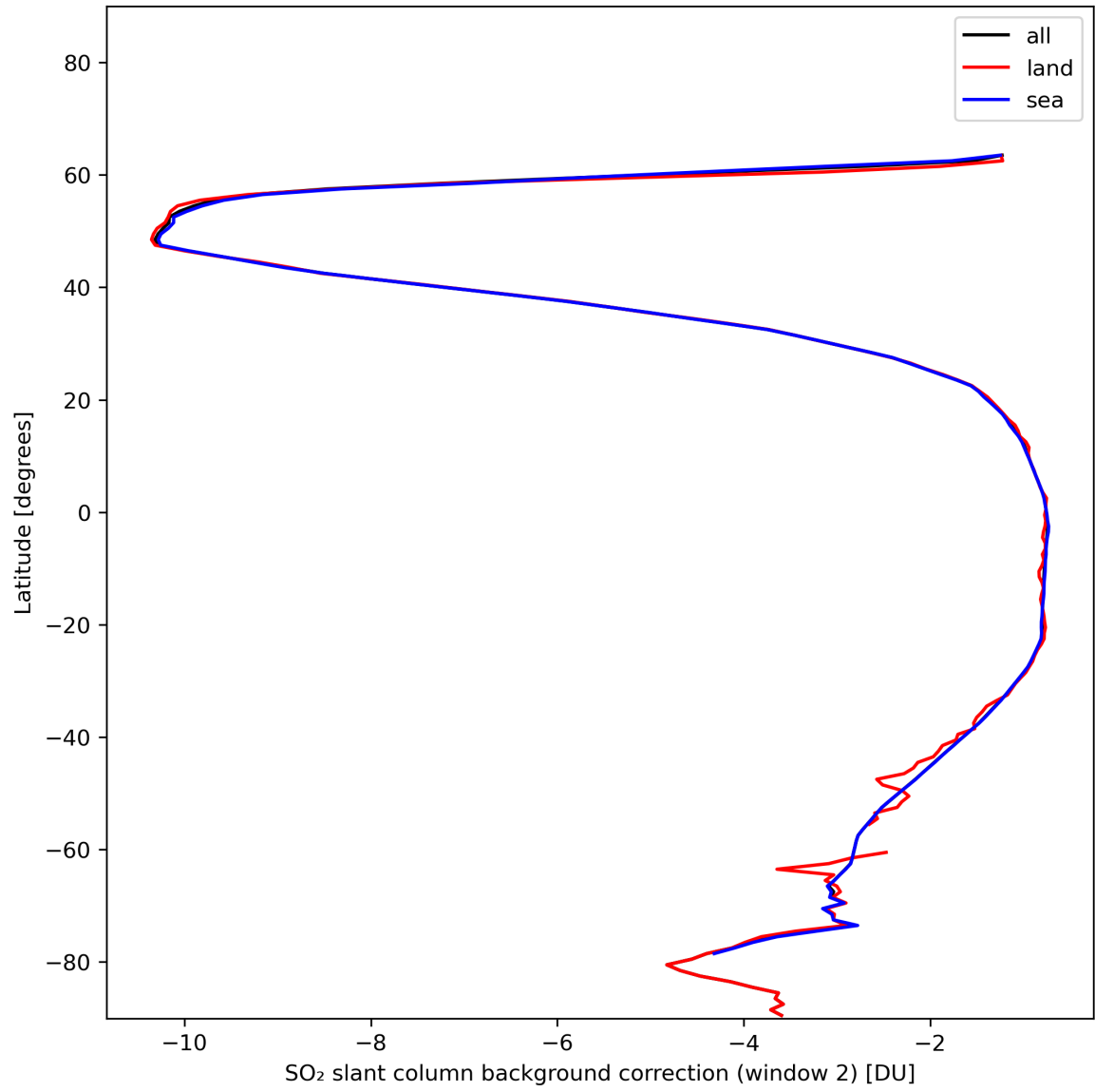
Figure 40: Zonal average of “SO 2 slant column background correction (window 2)” for 2024-01-11 to 2024-01-13.
