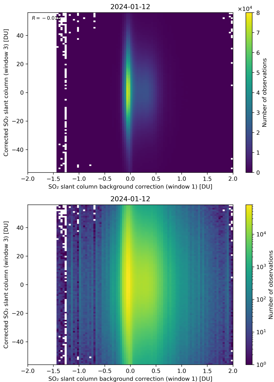
Figure 105: Scatter density plot of “SO 2 slant column background correction (window 1)” against “Corrected SO 2 slant column (window 3)” for 2024-01-11 to 2024-01-13.
