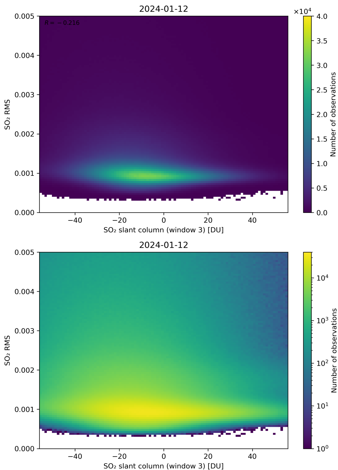
Figure 256: Scatter density plot of “SO 2 slant column (window 3)” against “SO 2 RMS” for 2024-01-11 to 2024-01-13.
