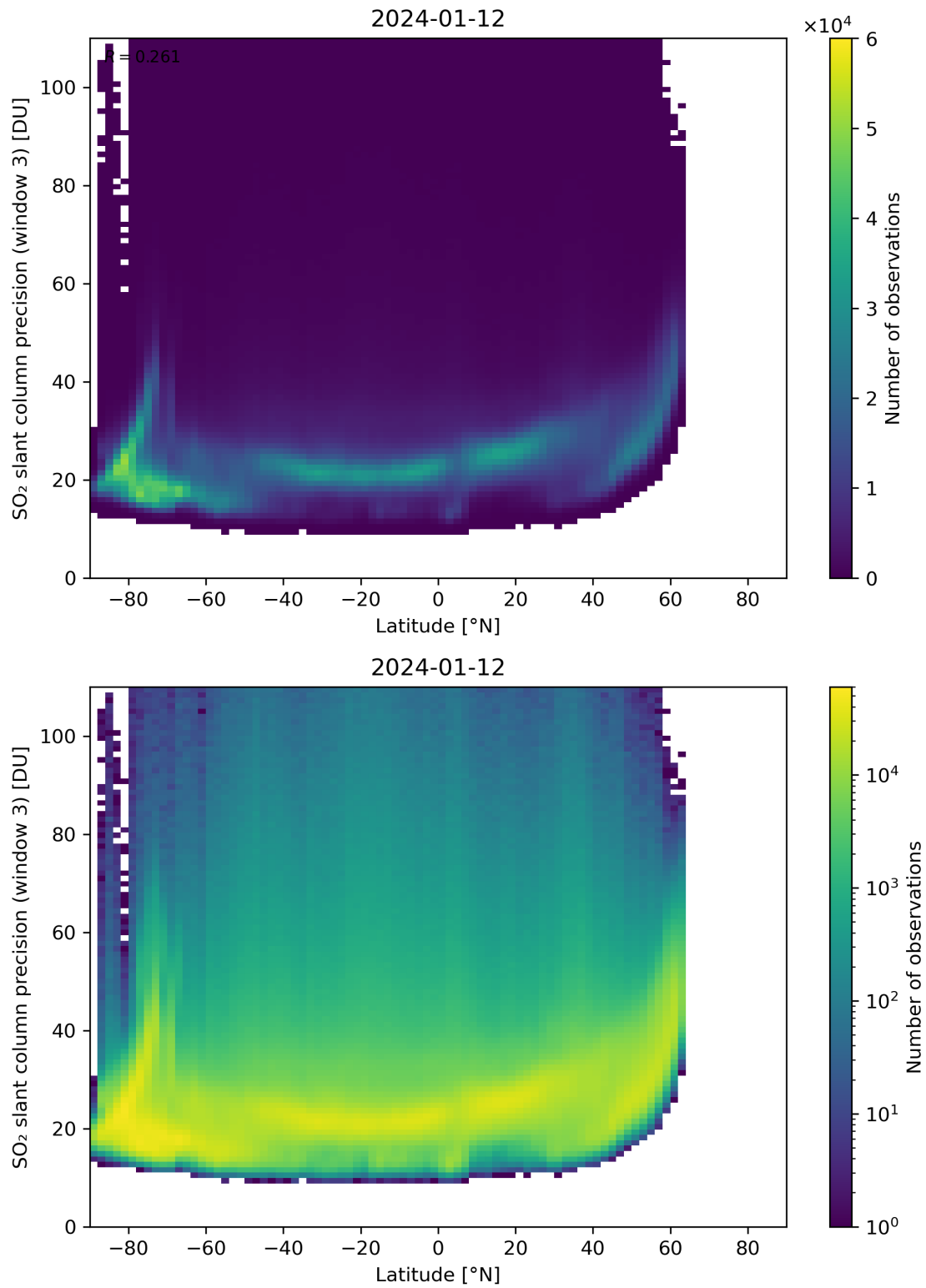
Figure 153: Scatter density plot of “Latitude” against “SO 2 slant column precision (window 3)” for 2024-01-11 to 2024-01-13.
