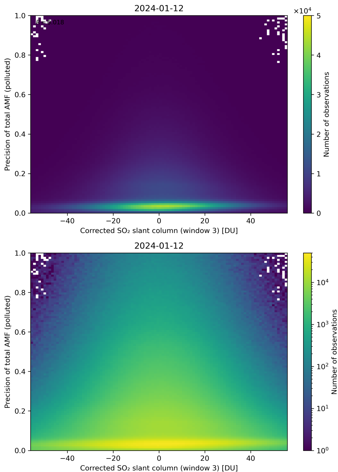
Figure 211: Scatter density plot of “Corrected SO 2 slant column (window 3)” against “Precision of total AMF (polluted)” for 2024-01-11 to 2024-01-13.
