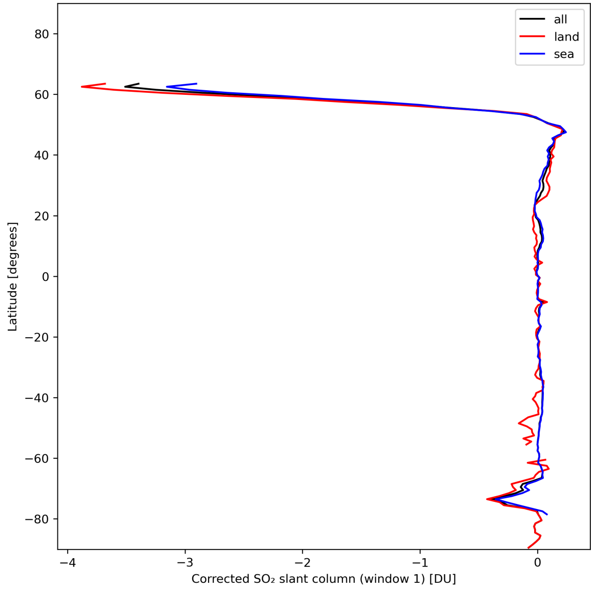
Figure 35: Zonal average of “Corrected SO 2 slant column (window 1)” for 2024-01-11 to 2024-01-13.
