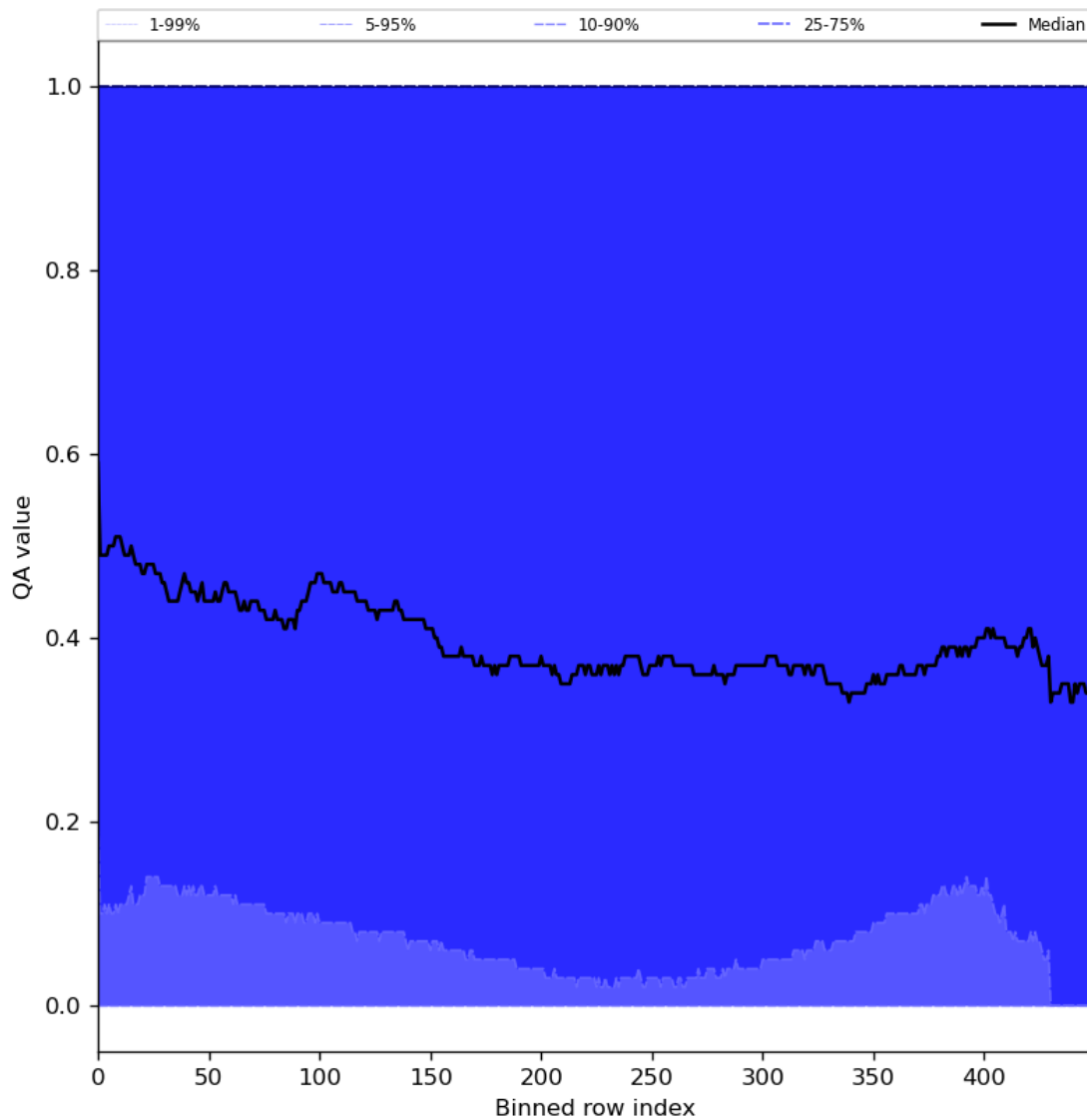
Figure 75: Along track statistics of “QA value” for 2024-01-11 to 2024-01-13
