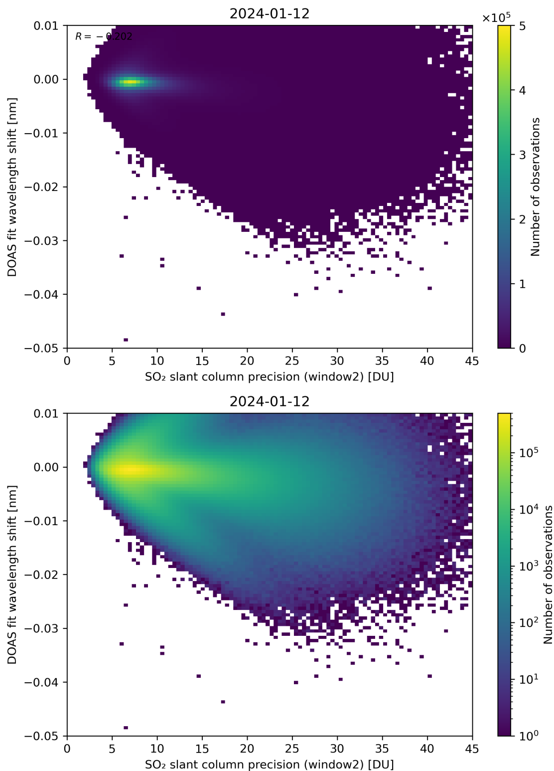
Figure 243: Scatter density plot of “SO 2 slant column precision (window2)” against “DOAS fit wavelength shift” for 2024-01-11 to 2024-01-13.
