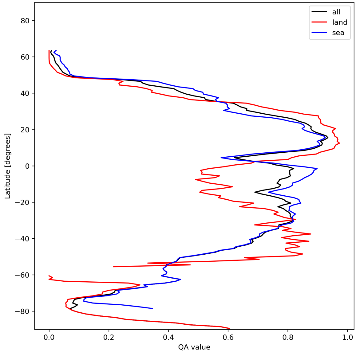
Figure 29: Zonal average of “QA value” for 2024-01-11 to 2024-01-13.
