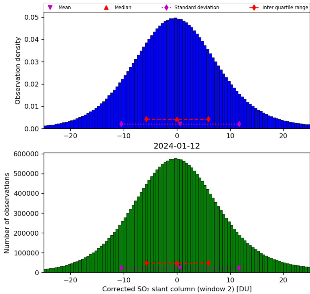
Figure 62: Histogram of “Corrected SO 2 slant column (window 2)” for 2024-01-11 to 2024-01-13
