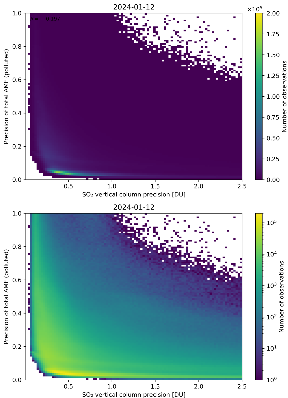
Figure 295: Scatter density plot of “SO 2 vertical column precision” against “Precision of total AMF (polluted)” for 2024-01-11 to 2024-01-13.
