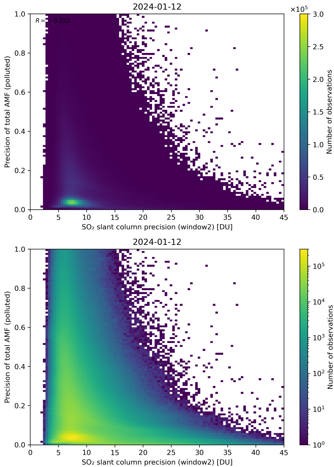
Figure 252: Scatter density plot of “SO 2 slant column precision (window2)” against “Precision of total AMF (polluted)” for 2024-01-11 to 2024-01-13.
