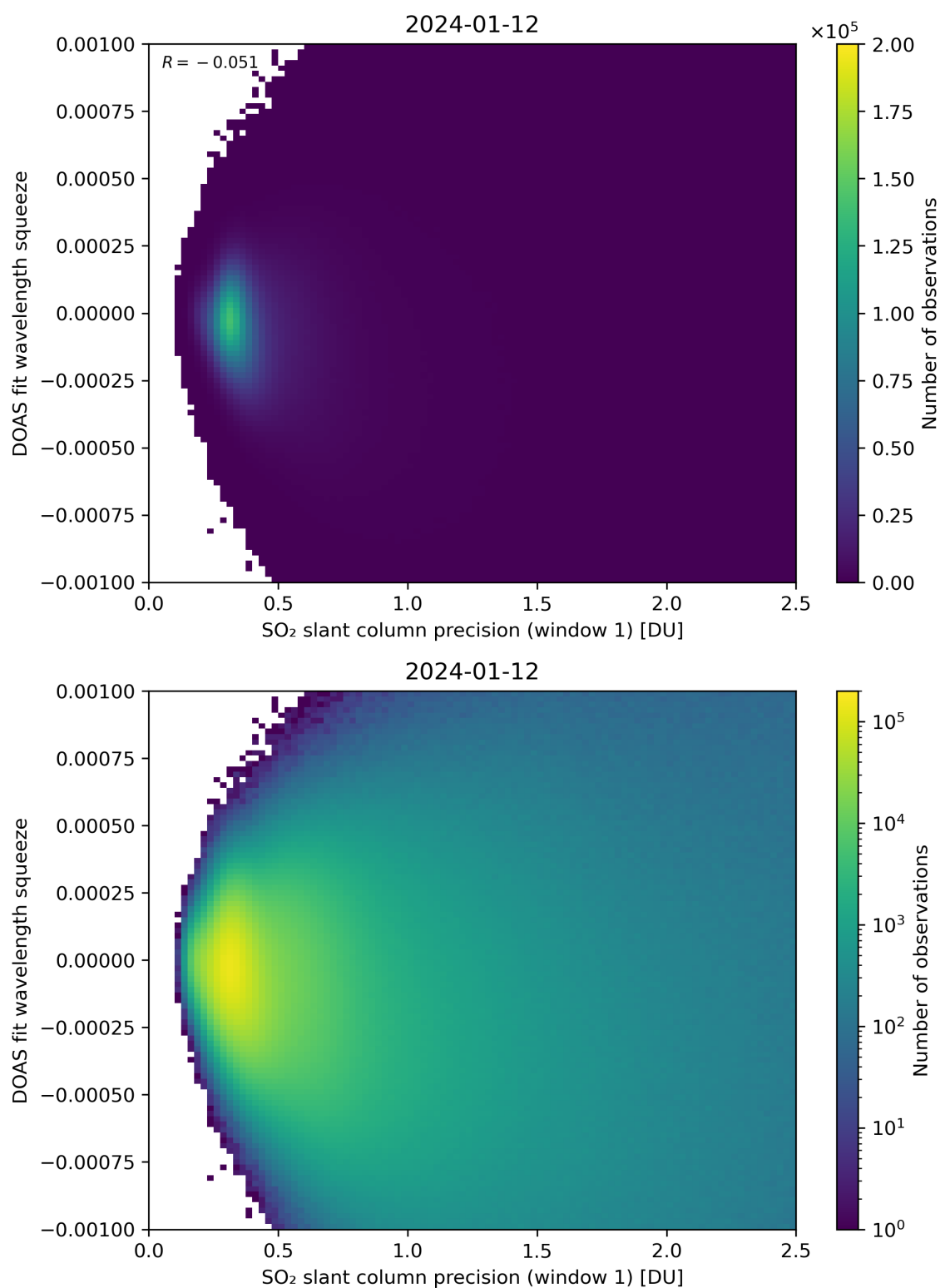
Figure 222: Scatter density plot of “SO 2 slant column precision (window 1)” against “DOAS fit wavelength squeeze” for 2024-01-11 to 2024-01-13.
