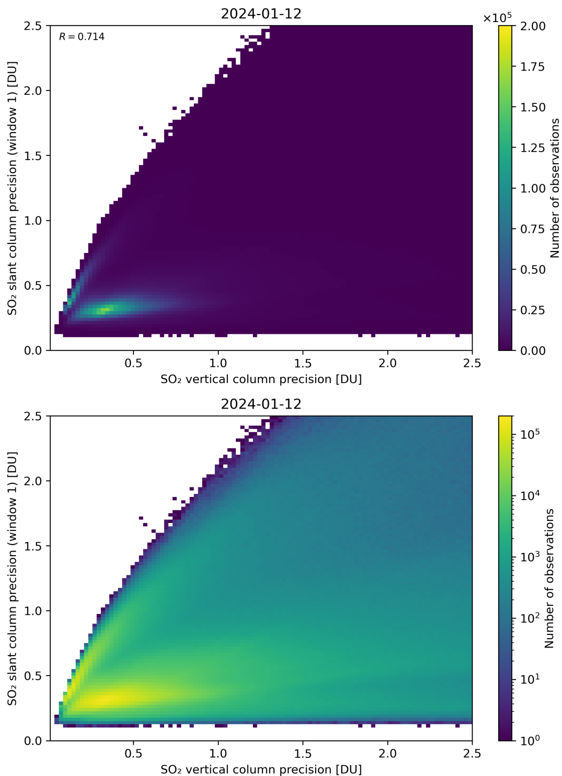
Figure 290: Scatter density plot of “SO 2 vertical column precision” against “SO 2 slant column precision (window 1)” for 2024-01-11 to 2024-01-13.
