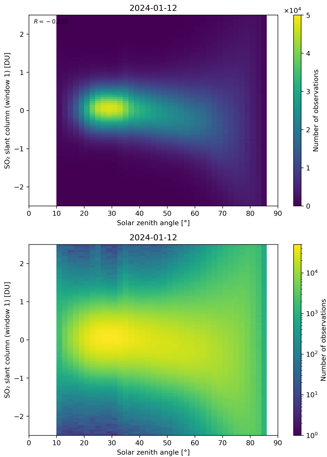
Figure 169: Scatter density plot of “Solar zenith angle” against “SO 2 slant column (window 1)” for 2024-01-11 to 2024-01-13.
