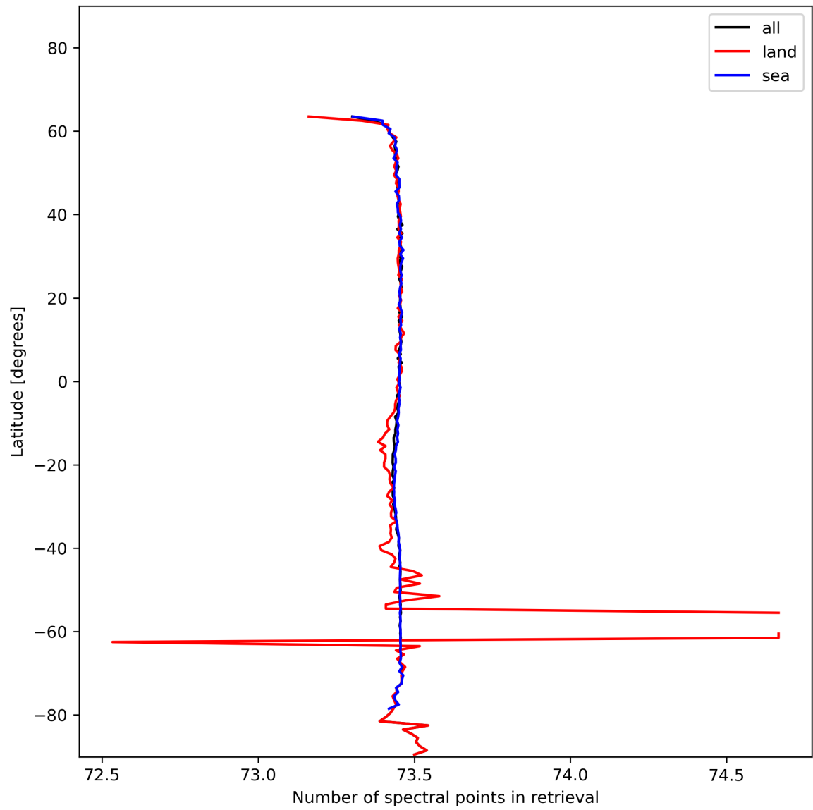
Figure 51: Zonal average of “Number of spectral points in retrieval” for 2024-01-11 to 2024-01-13.
