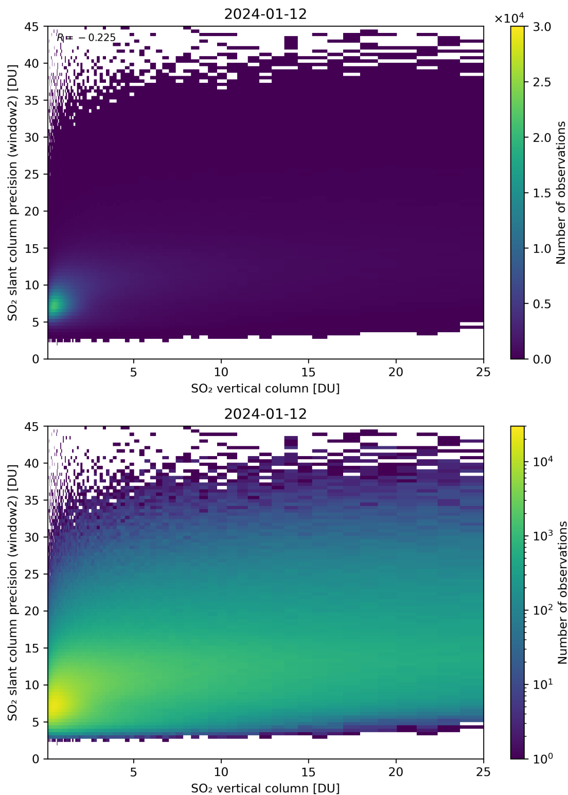
Figure 302: Scatter density plot of “SO 2 vertical column” against “SO 2 slant column precision (window2)” for 2024-01-11 to 2024-01-13.
