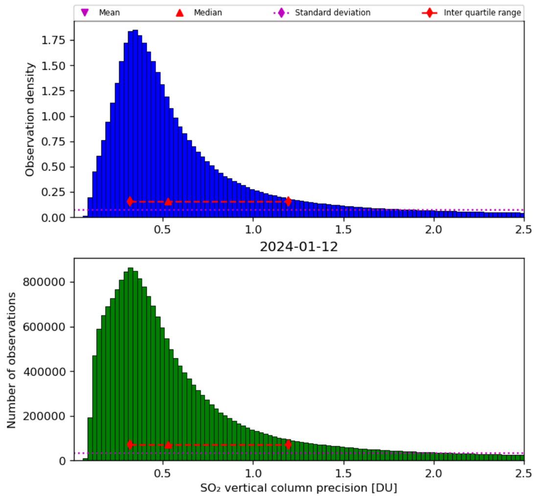
Figure 54: Histogram of “SO 2 vertical column precision” for 2024-01-11 to 2024-01-13
