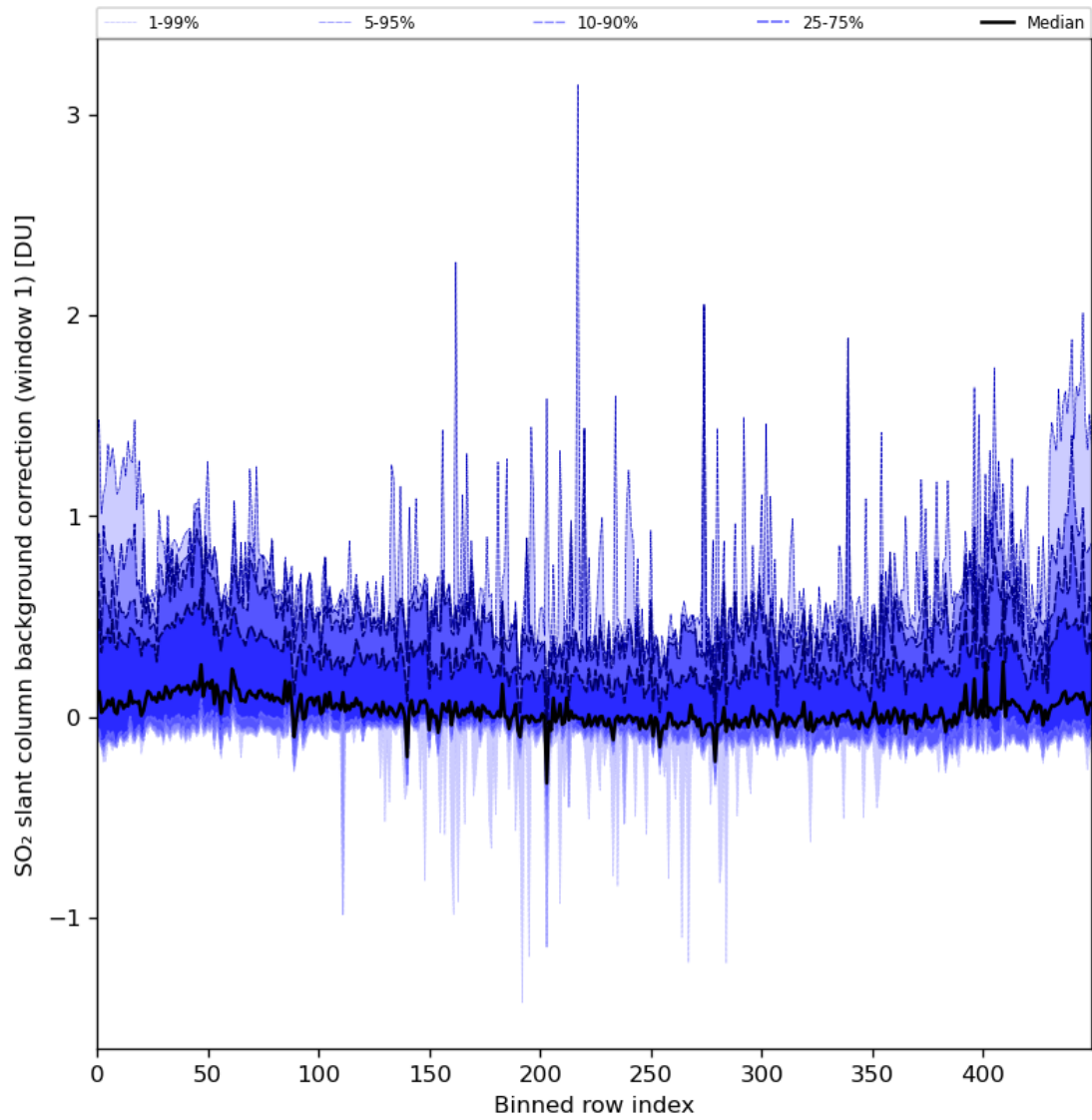
Figure 82: Along track statistics of “SO 2 slant column background correction (window 1)” for 2024-01-11 to 2024-01-13
