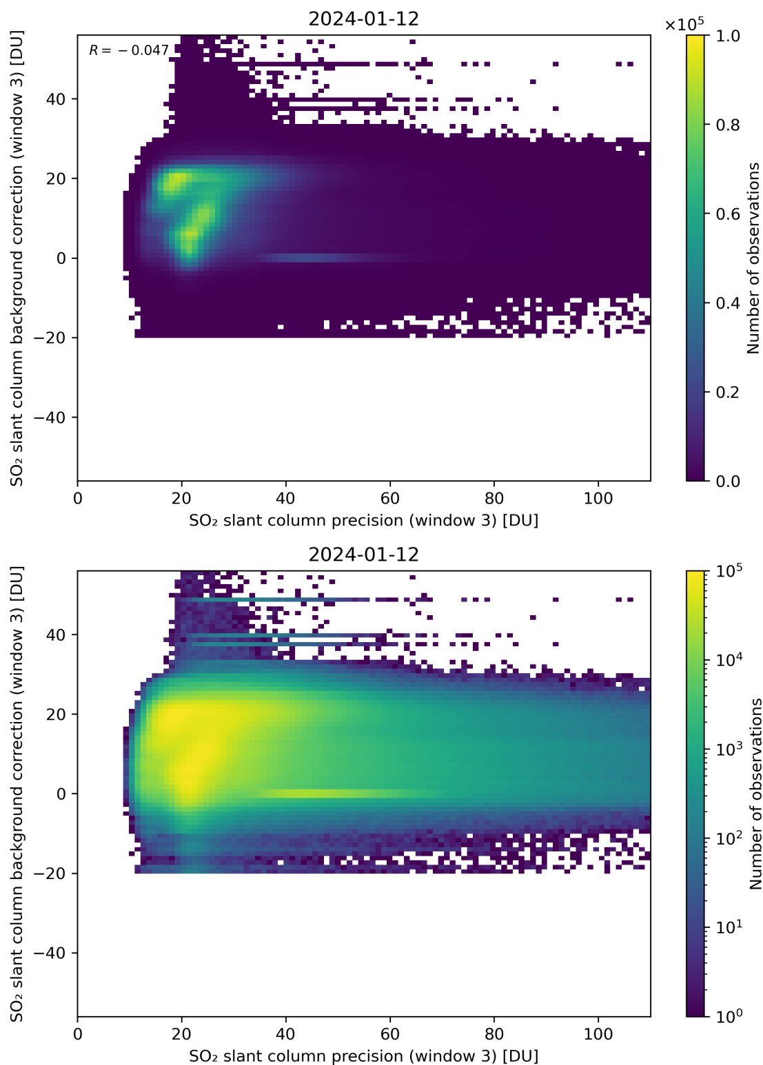
Figure 257: Scatter density plot of “SO 2 slant column precision (window 3)” against “SO 2 slant column background correction (window 3)” for 2024-01-11 to 2024-01-13.
