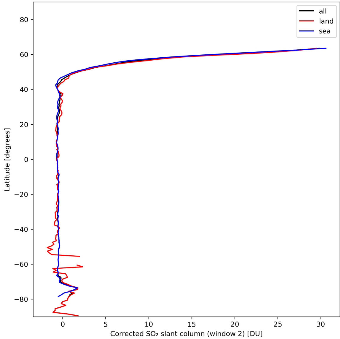
Figure 39: Zonal average of “Corrected SO 2 slant column (window 2)” for 2024-01-11 to 2024-01-13.
