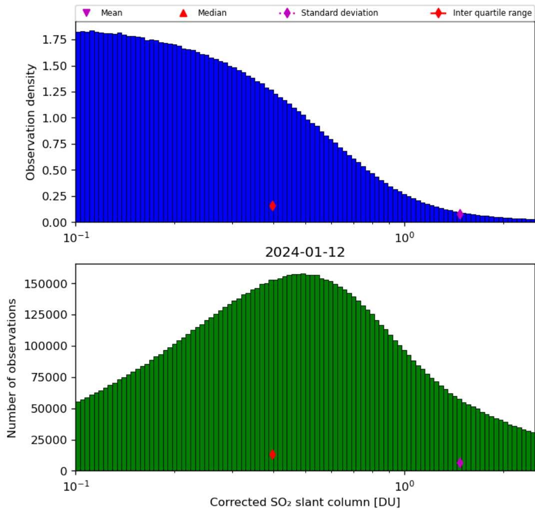
Figure 55: Histogram of “Corrected SO 2 slant column” for 2024-01-11 to 2024-01-13
