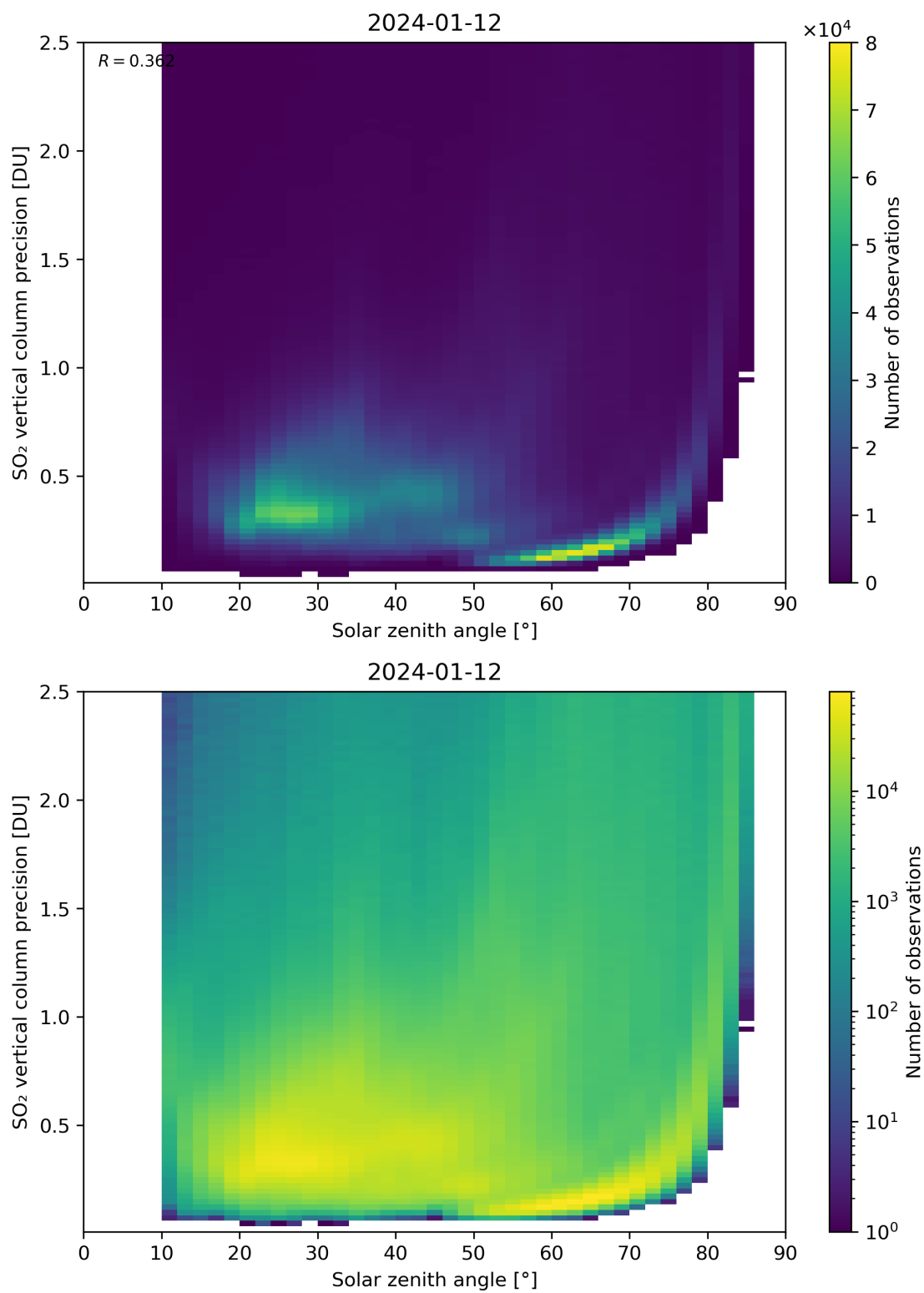
Figure 177: Scatter density plot of “Solar zenith angle” against “SO 2 vertical column precision” for 2024-01-11 to 2024-01-13.
