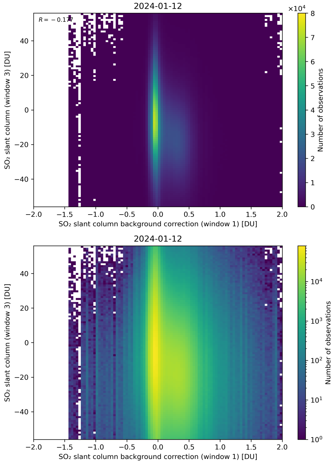
Figure 107: Scatter density plot of “SO 2 slant column background correction (window 1)” against “SO 2 slant column (window 3)” for 2024-01-11 to 2024-01-13.
