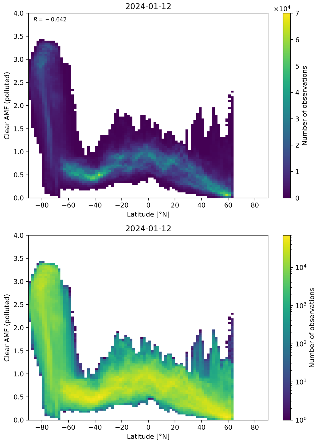
Figure 145: Scatter density plot of “Latitude” against “Clear AMF (polluted)” for 2024-01-11 to 2024-01-13.
