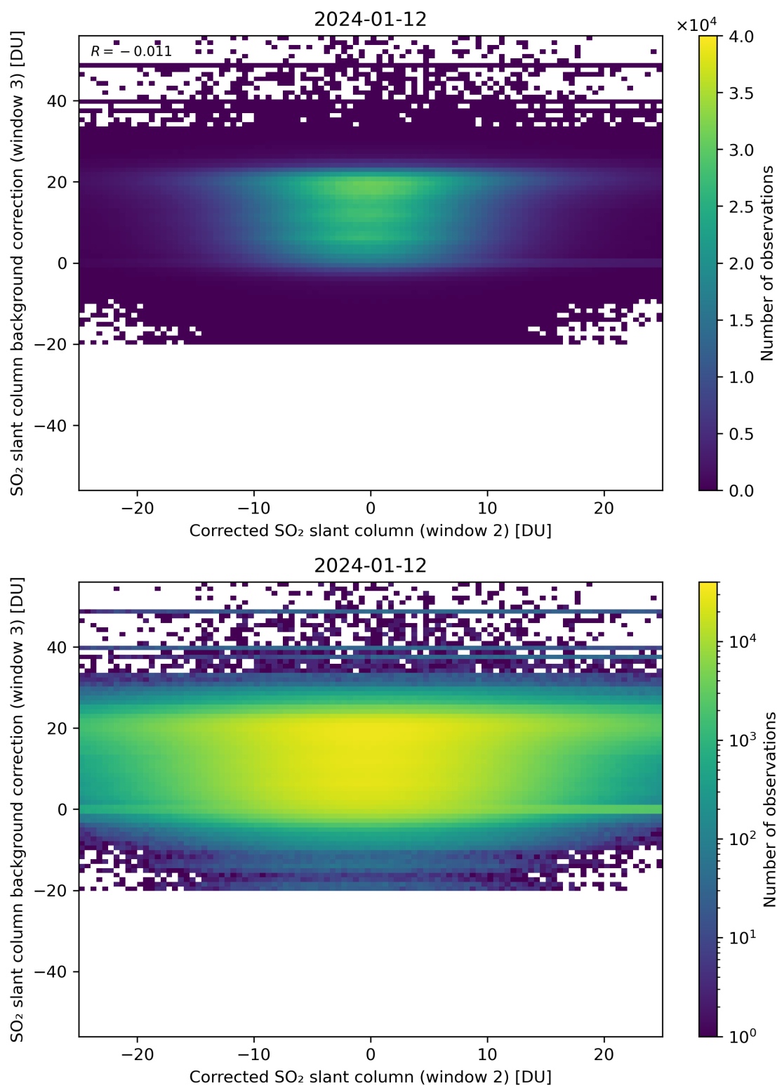
Figure 195: Scatter density plot of “Corrected SO 2 slant column (window 2)” against “SO 2 slant column background correction (window 3)” for 2024-01-11 to 2024-01-13.
