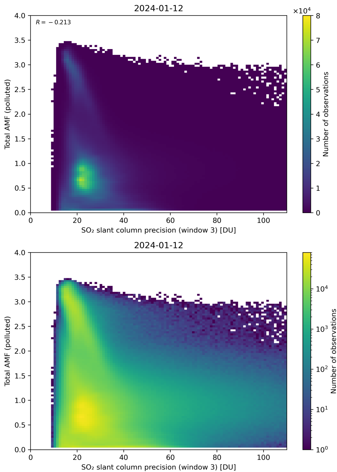
Figure 263: Scatter density plot of “SO 2 slant column precision (window 3)” against “Total AMF (polluted)” for 2024-01-11 to 2024-01-13.
