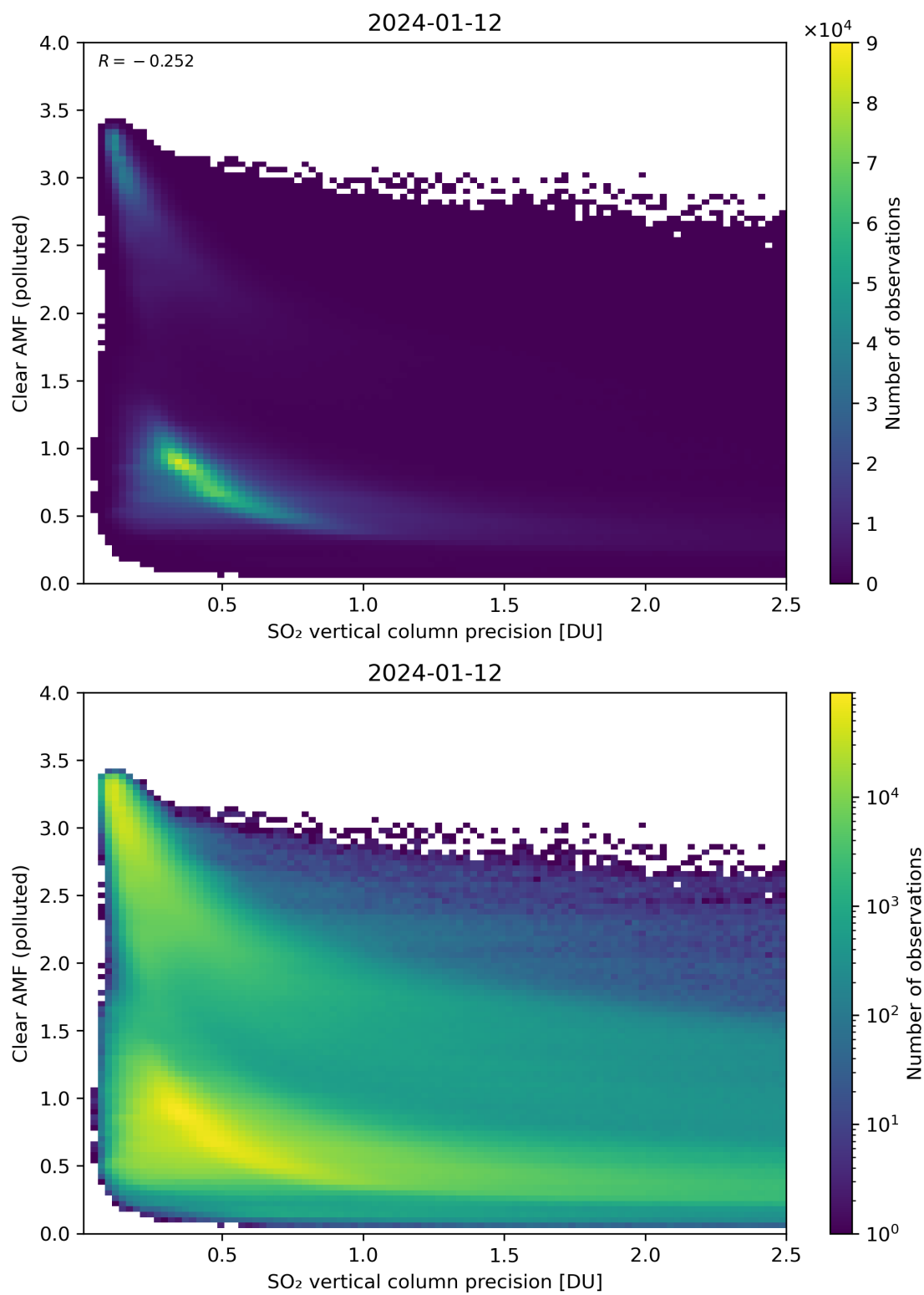
Figure 285: Scatter density plot of “SO 2 vertical column precision” against “Clear AMF (polluted)” for 2024-01-11 to 2024-01-13.
