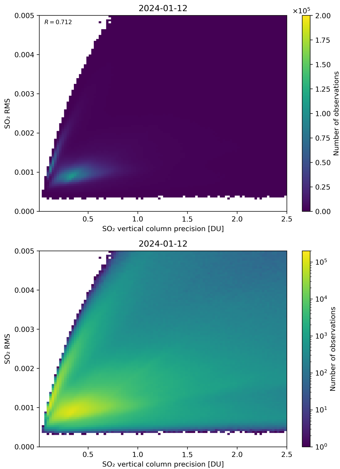
Figure 284: Scatter density plot of “SO 2 vertical column precision” against “SO 2 RMS” for 2024-01-11 to 2024-01-13.
