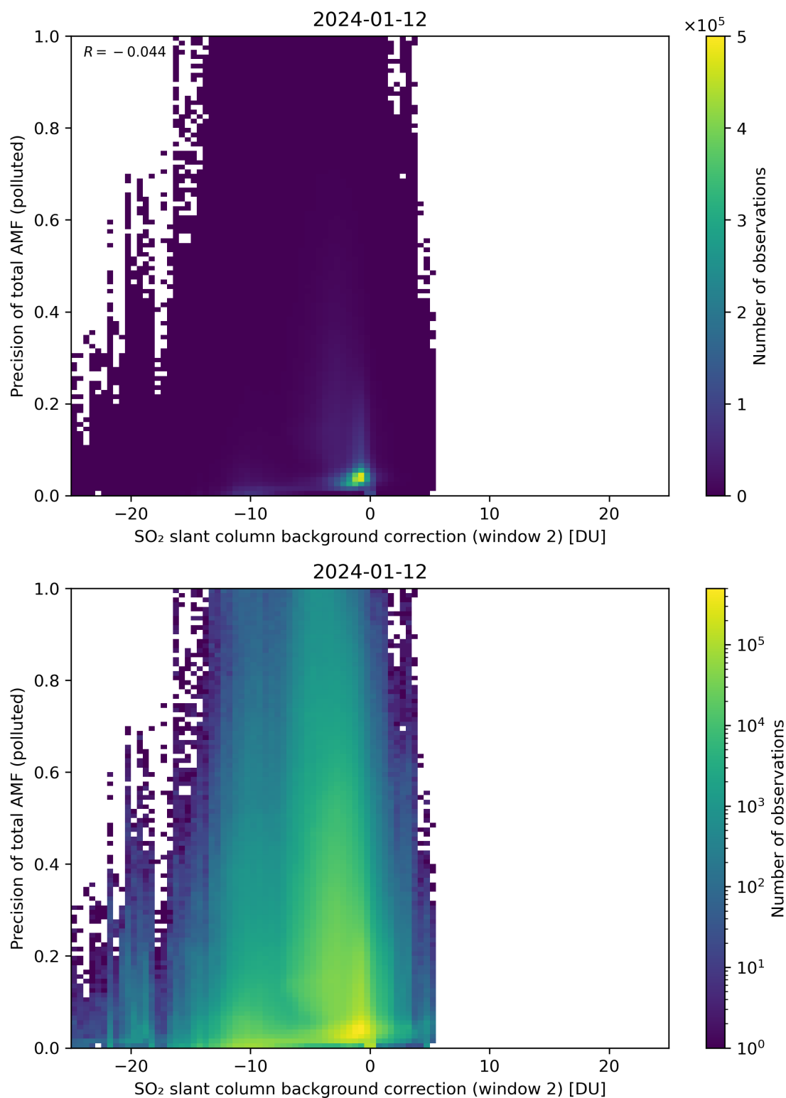
Figure 120: Scatter density plot of “SO 2 slant column background correction (window 2)” against “Precision of total AMF (polluted)” for 2024-01-11 to 2024-01-13.
