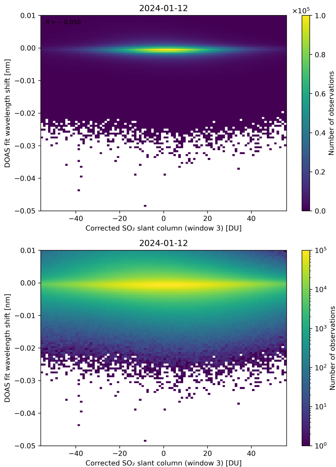
Figure 206: Scatter density plot of “Corrected SO 2 slant column (window 3)” against “DOAS fit wavelength shift” for 2024-01-11 to 2024-01-13.
