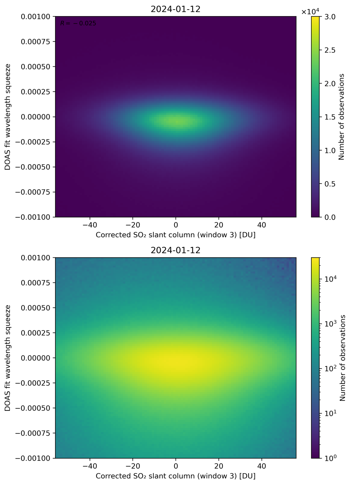
Figure 207: Scatter density plot of “Corrected SO 2 slant column (window 3)” against “DOAS fit wavelength squeeze” for 2024-01-11 to 2024-01-13.
