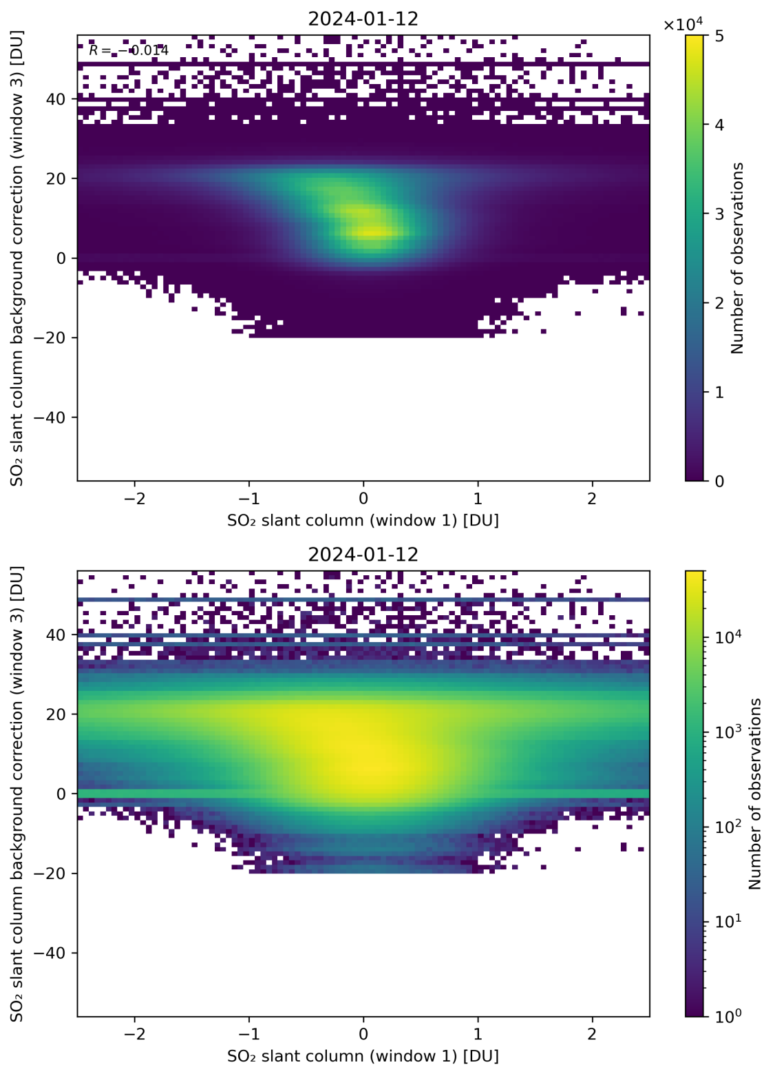
Figure 214: Scatter density plot of “SO 2 slant column (window 1)” against “SO 2 slant column background correction (window 3)” for 2024-01-11 to 2024-01-13.
