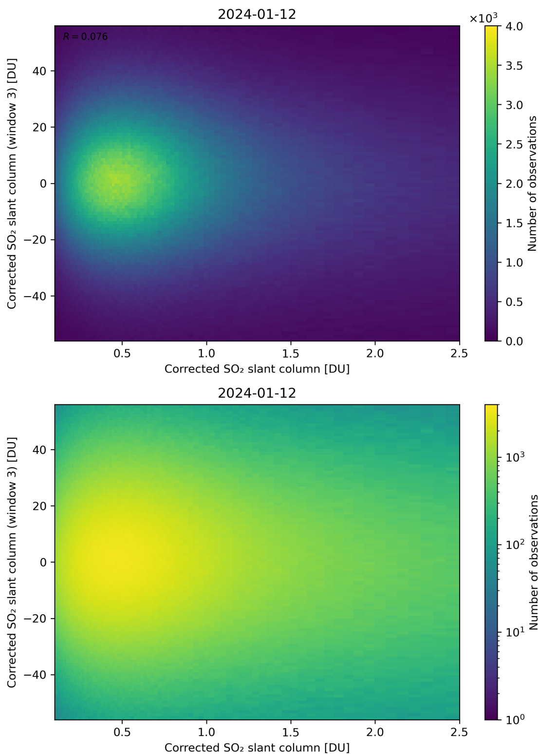
Figure 186: Scatter density plot of “Corrected SO 2 slant column” against “Corrected SO 2 slant column (window 3)” for 2024-01-11 to 2024-01-13.
