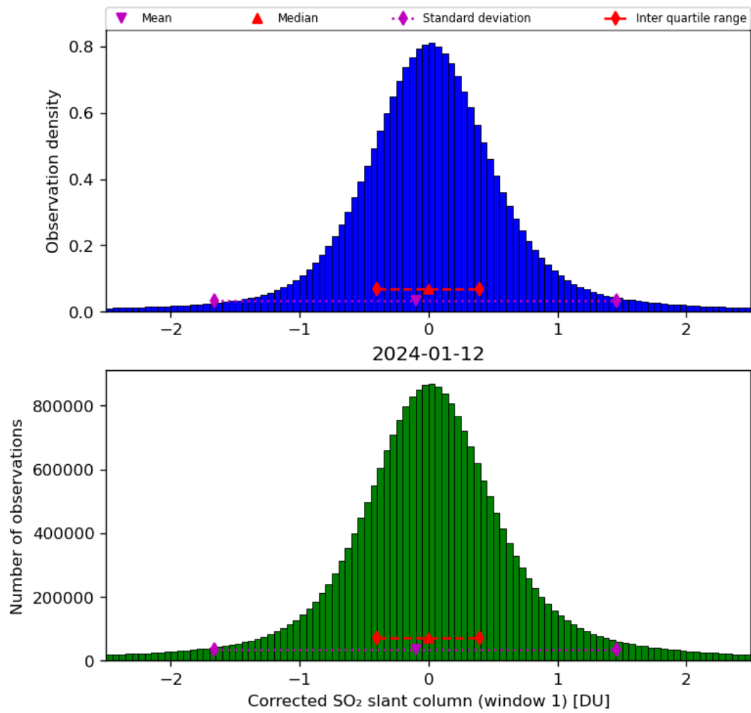
Figure 58: Histogram of “Corrected SO 2 slant column (window 1)” for 2024-01-11 to 2024-01-13
