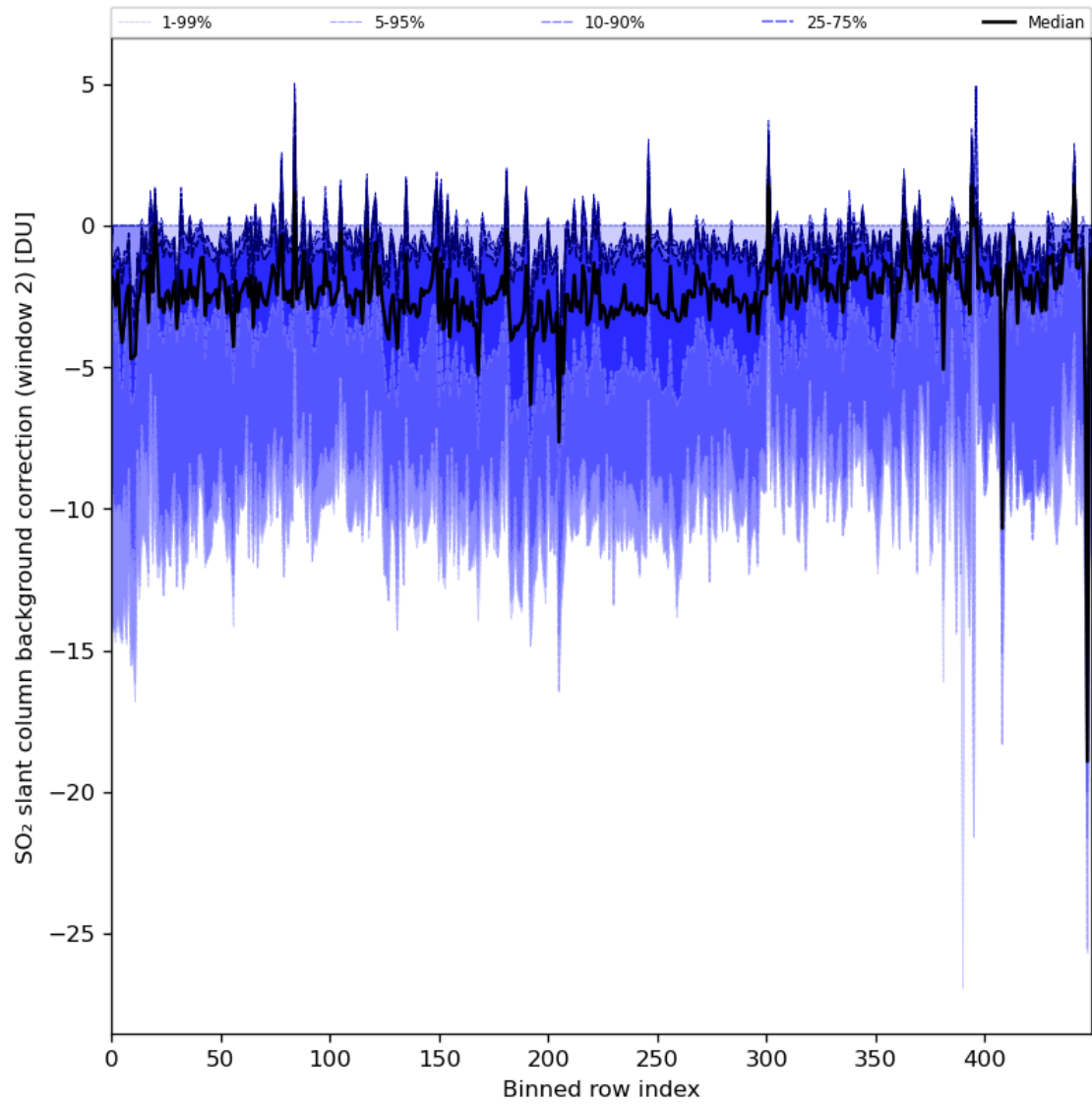
Figure 86: Along track statistics of “SO 2 slant column background correction (window 2)” for 2024-01-11 to 2024-01-13
