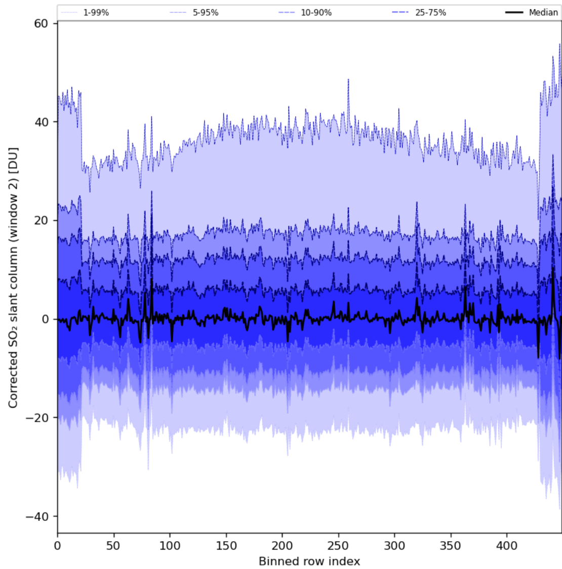
Figure 85: Along track statistics of “Corrected SO 2 slant column (window 2)” for 2024-01-11 to 2024-01-13
