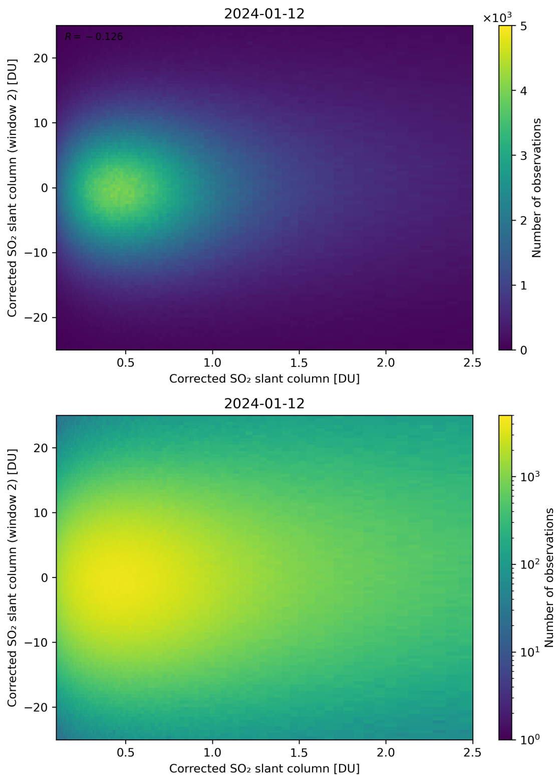
Figure 185: Scatter density plot of “Corrected SO 2 slant column” against “Corrected SO 2 slant column (window 2)” for 2024-01-11 to 2024-01-13.
