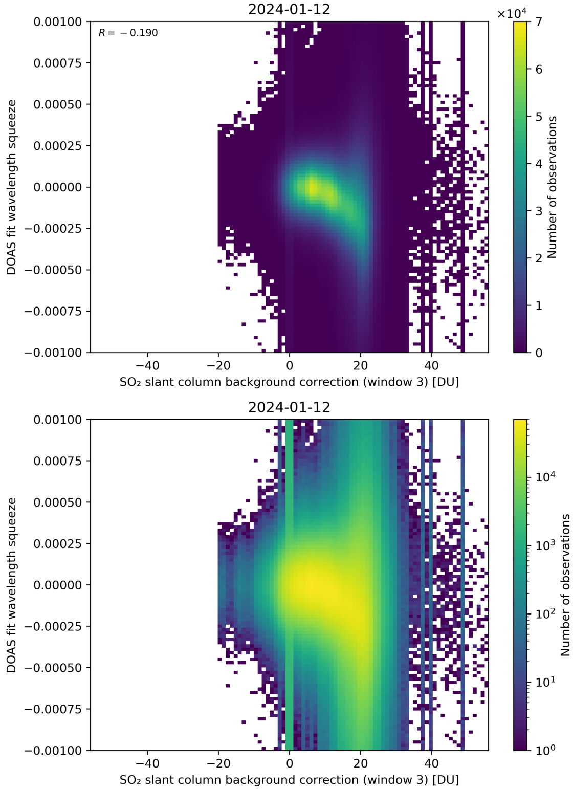
Figure 122: Scatter density plot of “SO 2 slant column background correction (window 3)” against “DOAS fit wavelength squeeze” for 2024-01-11 to 2024-01-13.
