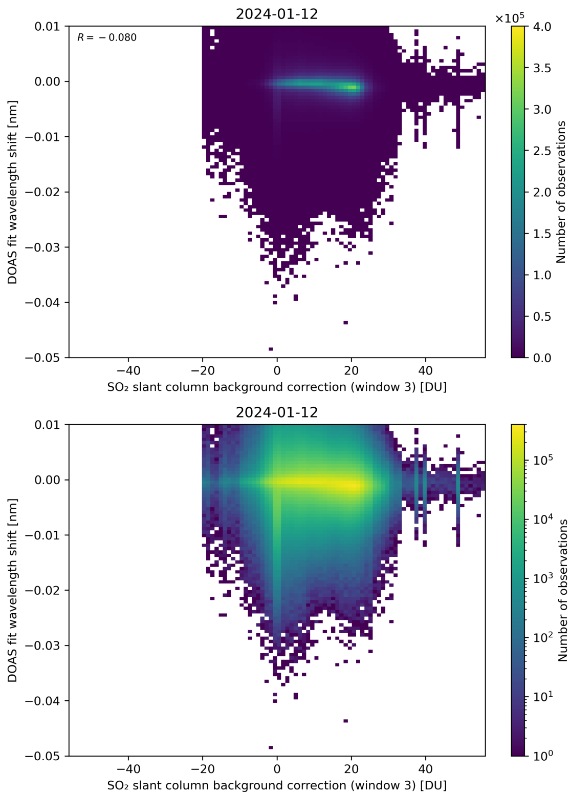
Figure 121: Scatter density plot of “SO 2 slant column background correction (window 3)” against “DOAS fit wavelength shift” for 2024-01-11 to 2024-01-13.
