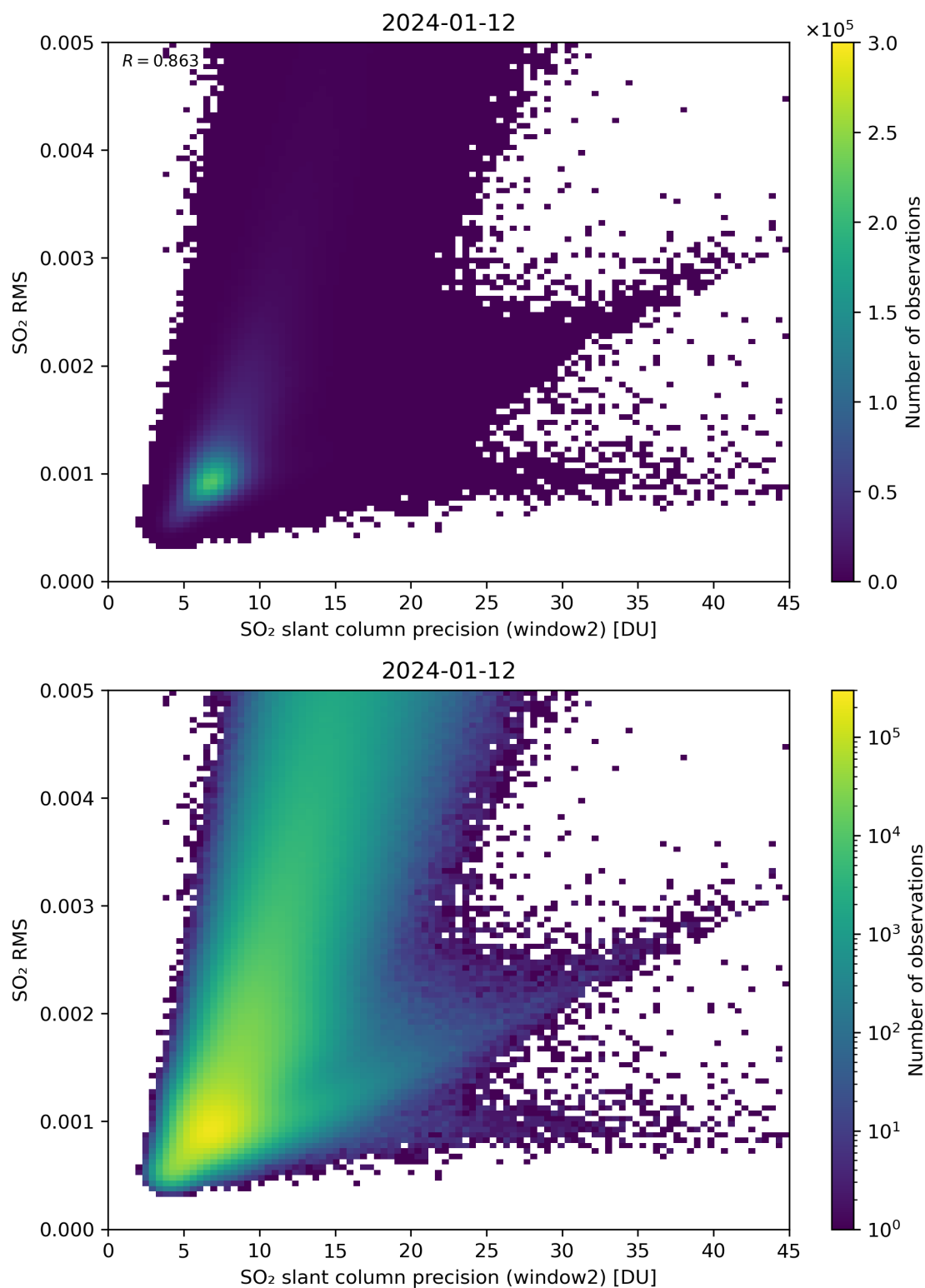
Figure 245: Scatter density plot of “SO 2 slant column precision (window2)” against “SO 2 RMS” for 2024-01-11 to 2024-01-13.
