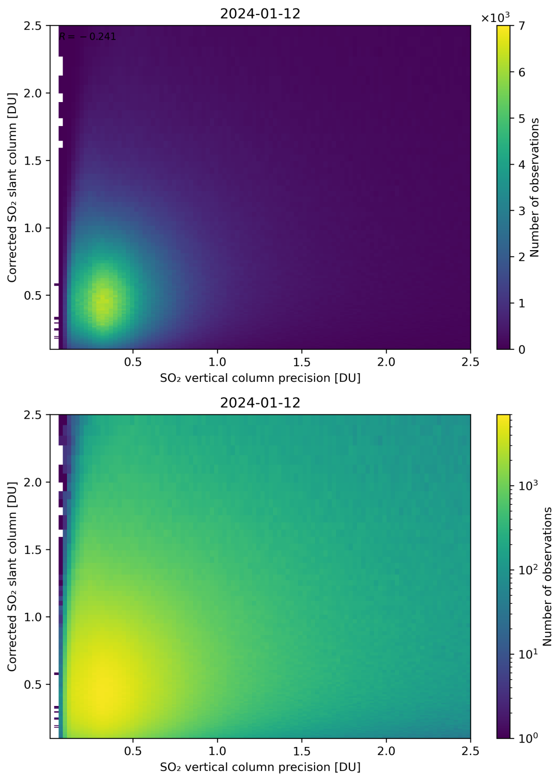
Figure 286: Scatter density plot of “SO 2 vertical column precision” against “Corrected SO 2 slant column” for 2024-01-11 to 2024-01-13.
