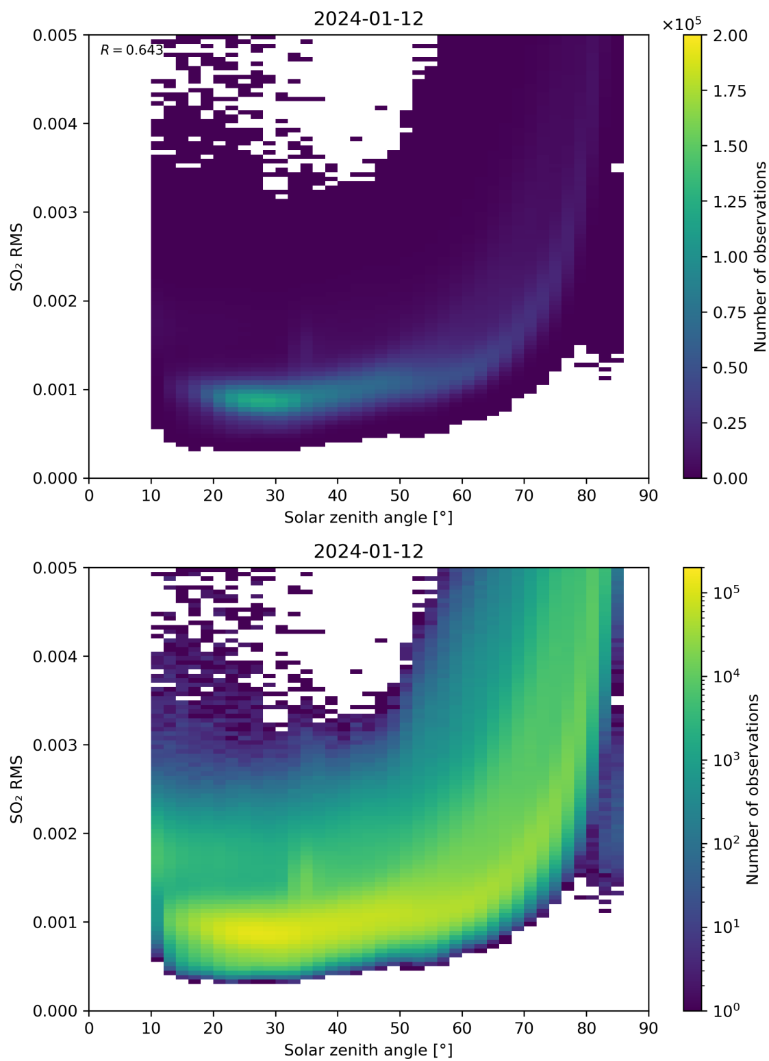
Figure 163: Scatter density plot of “Solar zenith angle” against “SO 2 RMS” for 2024-01-11 to 2024-01-13.
