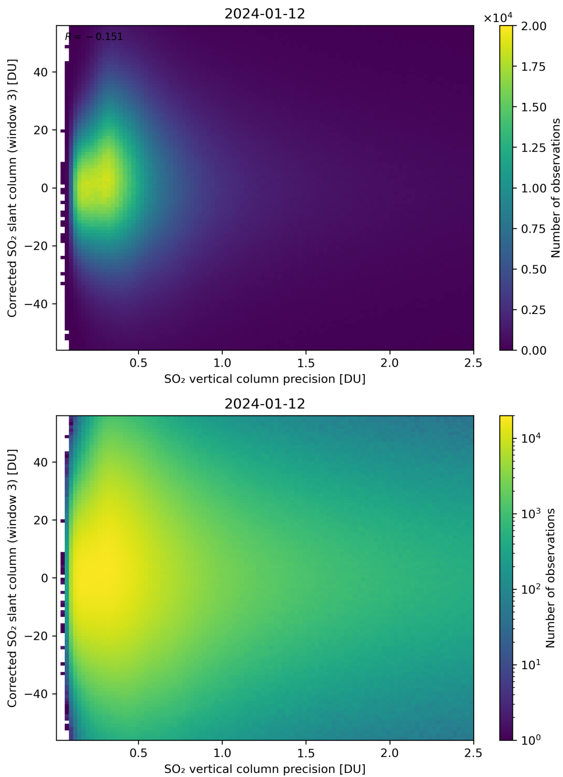
Figure 288: Scatter density plot of “SO 2 vertical column precision” against “Corrected SO 2 slant column (window 3)” for 2024-01-11 to 2024-01-13.
