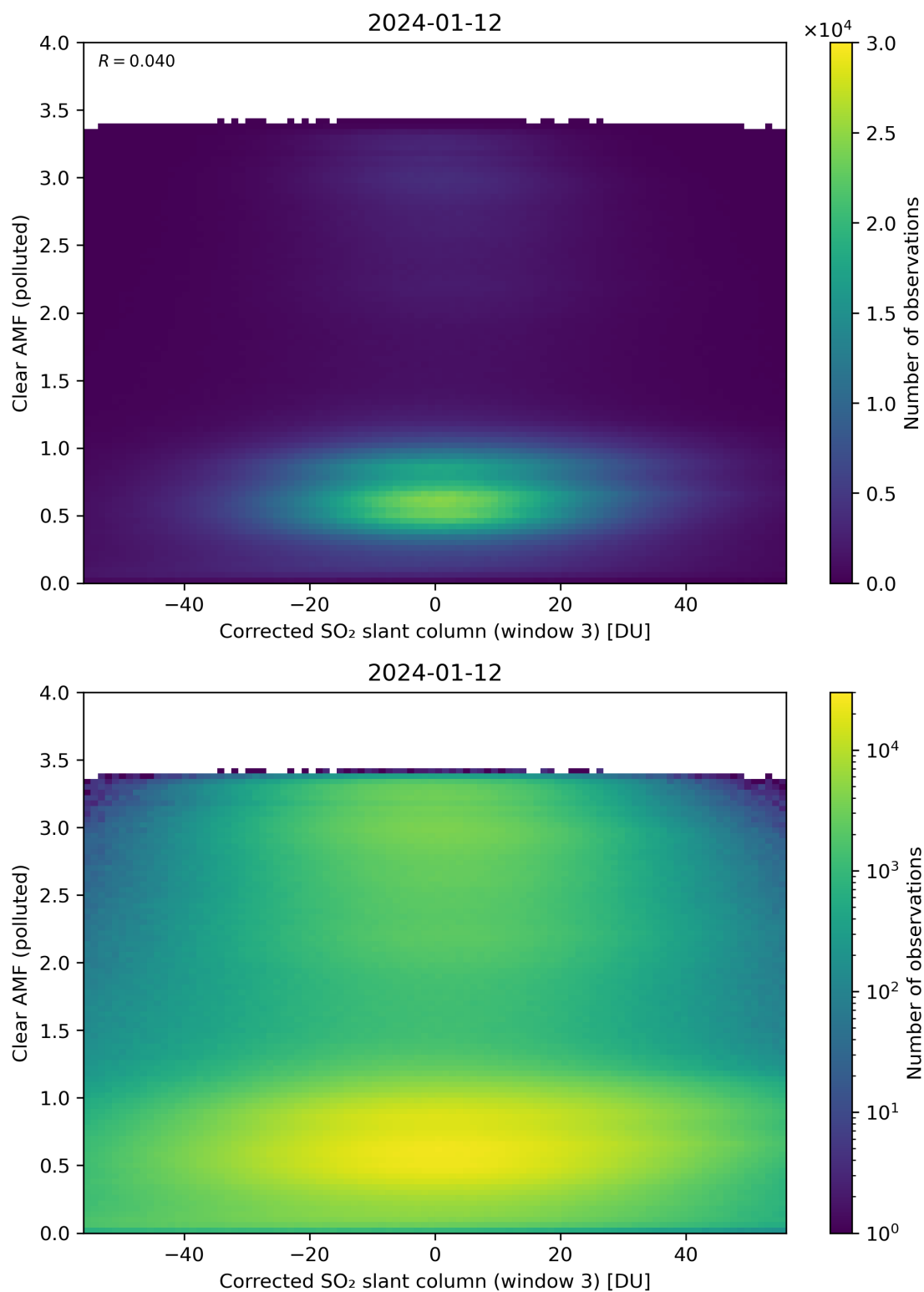
Figure 209: Scatter density plot of “Corrected SO 2 slant column (window 3)” against “Clear AMF (polluted)” for 2024-01-11 to 2024-01-13.
