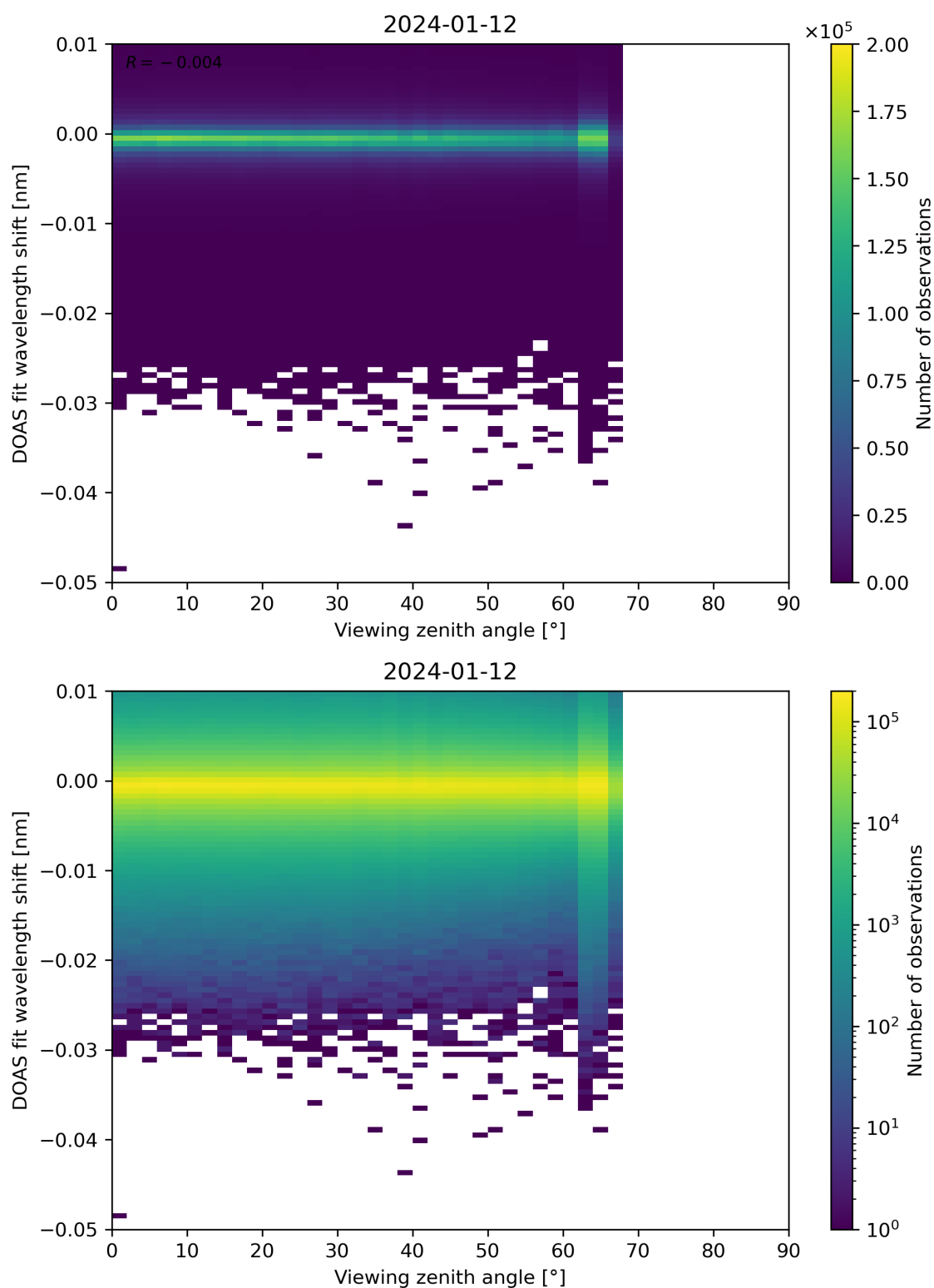
Figure 311: Scatter density plot of “Viewing zenith angle” against “DOAS fit wavelength shift” for 2024-01-11 to 2024-01-13.
