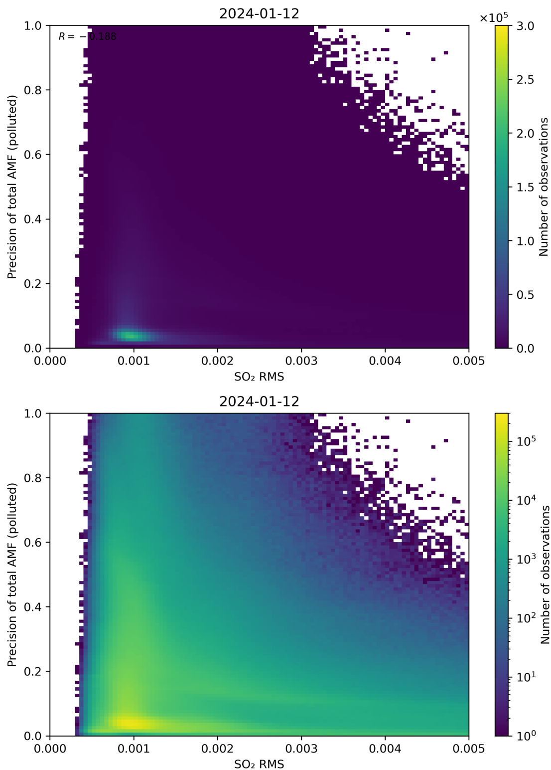
Figure 138: Scatter density plot of “SO 2 RMS” against “Precision of total AMF (polluted)” for 2024-01-11 to 2024-01-13.
