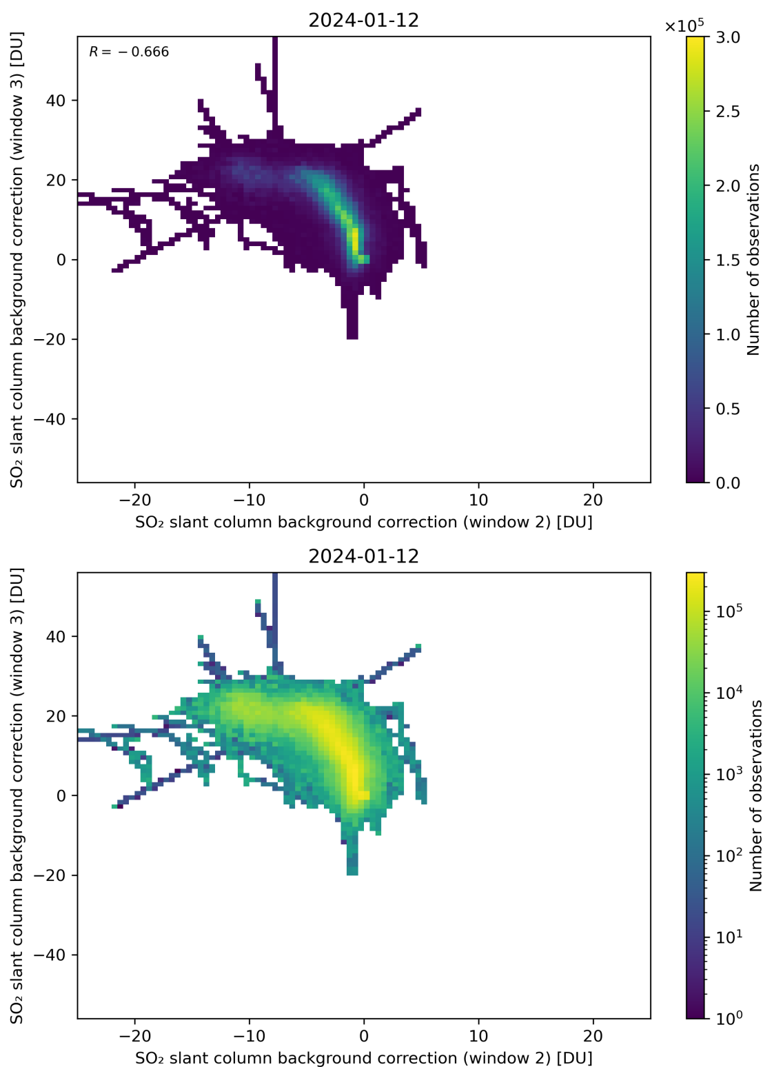
Figure 111: Scatter density plot of “SO 2 slant column background correction (window 2)” against “SO 2 slant column background correction (window 3)” for 2024-01-11 to 2024-01-13.
