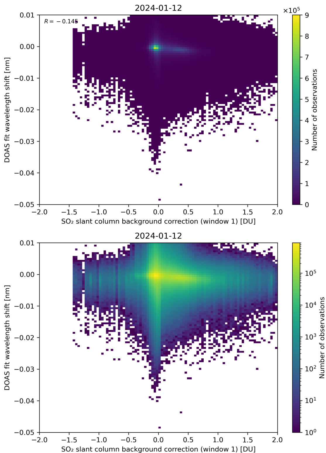
Figure 100: Scatter density plot of “SO 2 slant column background correction (window 1)” against “DOAS fit wavelength shift” for 2024-01-11 to 2024-01-13.
