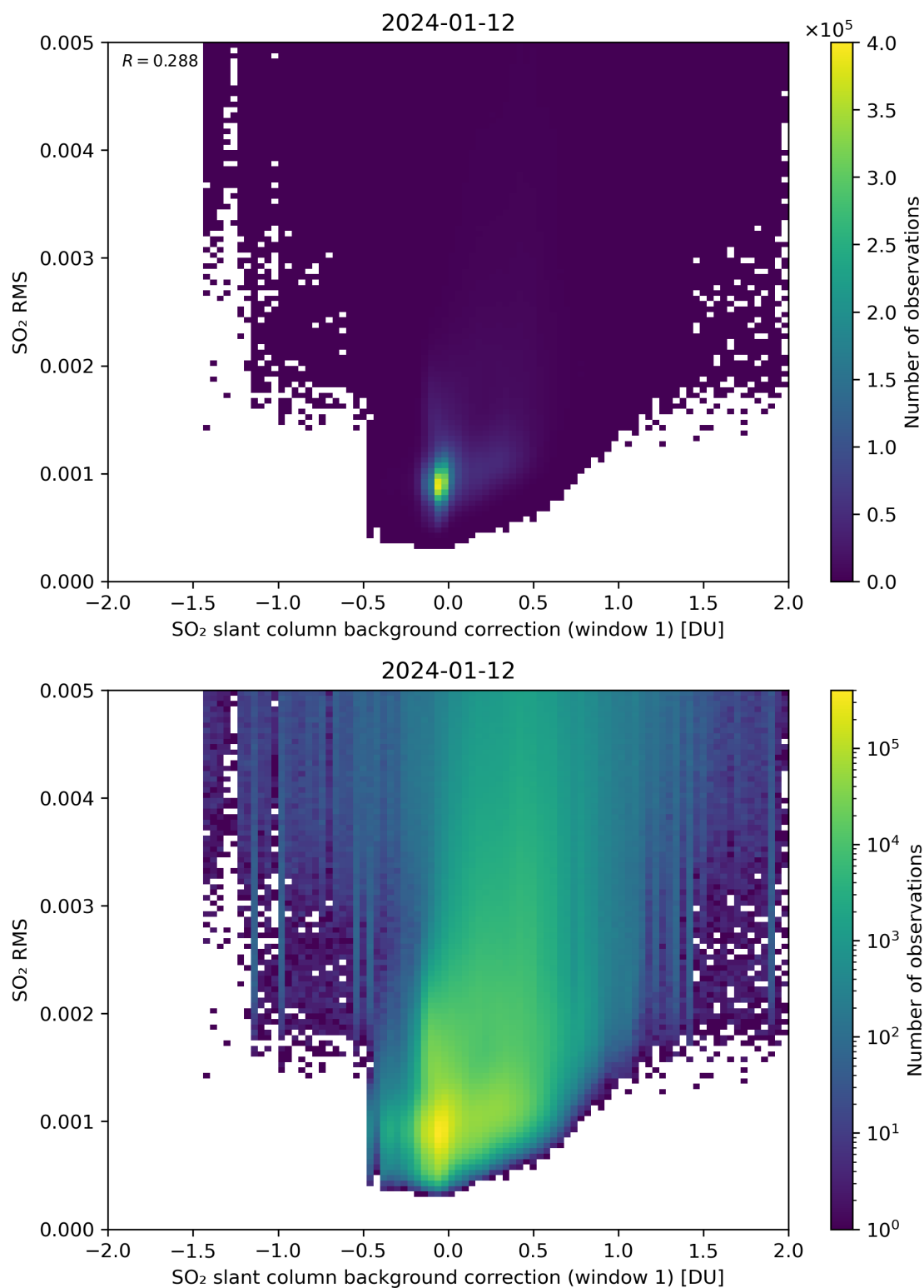
Figure 102: Scatter density plot of “SO 2 slant column background correction (window 1)” against “SO 2 RMS” for 2024-01-11 to 2024-01-13.
