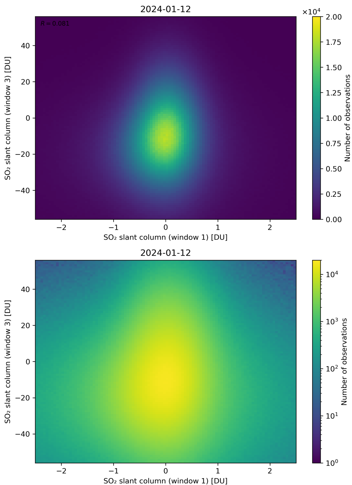
Figure 237: Scatter density plot of “SO 2 slant column (window 1)” against “SO 2 slant column (window 3)” for 2024-01-11 to 2024-01-13.
