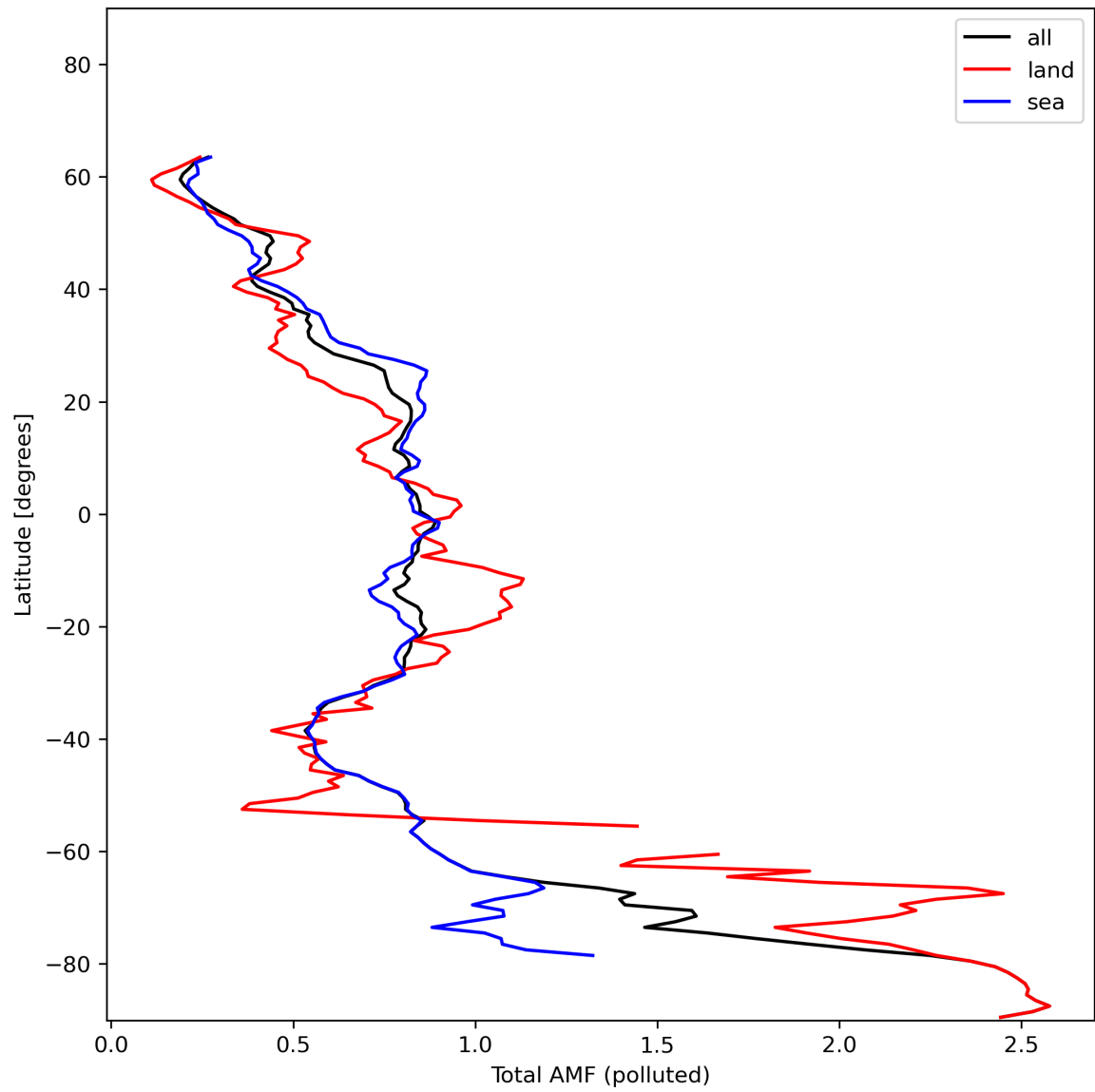
Figure 48: Zonal average of “Total AMF (polluted)” for 2024-01-11 to 2024-01-13.
