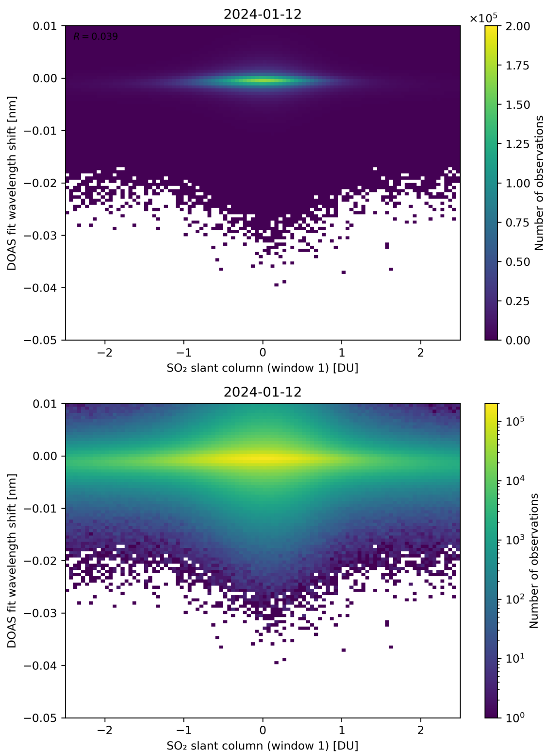
Figure 215: Scatter density plot of “SO 2 slant column (window 1)” against “DOAS fit wavelength shift” for 2024-01-11 to 2024-01-13.
