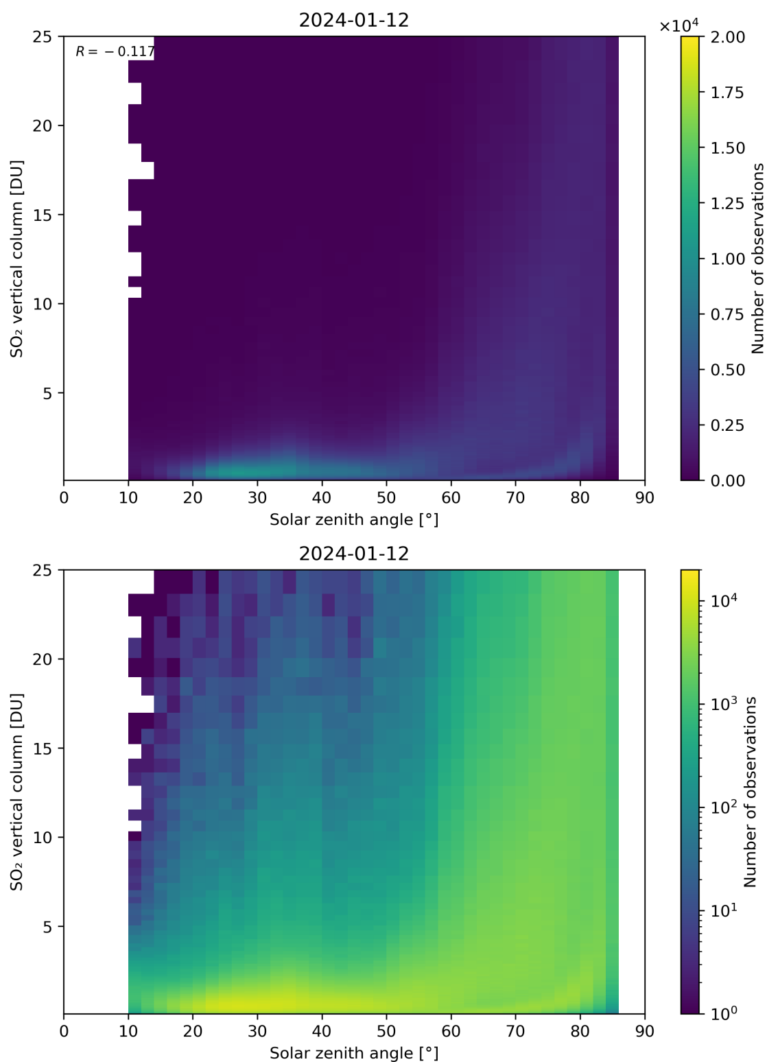
Figure 176: Scatter density plot of “Solar zenith angle” against “SO 2 vertical column” for 2024-01-11 to 2024-01-13.
