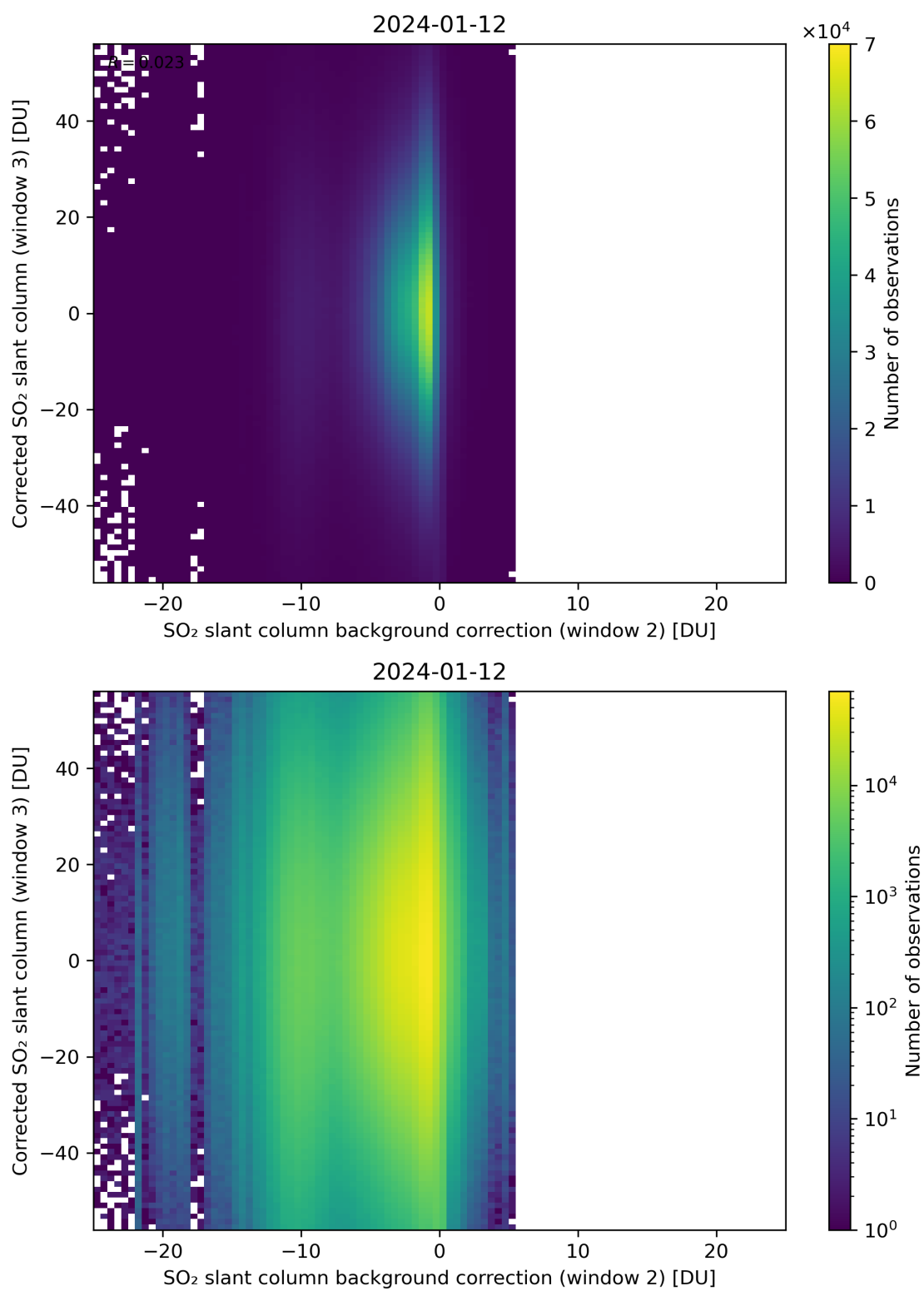
Figure 116: Scatter density plot of “SO 2 slant column background correction (window 2)” against “Corrected SO 2 slant column (window 3)” for 2024-01-11 to 2024-01-13.
