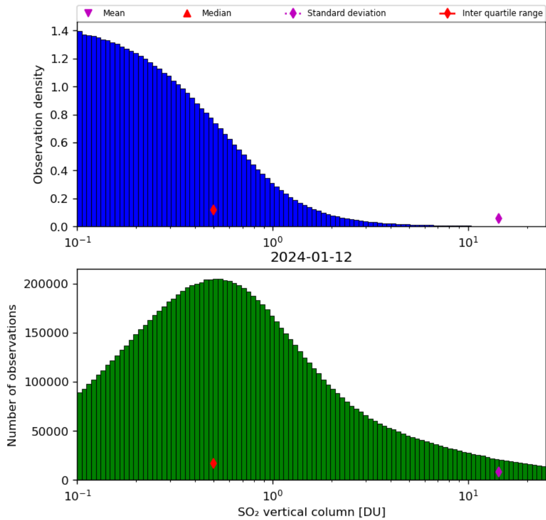
Figure 53: Histogram of “SO 2 vertical column” for 2024-01-11 to 2024-01-13
