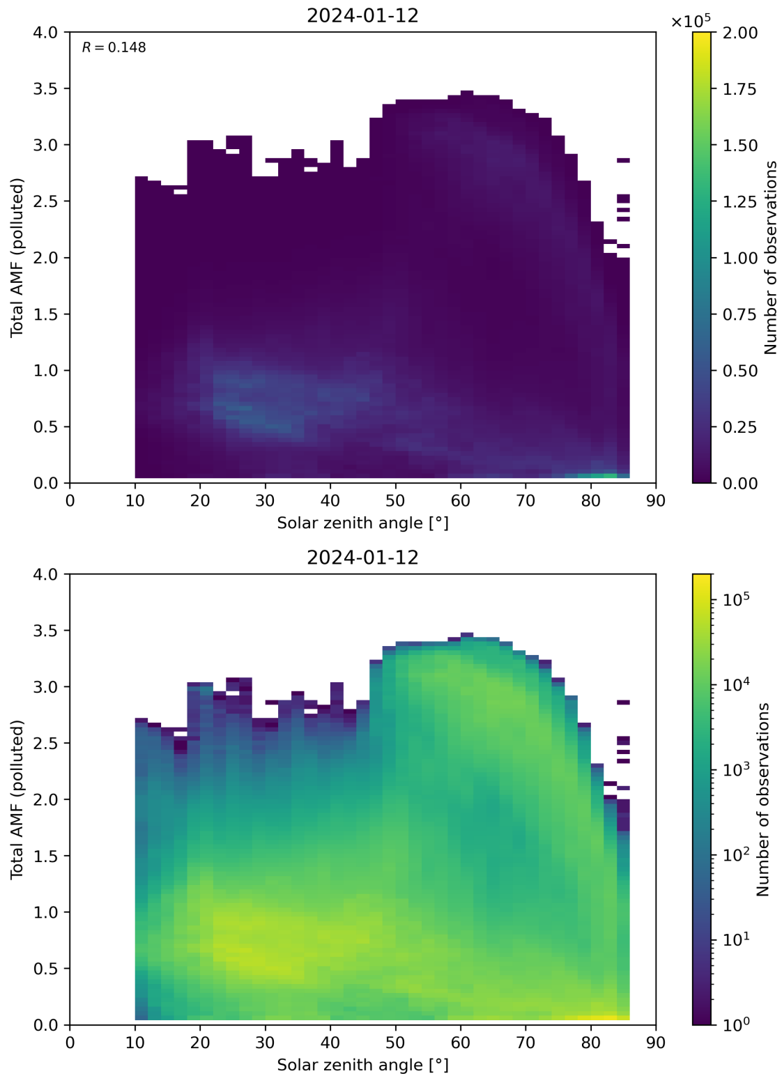
Figure 174: Scatter density plot of “Solar zenith angle” against “Total AMF (polluted)” for 2024-01-11 to 2024-01-13.
