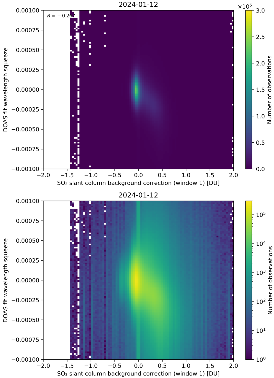
Figure 101: Scatter density plot of “SO 2 slant column background correction (window 1)” against “DOAS fit wavelength squeeze” for 2024-01-11 to 2024-01-13.
