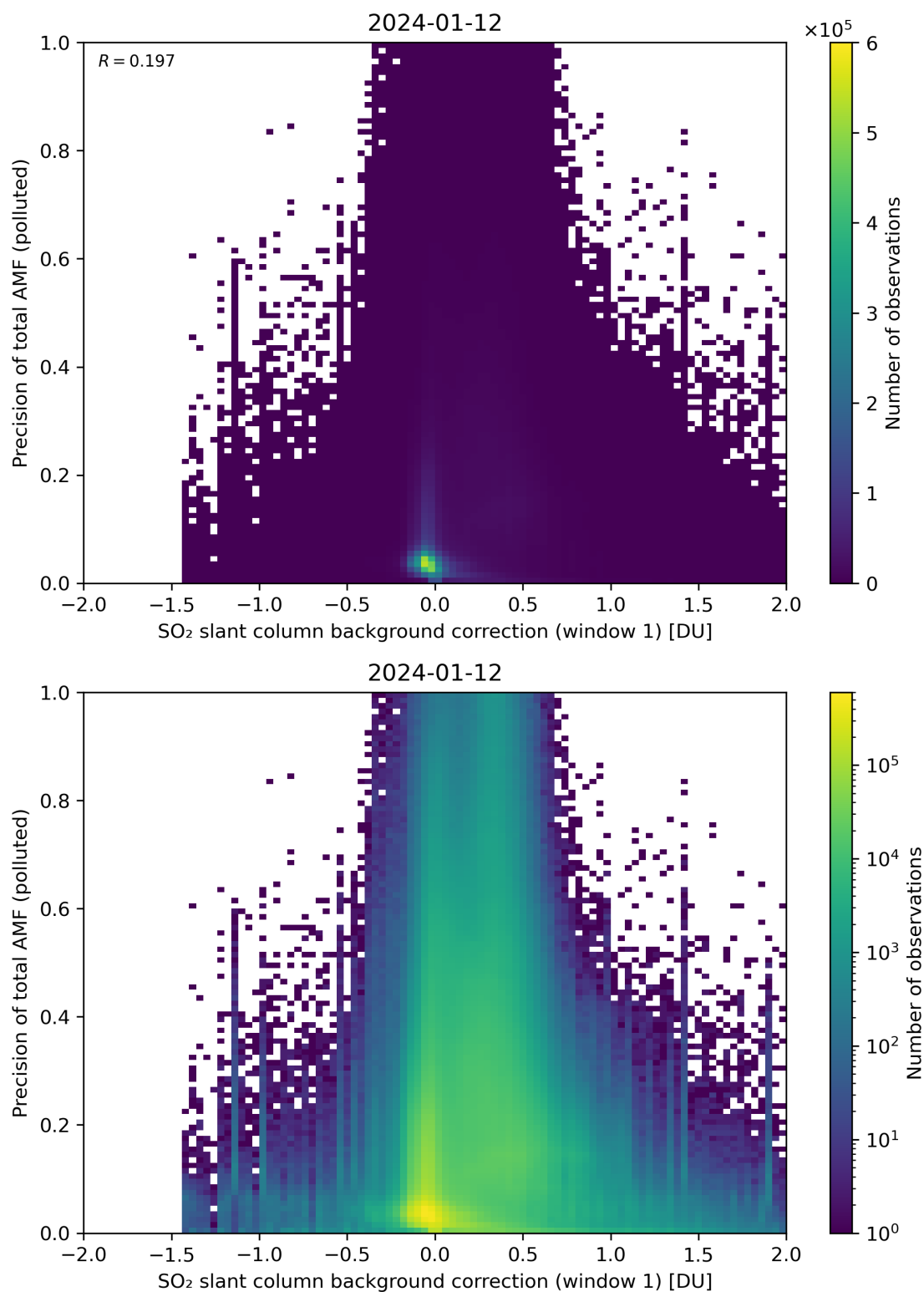
Figure 110: Scatter density plot of “SO 2 slant column background correction (window 1)” against “Precision of total AMF (polluted)” for 2024-01-11 to 2024-01-13.
