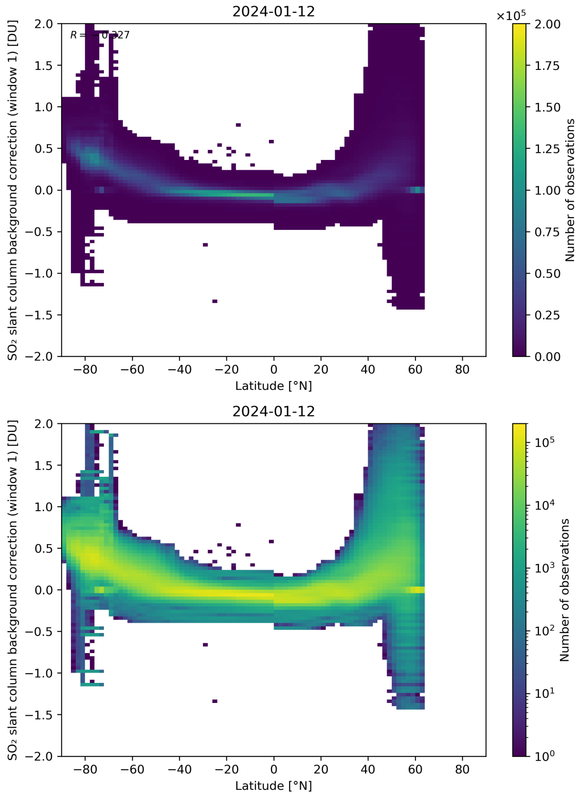
Figure 139: Scatter density plot of “Latitude” against “SO 2 slant column background correction (window 1)” for 2024-01-11 to 2024-01-13.
