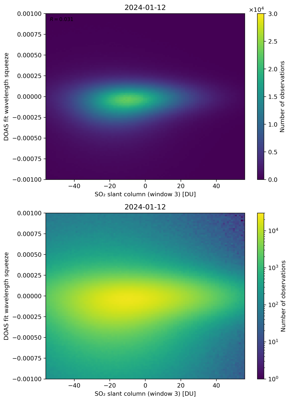
Figure 255: Scatter density plot of “SO 2 slant column (window 3)” against “DOAS fit wavelength squeeze” for 2024-01-11 to 2024-01-13.
