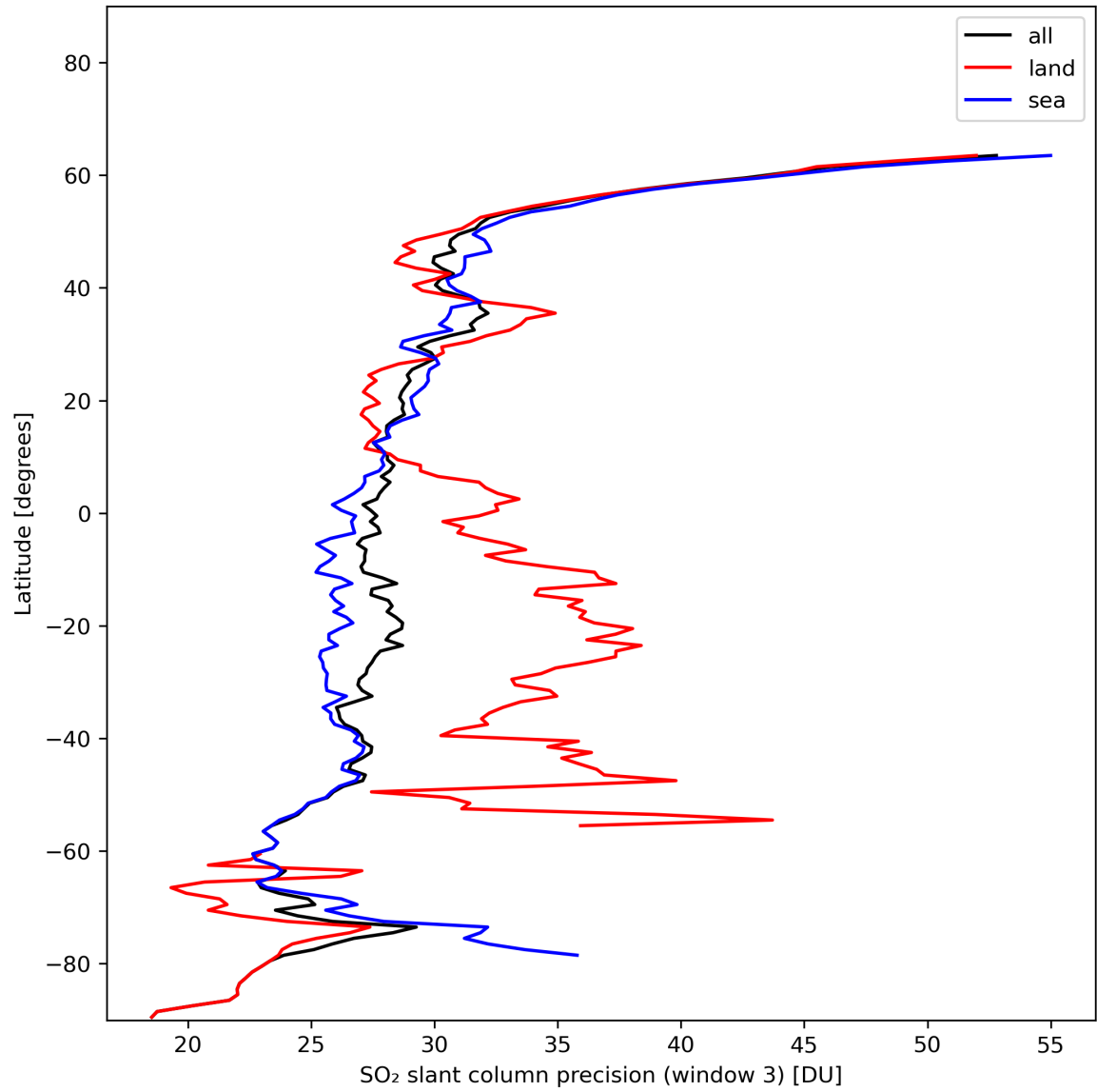
Figure 42: Zonal average of “SO 2 slant column precision (window 3)” for 2024-01-11 to 2024-01-13.
