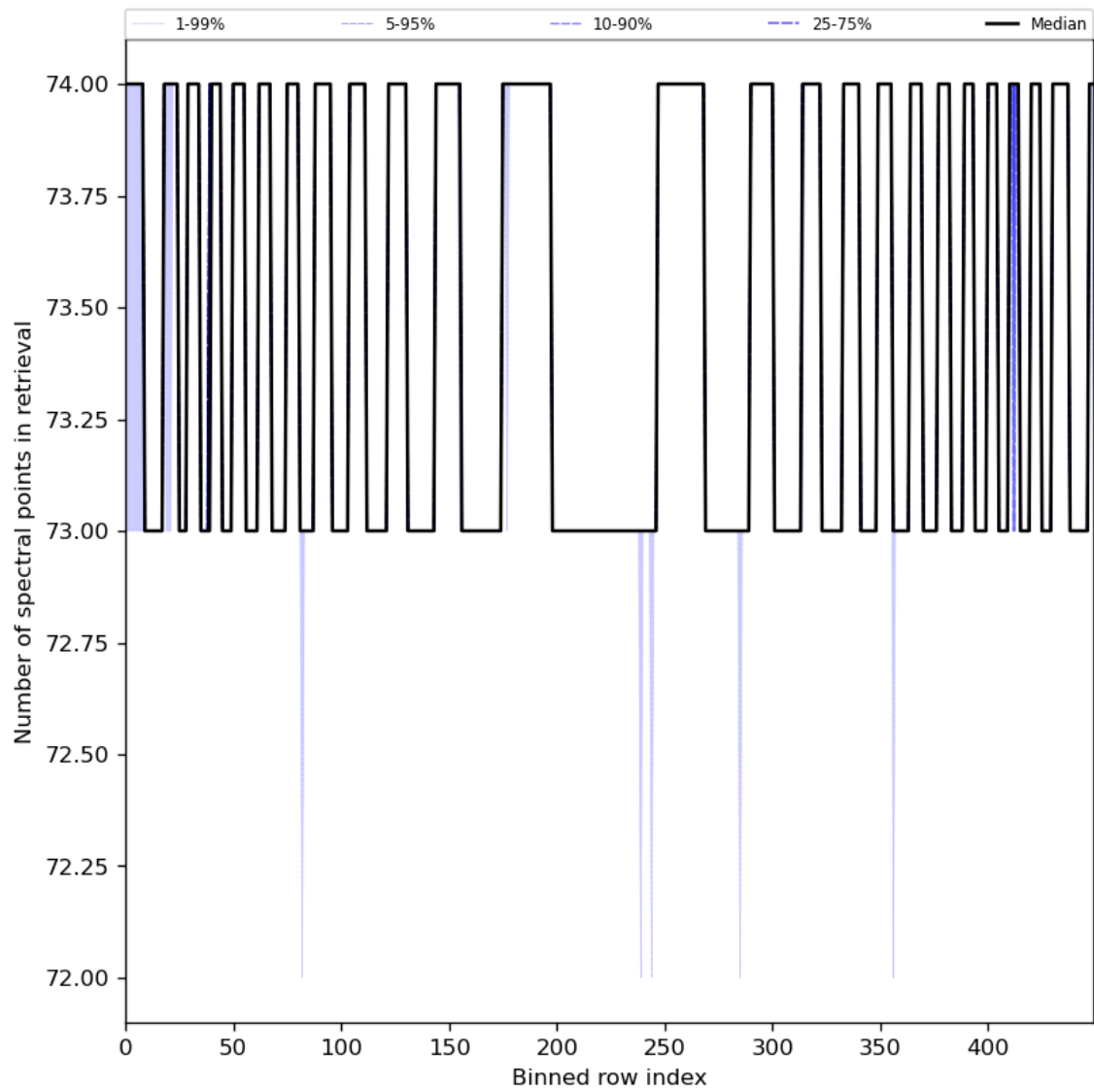
Figure 97: Along track statistics of “Number of spectral points in retrieval” for 2024-01-11 to 2024-01-13
