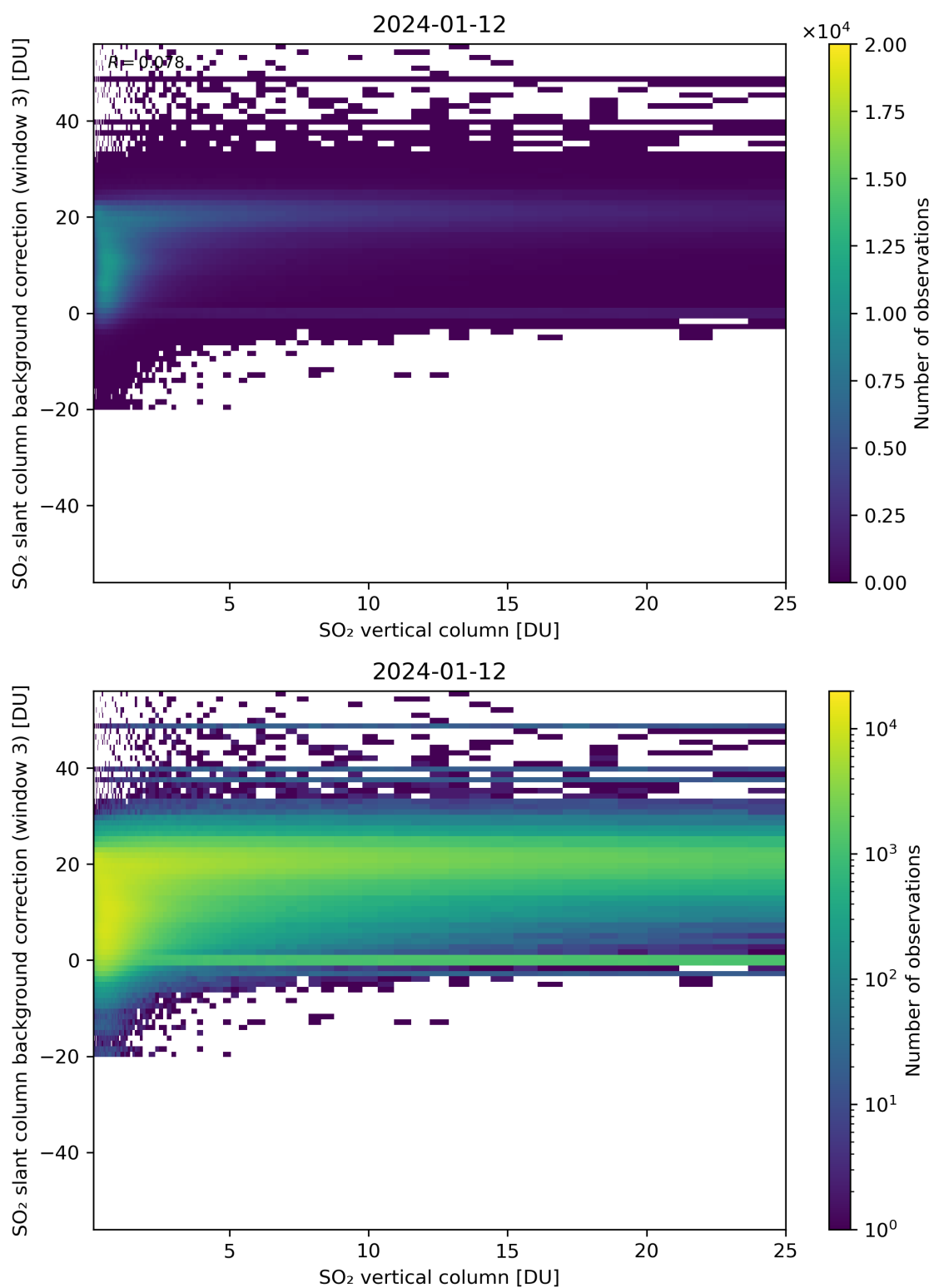
Figure 275: Scatter density plot of “SO 2 vertical column” against “SO 2 slant column background correction (window 3)” for 2024-01-11 to 2024-01-13.
