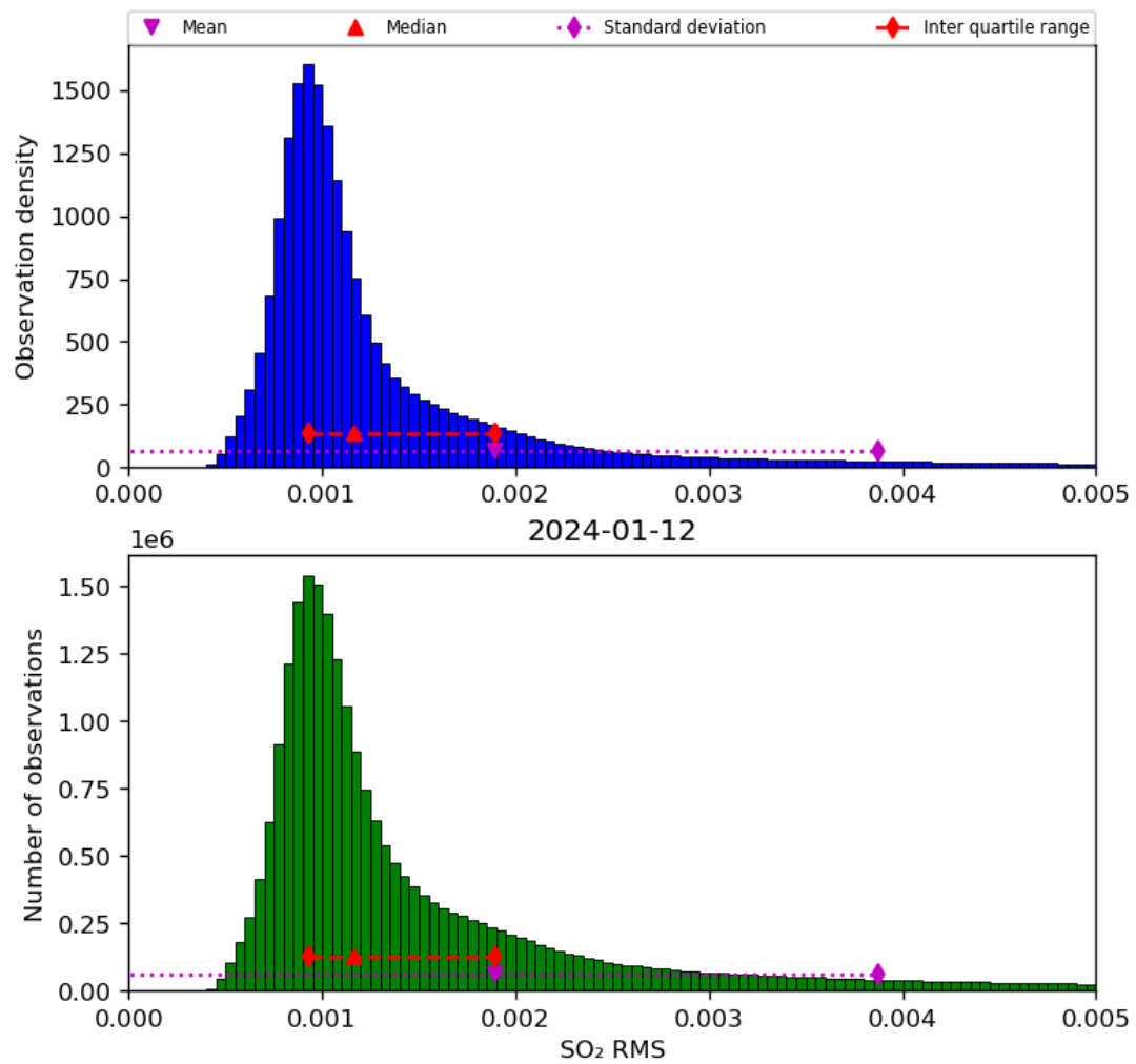
Figure 70: Histogram of “SO 2 RMS” for 2024-01-11 to 2024-01-13
