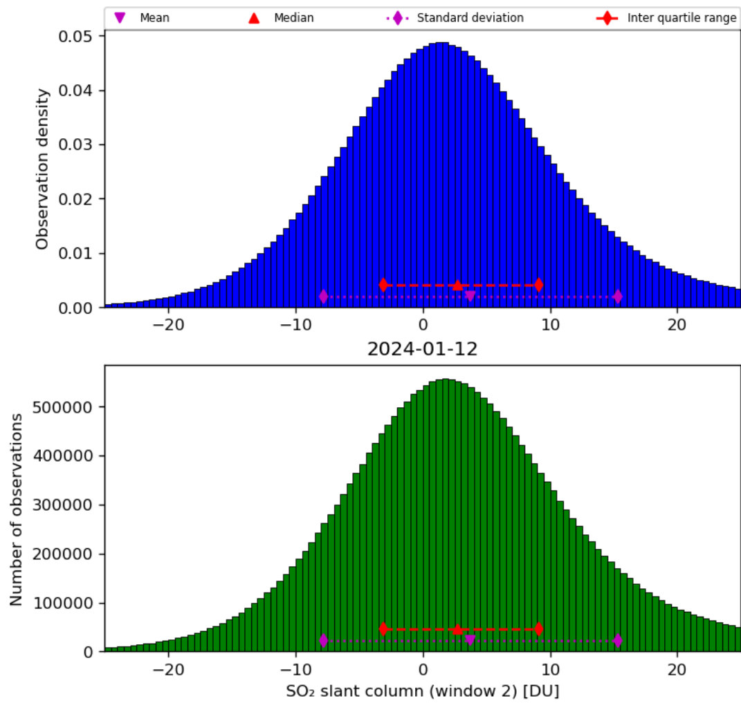
Figure 60: Histogram of “SO 2 slant column (window 2)” for 2024-01-11 to 2024-01-13
