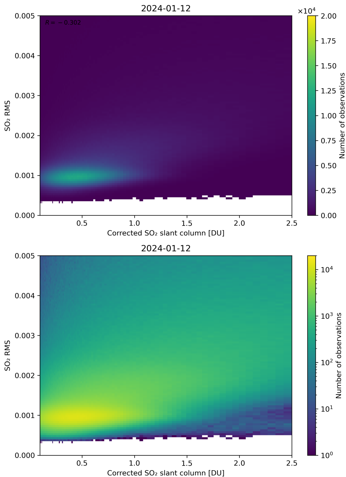
Figure 183: Scatter density plot of “Corrected SO 2 slant column” against “SO 2 RMS” for 2024-01-11 to 2024-01-13.
