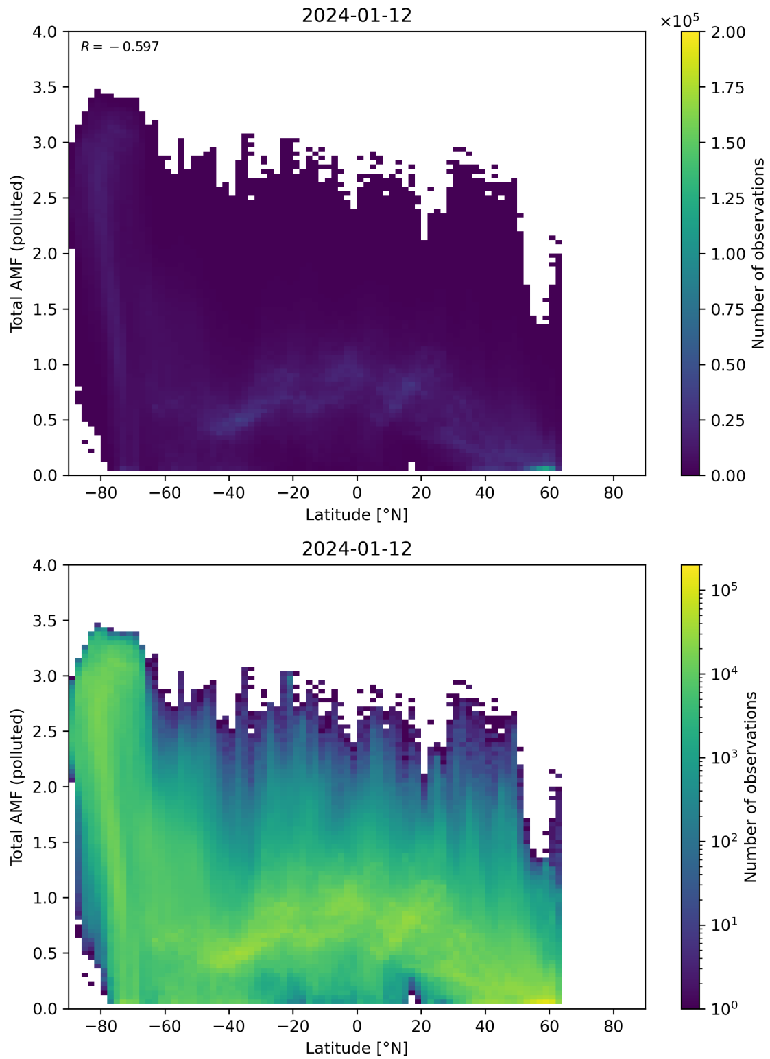
Figure 154: Scatter density plot of “Latitude” against “Total AMF (polluted)” for 2024-01-11 to 2024-01-13.
