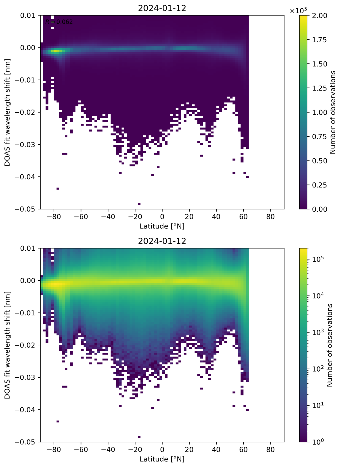
Figure 142: Scatter density plot of “Latitude” against “DOAS fit wavelength shift” for 2024-01-11 to 2024-01-13.
