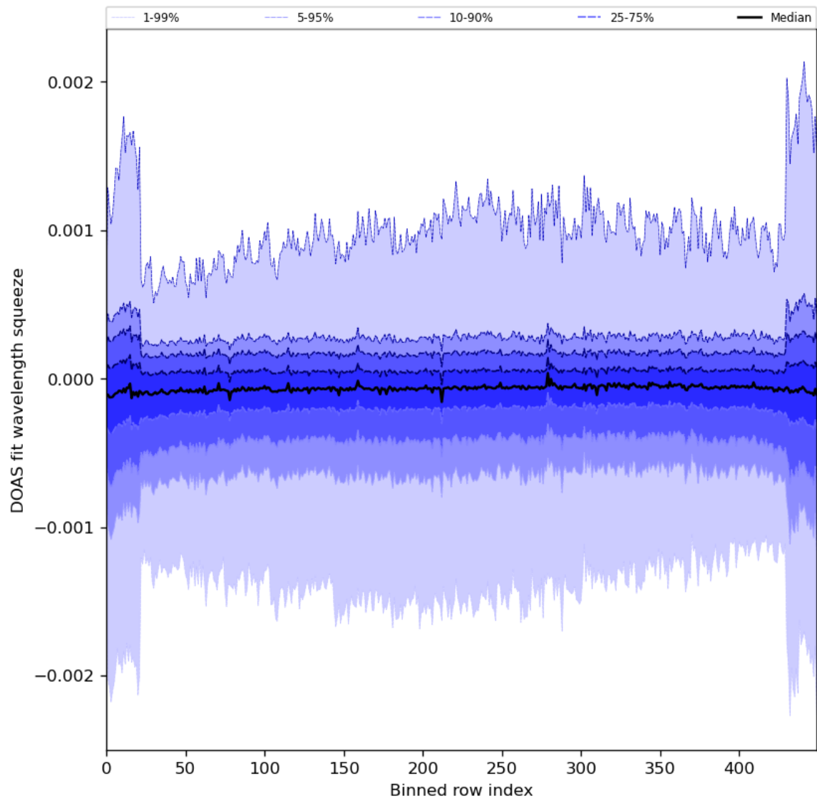
Figure 92: Along track statistics of “DOAS fit wavelength squeeze” for 2024-01-11 to 2024-01-13
