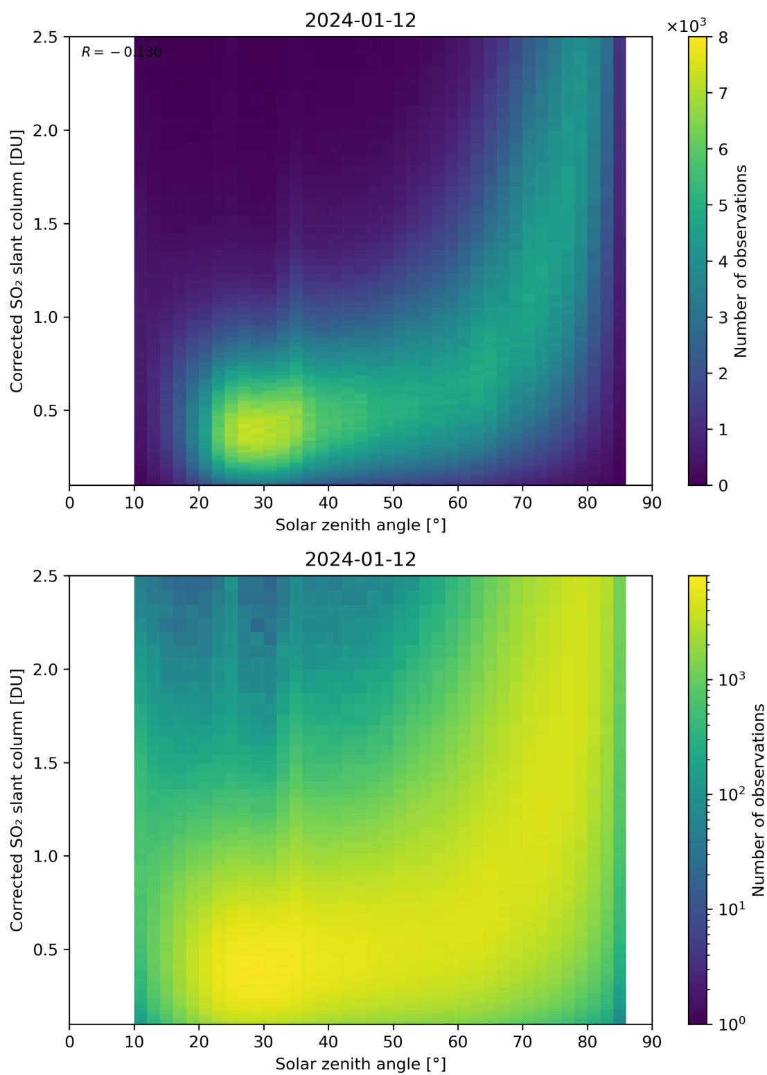
Figure 166: Scatter density plot of “Solar zenith angle” against “Corrected SO 2 slant column” for 2024-01-11 to 2024-01-13.
