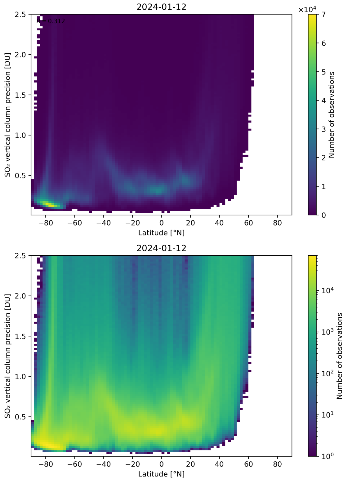
Figure 157: Scatter density plot of “Latitude” against “SO 2 vertical column precision” for 2024-01-11 to 2024-01-13.
