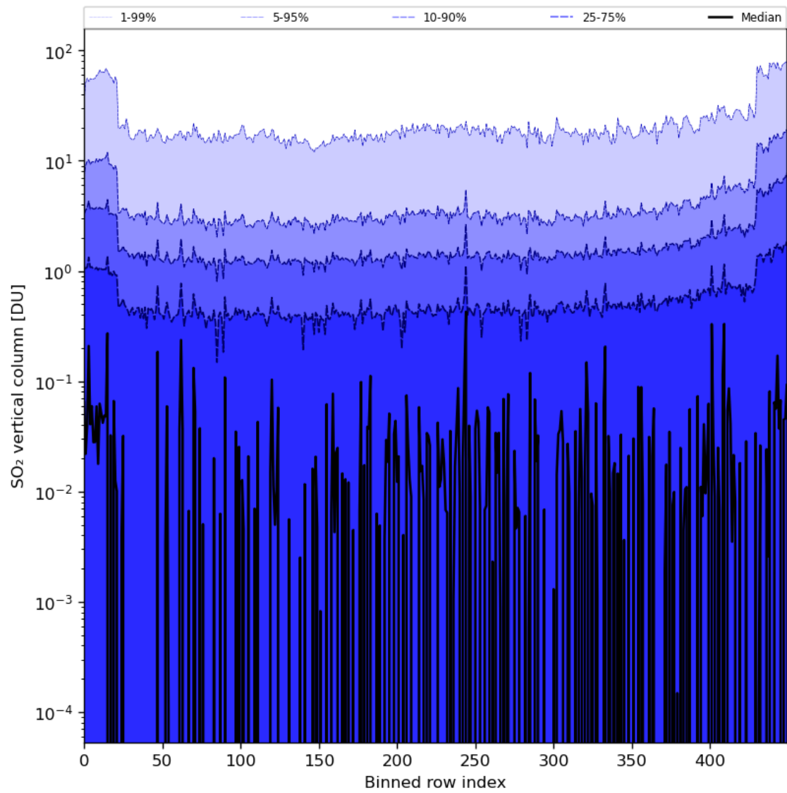
Figure 76: Along track statistics of “SO 2 vertical column” for 2024-01-11 to 2024-01-13
