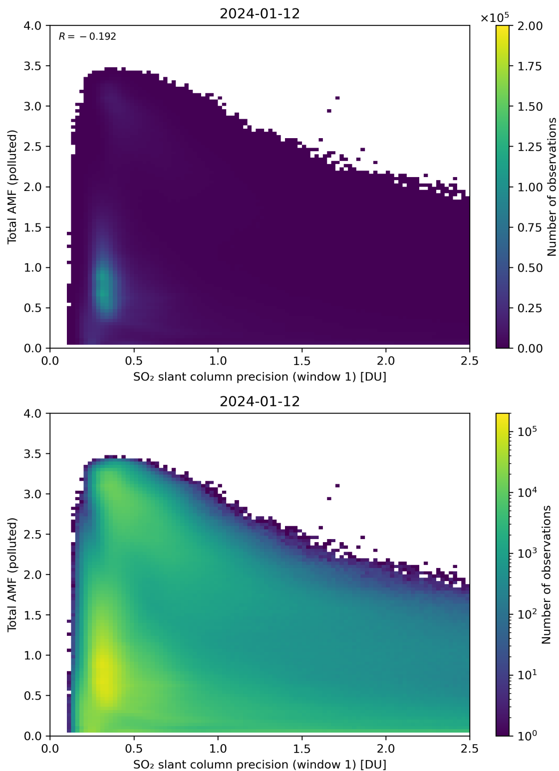
Figure 230: Scatter density plot of “SO 2 slant column precision (window 1)” against “Total AMF (polluted)” for 2024-01-11 to 2024-01-13.
