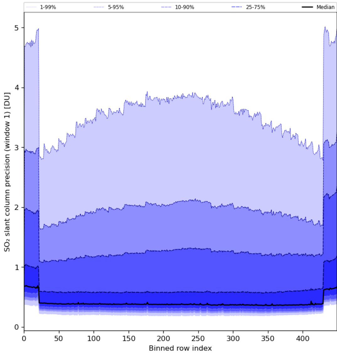
Figure 80: Along track statistics of “SO 2 slant column precision (window 1)” for 2024-01-11 to 2024-01-13
