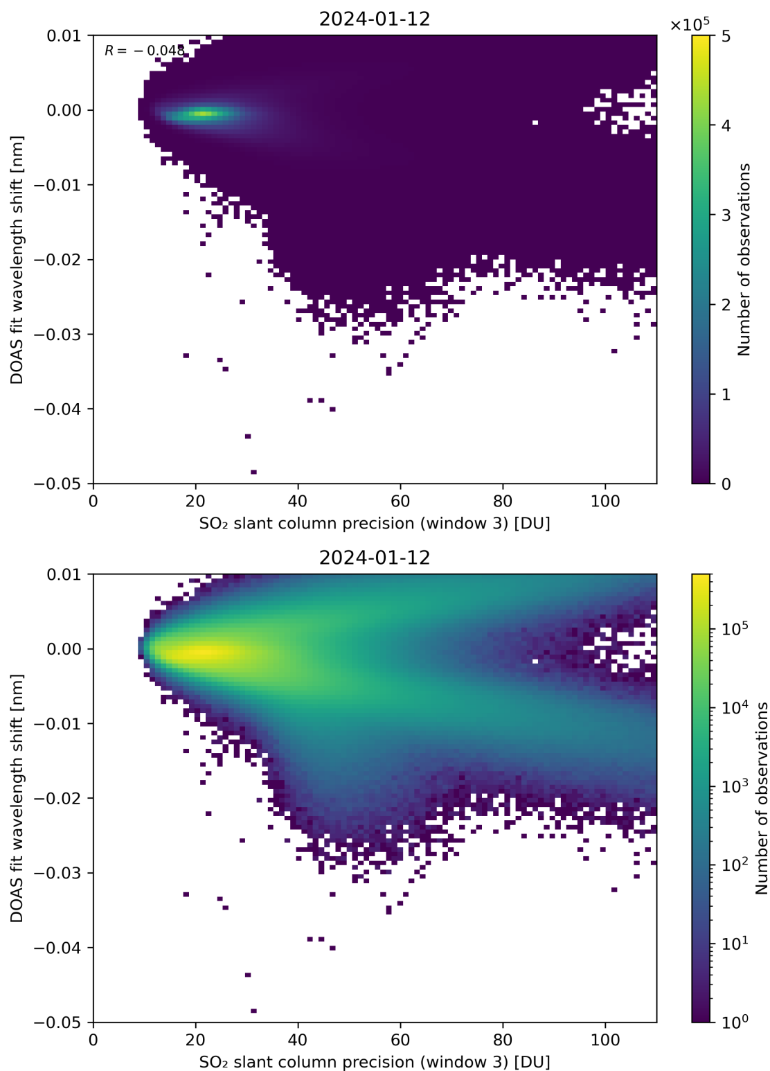
Figure 258: Scatter density plot of “SO 2 slant column precision (window 3)” against “DOAS fit wavelength shift” for 2024-01-11 to 2024-01-13.
