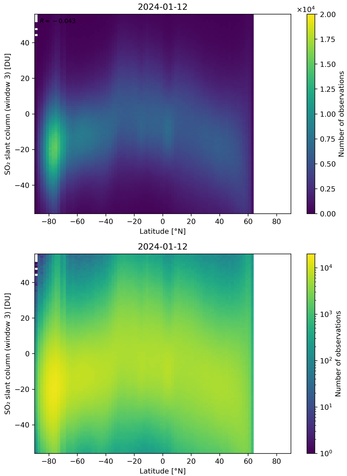
Figure 152: Scatter density plot of “Latitude” against “SO 2 slant column (window 3)” for 2024-01-11 to 2024-01-13.
