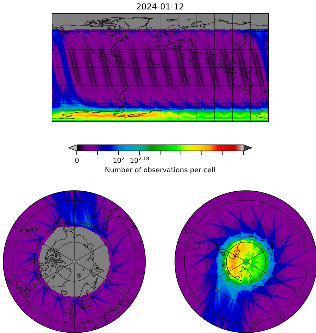
Figure 28: Map of the number of observations for 2024-01-11 to 2024-01-13
