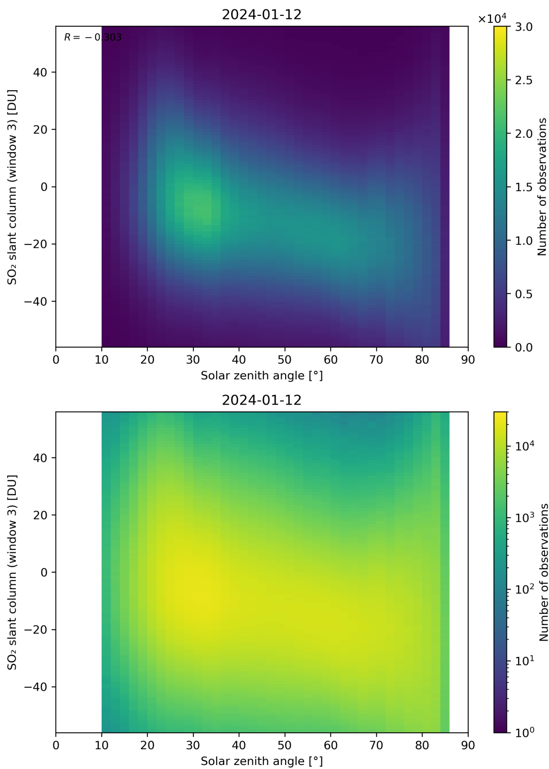
Figure 172: Scatter density plot of “Solar zenith angle” against “SO 2 slant column (window 3)” for 2024-01-11 to 2024-01-13.
