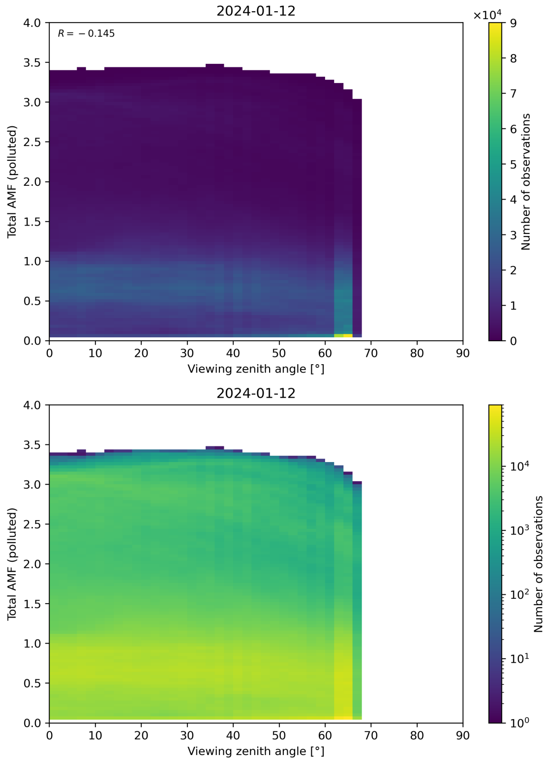
Figure 325: Scatter density plot of “Viewing zenith angle” against “Total AMF (polluted)” for 2024-01-11 to 2024-01-13.
