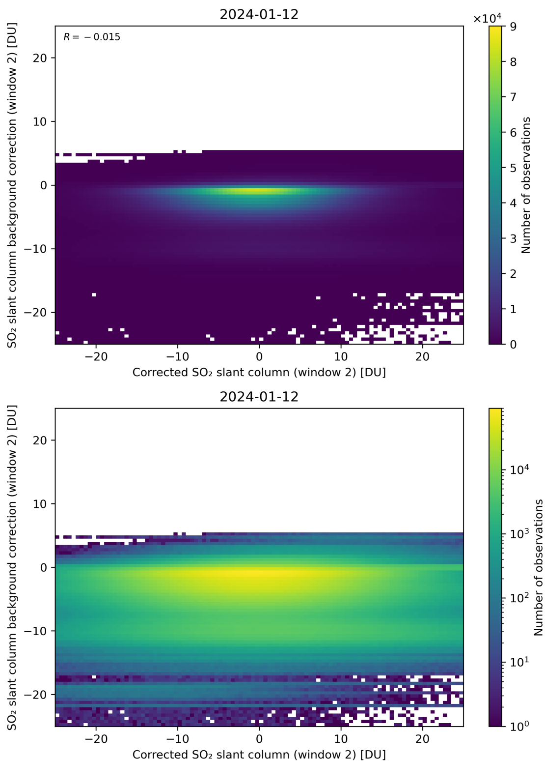
Figure 194: Scatter density plot of “Corrected SO 2 slant column (window 2)” against “SO 2 slant column background correction (window 2)” for 2024-01-11 to 2024-01-13.
