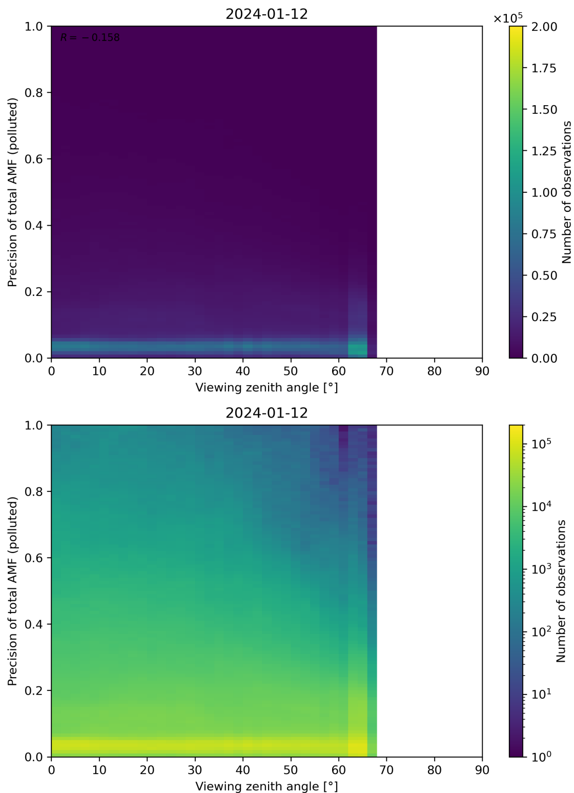
Figure 326: Scatter density plot of “Viewing zenith angle” against “Precision of total AMF (polluted)” for 2024-01-11 to 2024-01-13.
