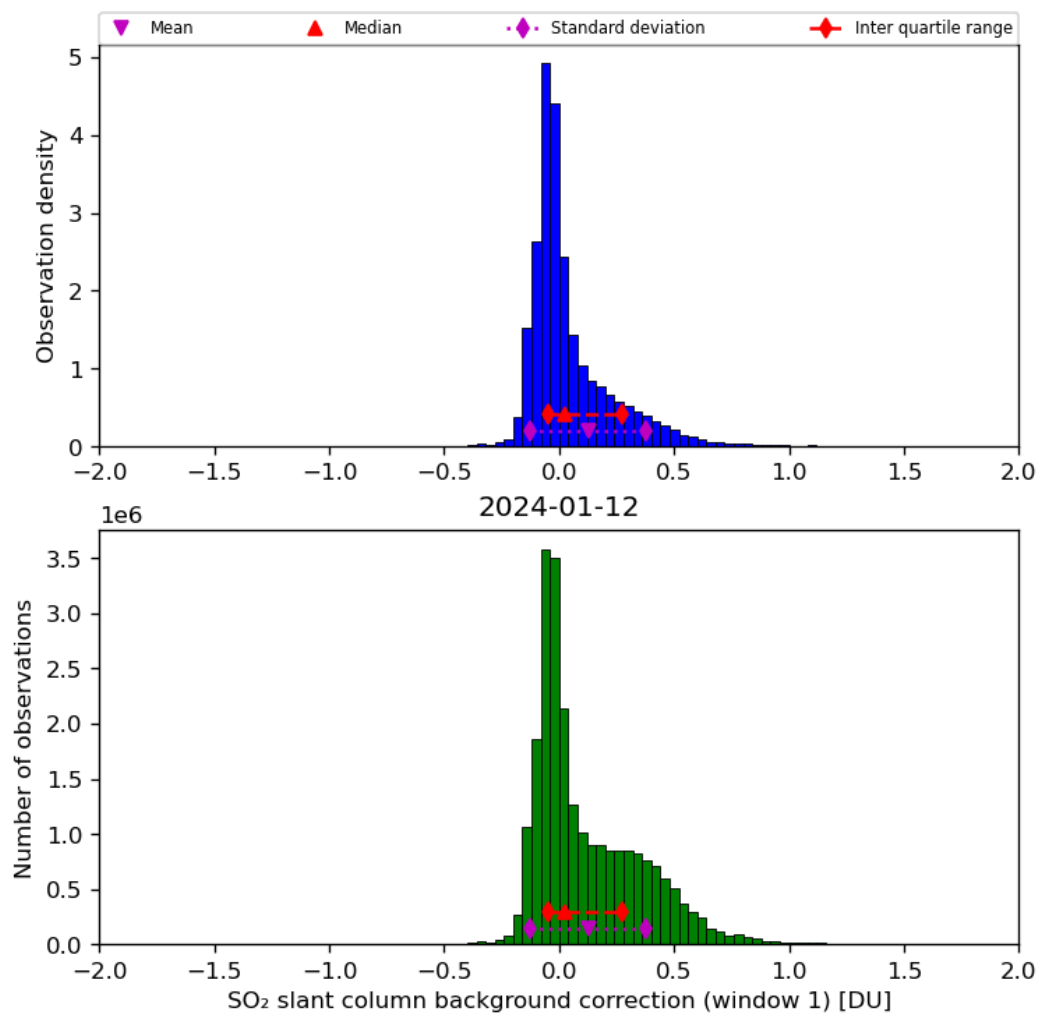
Figure 59: Histogram of “SO 2 slant column background correction (window 1)” for 2024-01-11 to 2024-01-13
