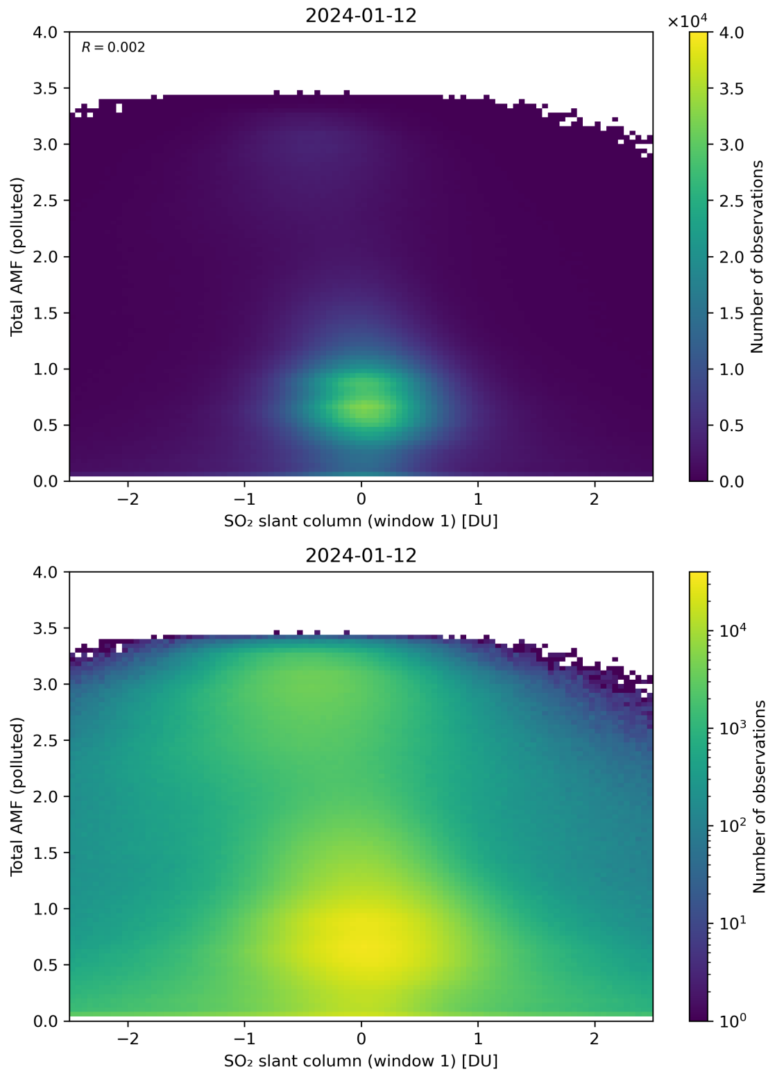
Figure 239: Scatter density plot of “SO 2 slant column (window 1)” against “Total AMF (polluted)” for 2024-01-11 to 2024-01-13.
