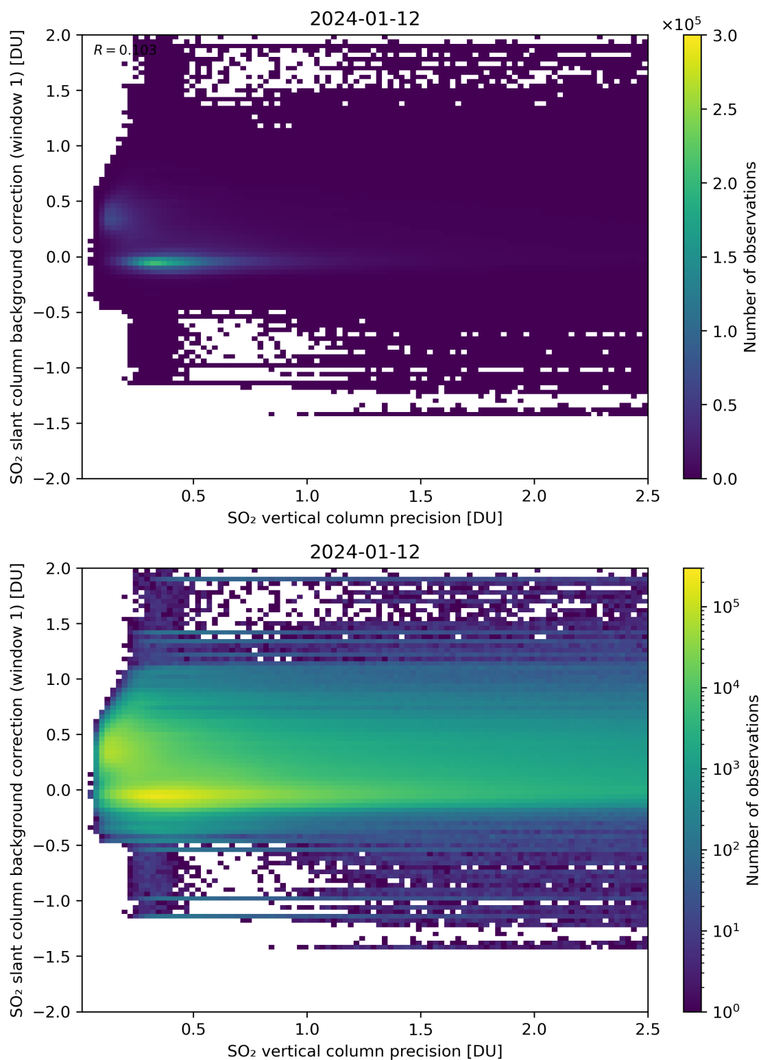
Figure 279: Scatter density plot of “SO 2 vertical column precision” against “SO 2 slant column background correction (window 1)” for 2024-01-11 to 2024-01-13.
