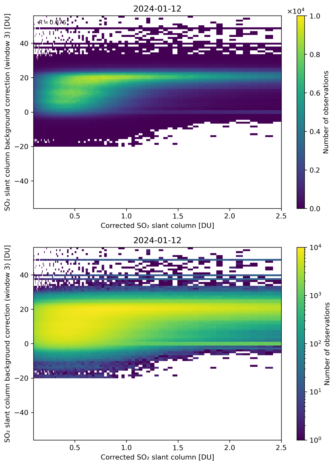
Figure 180: Scatter density plot of “Corrected SO 2 slant column” against “SO 2 slant column background correction (window 3)” for 2024-01-11 to 2024-01-13.
