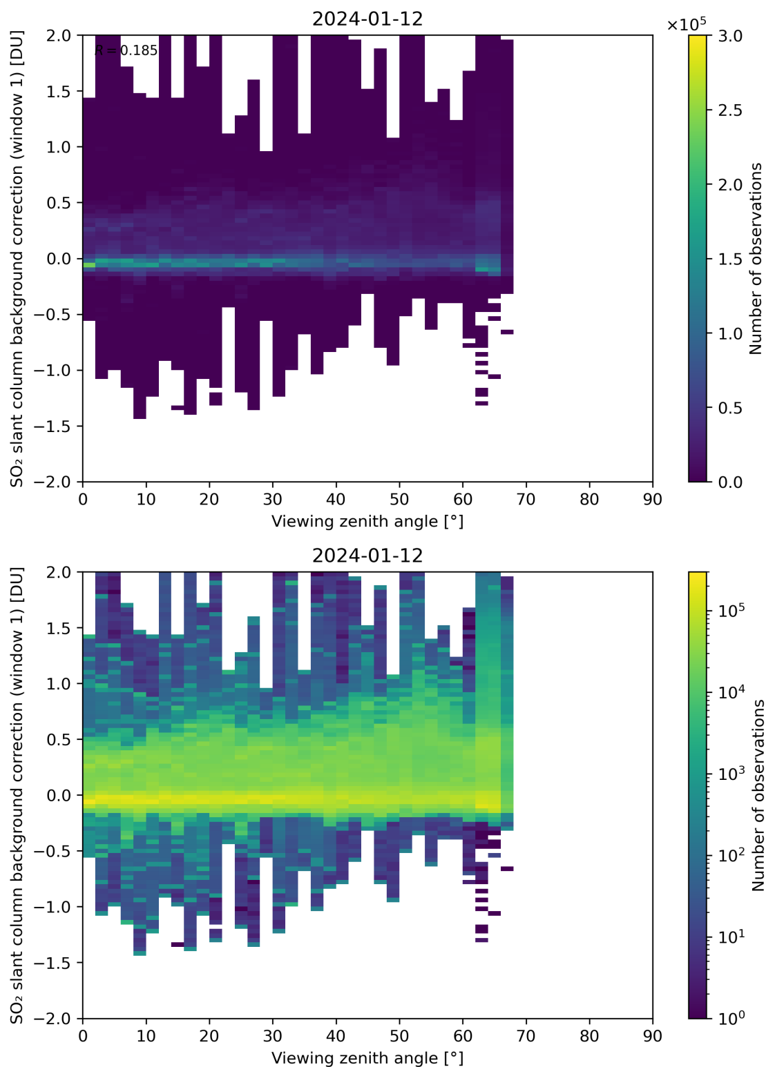
Figure 308: Scatter density plot of “Viewing zenith angle” against “SO 2 slant column background correction (window 1)” for 2024-01-11 to 2024-01-13.
