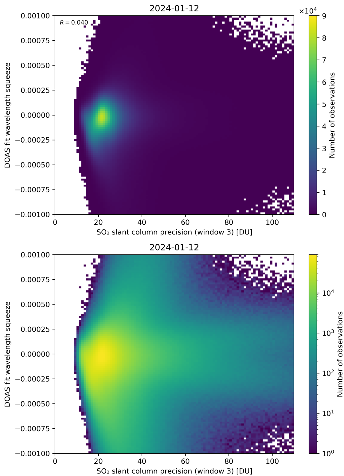
Figure 259: Scatter density plot of “SO 2 slant column precision (window 3)” against “DOAS fit wavelength squeeze” for 2024-01-11 to 2024-01-13.
