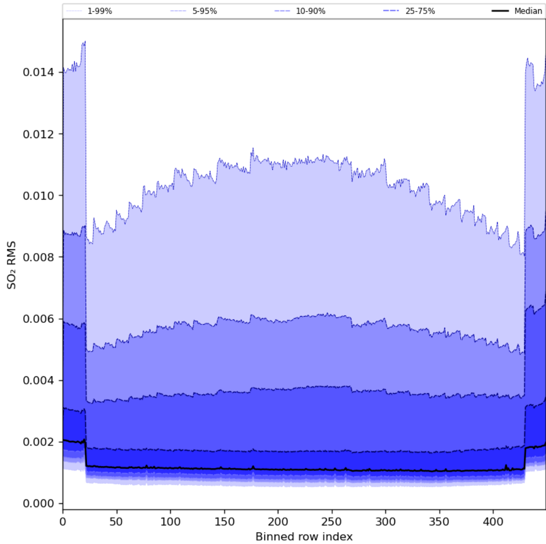
Figure 93: Along track statistics of “SO 2 RMS” for 2024-01-11 to 2024-01-13
