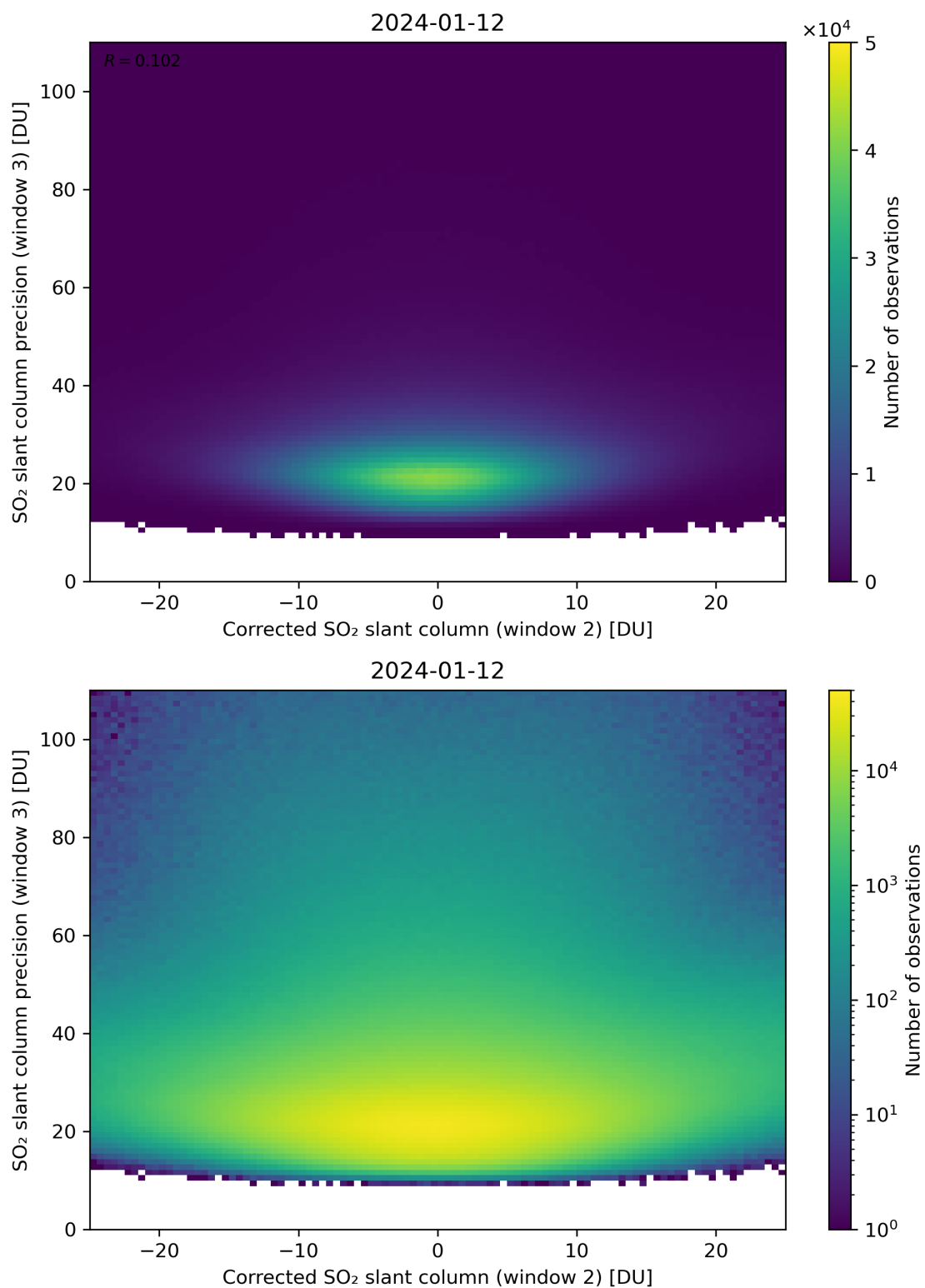
Figure 202: Scatter density plot of “Corrected SO 2 slant column (window 2)” against “SO 2 slant column precision (window 3)” for 2024-01-11 to 2024-01-13.
