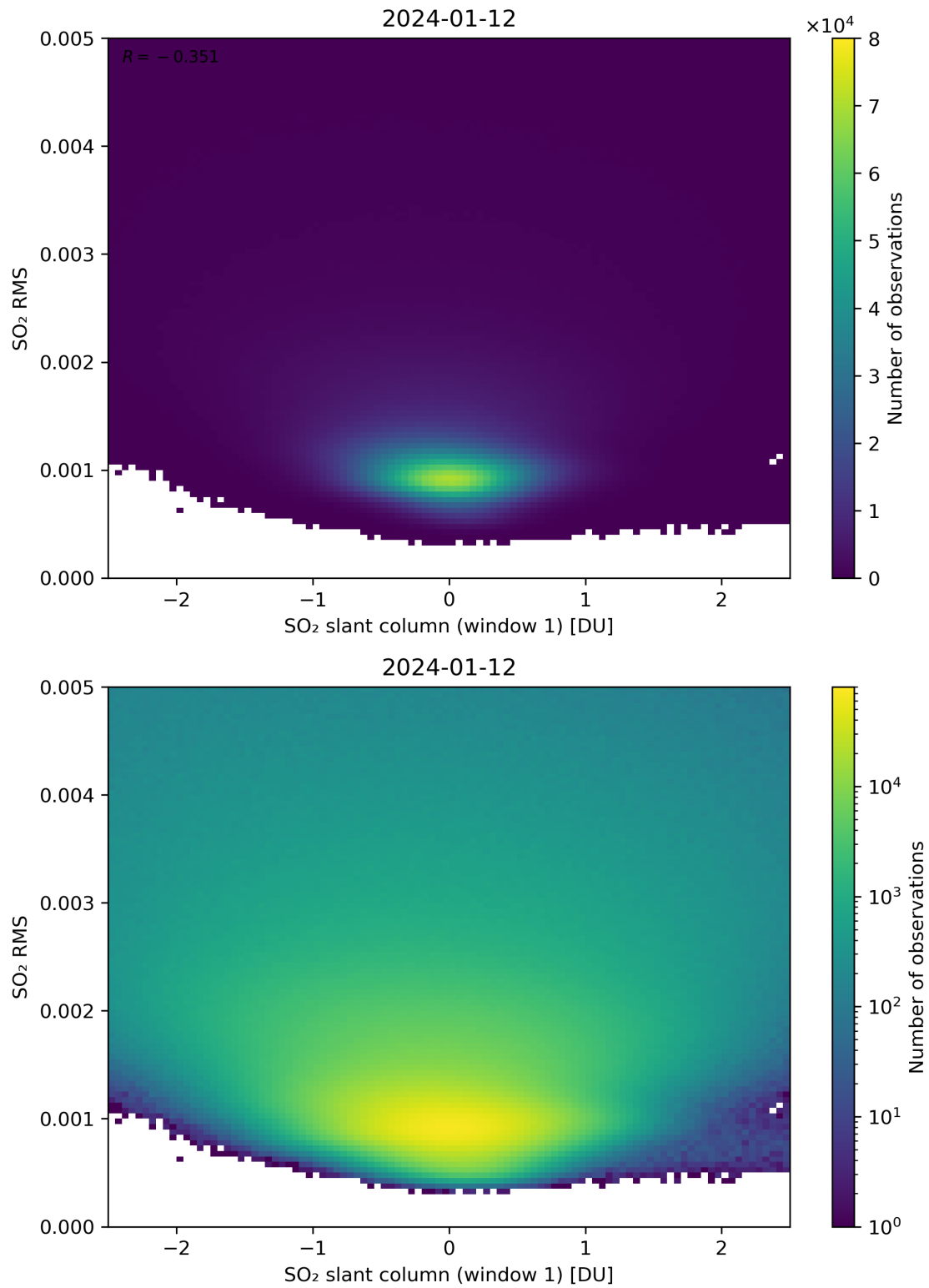
Figure 217: Scatter density plot of “SO 2 slant column (window 1)” against “SO 2 RMS” for 2024-01-11 to 2024-01-13.
