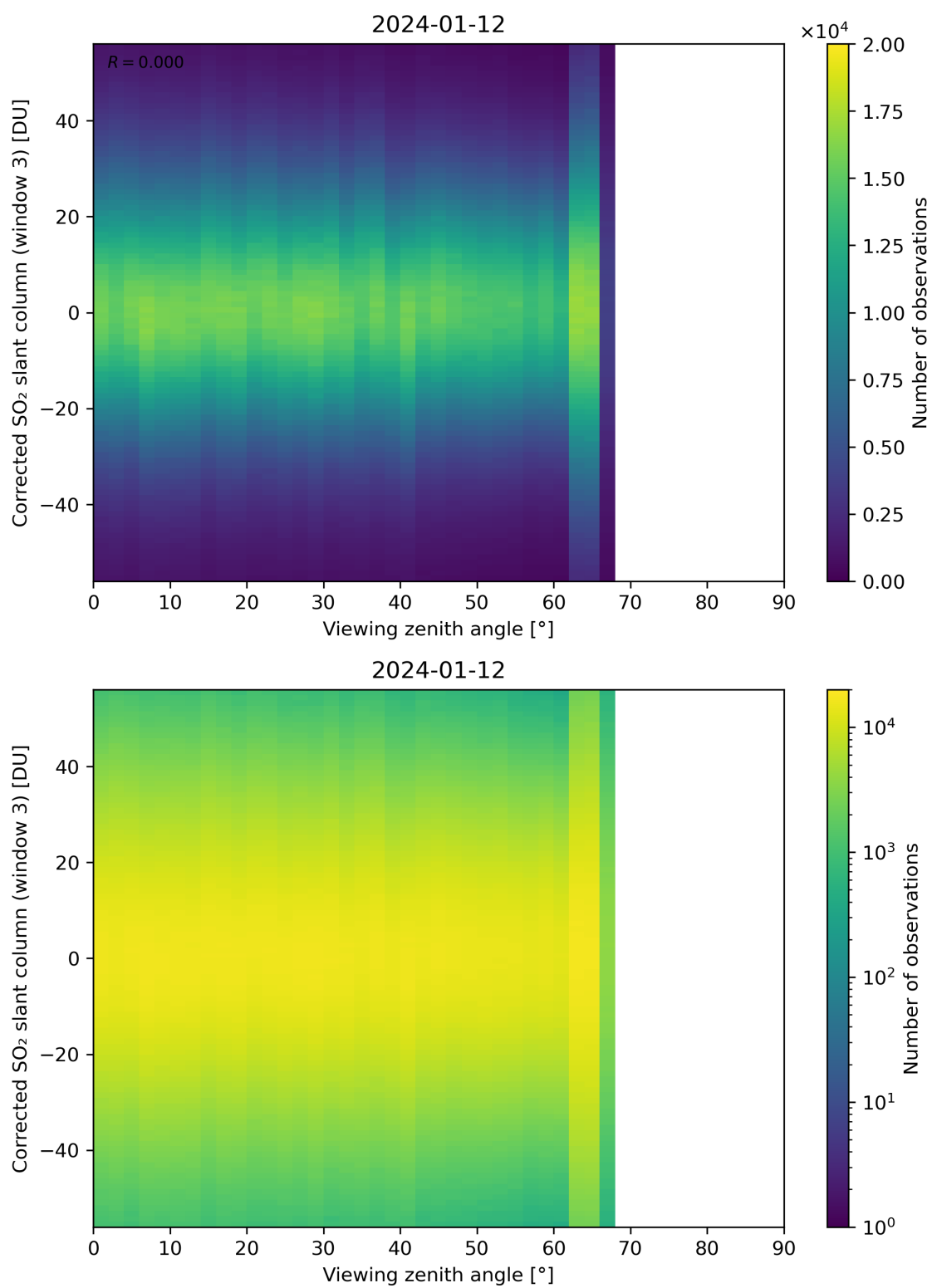
Figure 319: Scatter density plot of “Viewing zenith angle” against “Corrected SO 2 slant column (window 3)” for 2024-01-11 to 2024-01-13.
