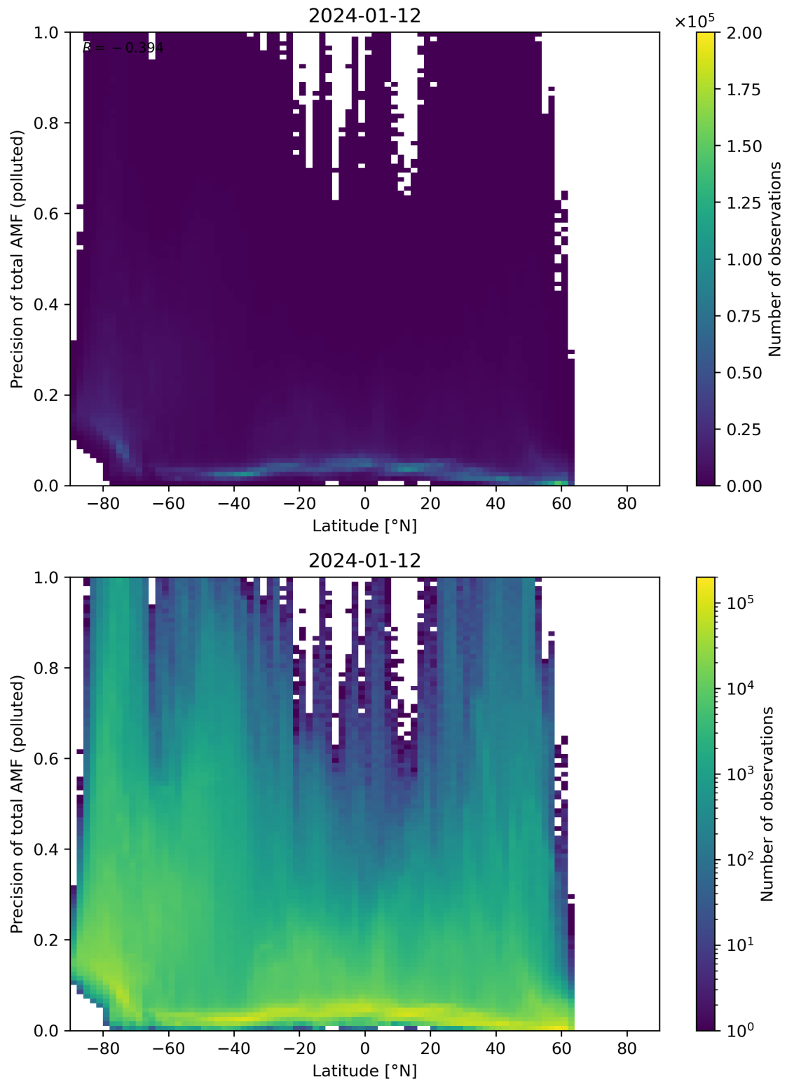
Figure 155: Scatter density plot of “Latitude” against “Precision of total AMF (polluted)” for 2024-01-11 to 2024-01-13.
