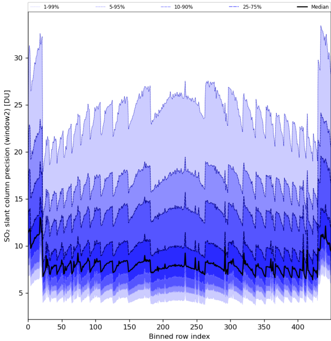
Figure 84: Along track statistics of “SO 2 slant column precision (window2)” for 2024-01-11 to 2024-01-13
