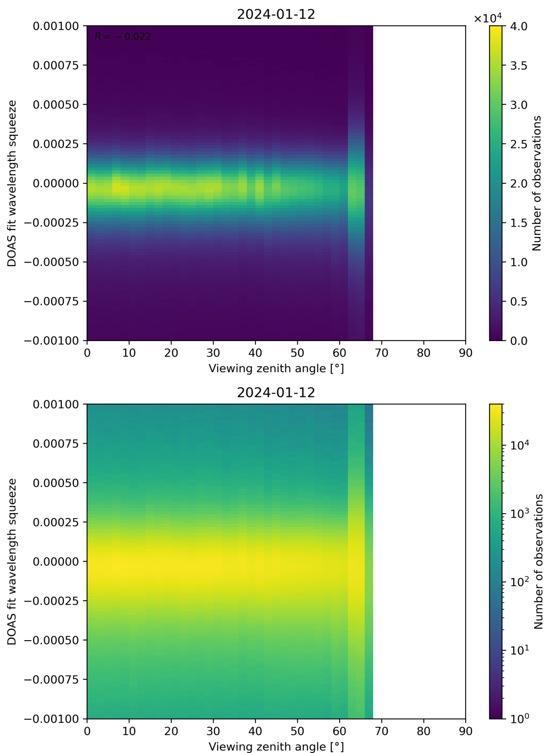
Figure 312: Scatter density plot of “Viewing zenith angle” against “DOAS fit wavelength squeeze” for 2024-01-11 to 2024-01-13.
