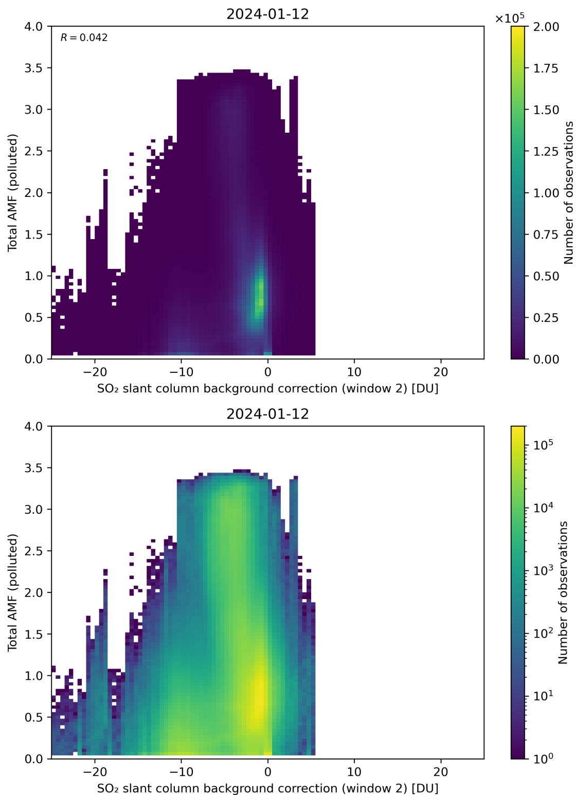
Figure 119: Scatter density plot of “SO 2 slant column background correction (window 2)” against “Total AMF (polluted)” for 2024-01-11 to 2024-01-13.
