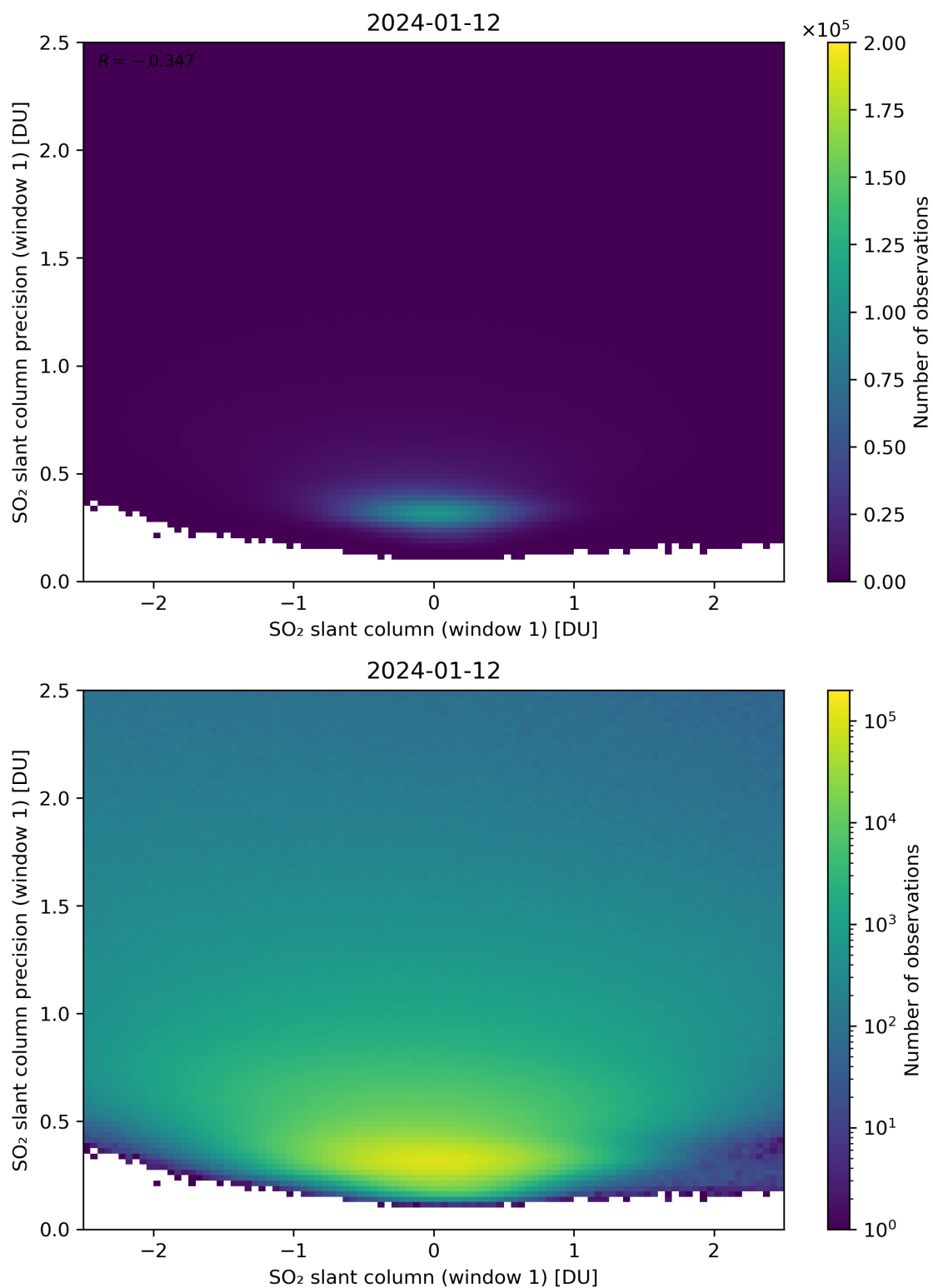
Figure 235: Scatter density plot of “SO 2 slant column (window 1)” against “SO 2 slant column precision (window 1)” for 2024-01-11 to 2024-01-13.
