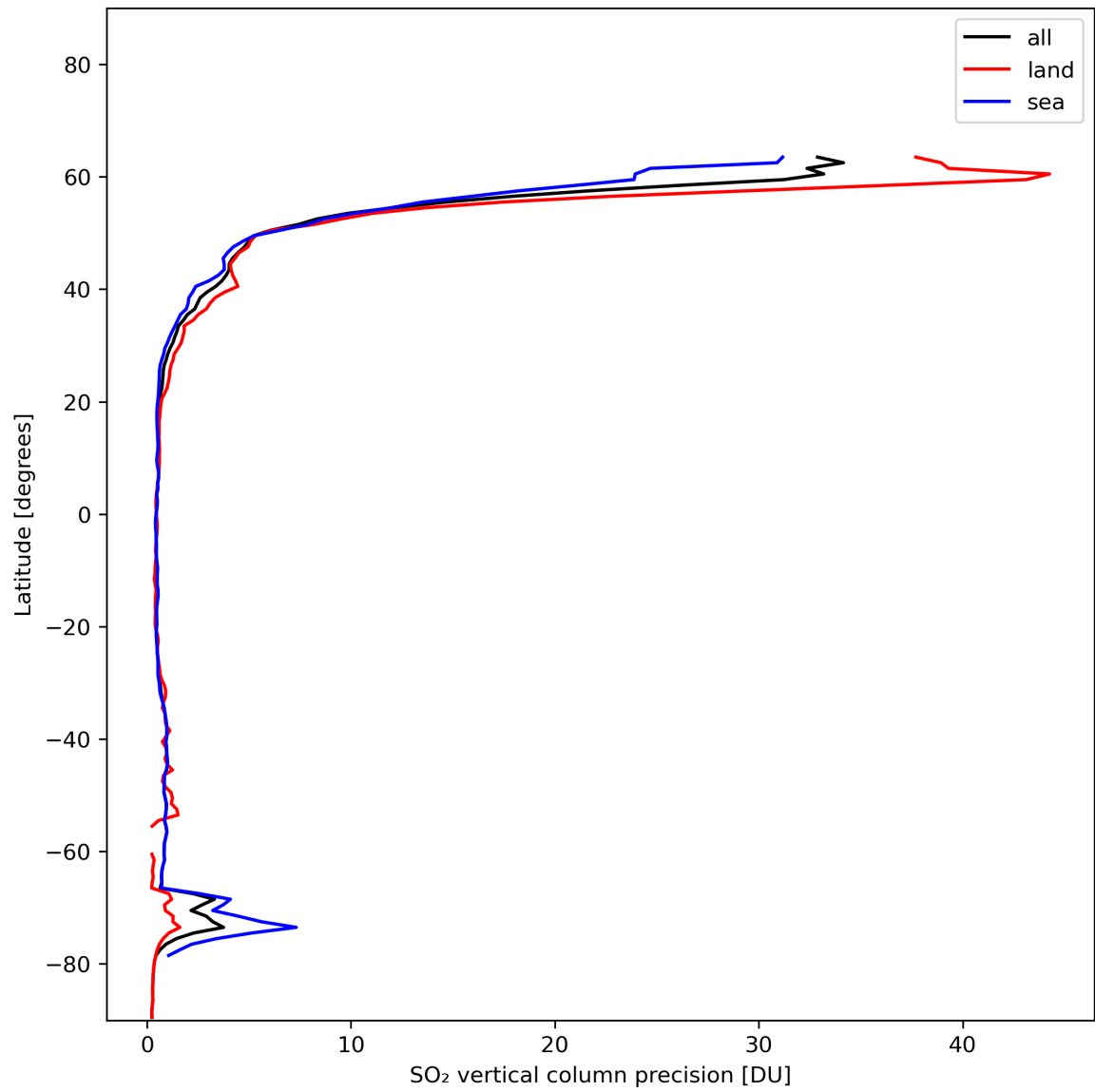
Figure 31: Zonal average of “SO 2 vertical column precision” for 2024-01-11 to 2024-01-13.
