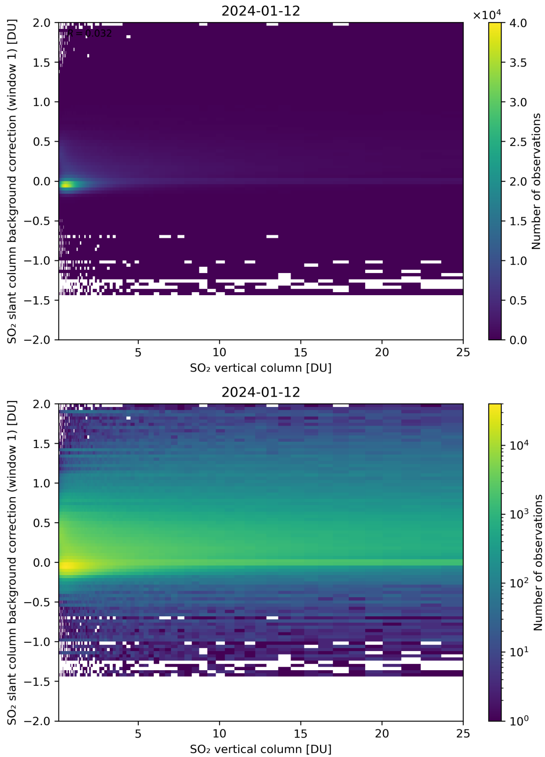
Figure 273: Scatter density plot of “SO 2 vertical column” against “SO 2 slant column background correction (window 1)” for 2024-01-11 to 2024-01-13.
