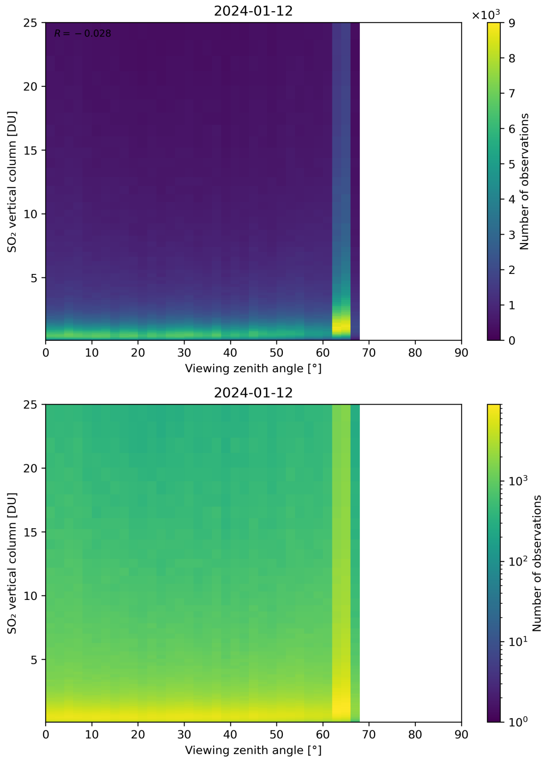
Figure 327: Scatter density plot of “Viewing zenith angle” against “SO 2 vertical column” for 2024-01-11 to 2024-01-13.
