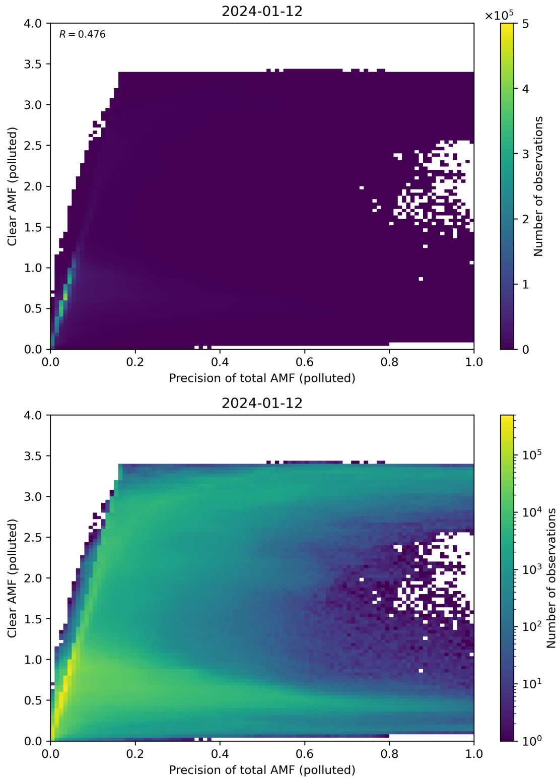
Figure 270: Scatter density plot of “Precision of total AMF (polluted)” against “Clear AMF (polluted)” for 2024-01-11 to 2024-01-13.
