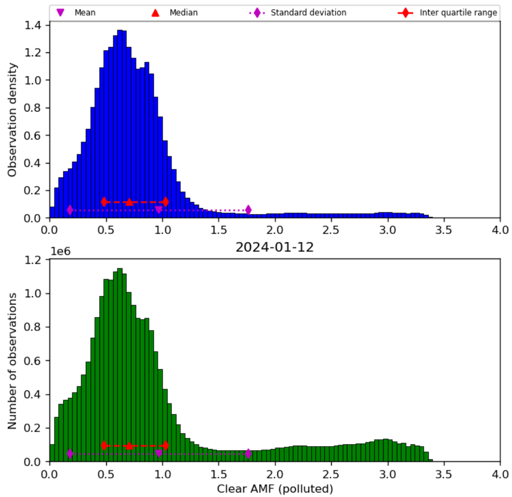
Figure 73: Histogram of “Clear AMF (polluted)” for 2024-01-11 to 2024-01-13
