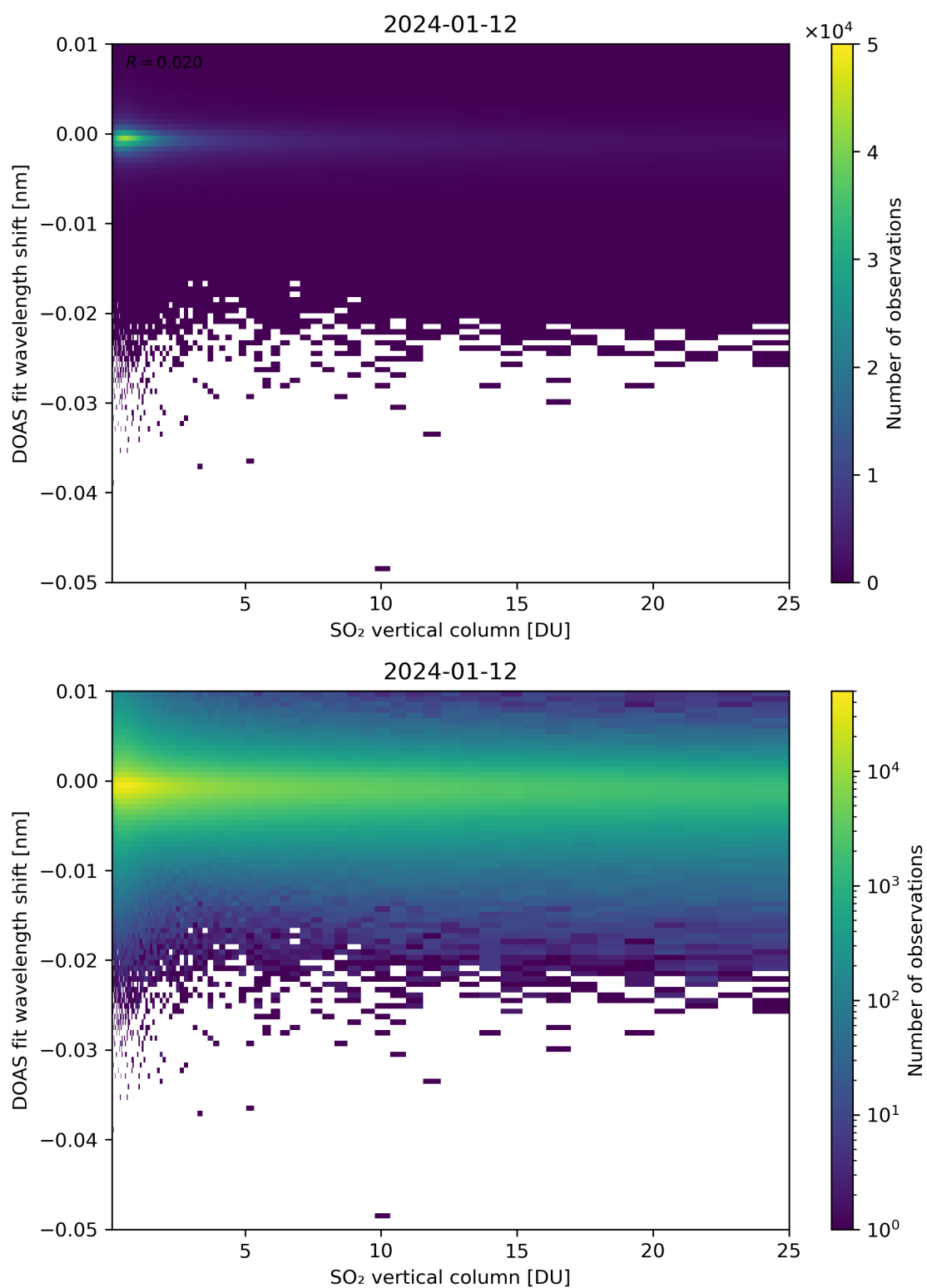
Figure 276: Scatter density plot of “SO 2 vertical column” against “DOAS fit wavelength shift” for 2024-01-11 to 2024-01-13.
