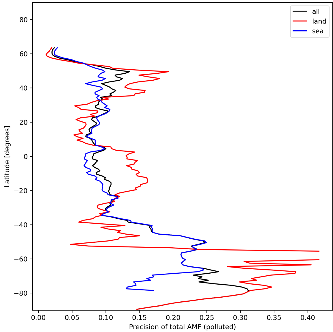
Figure 49: Zonal average of “Precision of total AMF (polluted)” for 2024-01-11 to 2024-01-13.
