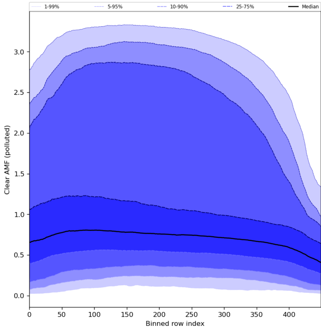
Figure 96: Along track statistics of “Clear AMF (polluted)” for 2024-01-11 to 2024-01-13
