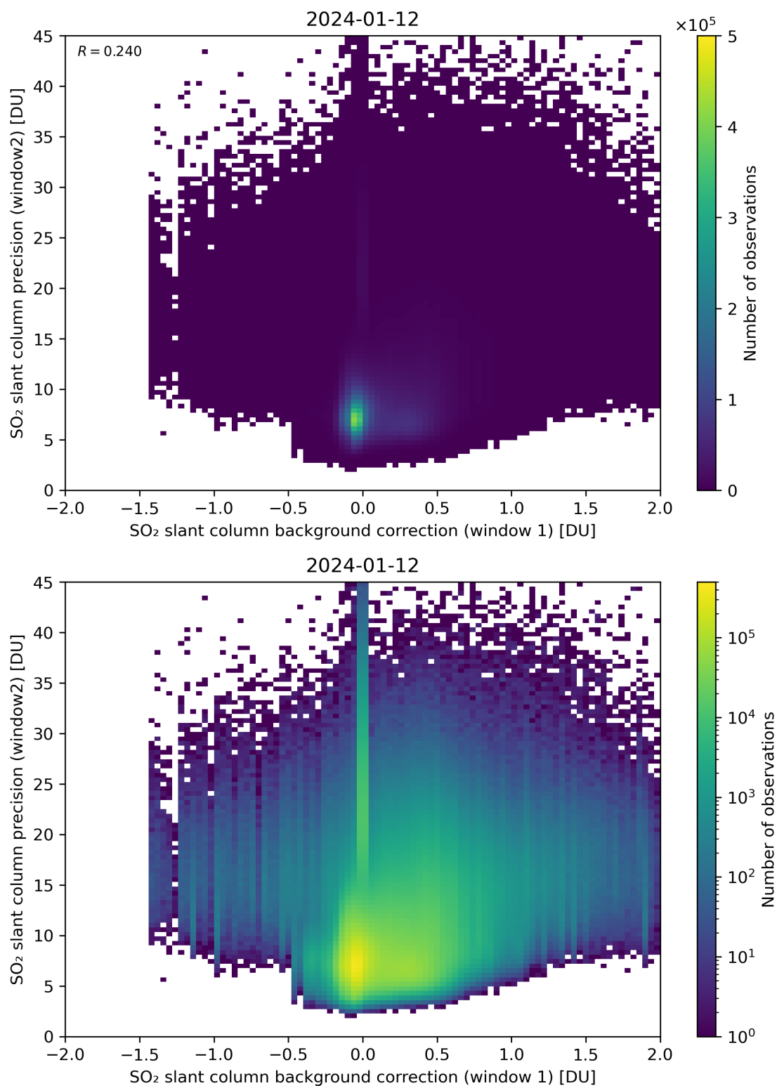
Figure 106: Scatter density plot of “SO 2 slant column background correction (window 1)” against “SO 2 slant column precision (window2)” for 2024-01-11 to 2024-01-13.
