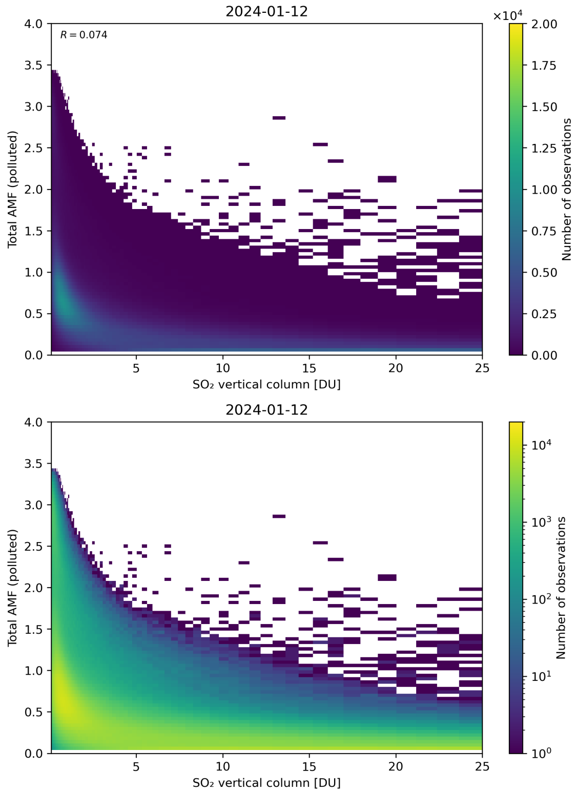
Figure 305: Scatter density plot of “SO 2 vertical column” against “Total AMF (polluted)” for 2024-01-11 to 2024-01-13.
