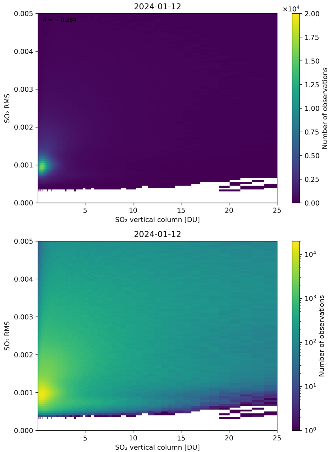
Figure 278: Scatter density plot of “SO 2 vertical column” against “SO 2 RMS” for 2024-01-11 to 2024-01-13.
