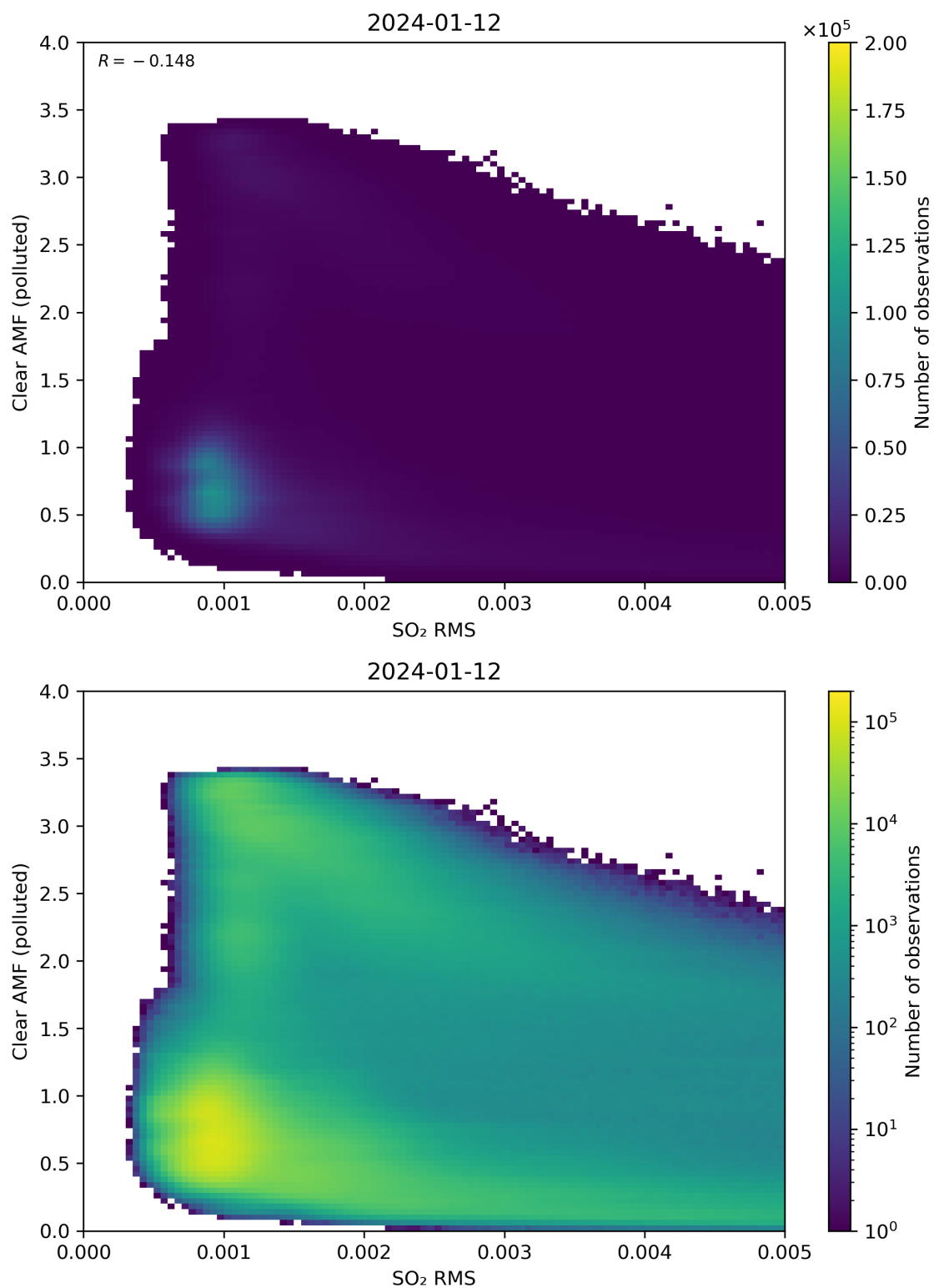
Figure 136: Scatter density plot of “SO 2 RMS” against “Clear AMF (polluted)” for 2024-01-11 to 2024-01-13.
