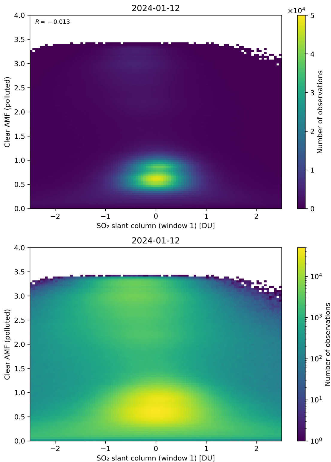
Figure 232: Scatter density plot of “SO 2 slant column (window 1)” against “Clear AMF (polluted)” for 2024-01-11 to 2024-01-13.
