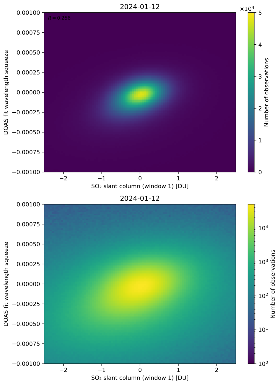
Figure 216: Scatter density plot of “SO 2 slant column (window 1)” against “DOAS fit wavelength squeeze” for 2024-01-11 to 2024-01-13.
