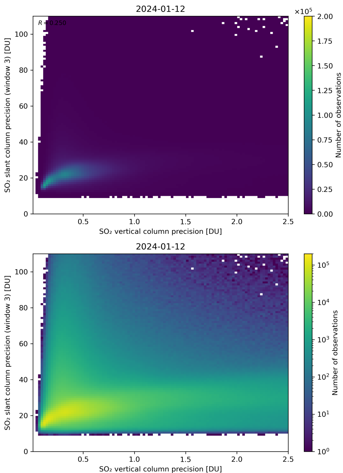
Figure 293: Scatter density plot of “SO 2 vertical column precision” against “SO 2 slant column precision (window 3)” for 2024-01-11 to 2024-01-13.
