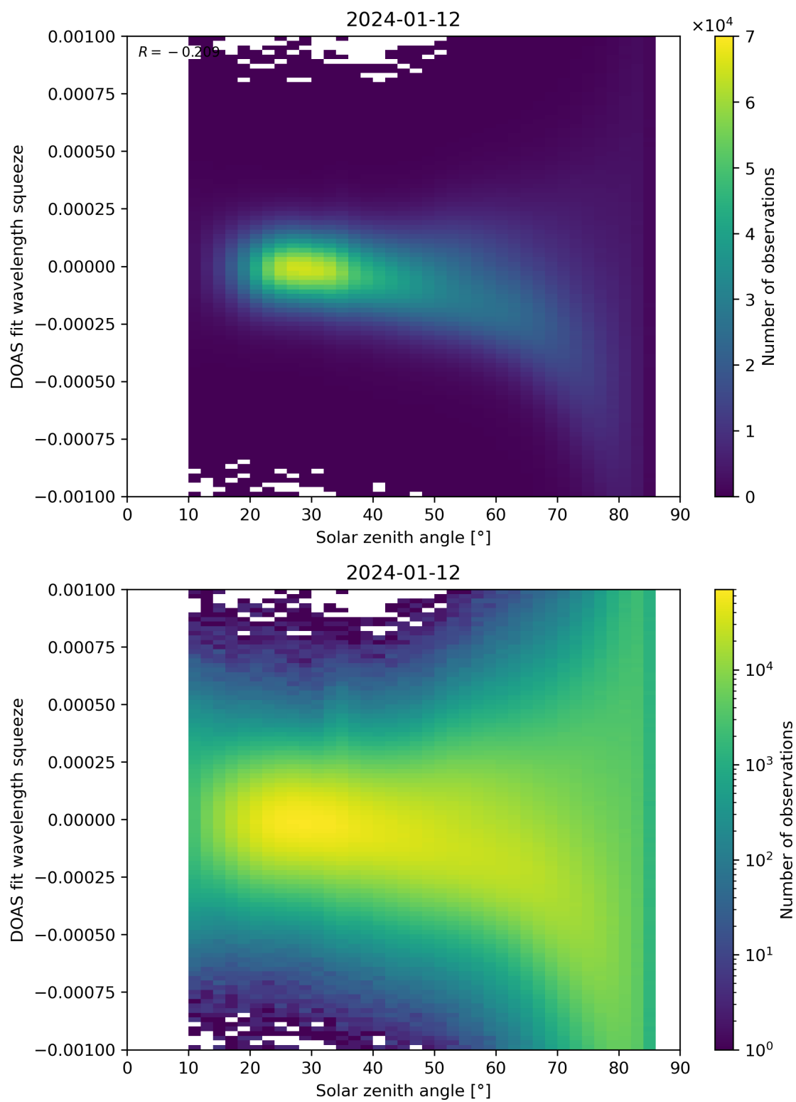
Figure 162: Scatter density plot of “Solar zenith angle” against “DOAS fit wavelength squeeze” for 2024-01-11 to 2024-01-13.
