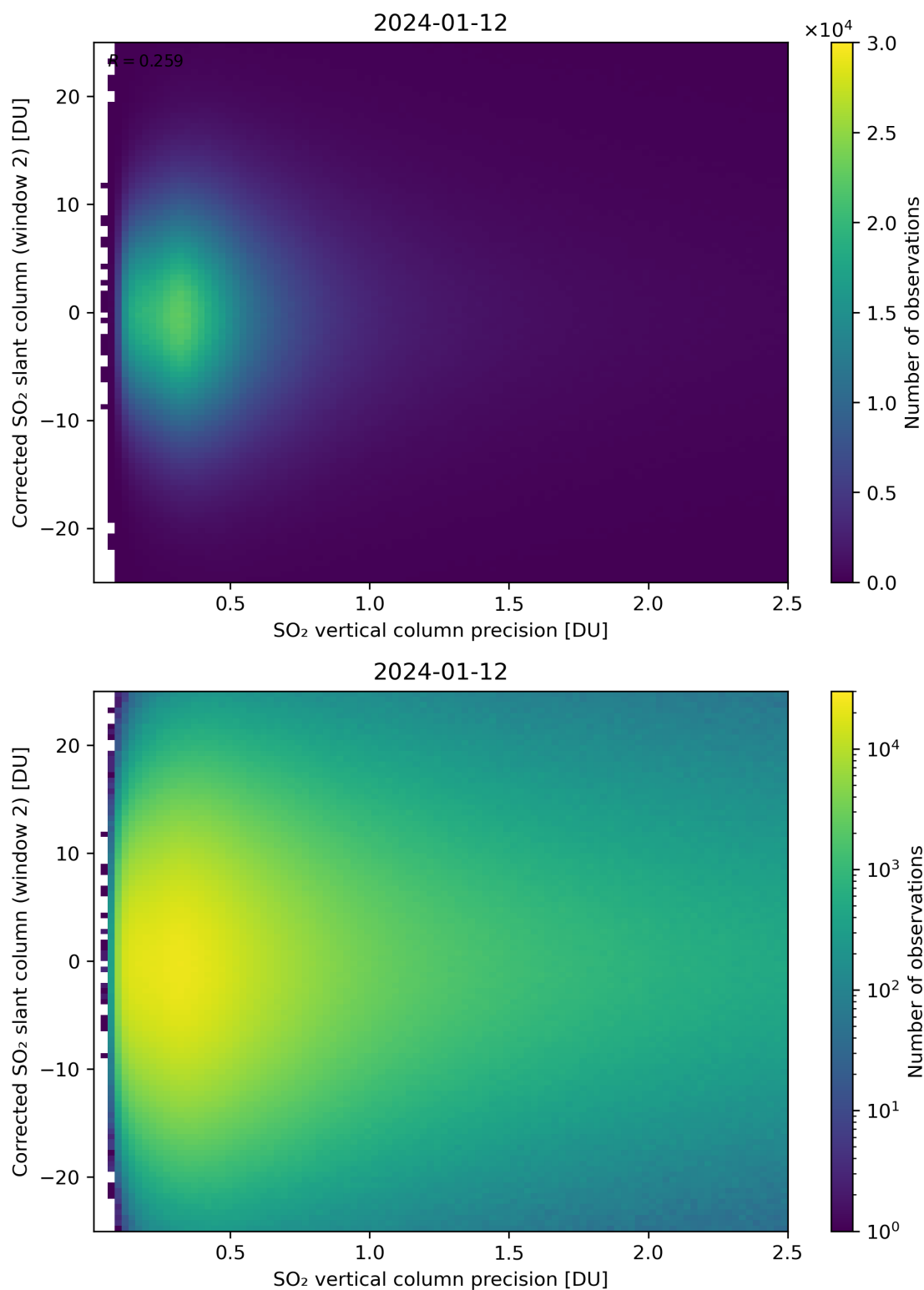
Figure 287: Scatter density plot of “SO 2 vertical column precision” against “Corrected SO 2 slant column (window 2)” for 2024-01-11 to 2024-01-13.
