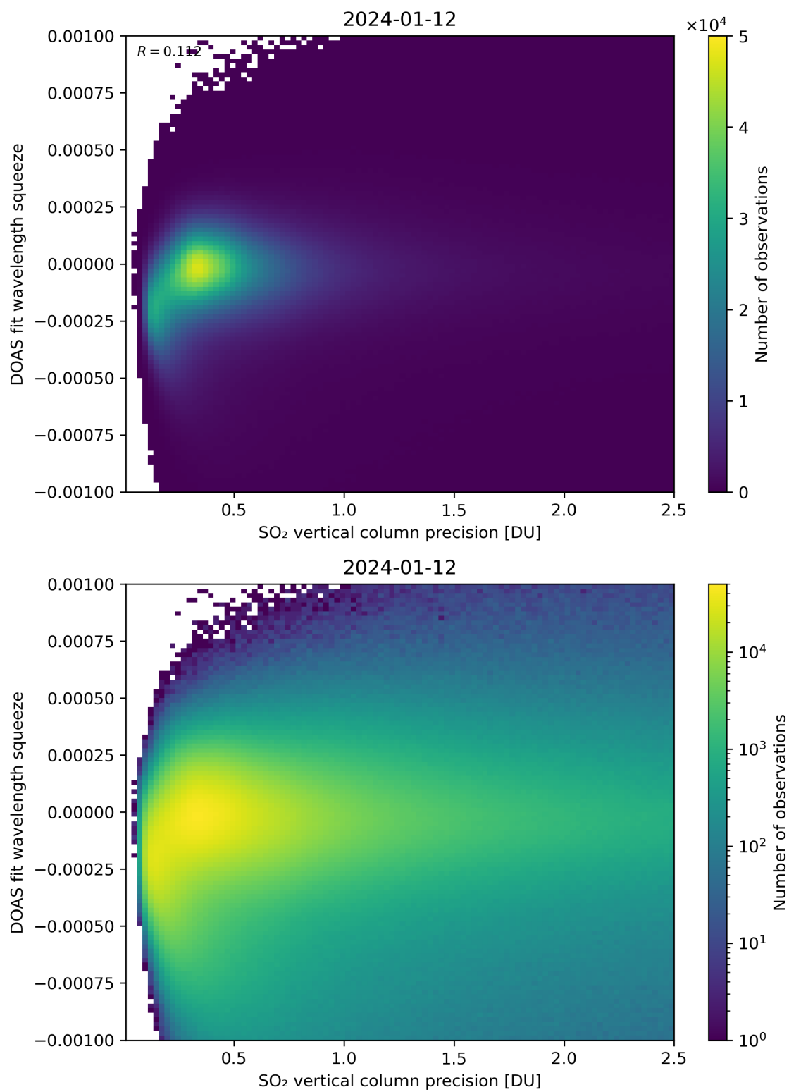
Figure 283: Scatter density plot of “SO 2 vertical column precision” against “DOAS fit wavelength squeeze” for 2024-01-11 to 2024-01-13.
