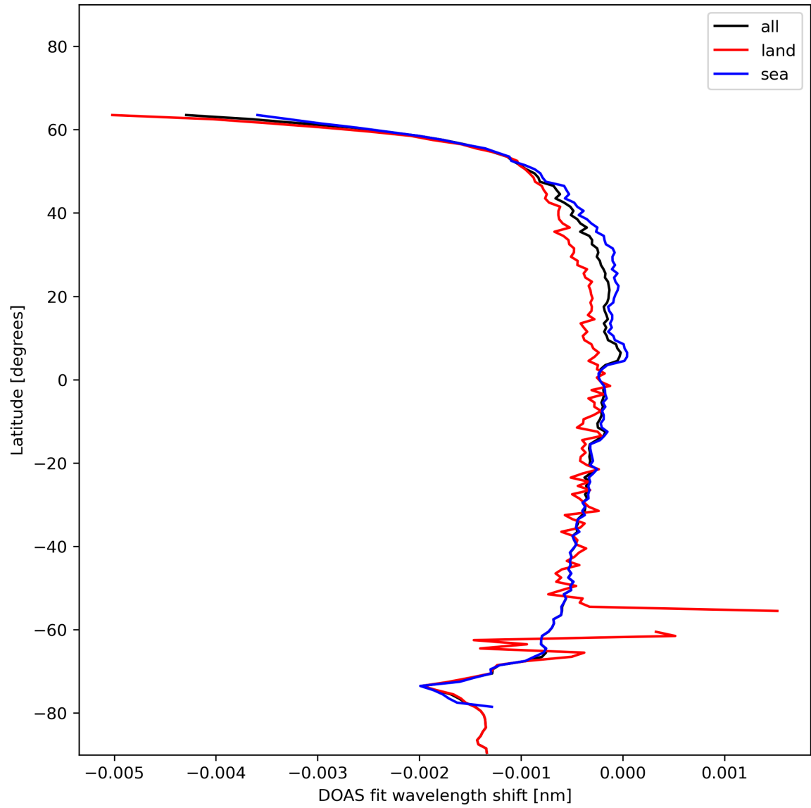
Figure 45: Zonal average of “DOAS fit wavelength shift” for 2024-01-11 to 2024-01-13.
