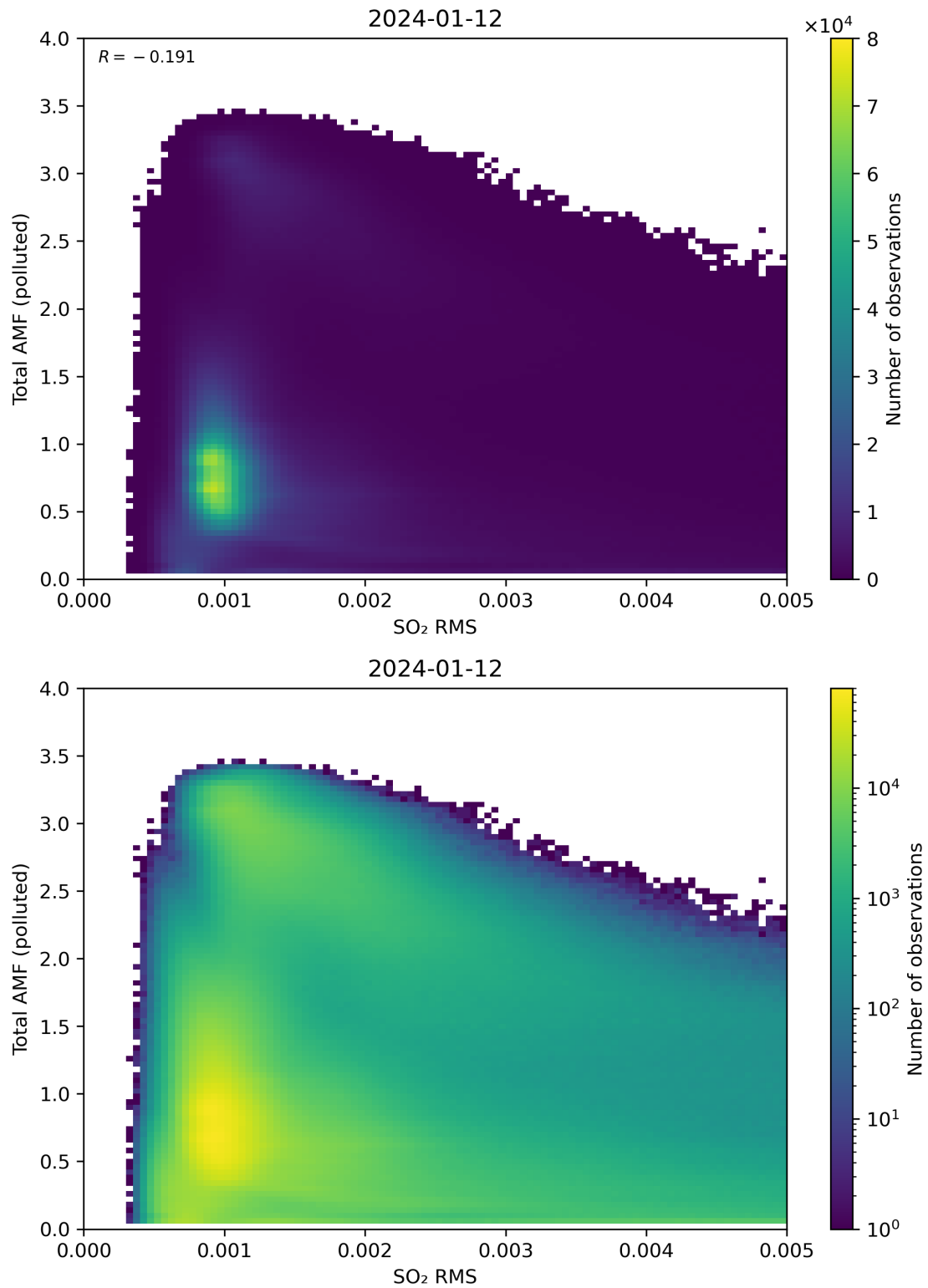
Figure 137: Scatter density plot of “SO 2 RMS” against “Total AMF (polluted)” for 2024-01-11 to 2024-01-13.
