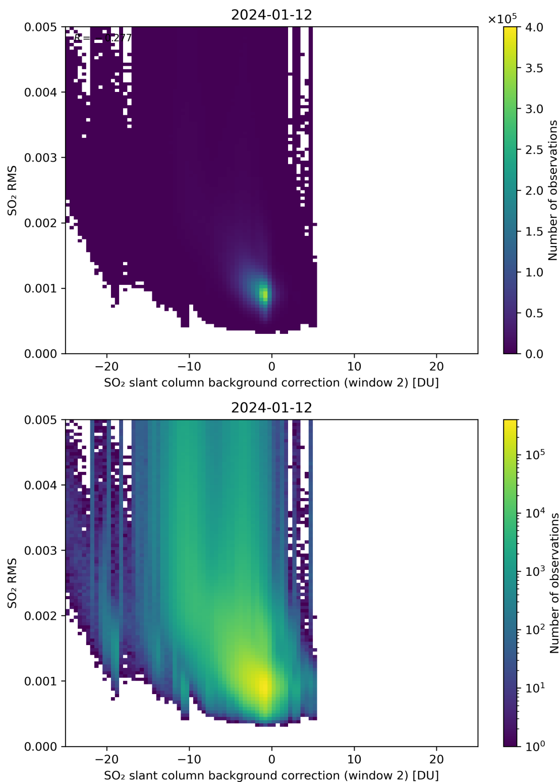
Figure 114: Scatter density plot of “SO 2 slant column background correction (window 2)” against “SO 2 RMS” for 2024-01-11 to 2024-01-13.
