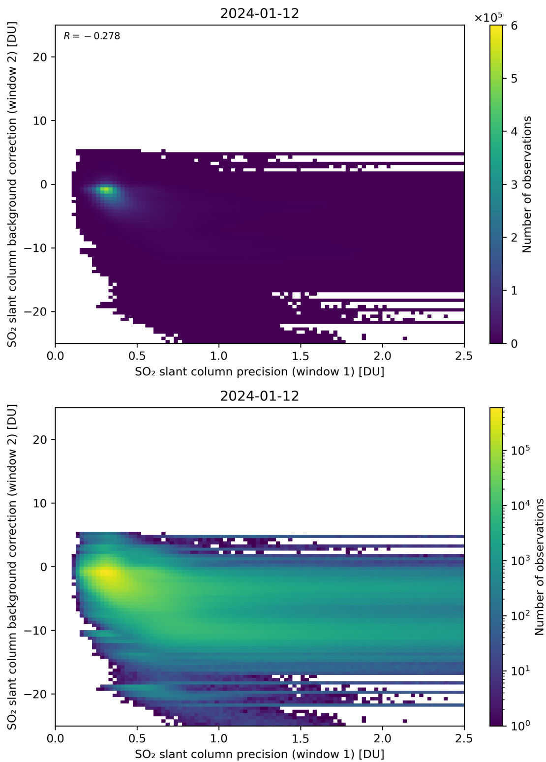
Figure 219: Scatter density plot of “SO 2 slant column precision (window 1)” against “SO 2 slant column background correction (window 2)” for 2024-01-11 to 2024-01-13.
