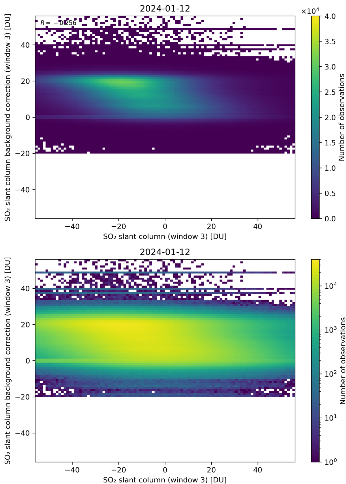
Figure 253: Scatter density plot of “SO 2 slant column (window 3)” against “SO 2 slant column background correction (window 3)” for 2024-01-11 to 2024-01-13.
