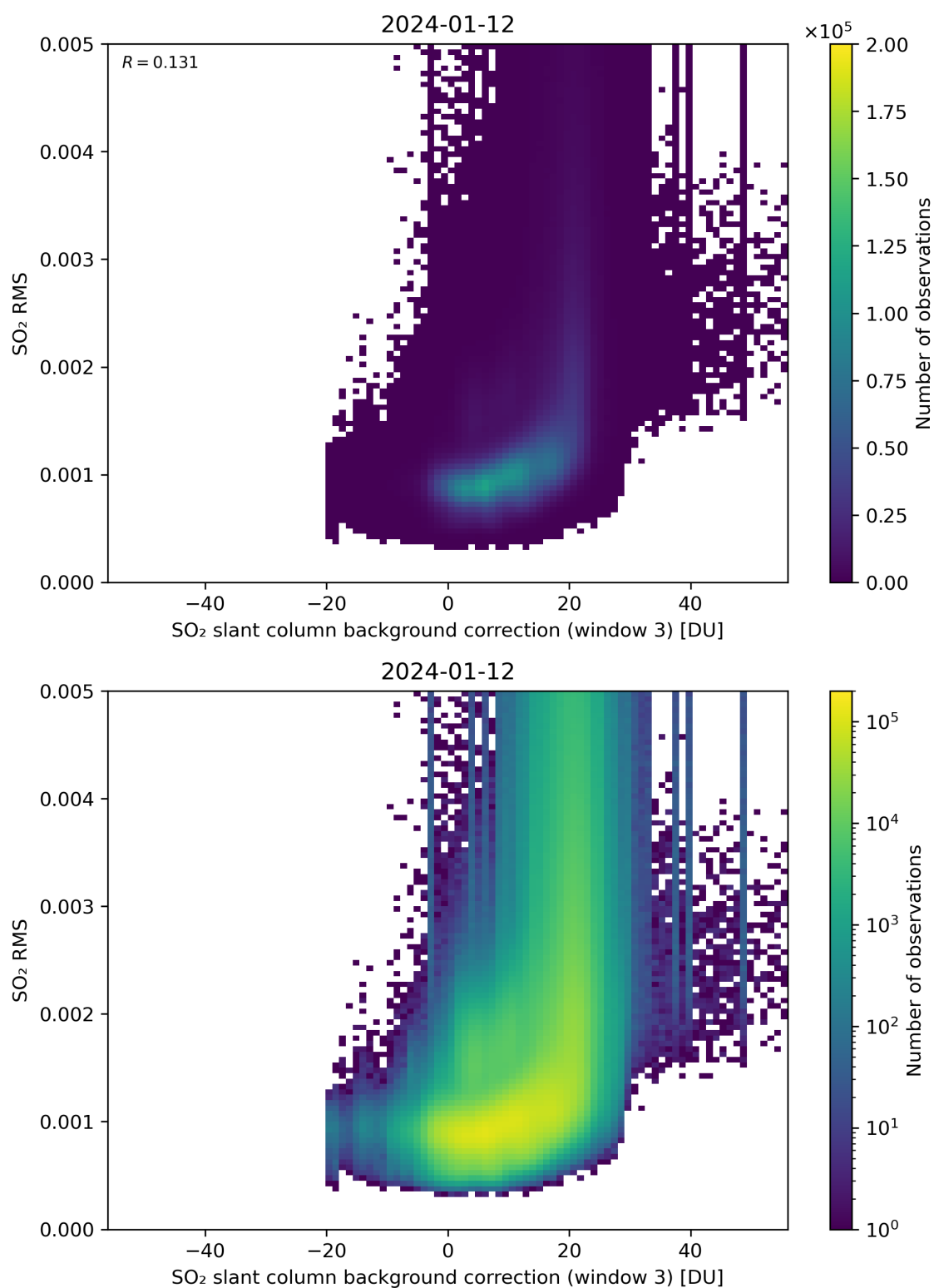
Figure 123: Scatter density plot of “SO 2 slant column background correction (window 3)” against “SO 2 RMS” for 2024-01-11 to 2024-01-13.
