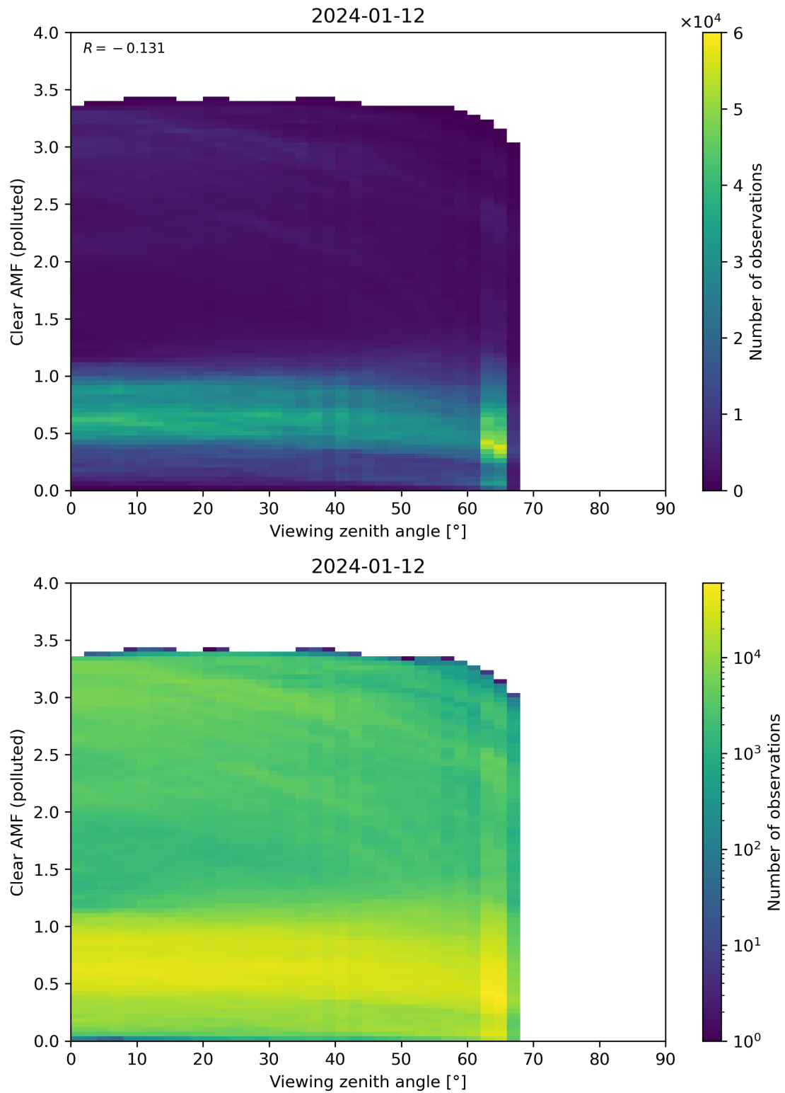
Figure 316: Scatter density plot of “Viewing zenith angle” against “Clear AMF (polluted)” for 2024-01-11 to 2024-01-13.
