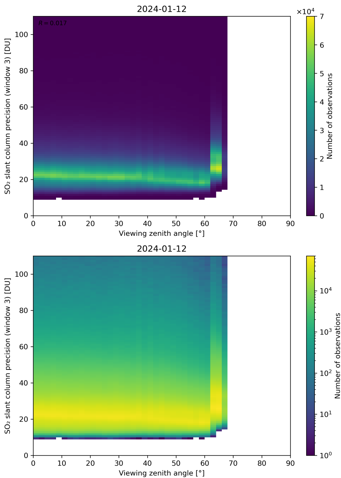
Figure 324: Scatter density plot of “Viewing zenith angle” against “SO 2 slant column precision (window 3)” for 2024-01-11 to 2024-01-13.
