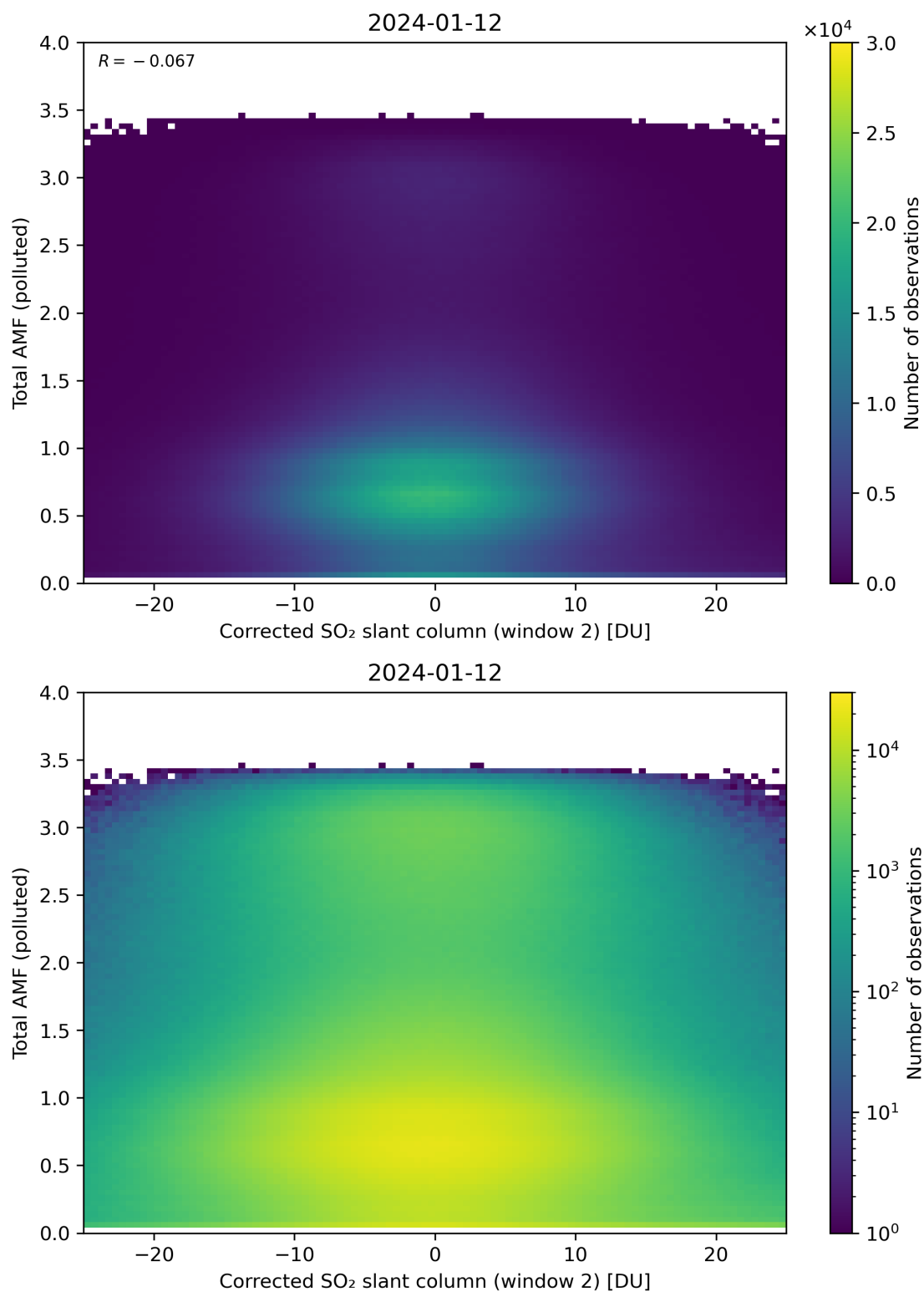
Figure 203: Scatter density plot of “Corrected SO 2 slant column (window 2)” against “Total AMF (polluted)” for 2024-01-11 to 2024-01-13.
