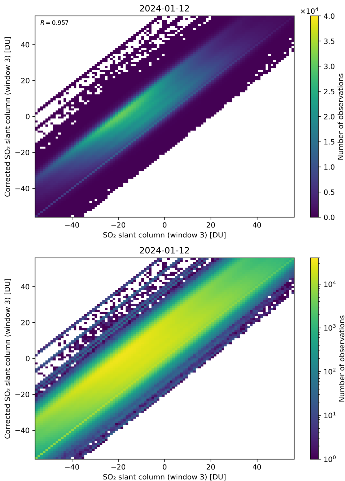
Figure 266: Scatter density plot of “SO 2 slant column (window 3)” against “Corrected SO 2 slant column (window 3)” for 2024-01-11 to 2024-01-13.
