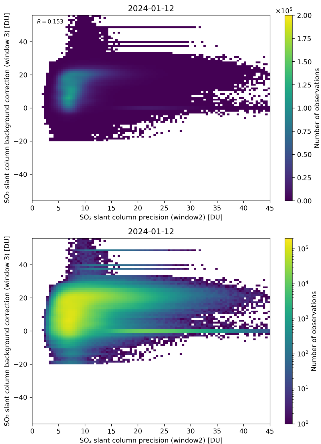
Figure 242: Scatter density plot of “SO 2 slant column precision (window2)” against “SO 2 slant column background correction (window 3)” for 2024-01-11 to 2024-01-13.
