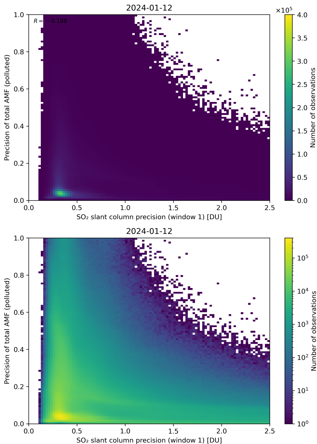
Figure 231: Scatter density plot of “SO 2 slant column precision (window 1)” against “Precision of total AMF (polluted)” for 2024-01-11 to 2024-01-13.
