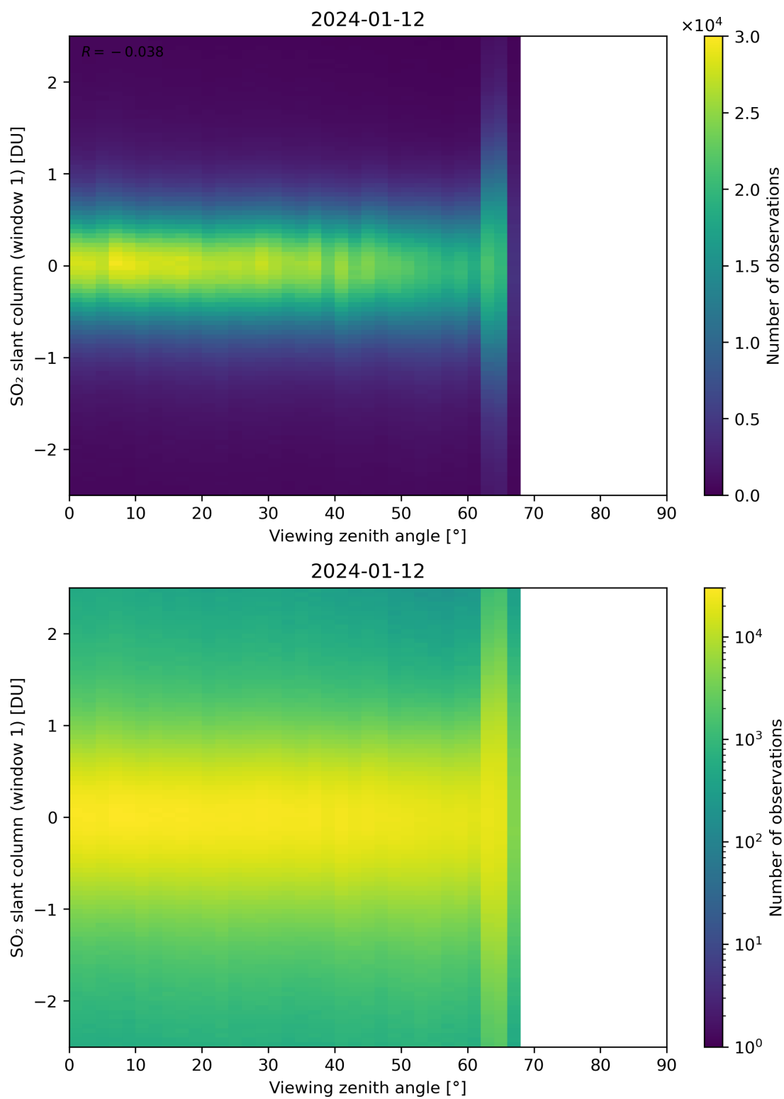
Figure 320: Scatter density plot of “Viewing zenith angle” against “SO 2 slant column (window 1)” for 2024-01-11 to 2024-01-13.
