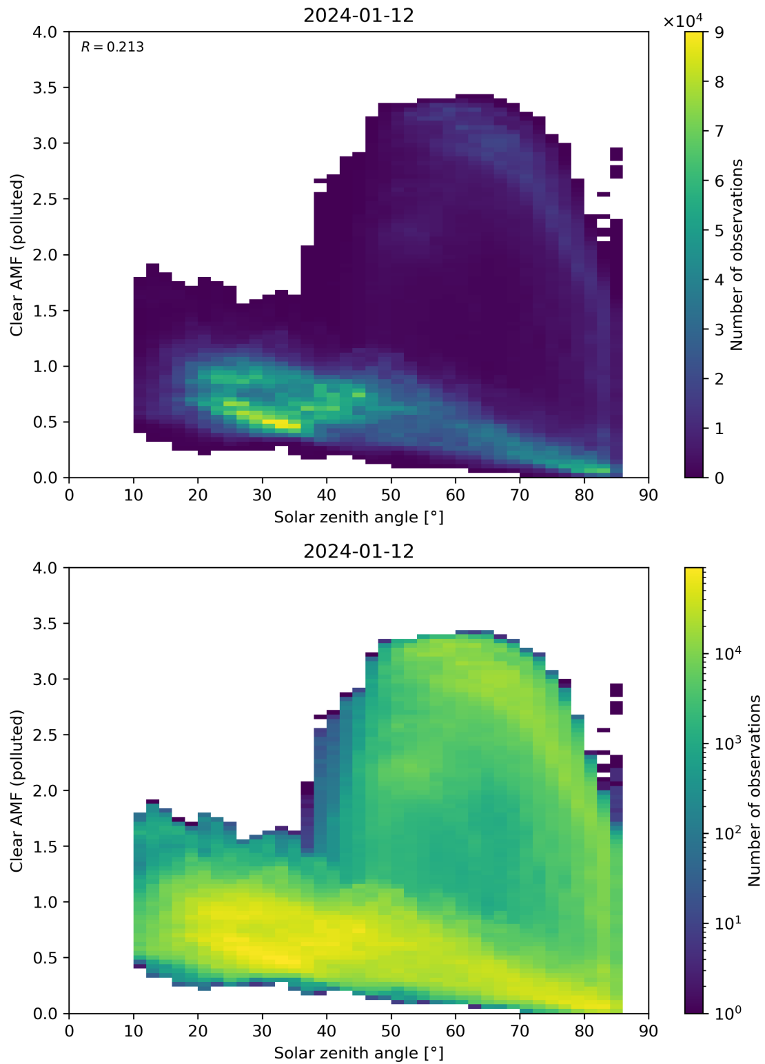
Figure 165: Scatter density plot of “Solar zenith angle” against “Clear AMF (polluted)” for 2024-01-11 to 2024-01-13.
