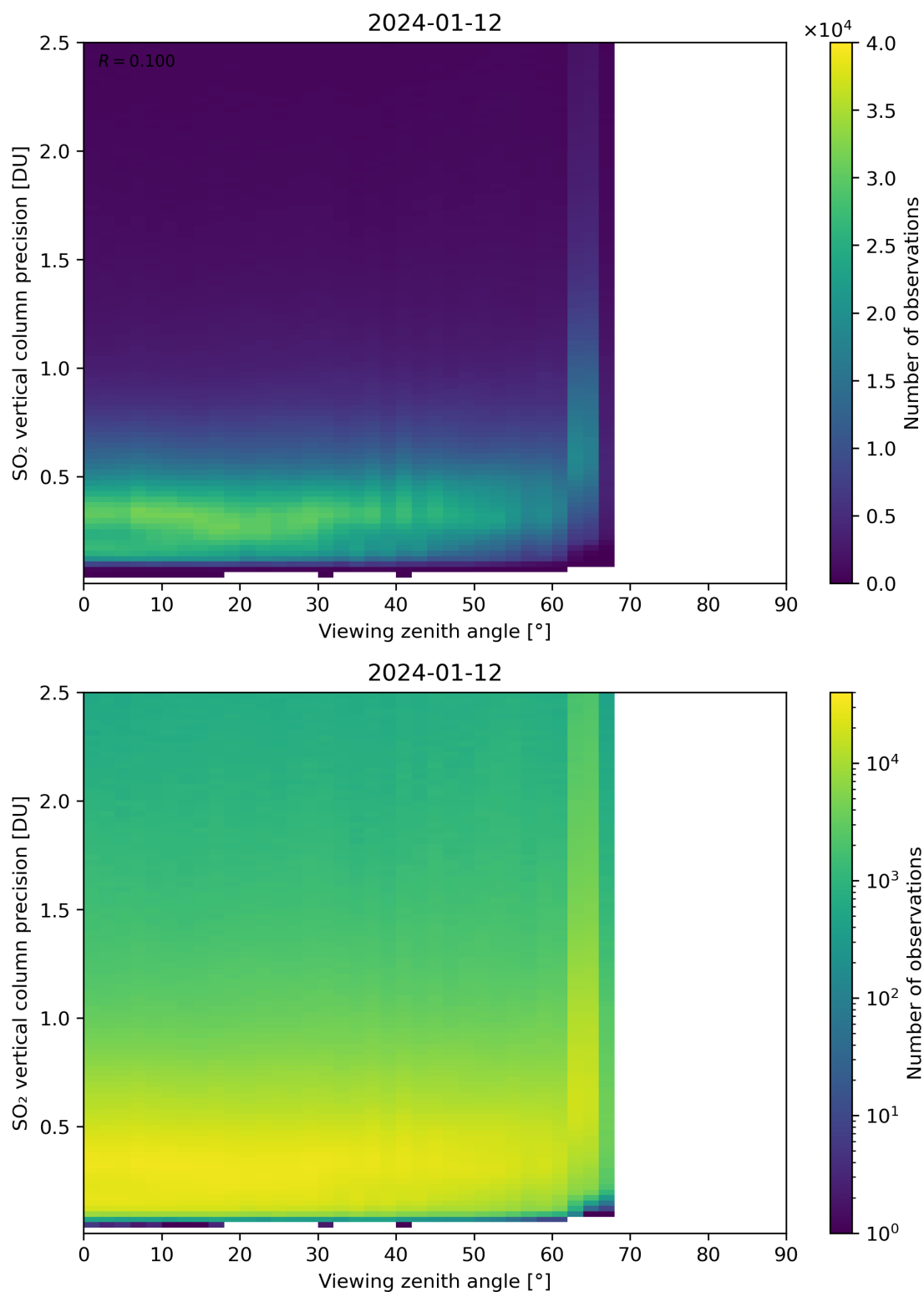
Figure 328: Scatter density plot of “Viewing zenith angle” against “SO 2 vertical column precision” for 2024-01-11 to 2024-01-13.
