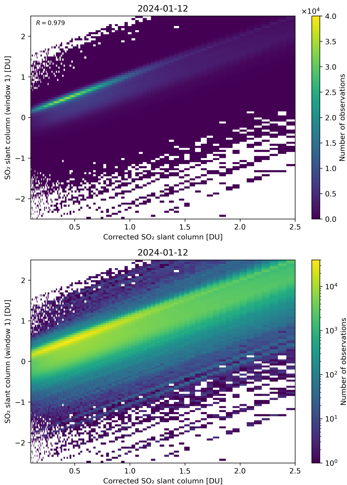
Figure 187: Scatter density plot of “Corrected SO 2 slant column” against “SO 2 slant column (window 1)” for 2024-01-11 to 2024-01-13.
