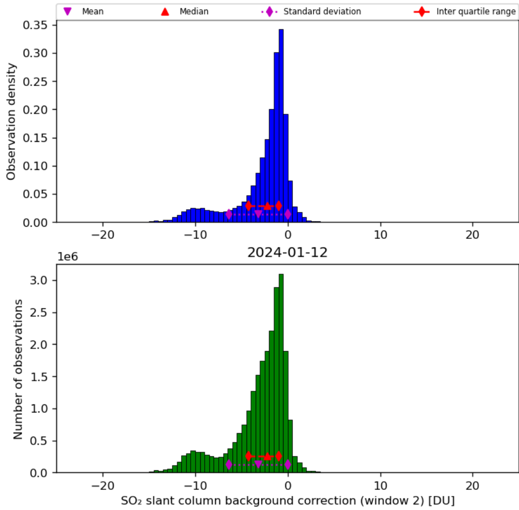
Figure 63: Histogram of “SO 2 slant column background correction (window 2)” for 2024-01-11 to 2024-01-13
