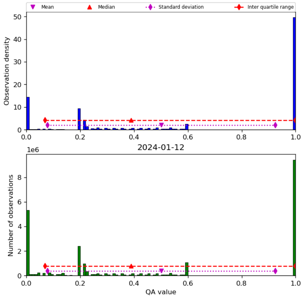
Figure 52: Histogram of “QA value” for 2024-01-11 to 2024-01-13
