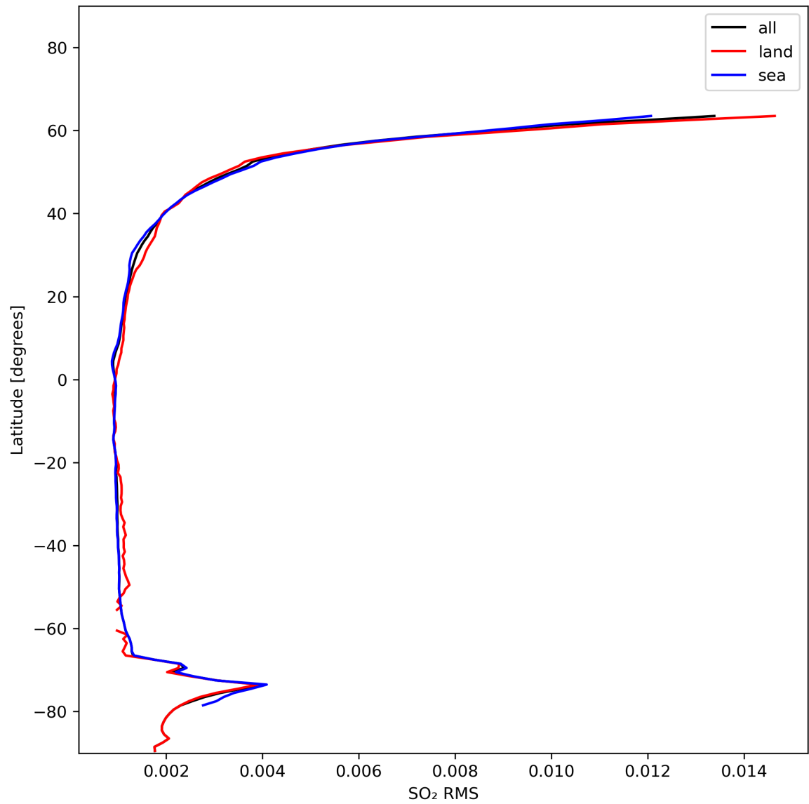
Figure 47: Zonal average of “SO 2 RMS” for 2024-01-11 to 2024-01-13.
