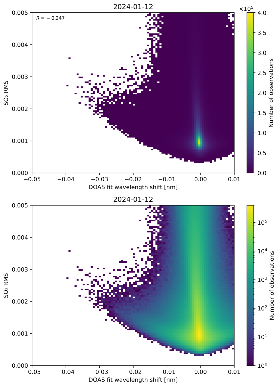
Figure 128: Scatter density plot of “DOAS fit wavelength shift” against “SO 2 RMS” for 2024-01-11 to 2024-01-13.
