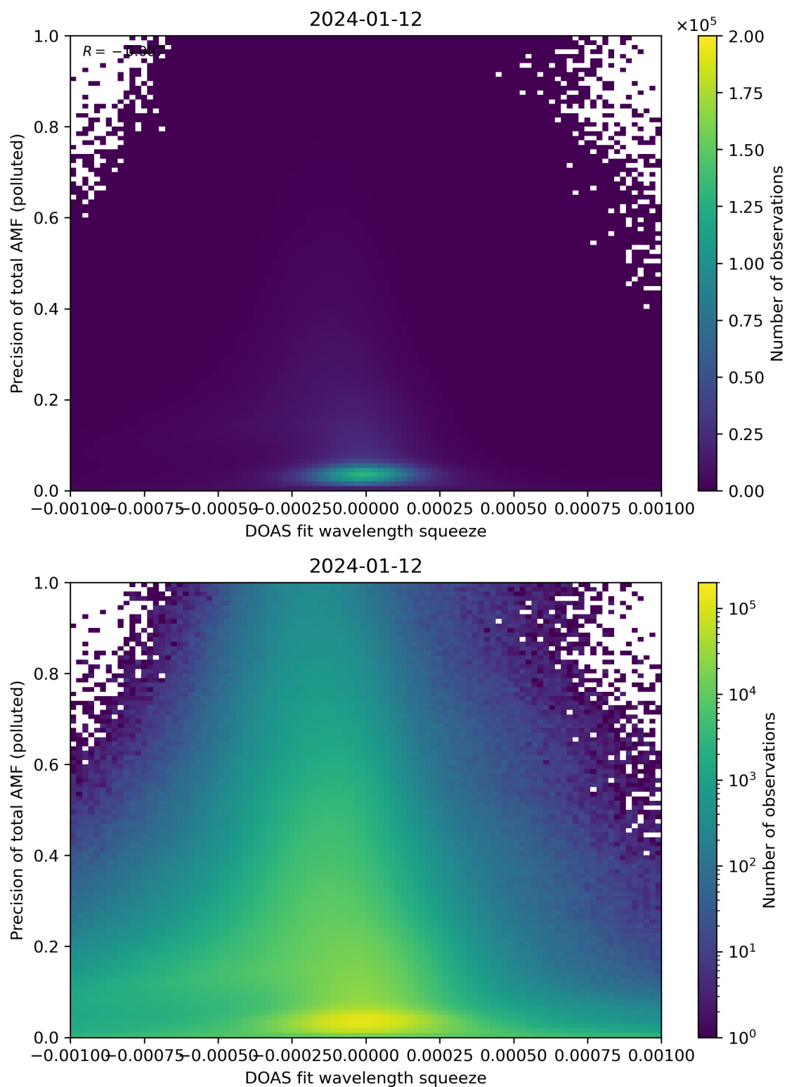
Figure 135: Scatter density plot of “DOAS fit wavelength squeeze” against “Precision of total AMF (polluted)” for 2024-01-11 to 2024-01-13.
