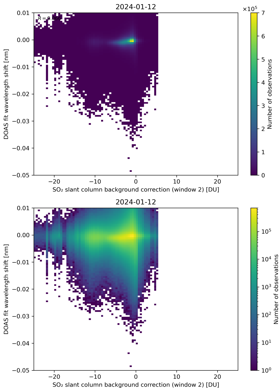
Figure 112: Scatter density plot of “SO 2 slant column background correction (window 2)” against “DOAS fit wavelength shift” for 2024-01-11 to 2024-01-13.
