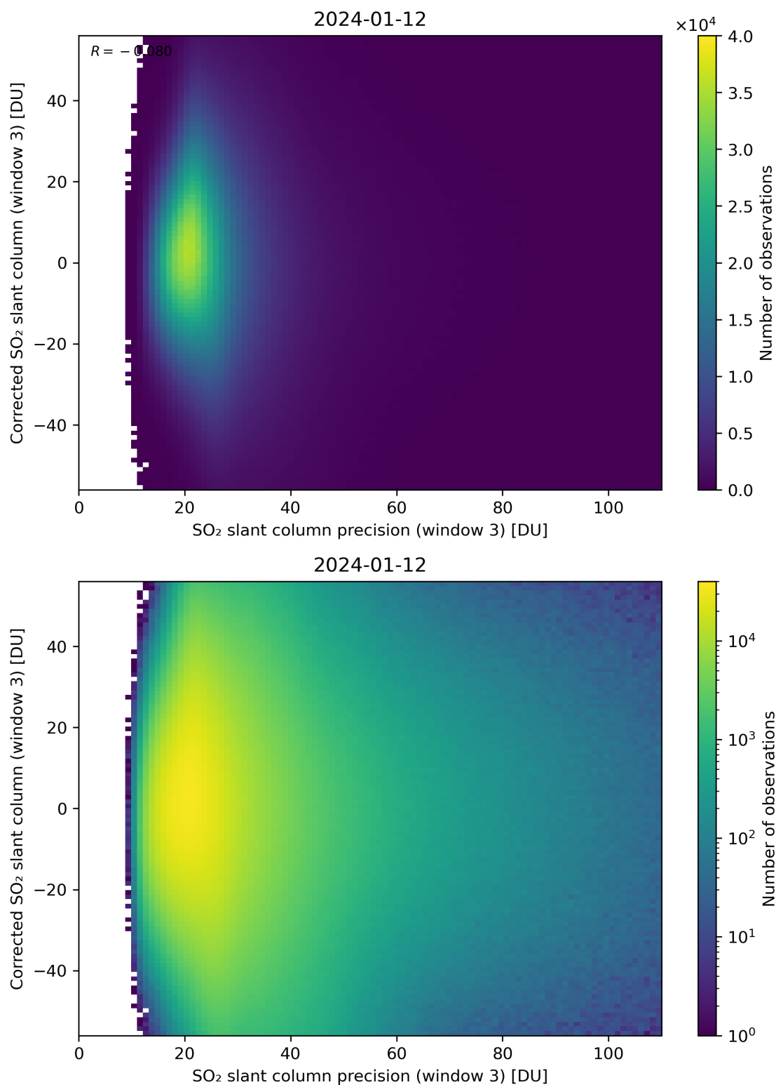
Figure 262: Scatter density plot of “SO 2 slant column precision (window 3)” against “Corrected SO 2 slant column (window 3)” for 2024-01-11 to 2024-01-13.
