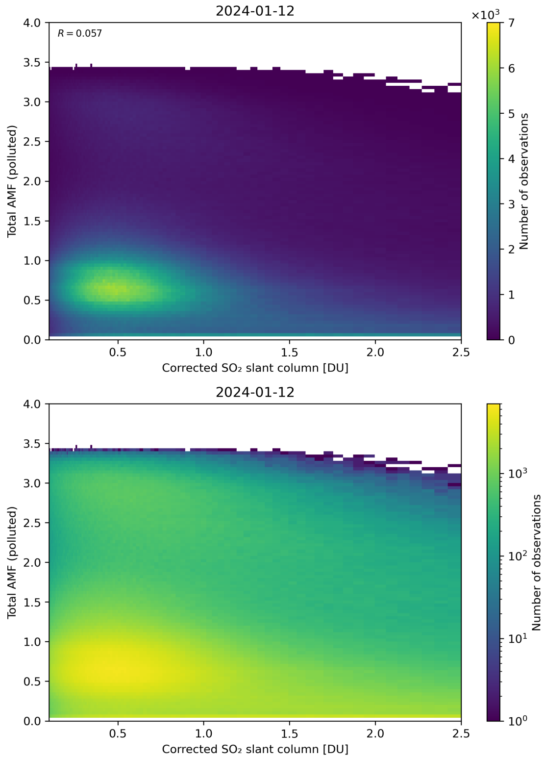
Figure 192: Scatter density plot of “Corrected SO 2 slant column” against “Total AMF (polluted)” for 2024-01-11 to 2024-01-13.
