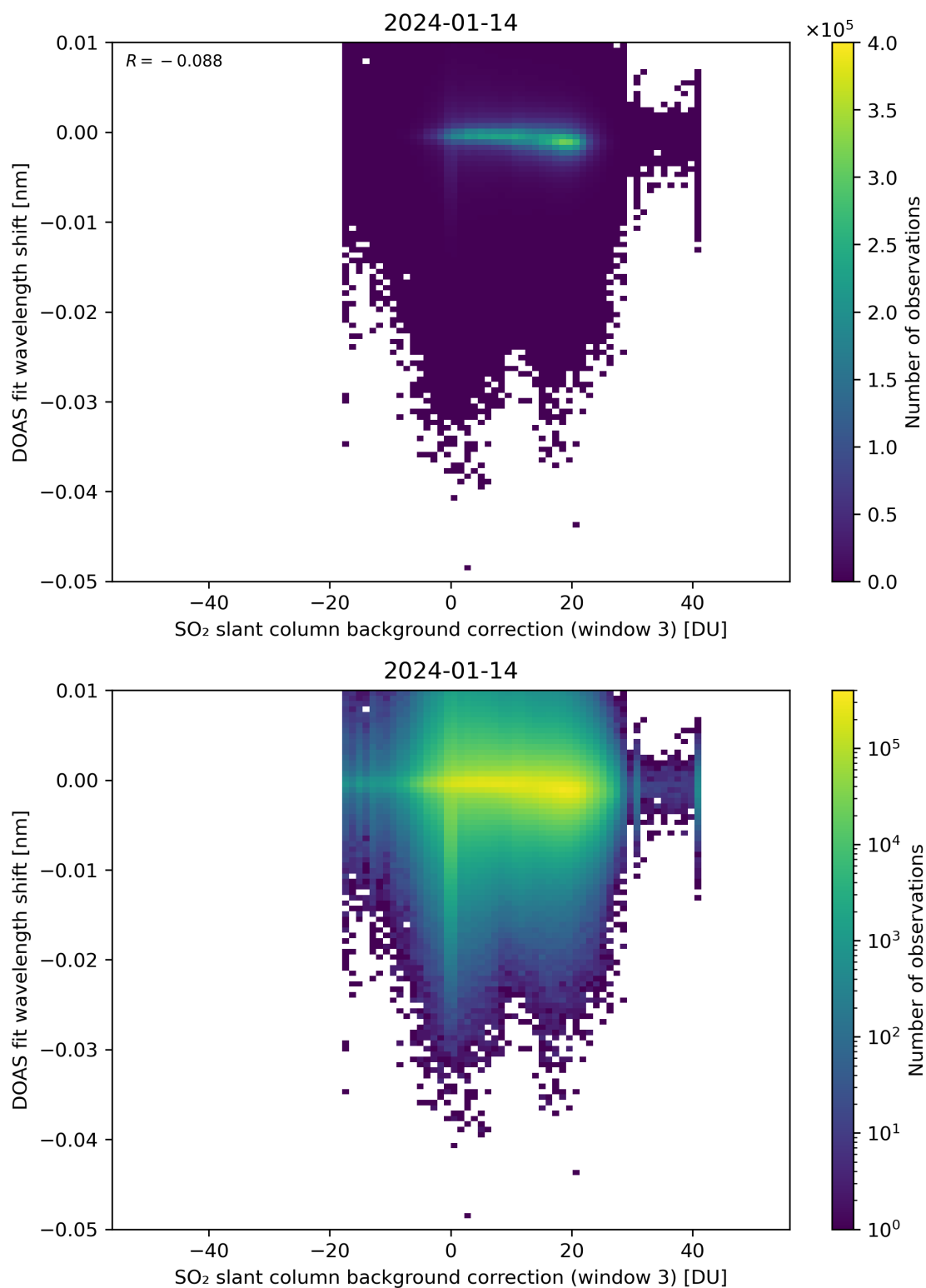
Figure 121: Scatter density plot of “SO 2 slant column background correction (window 3)” against “DOAS fit wavelength shift” for 2024-01-13 to 2024-01-15.
