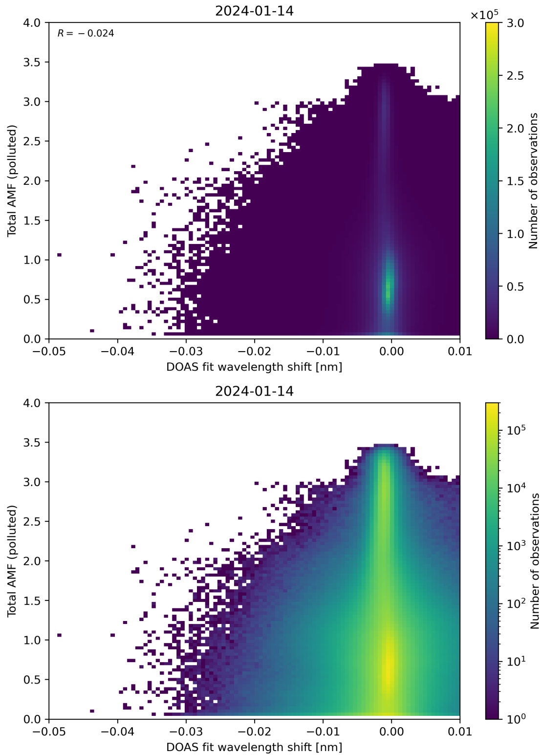
Figure 130: Scatter density plot of “DOAS fit wavelength shift” against “Total AMF (polluted)” for 2024-01-13 to 2024-01-15.
