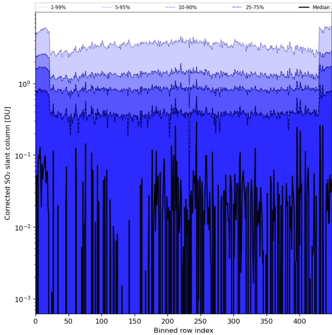
Figure 78: Along track statistics of “Corrected SO 2 slant column” for 2024-01-13 to 2024-01-15
