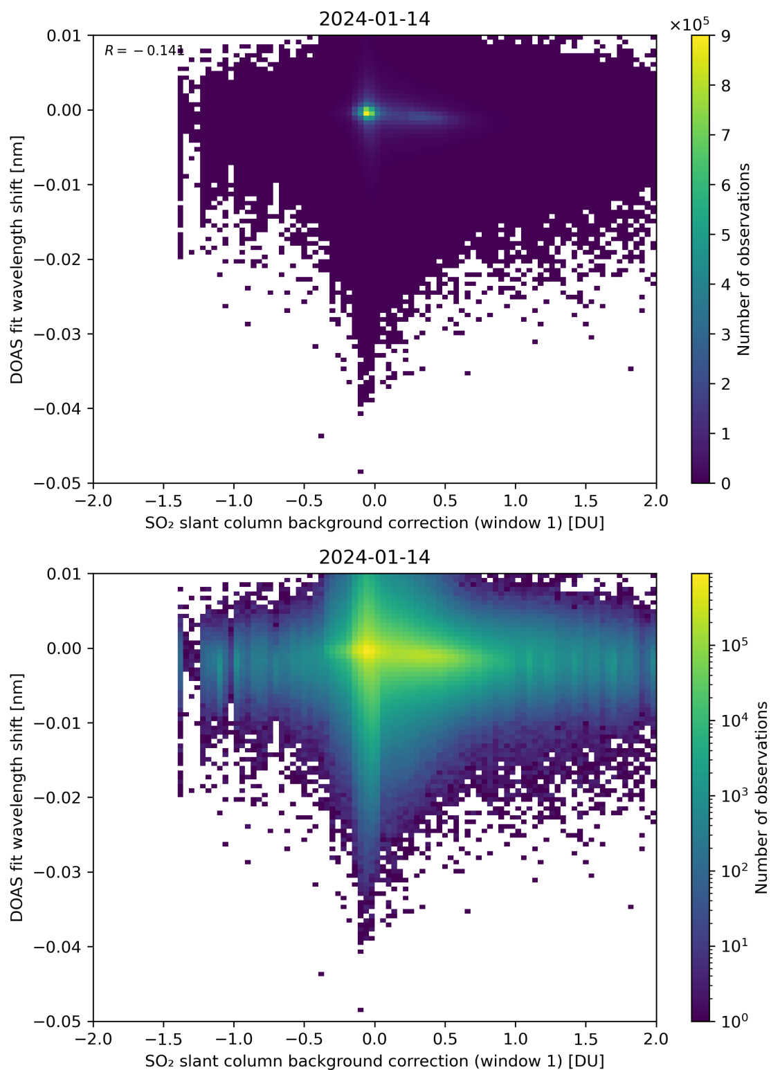
Figure 100: Scatter density plot of “SO 2 slant column background correction (window 1)” against “DOAS fit wavelength shift” for 2024-01-13 to 2024-01-15.
