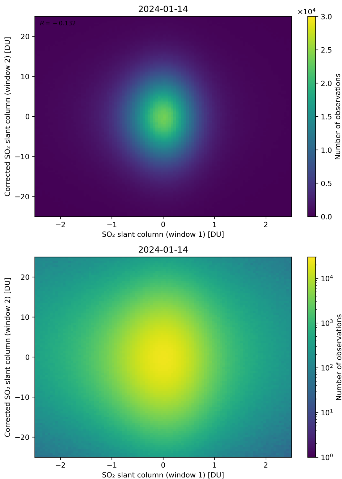
Figure 233: Scatter density plot of “SO 2 slant column (window 1)” against “Corrected SO 2 slant column (window 2)” for 2024-01-13 to 2024-01-15.
