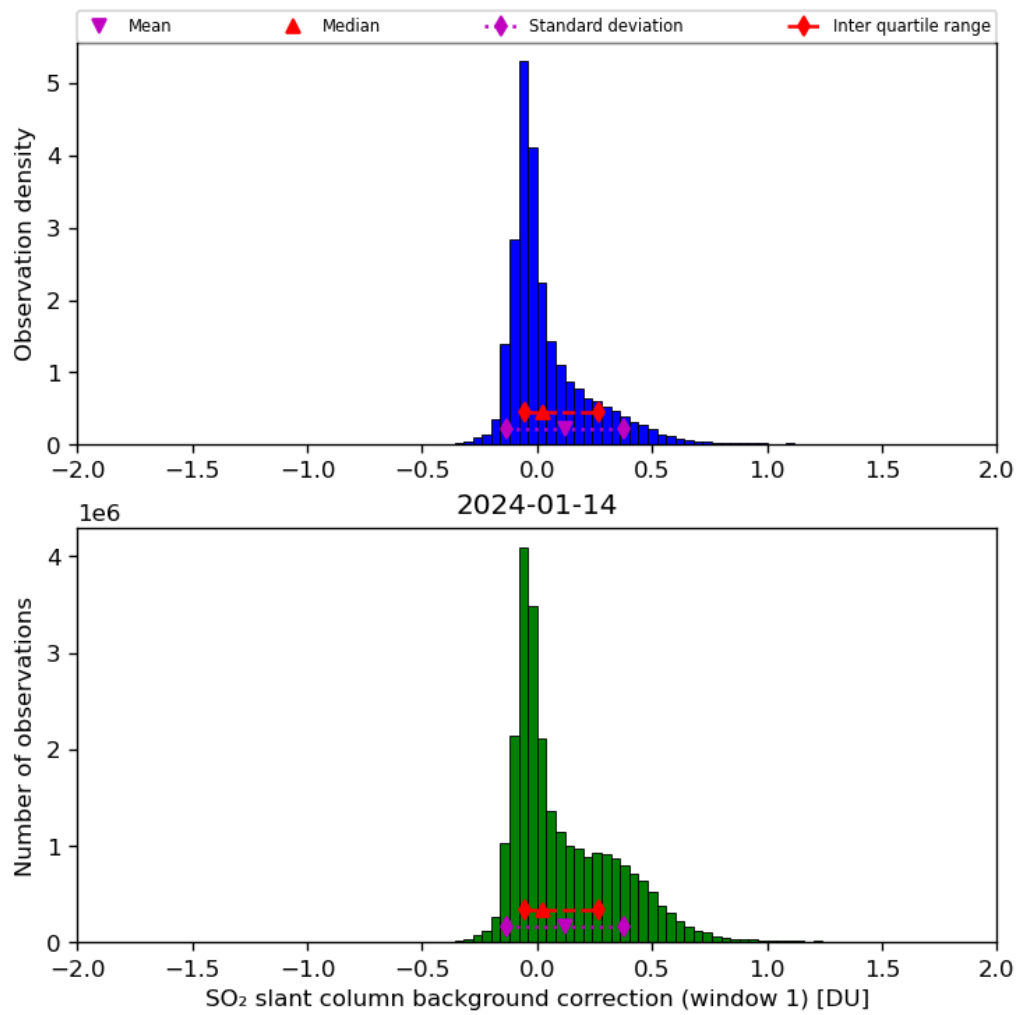
Figure 59: Histogram of “SO 2 slant column background correction (window 1)” for 2024-01-13 to 2024-01-15
