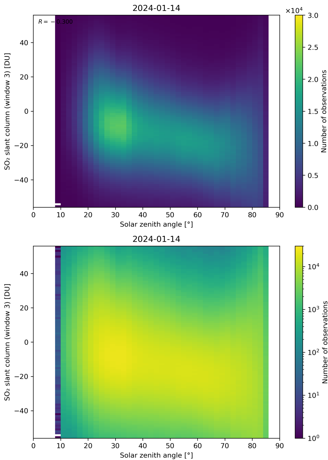
Figure 172: Scatter density plot of “Solar zenith angle” against “SO 2 slant column (window 3)” for 2024-01-13 to 2024-01-15.
