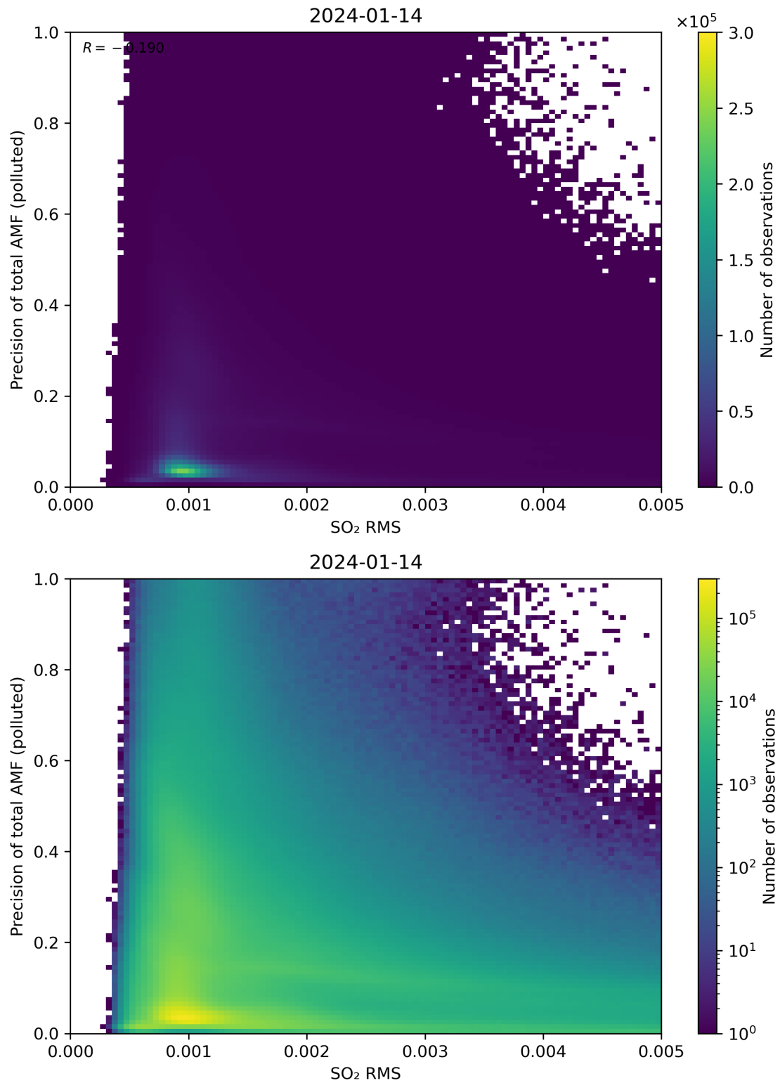
Figure 138: Scatter density plot of “SO 2 RMS” against “Precision of total AMF (polluted)” for 2024-01-13 to 2024-01-15.
