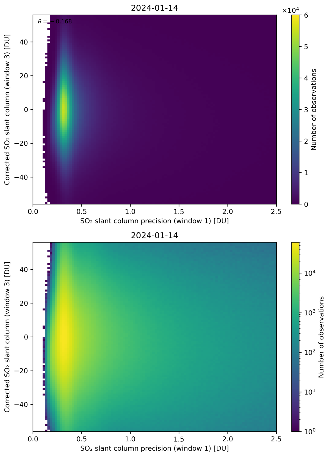
Figure 226: Scatter density plot of “SO 2 slant column precision (window 1)” against “Corrected SO 2 slant column (window 3)” for 2024-01-13 to 2024-01-15.
