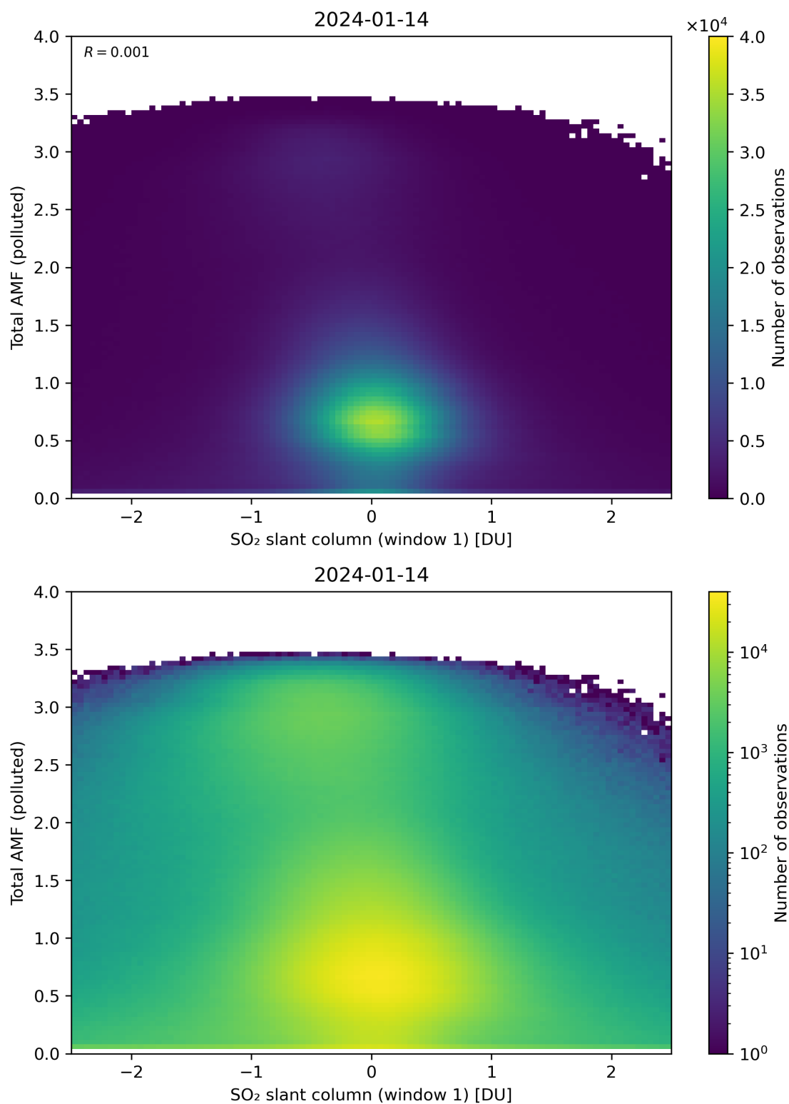
Figure 239: Scatter density plot of “SO 2 slant column (window 1)” against “Total AMF (polluted)” for 2024-01-13 to 2024-01-15.
