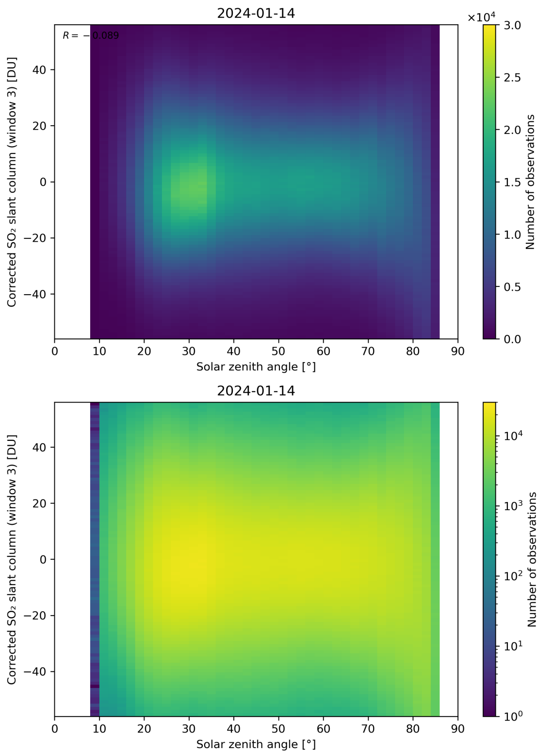
Figure 168: Scatter density plot of “Solar zenith angle” against “Corrected SO 2 slant column (window 3)” for 2024-01-13 to 2024-01-15.
