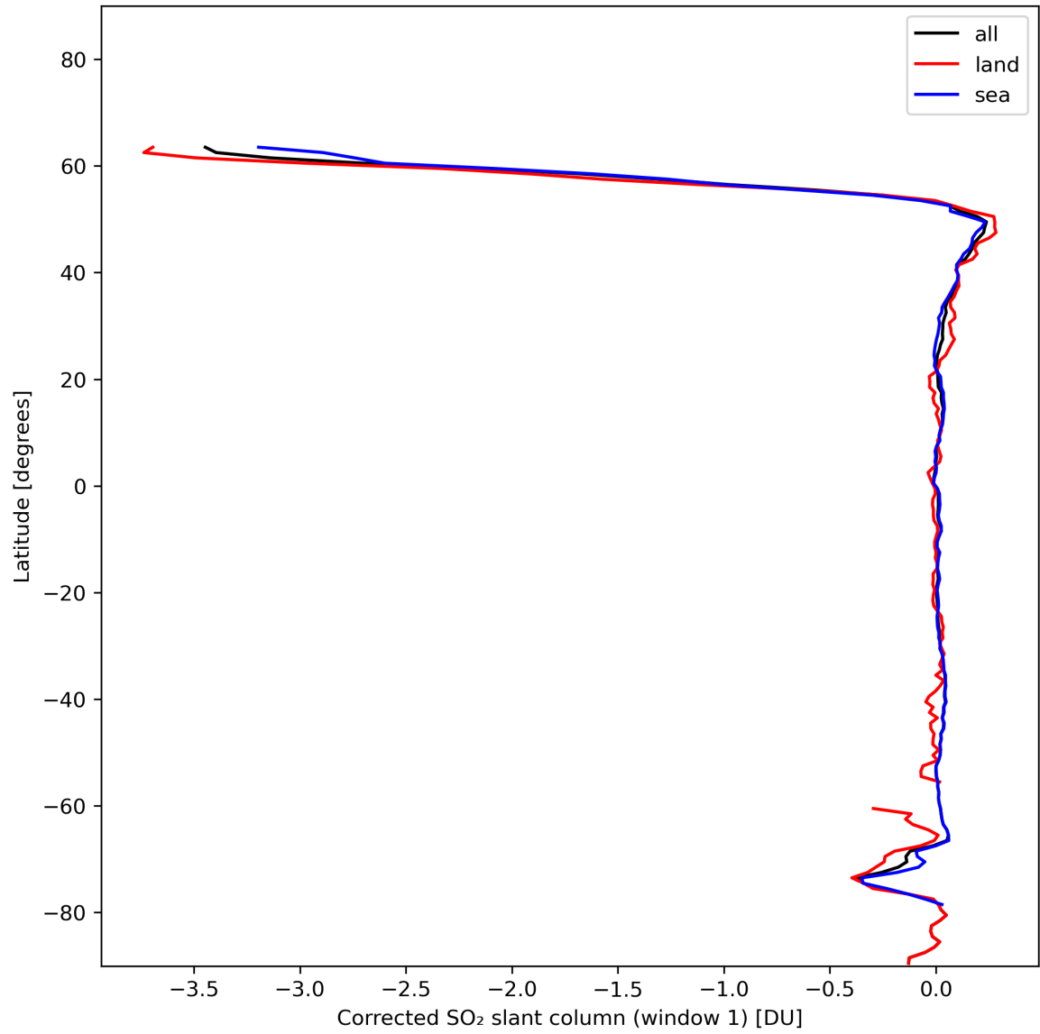
Figure 35: Zonal average of “Corrected SO 2 slant column (window 1)” for 2024-01-13 to 2024-01-15.
