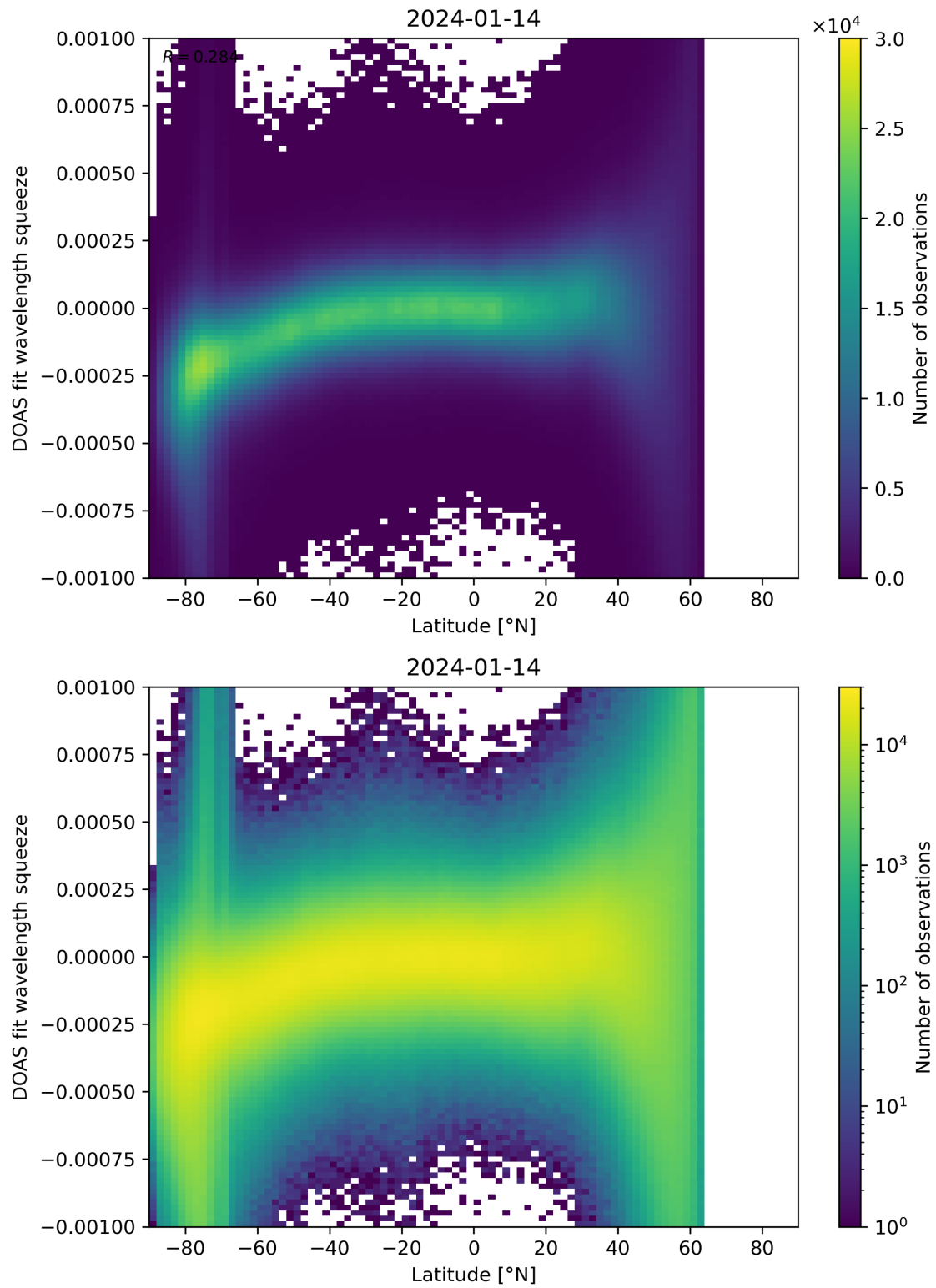
Figure 143: Scatter density plot of “Latitude” against “DOAS fit wavelength squeeze” for 2024-01-13 to 2024-01-15.
