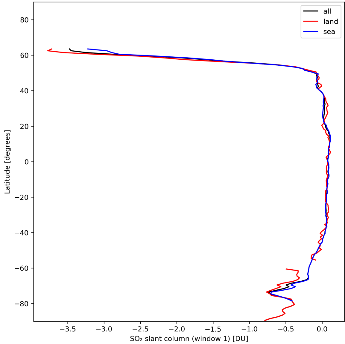
Figure 33: Zonal average of “SO 2 slant column (window 1)” for 2024-01-13 to 2024-01-15.
