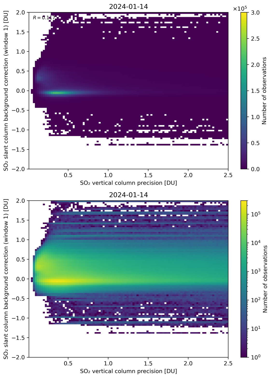
Figure 279: Scatter density plot of “SO 2 vertical column precision” against “SO 2 slant column background correction (window 1)” for 2024-01-13 to 2024-01-15.
