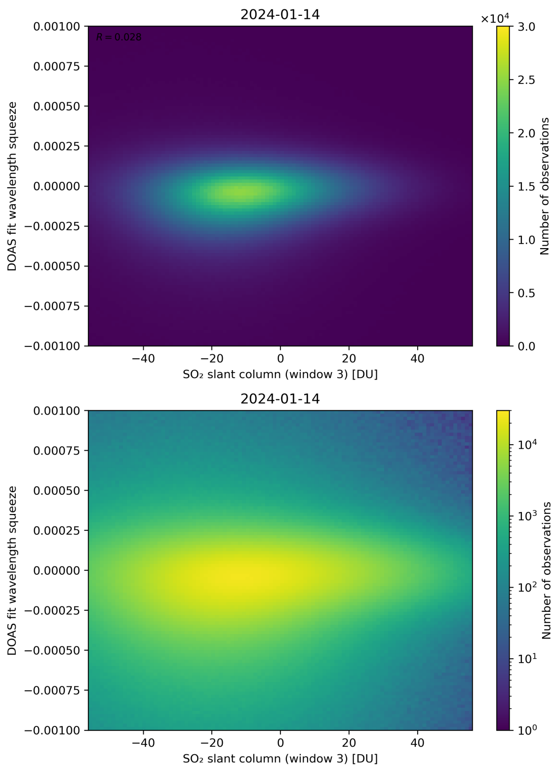
Figure 255: Scatter density plot of “SO 2 slant column (window 3)” against “DOAS fit wavelength squeeze” for 2024-01-13 to 2024-01-15.
