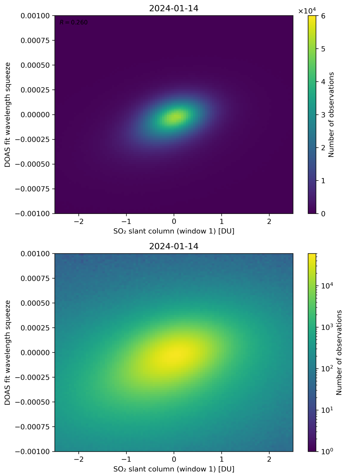
Figure 216: Scatter density plot of “SO 2 slant column (window 1)” against “DOAS fit wavelength squeeze” for 2024-01-13 to 2024-01-15.
