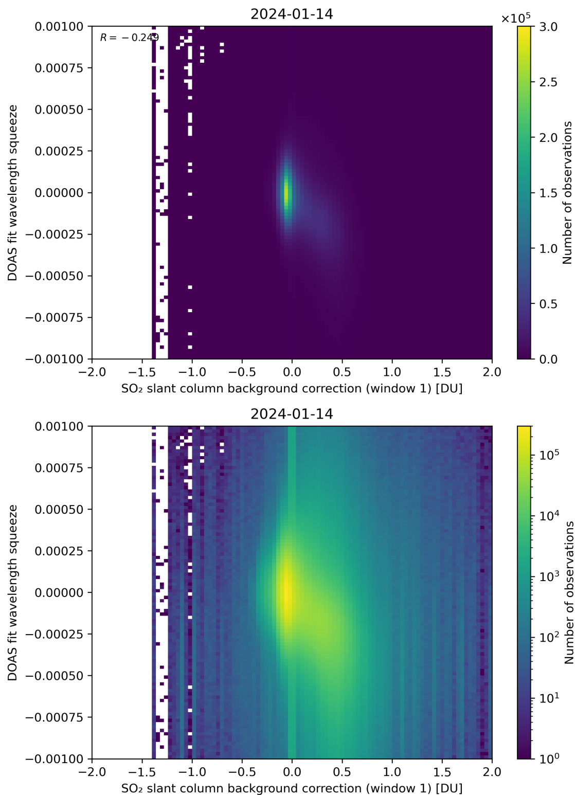
Figure 101: Scatter density plot of “SO 2 slant column background correction (window 1)” against “DOAS fit wavelength squeeze” for 2024-01-13 to 2024-01-15.
