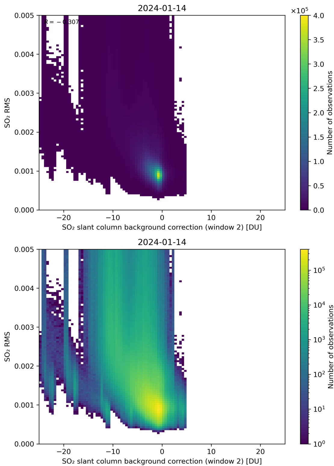
Figure 114: Scatter density plot of “SO 2 slant column background correction (window 2)” against “SO 2 RMS” for 2024-01-13 to 2024-01-15.
