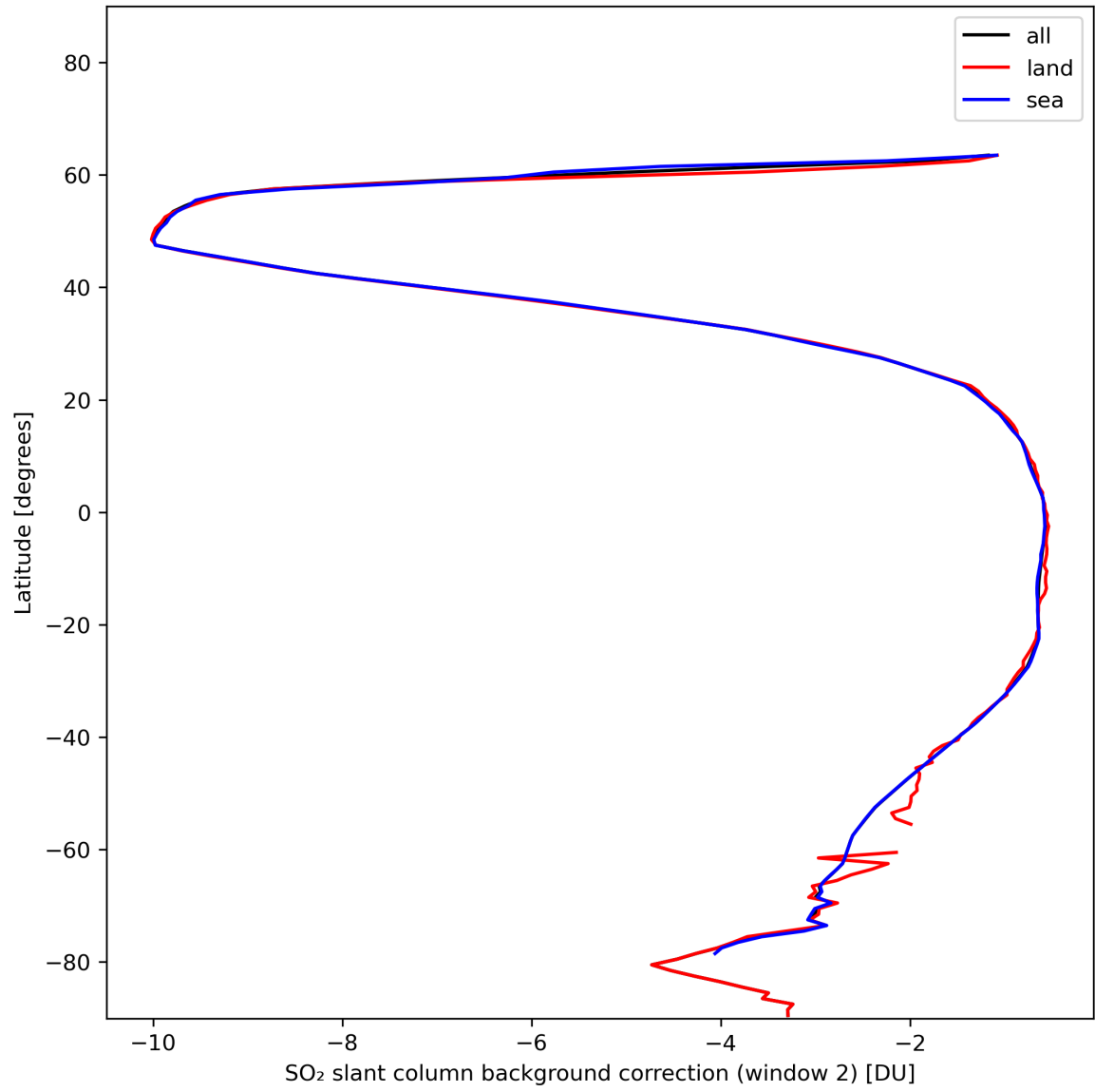
Figure 40: Zonal average of “SO 2 slant column background correction (window 2)” for 2024-01-13 to 2024-01-15.
