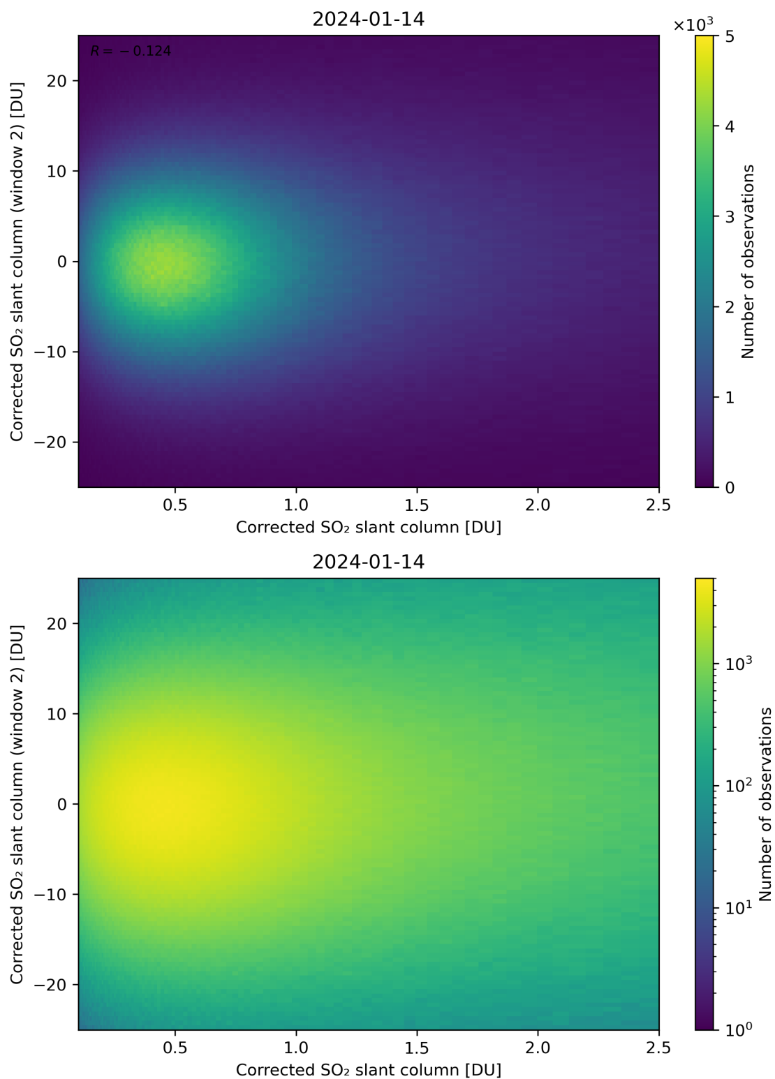
Figure 185: Scatter density plot of “Corrected SO 2 slant column” against “Corrected SO 2 slant column (window 2)” for 2024-01-13 to 2024-01-15.
