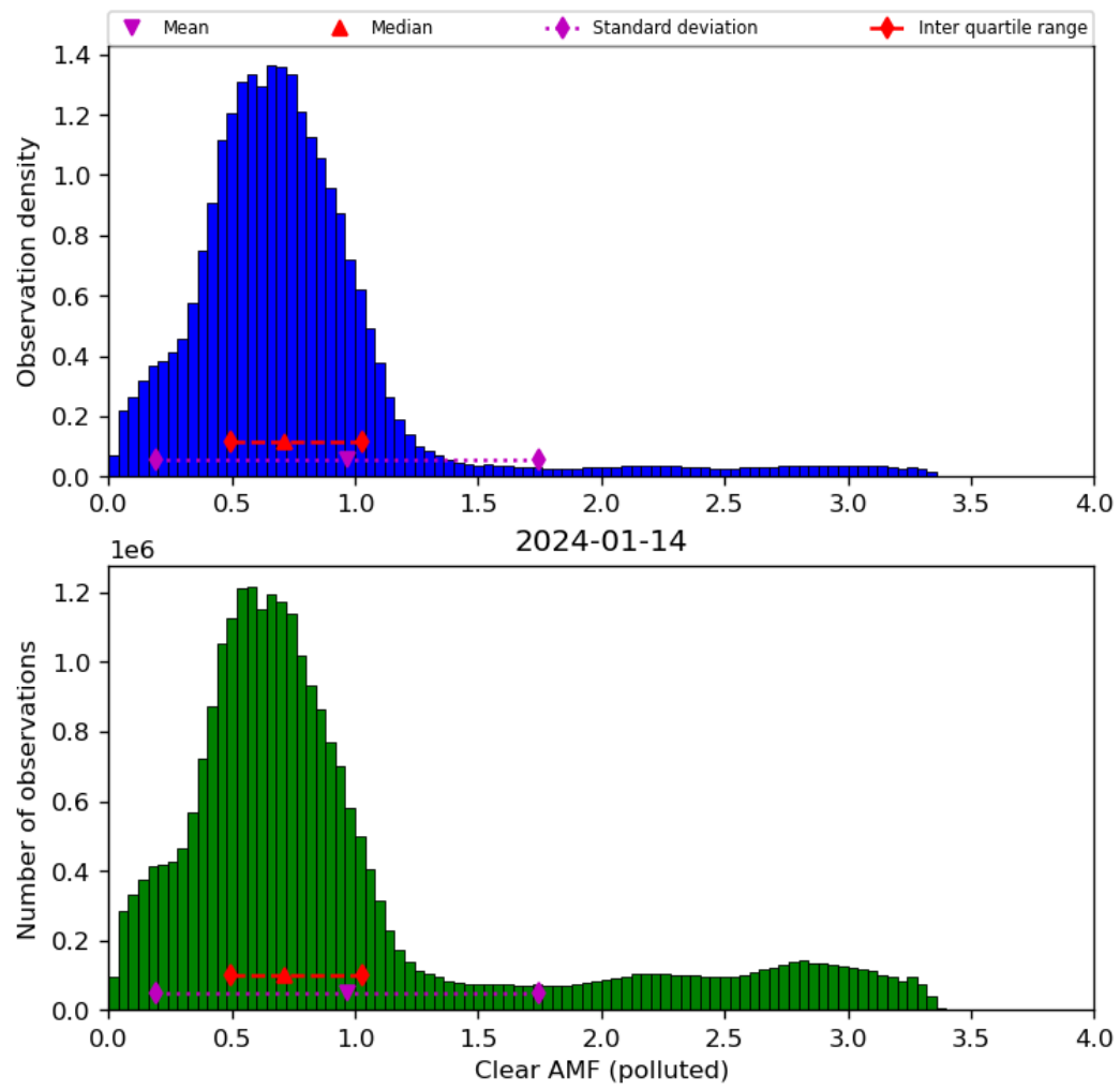
Figure 73: Histogram of “Clear AMF (polluted)” for 2024-01-13 to 2024-01-15
