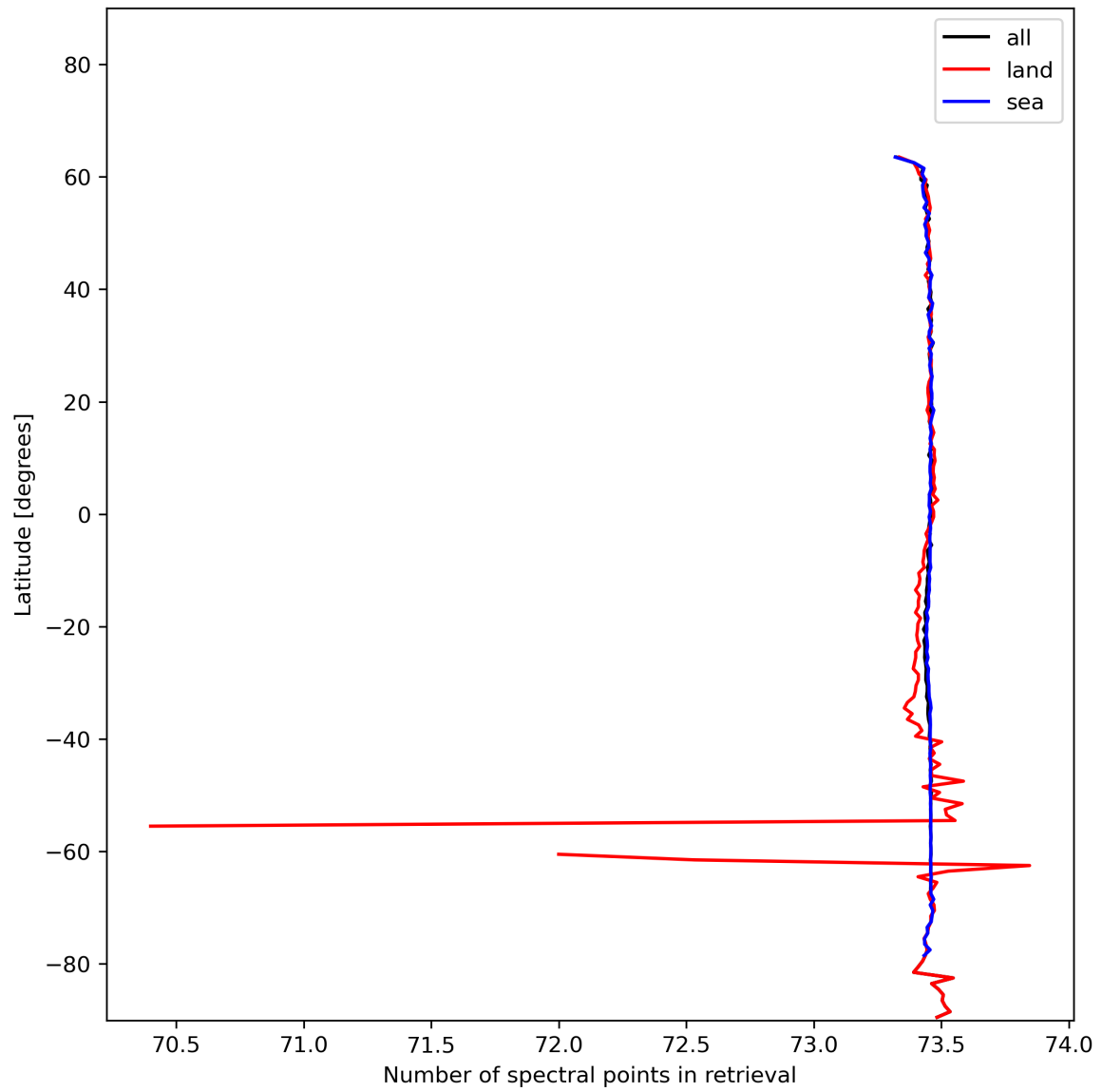
Figure 51: Zonal average of “Number of spectral points in retrieval” for 2024-01-13 to 2024-01-15.
