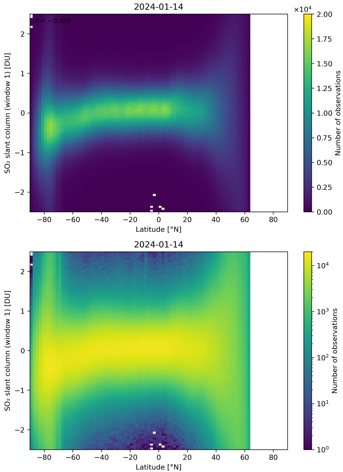
Figure 149: Scatter density plot of “Latitude” against “SO 2 slant column (window 1)” for 2024-01-13 to 2024-01-15.
