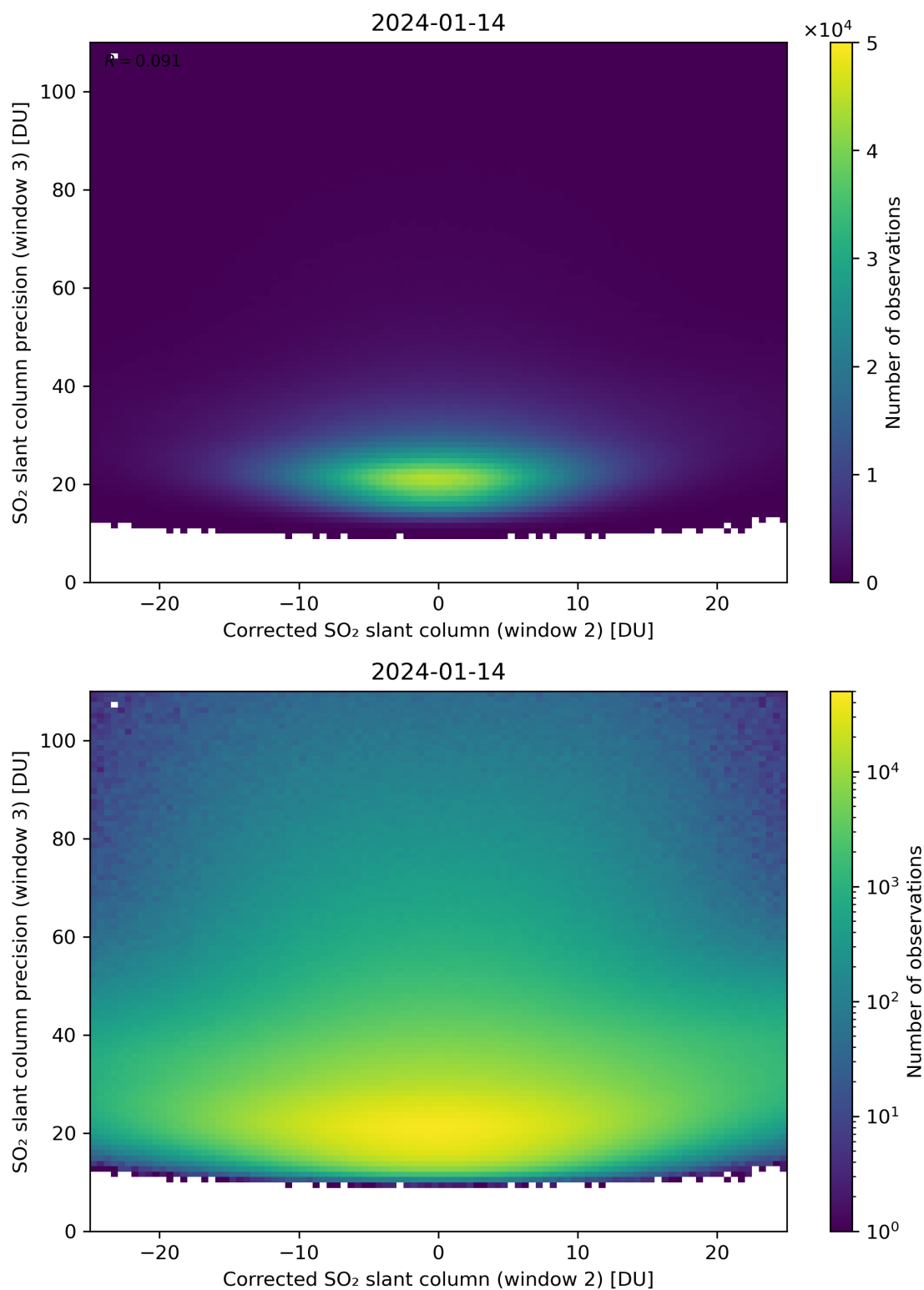
Figure 202: Scatter density plot of “Corrected SO 2 slant column (window 2)” against “SO 2 slant column precision (window 3)” for 2024-01-13 to 2024-01-15.
