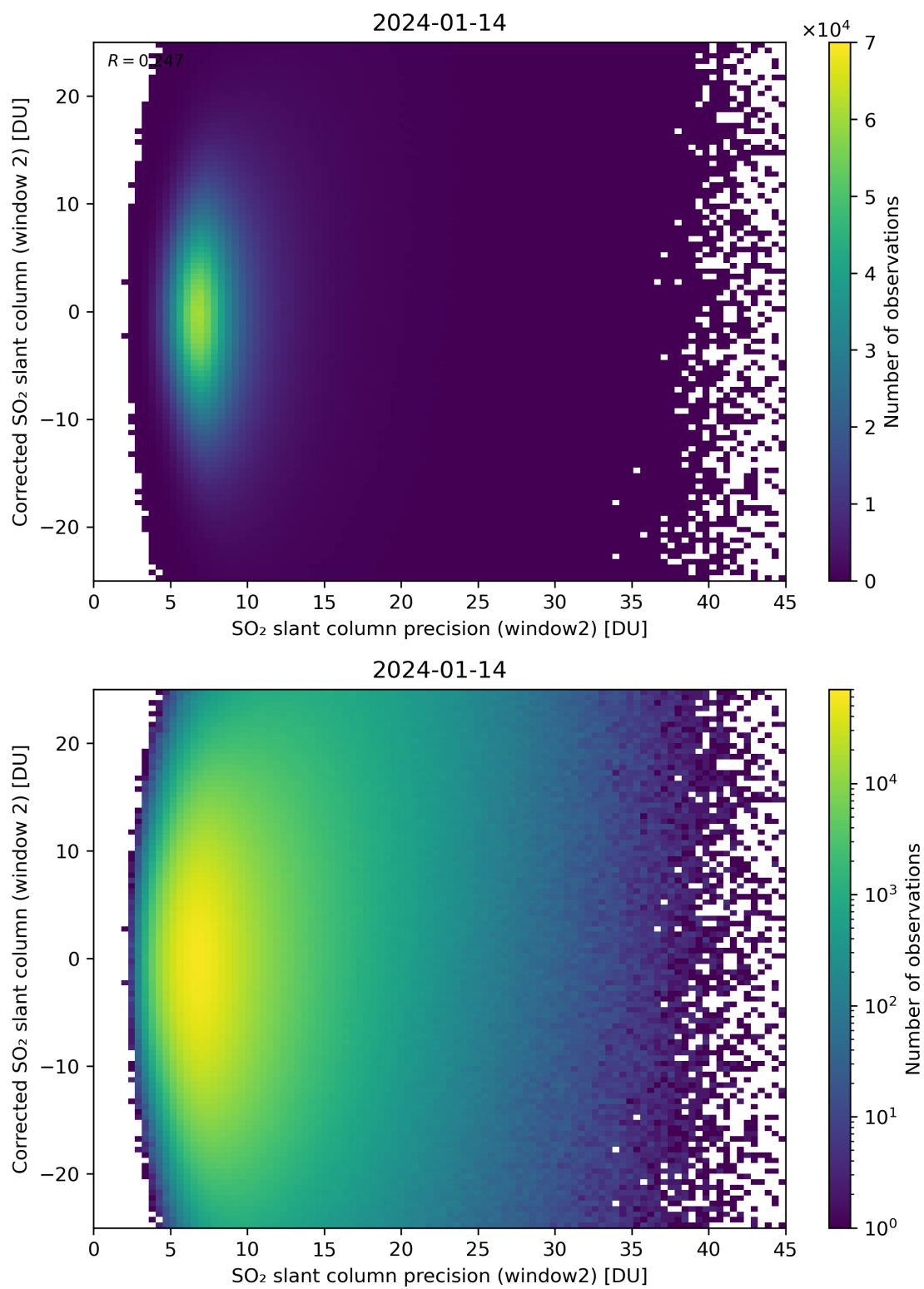
Figure 247: Scatter density plot of “SO 2 slant column precision (window2)” against “Corrected SO 2 slant column (window 2)” for 2024-01-13 to 2024-01-15.
