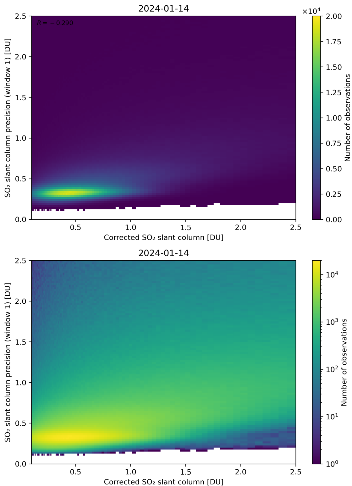
Figure 188: Scatter density plot of “Corrected SO 2 slant column” against “SO 2 slant column precision (window 1)” for 2024-01-13 to 2024-01-15.
