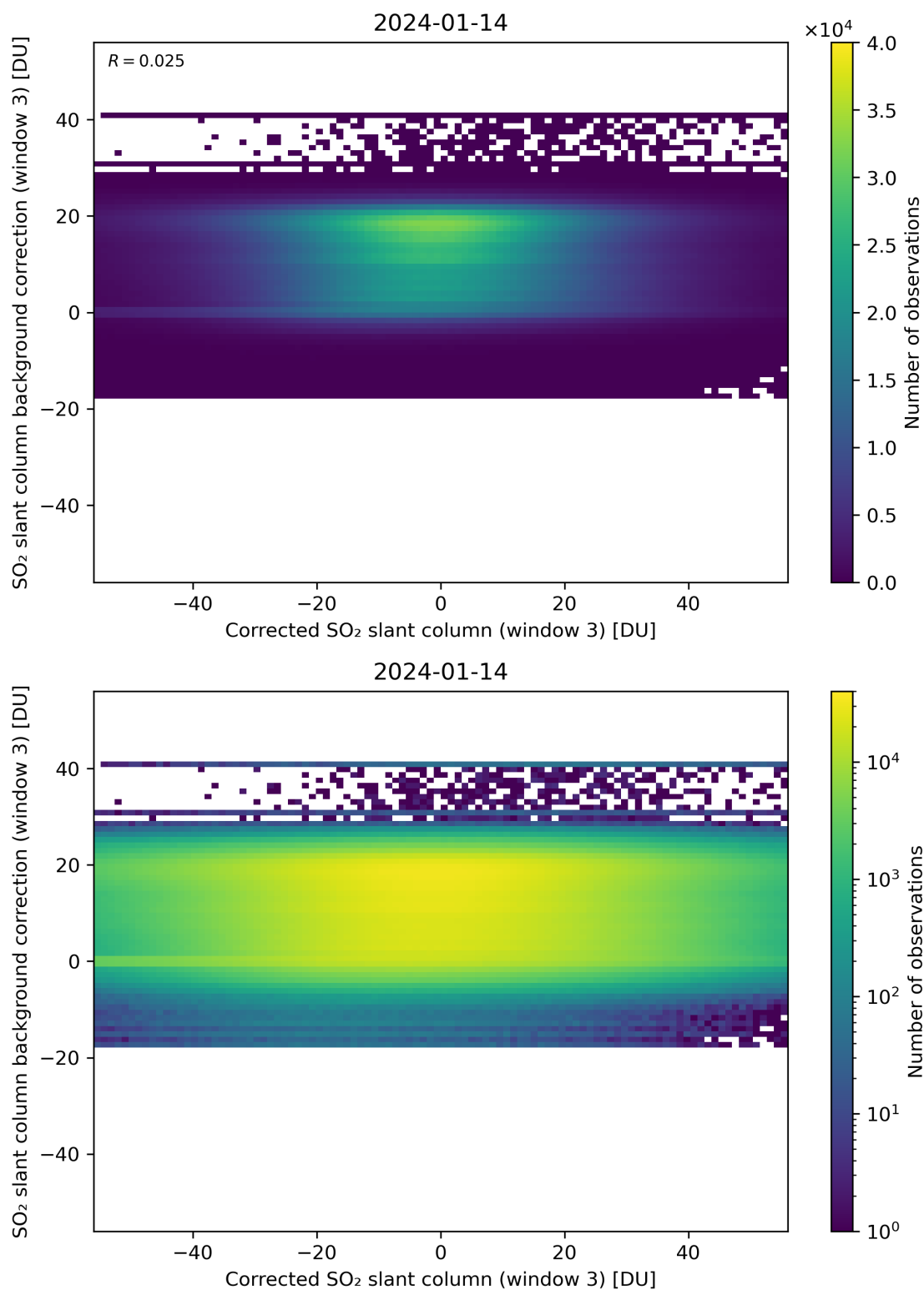
Figure 205: Scatter density plot of “Corrected SO 2 slant column (window 3)” against “SO 2 slant column background correction (window 3)” for 2024-01-13 to 2024-01-15.
