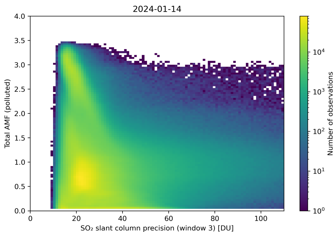
Figure 263: Scatter density plot of “SO 2 slant column precision (window 3)” against “Total AMF (polluted)” for 2024-01-13 to 2024-01-15.
