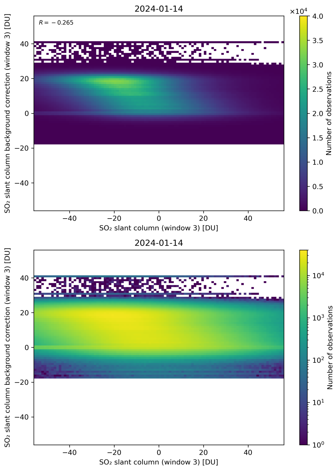
Figure 253: Scatter density plot of “SO 2 slant column (window 3)” against “SO 2 slant column background correction (window 3)” for 2024-01-13 to 2024-01-15.
