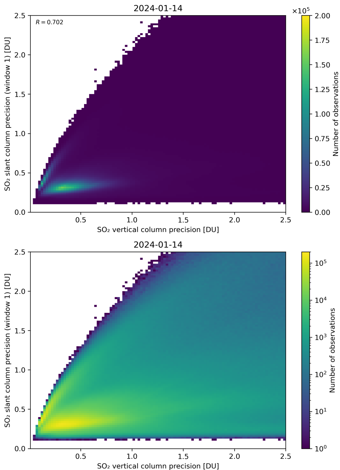
Figure 290: Scatter density plot of “SO 2 vertical column precision” against “SO 2 slant column precision (window 1)” for 2024-01-13 to 2024-01-15.
