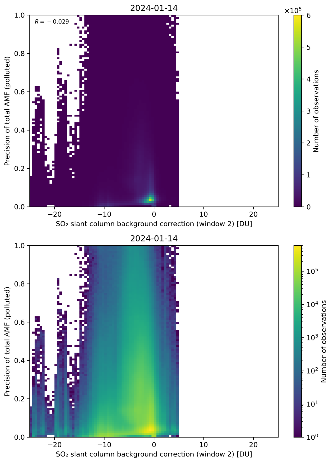
Figure 120: Scatter density plot of “SO 2 slant column background correction (window 2)” against “Precision of total AMF (polluted)” for 2024-01-13 to 2024-01-15.
