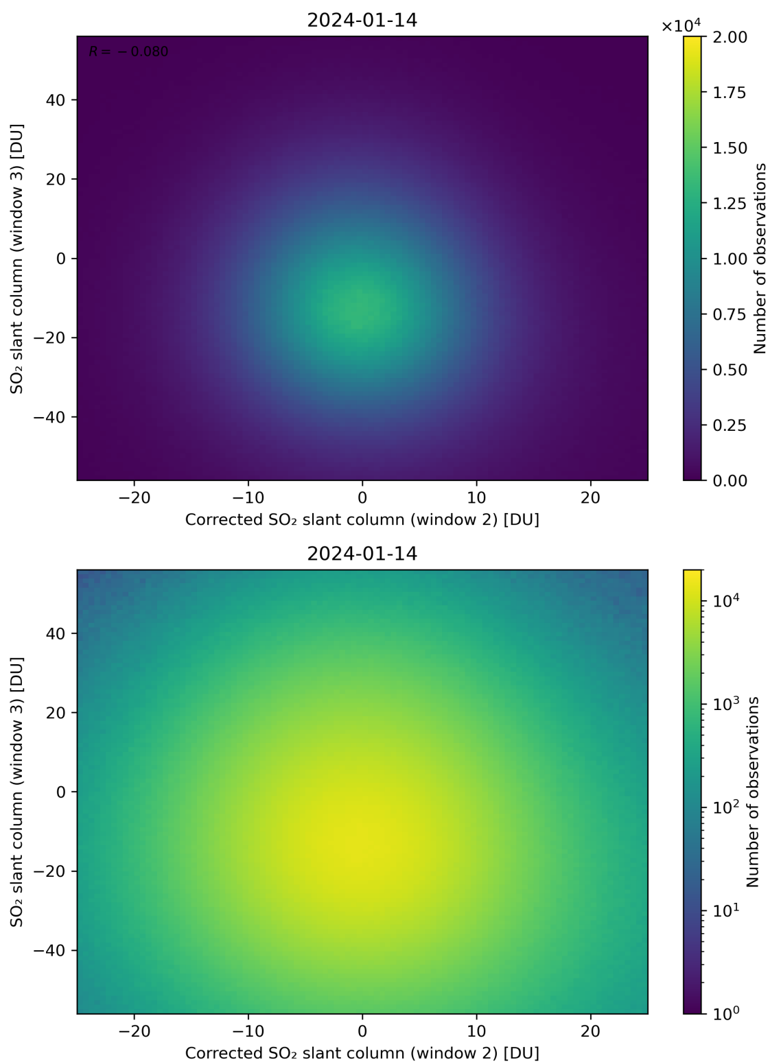
Figure 201: Scatter density plot of “Corrected SO 2 slant column (window 2)” against “SO 2 slant column (window 3)” for 2024-01-13 to 2024-01-15.
