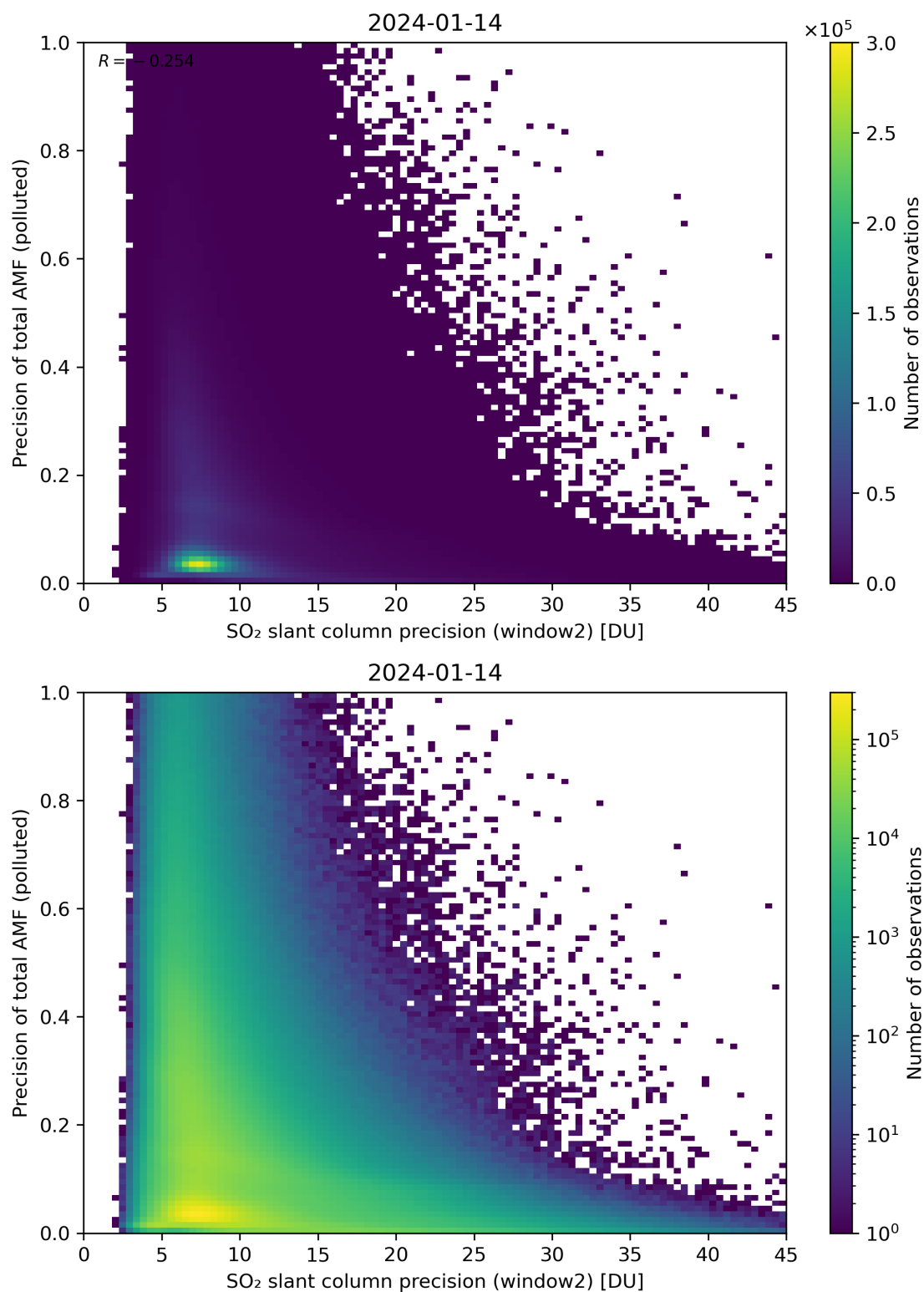
Figure 252: Scatter density plot of “SO 2 slant column precision (window2)” against “Precision of total AMF (polluted)” for 2024-01-13 to 2024-01-15.
