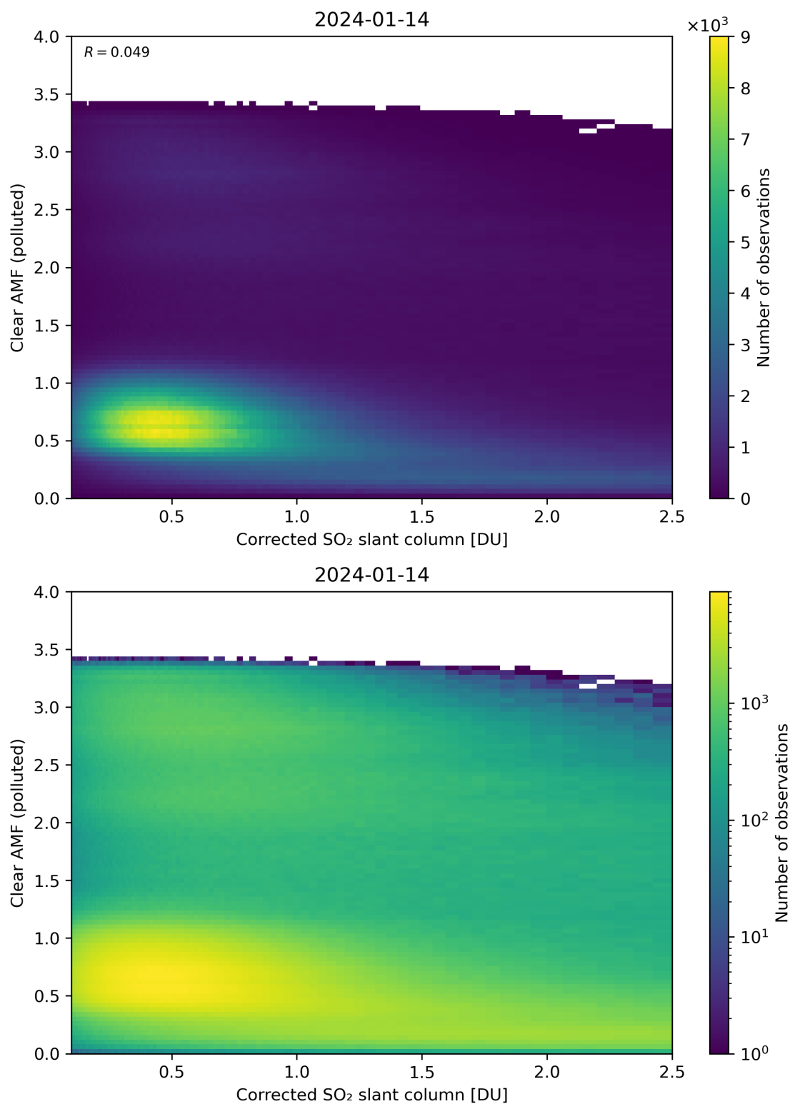
Figure 184: Scatter density plot of “Corrected SO 2 slant column” against “Clear AMF (polluted)” for 2024-01-13 to 2024-01-15.
