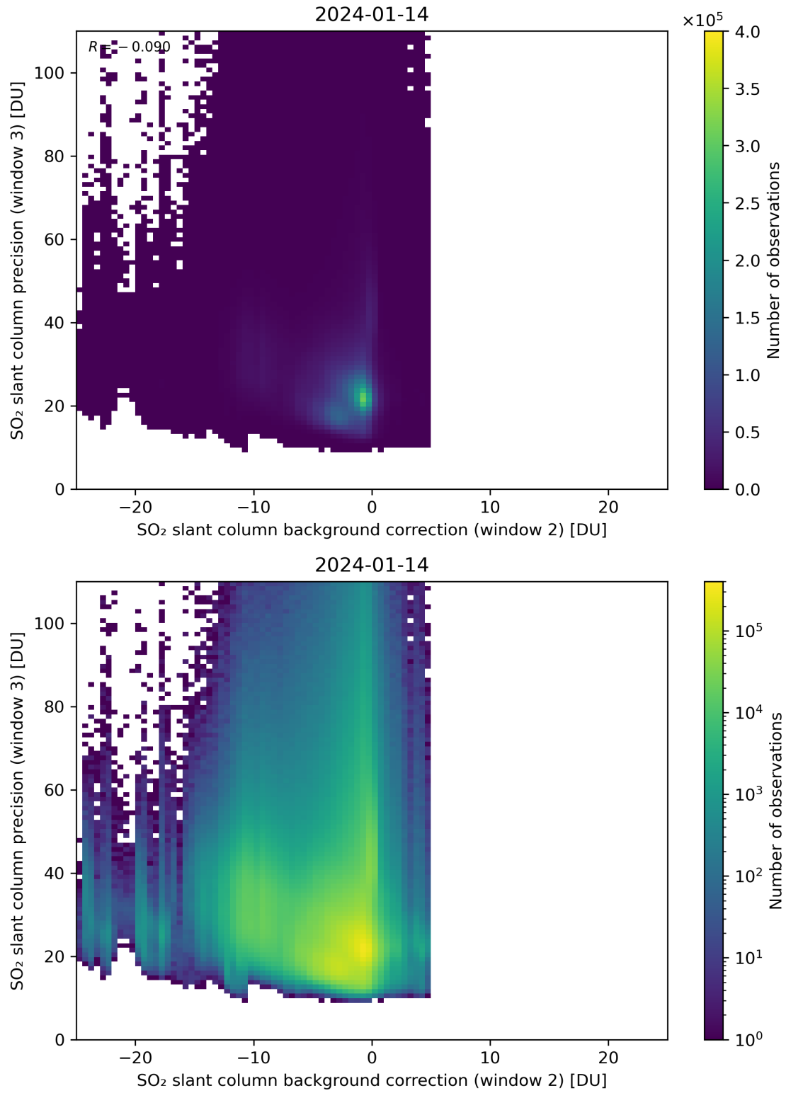
Figure 118: Scatter density plot of “SO 2 slant column background correction (window 2)” against “SO 2 slant column precision (window 3)” for 2024-01-13 to 2024-01-15.
