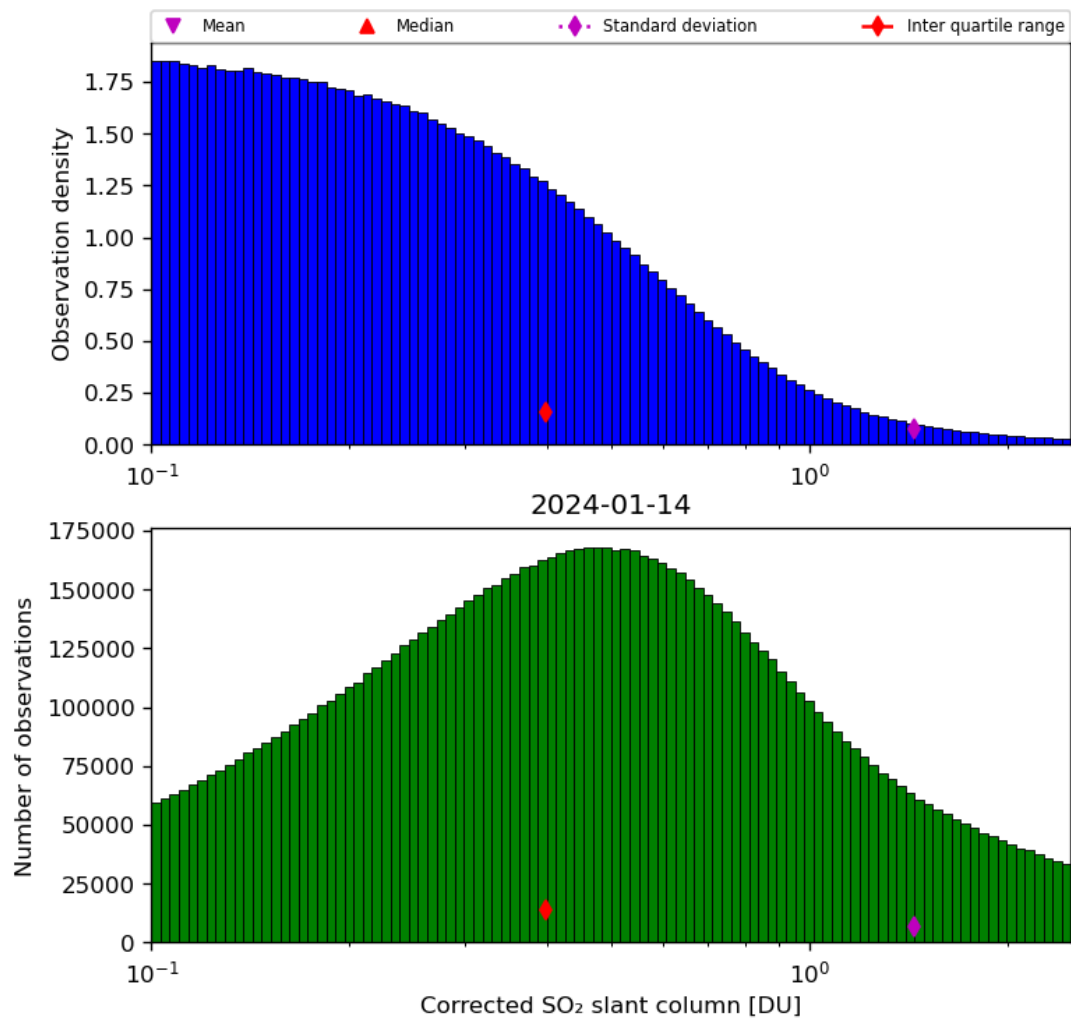
Figure 55: Histogram of “Corrected SO 2 slant column” for 2024-01-13 to 2024-01-15
