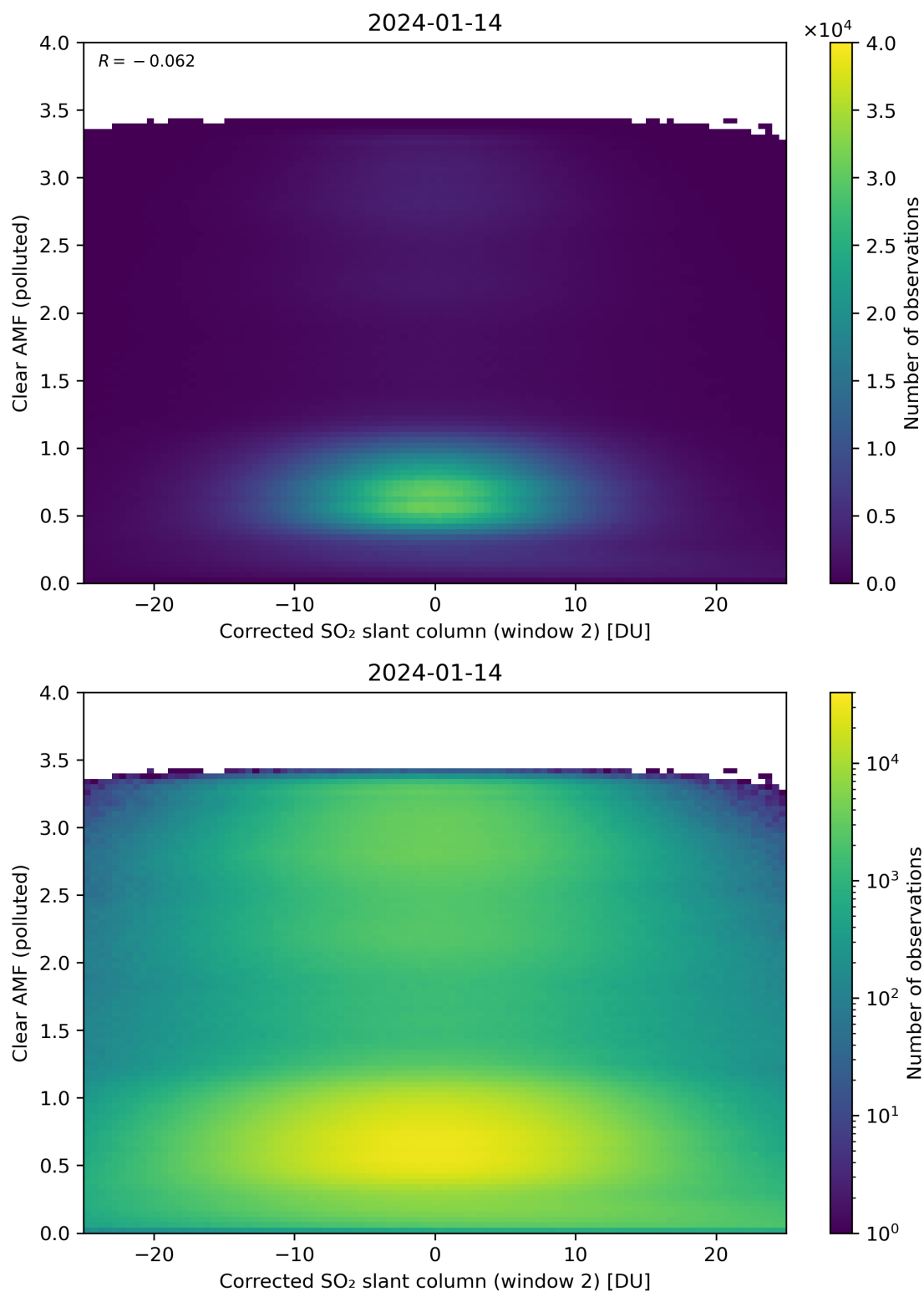
Figure 199: Scatter density plot of “Corrected SO 2 slant column (window 2)” against “Clear AMF (polluted)” for 2024-01-13 to 2024-01-15.
