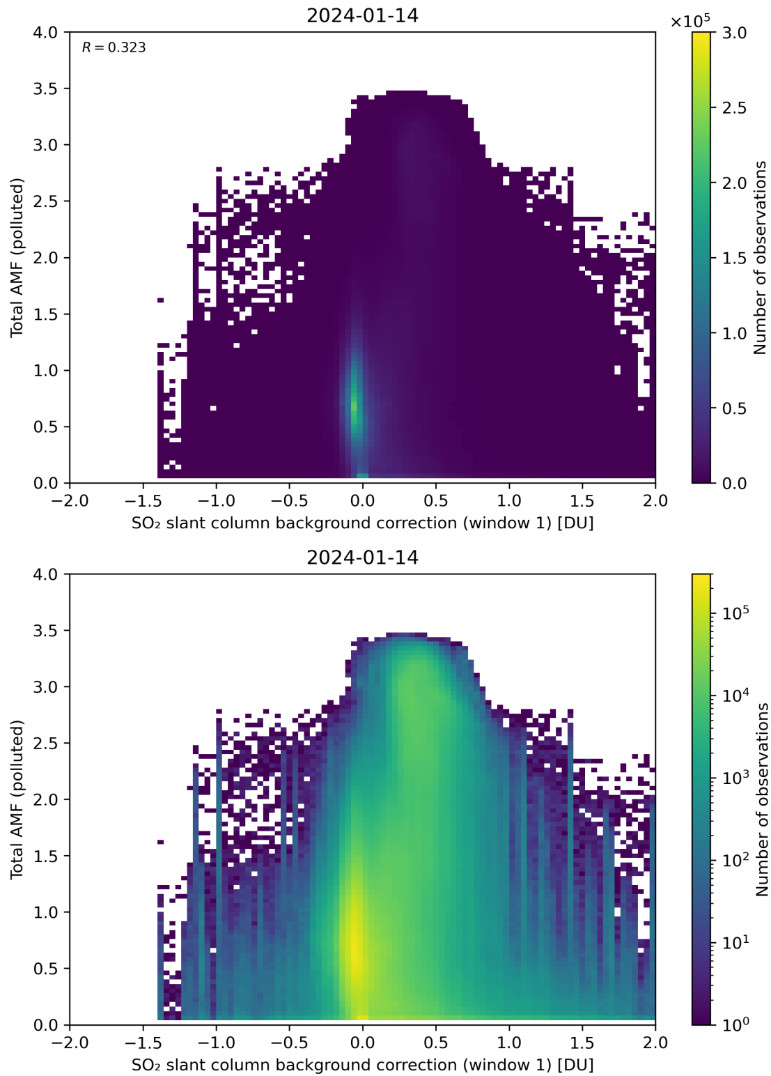
Figure 109: Scatter density plot of “SO 2 slant column background correction (window 1)” against “Total AMF (polluted)” for 2024-01-13 to 2024-01-15.
