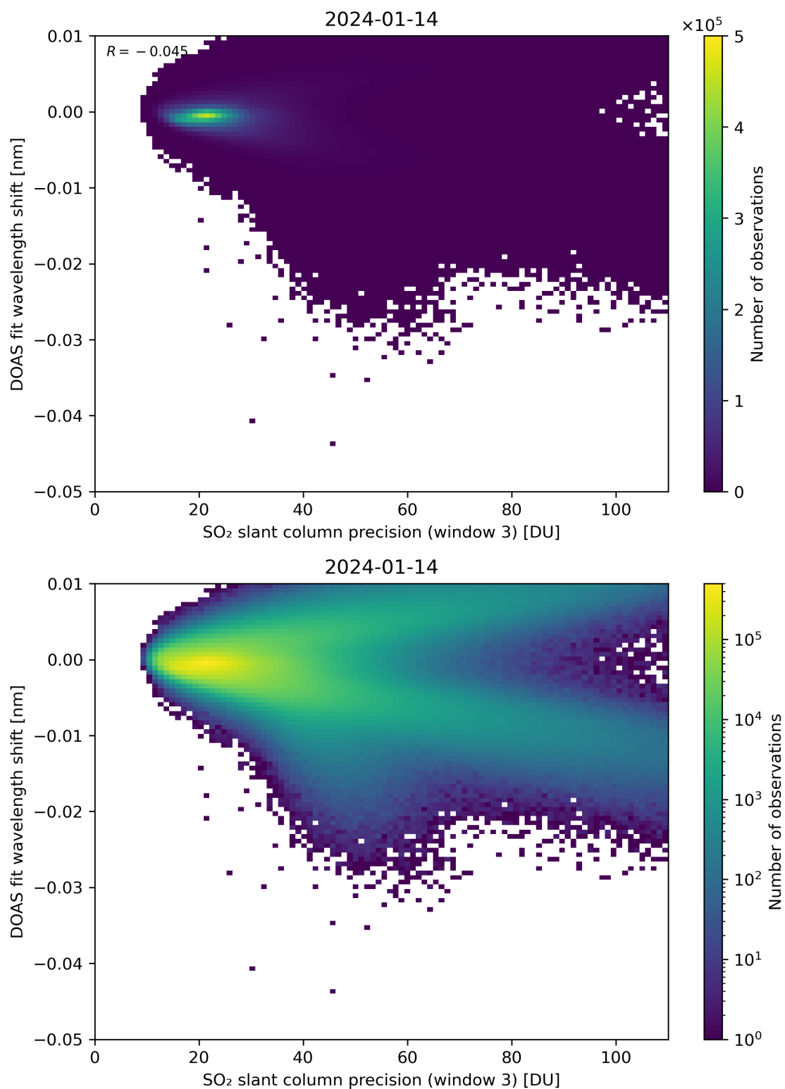
Figure 258: Scatter density plot of “SO 2 slant column precision (window 3)” against “DOAS fit wavelength shift” for 2024-01-13 to 2024-01-15.
