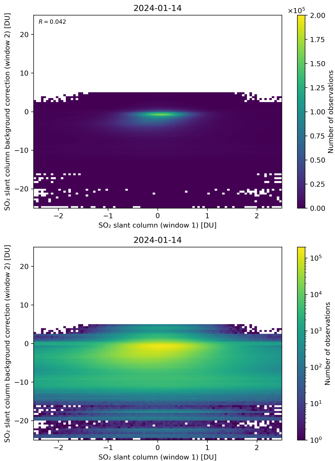
Figure 213: Scatter density plot of “SO 2 slant column (window 1)” against “SO 2 slant column background correction (window 2)” for 2024-01-13 to 2024-01-15.
