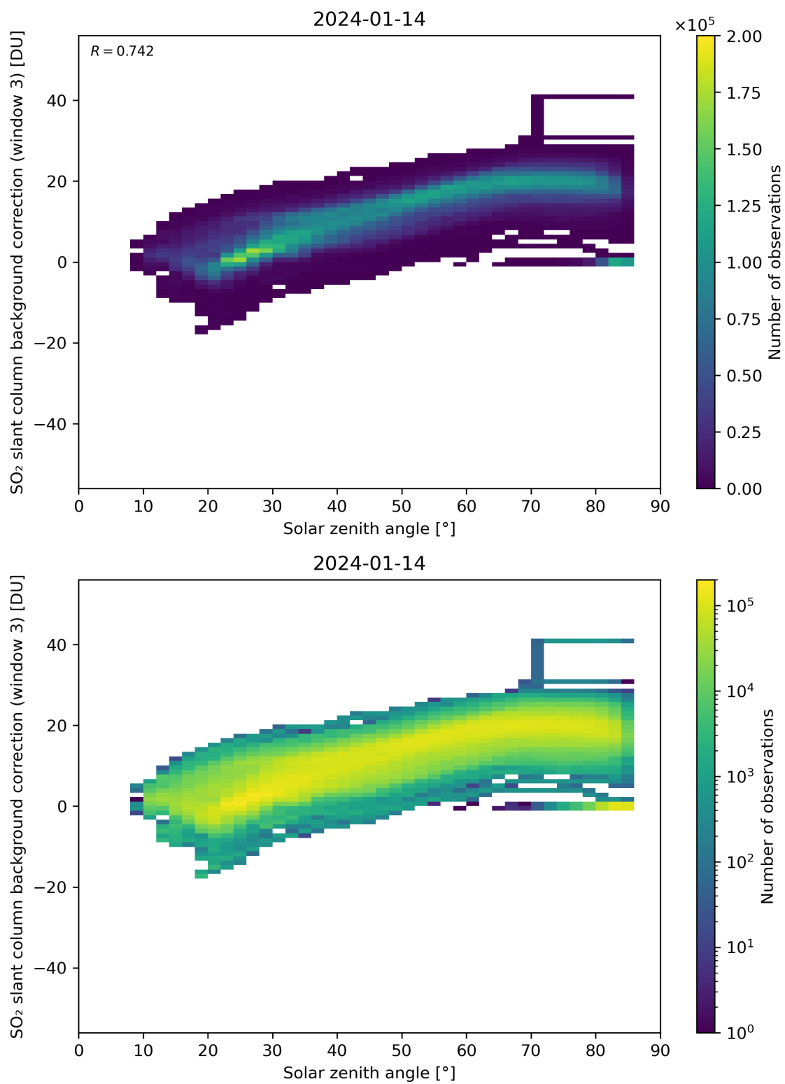
Figure 160: Scatter density plot of “Solar zenith angle” against “SO 2 slant column background correction (window 3)” for 2024-01-13 to 2024-01-15.
