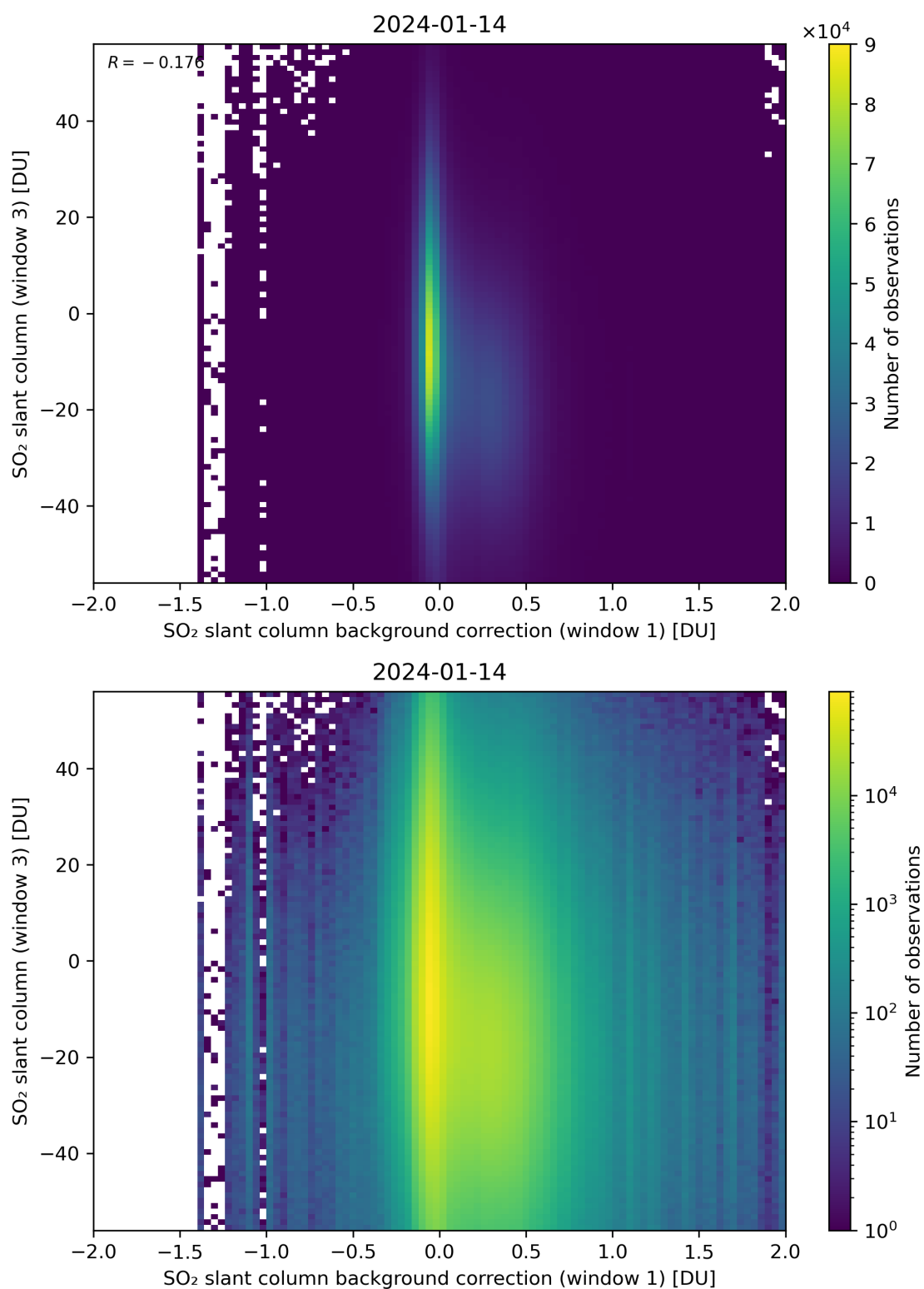
Figure 107: Scatter density plot of “SO 2 slant column background correction (window 1)” against “SO 2 slant column (window 3)” for 2024-01-13 to 2024-01-15.
