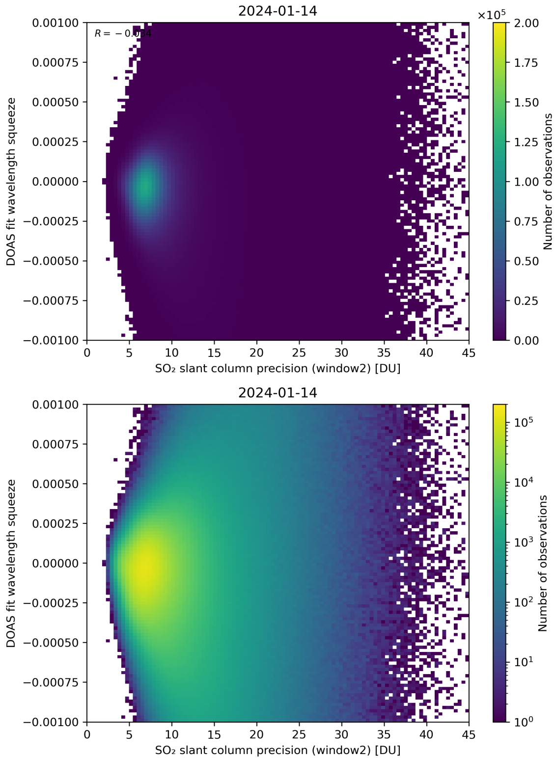
Figure 244: Scatter density plot of “SO 2 slant column precision (window2)” against “DOAS fit wavelength squeeze” for 2024-01-13 to 2024-01-15.
