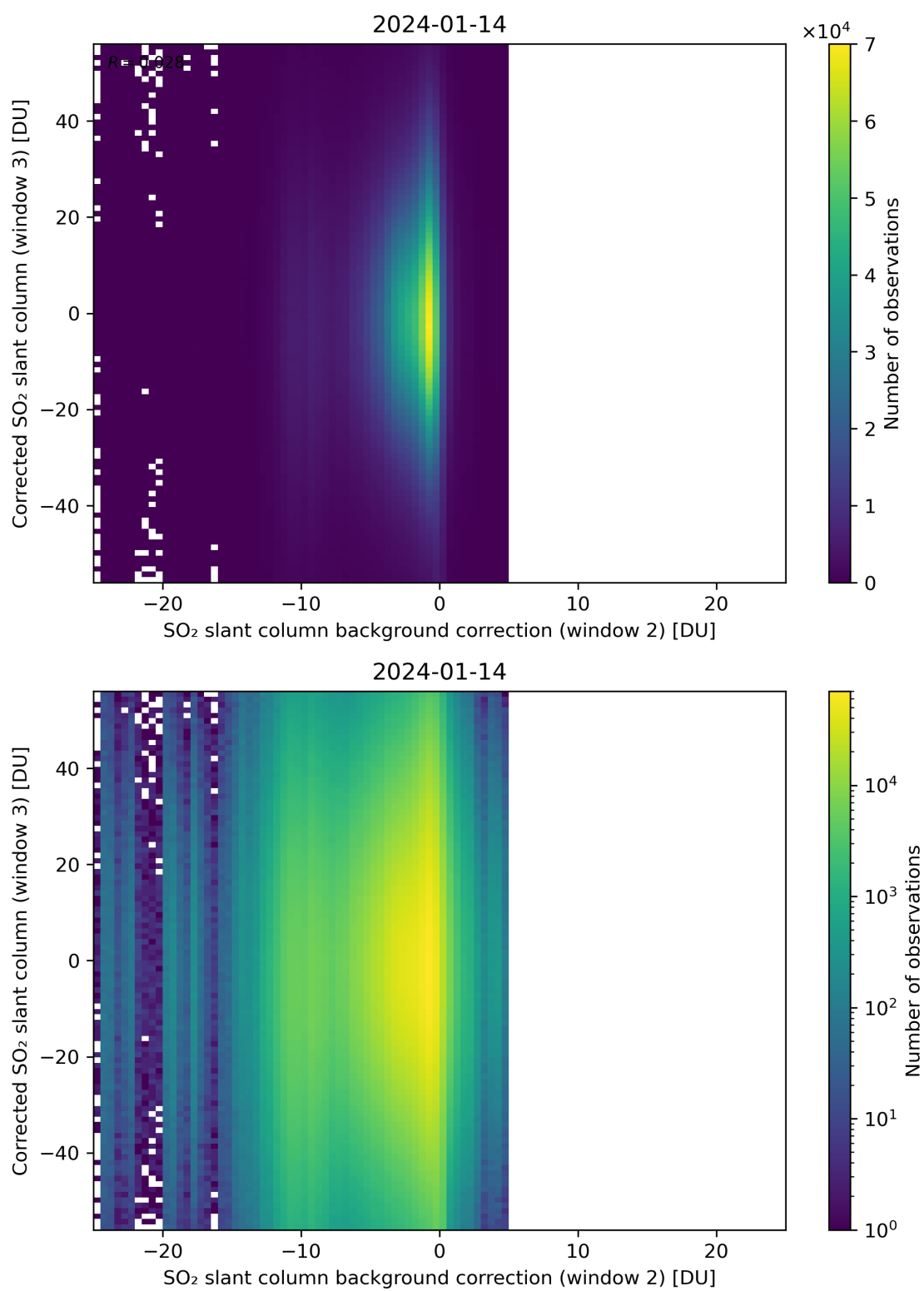
Figure 116: Scatter density plot of “SO 2 slant column background correction (window 2)” against “Corrected SO 2 slant column (window 3)” for 2024-01-13 to 2024-01-15.
