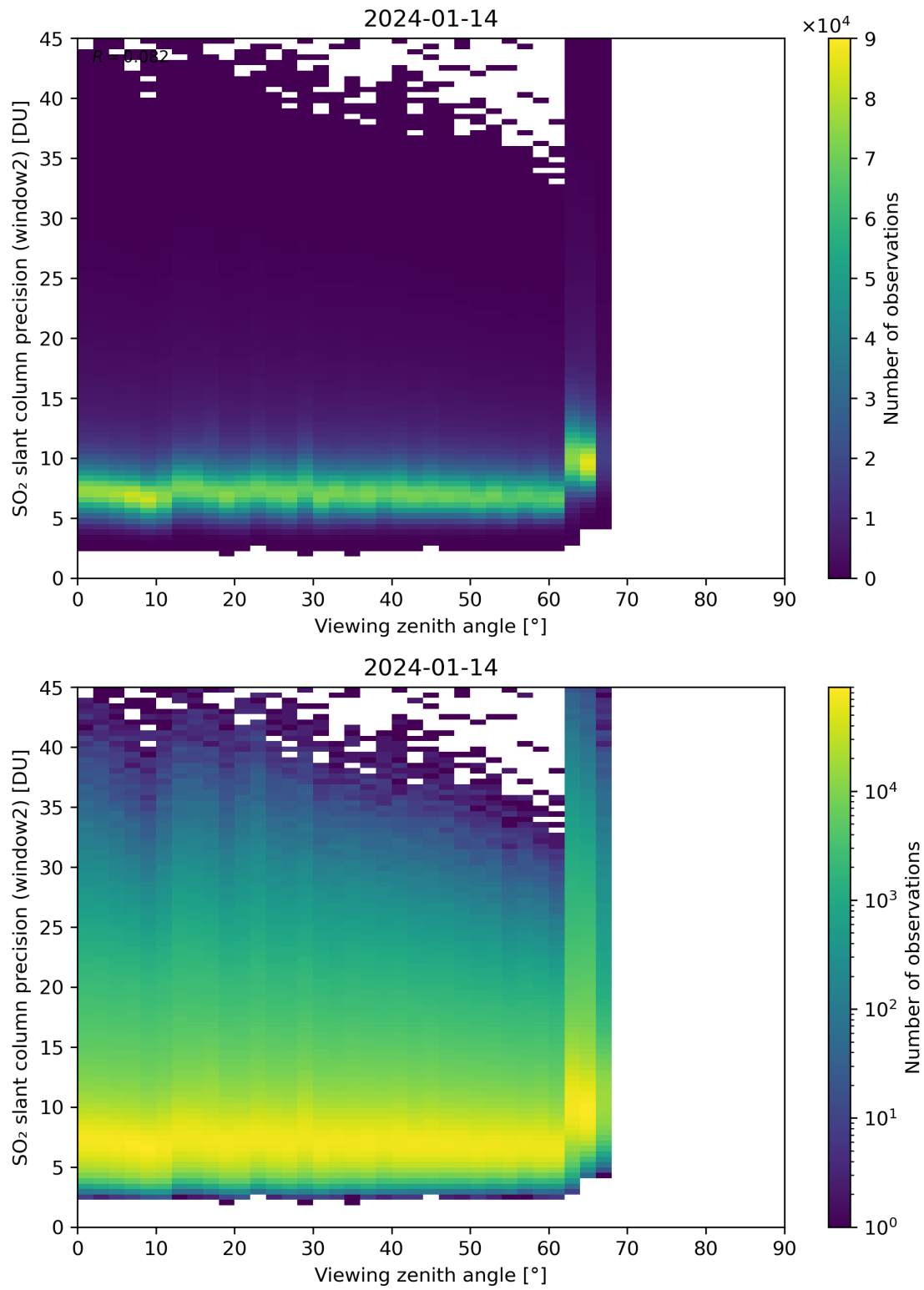
Figure 322: Scatter density plot of “Viewing zenith angle” against “SO 2 slant column precision (window2)” for 2024-01-13 to 2024-01-15.
