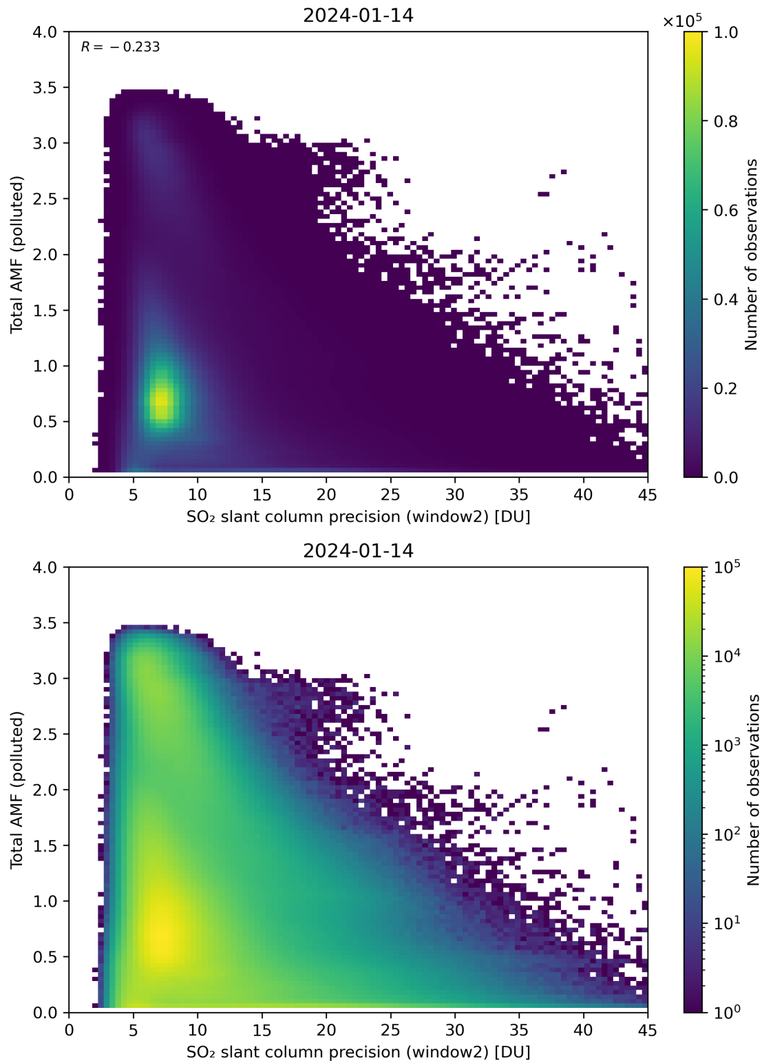
Figure 251: Scatter density plot of “SO 2 slant column precision (window2)” against “Total AMF (polluted)” for 2024-01-13 to 2024-01-15.
