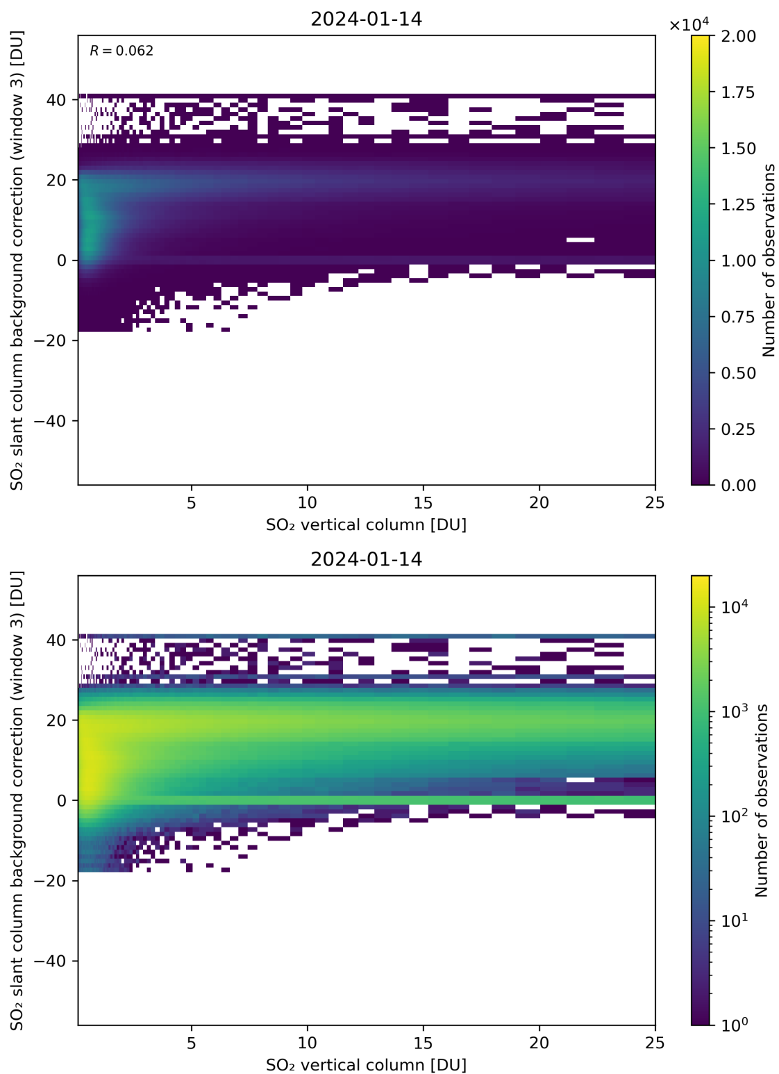
Figure 275: Scatter density plot of “SO 2 vertical column” against “SO 2 slant column background correction (window 3)” for 2024-01-13 to 2024-01-15.
