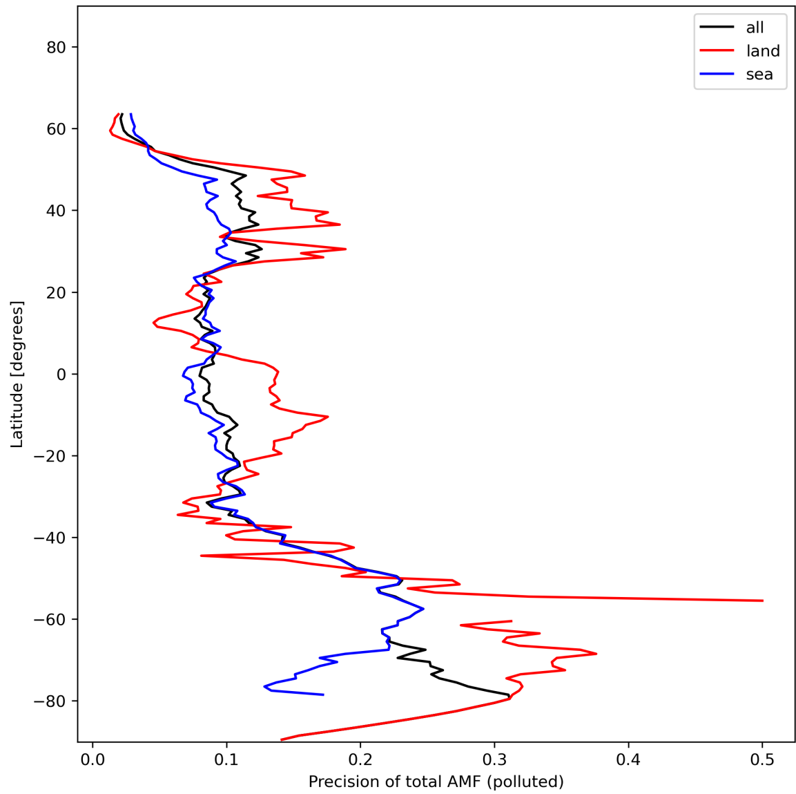
Figure 49: Zonal average of “Precision of total AMF (polluted)” for 2024-01-13 to 2024-01-15.
