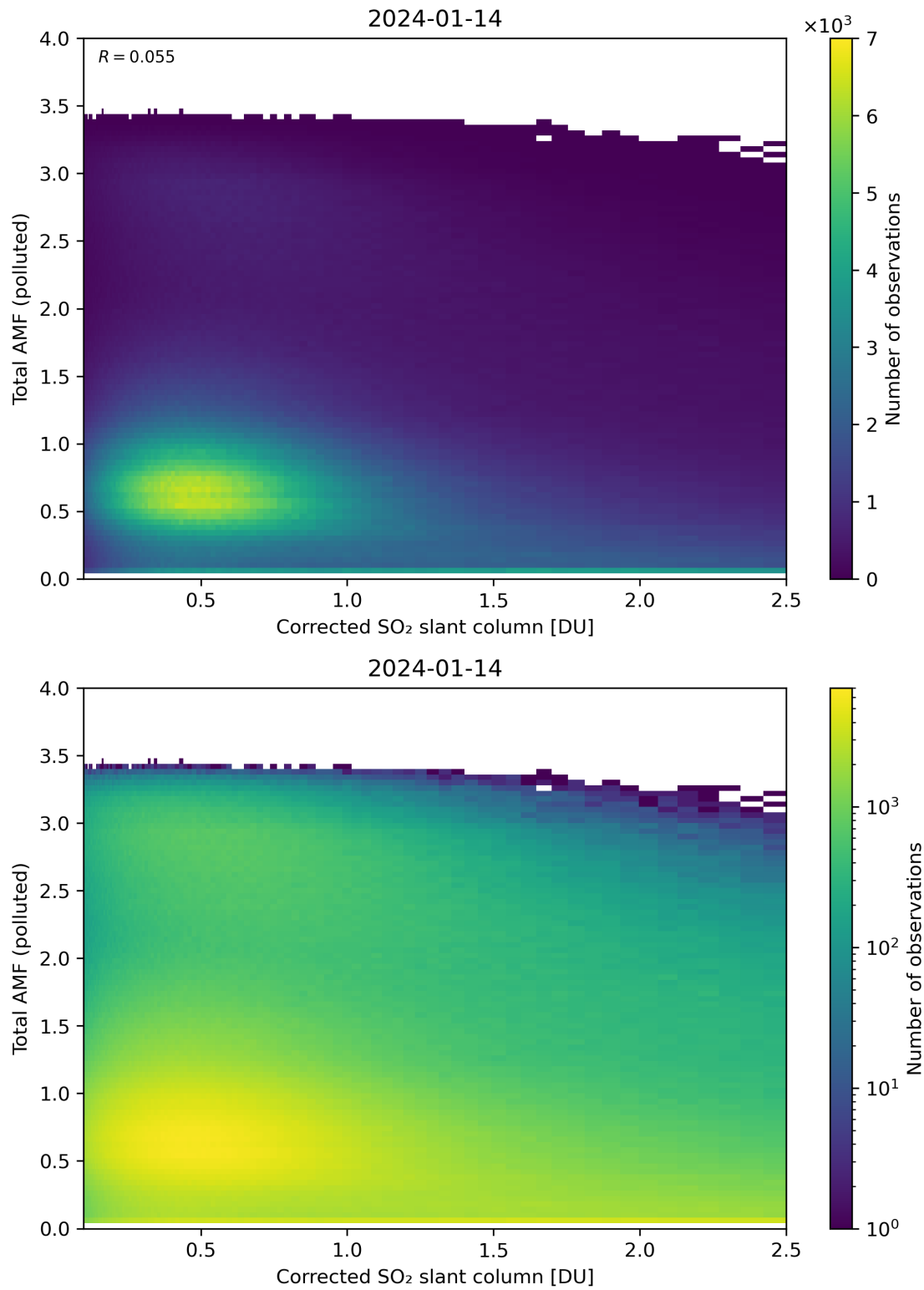
Figure 192: Scatter density plot of “Corrected SO 2 slant column” against “Total AMF (polluted)” for 2024-01-13 to 2024-01-15.
