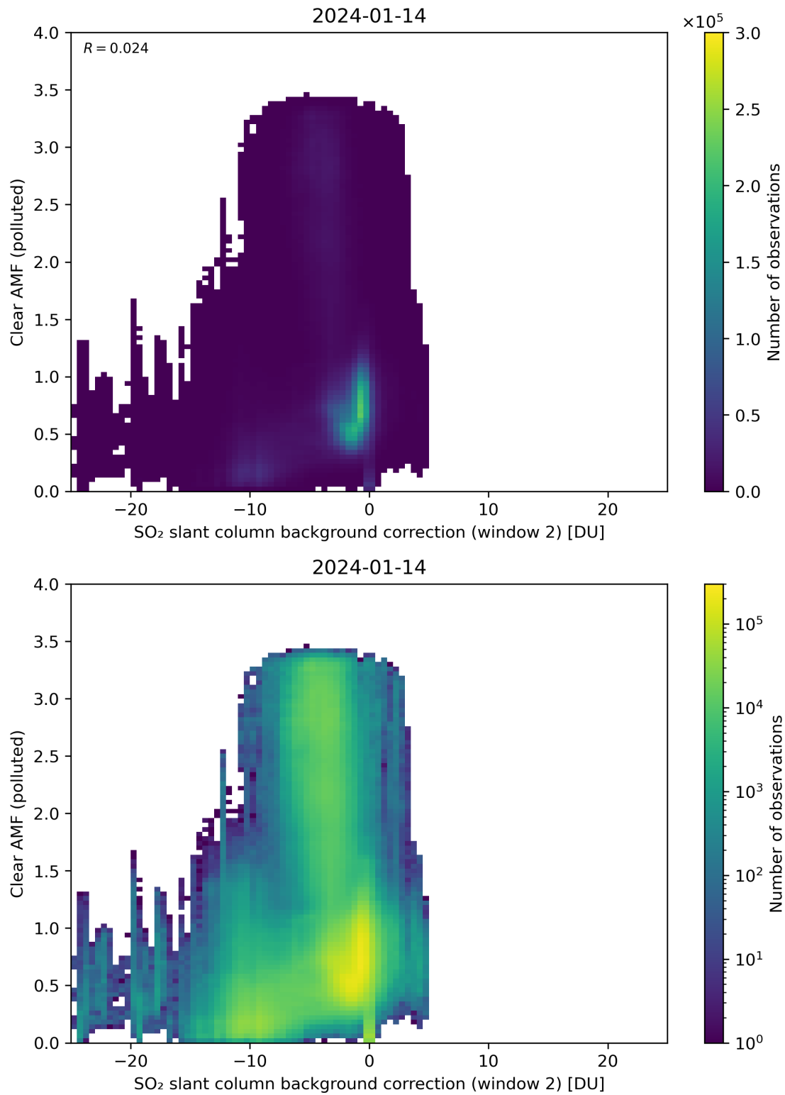
Figure 115: Scatter density plot of “SO 2 slant column background correction (window 2)” against “Clear AMF (polluted)” for 2024-01-13 to 2024-01-15.
