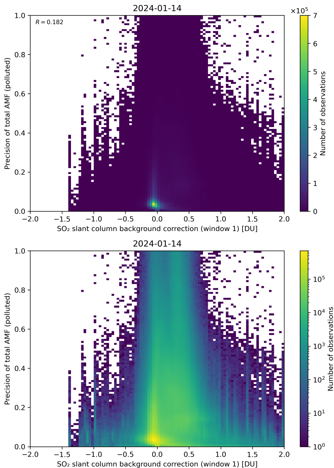
Figure 110: Scatter density plot of “SO 2 slant column background correction (window 1)” against “Precision of total AMF (polluted)” for 2024-01-13 to 2024-01-15.
