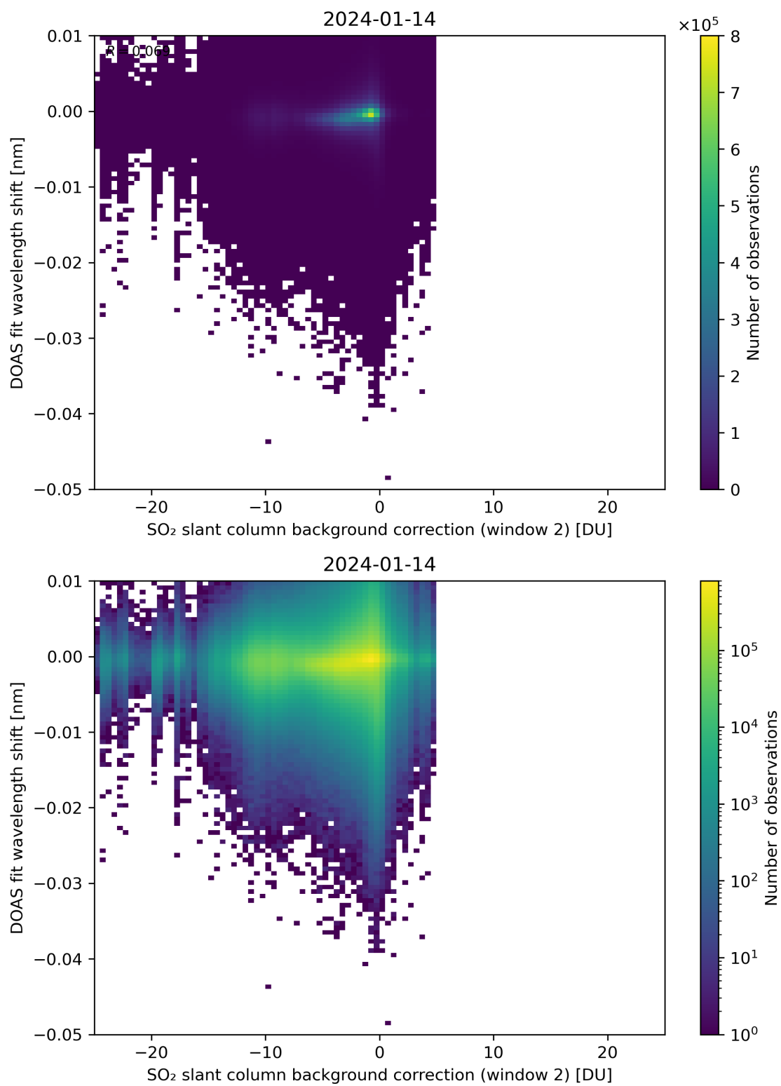
Figure 112: Scatter density plot of “SO 2 slant column background correction (window 2)” against “DOAS fit wavelength shift” for 2024-01-13 to 2024-01-15.
