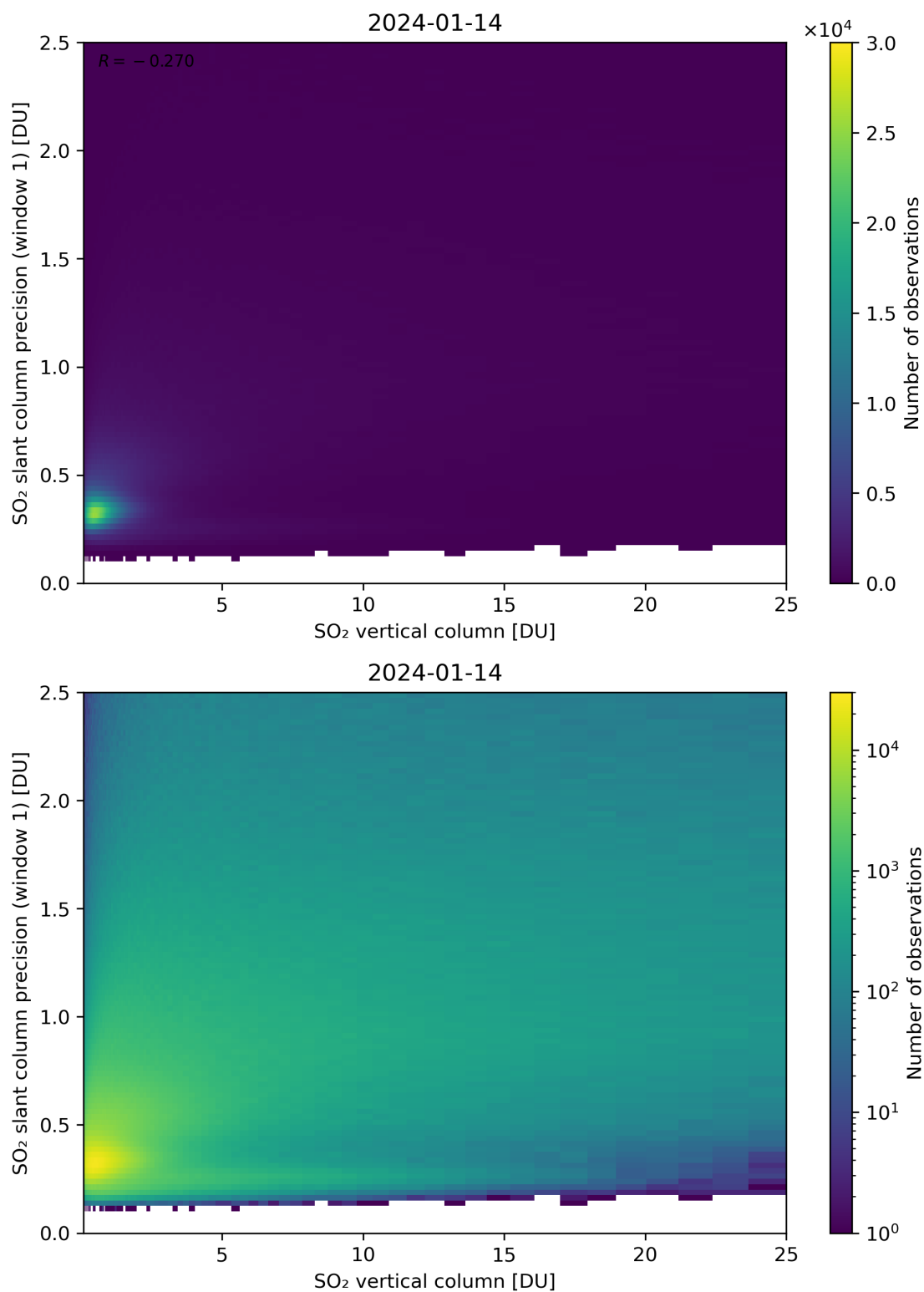
Figure 301: Scatter density plot of “SO 2 vertical column” against “SO 2 slant column precision (window 1)” for 2024-01-13 to 2024-01-15.
