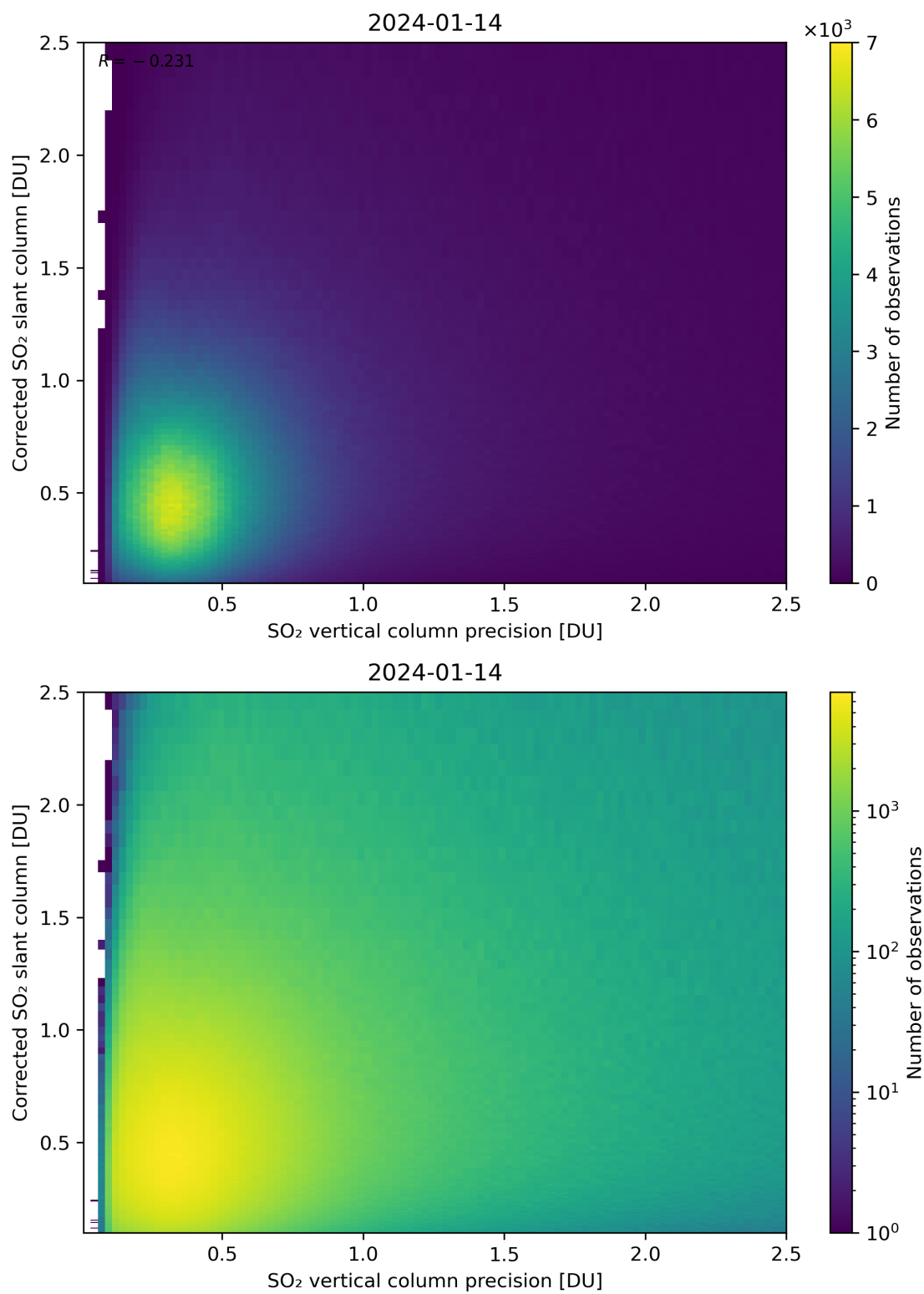
Figure 286: Scatter density plot of “SO 2 vertical column precision” against “Corrected SO 2 slant column” for 2024-01-13 to 2024-01-15.
