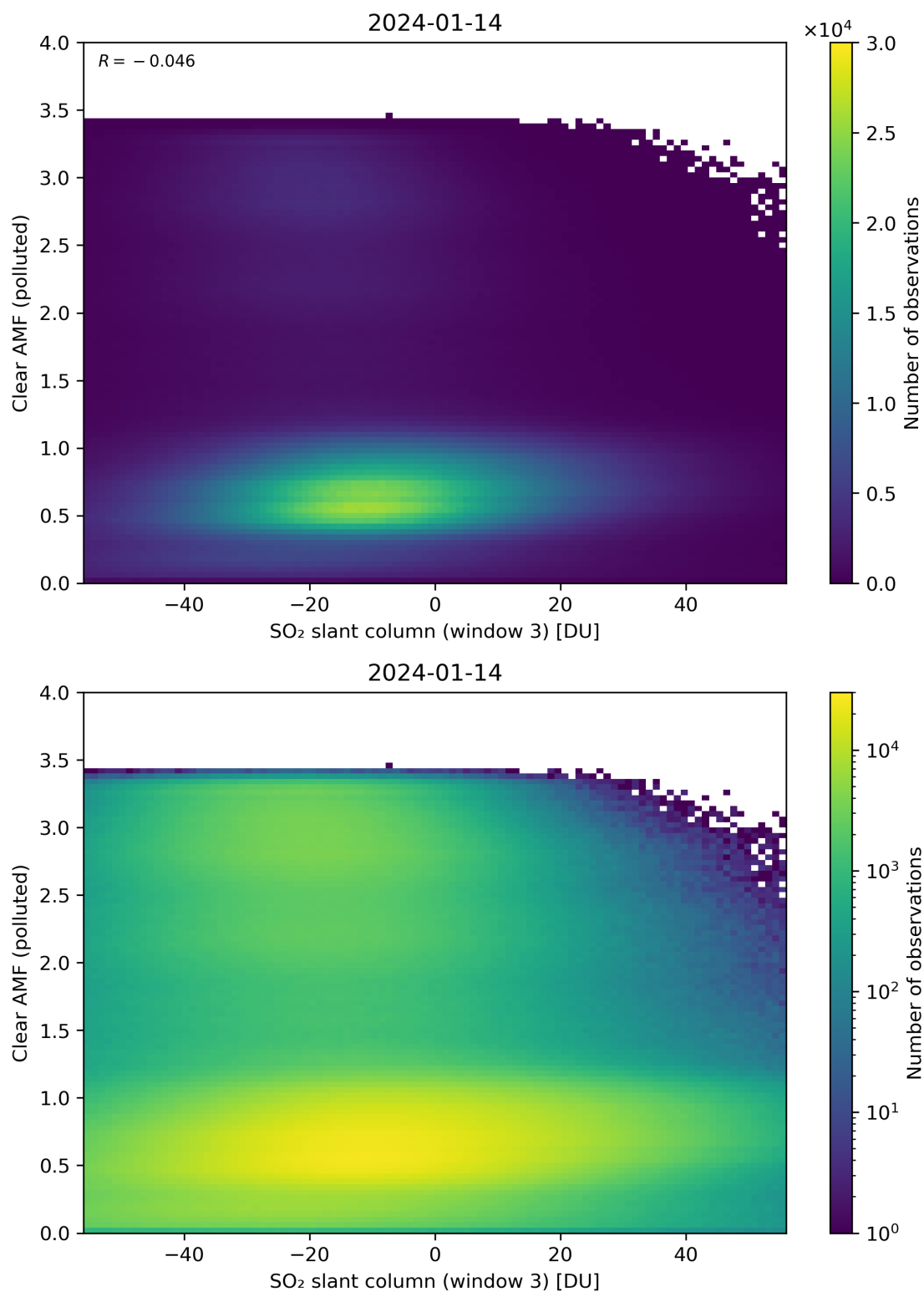
Figure 265: Scatter density plot of “SO 2 slant column (window 3)” against “Clear AMF (polluted)” for 2024-01-13 to 2024-01-15.
