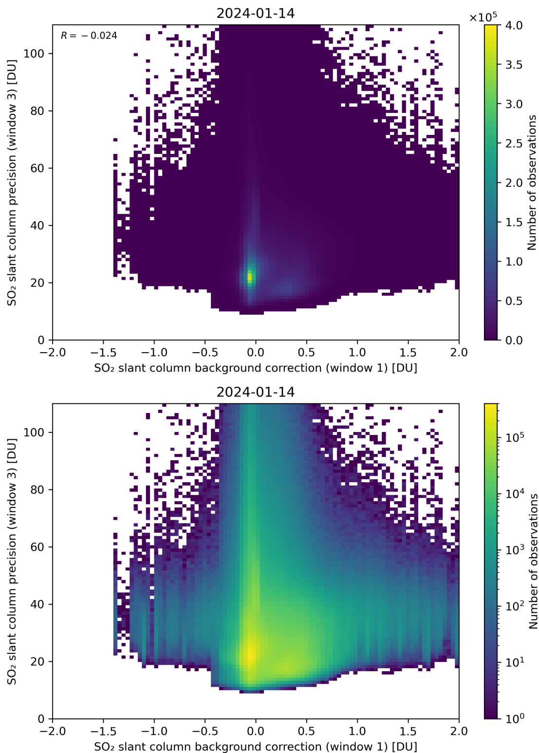
Figure 108: Scatter density plot of “SO 2 slant column background correction (window 1)” against “SO 2 slant column precision (window 3)” for 2024-01-13 to 2024-01-15.
