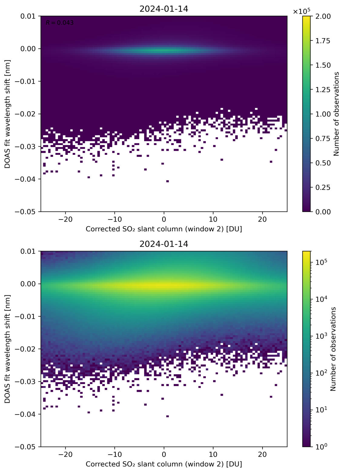
Figure 196: Scatter density plot of “Corrected SO 2 slant column (window 2)” against “DOAS fit wavelength shift” for 2024-01-13 to 2024-01-15.
