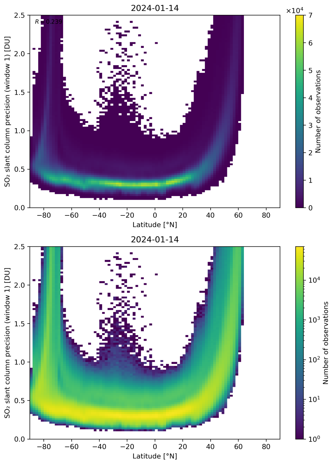
Figure 150: Scatter density plot of “Latitude” against “SO 2 slant column precision (window 1)” for 2024-01-13 to 2024-01-15.
