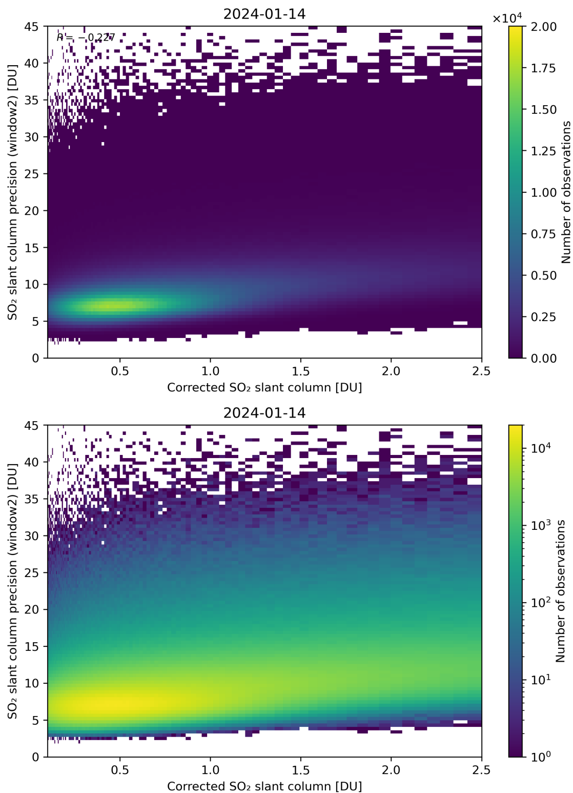
Figure 189: Scatter density plot of “Corrected SO 2 slant column” against “SO 2 slant column precision (window2)” for 2024-01-13 to 2024-01-15.
