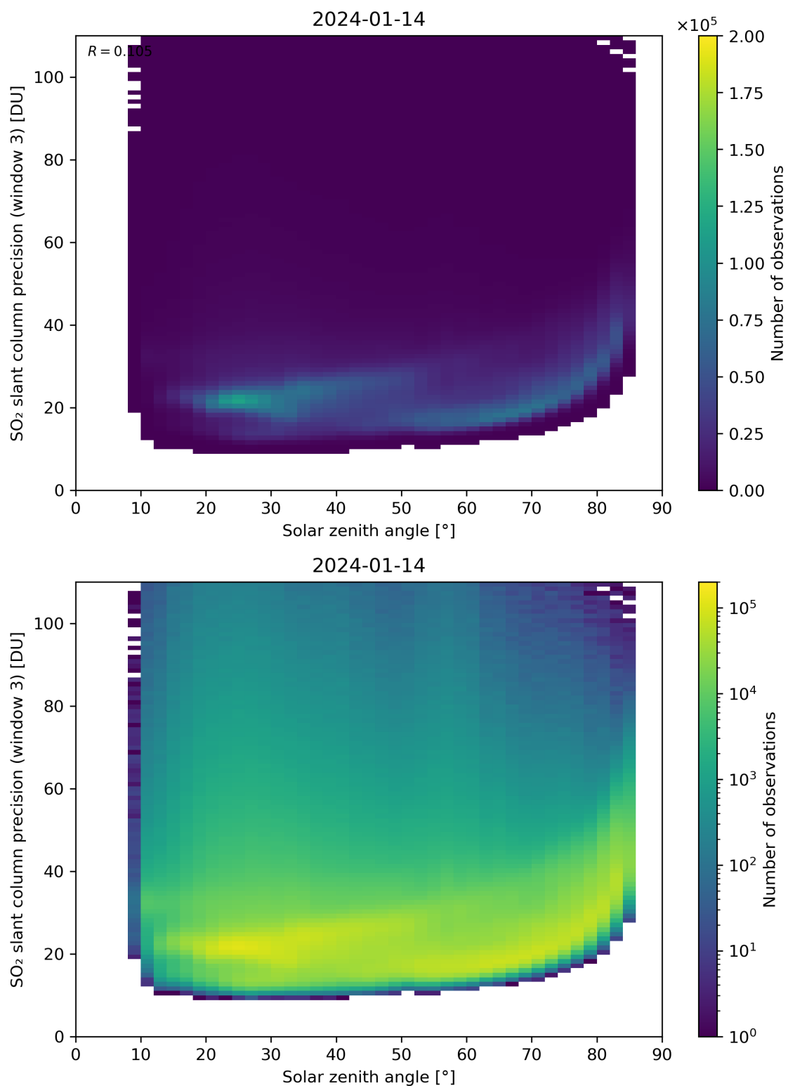
Figure 173: Scatter density plot of “Solar zenith angle” against “SO 2 slant column precision (window 3)” for 2024-01-13 to 2024-01-15.
