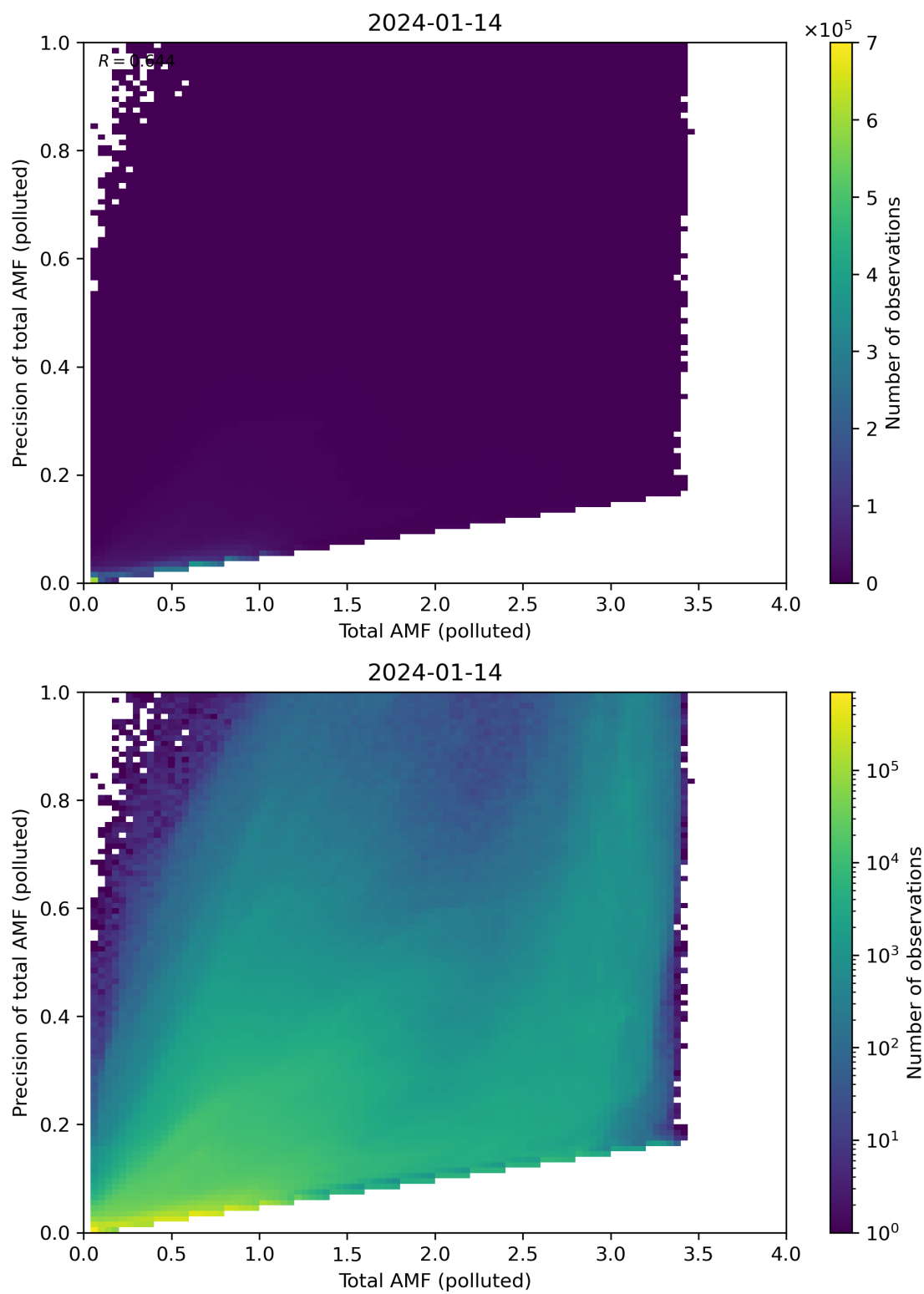
Figure 272: Scatter density plot of “Total AMF (polluted)” against “Precision of total AMF (polluted)” for 2024-01-13 to 2024-01-15.
