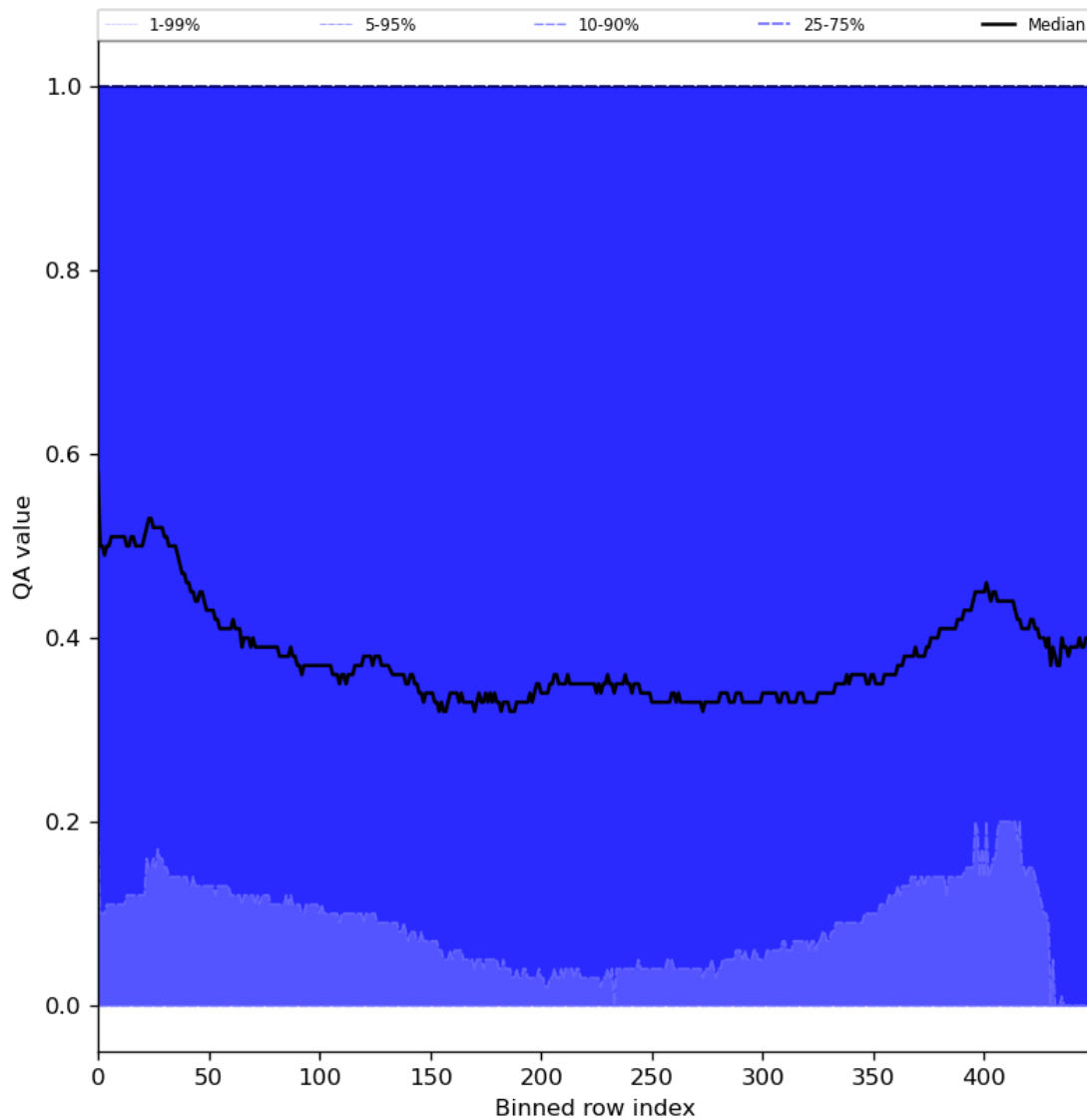
Figure 75: Along track statistics of “QA value” for 2024-01-13 to 2024-01-15
