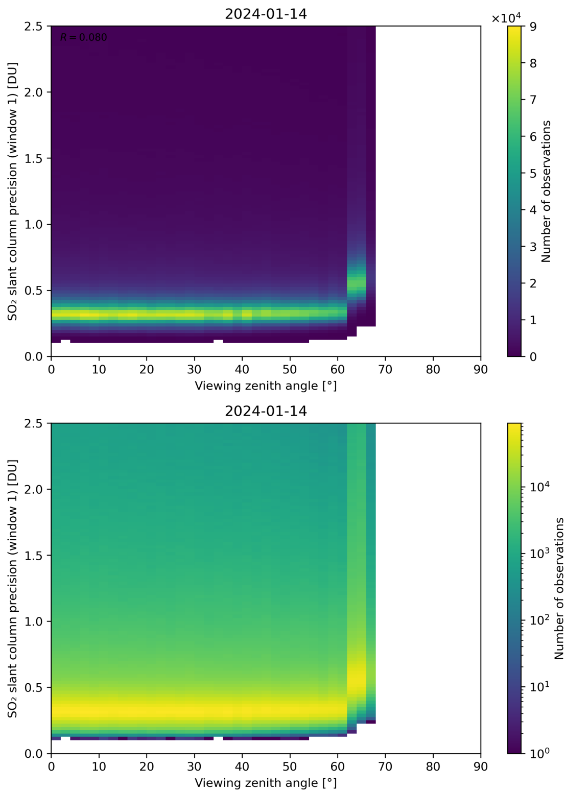
Figure 321: Scatter density plot of “Viewing zenith angle” against “SO 2 slant column precision (window 1)” for 2024-01-13 to 2024-01-15.
