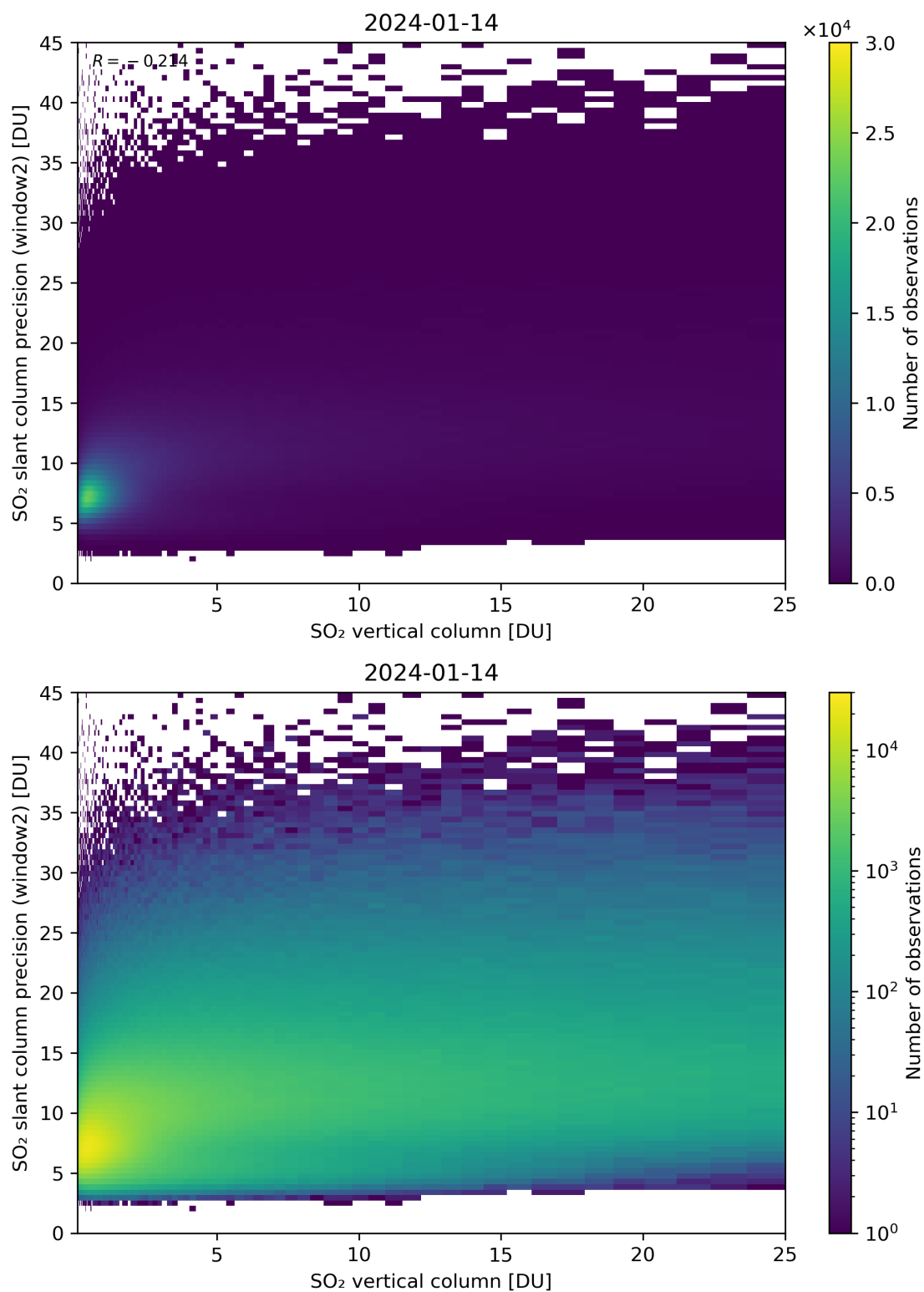
Figure 302: Scatter density plot of “SO 2 vertical column” against “SO 2 slant column precision (window2)” for 2024-01-13 to 2024-01-15.
