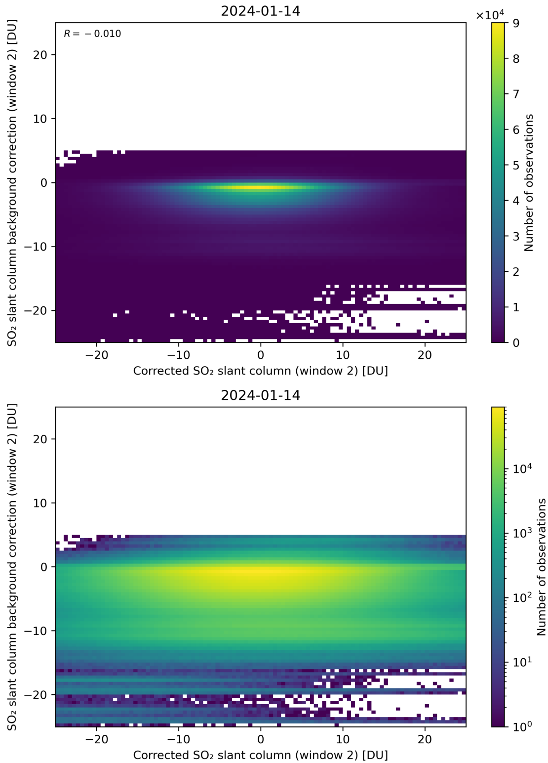
Figure 194: Scatter density plot of “Corrected SO 2 slant column (window 2)” against “SO 2 slant column background correction (window 2)” for 2024-01-13 to 2024-01-15.
