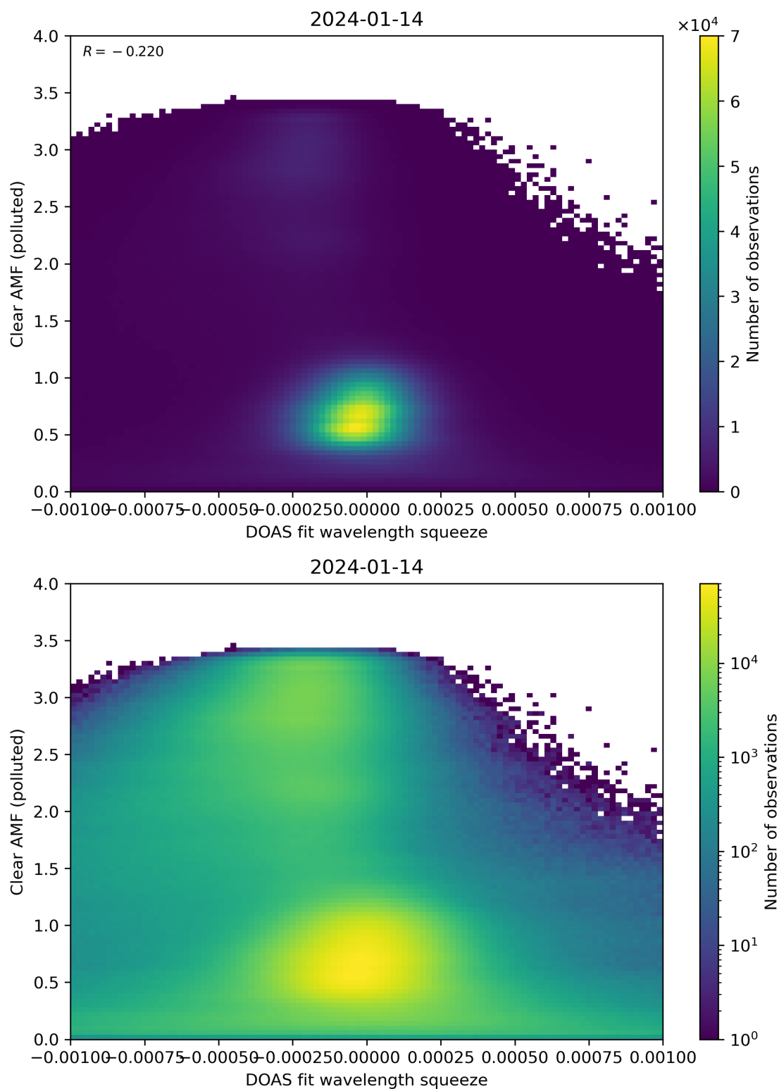
Figure 133: Scatter density plot of “DOAS fit wavelength squeeze” against “Clear AMF (polluted)” for 2024-01-13 to 2024-01-15.
