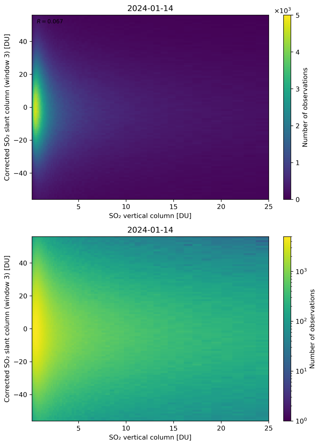
Figure 299: Scatter density plot of “SO 2 vertical column” against “Corrected SO 2 slant column (window 3)” for 2024-01-13 to 2024-01-15.
