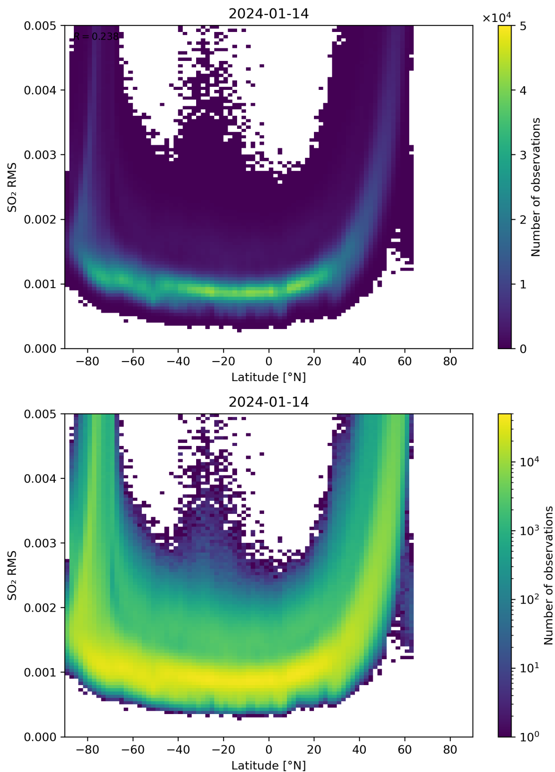
Figure 144: Scatter density plot of “Latitude” against “SO 2 RMS” for 2024-01-13 to 2024-01-15.
