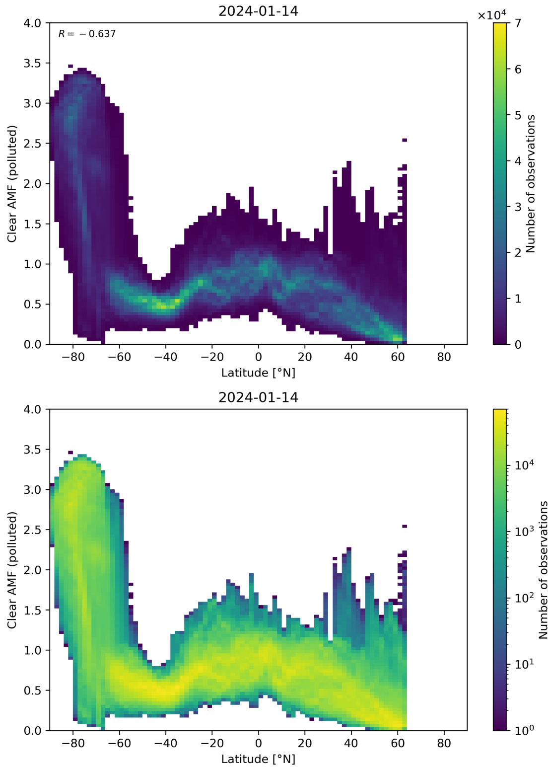
Figure 145: Scatter density plot of “Latitude” against “Clear AMF (polluted)” for 2024-01-13 to 2024-01-15.
