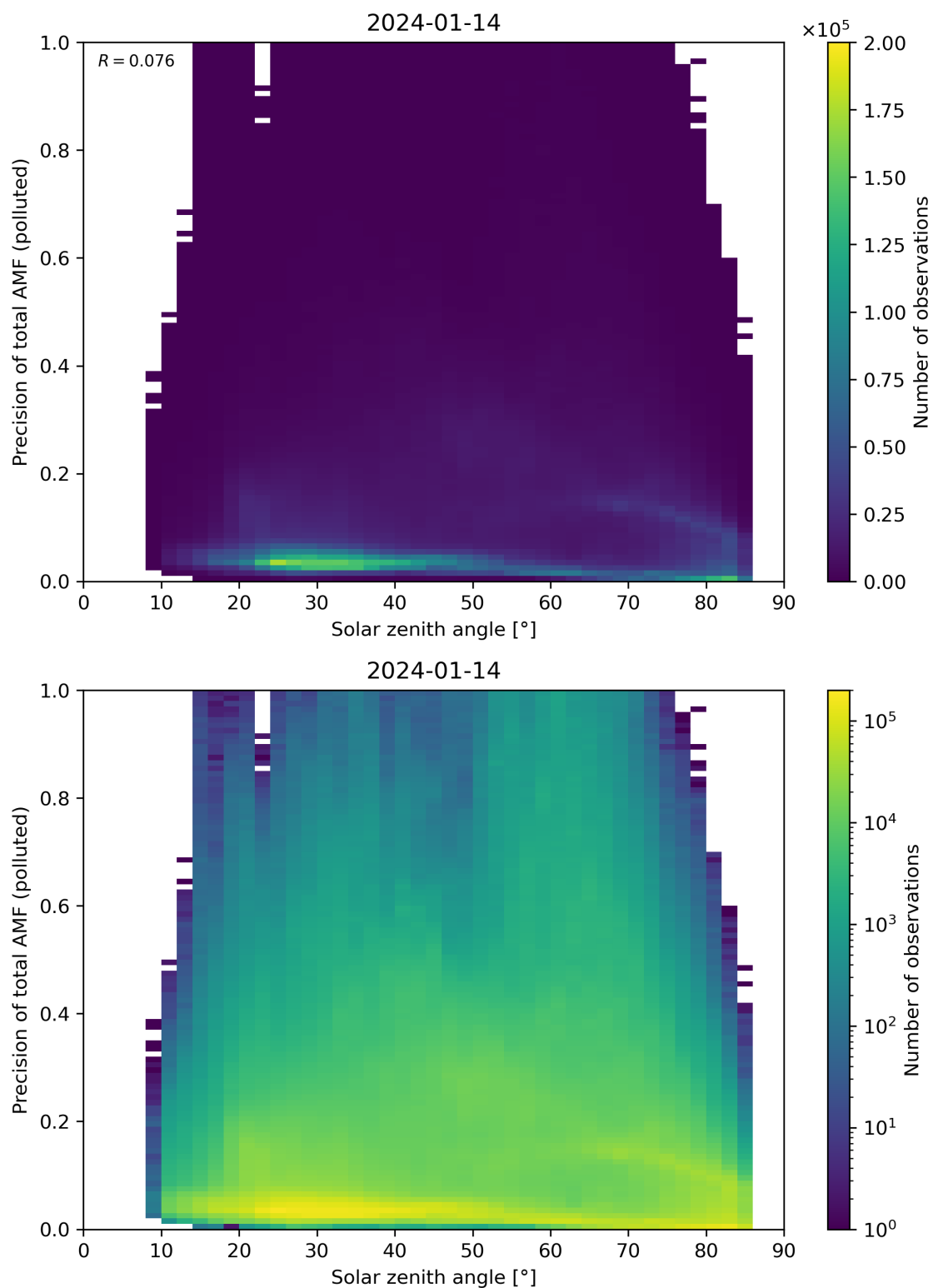
Figure 175: Scatter density plot of “Solar zenith angle” against “Precision of total AMF (polluted)” for 2024-01-13 to 2024-01-15.
