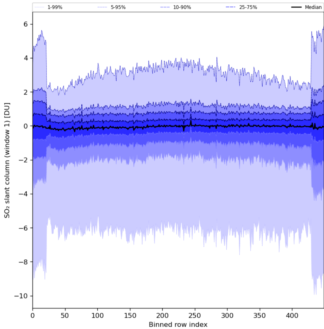
Figure 79: Along track statistics of “SO 2 slant column (window 1)” for 2024-01-13 to 2024-01-15
