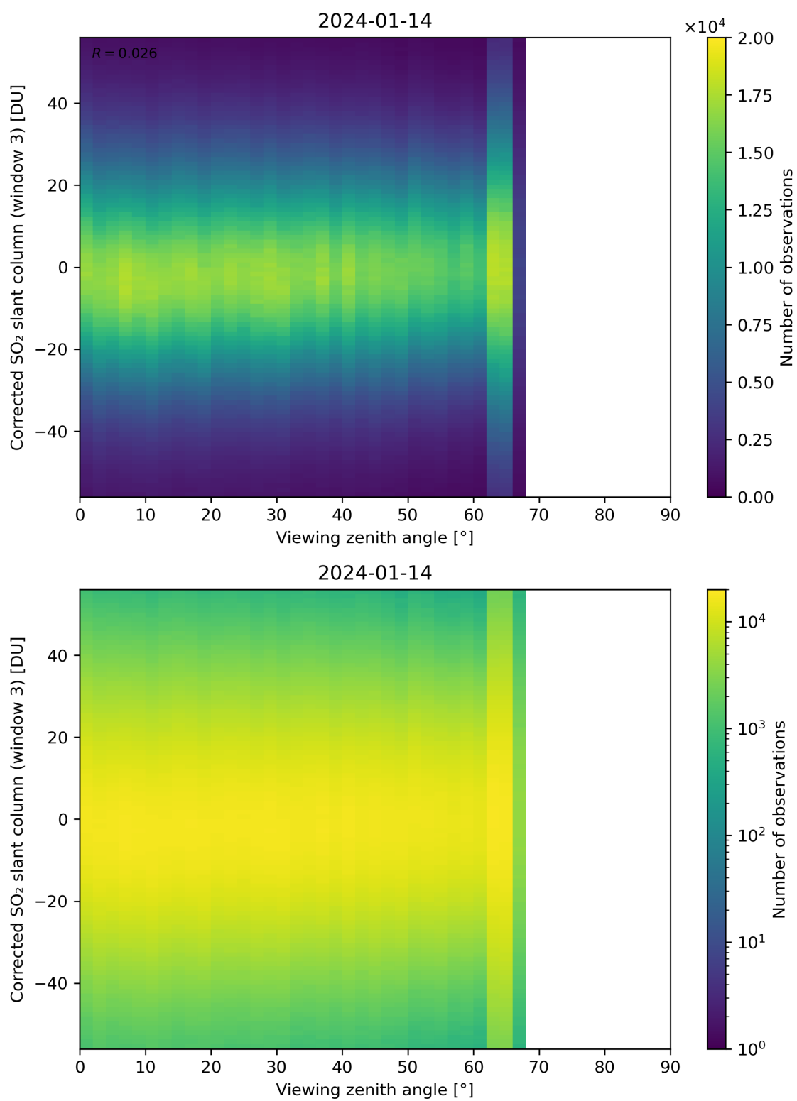
Figure 319: Scatter density plot of “Viewing zenith angle” against “Corrected SO 2 slant column (window 3)” for 2024-01-13 to 2024-01-15.
