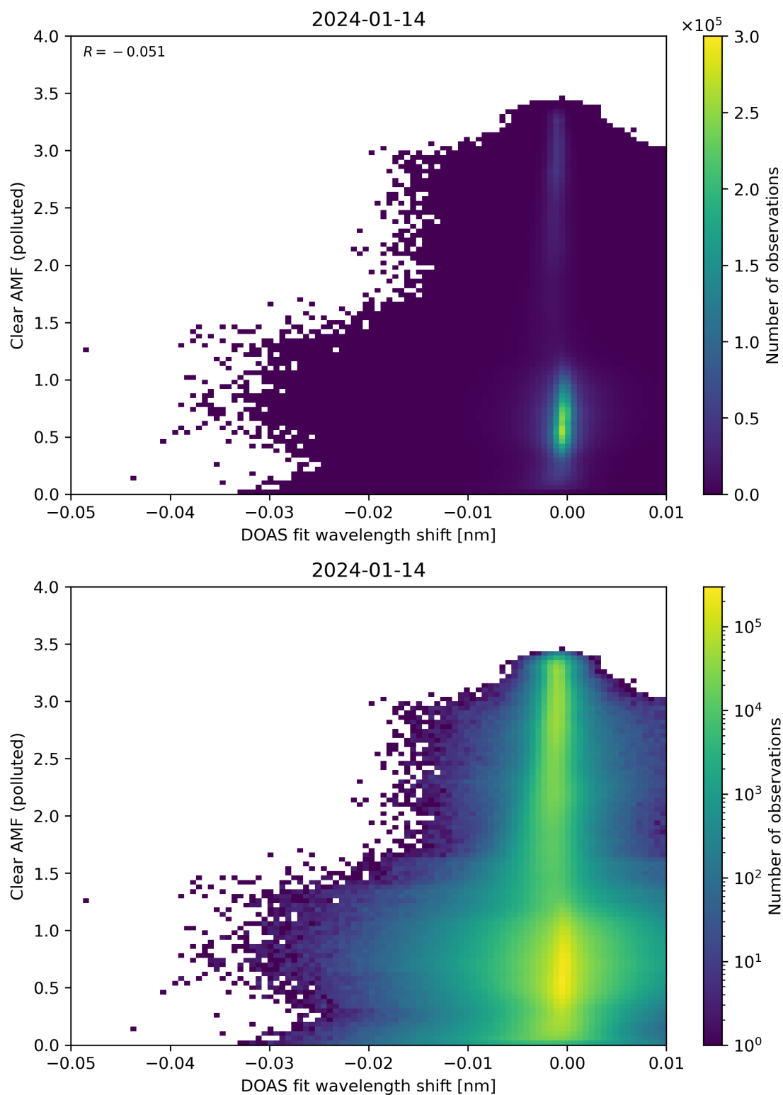
Figure 129: Scatter density plot of “DOAS fit wavelength shift” against “Clear AMF (polluted)” for 2024-01-13 to 2024-01-15.
