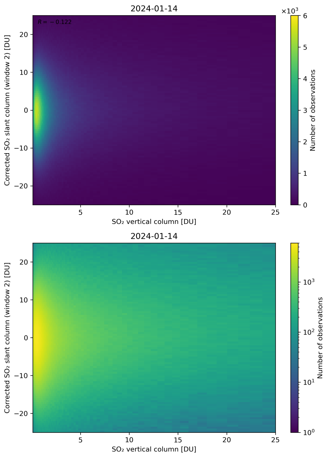
Figure 298: Scatter density plot of “SO 2 vertical column” against “Corrected SO 2 slant column (window 2)” for 2024-01-13 to 2024-01-15.
