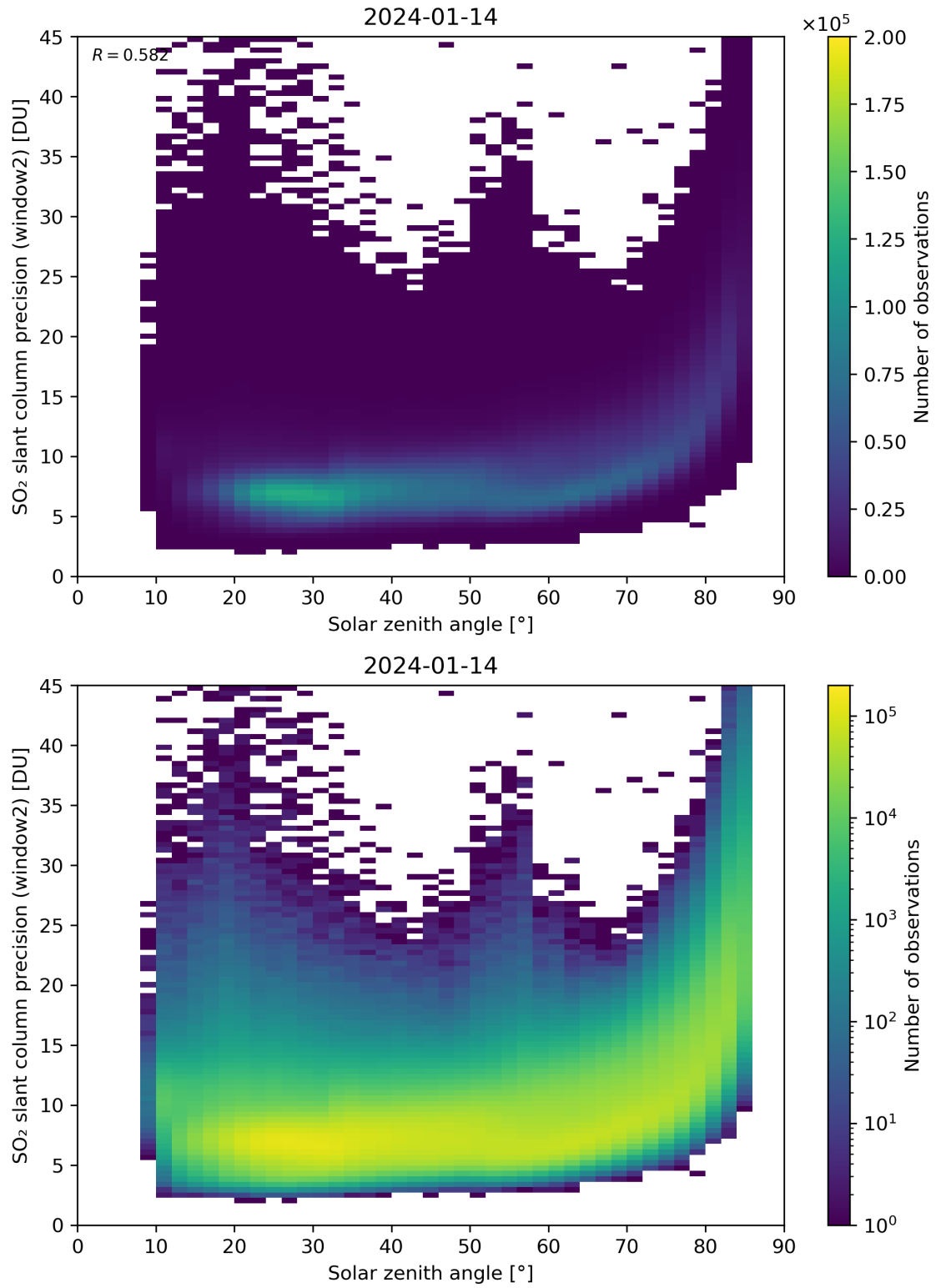
Figure 171: Scatter density plot of “Solar zenith angle” against “SO 2 slant column precision (window2)” for 2024-01-13 to 2024-01-15.
