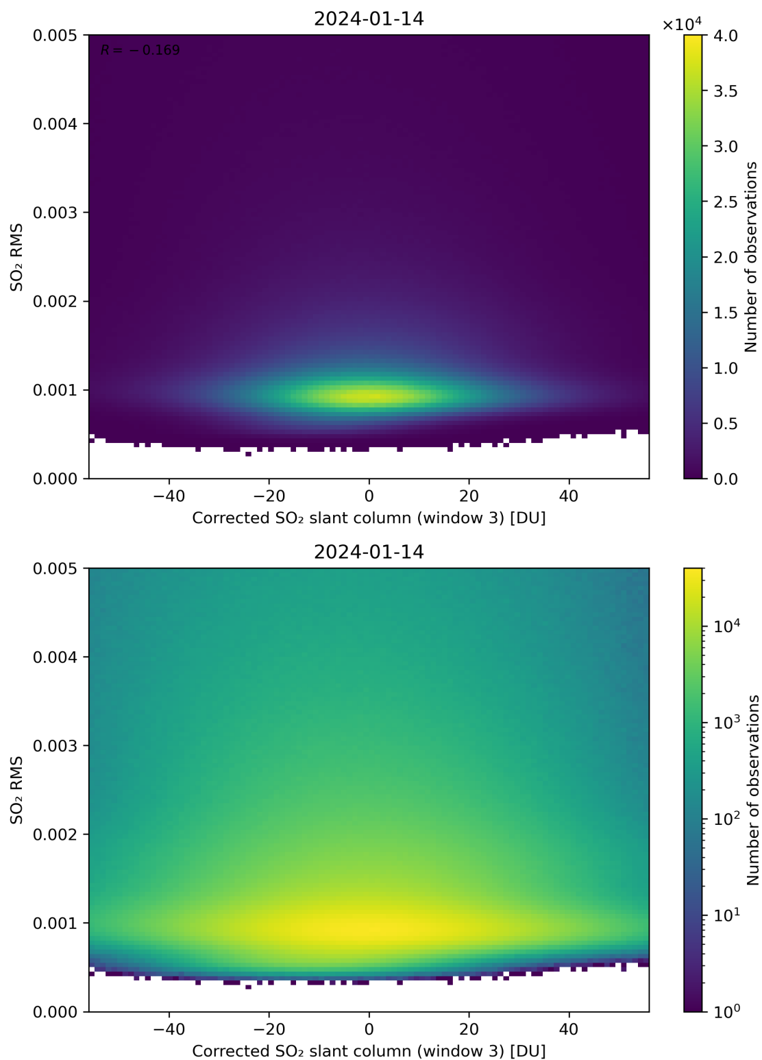
Figure 208: Scatter density plot of “Corrected SO 2 slant column (window 3)” against “SO 2 RMS” for 2024-01-13 to 2024-01-15.
