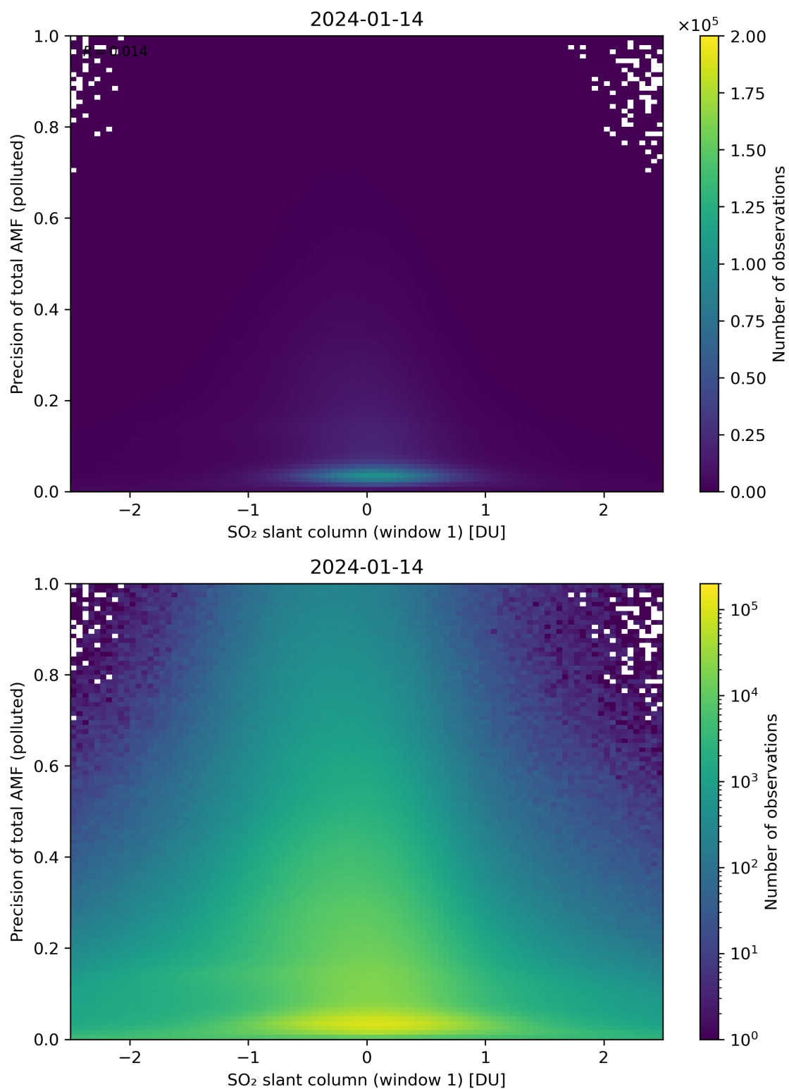
Figure 240: Scatter density plot of “SO 2 slant column (window 1)” against “Precision of total AMF (polluted)” for 2024-01-13 to 2024-01-15.
