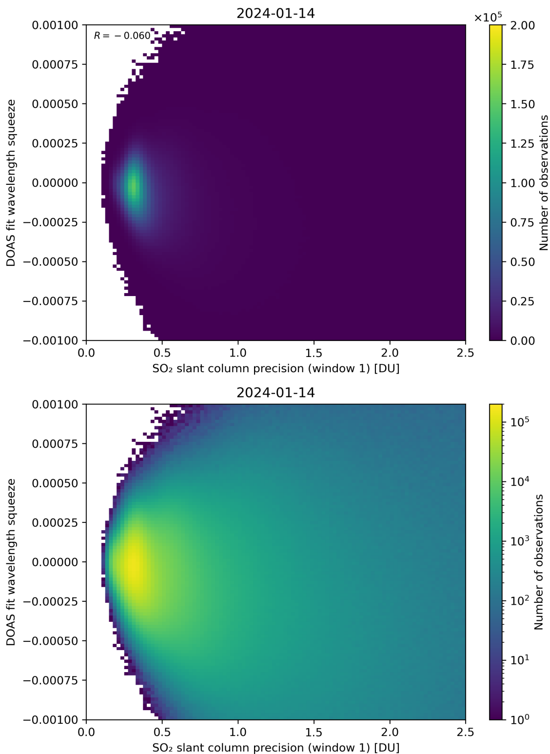
Figure 222: Scatter density plot of “SO 2 slant column precision (window 1)” against “DOAS fit wavelength squeeze” for 2024-01-13 to 2024-01-15.
