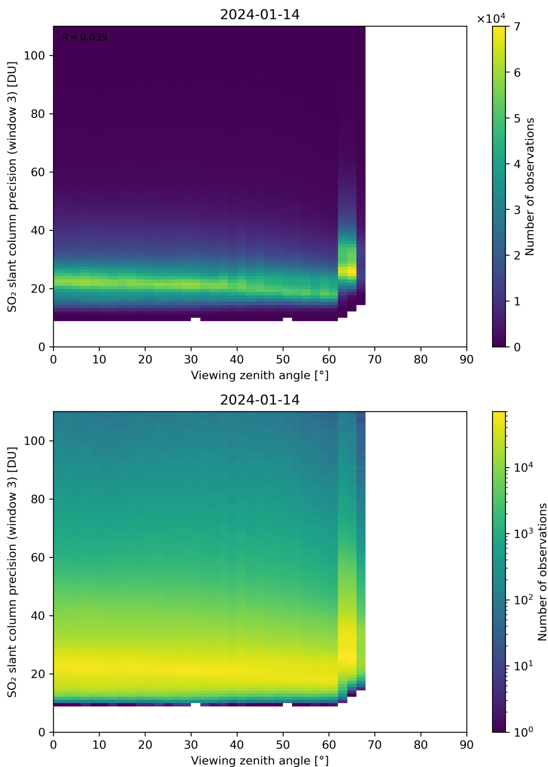
Figure 324: Scatter density plot of “Viewing zenith angle” against “SO 2 slant column precision (window 3)” for 2024-01-13 to 2024-01-15.
