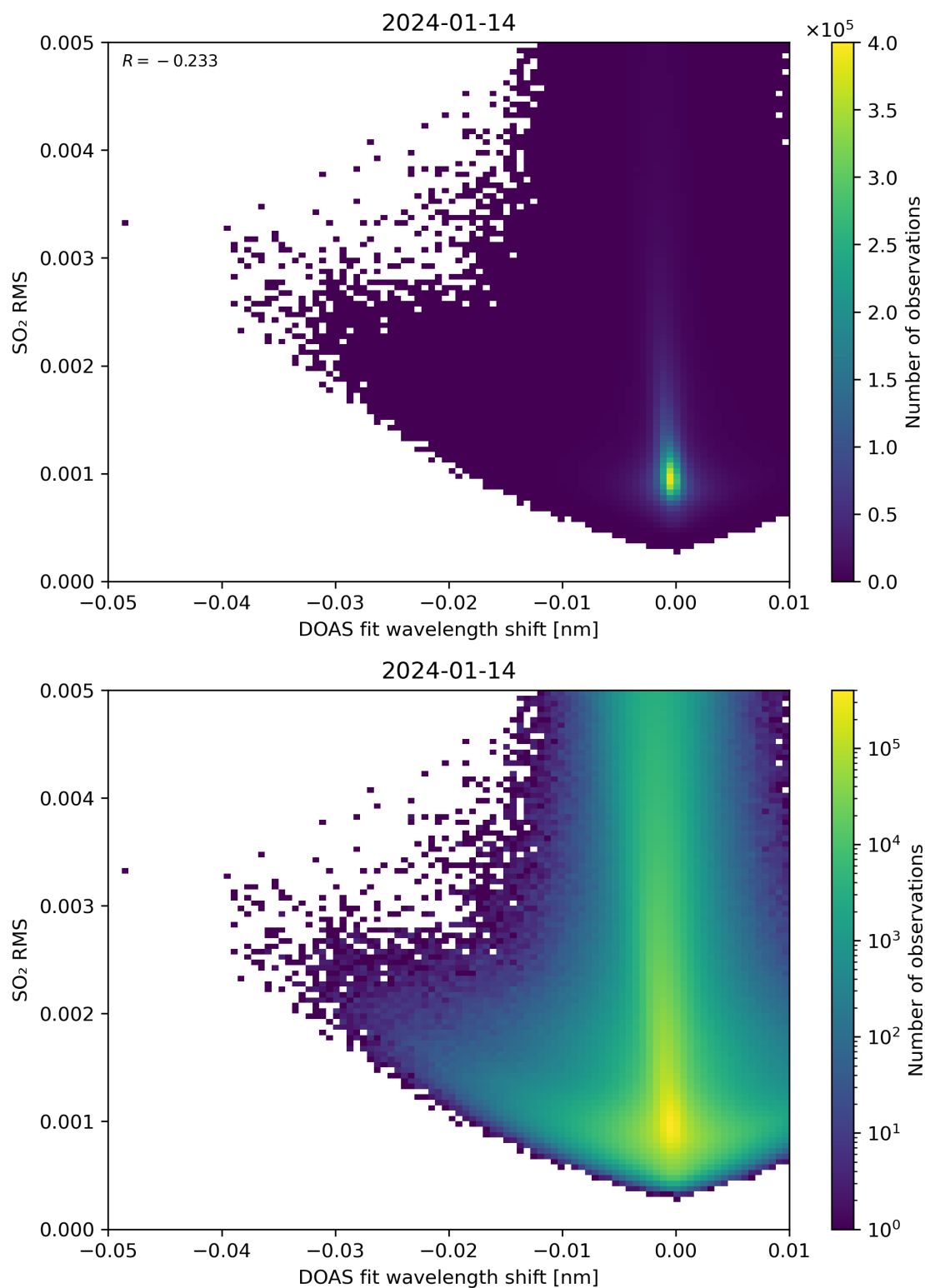
Figure 128: Scatter density plot of “DOAS fit wavelength shift” against “SO 2 RMS” for 2024-01-13 to 2024-01-15.
