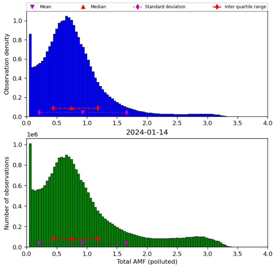
Figure 71: Histogram of “Total AMF (polluted)” for 2024-01-13 to 2024-01-15
