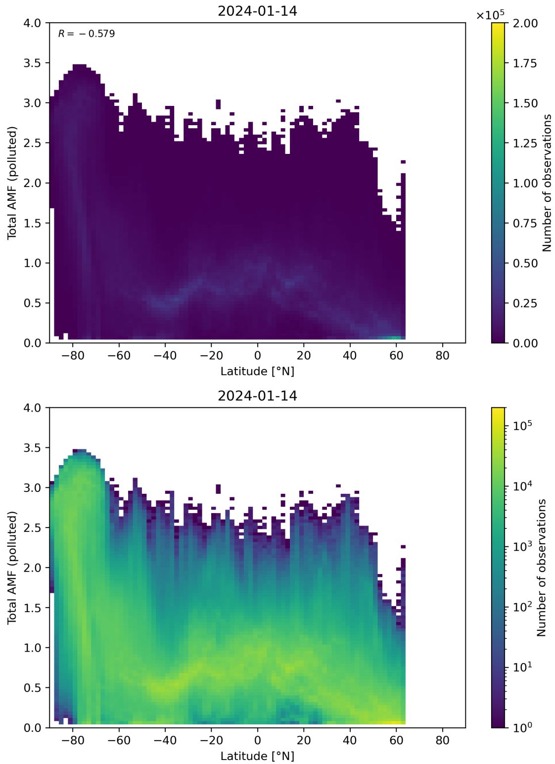
Figure 154: Scatter density plot of “Latitude” against “Total AMF (polluted)” for 2024-01-13 to 2024-01-15.
