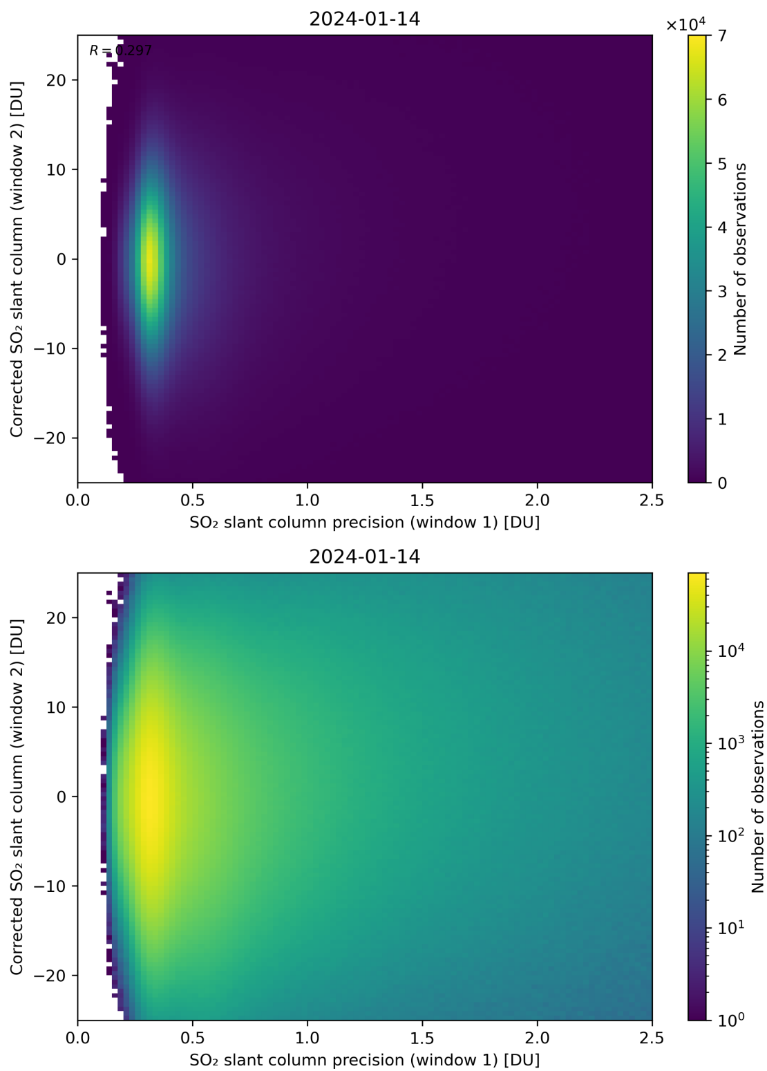
Figure 225: Scatter density plot of “SO 2 slant column precision (window 1)” against “Corrected SO 2 slant column (window 2)” for 2024-01-13 to 2024-01-15.
