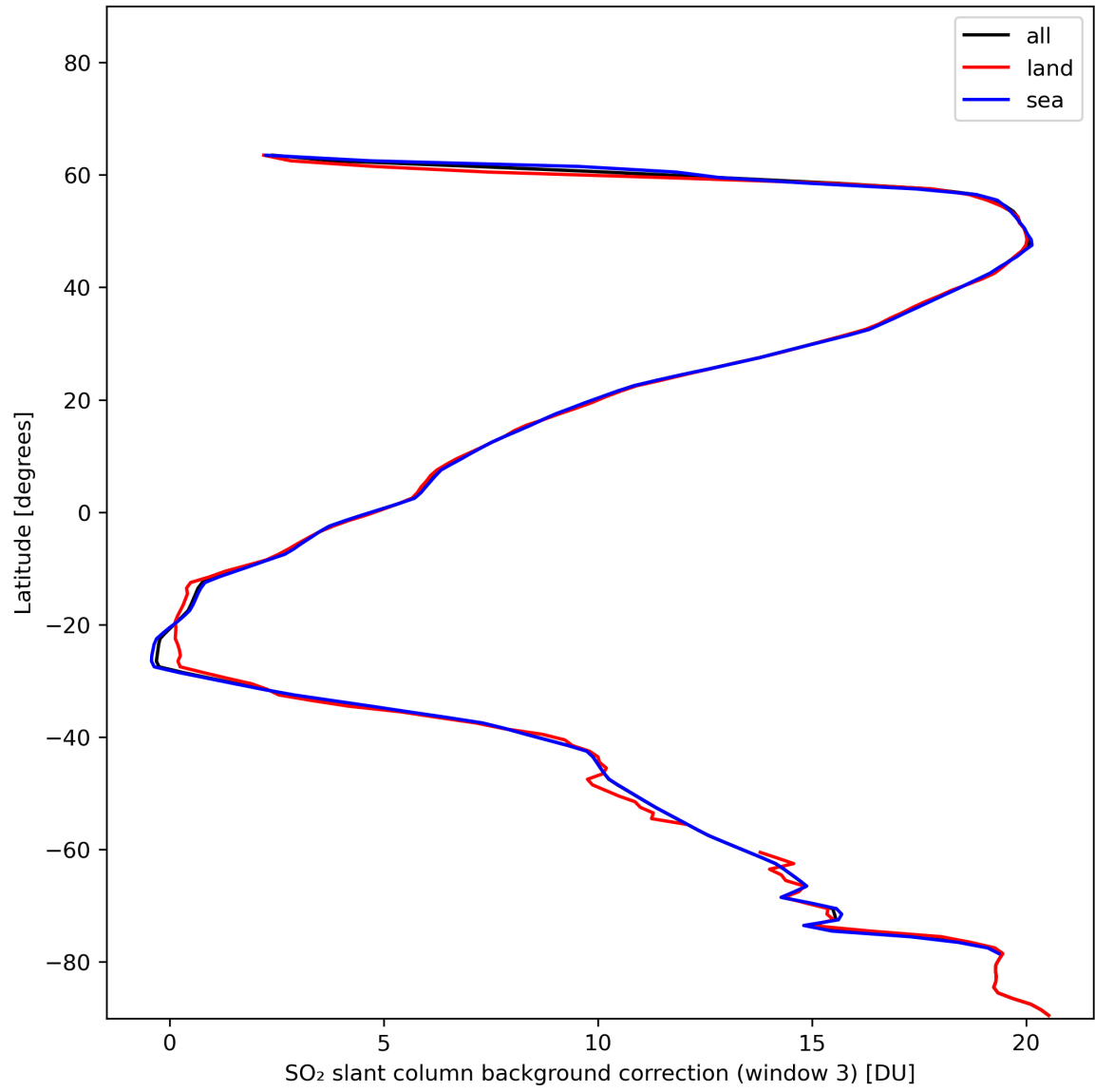
Figure 44: Zonal average of “SO 2 slant column background correction (window 3)” for 2024-01-13 to 2024-01-15.
