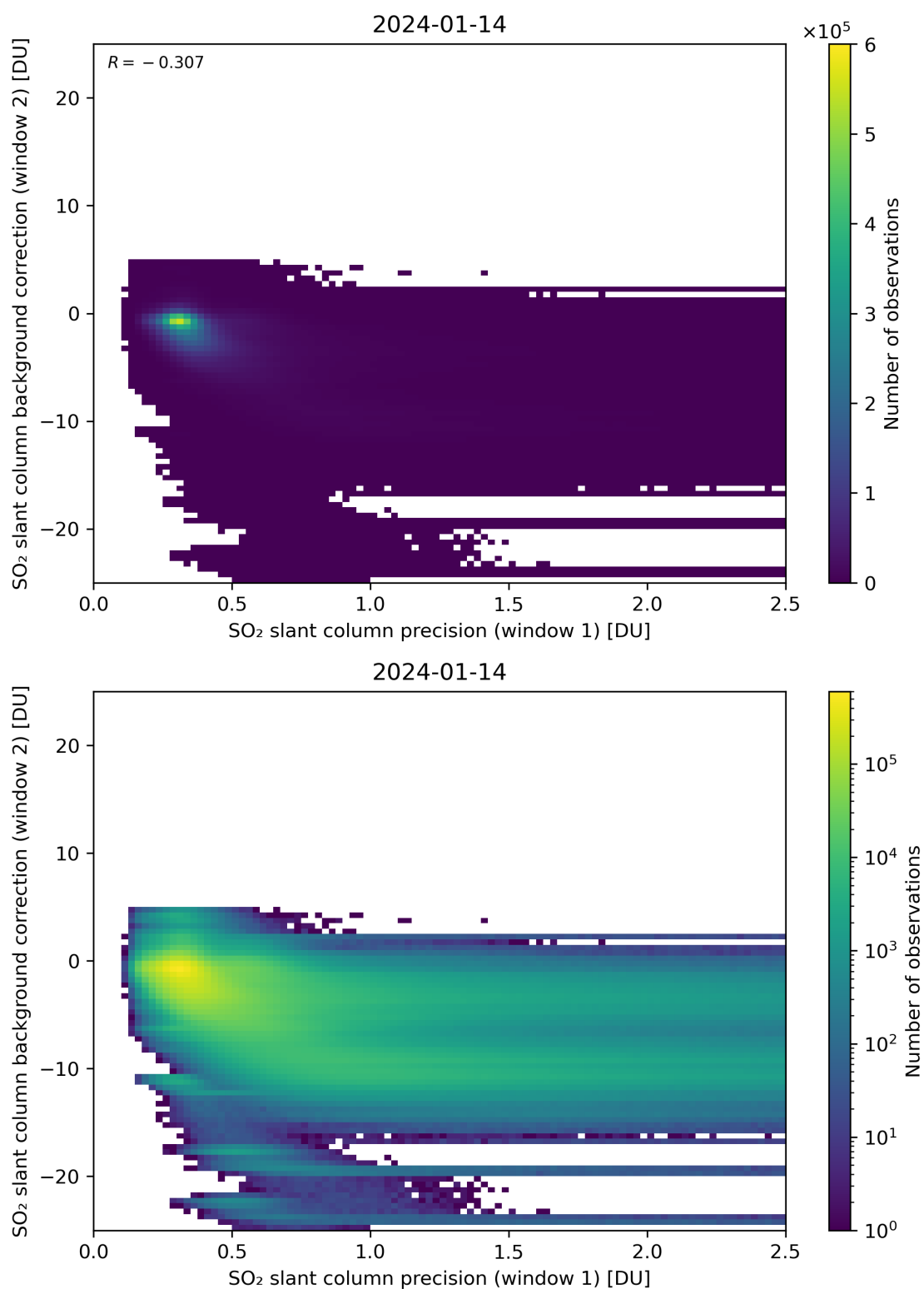
Figure 219: Scatter density plot of “SO 2 slant column precision (window 1)” against “SO 2 slant column background correction (window 2)” for 2024-01-13 to 2024-01-15.
