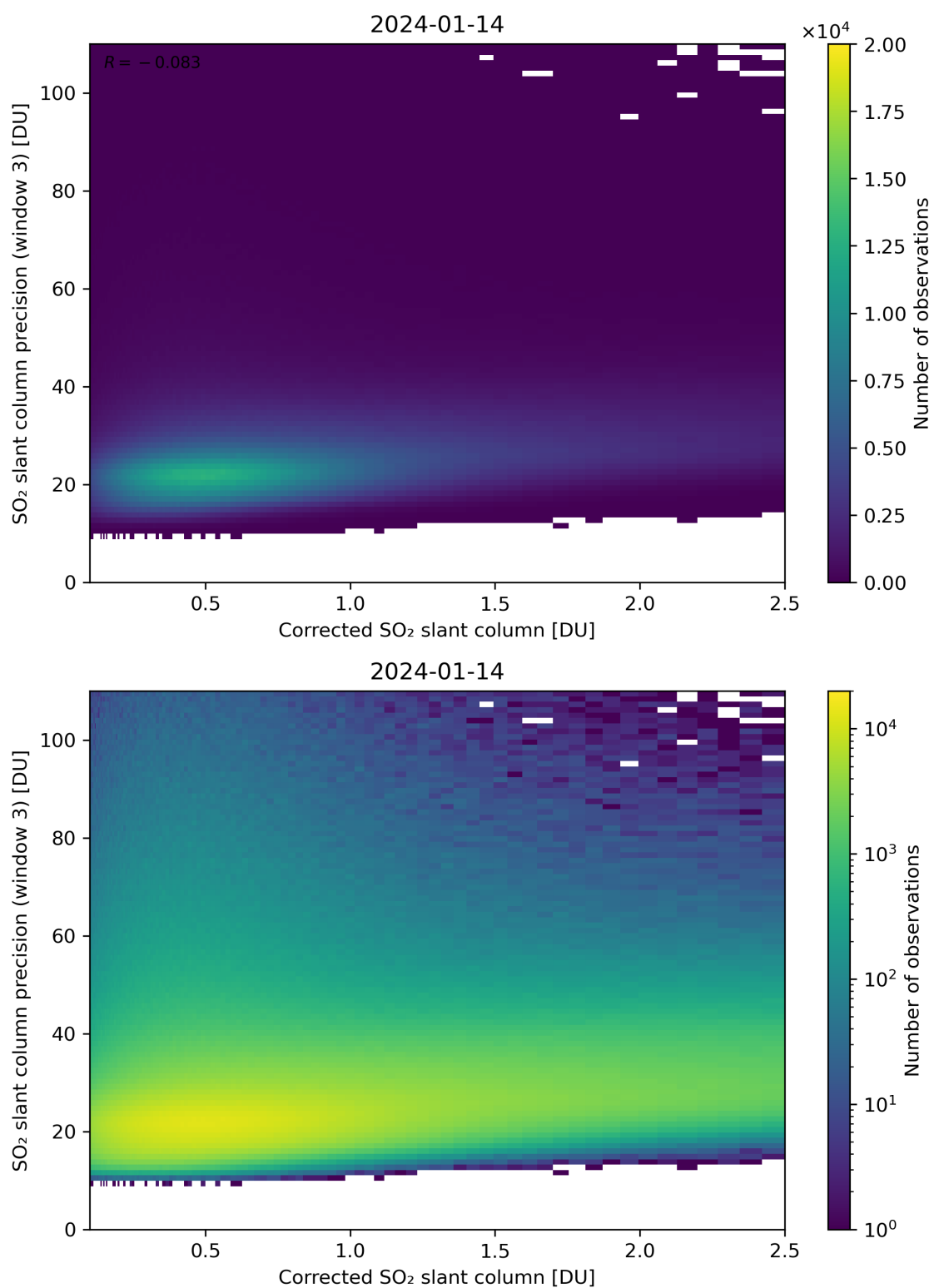
Figure 191: Scatter density plot of “Corrected SO 2 slant column” against “SO 2 slant column precision (window 3)” for 2024-01-13 to 2024-01-15.
