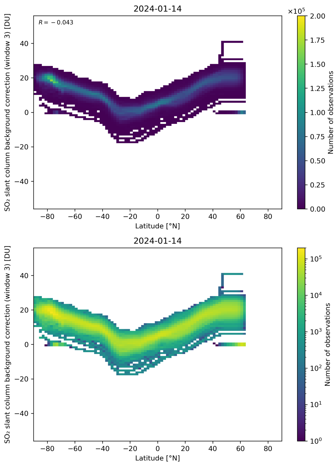
Figure 141: Scatter density plot of “Latitude” against “SO 2 slant column background correction (window 3)” for 2024-01-13 to 2024-01-15.
