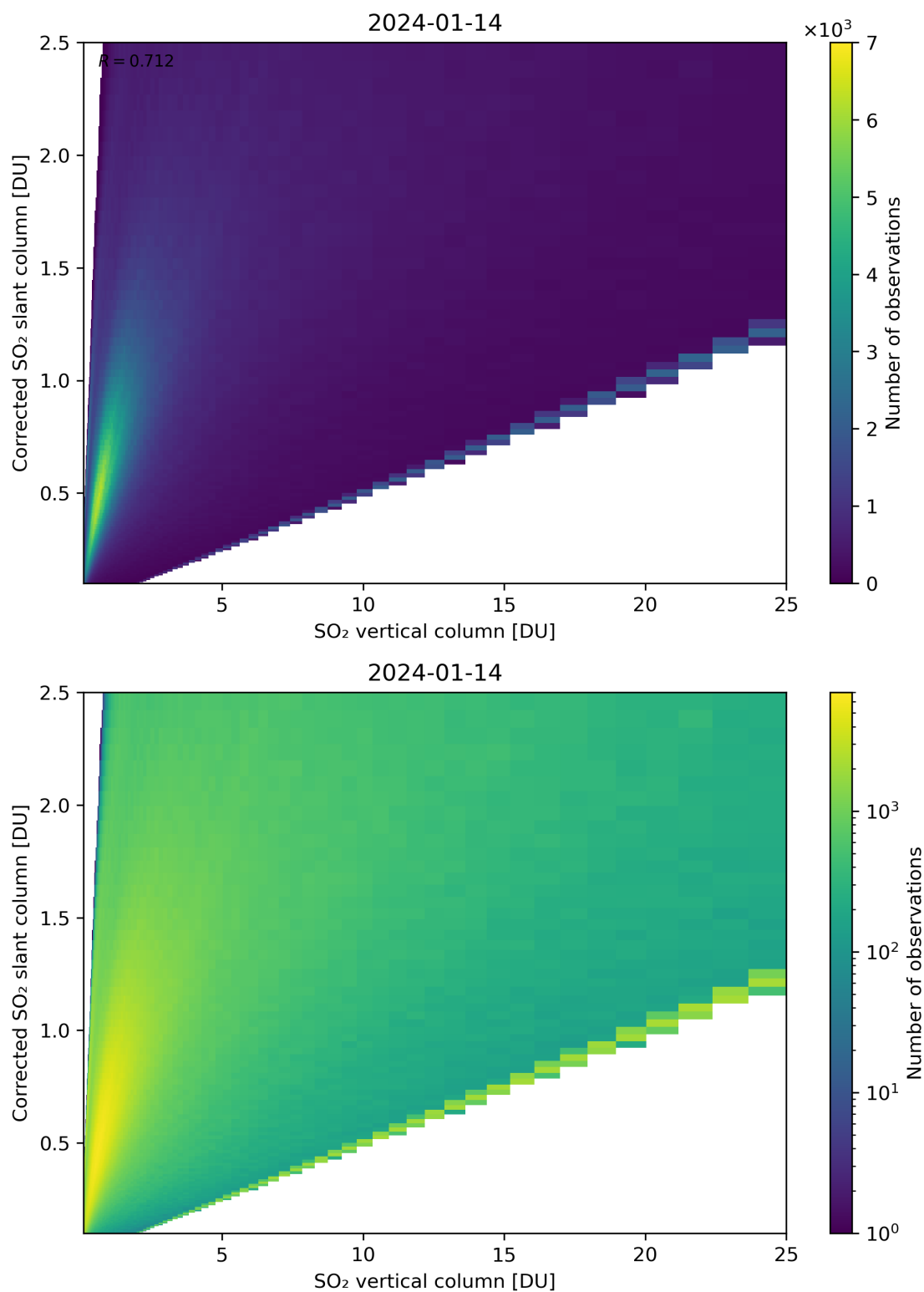
Figure 297: Scatter density plot of “SO 2 vertical column” against “Corrected SO 2 slant column” for 2024-01-13 to 2024-01-15.
