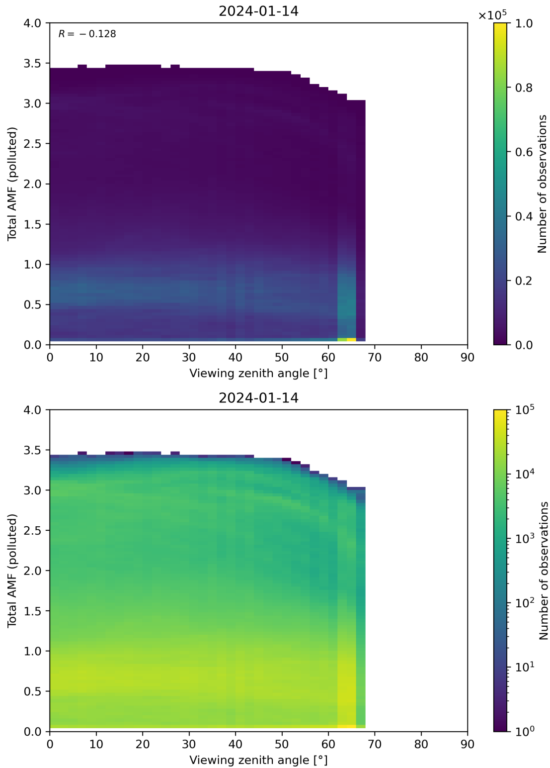
Figure 325: Scatter density plot of “Viewing zenith angle” against “Total AMF (polluted)” for 2024-01-13 to 2024-01-15.
