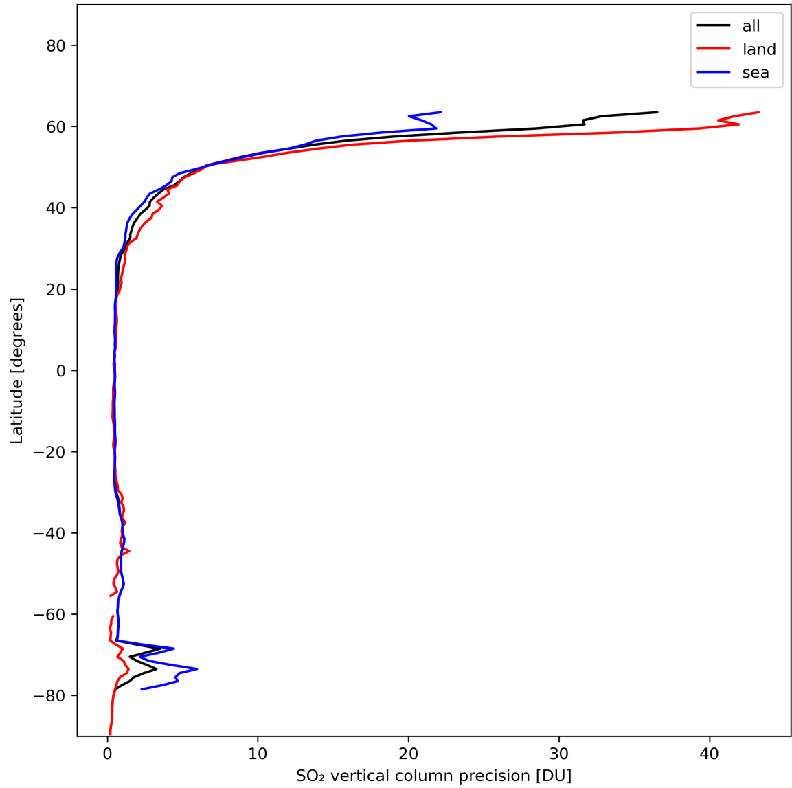
Figure 31: Zonal average of “SO 2 vertical column precision” for 2024-01-13 to 2024-01-15.
