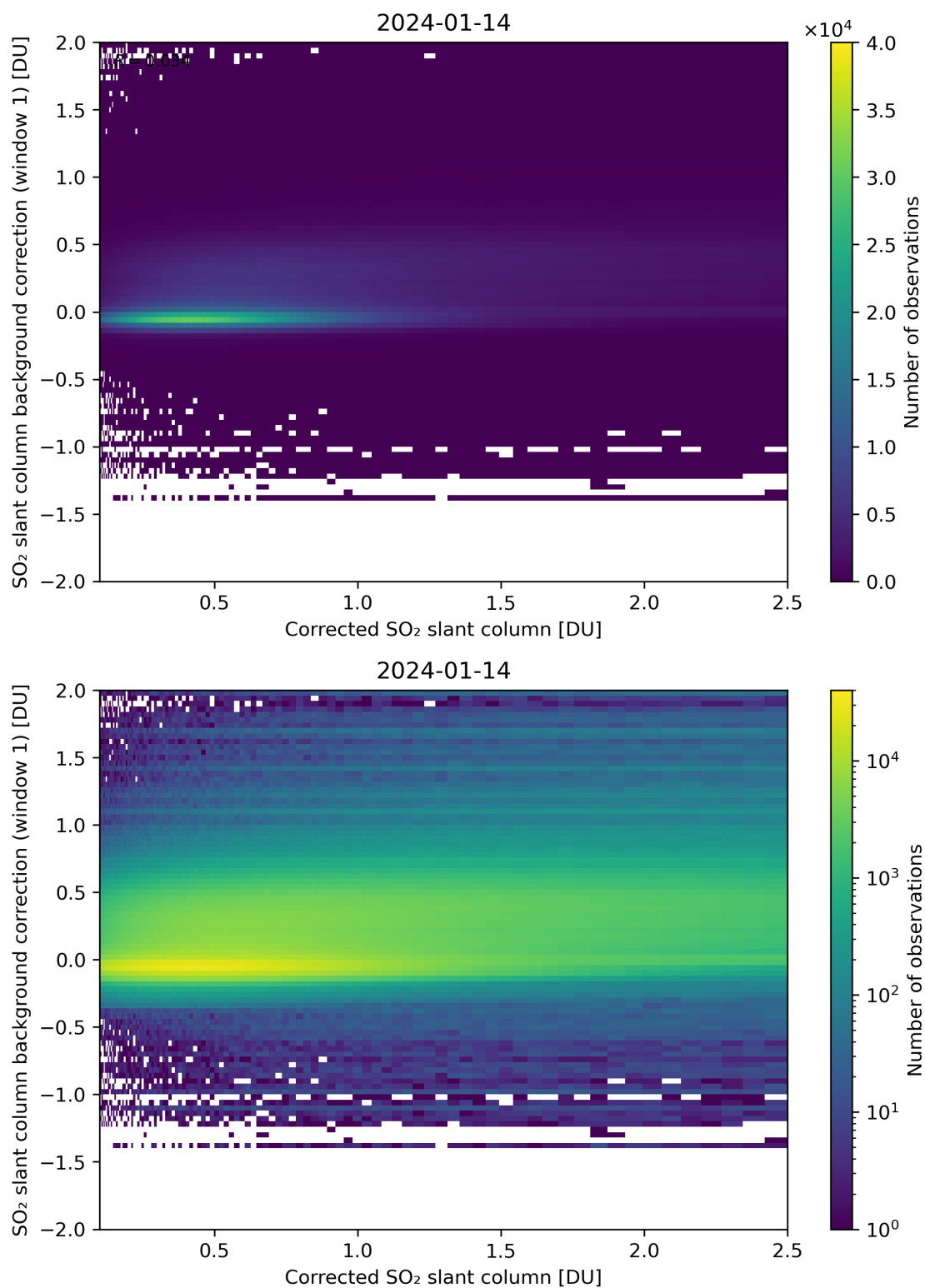
Figure 178: Scatter density plot of “Corrected SO 2 slant column” against “SO 2 slant column background correction (window 1)” for 2024-01-13 to 2024-01-15.
