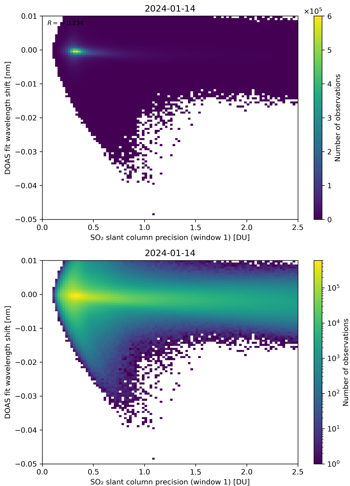
Figure 221: Scatter density plot of “SO 2 slant column precision (window 1)” against “DOAS fit wavelength shift” for 2024-01-13 to 2024-01-15.
