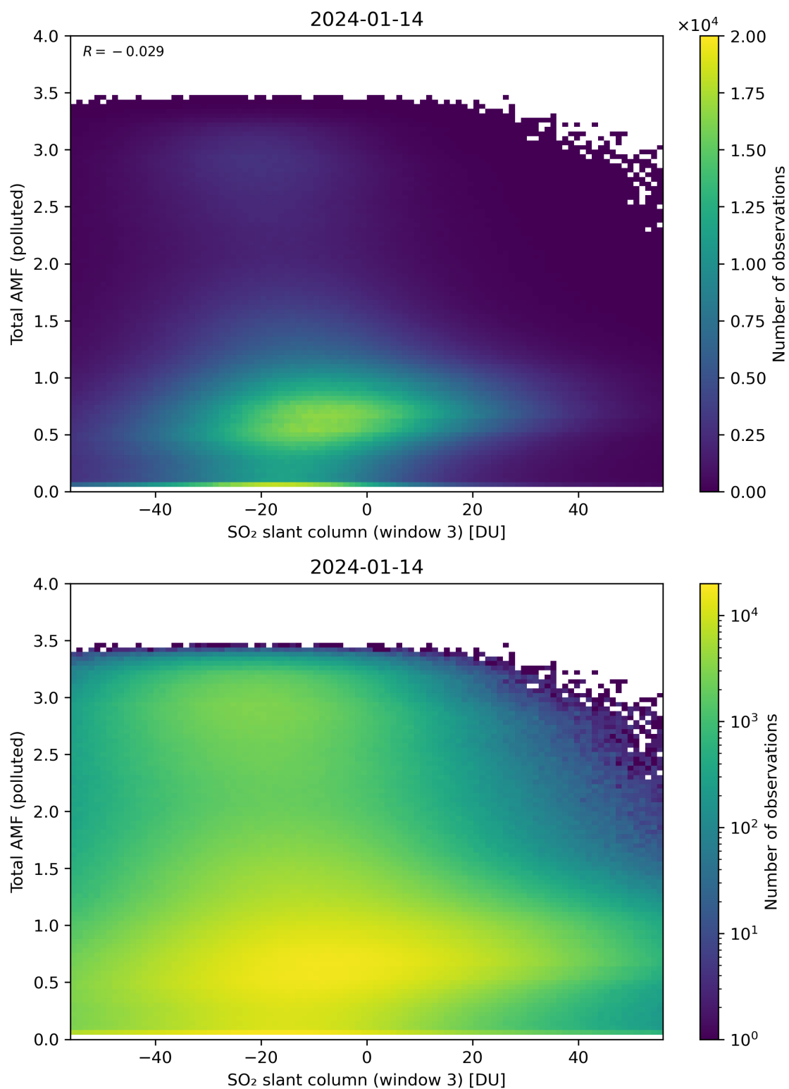
Figure 268: Scatter density plot of “SO 2 slant column (window 3)” against “Total AMF (polluted)” for 2024-01-13 to 2024-01-15.
