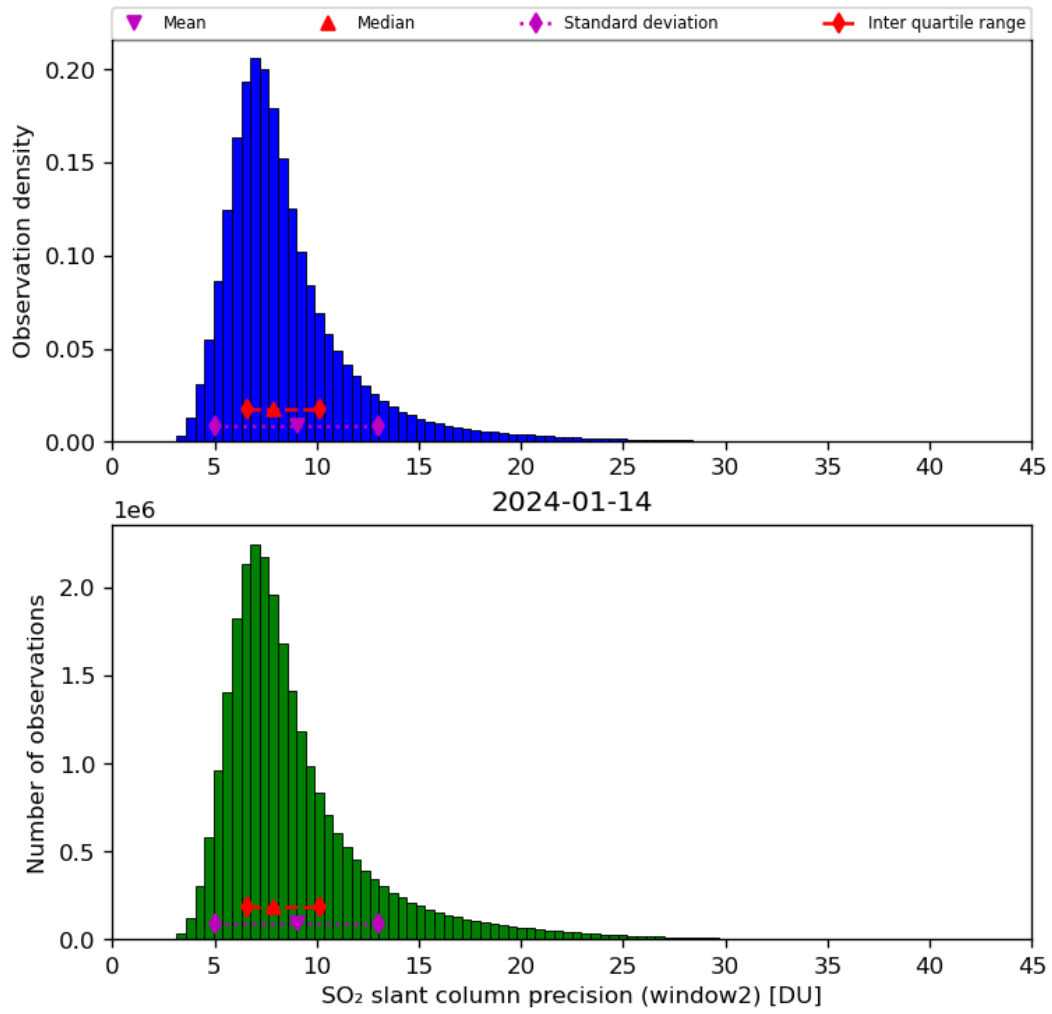
Figure 61: Histogram of “SO 2 slant column precision (window2)” for 2024-01-13 to 2024-01-15
