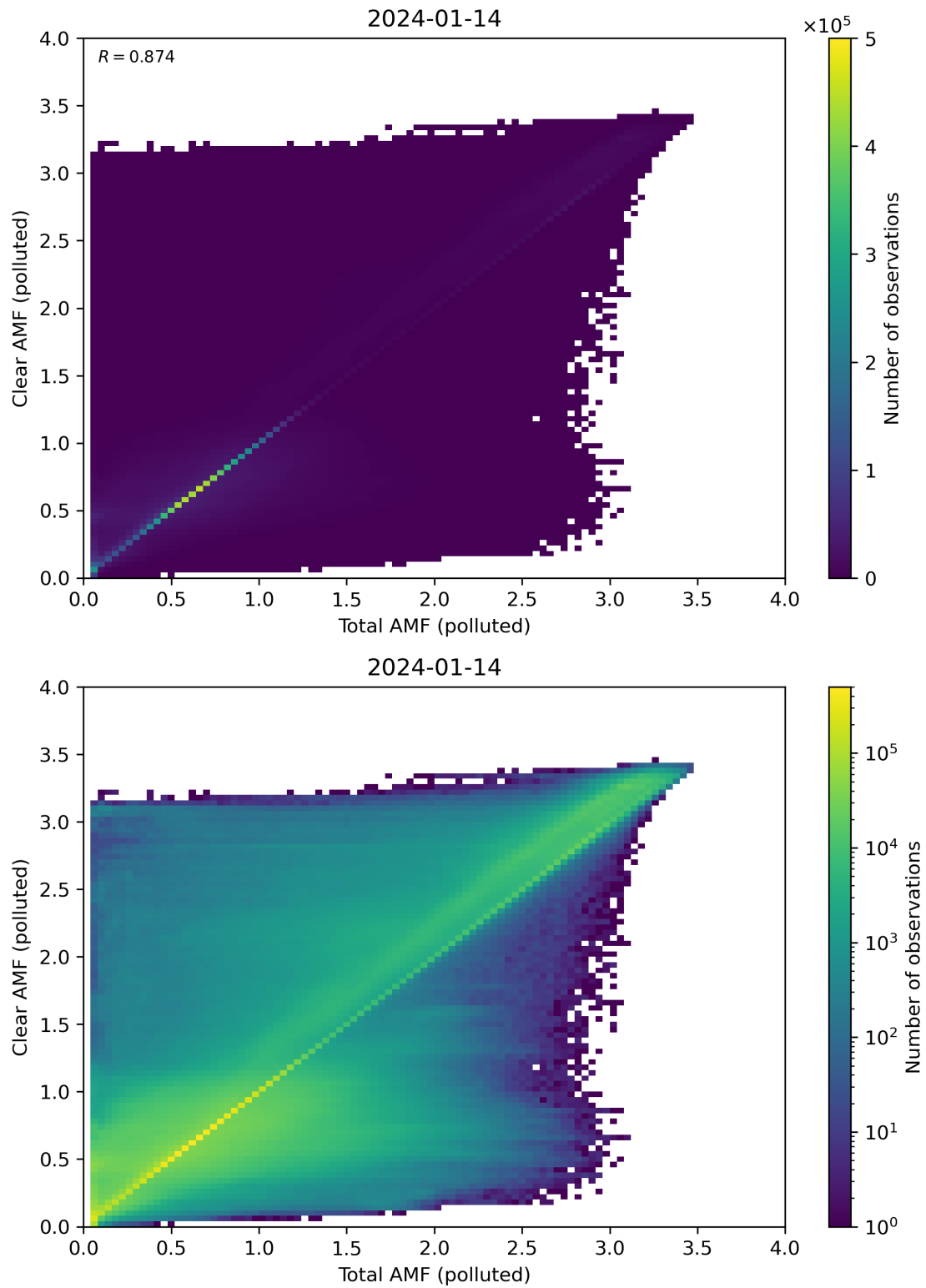
Figure 271: Scatter density plot of “Total AMF (polluted)” against “Clear AMF (polluted)” for 2024-01-13 to 2024-01-15.
