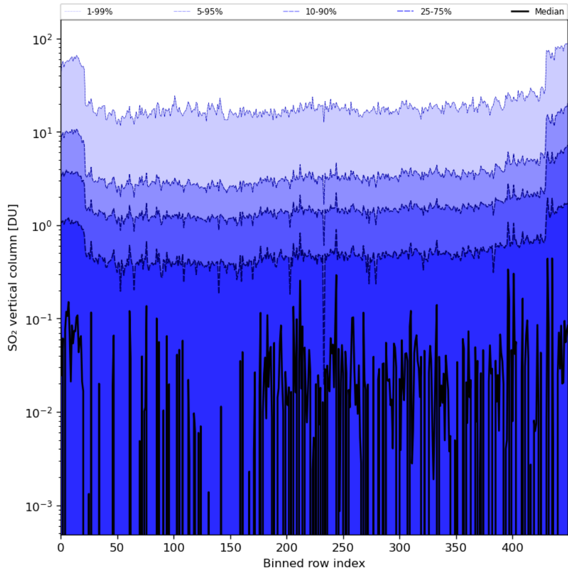
Figure 76: Along track statistics of “SO 2 vertical column” for 2024-01-13 to 2024-01-15
