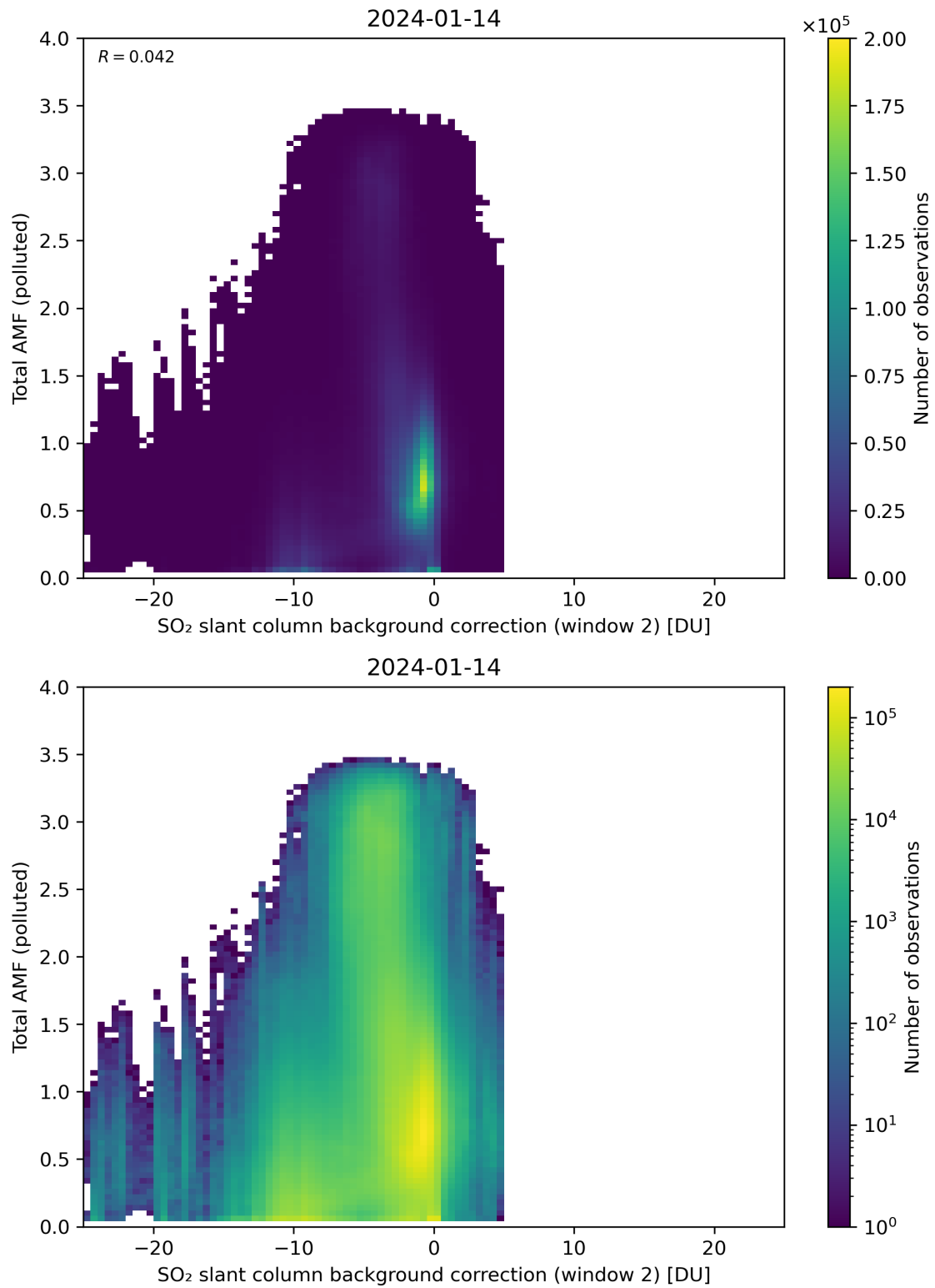
Figure 119: Scatter density plot of “SO 2 slant column background correction (window 2)” against “Total AMF (polluted)” for 2024-01-13 to 2024-01-15.
