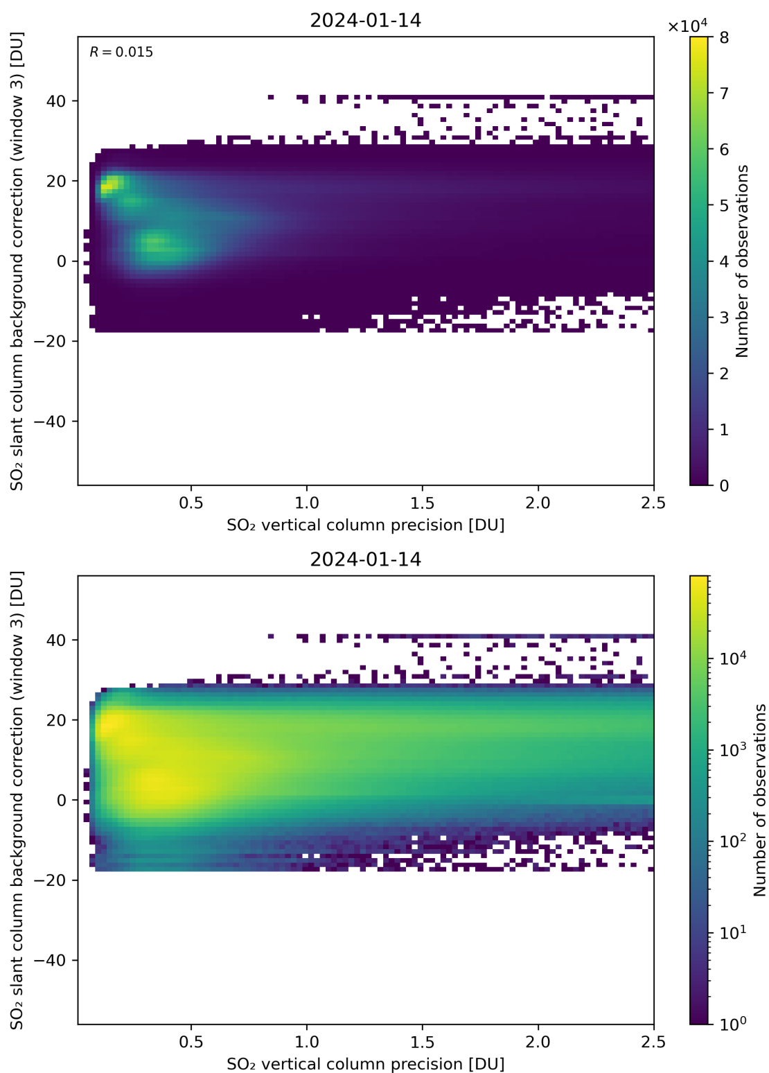
Figure 281: Scatter density plot of “SO 2 vertical column precision” against “SO 2 slant column background correction (window 3)” for 2024-01-13 to 2024-01-15.
