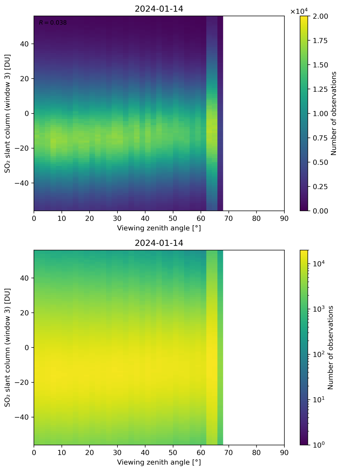
Figure 323: Scatter density plot of “Viewing zenith angle” against “SO 2 slant column (window 3)” for 2024-01-13 to 2024-01-15.
