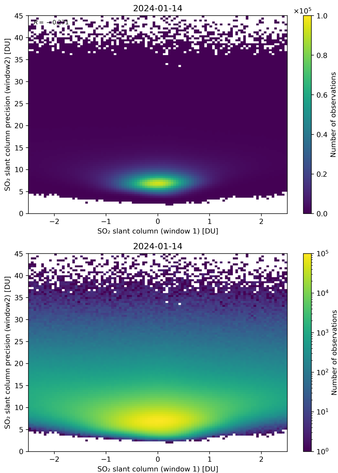
Figure 236: Scatter density plot of “SO 2 slant column (window 1)” against “SO 2 slant column precision (window2)” for 2024-01-13 to 2024-01-15.
