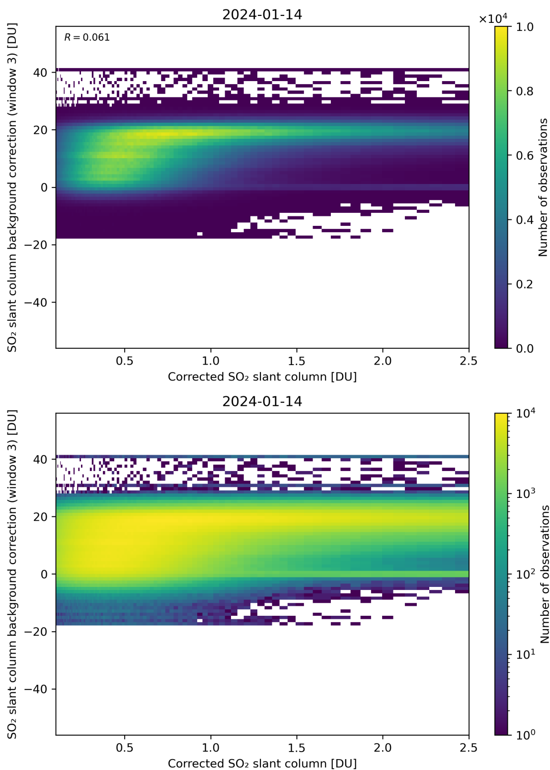
Figure 180: Scatter density plot of “Corrected SO 2 slant column” against “SO 2 slant column background correction (window 3)” for 2024-01-13 to 2024-01-15.
