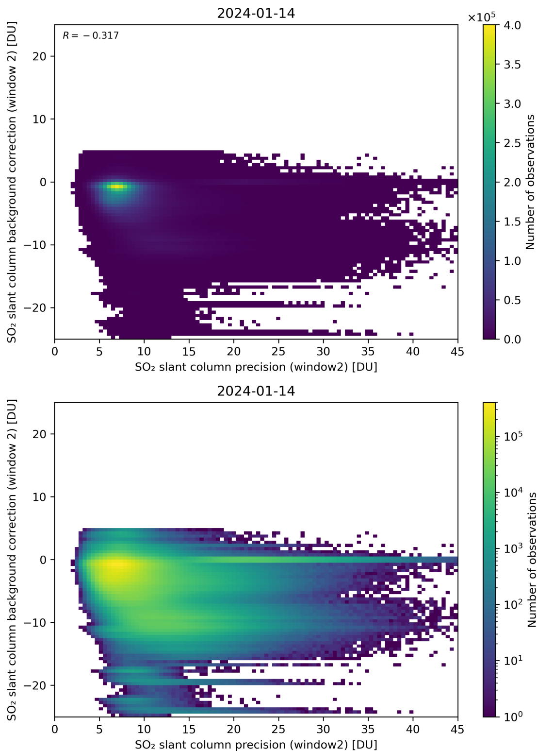
Figure 241: Scatter density plot of “SO 2 slant column precision (window2)” against “SO 2 slant column background correction (window 2)” for 2024-01-13 to 2024-01-15.
