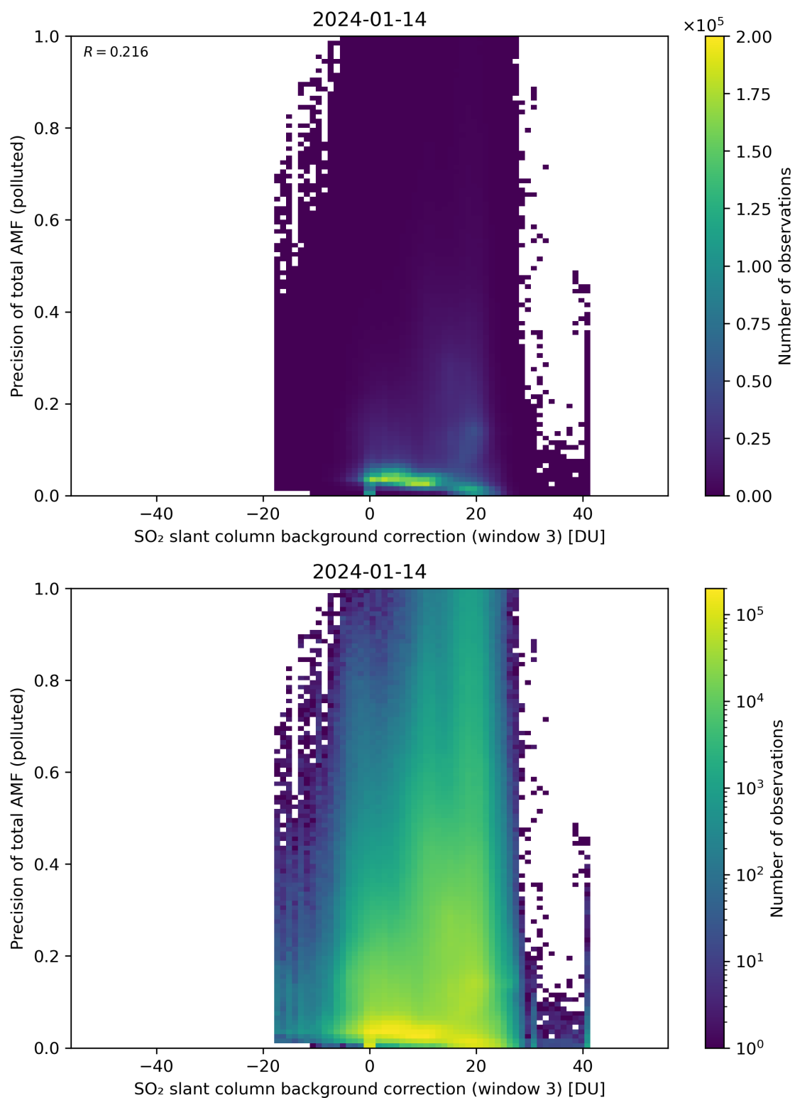
Figure 126: Scatter density plot of “SO 2 slant column background correction (window 3)” against “Precision of total AMF (polluted)” for 2024-01-13 to 2024-01-15.
