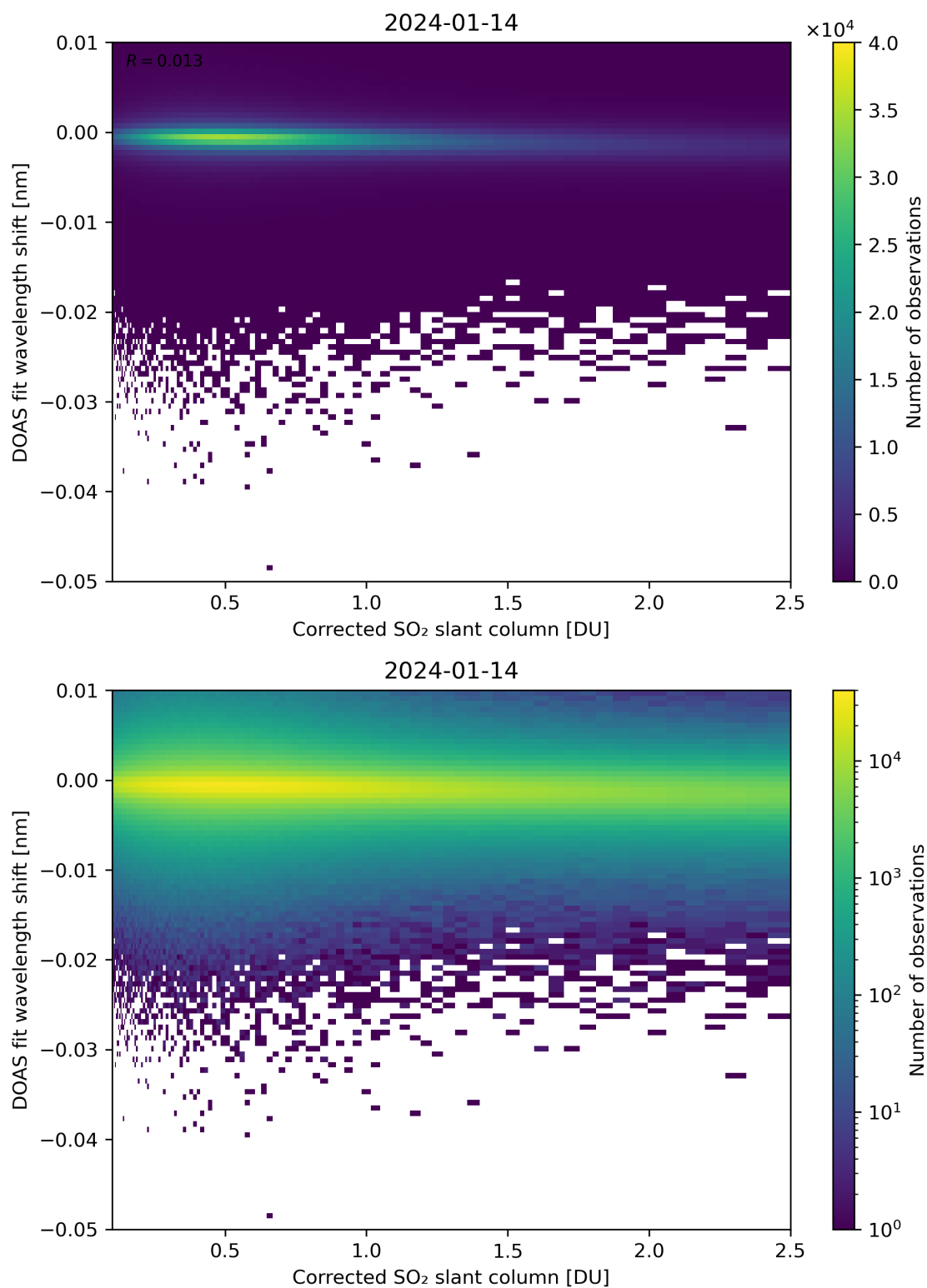
Figure 181: Scatter density plot of “Corrected SO 2 slant column” against “DOAS fit wavelength shift” for 2024-01-13 to 2024-01-15.
