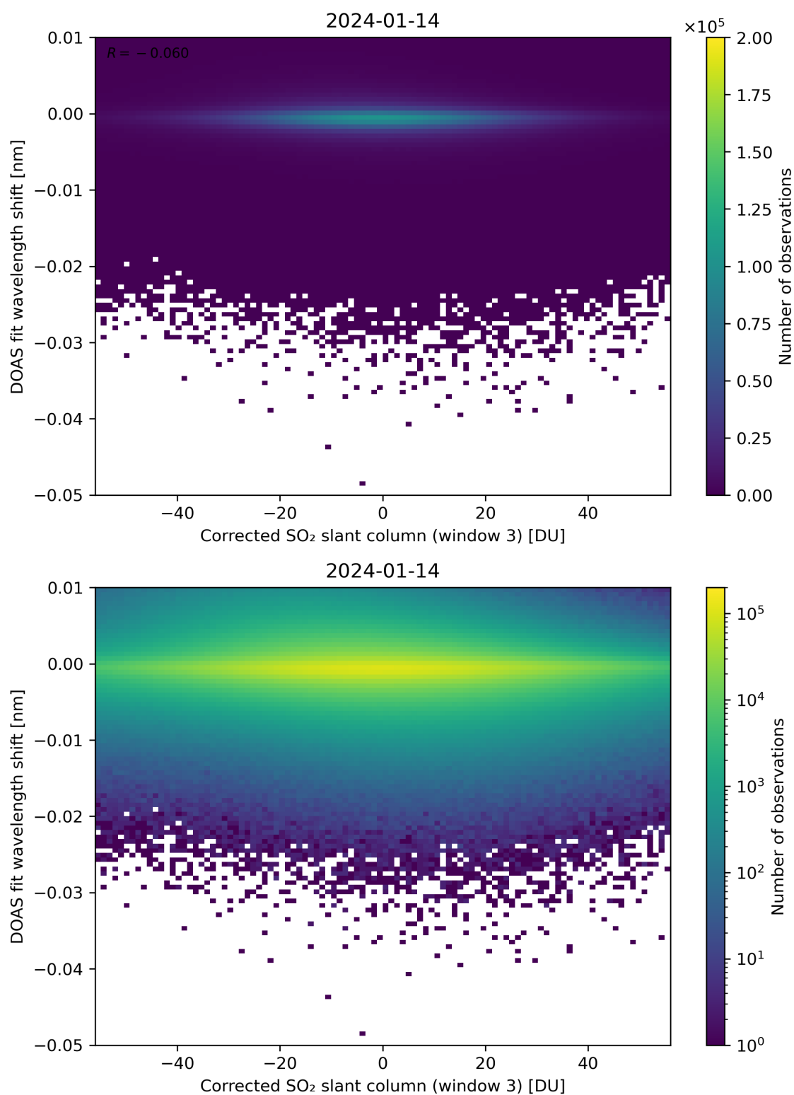
Figure 206: Scatter density plot of “Corrected SO 2 slant column (window 3)” against “DOAS fit wavelength shift” for 2024-01-13 to 2024-01-15.
