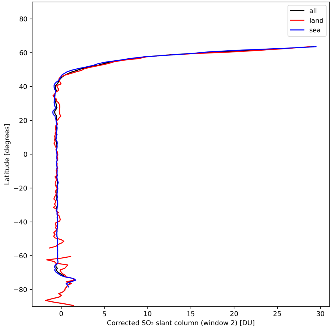
Figure 39: Zonal average of “Corrected SO 2 slant column (window 2)” for 2024-01-13 to 2024-01-15.
