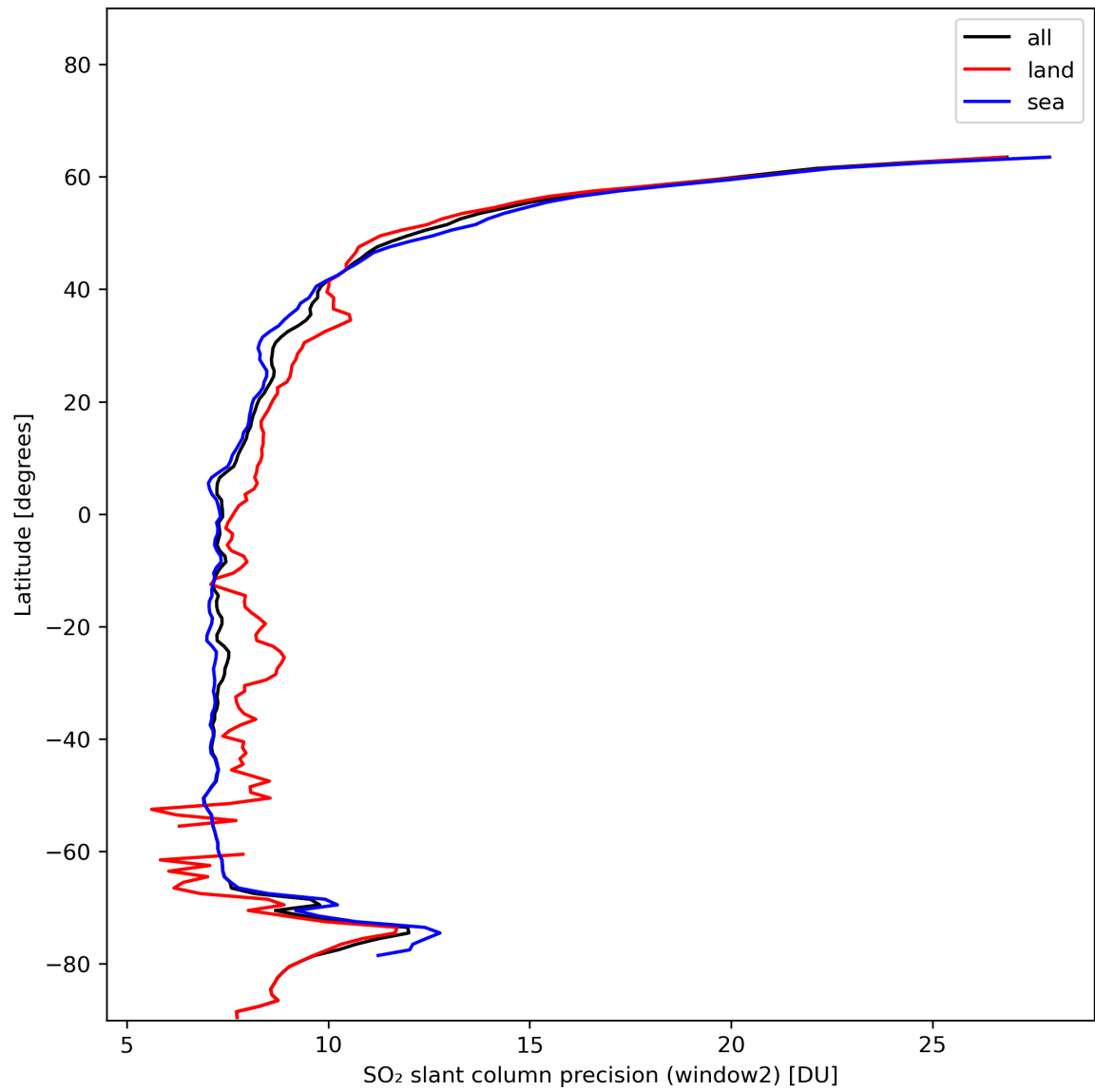
Figure 38: Zonal average of “SO 2 slant column precision (window2)” for 2024-01-13 to 2024-01-15.
