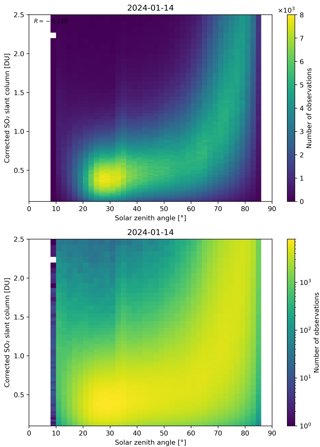
Figure 166: Scatter density plot of “Solar zenith angle” against “Corrected SO 2 slant column” for 2024-01-13 to 2024-01-15.
