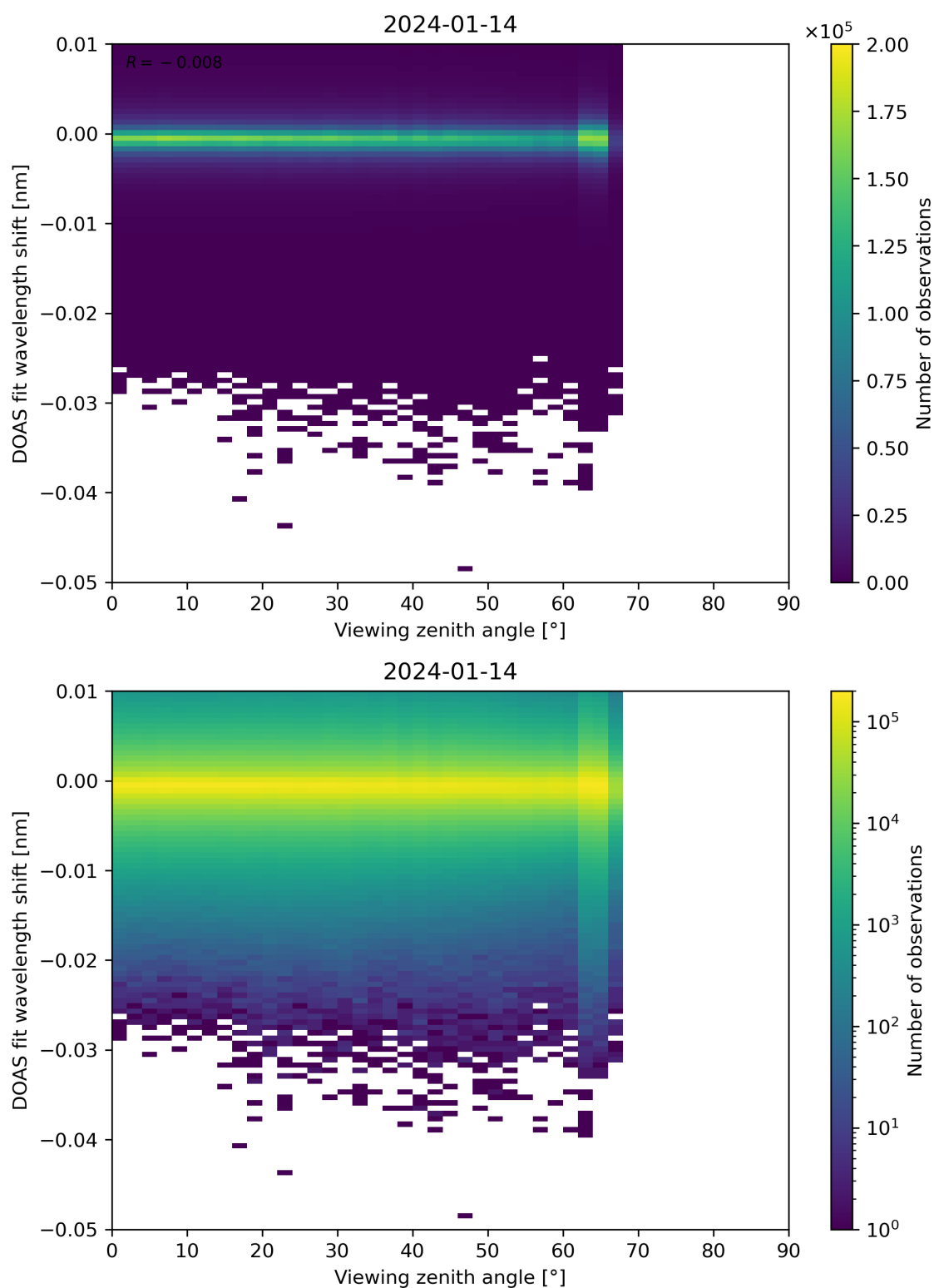
Figure 311: Scatter density plot of “Viewing zenith angle” against “DOAS fit wavelength shift” for 2024-01-13 to 2024-01-15.
