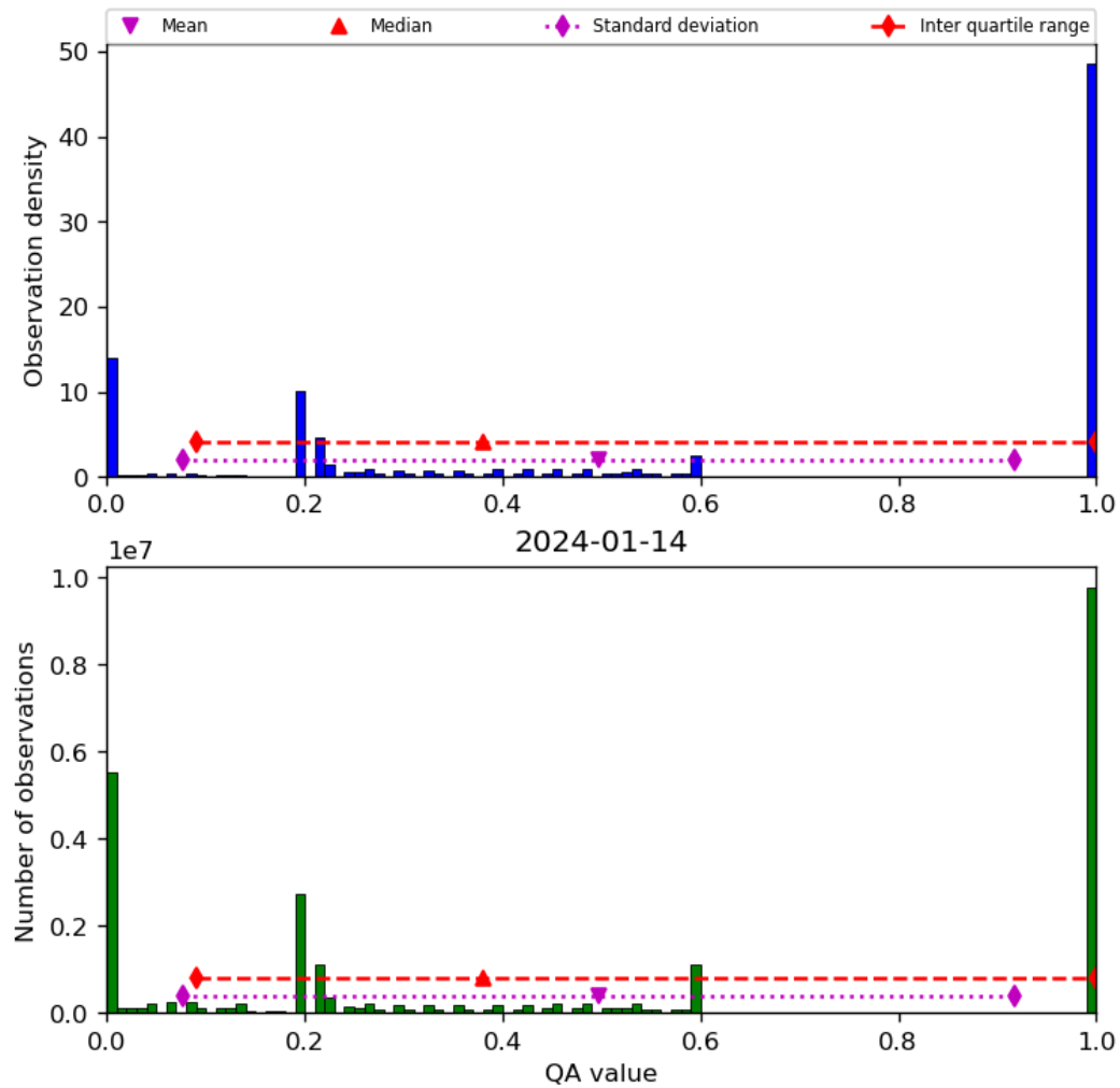
Figure 52: Histogram of “QA value” for 2024-01-13 to 2024-01-15
