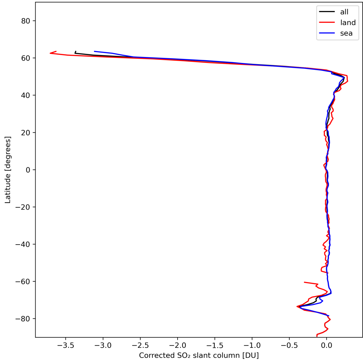
Figure 32: Zonal average of “Corrected SO 2 slant column” for 2024-01-13 to 2024-01-15.
