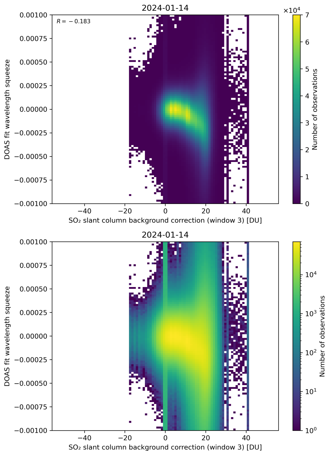
Figure 122: Scatter density plot of “SO 2 slant column background correction (window 3)” against “DOAS fit wavelength squeeze” for 2024-01-13 to 2024-01-15.
