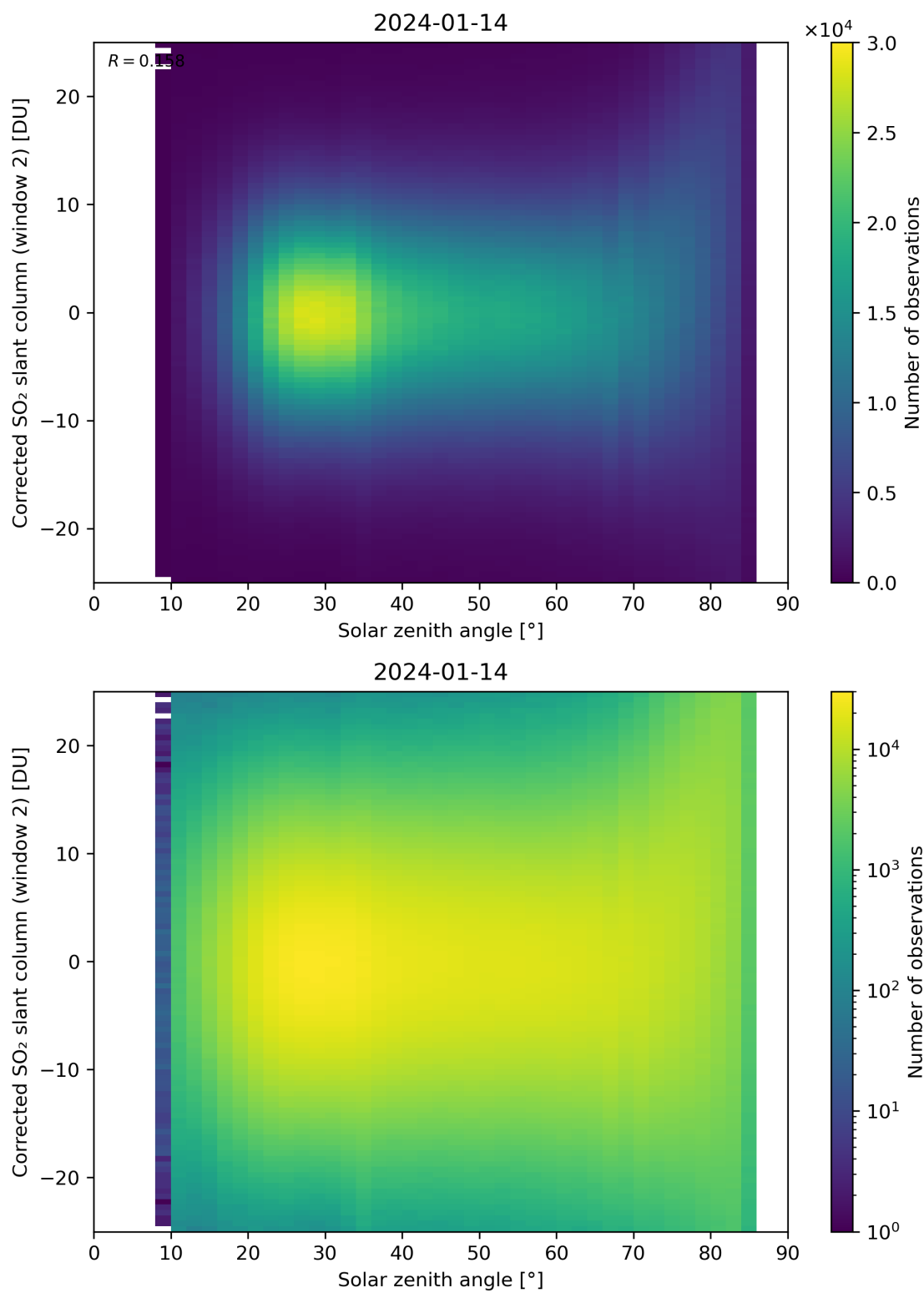
Figure 167: Scatter density plot of “Solar zenith angle” against “Corrected SO 2 slant column (window 2)” for 2024-01-13 to 2024-01-15.
