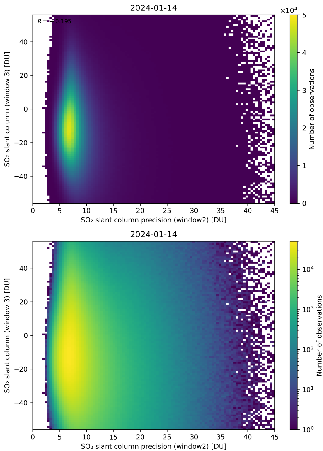
Figure 249: Scatter density plot of “SO 2 slant column precision (window2)” against “SO 2 slant column (window 3)” for 2024-01-13 to 2024-01-15.
