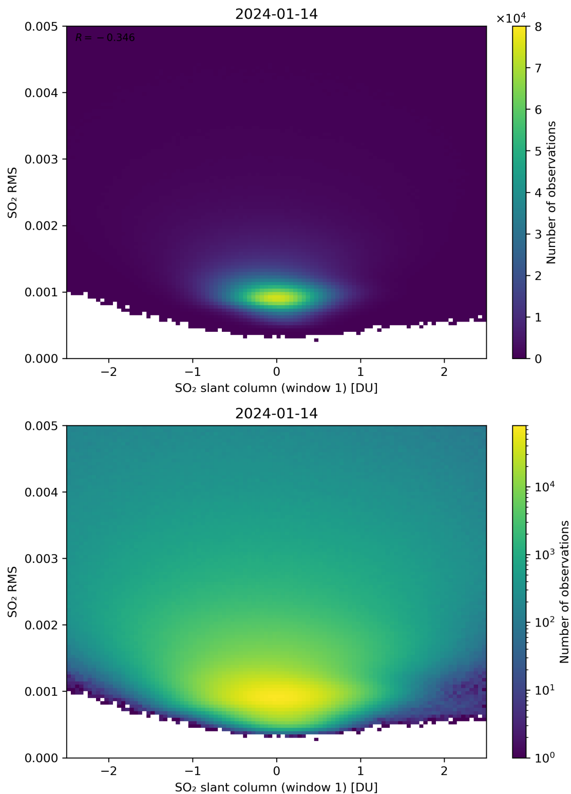
Figure 217: Scatter density plot of “SO 2 slant column (window 1)” against “SO 2 RMS” for 2024-01-13 to 2024-01-15.
