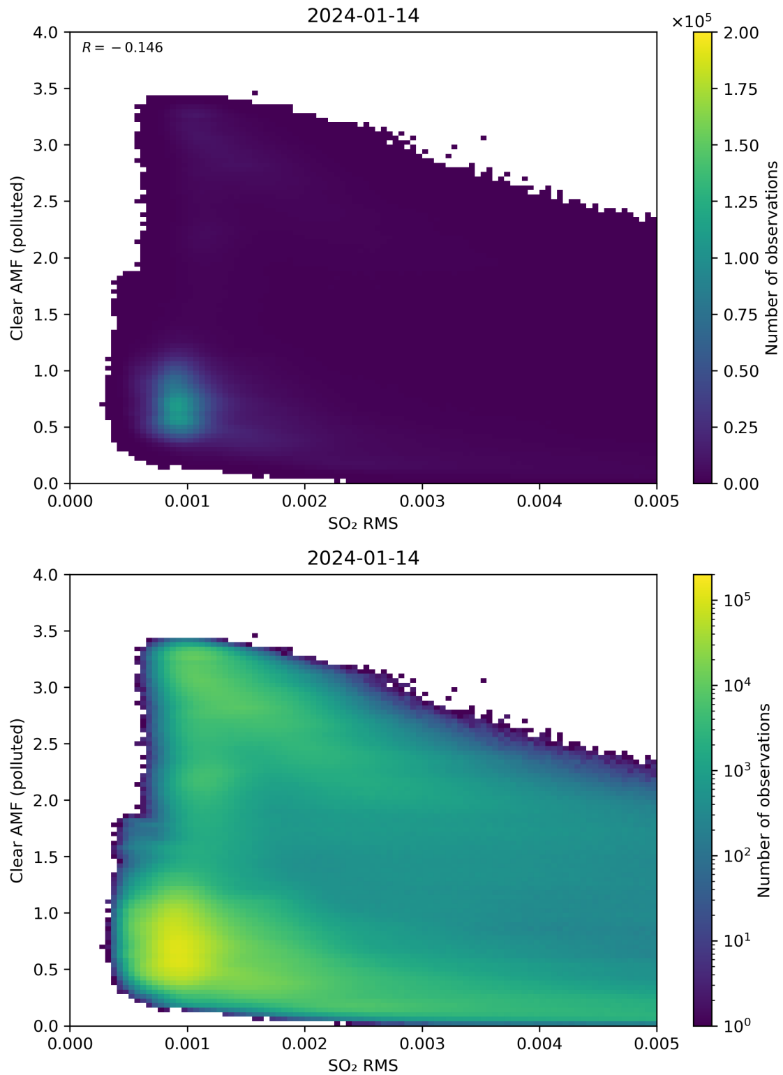
Figure 136: Scatter density plot of “SO 2 RMS” against “Clear AMF (polluted)” for 2024-01-13 to 2024-01-15.
