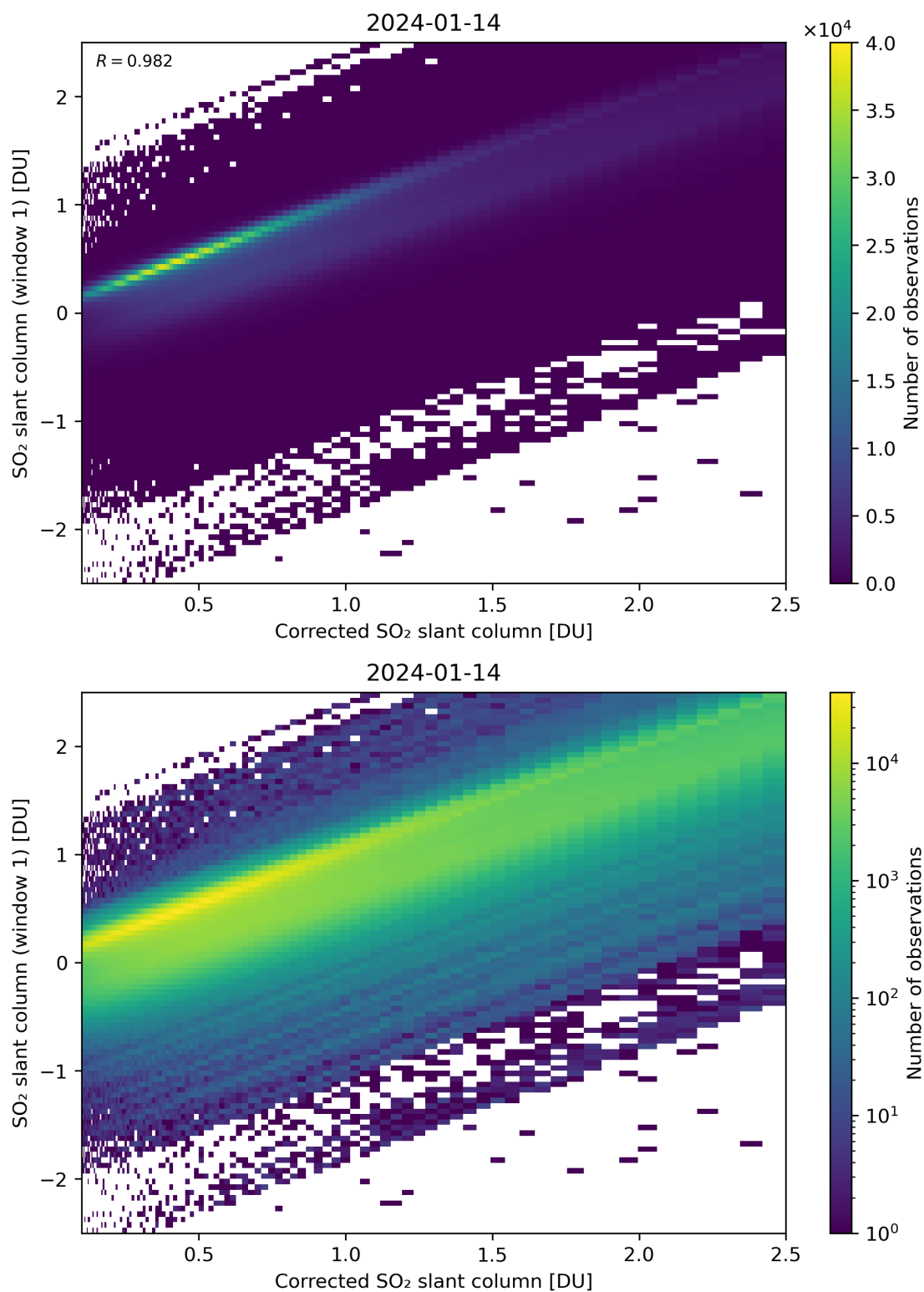
Figure 187: Scatter density plot of “Corrected SO 2 slant column” against “SO 2 slant column (window 1)” for 2024-01-13 to 2024-01-15.
