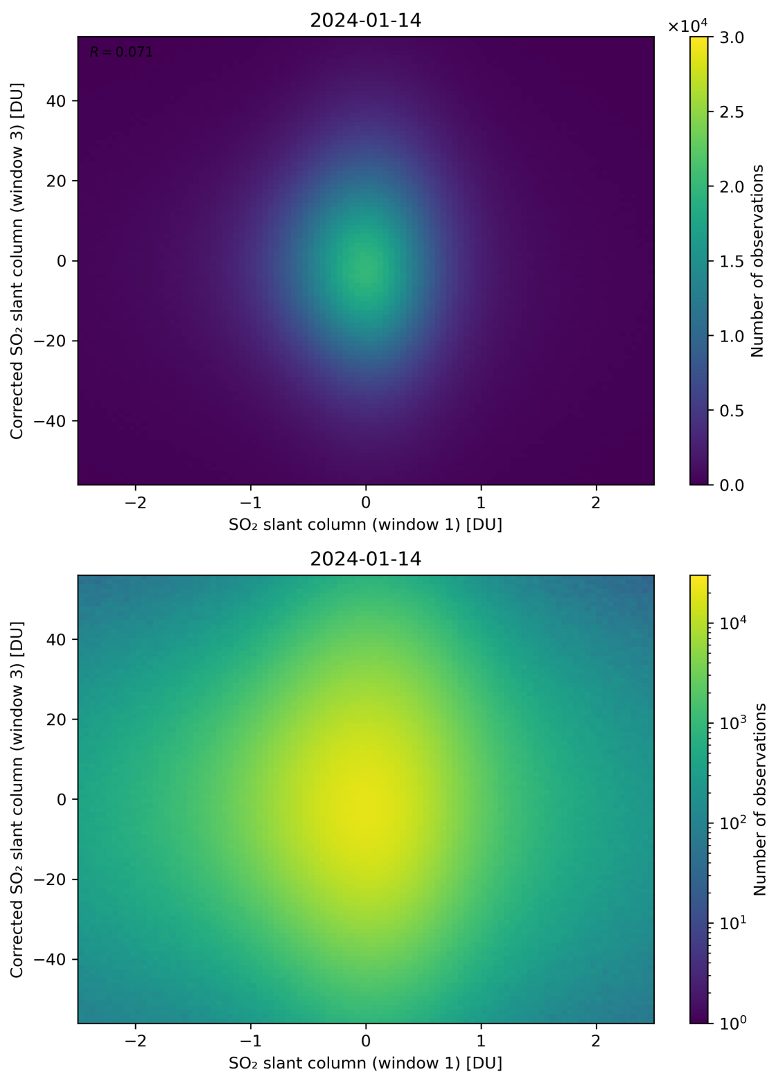
Figure 234: Scatter density plot of “SO 2 slant column (window 1)” against “Corrected SO 2 slant column (window 3)” for 2024-01-13 to 2024-01-15.
