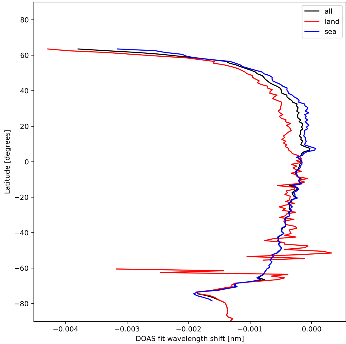
Figure 45: Zonal average of “DOAS fit wavelength shift” for 2024-01-13 to 2024-01-15.
