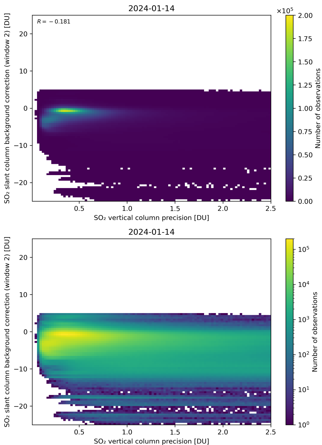
Figure 280: Scatter density plot of “SO 2 vertical column precision” against “SO 2 slant column background correction (window 2)” for 2024-01-13 to 2024-01-15.
