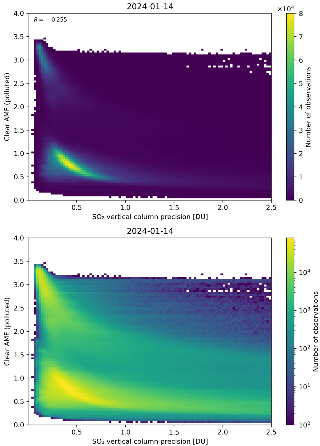
Figure 285: Scatter density plot of “SO 2 vertical column precision” against “Clear AMF (polluted)” for 2024-01-13 to 2024-01-15.
