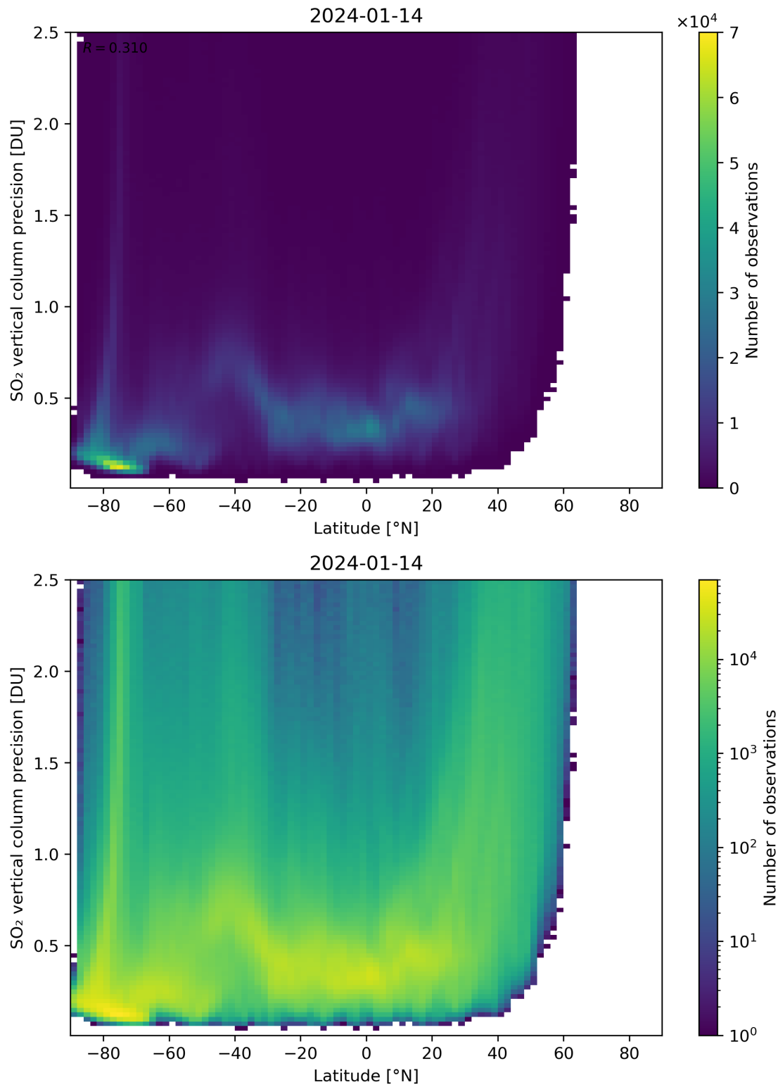
Figure 157: Scatter density plot of “Latitude” against “SO 2 vertical column precision” for 2024-01-13 to 2024-01-15.
