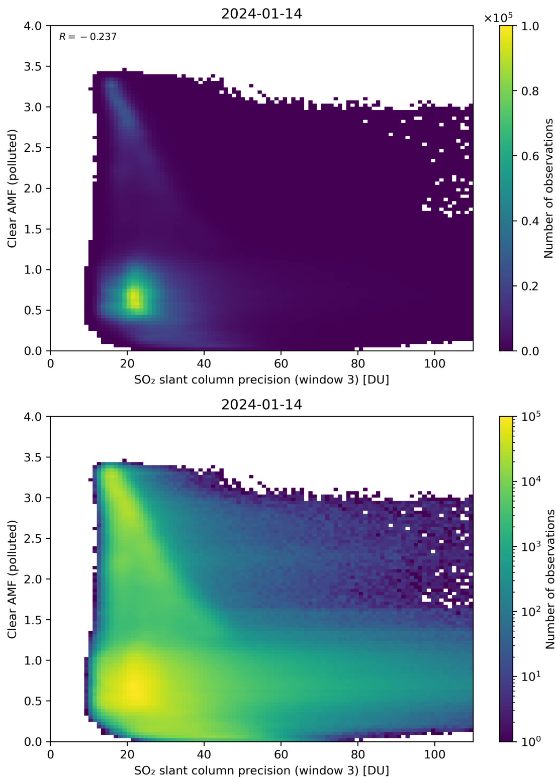
Figure 261: Scatter density plot of “SO 2 slant column precision (window 3)” against “Clear AMF (polluted)” for 2024-01-13 to 2024-01-15.
