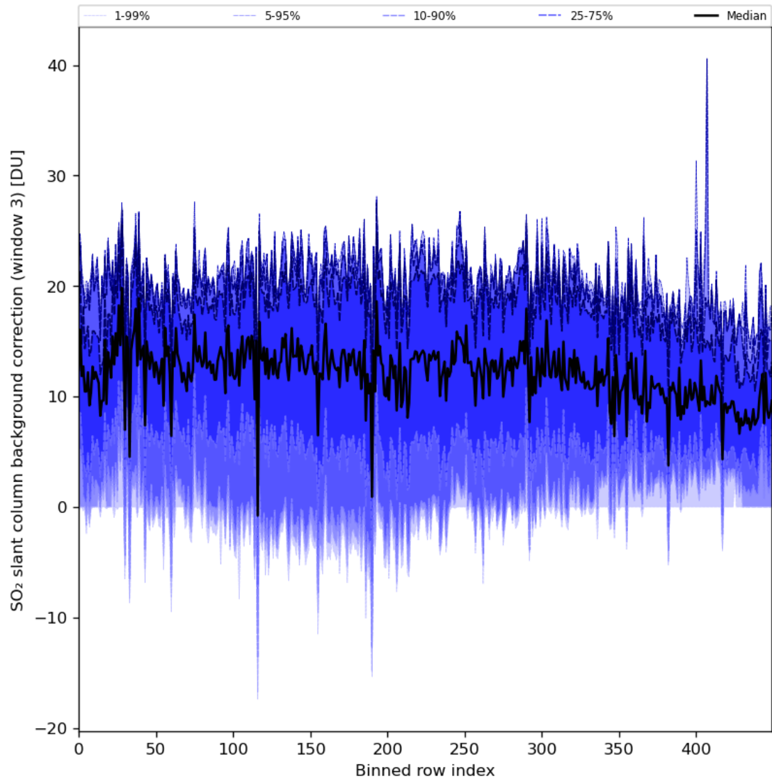
Figure 90: Along track statistics of “SO 2 slant column background correction (window 3)” for 2024-01-13 to 2024-01-15
