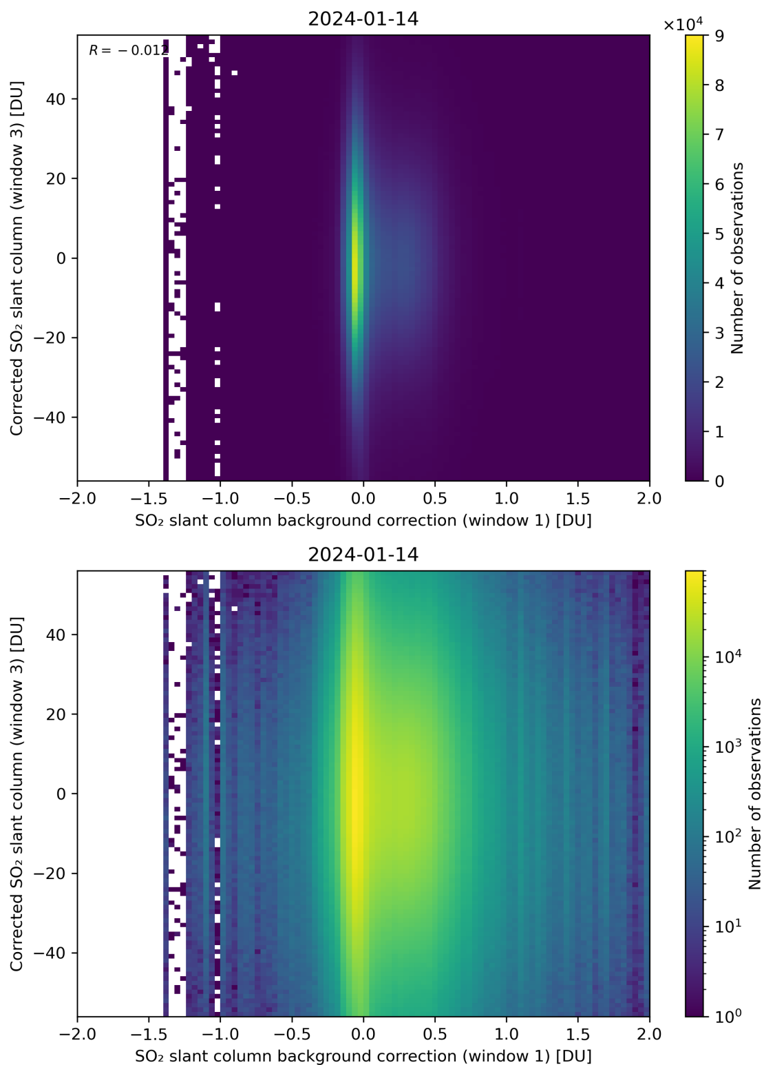
Figure 105: Scatter density plot of “SO 2 slant column background correction (window 1)” against “Corrected SO 2 slant column (window 3)” for 2024-01-13 to 2024-01-15.
