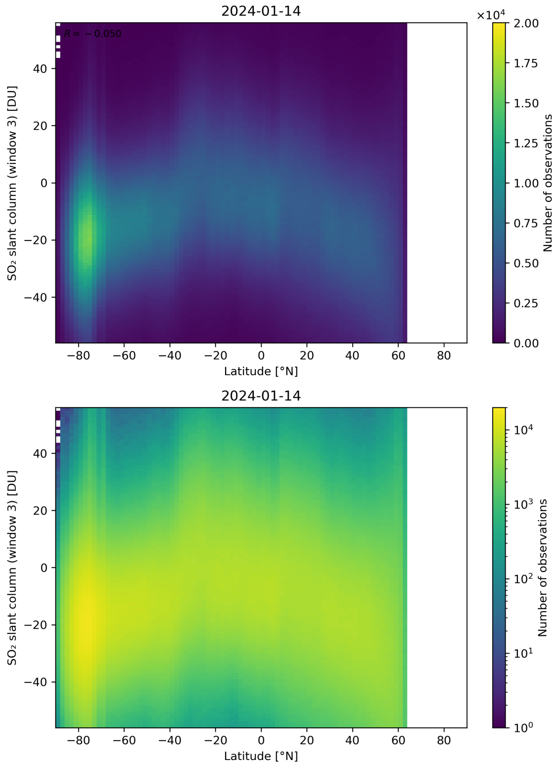
Figure 152: Scatter density plot of “Latitude” against “SO 2 slant column (window 3)” for 2024-01-13 to 2024-01-15.
