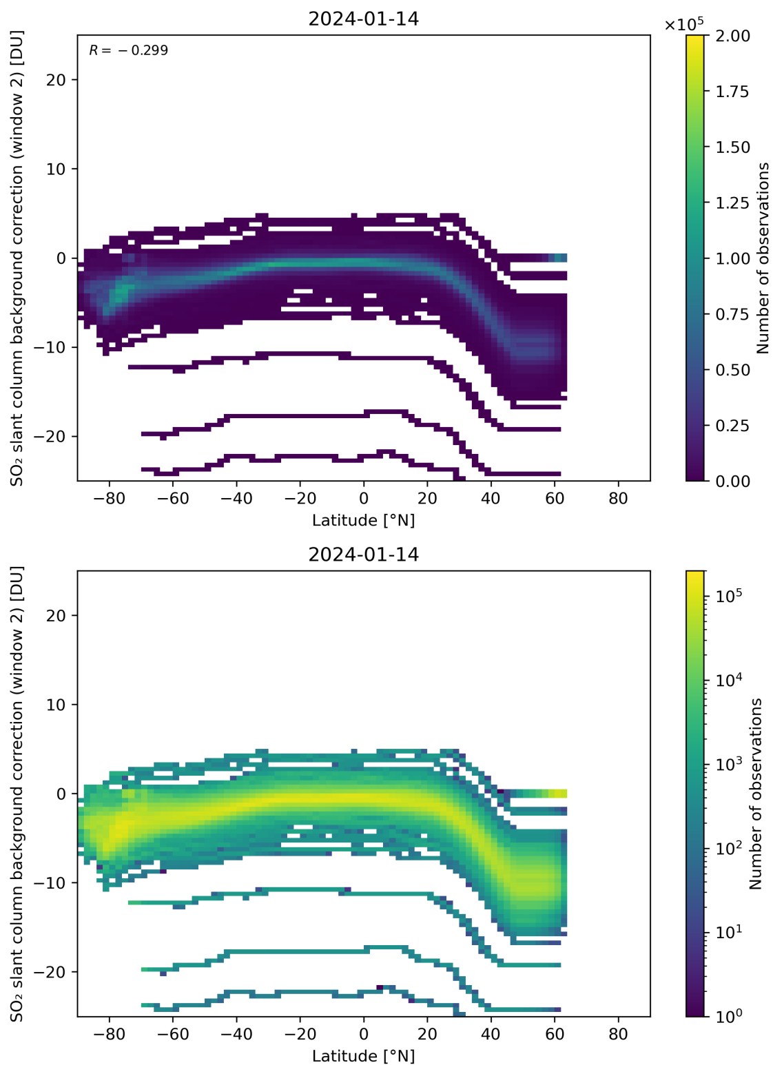
Figure 140: Scatter density plot of “Latitude” against “SO 2 slant column background correction (window 2)” for 2024-01-13 to 2024-01-15.
