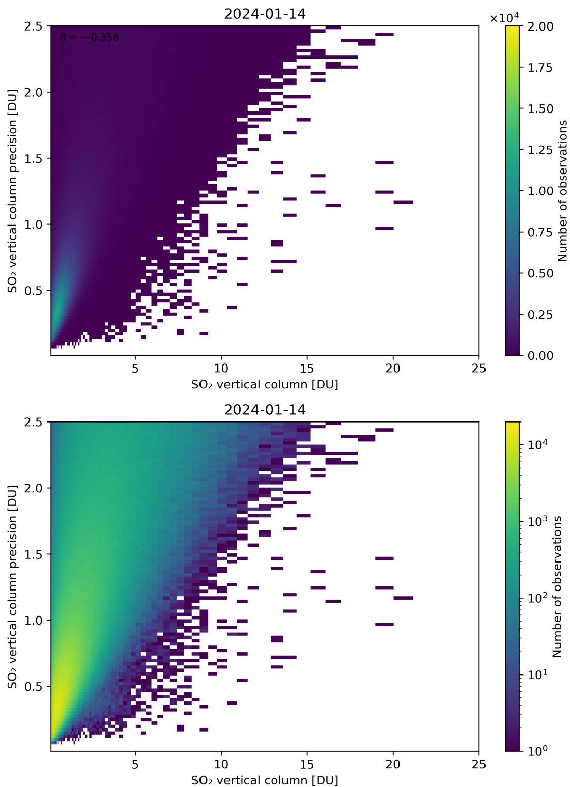
Figure 307: Scatter density plot of “SO 2 vertical column” against “SO 2 vertical column precision” for 2024-01-13 to 2024-01-15.
