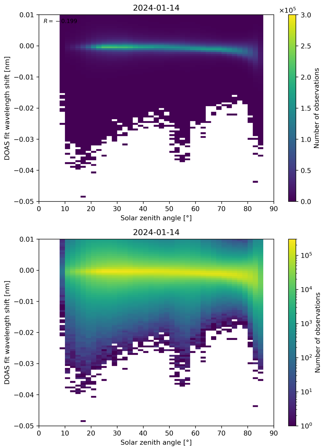
Figure 161: Scatter density plot of “Solar zenith angle” against “DOAS fit wavelength shift” for 2024-01-13 to 2024-01-15.
