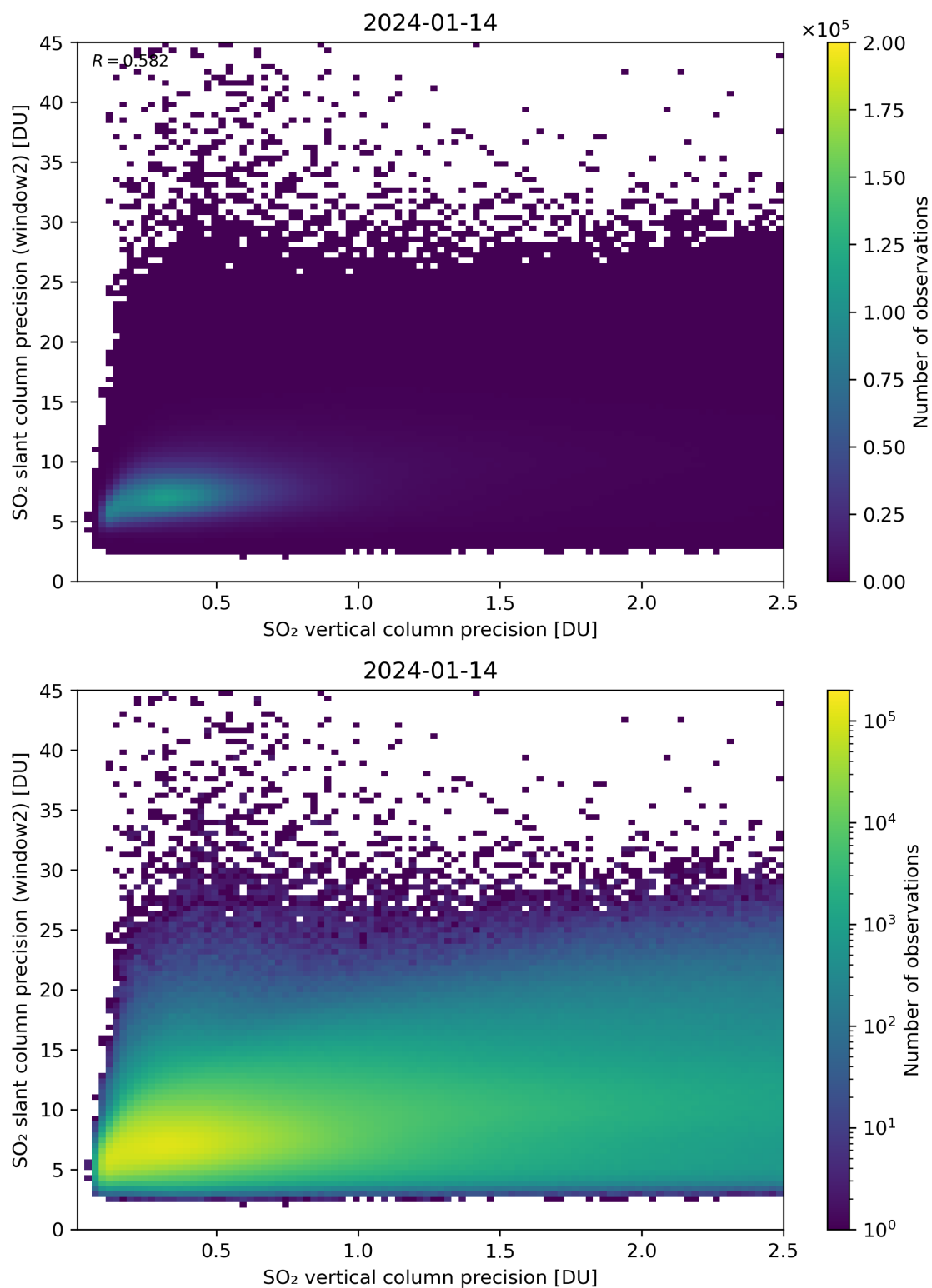
Figure 291: Scatter density plot of “SO 2 vertical column precision” against “SO 2 slant column precision (window2)” for 2024-01-13 to 2024-01-15.
