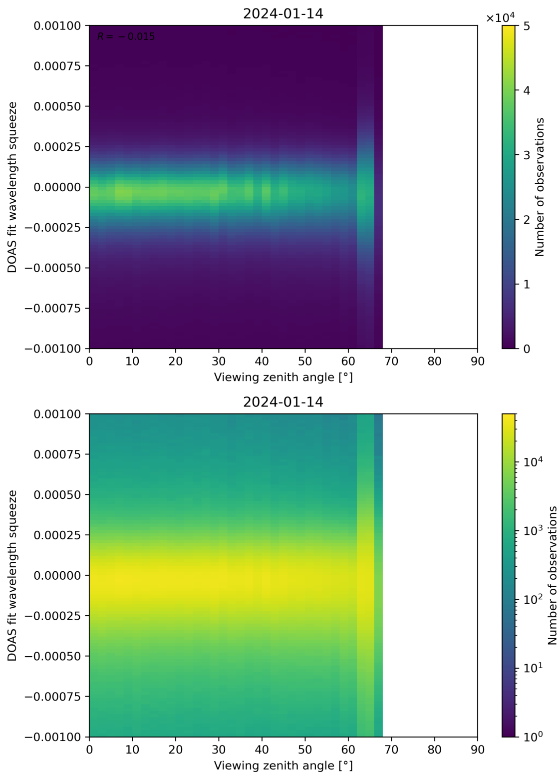
Figure 312: Scatter density plot of “Viewing zenith angle” against “DOAS fit wavelength squeeze” for 2024-01-13 to 2024-01-15.
