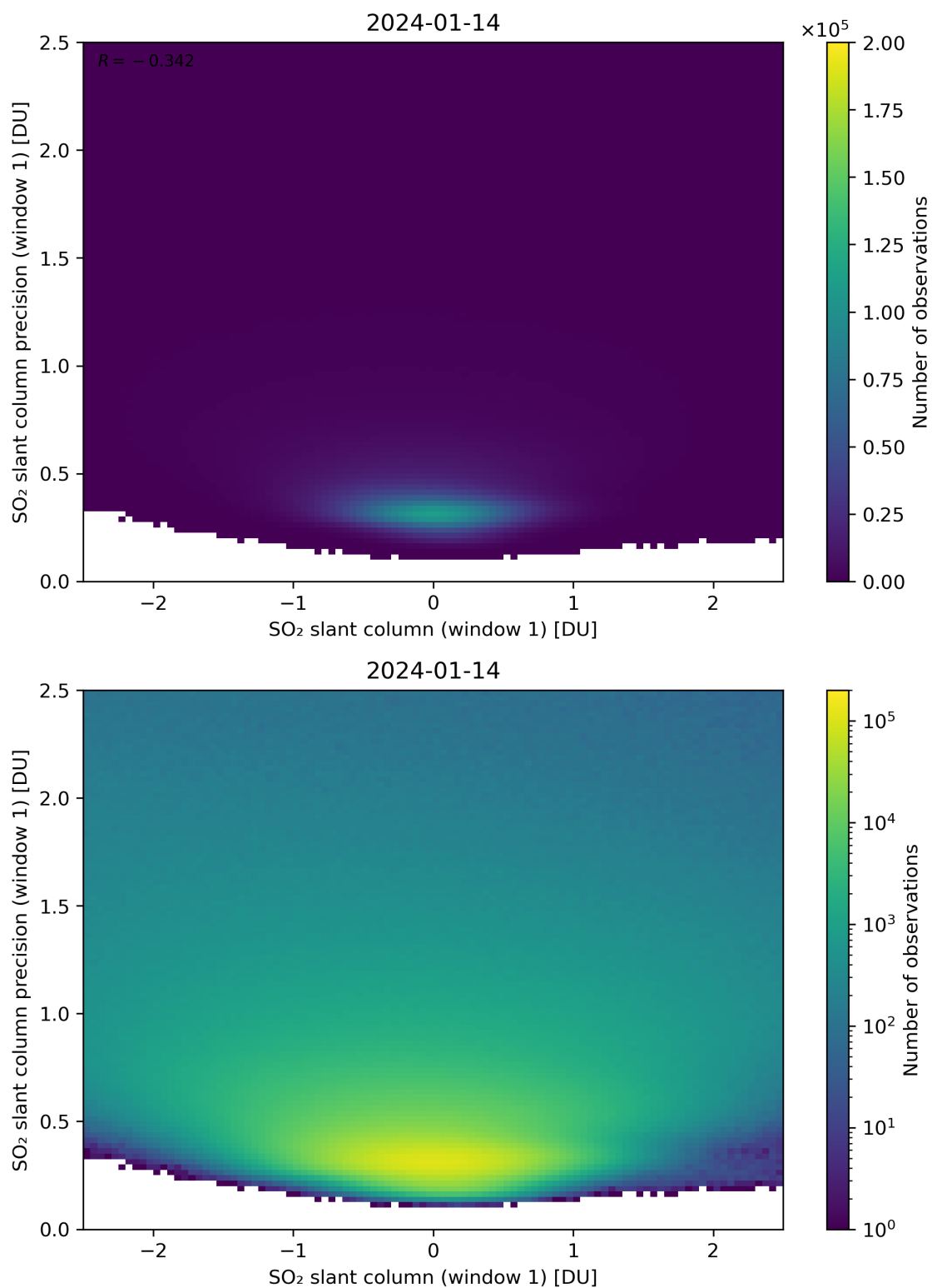
Figure 235: Scatter density plot of “SO 2 slant column (window 1)” against “SO 2 slant column precision (window 1)” for 2024-01-13 to 2024-01-15.
