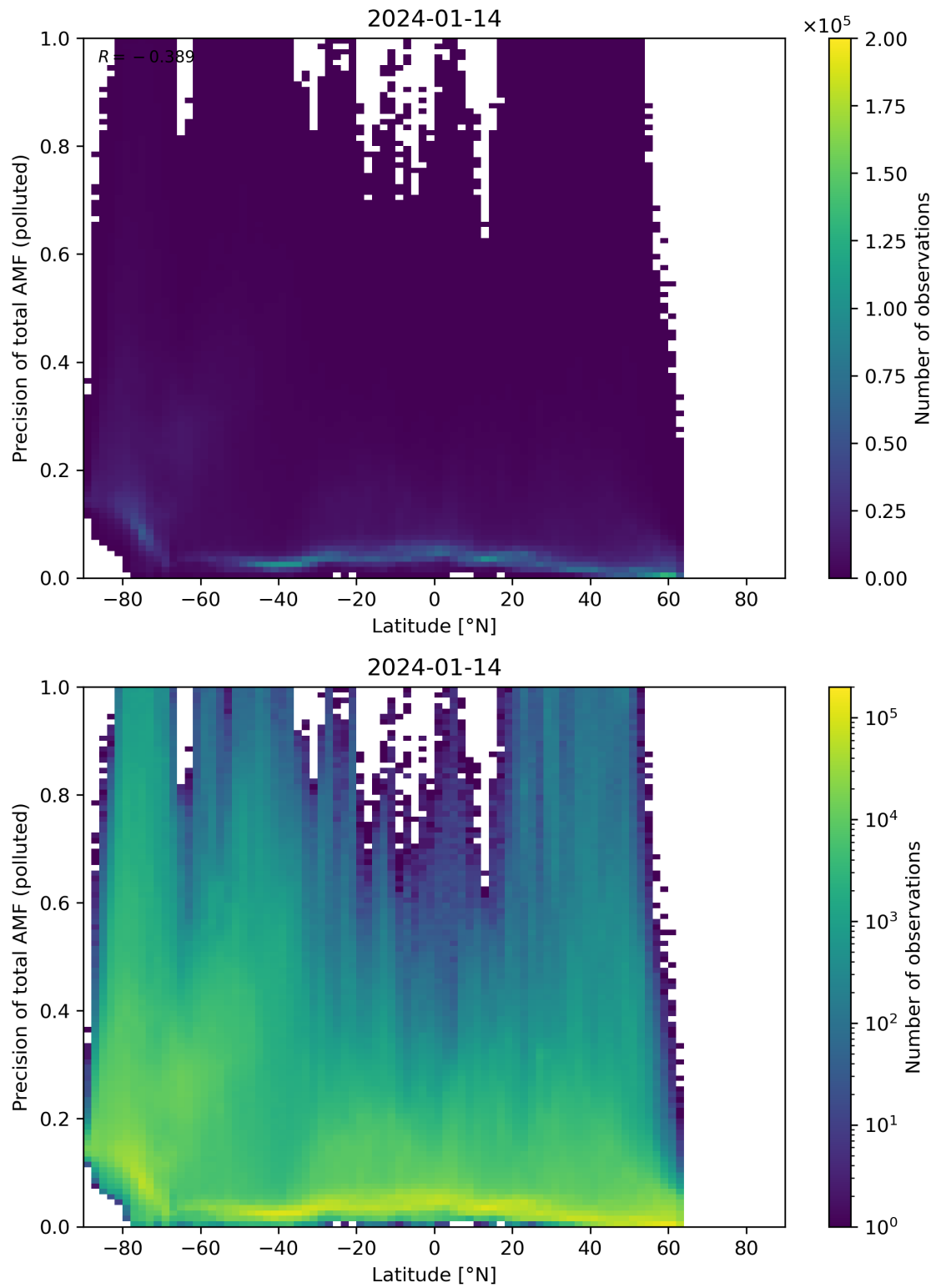
Figure 155: Scatter density plot of “Latitude” against “Precision of total AMF (polluted)” for 2024-01-13 to 2024-01-15.
