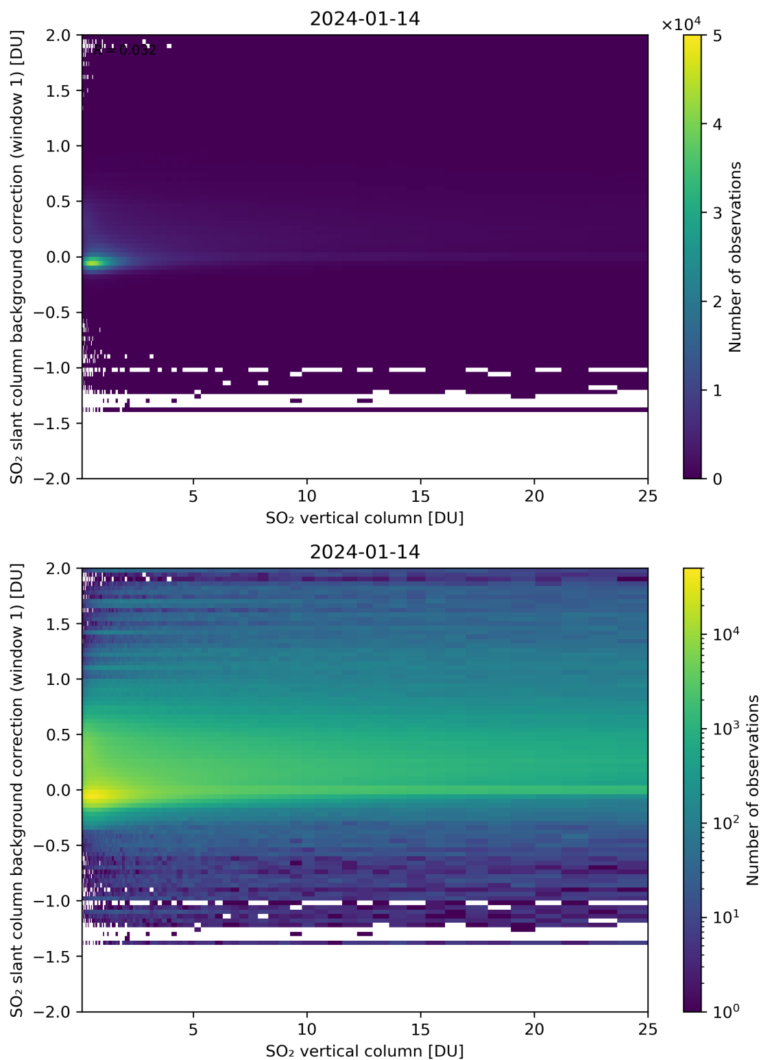
Figure 273: Scatter density plot of “SO 2 vertical column” against “SO 2 slant column background correction (window 1)” for 2024-01-13 to 2024-01-15.
