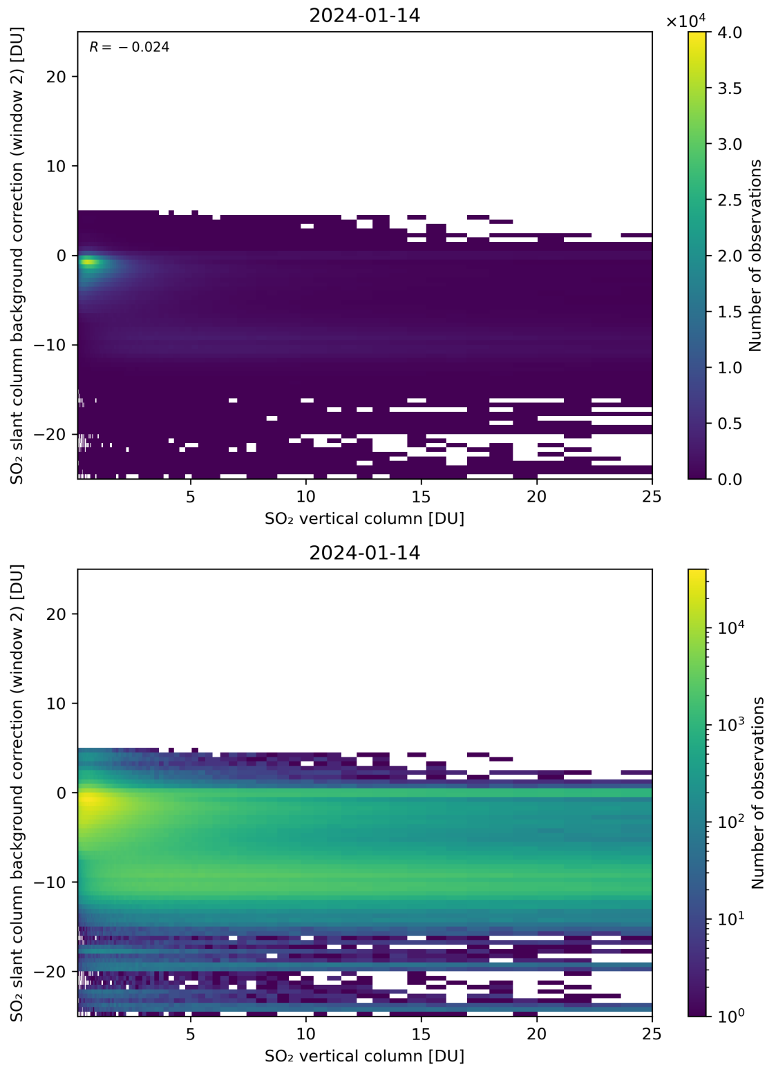
Figure 274: Scatter density plot of “SO 2 vertical column” against “SO 2 slant column background correction (window 2)” for 2024-01-13 to 2024-01-15.
