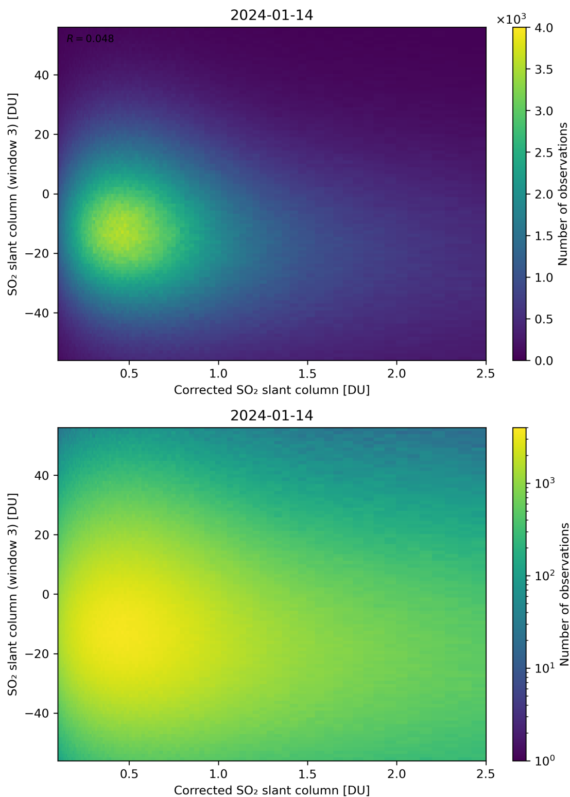
Figure 190: Scatter density plot of “Corrected SO 2 slant column” against “SO 2 slant column (window 3)” for 2024-01-13 to 2024-01-15.
