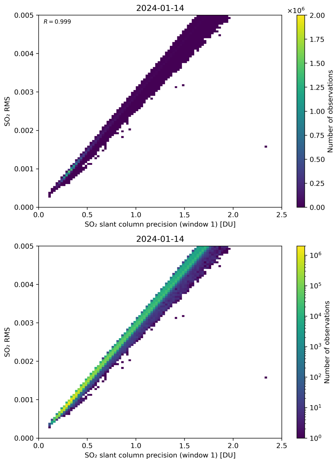
Figure 223: Scatter density plot of “SO 2 slant column precision (window 1)” against “SO 2 RMS” for 2024-01-13 to 2024-01-15.
