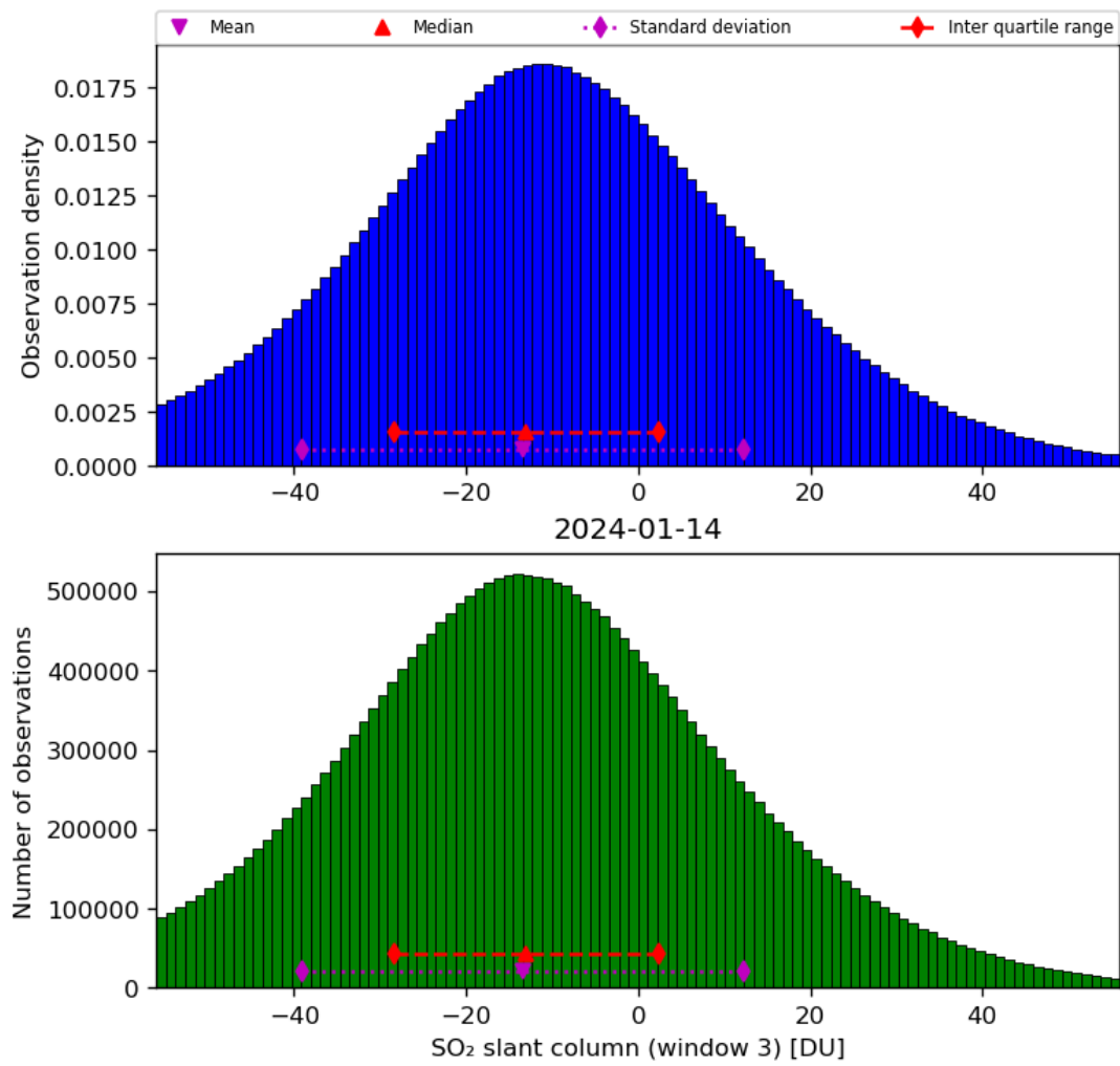
Figure 64: Histogram of “SO 2 slant column (window 3)” for 2024-01-13 to 2024-01-15
