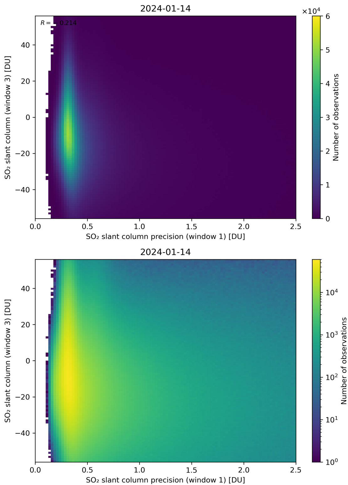
Figure 228: Scatter density plot of “SO 2 slant column precision (window 1)” against “SO 2 slant column (window 3)” for 2024-01-13 to 2024-01-15.
