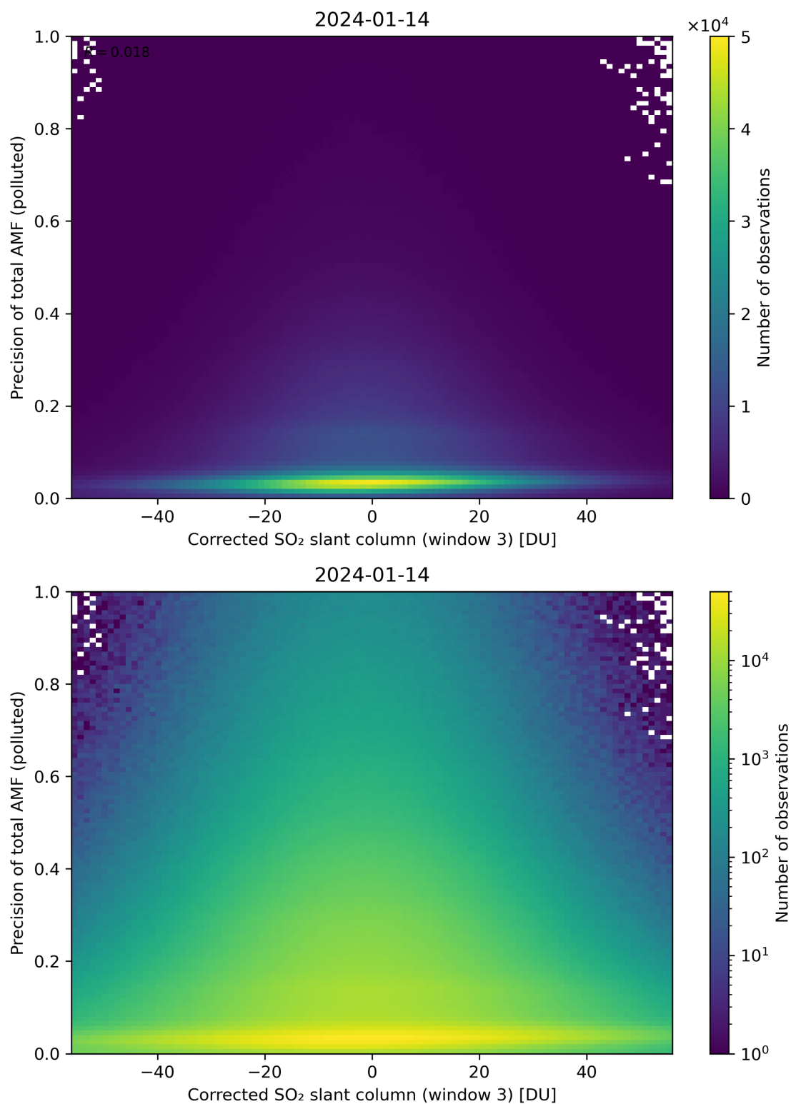
Figure 211: Scatter density plot of “Corrected SO 2 slant column (window 3)” against “Precision of total AMF (polluted)” for 2024-01-13 to 2024-01-15.
