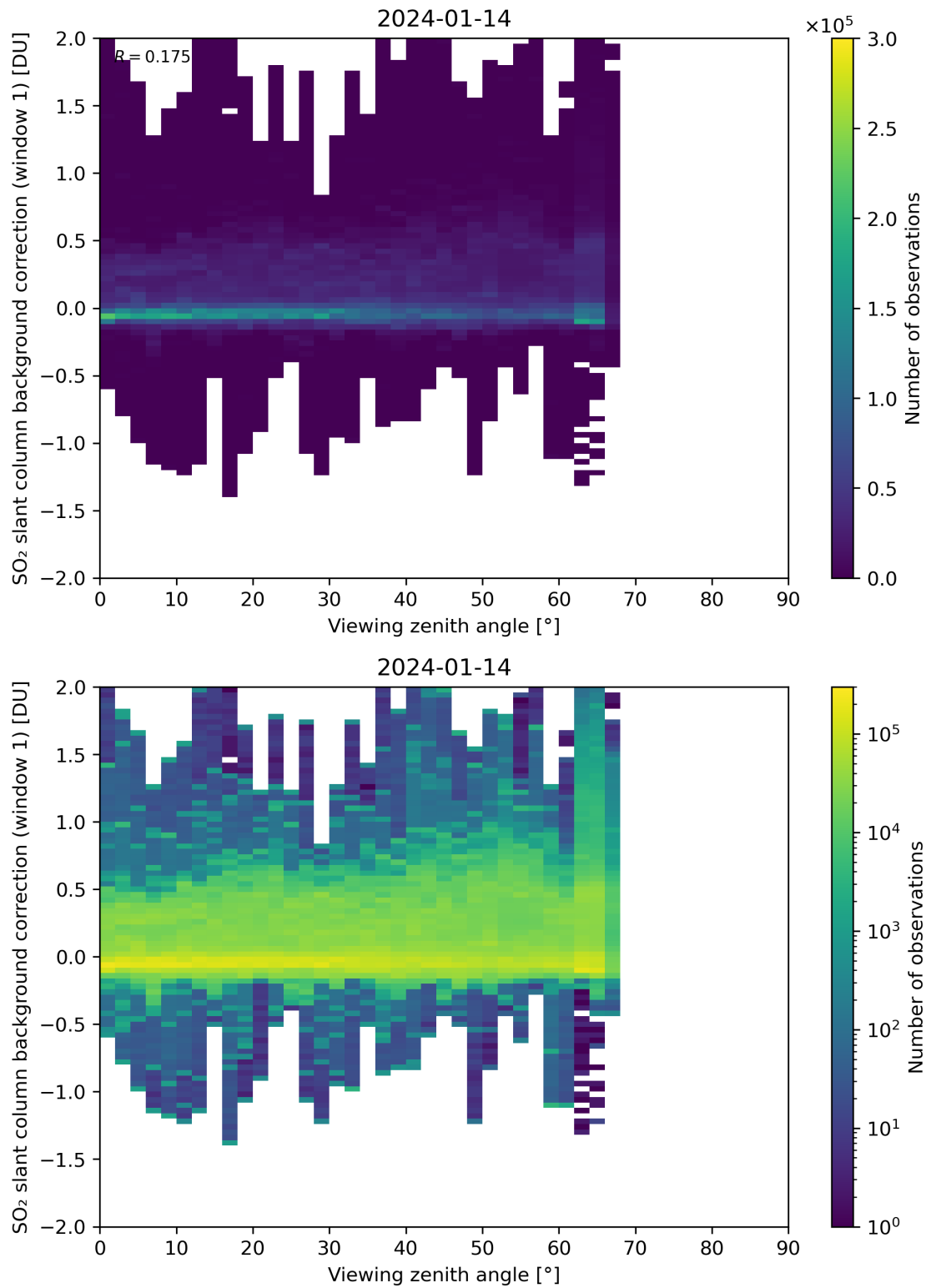
Figure 308: Scatter density plot of “Viewing zenith angle” against “SO 2 slant column background correction (window 1)” for 2024-01-13 to 2024-01-15.
