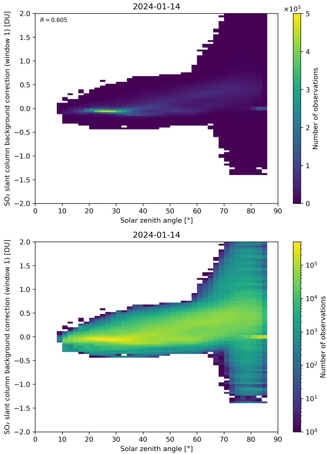
Figure 158: Scatter density plot of “Solar zenith angle” against “SO 2 slant column background correction (window 1)” for 2024-01-13 to 2024-01-15.
