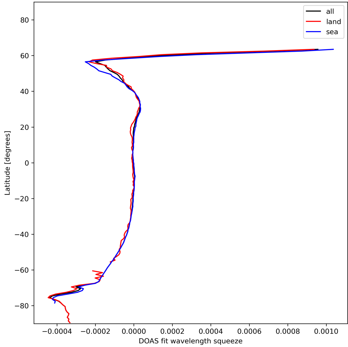
Figure 46: Zonal average of “DOAS fit wavelength squeeze” for 2024-01-13 to 2024-01-15.
