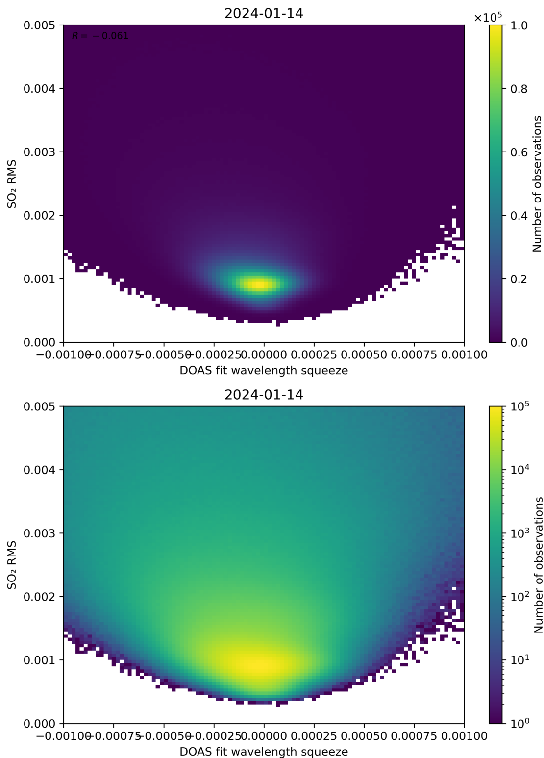
Figure 132: Scatter density plot of “DOAS fit wavelength squeeze” against “SO 2 RMS” for 2024-01-13 to 2024-01-15.
