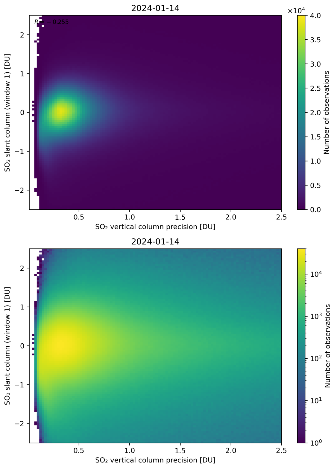
Figure 289: Scatter density plot of “SO 2 vertical column precision” against “SO 2 slant column (window 1)” for 2024-01-13 to 2024-01-15.
