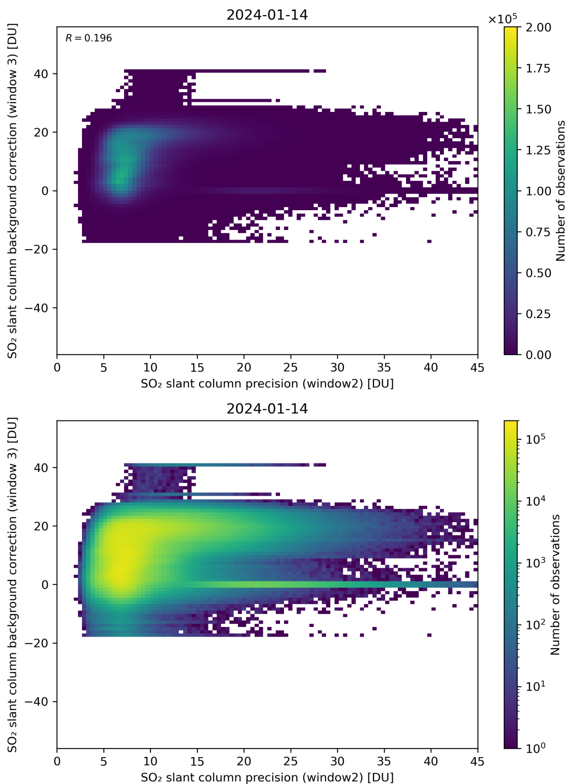
Figure 242: Scatter density plot of “SO 2 slant column precision (window2)” against “SO 2 slant column background correction (window 3)” for 2024-01-13 to 2024-01-15.
