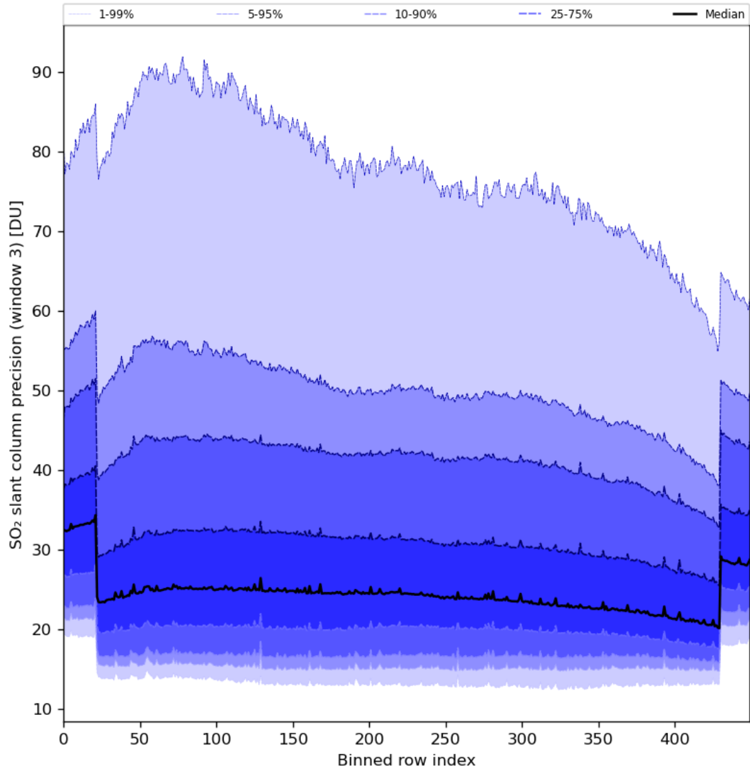
Figure 88: Along track statistics of “SO 2 slant column precision (window 3)” for 2024-01-13 to 2024-01-15
