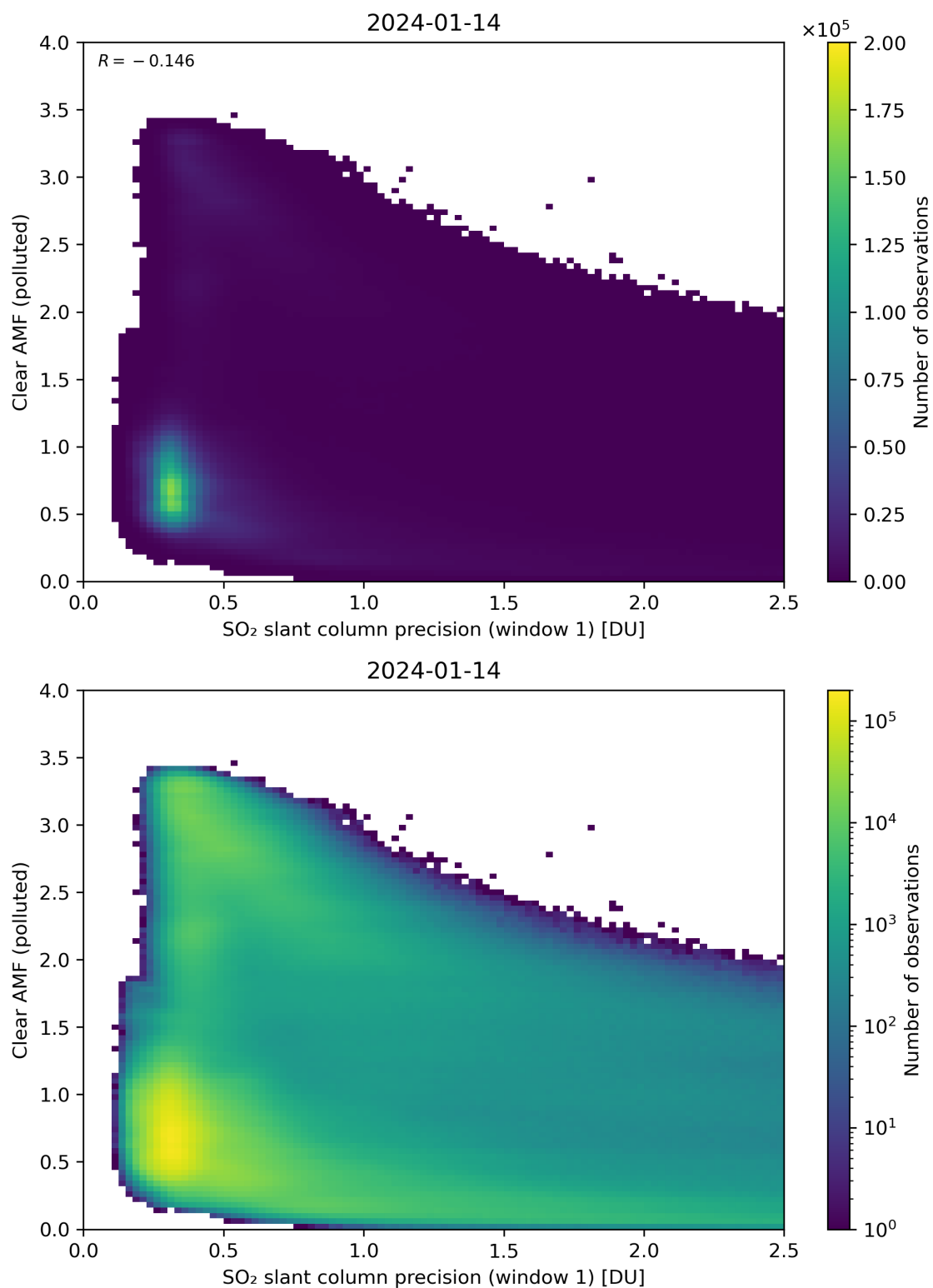
Figure 224: Scatter density plot of “SO 2 slant column precision (window 1)” against “Clear AMF (polluted)” for 2024-01-13 to 2024-01-15.
