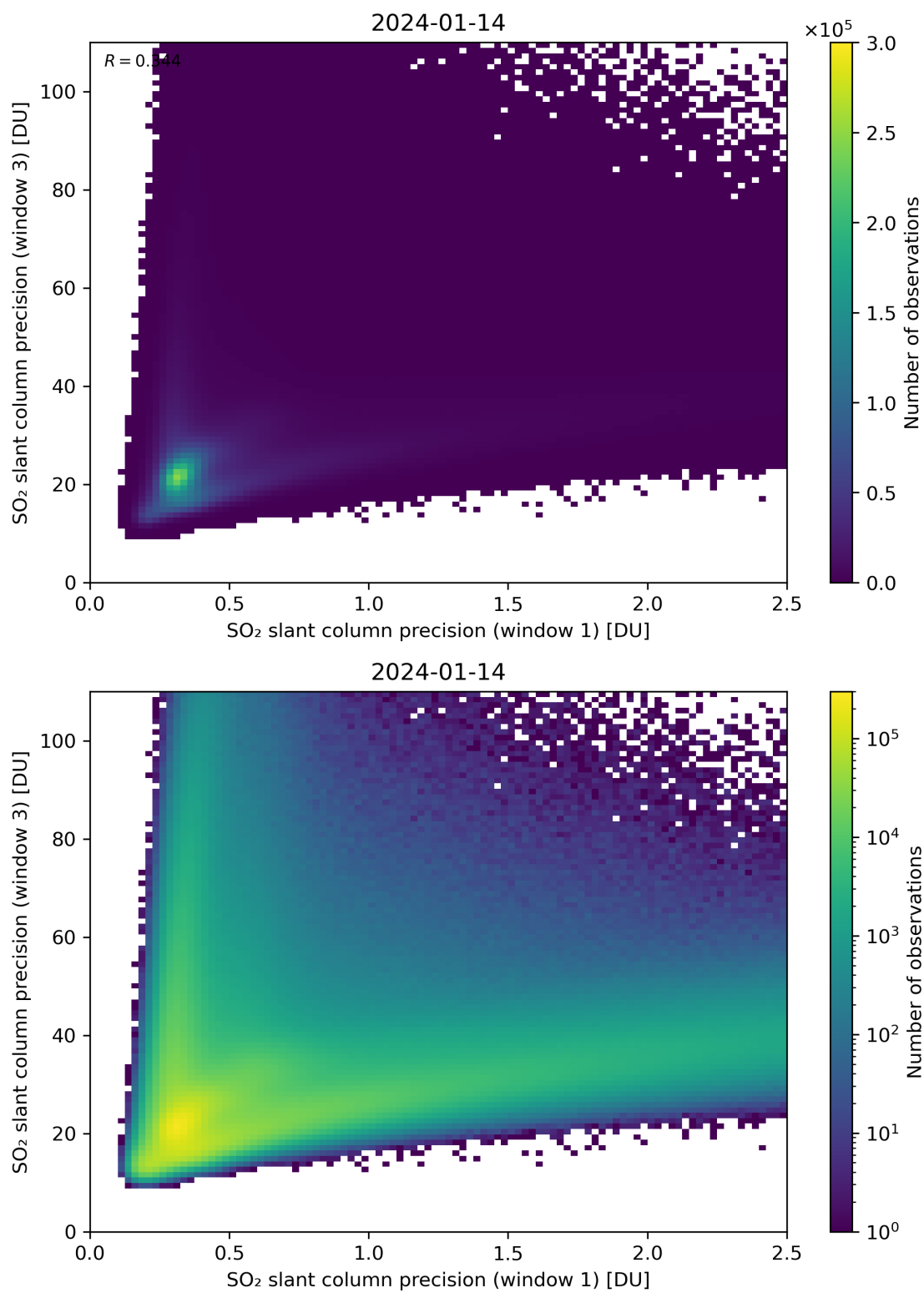
Figure 229: Scatter density plot of “SO 2 slant column precision (window 1)” against “SO 2 slant column precision (window 3)” for 2024-01-13 to 2024-01-15.
