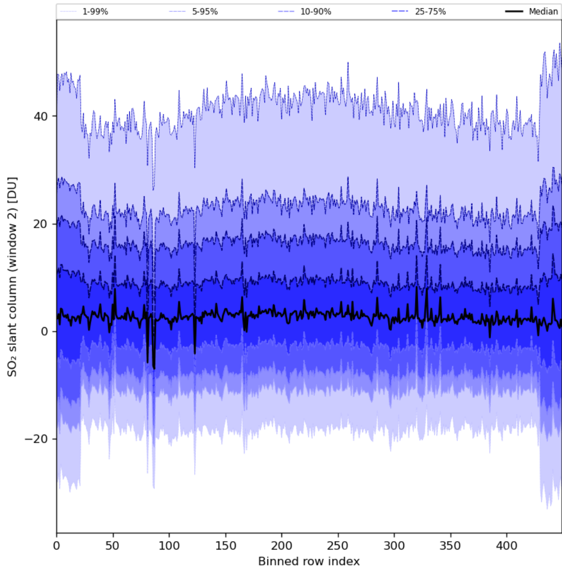
Figure 83: Along track statistics of “SO 2 slant column (window 2)” for 2024-01-13 to 2024-01-15
