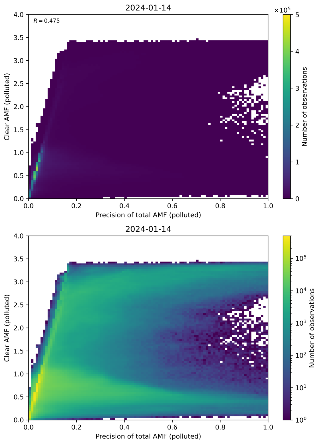
Figure 270: Scatter density plot of “Precision of total AMF (polluted)” against “Clear AMF (polluted)” for 2024-01-13 to 2024-01-15.
