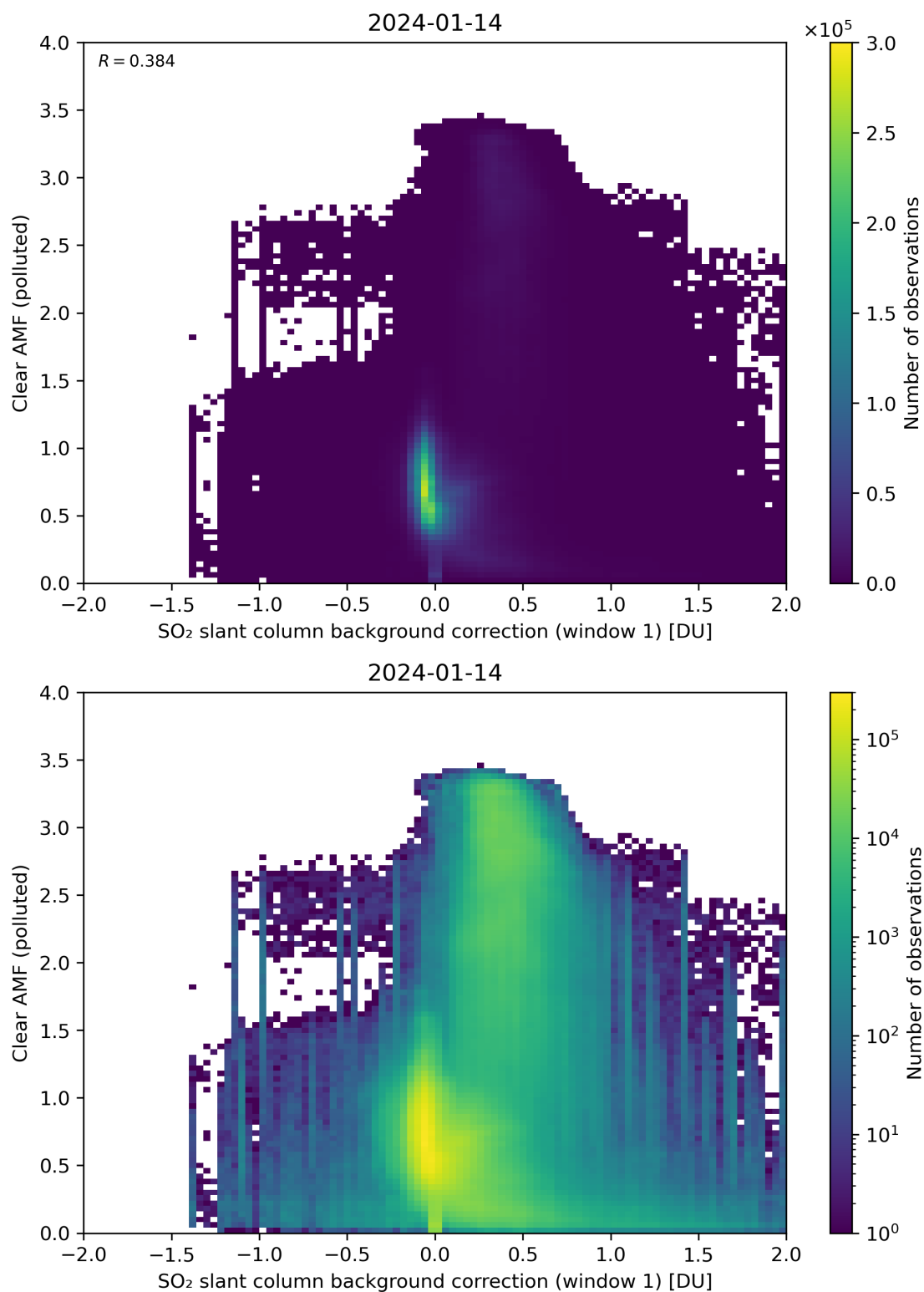
Figure 103: Scatter density plot of “SO 2 slant column background correction (window 1)” against “Clear AMF (polluted)” for 2024-01-13 to 2024-01-15.
