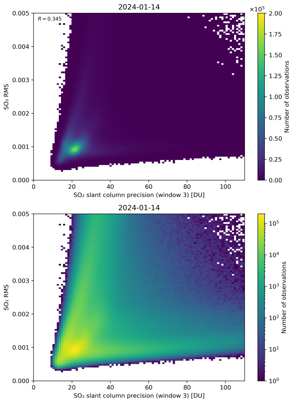
Figure 260: Scatter density plot of “SO 2 slant column precision (window 3)” against “SO 2 RMS” for 2024-01-13 to 2024-01-15.
