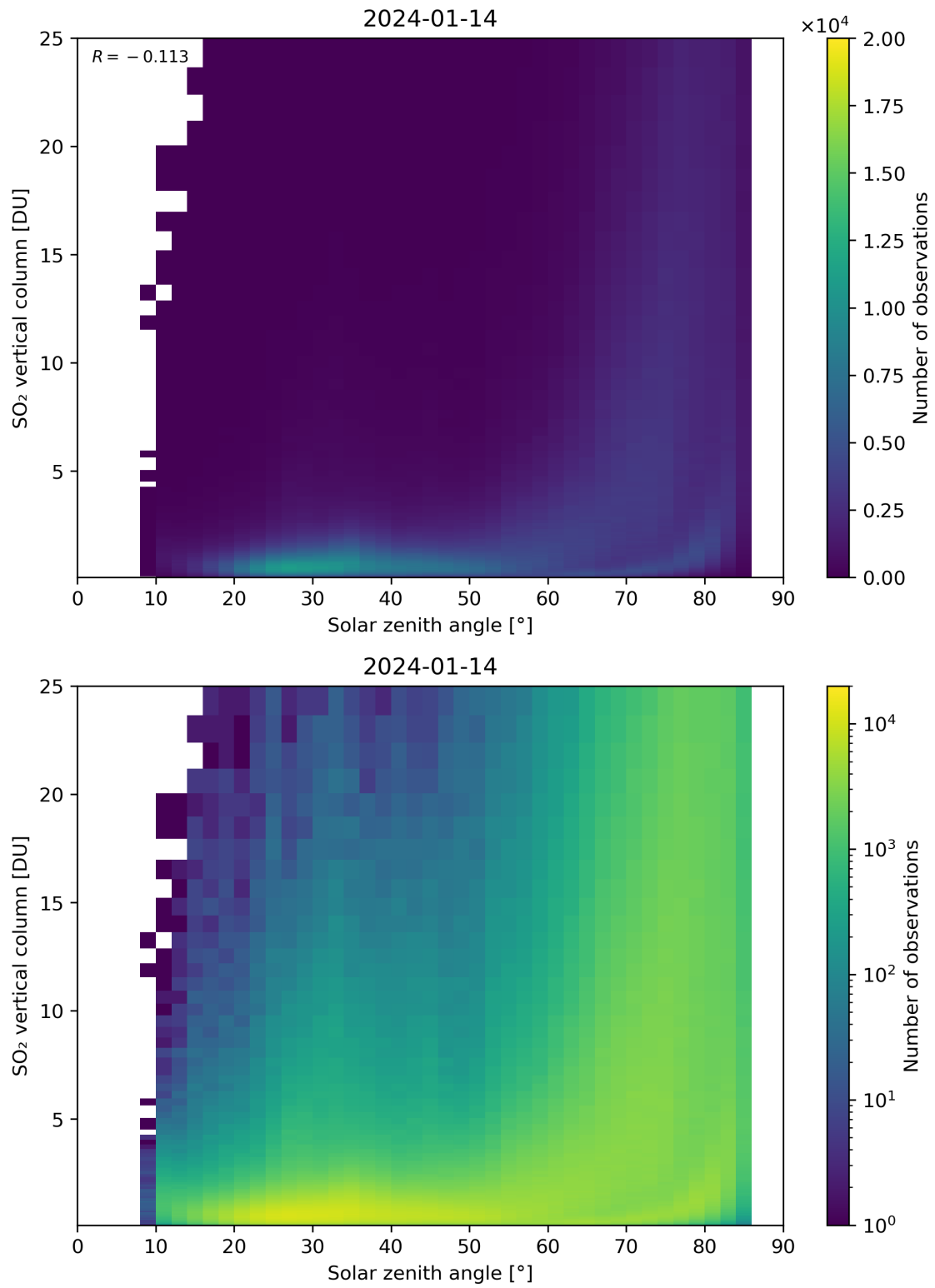
Figure 176: Scatter density plot of “Solar zenith angle” against “SO 2 vertical column” for 2024-01-13 to 2024-01-15.
