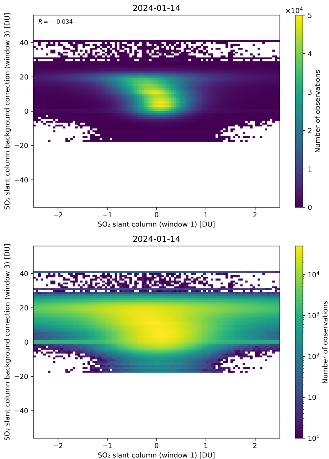
Figure 214: Scatter density plot of “SO 2 slant column (window 1)” against “SO 2 slant column background correction (window 3)” for 2024-01-13 to 2024-01-15.
