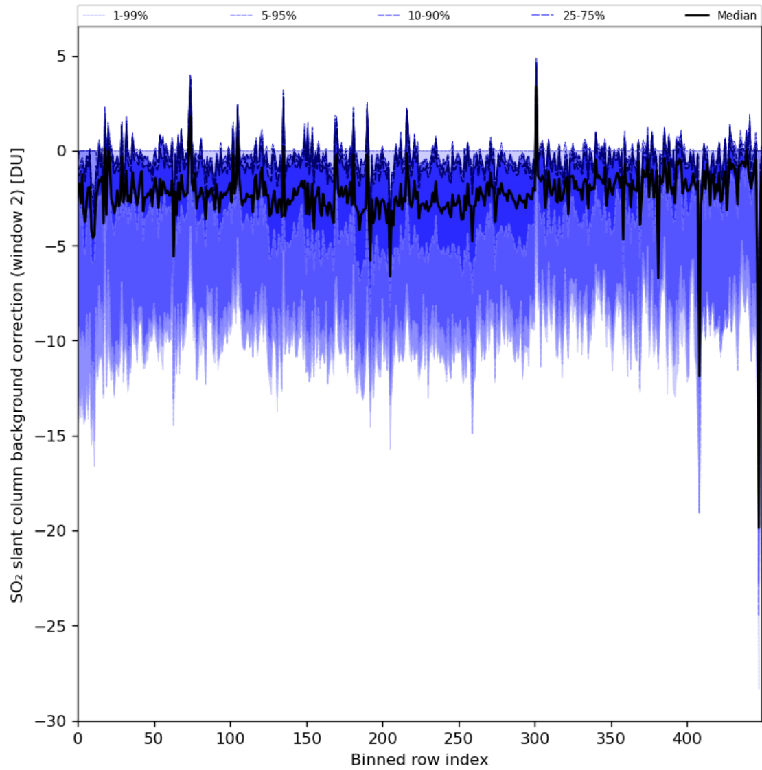
Figure 86: Along track statistics of “SO 2 slant column background correction (window 2)” for 2024-01-13 to 2024-01-15
