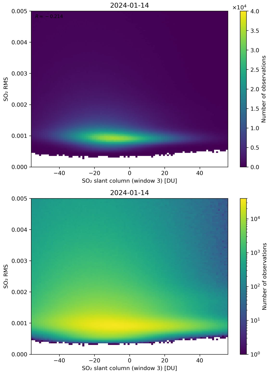
Figure 256: Scatter density plot of “SO 2 slant column (window 3)” against “SO 2 RMS” for 2024-01-13 to 2024-01-15.
