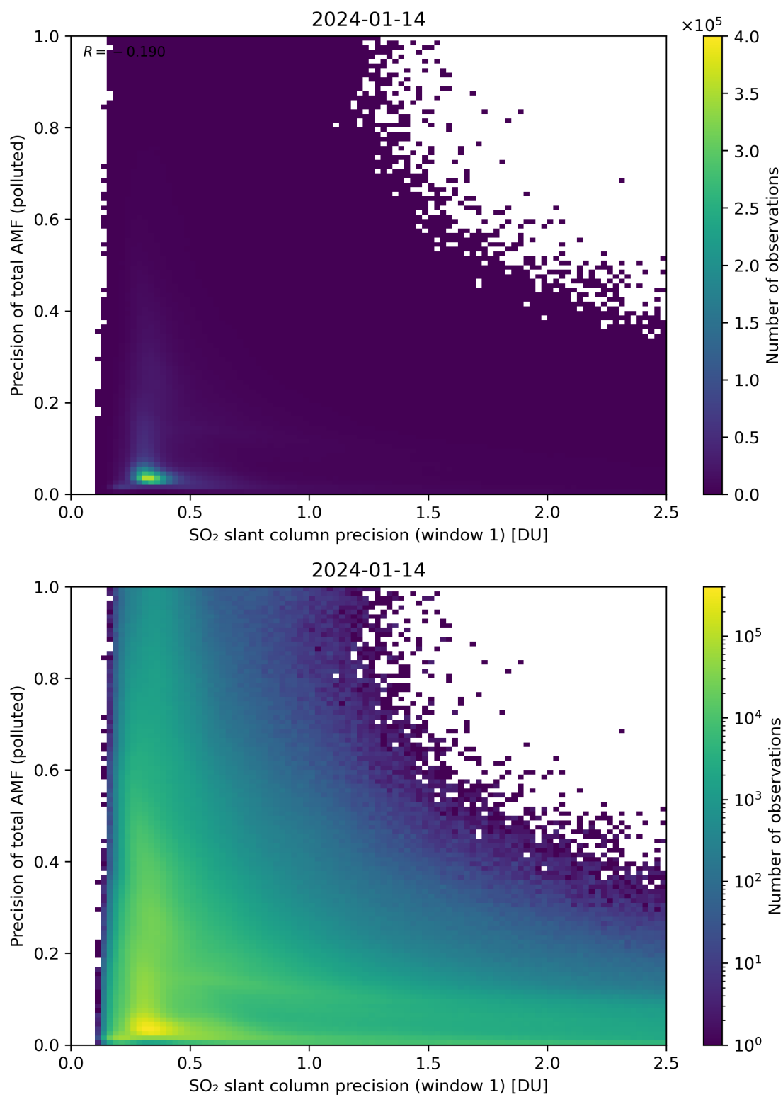
Figure 231: Scatter density plot of “SO 2 slant column precision (window 1)” against “Precision of total AMF (polluted)” for 2024-01-13 to 2024-01-15.
