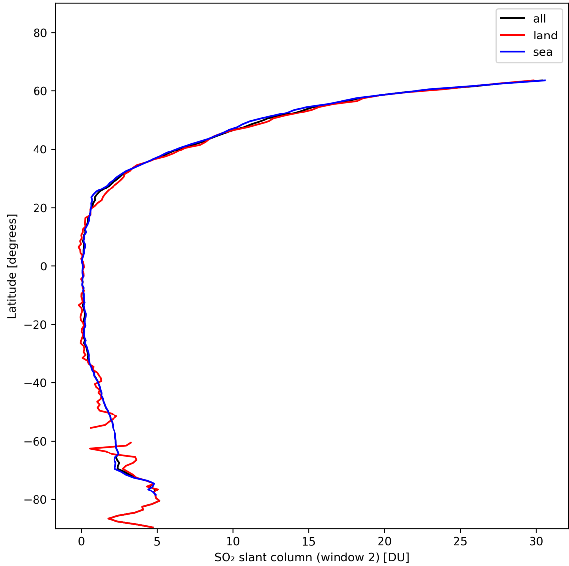
Figure 37: Zonal average of “SO 2 slant column (window 2)” for 2024-01-13 to 2024-01-15.
