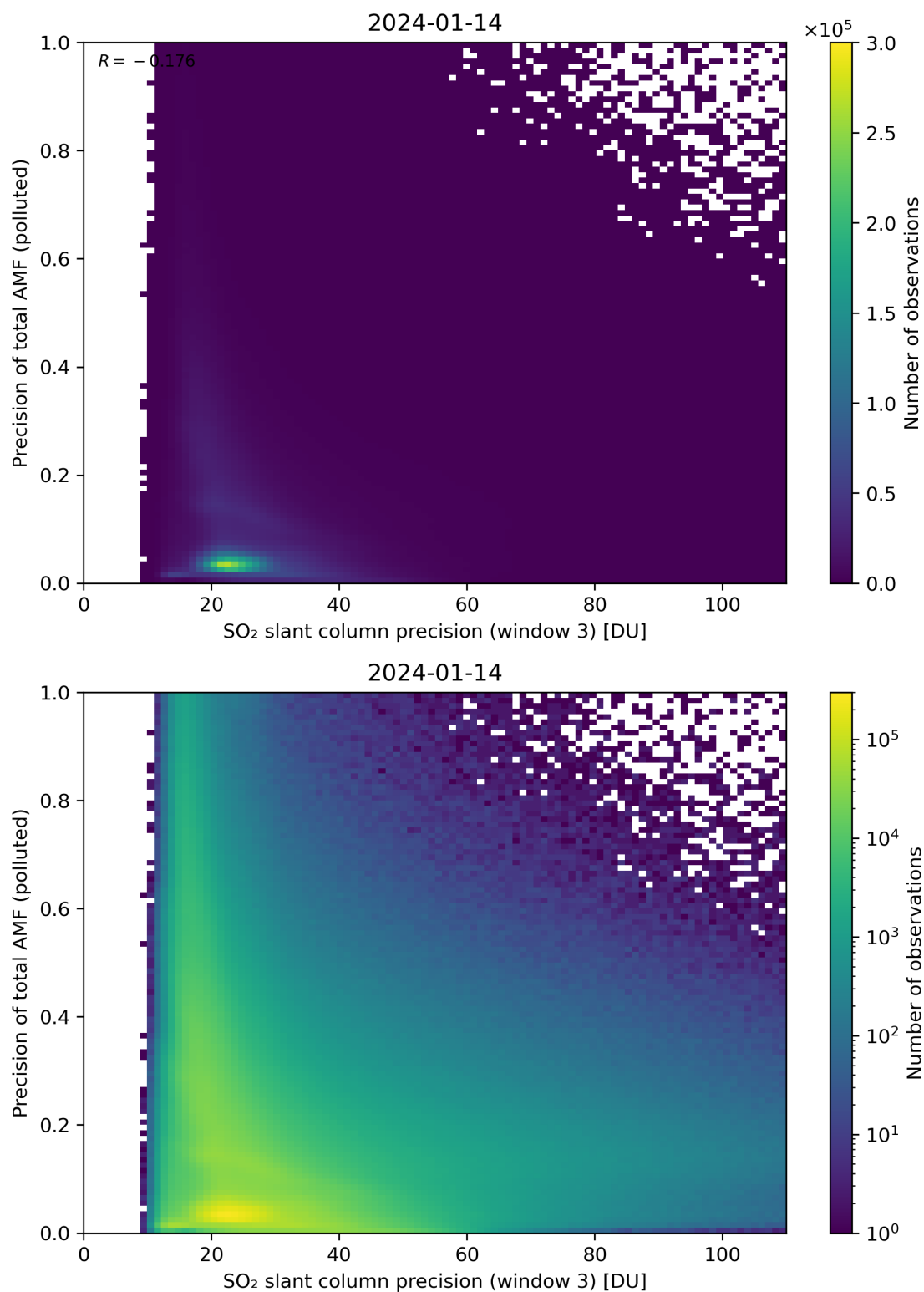
Figure 264: Scatter density plot of “SO 2 slant column precision (window 3)” against “Precision of total AMF (polluted)” for 2024-01-13 to 2024-01-15.
