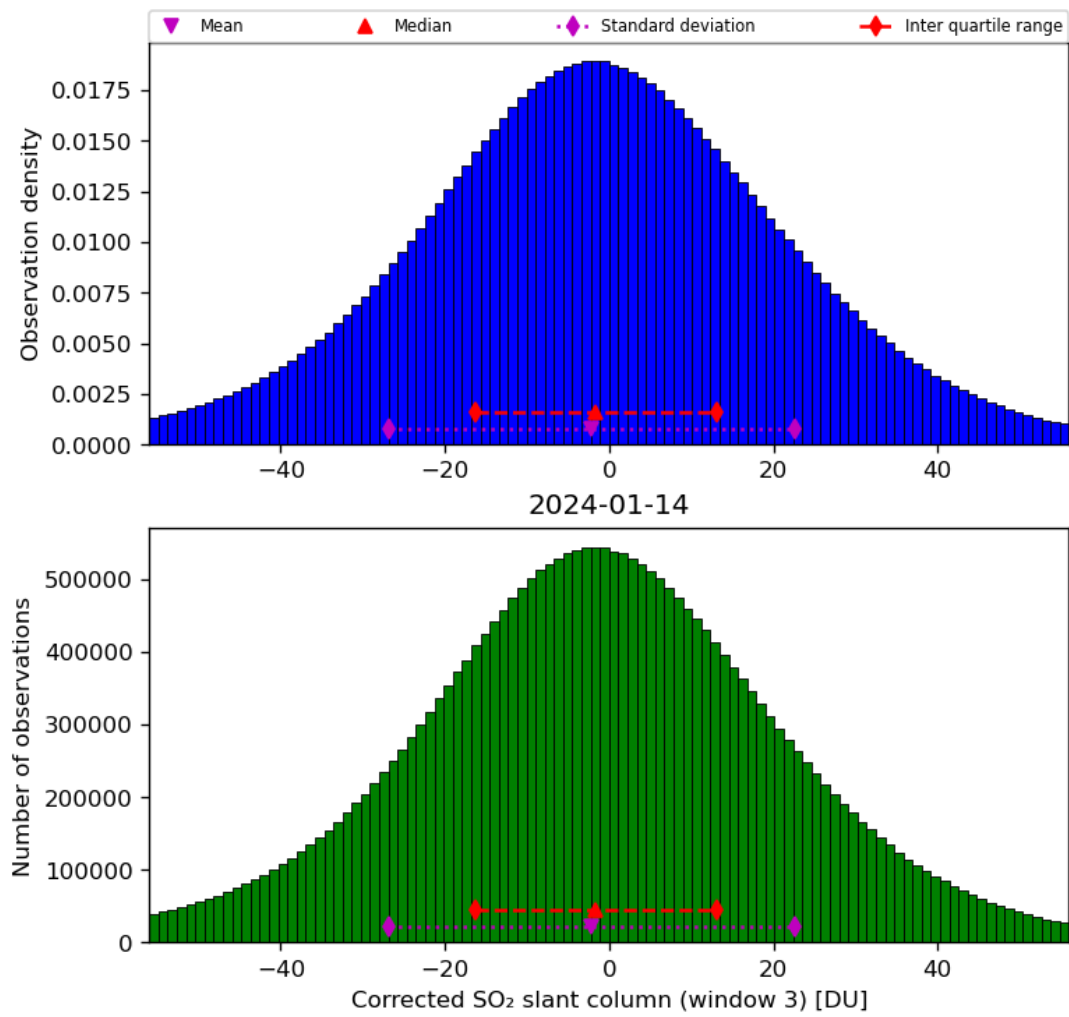
Figure 66: Histogram of “Corrected SO 2 slant column (window 3)” for 2024-01-13 to 2024-01-15
