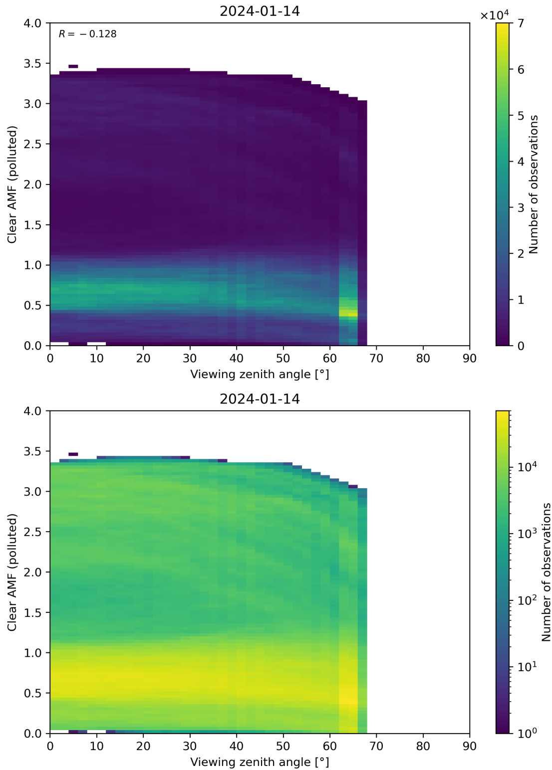
Figure 316: Scatter density plot of “Viewing zenith angle” against “Clear AMF (polluted)” for 2024-01-13 to 2024-01-15.
