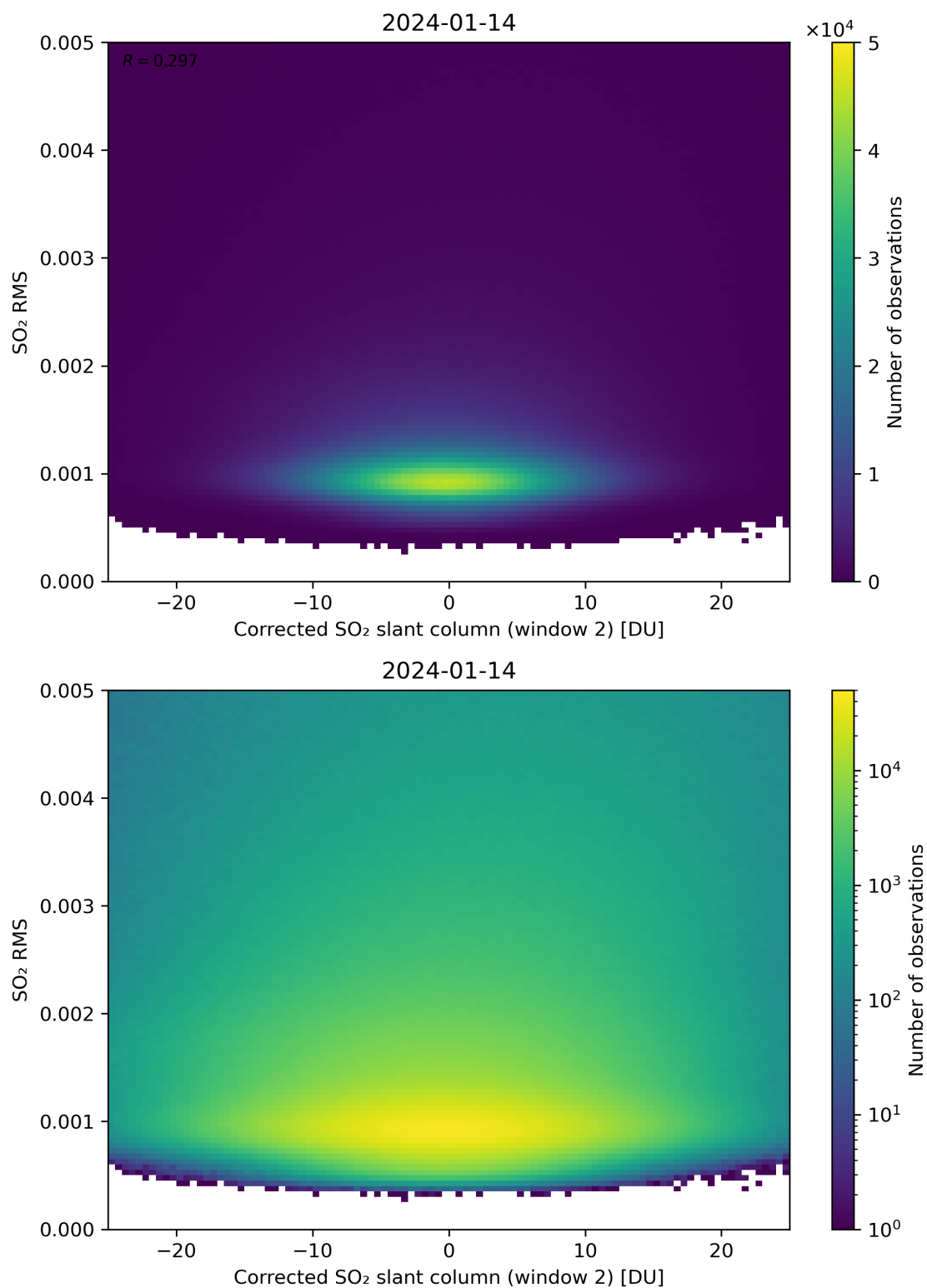
Figure 198: Scatter density plot of “Corrected SO 2 slant column (window 2)” against “SO 2 RMS” for 2024-01-13 to 2024-01-15.
