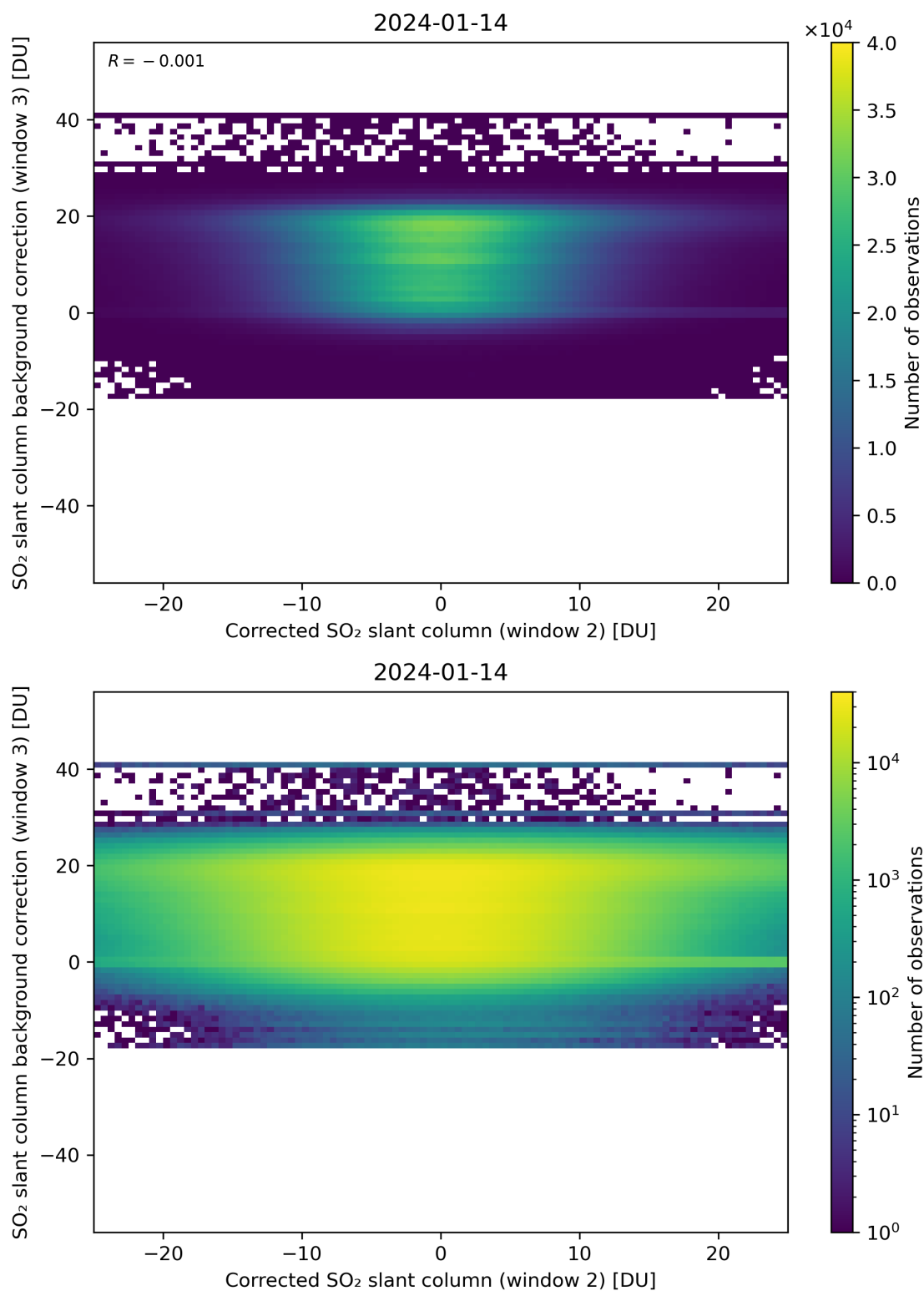
Figure 195: Scatter density plot of “Corrected SO 2 slant column (window 2)” against “SO 2 slant column background correction (window 3)” for 2024-01-13 to 2024-01-15.
