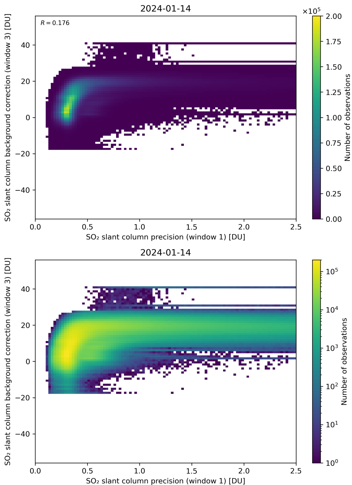
Figure 220: Scatter density plot of “SO 2 slant column precision (window 1)” against “SO 2 slant column background correction (window 3)” for 2024-01-13 to 2024-01-15.
