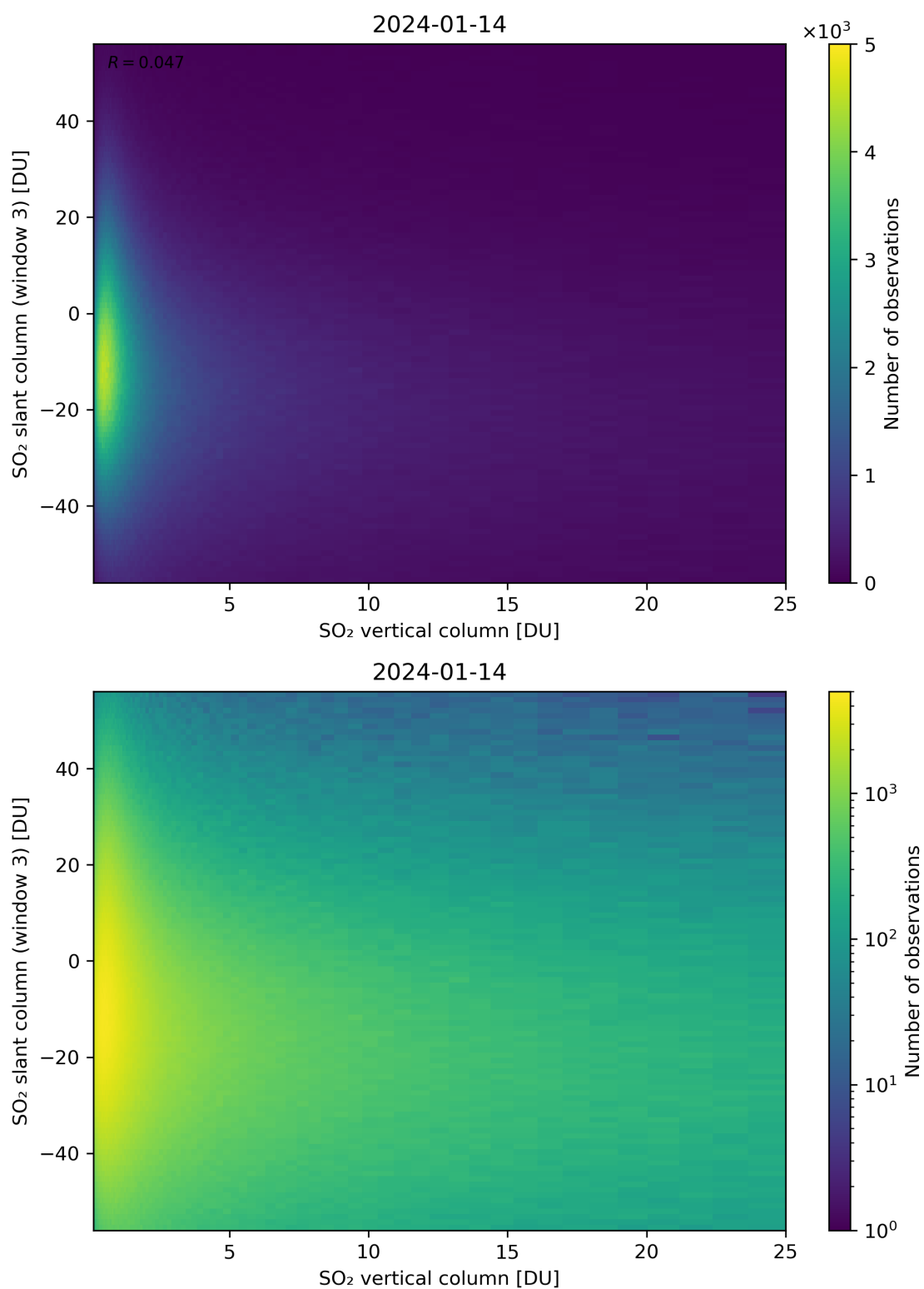
Figure 303: Scatter density plot of “SO 2 vertical column” against “SO 2 slant column (window 3)” for 2024-01-13 to 2024-01-15.
