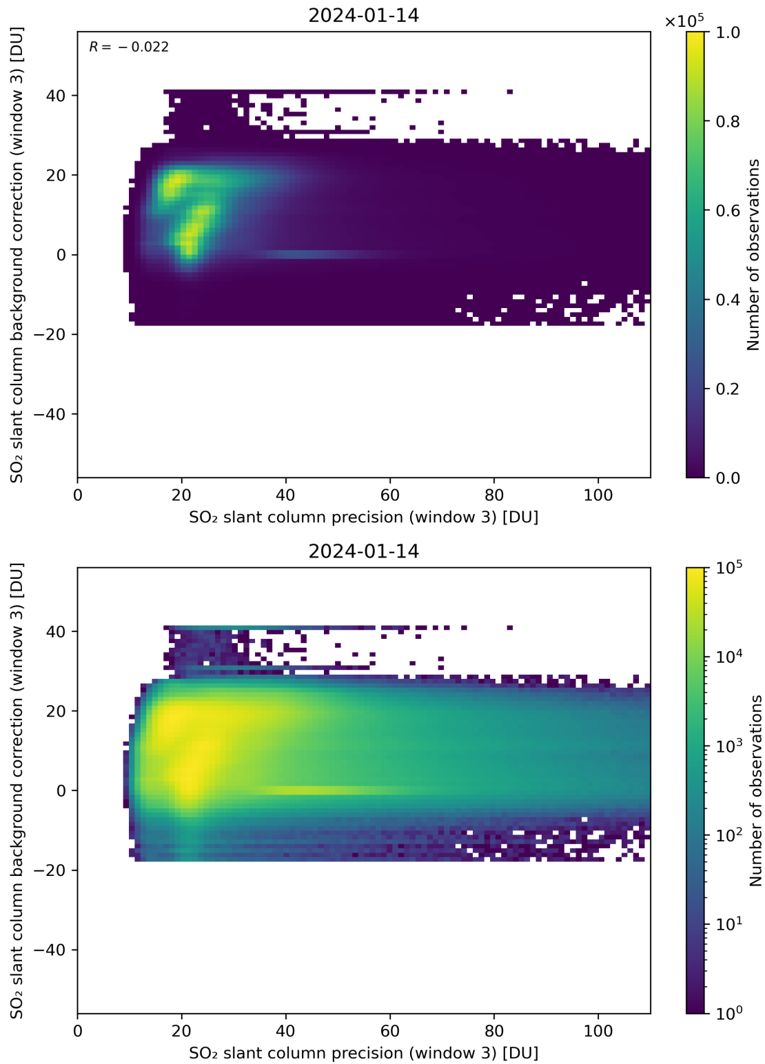
Figure 257: Scatter density plot of “SO 2 slant column precision (window 3)” against “SO 2 slant column background correction (window 3)” for 2024-01-13 to 2024-01-15.
