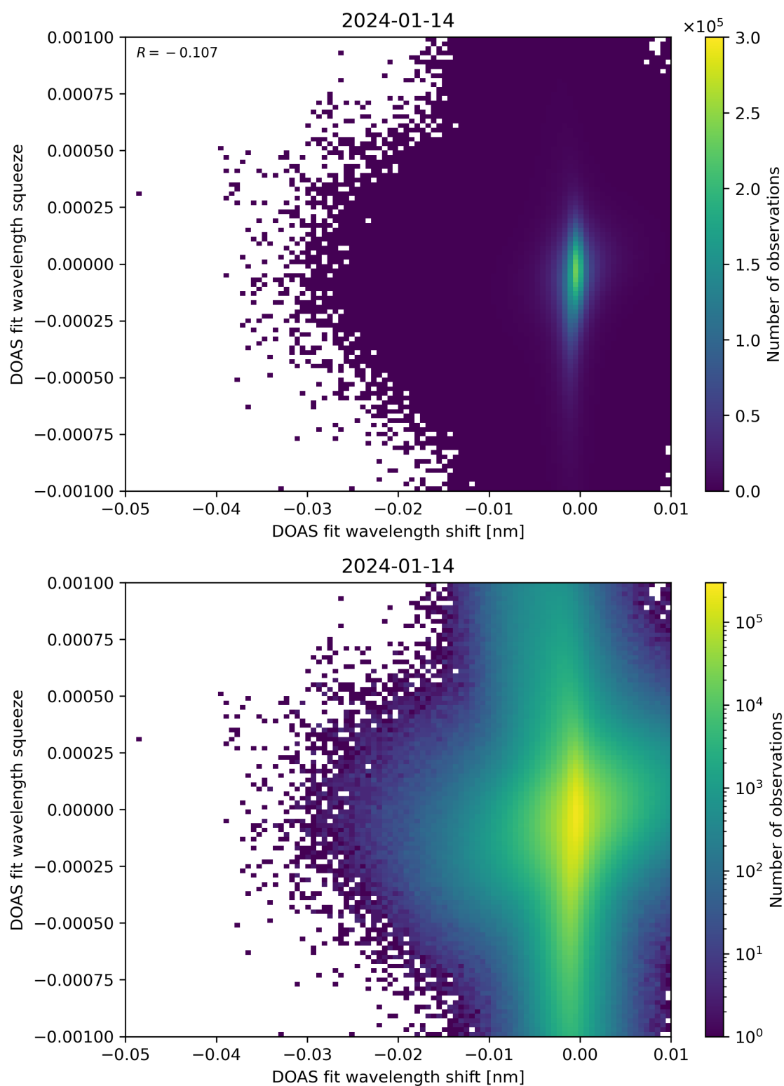
Figure 127: Scatter density plot of “DOAS fit wavelength shift” against “DOAS fit wavelength squeeze” for 2024-01-13 to 2024-01-15.
