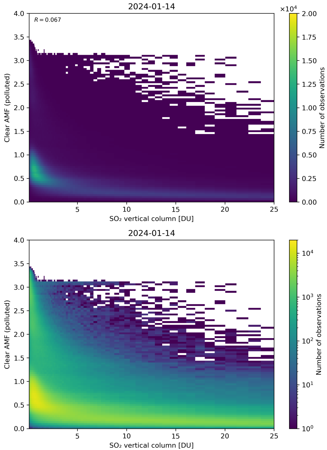
Figure 296: Scatter density plot of “SO 2 vertical column” against “Clear AMF (polluted)” for 2024-01-13 to 2024-01-15.
