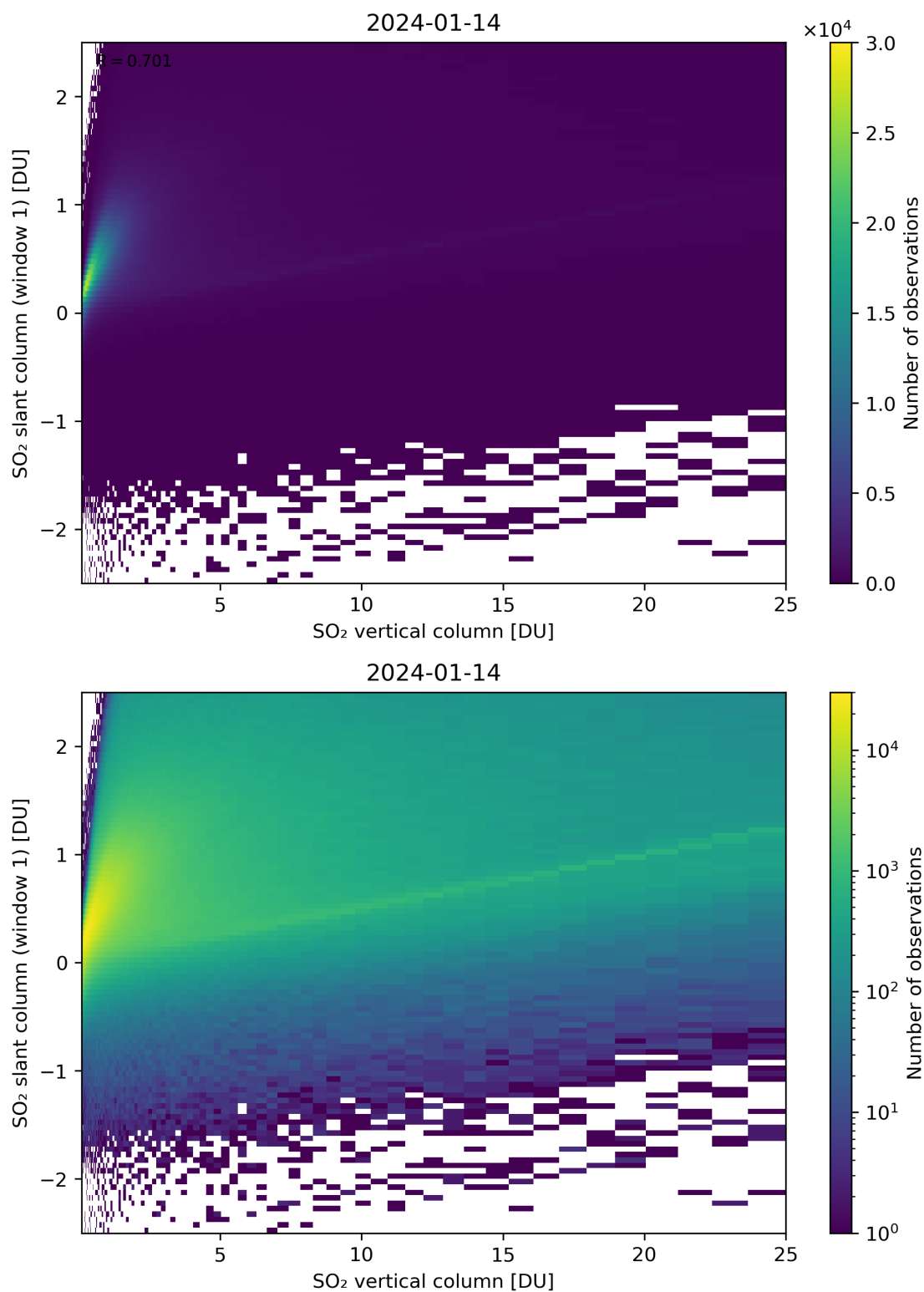
Figure 300: Scatter density plot of “SO 2 vertical column” against “SO 2 slant column (window 1)” for 2024-01-13 to 2024-01-15.
