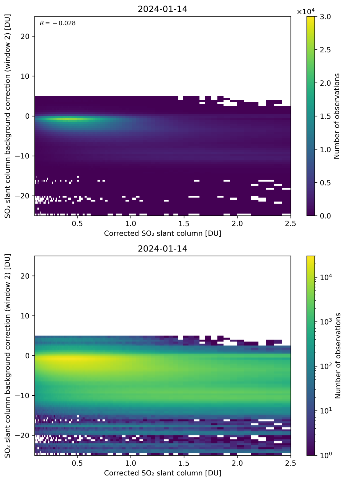
Figure 179: Scatter density plot of “Corrected SO 2 slant column” against “SO 2 slant column background correction (window 2)” for 2024-01-13 to 2024-01-15.
