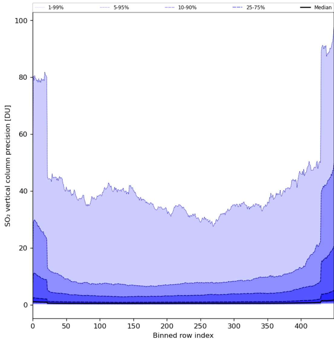
Figure 77: Along track statistics of “SO 2 vertical column precision” for 2024-01-13 to 2024-01-15
