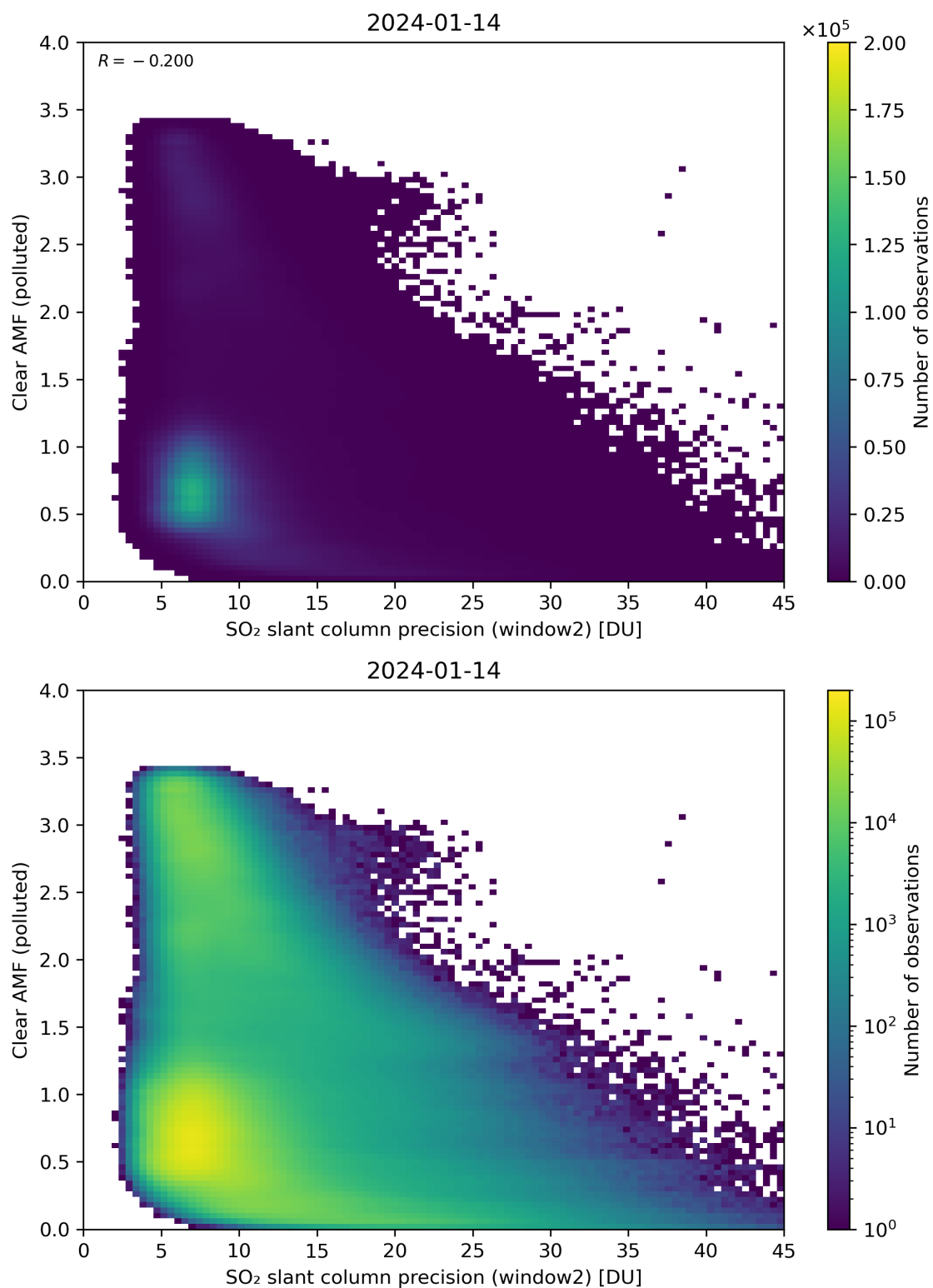
Figure 246: Scatter density plot of “SO 2 slant column precision (window2)” against “Clear AMF (polluted)” for 2024-01-13 to 2024-01-15.
