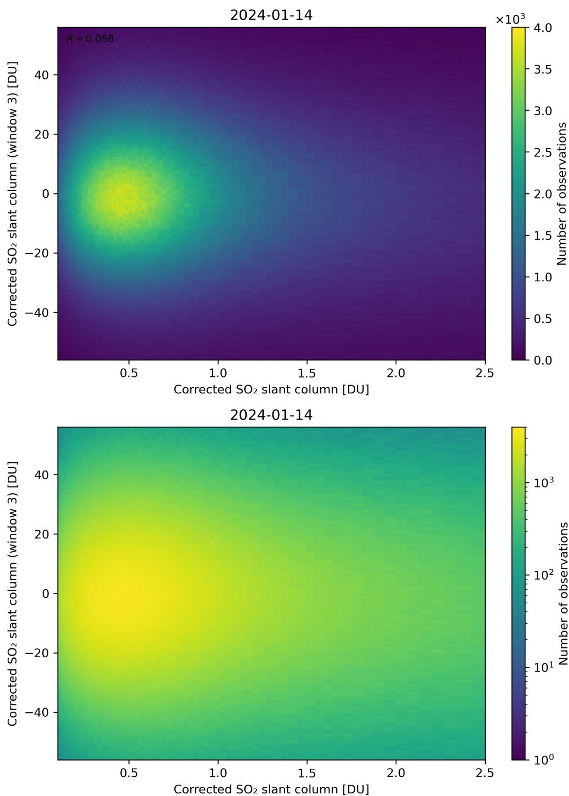
Figure 186: Scatter density plot of “Corrected SO 2 slant column” against “Corrected SO 2 slant column (window 3)” for 2024-01-13 to 2024-01-15.
