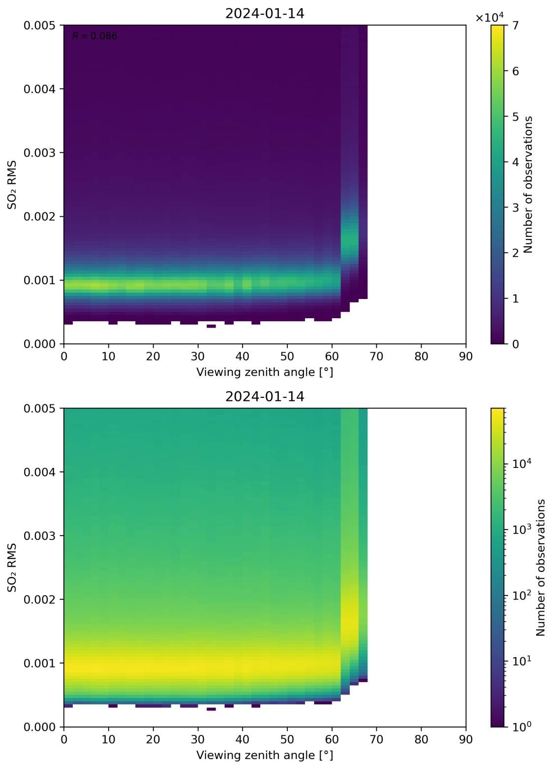
Figure 313: Scatter density plot of “Viewing zenith angle” against “SO 2 RMS” for 2024-01-13 to 2024-01-15.
