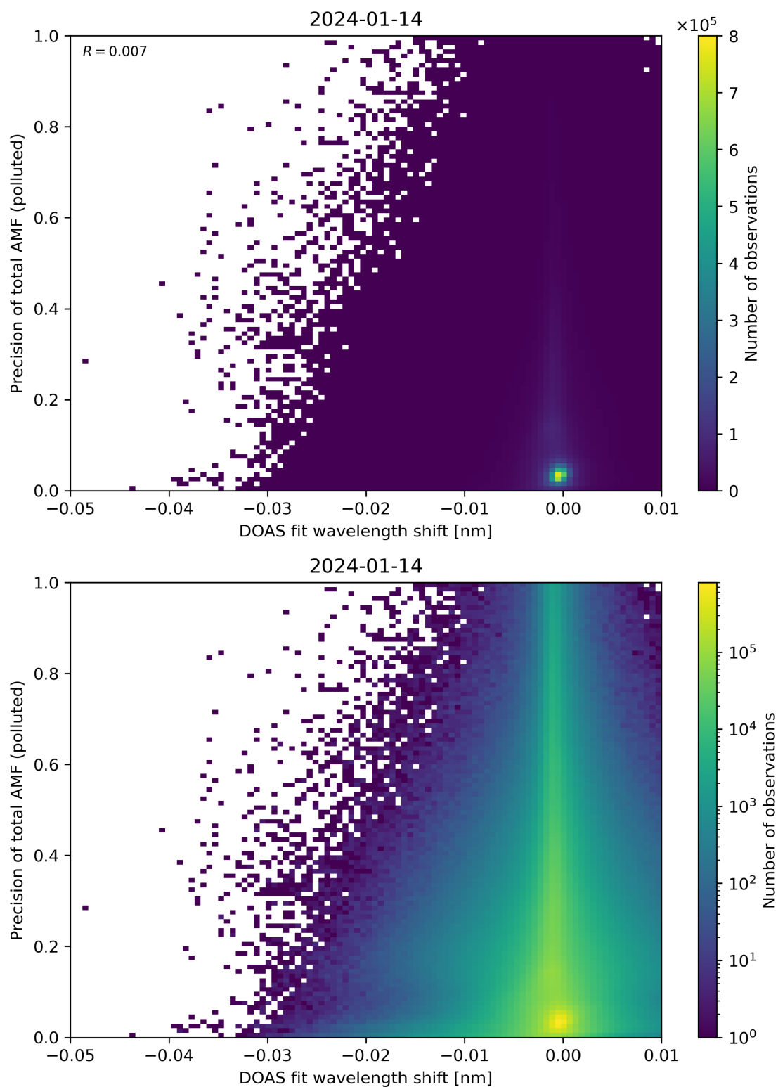
Figure 131: Scatter density plot of “DOAS fit wavelength shift” against “Precision of total AMF (polluted)” for 2024-01-13 to 2024-01-15.
