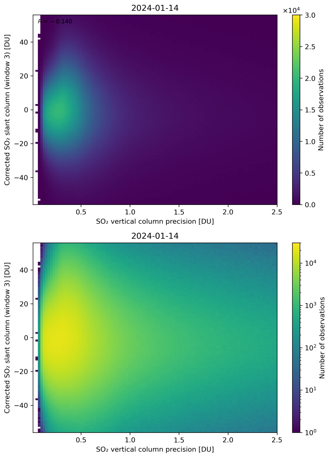
Figure 288: Scatter density plot of “SO 2 vertical column precision” against “Corrected SO 2 slant column (window 3)” for 2024-01-13 to 2024-01-15.
