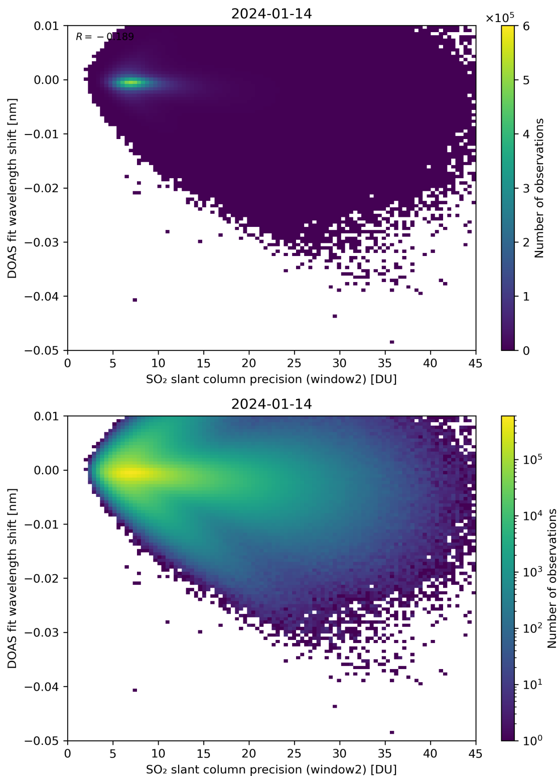
Figure 243: Scatter density plot of “SO 2 slant column precision (window2)” against “DOAS fit wavelength shift” for 2024-01-13 to 2024-01-15.
