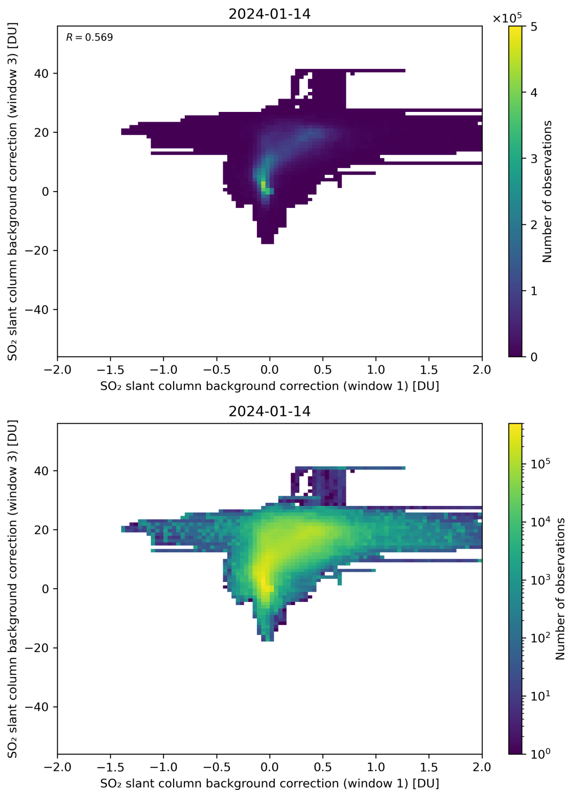
Figure 99: Scatter density plot of “SO 2 slant column background correction (window 1)” against “SO 2 slant column background correction (window 3)” for 2024-01-13 to 2024-01-15.
