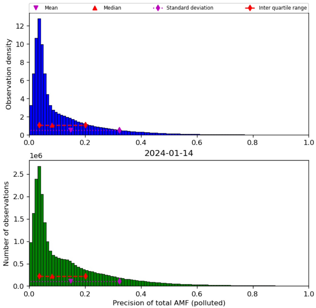
Figure 72: Histogram of “Precision of total AMF (polluted)” for 2024-01-13 to 2024-01-15
