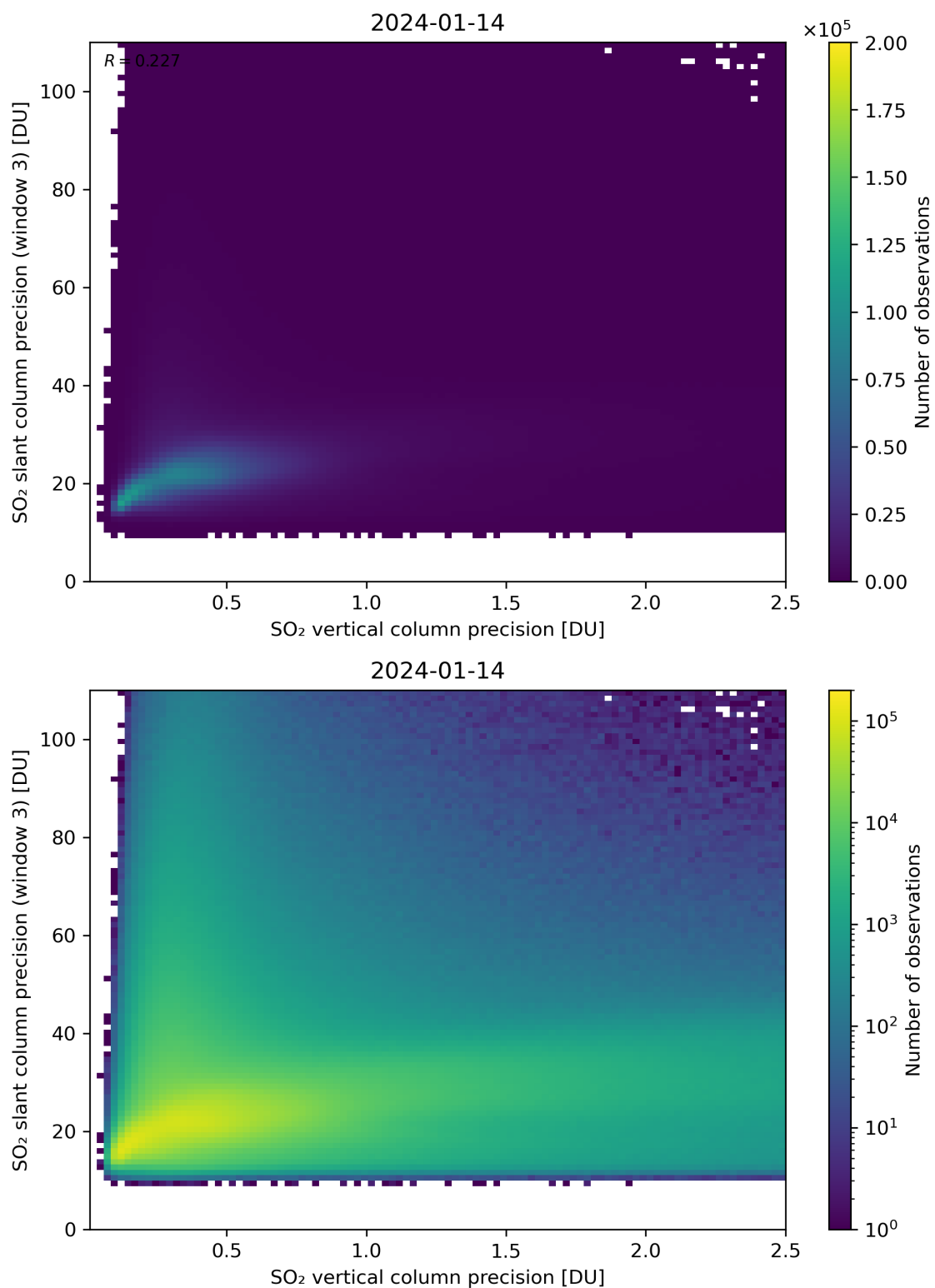
Figure 293: Scatter density plot of “SO 2 vertical column precision” against “SO 2 slant column precision (window 3)” for 2024-01-13 to 2024-01-15.
