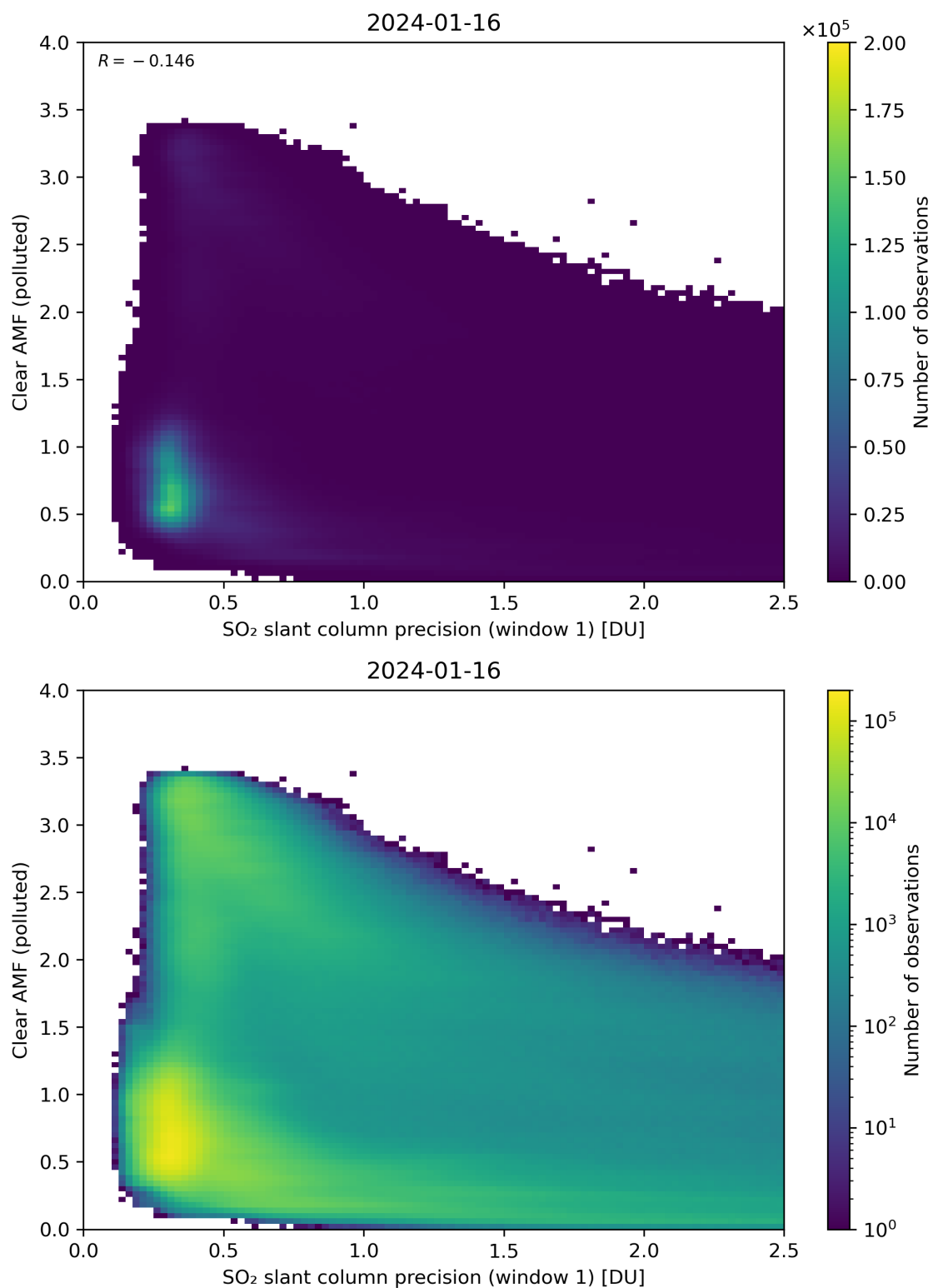
Figure 224: Scatter density plot of “SO 2 slant column precision (window 1)” against “Clear AMF (polluted)” for 2024-01-15 to 2024-01-17.
