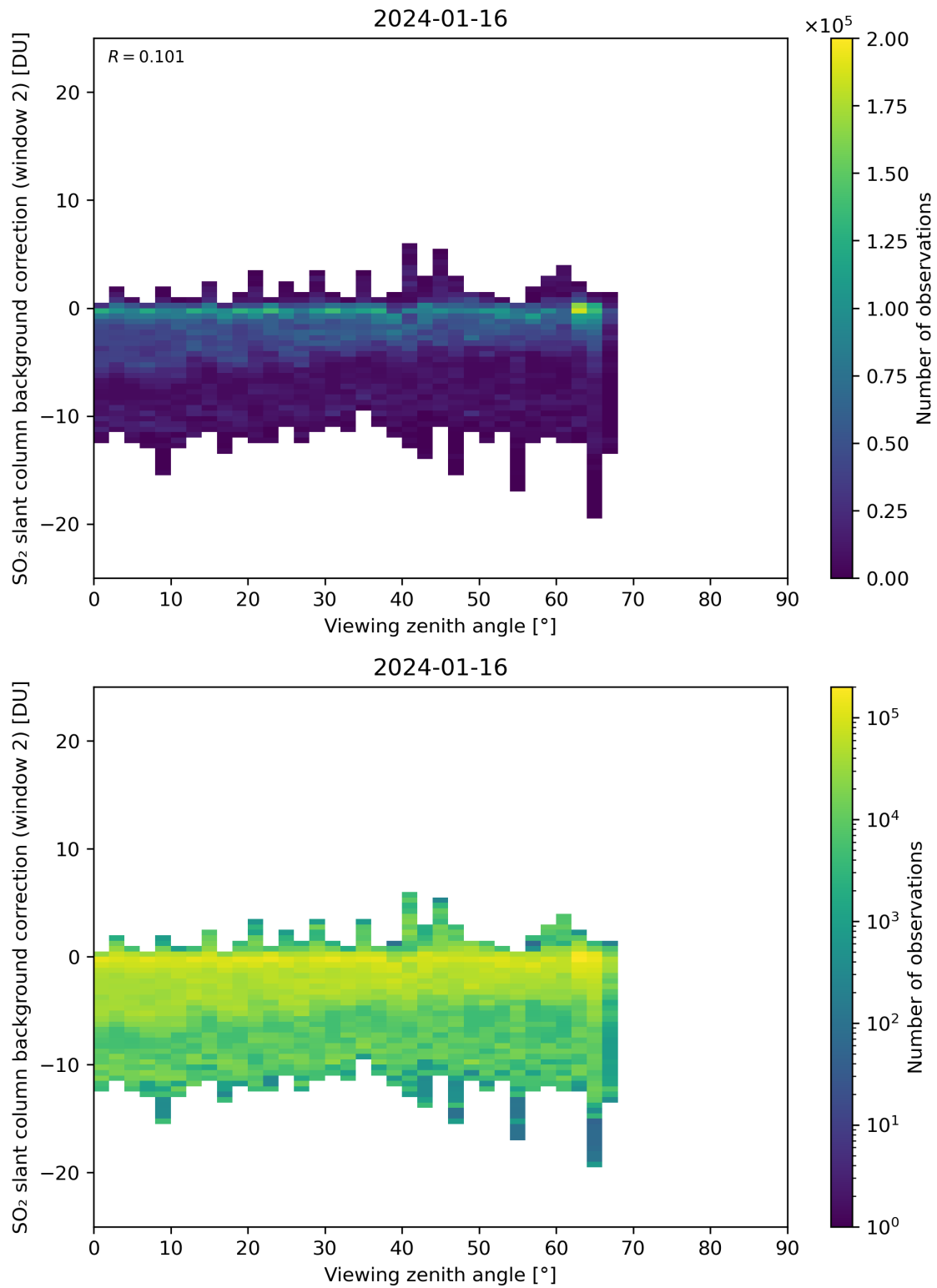
Figure 309: Scatter density plot of “Viewing zenith angle” against “SO 2 slant column background correction (window 2)” for 2024-01-15 to 2024-01-17.
