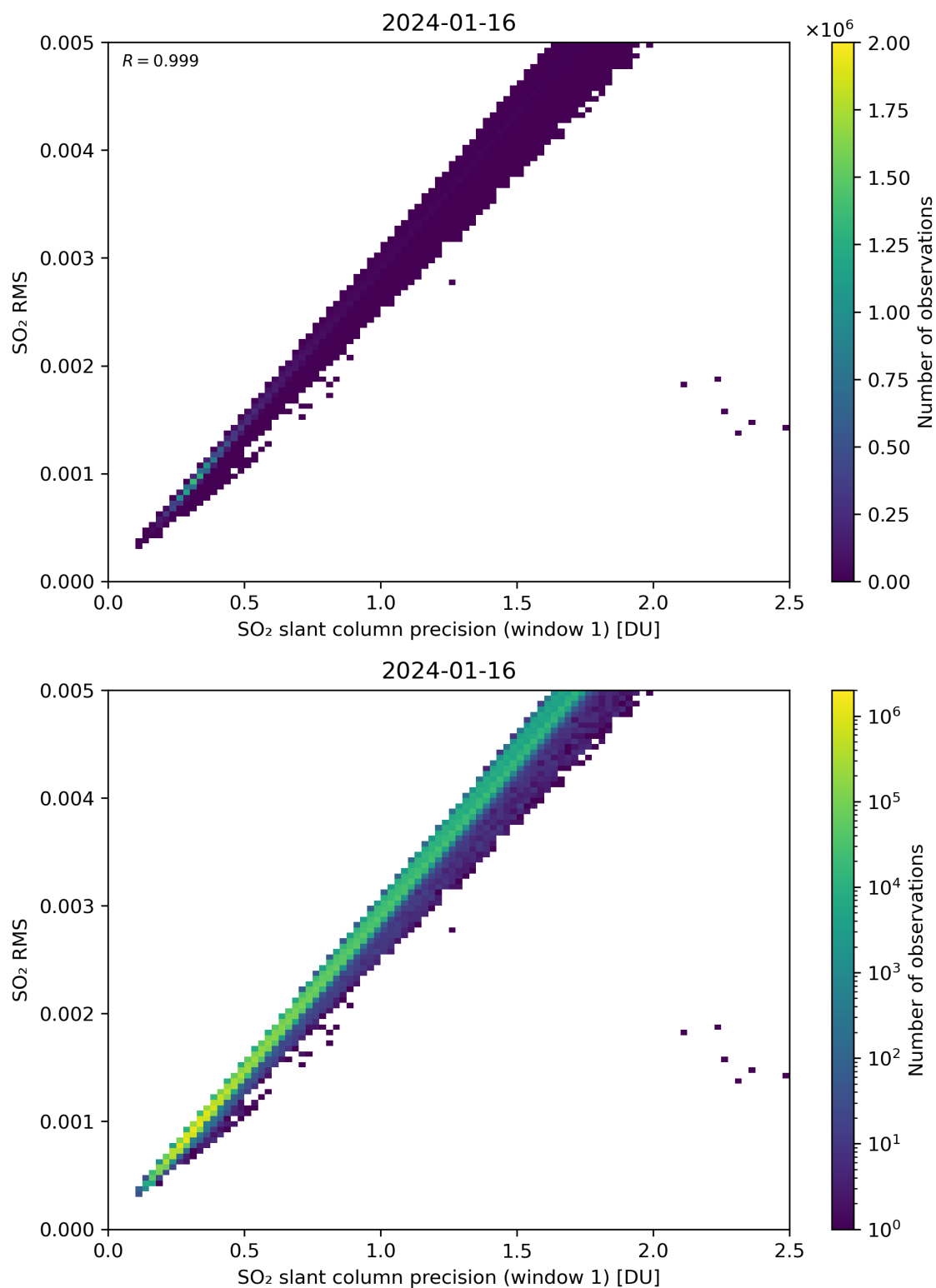
Figure 223: Scatter density plot of “SO 2 slant column precision (window 1)” against “SO 2 RMS” for 2024-01-15 to 2024-01-17.
