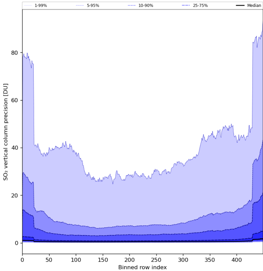
Figure 77: Along track statistics of “SO 2 vertical column precision” for 2024-01-15 to 2024-01-17
