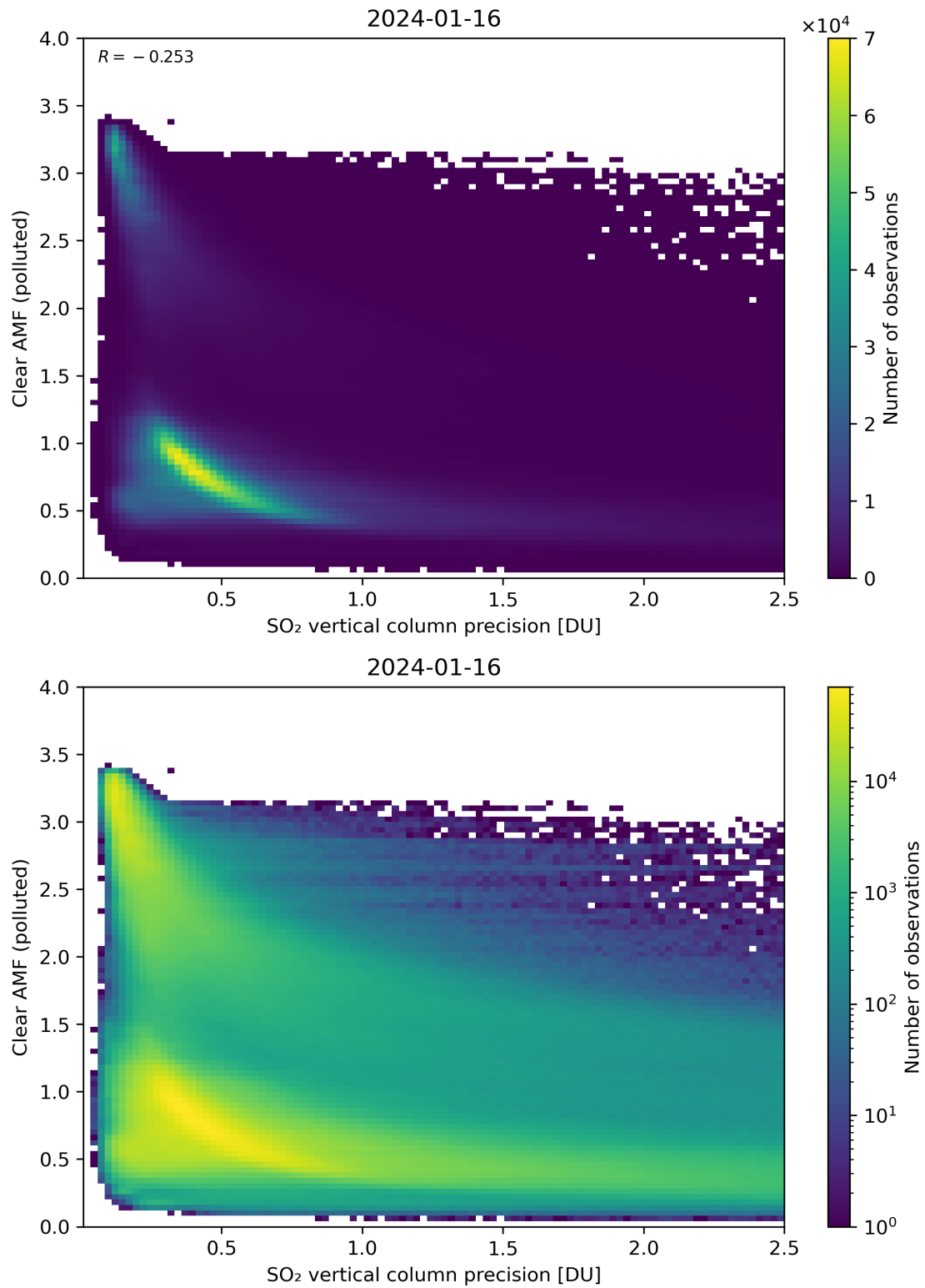
Figure 285: Scatter density plot of “SO 2 vertical column precision” against “Clear AMF (polluted)” for 2024-01-15 to 2024-01-17.
