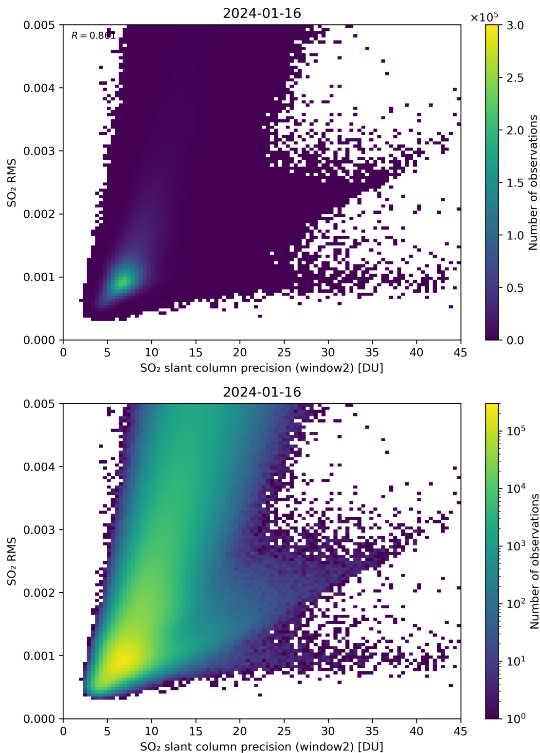
Figure 245: Scatter density plot of “SO 2 slant column precision (window2)” against “SO 2 RMS” for 2024-01-15 to 2024-01-17.
