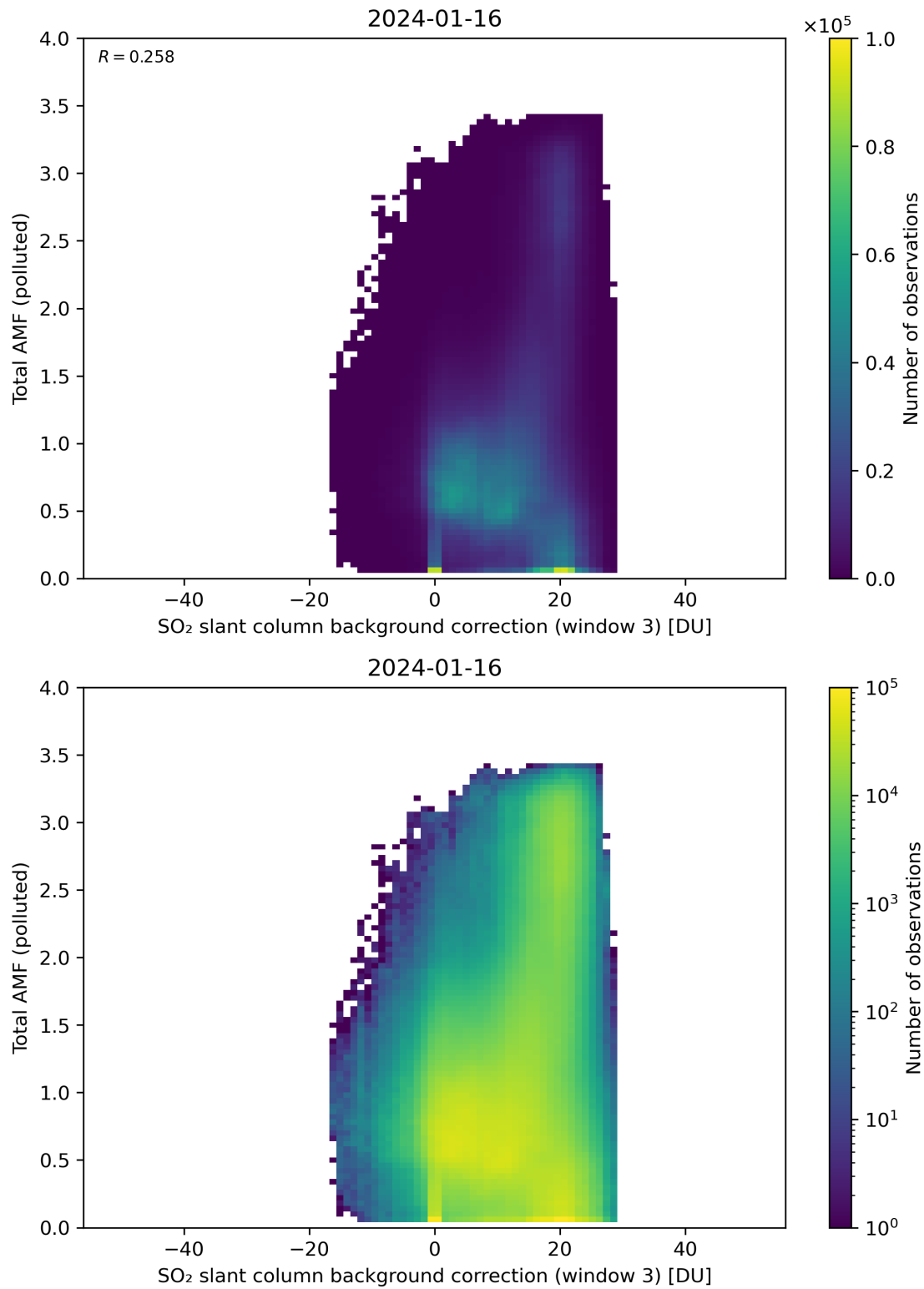
Figure 125: Scatter density plot of “SO 2 slant column background correction (window 3)” against “Total AMF (polluted)” for 2024-01-15 to 2024-01-17.
