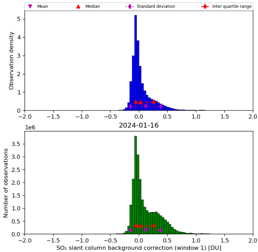
Figure 59: Histogram of “SO 2 slant column background correction (window 1)” for 2024-01-15 to 2024-01-17
