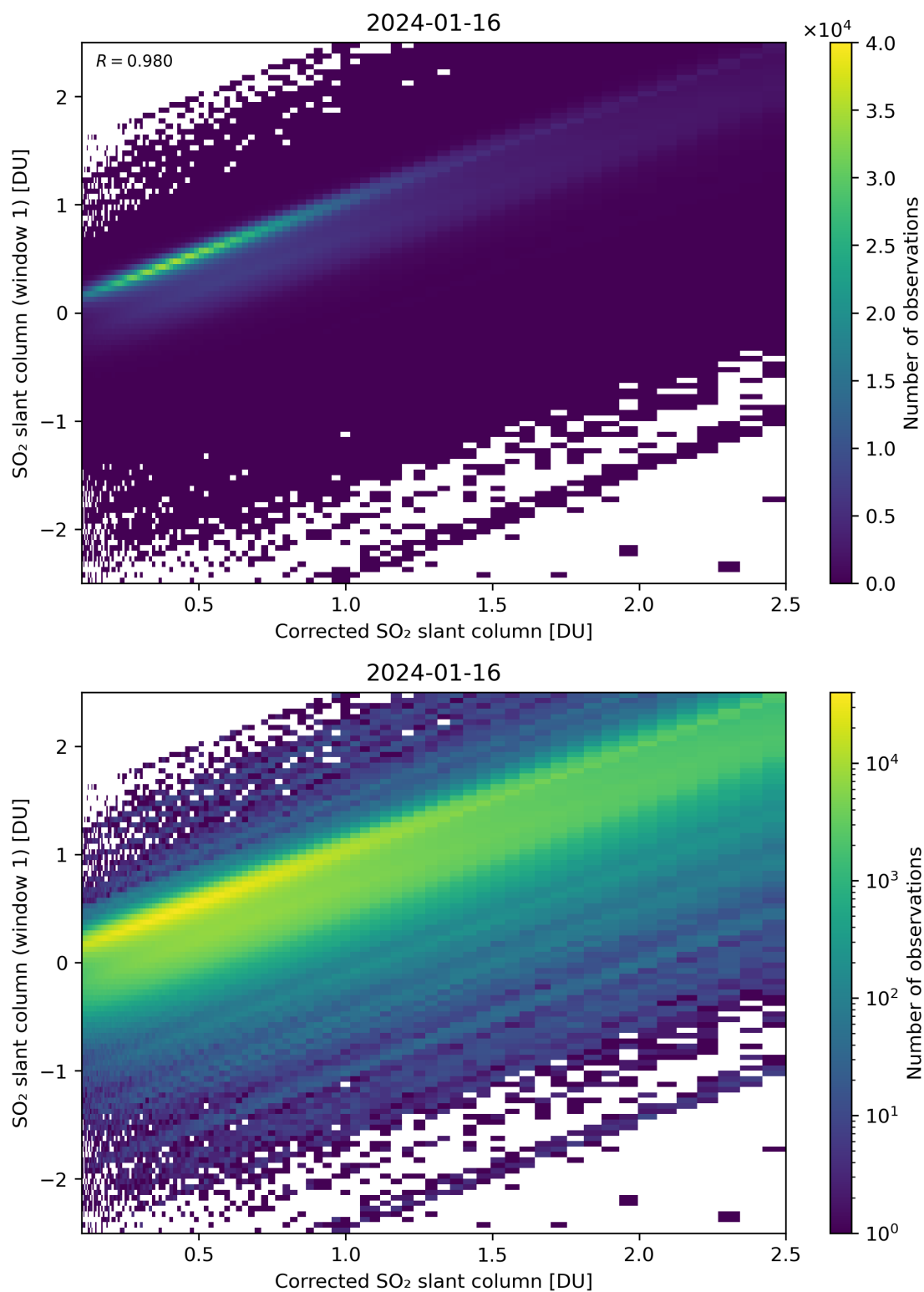
Figure 187: Scatter density plot of “Corrected SO 2 slant column” against “SO 2 slant column (window 1)” for 2024-01-15 to 2024-01-17.
