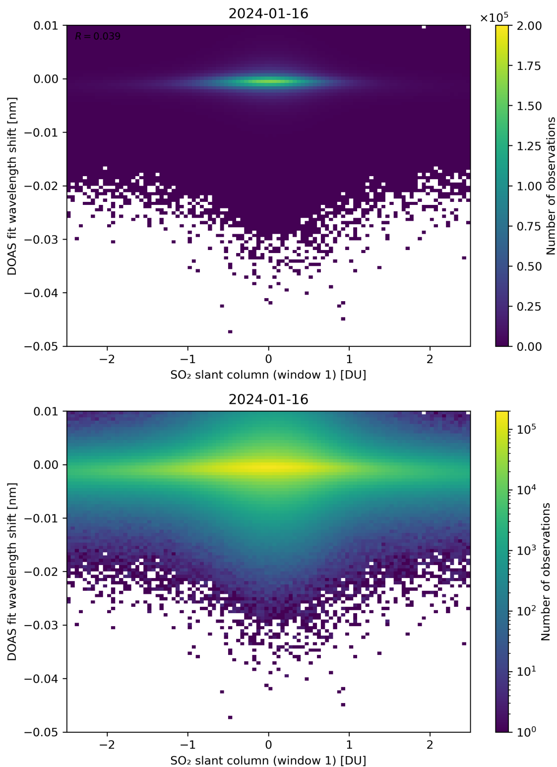
Figure 215: Scatter density plot of “SO 2 slant column (window 1)” against “DOAS fit wavelength shift” for 2024-01-15 to 2024-01-17.
