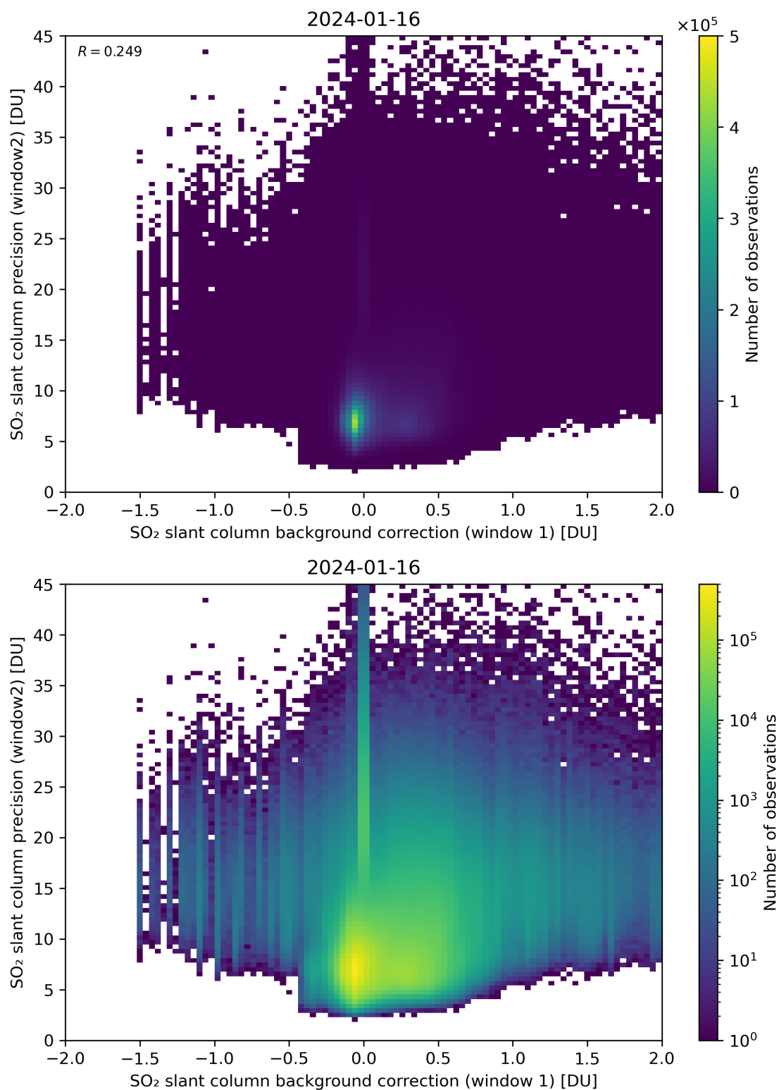
Figure 106: Scatter density plot of “SO 2 slant column background correction (window 1)” against “SO 2 slant column precision (window2)” for 2024-01-15 to 2024-01-17.
