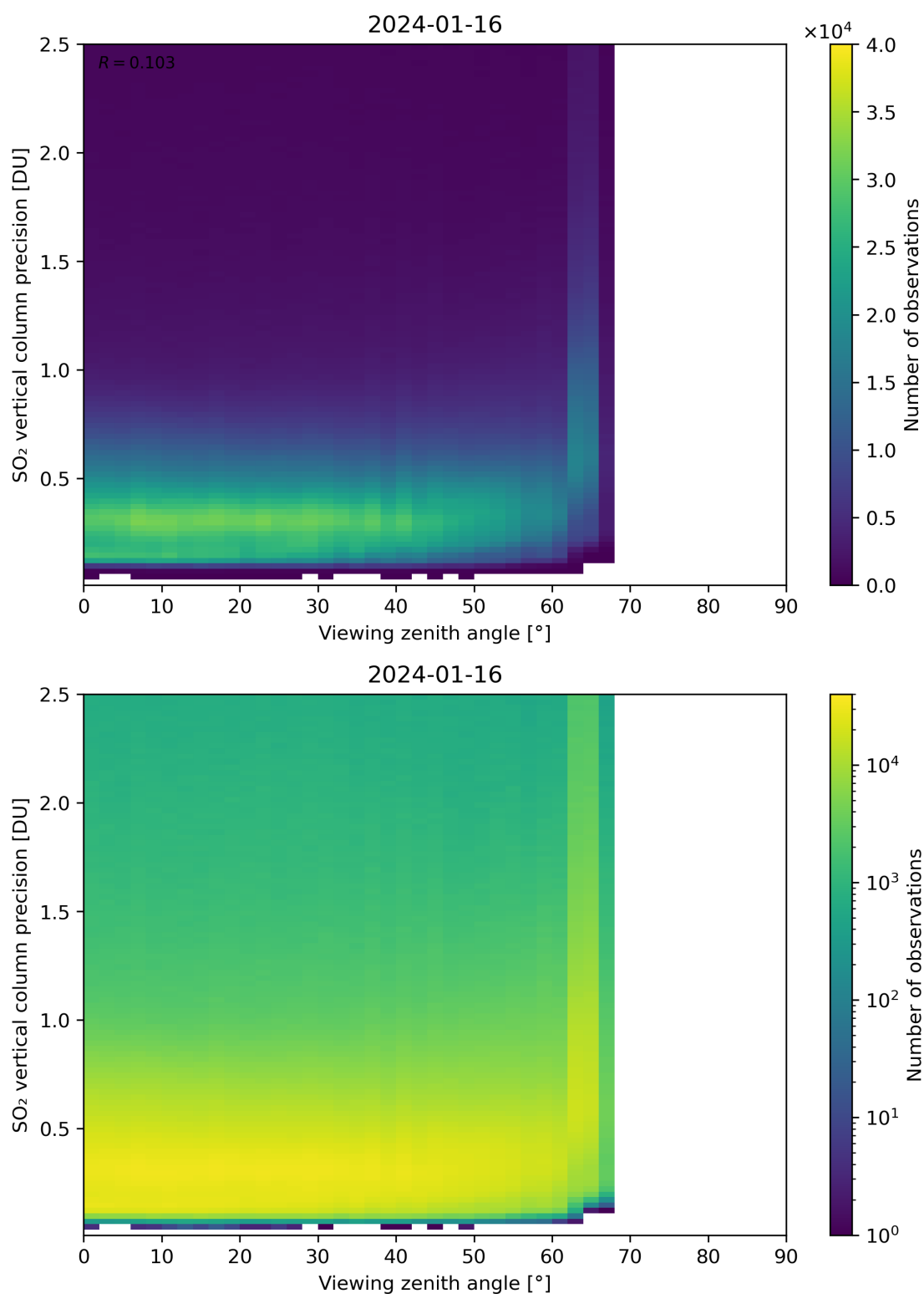
Figure 328: Scatter density plot of “Viewing zenith angle” against “SO 2 vertical column precision” for 2024-01-15 to 2024-01-17.
