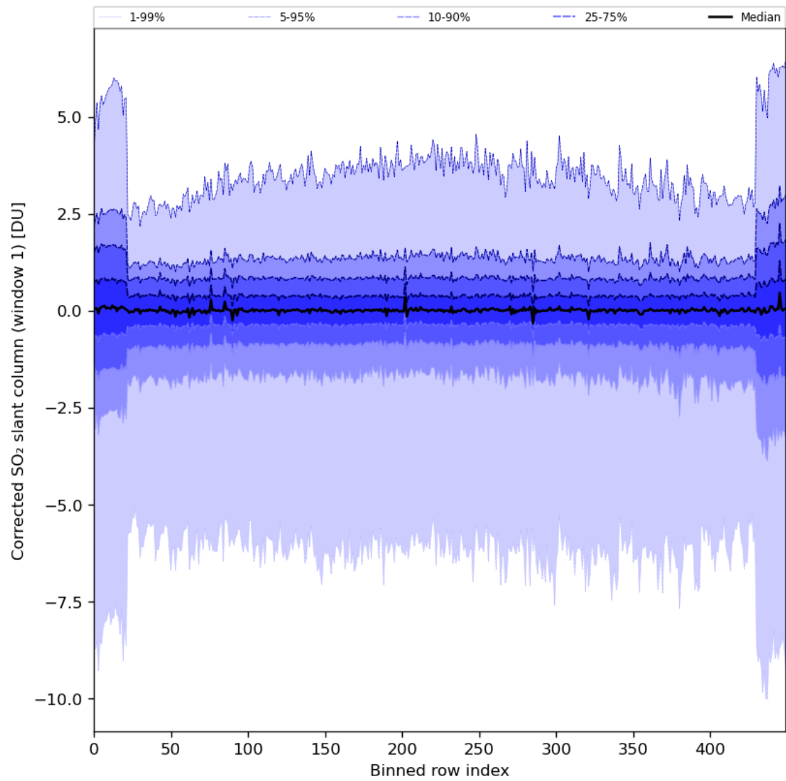
Figure 81: Along track statistics of “Corrected SO 2 slant column (window 1)” for 2024-01-15 to 2024-01-17
