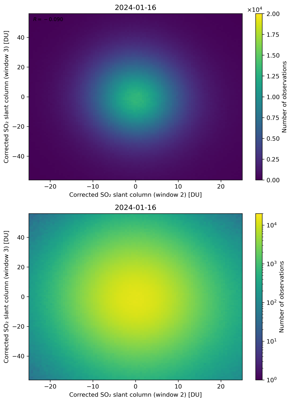
Figure 200: Scatter density plot of “Corrected SO 2 slant column (window 2)” against “Corrected SO 2 slant column (window 3)” for 2024-01-15 to 2024-01-17.
