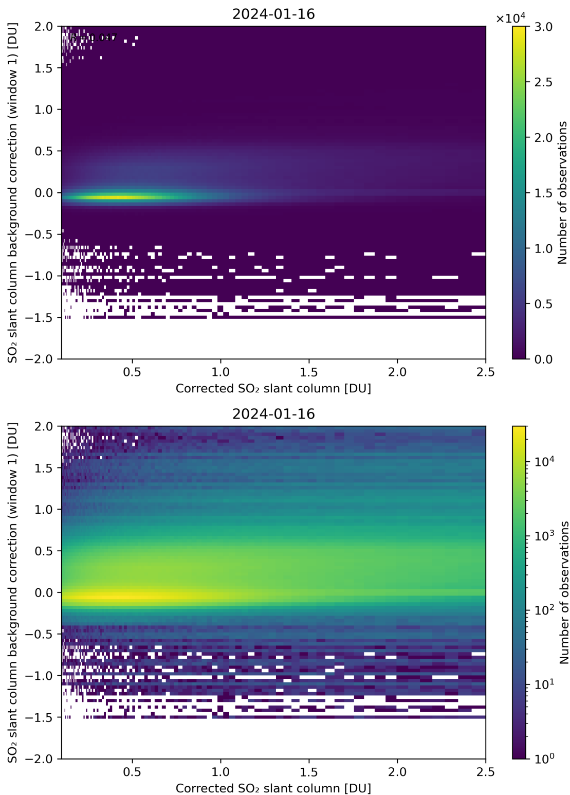
Figure 178: Scatter density plot of “Corrected SO 2 slant column” against “SO 2 slant column background correction (window 1)” for 2024-01-15 to 2024-01-17.
