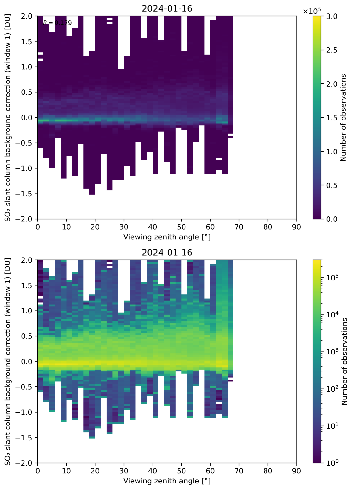
Figure 308: Scatter density plot of “Viewing zenith angle” against “SO 2 slant column background correction (window 1)” for 2024-01-15 to 2024-01-17.
