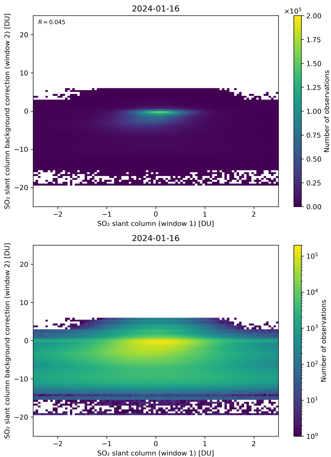
Figure 213: Scatter density plot of “SO 2 slant column (window 1)” against “SO 2 slant column background correction (window 2)” for 2024-01-15 to 2024-01-17.
