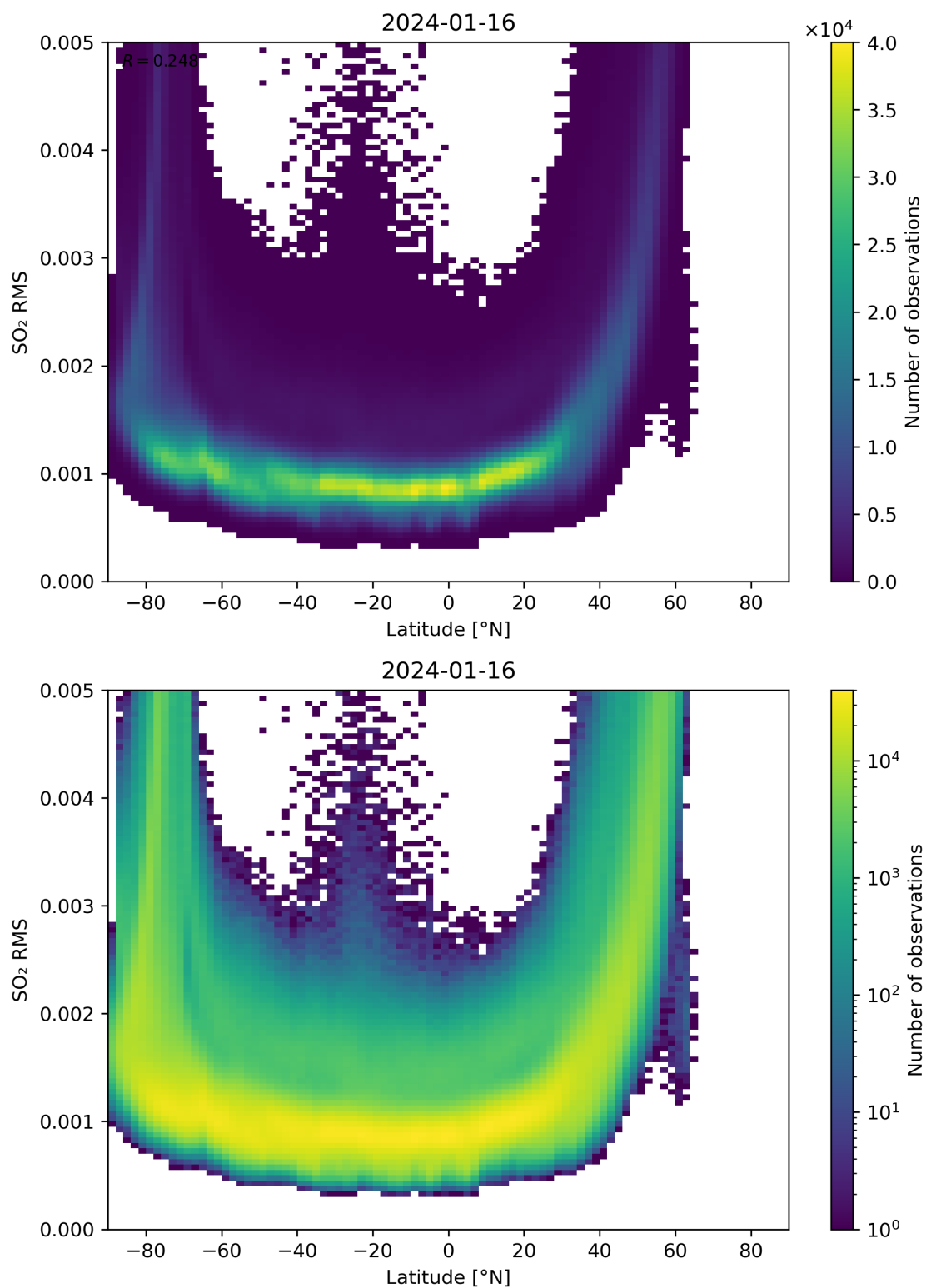
Figure 144: Scatter density plot of “Latitude” against “SO 2 RMS” for 2024-01-15 to 2024-01-17.
