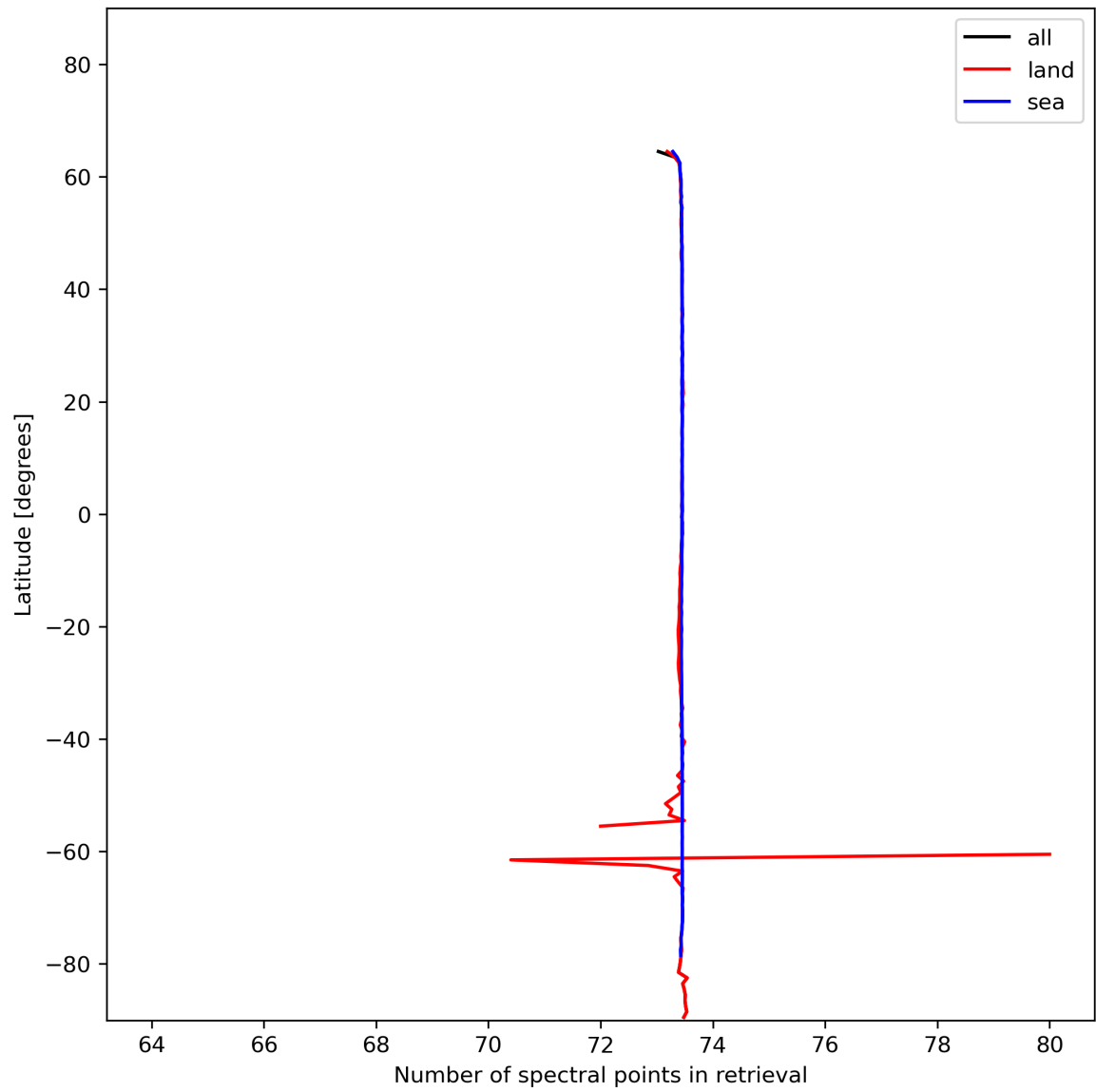
Figure 51: Zonal average of “Number of spectral points in retrieval” for 2024-01-15 to 2024-01-17.
