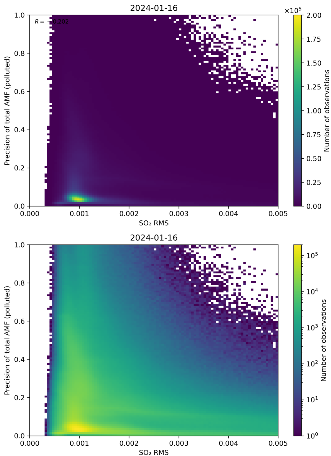
Figure 138: Scatter density plot of “SO 2 RMS” against “Precision of total AMF (polluted)” for 2024-01-15 to 2024-01-17.
