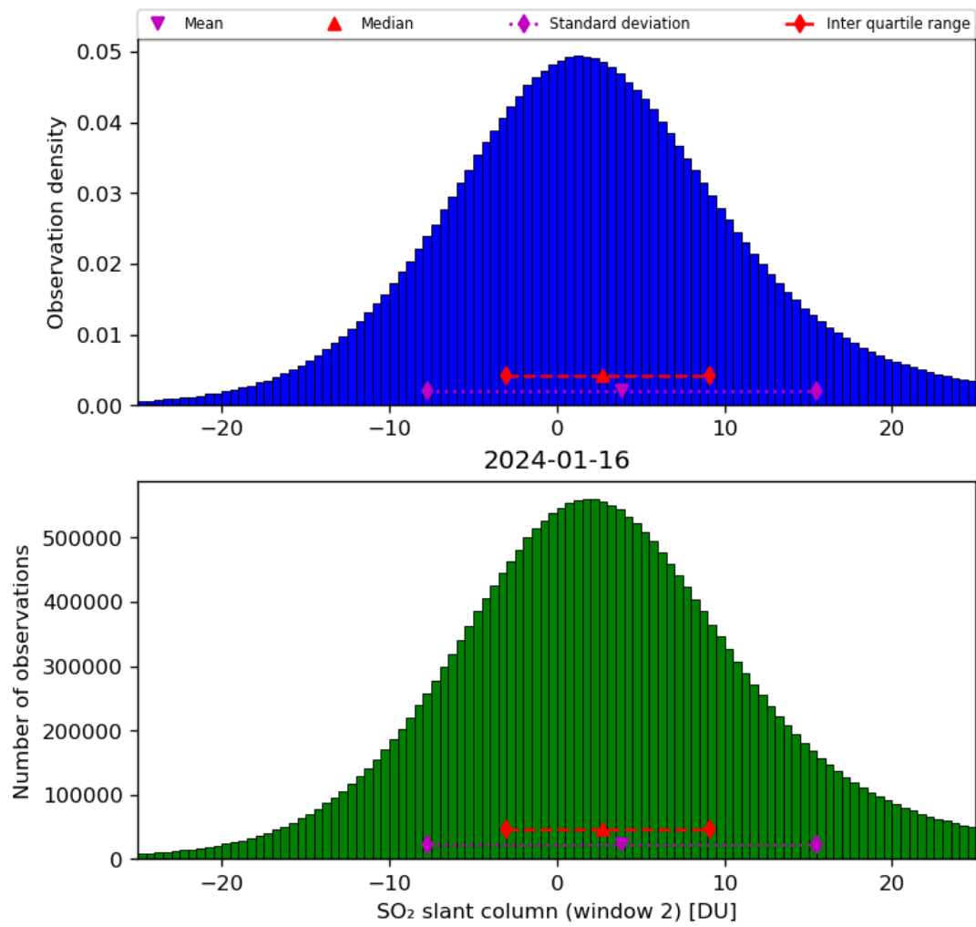
Figure 60: Histogram of “SO 2 slant column (window 2)” for 2024-01-15 to 2024-01-17
