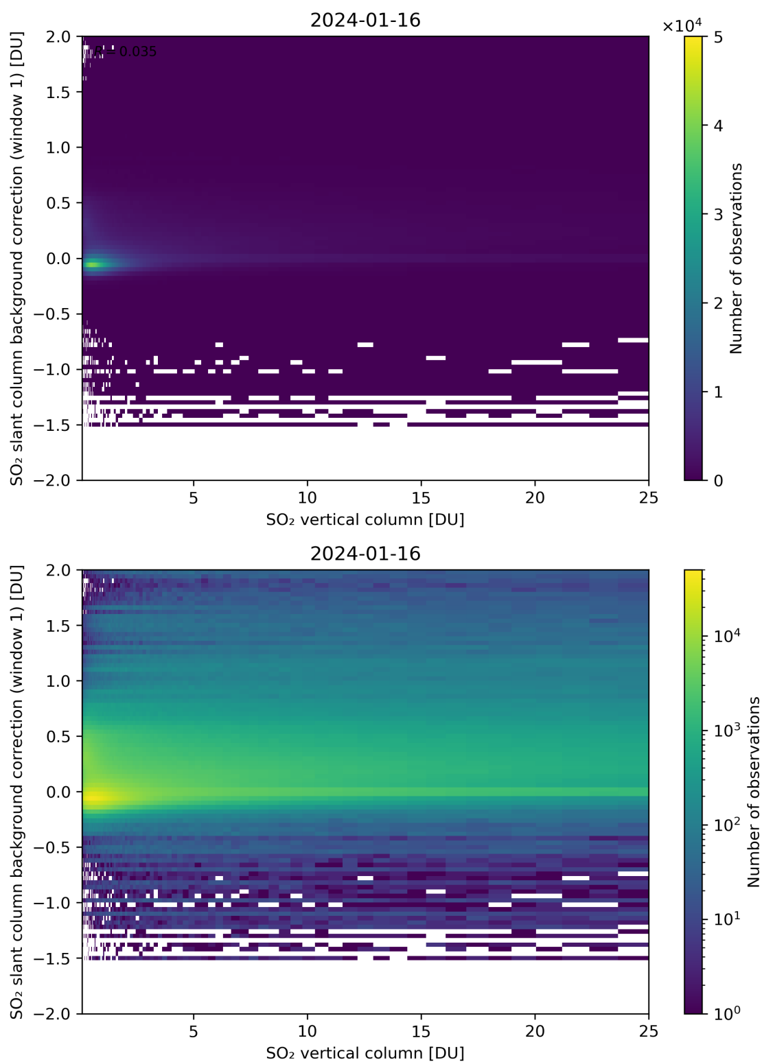
Figure 273: Scatter density plot of “SO 2 vertical column” against “SO 2 slant column background correction (window 1)” for 2024-01-15 to 2024-01-17.
