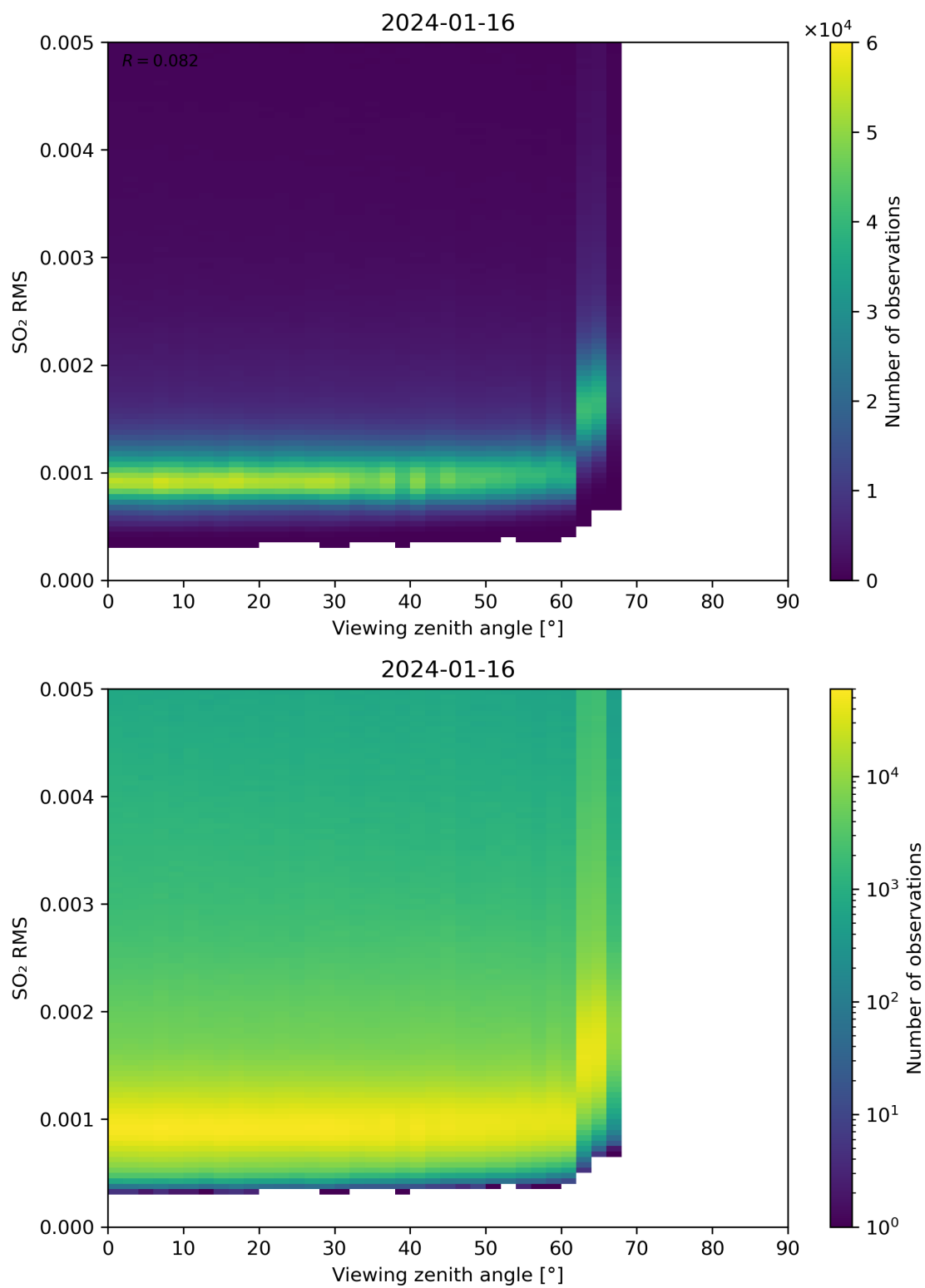
Figure 313: Scatter density plot of “Viewing zenith angle” against “SO 2 RMS” for 2024-01-15 to 2024-01-17.
