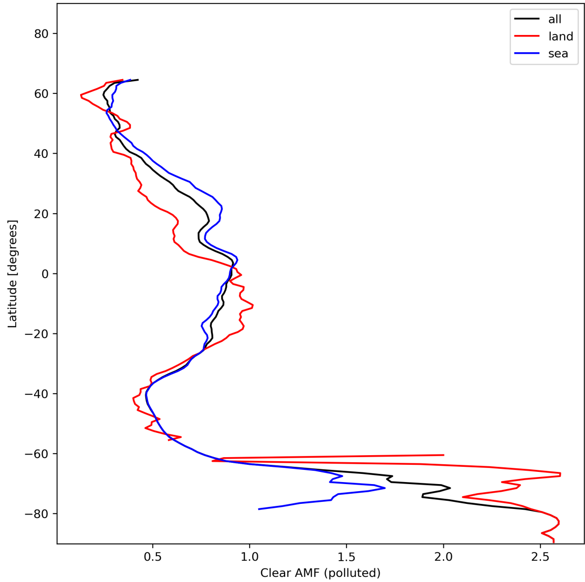
Figure 50: Zonal average of “Clear AMF (polluted)” for 2024-01-15 to 2024-01-17.
