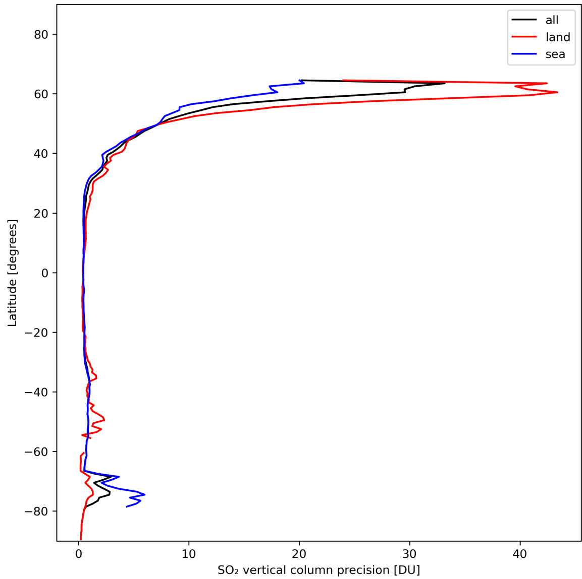
Figure 31: Zonal average of “SO 2 vertical column precision” for 2024-01-15 to 2024-01-17.
