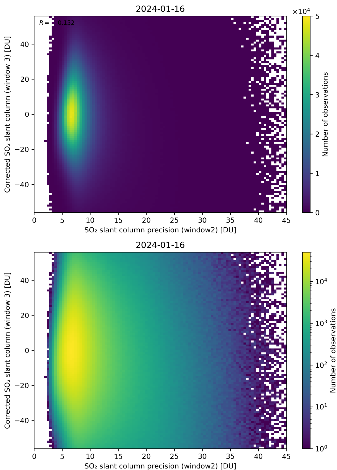
Figure 248: Scatter density plot of “SO 2 slant column precision (window2)” against “Corrected SO 2 slant column (window 3)” for 2024-01-15 to 2024-01-17.
