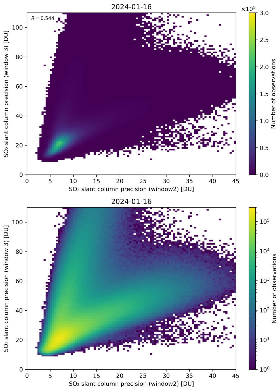
Figure 250: Scatter density plot of “SO 2 slant column precision (window2)” against “SO 2 slant column precision (window 3)” for 2024-01-15 to 2024-01-17.
