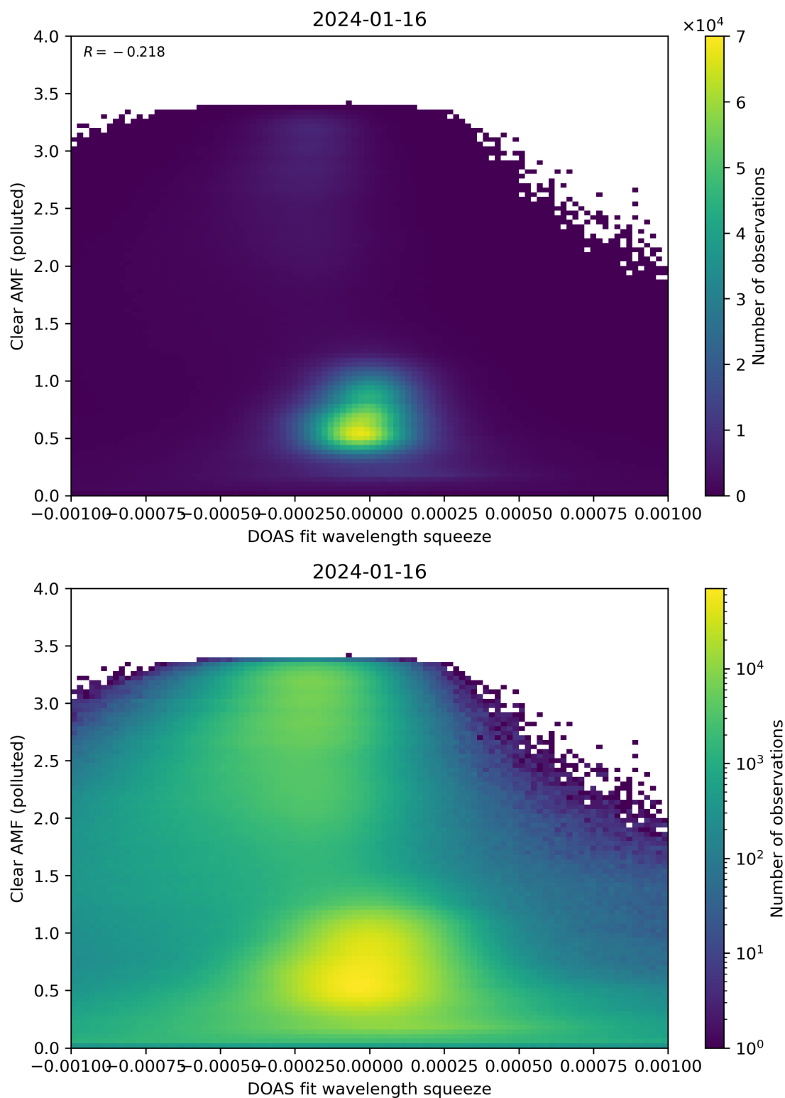
Figure 133: Scatter density plot of “DOAS fit wavelength squeeze” against “Clear AMF (polluted)” for 2024-01-15 to 2024-01-17.
