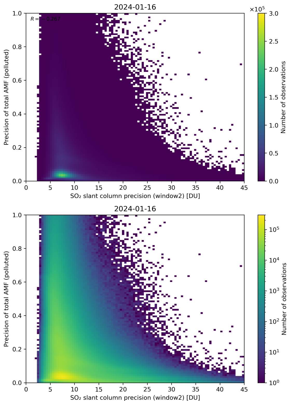
Figure 252: Scatter density plot of “SO 2 slant column precision (window2)” against “Precision of total AMF (polluted)” for 2024-01-15 to 2024-01-17.
