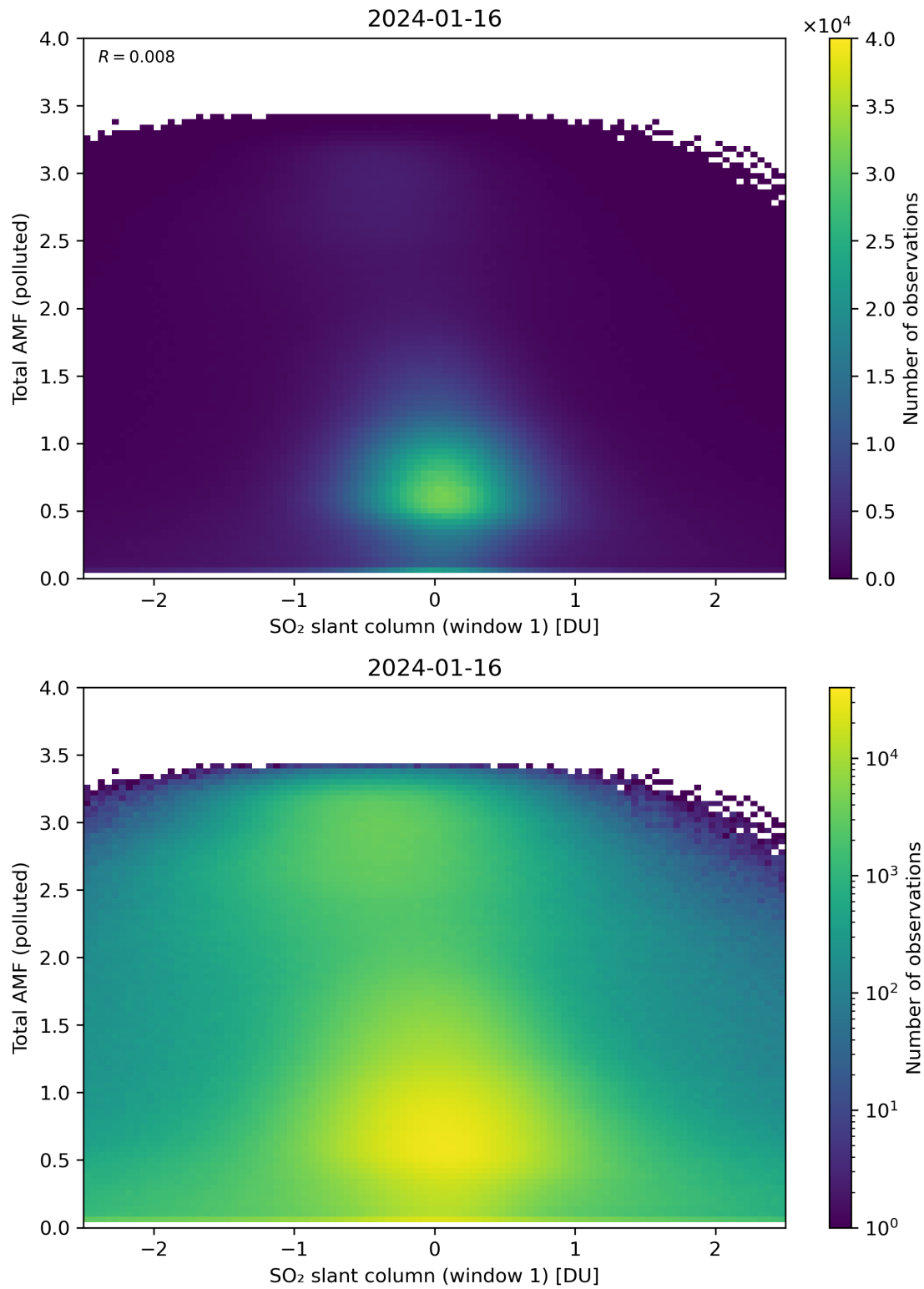
Figure 239: Scatter density plot of “SO 2 slant column (window 1)” against “Total AMF (polluted)” for 2024-01-15 to 2024-01-17.
