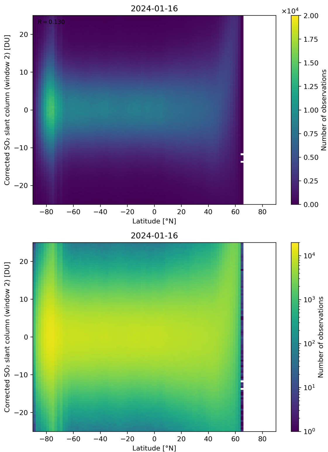
Figure 147: Scatter density plot of “Latitude” against “Corrected SO 2 slant column (window 2)” for 2024-01-15 to 2024-01-17.
