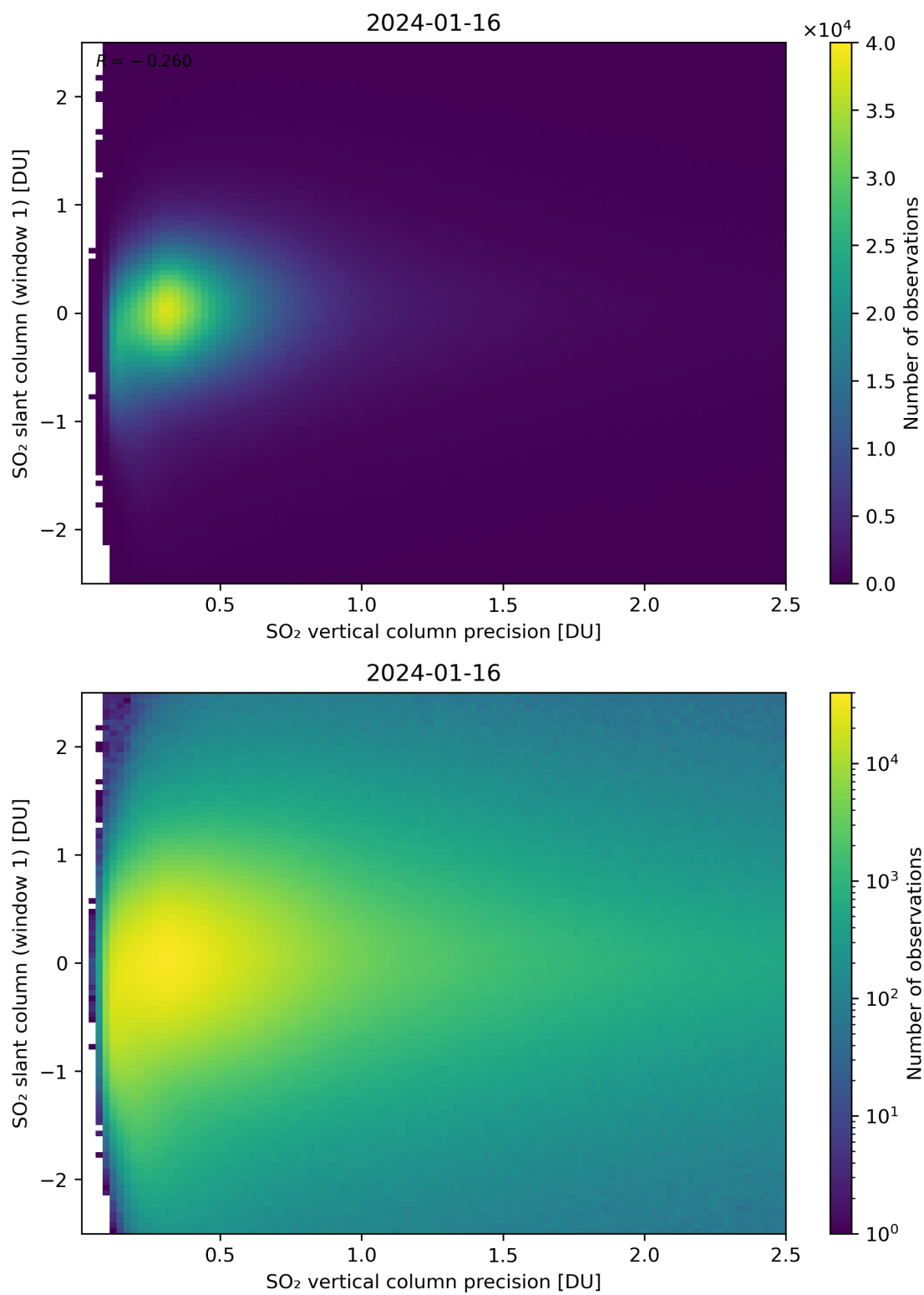
Figure 289: Scatter density plot of “SO 2 vertical column precision” against “SO 2 slant column (window 1)” for 2024-01-15 to 2024-01-17.
