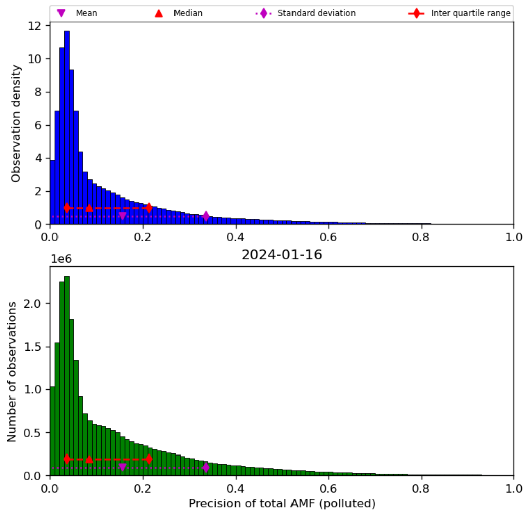
Figure 72: Histogram of “Precision of total AMF (polluted)” for 2024-01-15 to 2024-01-17
