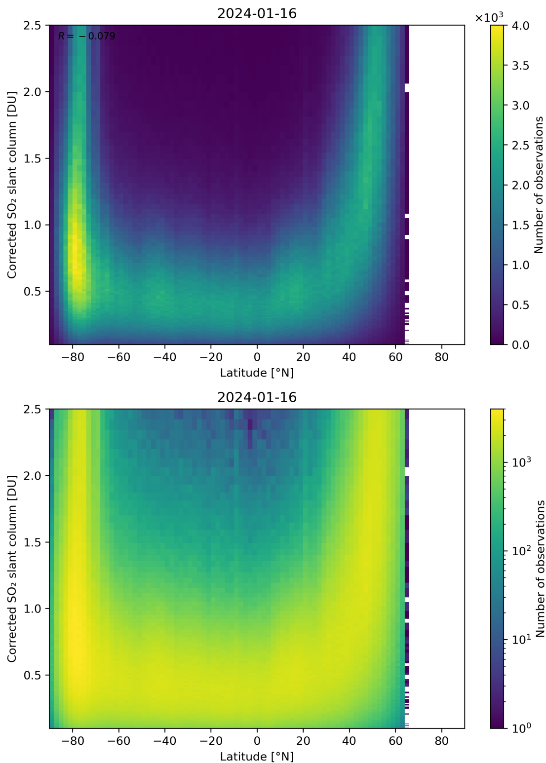
Figure 146: Scatter density plot of “Latitude” against “Corrected SO 2 slant column” for 2024-01-15 to 2024-01-17.
