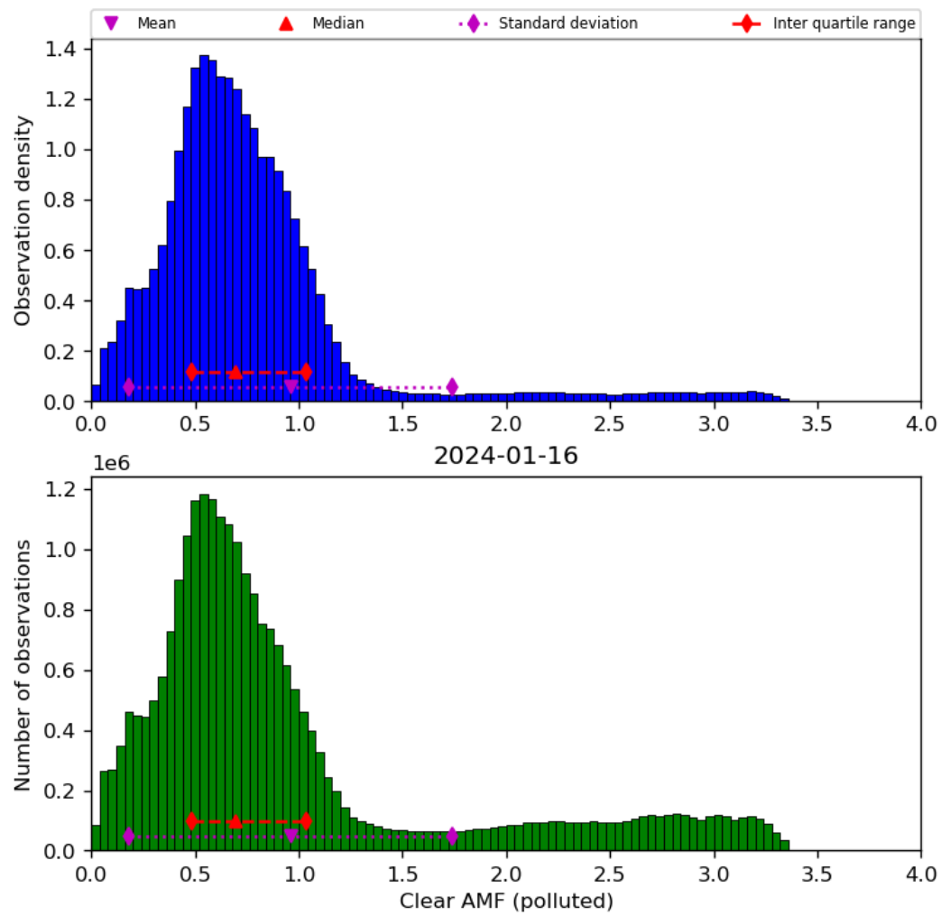
Figure 73: Histogram of “Clear AMF (polluted)” for 2024-01-15 to 2024-01-17
