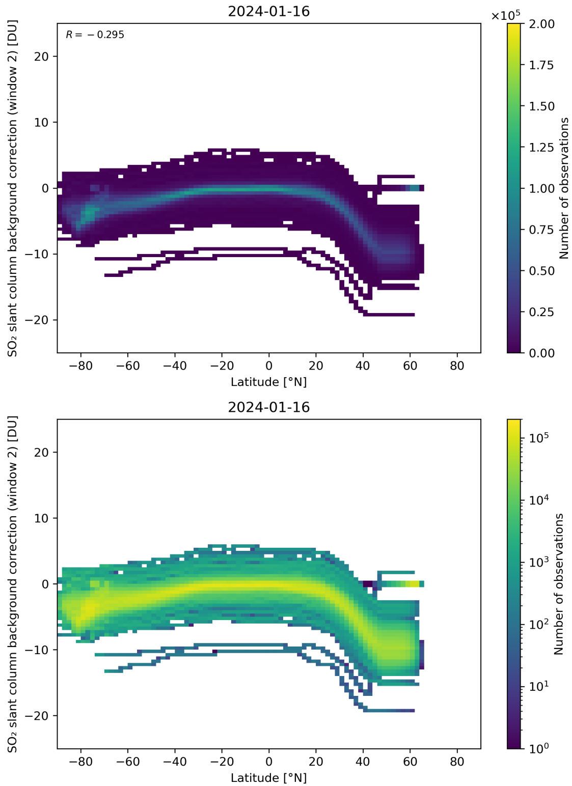
Figure 140: Scatter density plot of “Latitude” against “SO 2 slant column background correction (window 2)” for 2024-01-15 to 2024-01-17.
