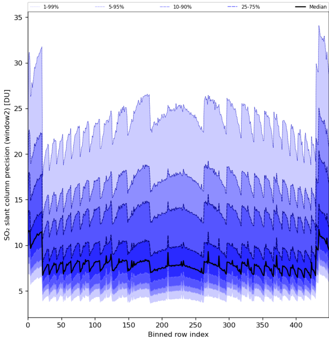
Figure 84: Along track statistics of “SO 2 slant column precision (window2)” for 2024-01-15 to 2024-01-17
