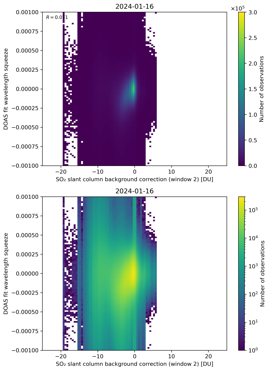
Figure 113: Scatter density plot of “SO 2 slant column background correction (window 2)” against “DOAS fit wavelength squeeze” for 2024-01-15 to 2024-01-17.
