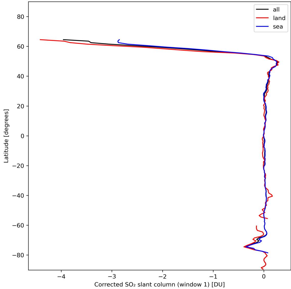
Figure 35: Zonal average of “Corrected SO 2 slant column (window 1)” for 2024-01-15 to 2024-01-17.
