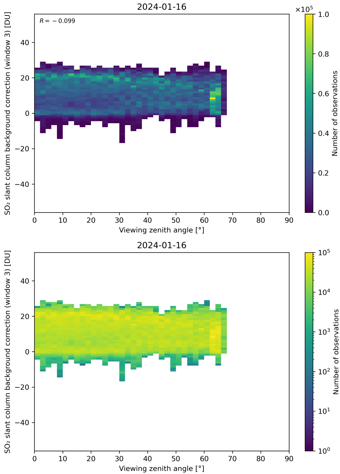
Figure 310: Scatter density plot of “Viewing zenith angle” against “SO 2 slant column background correction (window 3)” for 2024-01-15 to 2024-01-17.
