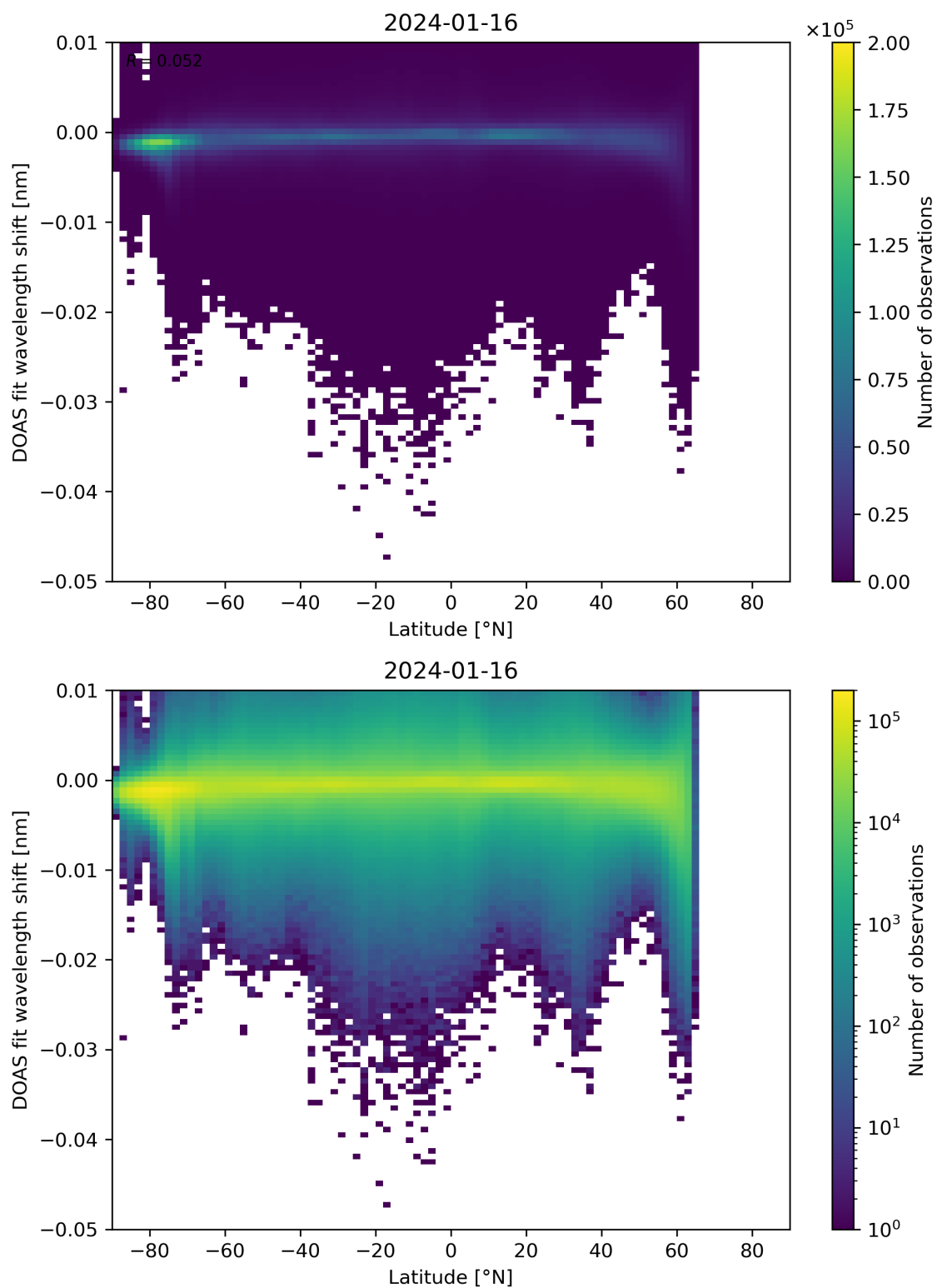
Figure 142: Scatter density plot of “Latitude” against “DOAS fit wavelength shift” for 2024-01-15 to 2024-01-17.
