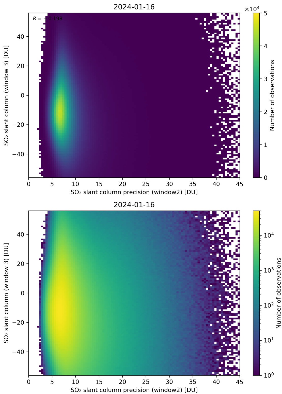
Figure 249: Scatter density plot of “SO 2 slant column precision (window2)” against “SO 2 slant column (window 3)” for 2024-01-15 to 2024-01-17.
