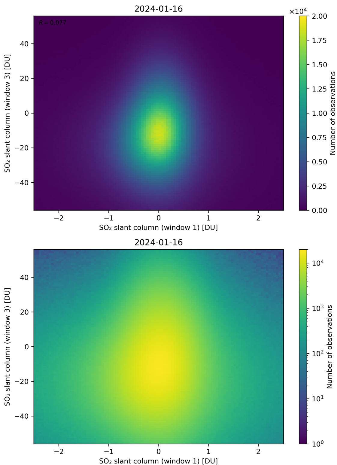
Figure 237: Scatter density plot of “SO 2 slant column (window 1)” against “SO 2 slant column (window 3)” for 2024-01-15 to 2024-01-17.
