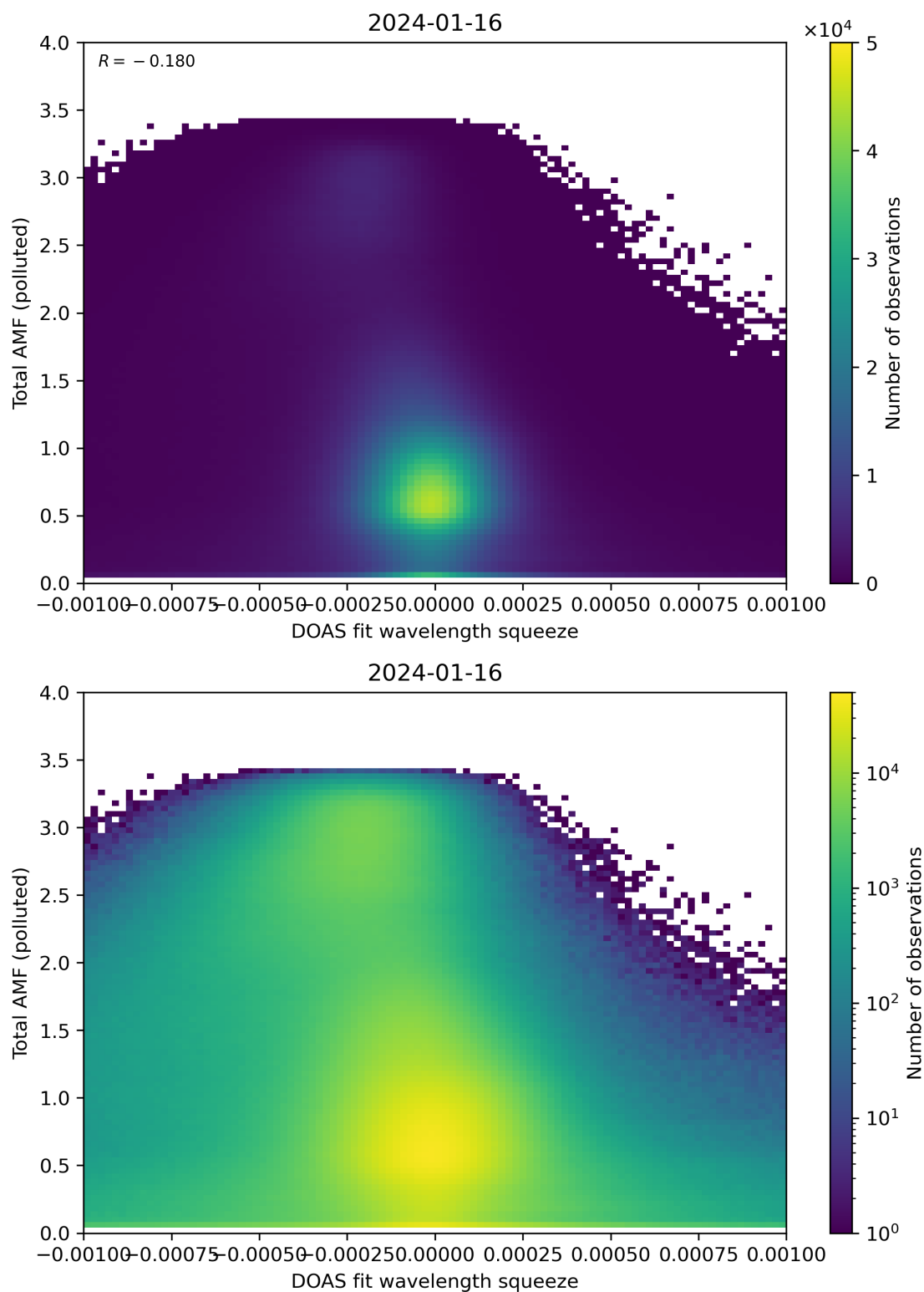
Figure 134: Scatter density plot of “DOAS fit wavelength squeeze” against “Total AMF (polluted)” for 2024-01-15 to 2024-01-17.
