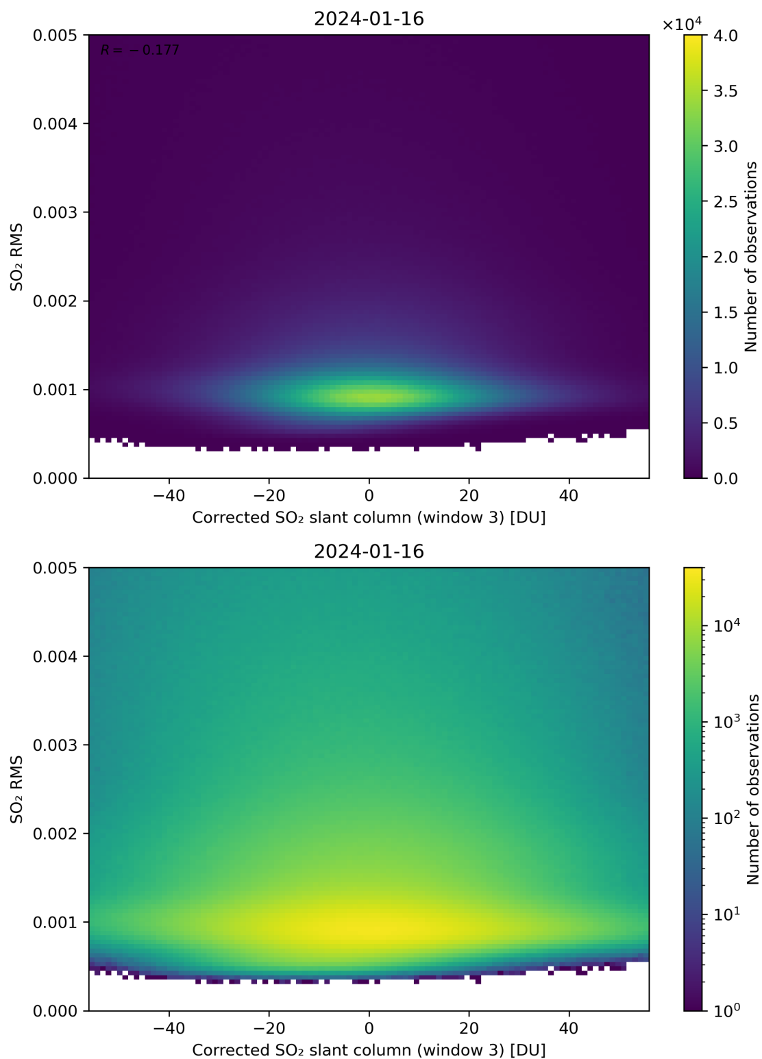
Figure 208: Scatter density plot of “Corrected SO 2 slant column (window 3)” against “SO 2 RMS” for 2024-01-15 to 2024-01-17.
