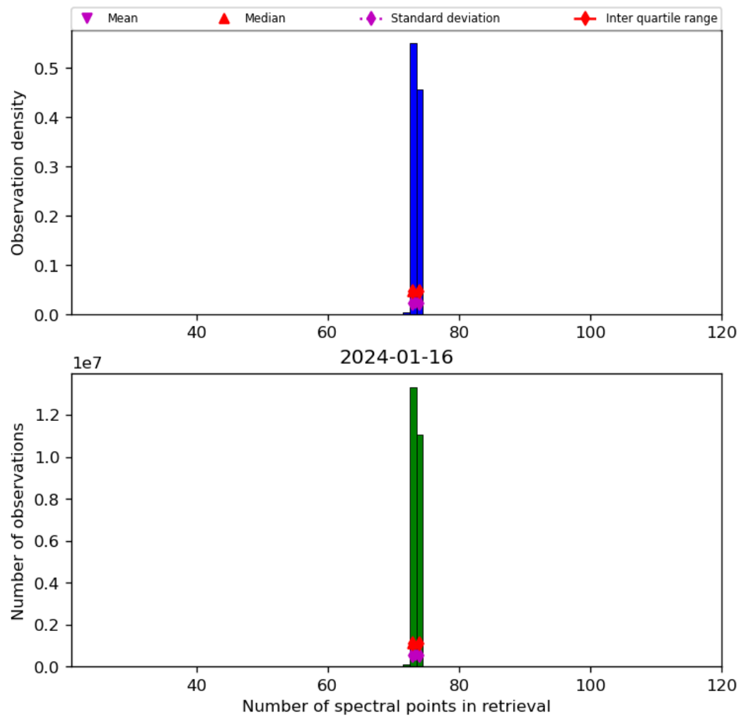
Figure 74: Histogram of “Number of spectral points in retrieval” for 2024-01-15 to 2024-01-17
