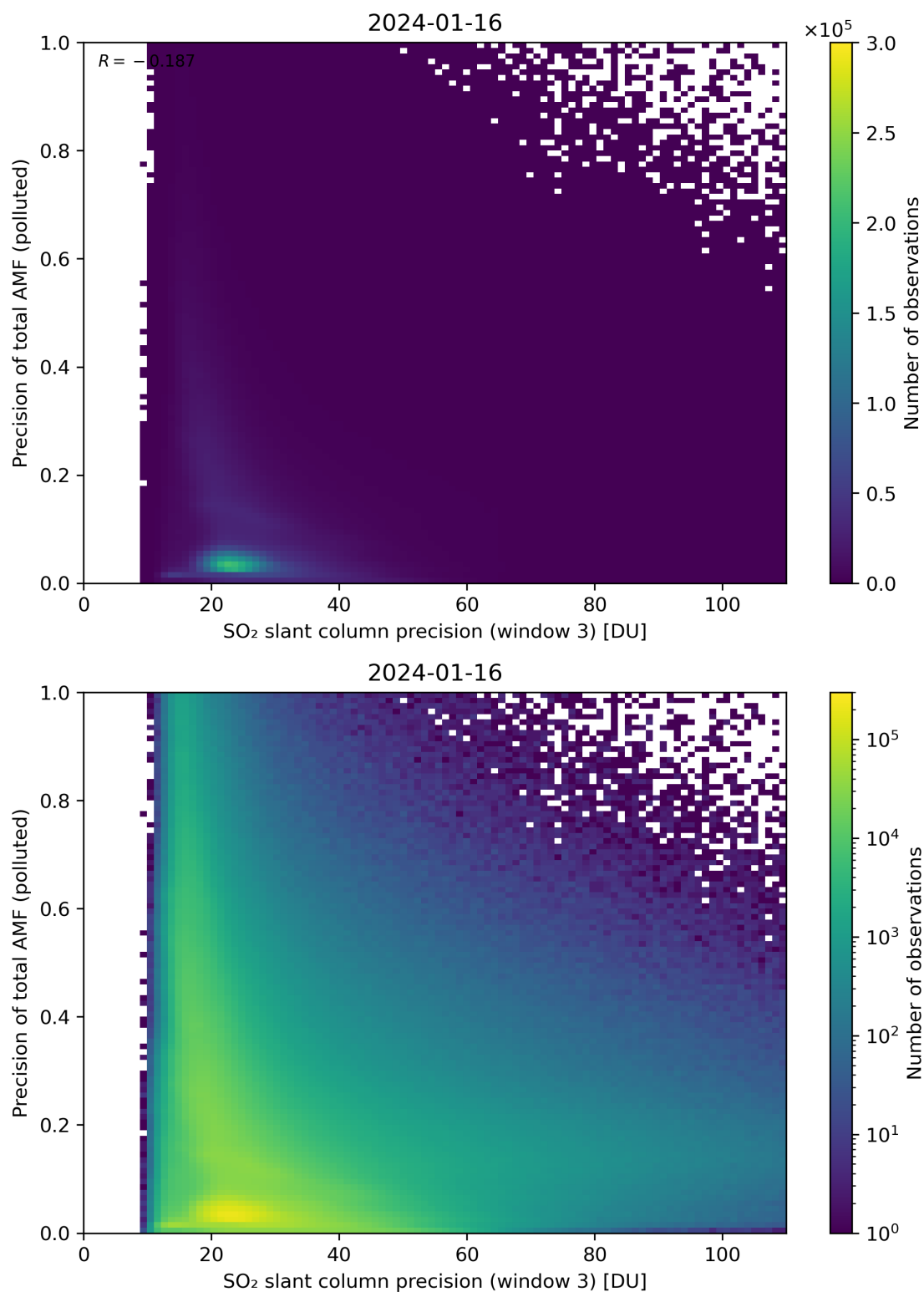
Figure 264: Scatter density plot of “SO 2 slant column precision (window 3)” against “Precision of total AMF (polluted)” for 2024-01-15 to 2024-01-17.
