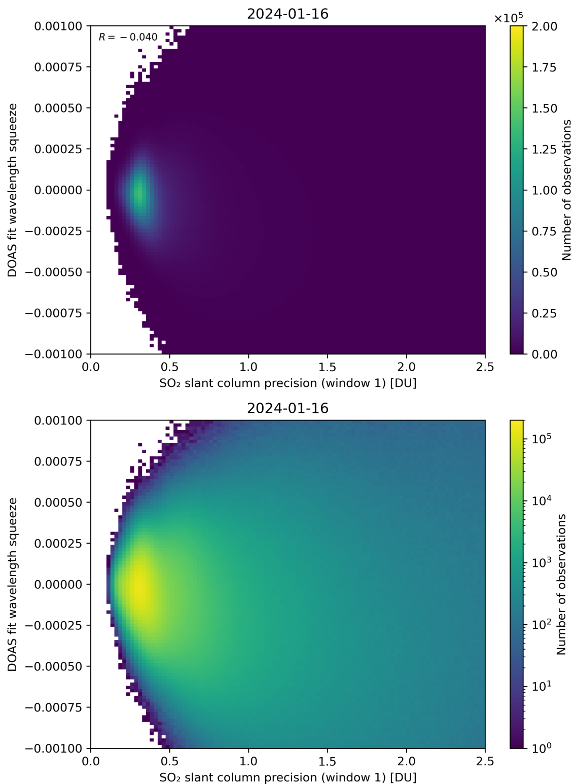
Figure 222: Scatter density plot of “SO 2 slant column precision (window 1)” against “DOAS fit wavelength squeeze” for 2024-01-15 to 2024-01-17.
