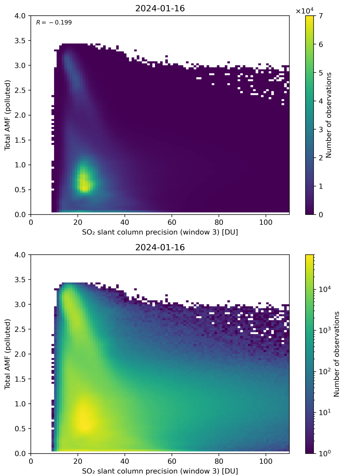
Figure 263: Scatter density plot of “SO 2 slant column precision (window 3)” against “Total AMF (polluted)” for 2024-01-15 to 2024-01-17.
