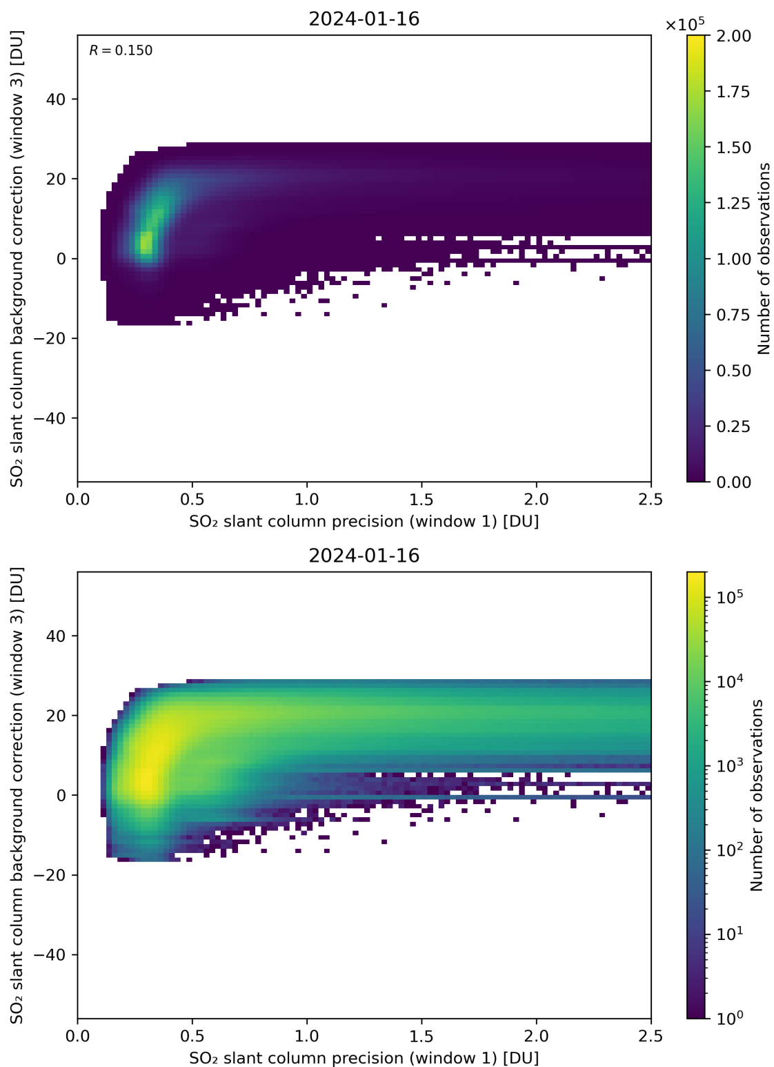
Figure 220: Scatter density plot of “SO 2 slant column precision (window 1)” against “SO 2 slant column background correction (window 3)” for 2024-01-15 to 2024-01-17.
