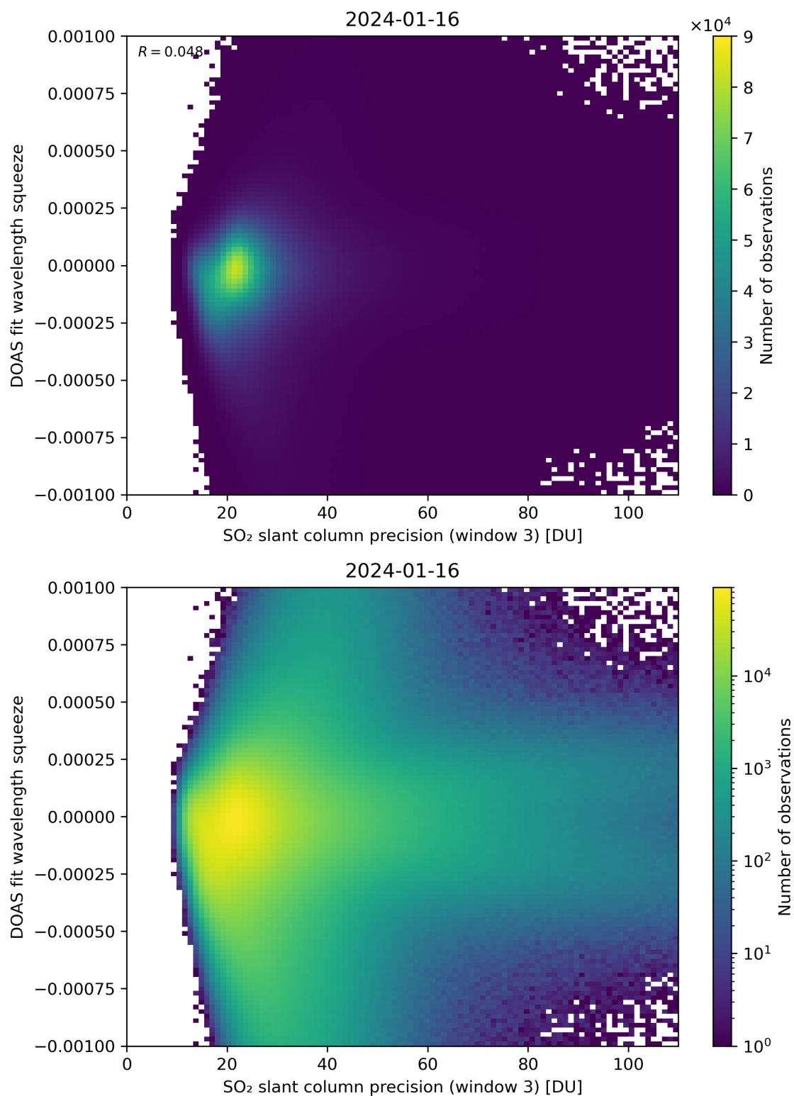
Figure 259: Scatter density plot of “SO 2 slant column precision (window 3)” against “DOAS fit wavelength squeeze” for 2024-01-15 to 2024-01-17.
