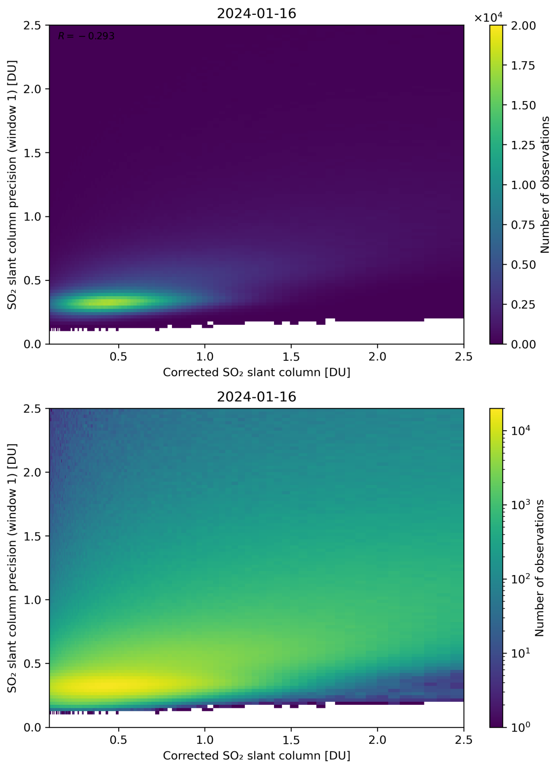
Figure 188: Scatter density plot of “Corrected SO 2 slant column” against “SO 2 slant column precision (window 1)” for 2024-01-15 to 2024-01-17.
