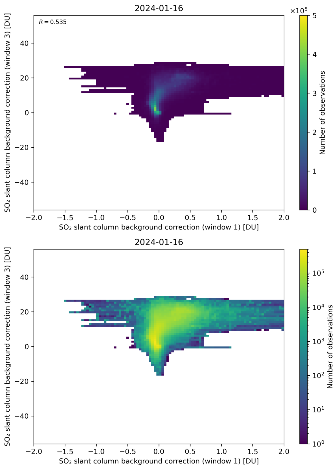
Figure 99: Scatter density plot of “SO 2 slant column background correction (window 1)” against “SO 2 slant column background correction (window 3)” for 2024-01-15 to 2024-01-17.
