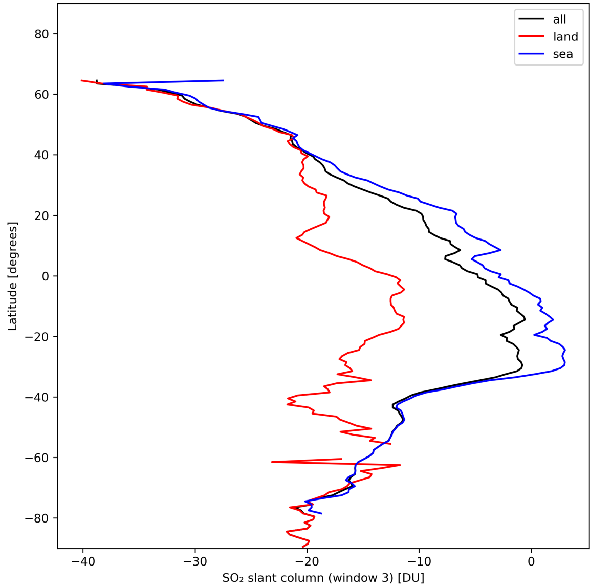
Figure 41: Zonal average of “SO 2 slant column (window 3)” for 2024-01-15 to 2024-01-17.
