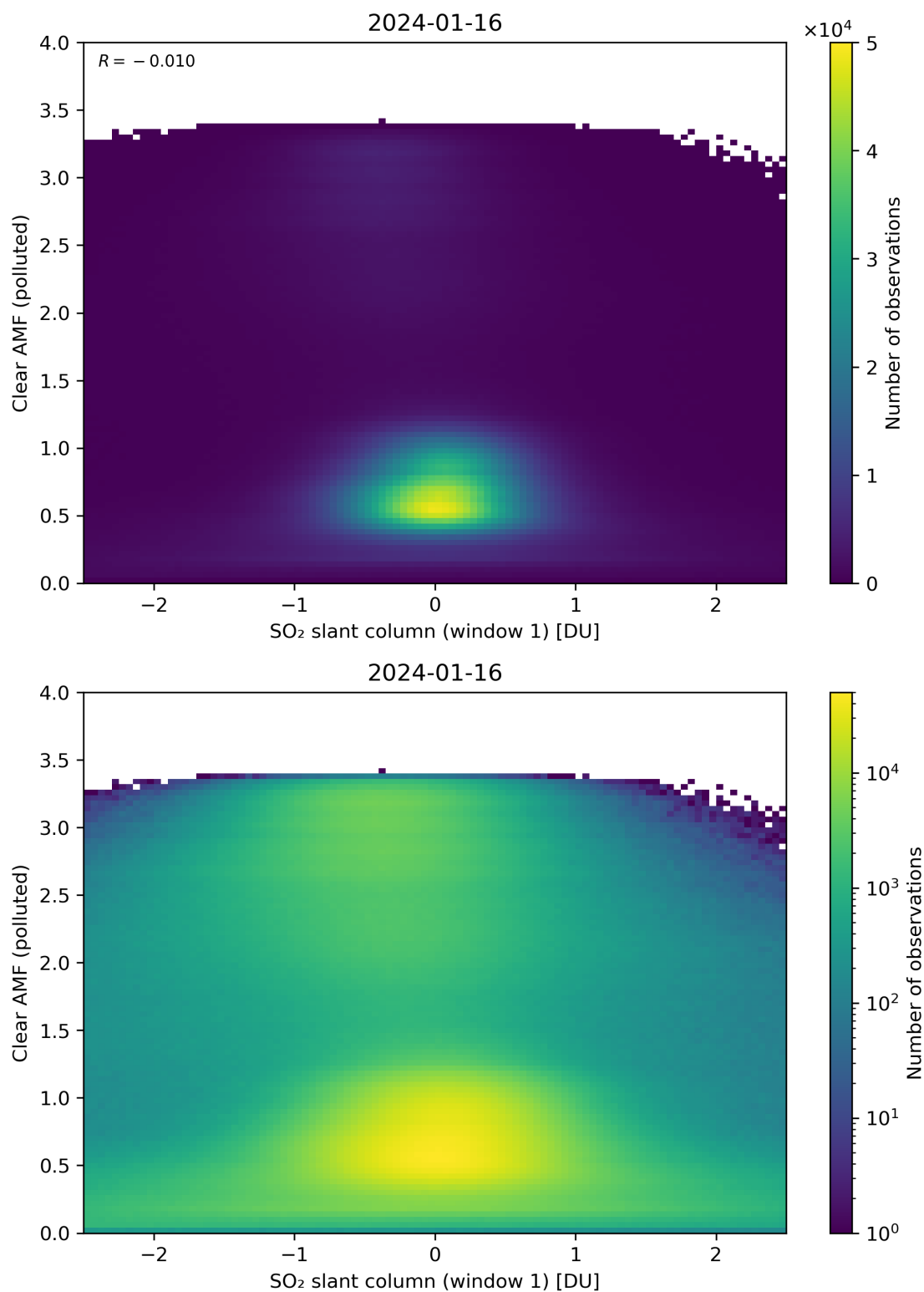
Figure 232: Scatter density plot of “SO 2 slant column (window 1)” against “Clear AMF (polluted)” for 2024-01-15 to 2024-01-17.
