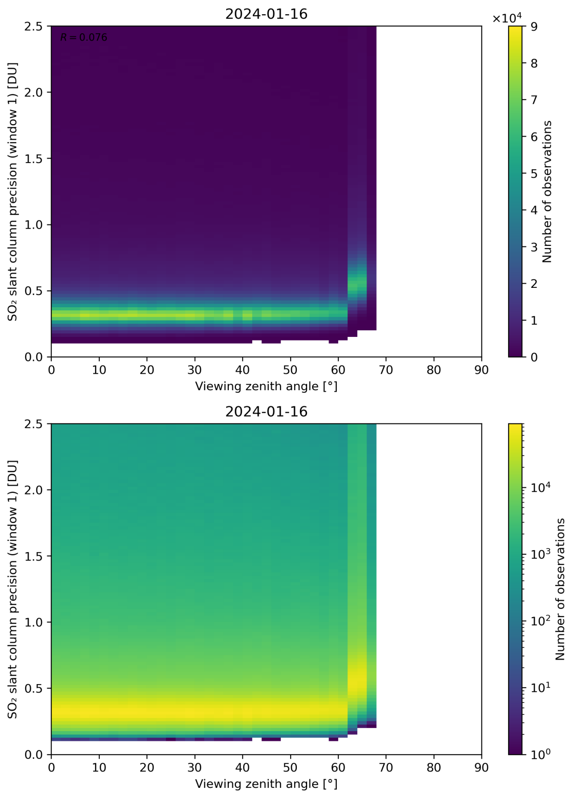
Figure 321: Scatter density plot of “Viewing zenith angle” against “SO 2 slant column precision (window 1)” for 2024-01-15 to 2024-01-17.
