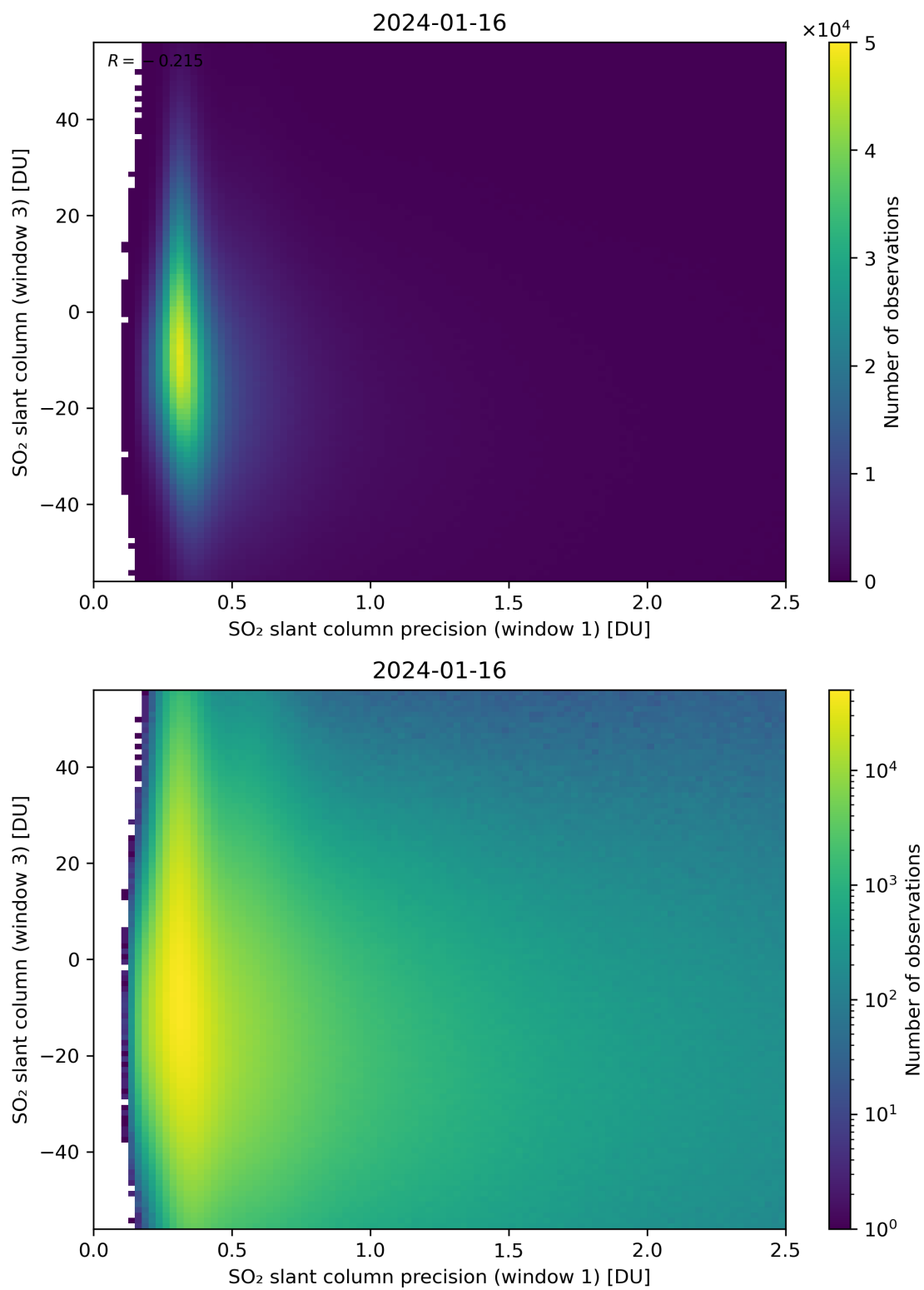
Figure 228: Scatter density plot of “SO 2 slant column precision (window 1)” against “SO 2 slant column (window 3)” for 2024-01-15 to 2024-01-17.
