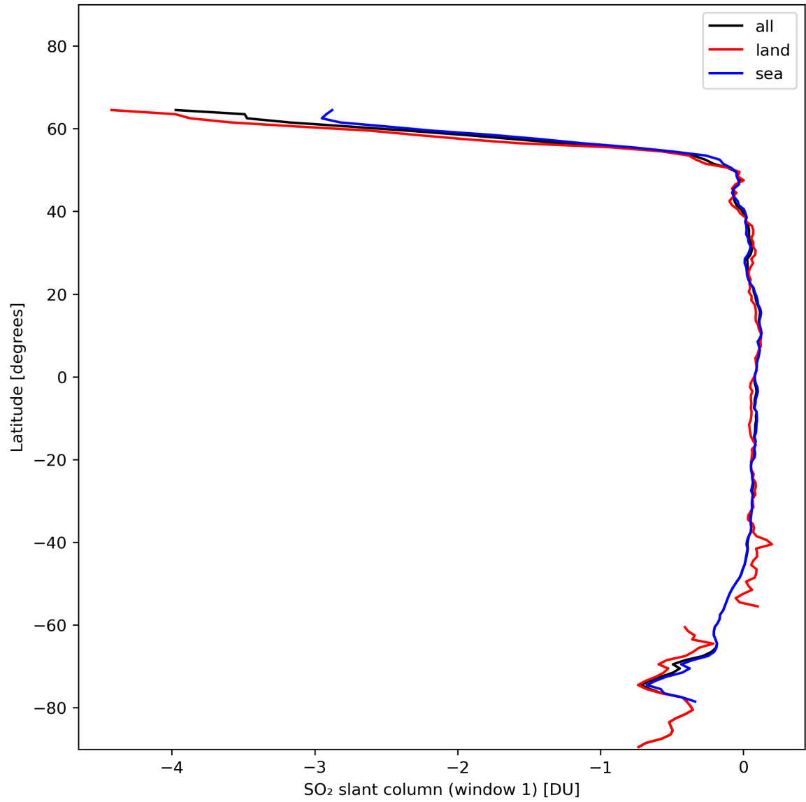
Figure 33: Zonal average of “SO 2 slant column (window 1)” for 2024-01-15 to 2024-01-17.
