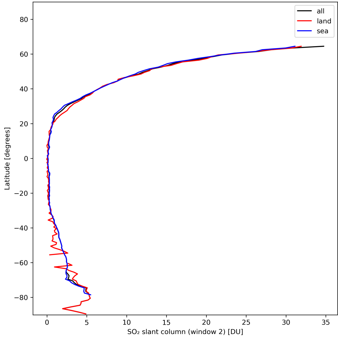
Figure 37: Zonal average of “SO 2 slant column (window 2)” for 2024-01-15 to 2024-01-17.
