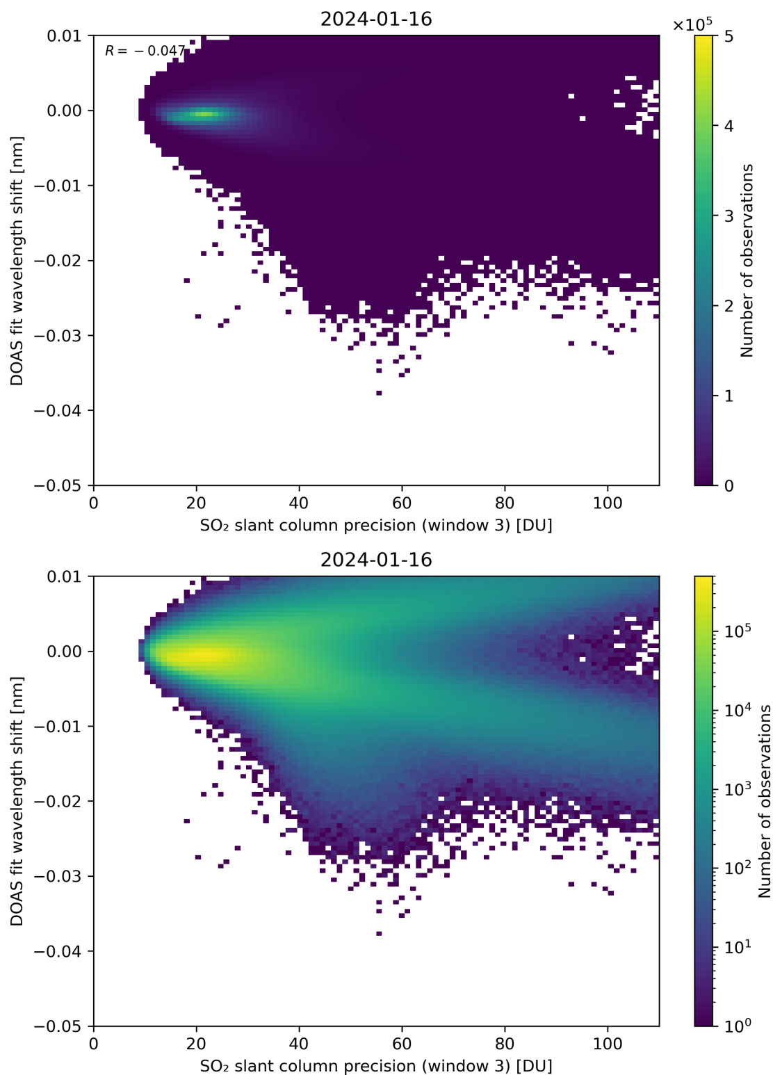
Figure 258: Scatter density plot of “SO 2 slant column precision (window 3)” against “DOAS fit wavelength shift” for 2024-01-15 to 2024-01-17.
