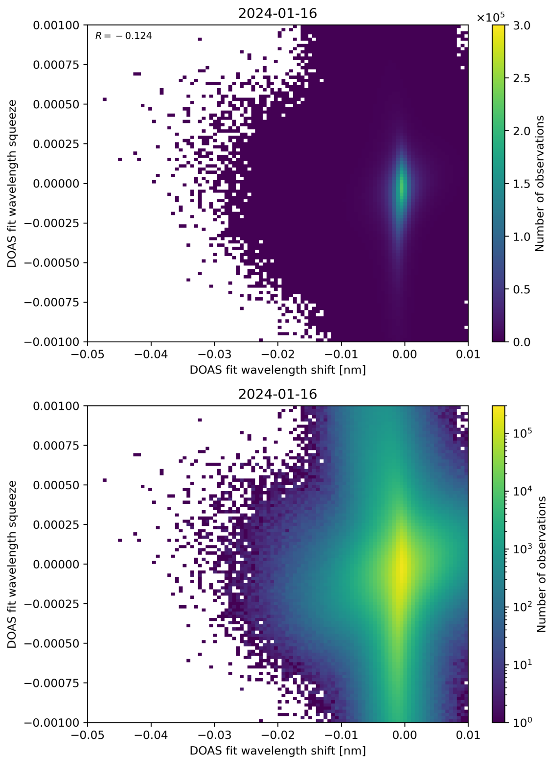
Figure 127: Scatter density plot of “DOAS fit wavelength shift” against “DOAS fit wavelength squeeze” for 2024-01-15 to 2024-01-17.
