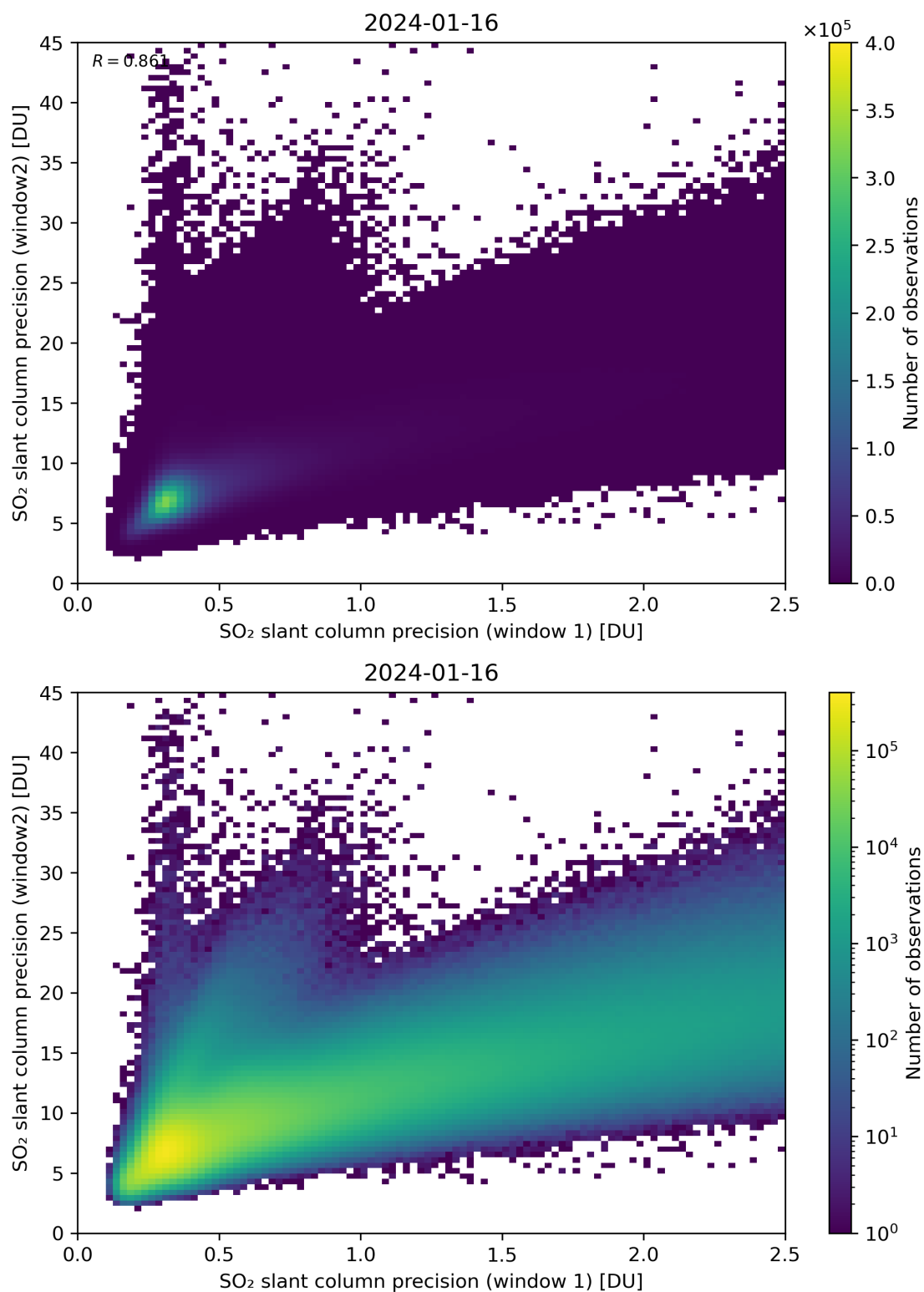
Figure 227: Scatter density plot of “SO 2 slant column precision (window 1)” against “SO 2 slant column precision (window2)” for 2024-01-15 to 2024-01-17.
