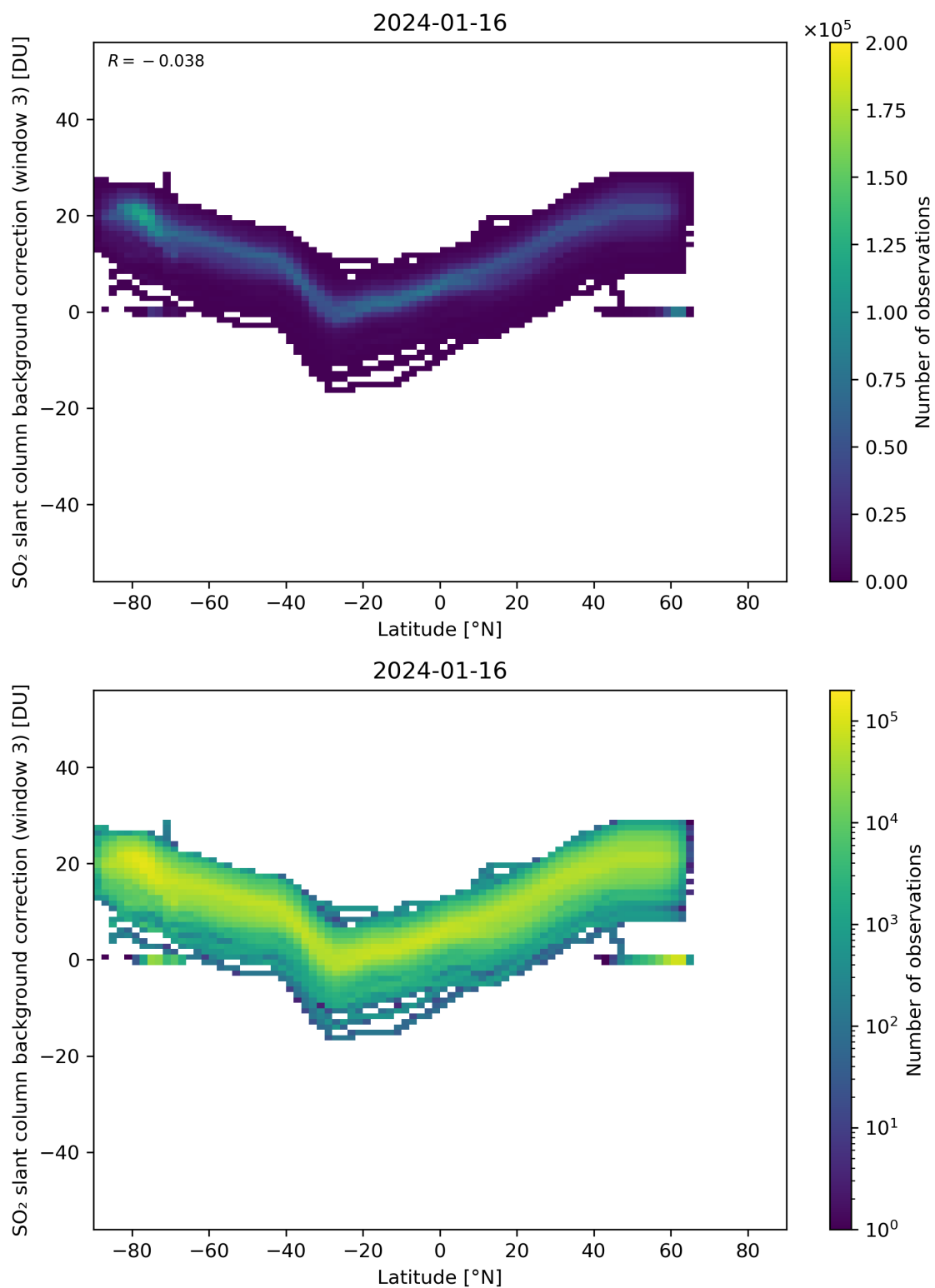
Figure 141: Scatter density plot of “Latitude” against “SO 2 slant column background correction (window 3)” for 2024-01-15 to 2024-01-17.
