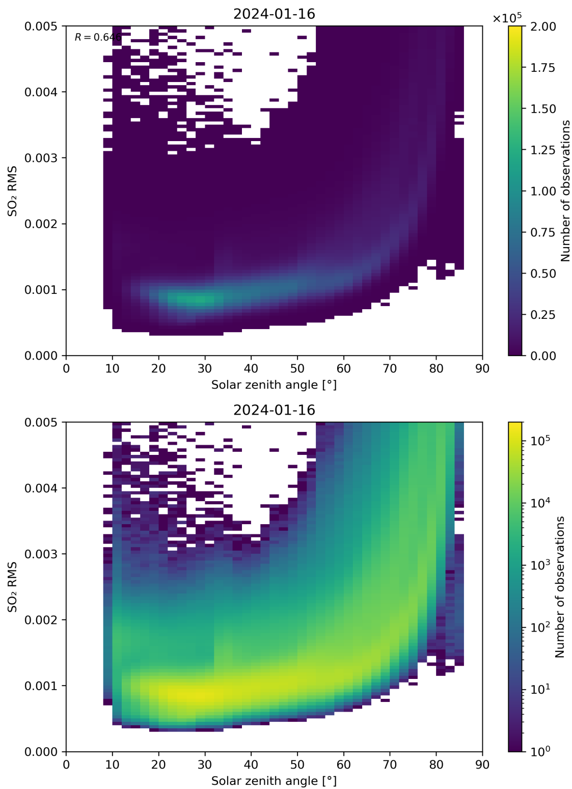
Figure 163: Scatter density plot of “Solar zenith angle” against “SO 2 RMS” for 2024-01-15 to 2024-01-17.
