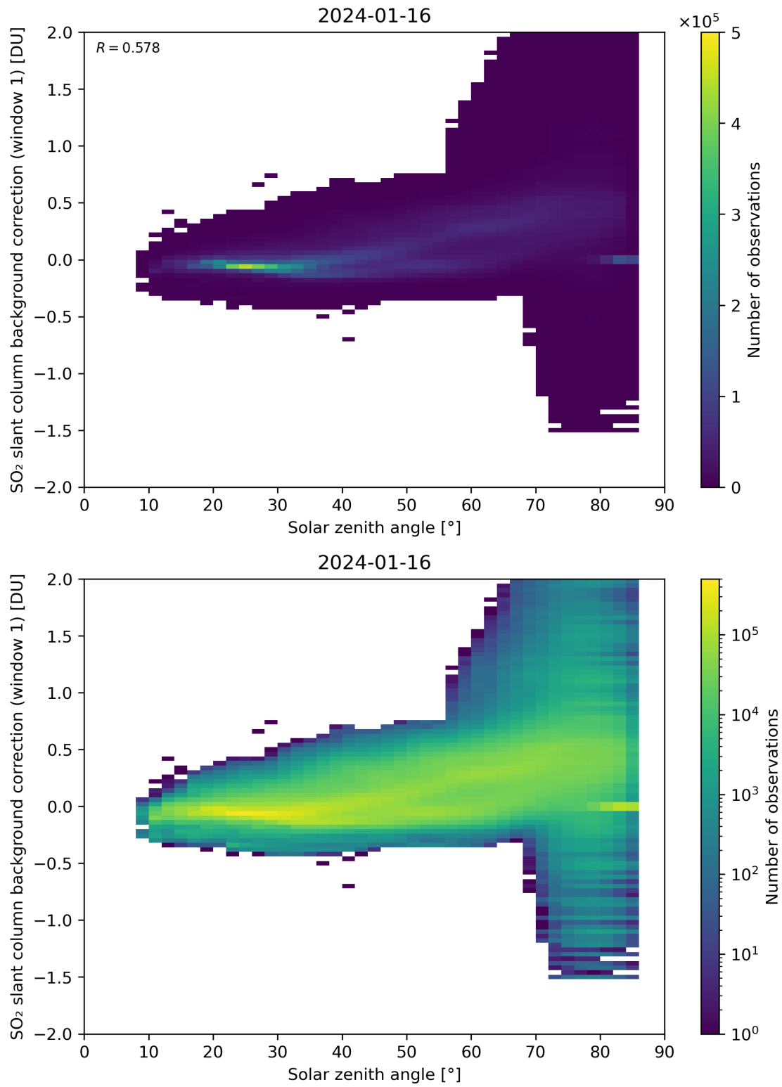
Figure 158: Scatter density plot of “Solar zenith angle” against “SO 2 slant column background correction (window 1)” for 2024-01-15 to 2024-01-17.
