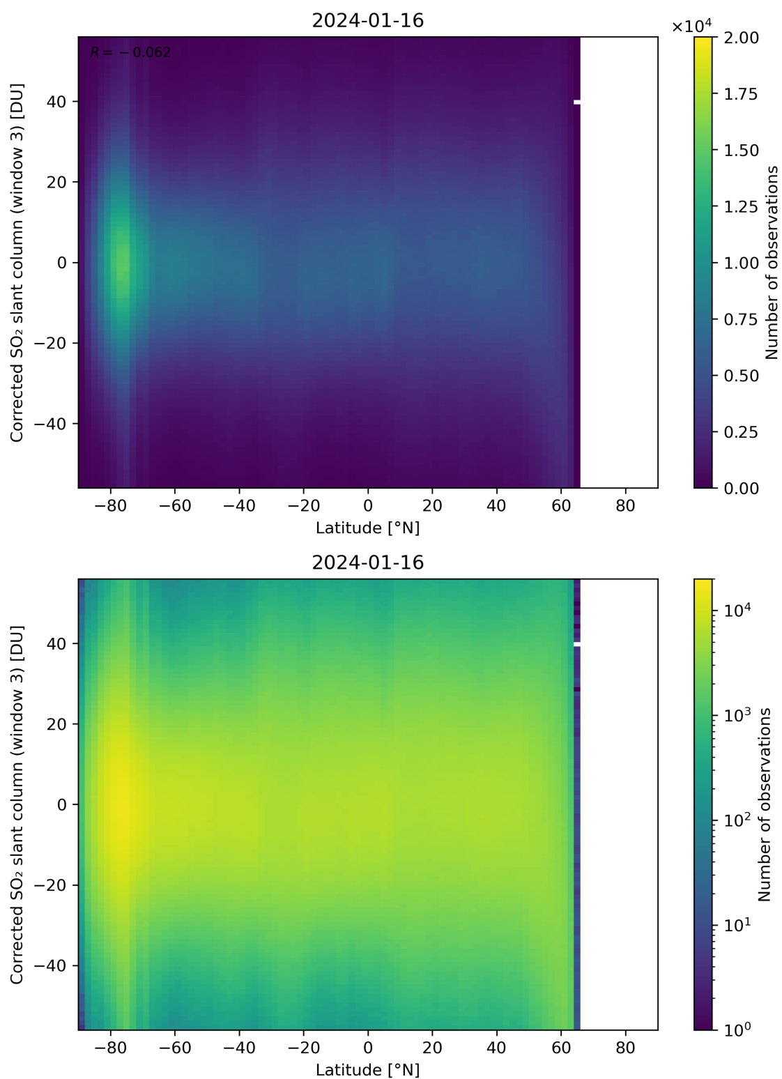
Figure 148: Scatter density plot of “Latitude” against “Corrected SO 2 slant column (window 3)” for 2024-01-15 to 2024-01-17.
