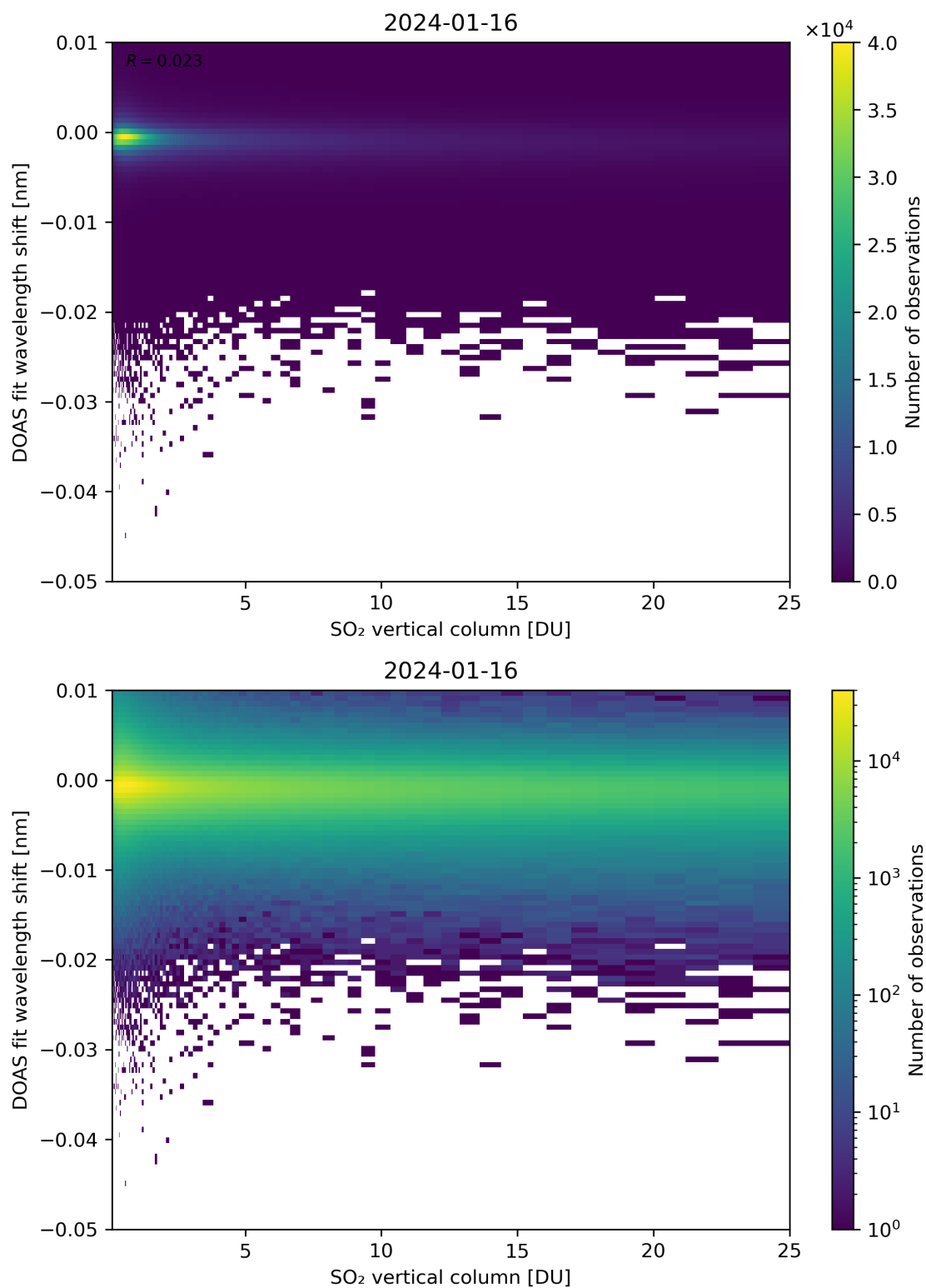
Figure 276: Scatter density plot of “SO 2 vertical column” against “DOAS fit wavelength shift” for 2024-01-15 to 2024-01-17.
