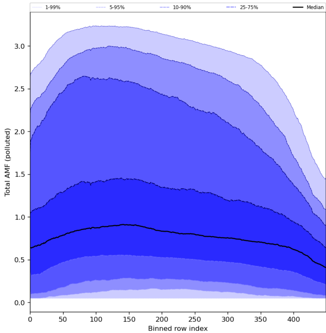
Figure 94: Along track statistics of “Total AMF (polluted)” for 2024-01-15 to 2024-01-17
