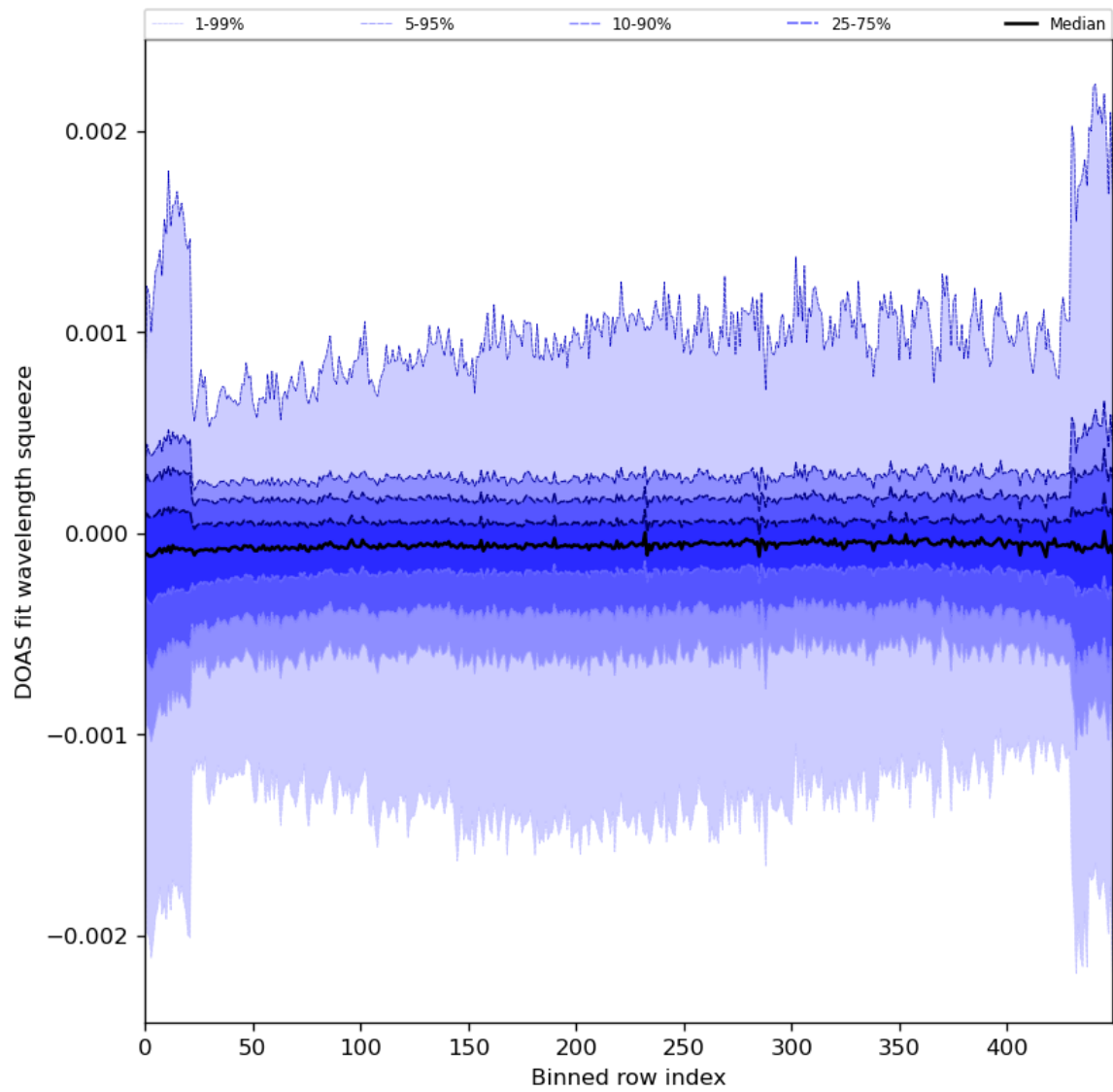
Figure 92: Along track statistics of “DOAS fit wavelength squeeze” for 2024-01-15 to 2024-01-17
