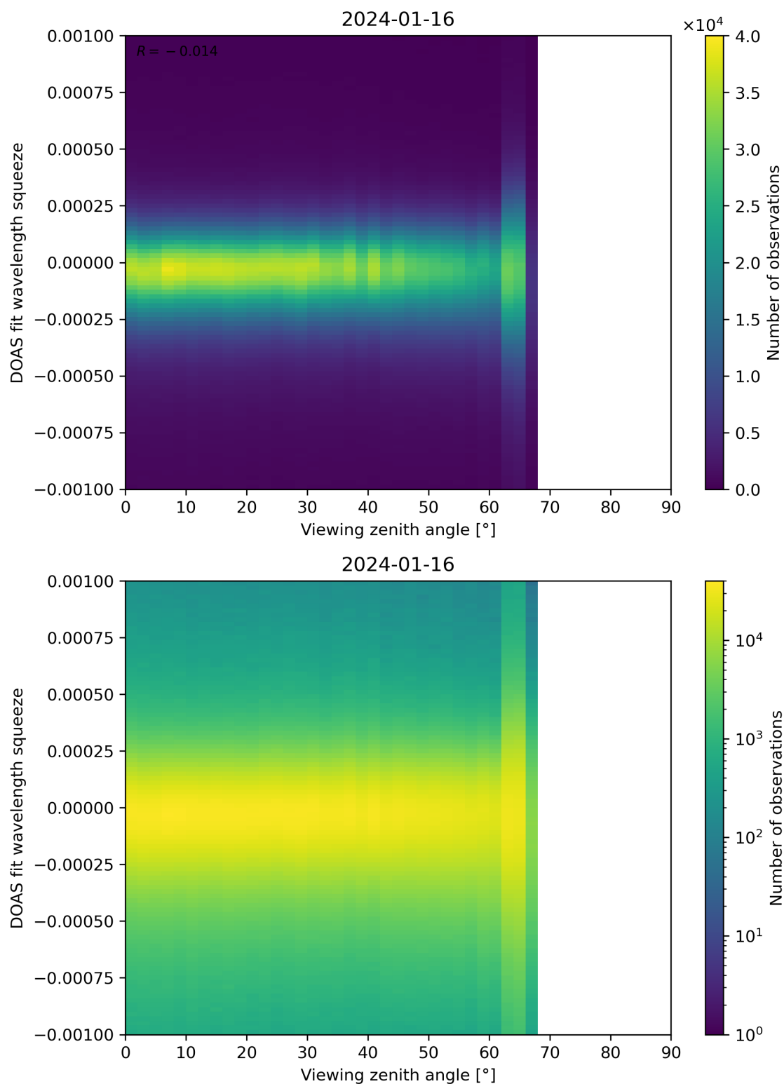
Figure 312: Scatter density plot of “Viewing zenith angle” against “DOAS fit wavelength squeeze” for 2024-01-15 to 2024-01-17.
