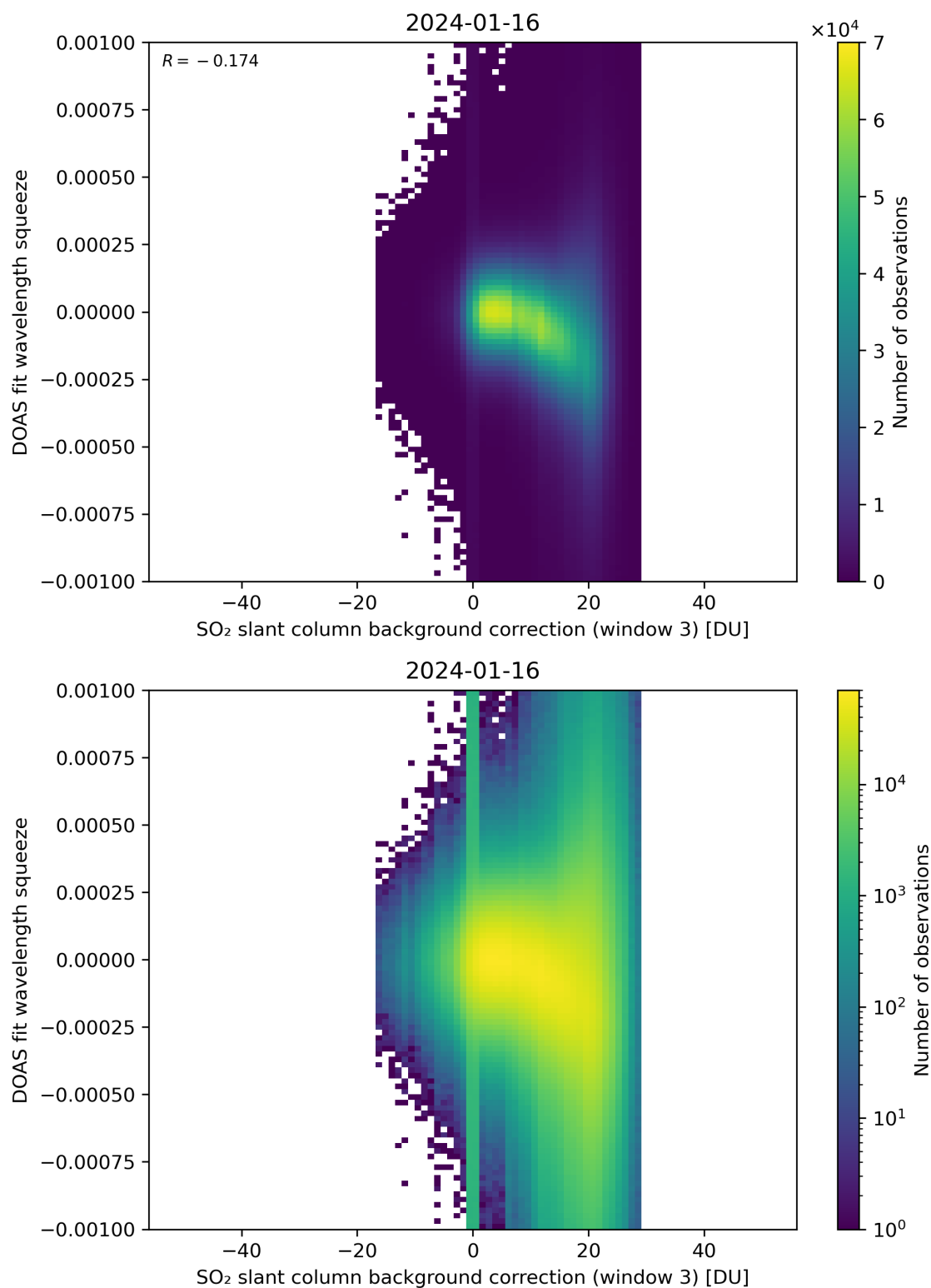
Figure 122: Scatter density plot of “SO 2 slant column background correction (window 3)” against “DOAS fit wavelength squeeze” for 2024-01-15 to 2024-01-17.
