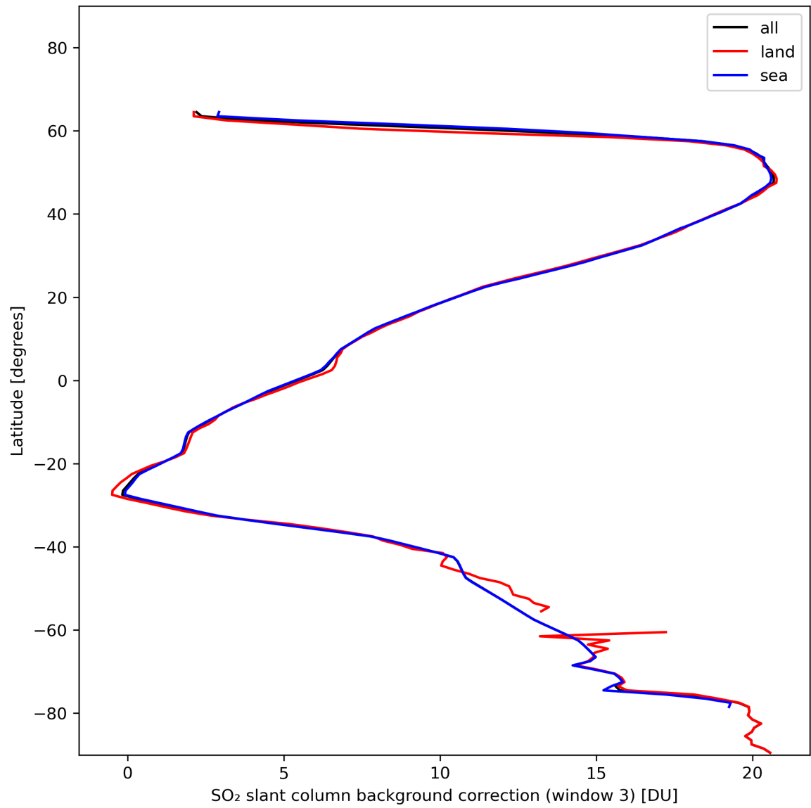
Figure 44: Zonal average of “SO 2 slant column background correction (window 3)” for 2024-01-15 to 2024-01-17.
