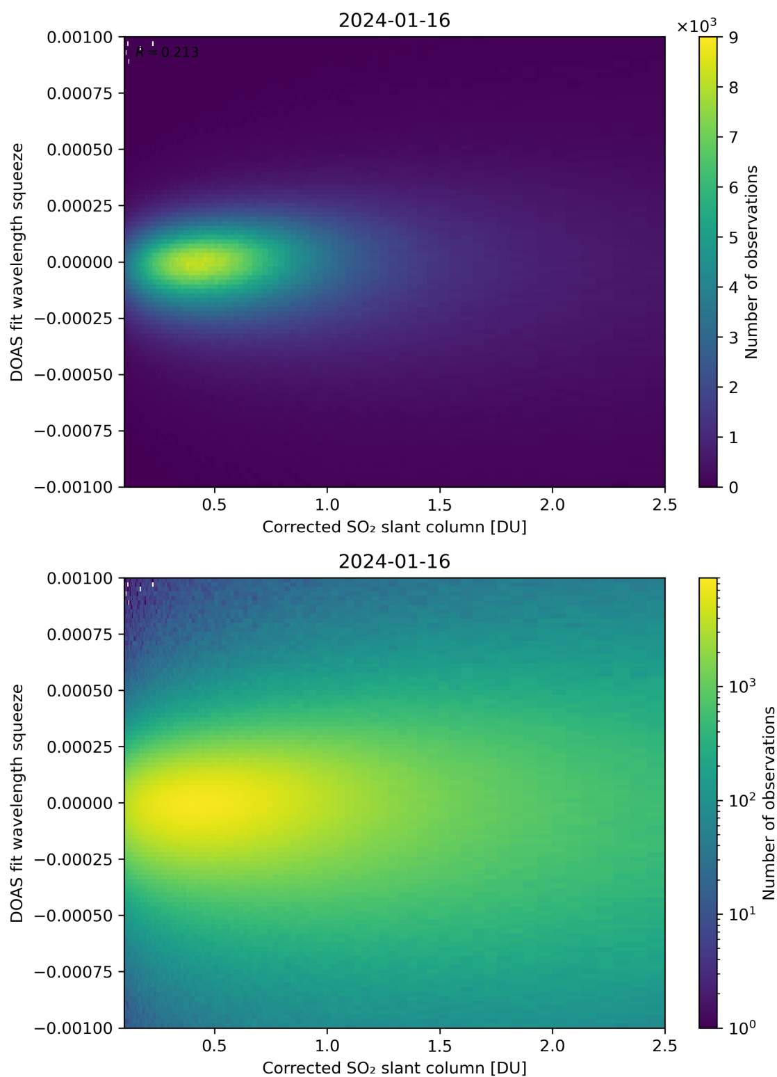
Figure 182: Scatter density plot of “Corrected SO 2 slant column” against “DOAS fit wavelength squeeze” for 2024-01-15 to 2024-01-17.
