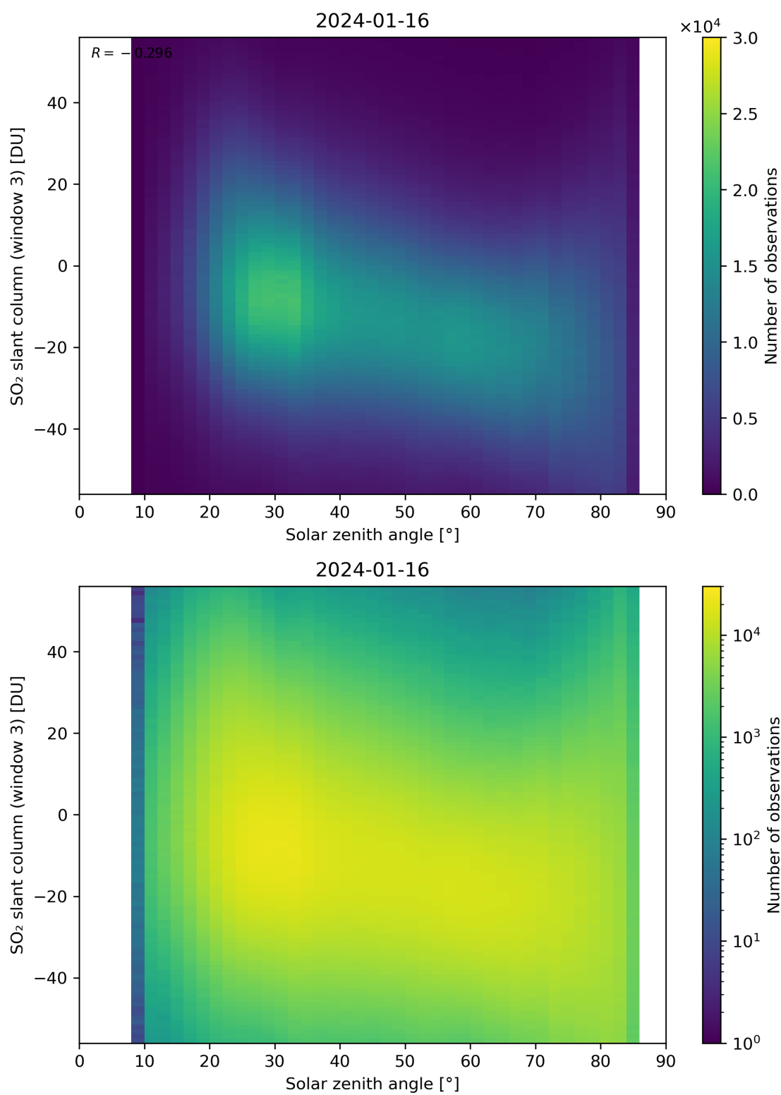
Figure 172: Scatter density plot of “Solar zenith angle” against “SO 2 slant column (window 3)” for 2024-01-15 to 2024-01-17.
