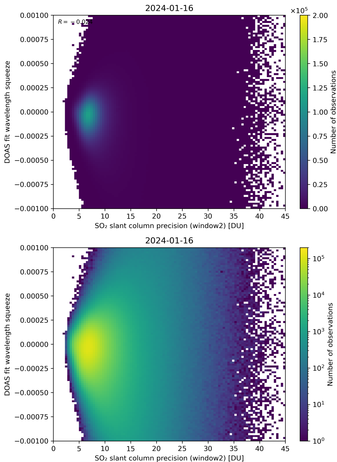
Figure 244: Scatter density plot of “SO 2 slant column precision (window2)” against “DOAS fit wavelength squeeze” for 2024-01-15 to 2024-01-17.
