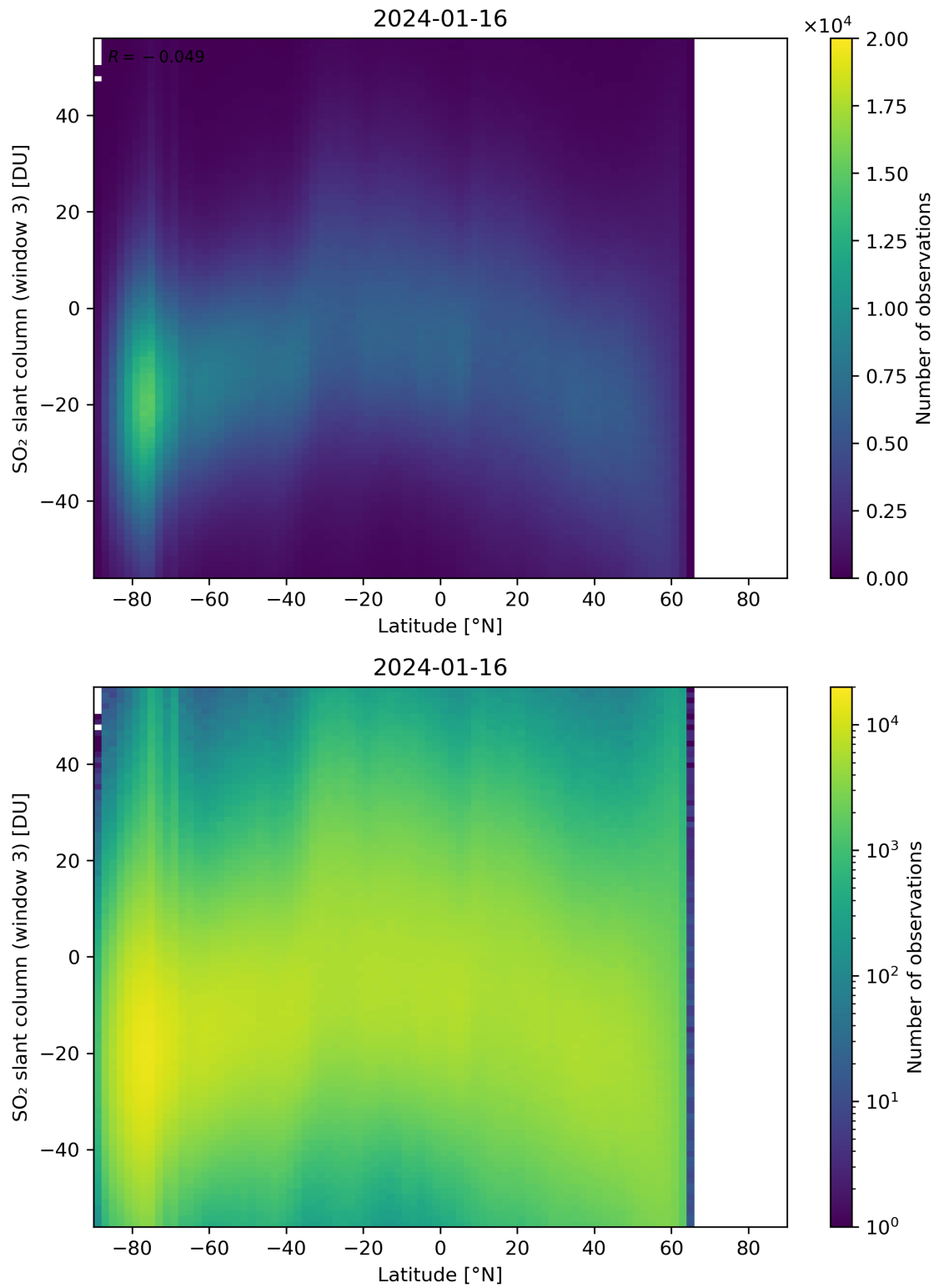
Figure 152: Scatter density plot of “Latitude” against “SO 2 slant column (window 3)” for 2024-01-15 to 2024-01-17.
