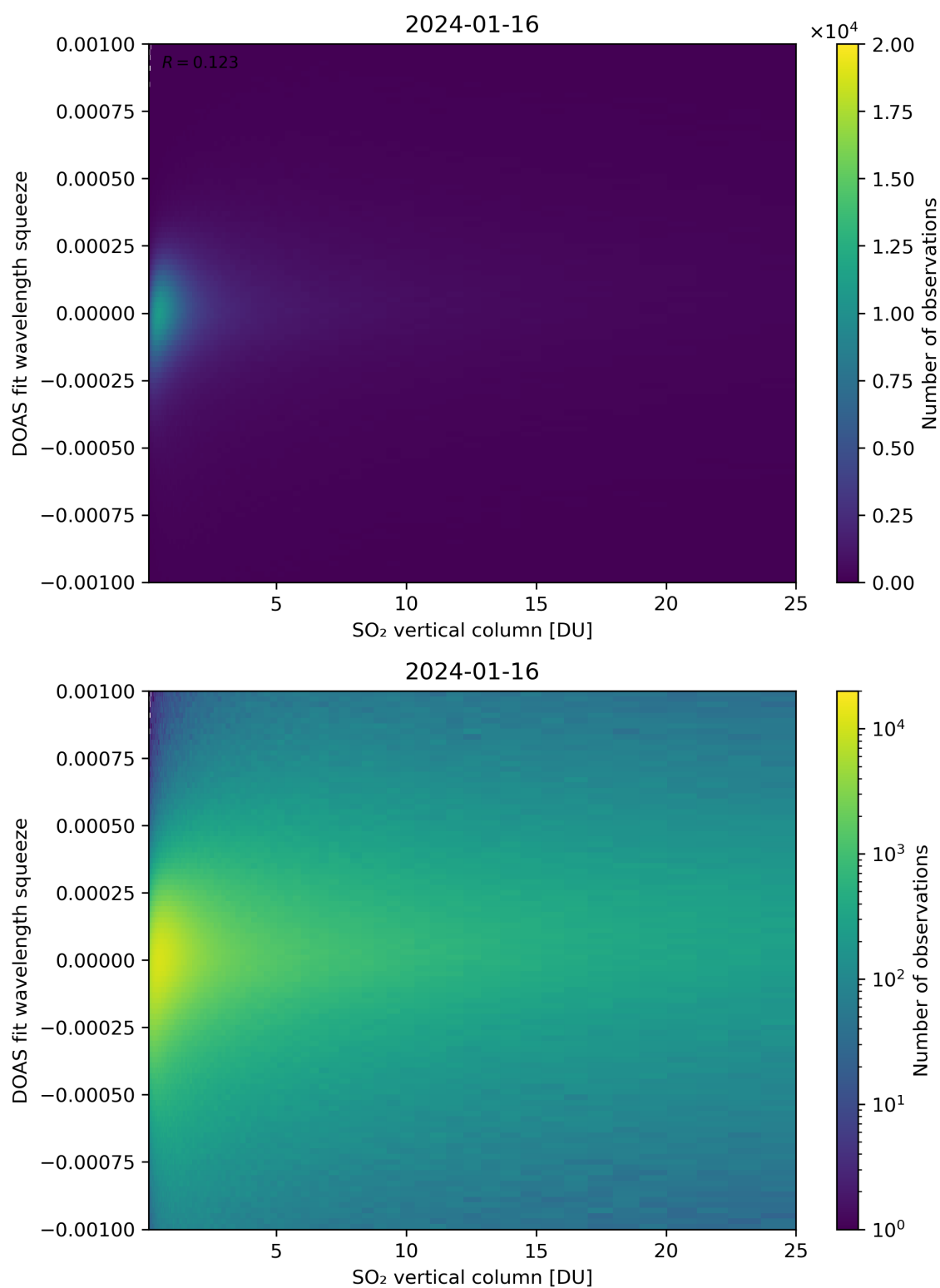
Figure 277: Scatter density plot of “SO 2 vertical column” against “DOAS fit wavelength squeeze” for 2024-01-15 to 2024-01-17.
