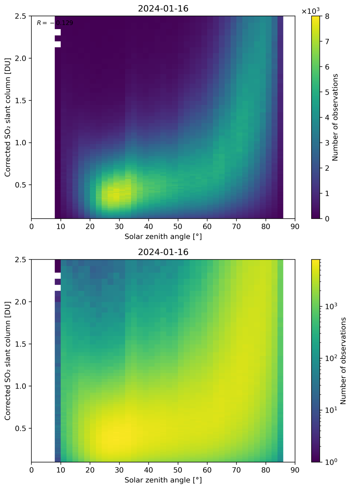
Figure 166: Scatter density plot of “Solar zenith angle” against “Corrected SO 2 slant column” for 2024-01-15 to 2024-01-17.
