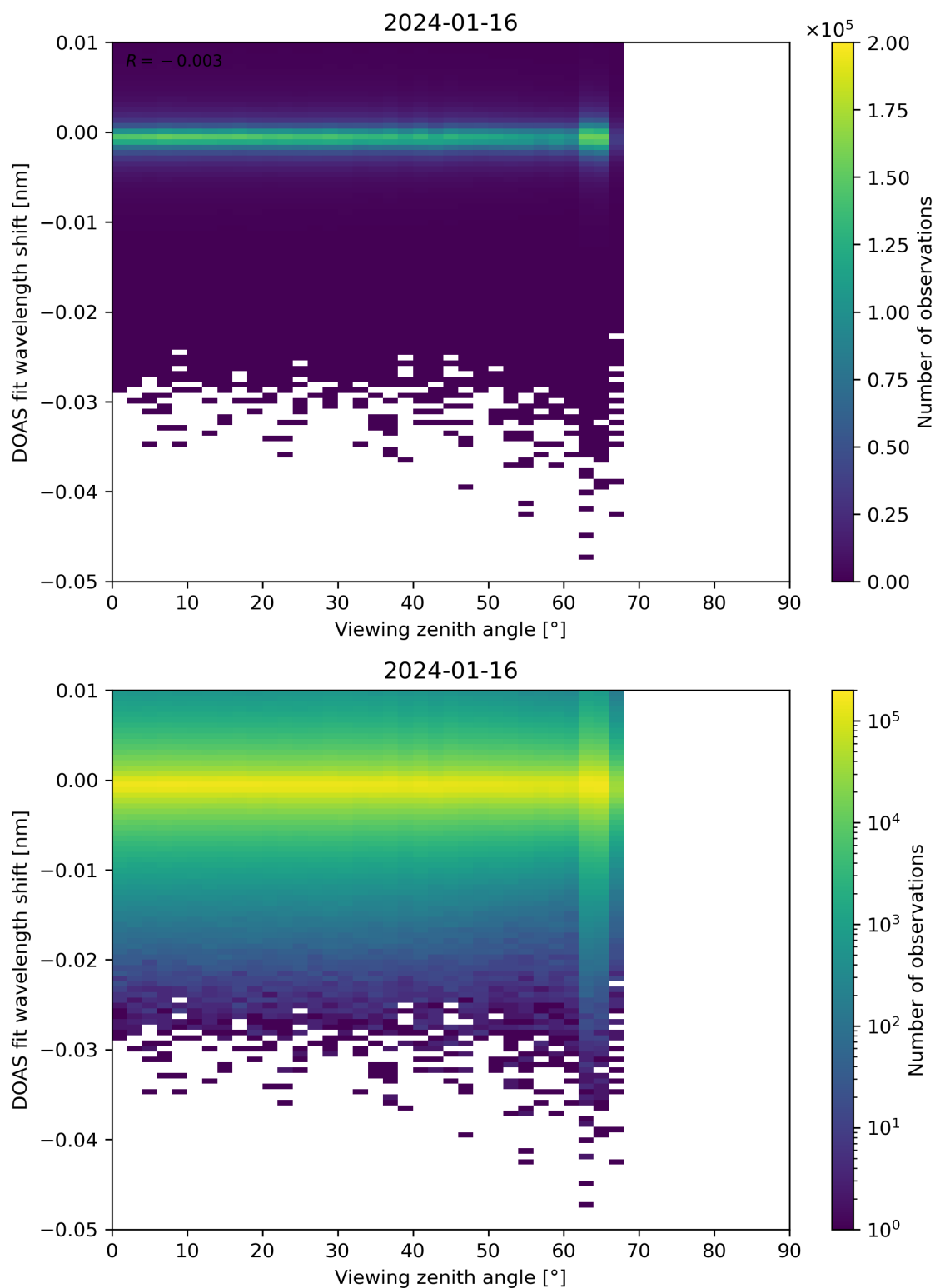
Figure 311: Scatter density plot of “Viewing zenith angle” against “DOAS fit wavelength shift” for 2024-01-15 to 2024-01-17.
