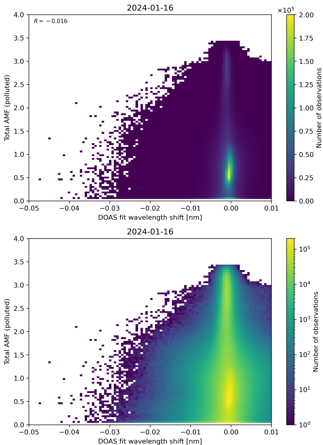
Figure 130: Scatter density plot of “DOAS fit wavelength shift” against “Total AMF (polluted)” for 2024-01-15 to 2024-01-17.
