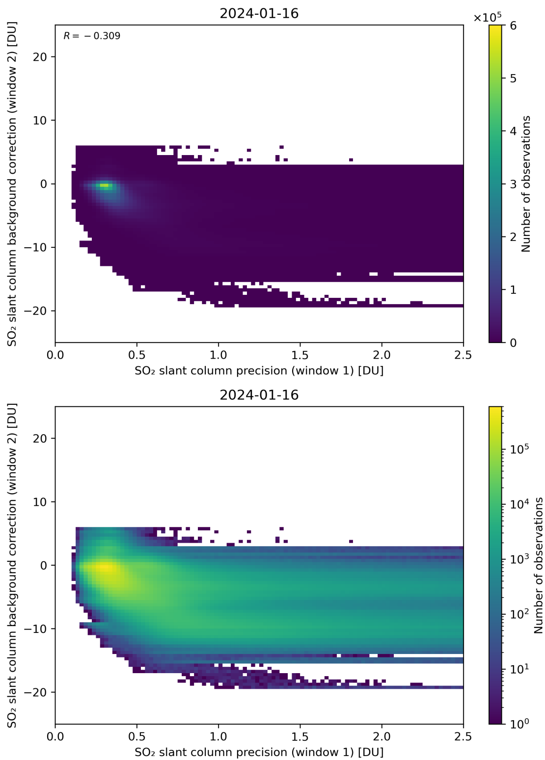
Figure 219: Scatter density plot of “SO 2 slant column precision (window 1)” against “SO 2 slant column background correction (window 2)” for 2024-01-15 to 2024-01-17.
