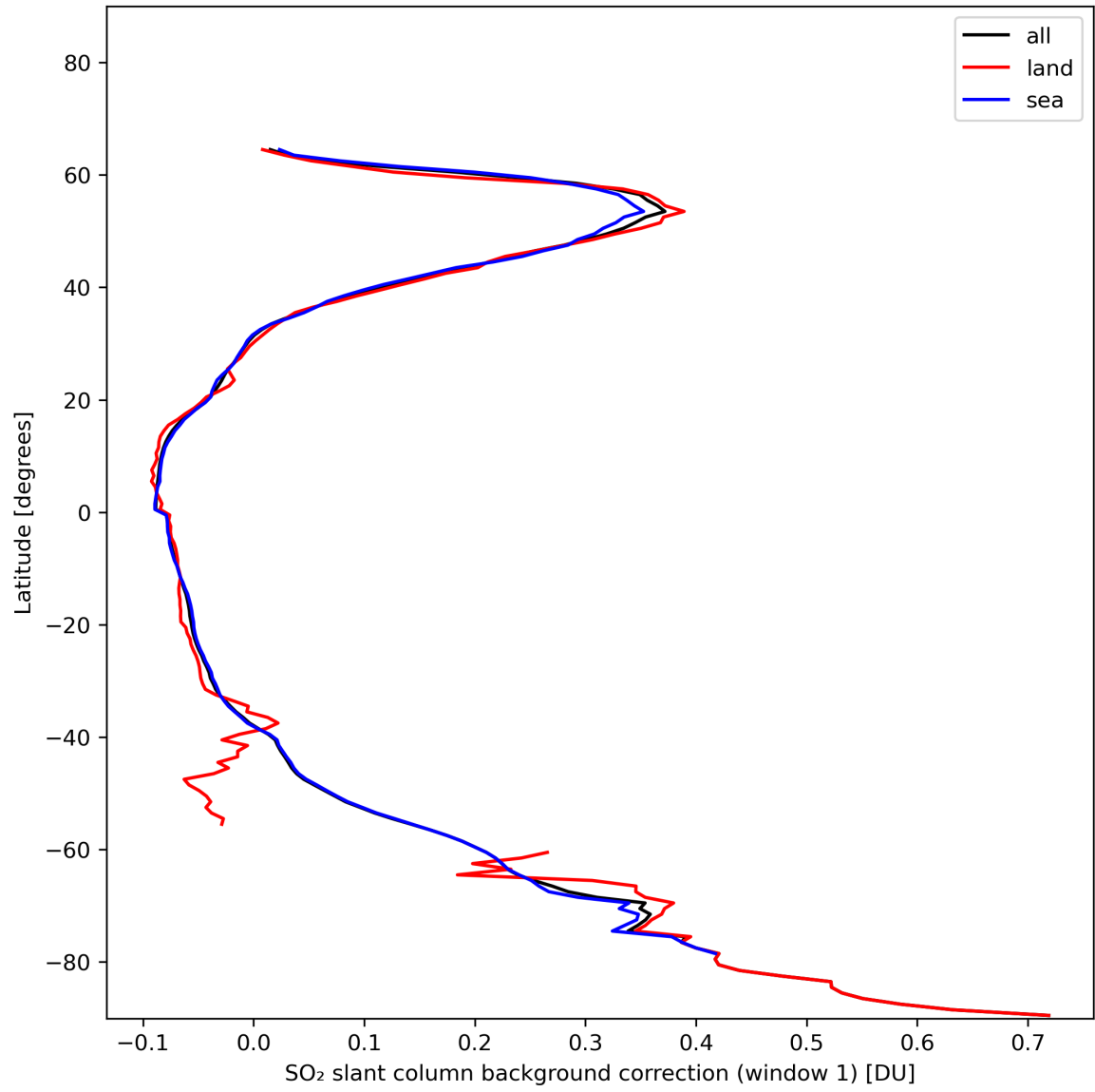
Figure 36: Zonal average of “SO 2 slant column background correction (window 1)” for 2024-01-15 to 2024-01-17.
