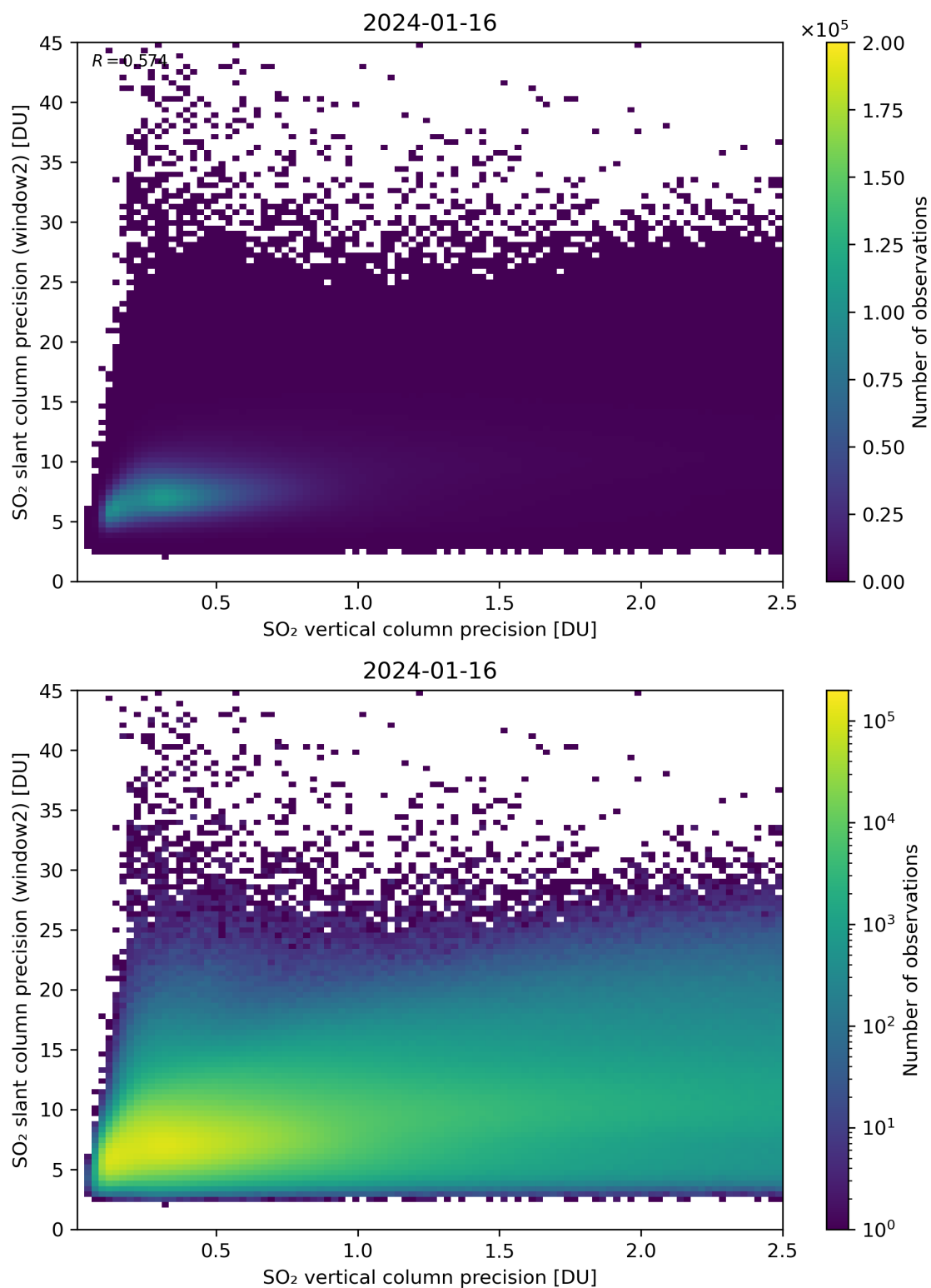
Figure 291: Scatter density plot of “SO 2 vertical column precision” against “SO 2 slant column precision (window2)” for 2024-01-15 to 2024-01-17.
