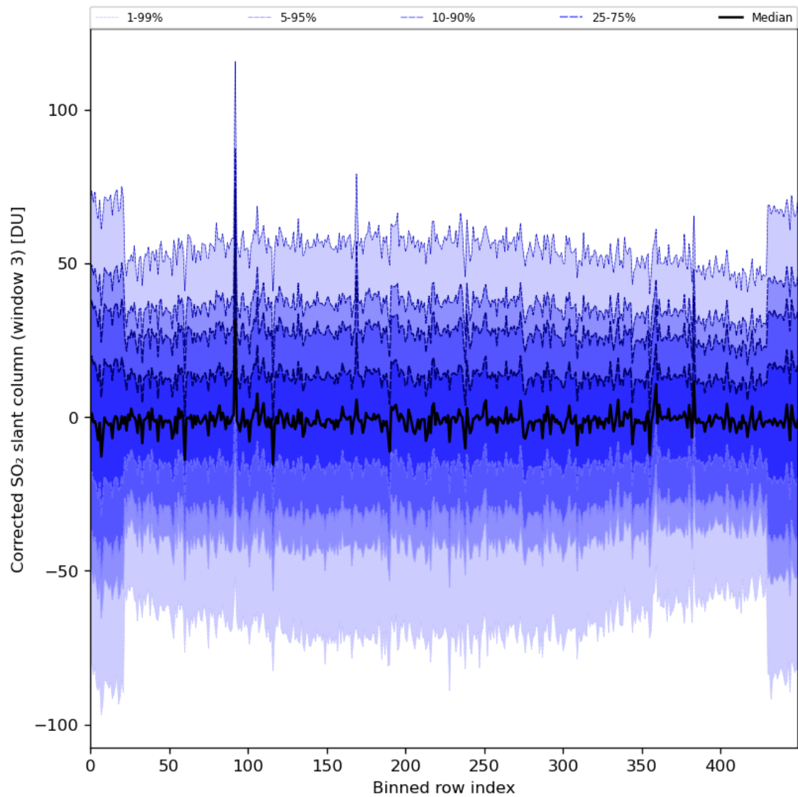
Figure 89: Along track statistics of “Corrected SO 2 slant column (window 3)” for 2024-01-15 to 2024-01-17
