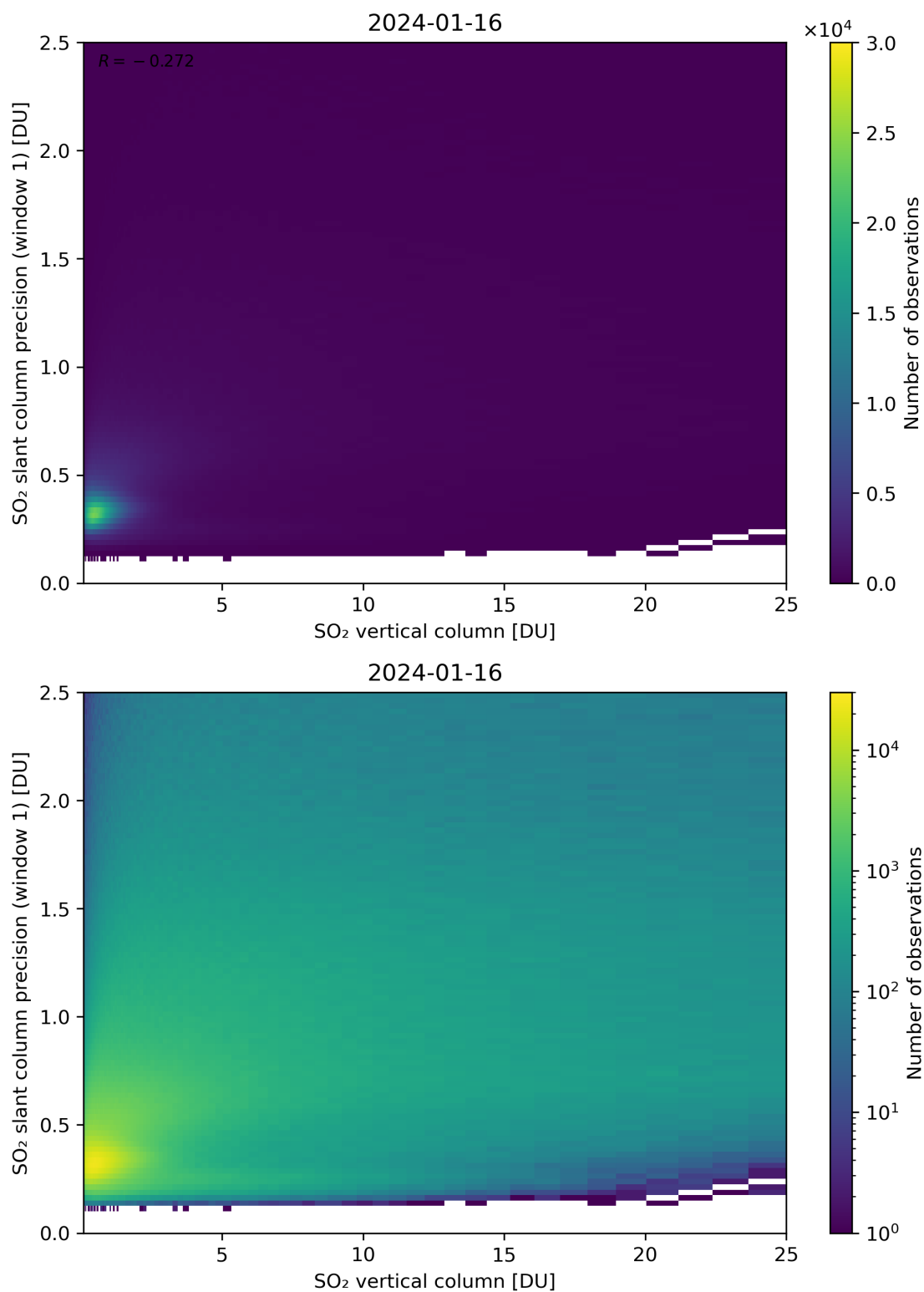
Figure 301: Scatter density plot of “SO 2 vertical column” against “SO 2 slant column precision (window 1)” for 2024-01-15 to 2024-01-17.
