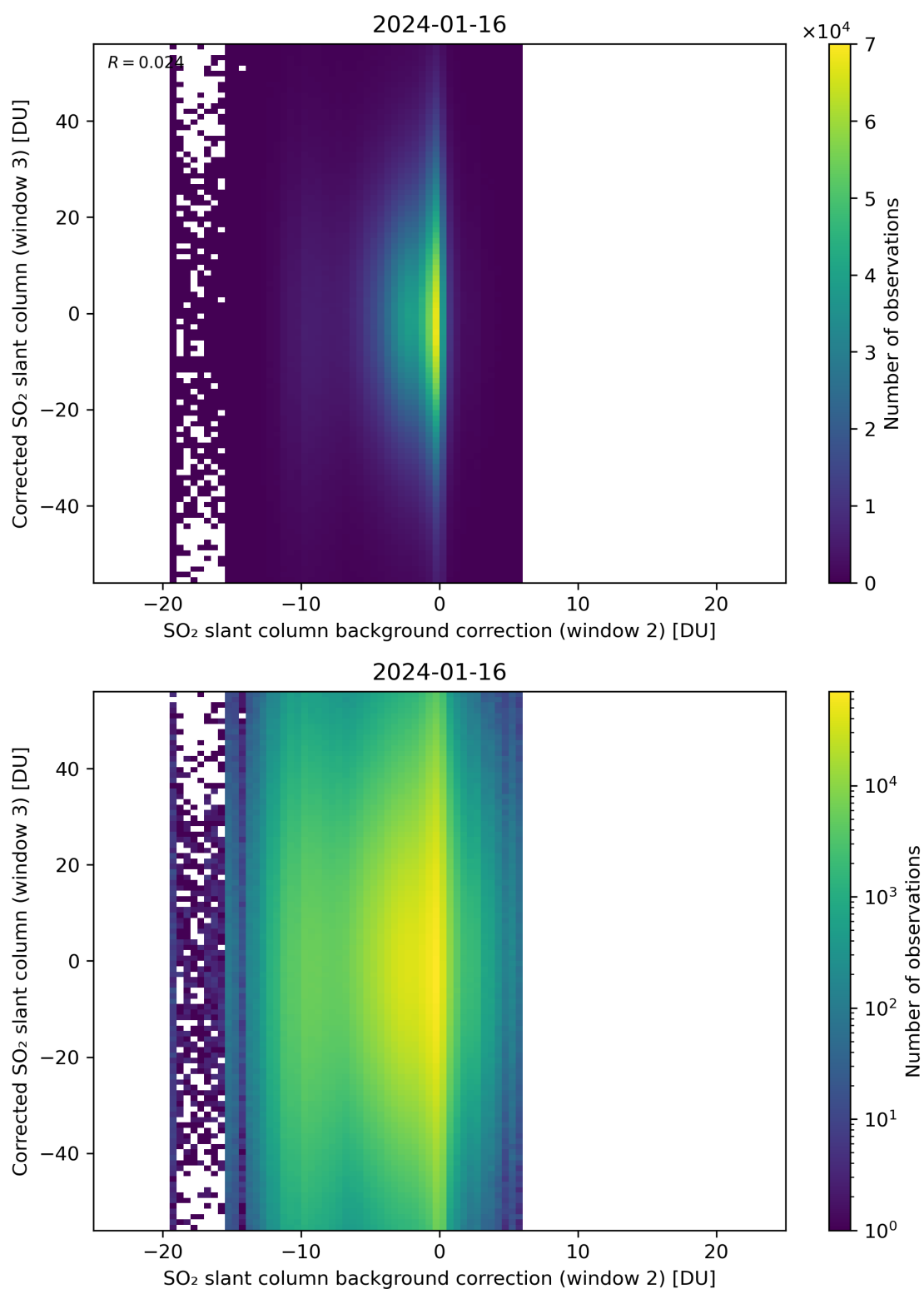
Figure 116: Scatter density plot of “SO 2 slant column background correction (window 2)” against “Corrected SO 2 slant column (window 3)” for 2024-01-15 to 2024-01-17.
