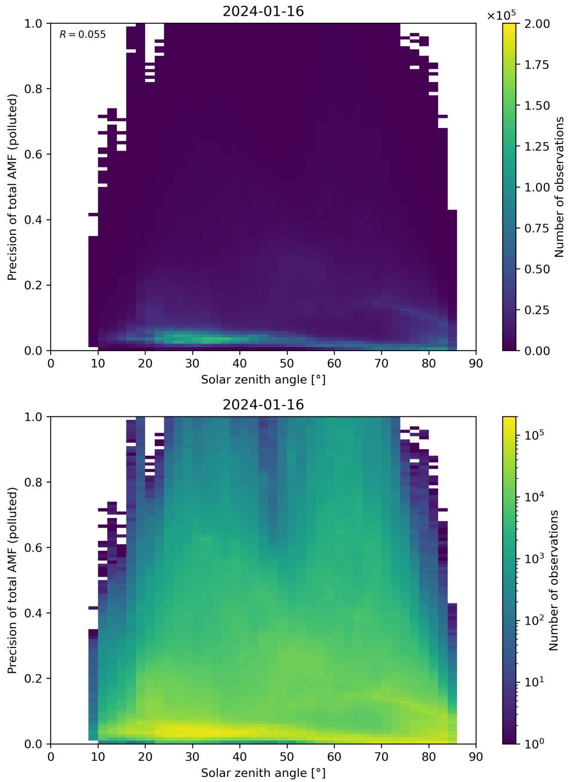
Figure 175: Scatter density plot of “Solar zenith angle” against “Precision of total AMF (polluted)” for 2024-01-15 to 2024-01-17.
