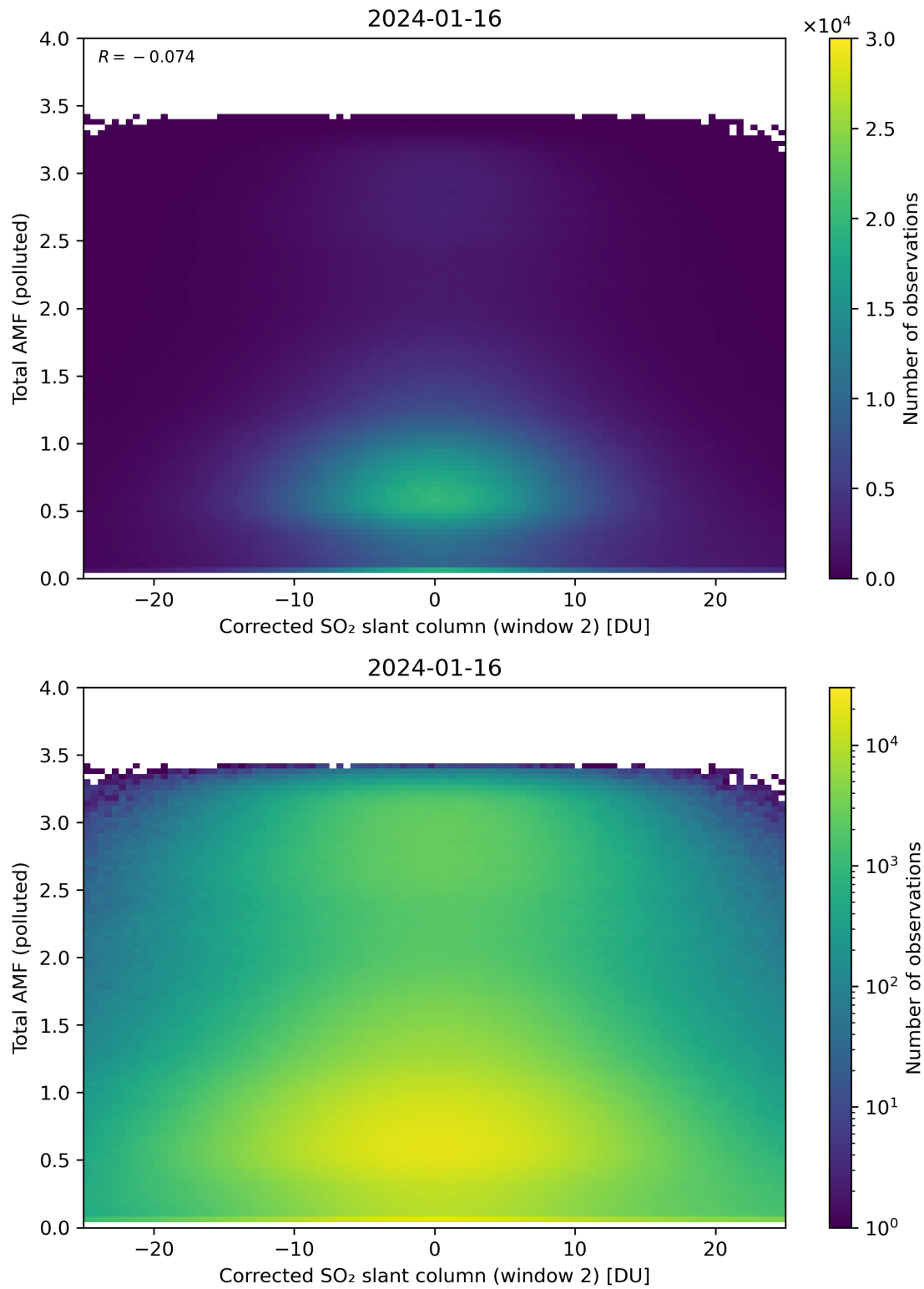
Figure 203: Scatter density plot of “Corrected SO 2 slant column (window 2)” against “Total AMF (polluted)” for 2024-01-15 to 2024-01-17.
