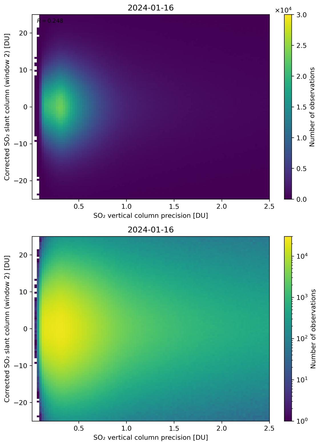
Figure 287: Scatter density plot of “SO 2 vertical column precision” against “Corrected SO 2 slant column (window 2)” for 2024-01-15 to 2024-01-17.
