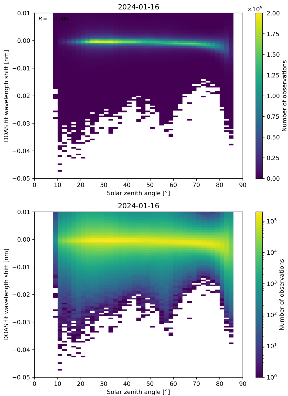
Figure 161: Scatter density plot of “Solar zenith angle” against “DOAS fit wavelength shift” for 2024-01-15 to 2024-01-17.
