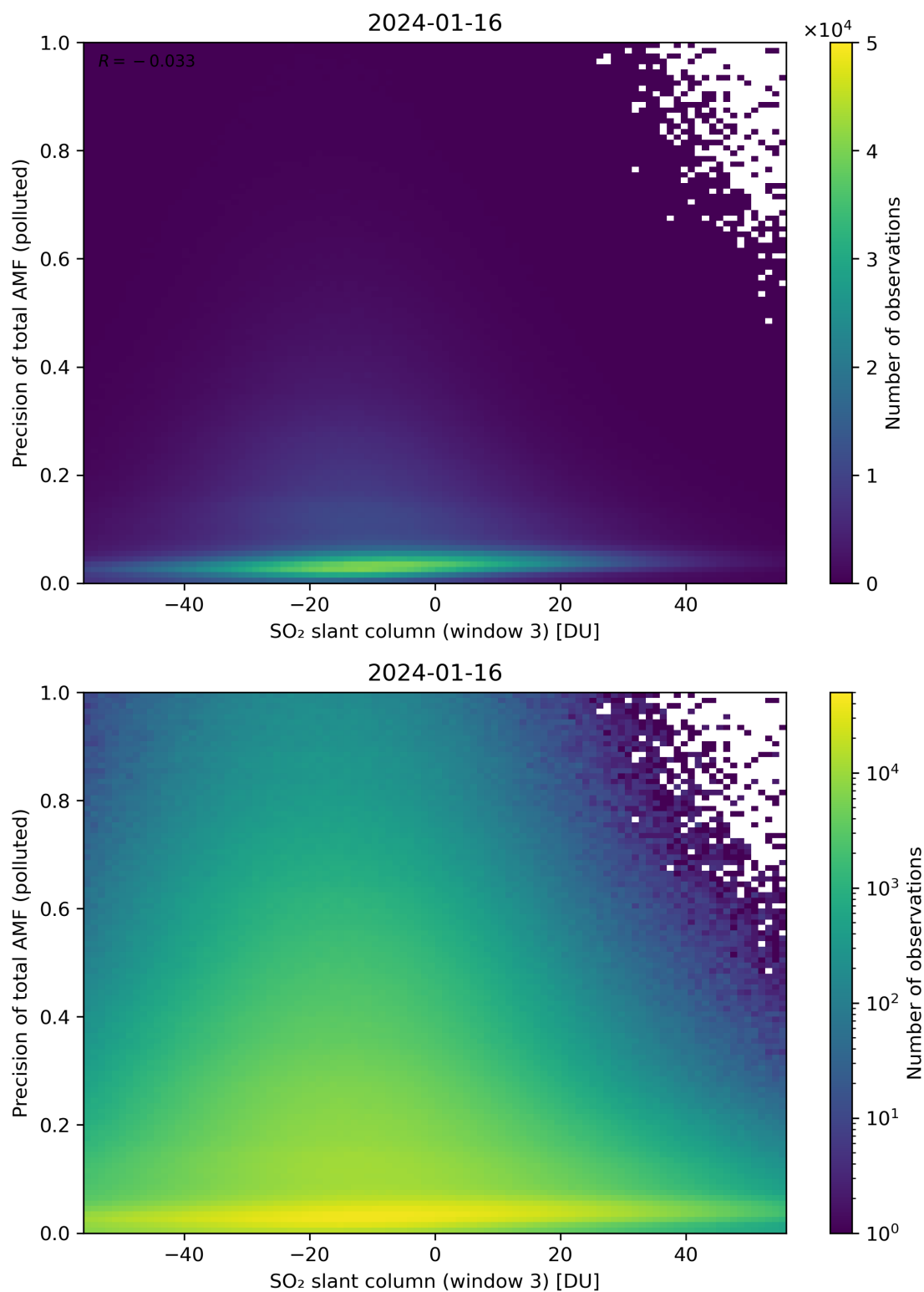
Figure 269: Scatter density plot of “SO 2 slant column (window 3)” against “Precision of total AMF (polluted)” for 2024-01-15 to 2024-01-17.
