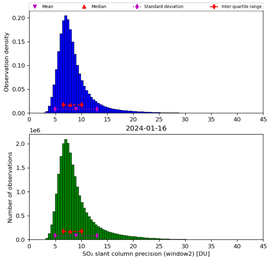
Figure 61: Histogram of “SO 2 slant column precision (window2)” for 2024-01-15 to 2024-01-17
