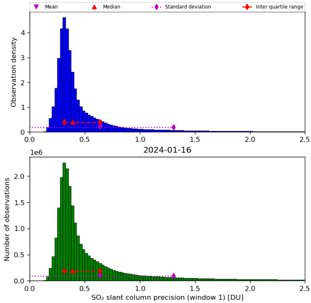
Figure 57: Histogram of “SO 2 slant column precision (window 1)” for 2024-01-15 to 2024-01-17
