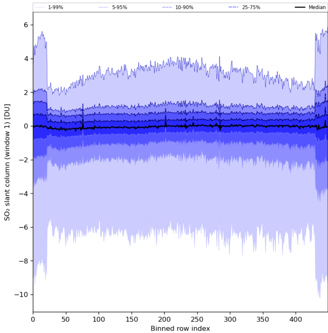
Figure 79: Along track statistics of “SO 2 slant column (window 1)” for 2024-01-15 to 2024-01-17
