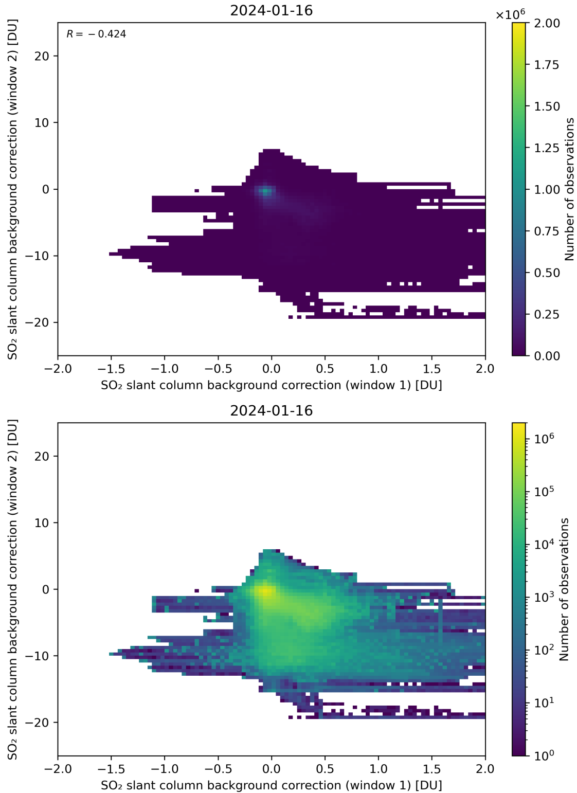
Figure 98: Scatter density plot of “SO 2 slant column background correction (window 1)” against “SO 2 slant column background correction (window 2)” for 2024-01-15 to 2024-01-17.
