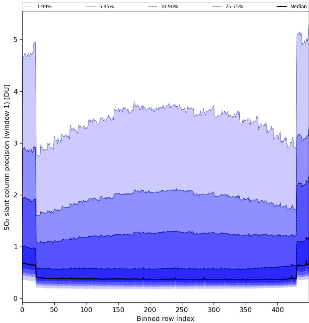
Figure 80: Along track statistics of “SO 2 slant column precision (window 1)” for 2024-01-15 to 2024-01-17
