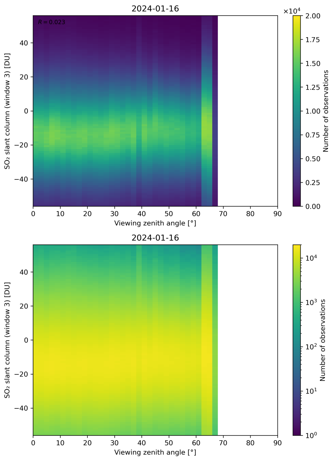
Figure 323: Scatter density plot of “Viewing zenith angle” against “SO 2 slant column (window 3)” for 2024-01-15 to 2024-01-17.
