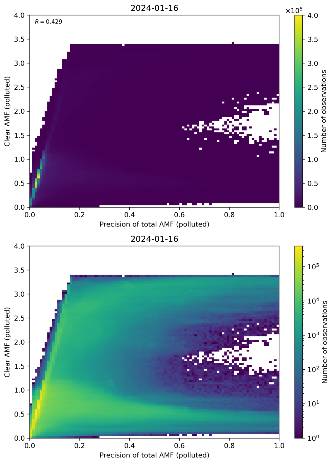
Figure 270: Scatter density plot of “Precision of total AMF (polluted)” against “Clear AMF (polluted)” for 2024-01-15 to 2024-01-17.
