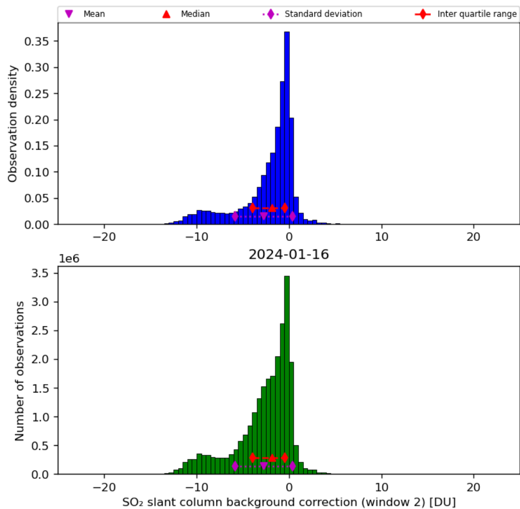
Figure 63: Histogram of “SO 2 slant column background correction (window 2)” for 2024-01-15 to 2024-01-17
