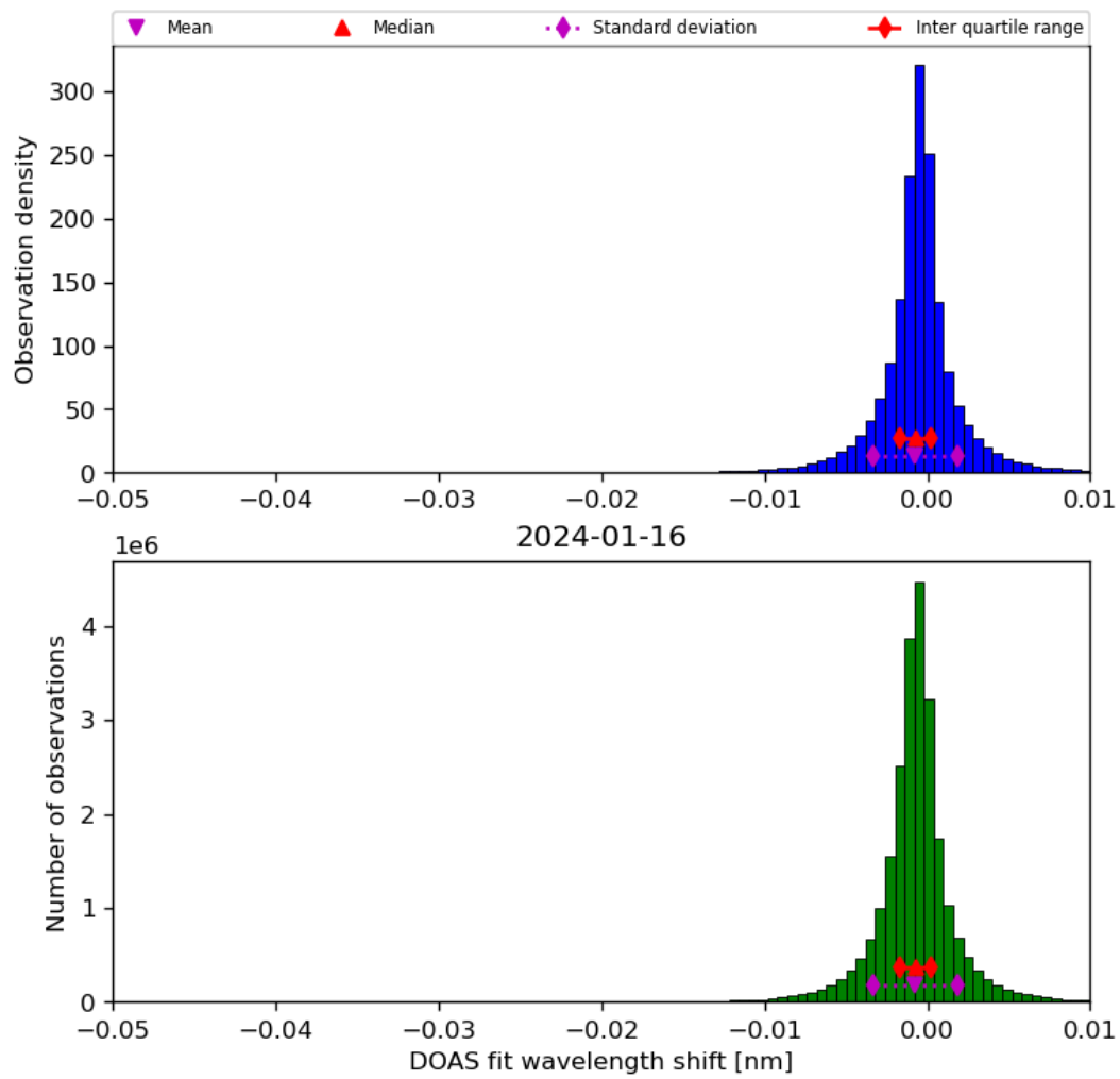
Figure 68: Histogram of “DOAS fit wavelength shift” for 2024-01-15 to 2024-01-17
