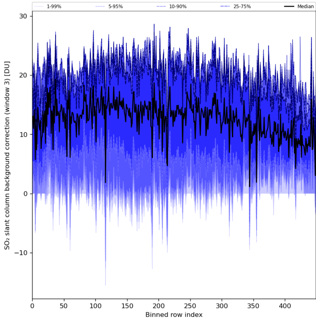
Figure 90: Along track statistics of “SO 2 slant column background correction (window 3)” for 2024-01-15 to 2024-01-17
