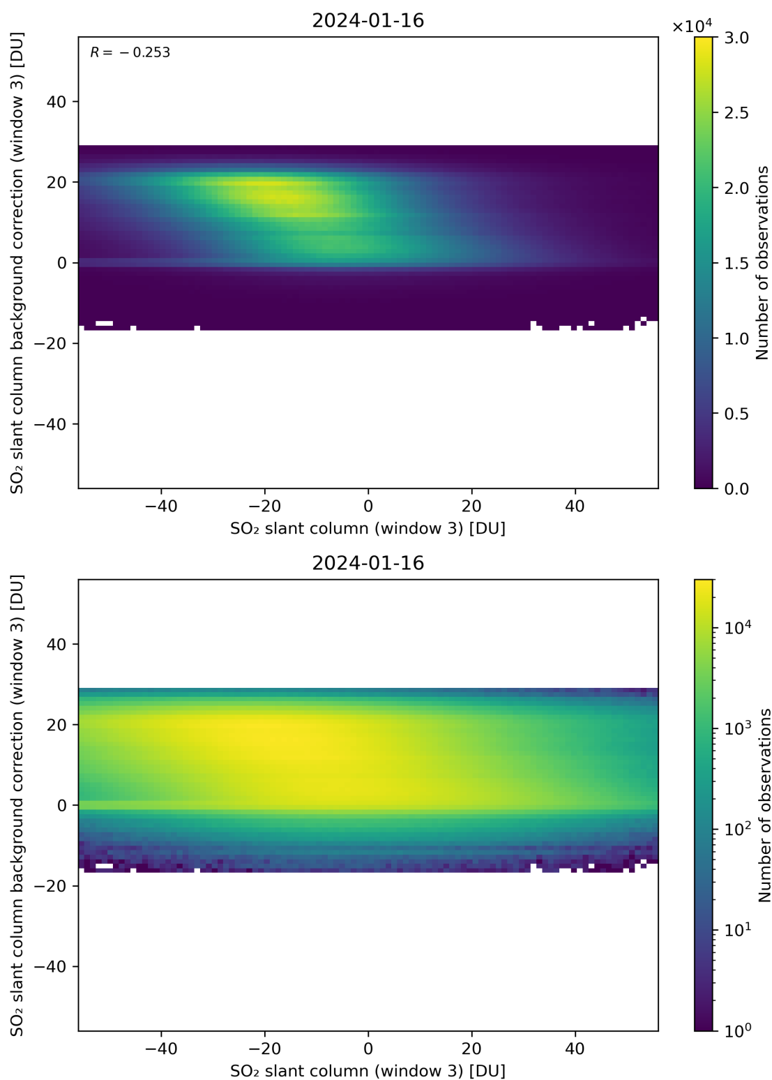
Figure 253: Scatter density plot of “SO 2 slant column (window 3)” against “SO 2 slant column background correction (window 3)” for 2024-01-15 to 2024-01-17.
