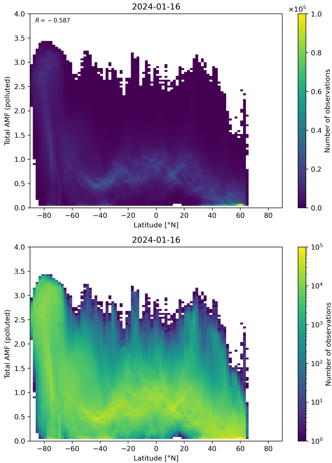
Figure 154: Scatter density plot of “Latitude” against “Total AMF (polluted)” for 2024-01-15 to 2024-01-17.
