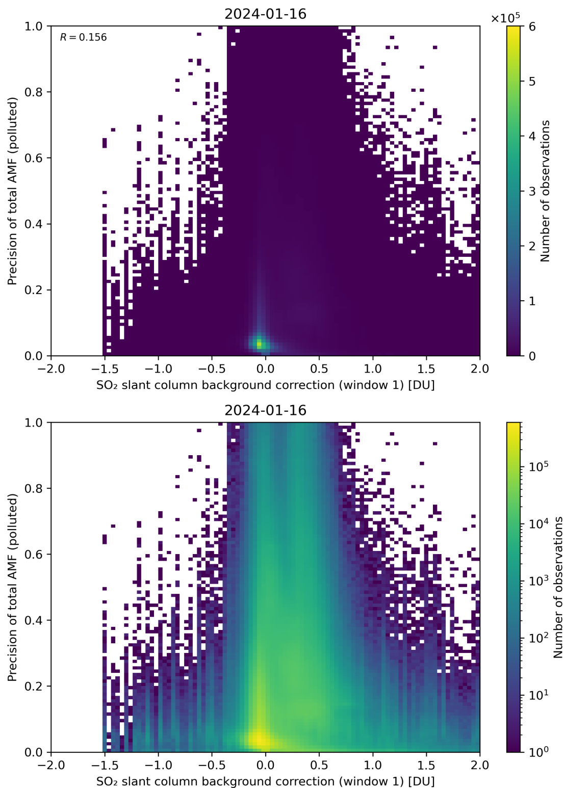
Figure 110: Scatter density plot of “SO 2 slant column background correction (window 1)” against “Precision of total AMF (polluted)” for 2024-01-15 to 2024-01-17.
