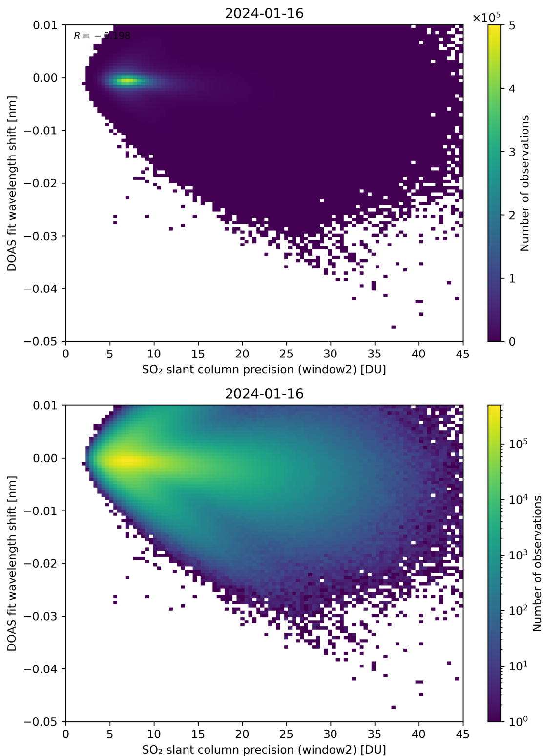
Figure 243: Scatter density plot of “SO 2 slant column precision (window2)” against “DOAS fit wavelength shift” for 2024-01-15 to 2024-01-17.
