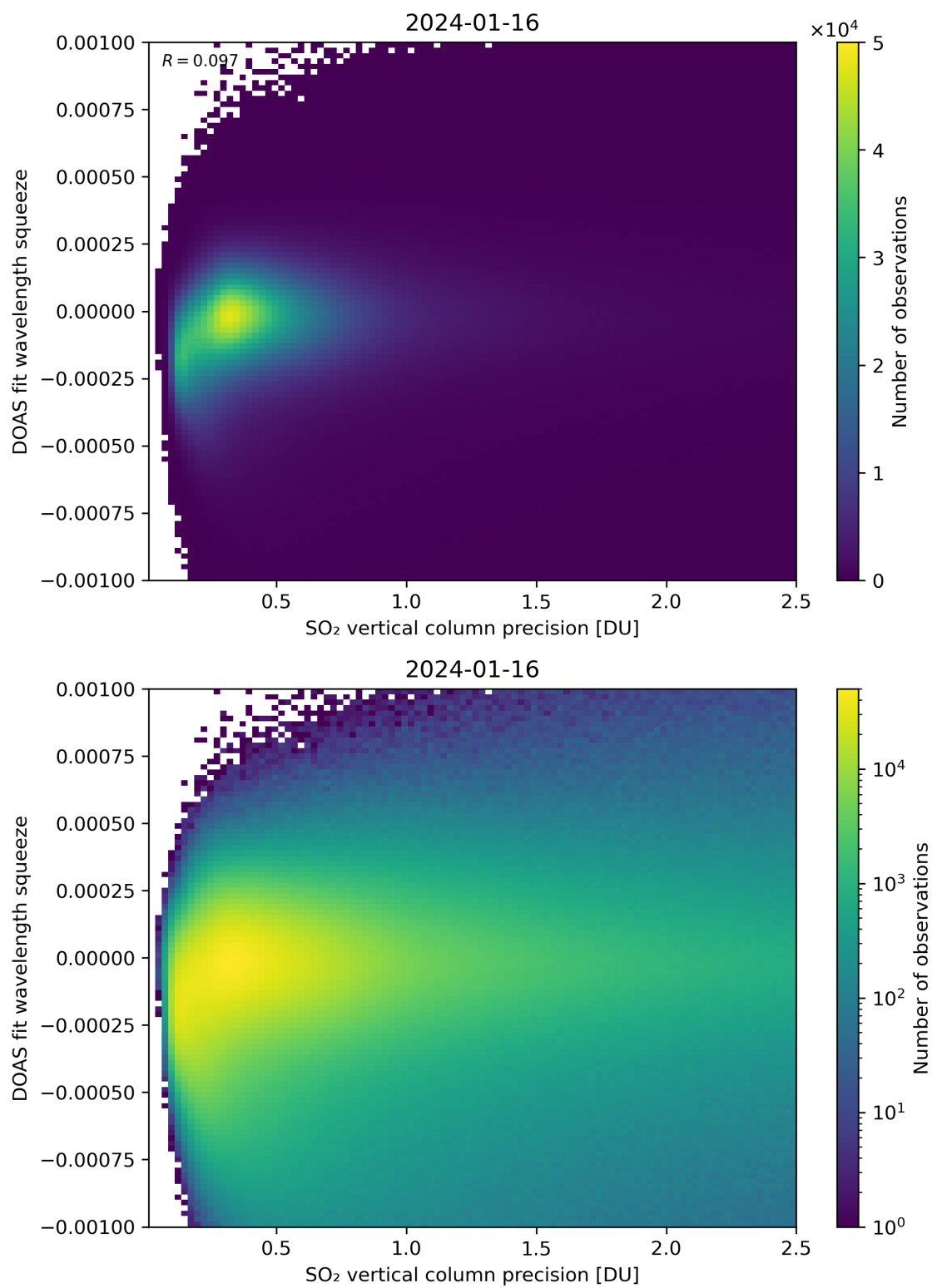
Figure 283: Scatter density plot of “SO 2 vertical column precision” against “DOAS fit wavelength squeeze” for 2024-01-15 to 2024-01-17.
