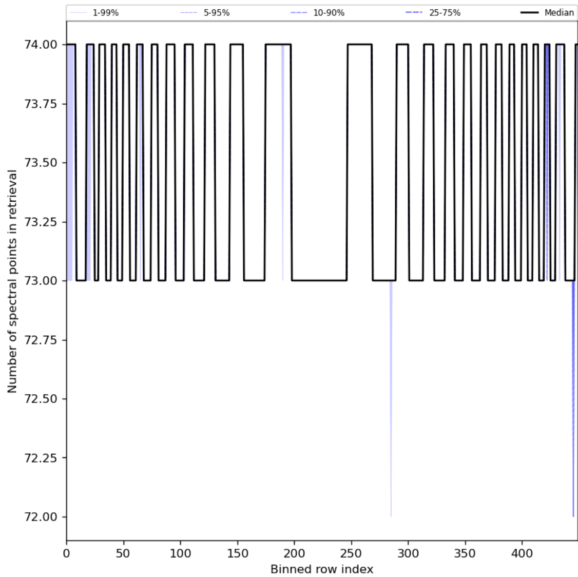
Figure 97: Along track statistics of “Number of spectral points in retrieval” for 2024-01-15 to 2024-01-17
