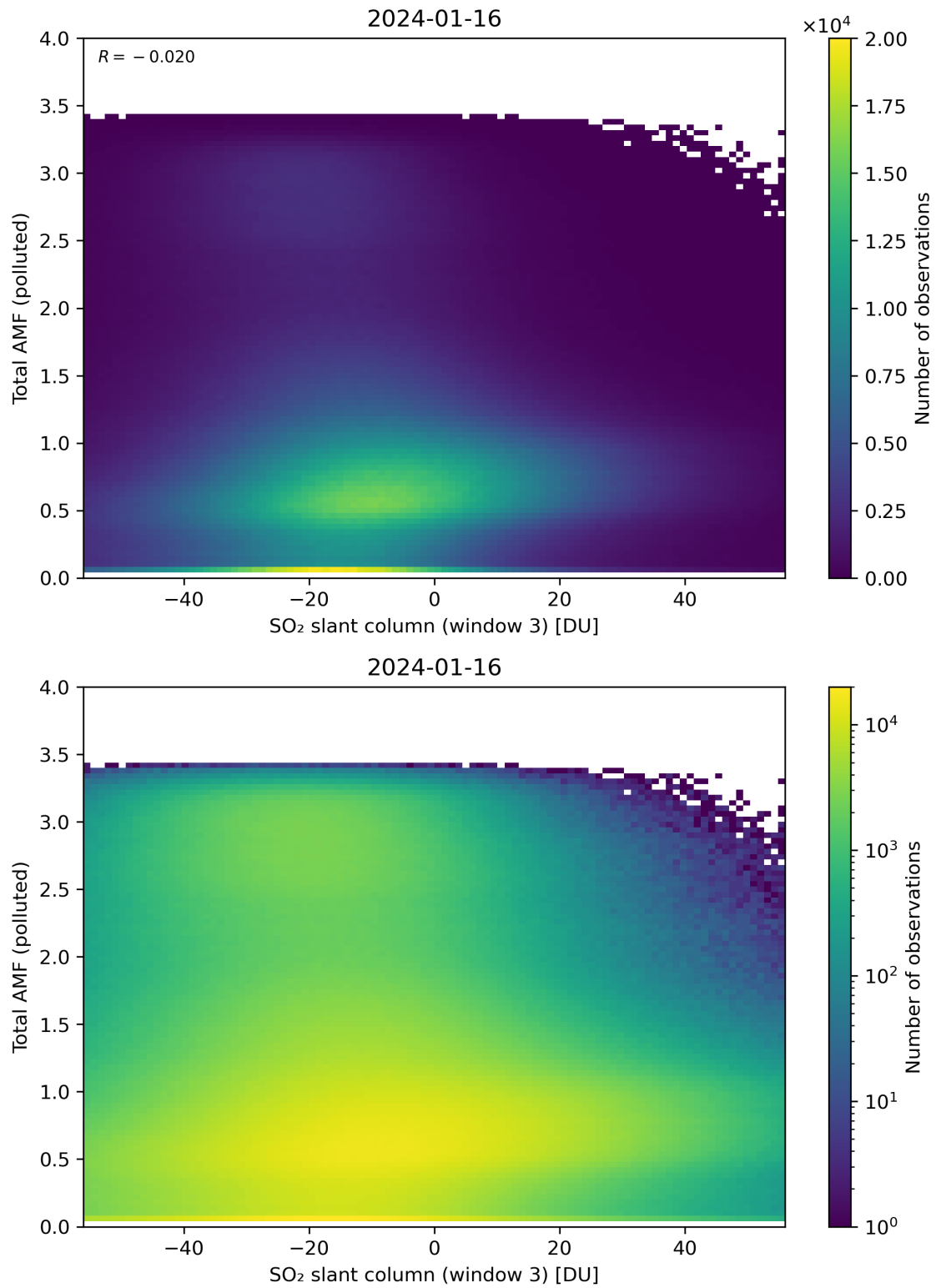
Figure 268: Scatter density plot of “SO 2 slant column (window 3)” against “Total AMF (polluted)” for 2024-01-15 to 2024-01-17.
