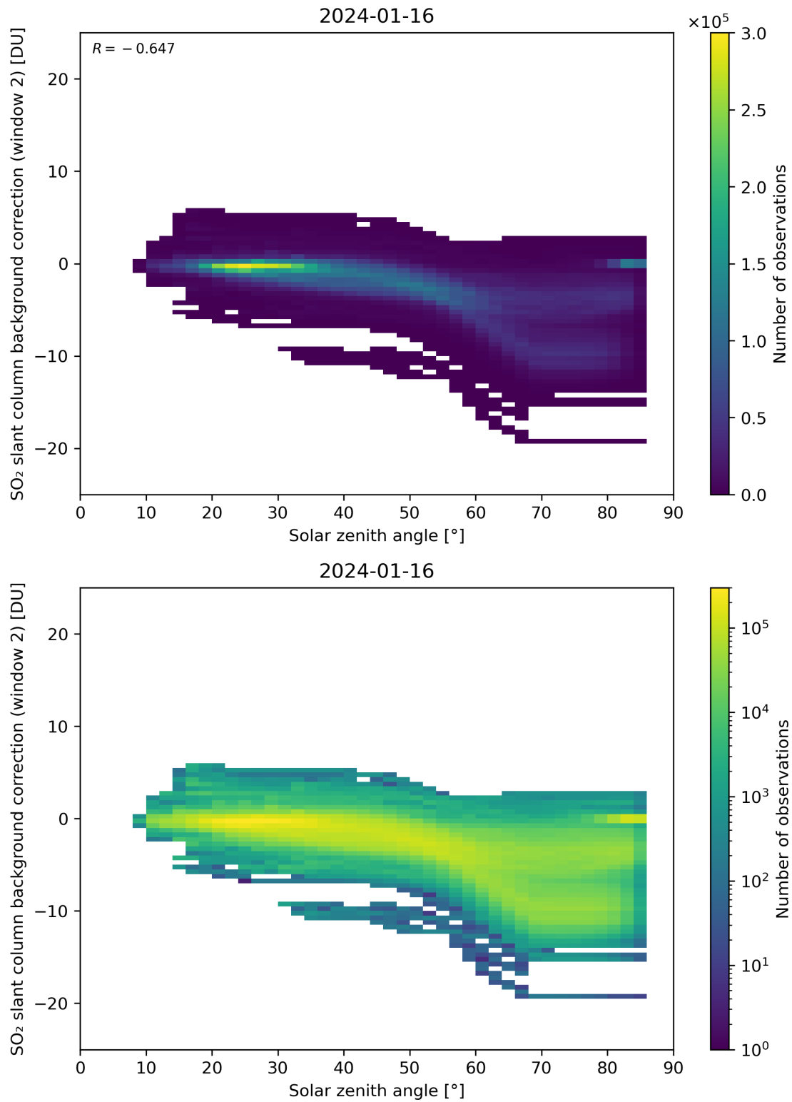
Figure 159: Scatter density plot of “Solar zenith angle” against “SO 2 slant column background correction (window 2)” for 2024-01-15 to 2024-01-17.
