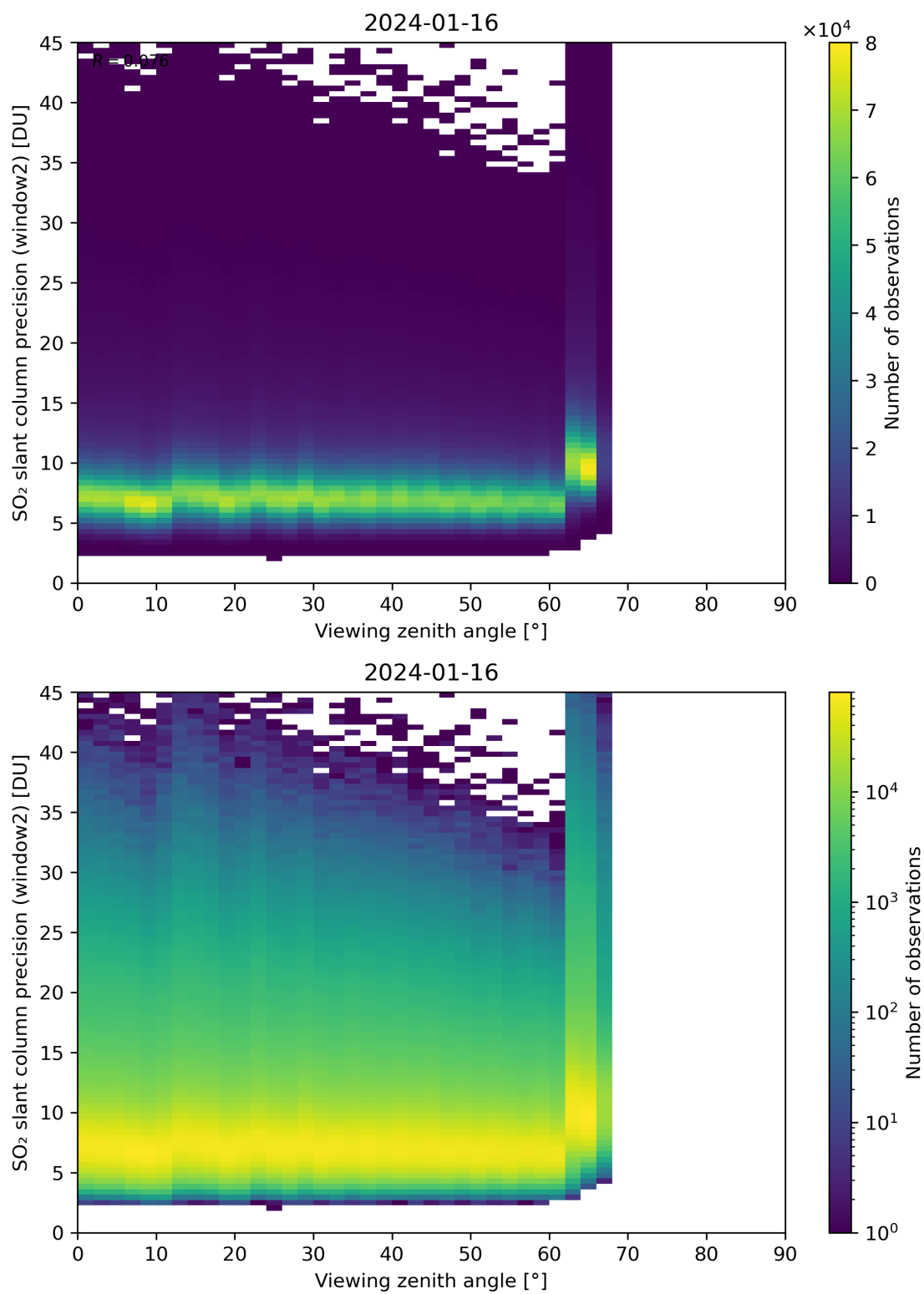
Figure 322: Scatter density plot of “Viewing zenith angle” against “SO 2 slant column precision (window2)” for 2024-01-15 to 2024-01-17.
