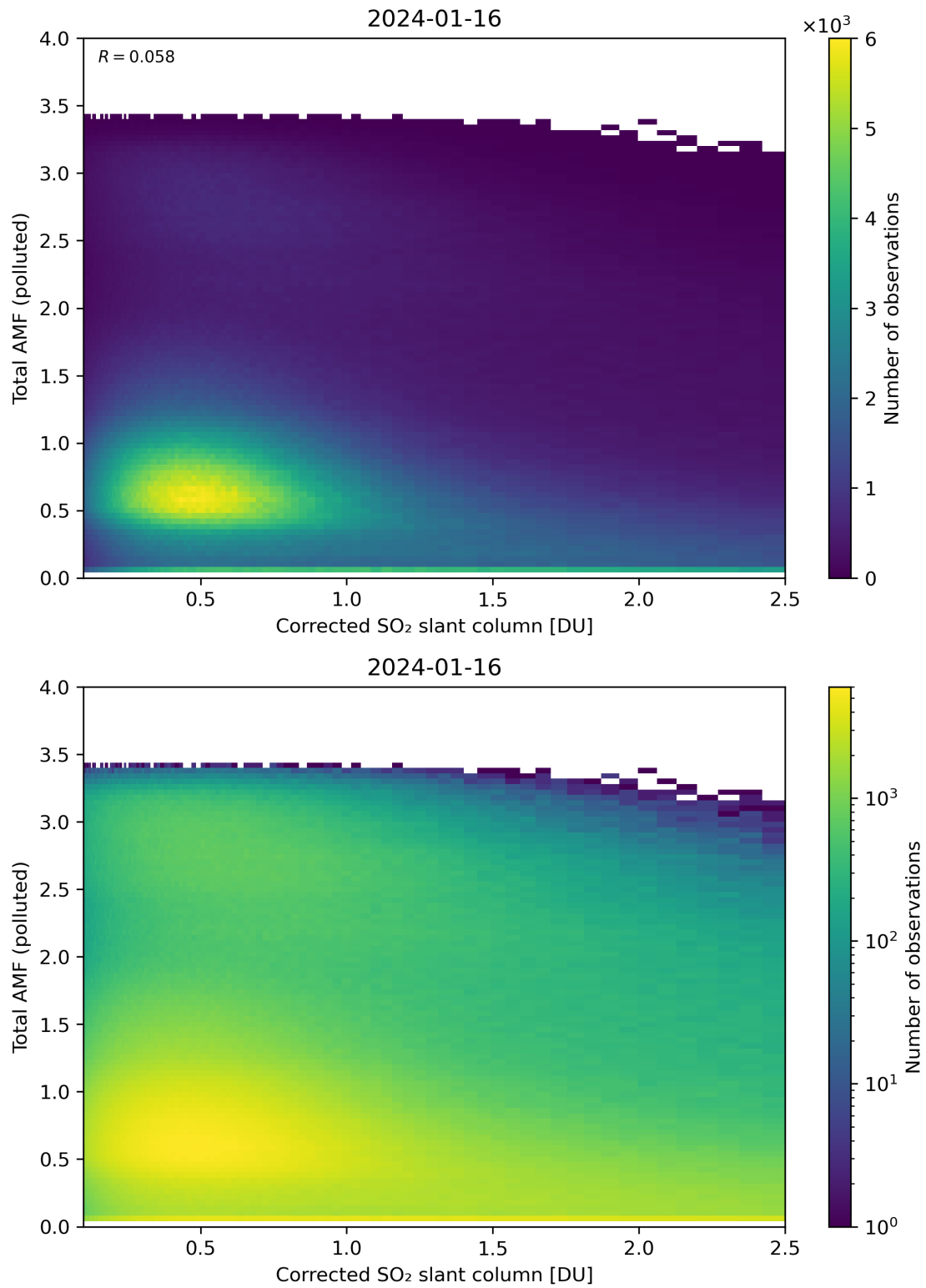
Figure 192: Scatter density plot of “Corrected SO 2 slant column” against “Total AMF (polluted)” for 2024-01-15 to 2024-01-17.
