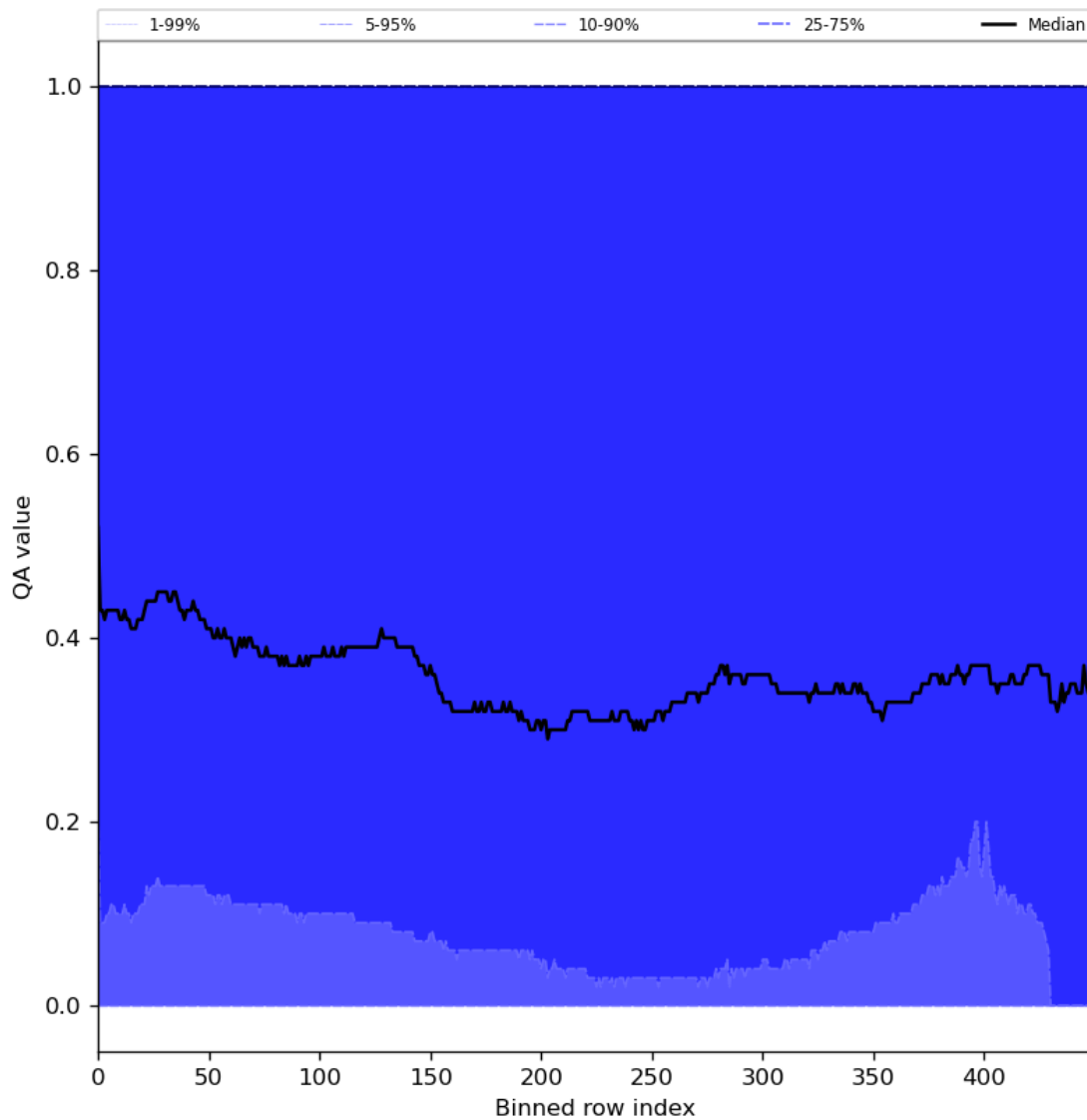
Figure 75: Along track statistics of “QA value” for 2024-01-15 to 2024-01-17
