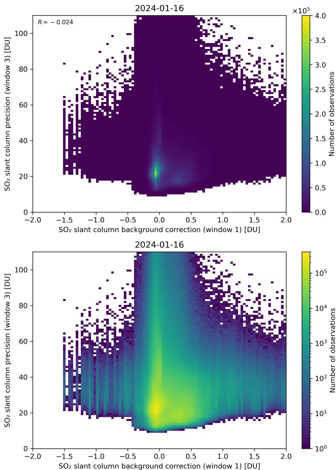
Figure 108: Scatter density plot of “SO 2 slant column background correction (window 1)” against “SO 2 slant column precision (window 3)” for 2024-01-15 to 2024-01-17.
