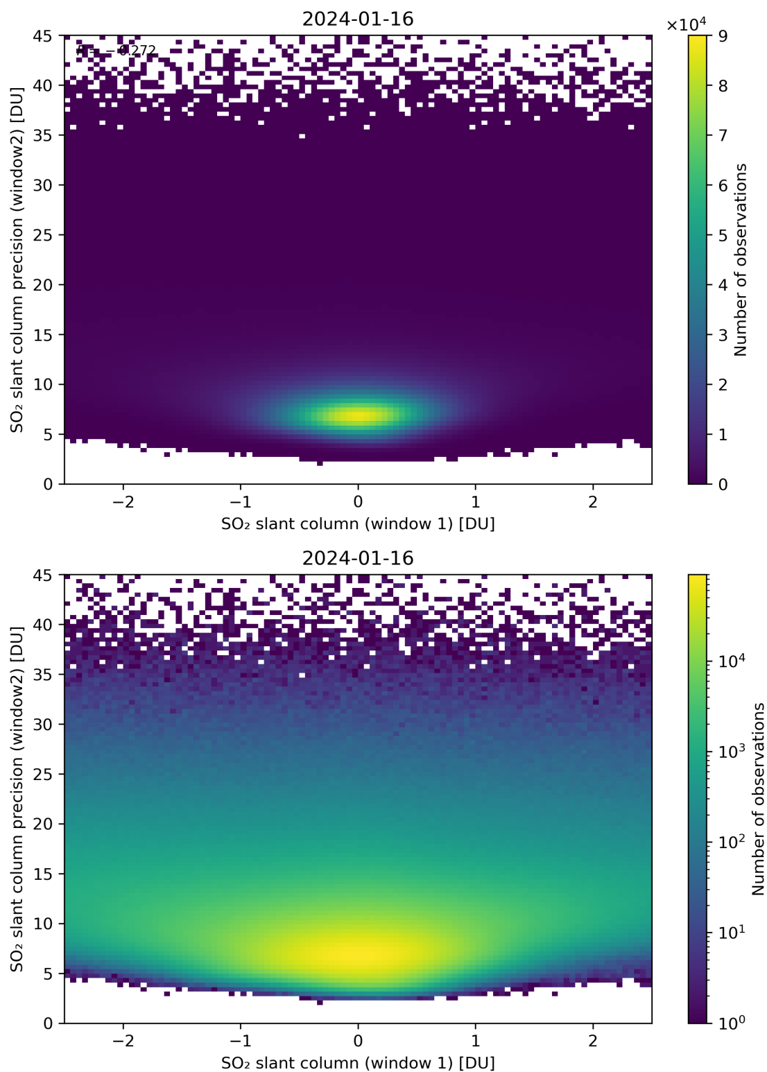
Figure 236: Scatter density plot of “SO 2 slant column (window 1)” against “SO 2 slant column precision (window2)” for 2024-01-15 to 2024-01-17.
