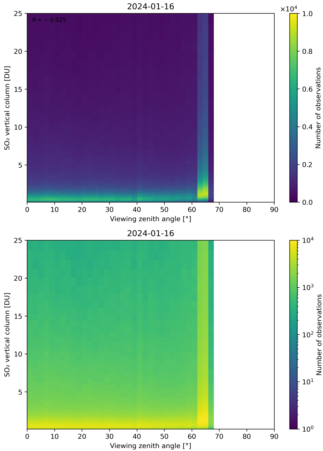
Figure 327: Scatter density plot of “Viewing zenith angle” against “SO 2 vertical column” for 2024-01-15 to 2024-01-17.
