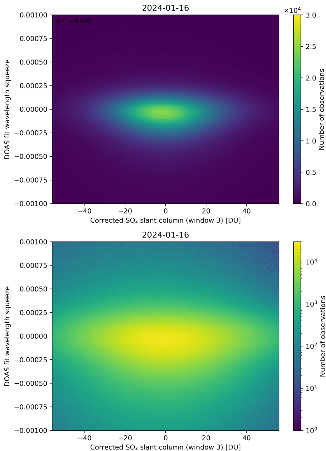
Figure 207: Scatter density plot of “Corrected SO 2 slant column (window 3)” against “DOAS fit wavelength squeeze” for 2024-01-15 to 2024-01-17.
