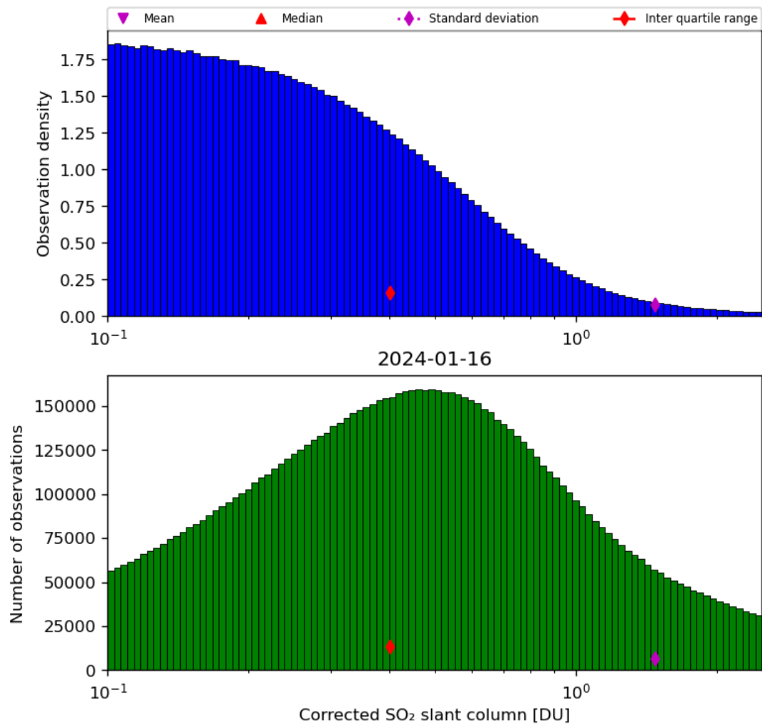
Figure 55: Histogram of “Corrected SO 2 slant column” for 2024-01-15 to 2024-01-17
