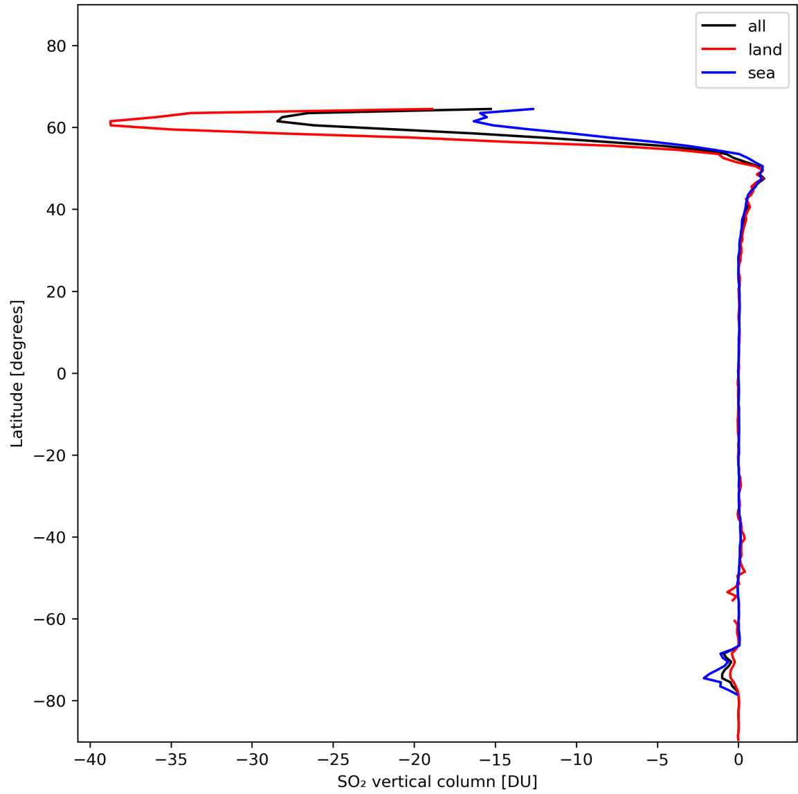
Figure 30: Zonal average of “SO 2 vertical column” for 2024-01-15 to 2024-01-17.
