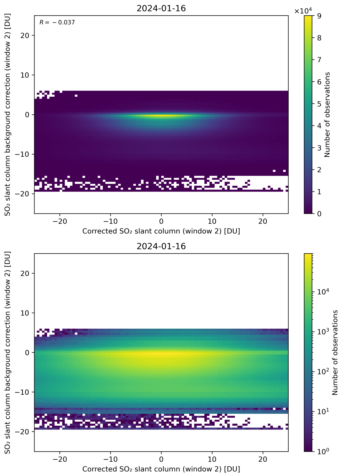
Figure 194: Scatter density plot of “Corrected SO 2 slant column (window 2)” against “SO 2 slant column background correction (window 2)” for 2024-01-15 to 2024-01-17.
