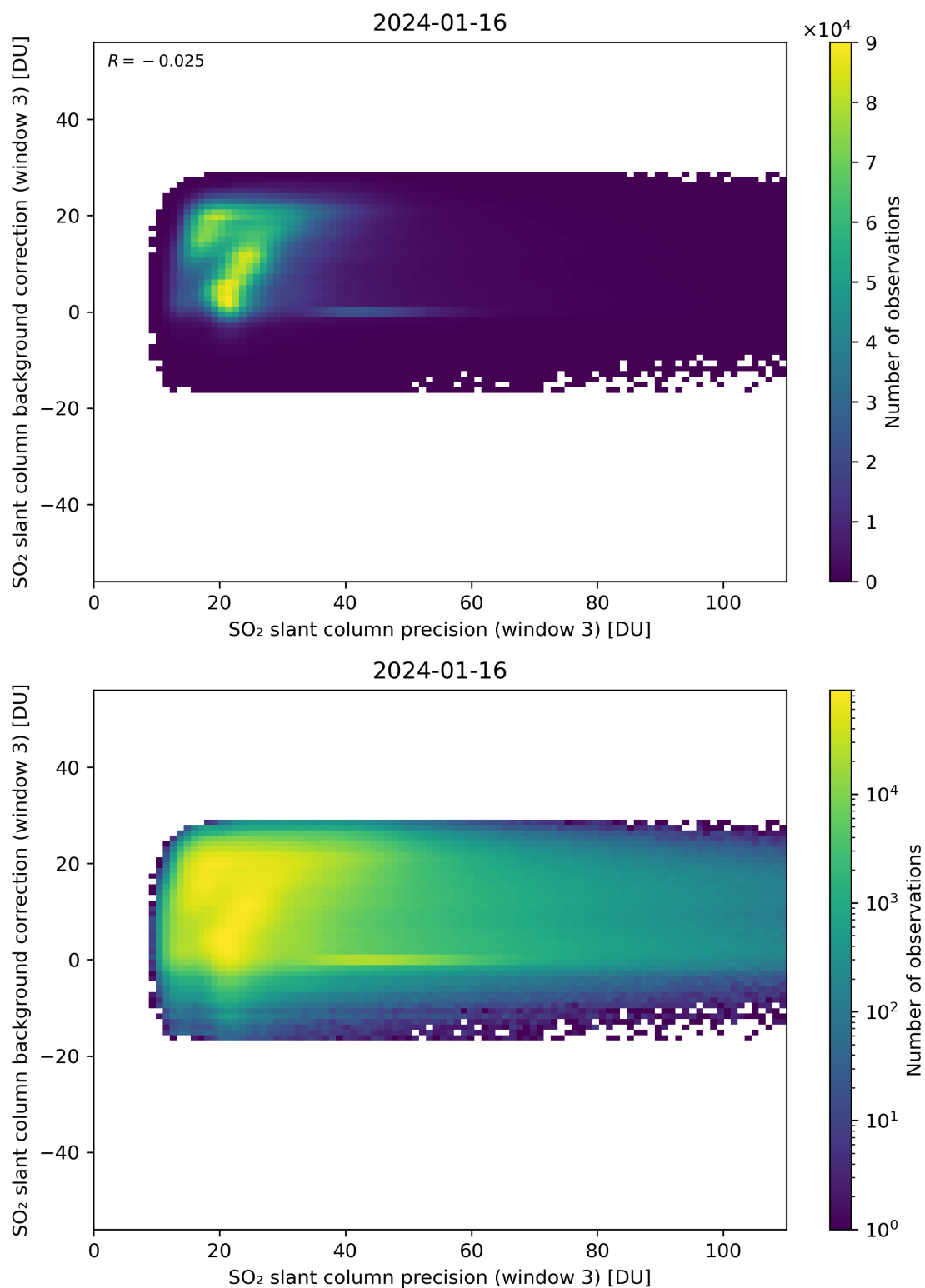
Figure 257: Scatter density plot of “SO 2 slant column precision (window 3)” against “SO 2 slant column background correction (window 3)” for 2024-01-15 to 2024-01-17.
