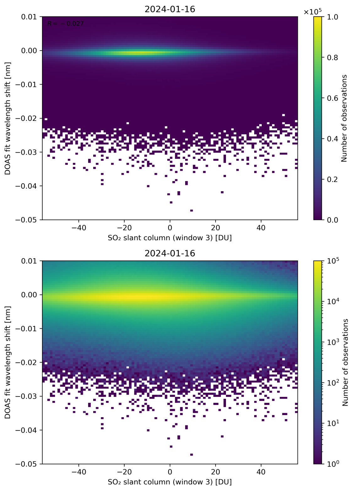
Figure 254: Scatter density plot of “SO 2 slant column (window 3)” against “DOAS fit wavelength shift” for 2024-01-15 to 2024-01-17.
