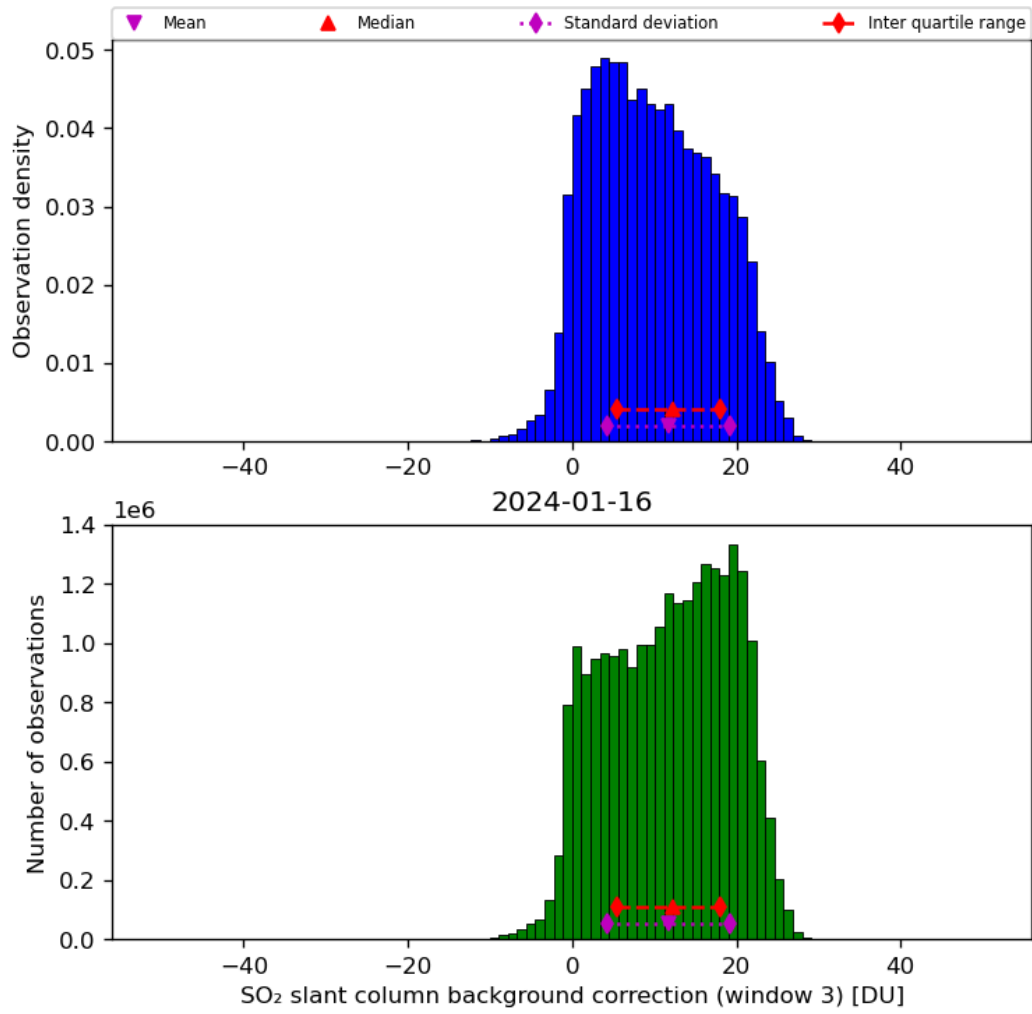
Figure 67: Histogram of “SO 2 slant column background correction (window 3)” for 2024-01-15 to 2024-01-17
