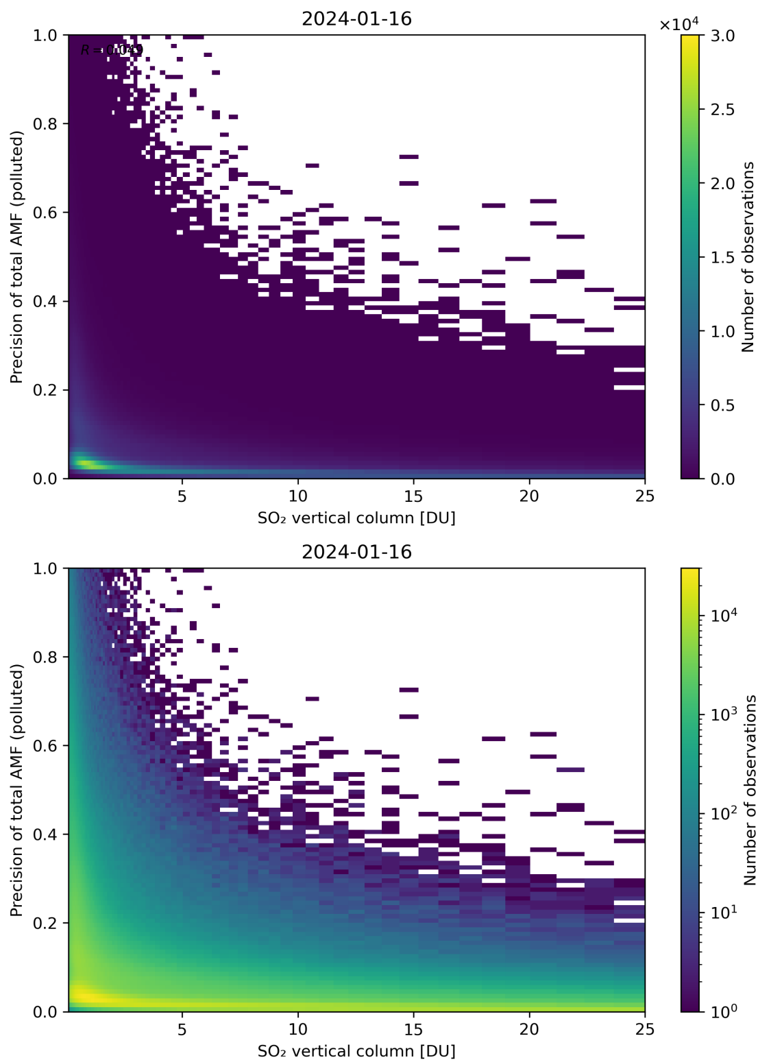
Figure 306: Scatter density plot of “SO 2 vertical column” against “Precision of total AMF (polluted)” for 2024-01-15 to 2024-01-17.
