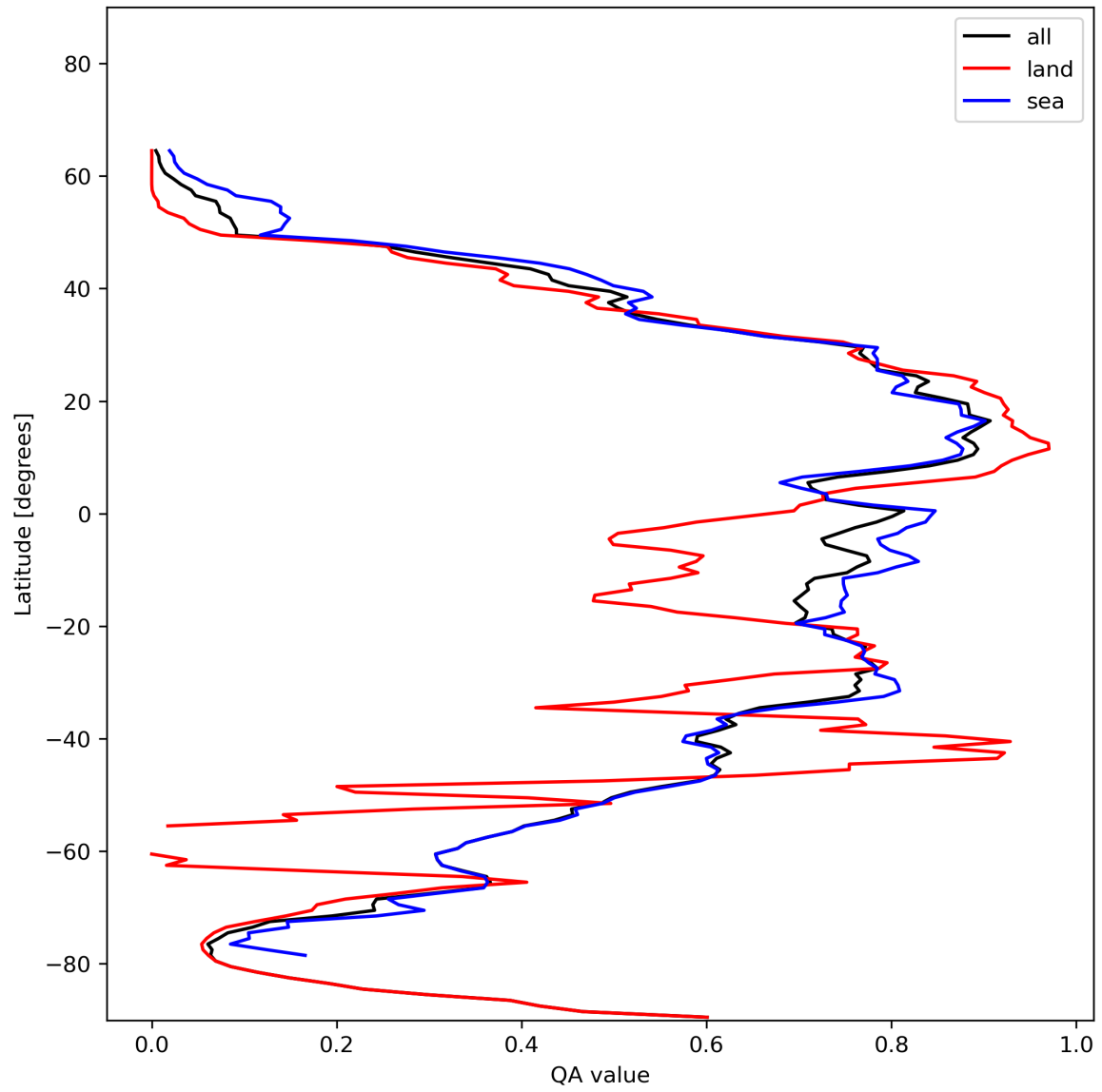
Figure 29: Zonal average of “QA value” for 2024-01-15 to 2024-01-17.
