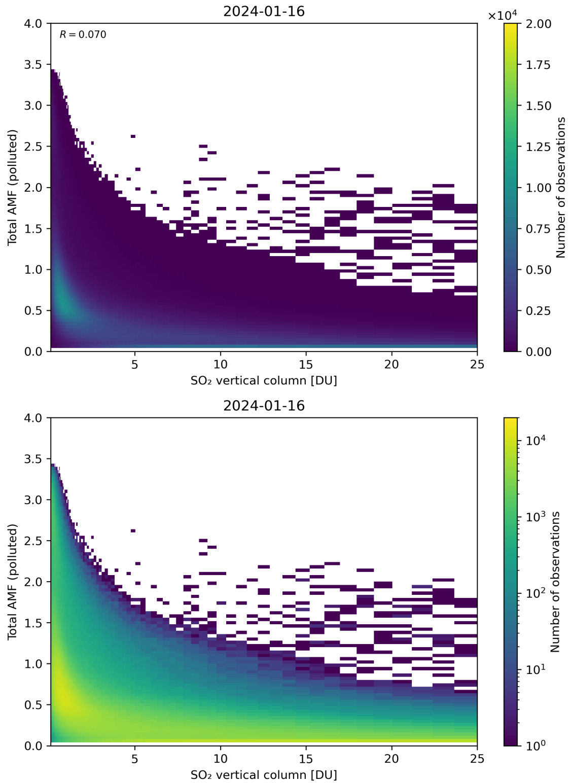
Figure 305: Scatter density plot of “SO 2 vertical column” against “Total AMF (polluted)” for 2024-01-15 to 2024-01-17.
