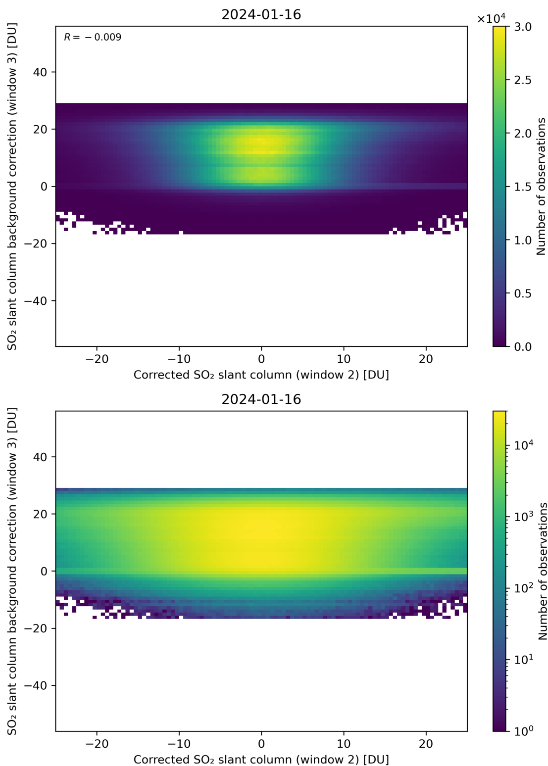
Figure 195: Scatter density plot of “Corrected SO 2 slant column (window 2)” against “SO 2 slant column background correction (window 3)” for 2024-01-15 to 2024-01-17.
