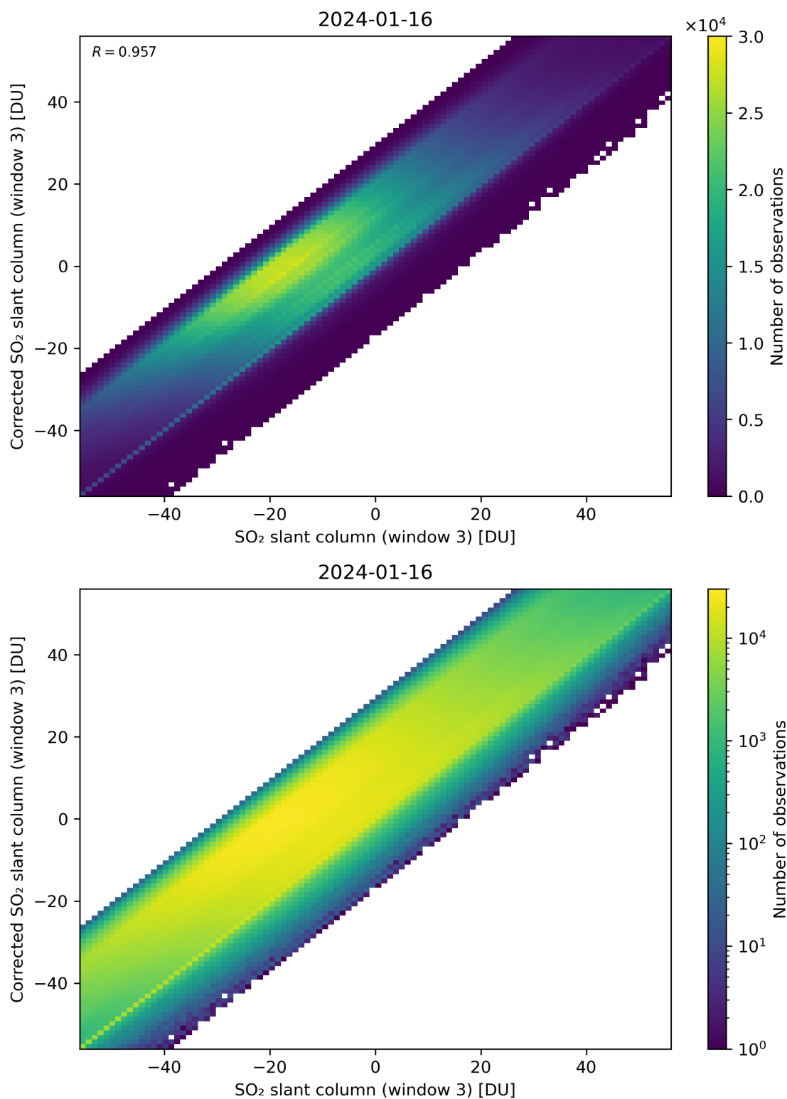
Figure 266: Scatter density plot of “SO 2 slant column (window 3)” against “Corrected SO 2 slant column (window 3)” for 2024-01-15 to 2024-01-17.
