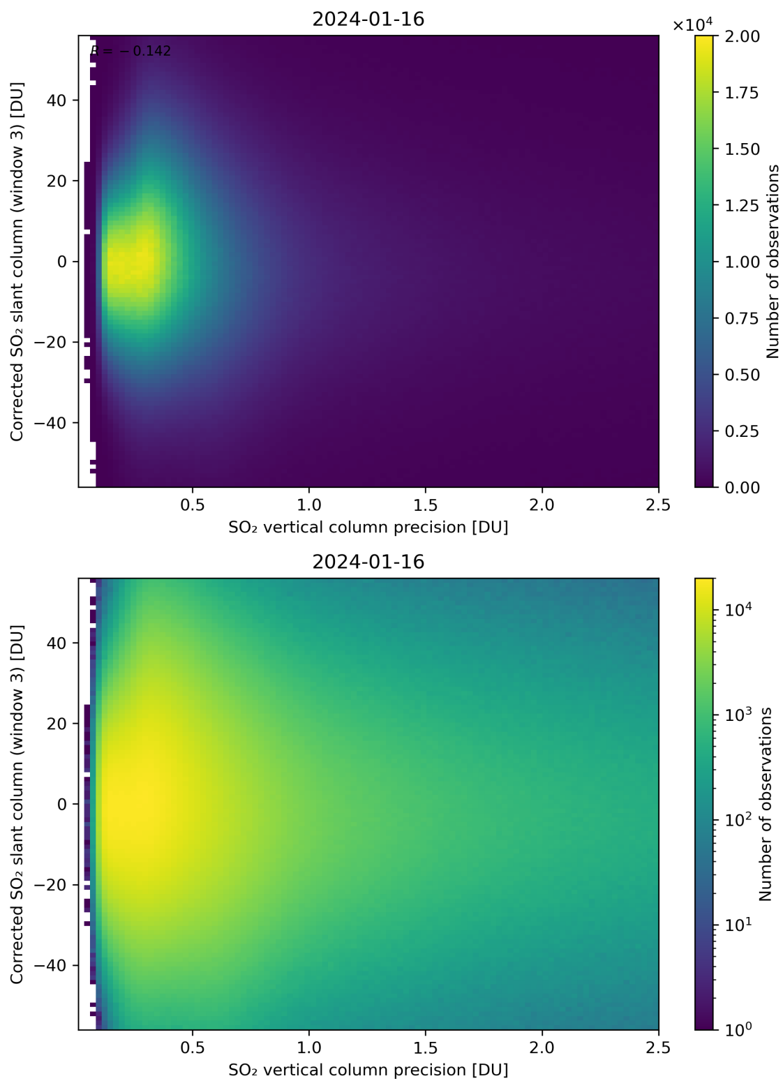
Figure 288: Scatter density plot of “SO 2 vertical column precision” against “Corrected SO 2 slant column (window 3)” for 2024-01-15 to 2024-01-17.
