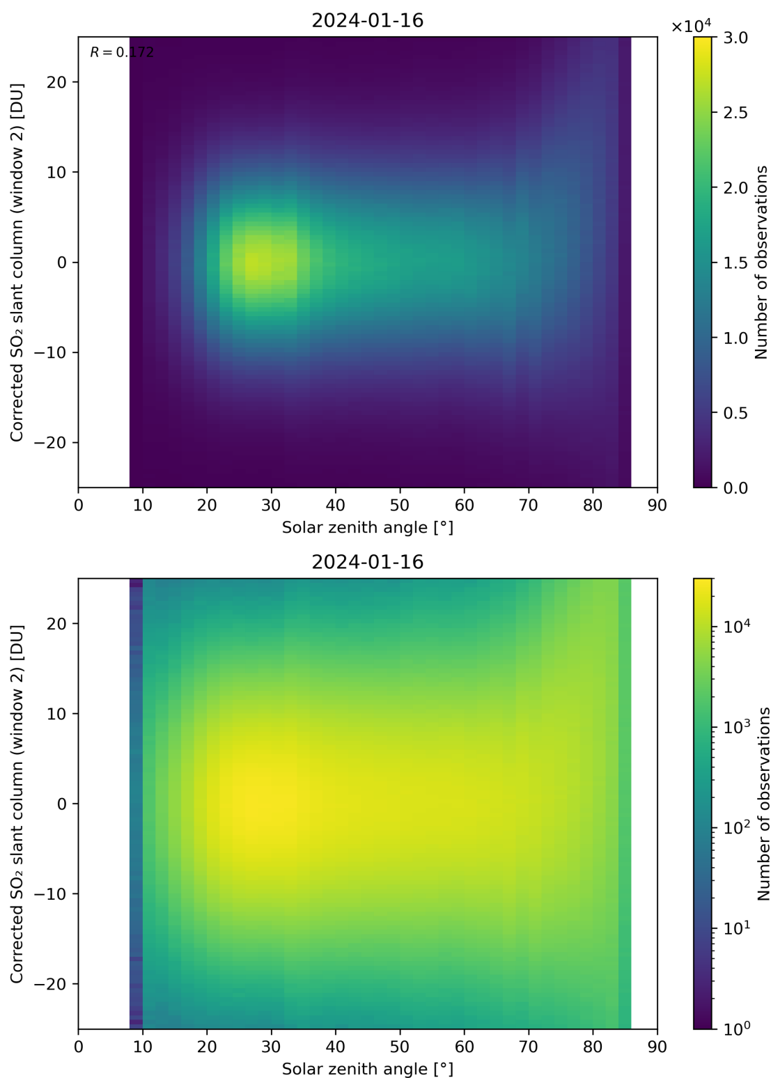
Figure 167: Scatter density plot of “Solar zenith angle” against “Corrected SO 2 slant column (window 2)” for 2024-01-15 to 2024-01-17.
