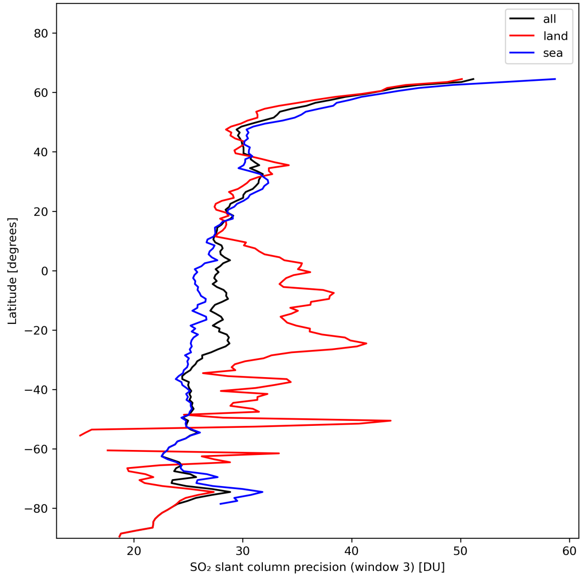
Figure 42: Zonal average of “SO 2 slant column precision (window 3)” for 2024-01-15 to 2024-01-17.
