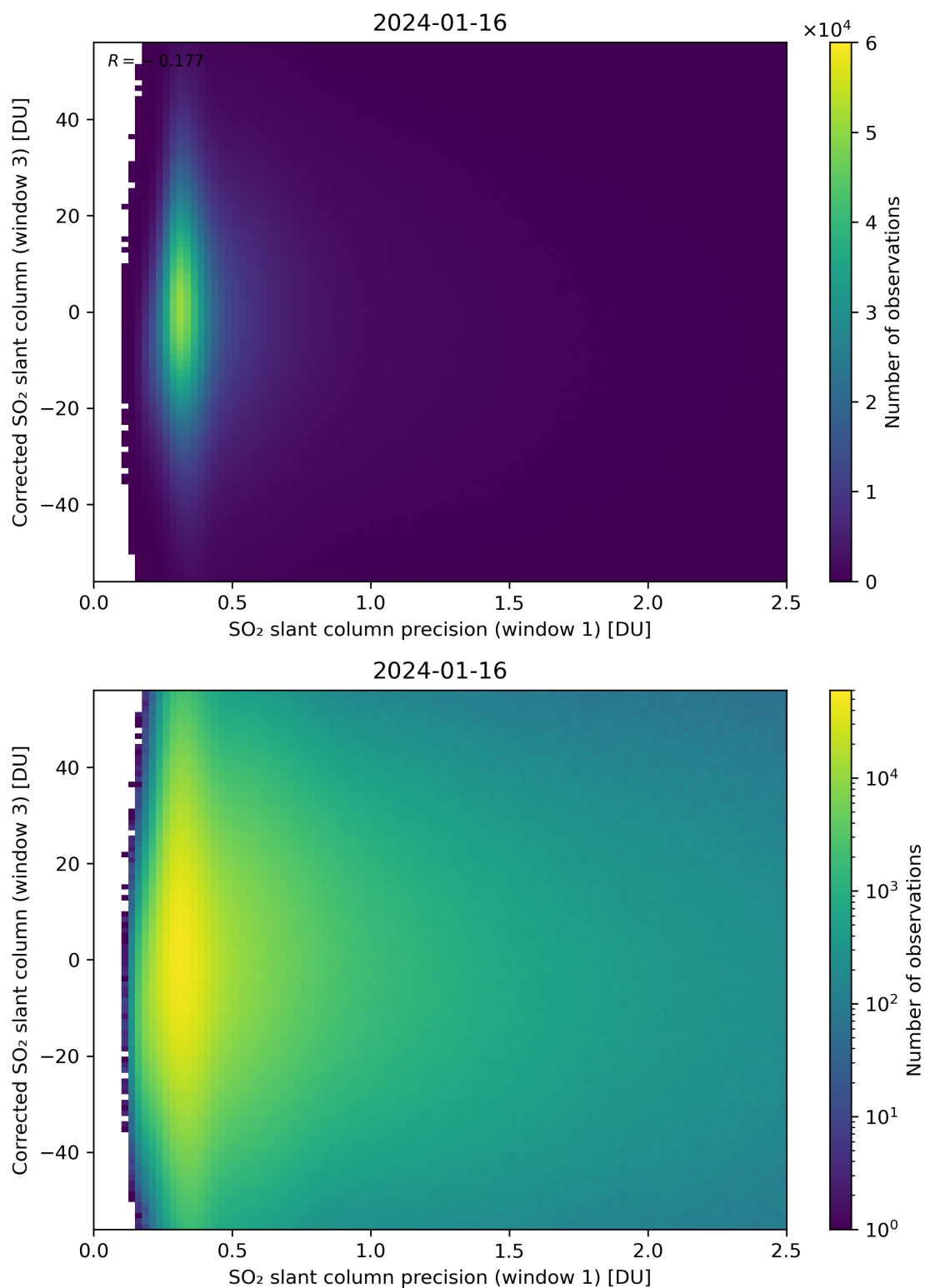
Figure 226: Scatter density plot of “SO 2 slant column precision (window 1)” against “Corrected SO 2 slant column (window 3)” for 2024-01-15 to 2024-01-17.
