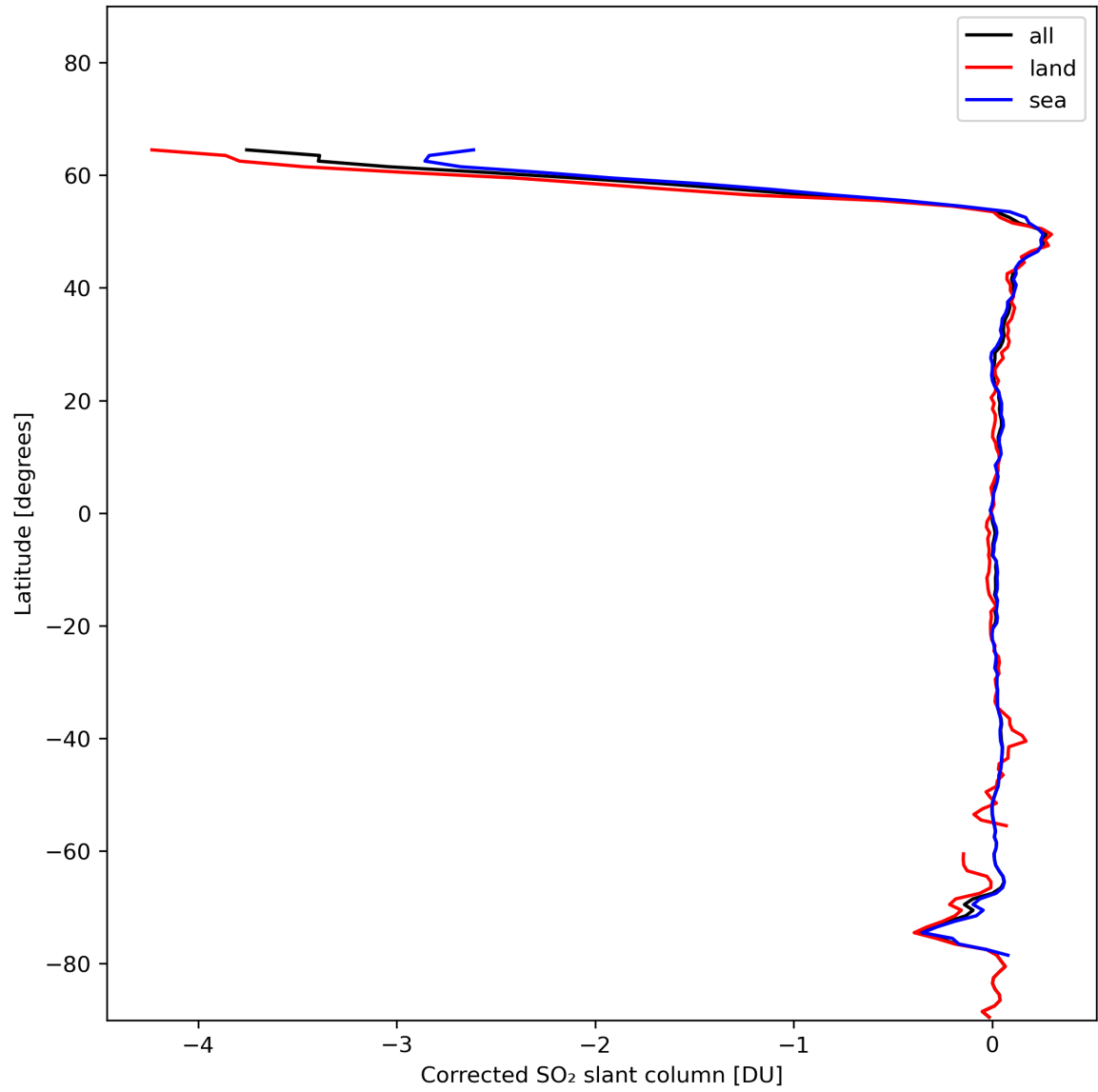
Figure 32: Zonal average of “Corrected SO 2 slant column” for 2024-01-15 to 2024-01-17.
