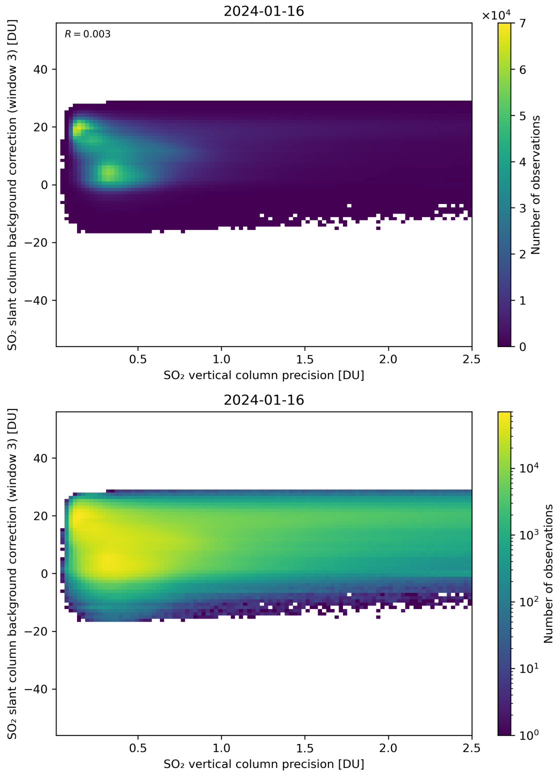
Figure 281: Scatter density plot of “SO 2 vertical column precision” against “SO 2 slant column background correction (window 3)” for 2024-01-15 to 2024-01-17.
