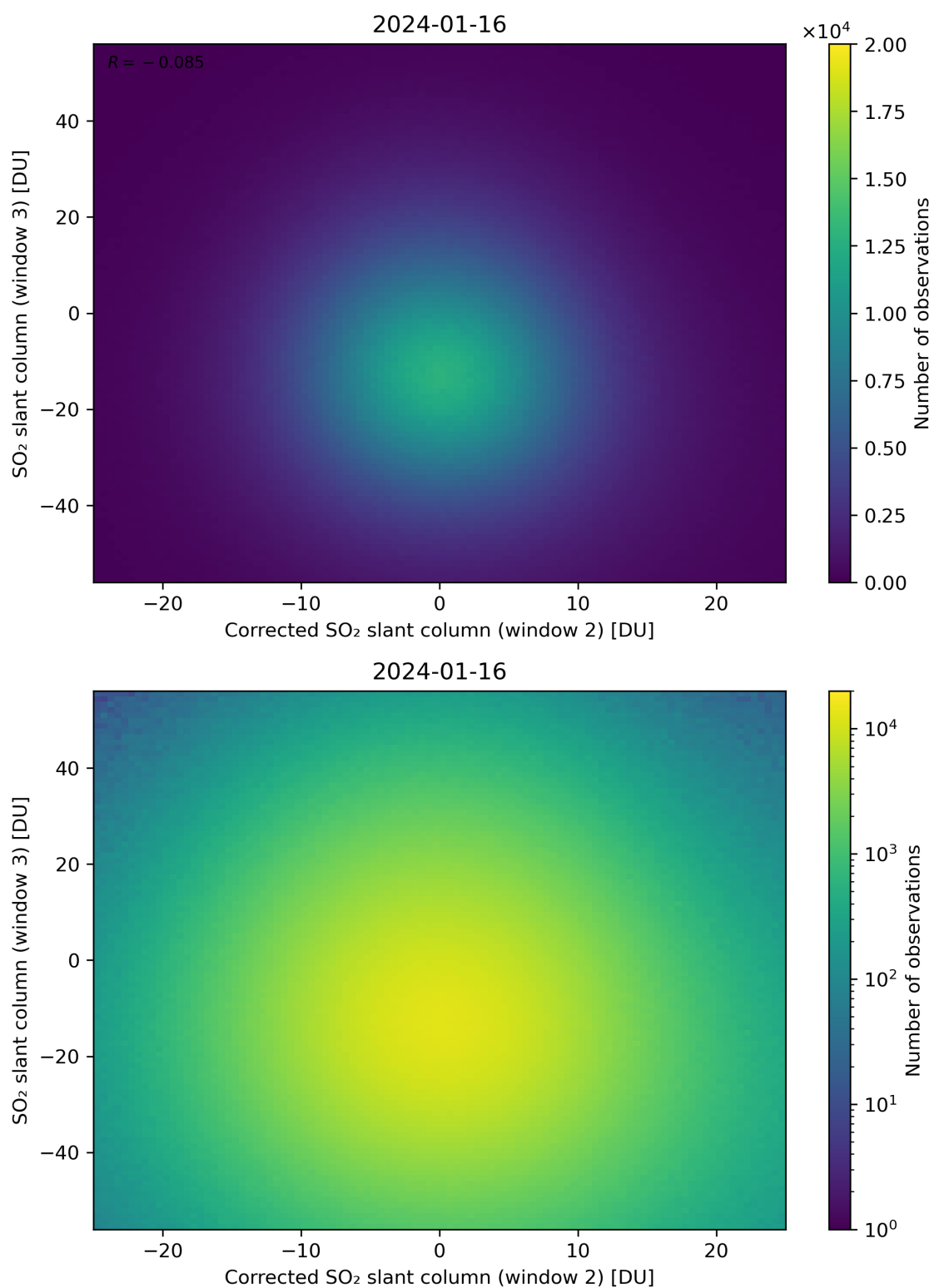
Figure 201: Scatter density plot of “Corrected SO 2 slant column (window 2)” against “SO 2 slant column (window 3)” for 2024-01-15 to 2024-01-17.
