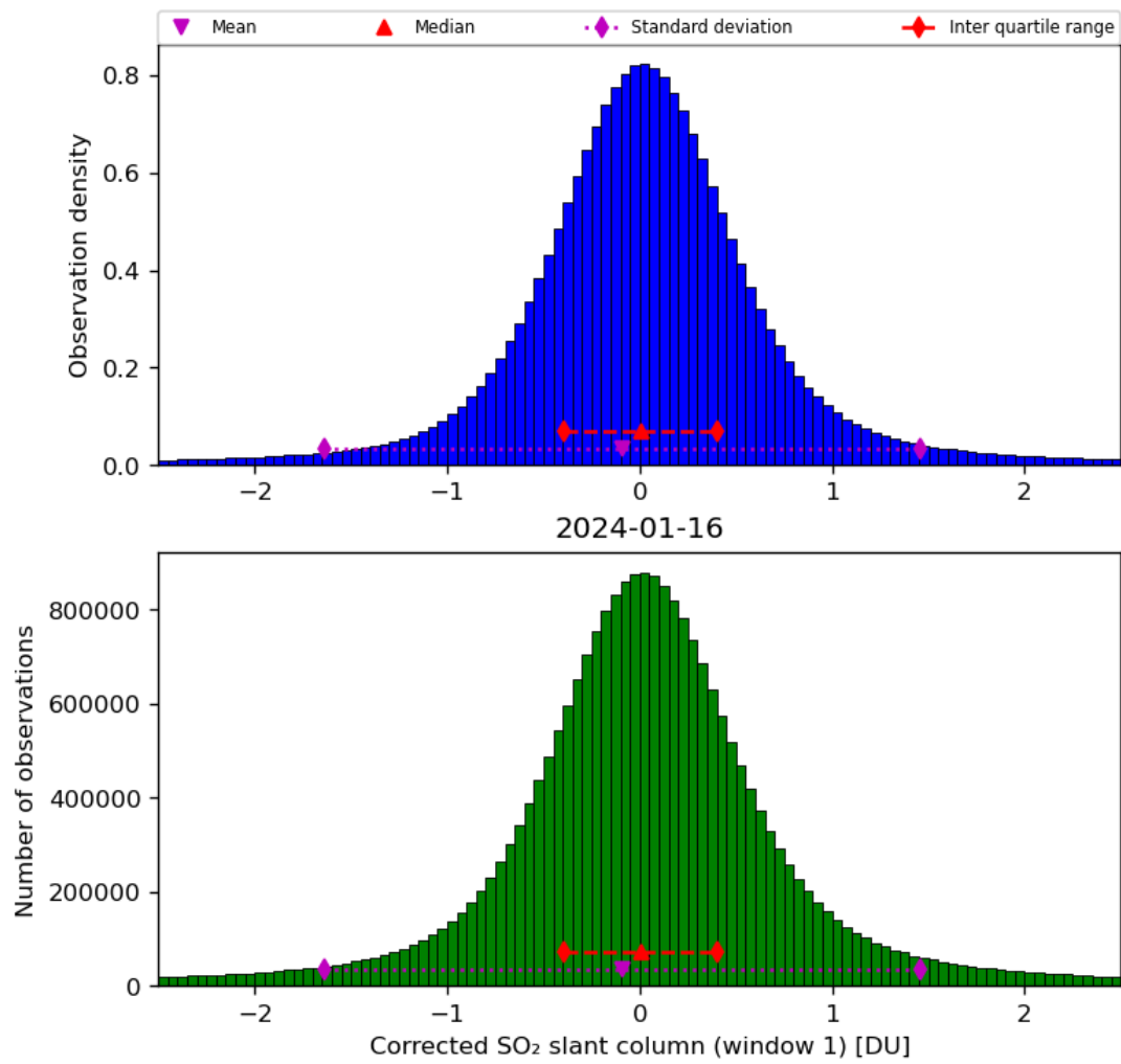
Figure 58: Histogram of “Corrected SO 2 slant column (window 1)” for 2024-01-15 to 2024-01-17
