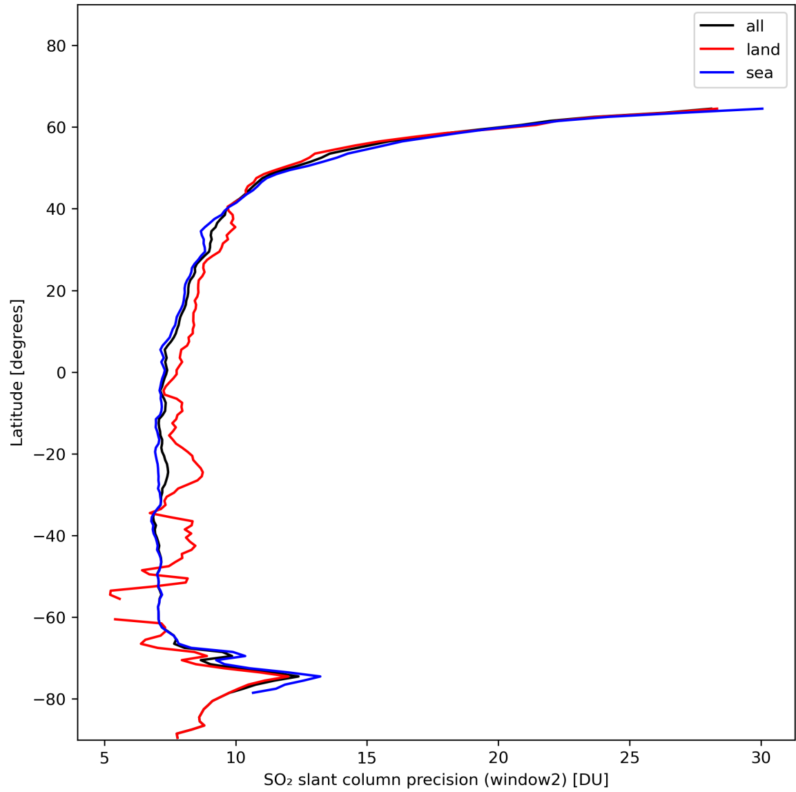
Figure 38: Zonal average of “SO 2 slant column precision (window2)” for 2024-01-15 to 2024-01-17.
