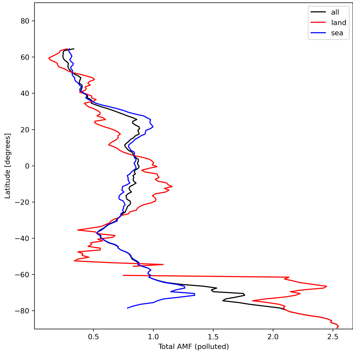
Figure 48: Zonal average of “Total AMF (polluted)” for 2024-01-15 to 2024-01-17.
