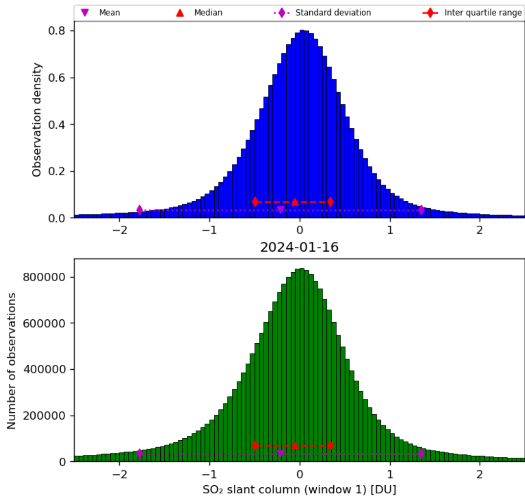
Figure 56: Histogram of “SO 2 slant column (window 1)” for 2024-01-15 to 2024-01-17
