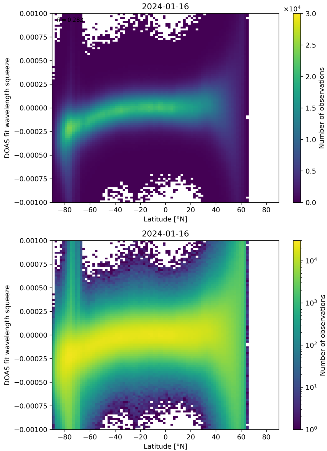
Figure 143: Scatter density plot of “Latitude” against “DOAS fit wavelength squeeze” for 2024-01-15 to 2024-01-17.
