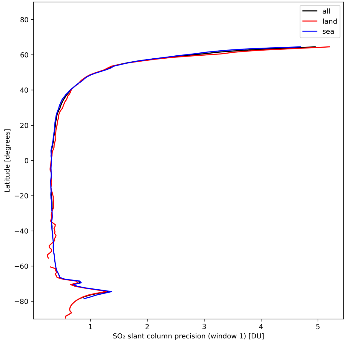
Figure 34: Zonal average of “SO 2 slant column precision (window 1)” for 2024-01-15 to 2024-01-17.
