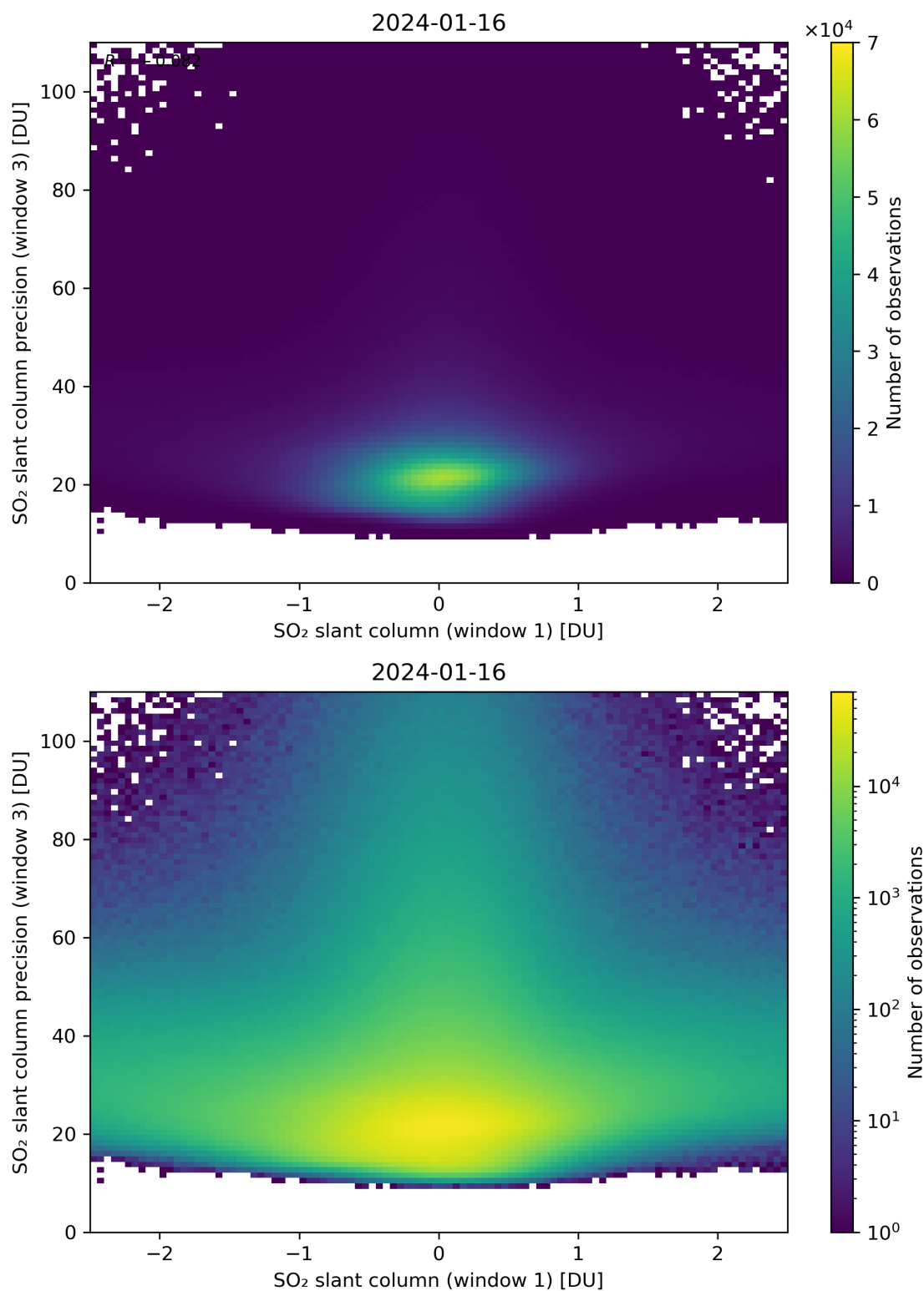
Figure 238: Scatter density plot of “SO 2 slant column (window 1)” against “SO 2 slant column precision (window 3)” for 2024-01-15 to 2024-01-17.
