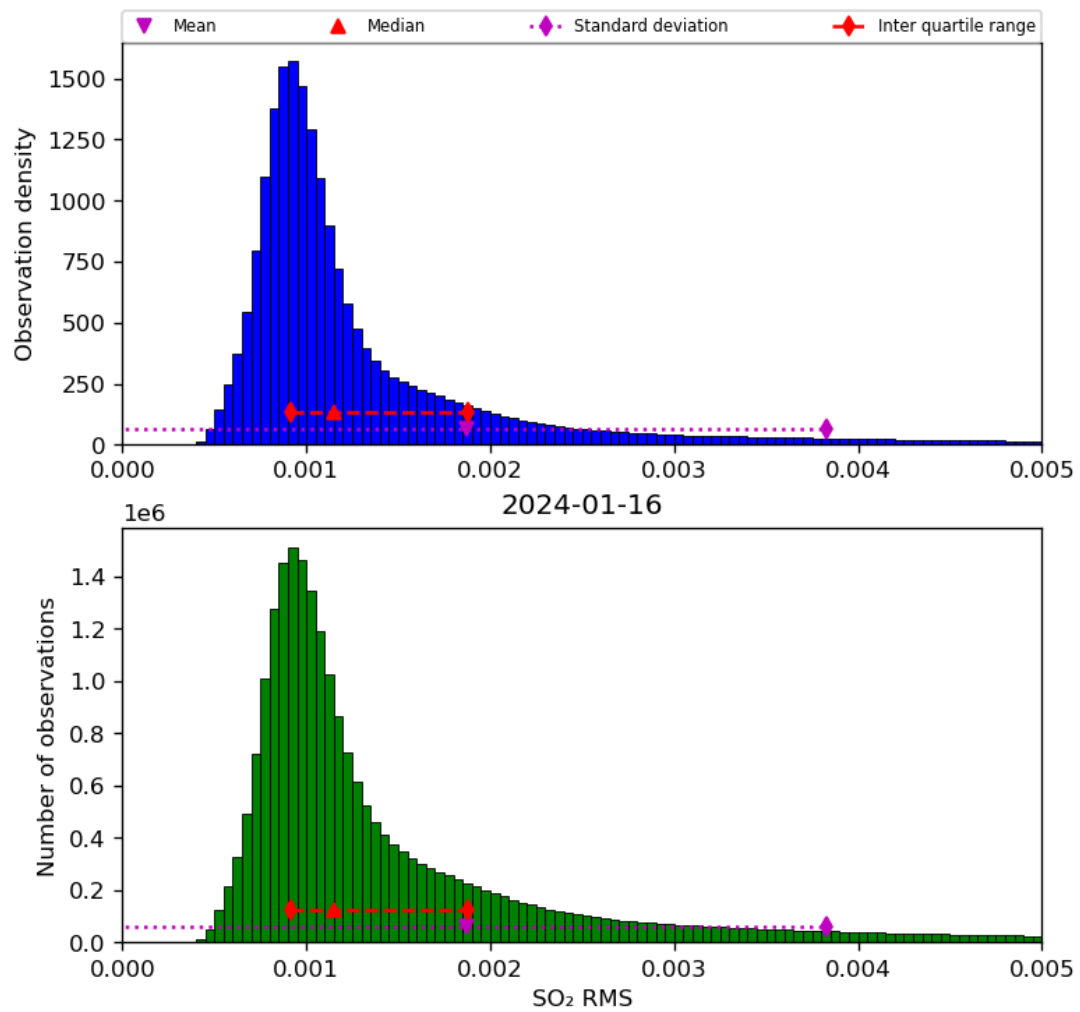
Figure 70: Histogram of “SO 2 RMS” for 2024-01-15 to 2024-01-17
