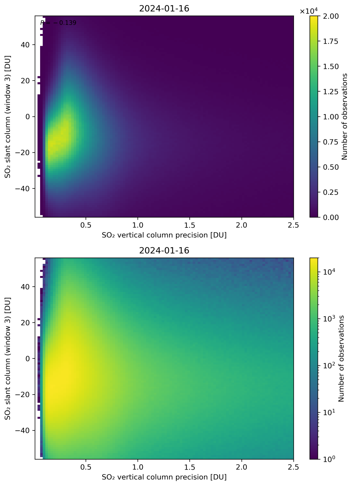
Figure 292: Scatter density plot of “SO 2 vertical column precision” against “SO 2 slant column (window 3)” for 2024-01-15 to 2024-01-17.
