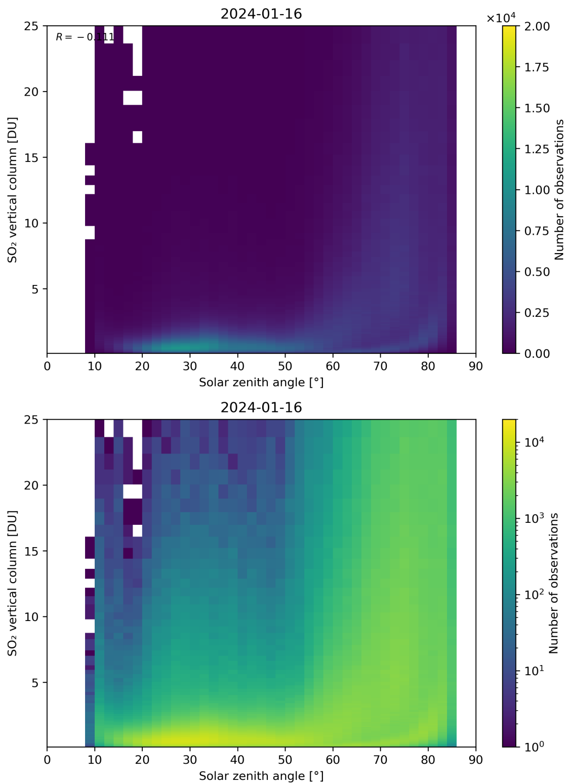
Figure 176: Scatter density plot of “Solar zenith angle” against “SO 2 vertical column” for 2024-01-15 to 2024-01-17.
