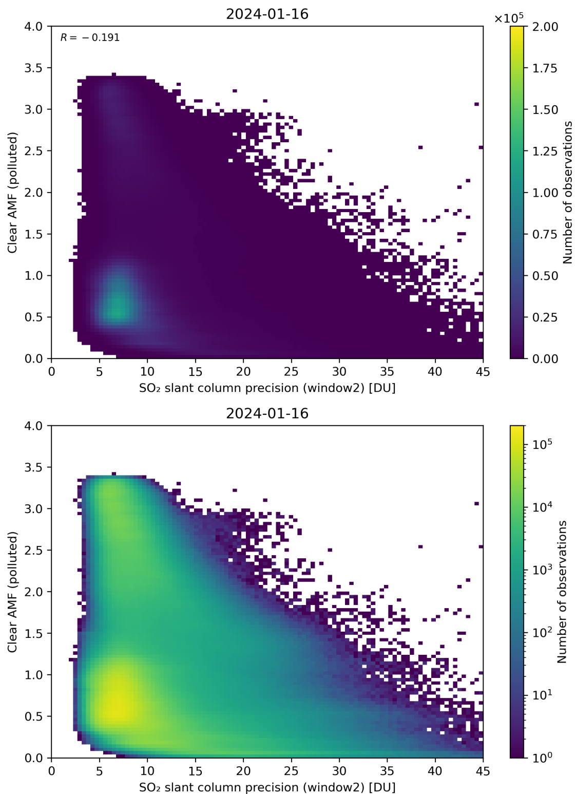
Figure 246: Scatter density plot of “SO 2 slant column precision (window2)” against “Clear AMF (polluted)” for 2024-01-15 to 2024-01-17.
