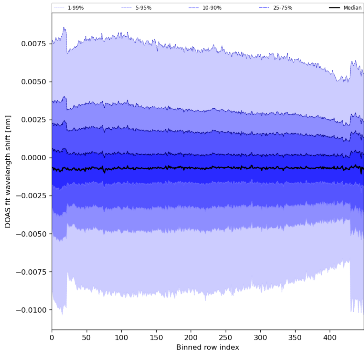
Figure 91: Along track statistics of “DOAS fit wavelength shift” for 2024-01-15 to 2024-01-17
