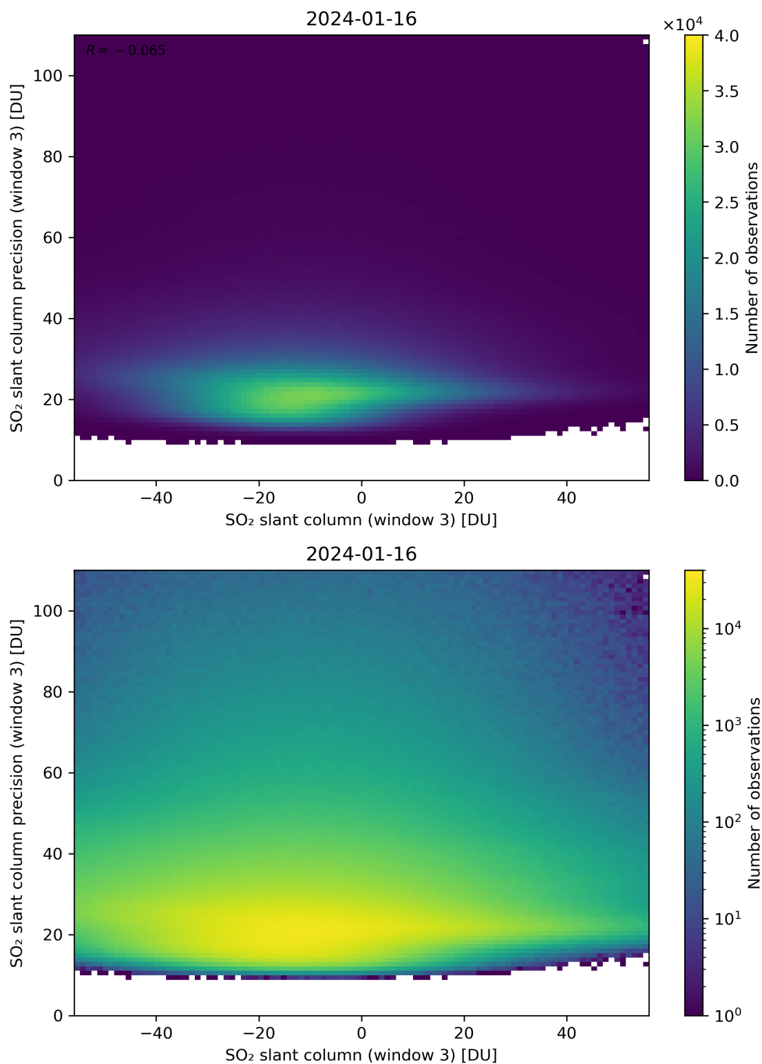
Figure 267: Scatter density plot of “SO 2 slant column (window 3)” against “SO 2 slant column precision (window 3)” for 2024-01-15 to 2024-01-17.
