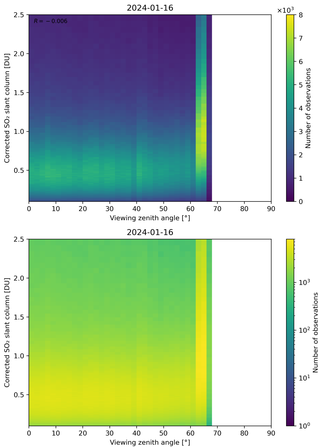
Figure 317: Scatter density plot of “Viewing zenith angle” against “Corrected SO 2 slant column” for 2024-01-15 to 2024-01-17.
