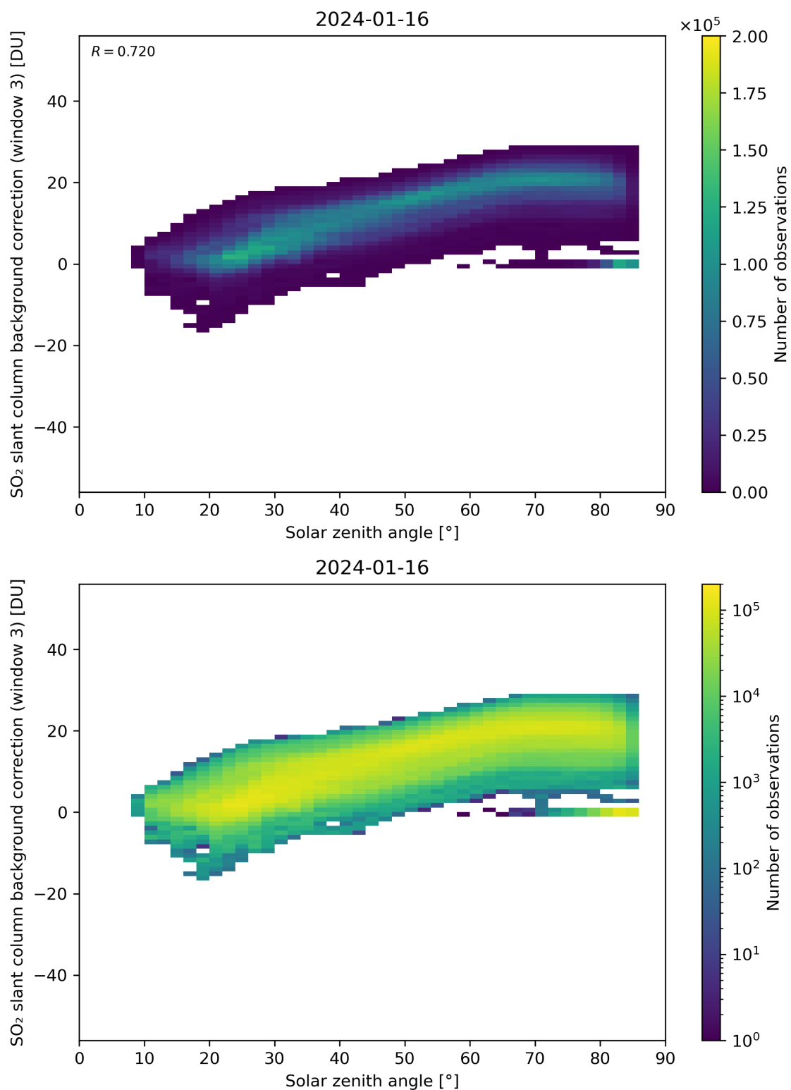
Figure 160: Scatter density plot of “Solar zenith angle” against “SO 2 slant column background correction (window 3)” for 2024-01-15 to 2024-01-17.
