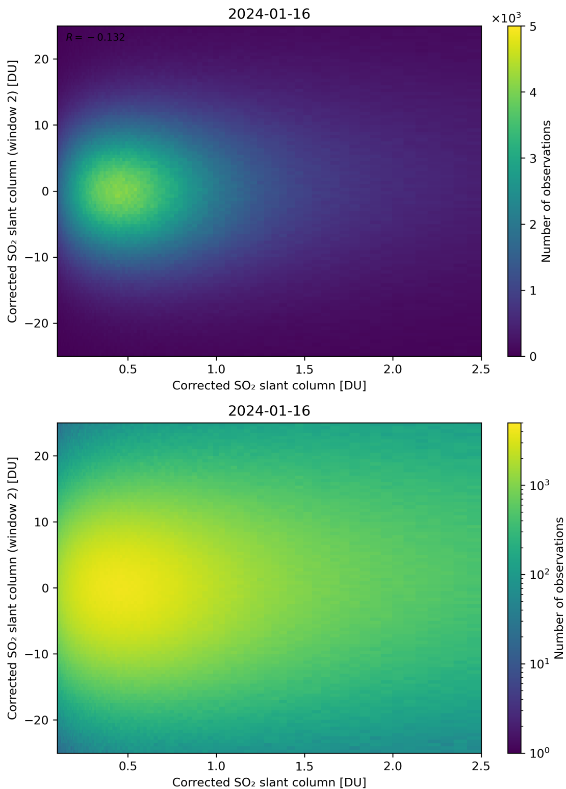
Figure 185: Scatter density plot of “Corrected SO 2 slant column” against “Corrected SO 2 slant column (window 2)” for 2024-01-15 to 2024-01-17.
