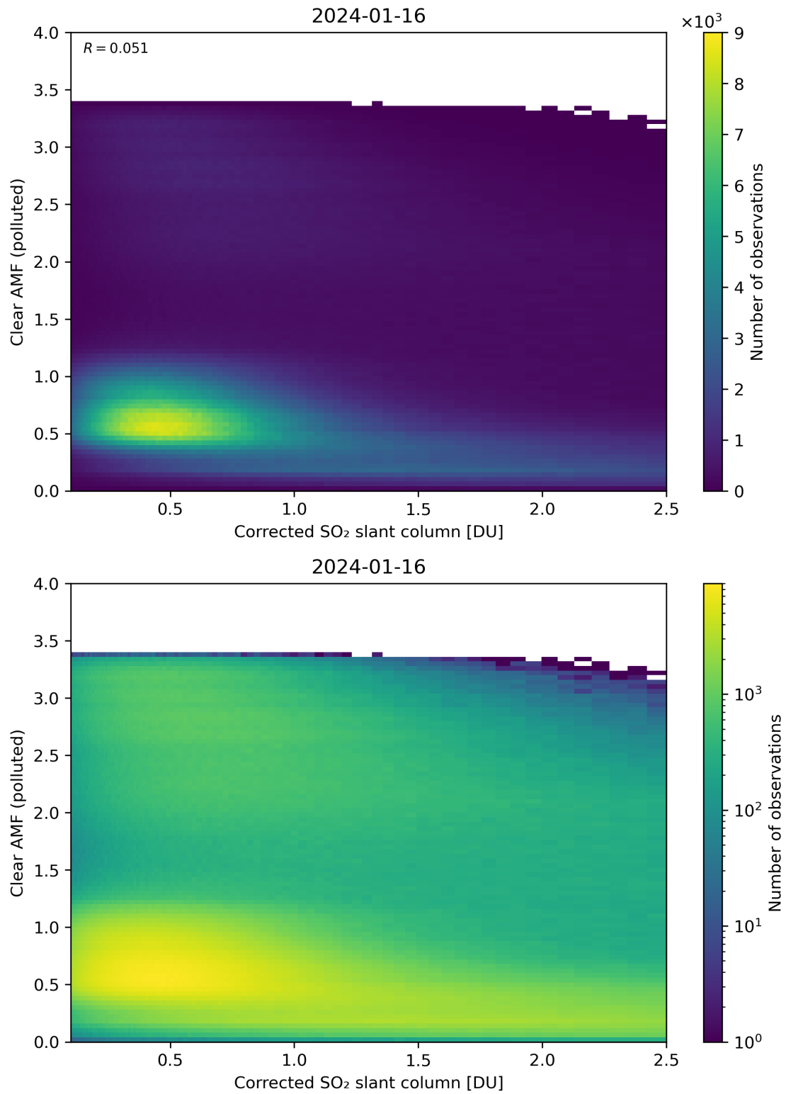
Figure 184: Scatter density plot of “Corrected SO 2 slant column” against “Clear AMF (polluted)” for 2024-01-15 to 2024-01-17.
