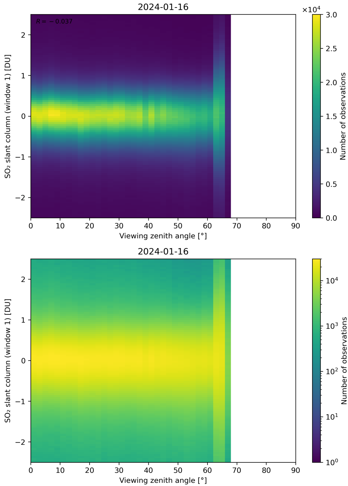
Figure 320: Scatter density plot of “Viewing zenith angle” against “SO 2 slant column (window 1)” for 2024-01-15 to 2024-01-17.
