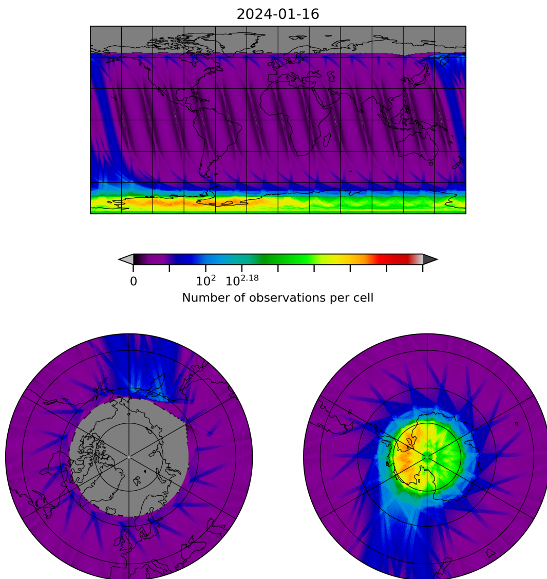
Figure 28: Map of the number of observations for 2024-01-15 to 2024-01-17
