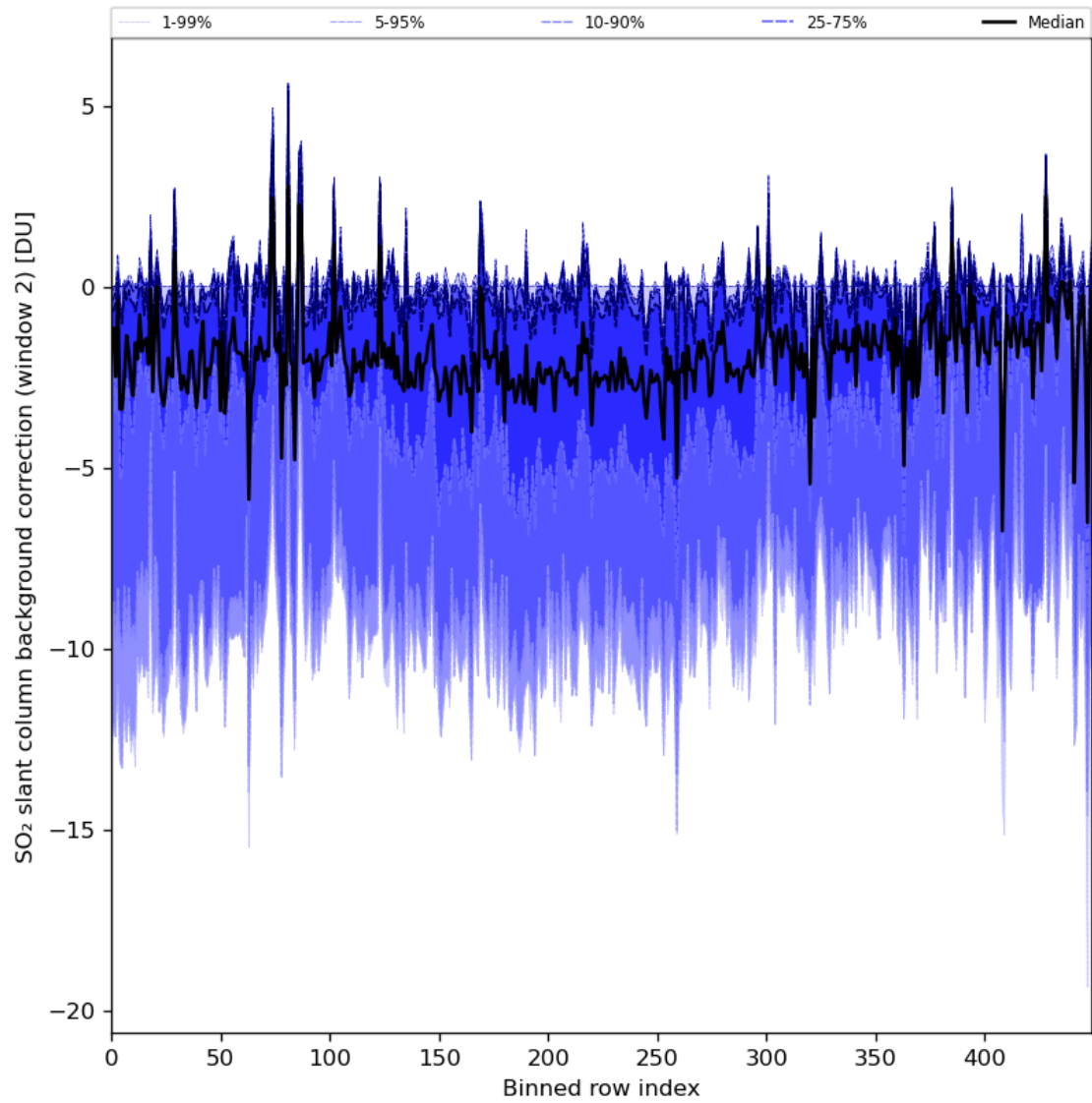
Figure 86: Along track statistics of “SO 2 slant column background correction (window 2)” for 2024-01-15 to 2024-01-17
