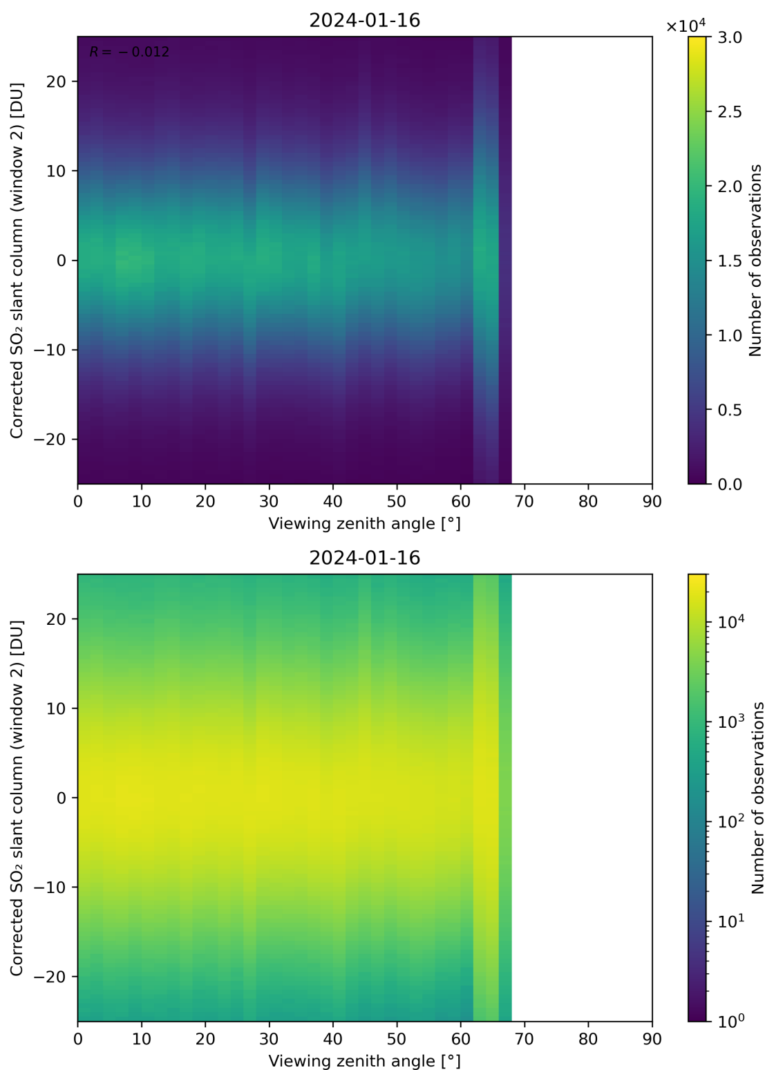
Figure 318: Scatter density plot of “Viewing zenith angle” against “Corrected SO 2 slant column (window 2)” for 2024-01-15 to 2024-01-17.
