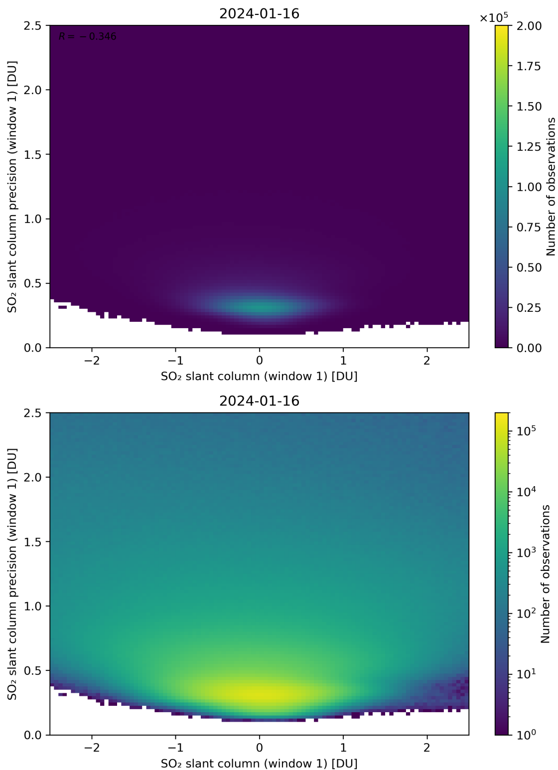
Figure 235: Scatter density plot of “SO 2 slant column (window 1)” against “SO 2 slant column precision (window 1)” for 2024-01-15 to 2024-01-17.
