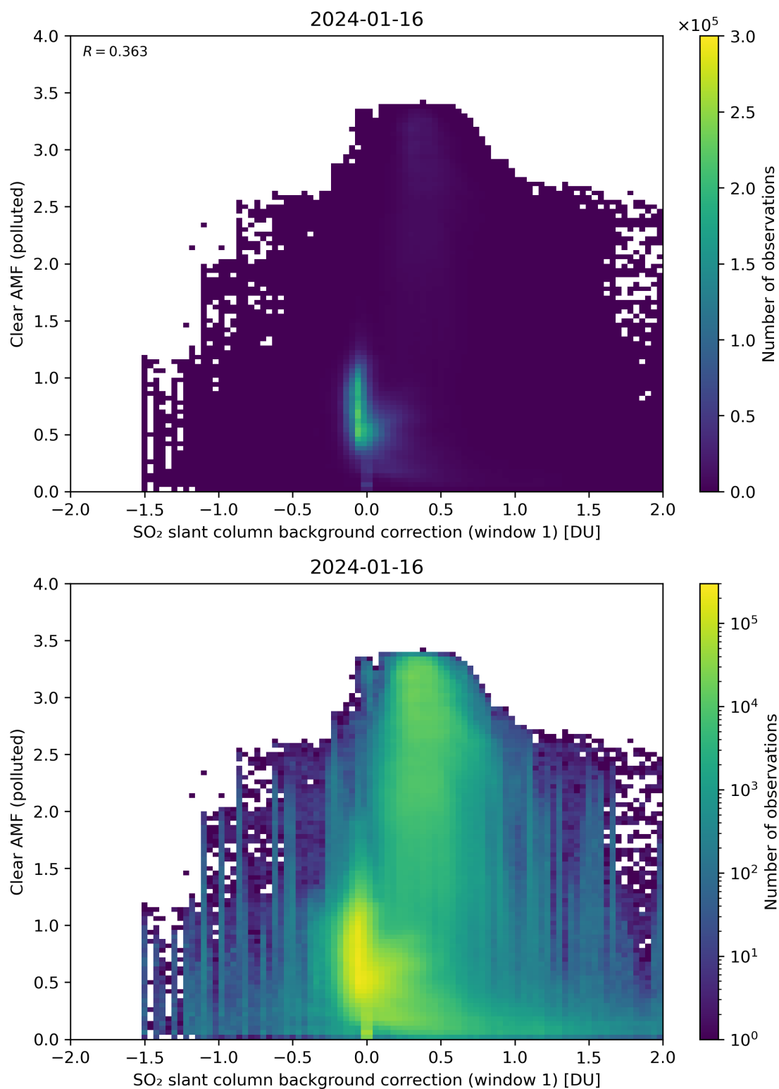
Figure 103: Scatter density plot of “SO 2 slant column background correction (window 1)” against “Clear AMF (polluted)” for 2024-01-15 to 2024-01-17.
