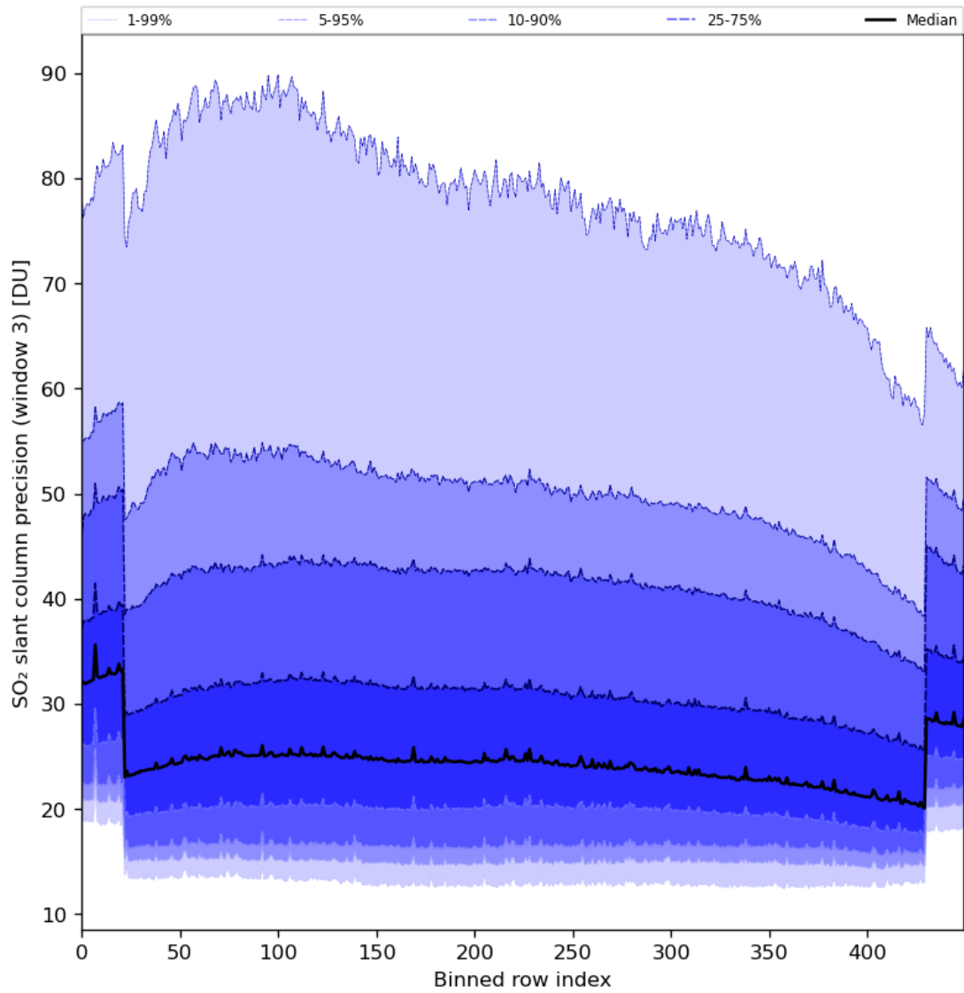
Figure 88: Along track statistics of “SO 2 slant column precision (window 3)” for 2024-01-15 to 2024-01-17
