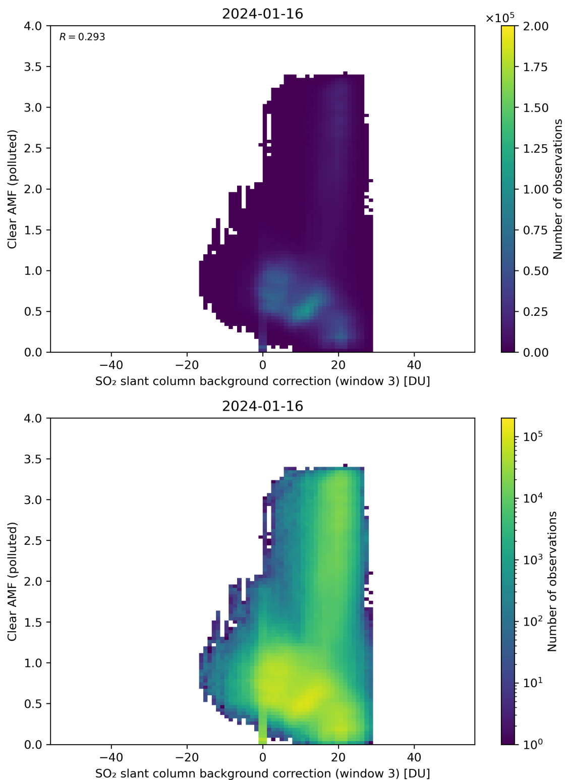
Figure 124: Scatter density plot of “SO 2 slant column background correction (window 3)” against “Clear AMF (polluted)” for 2024-01-15 to 2024-01-17.
