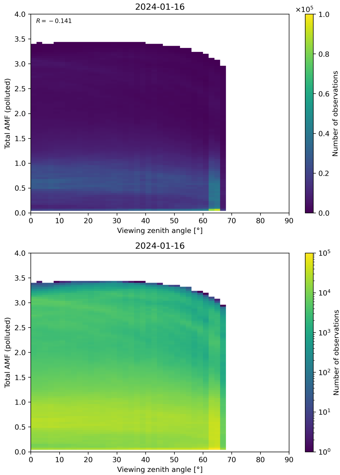
Figure 325: Scatter density plot of “Viewing zenith angle” against “Total AMF (polluted)” for 2024-01-15 to 2024-01-17.
