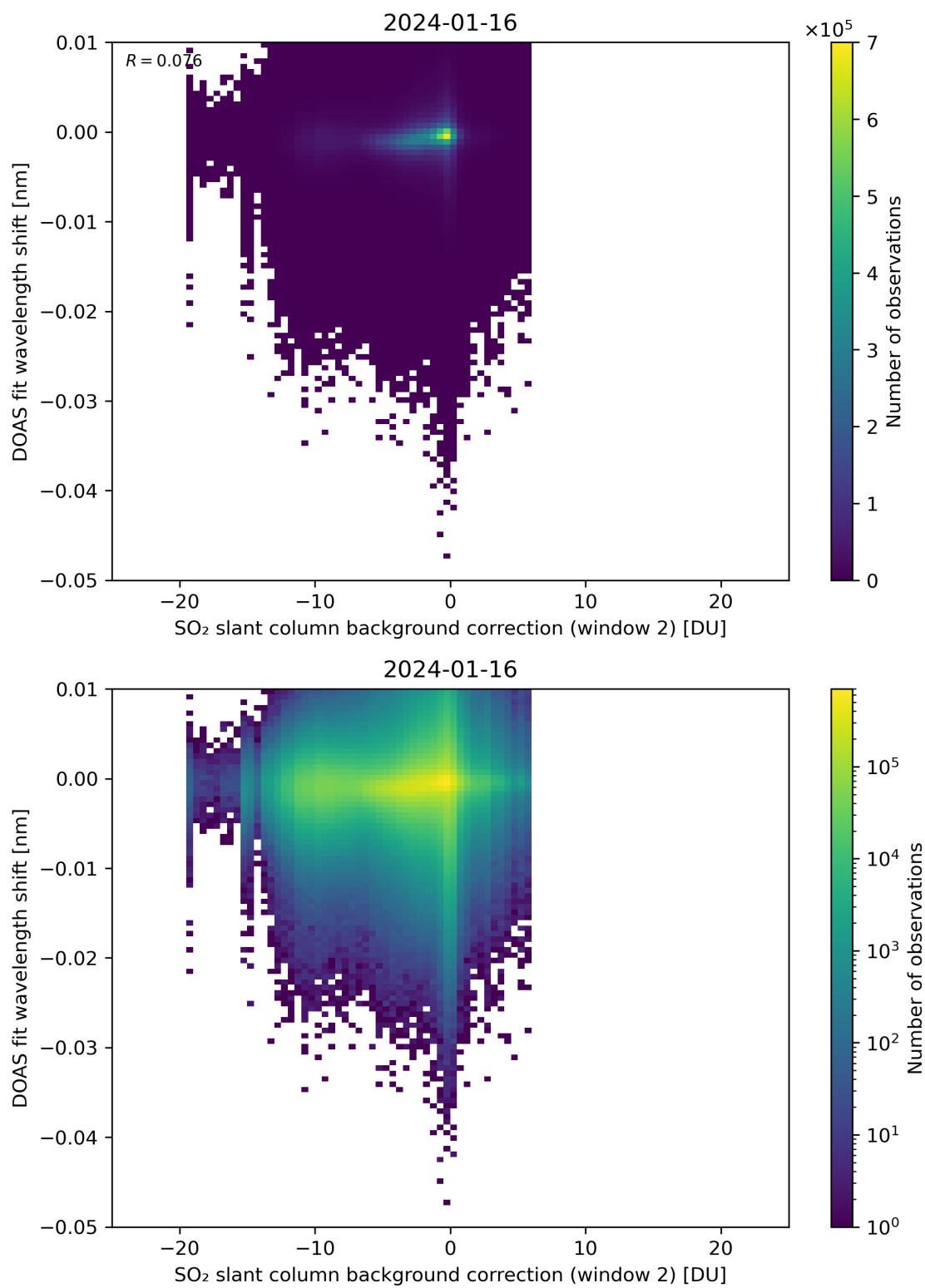
Figure 112: Scatter density plot of “SO 2 slant column background correction (window 2)” against “DOAS fit wavelength shift” for 2024-01-15 to 2024-01-17.
