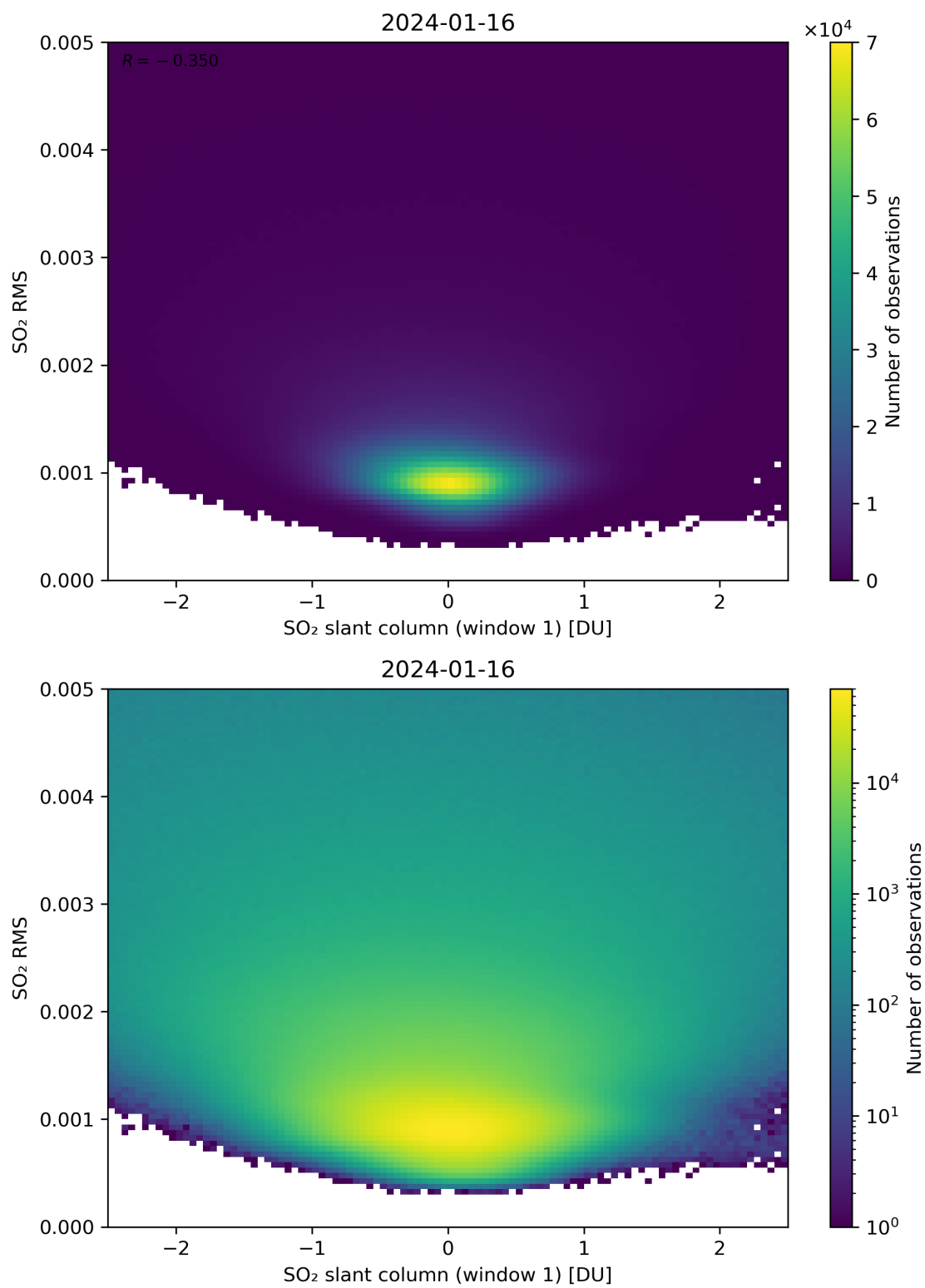
Figure 217: Scatter density plot of “SO 2 slant column (window 1)” against “SO 2 RMS” for 2024-01-15 to 2024-01-17.
