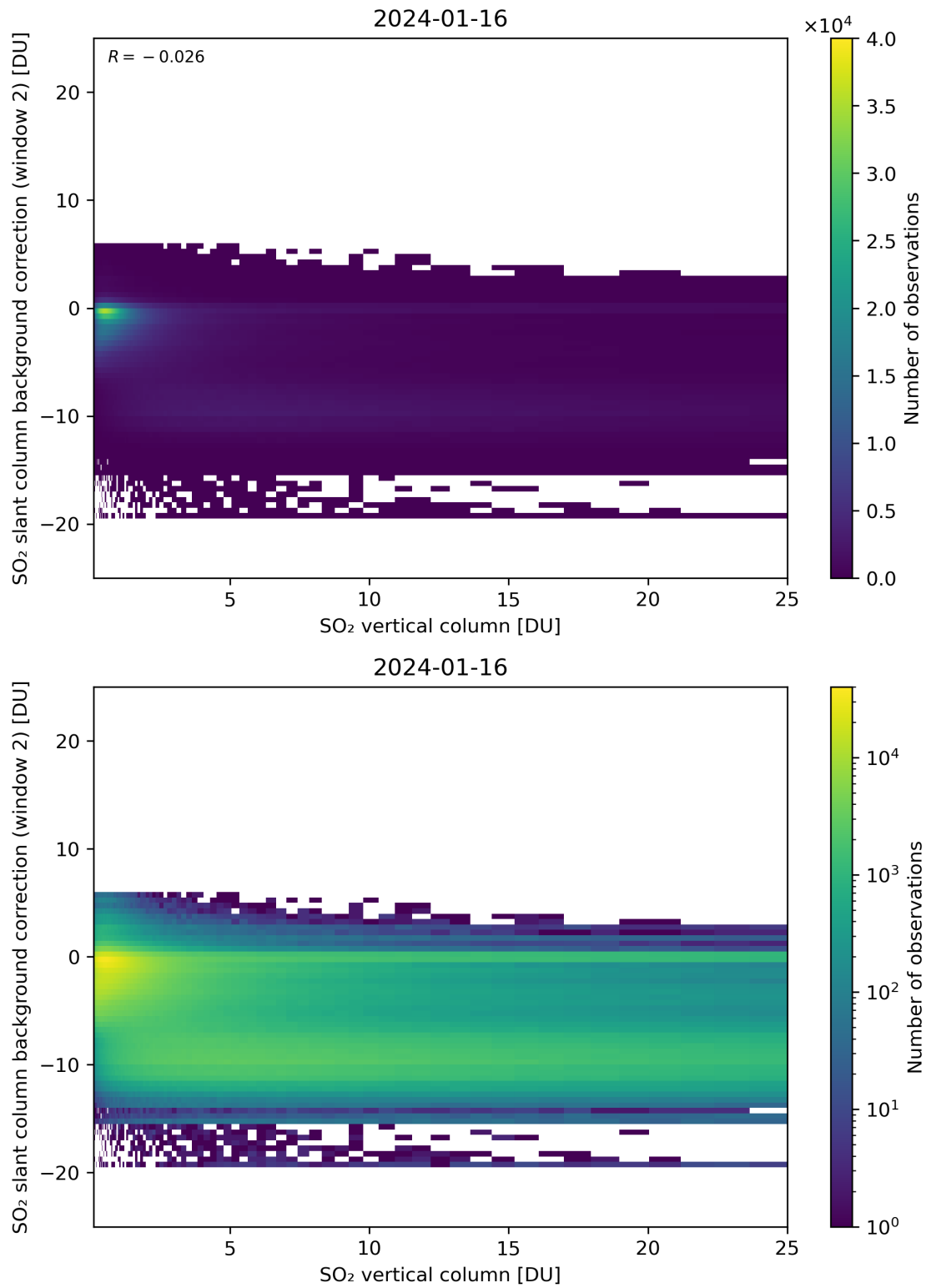
Figure 274: Scatter density plot of “SO 2 vertical column” against “SO 2 slant column background correction (window 2)” for 2024-01-15 to 2024-01-17.
