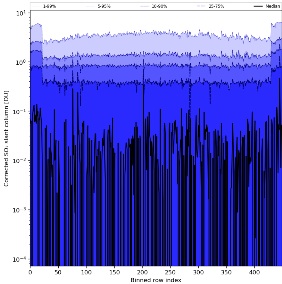
Figure 78: Along track statistics of “Corrected SO 2 slant column” for 2024-01-15 to 2024-01-17
