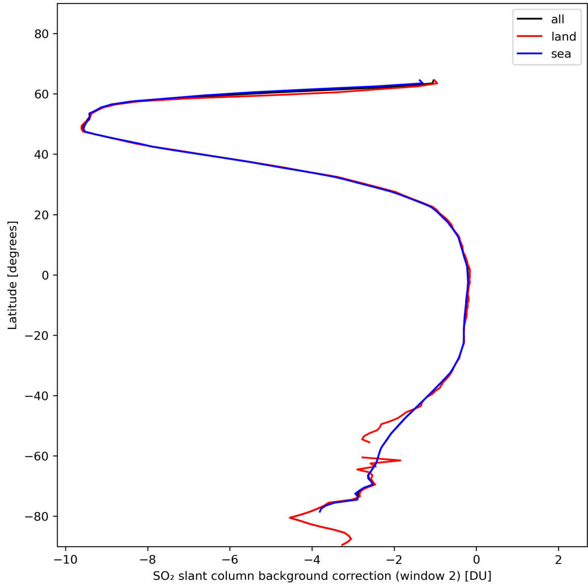
Figure 40: Zonal average of “SO 2 slant column background correction (window 2)” for 2024-01-15 to 2024-01-17.
