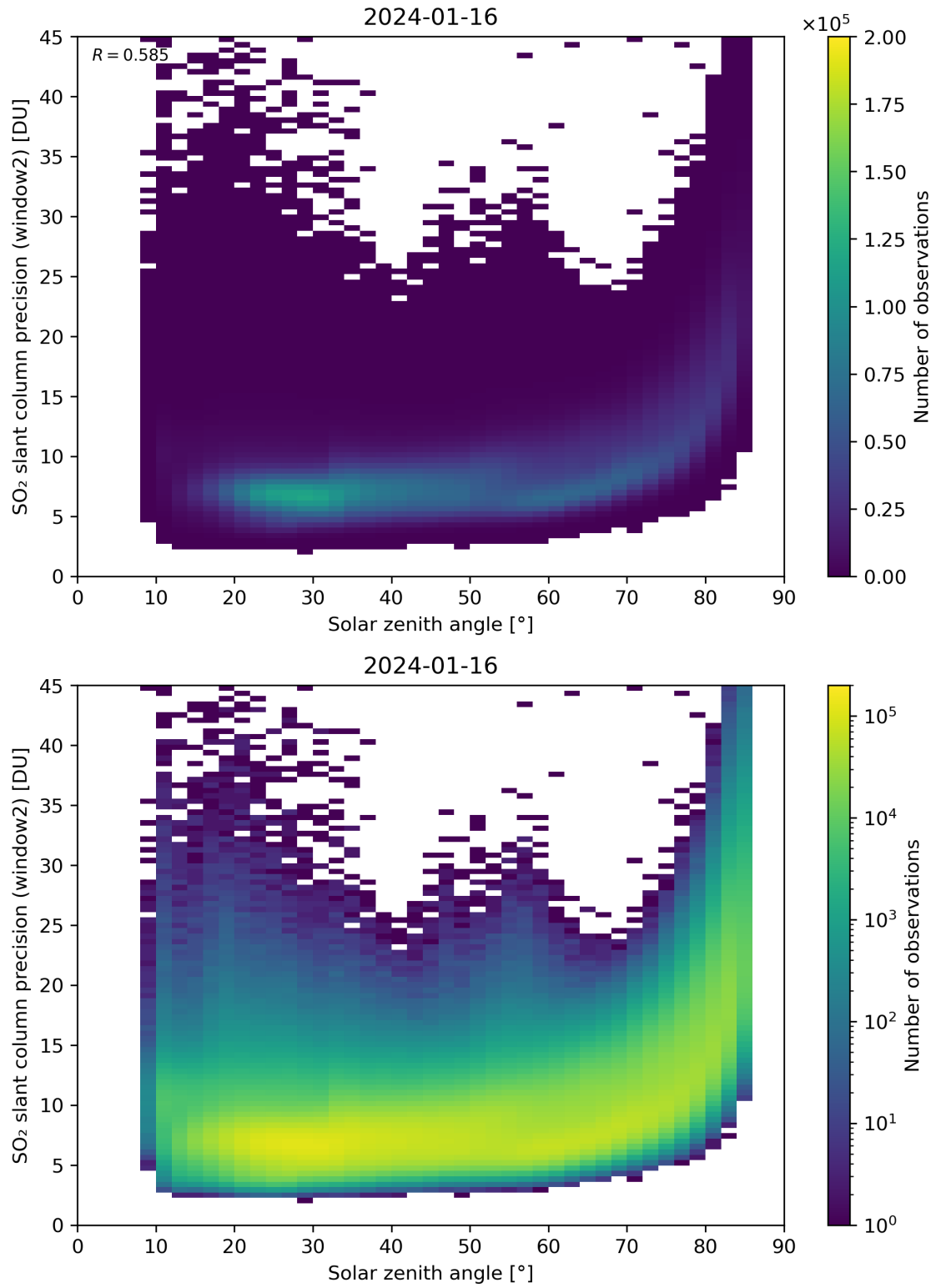
Figure 171: Scatter density plot of “Solar zenith angle” against “SO 2 slant column precision (window2)” for 2024-01-15 to 2024-01-17.
