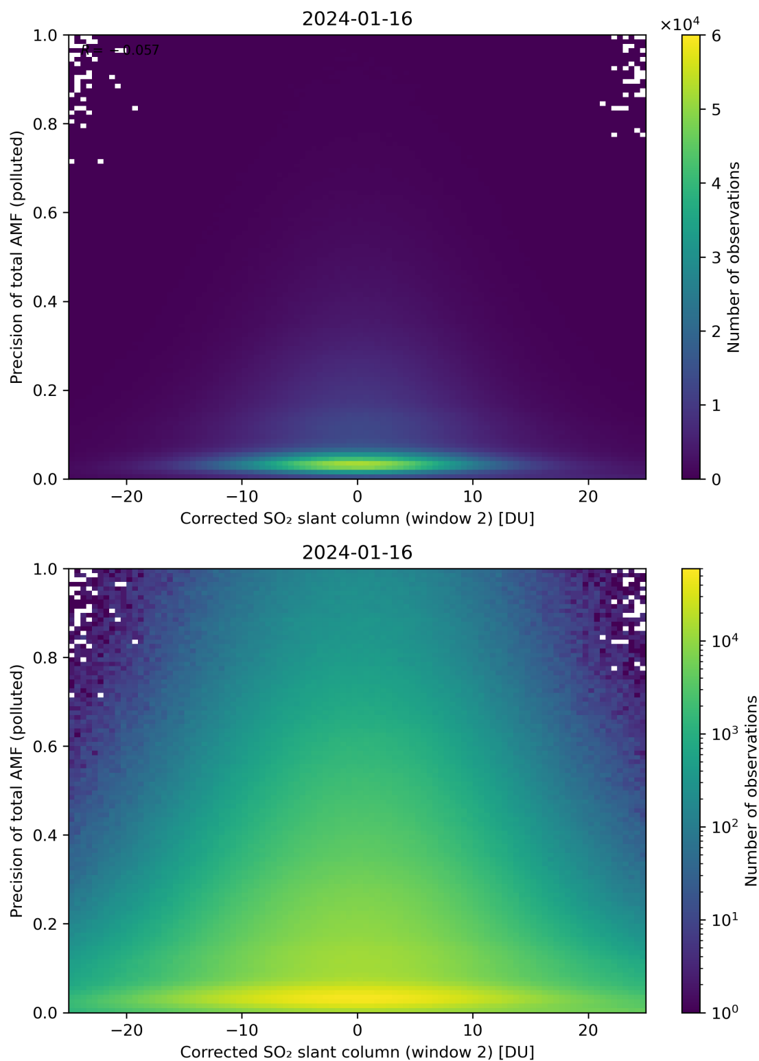
Figure 204: Scatter density plot of “Corrected SO 2 slant column (window 2)” against “Precision of total AMF (polluted)” for 2024-01-15 to 2024-01-17.
