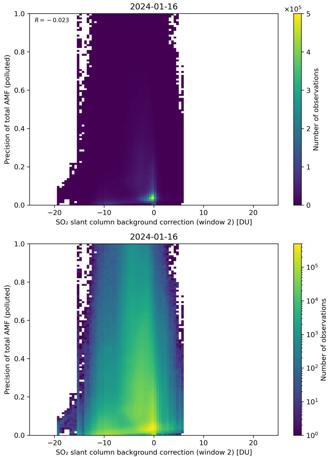
Figure 120: Scatter density plot of “SO 2 slant column background correction (window 2)” against “Precision of total AMF (polluted)” for 2024-01-15 to 2024-01-17.
