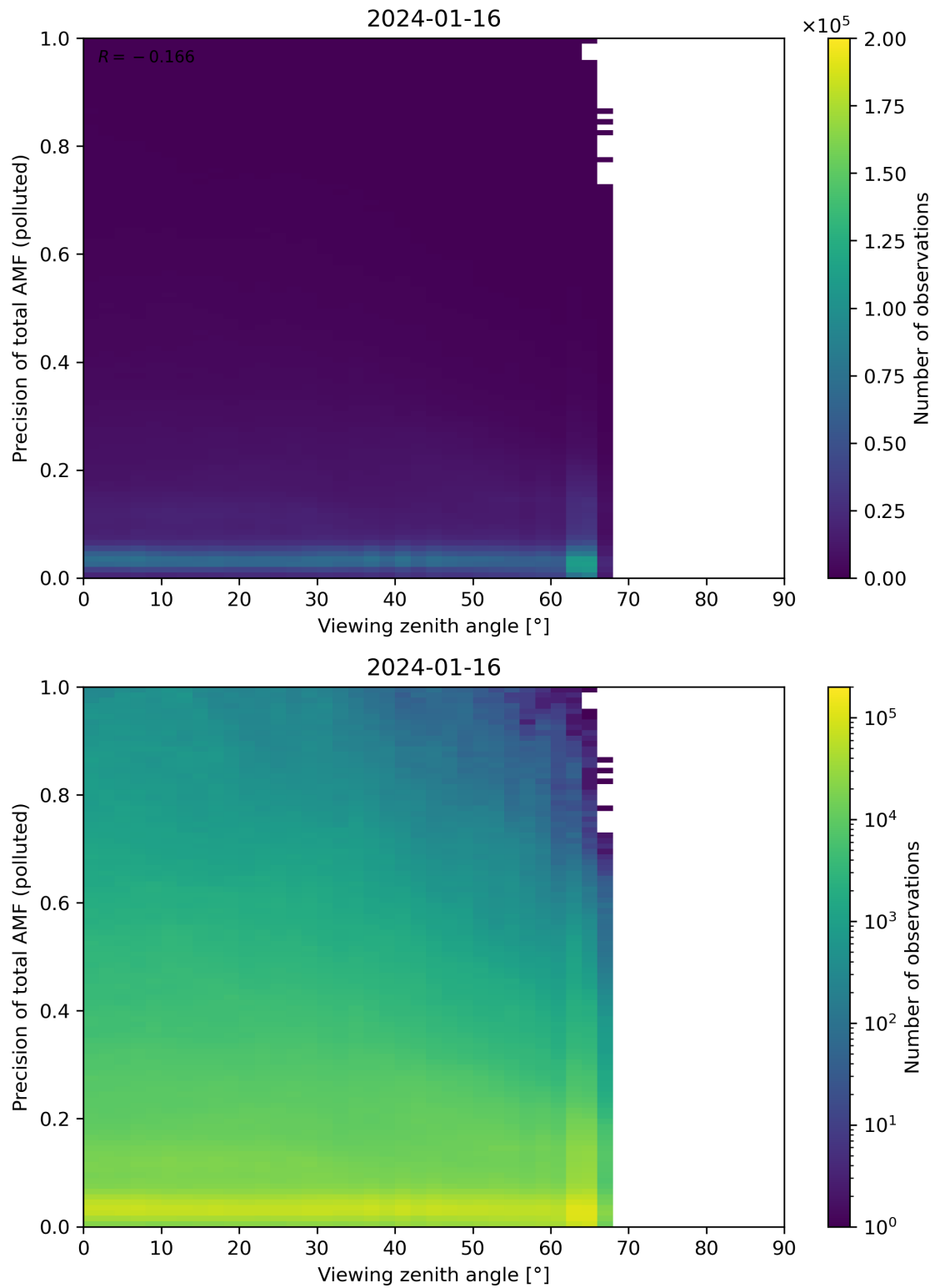
Figure 326: Scatter density plot of “Viewing zenith angle” against “Precision of total AMF (polluted)” for 2024-01-15 to 2024-01-17.
