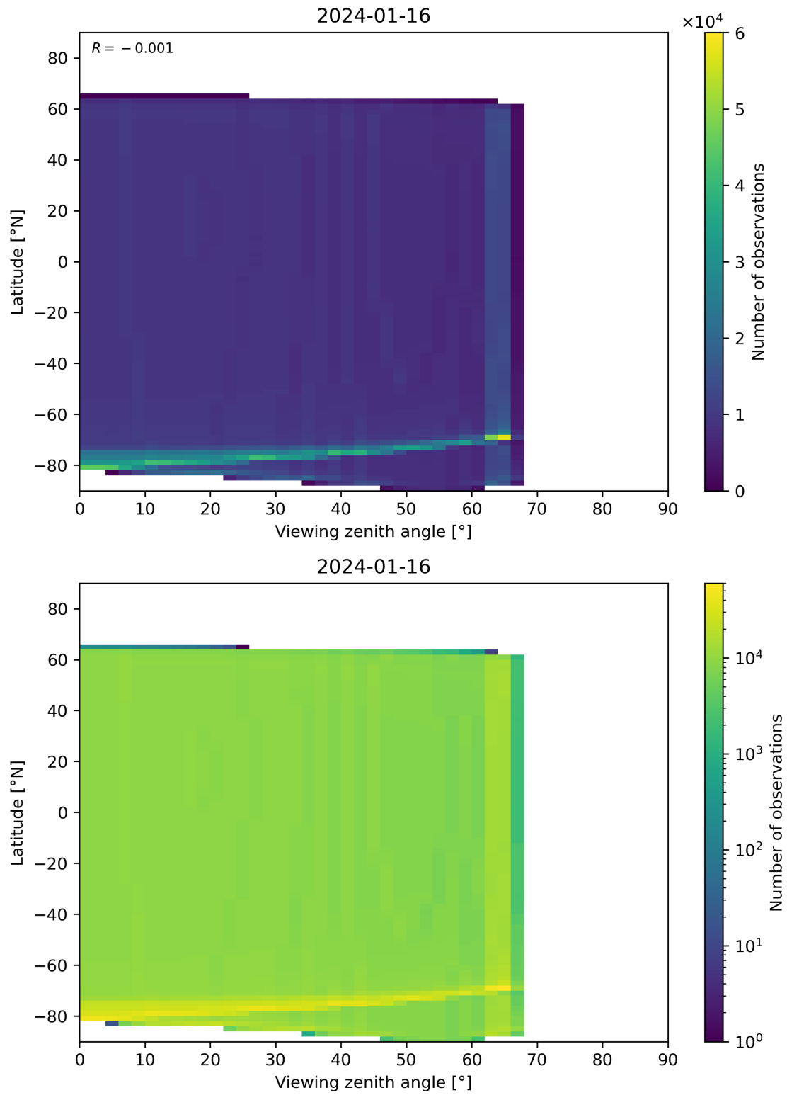
Figure 314: Scatter density plot of “Viewing zenith angle” against “Latitude” for 2024-01-15 to 2024-01-17.
