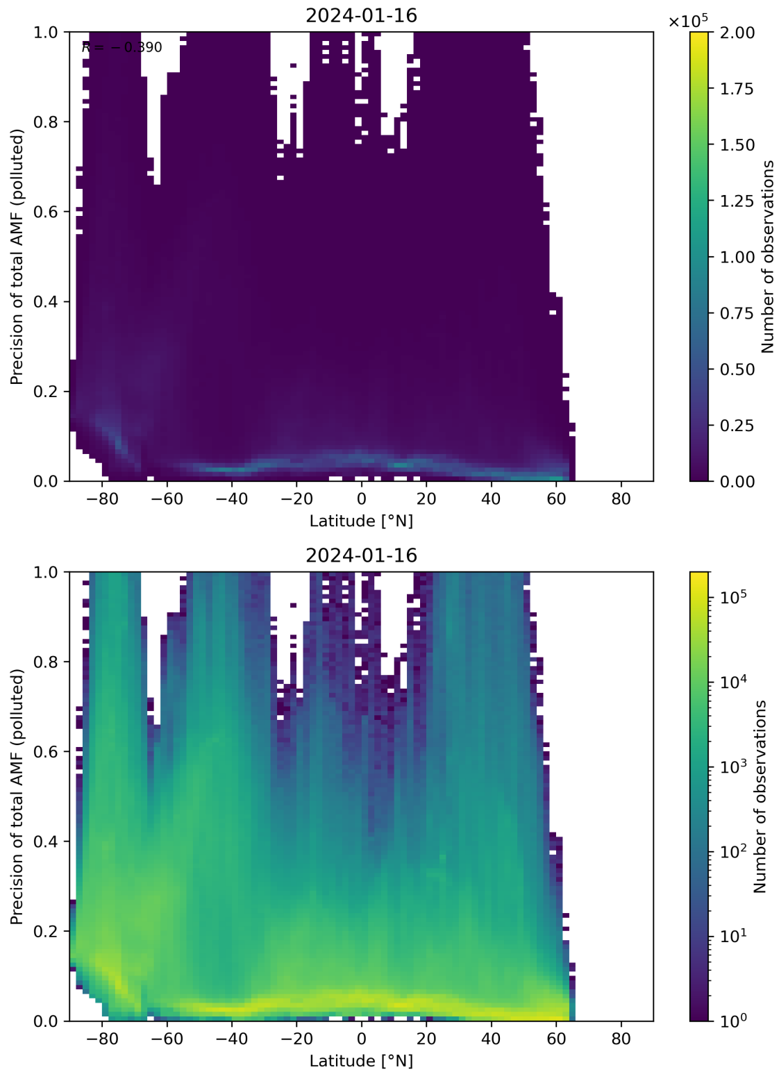
Figure 155: Scatter density plot of “Latitude” against “Precision of total AMF (polluted)” for 2024-01-15 to 2024-01-17.
