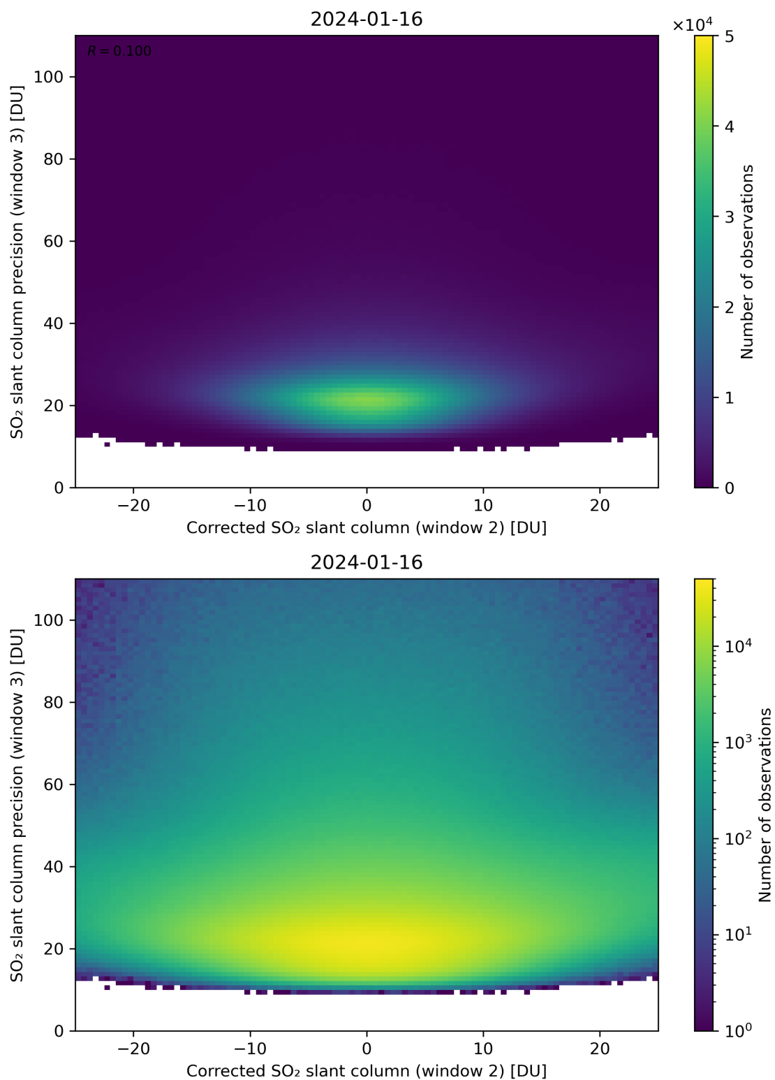
Figure 202: Scatter density plot of “Corrected SO 2 slant column (window 2)” against “SO 2 slant column precision (window 3)” for 2024-01-15 to 2024-01-17.
