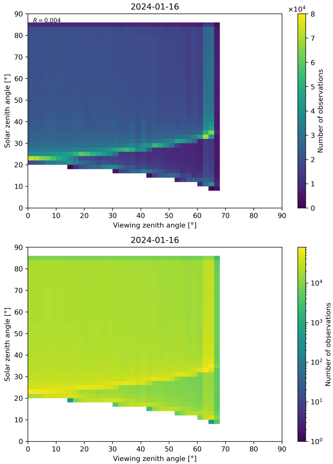
Figure 315: Scatter density plot of “Viewing zenith angle” against “Solar zenith angle” for 2024-01-15 to 2024-01-17.
