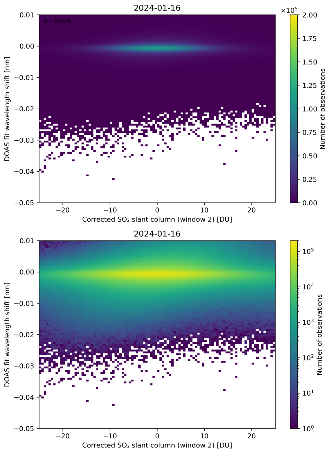
Figure 196: Scatter density plot of “Corrected SO 2 slant column (window 2)” against “DOAS fit wavelength shift” for 2024-01-15 to 2024-01-17.
