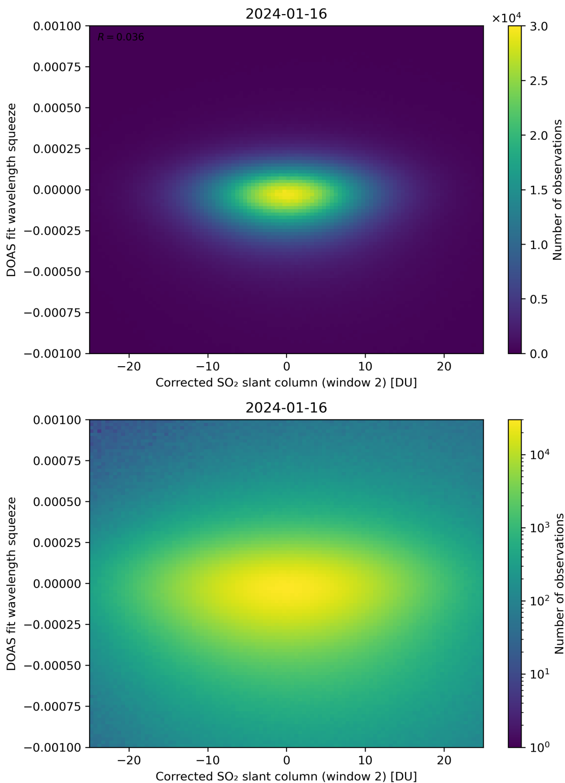
Figure 197: Scatter density plot of “Corrected SO 2 slant column (window 2)” against “DOAS fit wavelength squeeze” for 2024-01-15 to 2024-01-17.
