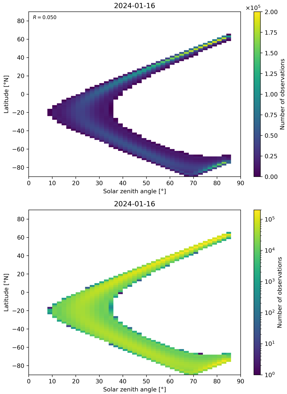
Figure 164: Scatter density plot of “Solar zenith angle” against “Latitude” for 2024-01-15 to 2024-01-17.
