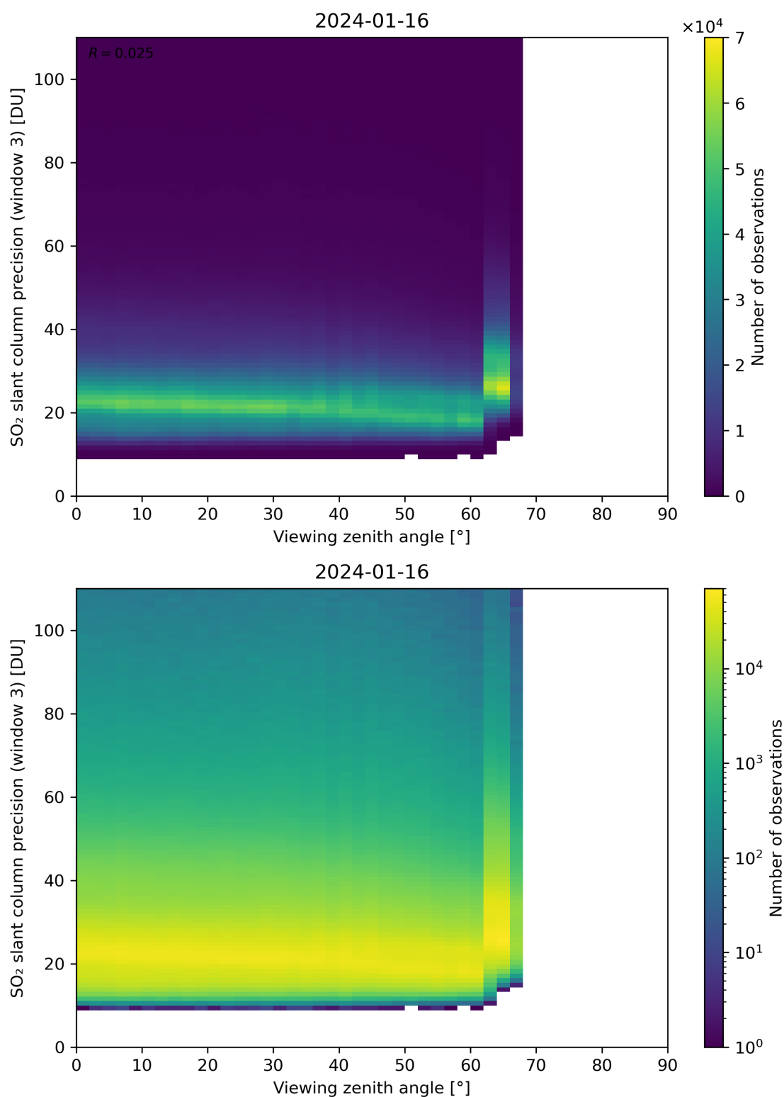
Figure 324: Scatter density plot of “Viewing zenith angle” against “SO 2 slant column precision (window 3)” for 2024-01-15 to 2024-01-17.
