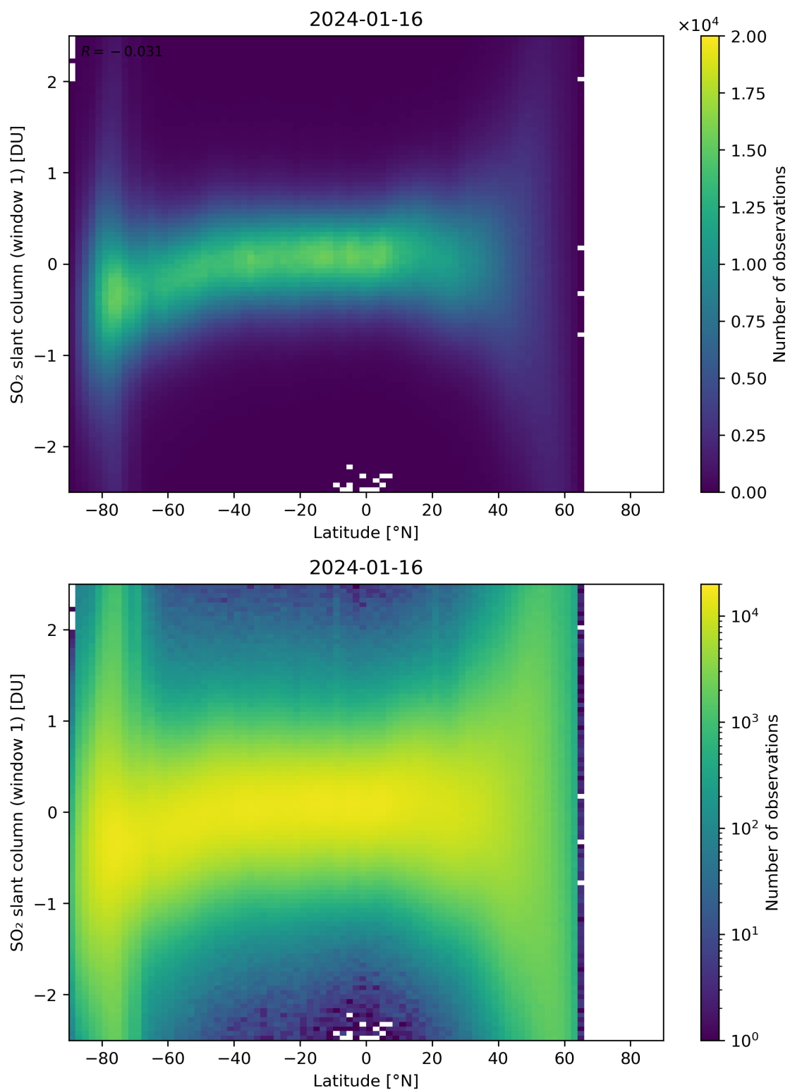
Figure 149: Scatter density plot of “Latitude” against “SO 2 slant column (window 1)” for 2024-01-15 to 2024-01-17.
