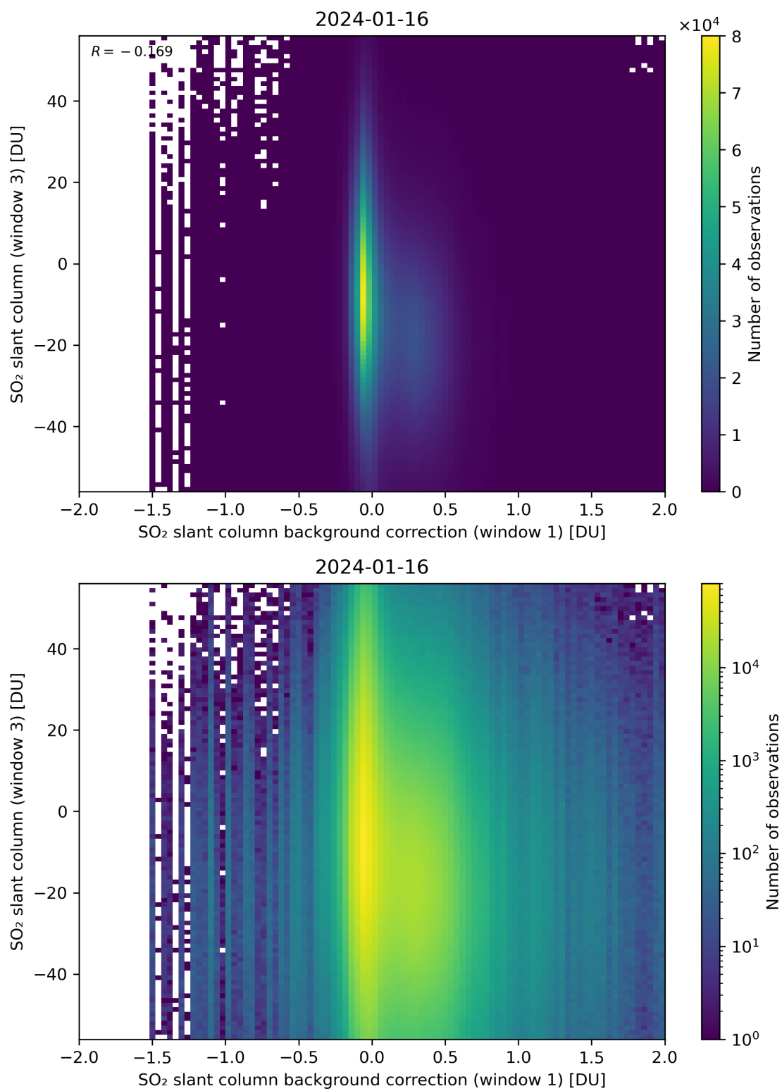
Figure 107: Scatter density plot of “SO 2 slant column background correction (window 1)” against “SO 2 slant column (window 3)” for 2024-01-15 to 2024-01-17.
