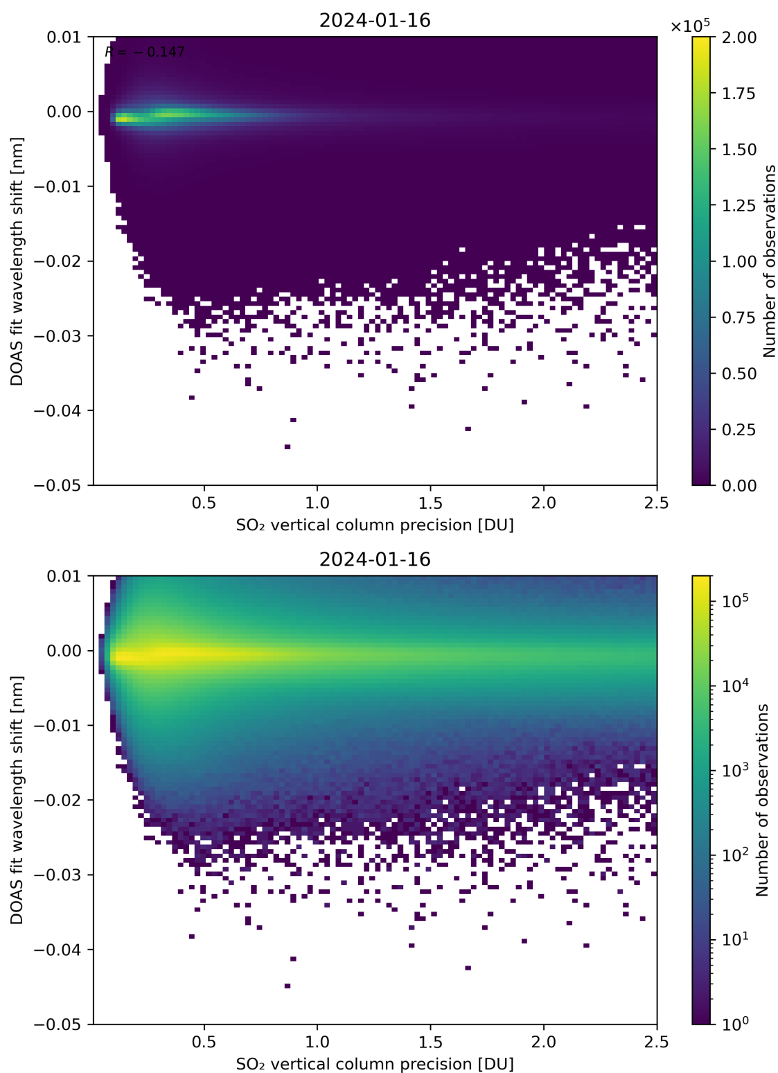
Figure 282: Scatter density plot of “SO 2 vertical column precision” against “DOAS fit wavelength shift” for 2024-01-15 to 2024-01-17.
