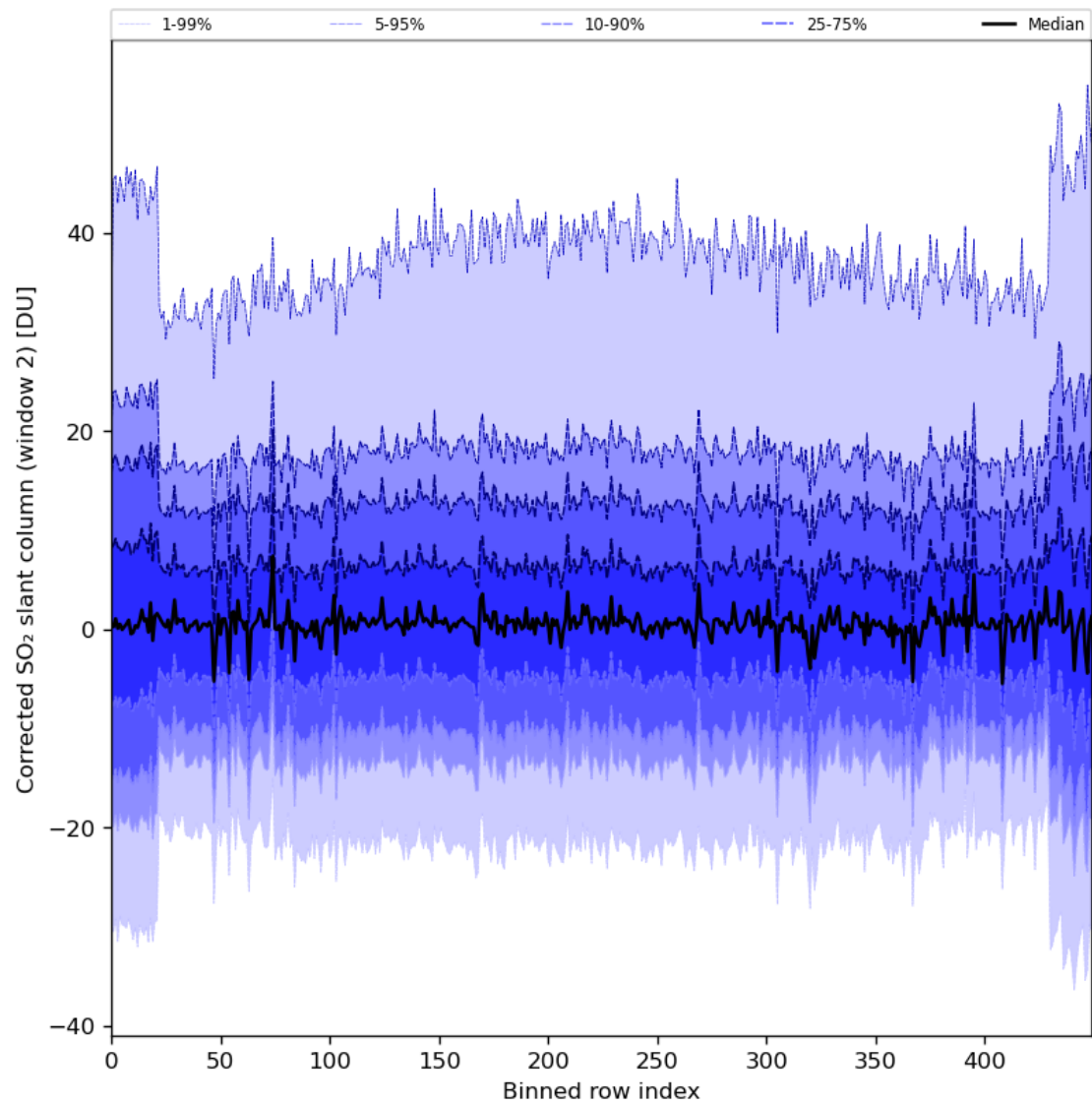
Figure 85: Along track statistics of “Corrected SO 2 slant column (window 2)” for 2024-01-15 to 2024-01-17
