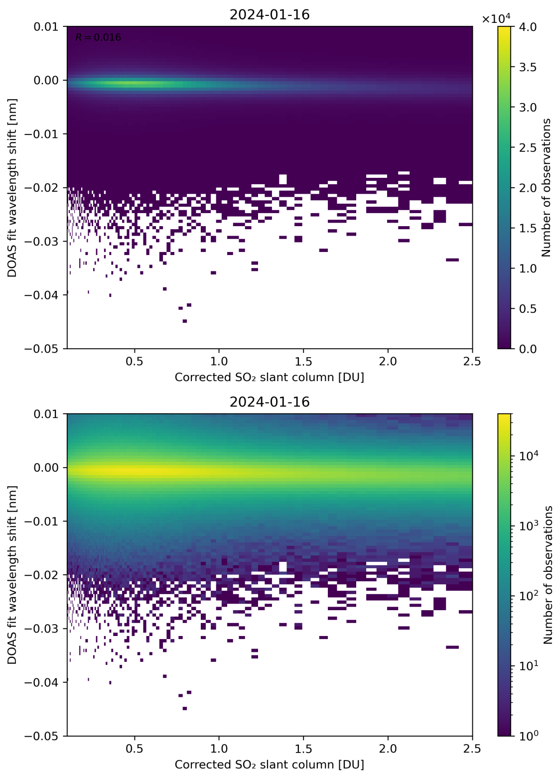
Figure 181: Scatter density plot of “Corrected SO 2 slant column” against “DOAS fit wavelength shift” for 2024-01-15 to 2024-01-17.
