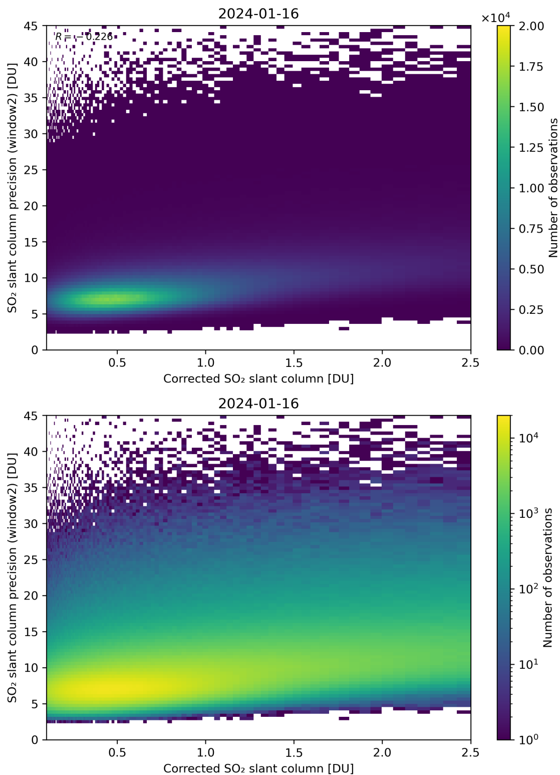
Figure 189: Scatter density plot of “Corrected SO 2 slant column” against “SO 2 slant column precision (window2)” for 2024-01-15 to 2024-01-17.
