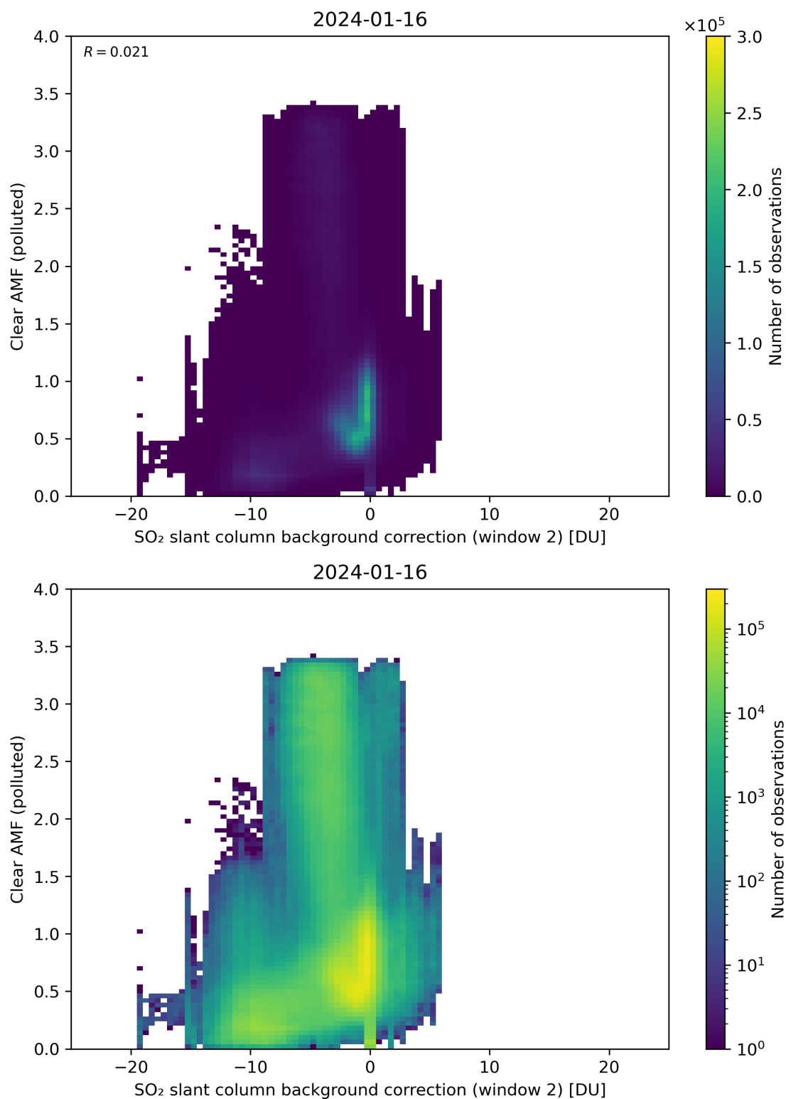
Figure 115: Scatter density plot of “SO 2 slant column background correction (window 2)” against “Clear AMF (polluted)” for 2024-01-15 to 2024-01-17.
