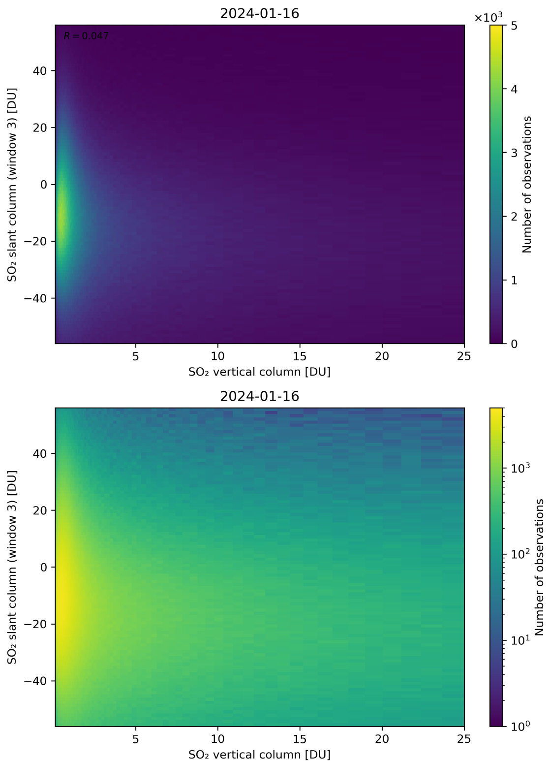
Figure 303: Scatter density plot of “SO 2 vertical column” against “SO 2 slant column (window 3)” for 2024-01-15 to 2024-01-17.
