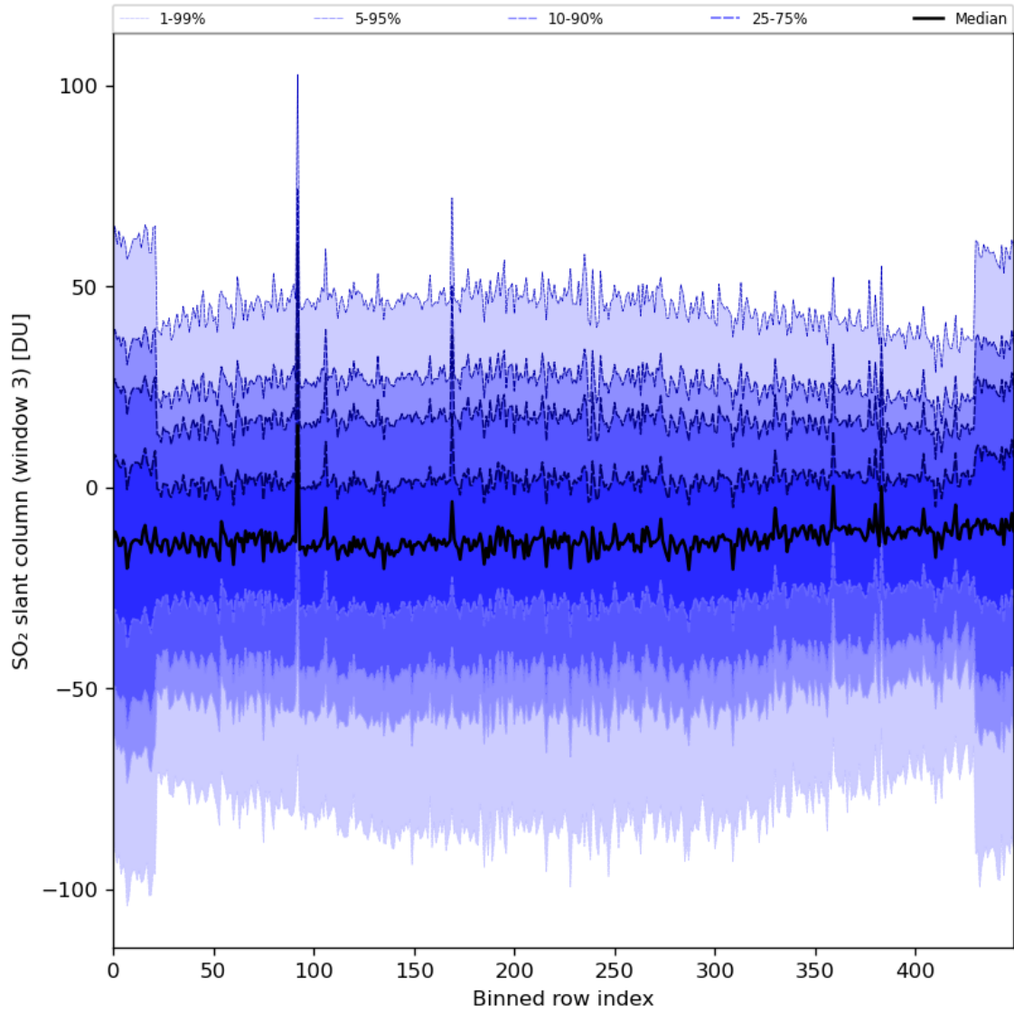
Figure 87: Along track statistics of “SO 2 slant column (window 3)” for 2024-01-15 to 2024-01-17
