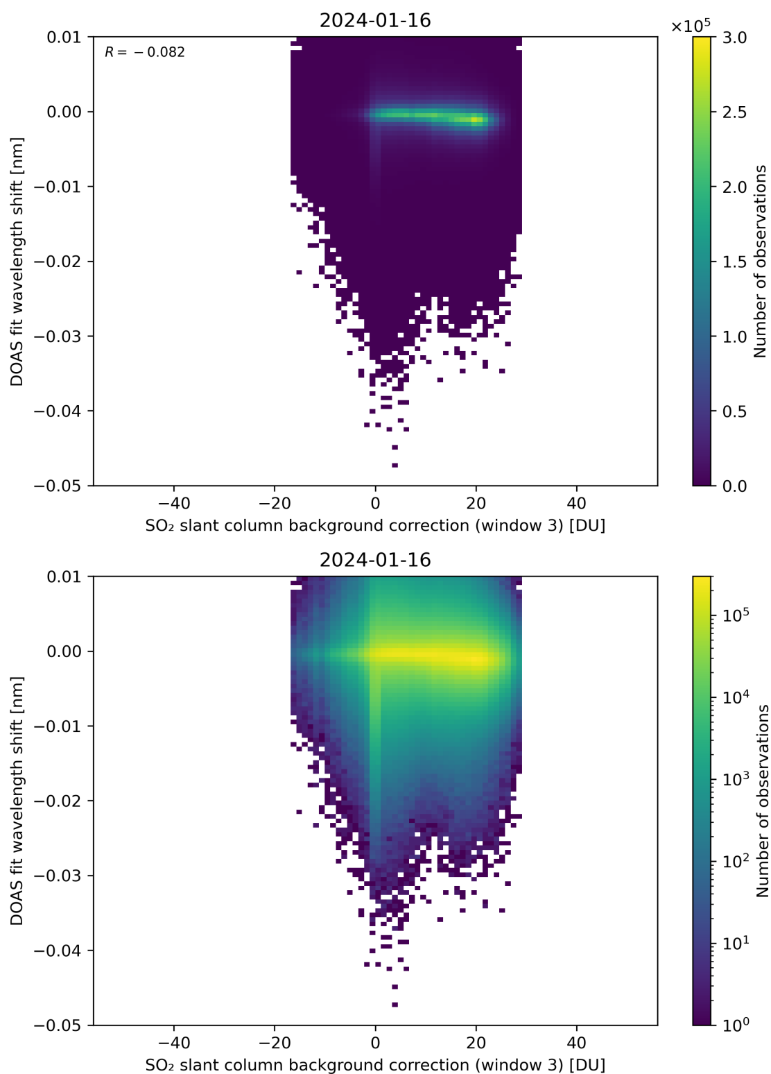
Figure 121: Scatter density plot of “SO 2 slant column background correction (window 3)” against “DOAS fit wavelength shift” for 2024-01-15 to 2024-01-17.
