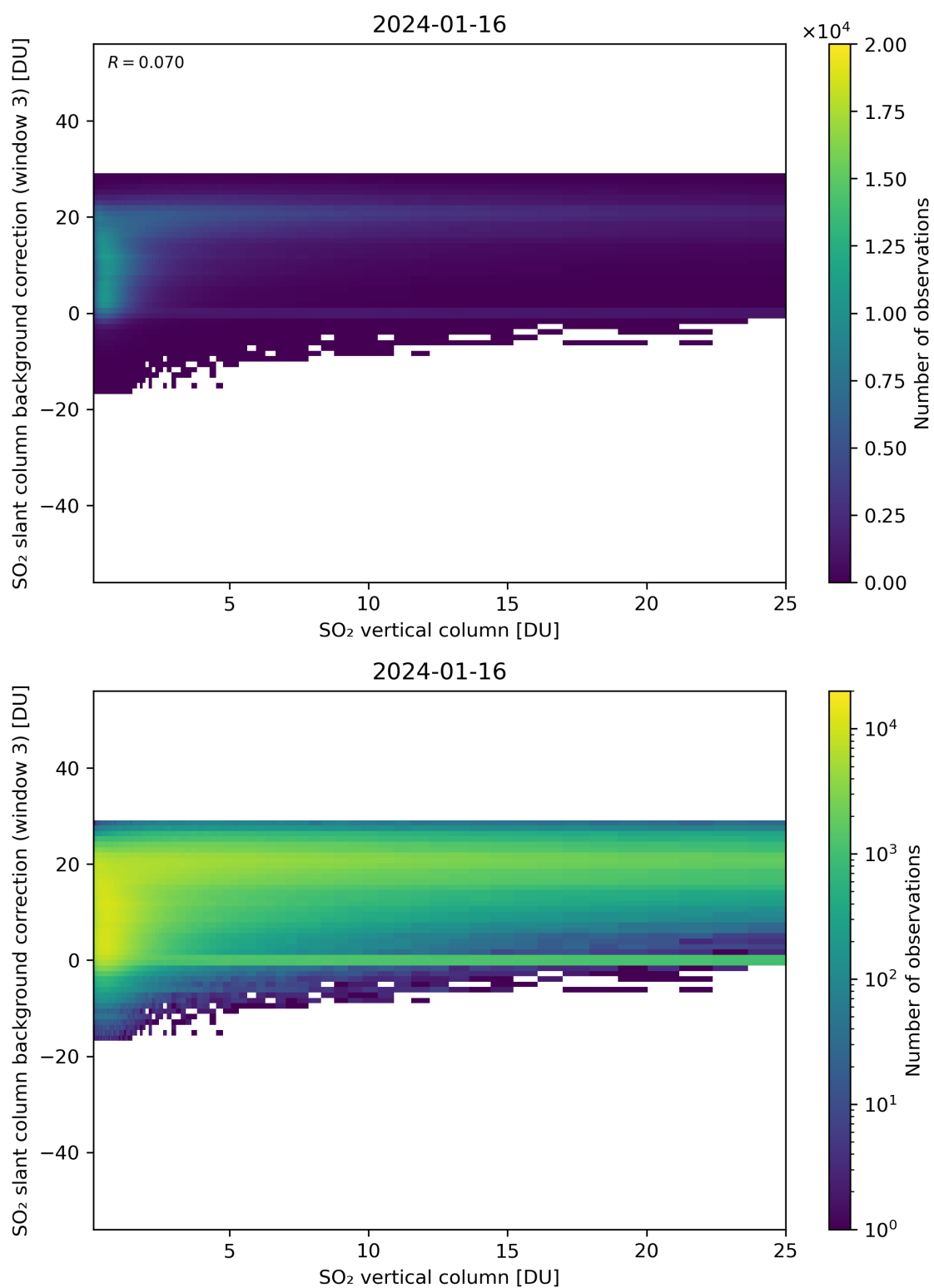
Figure 275: Scatter density plot of “SO 2 vertical column” against “SO 2 slant column background correction (window 3)” for 2024-01-15 to 2024-01-17.
