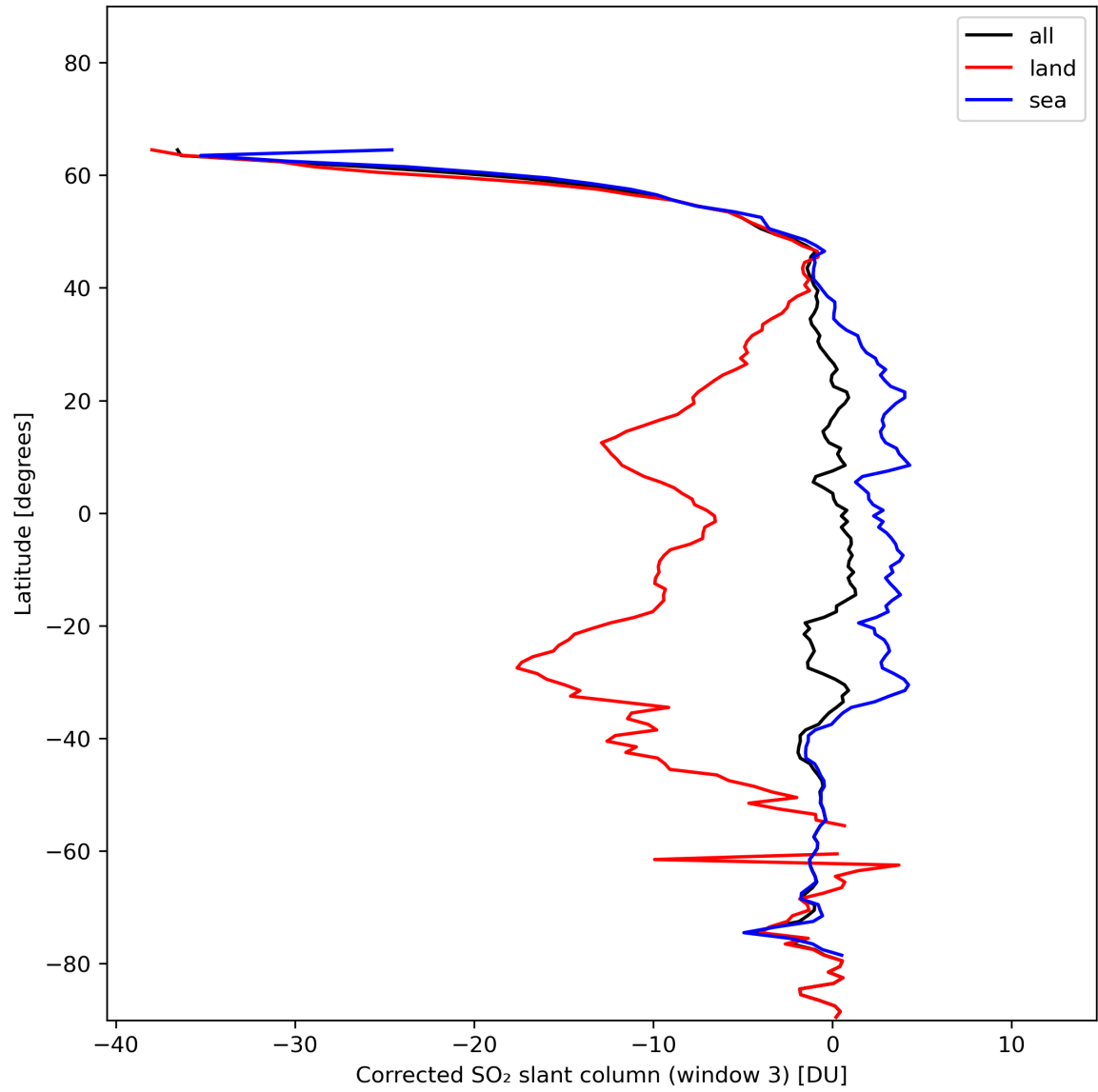
Figure 43: Zonal average of “Corrected SO 2 slant column (window 3)” for 2024-01-15 to 2024-01-17.
