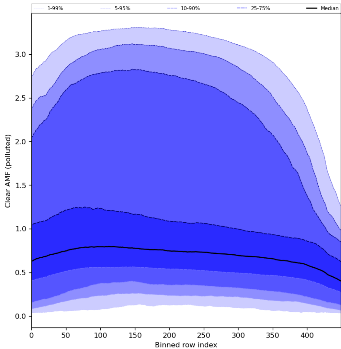
Figure 96: Along track statistics of “Clear AMF (polluted)” for 2024-01-15 to 2024-01-17
