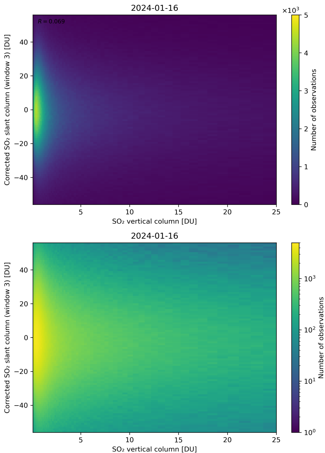
Figure 299: Scatter density plot of “SO 2 vertical column” against “Corrected SO 2 slant column (window 3)” for 2024-01-15 to 2024-01-17.
