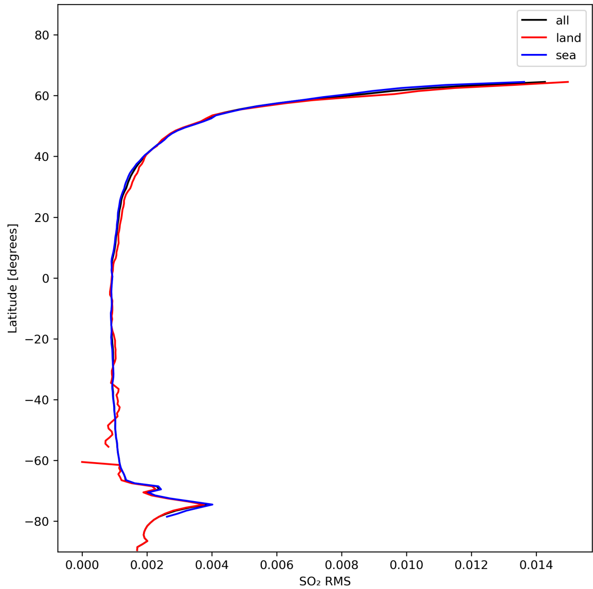
Figure 47: Zonal average of “SO 2 RMS” for 2024-01-15 to 2024-01-17.
