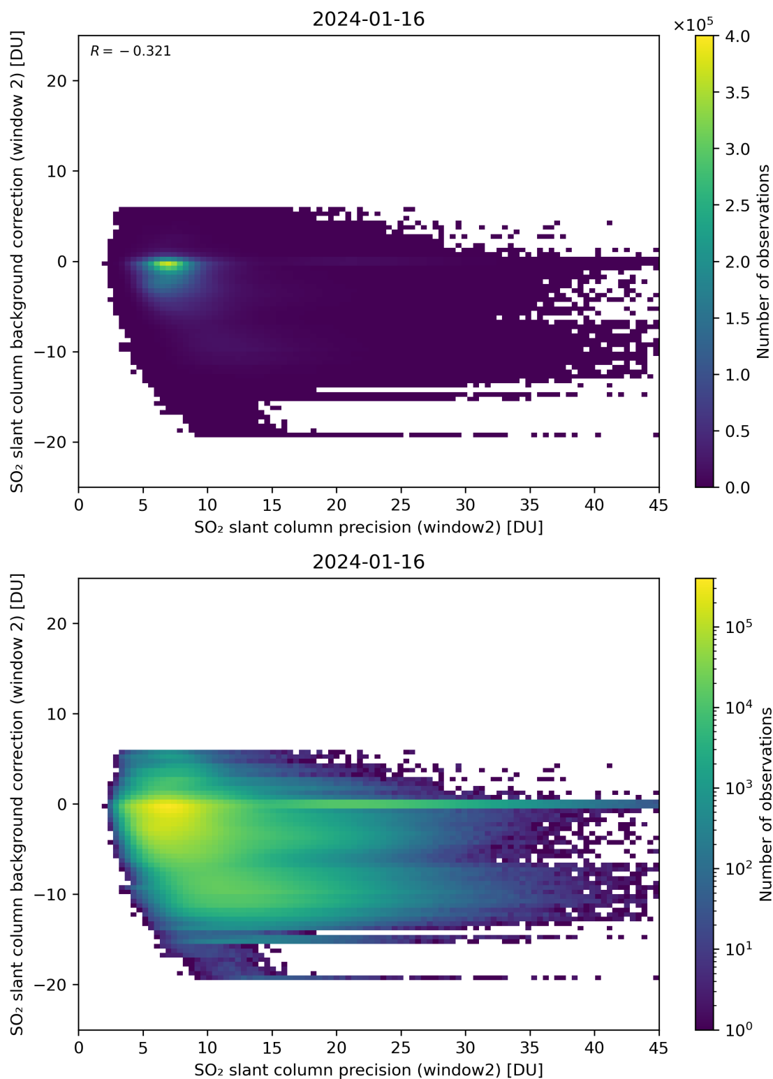
Figure 241: Scatter density plot of “SO 2 slant column precision (window2)” against “SO 2 slant column background correction (window 2)” for 2024-01-15 to 2024-01-17.
