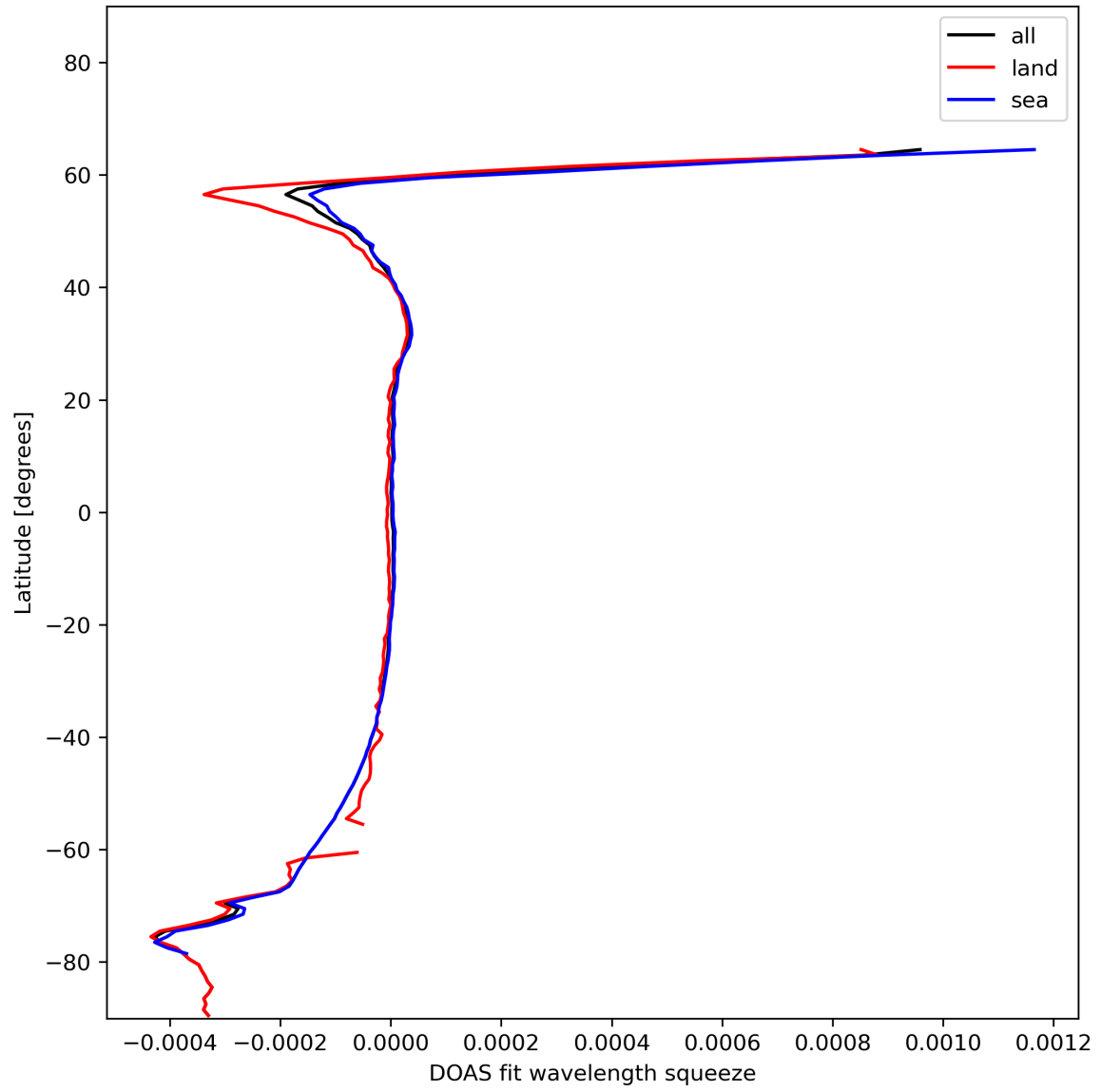
Figure 46: Zonal average of “DOAS fit wavelength squeeze” for 2024-01-15 to 2024-01-17.
