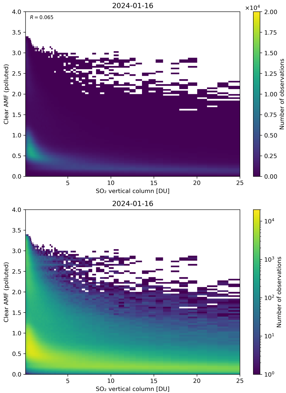
Figure 296: Scatter density plot of “SO 2 vertical column” against “Clear AMF (polluted)” for 2024-01-15 to 2024-01-17.
