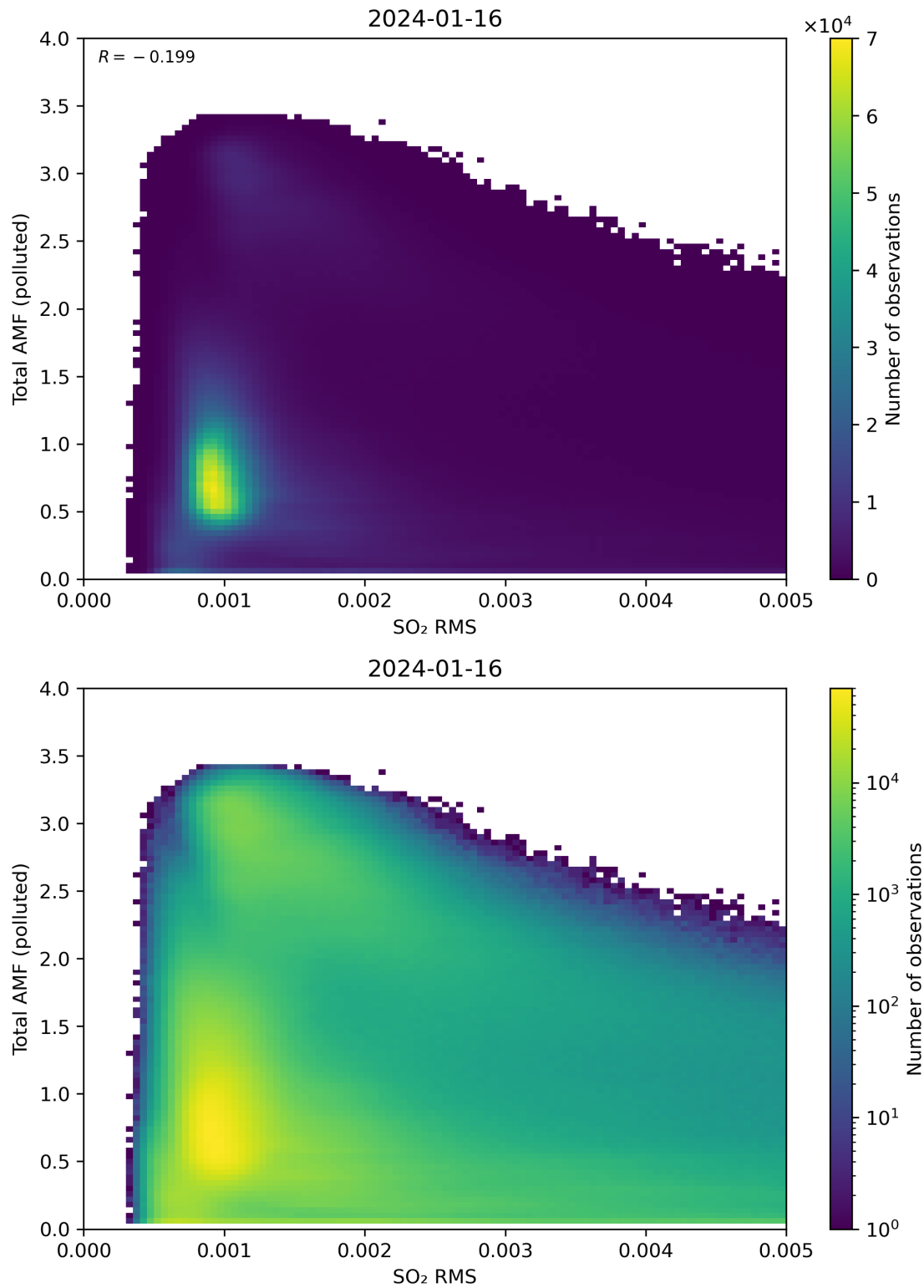
Figure 137: Scatter density plot of “SO 2 RMS” against “Total AMF (polluted)” for 2024-01-15 to 2024-01-17.
