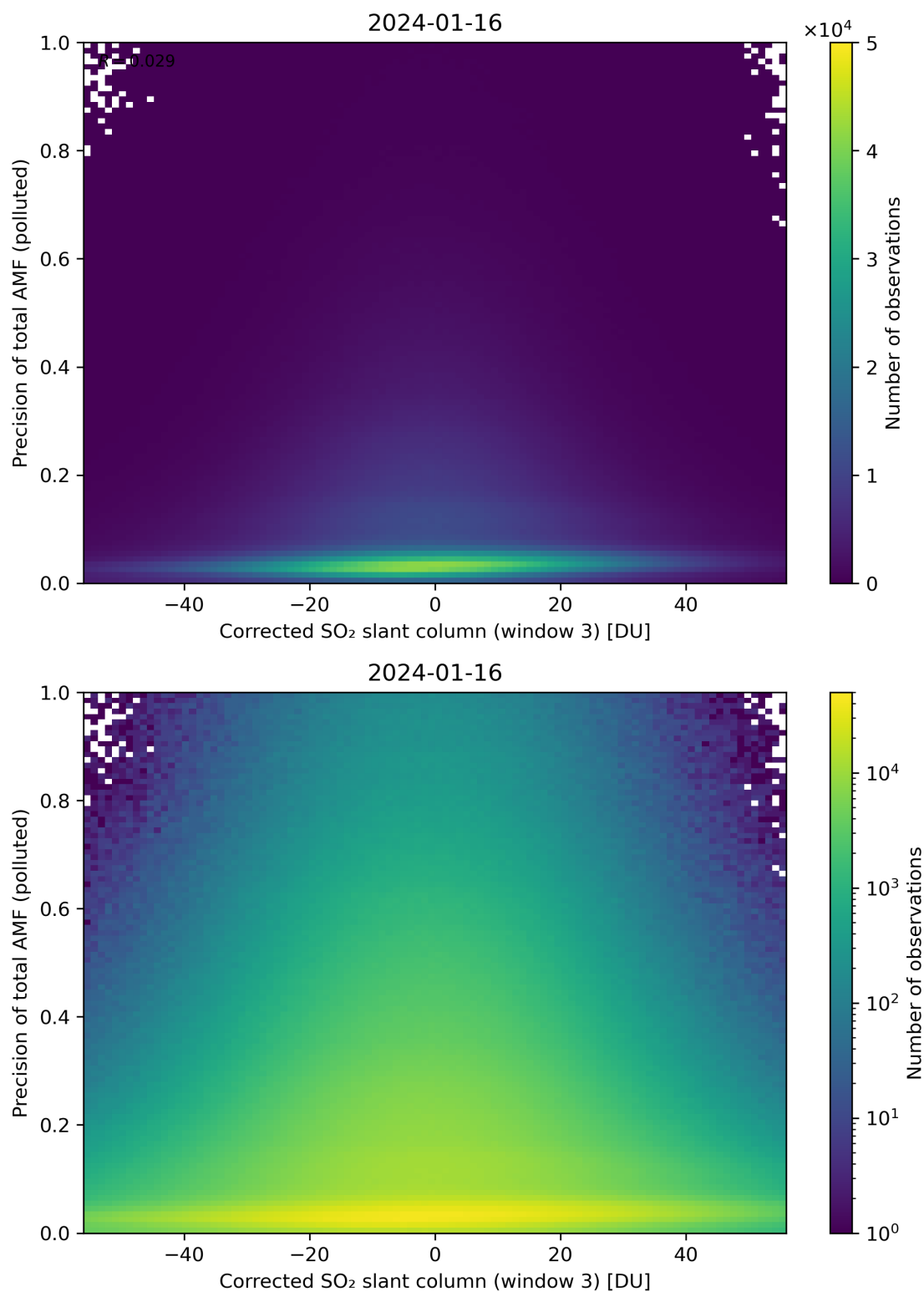
Figure 211: Scatter density plot of “Corrected SO 2 slant column (window 3)” against “Precision of total AMF (polluted)” for 2024-01-15 to 2024-01-17.
