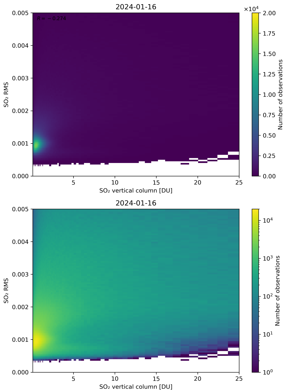
Figure 278: Scatter density plot of “SO 2 vertical column” against “SO 2 RMS” for 2024-01-15 to 2024-01-17.
