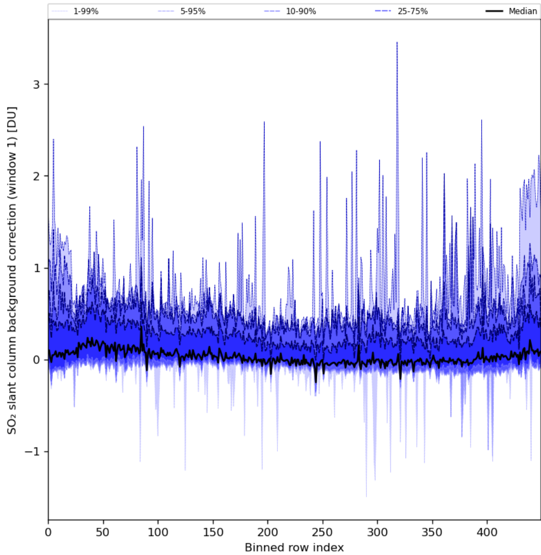
Figure 82: Along track statistics of “SO 2 slant column background correction (window 1)” for 2024-01-15 to 2024-01-17
