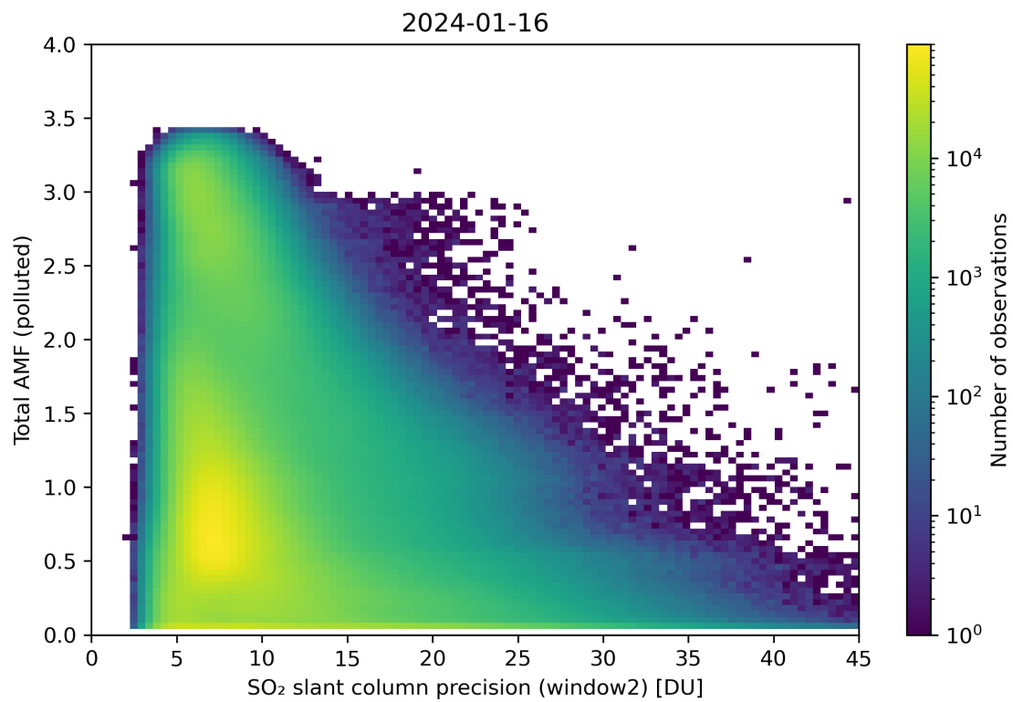
Figure 251: Scatter density plot of “SO 2 slant column precision (window2)” against “Total AMF (polluted)” for 2024-01-15 to 2024-01-17.
