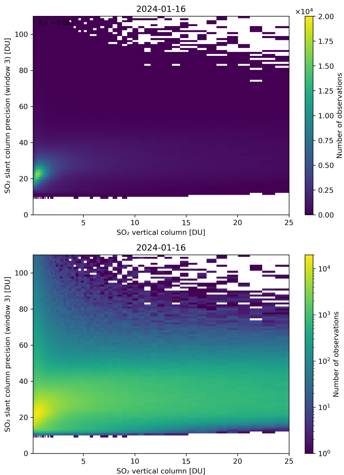
Figure 304: Scatter density plot of “SO 2 vertical column” against “SO 2 slant column precision (window 3)” for 2024-01-15 to 2024-01-17.
