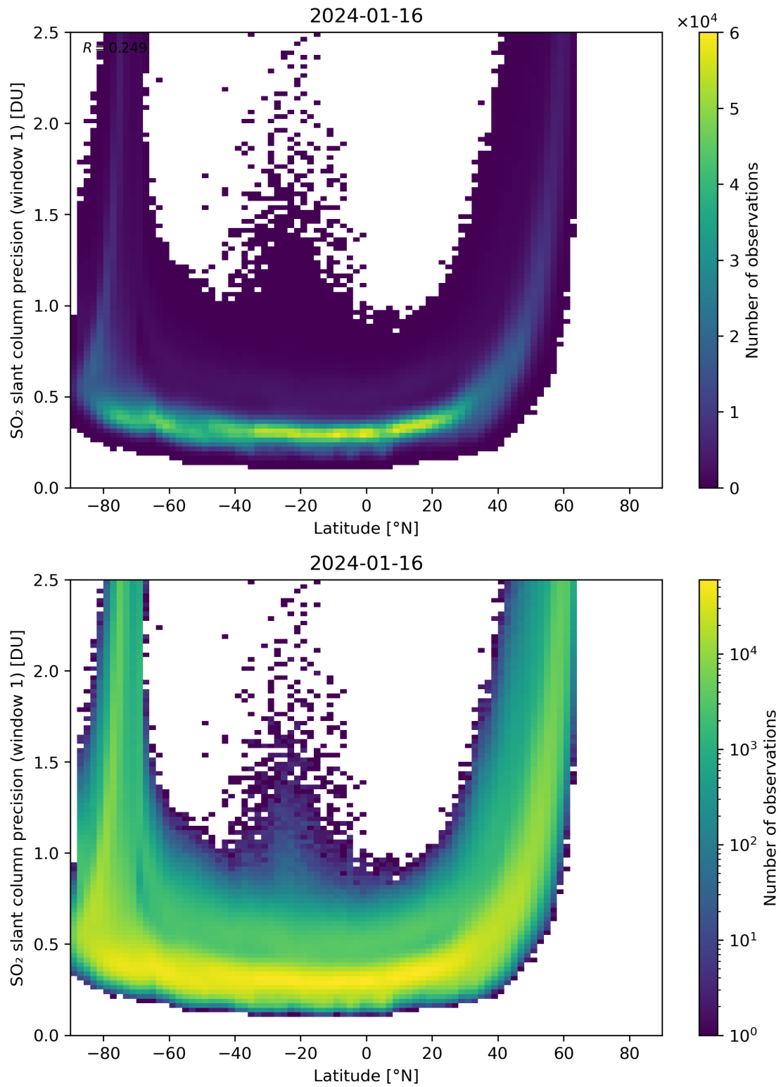
Figure 150: Scatter density plot of “Latitude” against “SO 2 slant column precision (window 1)” for 2024-01-15 to 2024-01-17.
