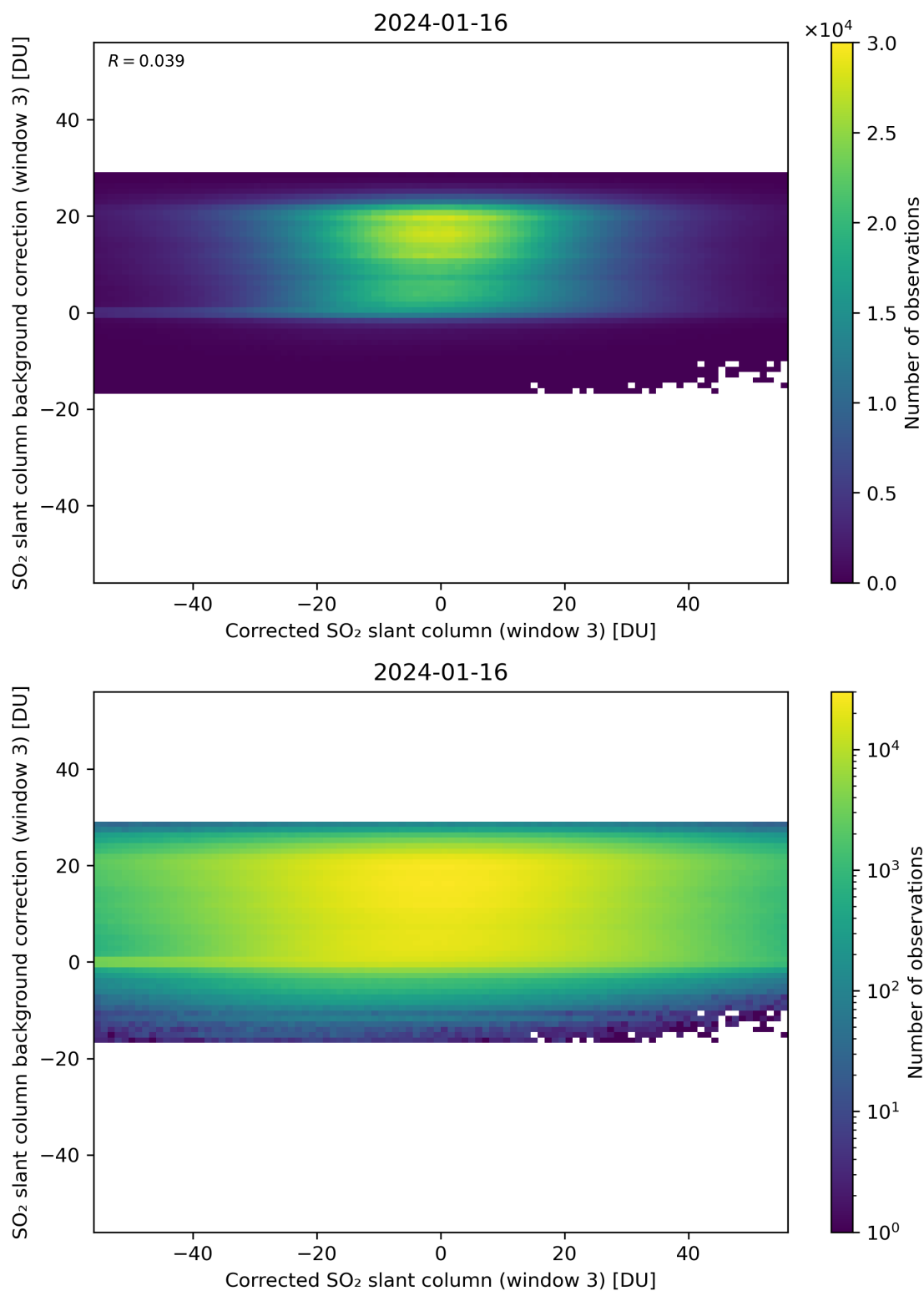
Figure 205: Scatter density plot of “Corrected SO 2 slant column (window 3)” against “SO 2 slant column background correction (window 3)” for 2024-01-15 to 2024-01-17.
