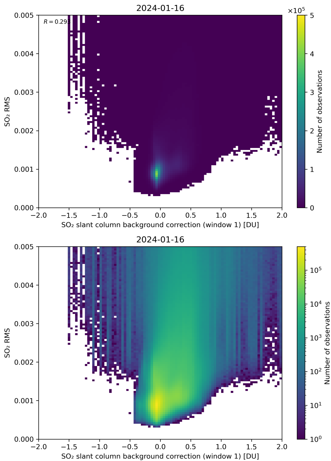
Figure 102: Scatter density plot of “SO 2 slant column background correction (window 1)” against “SO 2 RMS” for 2024-01-15 to 2024-01-17.
