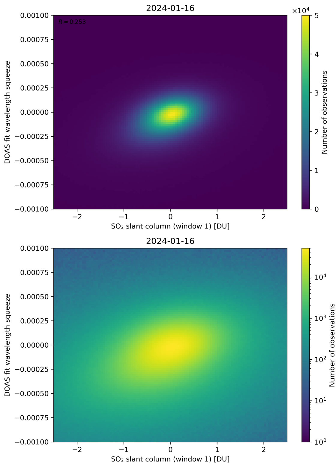
Figure 216: Scatter density plot of “SO 2 slant column (window 1)” against “DOAS fit wavelength squeeze” for 2024-01-15 to 2024-01-17.
