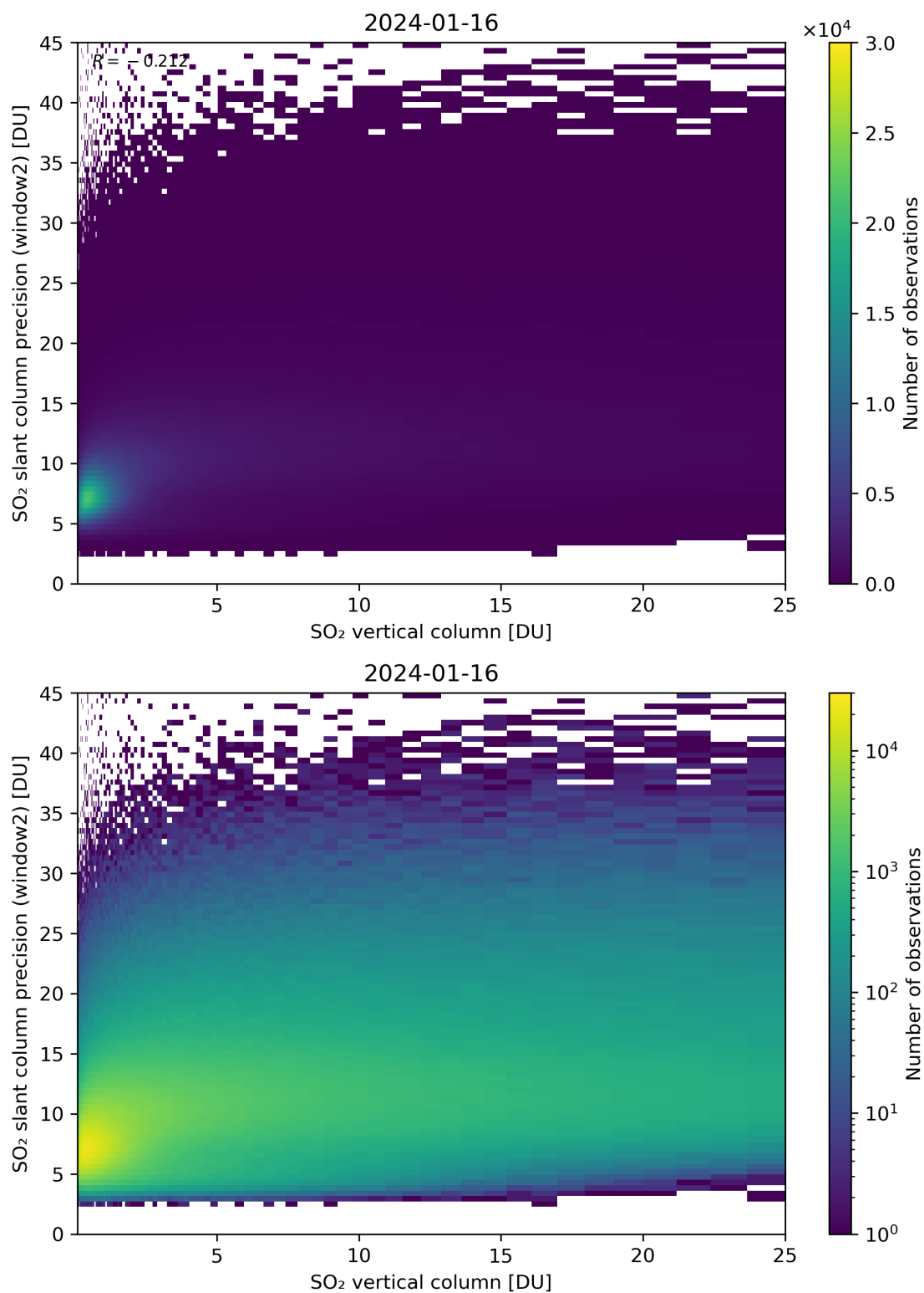
Figure 302: Scatter density plot of “SO 2 vertical column” against “SO 2 slant column precision (window2)” for 2024-01-15 to 2024-01-17.
