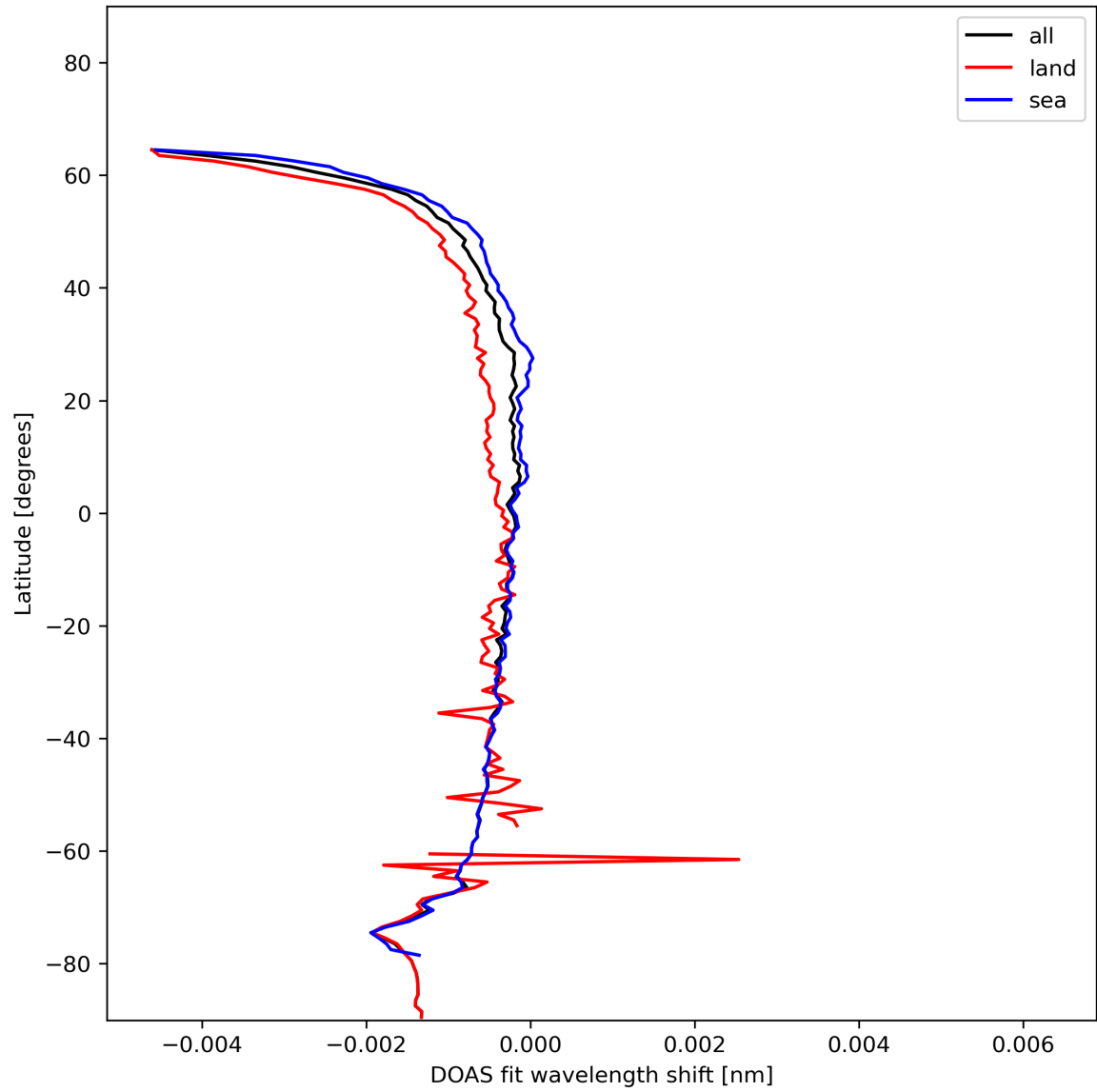
Figure 45: Zonal average of “DOAS fit wavelength shift” for 2024-01-15 to 2024-01-17.
