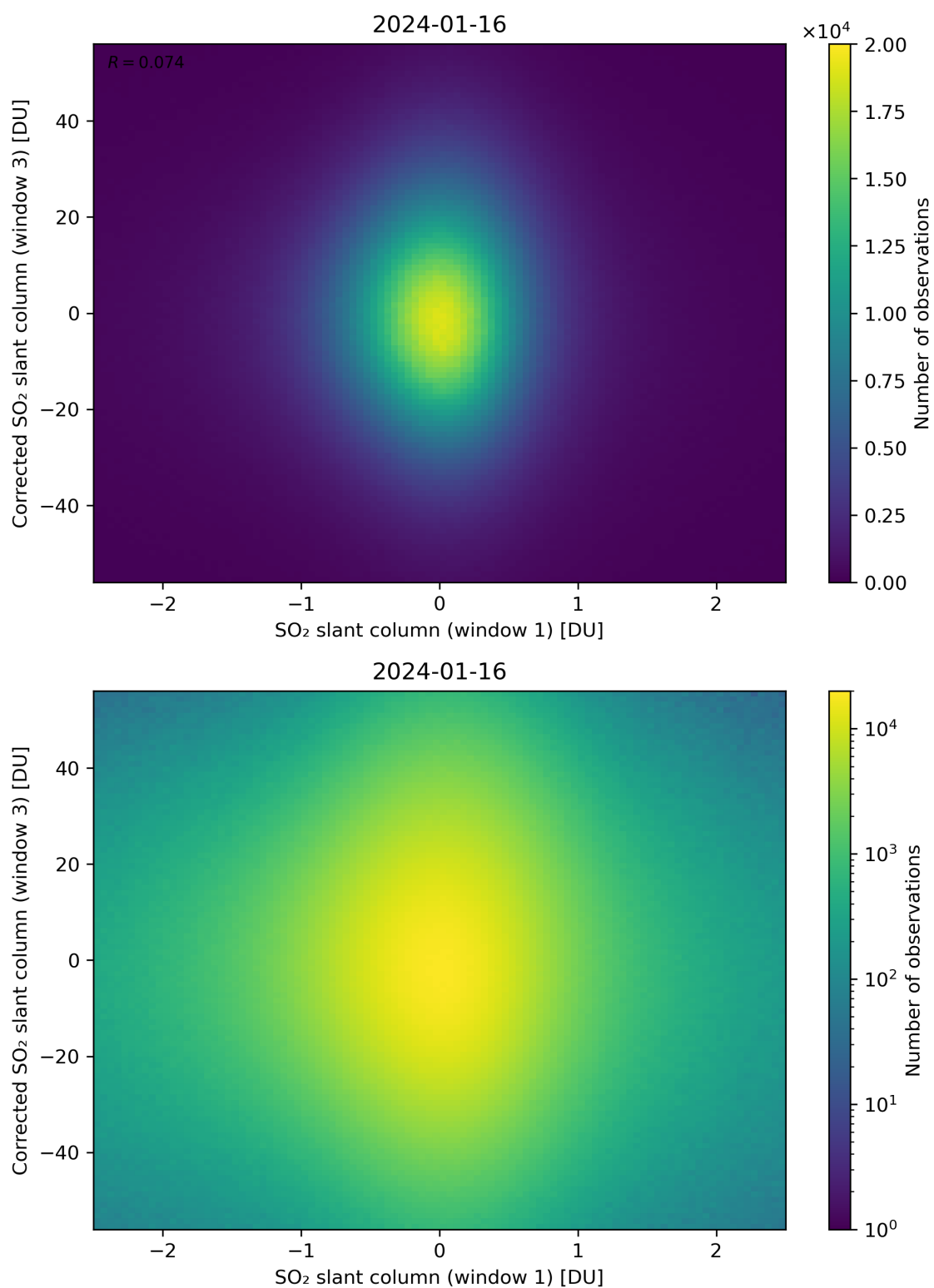
Figure 234: Scatter density plot of “SO 2 slant column (window 1)” against “Corrected SO 2 slant column (window 3)” for 2024-01-15 to 2024-01-17.
