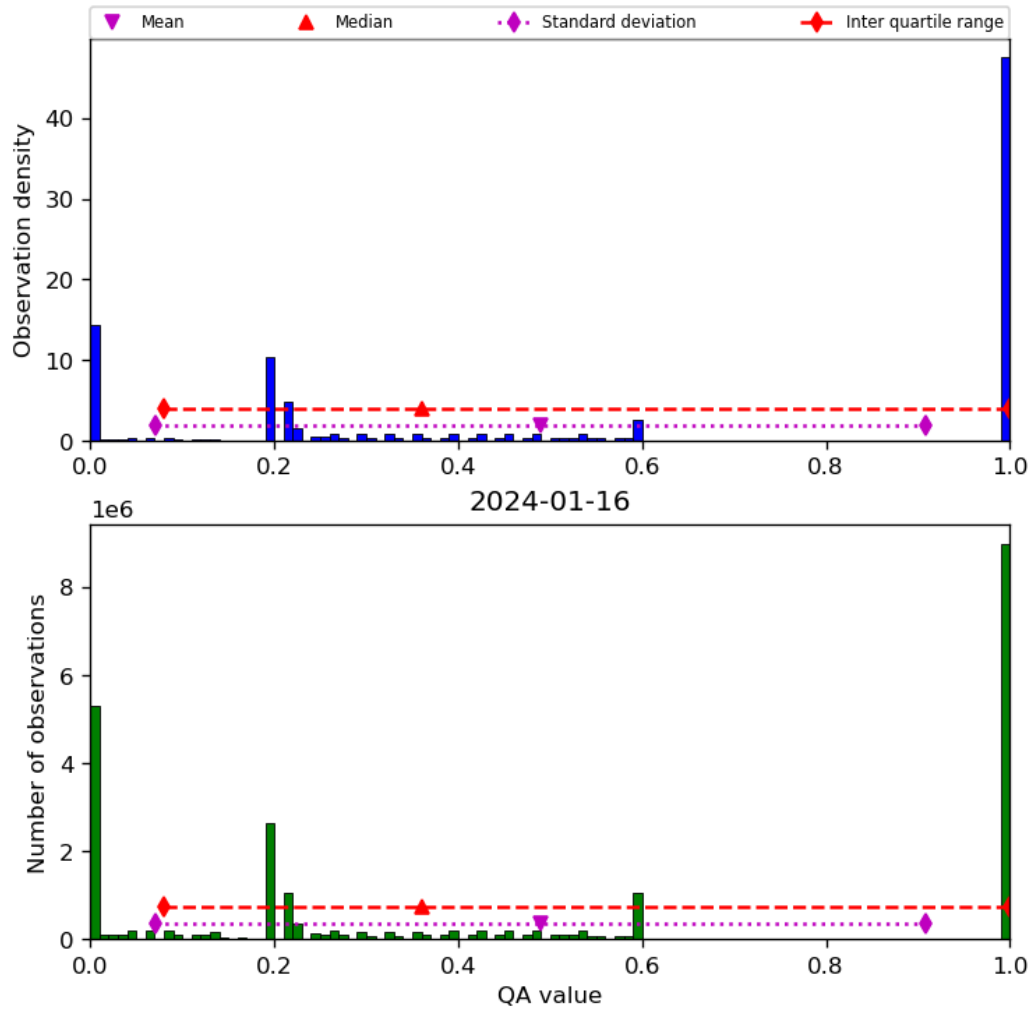
Figure 52: Histogram of “QA value” for 2024-01-15 to 2024-01-17
