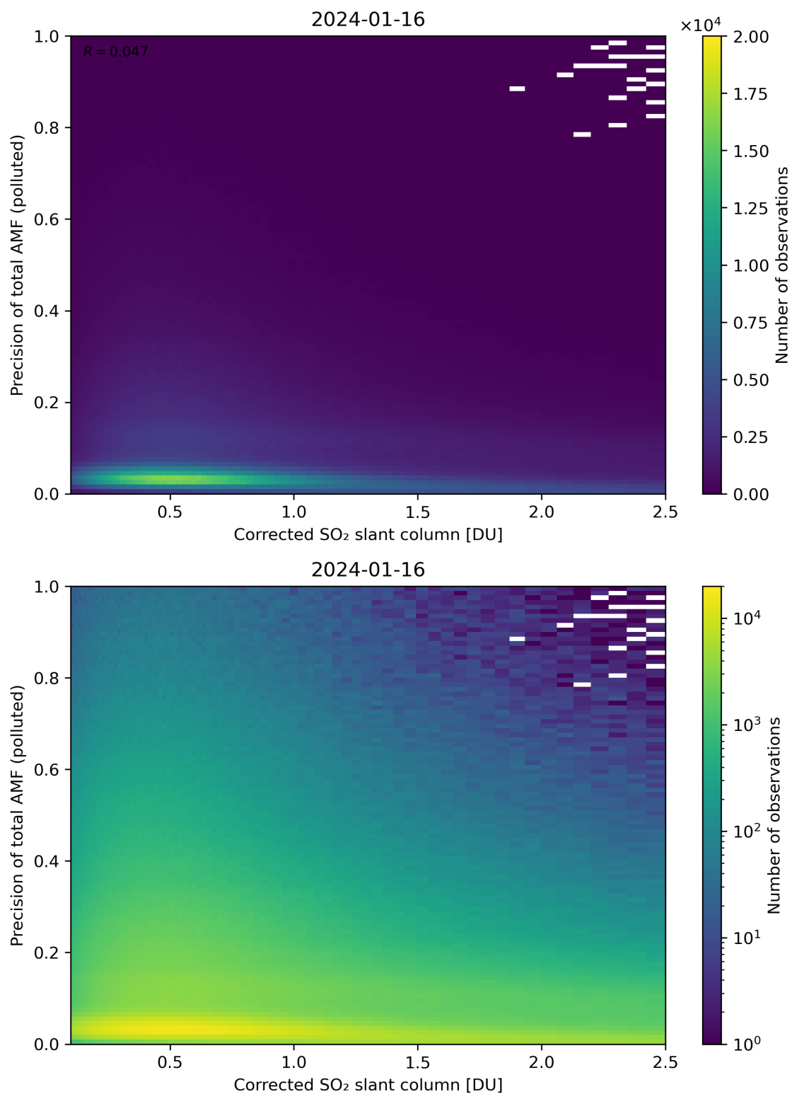
Figure 193: Scatter density plot of “Corrected SO 2 slant column” against “Precision of total AMF (polluted)” for 2024-01-15 to 2024-01-17.
