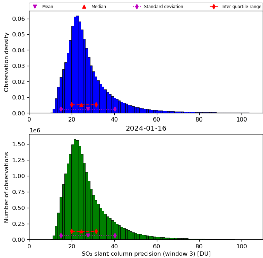
Figure 65: Histogram of “SO 2 slant column precision (window 3)” for 2024-01-15 to 2024-01-17
