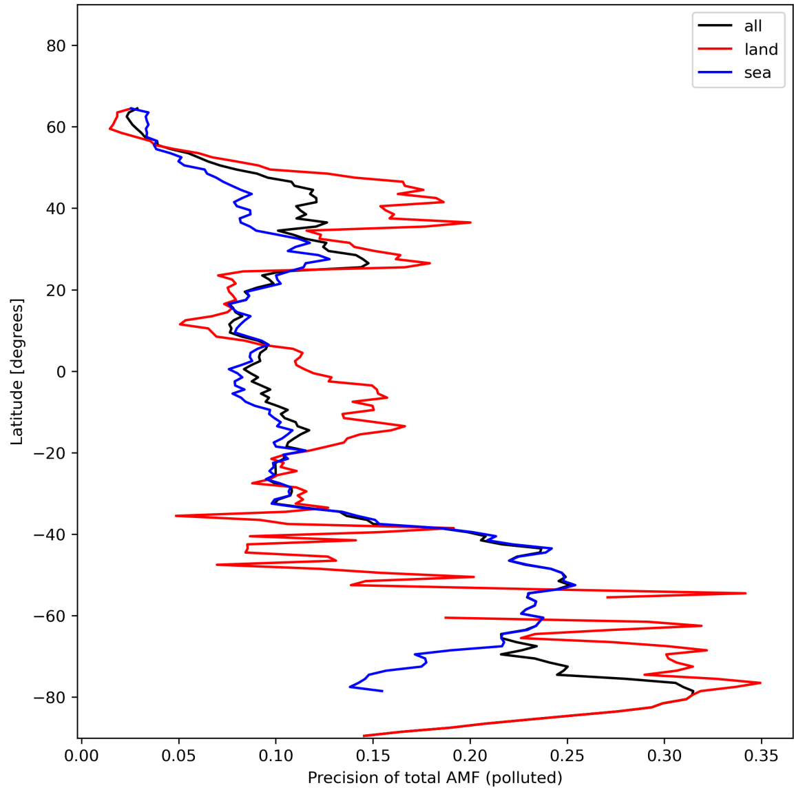
Figure 49: Zonal average of “Precision of total AMF (polluted)” for 2024-01-15 to 2024-01-17.
