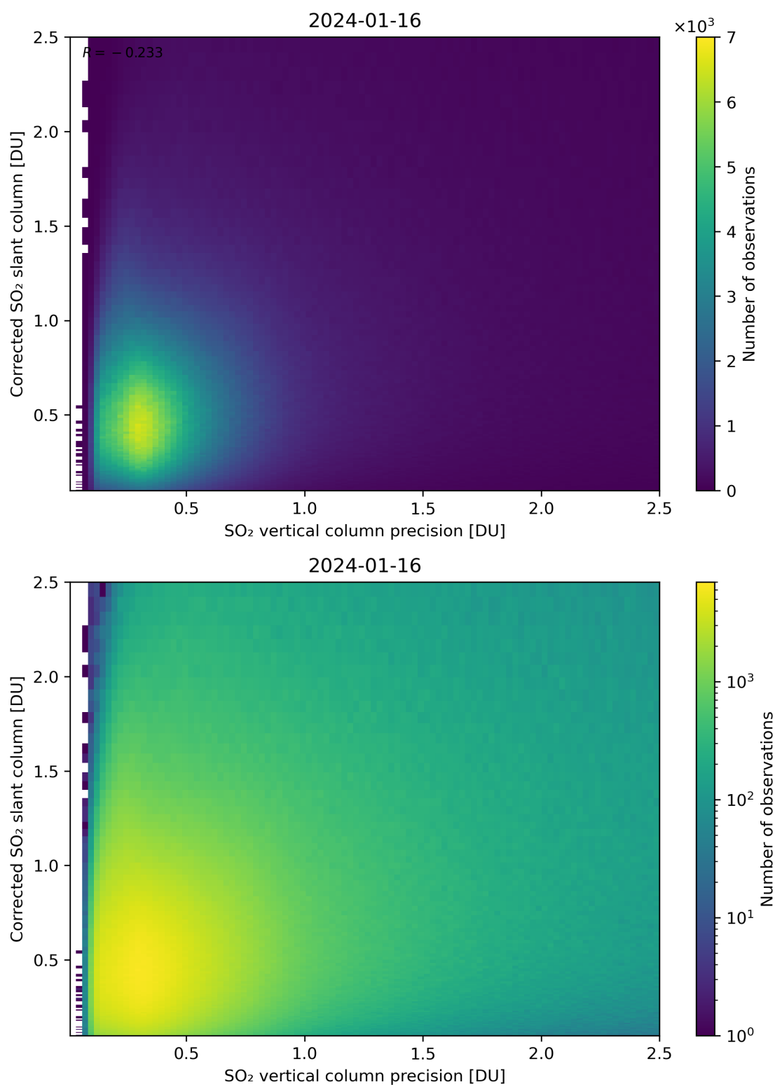
Figure 286: Scatter density plot of “SO 2 vertical column precision” against “Corrected SO 2 slant column” for 2024-01-15 to 2024-01-17.
