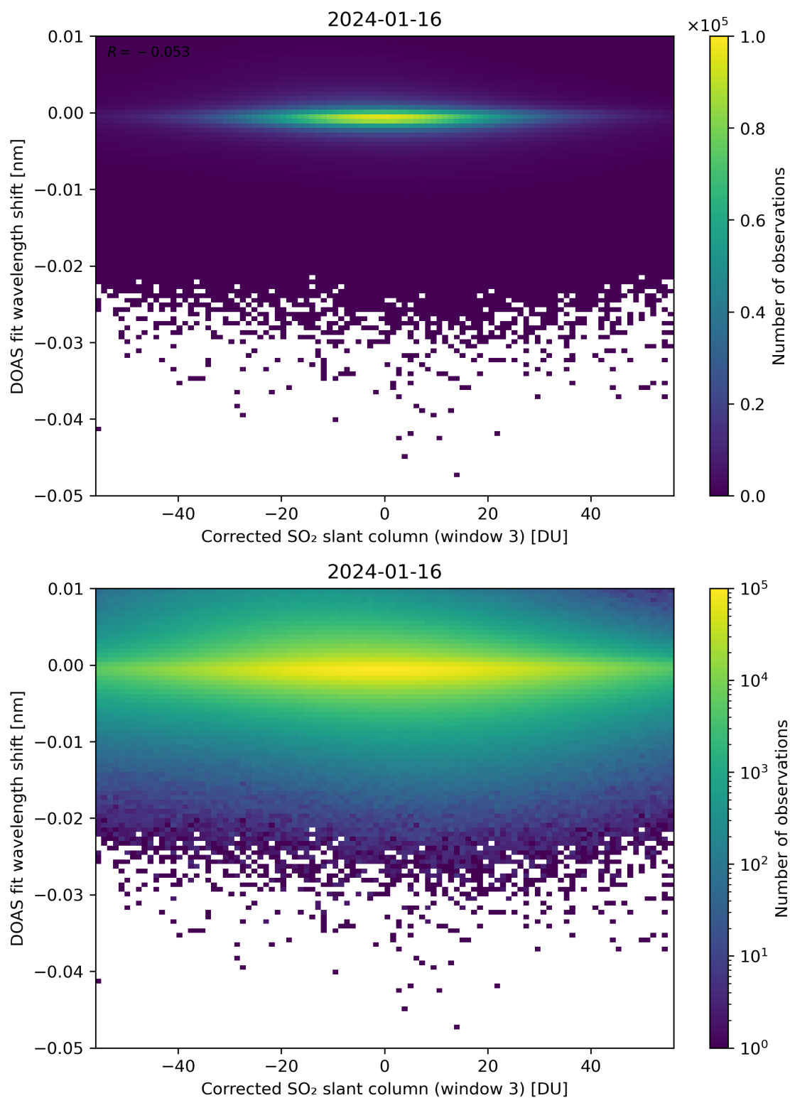
Figure 206: Scatter density plot of “Corrected SO 2 slant column (window 3)” against “DOAS fit wavelength shift” for 2024-01-15 to 2024-01-17.
