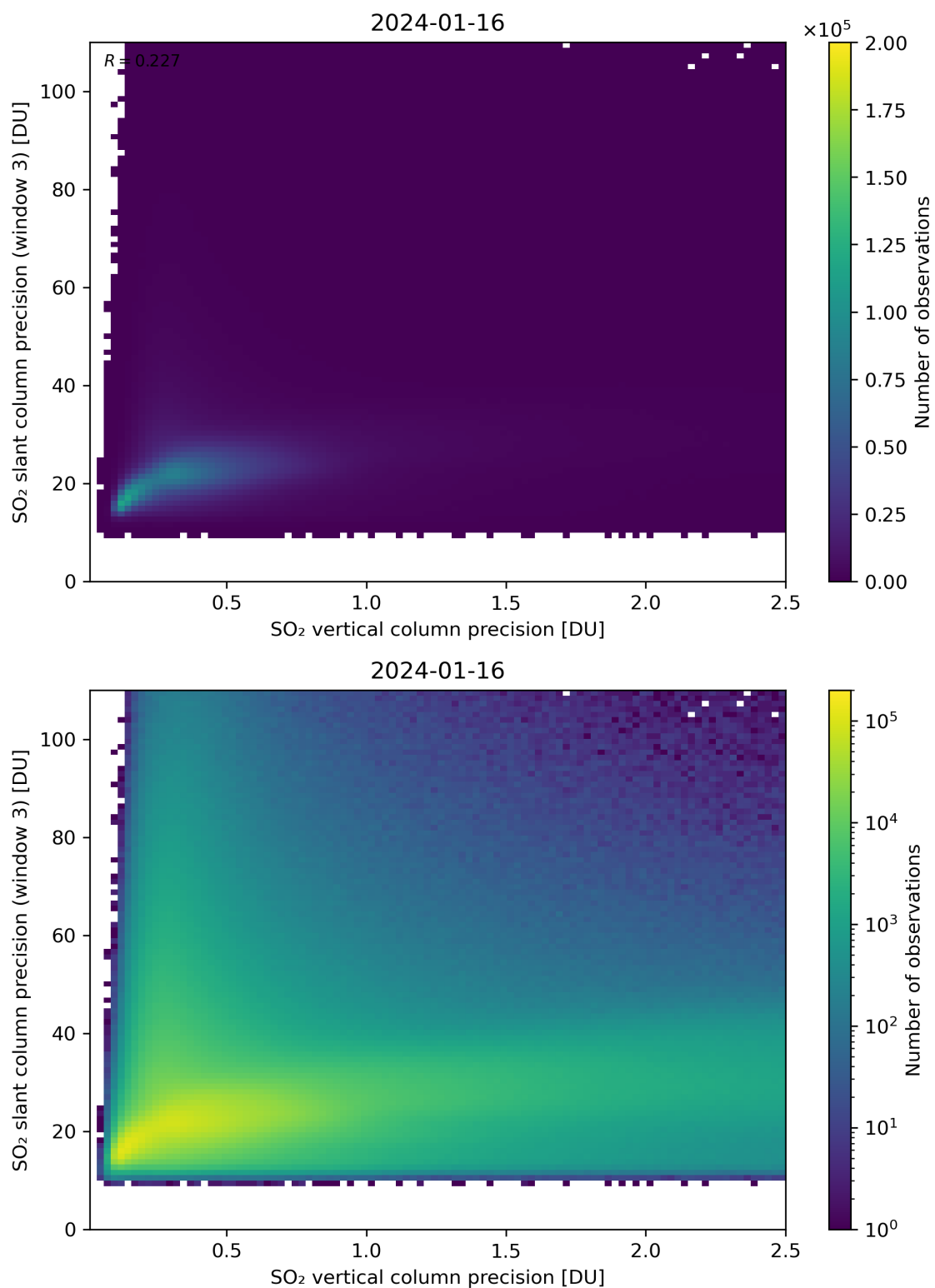
Figure 293: Scatter density plot of “SO 2 vertical column precision” against “SO 2 slant column precision (window 3)” for 2024-01-15 to 2024-01-17.
