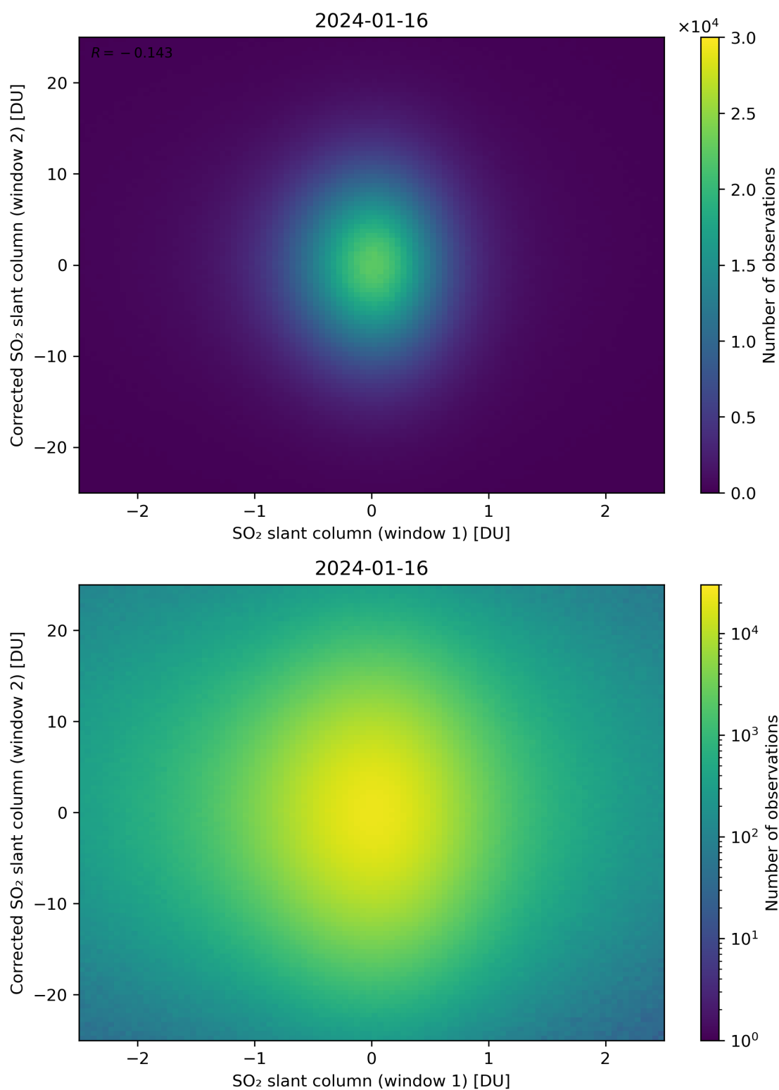
Figure 233: Scatter density plot of “SO 2 slant column (window 1)” against “Corrected SO 2 slant column (window 2)” for 2024-01-15 to 2024-01-17.
