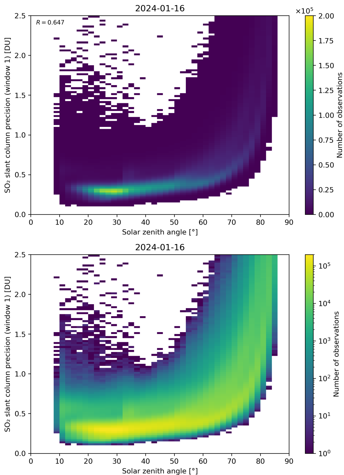
Figure 170: Scatter density plot of “Solar zenith angle” against “SO 2 slant column precision (window 1)” for 2024-01-15 to 2024-01-17.
