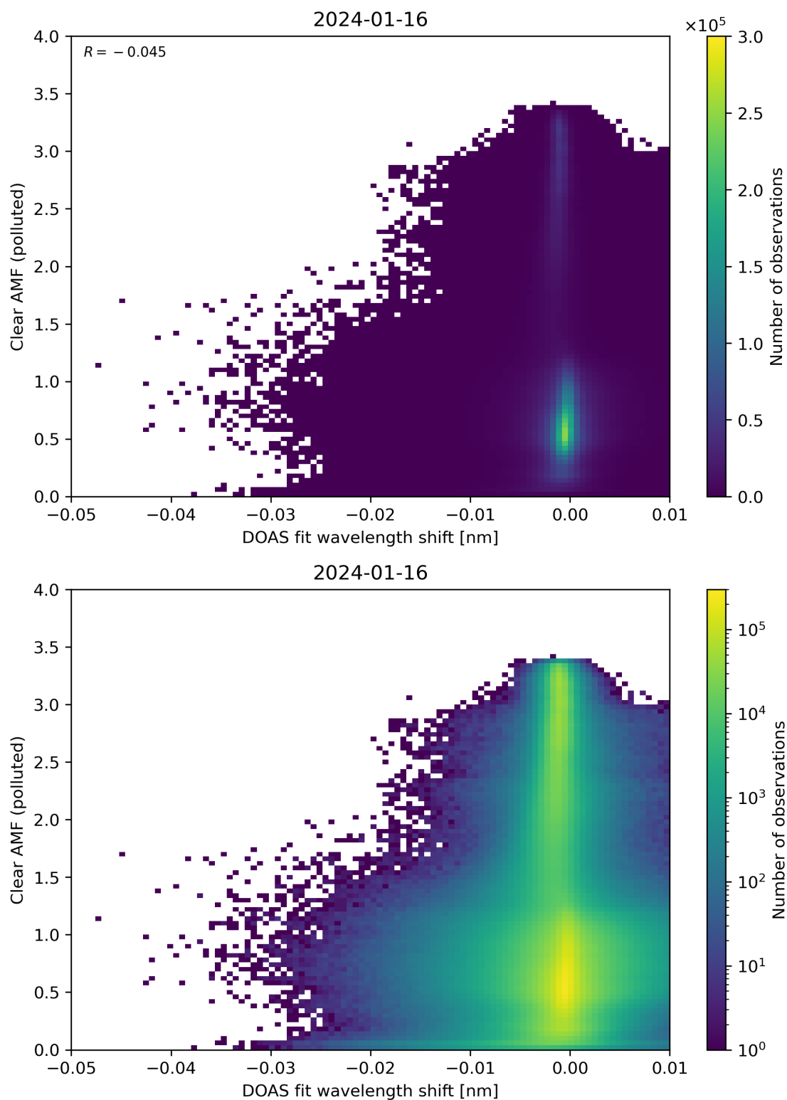
Figure 129: Scatter density plot of “DOAS fit wavelength shift” against “Clear AMF (polluted)” for 2024-01-15 to 2024-01-17.
