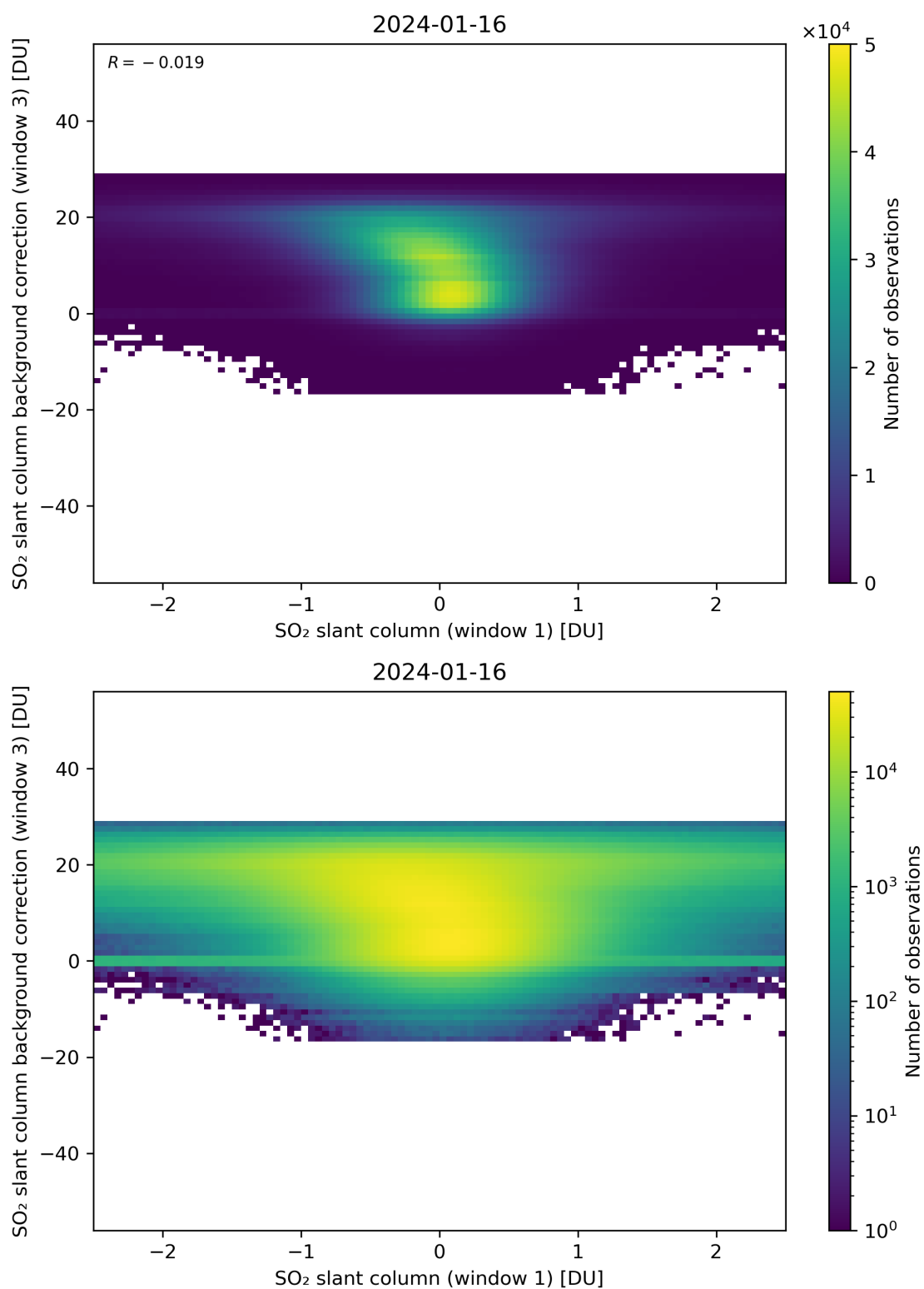
Figure 214: Scatter density plot of “SO 2 slant column (window 1)” against “SO 2 slant column background correction (window 3)” for 2024-01-15 to 2024-01-17.
