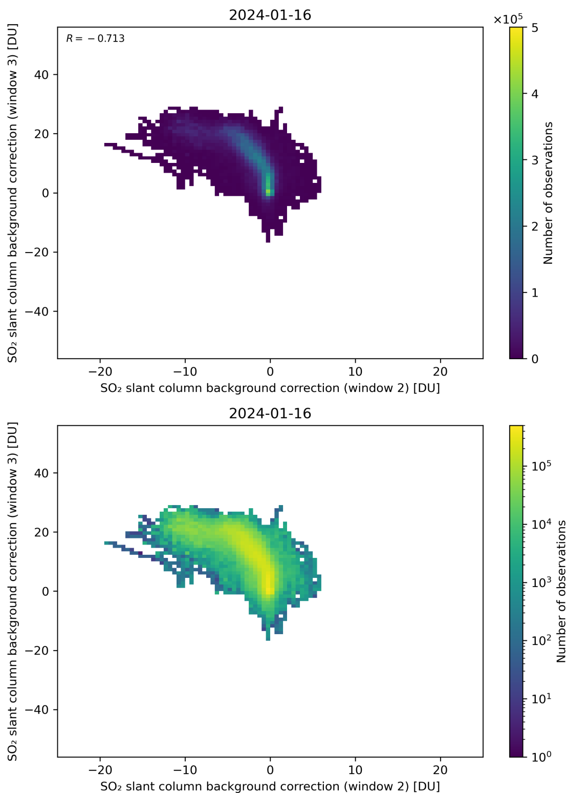
Figure 111: Scatter density plot of “SO 2 slant column background correction (window 2)” against “SO 2 slant column background correction (window 3)” for 2024-01-15 to 2024-01-17.
