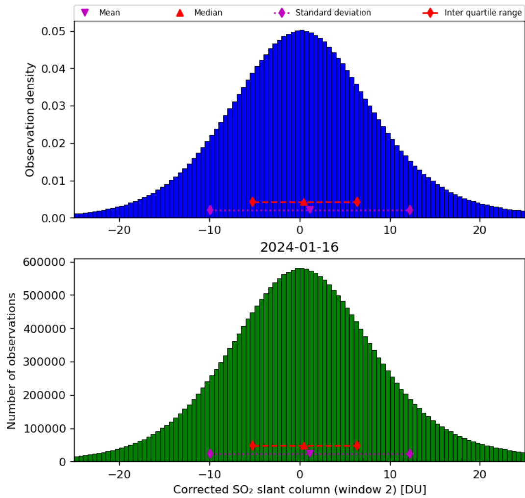
Figure 62: Histogram of “Corrected SO 2 slant column (window 2)” for 2024-01-15 to 2024-01-17
