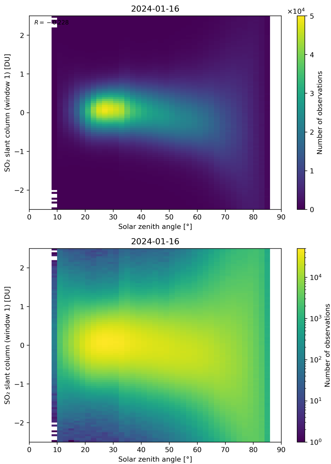
Figure 169: Scatter density plot of “Solar zenith angle” against “SO 2 slant column (window 1)” for 2024-01-15 to 2024-01-17.
