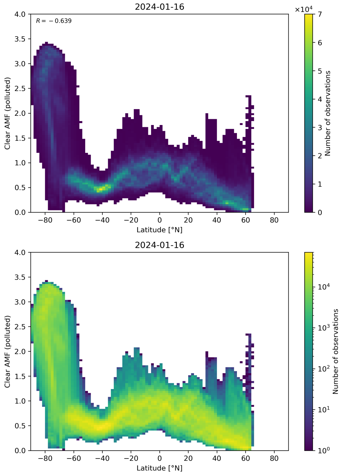
Figure 145: Scatter density plot of “Latitude” against “Clear AMF (polluted)” for 2024-01-15 to 2024-01-17.
