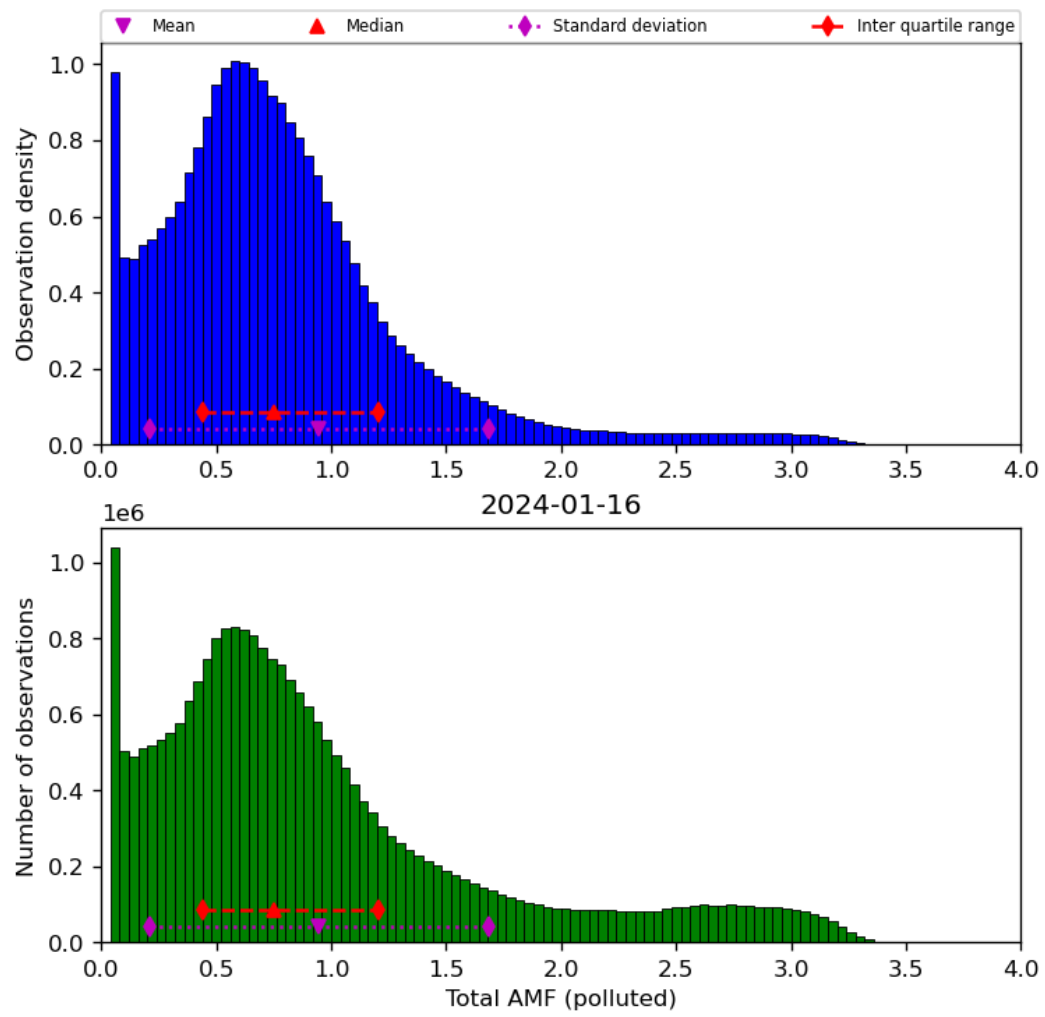
Figure 71: Histogram of “Total AMF (polluted)” for 2024-01-15 to 2024-01-17
