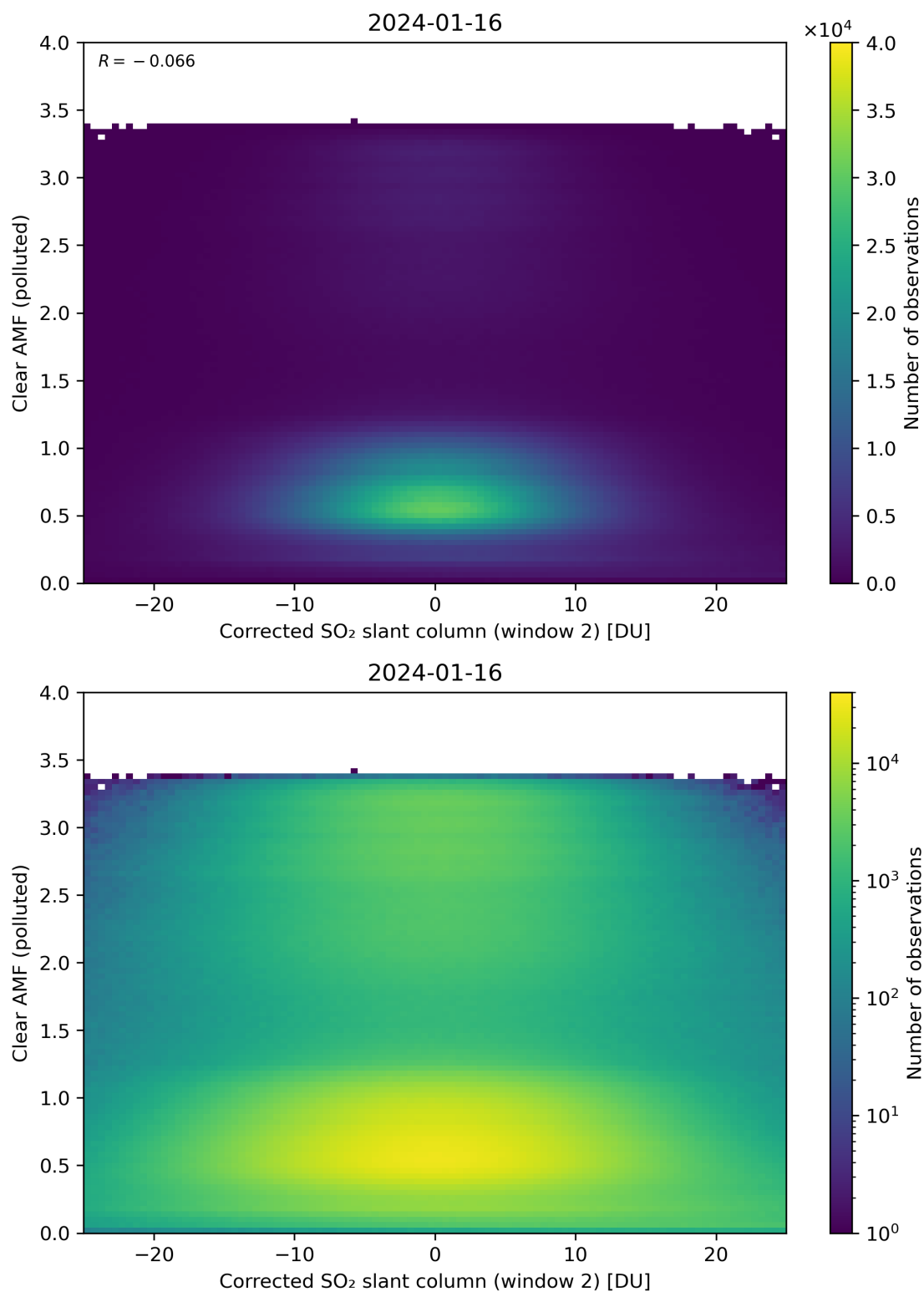
Figure 199: Scatter density plot of “Corrected SO 2 slant column (window 2)” against “Clear AMF (polluted)” for 2024-01-15 to 2024-01-17.
