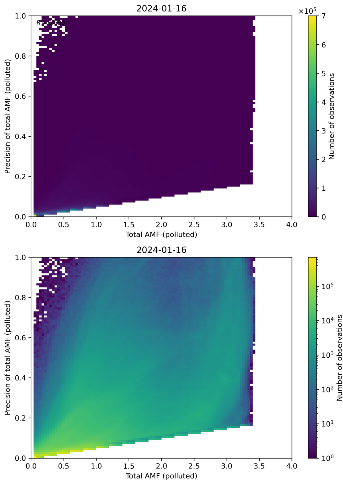
Figure 272: Scatter density plot of “Total AMF (polluted)” against “Precision of total AMF (polluted)” for 2024-01-15 to 2024-01-17.
