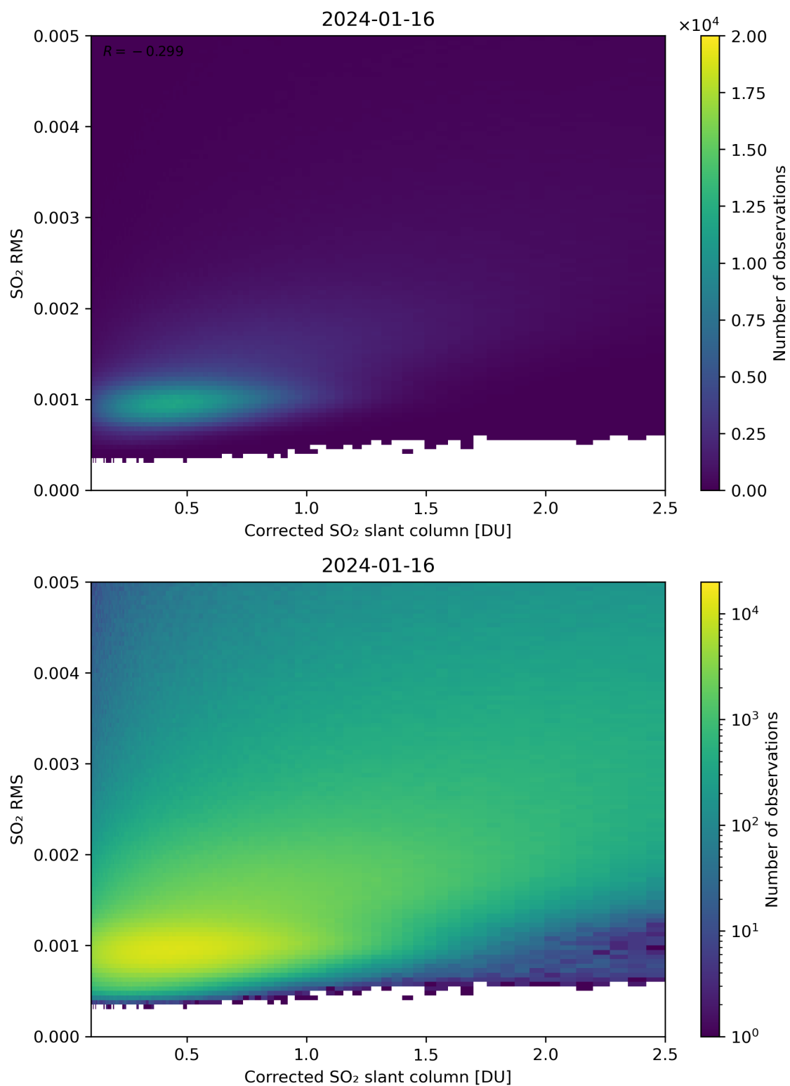
Figure 183: Scatter density plot of “Corrected SO 2 slant column” against “SO 2 RMS” for 2024-01-15 to 2024-01-17.
