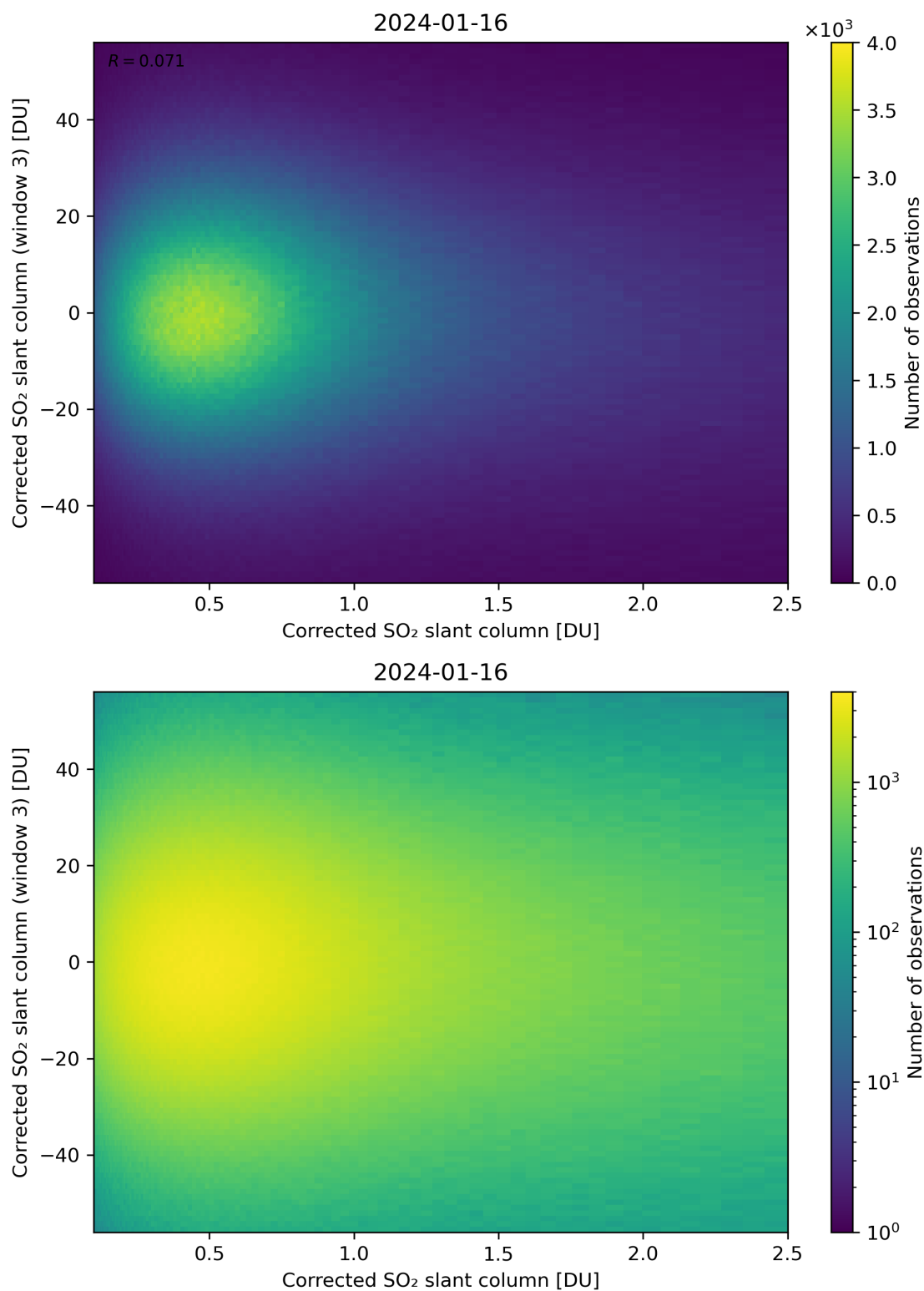
Figure 186: Scatter density plot of “Corrected SO 2 slant column” against “Corrected SO 2 slant column (window 3)” for 2024-01-15 to 2024-01-17.
