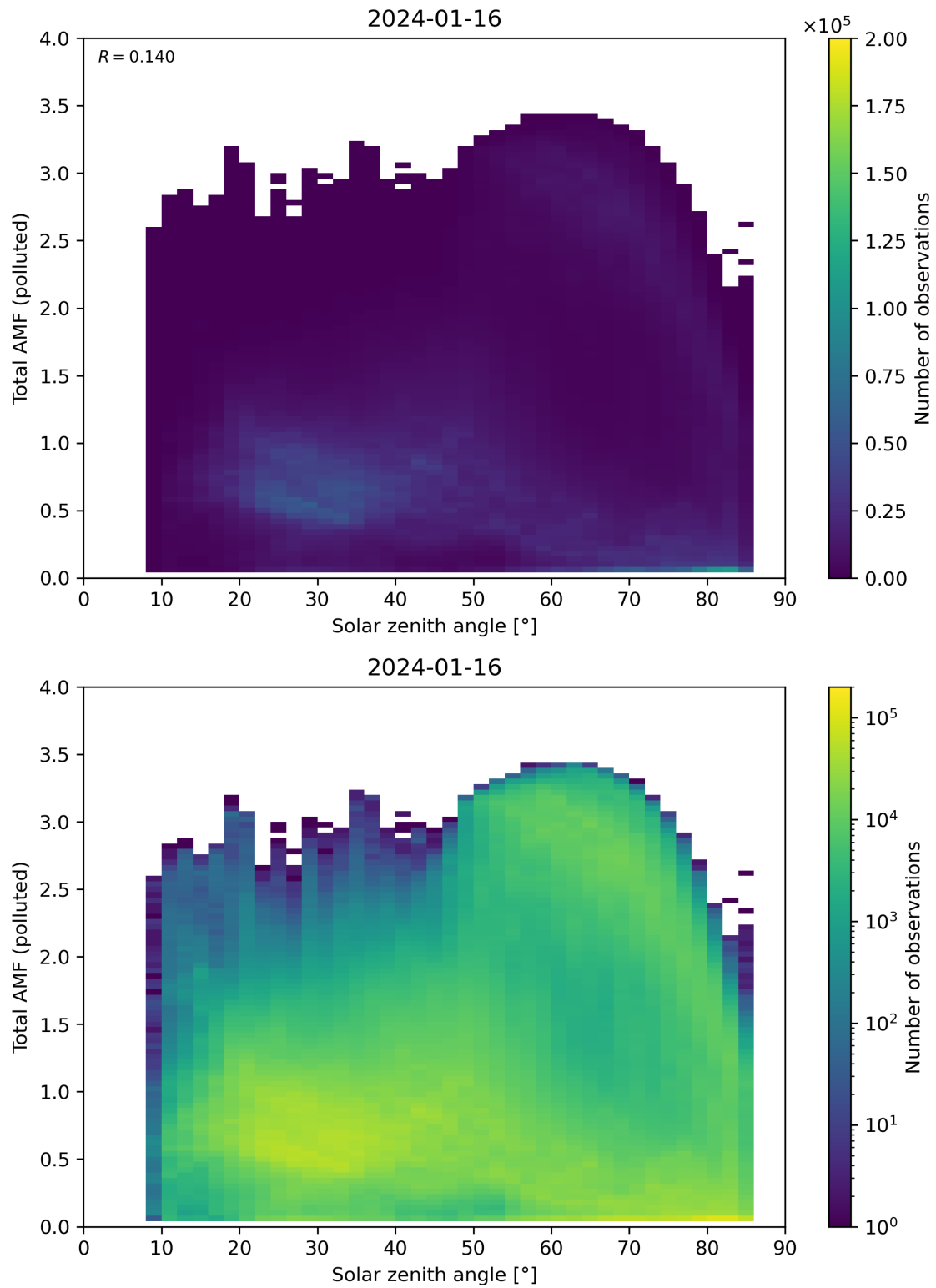
Figure 174: Scatter density plot of “Solar zenith angle” against “Total AMF (polluted)” for 2024-01-15 to 2024-01-17.
