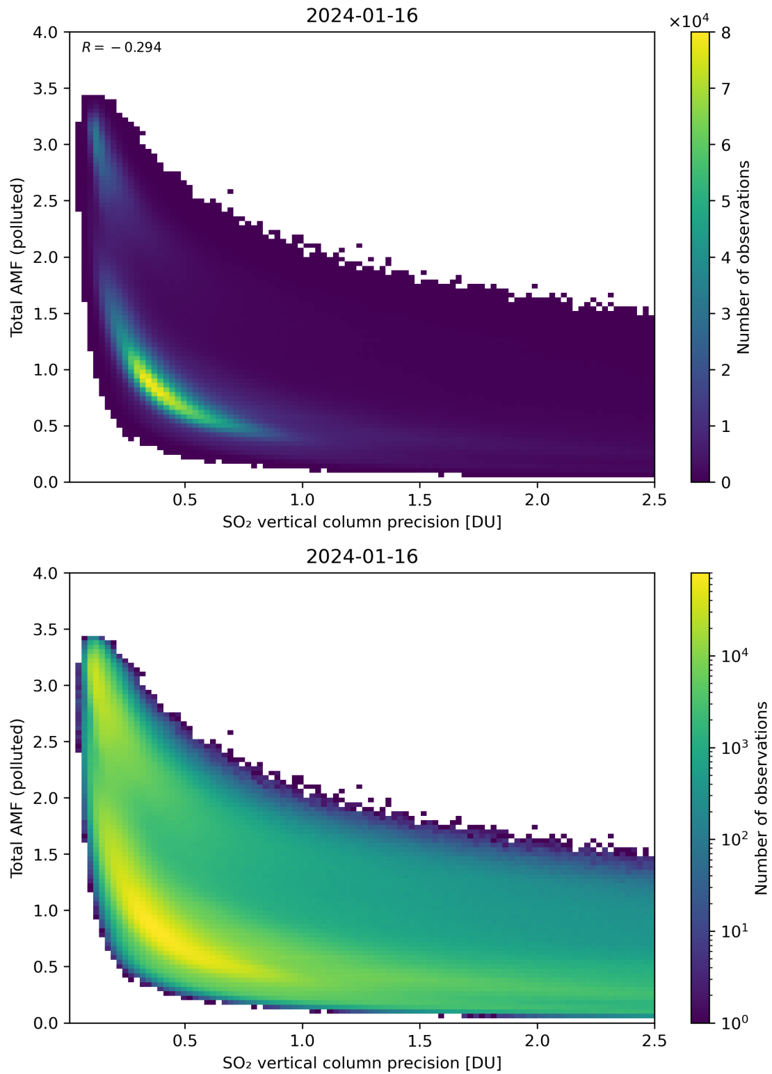
Figure 294: Scatter density plot of “SO 2 vertical column precision” against “Total AMF (polluted)” for 2024-01-15 to 2024-01-17.
