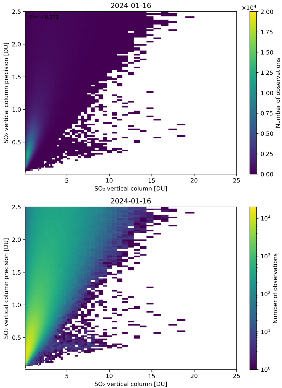
Figure 307: Scatter density plot of “SO 2 vertical column” against “SO 2 vertical column precision” for 2024-01-15 to 2024-01-17.
