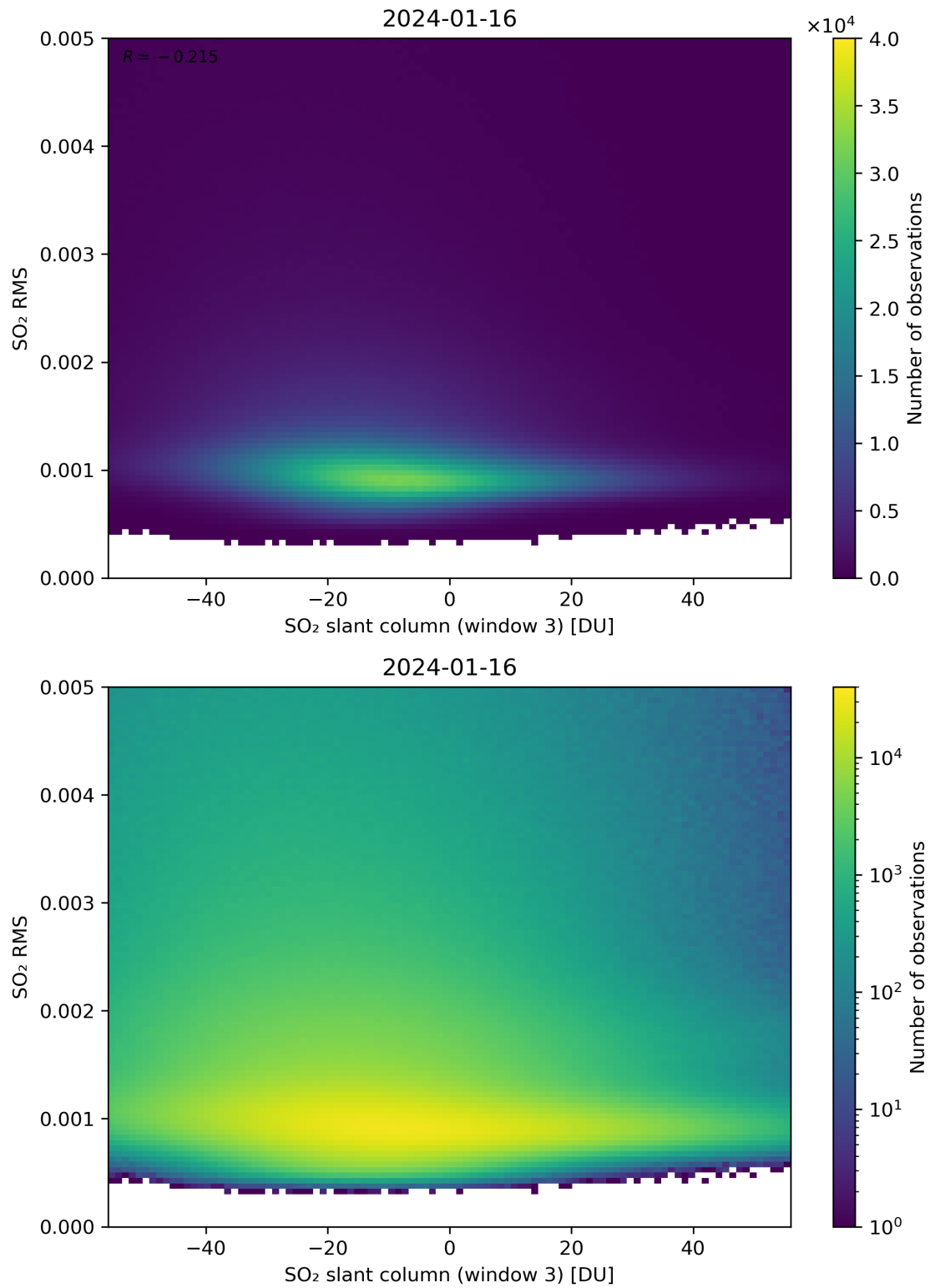
Figure 256: Scatter density plot of “SO 2 slant column (window 3)” against “SO 2 RMS” for 2024-01-15 to 2024-01-17.
