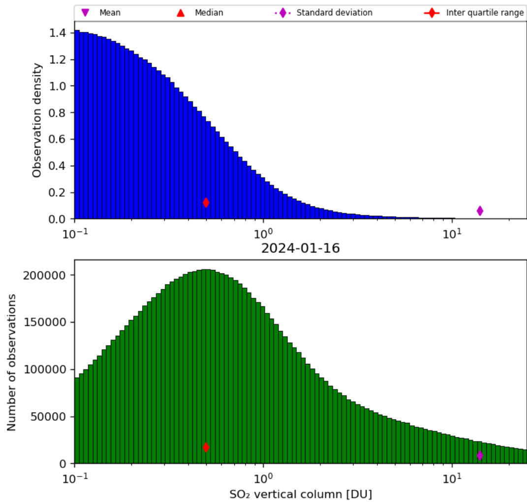
Figure 53: Histogram of “SO 2 vertical column” for 2024-01-15 to 2024-01-17
