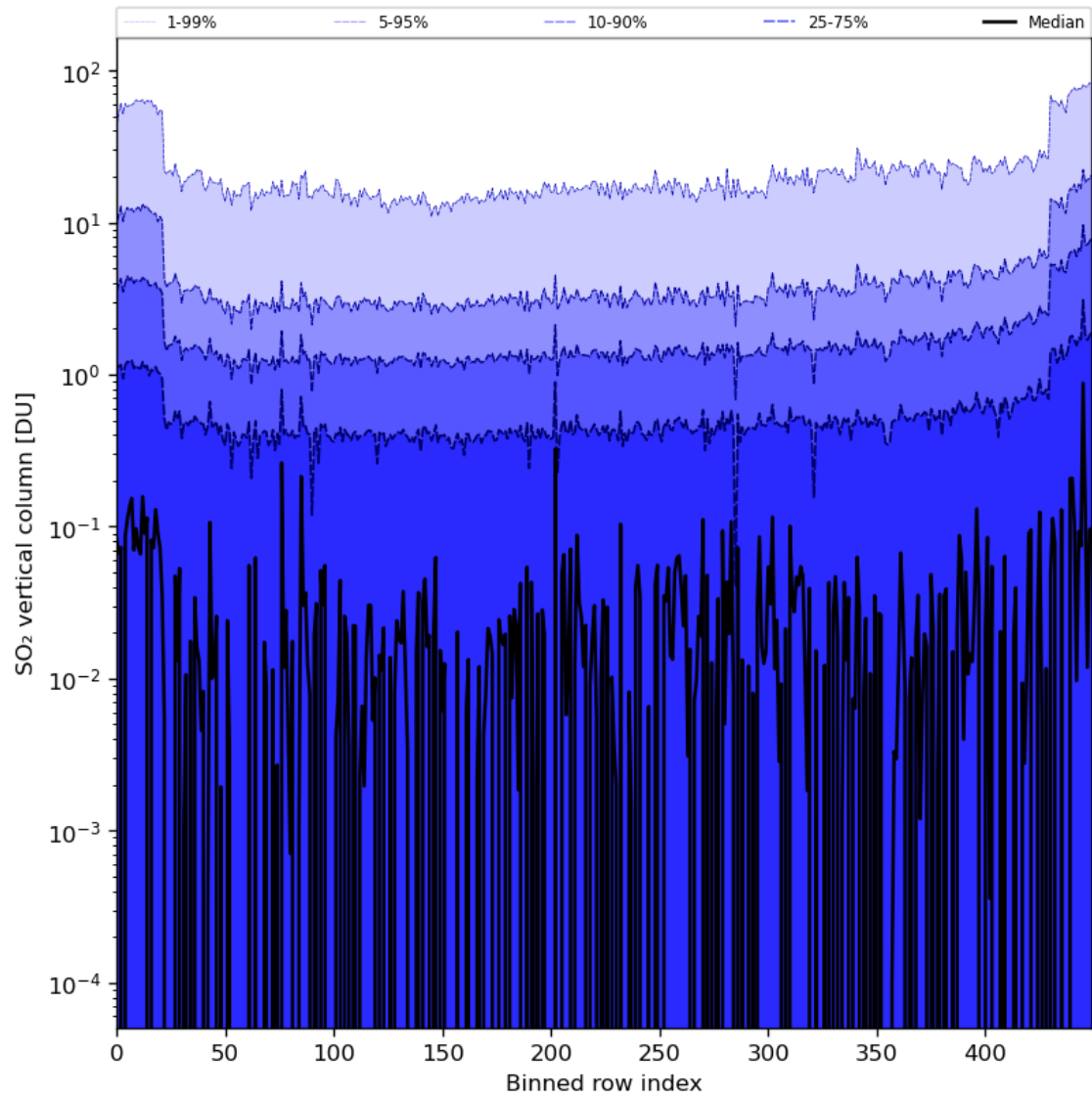
Figure 76: Along track statistics of “SO 2 vertical column” for 2024-01-15 to 2024-01-17
