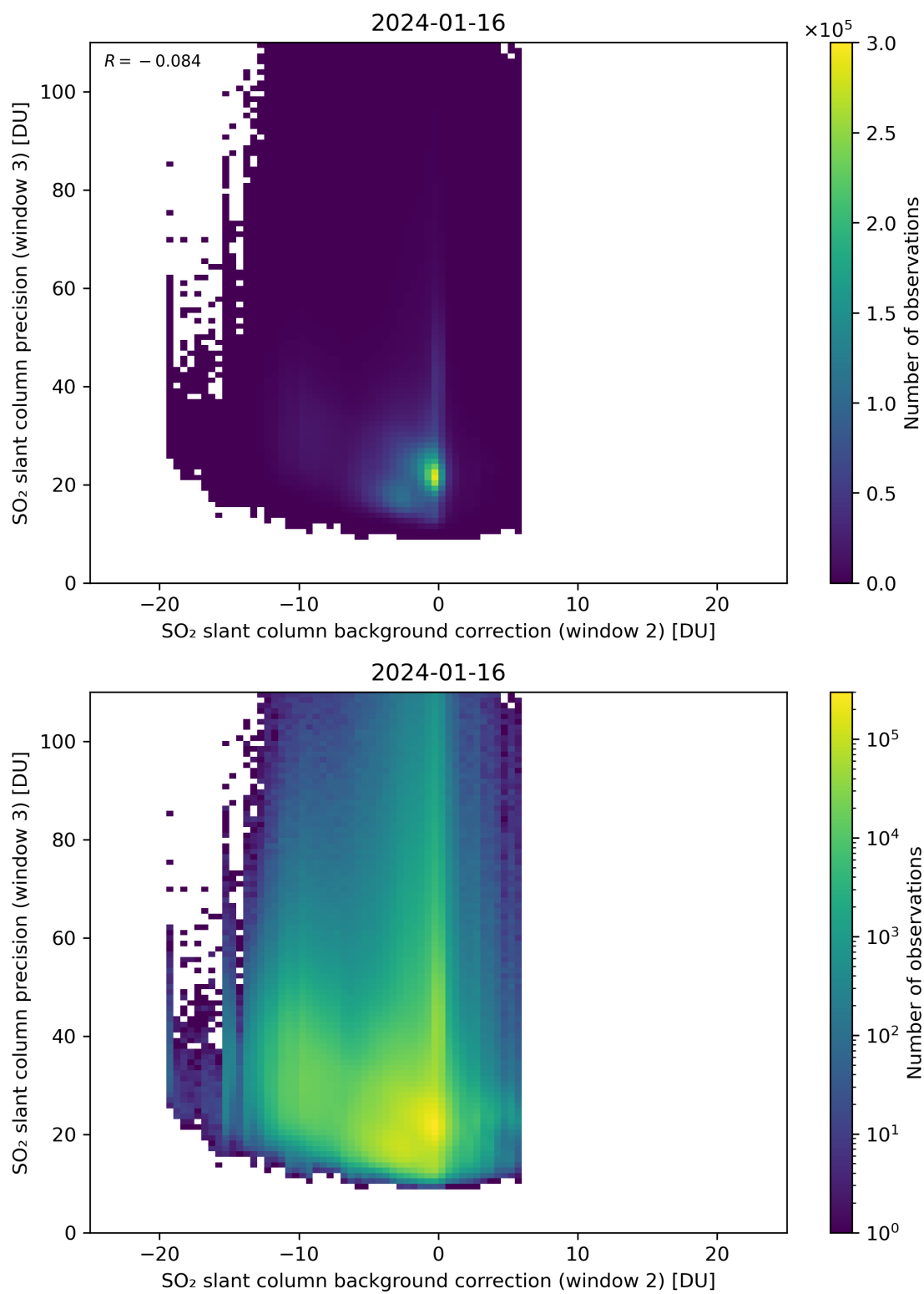
Figure 118: Scatter density plot of “SO 2 slant column background correction (window 2)” against “SO 2 slant column precision (window 3)” for 2024-01-15 to 2024-01-17.
