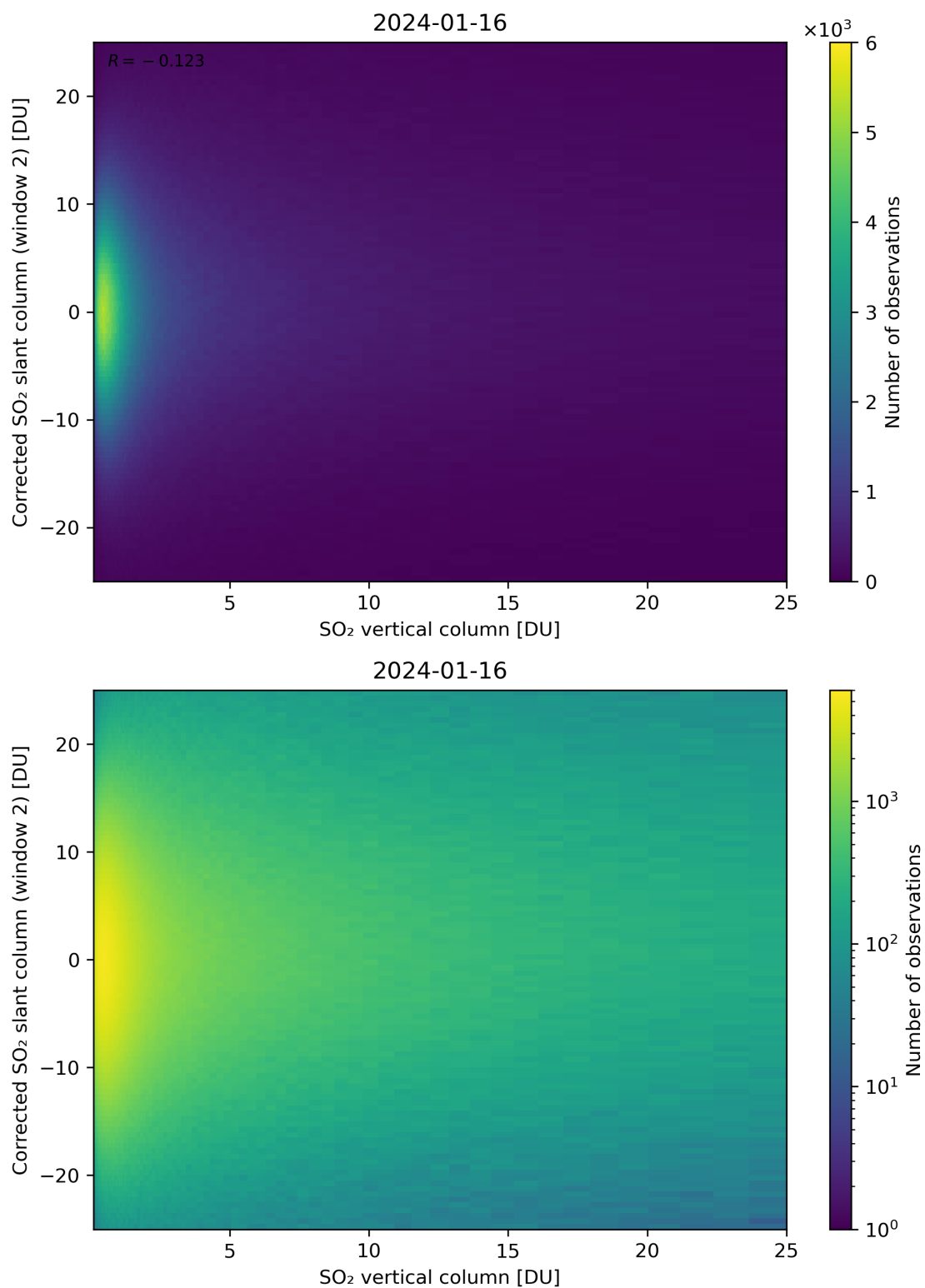
Figure 298: Scatter density plot of “SO 2 vertical column” against “Corrected SO 2 slant column (window 2)” for 2024-01-15 to 2024-01-17.
