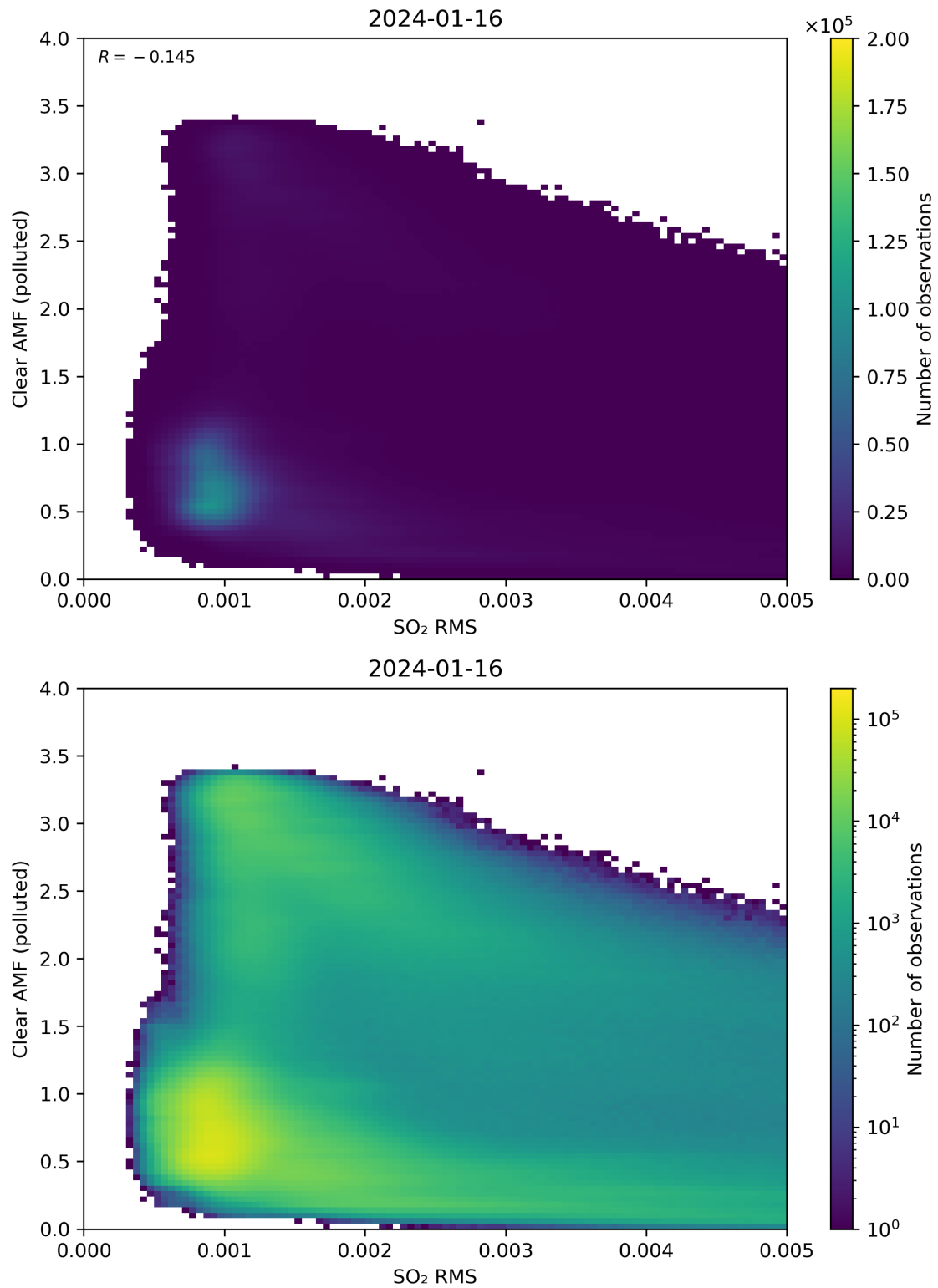
Figure 136: Scatter density plot of “SO 2 RMS” against “Clear AMF (polluted)” for 2024-01-15 to 2024-01-17.
