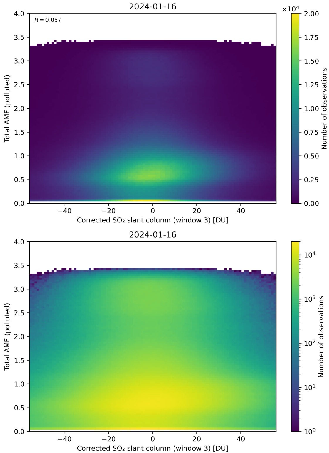
Figure 210: Scatter density plot of “Corrected SO 2 slant column (window 3)” against “Total AMF (polluted)” for 2024-01-15 to 2024-01-17.
