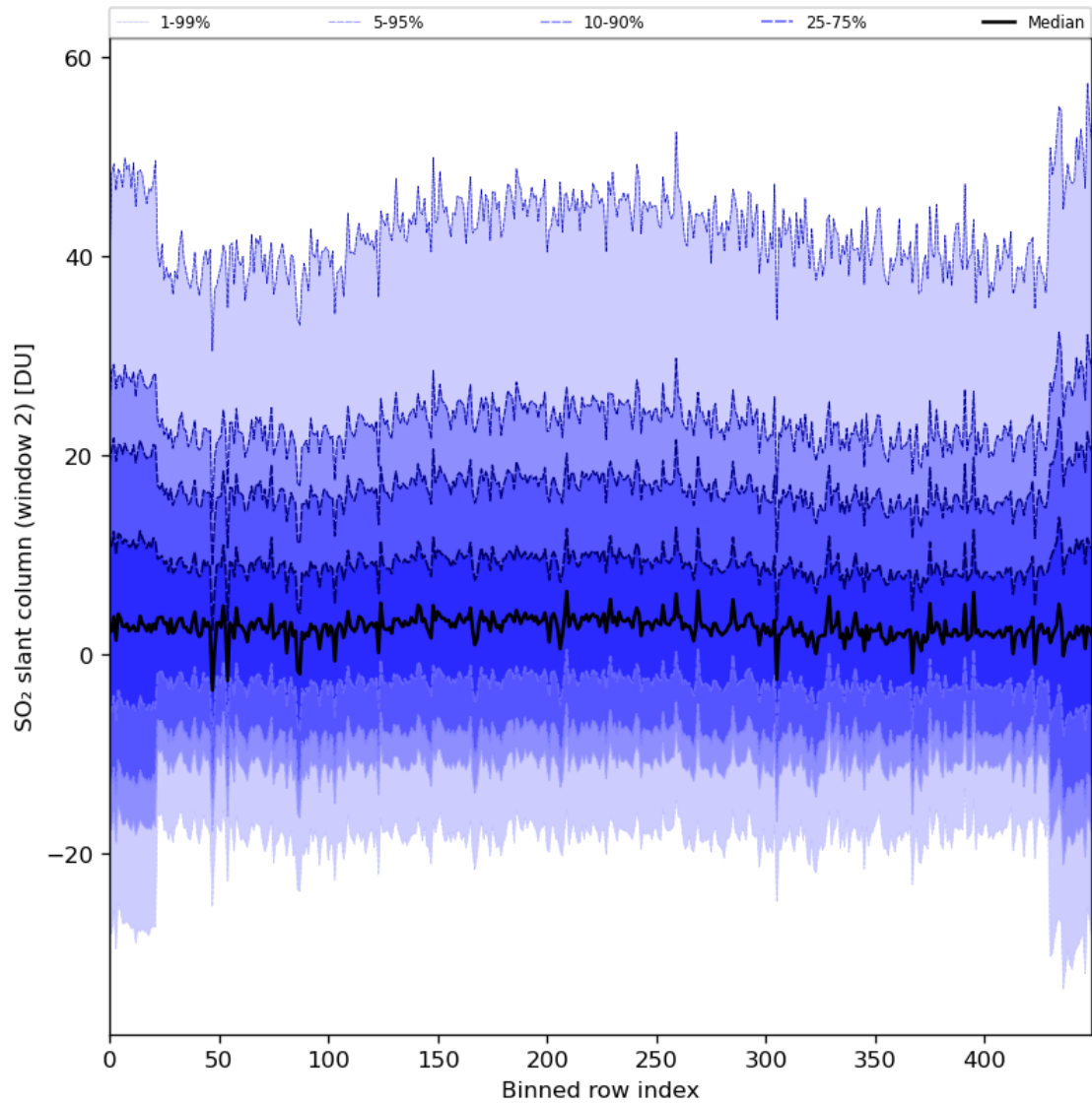
Figure 83: Along track statistics of “SO 2 slant column (window 2)” for 2024-01-15 to 2024-01-17
