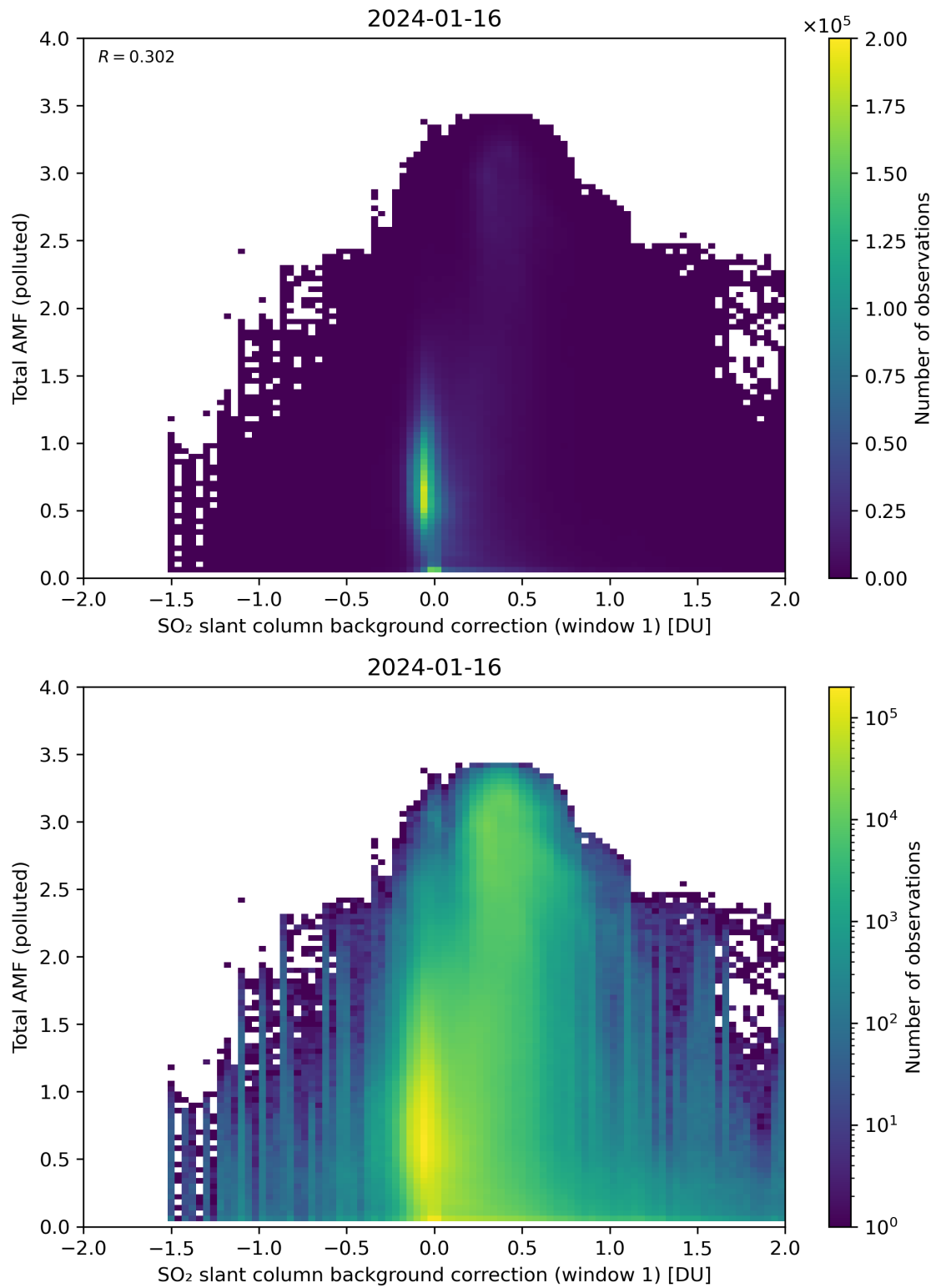
Figure 109: Scatter density plot of “SO 2 slant column background correction (window 1)” against “Total AMF (polluted)” for 2024-01-15 to 2024-01-17.
