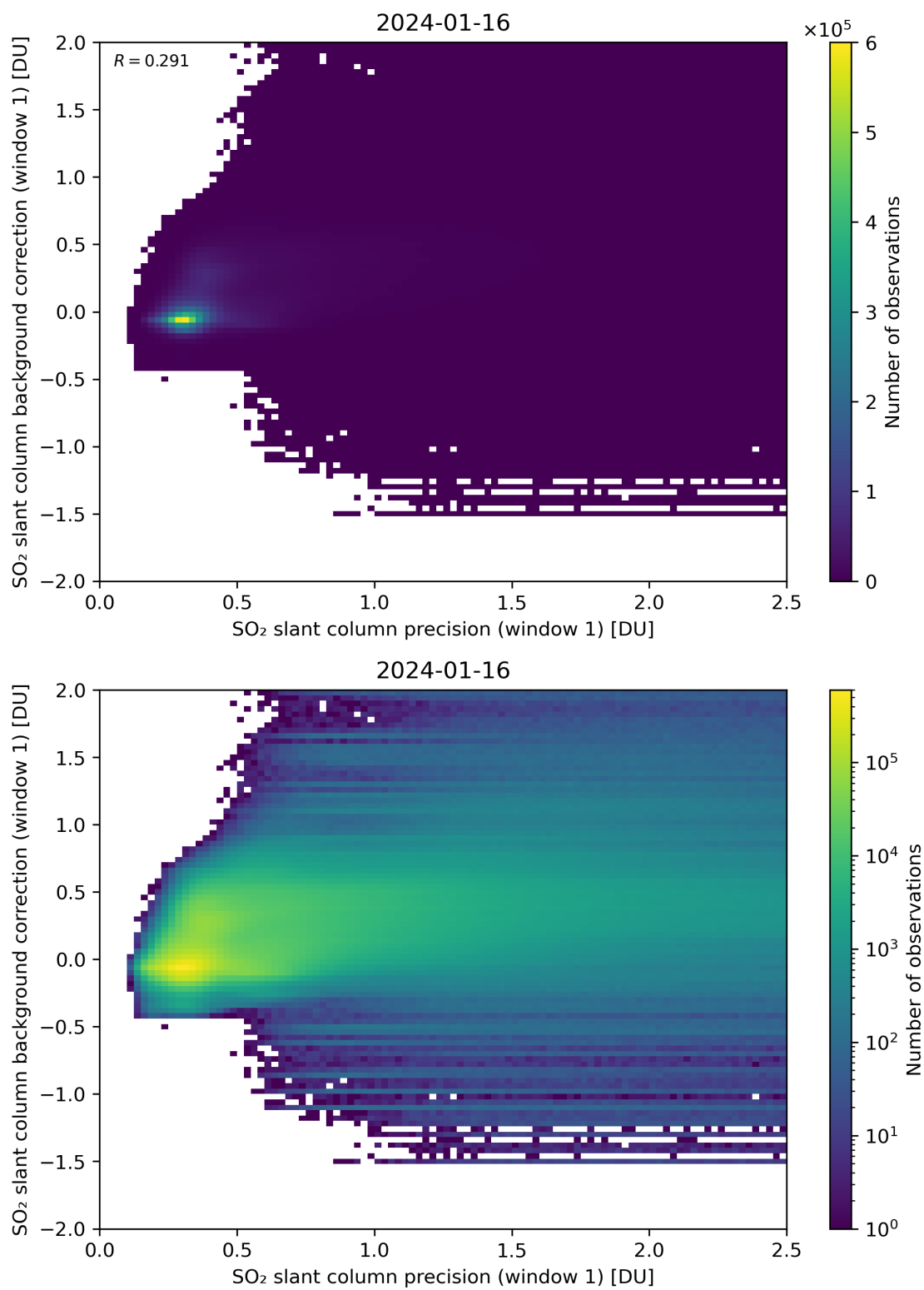
Figure 218: Scatter density plot of “SO 2 slant column precision (window 1)” against “SO 2 slant column background correction (window 1)” for 2024-01-15 to 2024-01-17.
