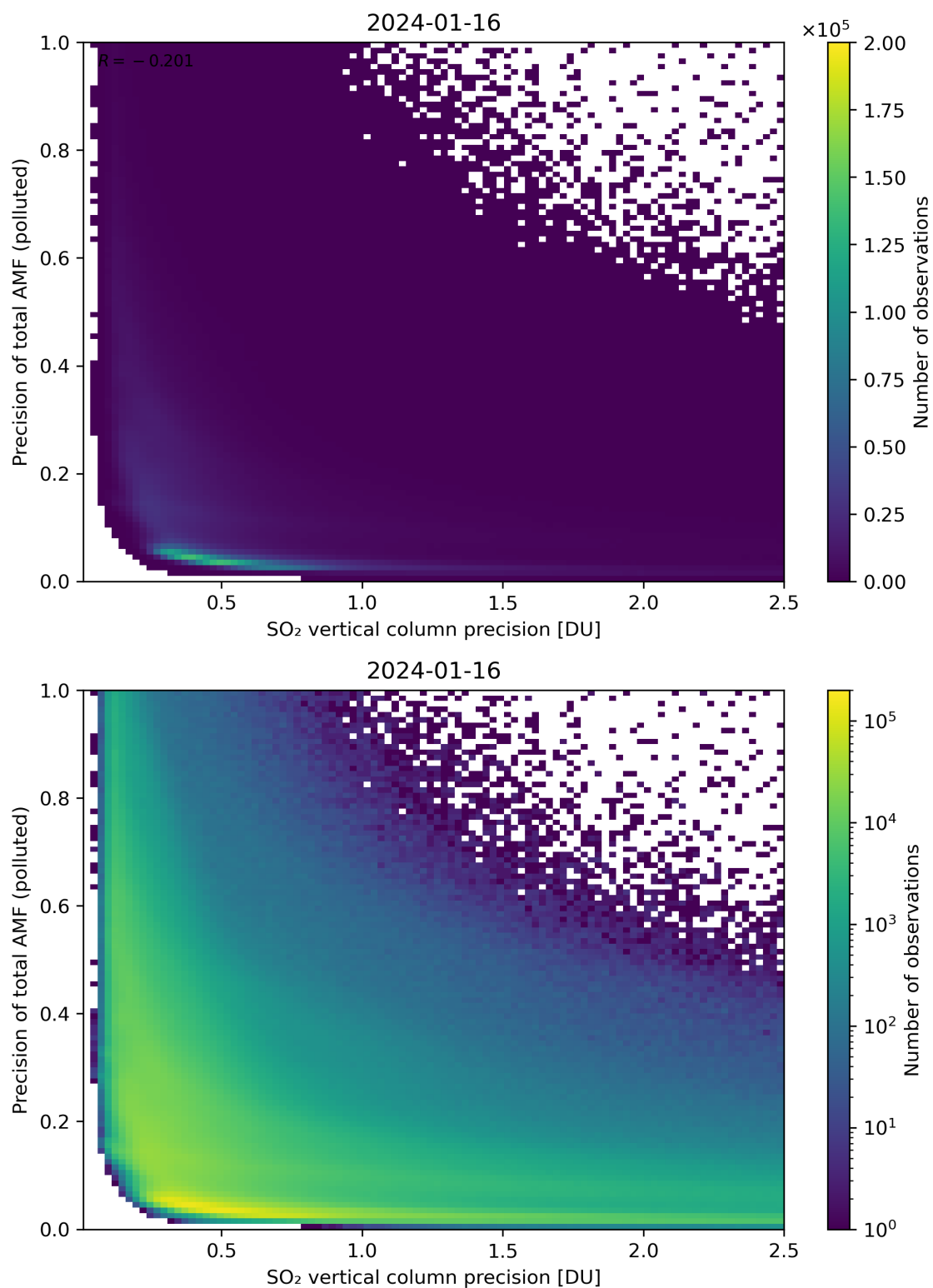
Figure 295: Scatter density plot of “SO 2 vertical column precision” against “Precision of total AMF (polluted)” for 2024-01-15 to 2024-01-17.
