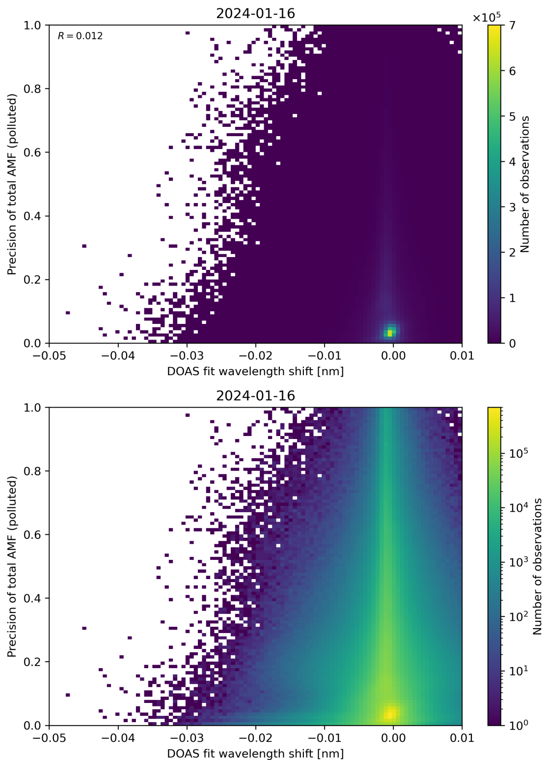
Figure 131: Scatter density plot of “DOAS fit wavelength shift” against “Precision of total AMF (polluted)” for 2024-01-15 to 2024-01-17.
