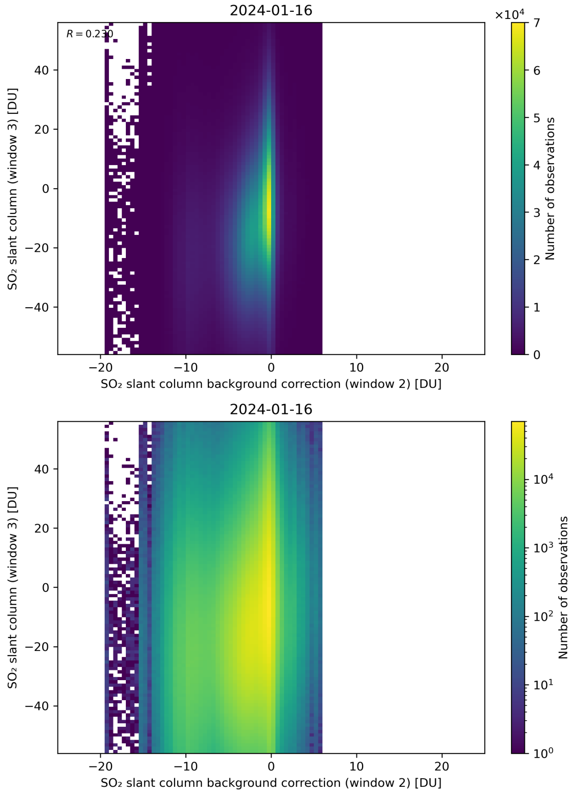
Figure 117: Scatter density plot of “SO 2 slant column background correction (window 2)” against “SO 2 slant column (window 3)” for 2024-01-15 to 2024-01-17.
