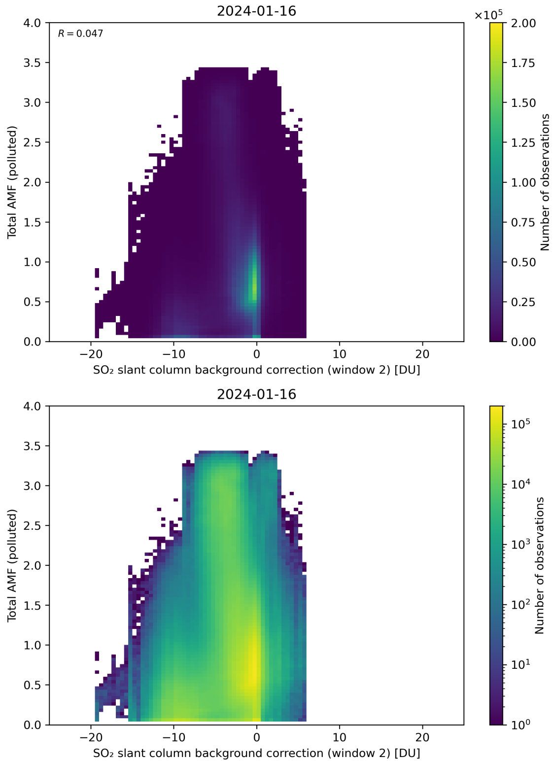
Figure 119: Scatter density plot of “SO 2 slant column background correction (window 2)” against “Total AMF (polluted)” for 2024-01-15 to 2024-01-17.
