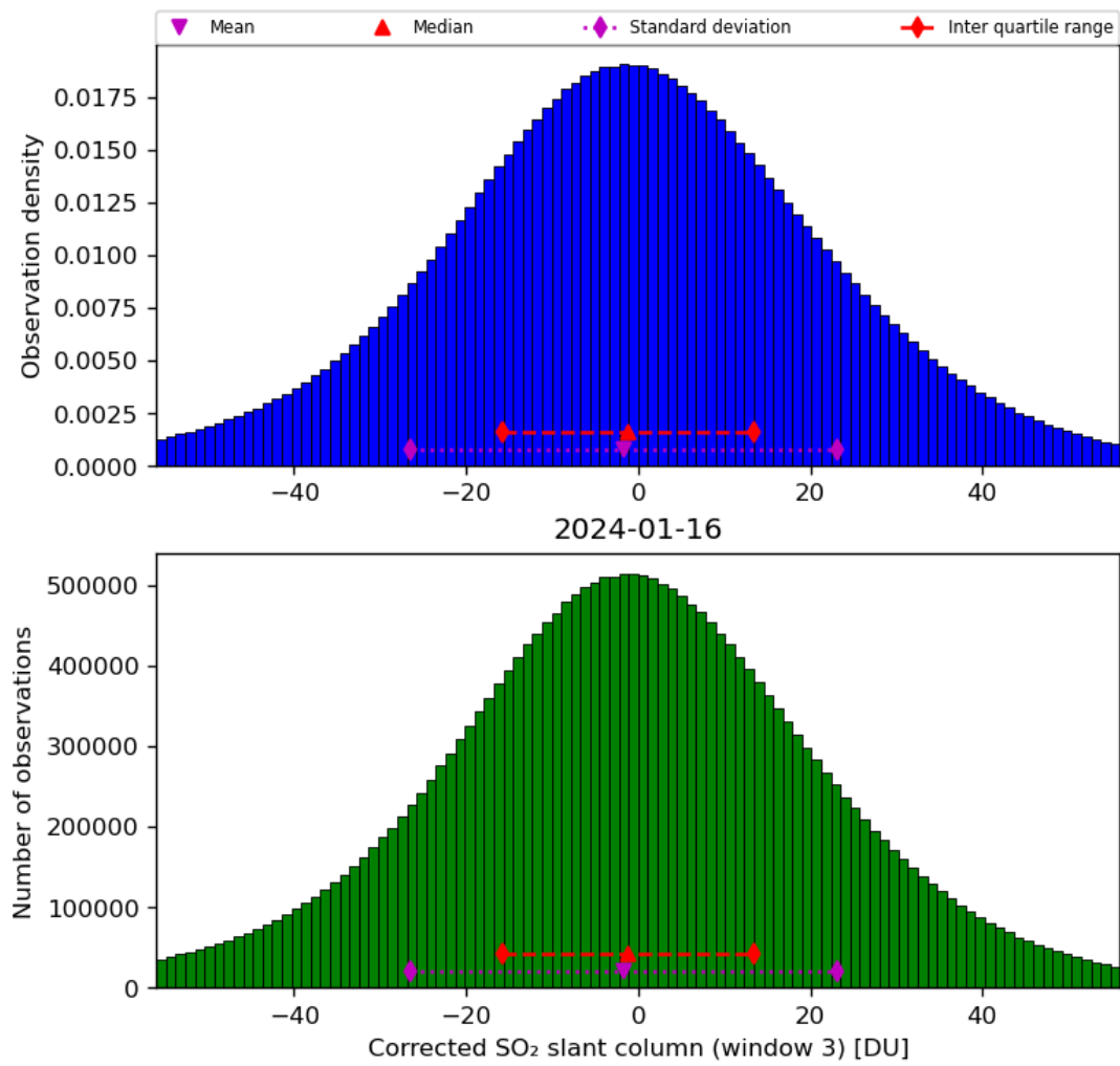
Figure 66: Histogram of "Corrected SO 2 slant column (window 3)" for 2024-01-15 to 2024-01-17
