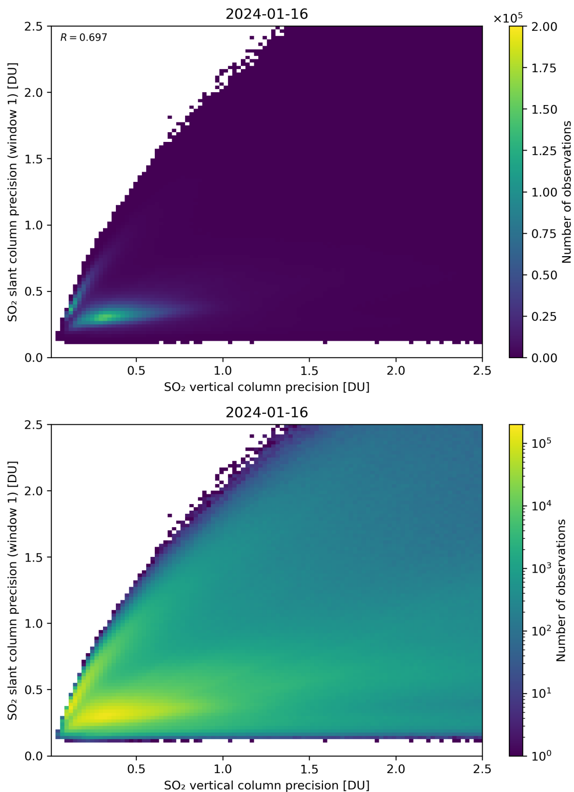
Figure 290: Scatter density plot of “SO 2 vertical column precision” against “SO 2 slant column precision (window 1)” for 2024-01-15 to 2024-01-17.
