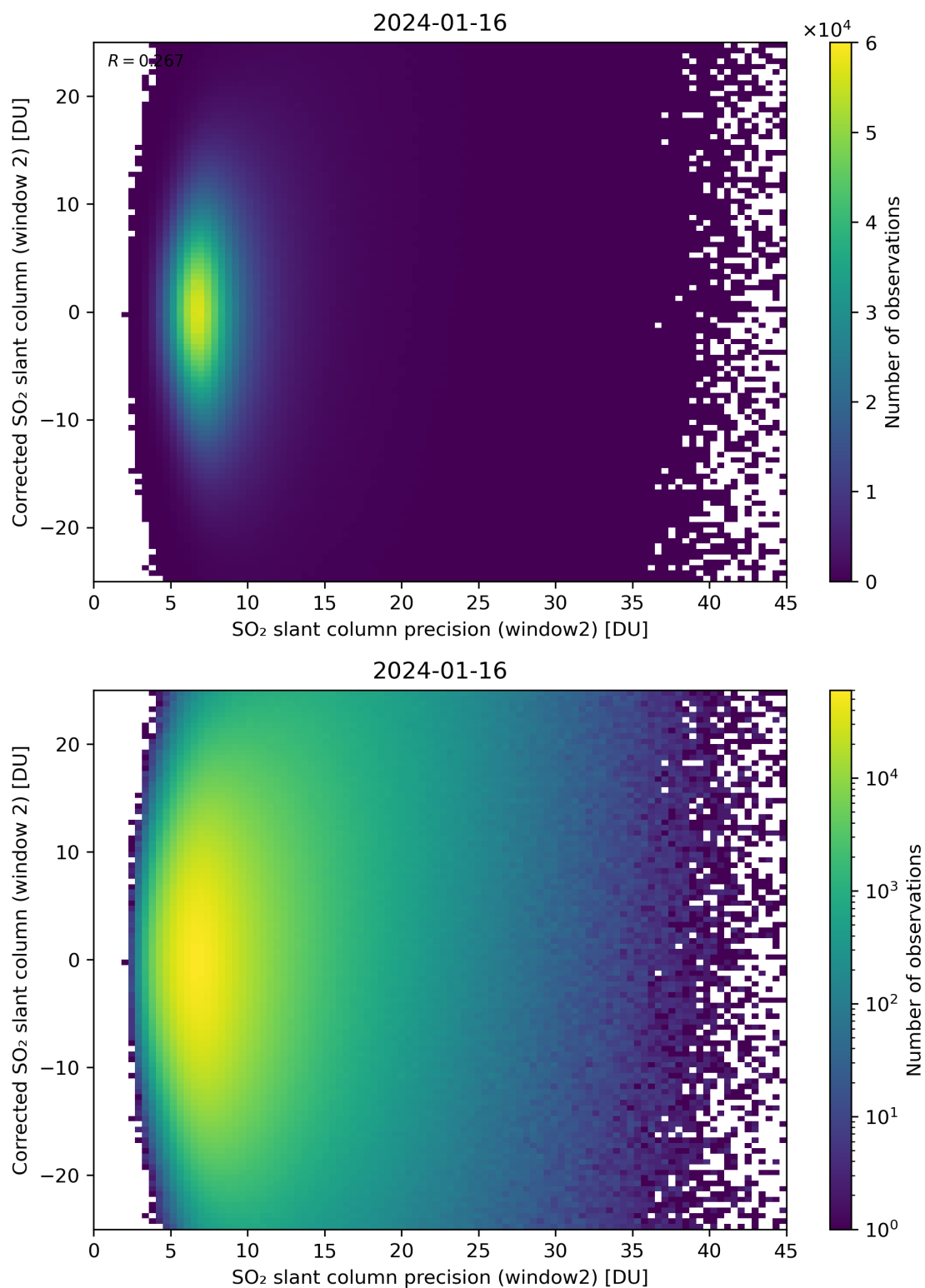
Figure 247: Scatter density plot of “SO 2 slant column precision (window2)” against “Corrected SO 2 slant column (window 2)” for 2024-01-15 to 2024-01-17.
