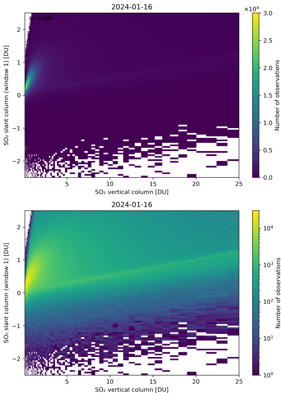
Figure 300: Scatter density plot of “SO 2 vertical column” against “SO 2 slant column (window 1)” for 2024-01-15 to 2024-01-17.
