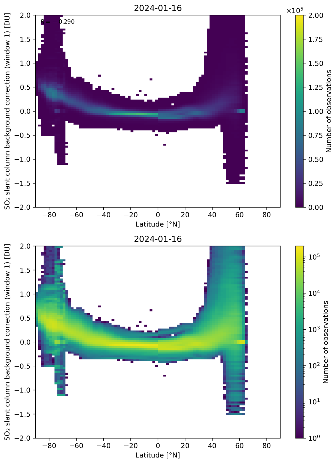
Figure 139: Scatter density plot of “Latitude” against “SO 2 slant column background correction (window 1)” for 2024-01-15 to 2024-01-17.
