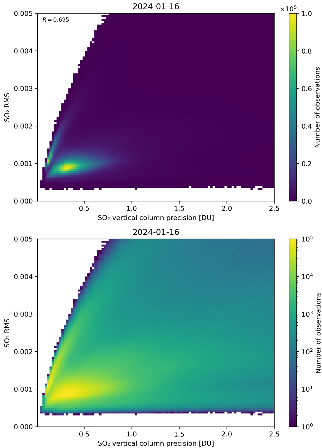
Figure 284: Scatter density plot of “SO 2 vertical column precision” against “SO 2 RMS” for 2024-01-15 to 2024-01-17.
