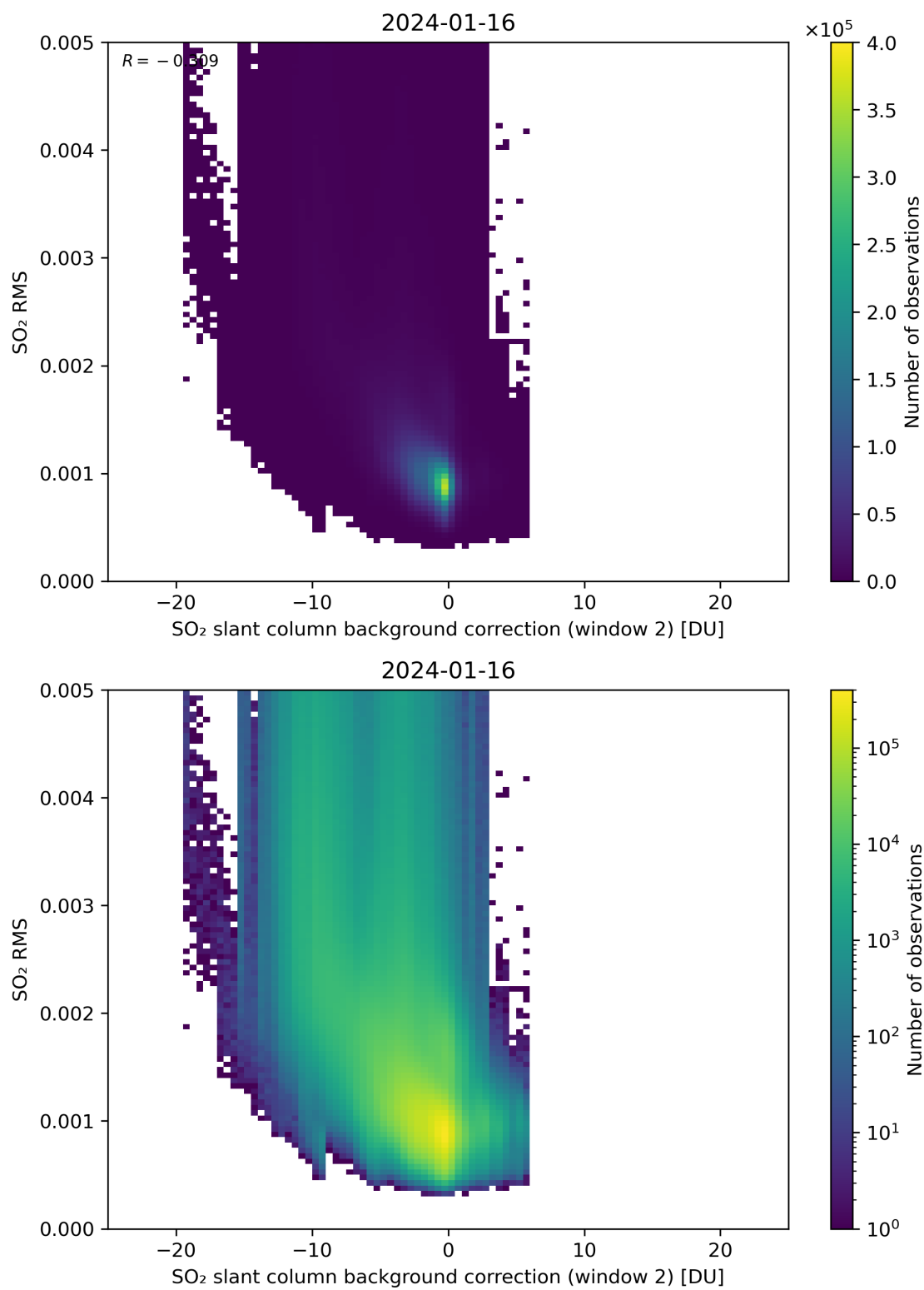
Figure 114: Scatter density plot of “SO 2 slant column background correction (window 2)” against “SO 2 RMS” for 2024-01-15 to 2024-01-17.
