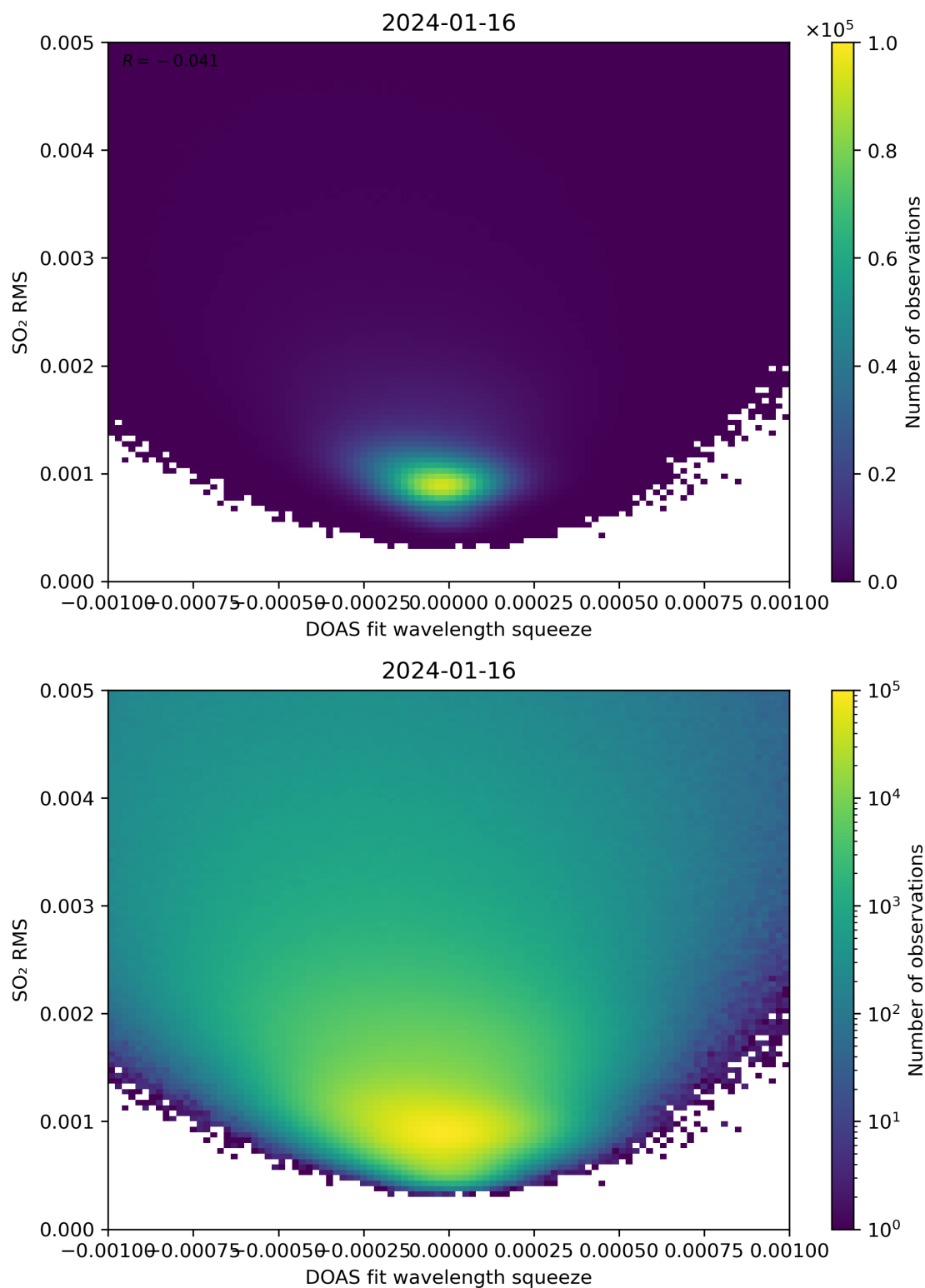
Figure 132: Scatter density plot of “DOAS fit wavelength squeeze” against “SO 2 RMS” for 2024-01-15 to 2024-01-17.
