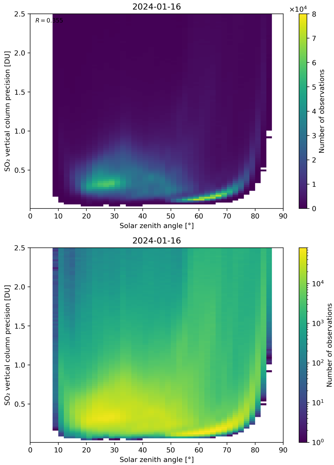
Figure 177: Scatter density plot of “Solar zenith angle” against “SO 2 vertical column precision” for 2024-01-15 to 2024-01-17.
