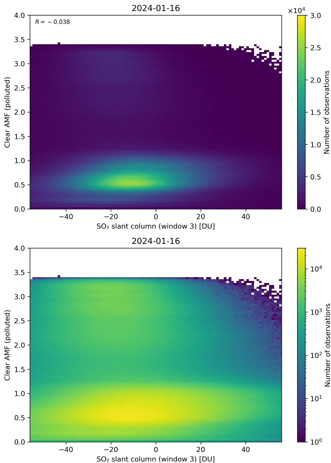
Figure 265: Scatter density plot of “SO 2 slant column (window 3)” against “Clear AMF (polluted)” for 2024-01-15 to 2024-01-17.
