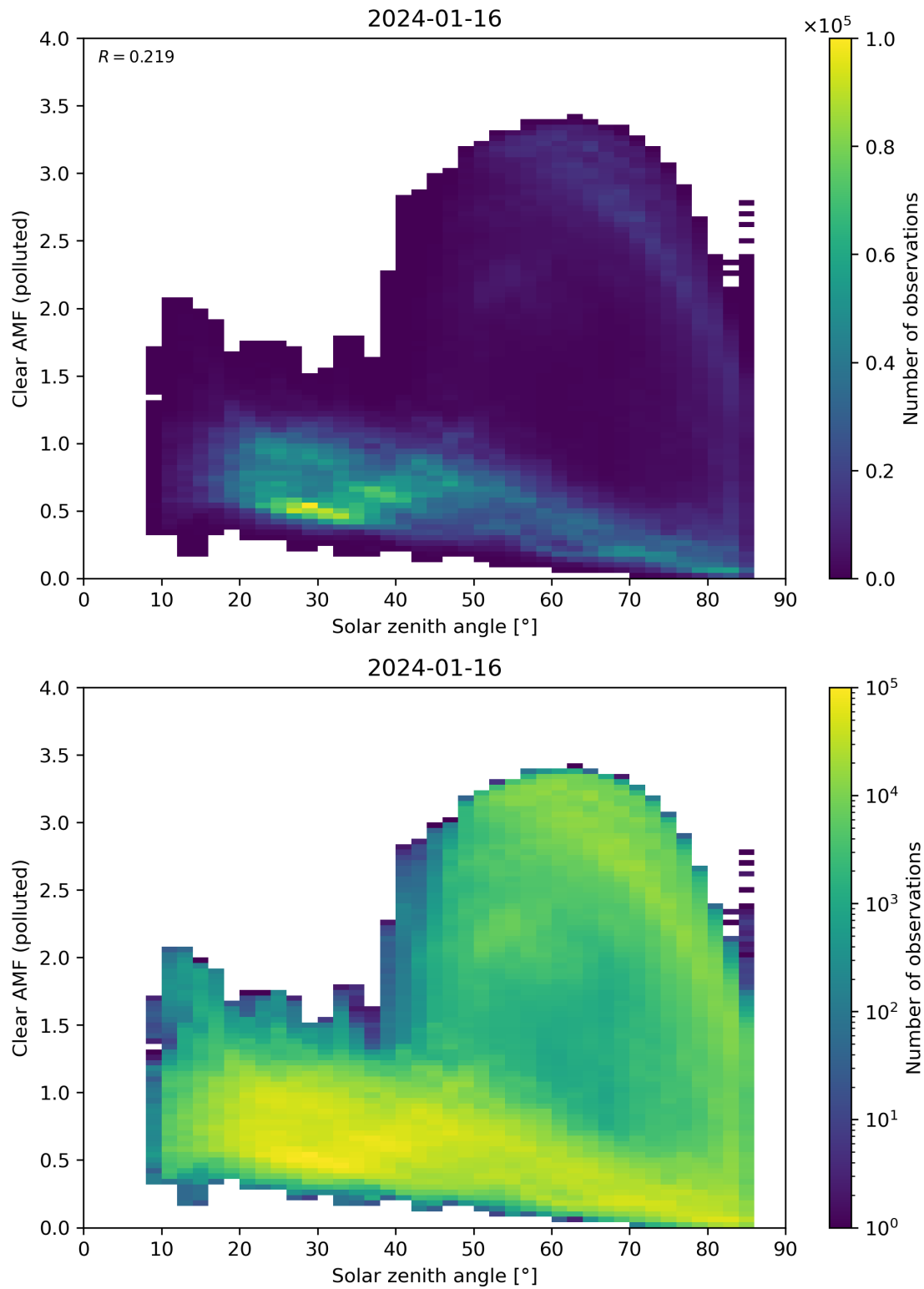
Figure 165: Scatter density plot of “Solar zenith angle” against “Clear AMF (polluted)” for 2024-01-15 to 2024-01-17.
