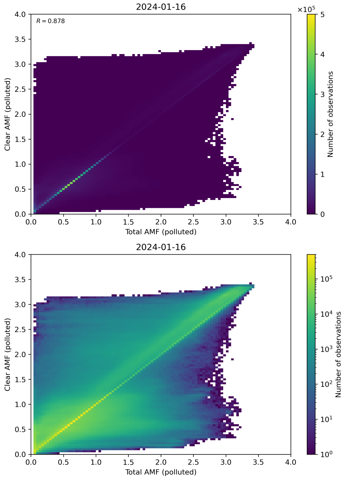
Figure 271: Scatter density plot of “Total AMF (polluted)” against “Clear AMF (polluted)” for 2024-01-15 to 2024-01-17.
