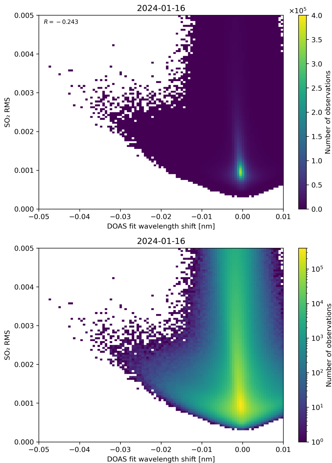
Figure 128: Scatter density plot of “DOAS fit wavelength shift” against “SO 2 RMS” for 2024-01-15 to 2024-01-17.
