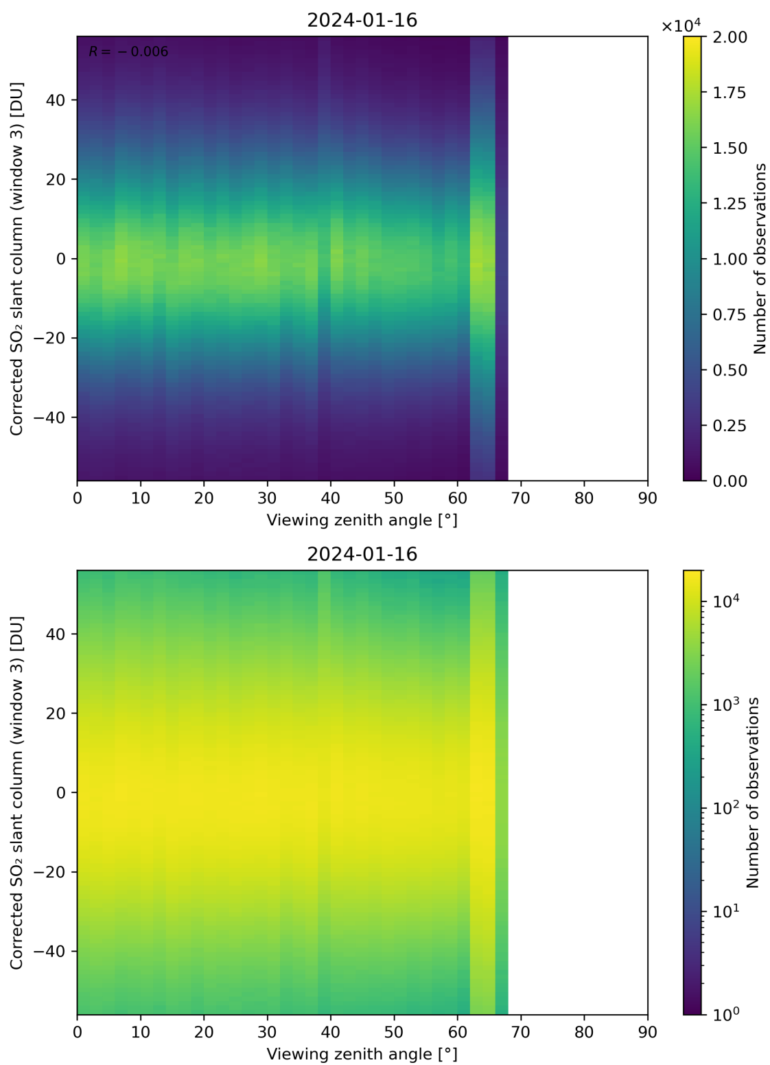
Figure 319: Scatter density plot of “Viewing zenith angle” against “Corrected SO 2 slant column (window 3)” for 2024-01-15 to 2024-01-17.
