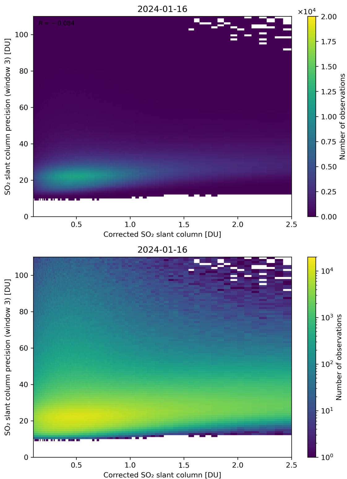
Figure 191: Scatter density plot of “Corrected SO 2 slant column” against “SO 2 slant column precision (window 3)” for 2024-01-15 to 2024-01-17.
