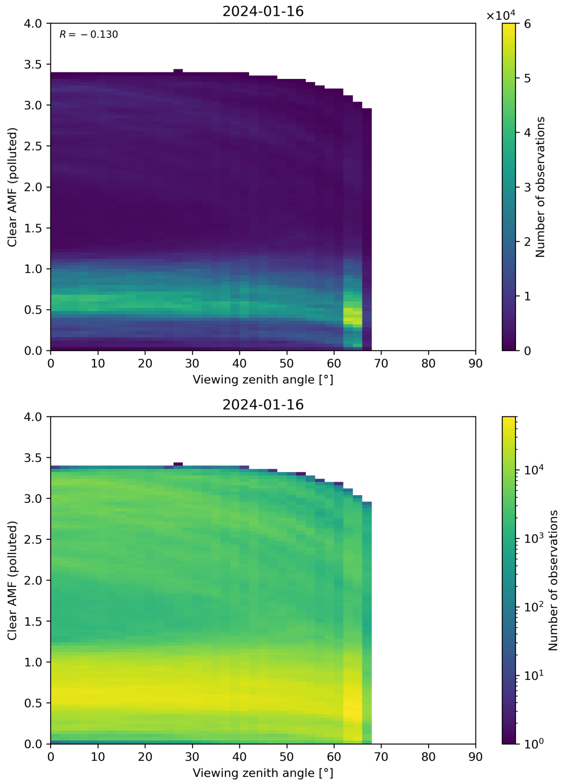
Figure 316: Scatter density plot of “Viewing zenith angle” against “Clear AMF (polluted)” for 2024-01-15 to 2024-01-17.
