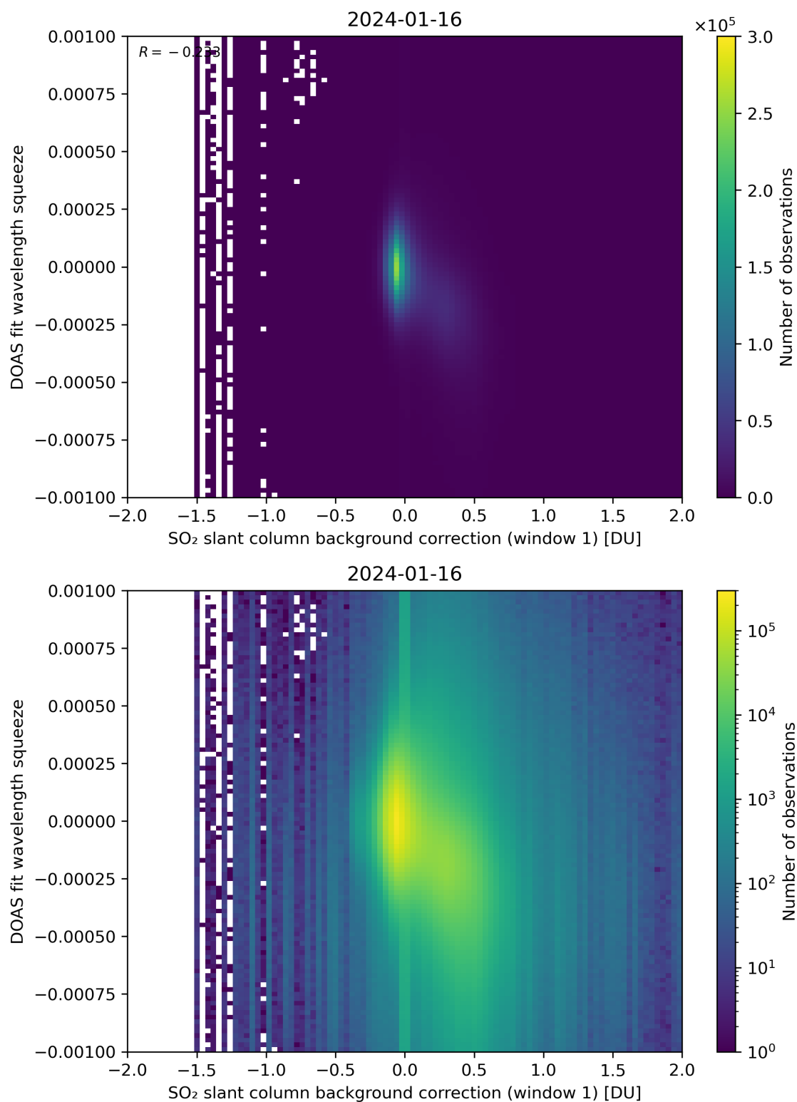
Figure 101: Scatter density plot of “SO 2 slant column background correction (window 1)” against “DOAS fit wavelength squeeze” for 2024-01-15 to 2024-01-17.
