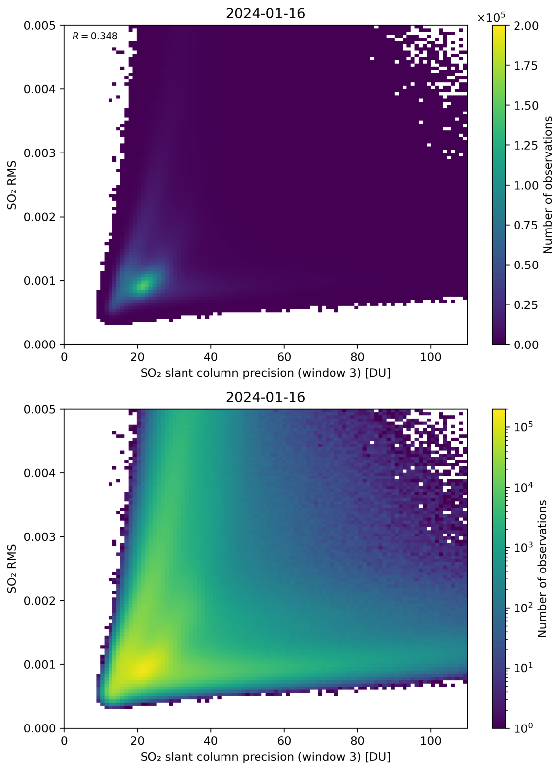
Figure 260: Scatter density plot of “SO 2 slant column precision (window 3)” against “SO 2 RMS” for 2024-01-15 to 2024-01-17.
