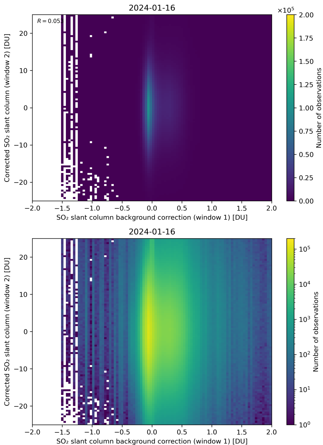
Figure 104: Scatter density plot of “SO 2 slant column background correction (window 1)” against “Corrected SO 2 slant column (window 2)” for 2024-01-15 to 2024-01-17.
