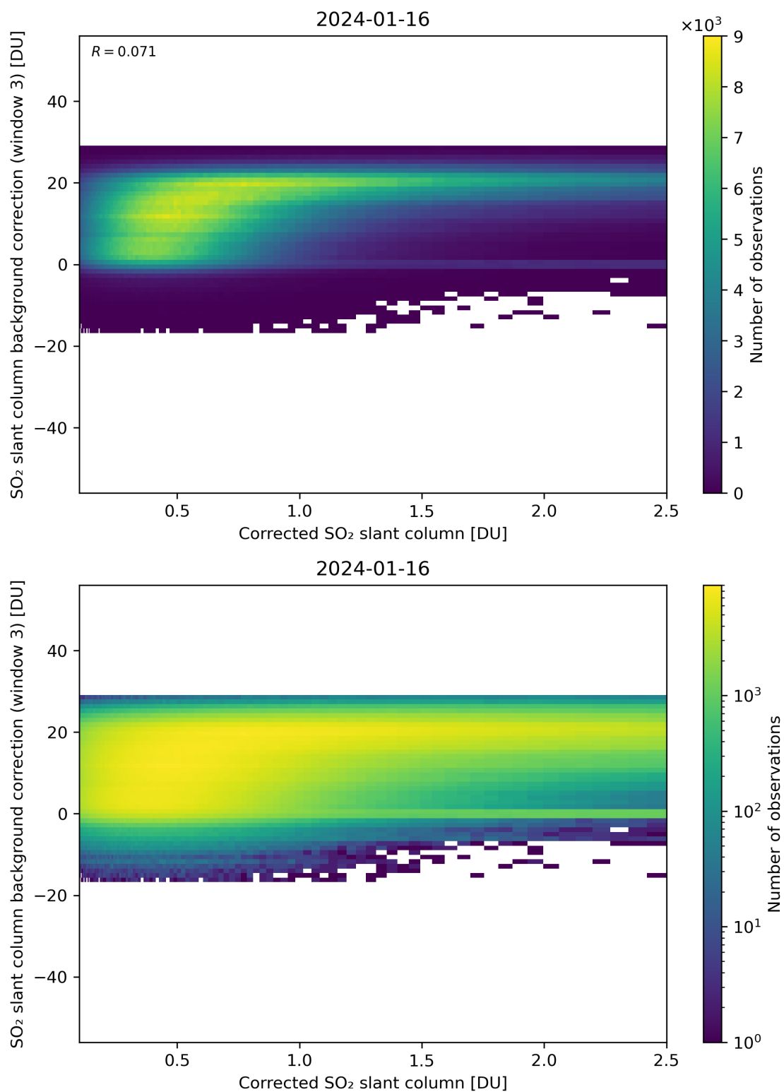
Figure 180: Scatter density plot of “Corrected SO 2 slant column” against “SO 2 slant column background correction (window 3)” for 2024-01-15 to 2024-01-17.
