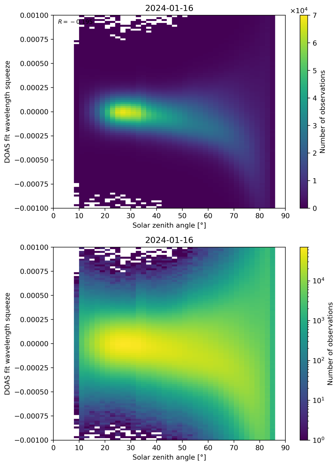
Figure 162: Scatter density plot of “Solar zenith angle” against “DOAS fit wavelength squeeze” for 2024-01-15 to 2024-01-17.
