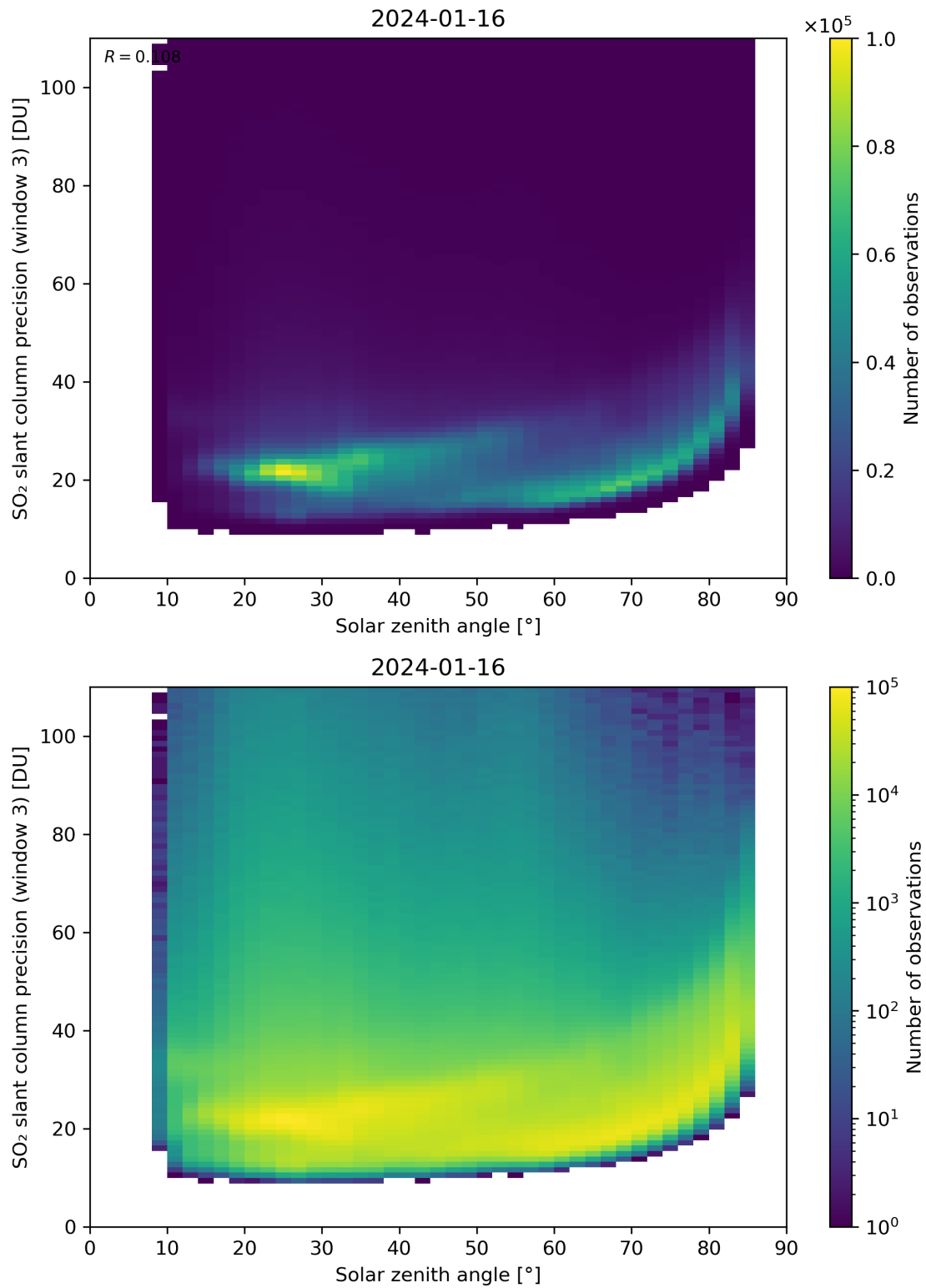
Figure 173: Scatter density plot of “Solar zenith angle” against “SO 2 slant column precision (window 3)” for 2024-01-15 to 2024-01-17.
