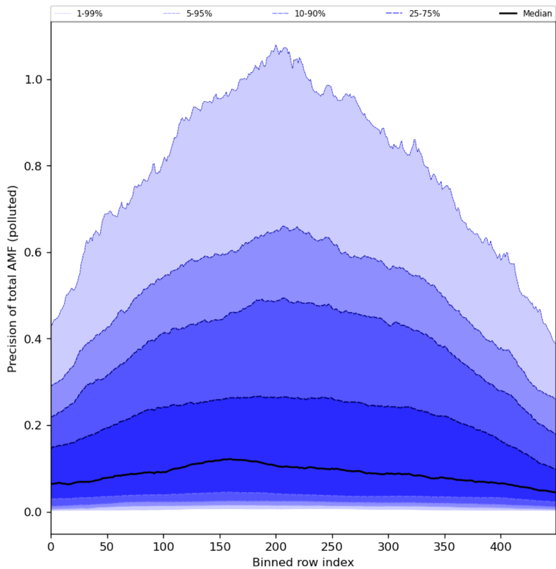
Figure 95: Along track statistics of “Precision of total AMF (polluted)” for 2024-01-15 to 2024-01-17
