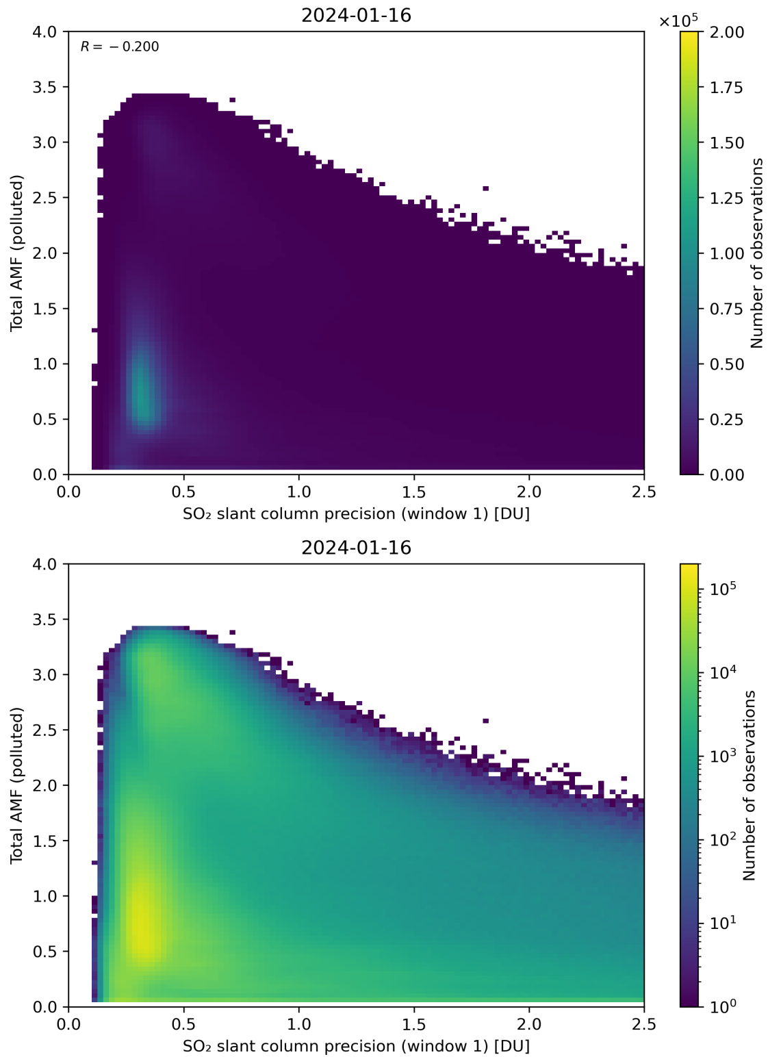
Figure 230: Scatter density plot of “SO 2 slant column precision (window 1)” against “Total AMF (polluted)” for 2024-01-15 to 2024-01-17.
