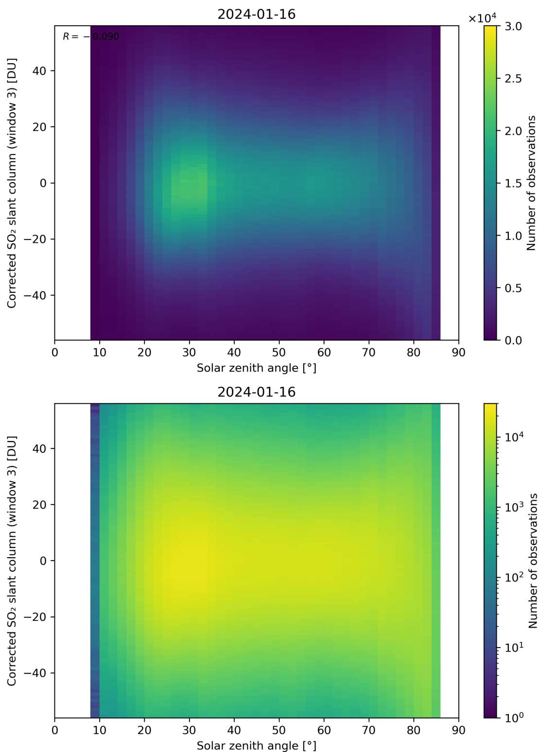
Figure 168: Scatter density plot of “Solar zenith angle” against “Corrected SO 2 slant column (window 3)” for 2024-01-15 to 2024-01-17.
