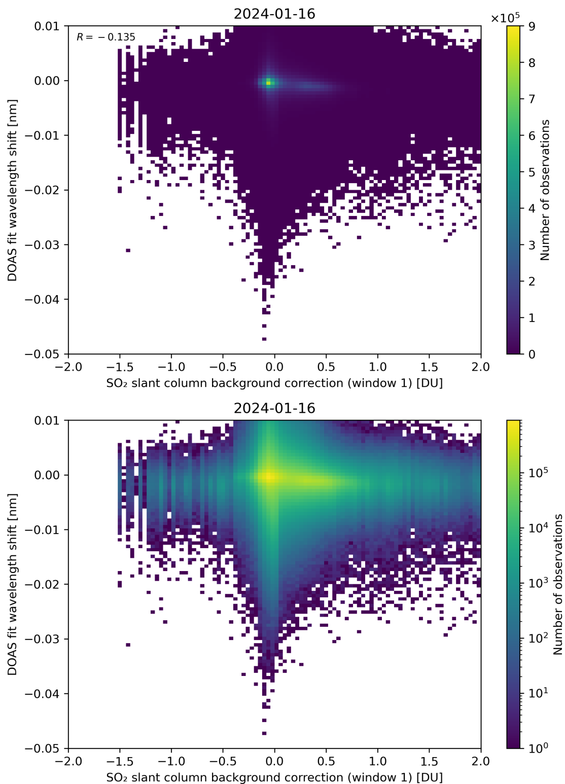
Figure 100: Scatter density plot of “SO 2 slant column background correction (window 1)” against “DOAS fit wavelength shift” for 2024-01-15 to 2024-01-17.
