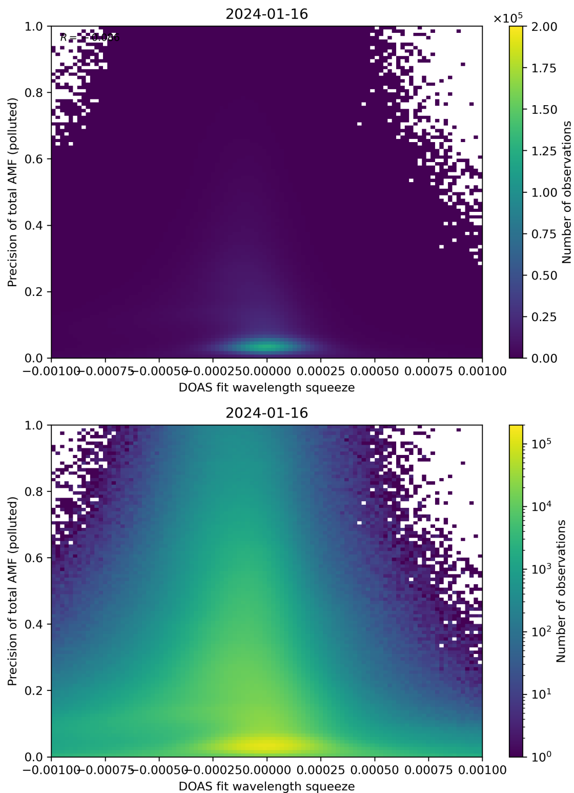
Figure 135: Scatter density plot of “DOAS fit wavelength squeeze” against “Precision of total AMF (polluted)” for 2024-01-15 to 2024-01-17.
