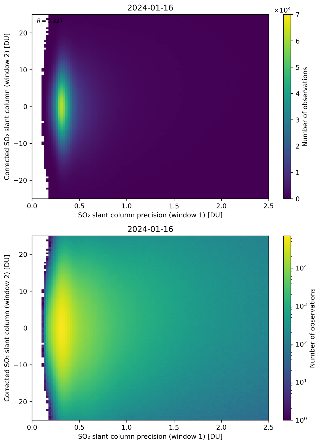
Figure 225: Scatter density plot of “SO 2 slant column precision (window 1)” against “Corrected SO 2 slant column (window 2)” for 2024-01-15 to 2024-01-17.
