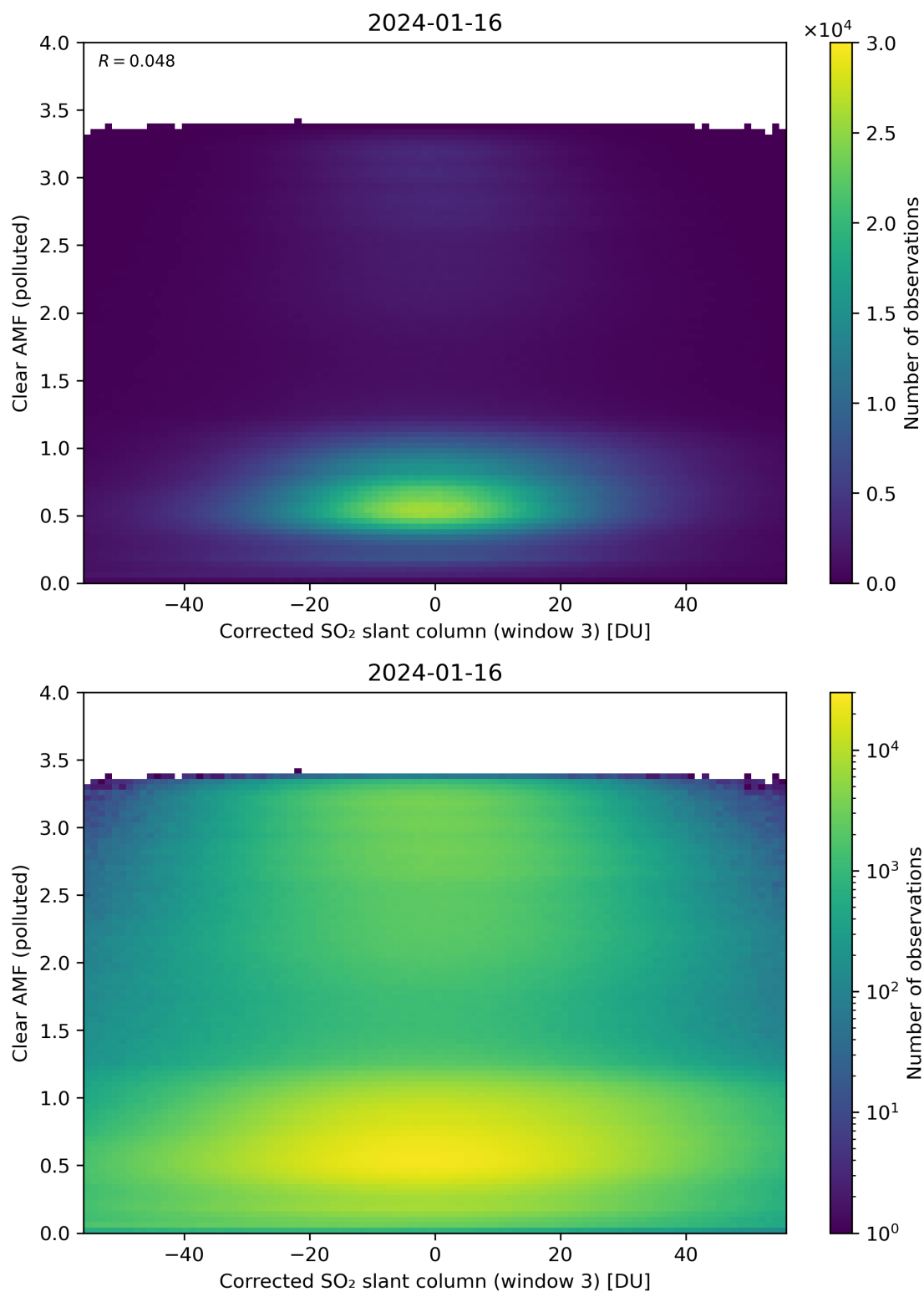
Figure 209: Scatter density plot of “Corrected SO 2 slant column (window 3)” against “Clear AMF (polluted)” for 2024-01-15 to 2024-01-17.
