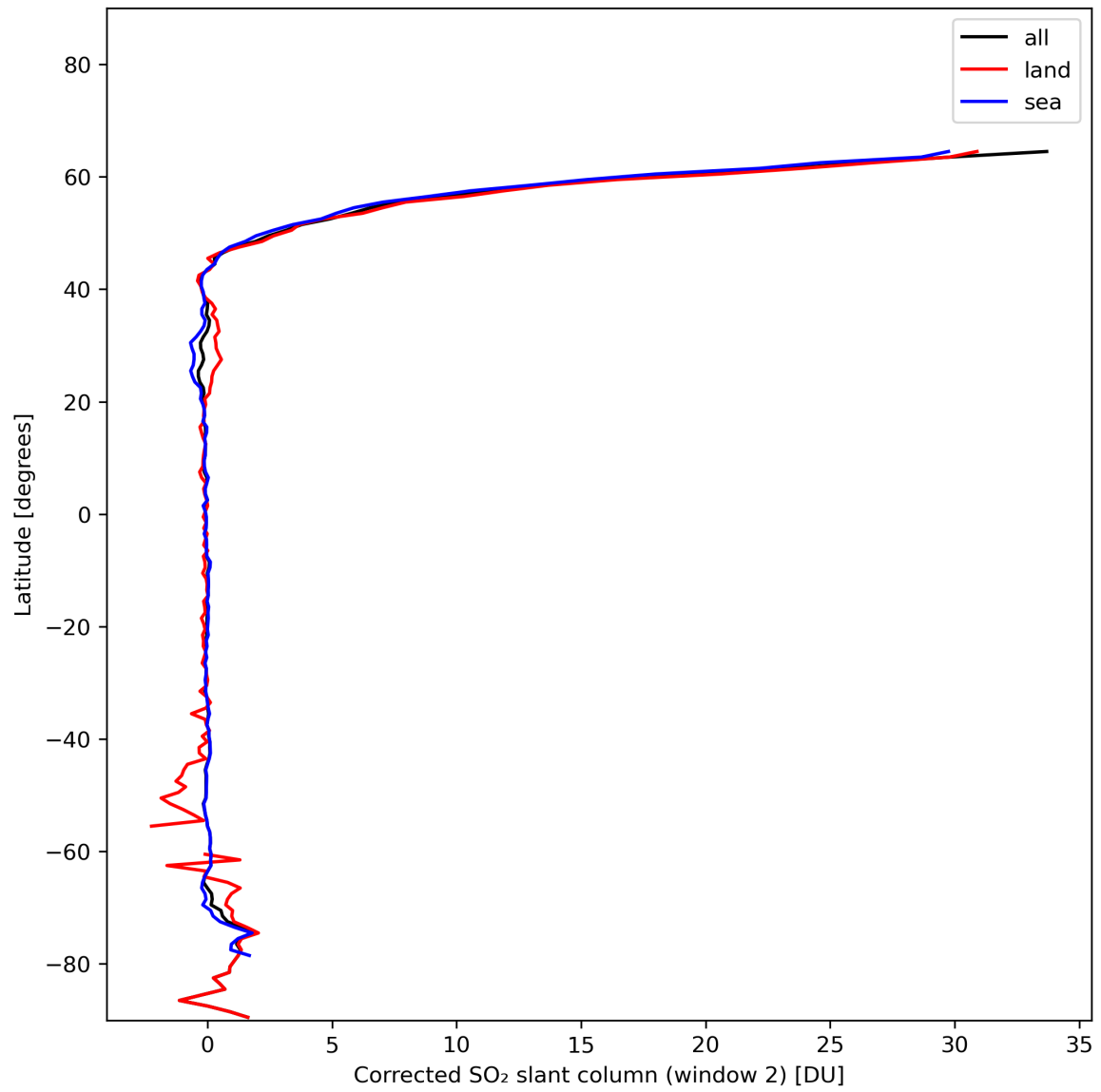
Figure 39: Zonal average of “Corrected SO 2 slant column (window 2)” for 2024-01-15 to 2024-01-17.
