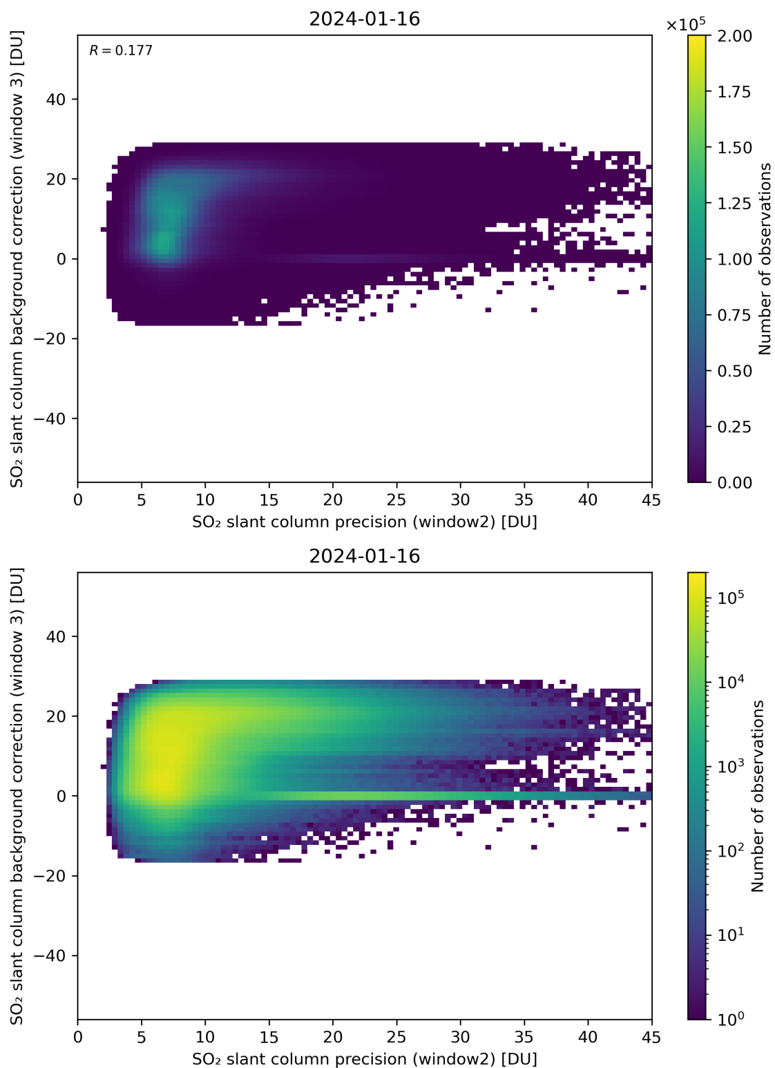
Figure 242: Scatter density plot of “SO 2 slant column precision (window2)” against “SO 2 slant column background correction (window 3)” for 2024-01-15 to 2024-01-17.
