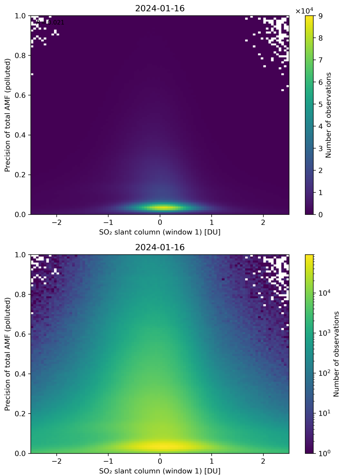
Figure 240: Scatter density plot of “SO 2 slant column (window 1)” against “Precision of total AMF (polluted)” for 2024-01-15 to 2024-01-17.
