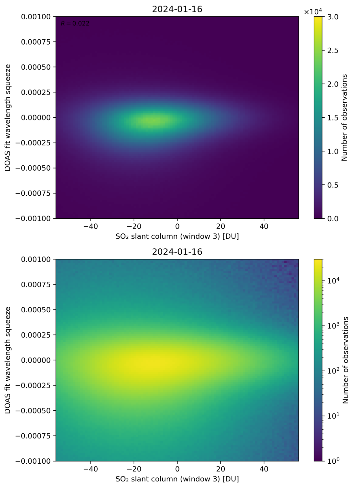
Figure 255: Scatter density plot of “SO 2 slant column (window 3)” against “DOAS fit wavelength squeeze” for 2024-01-15 to 2024-01-17.
