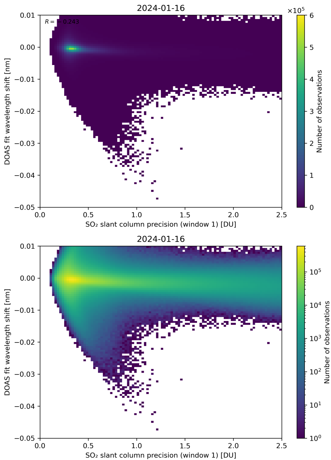
Figure 221: Scatter density plot of “SO 2 slant column precision (window 1)” against “DOAS fit wavelength shift” for 2024-01-15 to 2024-01-17.
