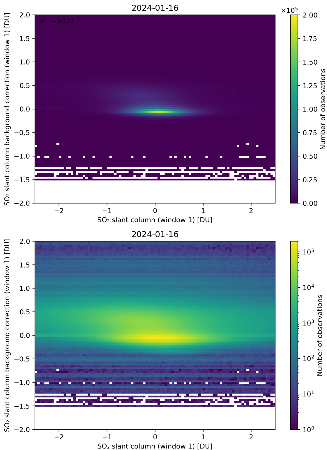
Figure 212: Scatter density plot of “SO 2 slant column (window 1)” against “SO 2 slant column background correction (window 1)” for 2024-01-15 to 2024-01-17.
