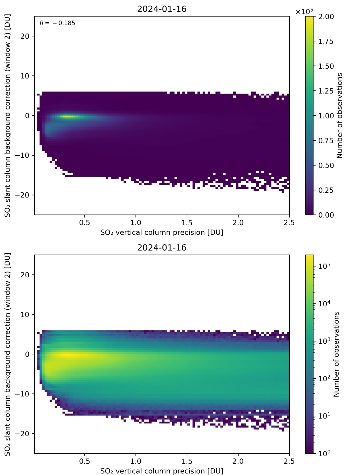
Figure 280: Scatter density plot of “SO 2 vertical column precision” against “SO 2 slant column background correction (window 2)” for 2024-01-15 to 2024-01-17.
