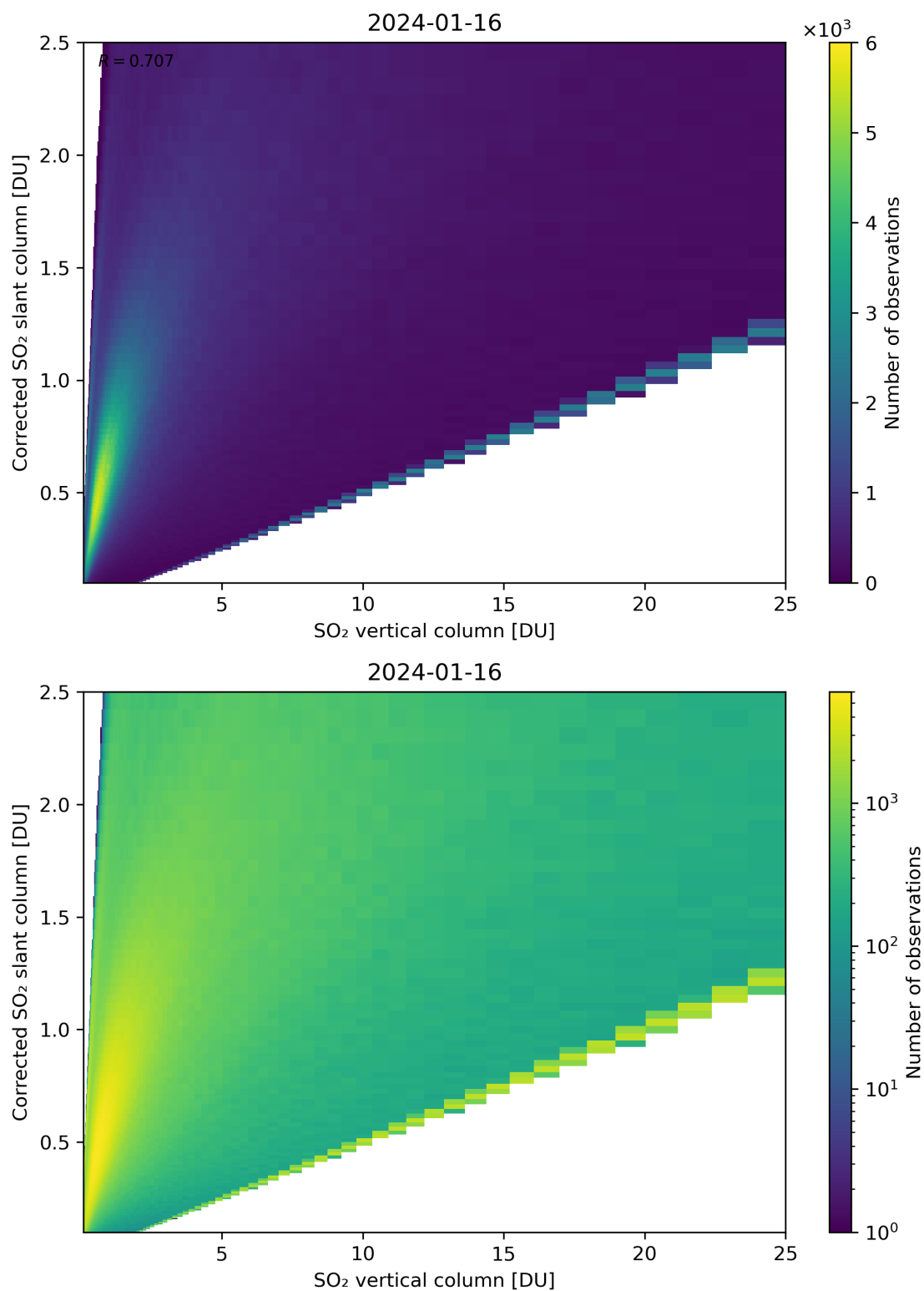
Figure 297: Scatter density plot of “SO 2 vertical column” against “Corrected SO 2 slant column” for 2024-01-15 to 2024-01-17.
