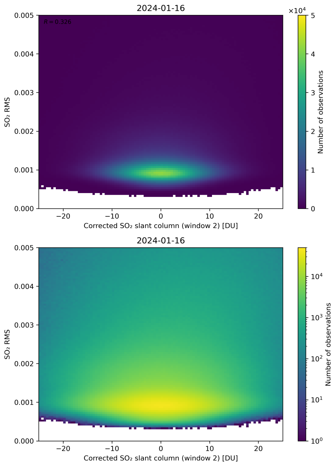
Figure 198: Scatter density plot of “Corrected SO 2 slant column (window 2)” against “SO 2 RMS” for 2024-01-15 to 2024-01-17.
