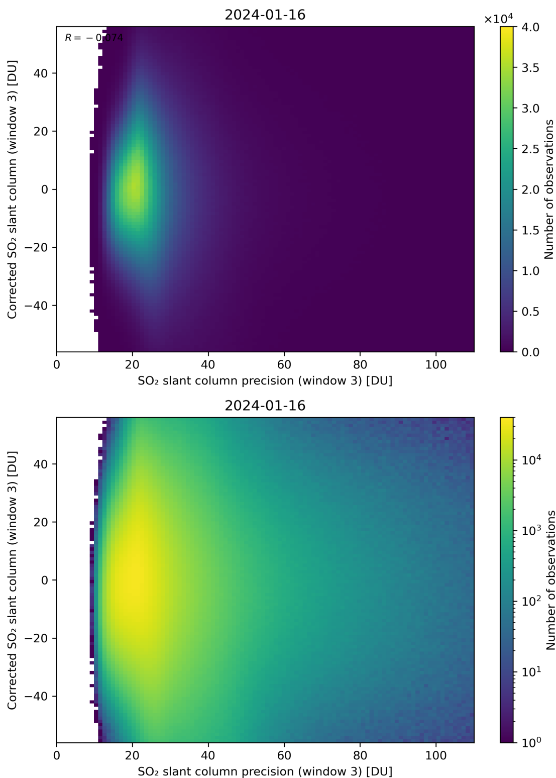
Figure 262: Scatter density plot of “SO 2 slant column precision (window 3)” against “Corrected SO 2 slant column (window 3)” for 2024-01-15 to 2024-01-17.
