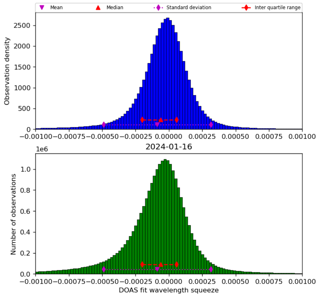
Figure 69: Histogram of “DOAS fit wavelength squeeze” for 2024-01-15 to 2024-01-17
