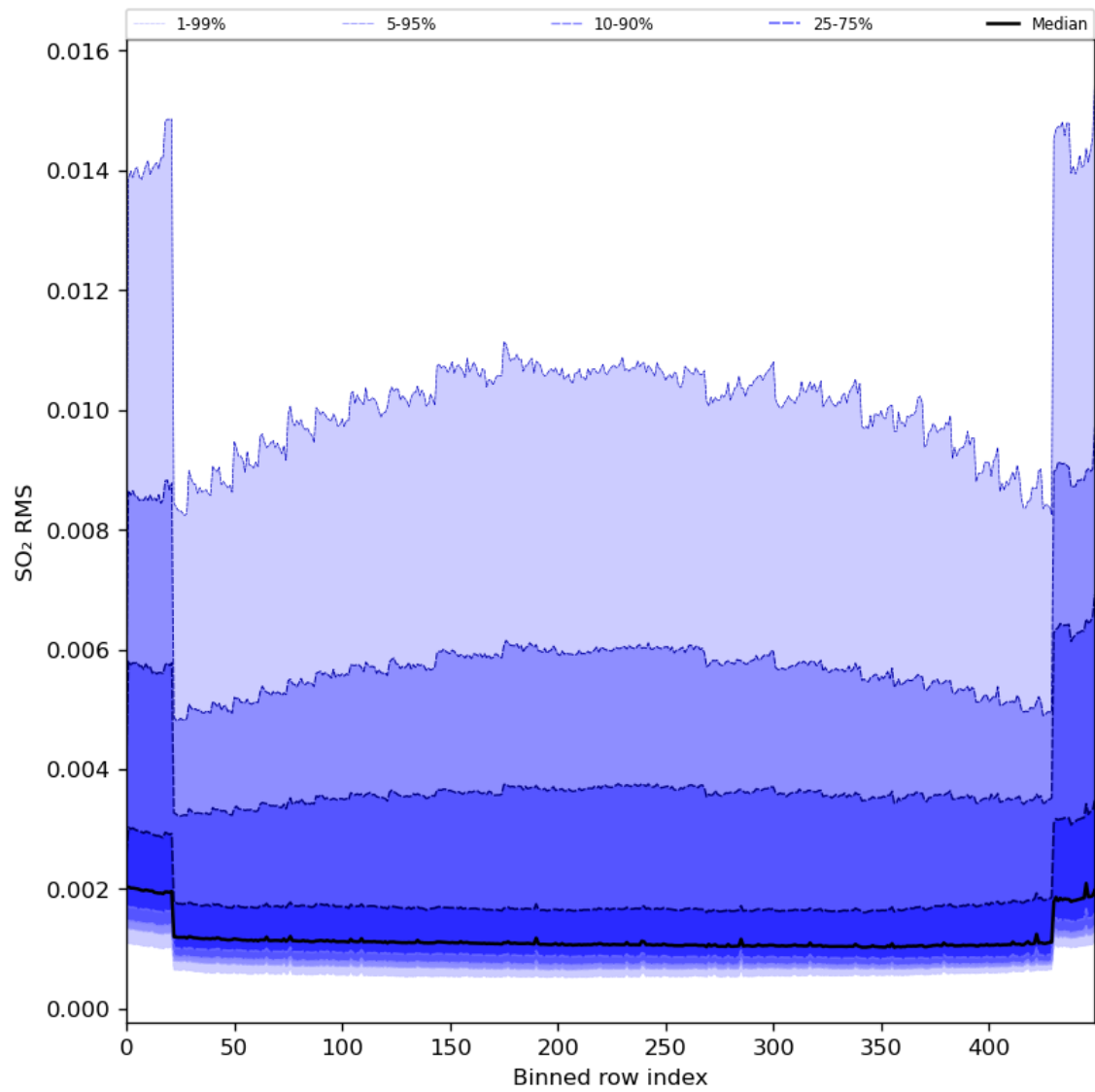
Figure 93: Along track statistics of “SO 2 RMS” for 2024-01-15 to 2024-01-17
