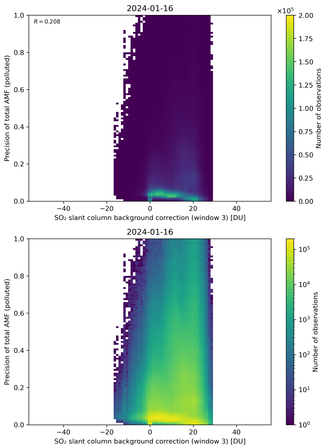
Figure 126: Scatter density plot of “SO 2 slant column background correction (window 3)” against “Precision of total AMF (polluted)” for 2024-01-15 to 2024-01-17.
