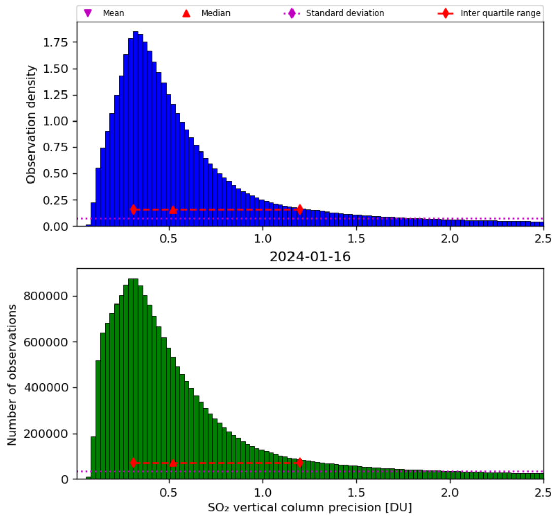
Figure 54: Histogram of “SO 2 vertical column precision” for 2024-01-15 to 2024-01-17
