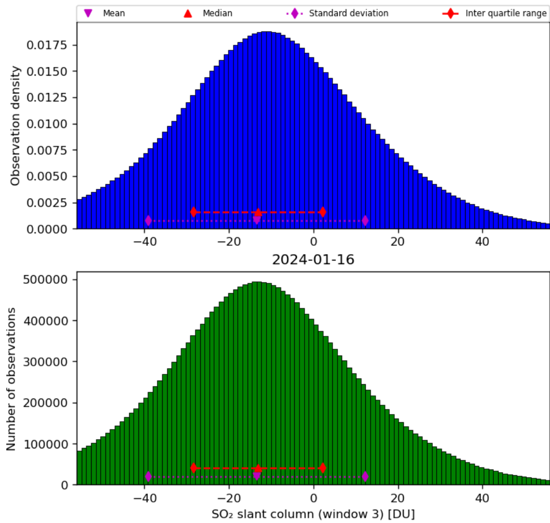
Figure 64: Histogram of “SO 2 slant column (window 3)” for 2024-01-15 to 2024-01-17
