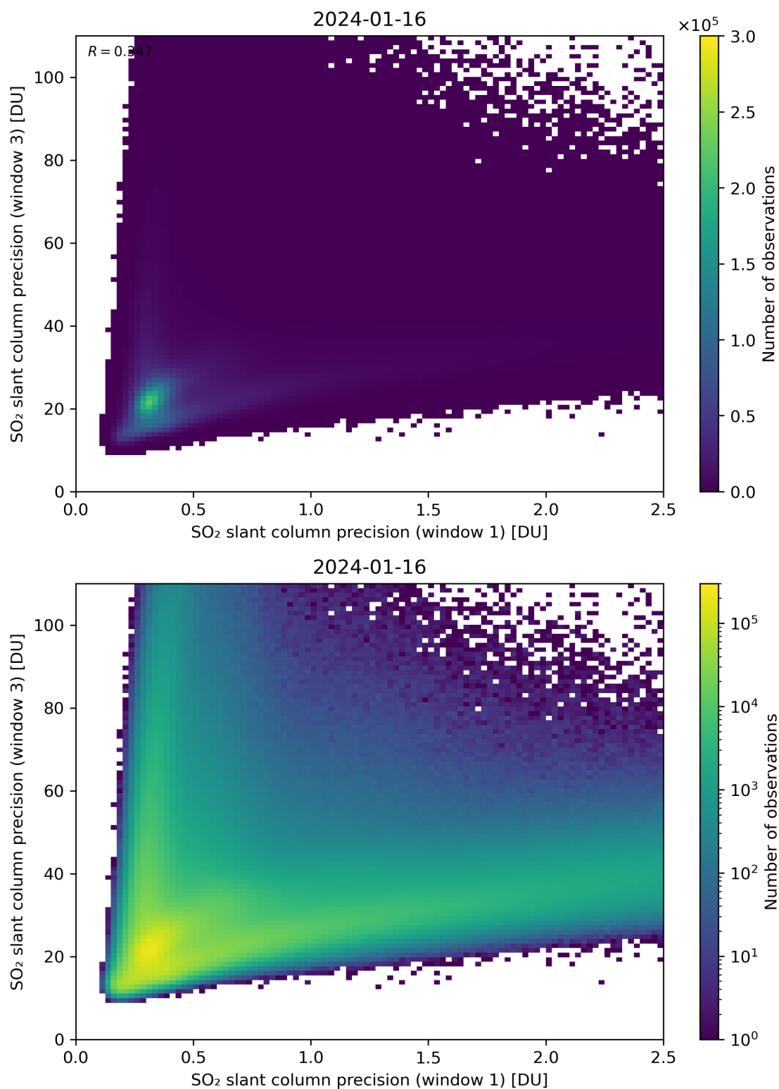
Figure 229: Scatter density plot of “SO 2 slant column precision (window 1)” against “SO 2 slant column precision (window 3)” for 2024-01-15 to 2024-01-17.
