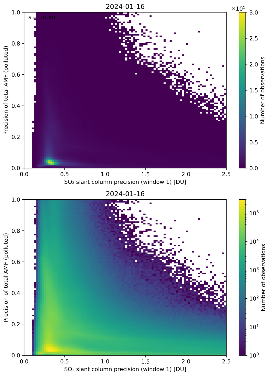
Figure 231: Scatter density plot of “SO 2 slant column precision (window 1)” against “Precision of total AMF (polluted)” for 2024-01-15 to 2024-01-17.
