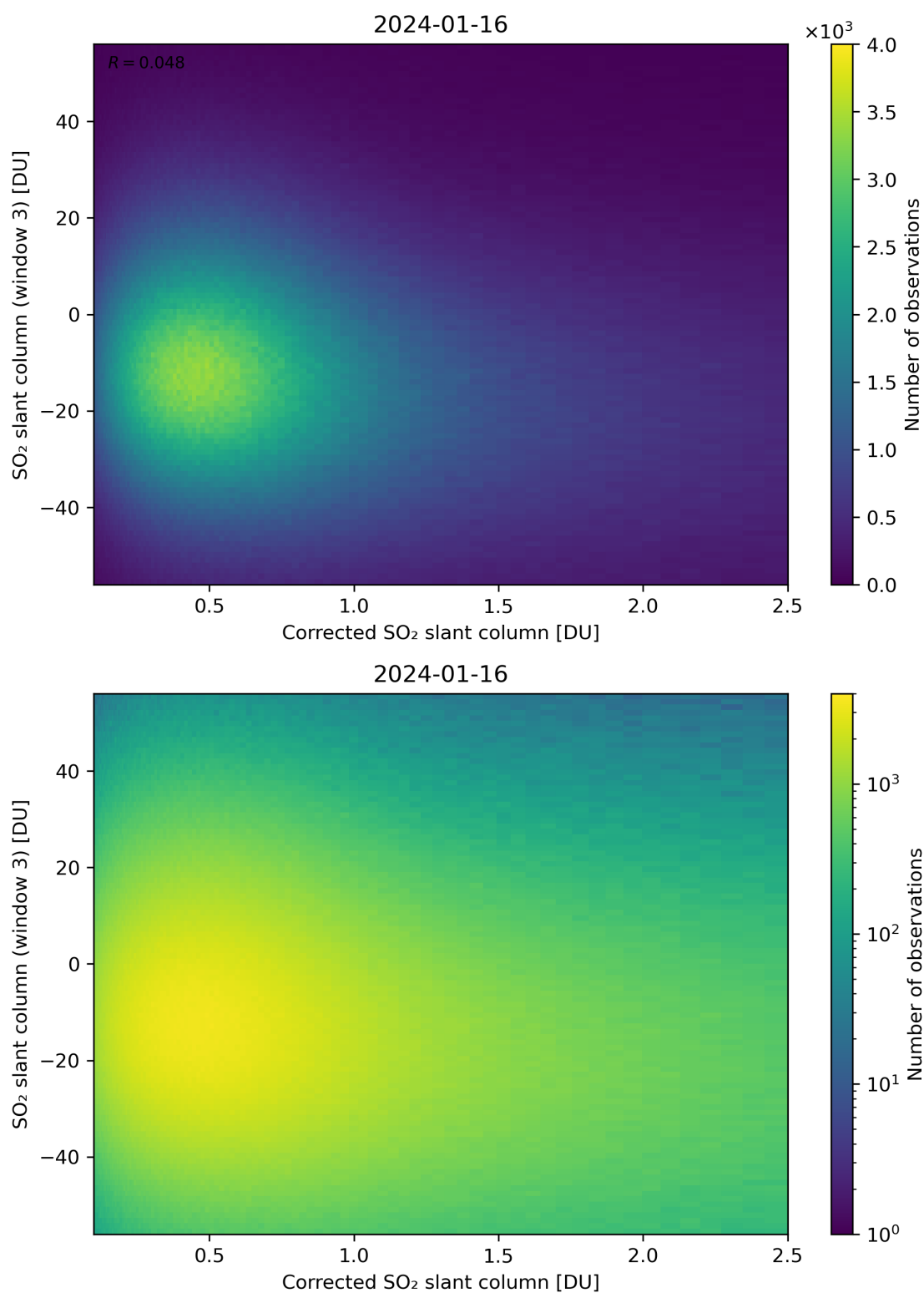
Figure 190: Scatter density plot of “Corrected SO 2 slant column” against “SO 2 slant column (window 3)” for 2024-01-15 to 2024-01-17.
