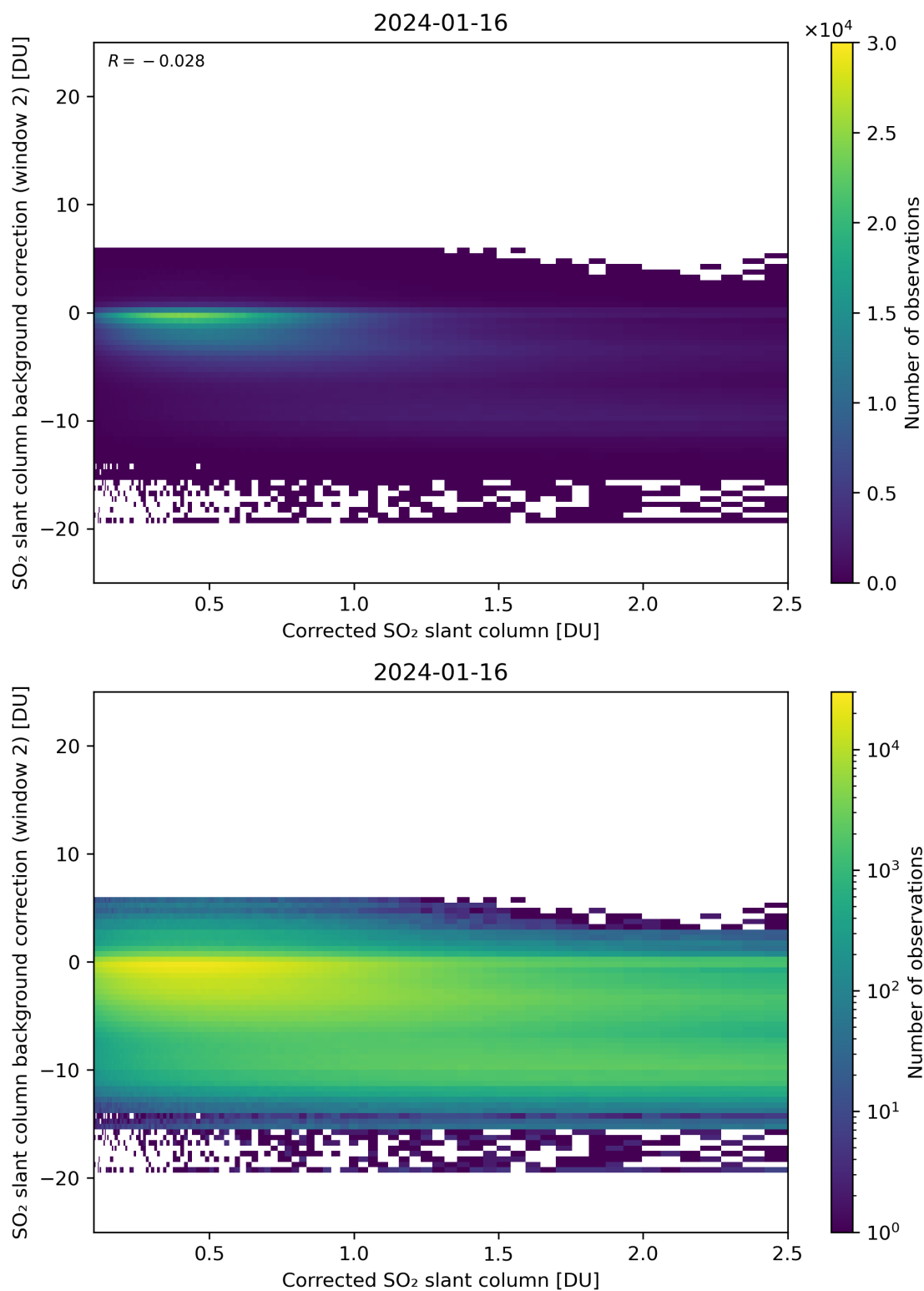
Figure 179: Scatter density plot of “Corrected SO 2 slant column” against “SO 2 slant column background correction (window 2)” for 2024-01-15 to 2024-01-17.
