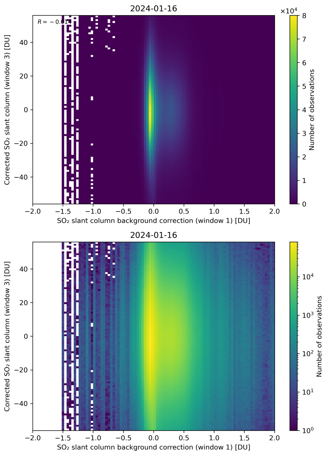
Figure 105: Scatter density plot of “SO 2 slant column background correction (window 1)” against “Corrected SO 2 slant column (window 3)” for 2024-01-15 to 2024-01-17.
