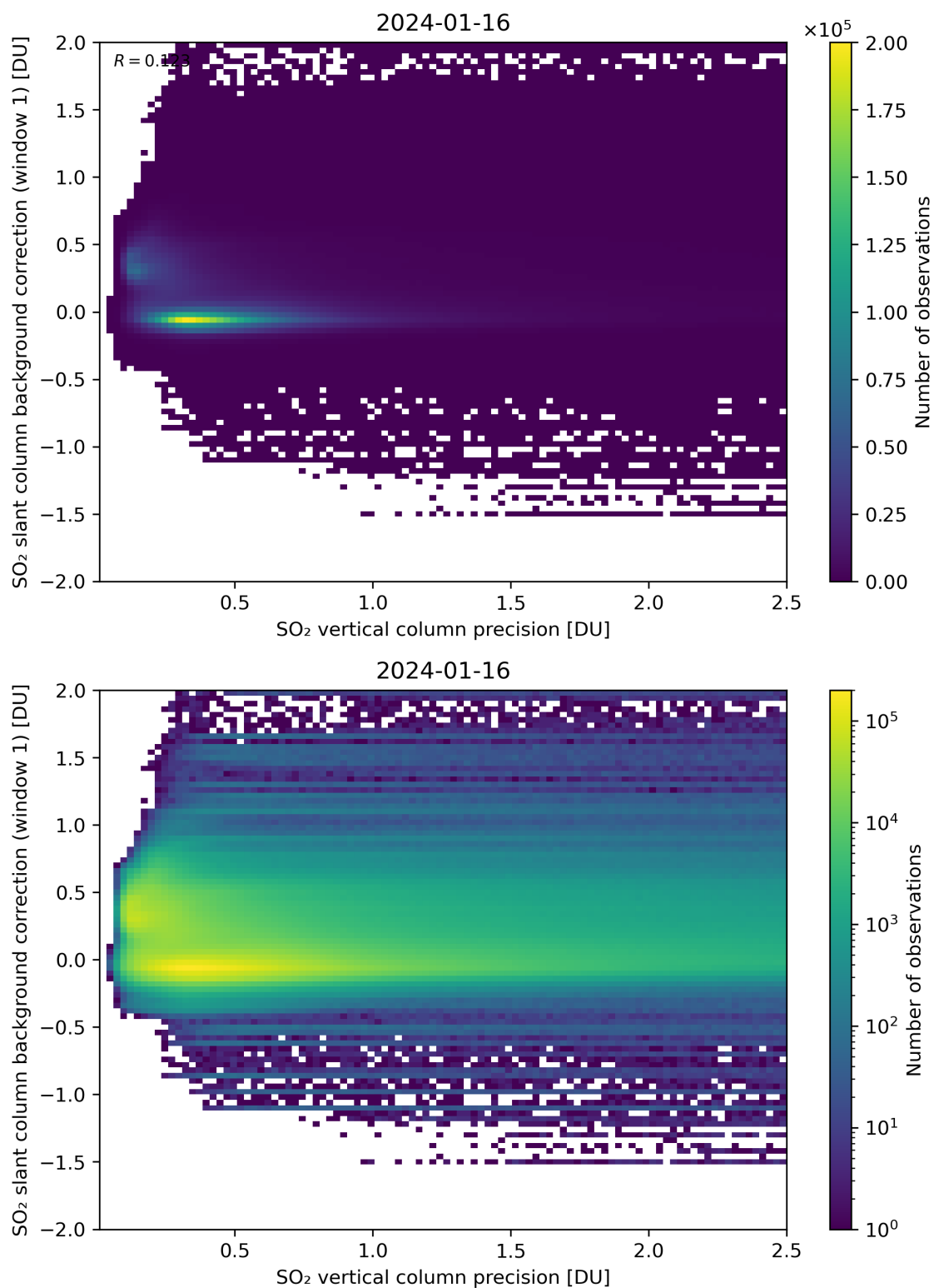
Figure 279: Scatter density plot of “SO 2 vertical column precision” against “SO 2 slant column background correction (window 1)” for 2024-01-15 to 2024-01-17.
