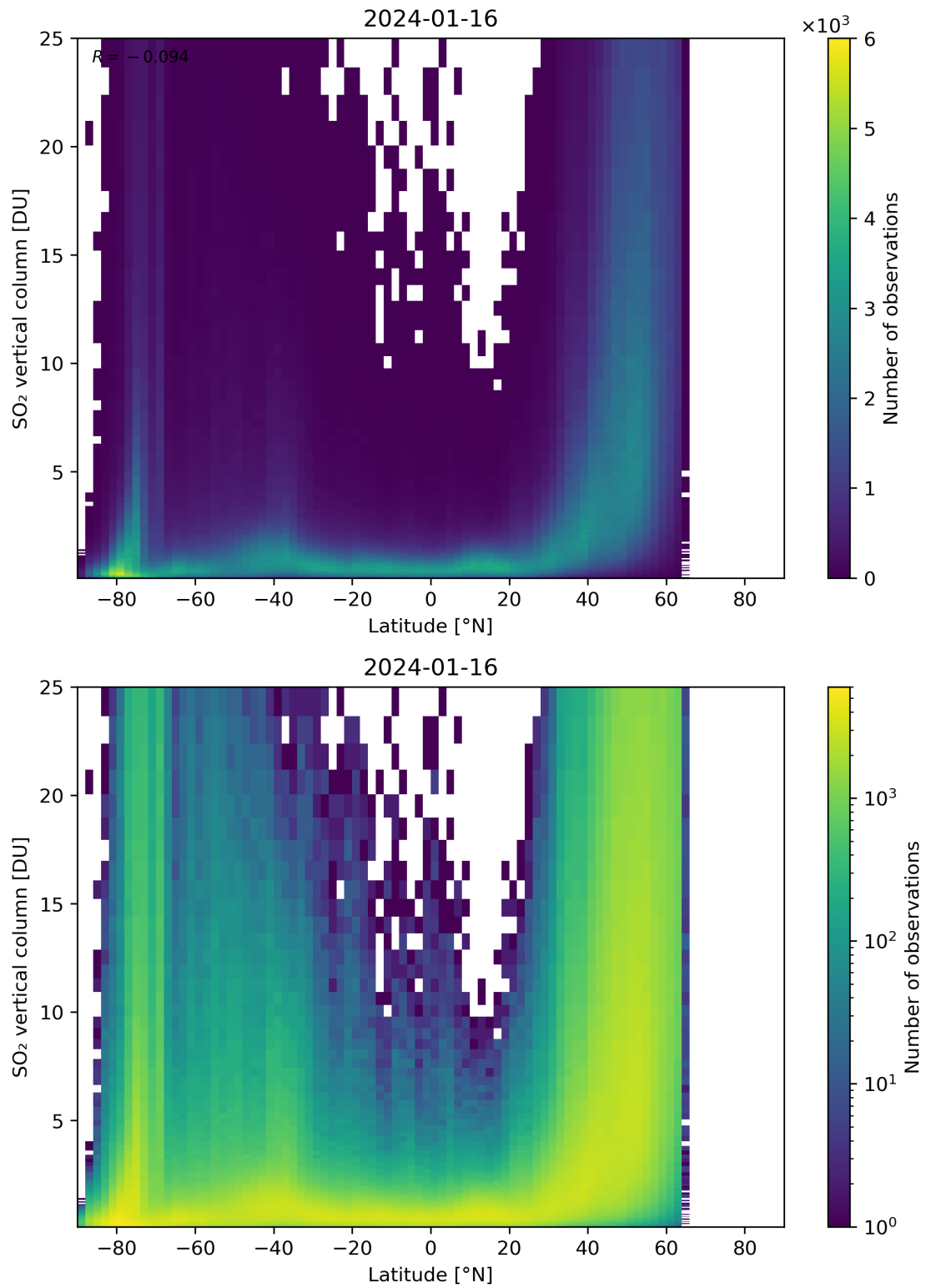
Figure 156: Scatter density plot of “Latitude” against “SO 2 vertical column” for 2024-01-15 to 2024-01-17.
