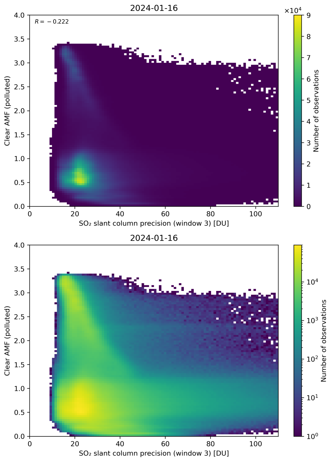
Figure 261: Scatter density plot of “SO 2 slant column precision (window 3)” against “Clear AMF (polluted)” for 2024-01-15 to 2024-01-17.
