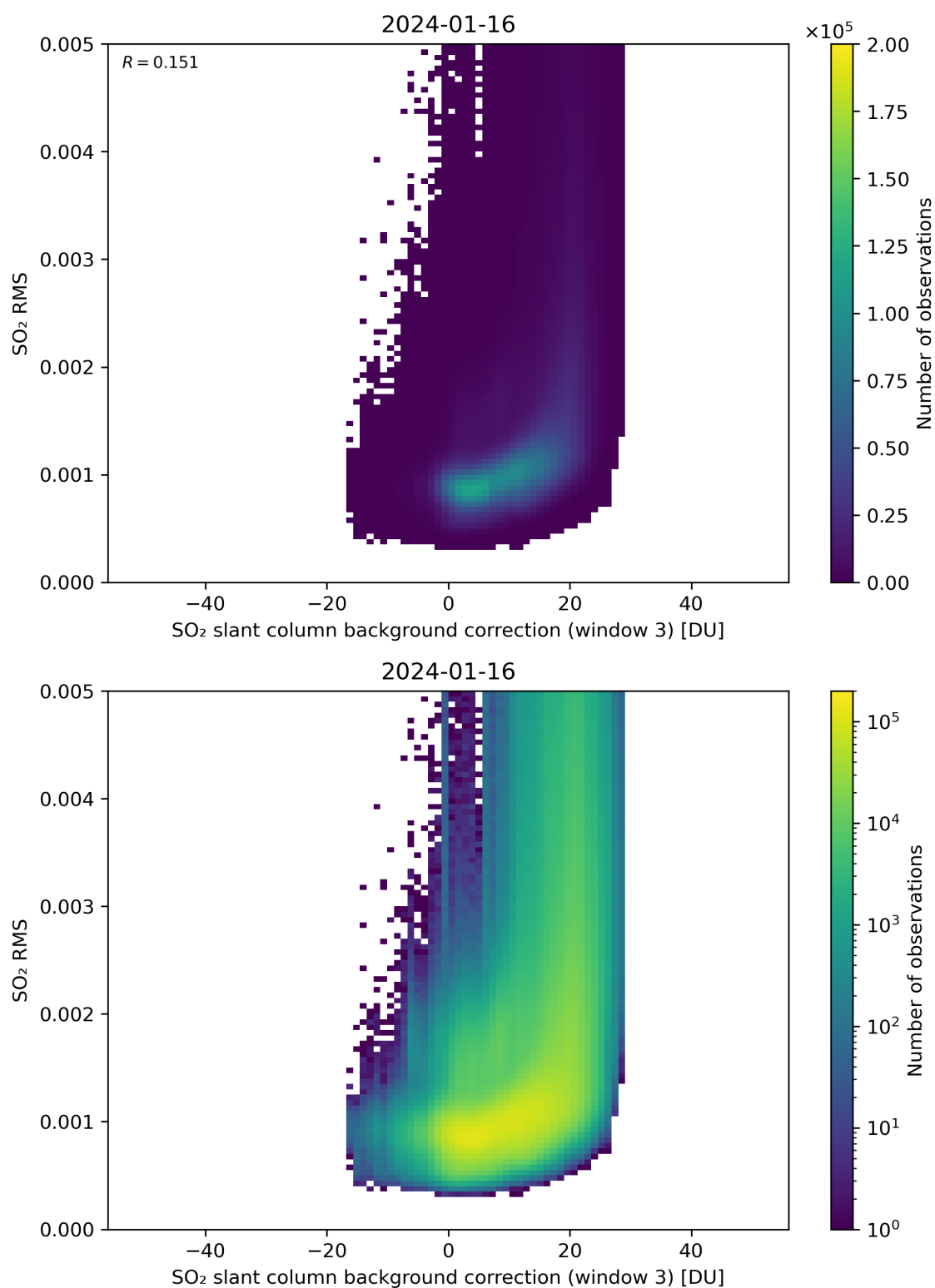
Figure 123: Scatter density plot of “SO 2 slant column background correction (window 3)” against “SO 2 RMS” for 2024-01-15 to 2024-01-17.
