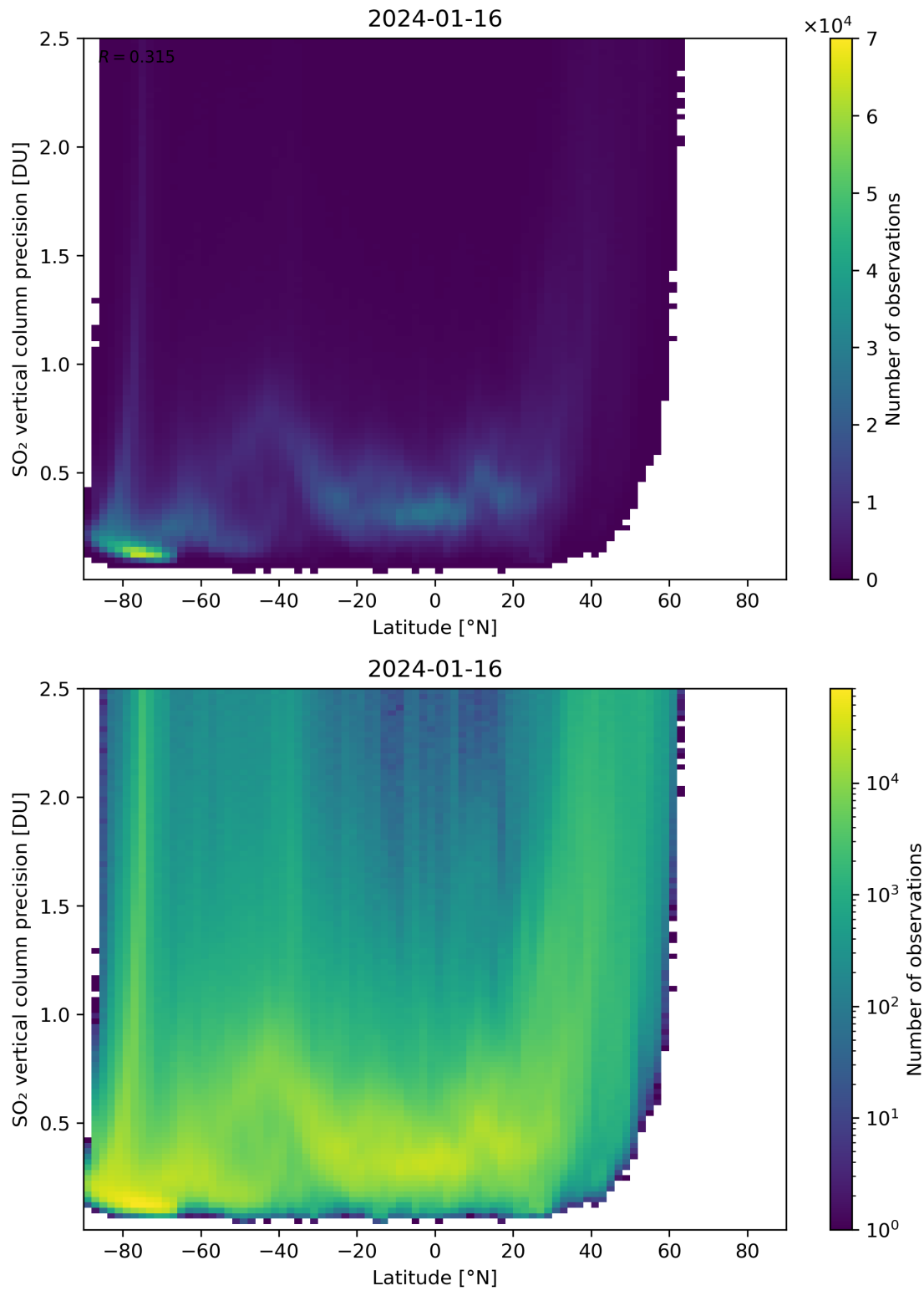
Figure 157: Scatter density plot of “Latitude” against “SO 2 vertical column precision” for 2024-01-15 to 2024-01-17.
