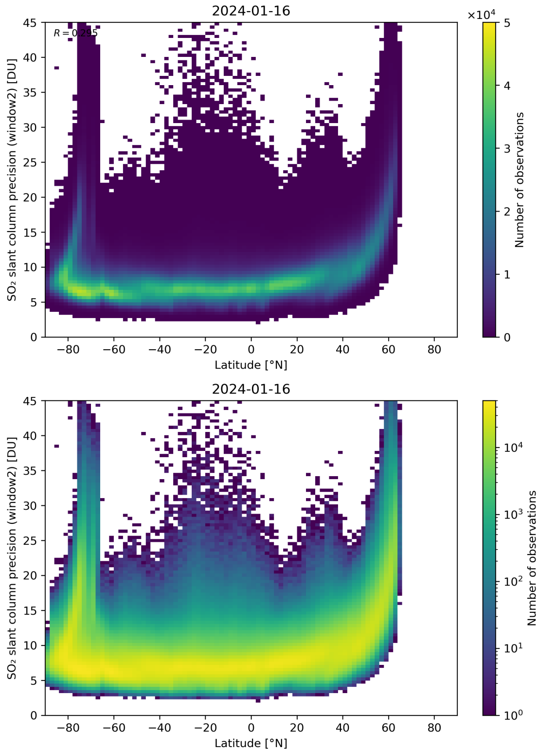
Figure 151: Scatter density plot of “Latitude” against “SO 2 slant column precision (window2)” for 2024-01-15 to 2024-01-17.
