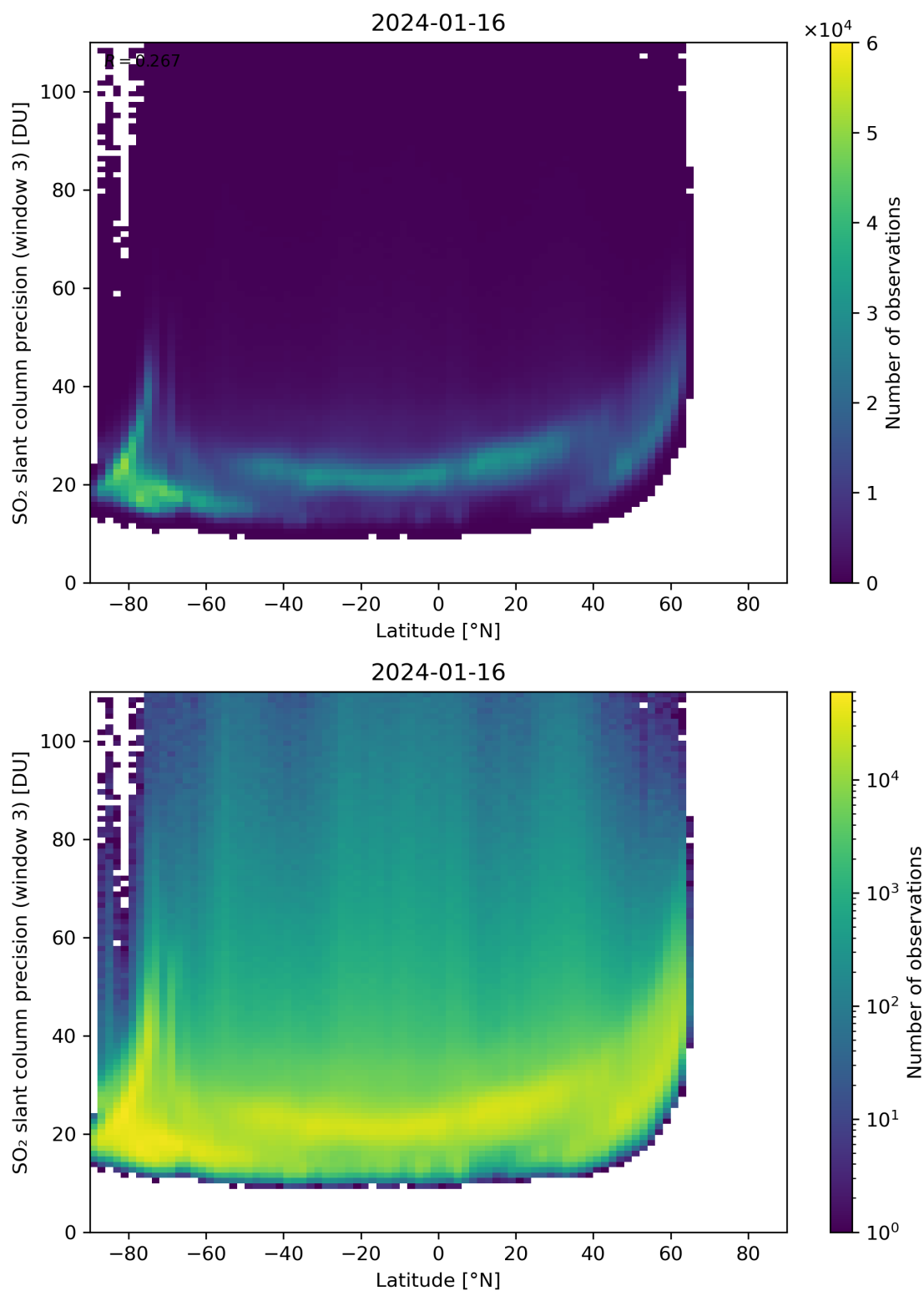
Figure 153: Scatter density plot of “Latitude” against “SO 2 slant column precision (window 3)” for 2024-01-15 to 2024-01-17.
