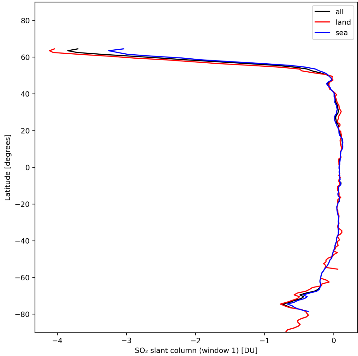
Figure 33: Zonal average of “SO 2 slant column (window 1)” for 2024-01-16 to 2024-01-18.
