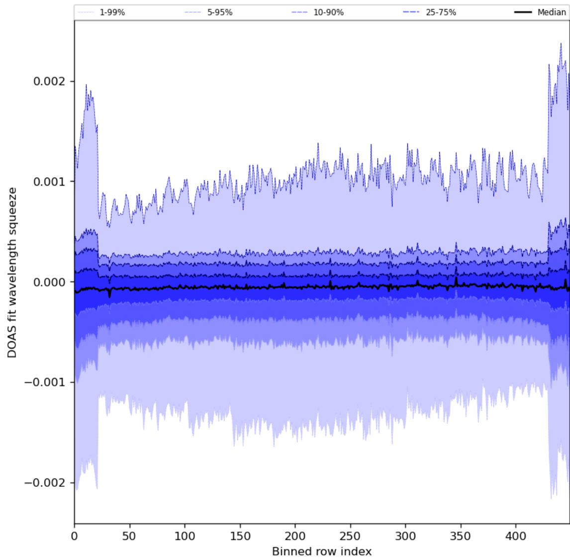
Figure 92: Along track statistics of “DOAS fit wavelength squeeze” for 2024-01-16 to 2024-01-18
