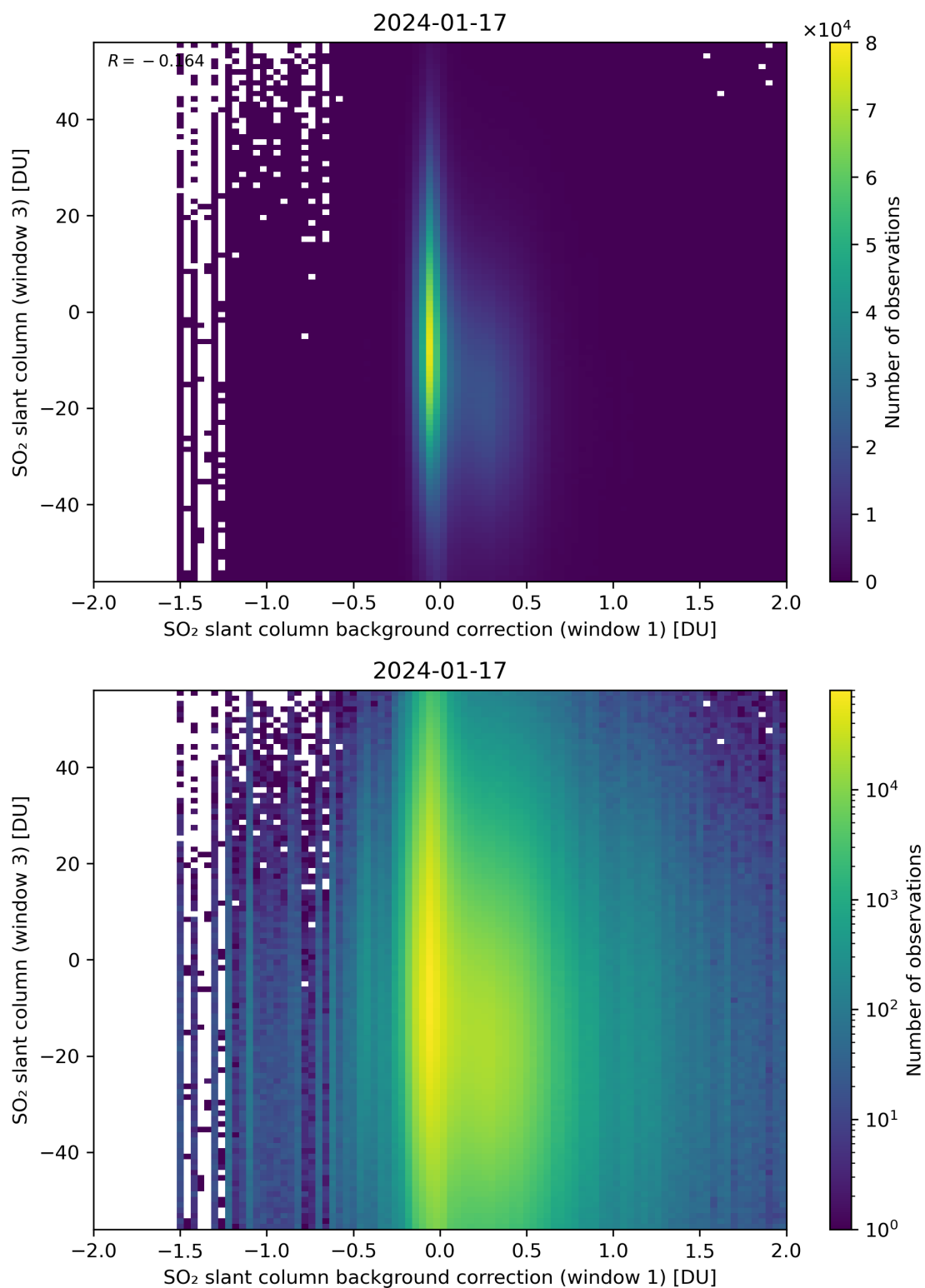
Figure 107: Scatter density plot of “SO 2 slant column background correction (window 1)” against “SO 2 slant column (window 3)” for 2024-01-16 to 2024-01-18.
