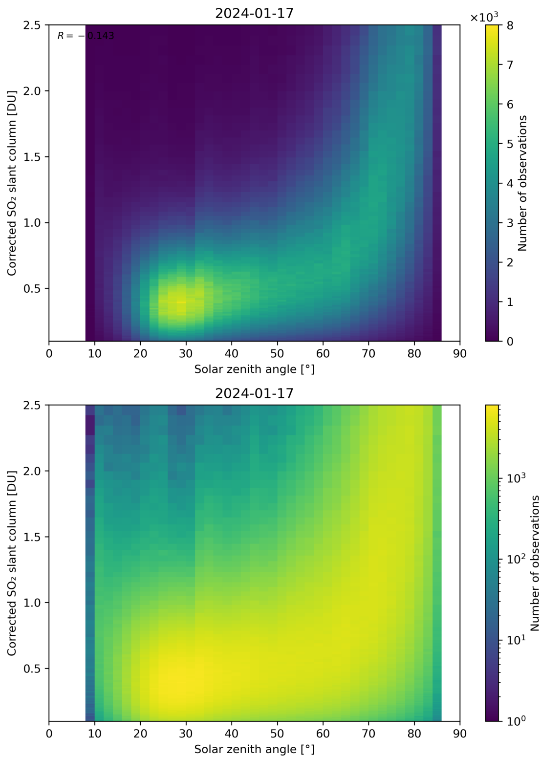
Figure 166: Scatter density plot of “Solar zenith angle” against “Corrected SO 2 slant column” for 2024-01-16 to 2024-01-18.
