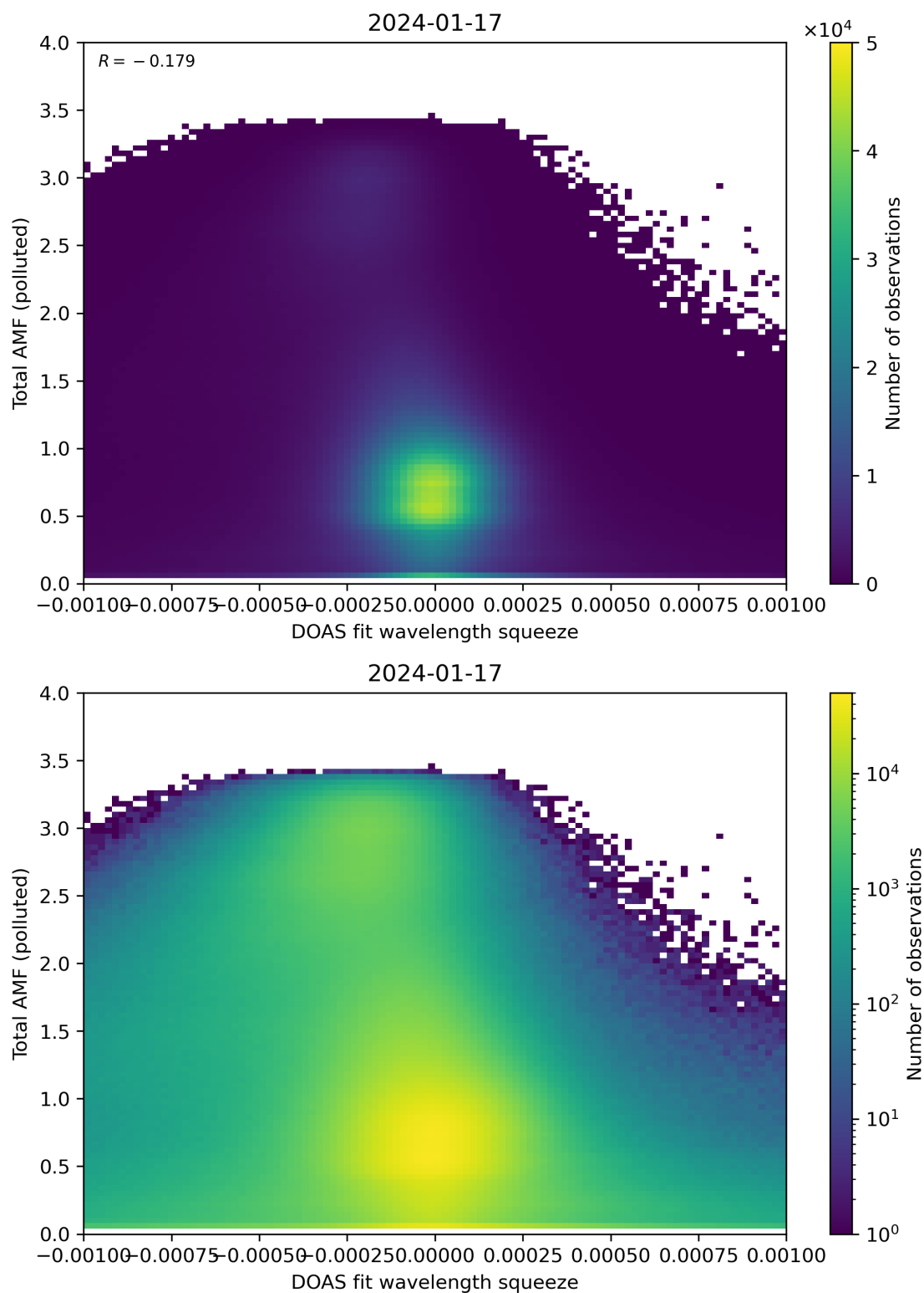
Figure 134: Scatter density plot of “DOAS fit wavelength squeeze” against “Total AMF (polluted)” for 2024-01-16 to 2024-01-18.
