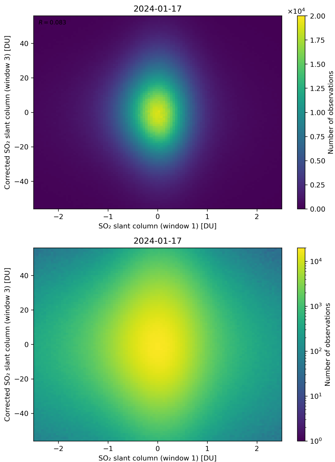
Figure 234: Scatter density plot of “SO 2 slant column (window 1)” against “Corrected SO 2 slant column (window 3)” for 2024-01-16 to 2024-01-18.
