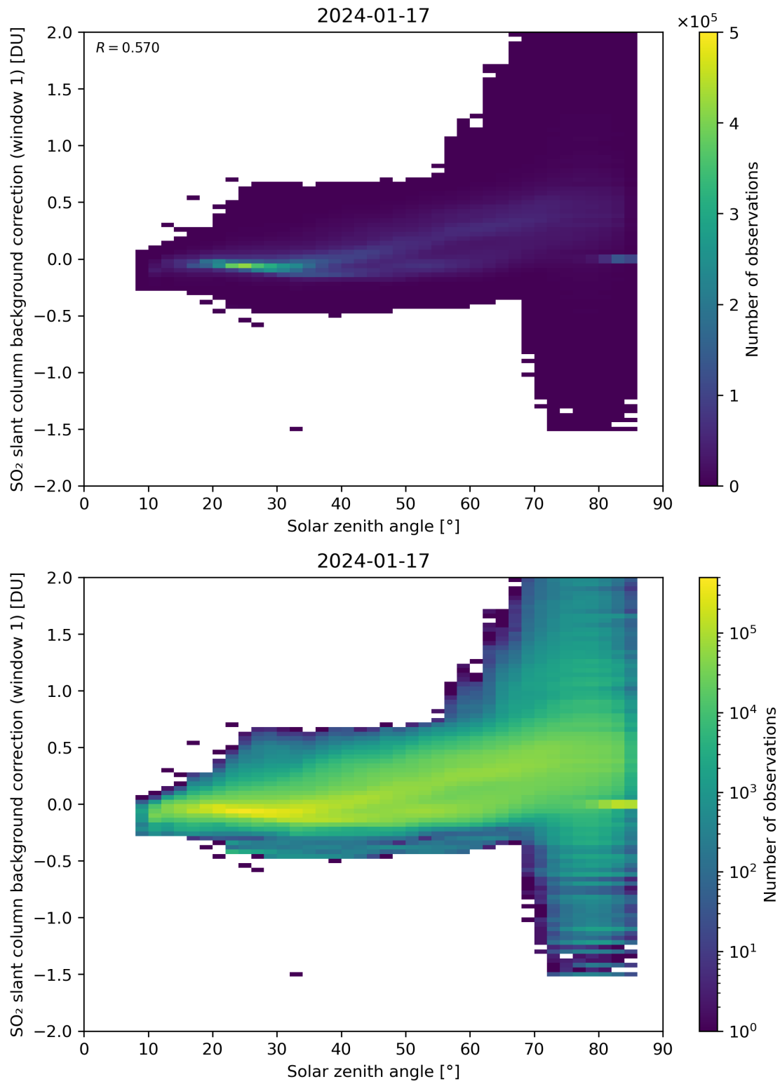
Figure 158: Scatter density plot of “Solar zenith angle” against “SO 2 slant column background correction (window 1)” for 2024-01-16 to 2024-01-18.
