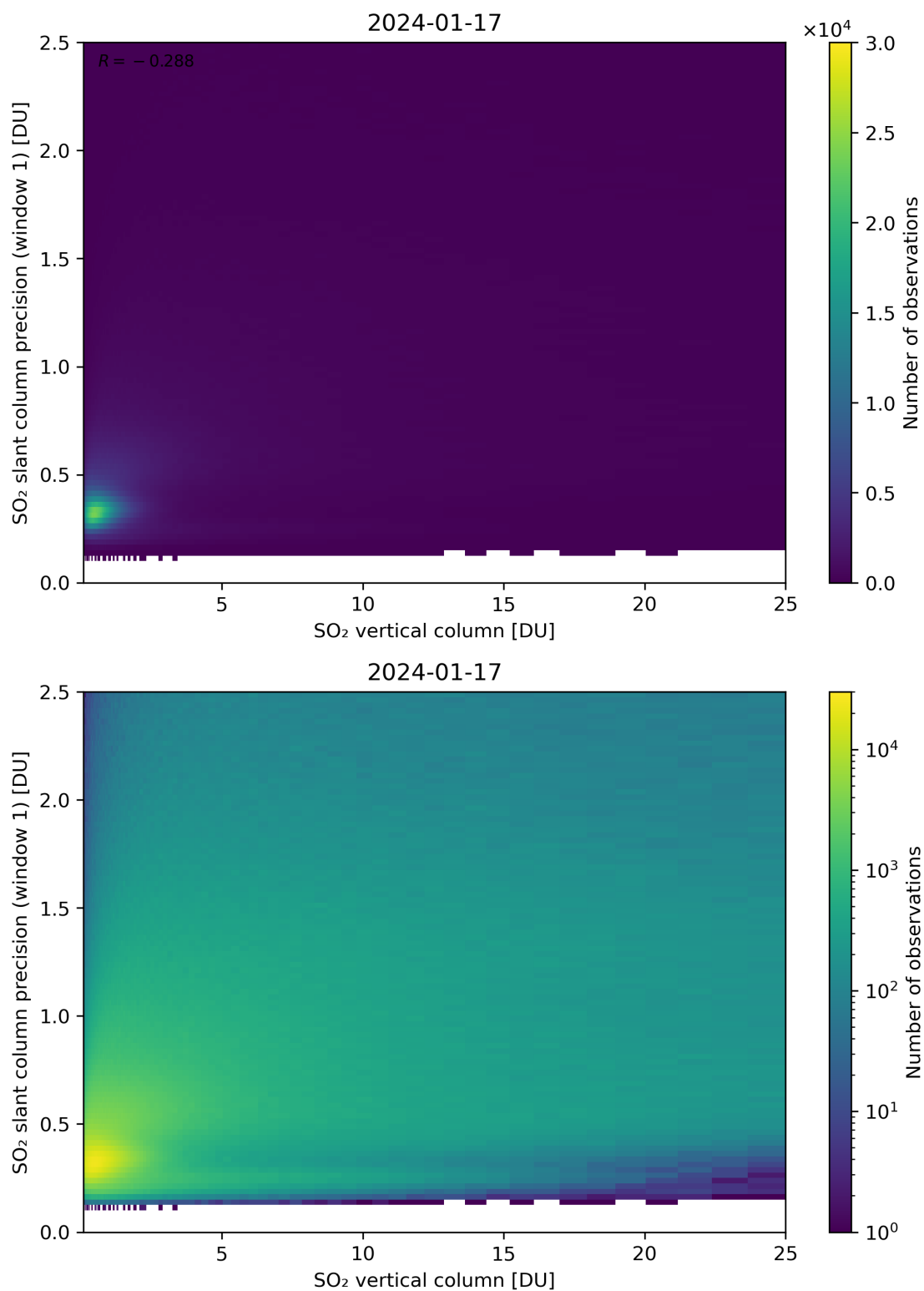
Figure 301: Scatter density plot of “SO 2 vertical column” against “SO 2 slant column precision (window 1)” for 2024-01-16 to 2024-01-18.
