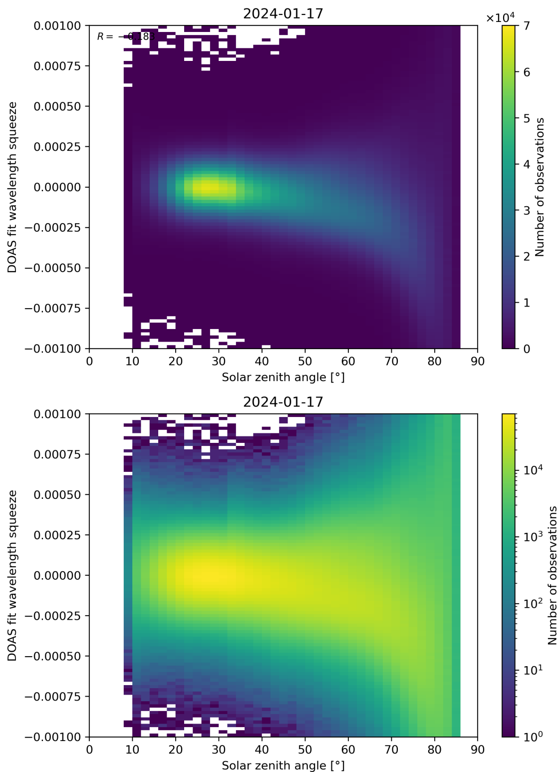
Figure 162: Scatter density plot of “Solar zenith angle” against “DOAS fit wavelength squeeze” for 2024-01-16 to 2024-01-18.
