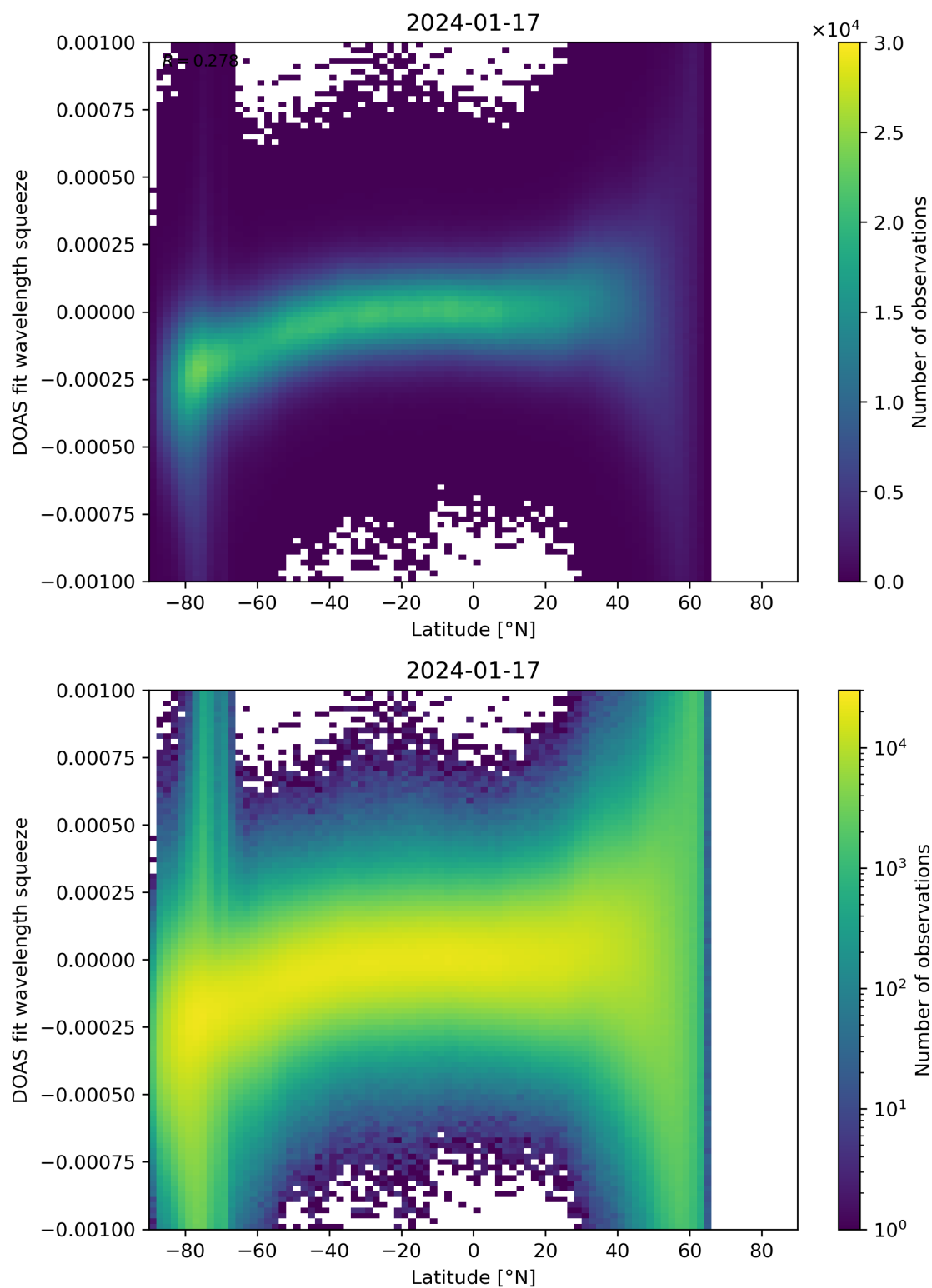
Figure 143: Scatter density plot of “Latitude” against “DOAS fit wavelength squeeze” for 2024-01-16 to 2024-01-18.
