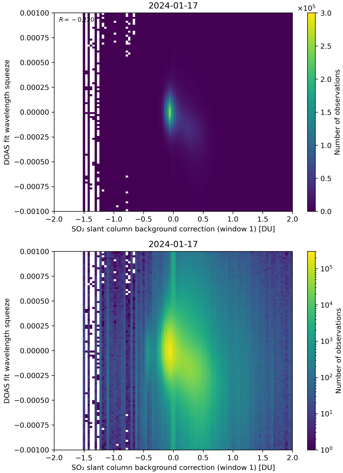
Figure 101: Scatter density plot of “SO 2 slant column background correction (window 1)” against “DOAS fit wavelength squeeze” for 2024-01-16 to 2024-01-18.
