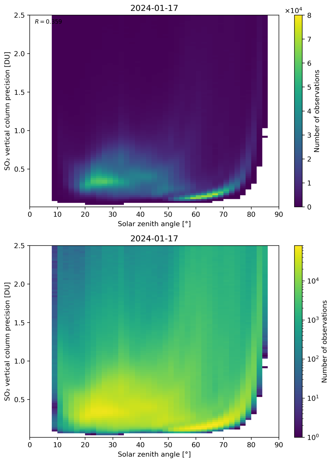
Figure 177: Scatter density plot of “Solar zenith angle” against “SO 2 vertical column precision” for 2024-01-16 to 2024-01-18.
