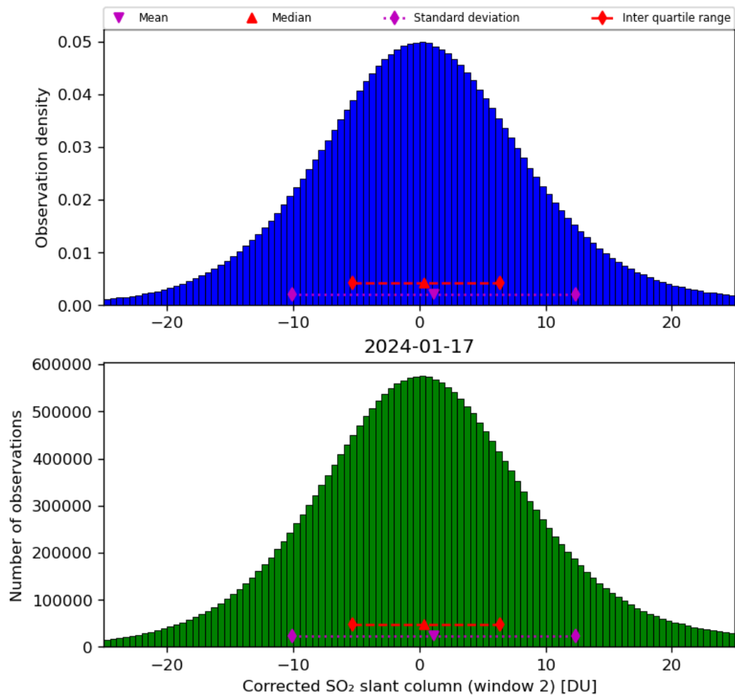
Figure 62: Histogram of “Corrected SO 2 slant column (window 2)” for 2024-01-16 to 2024-01-18
