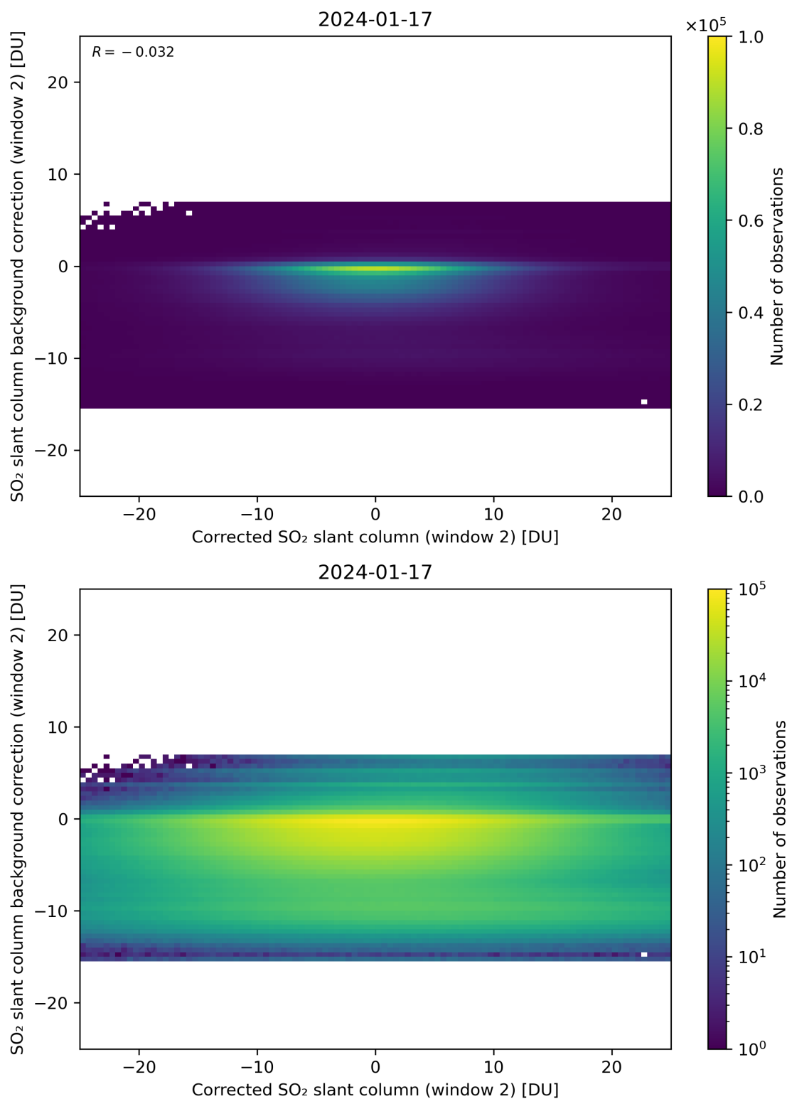
Figure 194: Scatter density plot of “Corrected SO 2 slant column (window 2)” against “SO 2 slant column background correction (window 2)” for 2024-01-16 to 2024-01-18.
