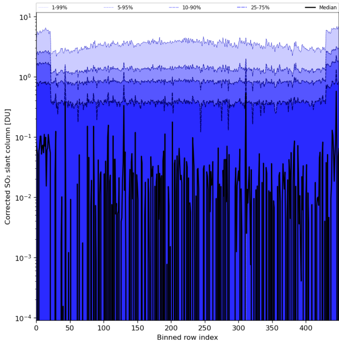
Figure 78: Along track statistics of “Corrected SO 2 slant column” for 2024-01-16 to 2024-01-18
