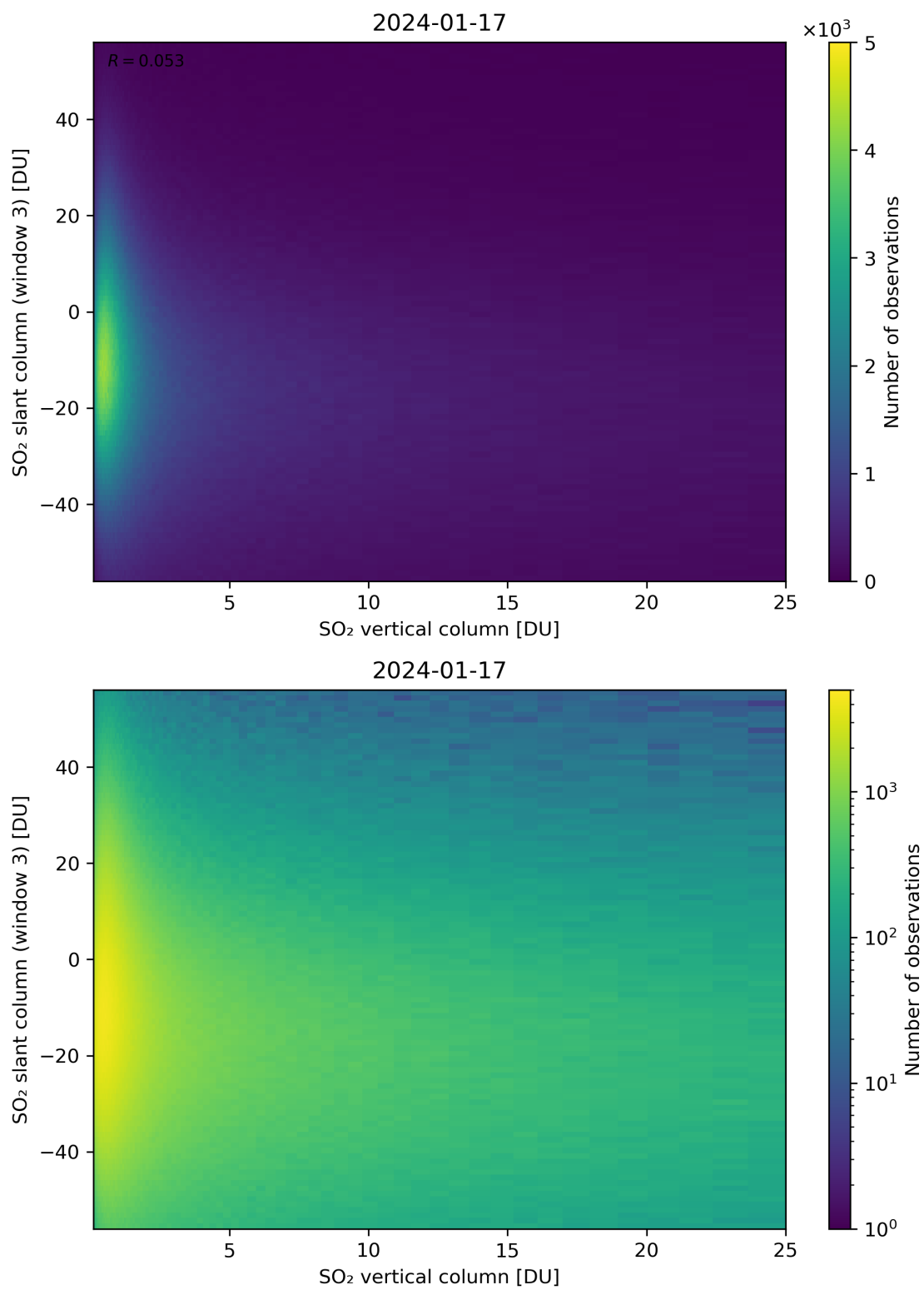
Figure 303: Scatter density plot of “SO 2 vertical column” against “SO 2 slant column (window 3)” for 2024-01-16 to 2024-01-18.
