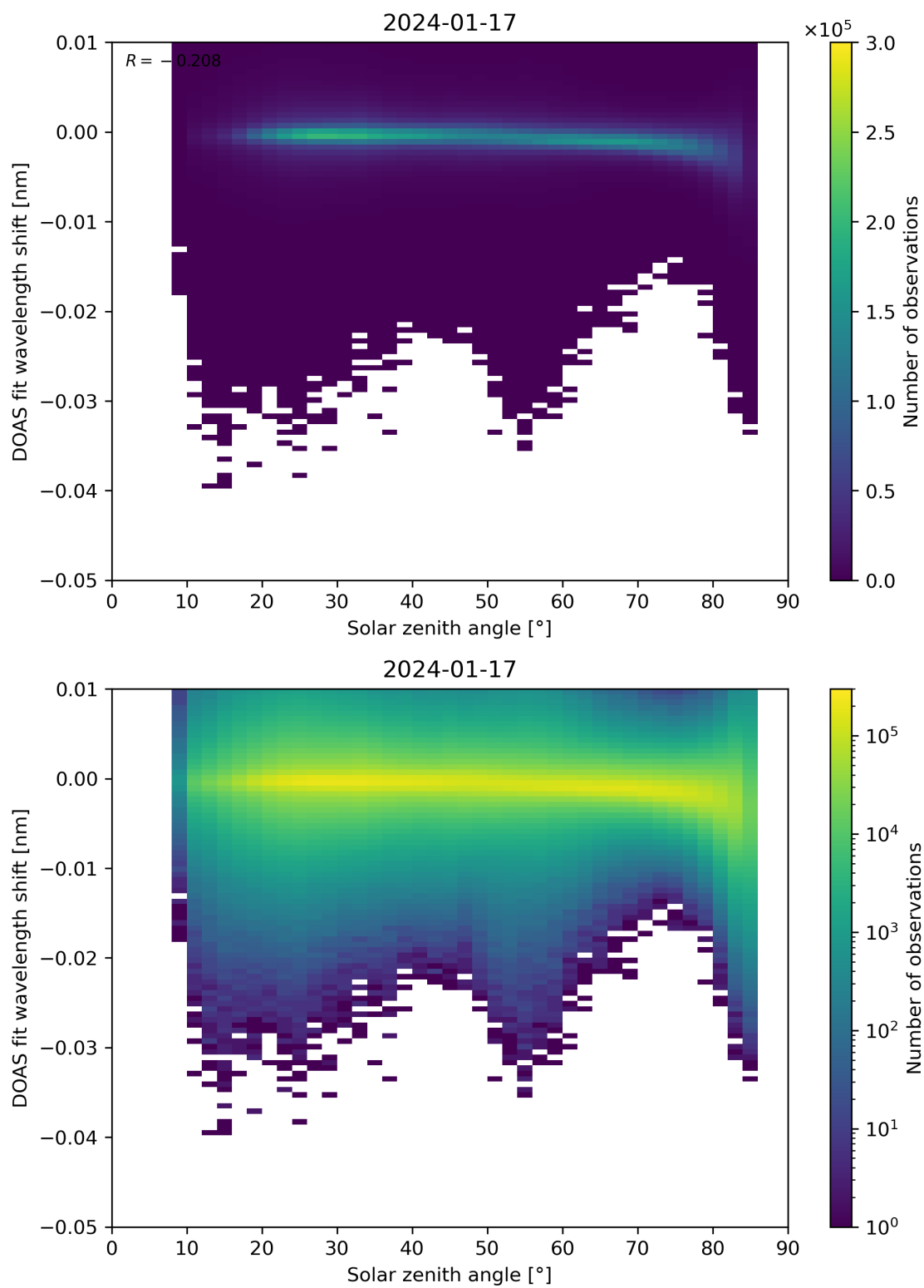
Figure 161: Scatter density plot of “Solar zenith angle” against “DOAS fit wavelength shift” for 2024-01-16 to 2024-01-18.
