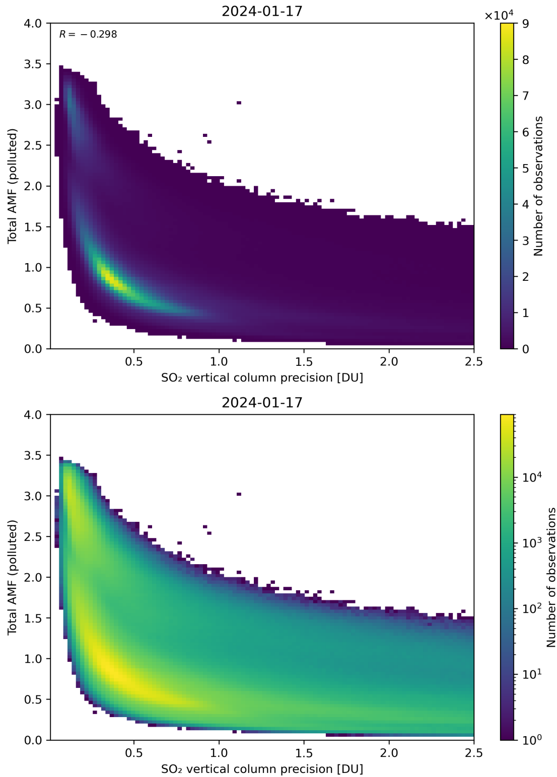
Figure 294: Scatter density plot of “SO 2 vertical column precision” against “Total AMF (polluted)” for 2024-01-16 to 2024-01-18.
