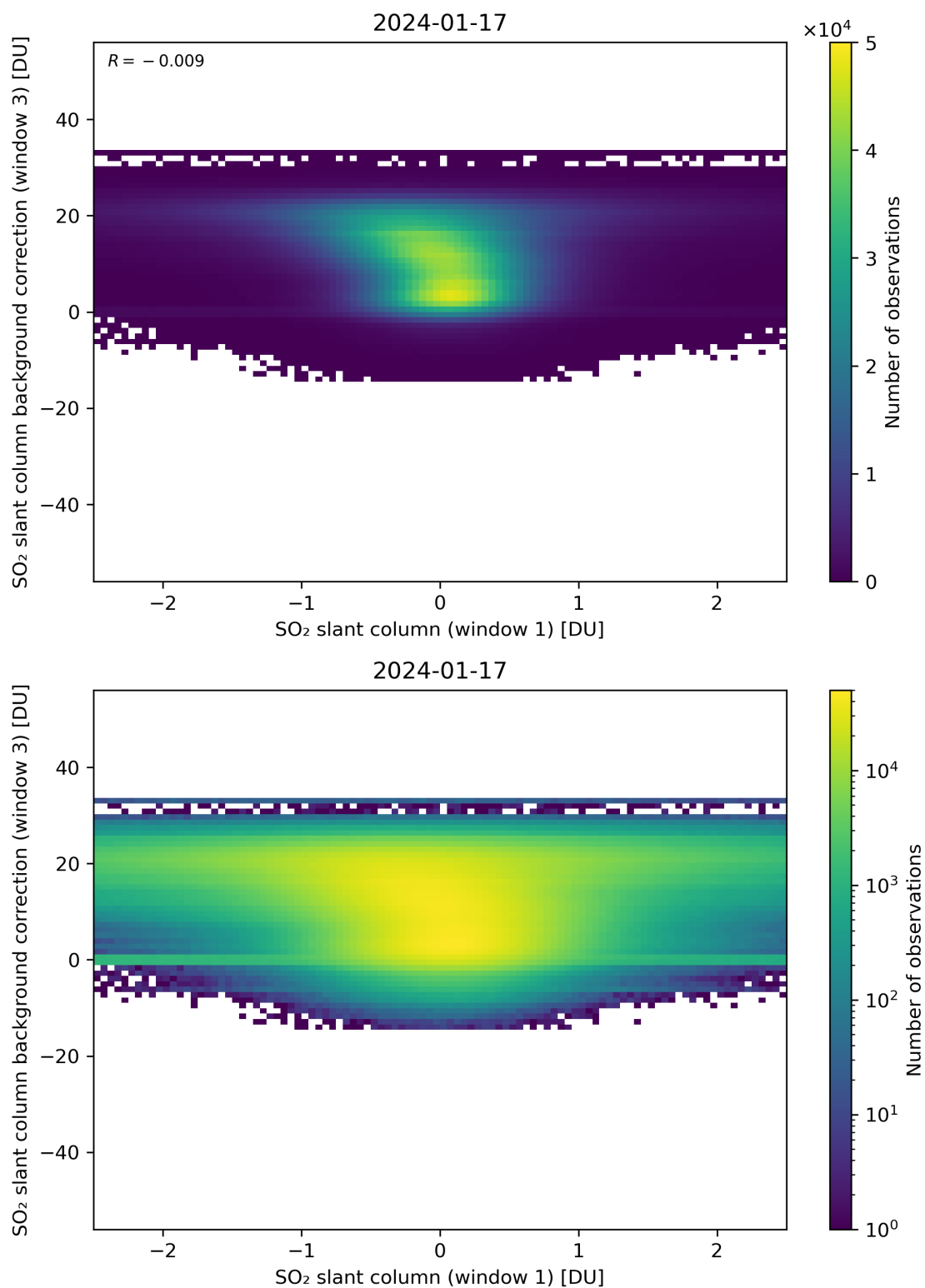
Figure 214: Scatter density plot of “SO 2 slant column (window 1)” against “SO 2 slant column background correction (window 3)” for 2024-01-16 to 2024-01-18.
