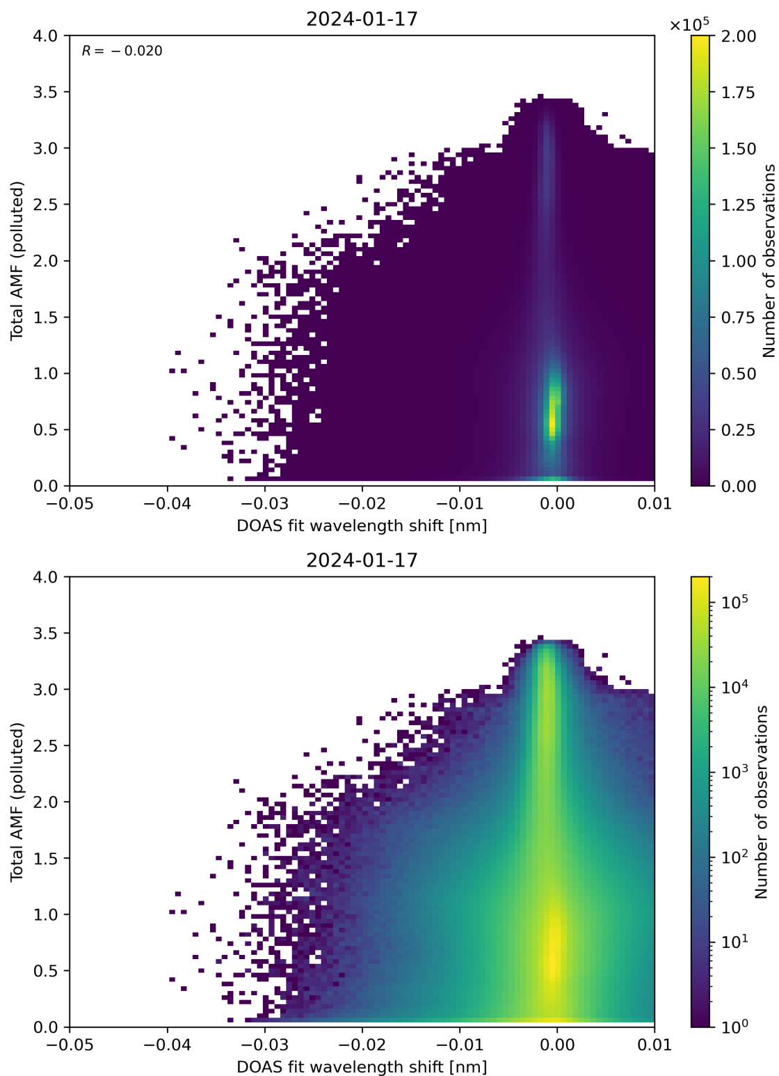
Figure 130: Scatter density plot of “DOAS fit wavelength shift” against “Total AMF (polluted)” for 2024-01-16 to 2024-01-18.
