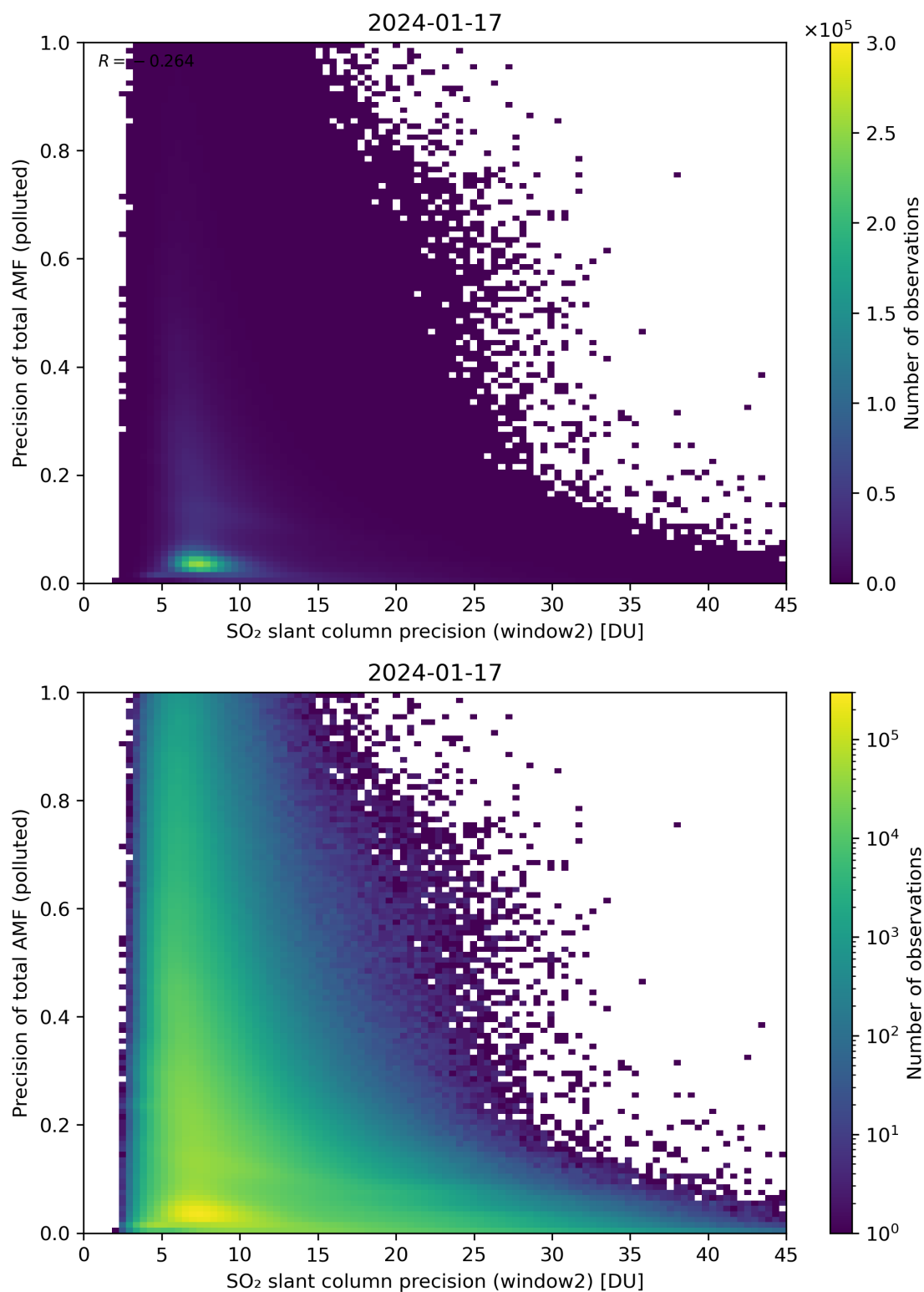
Figure 252: Scatter density plot of “SO 2 slant column precision (window2)” against “Precision of total AMF (polluted)” for 2024-01-16 to 2024-01-18.
