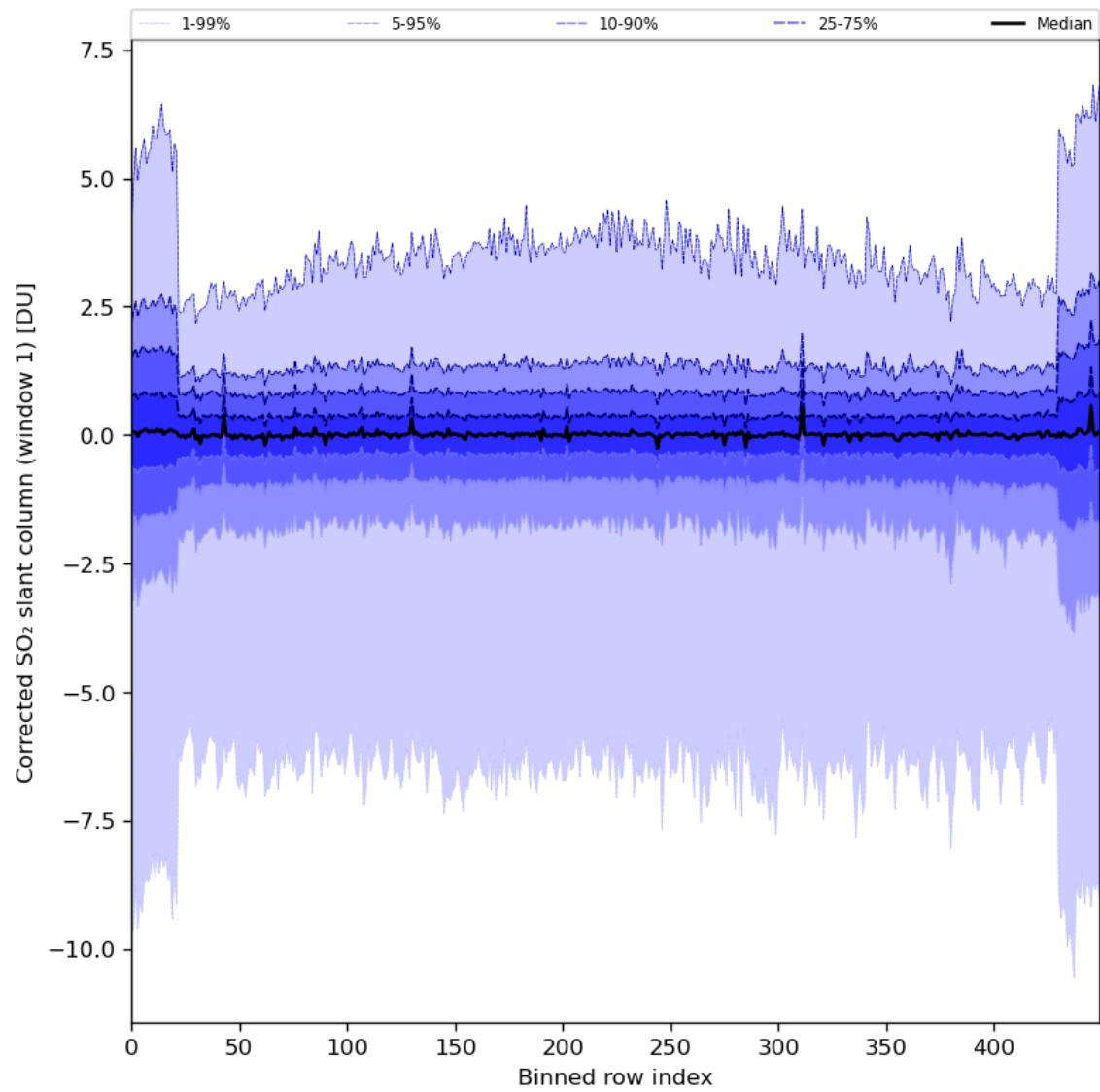
Figure 81: Along track statistics of “Corrected SO 2 slant column (window 1)” for 2024-01-16 to 2024-01-18
