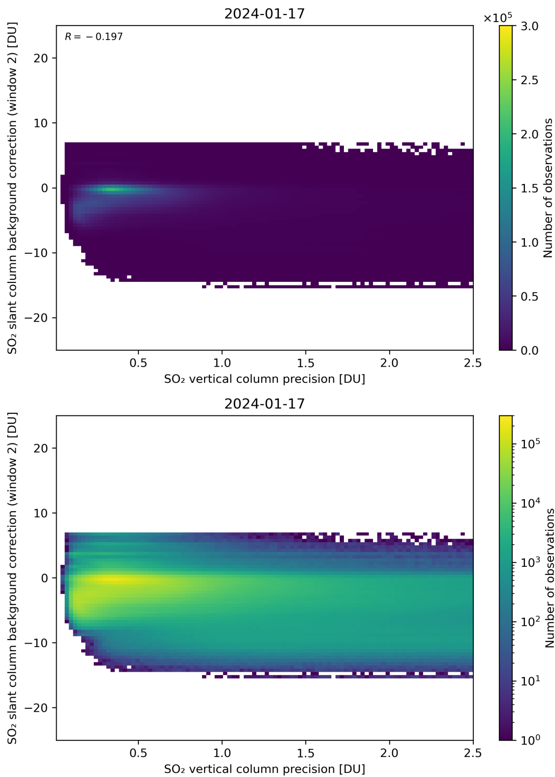
Figure 280: Scatter density plot of “SO 2 vertical column precision” against “SO 2 slant column background correction (window 2)” for 2024-01-16 to 2024-01-18.
