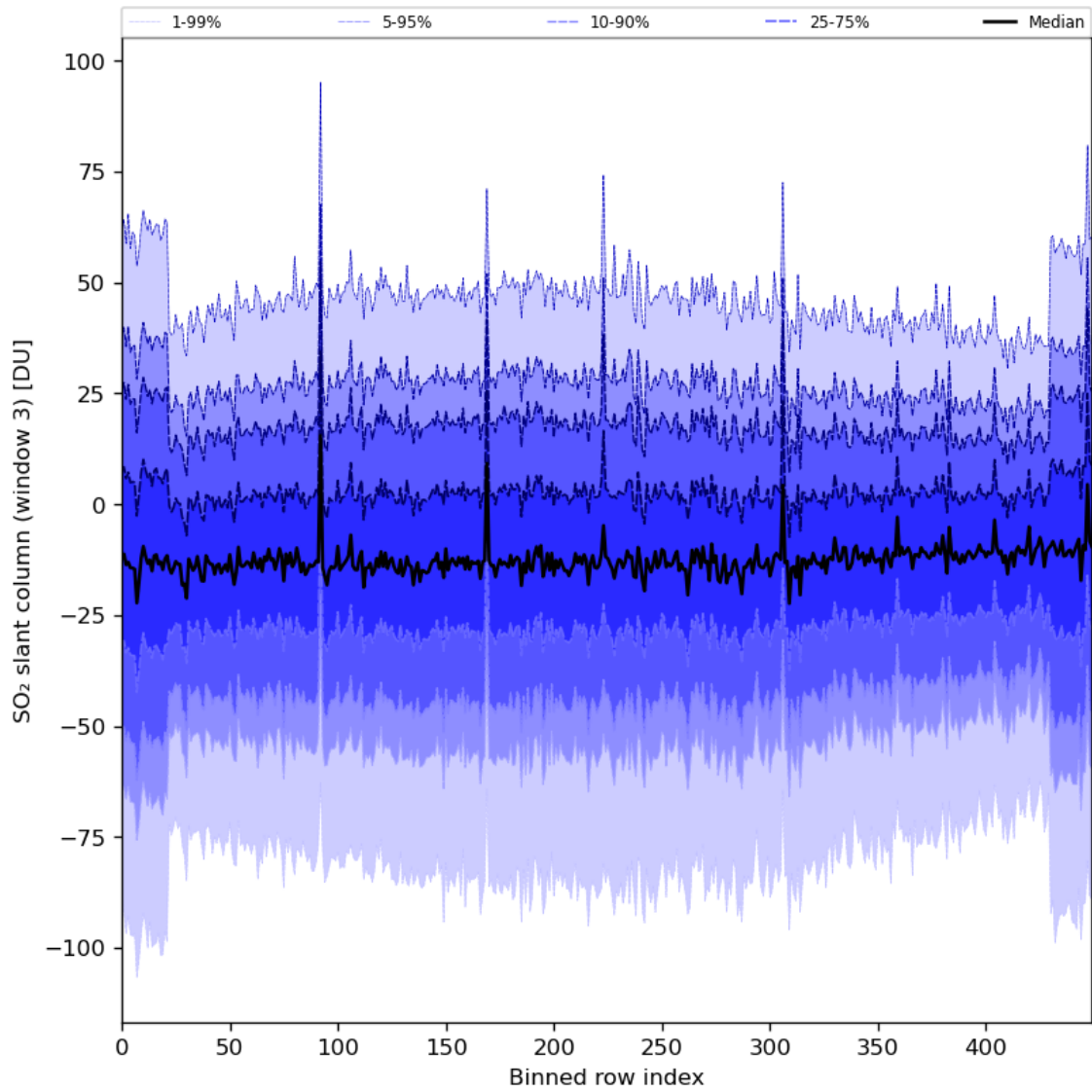
Figure 87: Along track statistics of “SO 2 slant column (window 3)” for 2024-01-16 to 2024-01-18
