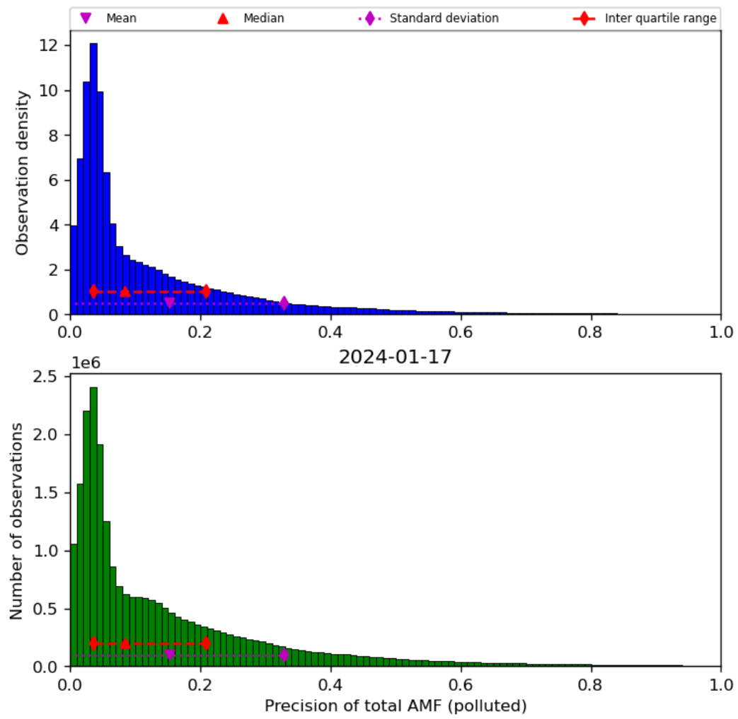
Figure 72: Histogram of “Precision of total AMF (polluted)” for 2024-01-16 to 2024-01-18
