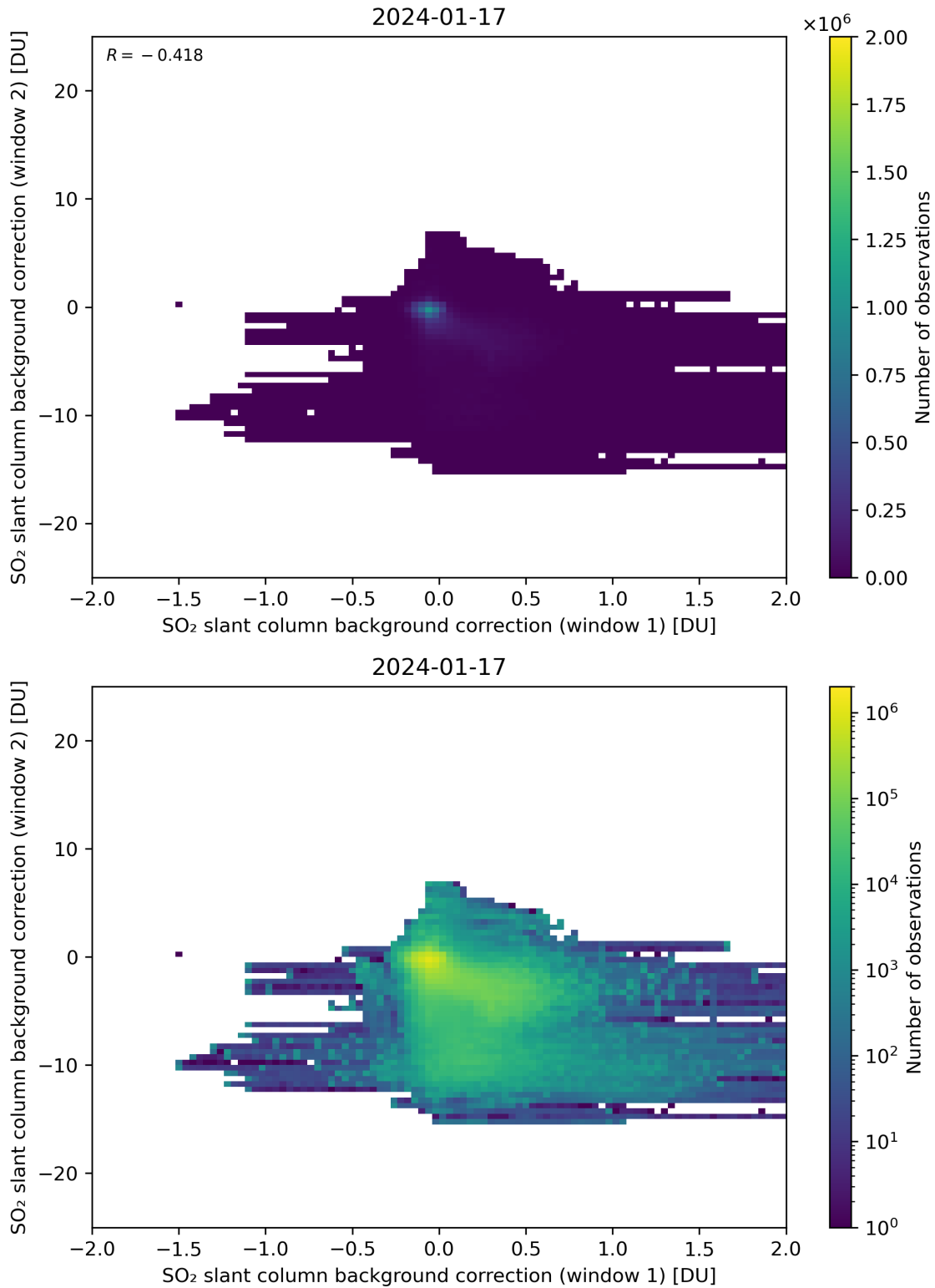
Figure 98: Scatter density plot of “SO 2 slant column background correction (window 1)” against “SO 2 slant column background correction (window 2)” for 2024-01-16 to 2024-01-18.
