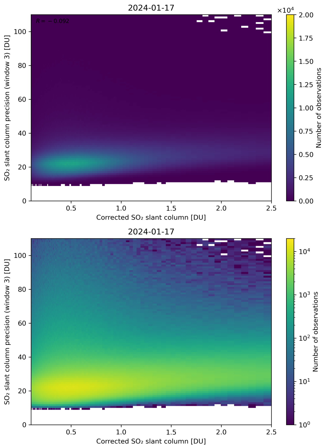
Figure 191: Scatter density plot of “Corrected SO 2 slant column” against “SO 2 slant column precision (window 3)” for 2024-01-16 to 2024-01-18.
