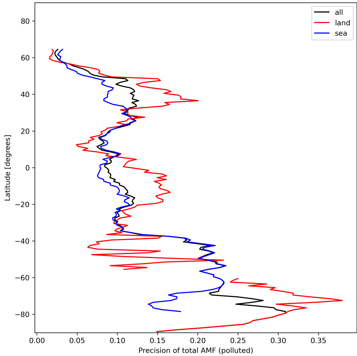
Figure 49: Zonal average of “Precision of total AMF (polluted)” for 2024-01-16 to 2024-01-18.
