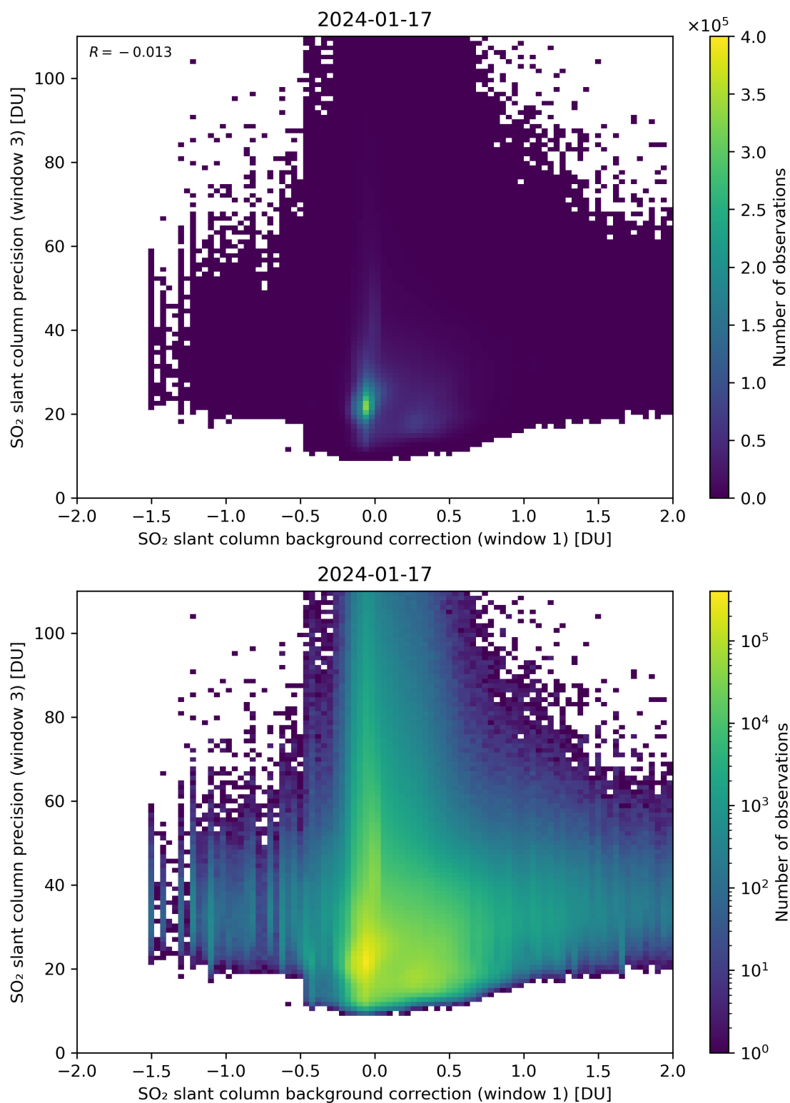
Figure 108: Scatter density plot of “SO 2 slant column background correction (window 1)” against “SO 2 slant column precision (window 3)” for 2024-01-16 to 2024-01-18.
