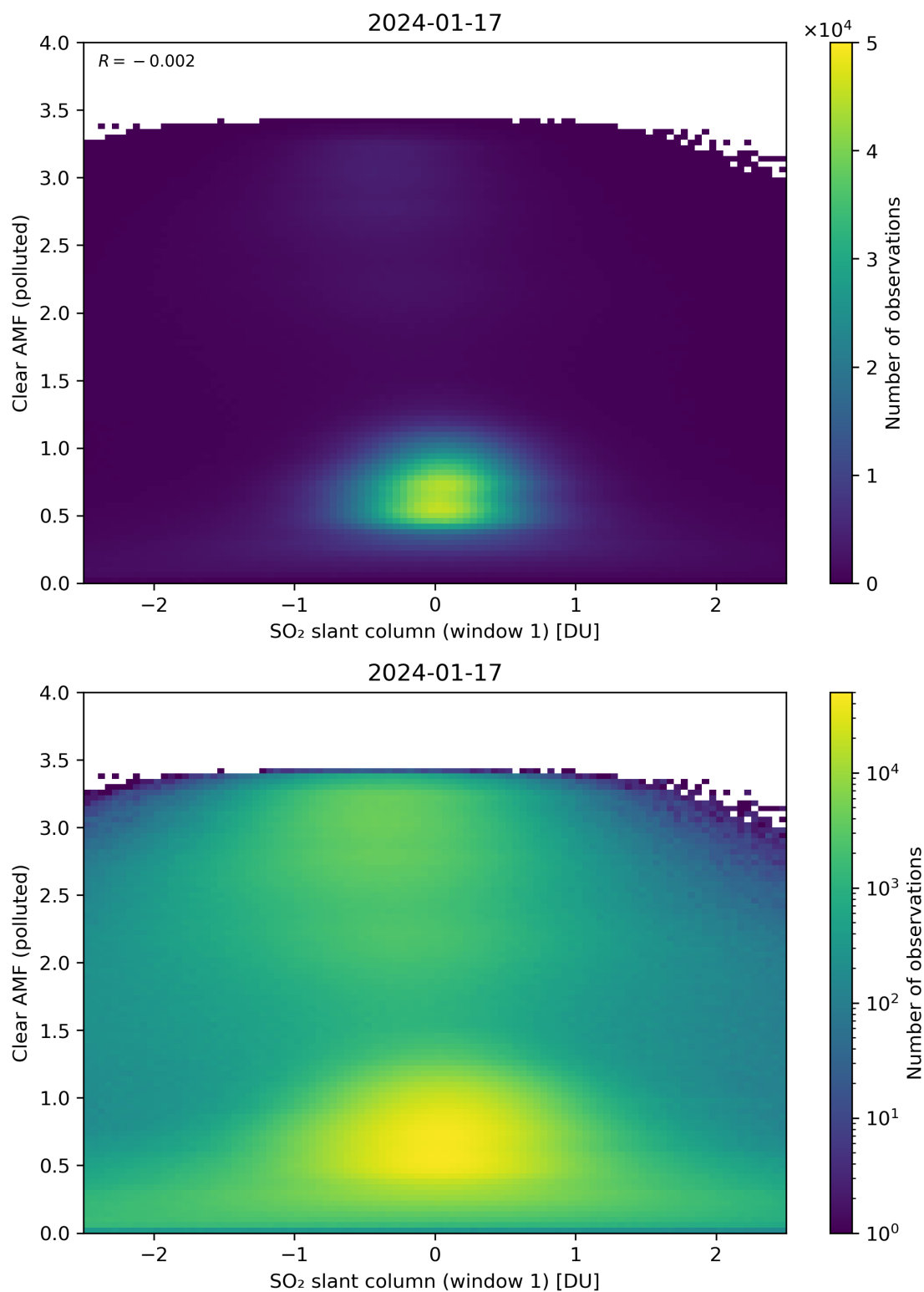
Figure 232: Scatter density plot of “SO 2 slant column (window 1)” against “Clear AMF (polluted)” for 2024-01-16 to 2024-01-18.
