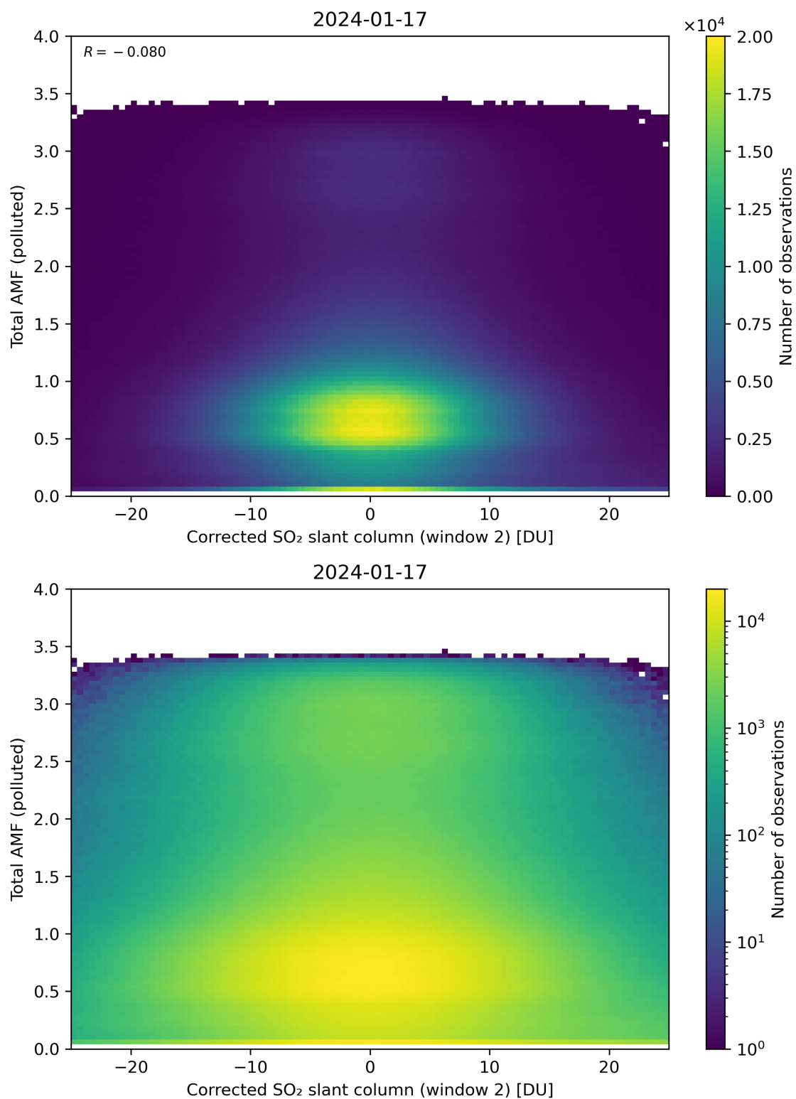
Figure 203: Scatter density plot of “Corrected SO 2 slant column (window 2)” against “Total AMF (polluted)” for 2024-01-16 to 2024-01-18.
