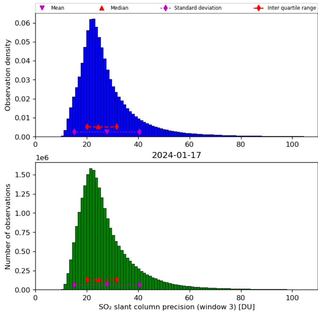
Figure 65: Histogram of “SO 2 slant column precision (window 3)” for 2024-01-16 to 2024-01-18
