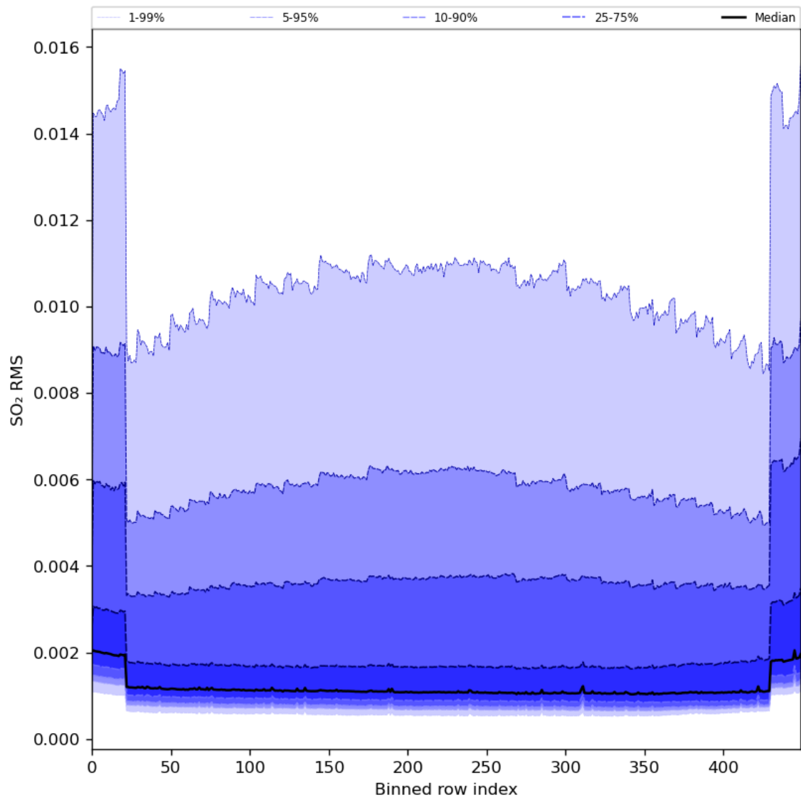
Figure 93: Along track statistics of “SO 2 RMS” for 2024-01-16 to 2024-01-18
