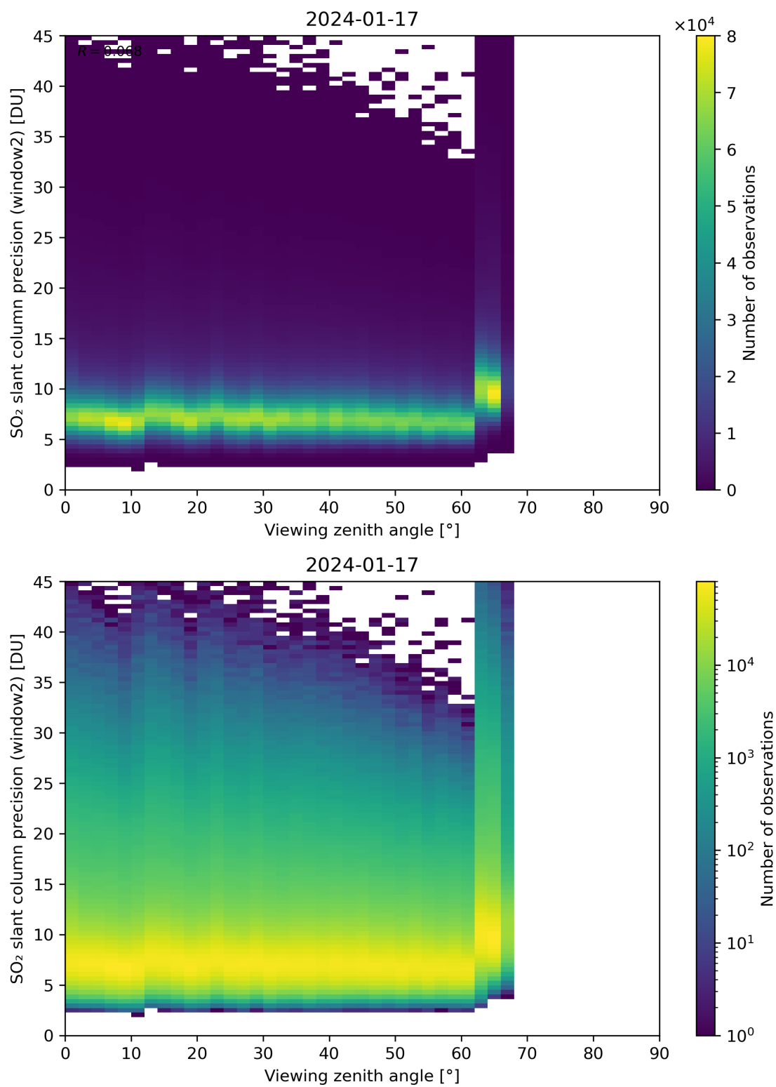
Figure 322: Scatter density plot of “Viewing zenith angle” against “SO 2 slant column precision (window2)” for 2024-01-16 to 2024-01-18.
