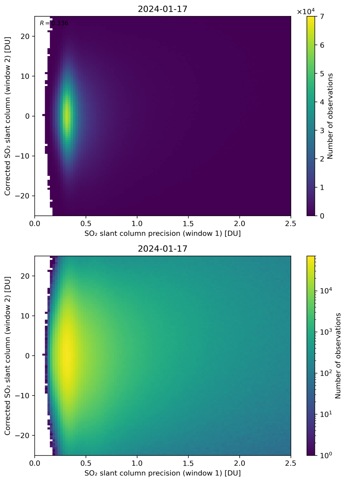
Figure 225: Scatter density plot of “SO 2 slant column precision (window 1)” against “Corrected SO 2 slant column (window 2)” for 2024-01-16 to 2024-01-18.
