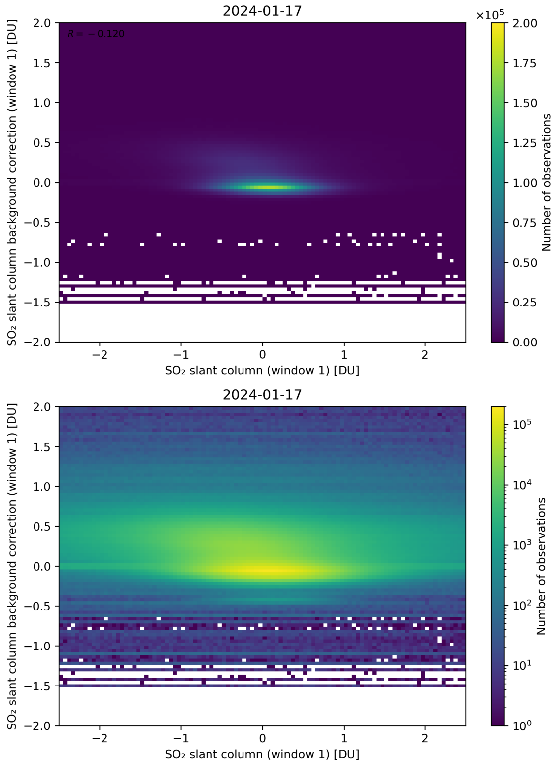
Figure 212: Scatter density plot of “SO 2 slant column (window 1)” against “SO 2 slant column background correction (window 1)” for 2024-01-16 to 2024-01-18.
