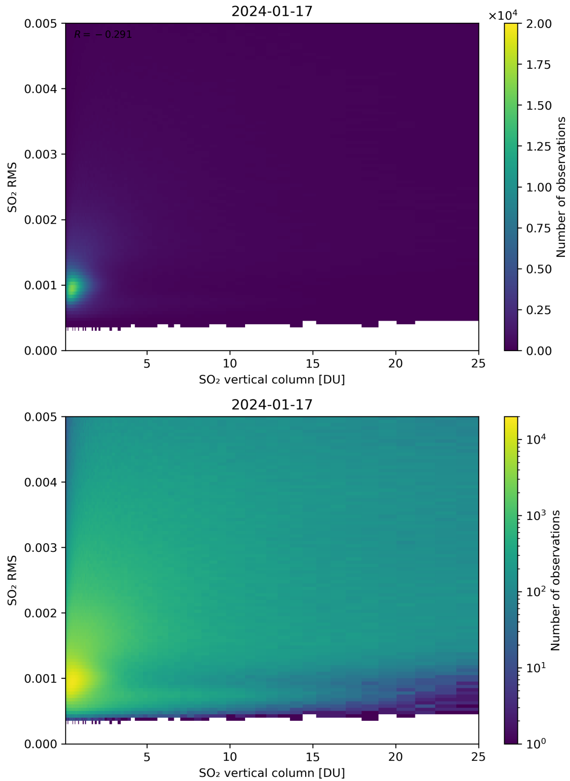
Figure 278: Scatter density plot of “SO 2 vertical column” against “SO 2 RMS” for 2024-01-16 to 2024-01-18.
