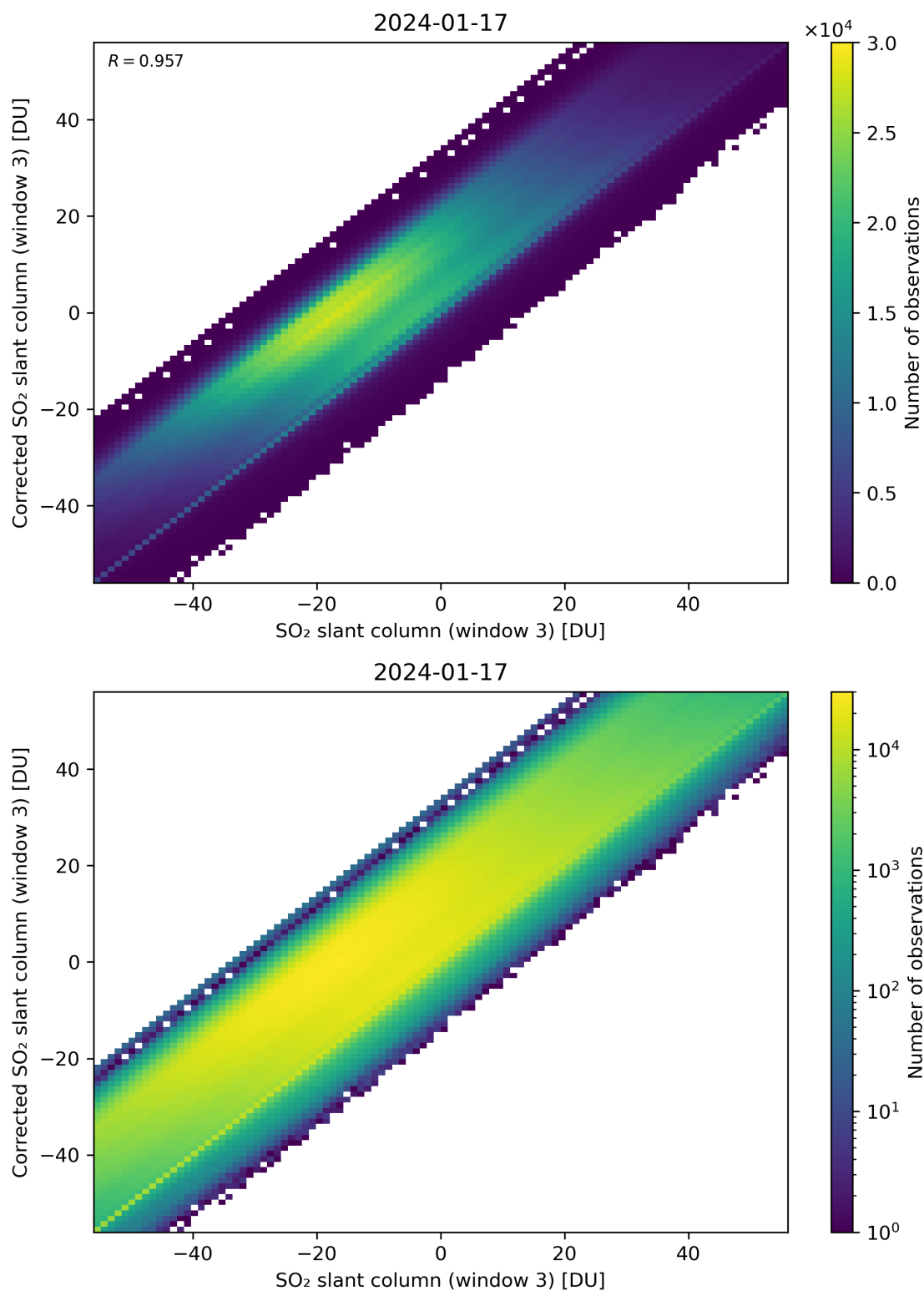
Figure 266: Scatter density plot of “SO 2 slant column (window 3)” against “Corrected SO 2 slant column (window 3)” for 2024-01-16 to 2024-01-18.
