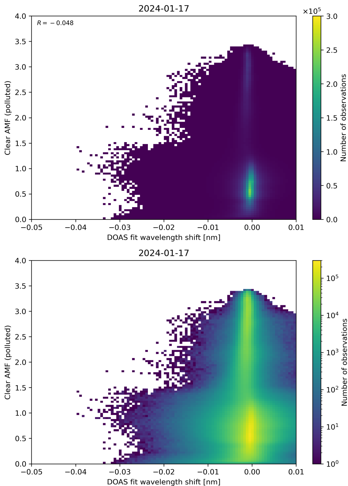
Figure 129: Scatter density plot of “DOAS fit wavelength shift” against “Clear AMF (polluted)” for 2024-01-16 to 2024-01-18.
