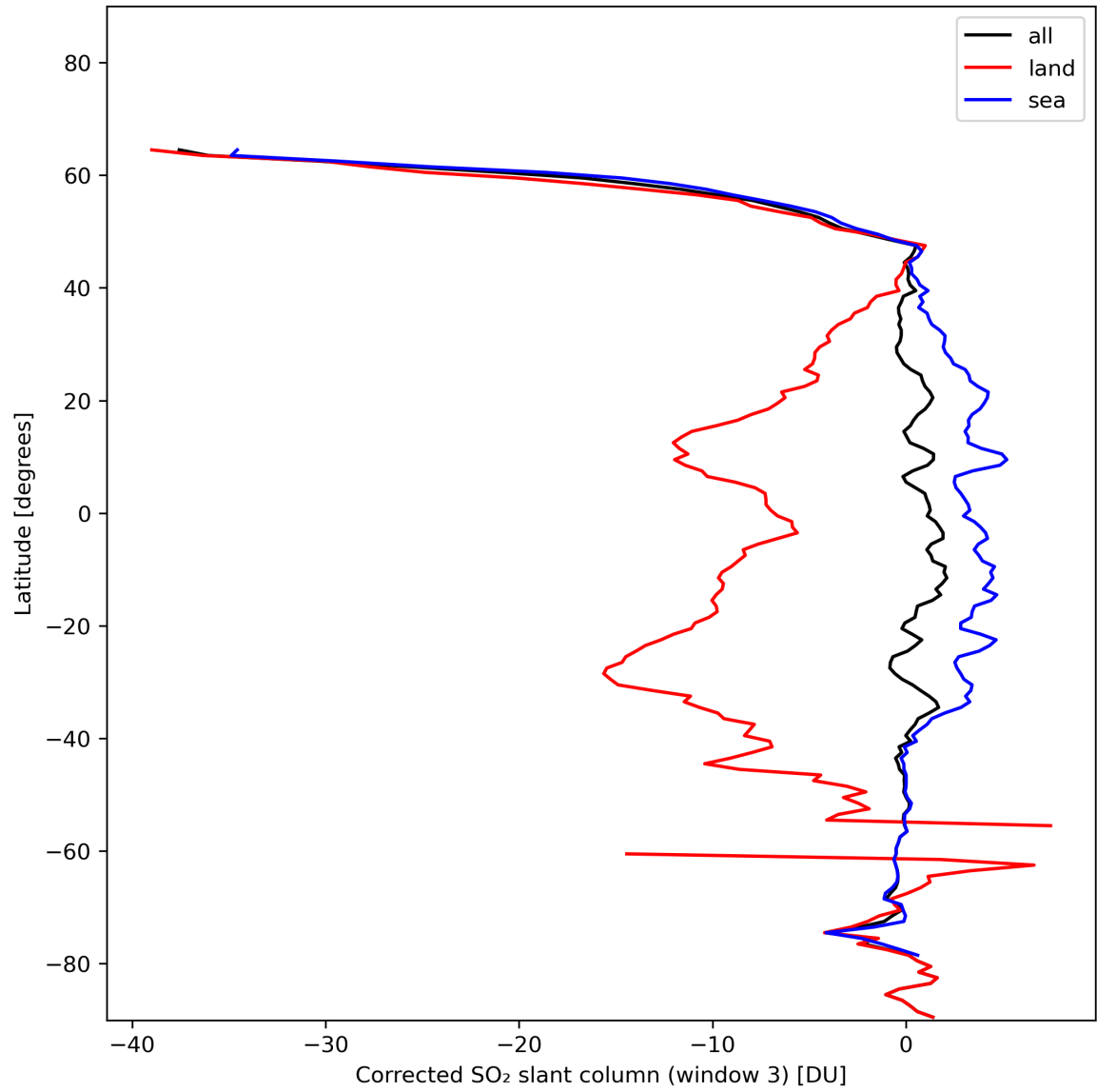
Figure 43: Zonal average of “Corrected SO 2 slant column (window 3)” for 2024-01-16 to 2024-01-18.
