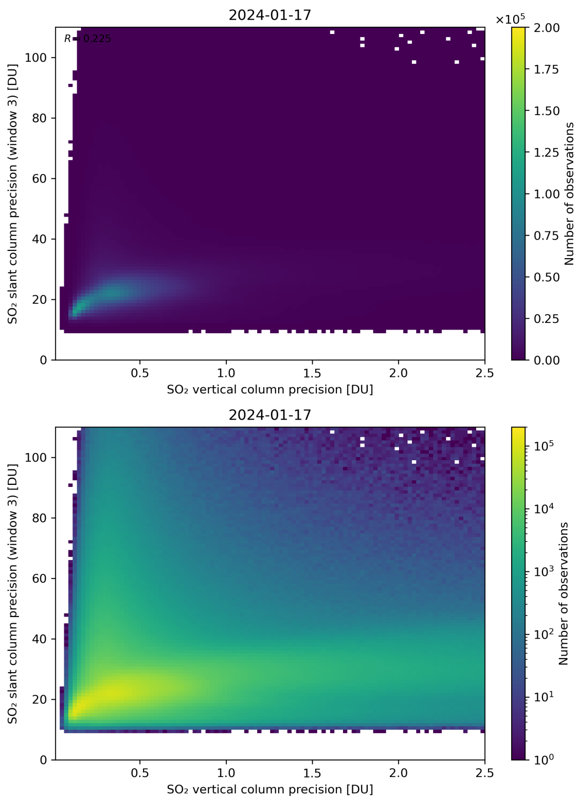
Figure 293: Scatter density plot of “SO 2 vertical column precision” against “SO 2 slant column precision (window 3)” for 2024-01-16 to 2024-01-18.
