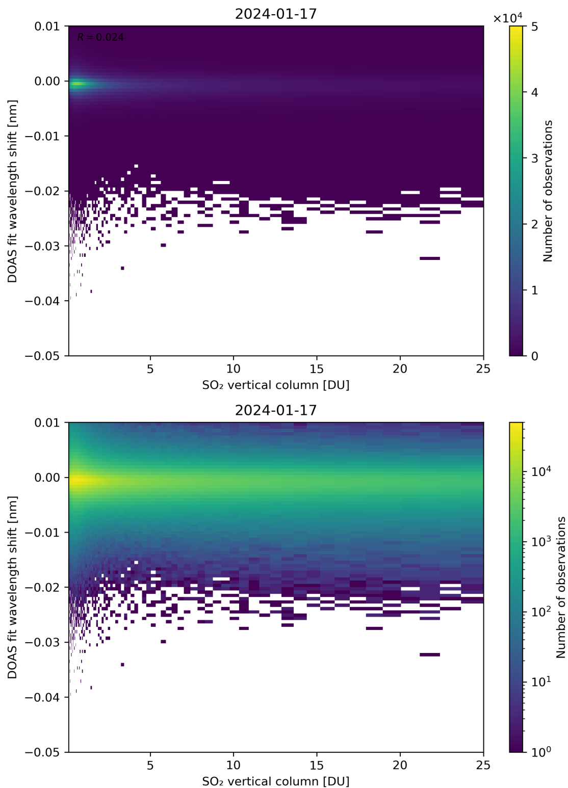
Figure 276: Scatter density plot of “SO 2 vertical column” against “DOAS fit wavelength shift” for 2024-01-16 to 2024-01-18.
