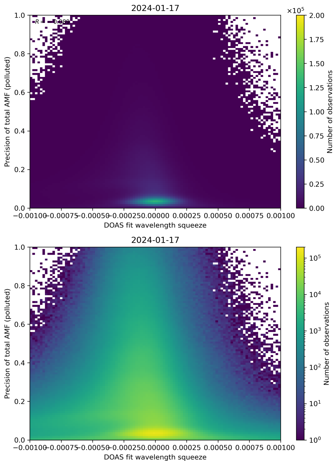
Figure 135: Scatter density plot of “DOAS fit wavelength squeeze” against “Precision of total AMF (polluted)” for 2024-01-16 to 2024-01-18.
