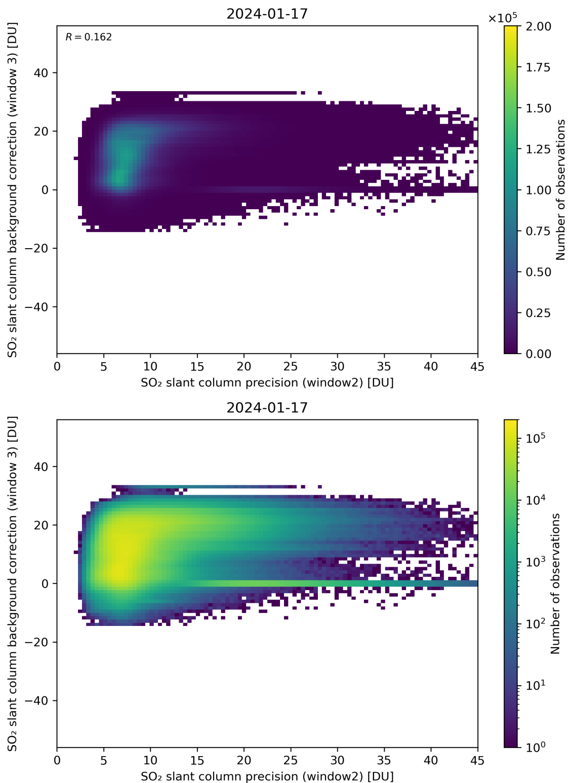
Figure 242: Scatter density plot of “SO 2 slant column precision (window2)” against “SO 2 slant column background correction (window 3)” for 2024-01-16 to 2024-01-18.
