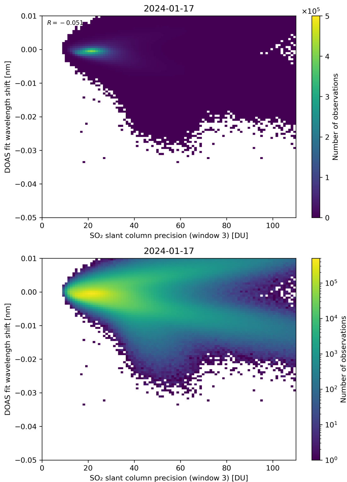
Figure 258: Scatter density plot of “SO 2 slant column precision (window 3)” against “DOAS fit wavelength shift” for 2024-01-16 to 2024-01-18.
