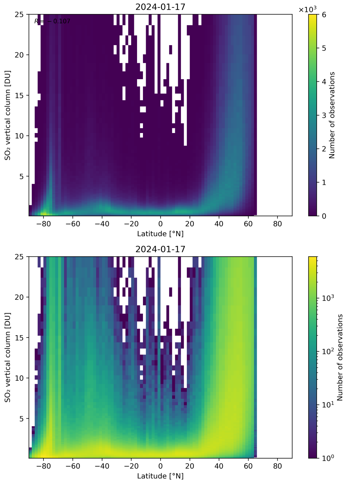
Figure 156: Scatter density plot of “Latitude” against “SO 2 vertical column” for 2024-01-16 to 2024-01-18.
