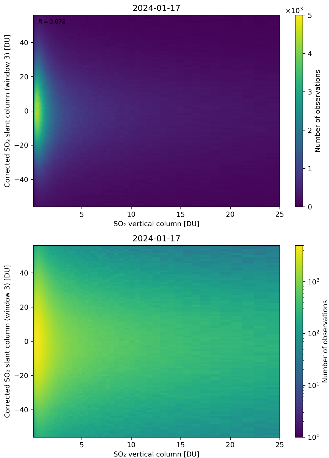
Figure 299: Scatter density plot of “SO 2 vertical column” against “Corrected SO 2 slant column (window 3)” for 2024-01-16 to 2024-01-18.
