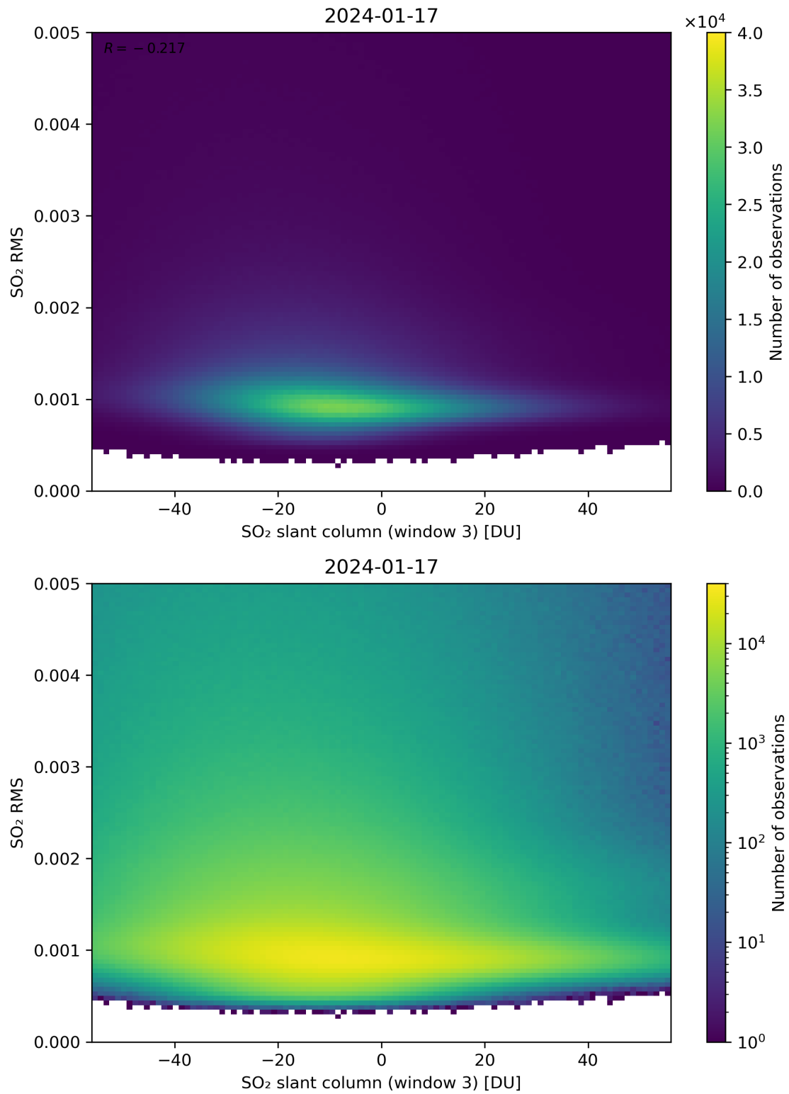
Figure 256: Scatter density plot of “SO 2 slant column (window 3)” against “SO 2 RMS” for 2024-01-16 to 2024-01-18.
