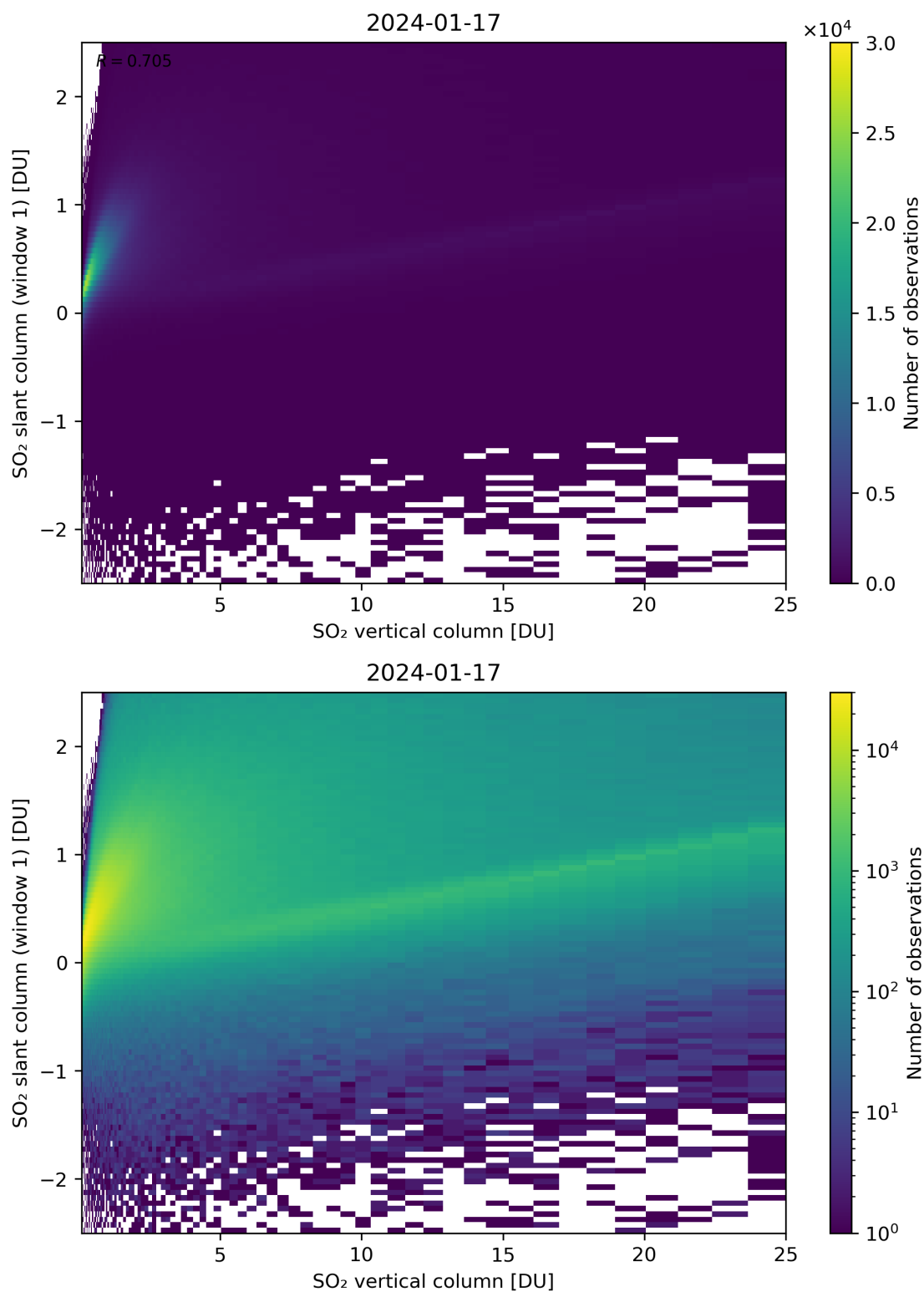
Figure 300: Scatter density plot of “SO 2 vertical column” against “SO 2 slant column (window 1)” for 2024-01-16 to 2024-01-18.
