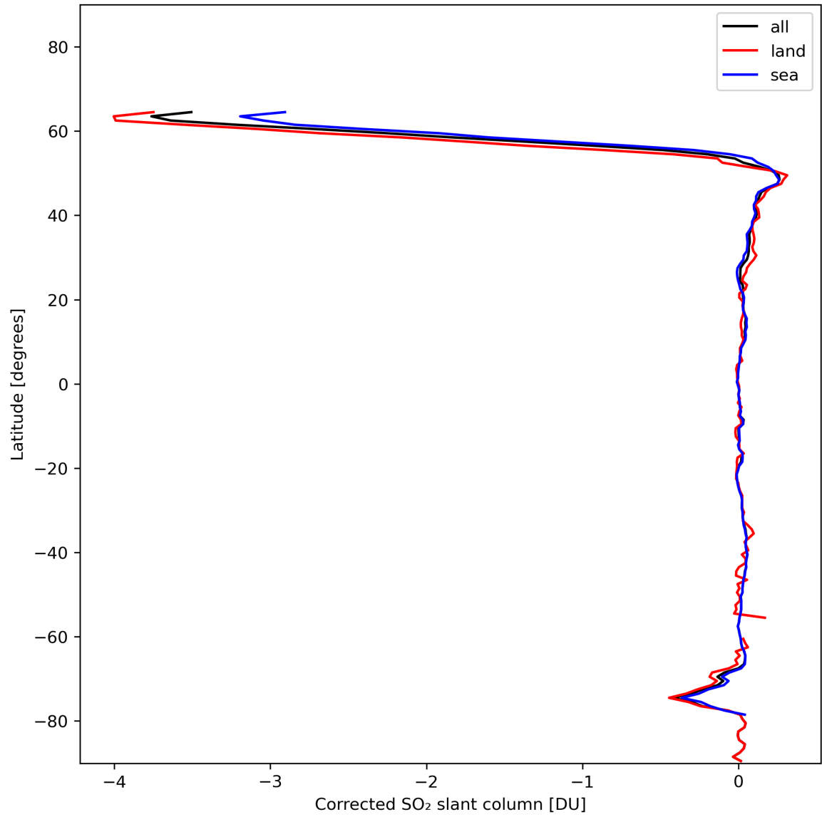
Figure 32: Zonal average of “Corrected SO 2 slant column” for 2024-01-16 to 2024-01-18.
