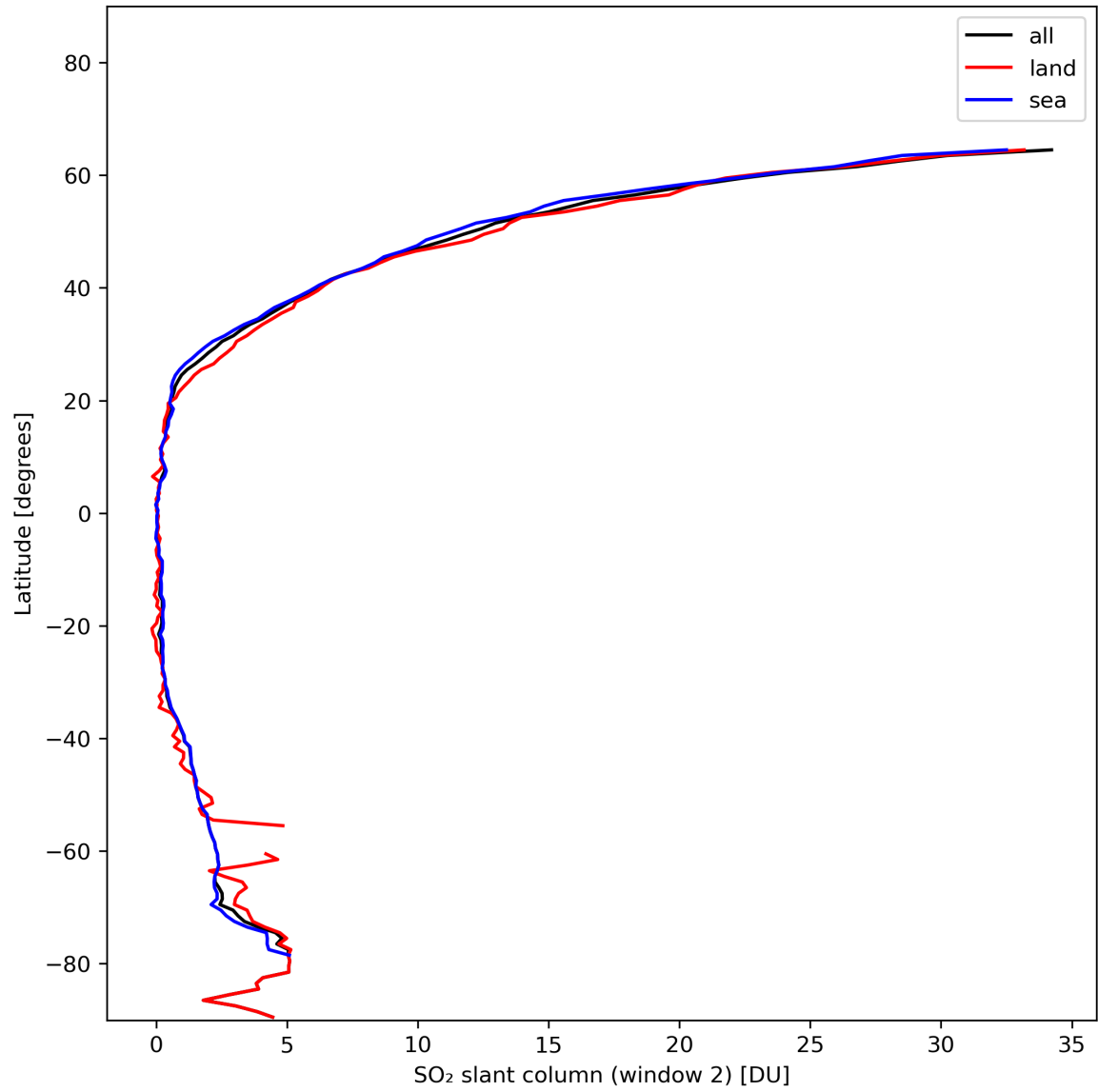
Figure 37: Zonal average of “SO 2 slant column (window 2)” for 2024-01-16 to 2024-01-18.
