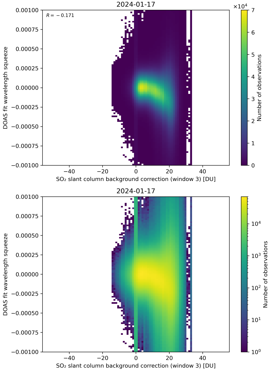
Figure 122: Scatter density plot of “SO 2 slant column background correction (window 3)” against “DOAS fit wavelength squeeze” for 2024-01-16 to 2024-01-18.
