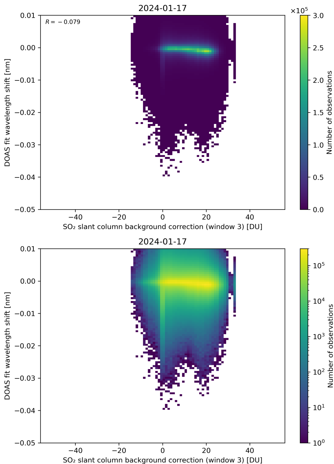
Figure 121: Scatter density plot of “SO 2 slant column background correction (window 3)” against “DOAS fit wavelength shift” for 2024-01-16 to 2024-01-18.
