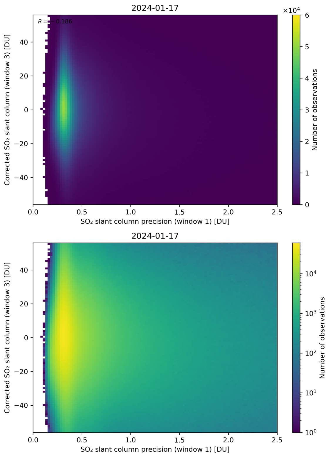
Figure 226: Scatter density plot of “SO 2 slant column precision (window 1)” against “Corrected SO 2 slant column (window 3)” for 2024-01-16 to 2024-01-18.
