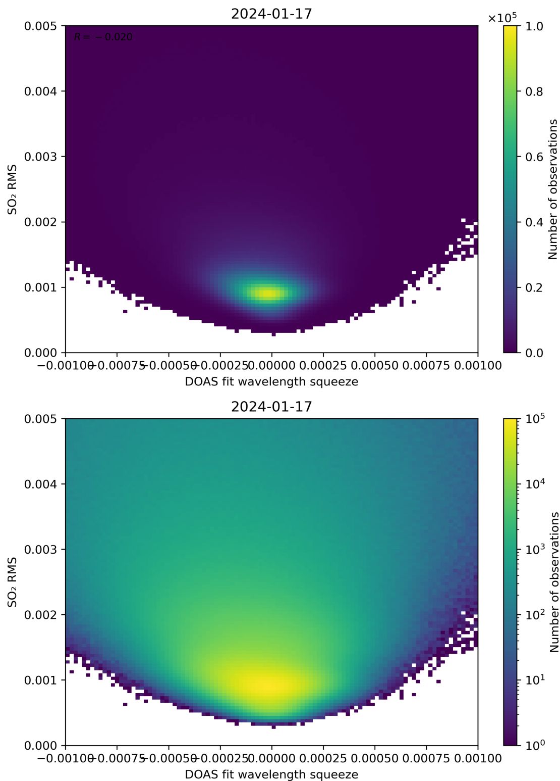
Figure 132: Scatter density plot of “DOAS fit wavelength squeeze” against “SO 2 RMS” for 2024-01-16 to 2024-01-18.
