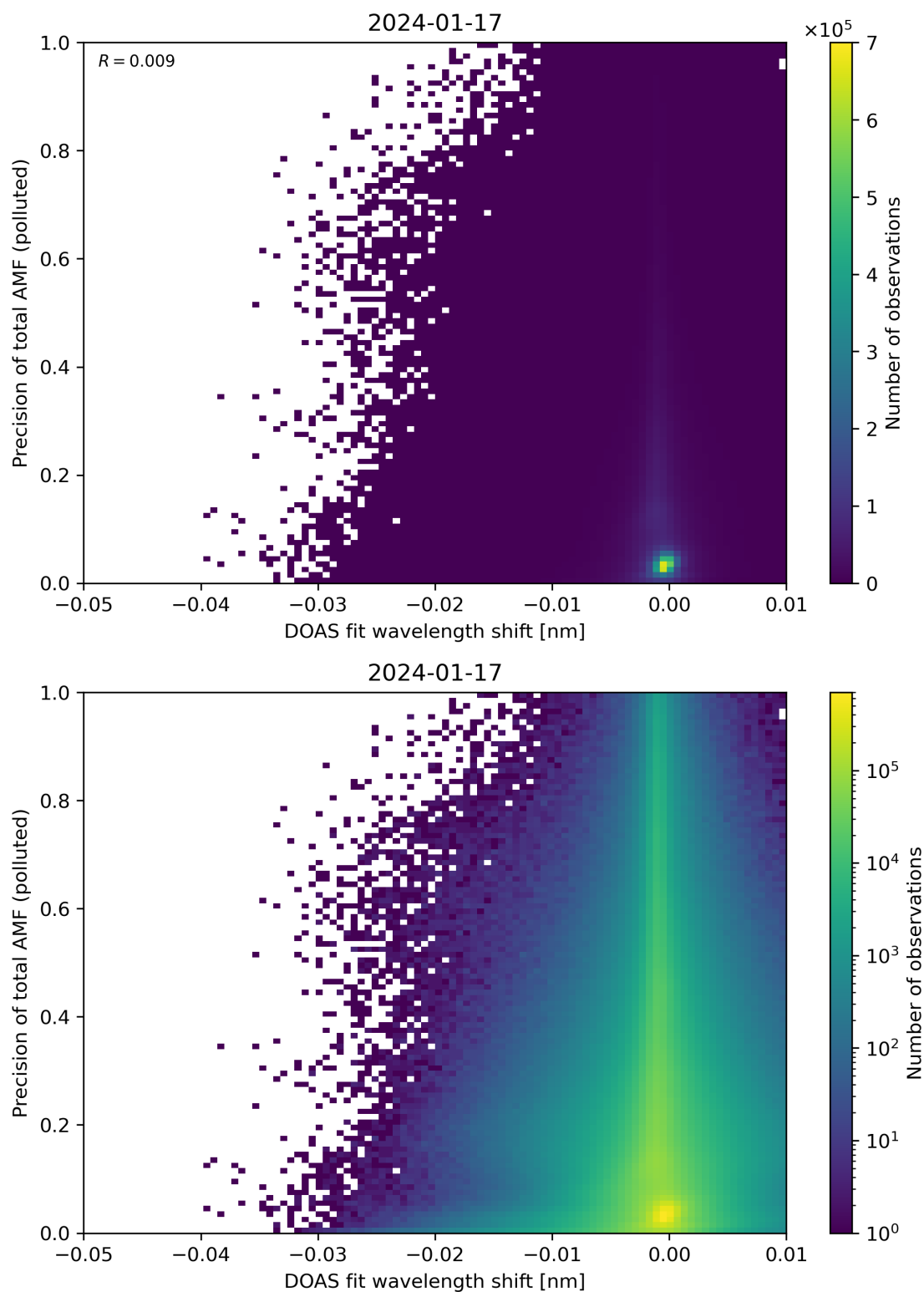
Figure 131: Scatter density plot of “DOAS fit wavelength shift” against “Precision of total AMF (polluted)” for 2024-01-16 to 2024-01-18.
