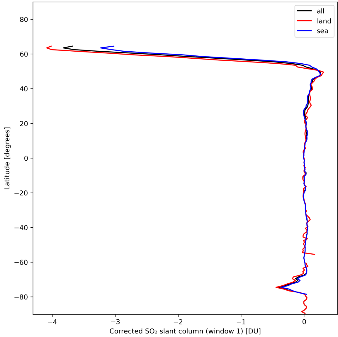
Figure 35: Zonal average of “Corrected SO 2 slant column (window 1)” for 2024-01-16 to 2024-01-18.
