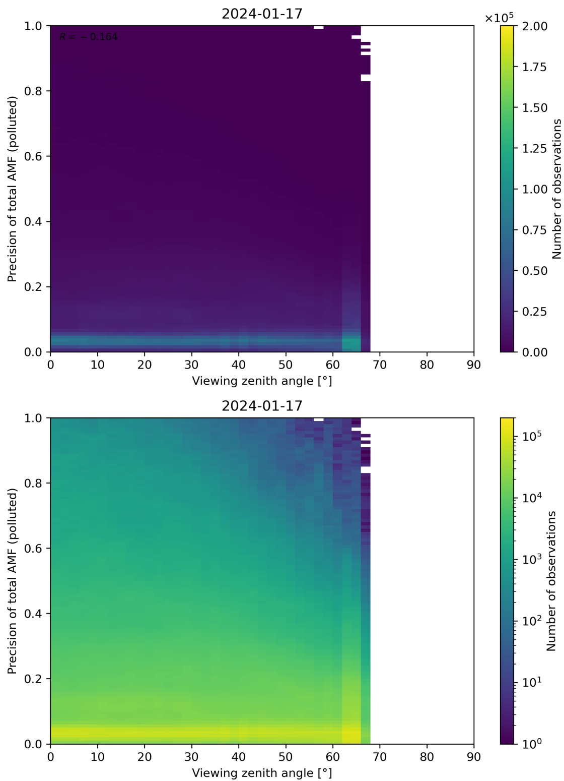
Figure 326: Scatter density plot of “Viewing zenith angle” against “Precision of total AMF (polluted)” for 2024-01-16 to 2024-01-18.
