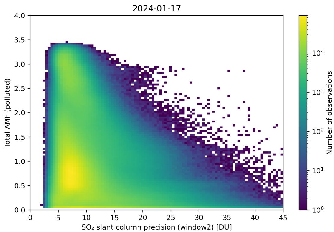
Figure 251: Scatter density plot of “SO 2 slant column precision (window2)” against “Total AMF (polluted)” for 2024-01-16 to 2024-01-18.
