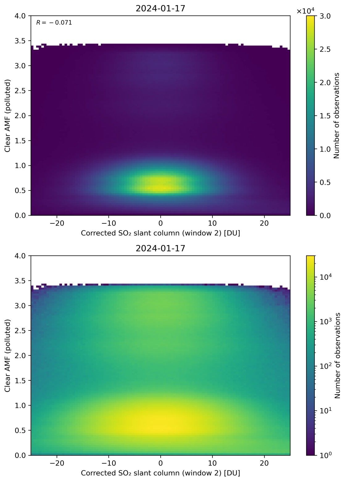
Figure 199: Scatter density plot of “Corrected SO 2 slant column (window 2)” against “Clear AMF (polluted)” for 2024-01-16 to 2024-01-18.
