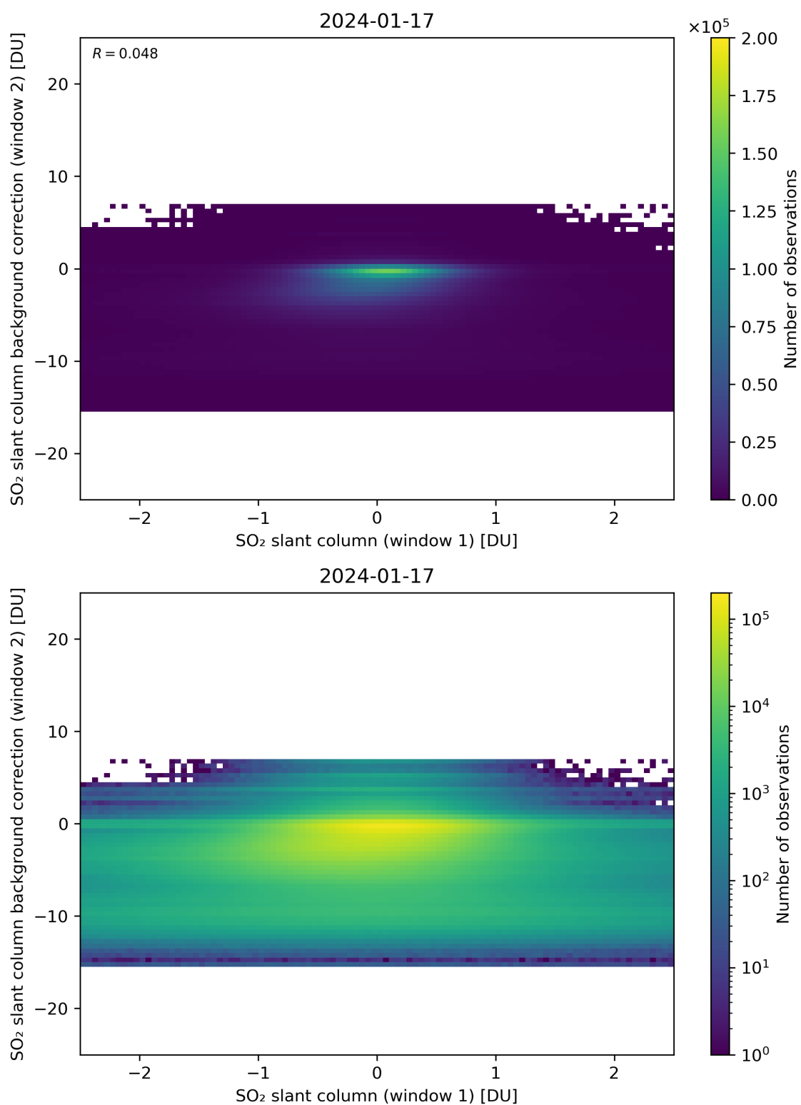
Figure 213: Scatter density plot of “SO 2 slant column (window 1)” against “SO 2 slant column background correction (window 2)” for 2024-01-16 to 2024-01-18.
