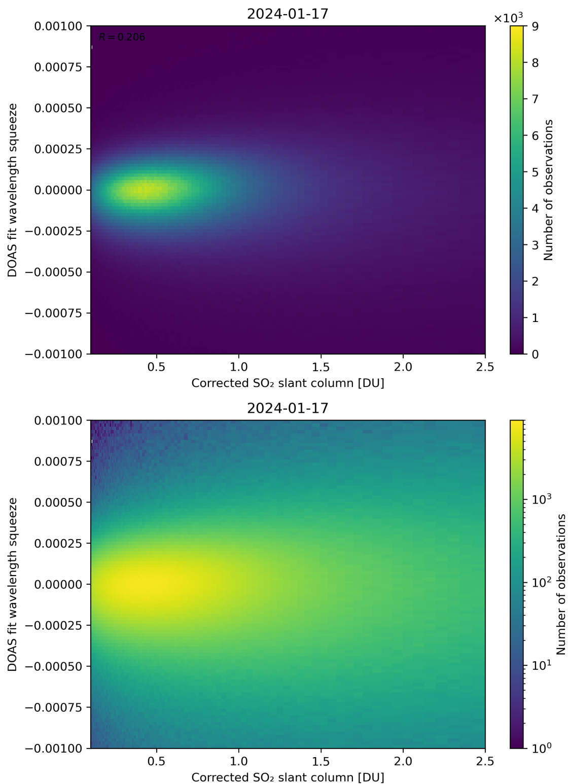
Figure 182: Scatter density plot of “Corrected SO 2 slant column” against “DOAS fit wavelength squeeze” for 2024-01-16 to 2024-01-18.
