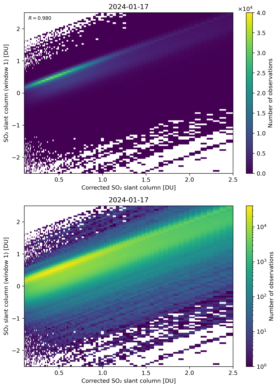
Figure 187: Scatter density plot of “Corrected SO 2 slant column” against “SO 2 slant column (window 1)” for 2024-01-16 to 2024-01-18.
