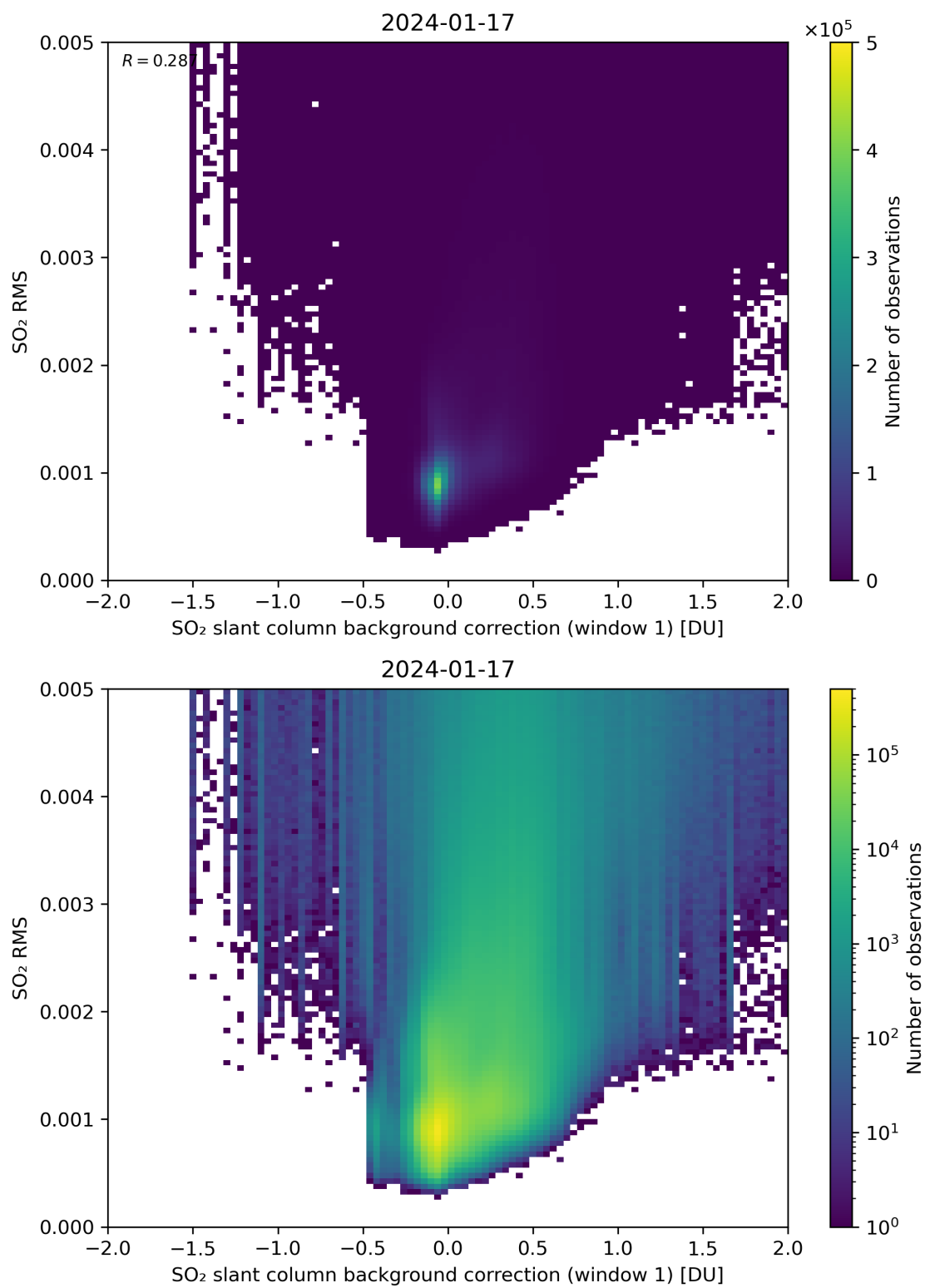
Figure 102: Scatter density plot of “SO 2 slant column background correction (window 1)” against “SO 2 RMS” for 2024-01-16 to 2024-01-18.
