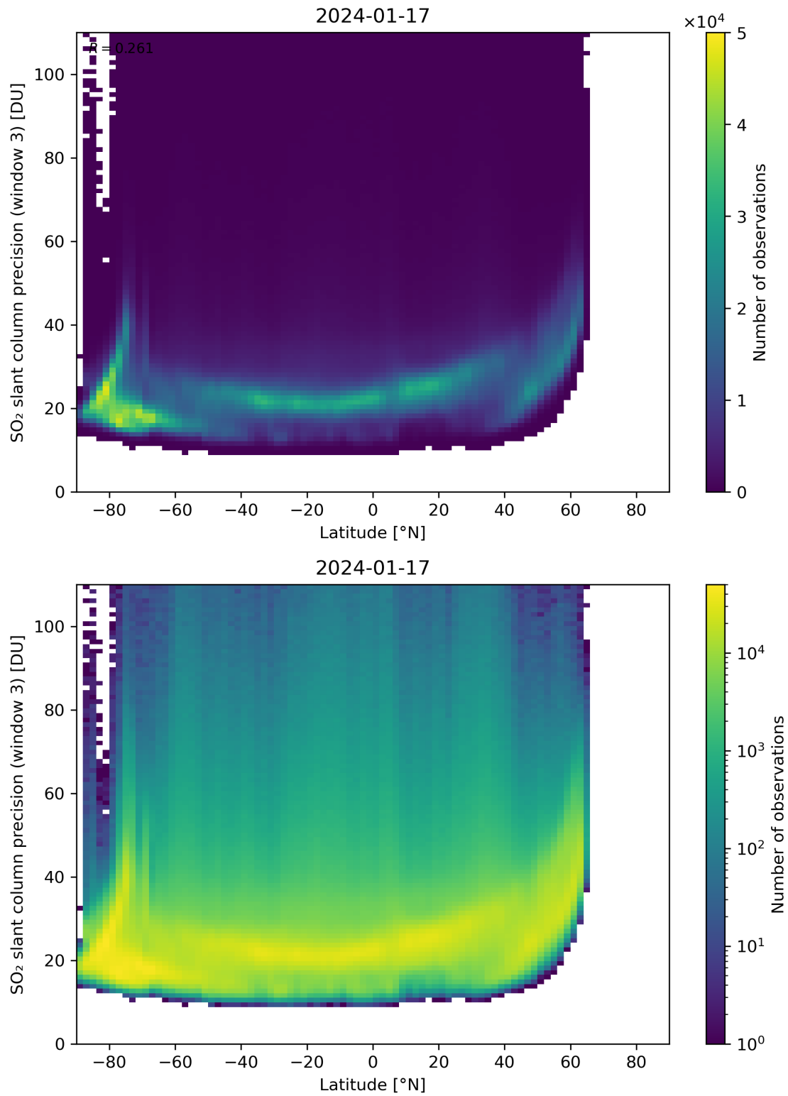
Figure 153: Scatter density plot of “Latitude” against “SO 2 slant column precision (window 3)” for 2024-01-16 to 2024-01-18.
