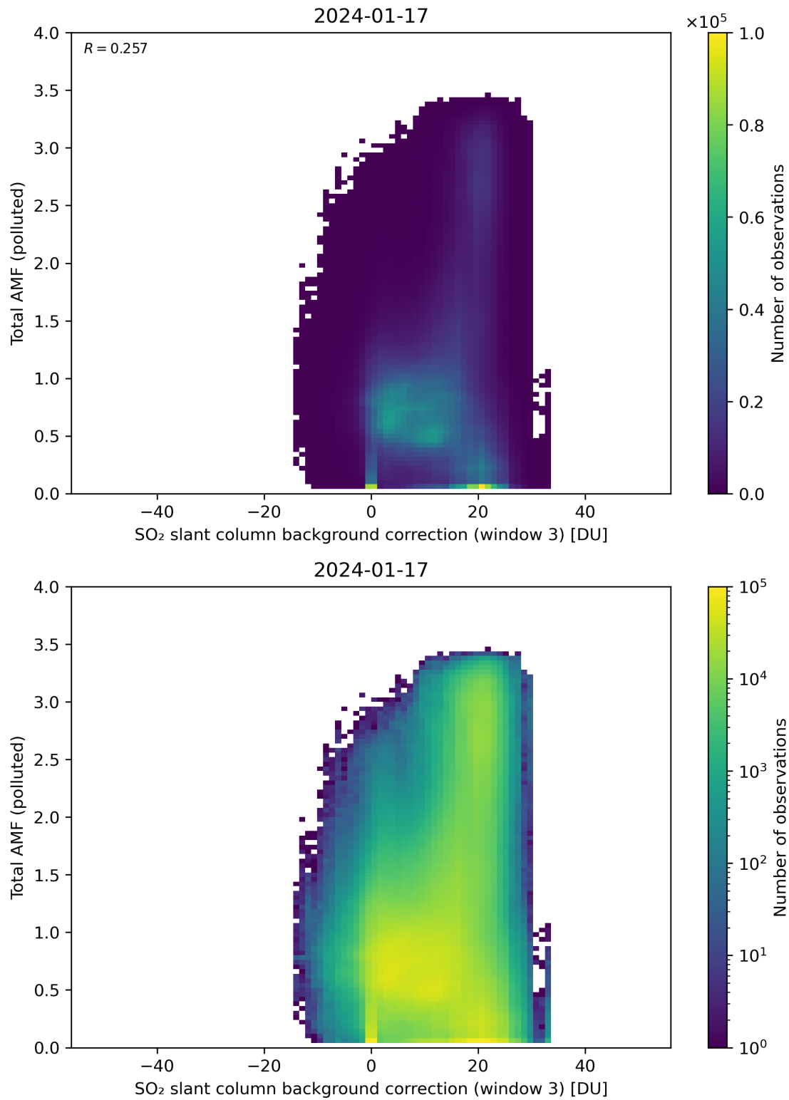
Figure 125: Scatter density plot of “SO 2 slant column background correction (window 3)” against “Total AMF (polluted)” for 2024-01-16 to 2024-01-18.
