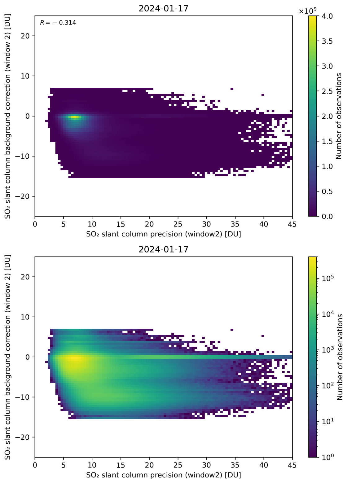
Figure 241: Scatter density plot of “SO 2 slant column precision (window2)” against “SO 2 slant column background correction (window 2)” for 2024-01-16 to 2024-01-18.
