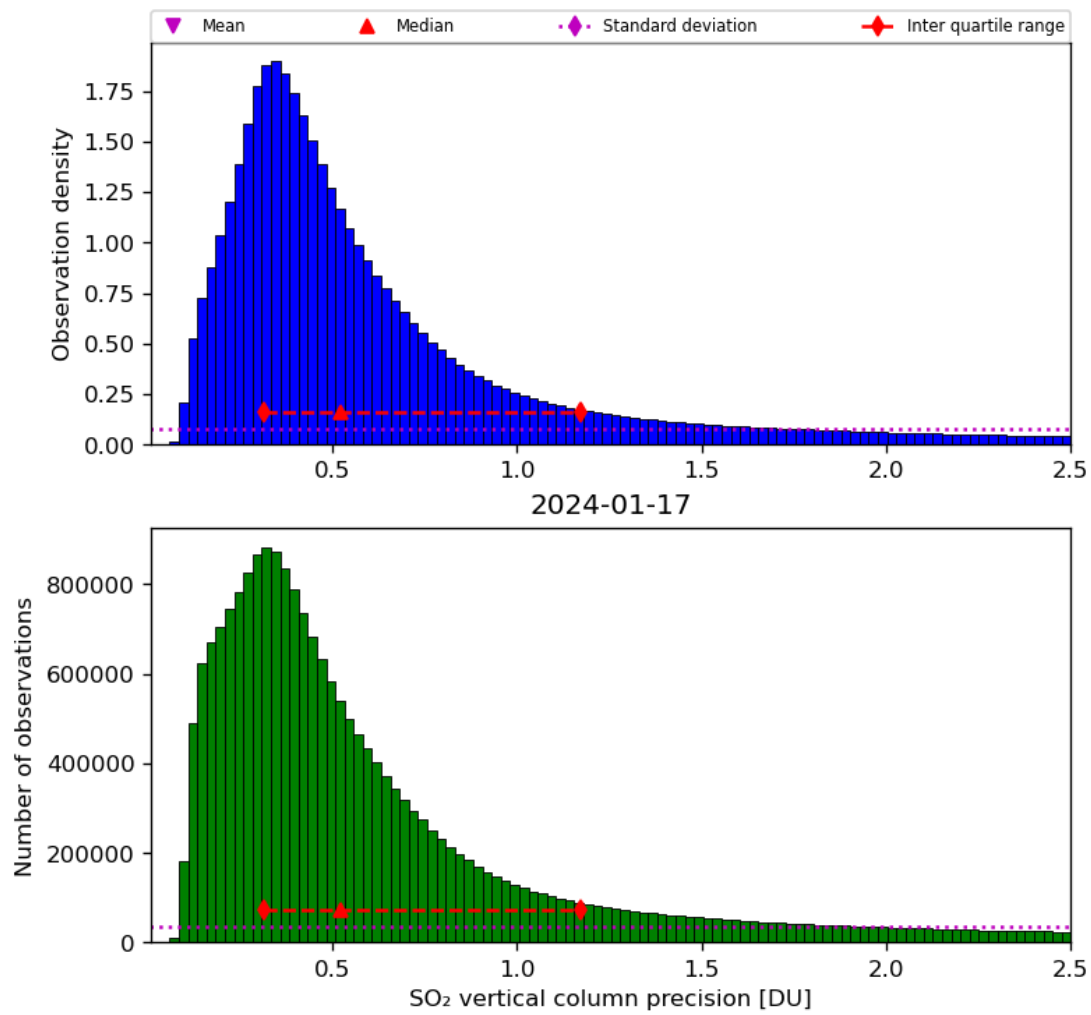
Figure 54: Histogram of “SO 2 vertical column precision” for 2024-01-16 to 2024-01-18
