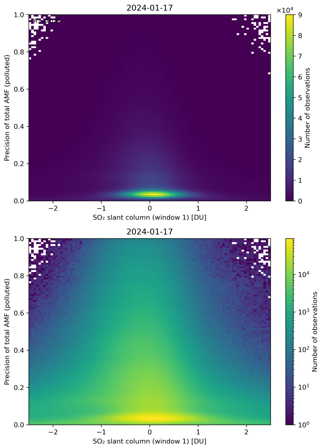
Figure 240: Scatter density plot of “SO 2 slant column (window 1)” against “Precision of total AMF (polluted)” for 2024-01-16 to 2024-01-18.
