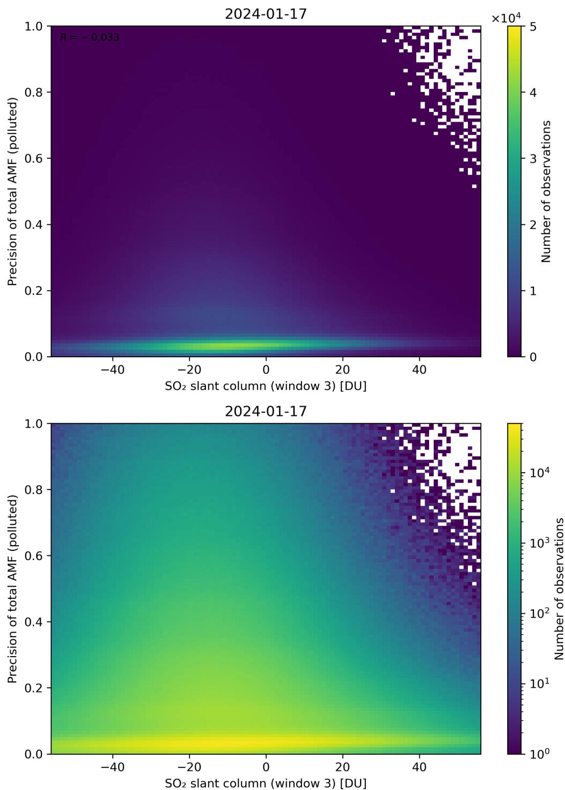
Figure 269: Scatter density plot of “SO 2 slant column (window 3)” against “Precision of total AMF (polluted)” for 2024-01-16 to 2024-01-18.
