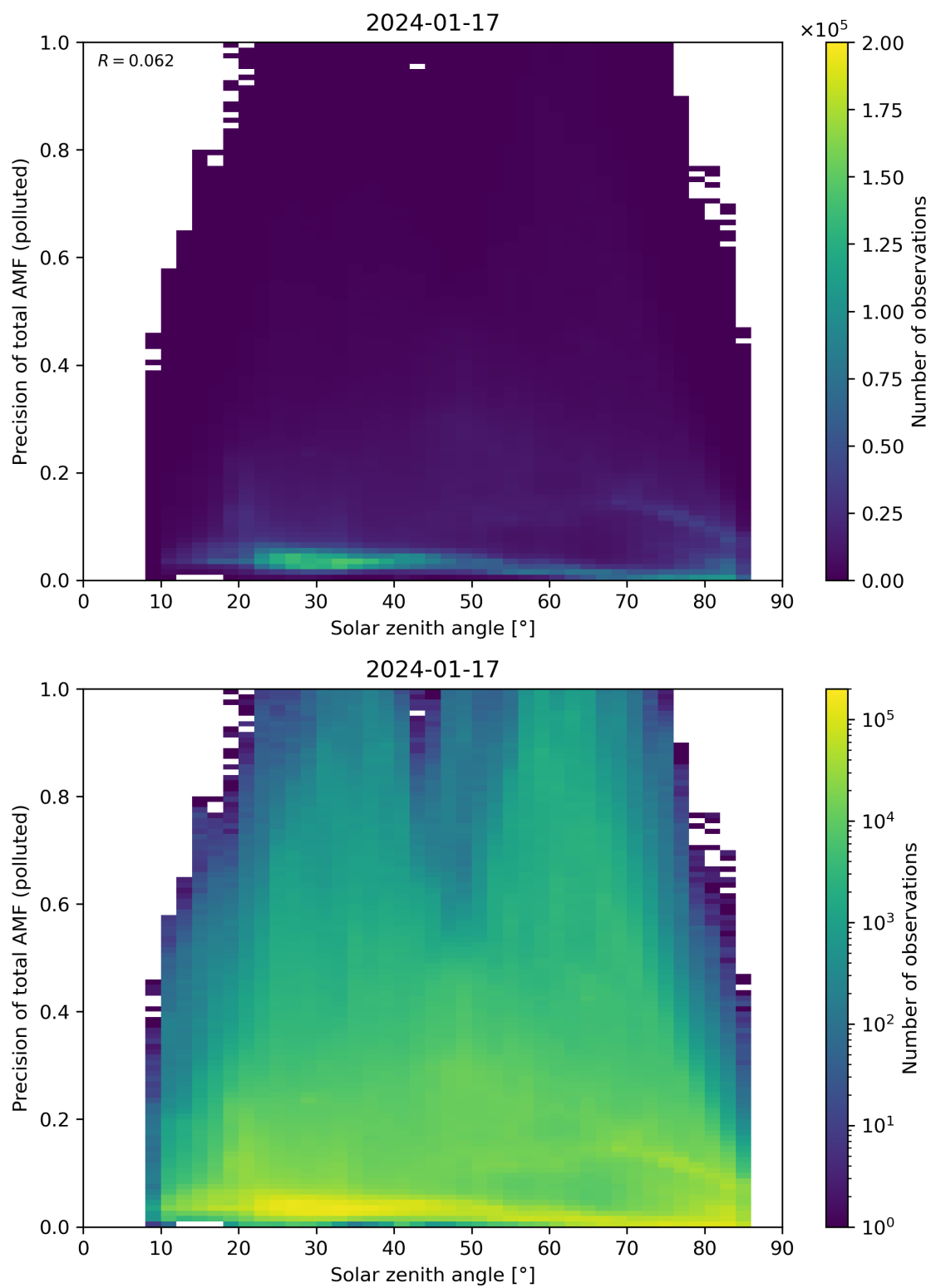
Figure 175: Scatter density plot of “Solar zenith angle” against “Precision of total AMF (polluted)” for 2024-01-16 to 2024-01-18.
