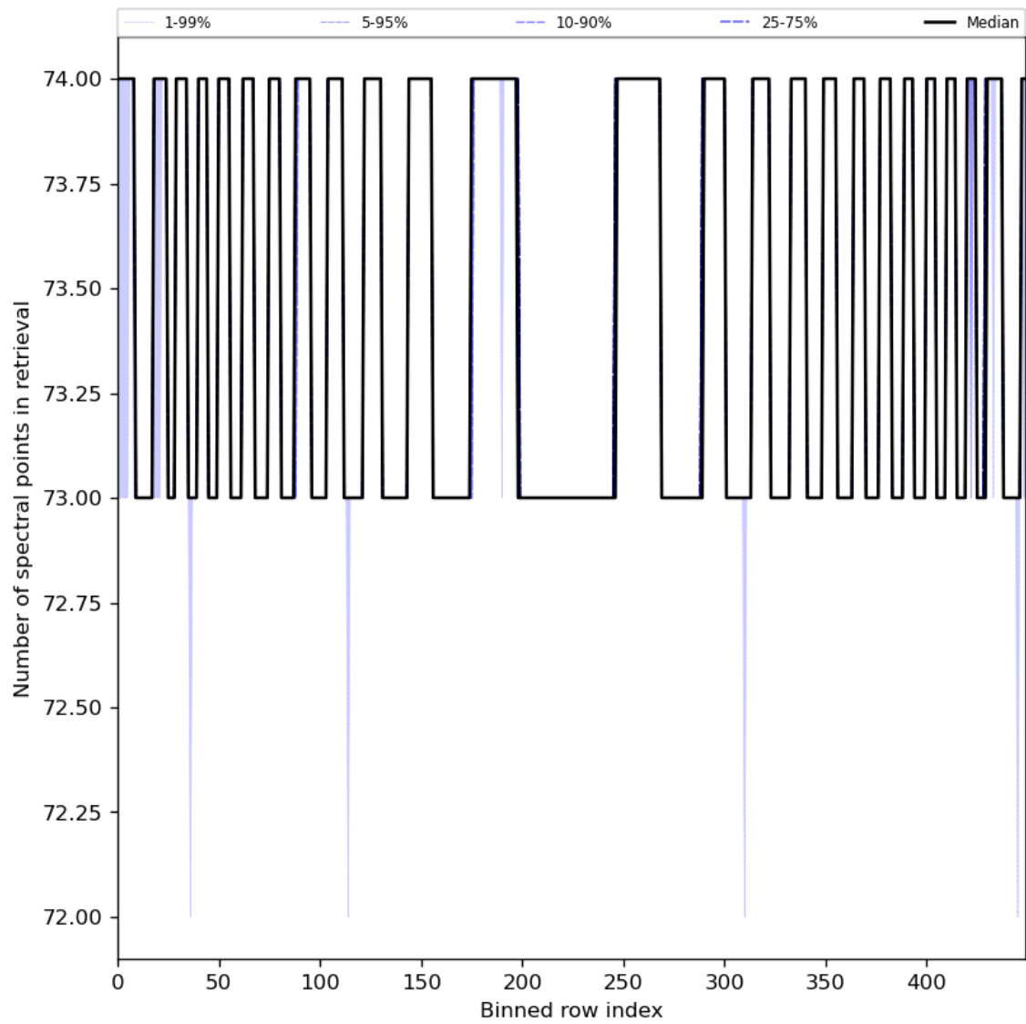
Figure 97: Along track statistics of “Number of spectral points in retrieval” for 2024-01-16 to 2024-01-18
