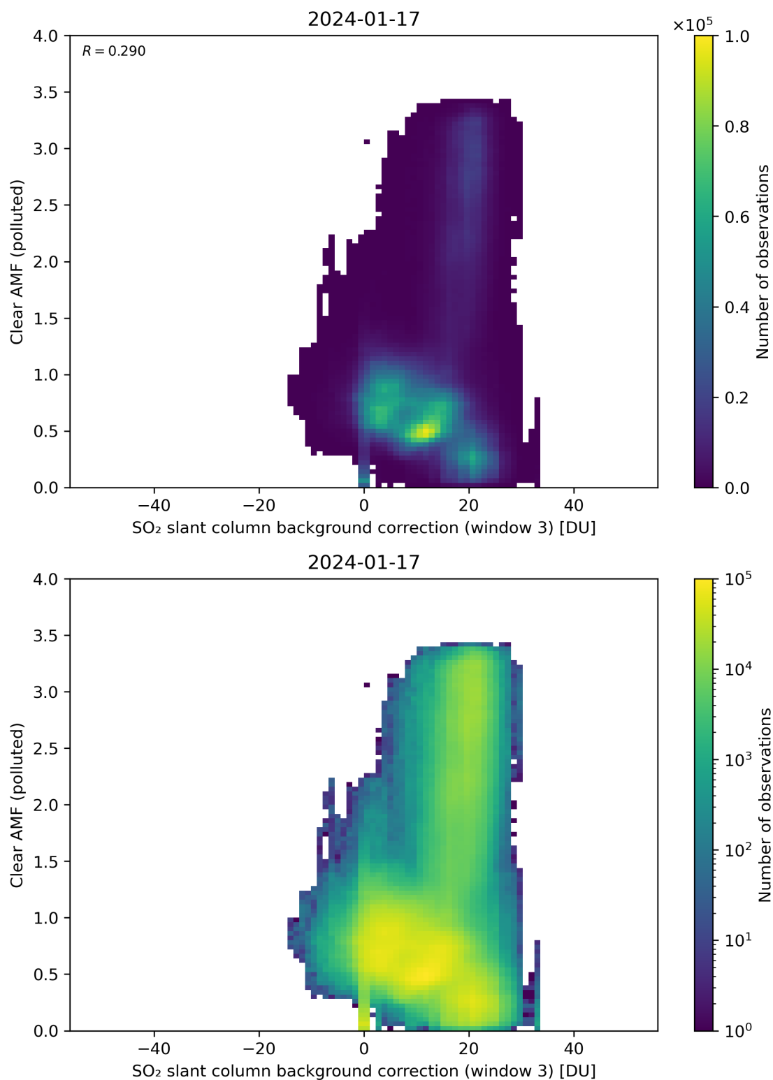
Figure 124: Scatter density plot of “SO 2 slant column background correction (window 3)” against “Clear AMF (polluted)” for 2024-01-16 to 2024-01-18.
