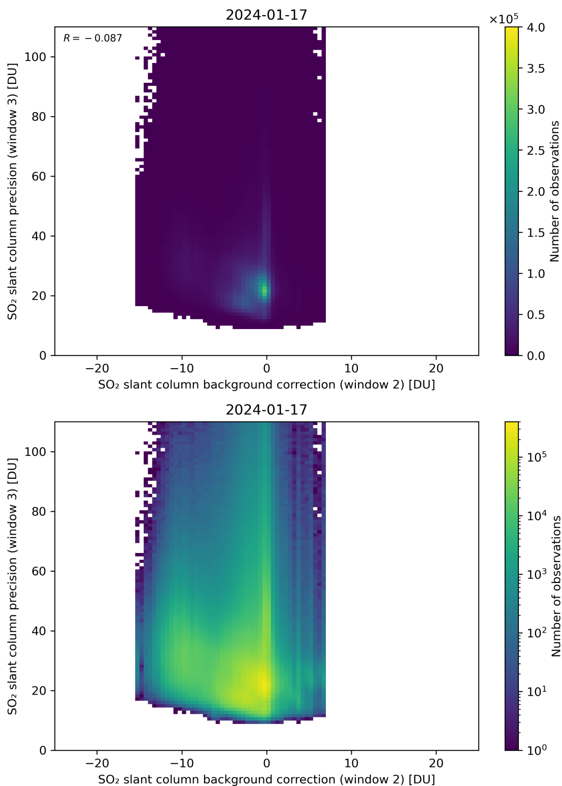
Figure 118: Scatter density plot of “SO 2 slant column background correction (window 2)” against “SO 2 slant column precision (window 3)” for 2024-01-16 to 2024-01-18.
