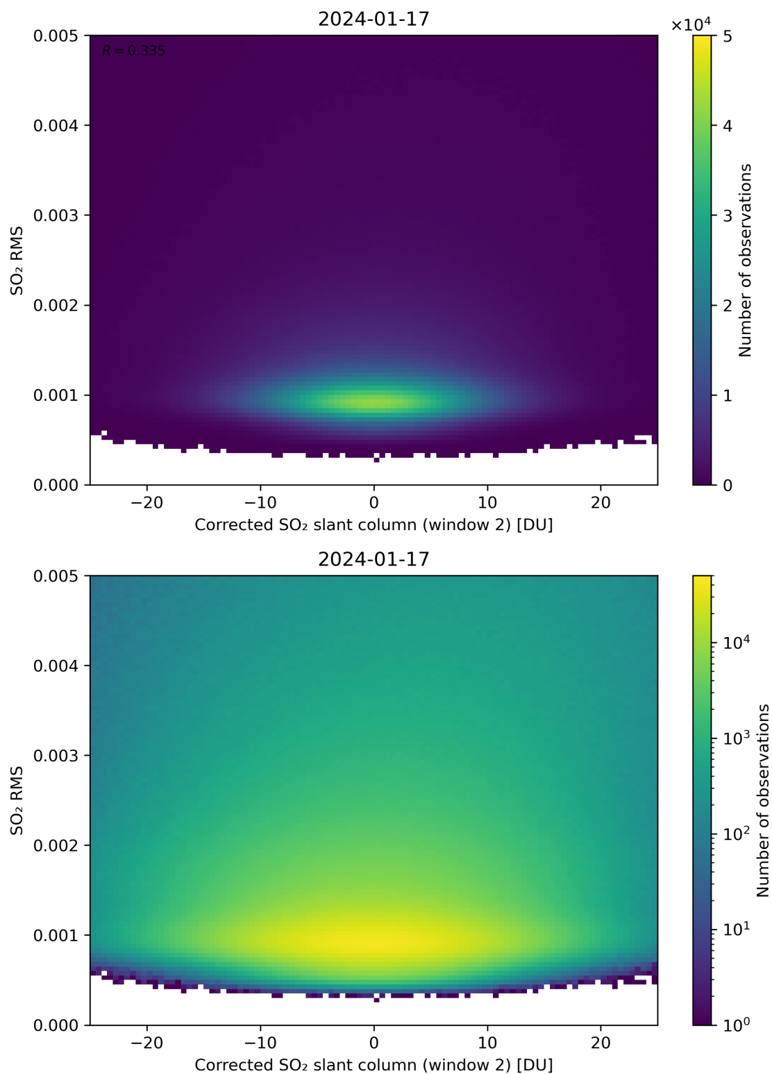
Figure 198: Scatter density plot of “Corrected SO 2 slant column (window 2)” against “SO 2 RMS” for 2024-01-16 to 2024-01-18.
