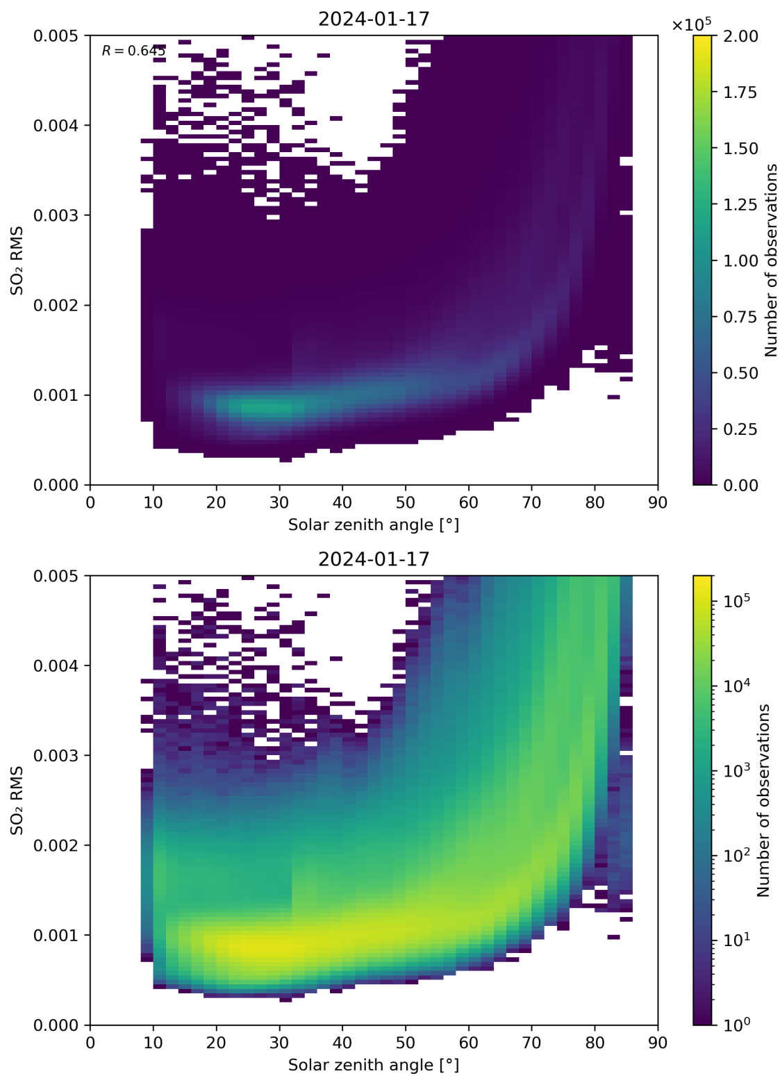
Figure 163: Scatter density plot of “Solar zenith angle” against “SO 2 RMS” for 2024-01-16 to 2024-01-18.
