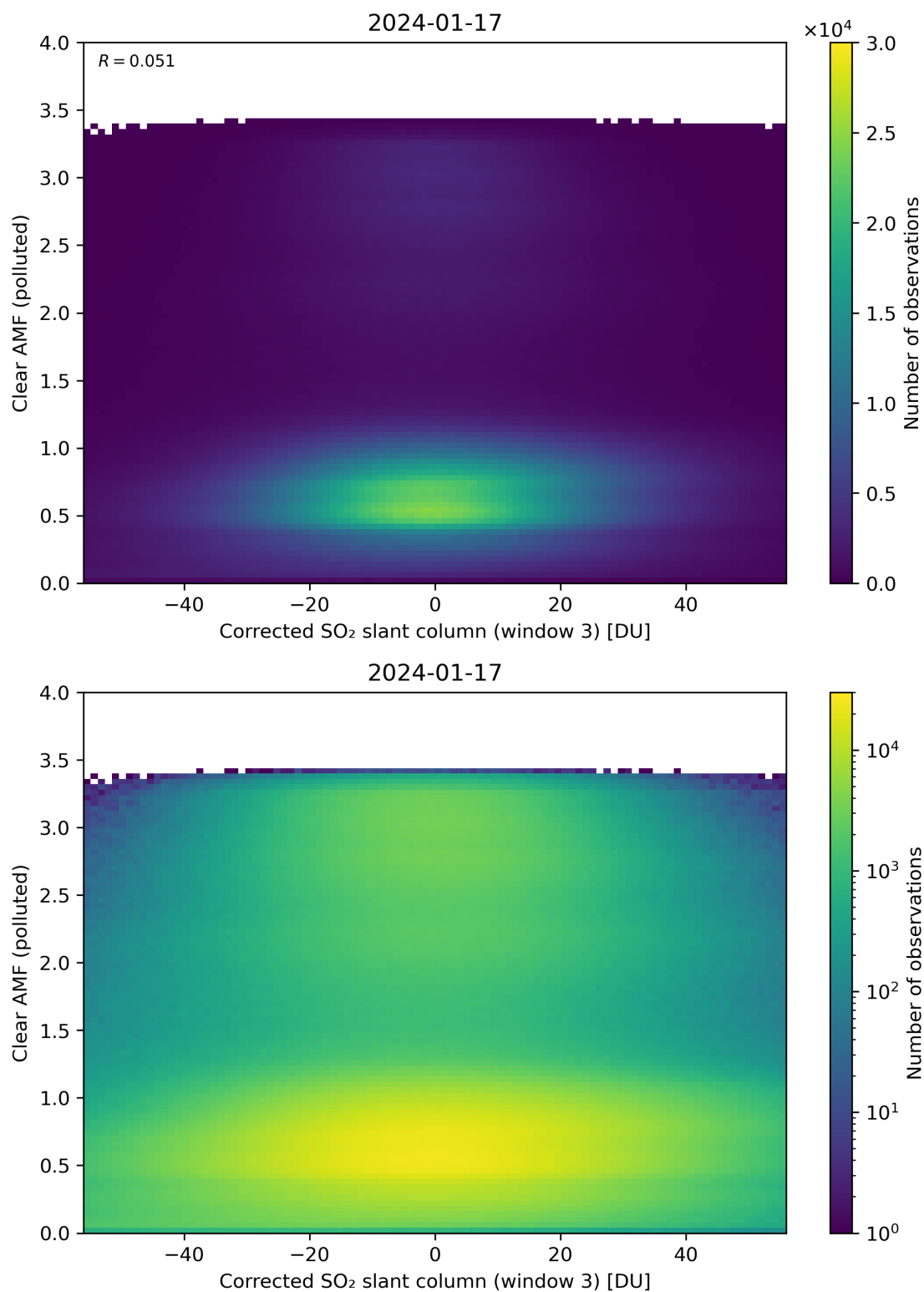
Figure 209: Scatter density plot of “Corrected SO 2 slant column (window 3)” against “Clear AMF (polluted)” for 2024-01-16 to 2024-01-18.
