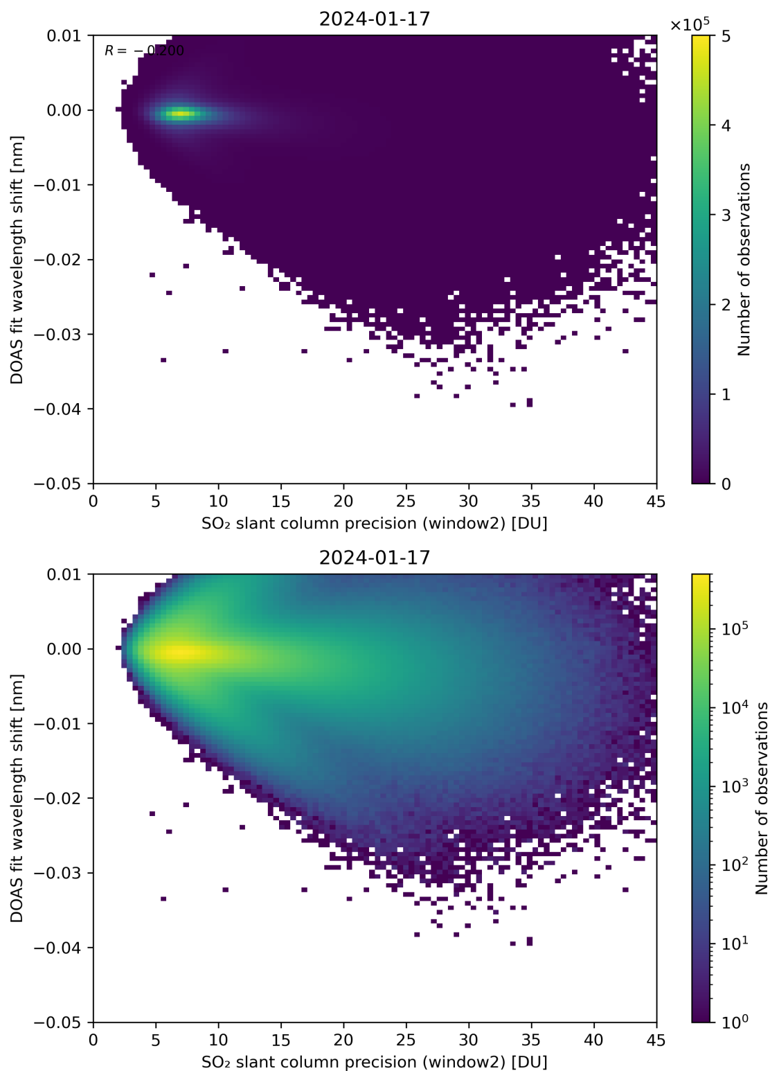
Figure 243: Scatter density plot of “SO 2 slant column precision (window2)” against “DOAS fit wavelength shift” for 2024-01-16 to 2024-01-18.
