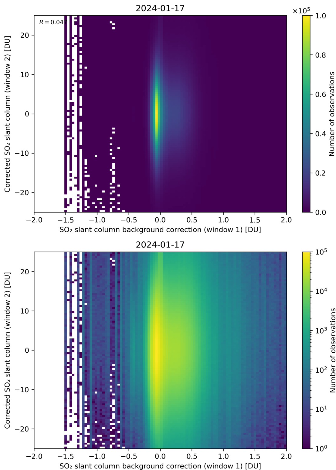
Figure 104: Scatter density plot of “SO 2 slant column background correction (window 1)” against “Corrected SO 2 slant column (window 2)” for 2024-01-16 to 2024-01-18.
