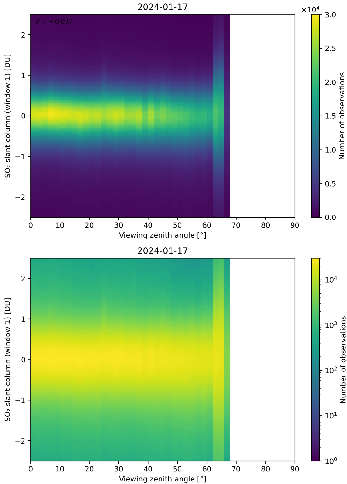
Figure 320: Scatter density plot of “Viewing zenith angle” against “SO 2 slant column (window 1)” for 2024-01-16 to 2024-01-18.
