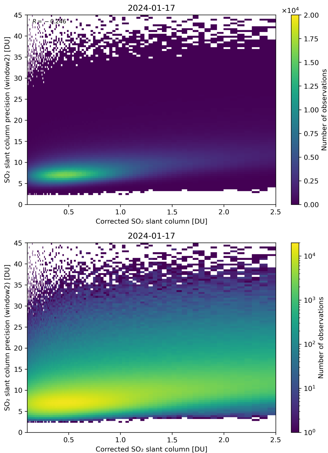
Figure 189: Scatter density plot of “Corrected SO 2 slant column” against “SO 2 slant column precision (window2)” for 2024-01-16 to 2024-01-18.
