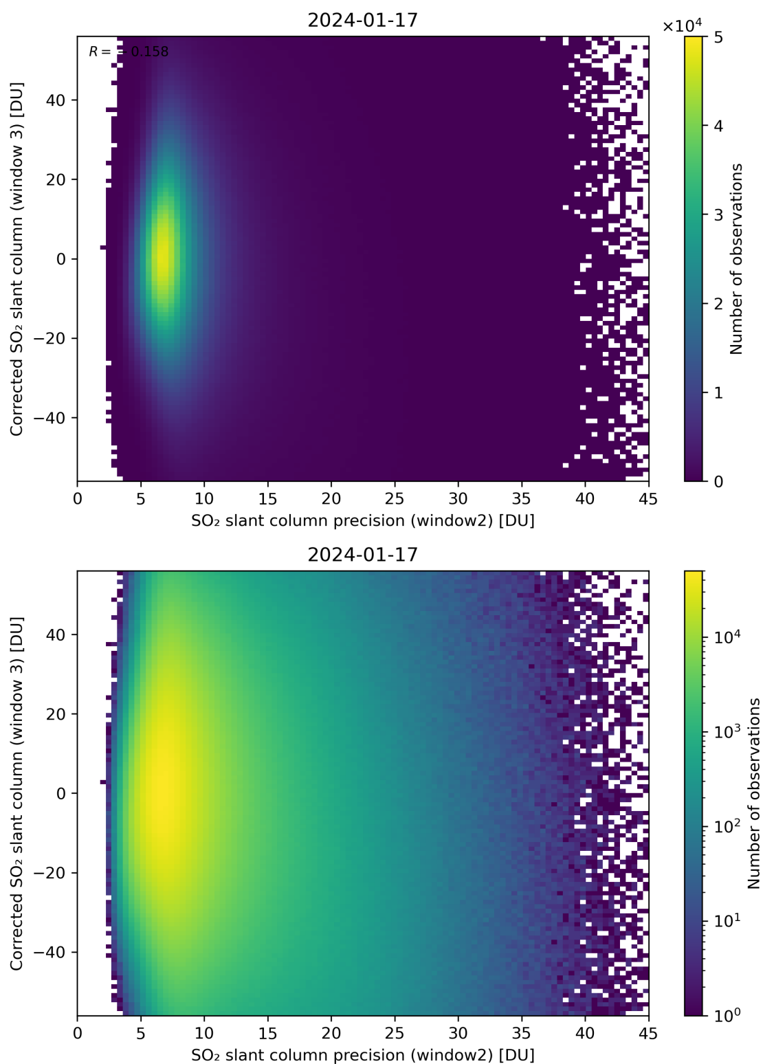
Figure 248: Scatter density plot of “SO 2 slant column precision (window2)” against “Corrected SO 2 slant column (window 3)” for 2024-01-16 to 2024-01-18.
