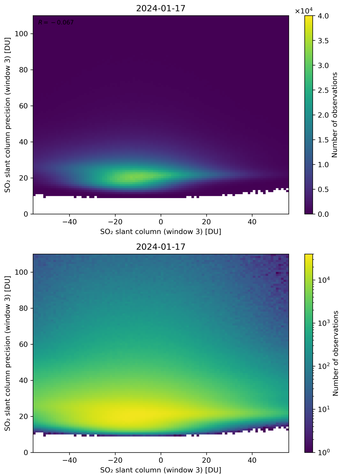
Figure 267: Scatter density plot of “SO 2 slant column (window 3)” against “SO 2 slant column precision (window 3)” for 2024-01-16 to 2024-01-18.
