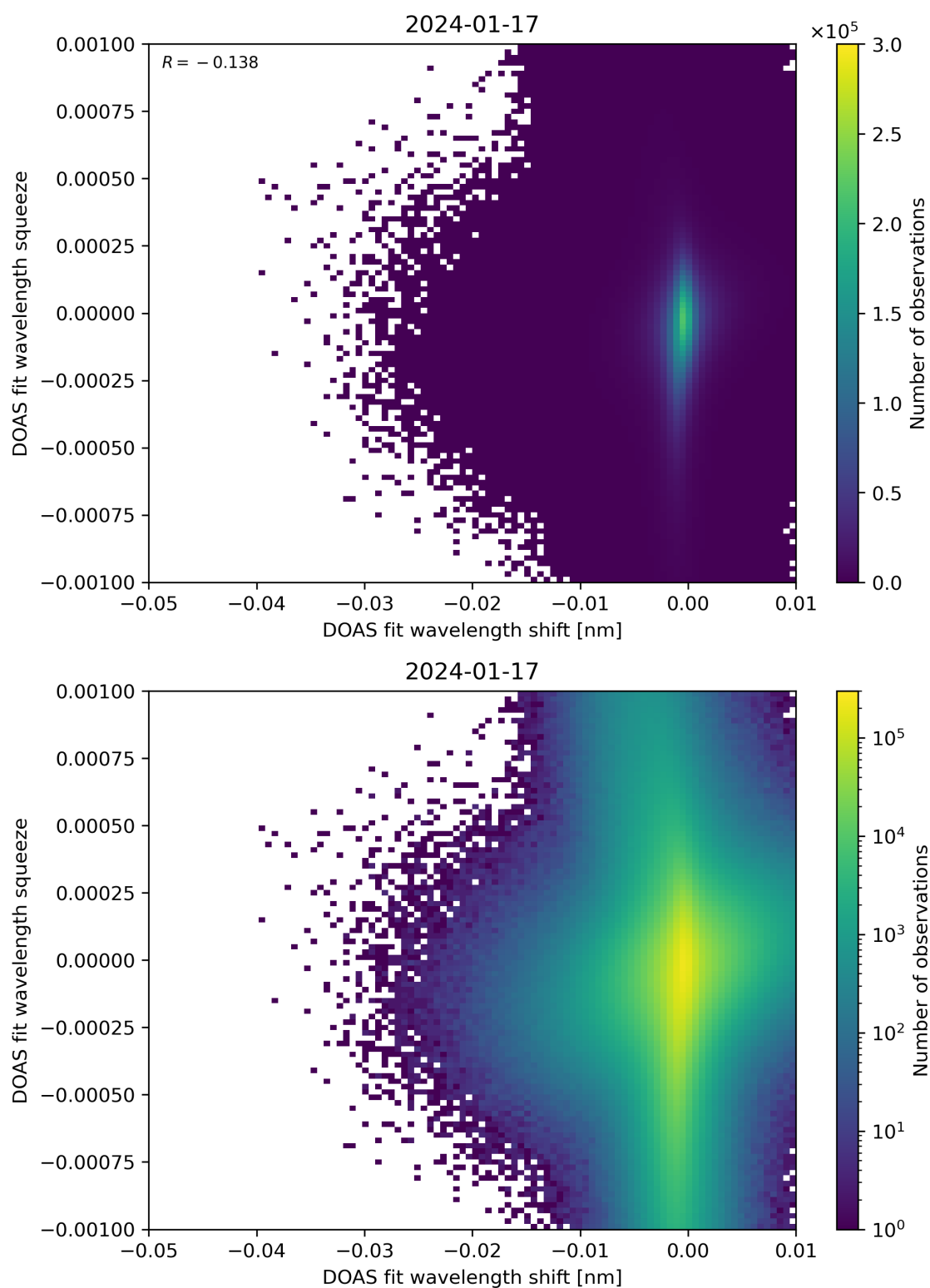
Figure 127: Scatter density plot of “DOAS fit wavelength shift” against “DOAS fit wavelength squeeze” for 2024-01-16 to 2024-01-18.
