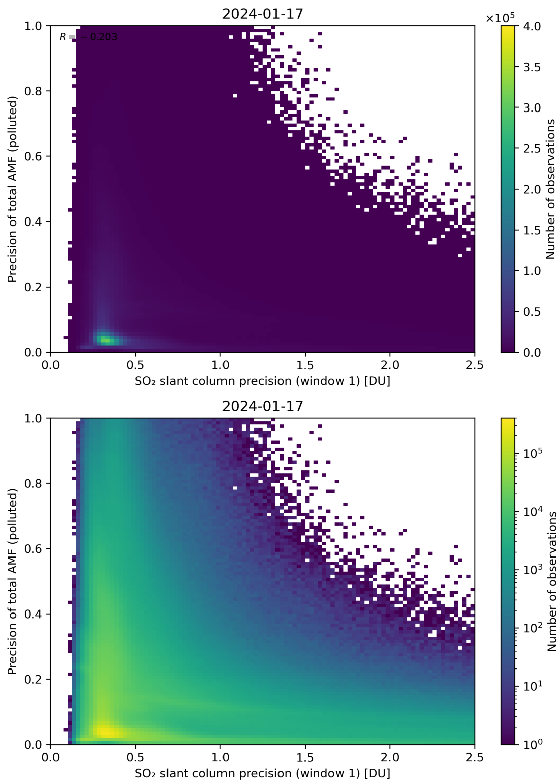
Figure 231: Scatter density plot of “SO 2 slant column precision (window 1)” against “Precision of total AMF (polluted)” for 2024-01-16 to 2024-01-18.
