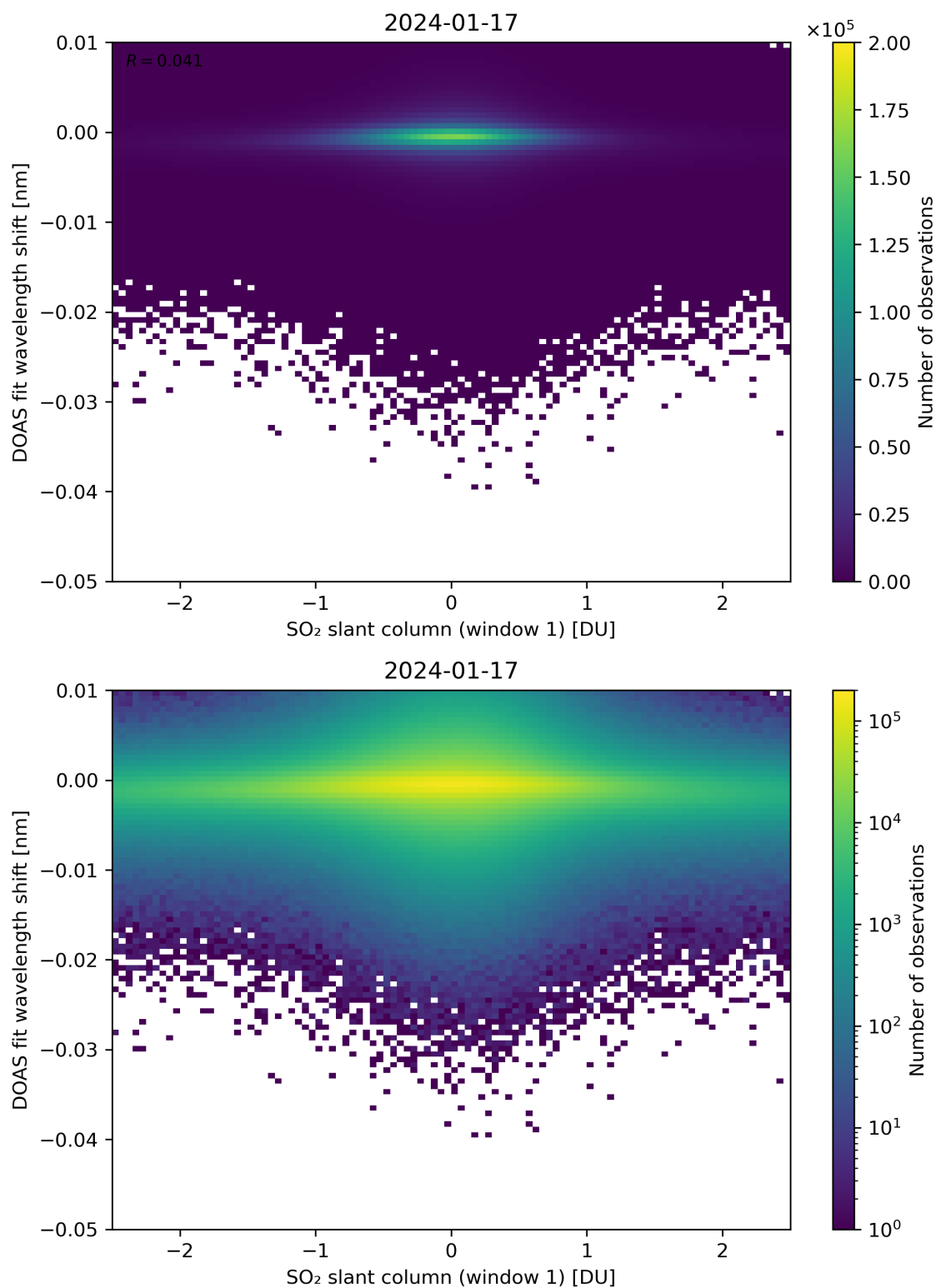
Figure 215: Scatter density plot of “SO 2 slant column (window 1)” against “DOAS fit wavelength shift” for 2024-01-16 to 2024-01-18.
