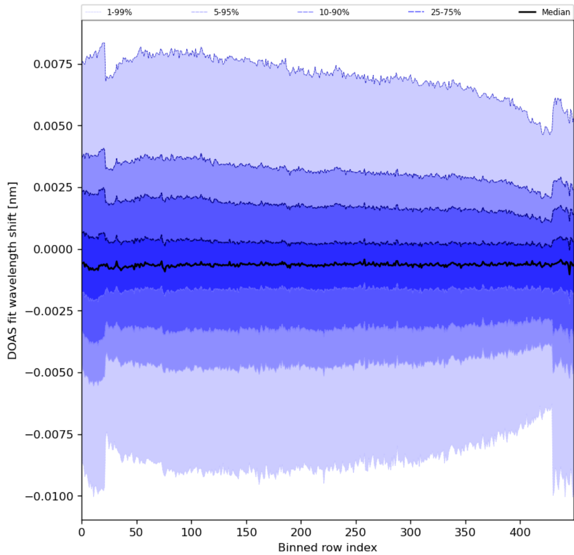
Figure 91: Along track statistics of “DOAS fit wavelength shift” for 2024-01-16 to 2024-01-18
