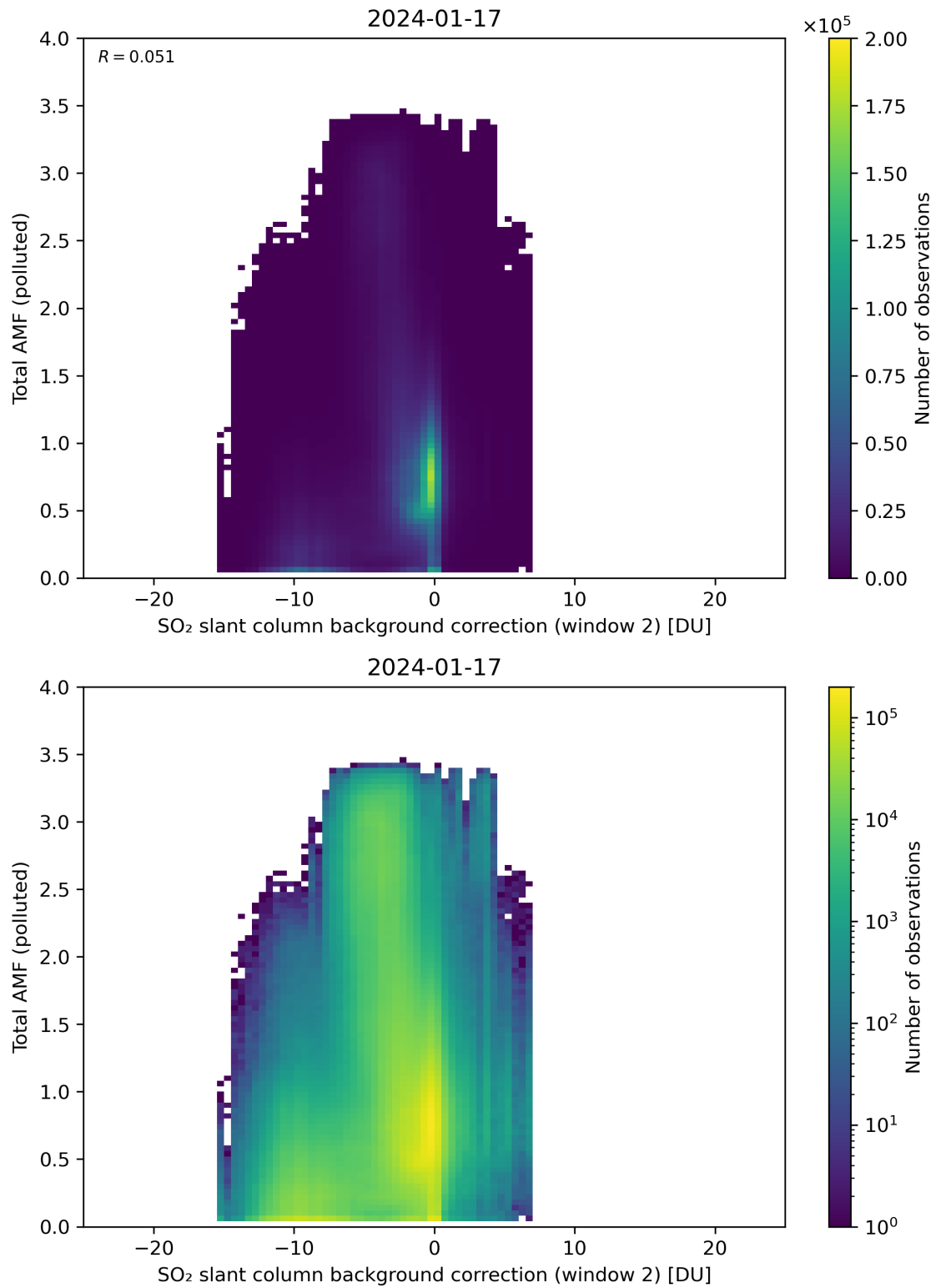
Figure 119: Scatter density plot of “SO 2 slant column background correction (window 2)” against “Total AMF (polluted)” for 2024-01-16 to 2024-01-18.
