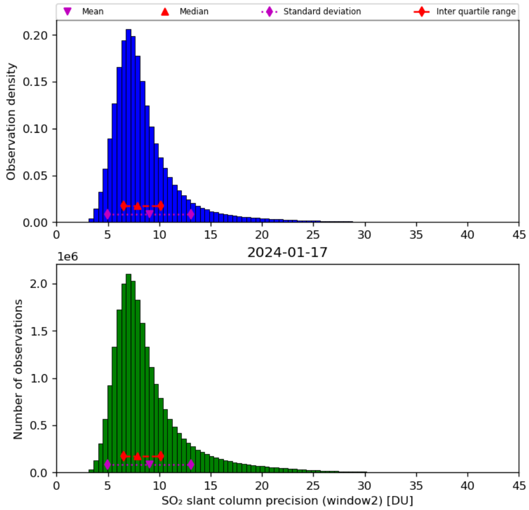
Figure 61: Histogram of “SO 2 slant column precision (window2)” for 2024-01-16 to 2024-01-18
