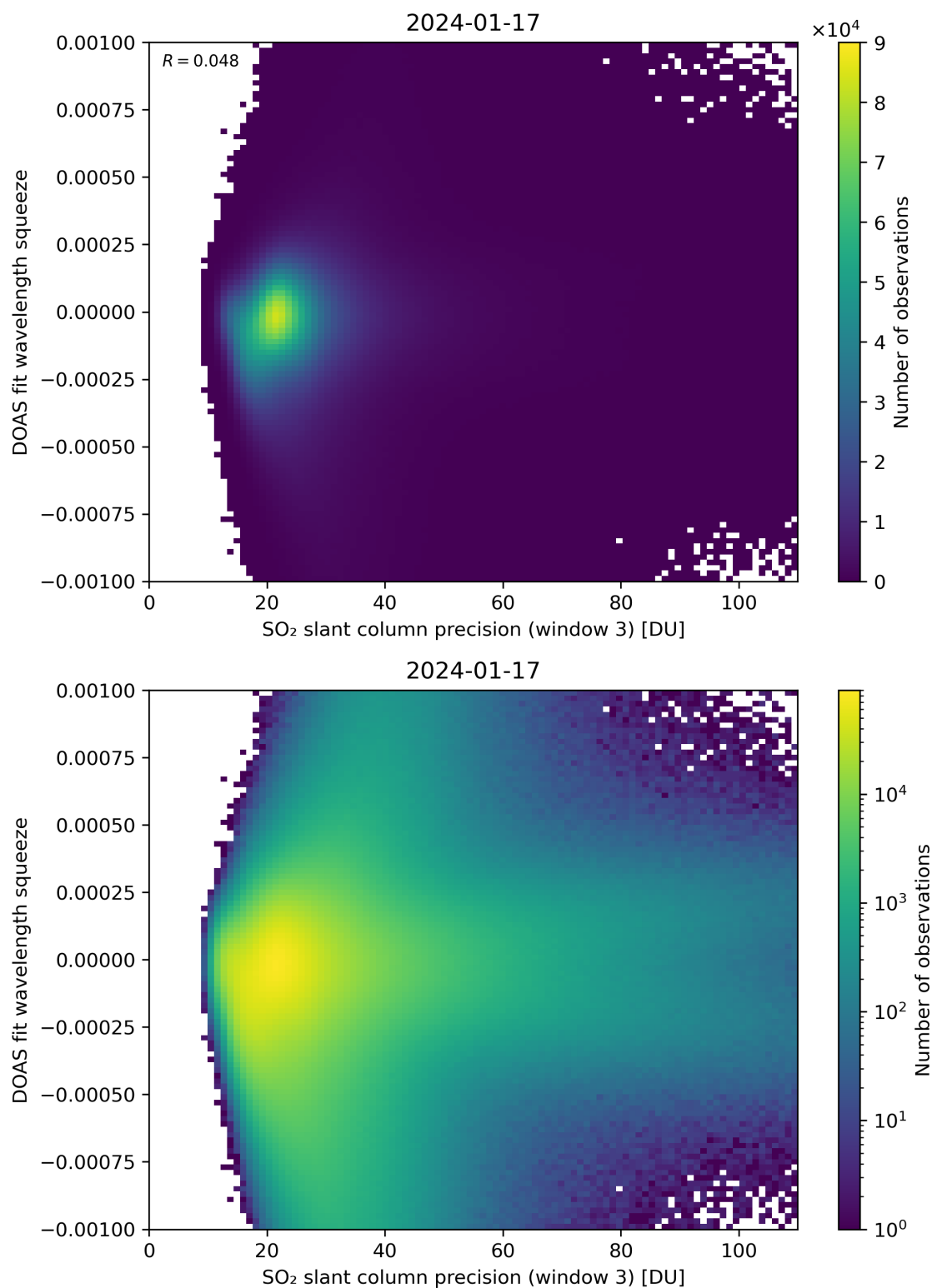
Figure 259: Scatter density plot of “SO 2 slant column precision (window 3)” against “DOAS fit wavelength squeeze” for 2024-01-16 to 2024-01-18.
