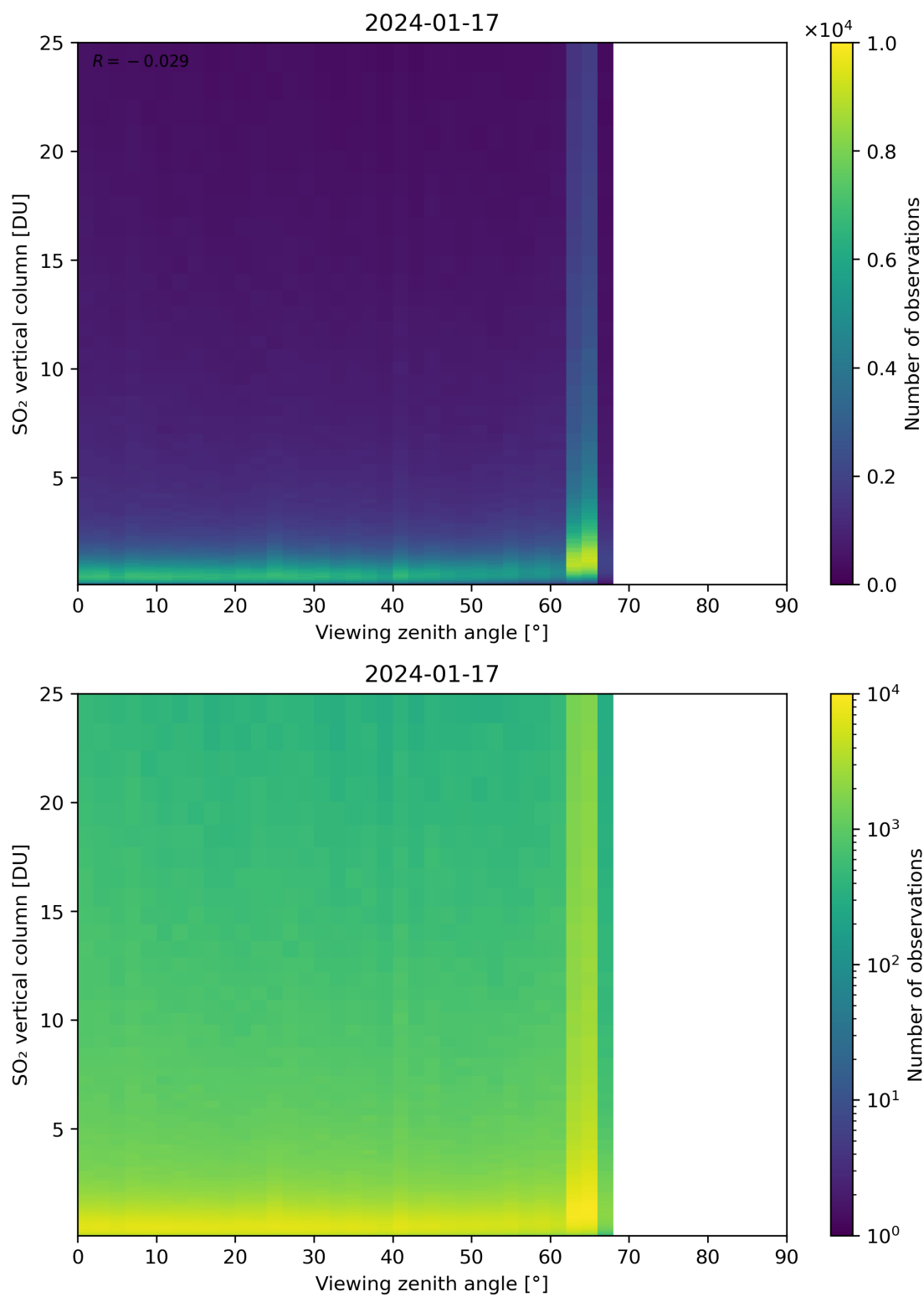
Figure 327: Scatter density plot of “Viewing zenith angle” against “SO 2 vertical column” for 2024-01-16 to 2024-01-18.
