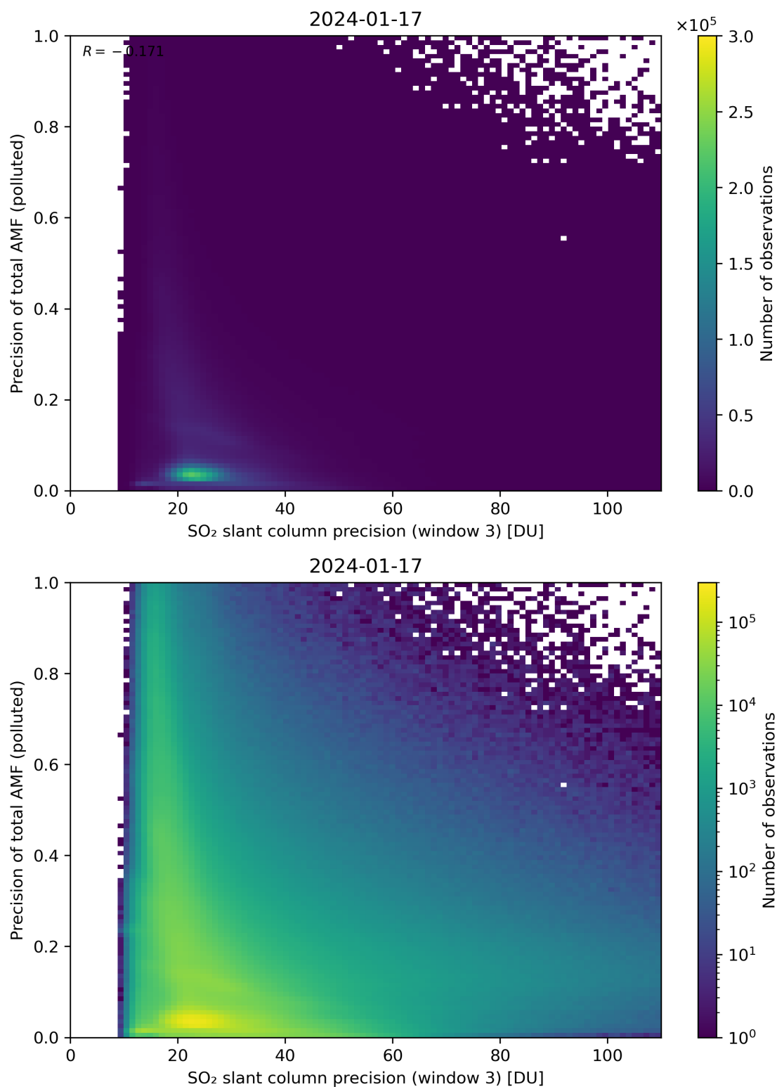
Figure 264: Scatter density plot of “SO 2 slant column precision (window 3)” against “Precision of total AMF (polluted)” for 2024-01-16 to 2024-01-18.
