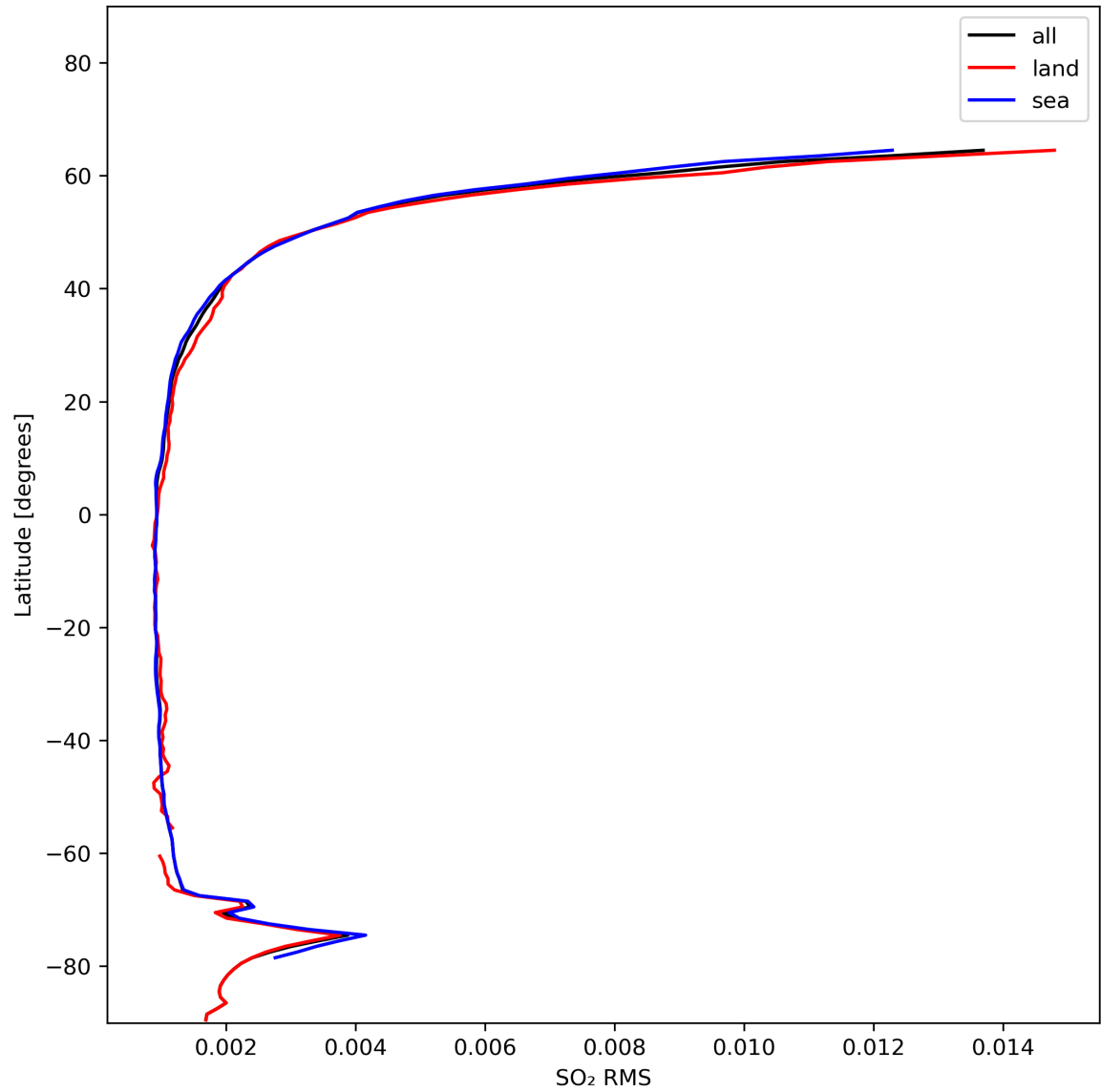
Figure 47: Zonal average of “SO 2 RMS” for 2024-01-16 to 2024-01-18.
