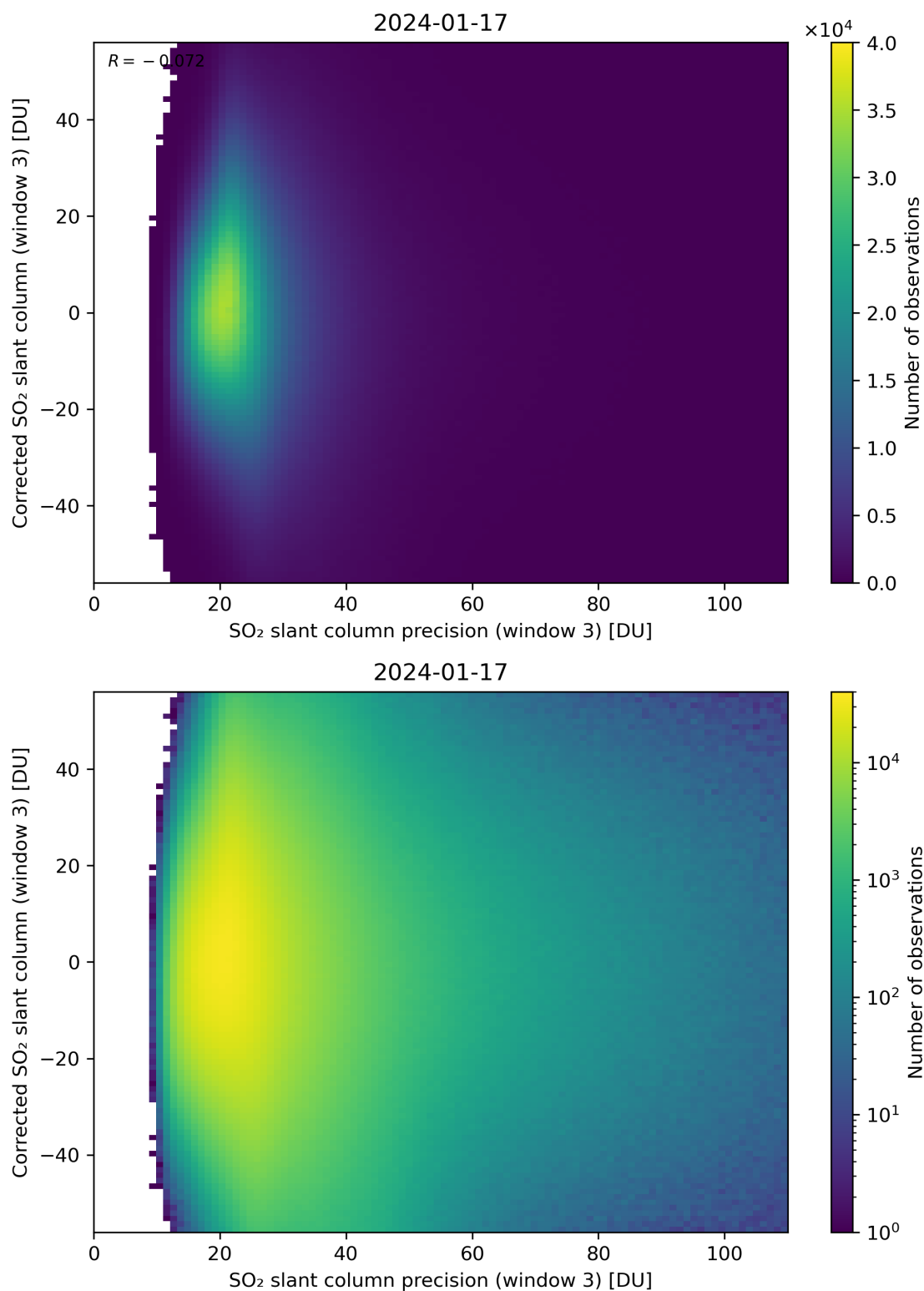
Figure 262: Scatter density plot of “SO 2 slant column precision (window 3)” against “Corrected SO 2 slant column (window 3)” for 2024-01-16 to 2024-01-18.
