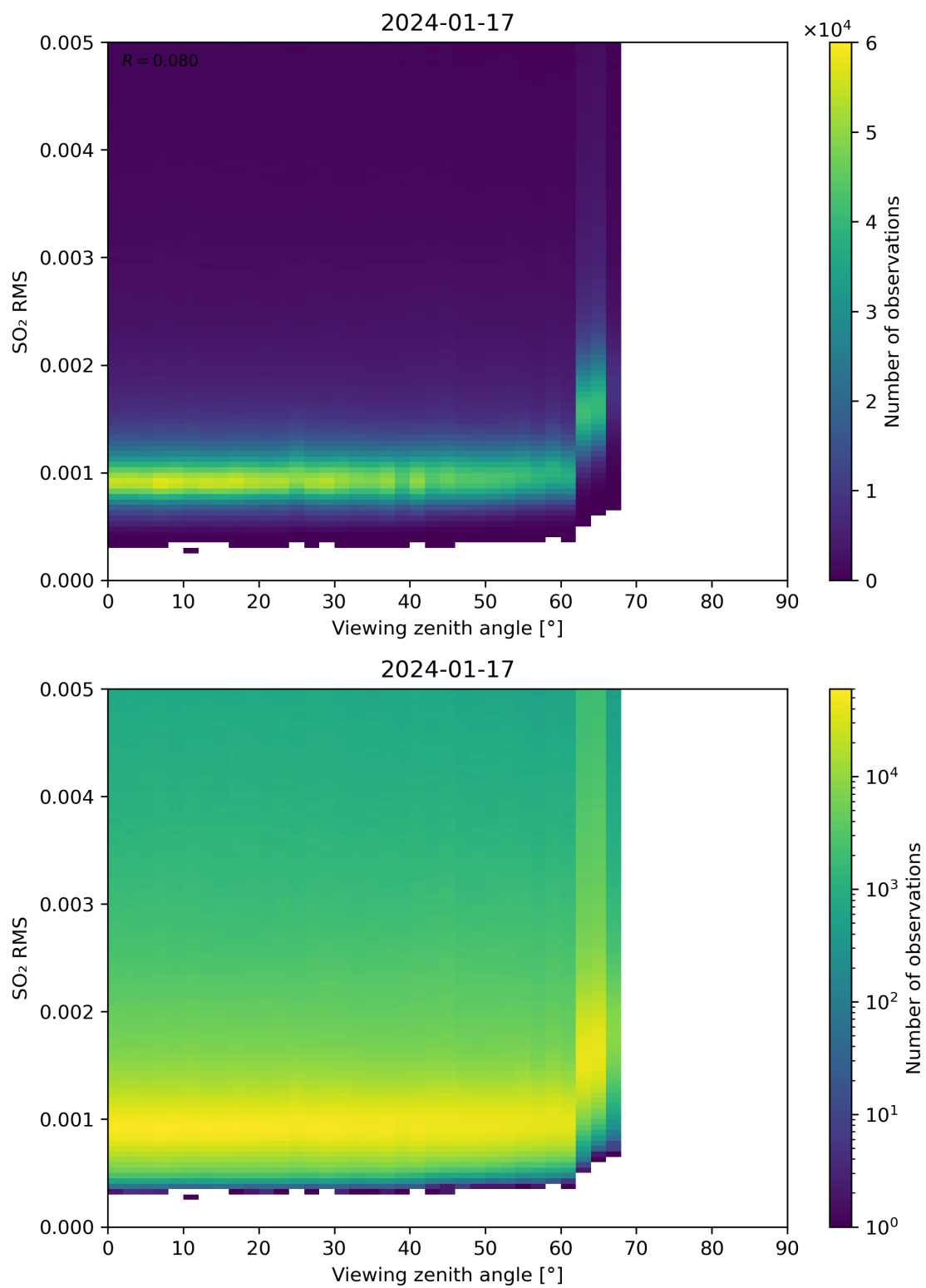
Figure 313: Scatter density plot of “Viewing zenith angle” against “SO 2 RMS” for 2024-01-16 to 2024-01-18.
