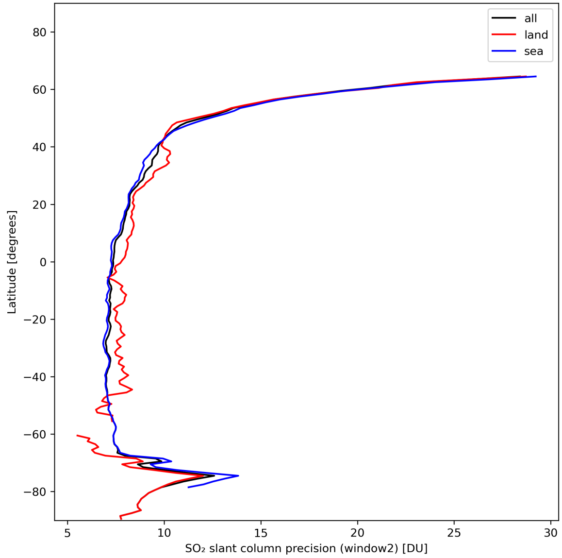
Figure 38: Zonal average of “SO 2 slant column precision (window2)” for 2024-01-16 to 2024-01-18.
