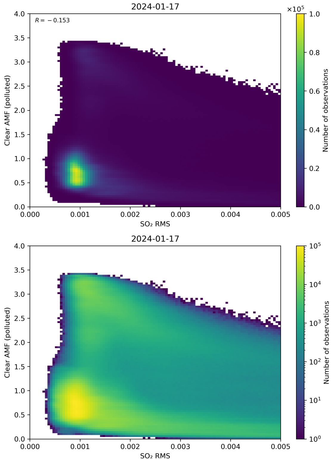
Figure 136: Scatter density plot of “SO 2 RMS” against “Clear AMF (polluted)” for 2024-01-16 to 2024-01-18.
