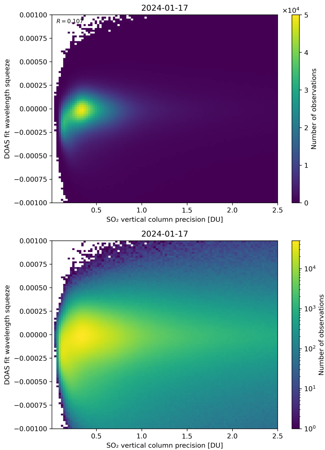
Figure 283: Scatter density plot of “SO 2 vertical column precision” against “DOAS fit wavelength squeeze” for 2024-01-16 to 2024-01-18.
