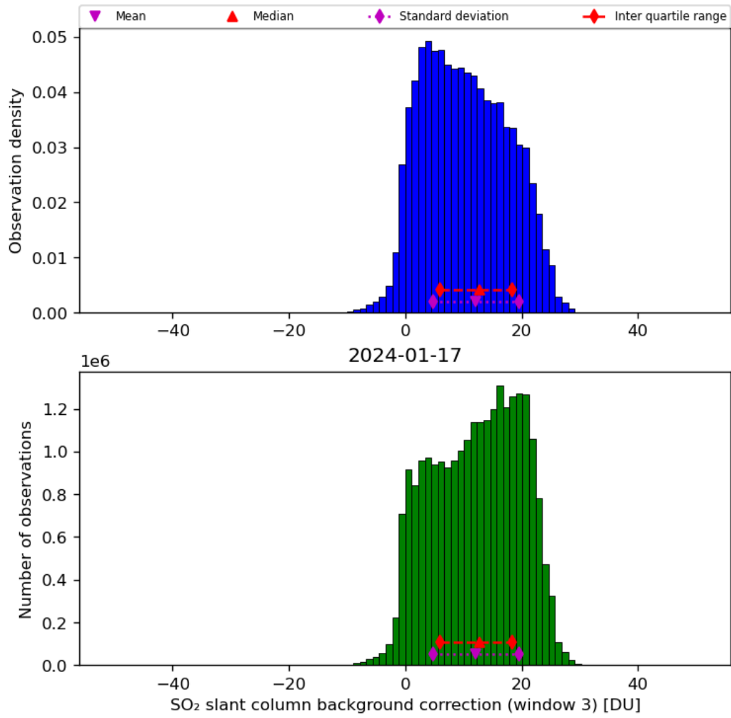
Figure 67: Histogram of “SO 2 slant column background correction (window 3)” for 2024-01-16 to 2024-01-18
