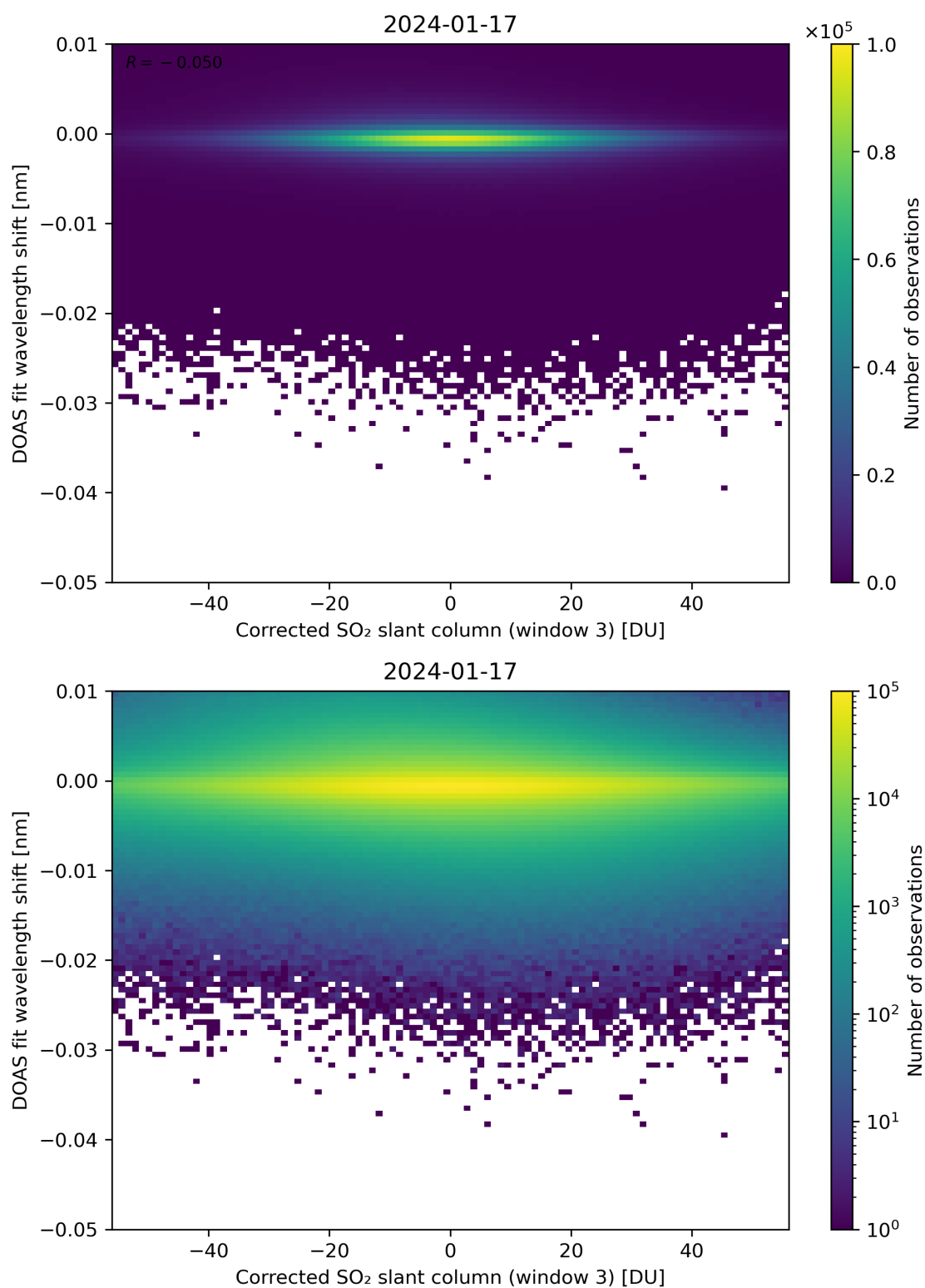
Figure 206: Scatter density plot of “Corrected SO 2 slant column (window 3)” against “DOAS fit wavelength shift” for 2024-01-16 to 2024-01-18.
