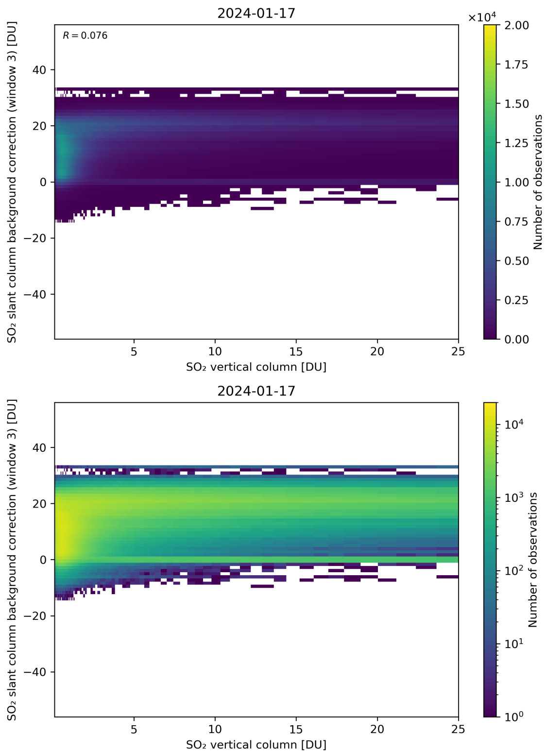
Figure 275: Scatter density plot of “SO 2 vertical column” against “SO 2 slant column background correction (window 3)” for 2024-01-16 to 2024-01-18.
