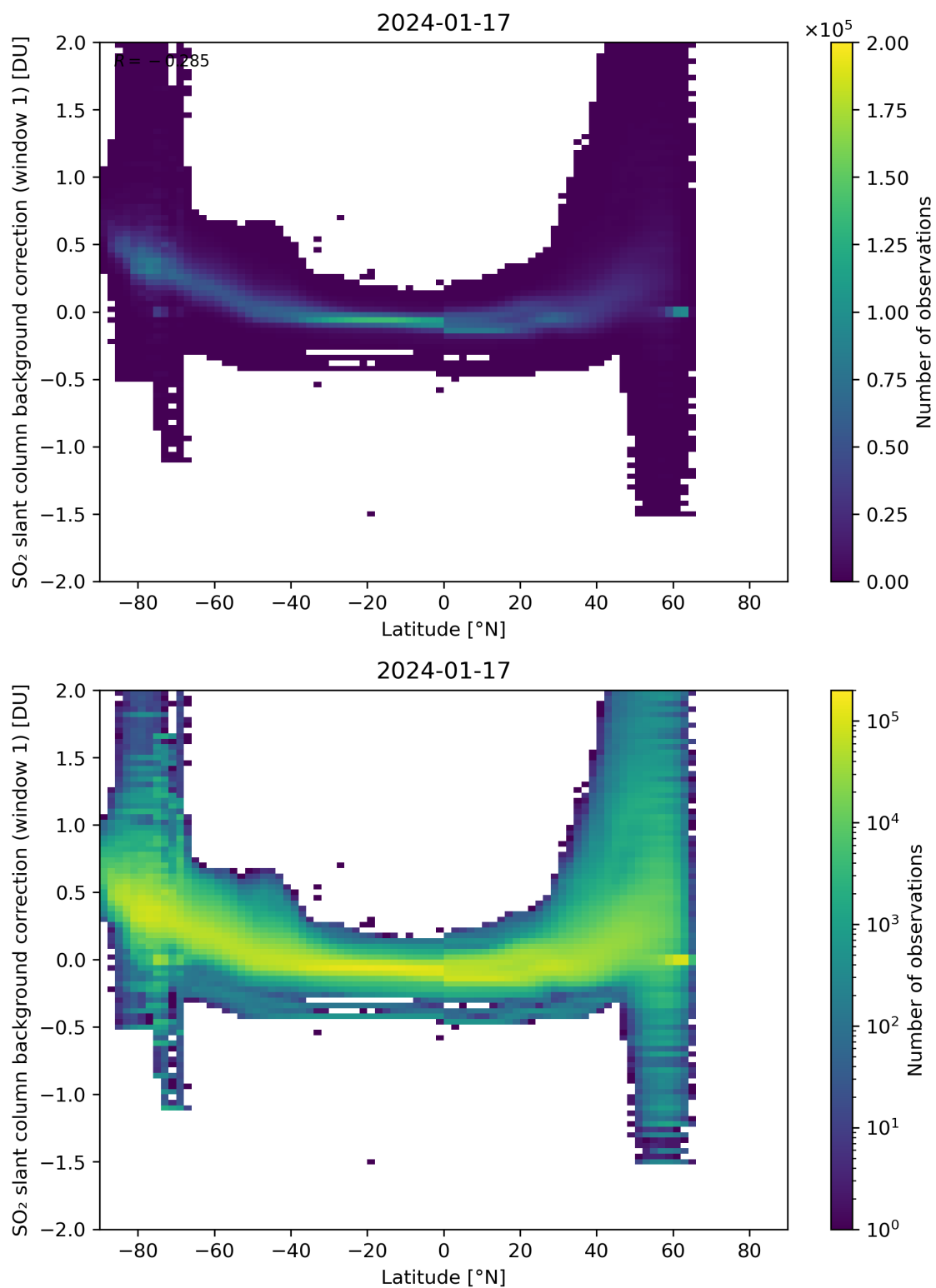
Figure 139: Scatter density plot of “Latitude” against “SO 2 slant column background correction (window 1)” for 2024-01-16 to 2024-01-18.
