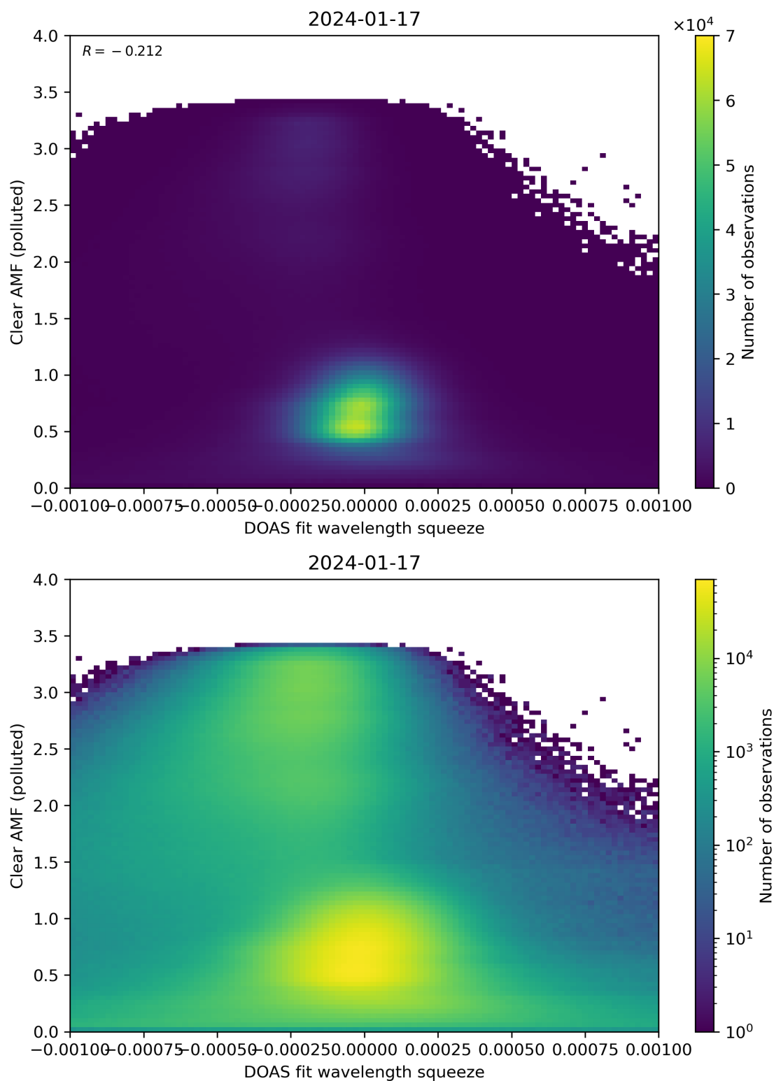
Figure 133: Scatter density plot of “DOAS fit wavelength squeeze” against “Clear AMF (polluted)” for 2024-01-16 to 2024-01-18.
