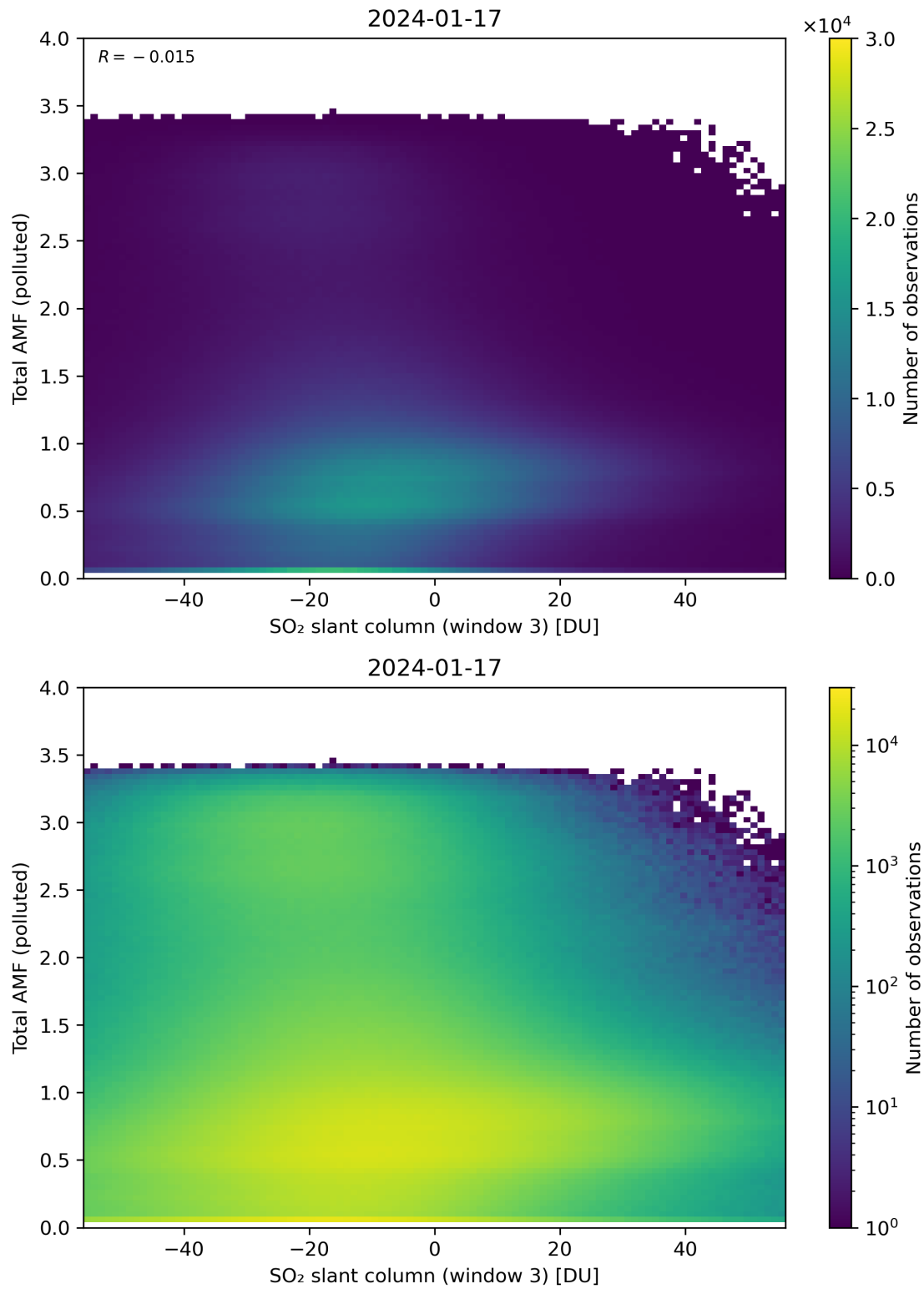
Figure 268: Scatter density plot of “SO 2 slant column (window 3)” against “Total AMF (polluted)” for 2024-01-16 to 2024-01-18.
