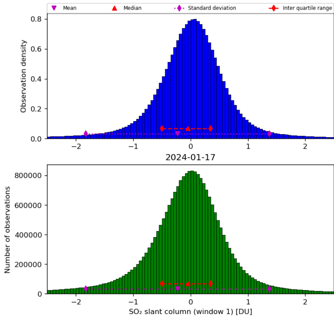
Figure 56: Histogram of “SO 2 slant column (window 1)” for 2024-01-16 to 2024-01-18
