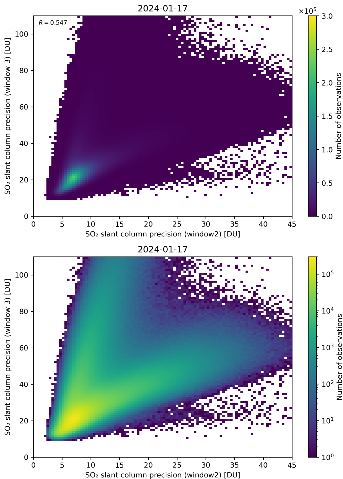
Figure 250: Scatter density plot of “SO 2 slant column precision (window2)” against “SO 2 slant column precision (window 3)” for 2024-01-16 to 2024-01-18.
