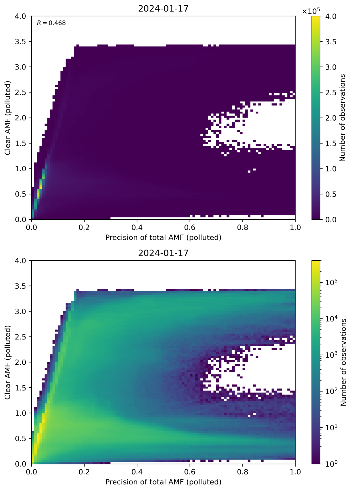
Figure 270: Scatter density plot of “Precision of total AMF (polluted)” against “Clear AMF (polluted)” for 2024-01-16 to 2024-01-18.
