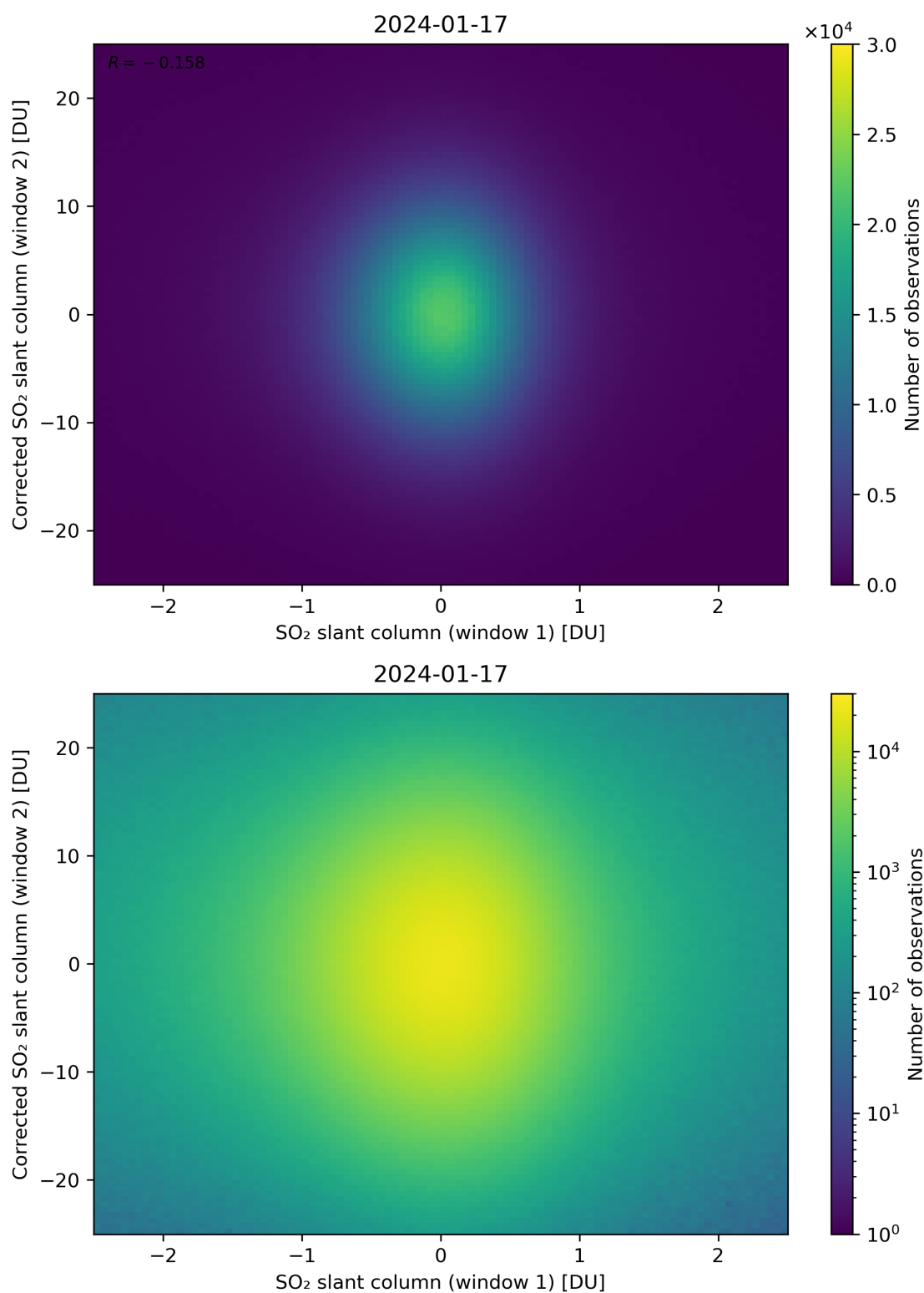
Figure 233: Scatter density plot of “SO 2 slant column (window 1)” against “Corrected SO 2 slant column (window 2)” for 2024-01-16 to 2024-01-18.
