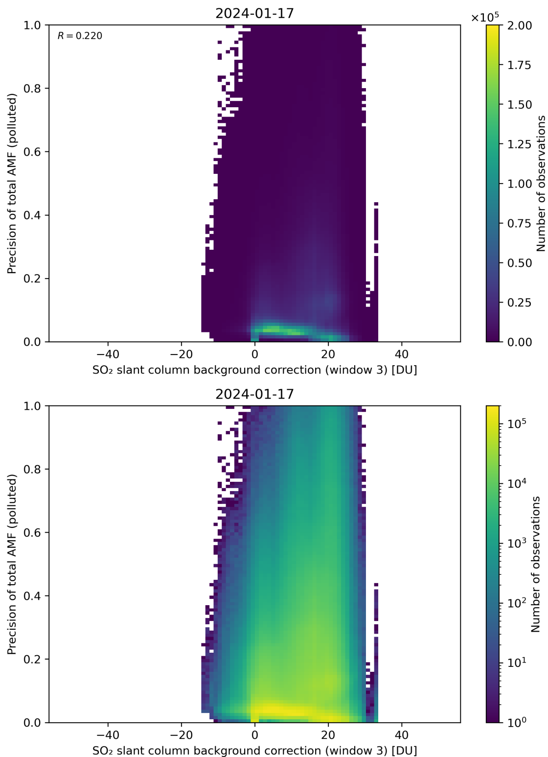
Figure 126: Scatter density plot of “SO 2 slant column background correction (window 3)” against “Precision of total AMF (polluted)” for 2024-01-16 to 2024-01-18.
