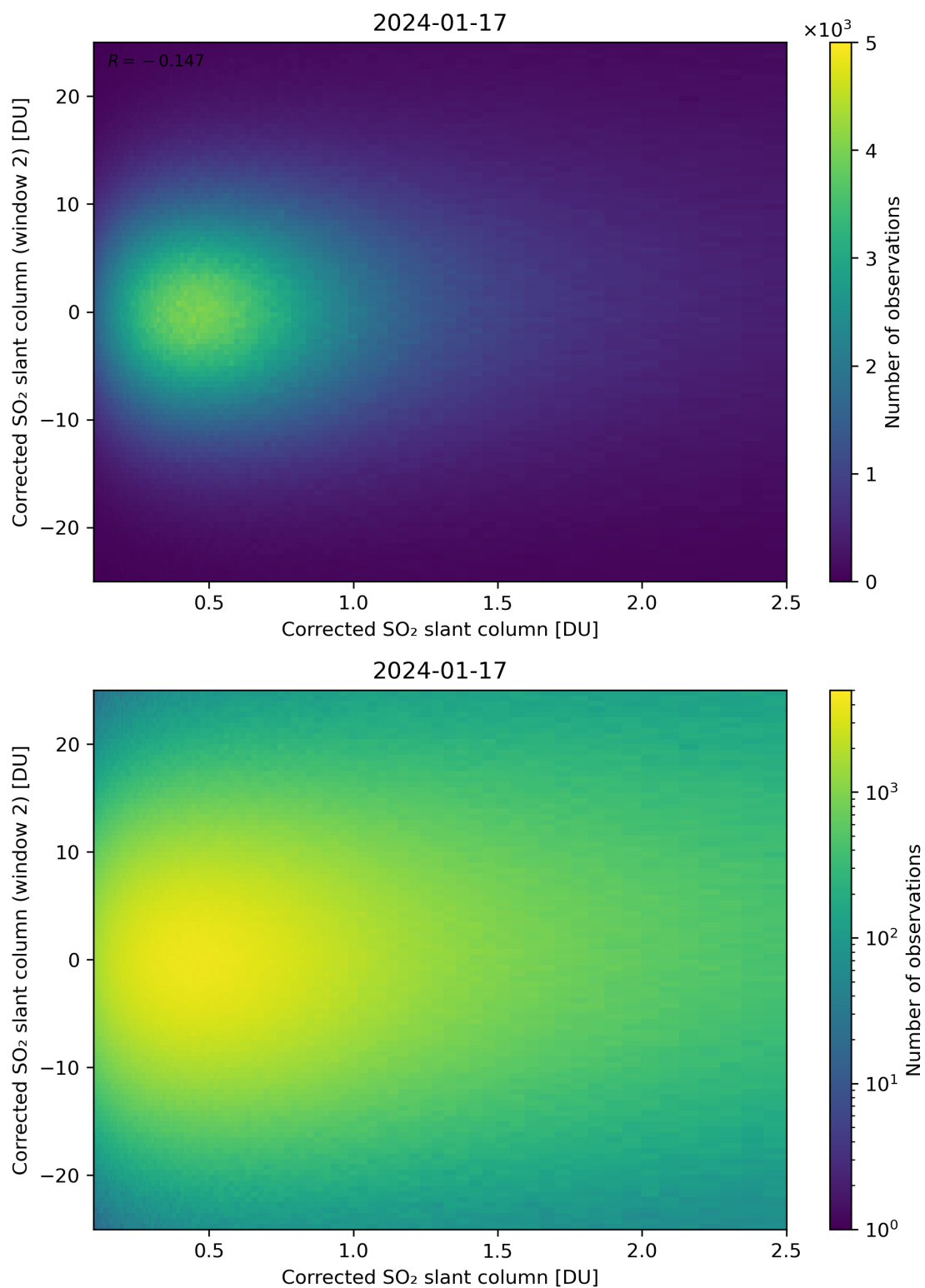
Figure 185: Scatter density plot of “Corrected SO 2 slant column” against “Corrected SO 2 slant column (window 2)” for 2024-01-16 to 2024-01-18.
