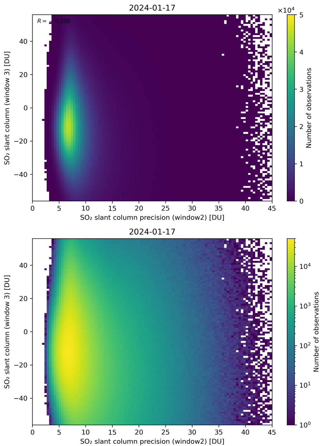
Figure 249: Scatter density plot of “SO 2 slant column precision (window2)” against “SO 2 slant column (window 3)” for 2024-01-16 to 2024-01-18.
