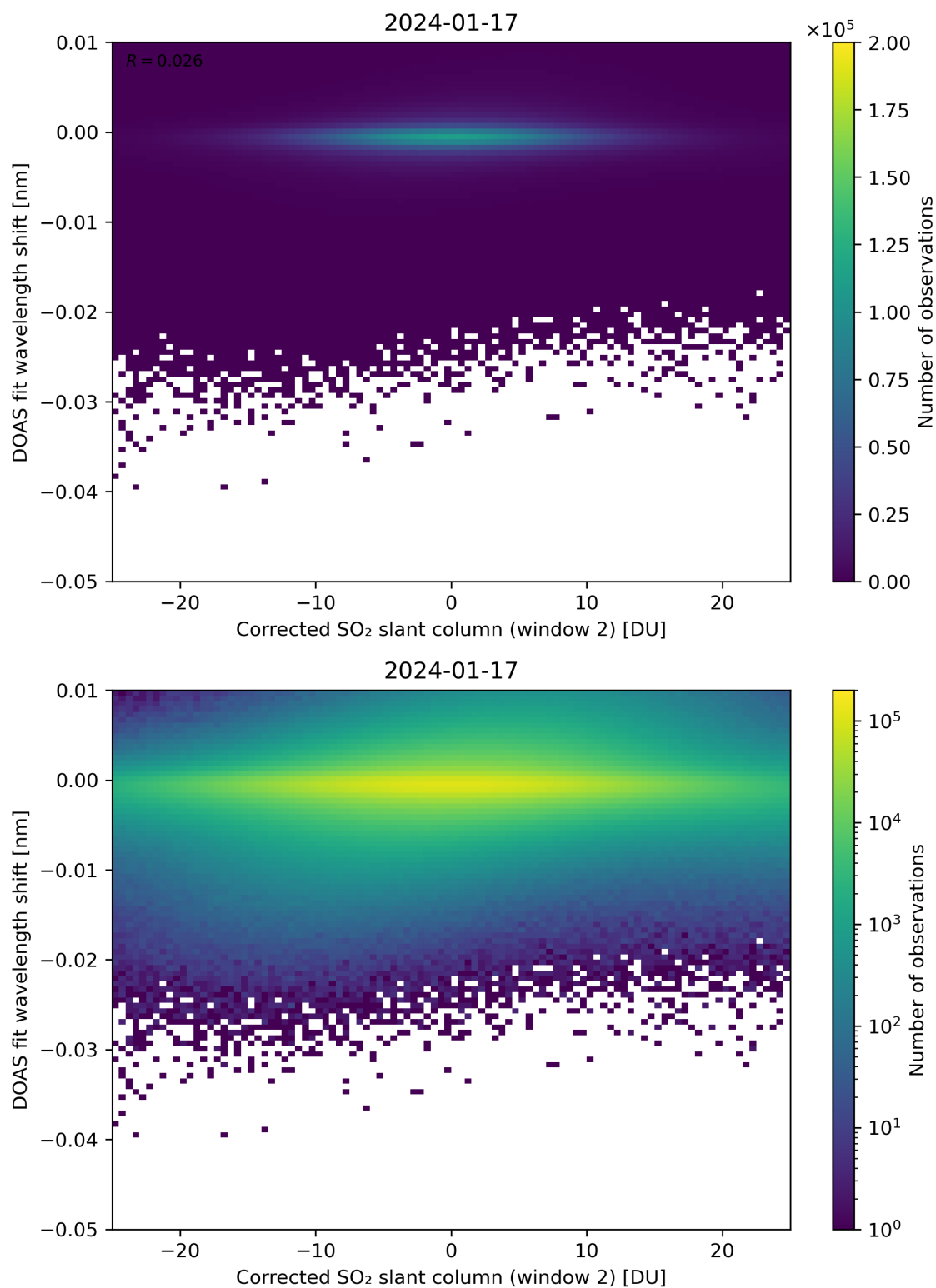
Figure 196: Scatter density plot of “Corrected SO 2 slant column (window 2)” against “DOAS fit wavelength shift” for 2024-01-16 to 2024-01-18.
