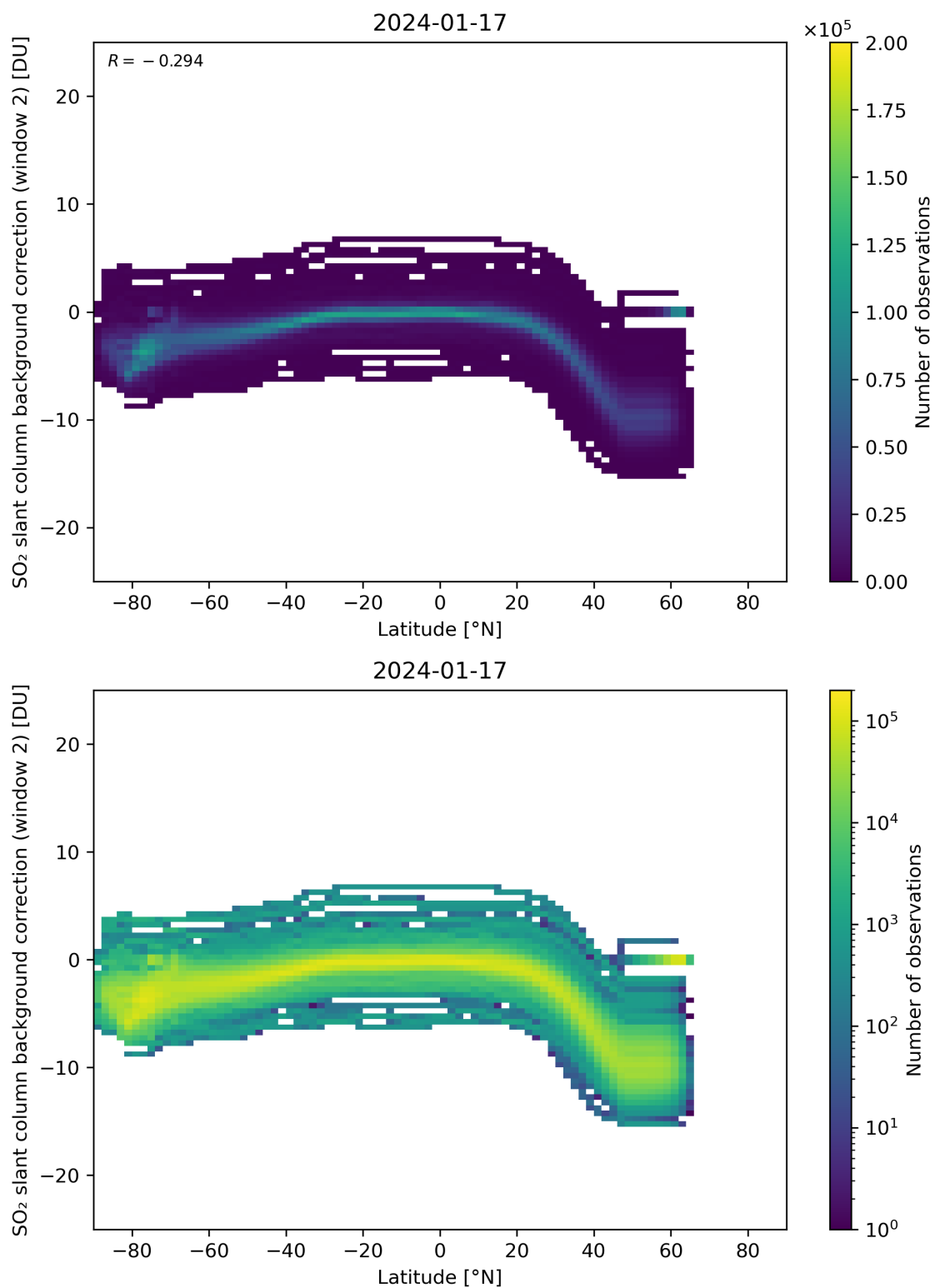
Figure 140: Scatter density plot of “Latitude” against “SO 2 slant column background correction (window 2)” for 2024-01-16 to 2024-01-18.
