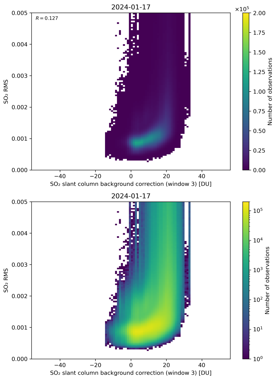
Figure 123: Scatter density plot of “SO 2 slant column background correction (window 3)” against “SO 2 RMS” for 2024-01-16 to 2024-01-18.
