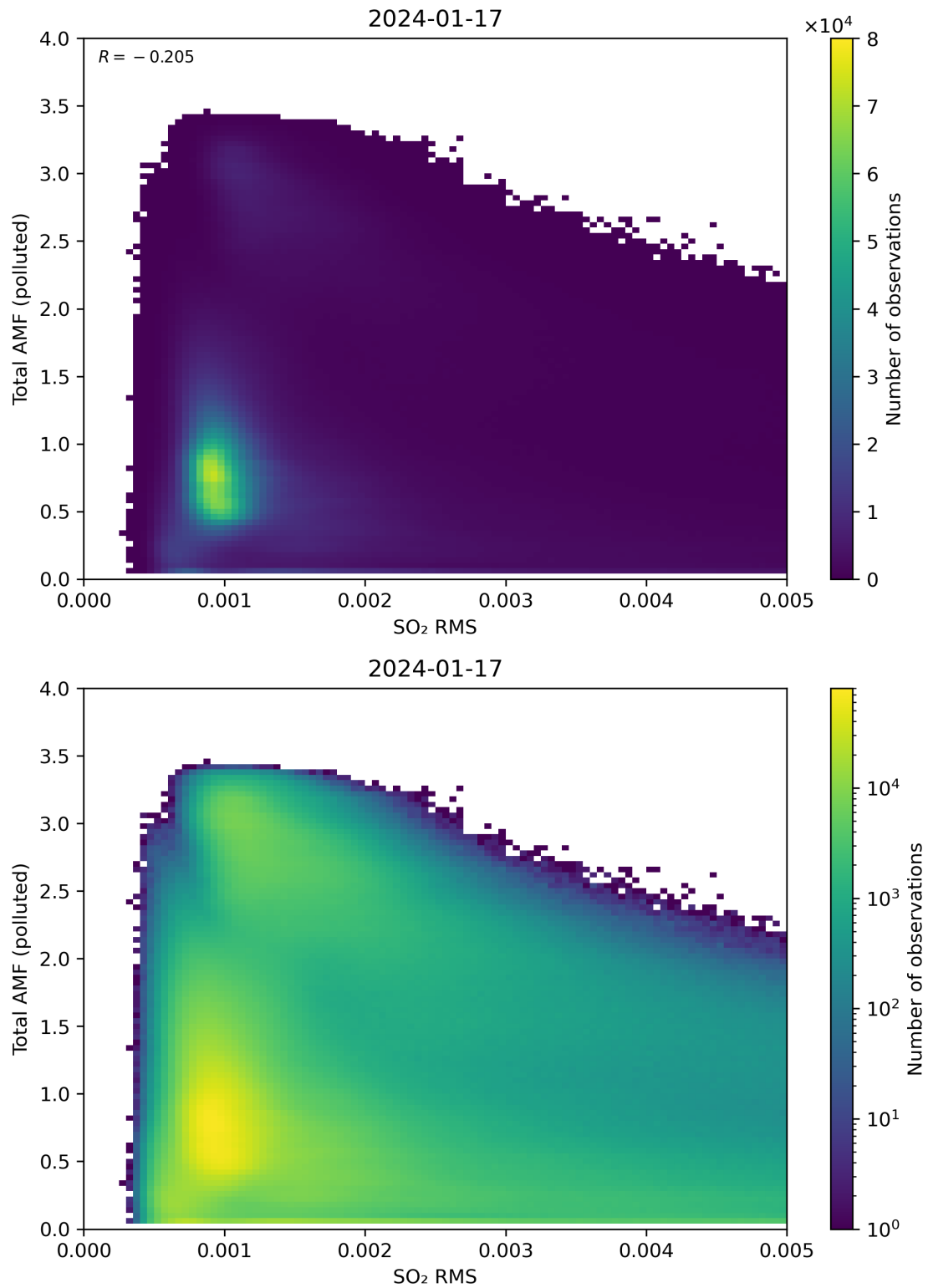
Figure 137: Scatter density plot of “SO 2 RMS” against “Total AMF (polluted)” for 2024-01-16 to 2024-01-18.
