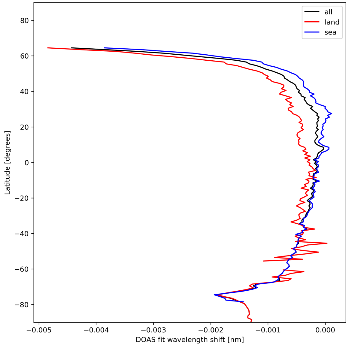
Figure 45: Zonal average of “DOAS fit wavelength shift” for 2024-01-16 to 2024-01-18.
