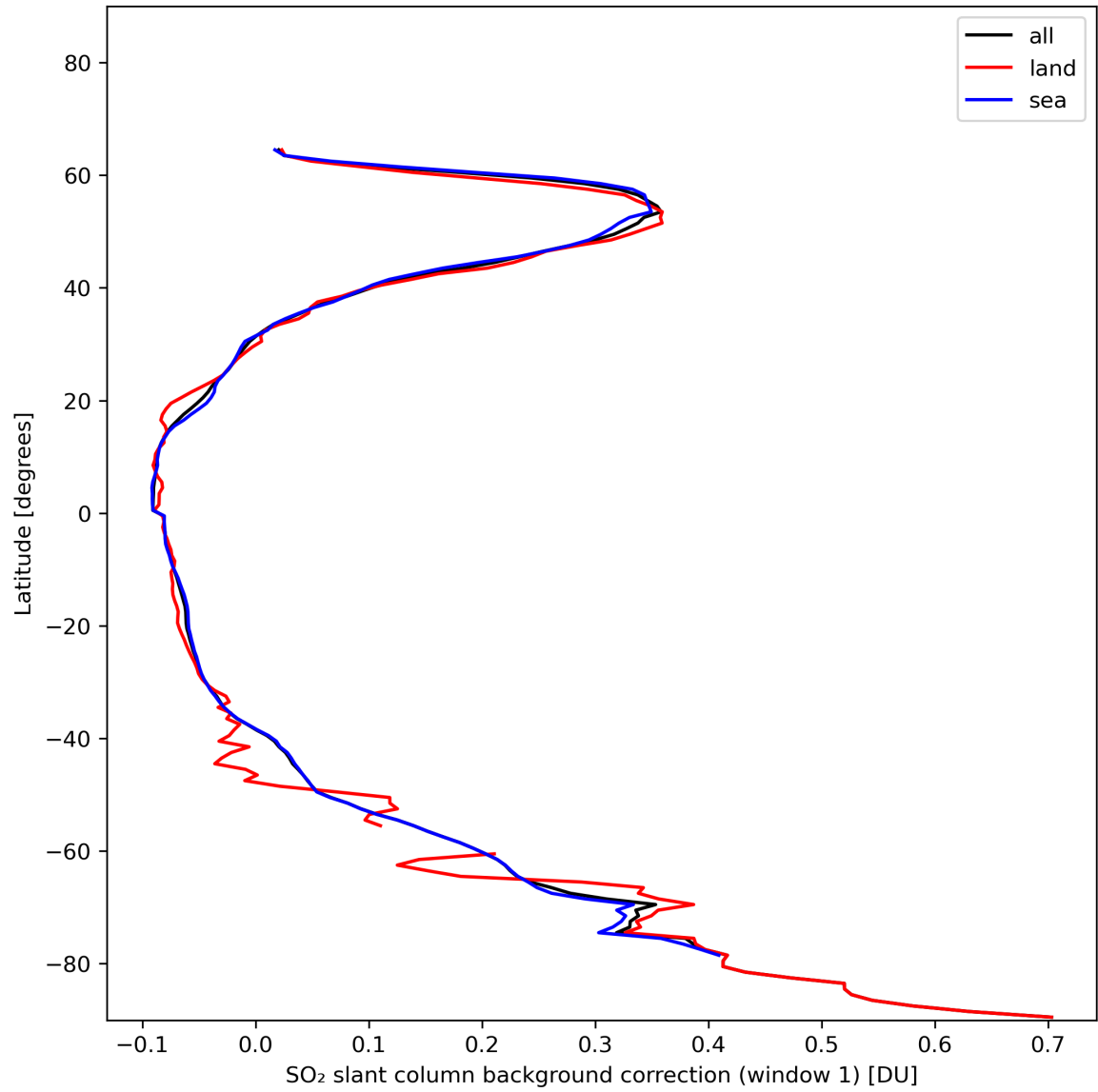
Figure 36: Zonal average of “SO 2 slant column background correction (window 1)” for 2024-01-16 to 2024-01-18.
