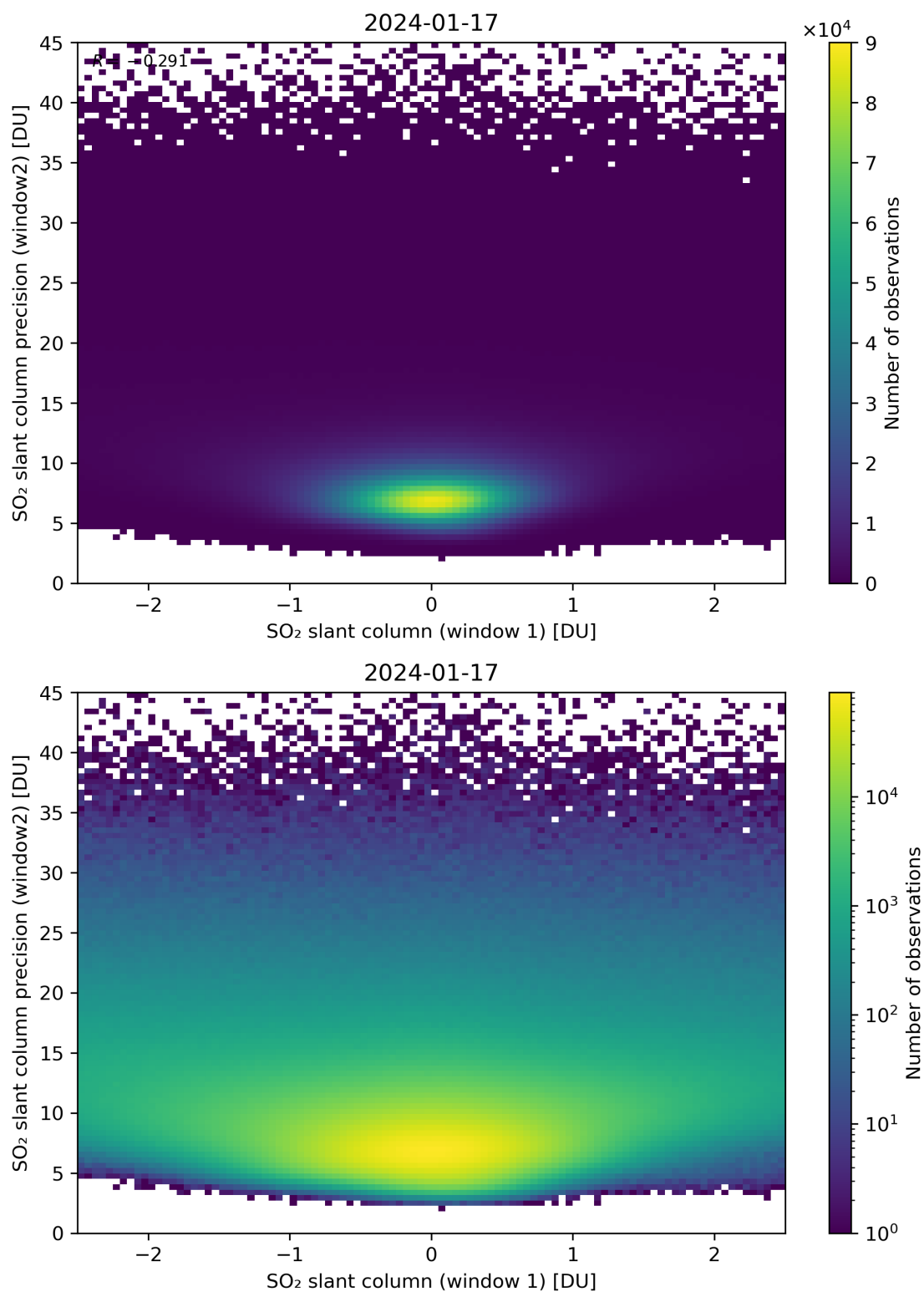
Figure 236: Scatter density plot of “SO 2 slant column (window 1)” against “SO 2 slant column precision (window2)” for 2024-01-16 to 2024-01-18.
