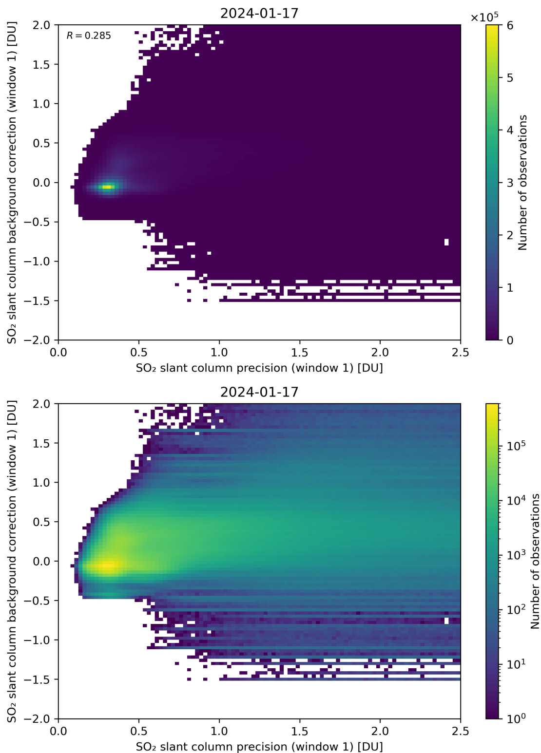
Figure 218: Scatter density plot of “SO 2 slant column precision (window 1)” against “SO 2 slant column background correction (window 1)” for 2024-01-16 to 2024-01-18.
