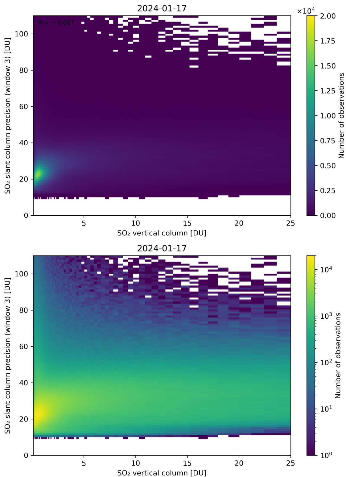
Figure 304: Scatter density plot of “SO 2 vertical column” against “SO 2 slant column precision (window 3)” for 2024-01-16 to 2024-01-18.
