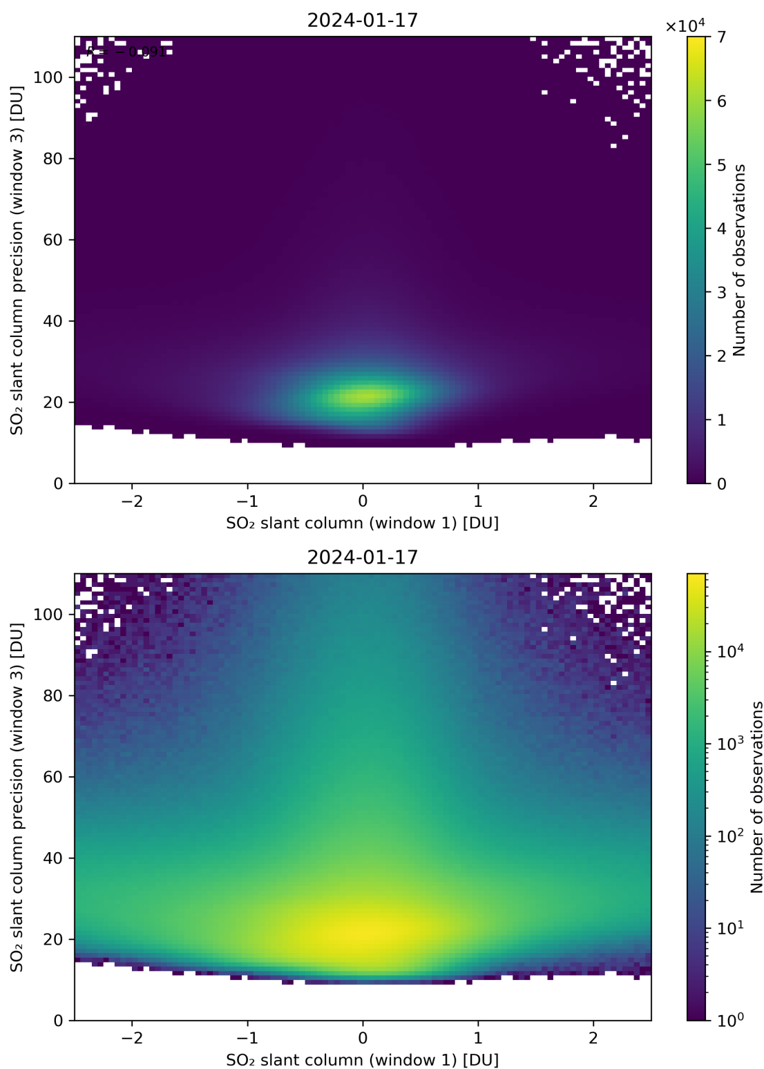
Figure 238: Scatter density plot of “SO 2 slant column (window 1)” against “SO 2 slant column precision (window 3)” for 2024-01-16 to 2024-01-18.
