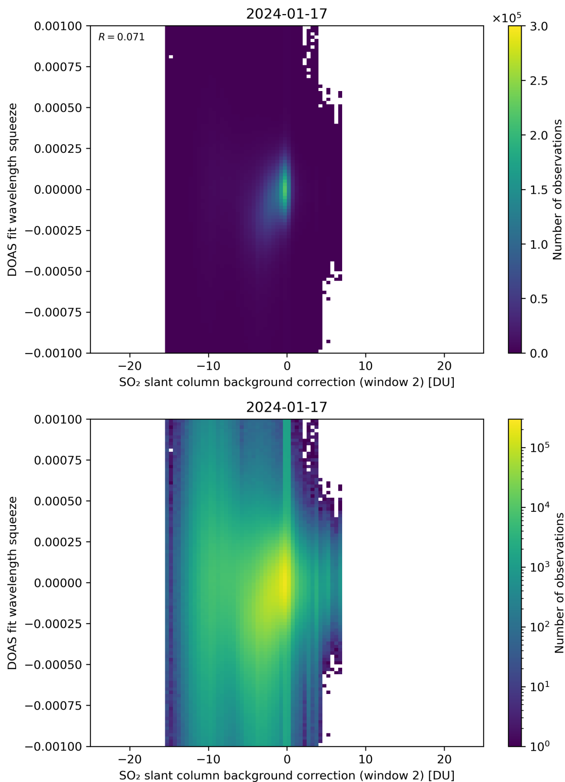
Figure 113: Scatter density plot of “SO 2 slant column background correction (window 2)” against “DOAS fit wavelength squeeze” for 2024-01-16 to 2024-01-18.
