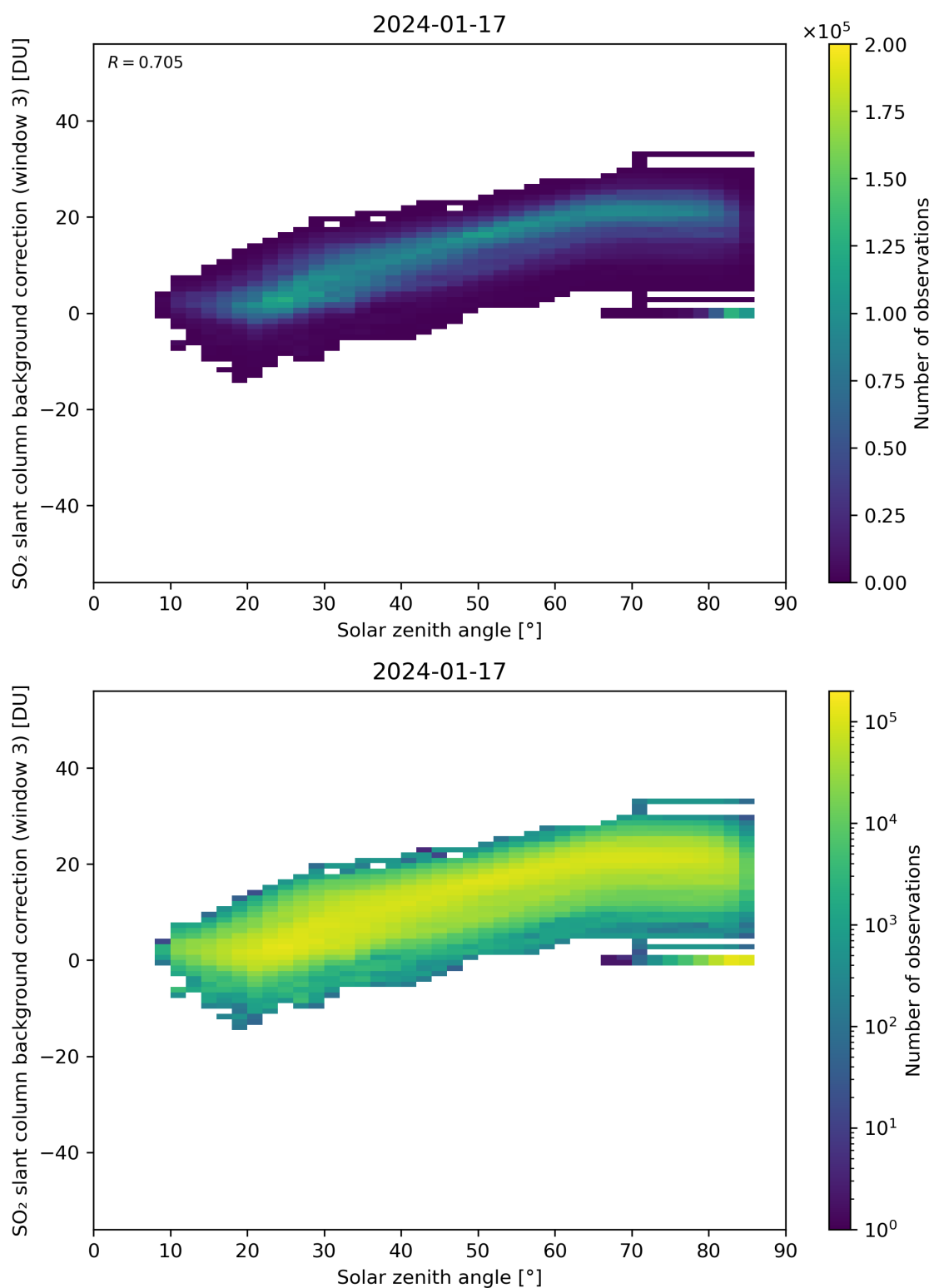
Figure 160: Scatter density plot of “Solar zenith angle” against “SO 2 slant column background correction (window 3)” for 2024-01-16 to 2024-01-18.
