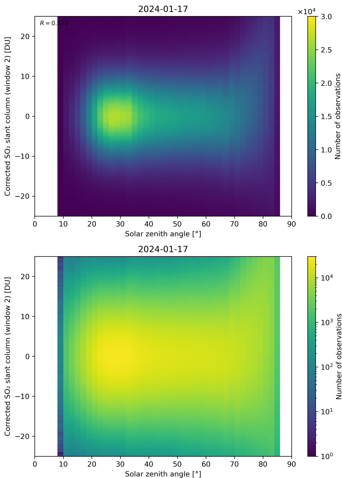
Figure 167: Scatter density plot of “Solar zenith angle” against “Corrected SO 2 slant column (window 2)” for 2024-01-16 to 2024-01-18.
