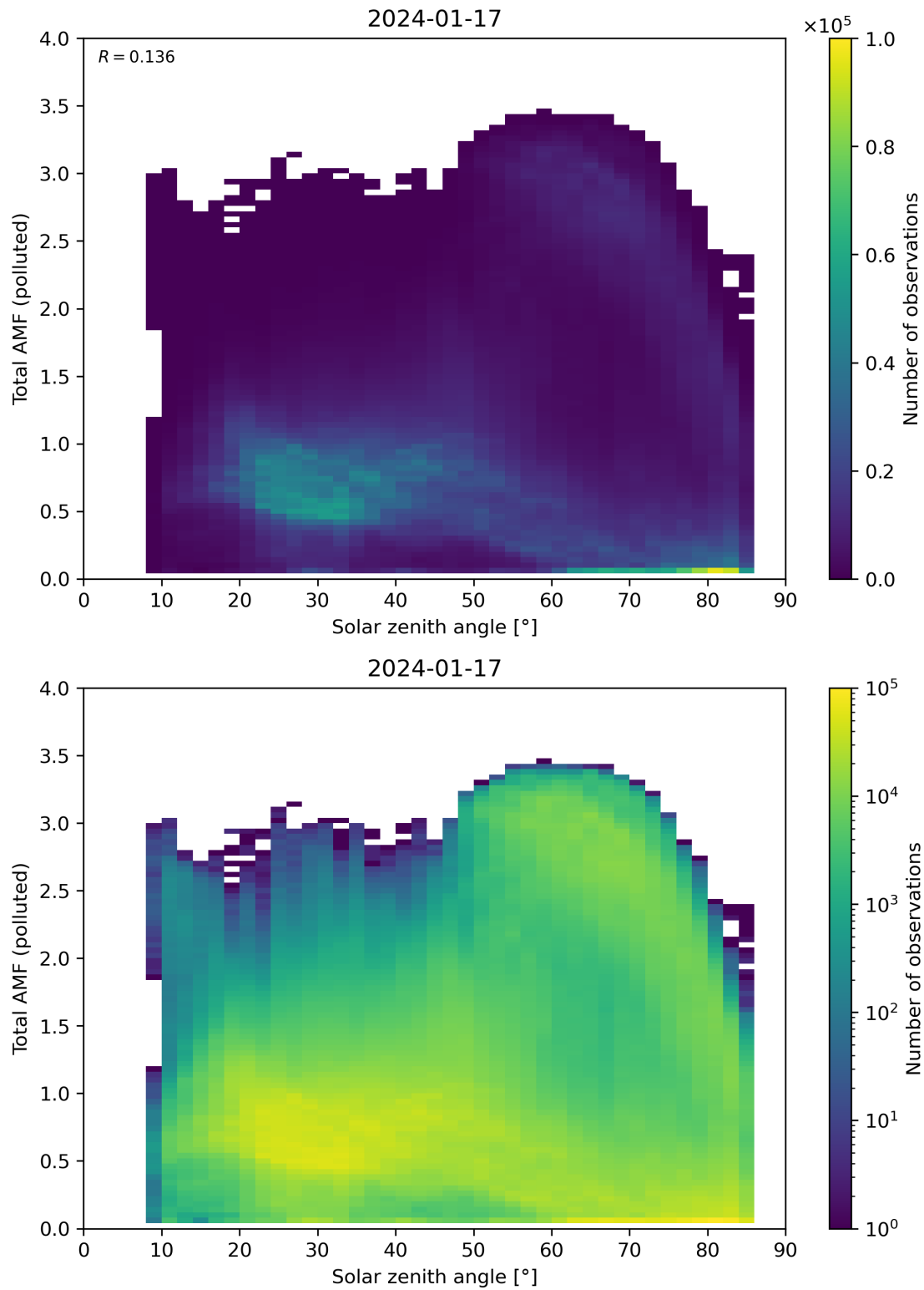
Figure 174: Scatter density plot of “Solar zenith angle” against “Total AMF (polluted)” for 2024-01-16 to 2024-01-18.
