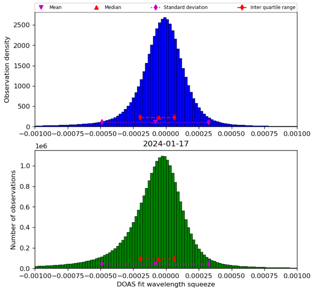
Figure 69: Histogram of “DOAS fit wavelength squeeze” for 2024-01-16 to 2024-01-18
