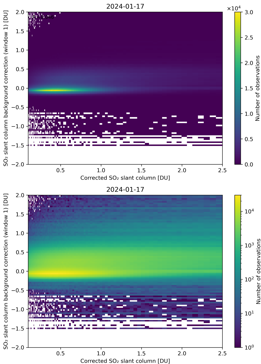
Figure 178: Scatter density plot of “Corrected SO 2 slant column” against “SO 2 slant column background correction (window 1)” for 2024-01-16 to 2024-01-18.
