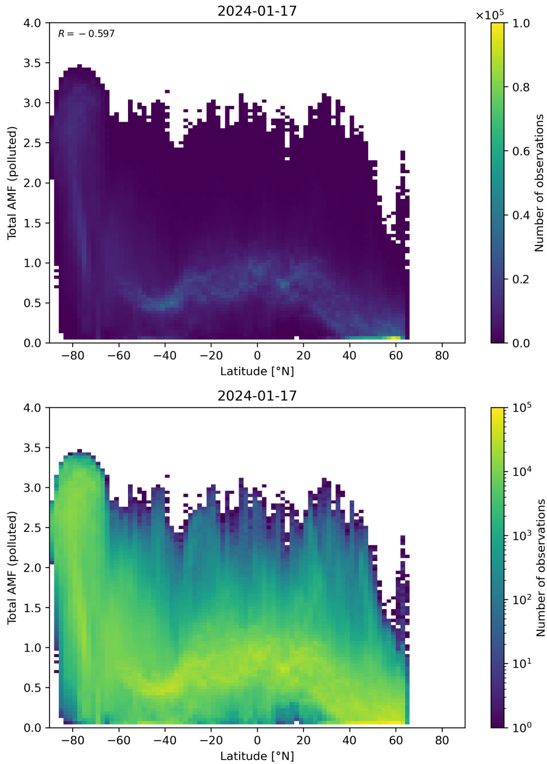
Figure 154: Scatter density plot of “Latitude” against “Total AMF (polluted)” for 2024-01-16 to 2024-01-18.
