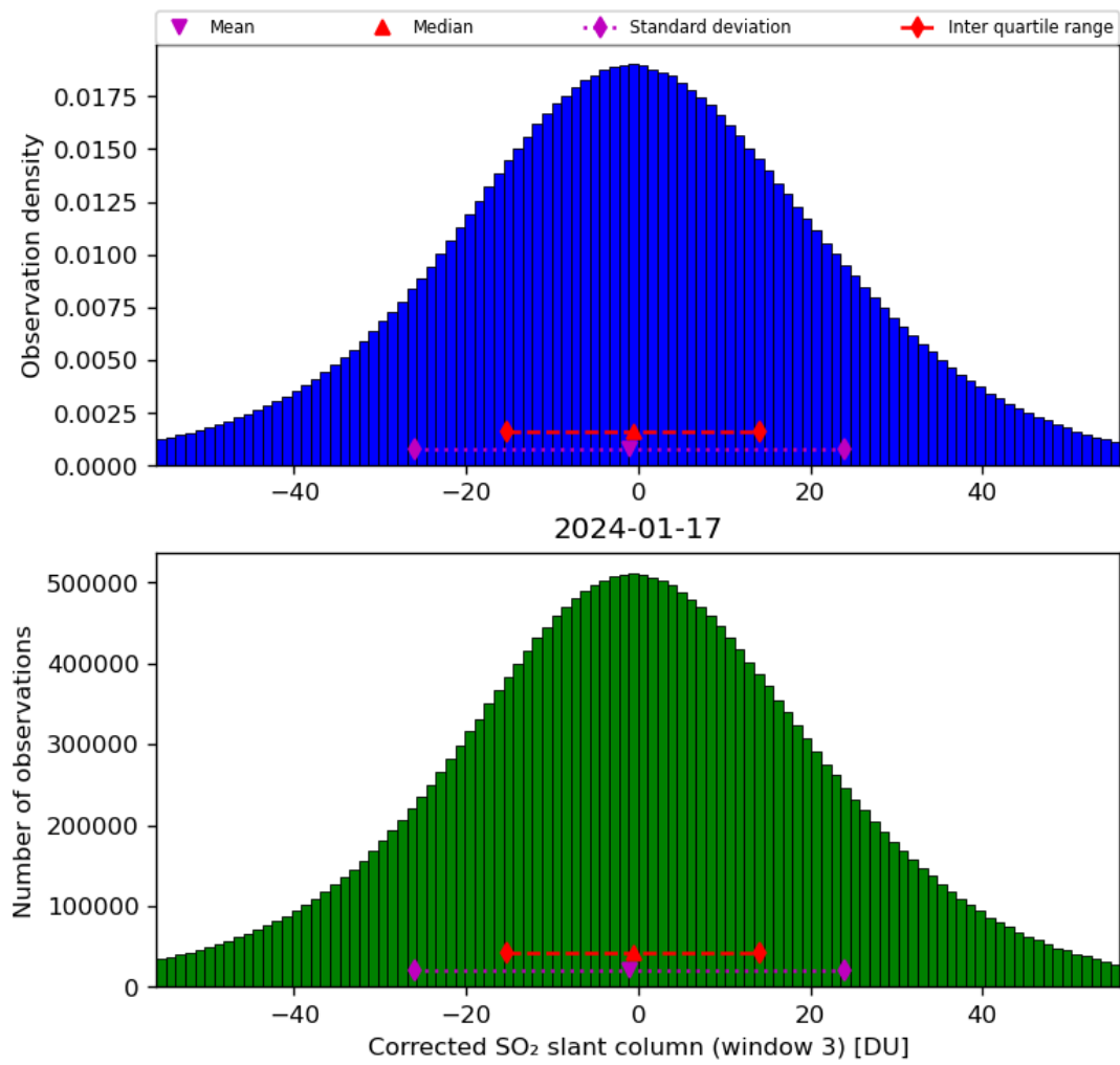
Figure 66: Histogram of "Corrected SO 2 slant column (window 3)" for 2024-01-16 to 2024-01-18
