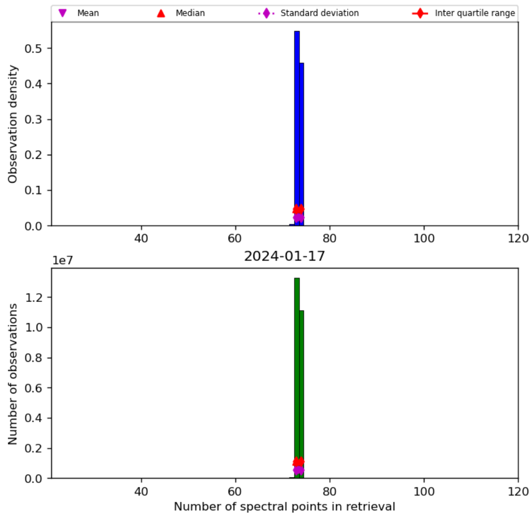
Figure 74: Histogram of “Number of spectral points in retrieval” for 2024-01-16 to 2024-01-18
