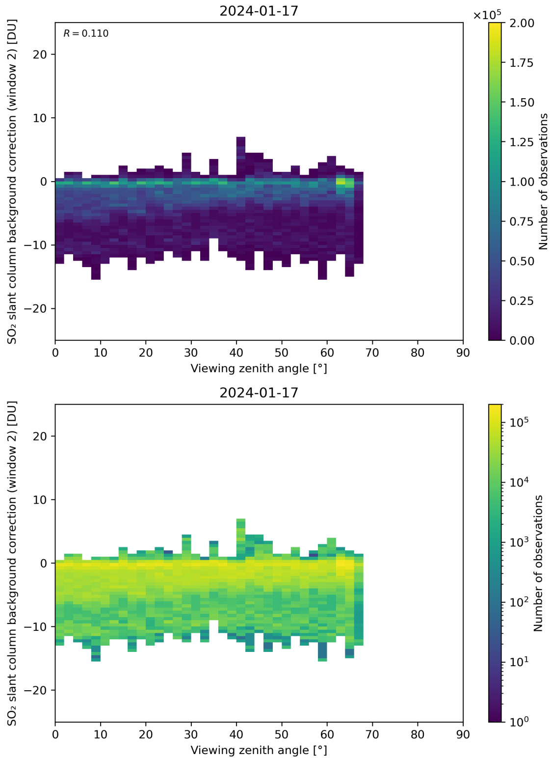
Figure 309: Scatter density plot of “Viewing zenith angle” against “SO 2 slant column background correction (window 2)” for 2024-01-16 to 2024-01-18.
