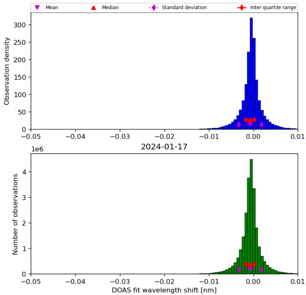
Figure 68: Histogram of “DOAS fit wavelength shift” for 2024-01-16 to 2024-01-18
