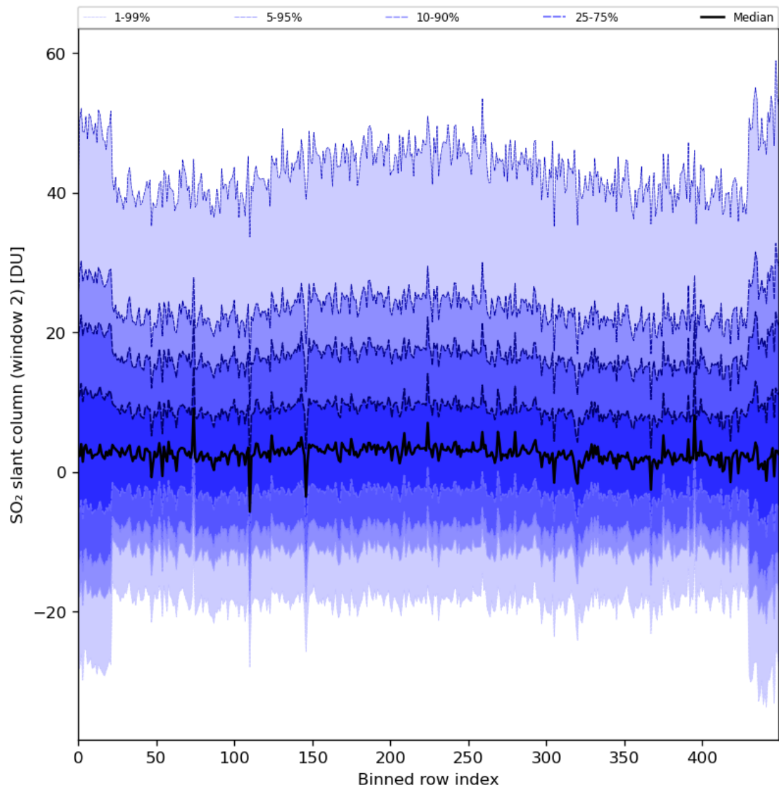
Figure 83: Along track statistics of “SO 2 slant column (window 2)” for 2024-01-16 to 2024-01-18
