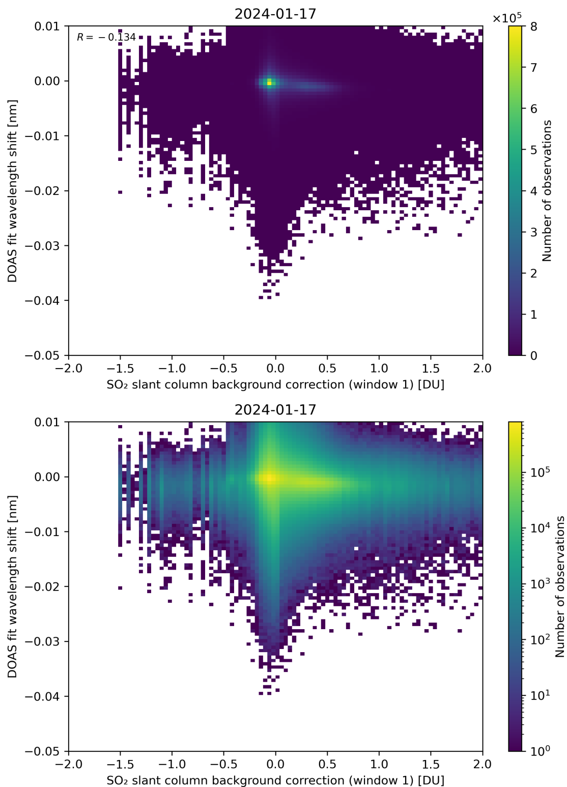
Figure 100: Scatter density plot of “SO 2 slant column background correction (window 1)” against “DOAS fit wavelength shift” for 2024-01-16 to 2024-01-18.
