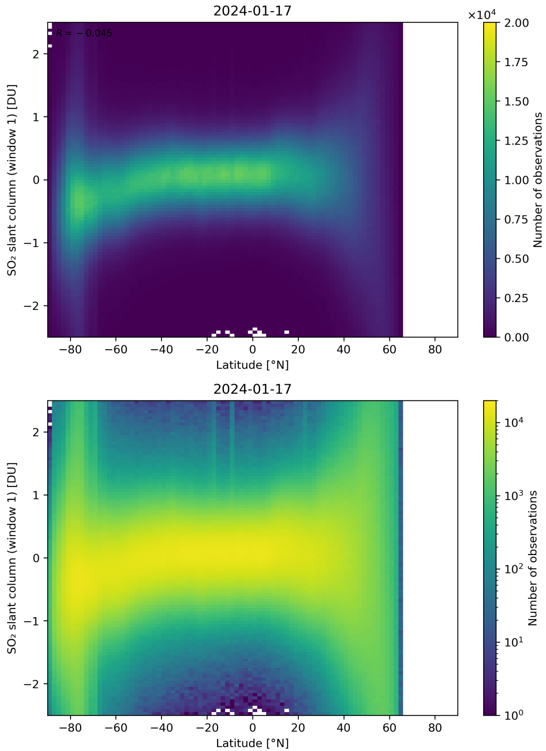
Figure 149: Scatter density plot of “Latitude” against “SO 2 slant column (window 1)” for 2024-01-16 to 2024-01-18.
