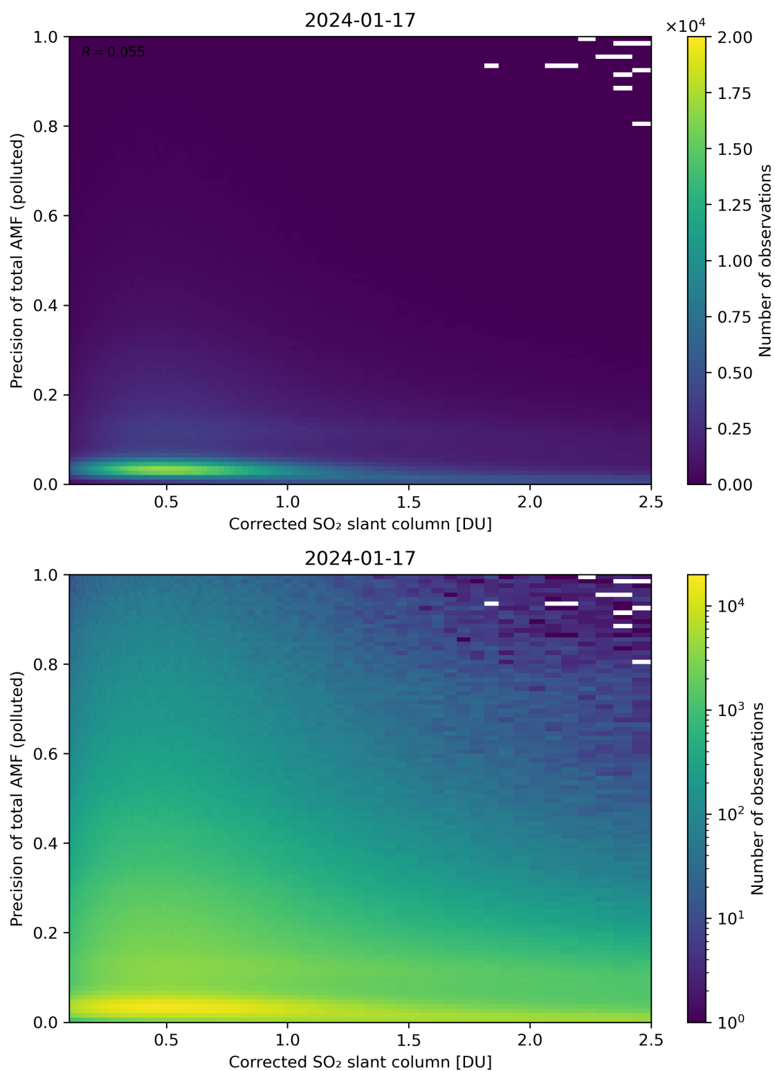
Figure 193: Scatter density plot of “Corrected SO 2 slant column” against “Precision of total AMF (polluted)” for 2024-01-16 to 2024-01-18.
