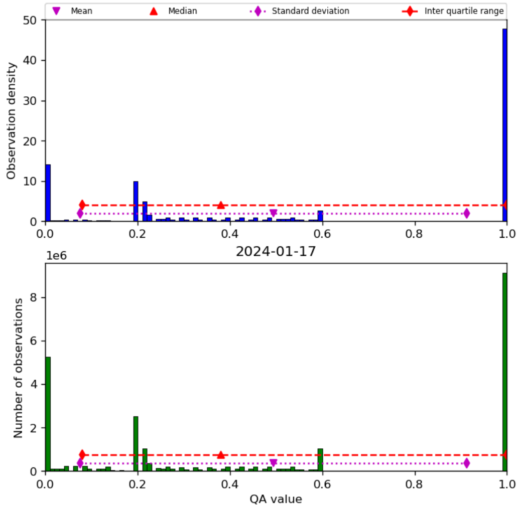
Figure 52: Histogram of “QA value” for 2024-01-16 to 2024-01-18
