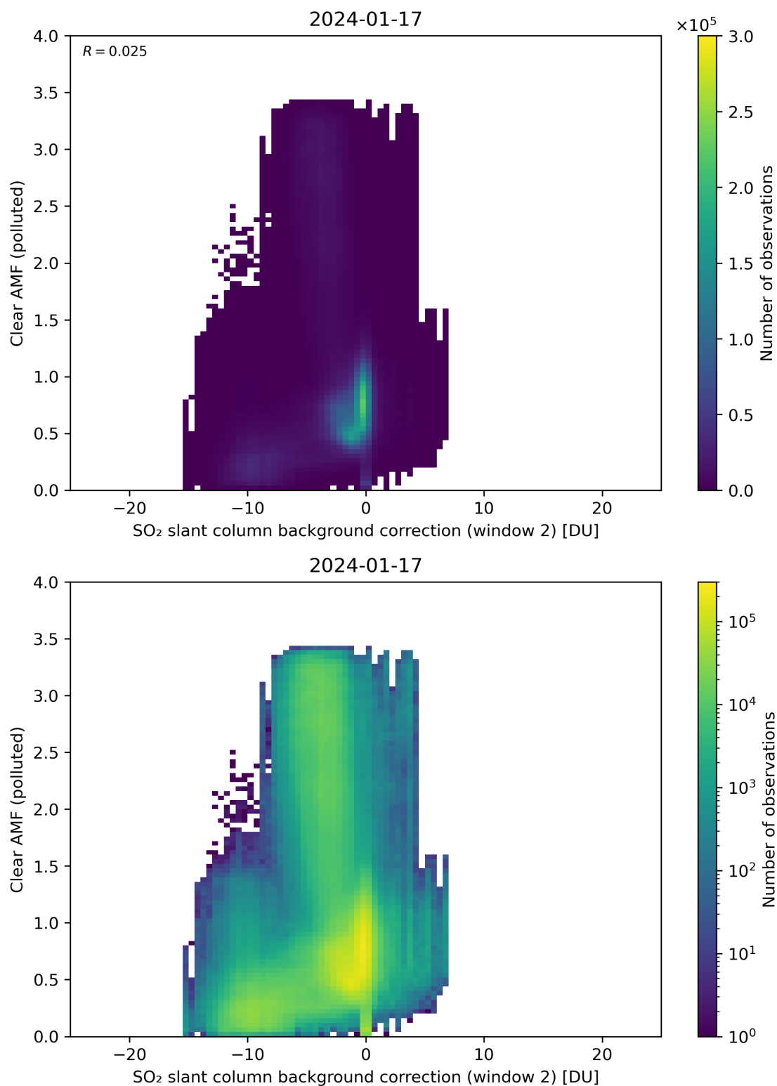
Figure 115: Scatter density plot of “SO 2 slant column background correction (window 2)” against “Clear AMF (polluted)” for 2024-01-16 to 2024-01-18.
