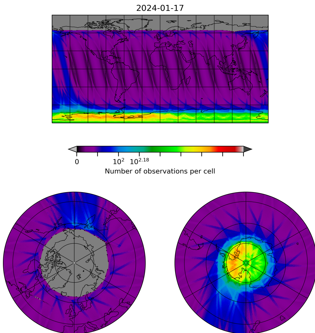
Figure 28: Map of the number of observations for 2024-01-16 to 2024-01-18
