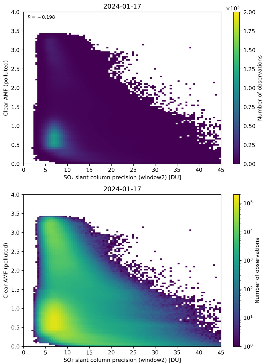
Figure 246: Scatter density plot of “SO 2 slant column precision (window2)” against “Clear AMF (polluted)” for 2024-01-16 to 2024-01-18.
