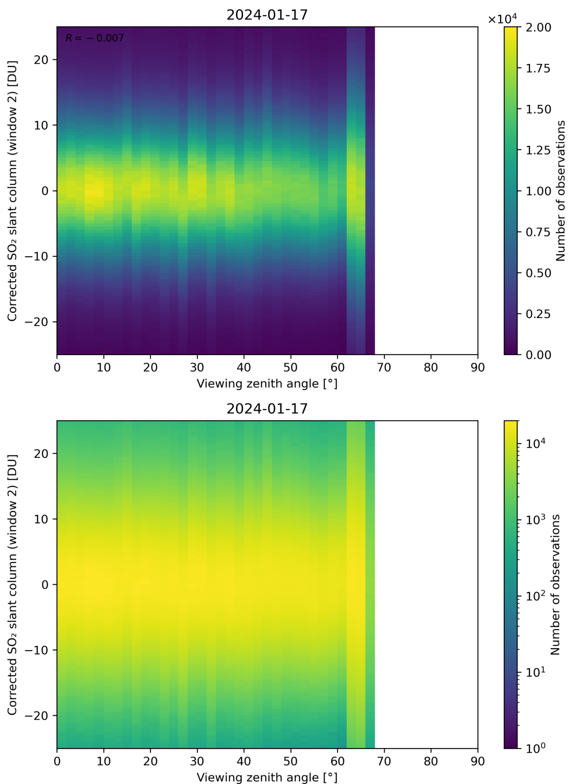
Figure 318: Scatter density plot of “Viewing zenith angle” against “Corrected SO 2 slant column (window 2)” for 2024-01-16 to 2024-01-18.
