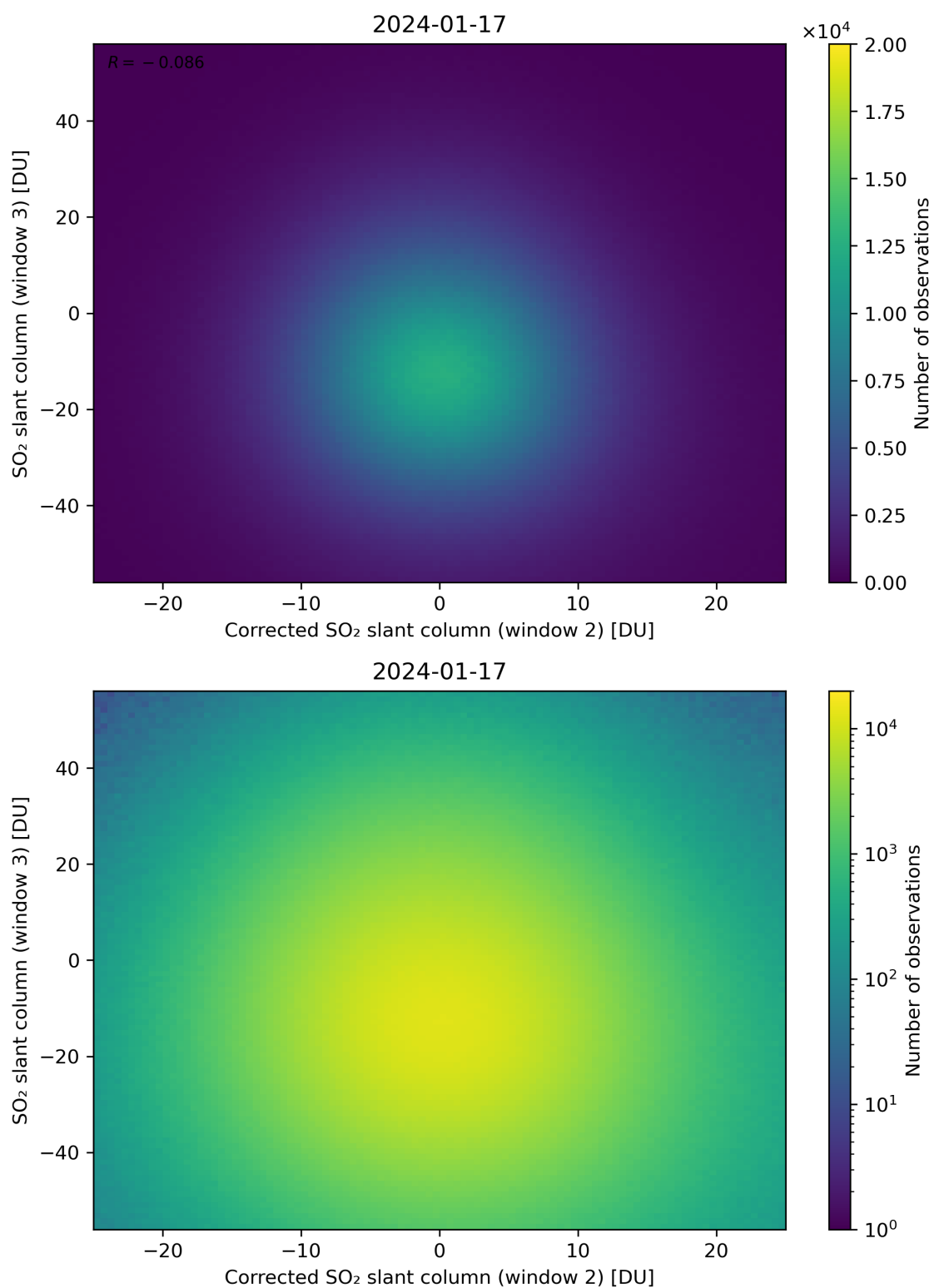
Figure 201: Scatter density plot of “Corrected SO 2 slant column (window 2)” against “SO 2 slant column (window 3)” for 2024-01-16 to 2024-01-18.
