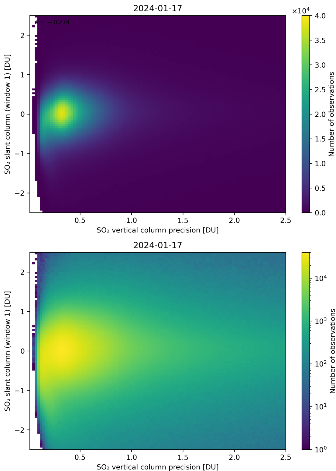
Figure 289: Scatter density plot of “SO 2 vertical column precision” against “SO 2 slant column (window 1)” for 2024-01-16 to 2024-01-18.
