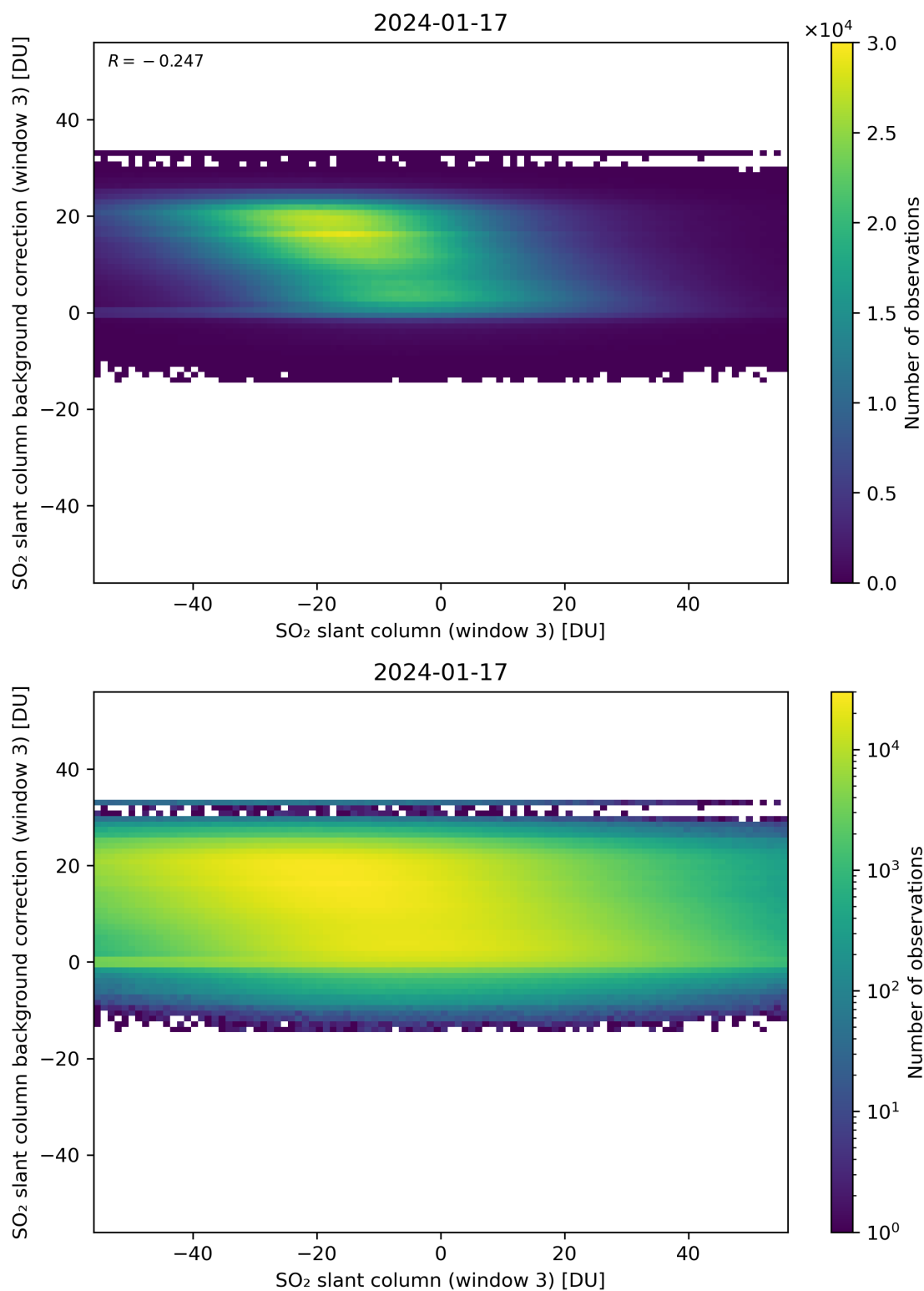
Figure 253: Scatter density plot of “SO 2 slant column (window 3)” against “SO 2 slant column background correction (window 3)” for 2024-01-16 to 2024-01-18.
