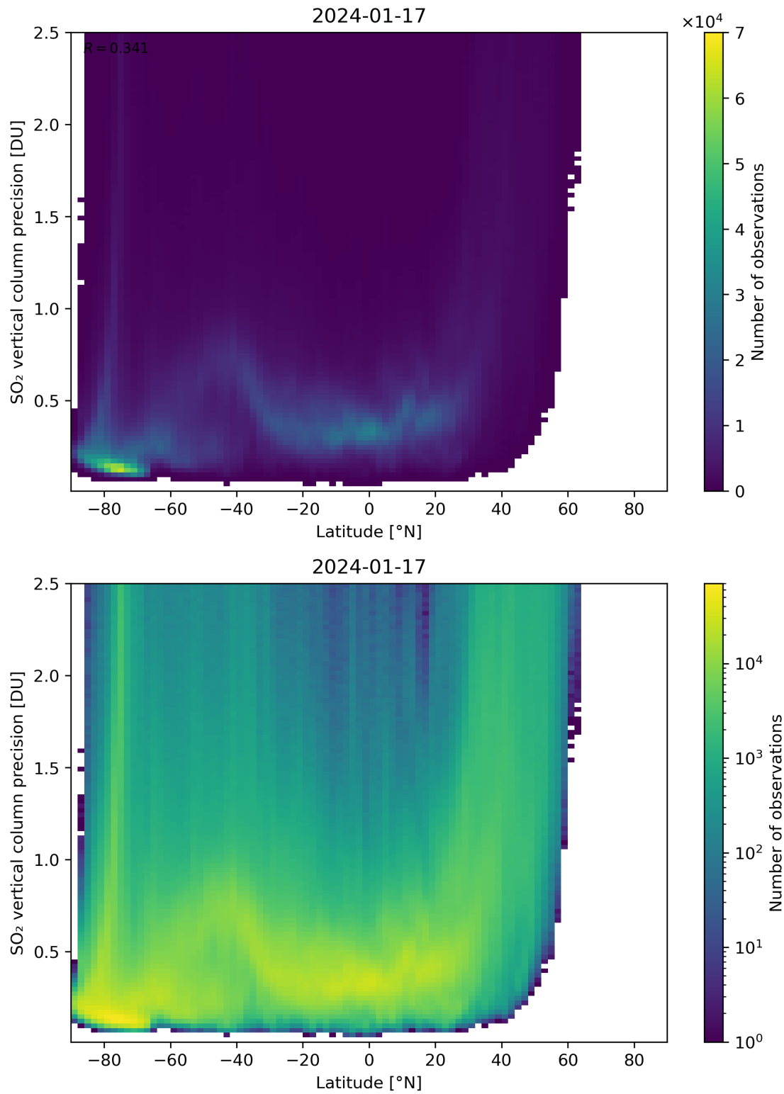
Figure 157: Scatter density plot of “Latitude” against “SO 2 vertical column precision” for 2024-01-16 to 2024-01-18.
