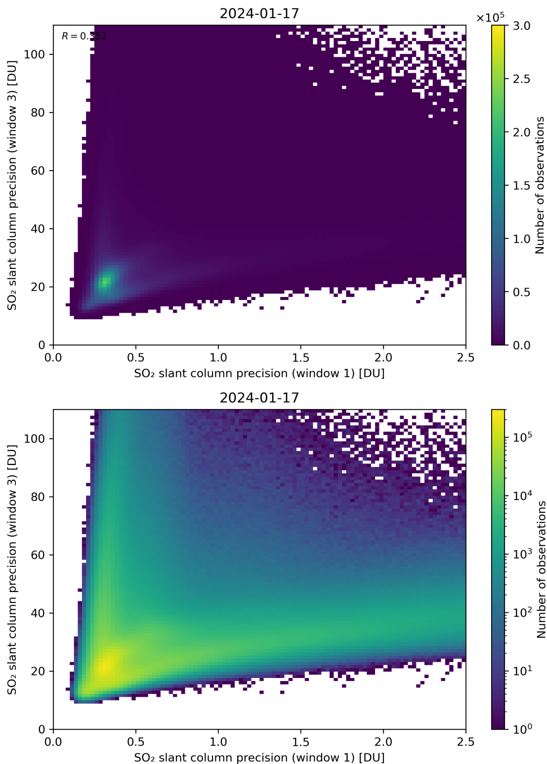
Figure 229: Scatter density plot of “SO 2 slant column precision (window 1)” against “SO 2 slant column precision (window 3)” for 2024-01-16 to 2024-01-18.
