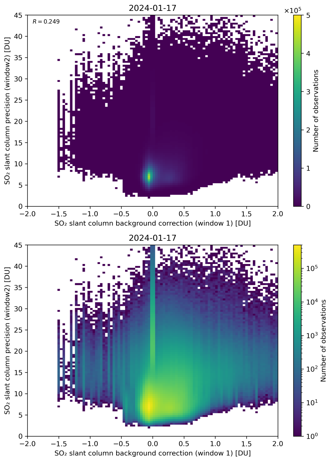
Figure 106: Scatter density plot of “SO 2 slant column background correction (window 1)” against “SO 2 slant column precision (window2)” for 2024-01-16 to 2024-01-18.
