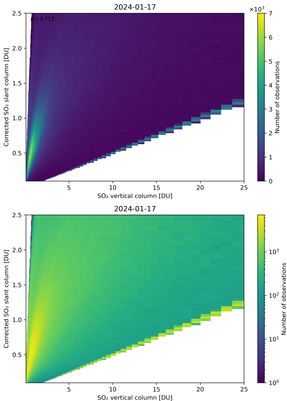
Figure 297: Scatter density plot of “SO 2 vertical column” against “Corrected SO 2 slant column” for 2024-01-16 to 2024-01-18.
