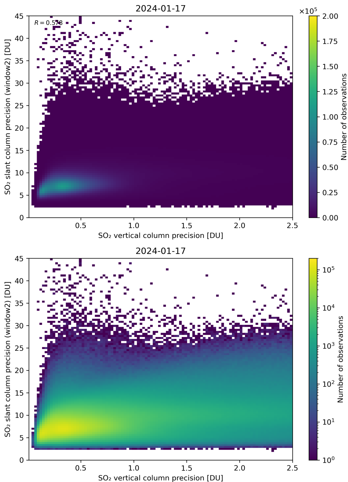
Figure 291: Scatter density plot of “SO 2 vertical column precision” against “SO 2 slant column precision (window2)” for 2024-01-16 to 2024-01-18.
