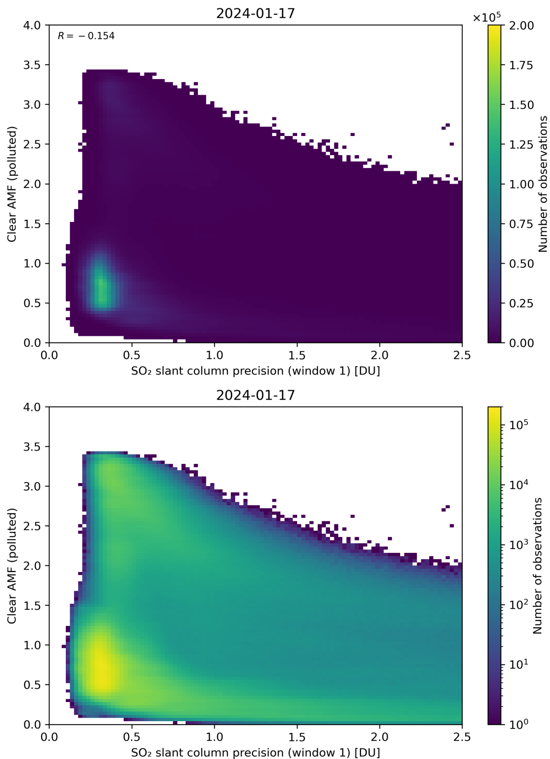
Figure 224: Scatter density plot of “SO 2 slant column precision (window 1)” against “Clear AMF (polluted)” for 2024-01-16 to 2024-01-18.
