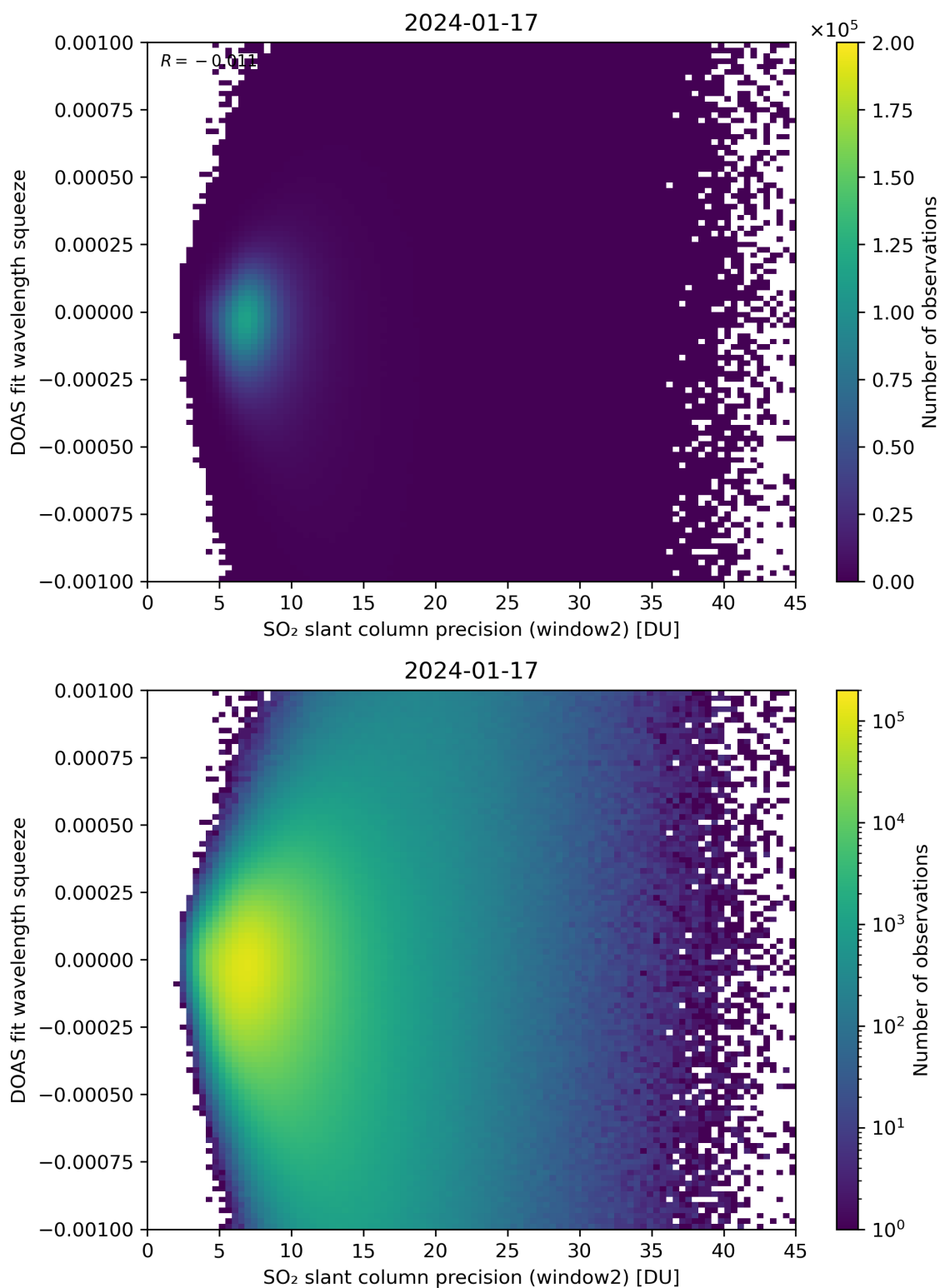
Figure 244: Scatter density plot of “SO 2 slant column precision (window2)” against “DOAS fit wavelength squeeze” for 2024-01-16 to 2024-01-18.
