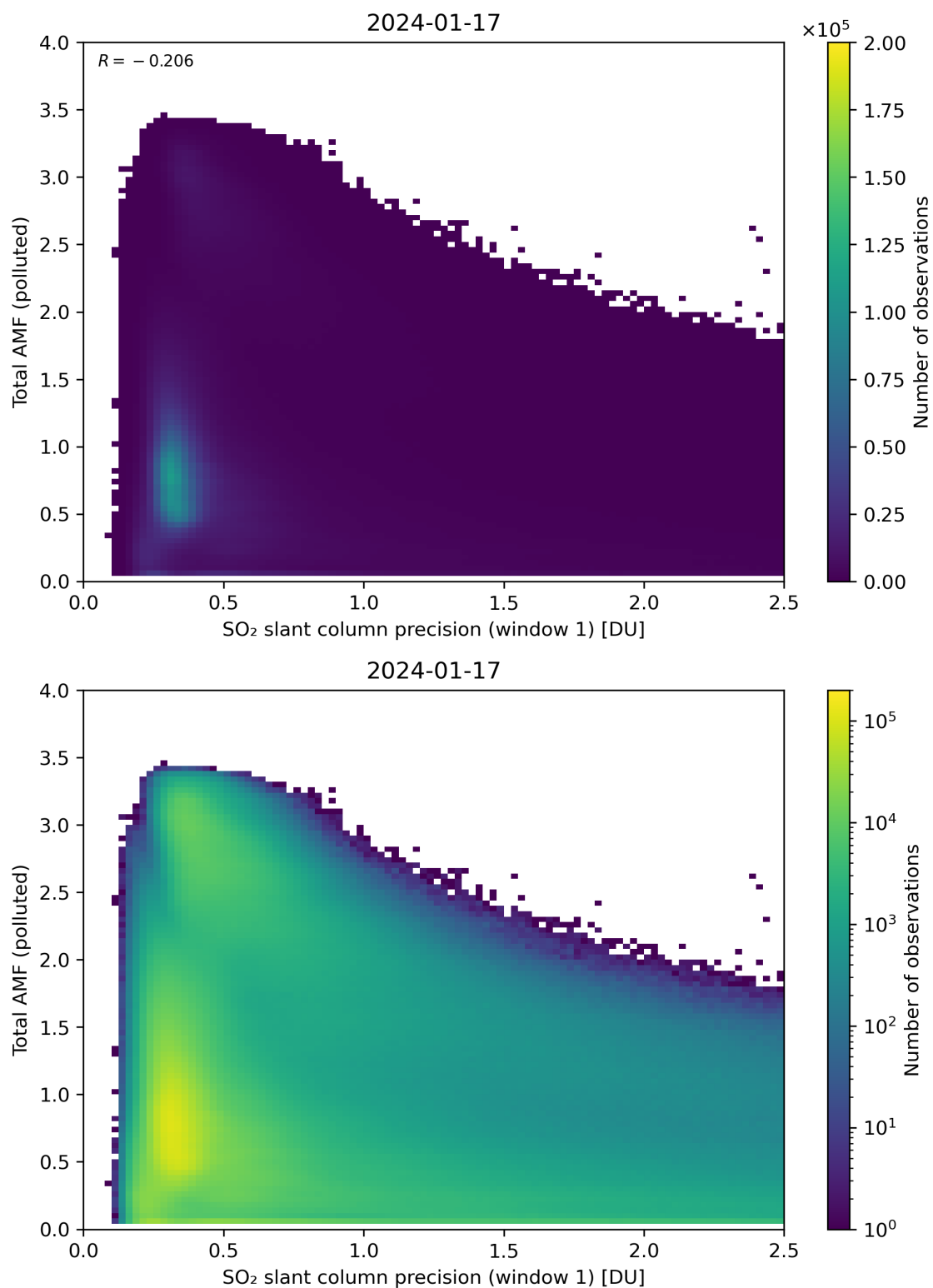
Figure 230: Scatter density plot of “SO 2 slant column precision (window 1)” against “Total AMF (polluted)” for 2024-01-16 to 2024-01-18.
