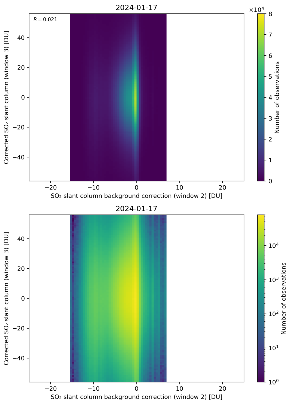
Figure 116: Scatter density plot of “SO 2 slant column background correction (window 2)” against “Corrected SO 2 slant column (window 3)” for 2024-01-16 to 2024-01-18.
