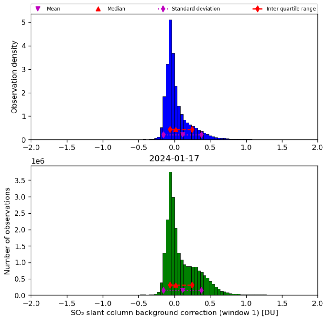
Figure 59: Histogram of “SO 2 slant column background correction (window 1)” for 2024-01-16 to 2024-01-18
