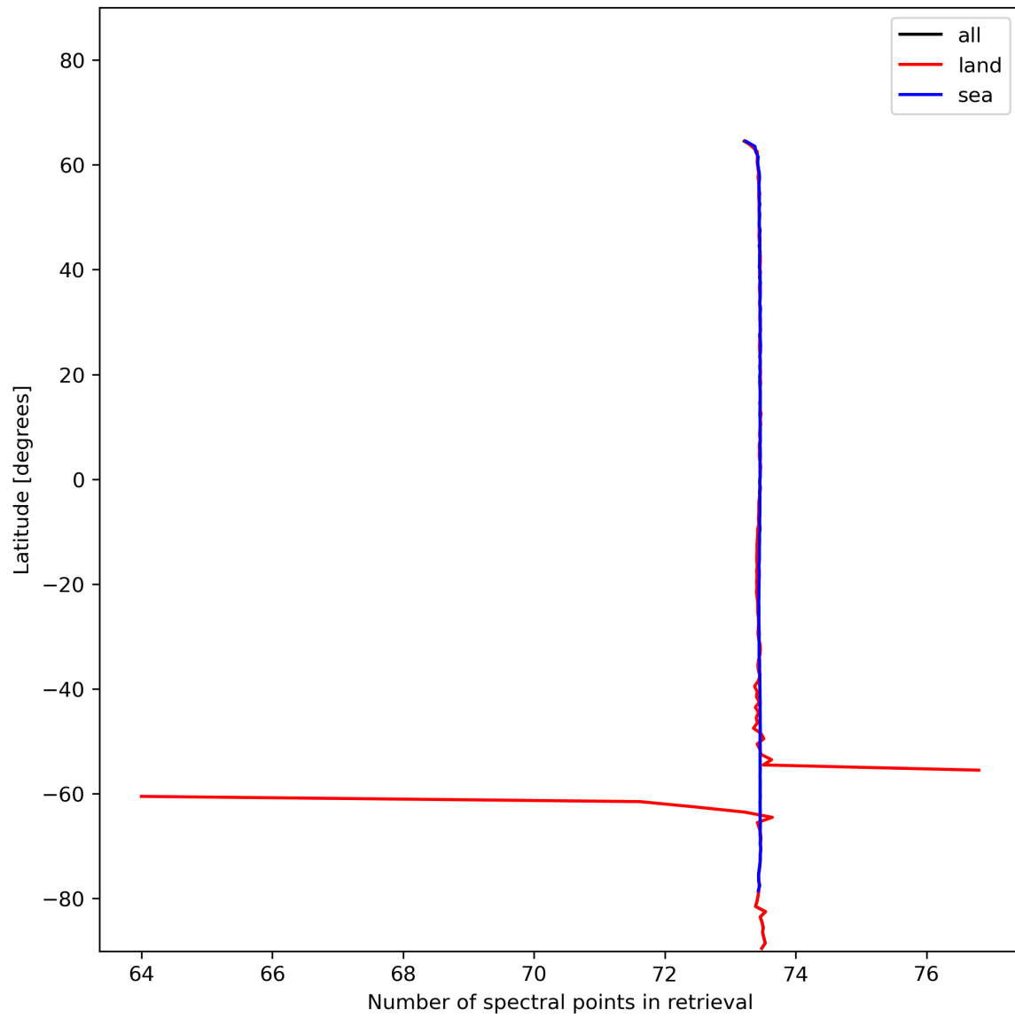
Figure 51: Zonal average of “Number of spectral points in retrieval” for 2024-01-16 to 2024-01-18.
