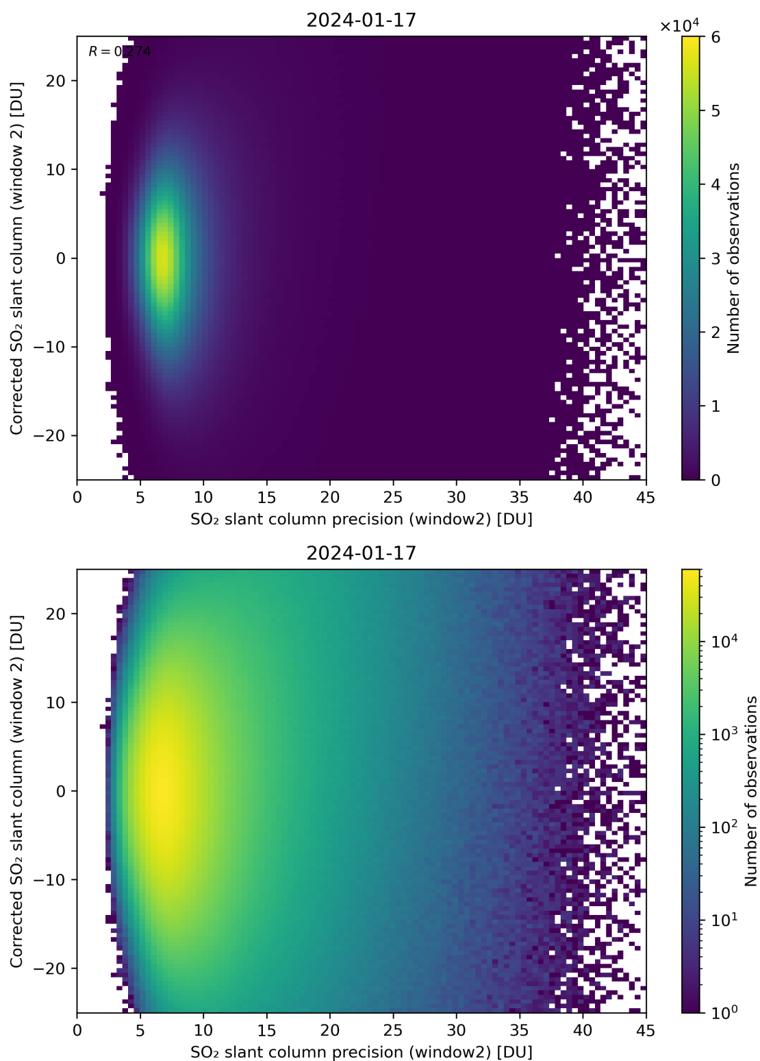
Figure 247: Scatter density plot of “SO 2 slant column precision (window2)” against “Corrected SO 2 slant column (window 2)” for 2024-01-16 to 2024-01-18.
