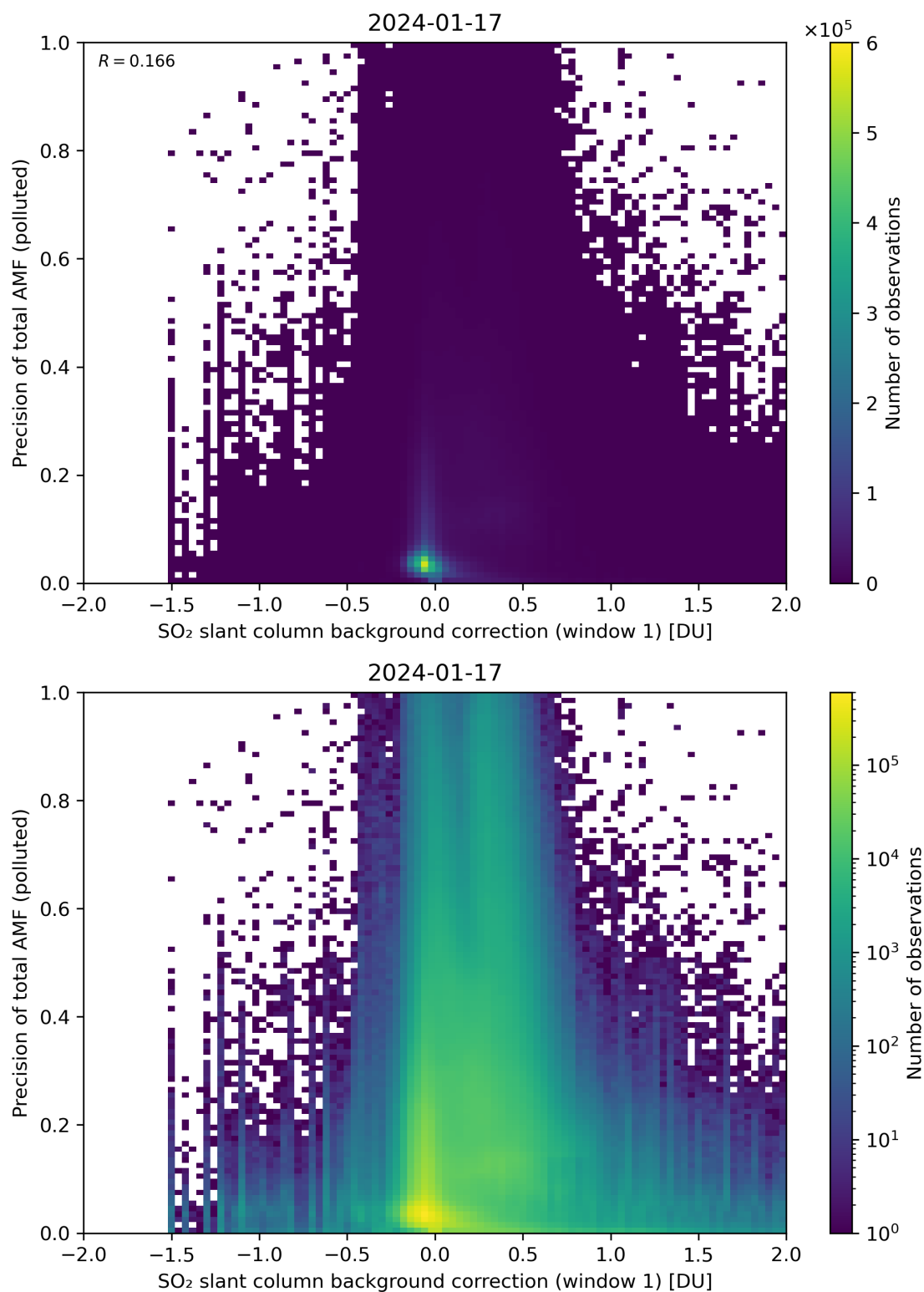
Figure 110: Scatter density plot of “SO 2 slant column background correction (window 1)” against “Precision of total AMF (polluted)” for 2024-01-16 to 2024-01-18.
