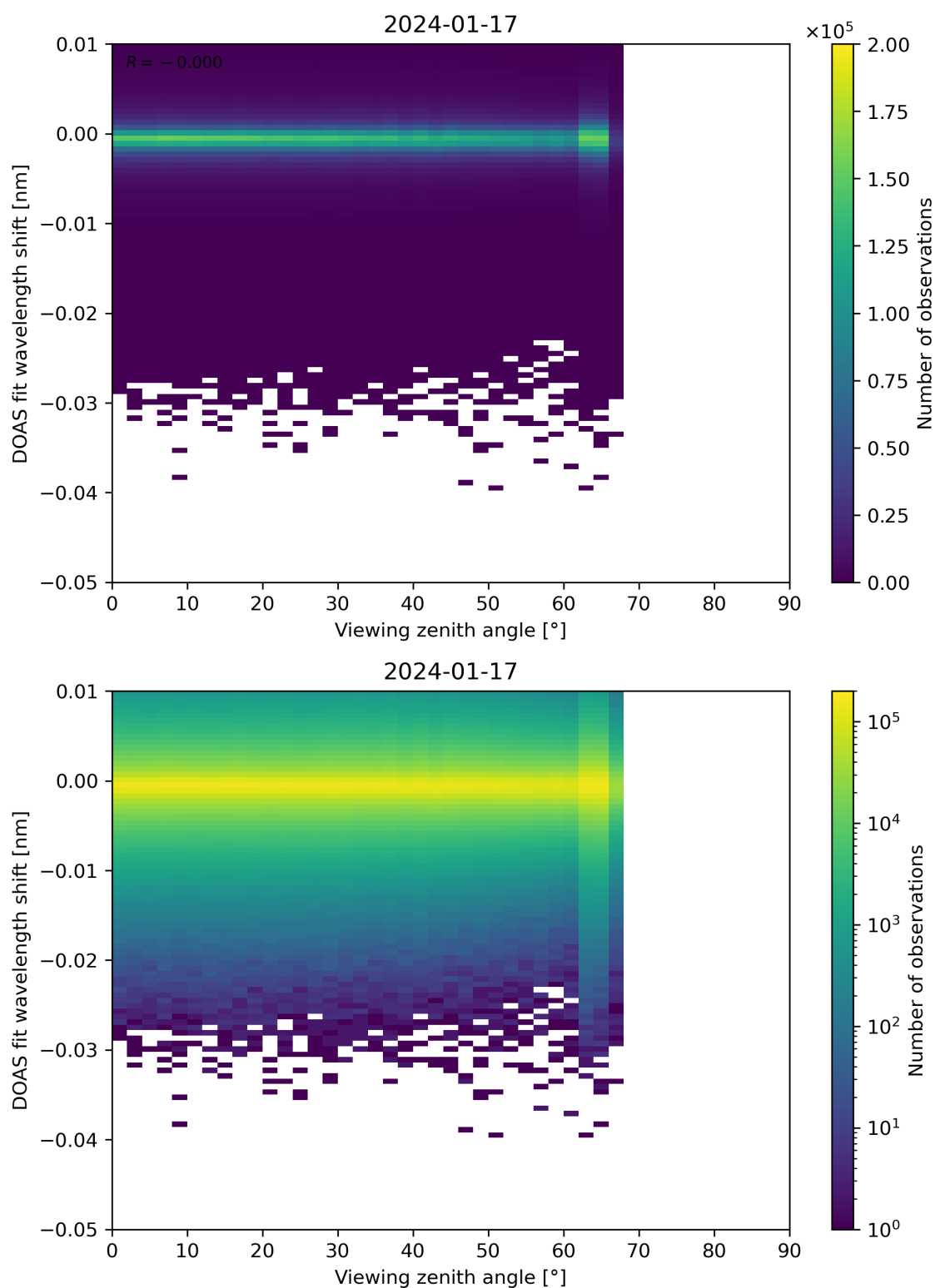
Figure 311: Scatter density plot of “Viewing zenith angle” against “DOAS fit wavelength shift” for 2024-01-16 to 2024-01-18.
