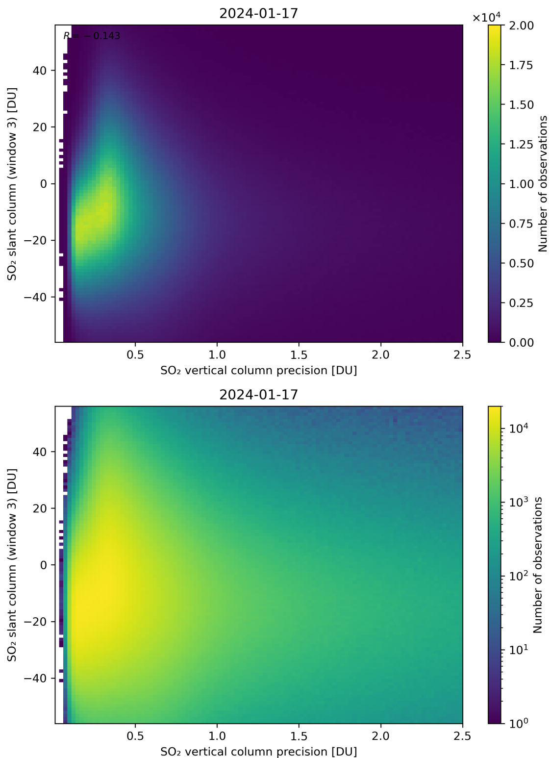
Figure 292: Scatter density plot of “SO 2 vertical column precision” against “SO 2 slant column (window 3)” for 2024-01-16 to 2024-01-18.
