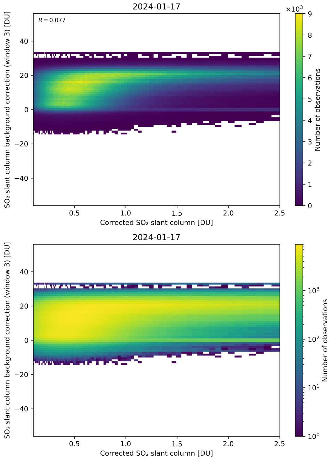
Figure 180: Scatter density plot of “Corrected SO 2 slant column” against “SO 2 slant column background correction (window 3)” for 2024-01-16 to 2024-01-18.
