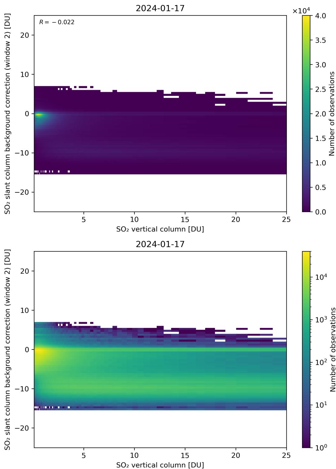
Figure 274: Scatter density plot of “SO 2 vertical column” against “SO 2 slant column background correction (window 2)” for 2024-01-16 to 2024-01-18.
