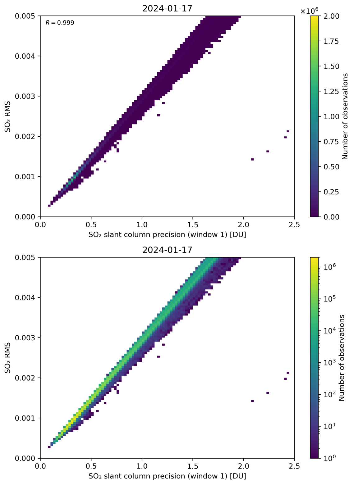
Figure 223: Scatter density plot of “SO 2 slant column precision (window 1)” against “SO 2 RMS” for 2024-01-16 to 2024-01-18.
