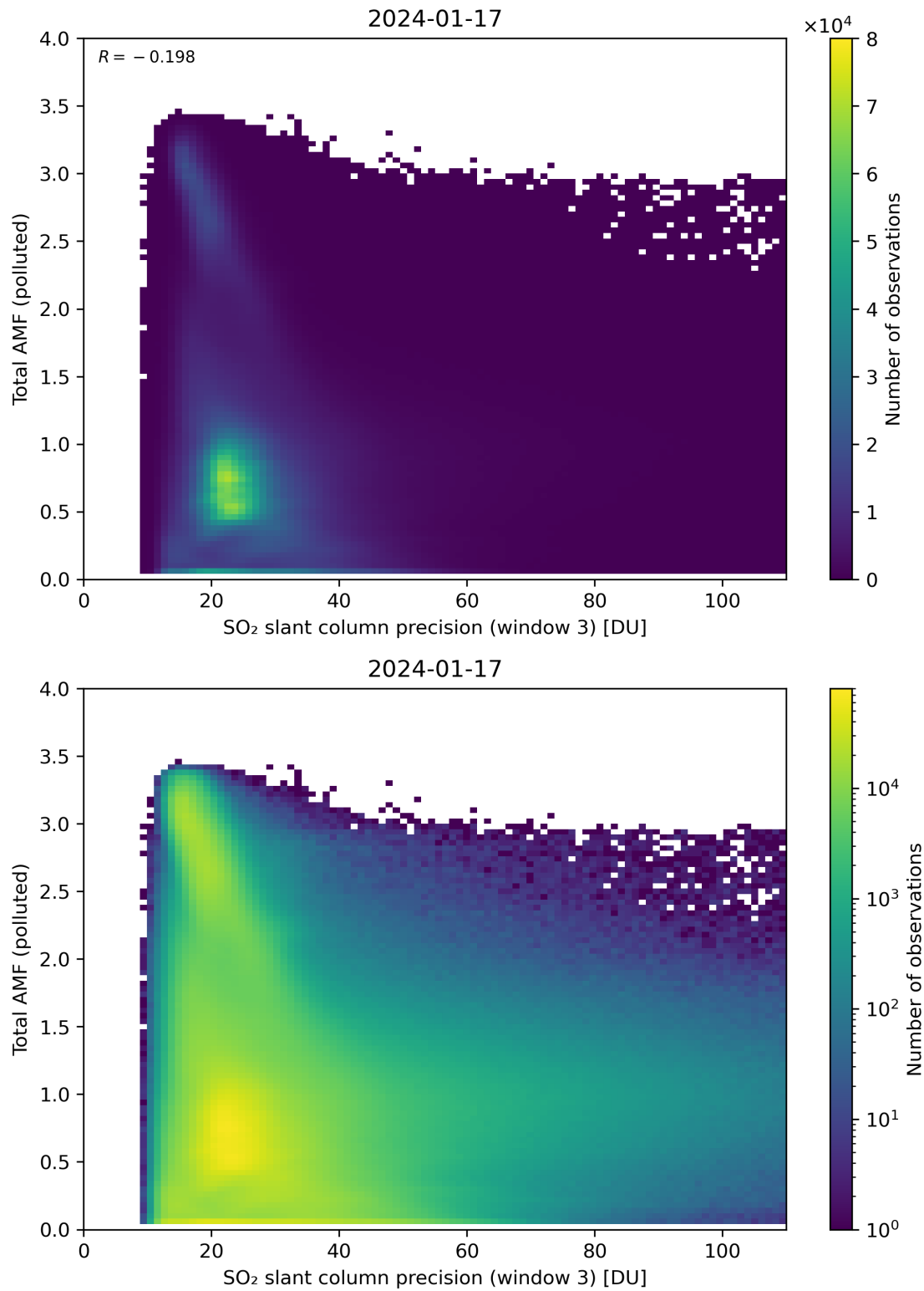
Figure 263: Scatter density plot of “SO 2 slant column precision (window 3)” against “Total AMF (polluted)” for 2024-01-16 to 2024-01-18.
