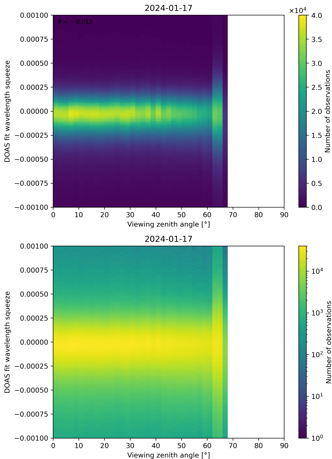
Figure 312: Scatter density plot of “Viewing zenith angle” against “DOAS fit wavelength squeeze” for 2024-01-16 to 2024-01-18.
