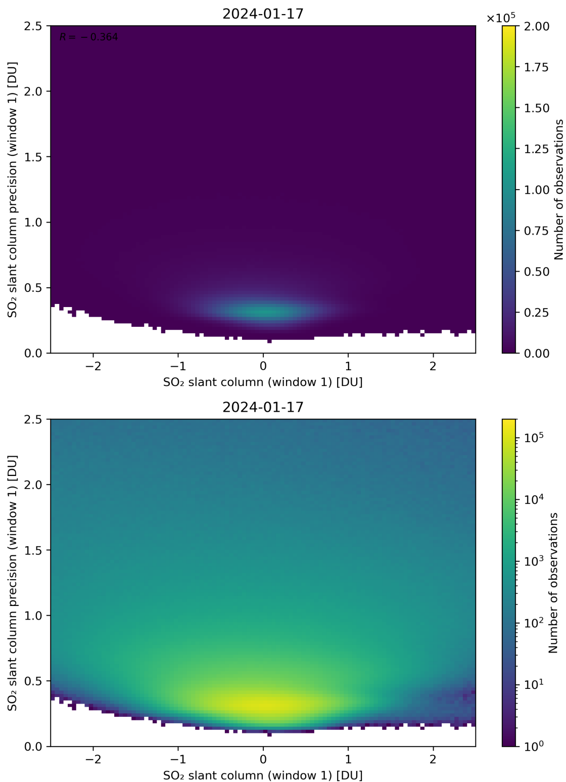
Figure 235: Scatter density plot of “SO 2 slant column (window 1)” against “SO 2 slant column precision (window 1)” for 2024-01-16 to 2024-01-18.
