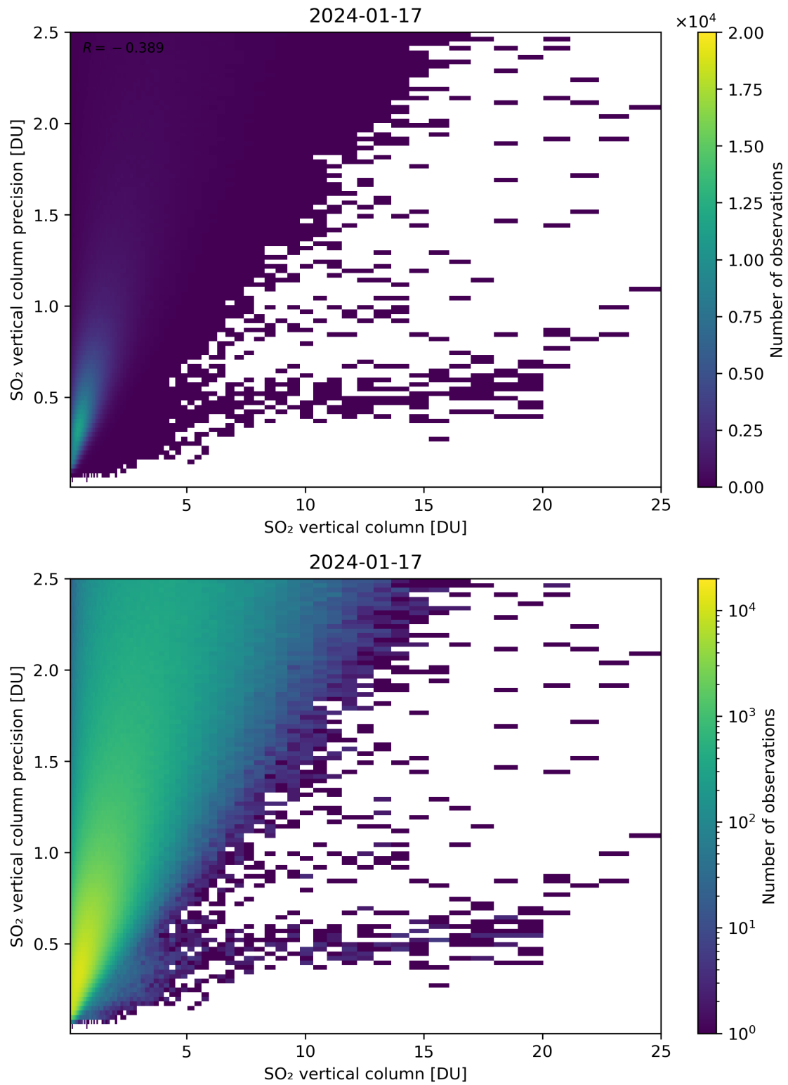
Figure 307: Scatter density plot of “SO 2 vertical column” against “SO 2 vertical column precision” for 2024-01-16 to 2024-01-18.
