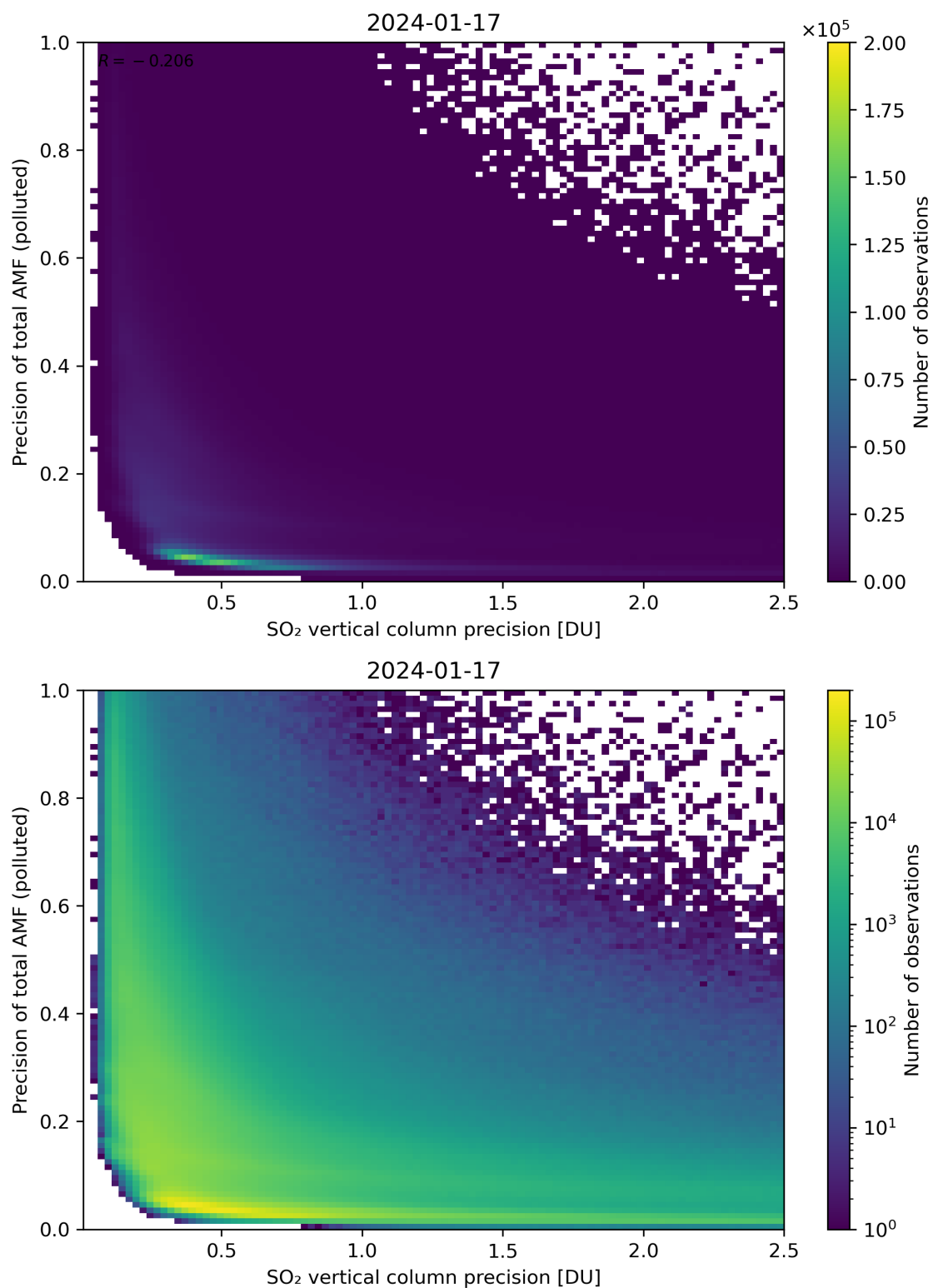
Figure 295: Scatter density plot of “SO 2 vertical column precision” against “Precision of total AMF (polluted)” for 2024-01-16 to 2024-01-18.
