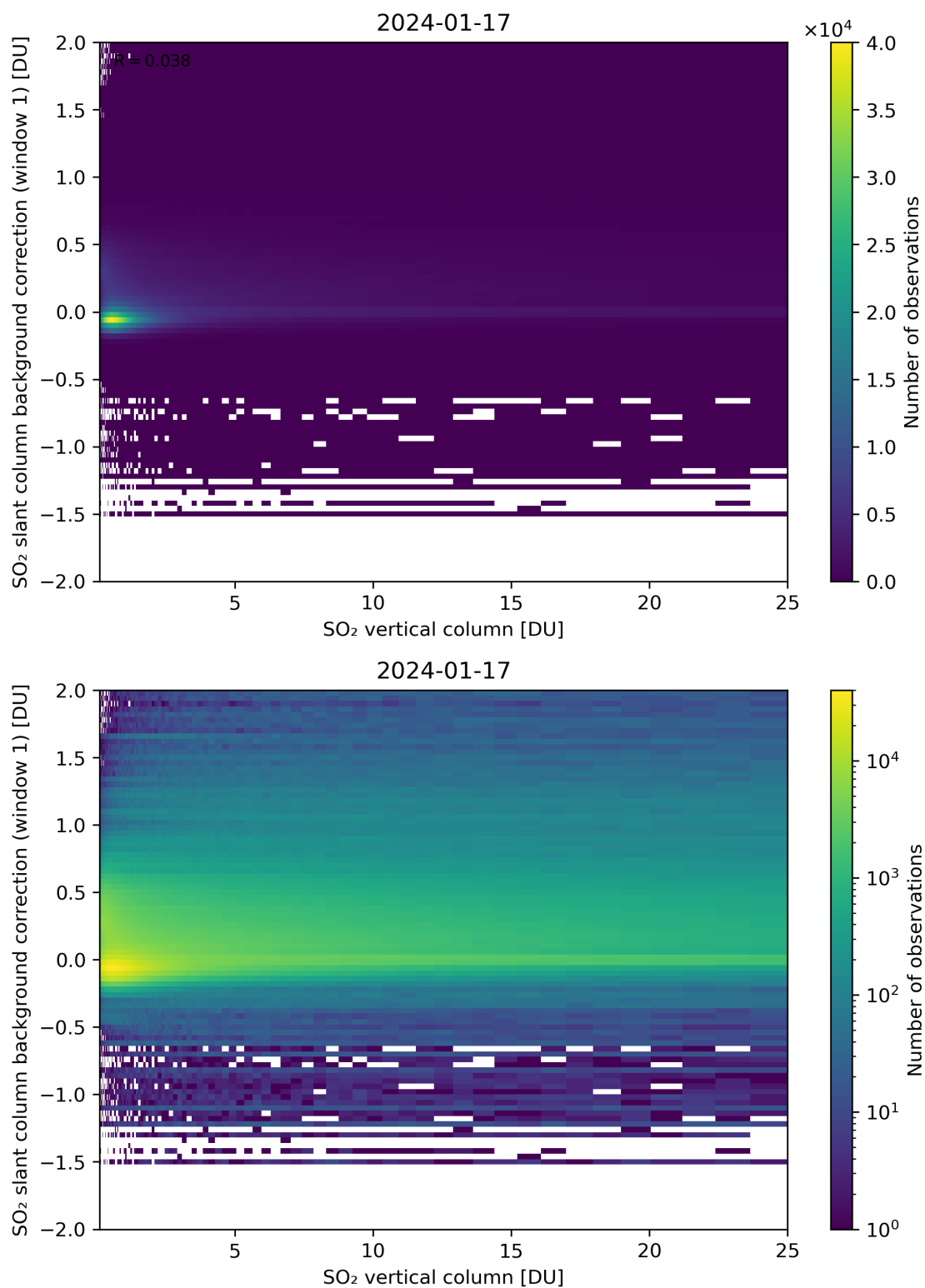
Figure 273: Scatter density plot of “SO 2 vertical column” against “SO 2 slant column background correction (window 1)” for 2024-01-16 to 2024-01-18.
