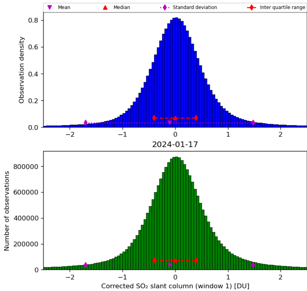
Figure 58: Histogram of “Corrected SO 2 slant column (window 1)” for 2024-01-16 to 2024-01-18
