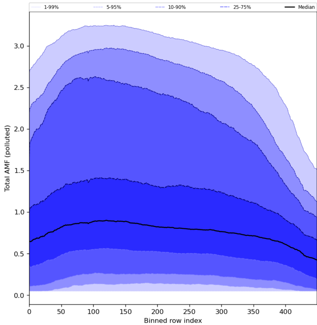
Figure 94: Along track statistics of “Total AMF (polluted)” for 2024-01-16 to 2024-01-18
