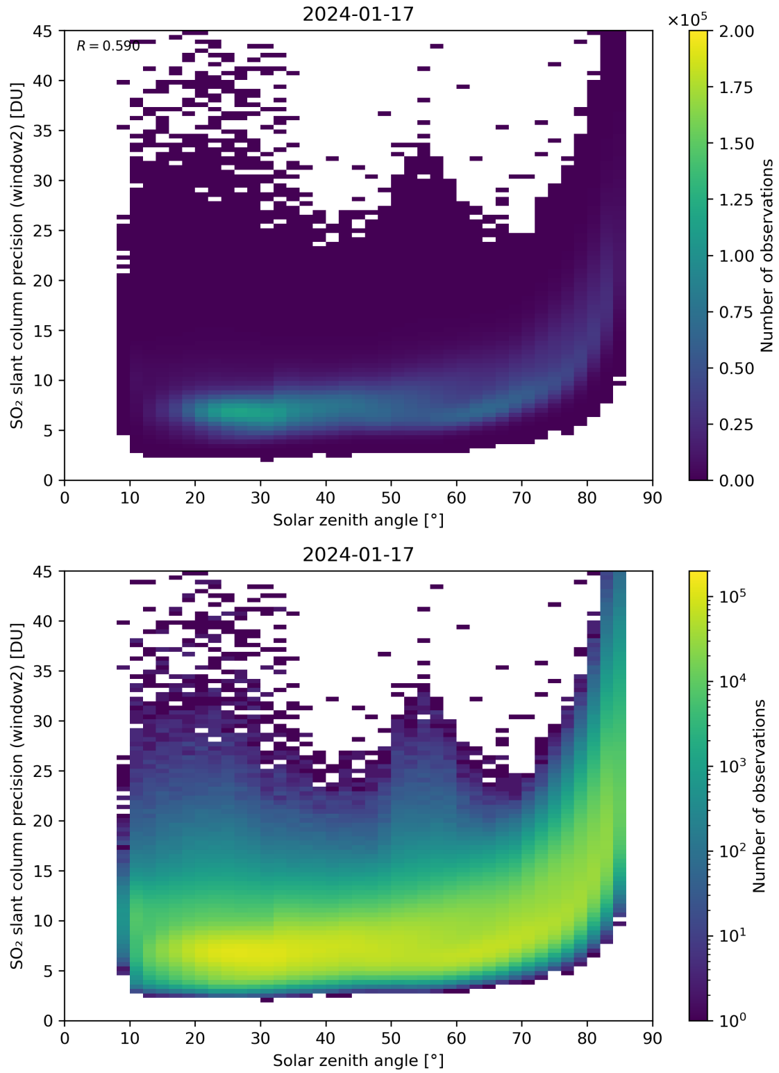
Figure 171: Scatter density plot of “Solar zenith angle” against “SO 2 slant column precision (window2)” for 2024-01-16 to 2024-01-18.
