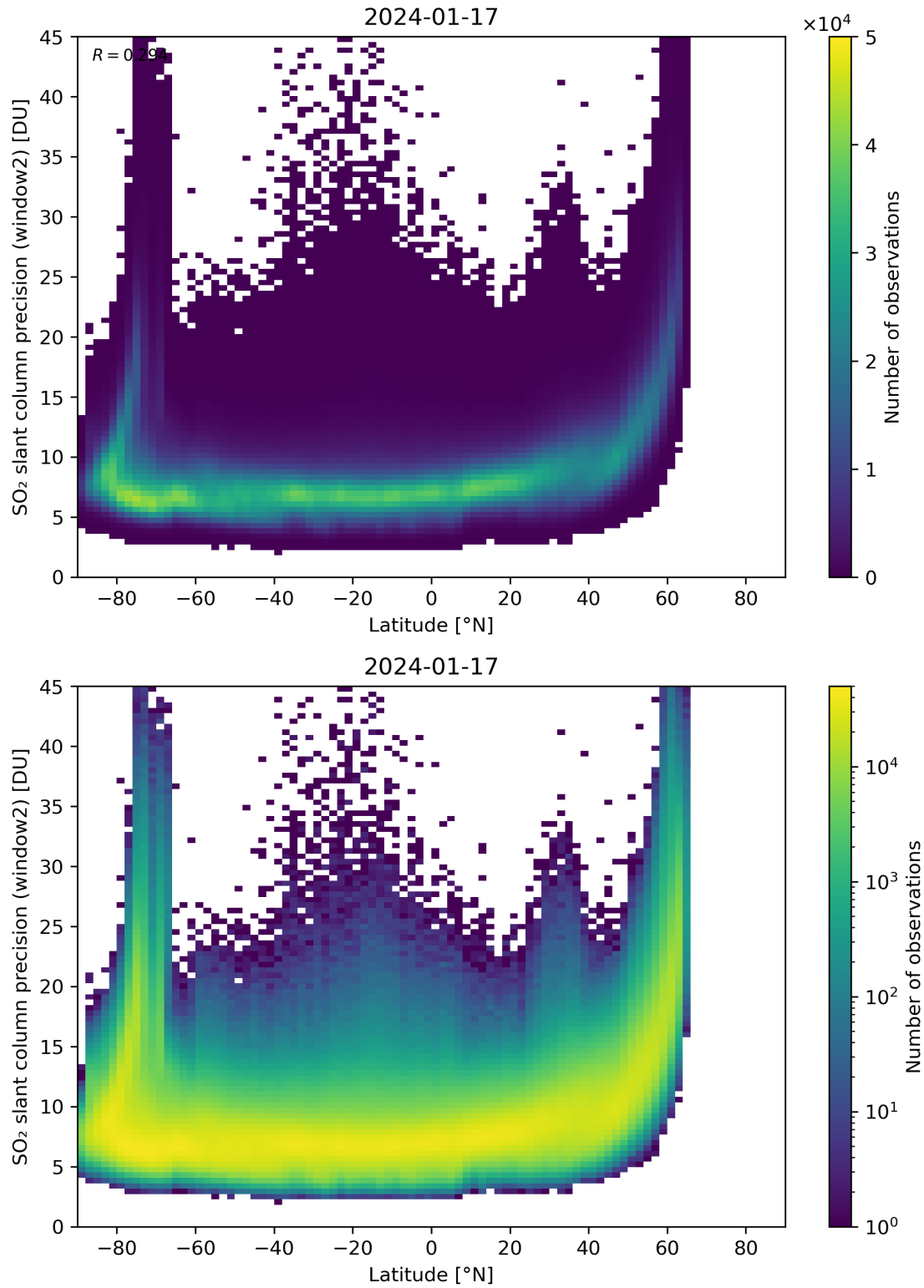
Figure 151: Scatter density plot of “Latitude” against “SO 2 slant column precision (window2)” for 2024-01-16 to 2024-01-18.
