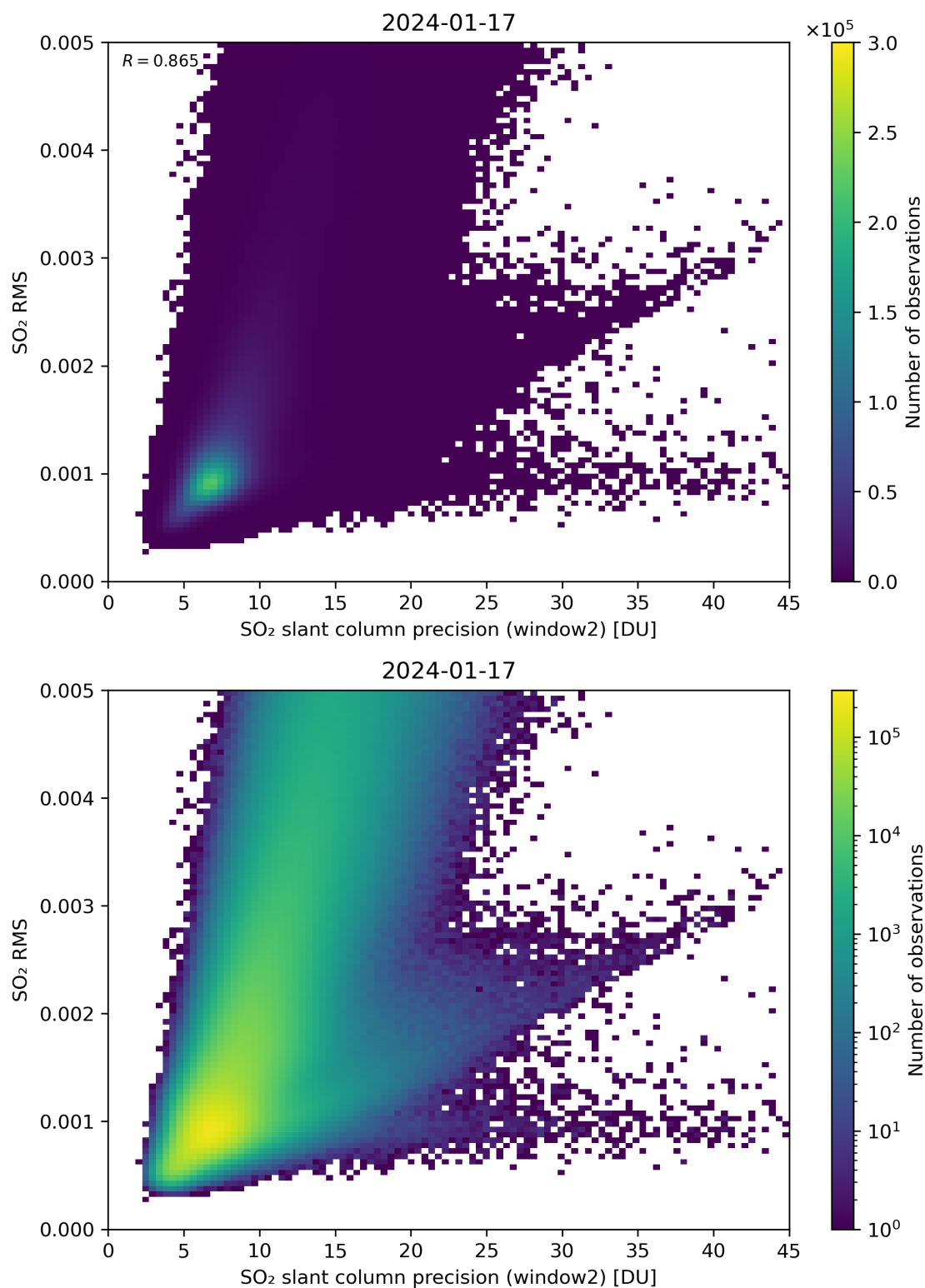
Figure 245: Scatter density plot of “SO 2 slant column precision (window2)” against “SO 2 RMS” for 2024-01-16 to 2024-01-18.
