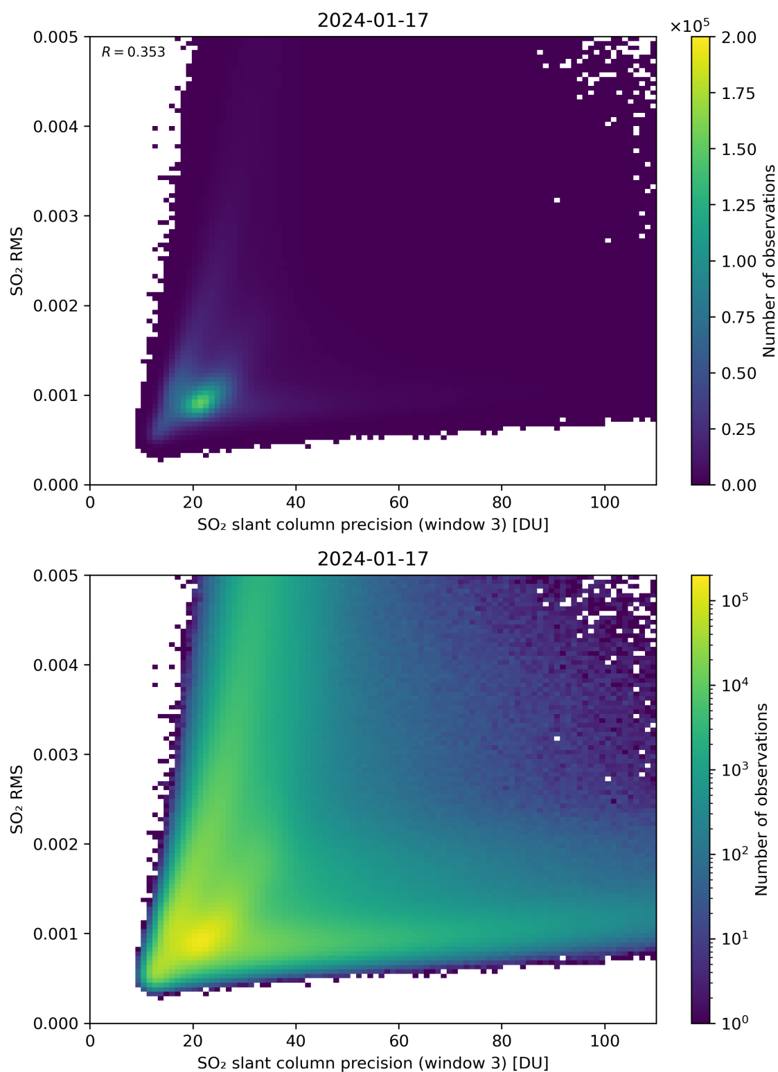
Figure 260: Scatter density plot of “SO 2 slant column precision (window 3)” against “SO 2 RMS” for 2024-01-16 to 2024-01-18.
