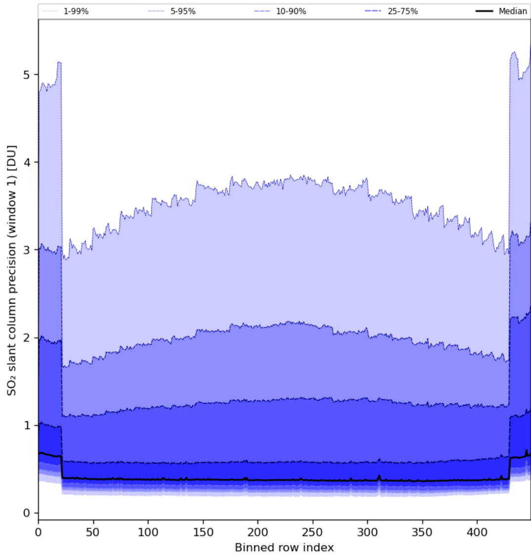
Figure 80: Along track statistics of “SO 2 slant column precision (window 1)” for 2024-01-16 to 2024-01-18
