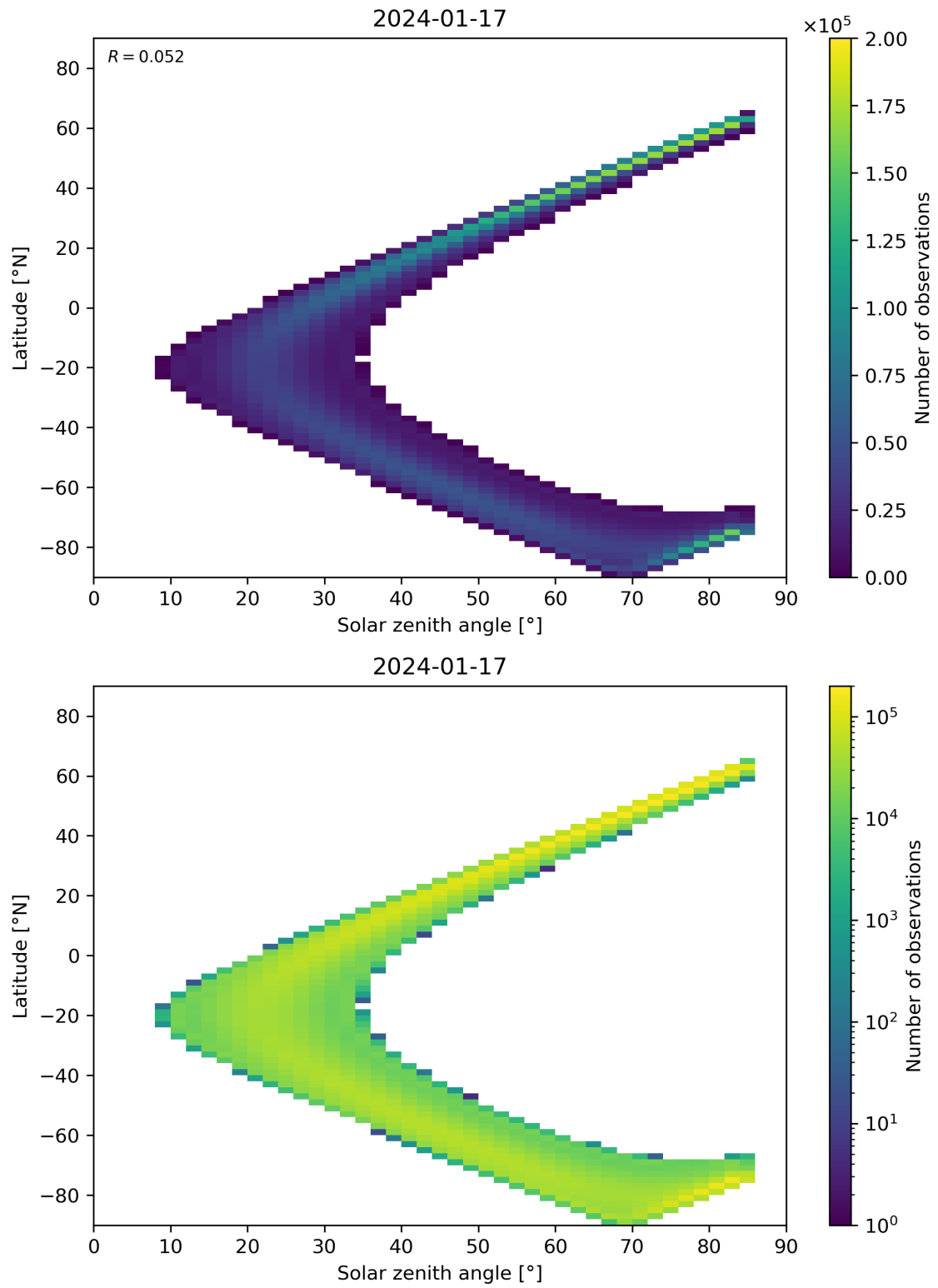
Figure 164: Scatter density plot of “Solar zenith angle” against “Latitude” for 2024-01-16 to 2024-01-18.
