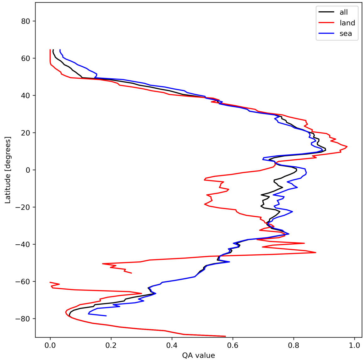
Figure 29: Zonal average of “QA value” for 2024-01-16 to 2024-01-18.
