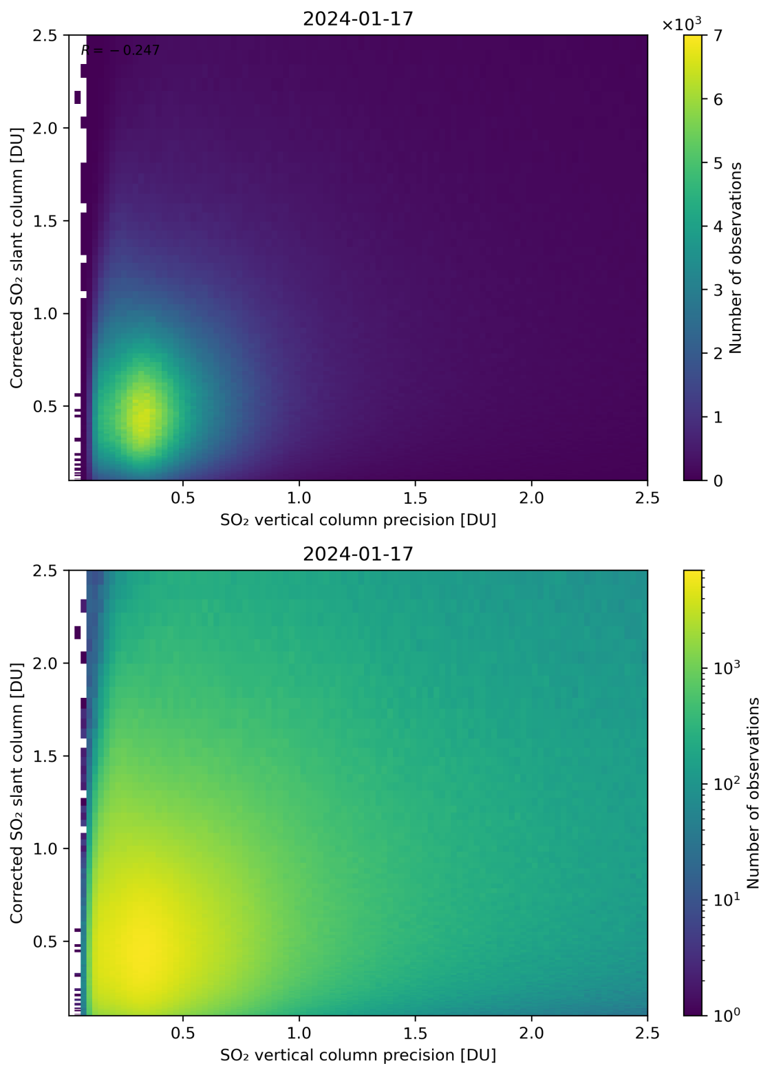
Figure 286: Scatter density plot of “SO 2 vertical column precision” against “Corrected SO 2 slant column” for 2024-01-16 to 2024-01-18.
