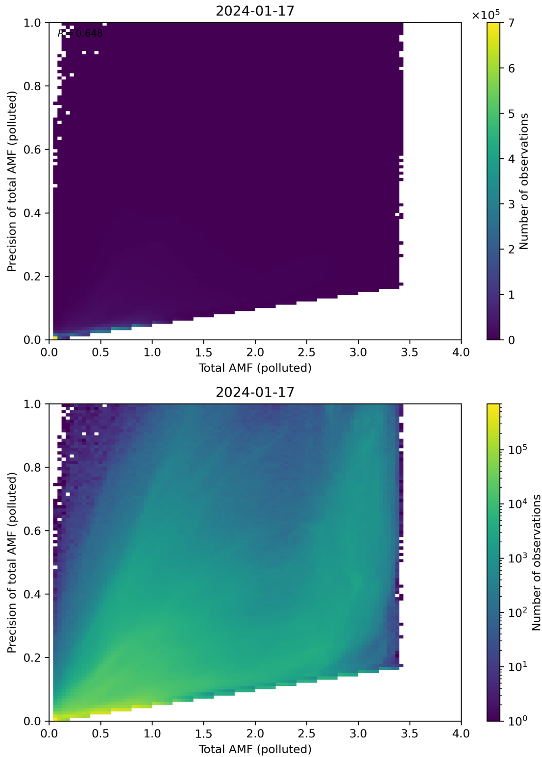
Figure 272: Scatter density plot of “Total AMF (polluted)” against “Precision of total AMF (polluted)” for 2024-01-16 to 2024-01-18.
