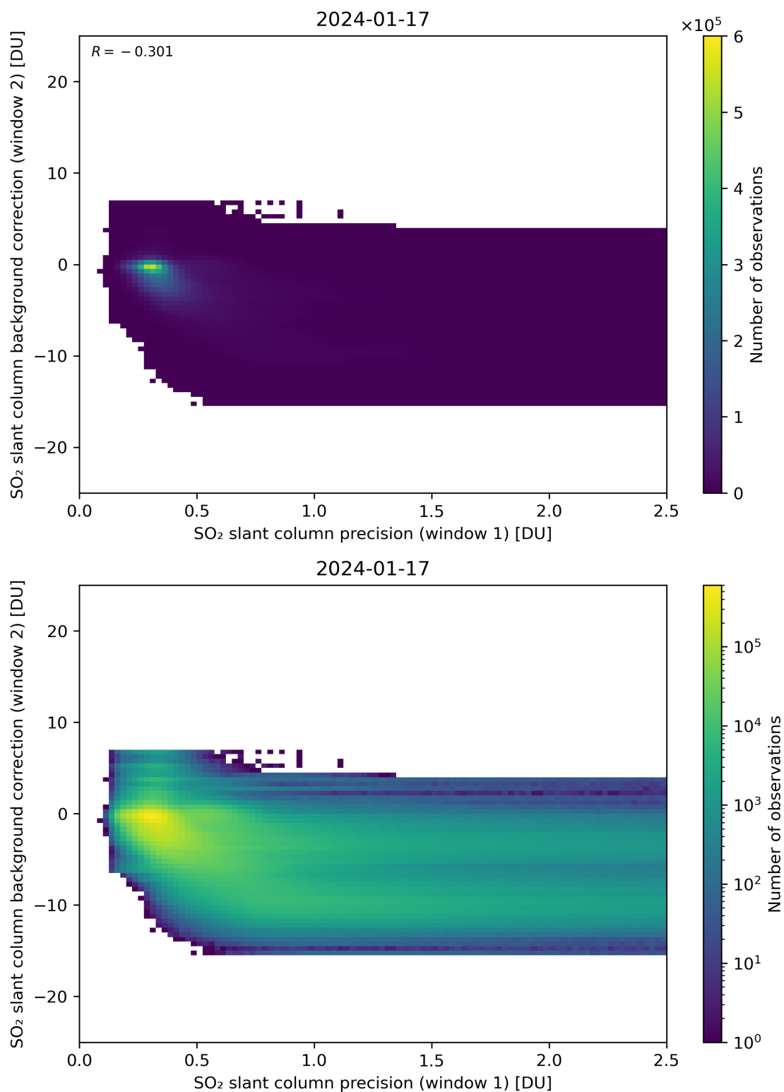
Figure 219: Scatter density plot of “SO 2 slant column precision (window 1)” against “SO 2 slant column background correction (window 2)” for 2024-01-16 to 2024-01-18.
