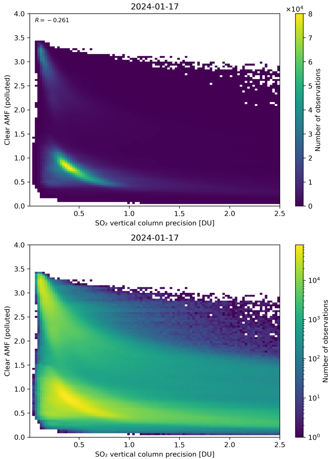
Figure 285: Scatter density plot of “SO 2 vertical column precision” against “Clear AMF (polluted)” for 2024-01-16 to 2024-01-18.
