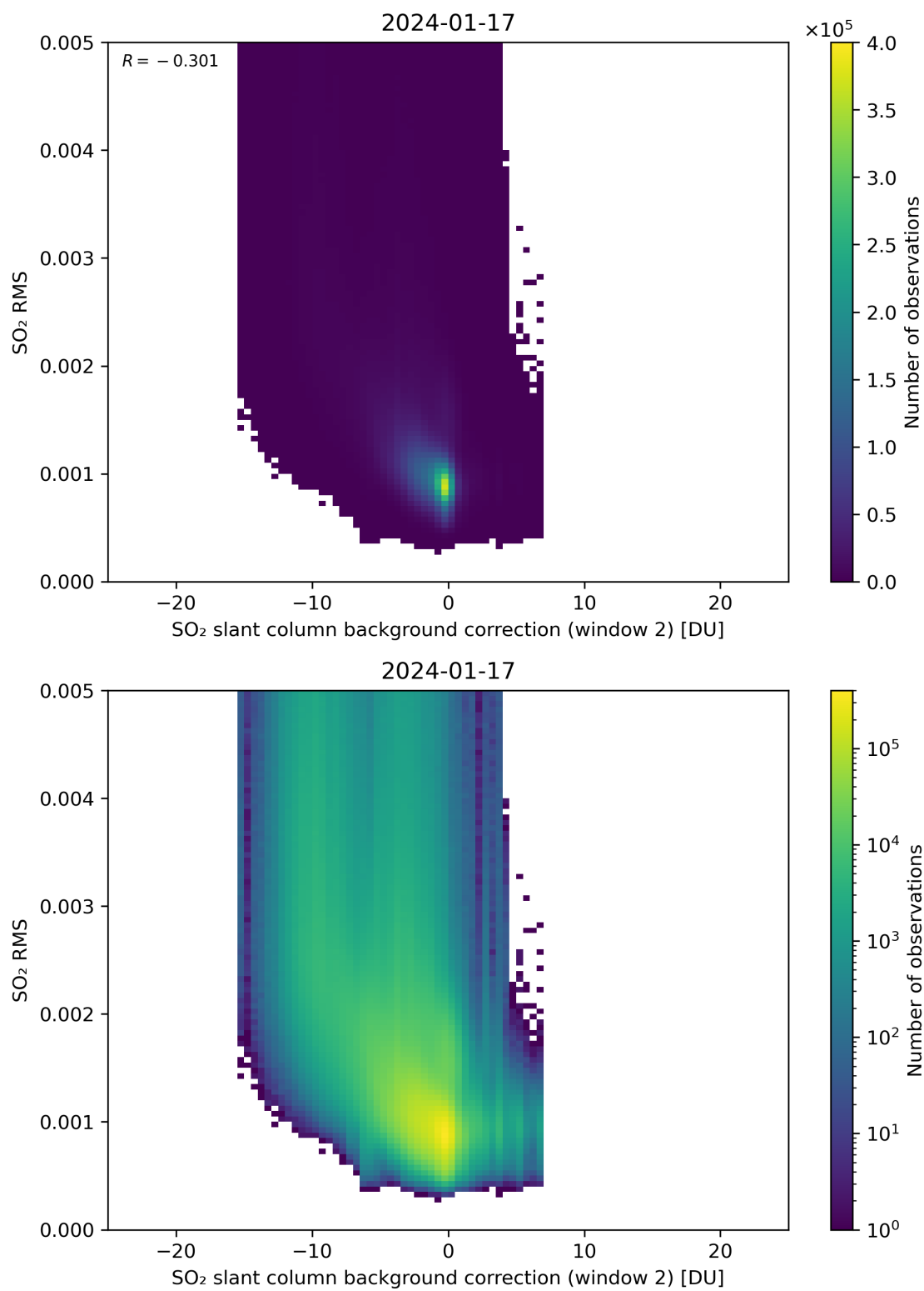
Figure 114: Scatter density plot of “SO 2 slant column background correction (window 2)” against “SO 2 RMS” for 2024-01-16 to 2024-01-18.
