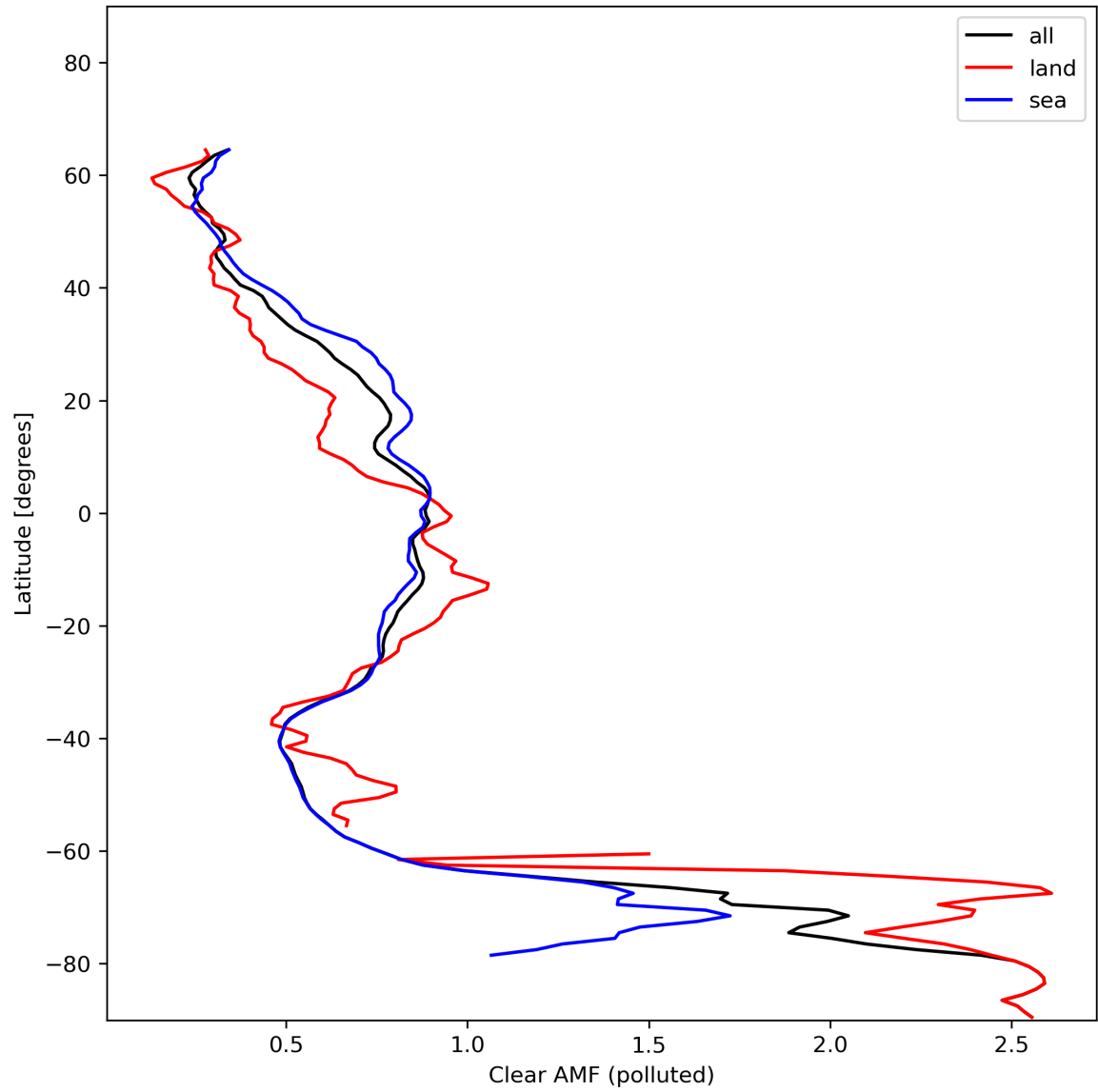
Figure 50: Zonal average of “Clear AMF (polluted)” for 2024-01-16 to 2024-01-18.
