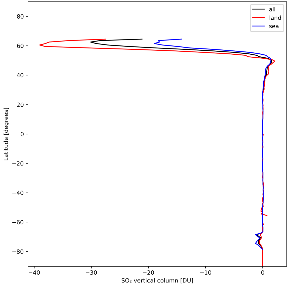
Figure 30: Zonal average of “SO 2 vertical column” for 2024-01-16 to 2024-01-18.
