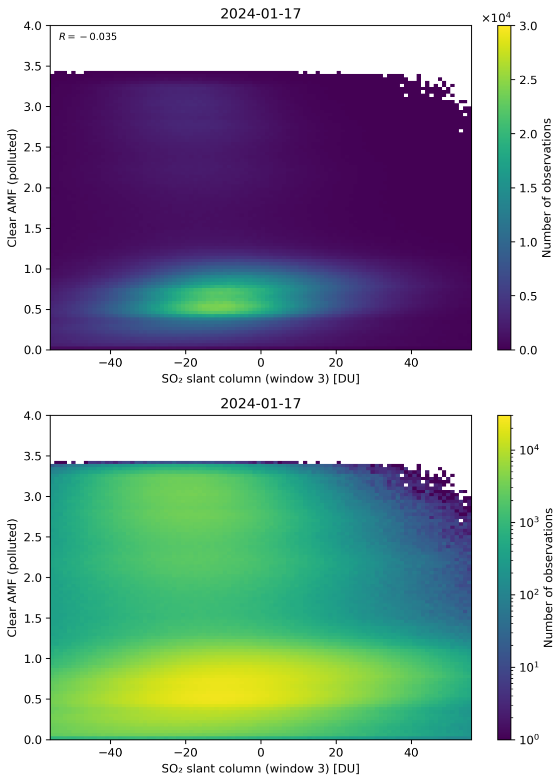
Figure 265: Scatter density plot of “SO 2 slant column (window 3)” against “Clear AMF (polluted)” for 2024-01-16 to 2024-01-18.
