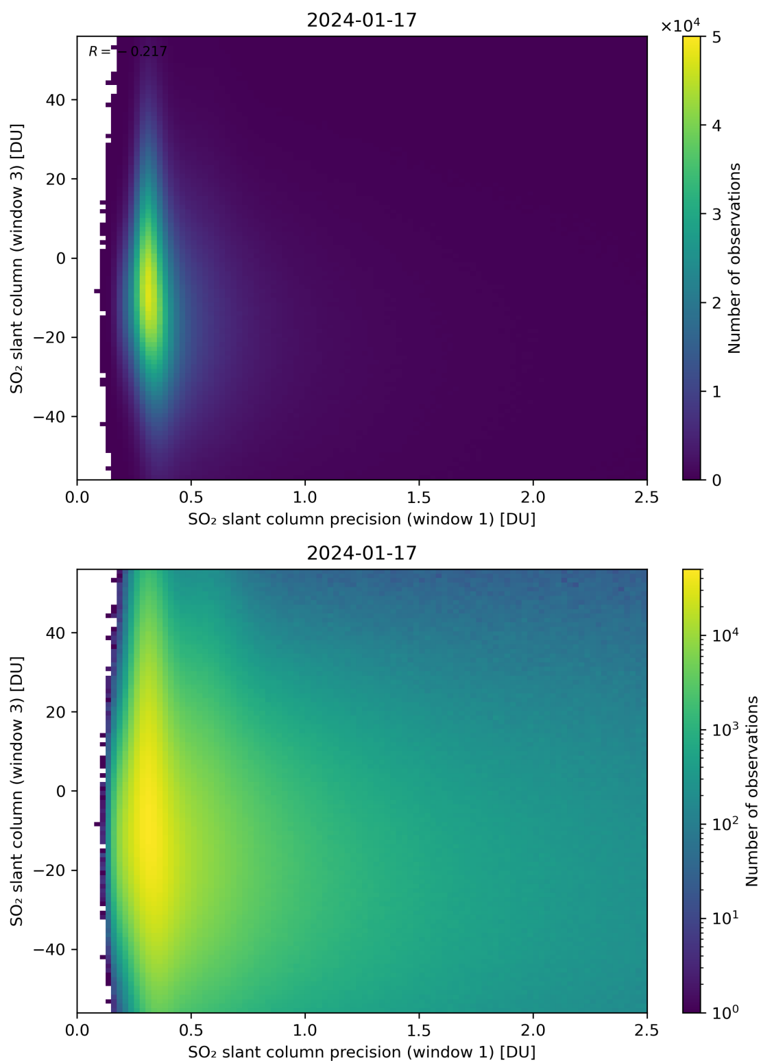
Figure 228: Scatter density plot of “SO 2 slant column precision (window 1)” against “SO 2 slant column (window 3)” for 2024-01-16 to 2024-01-18.
