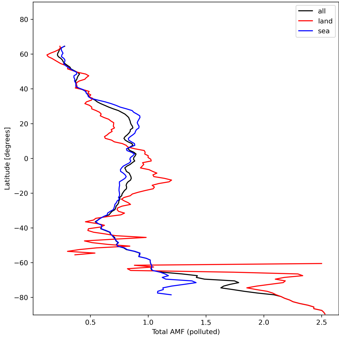
Figure 48: Zonal average of “Total AMF (polluted)” for 2024-01-16 to 2024-01-18.
