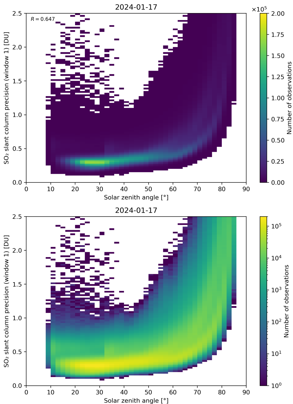
Figure 170: Scatter density plot of “Solar zenith angle” against “SO 2 slant column precision (window 1)” for 2024-01-16 to 2024-01-18.
