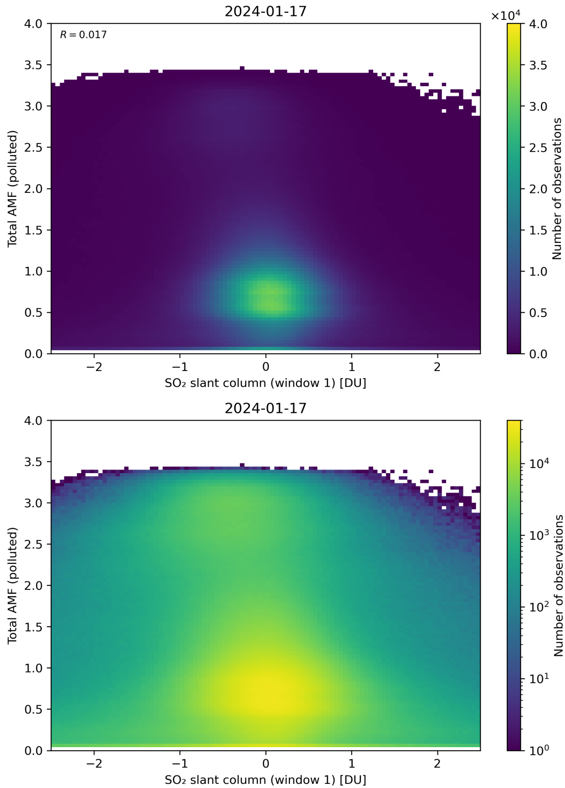
Figure 239: Scatter density plot of “SO 2 slant column (window 1)” against “Total AMF (polluted)” for 2024-01-16 to 2024-01-18.
