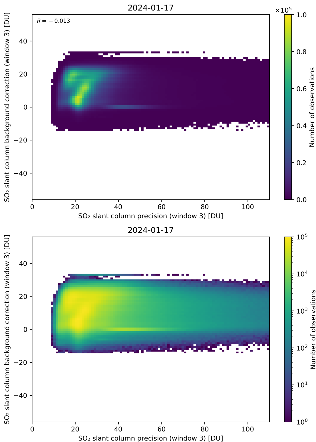
Figure 257: Scatter density plot of “SO 2 slant column precision (window 3)” against “SO 2 slant column background correction (window 3)” for 2024-01-16 to 2024-01-18.
