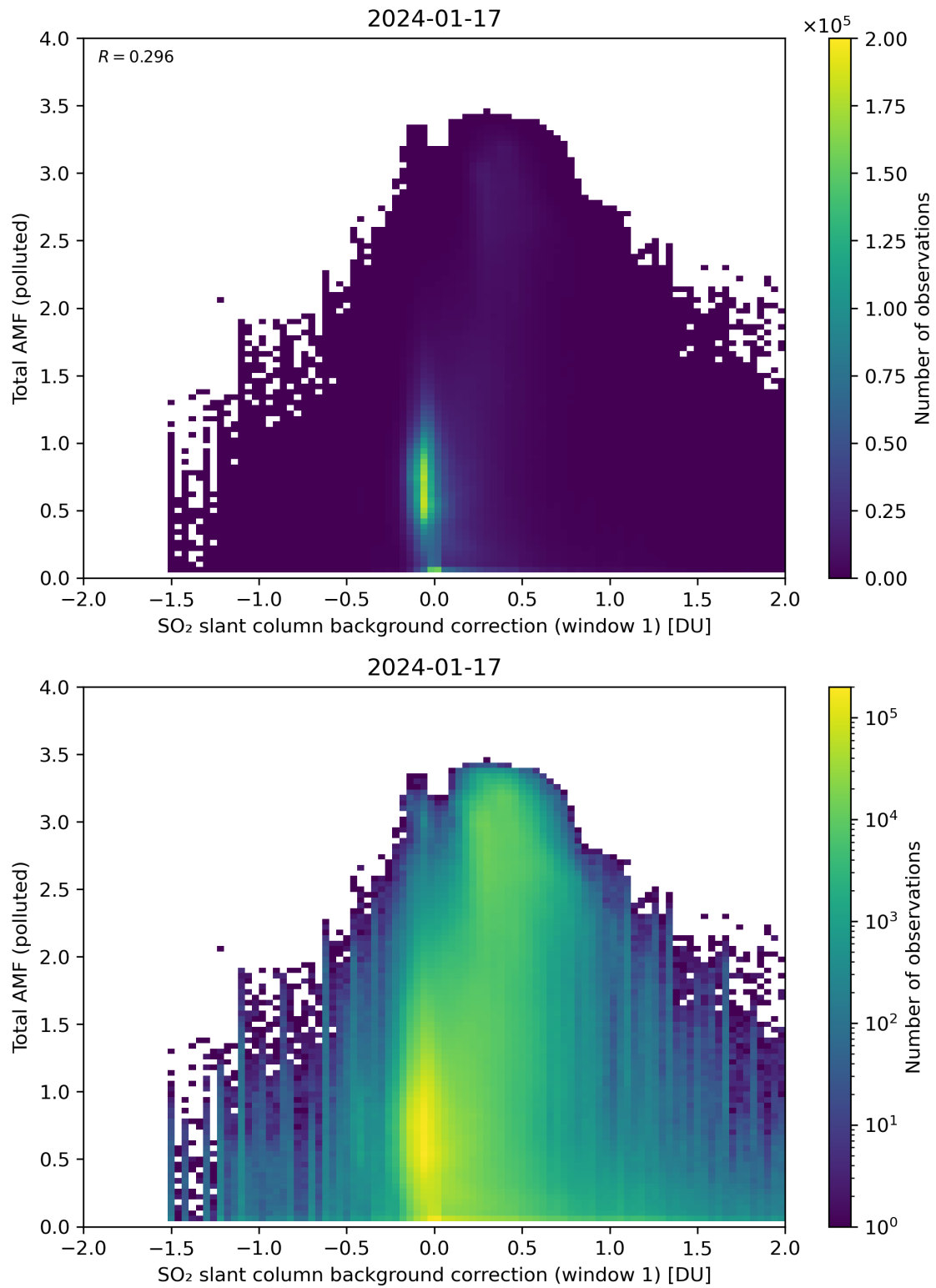
Figure 109: Scatter density plot of “SO 2 slant column background correction (window 1)” against “Total AMF (polluted)” for 2024-01-16 to 2024-01-18.
