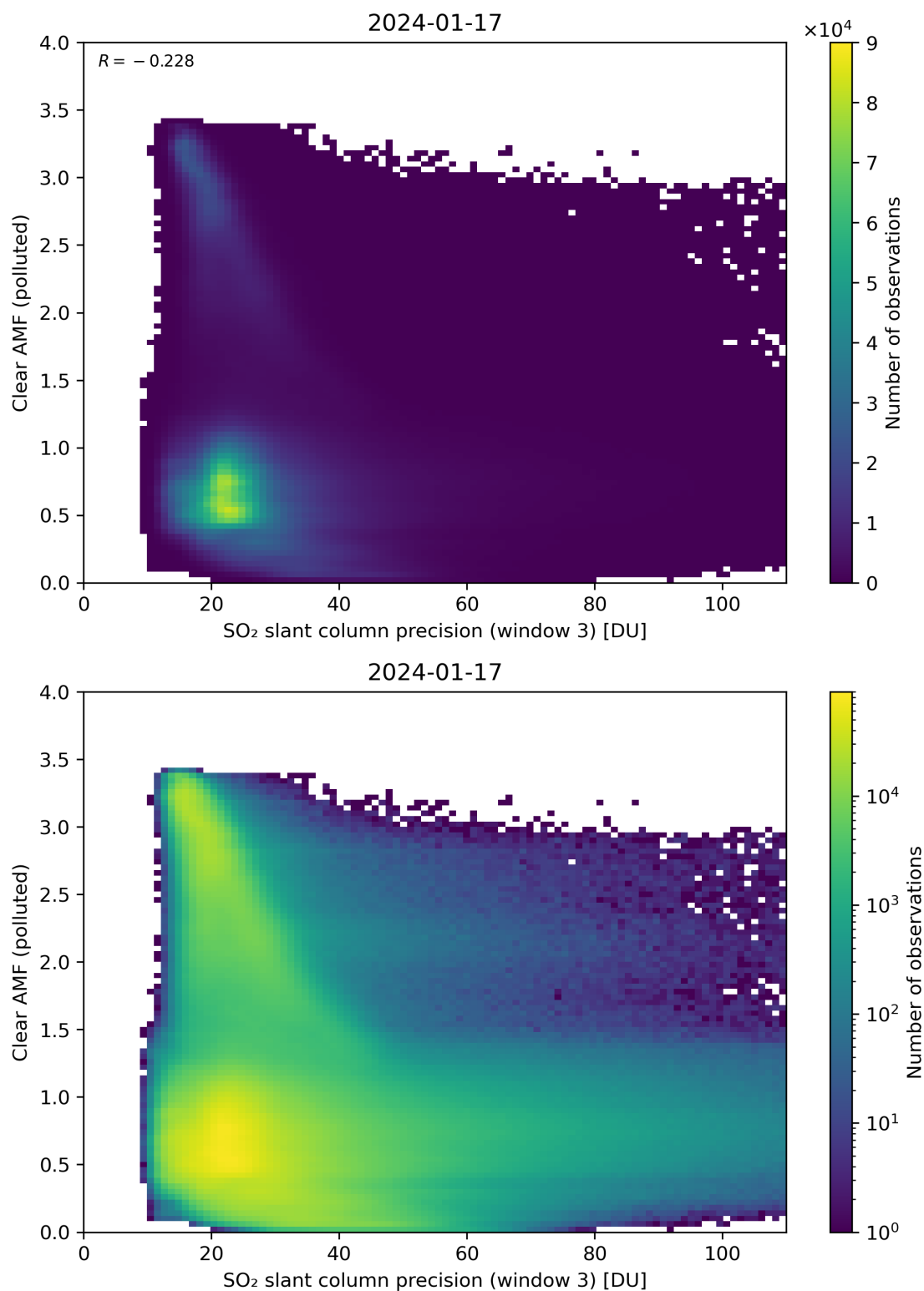
Figure 261: Scatter density plot of “SO 2 slant column precision (window 3)” against “Clear AMF (polluted)” for 2024-01-16 to 2024-01-18.
