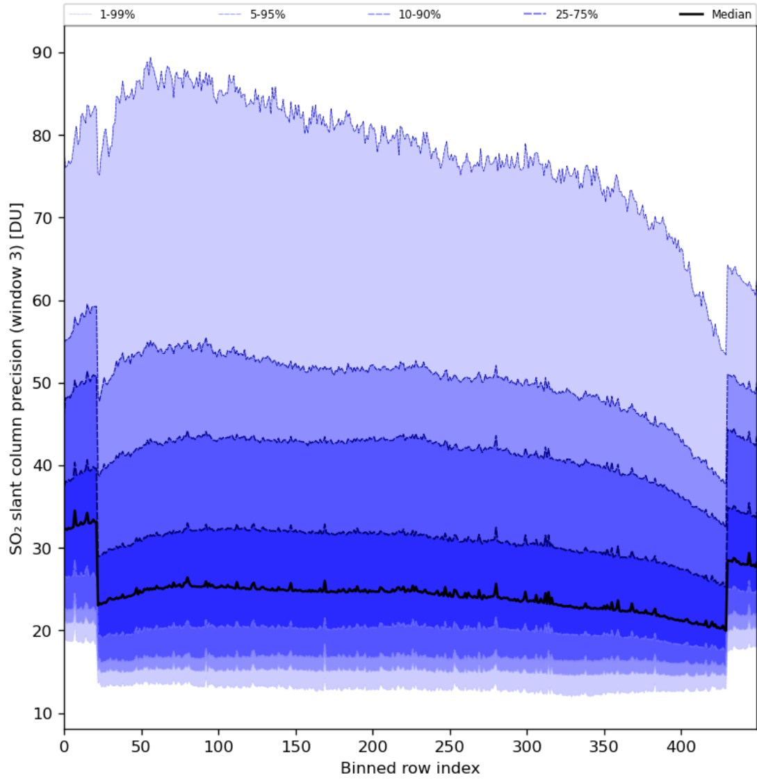
Figure 88: Along track statistics of “SO 2 slant column precision (window 3)” for 2024-01-16 to 2024-01-18
