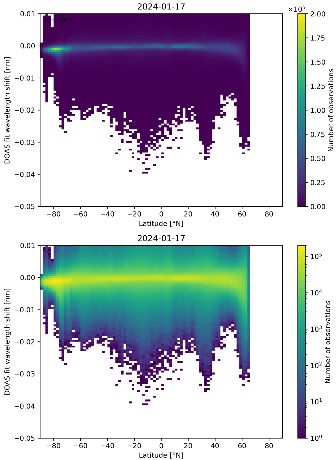
Figure 142: Scatter density plot of “Latitude” against “DOAS fit wavelength shift” for 2024-01-16 to 2024-01-18.
