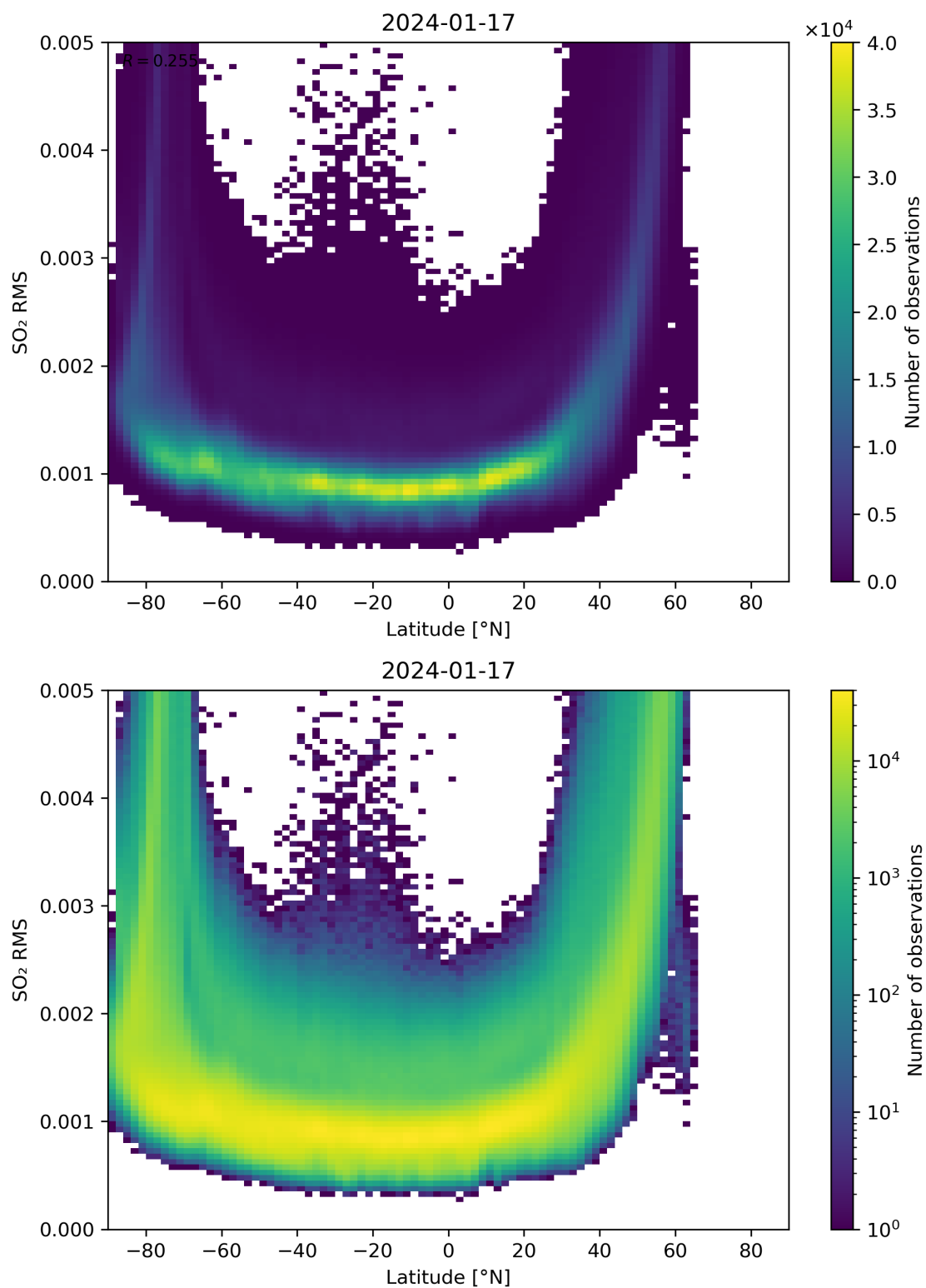
Figure 144: Scatter density plot of “Latitude” against “SO 2 RMS” for 2024-01-16 to 2024-01-18.
