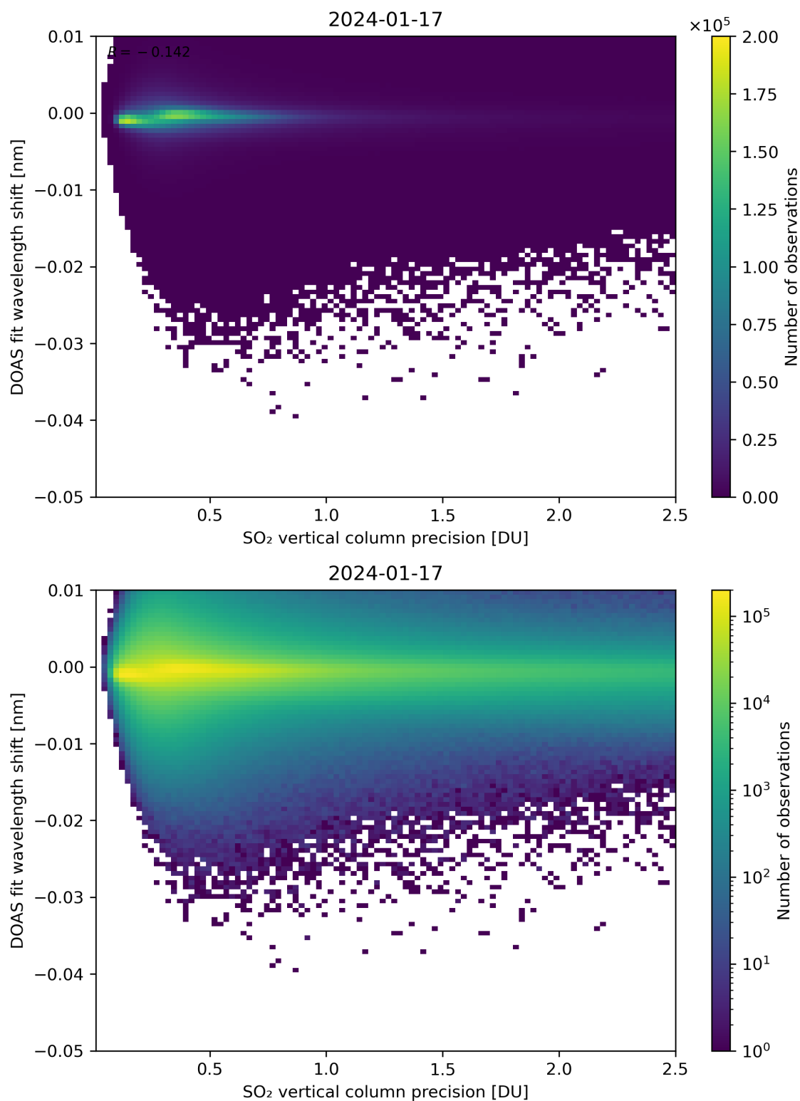
Figure 282: Scatter density plot of “SO 2 vertical column precision” against “DOAS fit wavelength shift” for 2024-01-16 to 2024-01-18.
