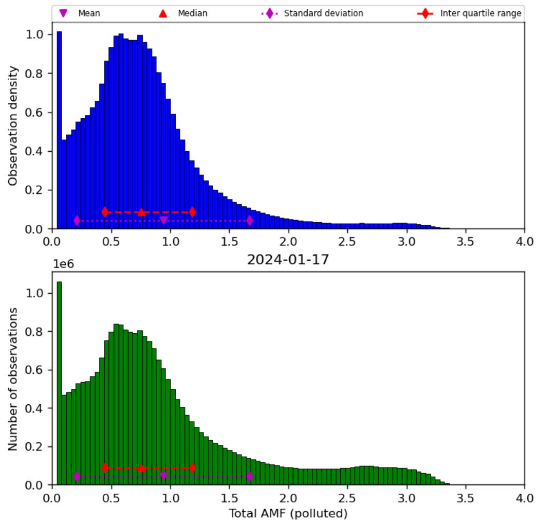
Figure 71: Histogram of “Total AMF (polluted)” for 2024-01-16 to 2024-01-18
