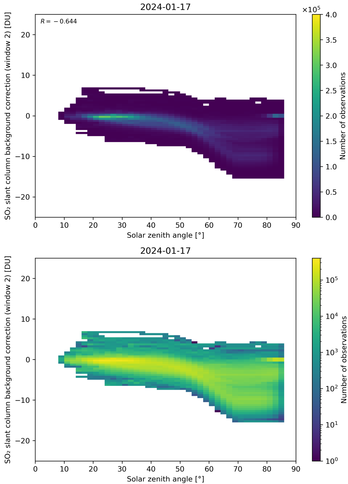
Figure 159: Scatter density plot of “Solar zenith angle” against “SO 2 slant column background correction (window 2)” for 2024-01-16 to 2024-01-18.
