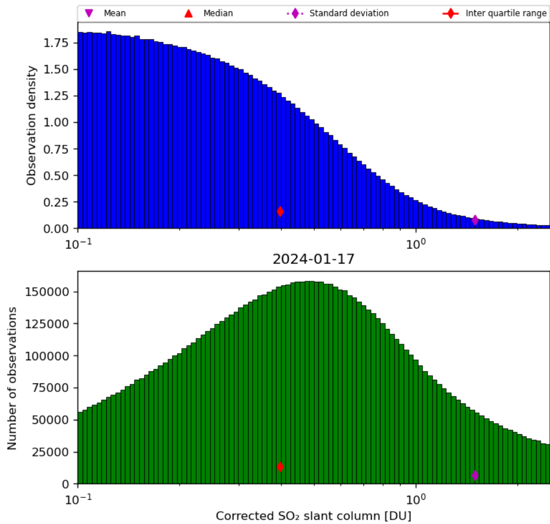
Figure 55: Histogram of “Corrected SO 2 slant column” for 2024-01-16 to 2024-01-18
