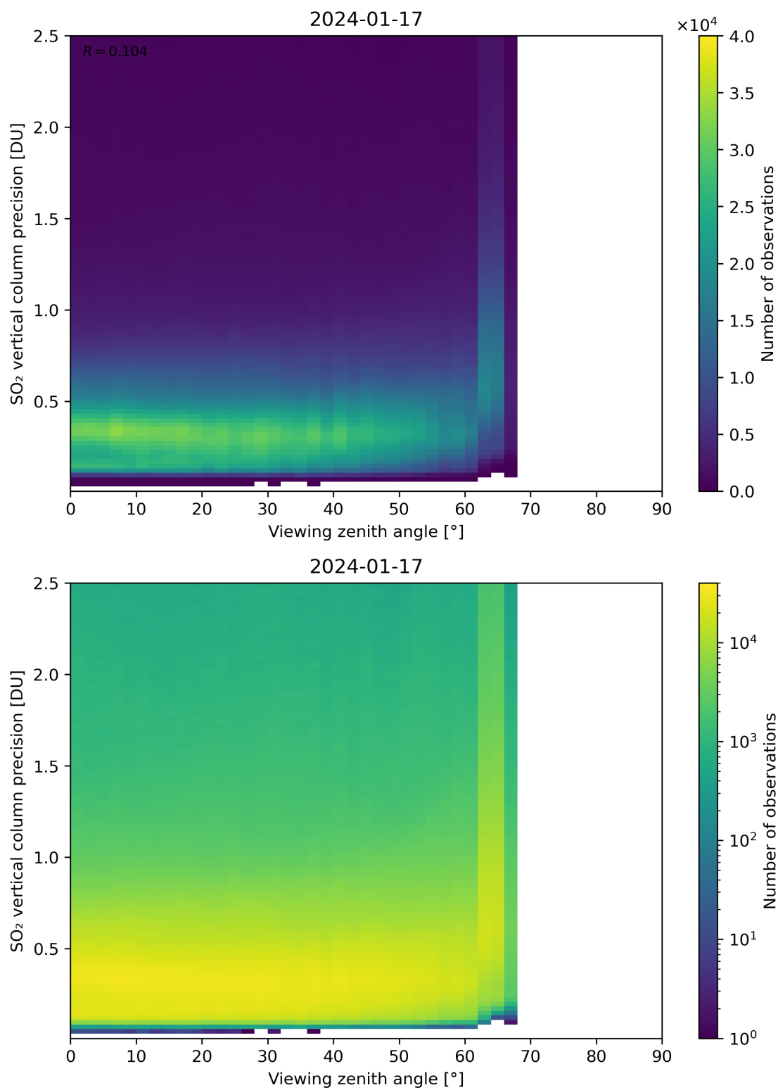
Figure 328: Scatter density plot of “Viewing zenith angle” against “SO 2 vertical column precision” for 2024-01-16 to 2024-01-18.
