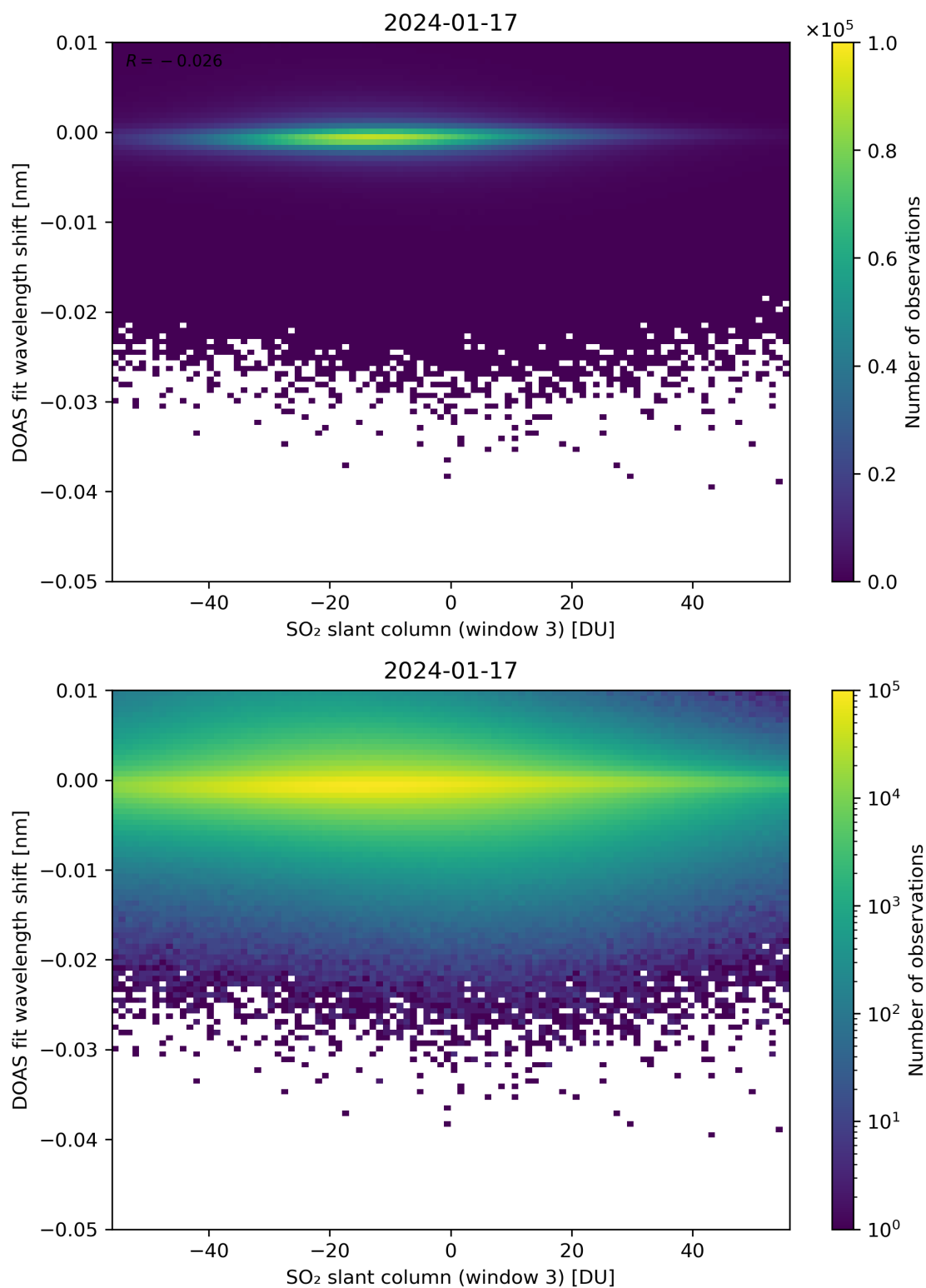
Figure 254: Scatter density plot of “SO 2 slant column (window 3)” against “DOAS fit wavelength shift” for 2024-01-16 to 2024-01-18.
