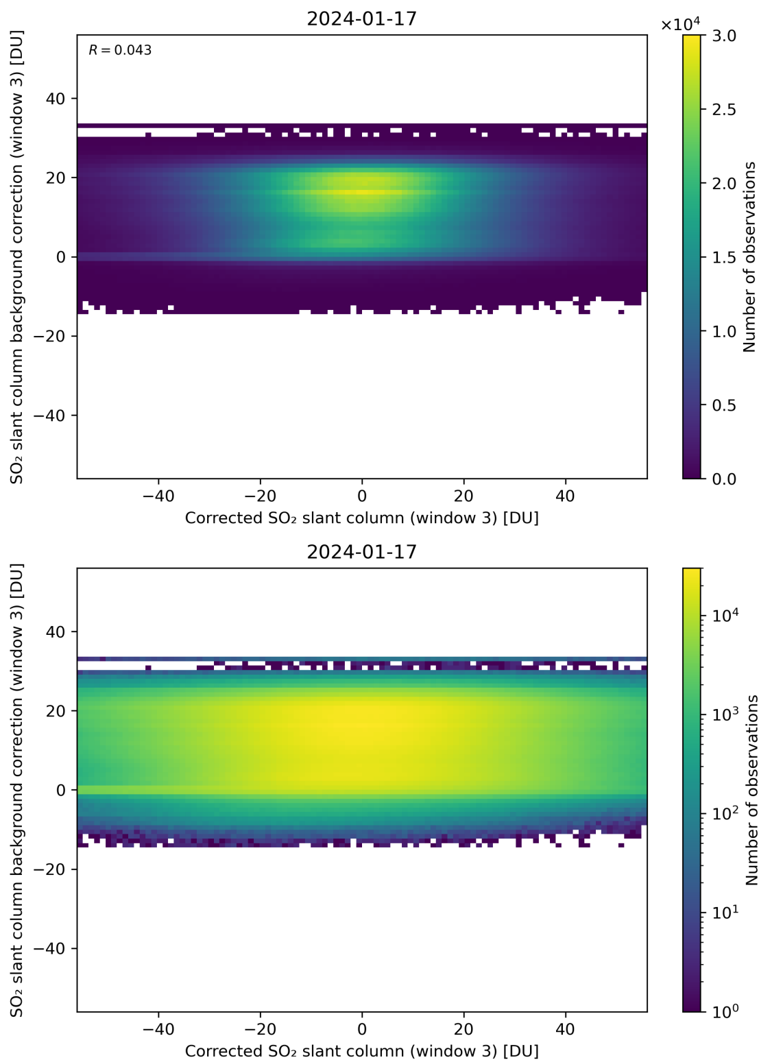
Figure 205: Scatter density plot of “Corrected SO 2 slant column (window 3)” against “SO 2 slant column background correction (window 3)” for 2024-01-16 to 2024-01-18.
