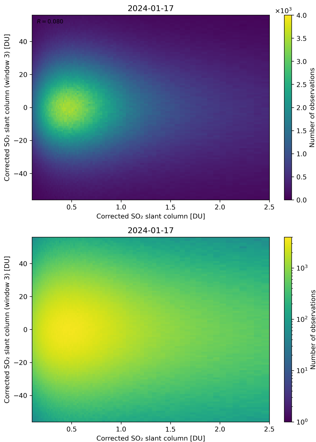
Figure 186: Scatter density plot of “Corrected SO 2 slant column” against “Corrected SO 2 slant column (window 3)” for 2024-01-16 to 2024-01-18.
