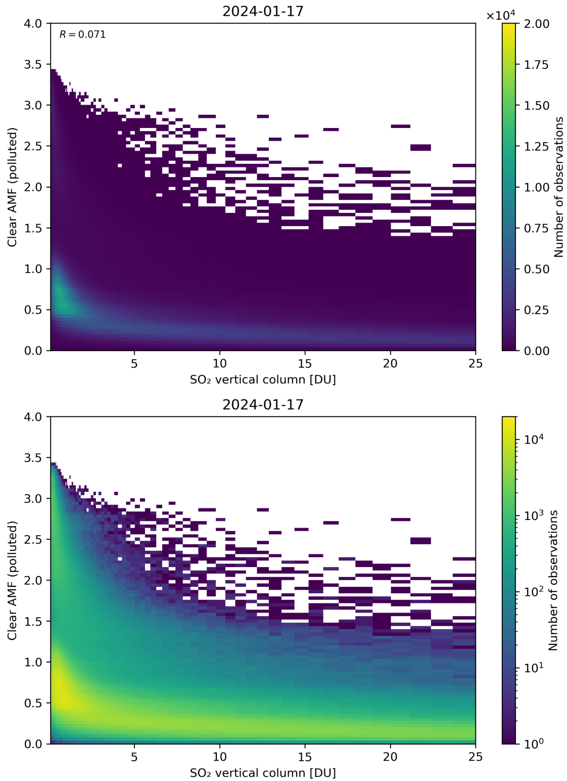
Figure 296: Scatter density plot of “SO 2 vertical column” against “Clear AMF (polluted)” for 2024-01-16 to 2024-01-18.
