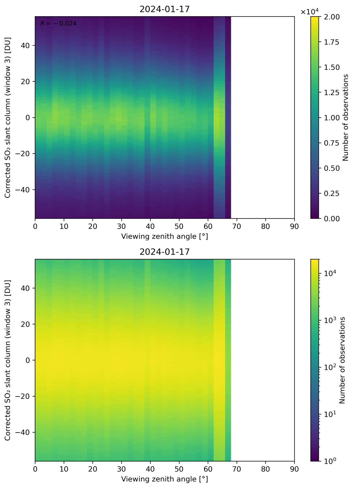
Figure 319: Scatter density plot of “Viewing zenith angle” against “Corrected SO 2 slant column (window 3)” for 2024-01-16 to 2024-01-18.
