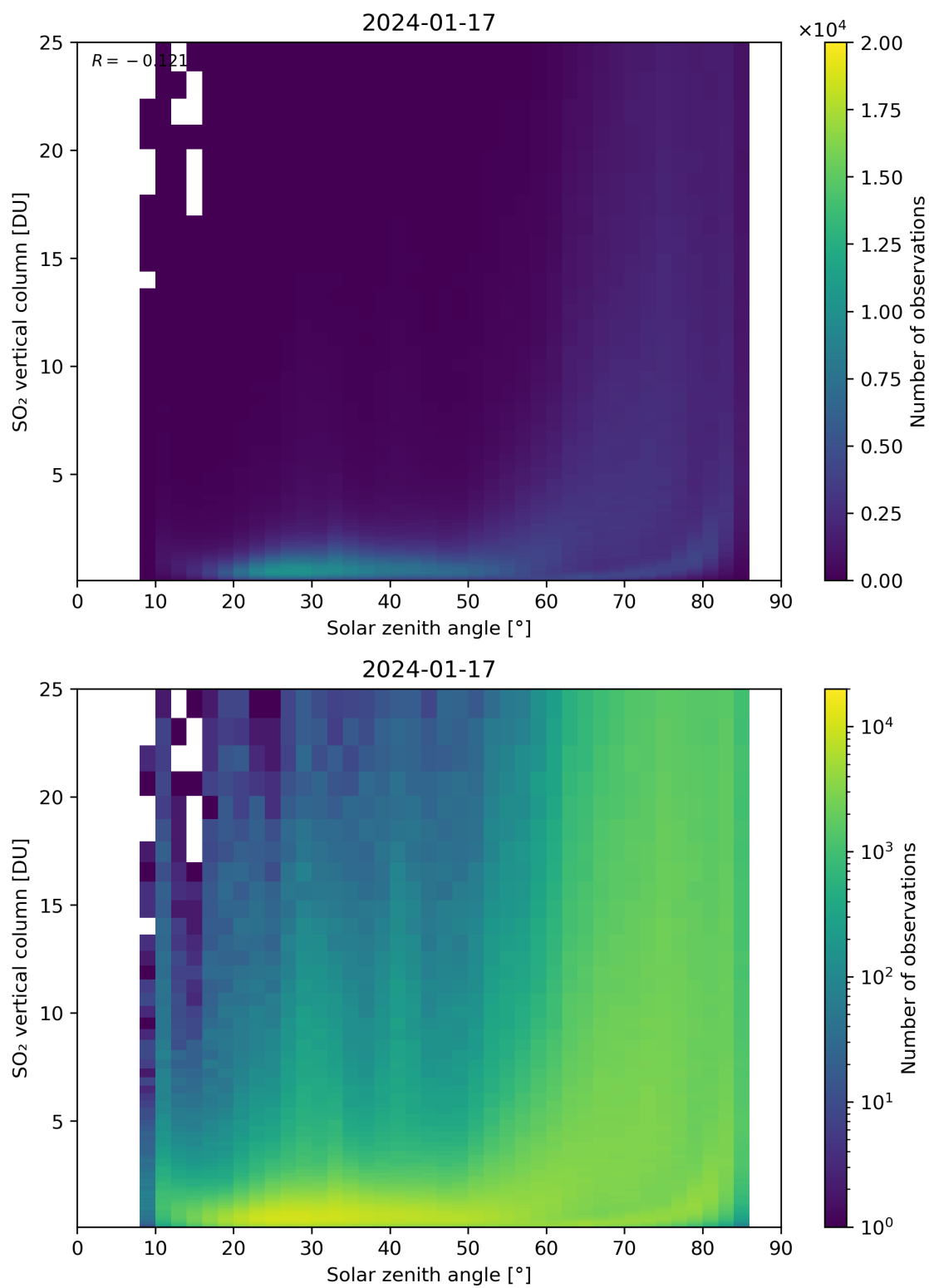
Figure 176: Scatter density plot of “Solar zenith angle” against “SO 2 vertical column” for 2024-01-16 to 2024-01-18.
