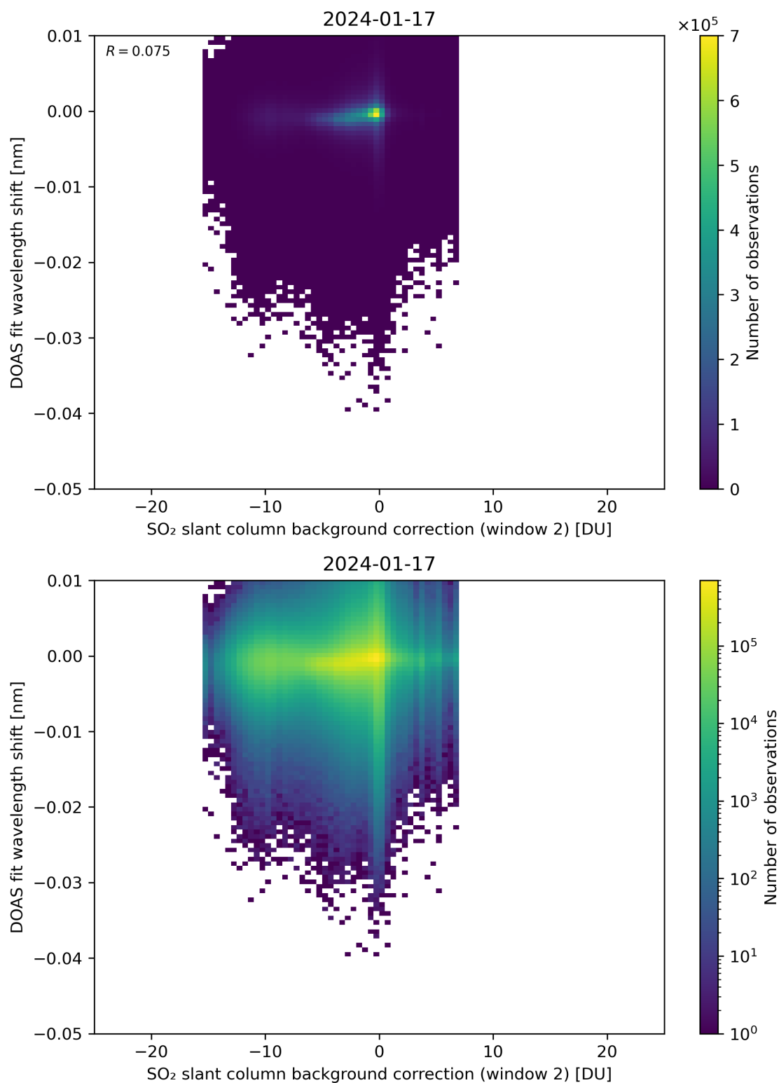
Figure 112: Scatter density plot of “SO 2 slant column background correction (window 2)” against “DOAS fit wavelength shift” for 2024-01-16 to 2024-01-18.
