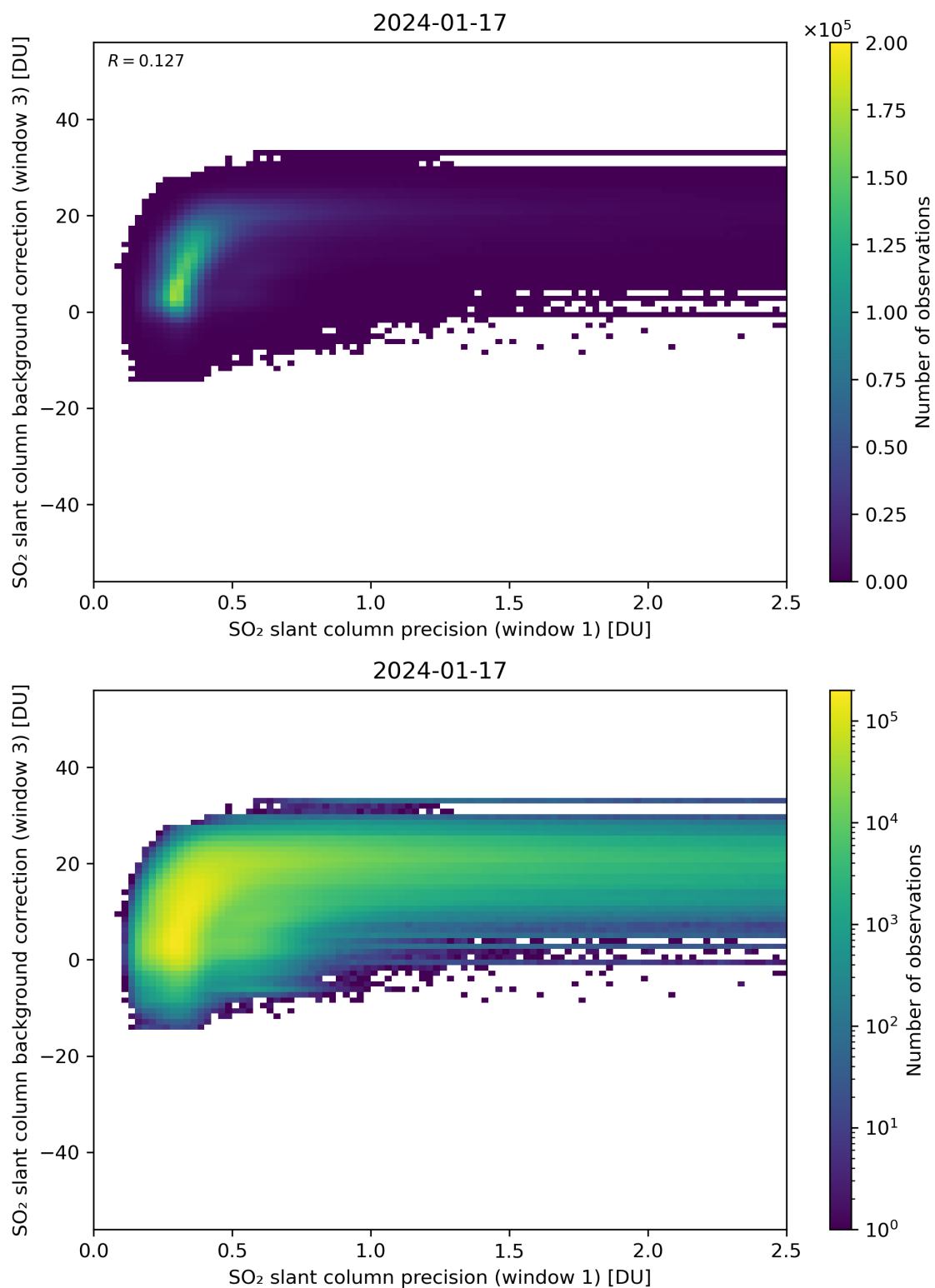
Figure 220: Scatter density plot of “SO 2 slant column precision (window 1)” against “SO 2 slant column background correction (window 3)” for 2024-01-16 to 2024-01-18.
