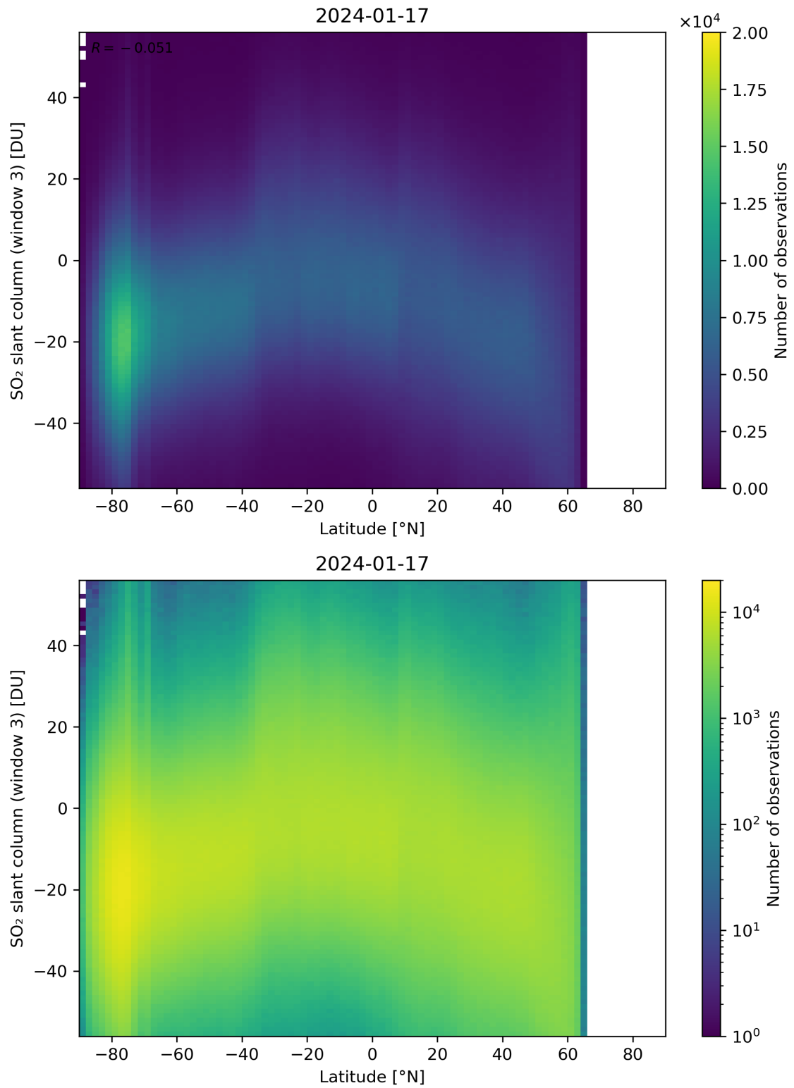
Figure 152: Scatter density plot of “Latitude” against “SO 2 slant column (window 3)” for 2024-01-16 to 2024-01-18.
