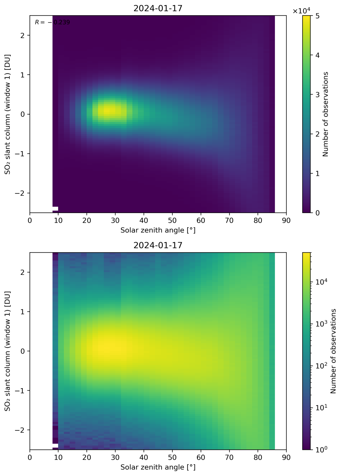
Figure 169: Scatter density plot of “Solar zenith angle” against “SO 2 slant column (window 1)” for 2024-01-16 to 2024-01-18.
