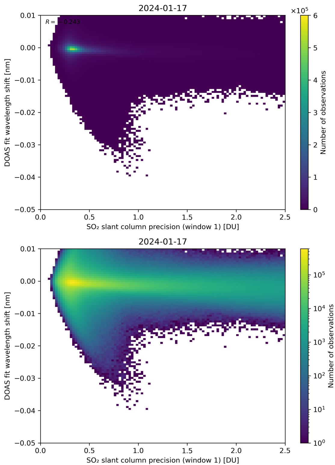
Figure 221: Scatter density plot of “SO 2 slant column precision (window 1)” against “DOAS fit wavelength shift” for 2024-01-16 to 2024-01-18.
