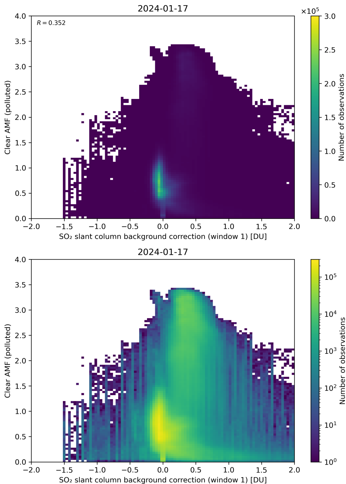
Figure 103: Scatter density plot of “SO 2 slant column background correction (window 1)” against “Clear AMF (polluted)” for 2024-01-16 to 2024-01-18.
