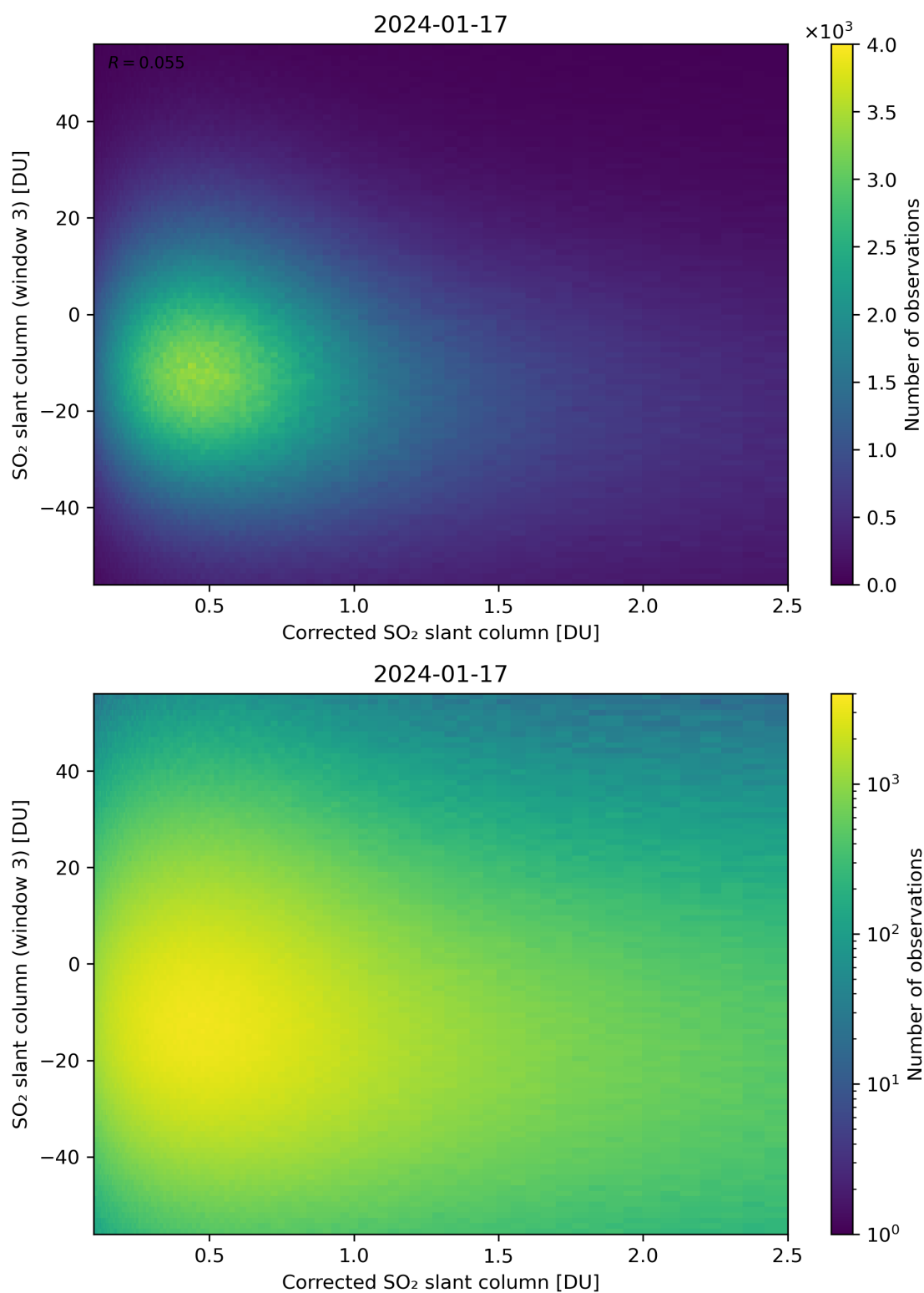
Figure 190: Scatter density plot of “Corrected SO 2 slant column” against “SO 2 slant column (window 3)” for 2024-01-16 to 2024-01-18.
