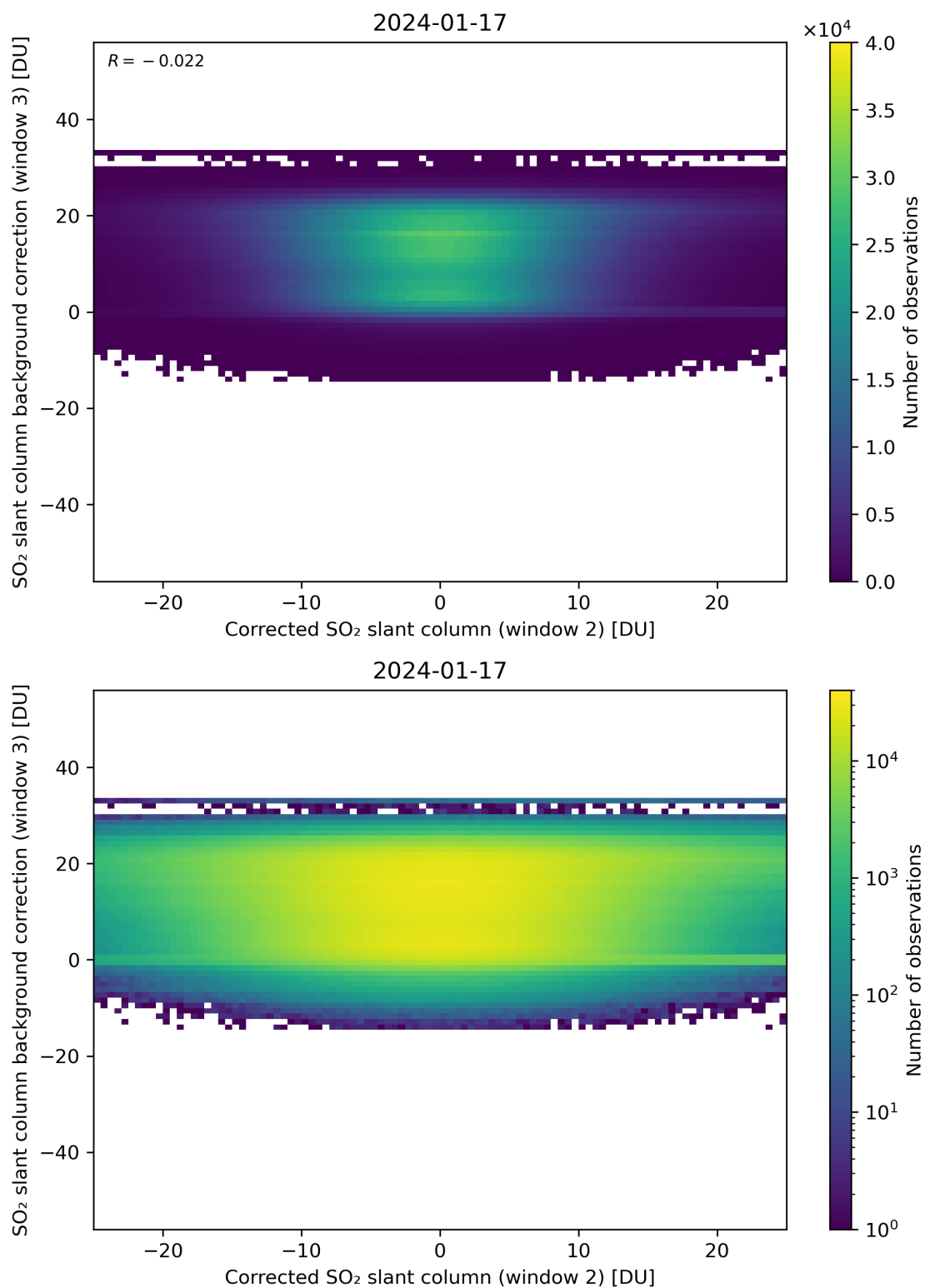
Figure 195: Scatter density plot of “Corrected SO 2 slant column (window 2)” against “SO 2 slant column background correction (window 3)” for 2024-01-16 to 2024-01-18.
