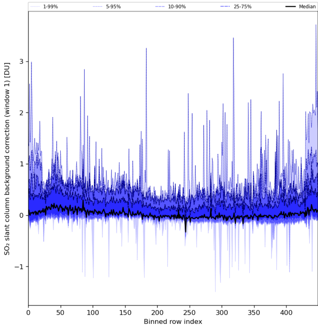
Figure 82: Along track statistics of “SO 2 slant column background correction (window 1)” for 2024-01-16 to 2024-01-18
