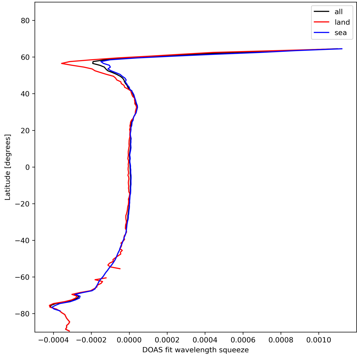
Figure 46: Zonal average of “DOAS fit wavelength squeeze” for 2024-01-16 to 2024-01-18.
