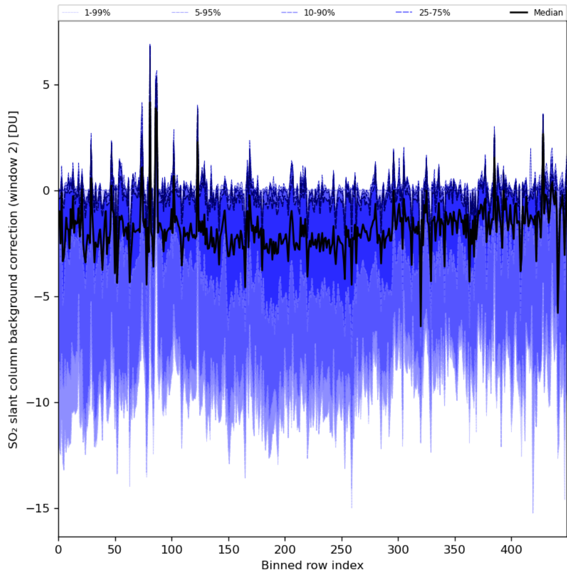
Figure 86: Along track statistics of “SO 2 slant column background correction (window 2)” for 2024-01-16 to 2024-01-18
