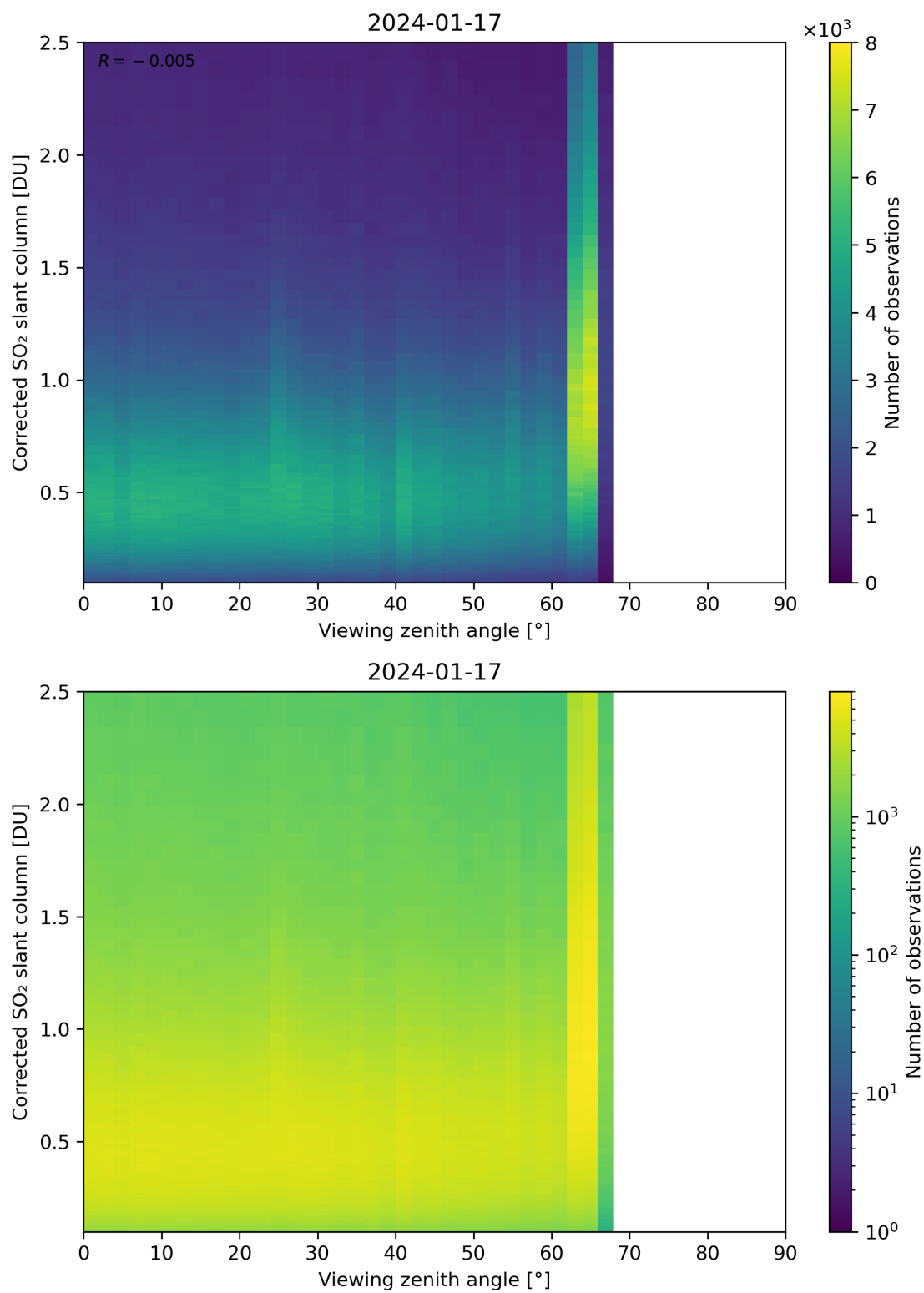
Figure 317: Scatter density plot of “Viewing zenith angle” against “Corrected SO 2 slant column” for 2024-01-16 to 2024-01-18.
