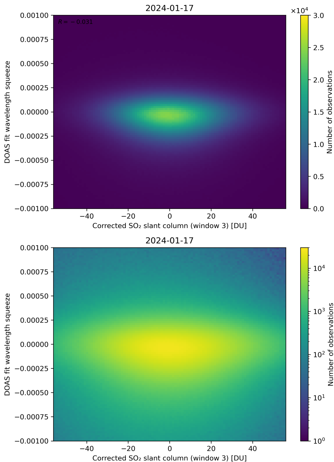
Figure 207: Scatter density plot of “Corrected SO 2 slant column (window 3)” against “DOAS fit wavelength squeeze” for 2024-01-16 to 2024-01-18.
