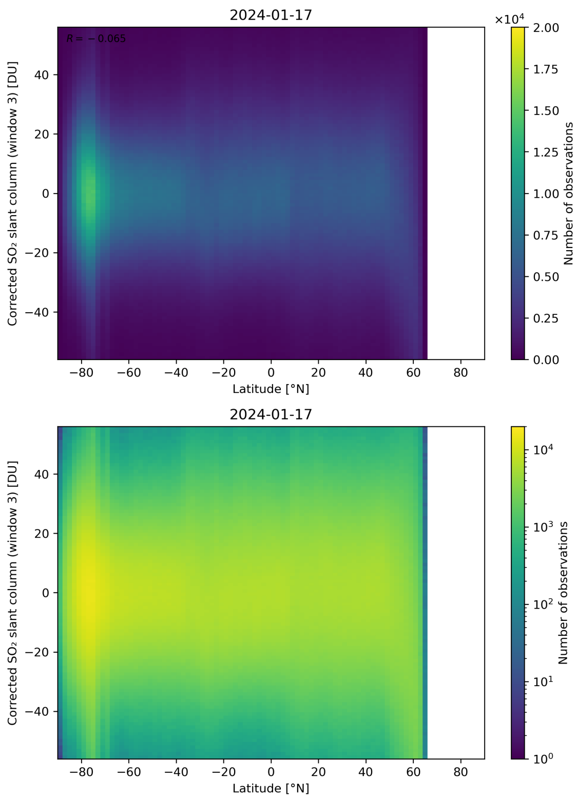
Figure 148: Scatter density plot of “Latitude” against “Corrected SO 2 slant column (window 3)” for 2024-01-16 to 2024-01-18.
