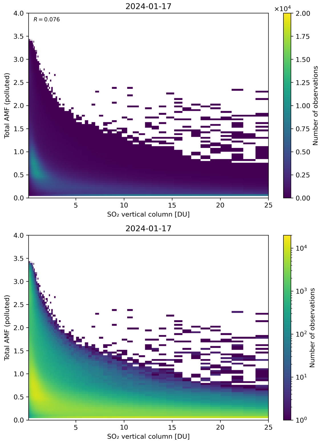
Figure 305: Scatter density plot of “SO 2 vertical column” against “Total AMF (polluted)” for 2024-01-16 to 2024-01-18.
