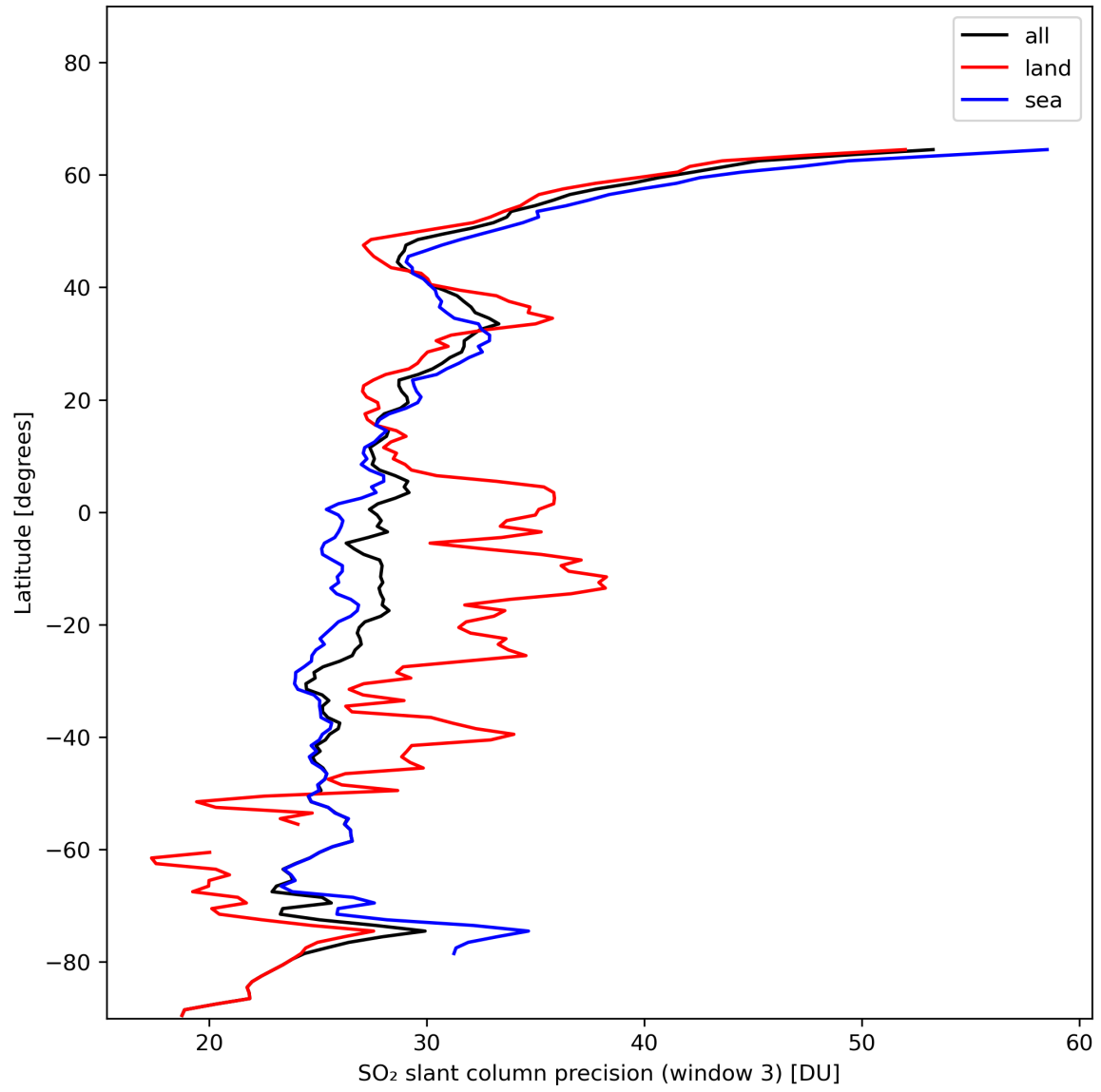
Figure 42: Zonal average of “SO 2 slant column precision (window 3)” for 2024-01-16 to 2024-01-18.
