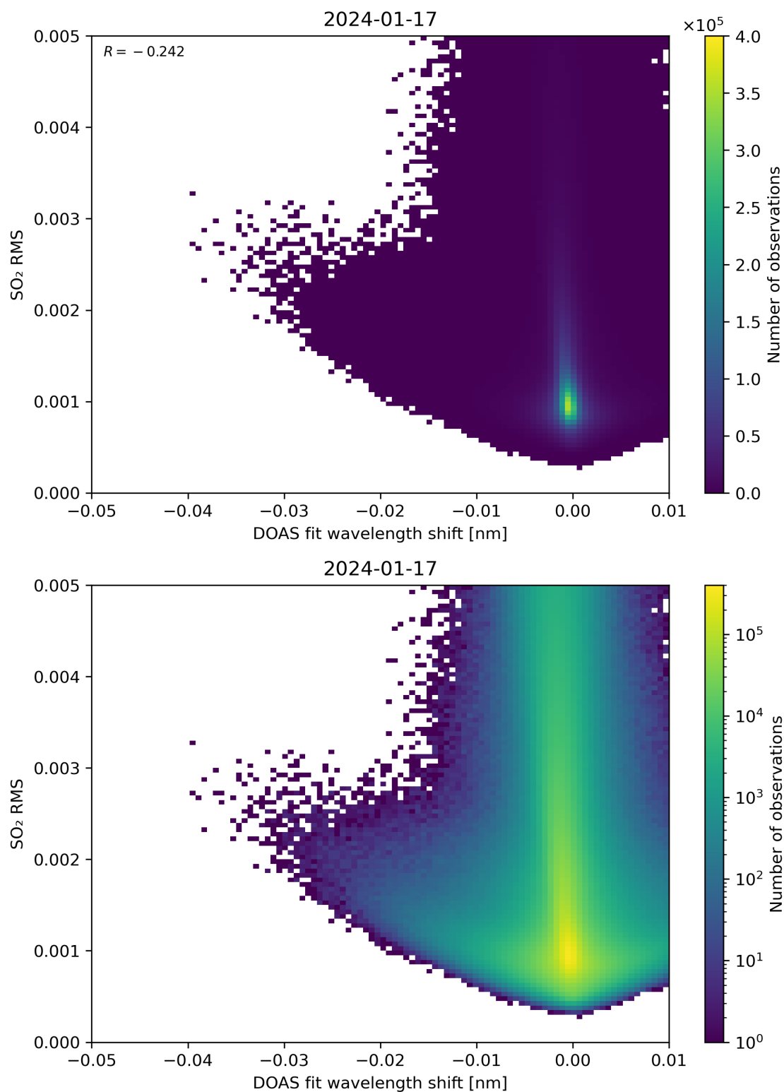
Figure 128: Scatter density plot of “DOAS fit wavelength shift” against “SO 2 RMS” for 2024-01-16 to 2024-01-18.
