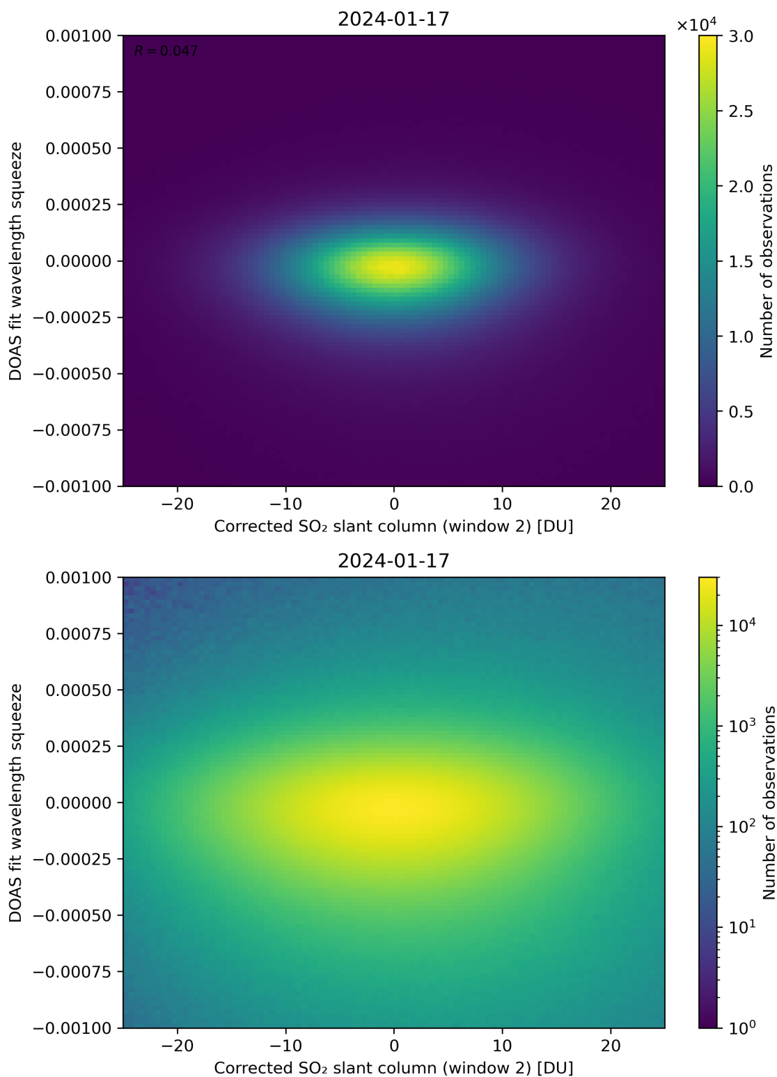
Figure 197: Scatter density plot of “Corrected SO 2 slant column (window 2)” against “DOAS fit wavelength squeeze” for 2024-01-16 to 2024-01-18.
