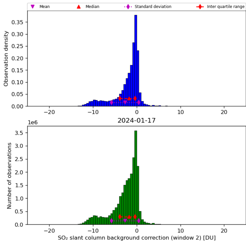
Figure 63: Histogram of “SO 2 slant column background correction (window 2)” for 2024-01-16 to 2024-01-18
