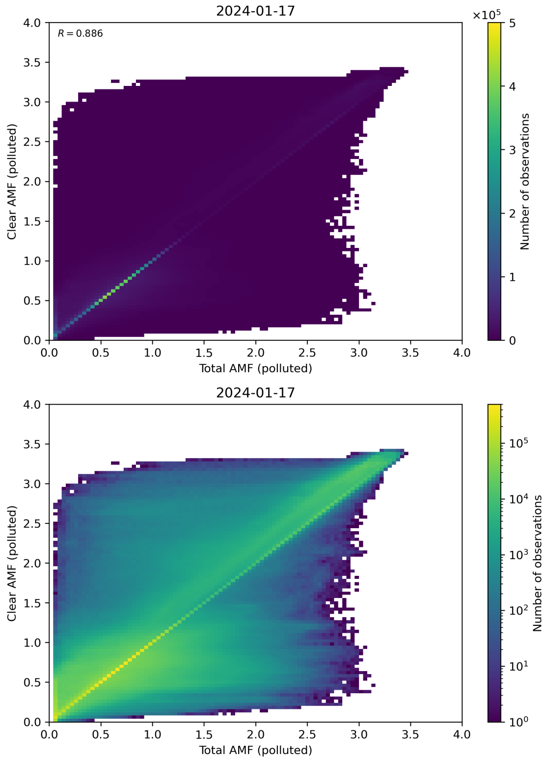
Figure 271: Scatter density plot of “Total AMF (polluted)” against “Clear AMF (polluted)” for 2024-01-16 to 2024-01-18.
