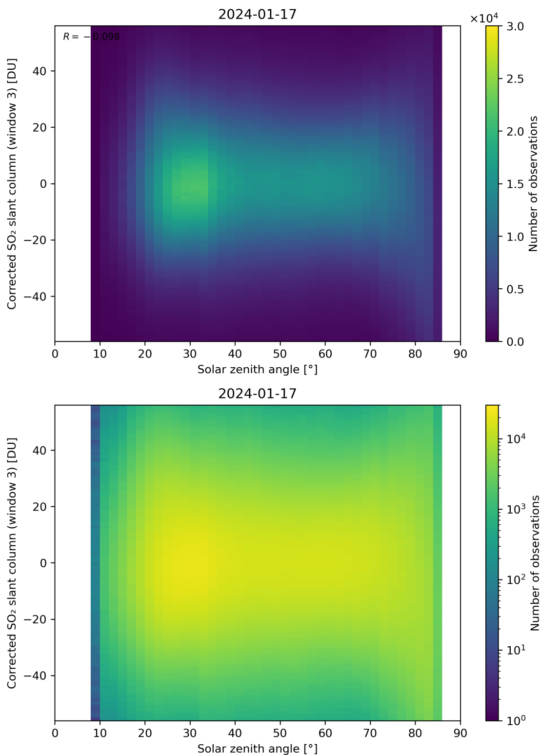
Figure 168: Scatter density plot of “Solar zenith angle” against “Corrected SO 2 slant column (window 3)” for 2024-01-16 to 2024-01-18.
