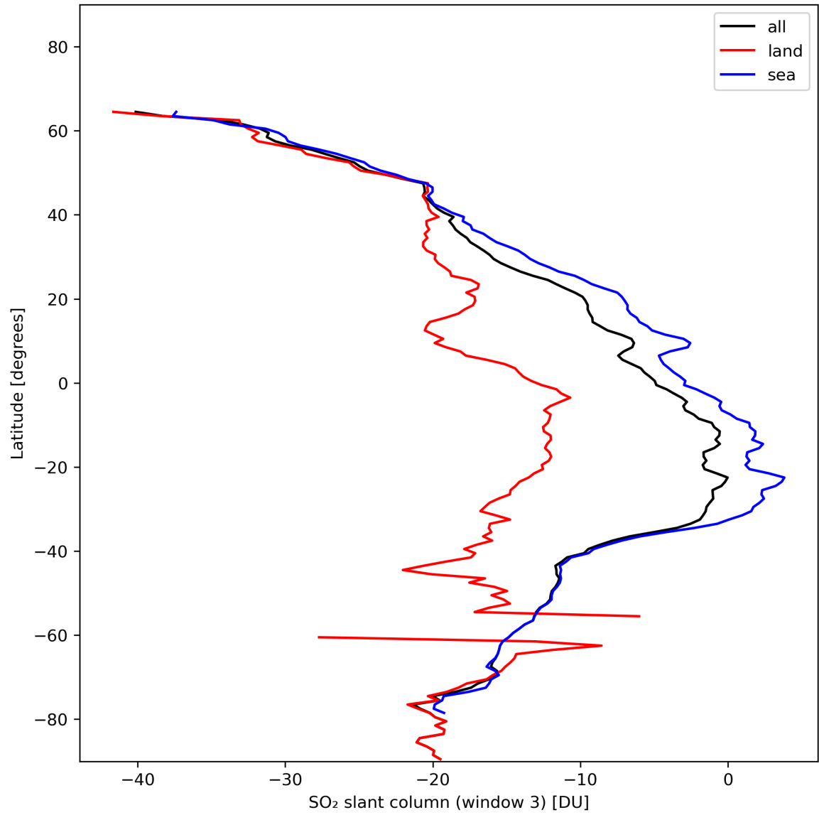
Figure 41: Zonal average of “SO 2 slant column (window 3)” for 2024-01-16 to 2024-01-18.
