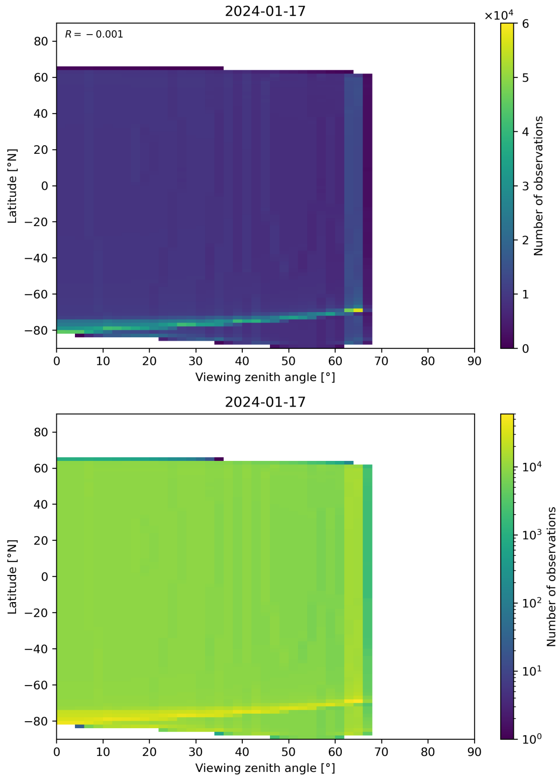
Figure 314: Scatter density plot of “Viewing zenith angle” against “Latitude” for 2024-01-16 to 2024-01-18.
