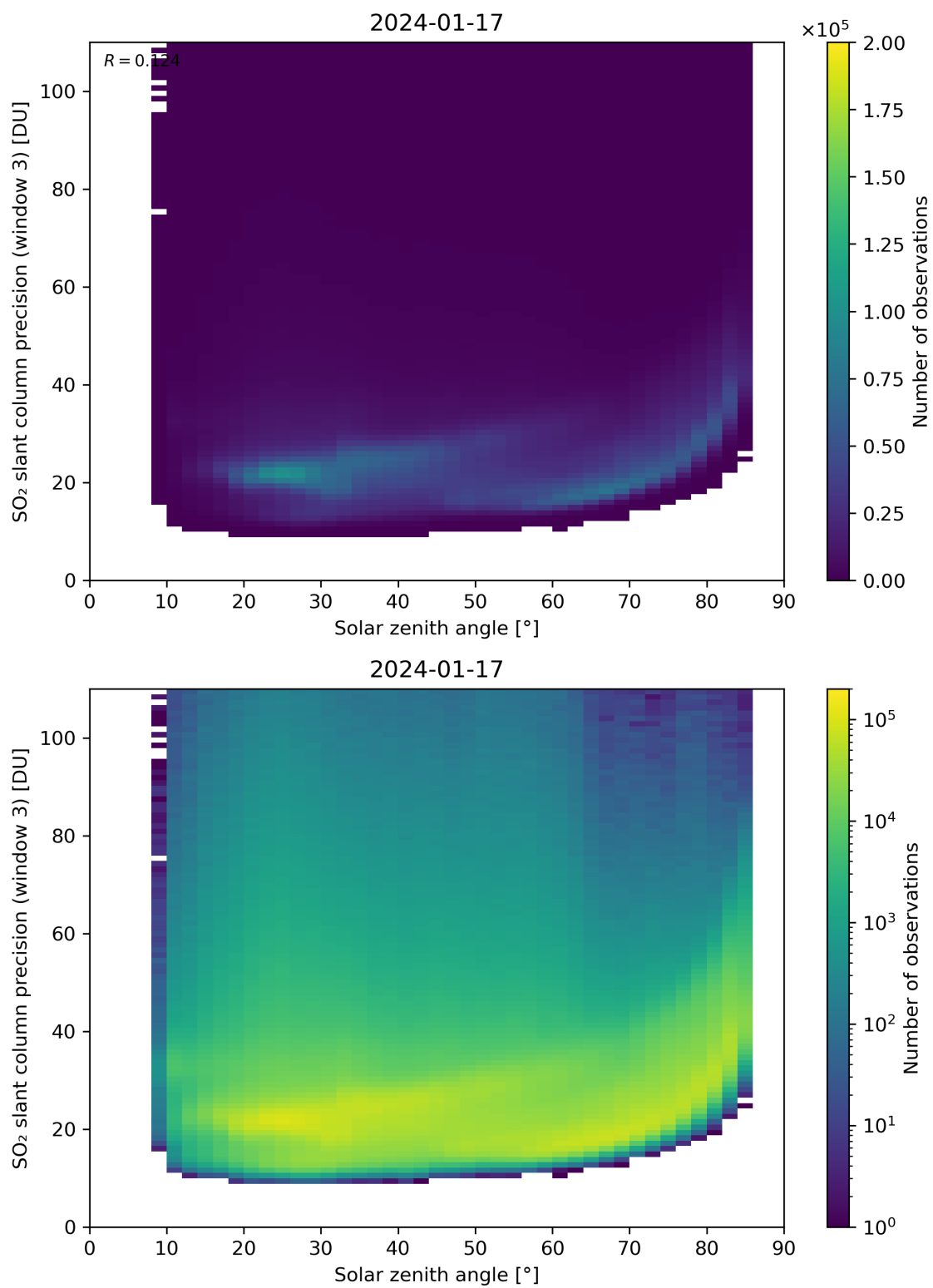
Figure 173: Scatter density plot of “Solar zenith angle” against “SO 2 slant column precision (window 3)” for 2024-01-16 to 2024-01-18.
