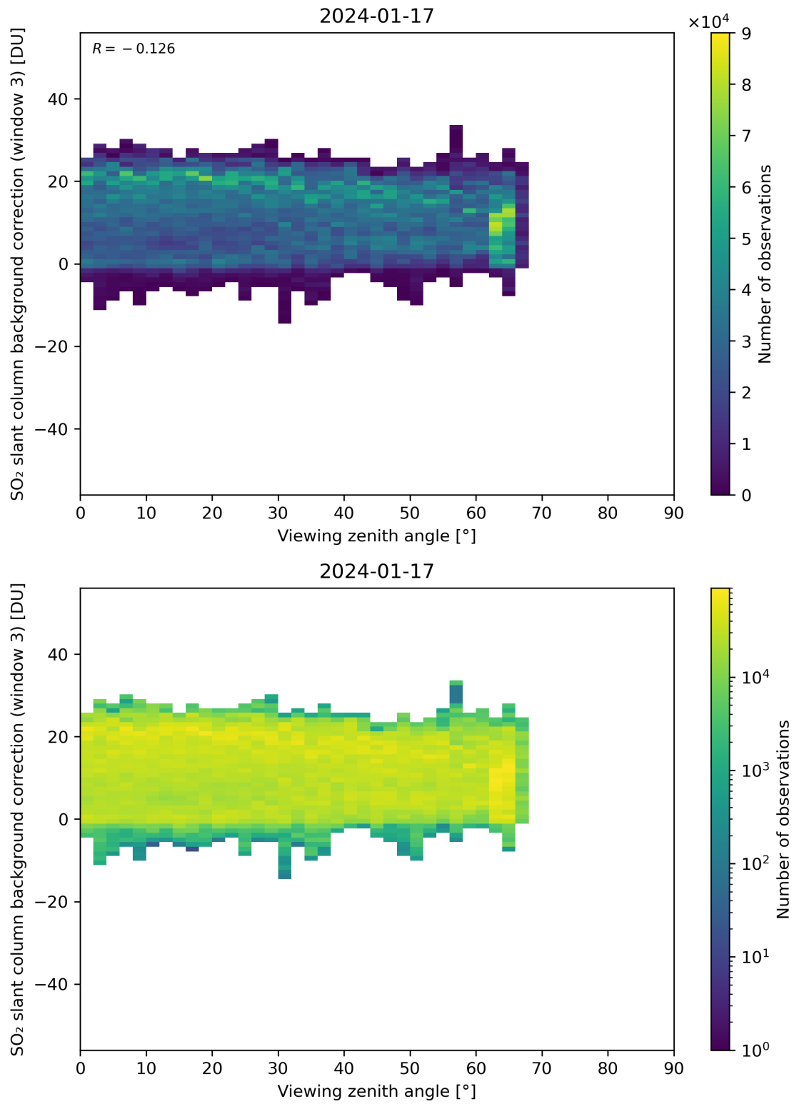
Figure 310: Scatter density plot of “Viewing zenith angle” against “SO 2 slant column background correction (window 3)” for 2024-01-16 to 2024-01-18.
