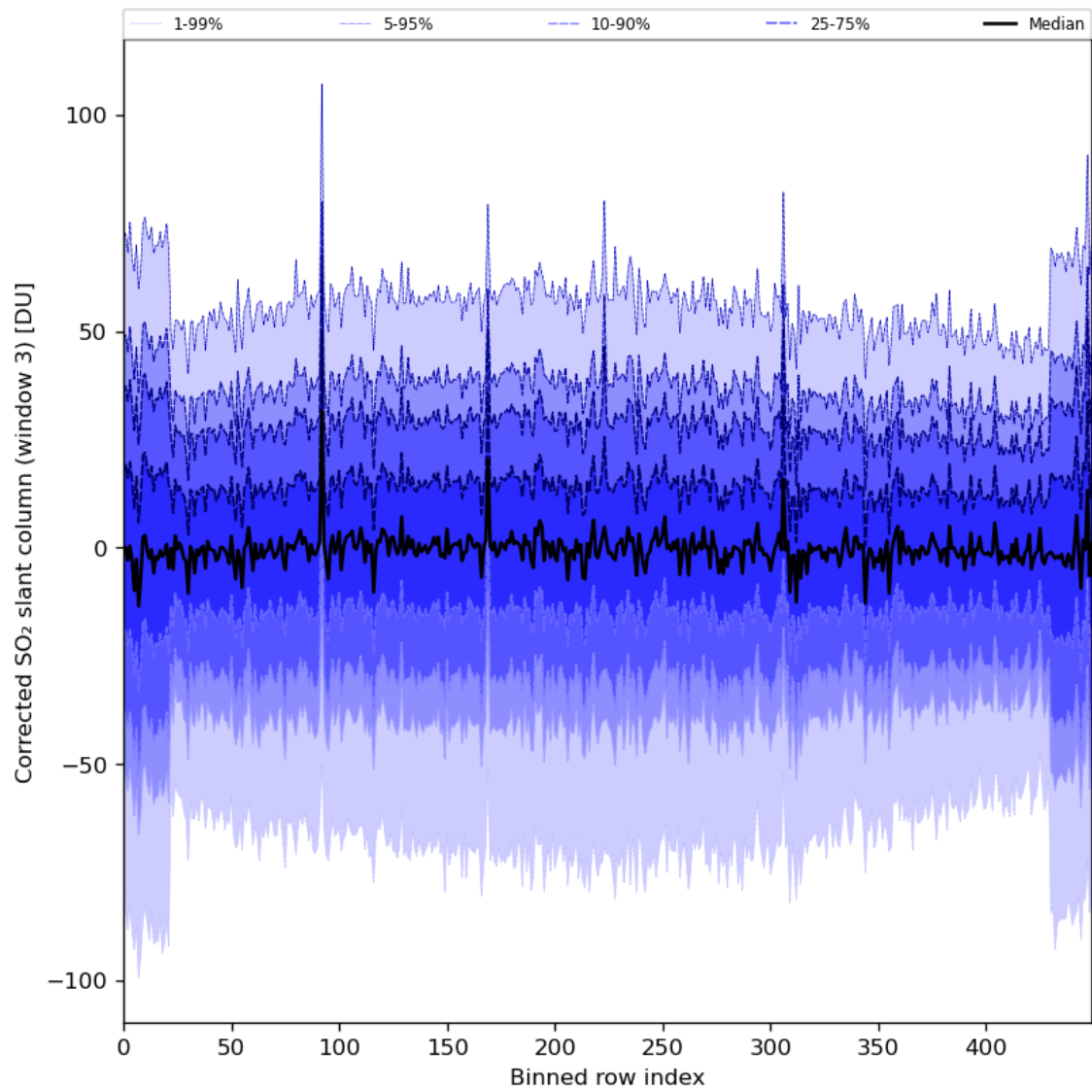
Figure 89: Along track statistics of “Corrected SO 2 slant column (window 3)” for 2024-01-16 to 2024-01-18
