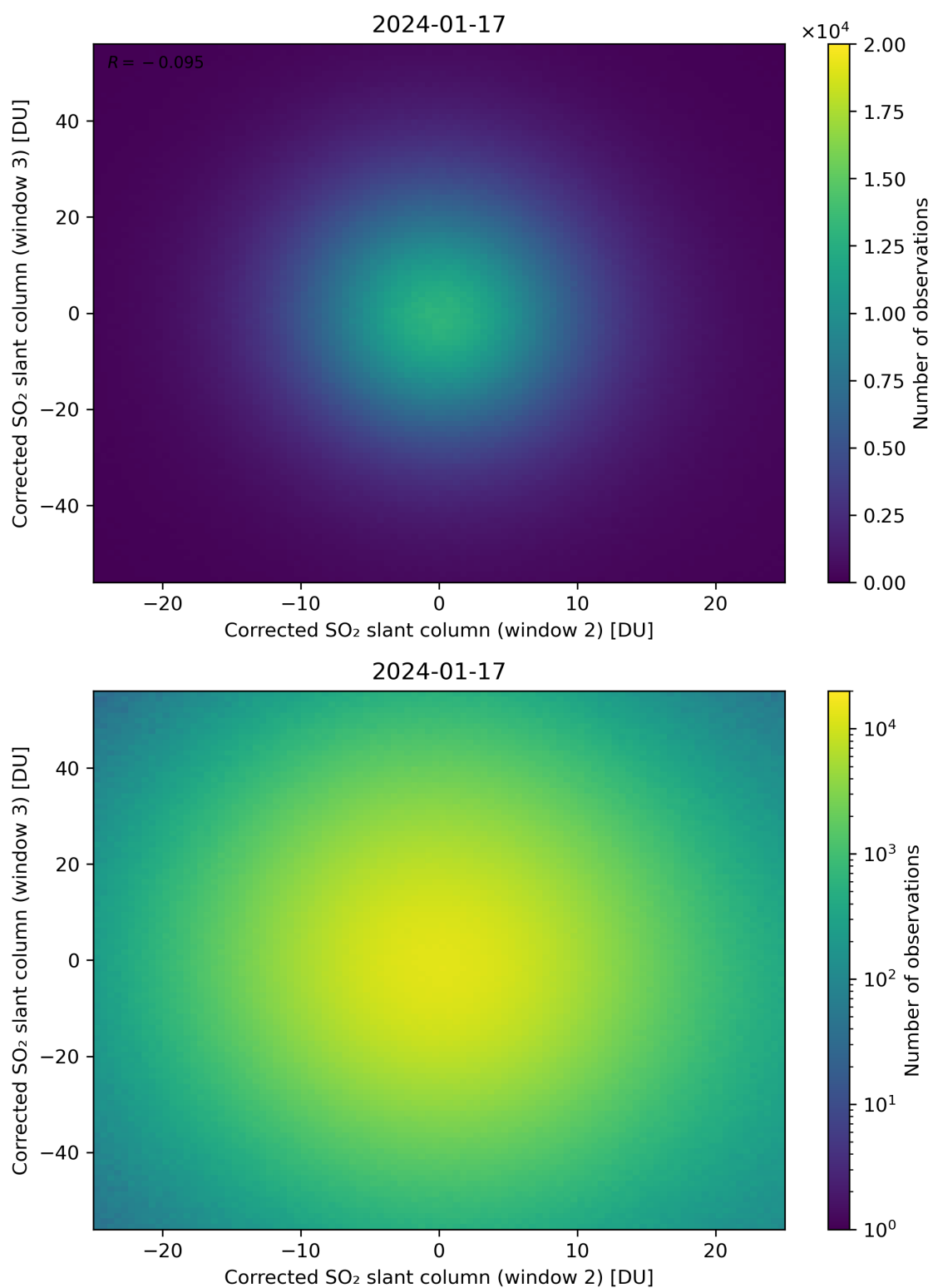
Figure 200: Scatter density plot of “Corrected SO 2 slant column (window 2)” against “Corrected SO 2 slant column (window 3)” for 2024-01-16 to 2024-01-18.
