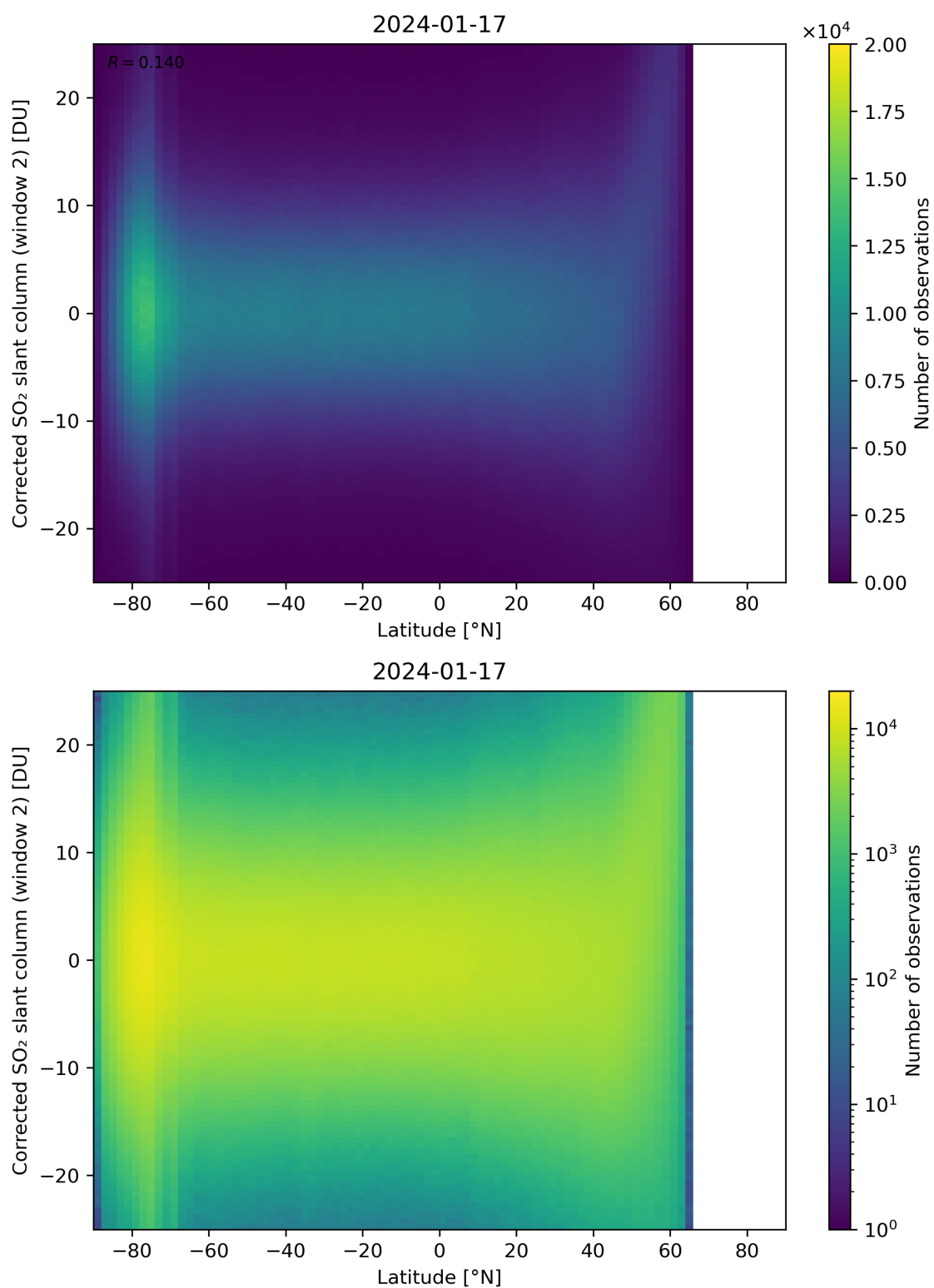
Figure 147: Scatter density plot of “Latitude” against “Corrected SO 2 slant column (window 2)” for 2024-01-16 to 2024-01-18.
