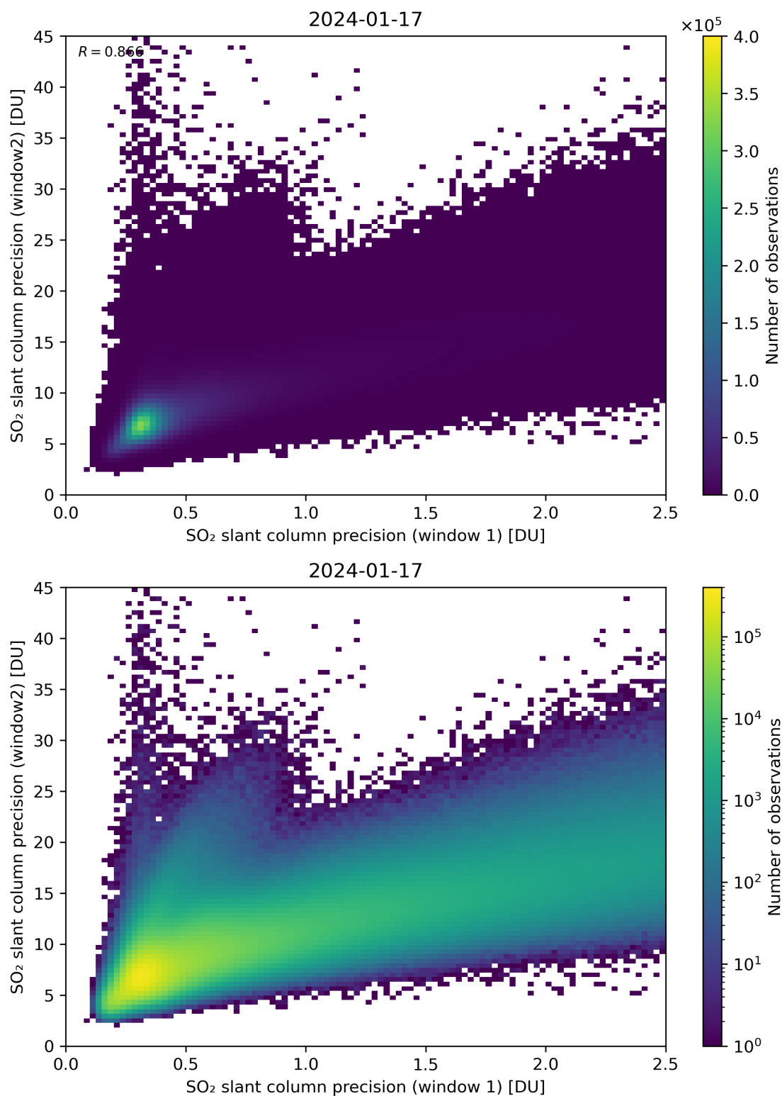
Figure 227: Scatter density plot of “SO 2 slant column precision (window 1)” against “SO 2 slant column precision (window 2)” for 2024-01-16 to 2024-01-18.
