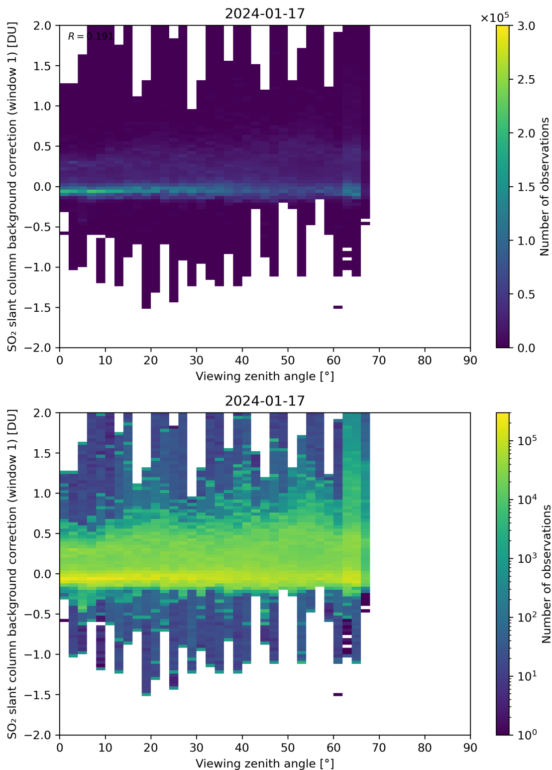
Figure 308: Scatter density plot of “Viewing zenith angle” against “SO 2 slant column background correction (window 1)” for 2024-01-16 to 2024-01-18.
