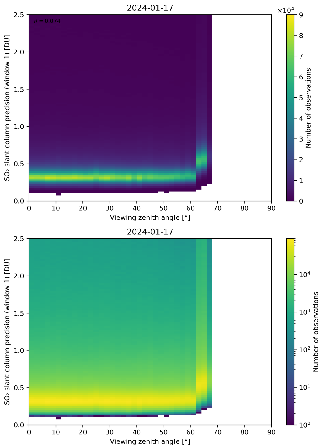
Figure 321: Scatter density plot of “Viewing zenith angle” against “SO 2 slant column precision (window 1)” for 2024-01-16 to 2024-01-18.
