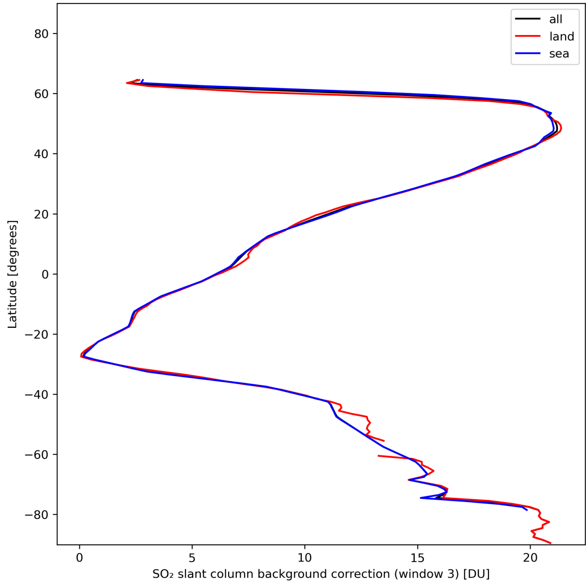
Figure 44: Zonal average of “SO 2 slant column background correction (window 3)” for 2024-01-16 to 2024-01-18.
