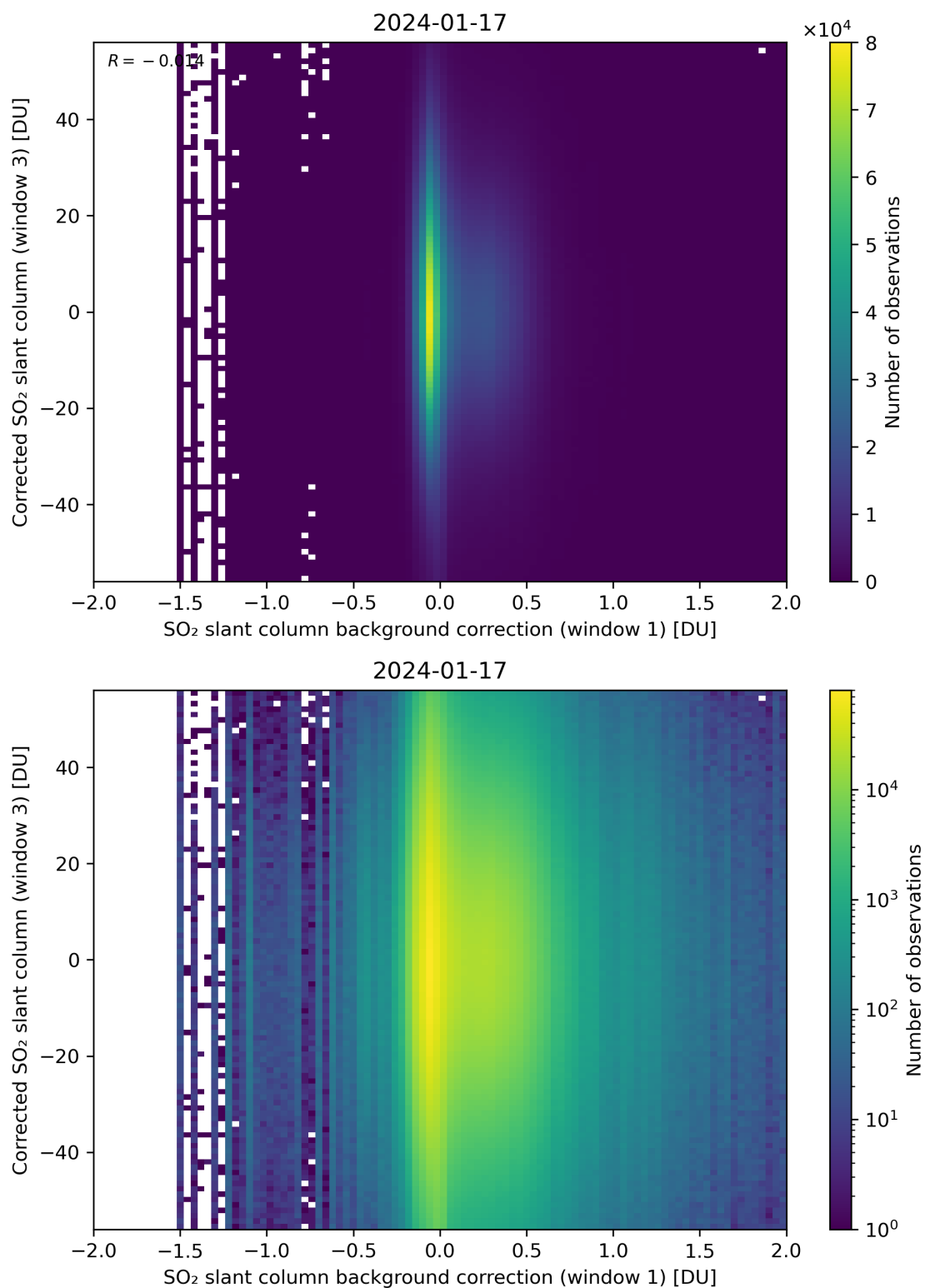
Figure 105: Scatter density plot of “SO 2 slant column background correction (window 1)” against “Corrected SO 2 slant column (window 3)” for 2024-01-16 to 2024-01-18.
