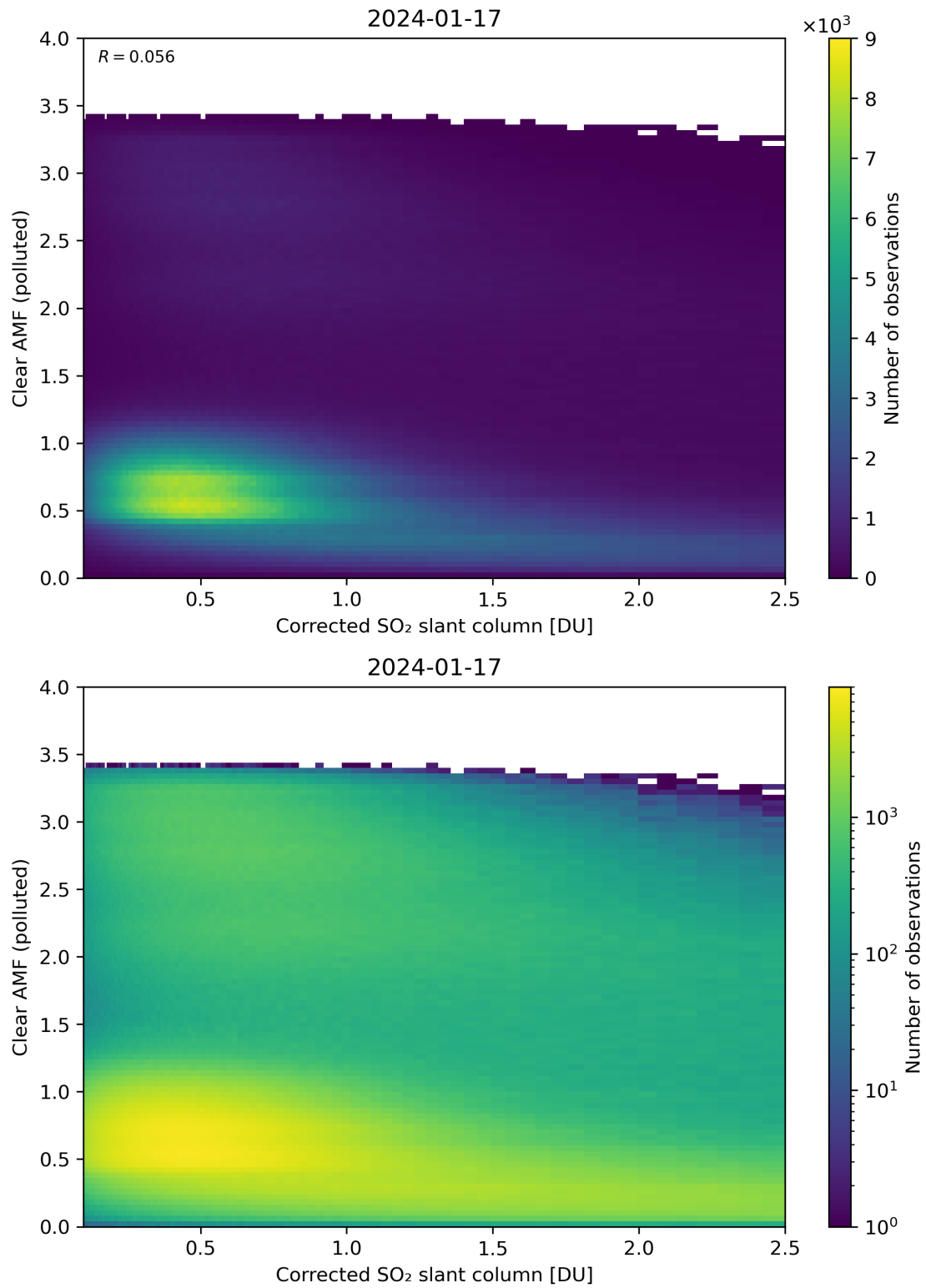
Figure 184: Scatter density plot of “Corrected SO 2 slant column” against “Clear AMF (polluted)” for 2024-01-16 to 2024-01-18.
