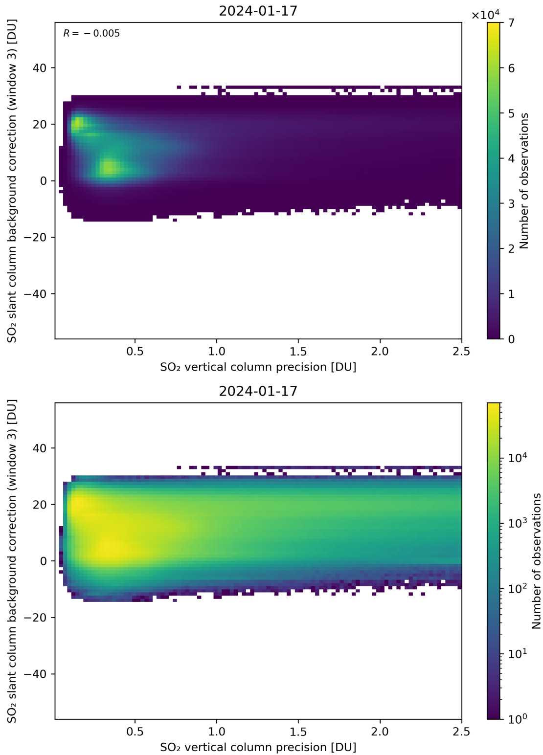
Figure 281: Scatter density plot of “SO 2 vertical column precision” against “SO 2 slant column background correction (window 3)” for 2024-01-16 to 2024-01-18.
