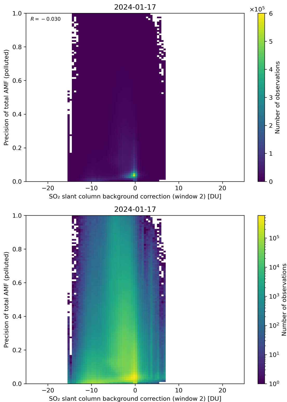
Figure 120: Scatter density plot of “SO 2 slant column background correction (window 2)” against “Precision of total AMF (polluted)” for 2024-01-16 to 2024-01-18.
