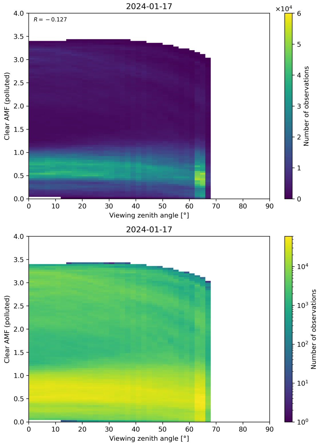
Figure 316: Scatter density plot of “Viewing zenith angle” against “Clear AMF (polluted)” for 2024-01-16 to 2024-01-18.
