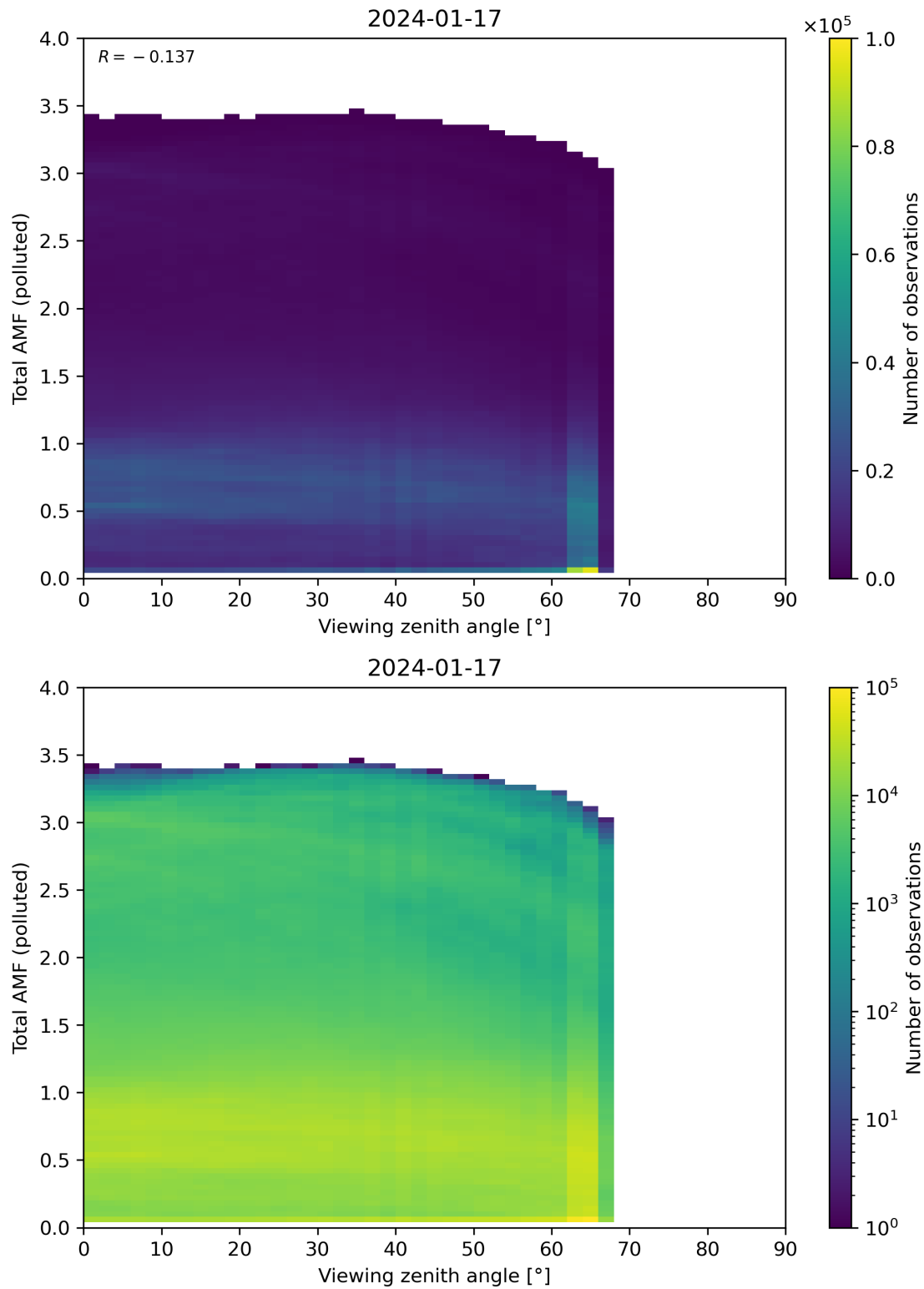
Figure 325: Scatter density plot of “Viewing zenith angle” against “Total AMF (polluted)” for 2024-01-16 to 2024-01-18.
