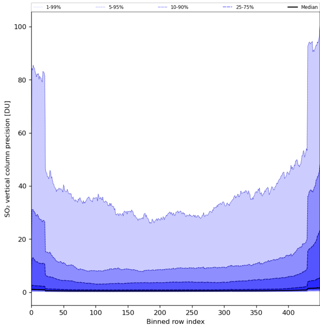
Figure 77: Along track statistics of “SO 2 vertical column precision” for 2024-01-16 to 2024-01-18
