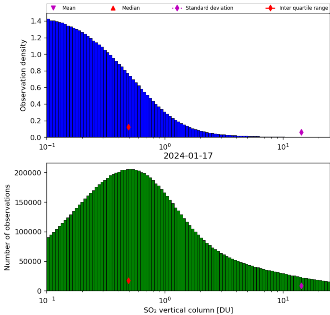
Figure 53: Histogram of “SO 2 vertical column” for 2024-01-16 to 2024-01-18
