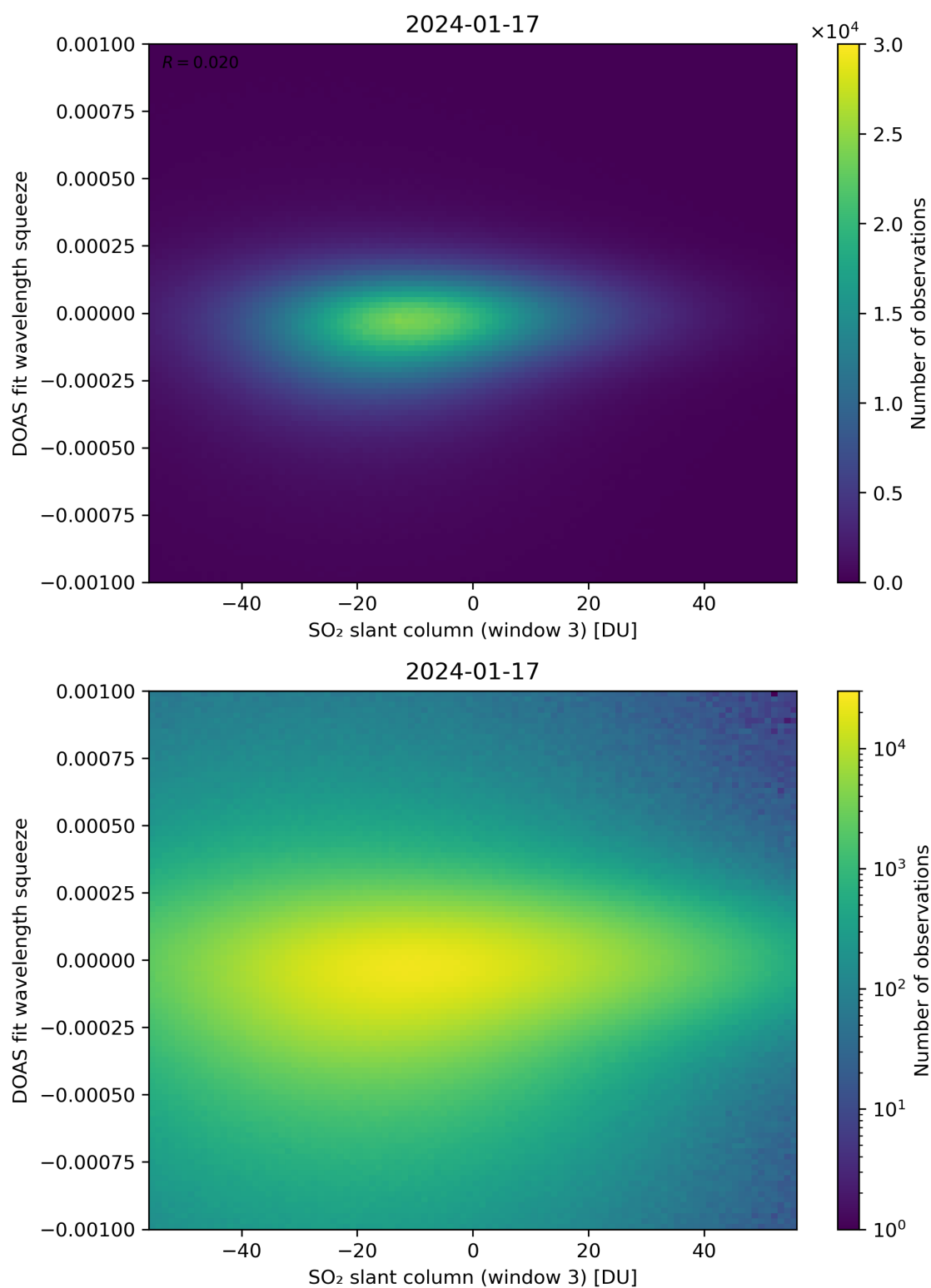
Figure 255: Scatter density plot of “SO 2 slant column (window 3)” against “DOAS fit wavelength squeeze” for 2024-01-16 to 2024-01-18.
