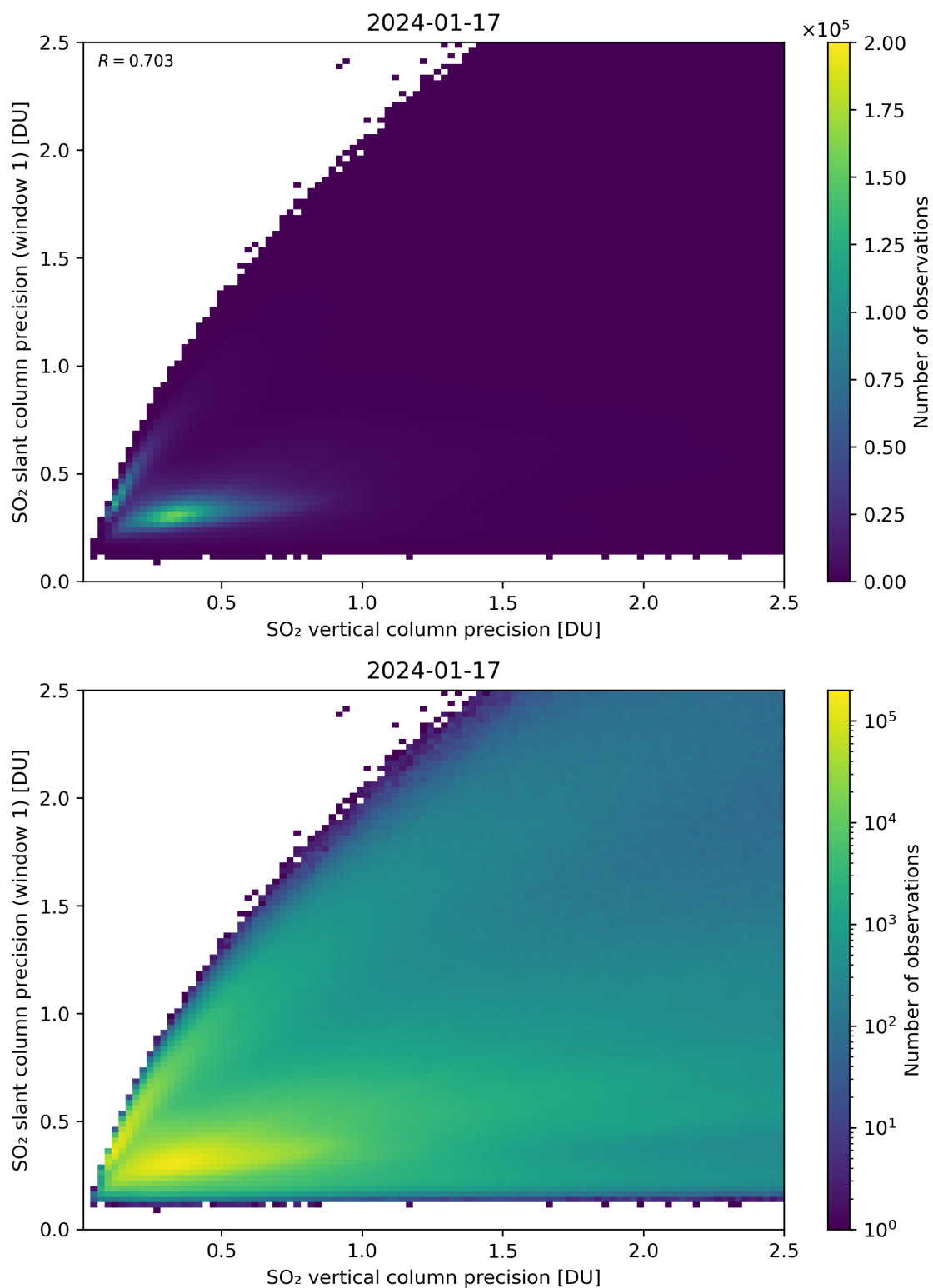
Figure 290: Scatter density plot of “SO 2 vertical column precision” against “SO 2 slant column precision (window 1)” for 2024-01-16 to 2024-01-18.
