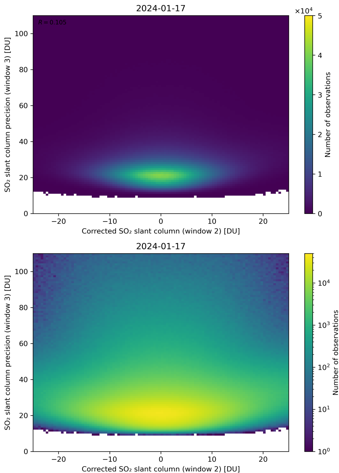
Figure 202: Scatter density plot of “Corrected SO 2 slant column (window 2)” against “SO 2 slant column precision (window 3)” for 2024-01-16 to 2024-01-18.
