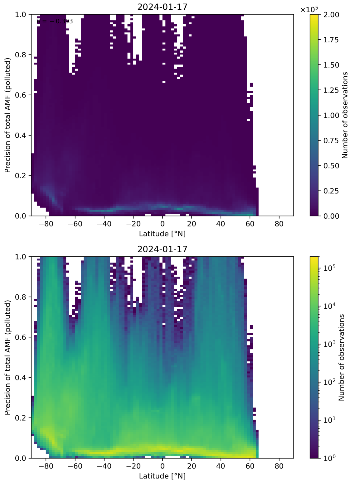
Figure 155: Scatter density plot of “Latitude” against “Precision of total AMF (polluted)” for 2024-01-16 to 2024-01-18.
