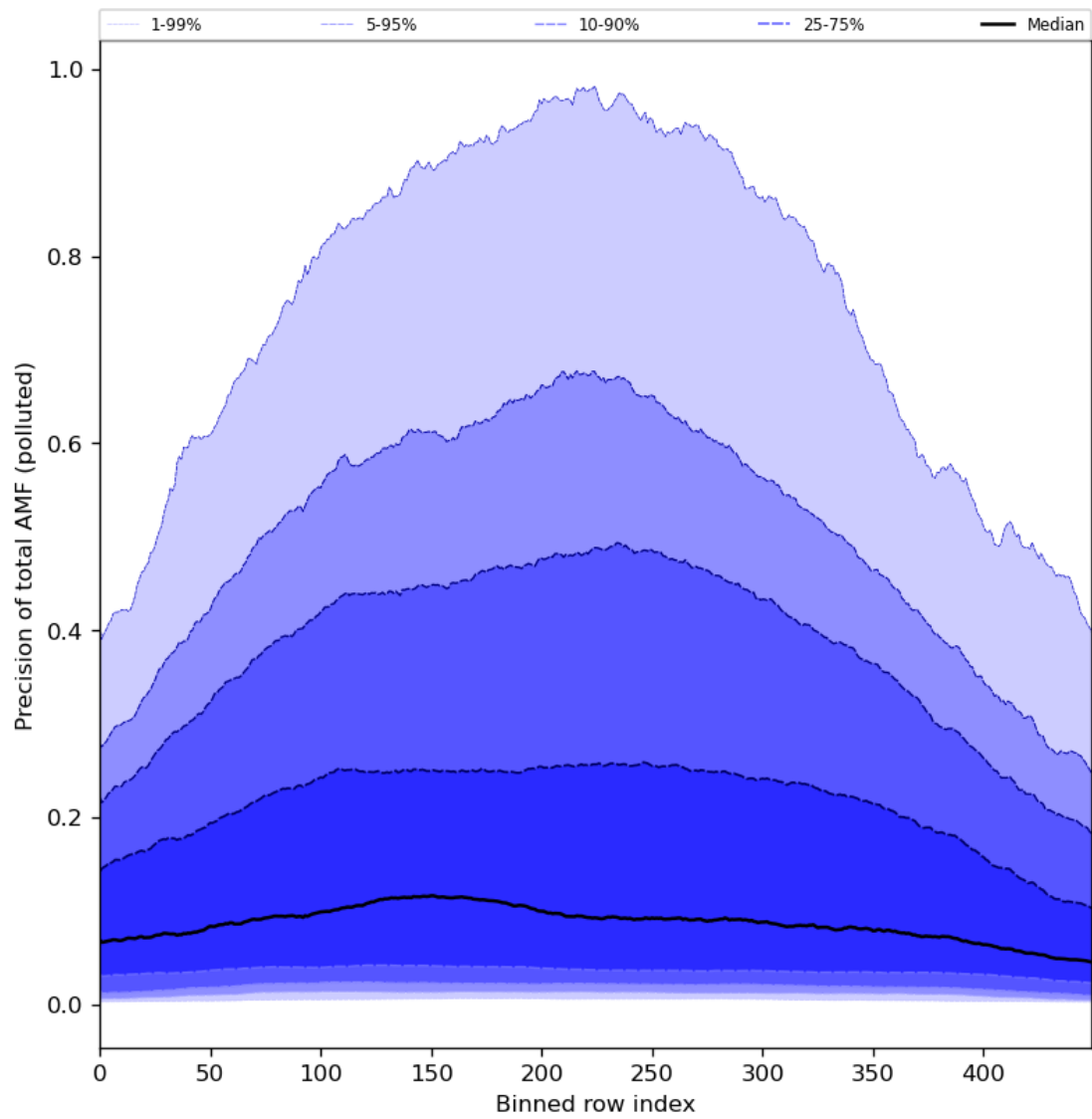
Figure 95: Along track statistics of “Precision of total AMF (polluted)” for 2024-01-16 to 2024-01-18
