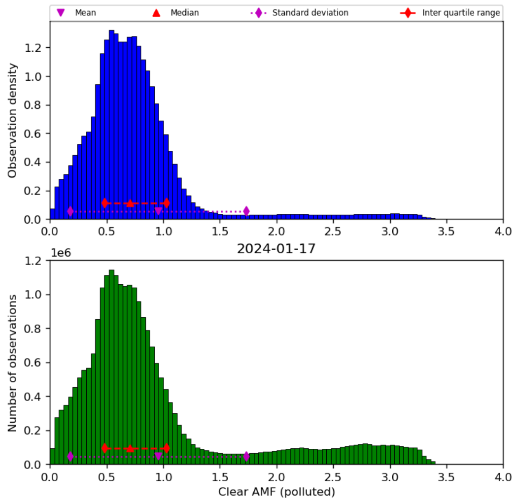
Figure 73: Histogram of “Clear AMF (polluted)” for 2024-01-16 to 2024-01-18
