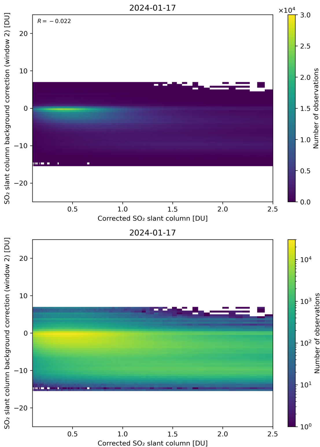
Figure 179: Scatter density plot of “Corrected SO 2 slant column” against “SO 2 slant column background correction (window 2)” for 2024-01-16 to 2024-01-18.
