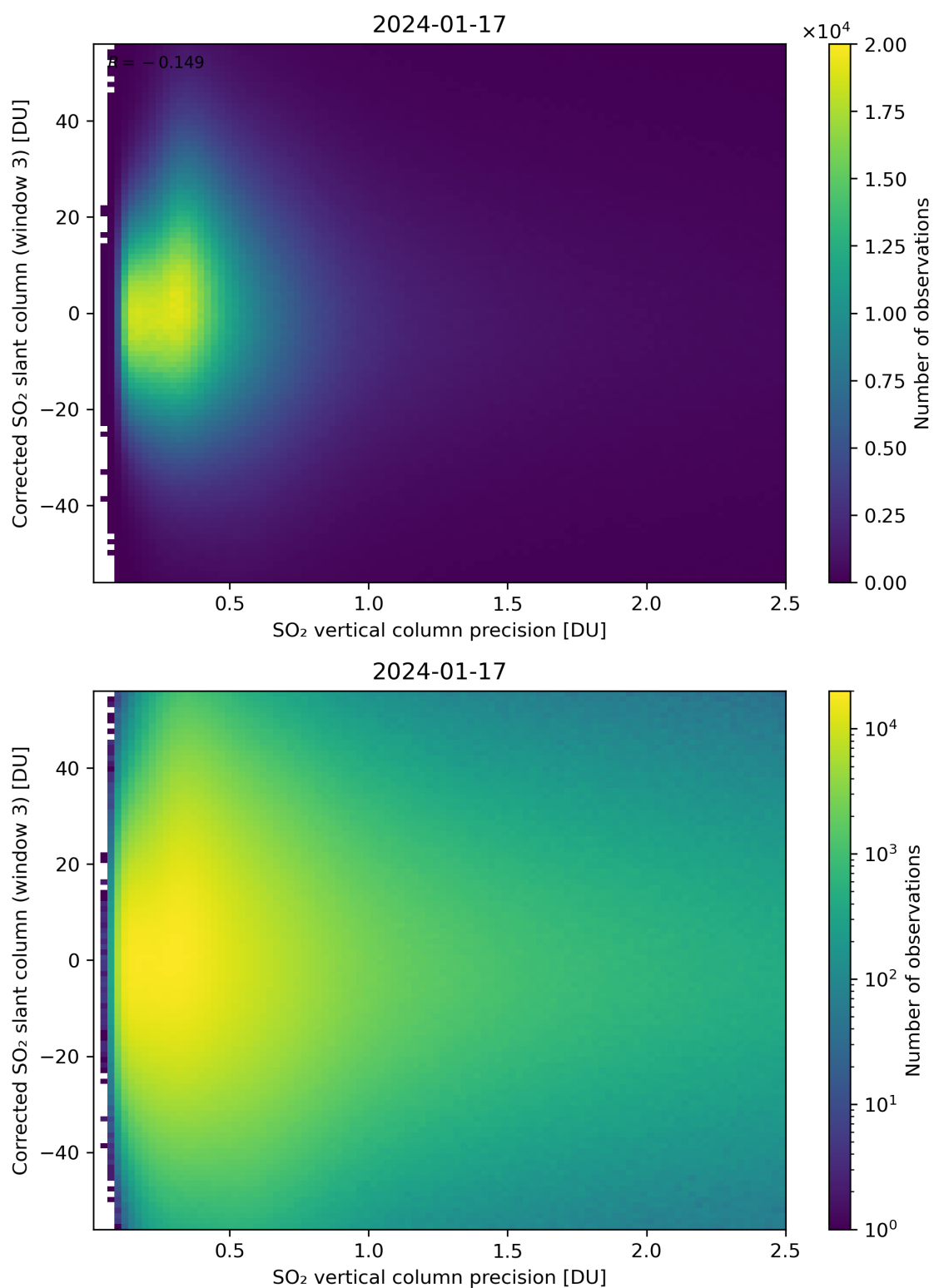
Figure 288: Scatter density plot of “SO 2 vertical column precision” against “Corrected SO 2 slant column (window 3)” for 2024-01-16 to 2024-01-18.
