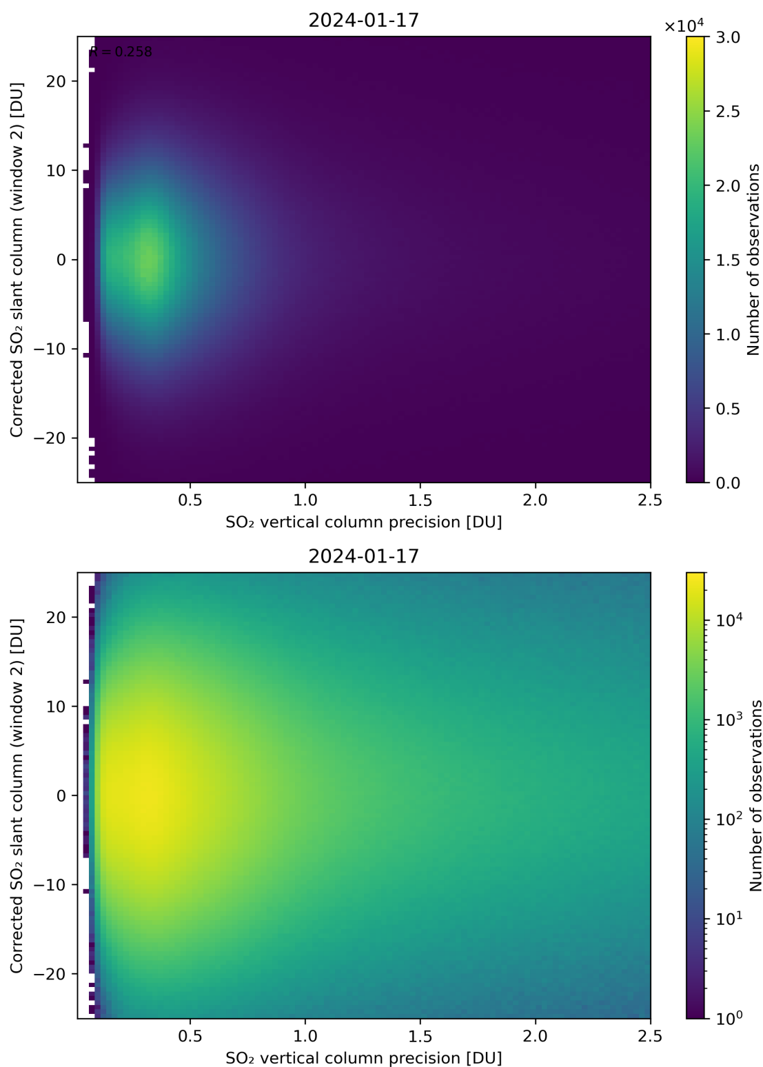
Figure 287: Scatter density plot of “SO 2 vertical column precision” against “Corrected SO 2 slant column (window 2)” for 2024-01-16 to 2024-01-18.
