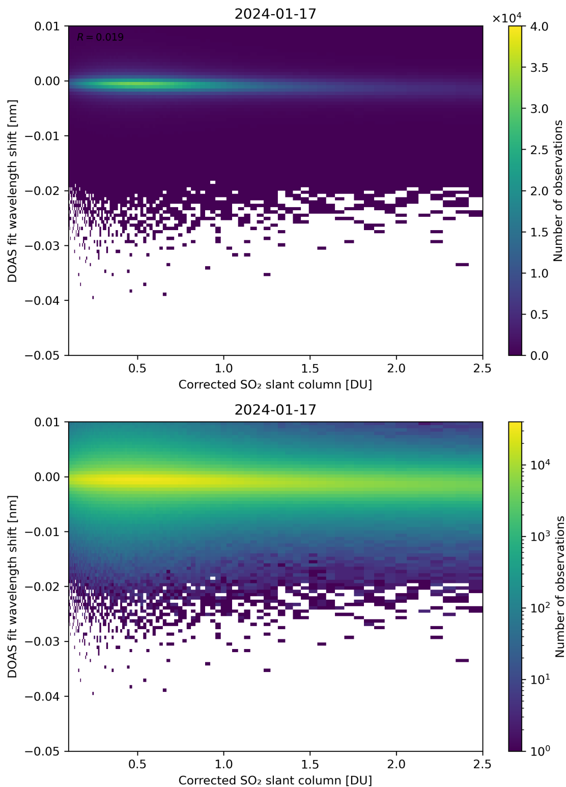
Figure 181: Scatter density plot of “Corrected SO 2 slant column” against “DOAS fit wavelength shift” for 2024-01-16 to 2024-01-18.
