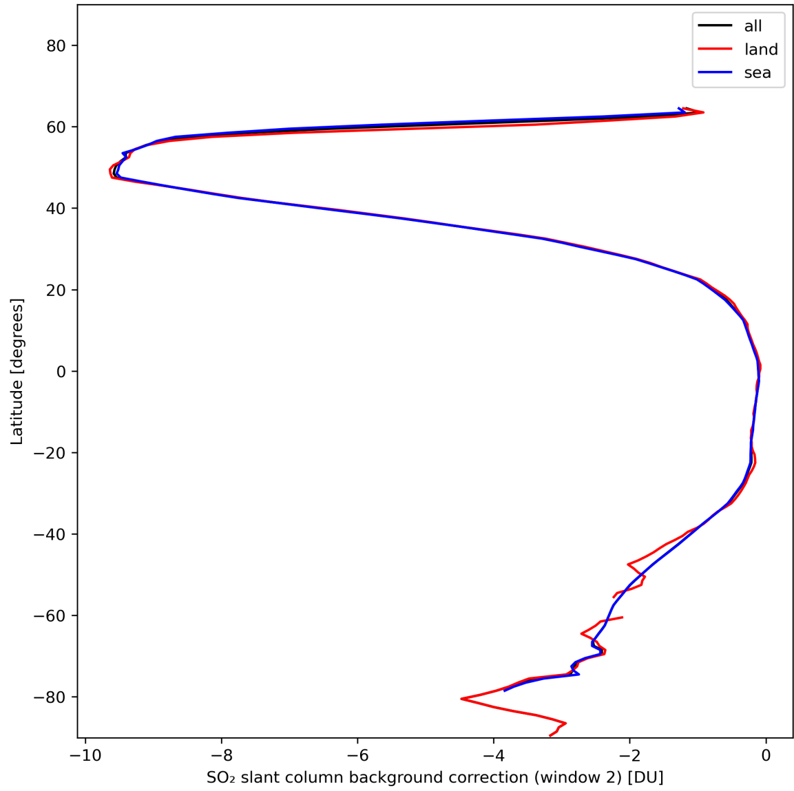
Figure 40: Zonal average of “SO 2 slant column background correction (window 2)” for 2024-01-16 to 2024-01-18.
