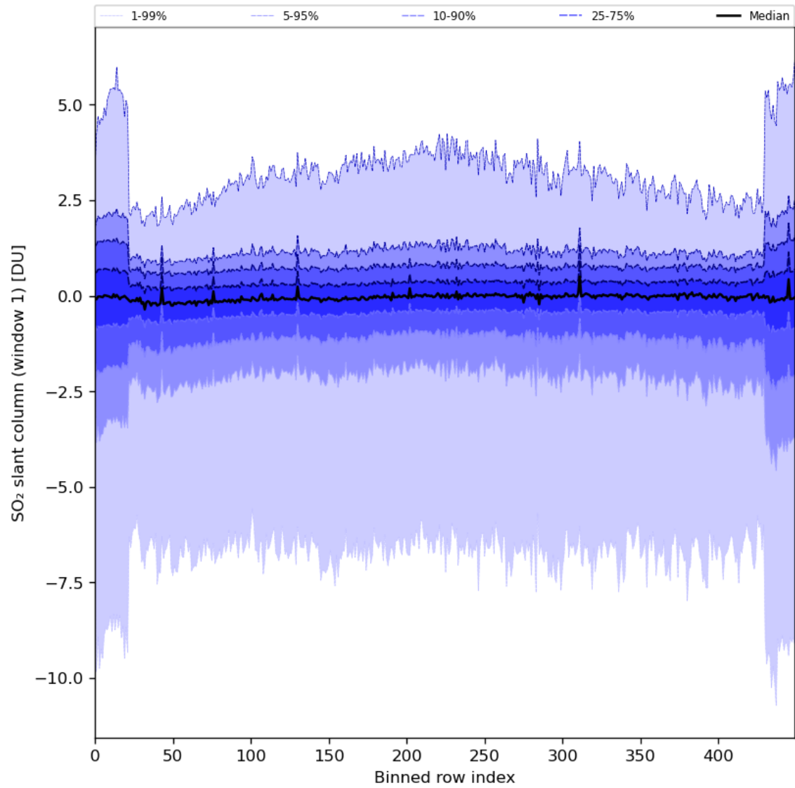
Figure 79: Along track statistics of “SO 2 slant column (window 1)” for 2024-01-16 to 2024-01-18
