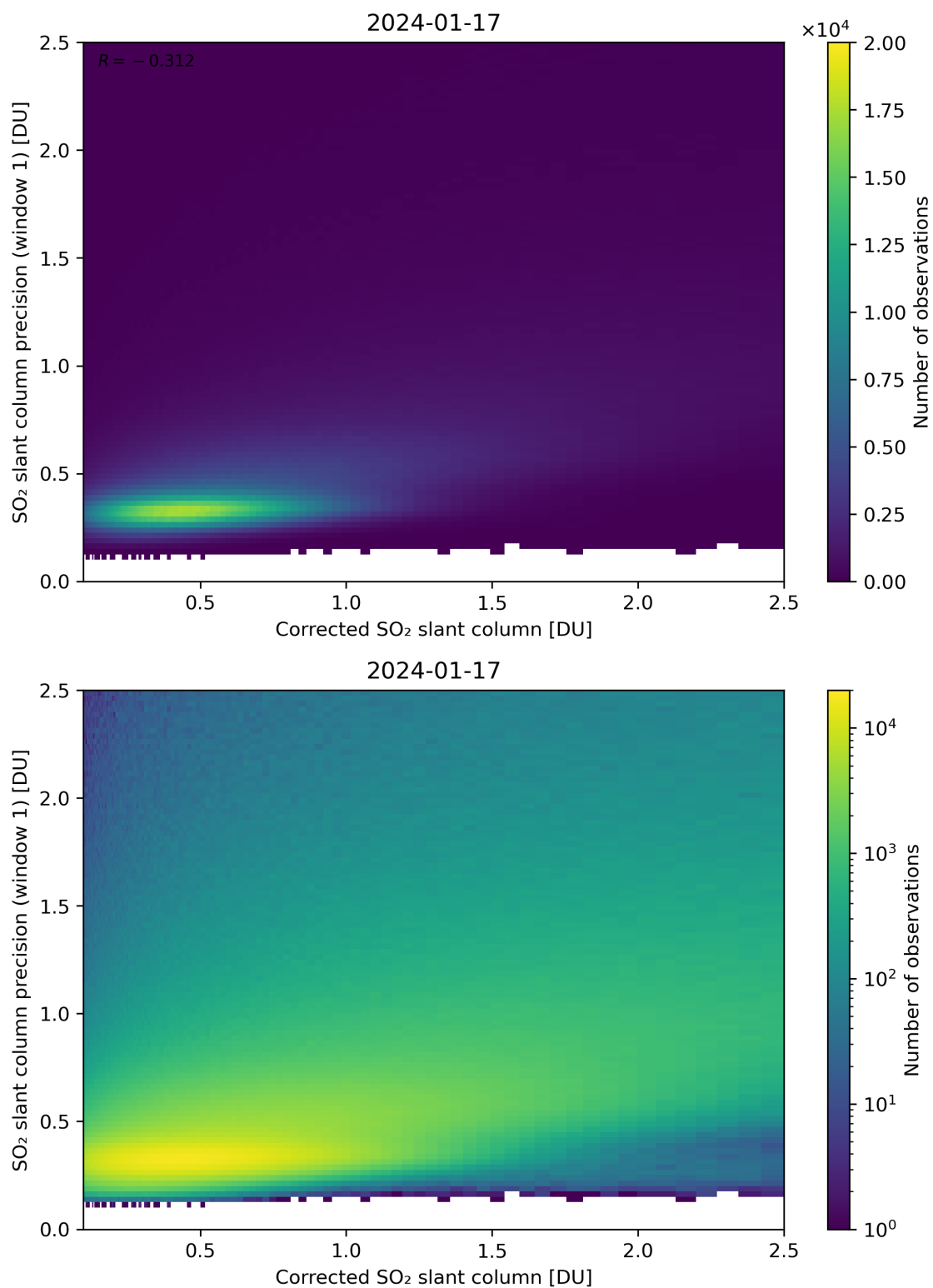
Figure 188: Scatter density plot of “Corrected SO 2 slant column” against “SO 2 slant column precision (window 1)” for 2024-01-16 to 2024-01-18.
