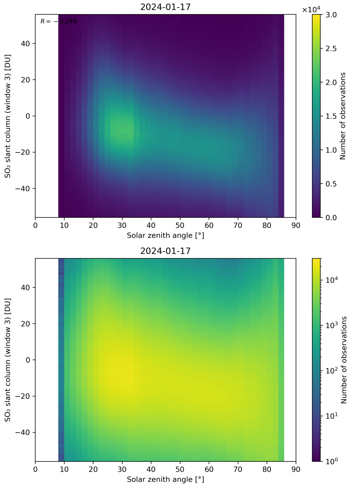
Figure 172: Scatter density plot of “Solar zenith angle” against “SO 2 slant column (window 3)” for 2024-01-16 to 2024-01-18.
