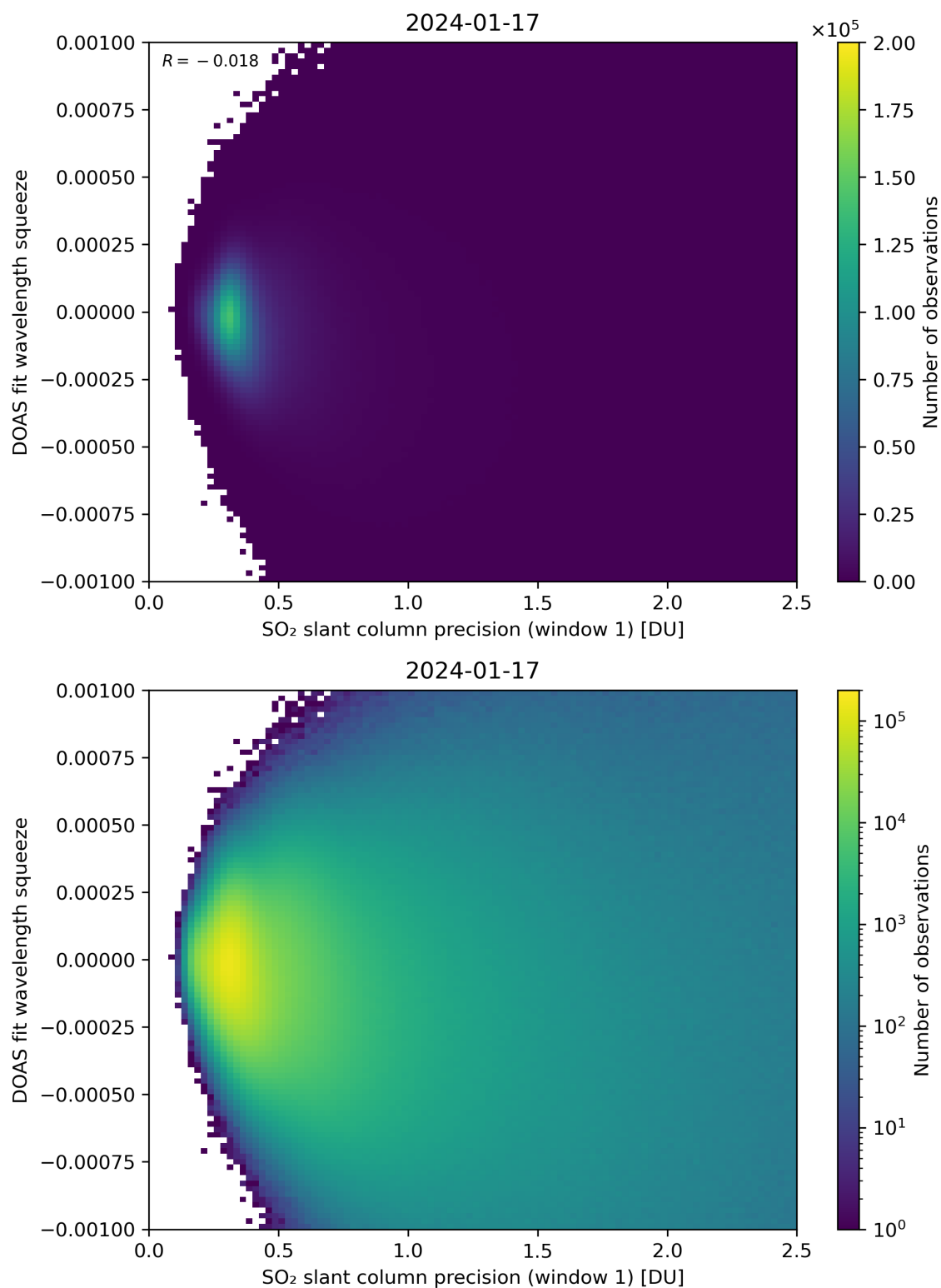
Figure 222: Scatter density plot of “SO 2 slant column precision (window 1)” against “DOAS fit wavelength squeeze” for 2024-01-16 to 2024-01-18.
