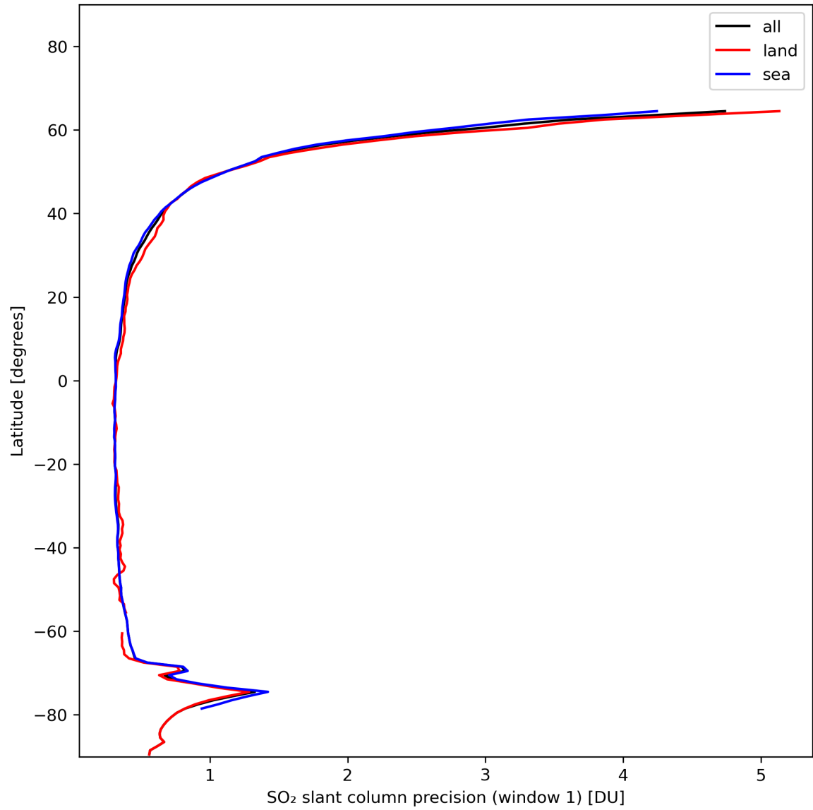
Figure 34: Zonal average of “SO 2 slant column precision (window 1)” for 2024-01-16 to 2024-01-18.
