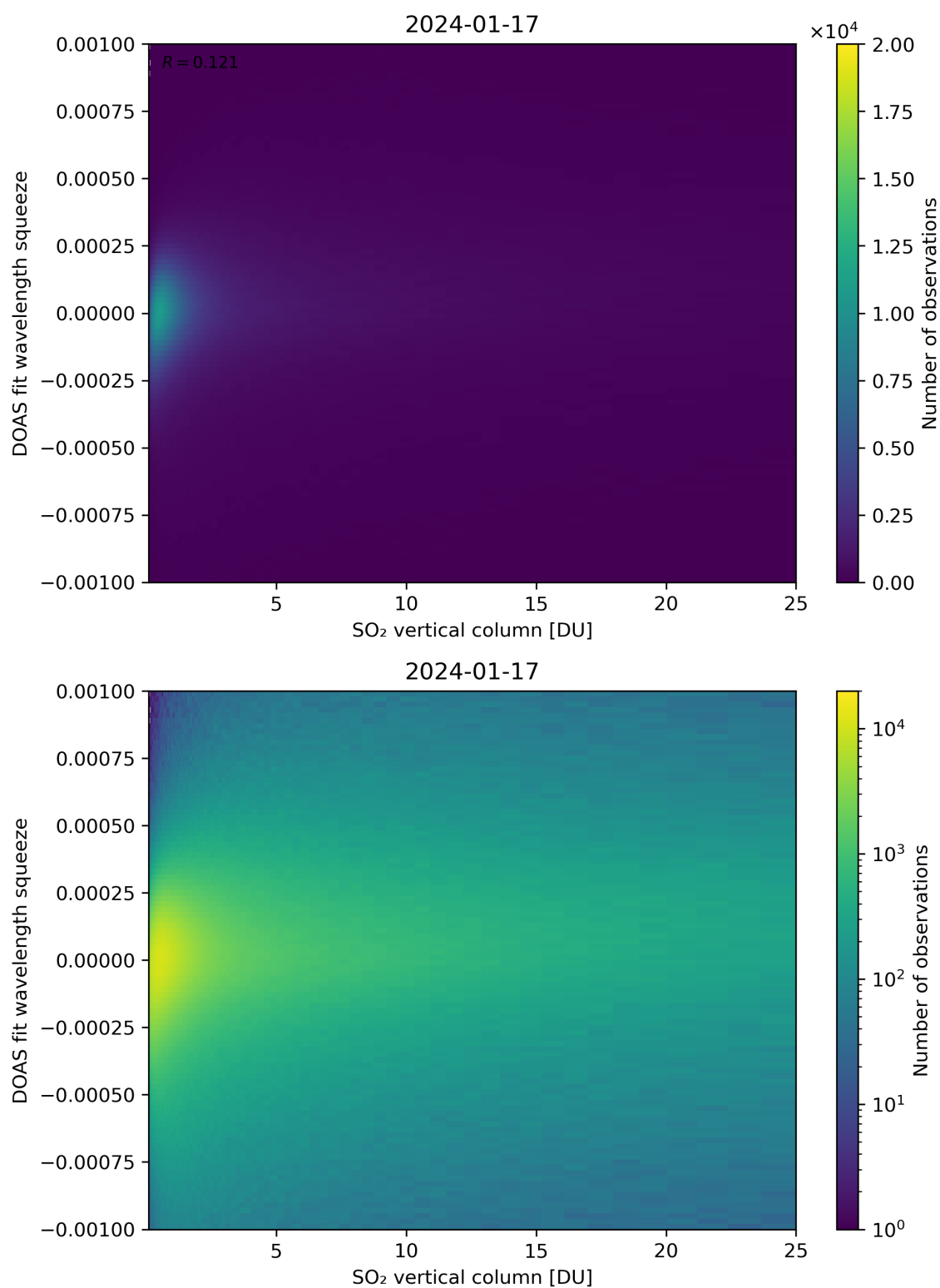
Figure 277: Scatter density plot of “SO 2 vertical column” against “DOAS fit wavelength squeeze” for 2024-01-16 to 2024-01-18.
