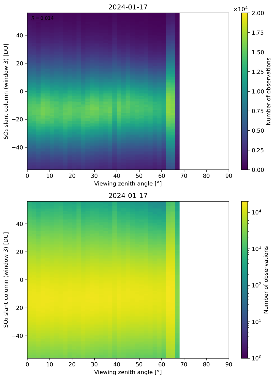
Figure 323: Scatter density plot of “Viewing zenith angle” against “SO 2 slant column (window 3)” for 2024-01-16 to 2024-01-18.
