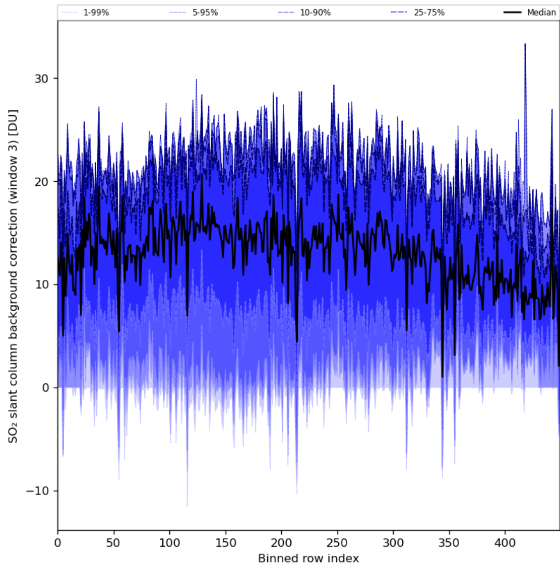
Figure 90: Along track statistics of “SO 2 slant column background correction (window 3)” for 2024-01-16 to 2024-01-18
