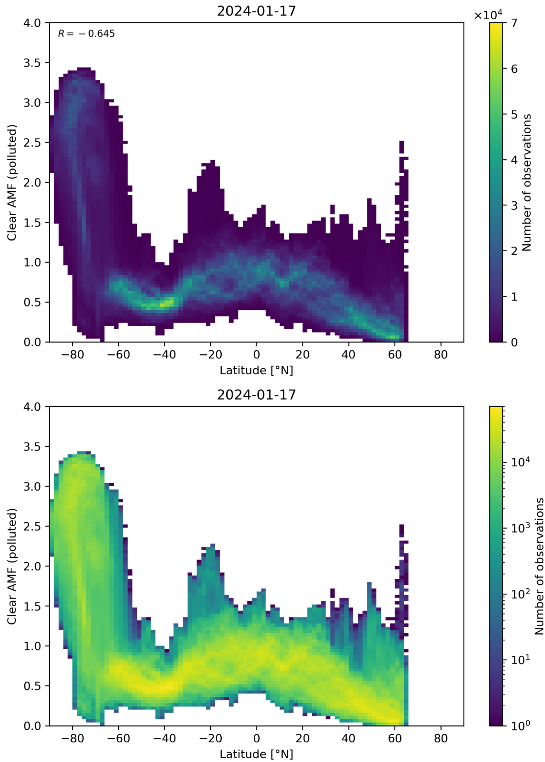
Figure 145: Scatter density plot of “Latitude” against “Clear AMF (polluted)” for 2024-01-16 to 2024-01-18.
