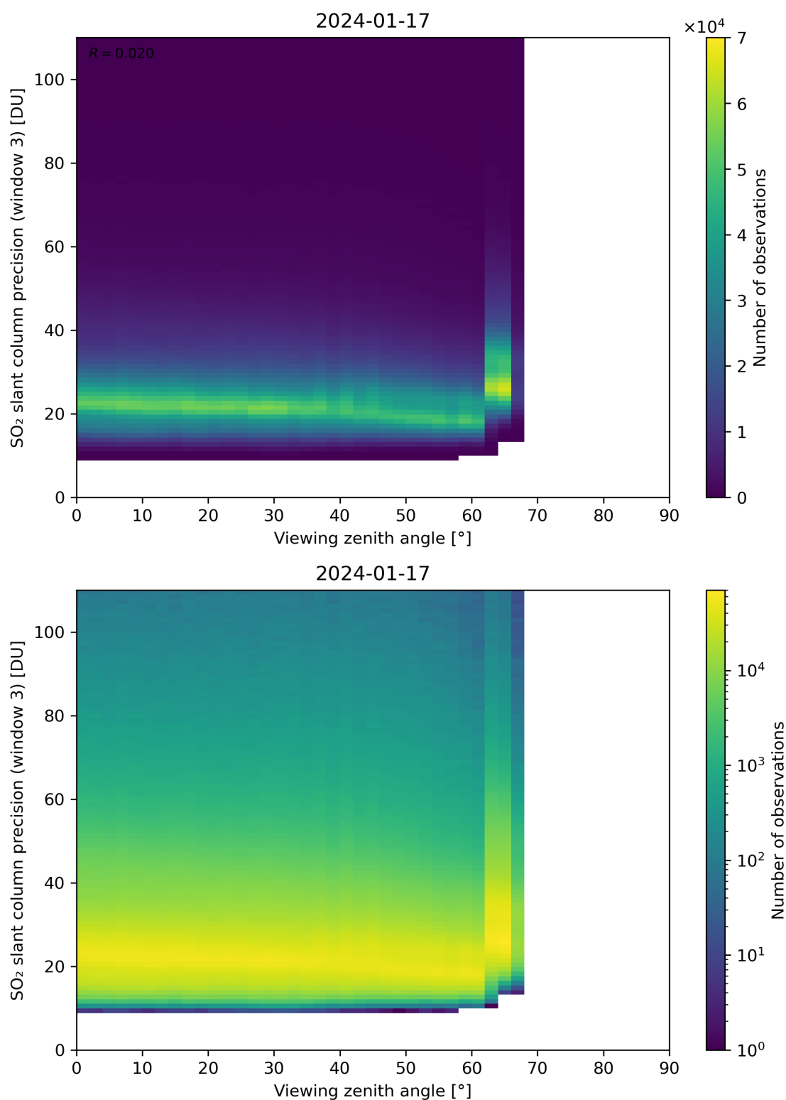
Figure 324: Scatter density plot of “Viewing zenith angle” against “SO 2 slant column precision (window 3)” for 2024-01-16 to 2024-01-18.
