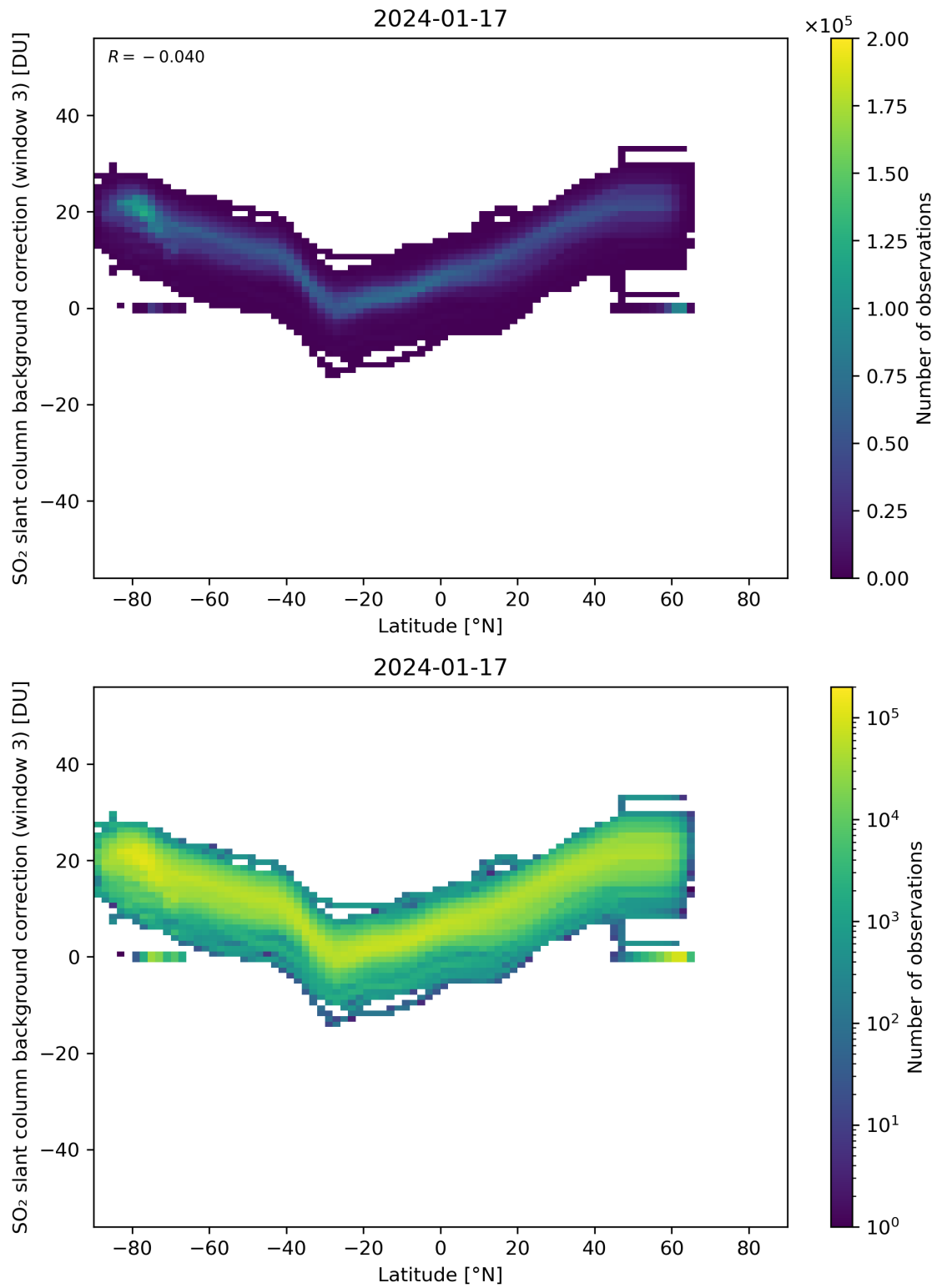
Figure 141: Scatter density plot of “Latitude” against “SO 2 slant column background correction (window 3)” for 2024-01-16 to 2024-01-18.
