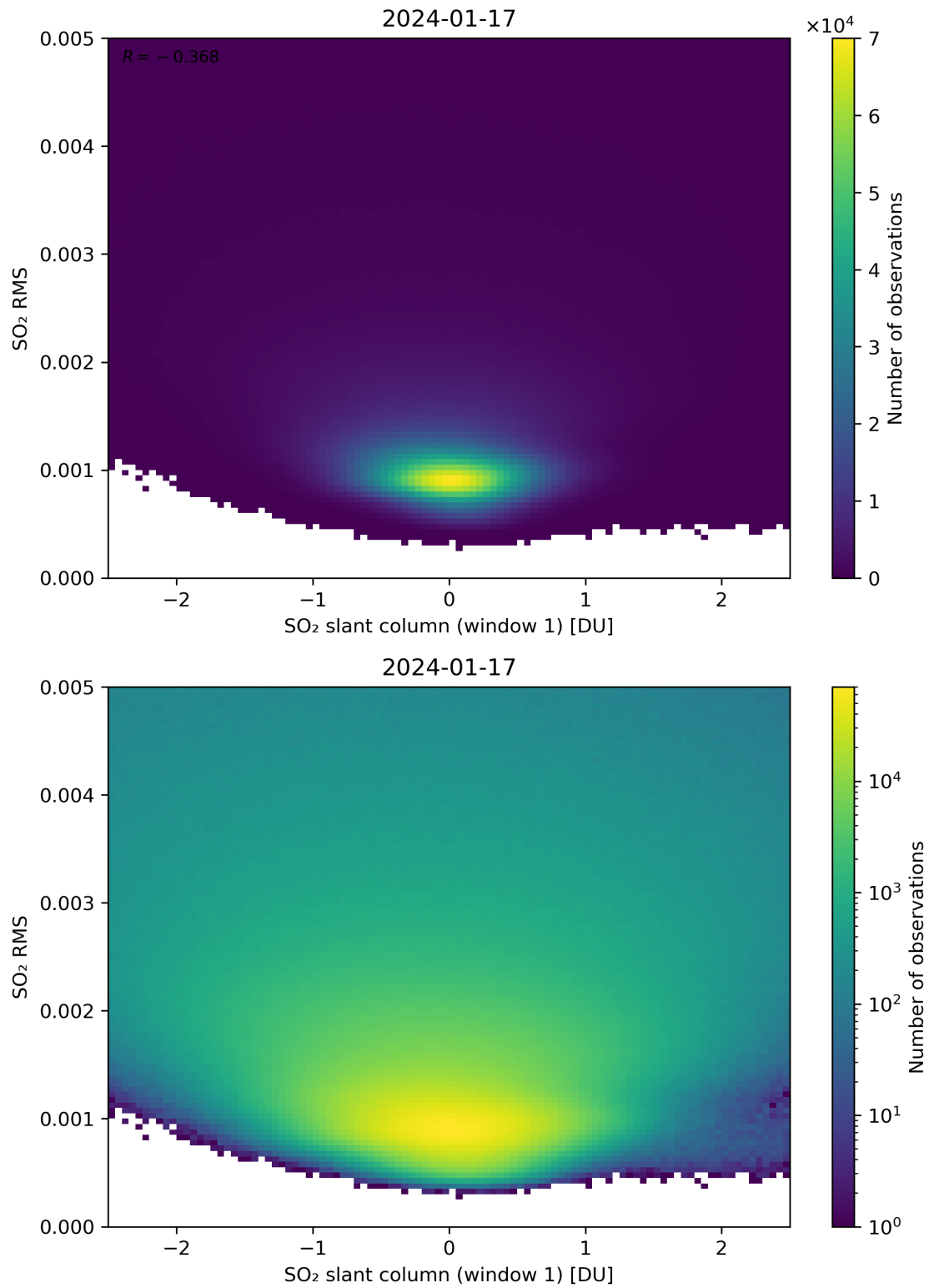
Figure 217: Scatter density plot of “SO 2 slant column (window 1)” against “SO 2 RMS” for 2024-01-16 to 2024-01-18.
