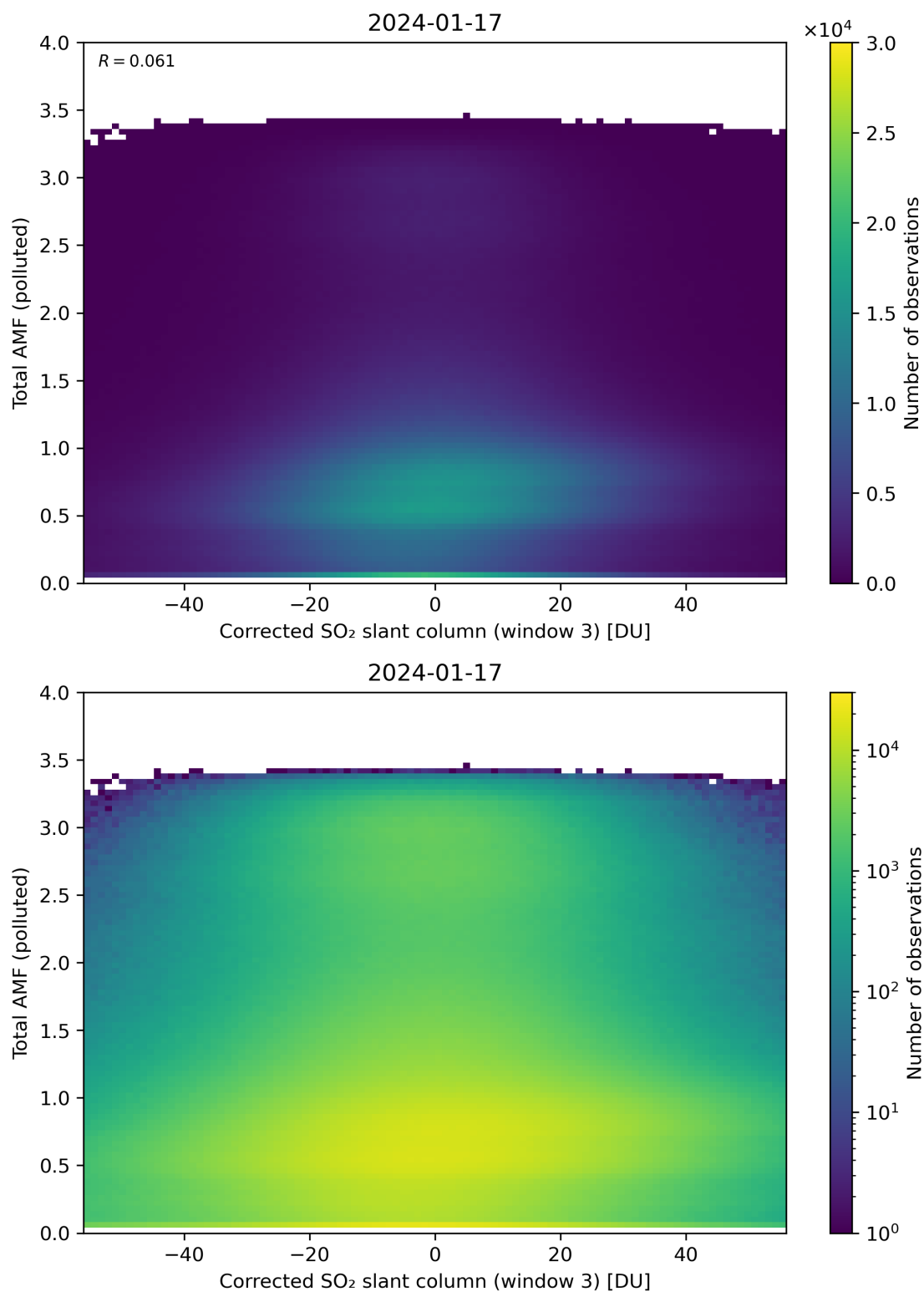
Figure 210: Scatter density plot of “Corrected SO 2 slant column (window 3)” against “Total AMF (polluted)” for 2024-01-16 to 2024-01-18.
