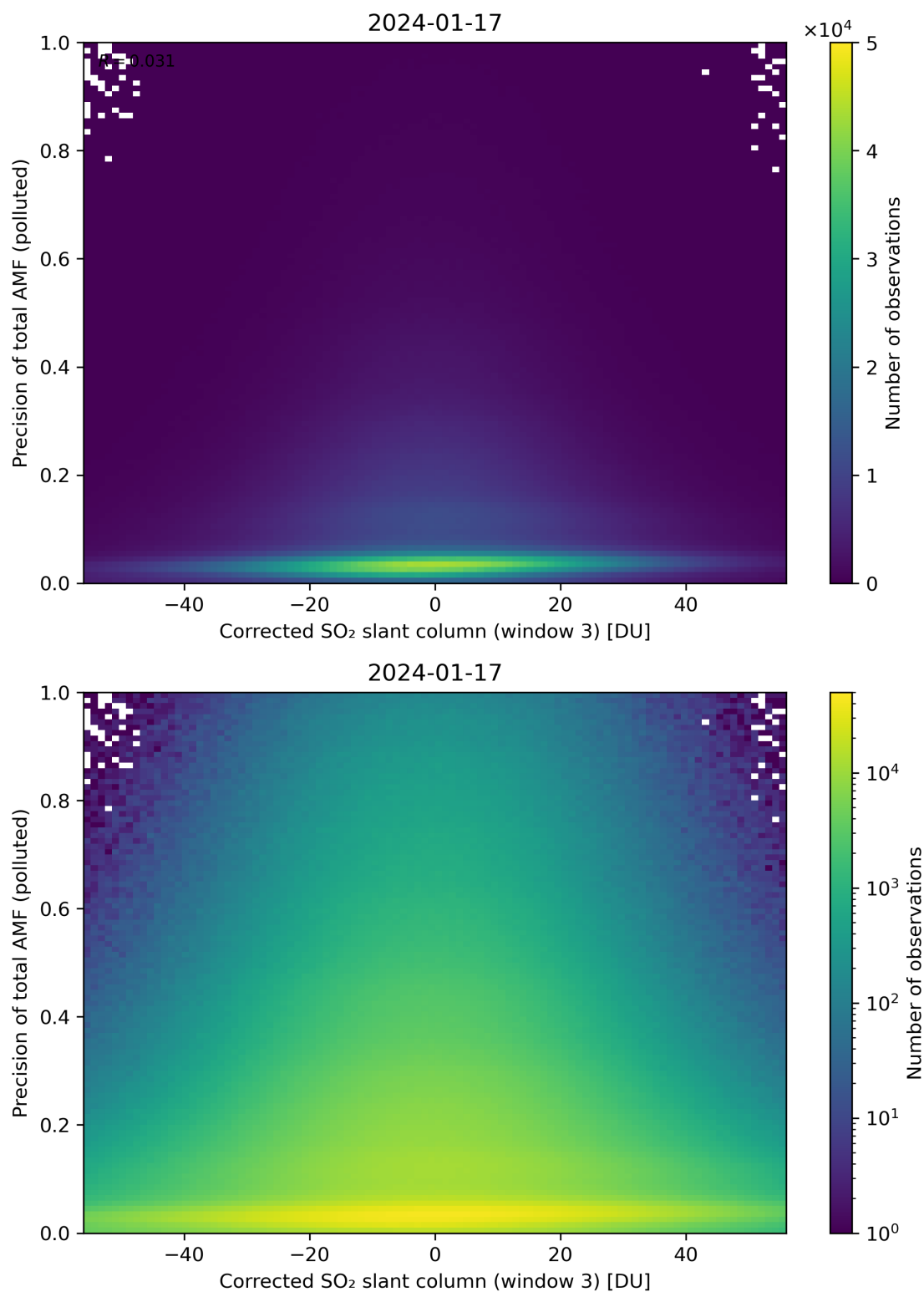
Figure 211: Scatter density plot of “Corrected SO 2 slant column (window 3)” against “Precision of total AMF (polluted)” for 2024-01-16 to 2024-01-18.
