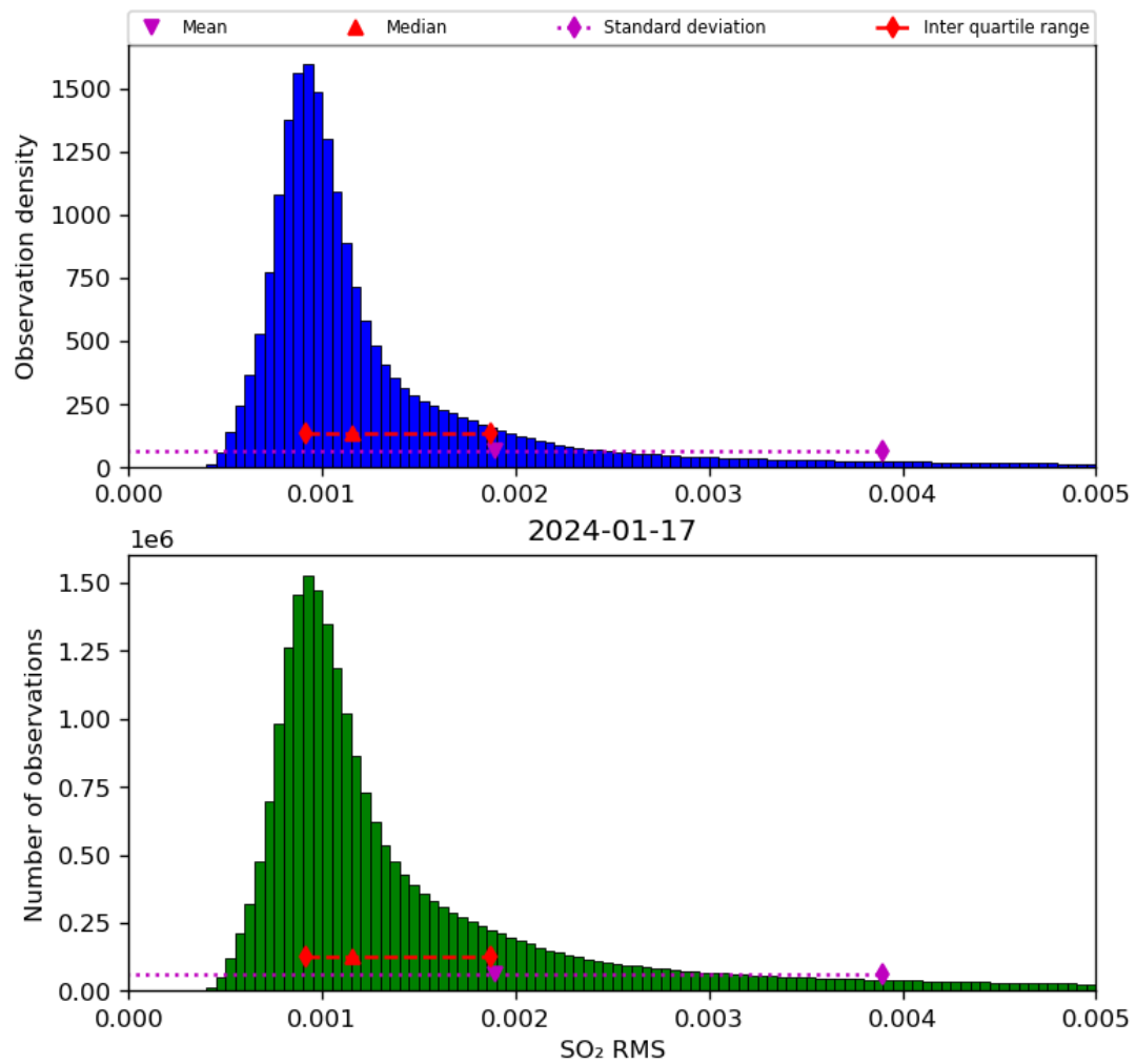
Figure 70: Histogram of “SO 2 RMS” for 2024-01-16 to 2024-01-18
