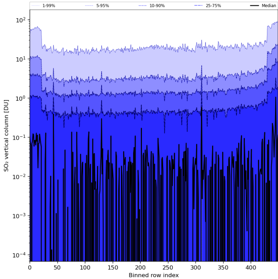
Figure 76: Along track statistics of “SO 2 vertical column” for 2024-01-16 to 2024-01-18
