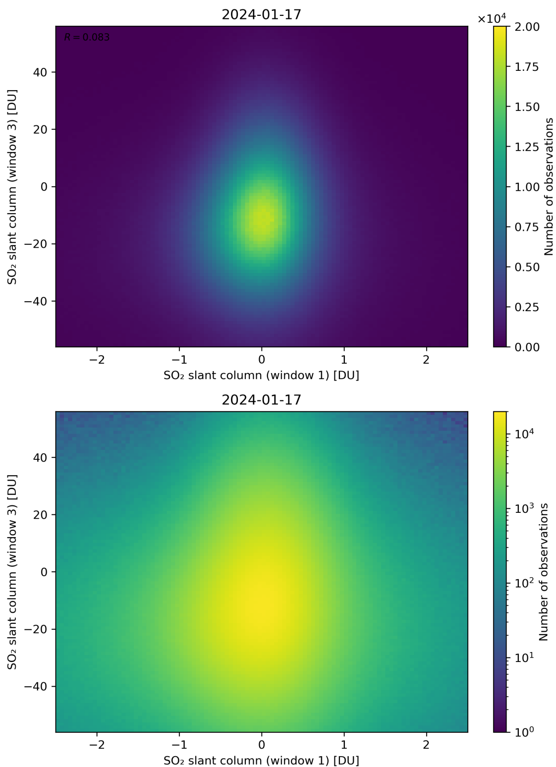
Figure 237: Scatter density plot of “SO 2 slant column (window 1)” against “SO 2 slant column (window 3)” for 2024-01-16 to 2024-01-18.
