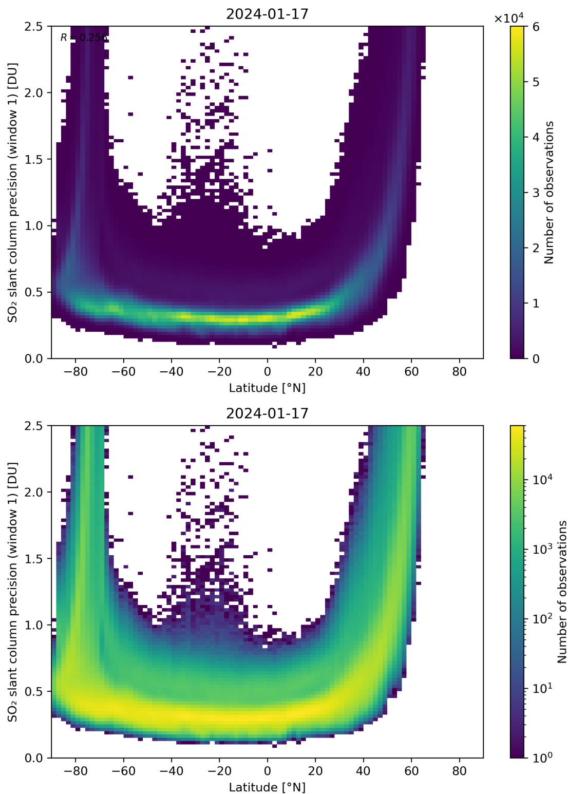
Figure 150: Scatter density plot of “Latitude” against “SO 2 slant column precision (window 1)” for 2024-01-16 to 2024-01-18.
