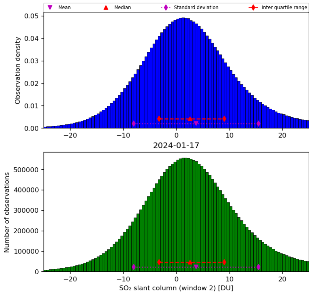
Figure 60: Histogram of “SO 2 slant column (window 2)” for 2024-01-16 to 2024-01-18
