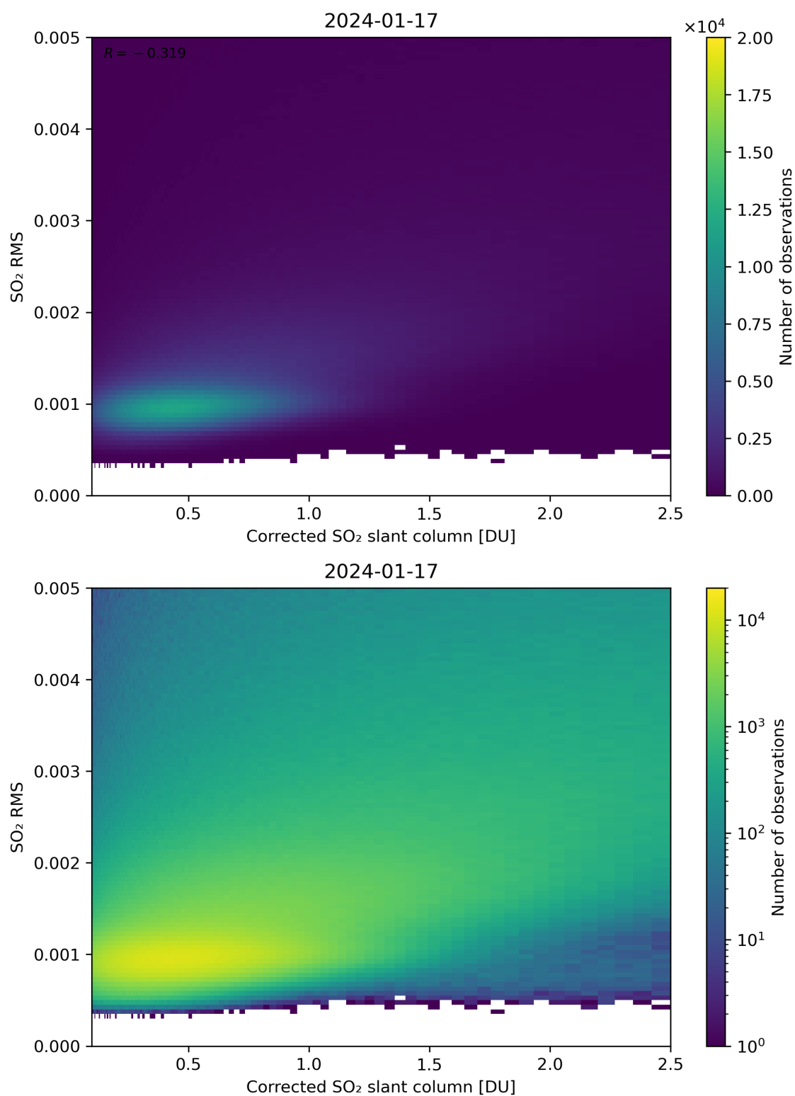
Figure 183: Scatter density plot of “Corrected SO 2 slant column” against “SO 2 RMS” for 2024-01-16 to 2024-01-18.
