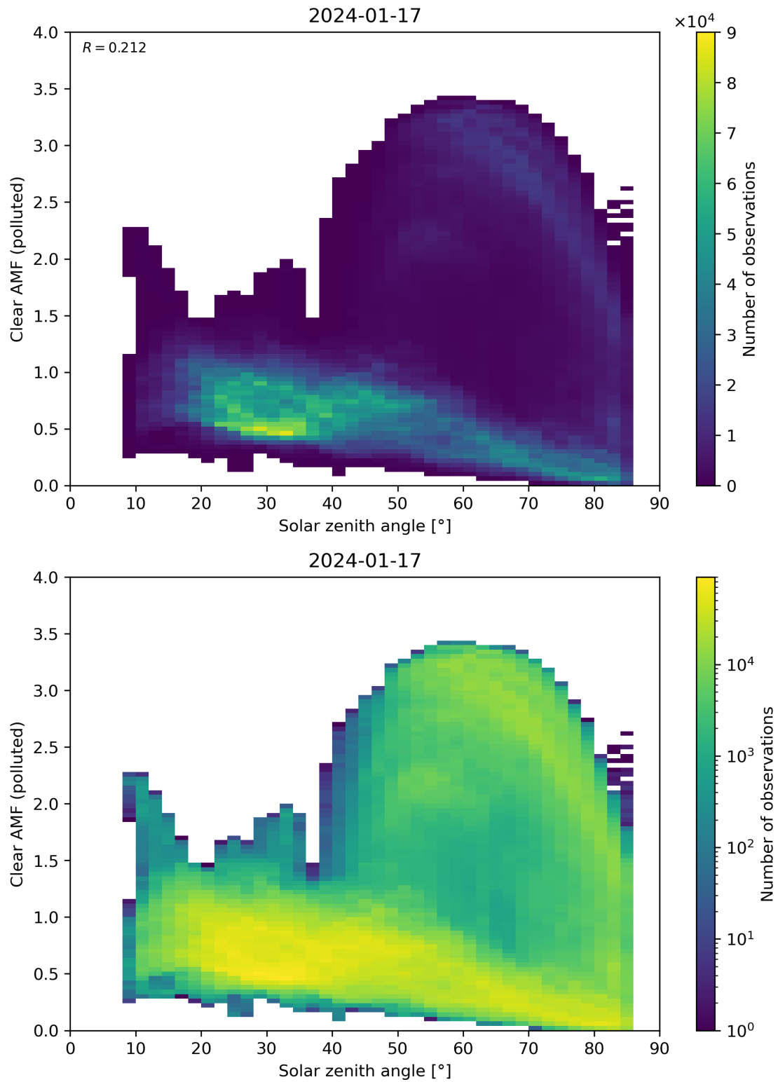
Figure 165: Scatter density plot of “Solar zenith angle” against “Clear AMF (polluted)” for 2024-01-16 to 2024-01-18.
