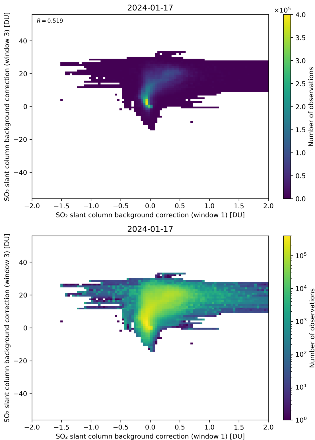
Figure 99: Scatter density plot of “SO 2 slant column background correction (window 1)” against “SO 2 slant column background correction (window 3)” for 2024-01-16 to 2024-01-18.
