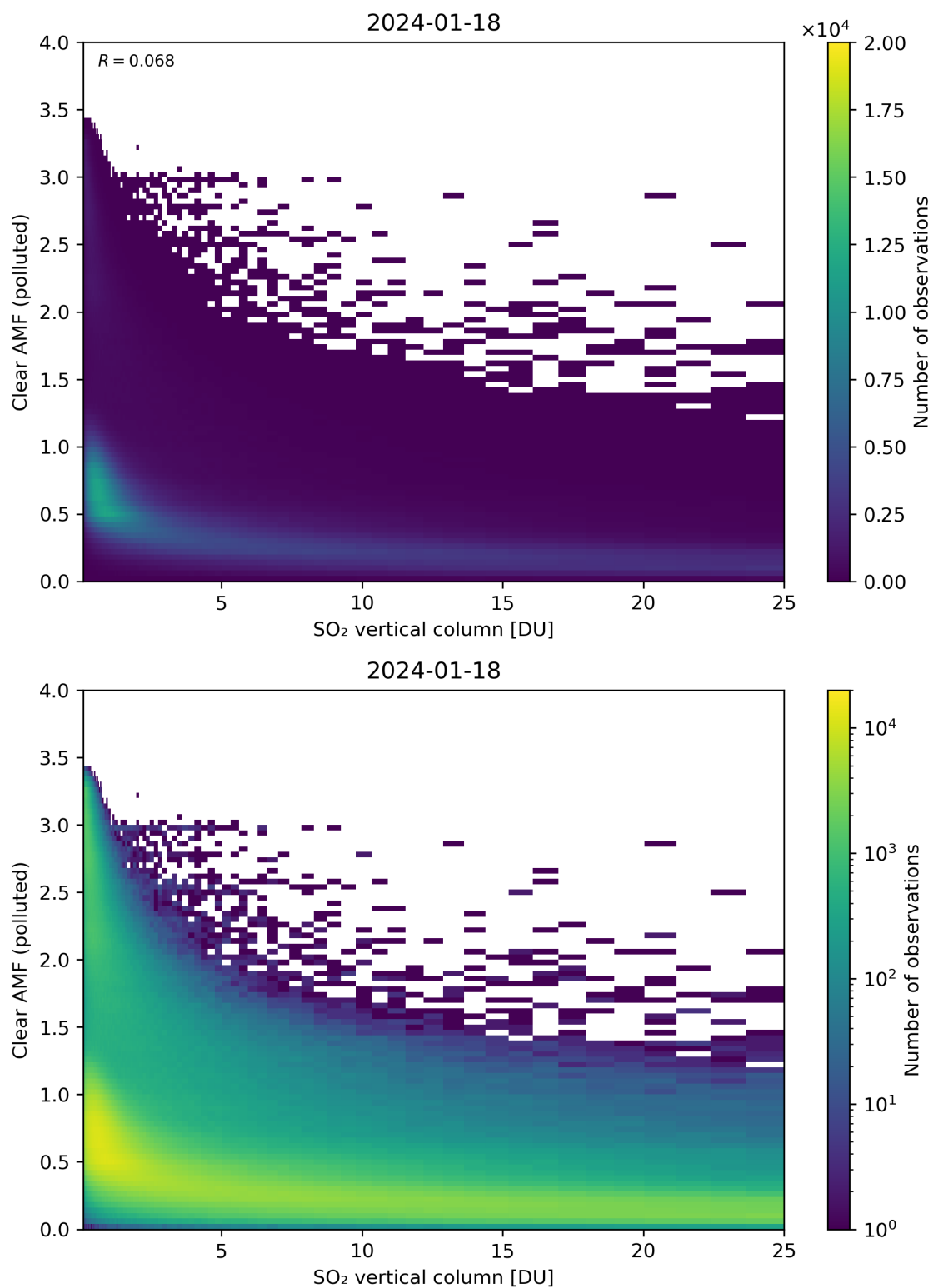
Figure 296: Scatter density plot of “SO 2 vertical column” against “Clear AMF (polluted)” for 2024-01-17 to 2024-01-19.
