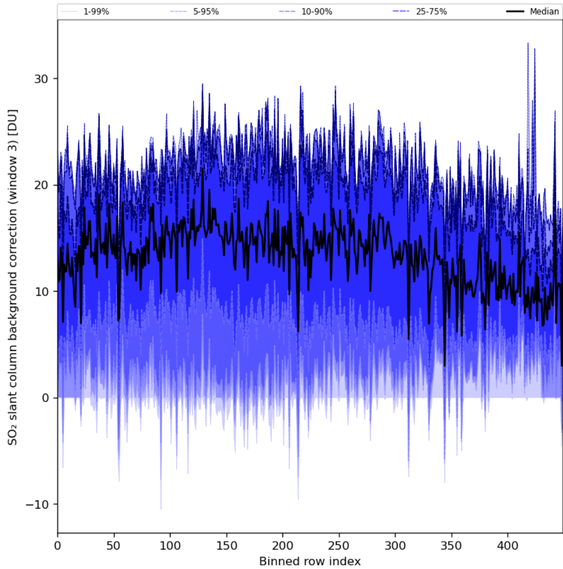
Figure 90: Along track statistics of “SO 2 slant column background correction (window 3)” for 2024-01-17 to 2024-01-19
