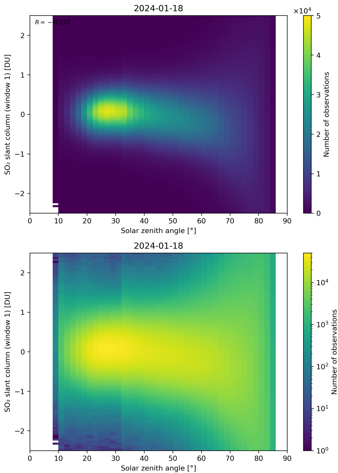
Figure 169: Scatter density plot of “Solar zenith angle” against “SO 2 slant column (window 1)” for 2024-01-17 to 2024-01-19.
