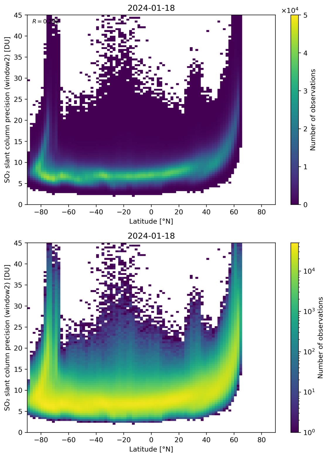
Figure 151: Scatter density plot of “Latitude” against “SO 2 slant column precision (window2)” for 2024-01-17 to 2024-01-19.
