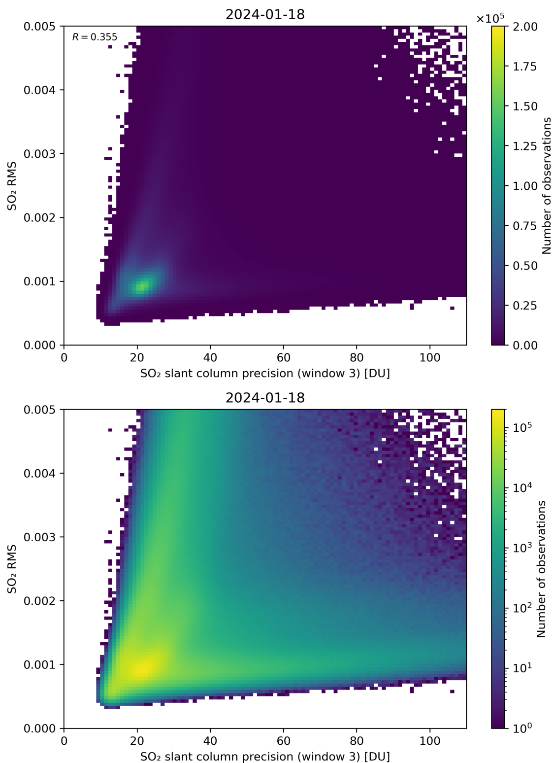
Figure 260: Scatter density plot of “SO 2 slant column precision (window 3)” against “SO 2 RMS” for 2024-01-17 to 2024-01-19.
