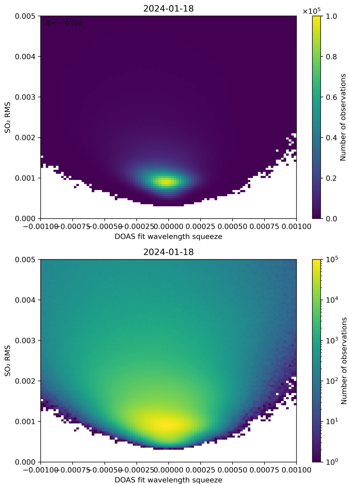
Figure 132: Scatter density plot of “DOAS fit wavelength squeeze” against “SO 2 RMS” for 2024-01-17 to 2024-01-19.
