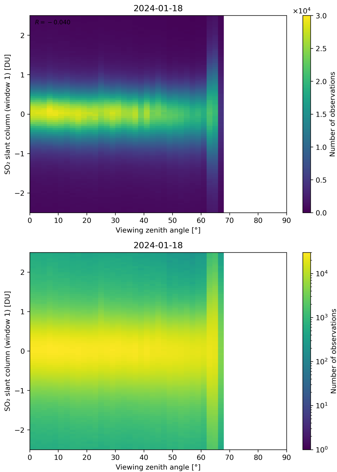
Figure 320: Scatter density plot of “Viewing zenith angle” against “SO 2 slant column (window 1)” for 2024-01-17 to 2024-01-19.
