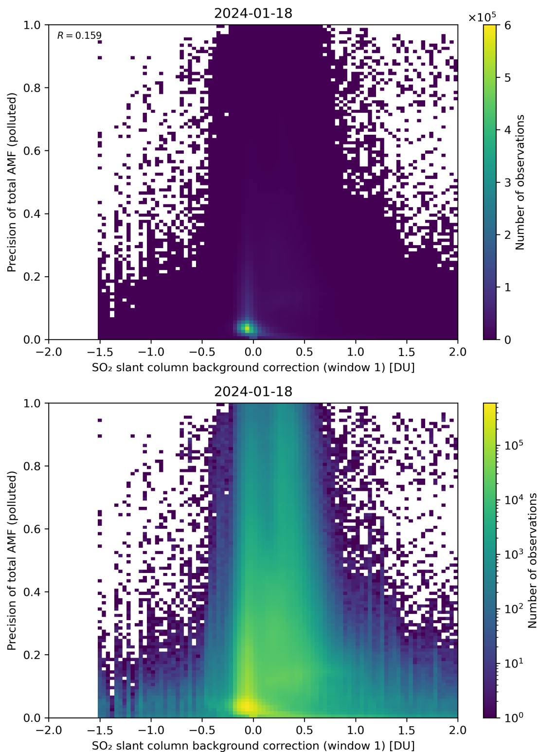
Figure 110: Scatter density plot of “SO 2 slant column background correction (window 1)” against “Precision of total AMF (polluted)” for 2024-01-17 to 2024-01-19.
