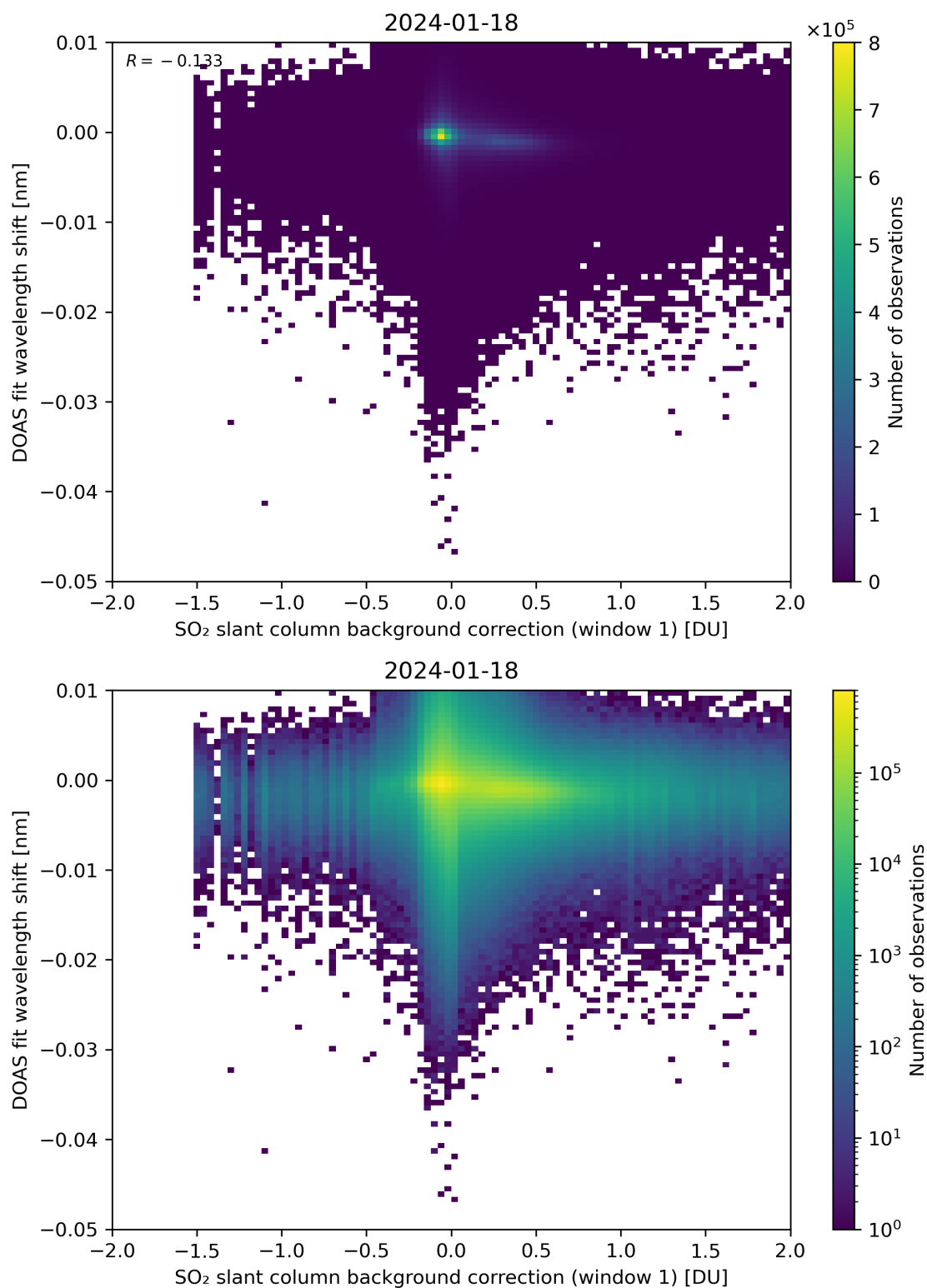
Figure 100: Scatter density plot of “SO 2 slant column background correction (window 1)” against “DOAS fit wavelength shift” for 2024-01-17 to 2024-01-19.
