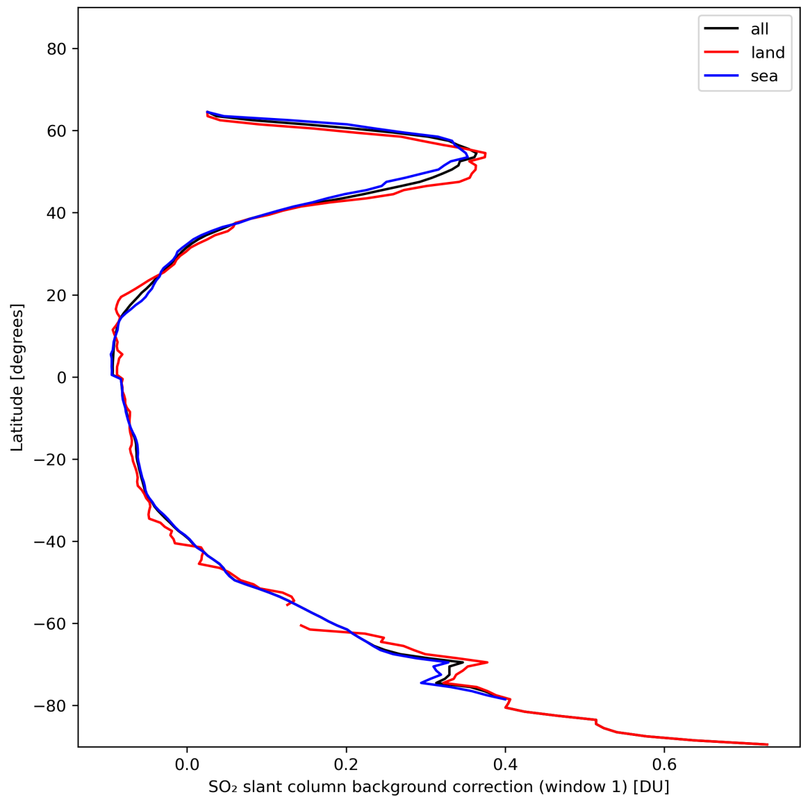
Figure 36: Zonal average of “SO 2 slant column background correction (window 1)” for 2024-01-17 to 2024-01-19.
