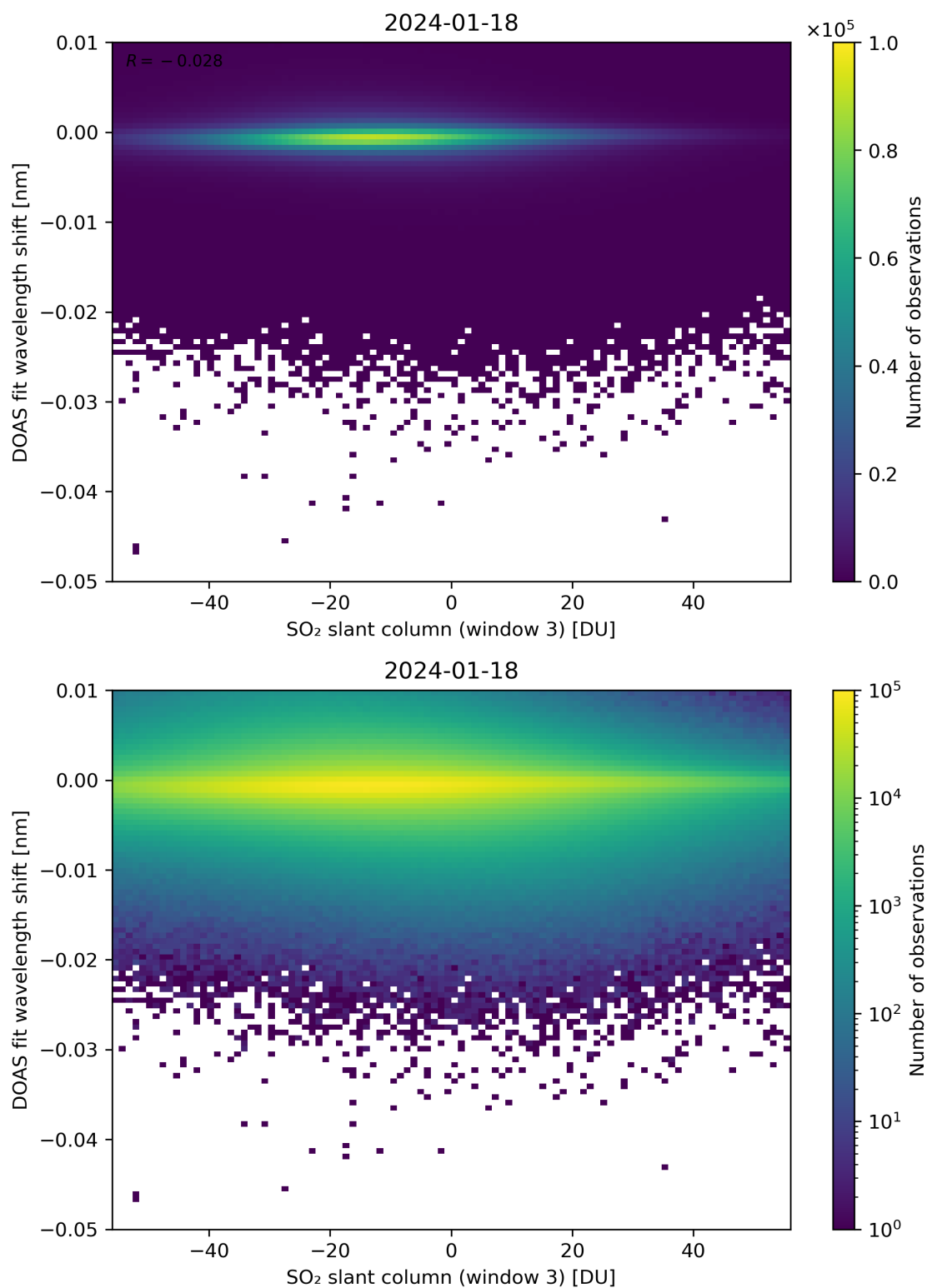
Figure 254: Scatter density plot of “SO 2 slant column (window 3)” against “DOAS fit wavelength shift” for 2024-01-17 to 2024-01-19.
