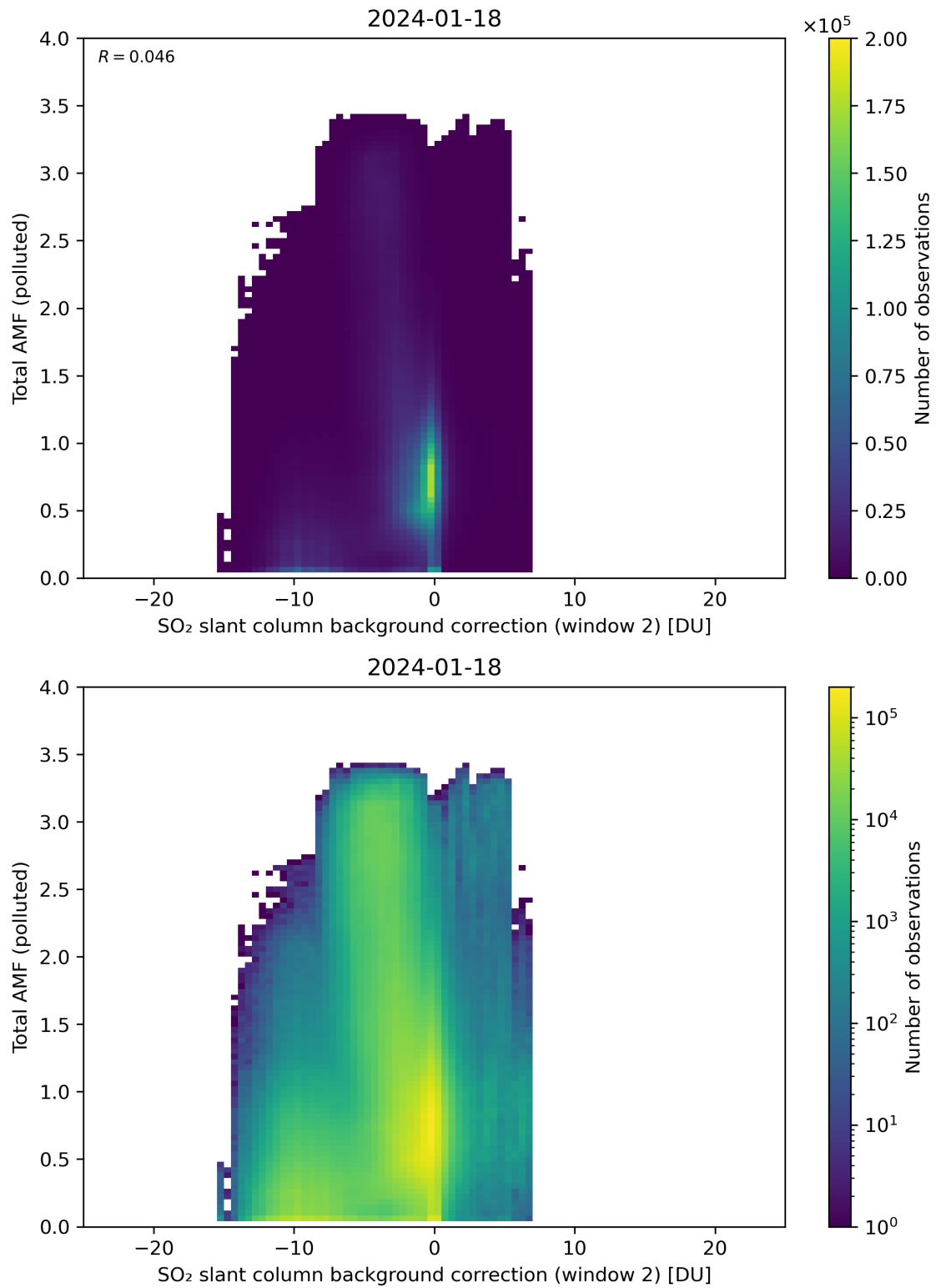
Figure 119: Scatter density plot of “SO 2 slant column background correction (window 2)” against “Total AMF (polluted)” for 2024-01-17 to 2024-01-19.
