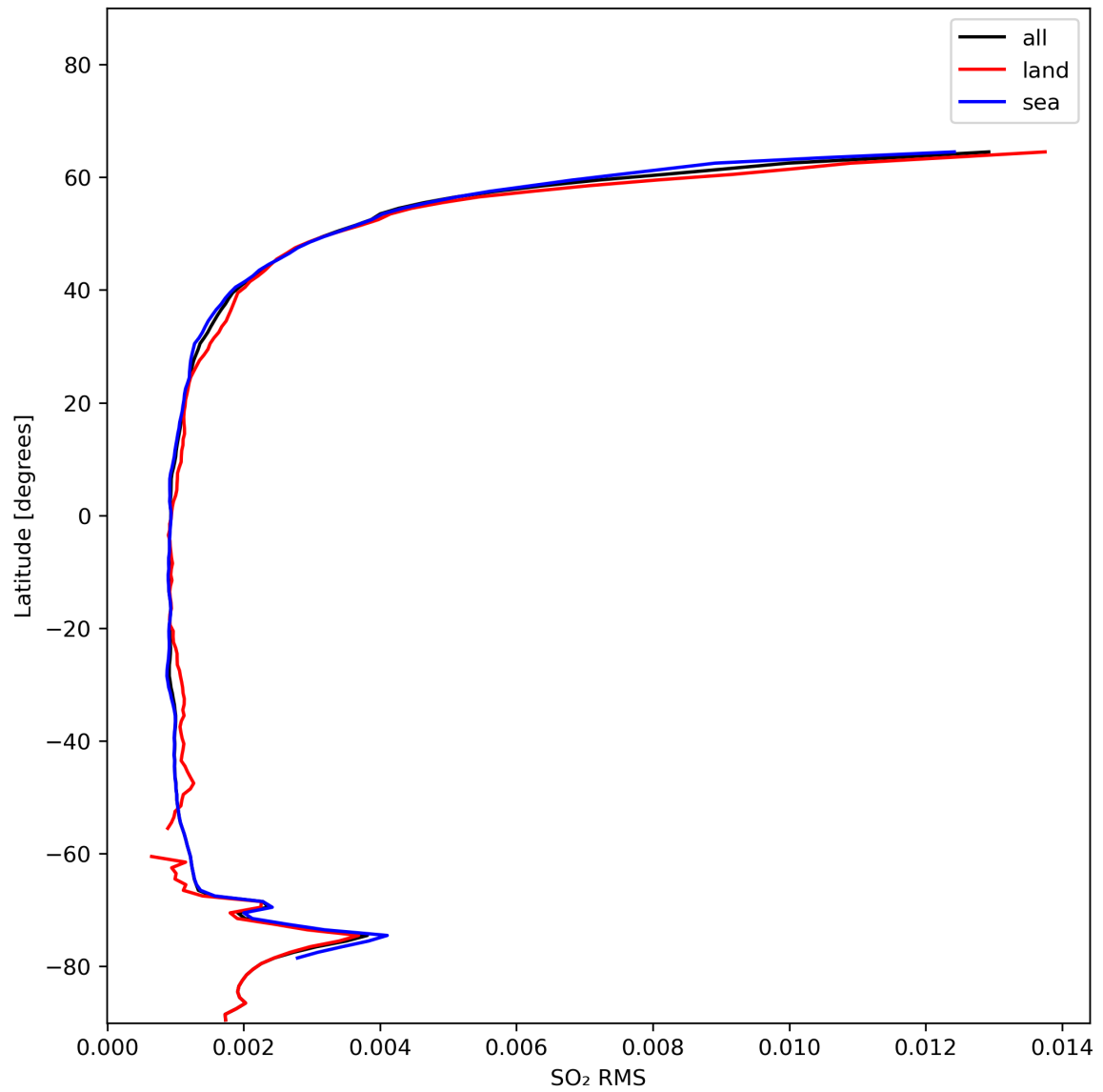
Figure 47: Zonal average of “SO 2 RMS” for 2024-01-17 to 2024-01-19.
