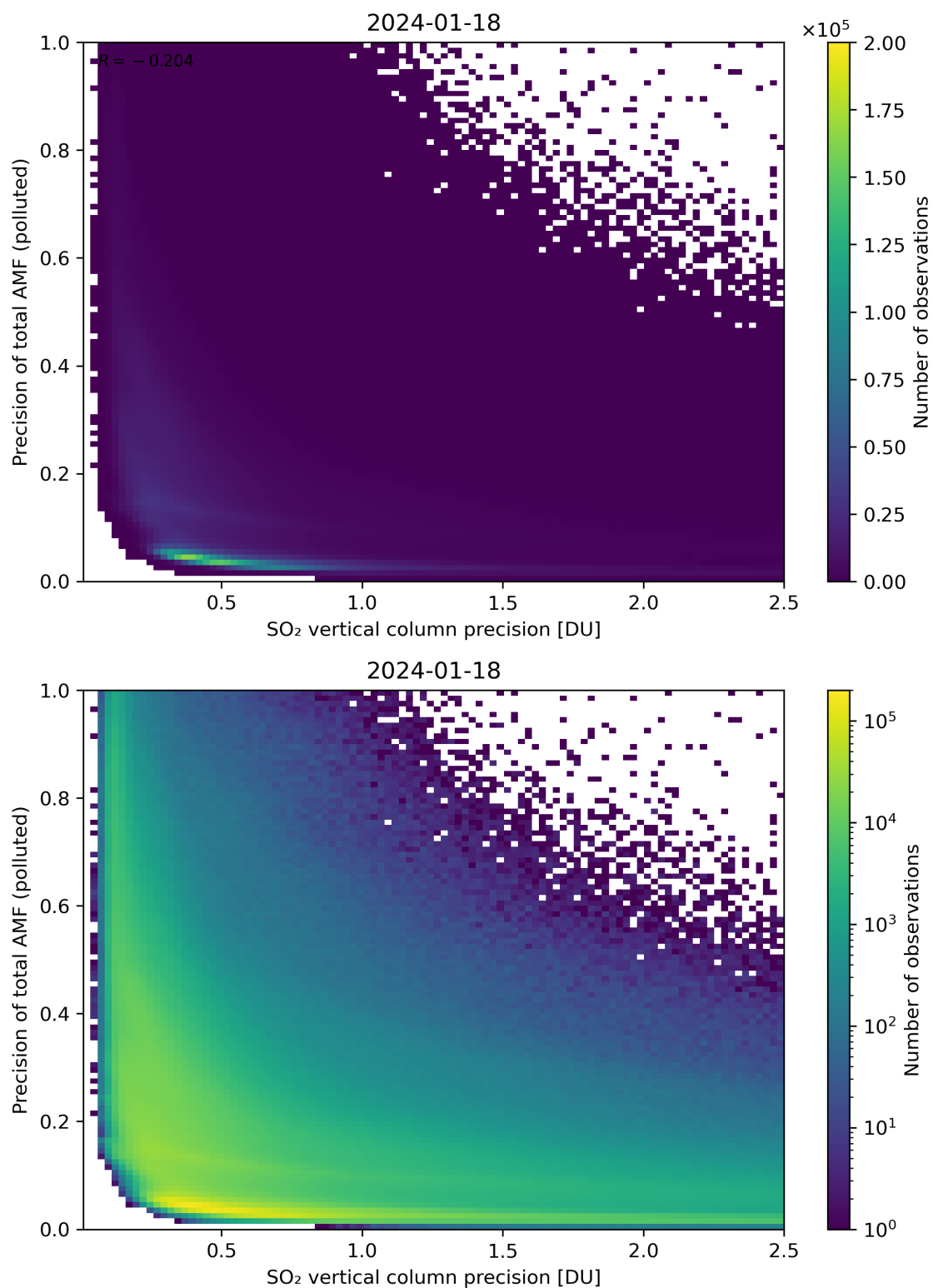
Figure 295: Scatter density plot of “SO 2 vertical column precision” against “Precision of total AMF (polluted)” for 2024-01-17 to 2024-01-19.
