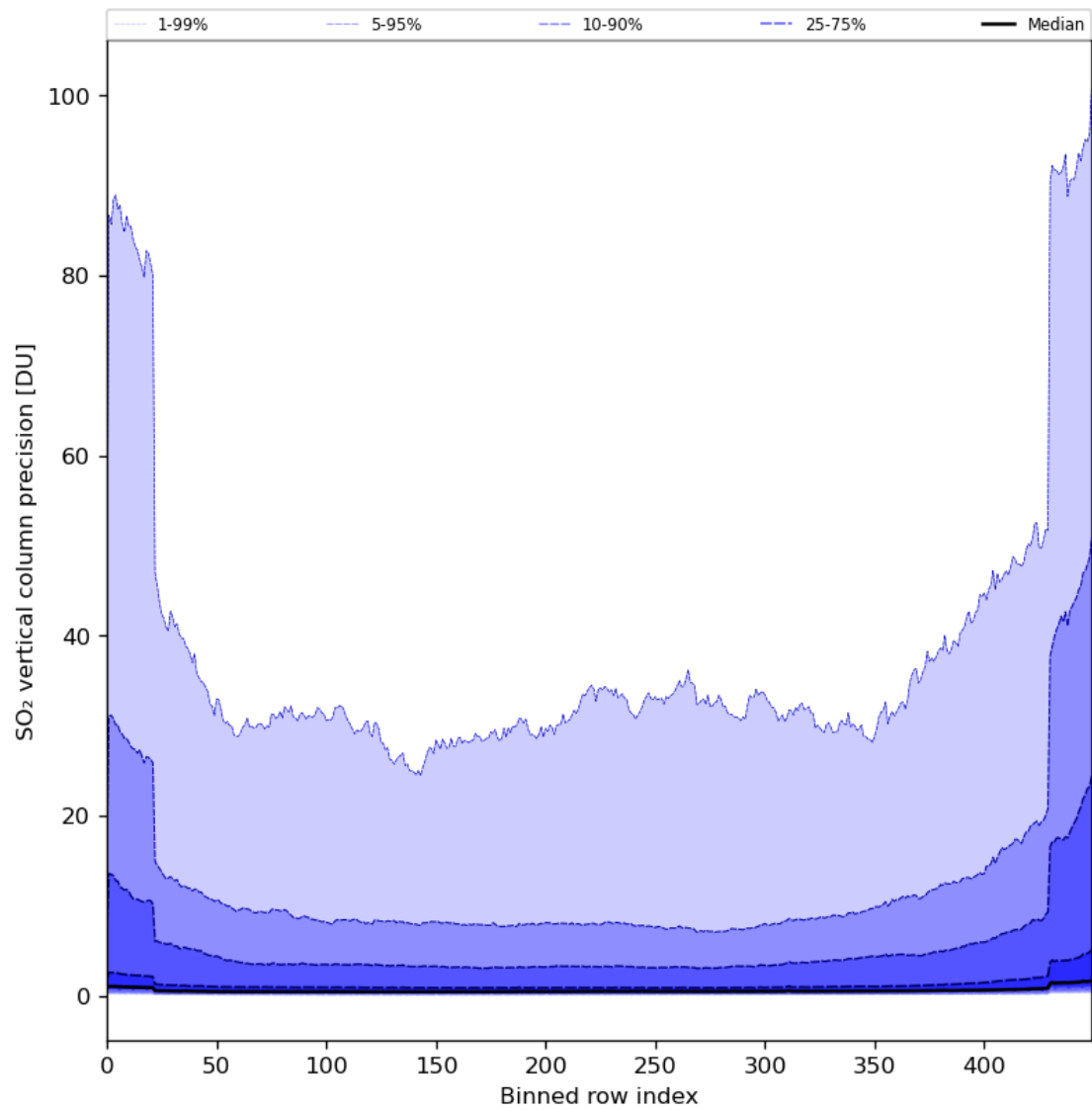
Figure 77: Along track statistics of “SO 2 vertical column precision” for 2024-01-17 to 2024-01-19
