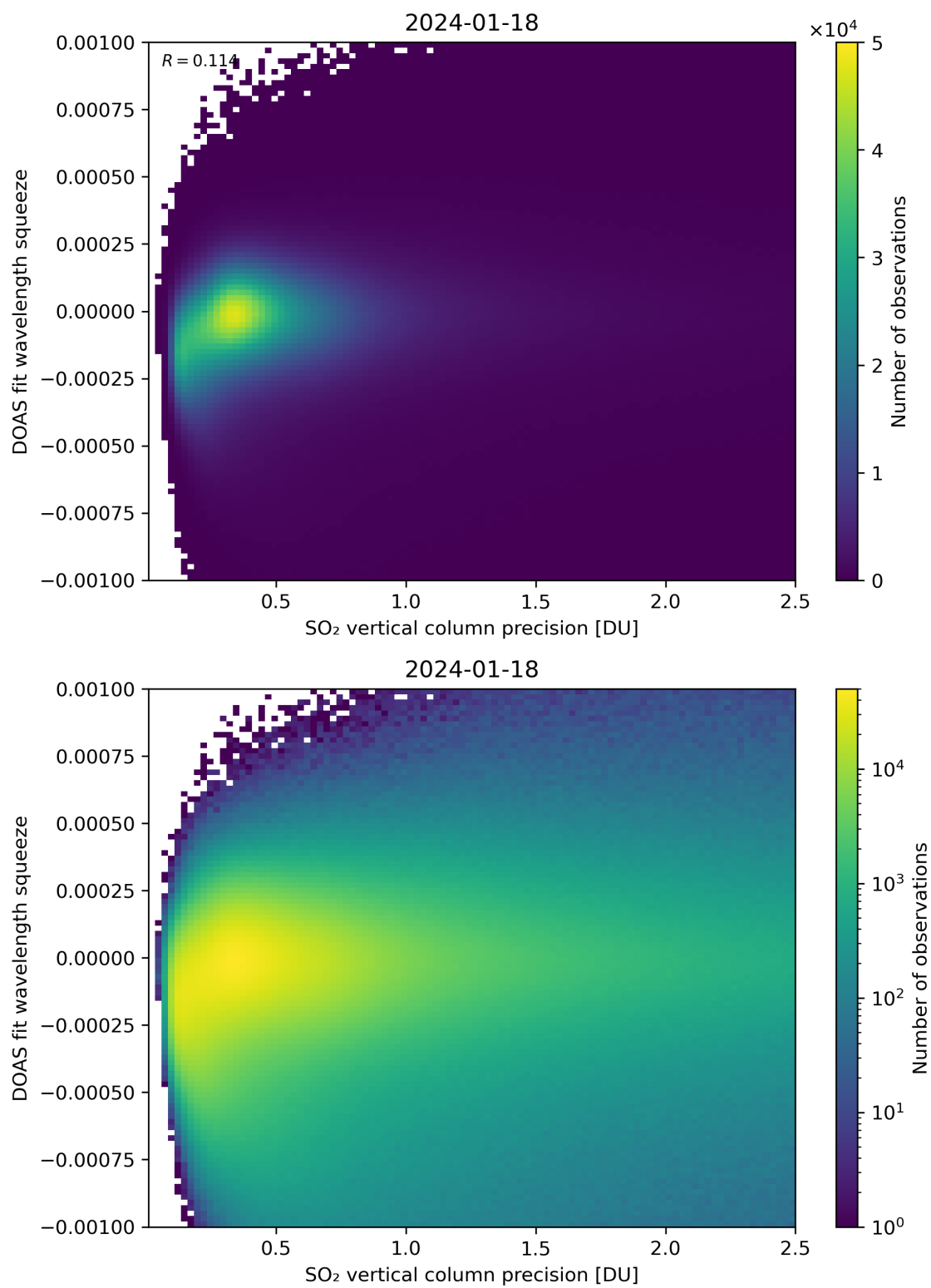
Figure 283: Scatter density plot of “SO 2 vertical column precision” against “DOAS fit wavelength squeeze” for 2024-01-17 to 2024-01-19.
