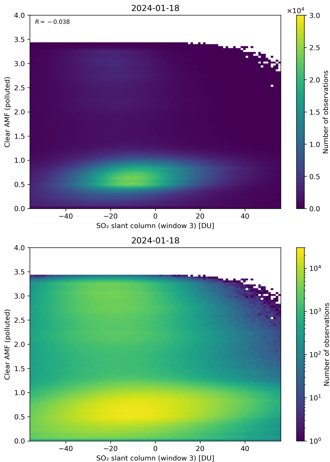
Figure 265: Scatter density plot of “SO 2 slant column (window 3)” against “Clear AMF (polluted)” for 2024-01-17 to 2024-01-19.
