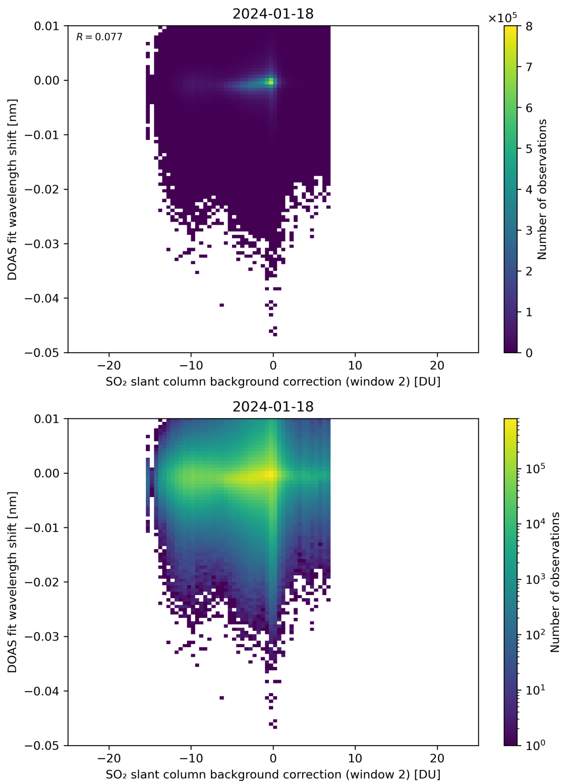
Figure 112: Scatter density plot of “SO 2 slant column background correction (window 2)” against “DOAS fit wavelength shift” for 2024-01-17 to 2024-01-19.
