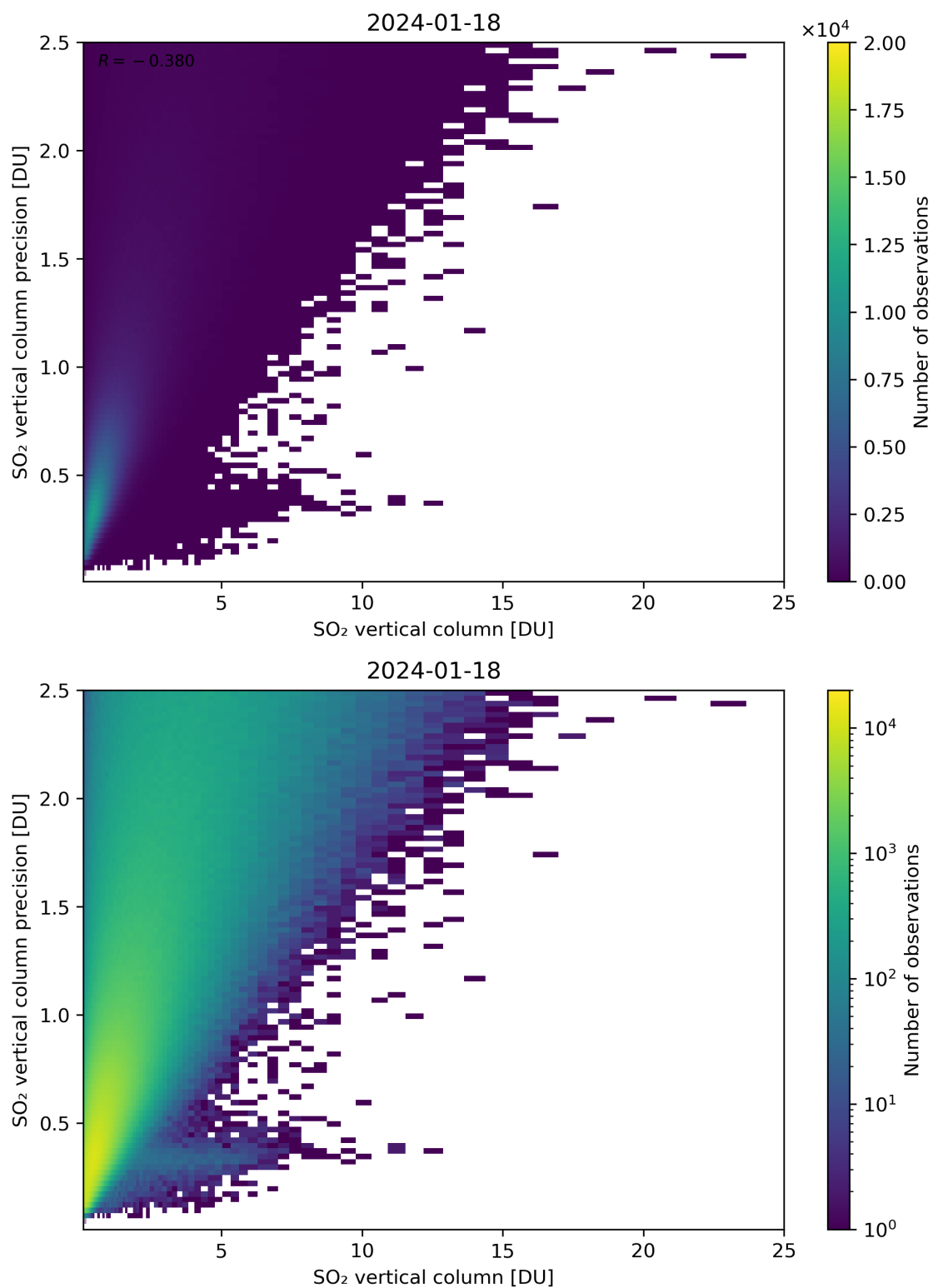
Figure 307: Scatter density plot of “SO 2 vertical column” against “SO 2 vertical column precision” for 2024-01-17 to 2024-01-19.
