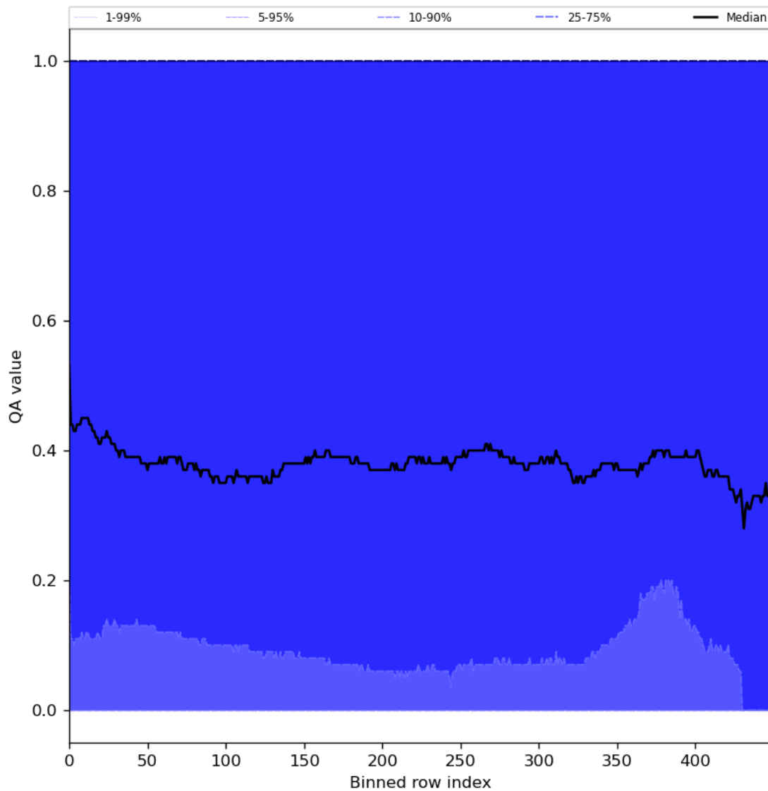
Figure 75: Along track statistics of “QA value” for 2024-01-17 to 2024-01-19
