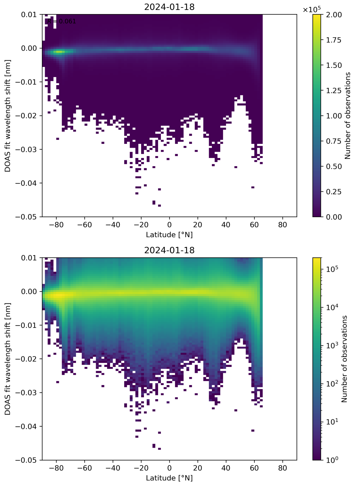
Figure 142: Scatter density plot of “Latitude” against “DOAS fit wavelength shift” for 2024-01-17 to 2024-01-19.
