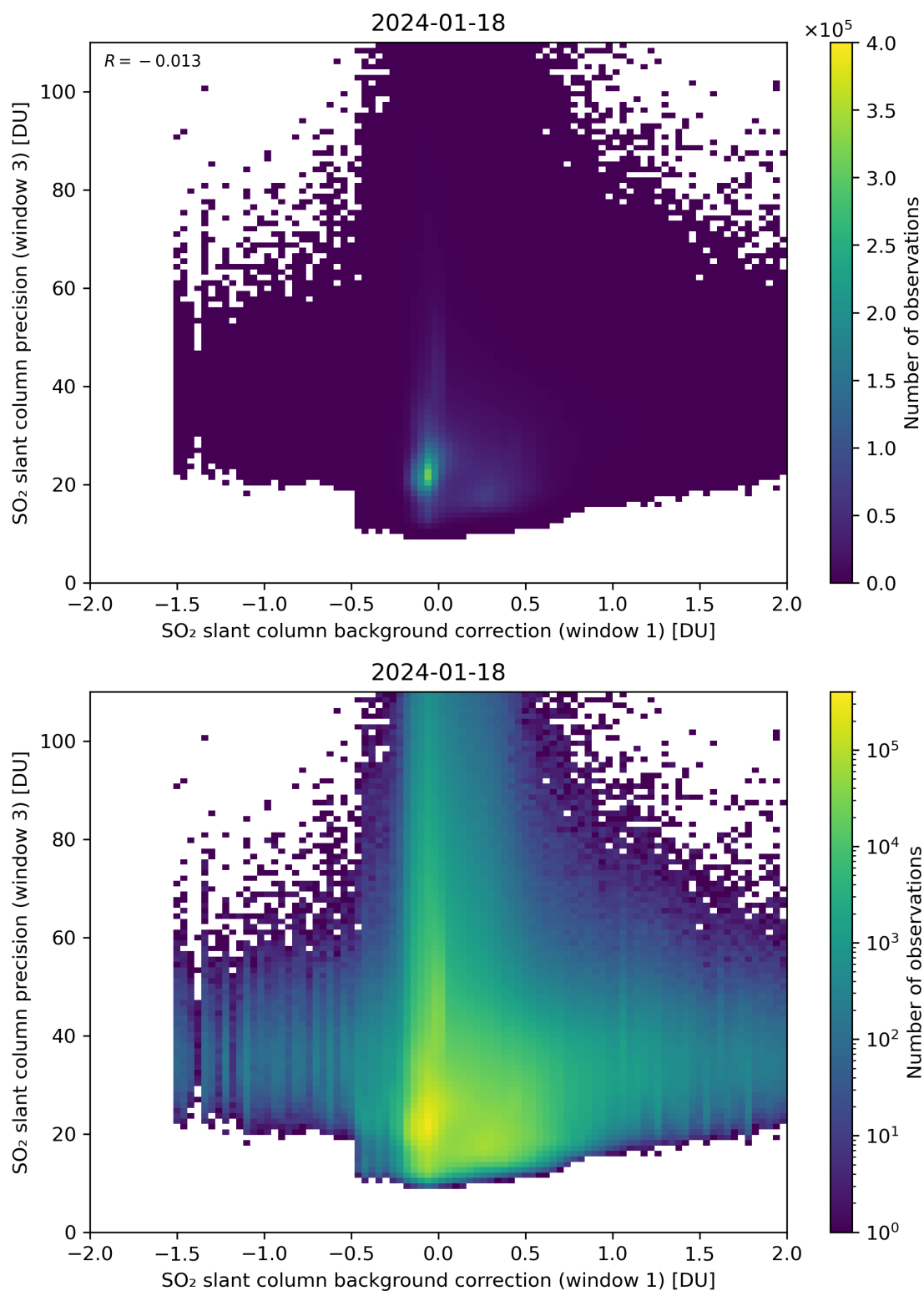
Figure 108: Scatter density plot of “SO 2 slant column background correction (window 1)” against “SO 2 slant column precision (window 3)” for 2024-01-17 to 2024-01-19.
