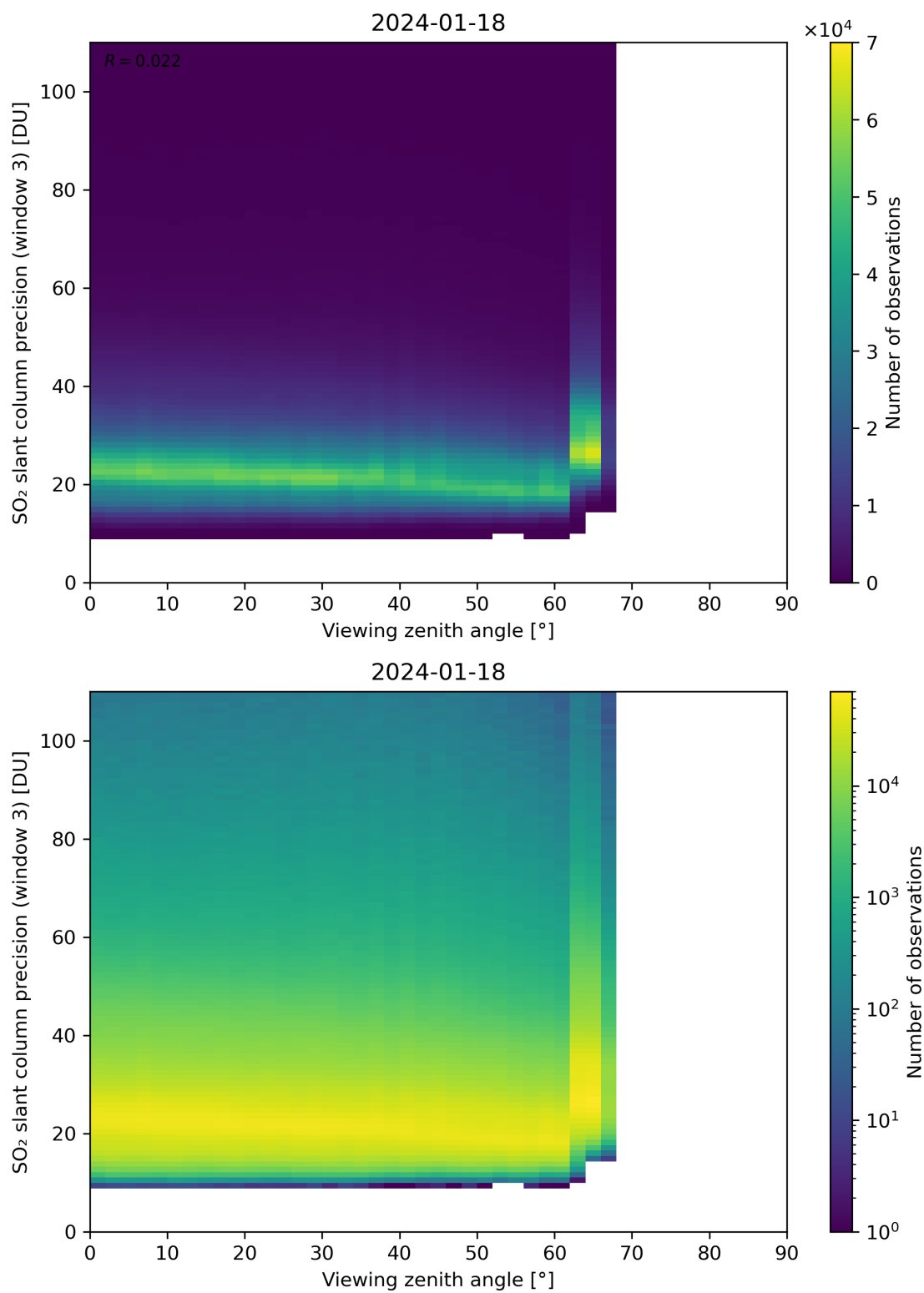
Figure 324: Scatter density plot of “Viewing zenith angle” against “SO 2 slant column precision (window 3)” for 2024-01-17 to 2024-01-19.
