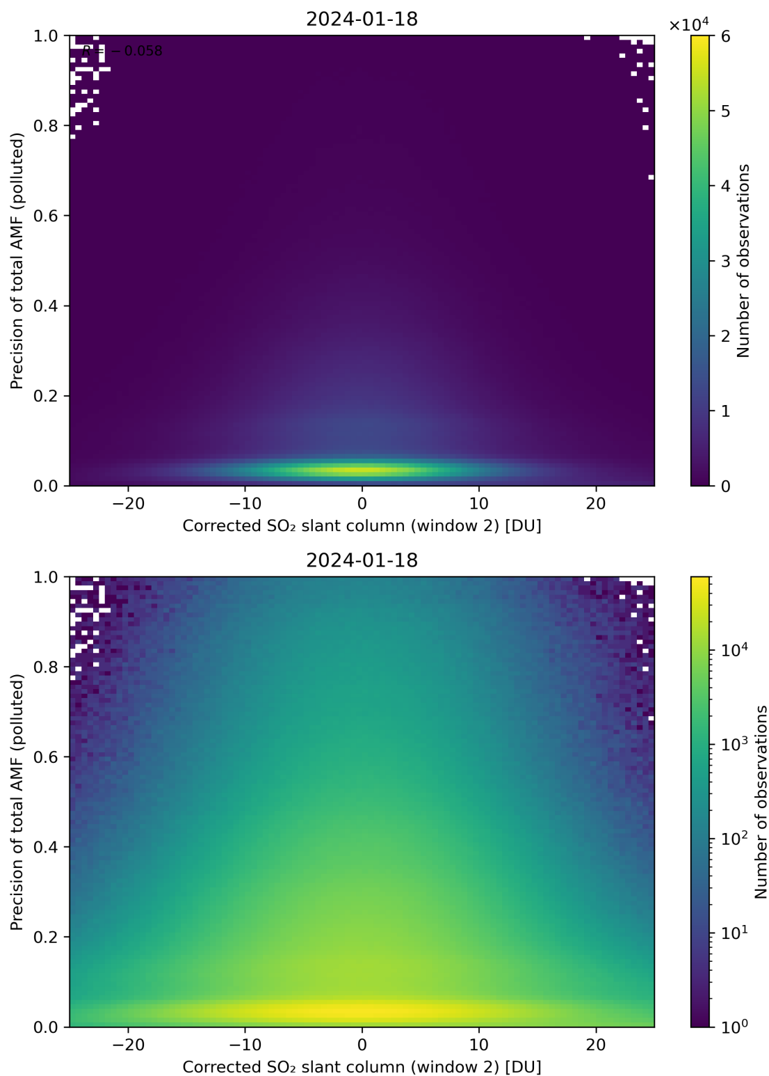
Figure 204: Scatter density plot of “Corrected SO 2 slant column (window 2)” against “Precision of total AMF (polluted)” for 2024-01-17 to 2024-01-19.
