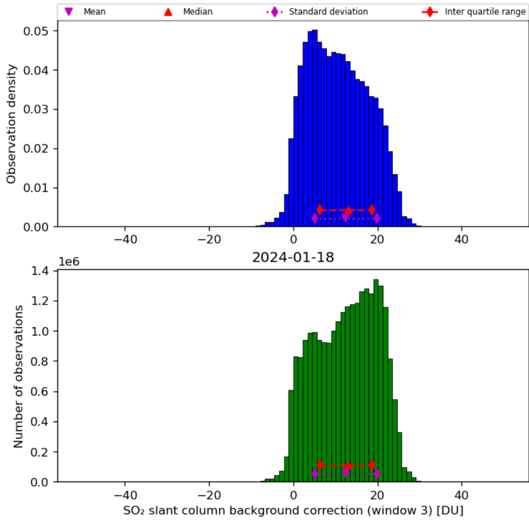
Figure 67: Histogram of “SO 2 slant column background correction (window 3)” for 2024-01-17 to 2024-01-19
