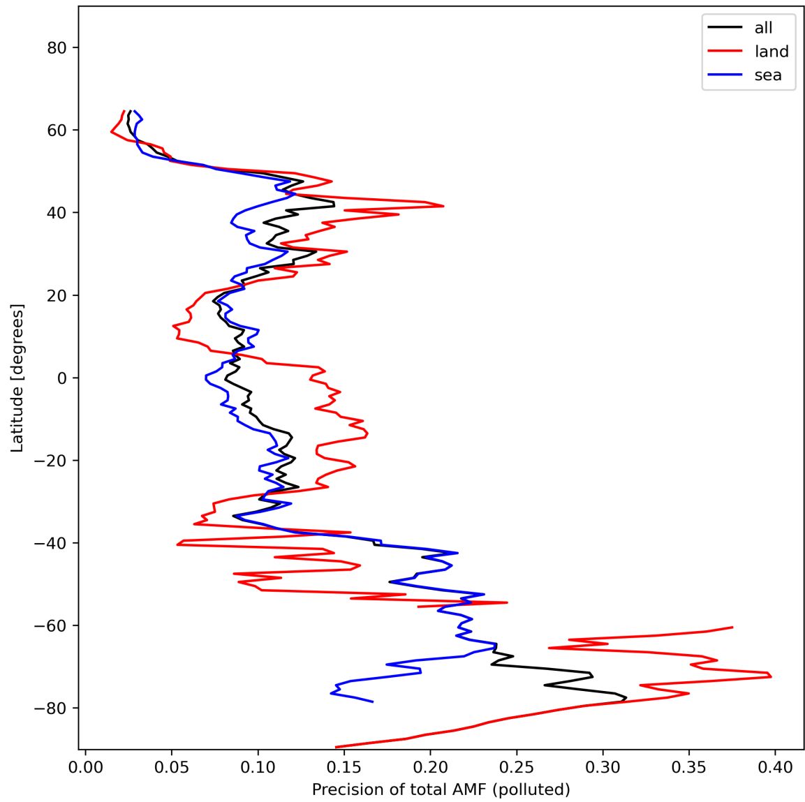
Figure 49: Zonal average of “Precision of total AMF (polluted)” for 2024-01-17 to 2024-01-19.
