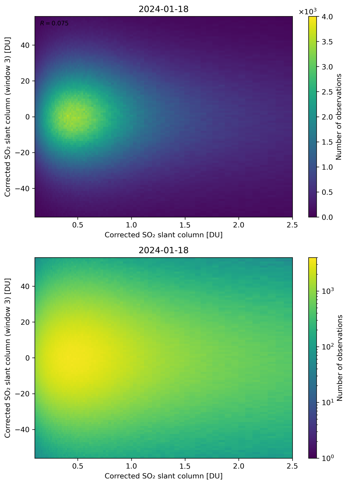
Figure 186: Scatter density plot of “Corrected SO 2 slant column” against “Corrected SO 2 slant column (window 3)” for 2024-01-17 to 2024-01-19.
