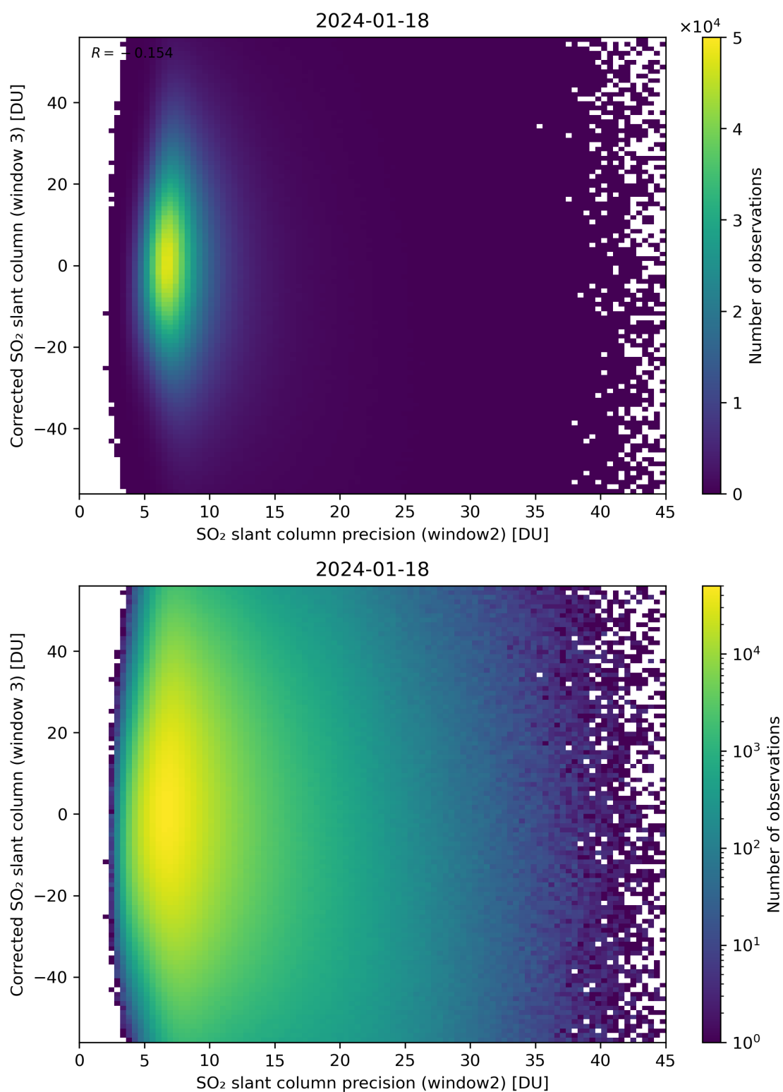
Figure 248: Scatter density plot of “SO 2 slant column precision (window2)” against “Corrected SO 2 slant column (window 3)” for 2024-01-17 to 2024-01-19.
