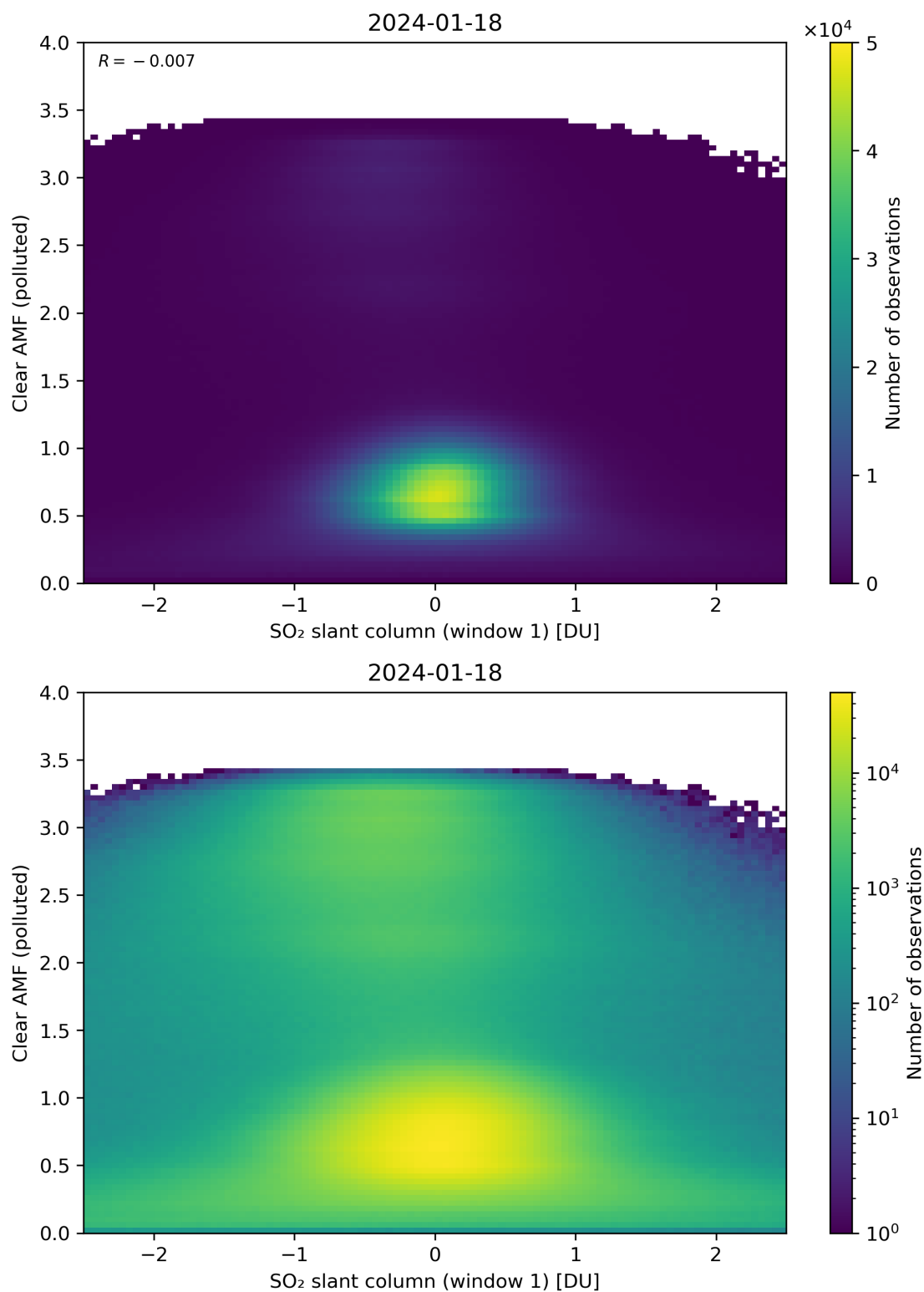
Figure 232: Scatter density plot of “SO 2 slant column (window 1)” against “Clear AMF (polluted)” for 2024-01-17 to 2024-01-19.
