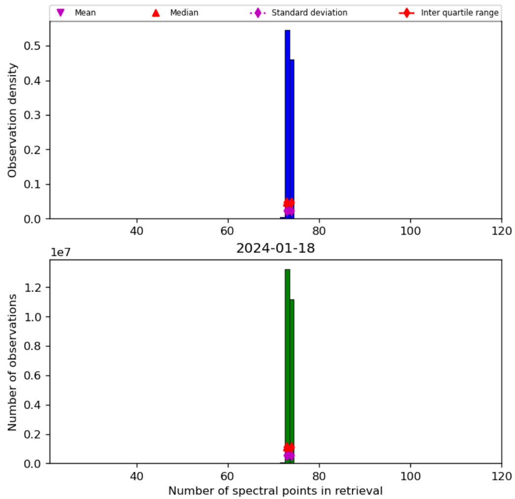
Figure 74: Histogram of “Number of spectral points in retrieval” for 2024-01-17 to 2024-01-19
