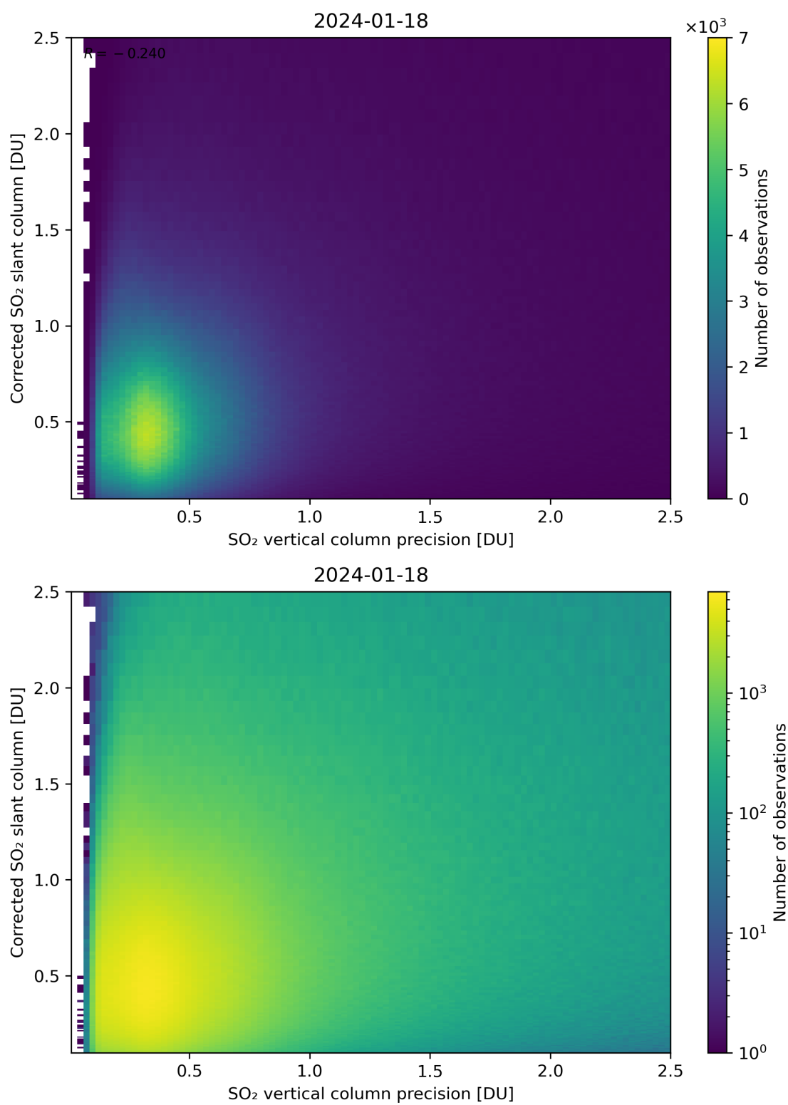
Figure 286: Scatter density plot of “SO 2 vertical column precision” against “Corrected SO 2 slant column” for 2024-01-17 to 2024-01-19.
