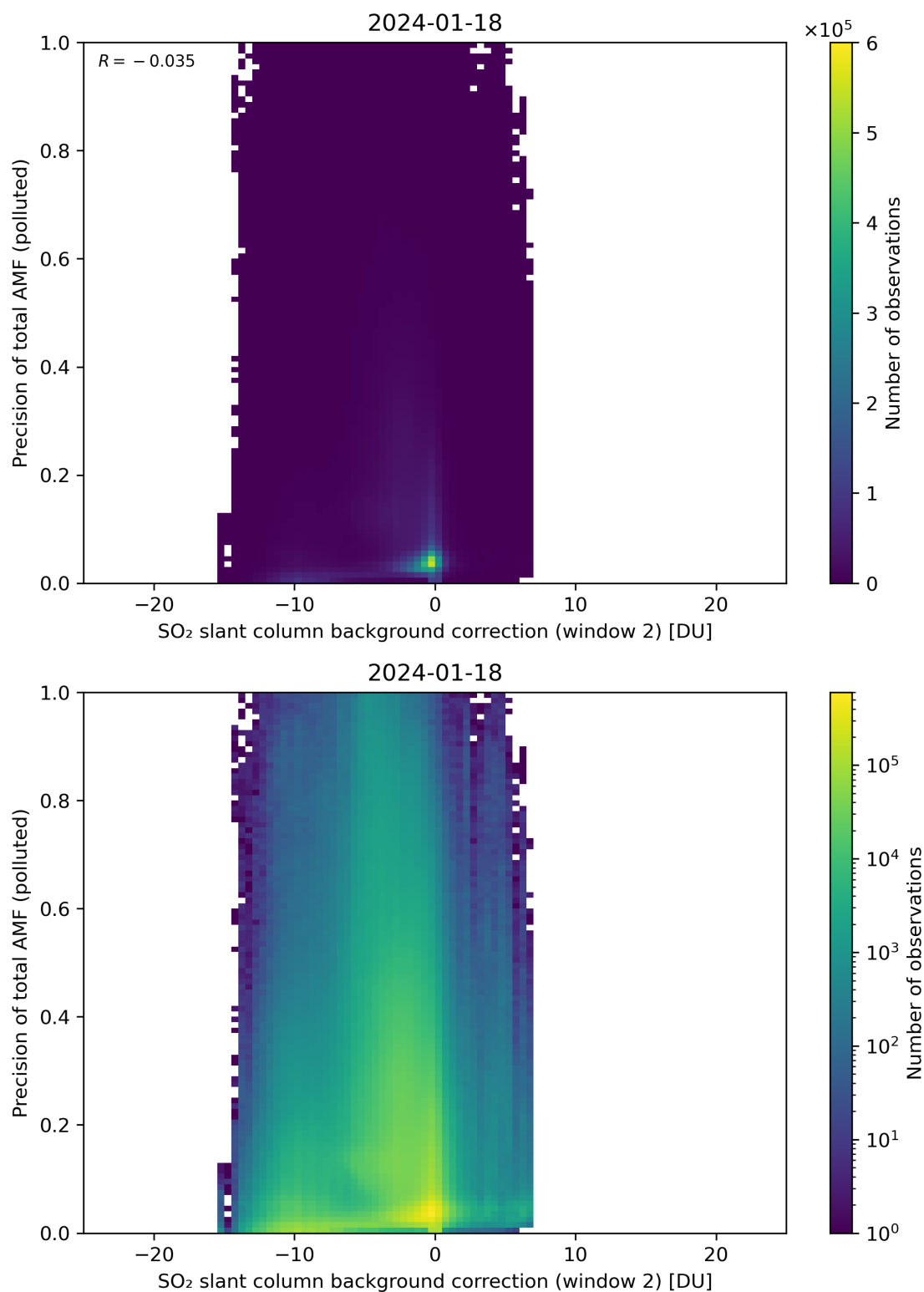
Figure 120: Scatter density plot of “SO 2 slant column background correction (window 2)” against “Precision of total AMF (polluted)” for 2024-01-17 to 2024-01-19.
