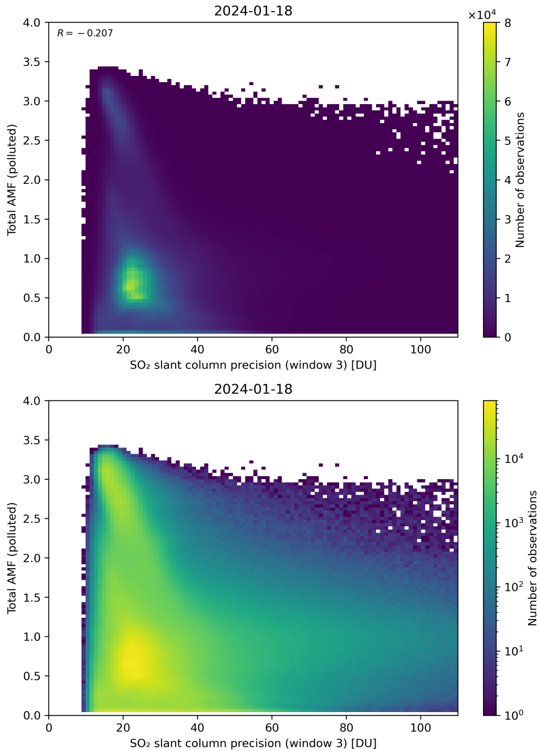
Figure 263: Scatter density plot of “SO 2 slant column precision (window 3)” against “Total AMF (polluted)” for 2024-01-17 to 2024-01-19.
