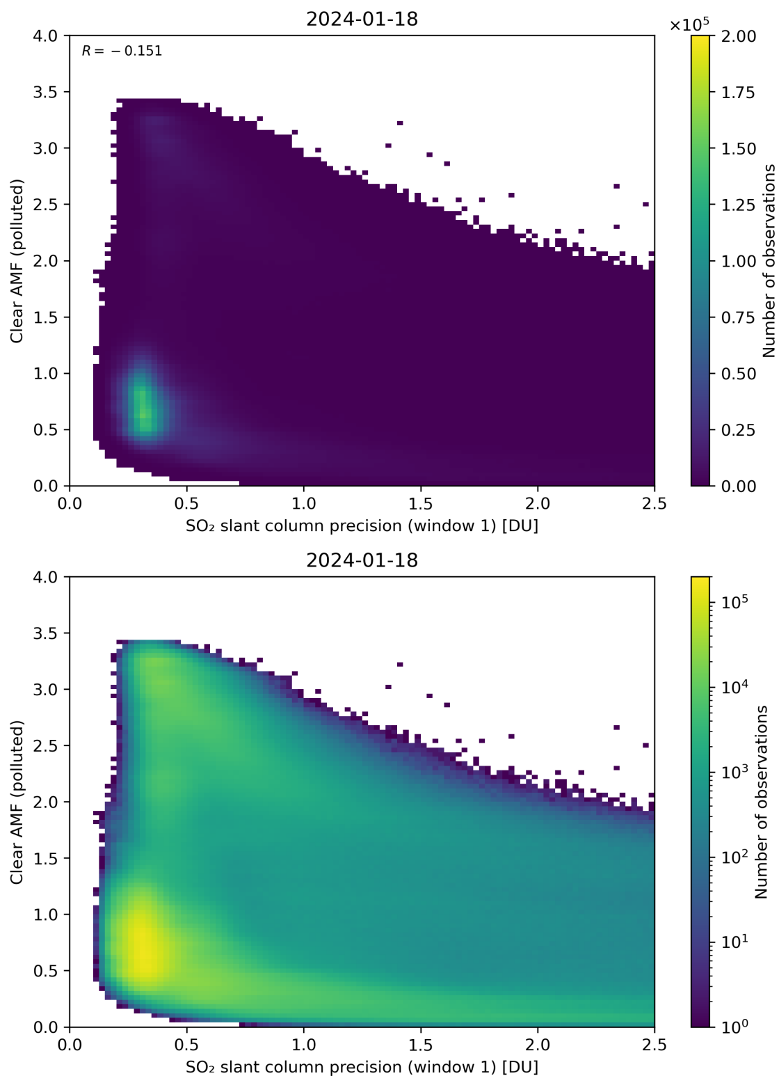
Figure 224: Scatter density plot of “SO 2 slant column precision (window 1)” against “Clear AMF (polluted)” for 2024-01-17 to 2024-01-19.
