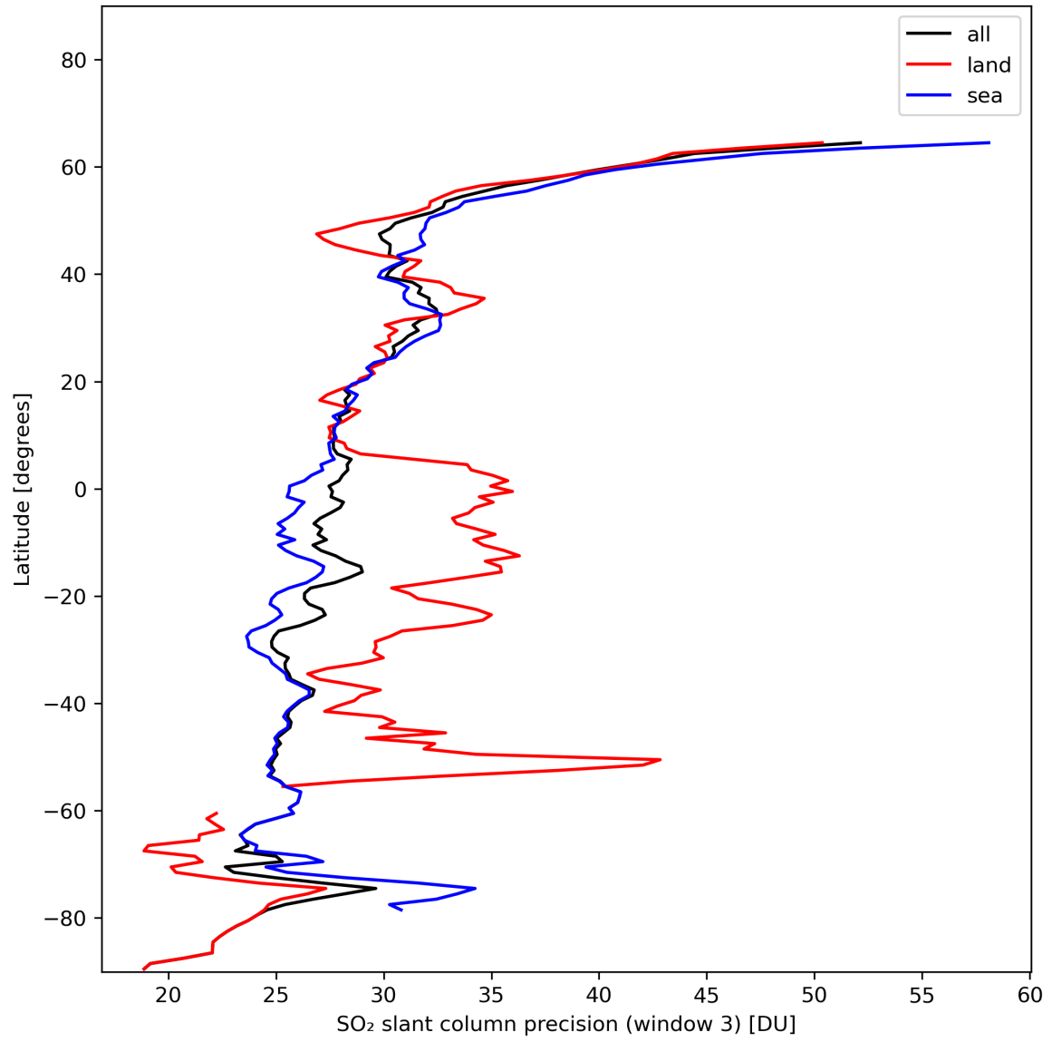
Figure 42: Zonal average of “SO 2 slant column precision (window 3)” for 2024-01-17 to 2024-01-19.
