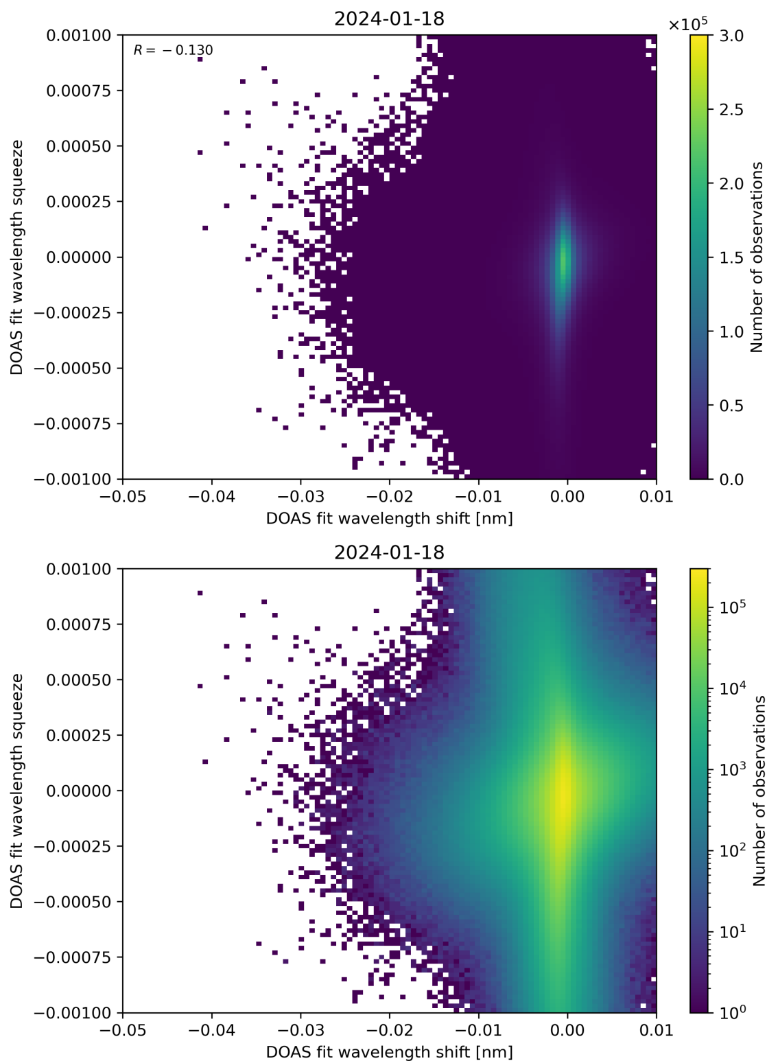
Figure 127: Scatter density plot of “DOAS fit wavelength shift” against “DOAS fit wavelength squeeze” for 2024-01-17 to 2024-01-19.
