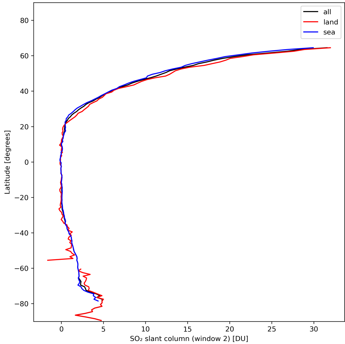
Figure 37: Zonal average of “SO 2 slant column (window 2)” for 2024-01-17 to 2024-01-19.
