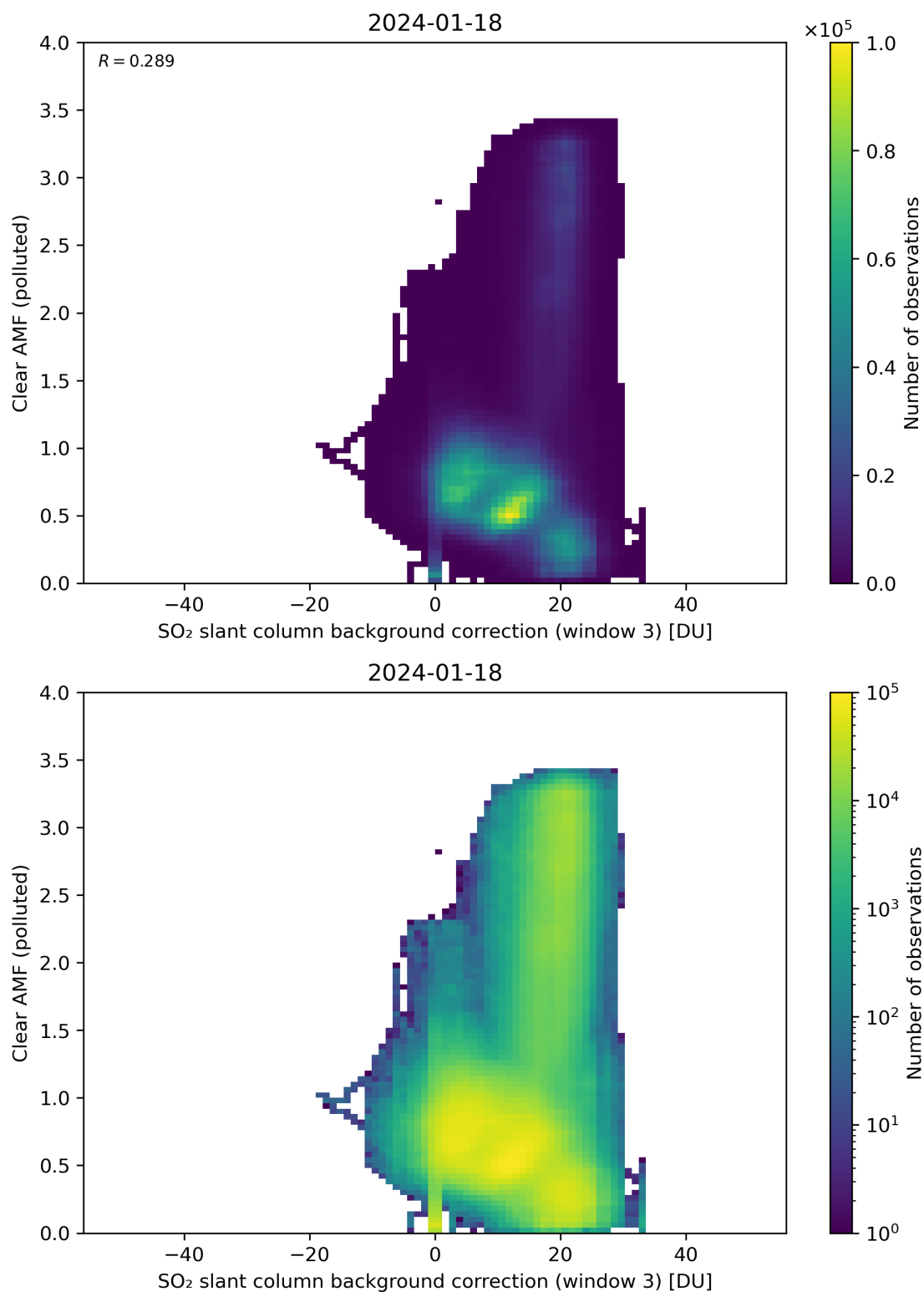
Figure 124: Scatter density plot of “SO 2 slant column background correction (window 3)” against “Clear AMF (polluted)” for 2024-01-17 to 2024-01-19.
