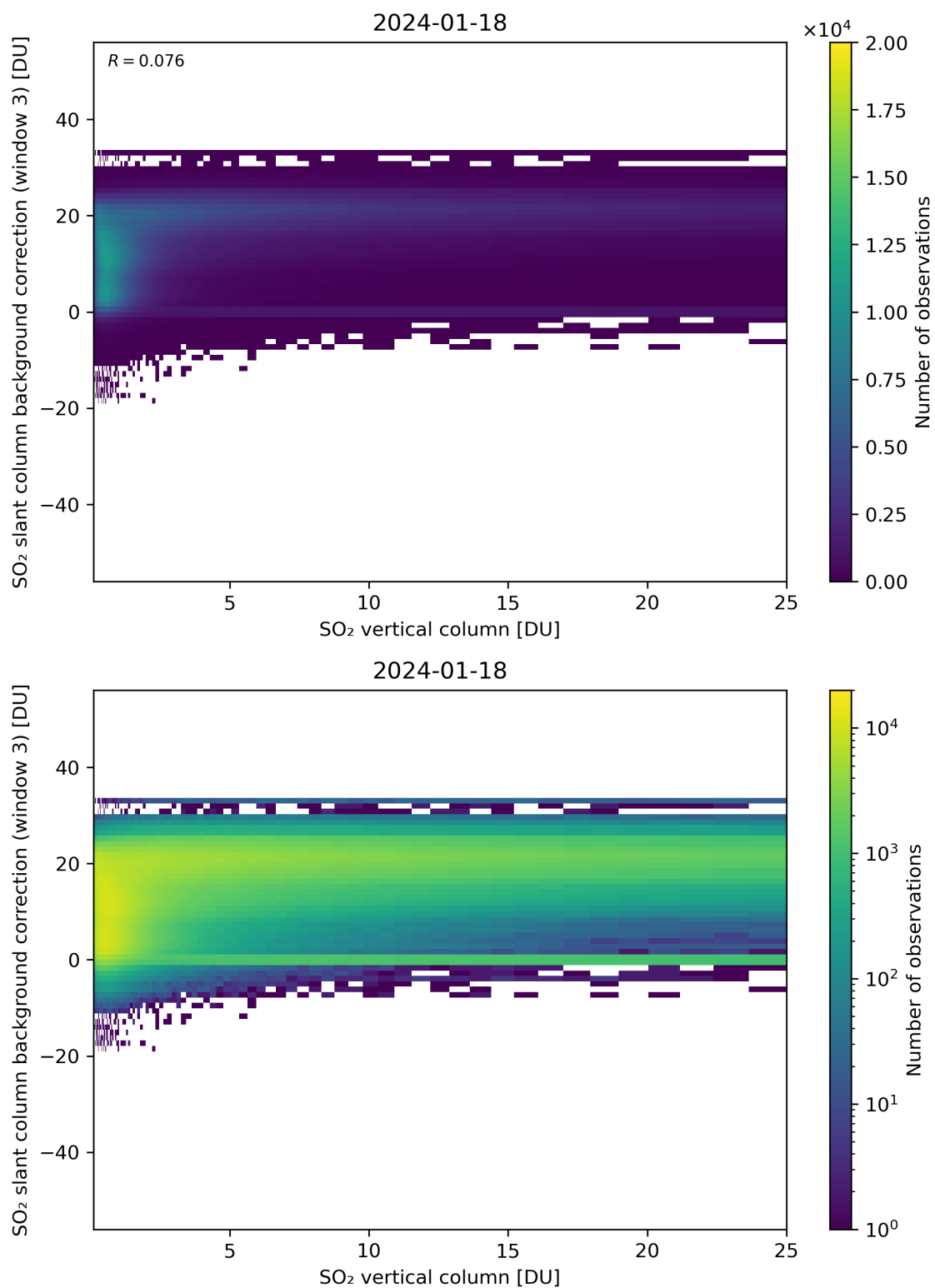
Figure 275: Scatter density plot of “SO 2 vertical column” against “SO 2 slant column background correction (window 3)” for 2024-01-17 to 2024-01-19.
