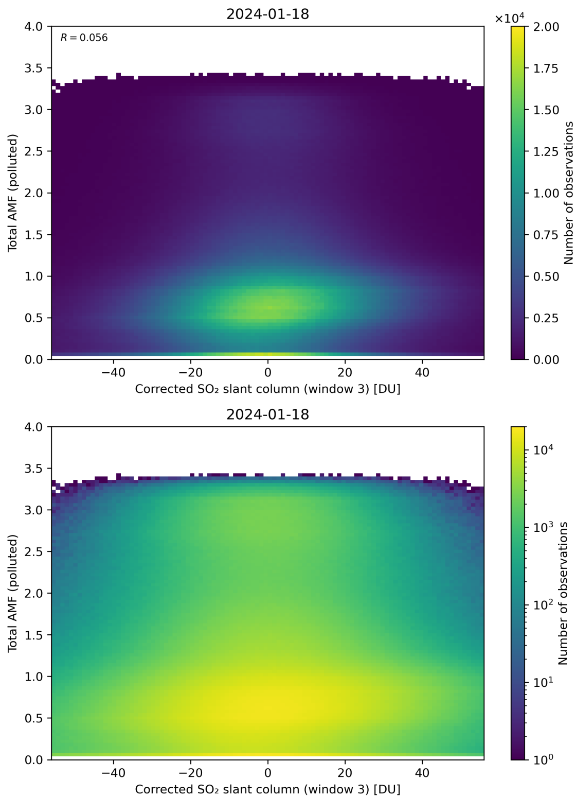
Figure 210: Scatter density plot of “Corrected SO 2 slant column (window 3)” against “Total AMF (polluted)” for 2024-01-17 to 2024-01-19.
