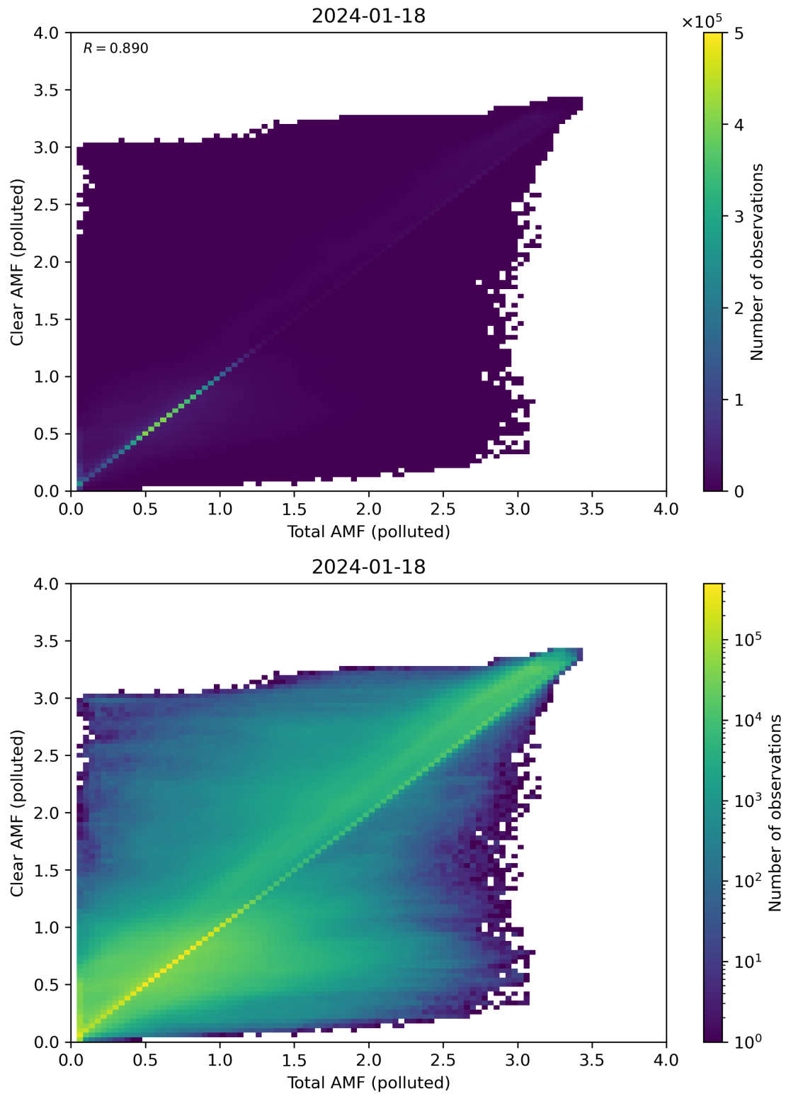
Figure 271: Scatter density plot of “Total AMF (polluted)” against “Clear AMF (polluted)” for 2024-01-17 to 2024-01-19.
