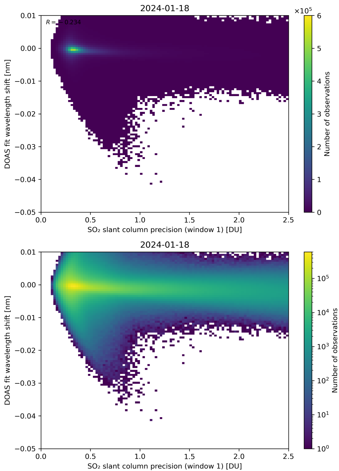
Figure 221: Scatter density plot of “SO 2 slant column precision (window 1)” against “DOAS fit wavelength shift” for 2024-01-17 to 2024-01-19.
