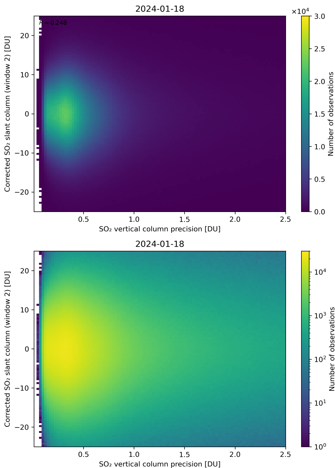
Figure 287: Scatter density plot of “SO 2 vertical column precision” against “Corrected SO 2 slant column (window 2)” for 2024-01-17 to 2024-01-19.
