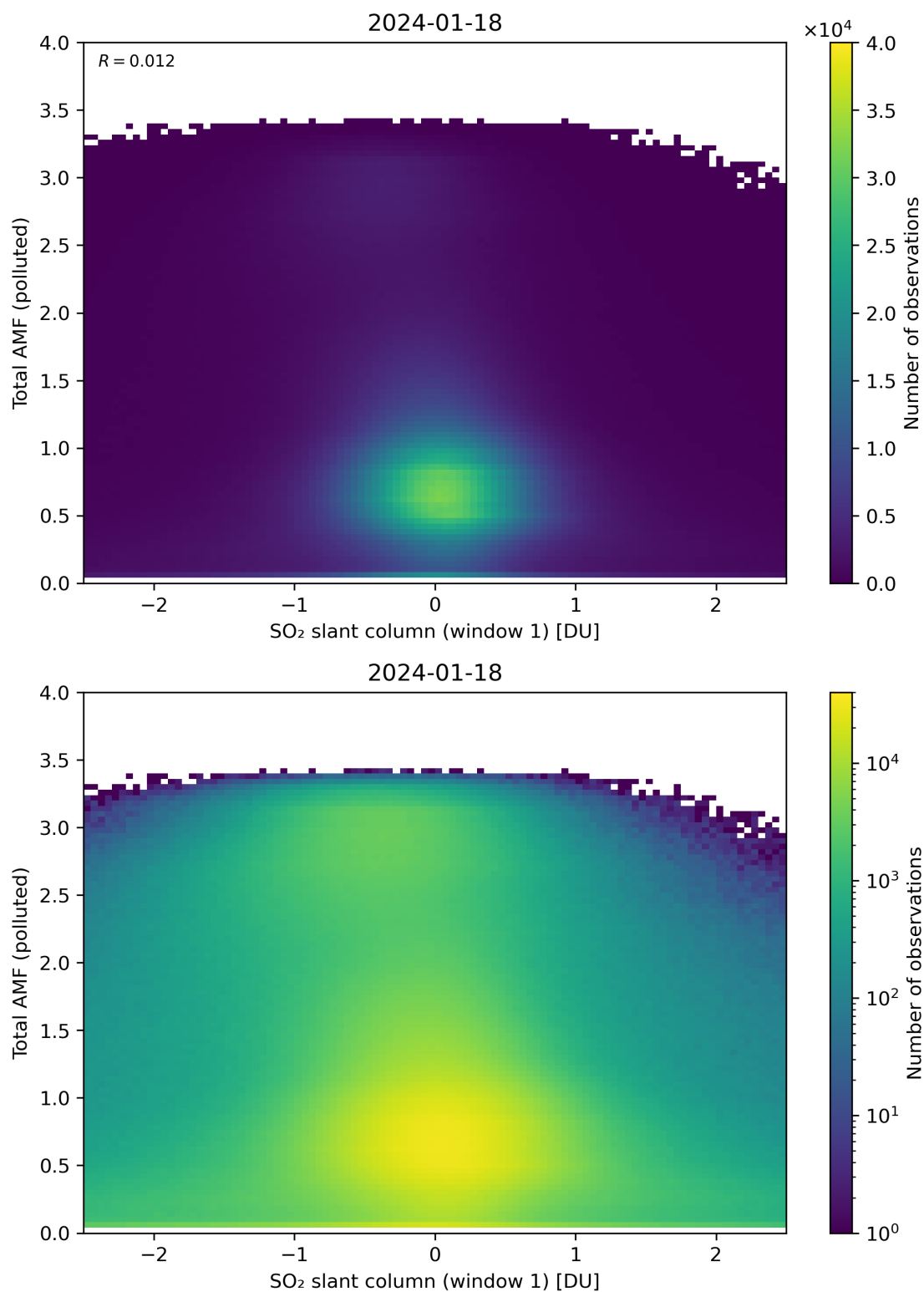
Figure 239: Scatter density plot of “SO 2 slant column (window 1)” against “Total AMF (polluted)” for 2024-01-17 to 2024-01-19.
