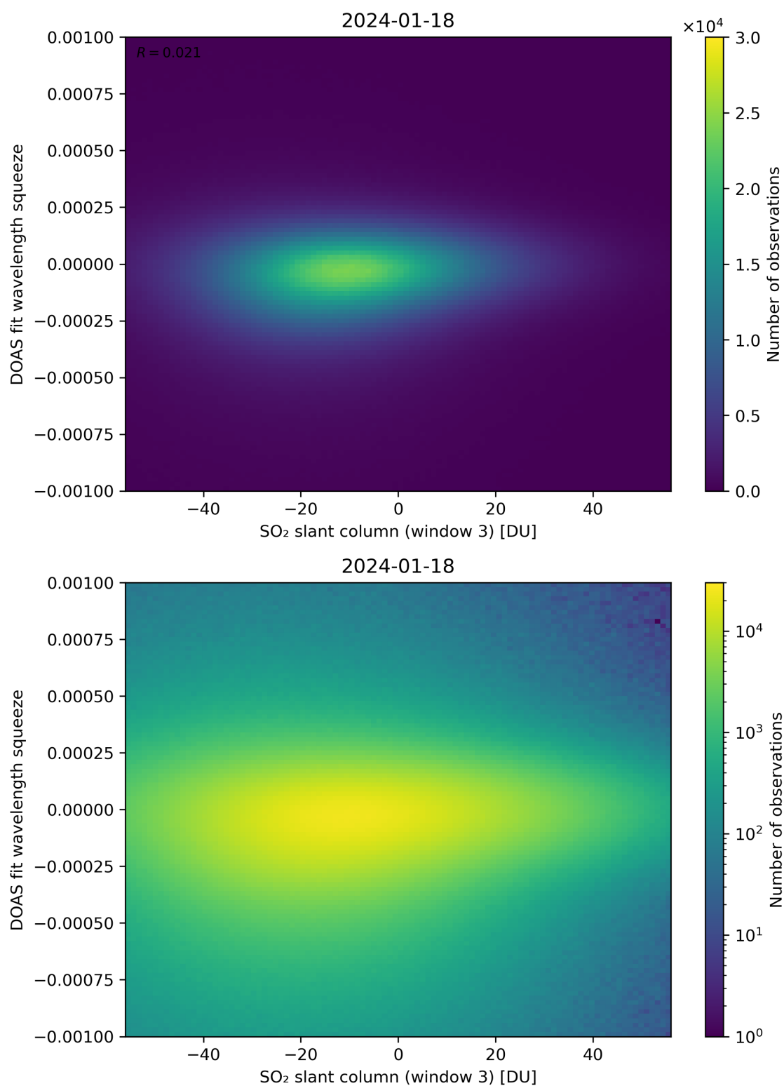
Figure 255: Scatter density plot of “SO 2 slant column (window 3)” against “DOAS fit wavelength squeeze” for 2024-01-17 to 2024-01-19.
