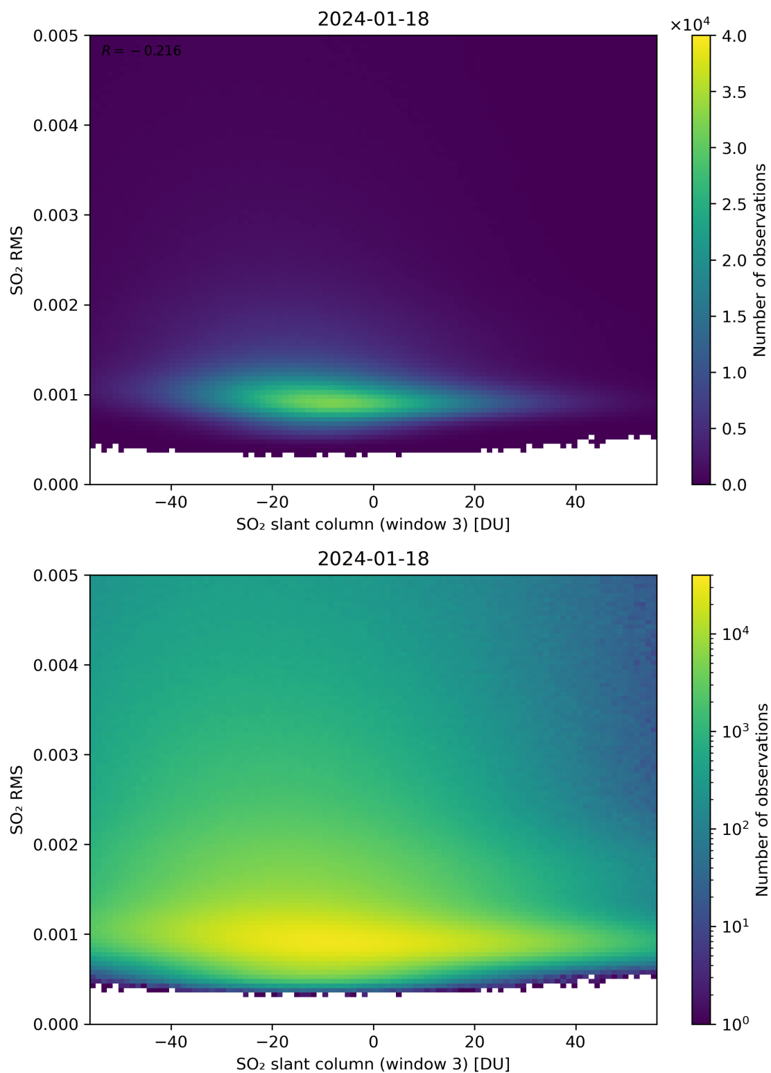
Figure 256: Scatter density plot of “SO 2 slant column (window 3)” against “SO 2 RMS” for 2024-01-17 to 2024-01-19.
