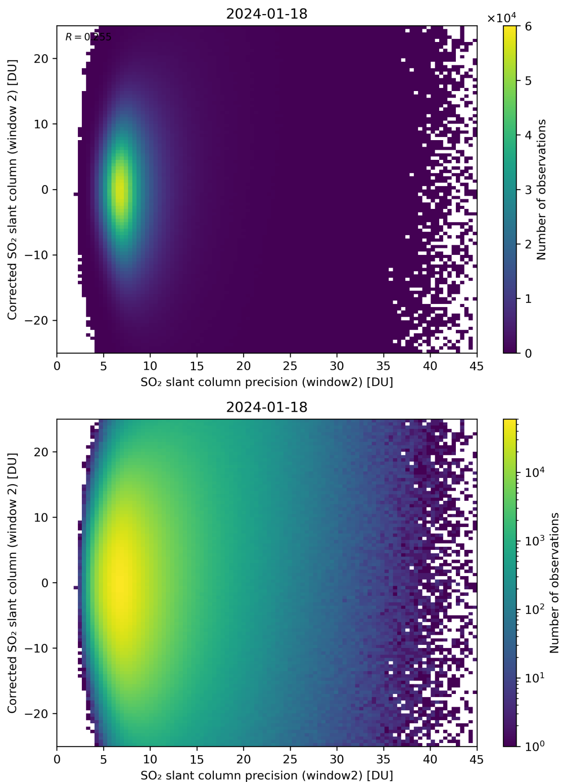
Figure 247: Scatter density plot of “SO 2 slant column precision (window2)” against “Corrected SO 2 slant column (window 2)” for 2024-01-17 to 2024-01-19.
