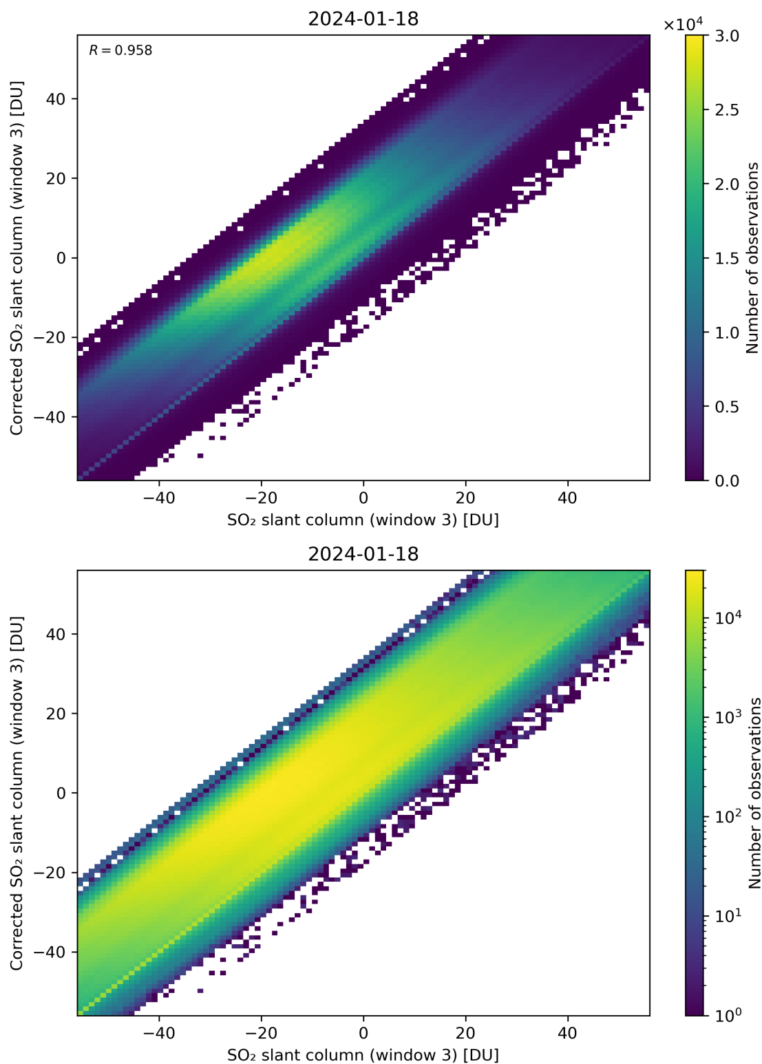
Figure 266: Scatter density plot of “SO 2 slant column (window 3)” against “Corrected SO 2 slant column (window 3)” for 2024-01-17 to 2024-01-19.
