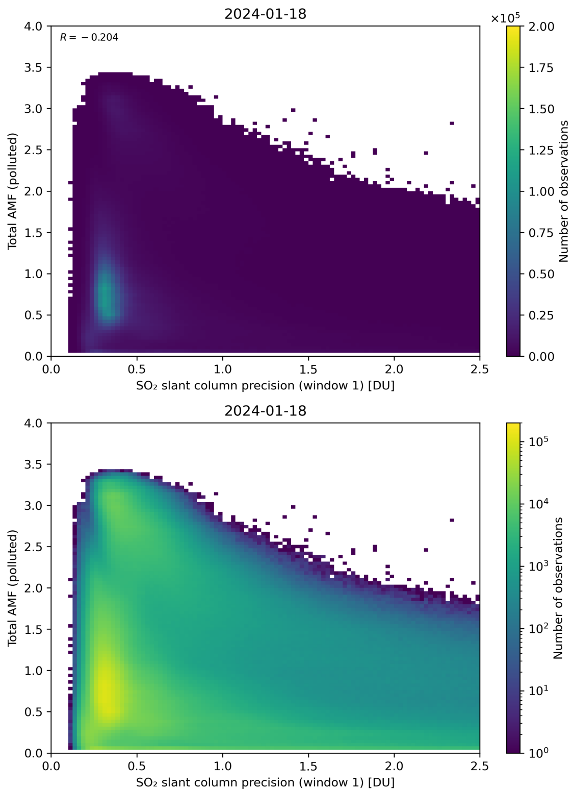
Figure 230: Scatter density plot of “SO 2 slant column precision (window 1)” against “Total AMF (polluted)” for 2024-01-17 to 2024-01-19.
