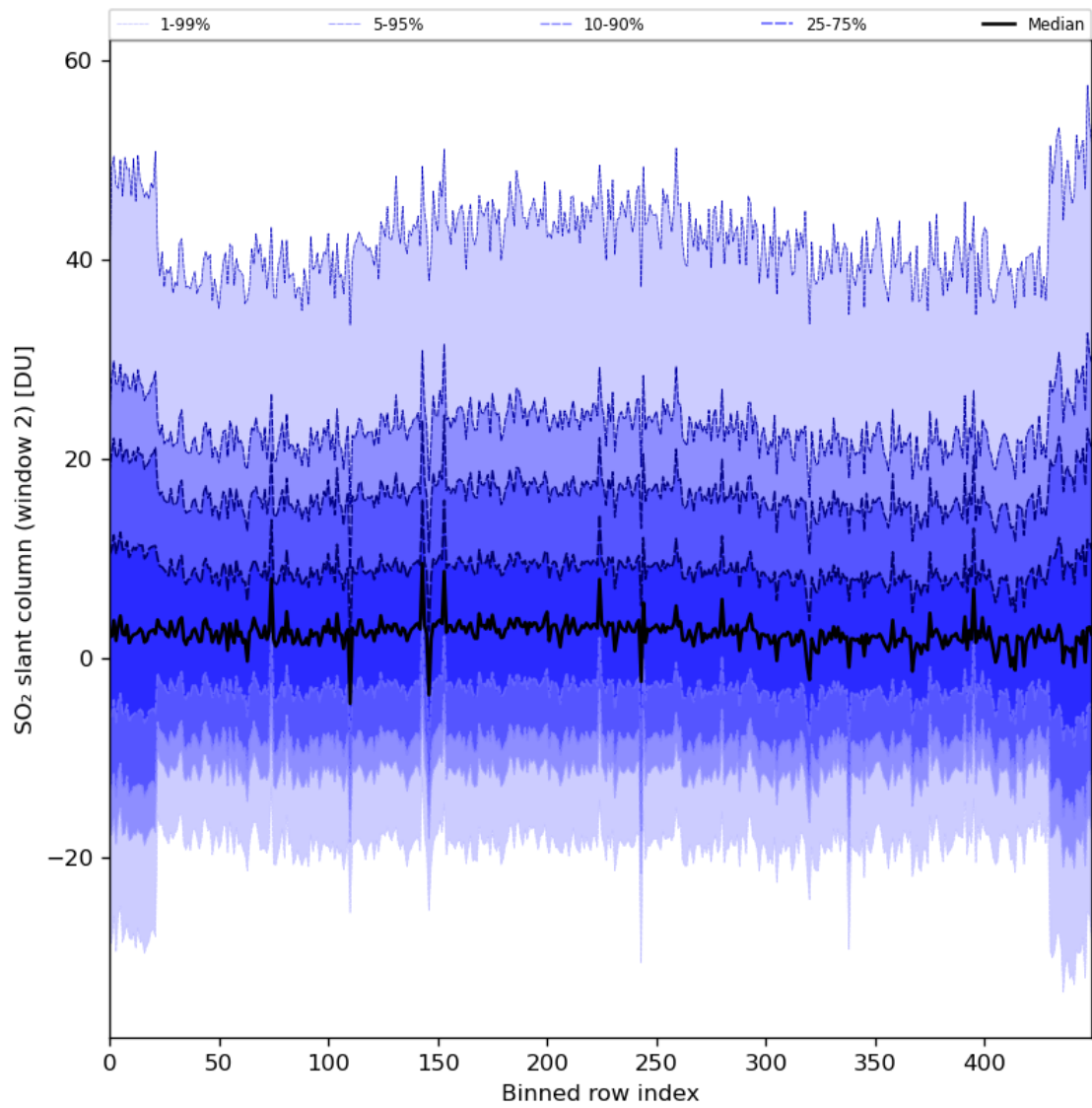
Figure 83: Along track statistics of “SO 2 slant column (window 2)” for 2024-01-17 to 2024-01-19
