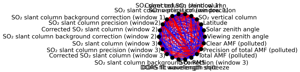
Figure 1: Map of correlation graph for 2024-01-17 to 2024-01-19.
