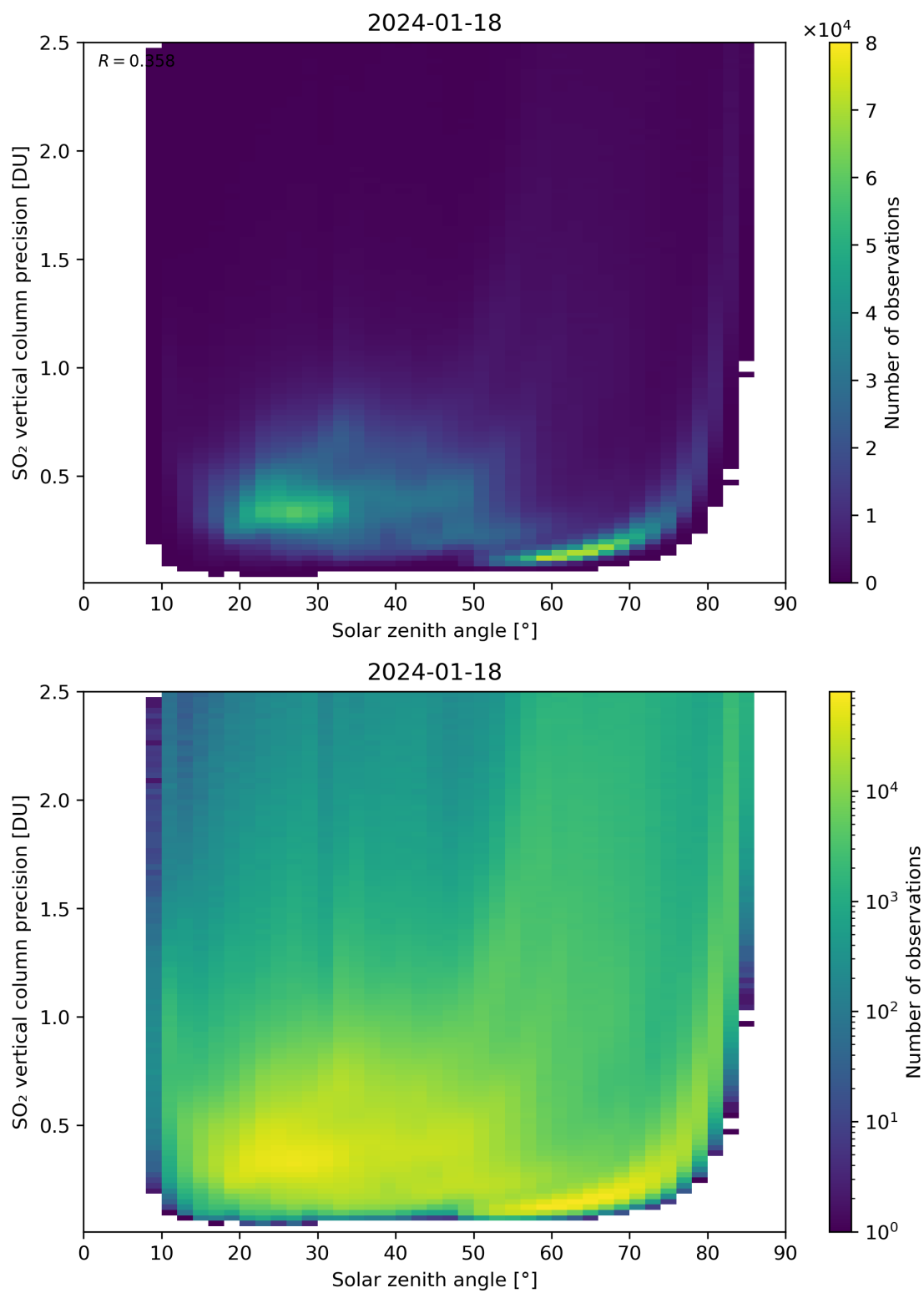
Figure 177: Scatter density plot of “Solar zenith angle” against “SO 2 vertical column precision” for 2024-01-17 to 2024-01-19.
