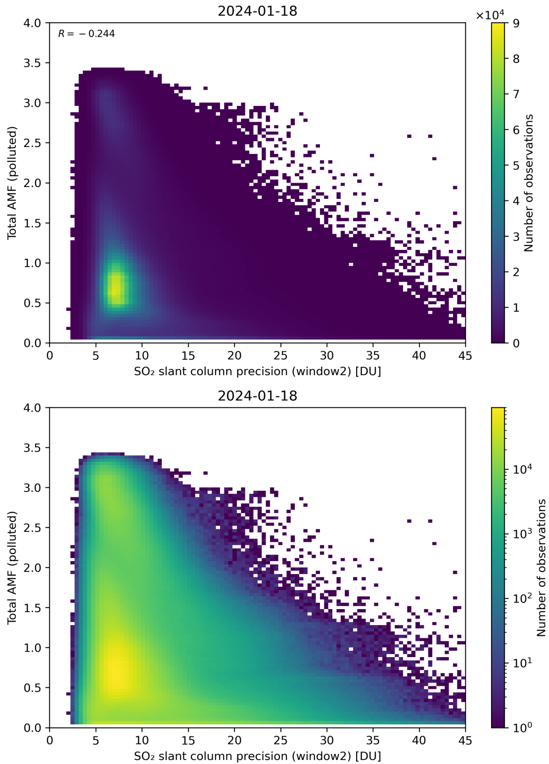
Figure 251: Scatter density plot of “SO 2 slant column precision (window2)” against “Total AMF (polluted)” for 2024-01-17 to 2024-01-19.
