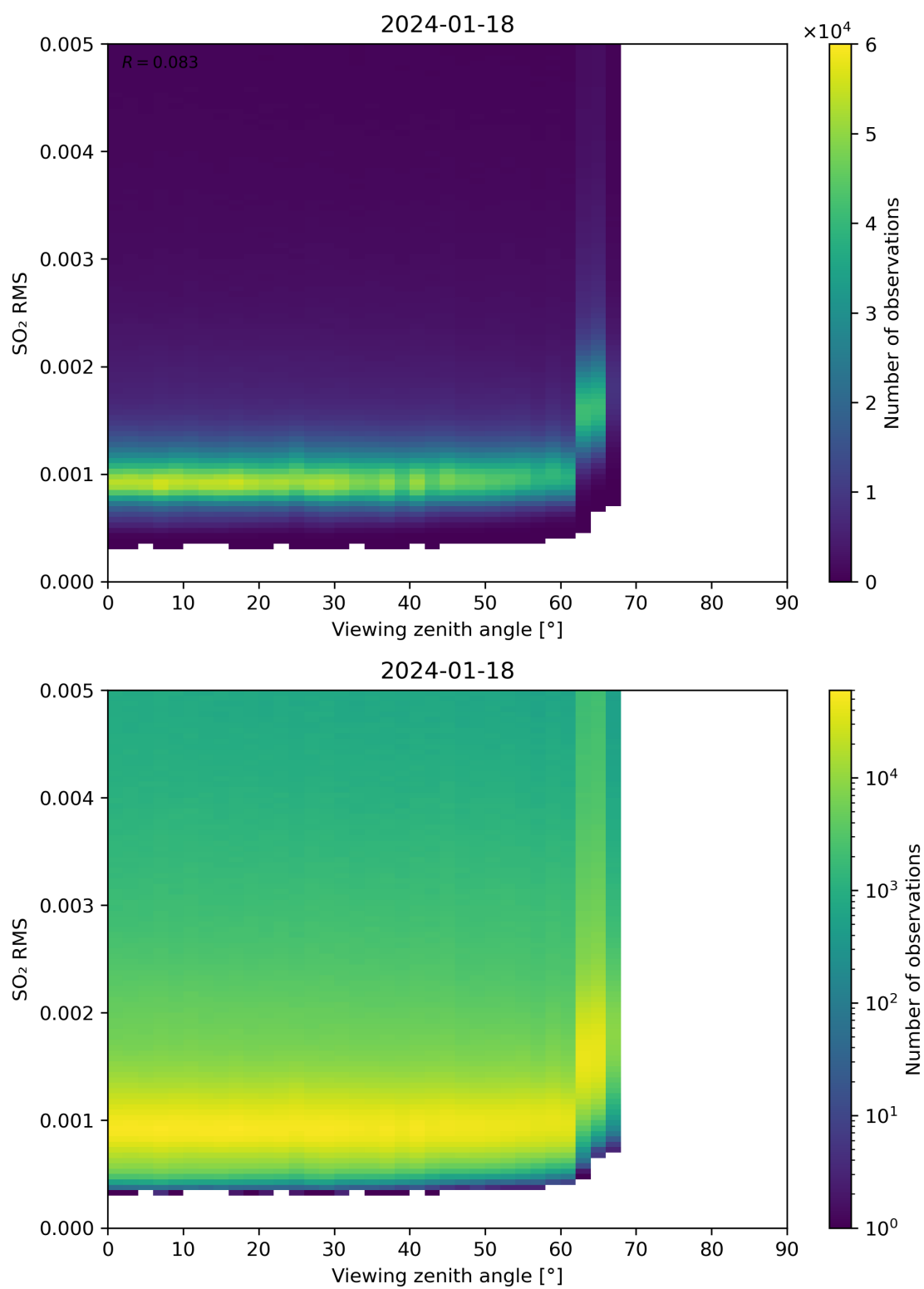
Figure 313: Scatter density plot of “Viewing zenith angle” against “SO 2 RMS” for 2024-01-17 to 2024-01-19.
