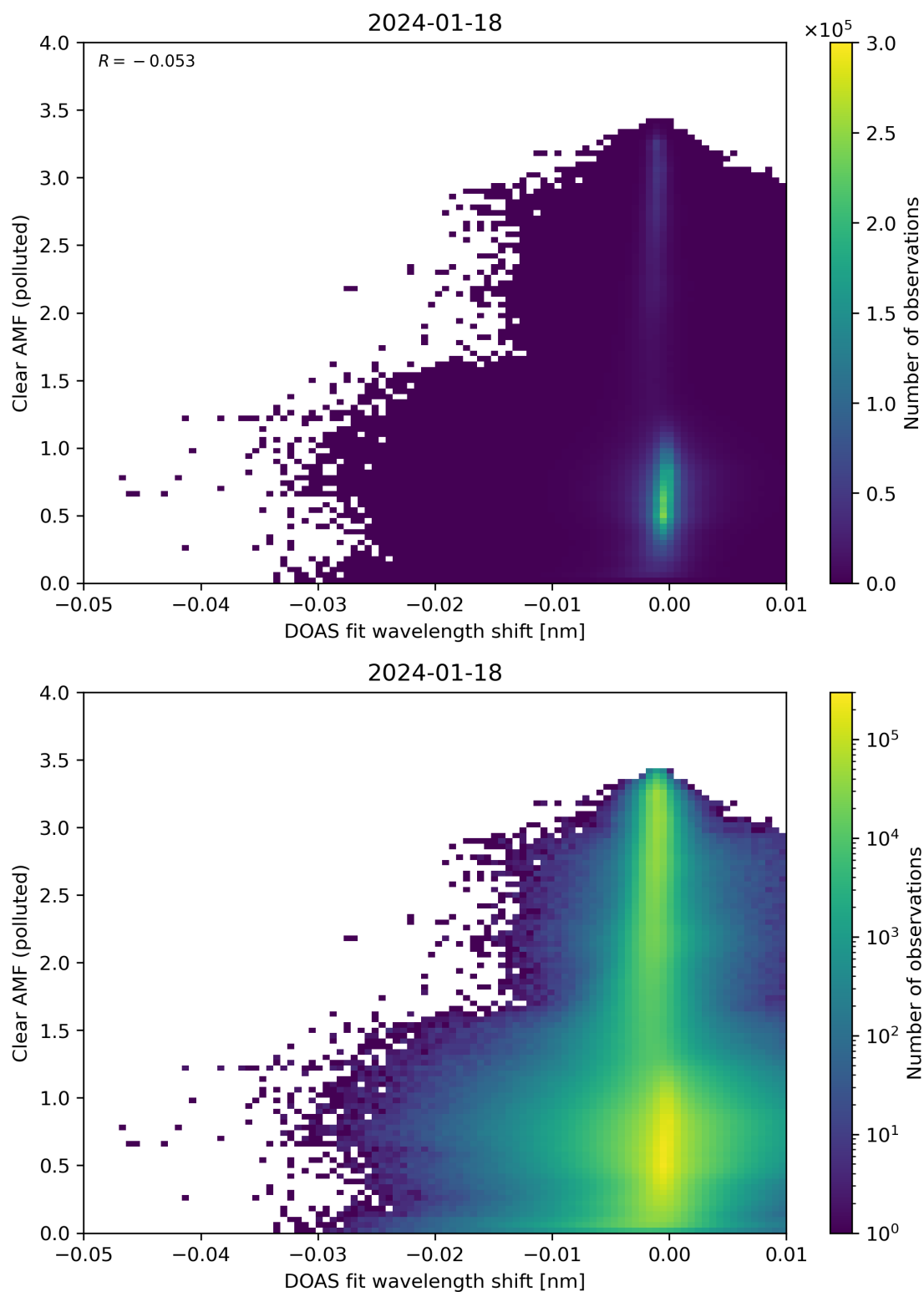
Figure 129: Scatter density plot of “DOAS fit wavelength shift” against “Clear AMF (polluted)” for 2024-01-17 to 2024-01-19.
