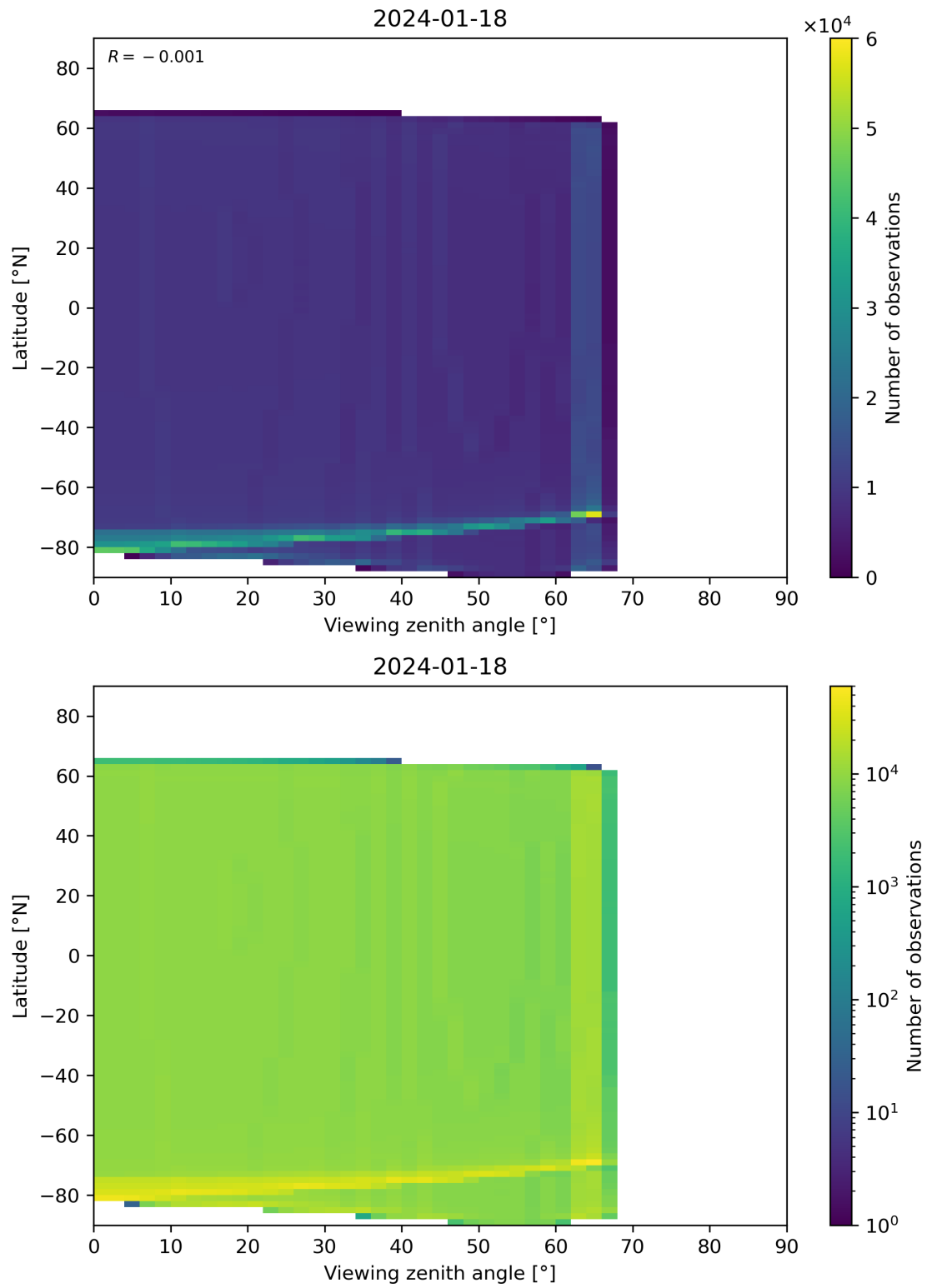
Figure 314: Scatter density plot of “Viewing zenith angle” against “Latitude” for 2024-01-17 to 2024-01-19.
