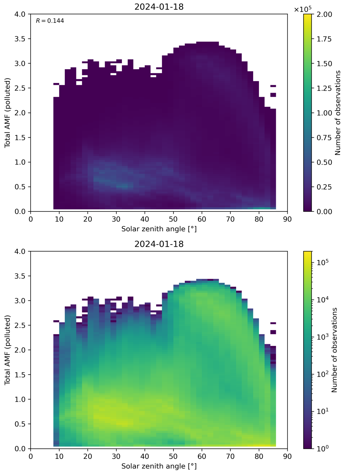
Figure 174: Scatter density plot of “Solar zenith angle” against “Total AMF (polluted)” for 2024-01-17 to 2024-01-19.
