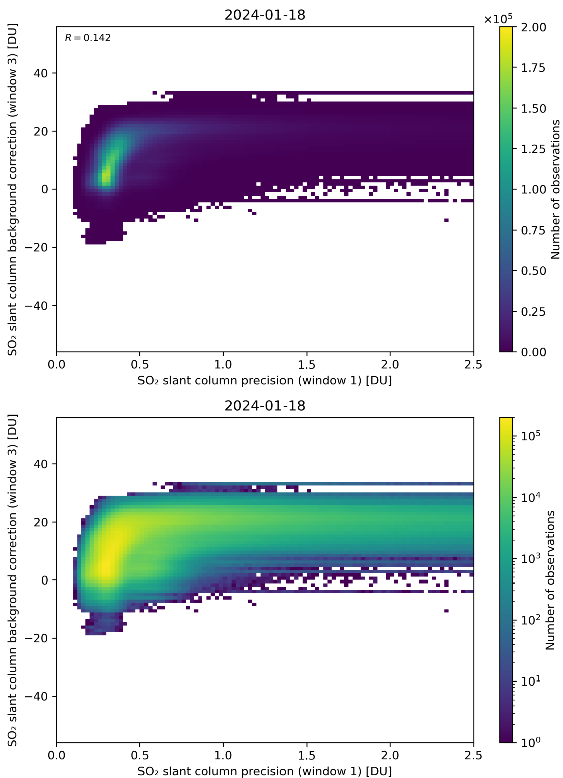
Figure 220: Scatter density plot of “SO 2 slant column precision (window 1)” against “SO 2 slant column background correction (window 3)” for 2024-01-17 to 2024-01-19.
