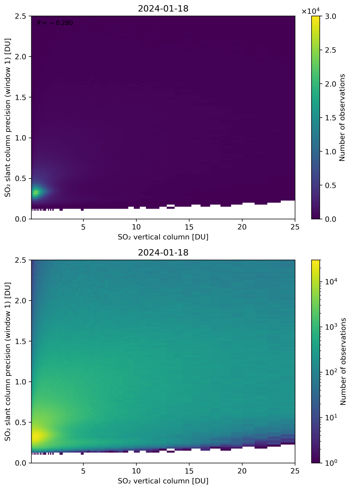
Figure 301: Scatter density plot of “SO 2 vertical column” against “SO 2 slant column precision (window 1)” for 2024-01-17 to 2024-01-19.
