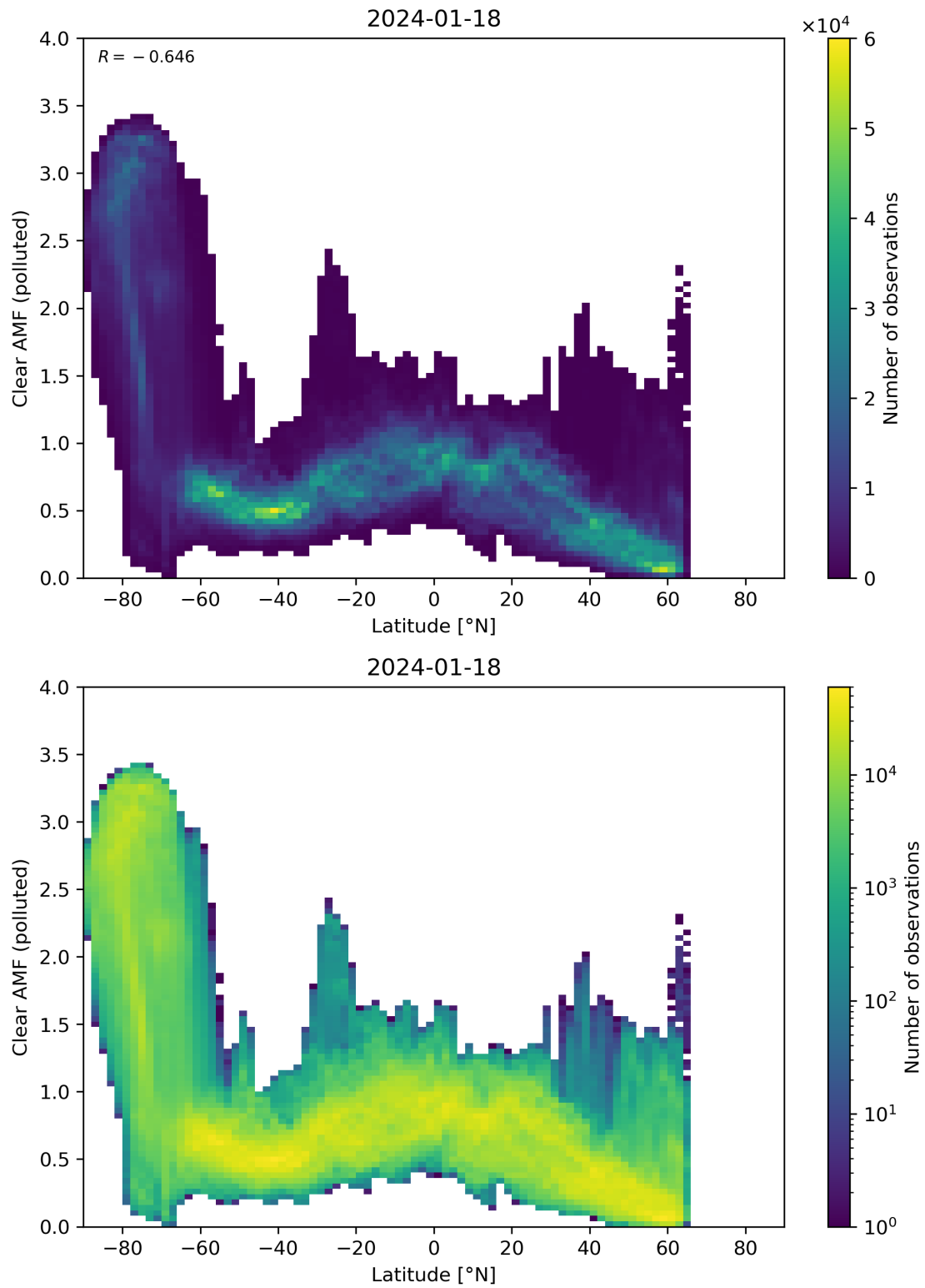
Figure 145: Scatter density plot of “Latitude” against “Clear AMF (polluted)” for 2024-01-17 to 2024-01-19.
