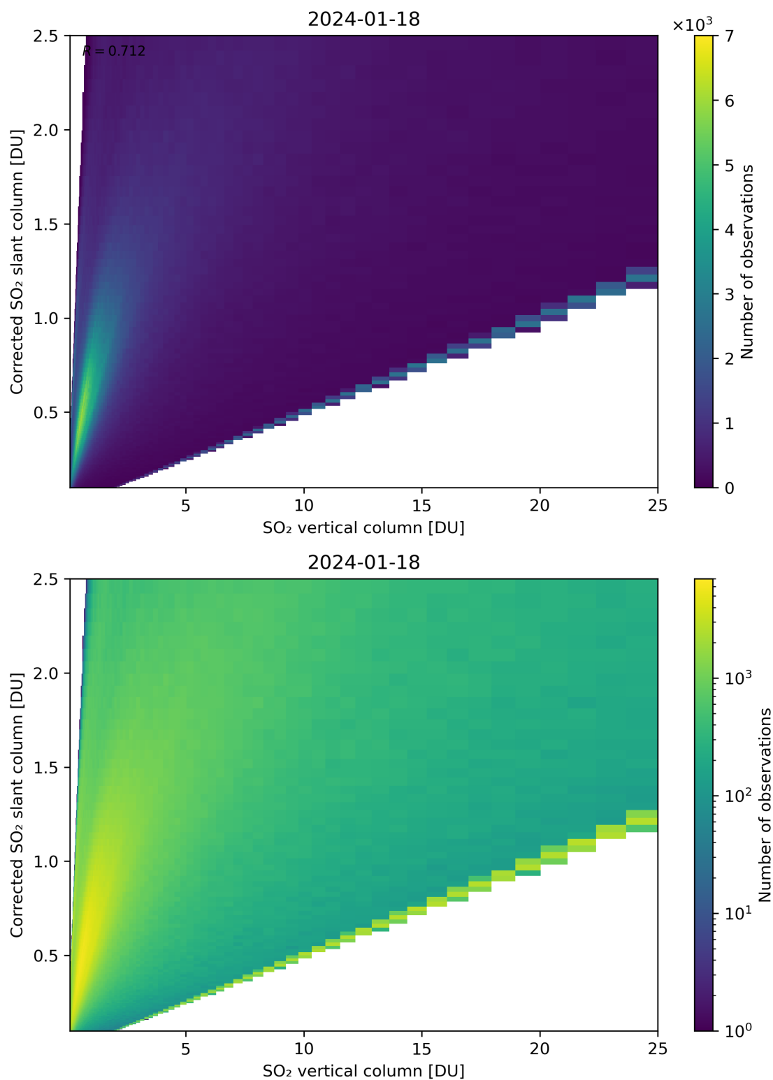
Figure 297: Scatter density plot of “SO 2 vertical column” against “Corrected SO 2 slant column” for 2024-01-17 to 2024-01-19.
