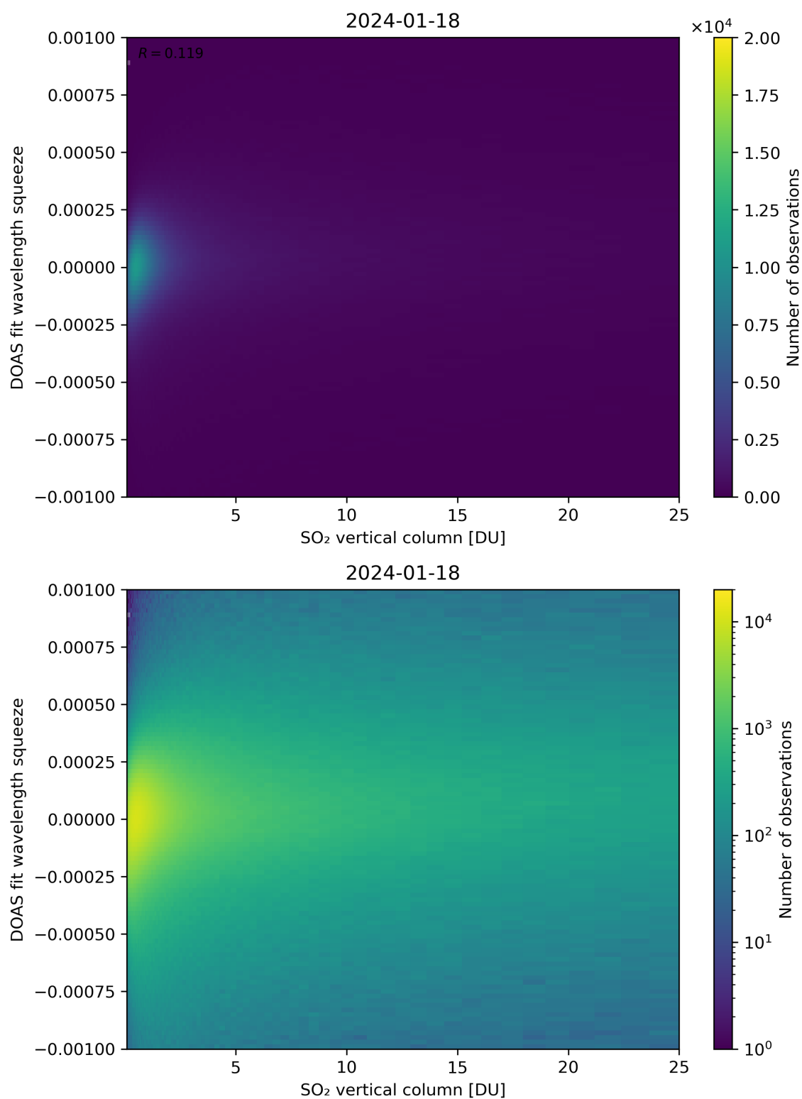
Figure 277: Scatter density plot of “SO 2 vertical column” against “DOAS fit wavelength squeeze” for 2024-01-17 to 2024-01-19.
