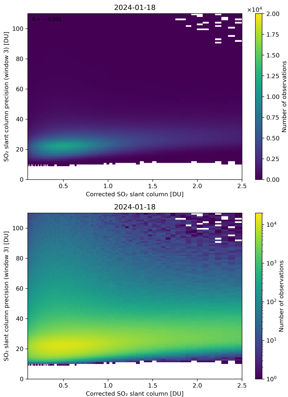
Figure 191: Scatter density plot of “Corrected SO 2 slant column” against “SO 2 slant column precision (window 3)” for 2024-01-17 to 2024-01-19.
