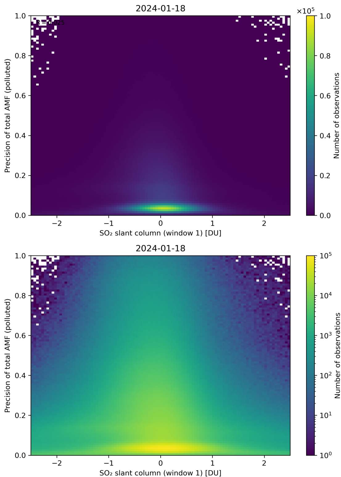
Figure 240: Scatter density plot of “SO 2 slant column (window 1)” against “Precision of total AMF (polluted)” for 2024-01-17 to 2024-01-19.
