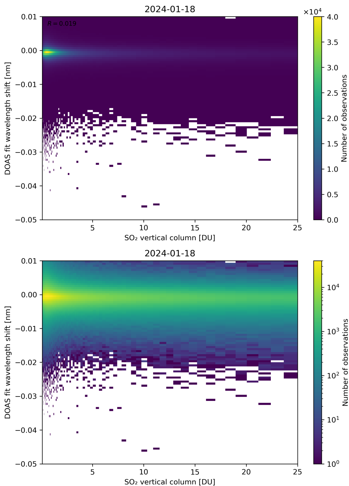
Figure 276: Scatter density plot of “SO 2 vertical column” against “DOAS fit wavelength shift” for 2024-01-17 to 2024-01-19.
