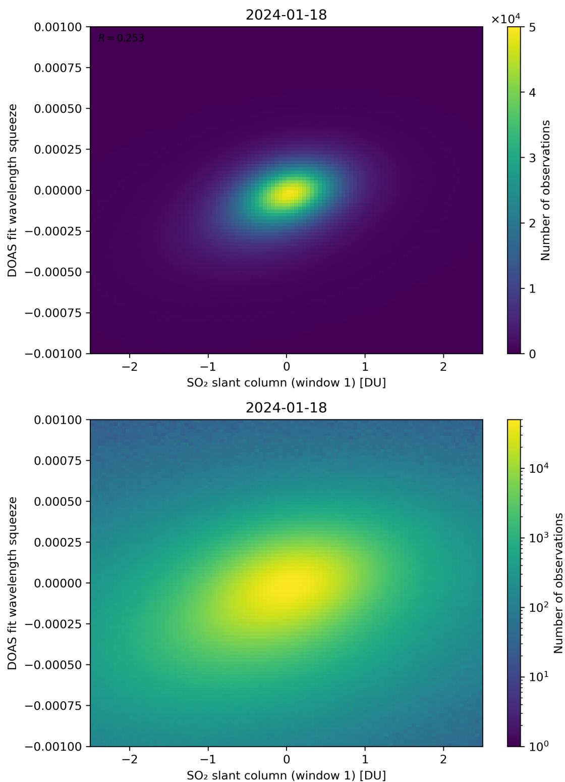
Figure 216: Scatter density plot of “SO 2 slant column (window 1)” against “DOAS fit wavelength squeeze” for 2024-01-17 to 2024-01-19.
