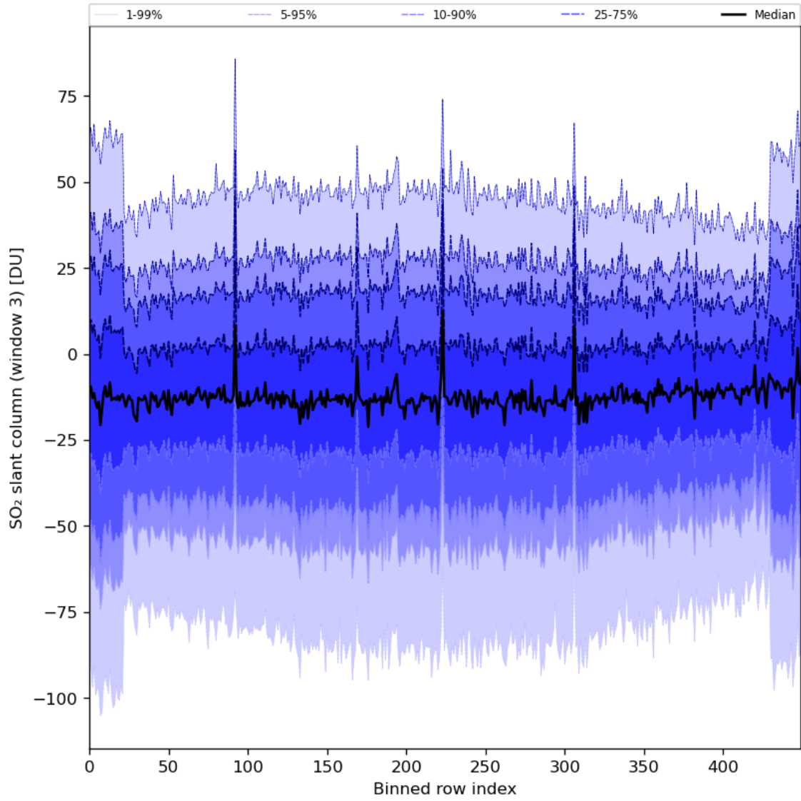
Figure 87: Along track statistics of “SO 2 slant column (window 3)” for 2024-01-17 to 2024-01-19
