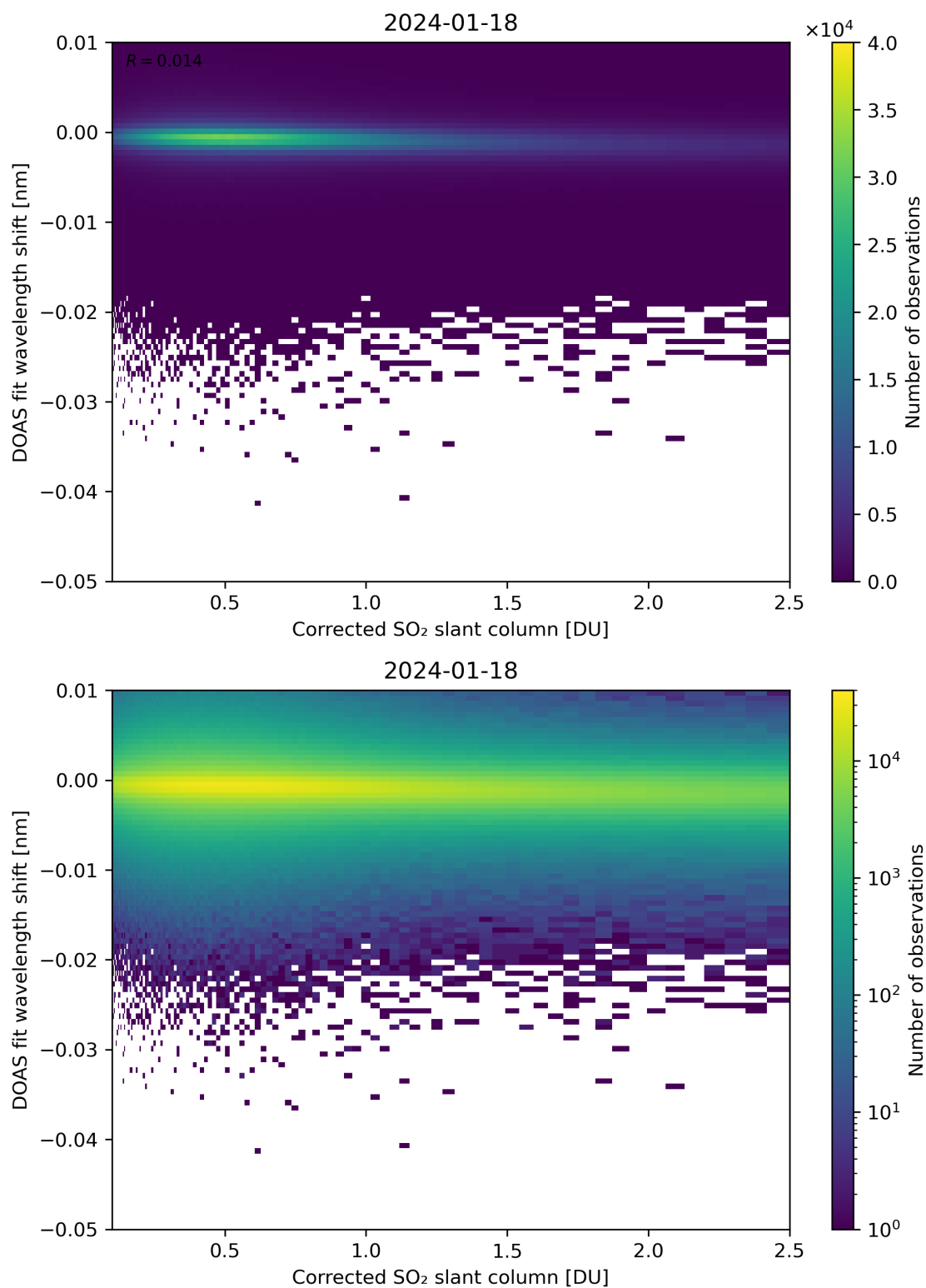
Figure 181: Scatter density plot of “Corrected SO 2 slant column” against “DOAS fit wavelength shift” for 2024-01-17 to 2024-01-19.
