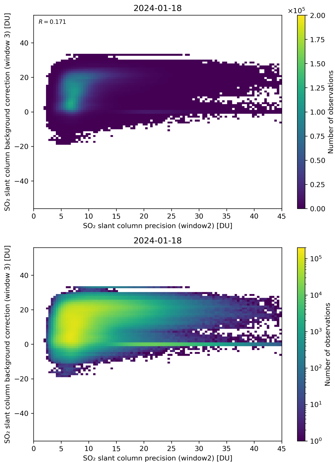
Figure 242: Scatter density plot of “SO 2 slant column precision (window2)” against “SO 2 slant column background correction (window 3)” for 2024-01-17 to 2024-01-19.
