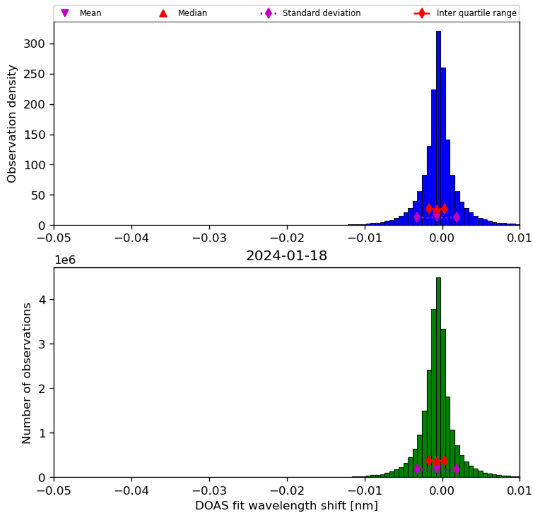
Figure 68: Histogram of “DOAS fit wavelength shift” for 2024-01-17 to 2024-01-19
