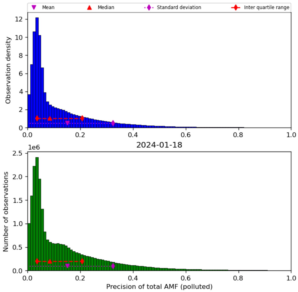
Figure 72: Histogram of “Precision of total AMF (polluted)” for 2024-01-17 to 2024-01-19
