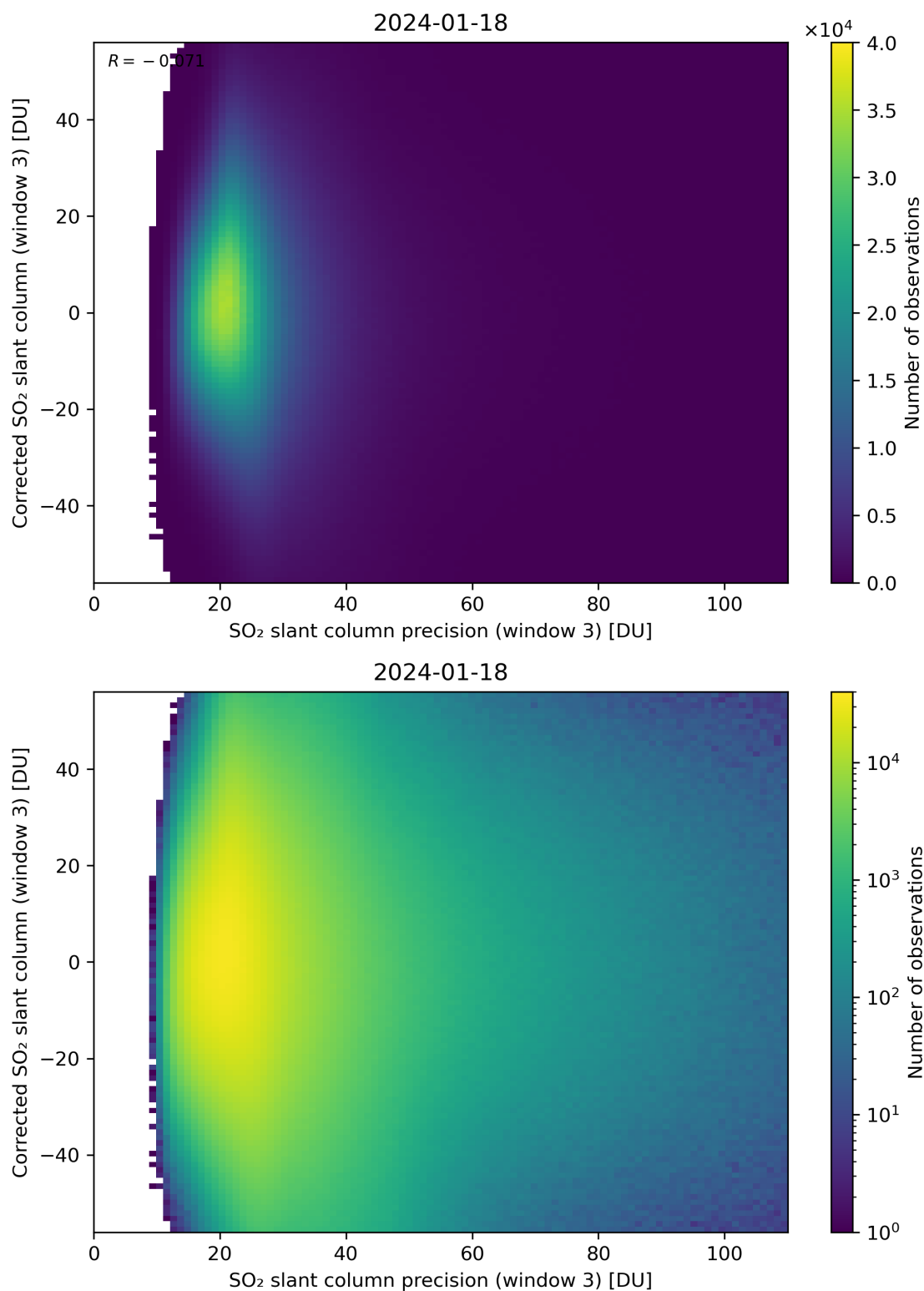
Figure 262: Scatter density plot of “SO 2 slant column precision (window 3)” against “Corrected SO 2 slant column (window 3)” for 2024-01-17 to 2024-01-19.
