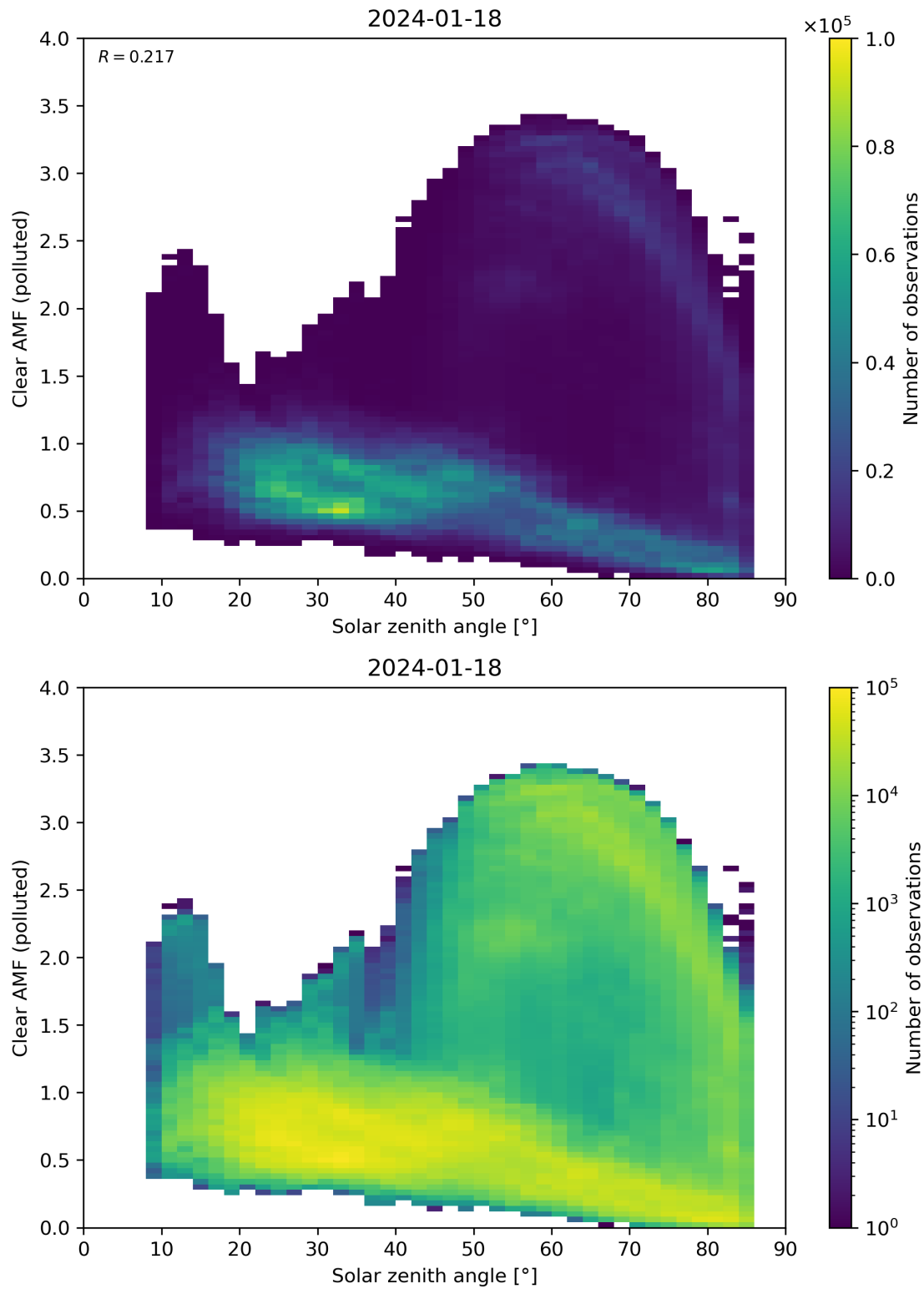
Figure 165: Scatter density plot of “Solar zenith angle” against “Clear AMF (polluted)” for 2024-01-17 to 2024-01-19.
