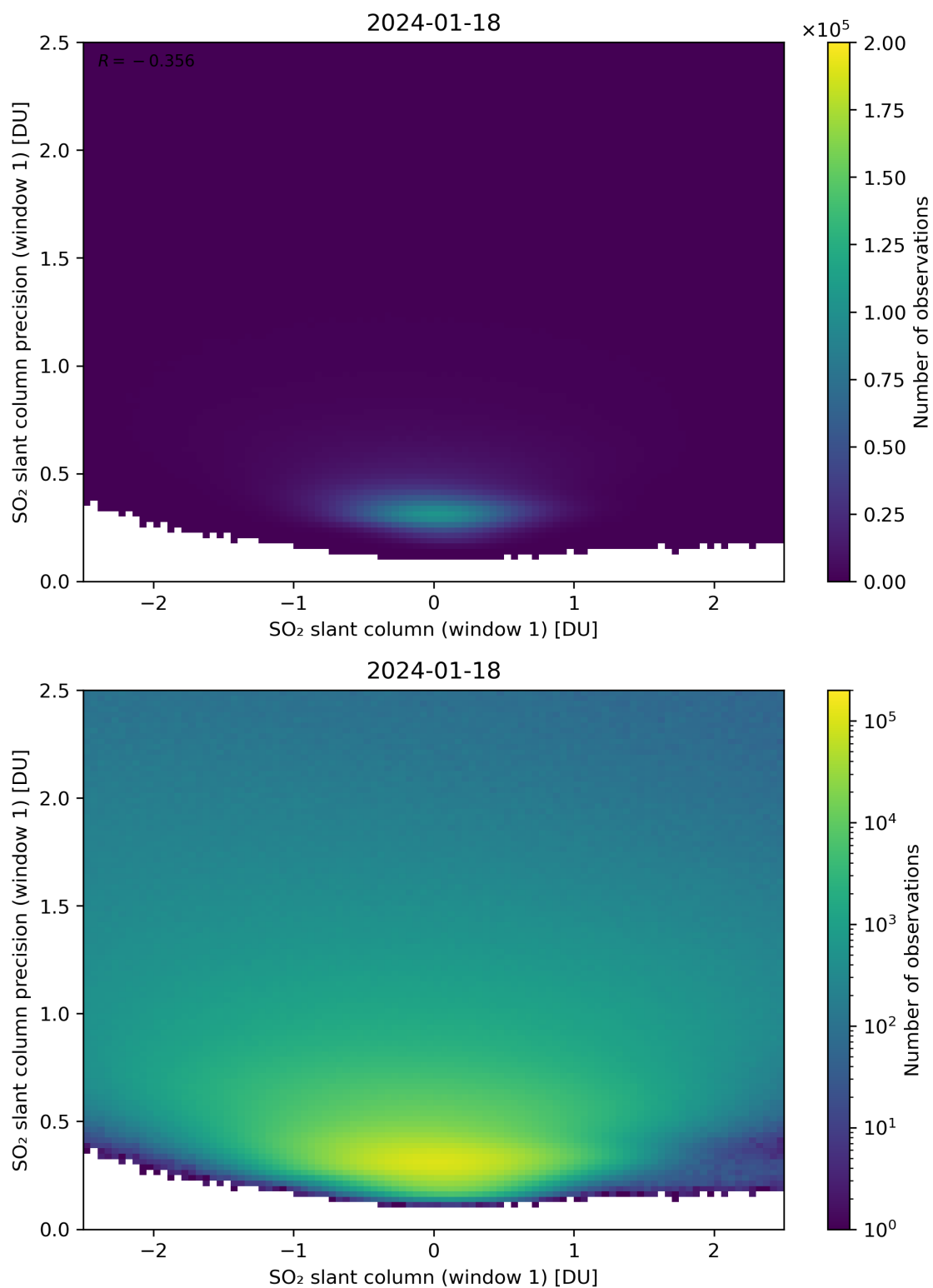
Figure 235: Scatter density plot of “SO 2 slant column (window 1)” against “SO 2 slant column precision (window 1)” for 2024-01-17 to 2024-01-19.
