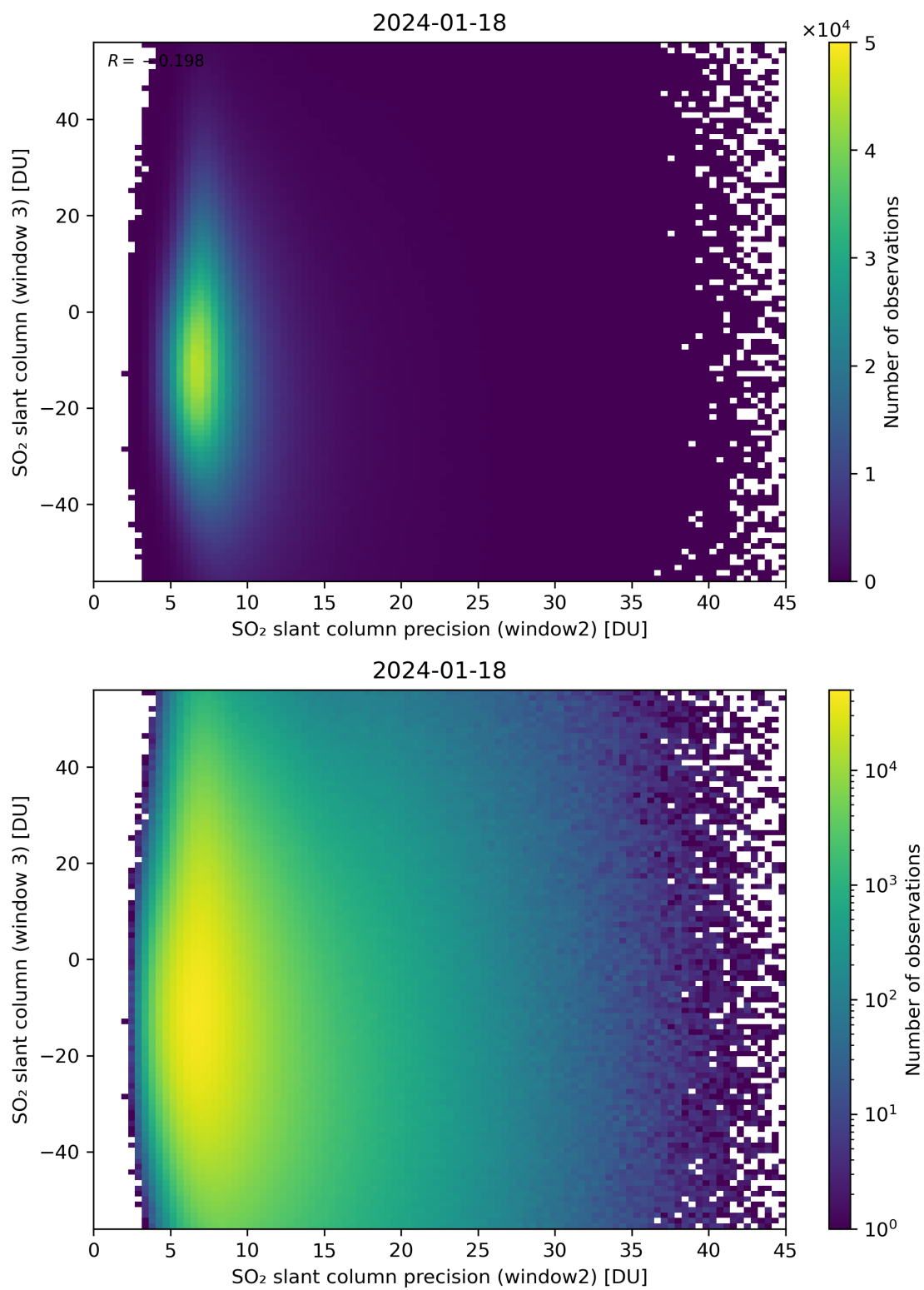
Figure 249: Scatter density plot of “SO 2 slant column precision (window2)” against “SO 2 slant column (window 3)” for 2024-01-17 to 2024-01-19.
