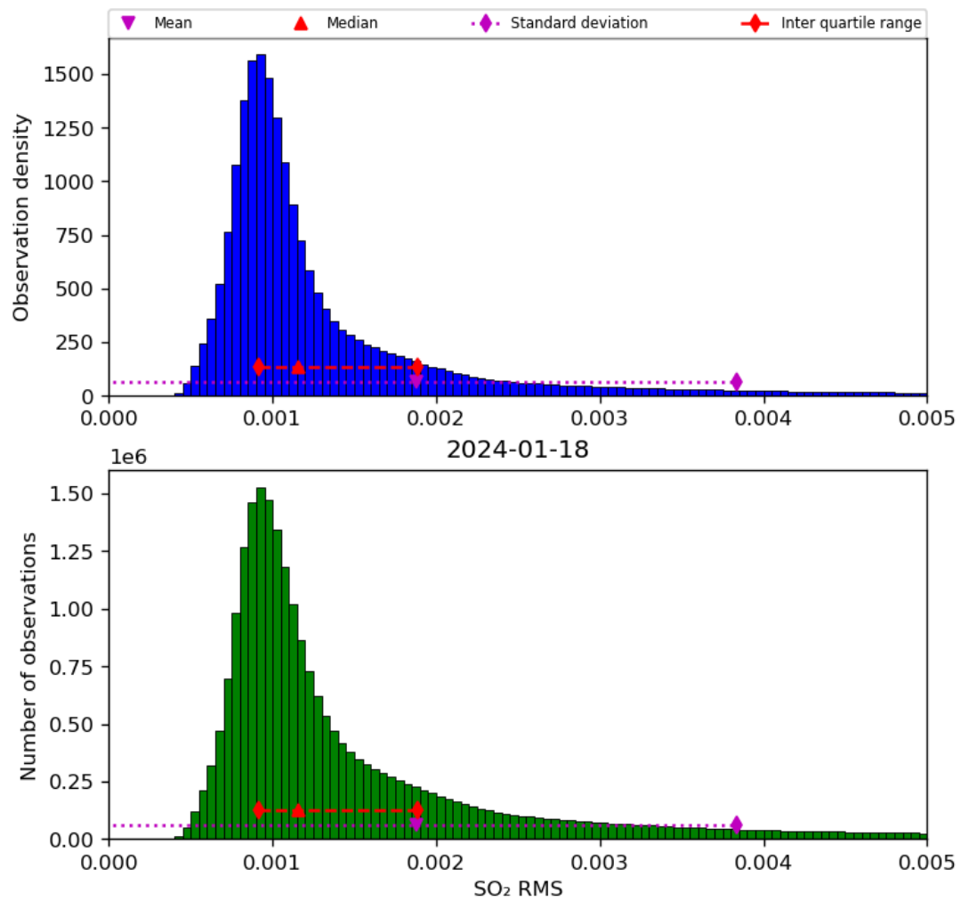
Figure 70: Histogram of “SO 2 RMS” for 2024-01-17 to 2024-01-19
