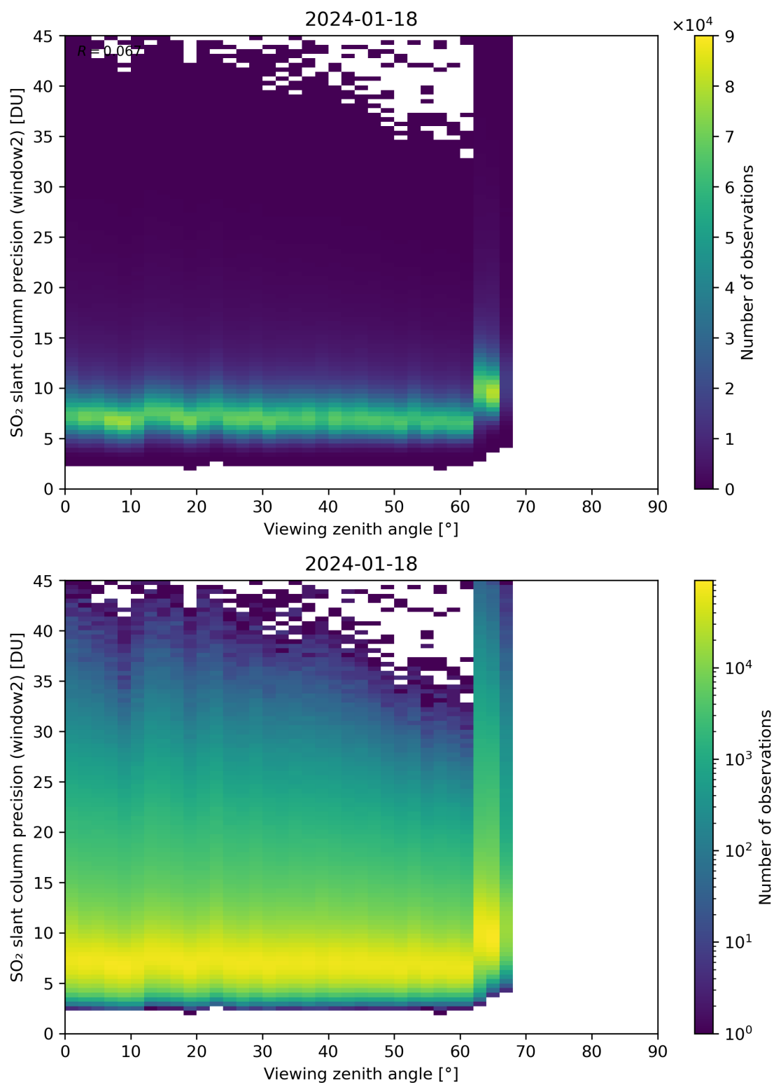
Figure 322: Scatter density plot of “Viewing zenith angle” against “SO 2 slant column precision (window2)” for 2024-01-17 to 2024-01-19.
