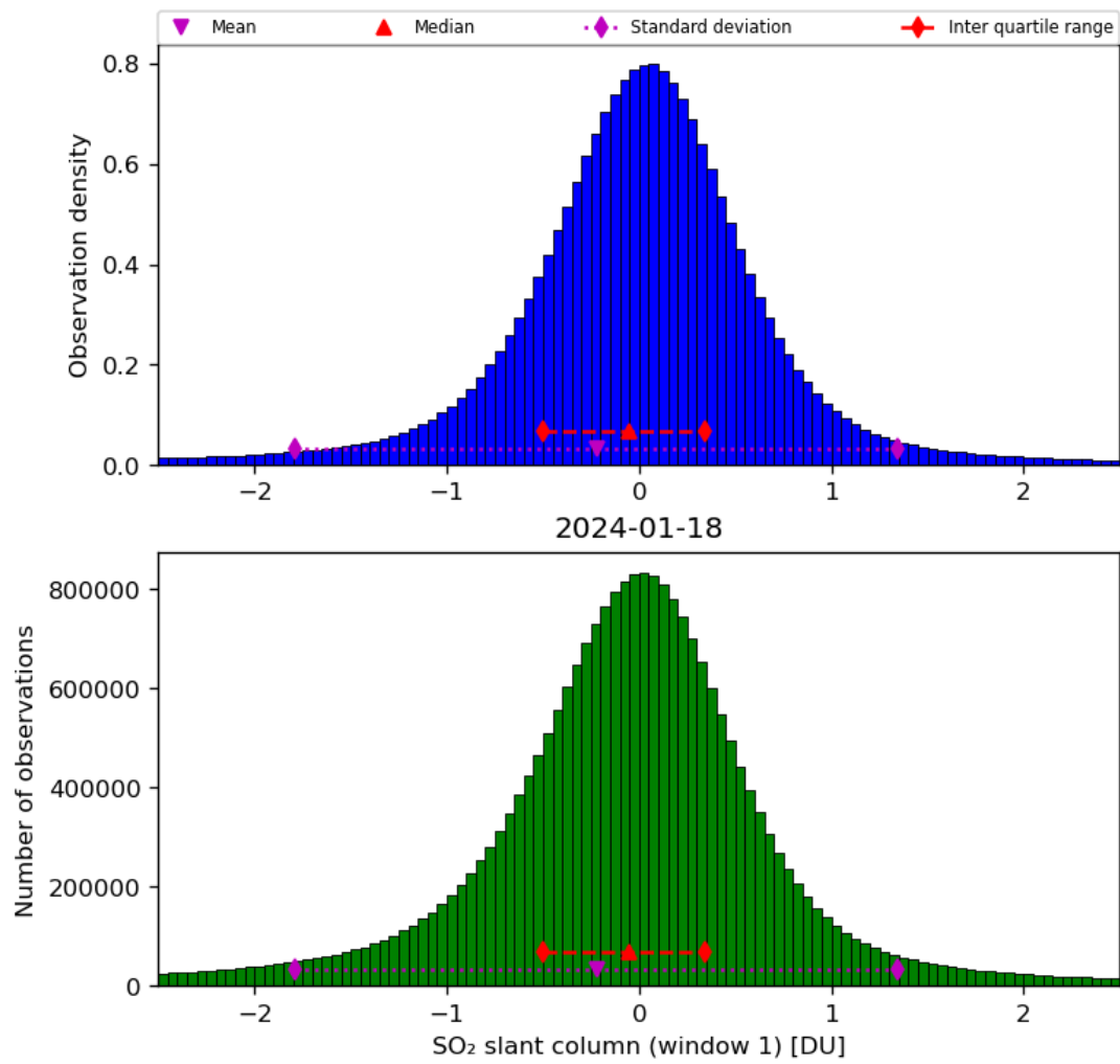
Figure 56: Histogram of “SO 2 slant column (window 1)” for 2024-01-17 to 2024-01-19
