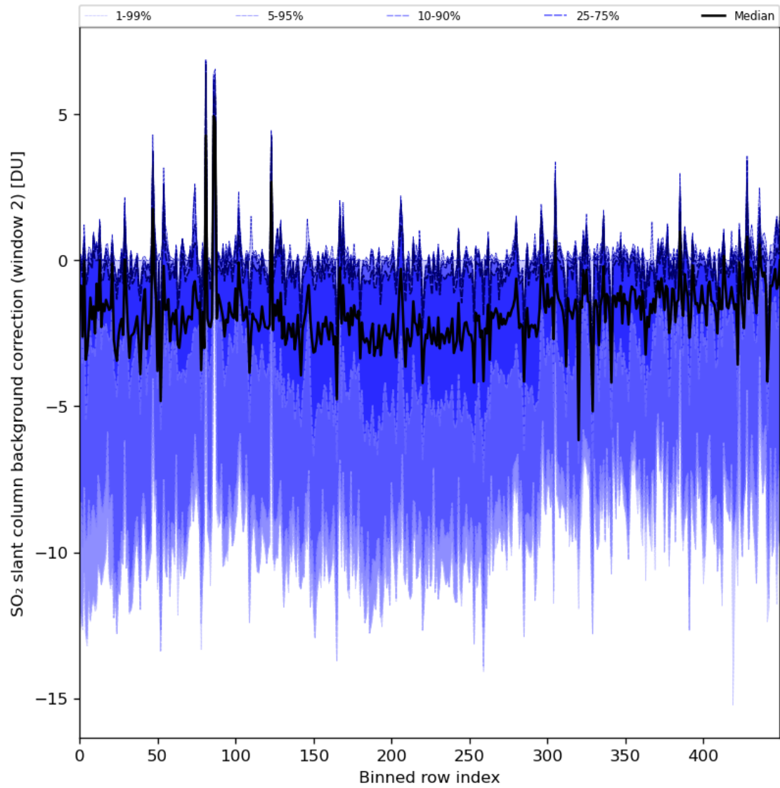
Figure 86: Along track statistics of “SO 2 slant column background correction (window 2)” for 2024-01-17 to 2024-01-19
