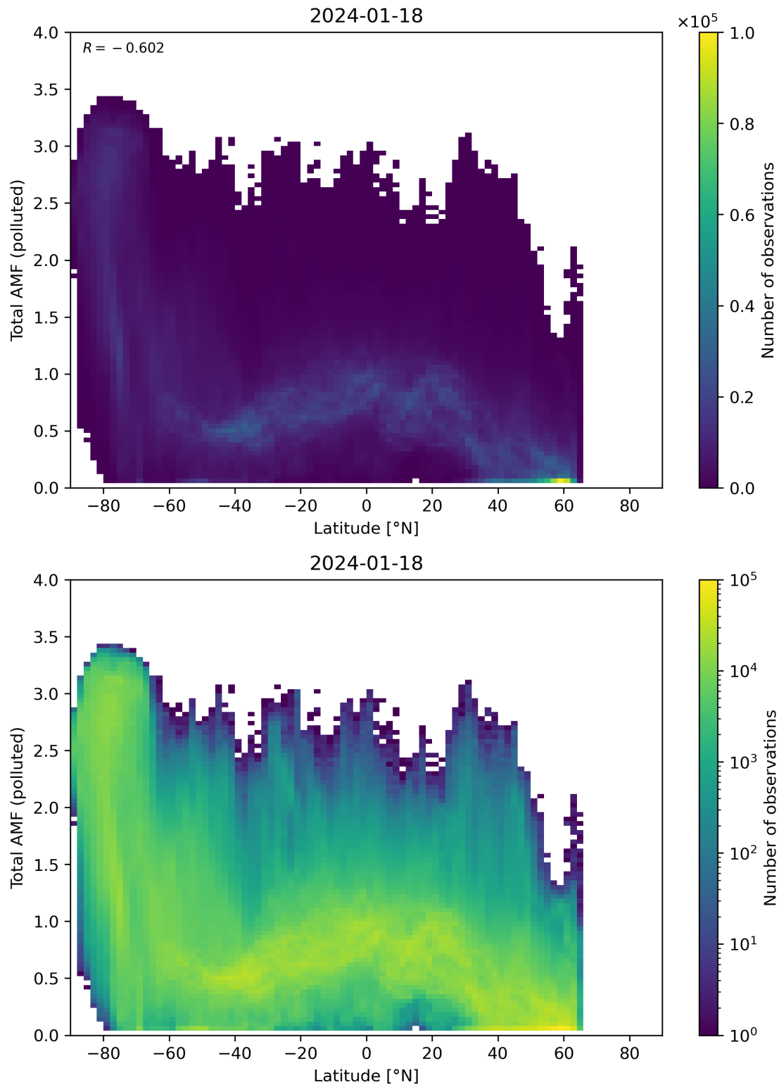
Figure 154: Scatter density plot of “Latitude” against “Total AMF (polluted)” for 2024-01-17 to 2024-01-19.
