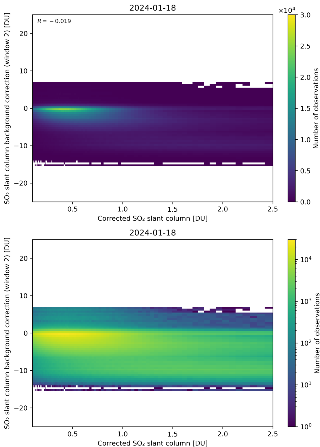
Figure 179: Scatter density plot of “Corrected SO 2 slant column” against “SO 2 slant column background correction (window 2)” for 2024-01-17 to 2024-01-19.
