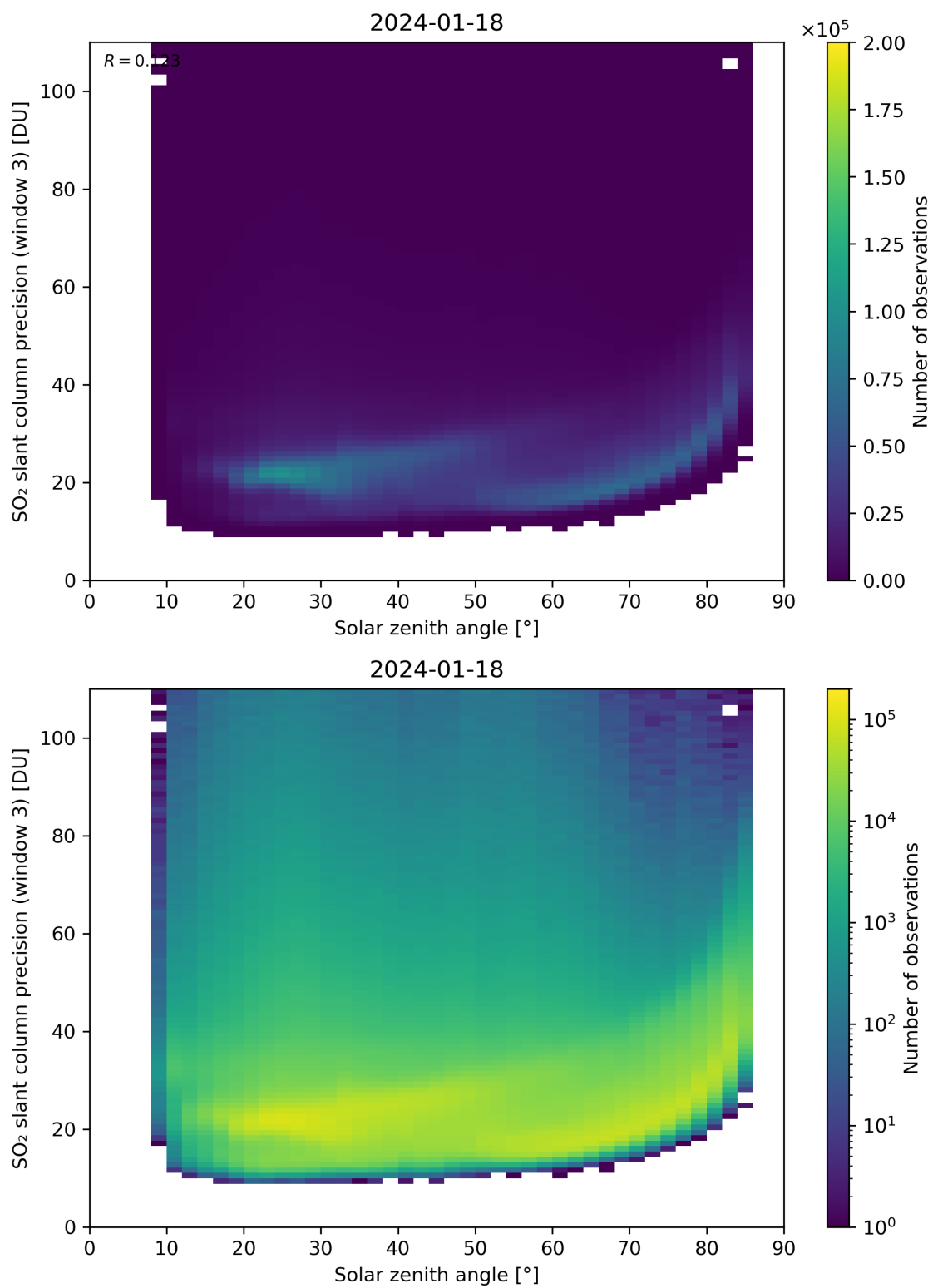
Figure 173: Scatter density plot of “Solar zenith angle” against “SO 2 slant column precision (window 3)” for 2024-01-17 to 2024-01-19.
