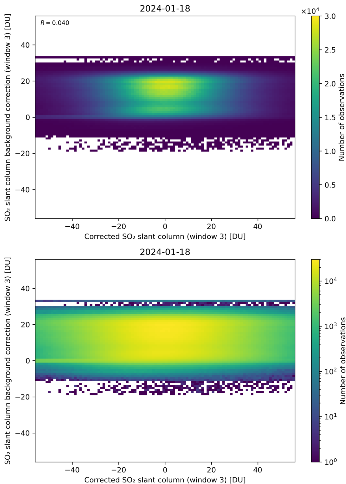
Figure 205: Scatter density plot of “Corrected SO 2 slant column (window 3)” against “SO 2 slant column background correction (window 3)” for 2024-01-17 to 2024-01-19.
