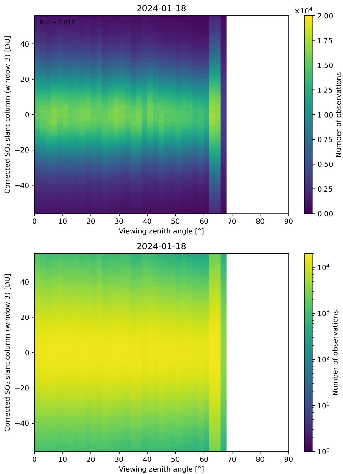
Figure 319: Scatter density plot of “Viewing zenith angle” against “Corrected SO 2 slant column (window 3)” for 2024-01-17 to 2024-01-19.
