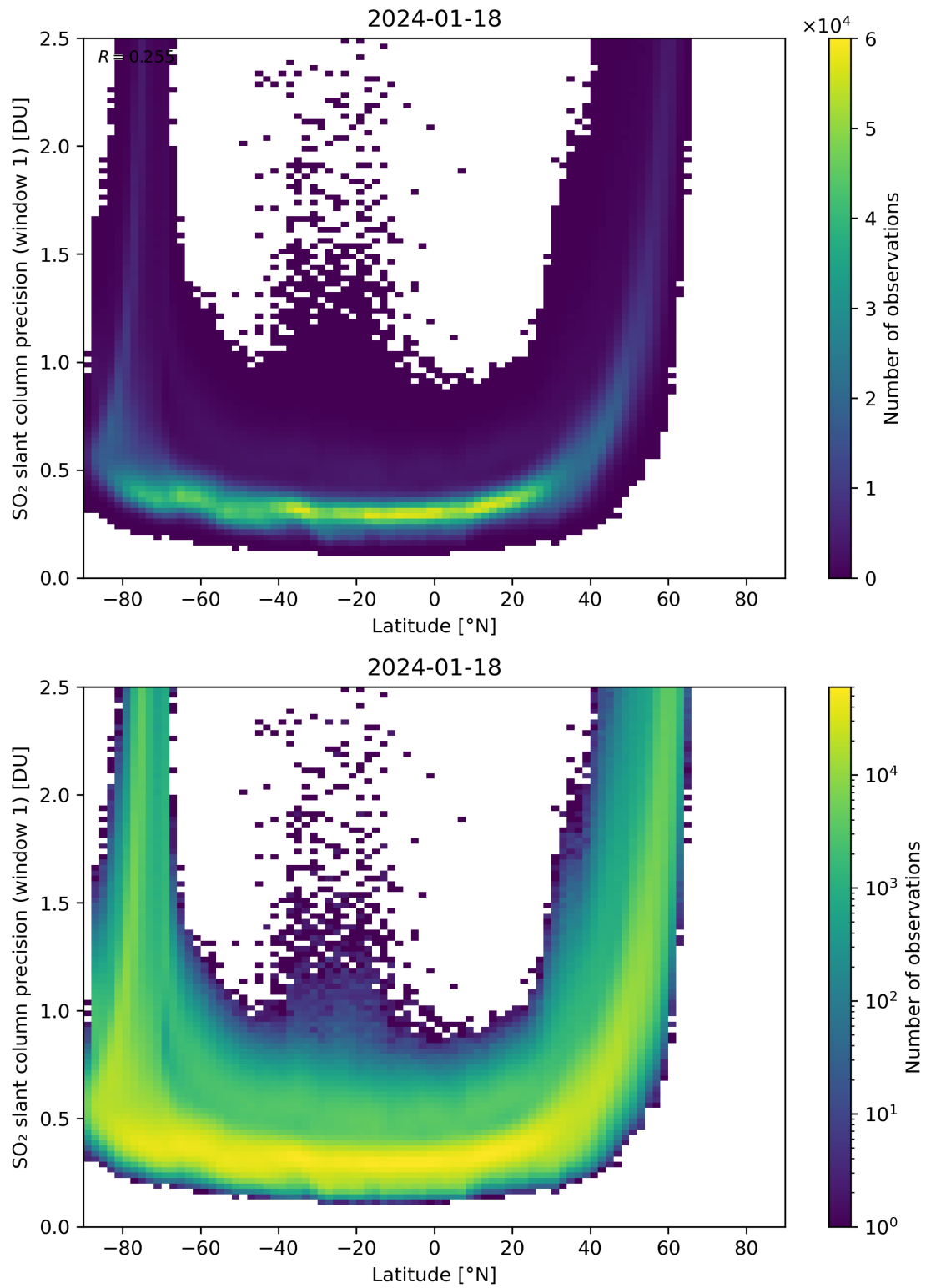
Figure 150: Scatter density plot of “Latitude” against “SO 2 slant column precision (window 1)” for 2024-01-17 to 2024-01-19.
