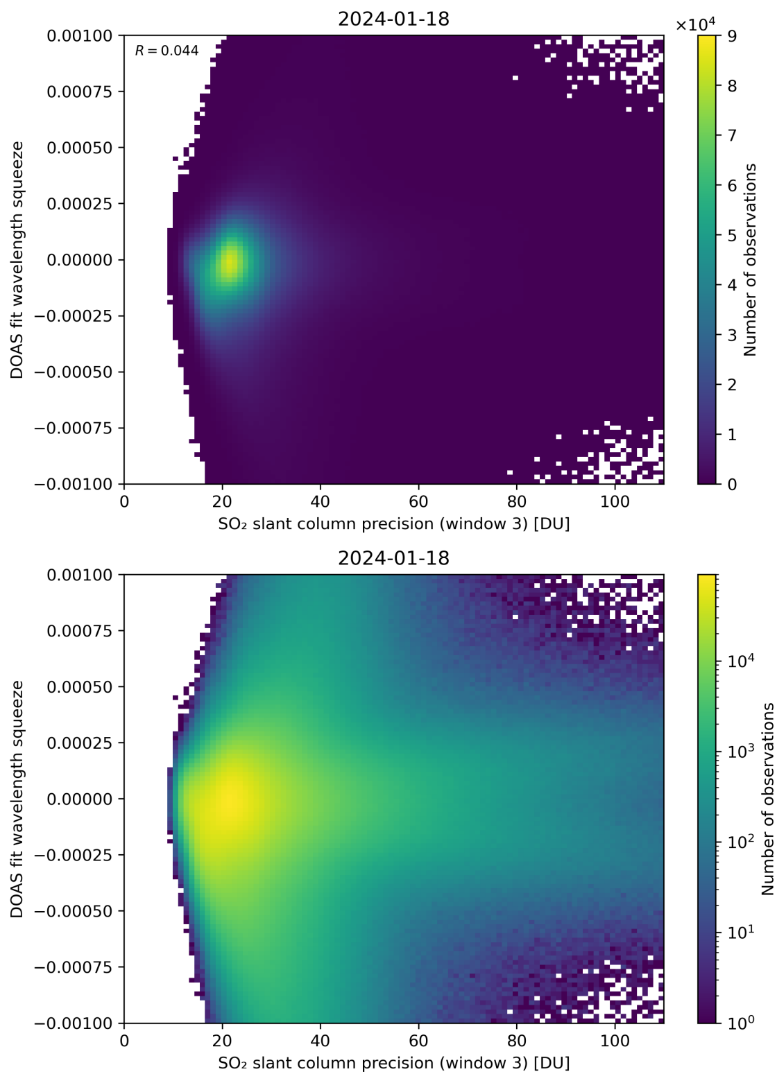
Figure 259: Scatter density plot of “SO 2 slant column precision (window 3)” against “DOAS fit wavelength squeeze” for 2024-01-17 to 2024-01-19.
