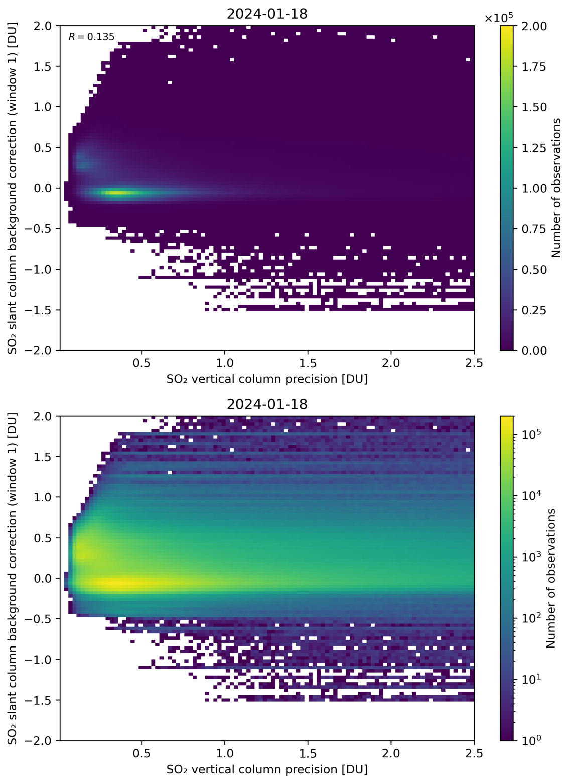
Figure 279: Scatter density plot of “SO 2 vertical column precision” against “SO 2 slant column background correction (window 1)” for 2024-01-17 to 2024-01-19.
