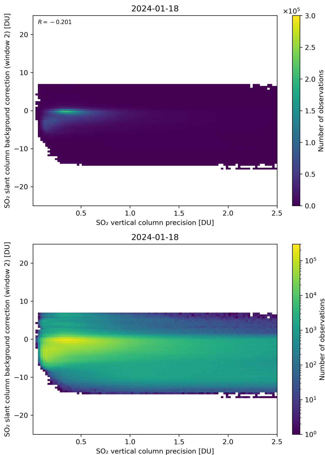
Figure 280: Scatter density plot of “SO 2 vertical column precision” against “SO 2 slant column background correction (window 2)” for 2024-01-17 to 2024-01-19.
