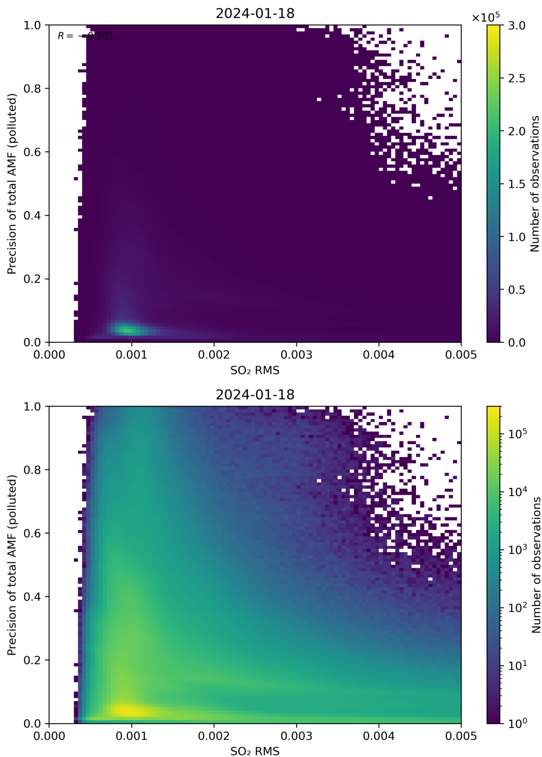
Figure 138: Scatter density plot of “SO 2 RMS” against “Precision of total AMF (polluted)” for 2024-01-17 to 2024-01-19.
