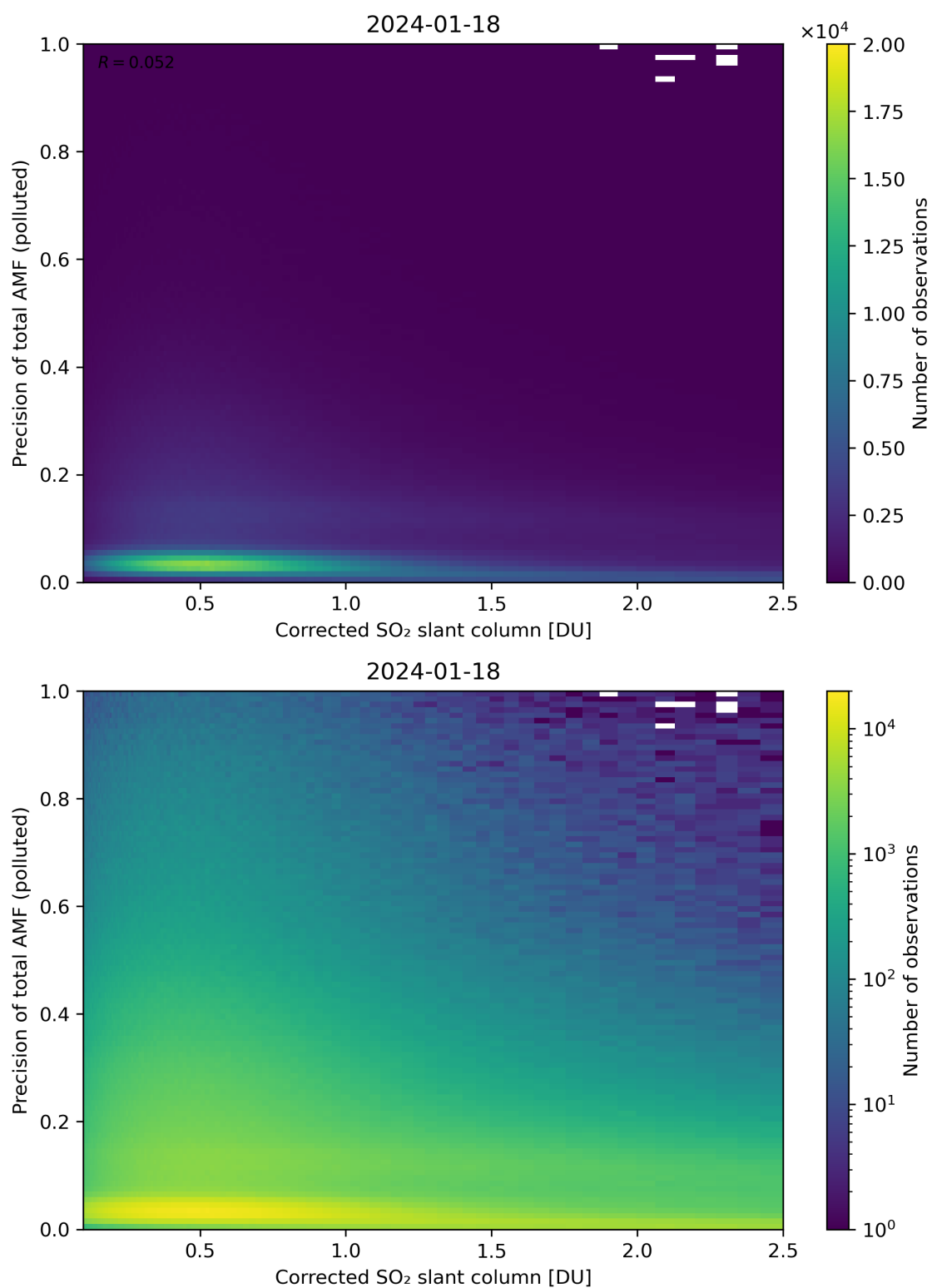
Figure 193: Scatter density plot of “Corrected SO 2 slant column” against “Precision of total AMF (polluted)” for 2024-01-17 to 2024-01-19.
