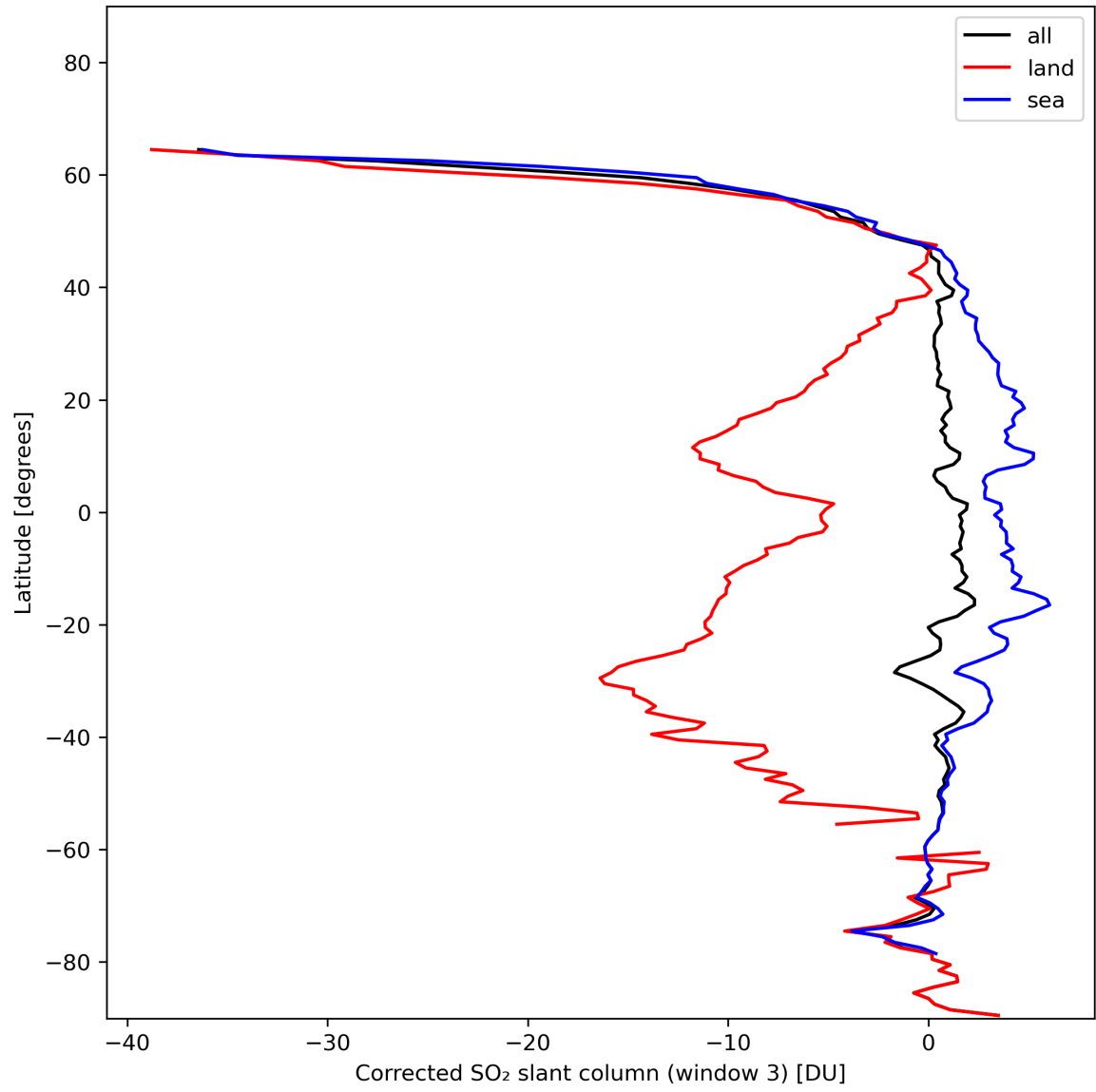
Figure 43: Zonal average of “Corrected SO 2 slant column (window 3)” for 2024-01-17 to 2024-01-19.
