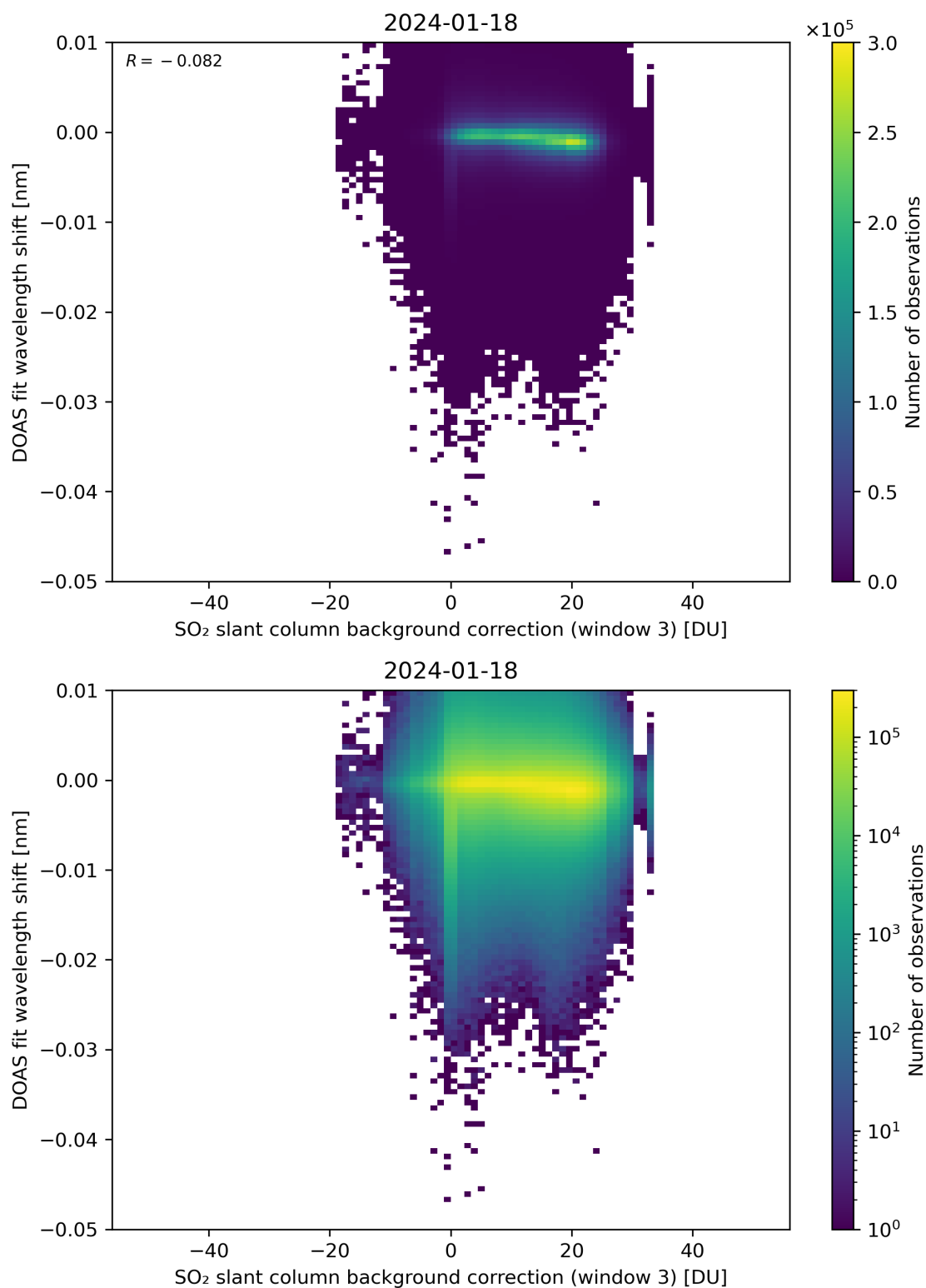
Figure 121: Scatter density plot of “SO 2 slant column background correction (window 3)” against “DOAS fit wavelength shift” for 2024-01-17 to 2024-01-19.
