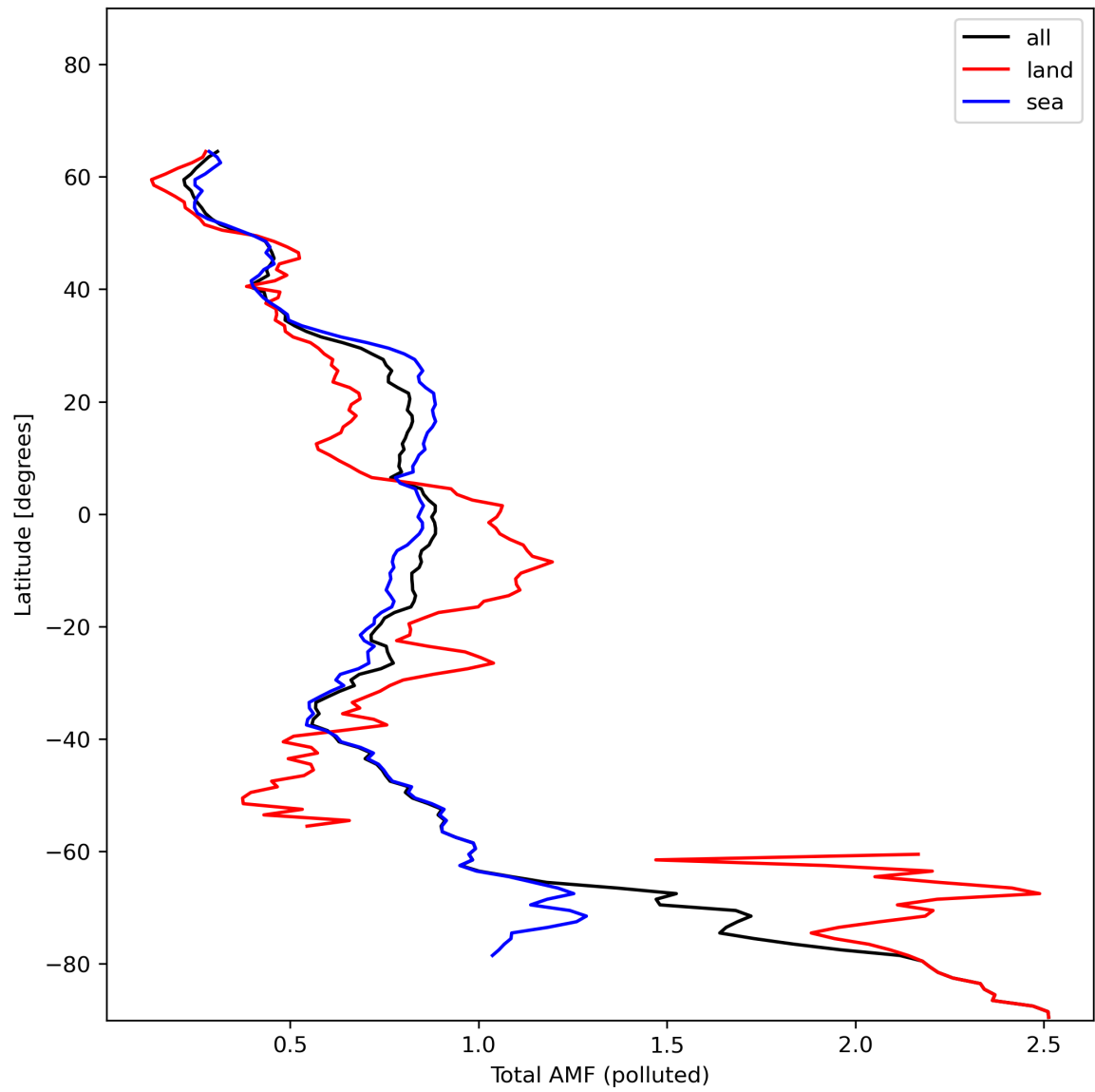
Figure 48: Zonal average of “Total AMF (polluted)” for 2024-01-17 to 2024-01-19.
