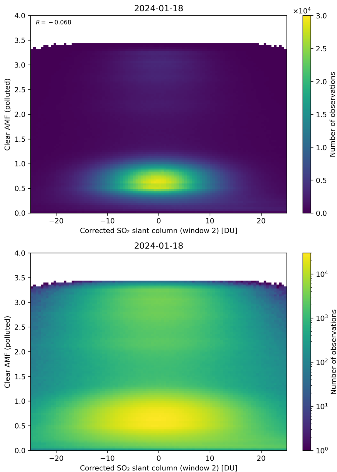
Figure 199: Scatter density plot of “Corrected SO 2 slant column (window 2)” against “Clear AMF (polluted)” for 2024-01-17 to 2024-01-19.
