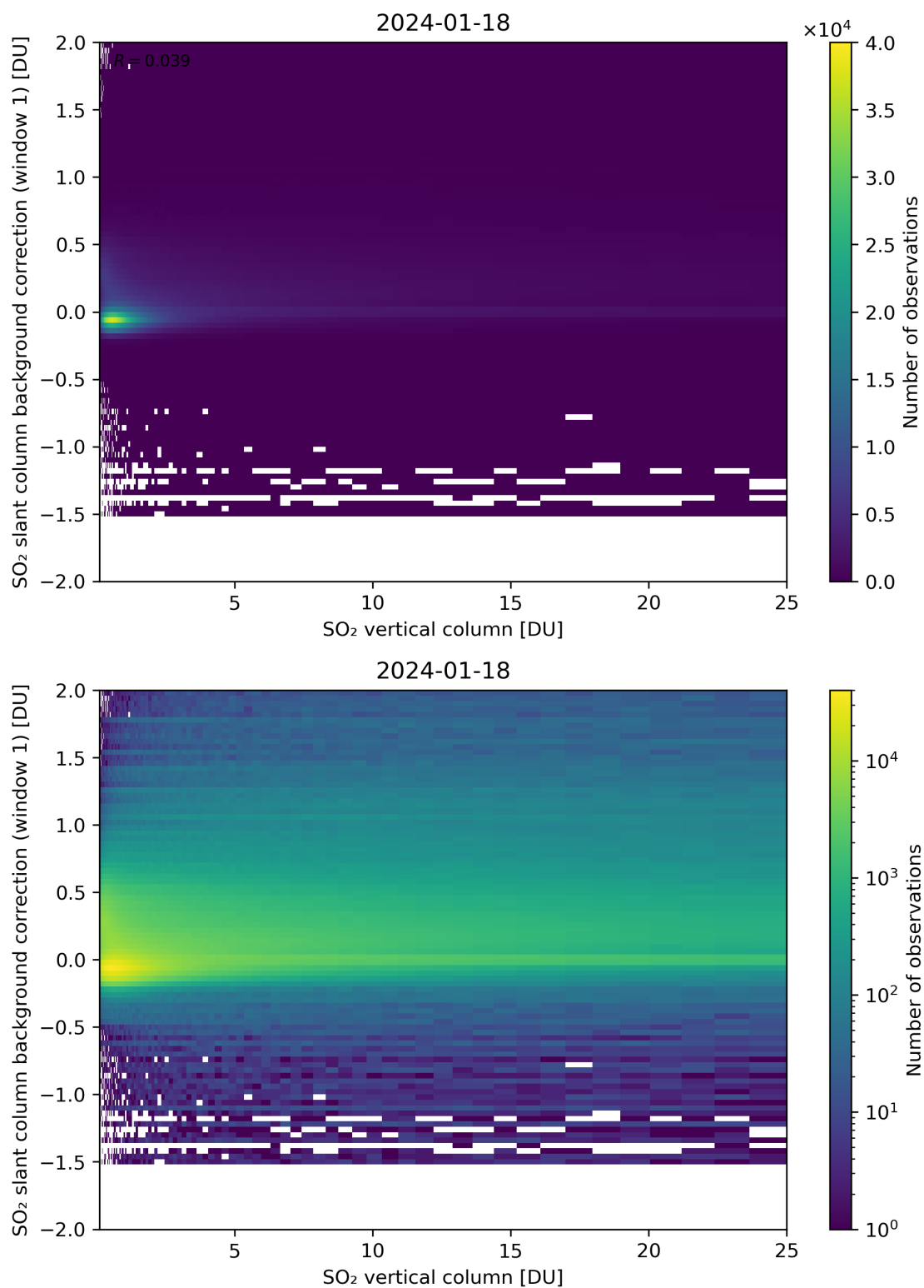
Figure 273: Scatter density plot of “SO 2 vertical column” against “SO 2 slant column background correction (window 1)” for 2024-01-17 to 2024-01-19.
