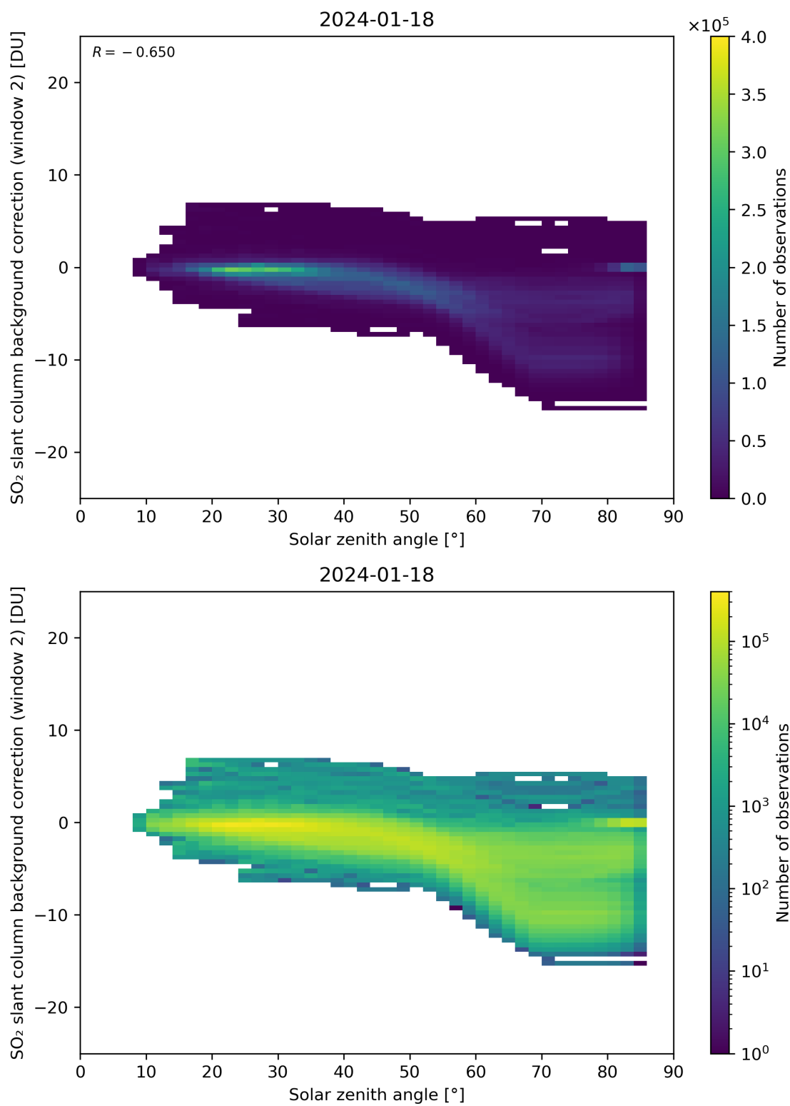
Figure 159: Scatter density plot of “Solar zenith angle” against “SO 2 slant column background correction (window 2)” for 2024-01-17 to 2024-01-19.
