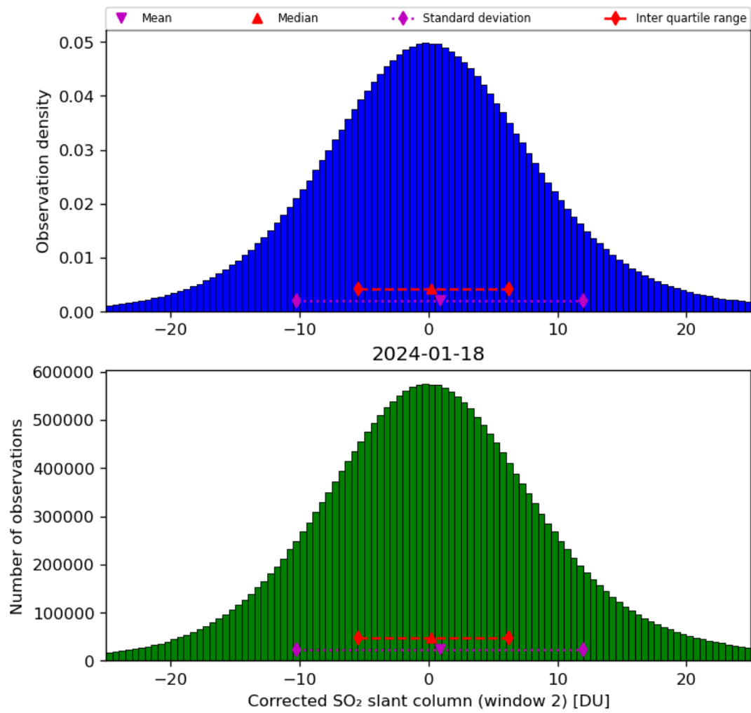
Figure 62: Histogram of “Corrected SO 2 slant column (window 2)” for 2024-01-17 to 2024-01-19
