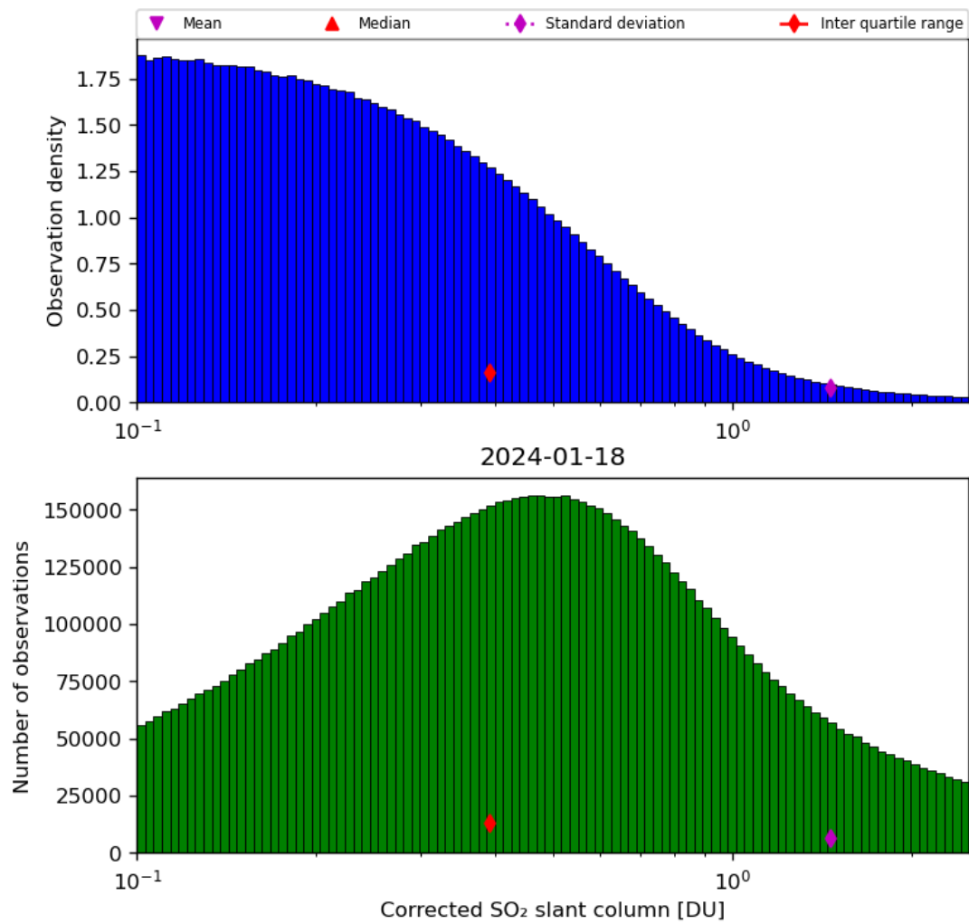
Figure 55: Histogram of “Corrected SO 2 slant column” for 2024-01-17 to 2024-01-19
