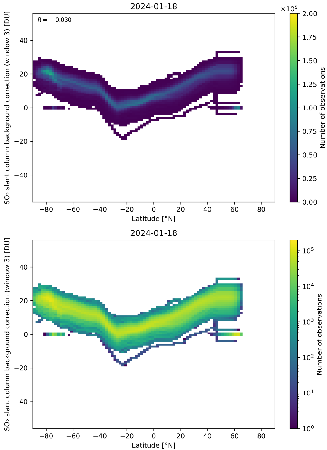
Figure 141: Scatter density plot of “Latitude” against “SO 2 slant column background correction (window 3)” for 2024-01-17 to 2024-01-19.
