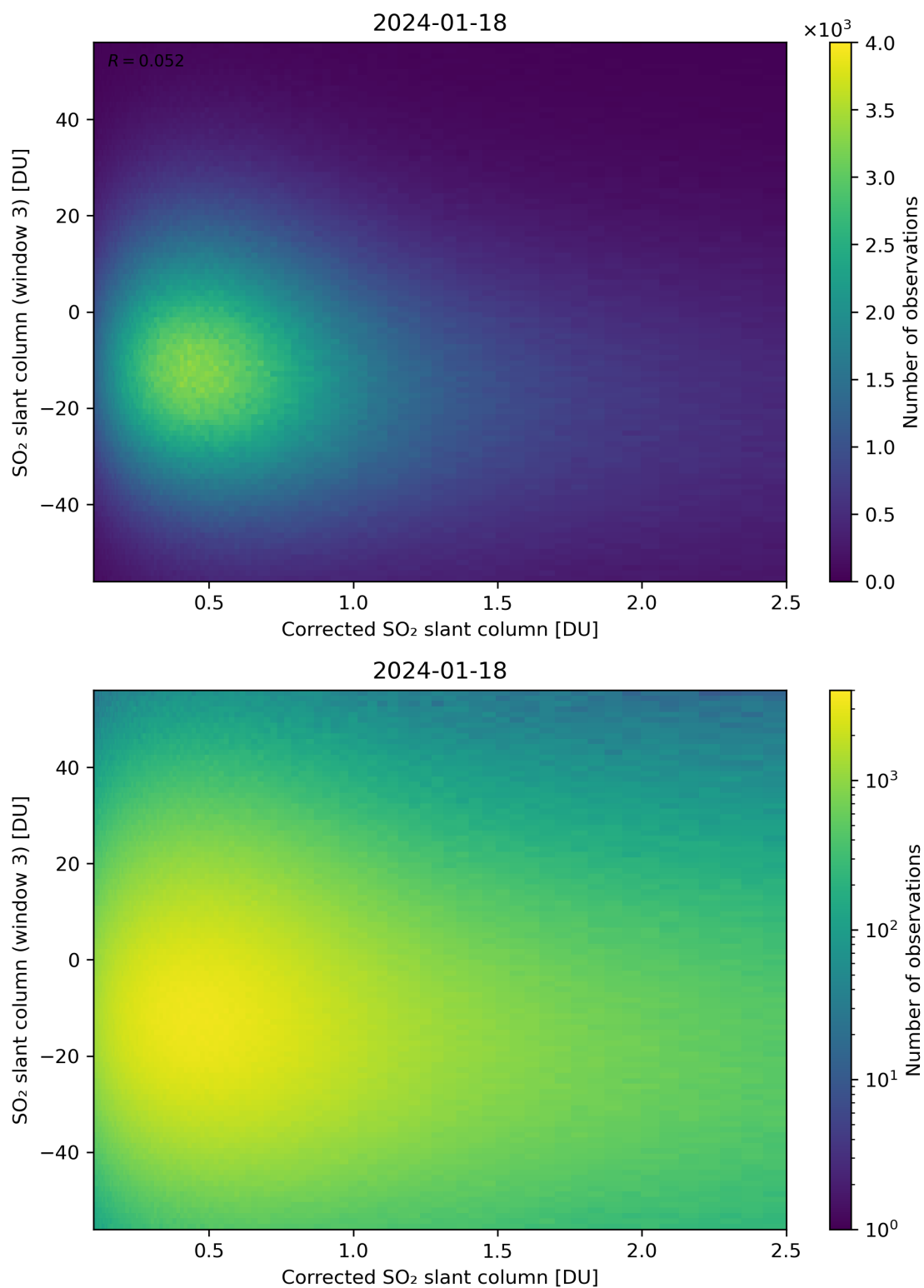
Figure 190: Scatter density plot of “Corrected SO 2 slant column” against “SO 2 slant column (window 3)” for 2024-01-17 to 2024-01-19.
