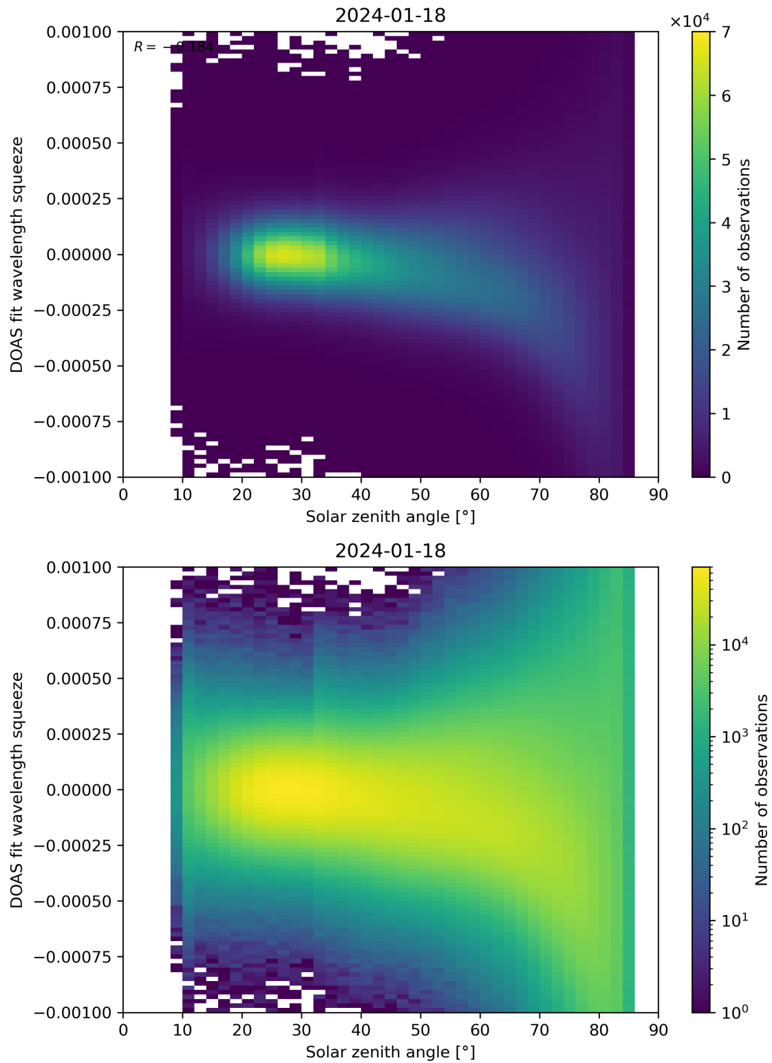
Figure 162: Scatter density plot of “Solar zenith angle” against “DOAS fit wavelength squeeze” for 2024-01-17 to 2024-01-19.
