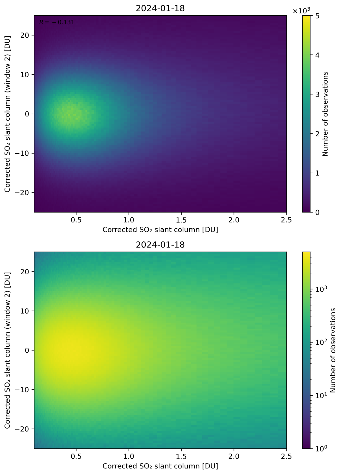
Figure 185: Scatter density plot of “Corrected SO 2 slant column” against “Corrected SO 2 slant column (window 2)” for 2024-01-17 to 2024-01-19.
