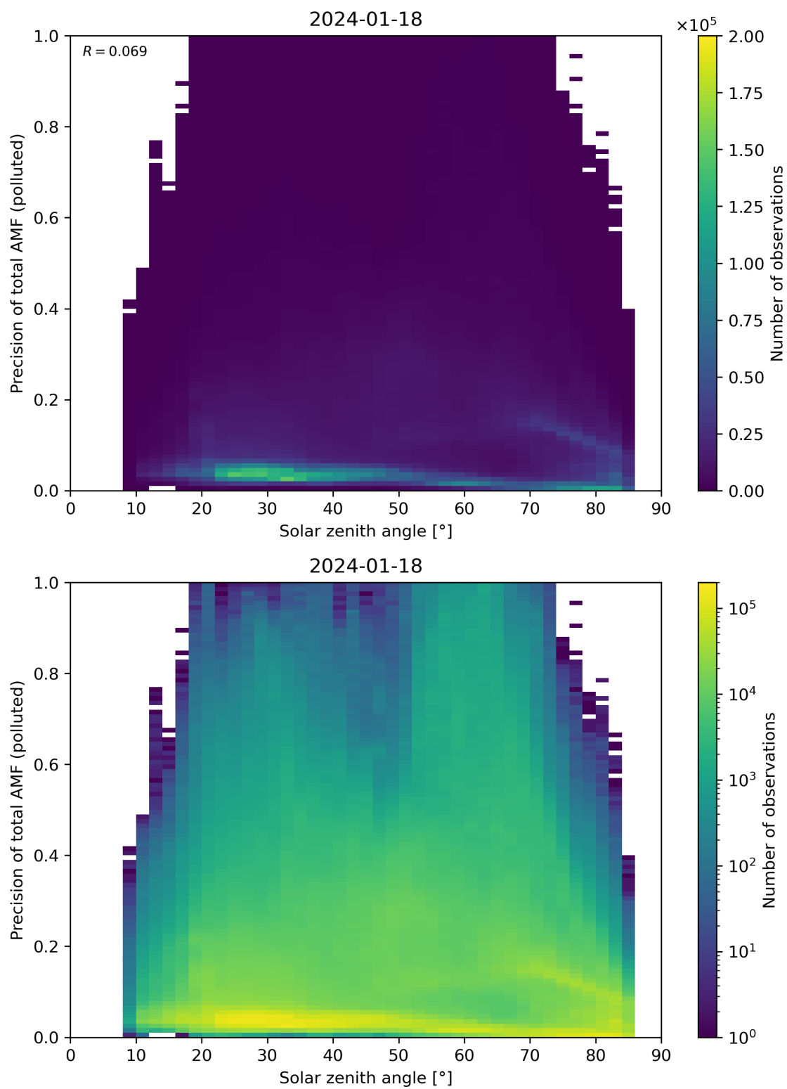
Figure 175: Scatter density plot of “Solar zenith angle” against “Precision of total AMF (polluted)” for 2024-01-17 to 2024-01-19.
