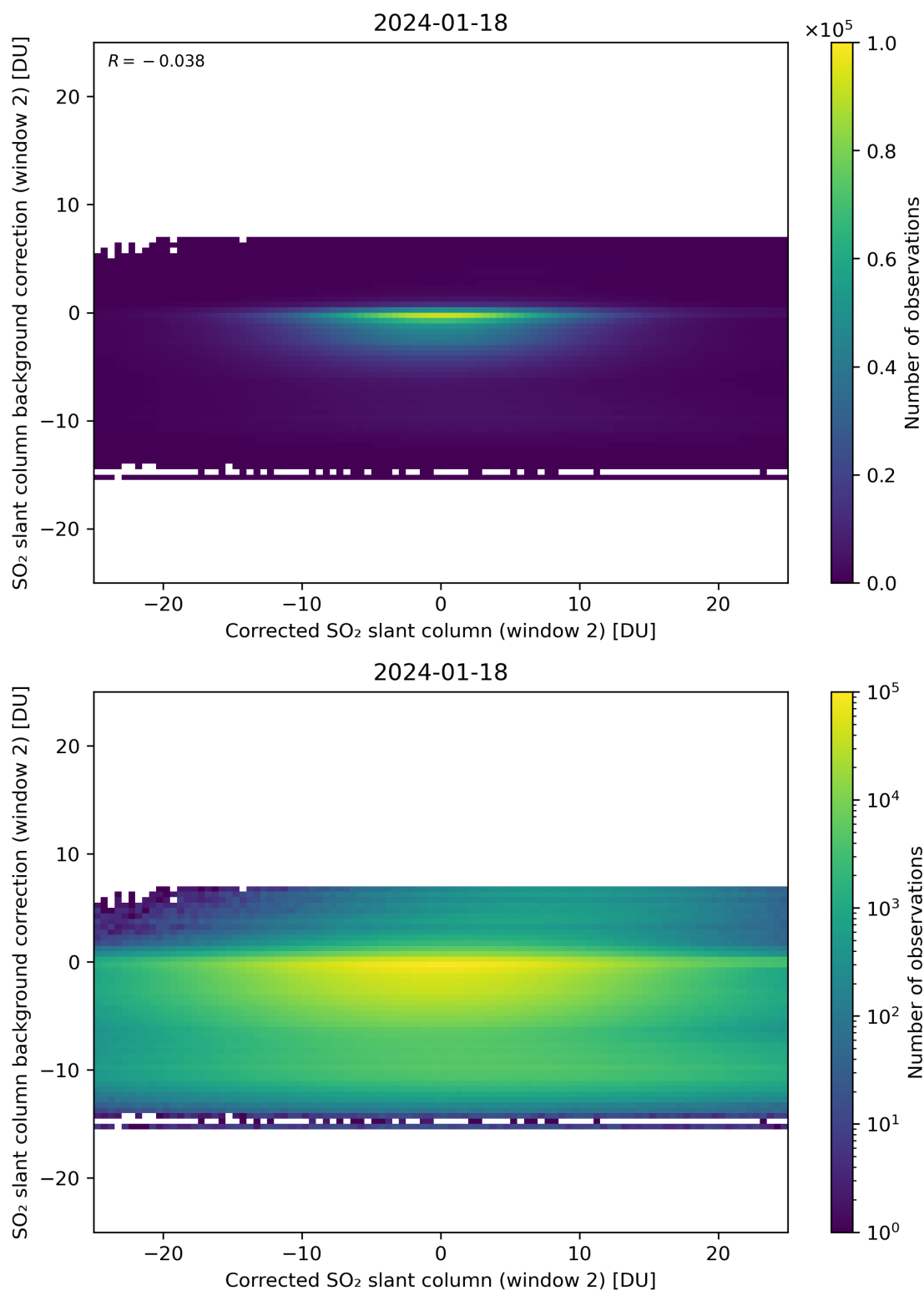
Figure 194: Scatter density plot of “Corrected SO 2 slant column (window 2)” against “SO 2 slant column background correction (window 2)” for 2024-01-17 to 2024-01-19.
