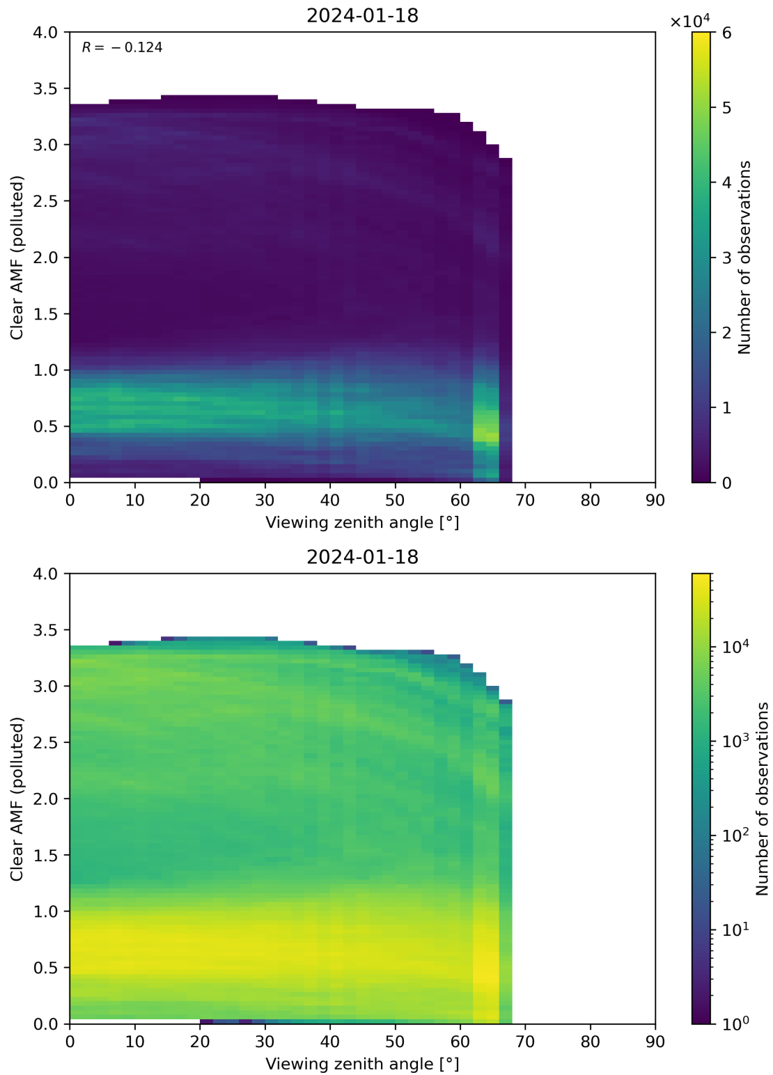
Figure 316: Scatter density plot of “Viewing zenith angle” against “Clear AMF (polluted)” for 2024-01-17 to 2024-01-19.
