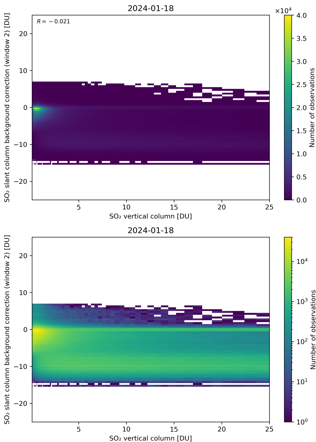
Figure 274: Scatter density plot of “SO 2 vertical column” against “SO 2 slant column background correction (window 2)” for 2024-01-17 to 2024-01-19.
