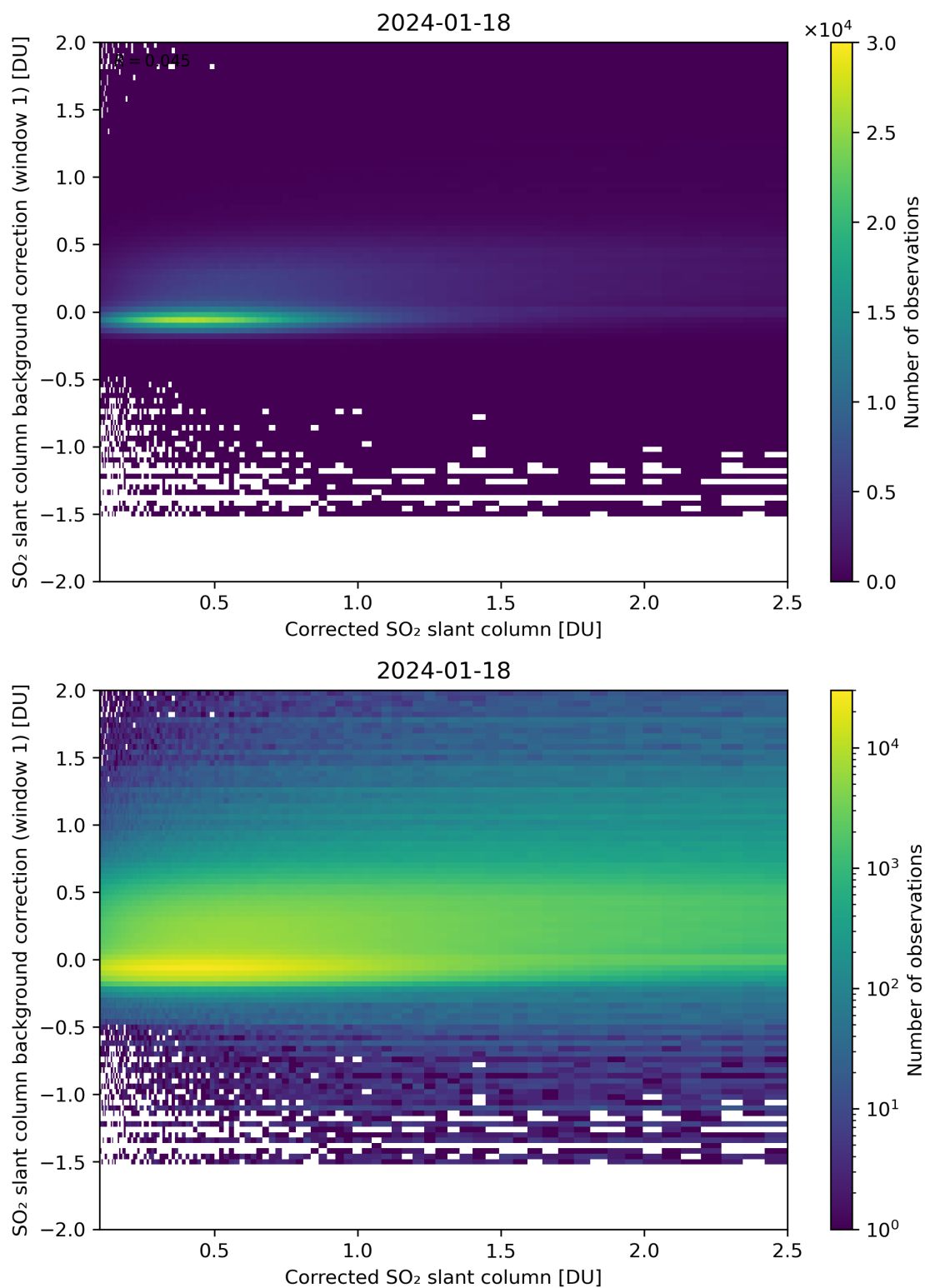
Figure 178: Scatter density plot of “Corrected SO 2 slant column” against “SO 2 slant column background correction (window 1)” for 2024-01-17 to 2024-01-19.
