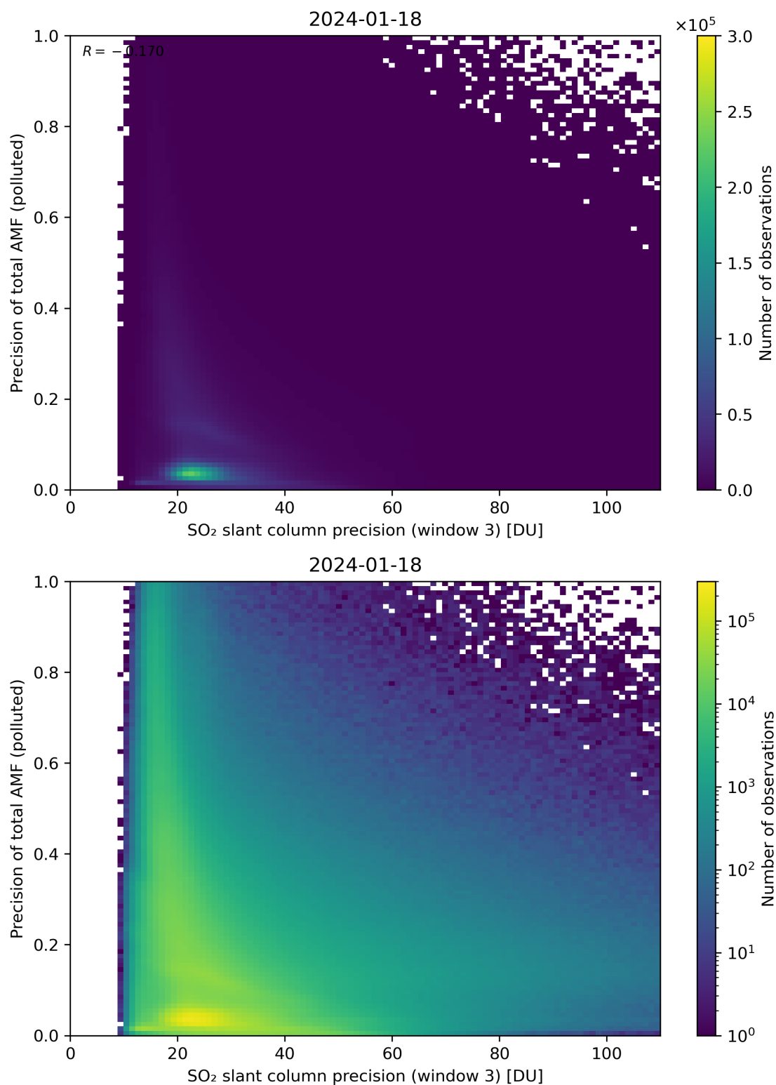
Figure 264: Scatter density plot of “SO 2 slant column precision (window 3)” against “Precision of total AMF (polluted)” for 2024-01-17 to 2024-01-19.
