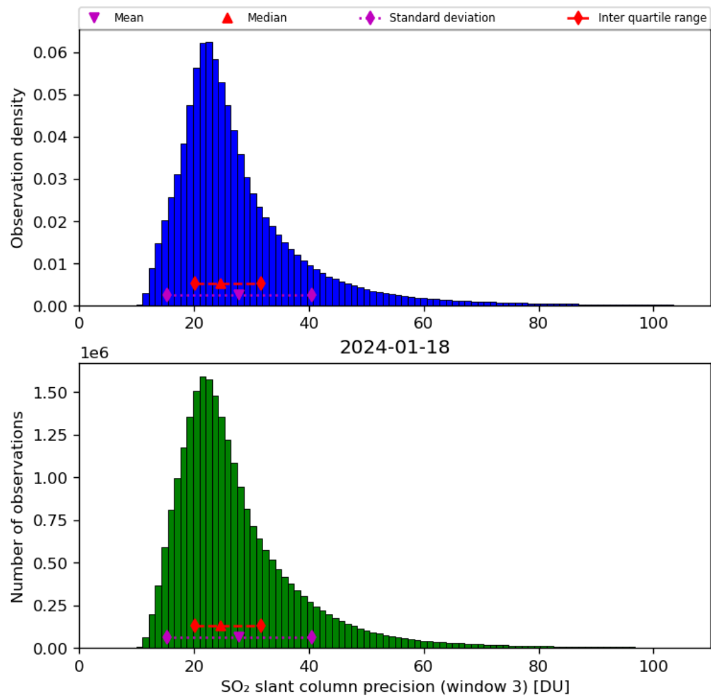
Figure 65: Histogram of “SO 2 slant column precision (window 3)” for 2024-01-17 to 2024-01-19
