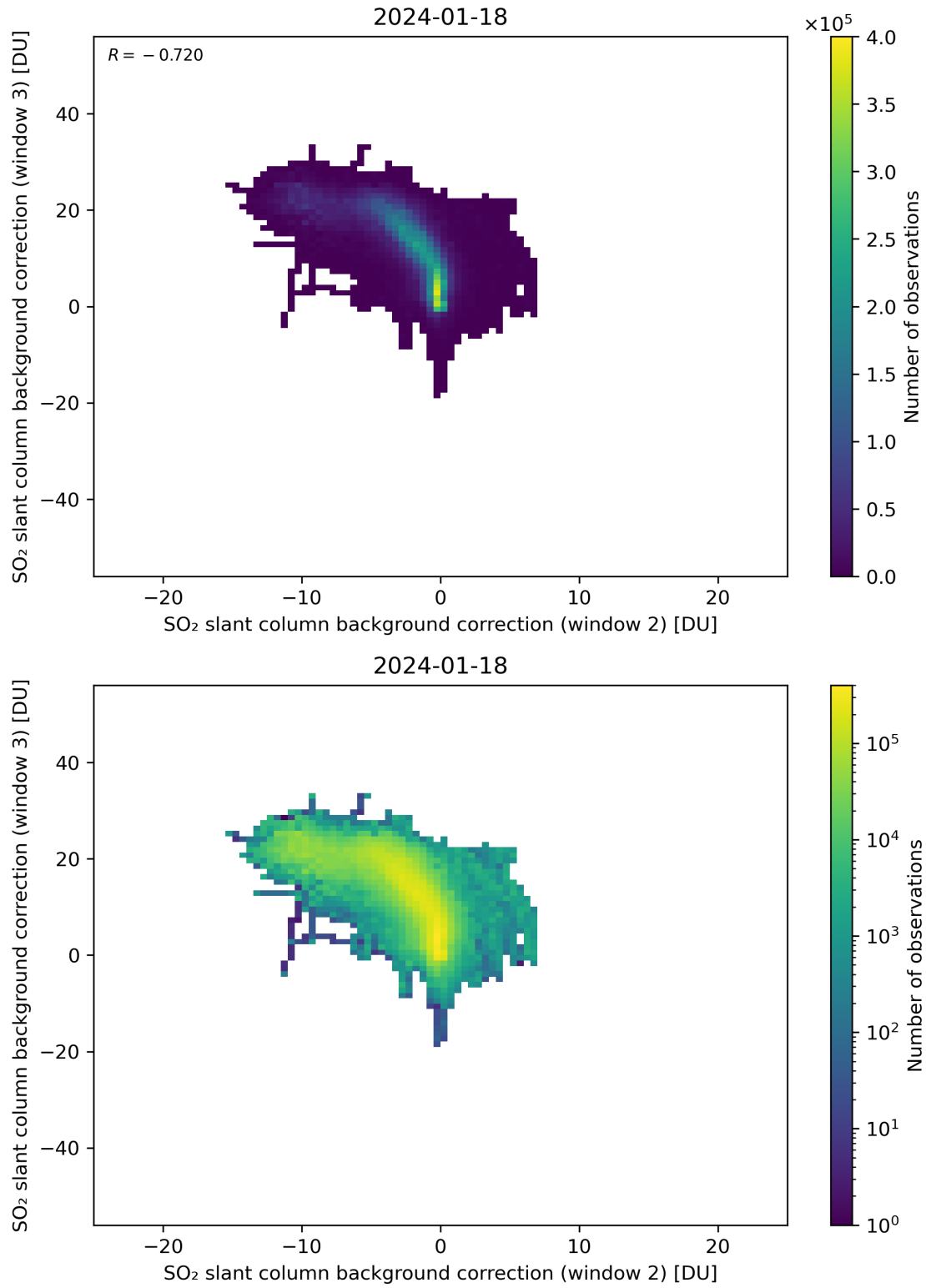
Figure 111: Scatter density plot of “SO 2 slant column background correction (window 2)” against “SO 2 slant column background correction (window 3)” for 2024-01-17 to 2024-01-19.
