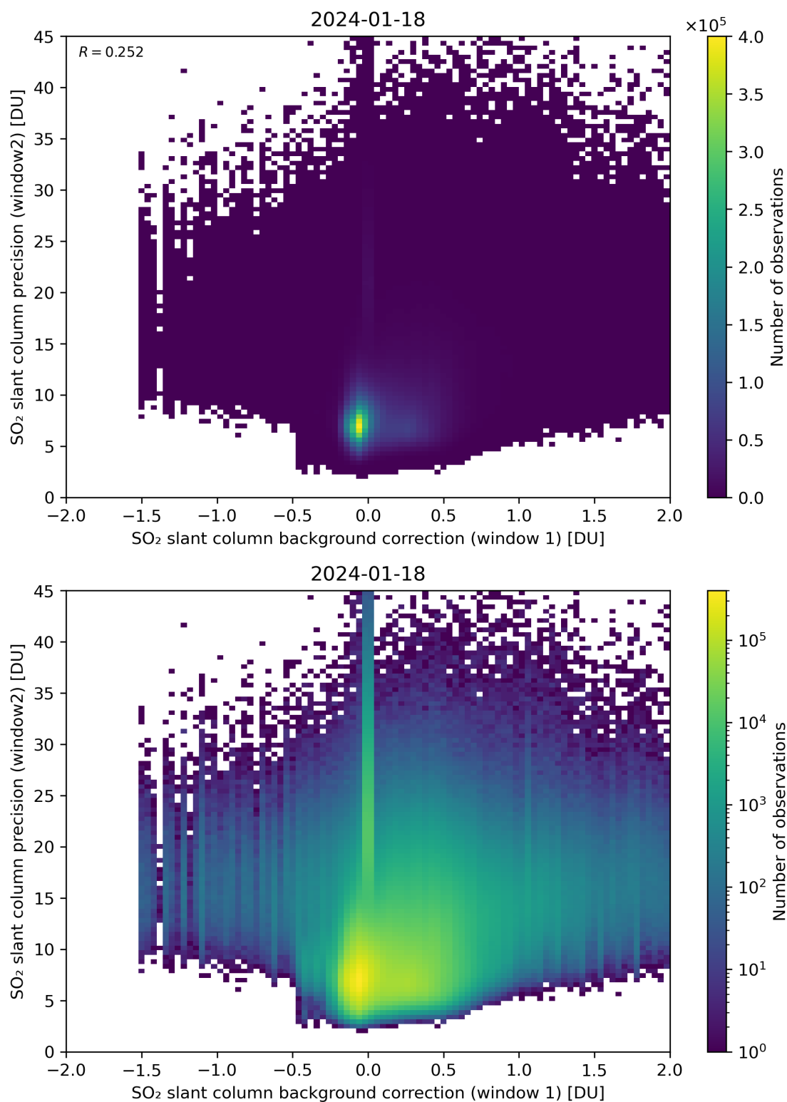
Figure 106: Scatter density plot of “SO 2 slant column background correction (window 1)” against “SO 2 slant column precision (window2)” for 2024-01-17 to 2024-01-19.
