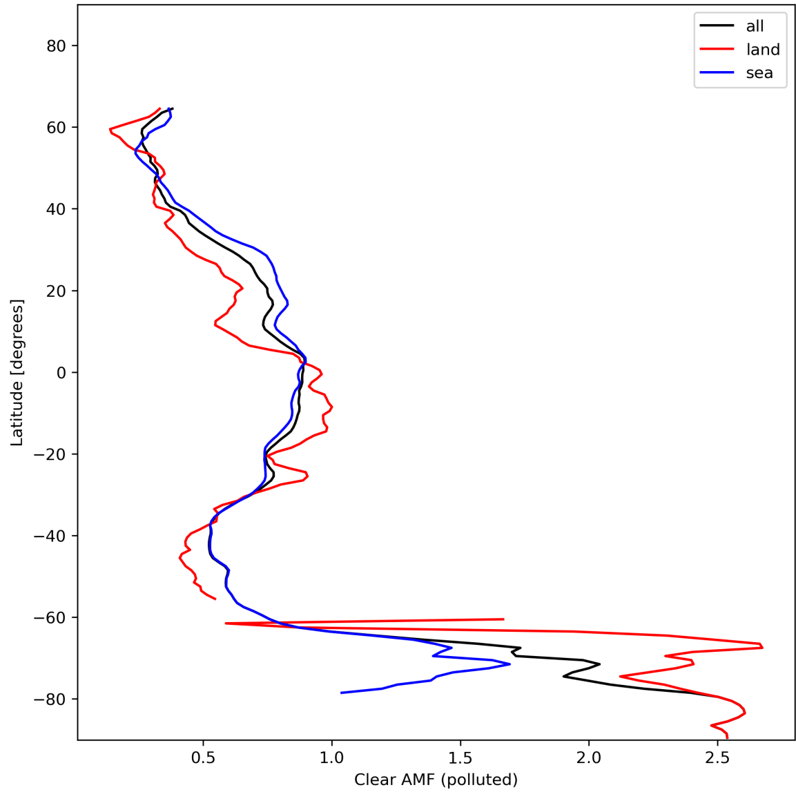
Figure 50: Zonal average of “Clear AMF (polluted)” for 2024-01-17 to 2024-01-19.
