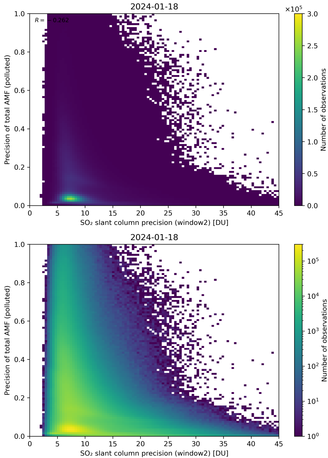
Figure 252: Scatter density plot of “SO 2 slant column precision (window2)” against “Precision of total AMF (polluted)” for 2024-01-17 to 2024-01-19.
