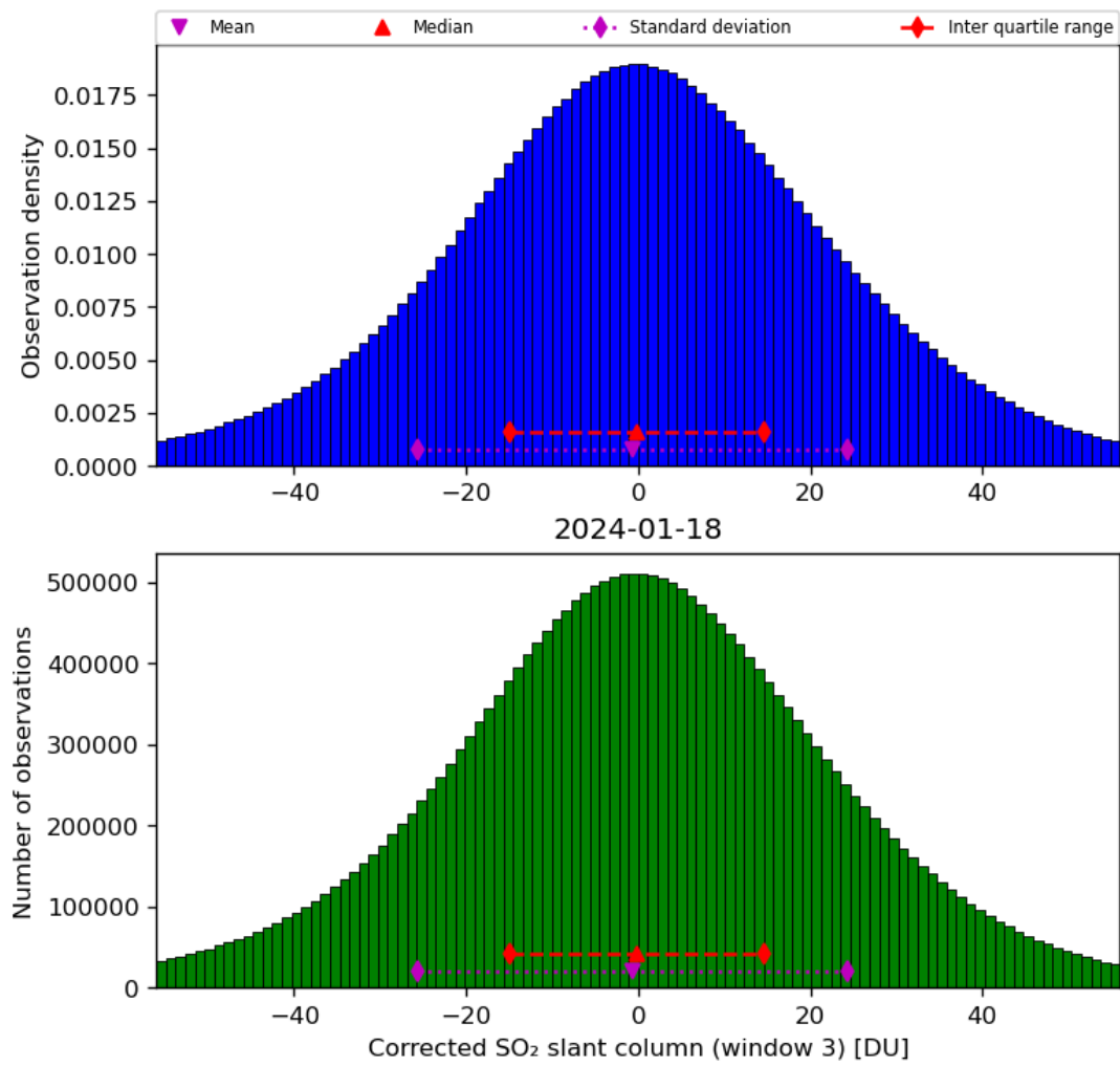
Figure 66: Histogram of “Corrected SO 2 slant column (window 3)” for 2024-01-17 to 2024-01-19
