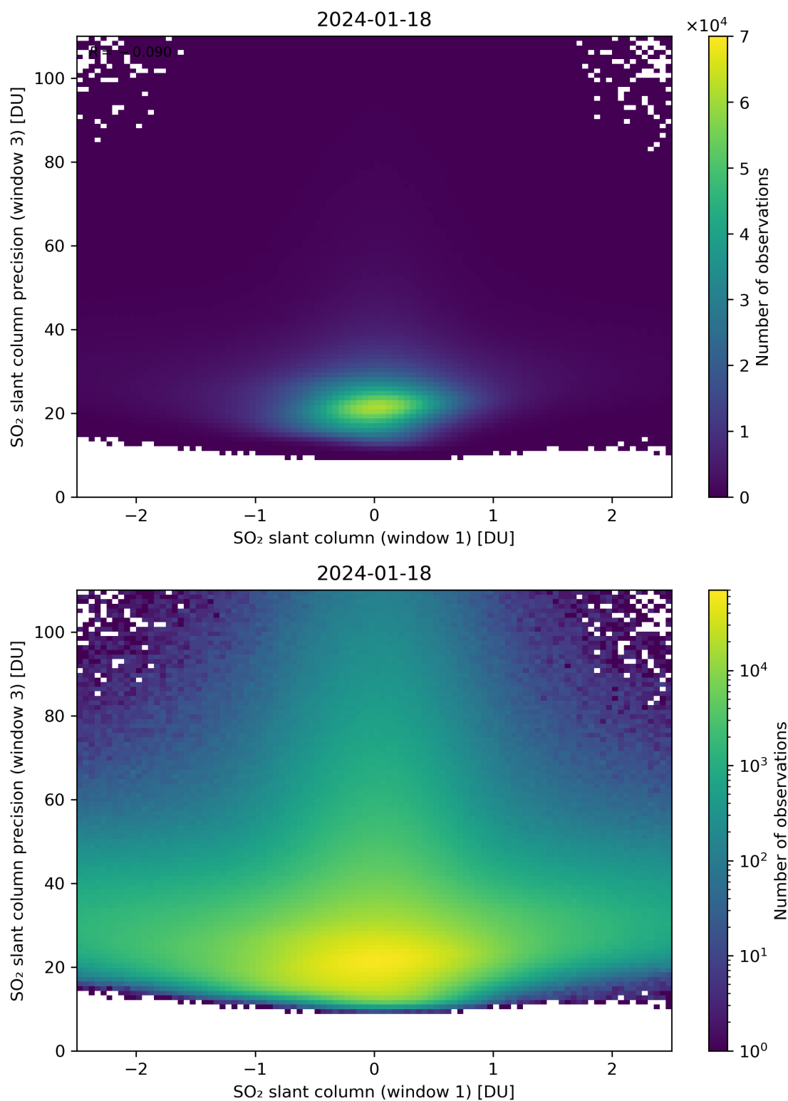
Figure 238: Scatter density plot of “SO 2 slant column (window 1)” against “SO 2 slant column precision (window 3)” for 2024-01-17 to 2024-01-19.
