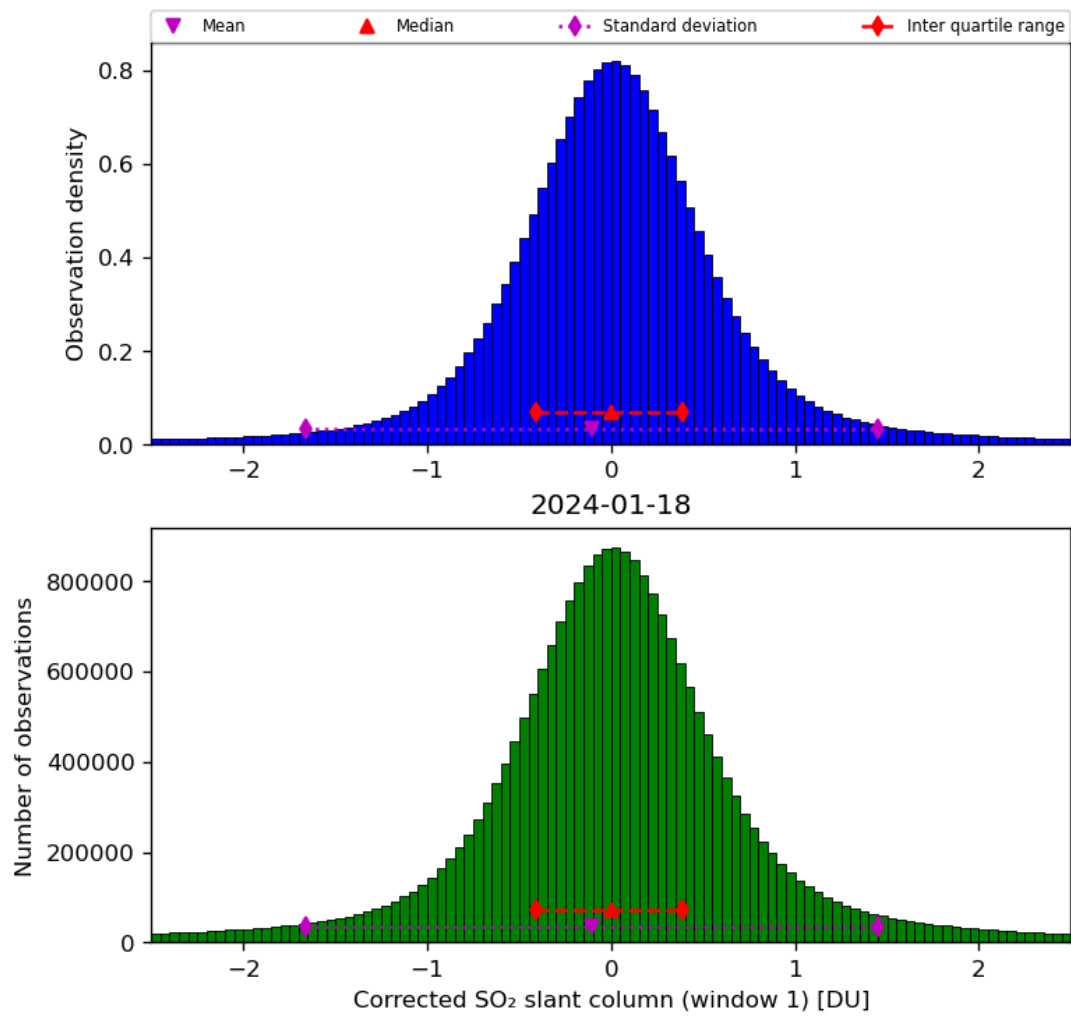
Figure 58: Histogram of “Corrected SO 2 slant column (window 1)” for 2024-01-17 to 2024-01-19
