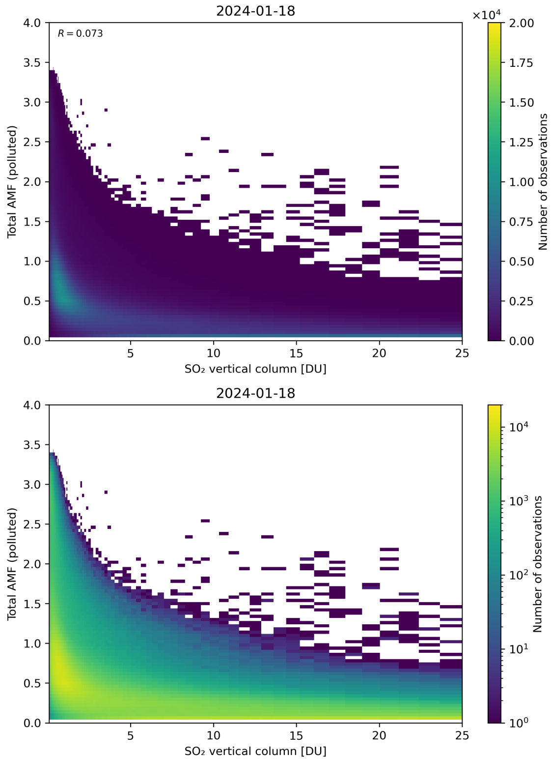
Figure 305: Scatter density plot of “SO 2 vertical column” against “Total AMF (polluted)” for 2024-01-17 to 2024-01-19.
