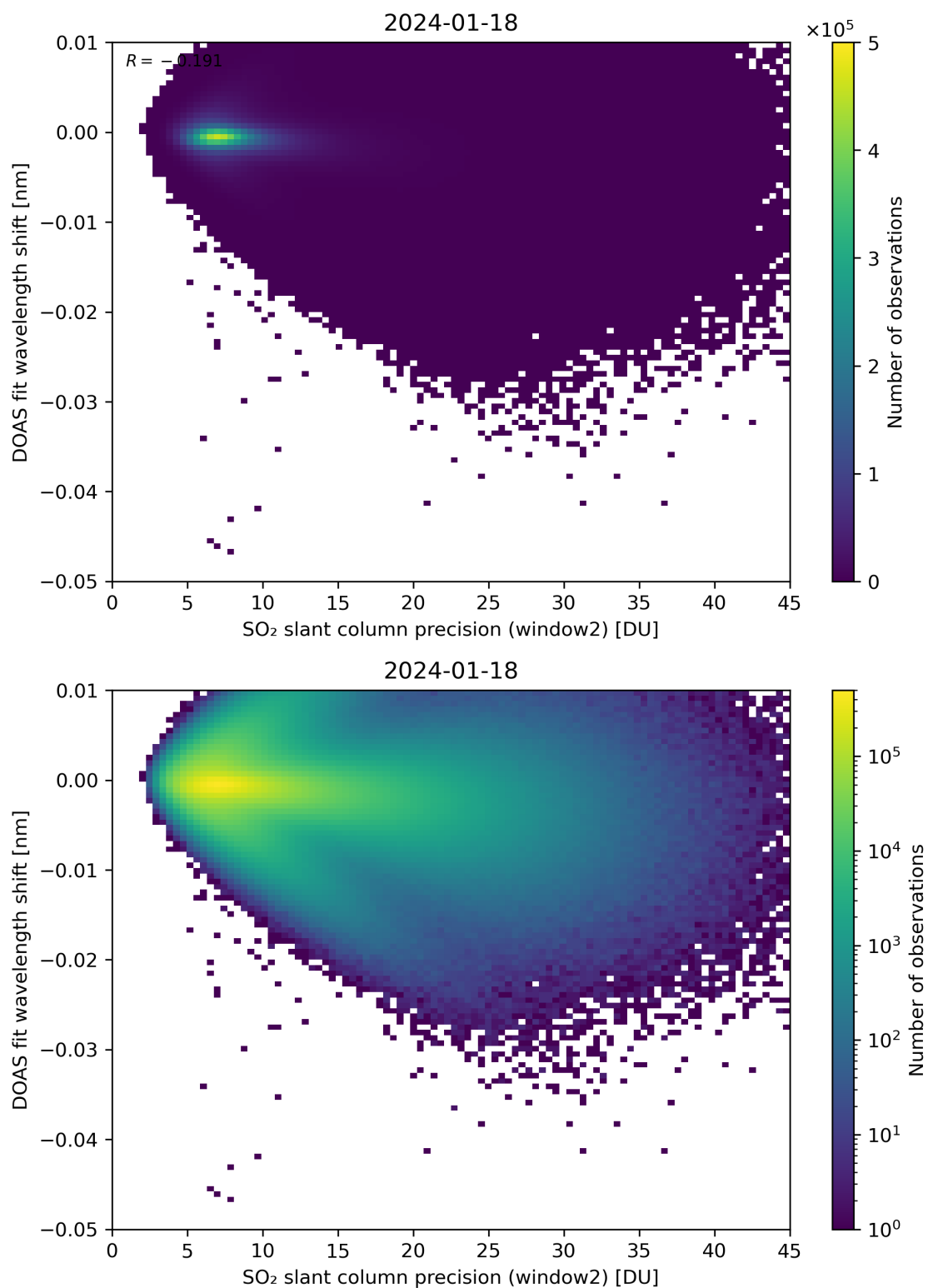
Figure 243: Scatter density plot of “SO 2 slant column precision (window2)” against “DOAS fit wavelength shift” for 2024-01-17 to 2024-01-19.
