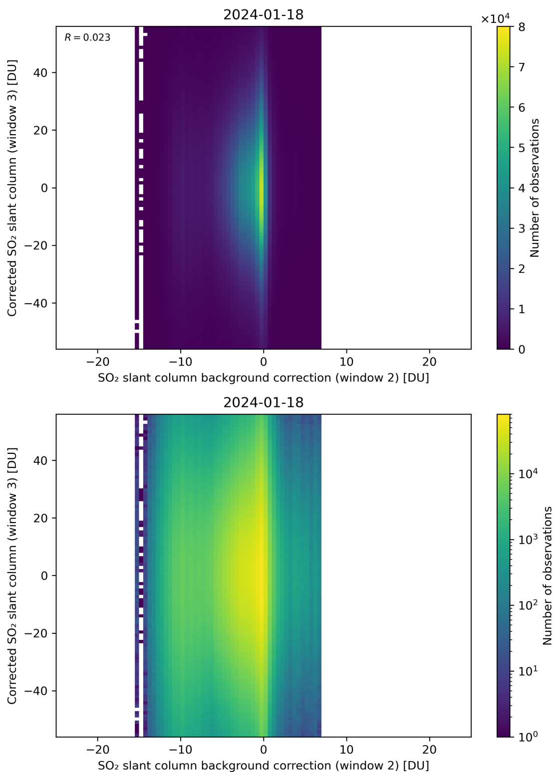
Figure 116: Scatter density plot of “SO 2 slant column background correction (window 2)” against “Corrected SO 2 slant column (window 3)” for 2024-01-17 to 2024-01-19.
