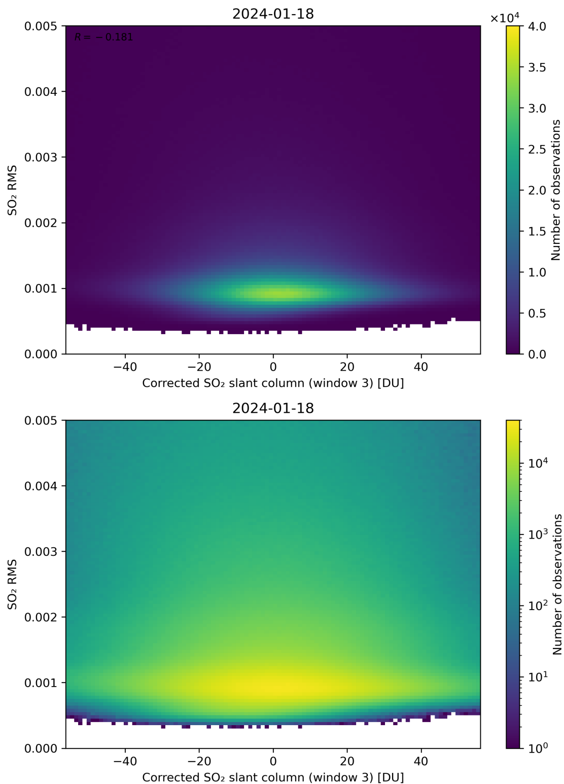
Figure 208: Scatter density plot of “Corrected SO 2 slant column (window 3)” against “SO 2 RMS” for 2024-01-17 to 2024-01-19.
