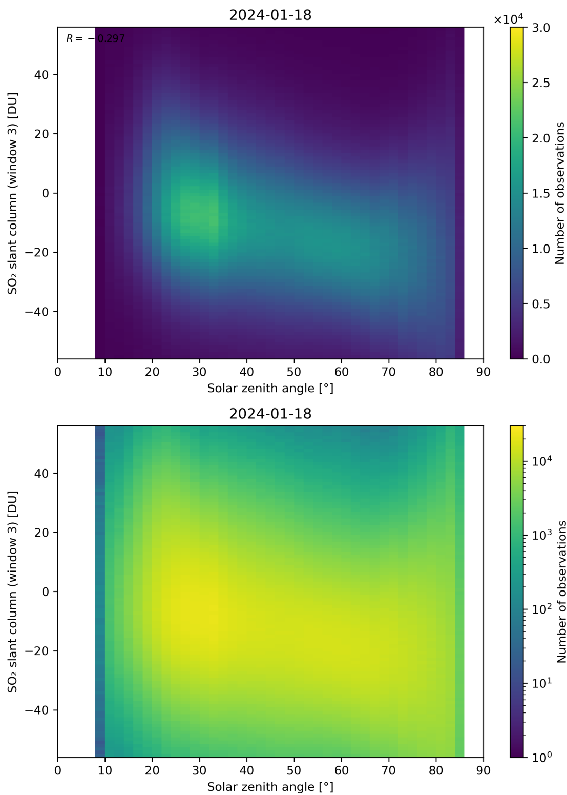
Figure 172: Scatter density plot of “Solar zenith angle” against “SO 2 slant column (window 3)” for 2024-01-17 to 2024-01-19.
