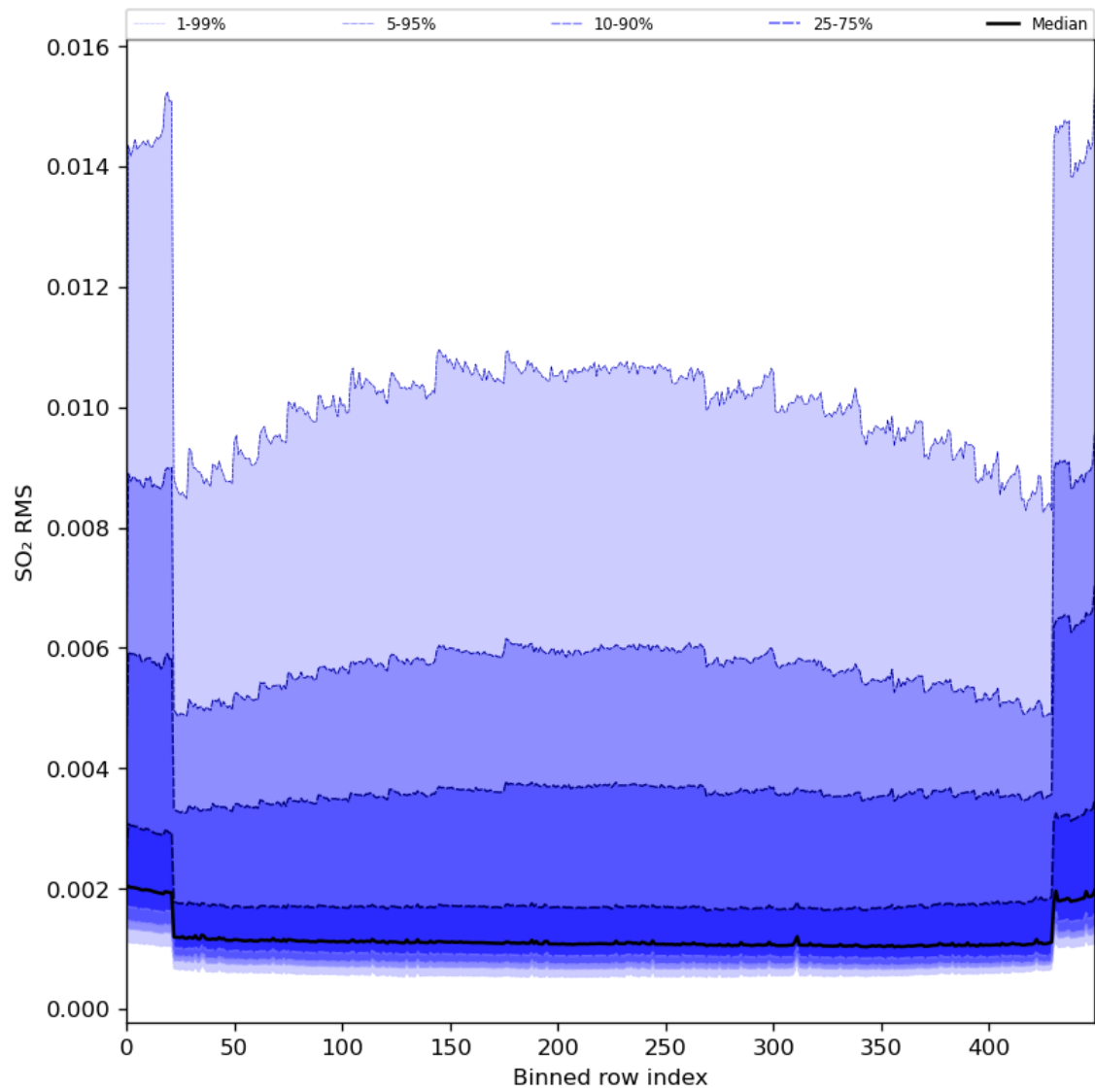
Figure 93: Along track statistics of “SO 2 RMS” for 2024-01-17 to 2024-01-19
