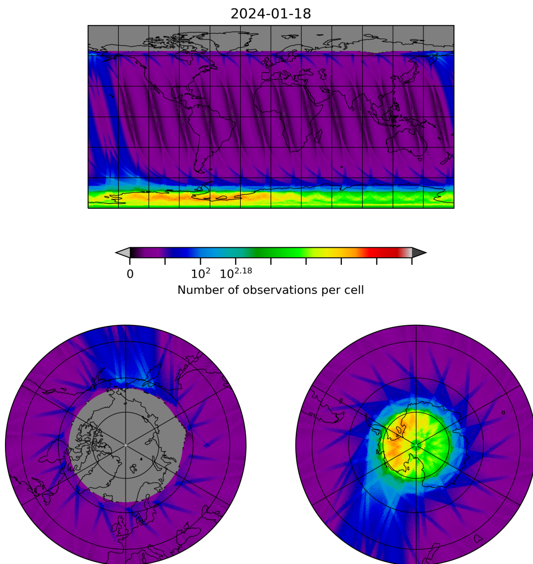
Figure 28: Map of the number of observations for 2024-01-17 to 2024-01-19
