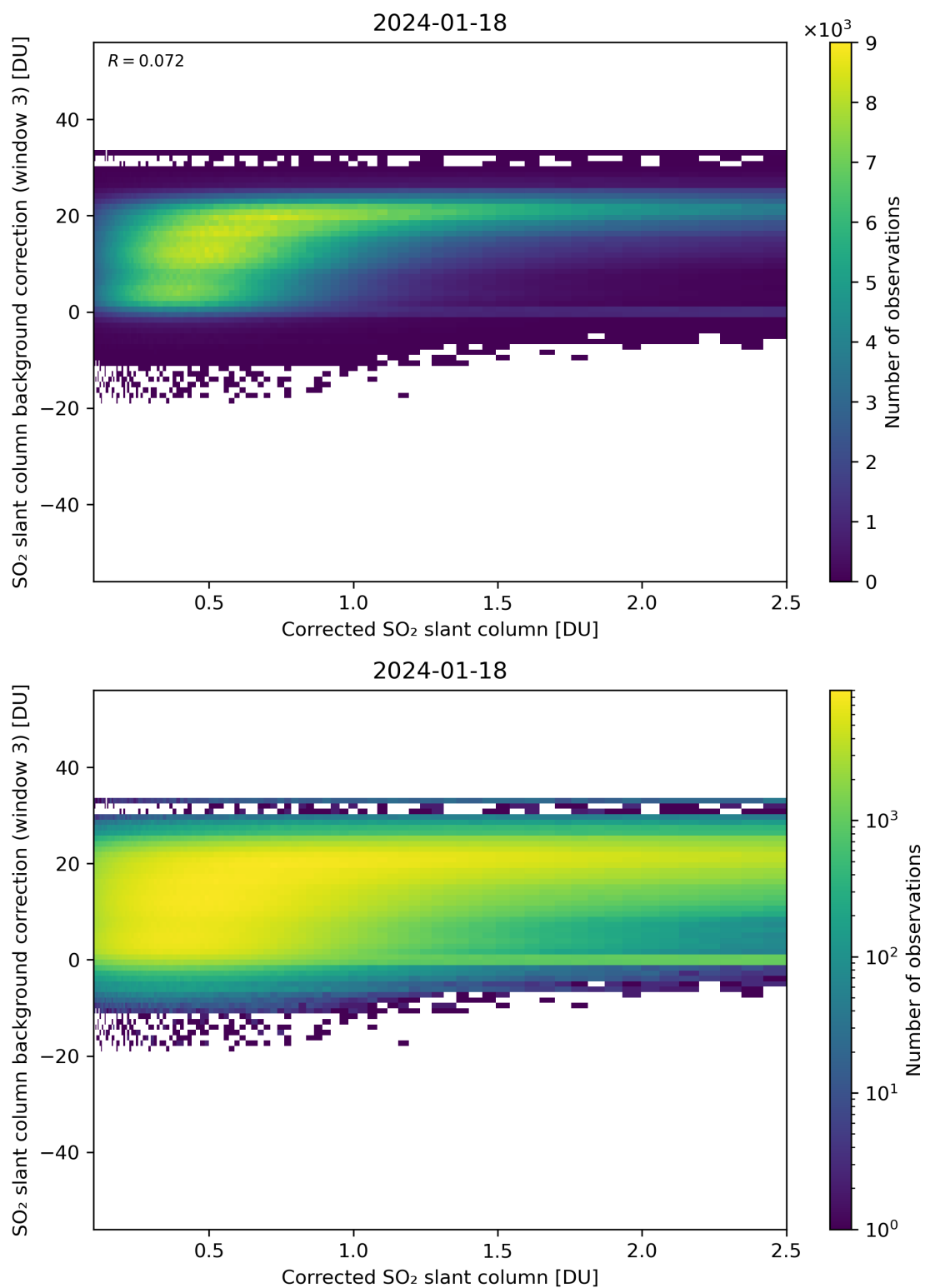
Figure 180: Scatter density plot of “Corrected SO 2 slant column” against “SO 2 slant column background correction (window 3)” for 2024-01-17 to 2024-01-19.
