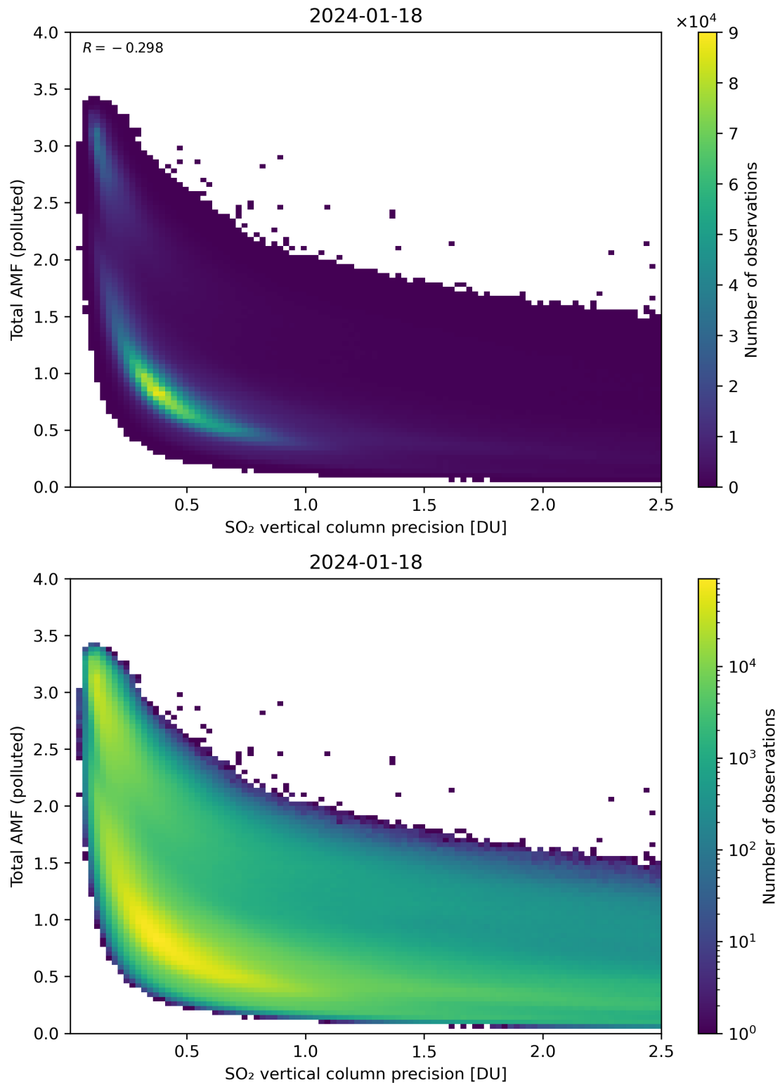
Figure 294: Scatter density plot of “SO 2 vertical column precision” against “Total AMF (polluted)” for 2024-01-17 to 2024-01-19.
