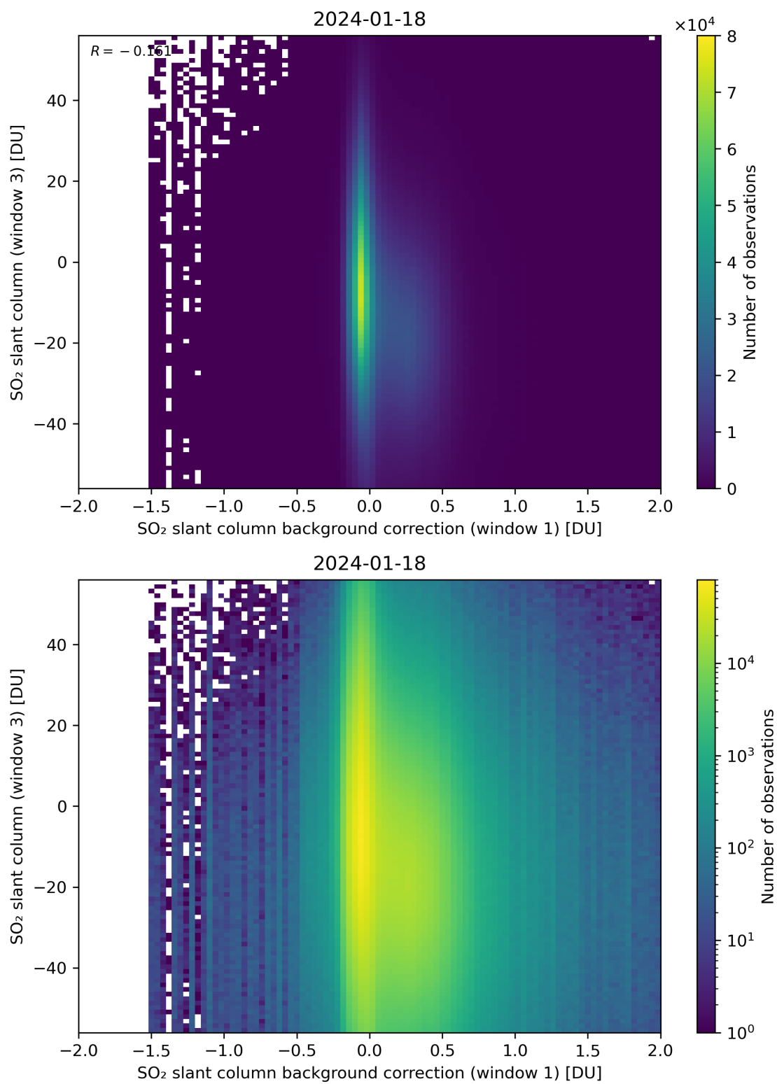
Figure 107: Scatter density plot of “SO 2 slant column background correction (window 1)” against “SO 2 slant column (window 3)” for 2024-01-17 to 2024-01-19.
