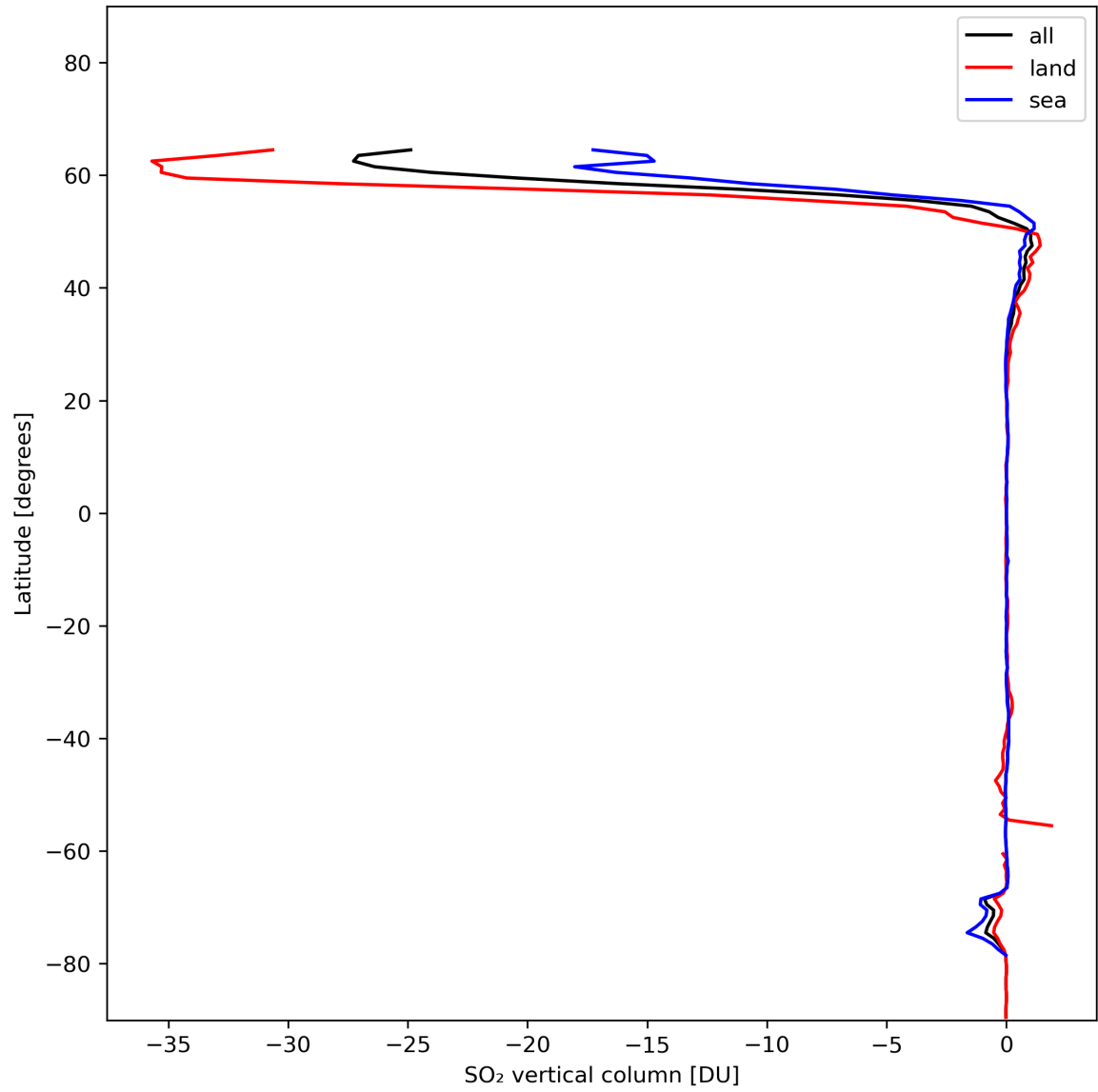
Figure 30: Zonal average of “SO 2 vertical column” for 2024-01-17 to 2024-01-19.
