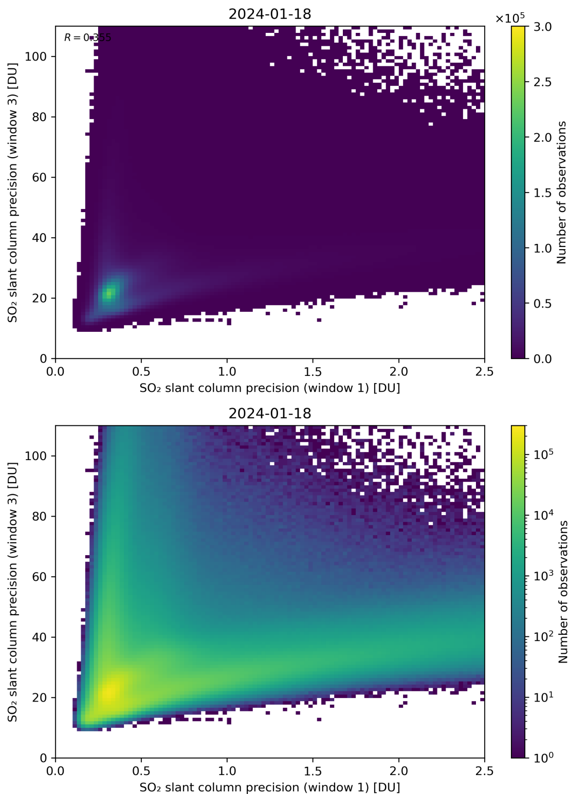
Figure 229: Scatter density plot of “SO 2 slant column precision (window 1)” against “SO 2 slant column precision (window 3)” for 2024-01-17 to 2024-01-19.
