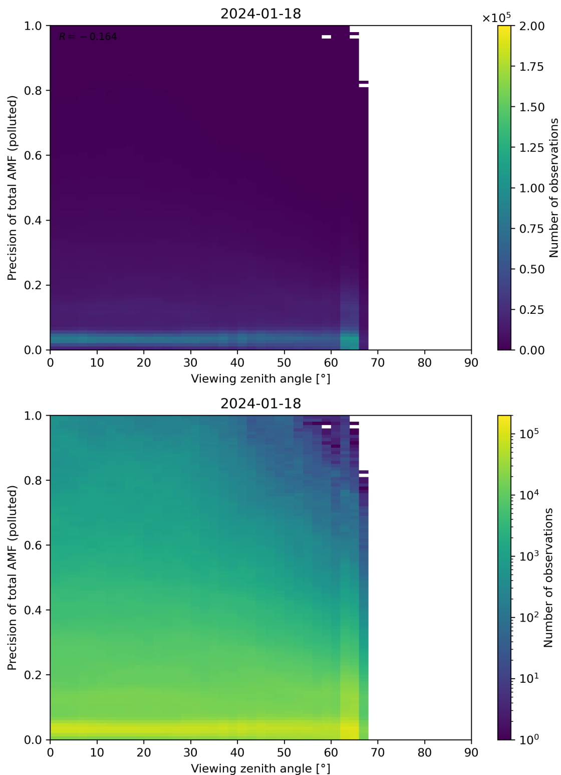
Figure 326: Scatter density plot of “Viewing zenith angle” against “Precision of total AMF (polluted)” for 2024-01-17 to 2024-01-19.
