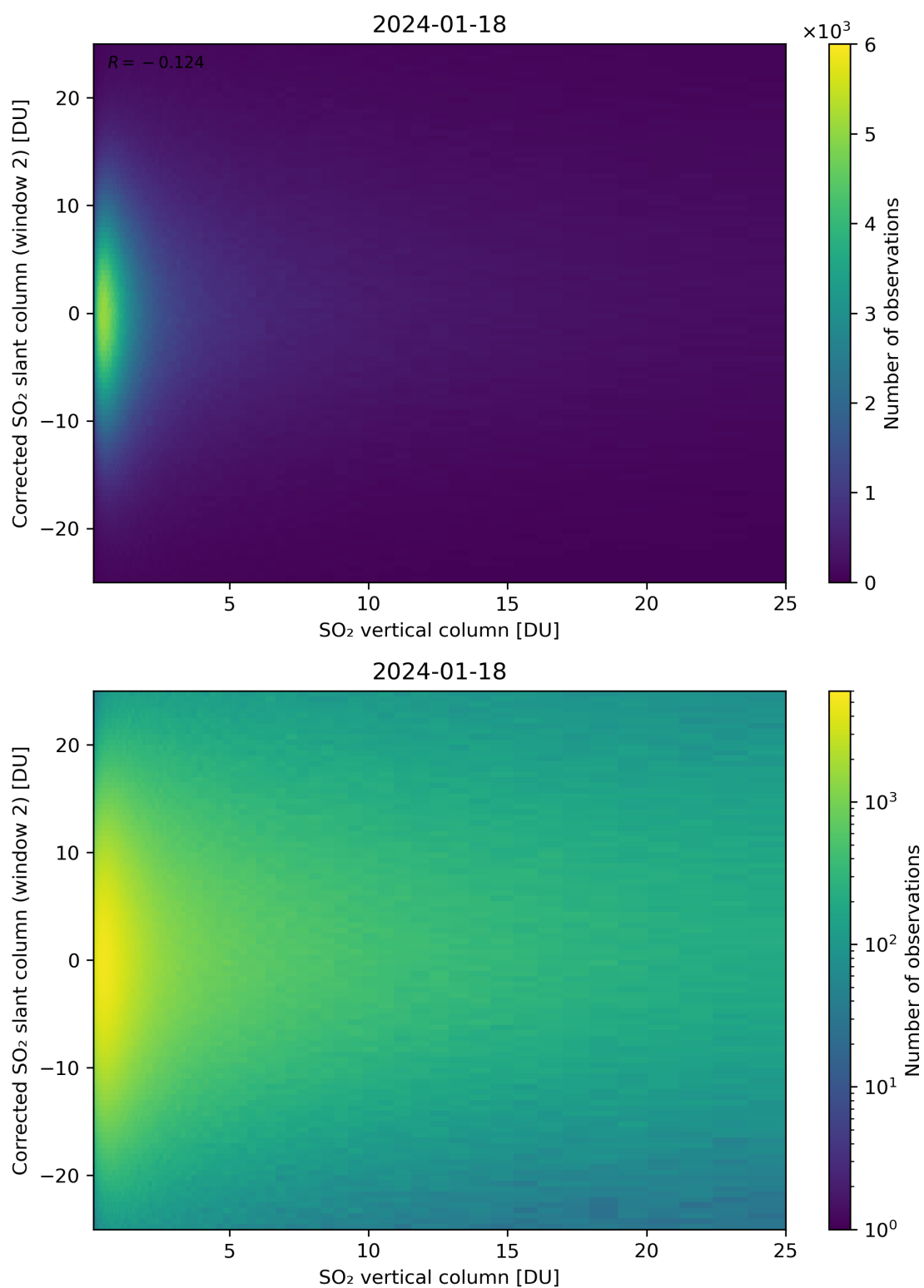
Figure 298: Scatter density plot of “SO 2 vertical column” against “Corrected SO 2 slant column (window 2)” for 2024-01-17 to 2024-01-19.
