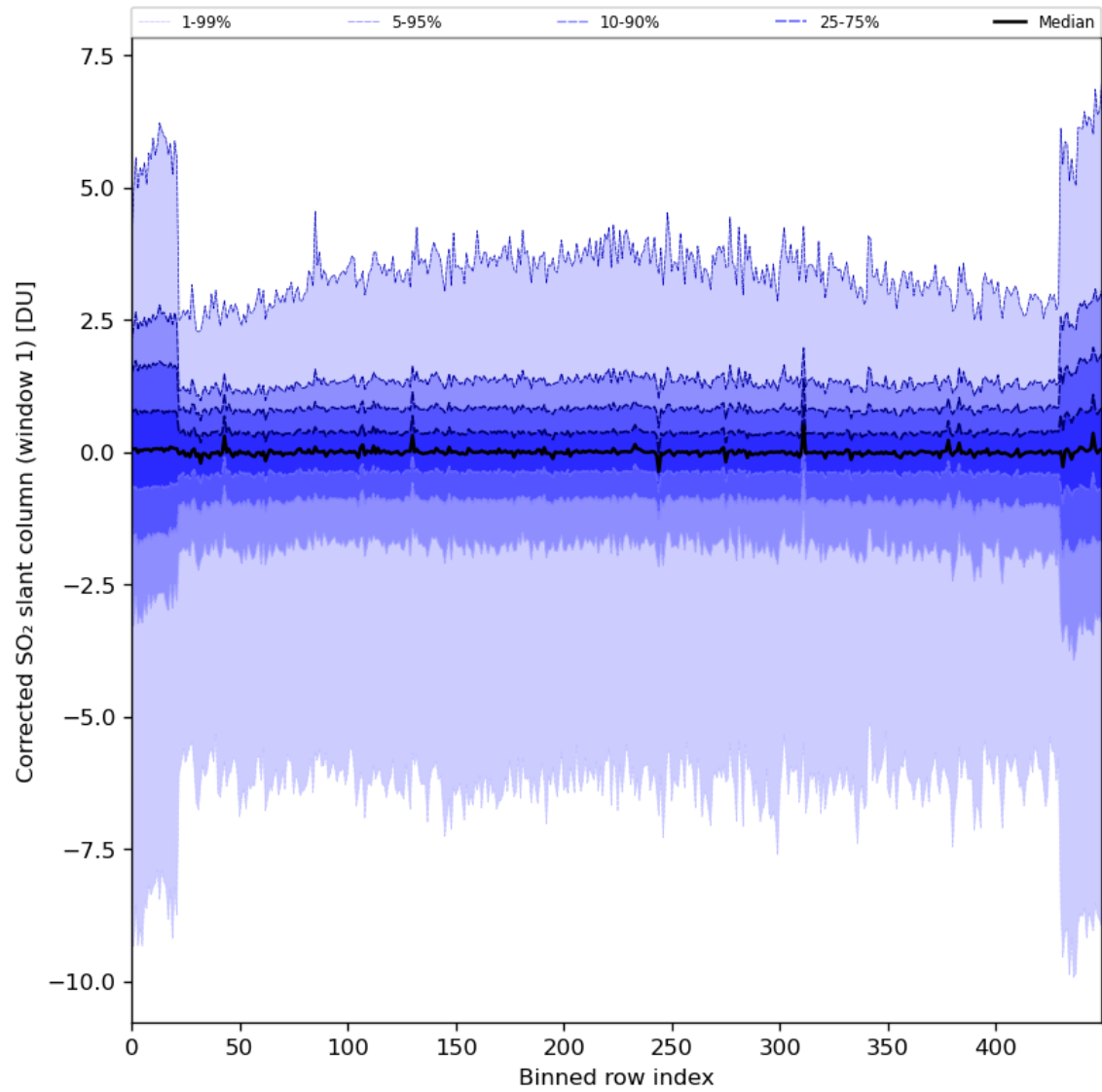
Figure 81: Along track statistics of “Corrected SO 2 slant column (window 1)” for 2024-01-17 to 2024-01-19
