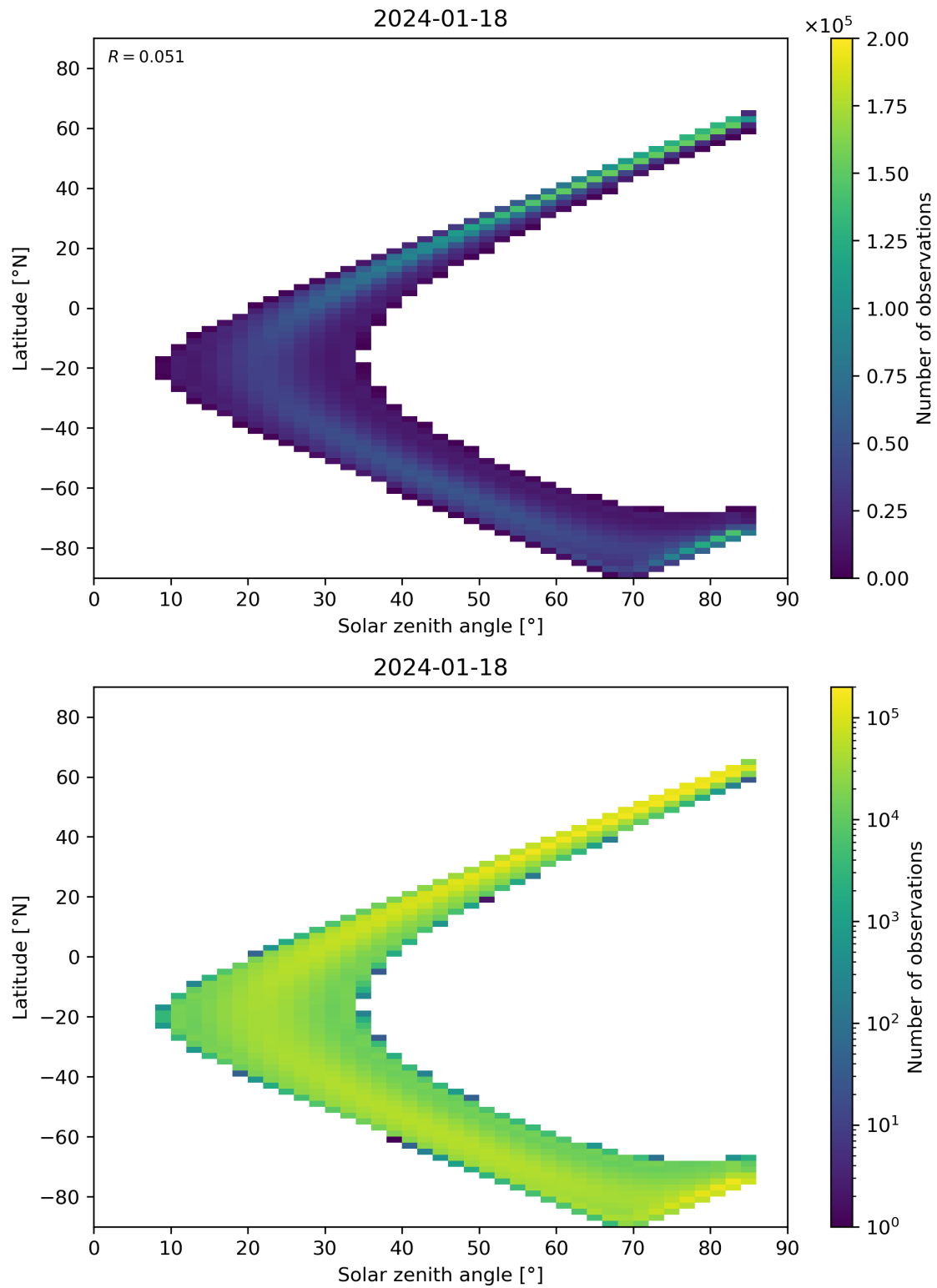
Figure 164: Scatter density plot of “Solar zenith angle” against “Latitude” for 2024-01-17 to 2024-01-19.
