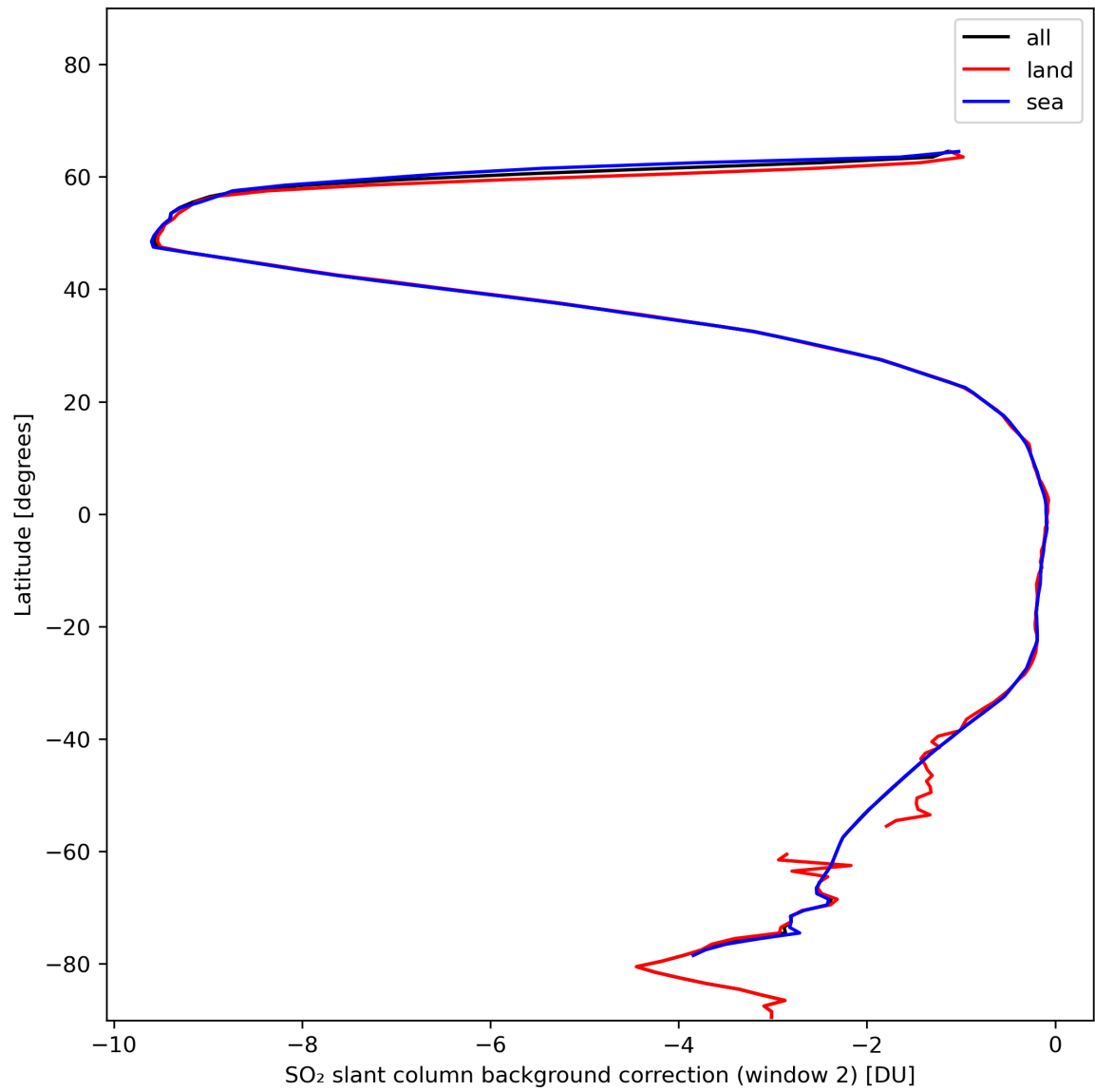
Figure 40: Zonal average of “SO 2 slant column background correction (window 2)” for 2024-01-17 to 2024-01-19.
