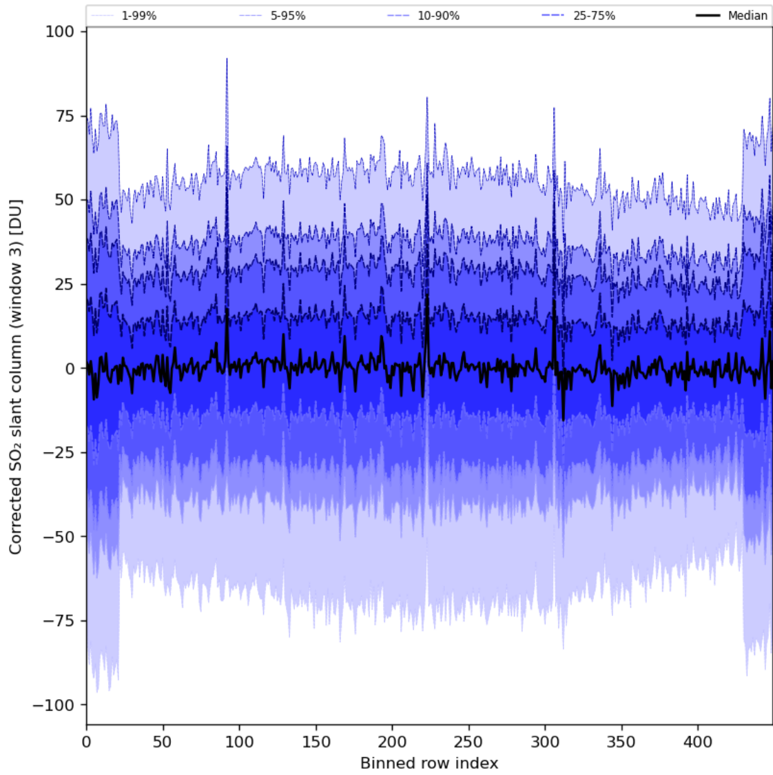
Figure 89: Along track statistics of "Corrected SO 2 slant column (window 3)" for 2024-01-17 to 2024-01-19
