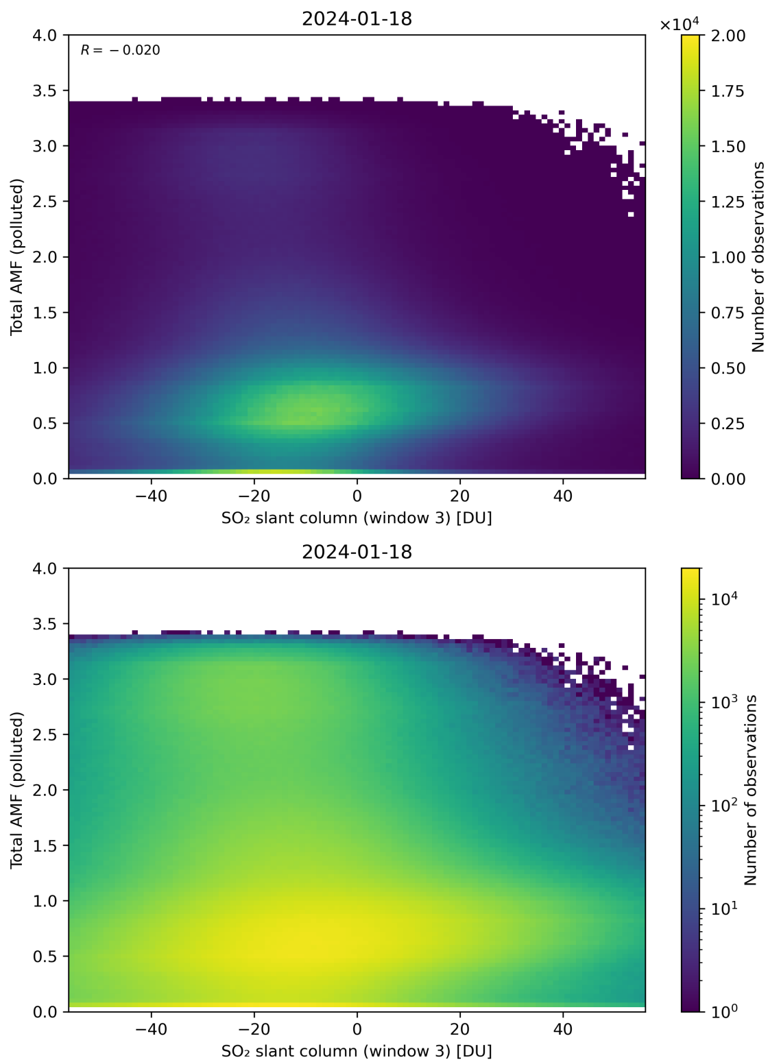
Figure 268: Scatter density plot of “SO 2 slant column (window 3)” against “Total AMF (polluted)” for 2024-01-17 to 2024-01-19.
