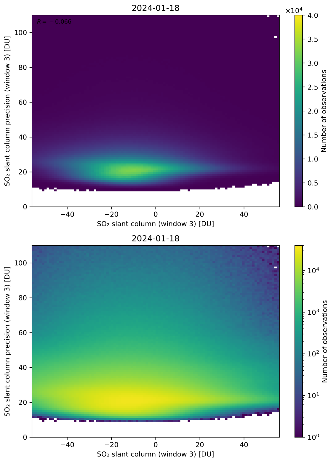
Figure 267: Scatter density plot of “SO 2 slant column (window 3)” against “SO 2 slant column precision (window 3)” for 2024-01-17 to 2024-01-19.
