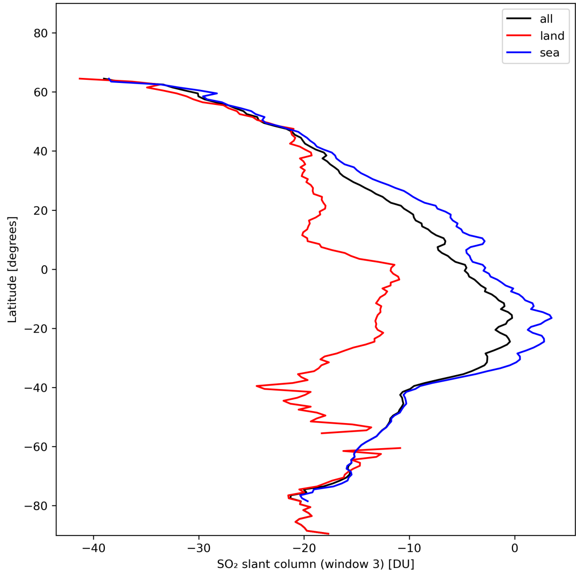
Figure 41: Zonal average of “SO 2 slant column (window 3)” for 2024-01-17 to 2024-01-19.
