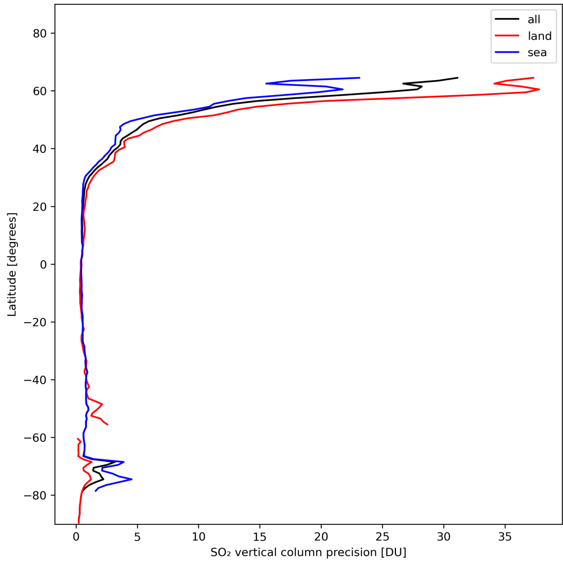
Figure 31: Zonal average of “SO 2 vertical column precision” for 2024-01-17 to 2024-01-19.
