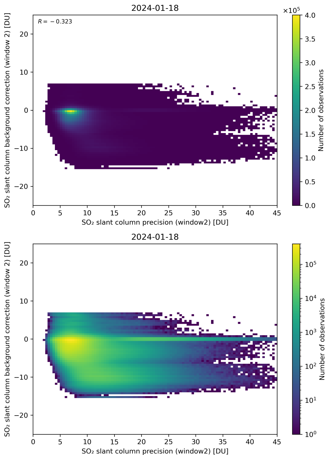
Figure 241: Scatter density plot of “SO 2 slant column precision (window2)” against “SO 2 slant column background correction (window 2)” for 2024-01-17 to 2024-01-19.
