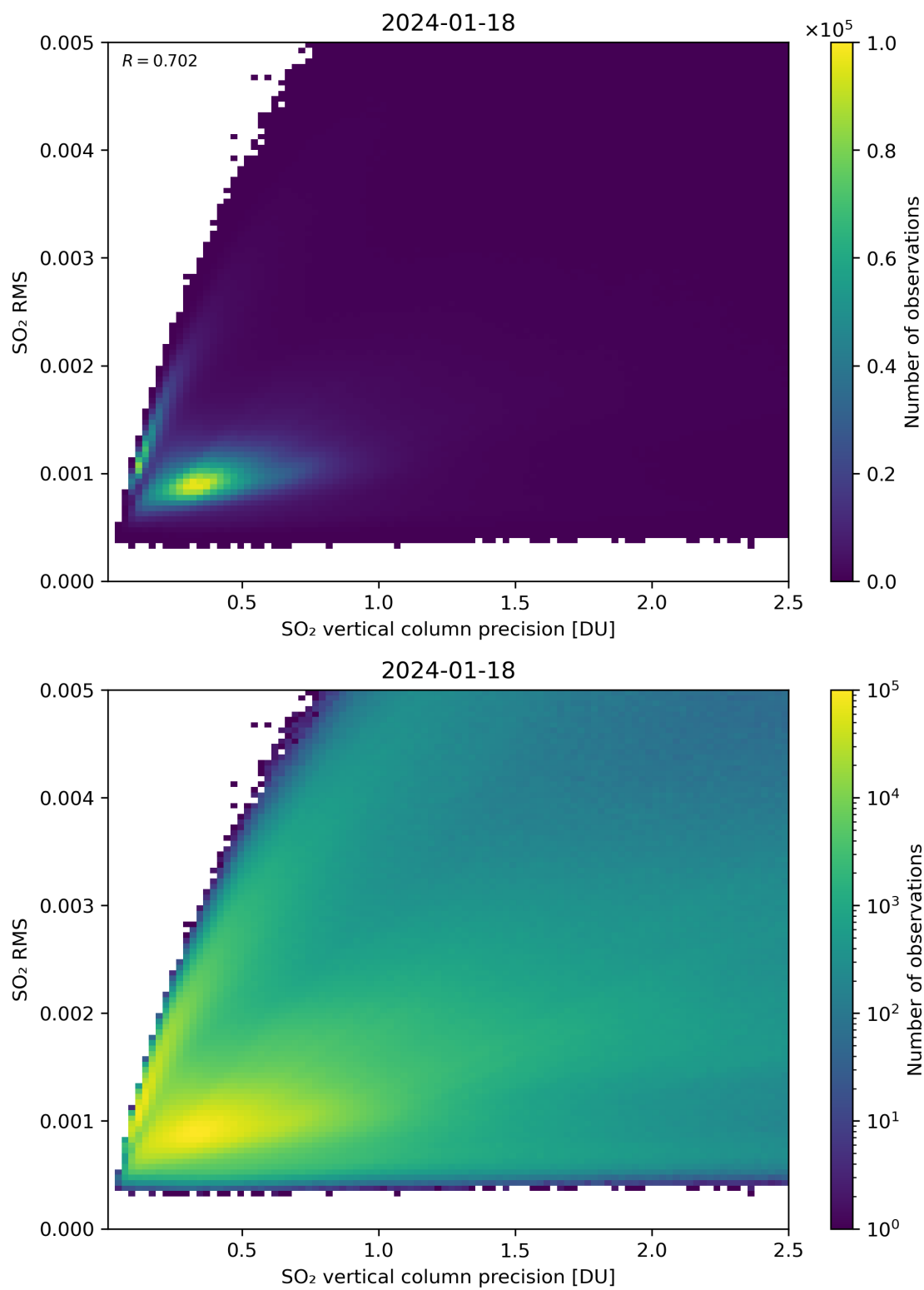
Figure 284: Scatter density plot of “SO 2 vertical column precision” against “SO 2 RMS” for 2024-01-17 to 2024-01-19.
