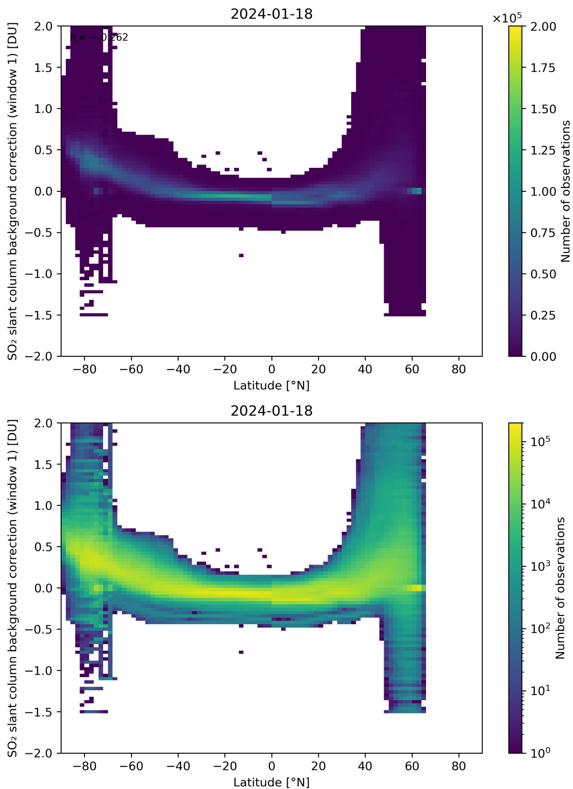
Figure 139: Scatter density plot of “Latitude” against “SO 2 slant column background correction (window 1)” for 2024-01-17 to 2024-01-19.
