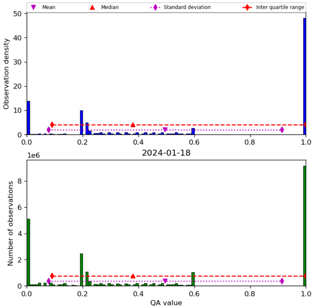
Figure 52: Histogram of “QA value” for 2024-01-17 to 2024-01-19
