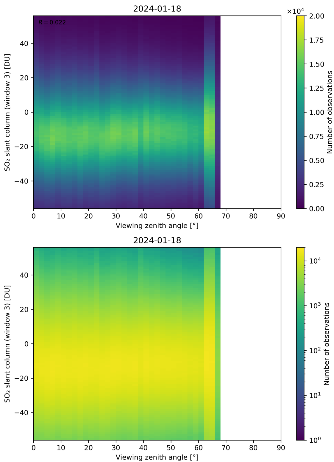
Figure 323: Scatter density plot of “Viewing zenith angle” against “SO 2 slant column (window 3)” for 2024-01-17 to 2024-01-19.
