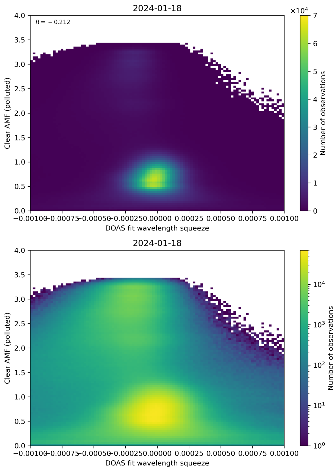
Figure 133: Scatter density plot of “DOAS fit wavelength squeeze” against “Clear AMF (polluted)” for 2024-01-17 to 2024-01-19.
