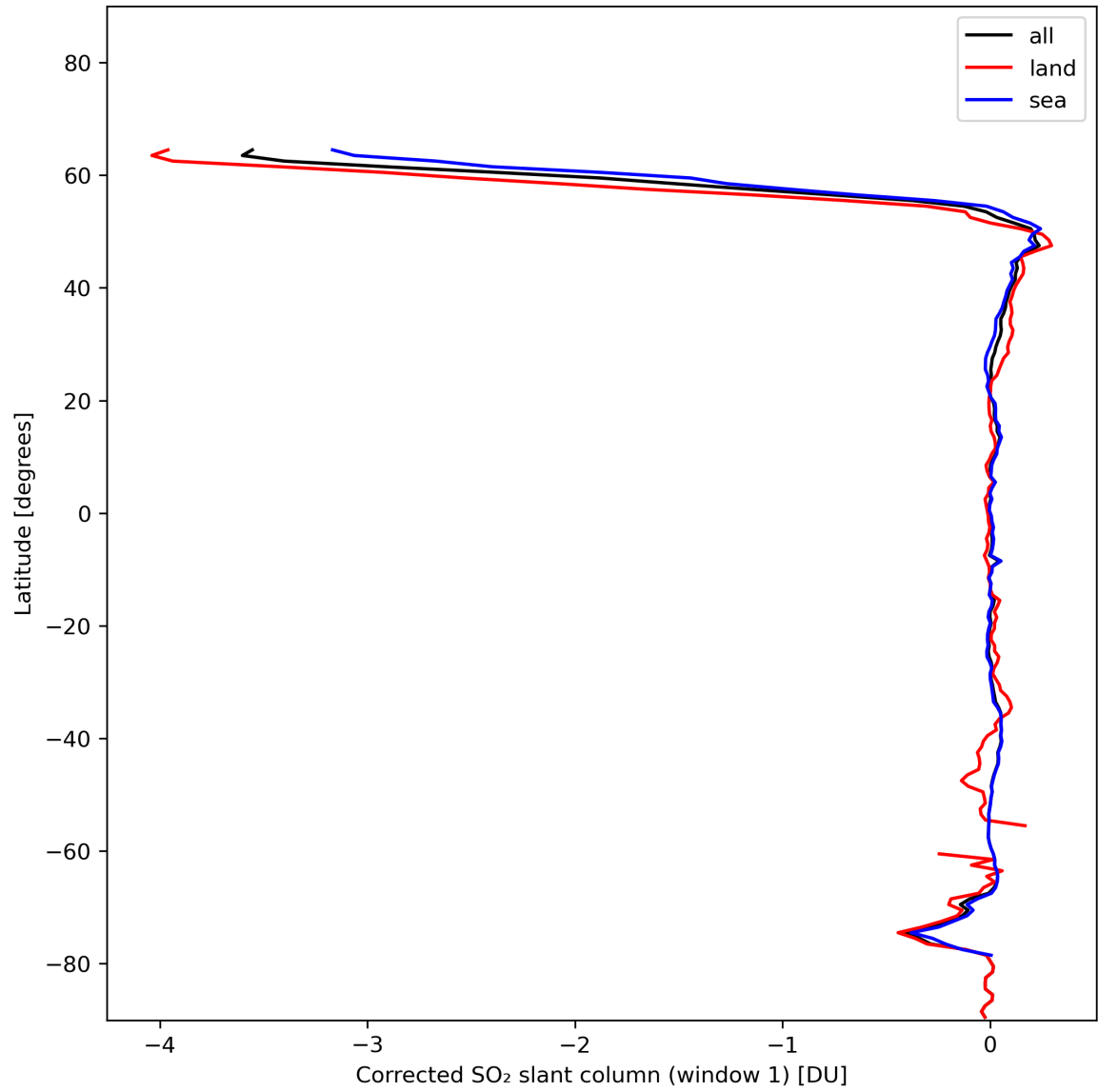
Figure 35: Zonal average of “Corrected SO 2 slant column (window 1)” for 2024-01-17 to 2024-01-19.
