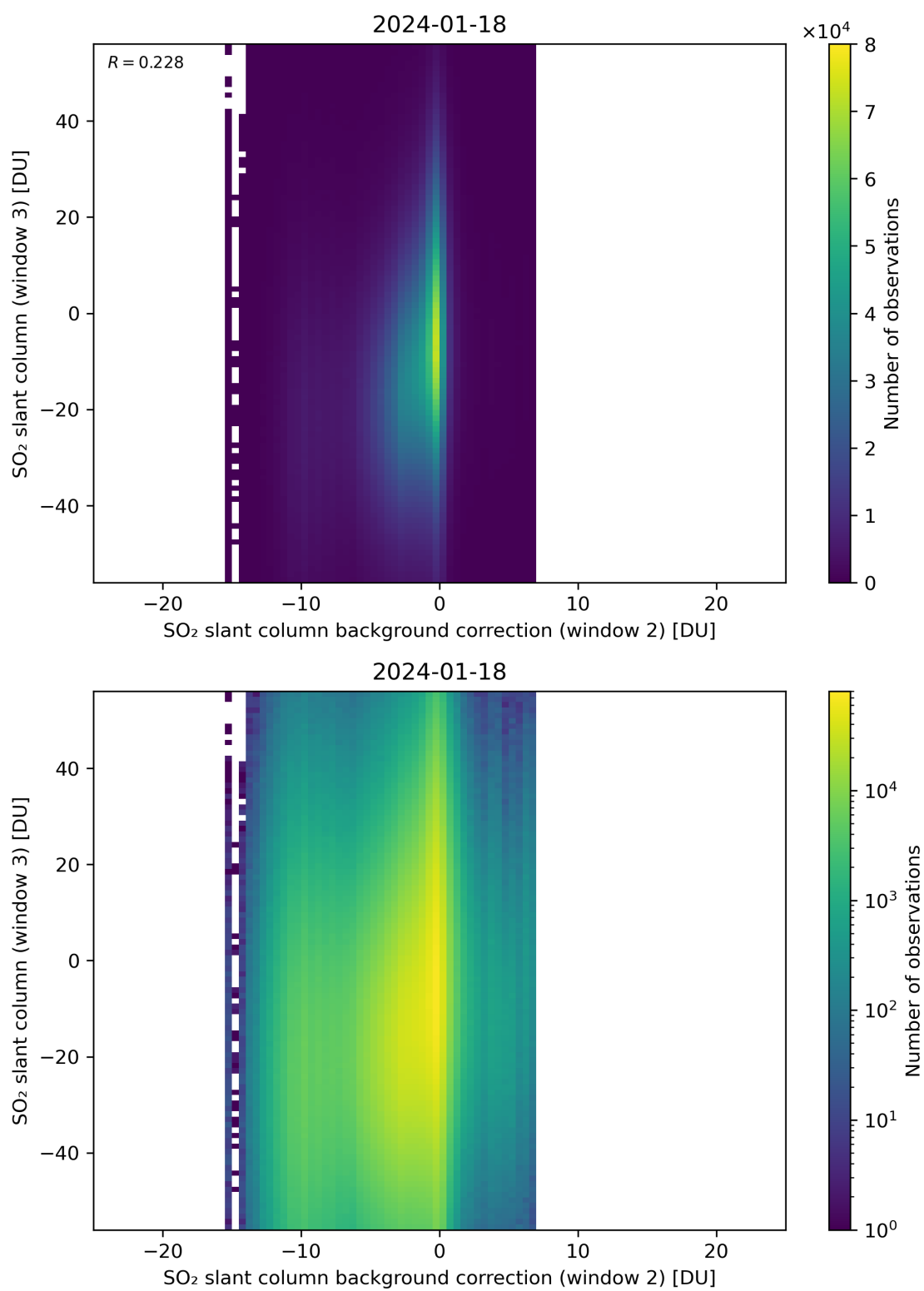
Figure 117: Scatter density plot of “SO 2 slant column background correction (window 2)” against “SO 2 slant column (window 3)” for 2024-01-17 to 2024-01-19.
