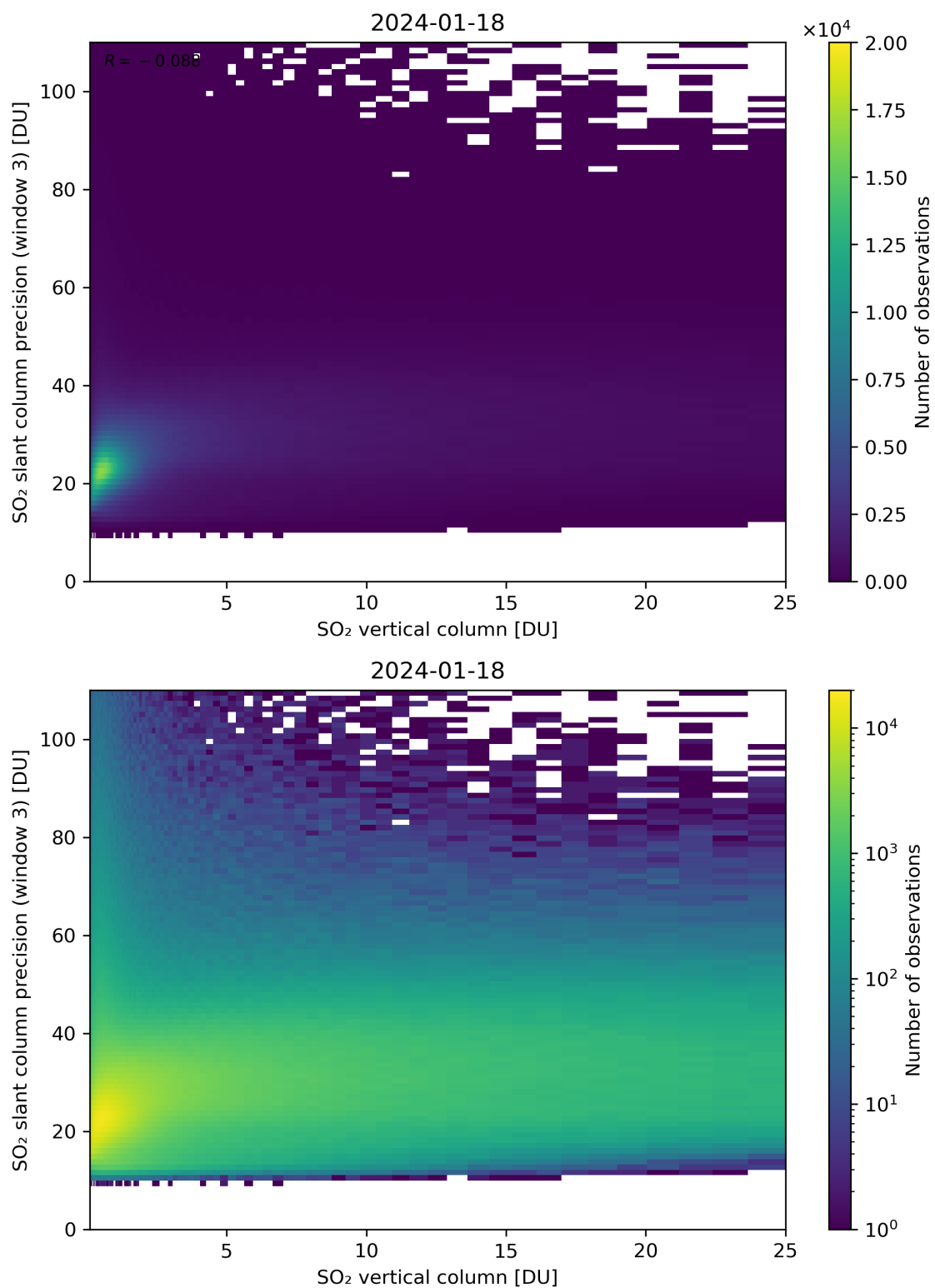
Figure 304: Scatter density plot of “SO 2 vertical column” against “SO 2 slant column precision (window 3)” for 2024-01-17 to 2024-01-19.
