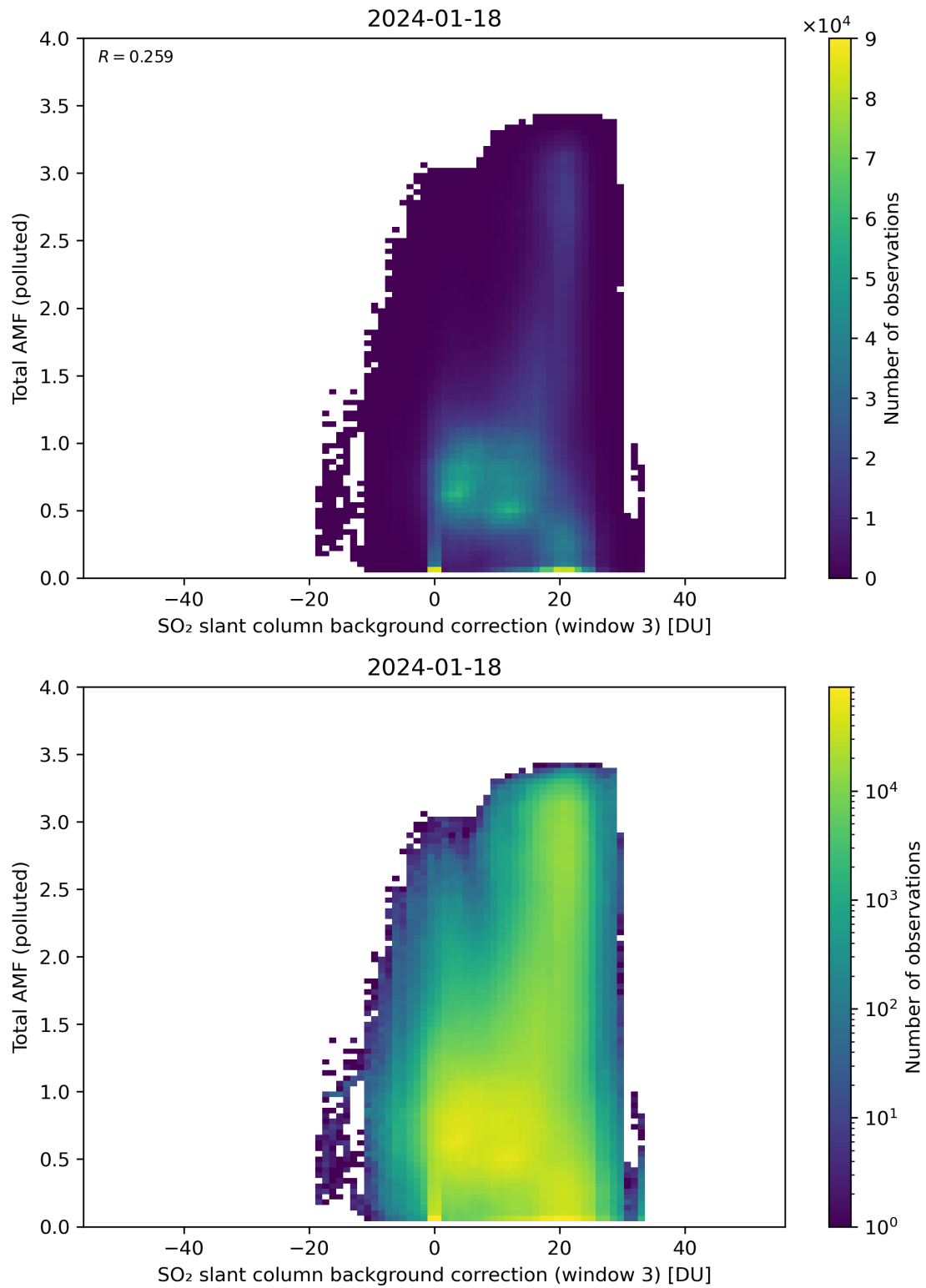
Figure 125: Scatter density plot of “SO 2 slant column background correction (window 3)” against “Total AMF (polluted)” for 2024-01-17 to 2024-01-19.
