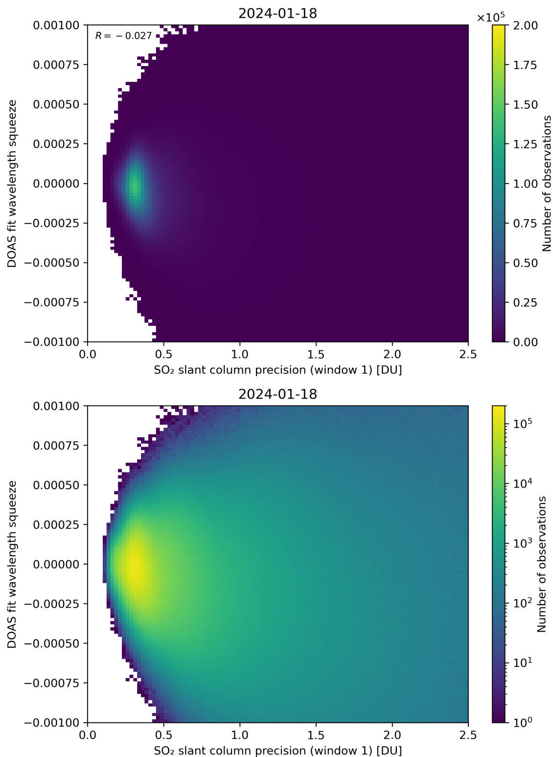
Figure 222: Scatter density plot of “SO 2 slant column precision (window 1)” against “DOAS fit wavelength squeeze” for 2024-01-17 to 2024-01-19.
