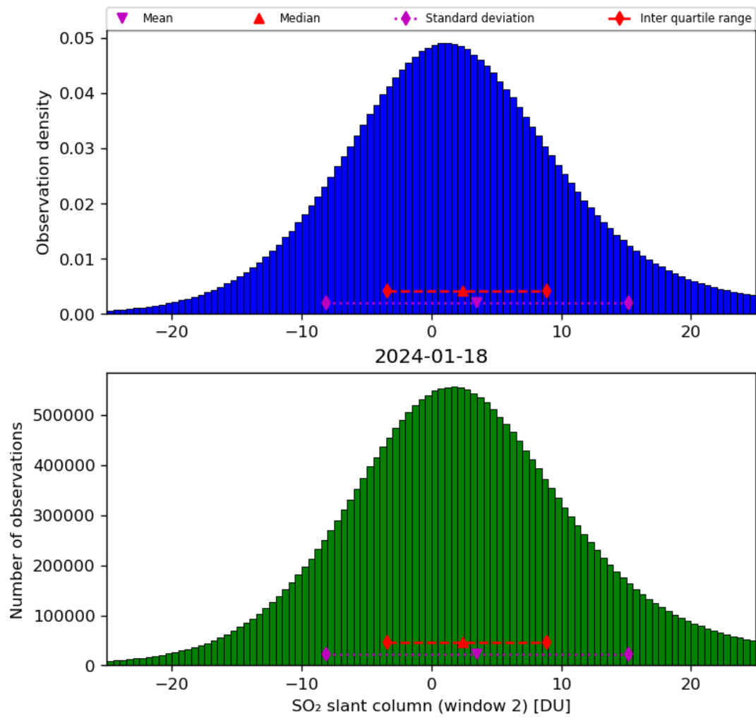
Figure 60: Histogram of “SO 2 slant column (window 2)” for 2024-01-17 to 2024-01-19
