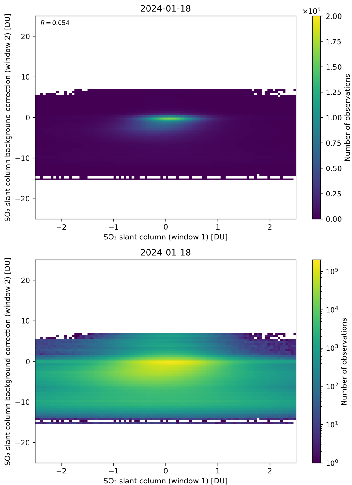
Figure 213: Scatter density plot of “SO 2 slant column (window 1)” against “SO 2 slant column background correction (window 2)” for 2024-01-17 to 2024-01-19.
