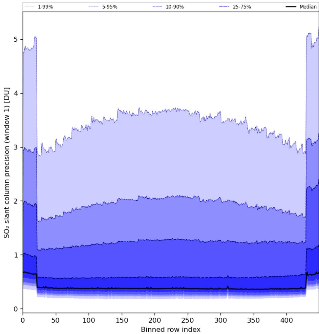
Figure 80: Along track statistics of “SO 2 slant column precision (window 1)” for 2024-01-17 to 2024-01-19
