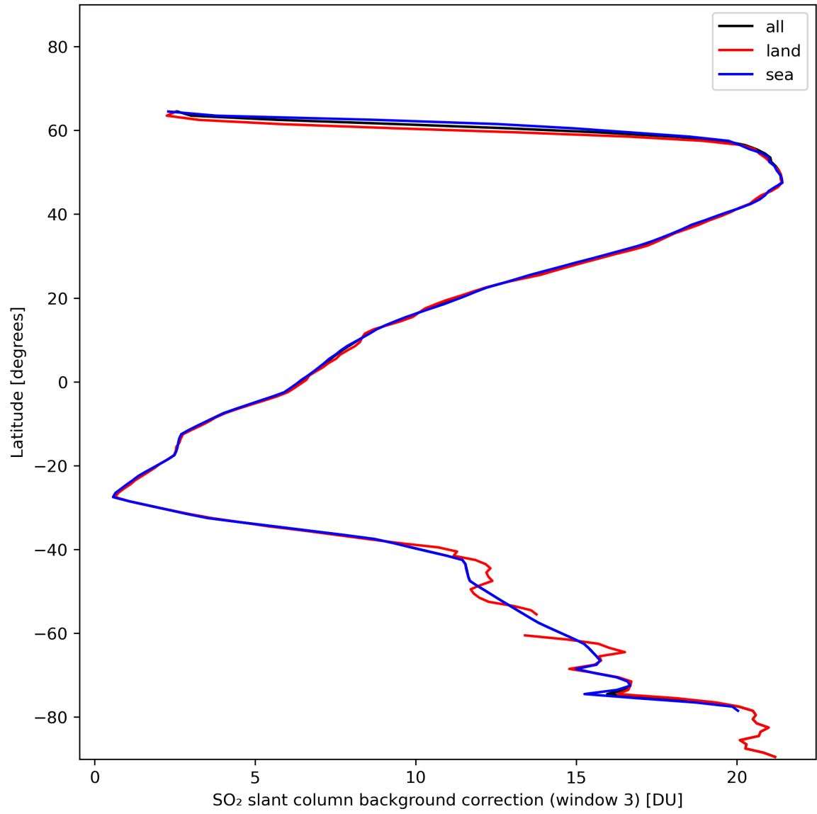
Figure 44: Zonal average of “SO 2 slant column background correction (window 3)” for 2024-01-17 to 2024-01-19.
