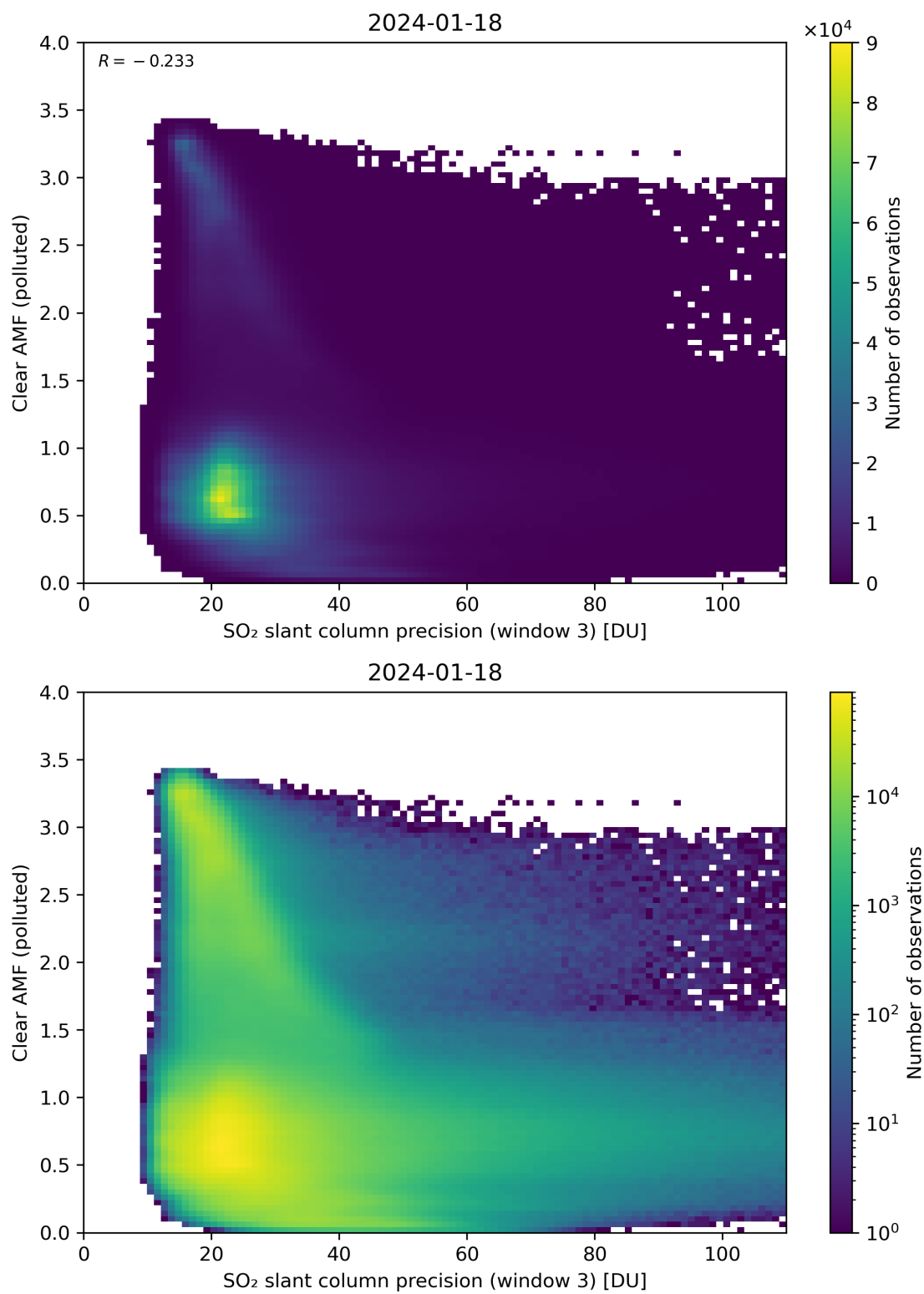
Figure 261: Scatter density plot of “SO 2 slant column precision (window 3)” against “Clear AMF (polluted)” for 2024-01-17 to 2024-01-19.
