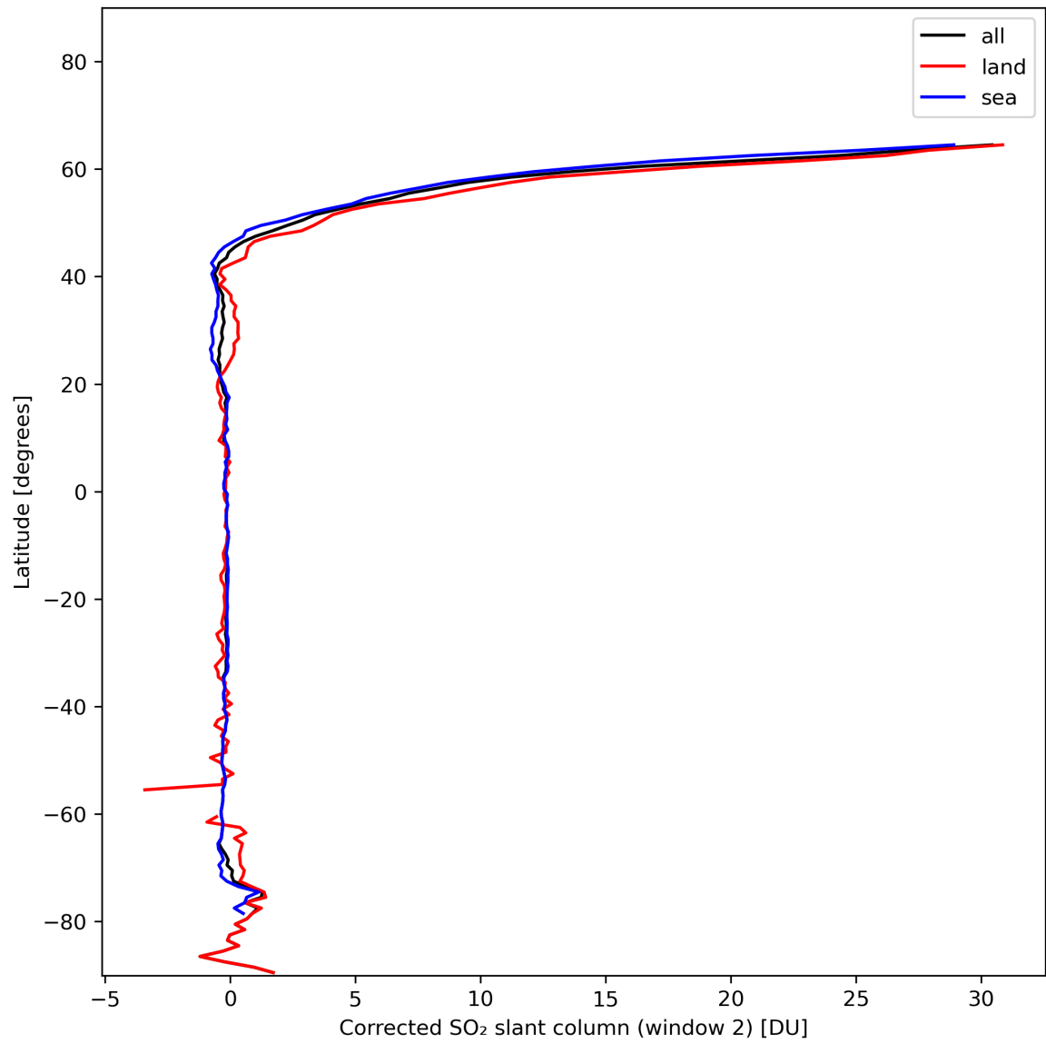
Figure 39: Zonal average of “Corrected SO 2 slant column (window 2)” for 2024-01-17 to 2024-01-19.
