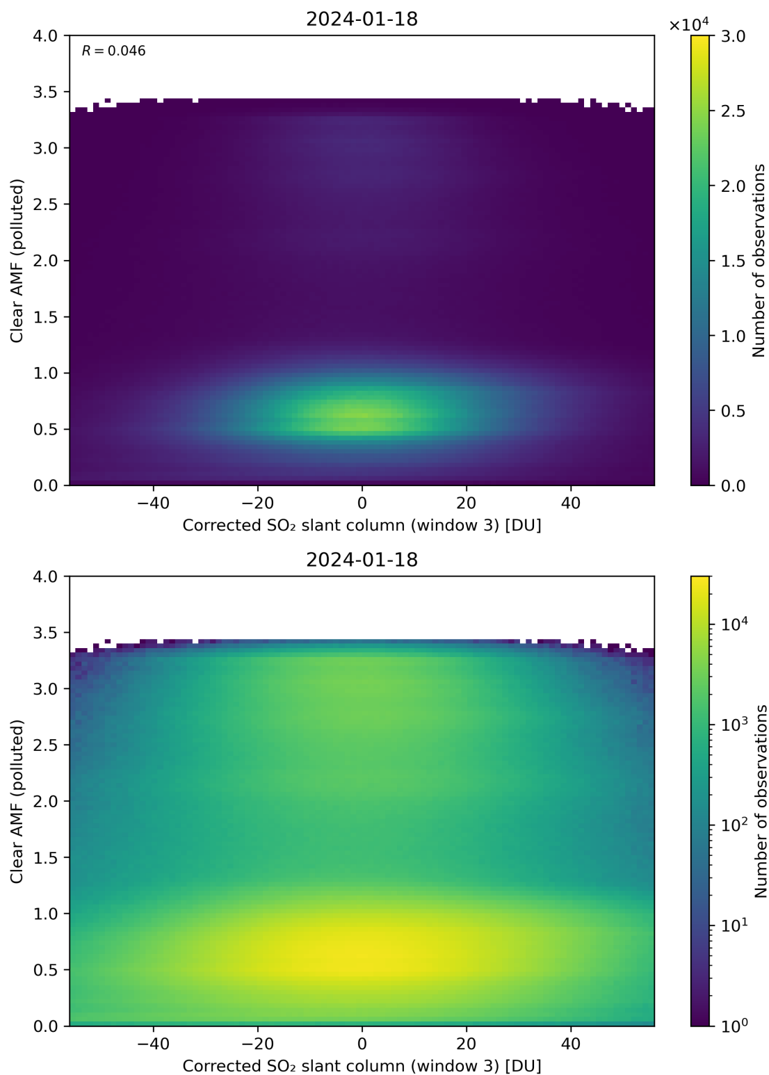
Figure 209: Scatter density plot of “Corrected SO 2 slant column (window 3)” against “Clear AMF (polluted)” for 2024-01-17 to 2024-01-19.
