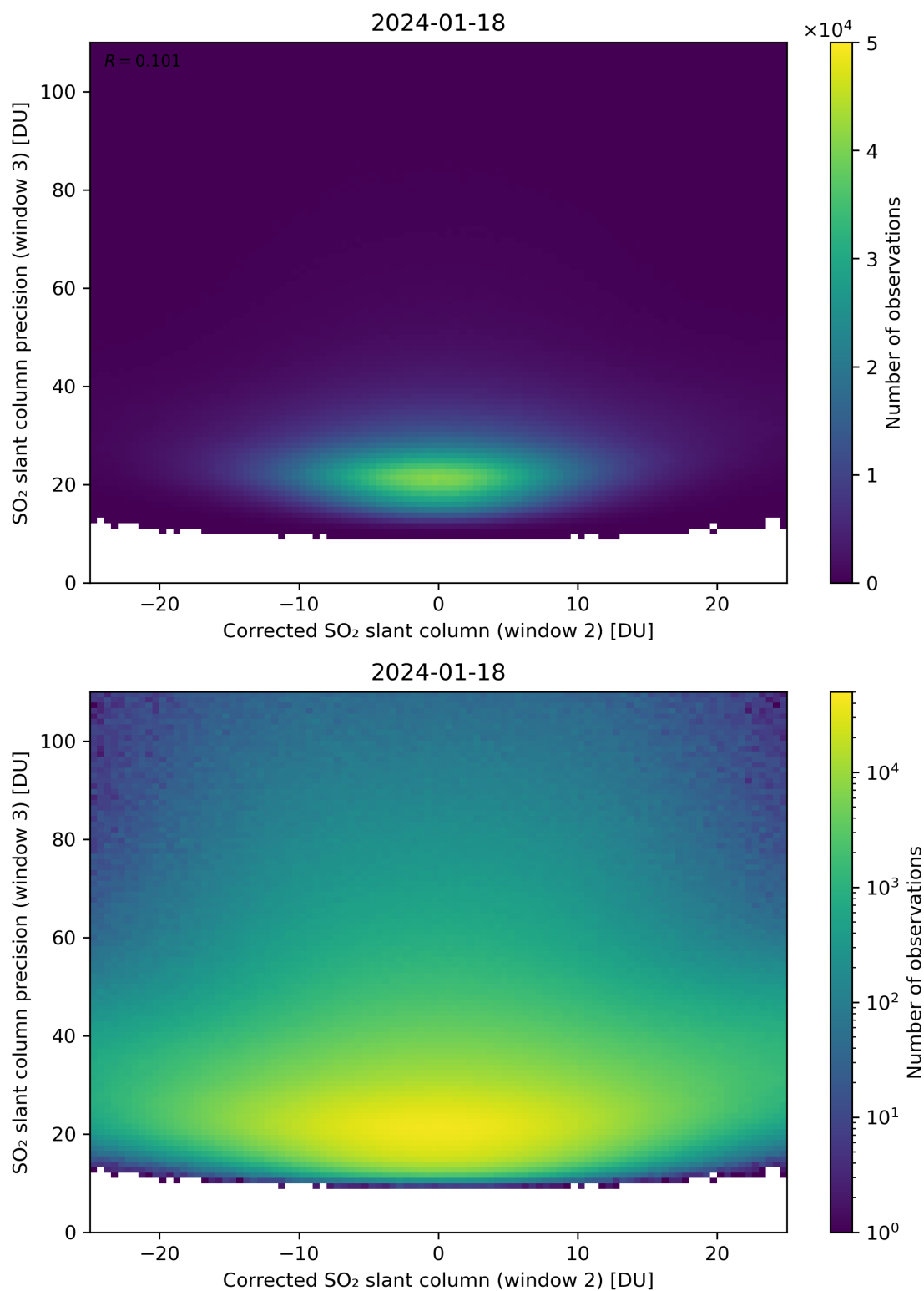
Figure 202: Scatter density plot of “Corrected SO 2 slant column (window 2)” against “SO 2 slant column precision (window 3)” for 2024-01-17 to 2024-01-19.
