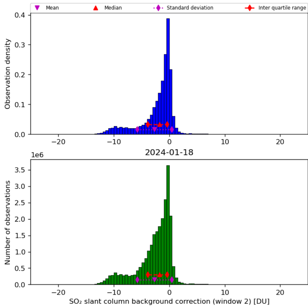
Figure 63: Histogram of “SO 2 slant column background correction (window 2)” for 2024-01-17 to 2024-01-19
