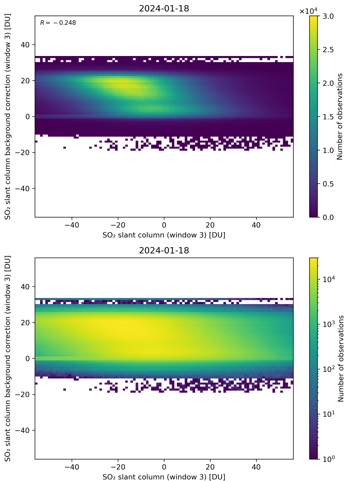
Figure 253: Scatter density plot of “SO 2 slant column (window 3)” against “SO 2 slant column background correction (window 3)” for 2024-01-17 to 2024-01-19.
