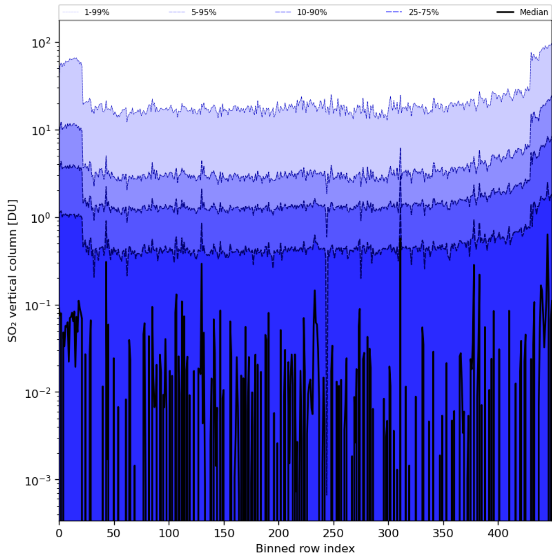
Figure 76: Along track statistics of “SO 2 vertical column” for 2024-01-17 to 2024-01-19
