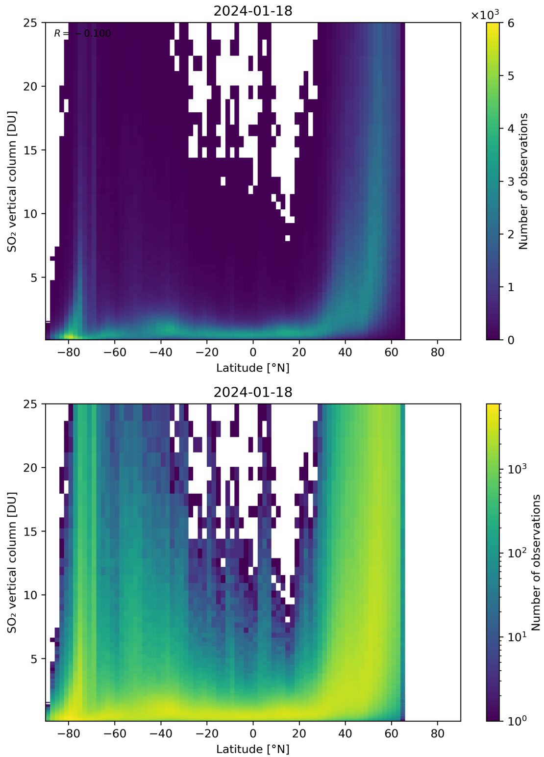
Figure 156: Scatter density plot of “Latitude” against “SO 2 vertical column” for 2024-01-17 to 2024-01-19.
