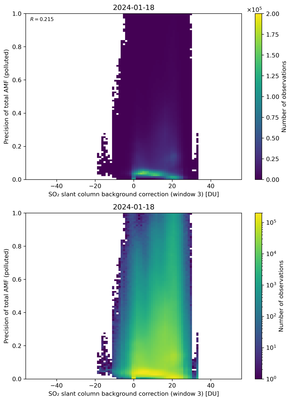
Figure 126: Scatter density plot of “SO 2 slant column background correction (window 3)” against “Precision of total AMF (polluted)” for 2024-01-17 to 2024-01-19.
