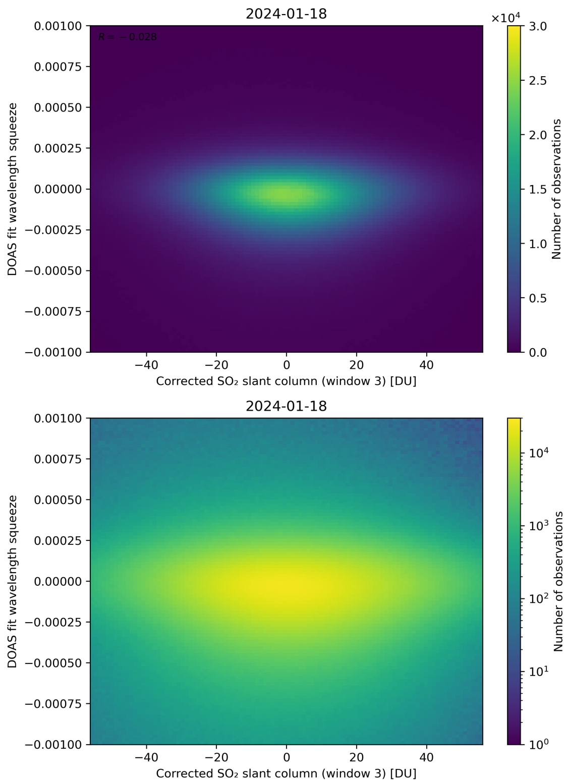
Figure 207: Scatter density plot of “Corrected SO 2 slant column (window 3)” against “DOAS fit wavelength squeeze” for 2024-01-17 to 2024-01-19.
