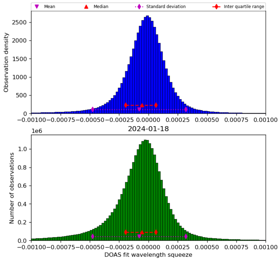
Figure 69: Histogram of “DOAS fit wavelength squeeze” for 2024-01-17 to 2024-01-19
