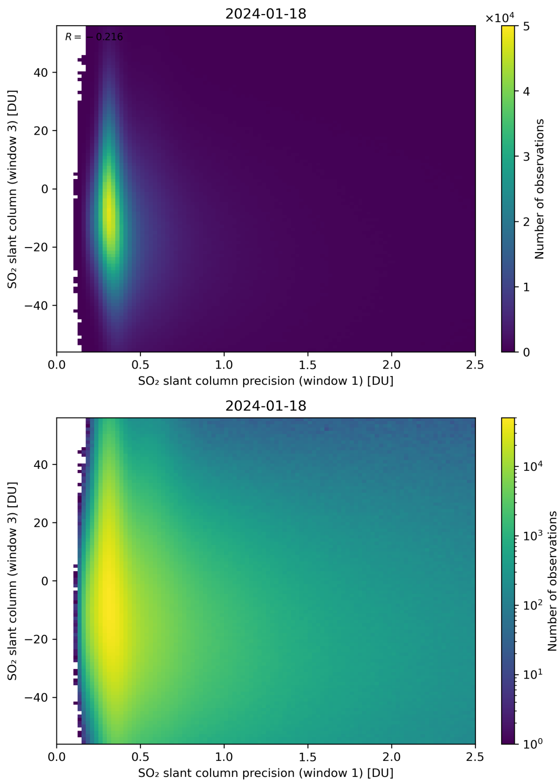
Figure 228: Scatter density plot of “SO 2 slant column precision (window 1)” against “SO 2 slant column (window 3)” for 2024-01-17 to 2024-01-19.
