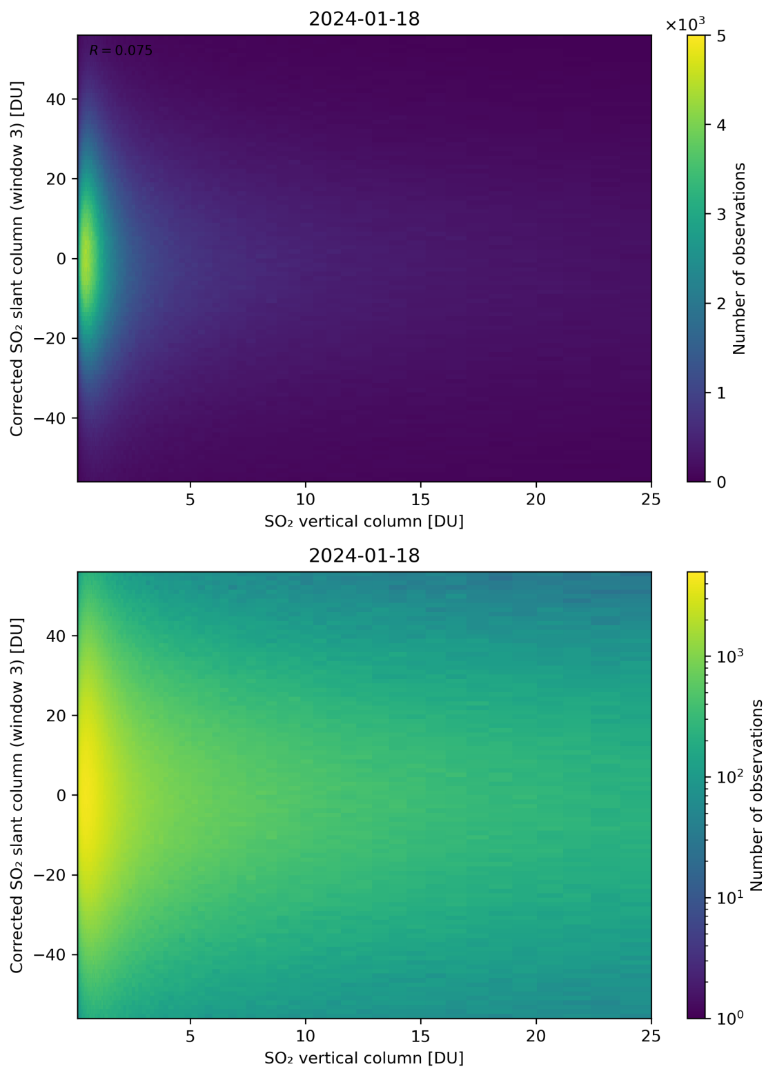
Figure 299: Scatter density plot of “SO 2 vertical column” against “Corrected SO 2 slant column (window 3)” for 2024-01-17 to 2024-01-19.
