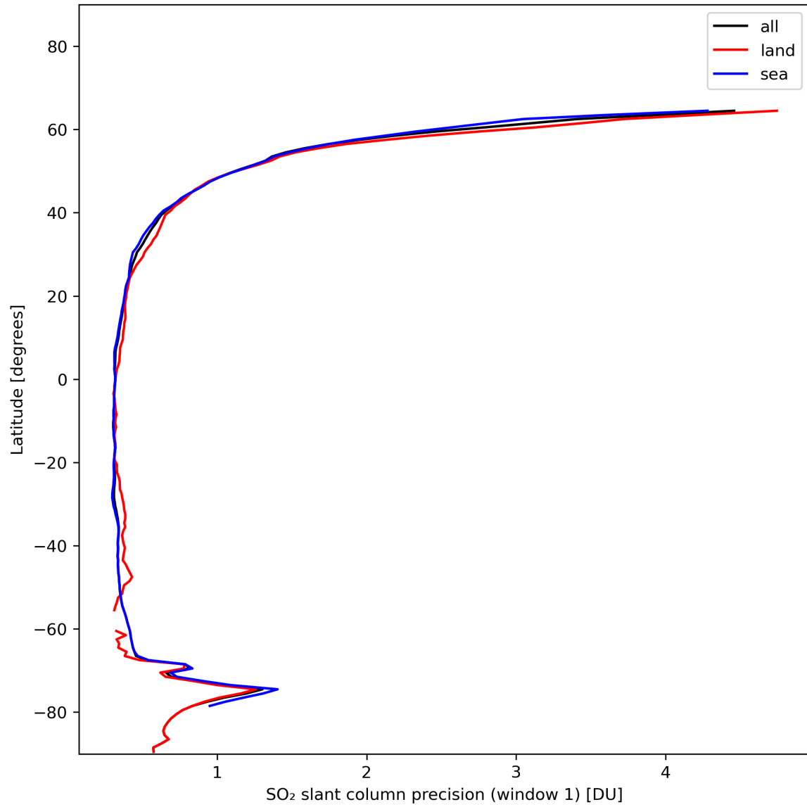
Figure 34: Zonal average of “SO 2 slant column precision (window 1)” for 2024-01-17 to 2024-01-19.
