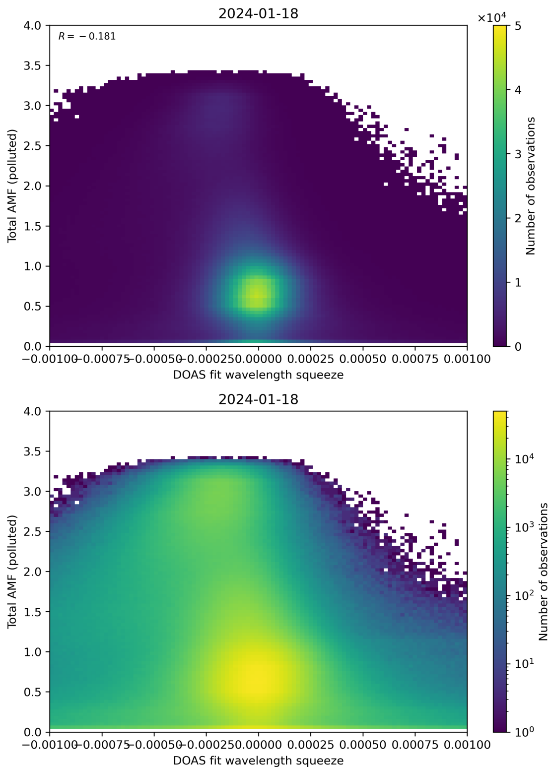
Figure 134: Scatter density plot of “DOAS fit wavelength squeeze” against “Total AMF (polluted)” for 2024-01-17 to 2024-01-19.
