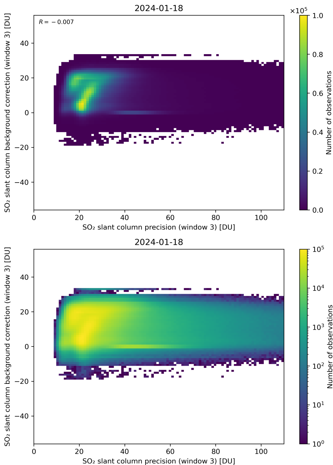
Figure 257: Scatter density plot of “SO 2 slant column precision (window 3)” against “SO 2 slant column background correction (window 3)” for 2024-01-17 to 2024-01-19.
