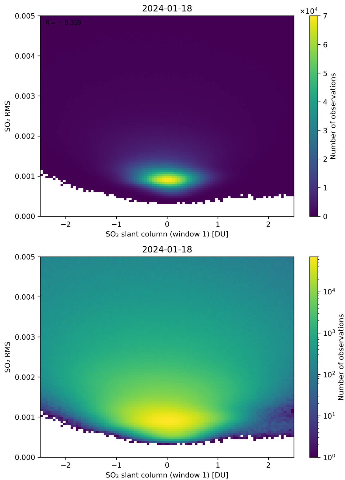
Figure 217: Scatter density plot of “SO 2 slant column (window 1)” against “SO 2 RMS” for 2024-01-17 to 2024-01-19.
