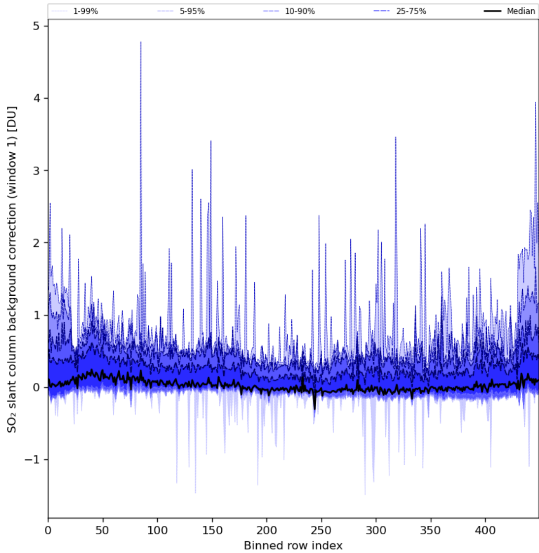
Figure 82: Along track statistics of “SO 2 slant column background correction (window 1)” for 2024-01-17 to 2024-01-19
