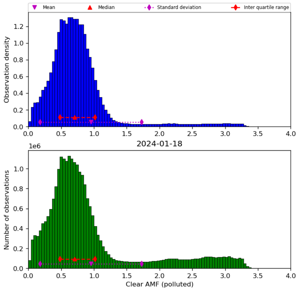
Figure 73: Histogram of “Clear AMF (polluted)” for 2024-01-17 to 2024-01-19
