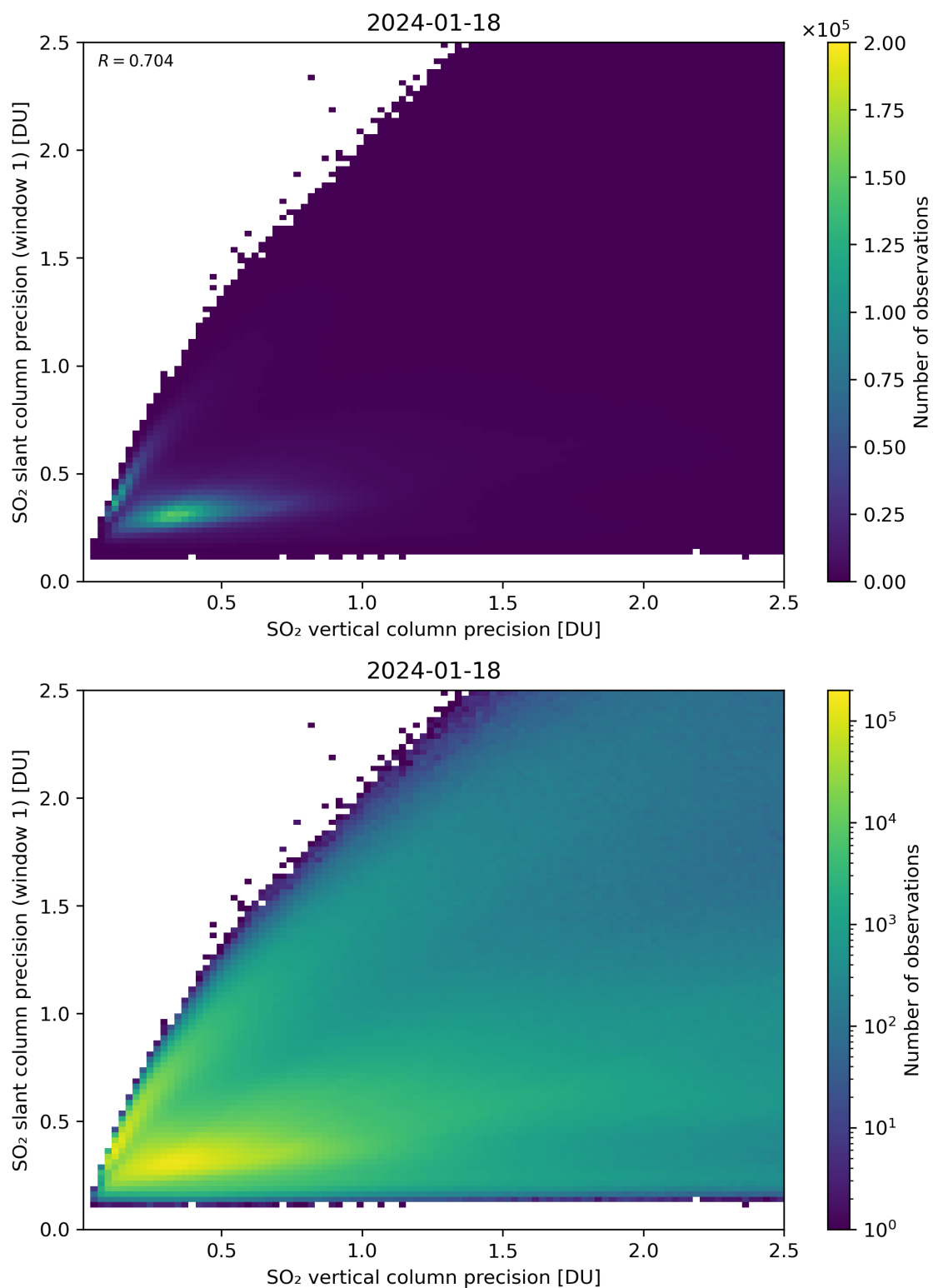
Figure 290: Scatter density plot of “SO 2 vertical column precision” against “SO 2 slant column precision (window 1)” for 2024-01-17 to 2024-01-19.
