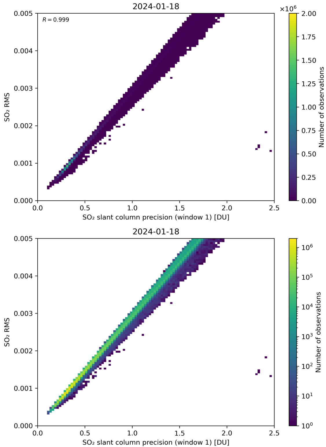
Figure 223: Scatter density plot of “SO 2 slant column precision (window 1)” against “SO 2 RMS” for 2024-01-17 to 2024-01-19.
