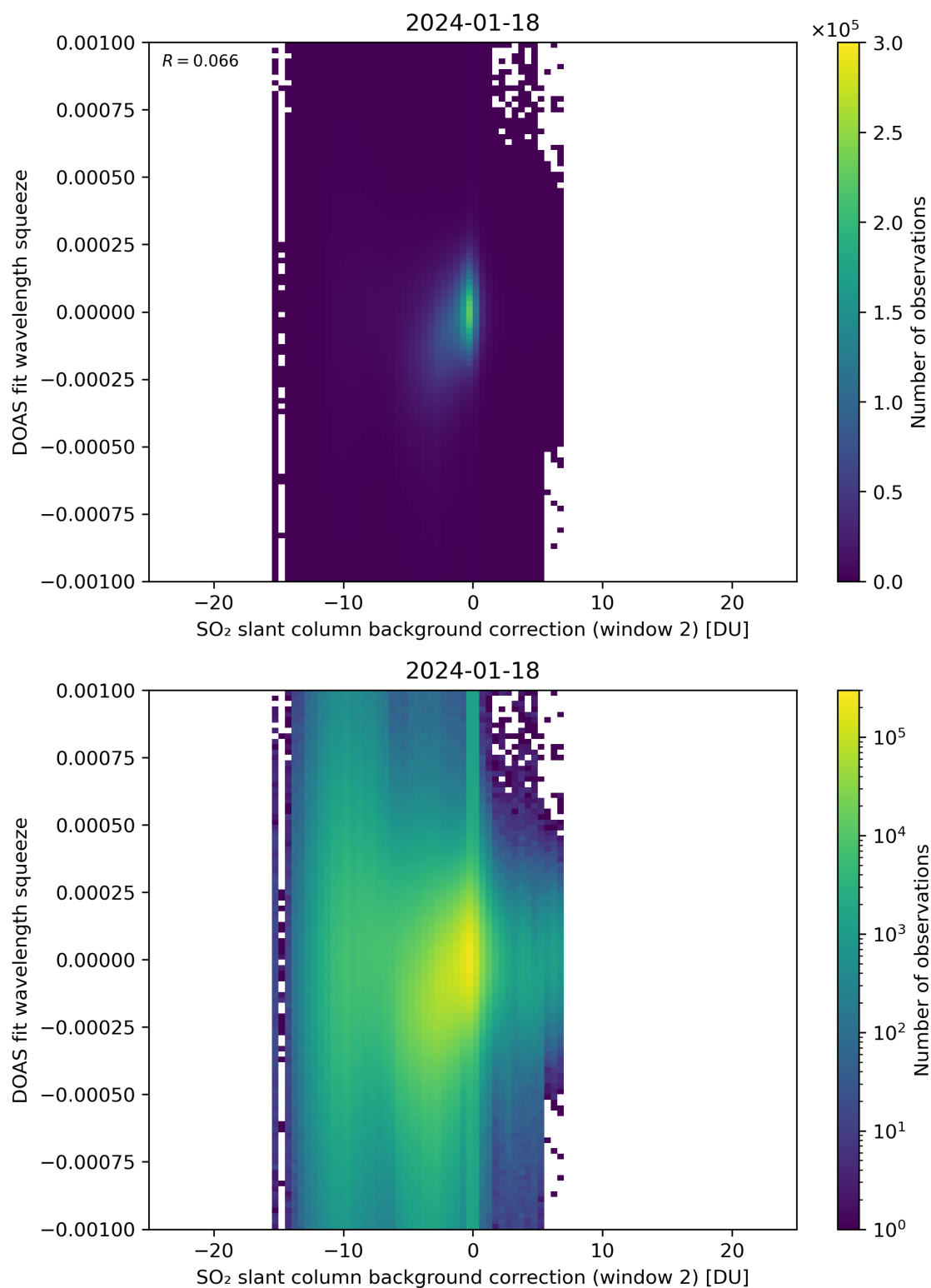
Figure 113: Scatter density plot of “SO 2 slant column background correction (window 2)” against “DOAS fit wavelength squeeze” for 2024-01-17 to 2024-01-19.
