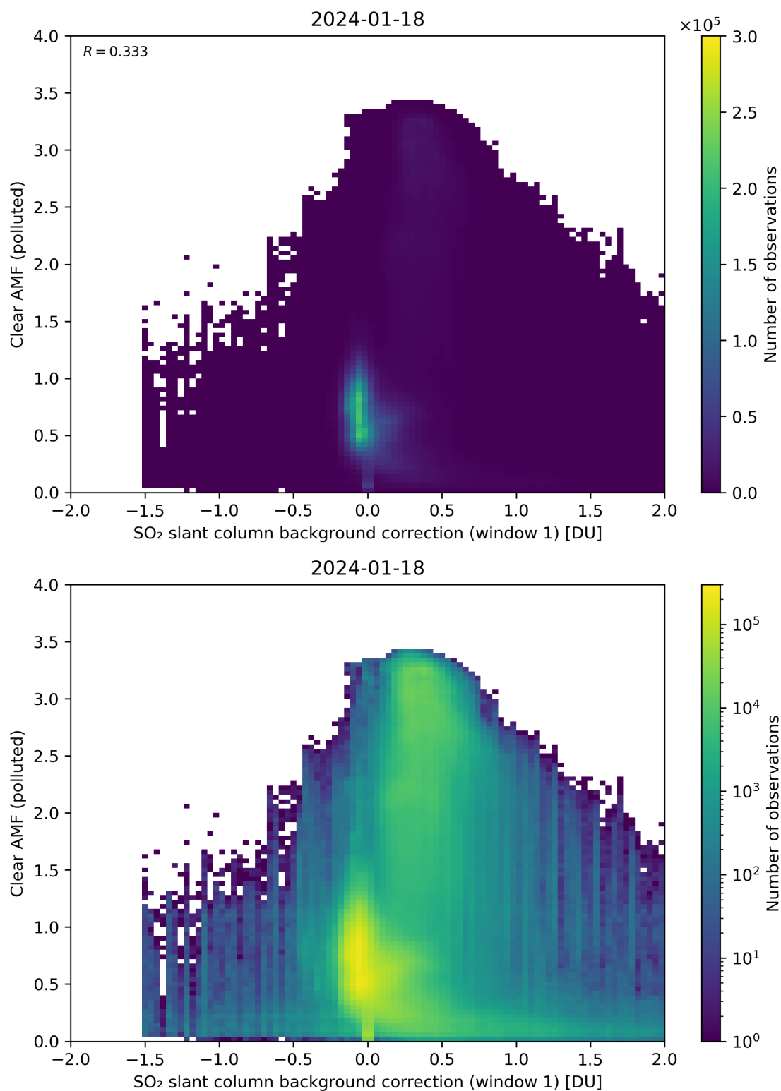
Figure 103: Scatter density plot of “SO 2 slant column background correction (window 1)” against “Clear AMF (polluted)” for 2024-01-17 to 2024-01-19.
