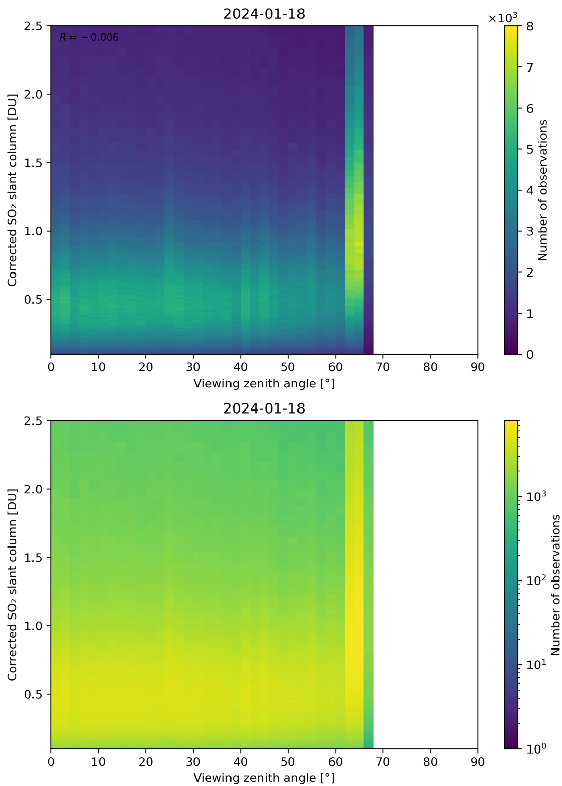
Figure 317: Scatter density plot of “Viewing zenith angle” against “Corrected SO 2 slant column” for 2024-01-17 to 2024-01-19.
