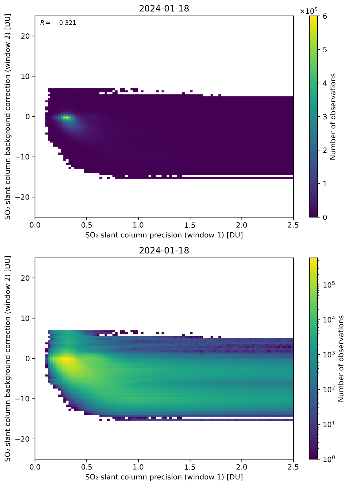
Figure 219: Scatter density plot of “SO 2 slant column precision (window 1)” against “SO 2 slant column background correction (window 2)” for 2024-01-17 to 2024-01-19.
