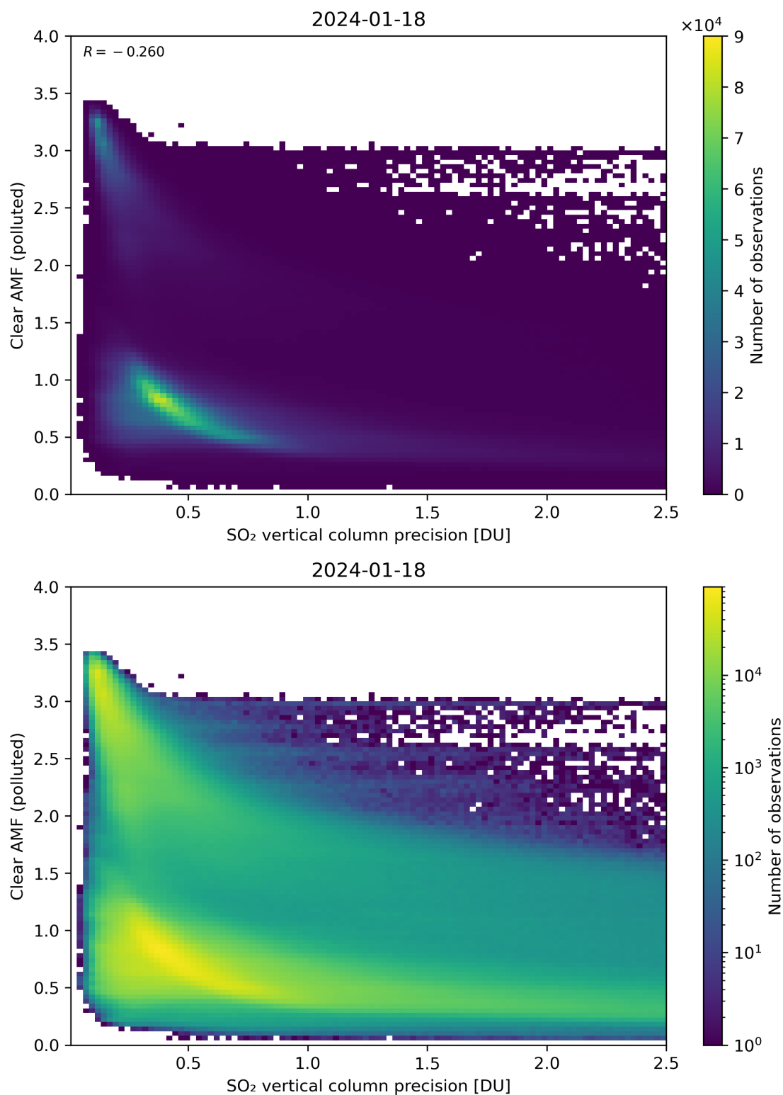
Figure 285: Scatter density plot of “SO 2 vertical column precision” against “Clear AMF (polluted)” for 2024-01-17 to 2024-01-19.
