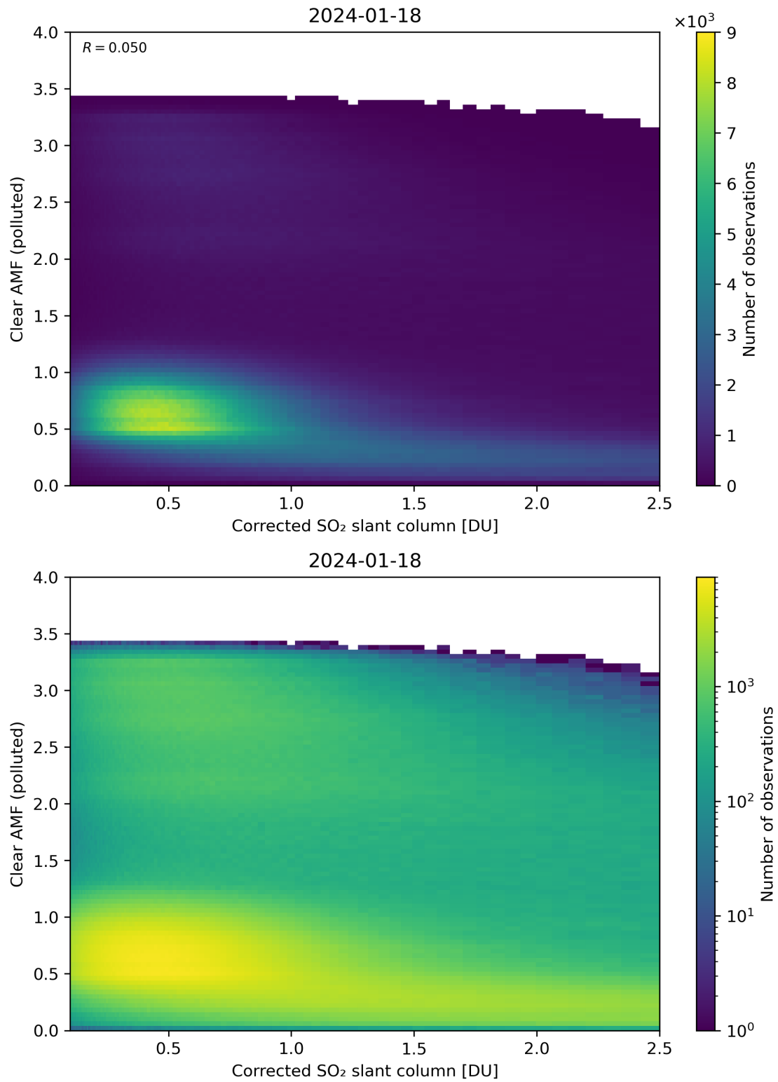
Figure 184: Scatter density plot of “Corrected SO 2 slant column” against “Clear AMF (polluted)” for 2024-01-17 to 2024-01-19.
