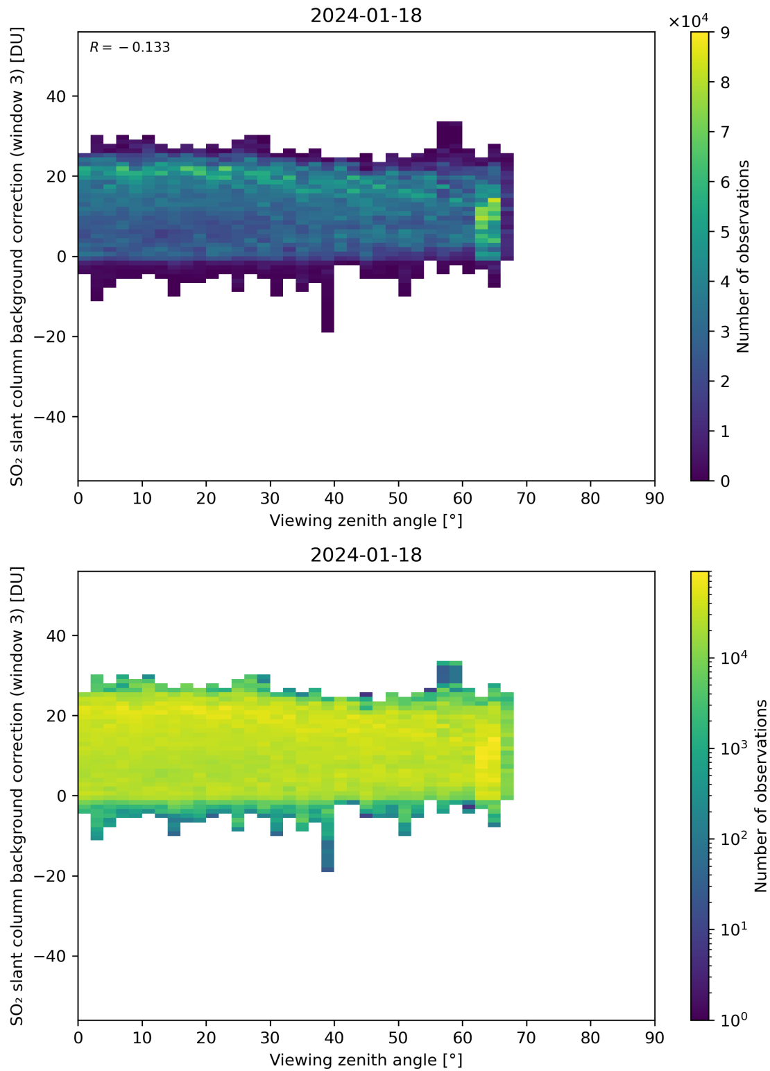
Figure 310: Scatter density plot of “Viewing zenith angle” against “SO 2 slant column background correction (window 3)” for 2024-01-17 to 2024-01-19.
