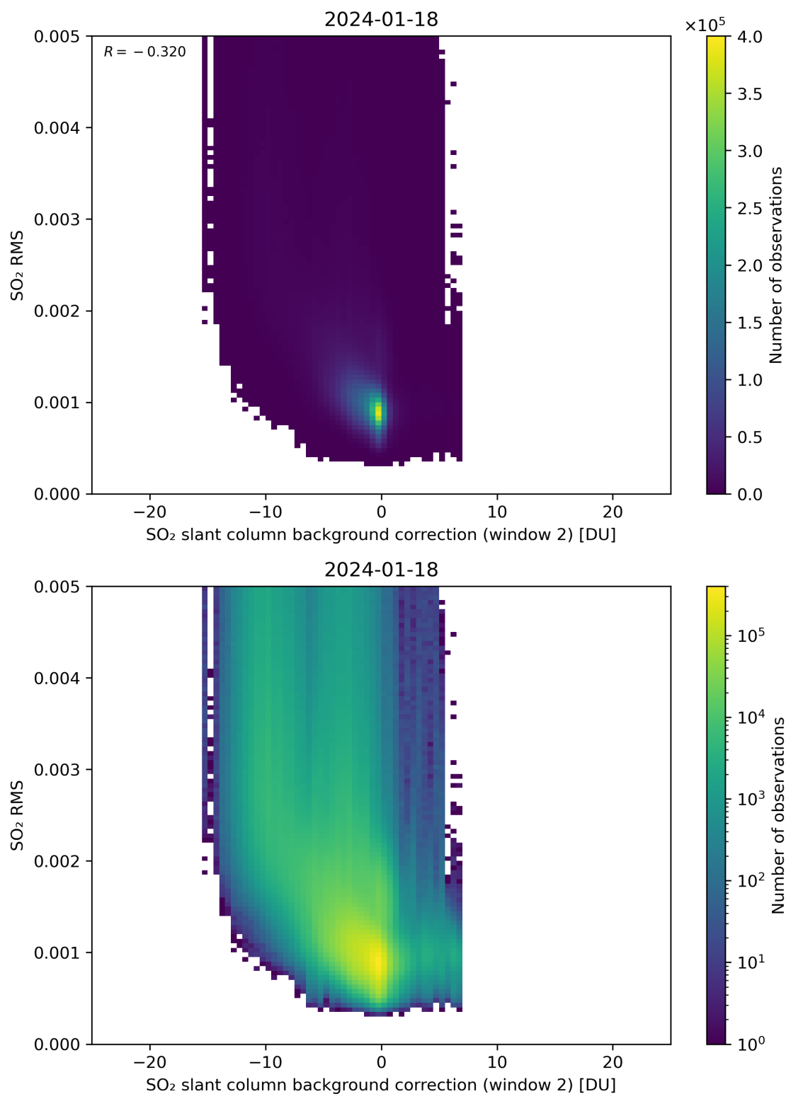
Figure 114: Scatter density plot of “SO 2 slant column background correction (window 2)” against “SO 2 RMS” for 2024-01-17 to 2024-01-19.
