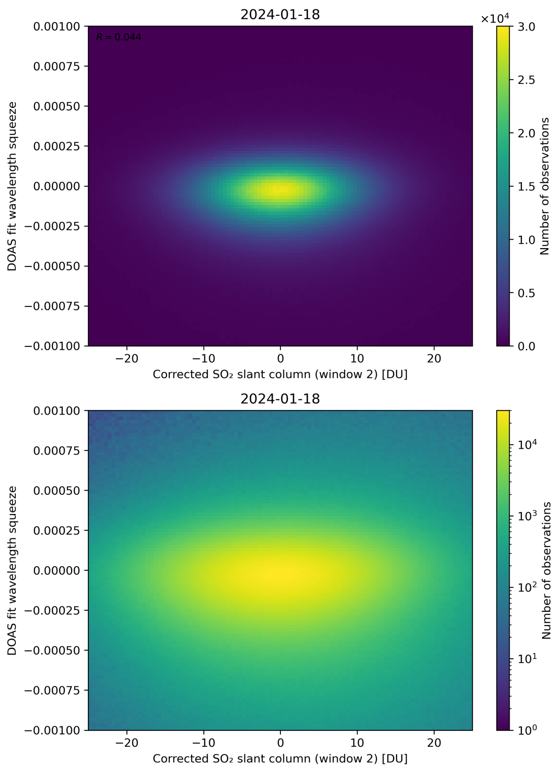
Figure 197: Scatter density plot of “Corrected SO 2 slant column (window 2)” against “DOAS fit wavelength squeeze” for 2024-01-17 to 2024-01-19.
