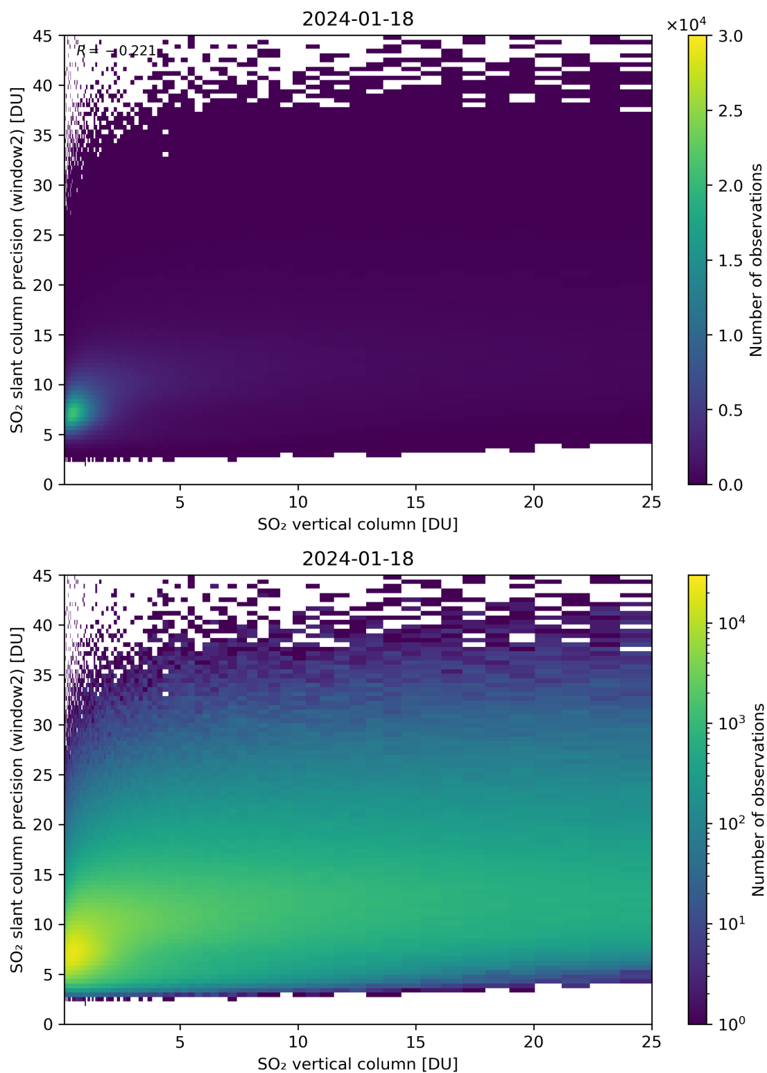
Figure 302: Scatter density plot of “SO 2 vertical column” against “SO 2 slant column precision (window2)” for 2024-01-17 to 2024-01-19.
