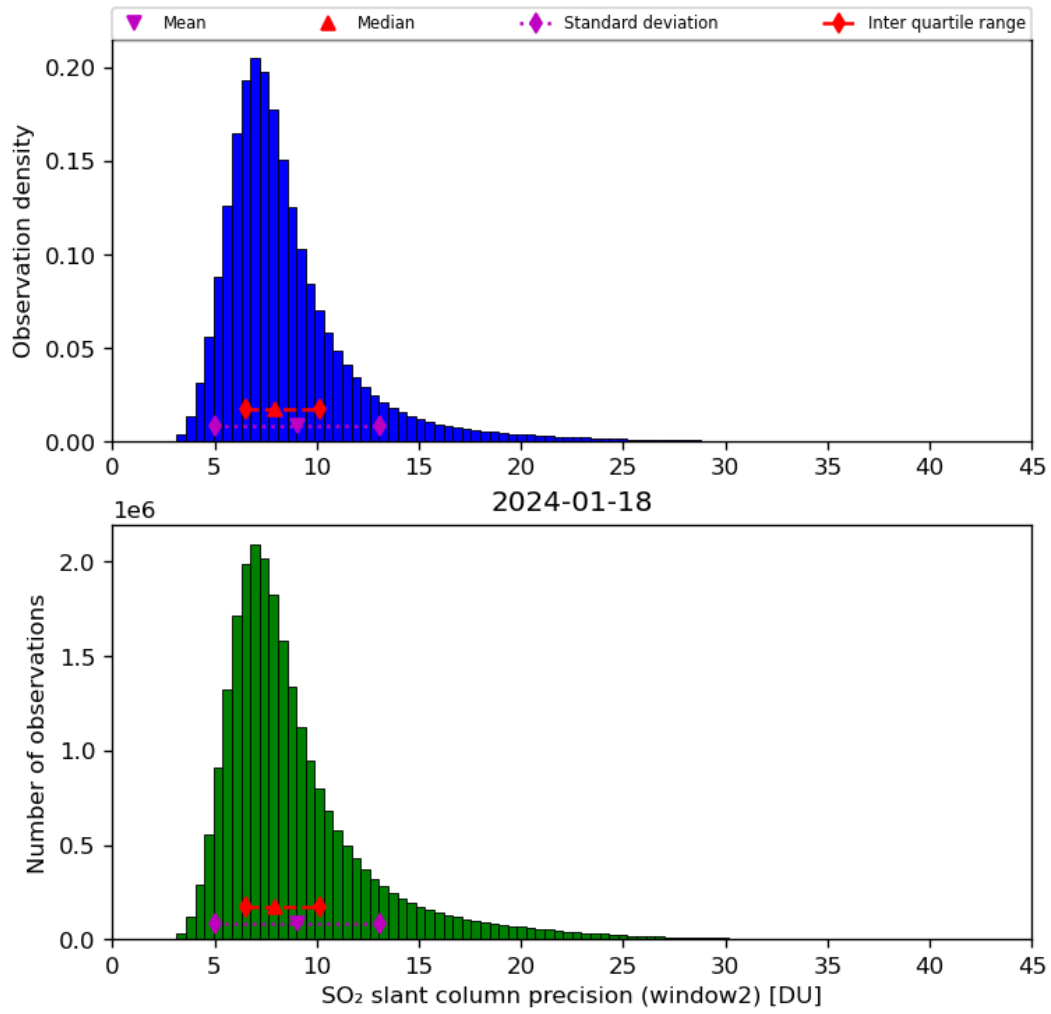
Figure 61: Histogram of “SO 2 slant column precision (window2)” for 2024-01-17 to 2024-01-19
