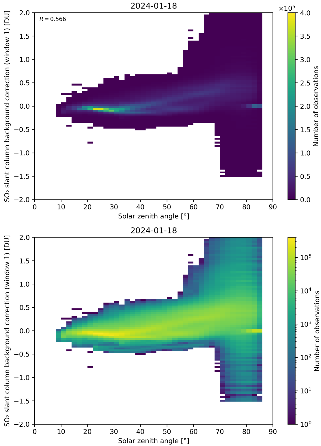
Figure 158: Scatter density plot of “Solar zenith angle” against “SO 2 slant column background correction (window 1)” for 2024-01-17 to 2024-01-19.
