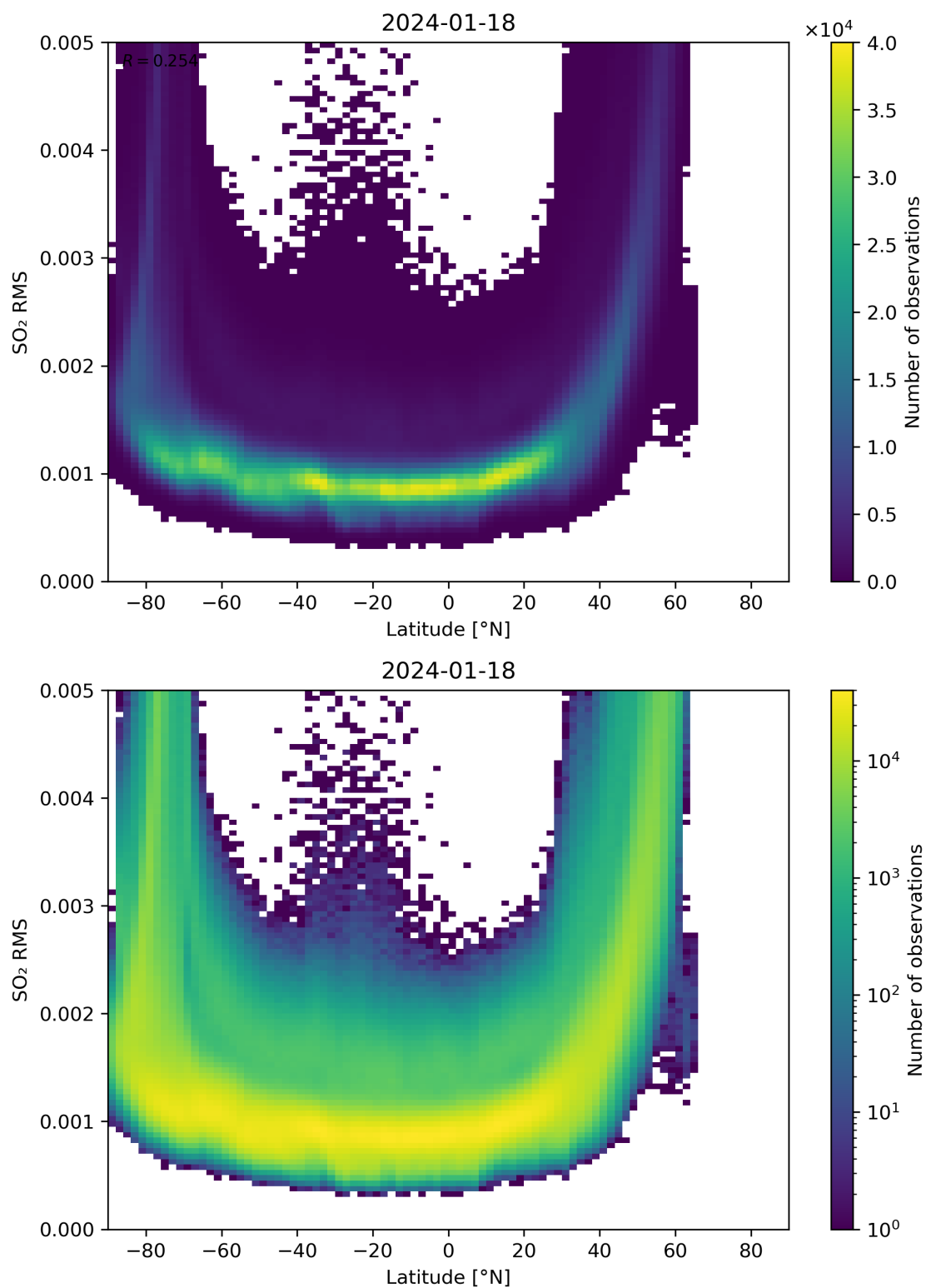
Figure 144: Scatter density plot of “Latitude” against “SO 2 RMS” for 2024-01-17 to 2024-01-19.
