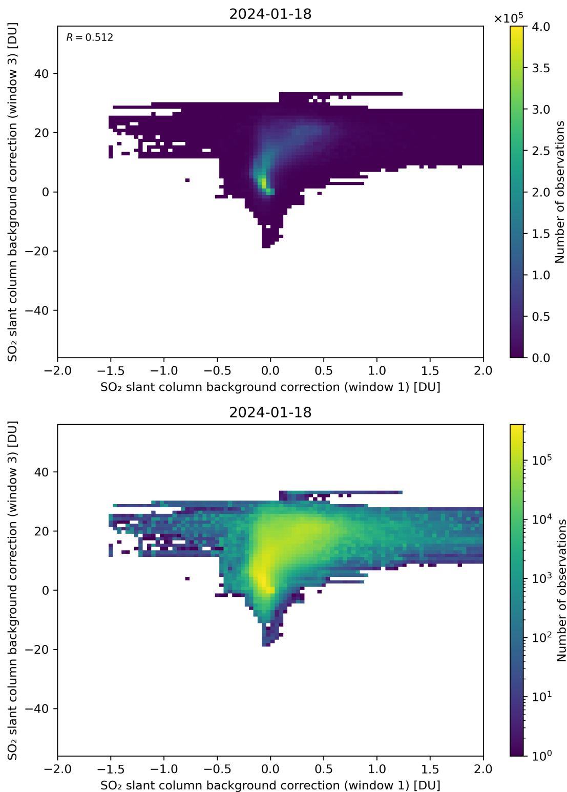
Figure 99: Scatter density plot of “SO 2 slant column background correction (window 1)” against “SO 2 slant column background correction (window 3)” for 2024-01-17 to 2024-01-19.
