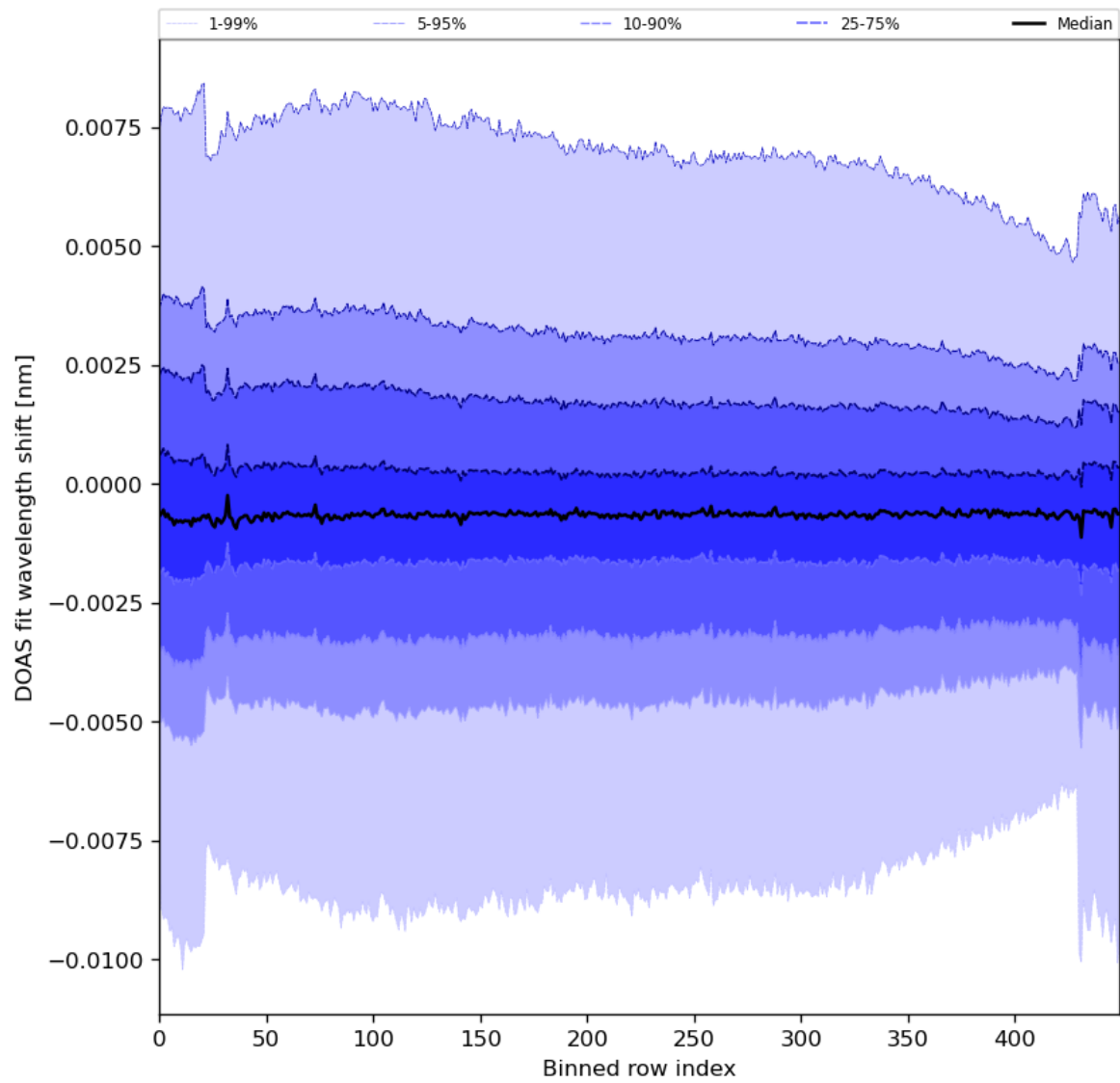
Figure 91: Along track statistics of “DOAS fit wavelength shift” for 2024-01-17 to 2024-01-19
