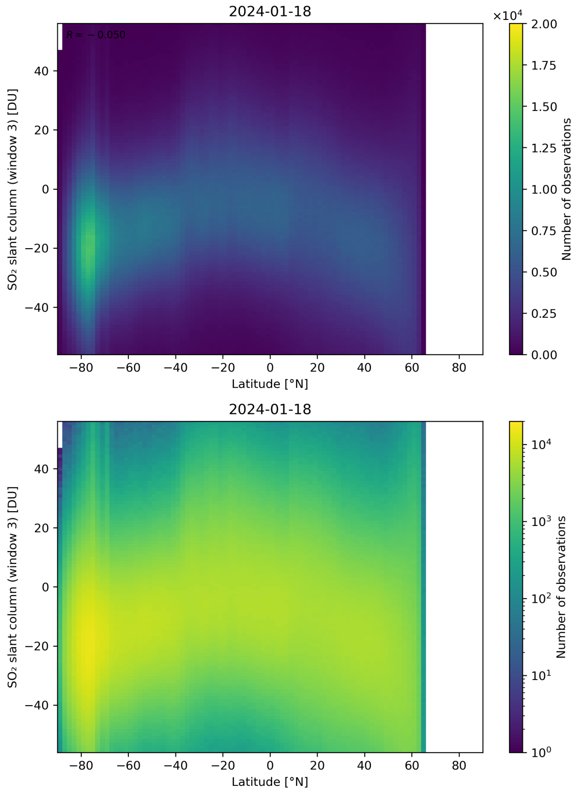
Figure 152: Scatter density plot of “Latitude” against “SO 2 slant column (window 3)” for 2024-01-17 to 2024-01-19.
