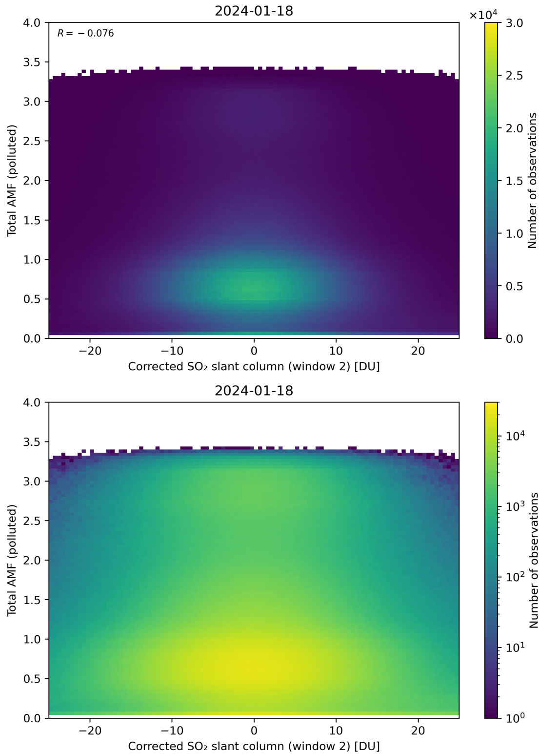
Figure 203: Scatter density plot of “Corrected SO 2 slant column (window 2)” against “Total AMF (polluted)” for 2024-01-17 to 2024-01-19.
