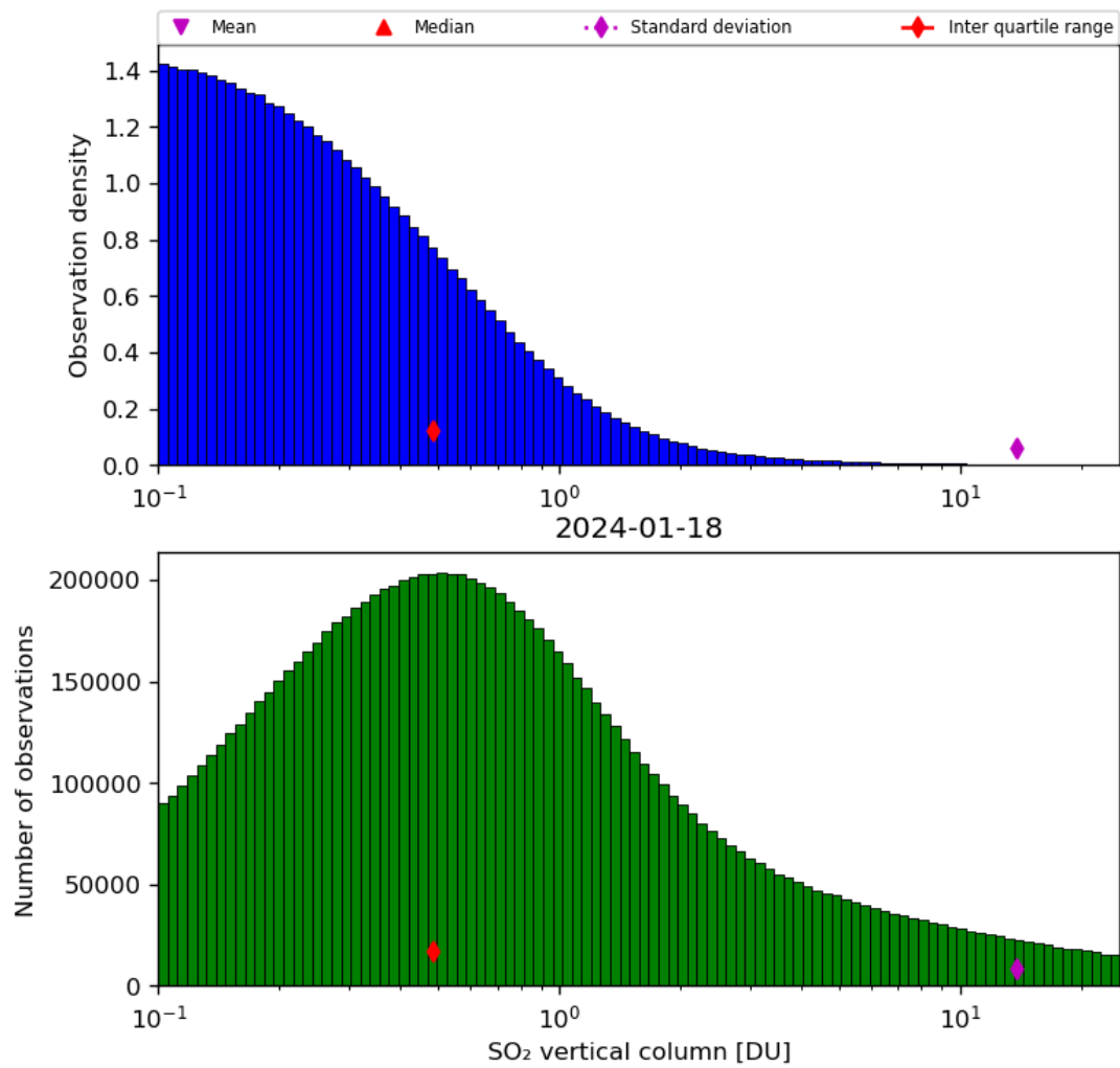
Figure 53: Histogram of “SO 2 vertical column” for 2024-01-17 to 2024-01-19
