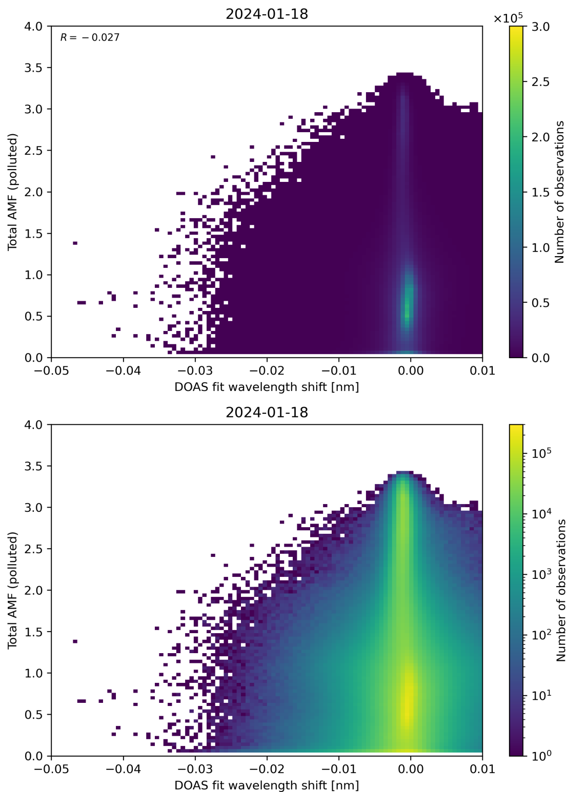
Figure 130: Scatter density plot of “DOAS fit wavelength shift” against “Total AMF (polluted)” for 2024-01-17 to 2024-01-19.
