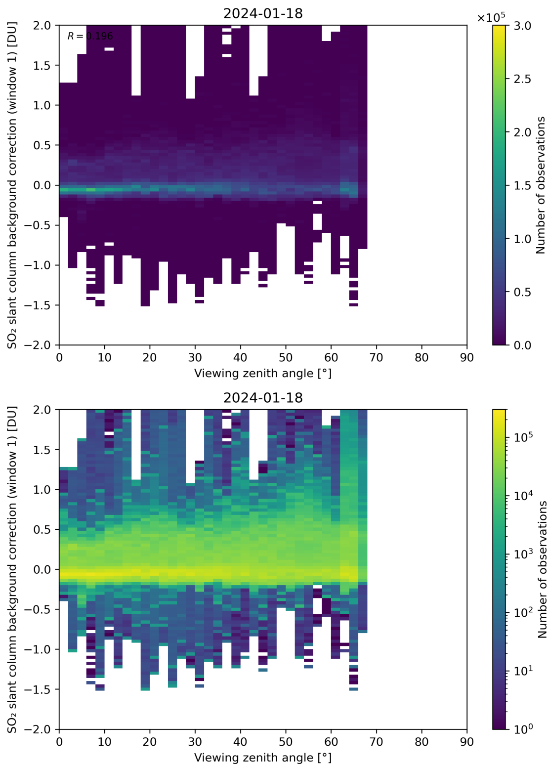
Figure 308: Scatter density plot of “Viewing zenith angle” against “SO 2 slant column background correction (window 1)” for 2024-01-17 to 2024-01-19.
