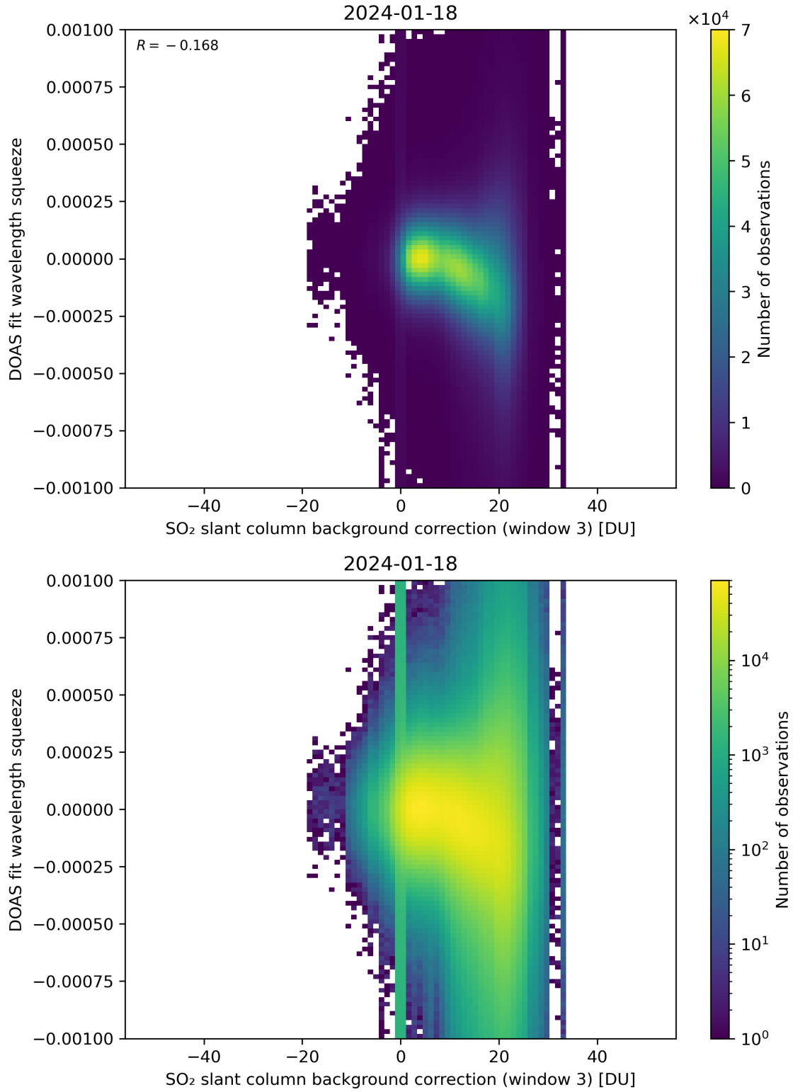
Figure 122: Scatter density plot of “SO 2 slant column background correction (window 3)” against “DOAS fit wavelength squeeze” for 2024-01-17 to 2024-01-19.
