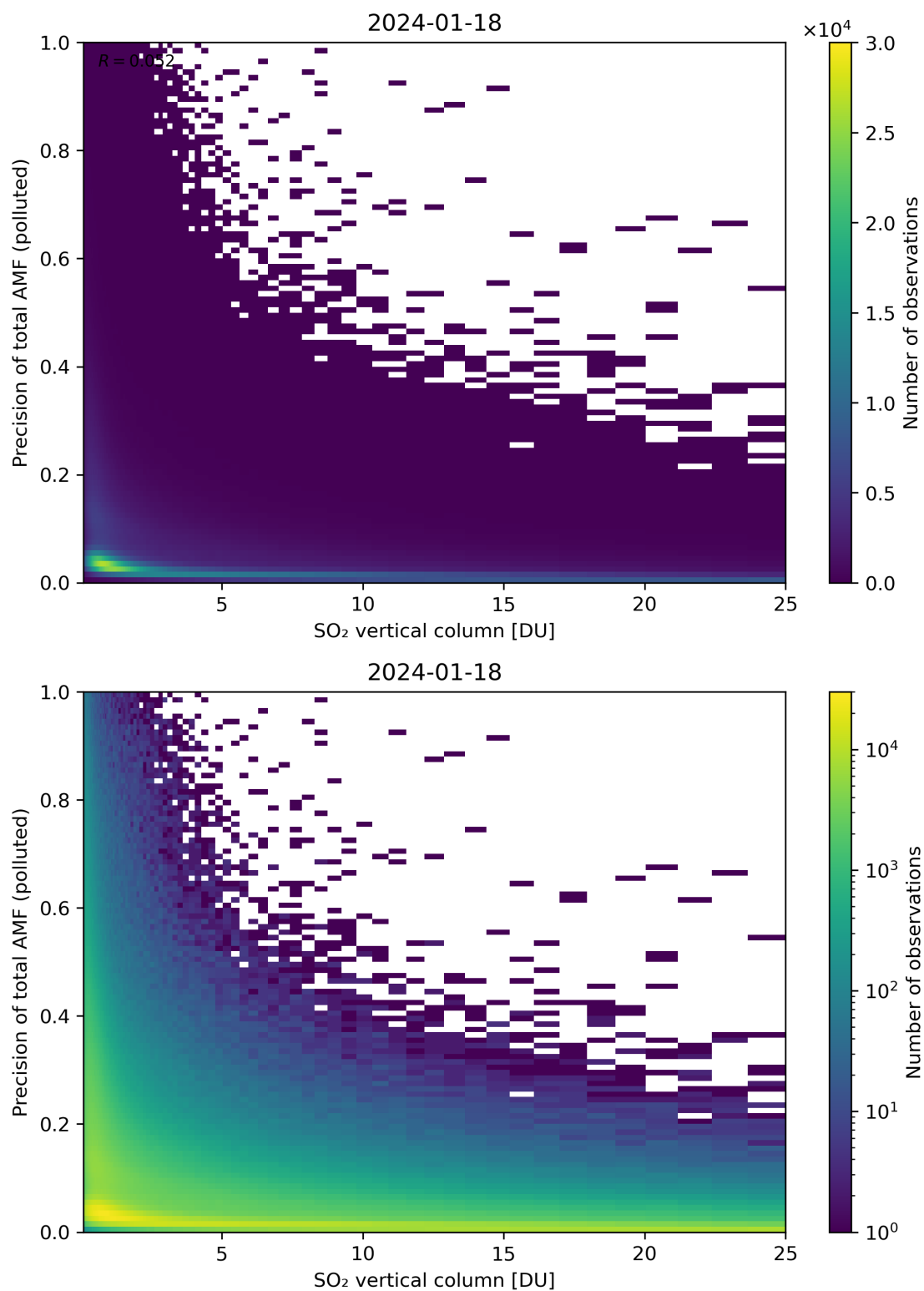
Figure 306: Scatter density plot of “SO 2 vertical column” against “Precision of total AMF (polluted)” for 2024-01-17 to 2024-01-19.
