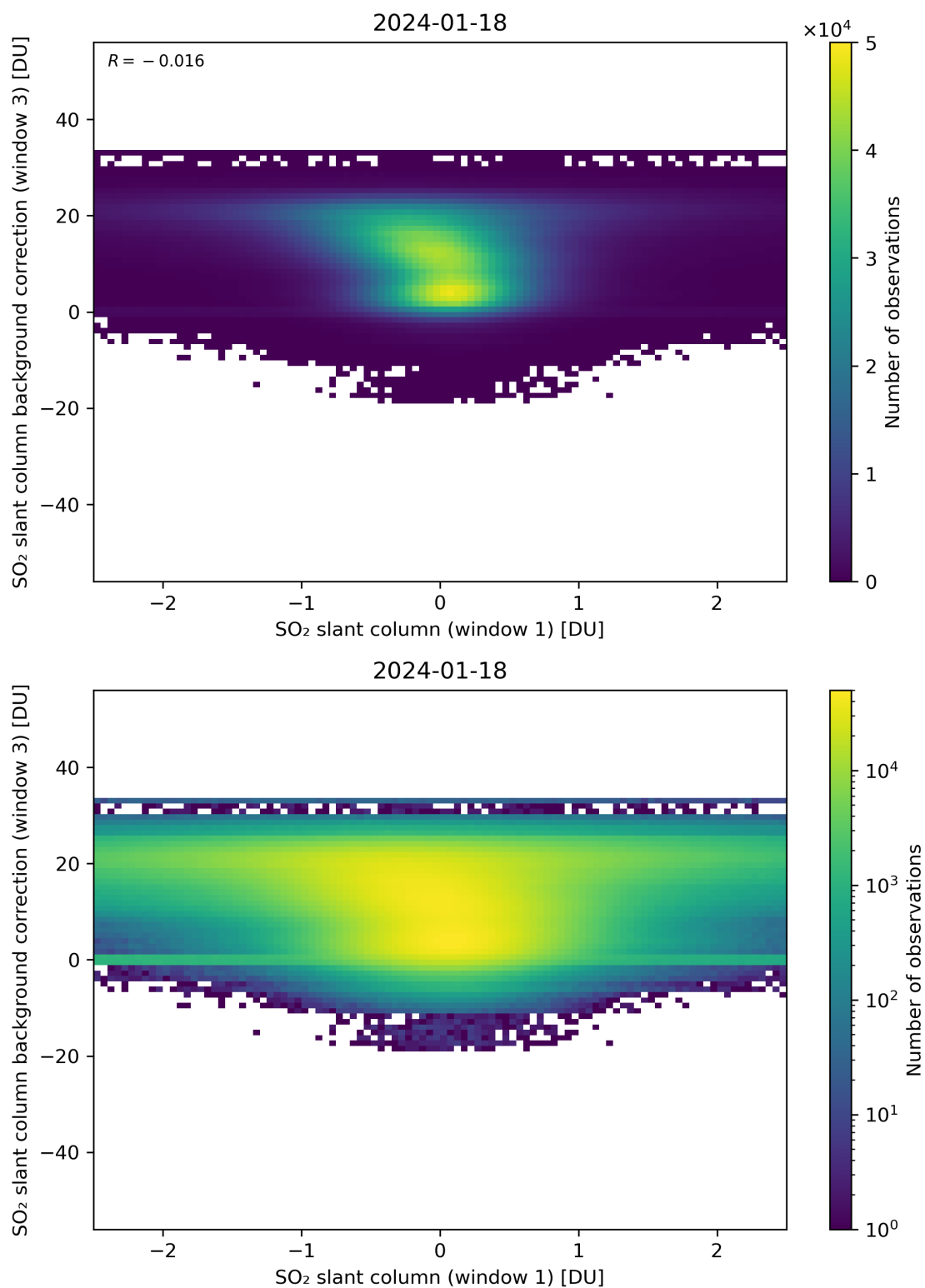
Figure 214: Scatter density plot of “SO 2 slant column (window 1)” against “SO 2 slant column background correction (window 3)” for 2024-01-17 to 2024-01-19.
