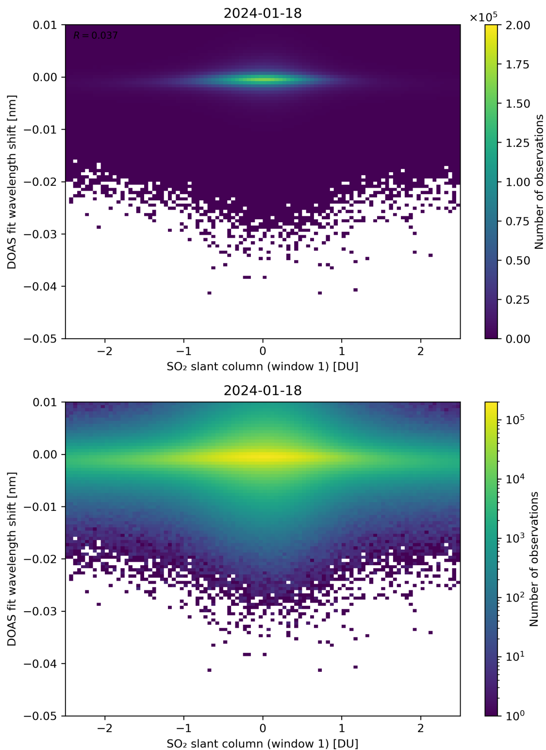
Figure 215: Scatter density plot of “SO 2 slant column (window 1)” against “DOAS fit wavelength shift” for 2024-01-17 to 2024-01-19.
