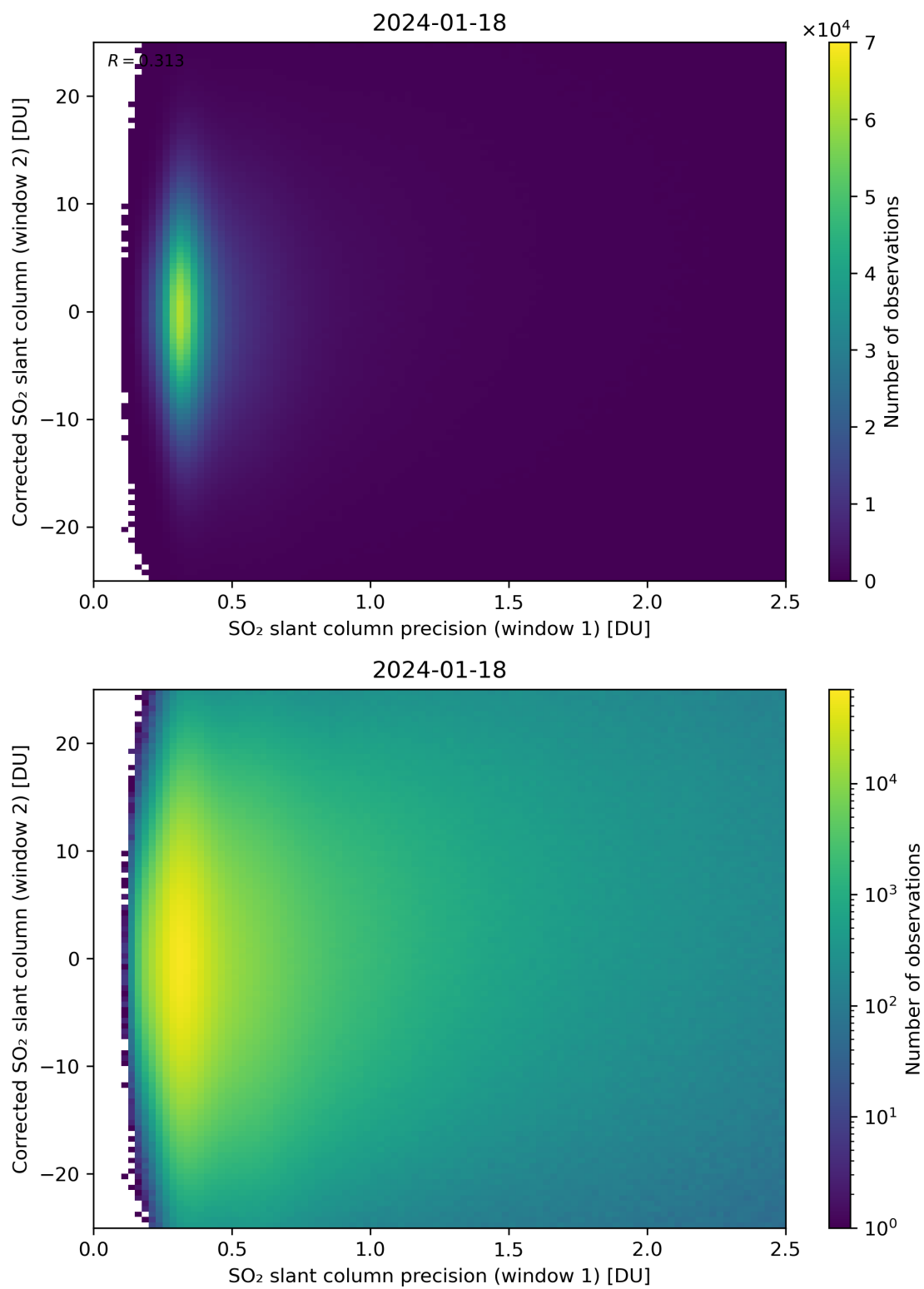
Figure 225: Scatter density plot of “SO 2 slant column precision (window 1)” against “Corrected SO 2 slant column (window 2)” for 2024-01-17 to 2024-01-19.
