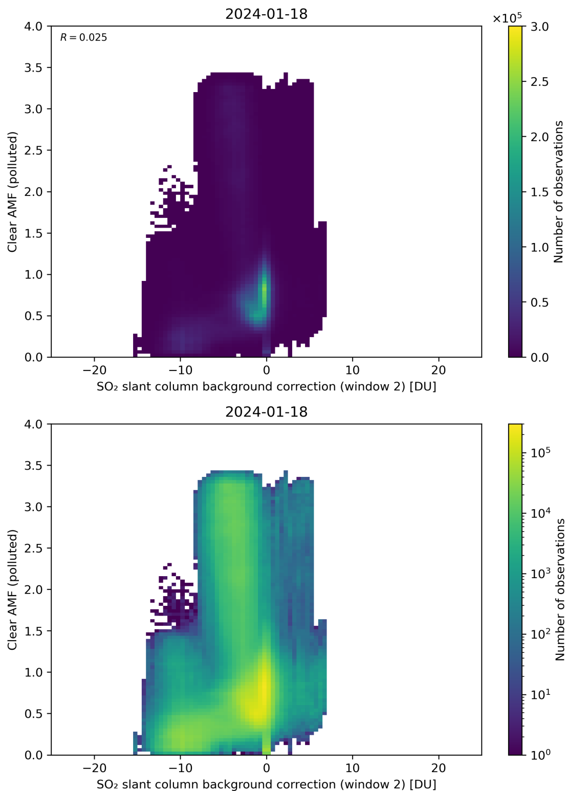
Figure 115: Scatter density plot of “SO 2 slant column background correction (window 2)” against “Clear AMF (polluted)” for 2024-01-17 to 2024-01-19.
