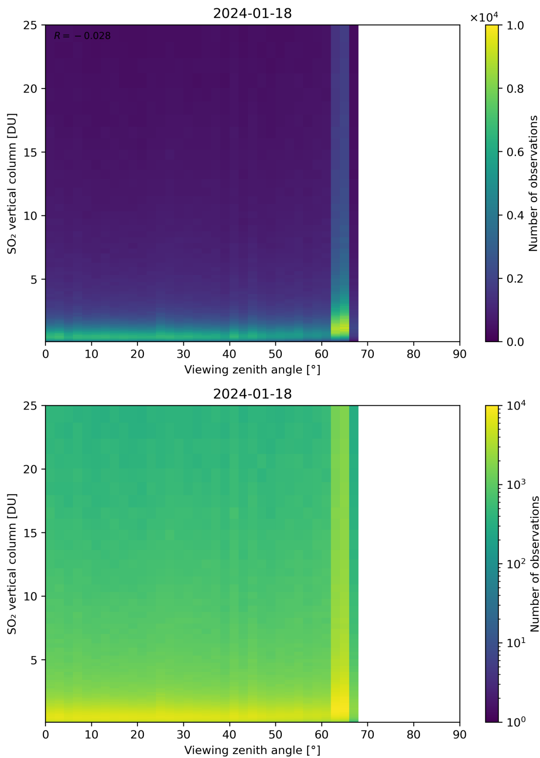
Figure 327: Scatter density plot of “Viewing zenith angle” against “SO 2 vertical column” for 2024-01-17 to 2024-01-19.
