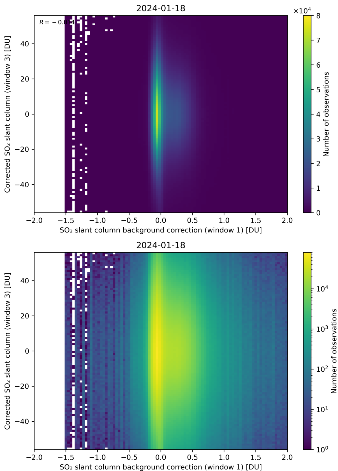
Figure 105: Scatter density plot of “SO 2 slant column background correction (window 1)” against “Corrected SO 2 slant column (window 3)” for 2024-01-17 to 2024-01-19.
