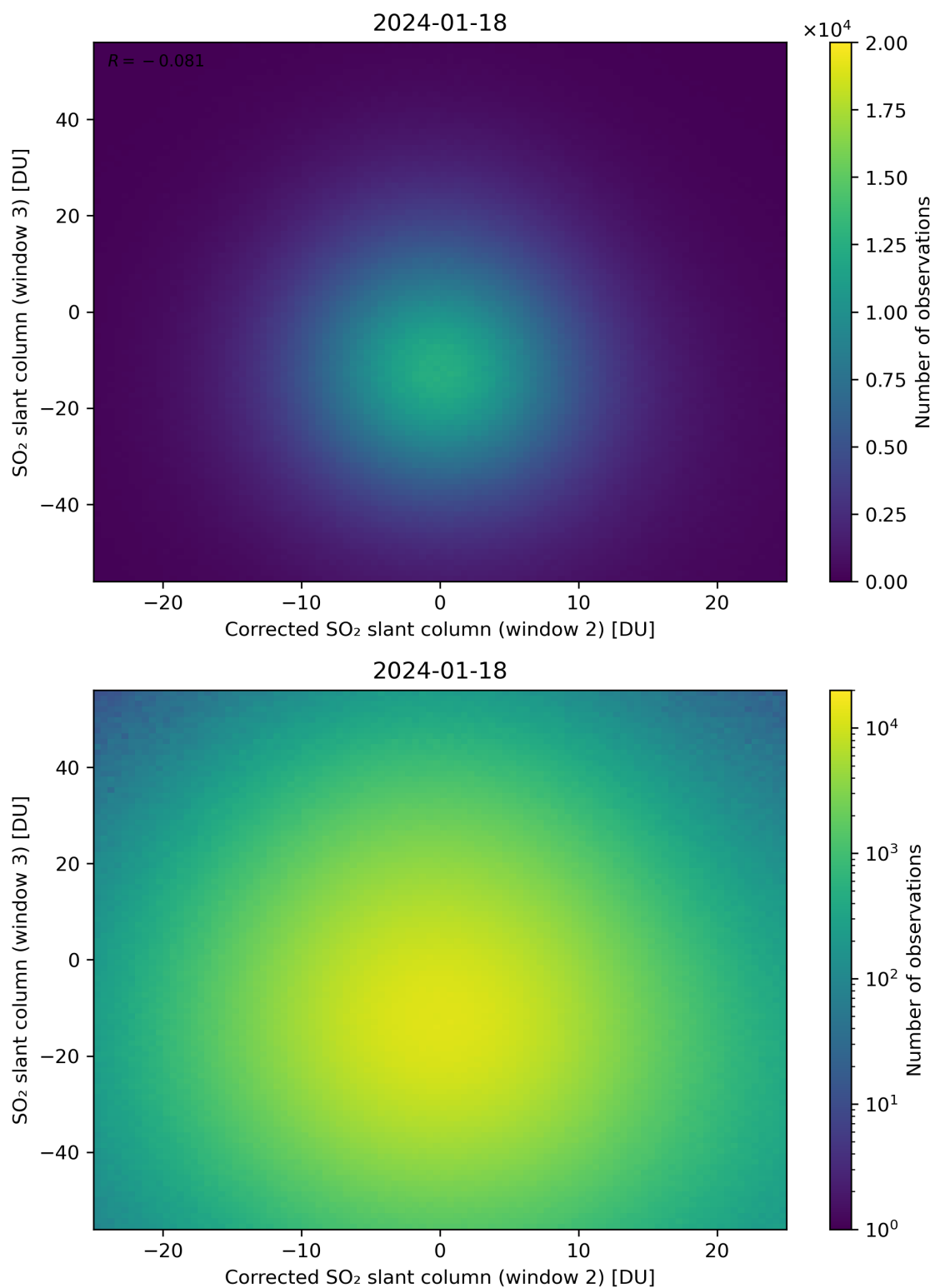
Figure 201: Scatter density plot of “Corrected SO 2 slant column (window 2)” against “SO 2 slant column (window 3)” for 2024-01-17 to 2024-01-19.
