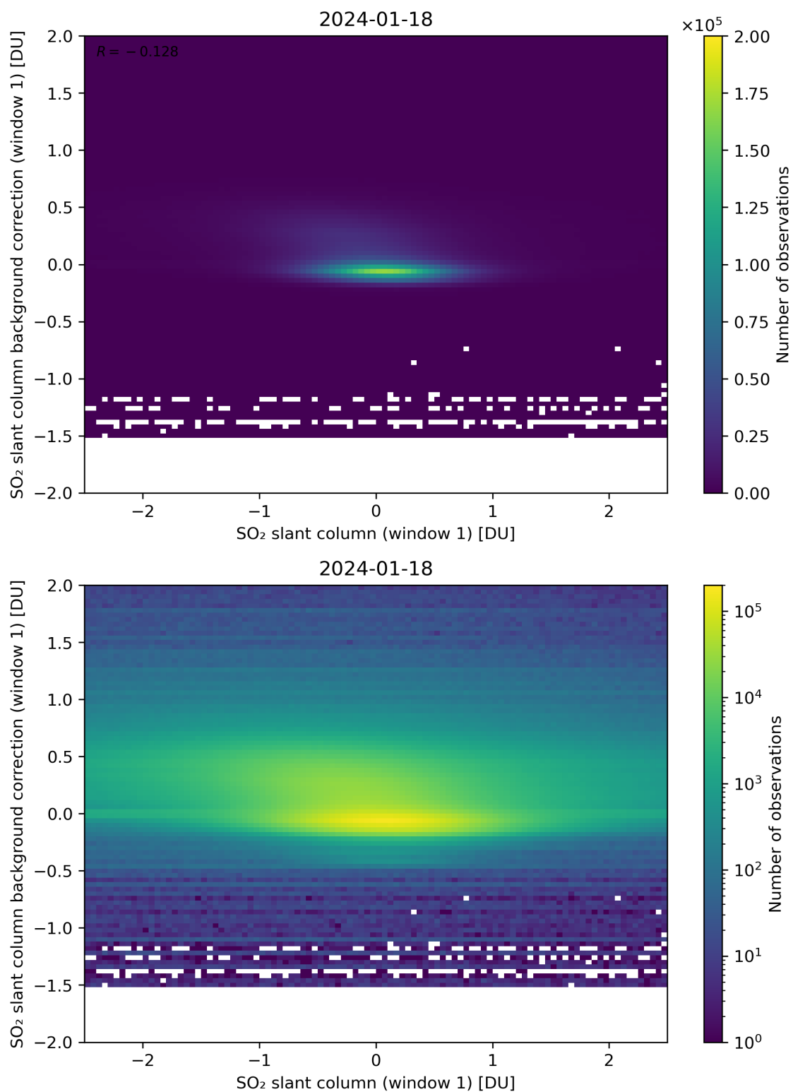
Figure 212: Scatter density plot of “SO 2 slant column (window 1)” against “SO 2 slant column background correction (window 1)” for 2024-01-17 to 2024-01-19.
