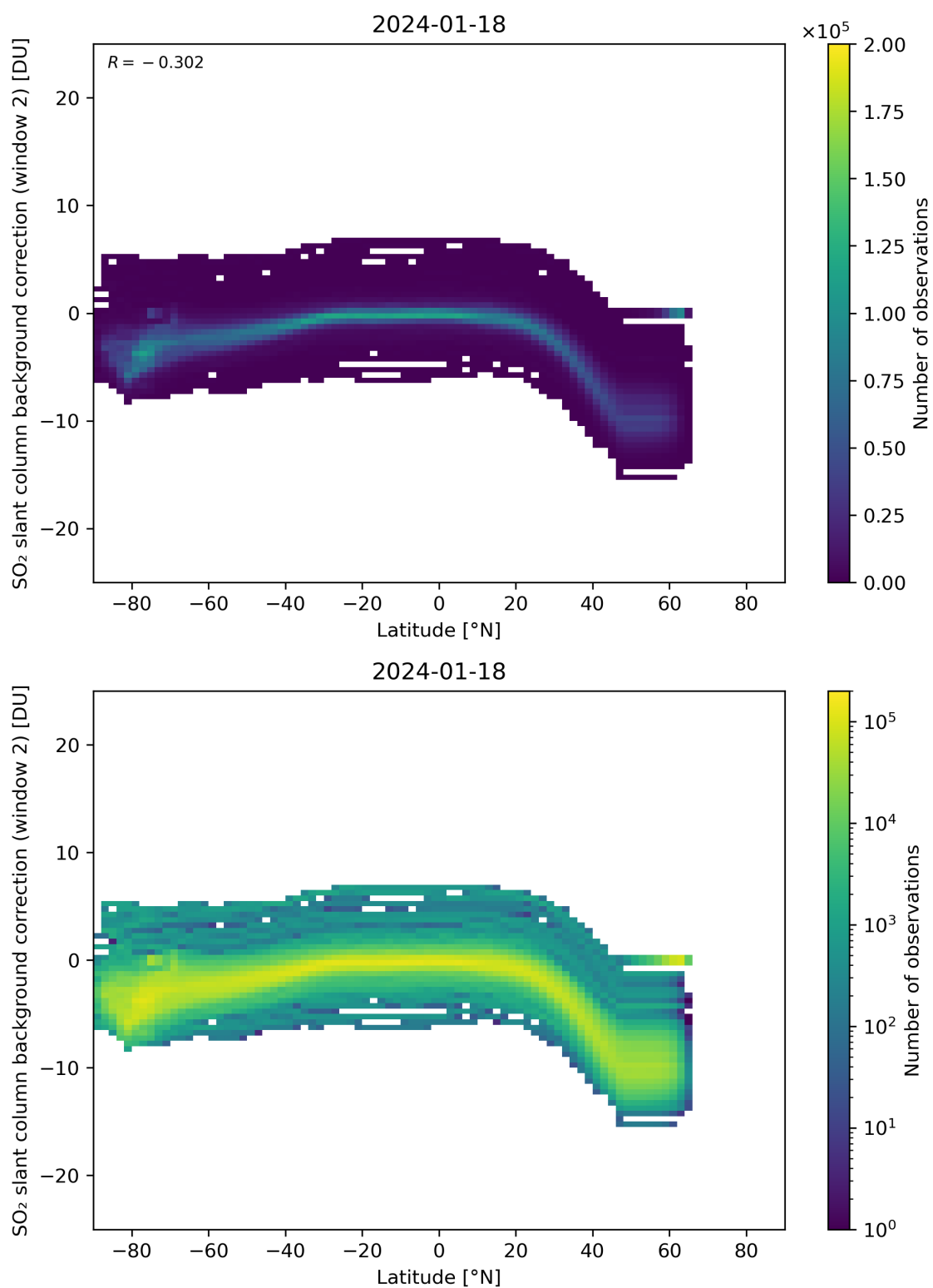
Figure 140: Scatter density plot of “Latitude” against “SO 2 slant column background correction (window 2)” for 2024-01-17 to 2024-01-19.
