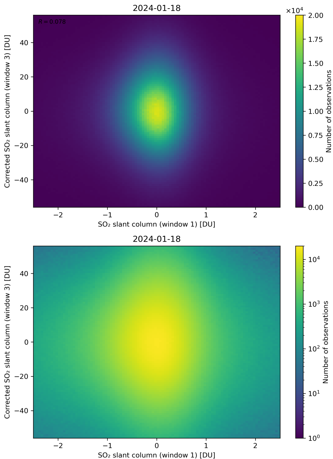
Figure 234: Scatter density plot of “SO 2 slant column (window 1)” against “Corrected SO 2 slant column (window 3)” for 2024-01-17 to 2024-01-19.
