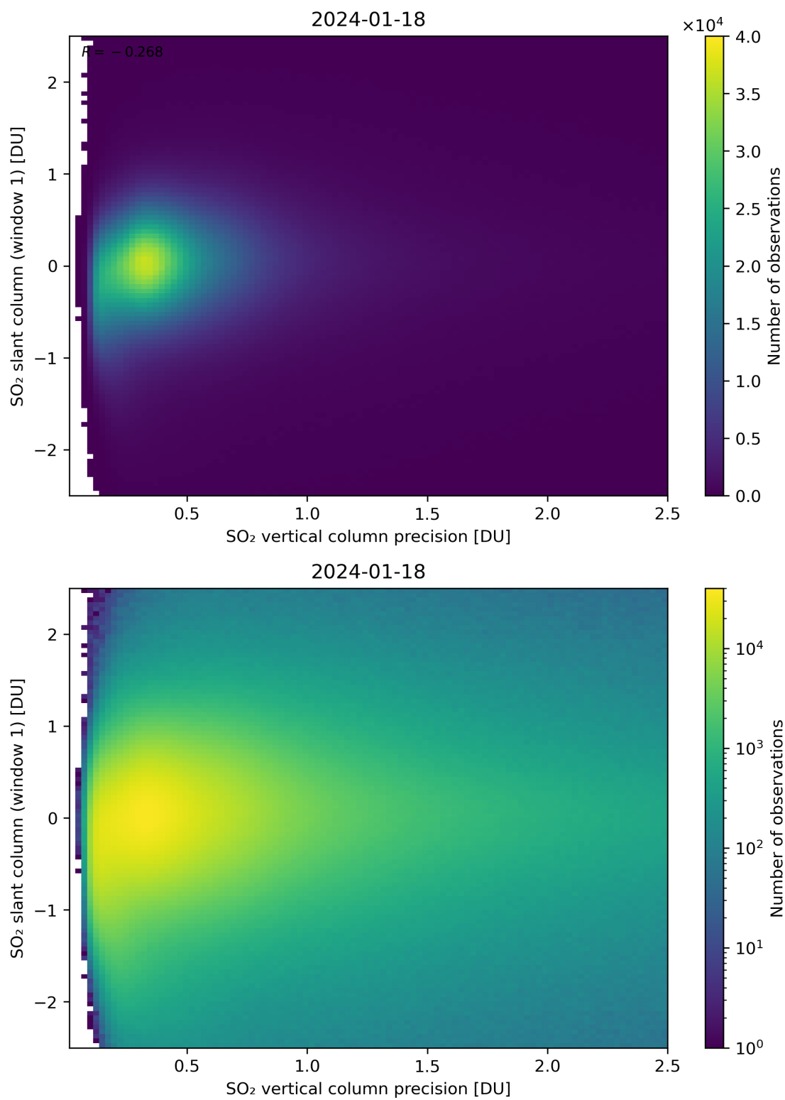
Figure 289: Scatter density plot of “SO 2 vertical column precision” against “SO 2 slant column (window 1)” for 2024-01-17 to 2024-01-19.
