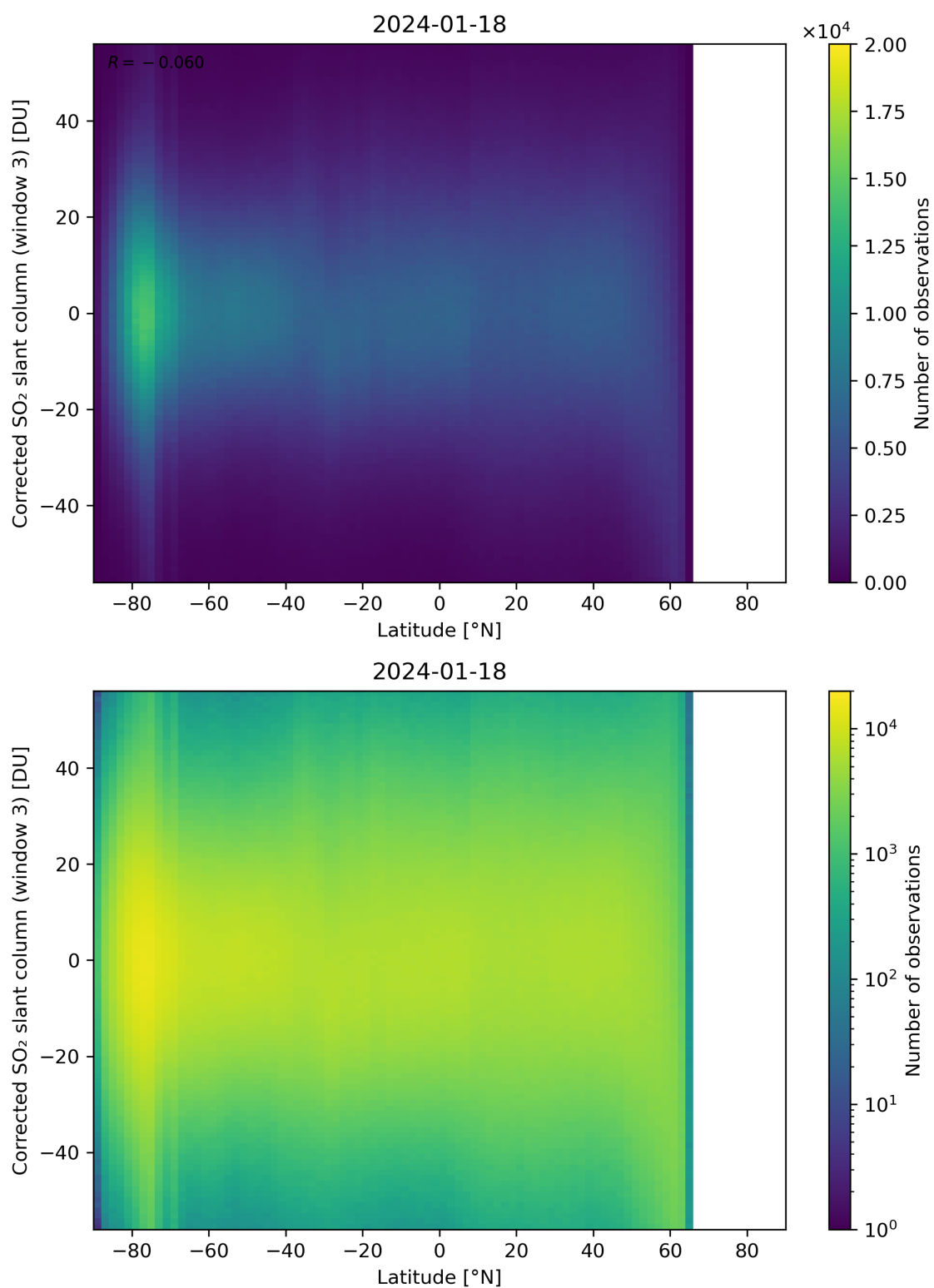
Figure 148: Scatter density plot of “Latitude” against “Corrected SO 2 slant column (window 3)” for 2024-01-17 to 2024-01-19.
