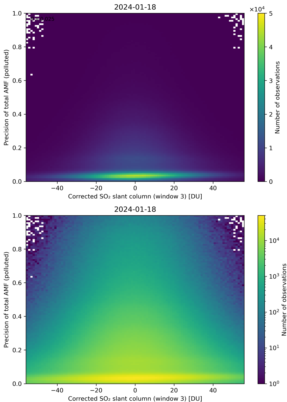
Figure 211: Scatter density plot of “Corrected SO 2 slant column (window 3)” against “Precision of total AMF (polluted)” for 2024-01-17 to 2024-01-19.
