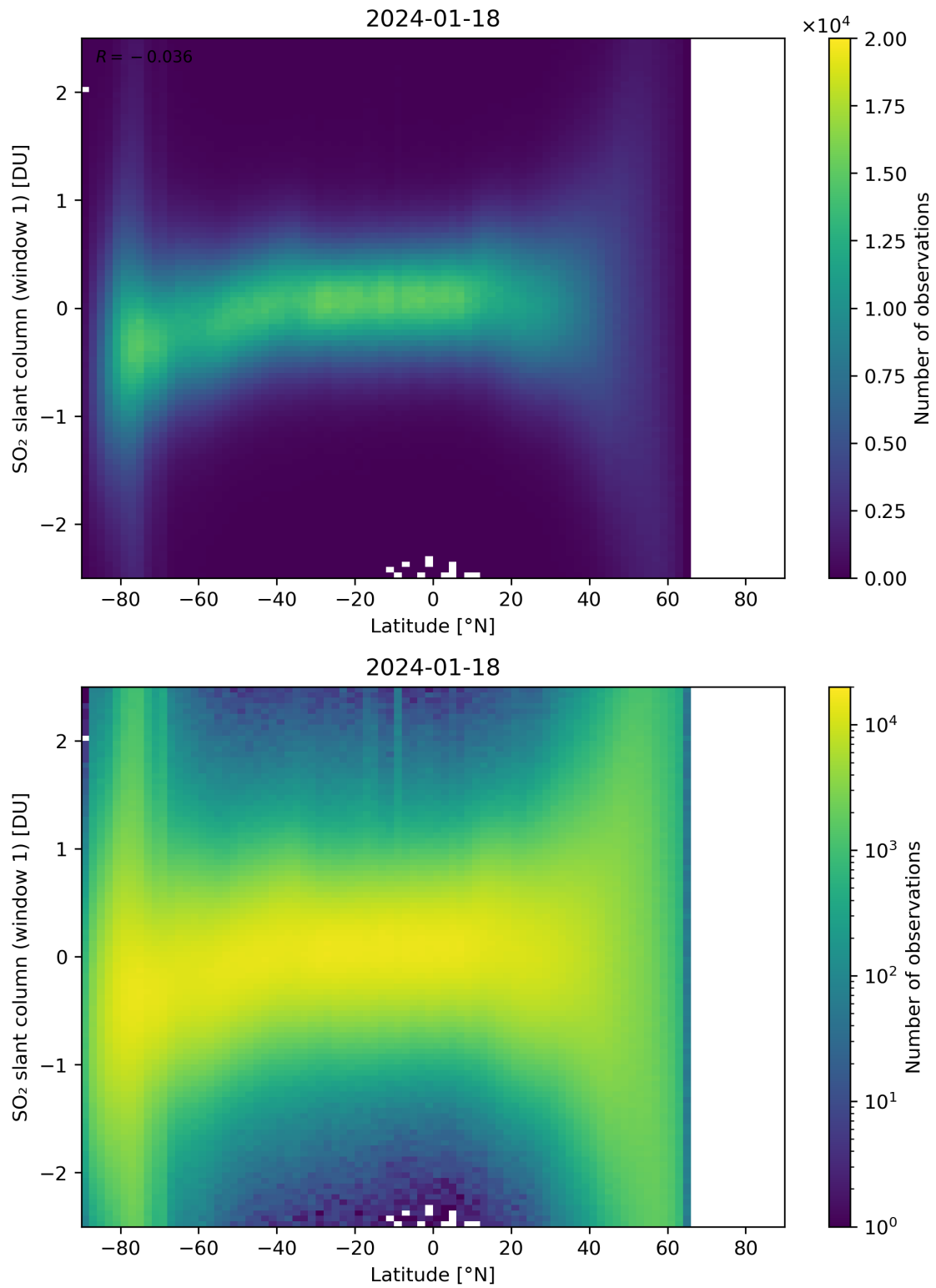
Figure 149: Scatter density plot of “Latitude” against “SO 2 slant column (window 1)” for 2024-01-17 to 2024-01-19.
