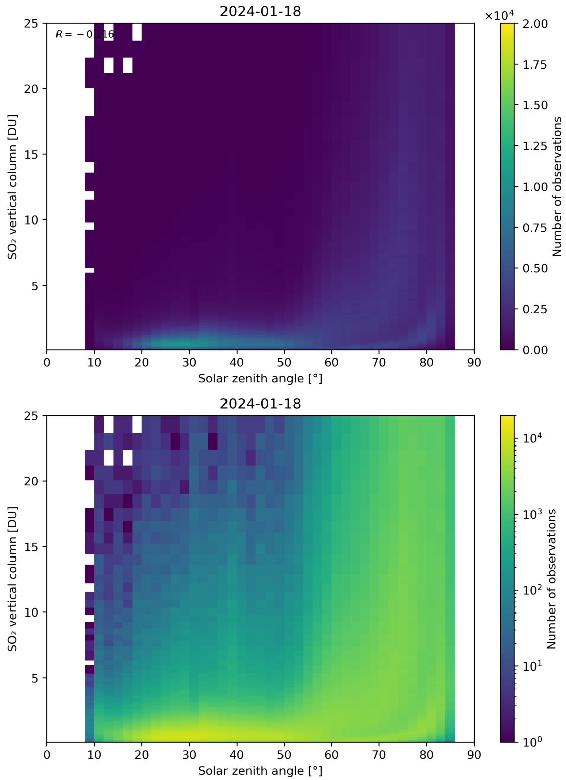
Figure 176: Scatter density plot of “Solar zenith angle” against “SO 2 vertical column” for 2024-01-17 to 2024-01-19.
