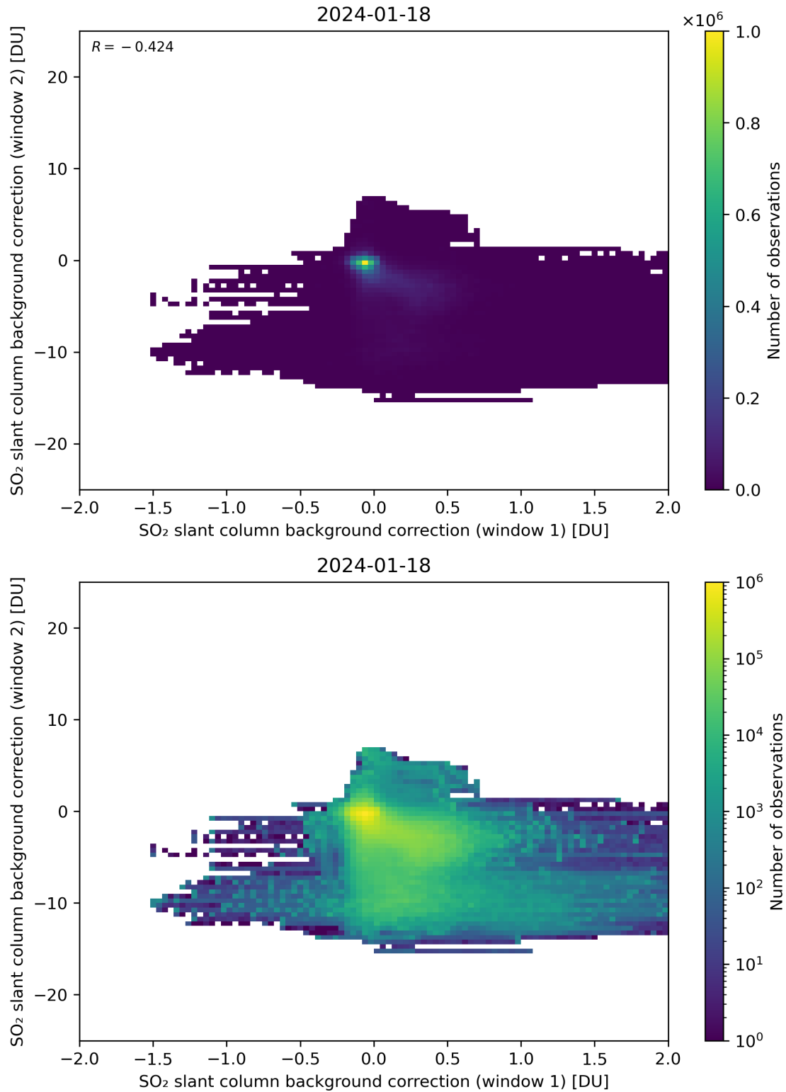
Figure 98: Scatter density plot of “SO 2 slant column background correction (window 1)” against “SO 2 slant column background correction (window 2)” for 2024-01-17 to 2024-01-19.
