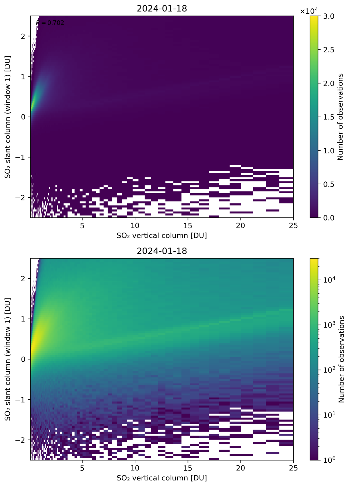
Figure 300: Scatter density plot of “SO 2 vertical column” against “SO 2 slant column (window 1)” for 2024-01-17 to 2024-01-19.
