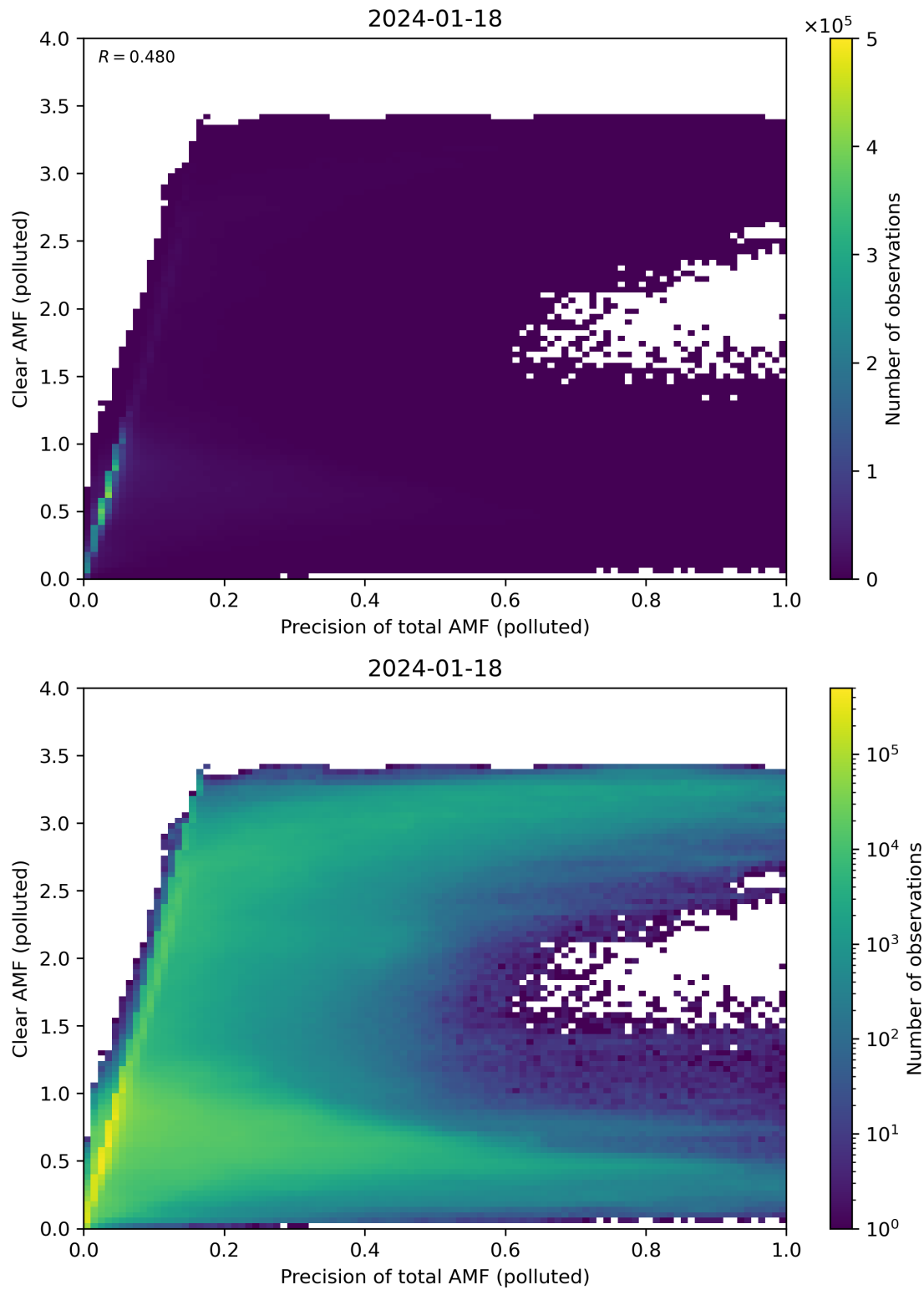
Figure 270: Scatter density plot of “Precision of total AMF (polluted)” against “Clear AMF (polluted)” for 2024-01-17 to 2024-01-19.
