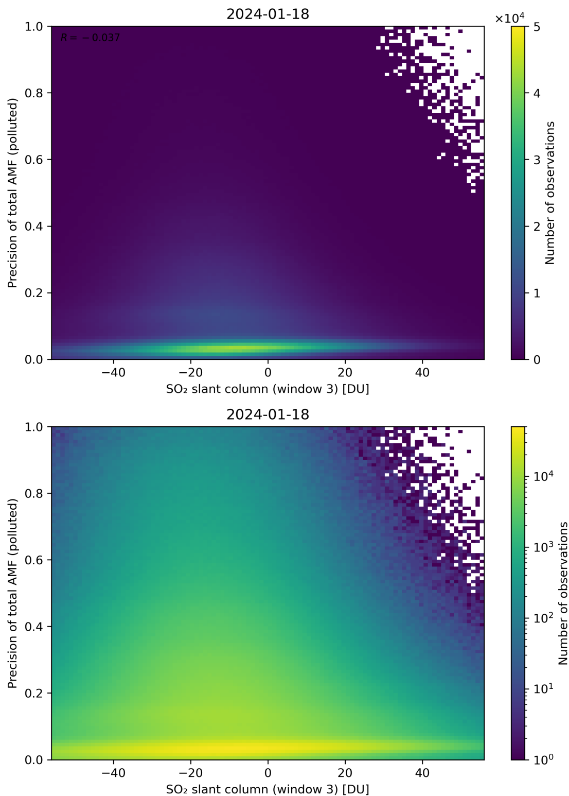
Figure 269: Scatter density plot of “SO 2 slant column (window 3)” against “Precision of total AMF (polluted)” for 2024-01-17 to 2024-01-19.
