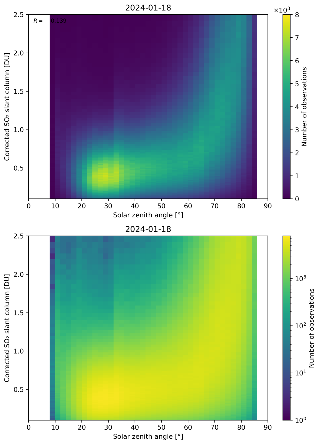
Figure 166: Scatter density plot of “Solar zenith angle” against “Corrected SO 2 slant column” for 2024-01-17 to 2024-01-19.
