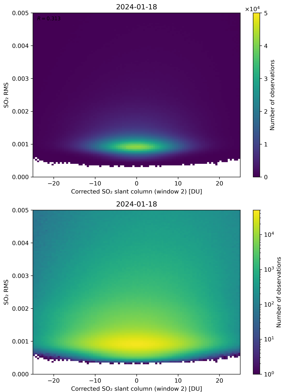
Figure 198: Scatter density plot of “Corrected SO 2 slant column (window 2)” against “SO 2 RMS” for 2024-01-17 to 2024-01-19.
