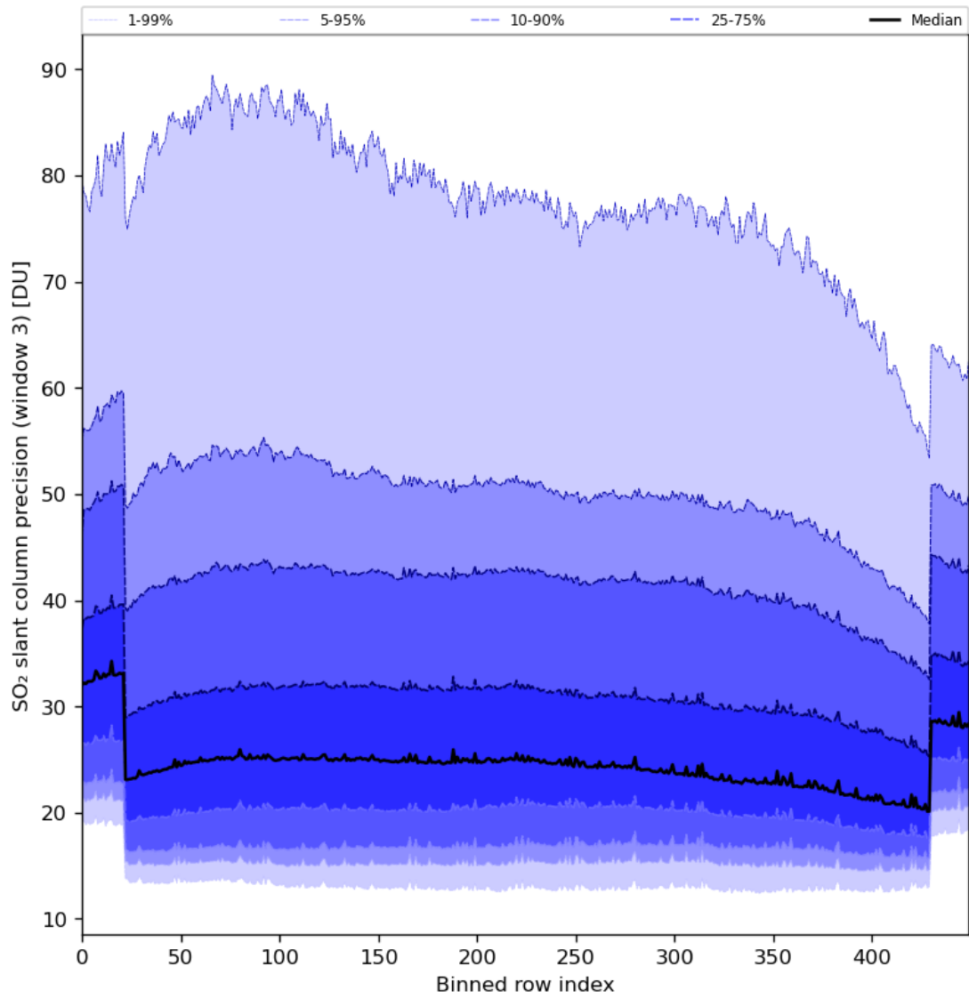
Figure 88: Along track statistics of “SO 2 slant column precision (window 3)” for 2024-01-17 to 2024-01-19
