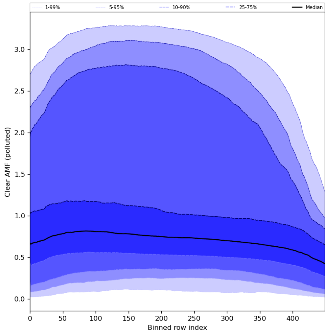
Figure 96: Along track statistics of “Clear AMF (polluted)” for 2024-01-17 to 2024-01-19
