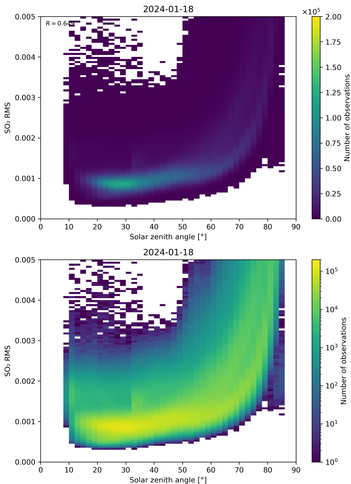
Figure 163: Scatter density plot of “Solar zenith angle” against “SO 2 RMS” for 2024-01-17 to 2024-01-19.
