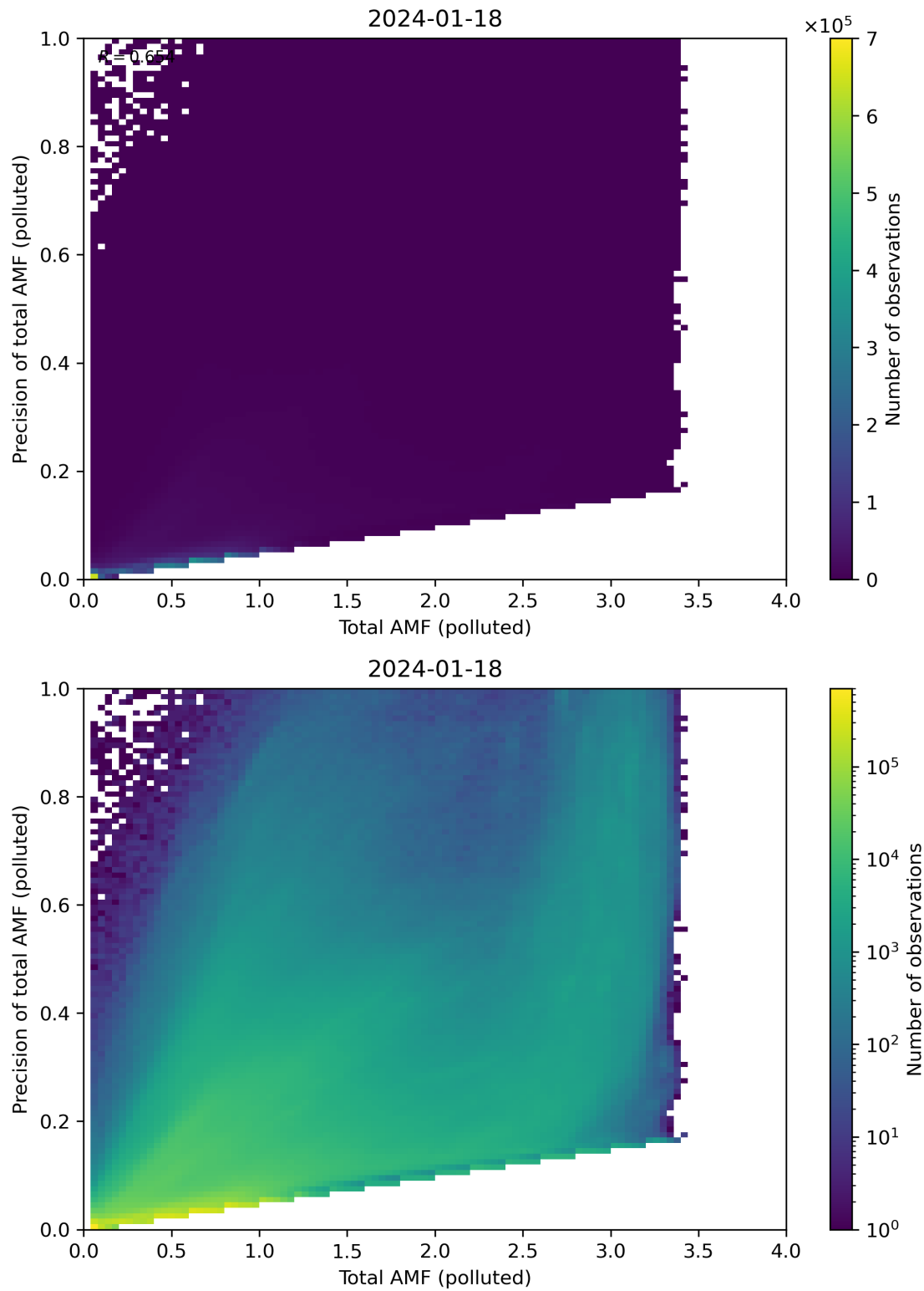
Figure 272: Scatter density plot of “Total AMF (polluted)” against “Precision of total AMF (polluted)” for 2024-01-17 to 2024-01-19.
