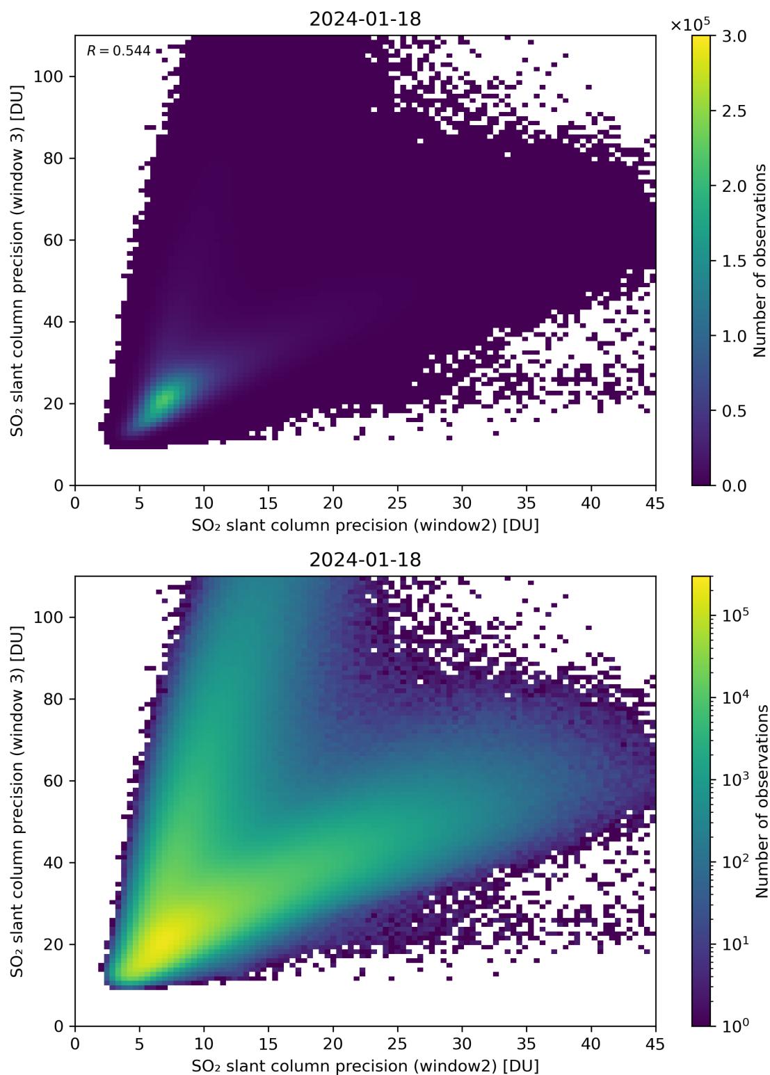
Figure 250: Scatter density plot of “SO 2 slant column precision (window2)” against “SO 2 slant column precision (window 3)” for 2024-01-17 to 2024-01-19.
