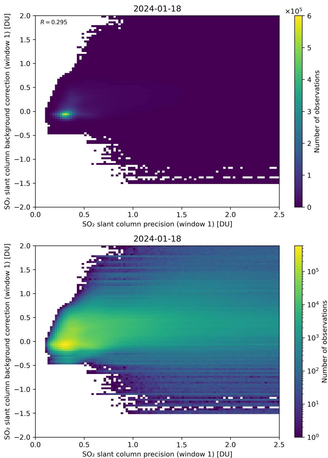
Figure 218: Scatter density plot of “SO 2 slant column precision (window 1)” against “SO 2 slant column background correction (window 1)” for 2024-01-17 to 2024-01-19.
