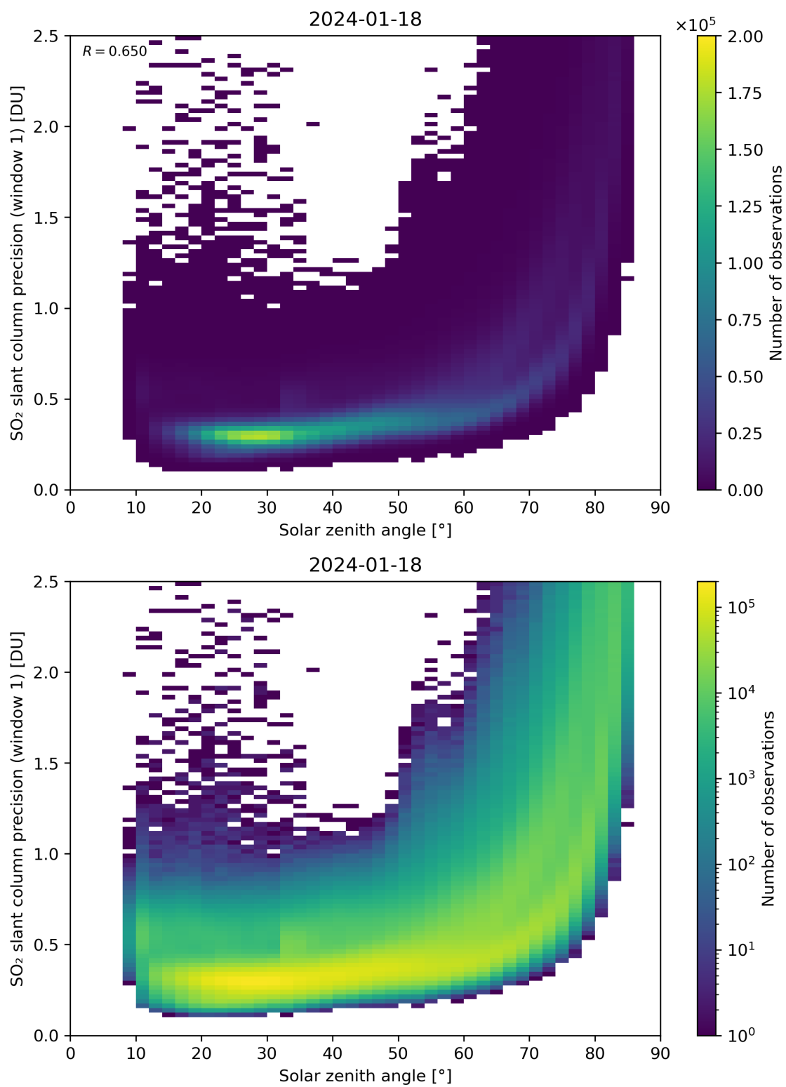
Figure 170: Scatter density plot of “Solar zenith angle” against “SO 2 slant column precision (window 1)” for 2024-01-17 to 2024-01-19.
