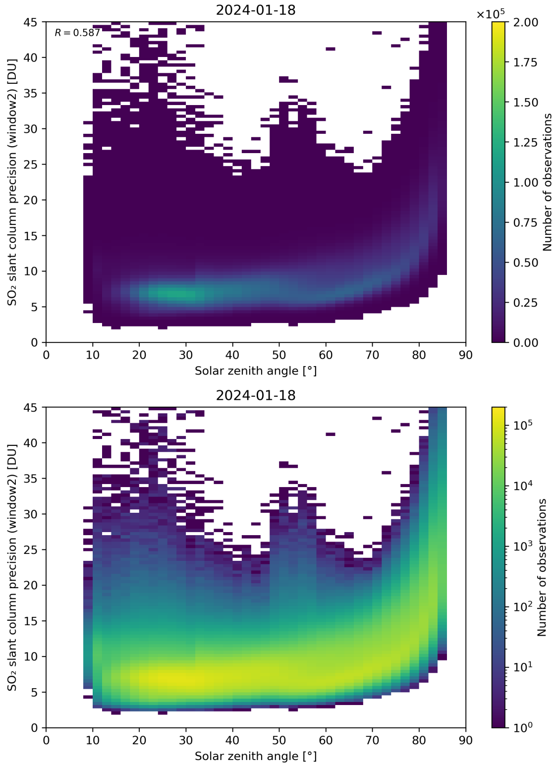
Figure 171: Scatter density plot of “Solar zenith angle” against “SO 2 slant column precision (window2)” for 2024-01-17 to 2024-01-19.
