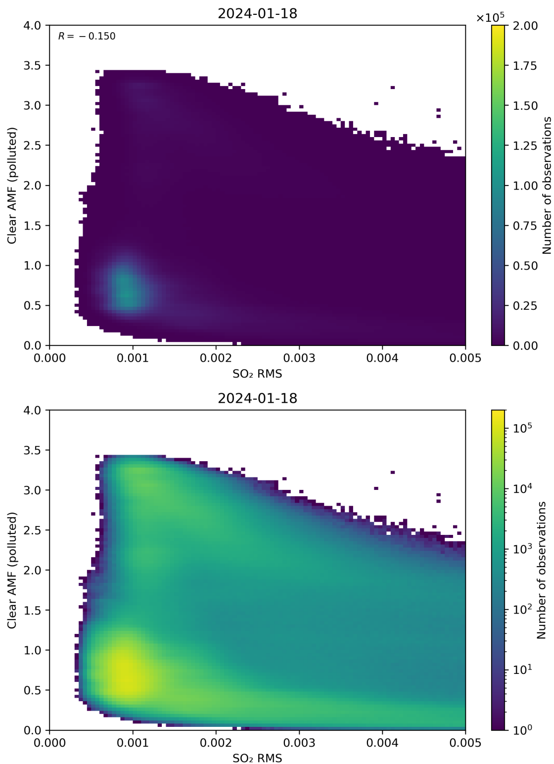
Figure 136: Scatter density plot of “SO 2 RMS” against “Clear AMF (polluted)” for 2024-01-17 to 2024-01-19.
