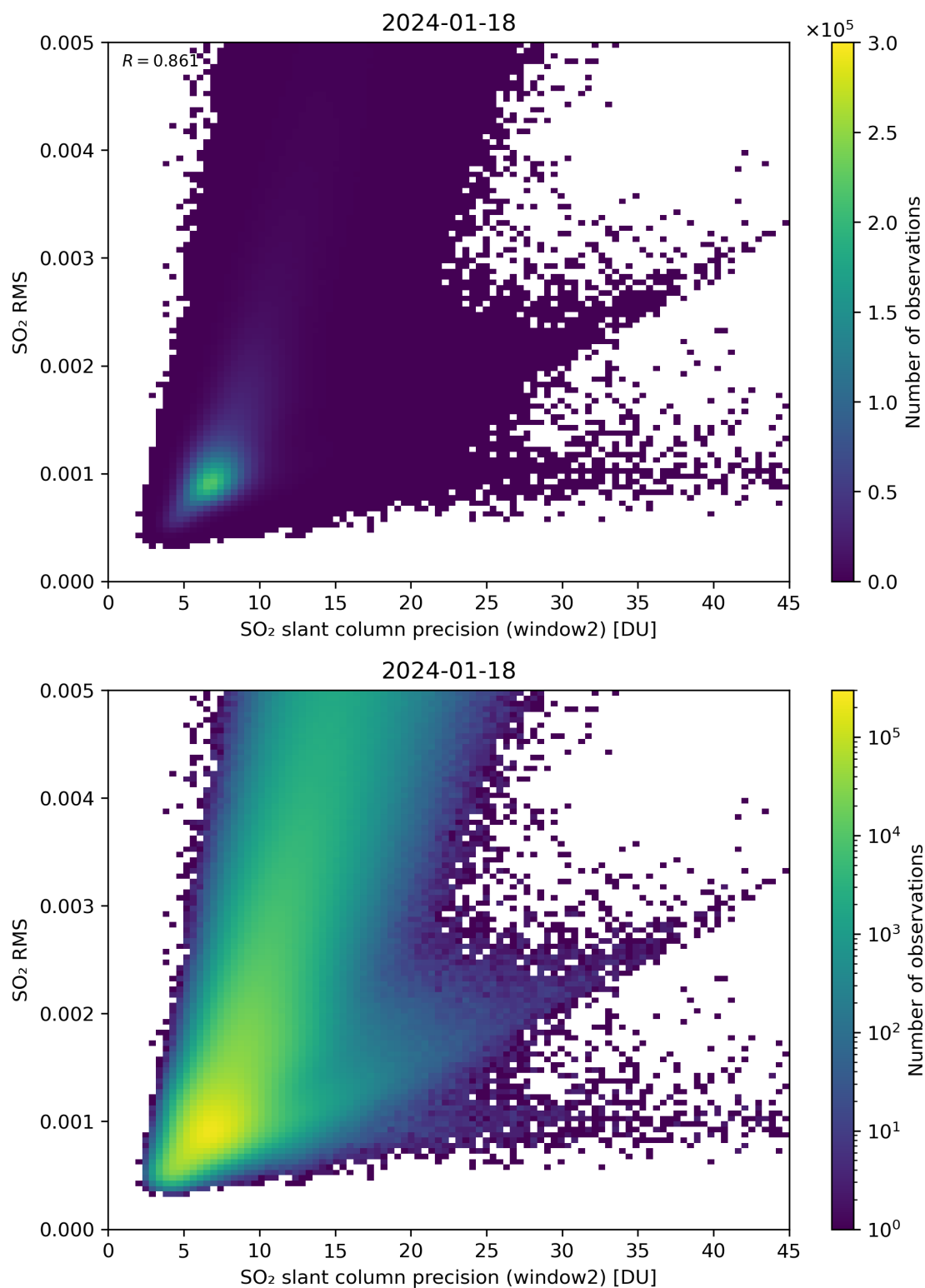
Figure 245: Scatter density plot of “SO 2 slant column precision (window2)” against “SO 2 RMS” for 2024-01-17 to 2024-01-19.
