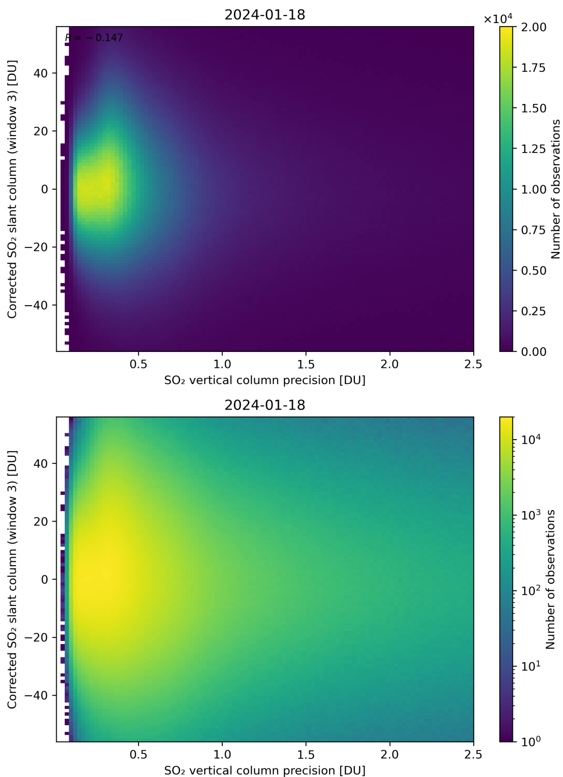
Figure 288: Scatter density plot of “SO 2 vertical column precision” against “Corrected SO 2 slant column (window 3)” for 2024-01-17 to 2024-01-19.
