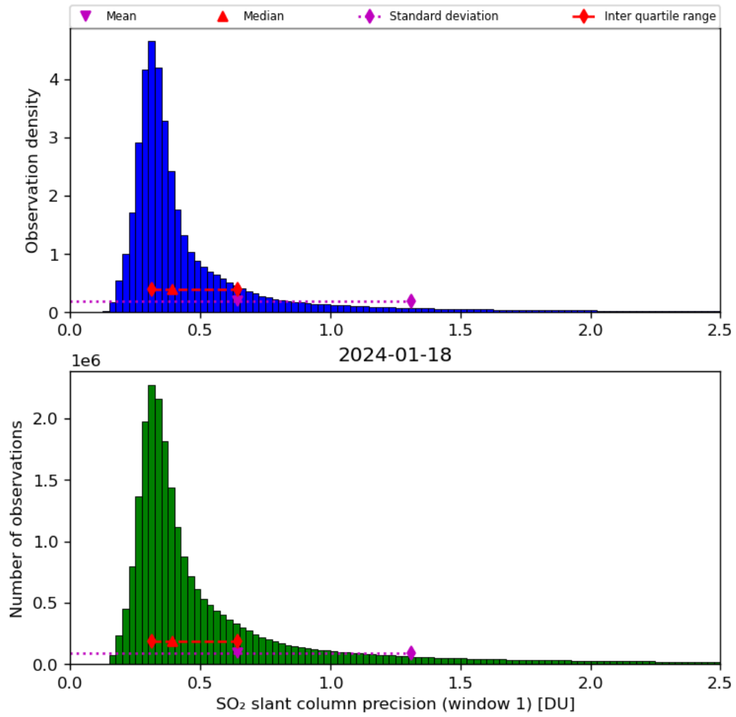
Figure 57: Histogram of “SO 2 slant column precision (window 1)” for 2024-01-17 to 2024-01-19
