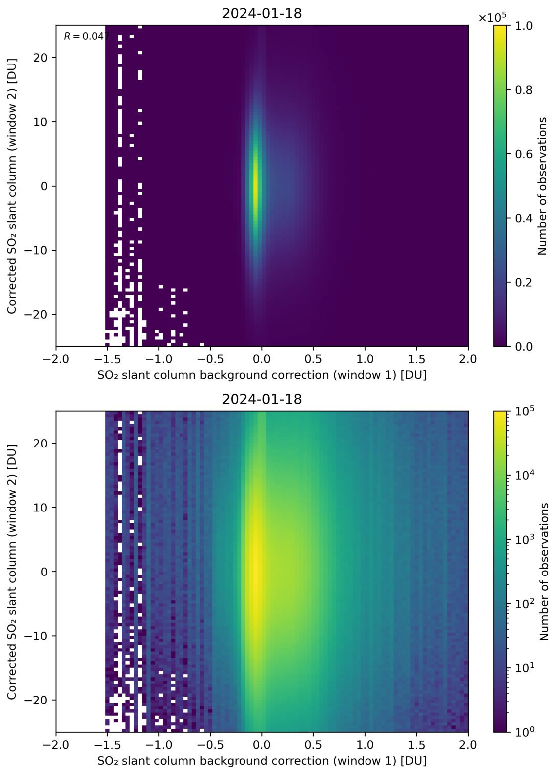
Figure 104: Scatter density plot of “SO 2 slant column background correction (window 1)” against “Corrected SO 2 slant column (window 2)” for 2024-01-17 to 2024-01-19.
