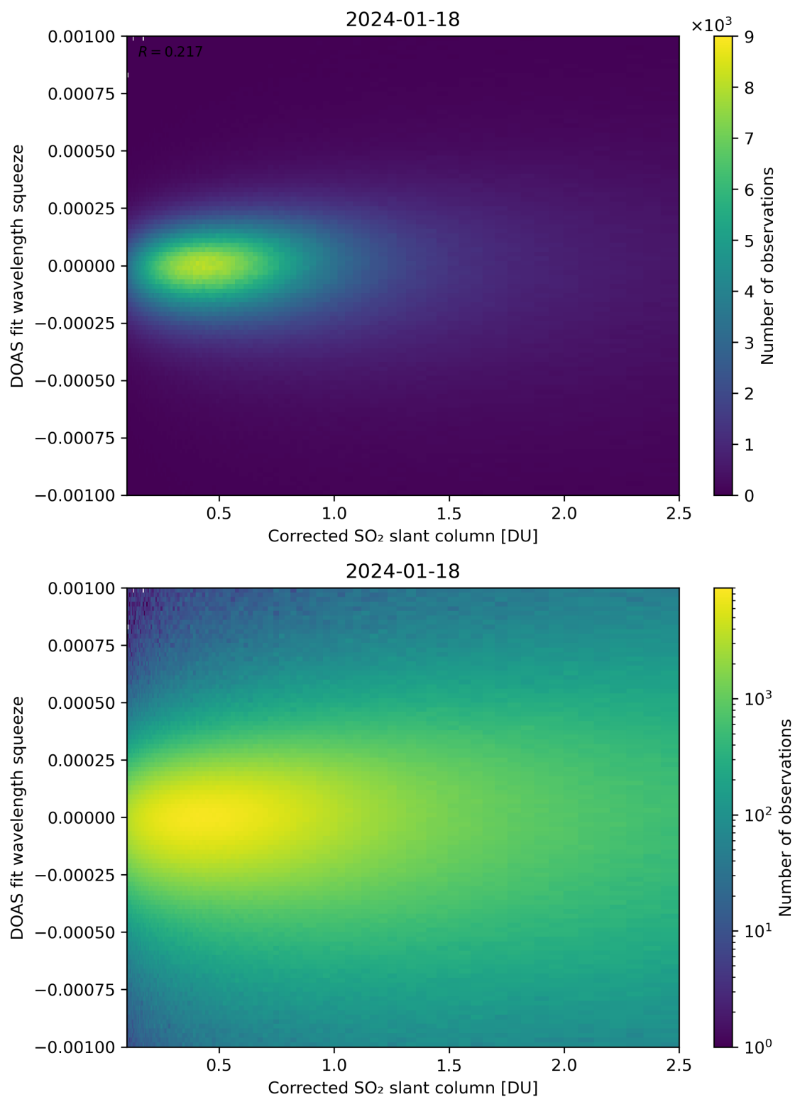
Figure 182: Scatter density plot of “Corrected SO 2 slant column” against “DOAS fit wavelength squeeze” for 2024-01-17 to 2024-01-19.
