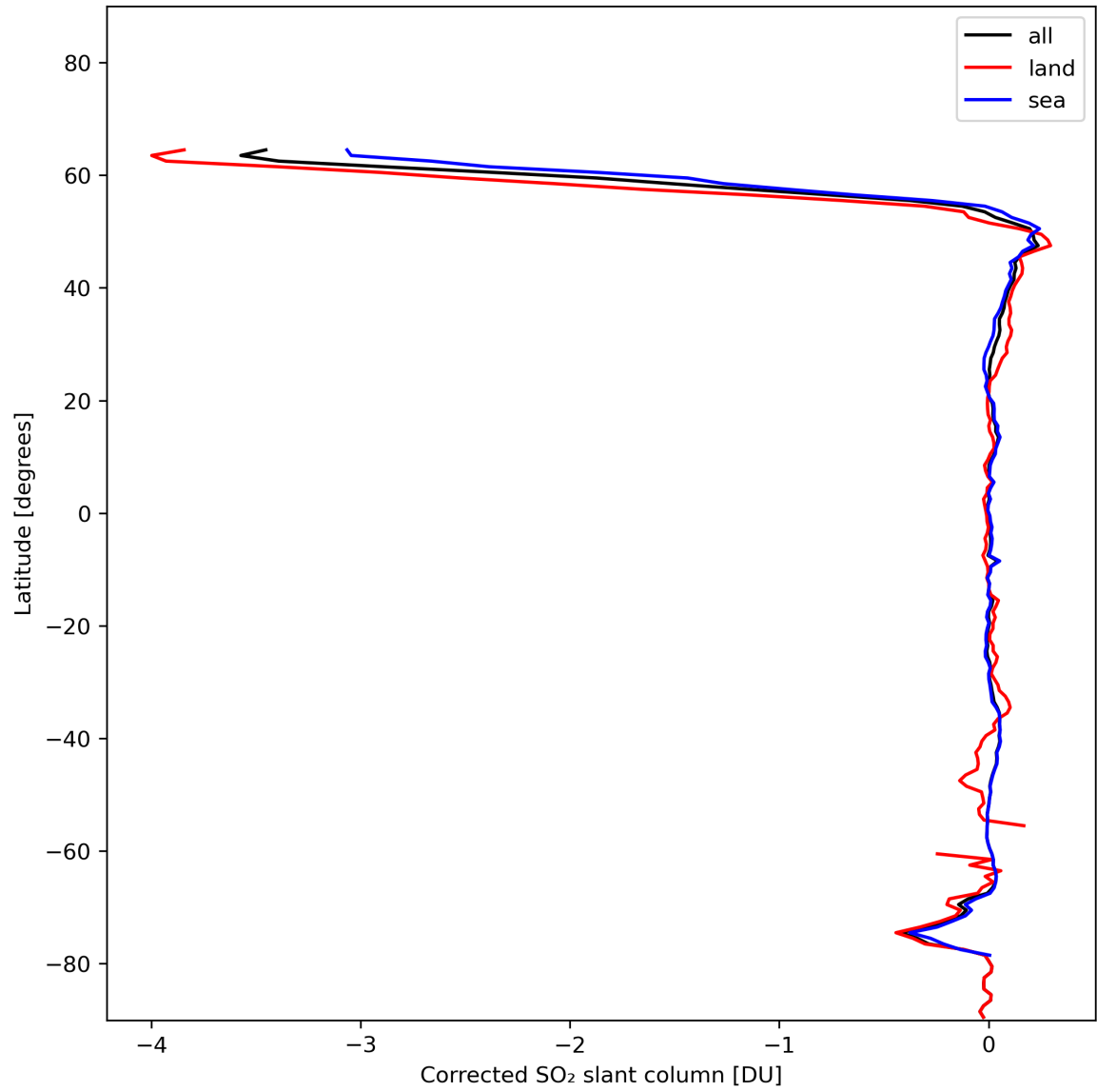
Figure 32: Zonal average of “Corrected SO 2 slant column” for 2024-01-17 to 2024-01-19.
