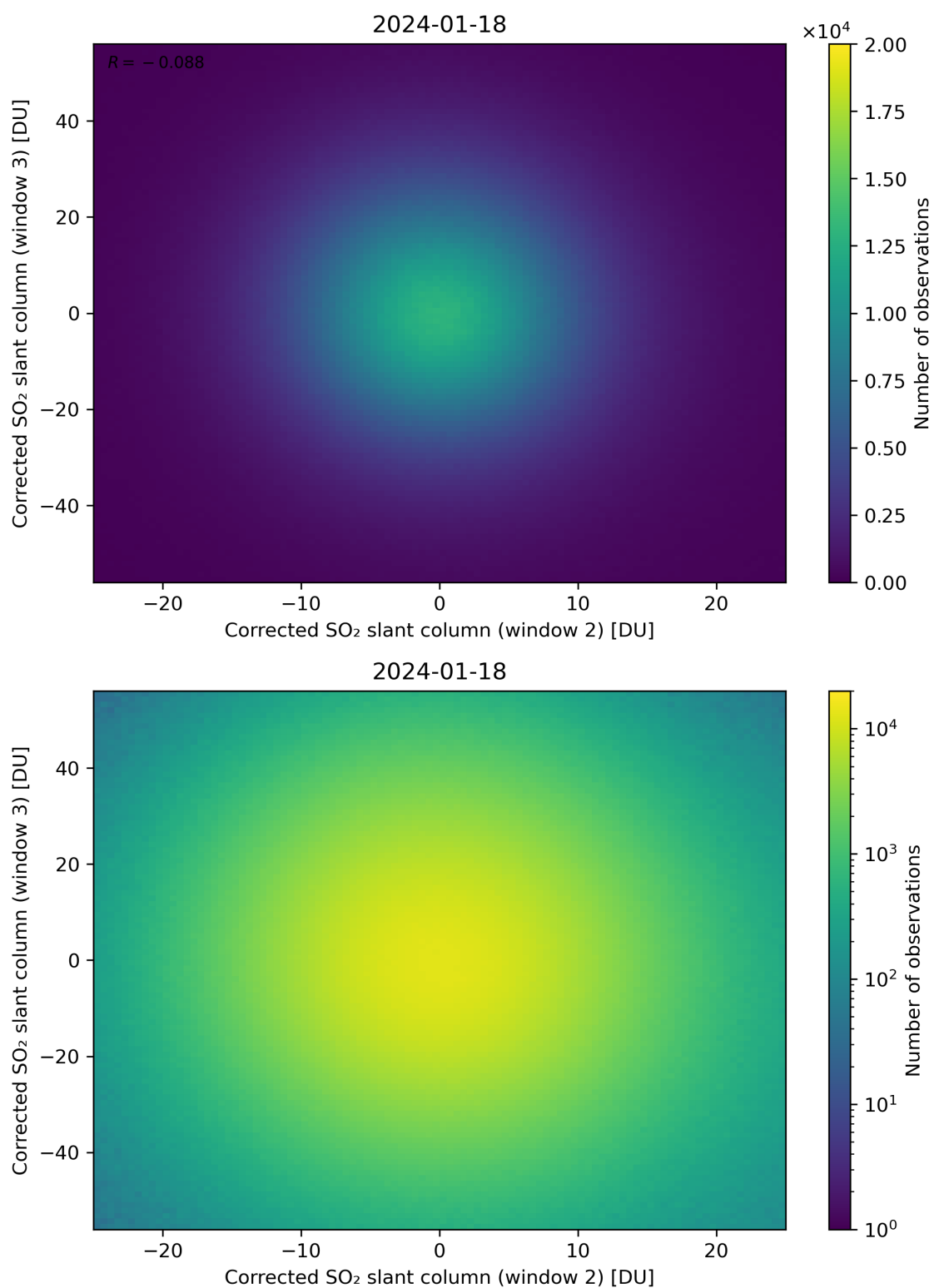
Figure 200: Scatter density plot of “Corrected SO 2 slant column (window 2)” against “Corrected SO 2 slant column (window 3)” for 2024-01-17 to 2024-01-19.
