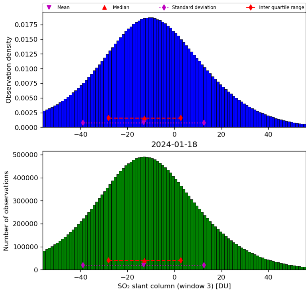
Figure 64: Histogram of “SO 2 slant column (window 3)” for 2024-01-17 to 2024-01-19
