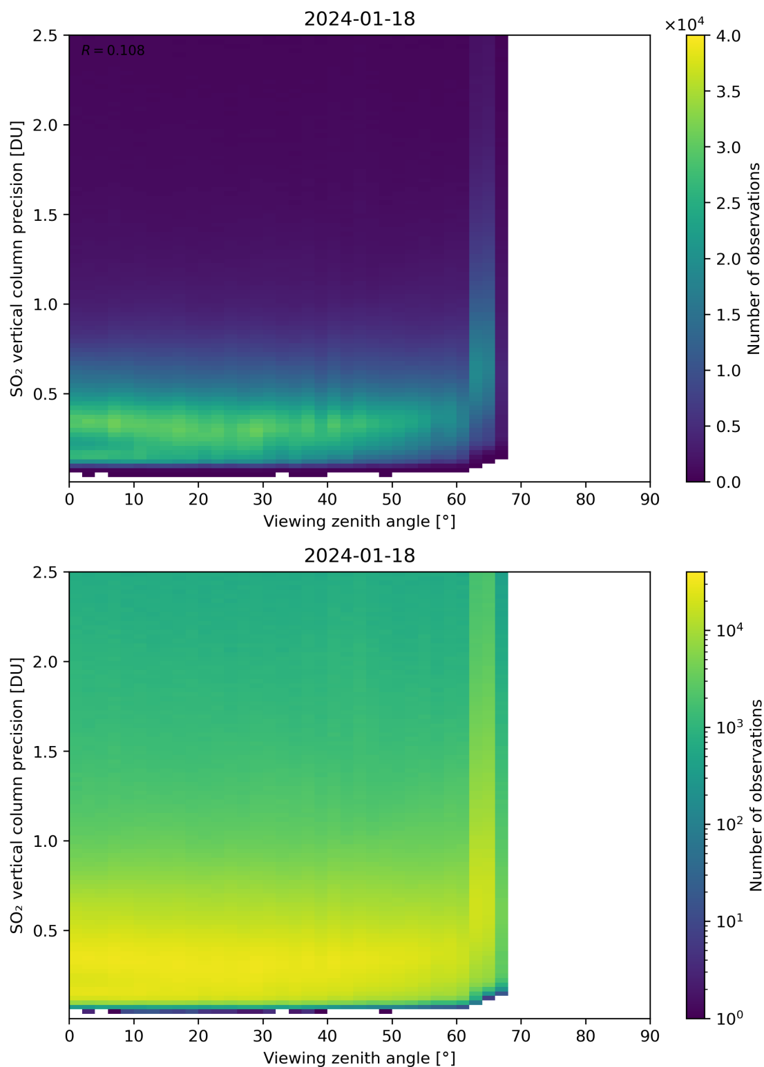
Figure 328: Scatter density plot of “Viewing zenith angle” against “SO 2 vertical column precision” for 2024-01-17 to 2024-01-19.
