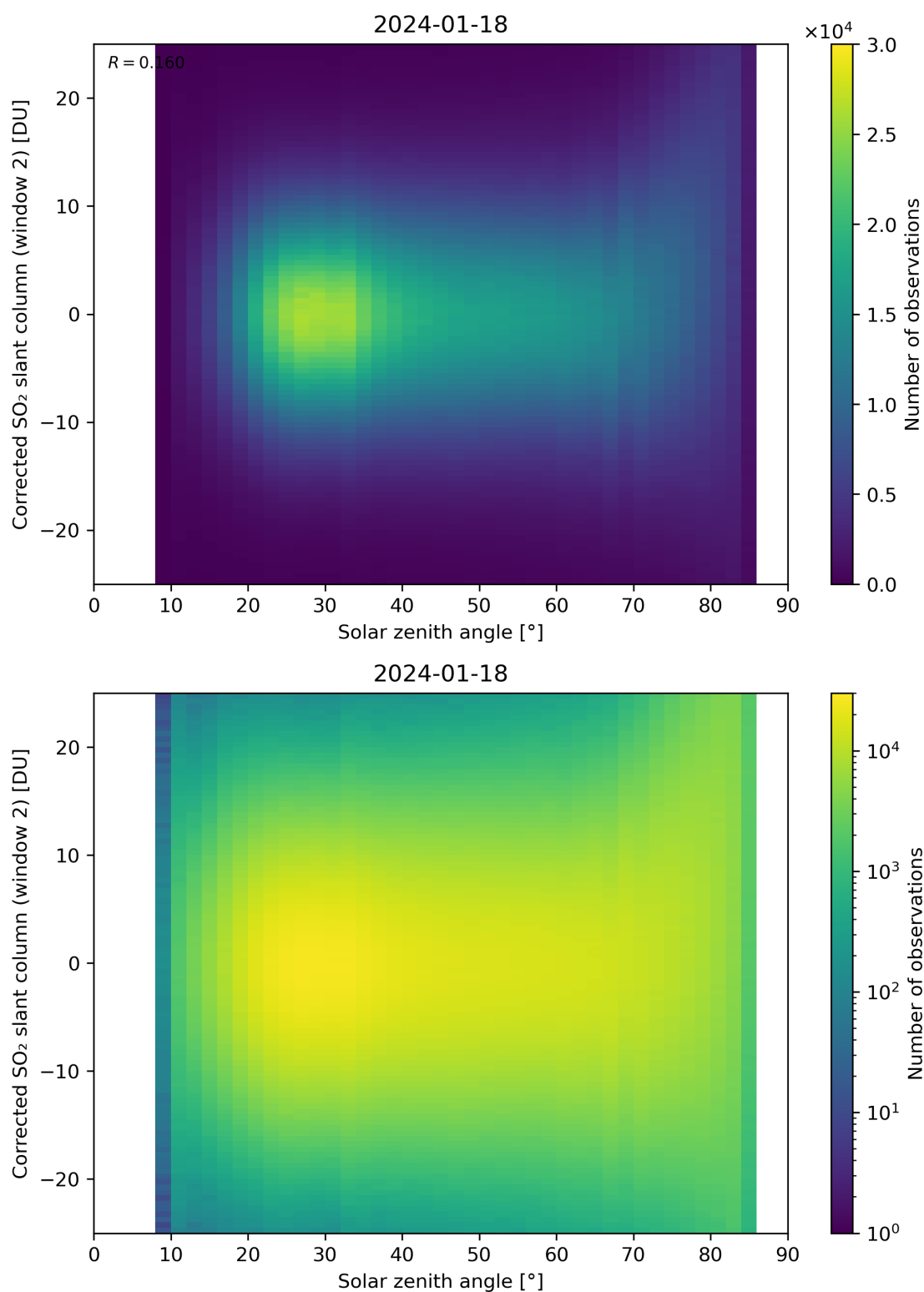
Figure 167: Scatter density plot of “Solar zenith angle” against “Corrected SO 2 slant column (window 2)” for 2024-01-17 to 2024-01-19.
