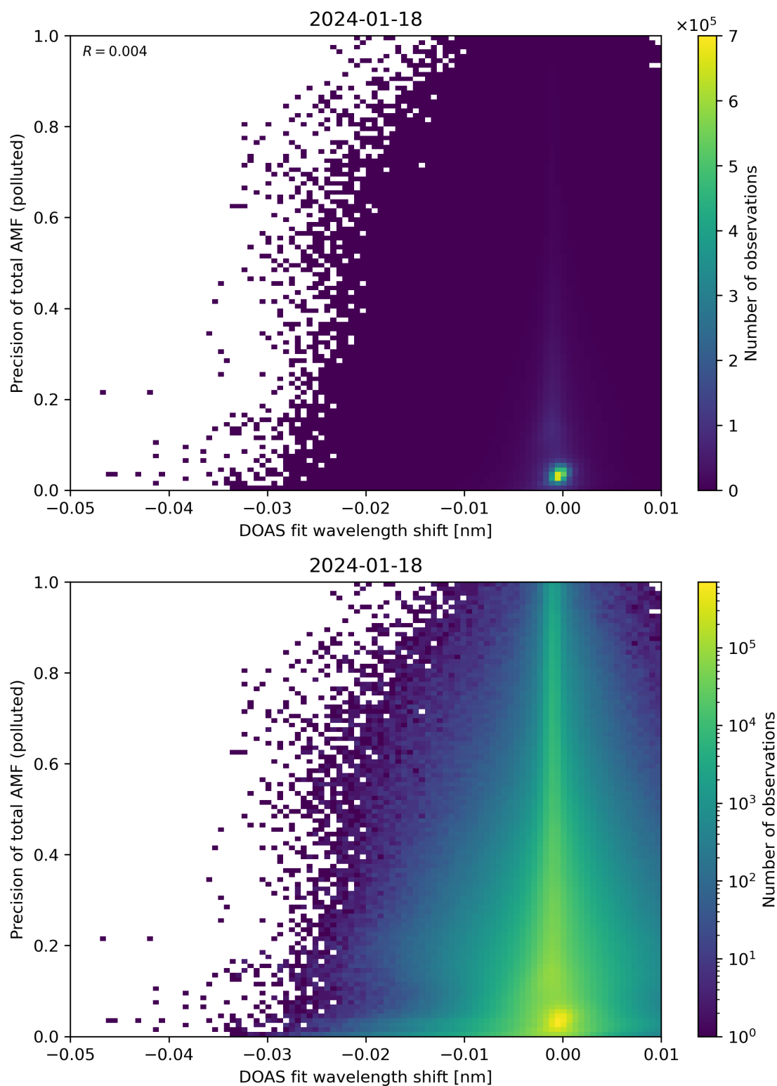
Figure 131: Scatter density plot of “DOAS fit wavelength shift” against “Precision of total AMF (polluted)” for 2024-01-17 to 2024-01-19.
