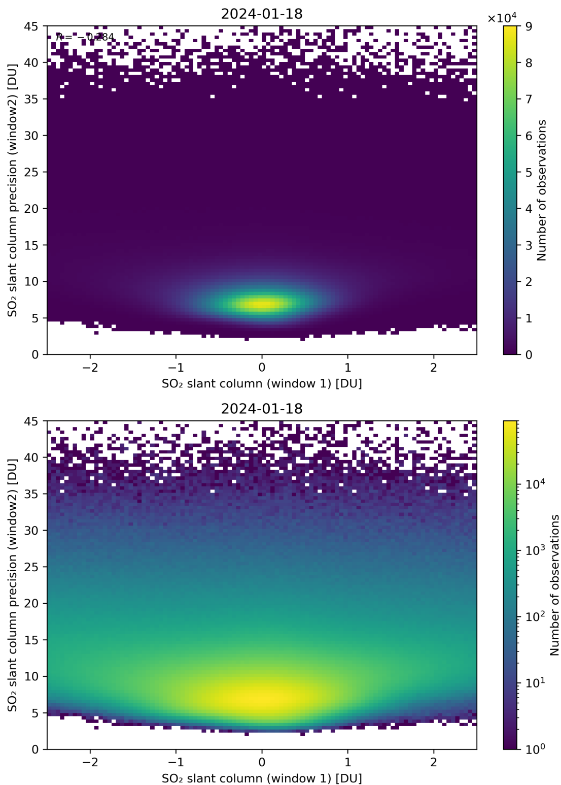
Figure 236: Scatter density plot of “SO 2 slant column (window 1)” against “SO 2 slant column precision (window2)” for 2024-01-17 to 2024-01-19.
