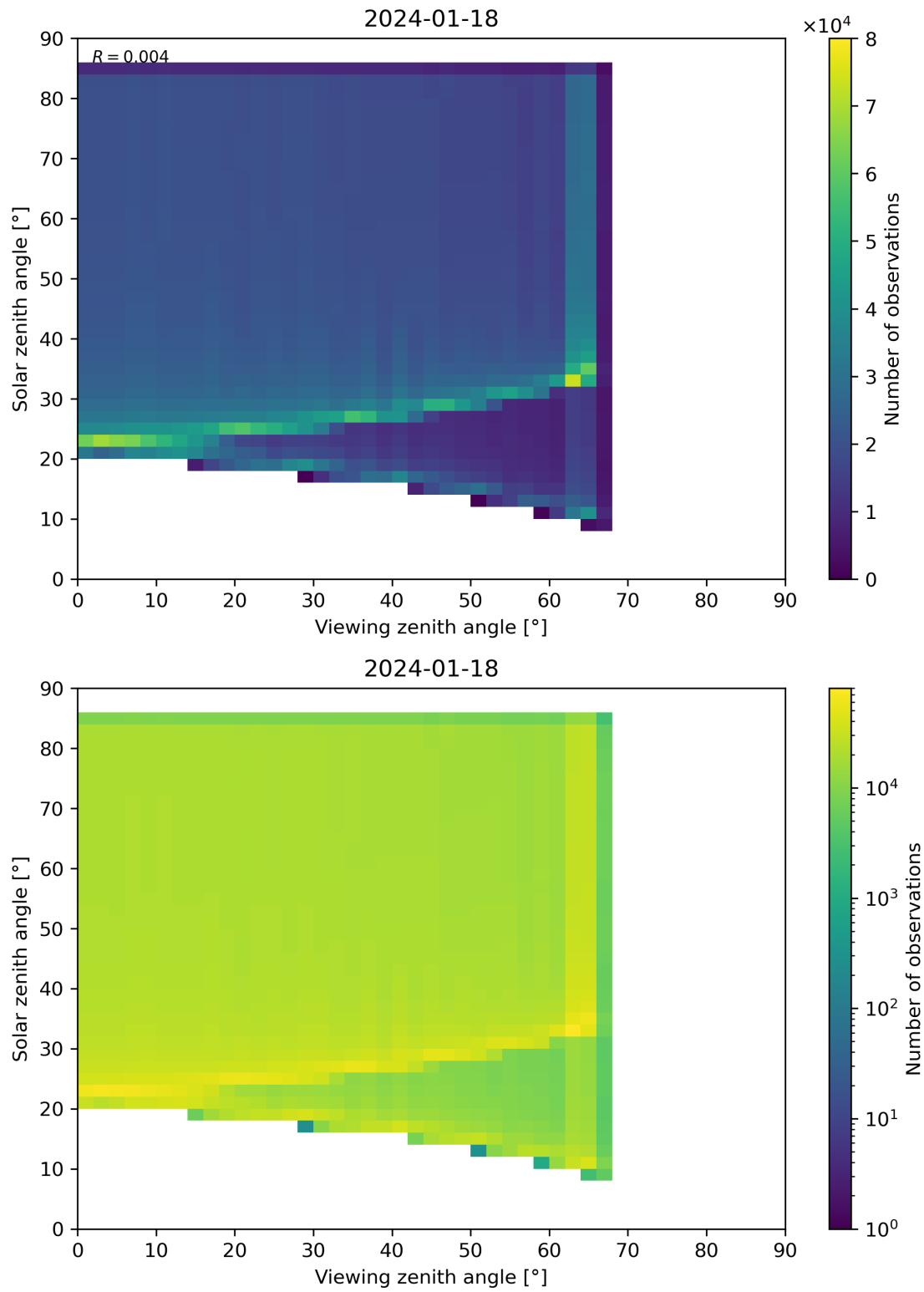
Figure 315: Scatter density plot of “Viewing zenith angle” against “Solar zenith angle” for 2024-01-17 to 2024-01-19.
