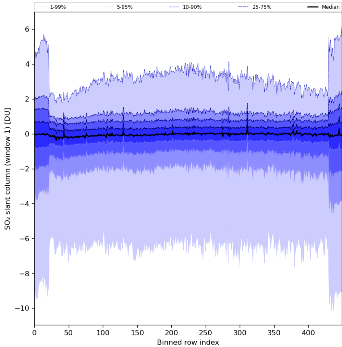
Figure 79: Along track statistics of “SO 2 slant column (window 1)” for 2024-01-17 to 2024-01-19
