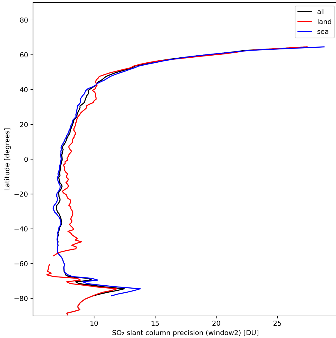
Figure 38: Zonal average of “SO 2 slant column precision (window2)” for 2024-01-17 to 2024-01-19.
