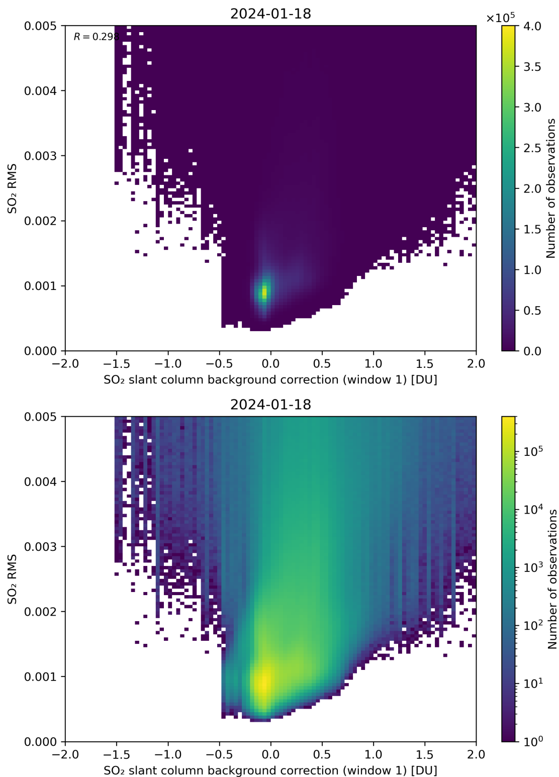
Figure 102: Scatter density plot of “SO 2 slant column background correction (window 1)” against “SO 2 RMS” for 2024-01-17 to 2024-01-19.
