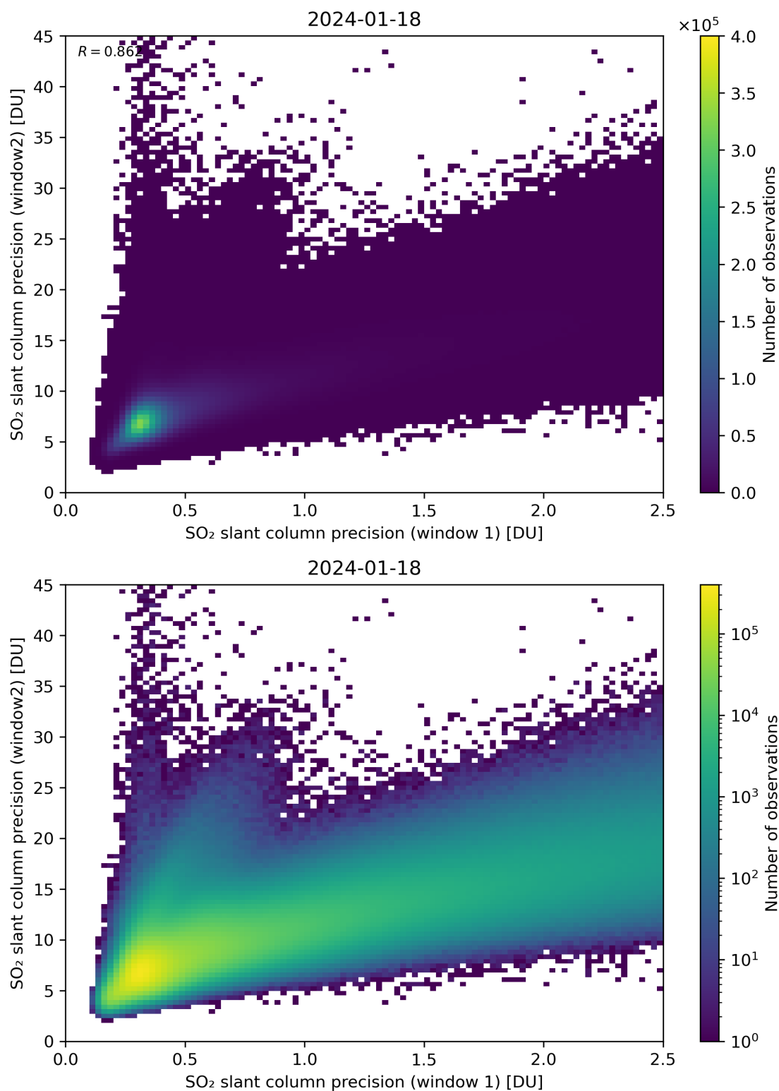
Figure 227: Scatter density plot of “SO 2 slant column precision (window 1)” against “SO 2 slant column precision (window2)” for 2024-01-17 to 2024-01-19.
