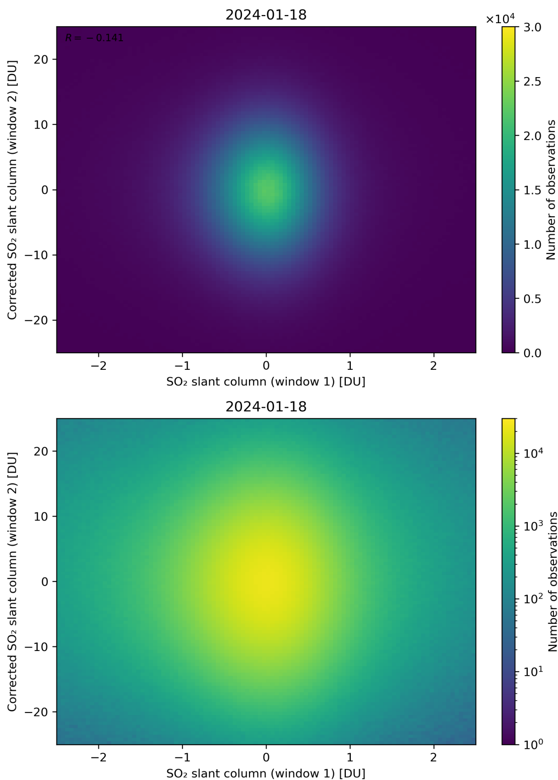
Figure 233: Scatter density plot of “SO 2 slant column (window 1)” against “Corrected SO 2 slant column (window 2)” for 2024-01-17 to 2024-01-19.
