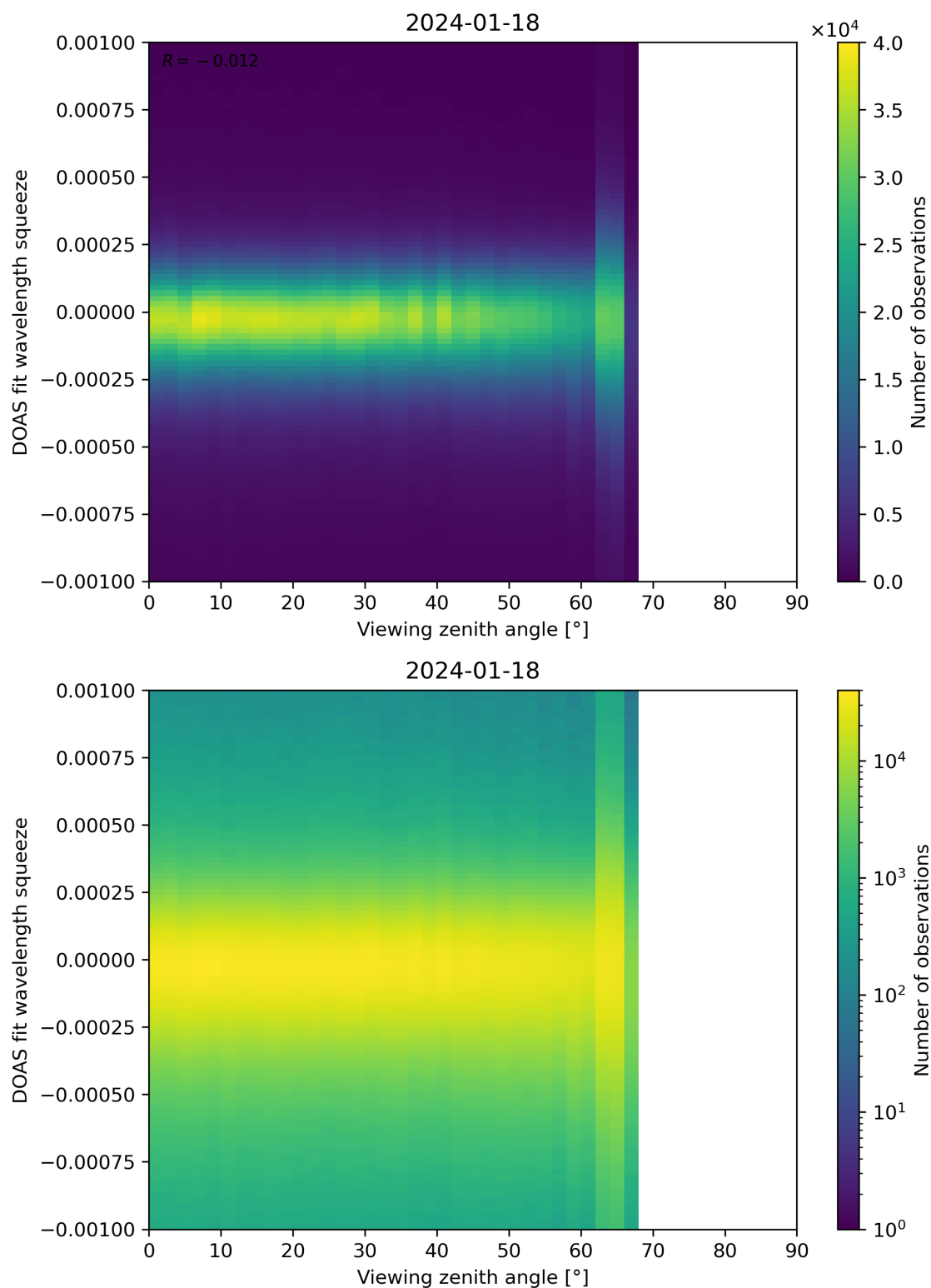
Figure 312: Scatter density plot of “Viewing zenith angle” against “DOAS fit wavelength squeeze” for 2024-01-17 to 2024-01-19.
