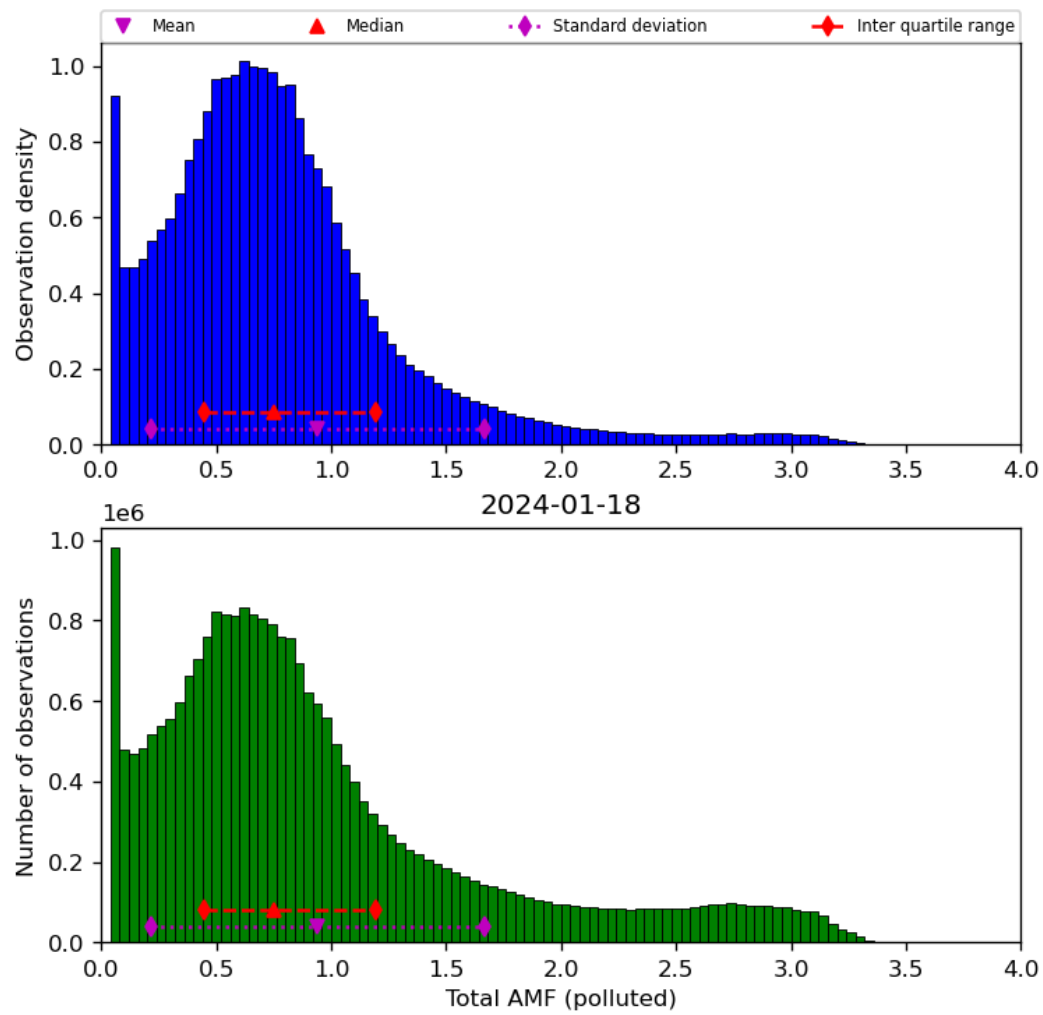
Figure 71: Histogram of “Total AMF (polluted)” for 2024-01-17 to 2024-01-19
