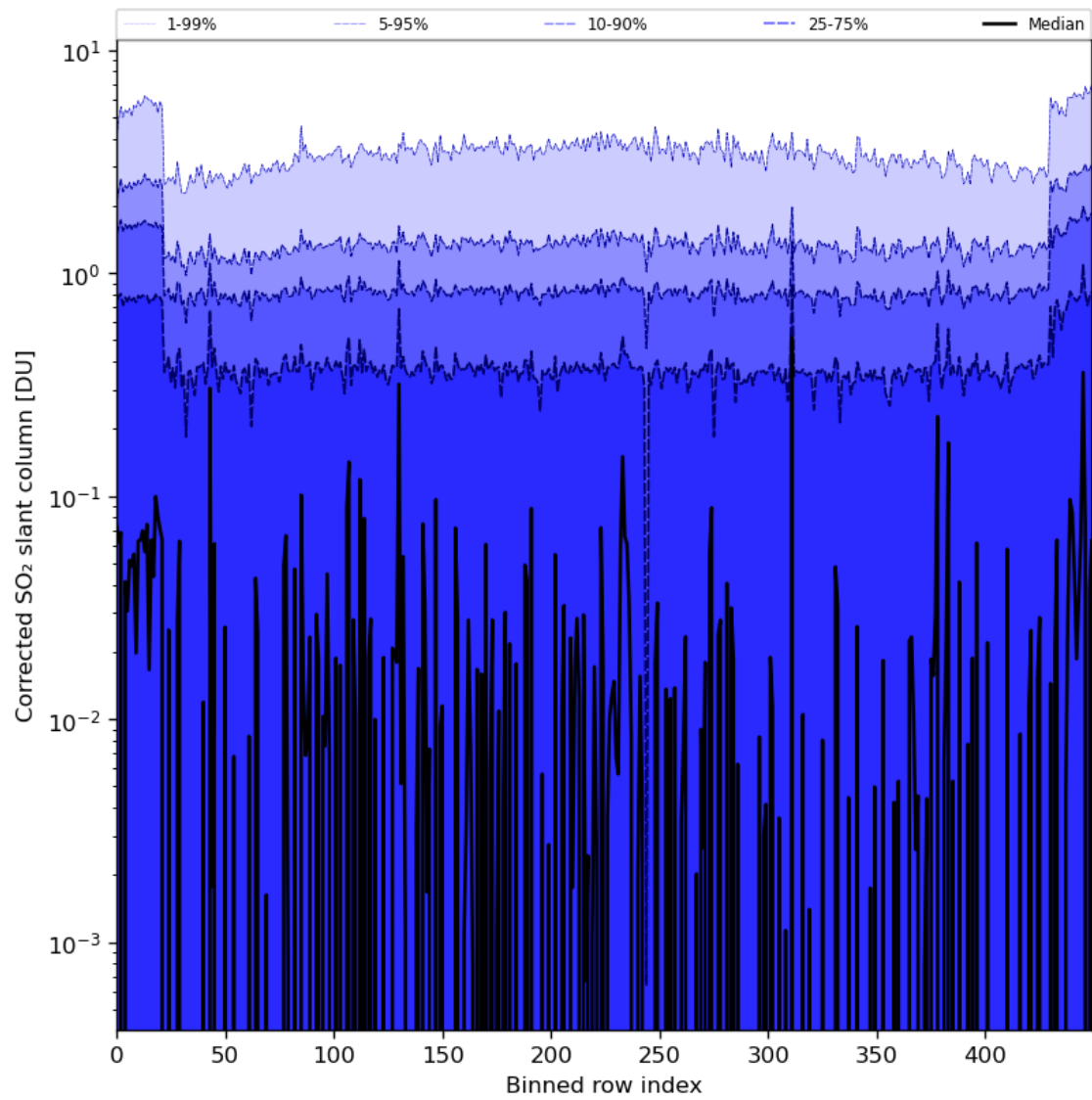
Figure 78: Along track statistics of “Corrected SO 2 slant column” for 2024-01-17 to 2024-01-19
