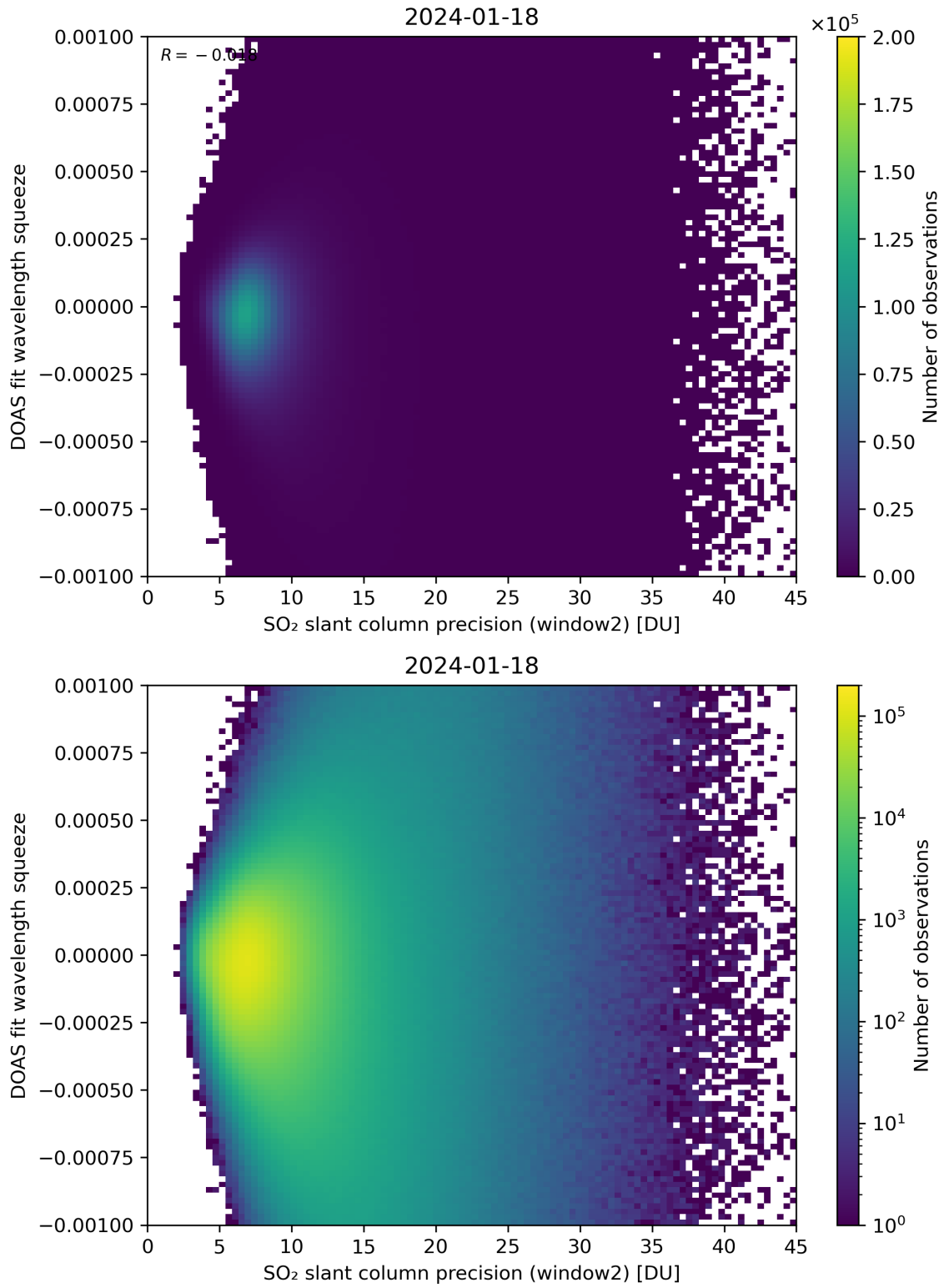
Figure 244: Scatter density plot of “SO 2 slant column precision (window2)” against “DOAS fit wavelength squeeze” for 2024-01-17 to 2024-01-19.
