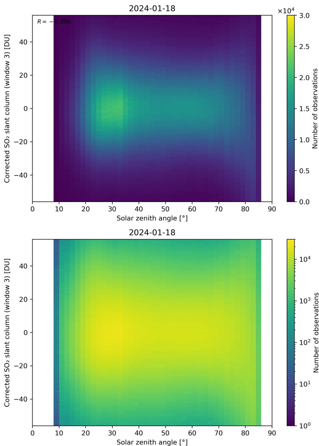
Figure 168: Scatter density plot of “Solar zenith angle” against “Corrected SO 2 slant column (window 3)” for 2024-01-17 to 2024-01-19.
