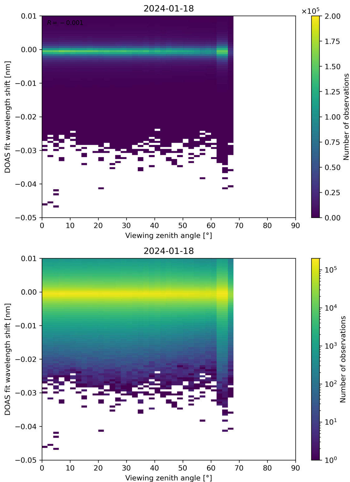
Figure 311: Scatter density plot of “Viewing zenith angle” against “DOAS fit wavelength shift” for 2024-01-17 to 2024-01-19.
