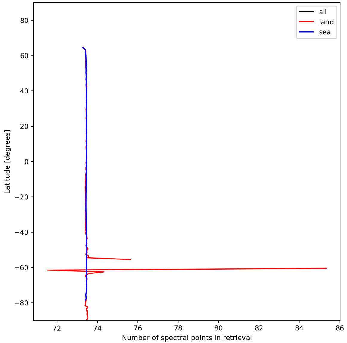
Figure 51: Zonal average of “Number of spectral points in retrieval” for 2024-01-17 to 2024-01-19.
