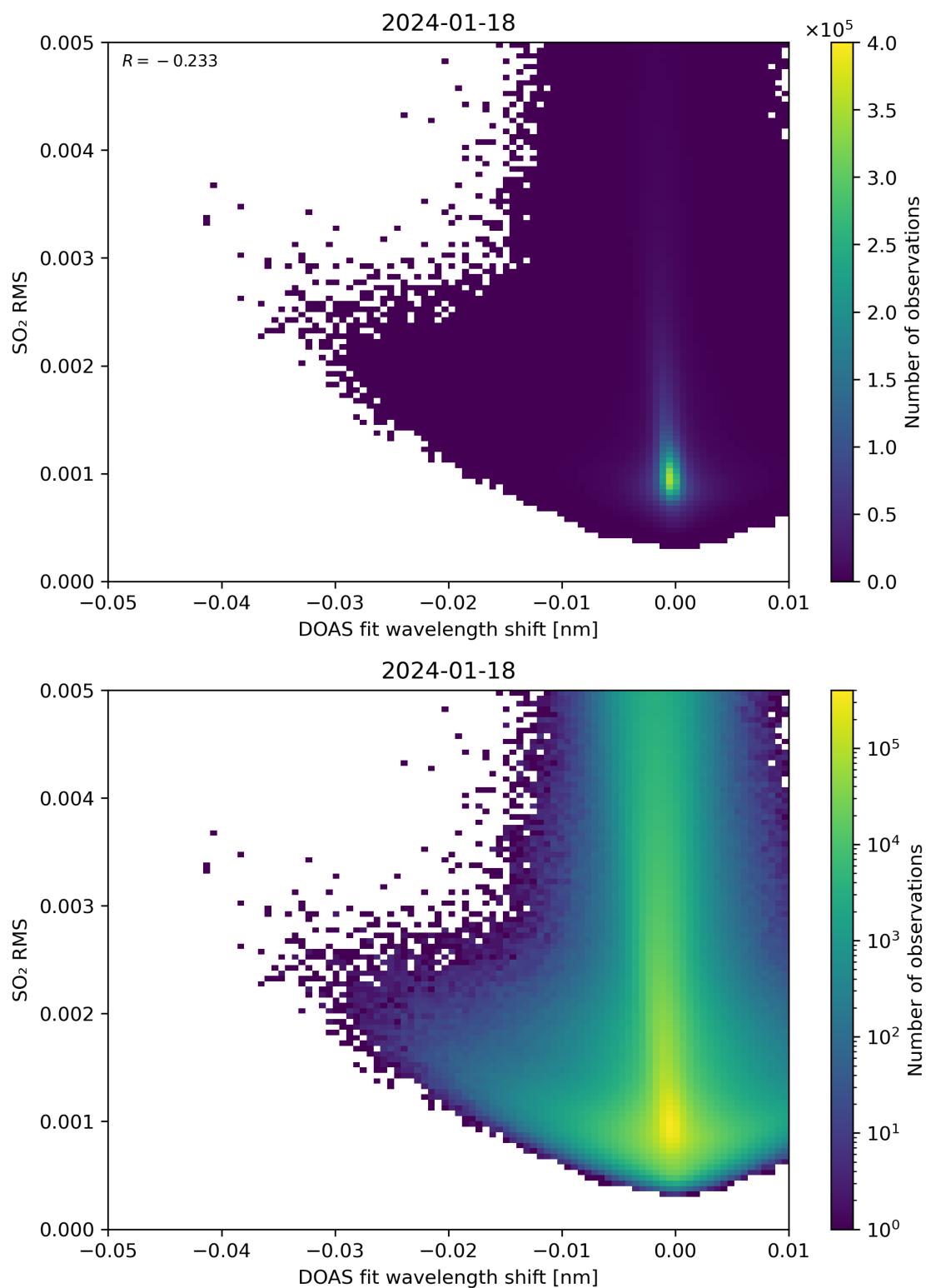
Figure 128: Scatter density plot of “DOAS fit wavelength shift” against “SO 2 RMS” for 2024-01-17 to 2024-01-19.
