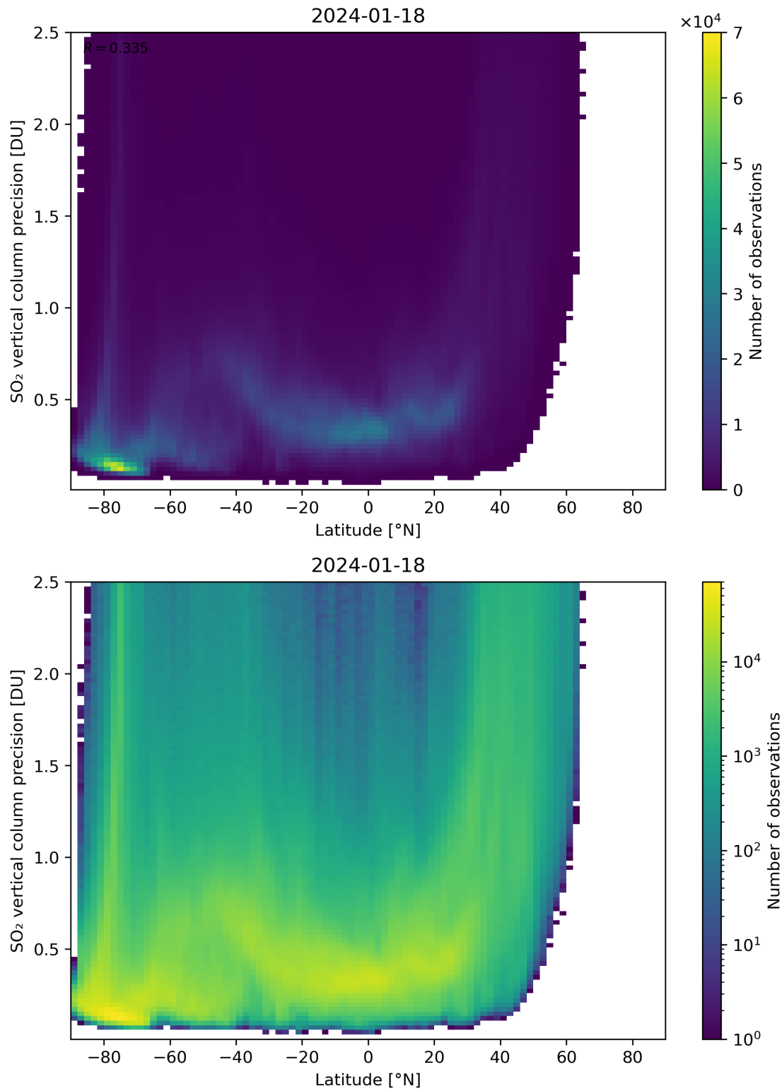
Figure 157: Scatter density plot of “Latitude” against “SO 2 vertical column precision” for 2024-01-17 to 2024-01-19.
