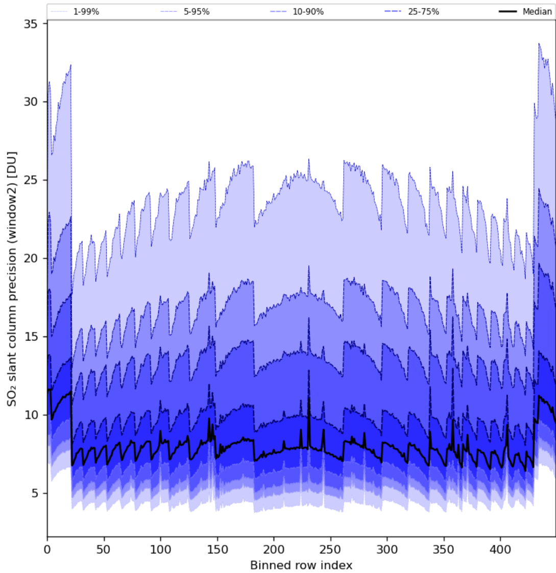
Figure 84: Along track statistics of “SO 2 slant column precision (window2)” for 2024-01-17 to 2024-01-19
