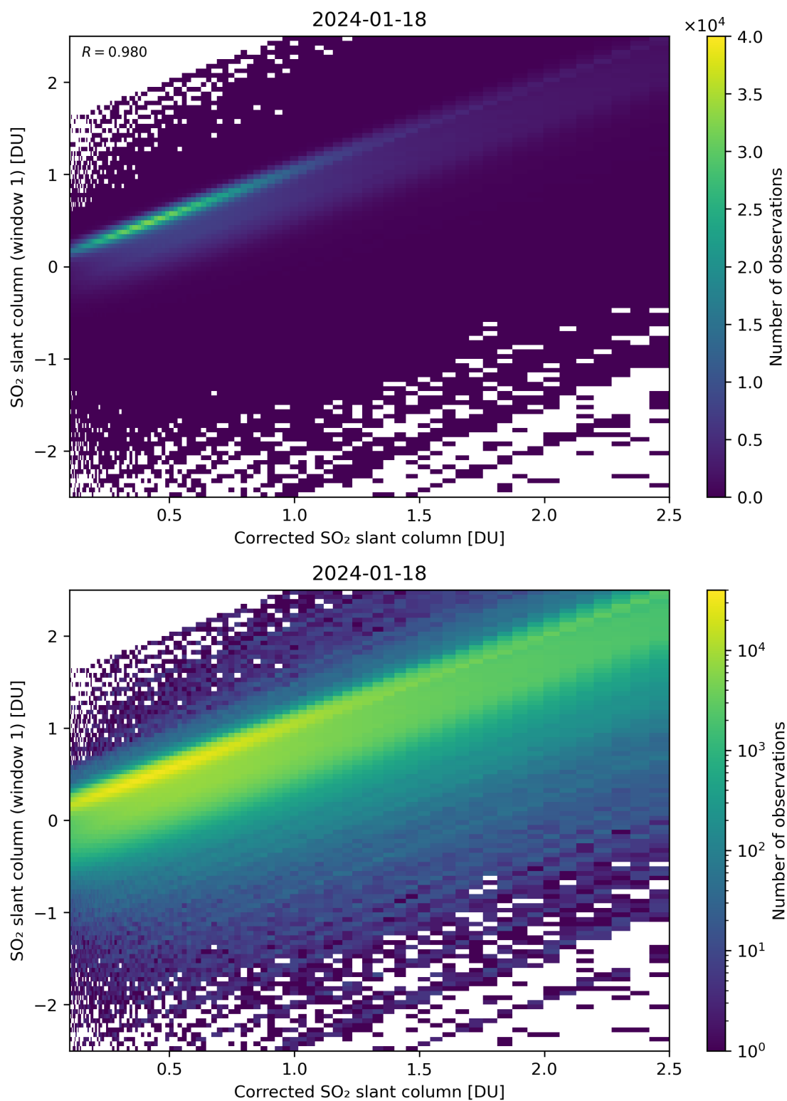
Figure 187: Scatter density plot of “Corrected SO 2 slant column” against “SO 2 slant column (window 1)” for 2024-01-17 to 2024-01-19.
