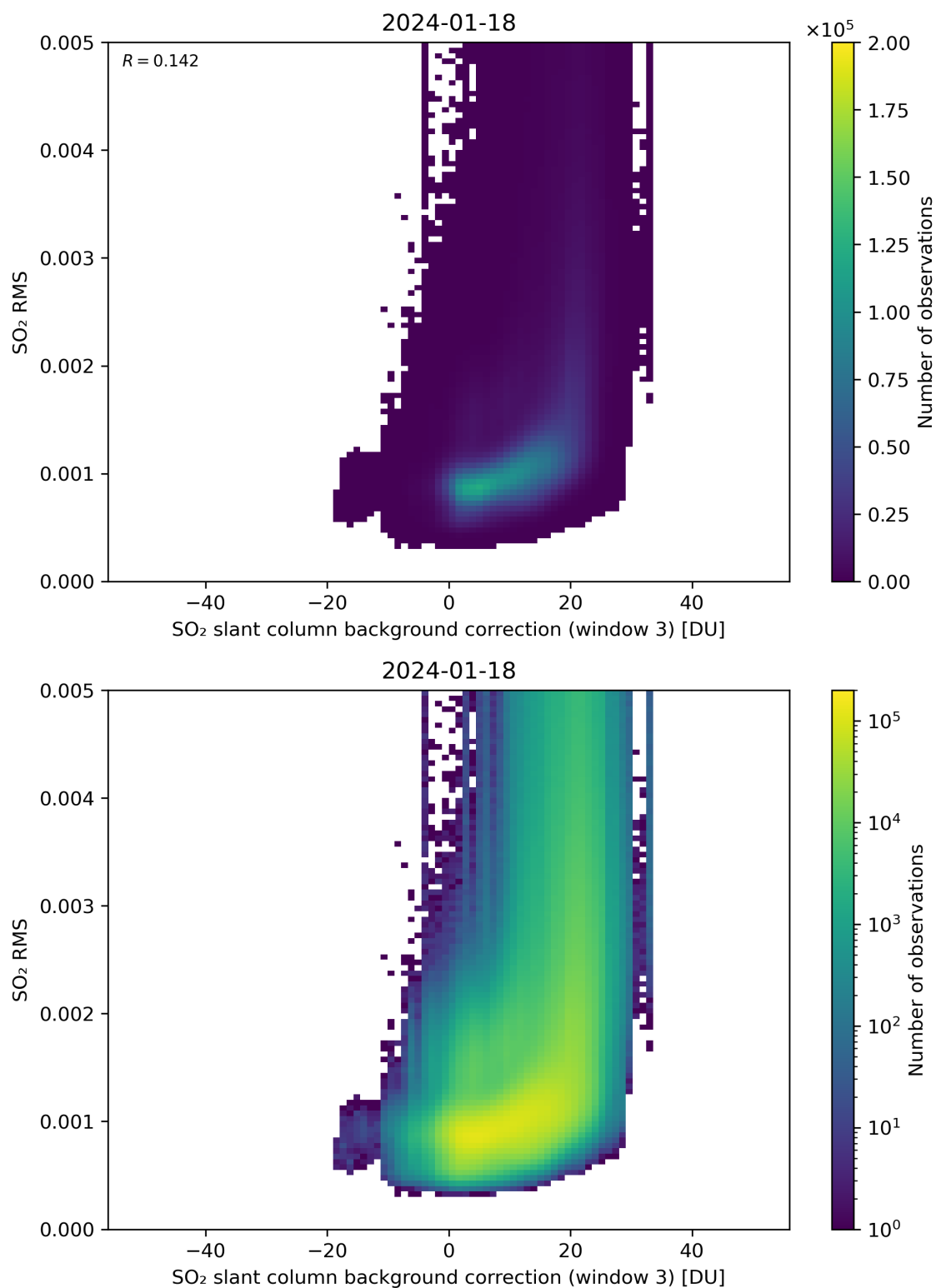
Figure 123: Scatter density plot of “SO 2 slant column background correction (window 3)” against “SO 2 RMS” for 2024-01-17 to 2024-01-19.
