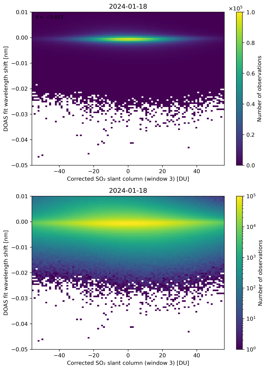
Figure 206: Scatter density plot of “Corrected SO 2 slant column (window 3)” against “DOAS fit wavelength shift” for 2024-01-17 to 2024-01-19.
