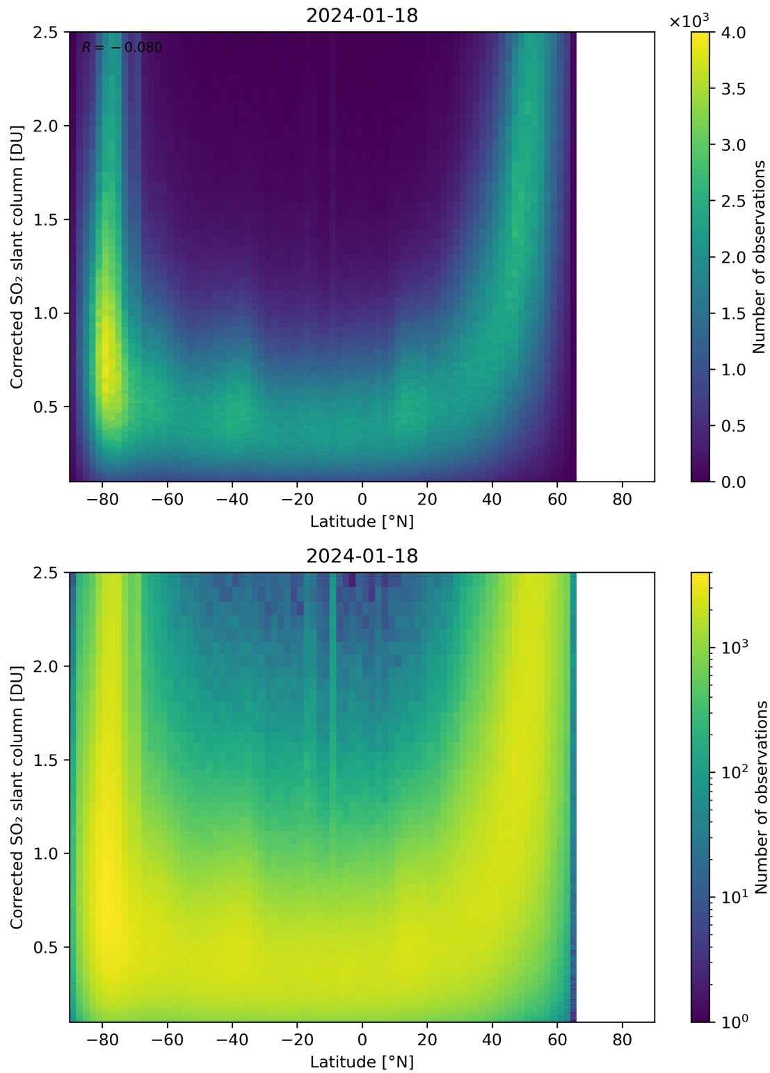
Figure 146: Scatter density plot of “Latitude” against “Corrected SO 2 slant column” for 2024-01-17 to 2024-01-19.
