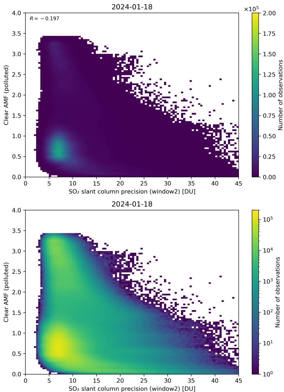
Figure 246: Scatter density plot of “SO 2 slant column precision (window2)” against “Clear AMF (polluted)” for 2024-01-17 to 2024-01-19.
