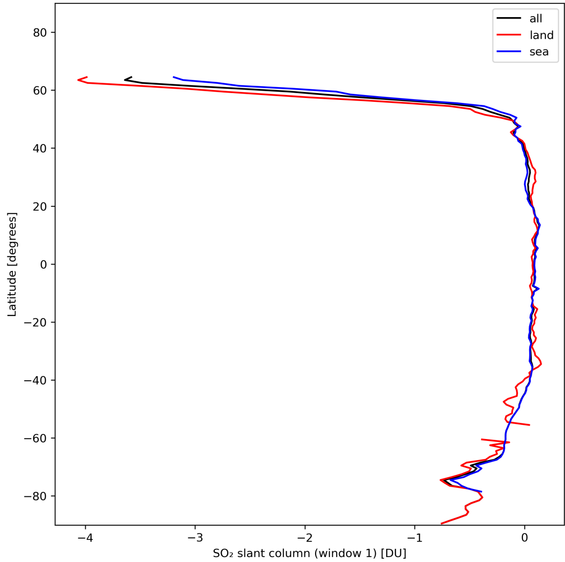
Figure 33: Zonal average of “SO 2 slant column (window 1)” for 2024-01-17 to 2024-01-19.
