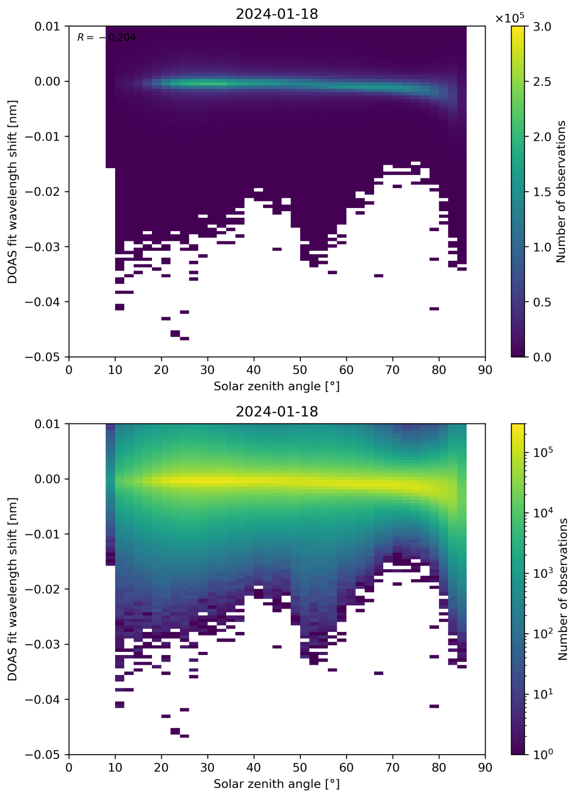
Figure 161: Scatter density plot of “Solar zenith angle” against “DOAS fit wavelength shift” for 2024-01-17 to 2024-01-19.
