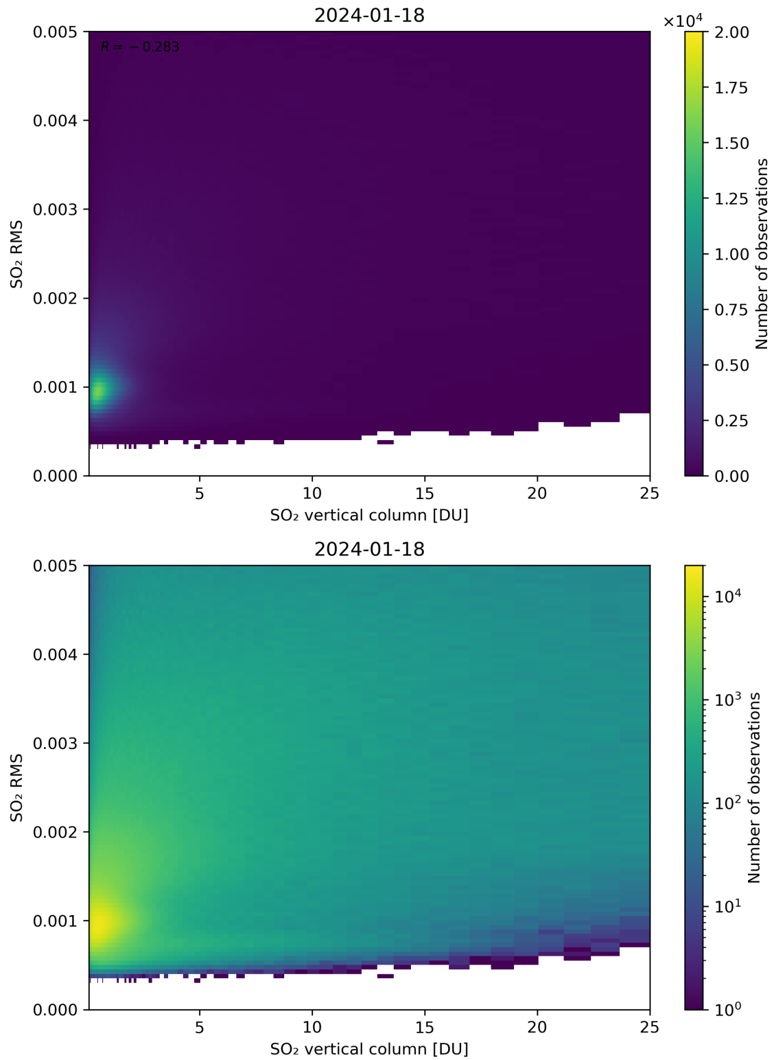
Figure 278: Scatter density plot of “SO 2 vertical column” against “SO 2 RMS” for 2024-01-17 to 2024-01-19.
