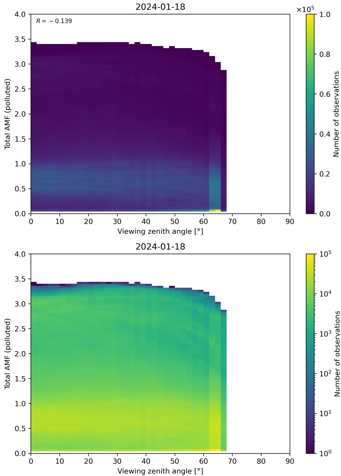
Figure 325: Scatter density plot of “Viewing zenith angle” against “Total AMF (polluted)” for 2024-01-17 to 2024-01-19.
