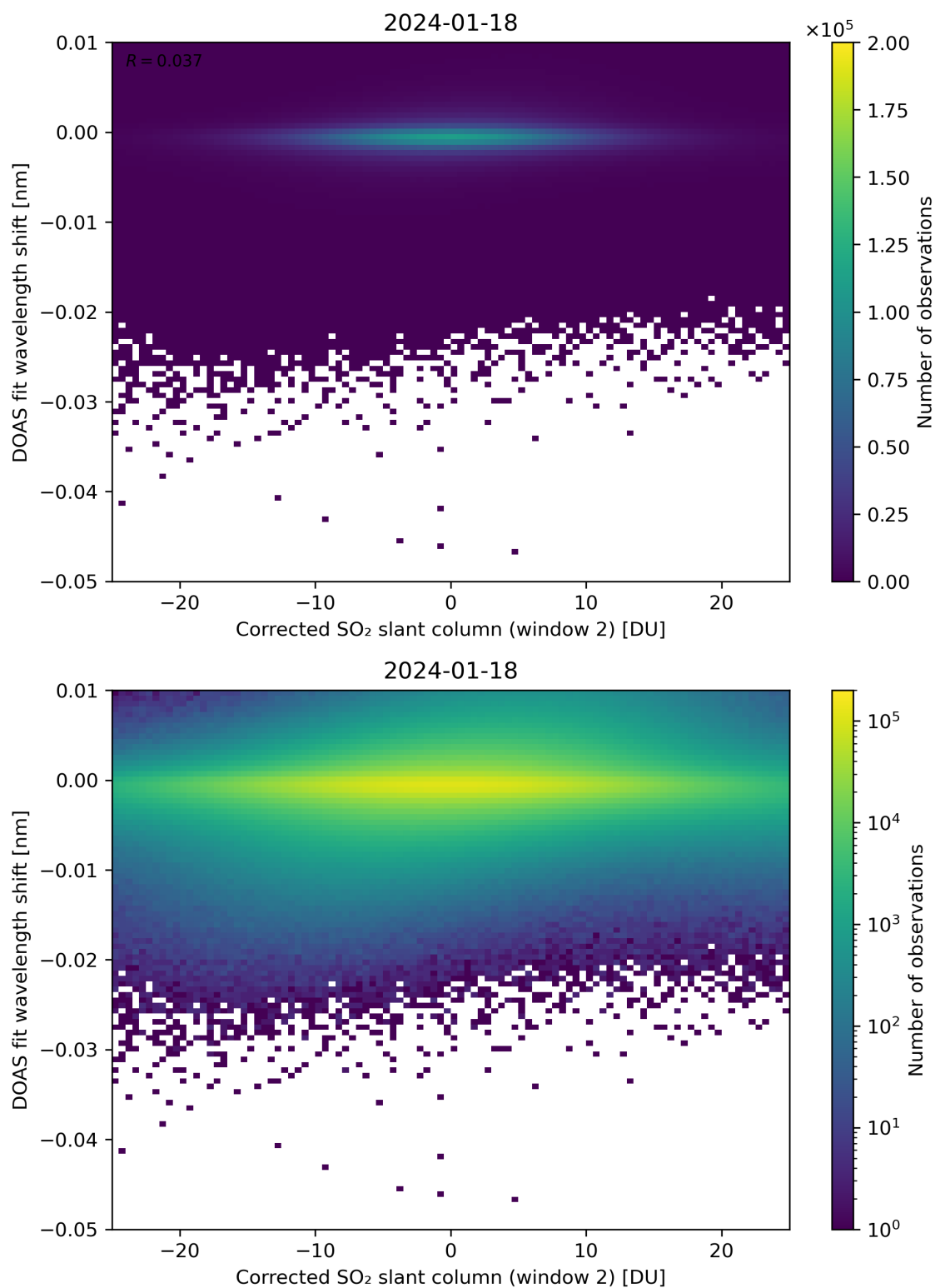
Figure 196: Scatter density plot of “Corrected SO 2 slant column (window 2)” against “DOAS fit wavelength shift” for 2024-01-17 to 2024-01-19.
