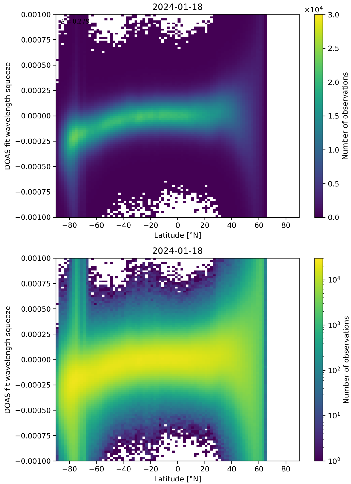
Figure 143: Scatter density plot of “Latitude” against “DOAS fit wavelength squeeze” for 2024-01-17 to 2024-01-19.
