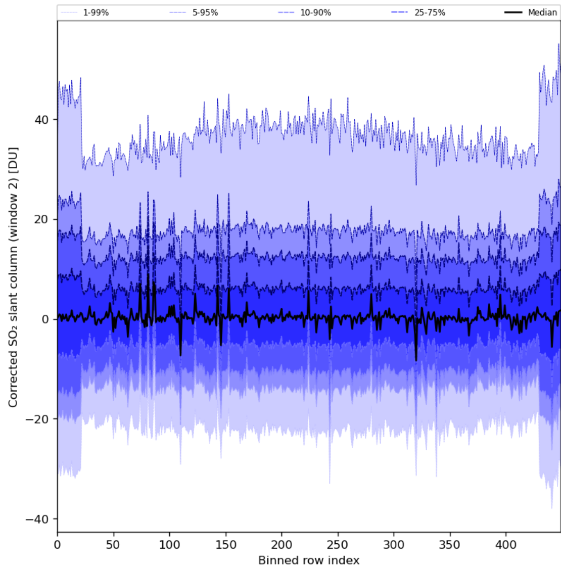
Figure 85: Along track statistics of “Corrected SO 2 slant column (window 2)” for 2024-01-17 to 2024-01-19
