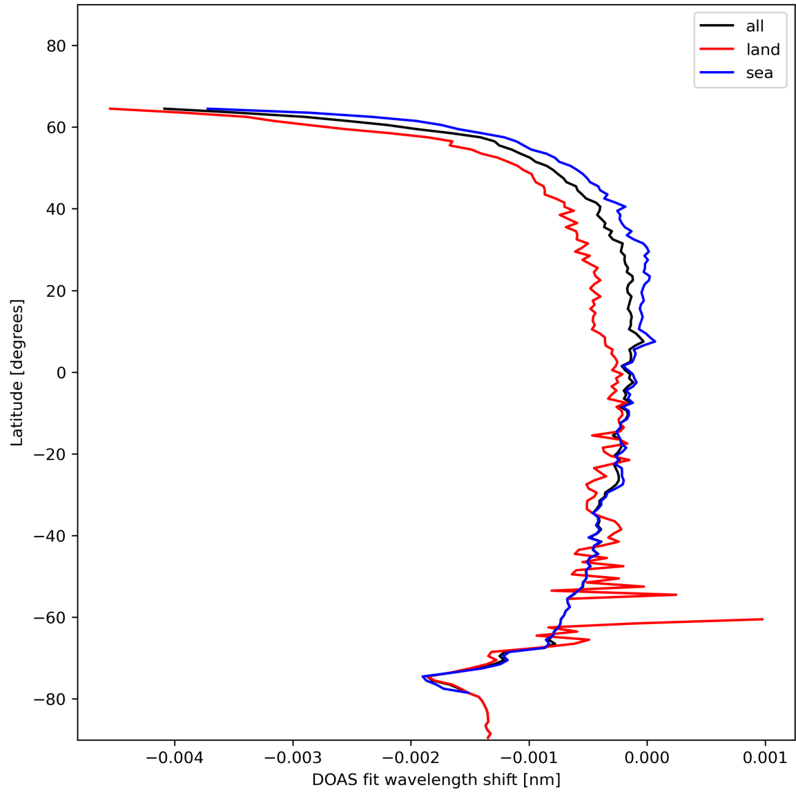
Figure 45: Zonal average of “DOAS fit wavelength shift” for 2024-01-17 to 2024-01-19.
