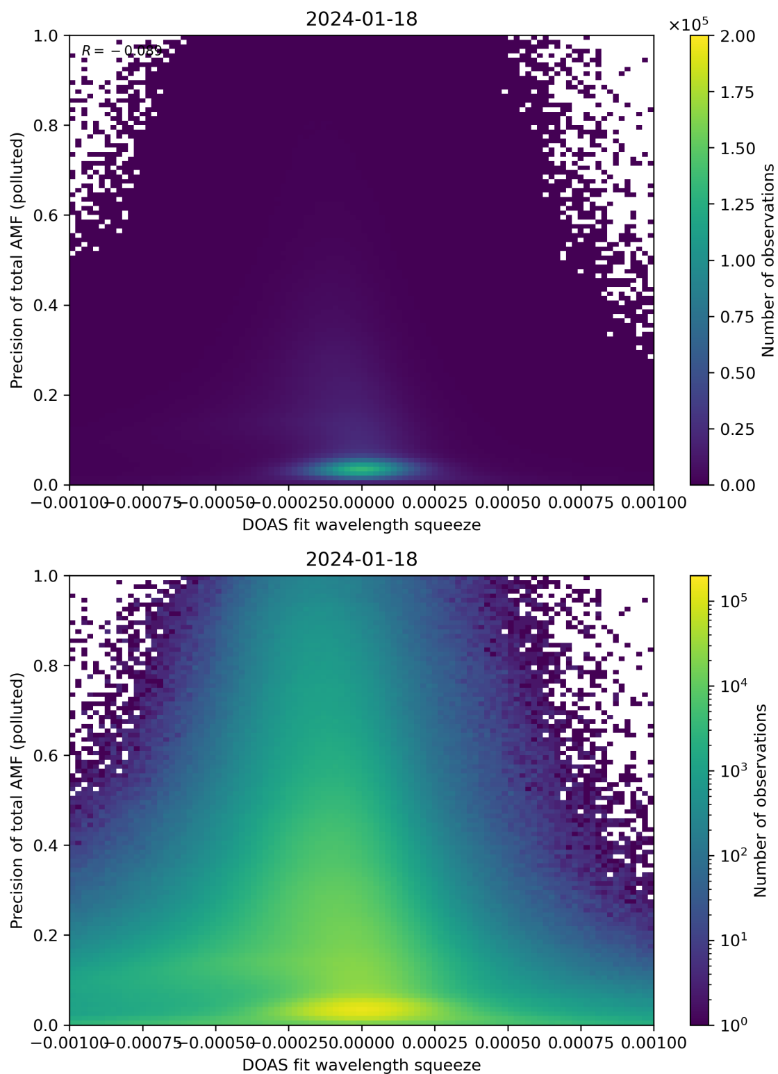
Figure 135: Scatter density plot of “DOAS fit wavelength squeeze” against “Precision of total AMF (polluted)” for 2024-01-17 to 2024-01-19.
