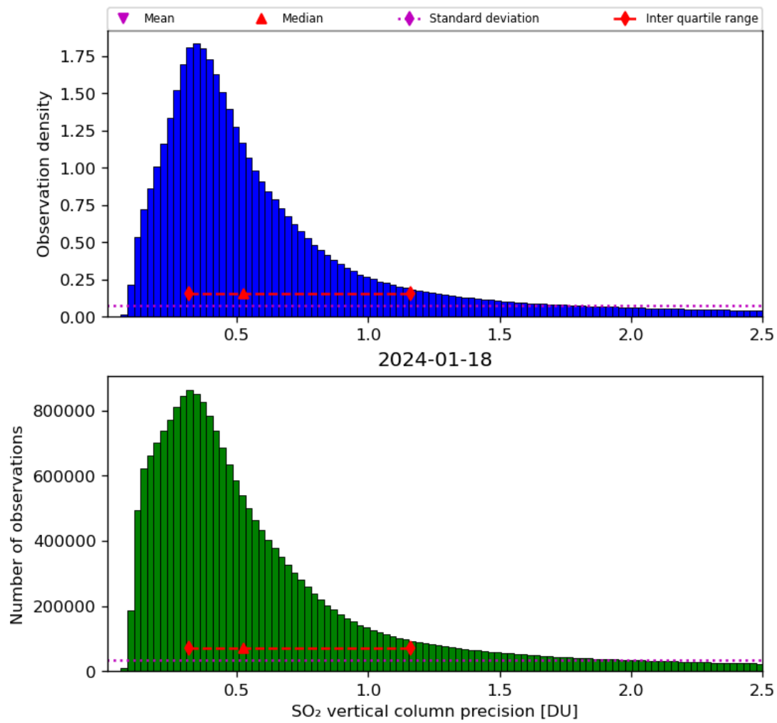
Figure 54: Histogram of “SO 2 vertical column precision” for 2024-01-17 to 2024-01-19
