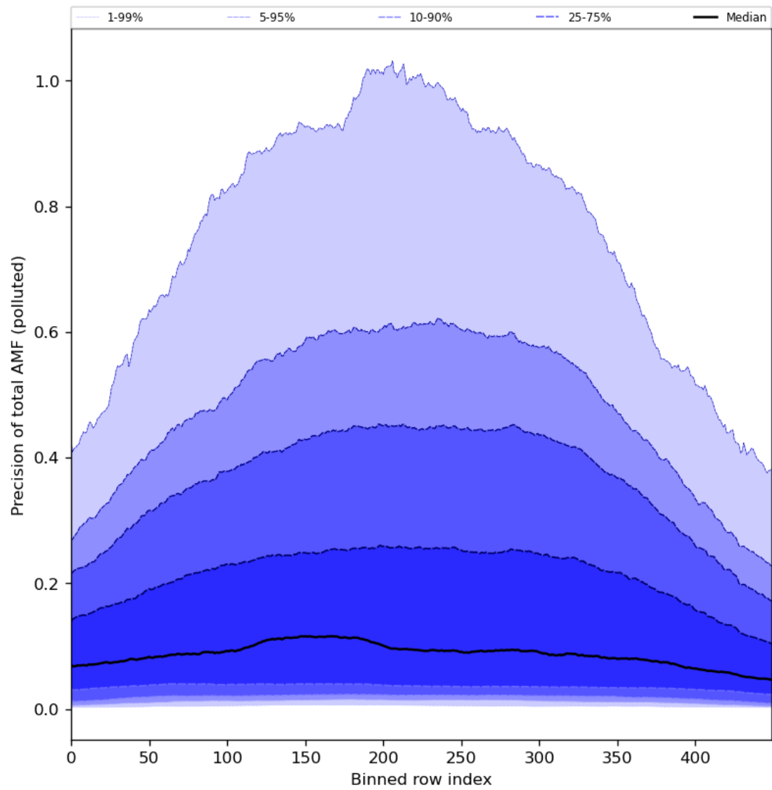
Figure 95: Along track statistics of “Precision of total AMF (polluted)” for 2024-01-17 to 2024-01-19
