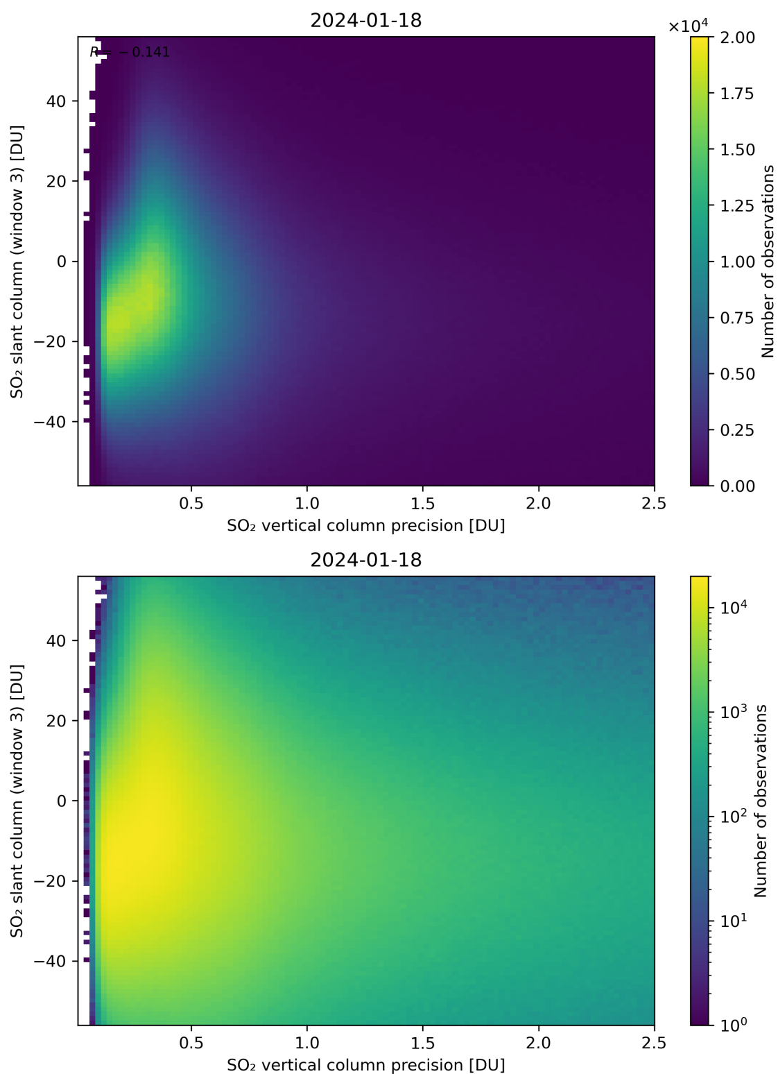
Figure 292: Scatter density plot of “SO 2 vertical column precision” against “SO 2 slant column (window 3)” for 2024-01-17 to 2024-01-19.
