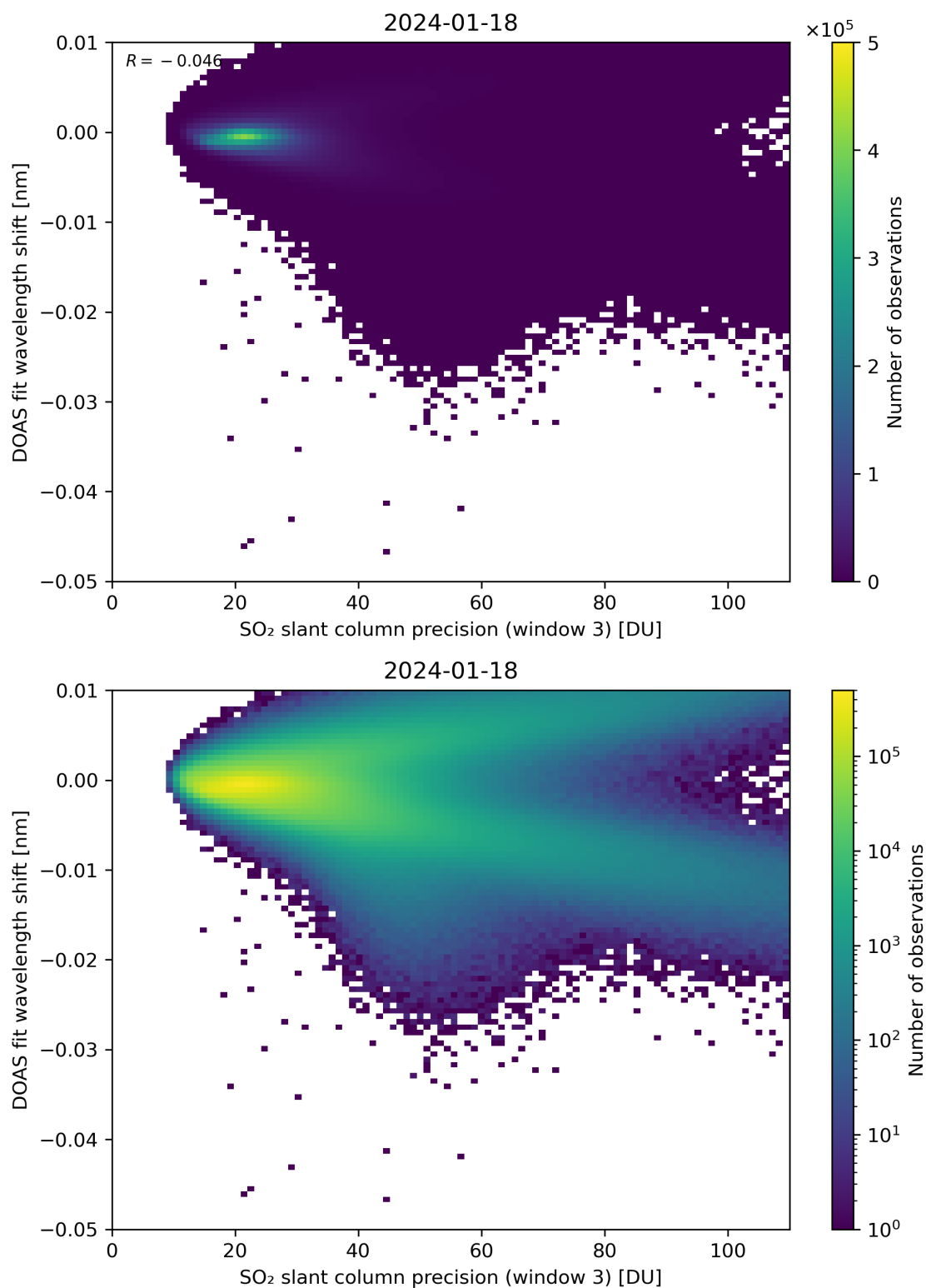
Figure 258: Scatter density plot of “SO 2 slant column precision (window 3)” against “DOAS fit wavelength shift” for 2024-01-17 to 2024-01-19.
