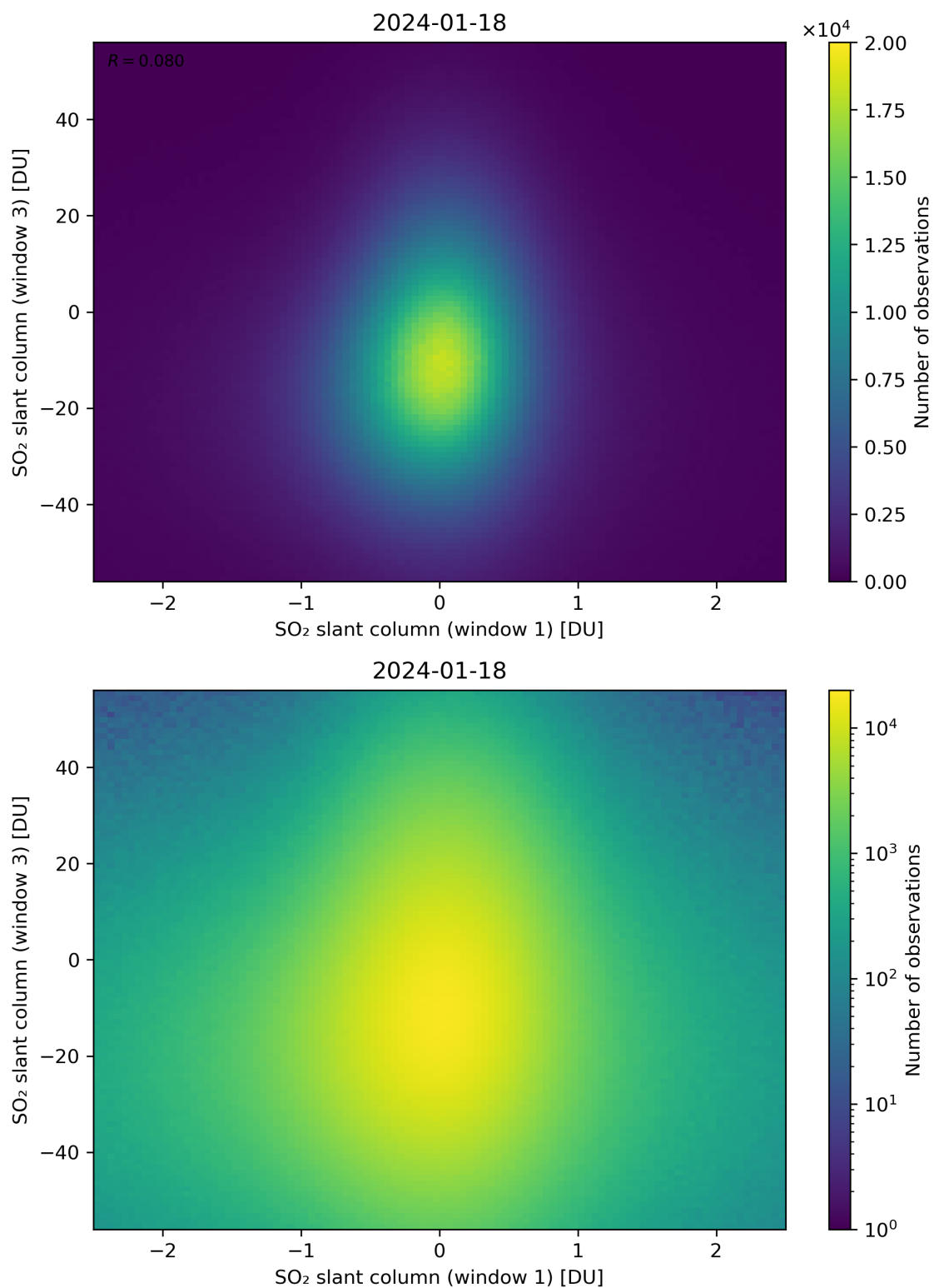
Figure 237: Scatter density plot of “SO 2 slant column (window 1)” against “SO 2 slant column (window 3)” for 2024-01-17 to 2024-01-19.
