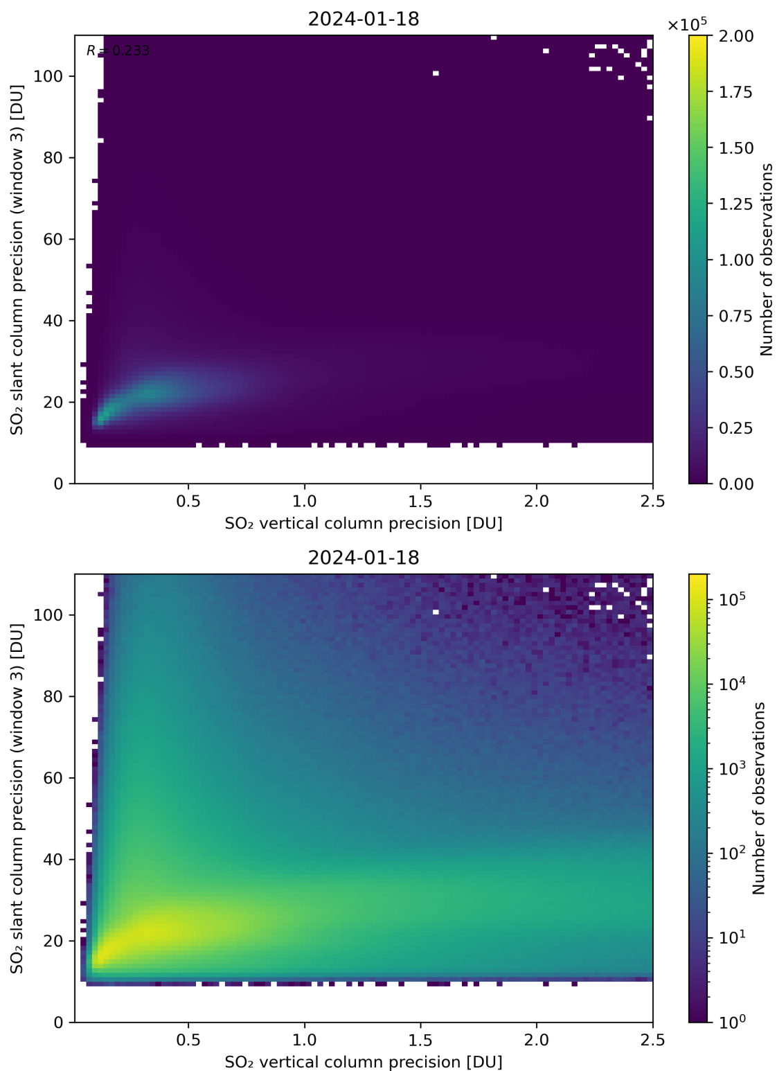
Figure 293: Scatter density plot of “SO 2 vertical column precision” against “SO 2 slant column precision (window 3)” for 2024-01-17 to 2024-01-19.
