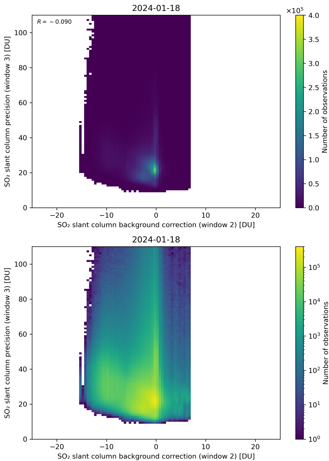
Figure 118: Scatter density plot of “SO 2 slant column background correction (window 2)” against “SO 2 slant column precision (window 3)” for 2024-01-17 to 2024-01-19.
