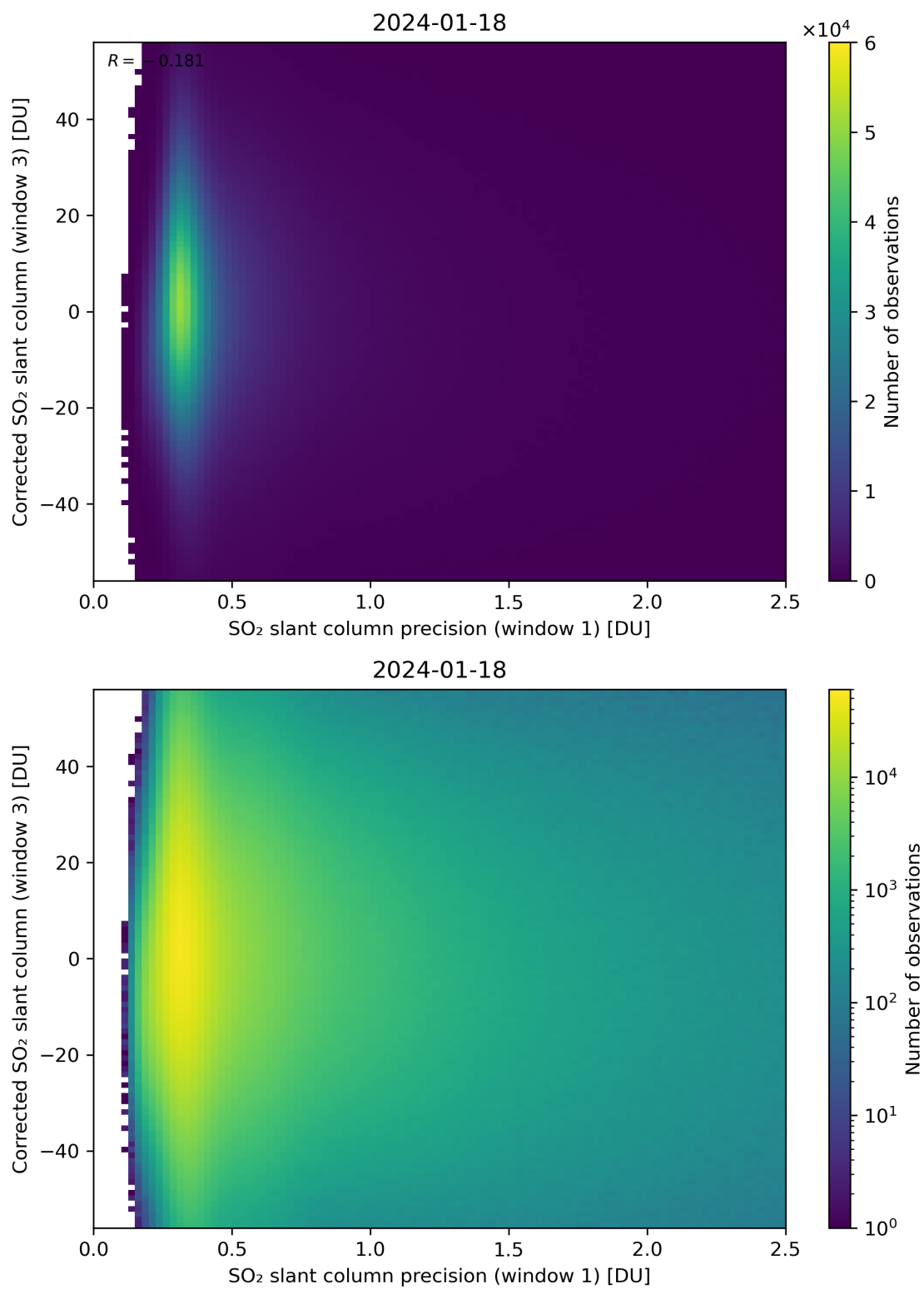
Figure 226: Scatter density plot of “SO 2 slant column precision (window 1)” against “Corrected SO 2 slant column (window 3)” for 2024-01-17 to 2024-01-19.
