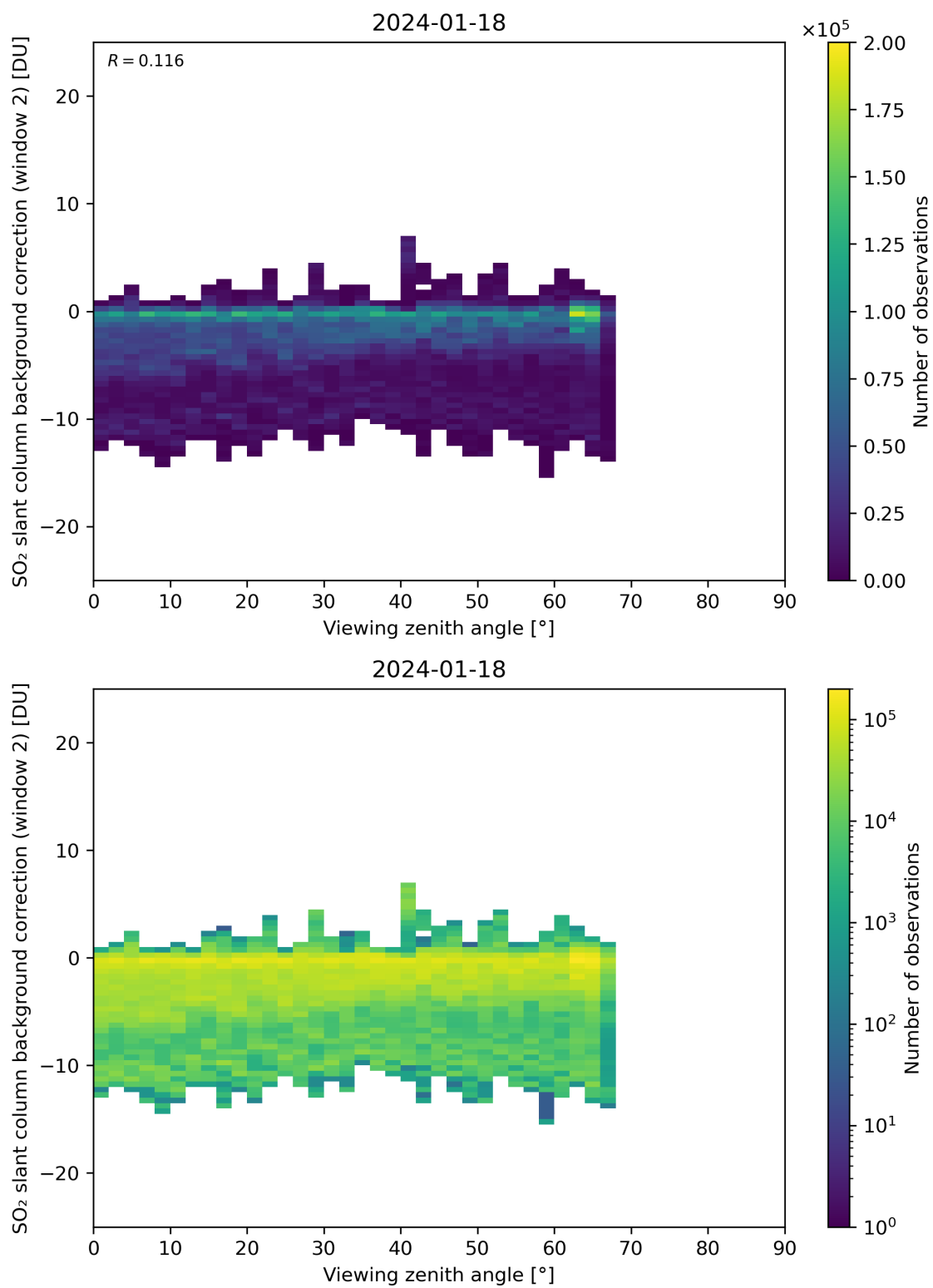
Figure 309: Scatter density plot of “Viewing zenith angle” against “SO 2 slant column background correction (window 2)” for 2024-01-17 to 2024-01-19.
