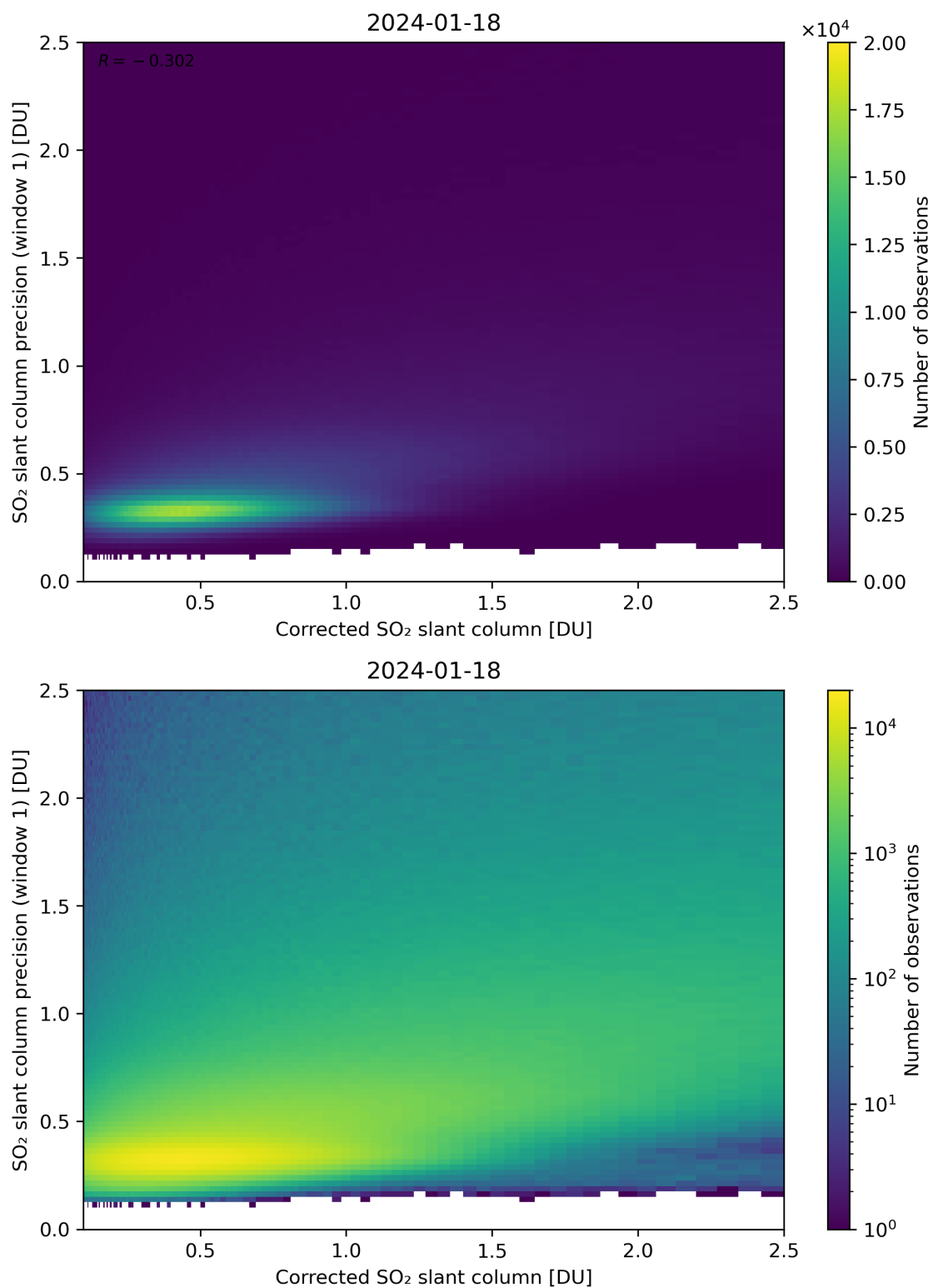
Figure 188: Scatter density plot of “Corrected SO 2 slant column” against “SO 2 slant column precision (window 1)” for 2024-01-17 to 2024-01-19.
