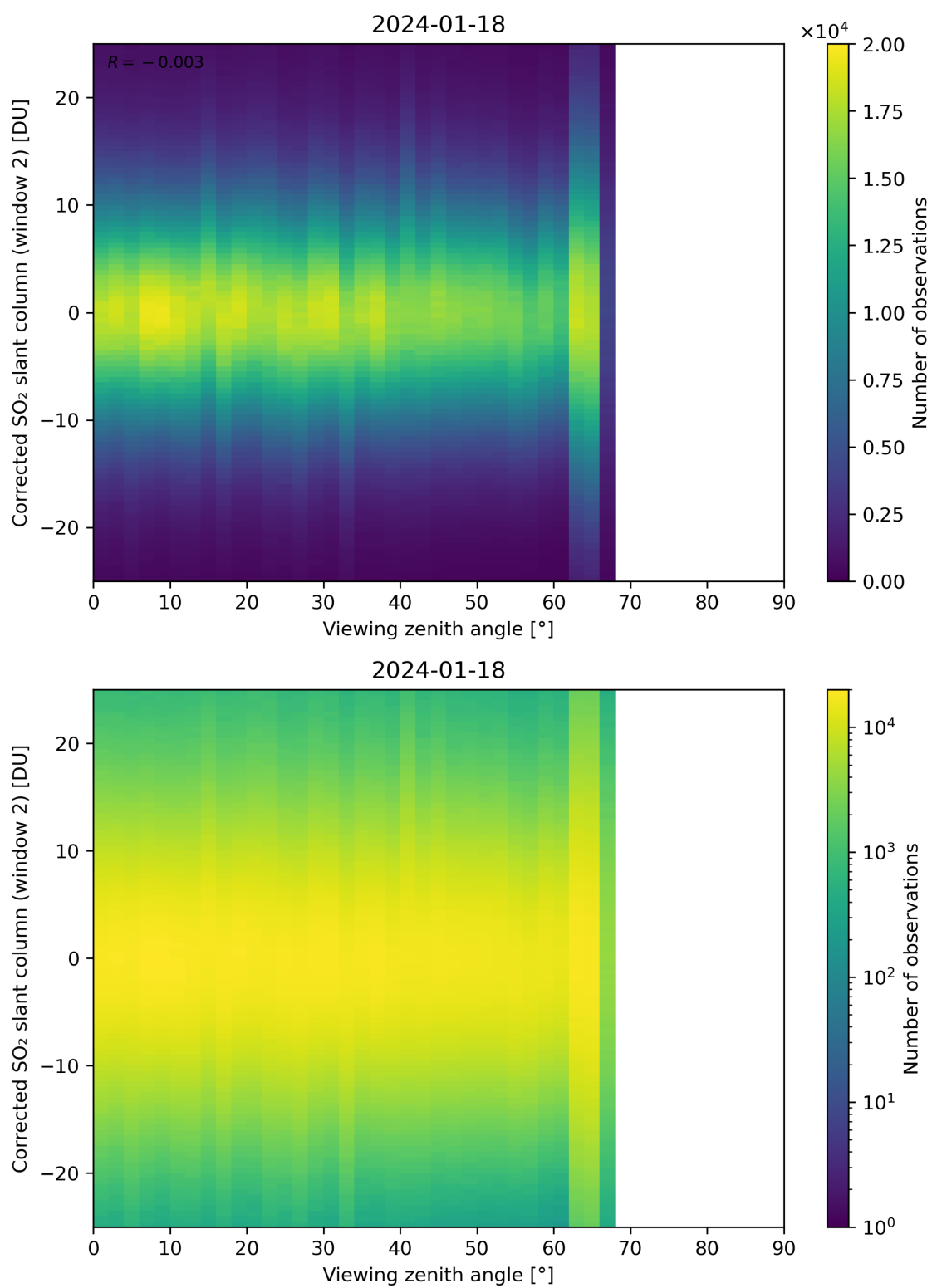
Figure 318: Scatter density plot of “Viewing zenith angle” against “Corrected SO 2 slant column (window 2)” for 2024-01-17 to 2024-01-19.
