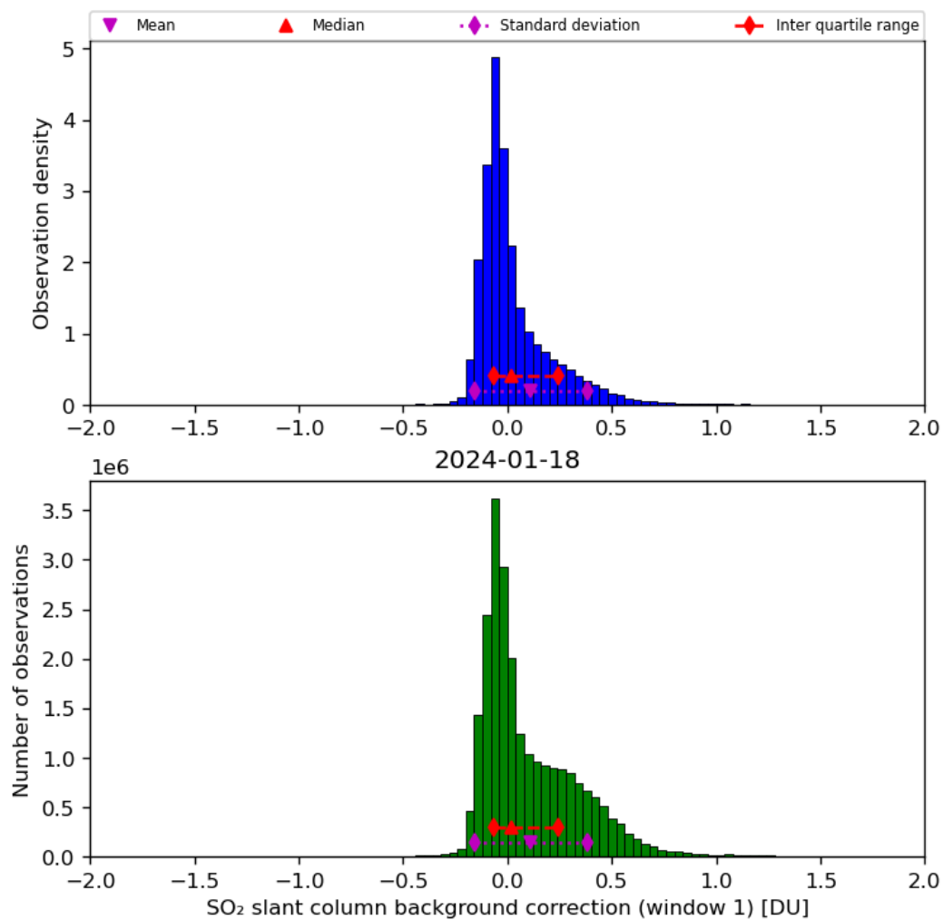
Figure 59: Histogram of “SO 2 slant column background correction (window 1)” for 2024-01-17 to 2024-01-19
