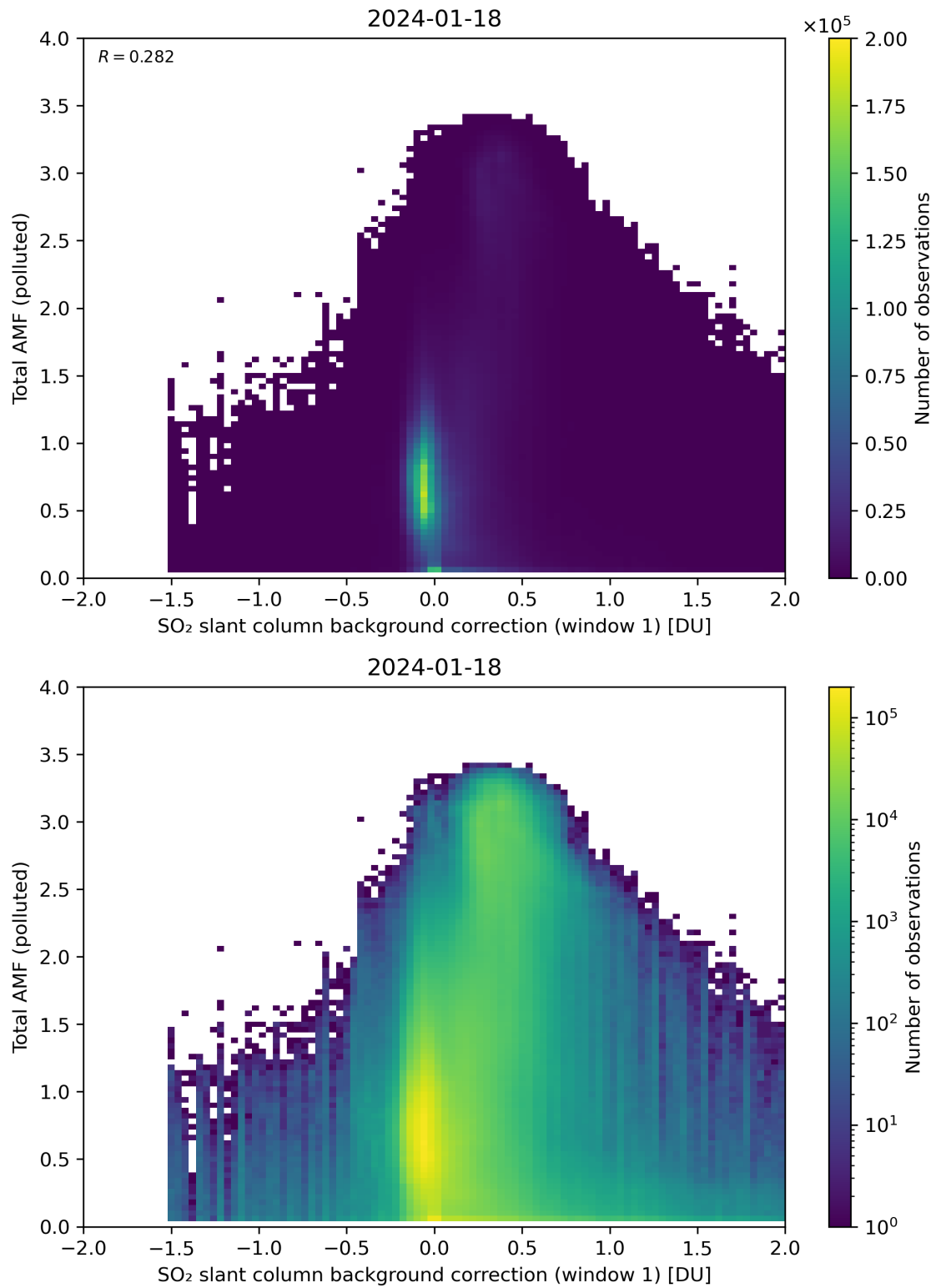
Figure 109: Scatter density plot of “SO 2 slant column background correction (window 1)” against “Total AMF (polluted)” for 2024-01-17 to 2024-01-19.
