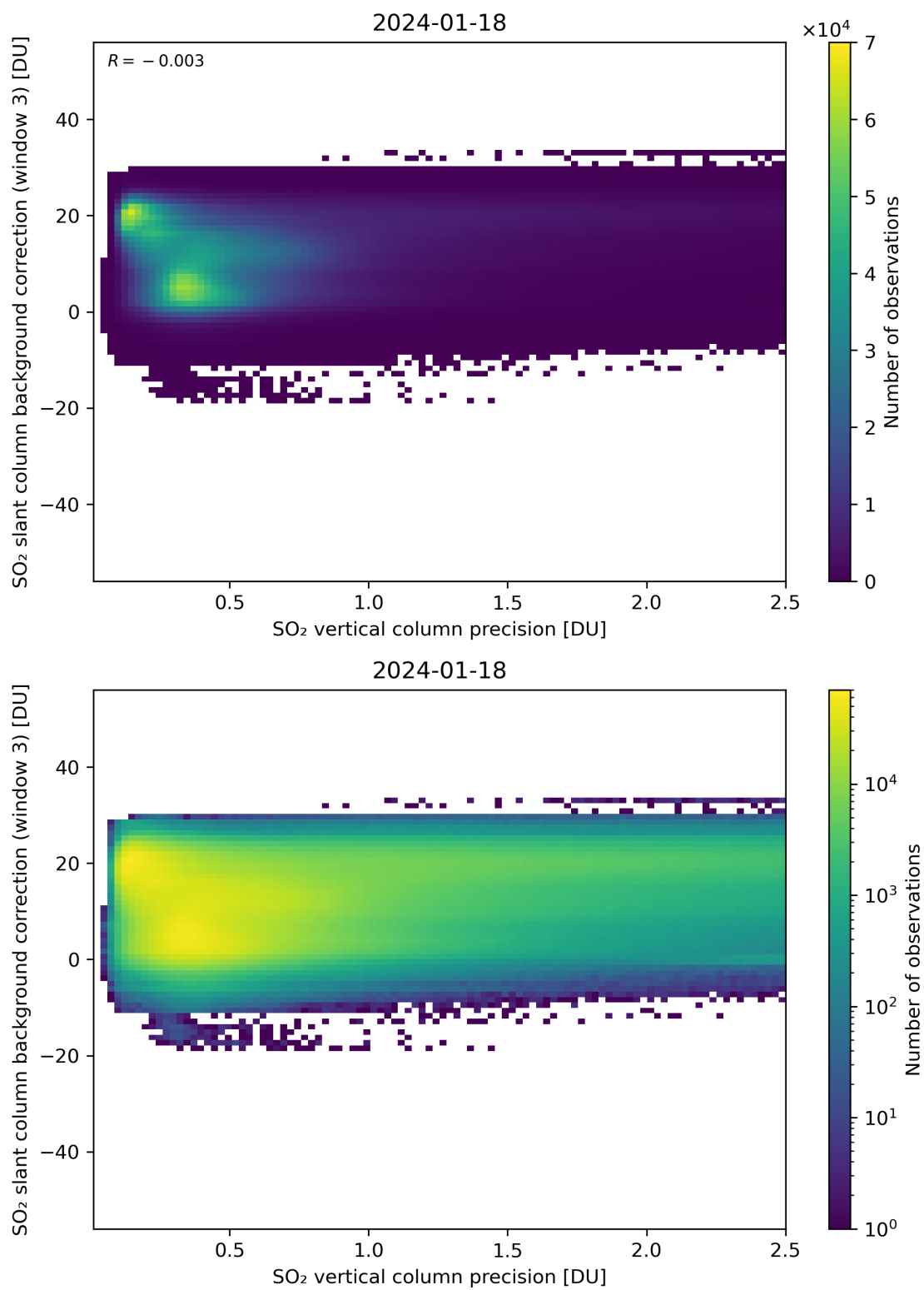
Figure 281: Scatter density plot of “SO 2 vertical column precision” against “SO 2 slant column background correction (window 3)” for 2024-01-17 to 2024-01-19.
