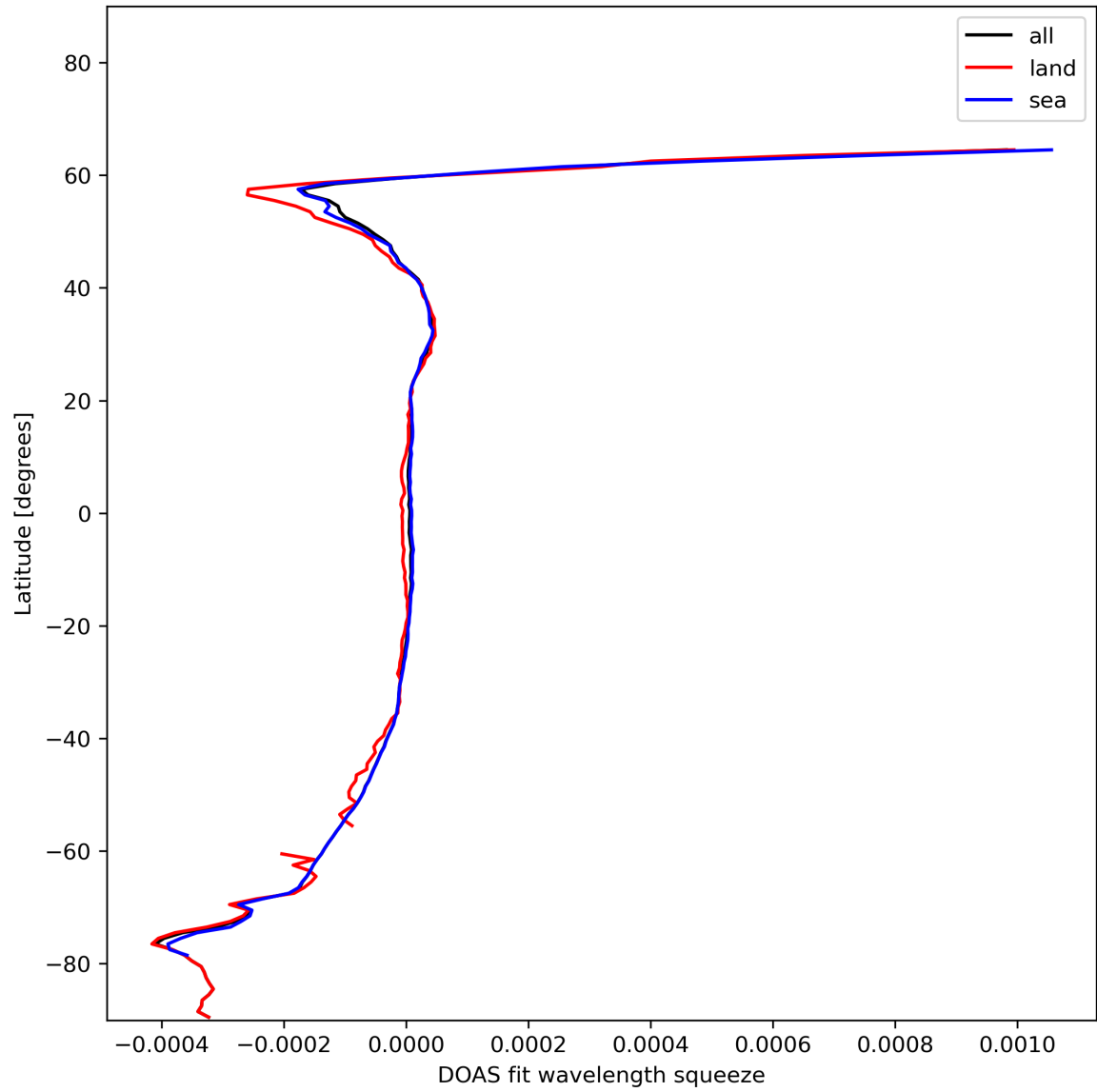
Figure 46: Zonal average of “DOAS fit wavelength squeeze” for 2024-01-17 to 2024-01-19.
