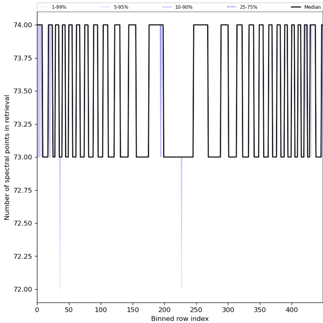
Figure 97: Along track statistics of “Number of spectral points in retrieval” for 2024-01-17 to 2024-01-19
