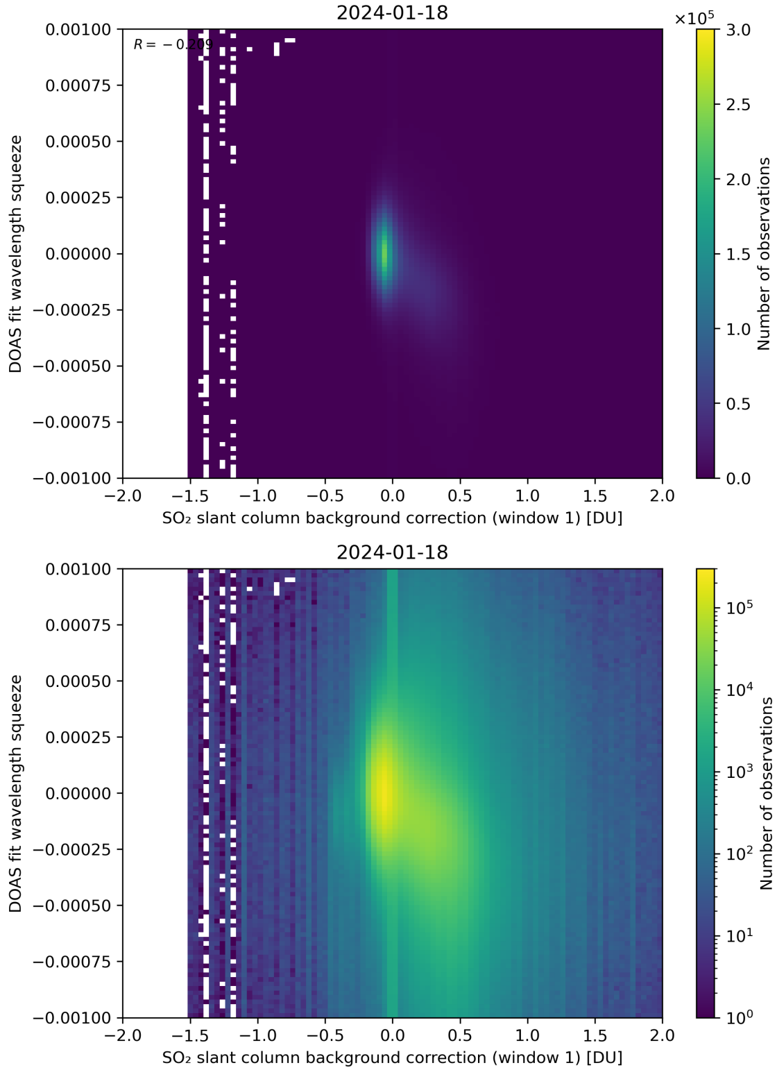
Figure 101: Scatter density plot of “SO 2 slant column background correction (window 1)” against “DOAS fit wavelength squeeze” for 2024-01-17 to 2024-01-19.
