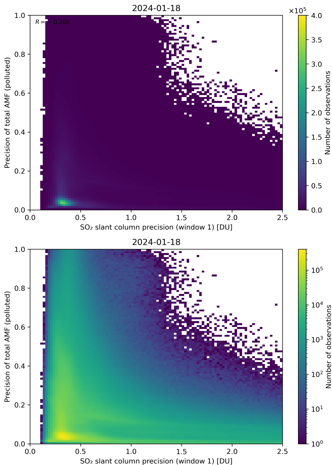
Figure 231: Scatter density plot of “SO 2 slant column precision (window 1)” against “Precision of total AMF (polluted)” for 2024-01-17 to 2024-01-19.
