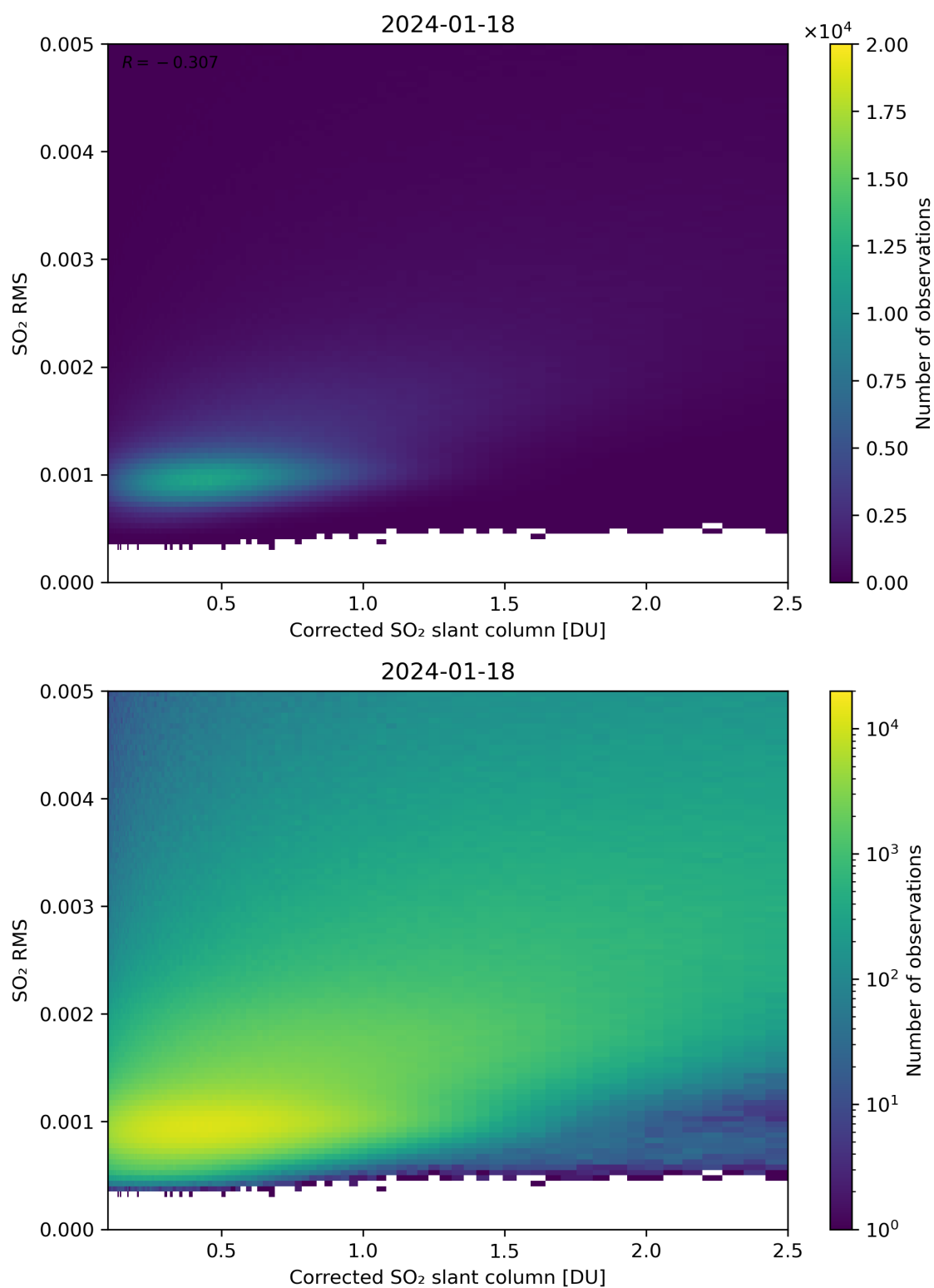
Figure 183: Scatter density plot of “Corrected SO 2 slant column” against “SO 2 RMS” for 2024-01-17 to 2024-01-19.
