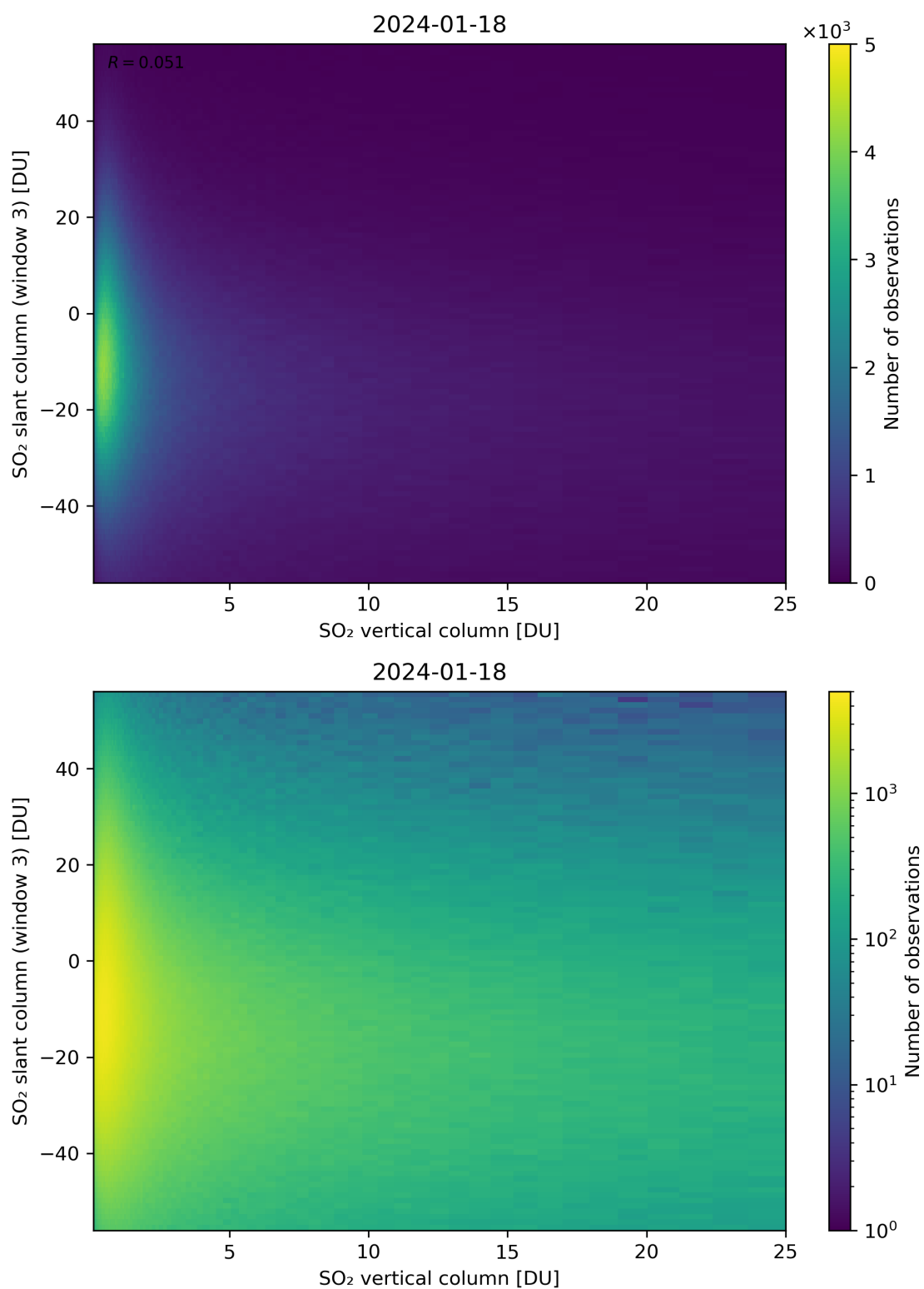
Figure 303: Scatter density plot of “SO 2 vertical column” against “SO 2 slant column (window 3)” for 2024-01-17 to 2024-01-19.
