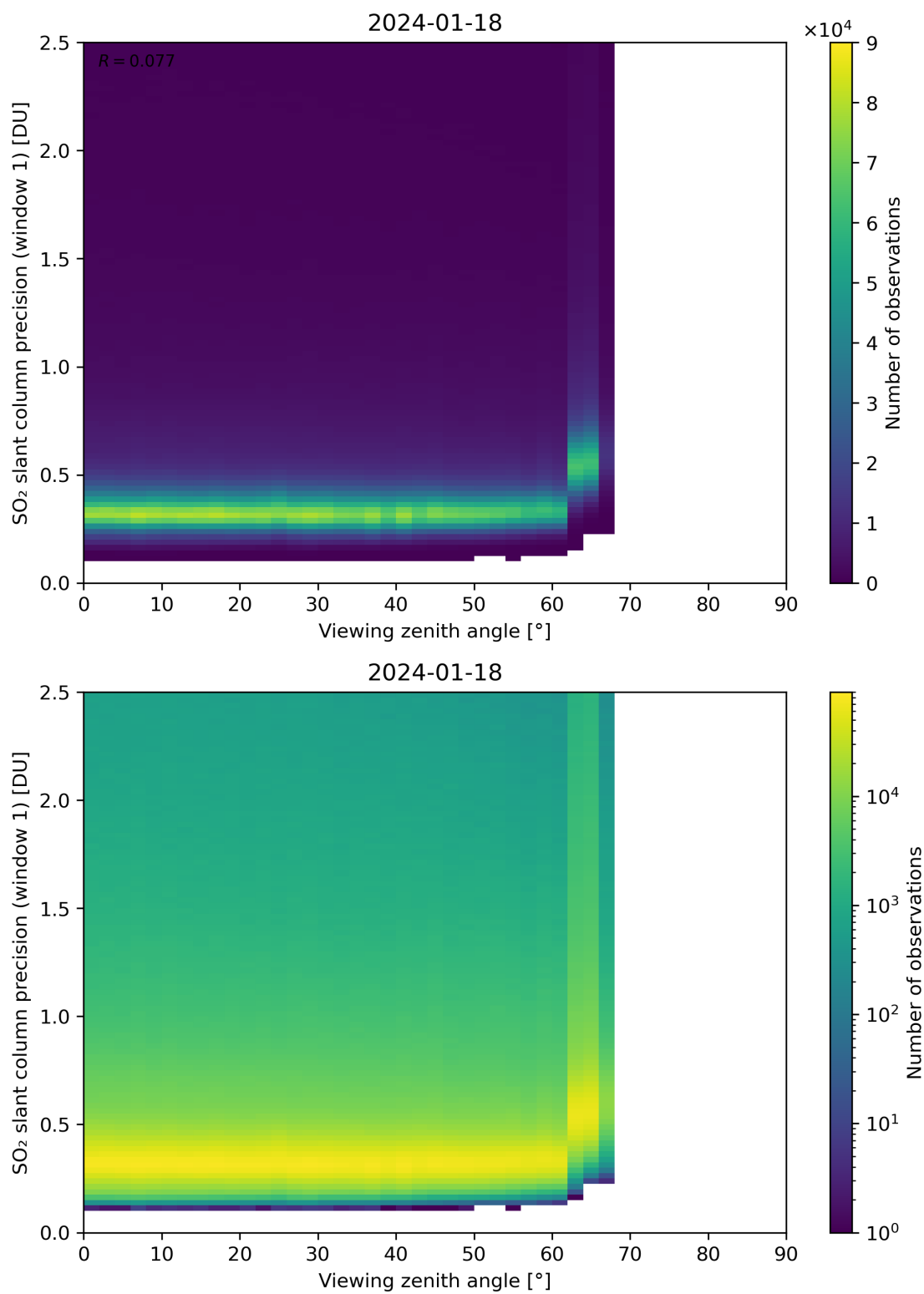
Figure 321: Scatter density plot of “Viewing zenith angle” against “SO 2 slant column precision (window 1)” for 2024-01-17 to 2024-01-19.
