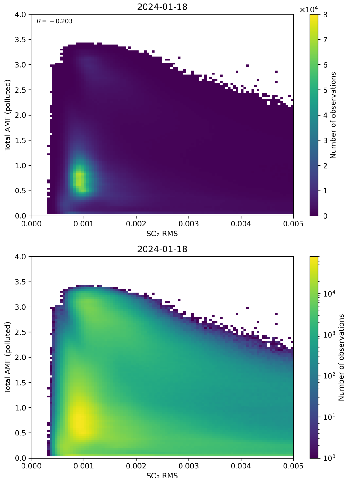
Figure 137: Scatter density plot of “SO 2 RMS” against “Total AMF (polluted)” for 2024-01-17 to 2024-01-19.
