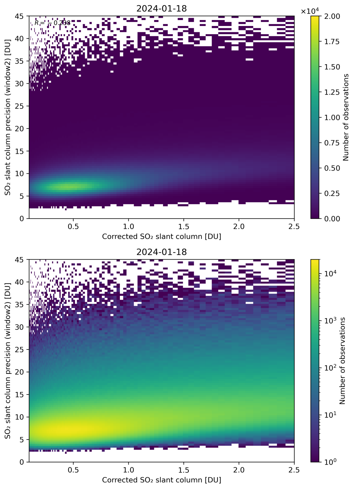
Figure 189: Scatter density plot of “Corrected SO 2 slant column” against “SO 2 slant column precision (window2)” for 2024-01-17 to 2024-01-19.
