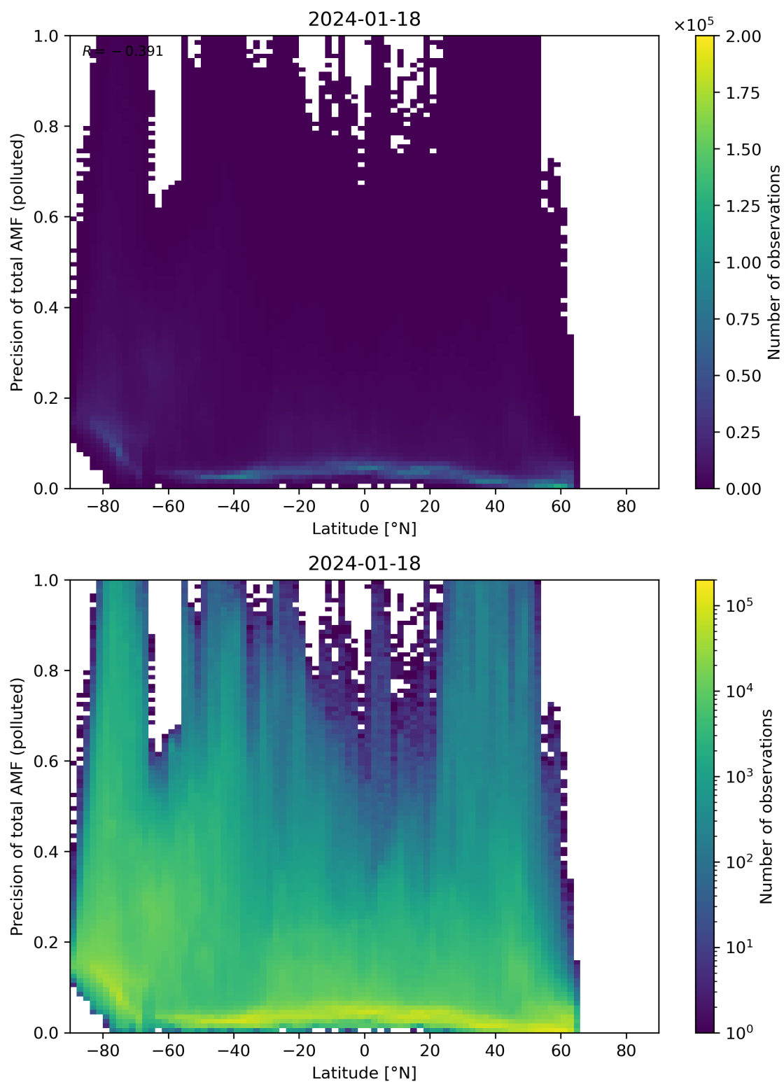
Figure 155: Scatter density plot of “Latitude” against “Precision of total AMF (polluted)” for 2024-01-17 to 2024-01-19.
