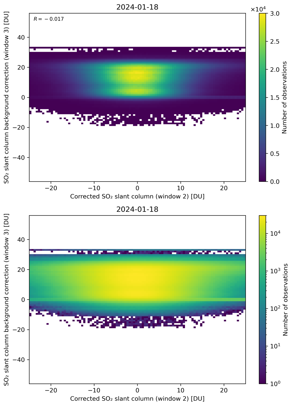
Figure 195: Scatter density plot of “Corrected SO 2 slant column (window 2)” against “SO 2 slant column background correction (window 3)” for 2024-01-17 to 2024-01-19.
