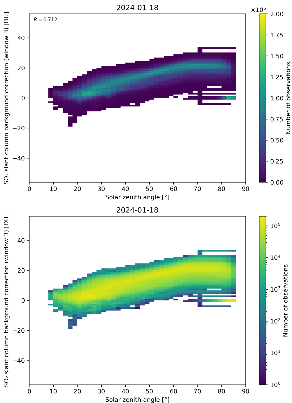
Figure 160: Scatter density plot of “Solar zenith angle” against “SO 2 slant column background correction (window 3)” for 2024-01-17 to 2024-01-19.
