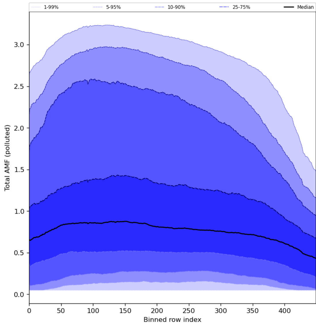
Figure 94: Along track statistics of “Total AMF (polluted)” for 2024-01-17 to 2024-01-19
