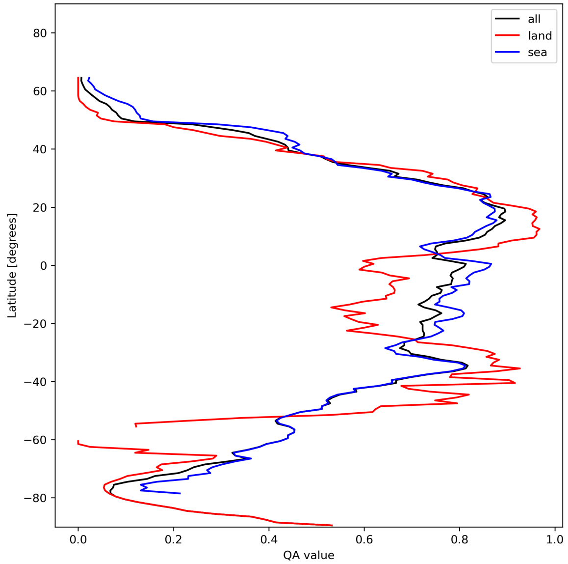
Figure 29: Zonal average of “QA value” for 2024-01-17 to 2024-01-19.
