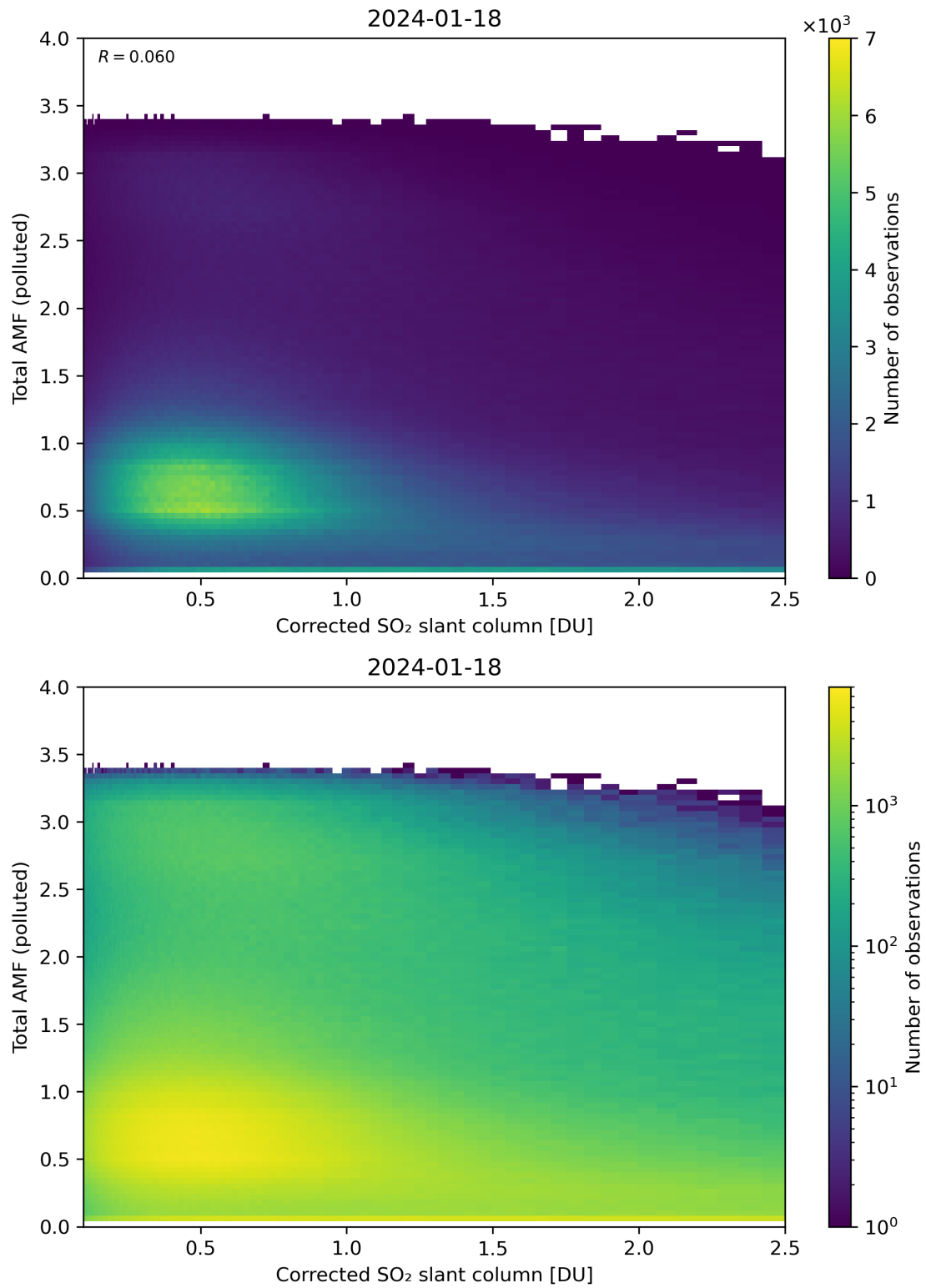
Figure 192: Scatter density plot of “Corrected SO 2 slant column” against “Total AMF (polluted)” for 2024-01-17 to 2024-01-19.
