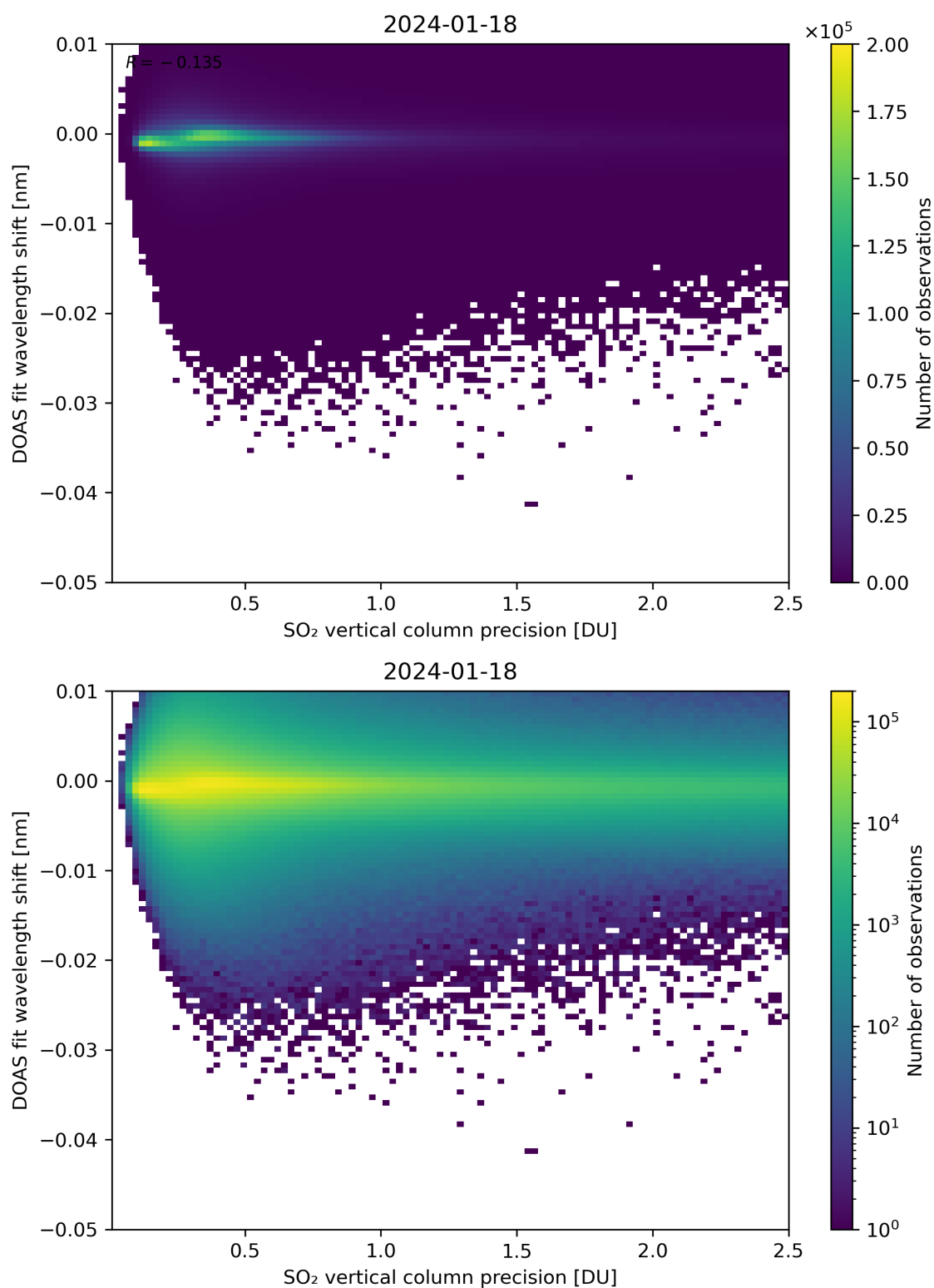
Figure 282: Scatter density plot of “SO 2 vertical column precision” against “DOAS fit wavelength shift” for 2024-01-17 to 2024-01-19.
