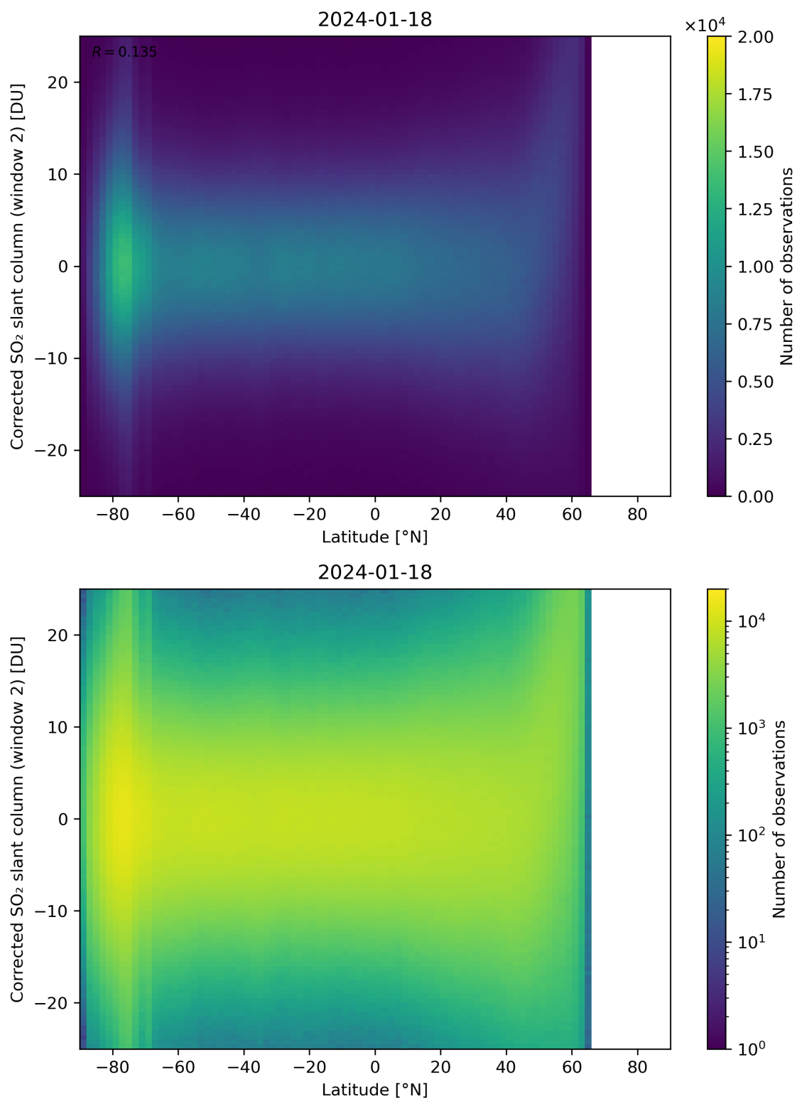
Figure 147: Scatter density plot of “Latitude” against “Corrected SO 2 slant column (window 2)” for 2024-01-17 to 2024-01-19.
