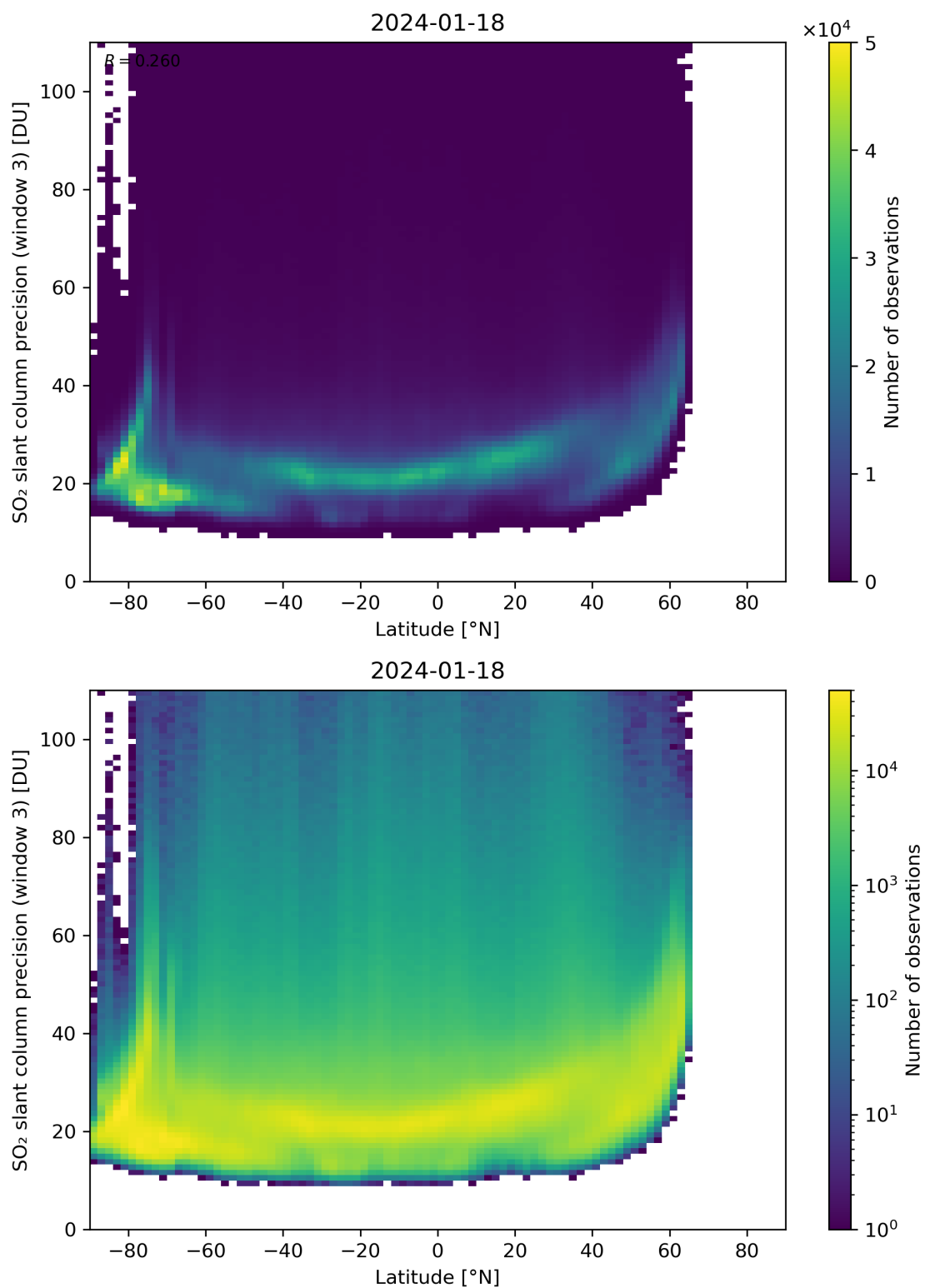
Figure 153: Scatter density plot of “Latitude” against “SO 2 slant column precision (window 3)” for 2024-01-17 to 2024-01-19.
