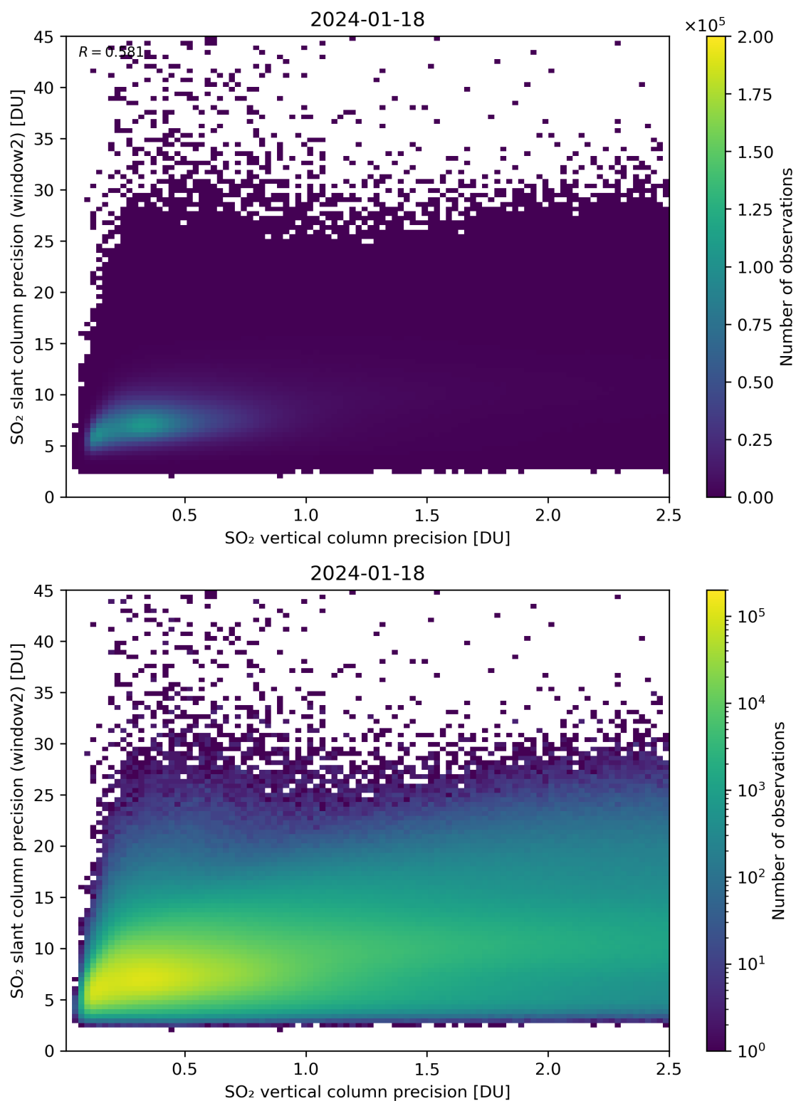
Figure 291: Scatter density plot of “SO 2 vertical column precision” against “SO 2 slant column precision (window2)” for 2024-01-17 to 2024-01-19.
