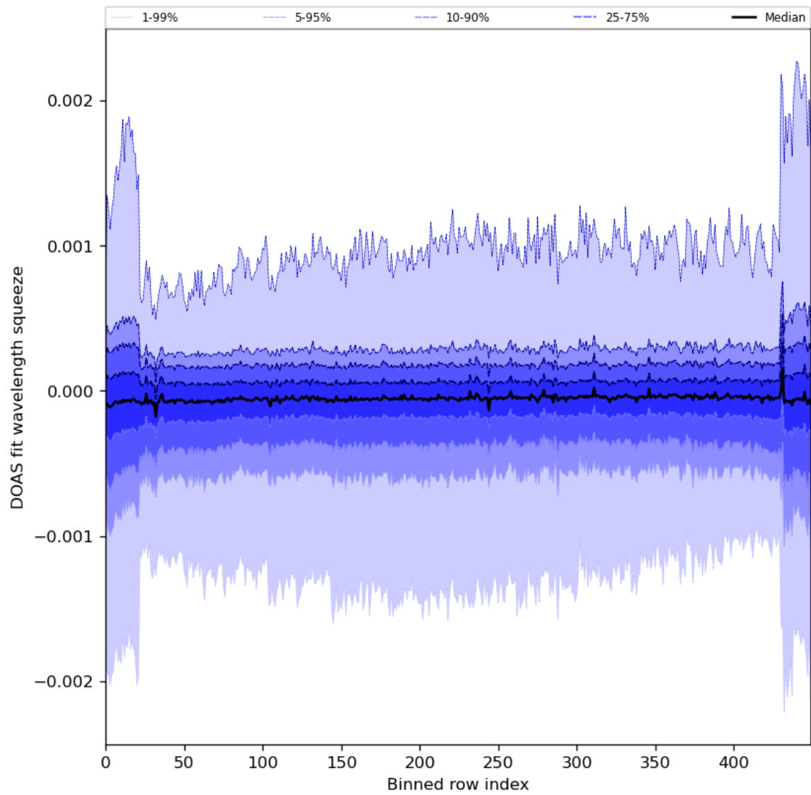
Figure 92: Along track statistics of “DOAS fit wavelength squeeze” for 2024-01-17 to 2024-01-19
