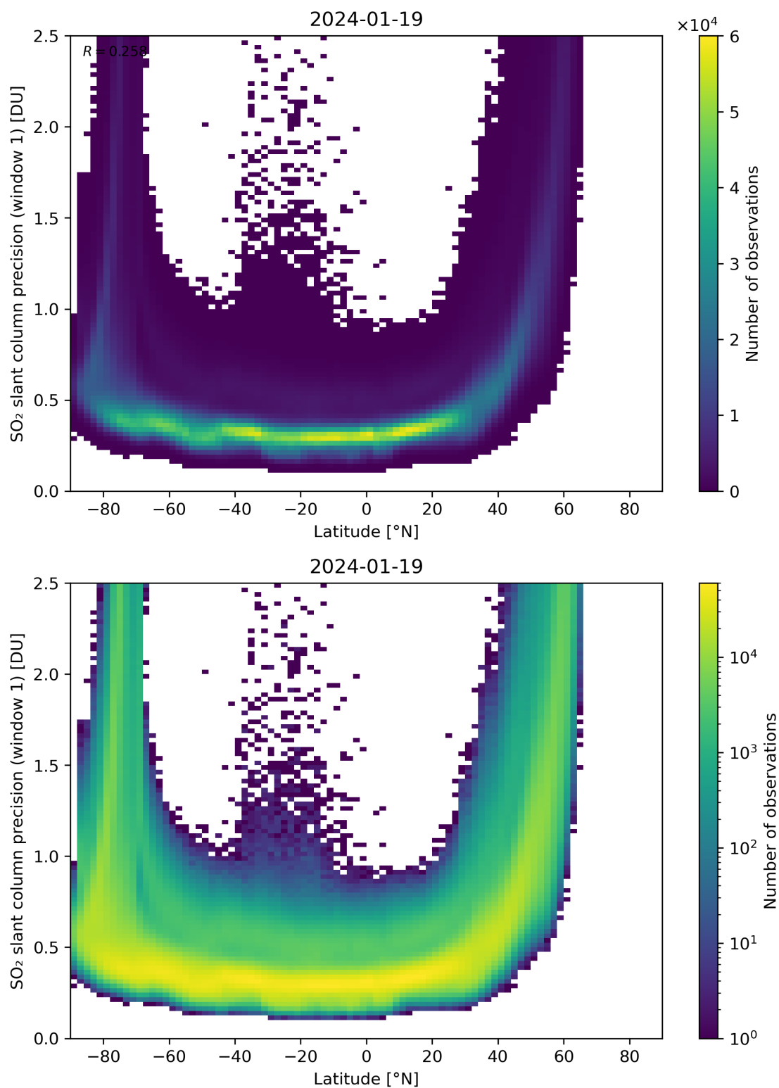
Figure 150: Scatter density plot of “Latitude” against “SO 2 slant column precision (window 1)” for 2024-01-18 to 2024-01-20.
