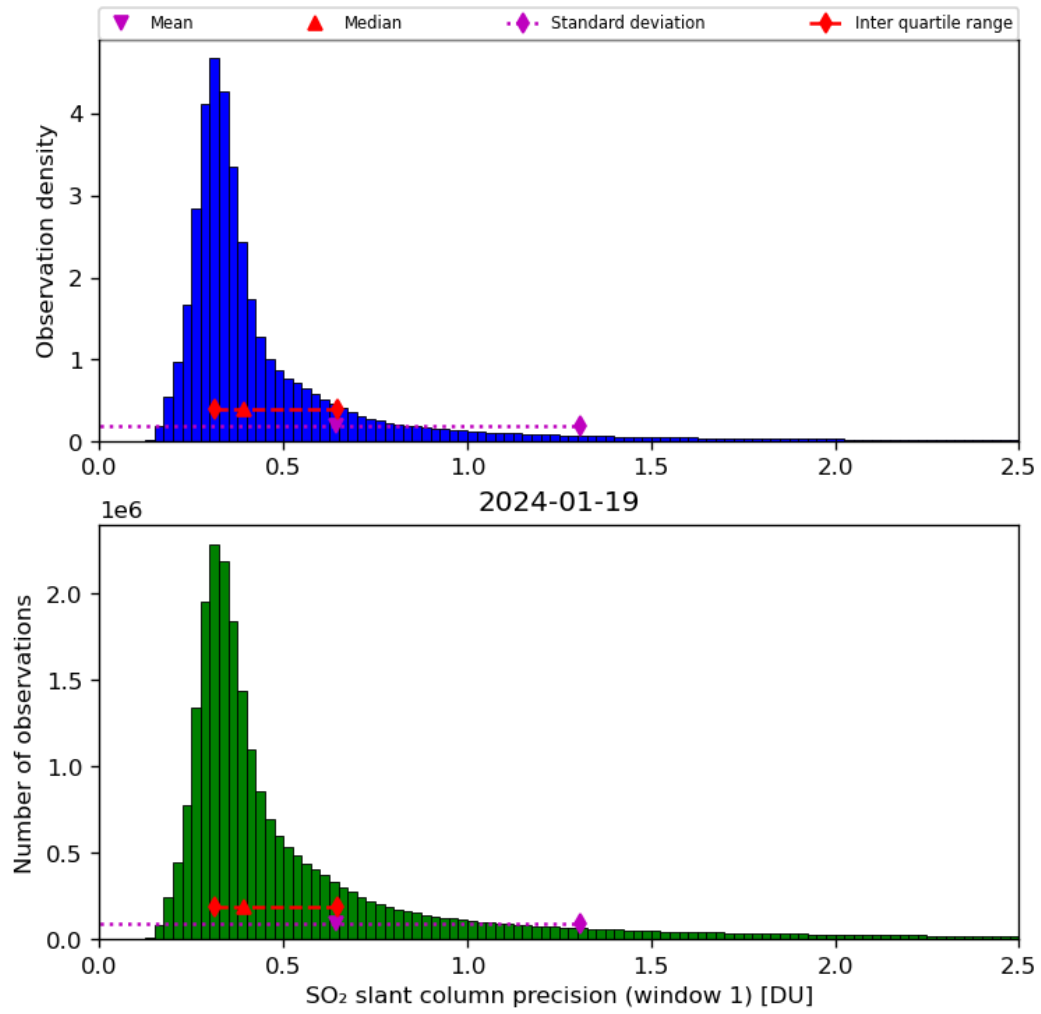
Figure 57: Histogram of “SO 2 slant column precision (window 1)” for 2024-01-18 to 2024-01-20
