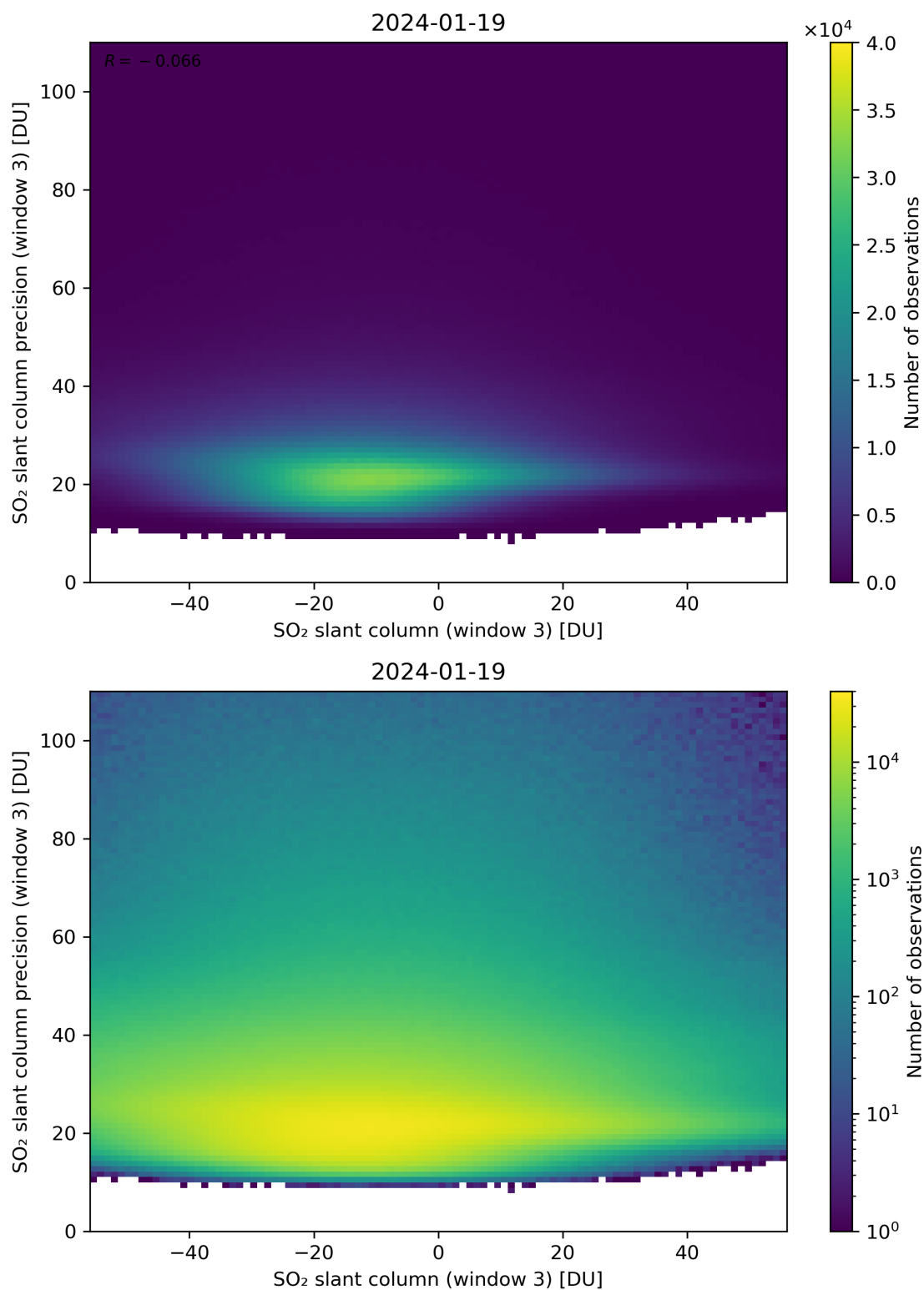
Figure 267: Scatter density plot of “SO 2 slant column (window 3)” against “SO 2 slant column precision (window 3)” for 2024-01-18 to 2024-01-20.
