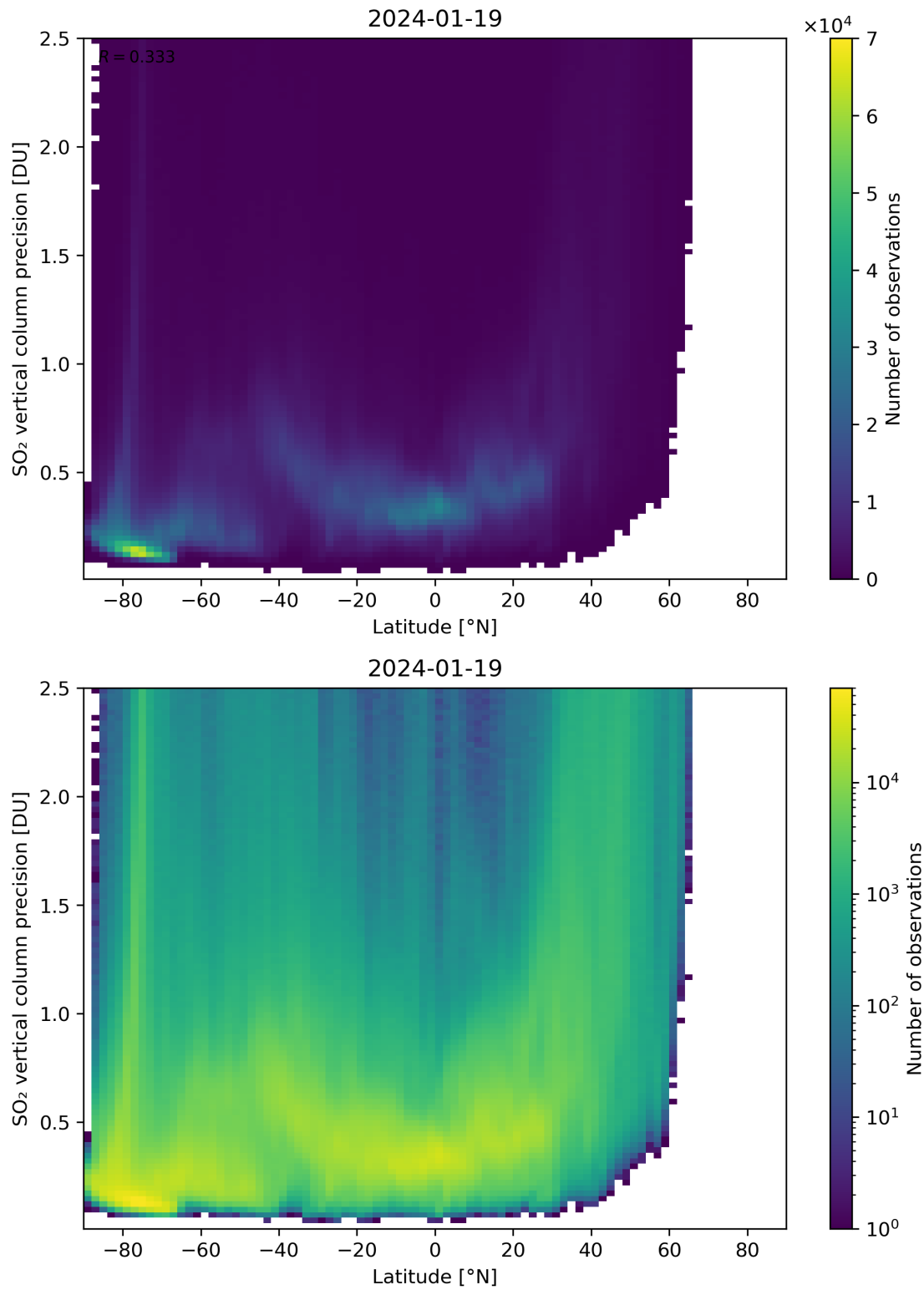
Figure 157: Scatter density plot of “Latitude” against “SO 2 vertical column precision” for 2024-01-18 to 2024-01-20.
