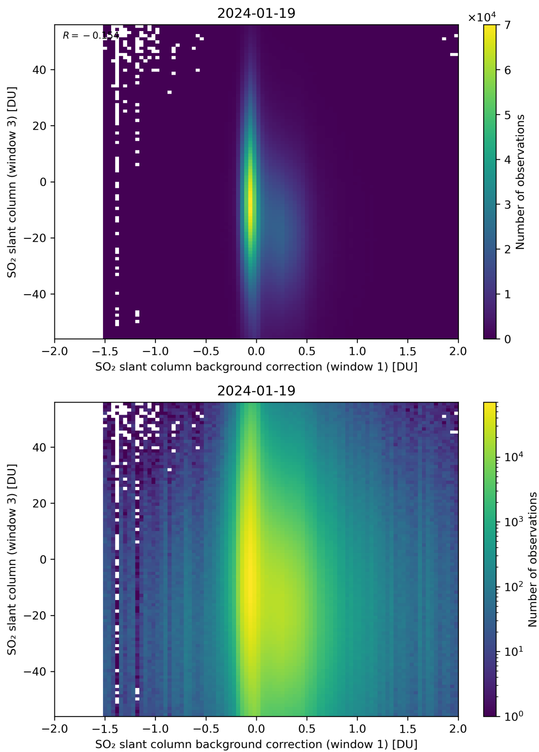
Figure 107: Scatter density plot of “SO 2 slant column background correction (window 1)” against “SO 2 slant column (window 3)” for 2024-01-18 to 2024-01-20.
