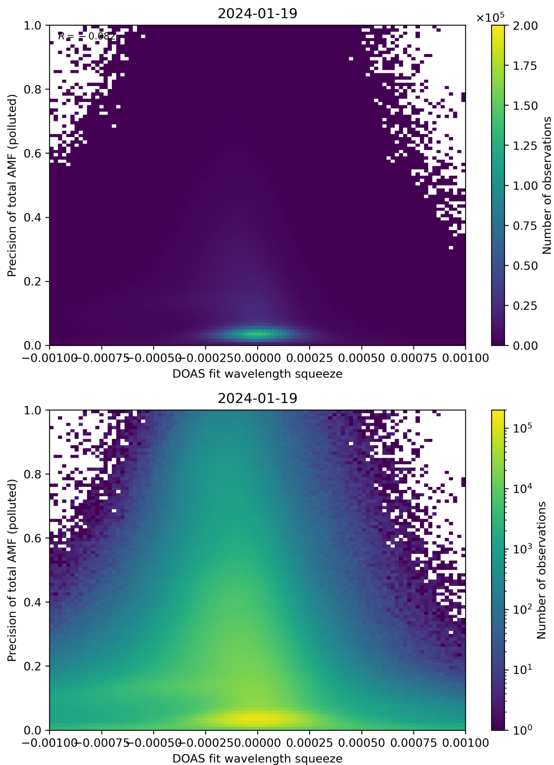
Figure 135: Scatter density plot of “DOAS fit wavelength squeeze” against “Precision of total AMF (polluted)” for 2024-01-18 to 2024-01-20.
