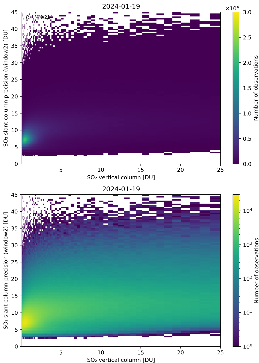
Figure 302: Scatter density plot of “SO 2 vertical column” against “SO 2 slant column precision (window2)” for 2024-01-18 to 2024-01-20.
