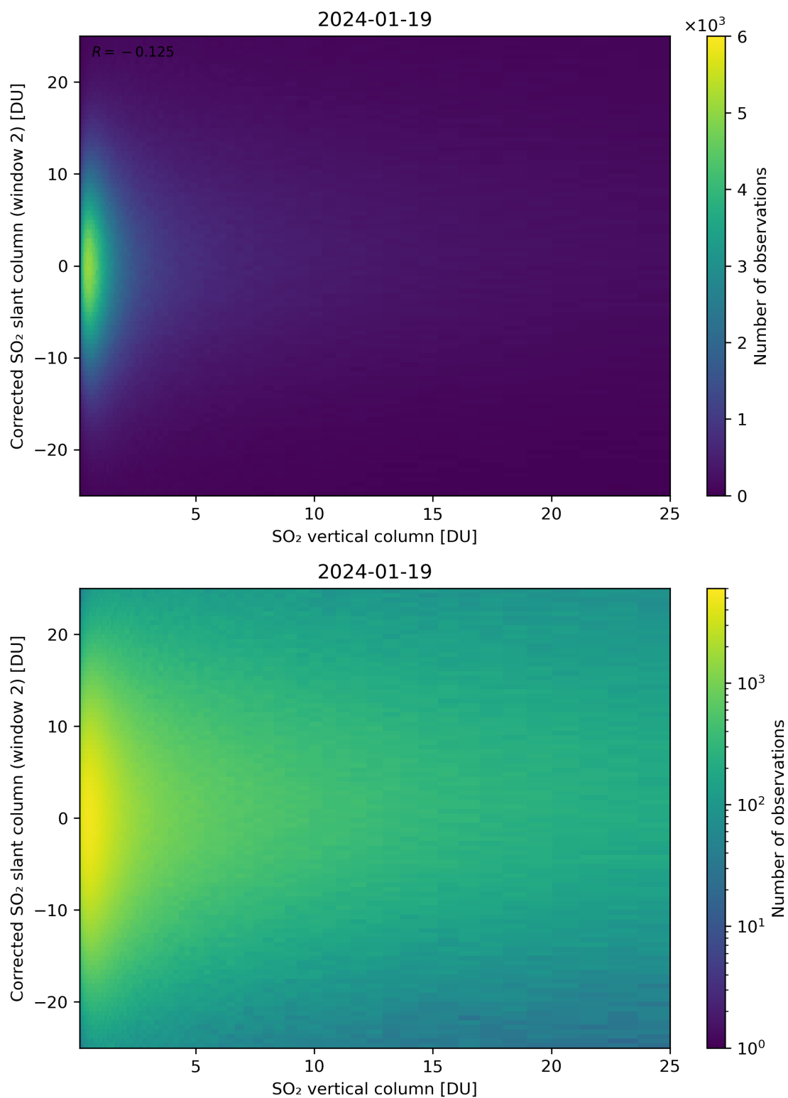
Figure 298: Scatter density plot of “SO 2 vertical column” against “Corrected SO 2 slant column (window 2)” for 2024-01-18 to 2024-01-20.
