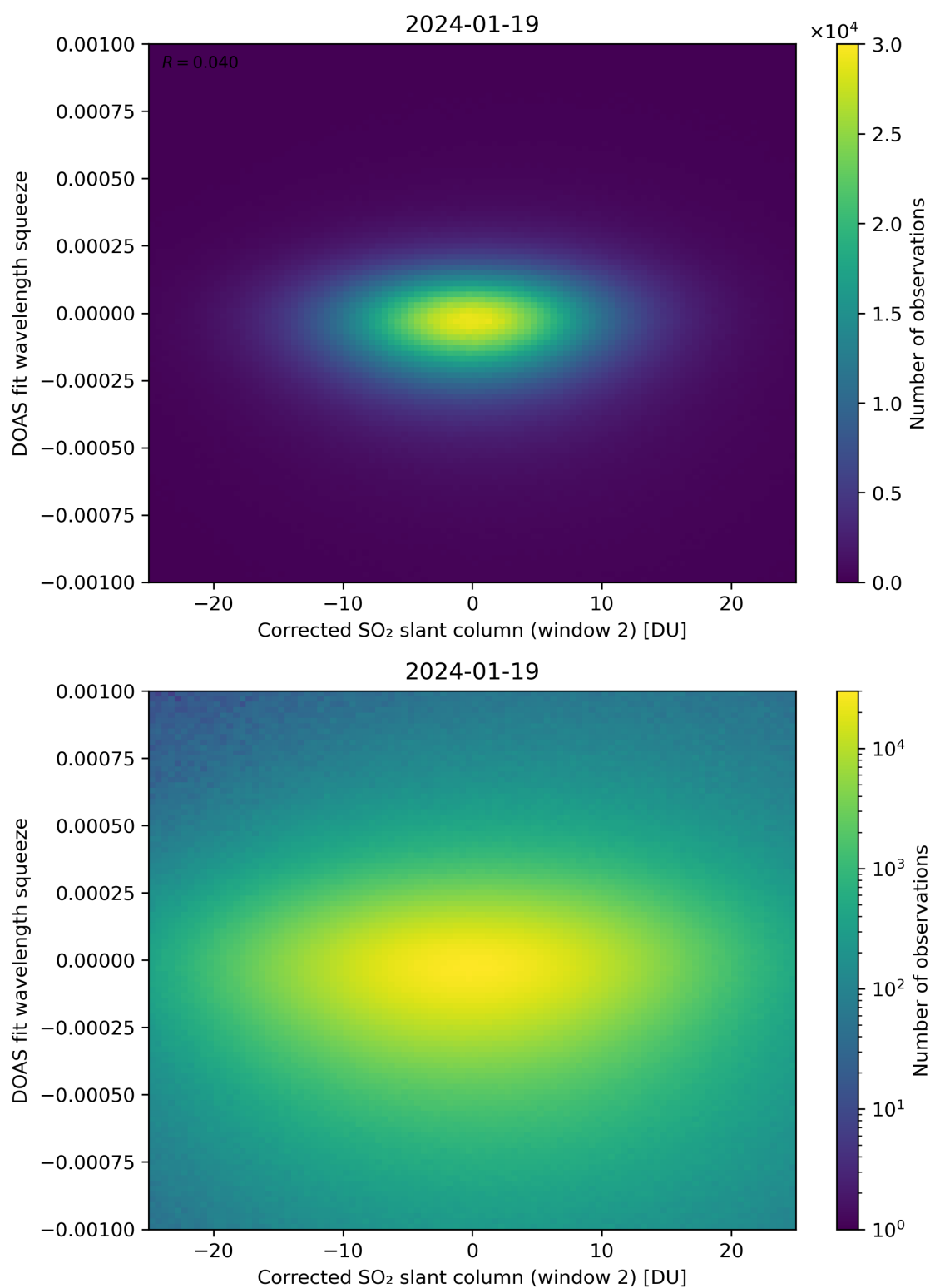
Figure 197: Scatter density plot of “Corrected SO 2 slant column (window 2)” against “DOAS fit wavelength squeeze” for 2024-01-18 to 2024-01-20.
