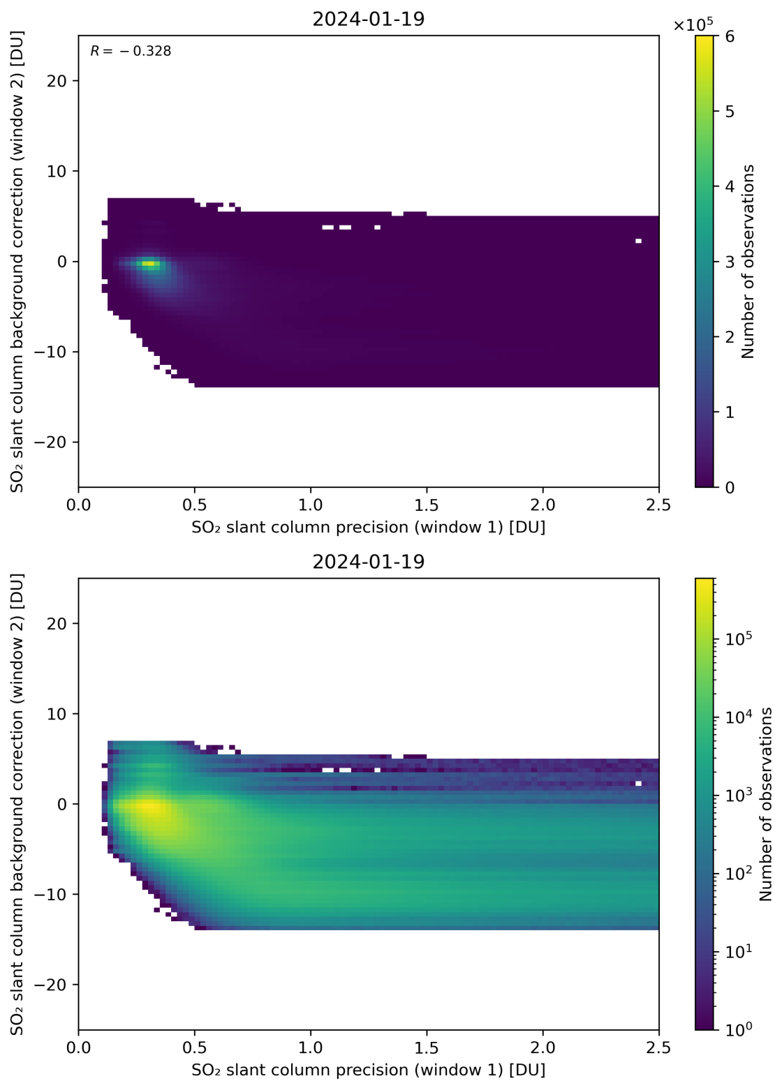
Figure 219: Scatter density plot of “SO 2 slant column precision (window 1)” against “SO 2 slant column background correction (window 2)” for 2024-01-18 to 2024-01-20.
