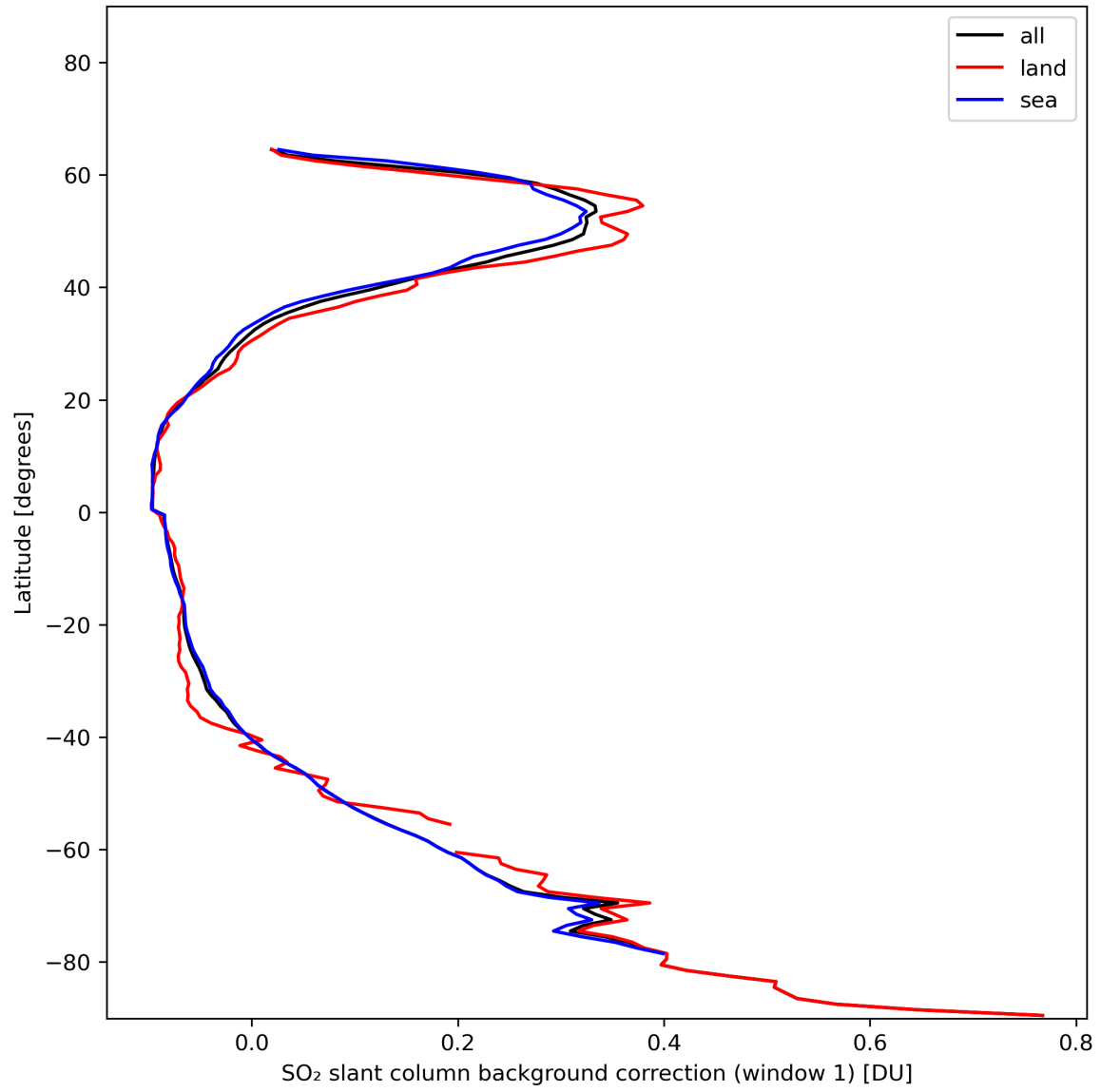
Figure 36: Zonal average of “SO 2 slant column background correction (window 1)” for 2024-01-18 to 2024-01-20.
