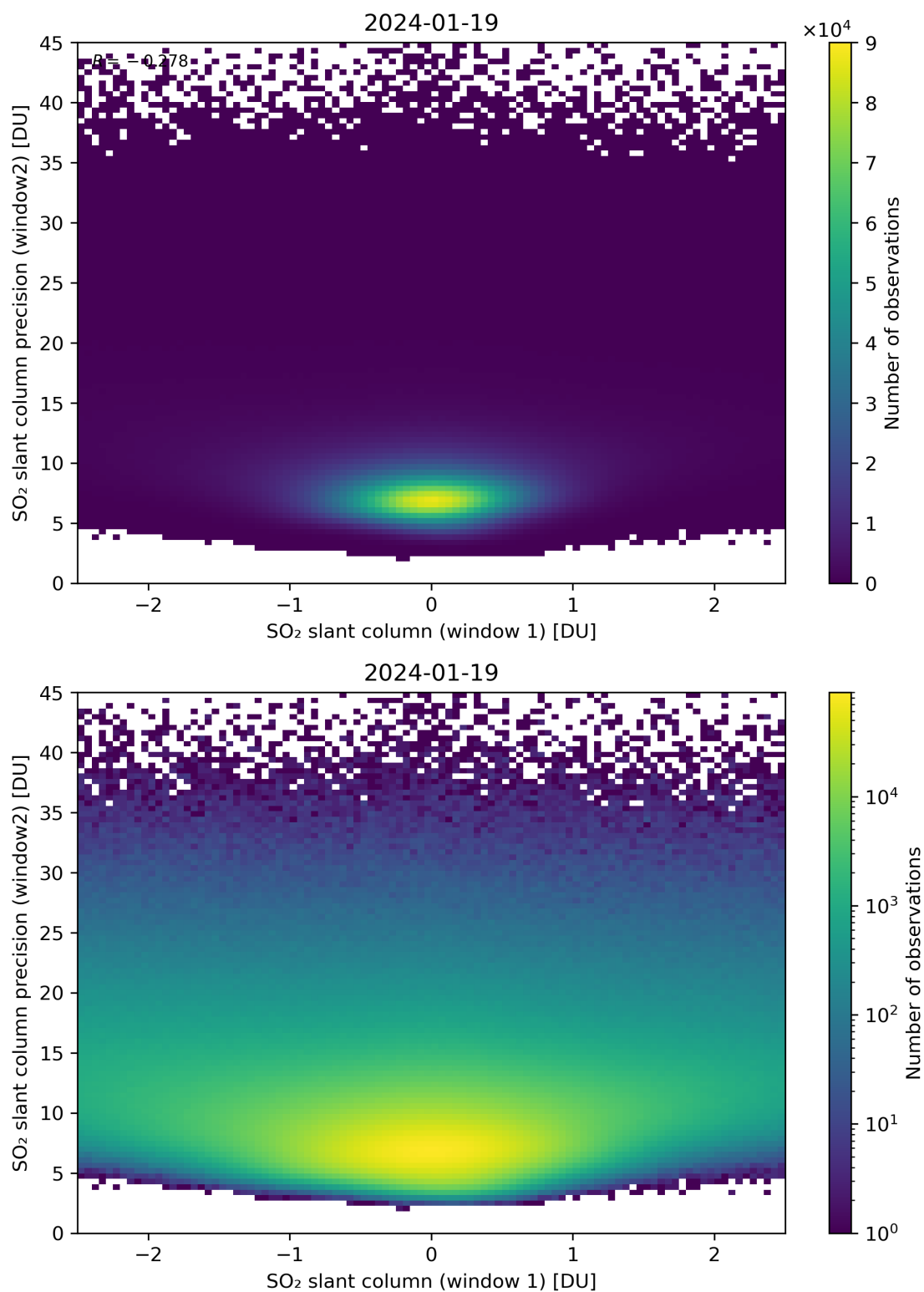
Figure 236: Scatter density plot of “SO 2 slant column (window 1)” against “SO 2 slant column precision (window2)” for 2024-01-18 to 2024-01-20.
