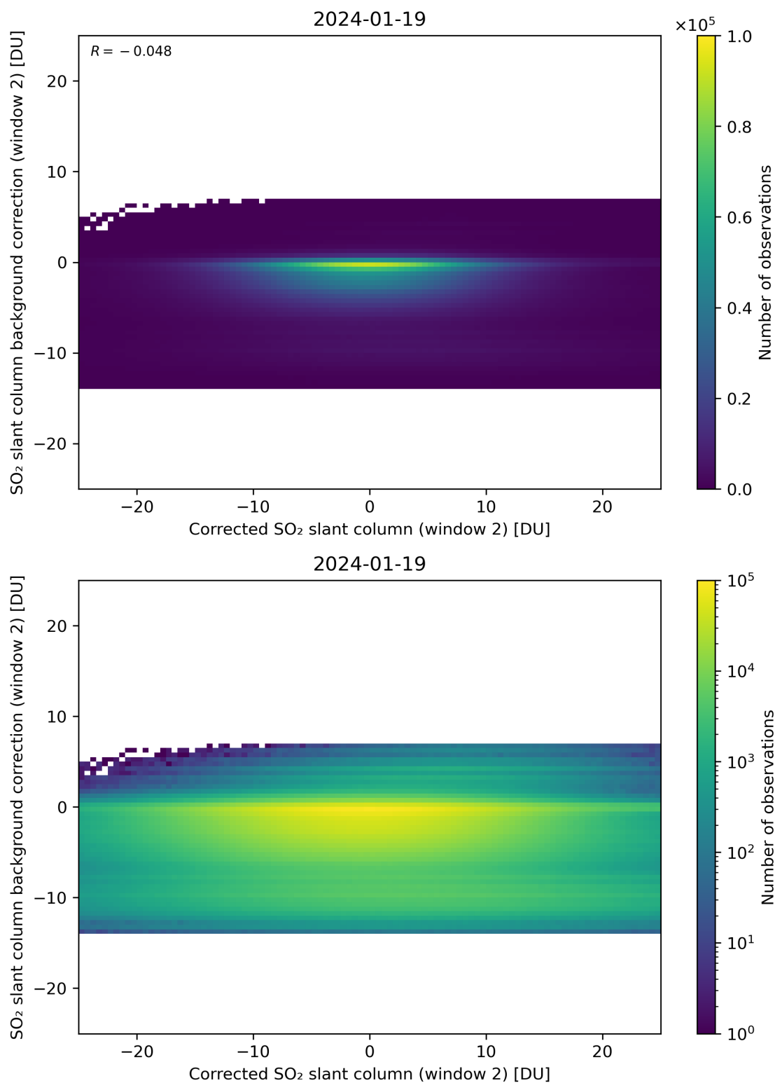
Figure 194: Scatter density plot of “Corrected SO 2 slant column (window 2)” against “SO 2 slant column background correction (window 2)” for 2024-01-18 to 2024-01-20.
