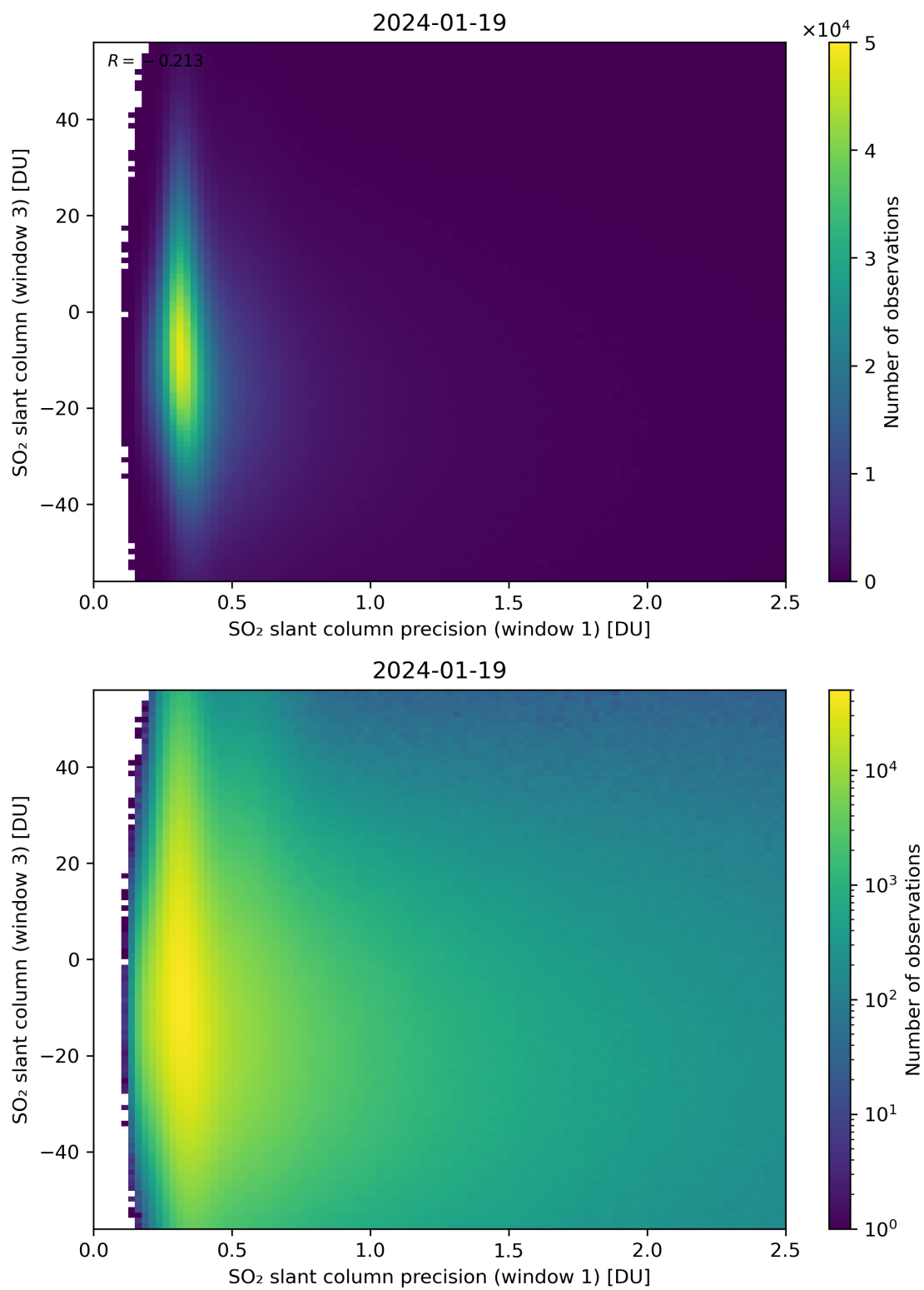
Figure 228: Scatter density plot of “SO 2 slant column precision (window 1)” against “SO 2 slant column (window 3)” for 2024-01-18 to 2024-01-20.
