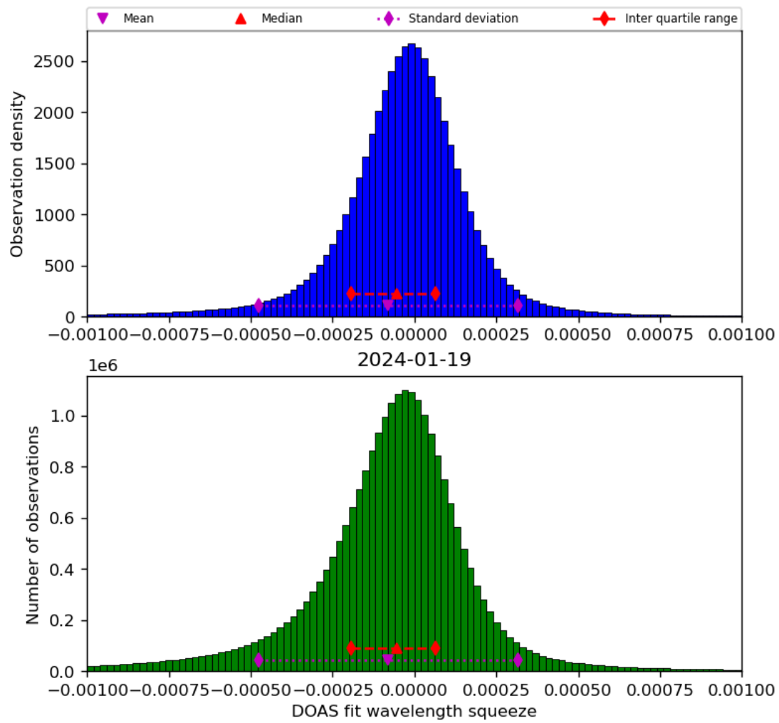
Figure 69: Histogram of “DOAS fit wavelength squeeze” for 2024-01-18 to 2024-01-20
