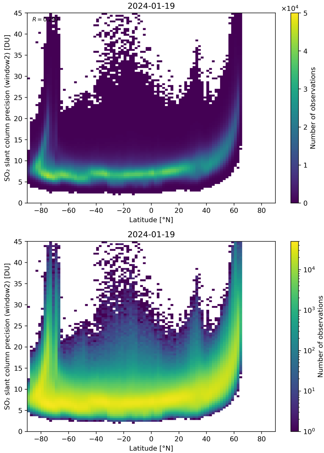
Figure 151: Scatter density plot of “Latitude” against “SO 2 slant column precision (window2)” for 2024-01-18 to 2024-01-20.
