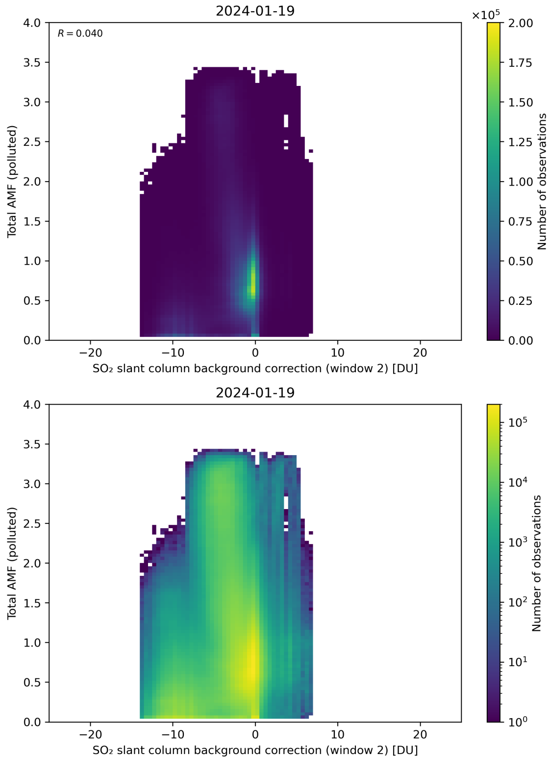
Figure 119: Scatter density plot of “SO 2 slant column background correction (window 2)” against “Total AMF (polluted)” for 2024-01-18 to 2024-01-20.
