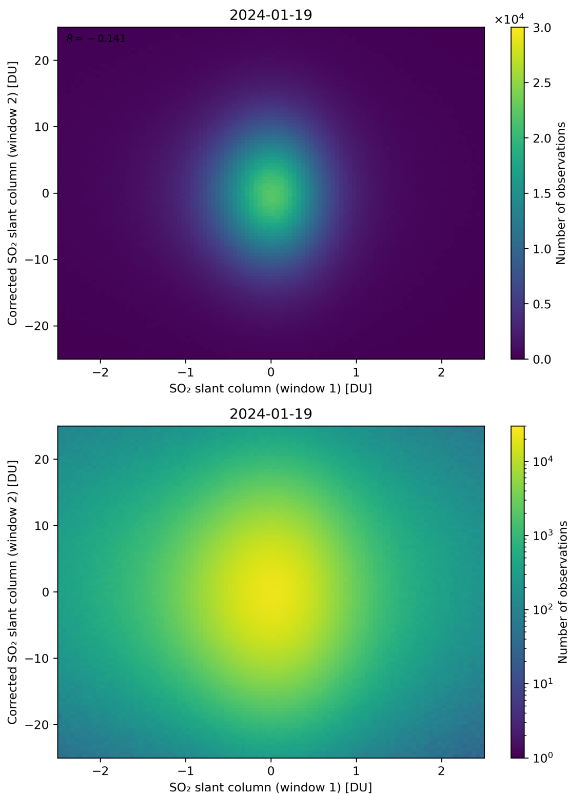
Figure 233: Scatter density plot of “SO 2 slant column (window 1)” against “Corrected SO 2 slant column (window 2)” for 2024-01-18 to 2024-01-20.
