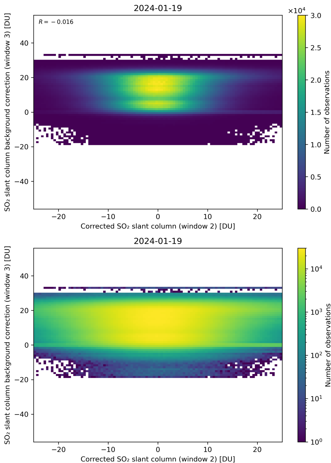
Figure 195: Scatter density plot of “Corrected SO 2 slant column (window 2)” against “SO 2 slant column background correction (window 3)” for 2024-01-18 to 2024-01-20.
