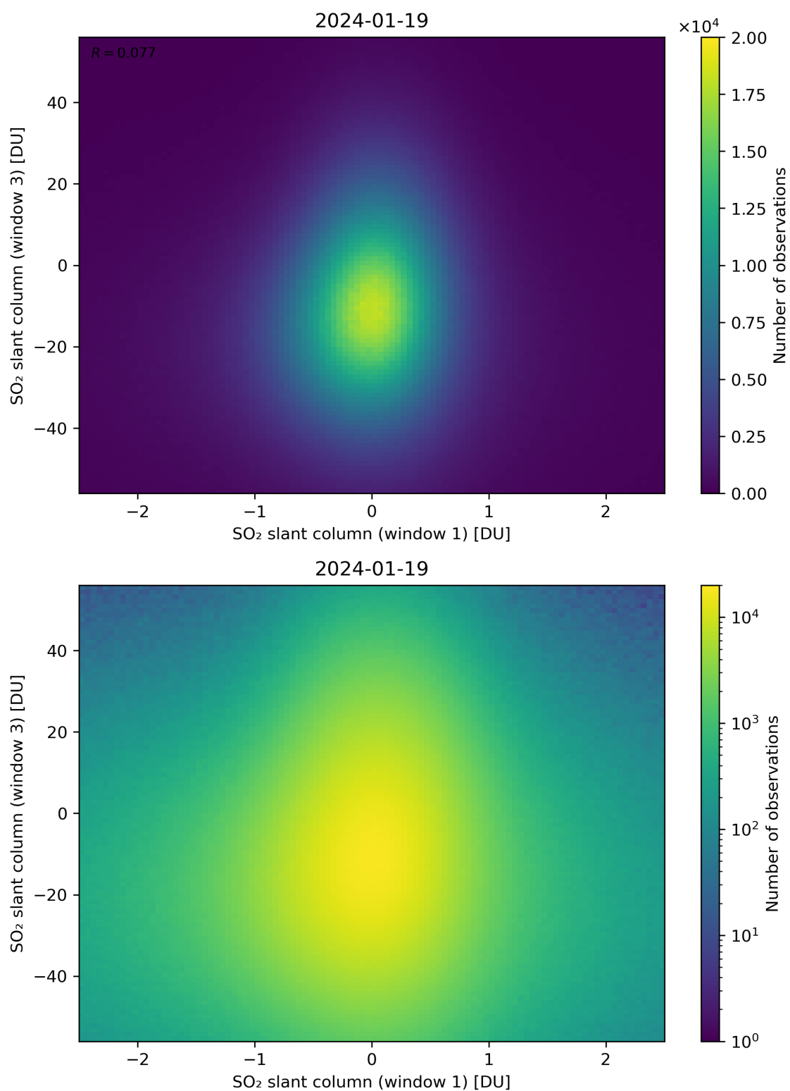
Figure 237: Scatter density plot of “SO 2 slant column (window 1)” against “SO 2 slant column (window 3)” for 2024-01-18 to 2024-01-20.
