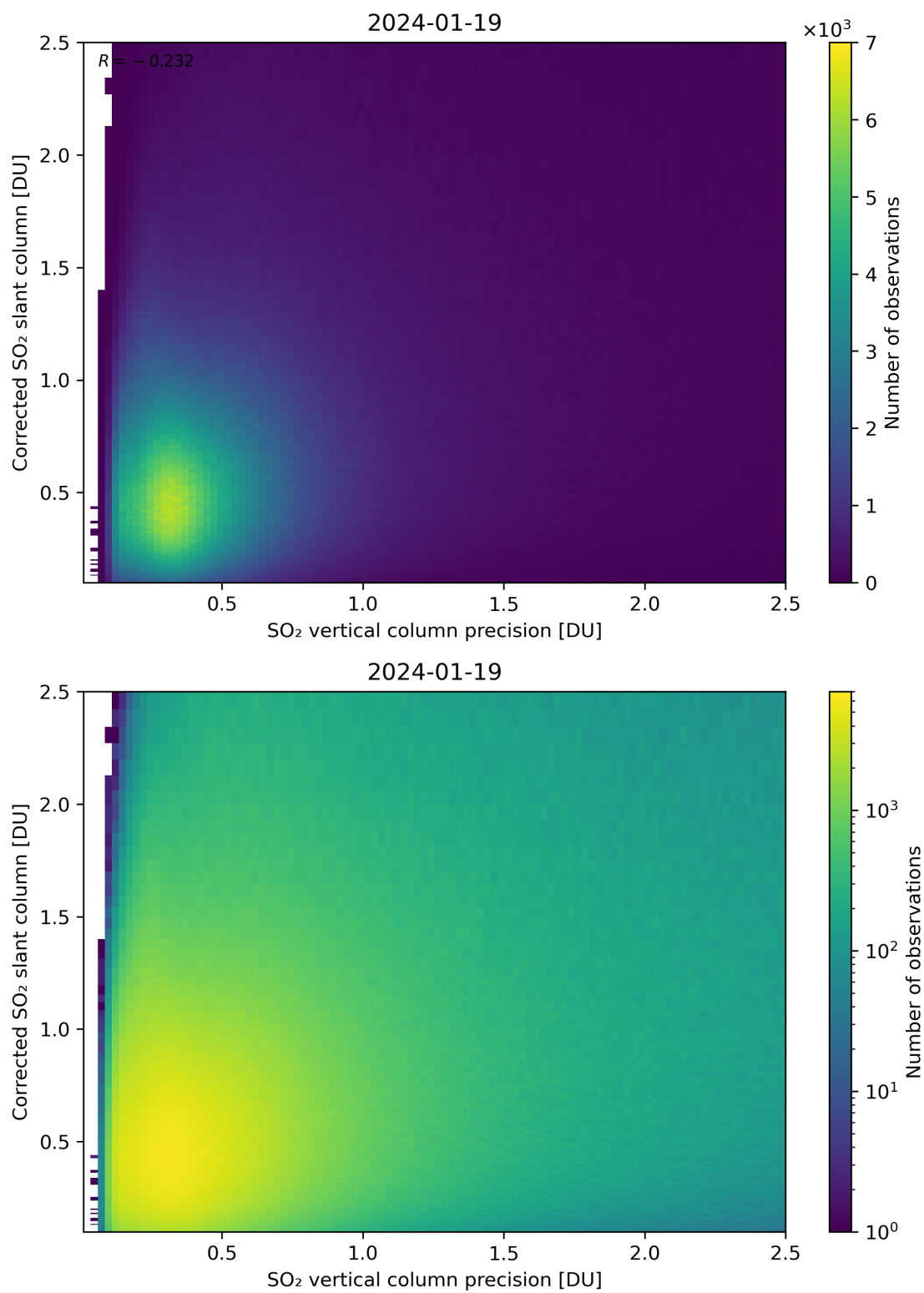
Figure 286: Scatter density plot of “SO 2 vertical column precision” against “Corrected SO 2 slant column” for 2024-01-18 to 2024-01-20.
