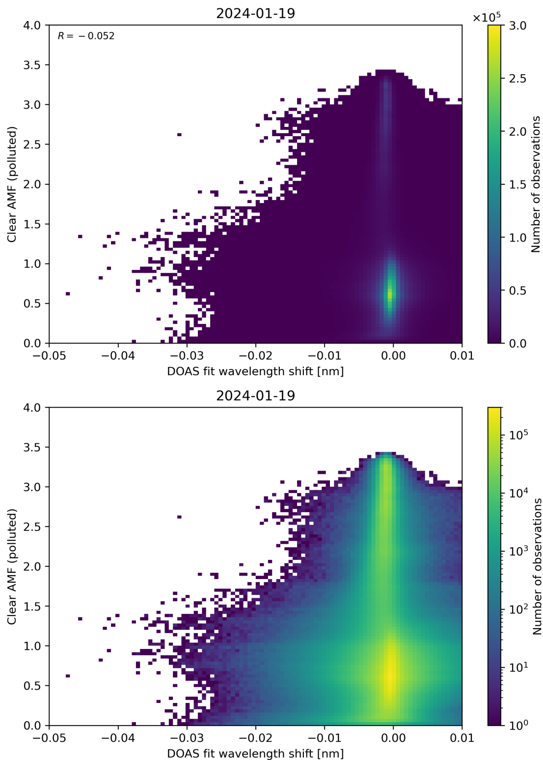
Figure 129: Scatter density plot of “DOAS fit wavelength shift” against “Clear AMF (polluted)” for 2024-01-18 to 2024-01-20.
