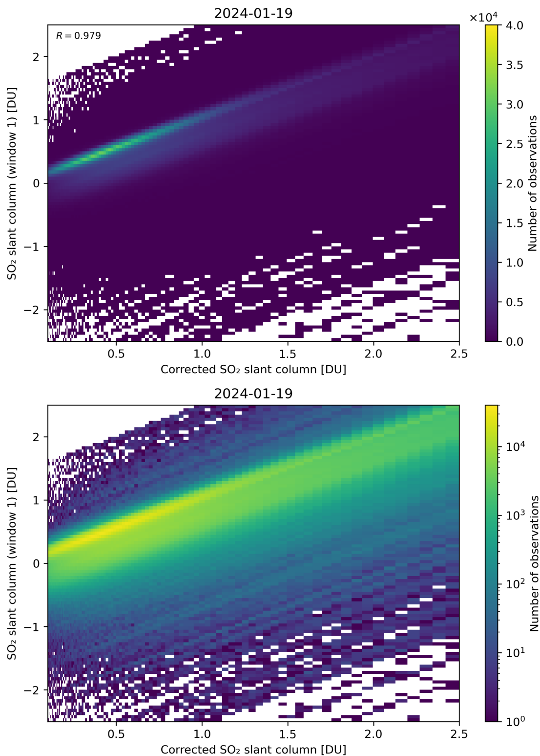
Figure 187: Scatter density plot of “Corrected SO 2 slant column” against “SO 2 slant column (window 1)” for 2024-01-18 to 2024-01-20.
