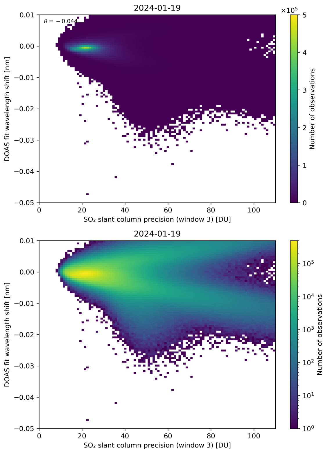
Figure 258: Scatter density plot of “SO 2 slant column precision (window 3)” against “DOAS fit wavelength shift” for 2024-01-18 to 2024-01-20.
