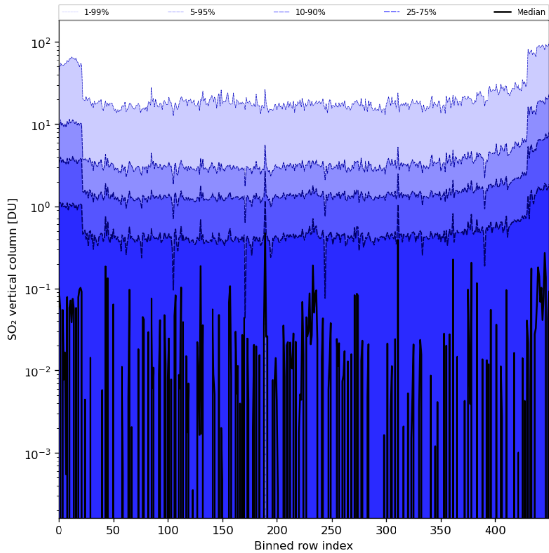
Figure 76: Along track statistics of “SO 2 vertical column” for 2024-01-18 to 2024-01-20
