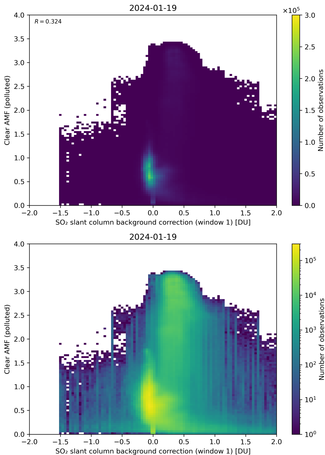
Figure 103: Scatter density plot of “SO 2 slant column background correction (window 1)” against “Clear AMF (polluted)” for 2024-01-18 to 2024-01-20.
