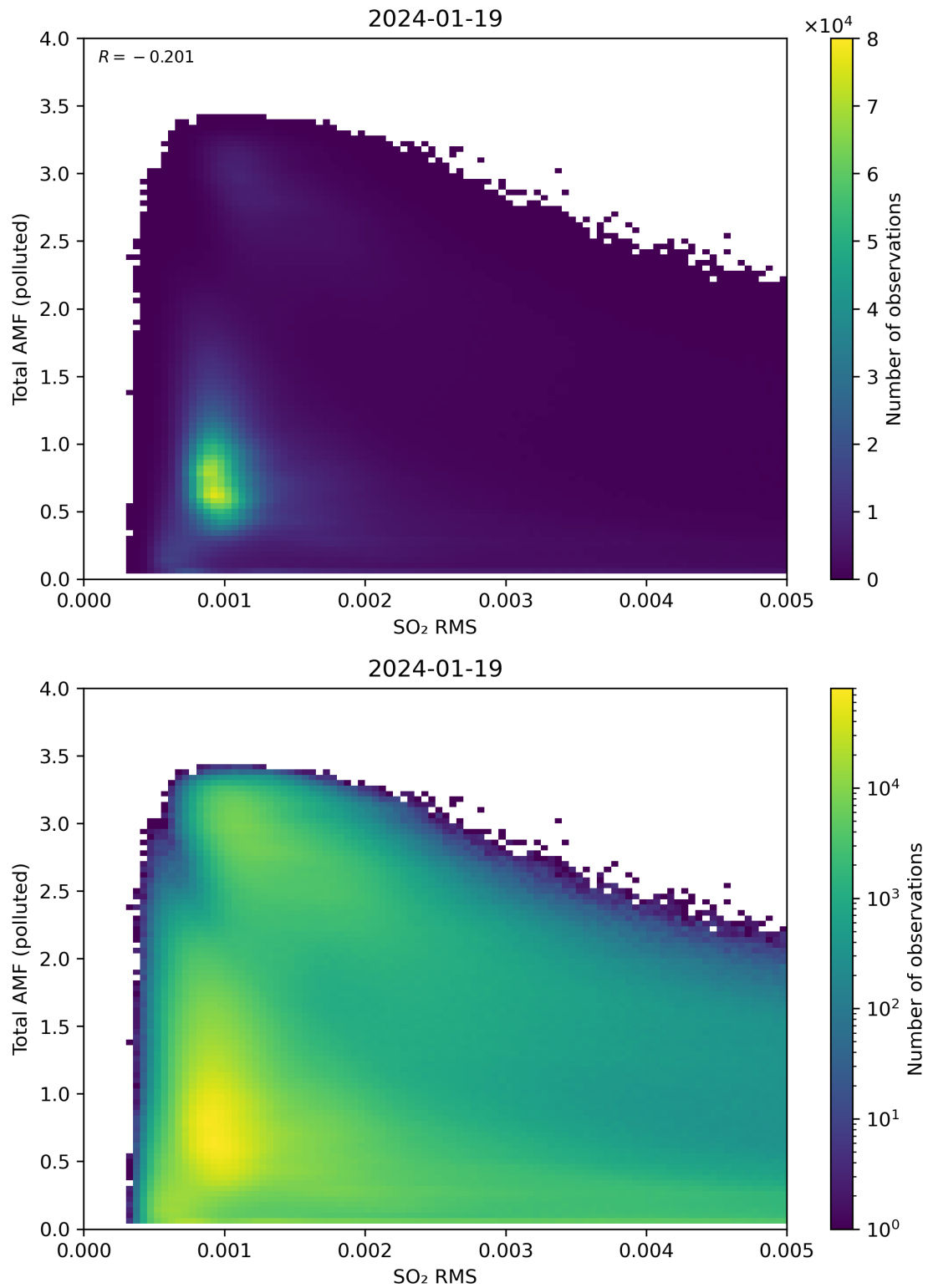
Figure 137: Scatter density plot of “SO 2 RMS” against “Total AMF (polluted)” for 2024-01-18 to 2024-01-20.
