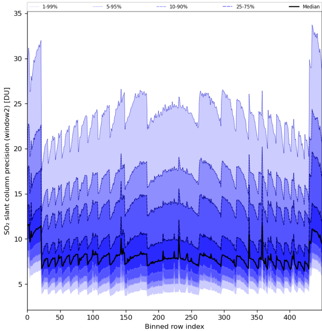
Figure 84: Along track statistics of “SO 2 slant column precision (window2)” for 2024-01-18 to 2024-01-20
