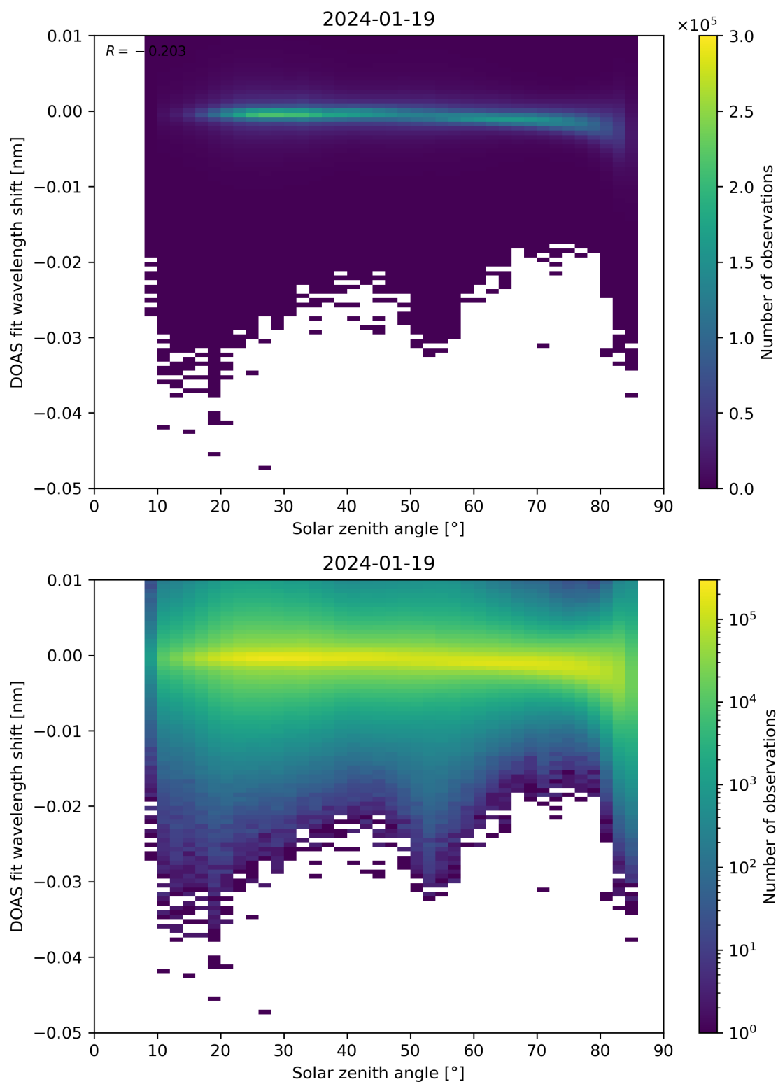
Figure 161: Scatter density plot of “Solar zenith angle” against “DOAS fit wavelength shift” for 2024-01-18 to 2024-01-20.
