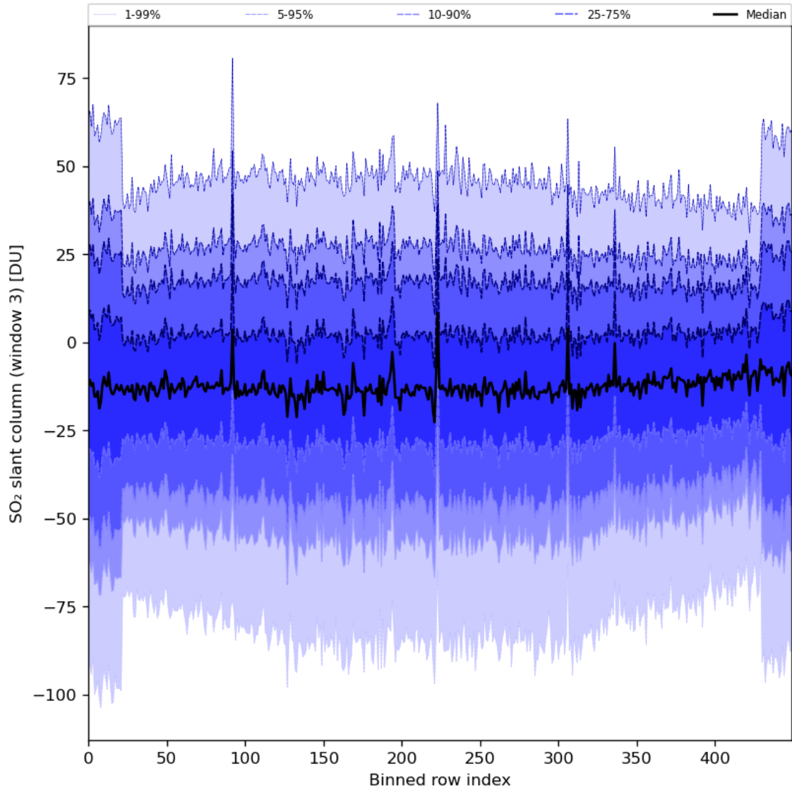
Figure 87: Along track statistics of “SO 2 slant column (window 3)” for 2024-01-18 to 2024-01-20
