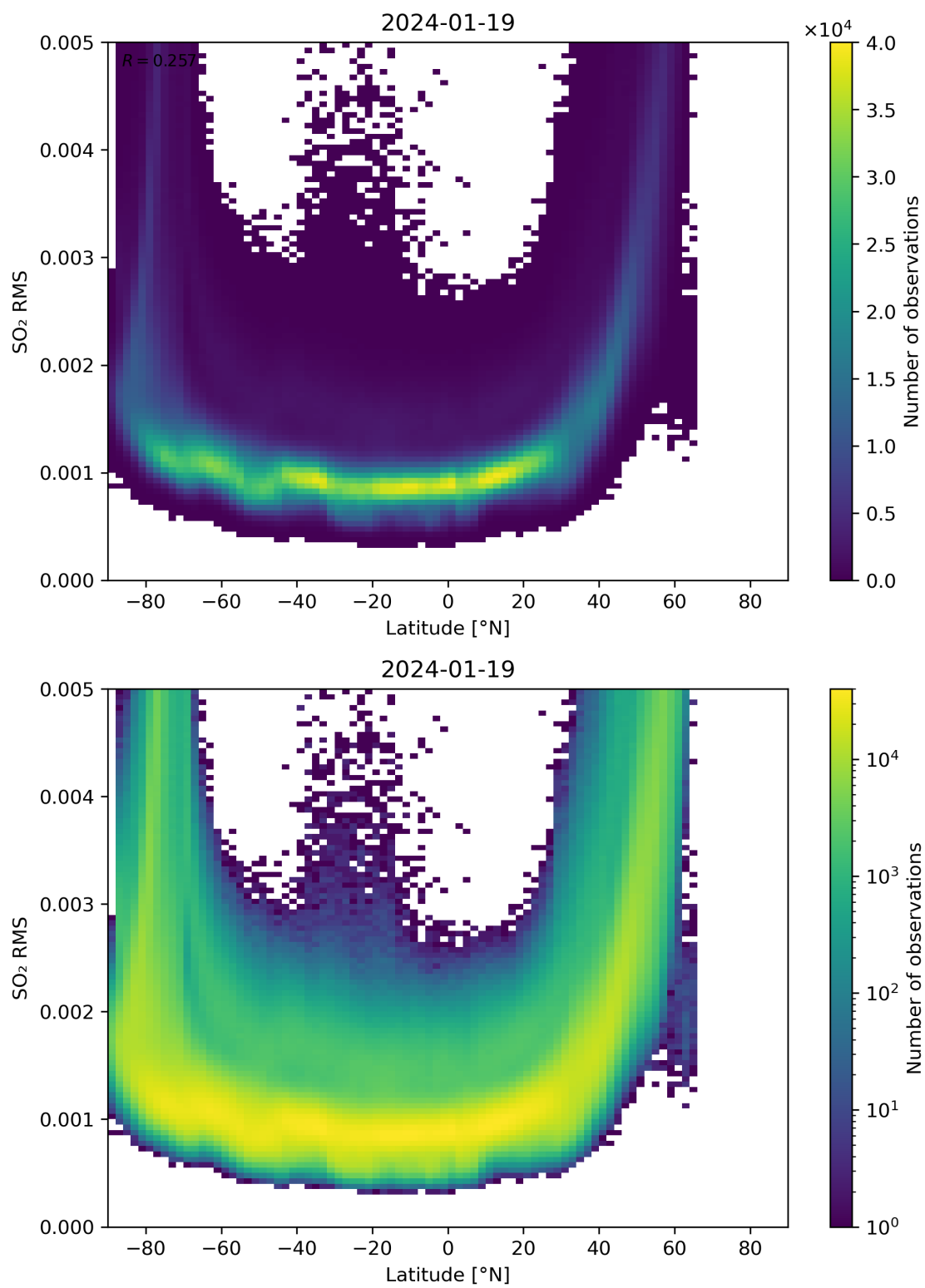
Figure 144: Scatter density plot of “Latitude” against “SO 2 RMS” for 2024-01-18 to 2024-01-20.
