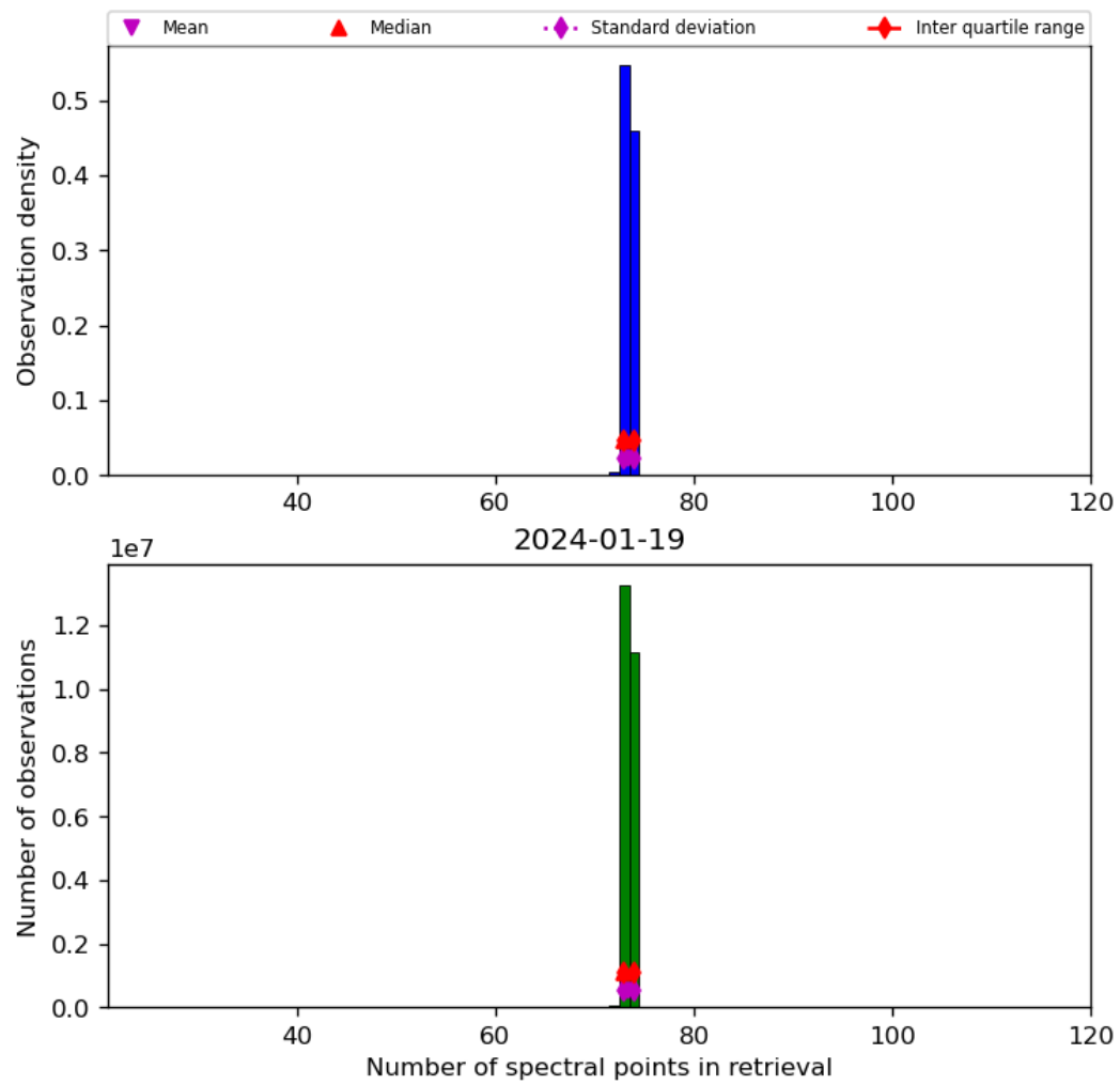
Figure 74: Histogram of “Number of spectral points in retrieval” for 2024-01-18 to 2024-01-20
