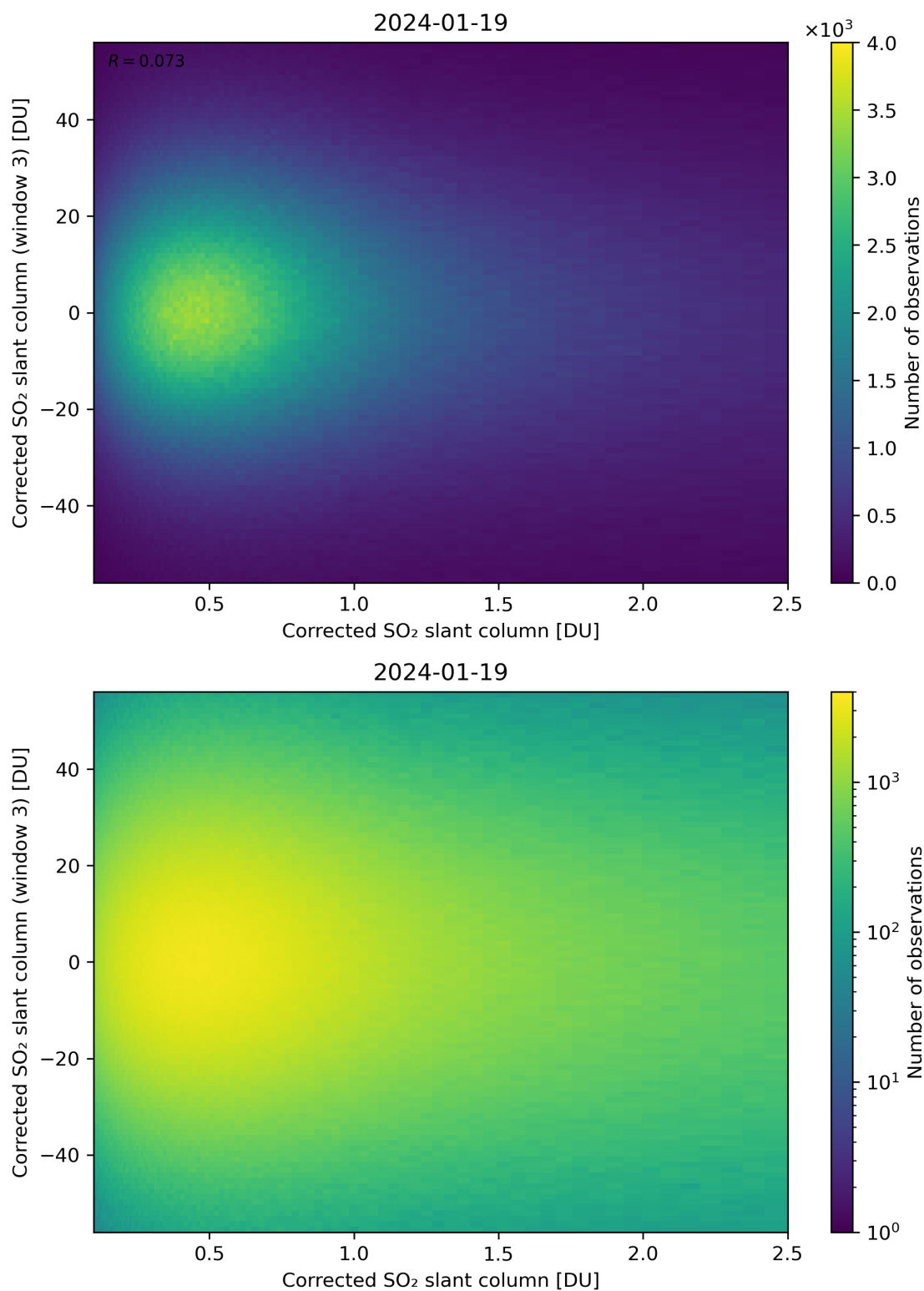
Figure 186: Scatter density plot of “Corrected SO 2 slant column” against “Corrected SO 2 slant column (window 3)” for 2024-01-18 to 2024-01-20.
