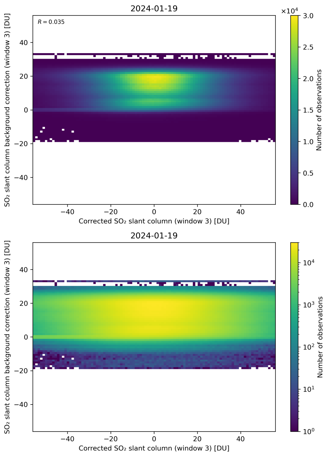
Figure 205: Scatter density plot of “Corrected SO 2 slant column (window 3)” against “SO 2 slant column background correction (window 3)” for 2024-01-18 to 2024-01-20.
