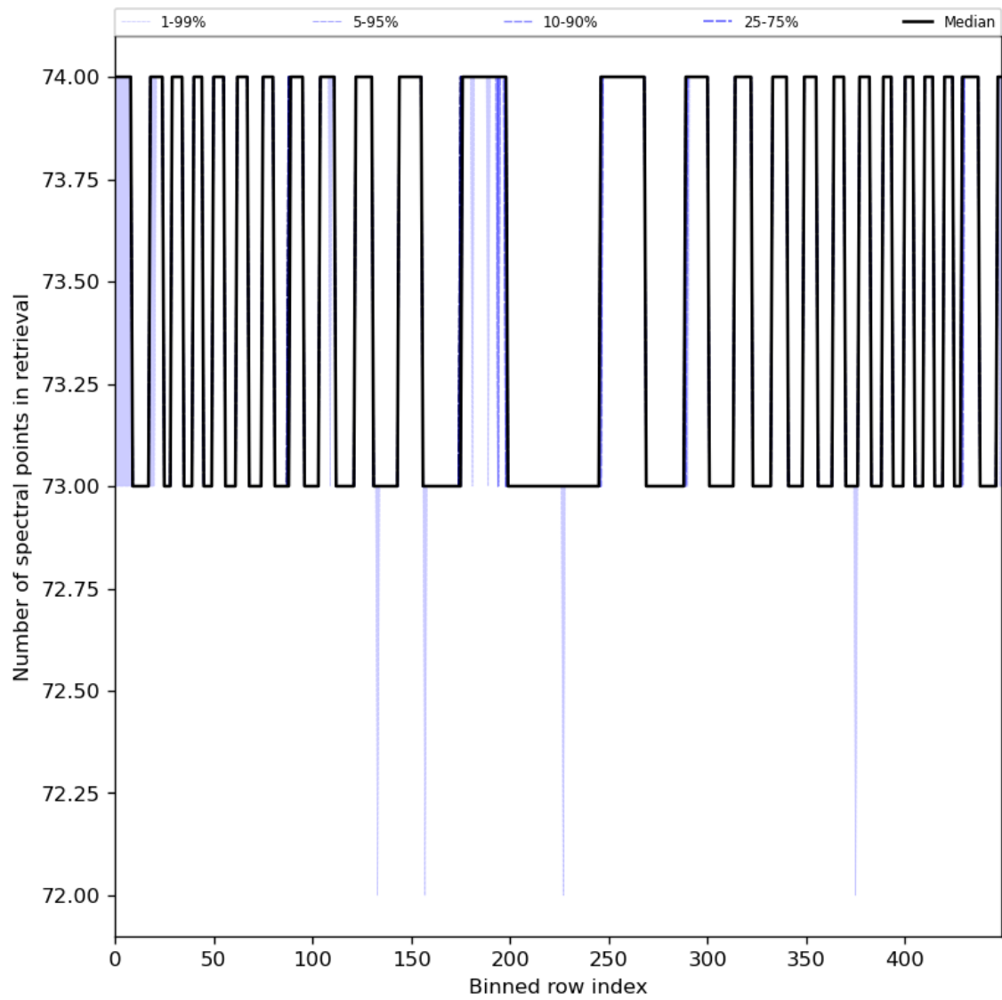
Figure 97: Along track statistics of “Number of spectral points in retrieval” for 2024-01-18 to 2024-01-20
