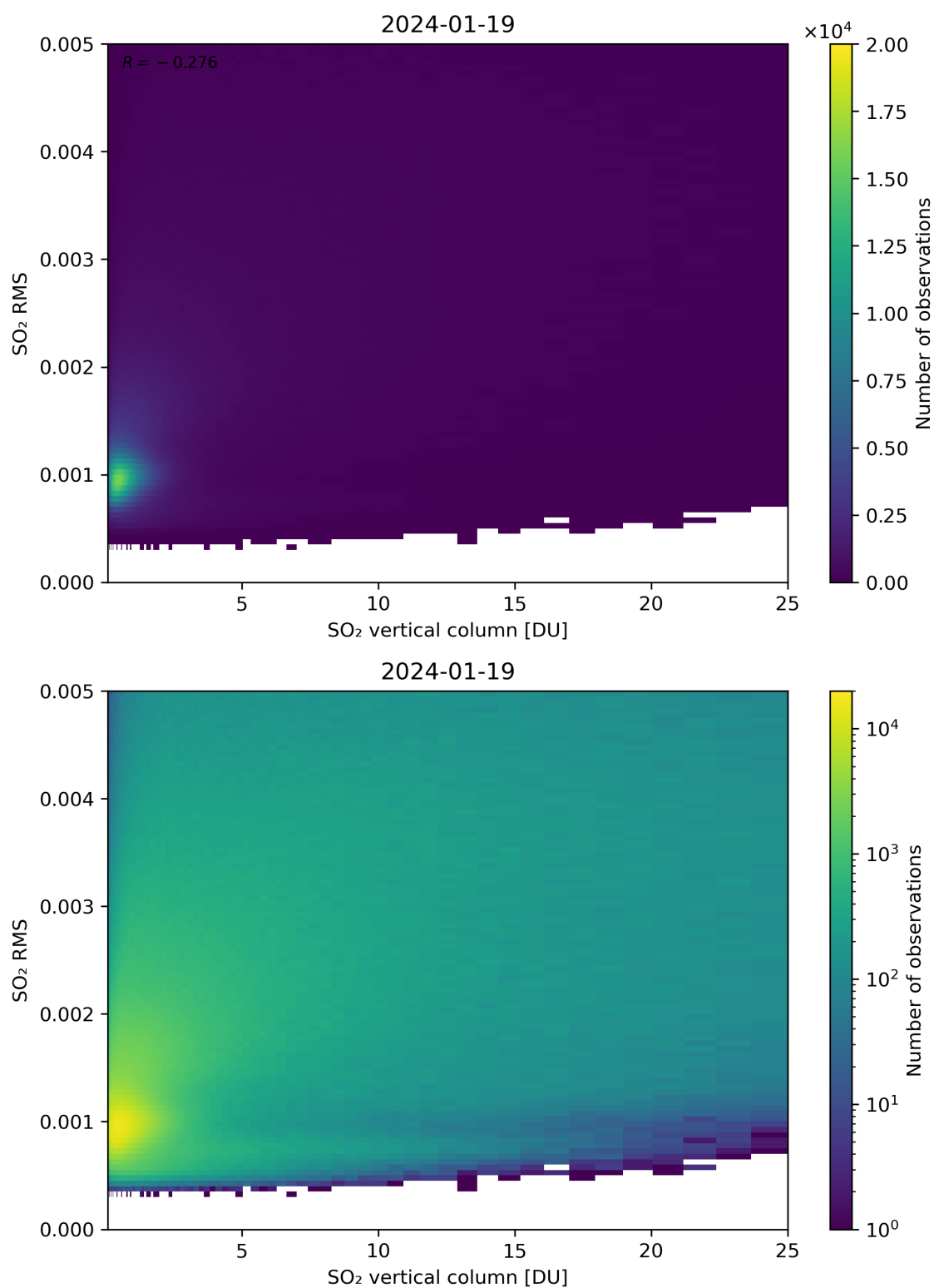
Figure 278: Scatter density plot of “SO 2 vertical column” against “SO 2 RMS” for 2024-01-18 to 2024-01-20.
