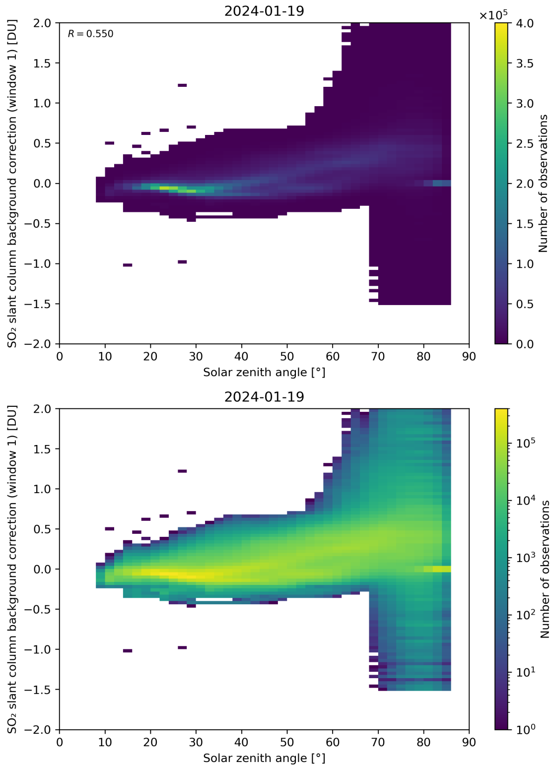
Figure 158: Scatter density plot of “Solar zenith angle” against “SO 2 slant column background correction (window 1)” for 2024-01-18 to 2024-01-20.
