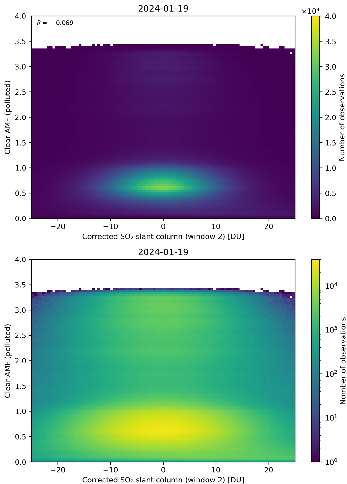
Figure 199: Scatter density plot of “Corrected SO 2 slant column (window 2)” against “Clear AMF (polluted)” for 2024-01-18 to 2024-01-20.
