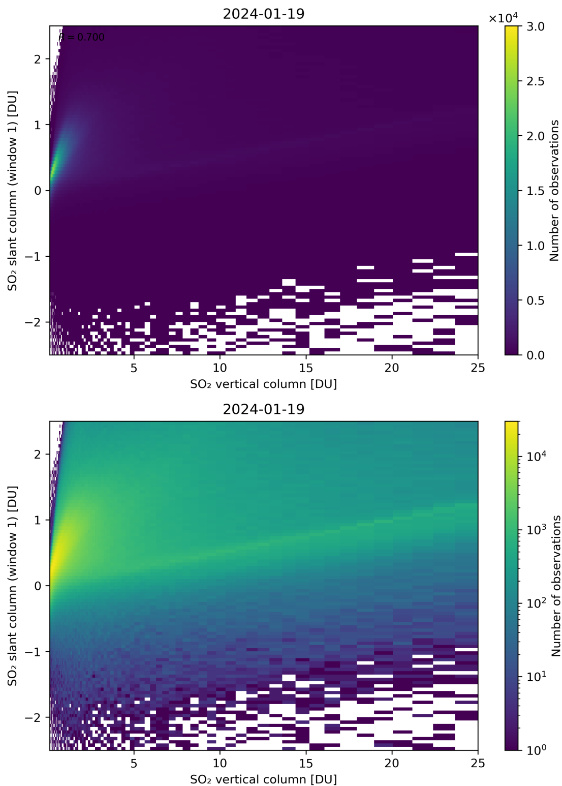
Figure 300: Scatter density plot of “SO 2 vertical column” against “SO 2 slant column (window 1)” for 2024-01-18 to 2024-01-20.
