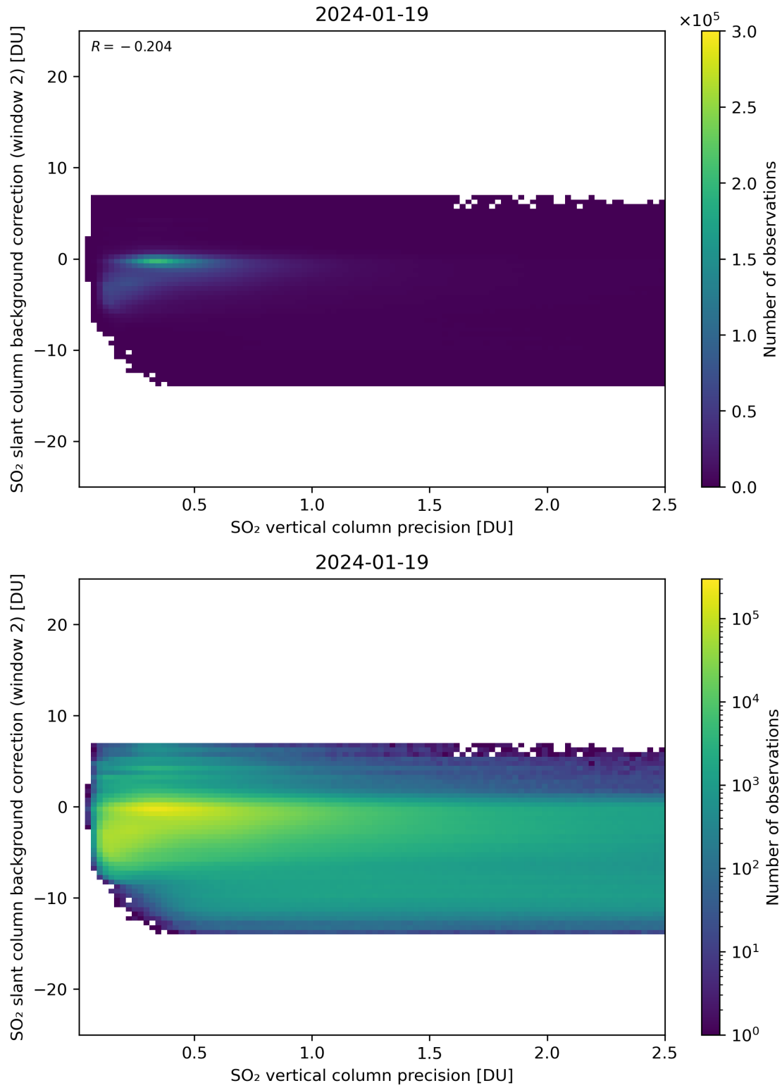
Figure 280: Scatter density plot of “SO 2 vertical column precision” against “SO 2 slant column background correction (window 2)” for 2024-01-18 to 2024-01-20.
