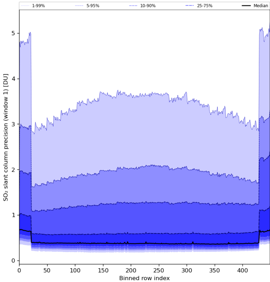
Figure 80: Along track statistics of “SO 2 slant column precision (window 1)” for 2024-01-18 to 2024-01-20
