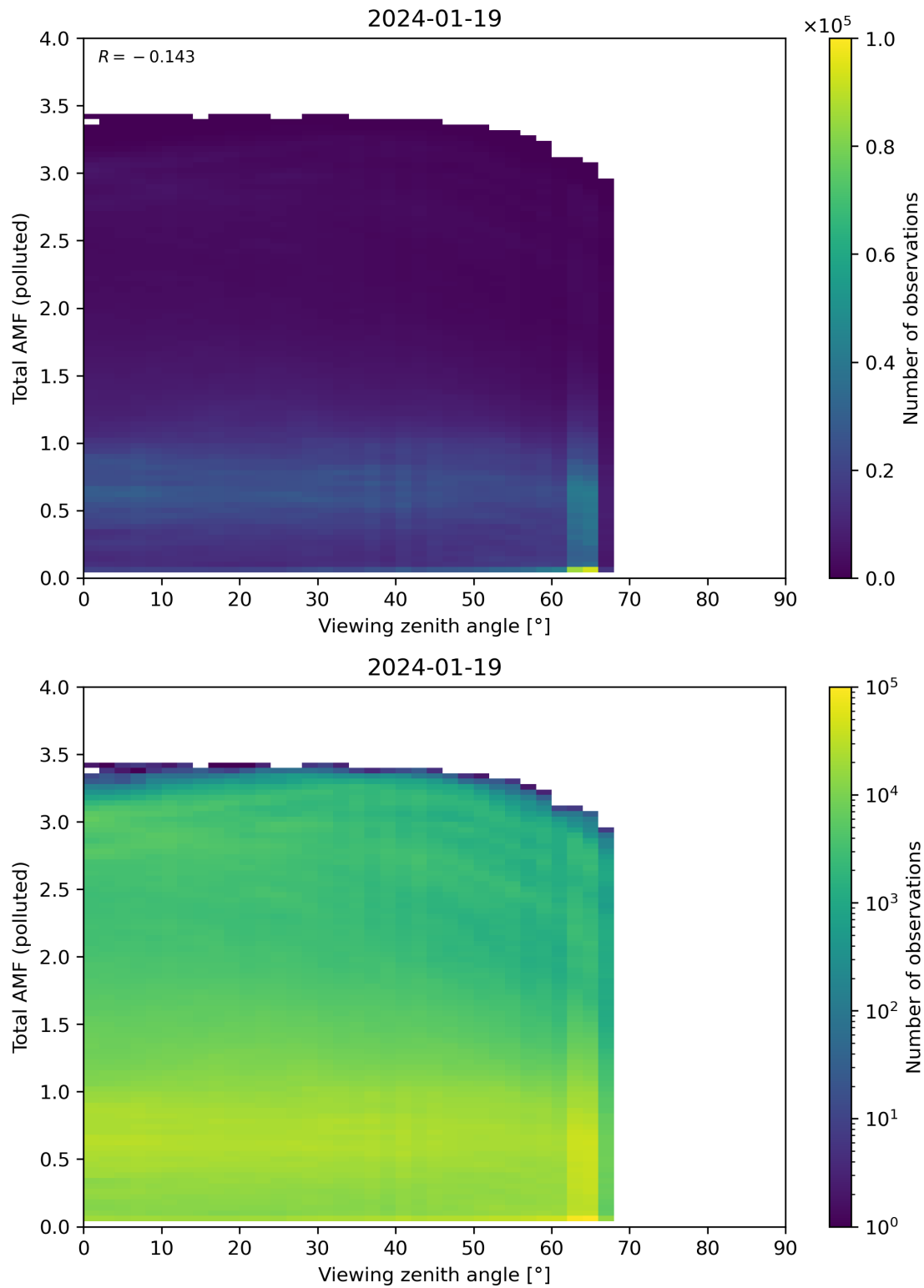
Figure 325: Scatter density plot of “Viewing zenith angle” against “Total AMF (polluted)” for 2024-01-18 to 2024-01-20.
