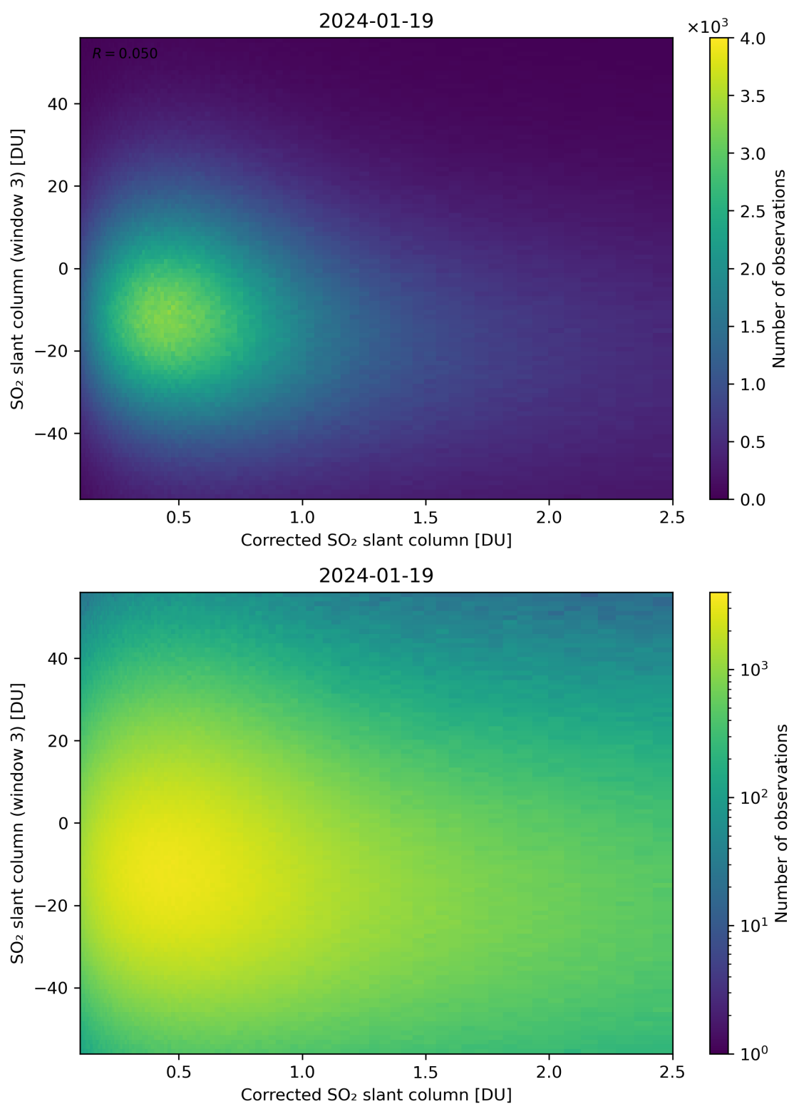
Figure 190: Scatter density plot of “Corrected SO 2 slant column” against “SO 2 slant column (window 3)” for 2024-01-18 to 2024-01-20.
