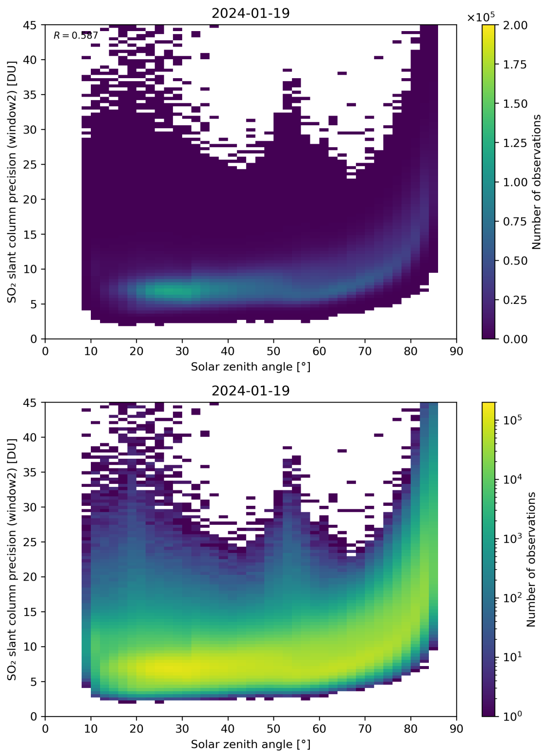
Figure 171: Scatter density plot of “Solar zenith angle” against “SO 2 slant column precision (window2)” for 2024-01-18 to 2024-01-20.
