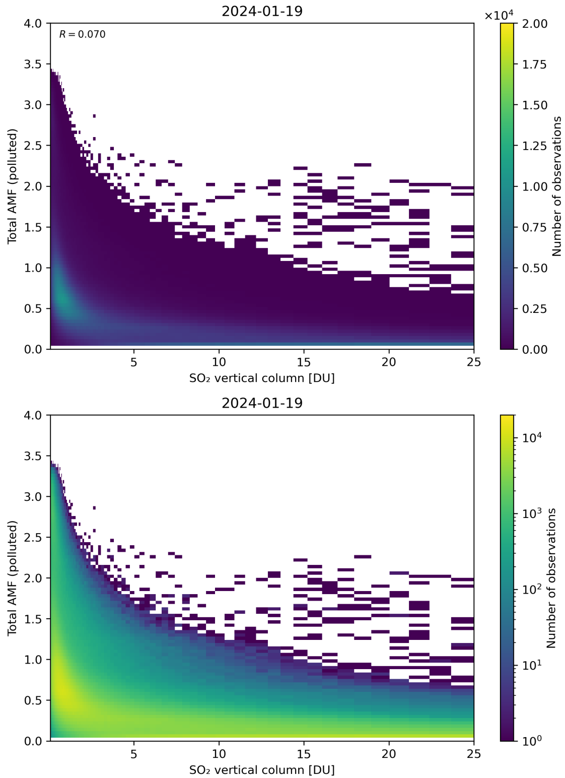
Figure 305: Scatter density plot of “SO 2 vertical column” against “Total AMF (polluted)” for 2024-01-18 to 2024-01-20.
