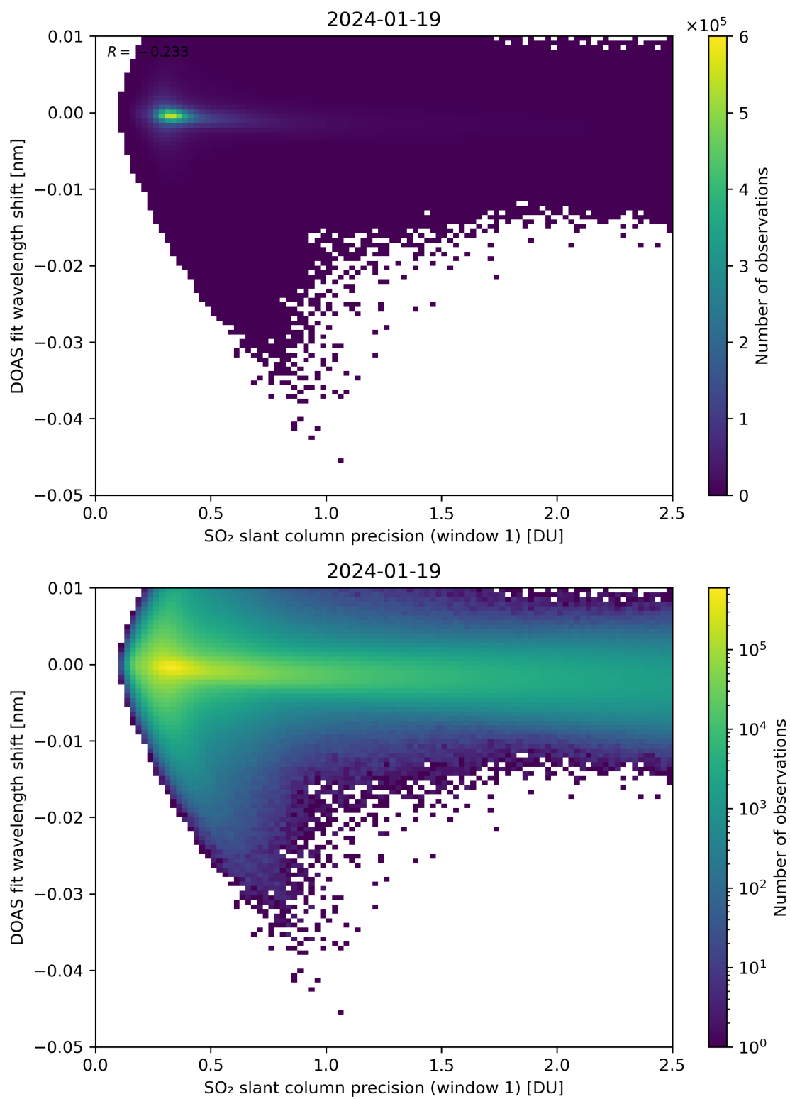
Figure 221: Scatter density plot of “SO 2 slant column precision (window 1)” against “DOAS fit wavelength shift” for 2024-01-18 to 2024-01-20.
