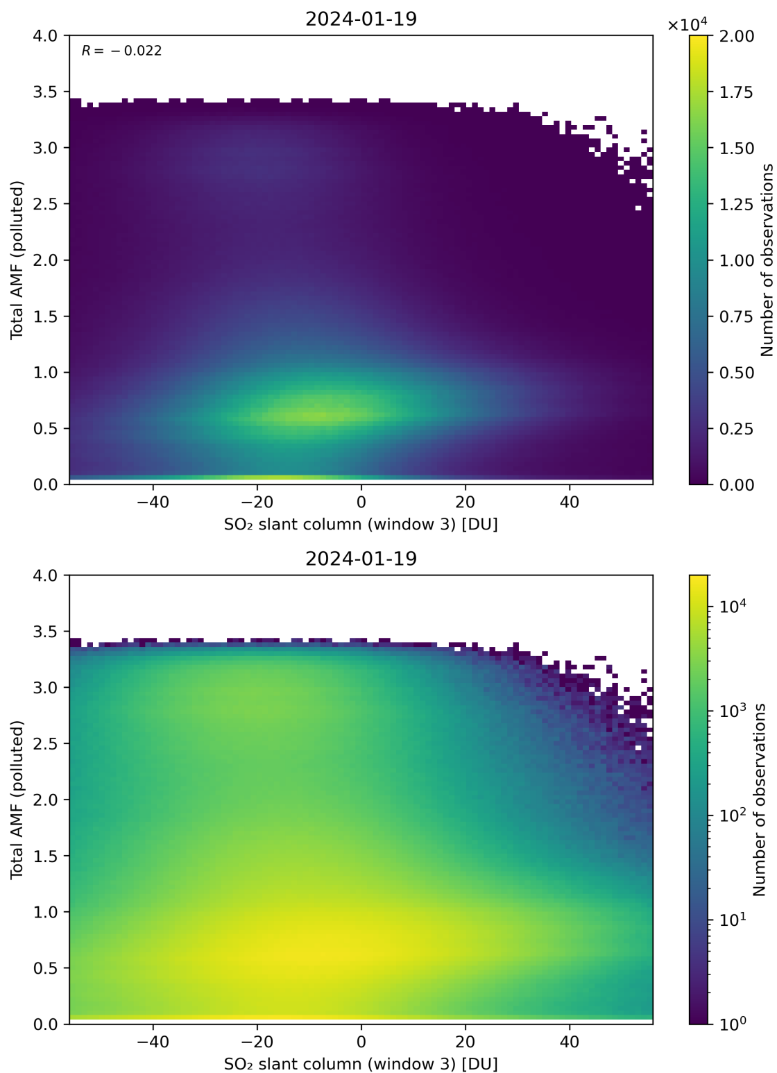
Figure 268: Scatter density plot of “SO 2 slant column (window 3)” against “Total AMF (polluted)” for 2024-01-18 to 2024-01-20.
