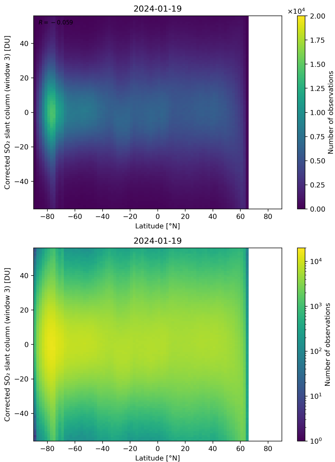
Figure 148: Scatter density plot of “Latitude” against “Corrected SO 2 slant column (window 3)” for 2024-01-18 to 2024-01-20.
