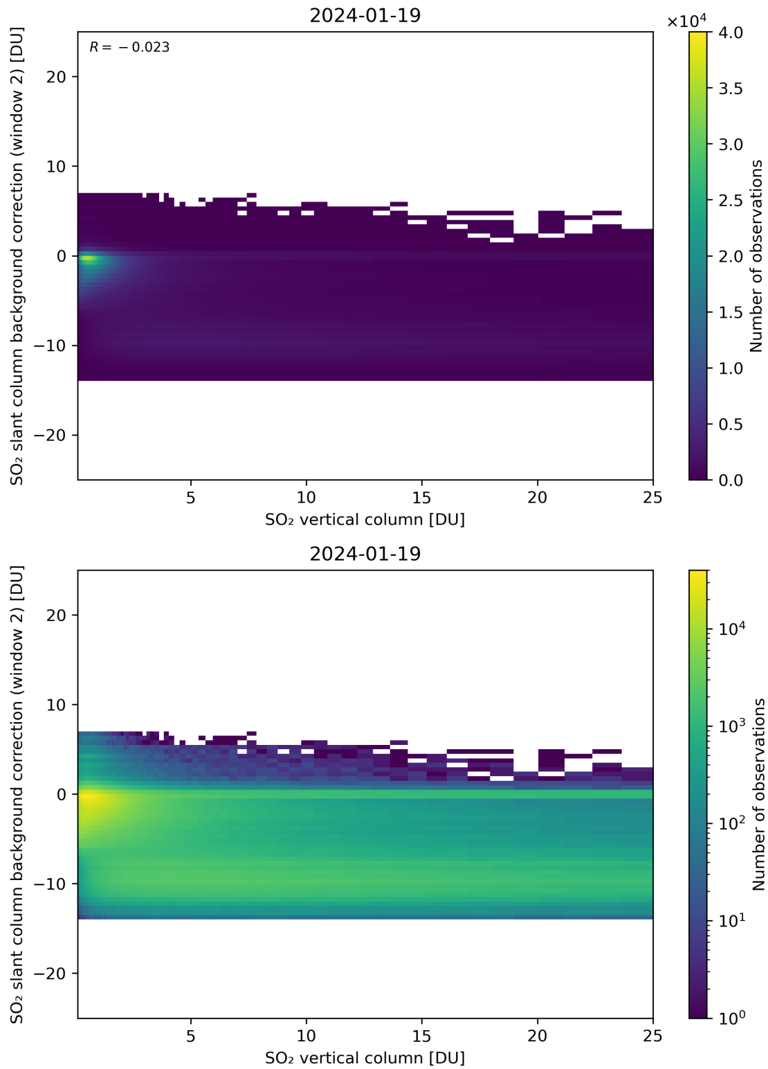
Figure 274: Scatter density plot of “SO 2 vertical column” against “SO 2 slant column background correction (window 2)” for 2024-01-18 to 2024-01-20.
