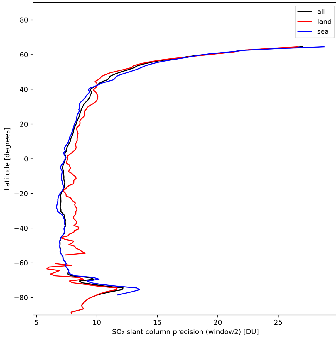
Figure 38: Zonal average of “SO 2 slant column precision (window2)” for 2024-01-18 to 2024-01-20.
