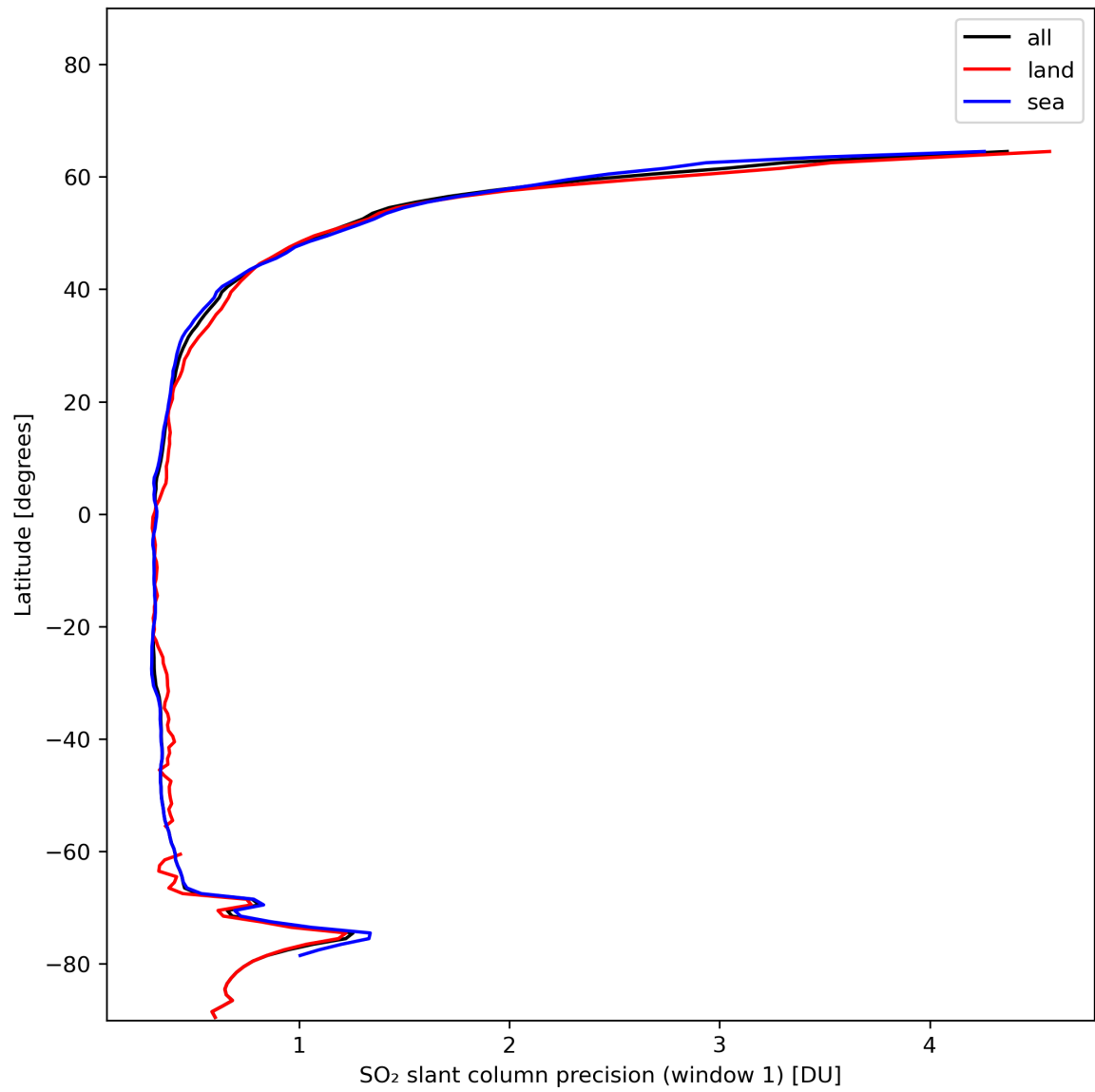
Figure 34: Zonal average of “SO 2 slant column precision (window 1)” for 2024-01-18 to 2024-01-20.
