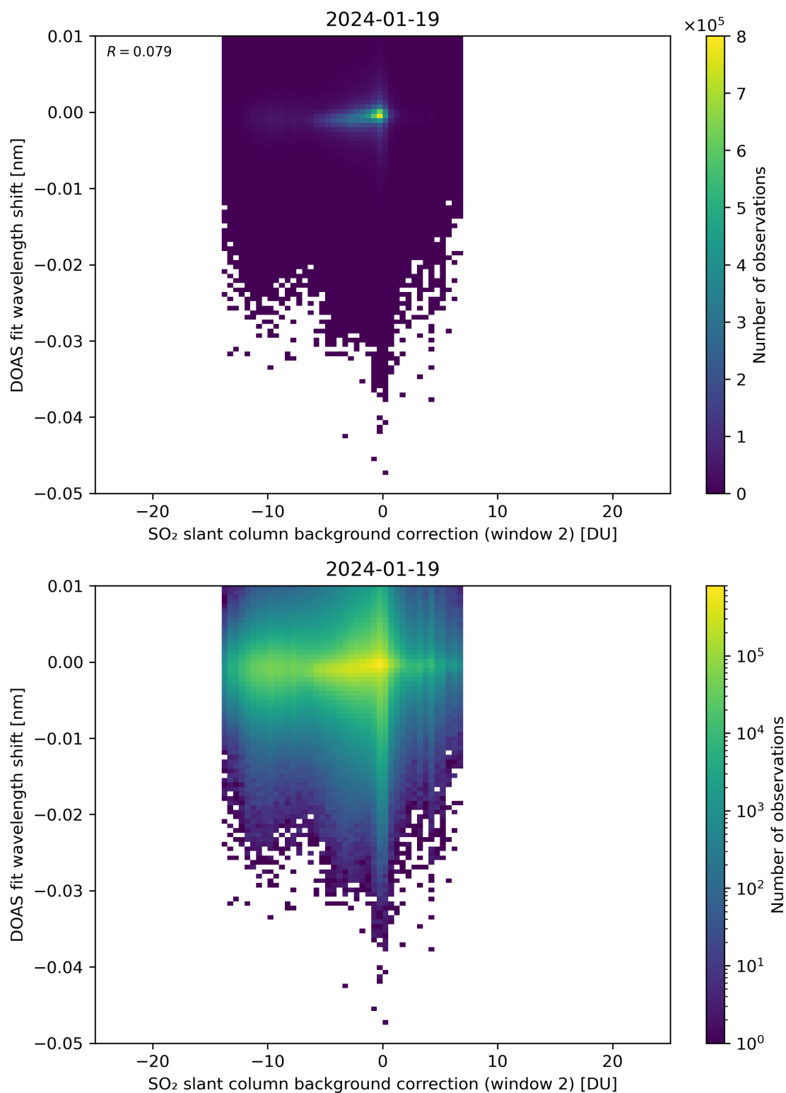
Figure 112: Scatter density plot of “SO 2 slant column background correction (window 2)” against “DOAS fit wavelength shift” for 2024-01-18 to 2024-01-20.
