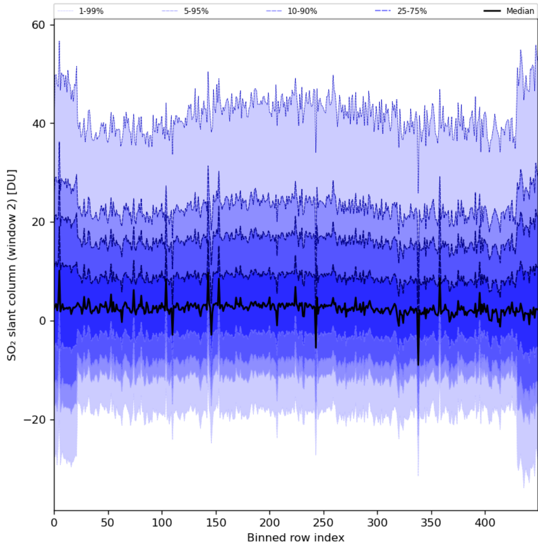
Figure 83: Along track statistics of “SO 2 slant column (window 2)” for 2024-01-18 to 2024-01-20
