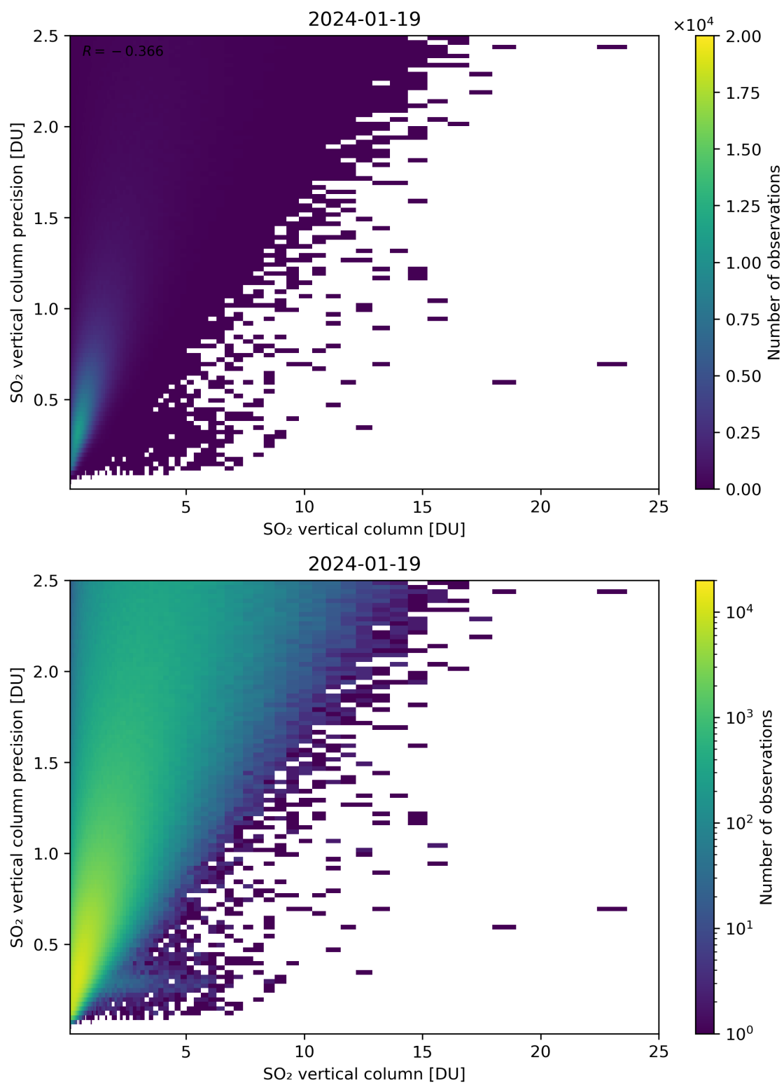
Figure 307: Scatter density plot of “SO 2 vertical column” against “SO 2 vertical column precision” for 2024-01-18 to 2024-01-20.
