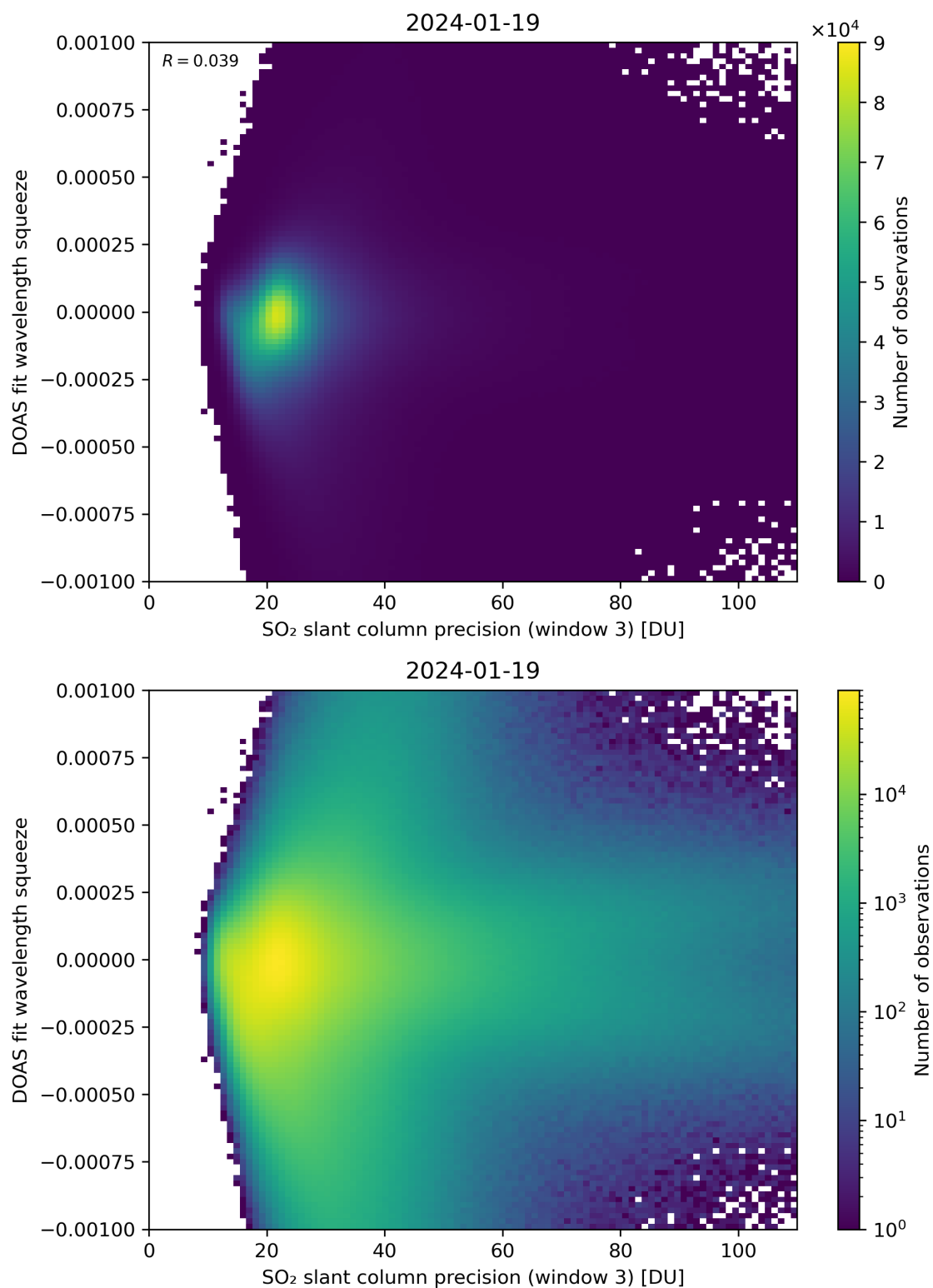
Figure 259: Scatter density plot of “SO 2 slant column precision (window 3)” against “DOAS fit wavelength squeeze” for 2024-01-18 to 2024-01-20.
