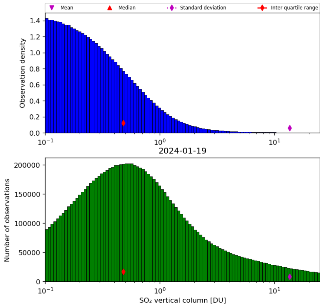
Figure 53: Histogram of “SO 2 vertical column” for 2024-01-18 to 2024-01-20
