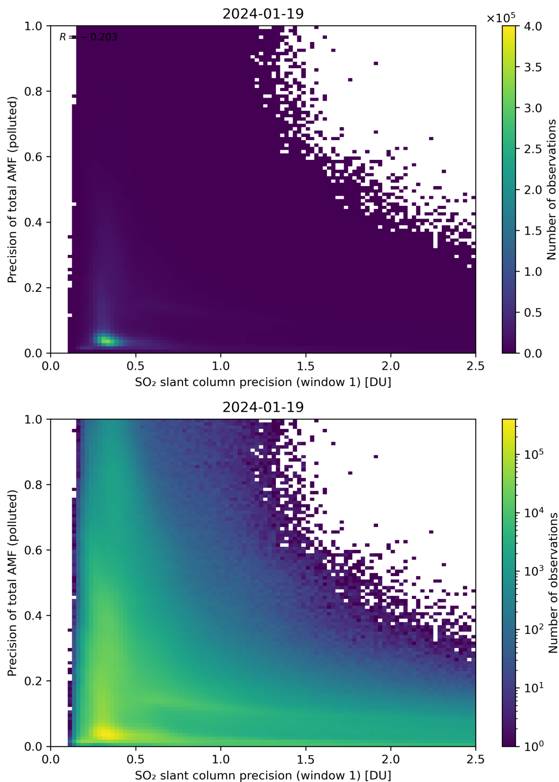
Figure 231: Scatter density plot of “SO 2 slant column precision (window 1)” against “Precision of total AMF (polluted)” for 2024-01-18 to 2024-01-20.
