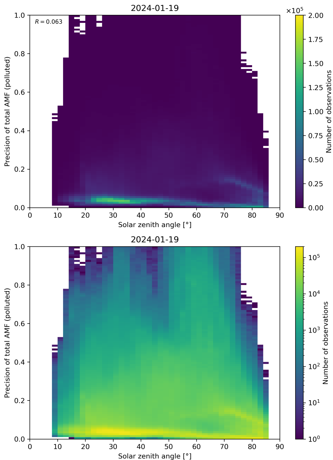
Figure 175: Scatter density plot of “Solar zenith angle” against “Precision of total AMF (polluted)” for 2024-01-18 to 2024-01-20.
