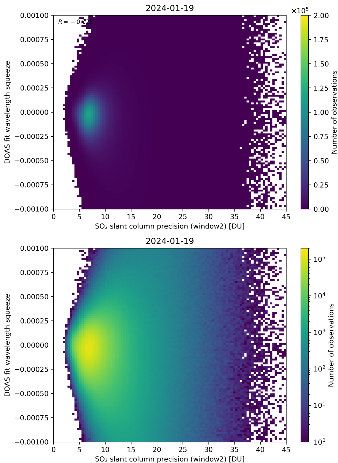
Figure 244: Scatter density plot of “SO 2 slant column precision (window2)” against “DOAS fit wavelength squeeze” for 2024-01-18 to 2024-01-20.
