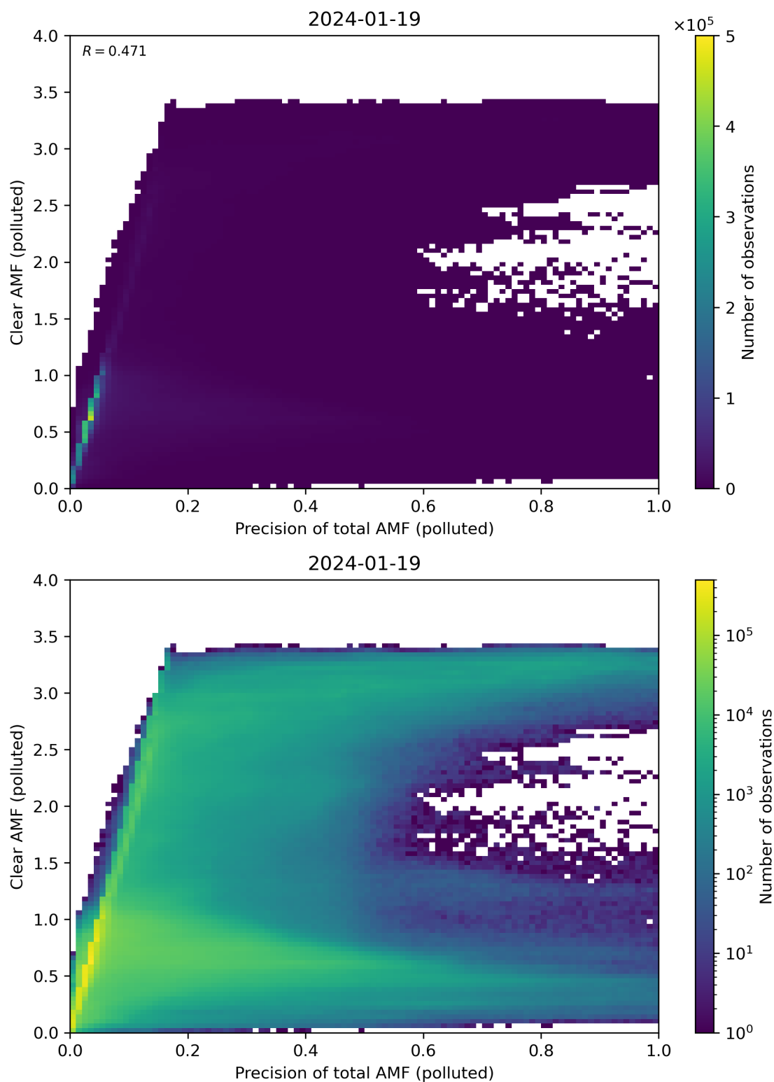
Figure 270: Scatter density plot of “Precision of total AMF (polluted)” against “Clear AMF (polluted)” for 2024-01-18 to 2024-01-20.
