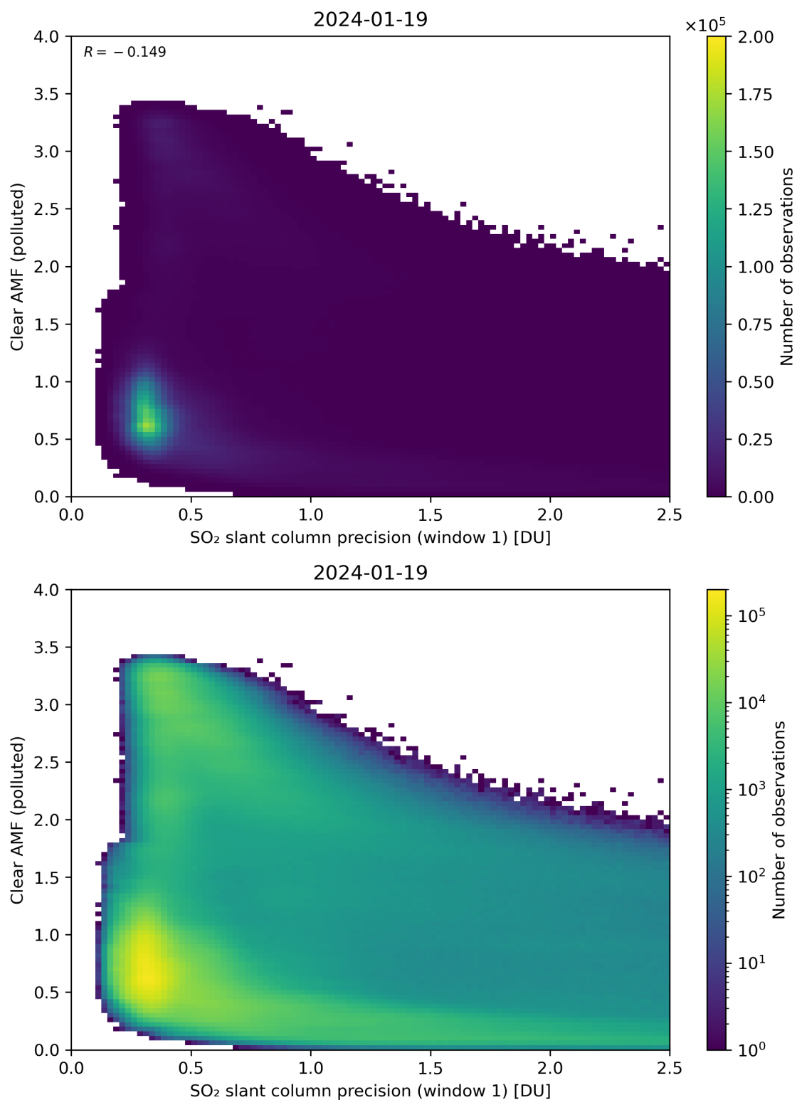
Figure 224: Scatter density plot of “SO 2 slant column precision (window 1)” against “Clear AMF (polluted)” for 2024-01-18 to 2024-01-20.
