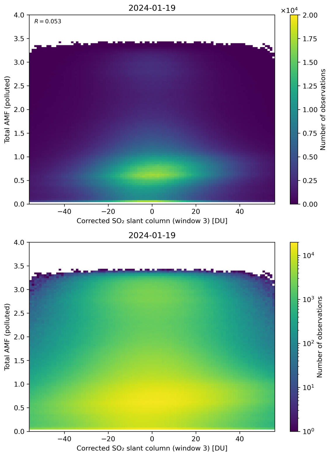
Figure 210: Scatter density plot of “Corrected SO 2 slant column (window 3)” against “Total AMF (polluted)” for 2024-01-18 to 2024-01-20.
