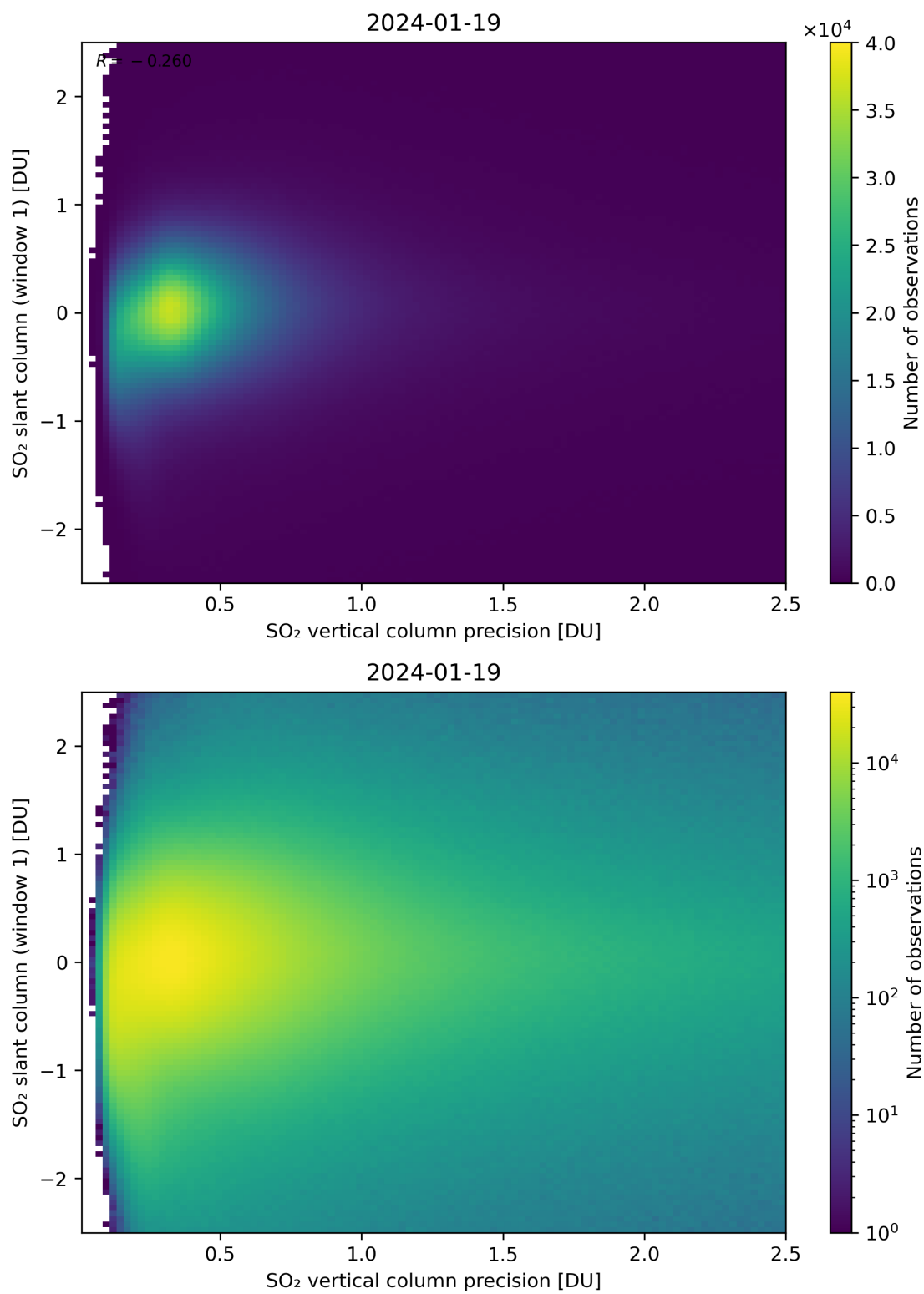
Figure 289: Scatter density plot of “SO 2 vertical column precision” against “SO 2 slant column (window 1)” for 2024-01-18 to 2024-01-20.
