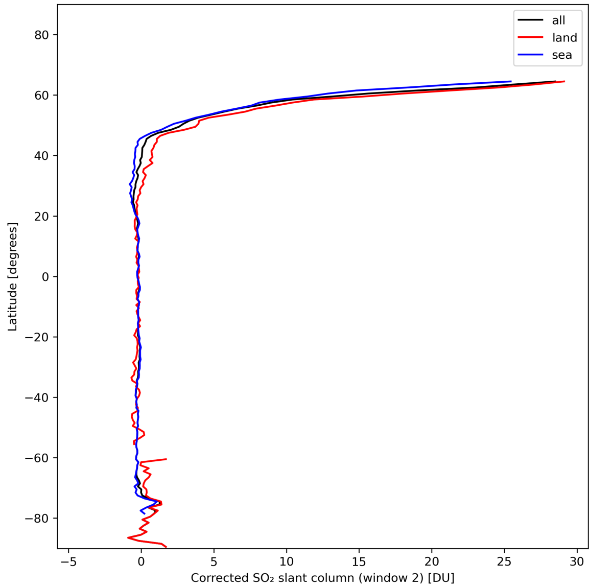
Figure 39: Zonal average of “Corrected SO 2 slant column (window 2)” for 2024-01-18 to 2024-01-20.
