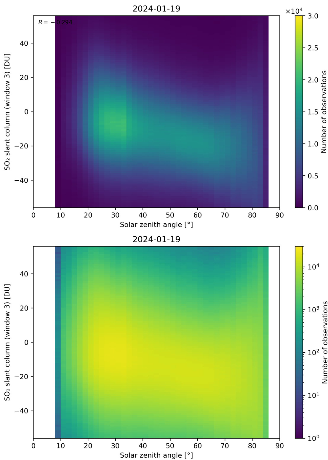
Figure 172: Scatter density plot of “Solar zenith angle” against “SO 2 slant column (window 3)” for 2024-01-18 to 2024-01-20.
