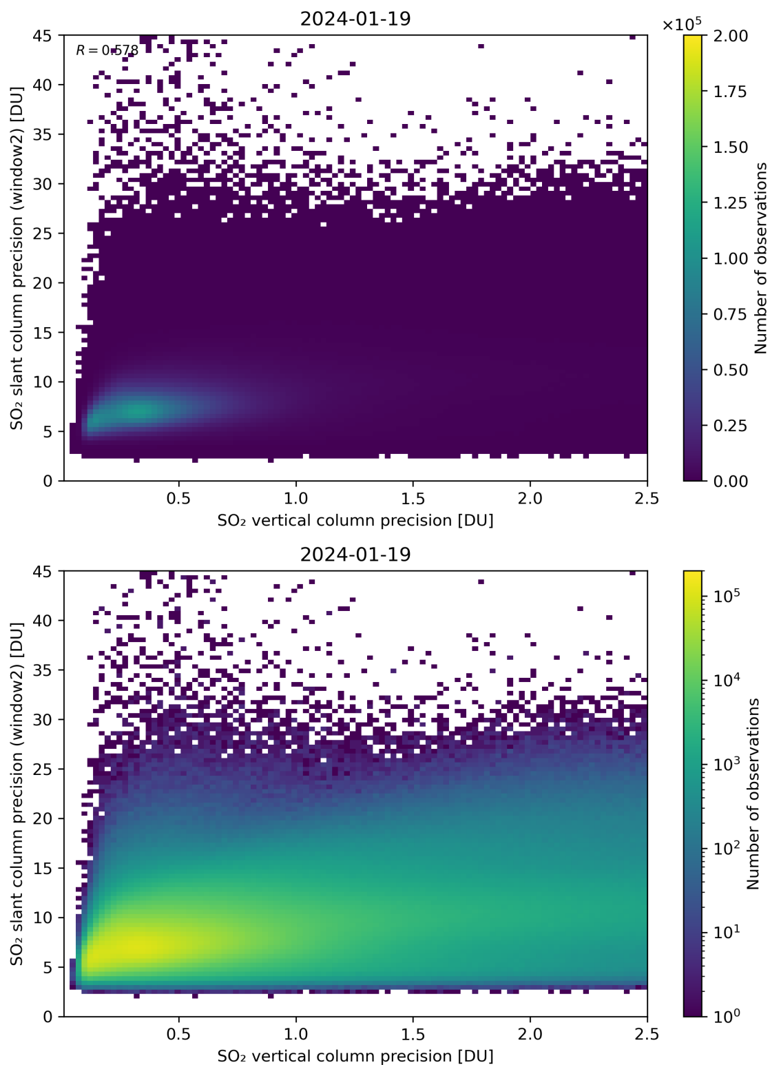
Figure 291: Scatter density plot of “SO 2 vertical column precision” against “SO 2 slant column precision (window2)” for 2024-01-18 to 2024-01-20.
