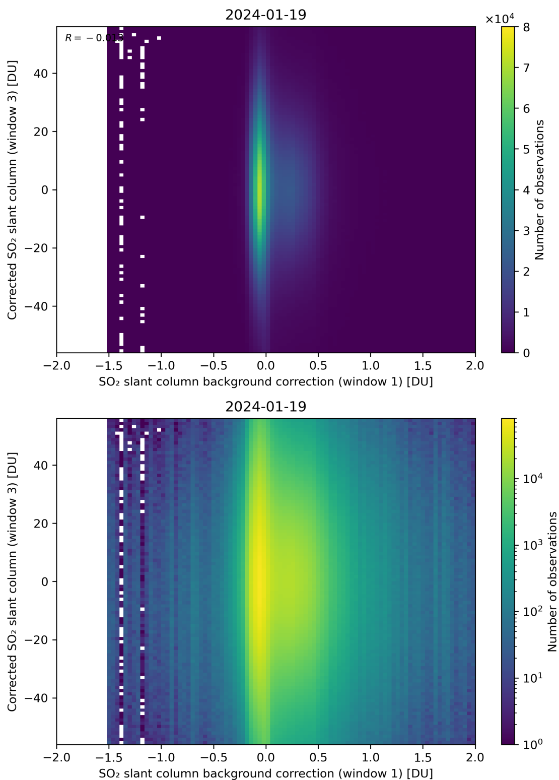
Figure 105: Scatter density plot of “SO 2 slant column background correction (window 1)” against “Corrected SO 2 slant column (window 3)” for 2024-01-18 to 2024-01-20.
