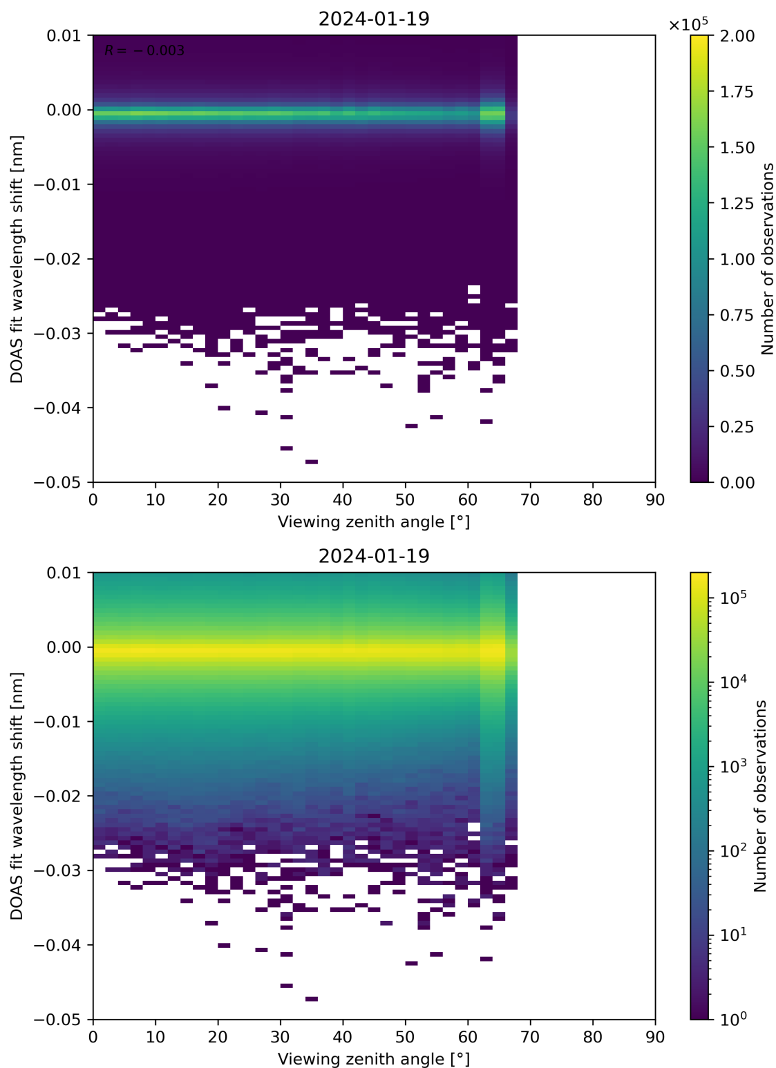
Figure 311: Scatter density plot of “Viewing zenith angle” against “DOAS fit wavelength shift” for 2024-01-18 to 2024-01-20.
