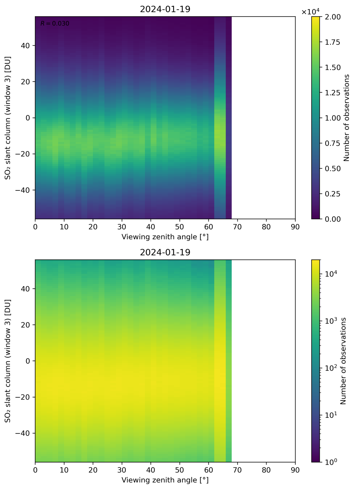
Figure 323: Scatter density plot of “Viewing zenith angle” against “SO 2 slant column (window 3)” for 2024-01-18 to 2024-01-20.
