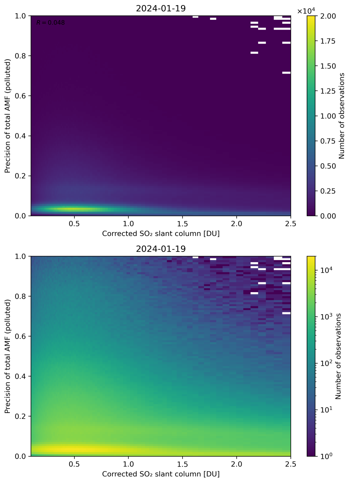
Figure 193: Scatter density plot of “Corrected SO 2 slant column” against “Precision of total AMF (polluted)” for 2024-01-18 to 2024-01-20.
