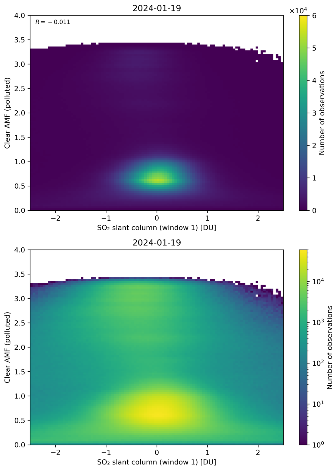
Figure 232: Scatter density plot of “SO 2 slant column (window 1)” against “Clear AMF (polluted)” for 2024-01-18 to 2024-01-20.
