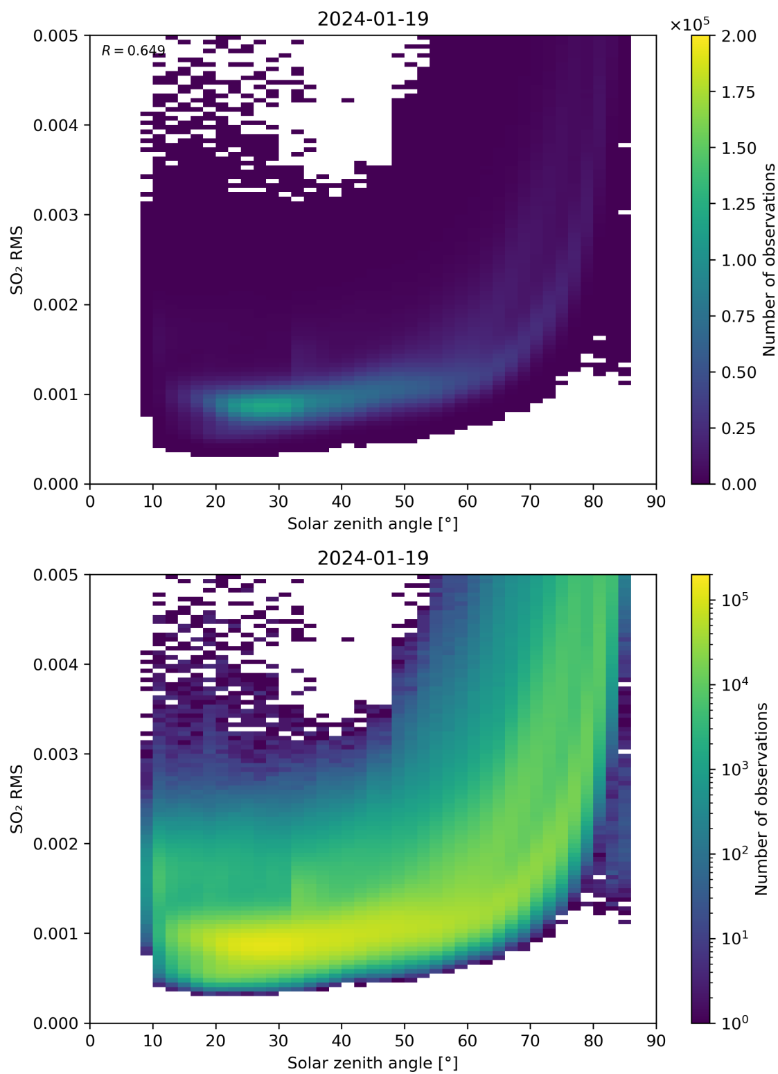
Figure 163: Scatter density plot of “Solar zenith angle” against “SO 2 RMS” for 2024-01-18 to 2024-01-20.
