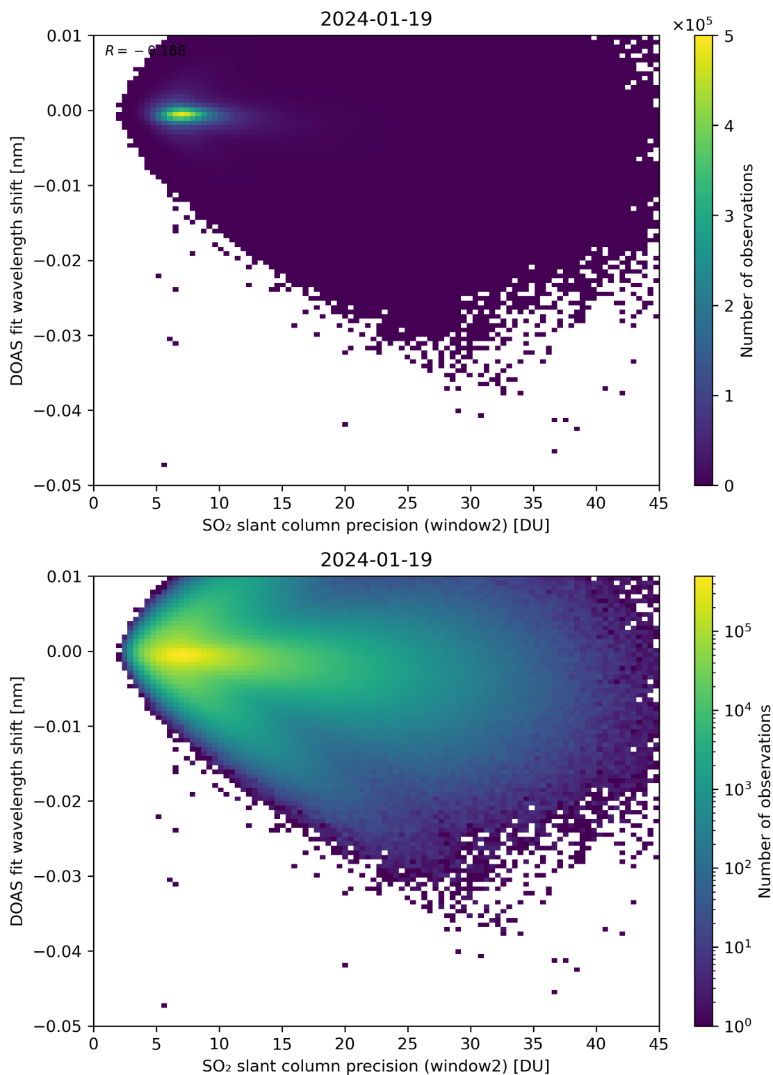
Figure 243: Scatter density plot of “SO 2 slant column precision (window2)” against “DOAS fit wavelength shift” for 2024-01-18 to 2024-01-20.
