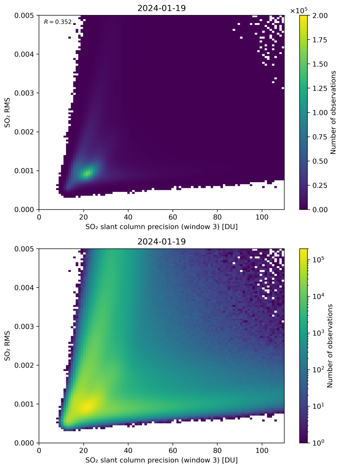
Figure 260: Scatter density plot of “SO 2 slant column precision (window 3)” against “SO 2 RMS” for 2024-01-18 to 2024-01-20.
