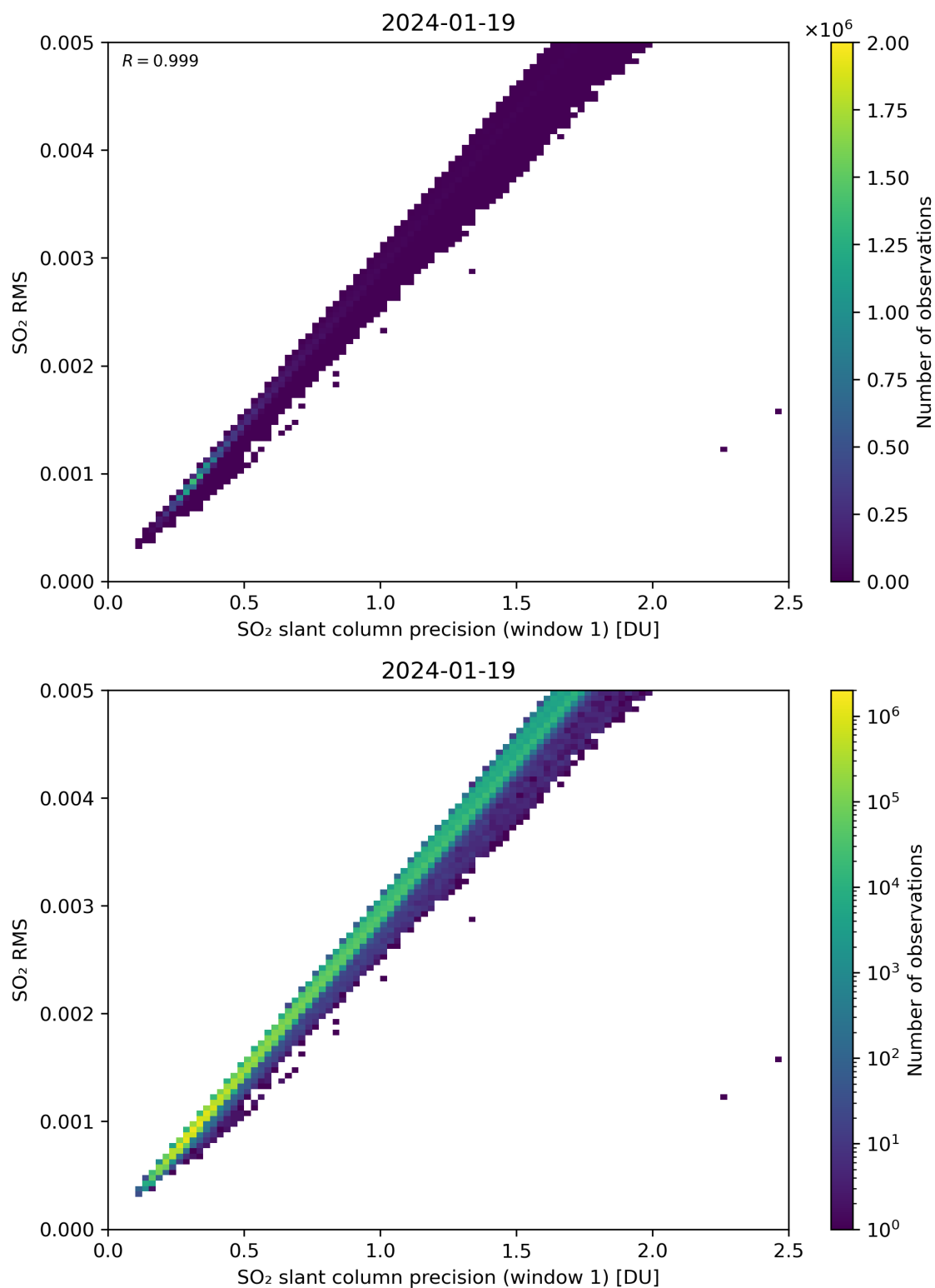
Figure 223: Scatter density plot of “SO 2 slant column precision (window 1)” against “SO 2 RMS” for 2024-01-18 to 2024-01-20.
