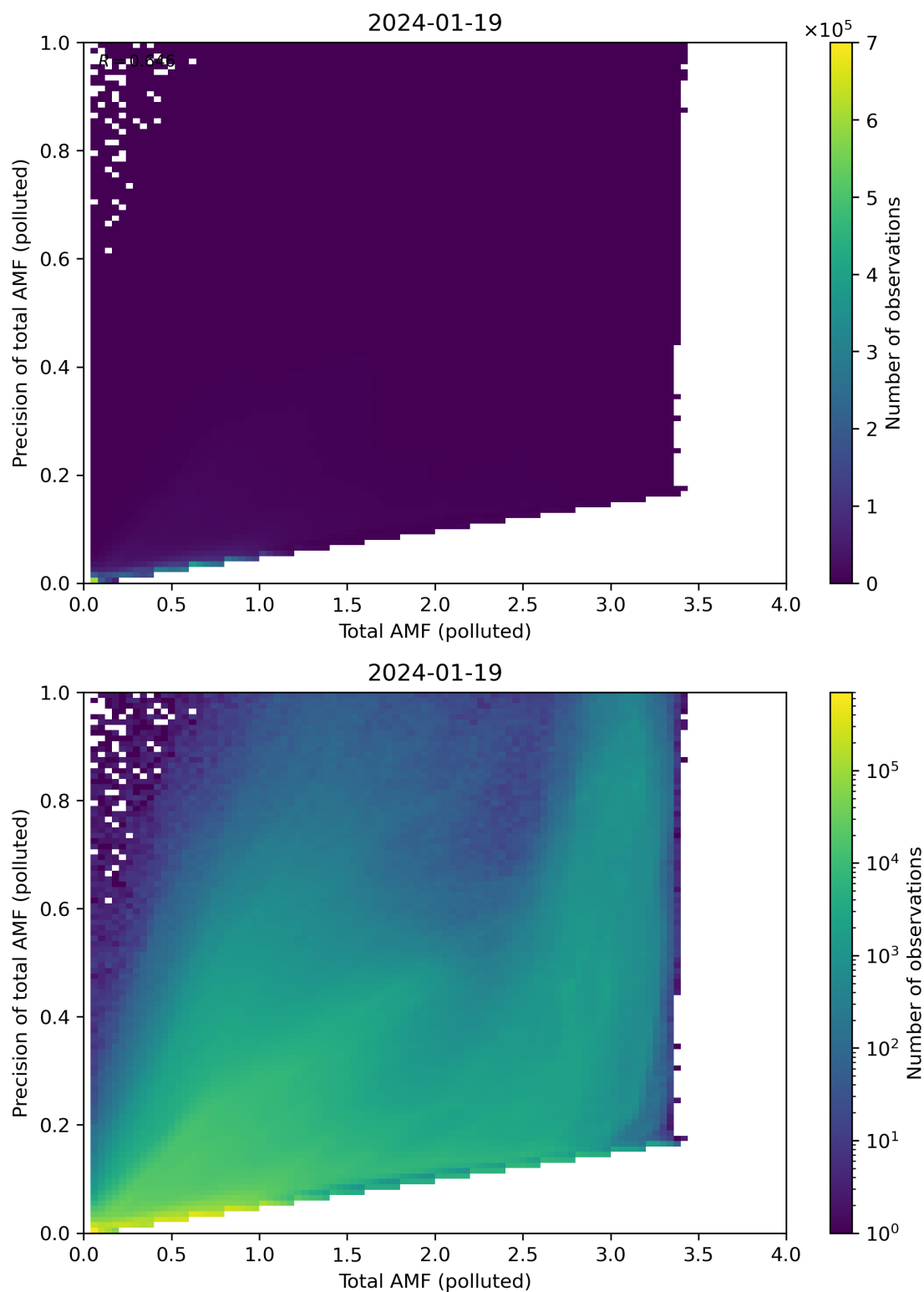
Figure 272: Scatter density plot of “Total AMF (polluted)” against “Precision of total AMF (polluted)” for 2024-01-18 to 2024-01-20.
