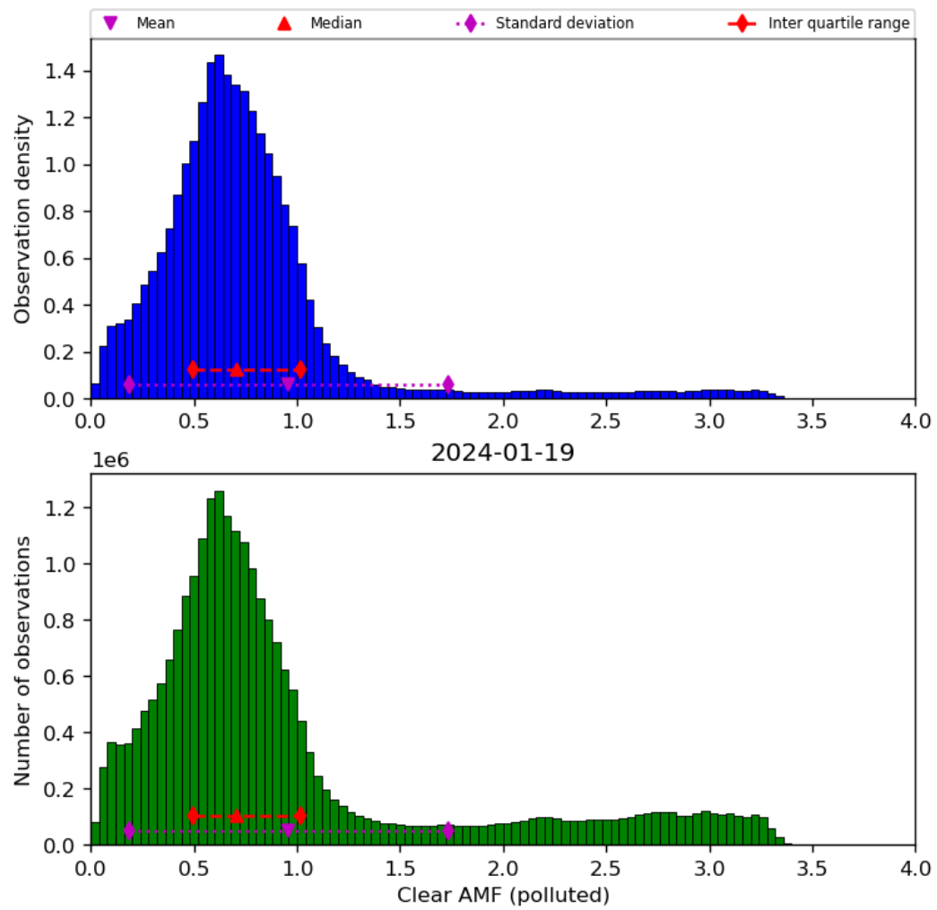
Figure 73: Histogram of “Clear AMF (polluted)” for 2024-01-18 to 2024-01-20
