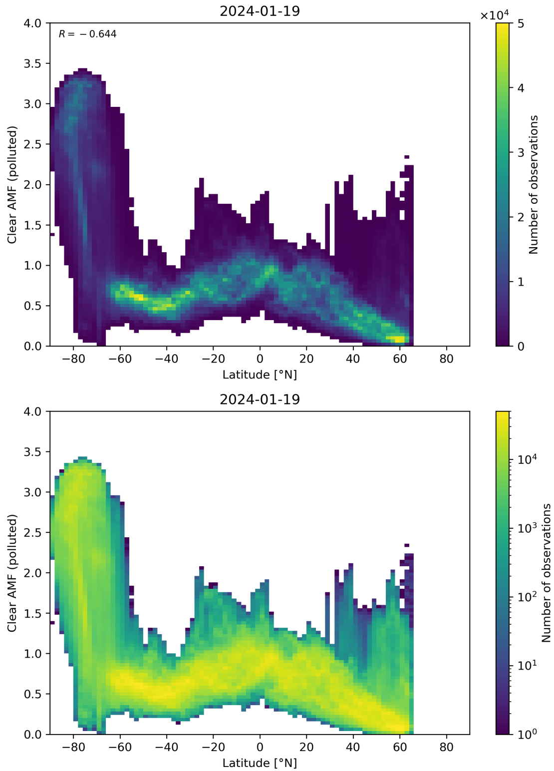
Figure 145: Scatter density plot of “Latitude” against “Clear AMF (polluted)” for 2024-01-18 to 2024-01-20.
