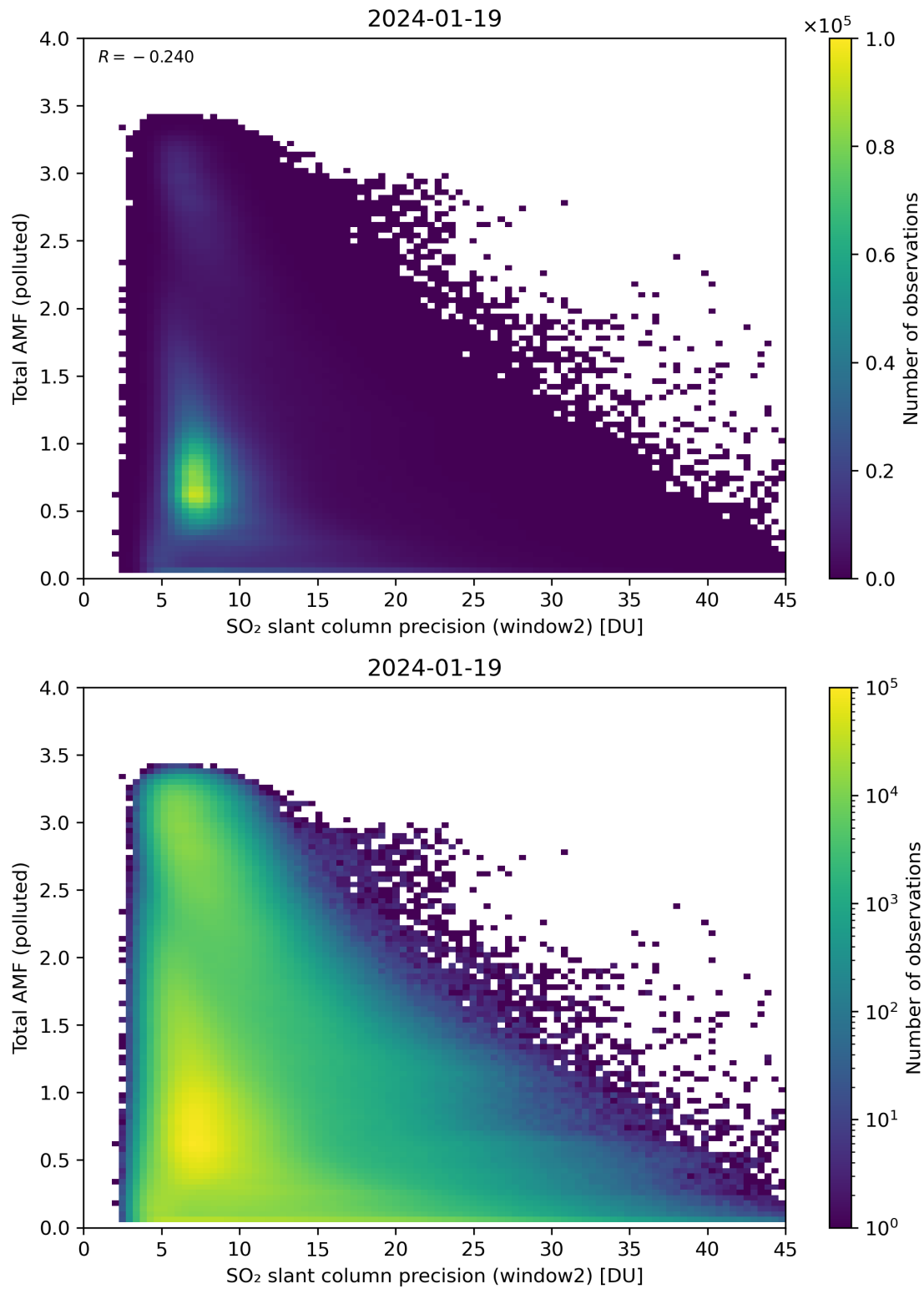
Figure 251: Scatter density plot of “SO 2 slant column precision (window2)” against “Total AMF (polluted)” for 2024-01-18 to 2024-01-20.
