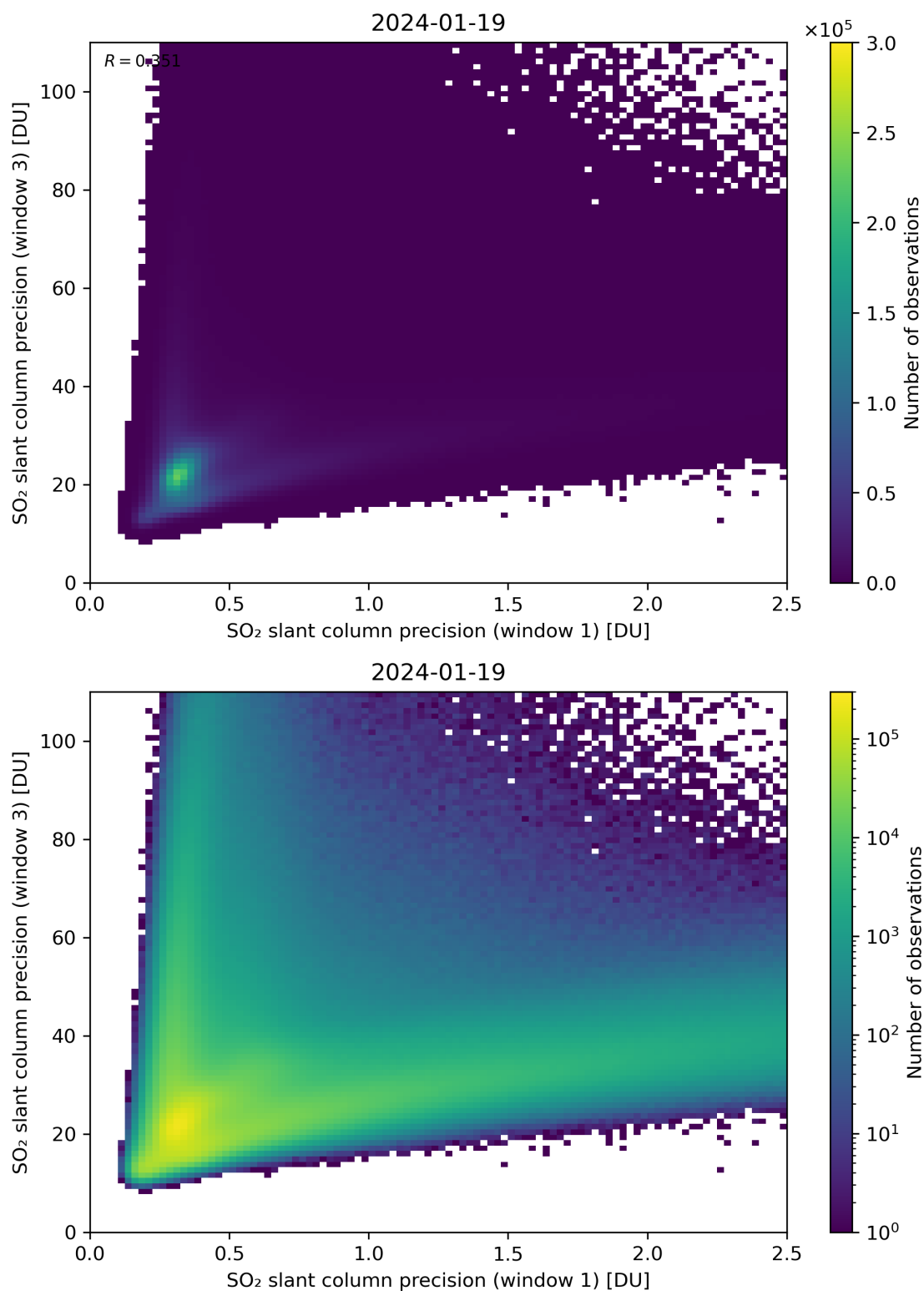
Figure 229: Scatter density plot of “SO 2 slant column precision (window 1)” against “SO 2 slant column precision (window 3)” for 2024-01-18 to 2024-01-20.
