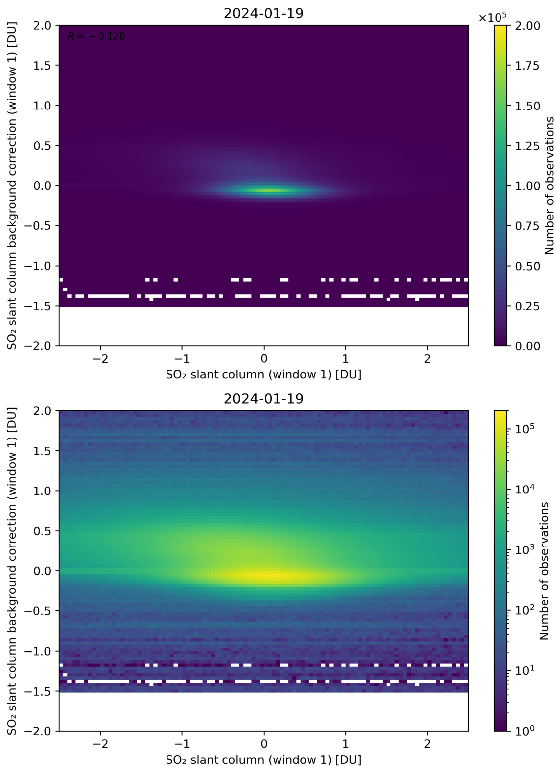
Figure 212: Scatter density plot of “SO 2 slant column (window 1)” against “SO 2 slant column background correction (window 1)” for 2024-01-18 to 2024-01-20.
