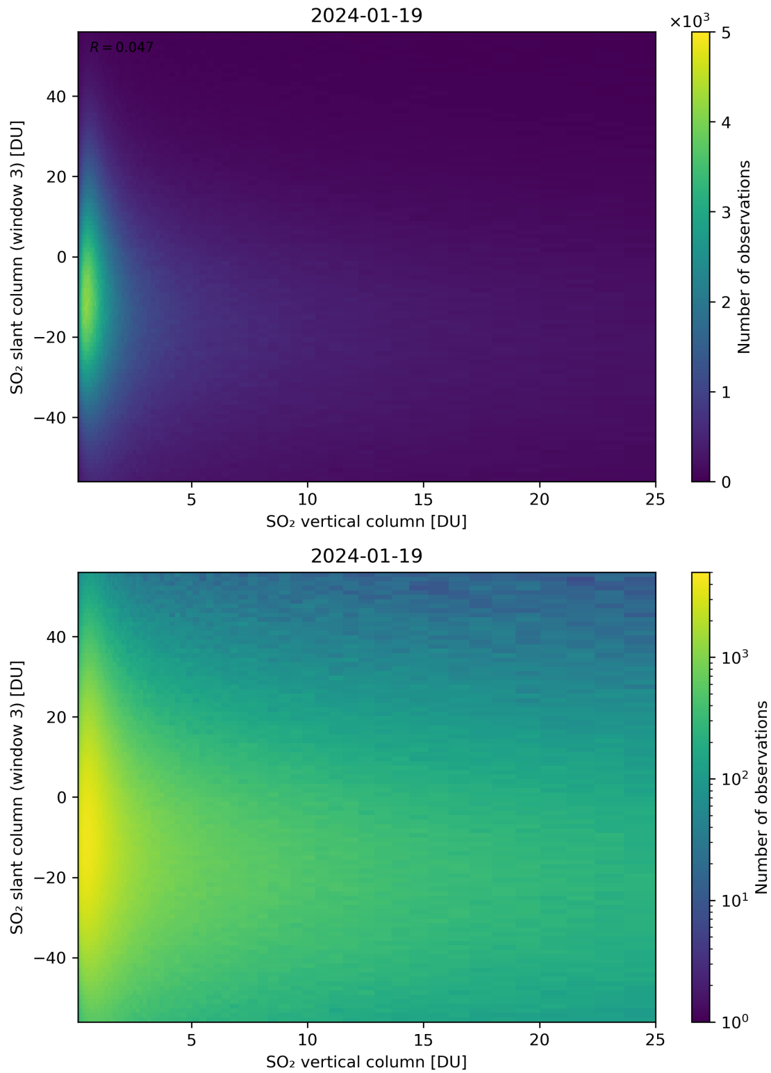
Figure 303: Scatter density plot of “SO 2 vertical column” against “SO 2 slant column (window 3)” for 2024-01-18 to 2024-01-20.
