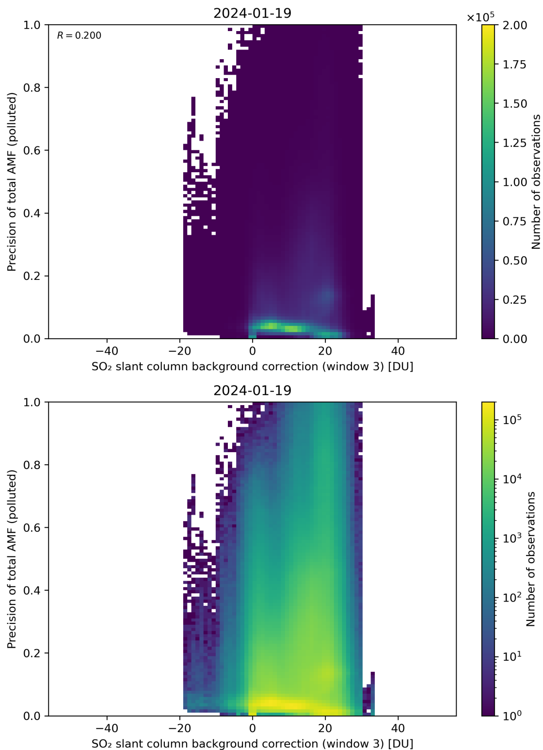
Figure 126: Scatter density plot of “SO 2 slant column background correction (window 3)” against “Precision of total AMF (polluted)” for 2024-01-18 to 2024-01-20.
