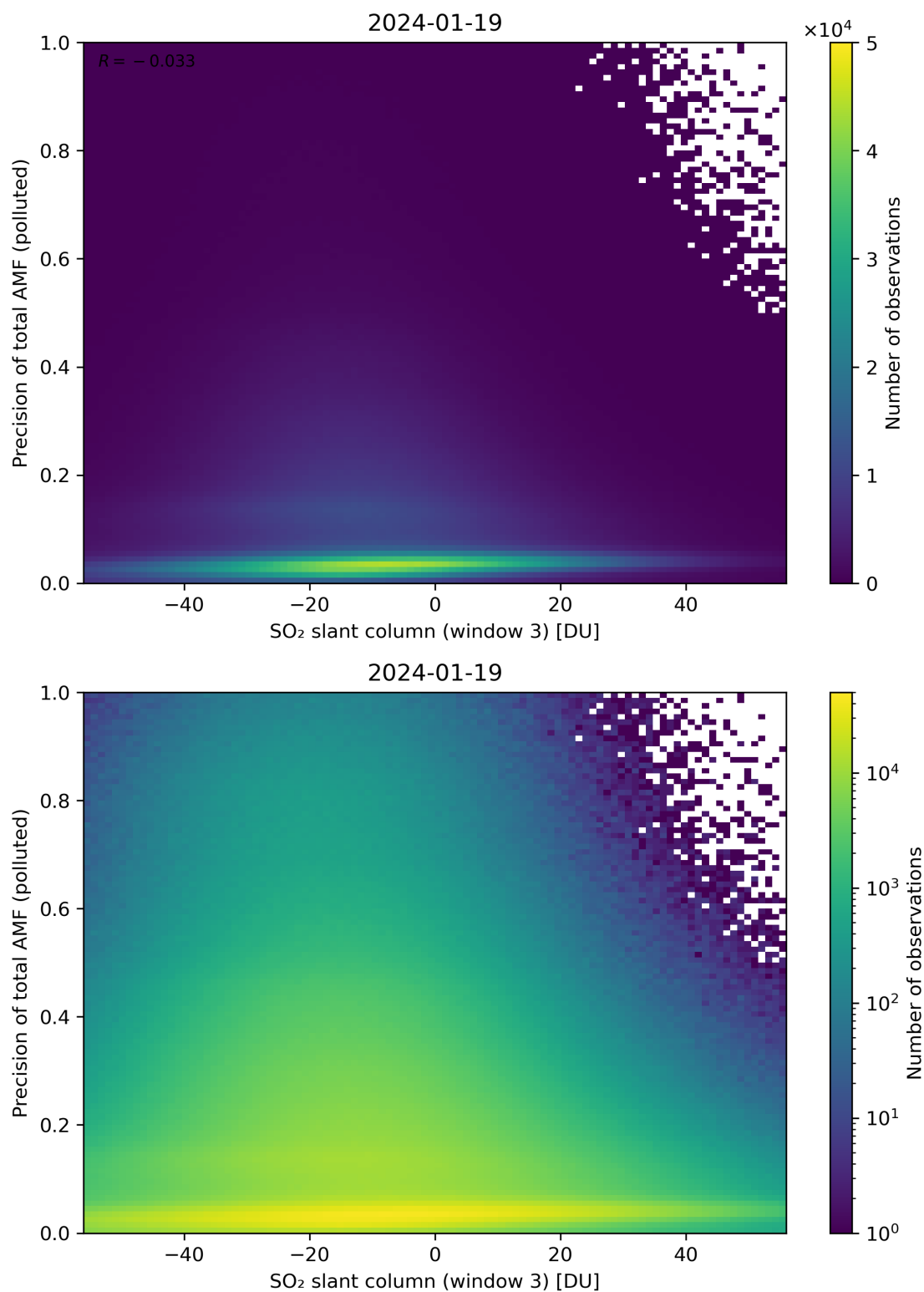
Figure 269: Scatter density plot of “SO 2 slant column (window 3)” against “Precision of total AMF (polluted)” for 2024-01-18 to 2024-01-20.
