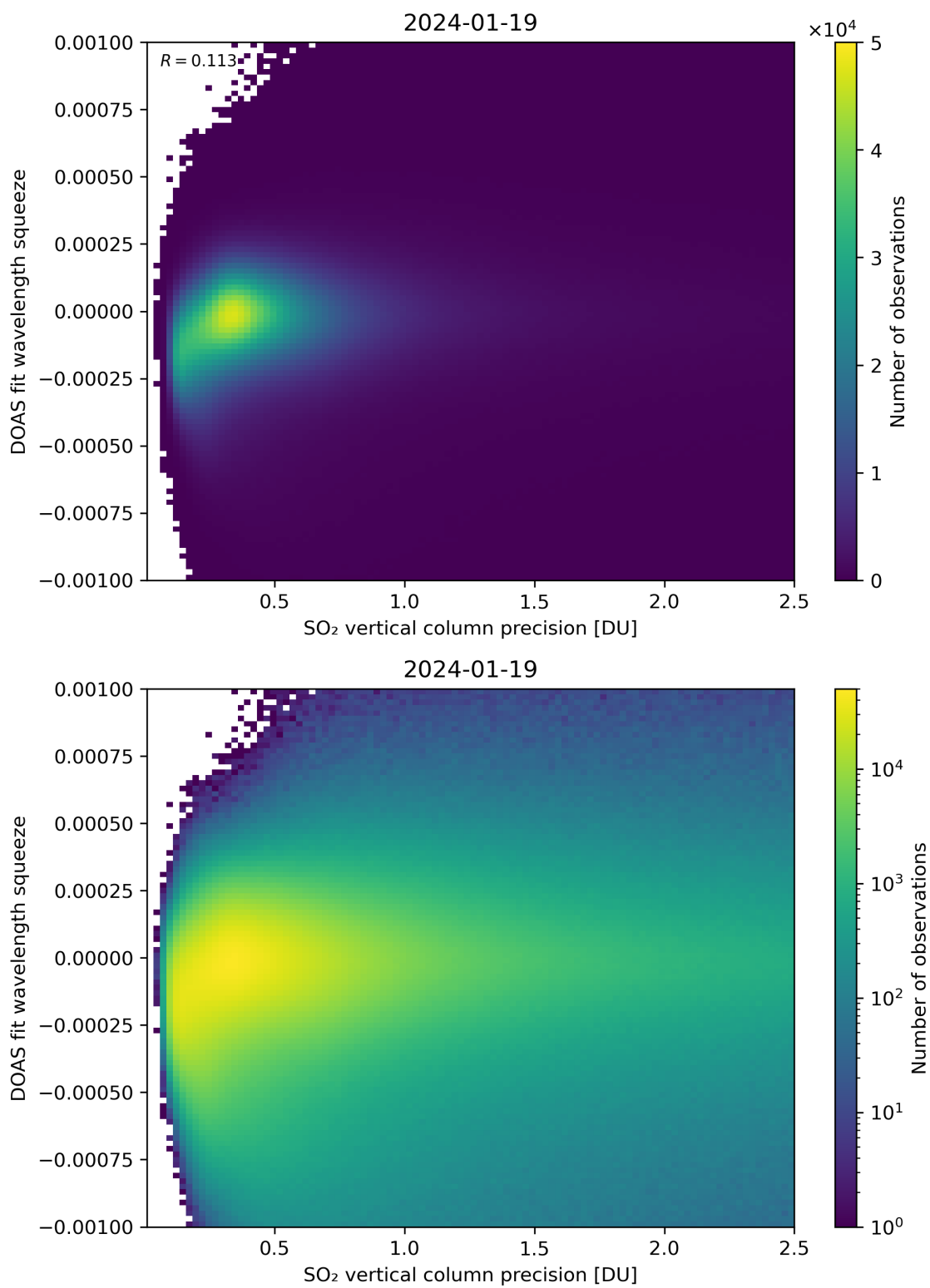
Figure 283: Scatter density plot of “SO 2 vertical column precision” against “DOAS fit wavelength squeeze” for 2024-01-18 to 2024-01-20.
