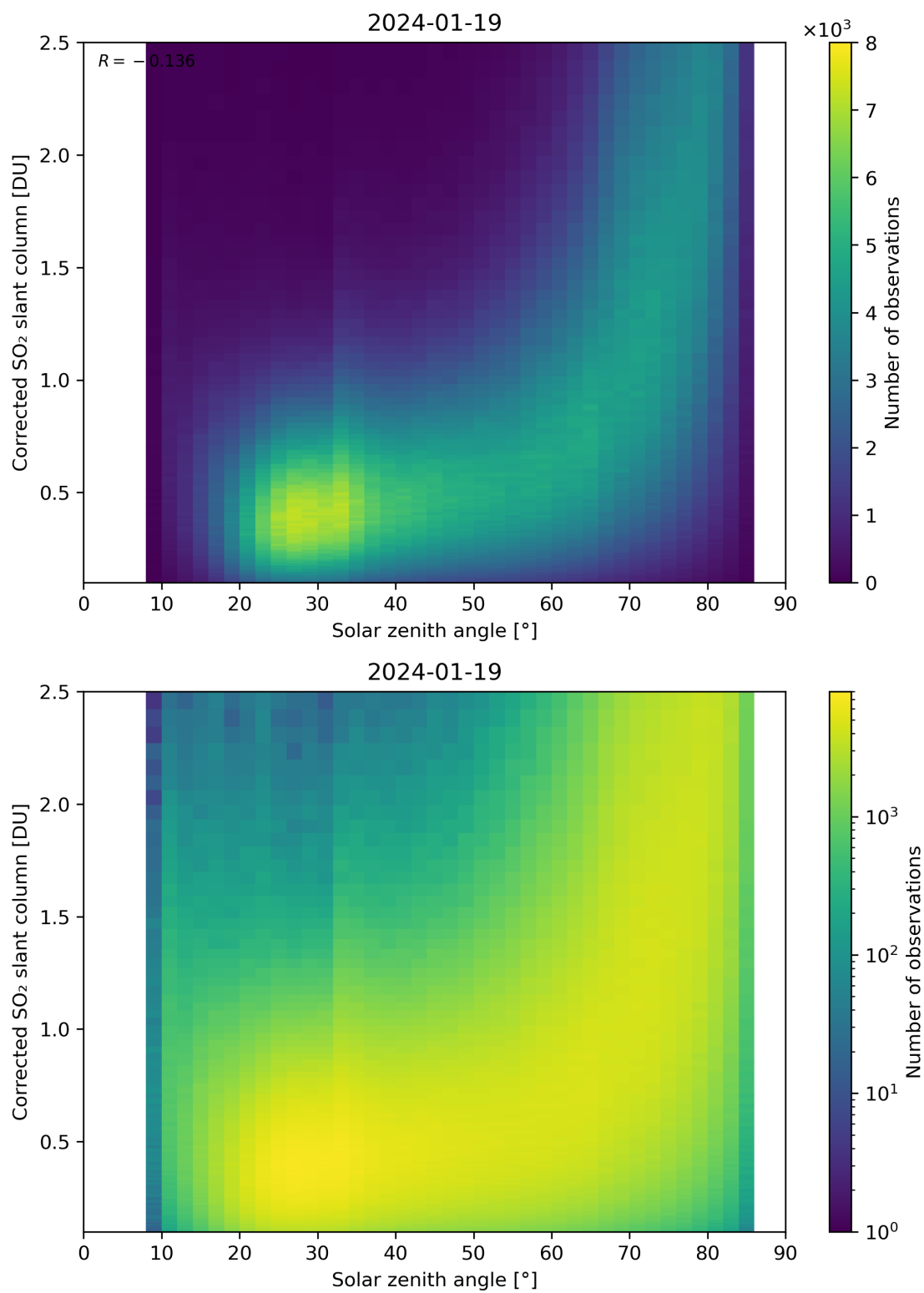
Figure 166: Scatter density plot of “Solar zenith angle” against “Corrected SO 2 slant column” for 2024-01-18 to 2024-01-20.
