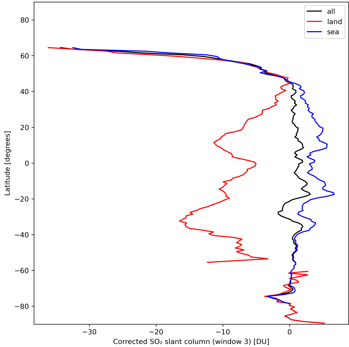
Figure 43: Zonal average of “Corrected SO 2 slant column (window 3)” for 2024-01-18 to 2024-01-20.
