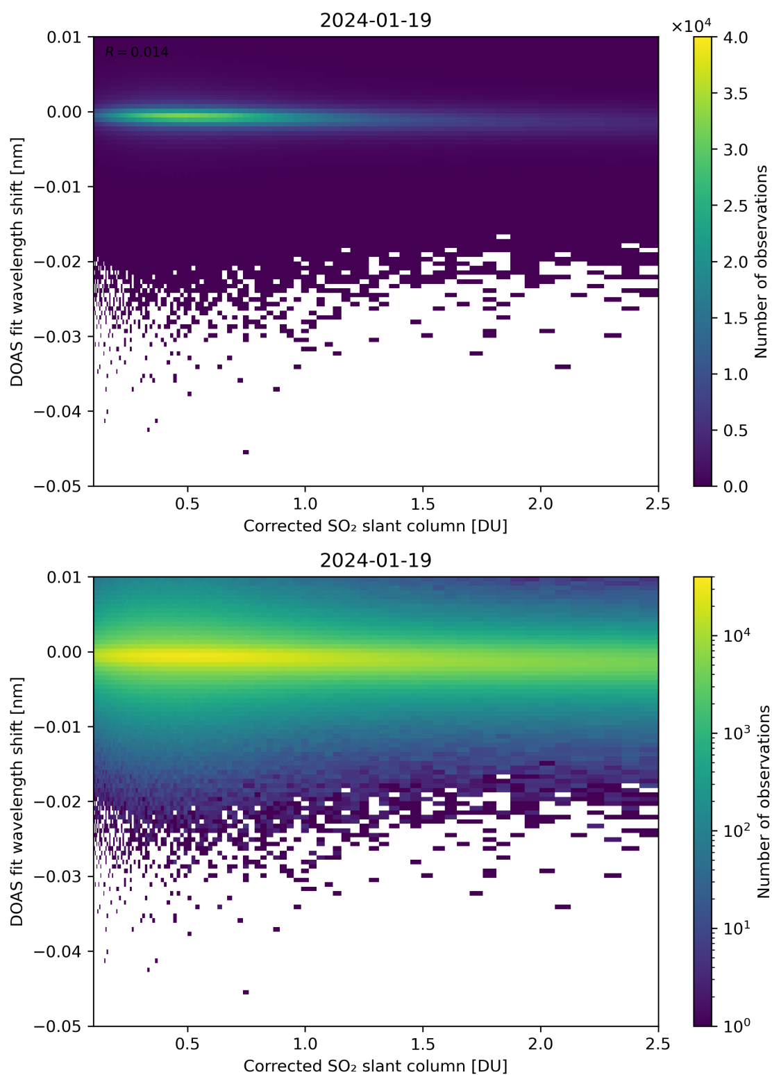
Figure 181: Scatter density plot of “Corrected SO 2 slant column” against “DOAS fit wavelength shift” for 2024-01-18 to 2024-01-20.
