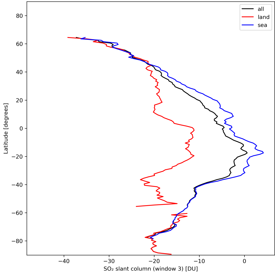
Figure 41: Zonal average of “SO 2 slant column (window 3)” for 2024-01-18 to 2024-01-20.
