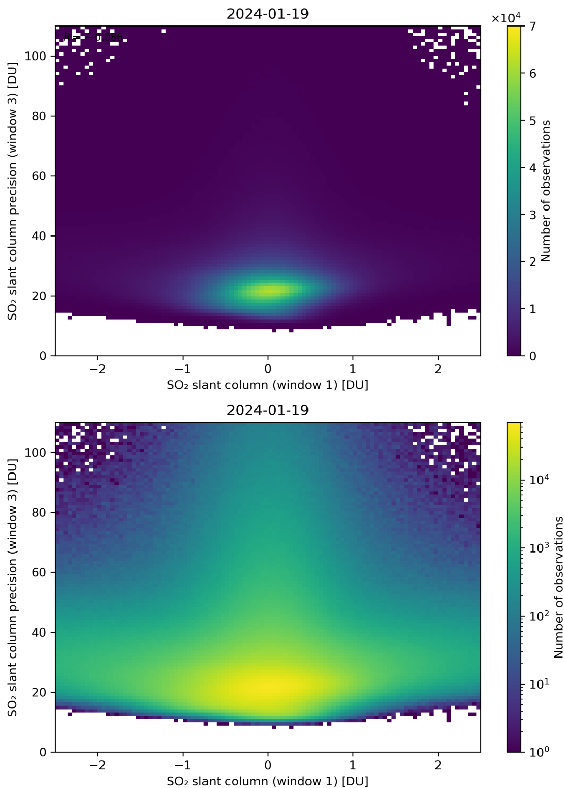
Figure 238: Scatter density plot of “SO 2 slant column (window 1)” against “SO 2 slant column precision (window 3)” for 2024-01-18 to 2024-01-20.
