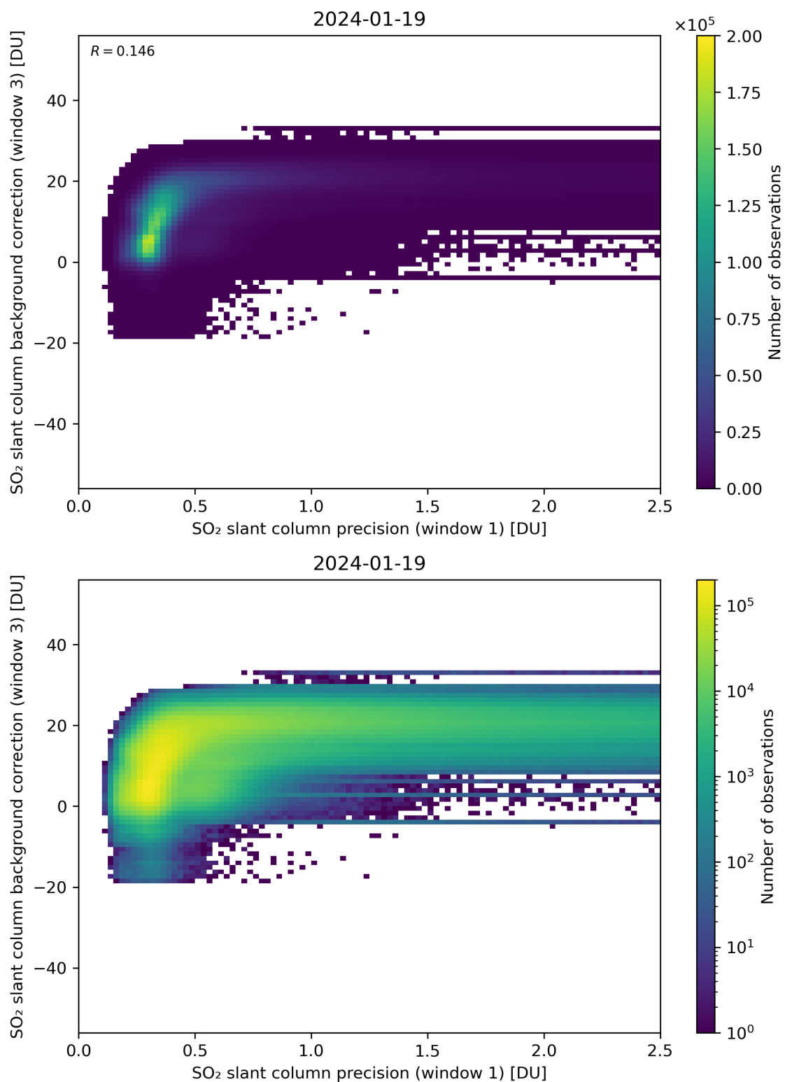
Figure 220: Scatter density plot of “SO 2 slant column precision (window 1)” against “SO 2 slant column background correction (window 3)” for 2024-01-18 to 2024-01-20.
