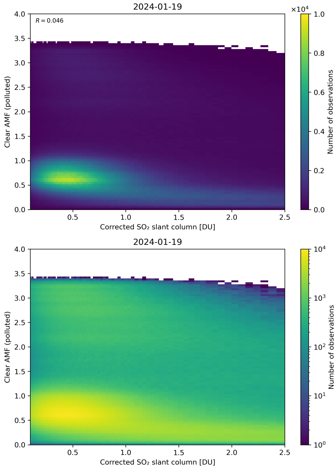
Figure 184: Scatter density plot of “Corrected SO 2 slant column” against “Clear AMF (polluted)” for 2024-01-18 to 2024-01-20.
