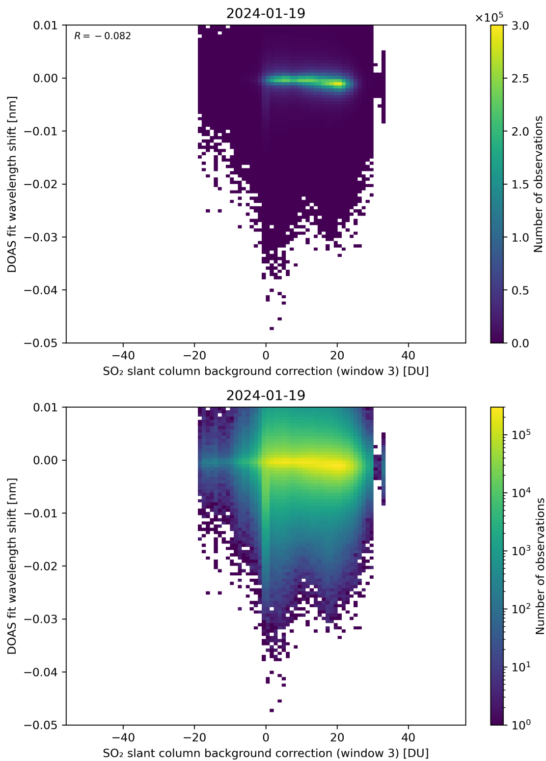
Figure 121: Scatter density plot of “SO 2 slant column background correction (window 3)” against “DOAS fit wavelength shift” for 2024-01-18 to 2024-01-20.
