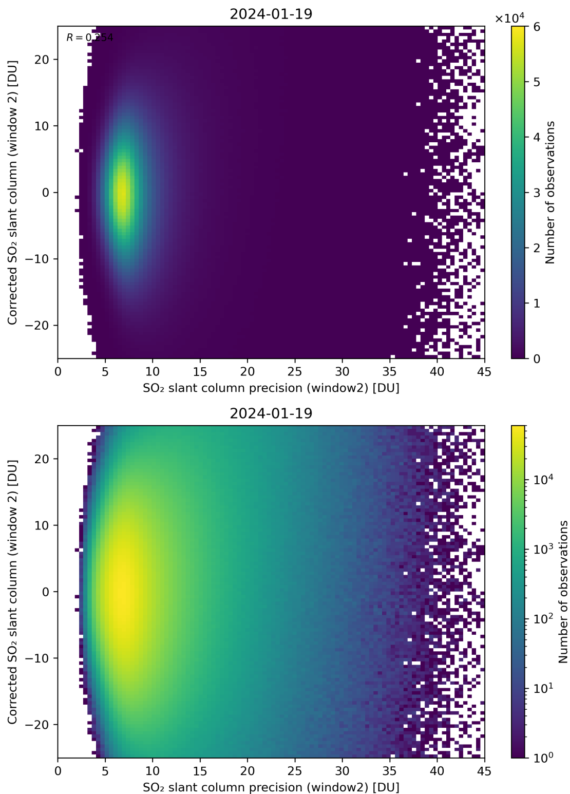
Figure 247: Scatter density plot of “SO 2 slant column precision (window2)” against “Corrected SO 2 slant column (window 2)” for 2024-01-18 to 2024-01-20.
