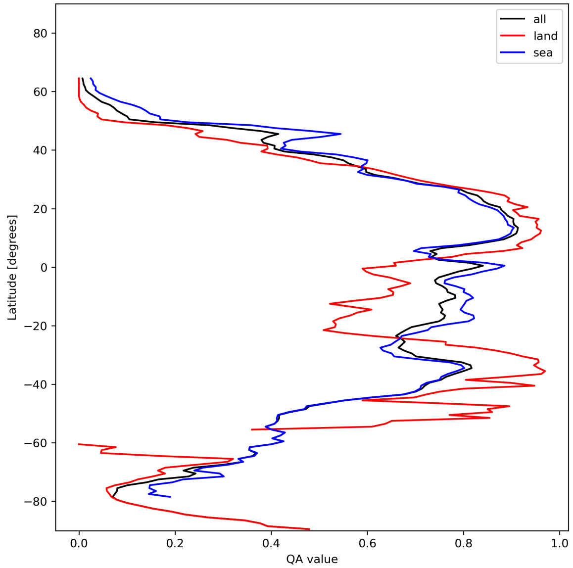
Figure 29: Zonal average of “QA value” for 2024-01-18 to 2024-01-20.
