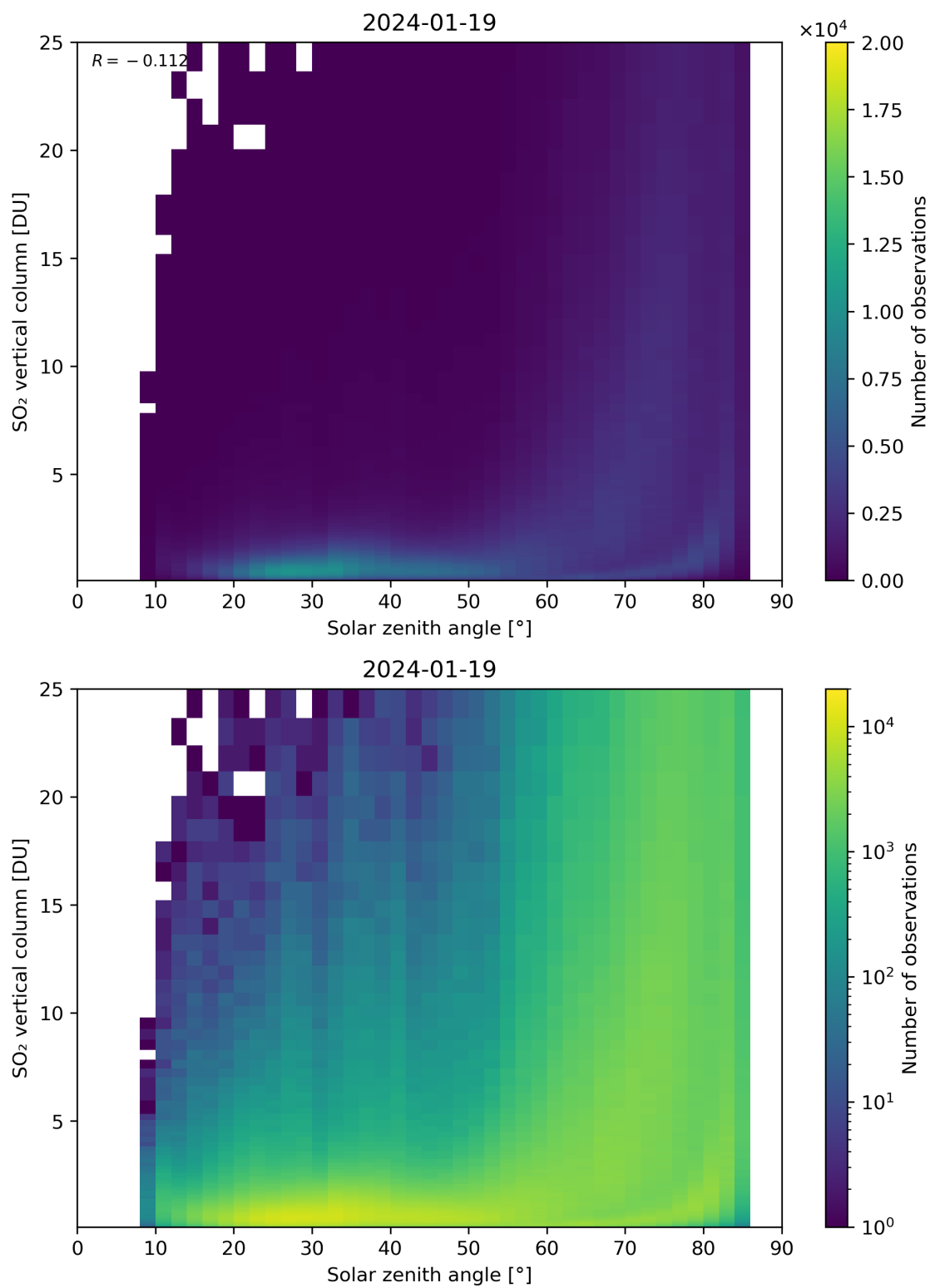
Figure 176: Scatter density plot of “Solar zenith angle” against “SO 2 vertical column” for 2024-01-18 to 2024-01-20.
