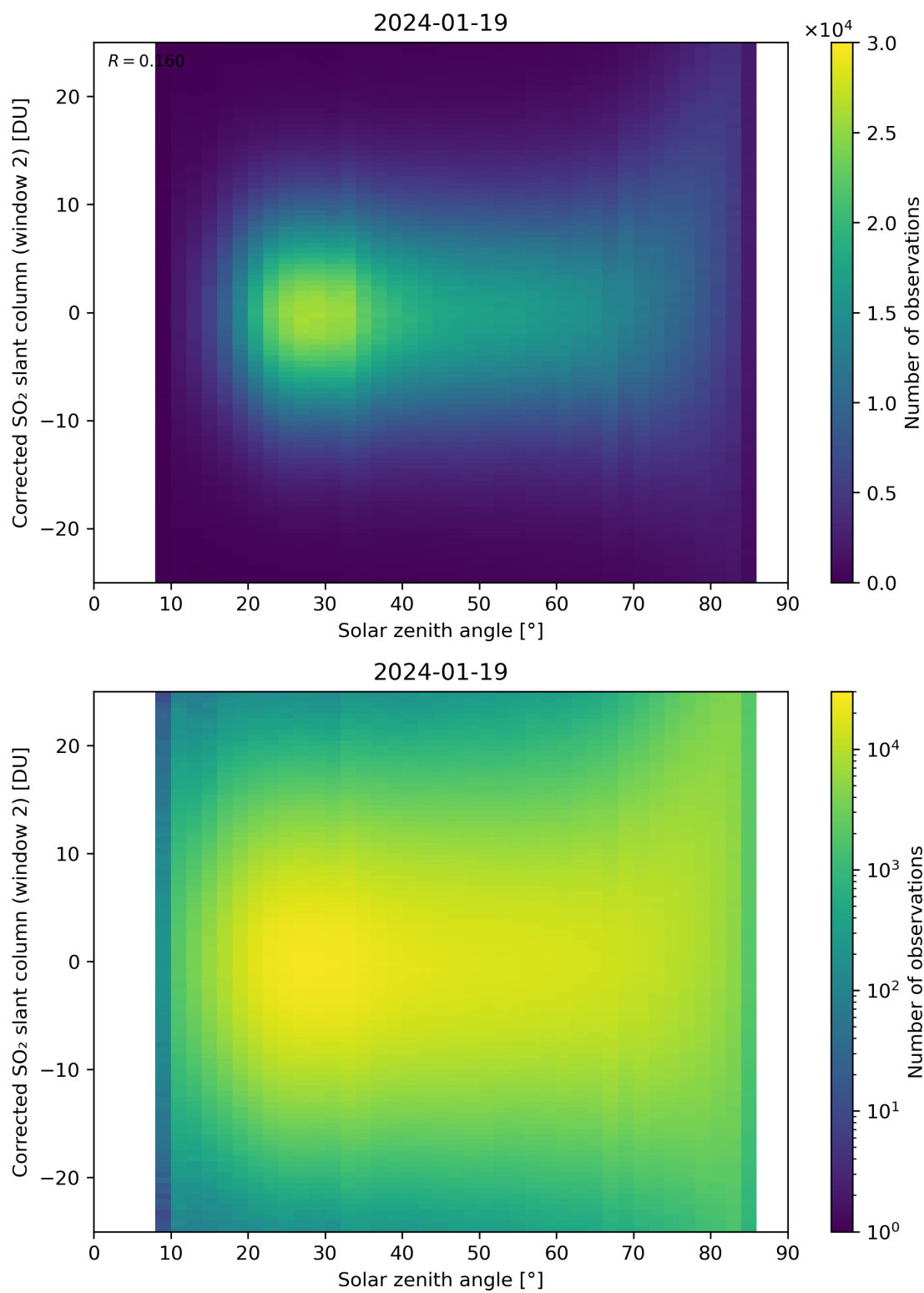
Figure 167: Scatter density plot of “Solar zenith angle” against “Corrected SO 2 slant column (window 2)” for 2024-01-18 to 2024-01-20.
