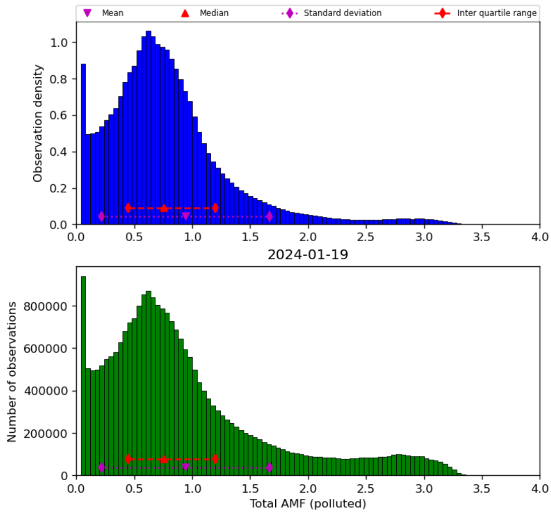
Figure 71: Histogram of “Total AMF (polluted)” for 2024-01-18 to 2024-01-20
