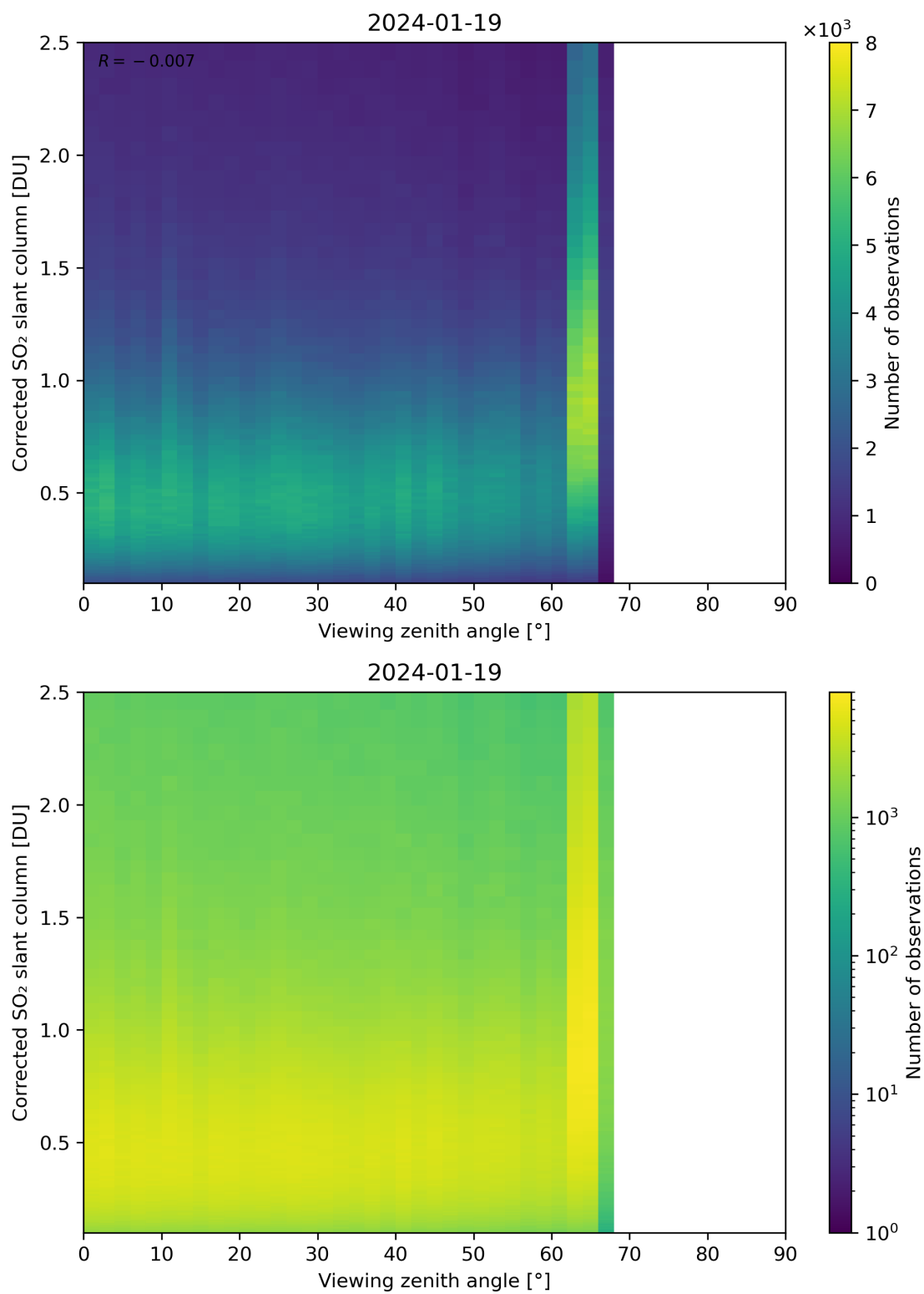
Figure 317: Scatter density plot of “Viewing zenith angle” against “Corrected SO 2 slant column” for 2024-01-18 to 2024-01-20.
