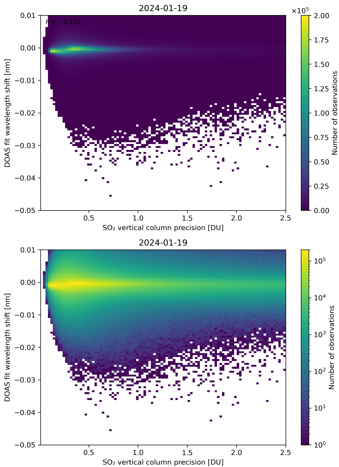
Figure 282: Scatter density plot of “SO 2 vertical column precision” against “DOAS fit wavelength shift” for 2024-01-18 to 2024-01-20.
