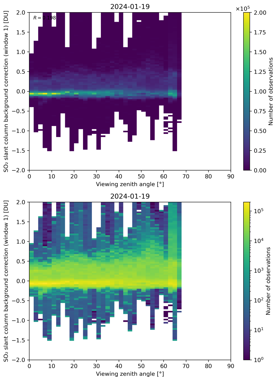
Figure 308: Scatter density plot of “Viewing zenith angle” against “SO 2 slant column background correction (window 1)” for 2024-01-18 to 2024-01-20.
