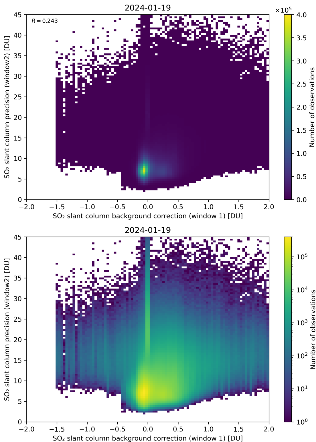
Figure 106: Scatter density plot of “SO 2 slant column background correction (window 1)” against “SO 2 slant column precision (window2)” for 2024-01-18 to 2024-01-20.
