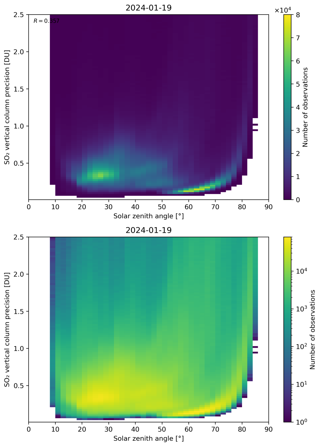
Figure 177: Scatter density plot of “Solar zenith angle” against “SO 2 vertical column precision” for 2024-01-18 to 2024-01-20.
