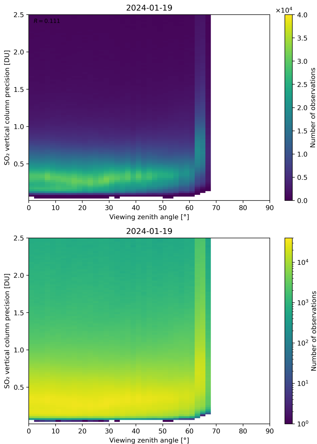
Figure 328: Scatter density plot of “Viewing zenith angle” against “SO 2 vertical column precision” for 2024-01-18 to 2024-01-20.
