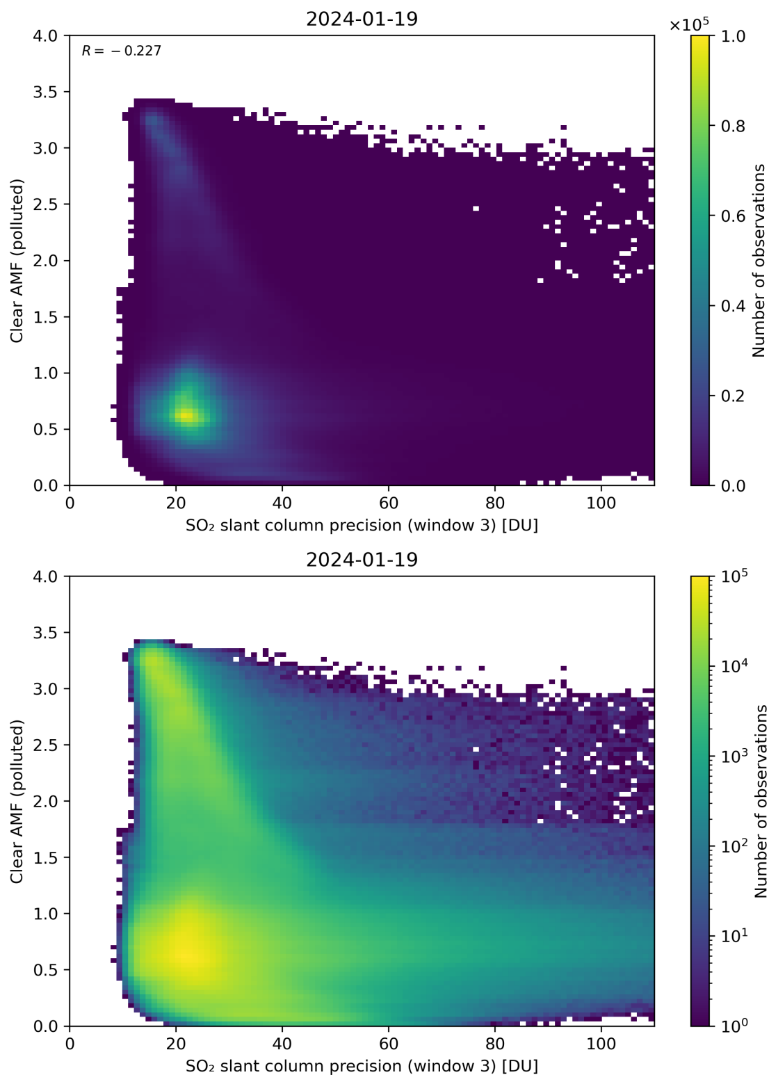
Figure 261: Scatter density plot of “SO 2 slant column precision (window 3)” against “Clear AMF (polluted)” for 2024-01-18 to 2024-01-20.
