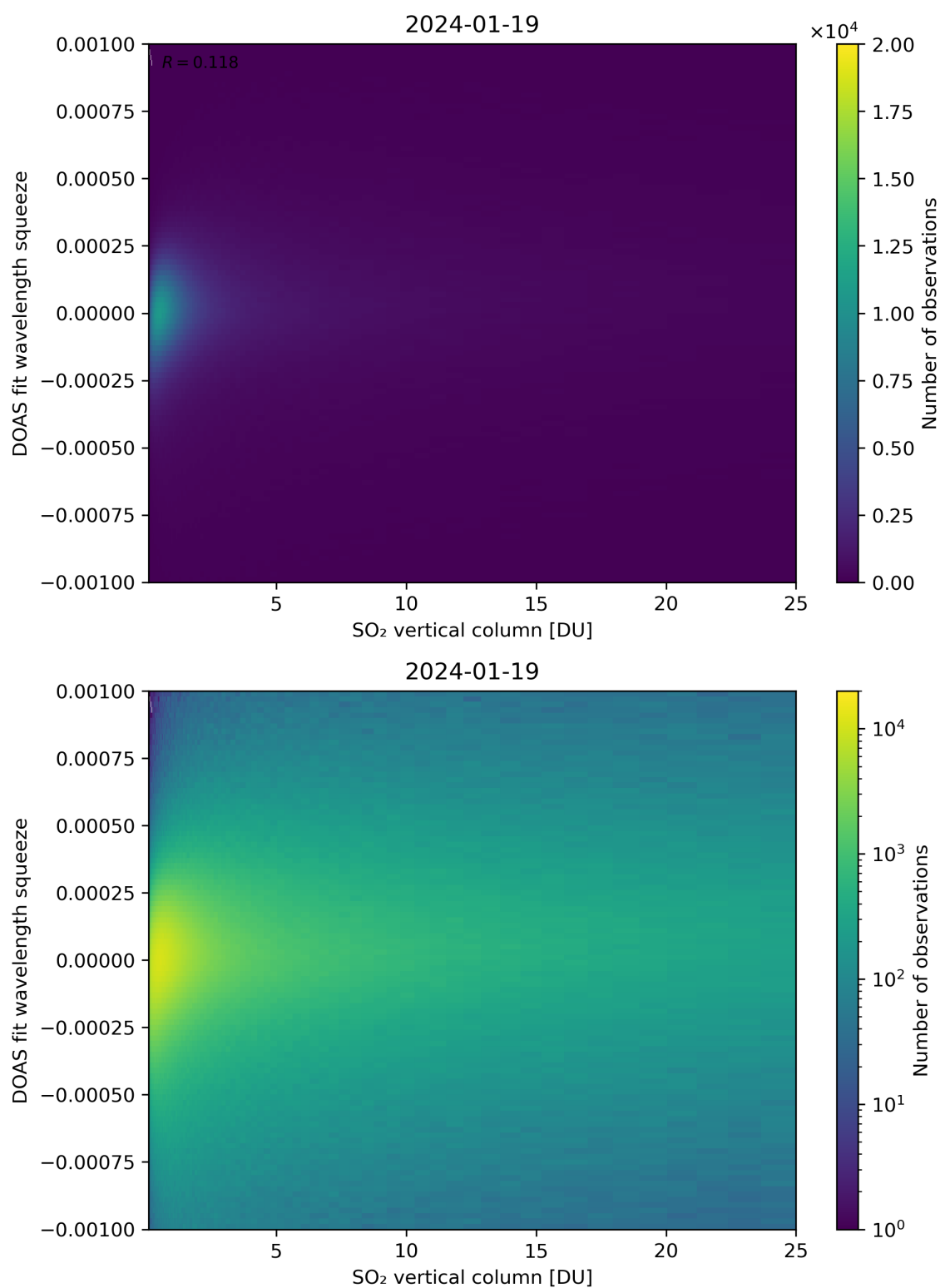
Figure 277: Scatter density plot of “SO 2 vertical column” against “DOAS fit wavelength squeeze” for 2024-01-18 to 2024-01-20.
