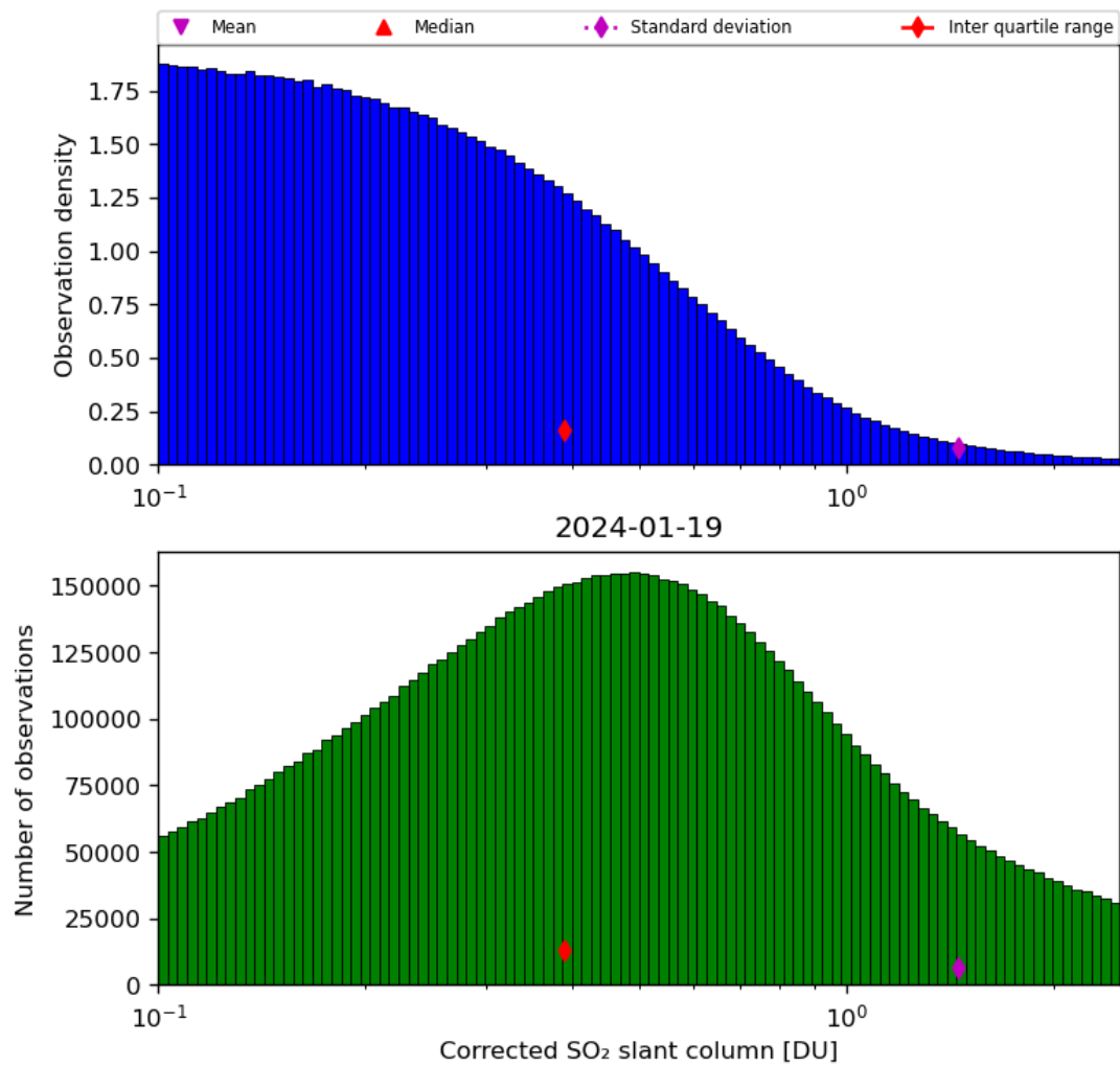
Figure 55: Histogram of “Corrected SO 2 slant column” for 2024-01-18 to 2024-01-20
