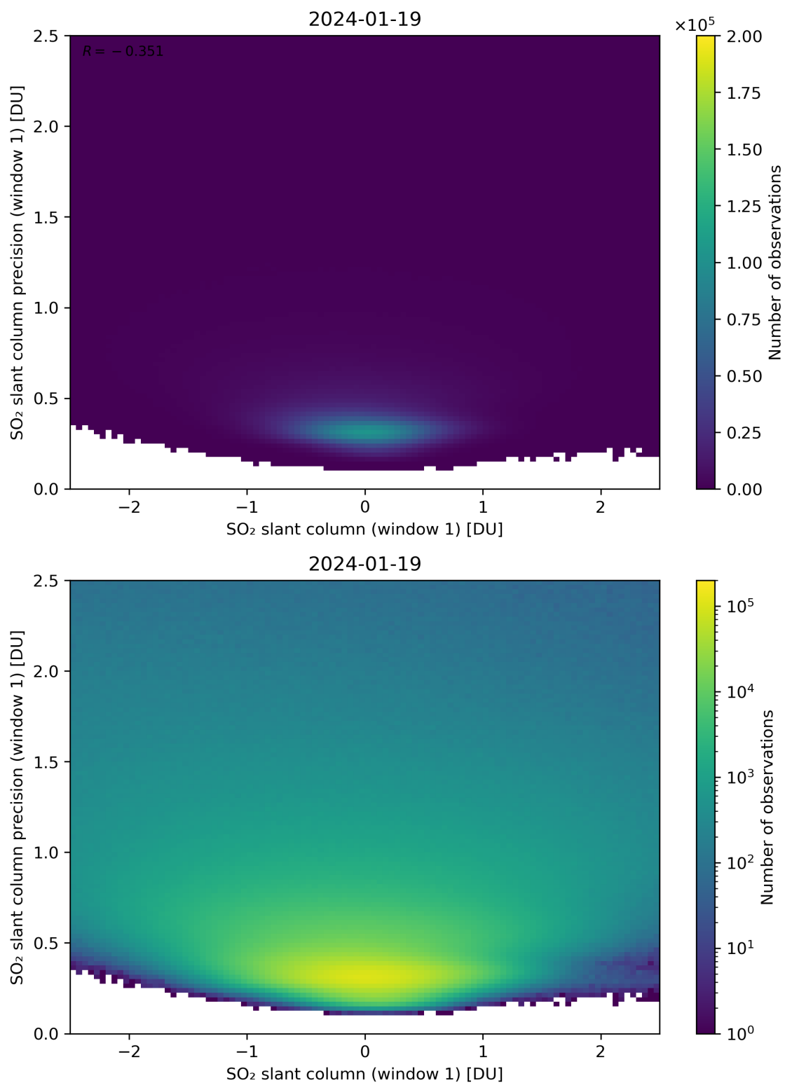
Figure 235: Scatter density plot of “SO 2 slant column (window 1)” against “SO 2 slant column precision (window 1)” for 2024-01-18 to 2024-01-20.
