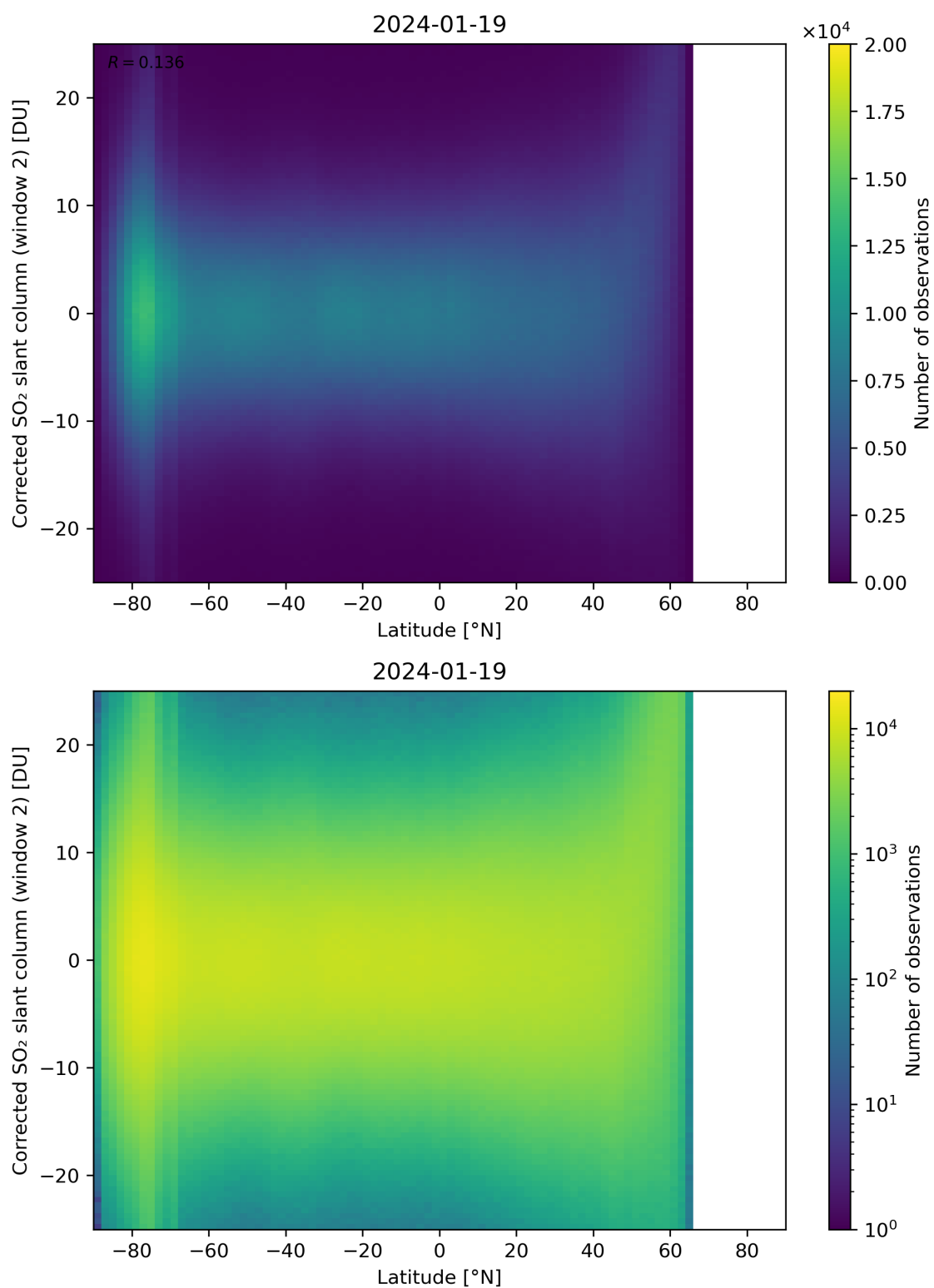
Figure 147: Scatter density plot of “Latitude” against “Corrected SO 2 slant column (window 2)” for 2024-01-18 to 2024-01-20.
