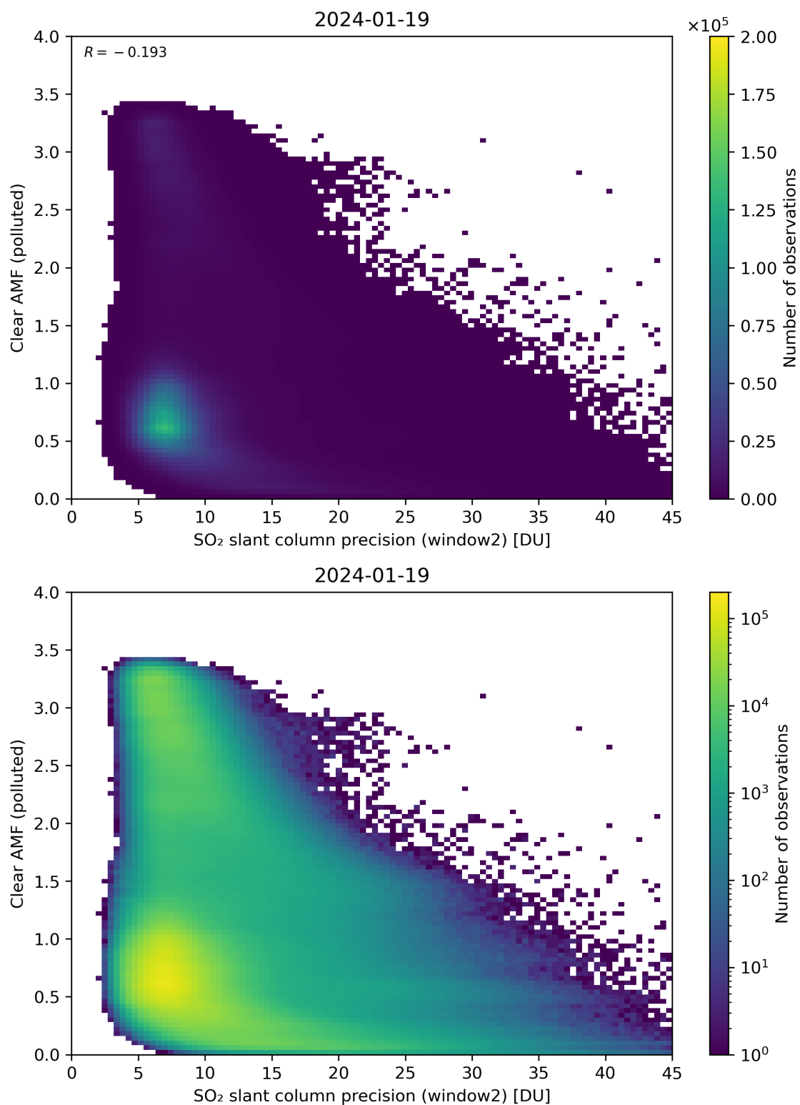
Figure 246: Scatter density plot of “SO 2 slant column precision (window2)” against “Clear AMF (polluted)” for 2024-01-18 to 2024-01-20.
