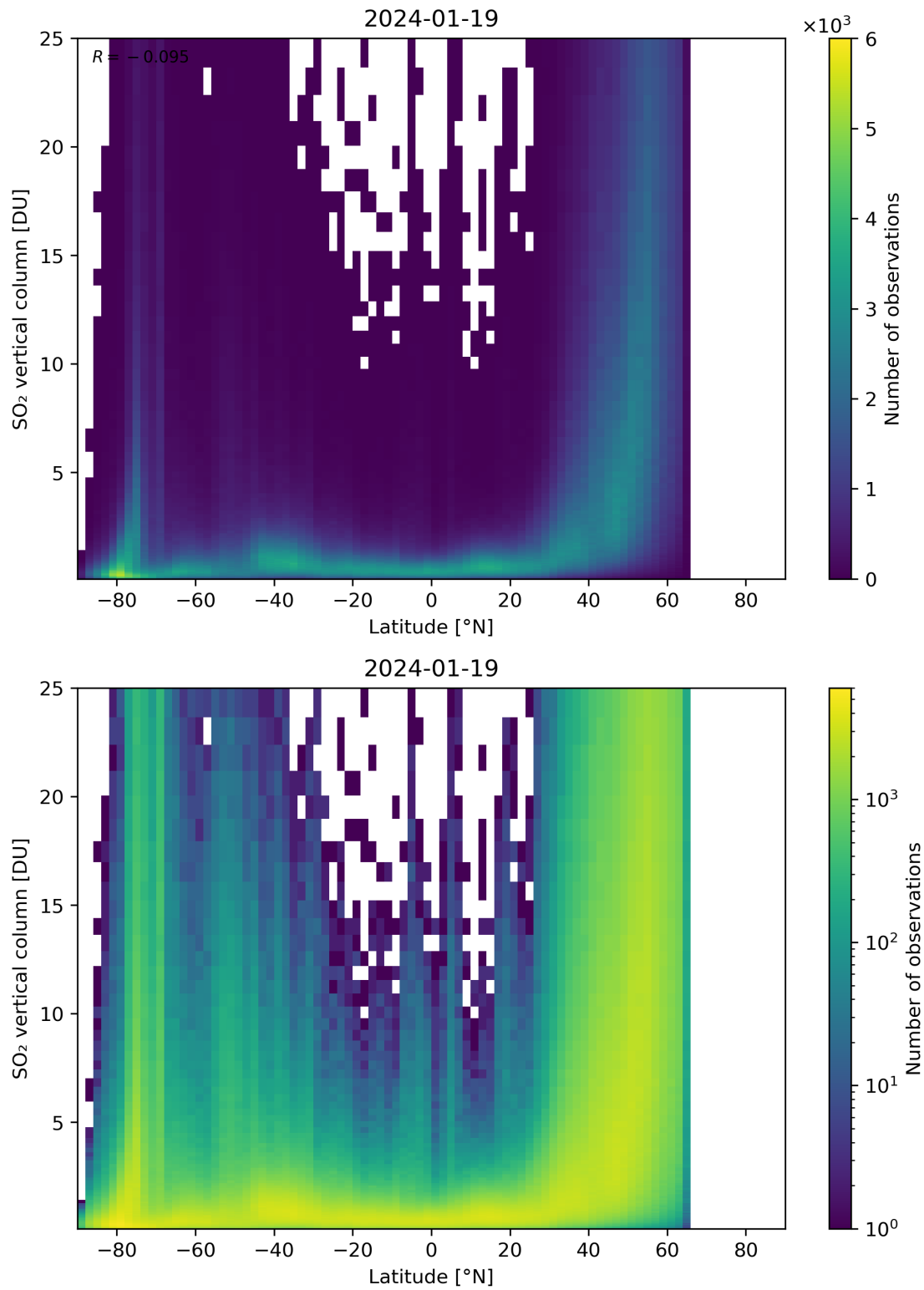
Figure 156: Scatter density plot of “Latitude” against “SO 2 vertical column” for 2024-01-18 to 2024-01-20.
