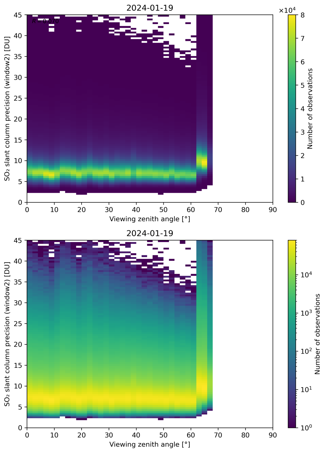
Figure 322: Scatter density plot of “Viewing zenith angle” against “SO 2 slant column precision (window2)” for 2024-01-18 to 2024-01-20.
