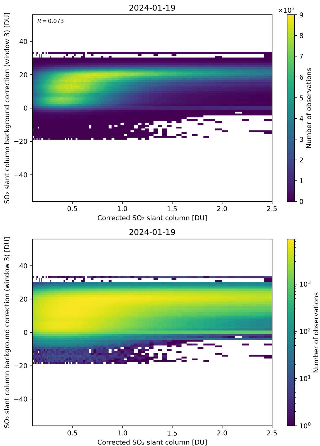
Figure 180: Scatter density plot of “Corrected SO 2 slant column” against “SO 2 slant column background correction (window 3)” for 2024-01-18 to 2024-01-20.
