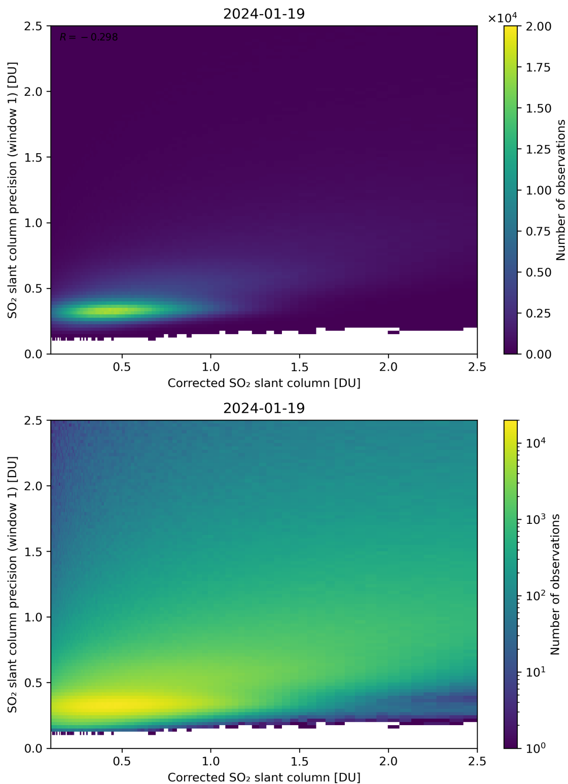
Figure 188: Scatter density plot of “Corrected SO 2 slant column” against “SO 2 slant column precision (window 1)” for 2024-01-18 to 2024-01-20.
