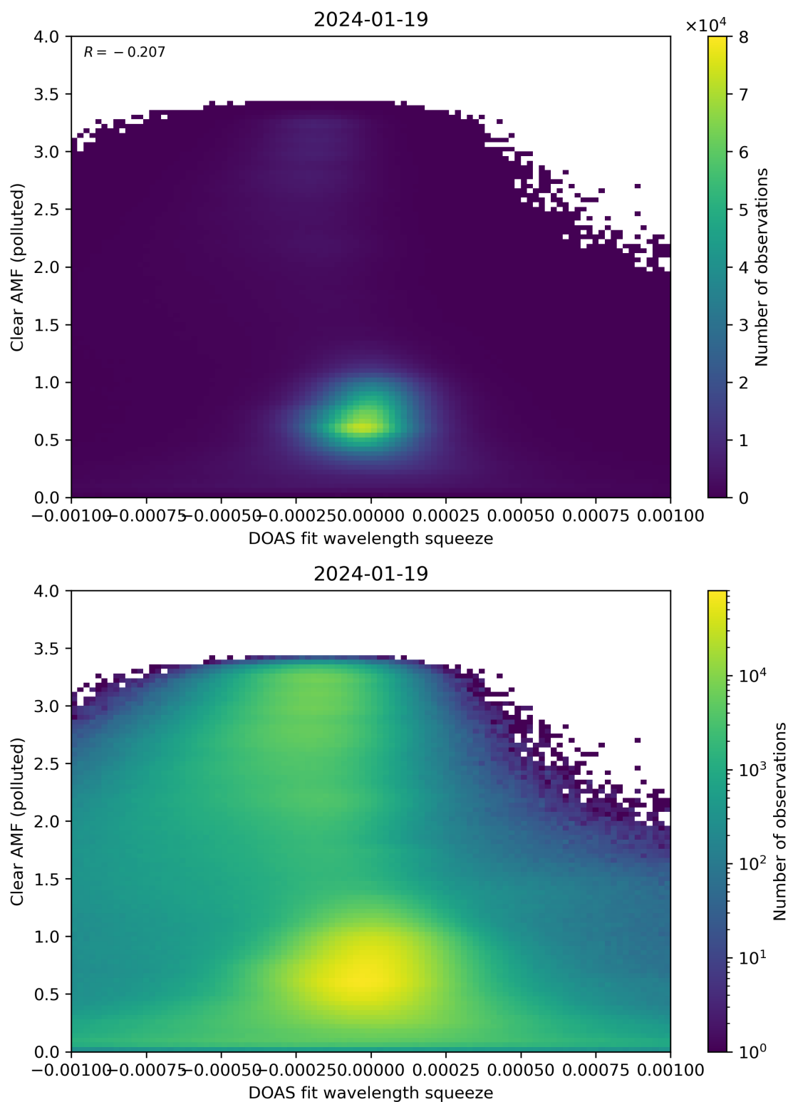
Figure 133: Scatter density plot of “DOAS fit wavelength squeeze” against “Clear AMF (polluted)” for 2024-01-18 to 2024-01-20.
