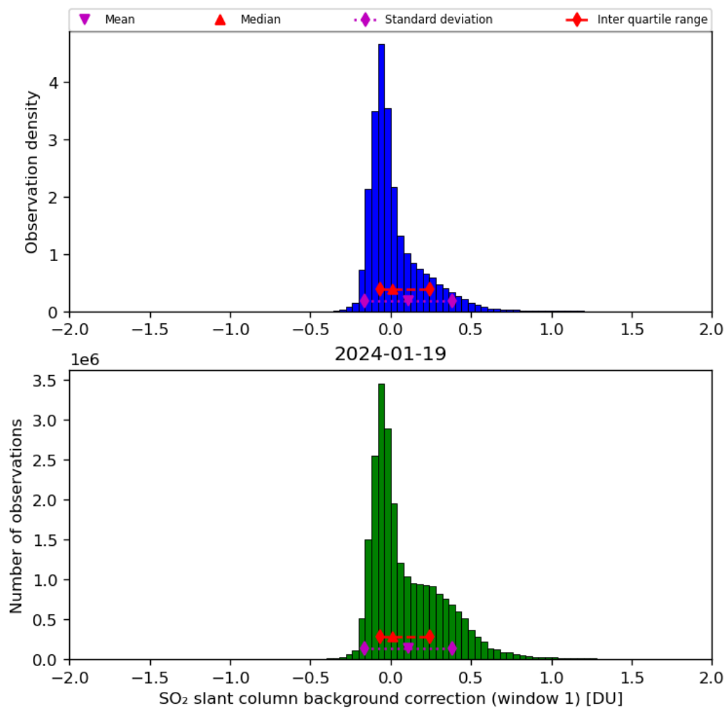
Figure 59: Histogram of “SO 2 slant column background correction (window 1)” for 2024-01-18 to 2024-01-20
