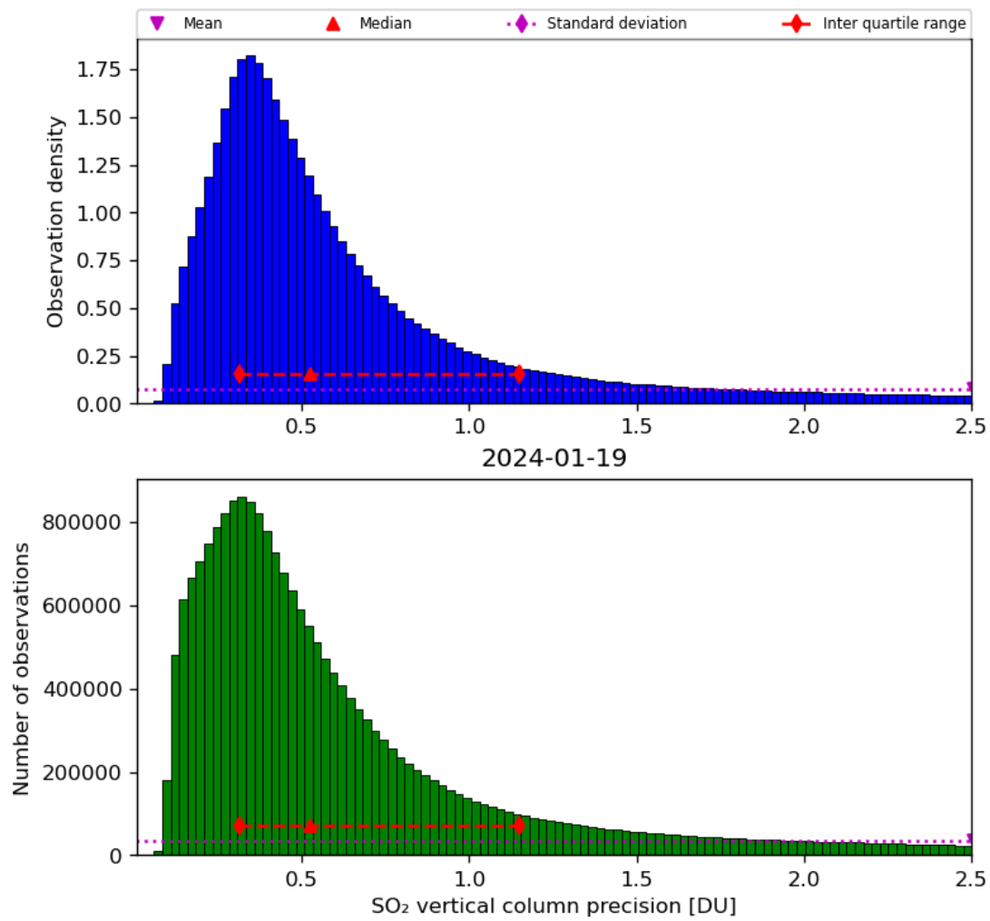
Figure 54: Histogram of “SO 2 vertical column precision” for 2024-01-18 to 2024-01-20
