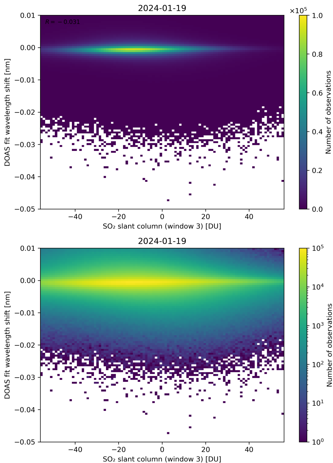
Figure 254: Scatter density plot of “SO 2 slant column (window 3)” against “DOAS fit wavelength shift” for 2024-01-18 to 2024-01-20.
