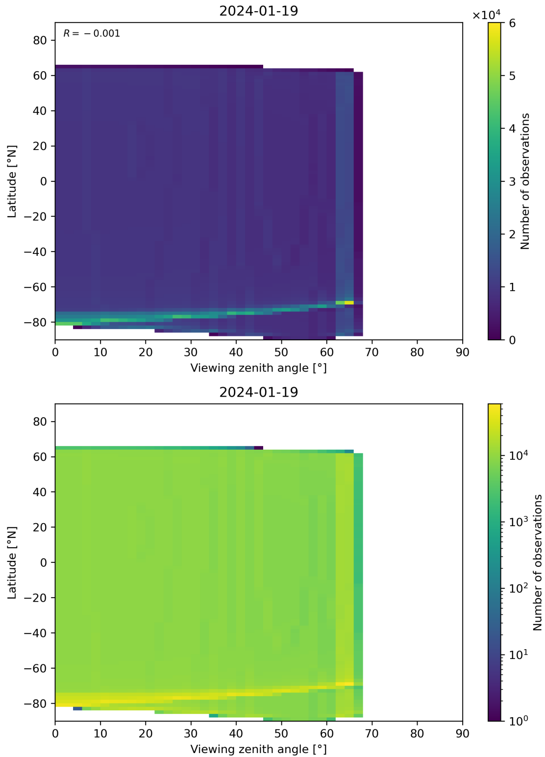
Figure 314: Scatter density plot of “Viewing zenith angle” against “Latitude” for 2024-01-18 to 2024-01-20.
