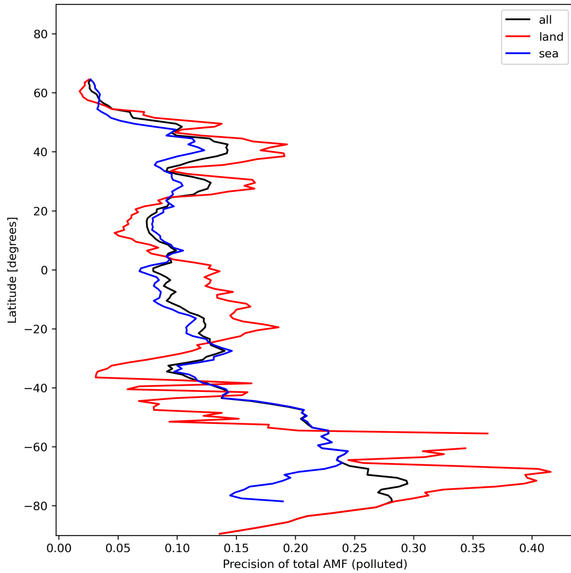
Figure 49: Zonal average of “Precision of total AMF (polluted)” for 2024-01-18 to 2024-01-20.
