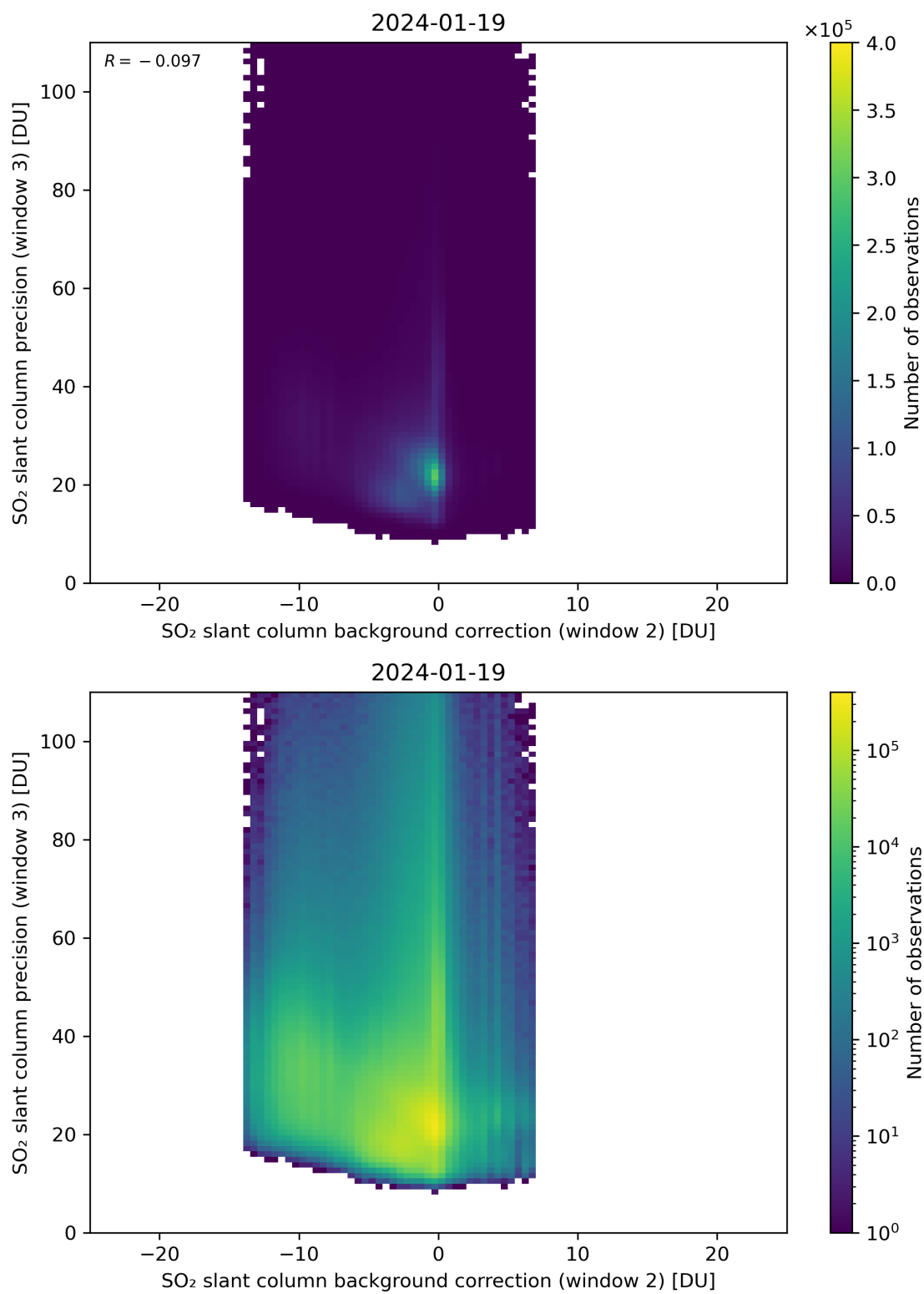
Figure 118: Scatter density plot of “SO 2 slant column background correction (window 2)” against “SO 2 slant column precision (window 3)” for 2024-01-18 to 2024-01-20.
