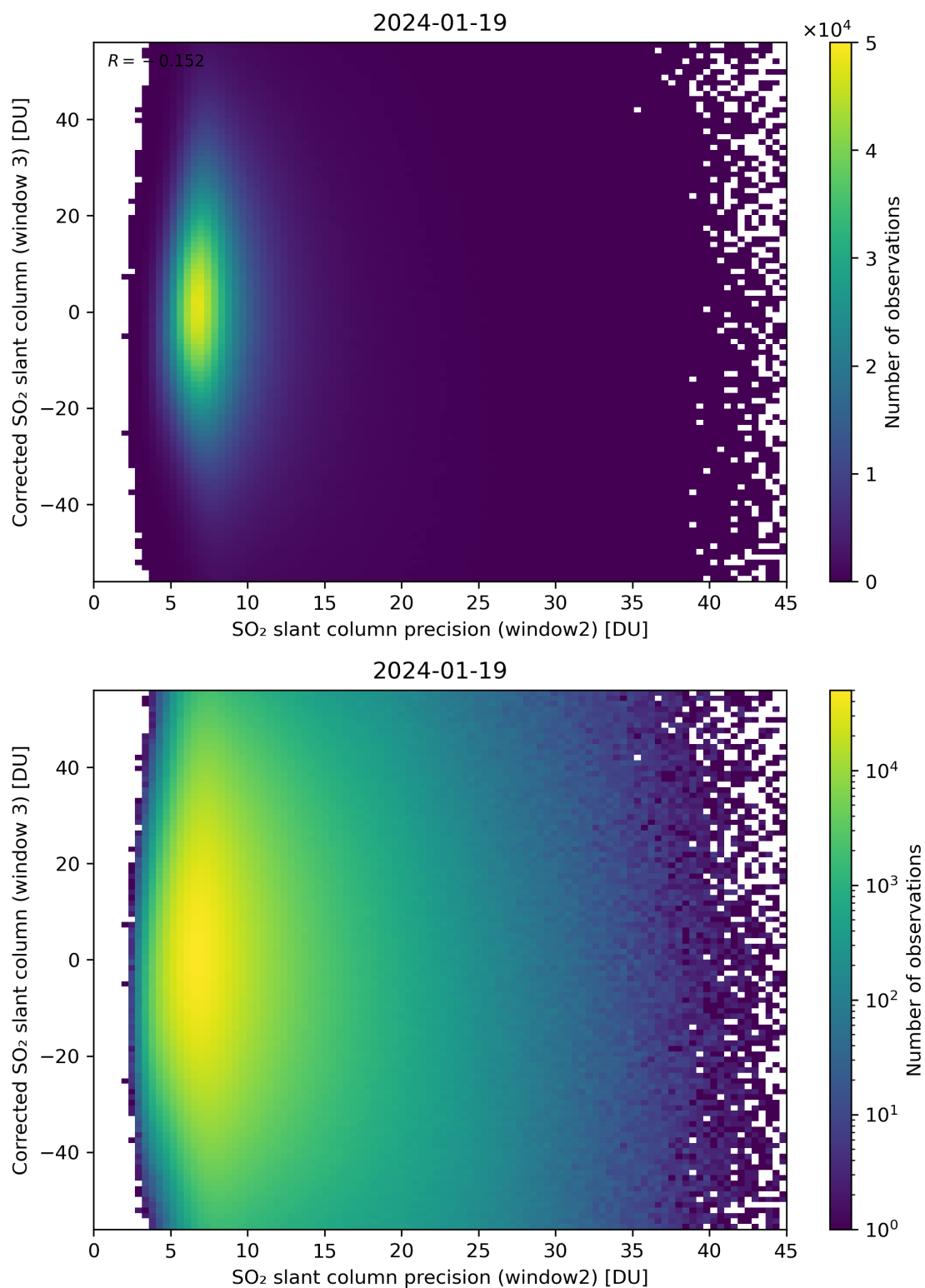
Figure 248: Scatter density plot of “SO 2 slant column precision (window2)” against “Corrected SO 2 slant column (window 3)” for 2024-01-18 to 2024-01-20.
