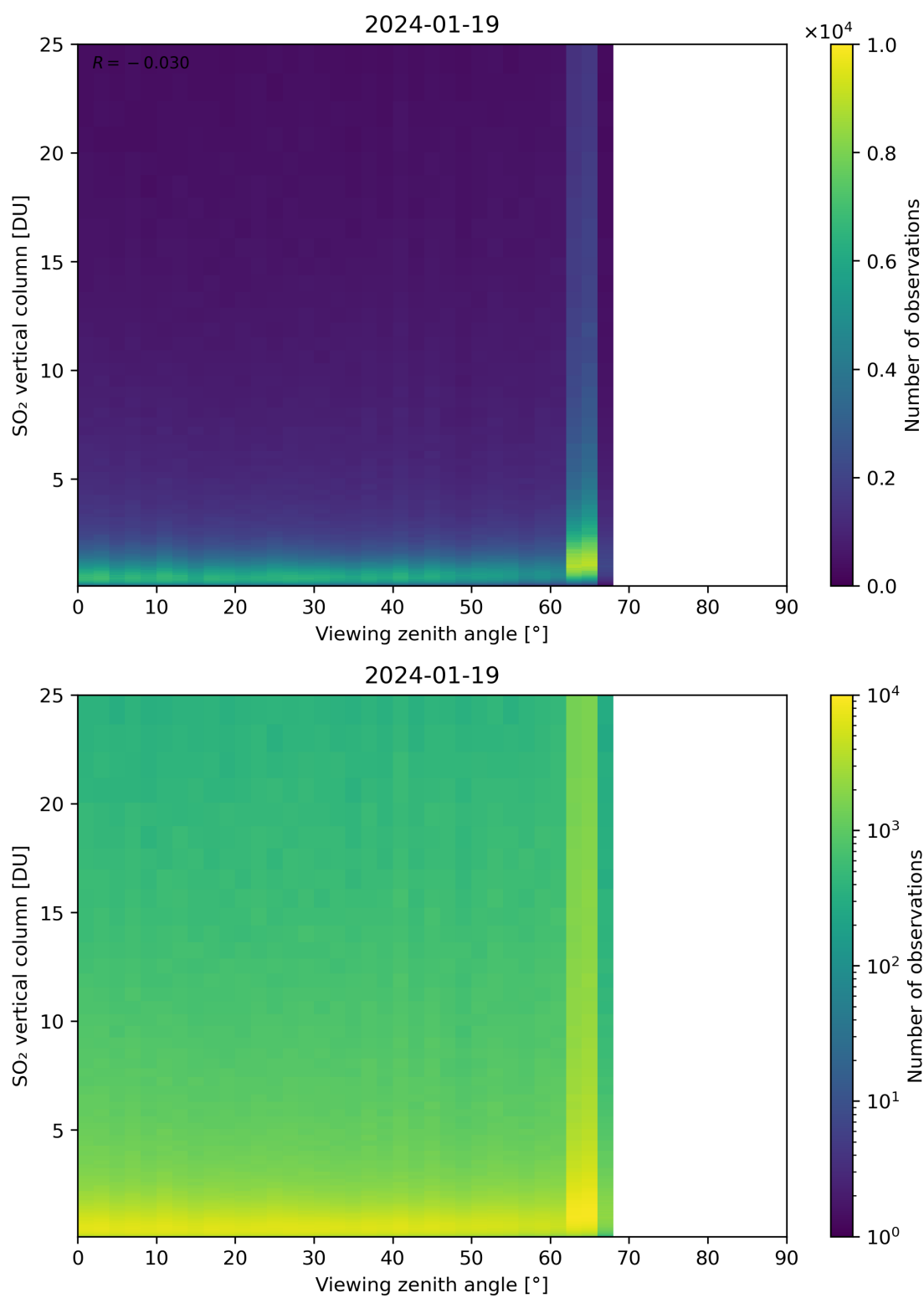
Figure 327: Scatter density plot of “Viewing zenith angle” against “SO 2 vertical column” for 2024-01-18 to 2024-01-20.
