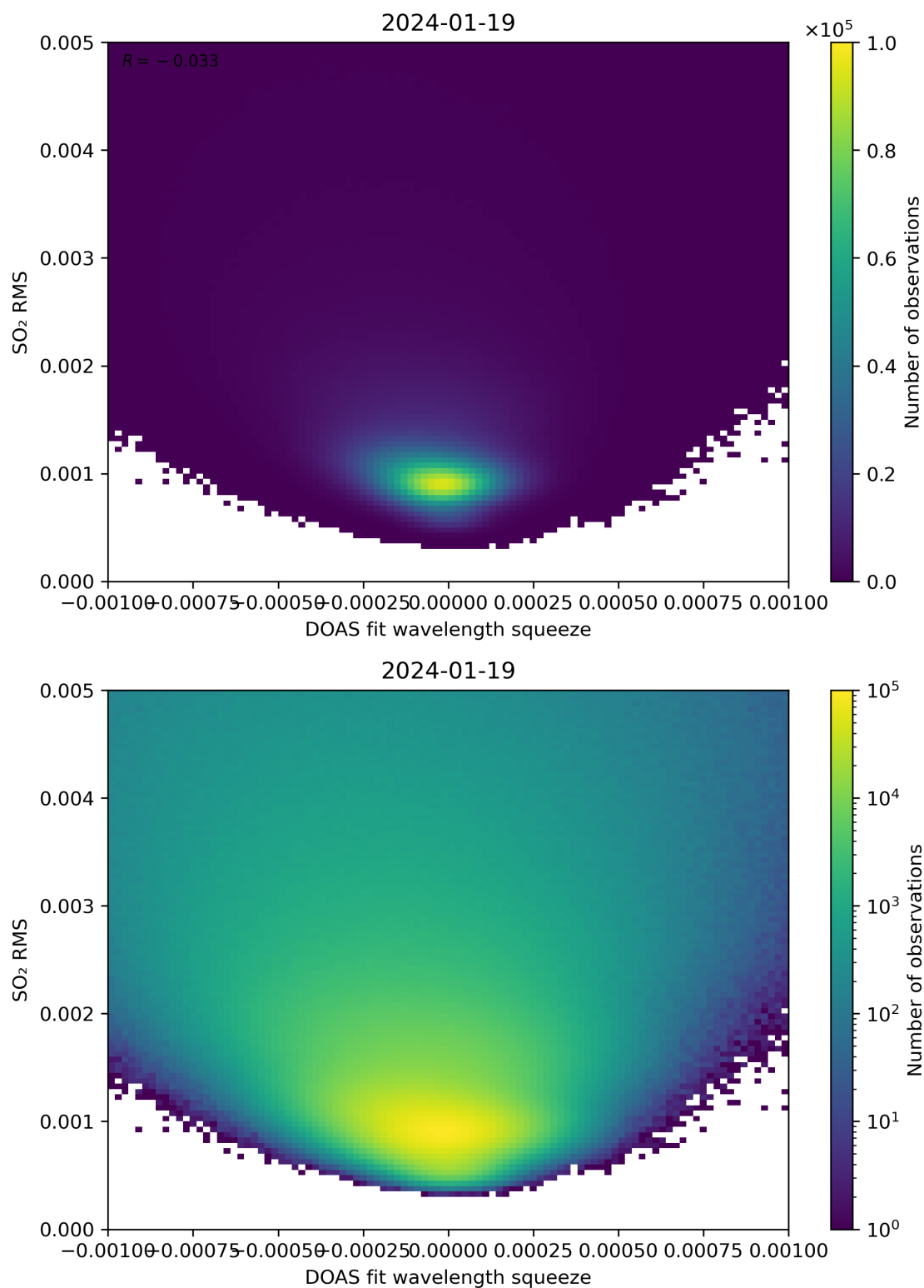
Figure 132: Scatter density plot of “DOAS fit wavelength squeeze” against “SO 2 RMS” for 2024-01-18 to 2024-01-20.
