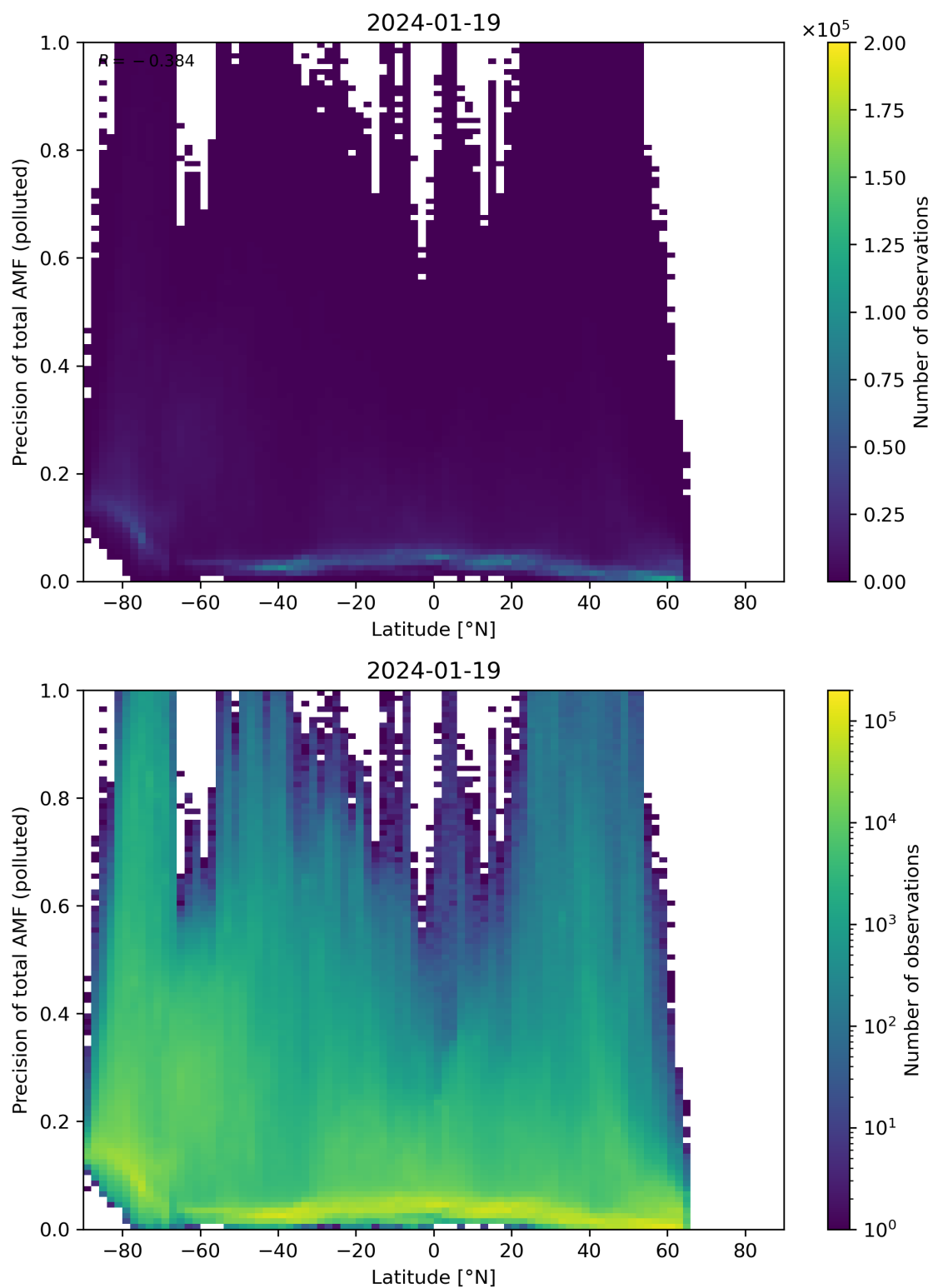
Figure 155: Scatter density plot of “Latitude” against “Precision of total AMF (polluted)” for 2024-01-18 to 2024-01-20.
