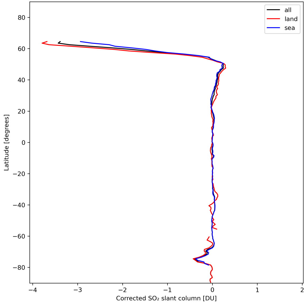
Figure 32: Zonal average of “Corrected SO 2 slant column” for 2024-01-18 to 2024-01-20.
