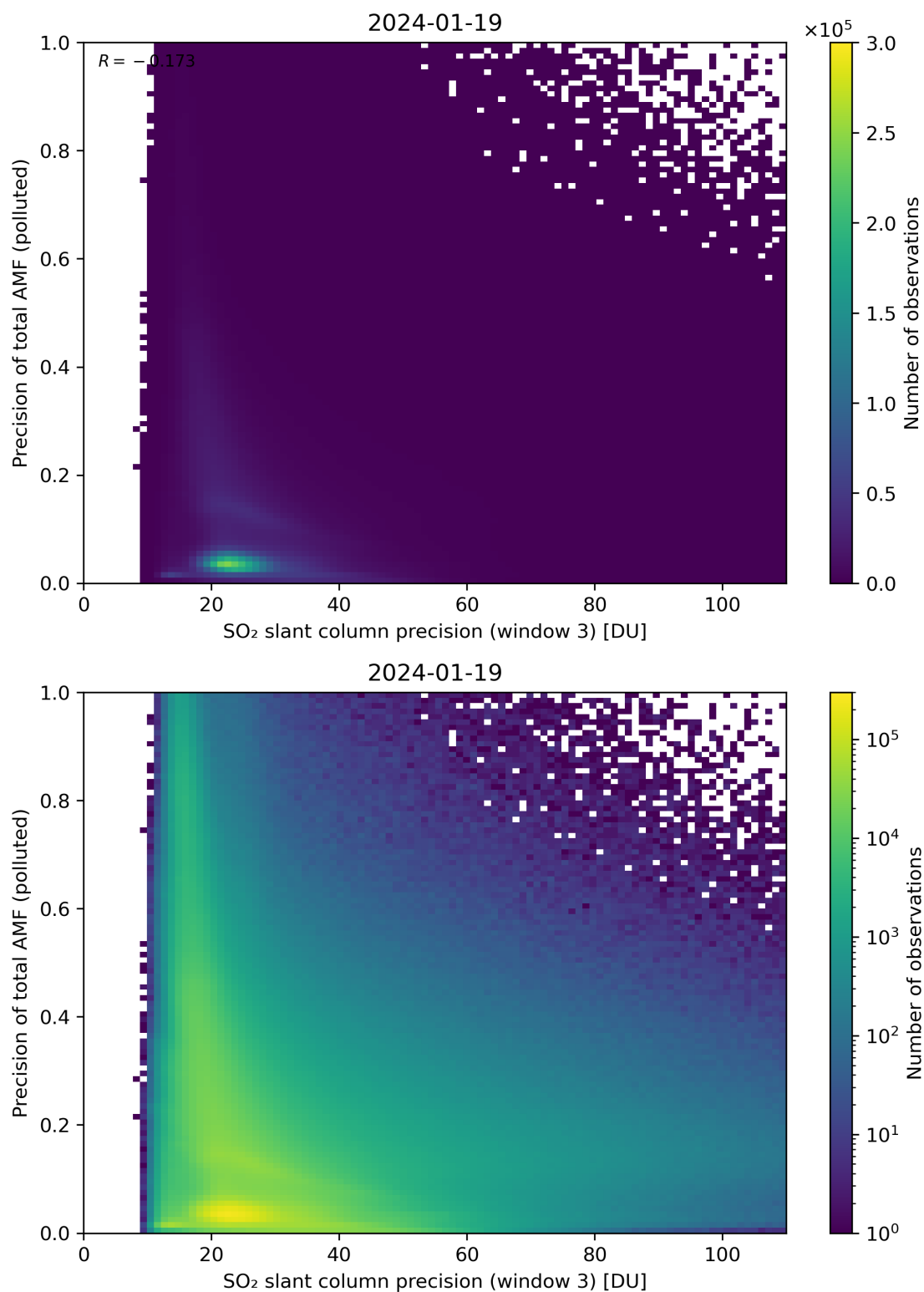
Figure 264: Scatter density plot of “SO 2 slant column precision (window 3)” against “Precision of total AMF (polluted)” for 2024-01-18 to 2024-01-20.
