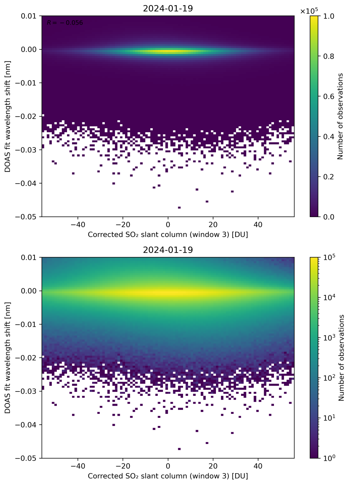
Figure 206: Scatter density plot of “Corrected SO 2 slant column (window 3)” against “DOAS fit wavelength shift” for 2024-01-18 to 2024-01-20.
