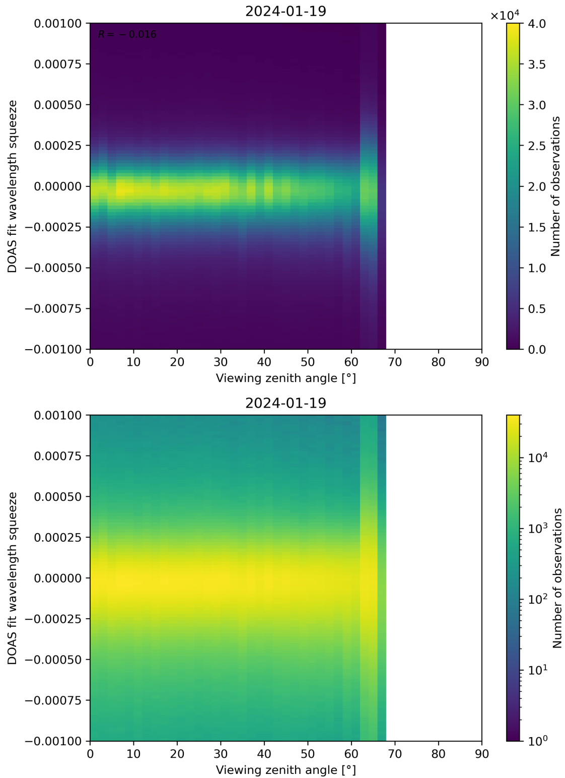
Figure 312: Scatter density plot of “Viewing zenith angle” against “DOAS fit wavelength squeeze” for 2024-01-18 to 2024-01-20.
