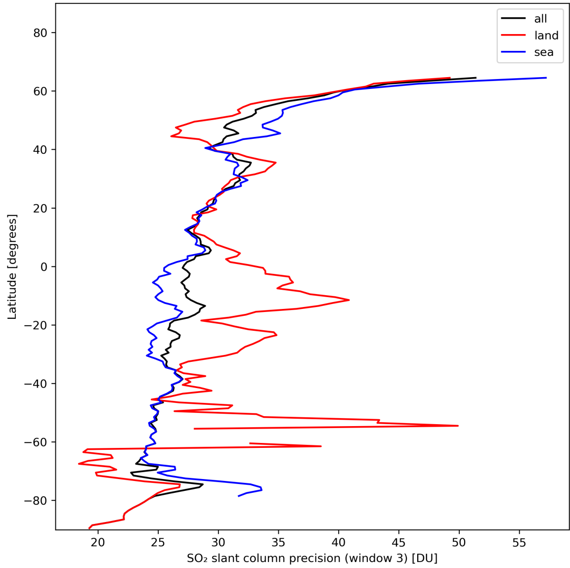
Figure 42: Zonal average of “SO 2 slant column precision (window 3)” for 2024-01-18 to 2024-01-20.
