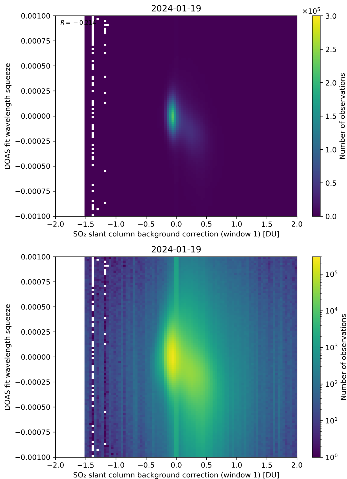
Figure 101: Scatter density plot of “SO 2 slant column background correction (window 1)” against “DOAS fit wavelength squeeze” for 2024-01-18 to 2024-01-20.
