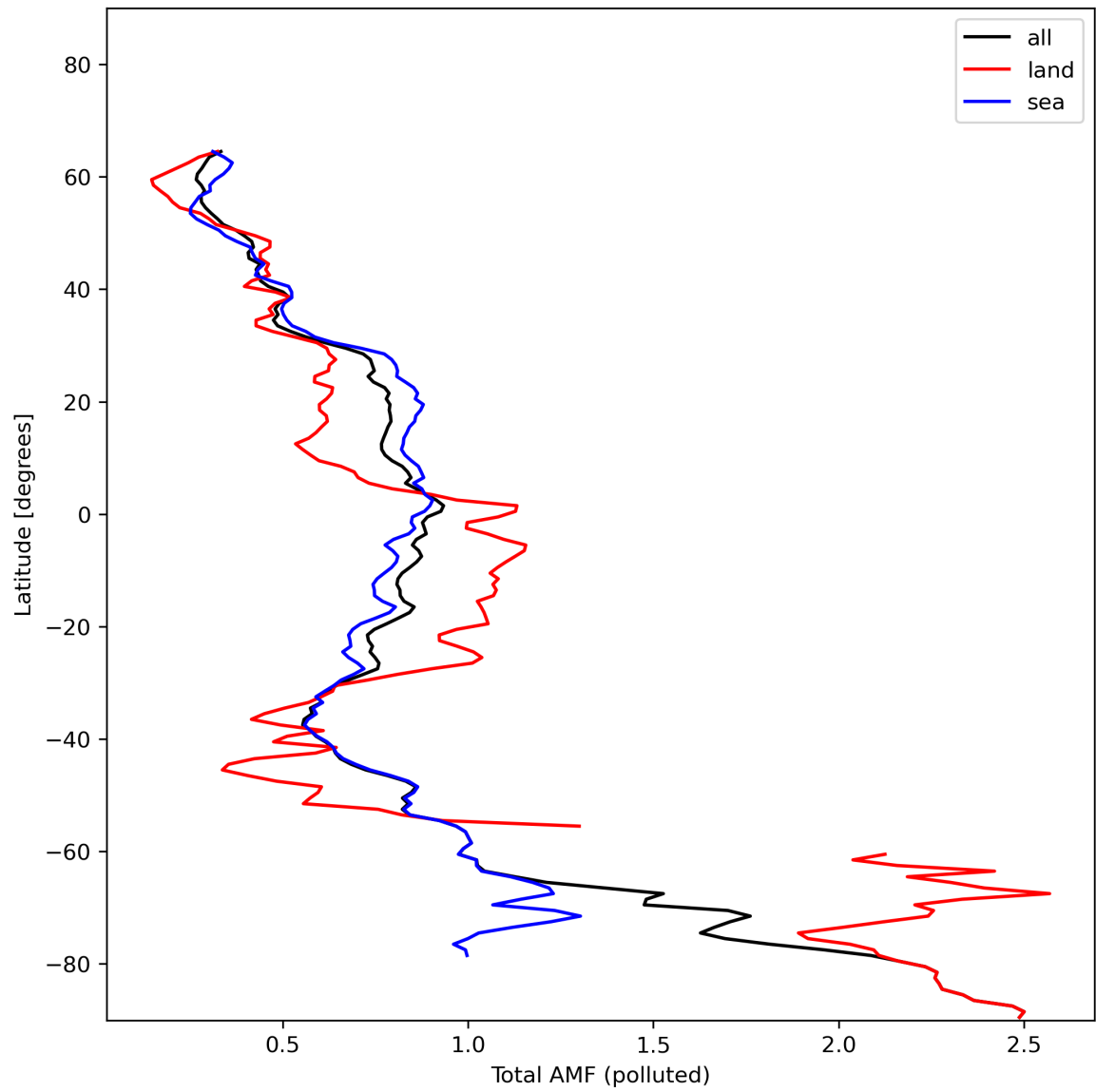
Figure 48: Zonal average of “Total AMF (polluted)” for 2024-01-18 to 2024-01-20.
