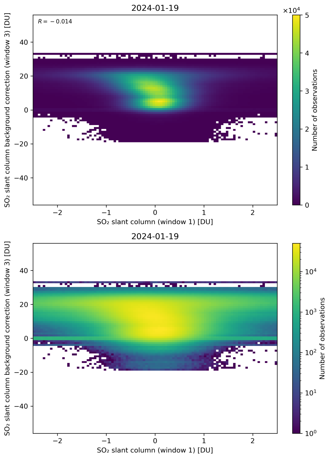
Figure 214: Scatter density plot of “SO 2 slant column (window 1)” against “SO 2 slant column background correction (window 3)” for 2024-01-18 to 2024-01-20.
