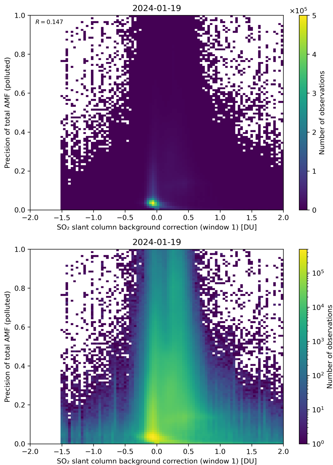
Figure 110: Scatter density plot of “SO 2 slant column background correction (window 1)” against “Precision of total AMF (polluted)” for 2024-01-18 to 2024-01-20.
