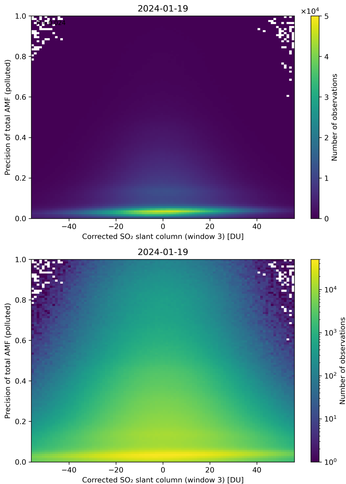
Figure 211: Scatter density plot of “Corrected SO 2 slant column (window 3)” against “Precision of total AMF (polluted)” for 2024-01-18 to 2024-01-20.
