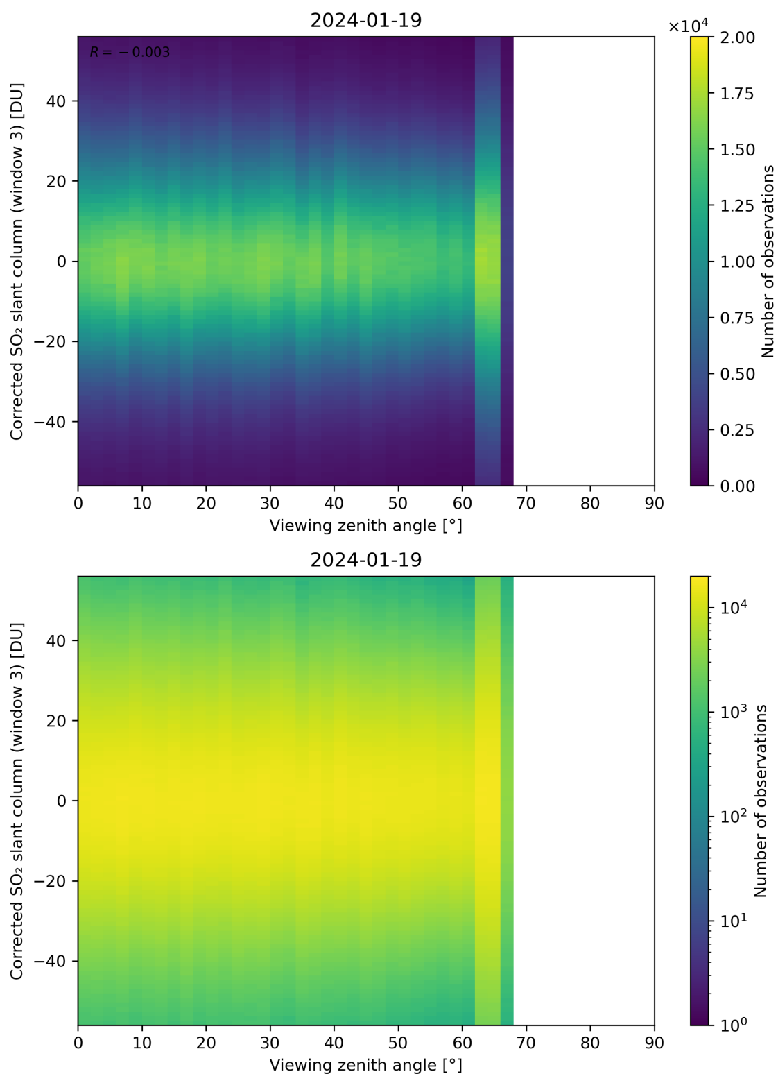
Figure 319: Scatter density plot of “Viewing zenith angle” against “Corrected SO 2 slant column (window 3)” for 2024-01-18 to 2024-01-20.
