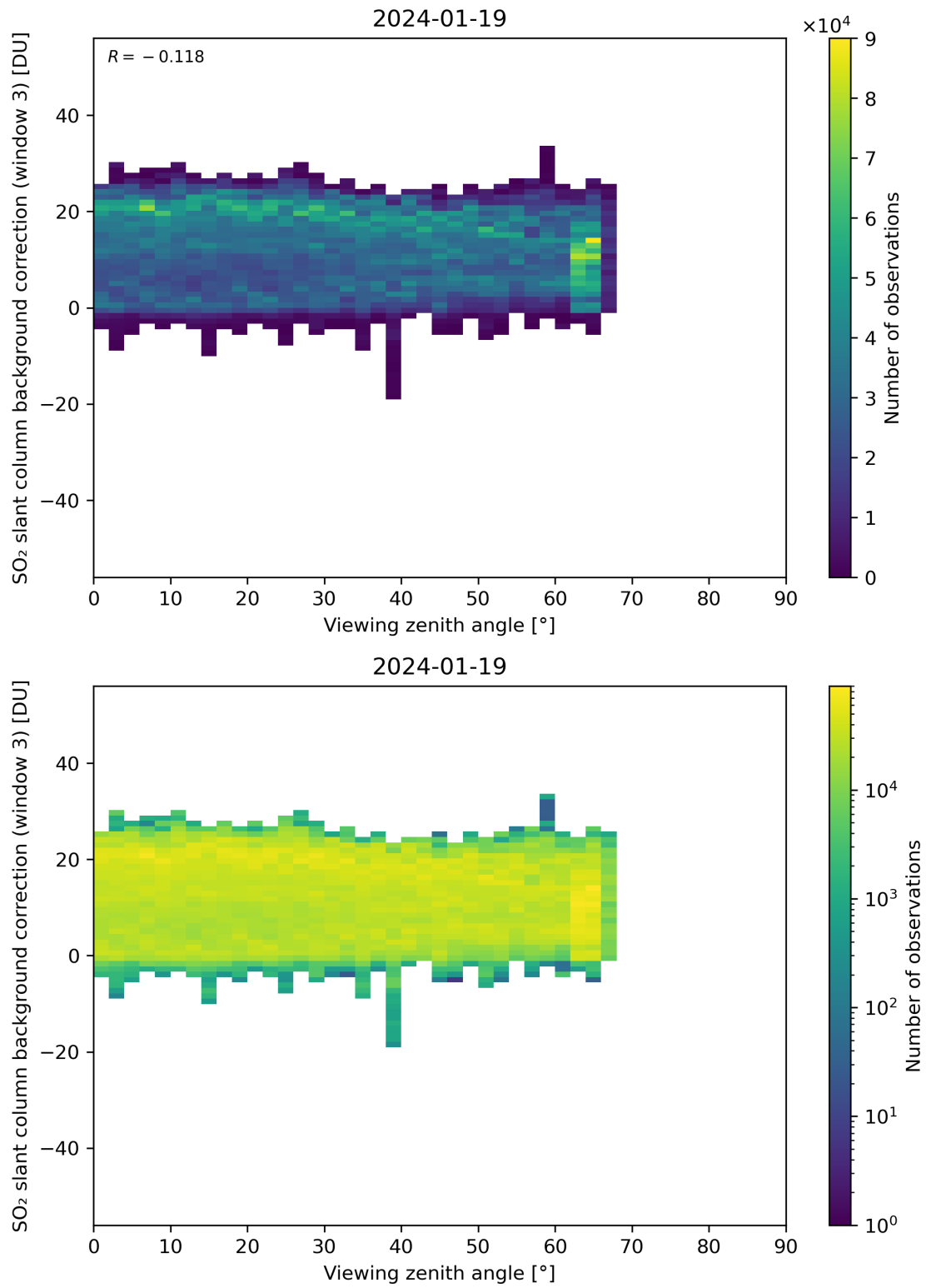
Figure 310: Scatter density plot of “Viewing zenith angle” against “SO 2 slant column background correction (window 3)” for 2024-01-18 to 2024-01-20.
