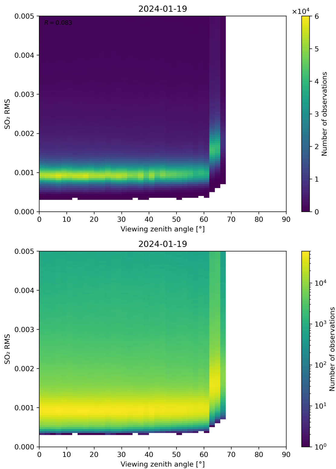
Figure 313: Scatter density plot of “Viewing zenith angle” against “SO 2 RMS” for 2024-01-18 to 2024-01-20.
