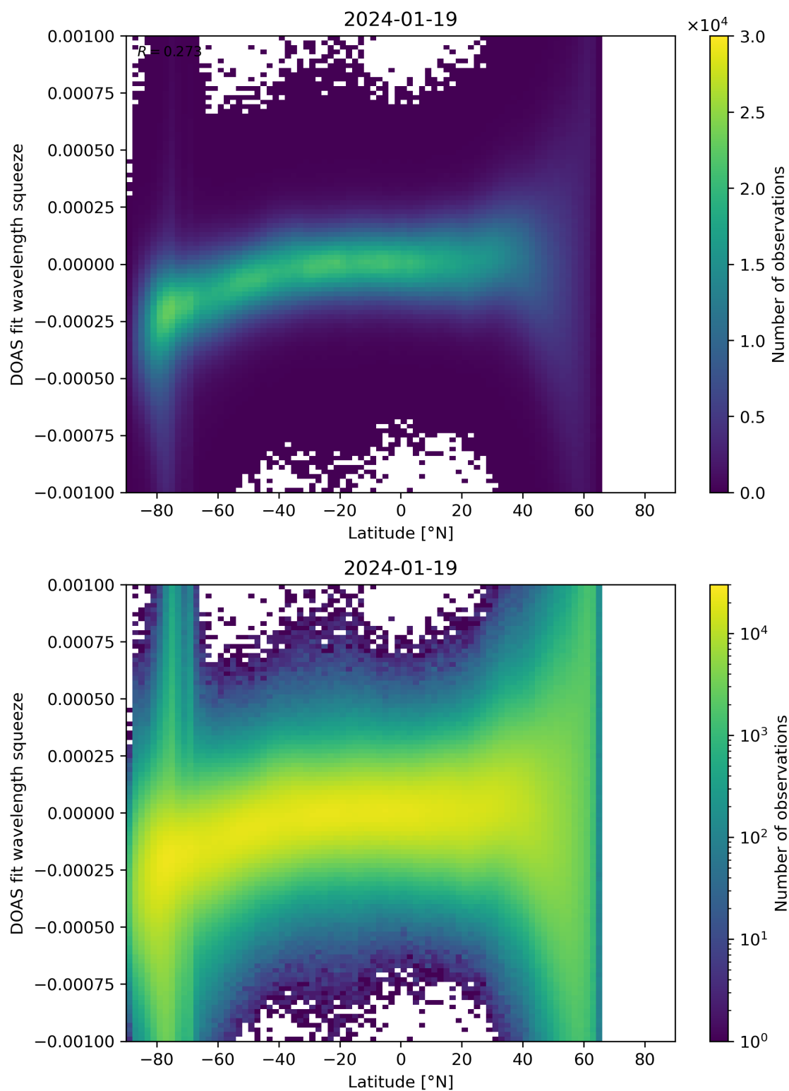
Figure 143: Scatter density plot of “Latitude” against “DOAS fit wavelength squeeze” for 2024-01-18 to 2024-01-20.
