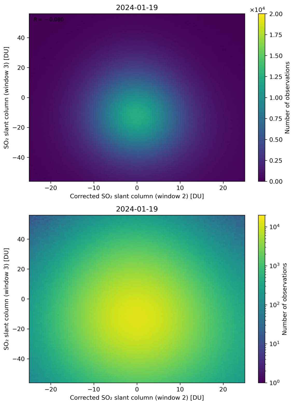
Figure 201: Scatter density plot of “Corrected SO 2 slant column (window 2)” against “SO 2 slant column (window 3)” for 2024-01-18 to 2024-01-20.
