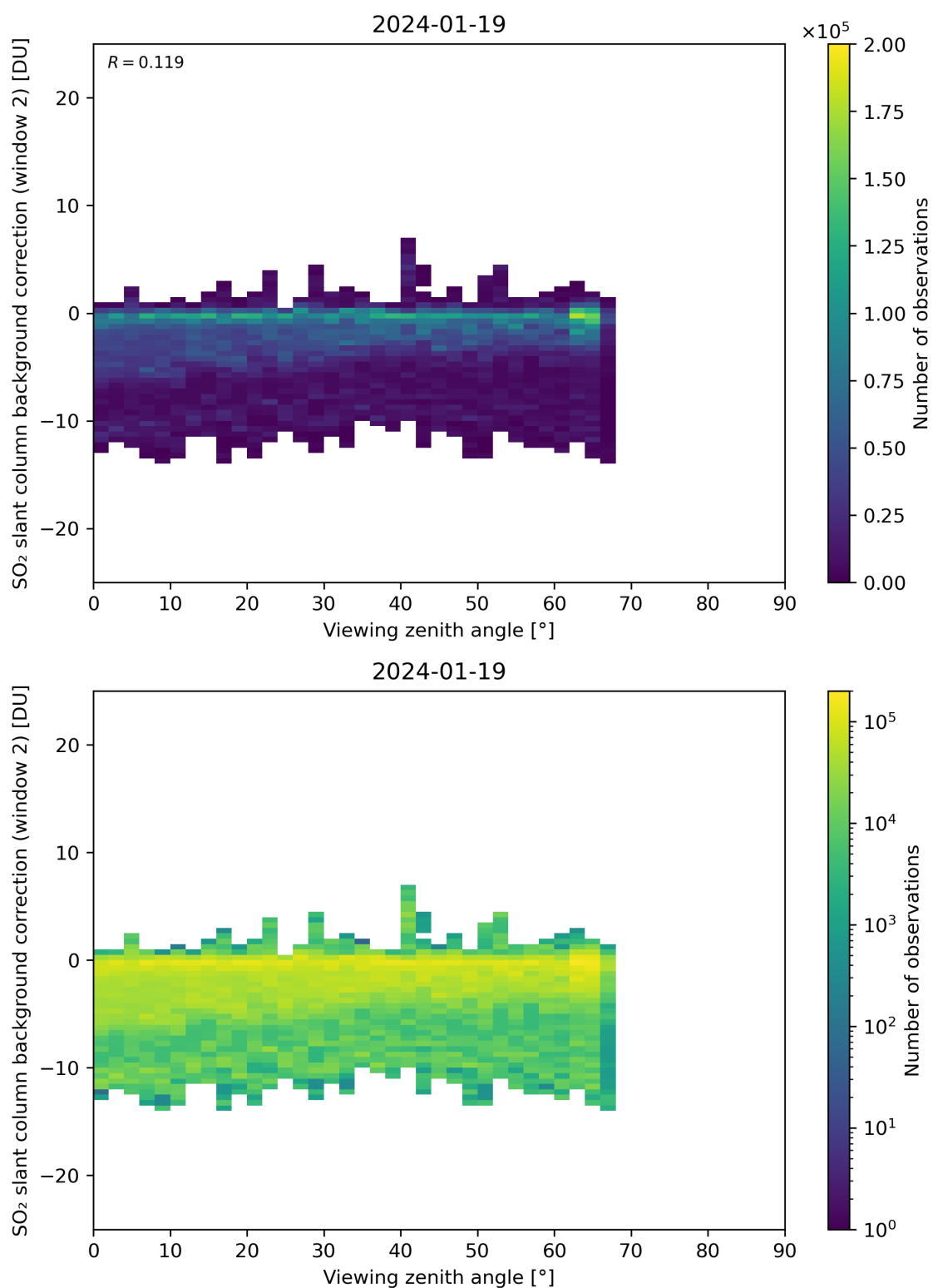
Figure 309: Scatter density plot of “Viewing zenith angle” against “SO 2 slant column background correction (window 2)” for 2024-01-18 to 2024-01-20.
