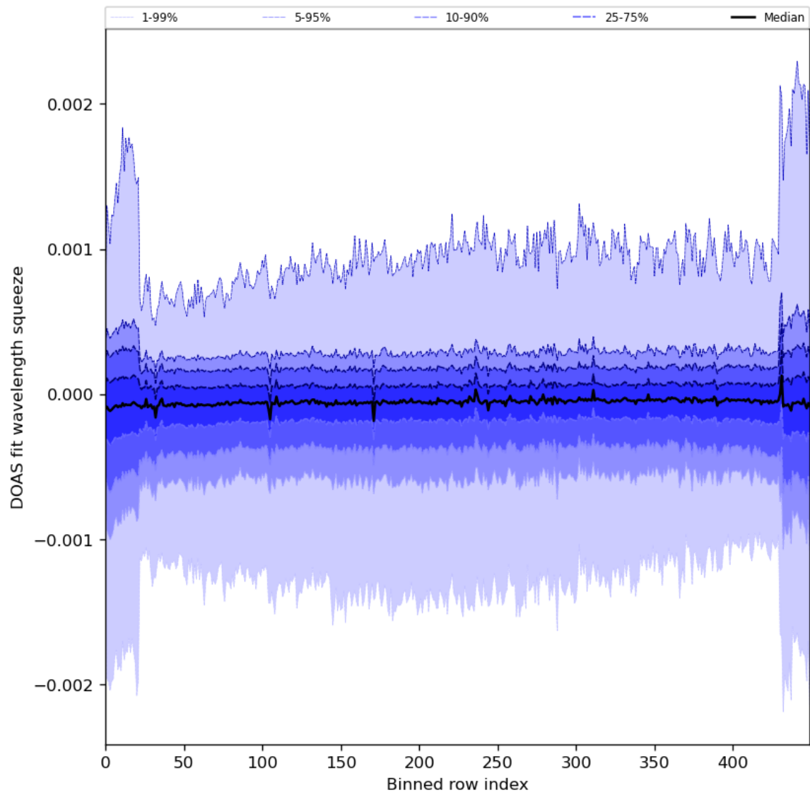
Figure 92: Along track statistics of “DOAS fit wavelength squeeze” for 2024-01-18 to 2024-01-20
