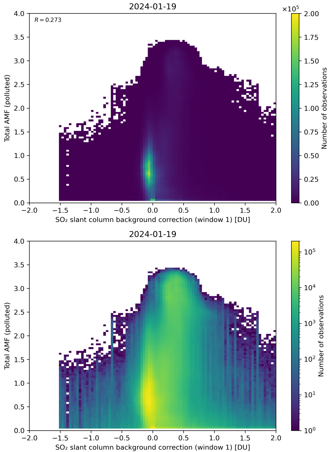
Figure 109: Scatter density plot of “SO 2 slant column background correction (window 1)” against “Total AMF (polluted)” for 2024-01-18 to 2024-01-20.
