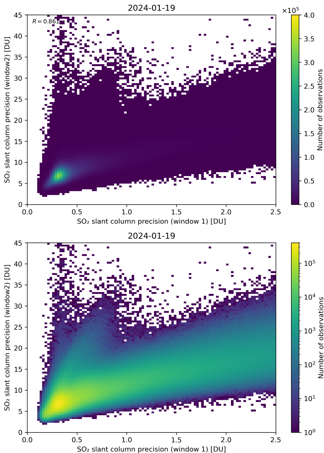
Figure 227: Scatter density plot of “SO 2 slant column precision (window 1)” against “SO 2 slant column precision (window2)” for 2024-01-18 to 2024-01-20.
