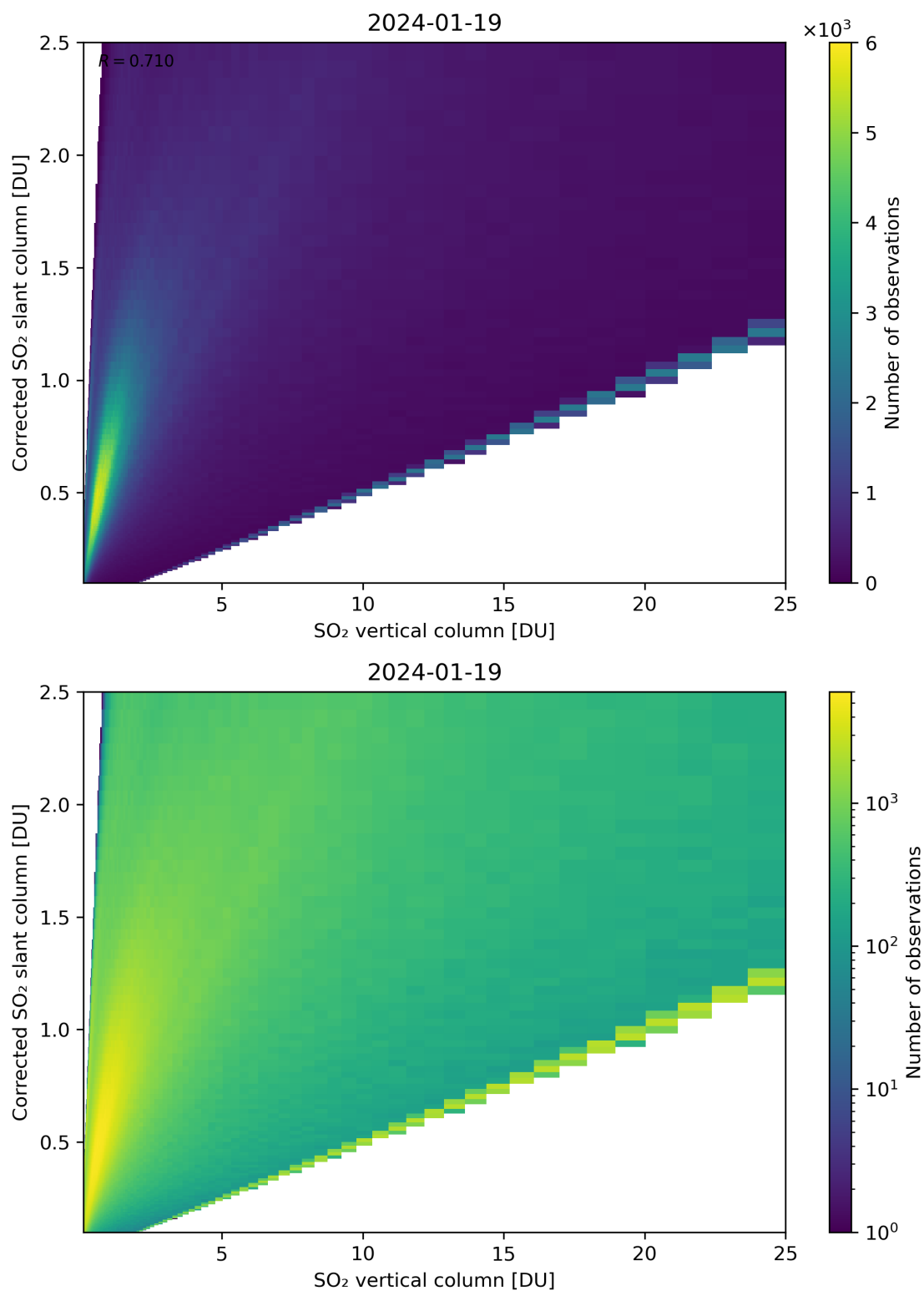
Figure 297: Scatter density plot of “SO 2 vertical column” against “Corrected SO 2 slant column” for 2024-01-18 to 2024-01-20.
