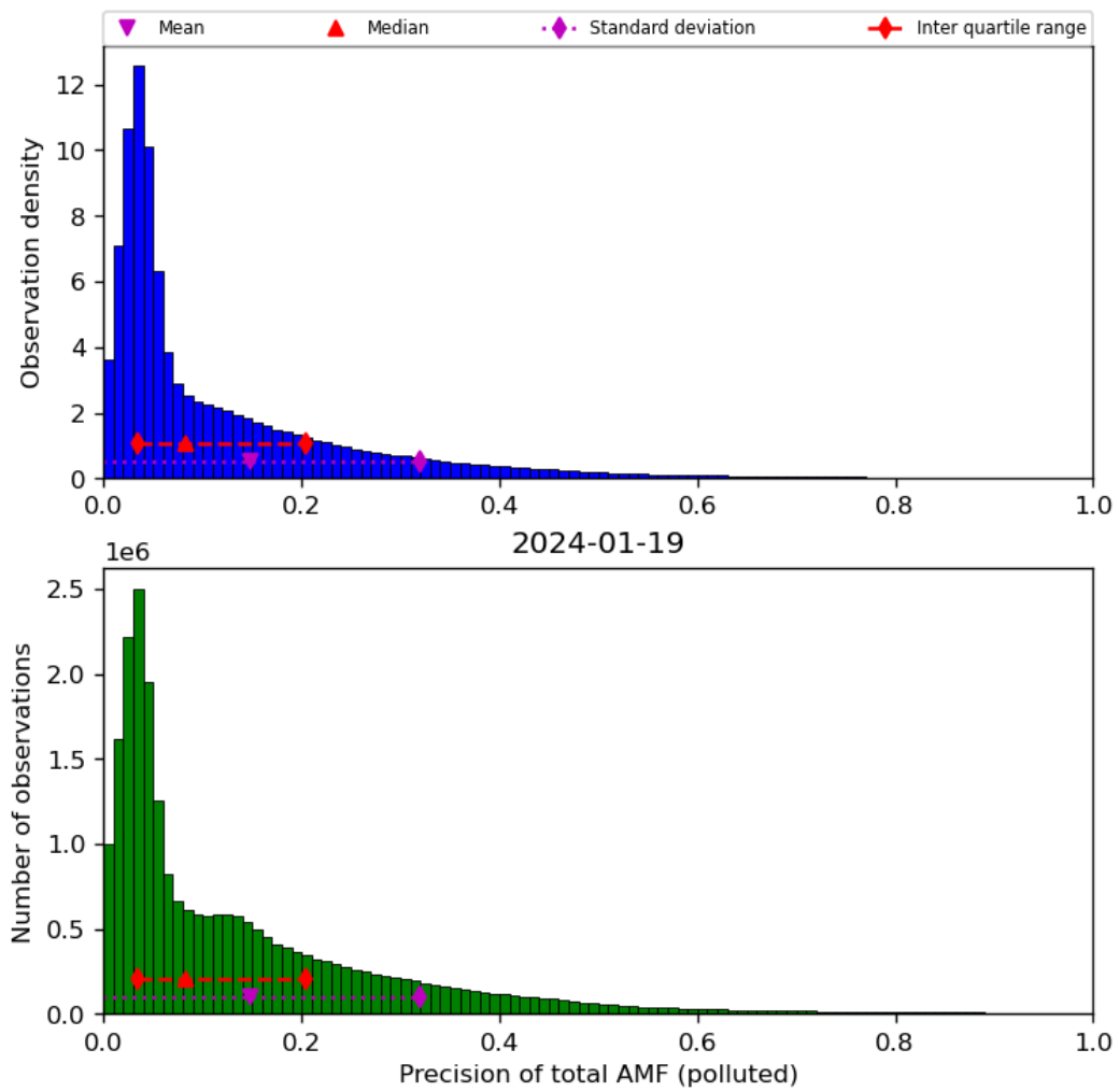
Figure 72: Histogram of “Precision of total AMF (polluted)” for 2024-01-18 to 2024-01-20
