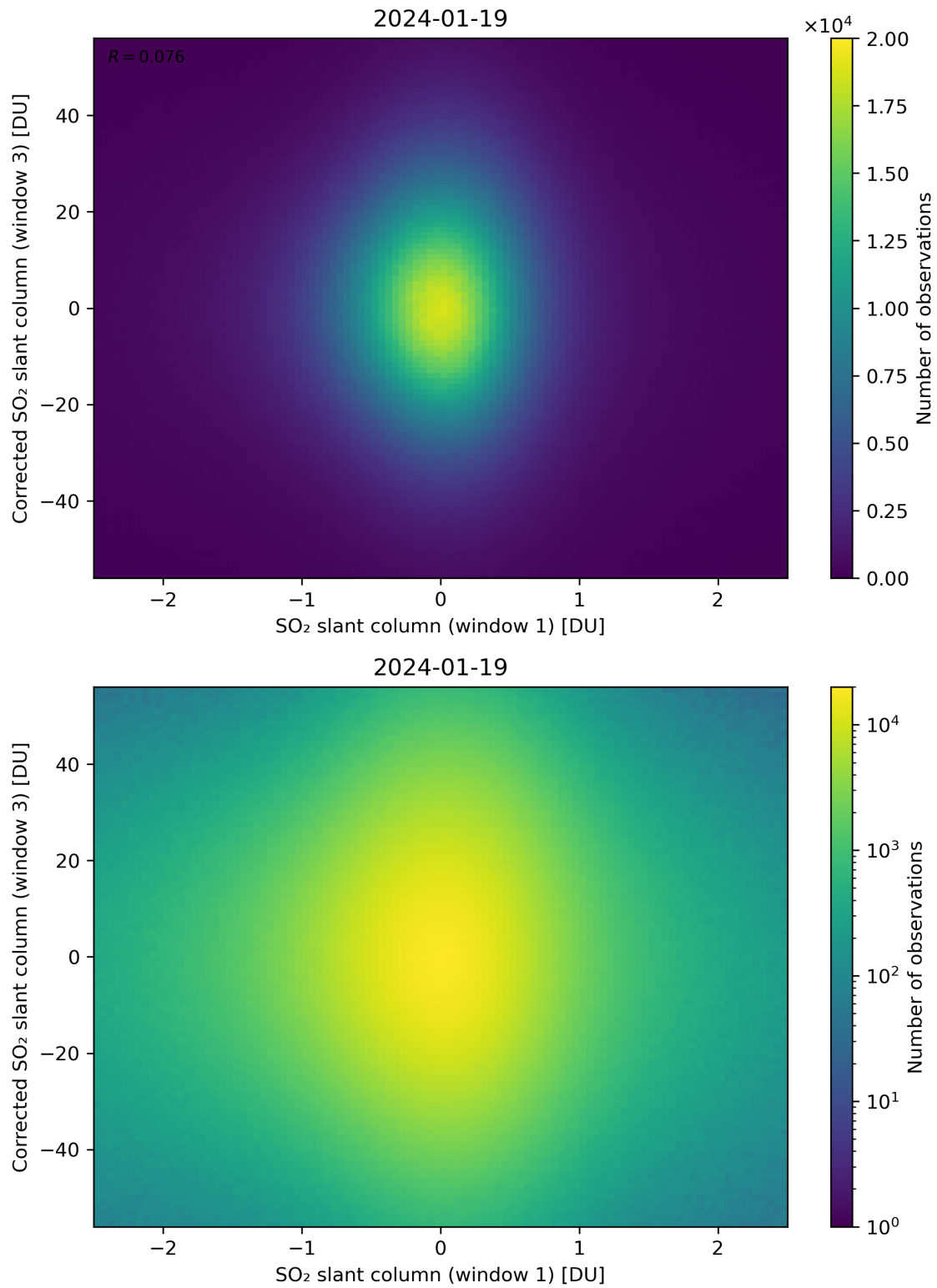
Figure 234: Scatter density plot of “SO 2 slant column (window 1)” against “Corrected SO 2 slant column (window 3)” for 2024-01-18 to 2024-01-20.
