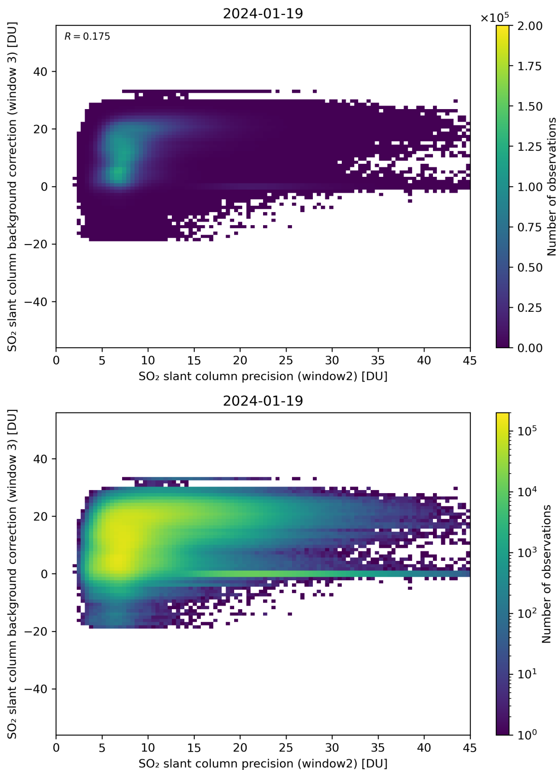
Figure 242: Scatter density plot of “SO 2 slant column precision (window2)” against “SO 2 slant column background correction (window 3)” for 2024-01-18 to 2024-01-20.
