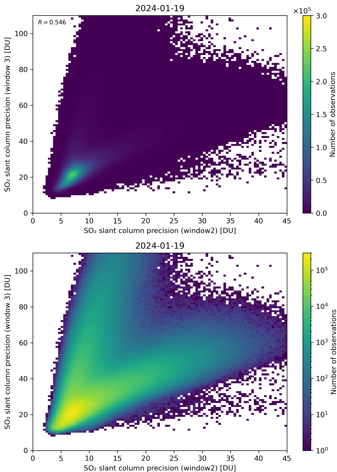
Figure 250: Scatter density plot of “SO 2 slant column precision (window2)” against “SO 2 slant column precision (window 3)” for 2024-01-18 to 2024-01-20.
