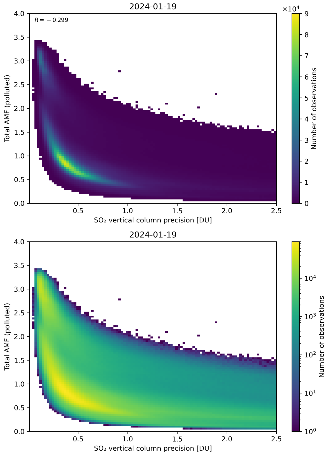
Figure 294: Scatter density plot of “SO 2 vertical column precision” against “Total AMF (polluted)” for 2024-01-18 to 2024-01-20.
