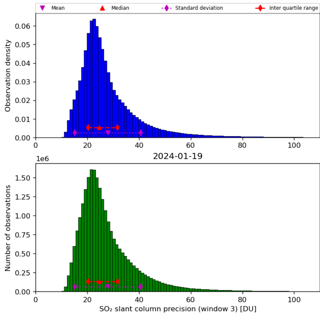
Figure 65: Histogram of “SO 2 slant column precision (window 3)” for 2024-01-18 to 2024-01-20
