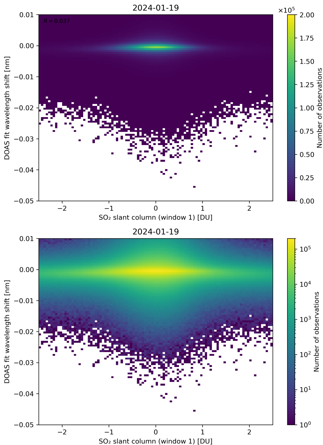
Figure 215: Scatter density plot of “SO 2 slant column (window 1)” against “DOAS fit wavelength shift” for 2024-01-18 to 2024-01-20.
