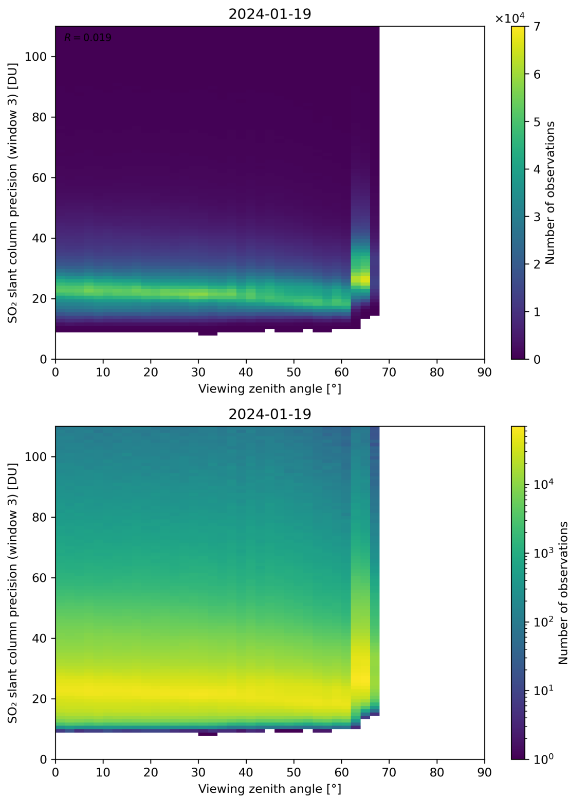
Figure 324: Scatter density plot of “Viewing zenith angle” against “SO 2 slant column precision (window 3)” for 2024-01-18 to 2024-01-20.
