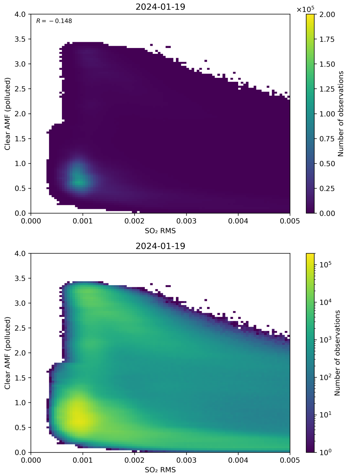
Figure 136: Scatter density plot of “SO 2 RMS” against “Clear AMF (polluted)” for 2024-01-18 to 2024-01-20.
