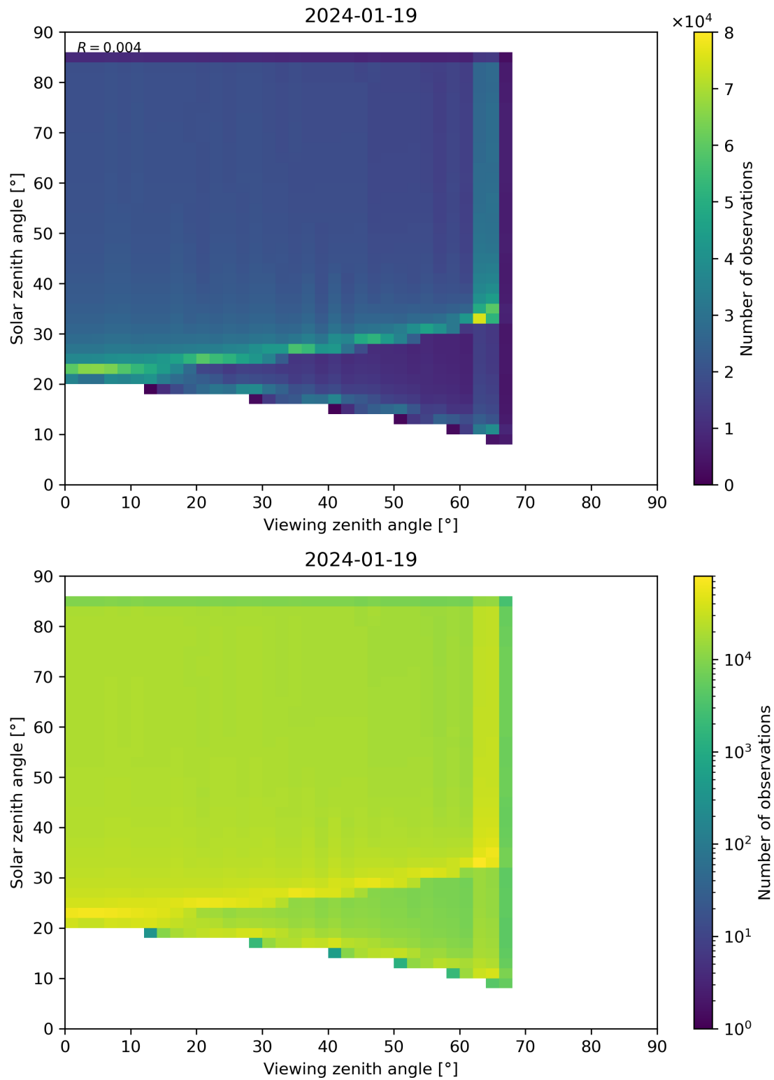
Figure 315: Scatter density plot of “Viewing zenith angle” against “Solar zenith angle” for 2024-01-18 to 2024-01-20.
