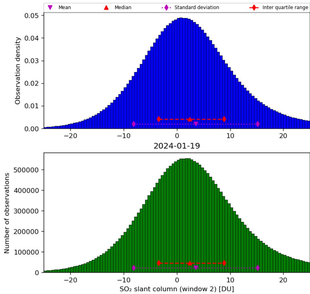
Figure 60: Histogram of “SO 2 slant column (window 2)” for 2024-01-18 to 2024-01-20
