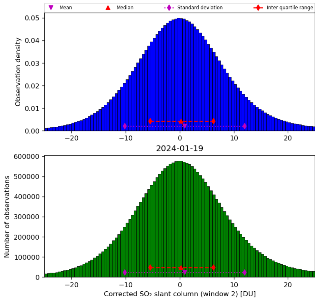
Figure 62: Histogram of “Corrected SO 2 slant column (window 2)” for 2024-01-18 to 2024-01-20
