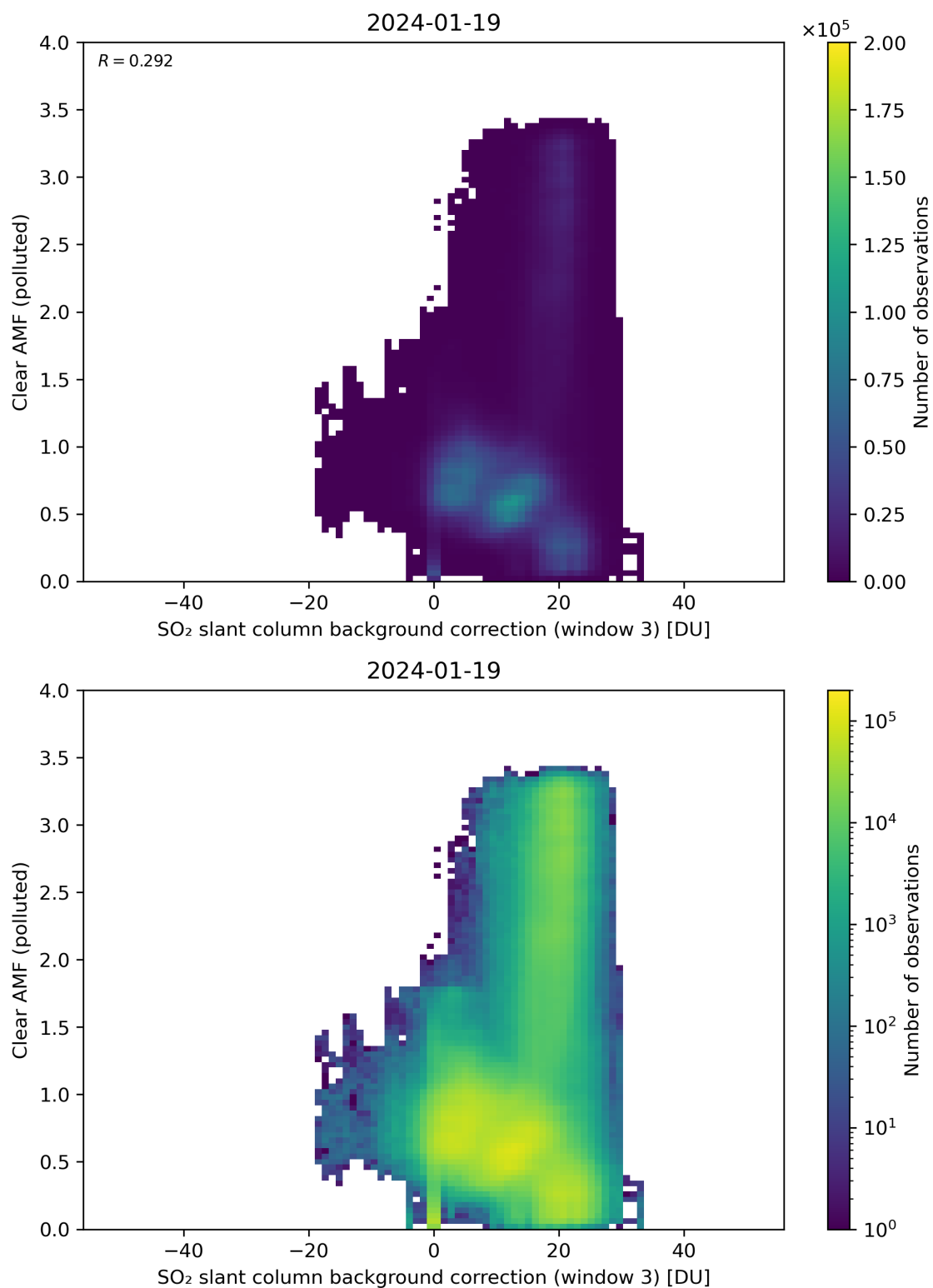
Figure 124: Scatter density plot of “SO 2 slant column background correction (window 3)” against “Clear AMF (polluted)” for 2024-01-18 to 2024-01-20.
