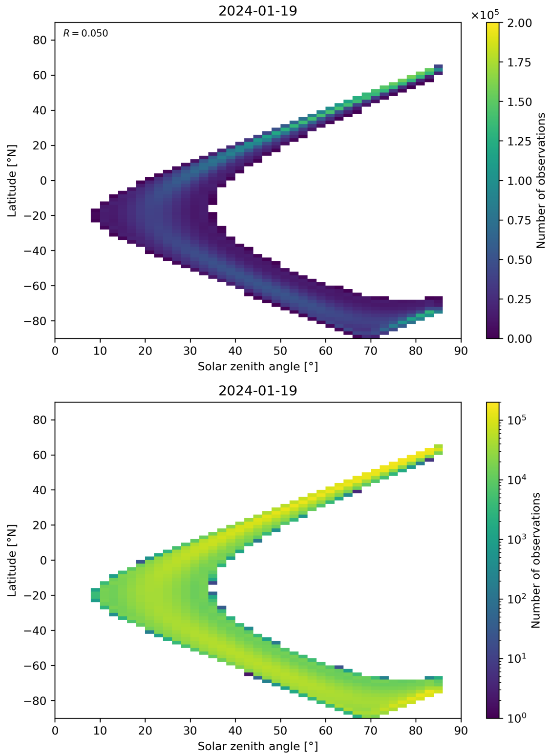
Figure 164: Scatter density plot of “Solar zenith angle” against “Latitude” for 2024-01-18 to 2024-01-20.
