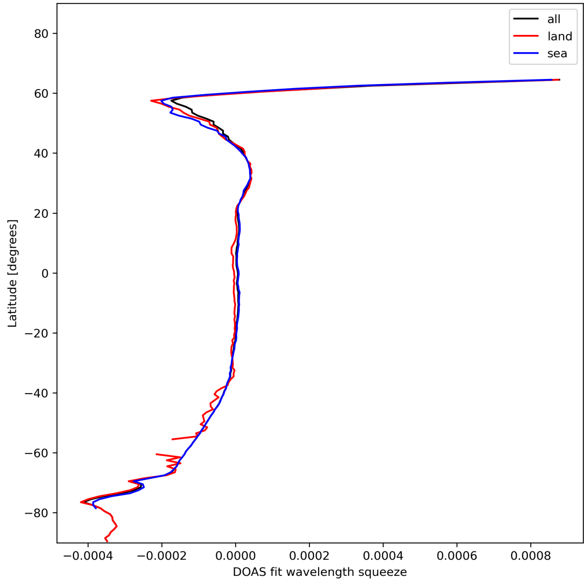
Figure 46: Zonal average of “DOAS fit wavelength squeeze” for 2024-01-18 to 2024-01-20.
