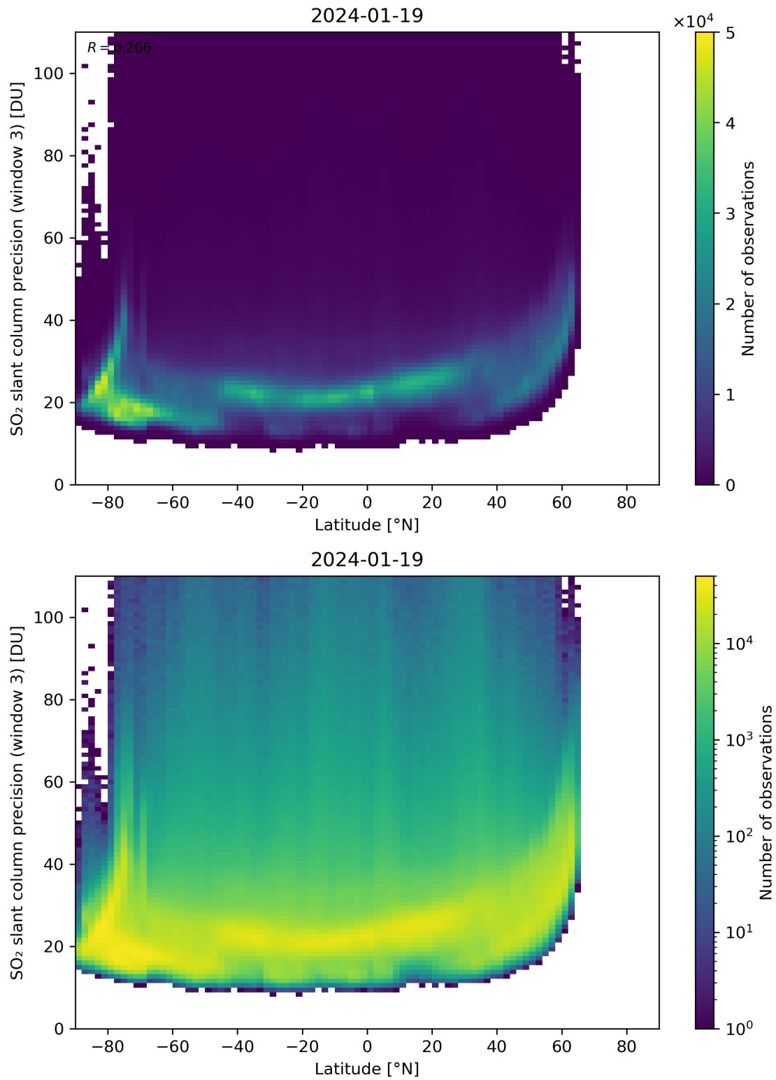
Figure 153: Scatter density plot of “Latitude” against “SO 2 slant column precision (window 3)” for 2024-01-18 to 2024-01-20.
