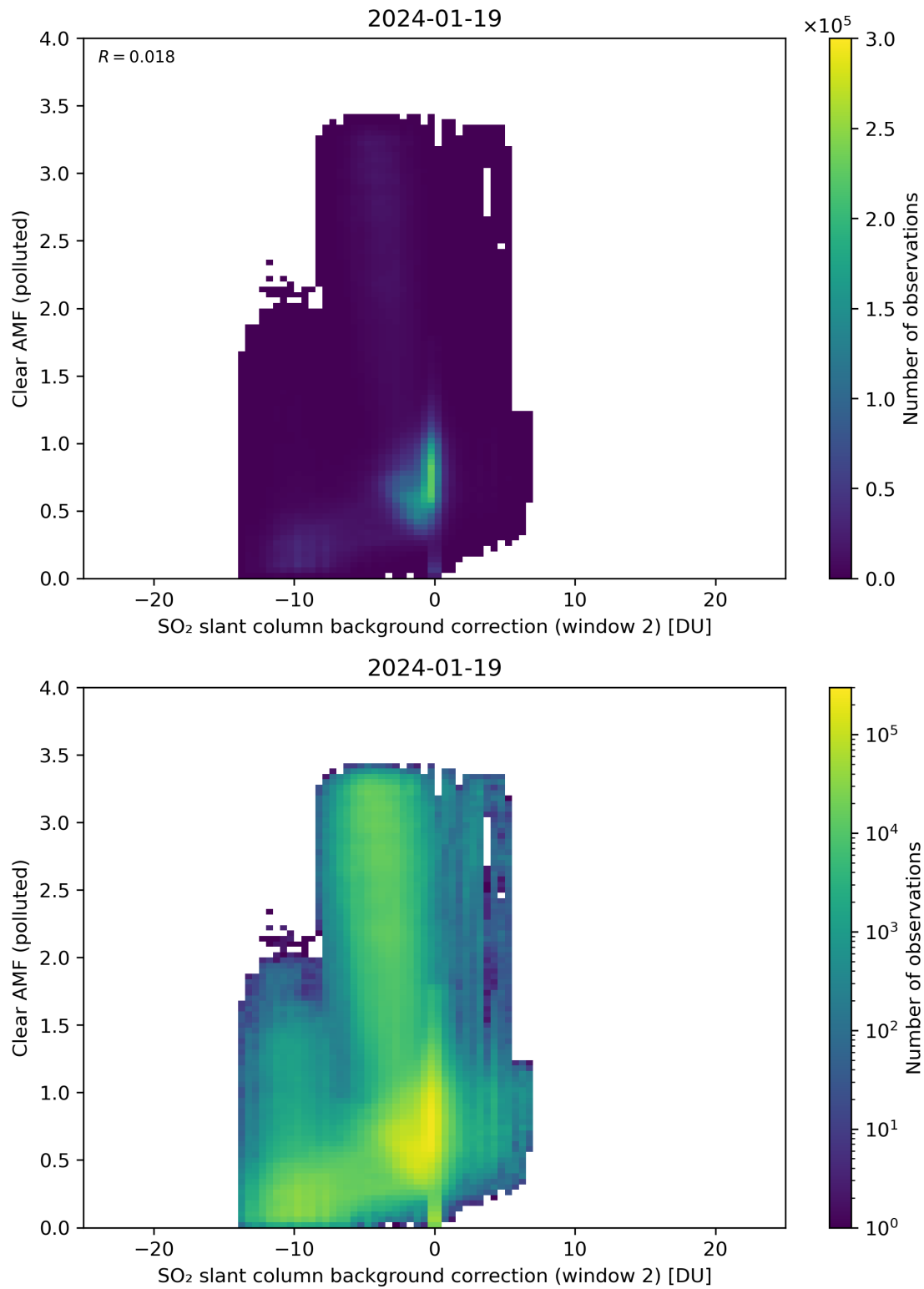
Figure 115: Scatter density plot of “SO 2 slant column background correction (window 2)” against “Clear AMF (polluted)” for 2024-01-18 to 2024-01-20.
