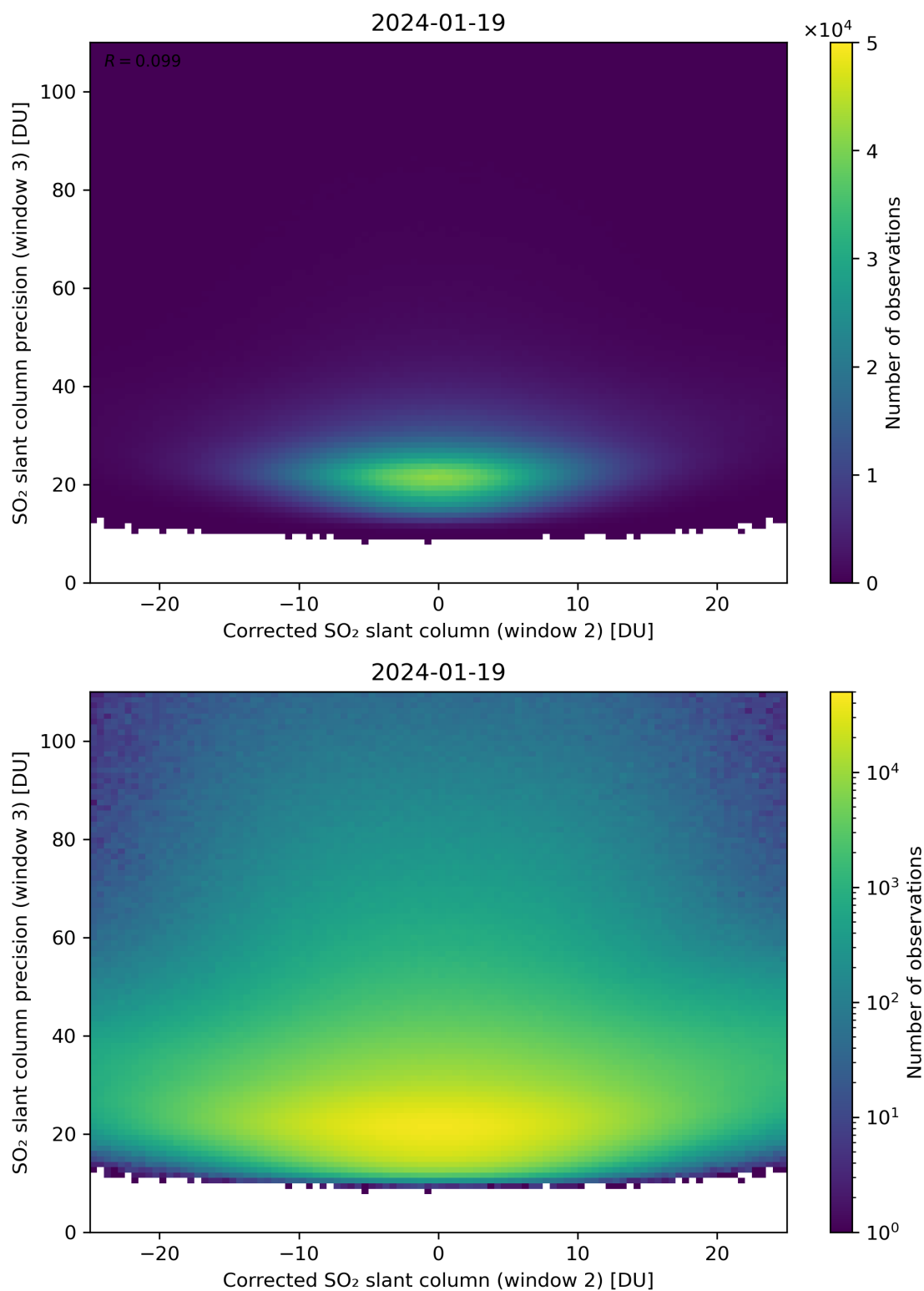
Figure 202: Scatter density plot of “Corrected SO 2 slant column (window 2)” against “SO 2 slant column precision (window 3)” for 2024-01-18 to 2024-01-20.
