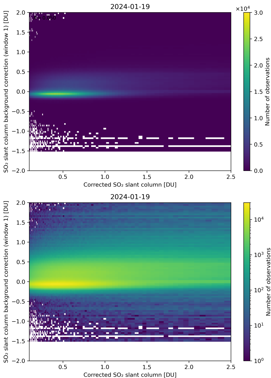
Figure 178: Scatter density plot of “Corrected SO 2 slant column” against “SO 2 slant column background correction (window 1)” for 2024-01-18 to 2024-01-20.
