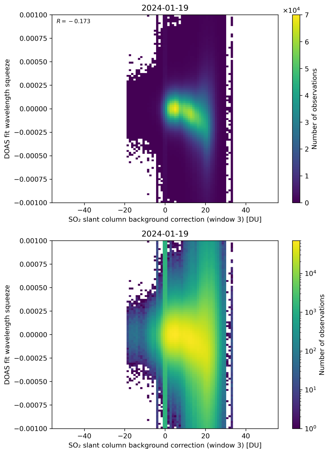
Figure 122: Scatter density plot of “SO 2 slant column background correction (window 3)” against “DOAS fit wavelength squeeze” for 2024-01-18 to 2024-01-20.
