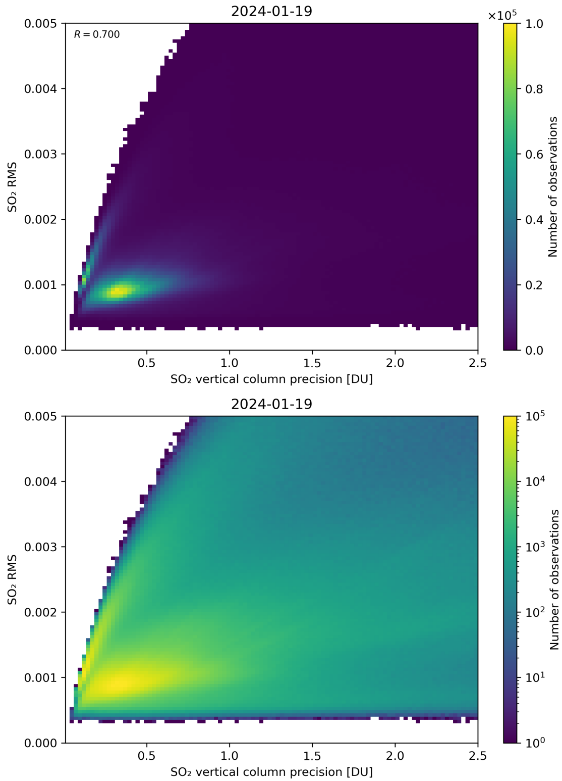
Figure 284: Scatter density plot of “SO 2 vertical column precision” against “SO 2 RMS” for 2024-01-18 to 2024-01-20.
