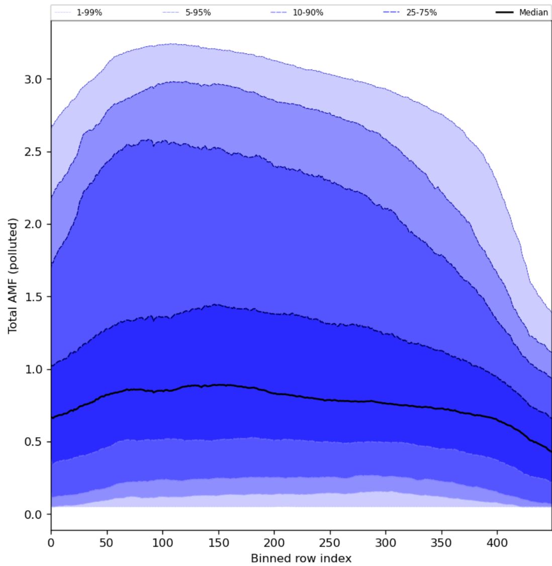
Figure 94: Along track statistics of “Total AMF (polluted)” for 2024-01-18 to 2024-01-20
