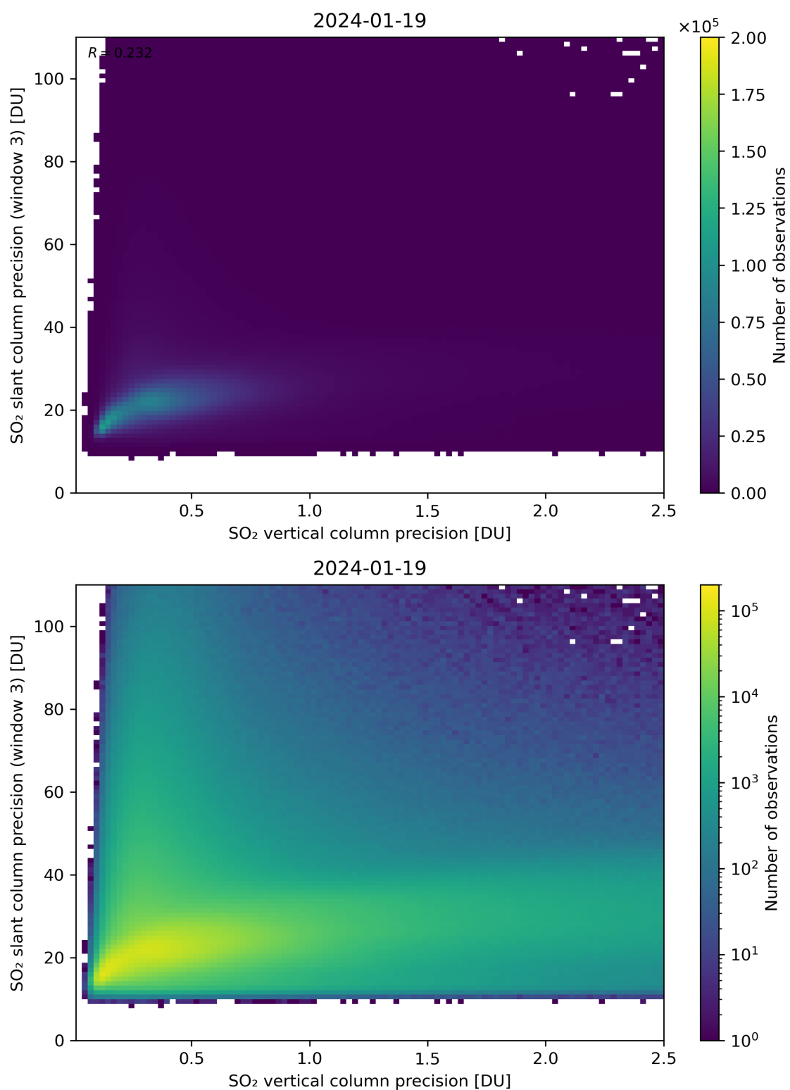
Figure 293: Scatter density plot of “SO 2 vertical column precision” against “SO 2 slant column precision (window 3)” for 2024-01-18 to 2024-01-20.
