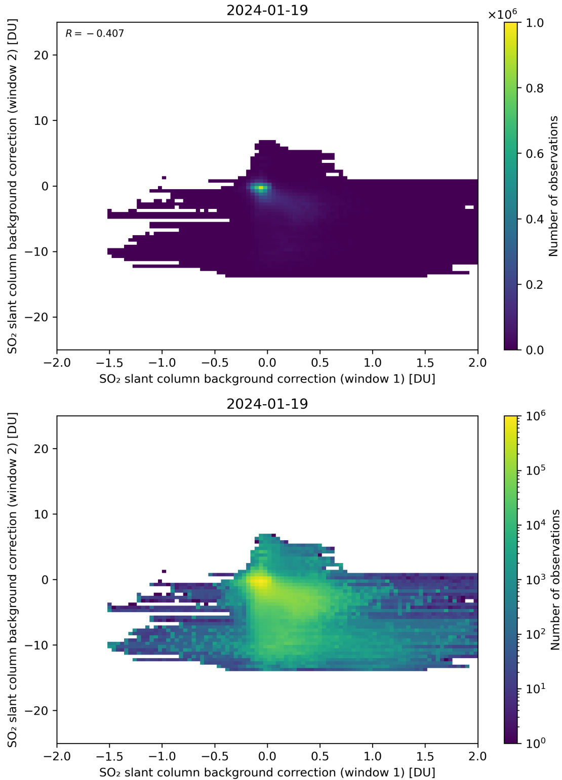
Figure 98: Scatter density plot of “SO 2 slant column background correction (window 1)” against “SO 2 slant column background correction (window 2)” for 2024-01-18 to 2024-01-20.
