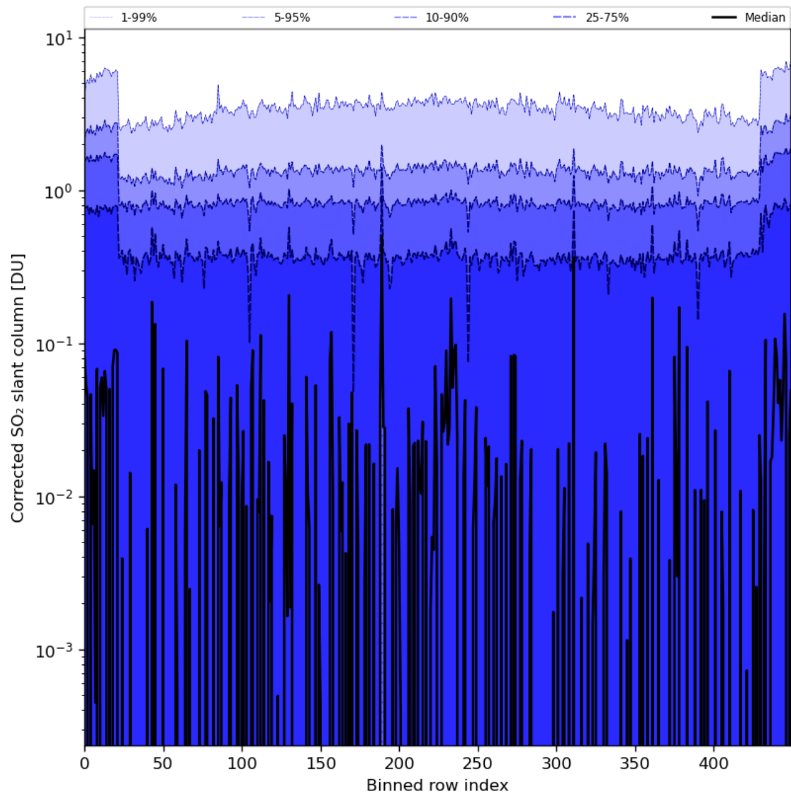
Figure 78: Along track statistics of "Corrected SO 2 slant column" for 2024-01-18 to 2024-01-20
