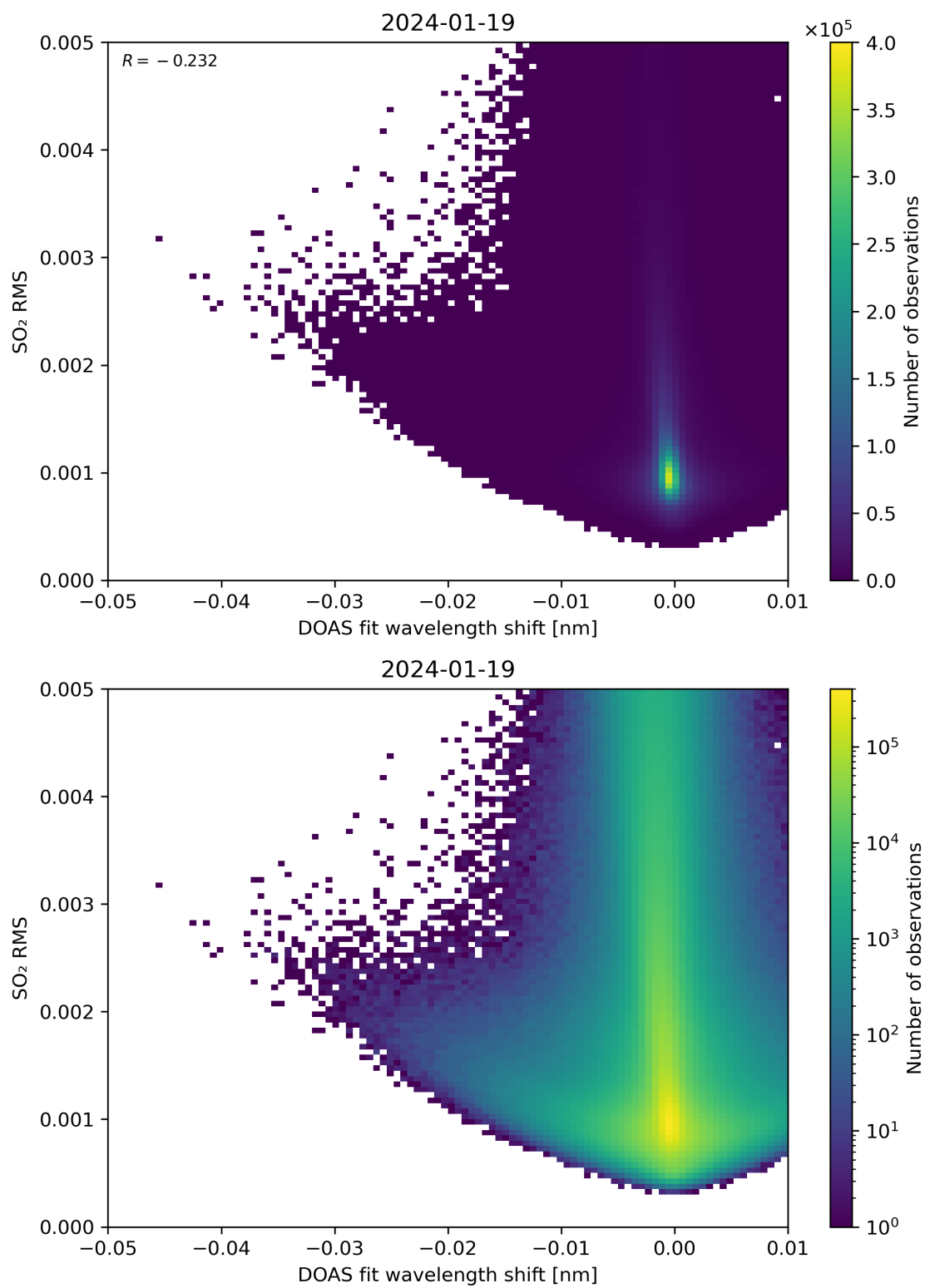
Figure 128: Scatter density plot of “DOAS fit wavelength shift” against “SO 2 RMS” for 2024-01-18 to 2024-01-20.
