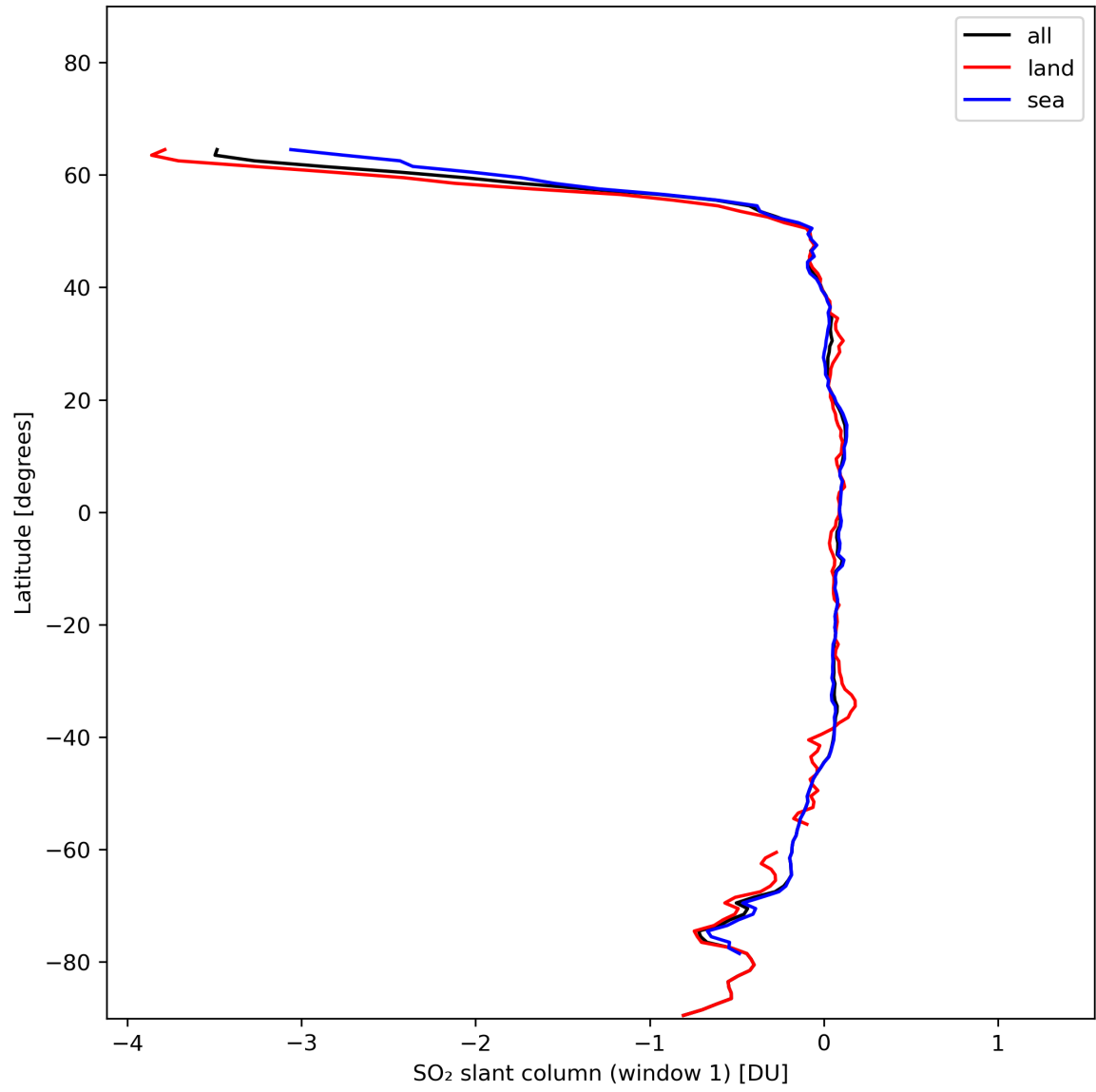
Figure 33: Zonal average of “SO 2 slant column (window 1)” for 2024-01-18 to 2024-01-20.
