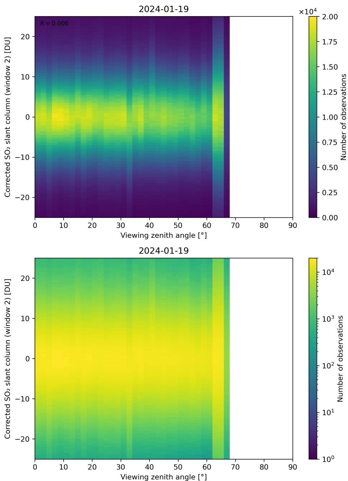
Figure 318: Scatter density plot of “Viewing zenith angle” against “Corrected SO 2 slant column (window 2)” for 2024-01-18 to 2024-01-20.
