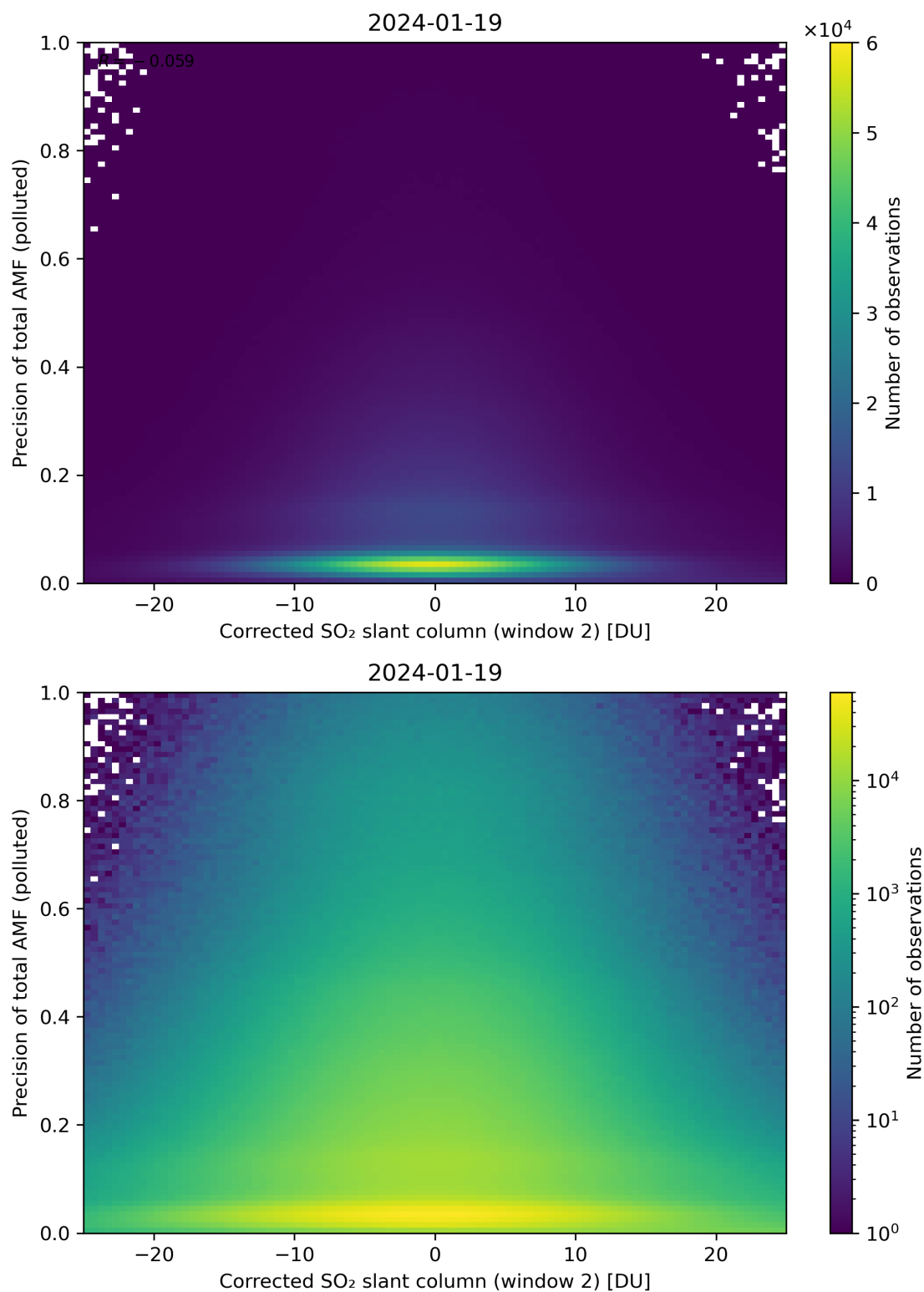
Figure 204: Scatter density plot of “Corrected SO 2 slant column (window 2)” against “Precision of total AMF (polluted)” for 2024-01-18 to 2024-01-20.
