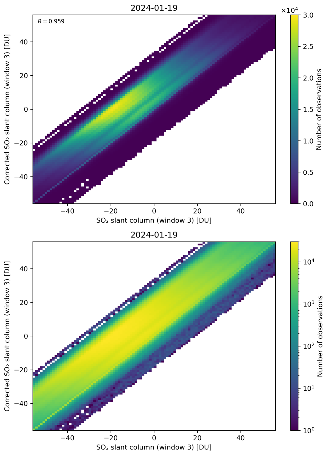
Figure 266: Scatter density plot of “SO 2 slant column (window 3)” against “Corrected SO 2 slant column (window 3)” for 2024-01-18 to 2024-01-20.
