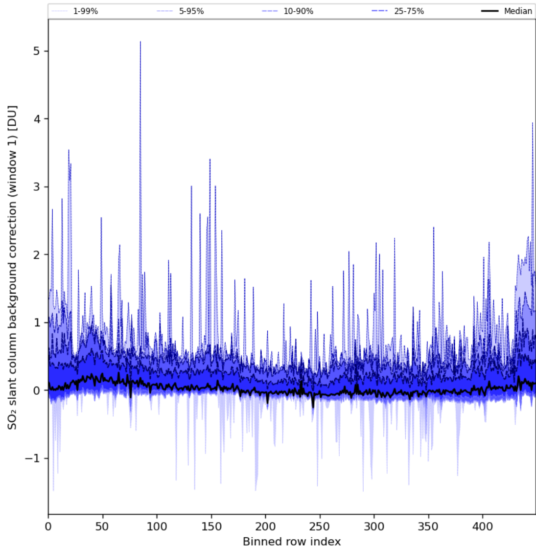
Figure 82: Along track statistics of “SO 2 slant column background correction (window 1)” for 2024-01-18 to 2024-01-20
