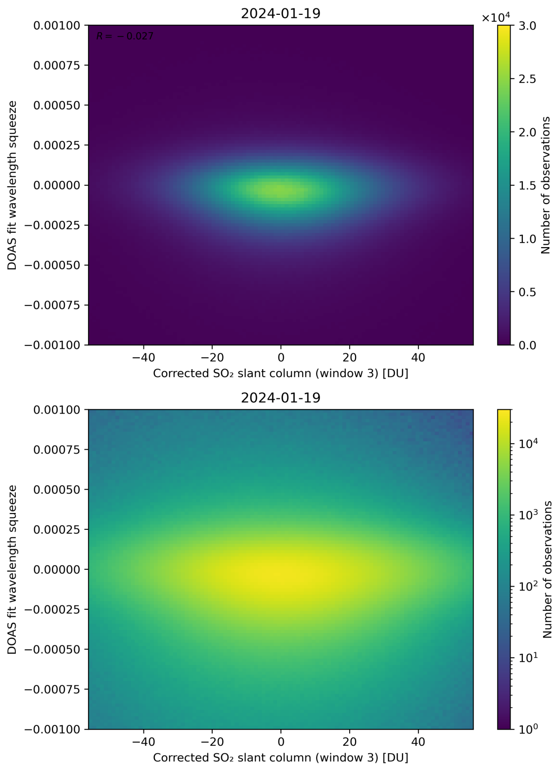
Figure 207: Scatter density plot of “Corrected SO 2 slant column (window 3)” against “DOAS fit wavelength squeeze” for 2024-01-18 to 2024-01-20.
