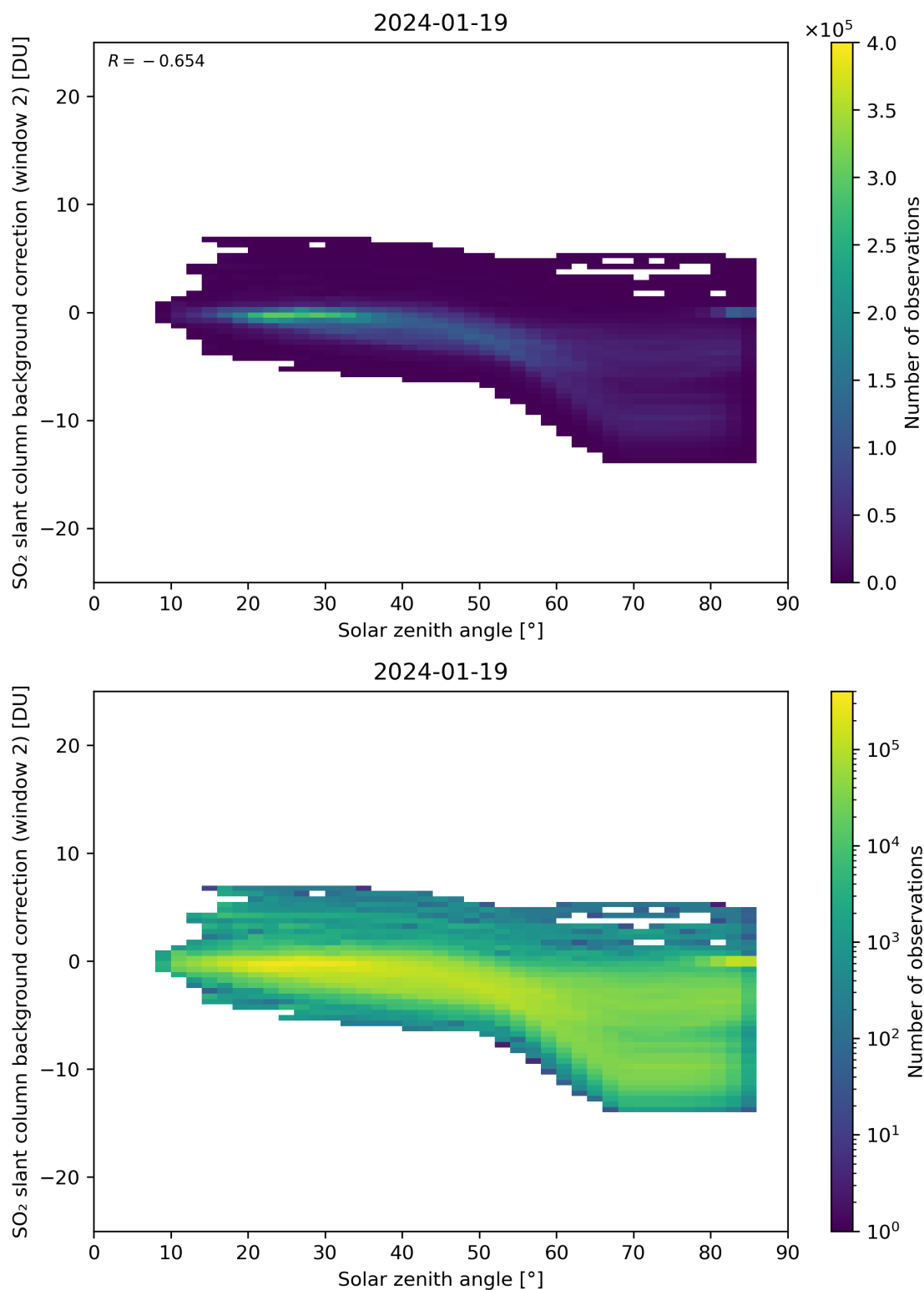
Figure 159: Scatter density plot of “Solar zenith angle” against “SO 2 slant column background correction (window 2)” for 2024-01-18 to 2024-01-20.
