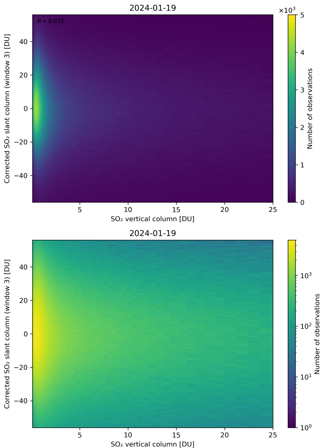
Figure 299: Scatter density plot of “SO 2 vertical column” against “Corrected SO 2 slant column (window 3)” for 2024-01-18 to 2024-01-20.
