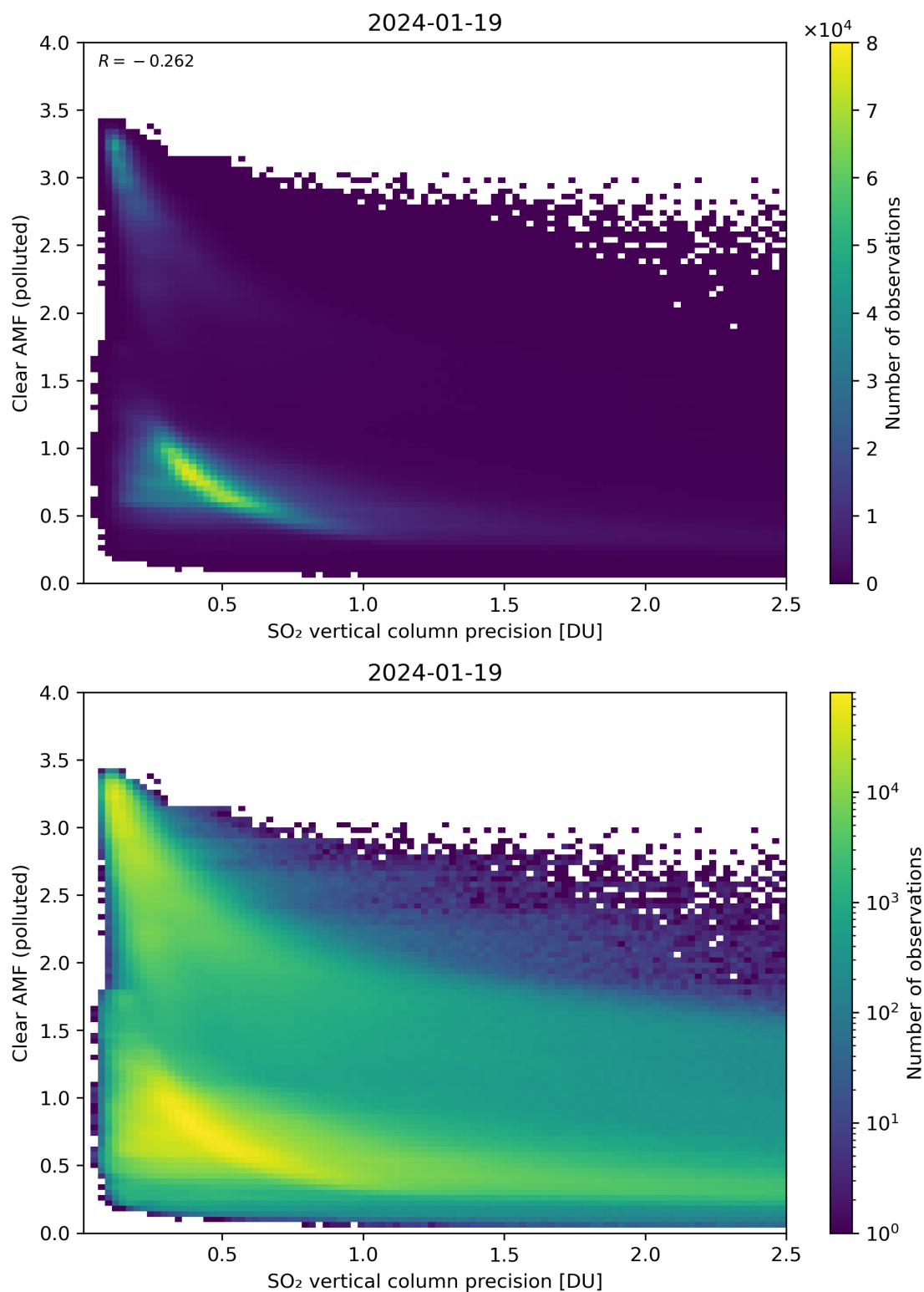
Figure 285: Scatter density plot of “SO 2 vertical column precision” against “Clear AMF (polluted)” for 2024-01-18 to 2024-01-20.
