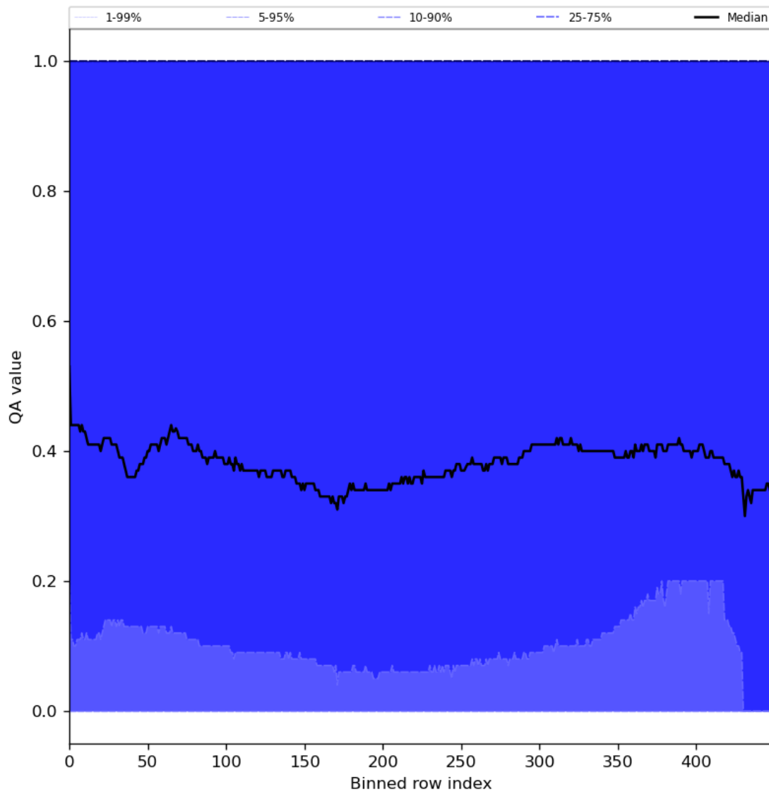
Figure 75: Along track statistics of “QA value” for 2024-01-18 to 2024-01-20
