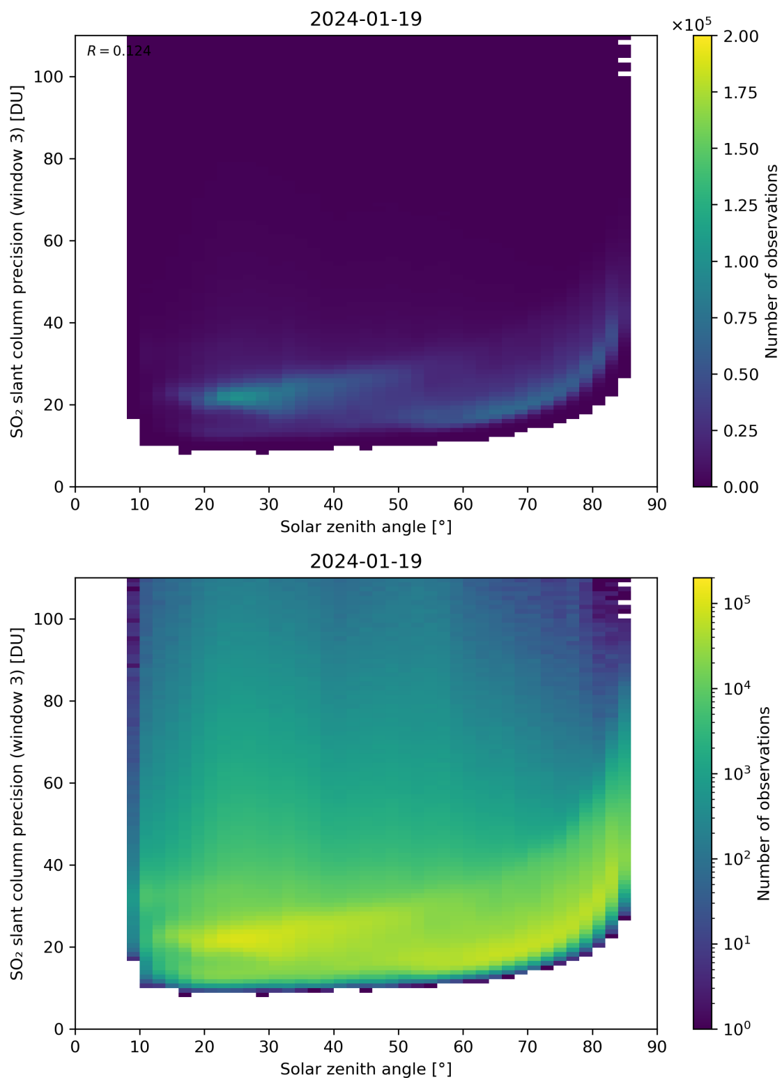
Figure 173: Scatter density plot of “Solar zenith angle” against “SO 2 slant column precision (window 3)” for 2024-01-18 to 2024-01-20.
