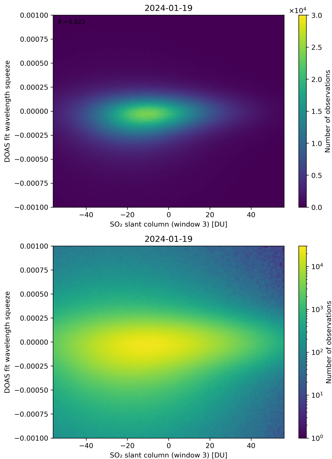
Figure 255: Scatter density plot of “SO 2 slant column (window 3)” against “DOAS fit wavelength squeeze” for 2024-01-18 to 2024-01-20.
