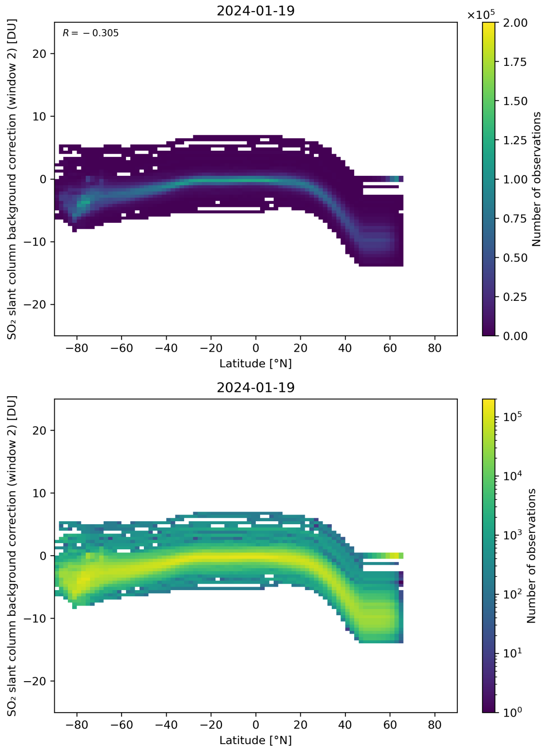
Figure 140: Scatter density plot of “Latitude” against “SO 2 slant column background correction (window 2)” for 2024-01-18 to 2024-01-20.
