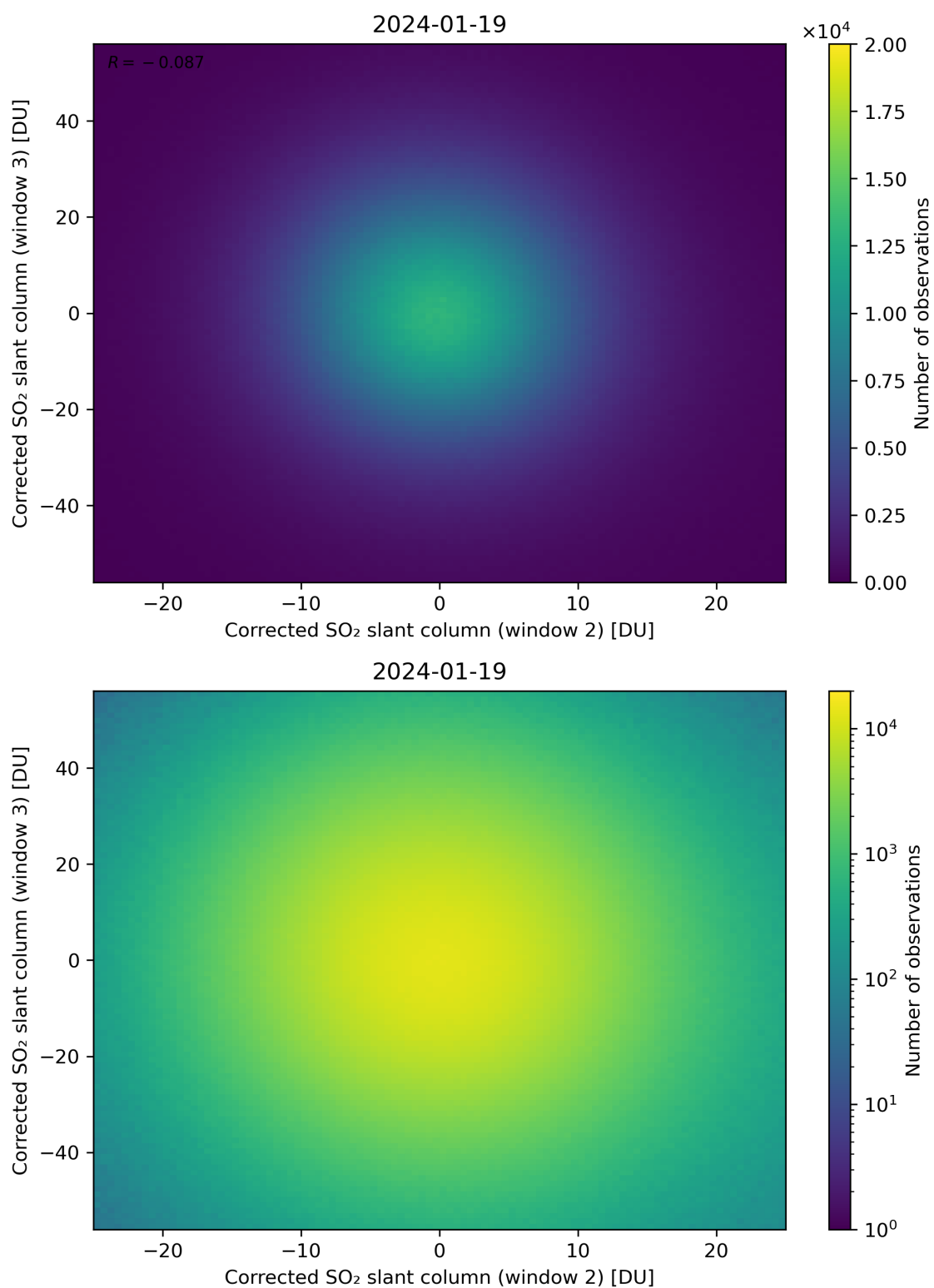
Figure 200: Scatter density plot of “Corrected SO 2 slant column (window 2)” against “Corrected SO 2 slant column (window 3)” for 2024-01-18 to 2024-01-20.
