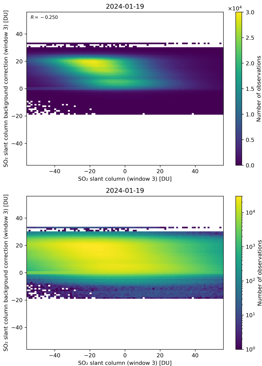
Figure 253: Scatter density plot of “SO 2 slant column (window 3)” against “SO 2 slant column background correction (window 3)” for 2024-01-18 to 2024-01-20.
