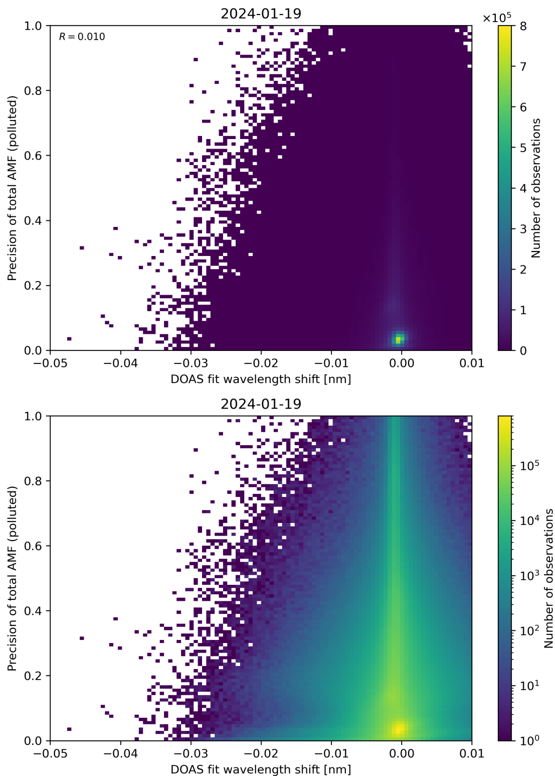
Figure 131: Scatter density plot of “DOAS fit wavelength shift” against “Precision of total AMF (polluted)” for 2024-01-18 to 2024-01-20.
