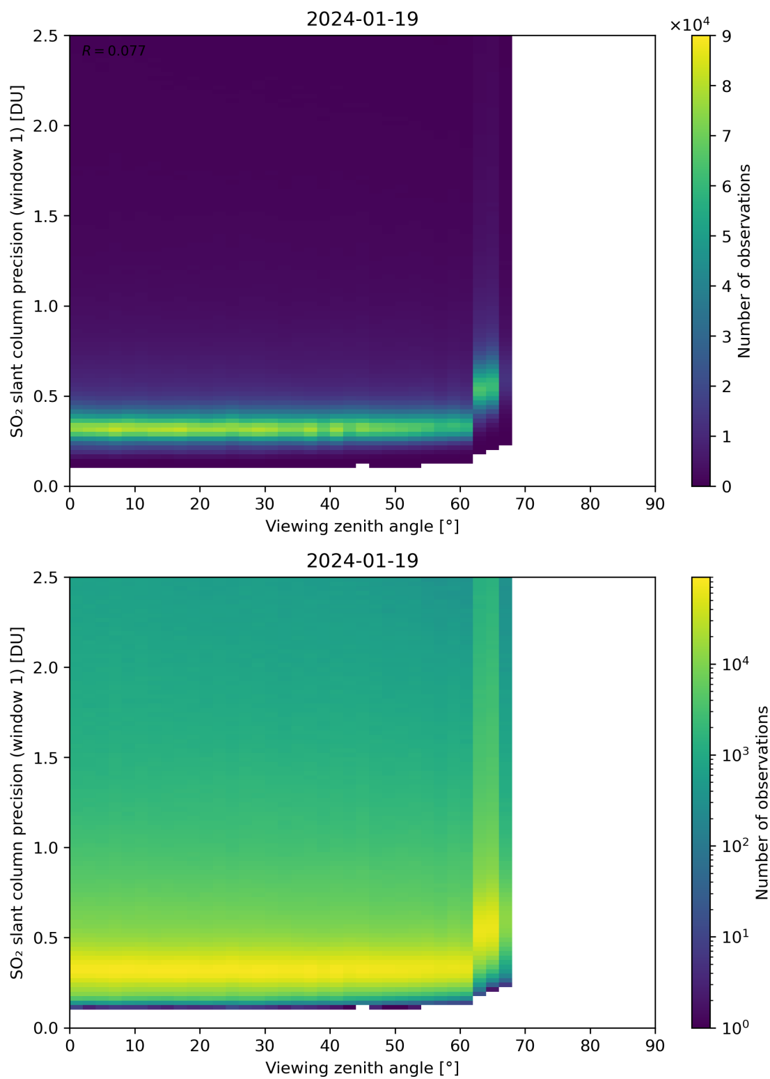
Figure 321: Scatter density plot of “Viewing zenith angle” against “SO 2 slant column precision (window 1)” for 2024-01-18 to 2024-01-20.
