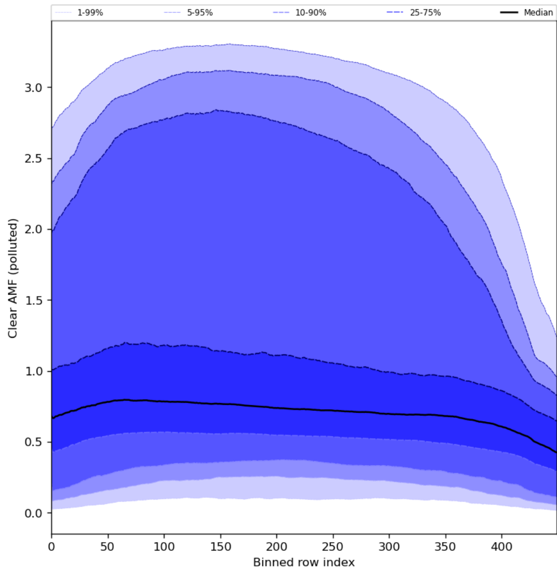
Figure 96: Along track statistics of “Clear AMF (polluted)” for 2024-01-18 to 2024-01-20
