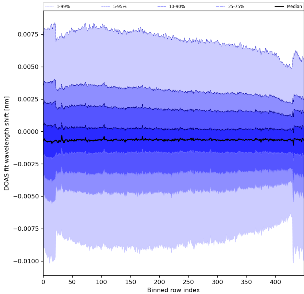
Figure 91: Along track statistics of “DOAS fit wavelength shift” for 2024-01-18 to 2024-01-20
