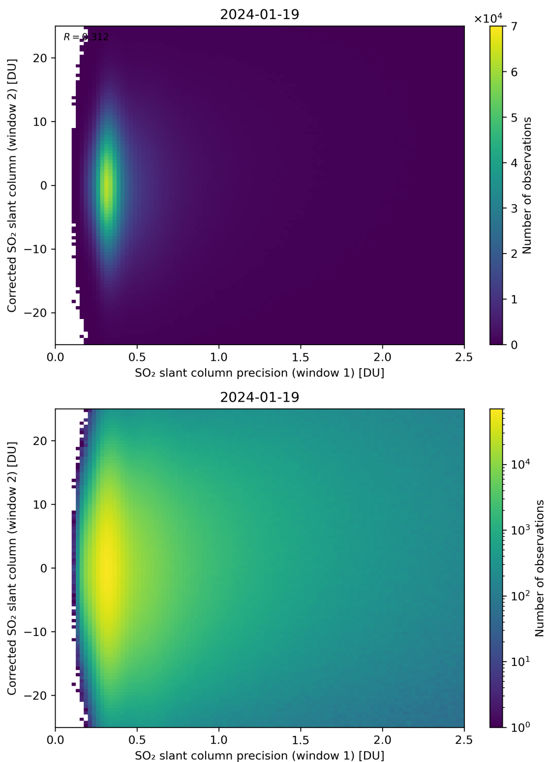
Figure 225: Scatter density plot of “SO 2 slant column precision (window 1)” against “Corrected SO 2 slant column (window 2)” for 2024-01-18 to 2024-01-20.
