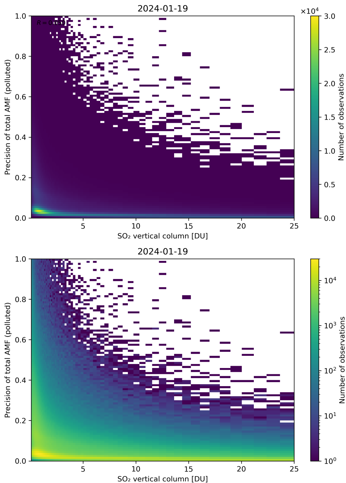
Figure 306: Scatter density plot of “SO 2 vertical column” against “Precision of total AMF (polluted)” for 2024-01-18 to 2024-01-20.
