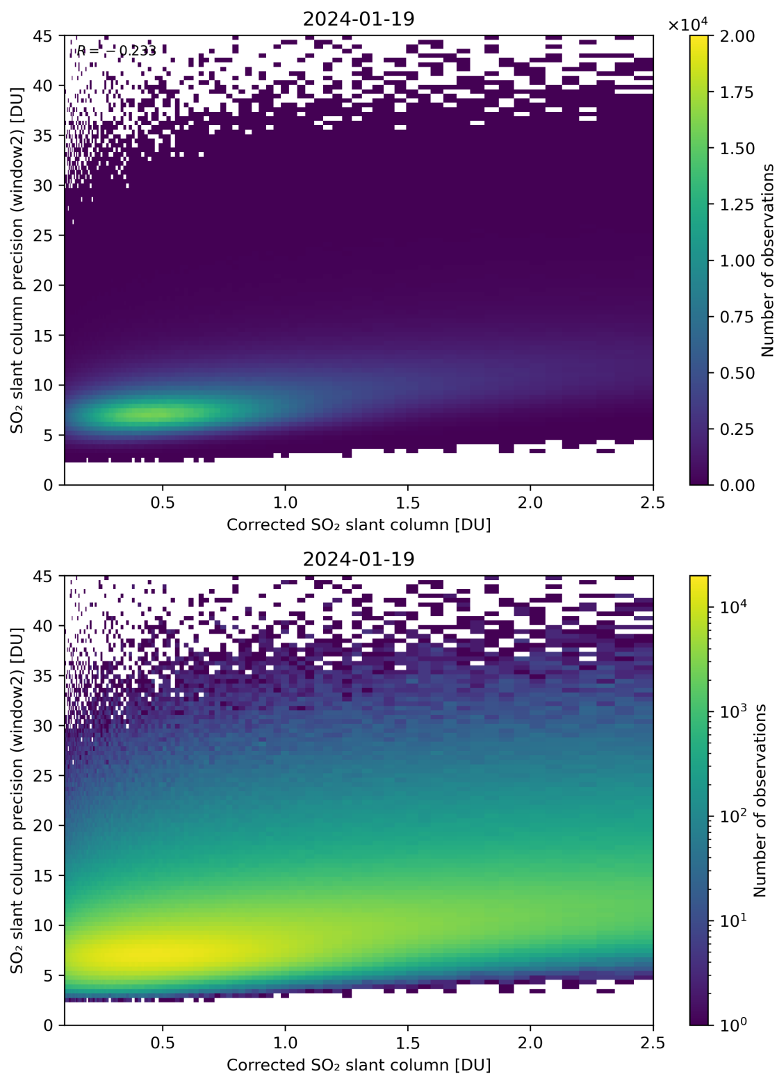
Figure 189: Scatter density plot of “Corrected SO 2 slant column” against “SO 2 slant column precision (window2)” for 2024-01-18 to 2024-01-20.
