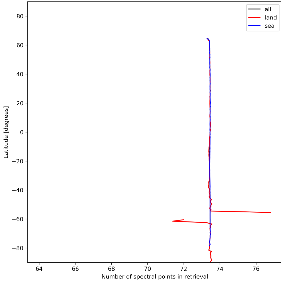
Figure 51: Zonal average of “Number of spectral points in retrieval” for 2024-01-18 to 2024-01-20.
