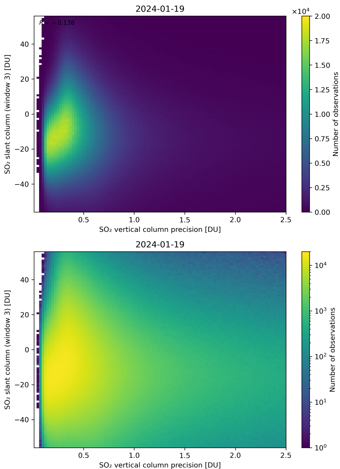
Figure 292: Scatter density plot of “SO 2 vertical column precision” against “SO 2 slant column (window 3)” for 2024-01-18 to 2024-01-20.
