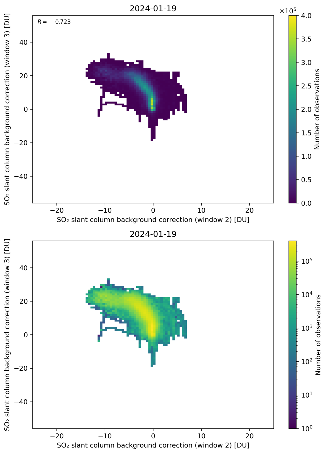
Figure 111: Scatter density plot of “SO 2 slant column background correction (window 2)” against “SO 2 slant column background correction (window 3)” for 2024-01-18 to 2024-01-20.
