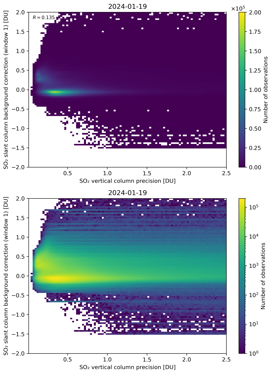
Figure 279: Scatter density plot of “SO 2 vertical column precision” against “SO 2 slant column background correction (window 1)” for 2024-01-18 to 2024-01-20.
