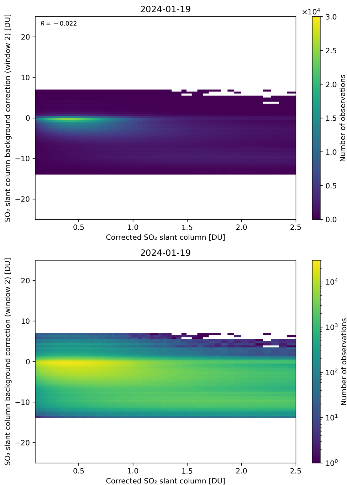
Figure 179: Scatter density plot of “Corrected SO 2 slant column” against “SO 2 slant column background correction (window 2)” for 2024-01-18 to 2024-01-20.
