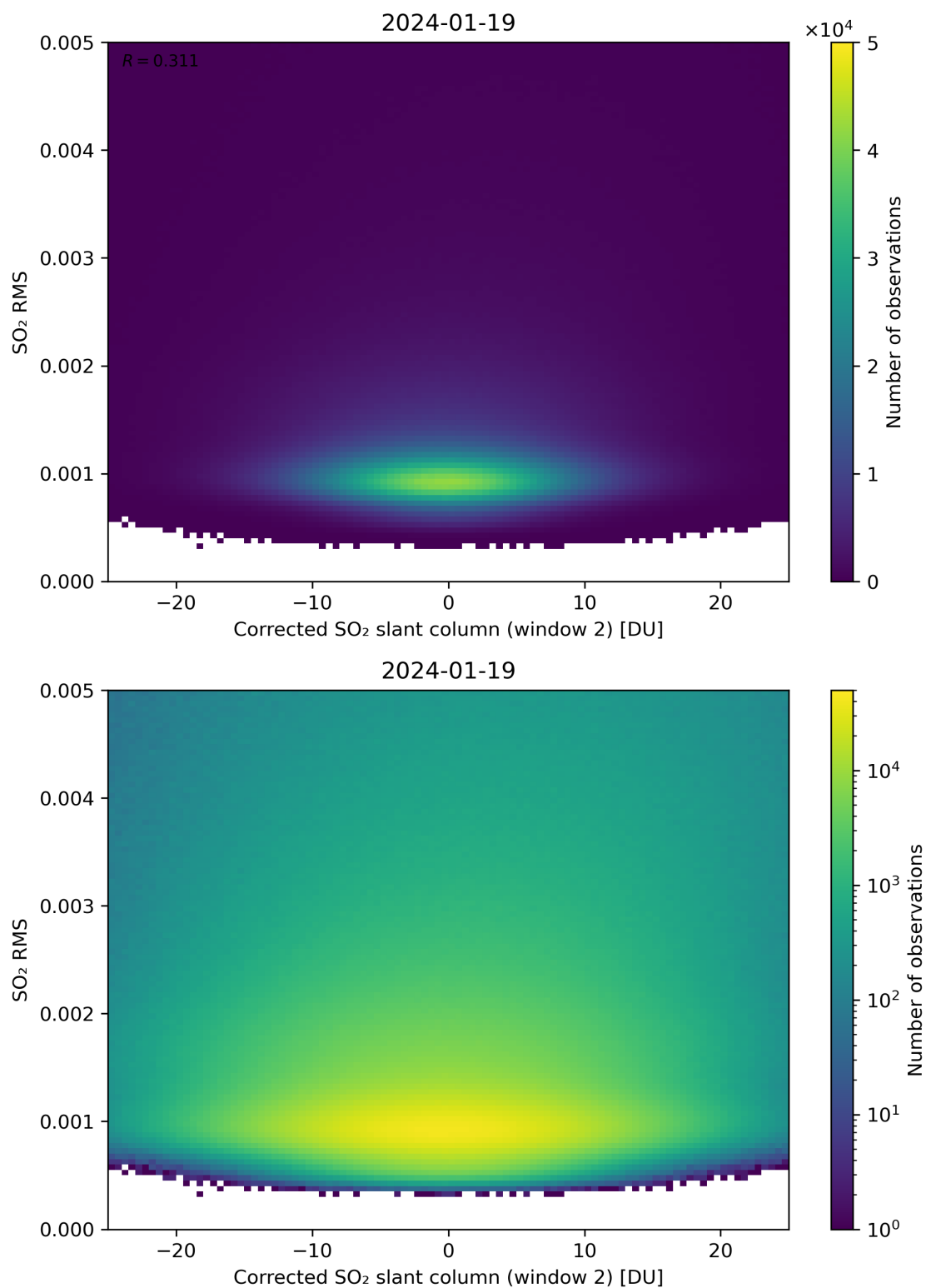
Figure 198: Scatter density plot of “Corrected SO 2 slant column (window 2)” against “SO 2 RMS” for 2024-01-18 to 2024-01-20.
