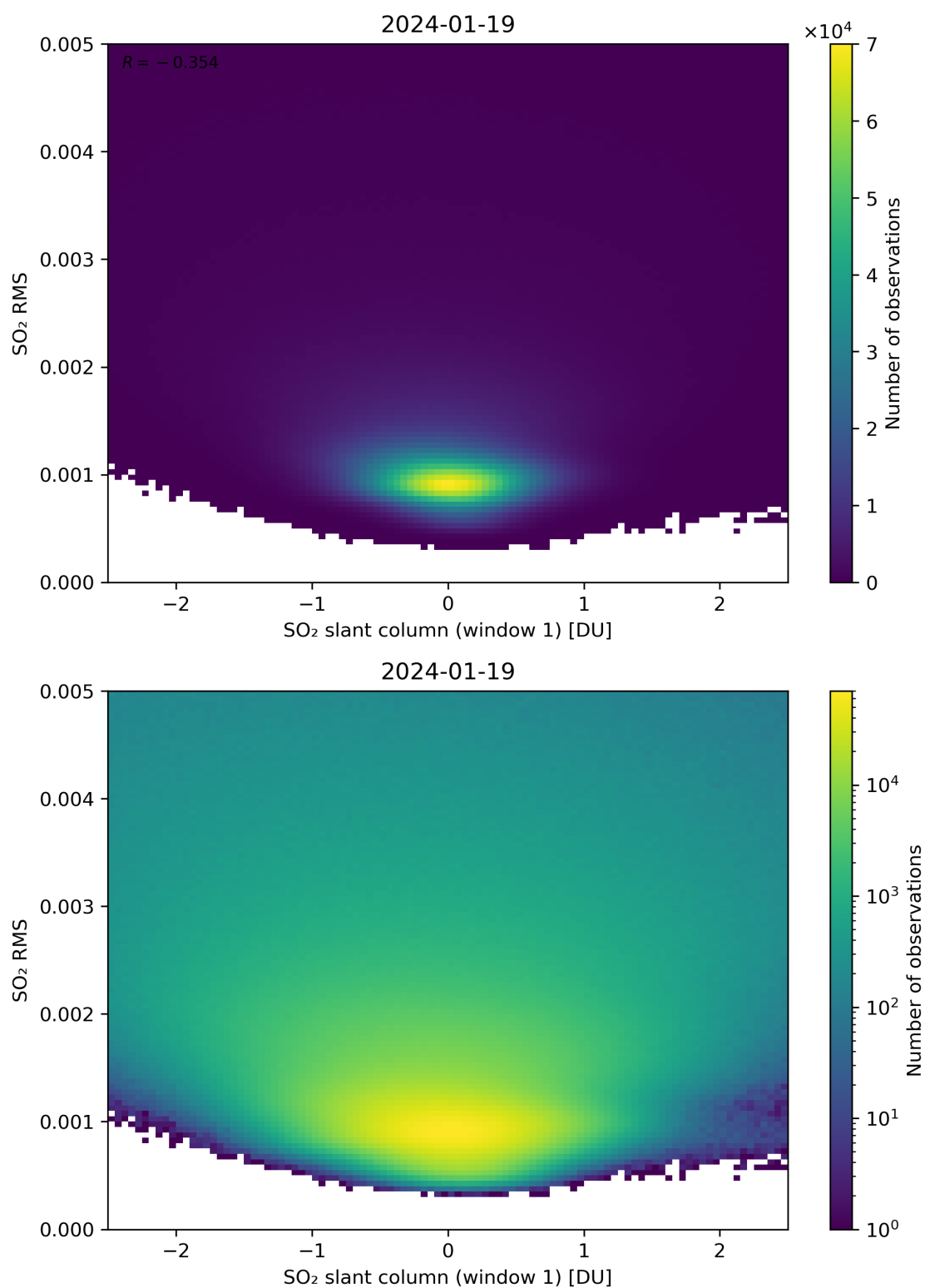
Figure 217: Scatter density plot of “SO 2 slant column (window 1)” against “SO 2 RMS” for 2024-01-18 to 2024-01-20.
