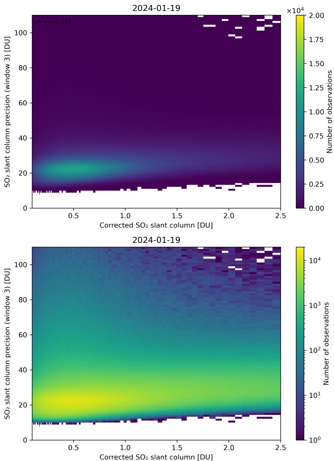
Figure 191: Scatter density plot of “Corrected SO 2 slant column” against “SO 2 slant column precision (window 3)” for 2024-01-18 to 2024-01-20.
