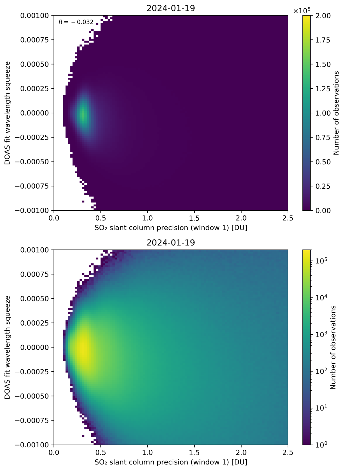
Figure 222: Scatter density plot of “SO 2 slant column precision (window 1)” against “DOAS fit wavelength squeeze” for 2024-01-18 to 2024-01-20.
