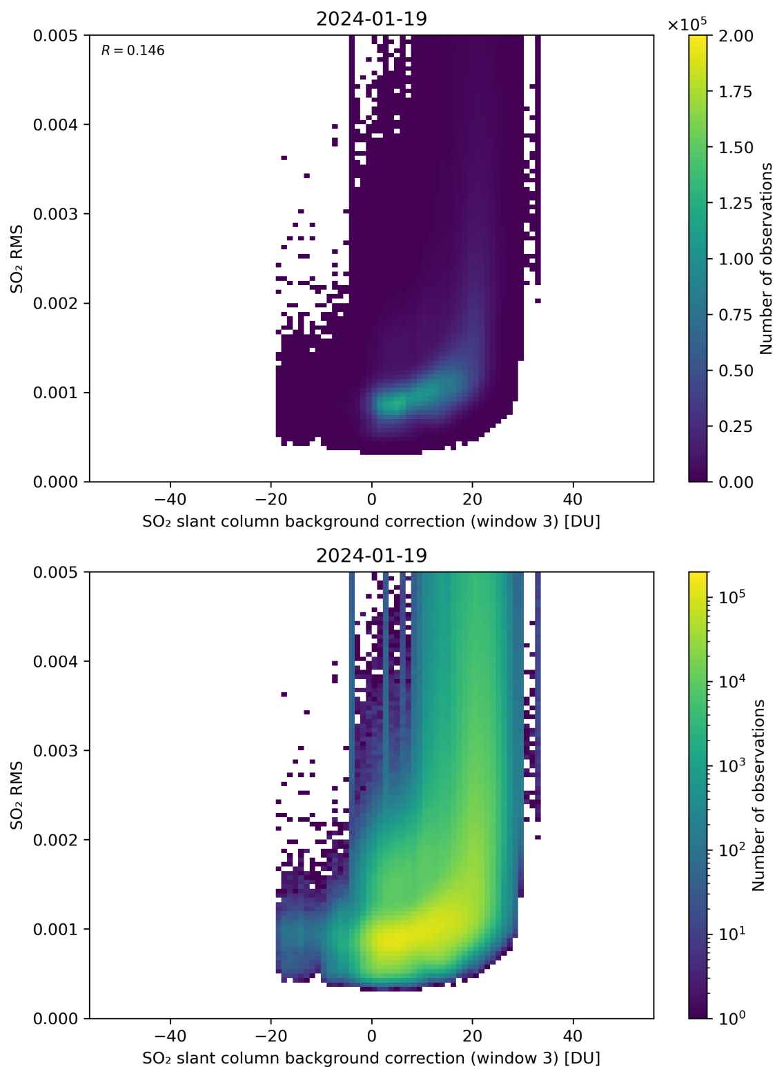
Figure 123: Scatter density plot of “SO 2 slant column background correction (window 3)” against “SO 2 RMS” for 2024-01-18 to 2024-01-20.
