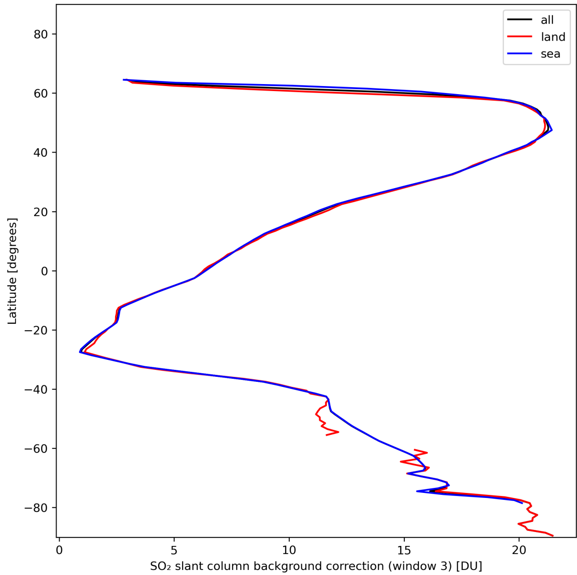
Figure 44: Zonal average of “SO 2 slant column background correction (window 3)” for 2024-01-18 to 2024-01-20.
