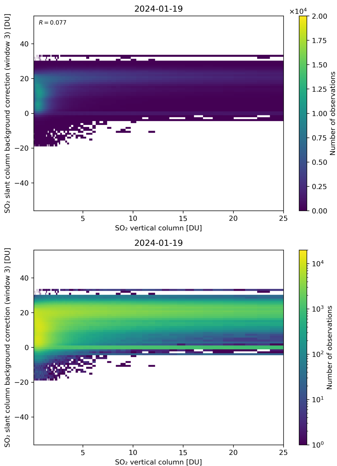
Figure 275: Scatter density plot of “SO 2 vertical column” against “SO 2 slant column background correction (window 3)” for 2024-01-18 to 2024-01-20.
