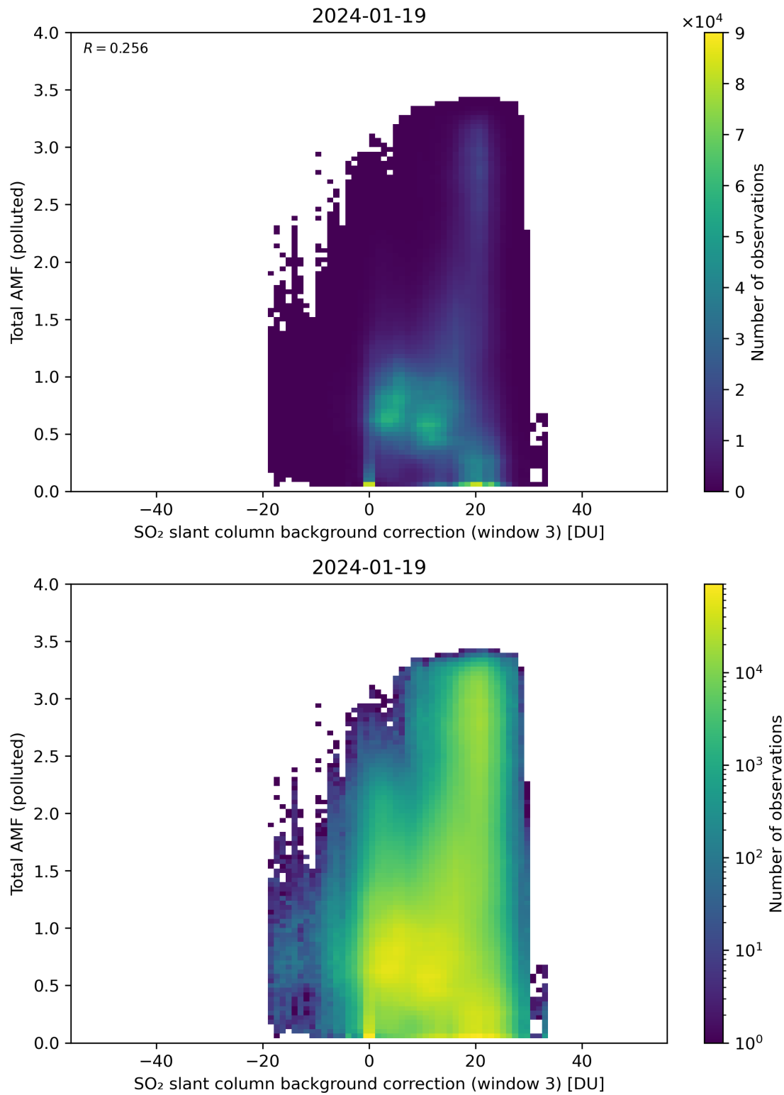
Figure 125: Scatter density plot of “SO 2 slant column background correction (window 3)” against “Total AMF (polluted)” for 2024-01-18 to 2024-01-20.
