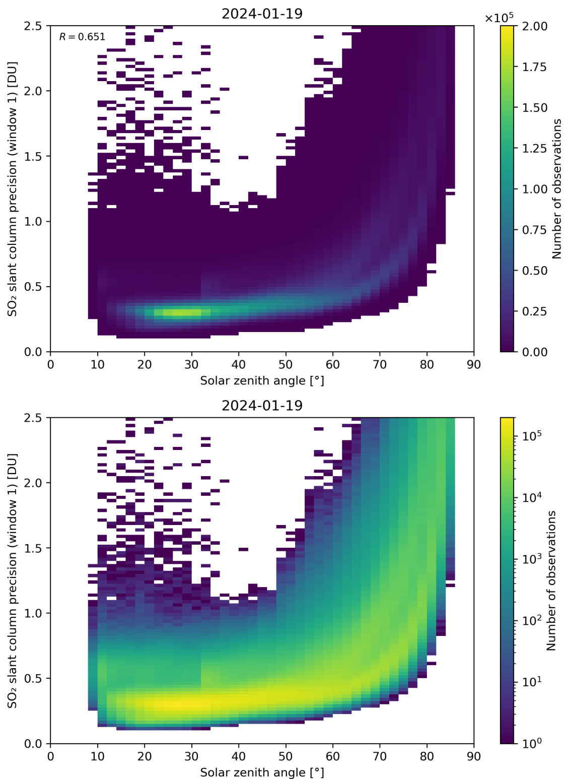
Figure 170: Scatter density plot of “Solar zenith angle” against “SO 2 slant column precision (window 1)” for 2024-01-18 to 2024-01-20.
