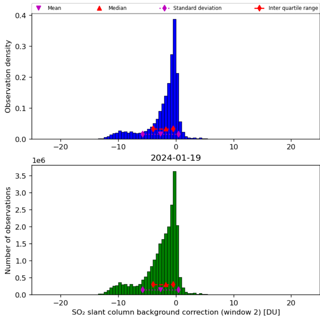
Figure 63: Histogram of “SO 2 slant column background correction (window 2)” for 2024-01-18 to 2024-01-20
