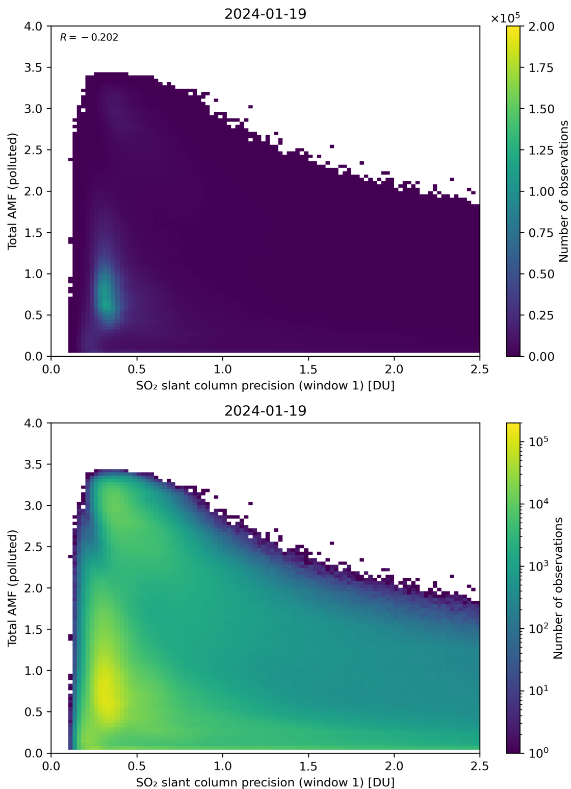
Figure 230: Scatter density plot of “SO 2 slant column precision (window 1)” against “Total AMF (polluted)” for 2024-01-18 to 2024-01-20.
