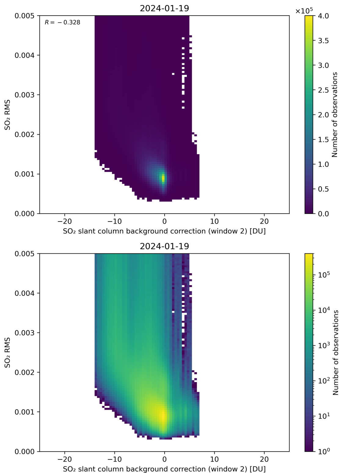
Figure 114: Scatter density plot of “SO 2 slant column background correction (window 2)” against “SO 2 RMS” for 2024-01-18 to 2024-01-20.
