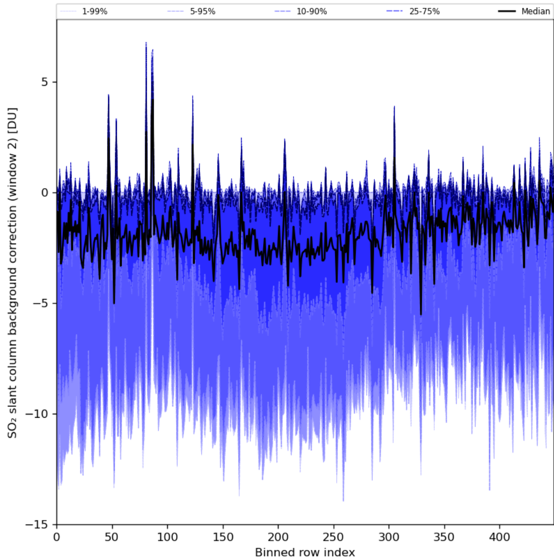
Figure 86: Along track statistics of “SO 2 slant column background correction (window 2)” for 2024-01-18 to 2024-01-20
