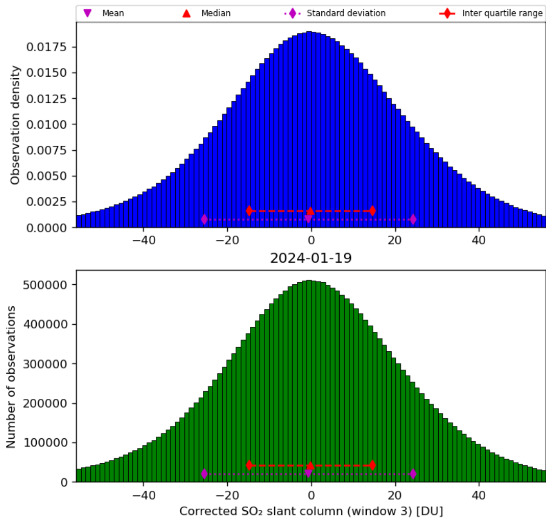
Figure 66: Histogram of “Corrected SO 2 slant column (window 3)” for 2024-01-18 to 2024-01-20
