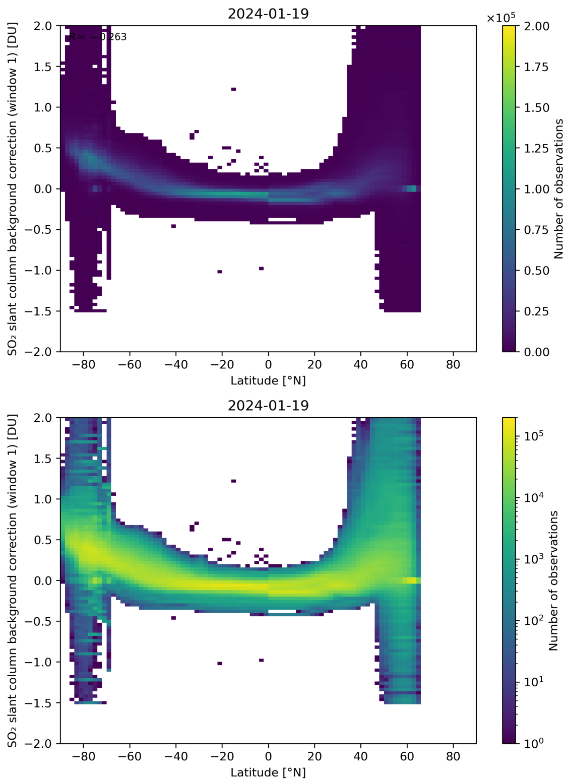
Figure 139: Scatter density plot of “Latitude” against “SO 2 slant column background correction (window 1)” for 2024-01-18 to 2024-01-20.
