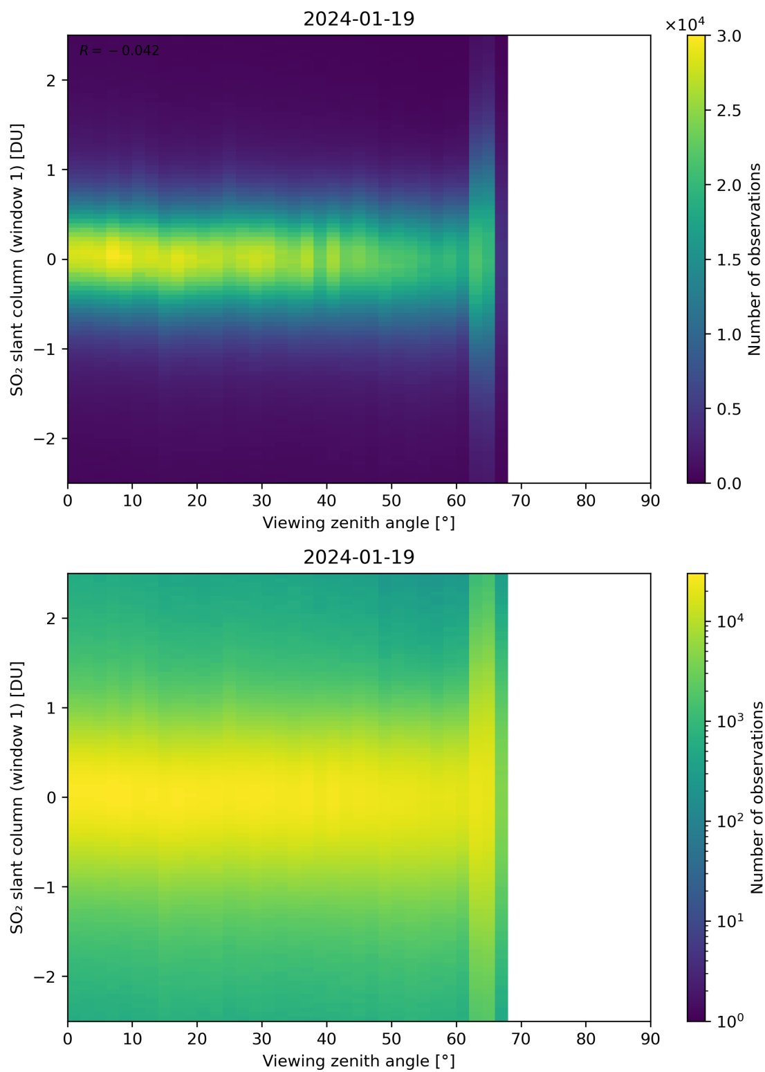
Figure 320: Scatter density plot of “Viewing zenith angle” against “SO 2 slant column (window 1)” for 2024-01-18 to 2024-01-20.
