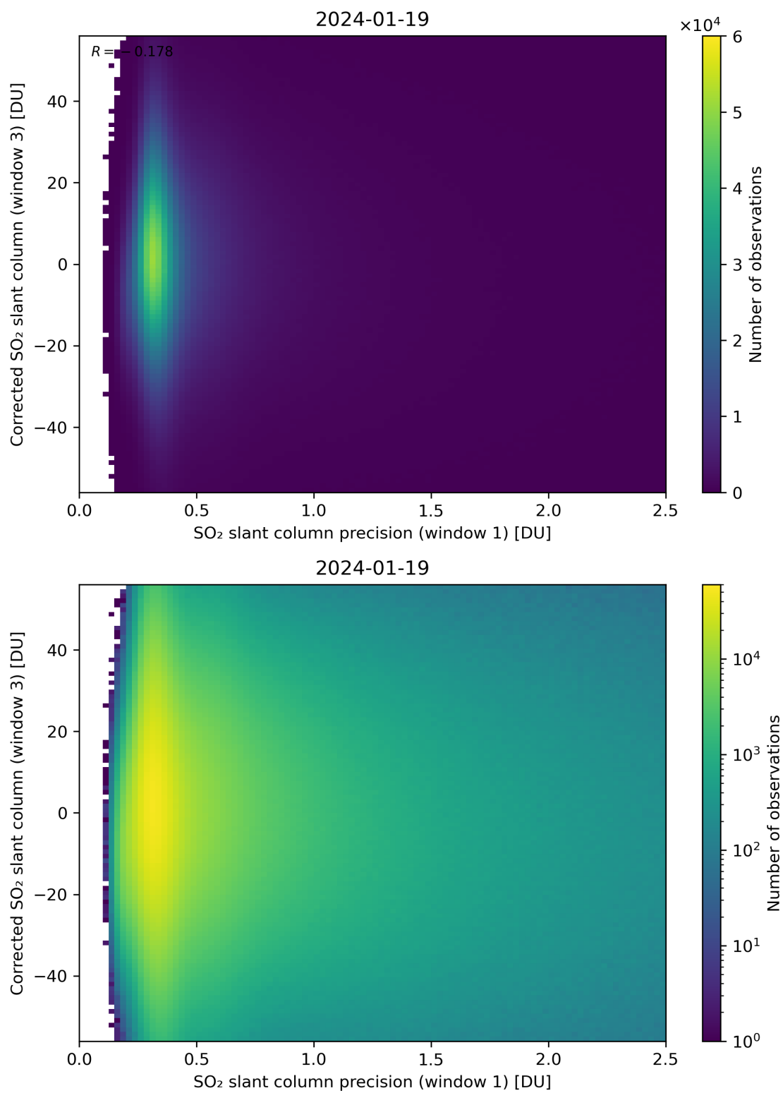
Figure 226: Scatter density plot of “SO 2 slant column precision (window 1)” against “Corrected SO 2 slant column (window 3)” for 2024-01-18 to 2024-01-20.
