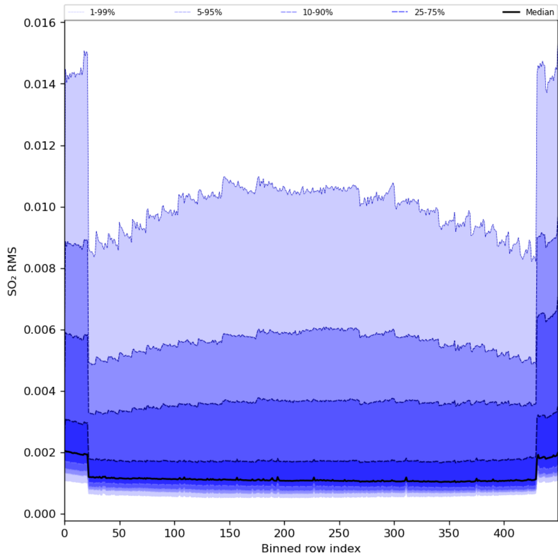
Figure 93: Along track statistics of “SO 2 RMS” for 2024-01-18 to 2024-01-20
