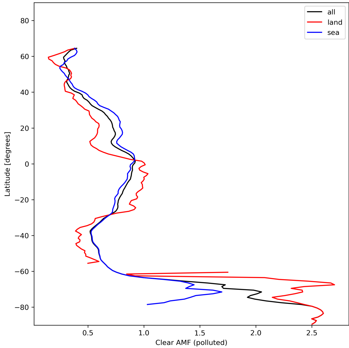
Figure 50: Zonal average of “Clear AMF (polluted)” for 2024-01-18 to 2024-01-20.
