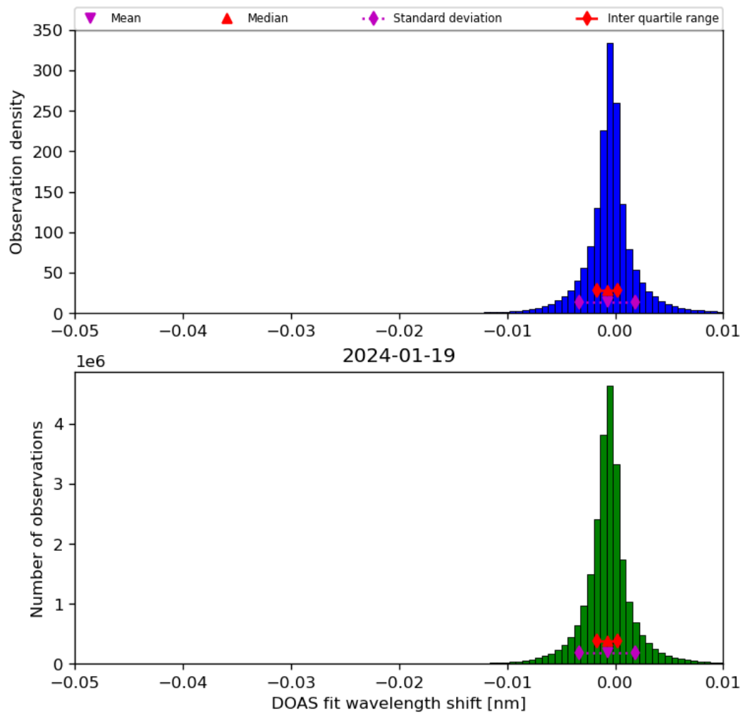
Figure 68: Histogram of “DOAS fit wavelength shift” for 2024-01-18 to 2024-01-20
