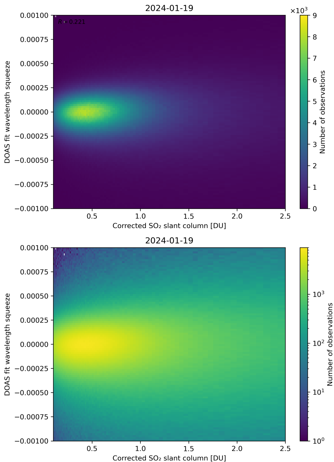
Figure 182: Scatter density plot of “Corrected SO 2 slant column” against “DOAS fit wavelength squeeze” for 2024-01-18 to 2024-01-20.
