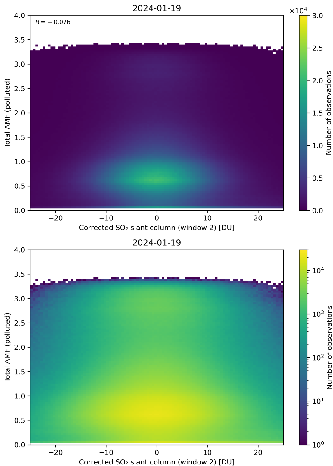
Figure 203: Scatter density plot of “Corrected SO 2 slant column (window 2)” against “Total AMF (polluted)” for 2024-01-18 to 2024-01-20.
