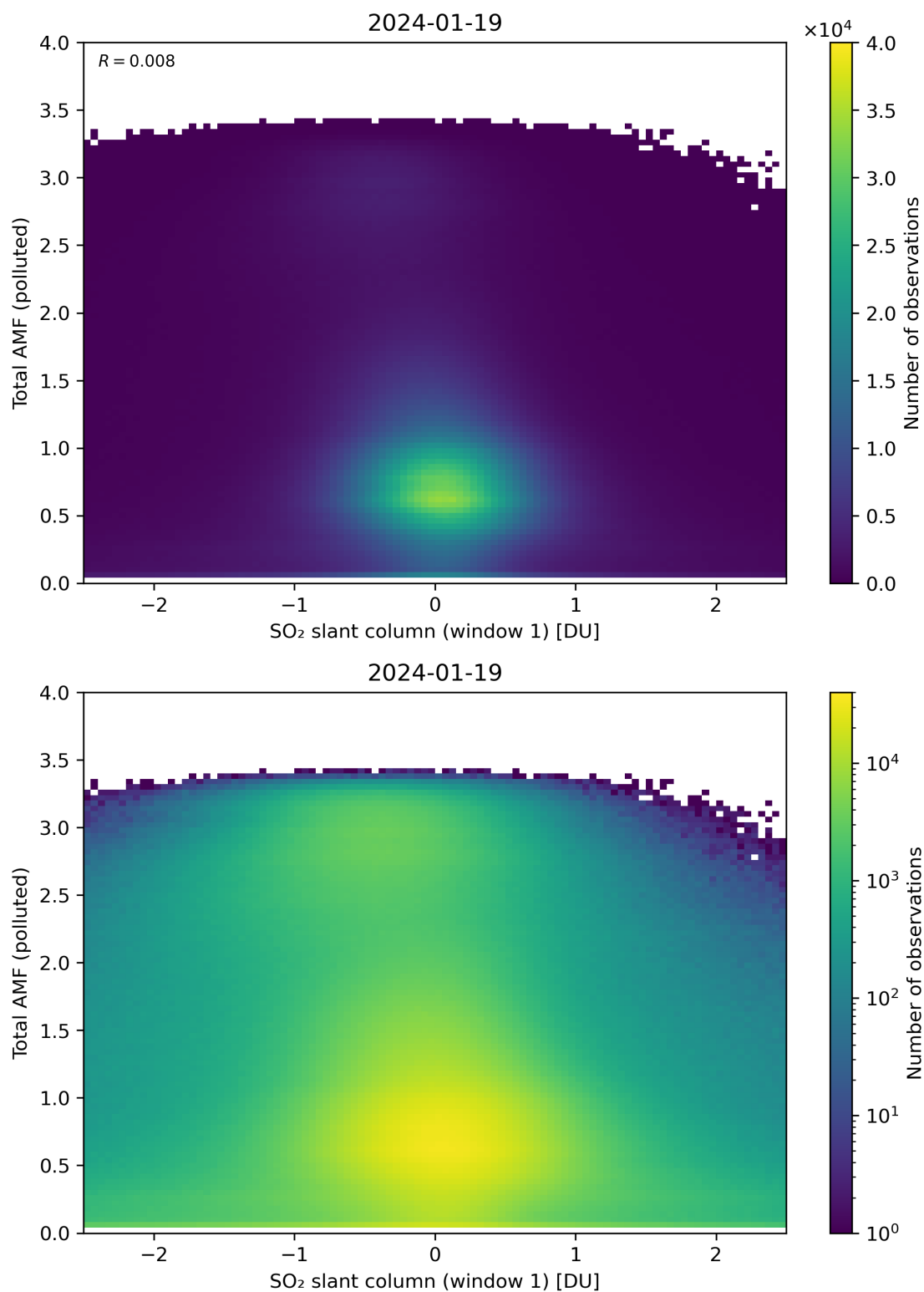
Figure 239: Scatter density plot of “SO 2 slant column (window 1)” against “Total AMF (polluted)” for 2024-01-18 to 2024-01-20.
