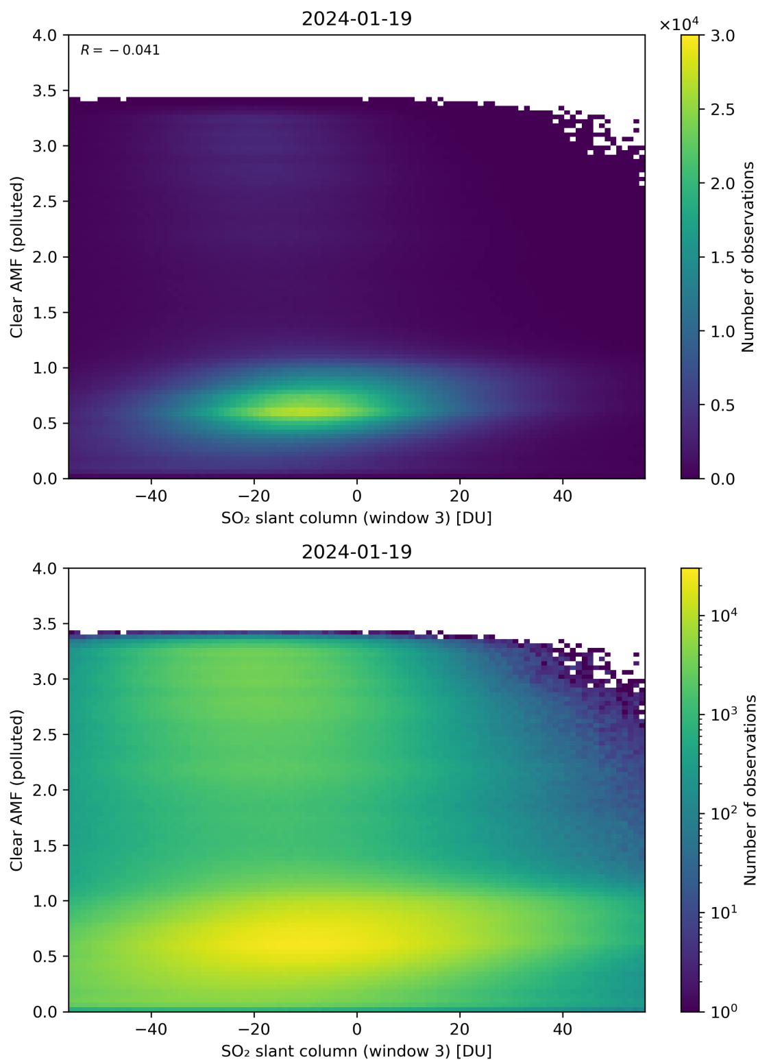
Figure 265: Scatter density plot of “SO 2 slant column (window 3)” against “Clear AMF (polluted)” for 2024-01-18 to 2024-01-20.
