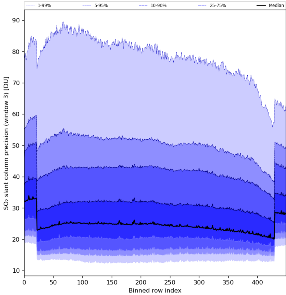
Figure 88: Along track statistics of “SO 2 slant column precision (window 3)” for 2024-01-18 to 2024-01-20
