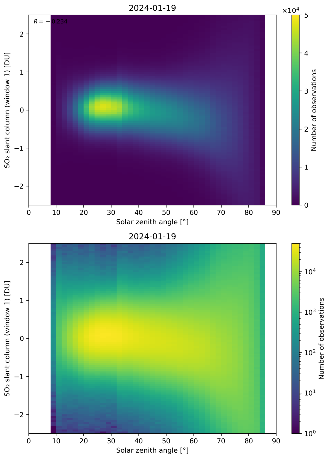
Figure 169: Scatter density plot of “Solar zenith angle” against “SO 2 slant column (window 1)” for 2024-01-18 to 2024-01-20.
