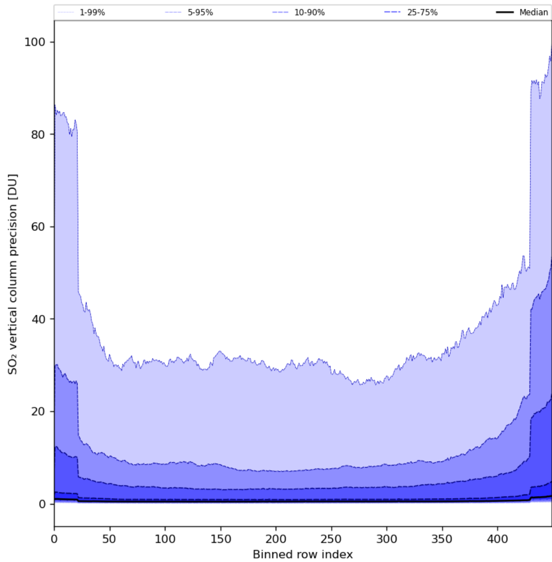
Figure 77: Along track statistics of “SO 2 vertical column precision” for 2024-01-18 to 2024-01-20
