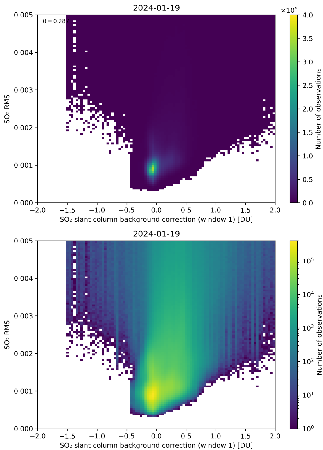
Figure 102: Scatter density plot of “SO 2 slant column background correction (window 1)” against “SO 2 RMS” for 2024-01-18 to 2024-01-20.
