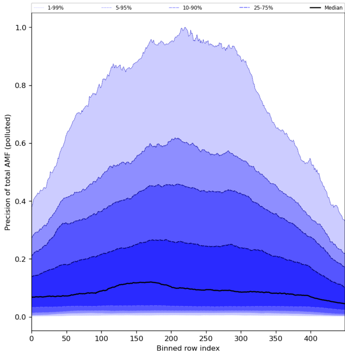
Figure 95: Along track statistics of “Precision of total AMF (polluted)” for 2024-01-18 to 2024-01-20
