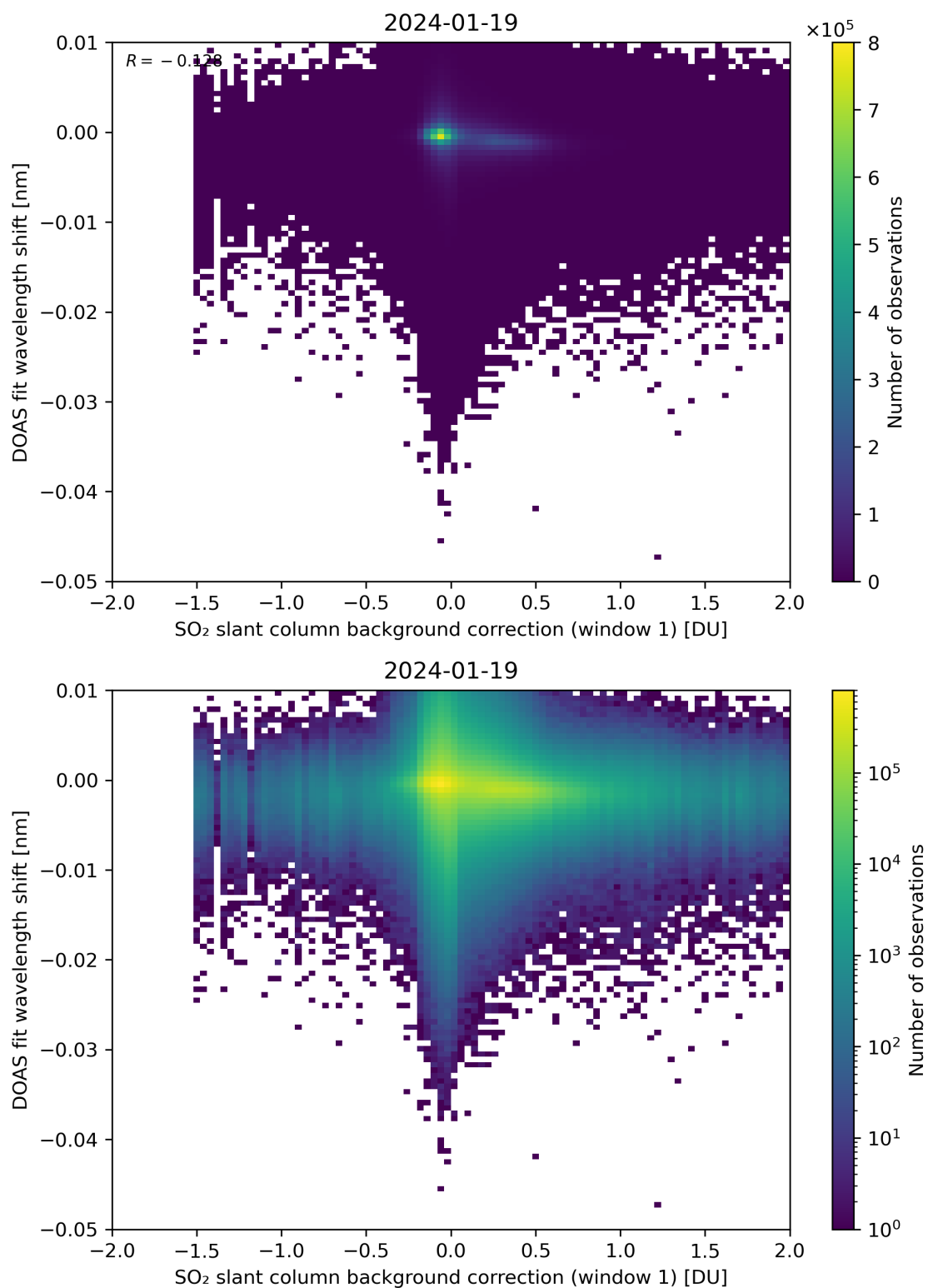
Figure 100: Scatter density plot of “SO 2 slant column background correction (window 1)” against “DOAS fit wavelength shift” for 2024-01-18 to 2024-01-20.
