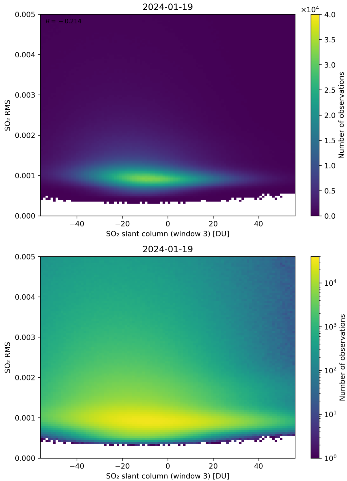
Figure 256: Scatter density plot of “SO 2 slant column (window 3)” against “SO 2 RMS” for 2024-01-18 to 2024-01-20.
