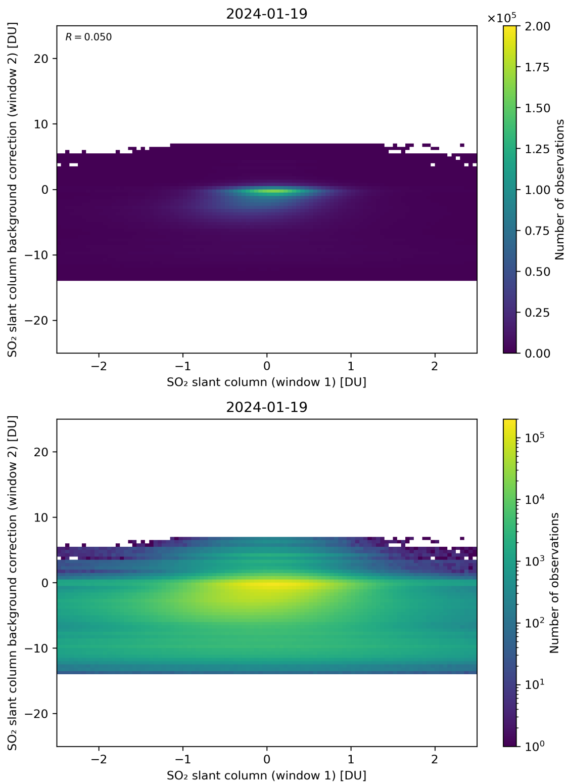
Figure 213: Scatter density plot of “SO 2 slant column (window 1)” against “SO 2 slant column background correction (window 2)” for 2024-01-18 to 2024-01-20.
