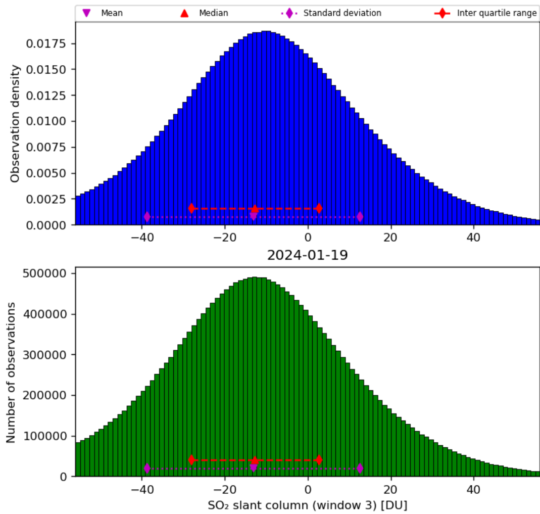
Figure 64: Histogram of “SO 2 slant column (window 3)” for 2024-01-18 to 2024-01-20
