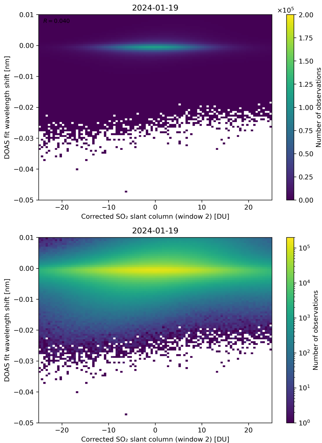
Figure 196: Scatter density plot of “Corrected SO 2 slant column (window 2)” against “DOAS fit wavelength shift” for 2024-01-18 to 2024-01-20.
