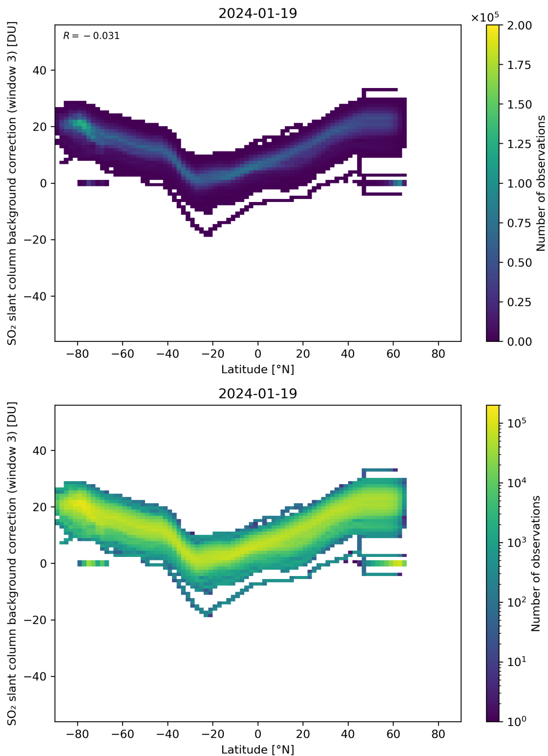
Figure 141: Scatter density plot of “Latitude” against “SO 2 slant column background correction (window 3)” for 2024-01-18 to 2024-01-20.
