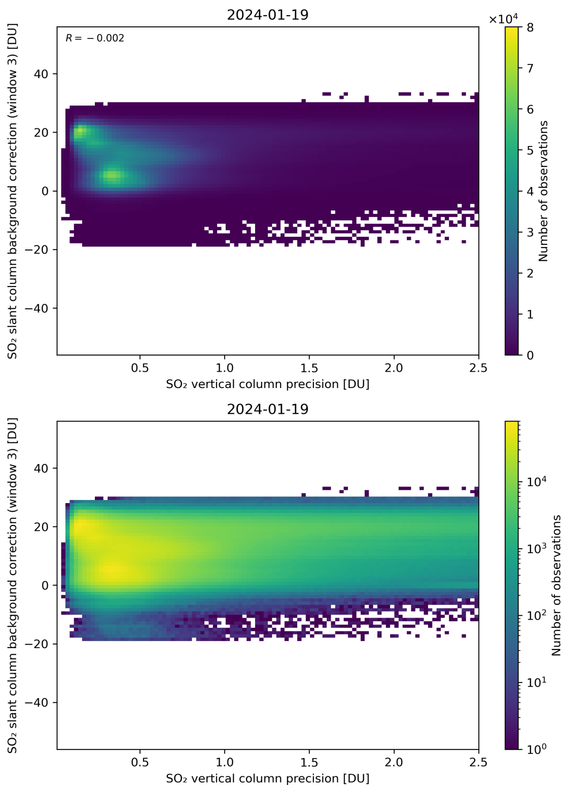
Figure 281: Scatter density plot of “SO 2 vertical column precision” against “SO 2 slant column background correction (window 3)” for 2024-01-18 to 2024-01-20.
