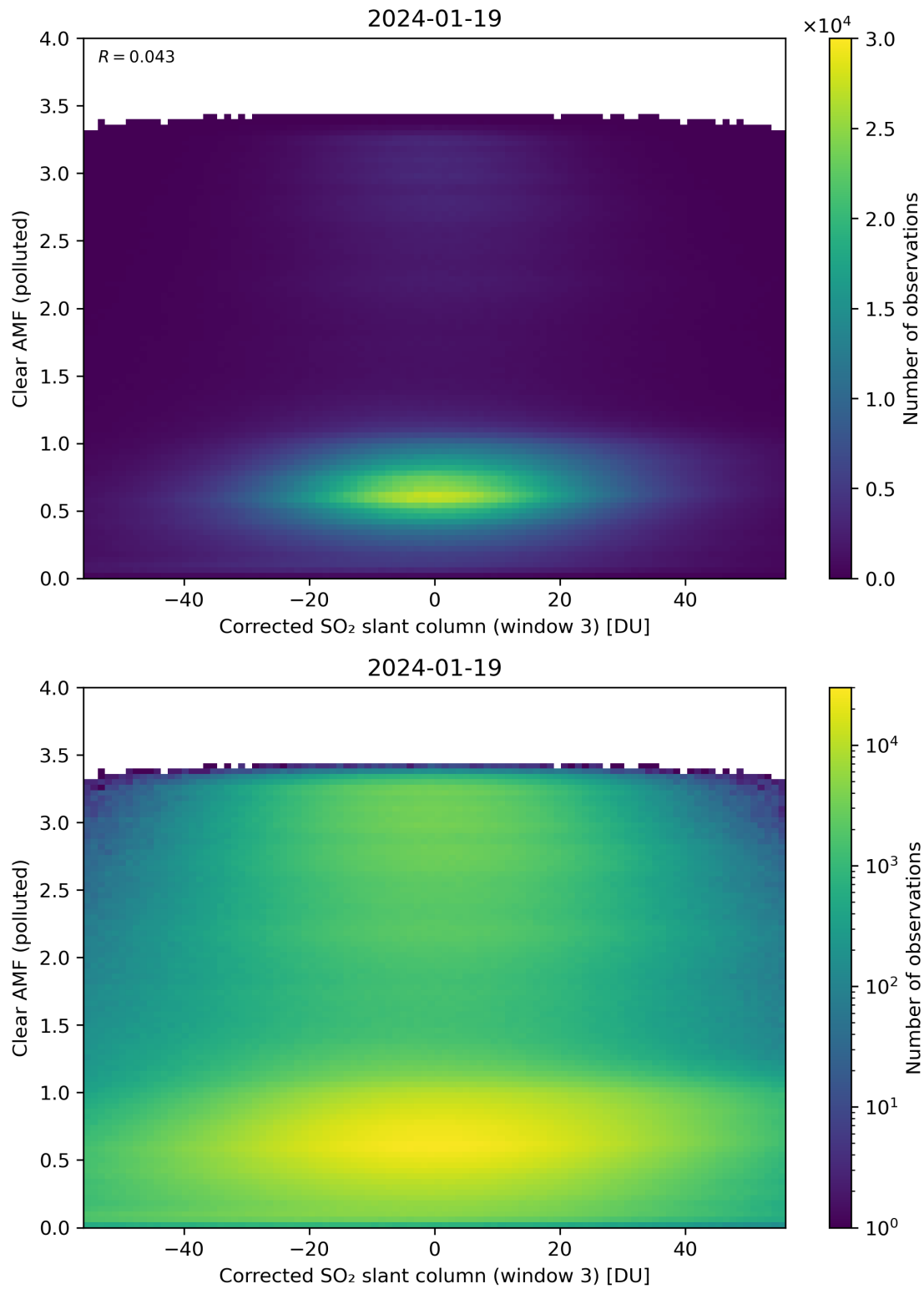
Figure 209: Scatter density plot of “Corrected SO 2 slant column (window 3)” against “Clear AMF (polluted)” for 2024-01-18 to 2024-01-20.
