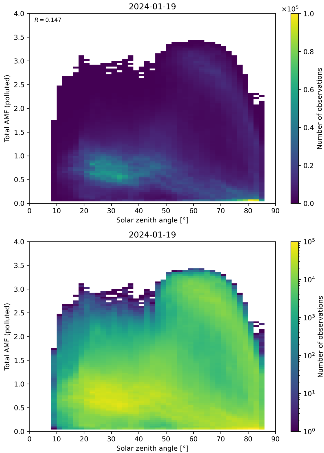
Figure 174: Scatter density plot of “Solar zenith angle” against “Total AMF (polluted)” for 2024-01-18 to 2024-01-20.
