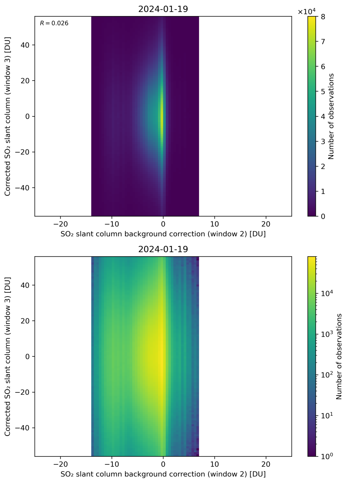
Figure 116: Scatter density plot of “SO 2 slant column background correction (window 2)” against “Corrected SO 2 slant column (window 3)” for 2024-01-18 to 2024-01-20.
