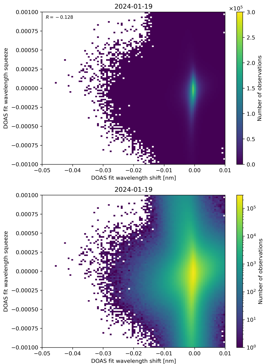
Figure 127: Scatter density plot of “DOAS fit wavelength shift” against “DOAS fit wavelength squeeze” for 2024-01-18 to 2024-01-20.
