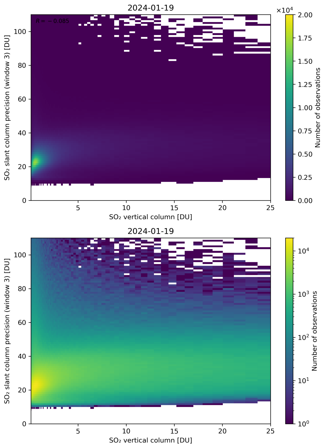
Figure 304: Scatter density plot of “SO 2 vertical column” against “SO 2 slant column precision (window 3)” for 2024-01-18 to 2024-01-20.
