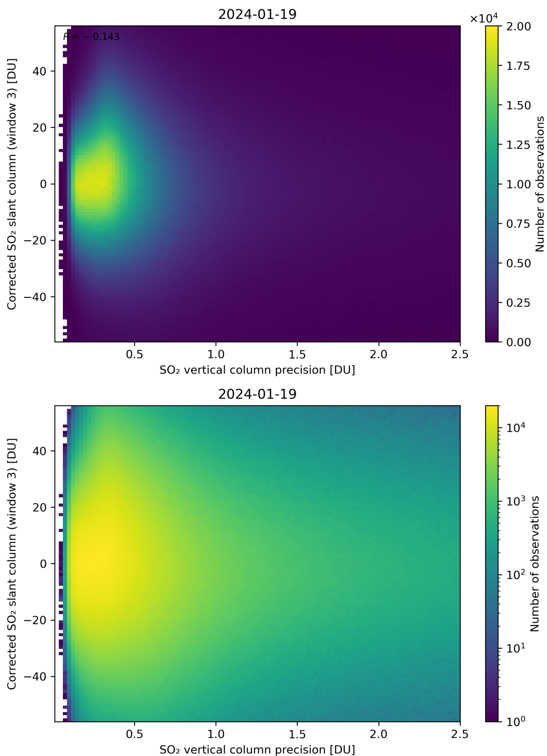
Figure 288: Scatter density plot of “SO 2 vertical column precision” against “Corrected SO 2 slant column (window 3)” for 2024-01-18 to 2024-01-20.
