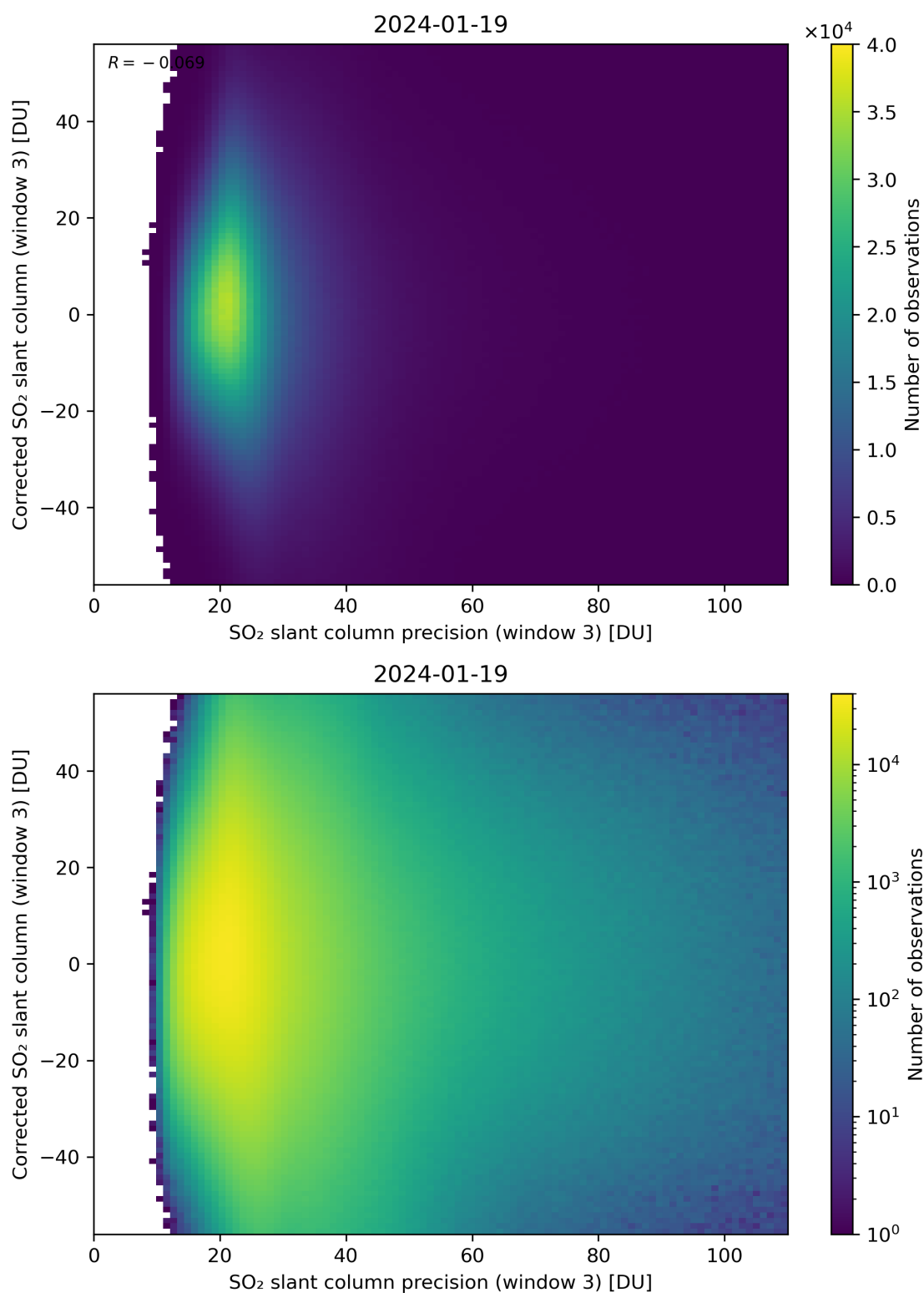
Figure 262: Scatter density plot of “SO 2 slant column precision (window 3)” against “Corrected SO 2 slant column (window 3)” for 2024-01-18 to 2024-01-20.
