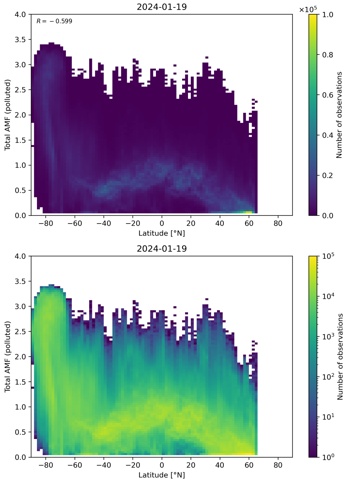
Figure 154: Scatter density plot of “Latitude” against “Total AMF (polluted)” for 2024-01-18 to 2024-01-20.
