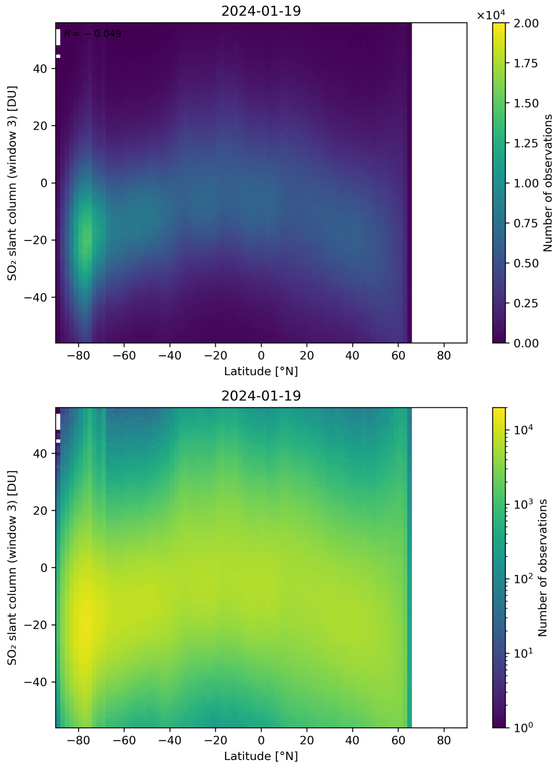
Figure 152: Scatter density plot of “Latitude” against “SO 2 slant column (window 3)” for 2024-01-18 to 2024-01-20.
