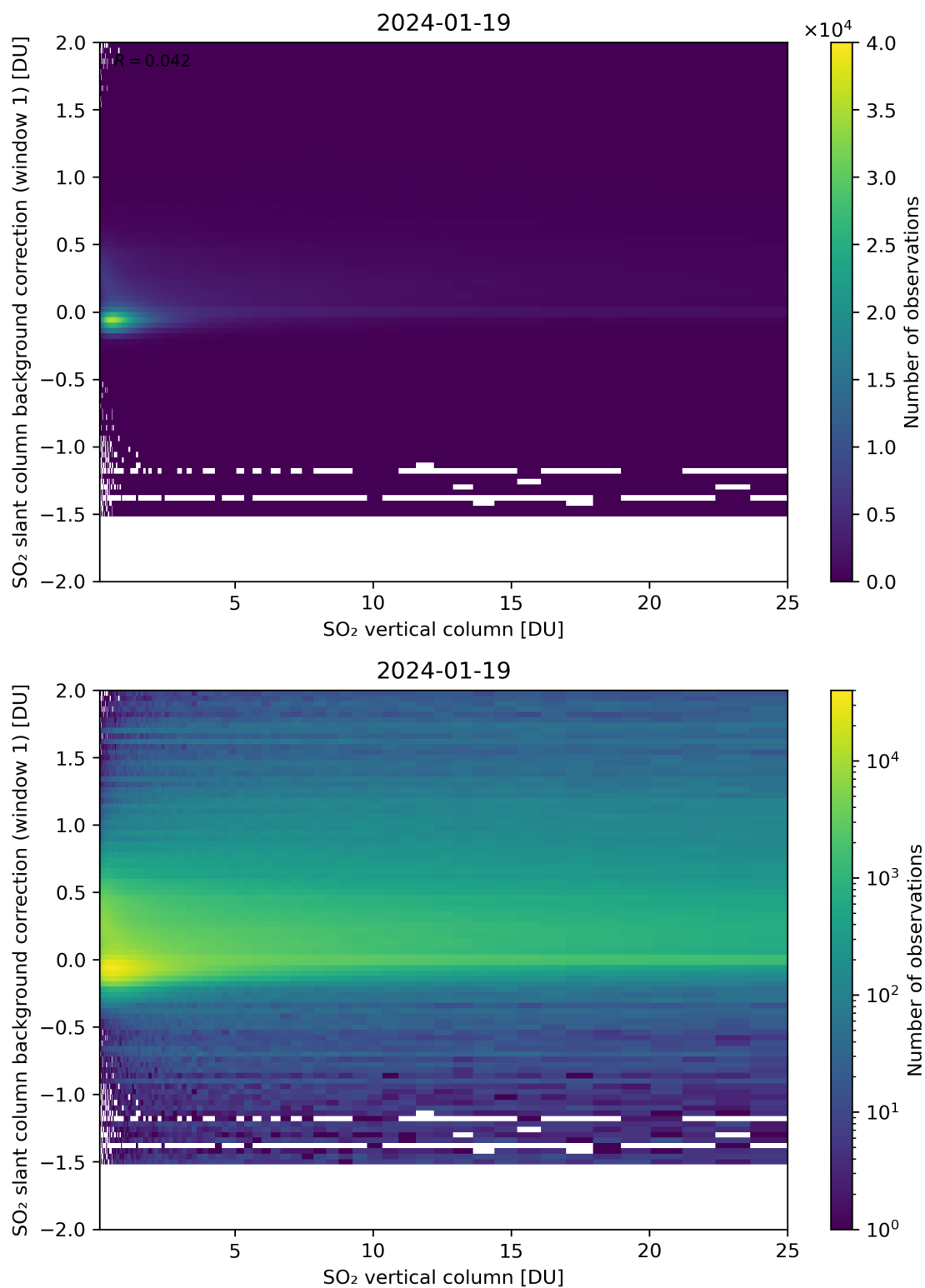
Figure 273: Scatter density plot of “SO 2 vertical column” against “SO 2 slant column background correction (window 1)” for 2024-01-18 to 2024-01-20.
