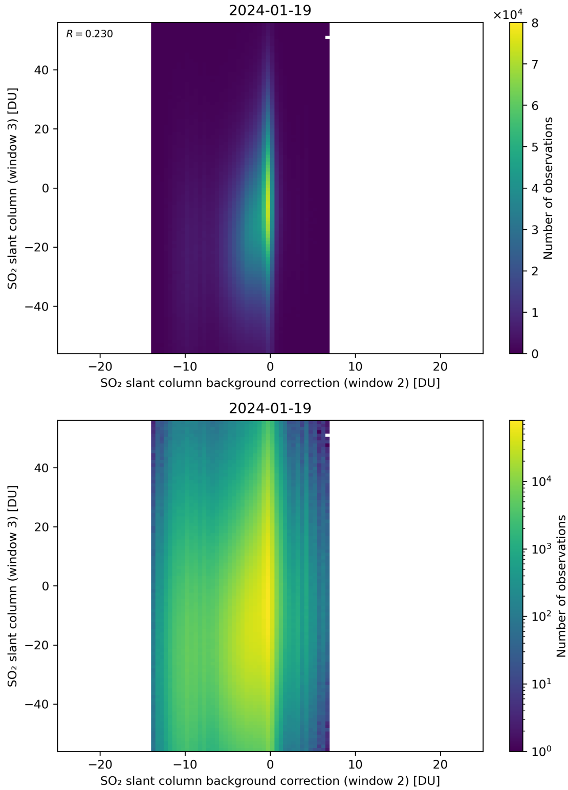
Figure 117: Scatter density plot of “SO 2 slant column background correction (window 2)” against “SO 2 slant column (window 3)” for 2024-01-18 to 2024-01-20.
