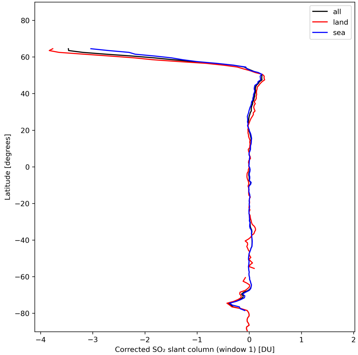
Figure 35: Zonal average of “Corrected SO 2 slant column (window 1)” for 2024-01-18 to 2024-01-20.
