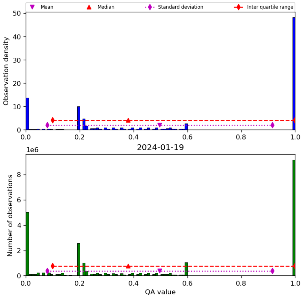
Figure 52: Histogram of “QA value” for 2024-01-18 to 2024-01-20
