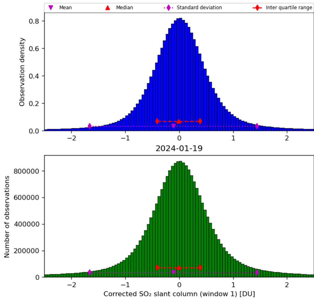
Figure 58: Histogram of “Corrected SO 2 slant column (window 1)” for 2024-01-18 to 2024-01-20
