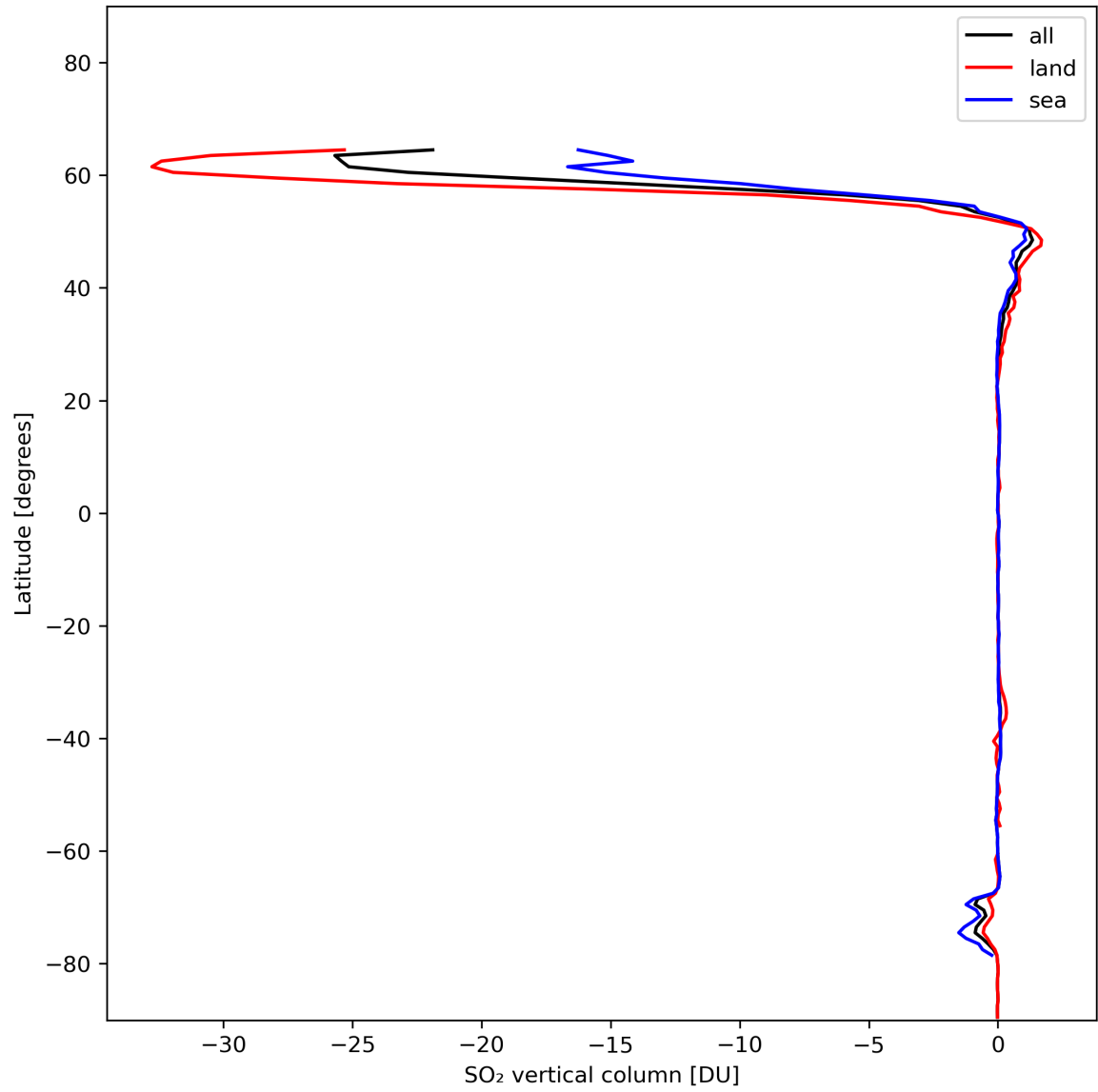
Figure 30: Zonal average of “SO 2 vertical column” for 2024-01-18 to 2024-01-20.
