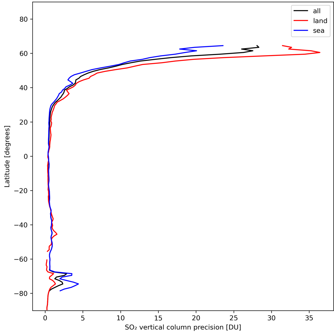
Figure 31: Zonal average of “SO 2 vertical column precision” for 2024-01-18 to 2024-01-20.
