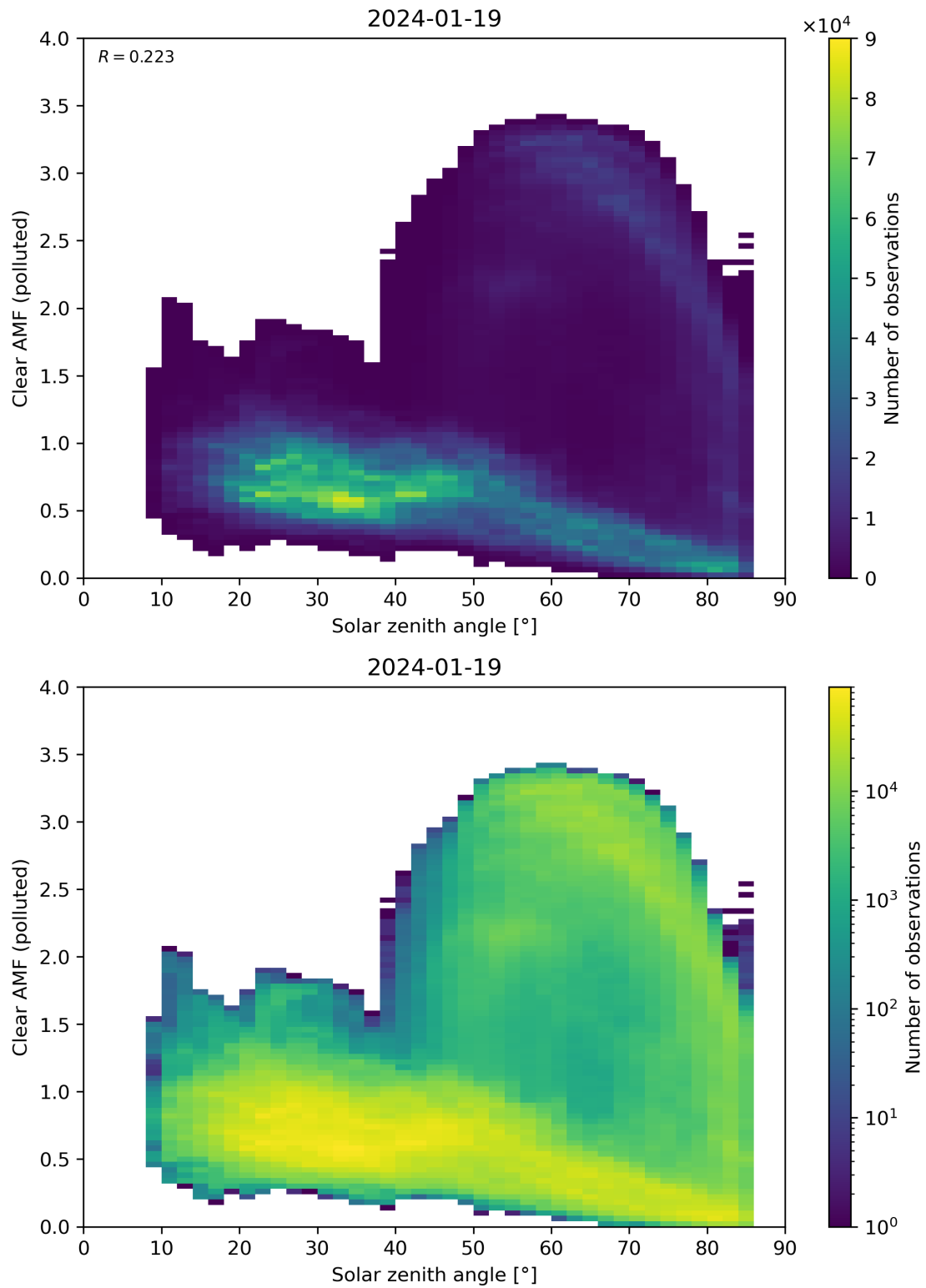
Figure 165: Scatter density plot of “Solar zenith angle” against “Clear AMF (polluted)” for 2024-01-18 to 2024-01-20.
