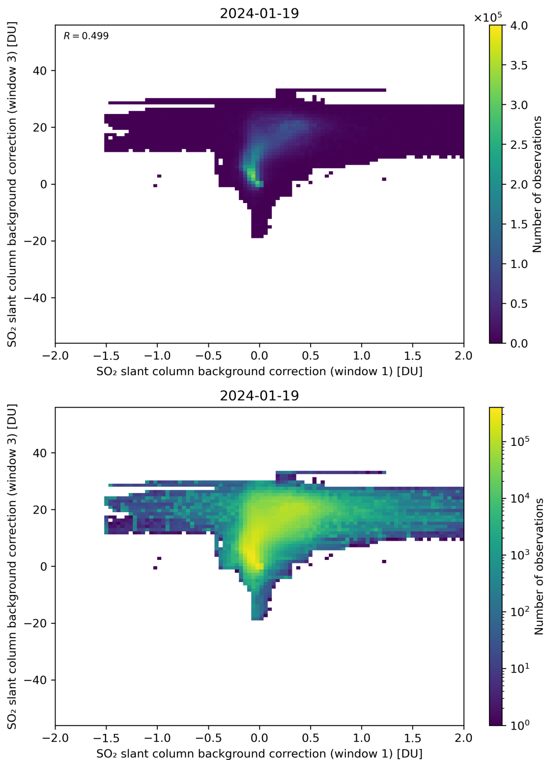
Figure 99: Scatter density plot of “SO 2 slant column background correction (window 1)” against “SO 2 slant column background correction (window 3)” for 2024-01-18 to 2024-01-20.
