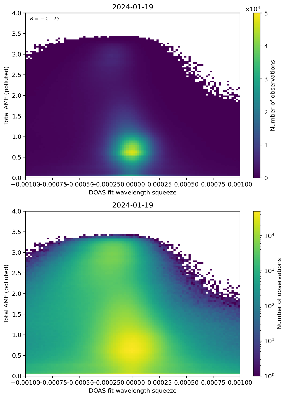
Figure 134: Scatter density plot of “DOAS fit wavelength squeeze” against “Total AMF (polluted)” for 2024-01-18 to 2024-01-20.
