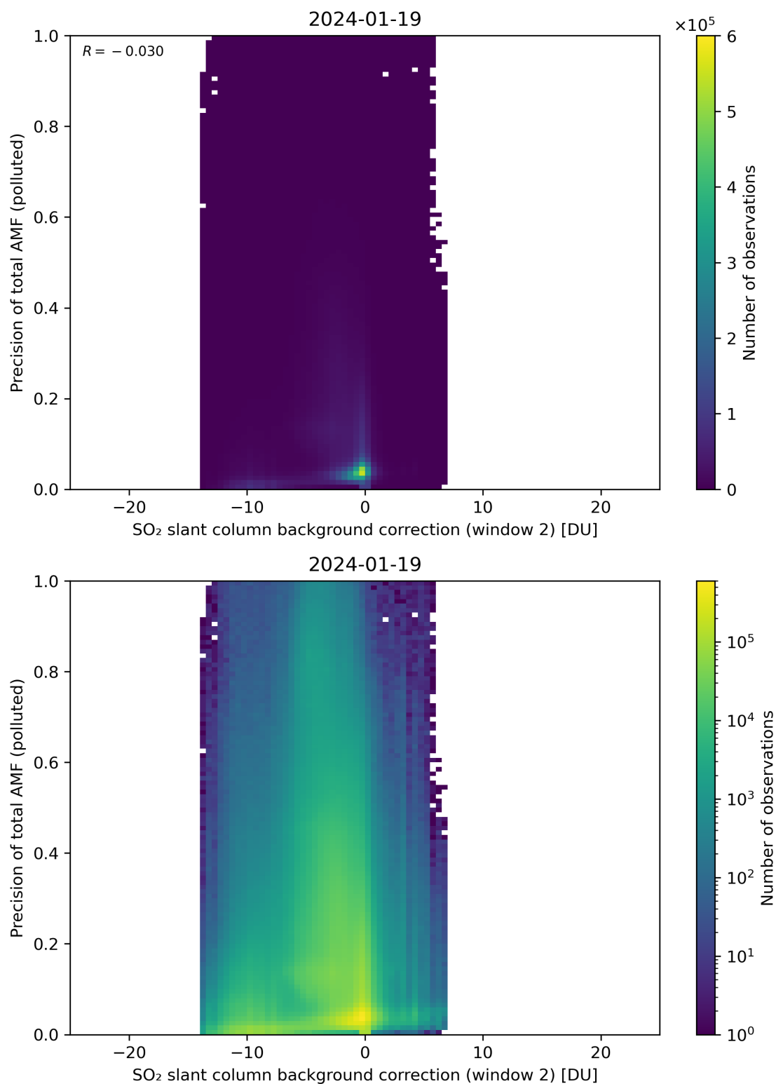
Figure 120: Scatter density plot of “SO 2 slant column background correction (window 2)” against “Precision of total AMF (polluted)” for 2024-01-18 to 2024-01-20.
