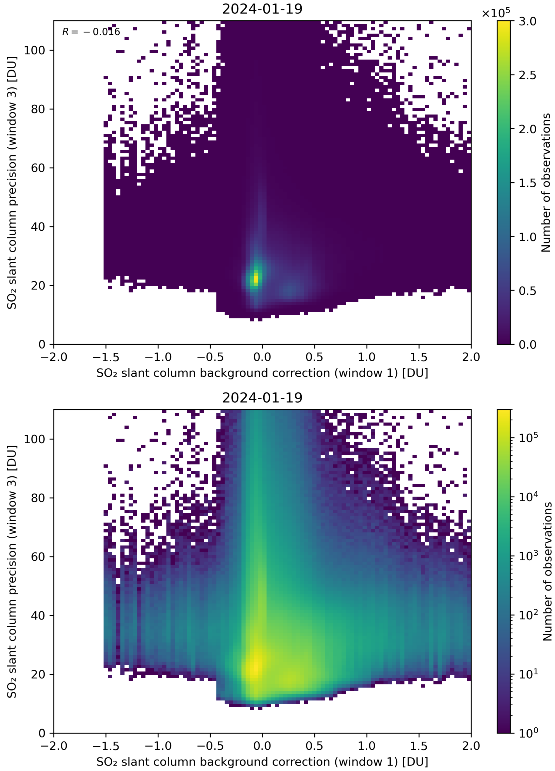
Figure 108: Scatter density plot of “SO 2 slant column background correction (window 1)” against “SO 2 slant column precision (window 3)” for 2024-01-18 to 2024-01-20.
