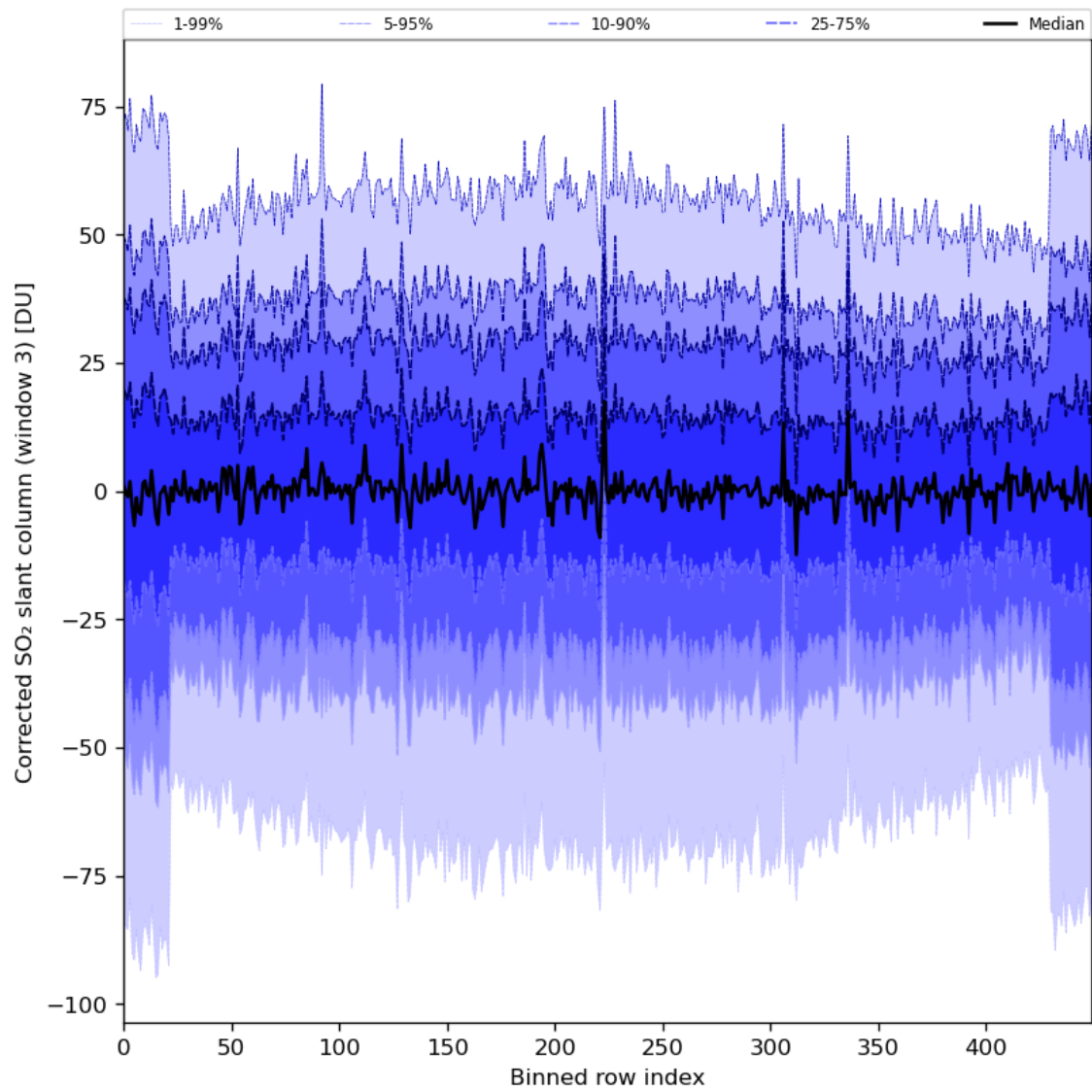
Figure 89: Along track statistics of “Corrected SO 2 slant column (window 3)” for 2024-01-18 to 2024-01-20
