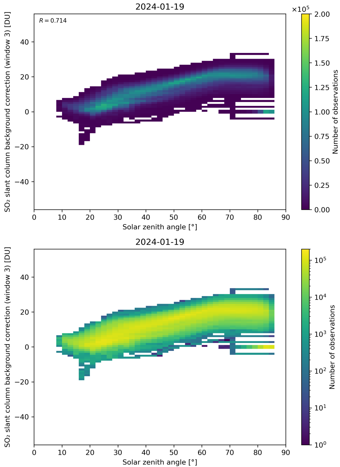
Figure 160: Scatter density plot of “Solar zenith angle” against “SO 2 slant column background correction (window 3)” for 2024-01-18 to 2024-01-20.
