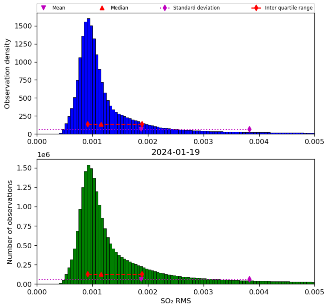
Figure 70: Histogram of “SO 2 RMS” for 2024-01-18 to 2024-01-20
