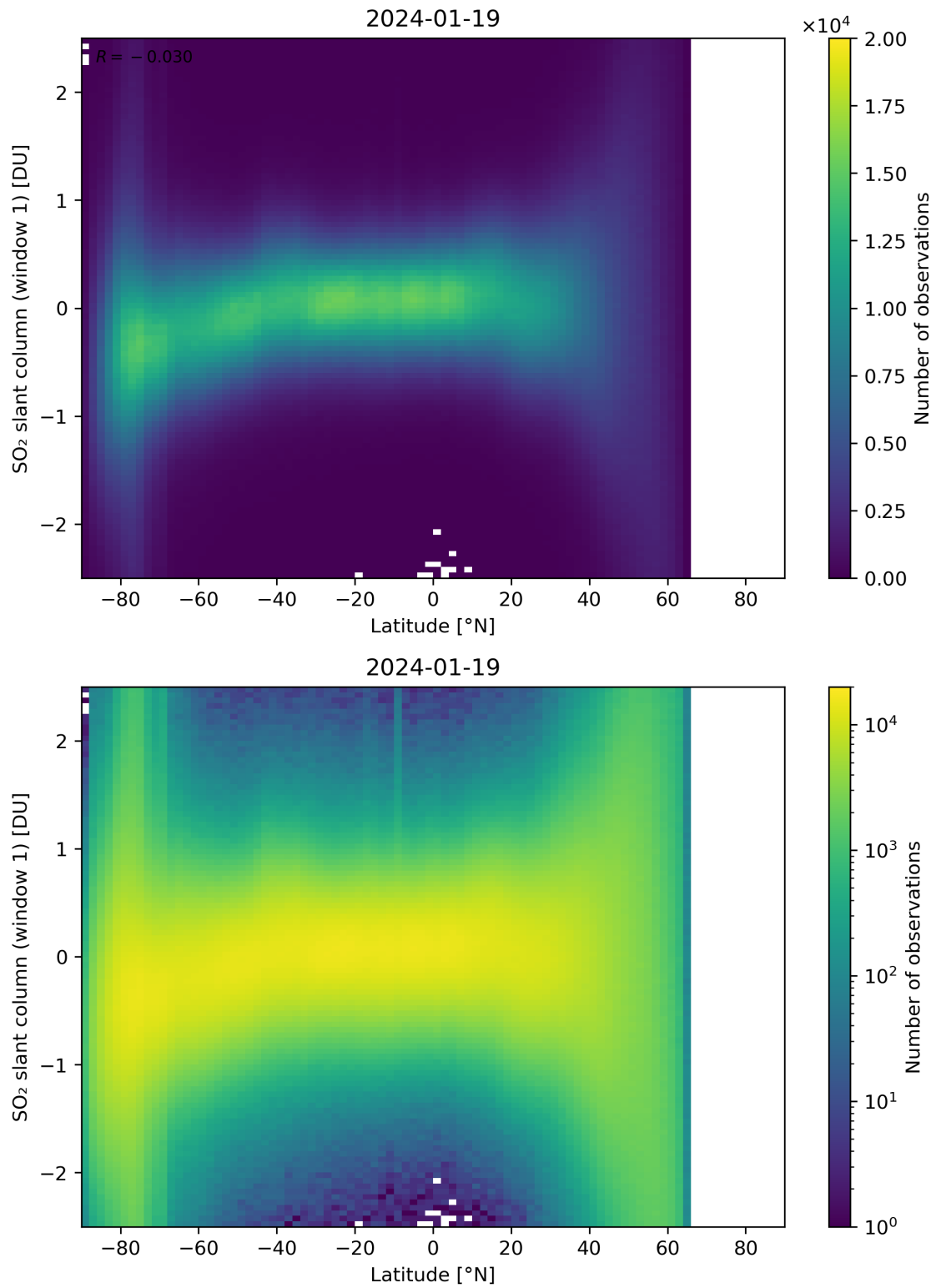
Figure 149: Scatter density plot of “Latitude” against “SO 2 slant column (window 1)” for 2024-01-18 to 2024-01-20.
