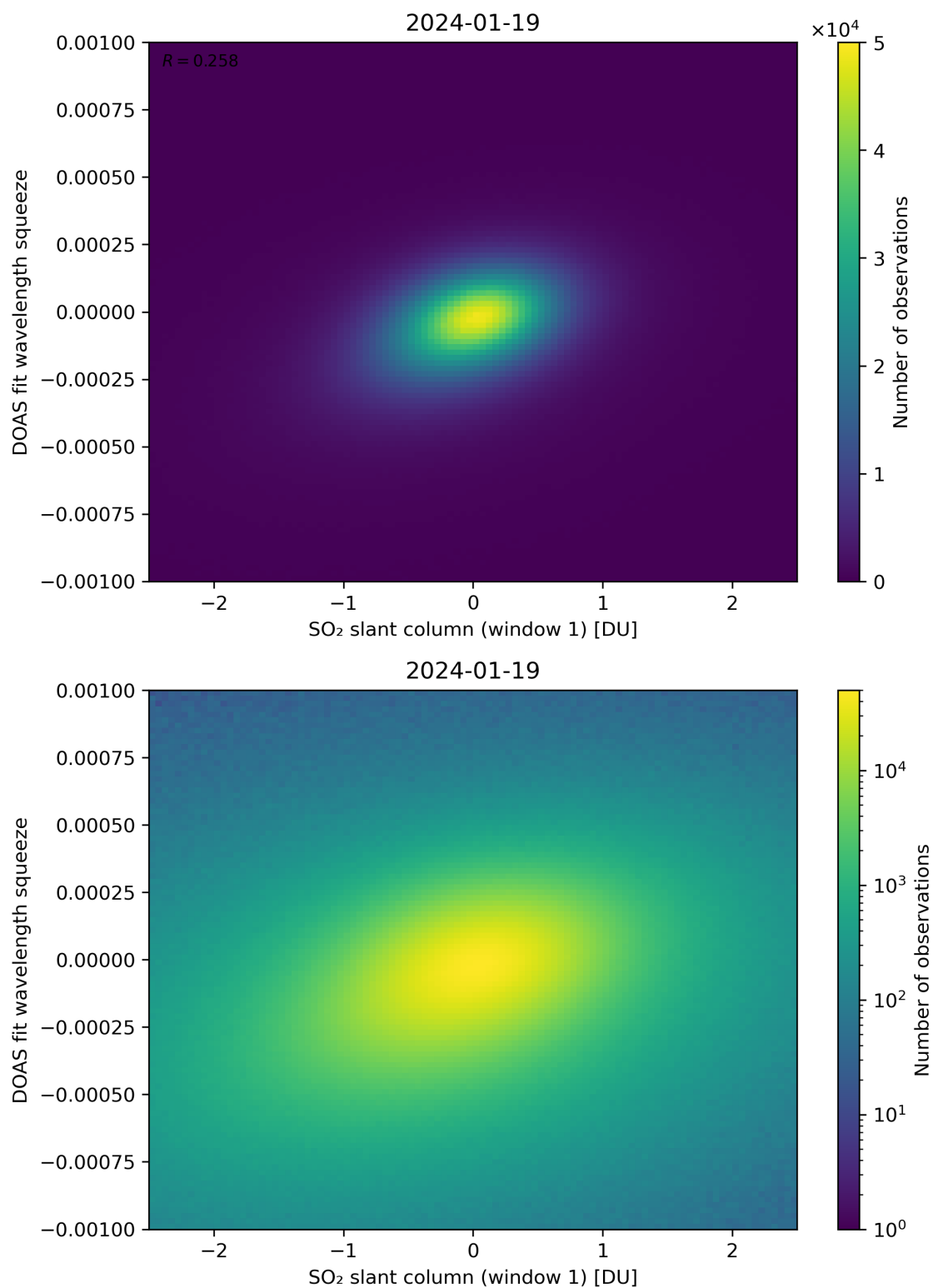
Figure 216: Scatter density plot of “SO 2 slant column (window 1)” against “DOAS fit wavelength squeeze” for 2024-01-18 to 2024-01-20.
