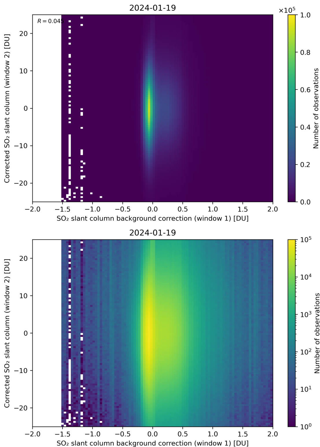
Figure 104: Scatter density plot of “SO 2 slant column background correction (window 1)” against “Corrected SO 2 slant column (window 2)” for 2024-01-18 to 2024-01-20.
