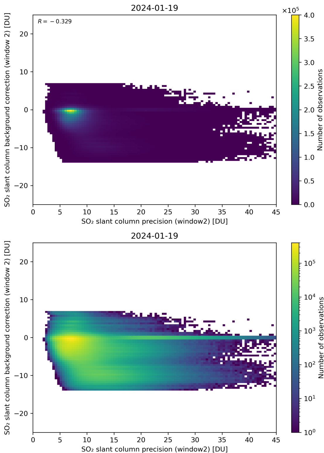
Figure 241: Scatter density plot of “SO 2 slant column precision (window2)” against “SO 2 slant column background correction (window 2)” for 2024-01-18 to 2024-01-20.
