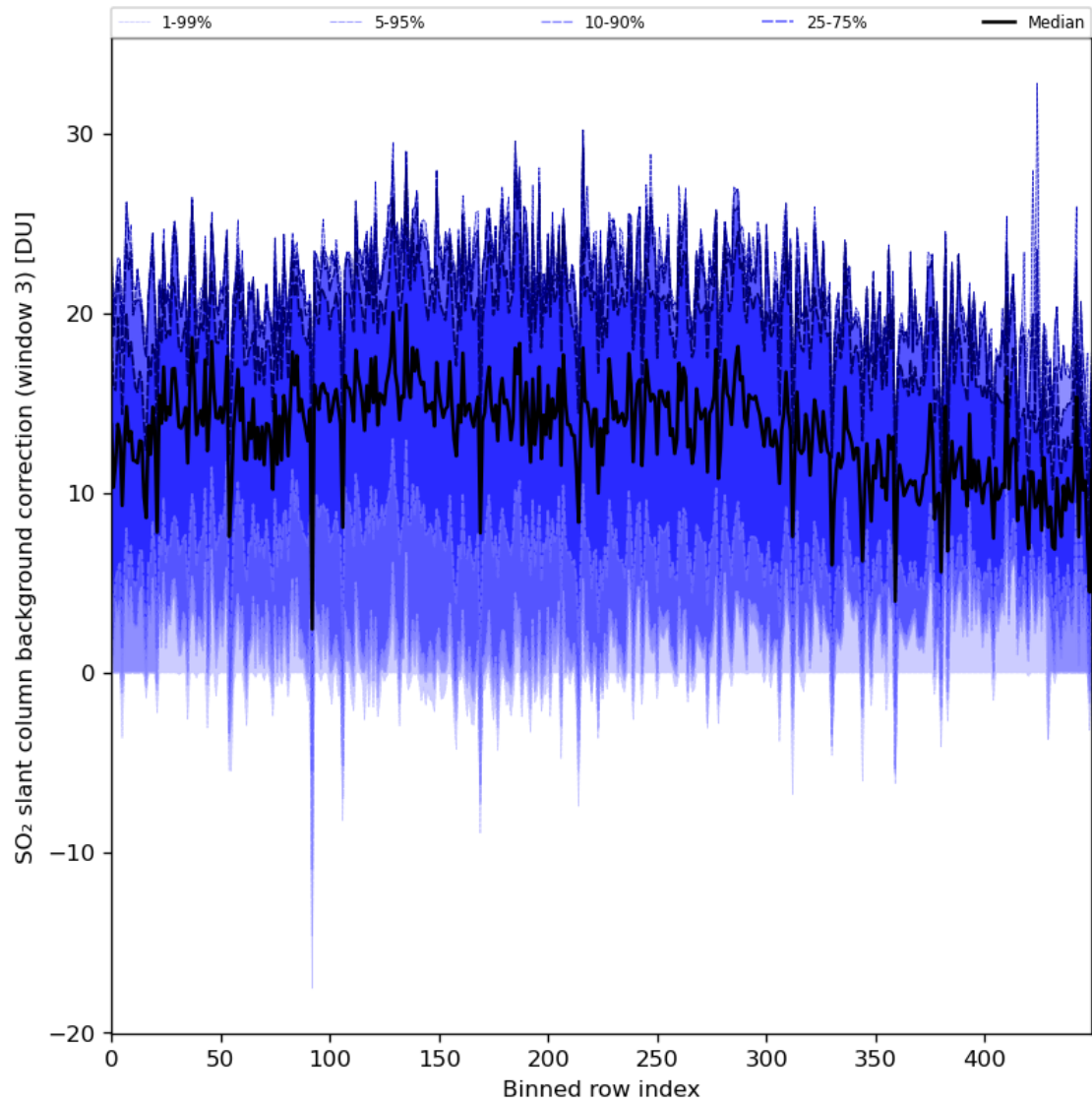
Figure 90: Along track statistics of “SO 2 slant column background correction (window 3)” for 2024-01-18 to 2024-01-20
