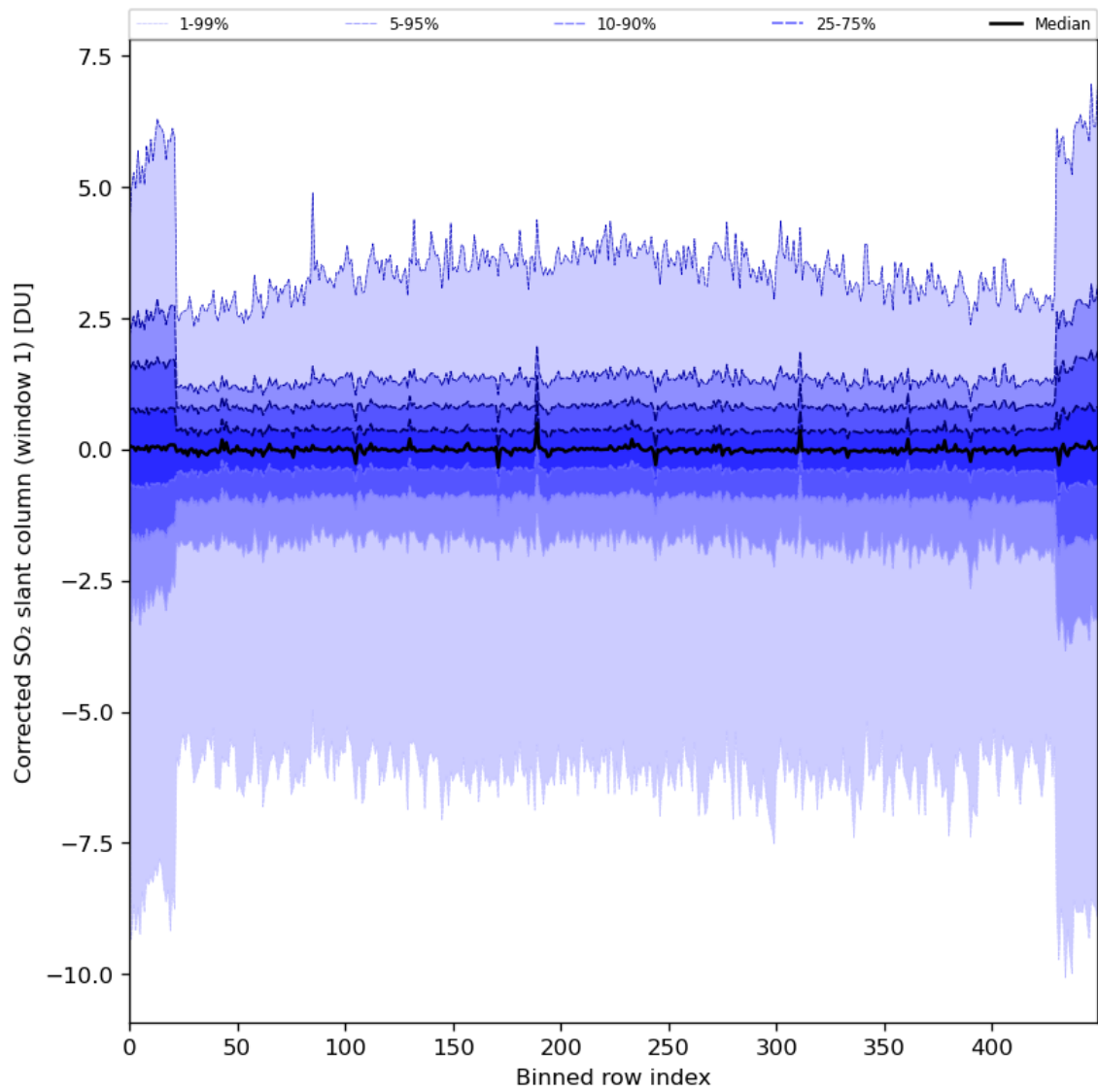
Figure 81: Along track statistics of “Corrected SO 2 slant column (window 1)” for 2024-01-18 to 2024-01-20
