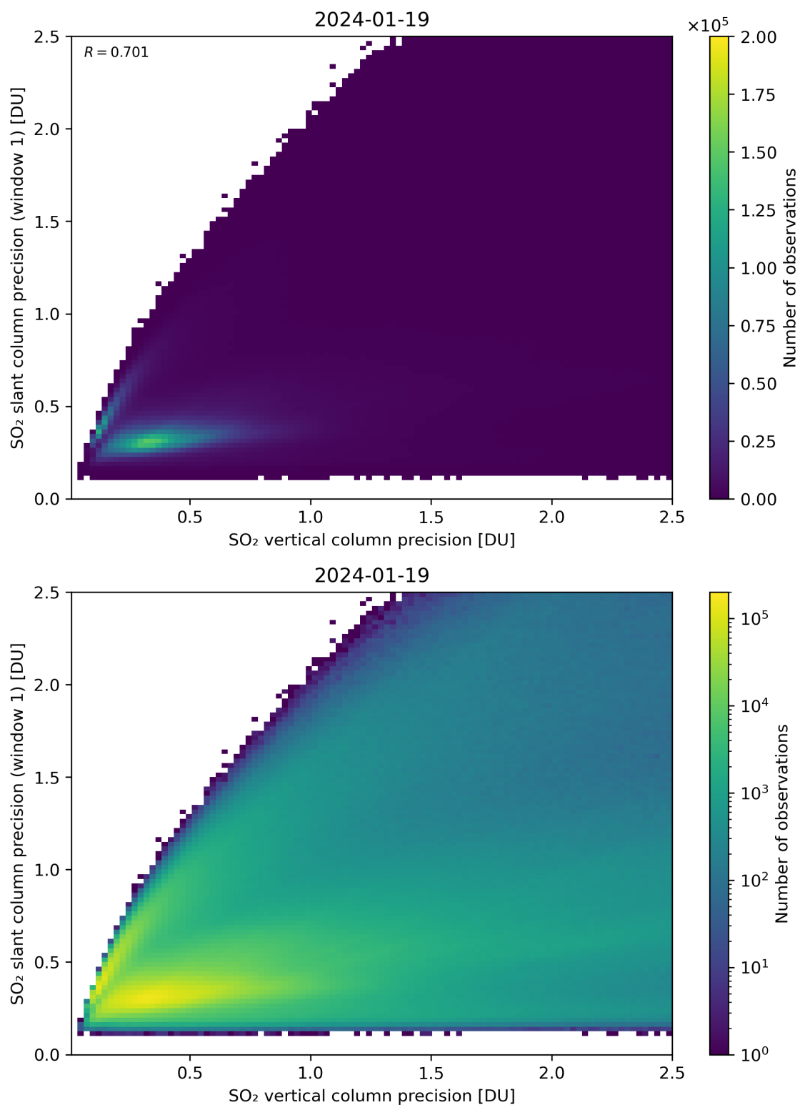
Figure 290: Scatter density plot of “SO 2 vertical column precision” against “SO 2 slant column precision (window 1)” for 2024-01-18 to 2024-01-20.
