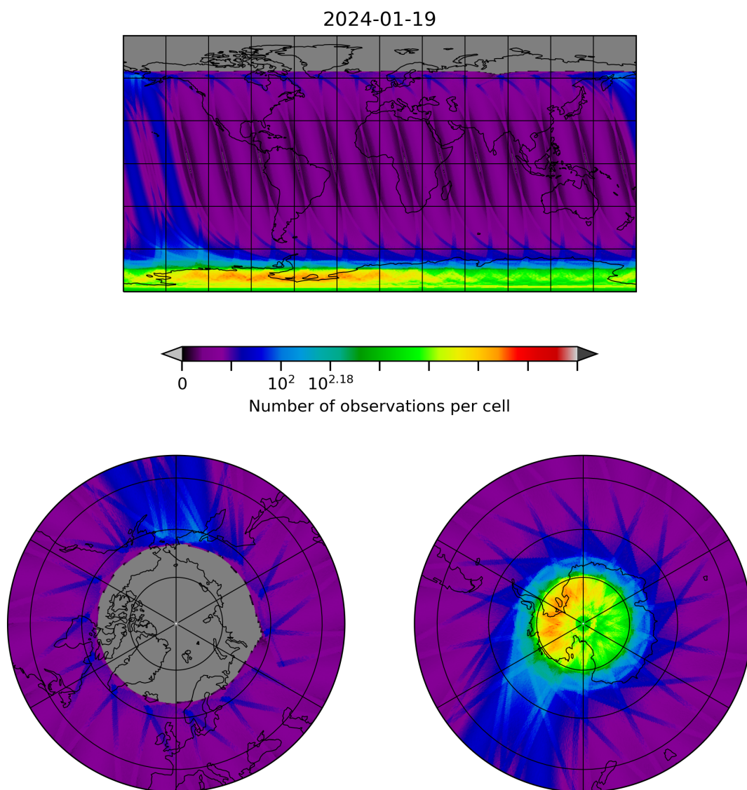
Figure 28: Map of the number of observations for 2024-01-18 to 2024-01-20
