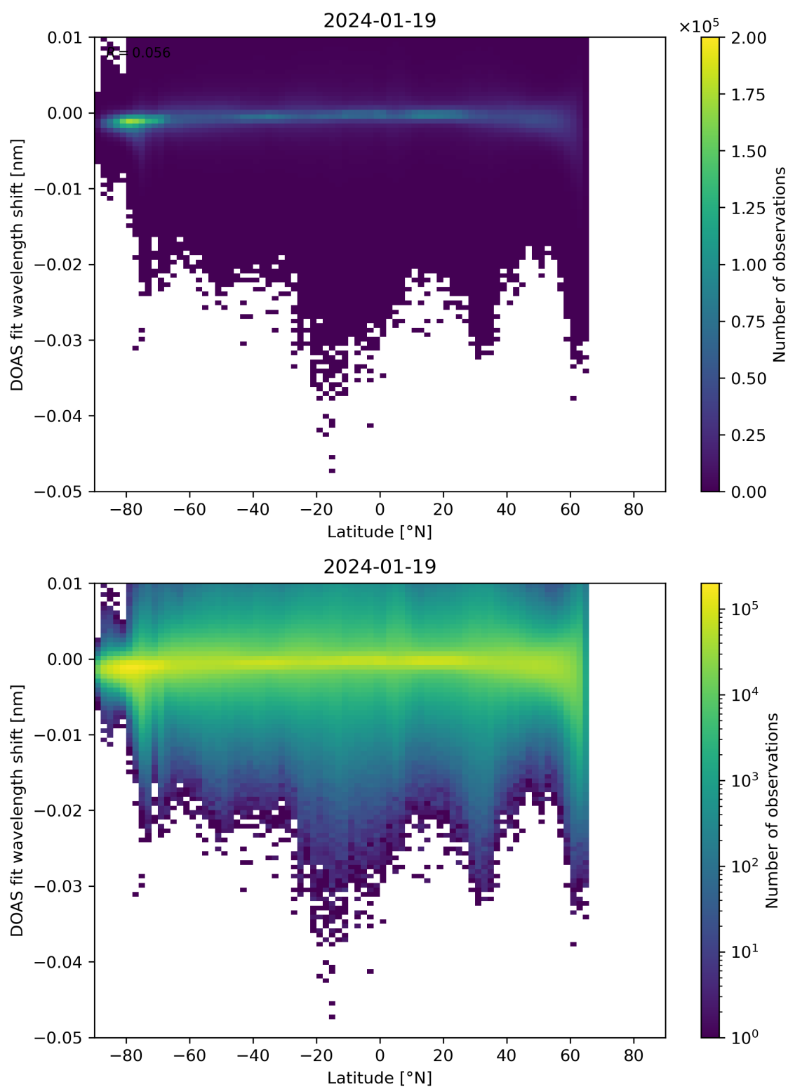
Figure 142: Scatter density plot of “Latitude” against “DOAS fit wavelength shift” for 2024-01-18 to 2024-01-20.
