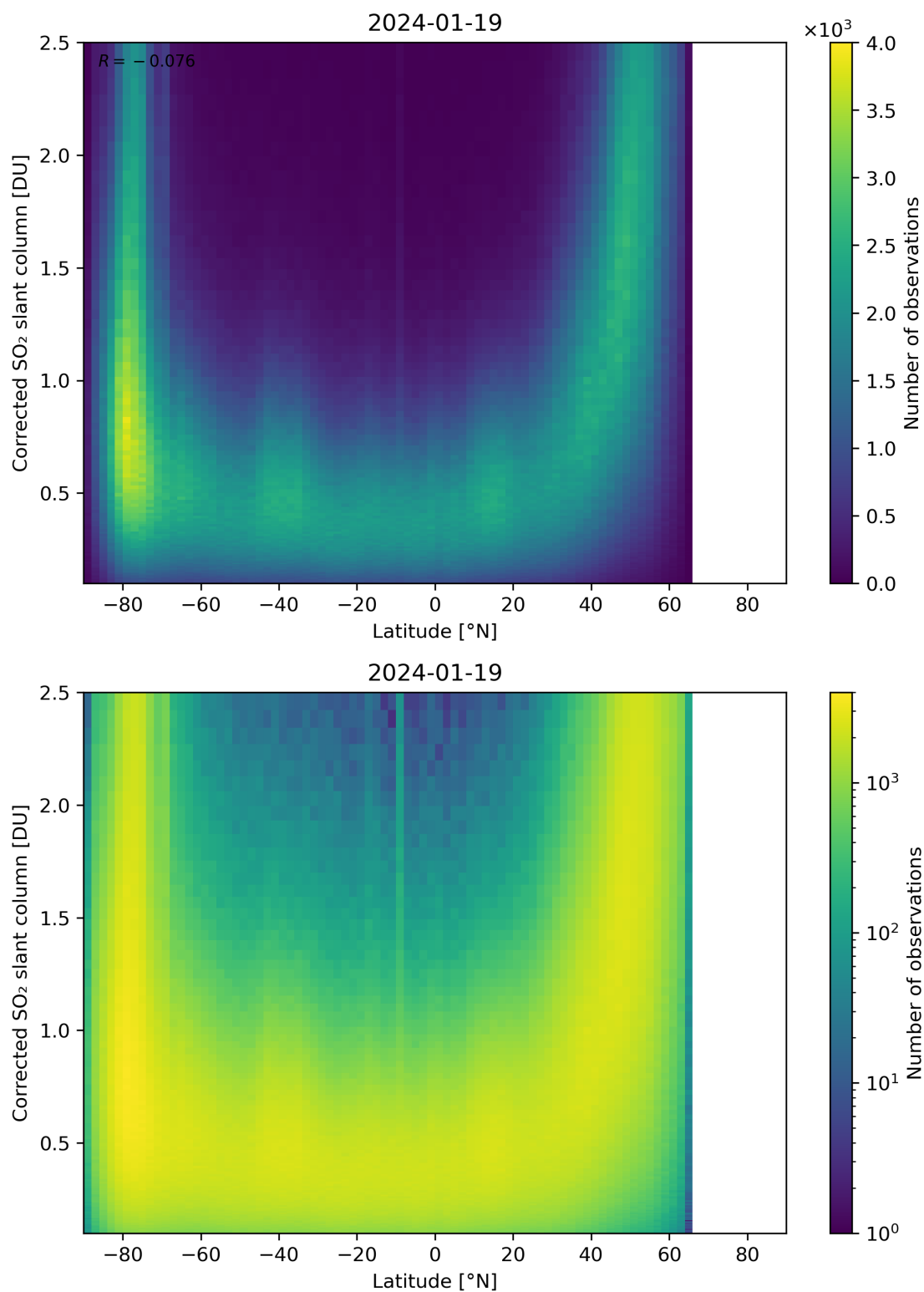
Figure 146: Scatter density plot of “Latitude” against “Corrected SO 2 slant column” for 2024-01-18 to 2024-01-20.
