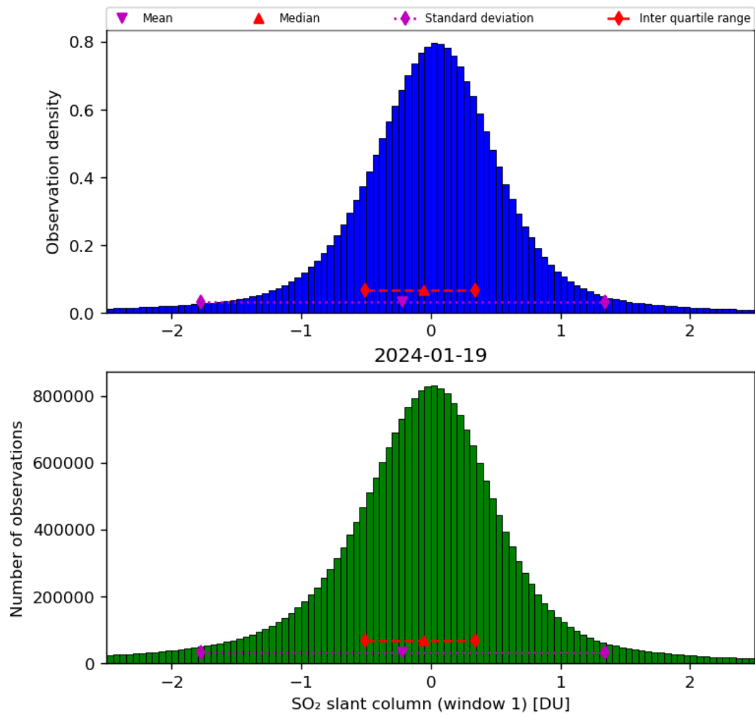
Figure 56: Histogram of “SO 2 slant column (window 1)” for 2024-01-18 to 2024-01-20
