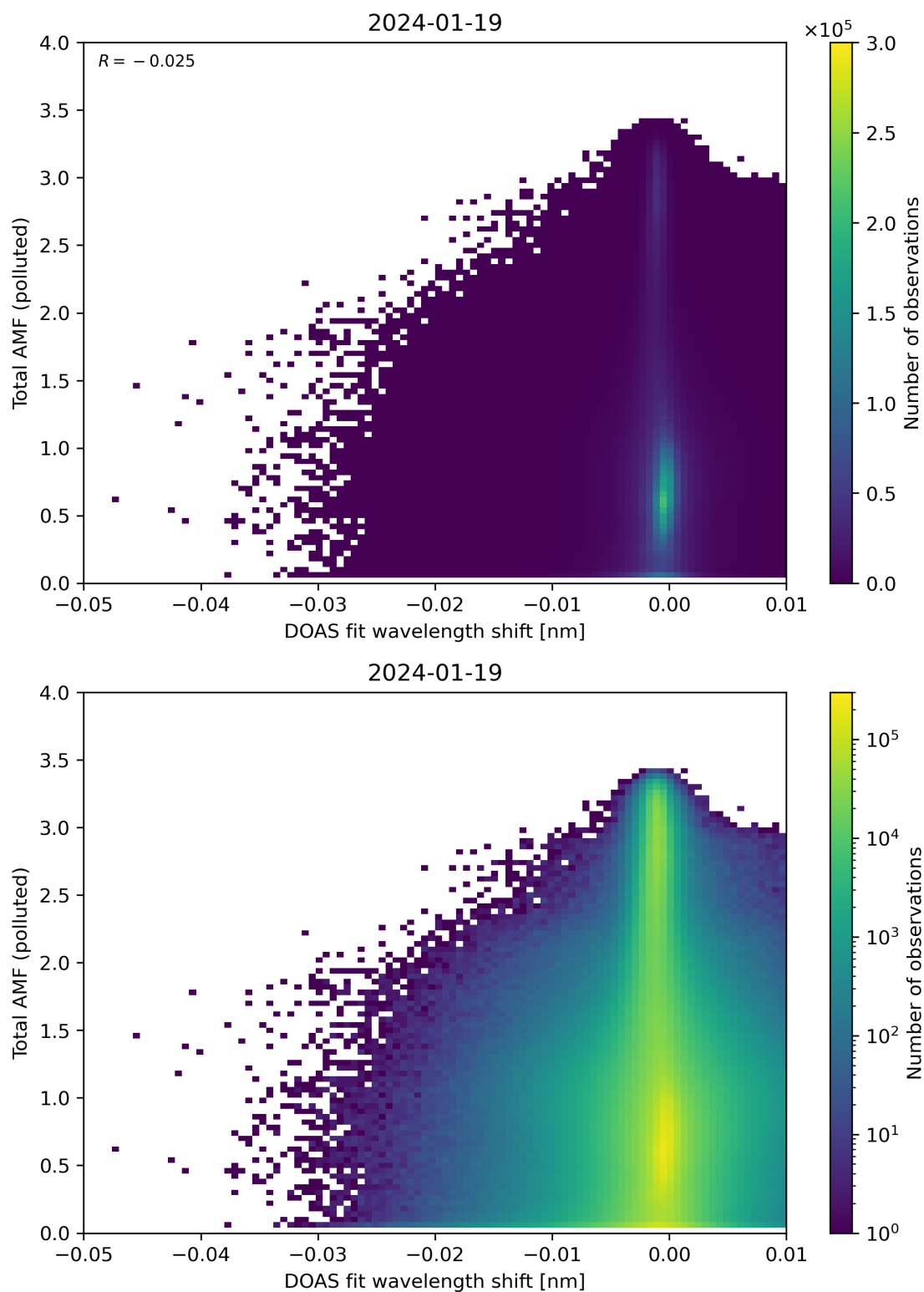
Figure 130: Scatter density plot of “DOAS fit wavelength shift” against “Total AMF (polluted)” for 2024-01-18 to 2024-01-20.
