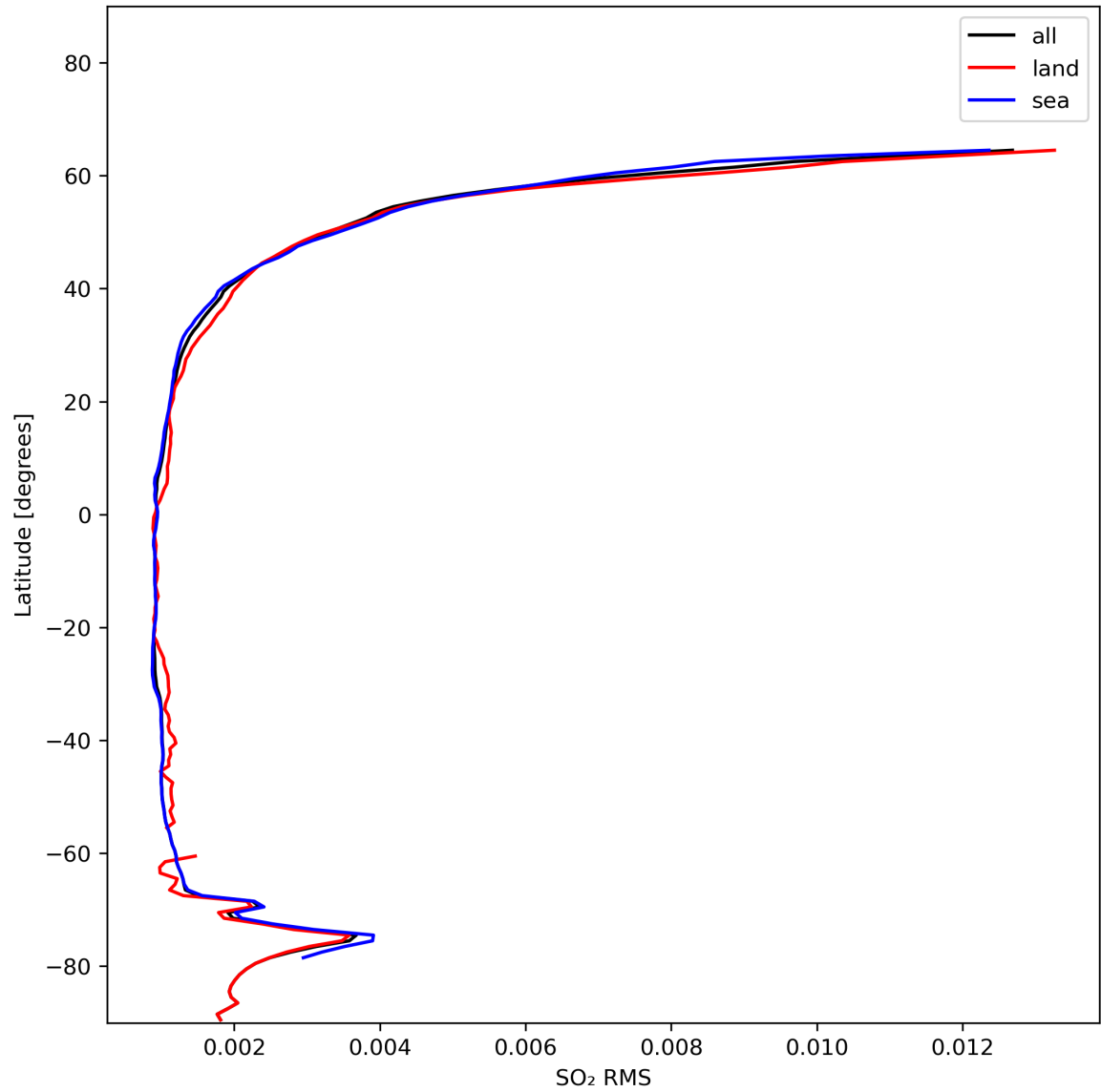
Figure 47: Zonal average of “SO 2 RMS” for 2024-01-18 to 2024-01-20.
