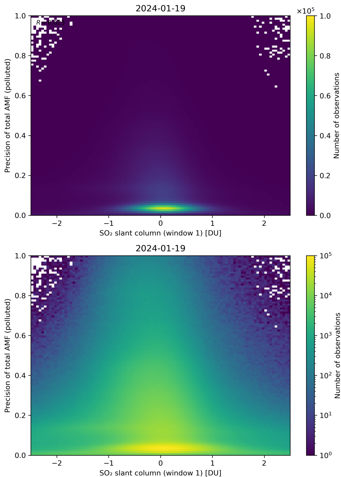
Figure 240: Scatter density plot of “SO 2 slant column (window 1)” against “Precision of total AMF (polluted)” for 2024-01-18 to 2024-01-20.
