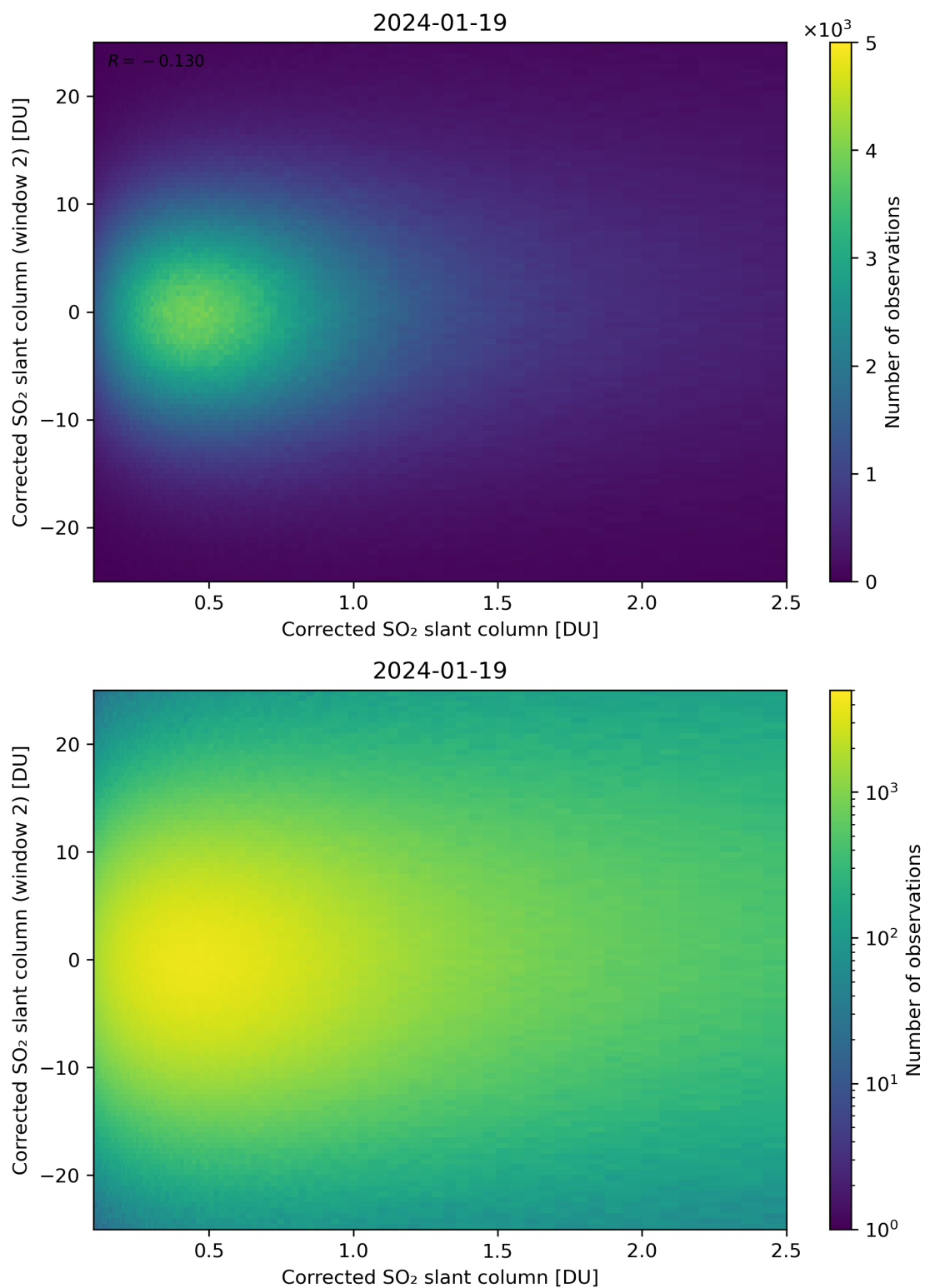
Figure 185: Scatter density plot of “Corrected SO 2 slant column” against “Corrected SO 2 slant column (window 2)” for 2024-01-18 to 2024-01-20.
