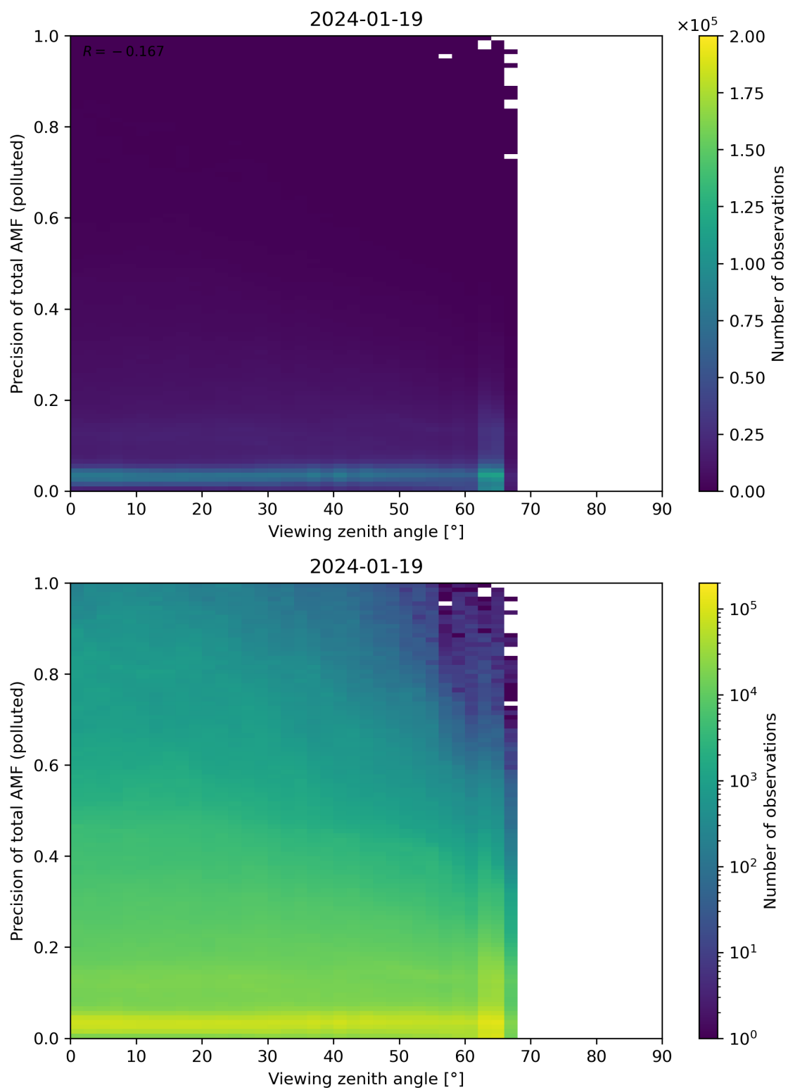
Figure 326: Scatter density plot of “Viewing zenith angle” against “Precision of total AMF (polluted)” for 2024-01-18 to 2024-01-20.
