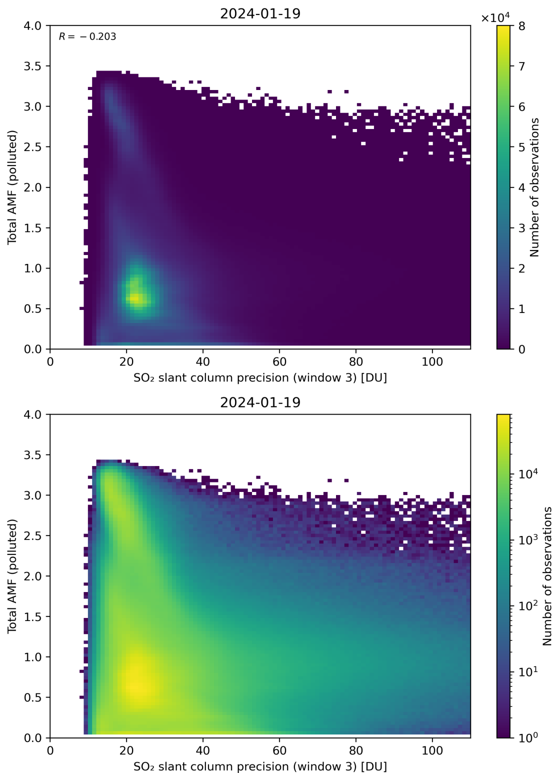
Figure 263: Scatter density plot of “SO 2 slant column precision (window 3)” against “Total AMF (polluted)” for 2024-01-18 to 2024-01-20.
