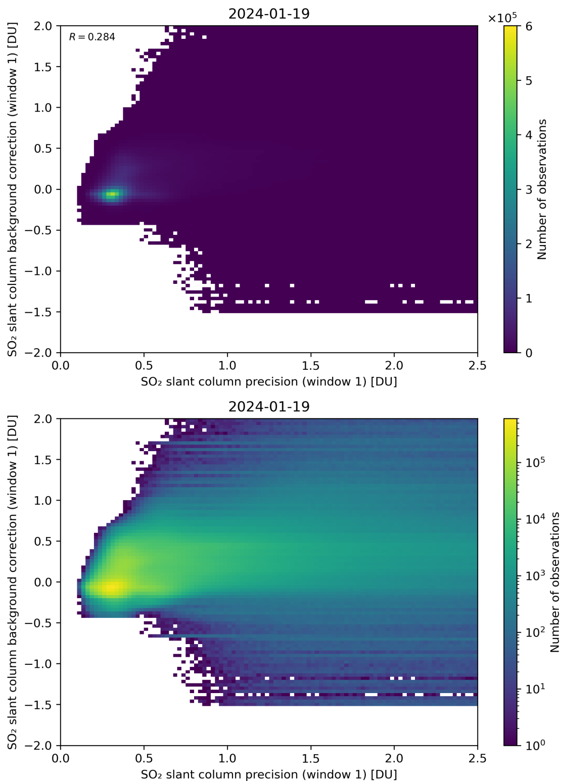
Figure 218: Scatter density plot of “SO 2 slant column precision (window 1)” against “SO 2 slant column background correction (window 1)” for 2024-01-18 to 2024-01-20.
