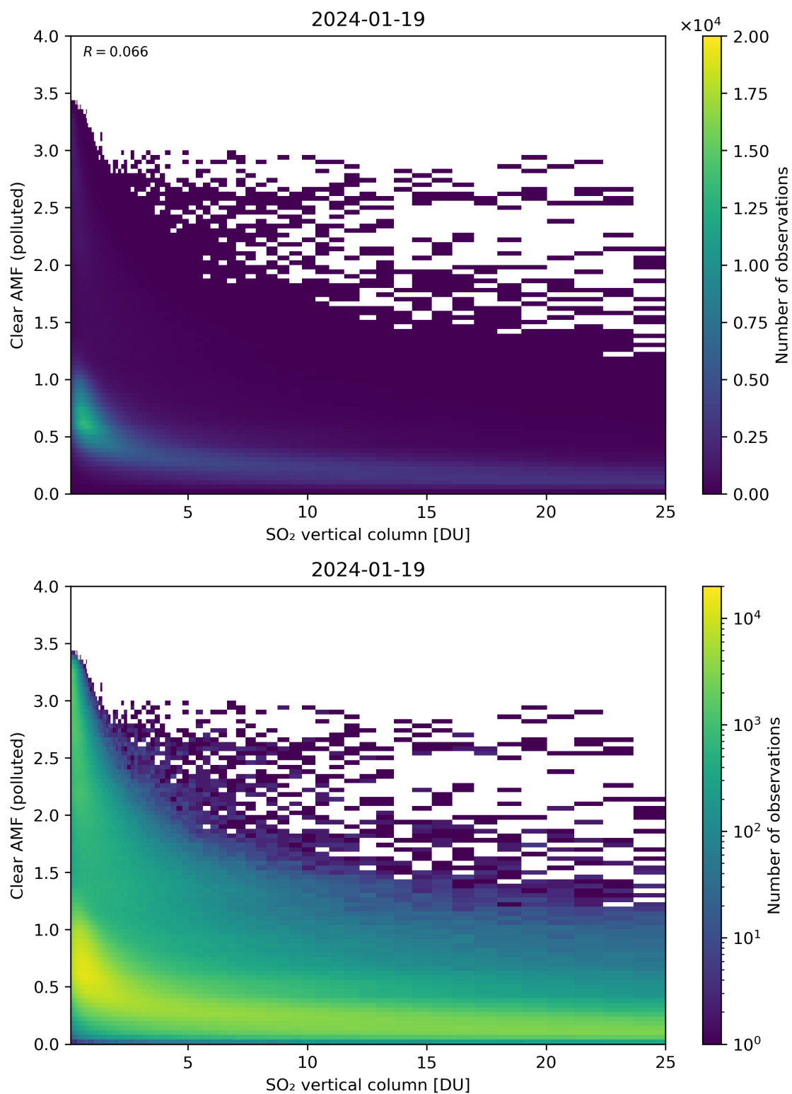
Figure 296: Scatter density plot of “SO 2 vertical column” against “Clear AMF (polluted)” for 2024-01-18 to 2024-01-20.
