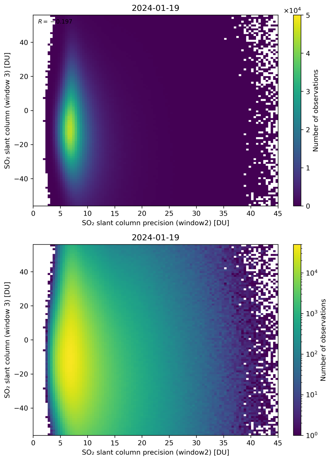
Figure 249: Scatter density plot of “SO 2 slant column precision (window2)” against “SO 2 slant column (window 3)” for 2024-01-18 to 2024-01-20.
