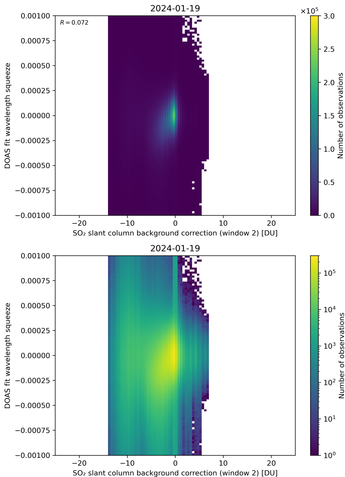
Figure 113: Scatter density plot of “SO 2 slant column background correction (window 2)” against “DOAS fit wavelength squeeze” for 2024-01-18 to 2024-01-20.
