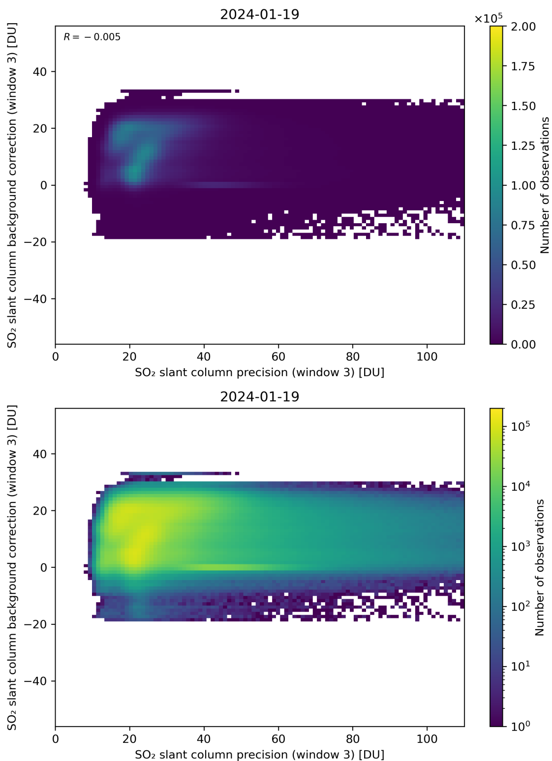
Figure 257: Scatter density plot of “SO 2 slant column precision (window 3)” against “SO 2 slant column background correction (window 3)” for 2024-01-18 to 2024-01-20.
