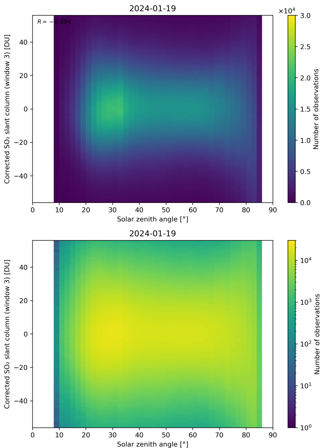
Figure 168: Scatter density plot of “Solar zenith angle” against “Corrected SO 2 slant column (window 3)” for 2024-01-18 to 2024-01-20.
