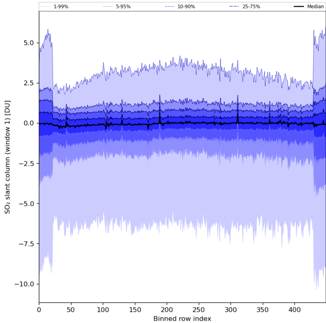
Figure 79: Along track statistics of “SO 2 slant column (window 1)” for 2024-01-18 to 2024-01-20
