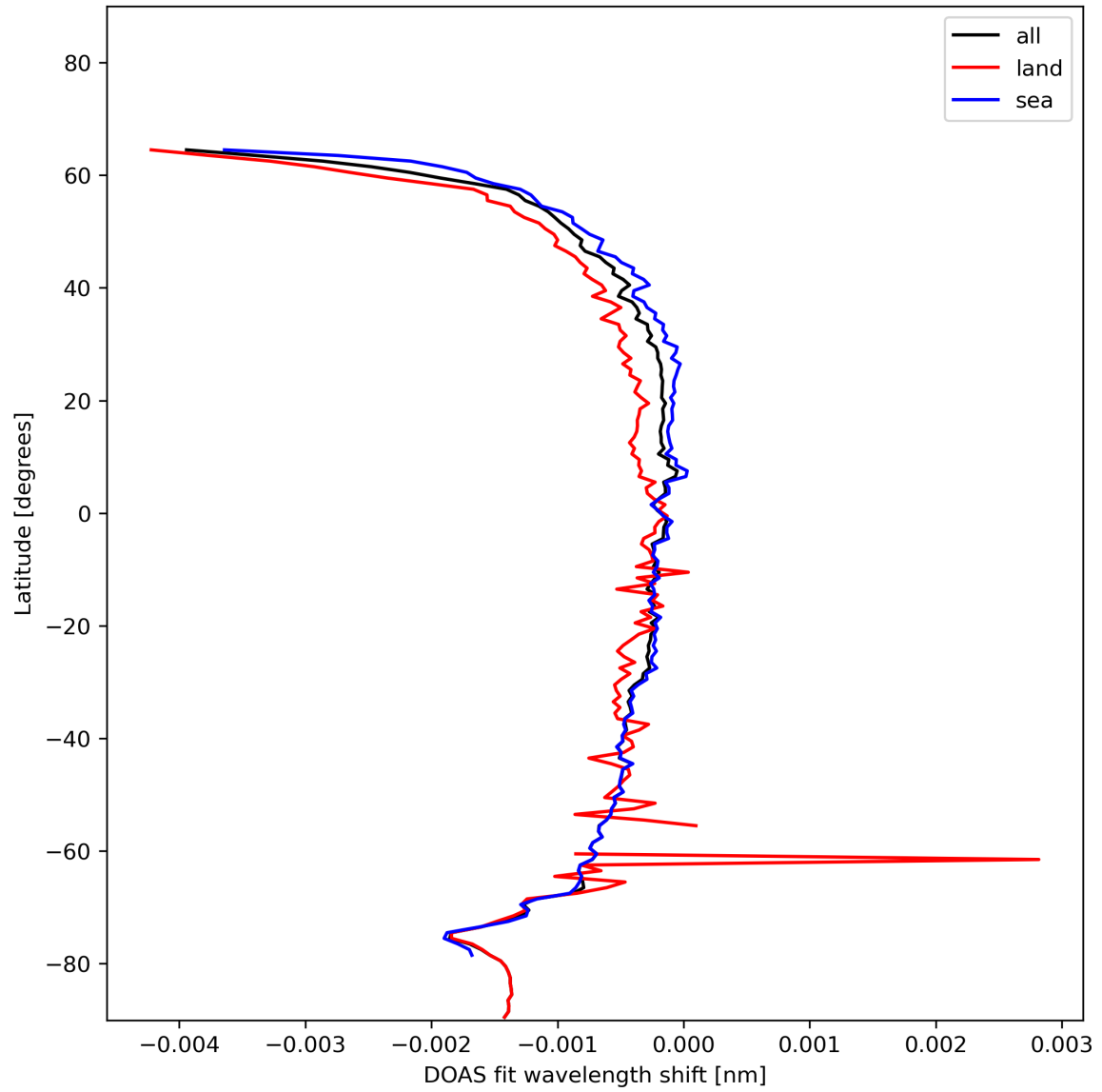
Figure 45: Zonal average of “DOAS fit wavelength shift” for 2024-01-18 to 2024-01-20.
