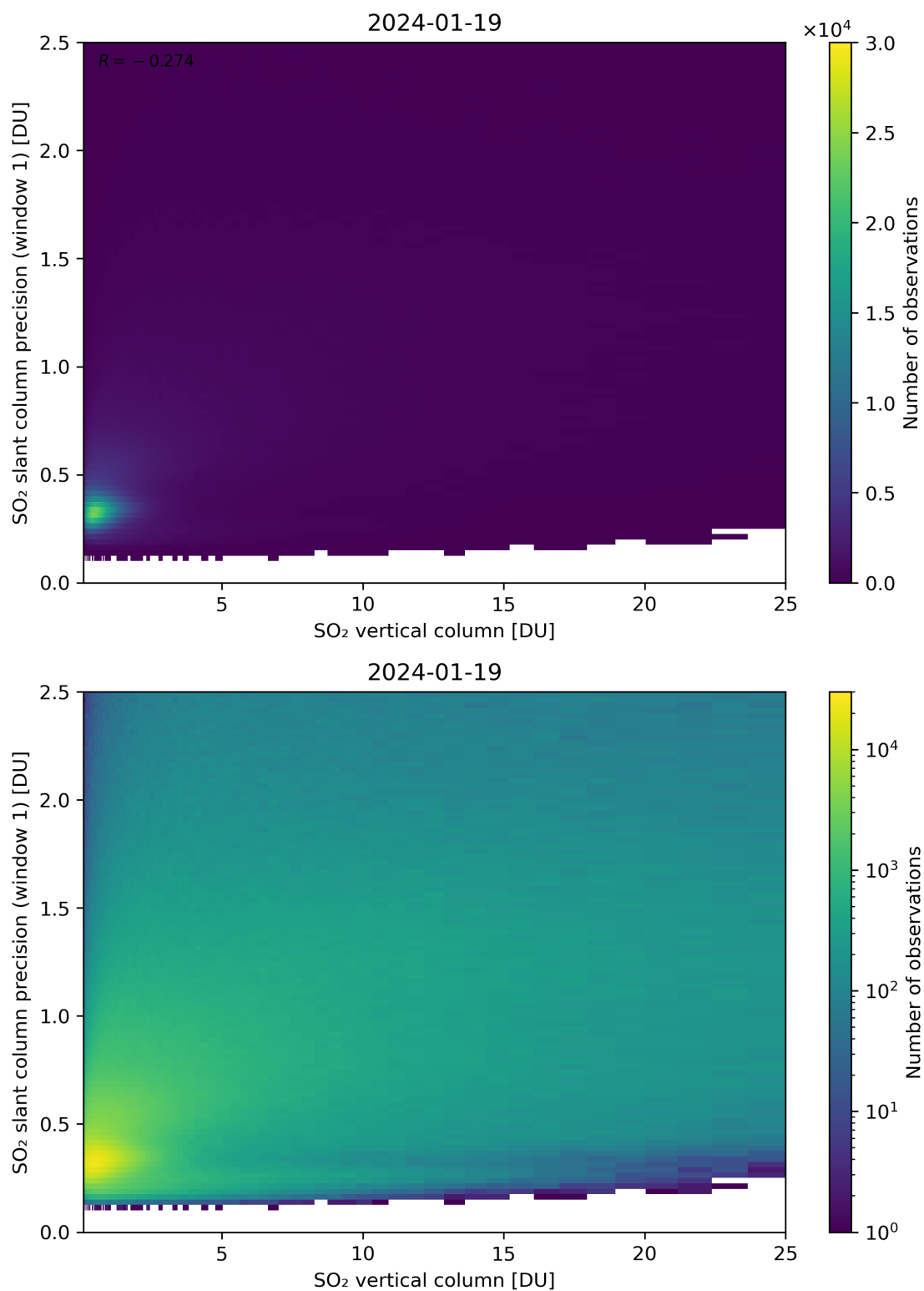
Figure 301: Scatter density plot of “SO 2 vertical column” against “SO 2 slant column precision (window 1)” for 2024-01-18 to 2024-01-20.
