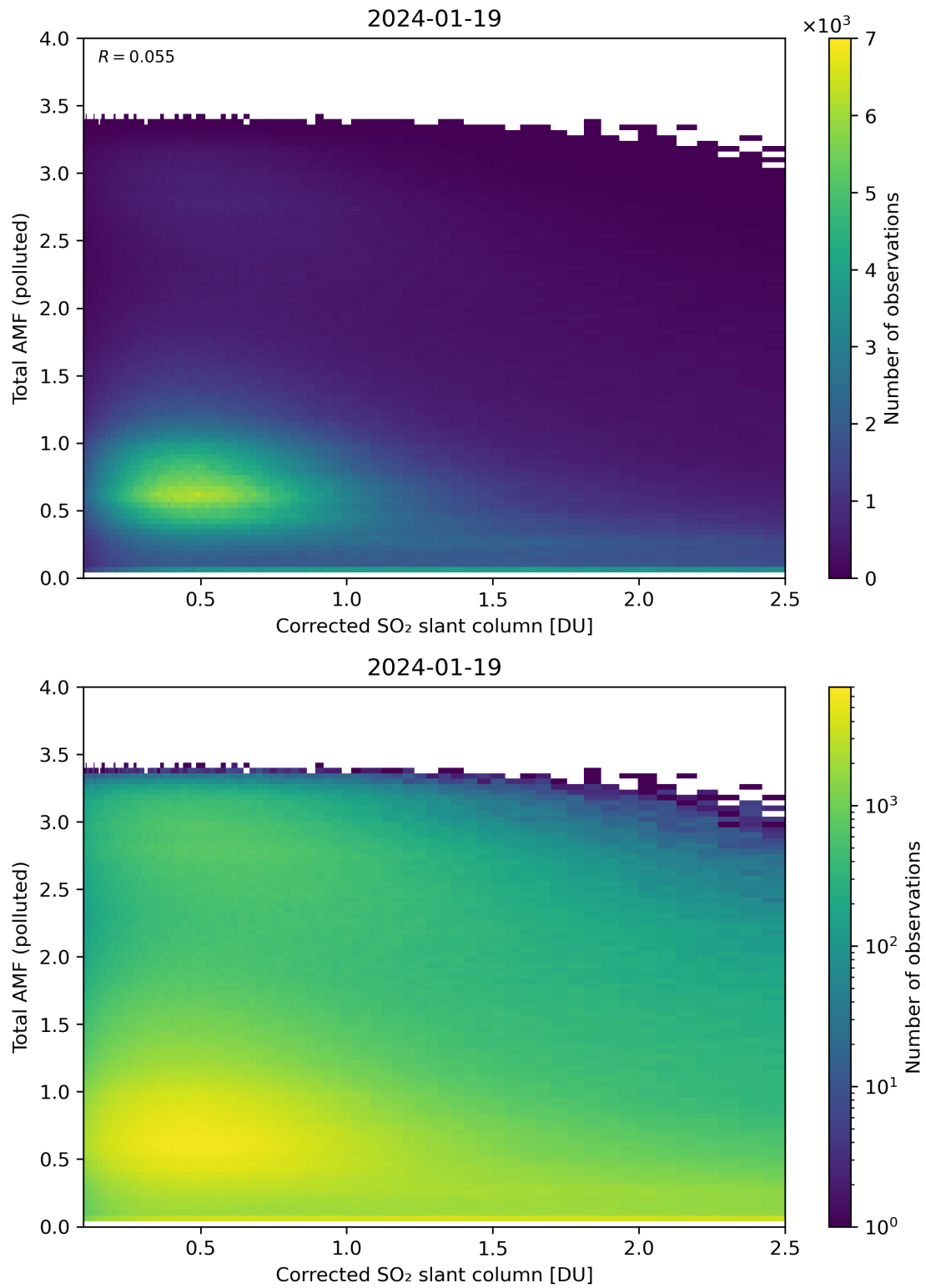
Figure 192: Scatter density plot of “Corrected SO 2 slant column” against “Total AMF (polluted)” for 2024-01-18 to 2024-01-20.
