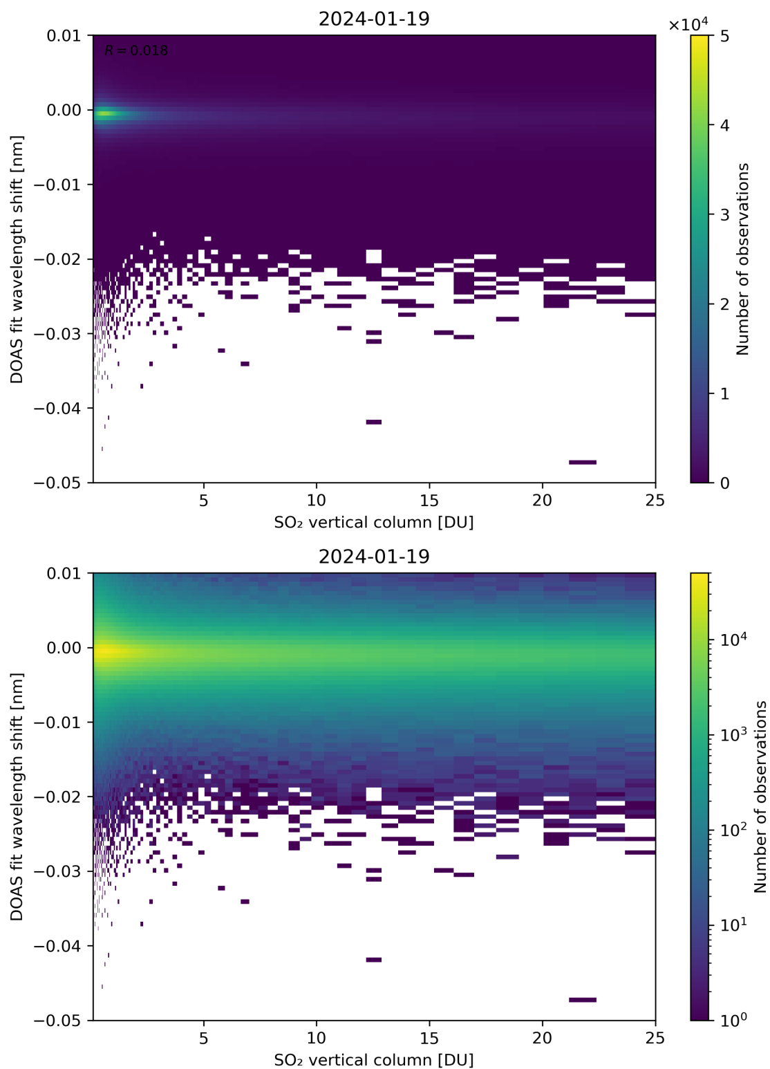
Figure 276: Scatter density plot of “SO 2 vertical column” against “DOAS fit wavelength shift” for 2024-01-18 to 2024-01-20.
