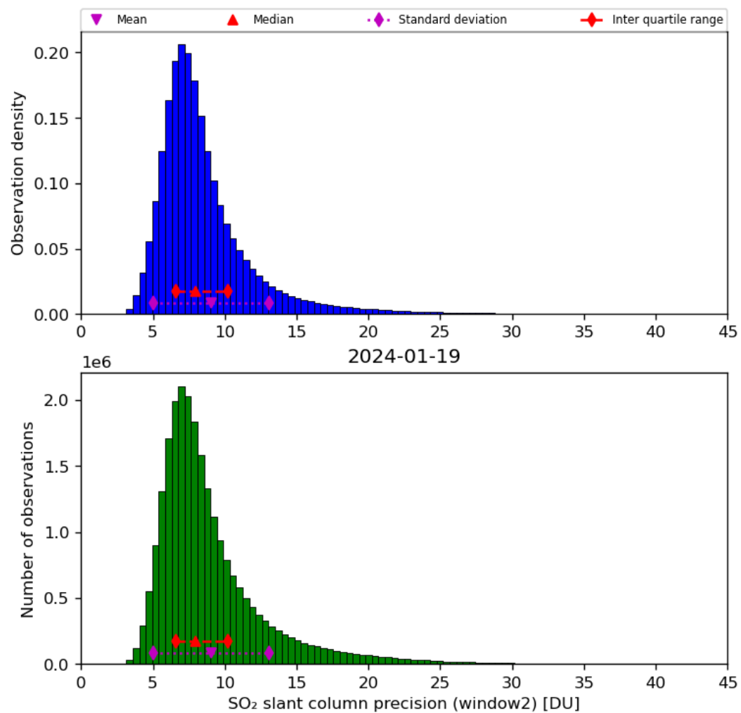
Figure 61: Histogram of “SO 2 slant column precision (window2)” for 2024-01-18 to 2024-01-20
