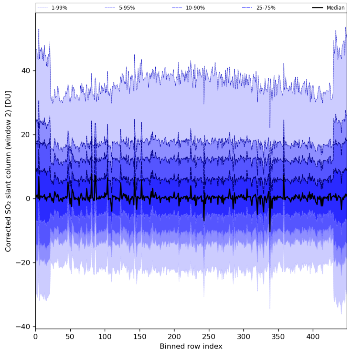
Figure 85: Along track statistics of “Corrected SO 2 slant column (window 2)” for 2024-01-18 to 2024-01-20
