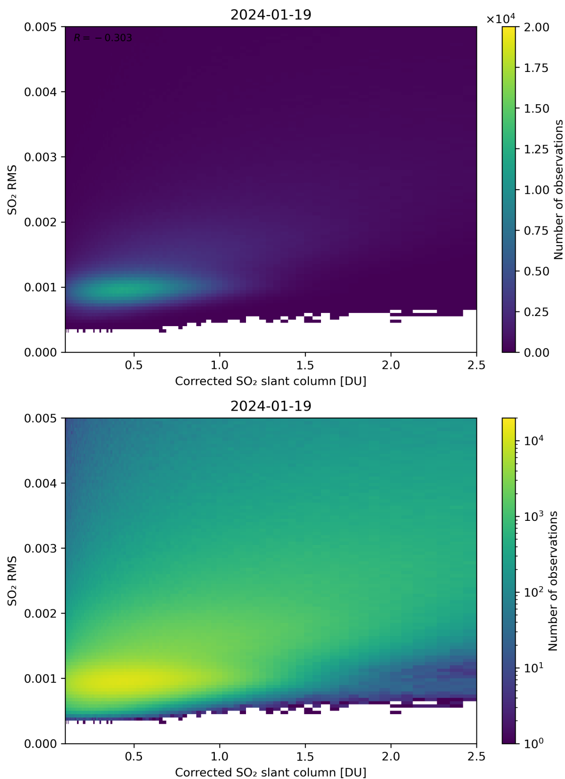
Figure 183: Scatter density plot of “Corrected SO 2 slant column” against “SO 2 RMS” for 2024-01-18 to 2024-01-20.
