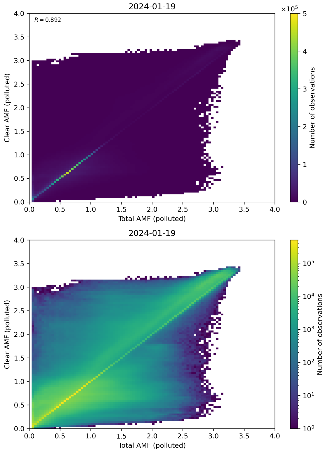
Figure 271: Scatter density plot of “Total AMF (polluted)” against “Clear AMF (polluted)” for 2024-01-18 to 2024-01-20.
