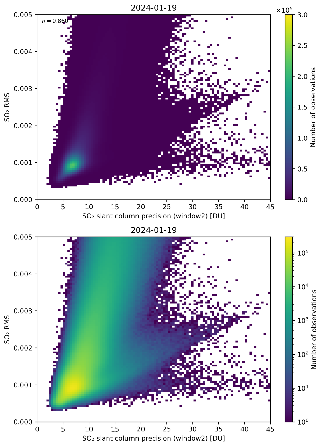
Figure 245: Scatter density plot of “SO 2 slant column precision (window2)” against “SO 2 RMS” for 2024-01-18 to 2024-01-20.
