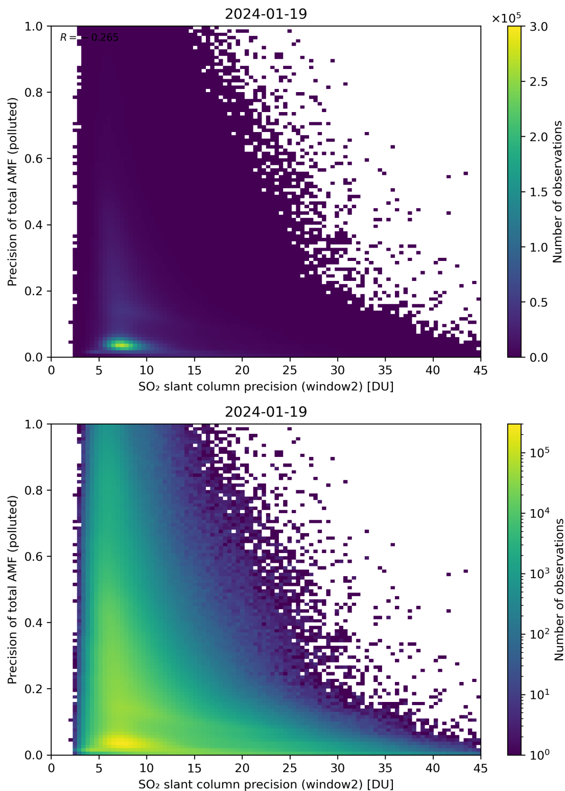
Figure 252: Scatter density plot of “SO 2 slant column precision (window2)” against “Precision of total AMF (polluted)” for 2024-01-18 to 2024-01-20.
