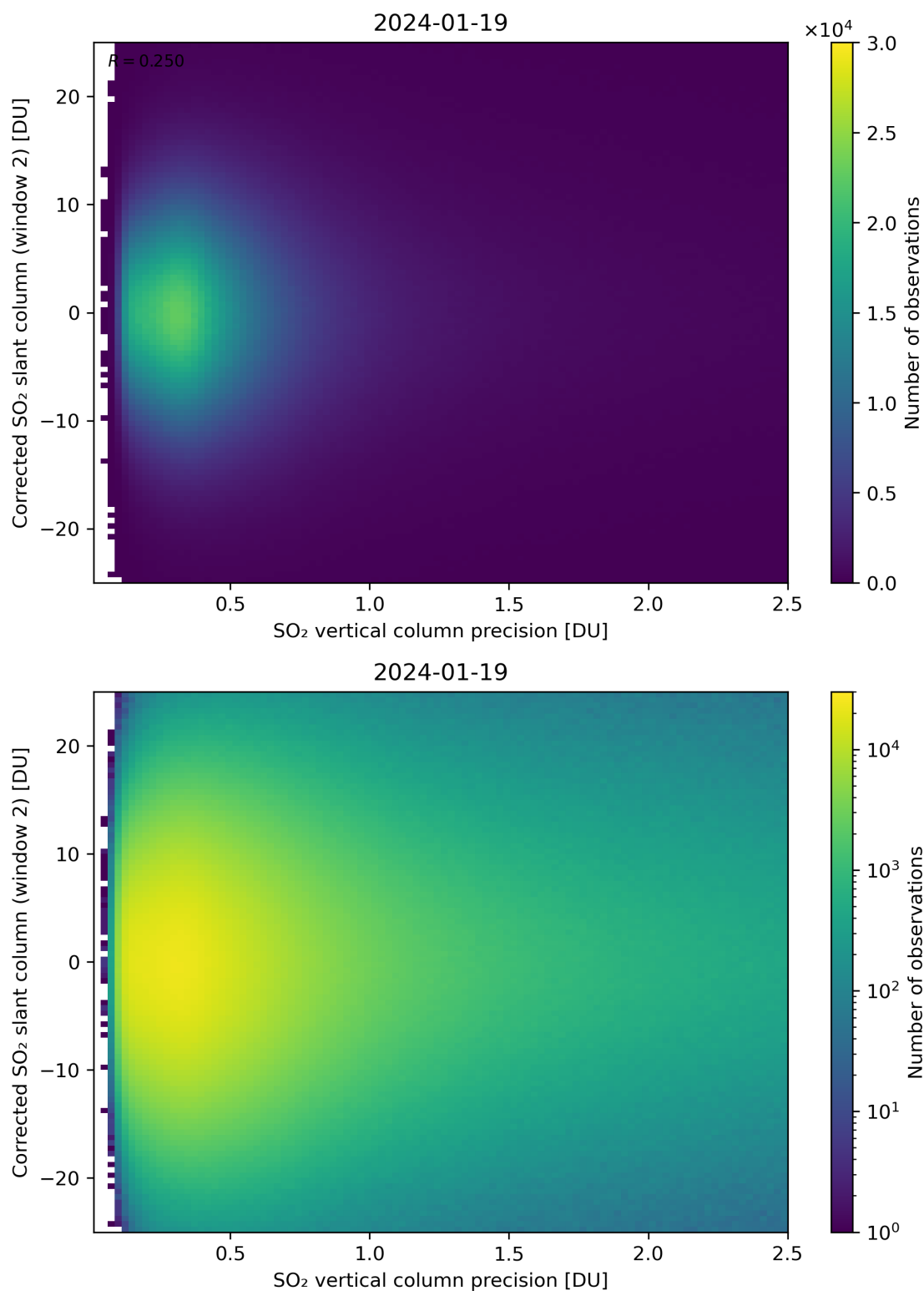
Figure 287: Scatter density plot of “SO 2 vertical column precision” against “Corrected SO 2 slant column (window 2)” for 2024-01-18 to 2024-01-20.
