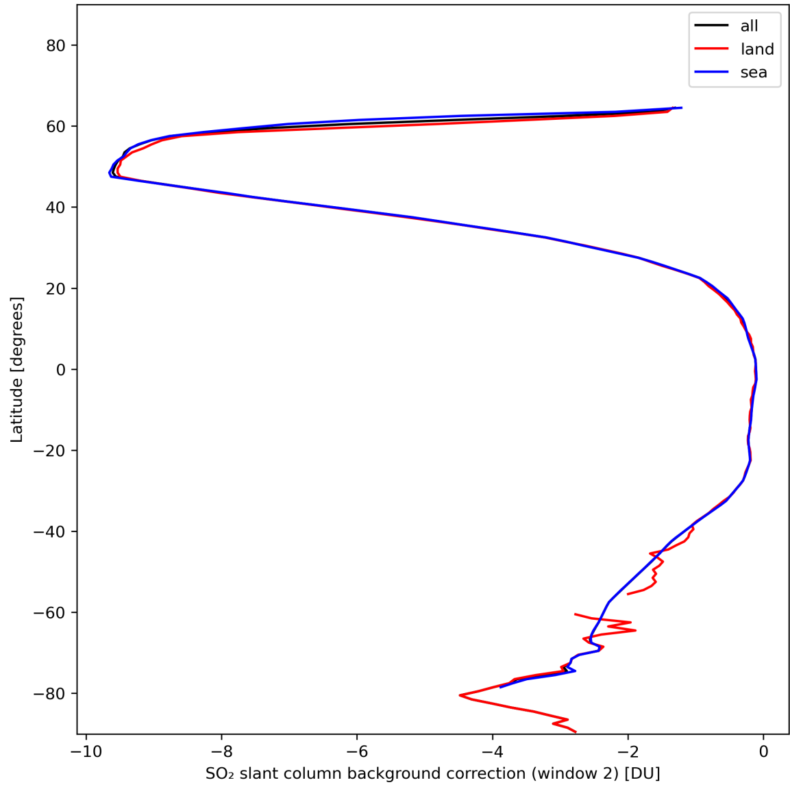
Figure 40: Zonal average of “SO 2 slant column background correction (window 2)” for 2024-01-18 to 2024-01-20.
