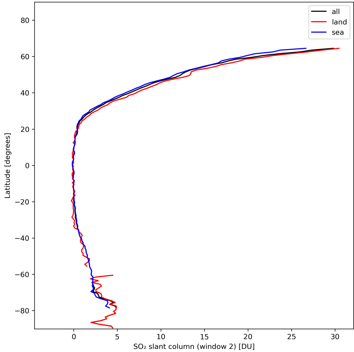
Figure 37: Zonal average of “SO 2 slant column (window 2)” for 2024-01-18 to 2024-01-20.
