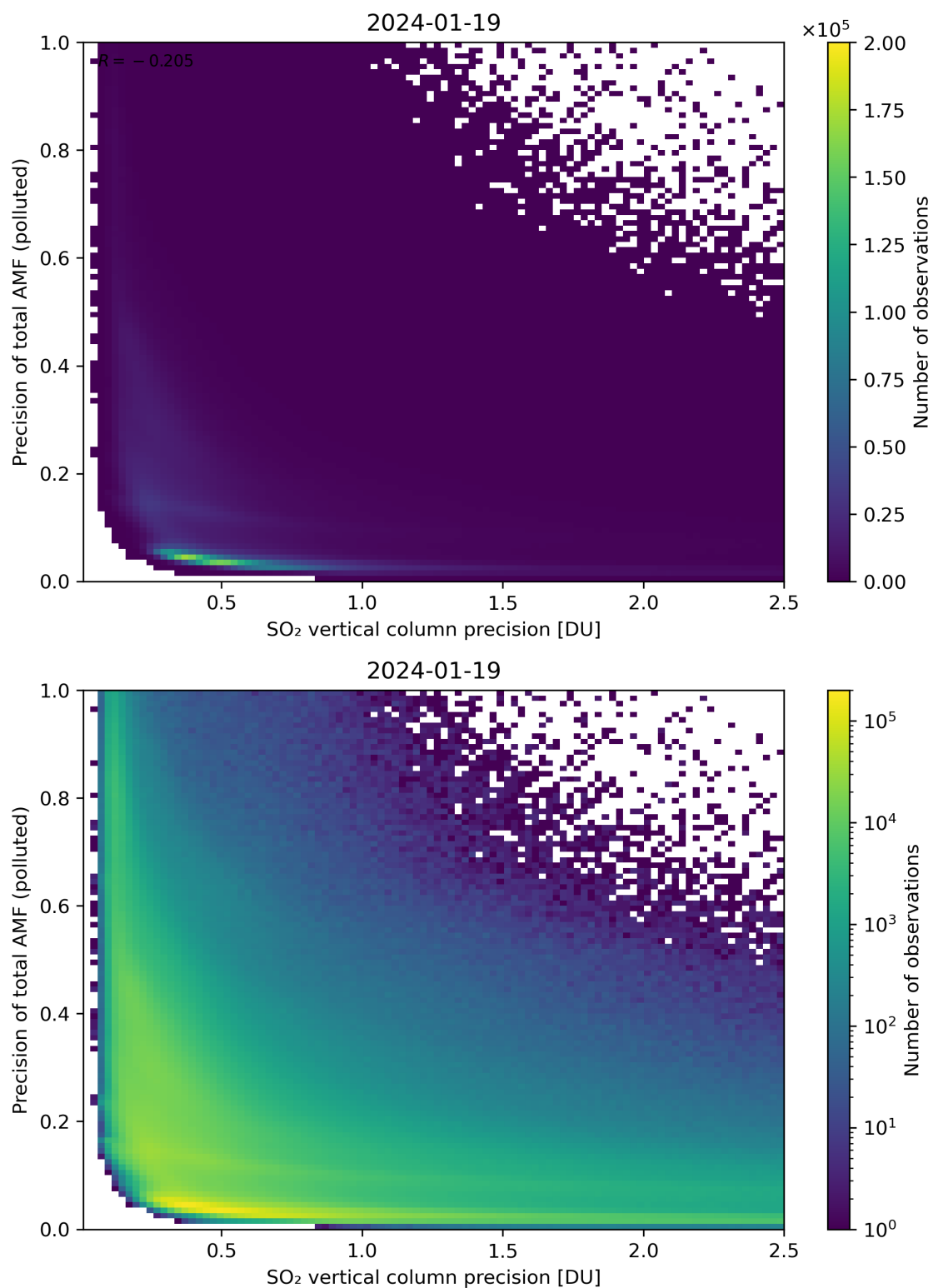
Figure 295: Scatter density plot of “SO 2 vertical column precision” against “Precision of total AMF (polluted)” for 2024-01-18 to 2024-01-20.
