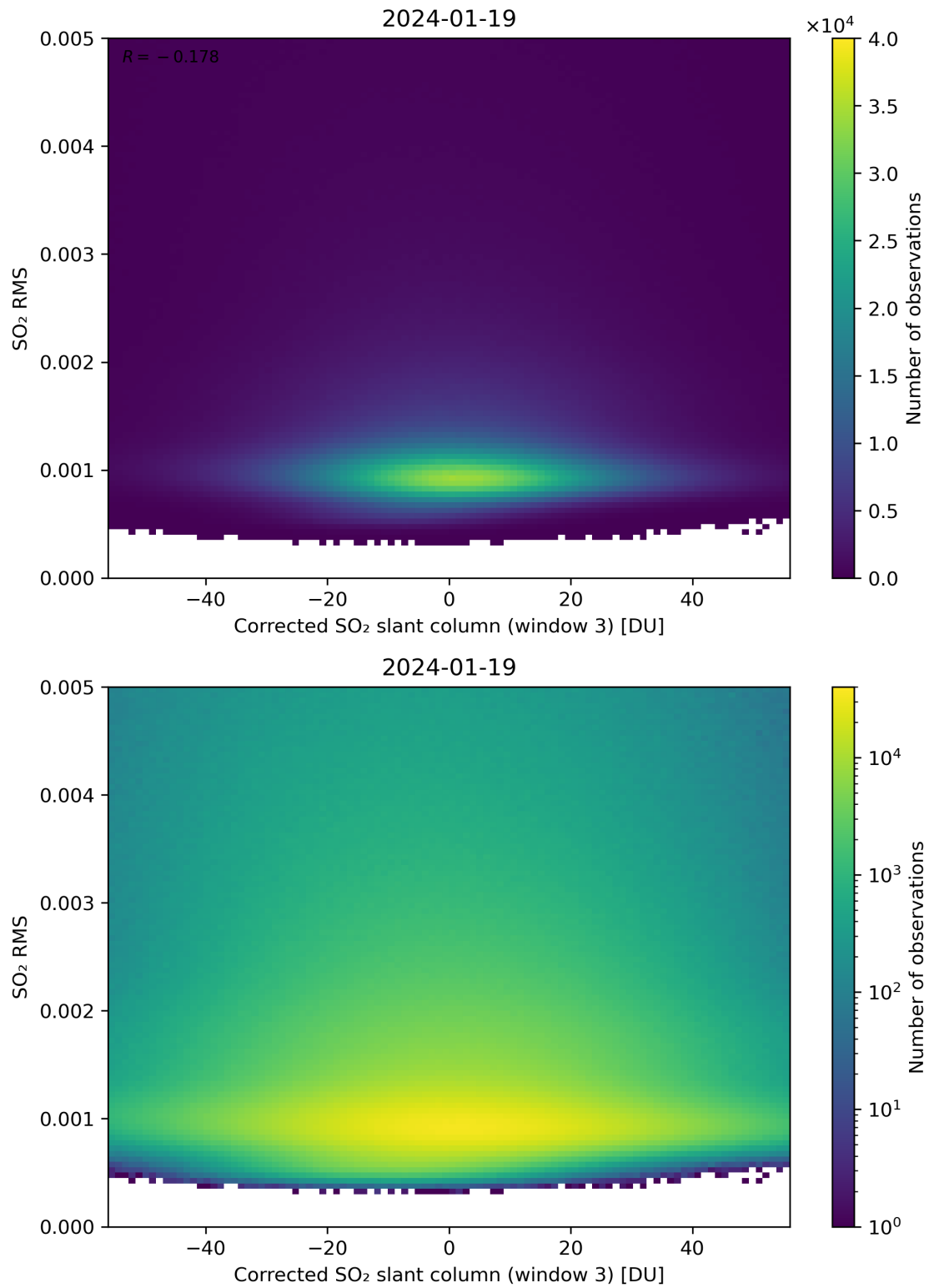
Figure 208: Scatter density plot of “Corrected SO 2 slant column (window 3)” against “SO 2 RMS” for 2024-01-18 to 2024-01-20.
