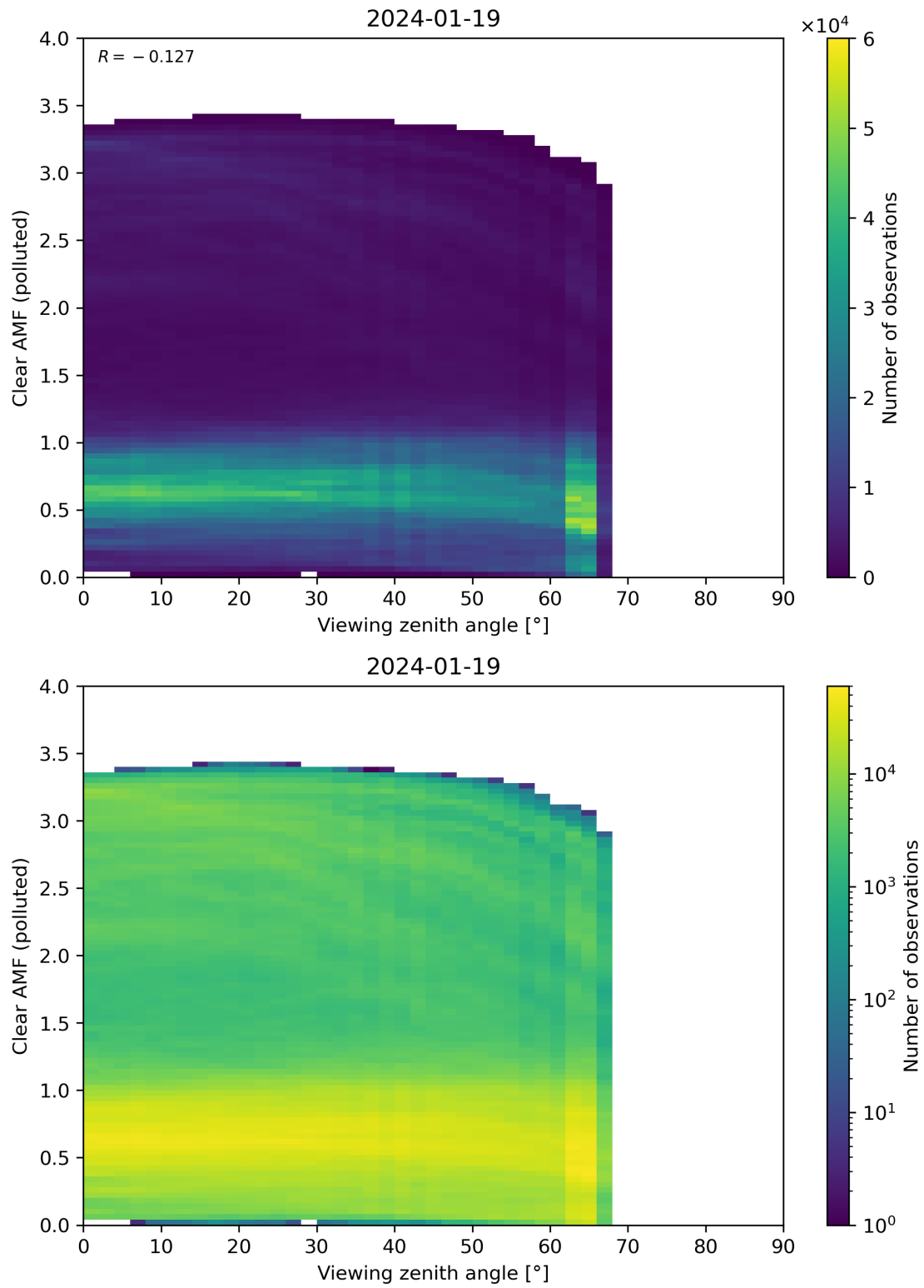
Figure 316: Scatter density plot of “Viewing zenith angle” against “Clear AMF (polluted)” for 2024-01-18 to 2024-01-20.
