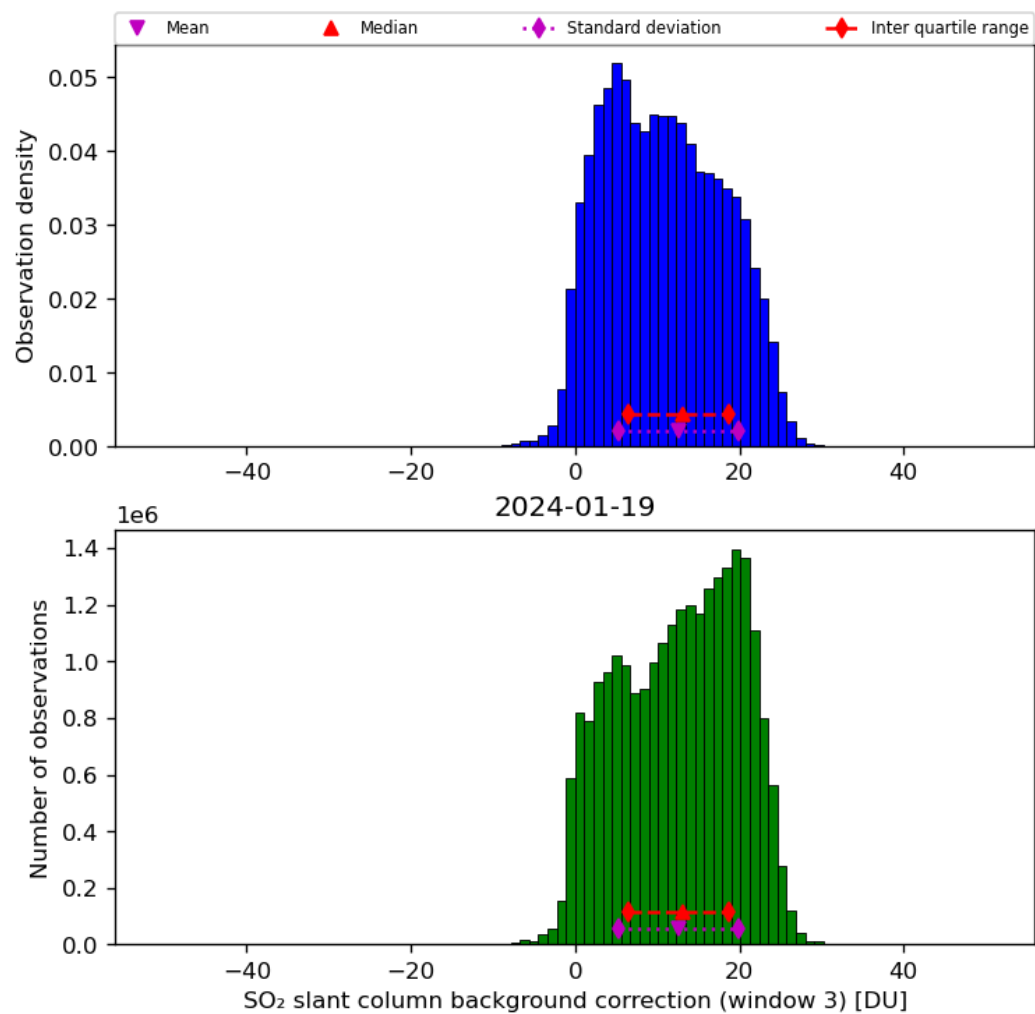
Figure 67: Histogram of “SO 2 slant column background correction (window 3)” for 2024-01-18 to 2024-01-20
