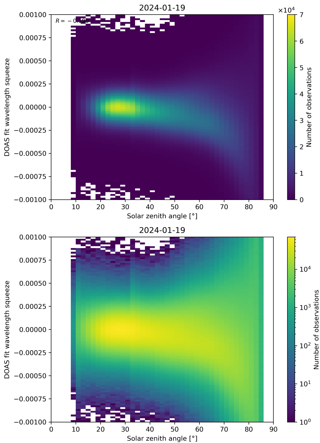
Figure 162: Scatter density plot of “Solar zenith angle” against “DOAS fit wavelength squeeze” for 2024-01-18 to 2024-01-20.
