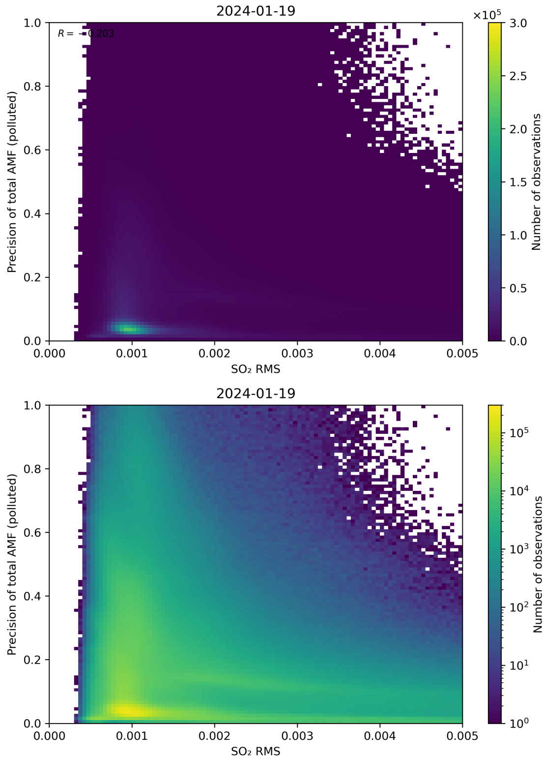
Figure 138: Scatter density plot of “SO 2 RMS” against “Precision of total AMF (polluted)” for 2024-01-18 to 2024-01-20.
