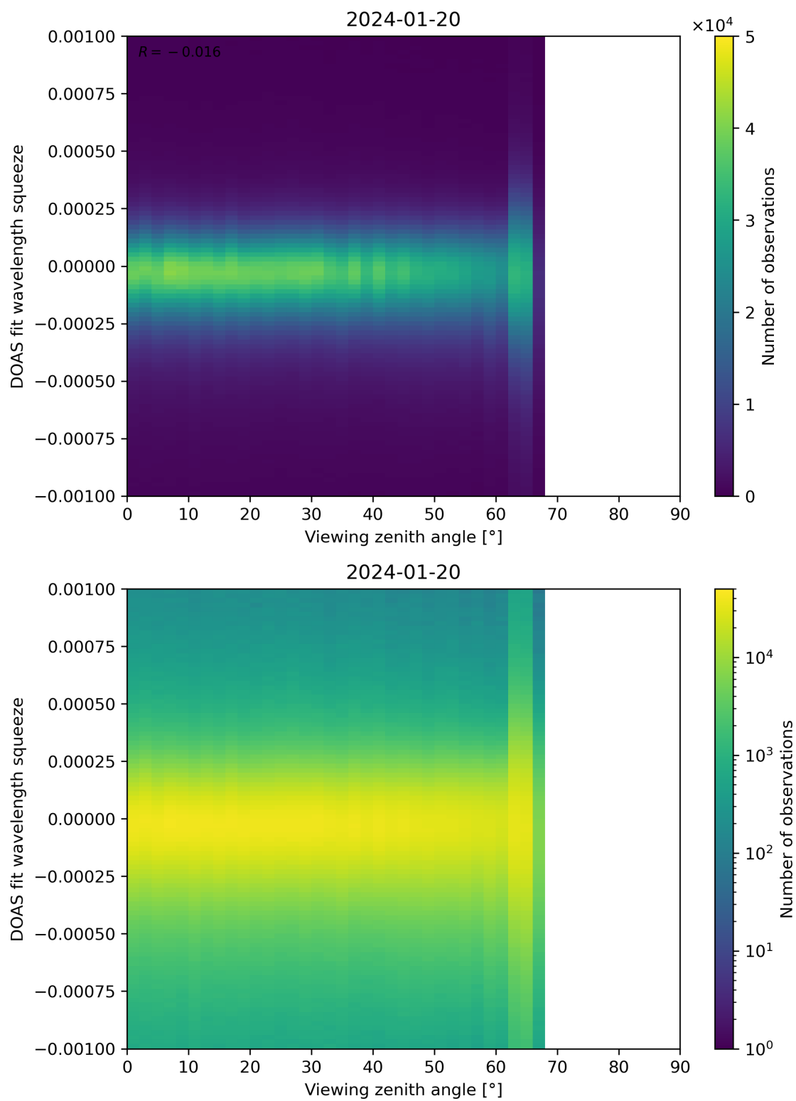
Figure 312: Scatter density plot of “Viewing zenith angle” against “DOAS fit wavelength squeeze” for 2024-01-19 to 2024-01-21.
