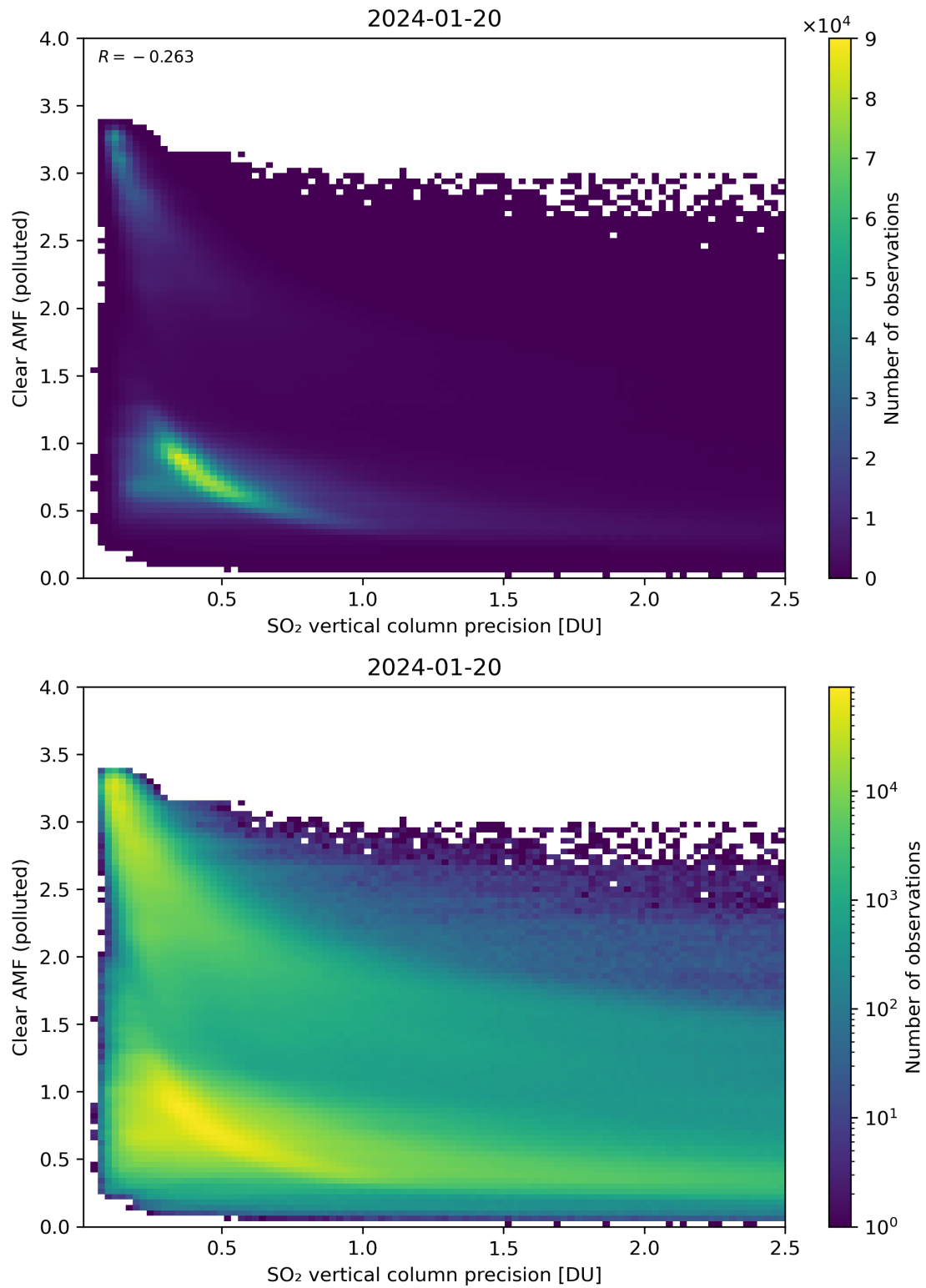
Figure 285: Scatter density plot of “SO 2 vertical column precision” against “Clear AMF (polluted)” for 2024-01-19 to 2024-01-21.
