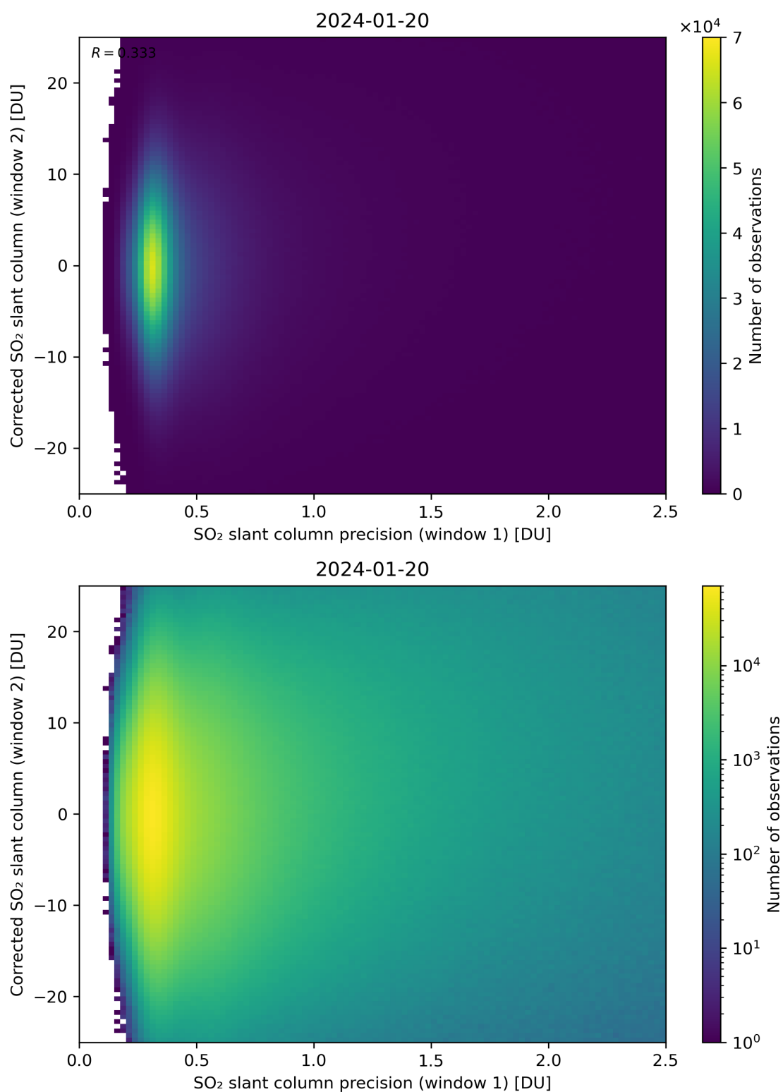
Figure 225: Scatter density plot of “SO 2 slant column precision (window 1)” against “Corrected SO 2 slant column (window 2)” for 2024-01-19 to 2024-01-21.
