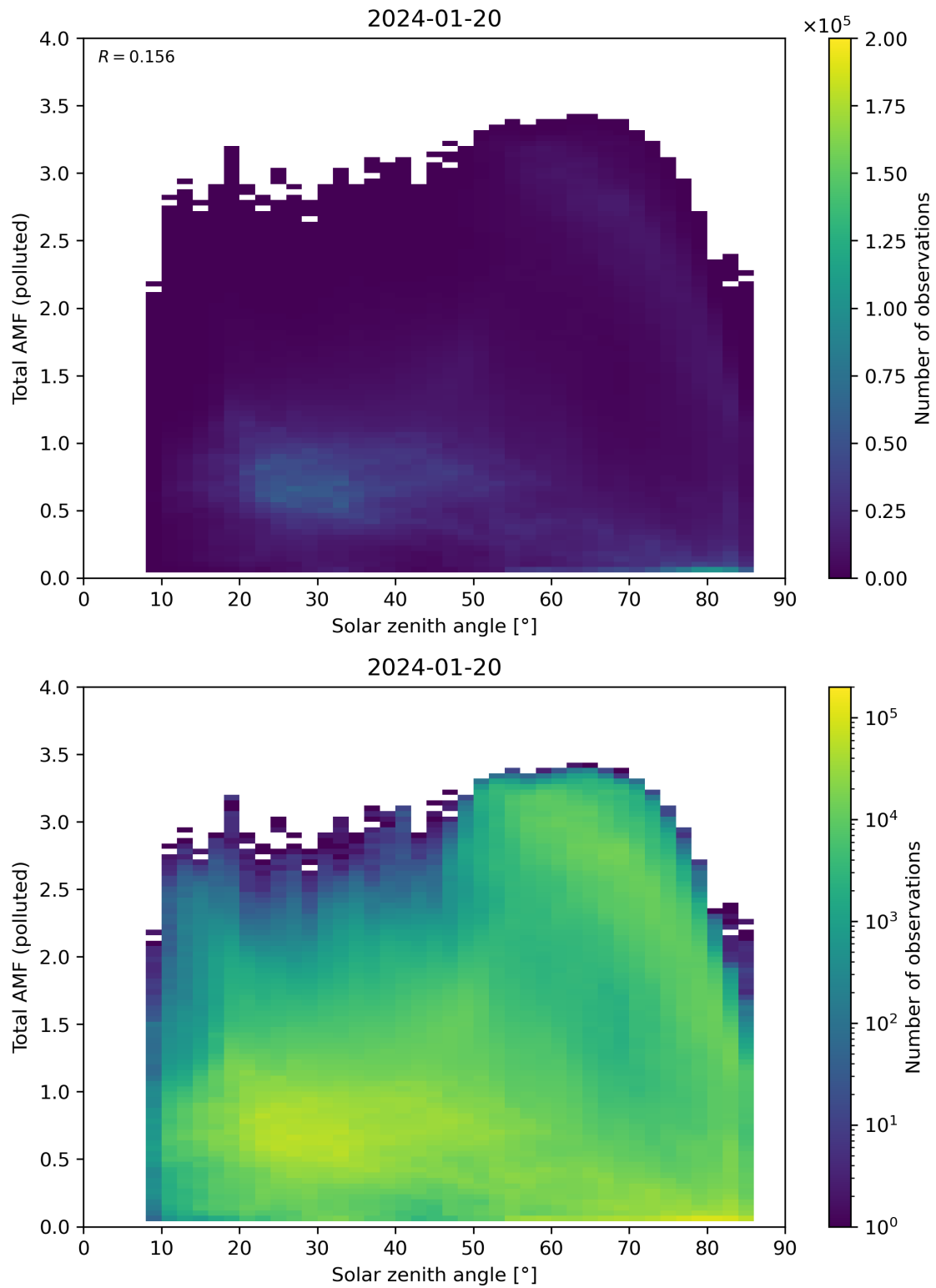
Figure 174: Scatter density plot of “Solar zenith angle” against “Total AMF (polluted)” for 2024-01-19 to 2024-01-21.
