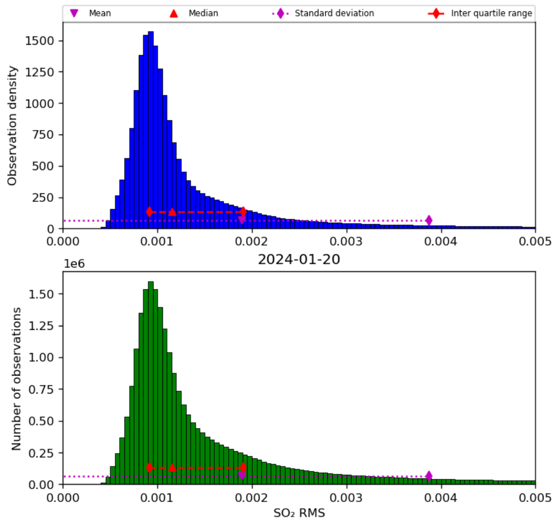
Figure 70: Histogram of “SO 2 RMS” for 2024-01-19 to 2024-01-21
