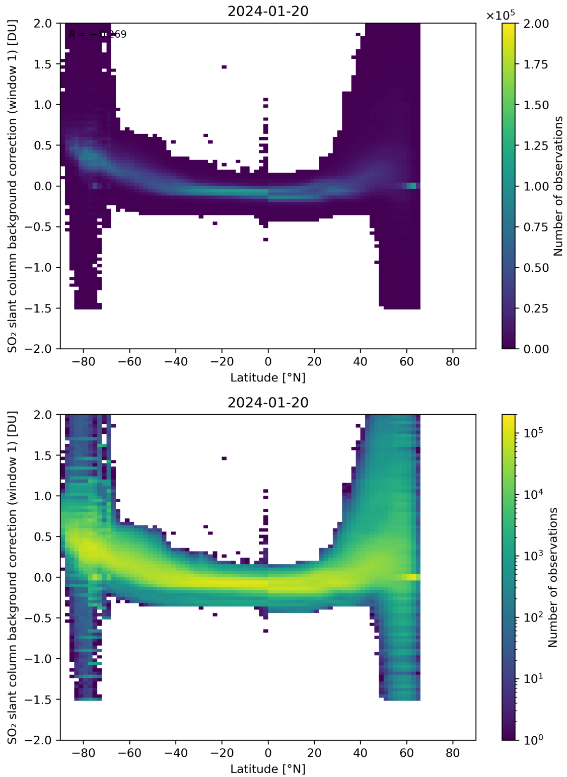
Figure 139: Scatter density plot of “Latitude” against “SO 2 slant column background correction (window 1)” for 2024-01-19 to 2024-01-21.
