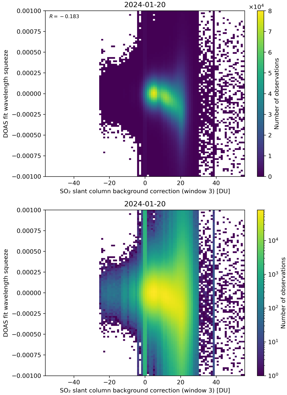
Figure 122: Scatter density plot of “SO 2 slant column background correction (window 3)” against “DOAS fit wavelength squeeze” for 2024-01-19 to 2024-01-21.
