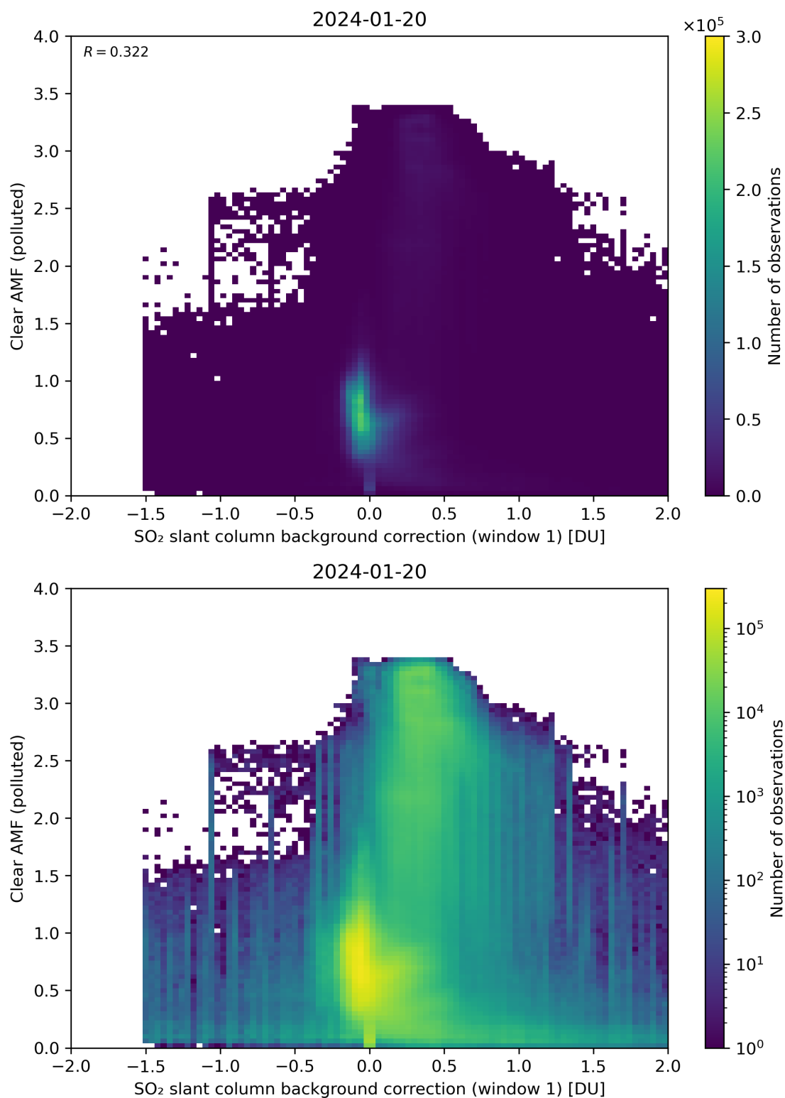
Figure 103: Scatter density plot of “SO 2 slant column background correction (window 1)” against “Clear AMF (polluted)” for 2024-01-19 to 2024-01-21.
