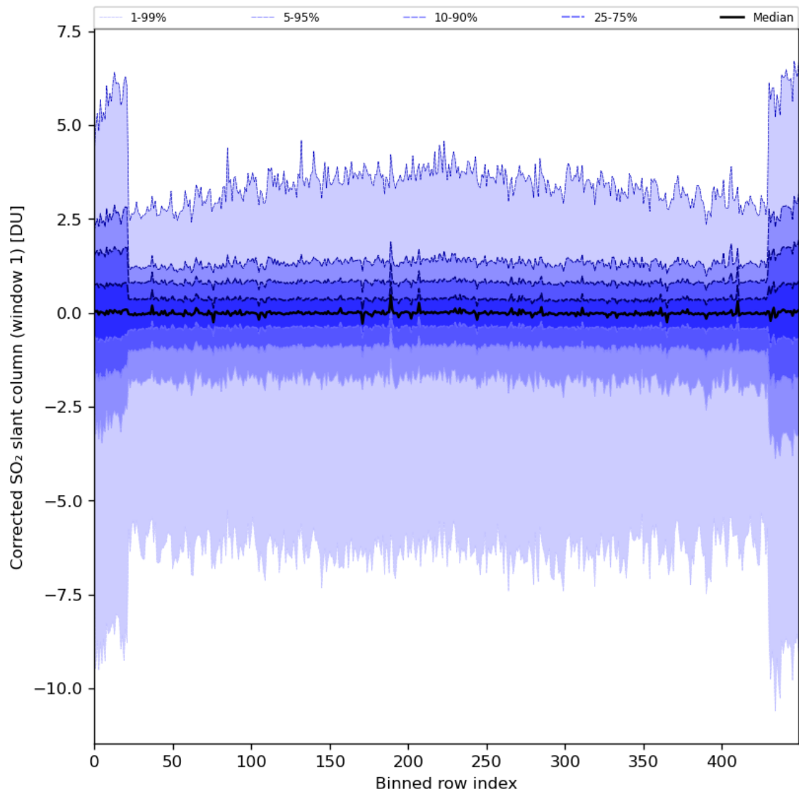
Figure 81: Along track statistics of “Corrected SO 2 slant column (window 1)” for 2024-01-19 to 2024-01-21
