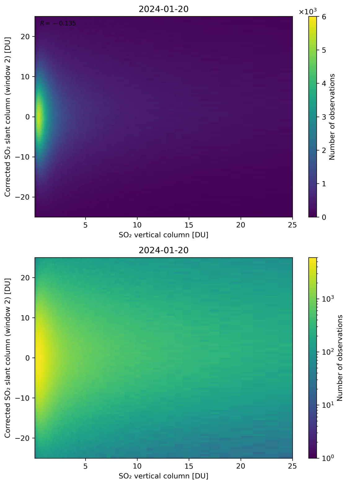
Figure 298: Scatter density plot of “SO 2 vertical column” against “Corrected SO 2 slant column (window 2)” for 2024-01-19 to 2024-01-21.
