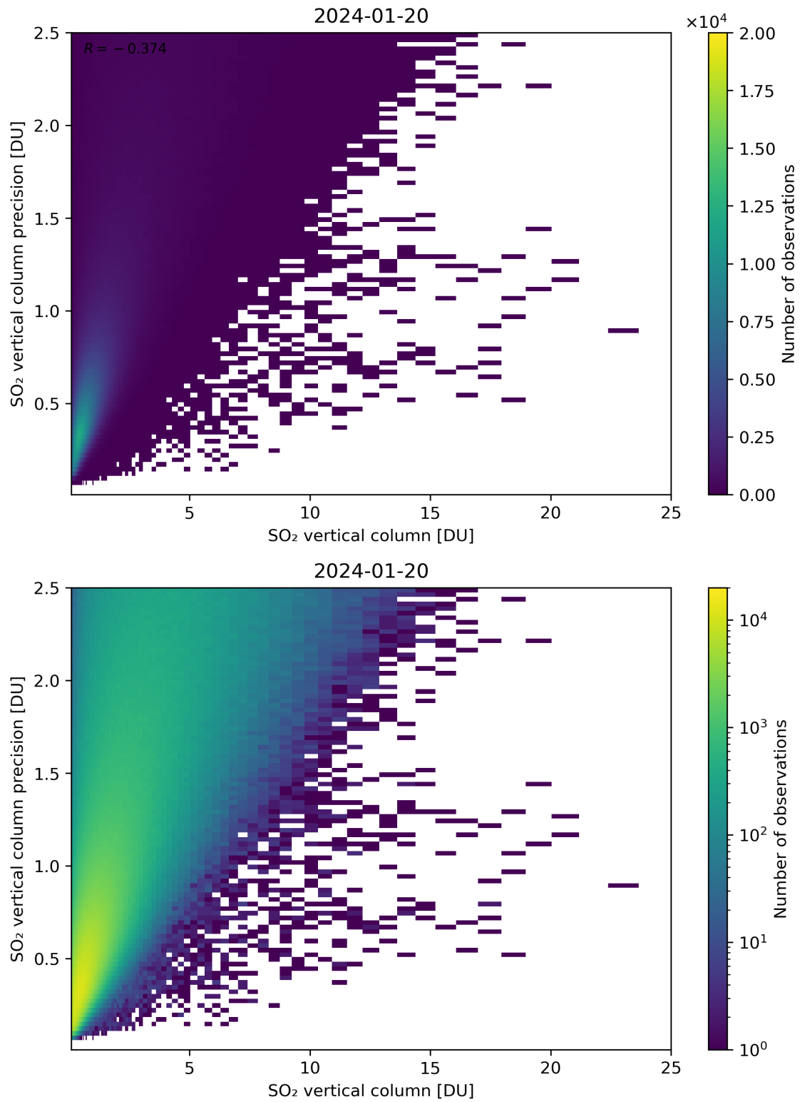
Figure 307: Scatter density plot of “SO 2 vertical column” against “SO 2 vertical column precision” for 2024-01-19 to 2024-01-21.
