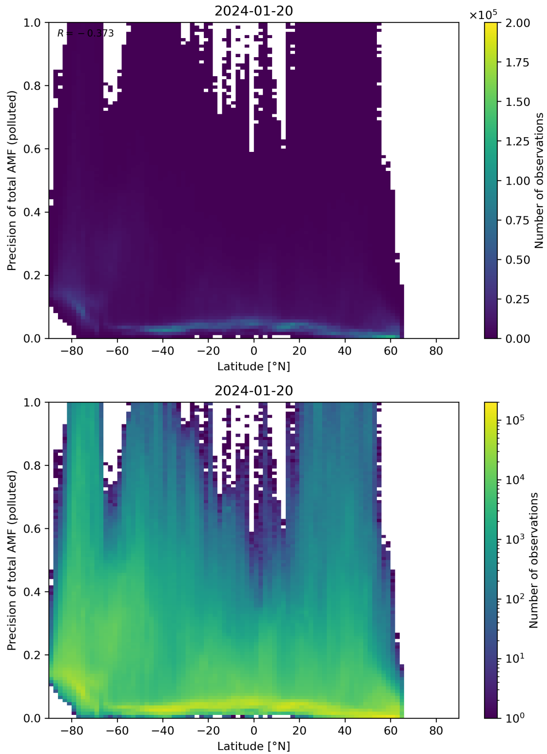
Figure 155: Scatter density plot of “Latitude” against “Precision of total AMF (polluted)” for 2024-01-19 to 2024-01-21.
