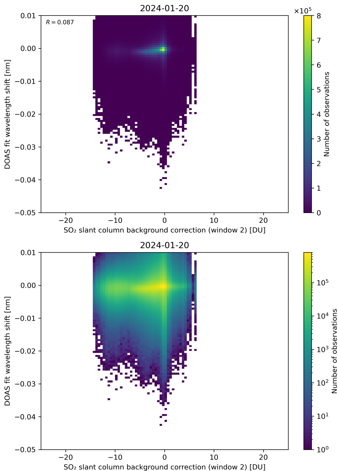
Figure 112: Scatter density plot of “SO 2 slant column background correction (window 2)” against “DOAS fit wavelength shift” for 2024-01-19 to 2024-01-21.
