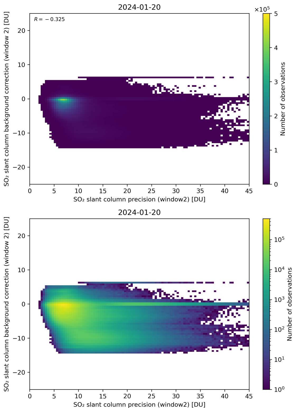
Figure 241: Scatter density plot of “SO 2 slant column precision (window2)” against “SO 2 slant column background correction (window 2)” for 2024-01-19 to 2024-01-21.
