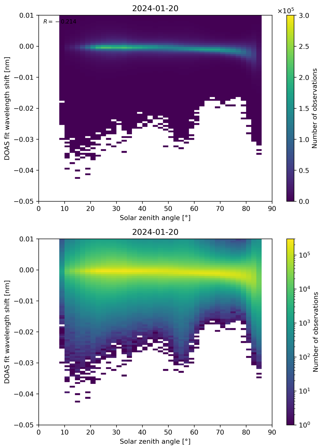
Figure 161: Scatter density plot of “Solar zenith angle” against “DOAS fit wavelength shift” for 2024-01-19 to 2024-01-21.
