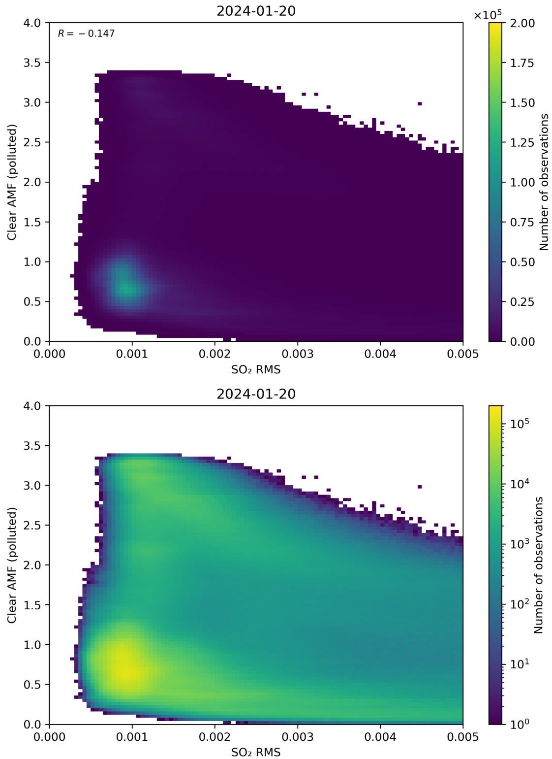
Figure 136: Scatter density plot of “SO 2 RMS” against “Clear AMF (polluted)” for 2024-01-19 to 2024-01-21.
