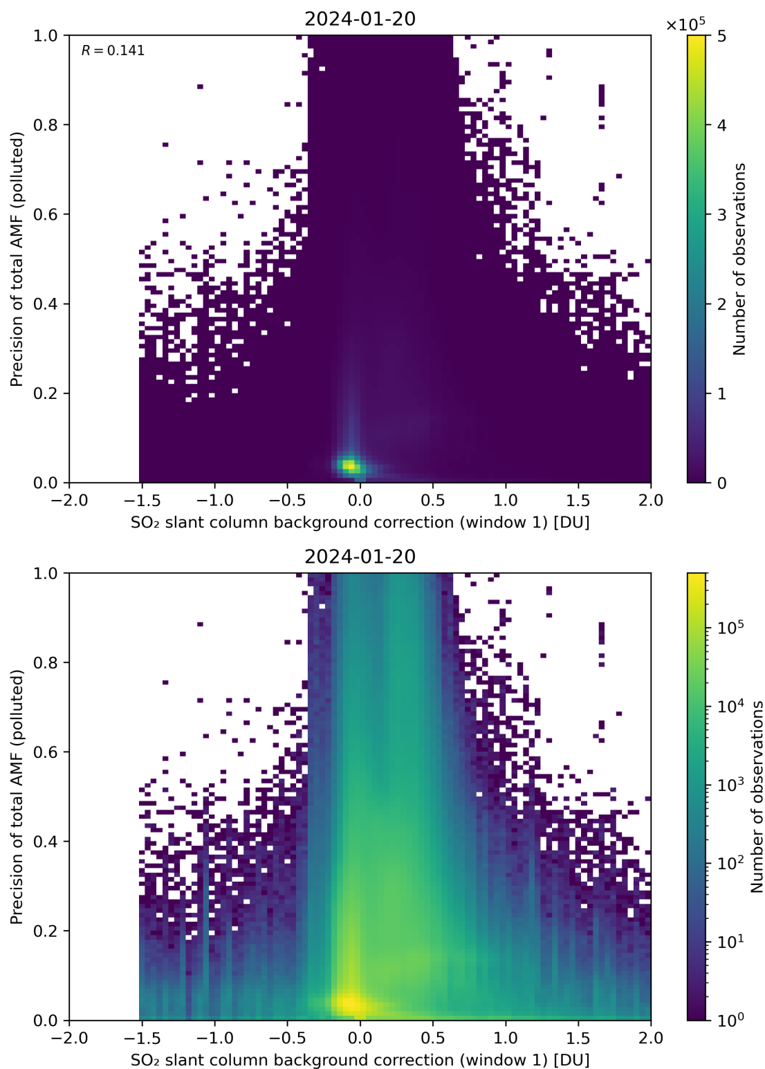
Figure 110: Scatter density plot of “SO 2 slant column background correction (window 1)” against “Precision of total AMF (polluted)” for 2024-01-19 to 2024-01-21.
