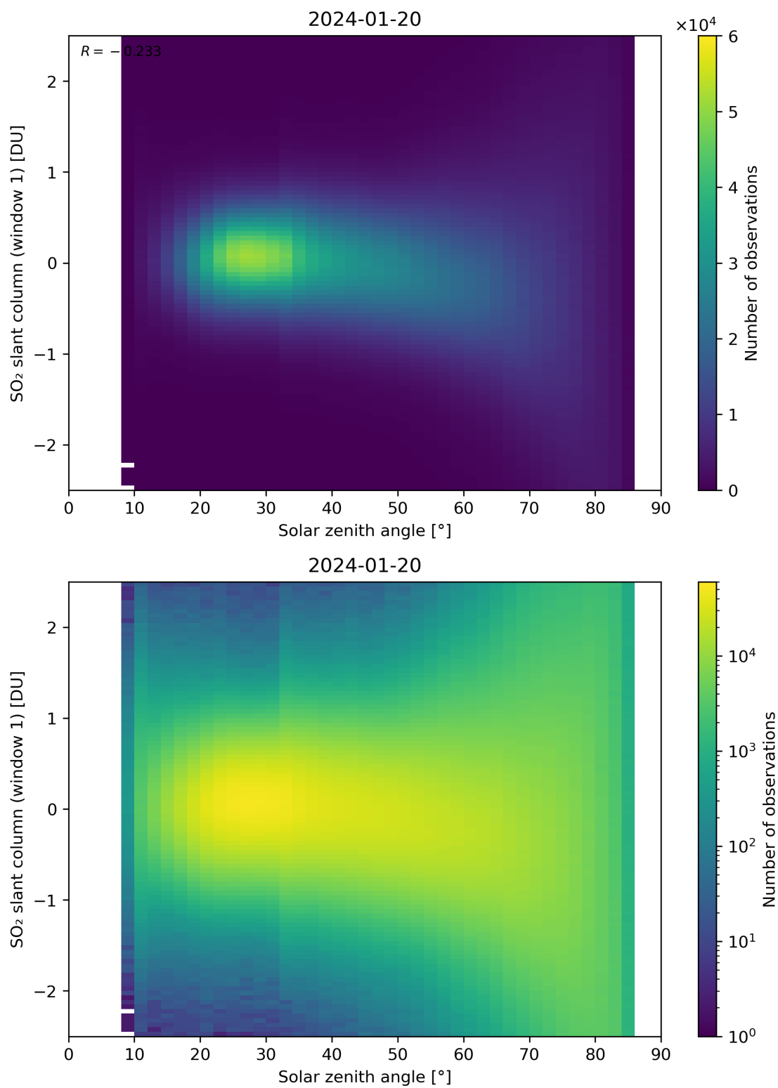
Figure 169: Scatter density plot of “Solar zenith angle” against “SO 2 slant column (window 1)” for 2024-01-19 to 2024-01-21.
