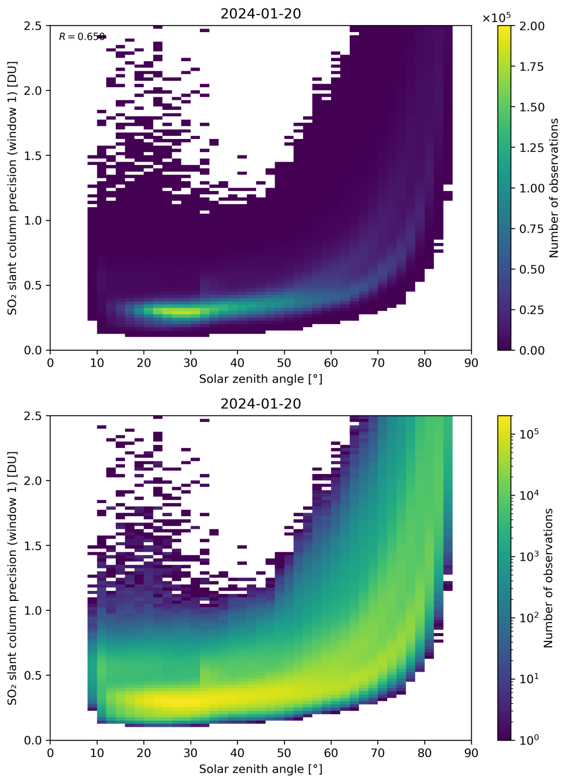
Figure 170: Scatter density plot of “Solar zenith angle” against “SO 2 slant column precision (window 1)” for 2024-01-19 to 2024-01-21.
