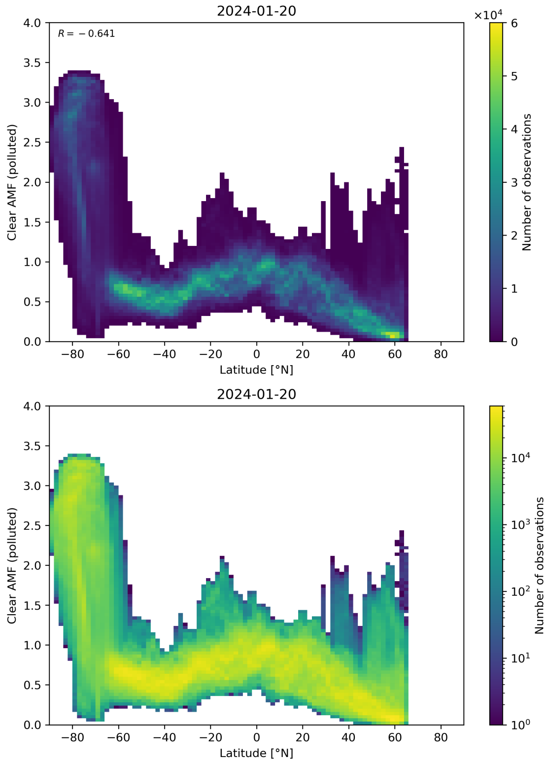
Figure 145: Scatter density plot of “Latitude” against “Clear AMF (polluted)” for 2024-01-19 to 2024-01-21.
