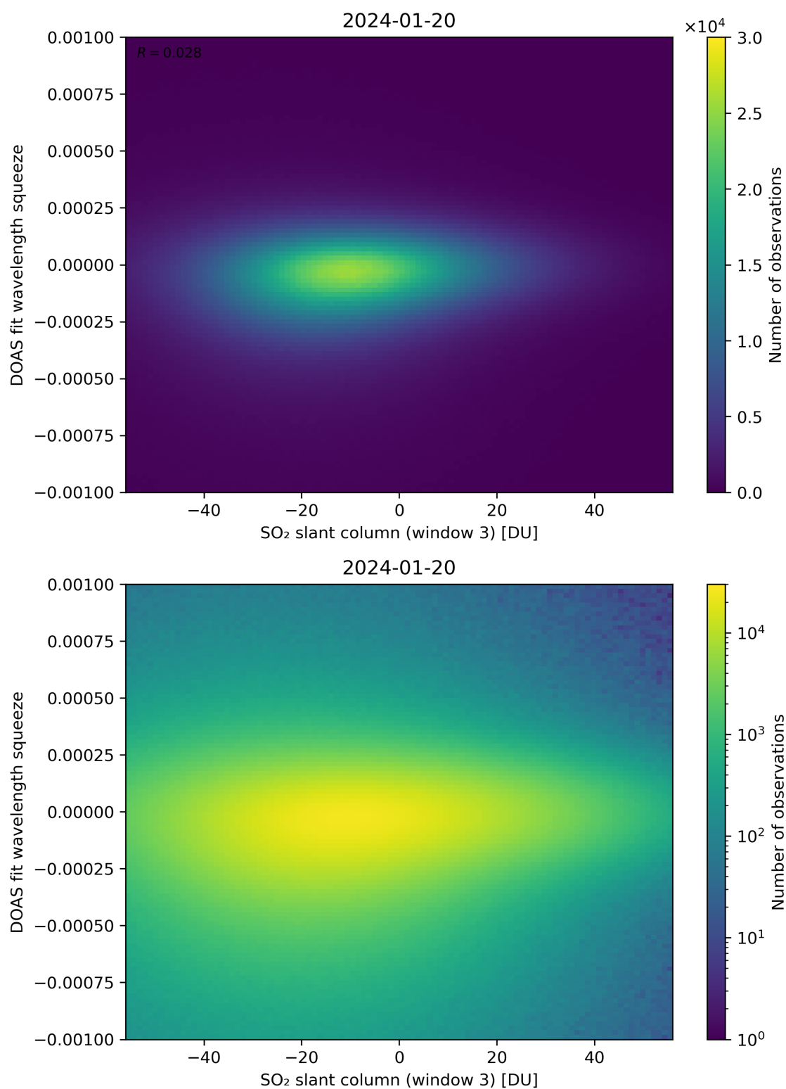
Figure 255: Scatter density plot of “SO 2 slant column (window 3)” against “DOAS fit wavelength squeeze” for 2024-01-19 to 2024-01-21.
