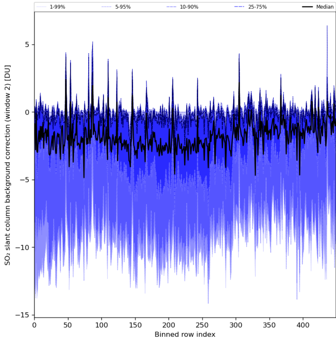
Figure 86: Along track statistics of “SO 2 slant column background correction (window 2)” for 2024-01-19 to 2024-01-21
