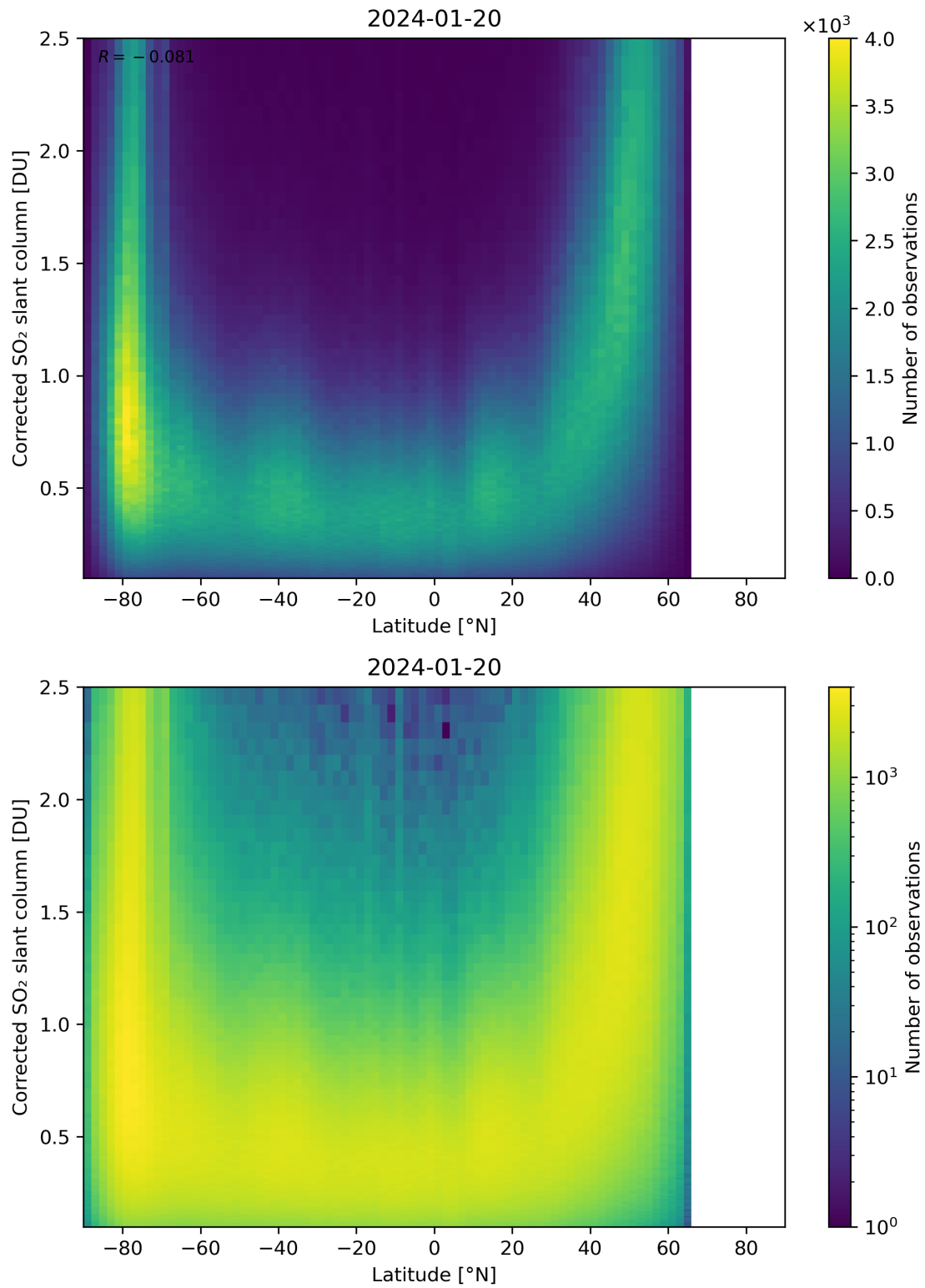
Figure 146: Scatter density plot of “Latitude” against “Corrected SO 2 slant column” for 2024-01-19 to 2024-01-21.
