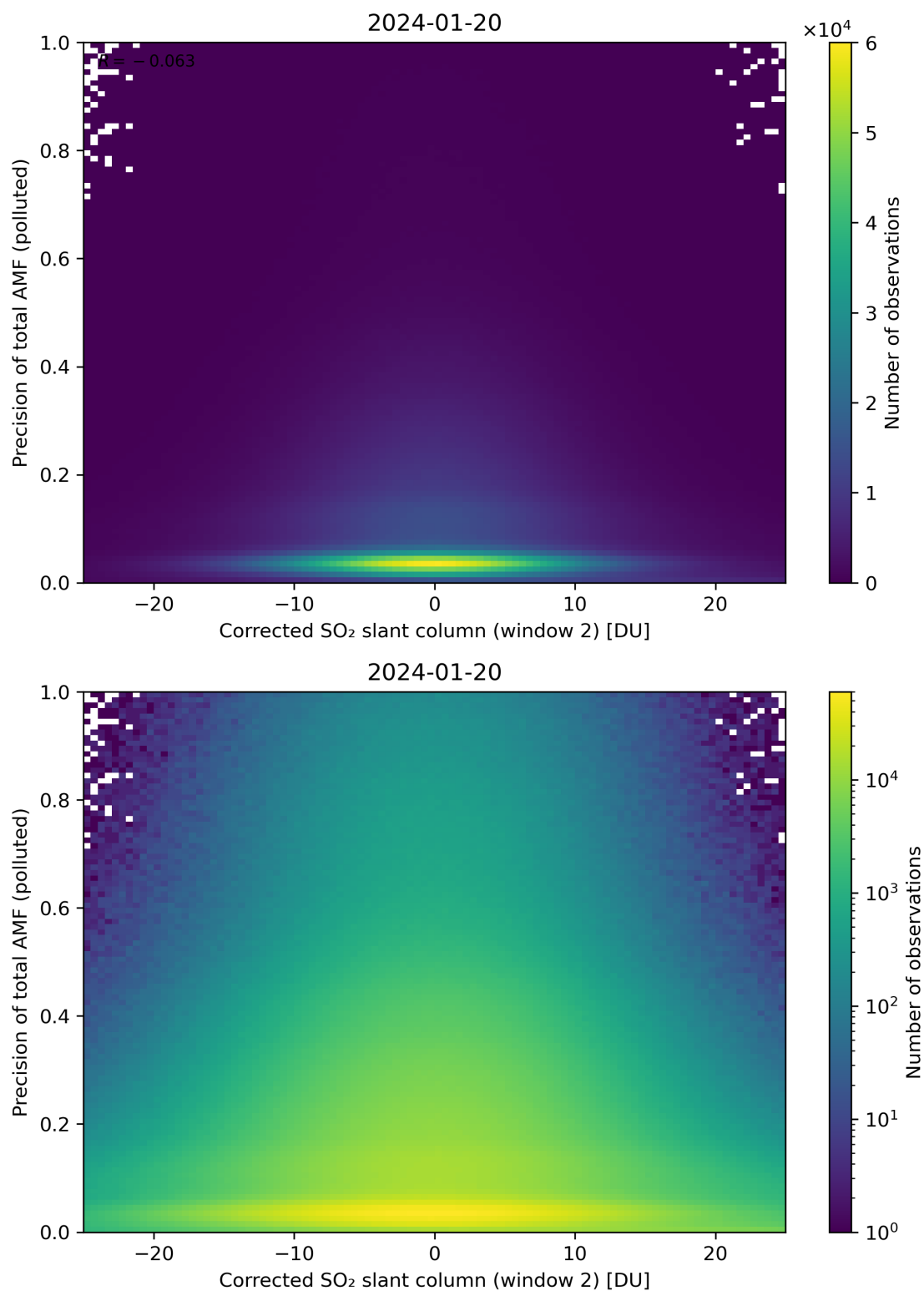
Figure 204: Scatter density plot of “Corrected SO 2 slant column (window 2)” against “Precision of total AMF (polluted)” for 2024-01-19 to 2024-01-21.
