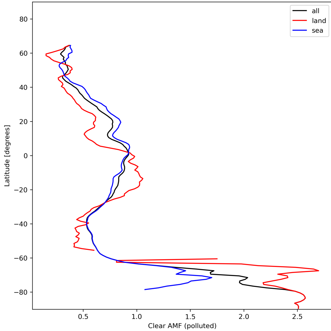
Figure 50: Zonal average of “Clear AMF (polluted)” for 2024-01-19 to 2024-01-21.
