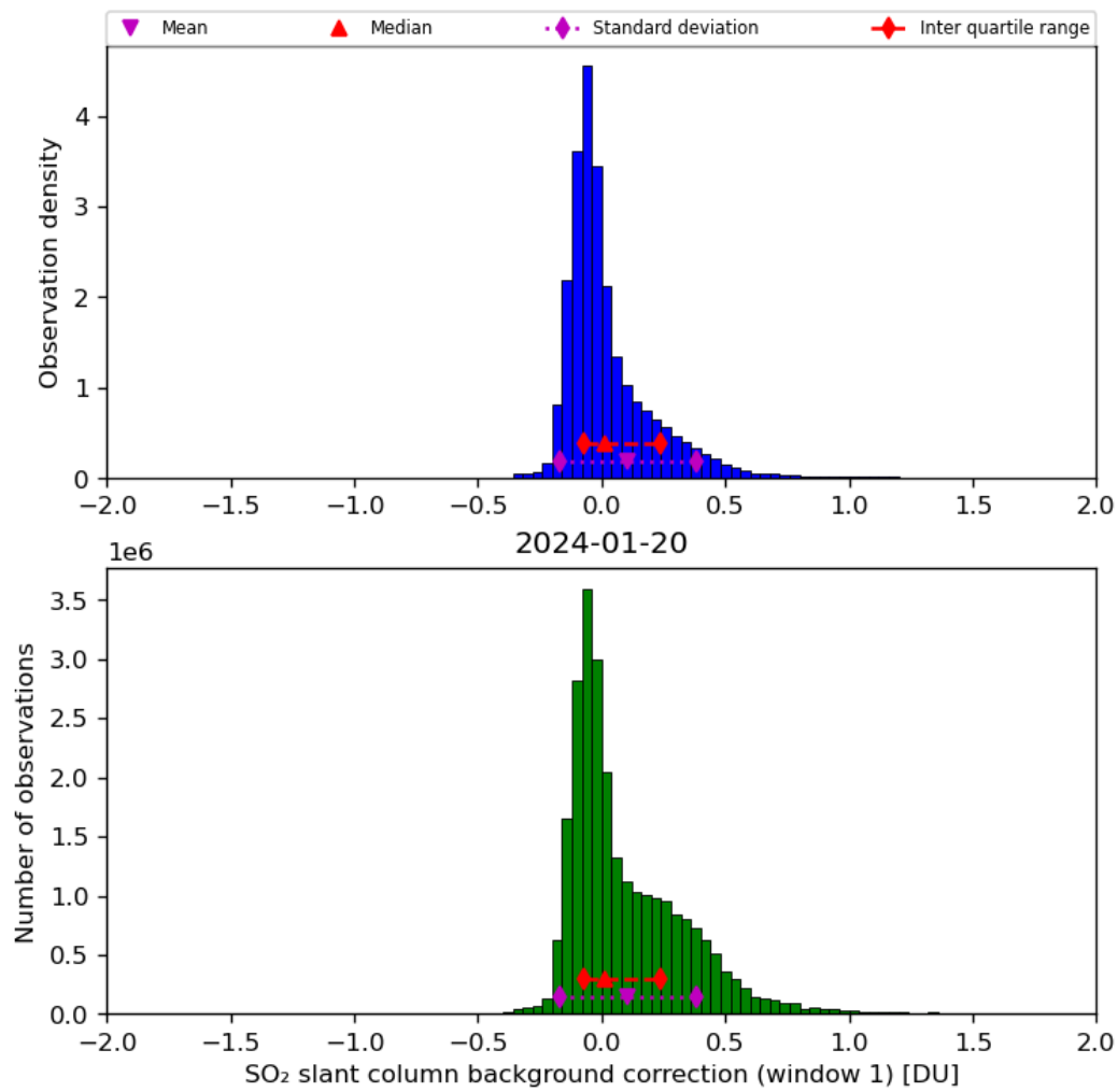
Figure 59: Histogram of “SO 2 slant column background correction (window 1)” for 2024-01-19 to 2024-01-21
