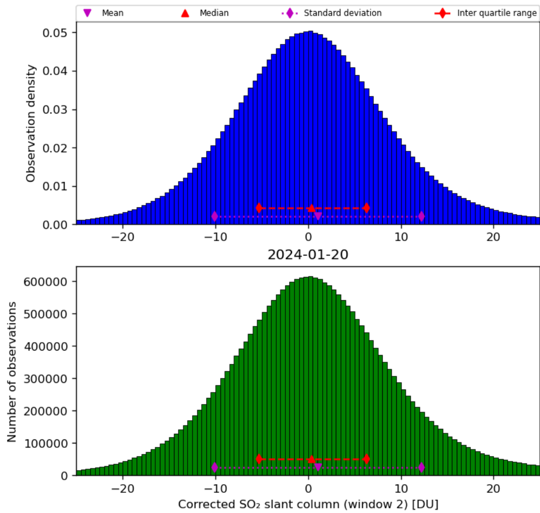
Figure 62: Histogram of “Corrected SO 2 slant column (window 2)” for 2024-01-19 to 2024-01-21
