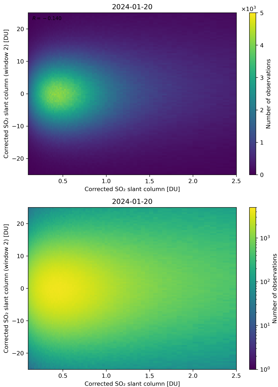
Figure 185: Scatter density plot of “Corrected SO 2 slant column” against “Corrected SO 2 slant column (window 2)” for 2024-01-19 to 2024-01-21.
