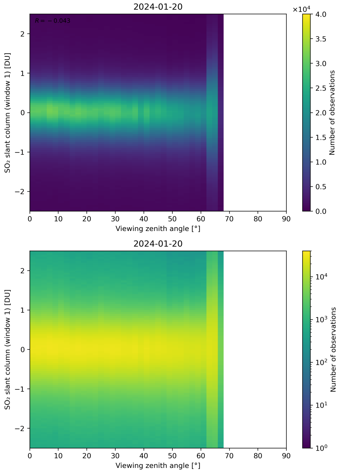
Figure 320: Scatter density plot of “Viewing zenith angle” against “SO 2 slant column (window 1)” for 2024-01-19 to 2024-01-21.
