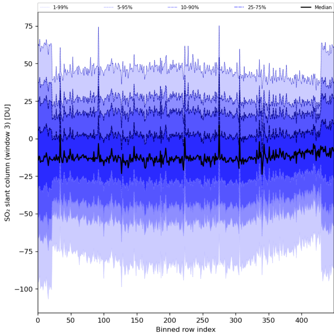
Figure 87: Along track statistics of “SO 2 slant column (window 3)” for 2024-01-19 to 2024-01-21
