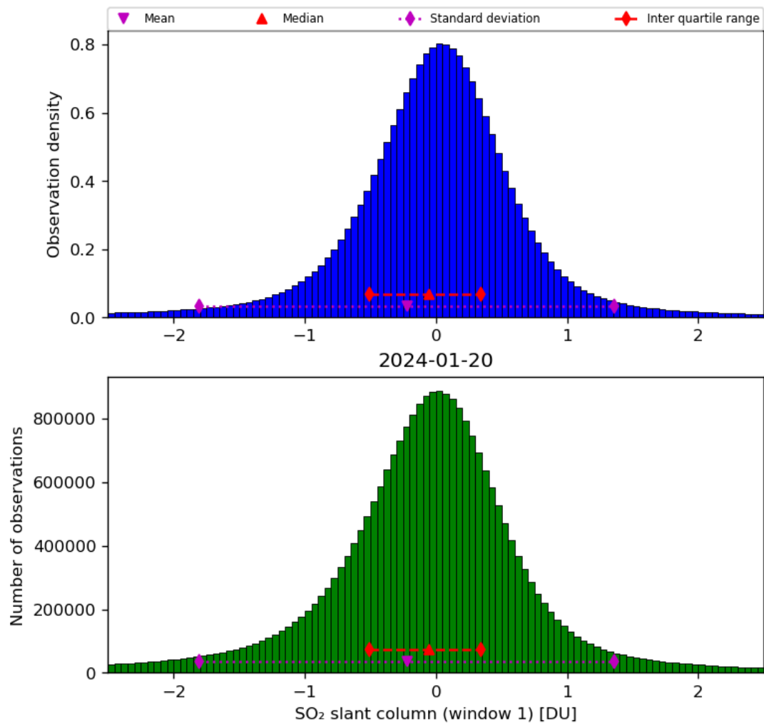
Figure 56: Histogram of “SO 2 slant column (window 1)” for 2024-01-19 to 2024-01-21
