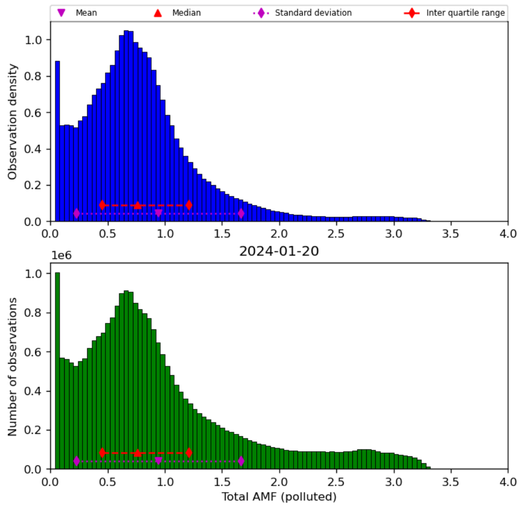
Figure 71: Histogram of “Total AMF (polluted)” for 2024-01-19 to 2024-01-21
