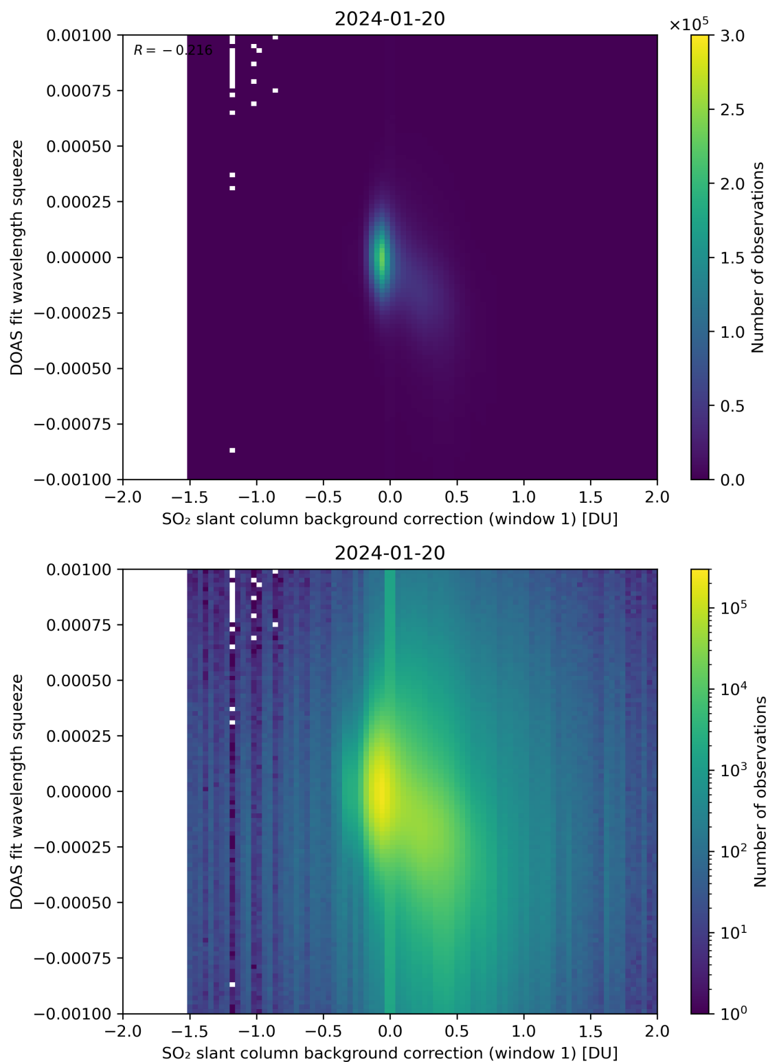
Figure 101: Scatter density plot of “SO 2 slant column background correction (window 1)” against “DOAS fit wavelength squeeze” for 2024-01-19 to 2024-01-21.
