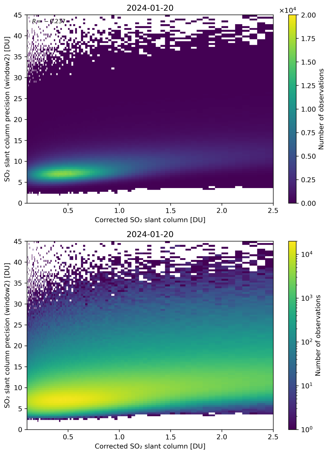
Figure 189: Scatter density plot of “Corrected SO 2 slant column” against “SO 2 slant column precision (window2)” for 2024-01-19 to 2024-01-21.
