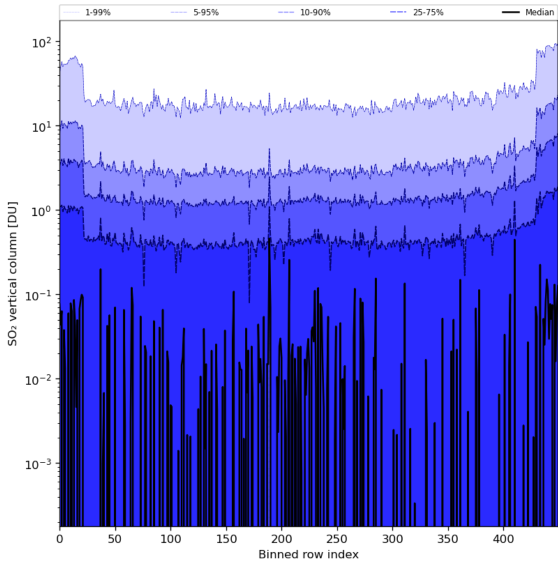
Figure 76: Along track statistics of “SO 2 vertical column” for 2024-01-19 to 2024-01-21
