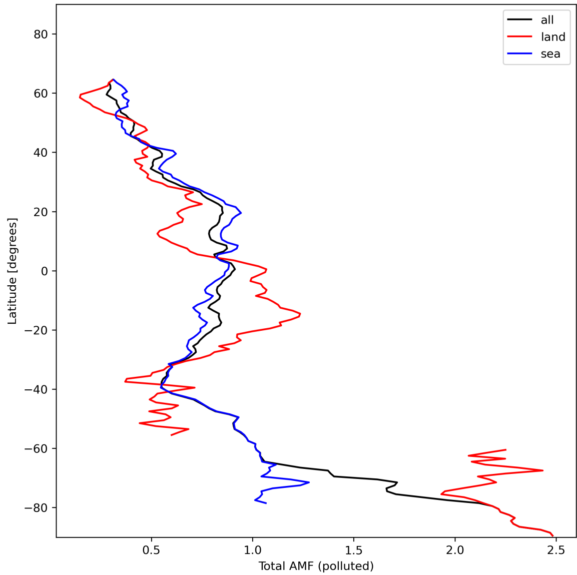
Figure 48: Zonal average of “Total AMF (polluted)” for 2024-01-19 to 2024-01-21.
