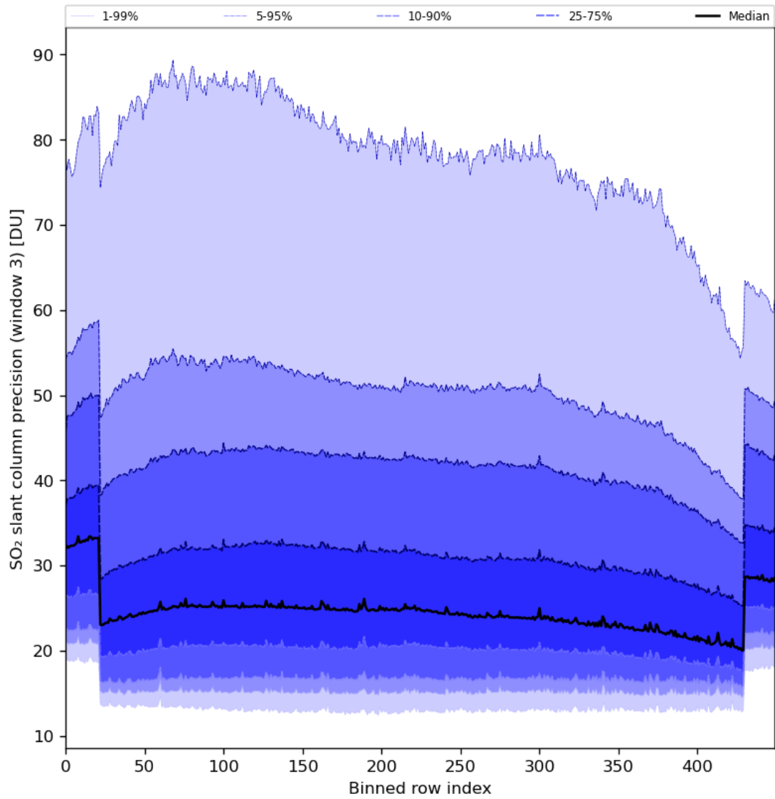
Figure 88: Along track statistics of “SO 2 slant column precision (window 3)” for 2024-01-19 to 2024-01-21
