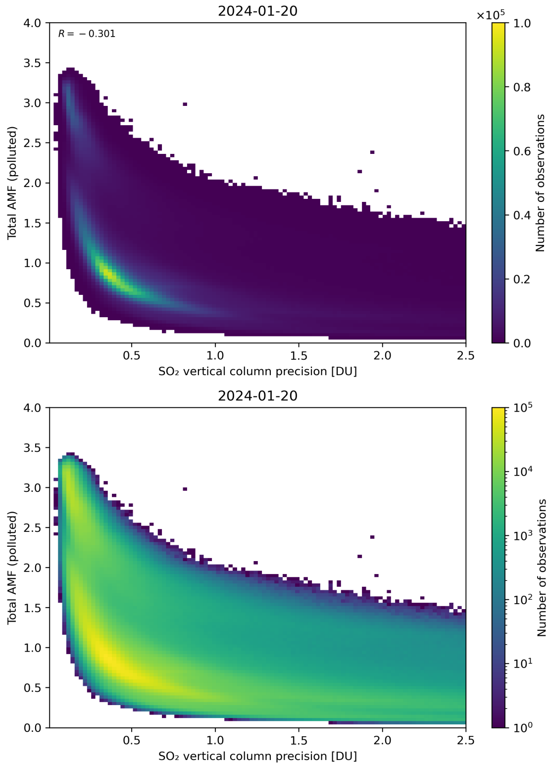
Figure 294: Scatter density plot of “SO 2 vertical column precision” against “Total AMF (polluted)” for 2024-01-19 to 2024-01-21.
