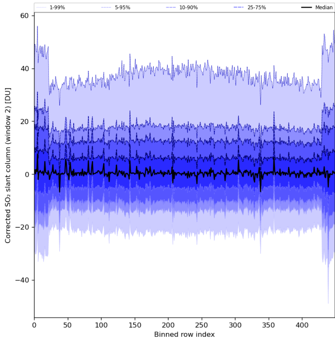
Figure 85: Along track statistics of “Corrected SO 2 slant column (window 2)” for 2024-01-19 to 2024-01-21
