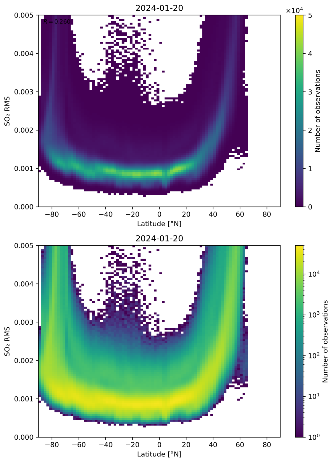
Figure 144: Scatter density plot of “Latitude” against “SO 2 RMS” for 2024-01-19 to 2024-01-21.
