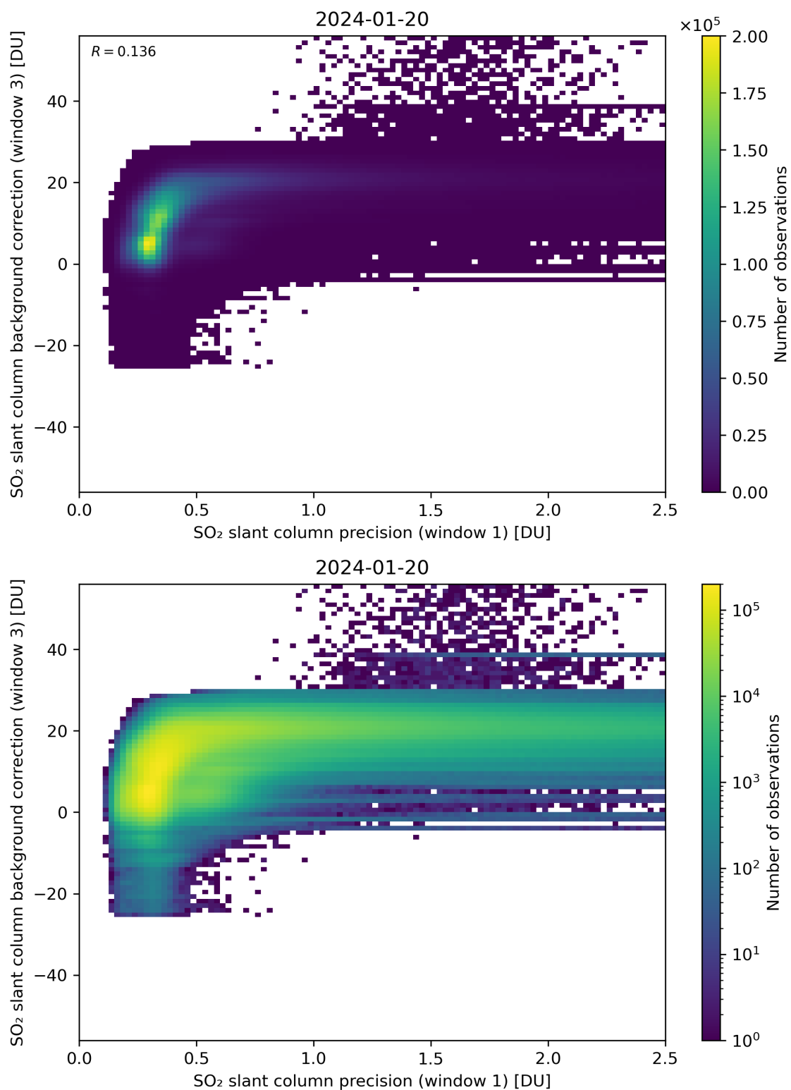
Figure 220: Scatter density plot of “SO 2 slant column precision (window 1)” against “SO 2 slant column background correction (window 3)” for 2024-01-19 to 2024-01-21.
