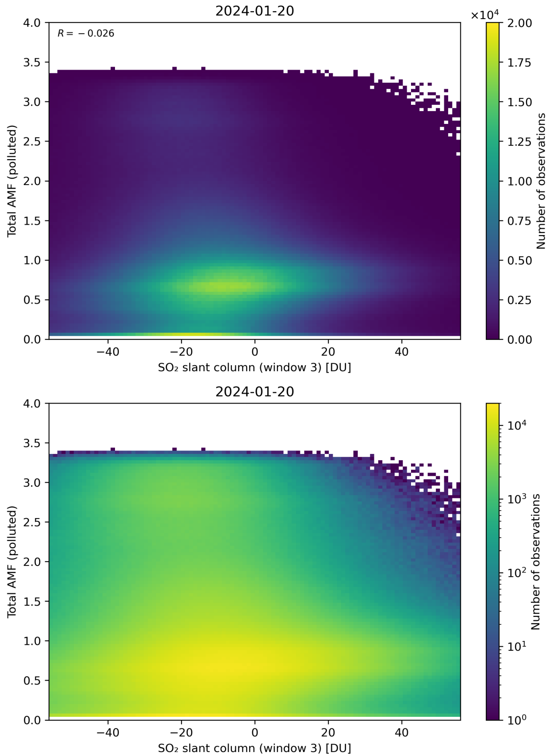
Figure 268: Scatter density plot of “SO 2 slant column (window 3)” against “Total AMF (polluted)” for 2024-01-19 to 2024-01-21.
