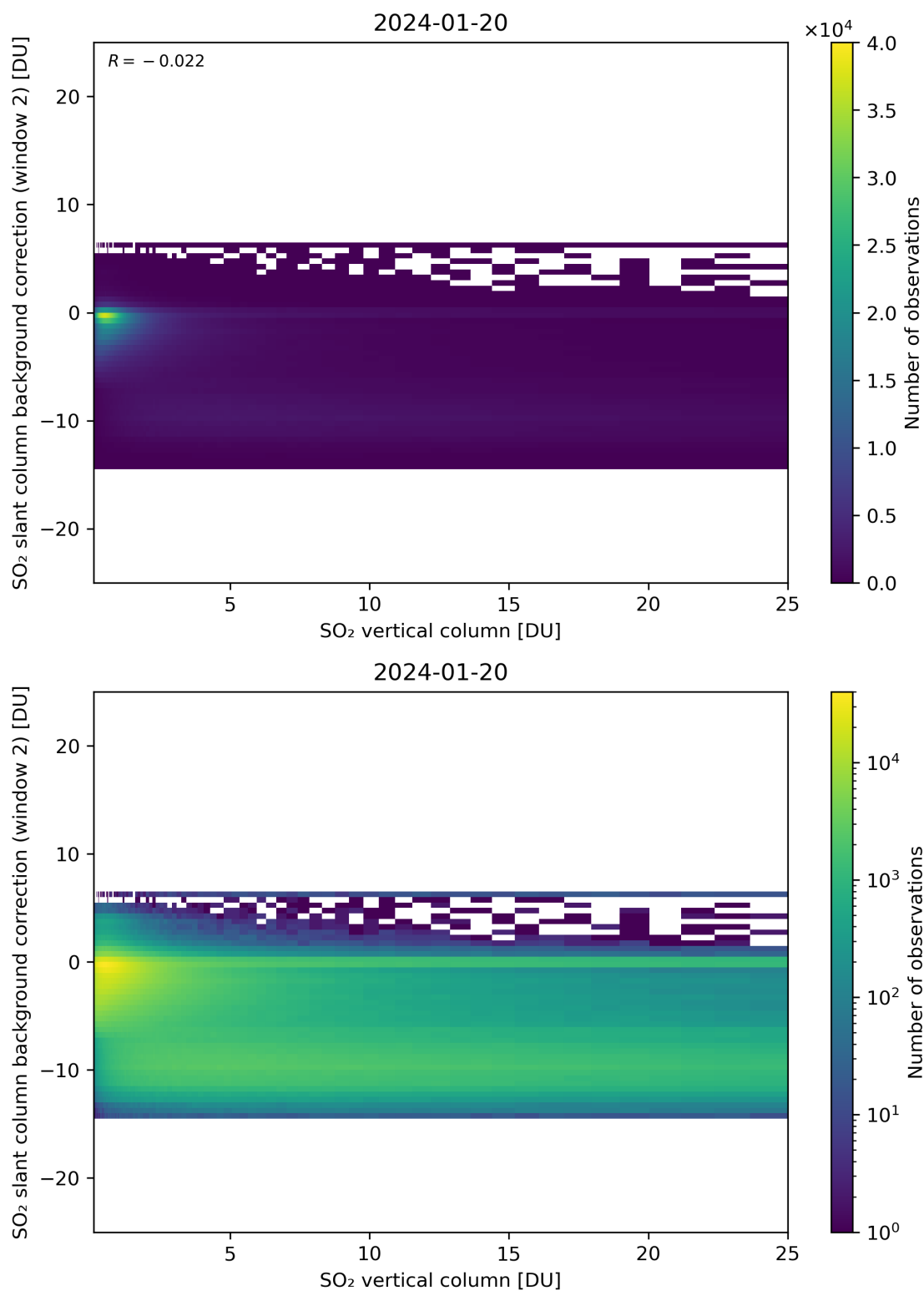
Figure 274: Scatter density plot of “SO 2 vertical column” against “SO 2 slant column background correction (window 2)” for 2024-01-19 to 2024-01-21.
