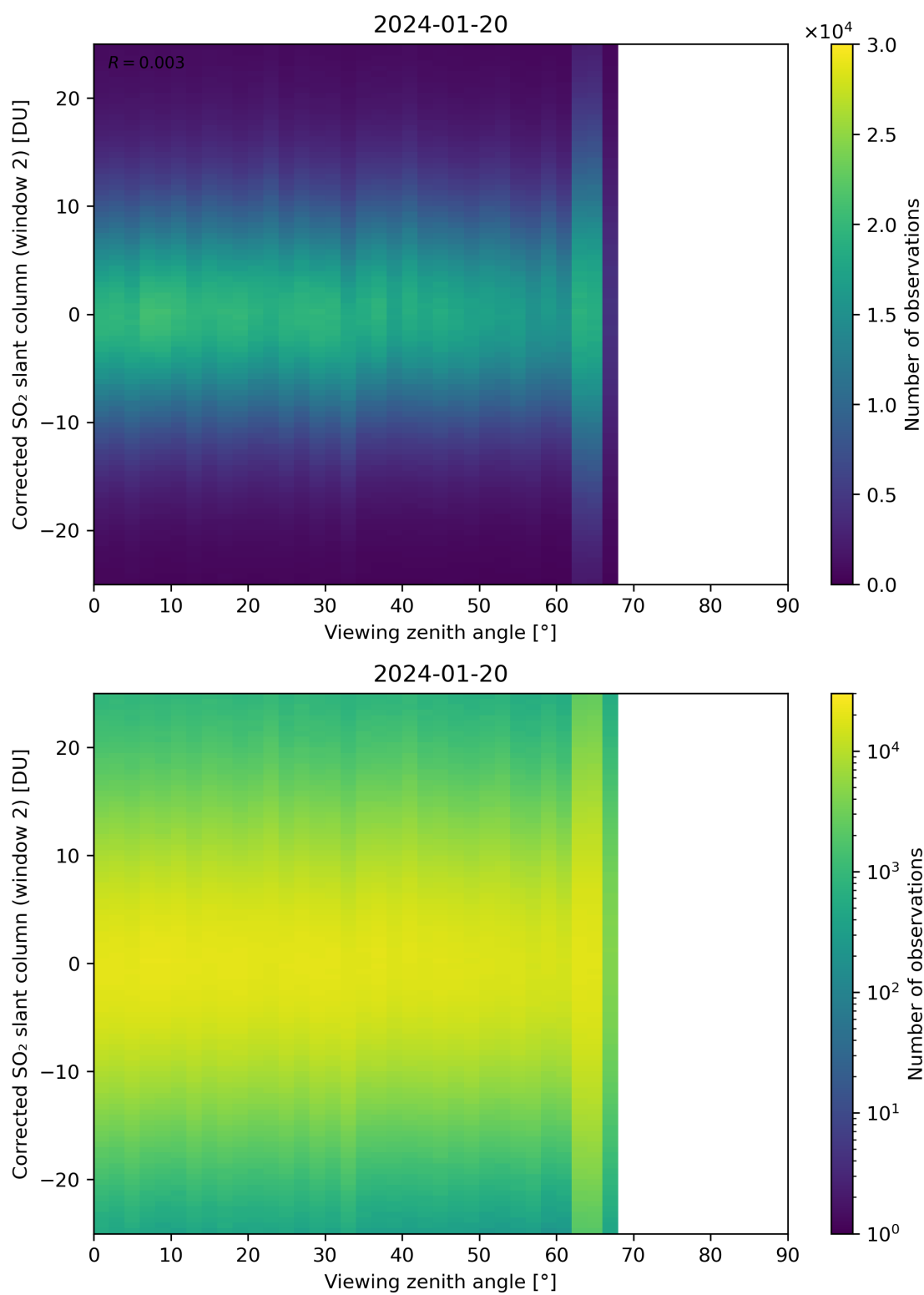
Figure 318: Scatter density plot of “Viewing zenith angle” against “Corrected SO 2 slant column (window 2)” for 2024-01-19 to 2024-01-21.
