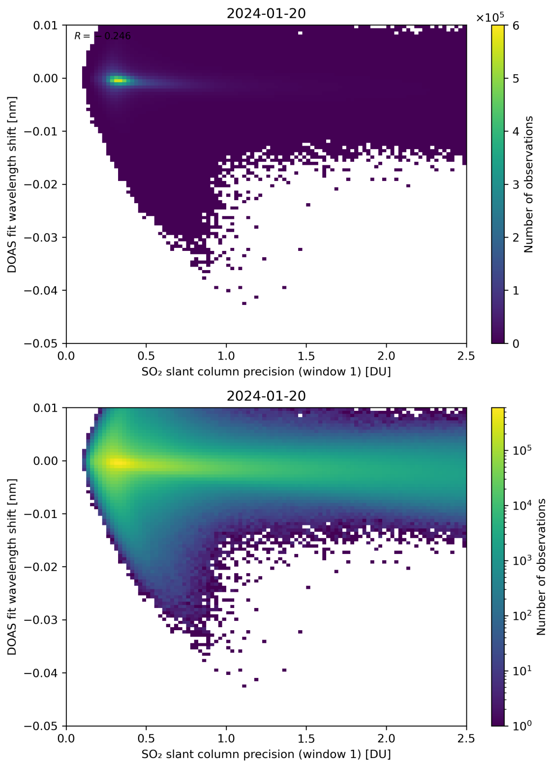
Figure 221: Scatter density plot of “SO 2 slant column precision (window 1)” against “DOAS fit wavelength shift” for 2024-01-19 to 2024-01-21.
