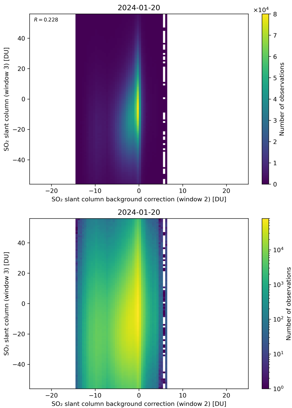
Figure 117: Scatter density plot of “SO 2 slant column background correction (window 2)” against “SO 2 slant column (window 3)” for 2024-01-19 to 2024-01-21.
