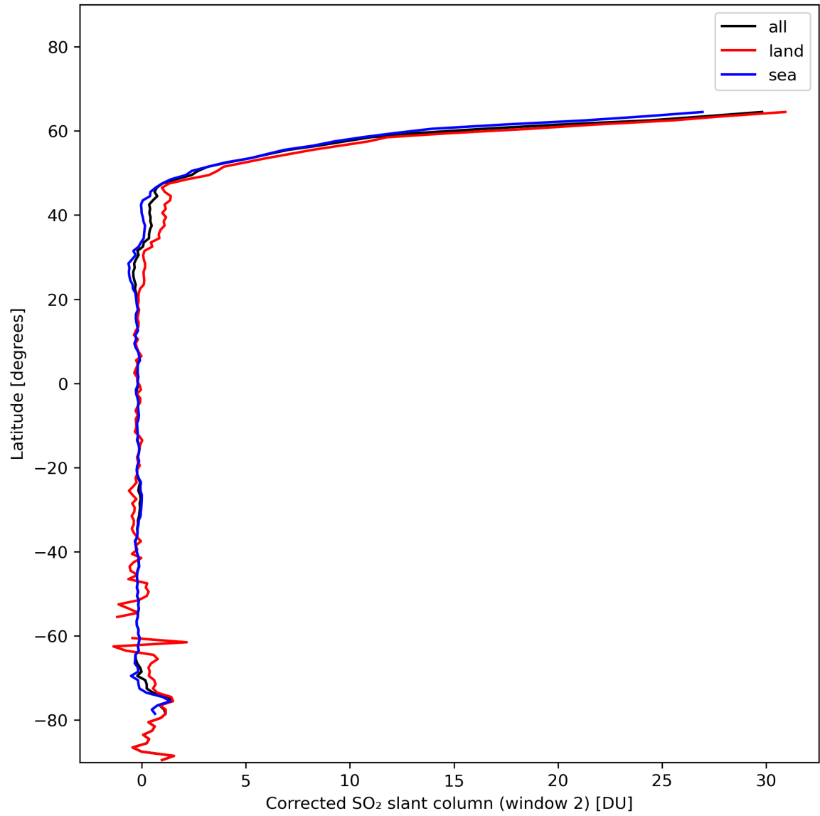
Figure 39: Zonal average of “Corrected SO 2 slant column (window 2)” for 2024-01-19 to 2024-01-21.
