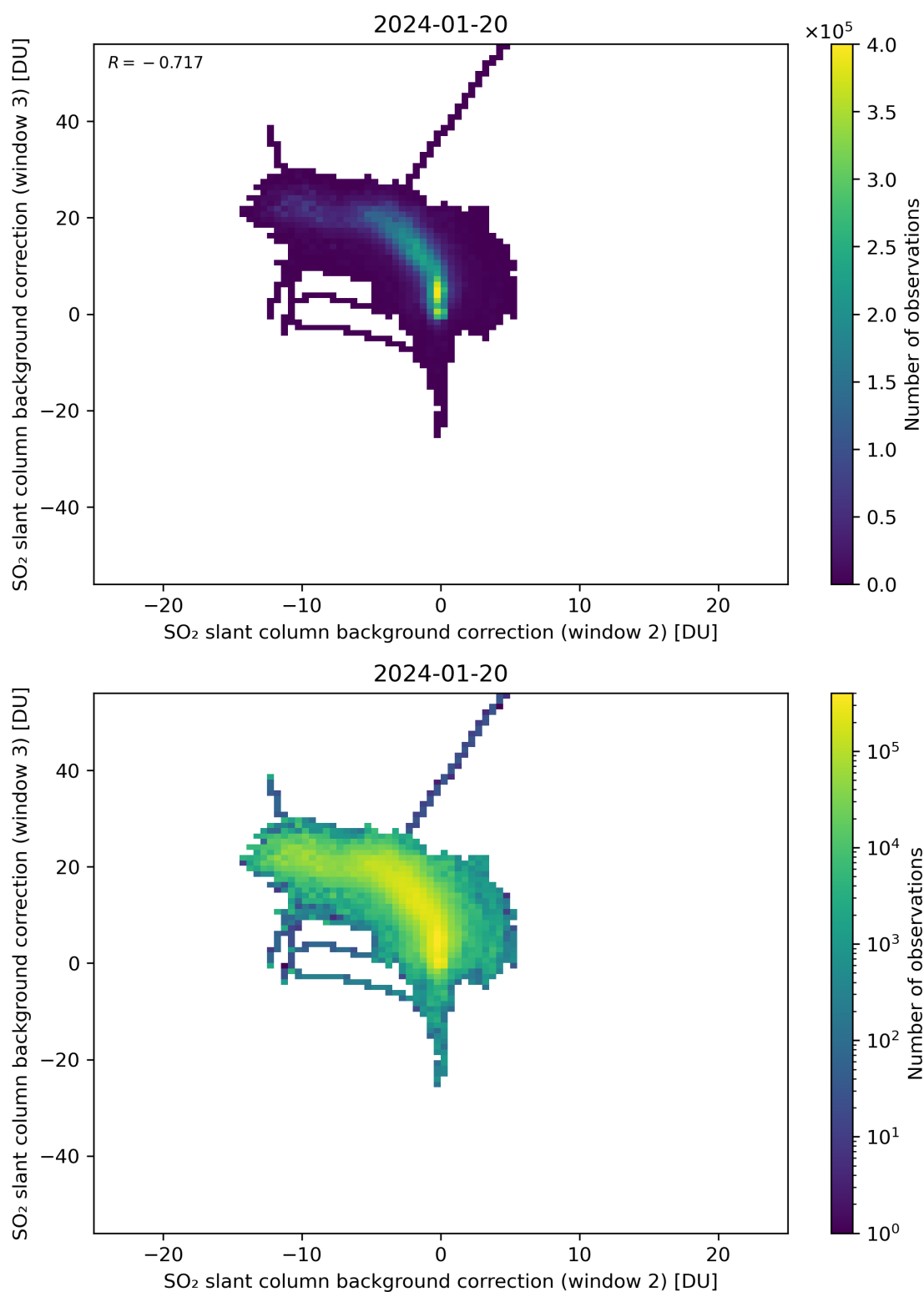
Figure 111: Scatter density plot of “SO 2 slant column background correction (window 2)” against “SO 2 slant column background correction (window 3)” for 2024-01-19 to 2024-01-21.
