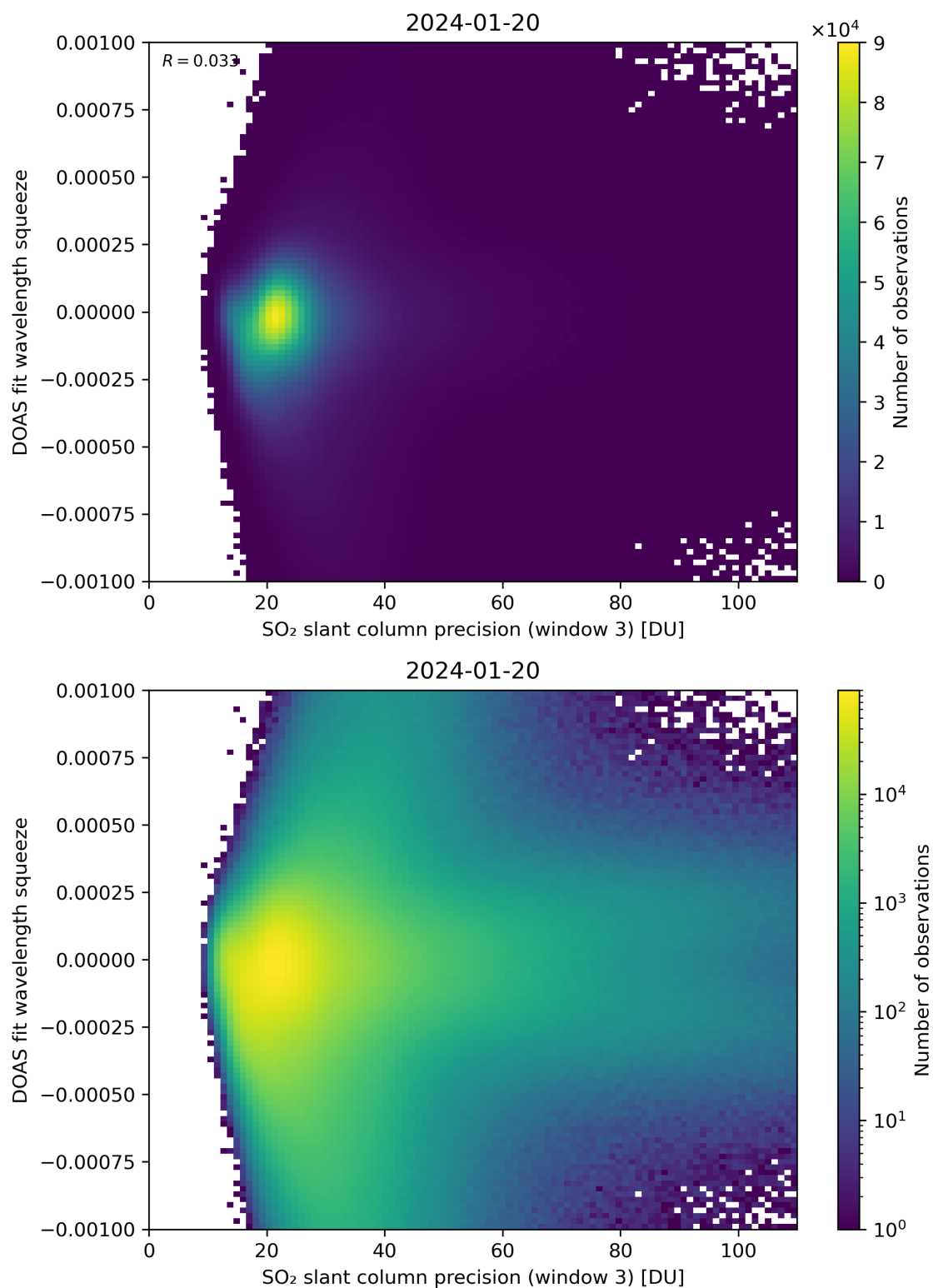
Figure 259: Scatter density plot of “SO 2 slant column precision (window 3)” against “DOAS fit wavelength squeeze” for 2024-01-19 to 2024-01-21.
