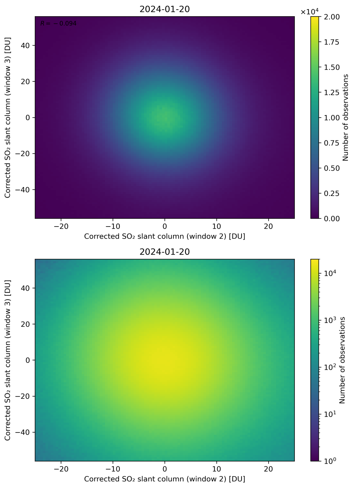
Figure 200: Scatter density plot of “Corrected SO 2 slant column (window 2)” against “Corrected SO 2 slant column (window 3)” for 2024-01-19 to 2024-01-21.
