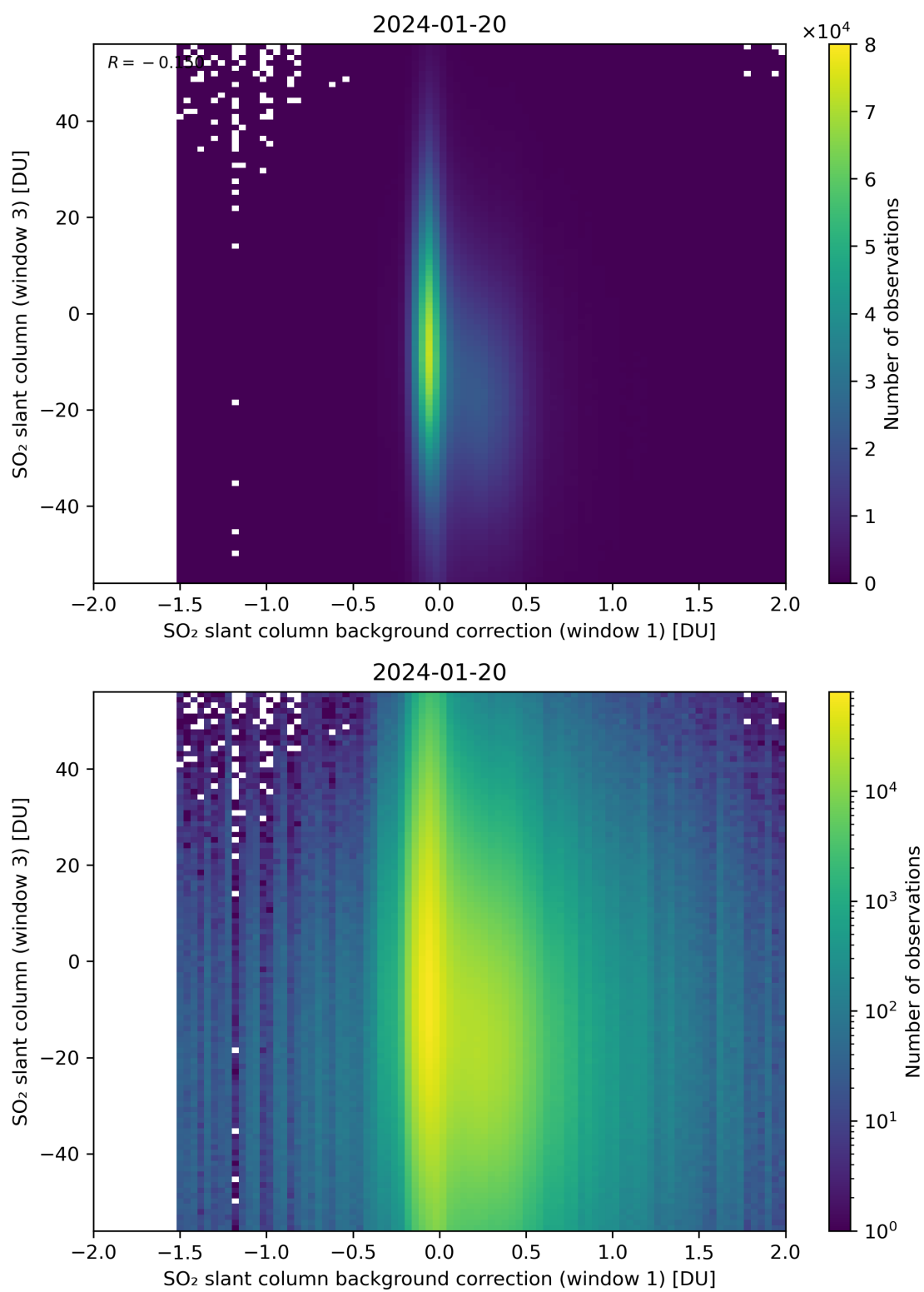
Figure 107: Scatter density plot of “SO 2 slant column background correction (window 1)” against “SO 2 slant column (window 3)” for 2024-01-19 to 2024-01-21.
