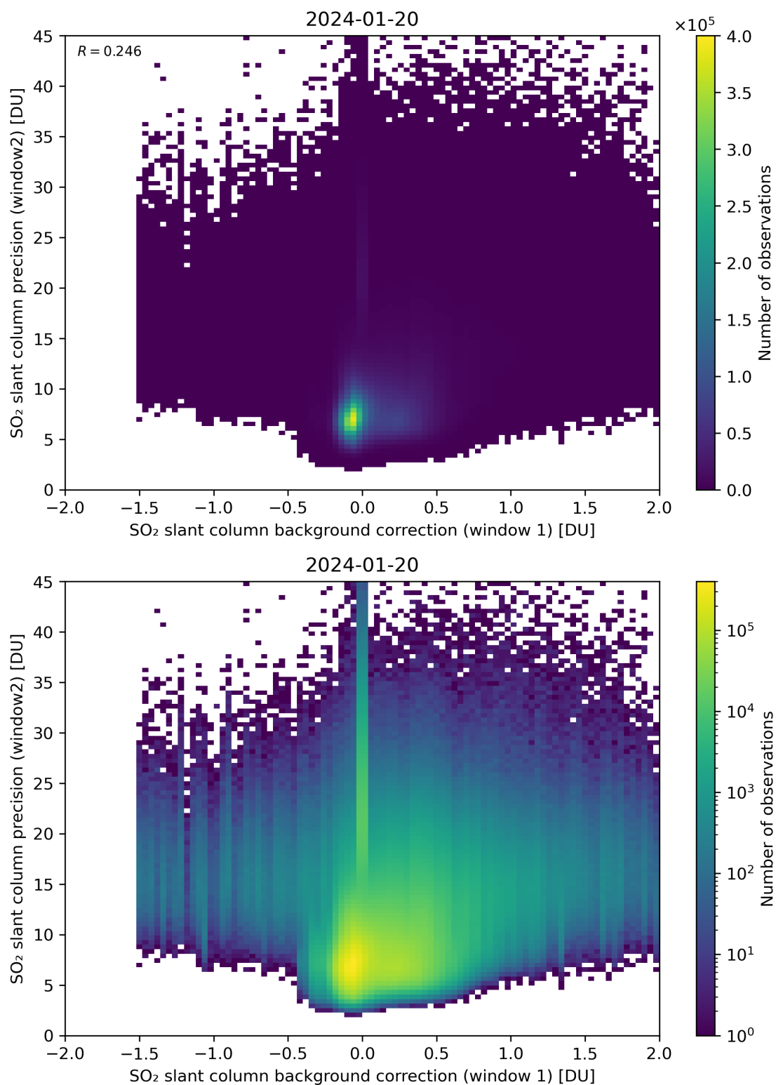
Figure 106: Scatter density plot of “SO 2 slant column background correction (window 1)” against “SO 2 slant column precision (window2)” for 2024-01-19 to 2024-01-21.
