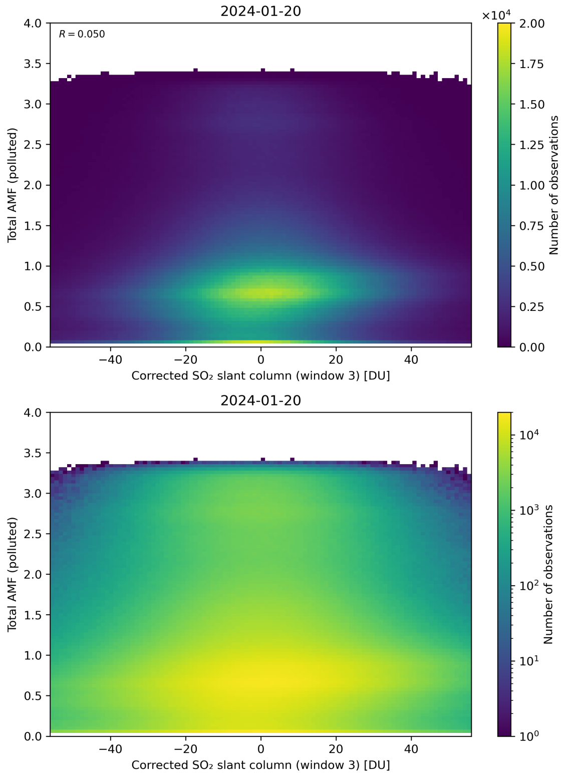
Figure 210: Scatter density plot of “Corrected SO 2 slant column (window 3)” against “Total AMF (polluted)” for 2024-01-19 to 2024-01-21.
