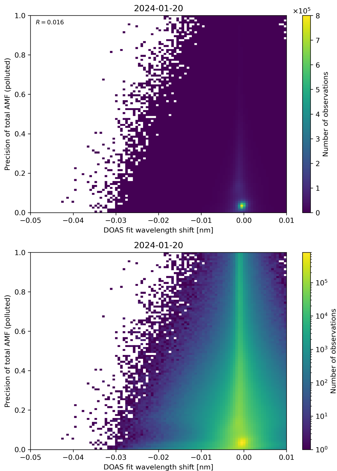
Figure 131: Scatter density plot of “DOAS fit wavelength shift” against “Precision of total AMF (polluted)” for 2024-01-19 to 2024-01-21.
