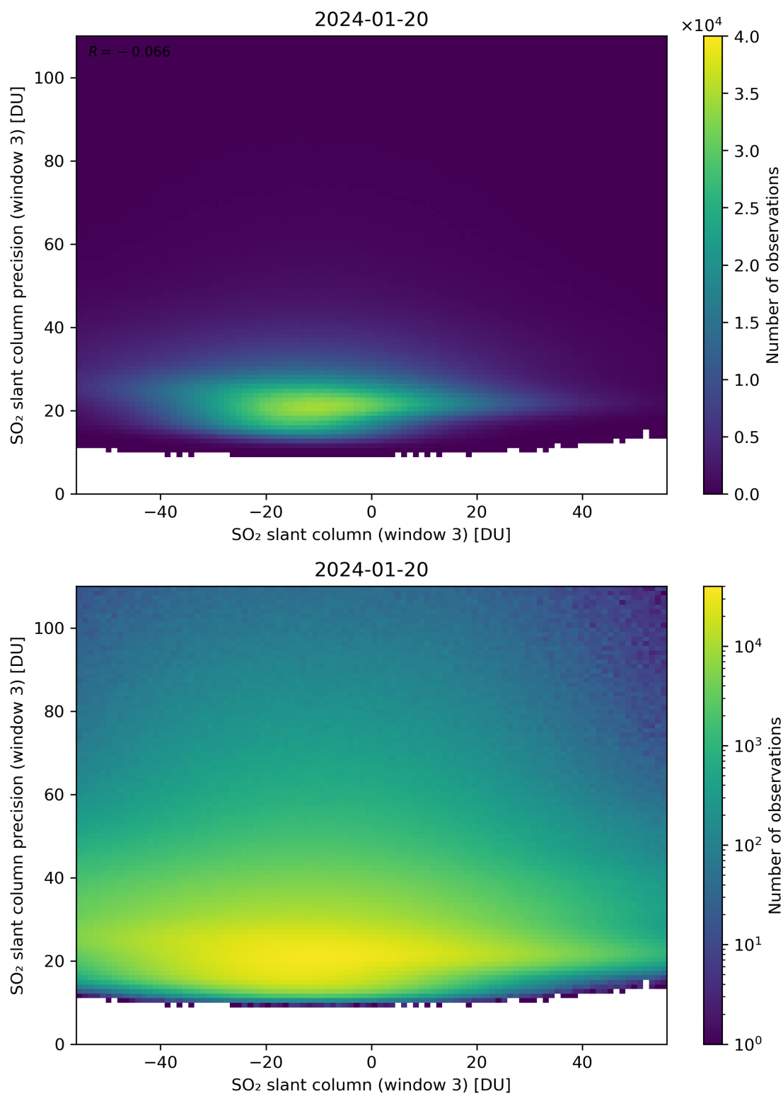
Figure 267: Scatter density plot of “SO 2 slant column (window 3)” against “SO 2 slant column precision (window 3)” for 2024-01-19 to 2024-01-21.
