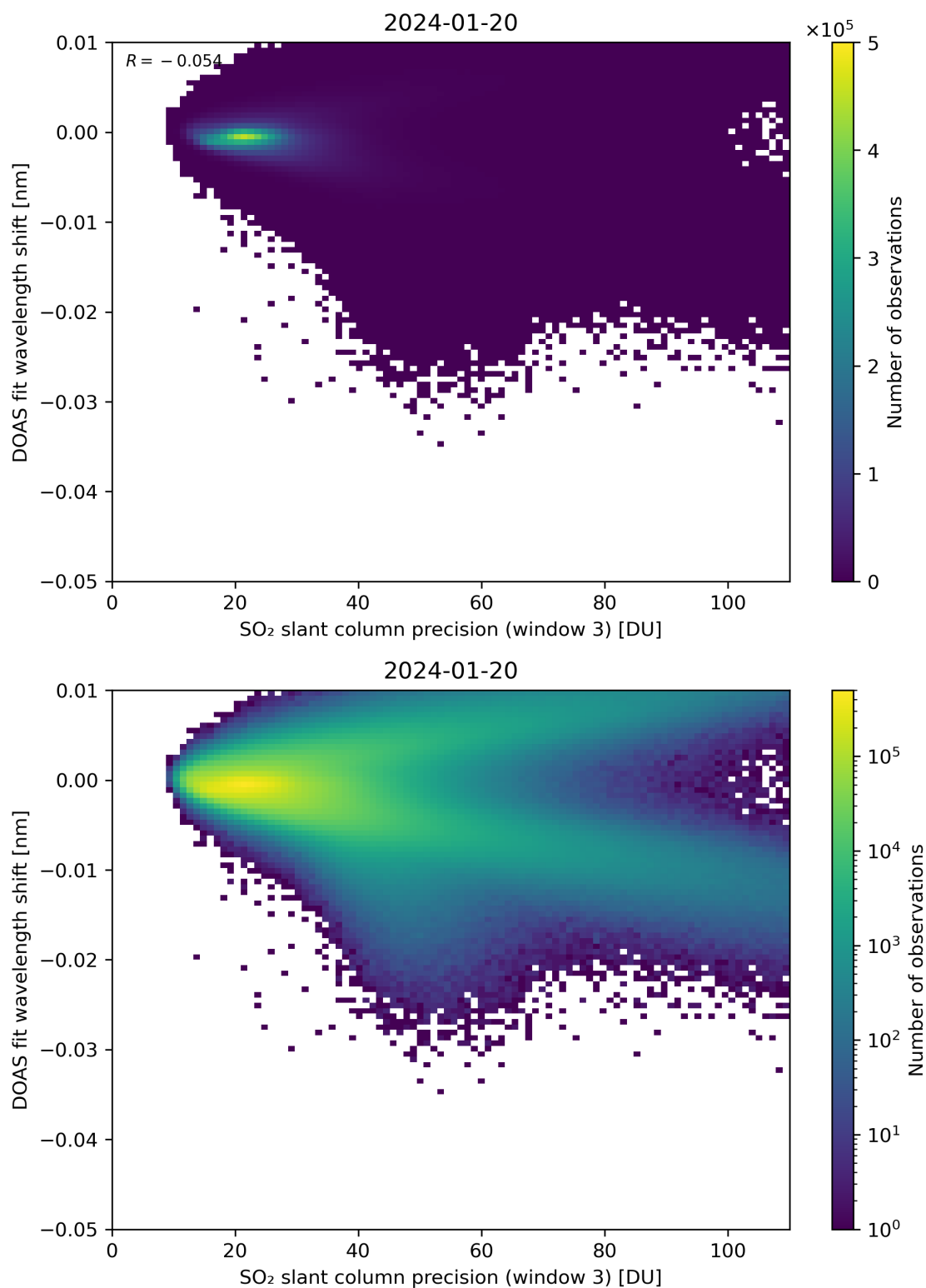
Figure 258: Scatter density plot of “SO 2 slant column precision (window 3)” against “DOAS fit wavelength shift” for 2024-01-19 to 2024-01-21.
