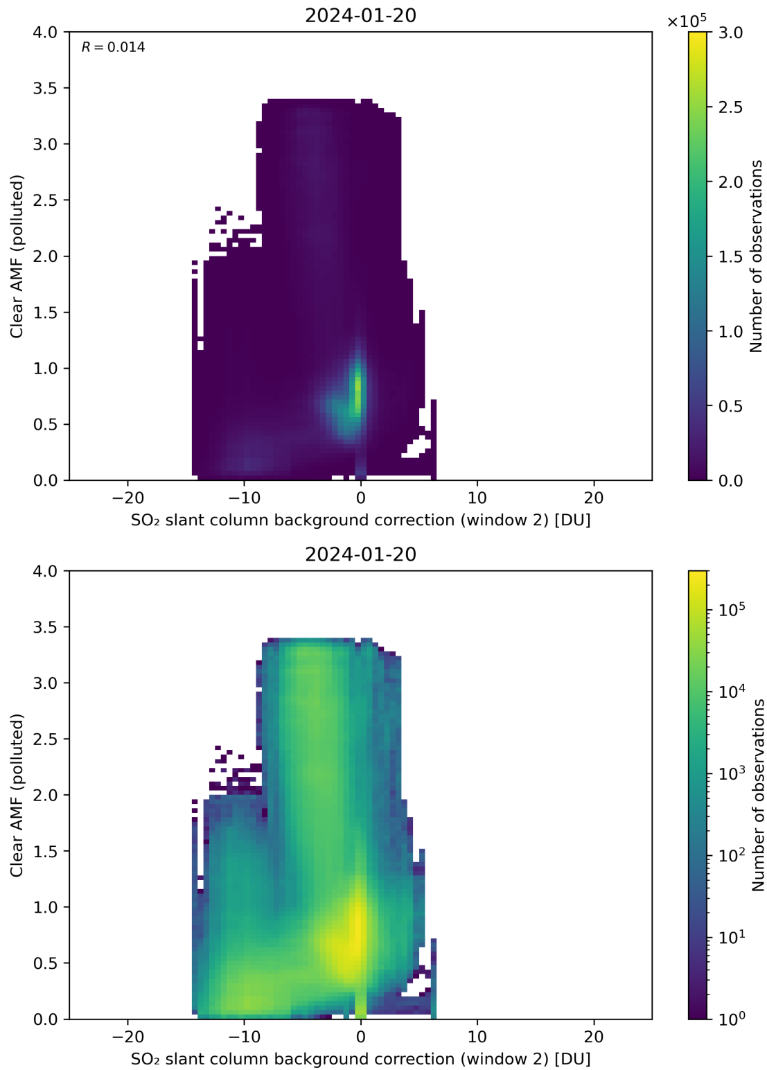
Figure 115: Scatter density plot of “SO 2 slant column background correction (window 2)” against “Clear AMF (polluted)” for 2024-01-19 to 2024-01-21.
