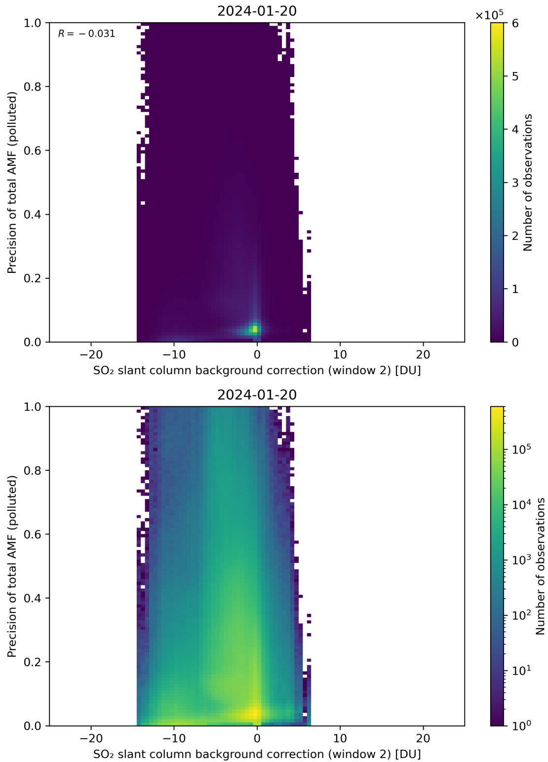
Figure 120: Scatter density plot of “SO 2 slant column background correction (window 2)” against “Precision of total AMF (polluted)” for 2024-01-19 to 2024-01-21.
