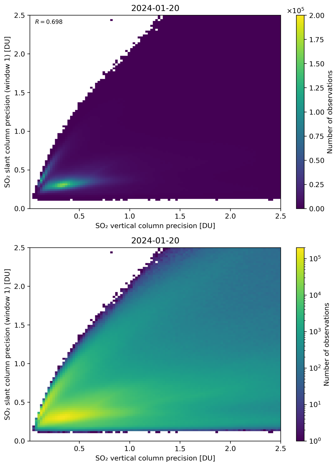
Figure 290: Scatter density plot of “SO 2 vertical column precision” against “SO 2 slant column precision (window 1)” for 2024-01-19 to 2024-01-21.
