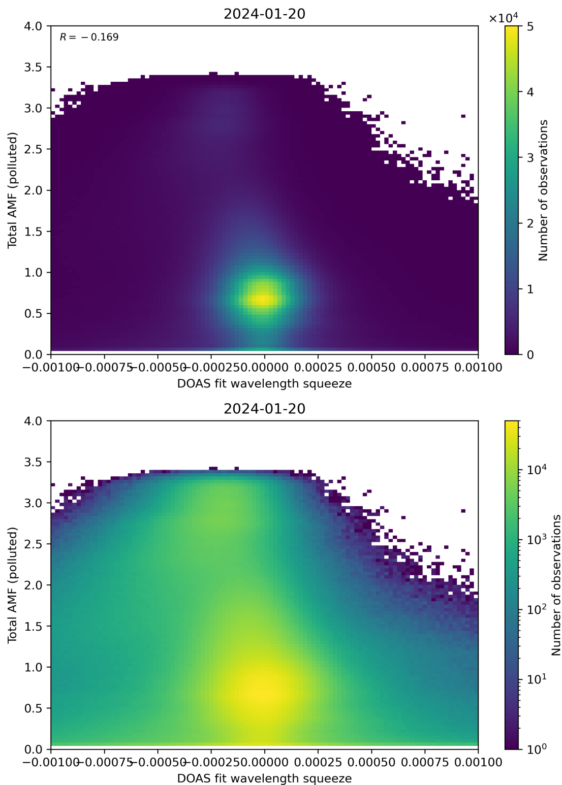
Figure 134: Scatter density plot of “DOAS fit wavelength squeeze” against “Total AMF (polluted)” for 2024-01-19 to 2024-01-21.
