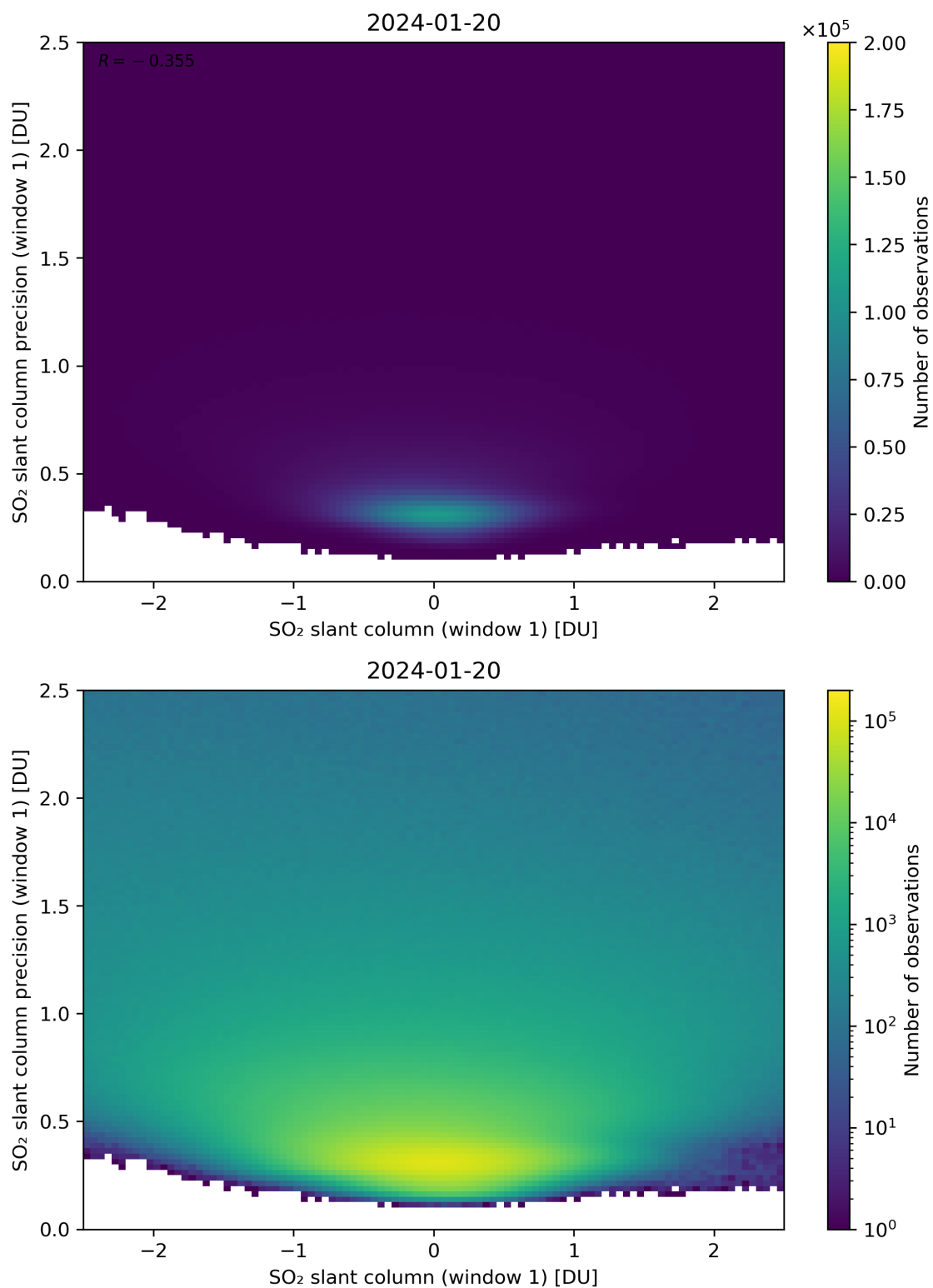
Figure 235: Scatter density plot of “SO 2 slant column (window 1)” against “SO 2 slant column precision (window 1)” for 2024-01-19 to 2024-01-21.
