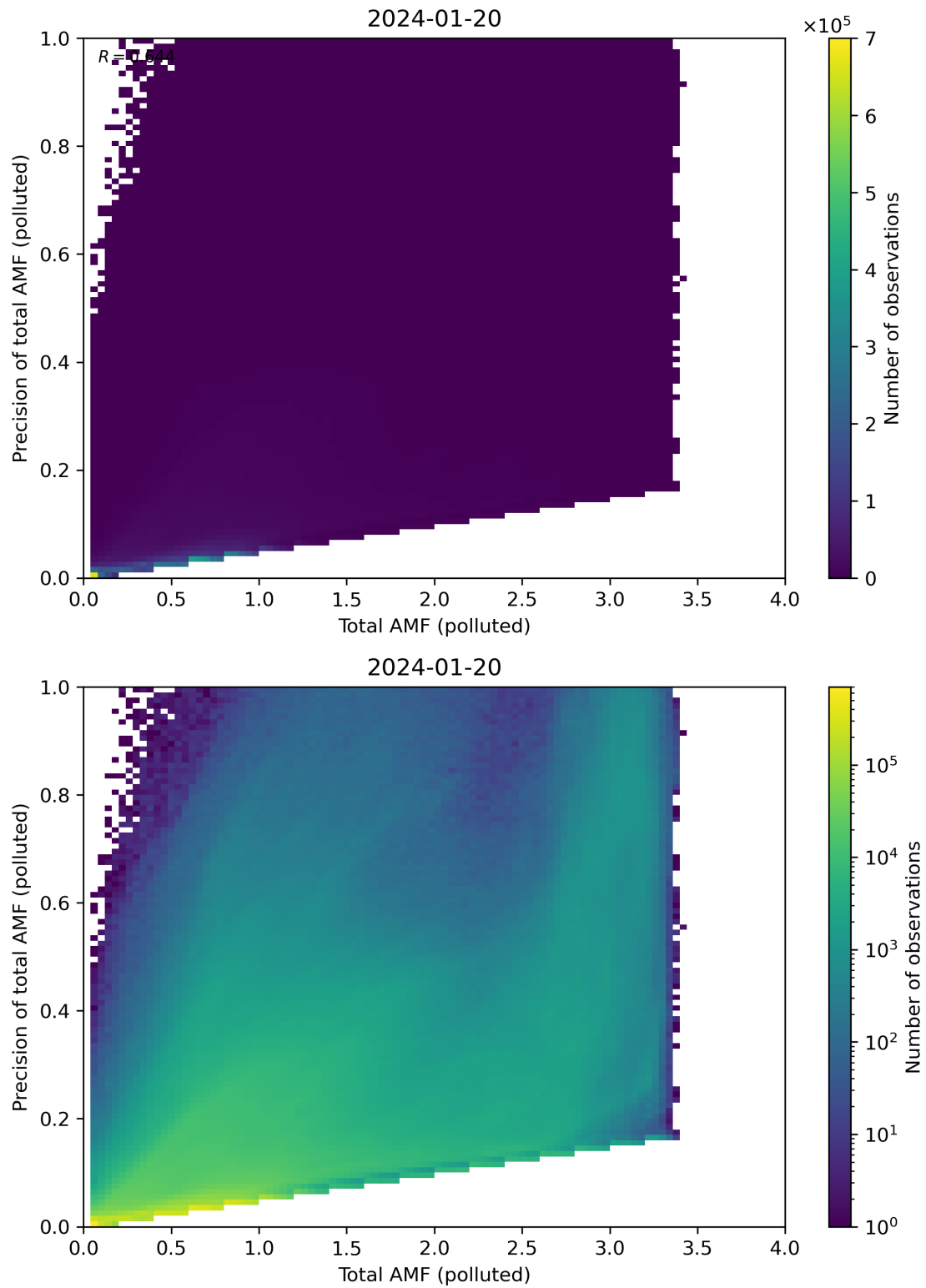
Figure 272: Scatter density plot of “Total AMF (polluted)” against “Precision of total AMF (polluted)” for 2024-01-19 to 2024-01-21.
