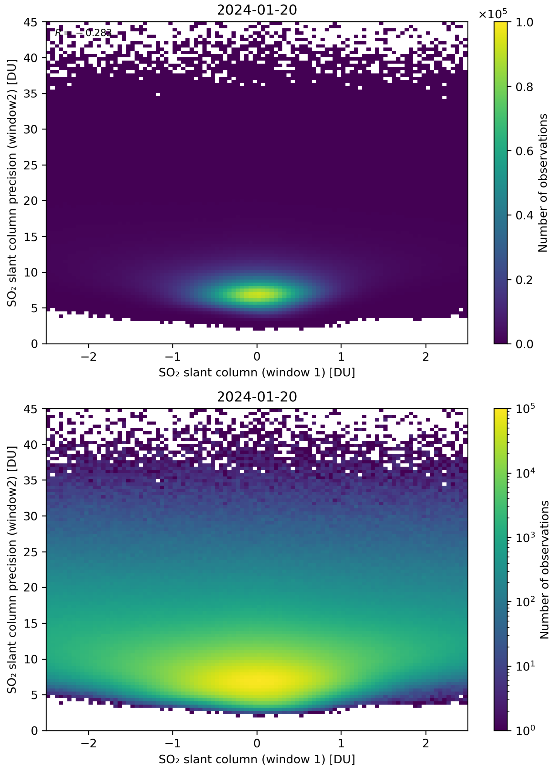
Figure 236: Scatter density plot of “SO 2 slant column (window 1)” against “SO 2 slant column precision (window2)” for 2024-01-19 to 2024-01-21.
