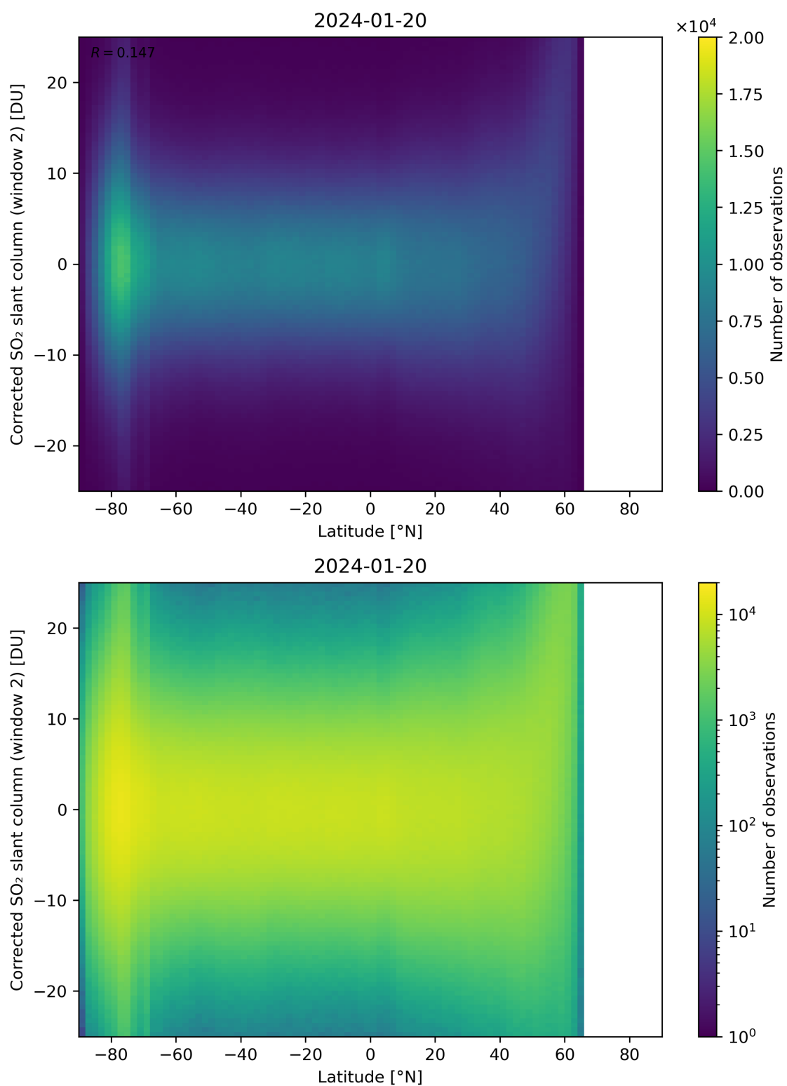
Figure 147: Scatter density plot of “Latitude” against “Corrected SO 2 slant column (window 2)” for 2024-01-19 to 2024-01-21.
