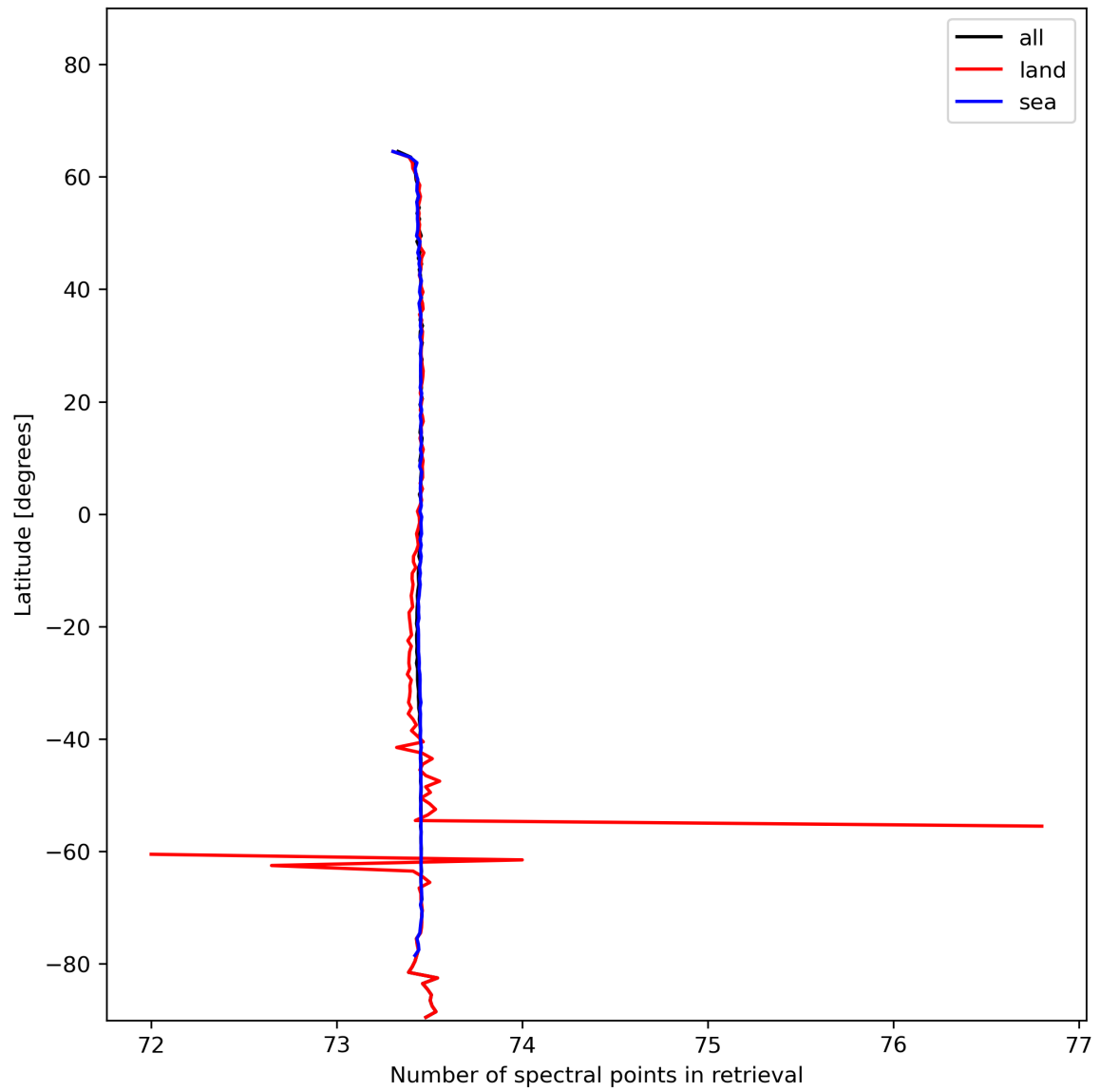
Figure 51: Zonal average of “Number of spectral points in retrieval” for 2024-01-19 to 2024-01-21.
