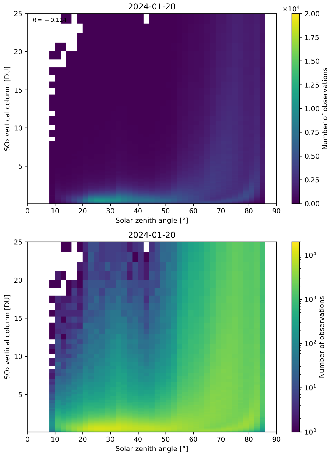
Figure 176: Scatter density plot of “Solar zenith angle” against “SO 2 vertical column” for 2024-01-19 to 2024-01-21.
