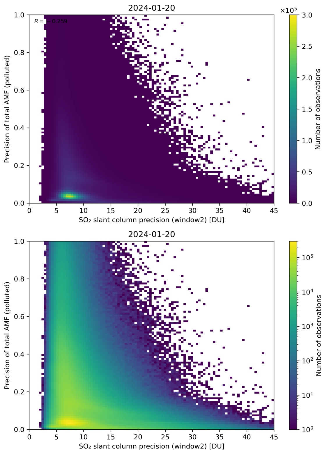
Figure 252: Scatter density plot of “SO 2 slant column precision (window2)” against “Precision of total AMF (polluted)” for 2024-01-19 to 2024-01-21.
