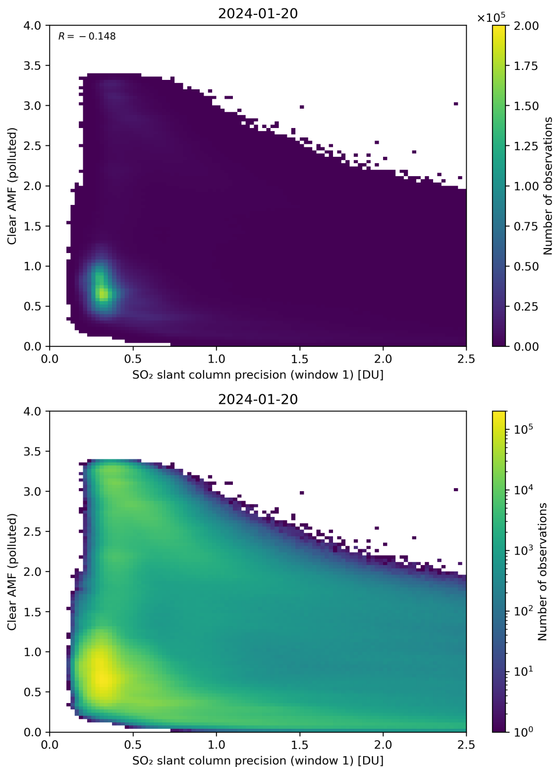
Figure 224: Scatter density plot of “SO 2 slant column precision (window 1)” against “Clear AMF (polluted)” for 2024-01-19 to 2024-01-21.
