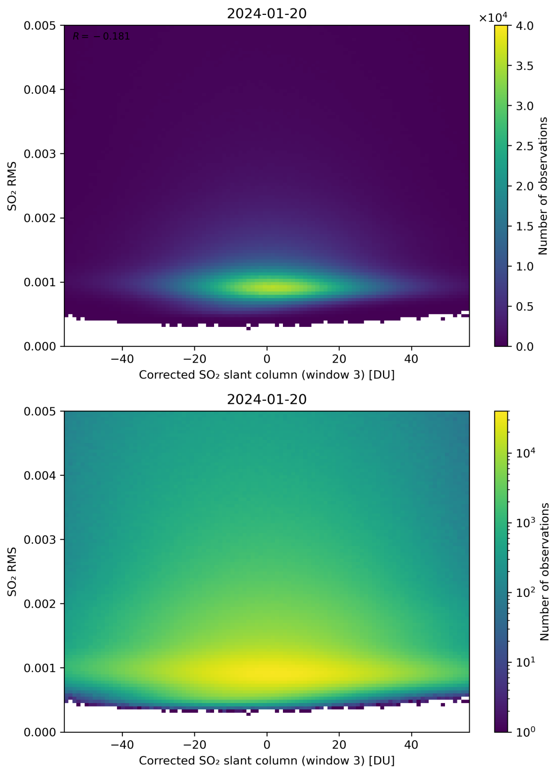
Figure 208: Scatter density plot of “Corrected SO 2 slant column (window 3)” against “SO 2 RMS” for 2024-01-19 to 2024-01-21.
