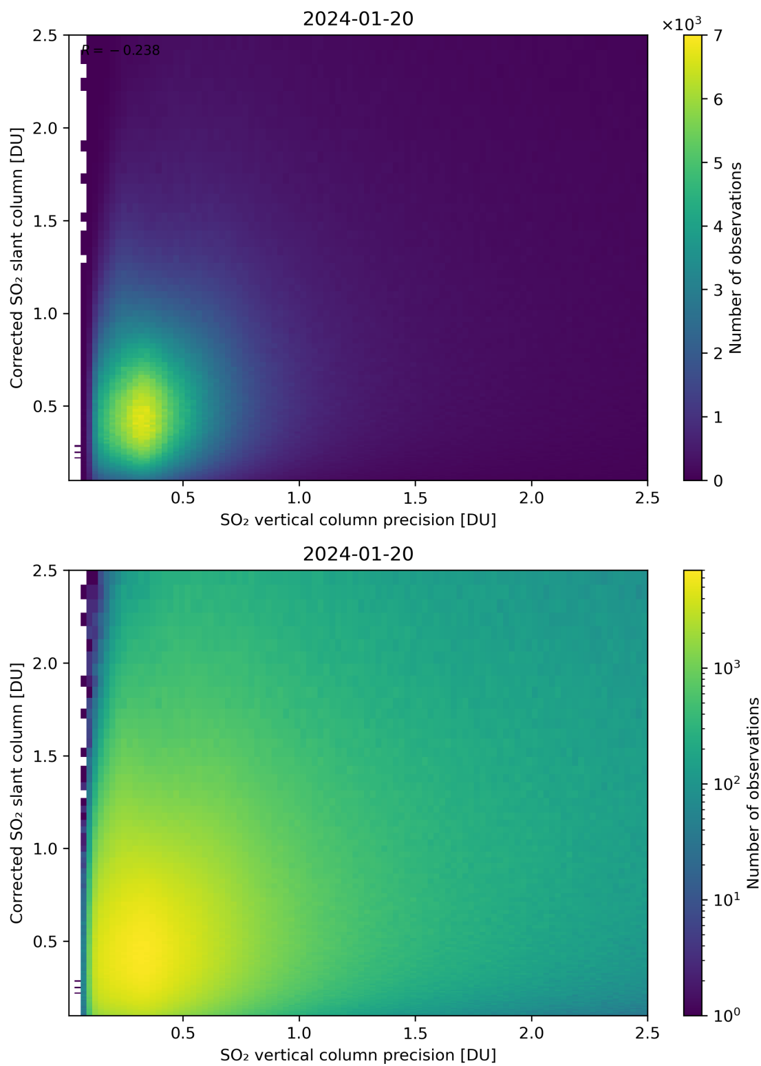
Figure 286: Scatter density plot of “SO 2 vertical column precision” against “Corrected SO 2 slant column” for 2024-01-19 to 2024-01-21.
