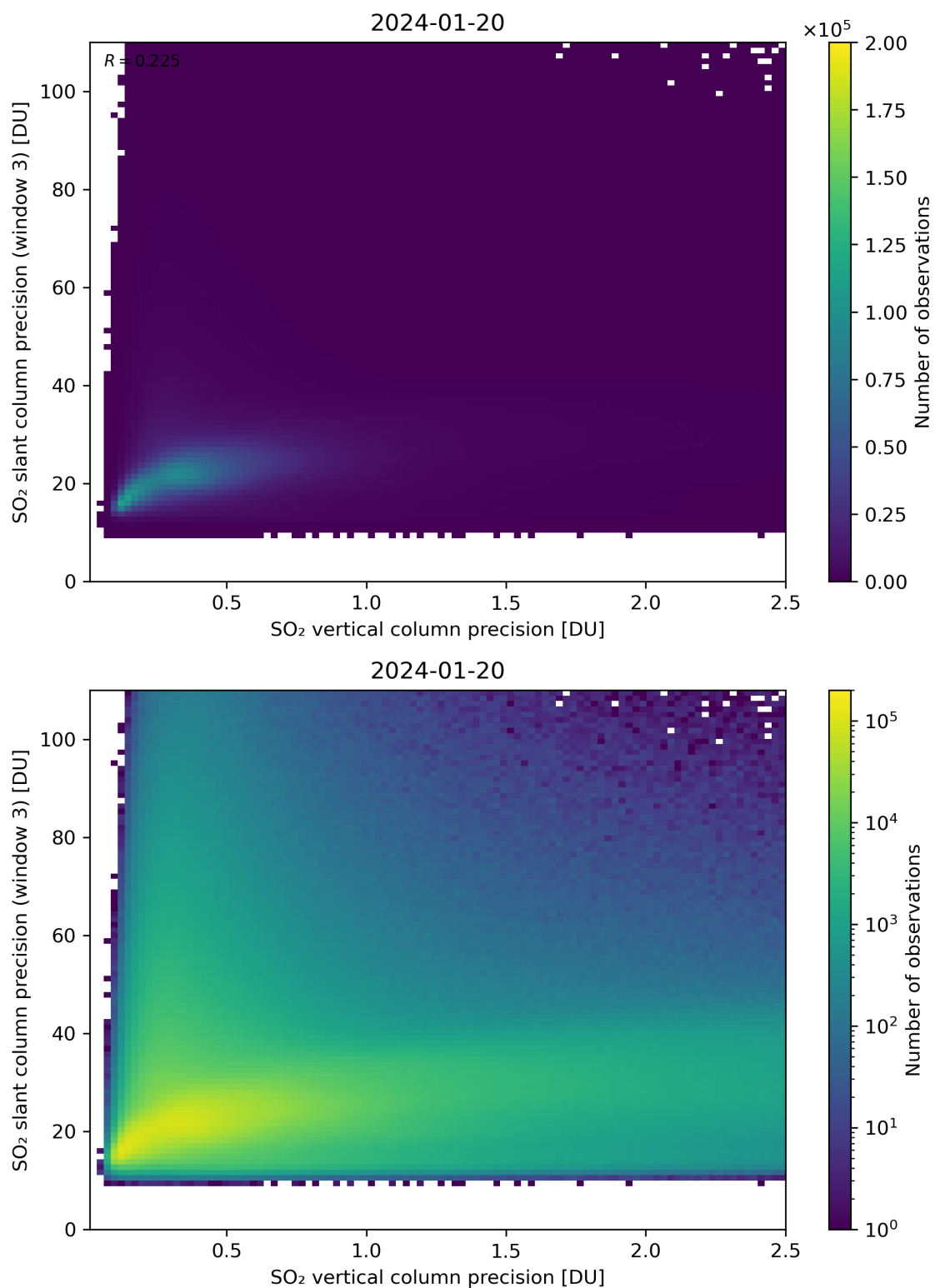
Figure 293: Scatter density plot of “SO 2 vertical column precision” against “SO 2 slant column precision (window 3)” for 2024-01-19 to 2024-01-21.
