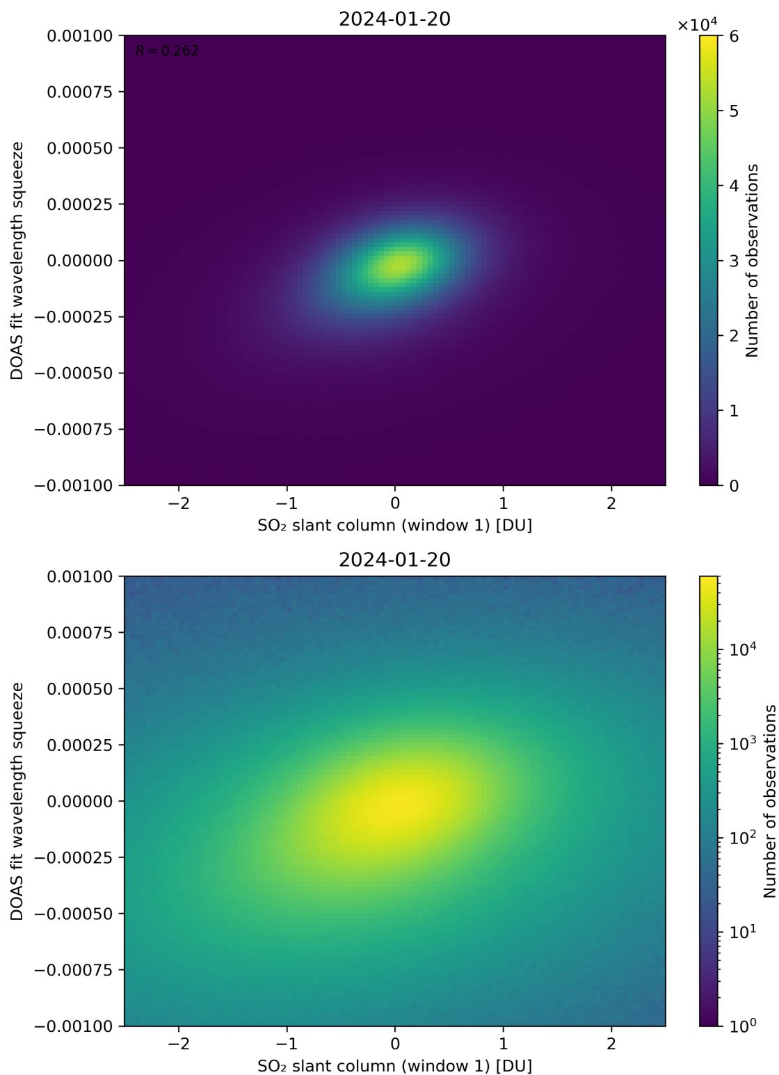
Figure 216: Scatter density plot of “SO 2 slant column (window 1)” against “DOAS fit wavelength squeeze” for 2024-01-19 to 2024-01-21.
