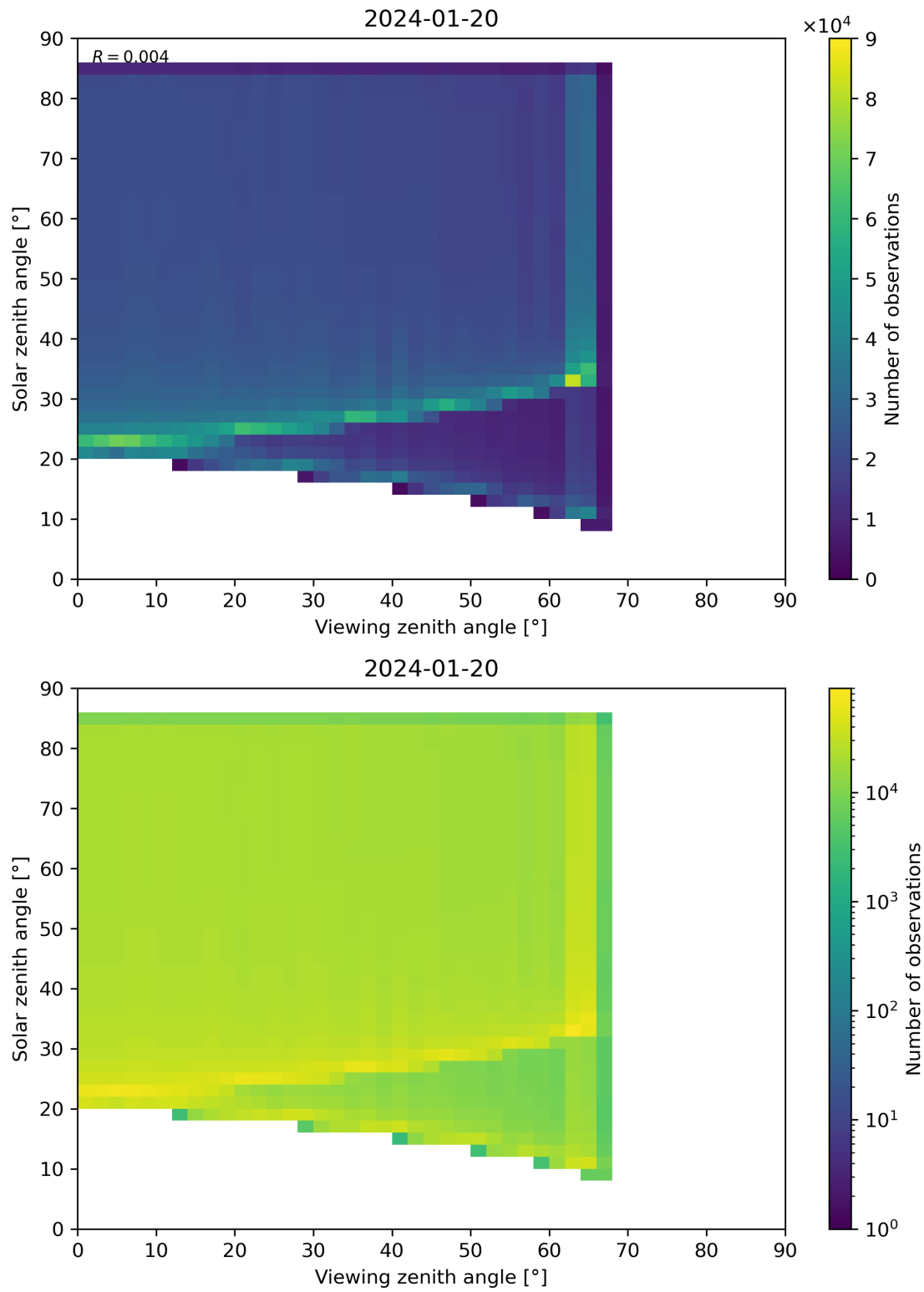
Figure 315: Scatter density plot of “Viewing zenith angle” against “Solar zenith angle” for 2024-01-19 to 2024-01-21.
