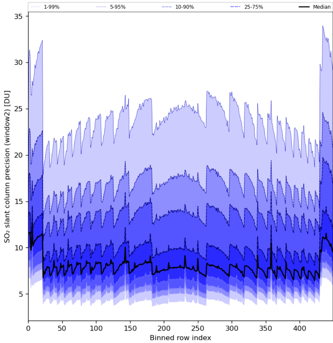
Figure 84: Along track statistics of “SO 2 slant column precision (window2)” for 2024-01-19 to 2024-01-21
