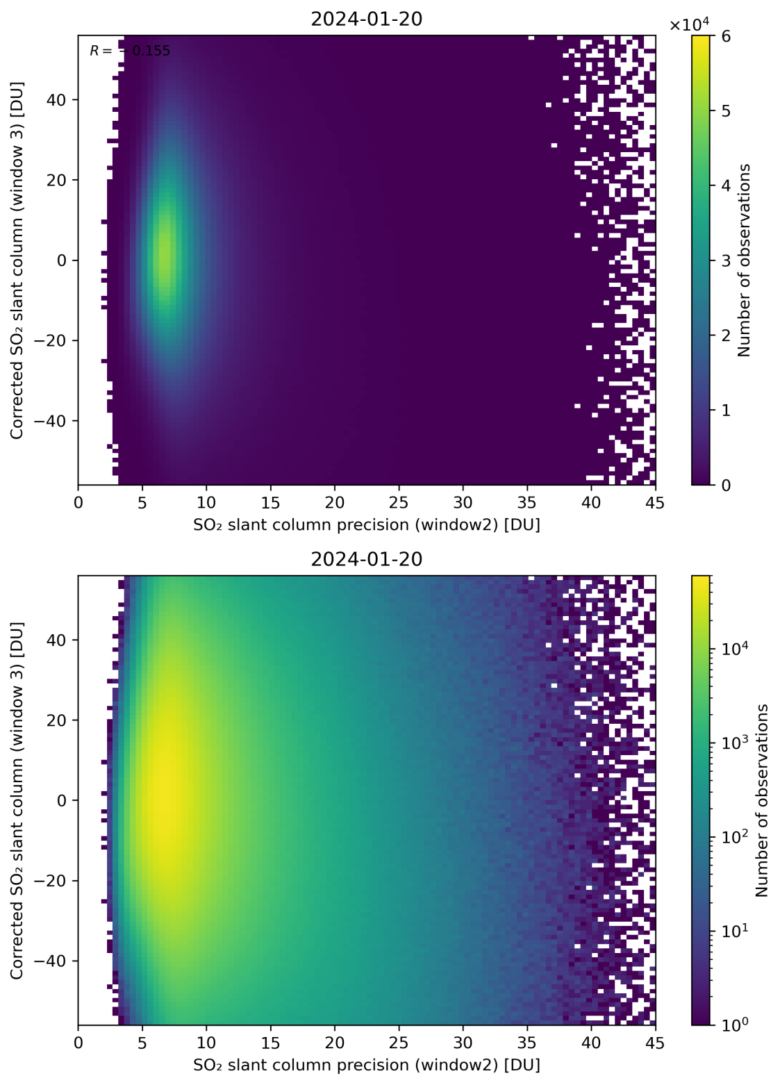
Figure 248: Scatter density plot of “SO 2 slant column precision (window2)” against “Corrected SO 2 slant column (window 3)” for 2024-01-19 to 2024-01-21.
