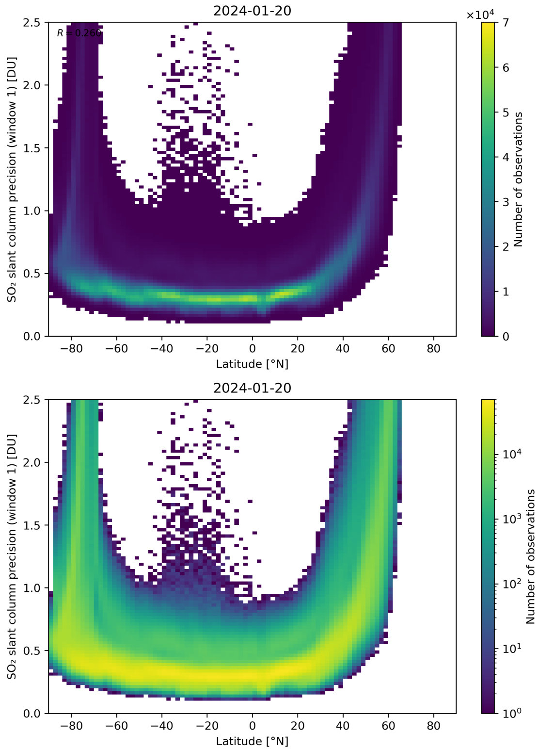
Figure 150: Scatter density plot of “Latitude” against “SO 2 slant column precision (window 1)” for 2024-01-19 to 2024-01-21.
