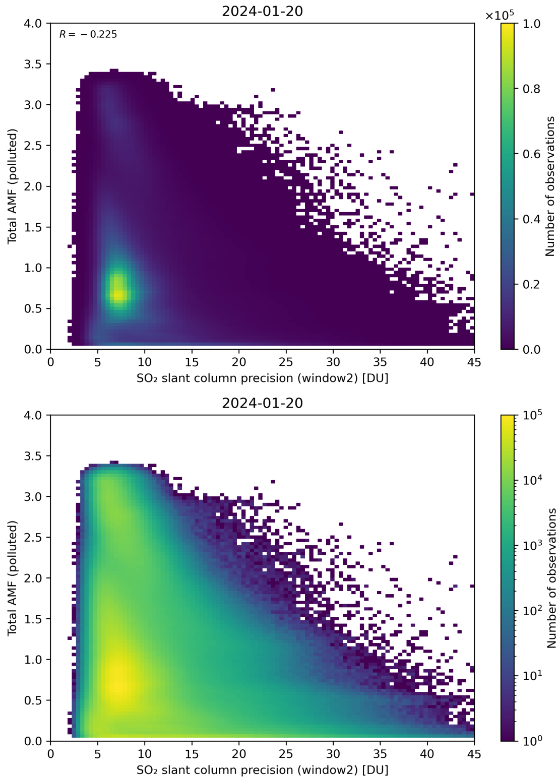
Figure 251: Scatter density plot of “SO 2 slant column precision (window2)” against “Total AMF (polluted)” for 2024-01-19 to 2024-01-21.
