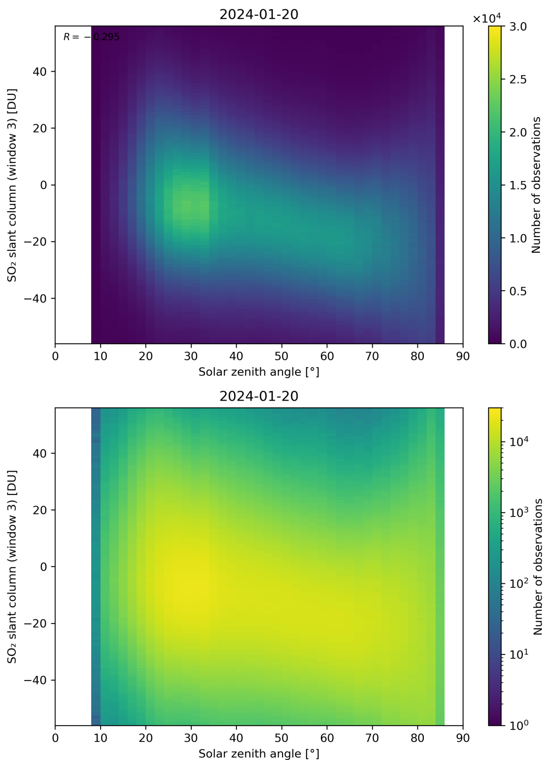
Figure 172: Scatter density plot of “Solar zenith angle” against “SO 2 slant column (window 3)” for 2024-01-19 to 2024-01-21.
