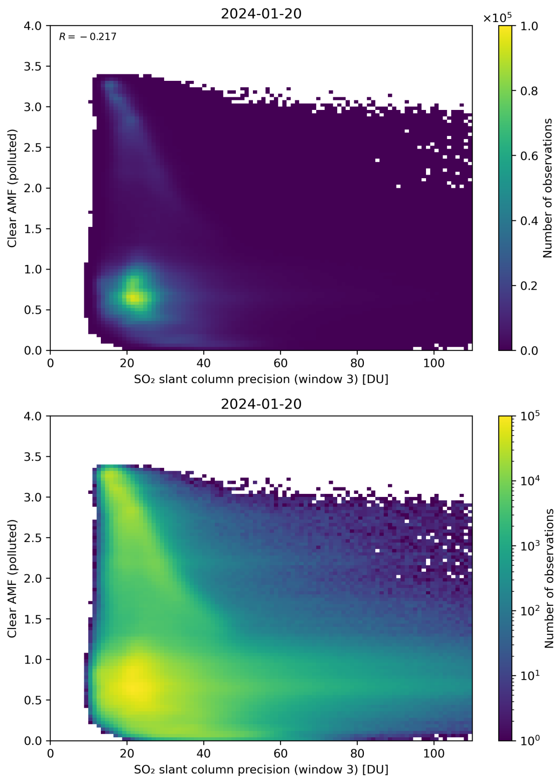
Figure 261: Scatter density plot of “SO 2 slant column precision (window 3)” against “Clear AMF (polluted)” for 2024-01-19 to 2024-01-21.
