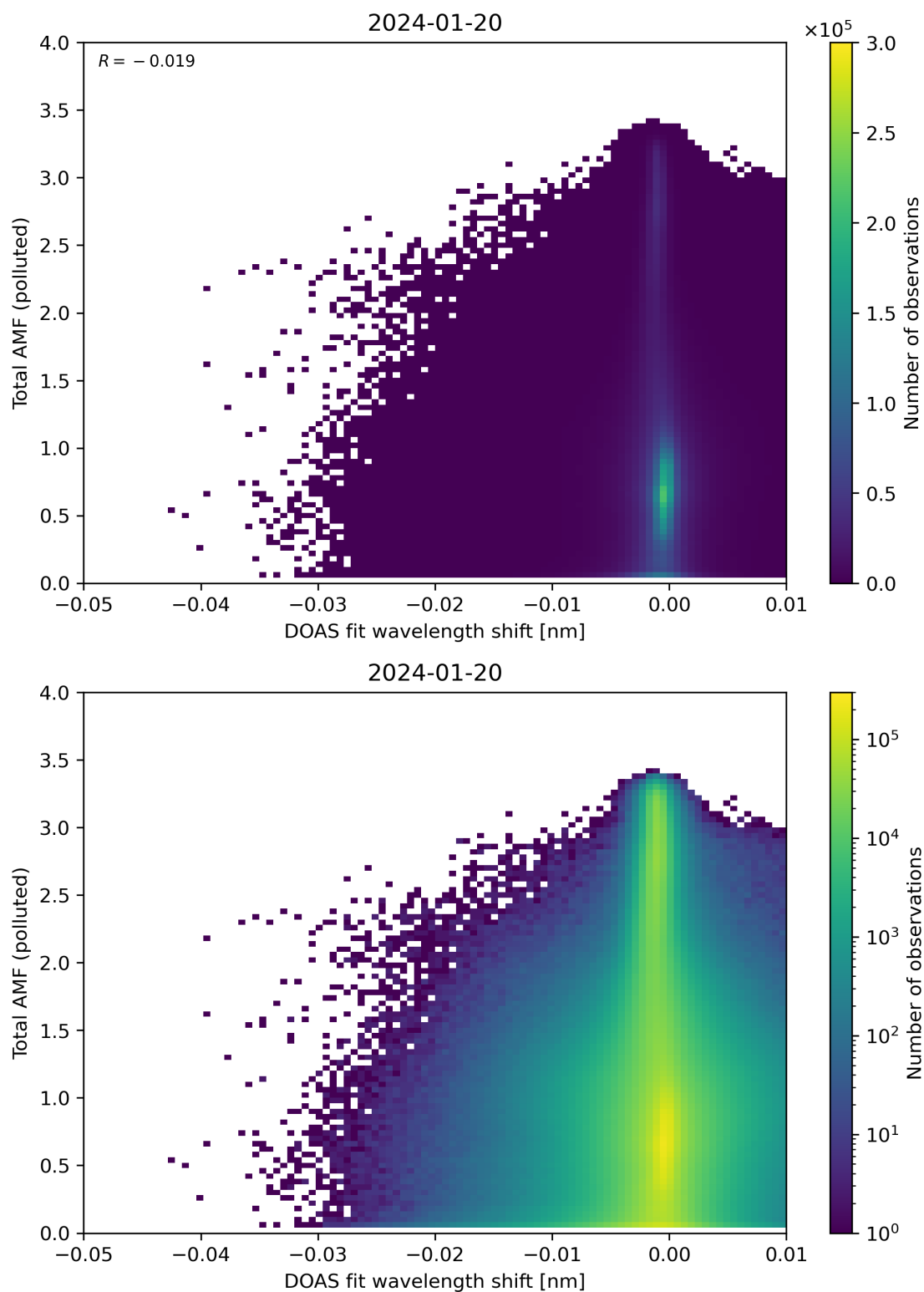
Figure 130: Scatter density plot of “DOAS fit wavelength shift” against “Total AMF (polluted)” for 2024-01-19 to 2024-01-21.
