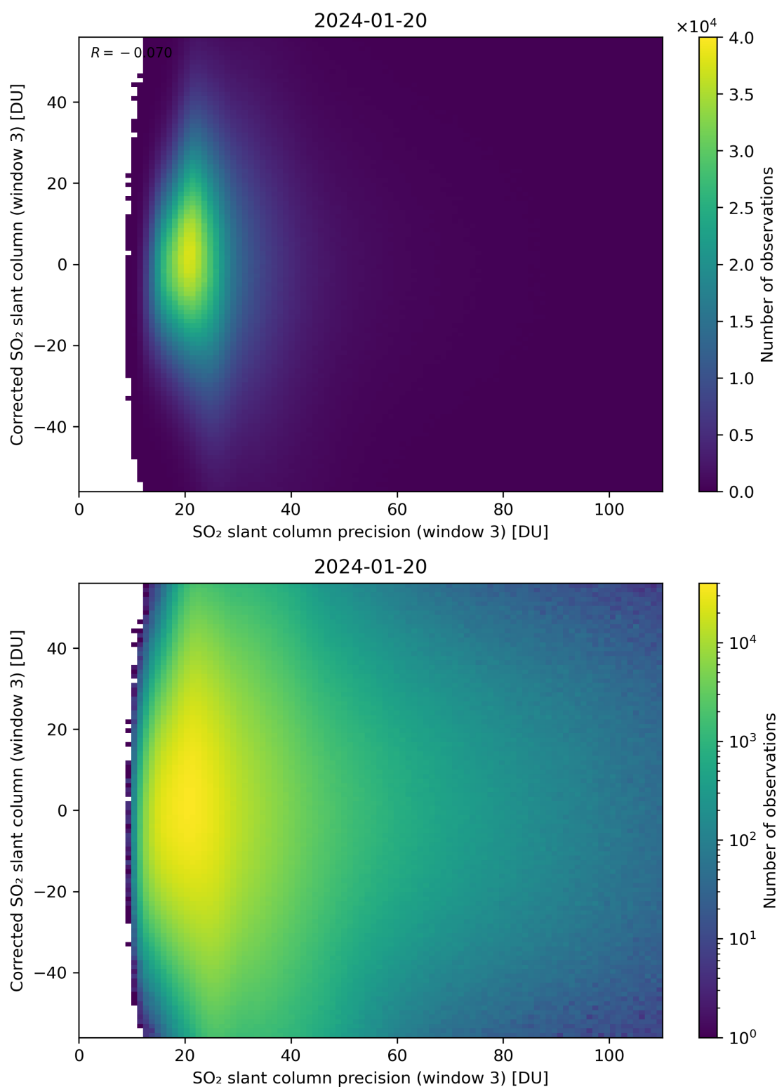
Figure 262: Scatter density plot of “SO 2 slant column precision (window 3)” against “Corrected SO 2 slant column (window 3)” for 2024-01-19 to 2024-01-21.
