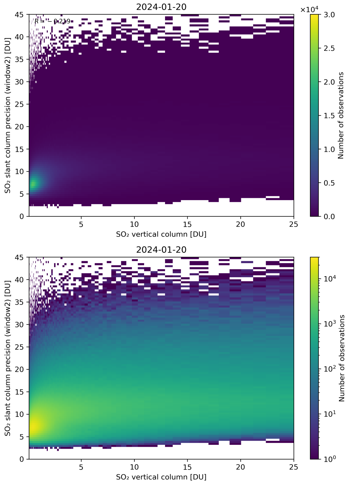
Figure 302: Scatter density plot of “SO 2 vertical column” against “SO 2 slant column precision (window2)” for 2024-01-19 to 2024-01-21.
