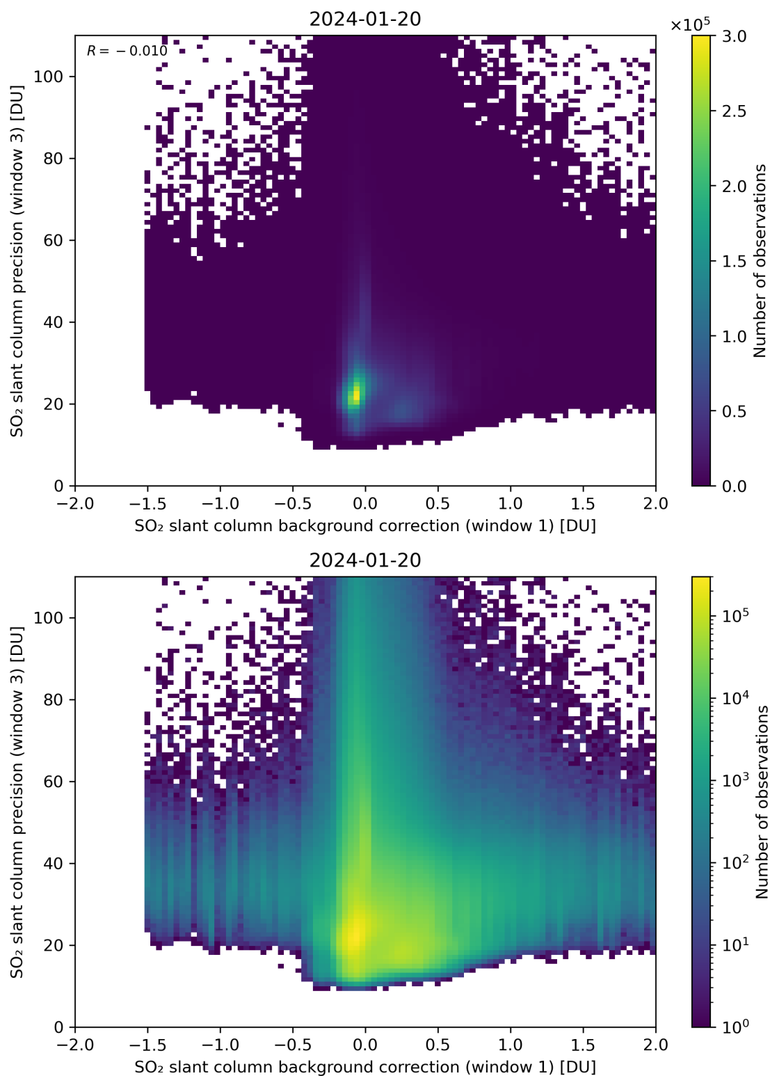
Figure 108: Scatter density plot of “SO 2 slant column background correction (window 1)” against “SO 2 slant column precision (window 3)” for 2024-01-19 to 2024-01-21.
