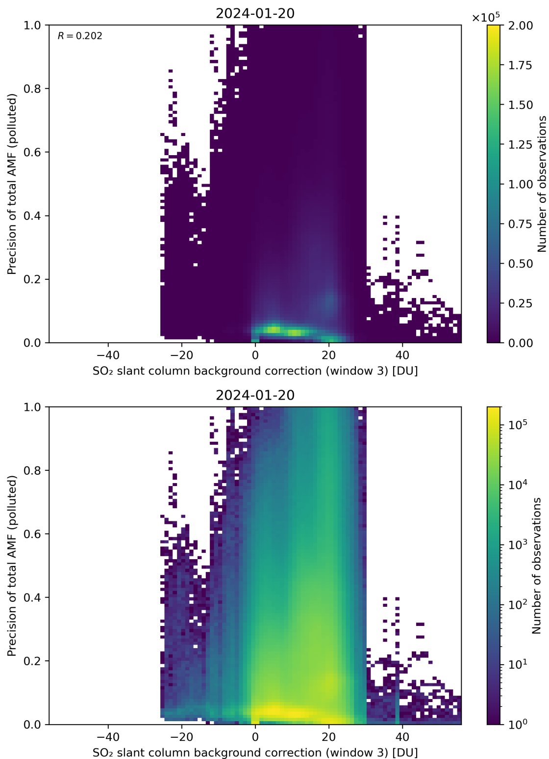
Figure 126: Scatter density plot of “SO 2 slant column background correction (window 3)” against “Precision of total AMF (polluted)” for 2024-01-19 to 2024-01-21.
