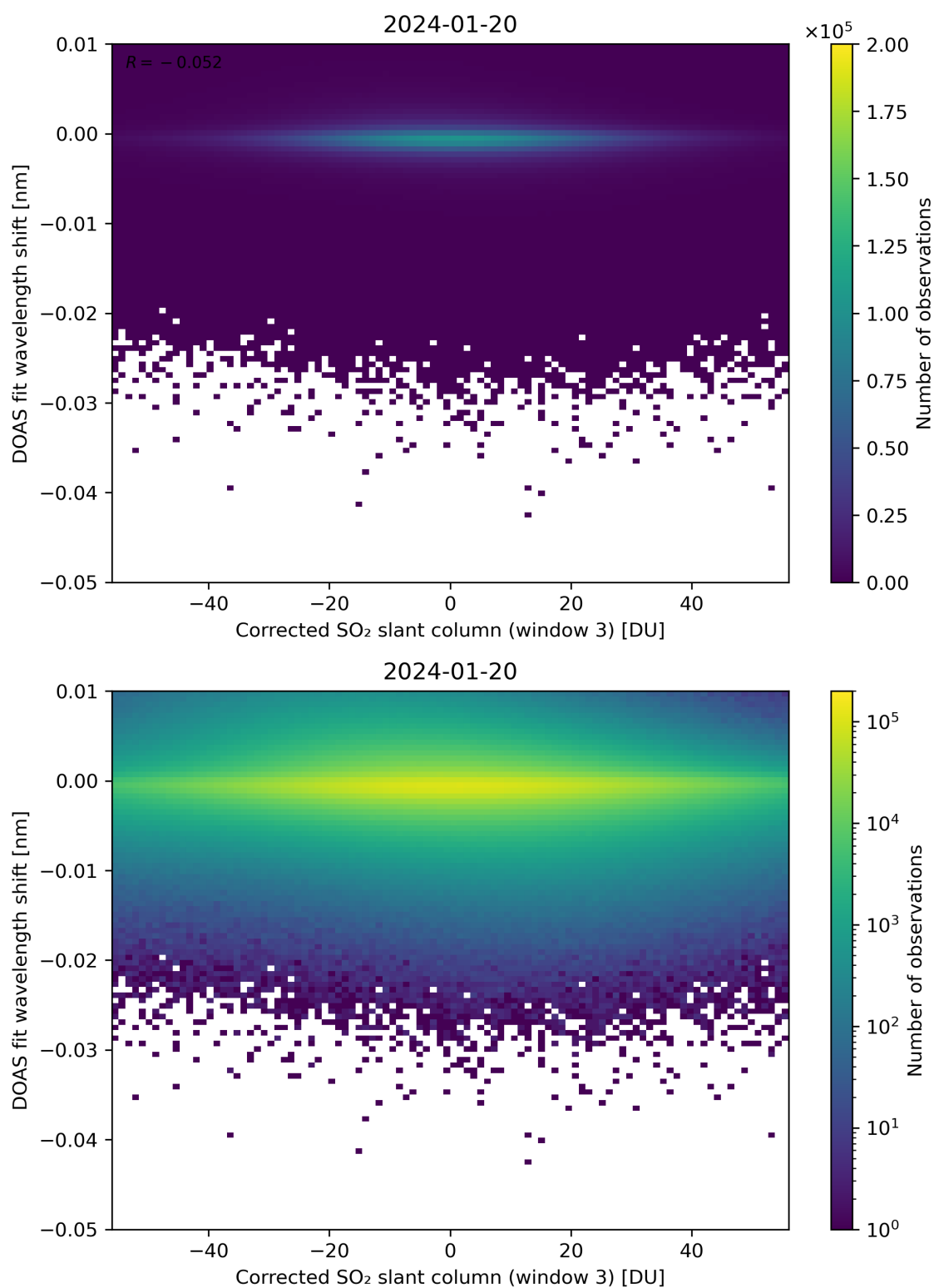
Figure 206: Scatter density plot of “Corrected SO 2 slant column (window 3)” against “DOAS fit wavelength shift” for 2024-01-19 to 2024-01-21.
