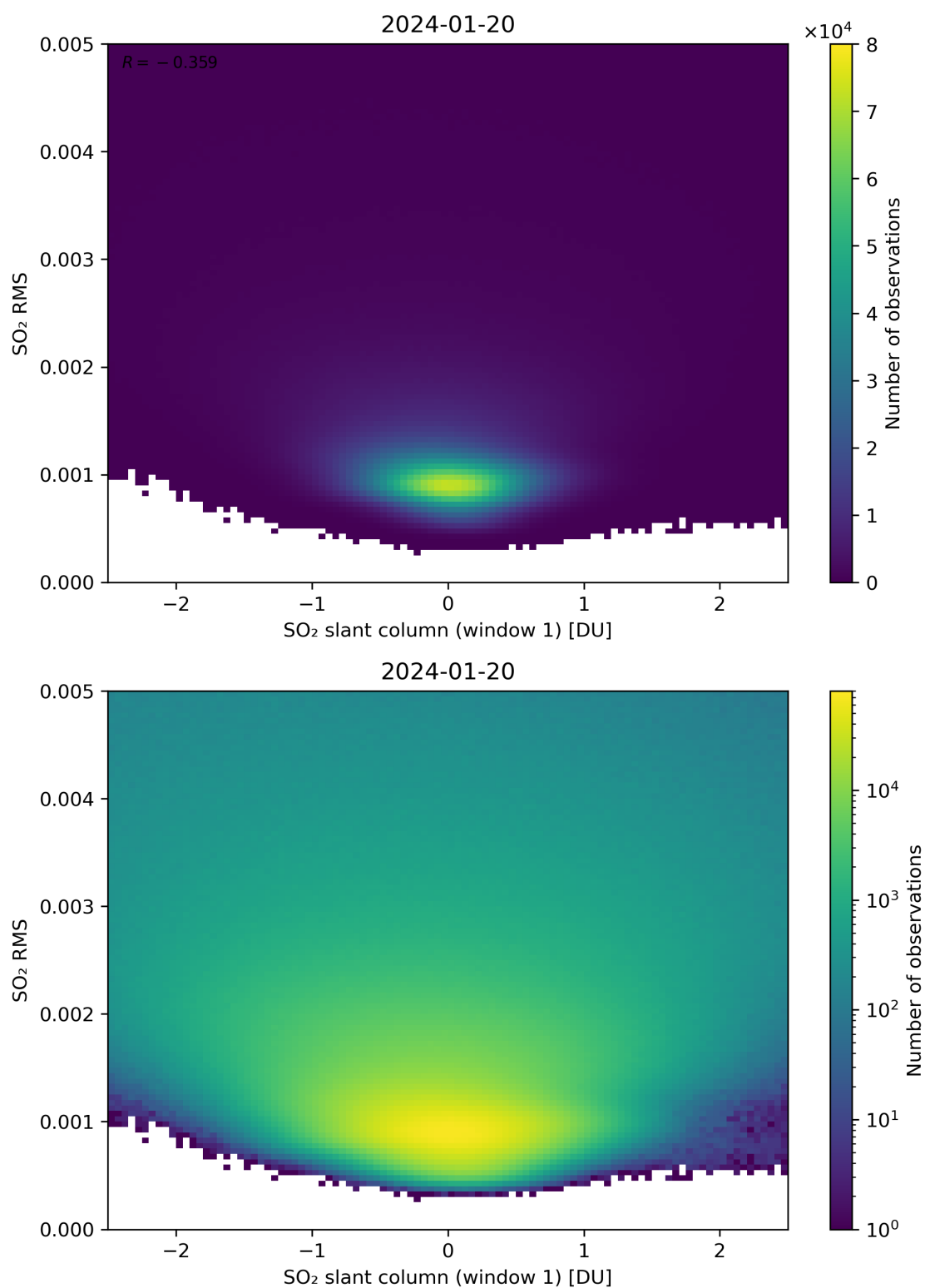
Figure 217: Scatter density plot of “SO 2 slant column (window 1)” against “SO 2 RMS” for 2024-01-19 to 2024-01-21.
