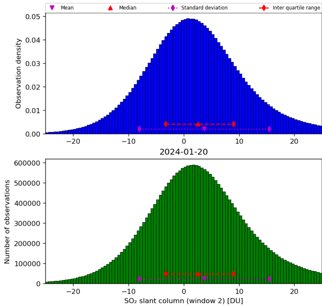
Figure 60: Histogram of “SO 2 slant column (window 2)” for 2024-01-19 to 2024-01-21
