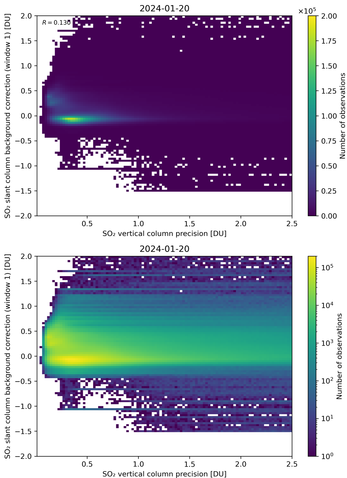
Figure 279: Scatter density plot of “SO 2 vertical column precision” against “SO 2 slant column background correction (window 1)” for 2024-01-19 to 2024-01-21.
