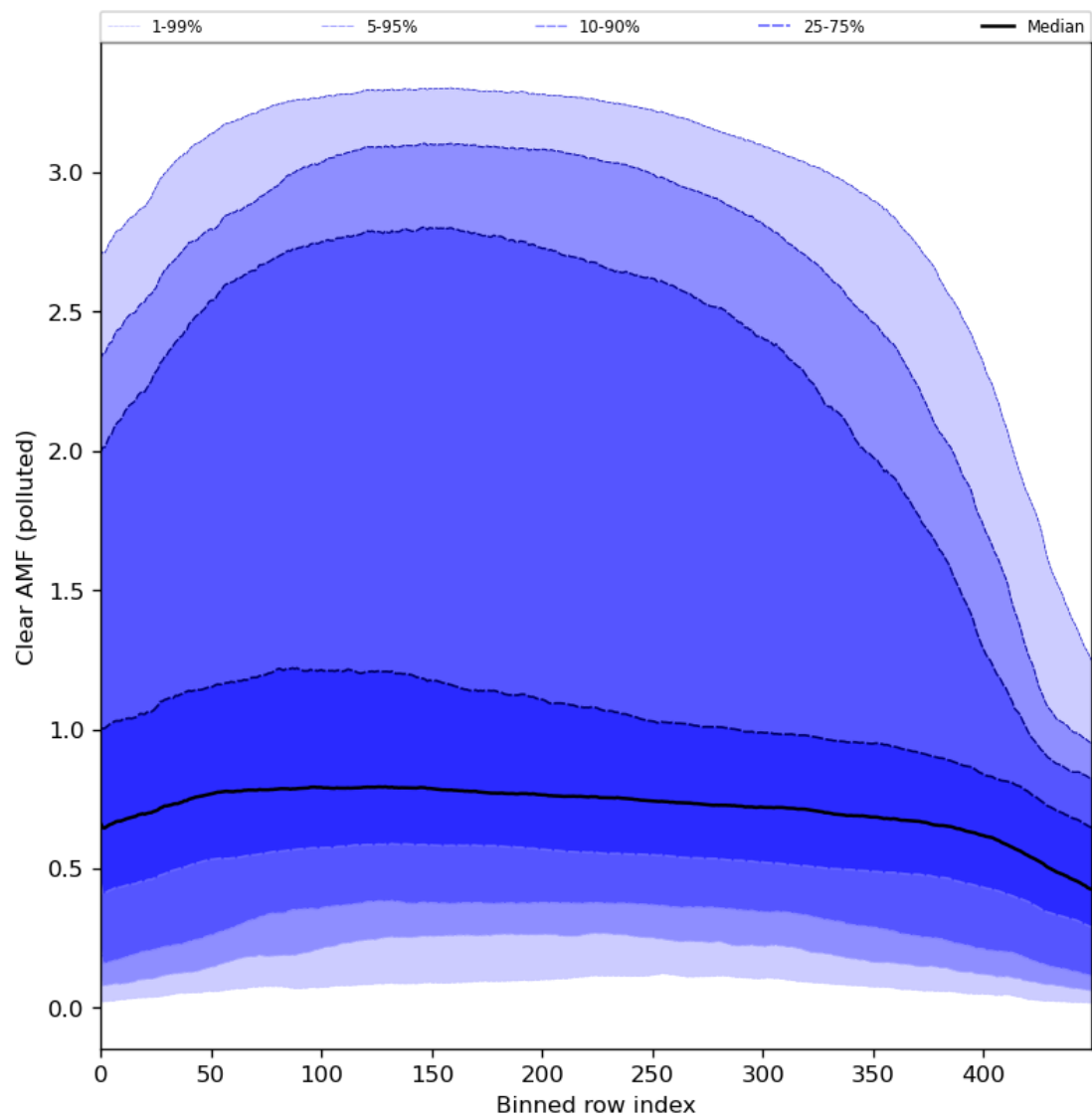
Figure 96: Along track statistics of “Clear AMF (polluted)” for 2024-01-19 to 2024-01-21
