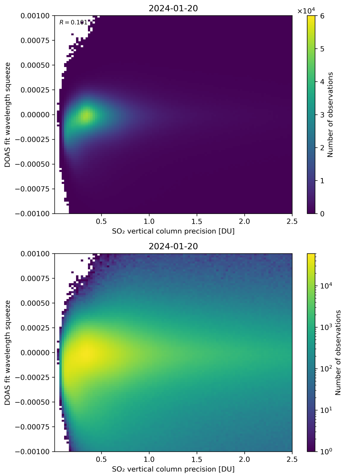
Figure 283: Scatter density plot of “SO 2 vertical column precision” against “DOAS fit wavelength squeeze” for 2024-01-19 to 2024-01-21.
