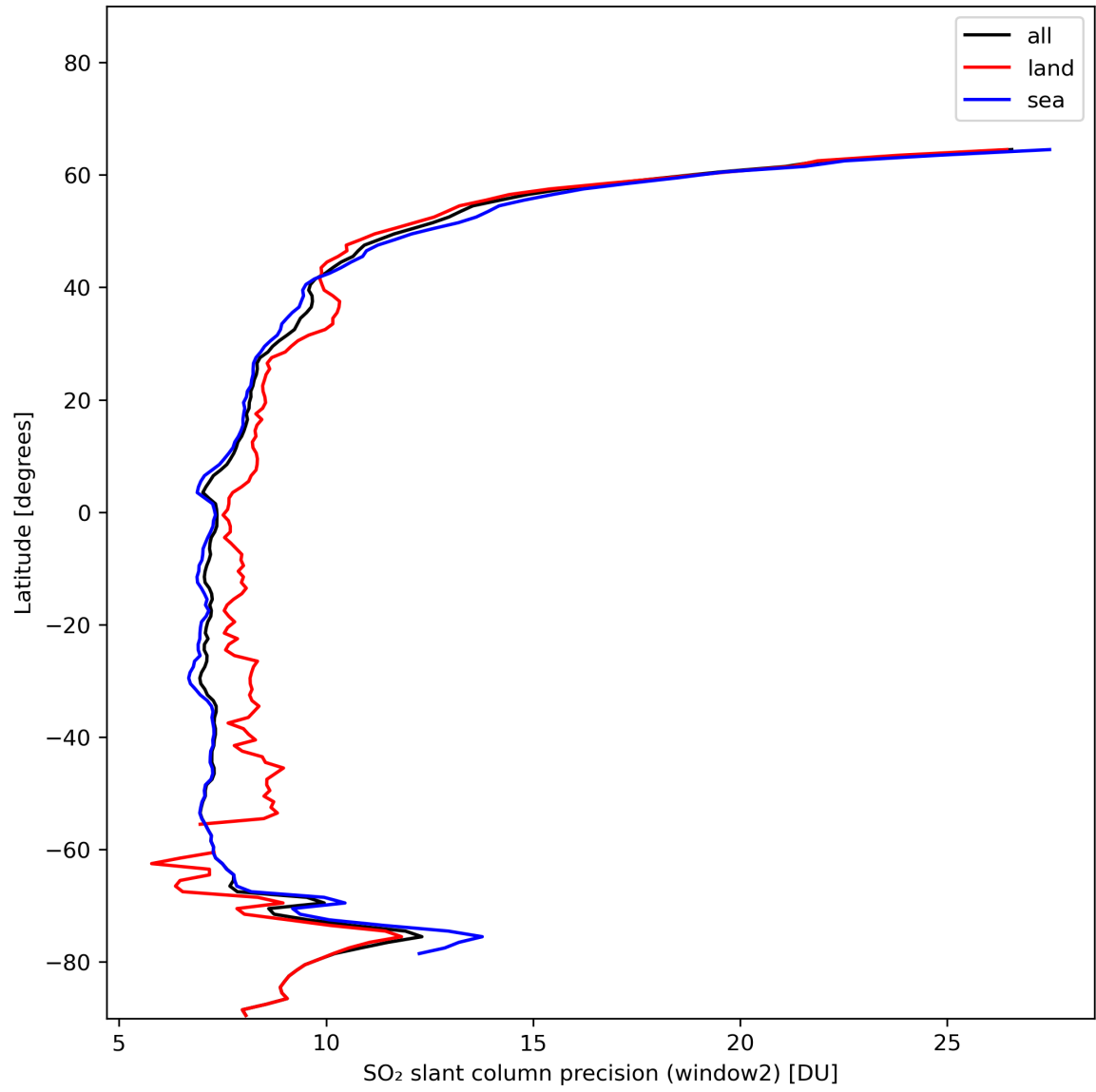
Figure 38: Zonal average of “SO 2 slant column precision (window2)” for 2024-01-19 to 2024-01-21.
