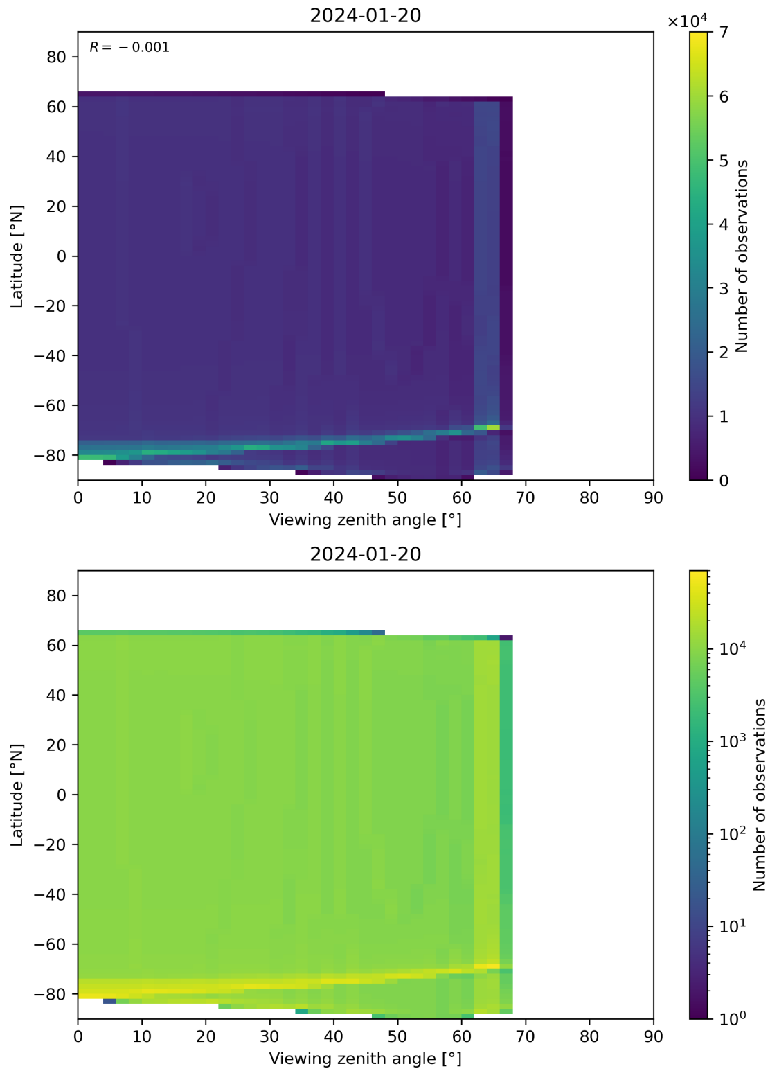
Figure 314: Scatter density plot of “Viewing zenith angle” against “Latitude” for 2024-01-19 to 2024-01-21.
