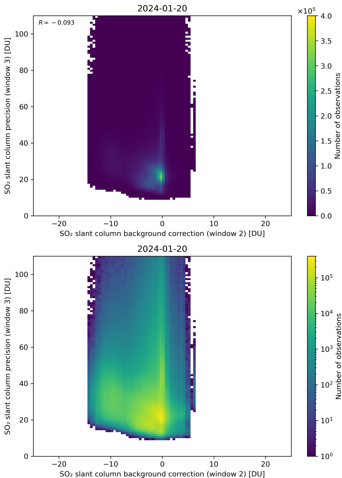
Figure 118: Scatter density plot of “SO 2 slant column background correction (window 2)” against “SO 2 slant column precision (window 3)” for 2024-01-19 to 2024-01-21.
