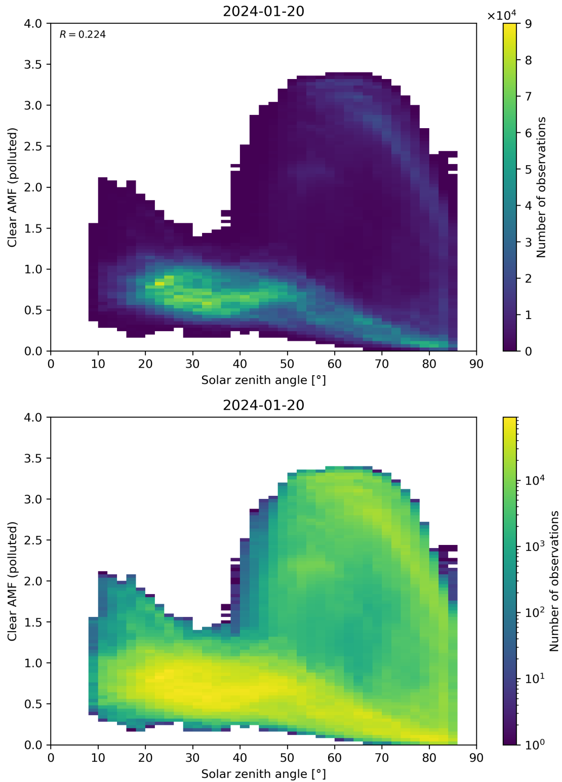
Figure 165: Scatter density plot of “Solar zenith angle” against “Clear AMF (polluted)” for 2024-01-19 to 2024-01-21.
