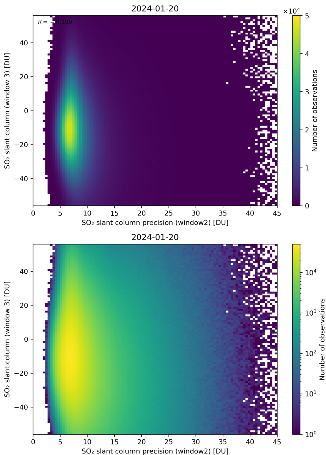
Figure 249: Scatter density plot of “SO 2 slant column precision (window2)” against “SO 2 slant column (window 3)” for 2024-01-19 to 2024-01-21.
