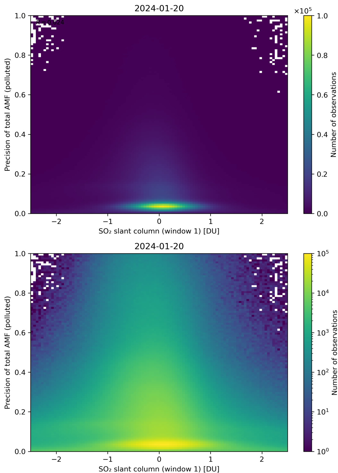
Figure 240: Scatter density plot of “SO 2 slant column (window 1)” against “Precision of total AMF (polluted)” for 2024-01-19 to 2024-01-21.
