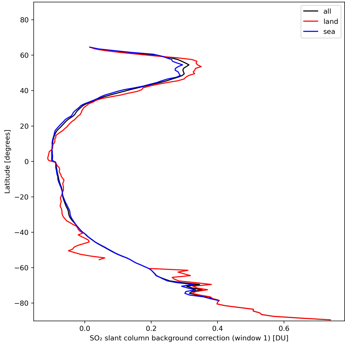
Figure 36: Zonal average of "SO 2 slant column background correction (window 1)" for 2024-01-19 to 2024-01-21.
