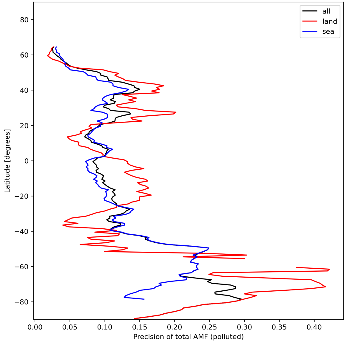
Figure 49: Zonal average of “Precision of total AMF (polluted)” for 2024-01-19 to 2024-01-21.
