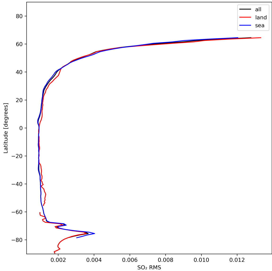
Figure 47: Zonal average of “SO 2 RMS” for 2024-01-19 to 2024-01-21.
