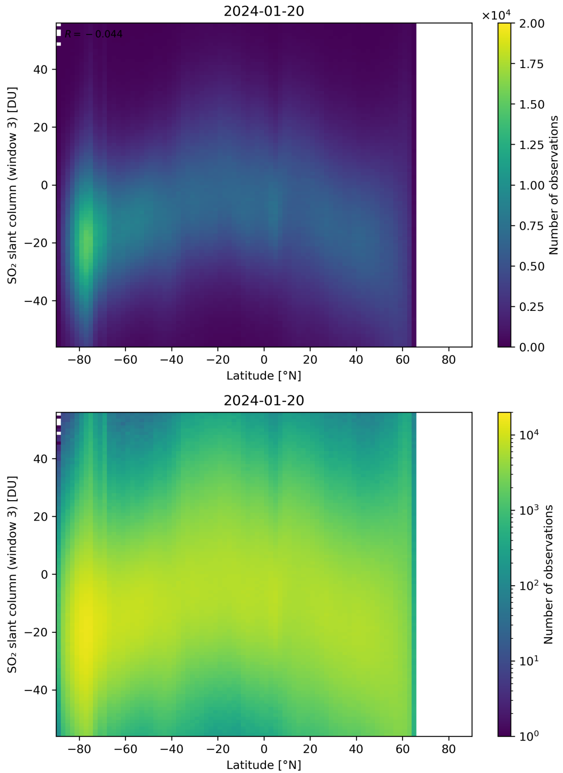
Figure 152: Scatter density plot of “Latitude” against “SO 2 slant column (window 3)” for 2024-01-19 to 2024-01-21.
