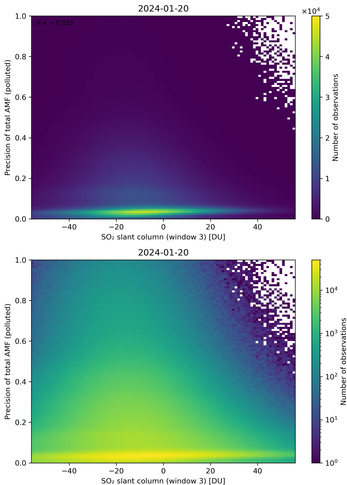
Figure 269: Scatter density plot of “SO 2 slant column (window 3)” against “Precision of total AMF (polluted)” for 2024-01-19 to 2024-01-21.
