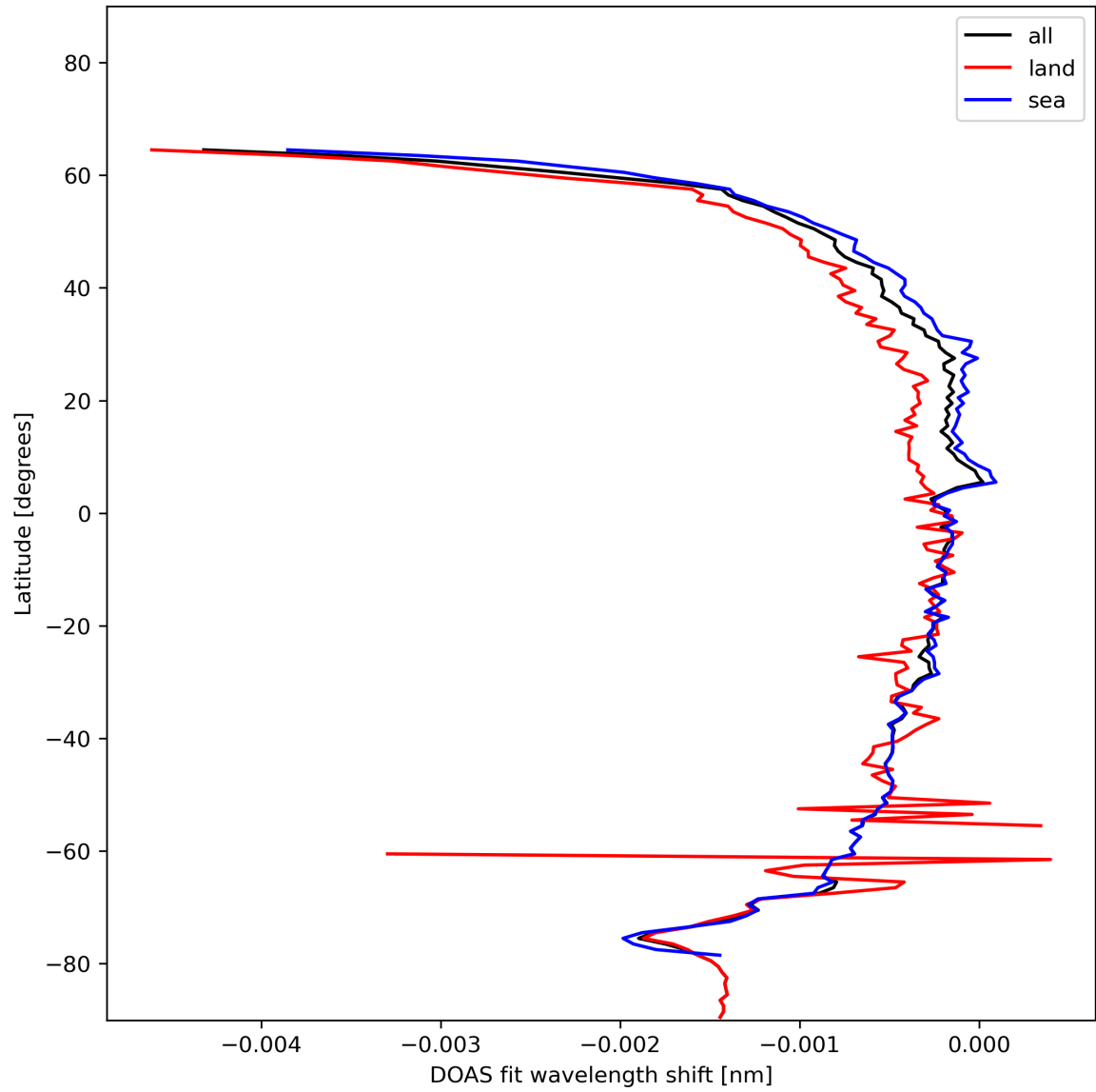
Figure 45: Zonal average of “DOAS fit wavelength shift” for 2024-01-19 to 2024-01-21.
