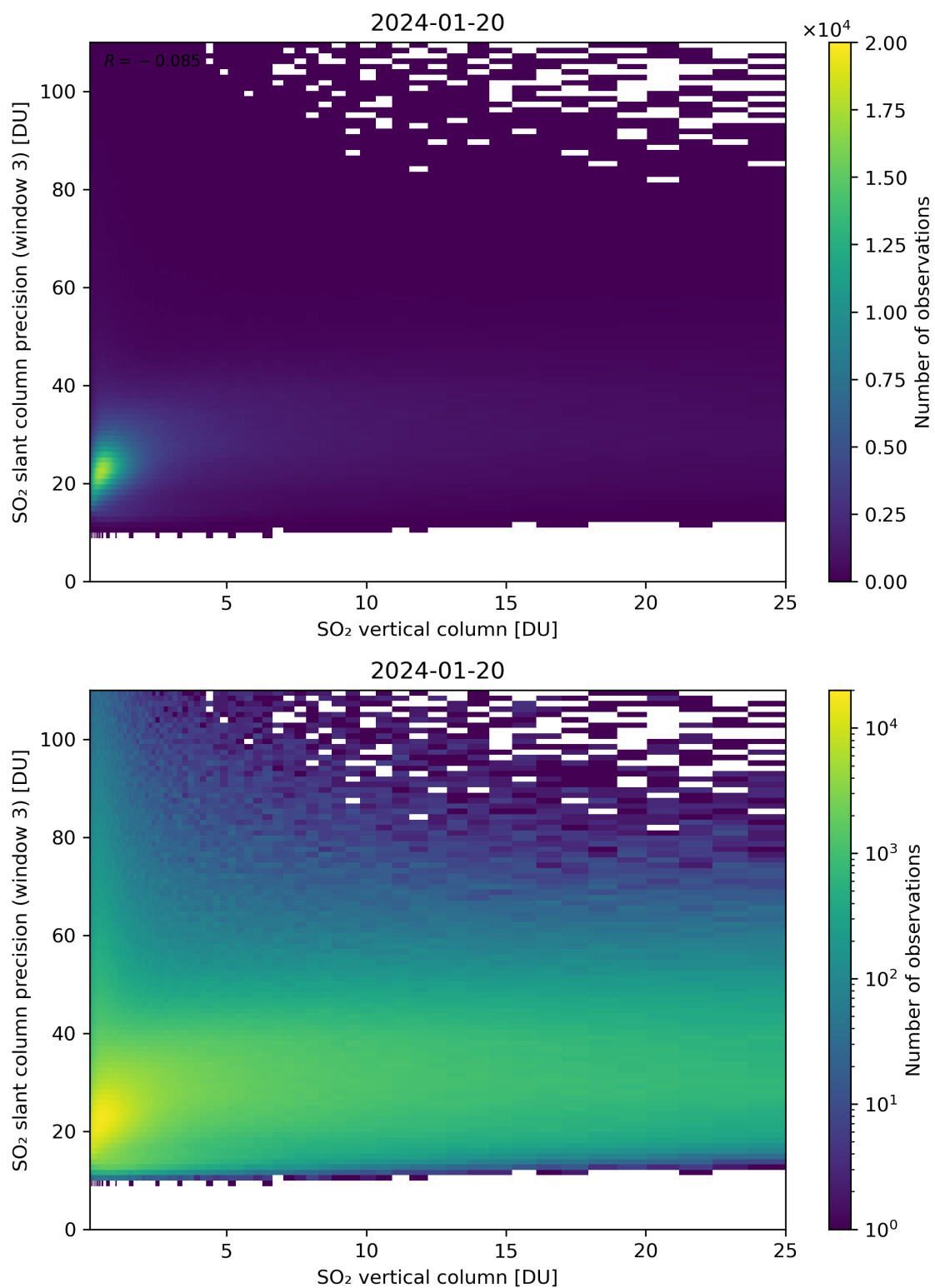
Figure 304: Scatter density plot of “SO 2 vertical column” against “SO 2 slant column precision (window 3)” for 2024-01-19 to 2024-01-21.
