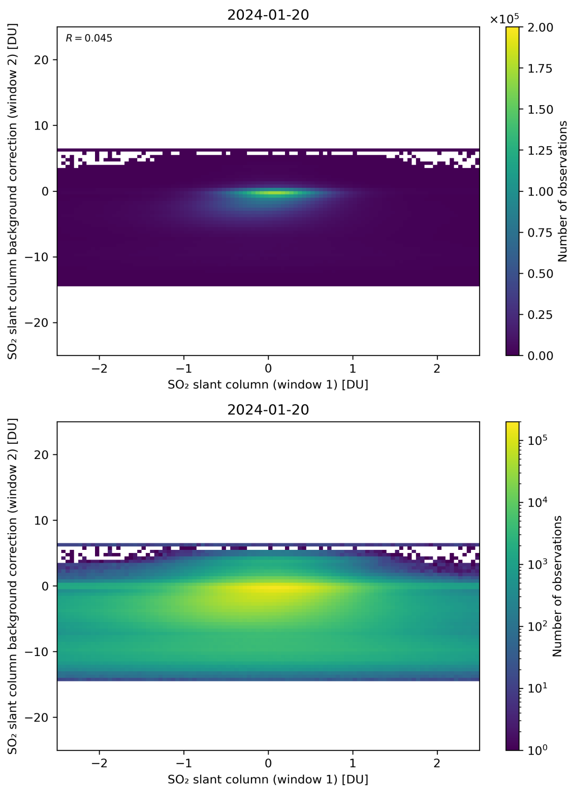
Figure 213: Scatter density plot of “SO 2 slant column (window 1)” against “SO 2 slant column background correction (window 2)” for 2024-01-19 to 2024-01-21.
