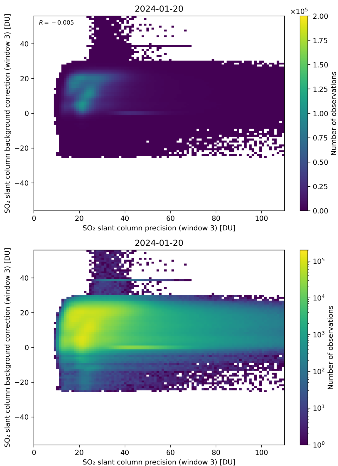
Figure 257: Scatter density plot of “SO 2 slant column precision (window 3)” against “SO 2 slant column background correction (window 3)” for 2024-01-19 to 2024-01-21.
