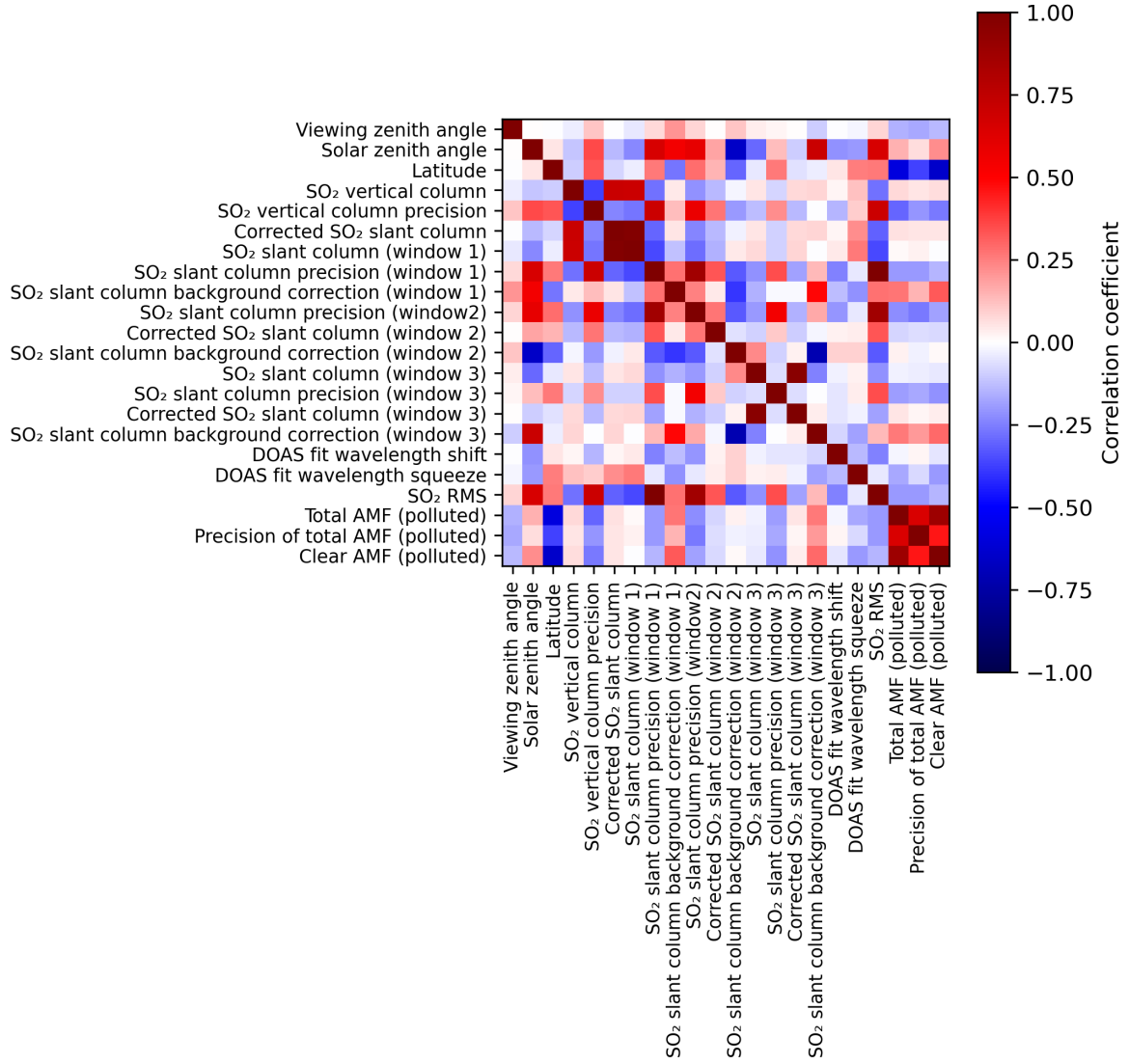
Figure 2: Map of correlation matrix for 2024-01-19 to 2024-01-21.
