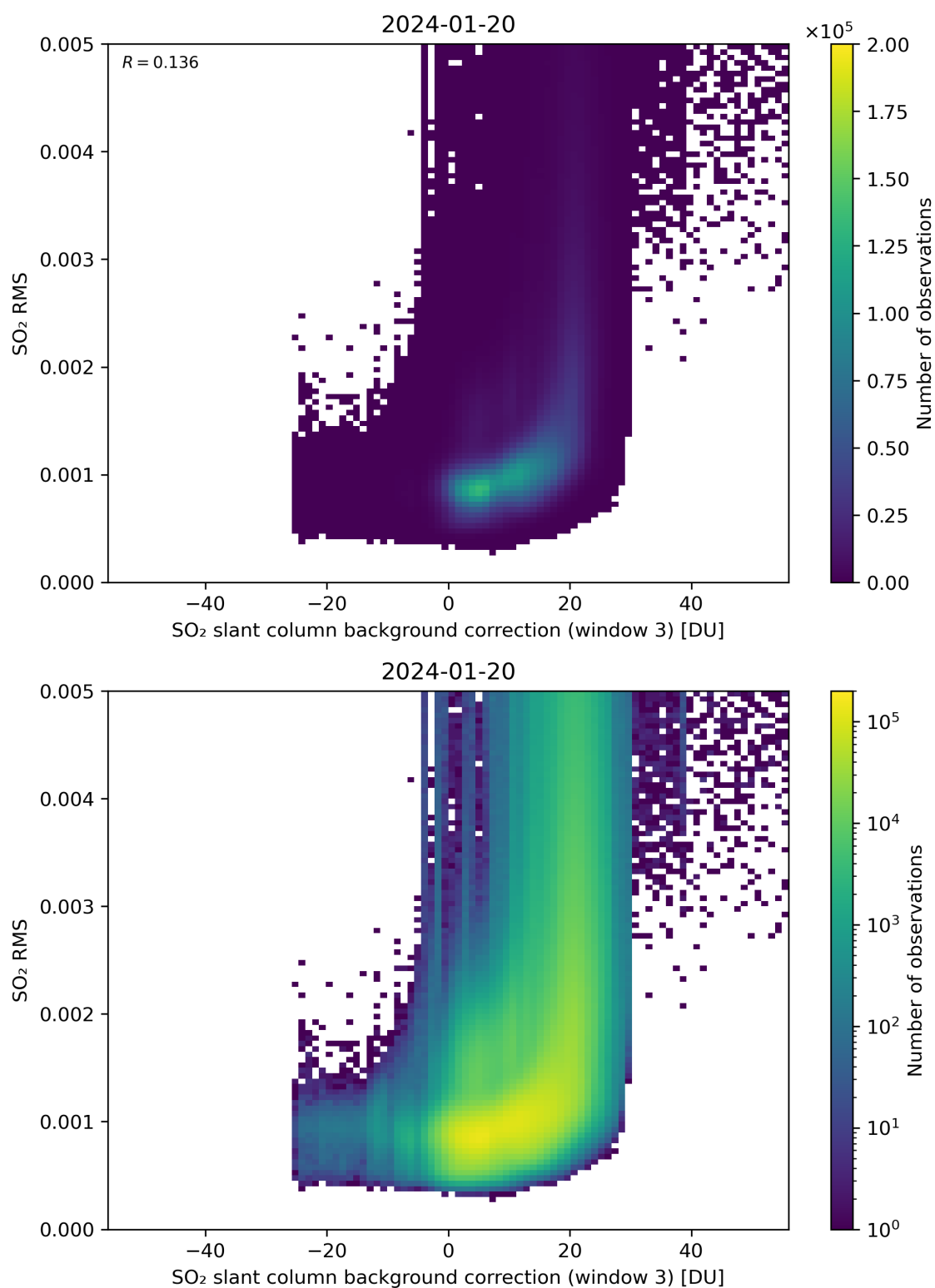
Figure 123: Scatter density plot of “SO 2 slant column background correction (window 3)” against “SO 2 RMS” for 2024-01-19 to 2024-01-21.
