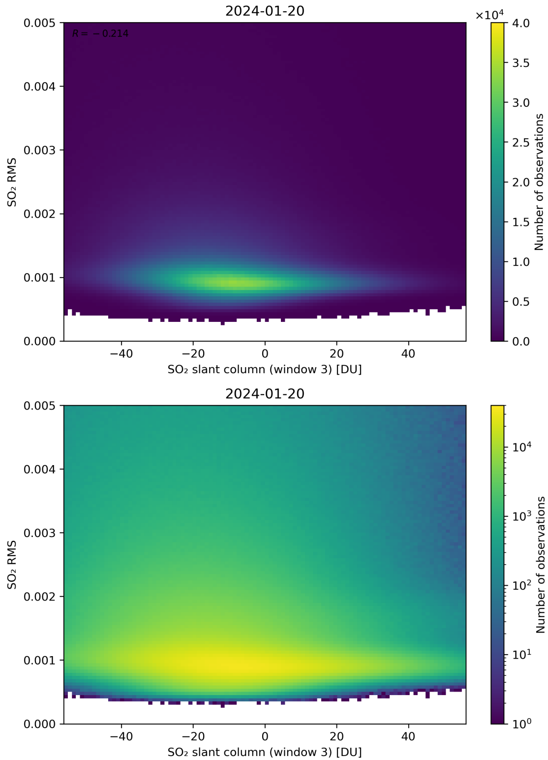
Figure 256: Scatter density plot of “SO 2 slant column (window 3)” against “SO 2 RMS” for 2024-01-19 to 2024-01-21.
