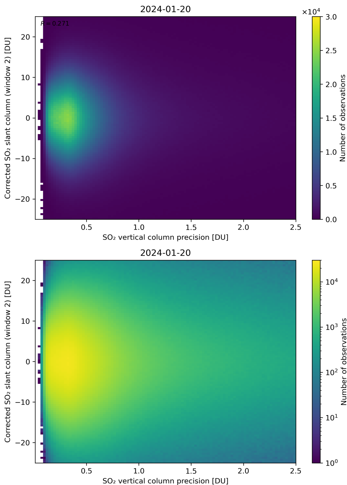
Figure 287: Scatter density plot of “SO 2 vertical column precision” against “Corrected SO 2 slant column (window 2)” for 2024-01-19 to 2024-01-21.
