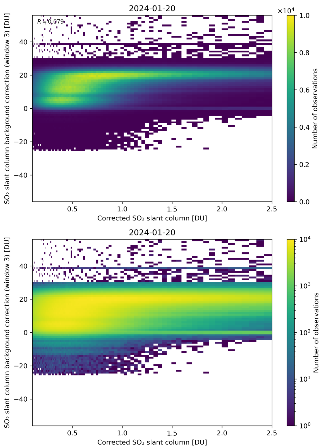
Figure 180: Scatter density plot of “Corrected SO 2 slant column” against “SO 2 slant column background correction (window 3)” for 2024-01-19 to 2024-01-21.
