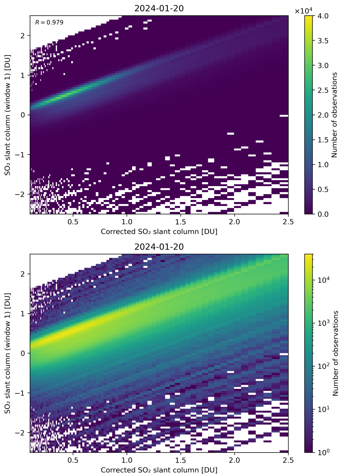
Figure 187: Scatter density plot of “Corrected SO 2 slant column” against “SO 2 slant column (window 1)” for 2024-01-19 to 2024-01-21.
