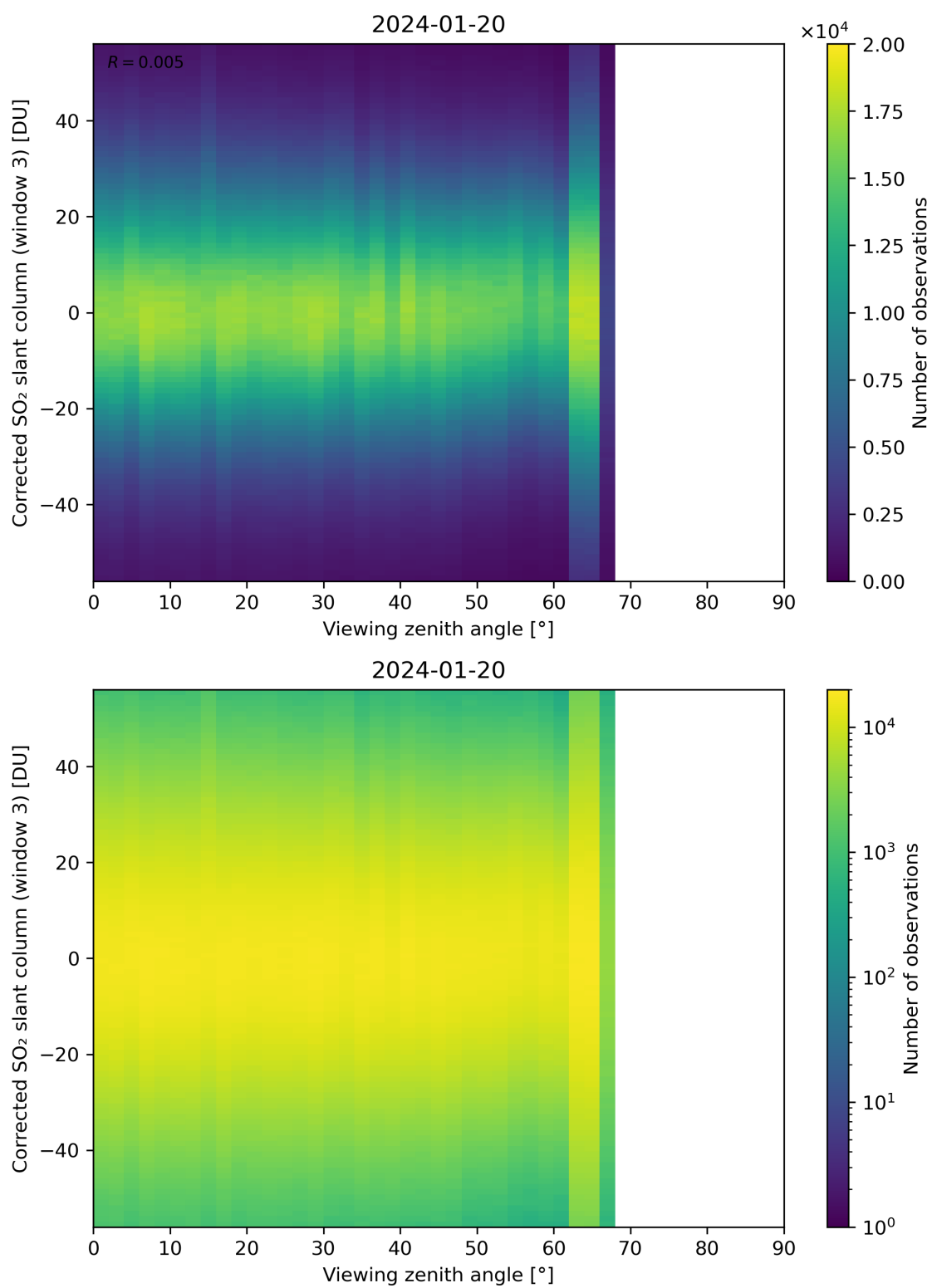
Figure 319: Scatter density plot of “Viewing zenith angle” against “Corrected SO 2 slant column (window 3)” for 2024-01-19 to 2024-01-21.
