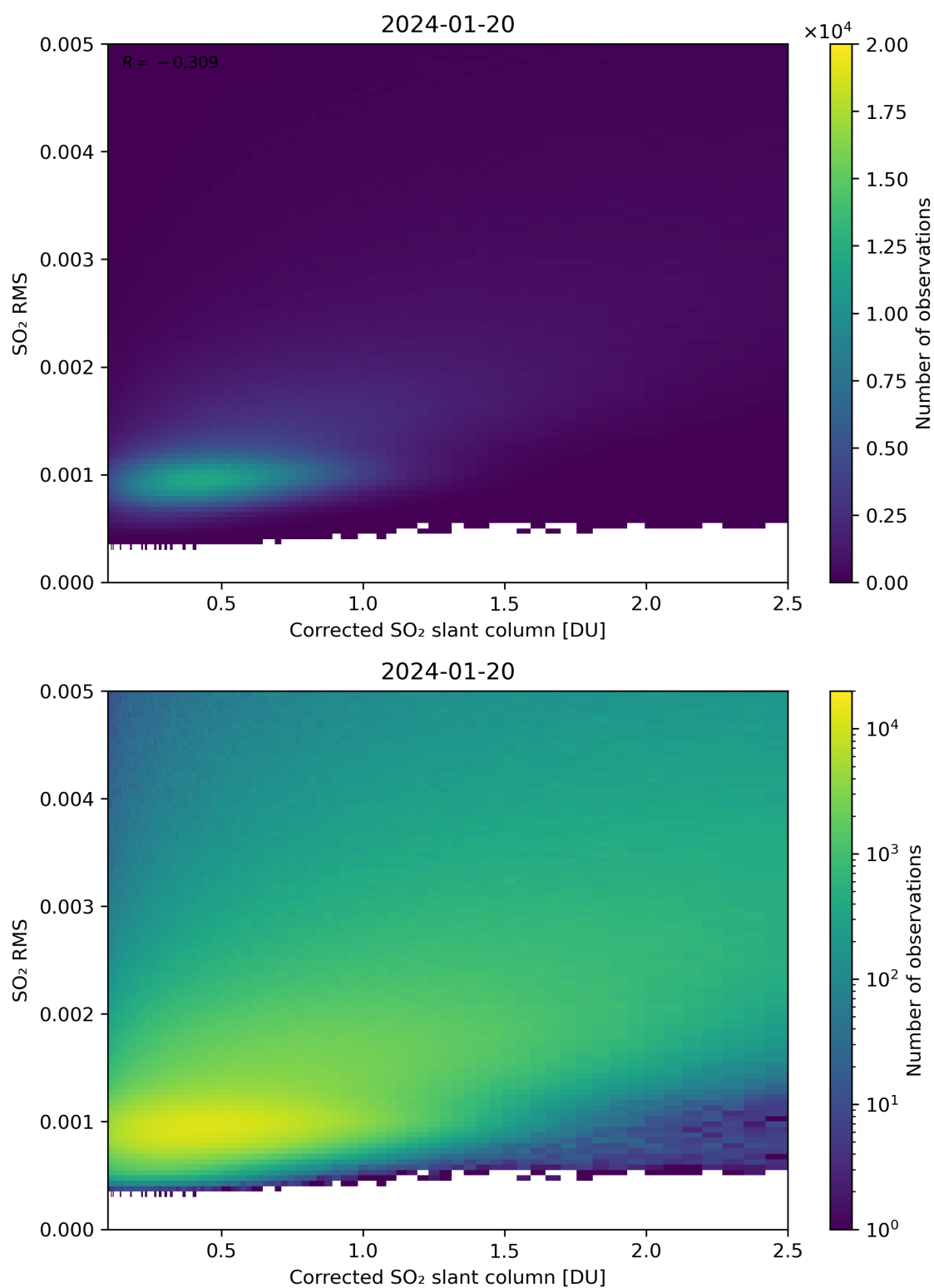
Figure 183: Scatter density plot of “Corrected SO 2 slant column” against “SO 2 RMS” for 2024-01-19 to 2024-01-21.
