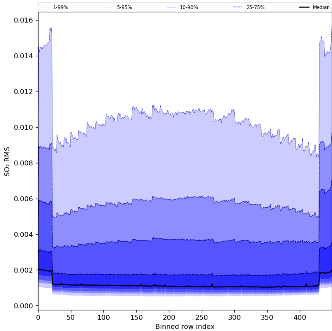
Figure 93: Along track statistics of “SO 2 RMS” for 2024-01-19 to 2024-01-21
