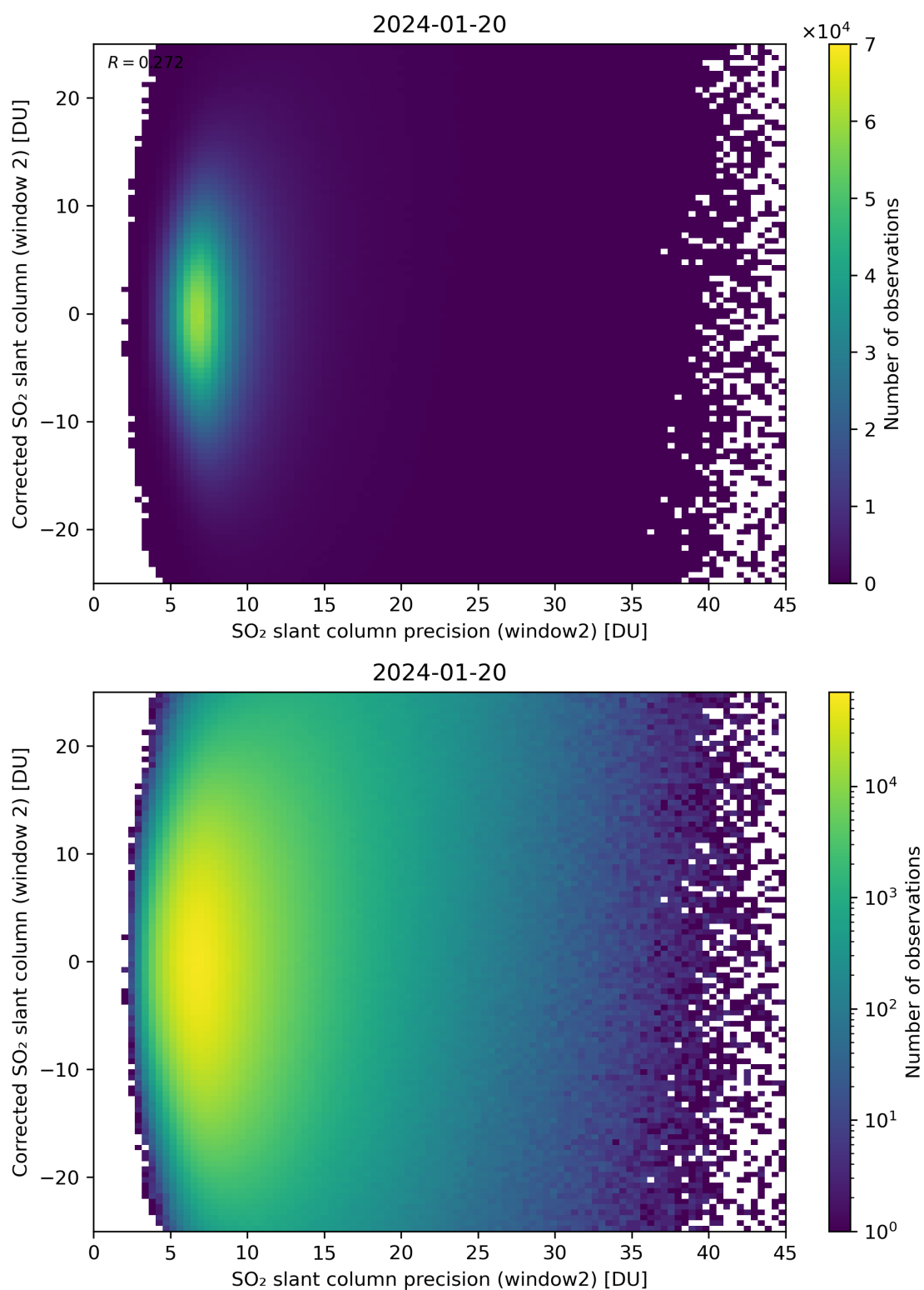
Figure 247: Scatter density plot of “SO 2 slant column precision (window2)” against “Corrected SO 2 slant column (window 2)” for 2024-01-19 to 2024-01-21.
