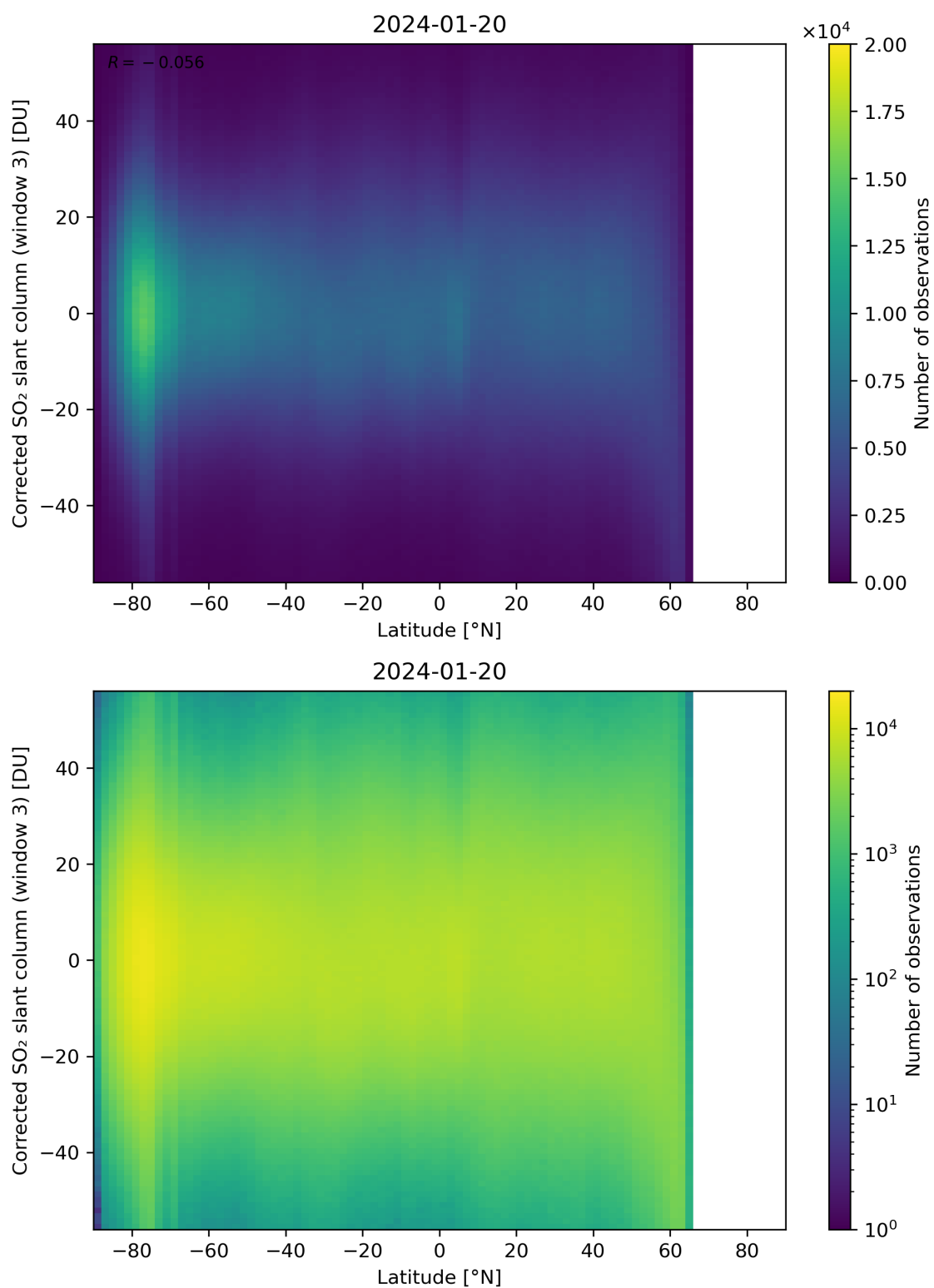
Figure 148: Scatter density plot of “Latitude” against “Corrected SO 2 slant column (window 3)” for 2024-01-19 to 2024-01-21.
