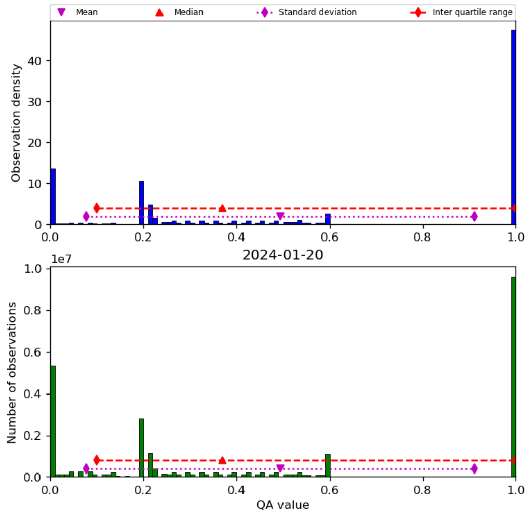
Figure 52: Histogram of “QA value” for 2024-01-19 to 2024-01-21
