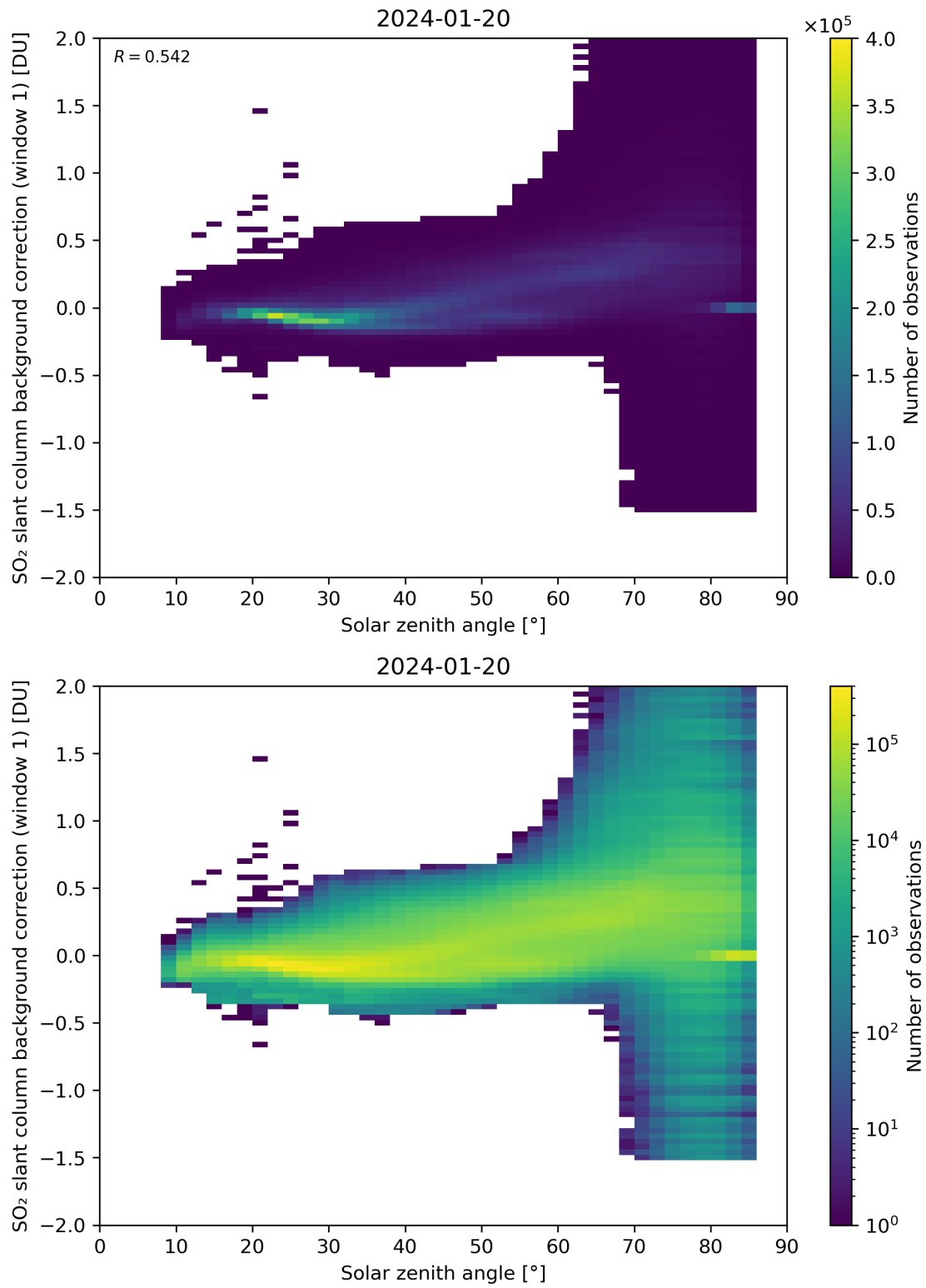
Figure 158: Scatter density plot of “Solar zenith angle” against “SO 2 slant column background correction (window 1)” for 2024-01-19 to 2024-01-21.
