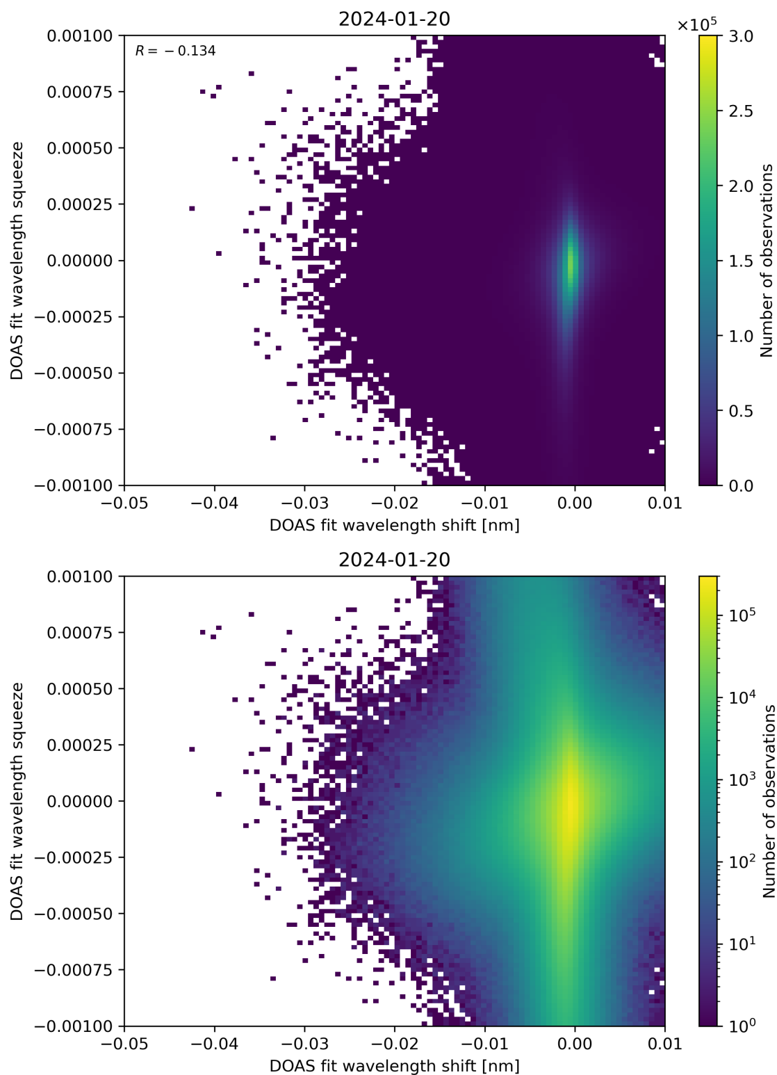
Figure 127: Scatter density plot of “DOAS fit wavelength shift” against “DOAS fit wavelength squeeze” for 2024-01-19 to 2024-01-21.
