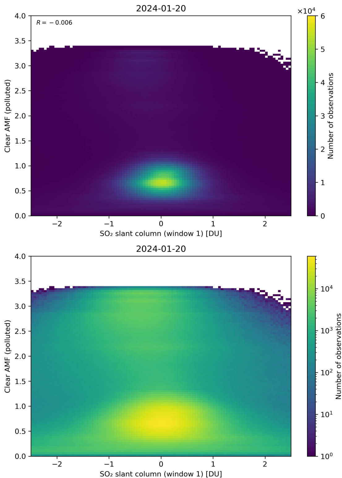
Figure 232: Scatter density plot of “SO 2 slant column (window 1)” against “Clear AMF (polluted)” for 2024-01-19 to 2024-01-21.
