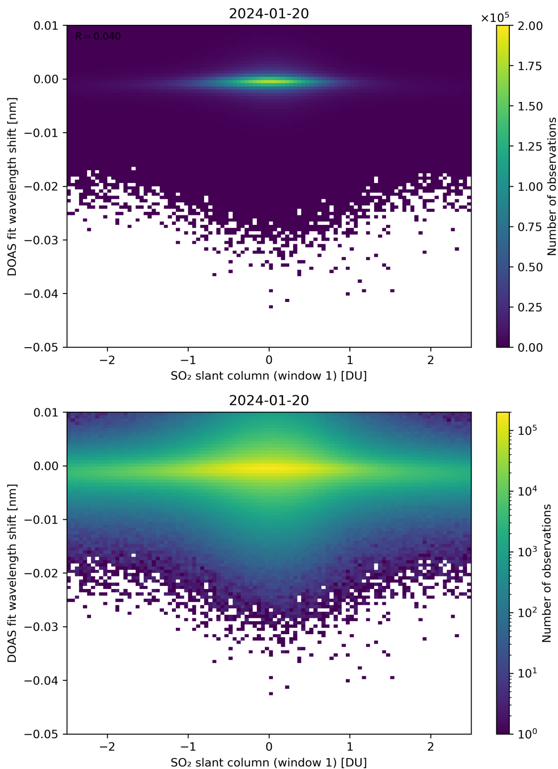
Figure 215: Scatter density plot of “SO 2 slant column (window 1)” against “DOAS fit wavelength shift” for 2024-01-19 to 2024-01-21.
