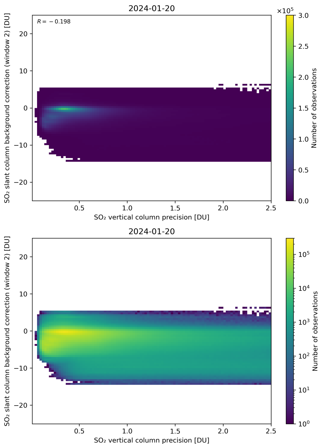
Figure 280: Scatter density plot of “SO 2 vertical column precision” against “SO 2 slant column background correction (window 2)” for 2024-01-19 to 2024-01-21.
