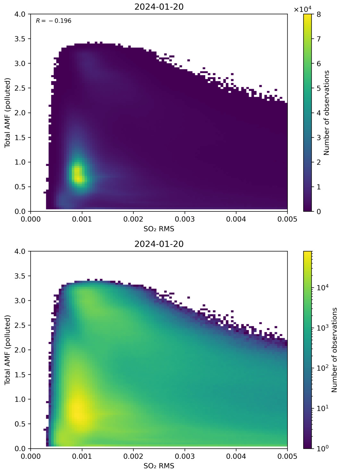
Figure 137: Scatter density plot of “SO 2 RMS” against “Total AMF (polluted)” for 2024-01-19 to 2024-01-21.
