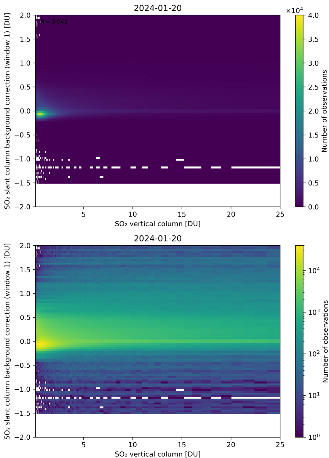
Figure 273: Scatter density plot of “SO 2 vertical column” against “SO 2 slant column background correction (window 1)” for 2024-01-19 to 2024-01-21.
