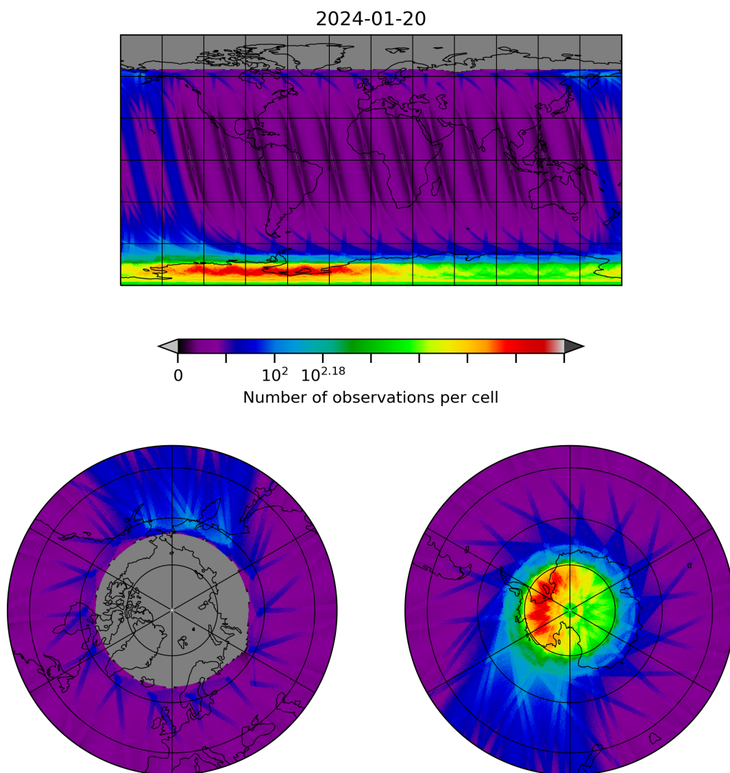
Figure 28: Map of the number of observations for 2024-01-19 to 2024-01-21
