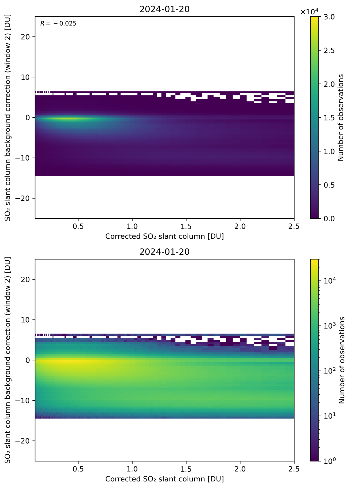
Figure 179: Scatter density plot of “Corrected SO 2 slant column” against “SO 2 slant column background correction (window 2)” for 2024-01-19 to 2024-01-21.
