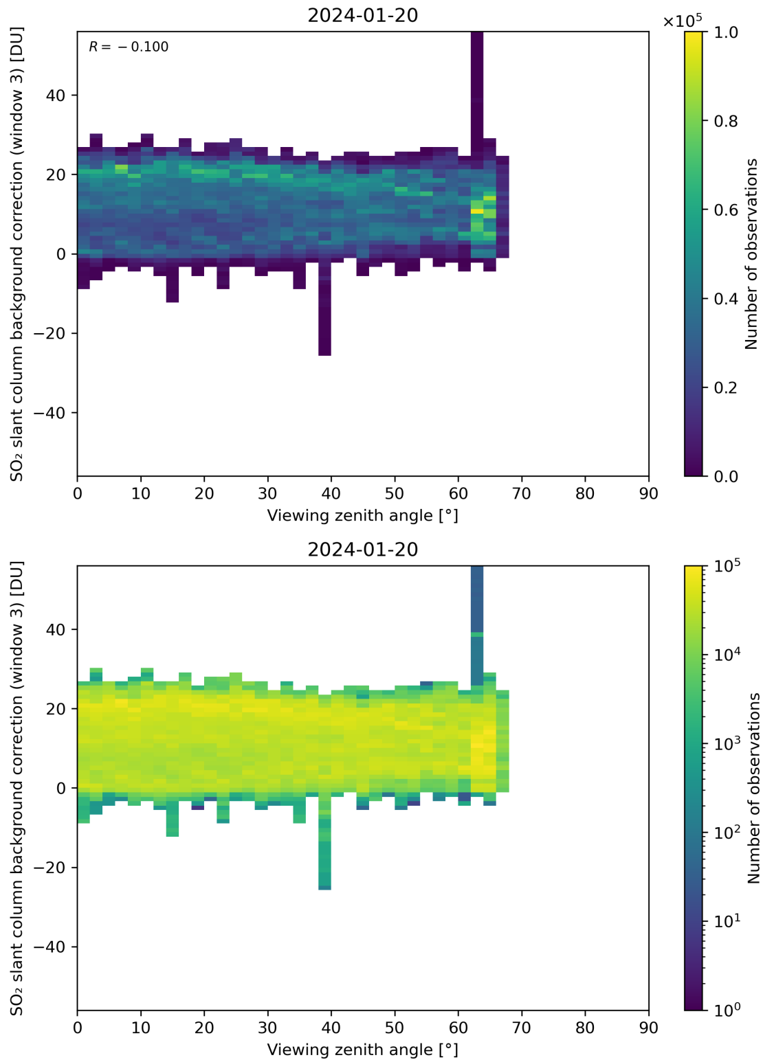
Figure 310: Scatter density plot of “Viewing zenith angle” against “SO 2 slant column background correction (window 3)” for 2024-01-19 to 2024-01-21.
