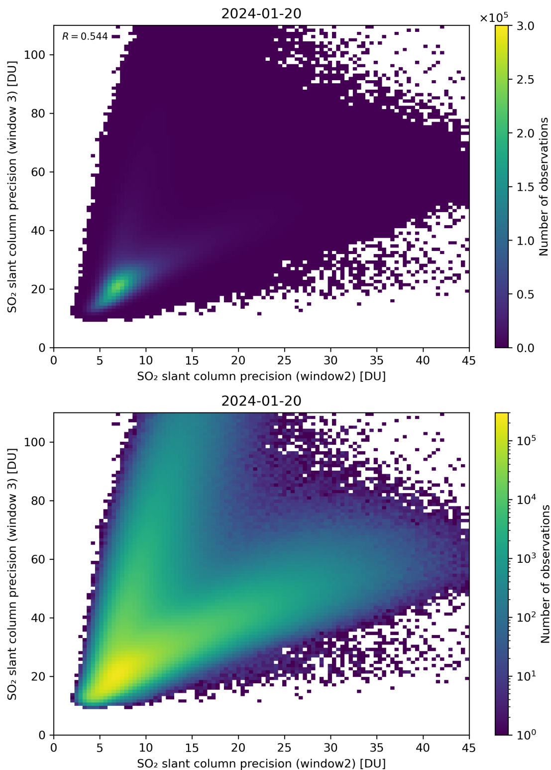
Figure 250: Scatter density plot of “SO 2 slant column precision (window2)” against “SO 2 slant column precision (window 3)” for 2024-01-19 to 2024-01-21.
