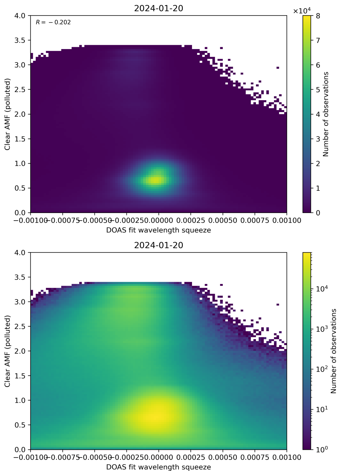
Figure 133: Scatter density plot of “DOAS fit wavelength squeeze” against “Clear AMF (polluted)” for 2024-01-19 to 2024-01-21.
