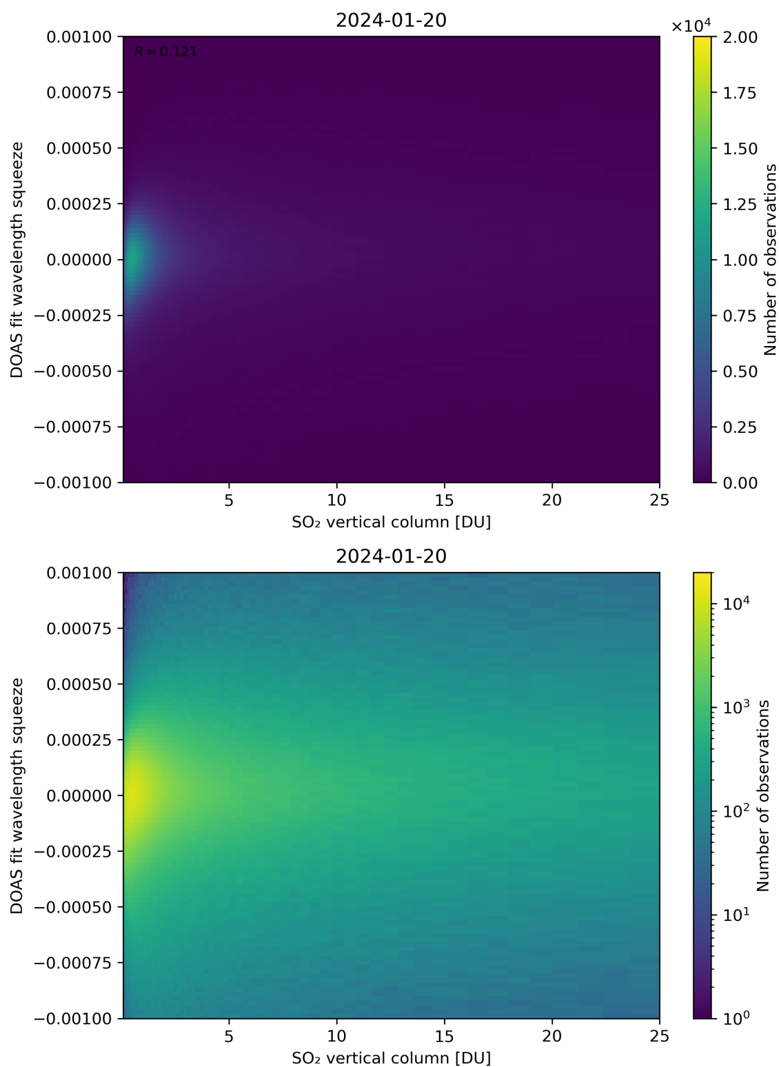
Figure 277: Scatter density plot of “SO 2 vertical column” against “DOAS fit wavelength squeeze” for 2024-01-19 to 2024-01-21.
