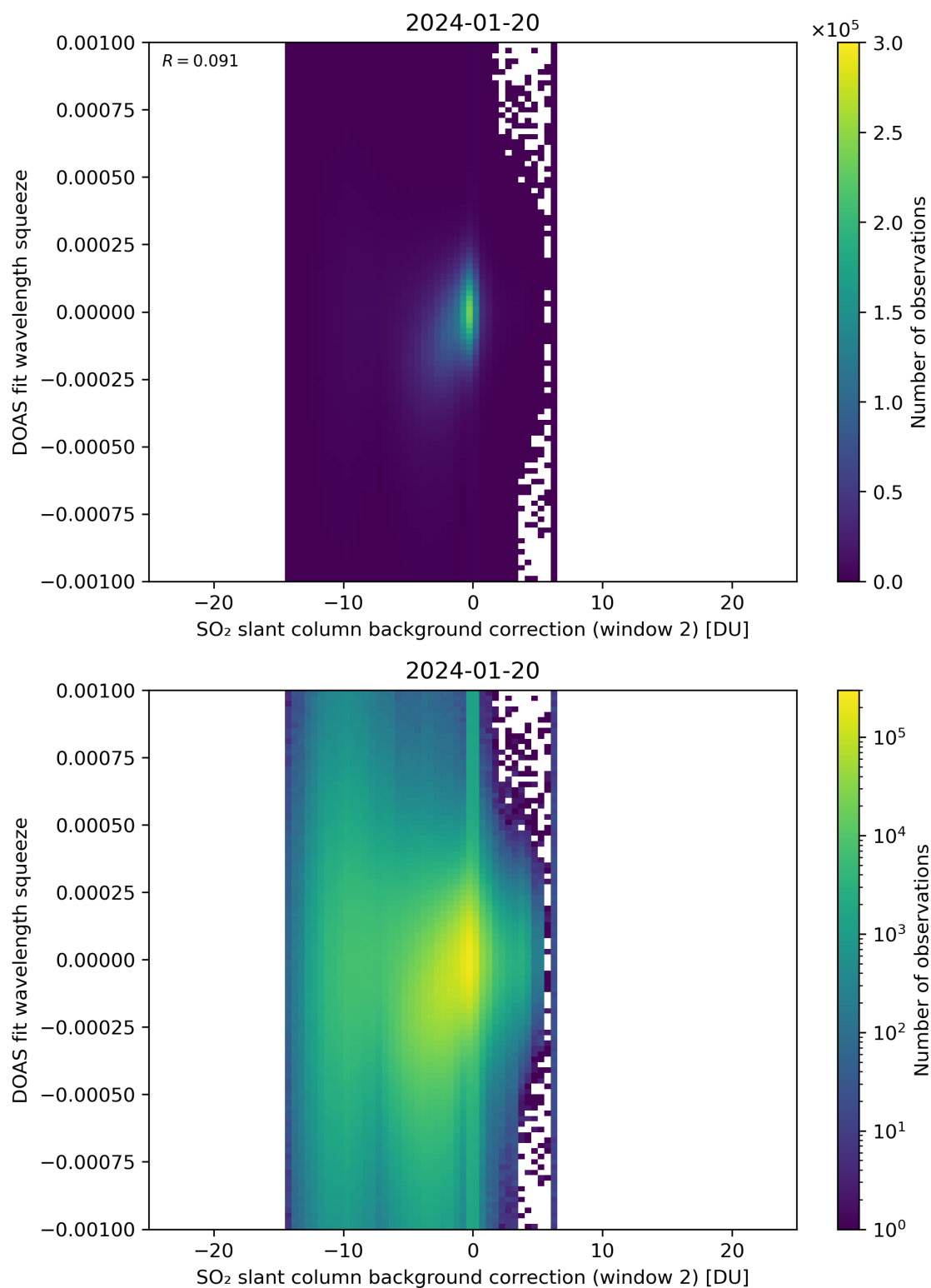
Figure 113: Scatter density plot of “SO 2 slant column background correction (window 2)” against “DOAS fit wavelength squeeze” for 2024-01-19 to 2024-01-21.
