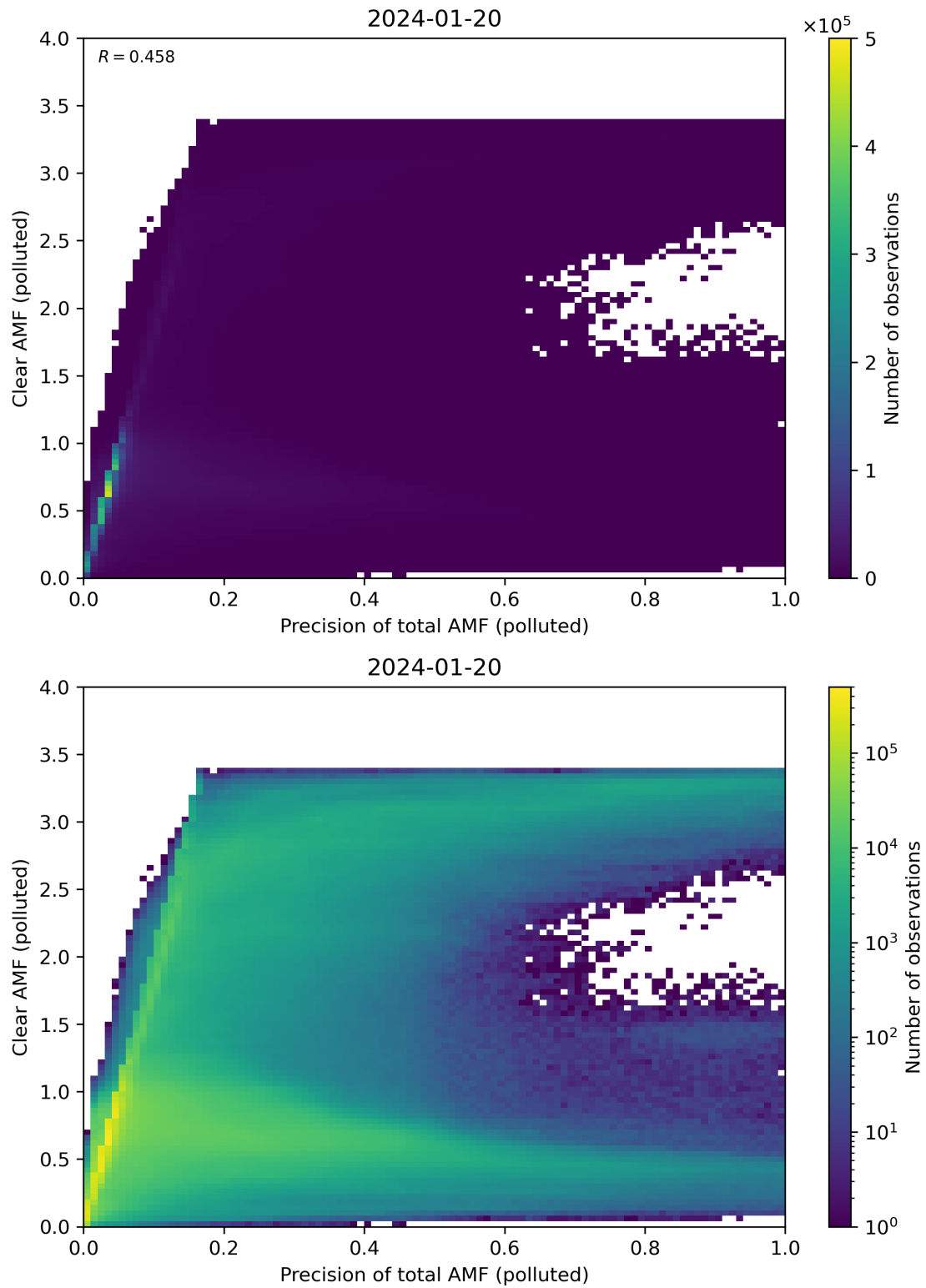
Figure 270: Scatter density plot of “Precision of total AMF (polluted)” against “Clear AMF (polluted)” for 2024-01-19 to 2024-01-21.
