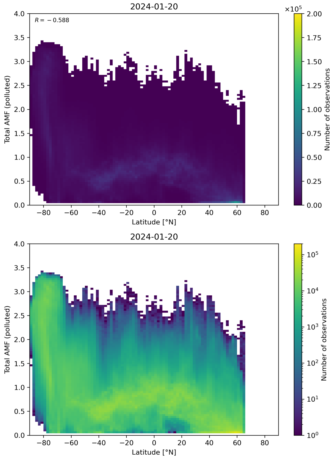
Figure 154: Scatter density plot of “Latitude” against “Total AMF (polluted)” for 2024-01-19 to 2024-01-21.
