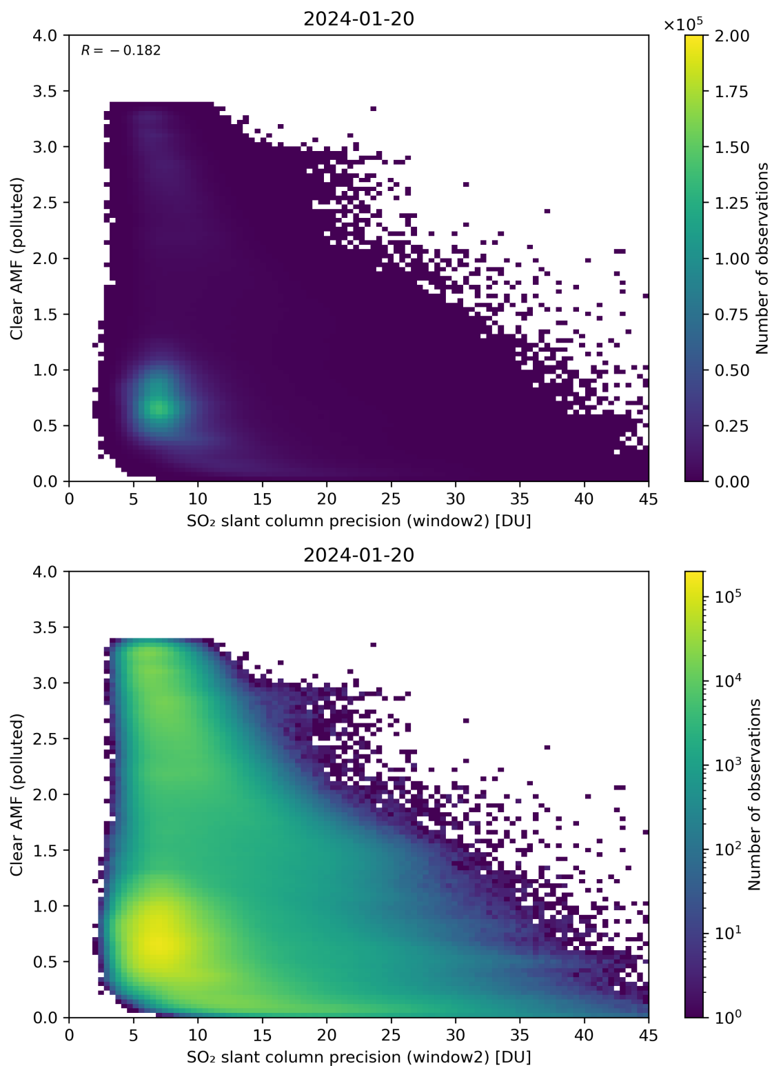
Figure 246: Scatter density plot of “SO 2 slant column precision (window2)” against “Clear AMF (polluted)” for 2024-01-19 to 2024-01-21.
