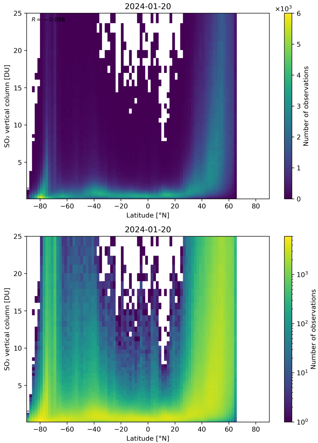
Figure 156: Scatter density plot of “Latitude” against “SO 2 vertical column” for 2024-01-19 to 2024-01-21.
