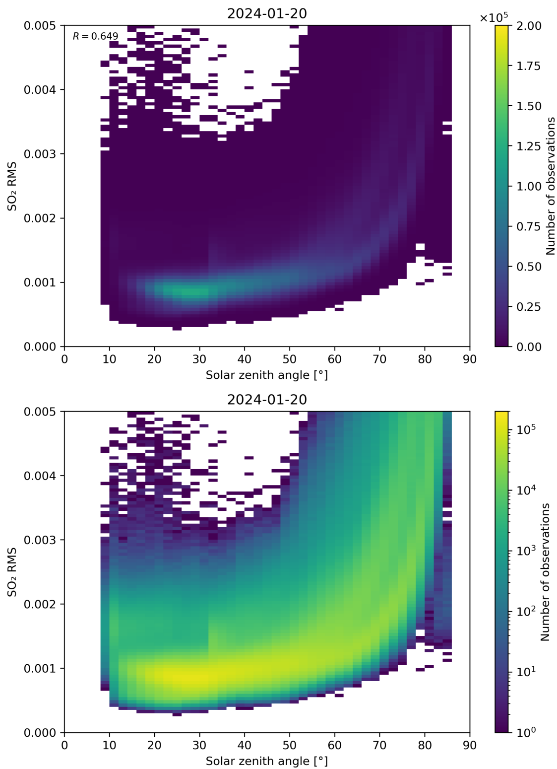
Figure 163: Scatter density plot of “Solar zenith angle” against “SO 2 RMS” for 2024-01-19 to 2024-01-21.
