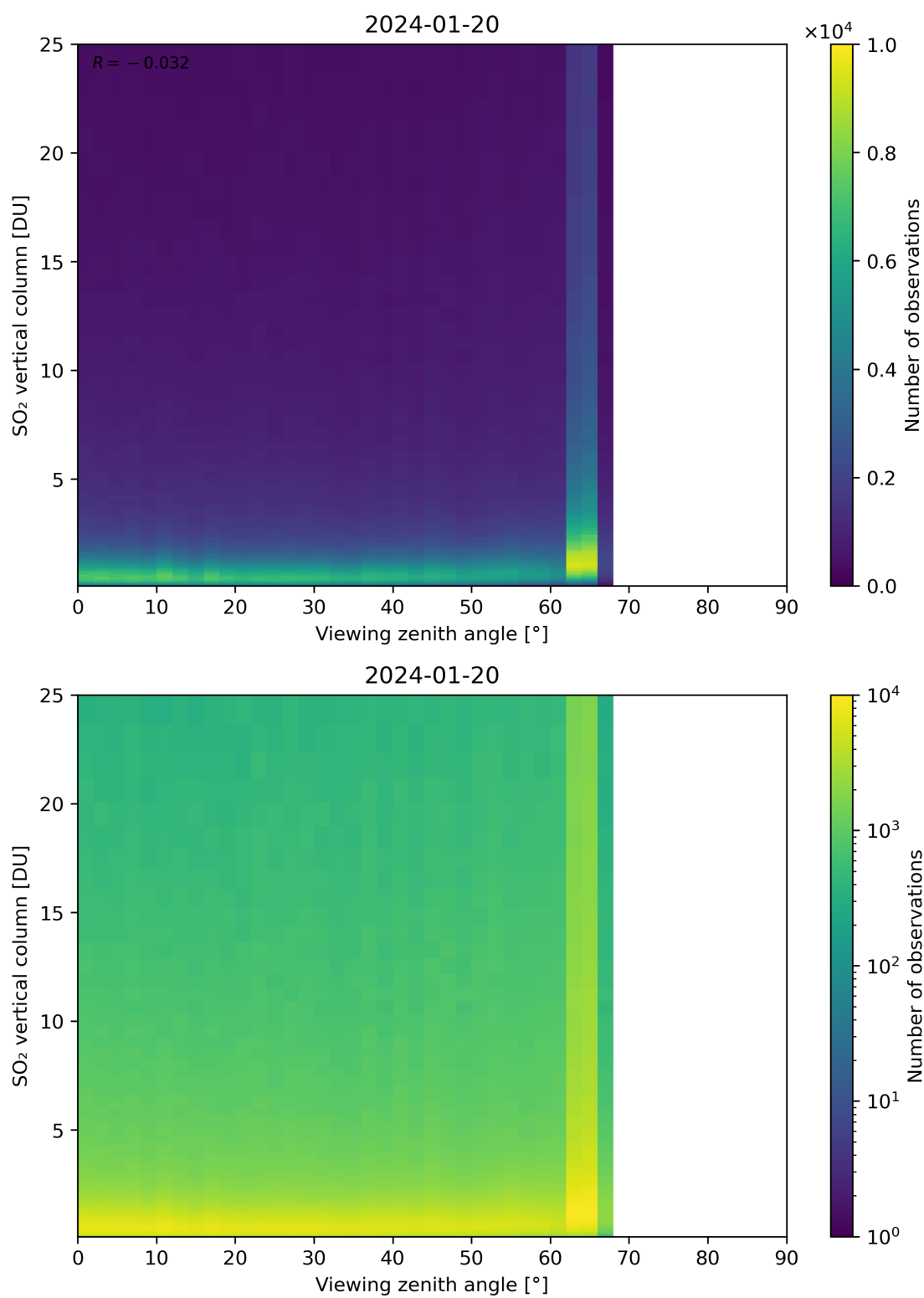
Figure 327: Scatter density plot of “Viewing zenith angle” against “SO 2 vertical column” for 2024-01-19 to 2024-01-21.
