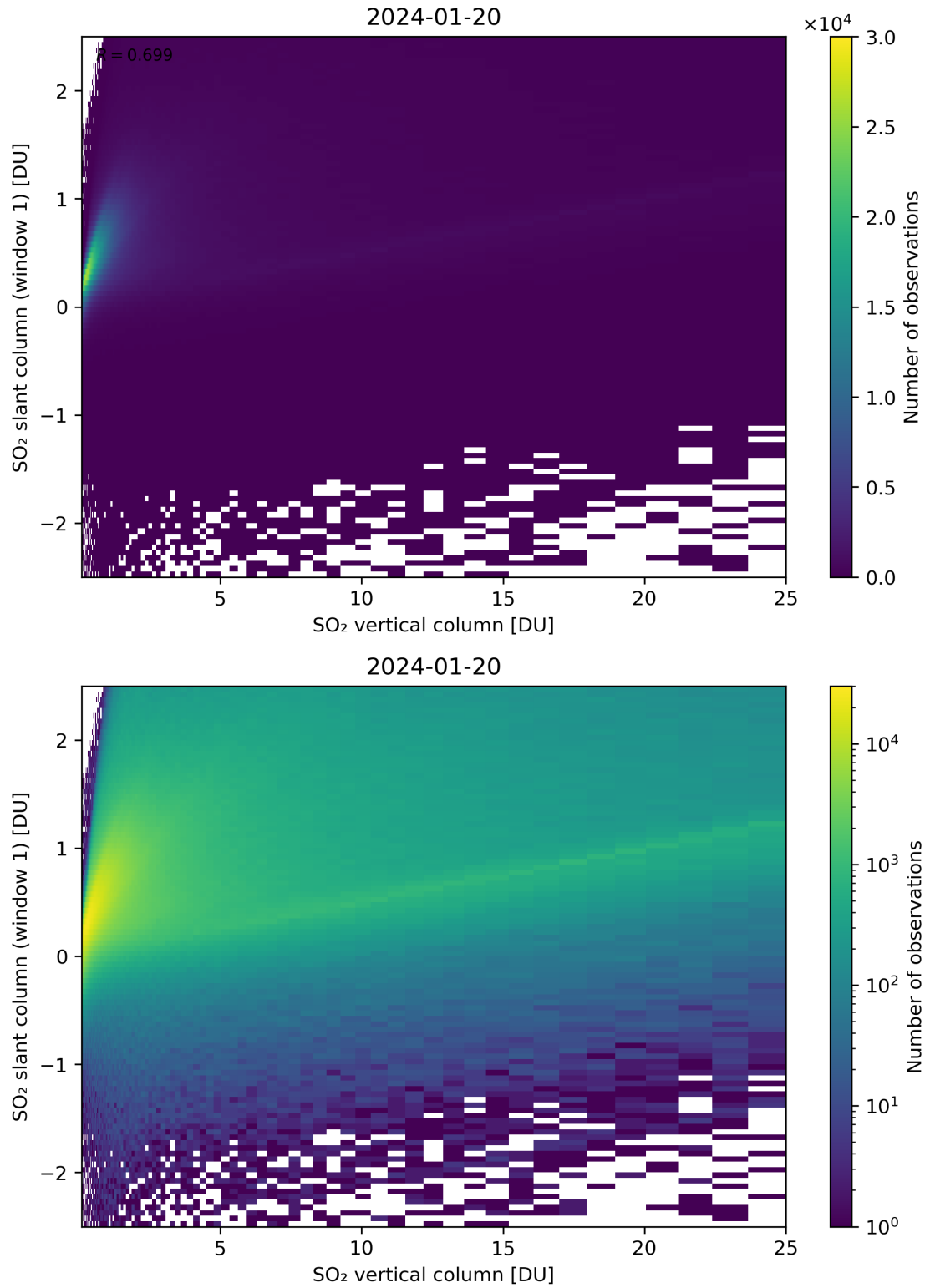
Figure 300: Scatter density plot of “SO 2 vertical column” against “SO 2 slant column (window 1)” for 2024-01-19 to 2024-01-21.
