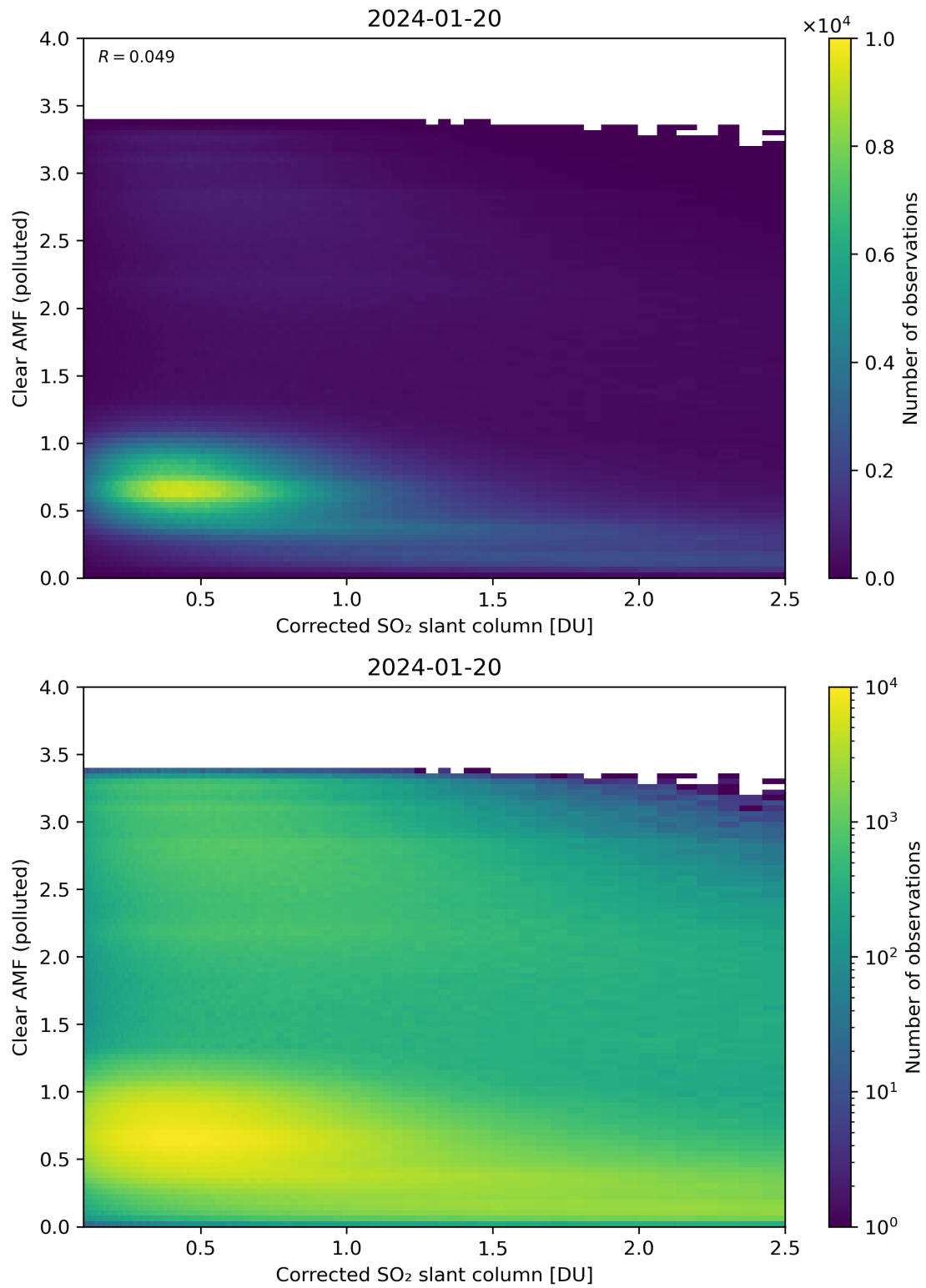
Figure 184: Scatter density plot of “Corrected SO 2 slant column” against “Clear AMF (polluted)” for 2024-01-19 to 2024-01-21.
