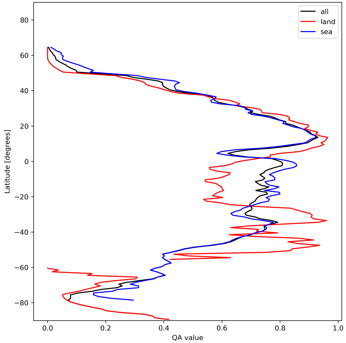
Figure 29: Zonal average of “QA value” for 2024-01-19 to 2024-01-21.
