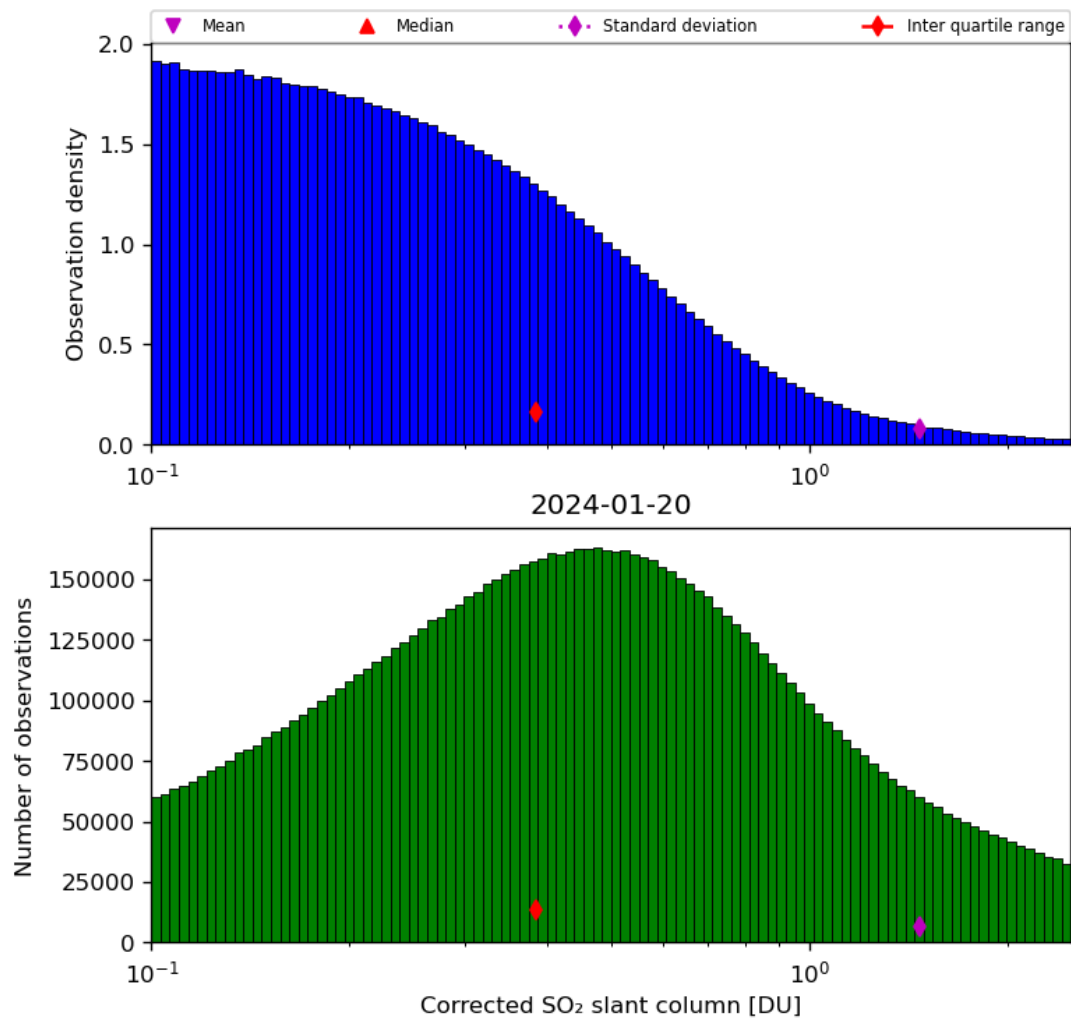
Figure 55: Histogram of “Corrected SO 2 slant column” for 2024-01-19 to 2024-01-21
