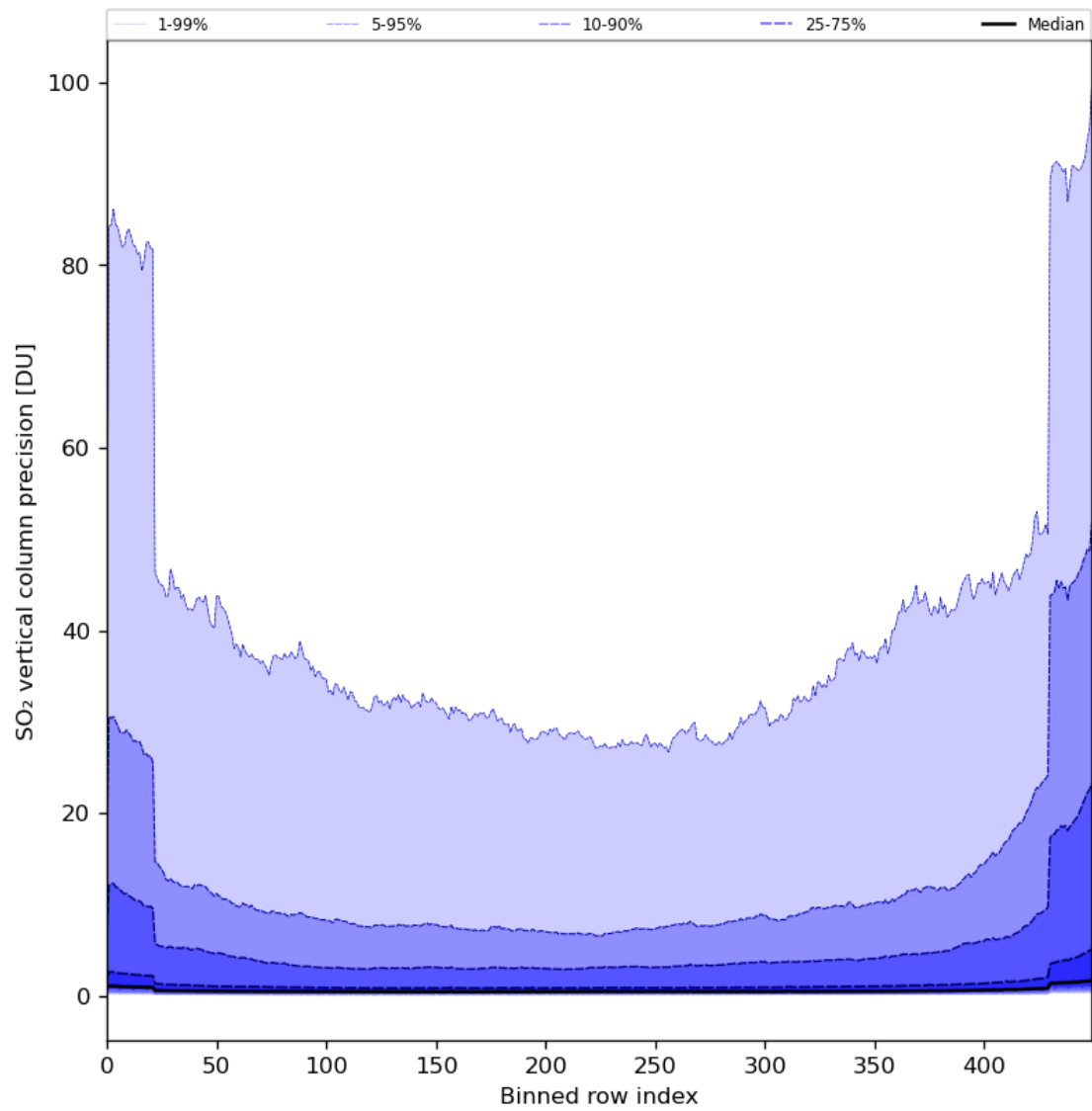
Figure 77: Along track statistics of “SO 2 vertical column precision” for 2024-01-19 to 2024-01-21
