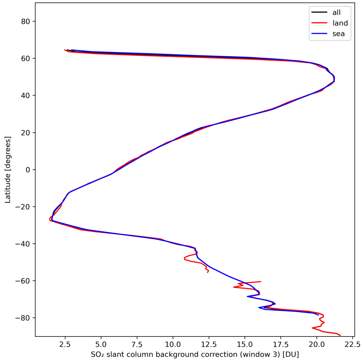
Figure 44: Zonal average of “SO 2 slant column background correction (window 3)” for 2024-01-19 to 2024-01-21.
