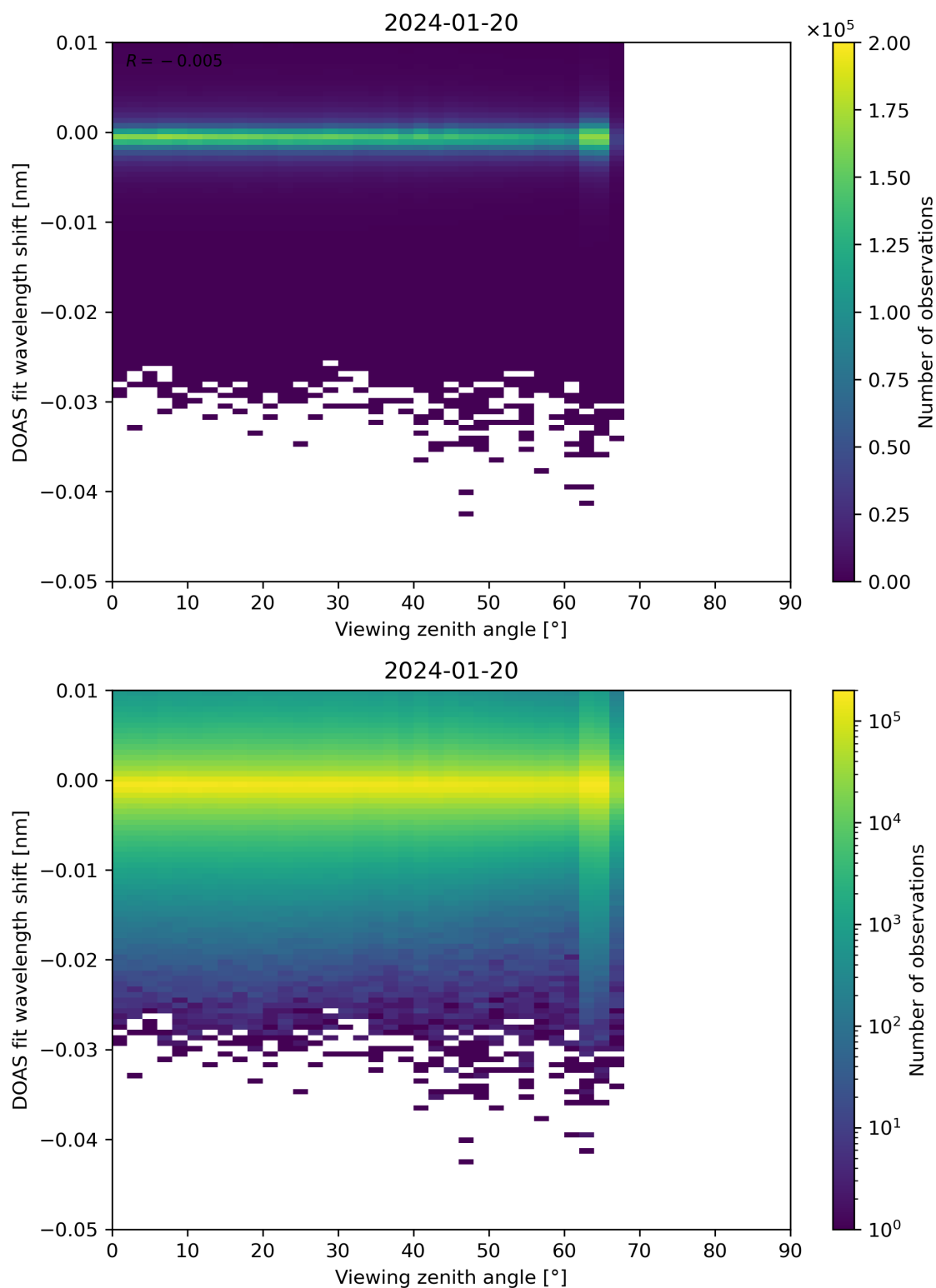
Figure 311: Scatter density plot of “Viewing zenith angle” against “DOAS fit wavelength shift” for 2024-01-19 to 2024-01-21.
