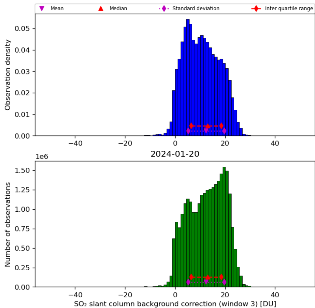
Figure 67: Histogram of “SO 2 slant column background correction (window 3)” for 2024-01-19 to 2024-01-21
