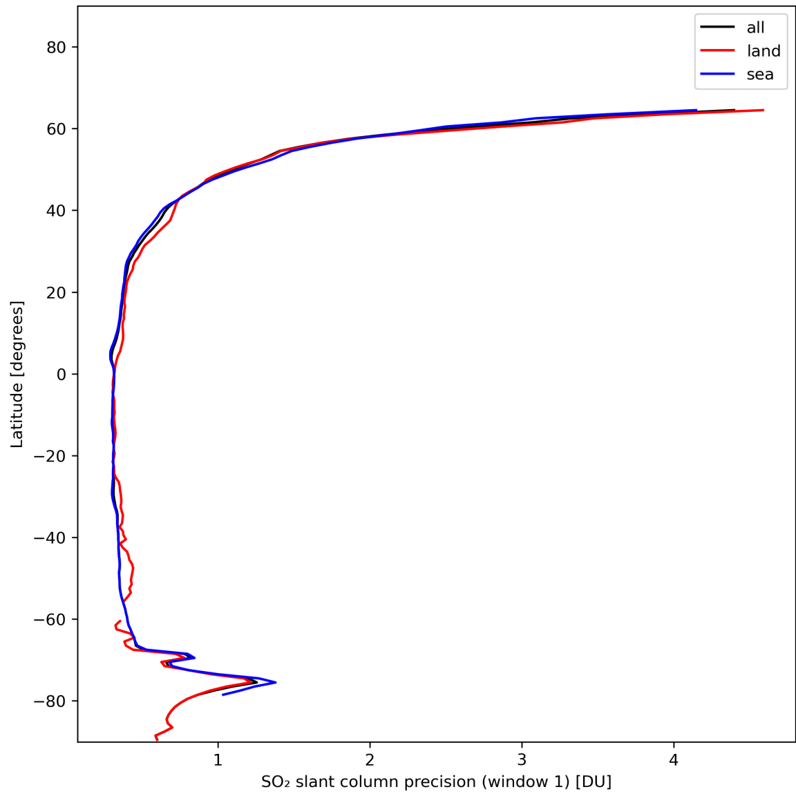
Figure 34: Zonal average of “SO 2 slant column precision (window 1)” for 2024-01-19 to 2024-01-21.
