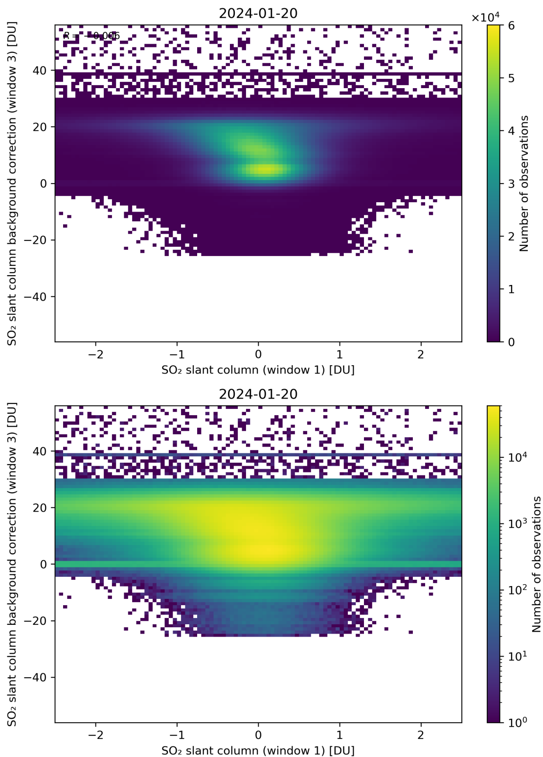
Figure 214: Scatter density plot of “SO 2 slant column (window 1)” against “SO 2 slant column background correction (window 3)” for 2024-01-19 to 2024-01-21.
