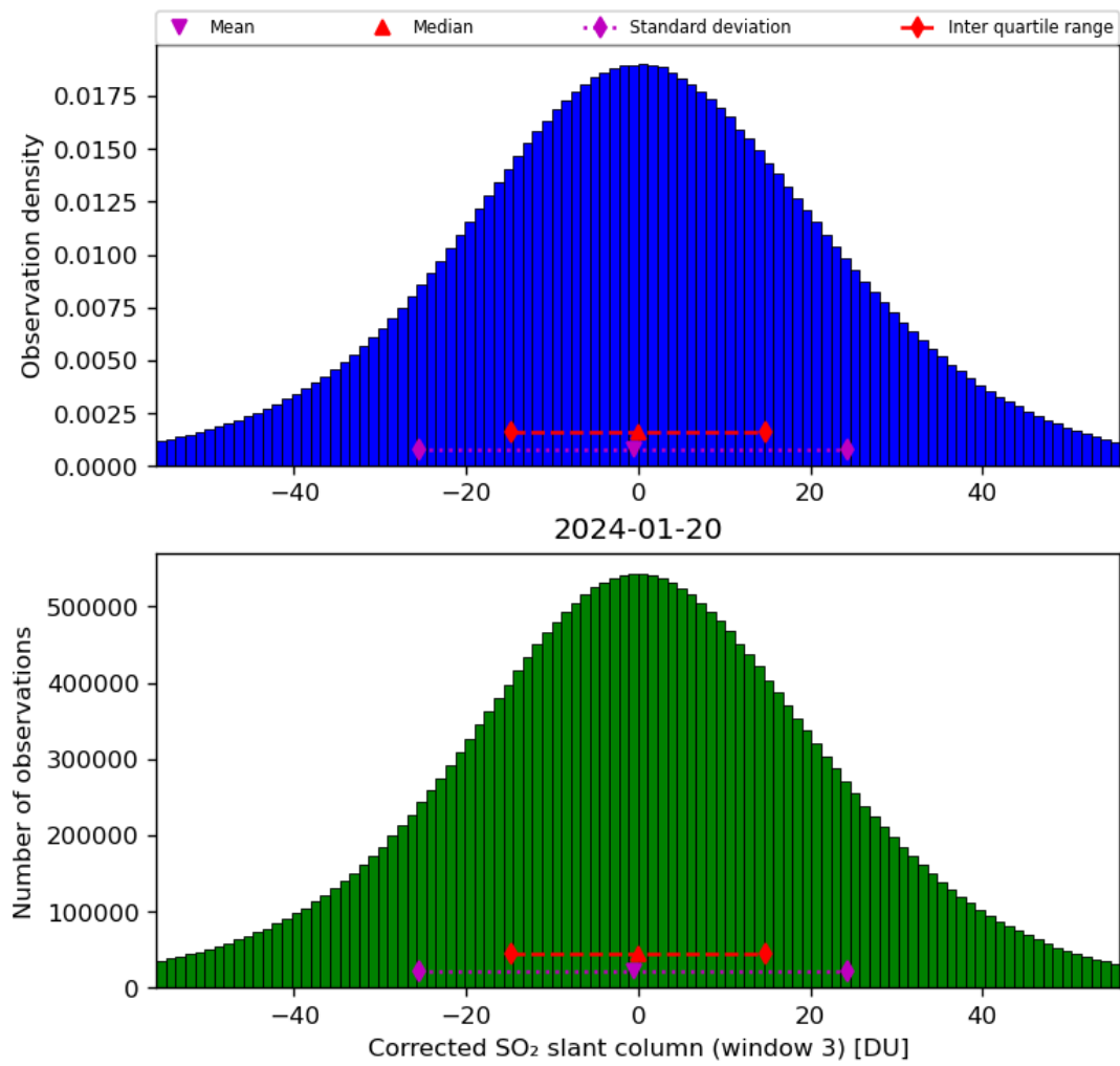
Figure 66: Histogram of “Corrected SO 2 slant column (window 3)” for 2024-01-19 to 2024-01-21
