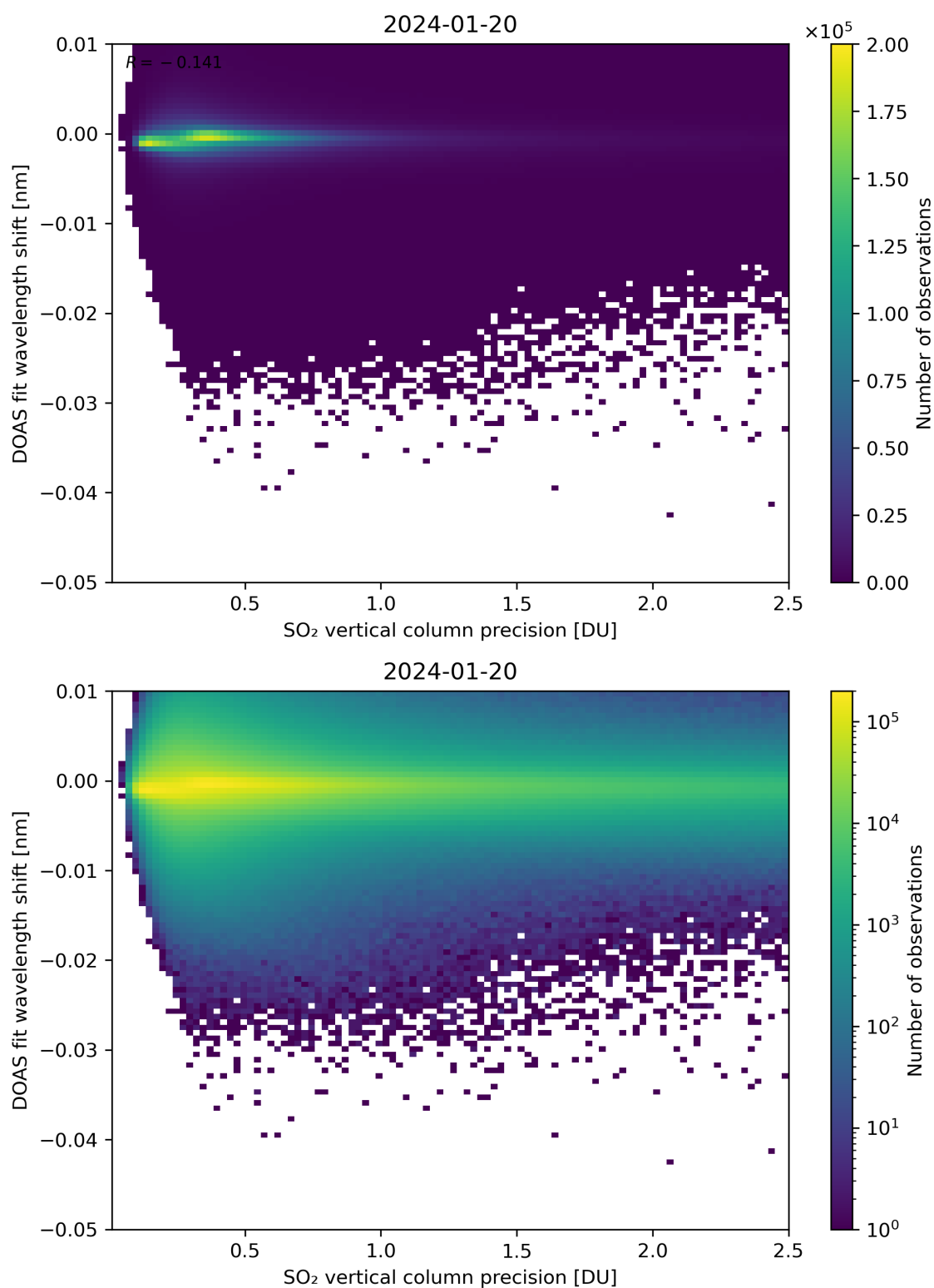
Figure 282: Scatter density plot of “SO 2 vertical column precision” against “DOAS fit wavelength shift” for 2024-01-19 to 2024-01-21.
