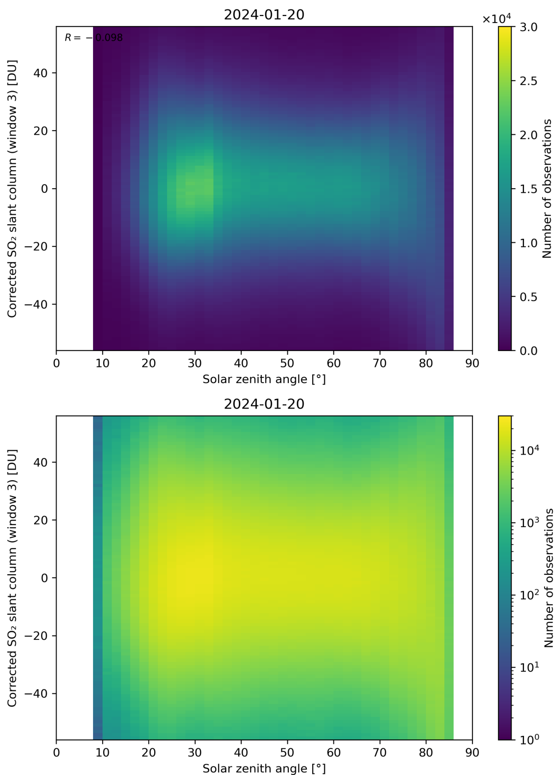
Figure 168: Scatter density plot of “Solar zenith angle” against “Corrected SO 2 slant column (window 3)” for 2024-01-19 to 2024-01-21.
