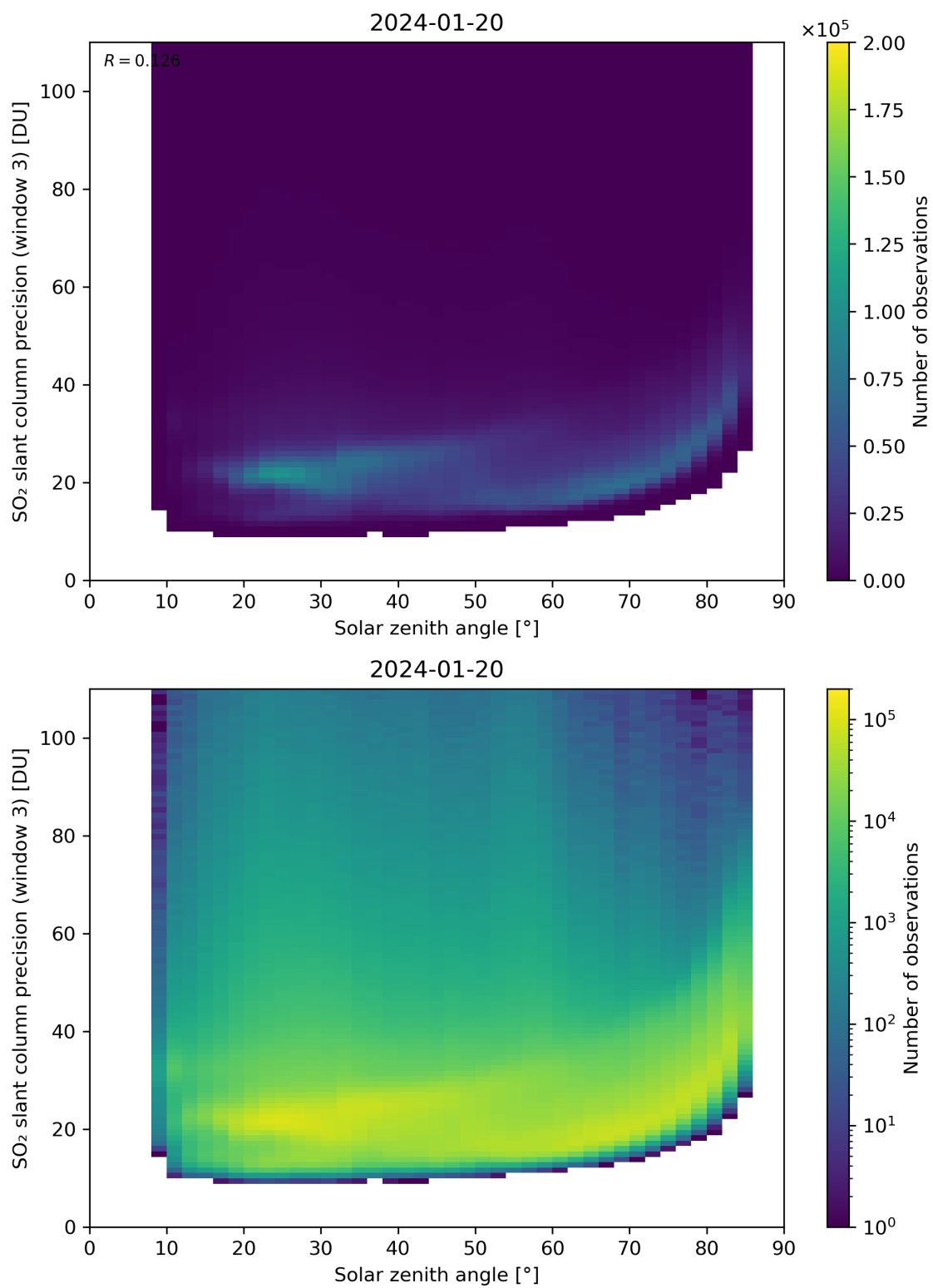
Figure 173: Scatter density plot of “Solar zenith angle” against “SO 2 slant column precision (window 3)” for 2024-01-19 to 2024-01-21.
