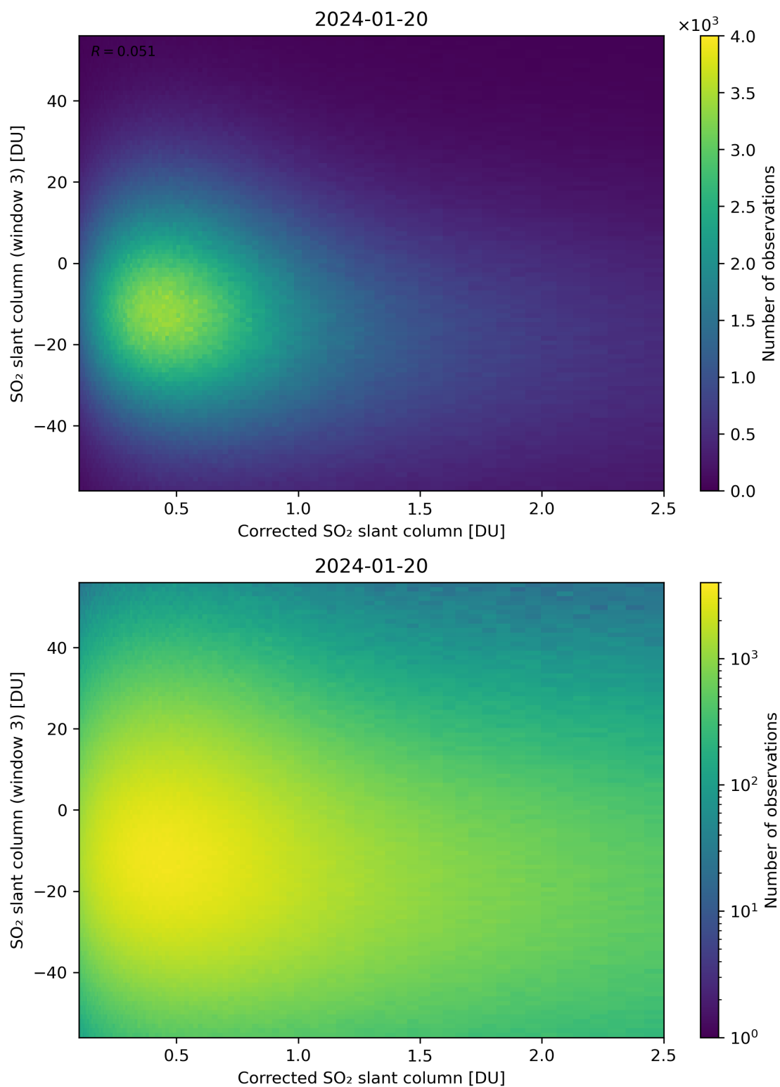
Figure 190: Scatter density plot of “Corrected SO 2 slant column” against “SO 2 slant column (window 3)” for 2024-01-19 to 2024-01-21.
