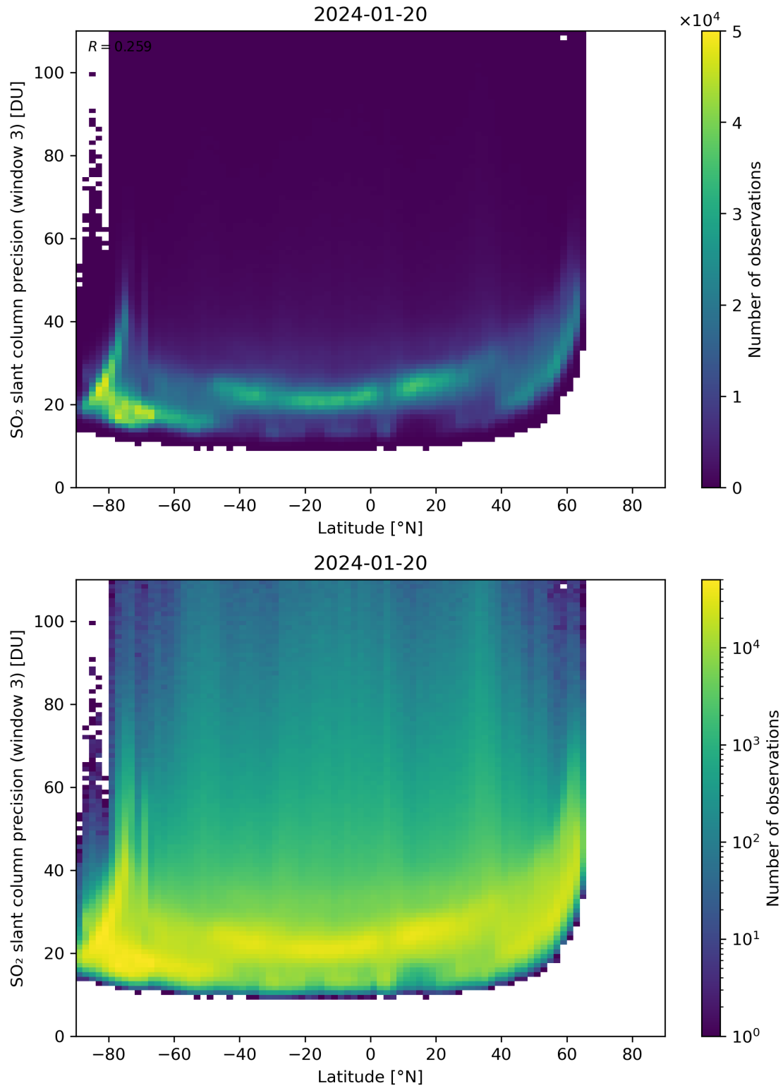
Figure 153: Scatter density plot of “Latitude” against “SO 2 slant column precision (window 3)” for 2024-01-19 to 2024-01-21.
