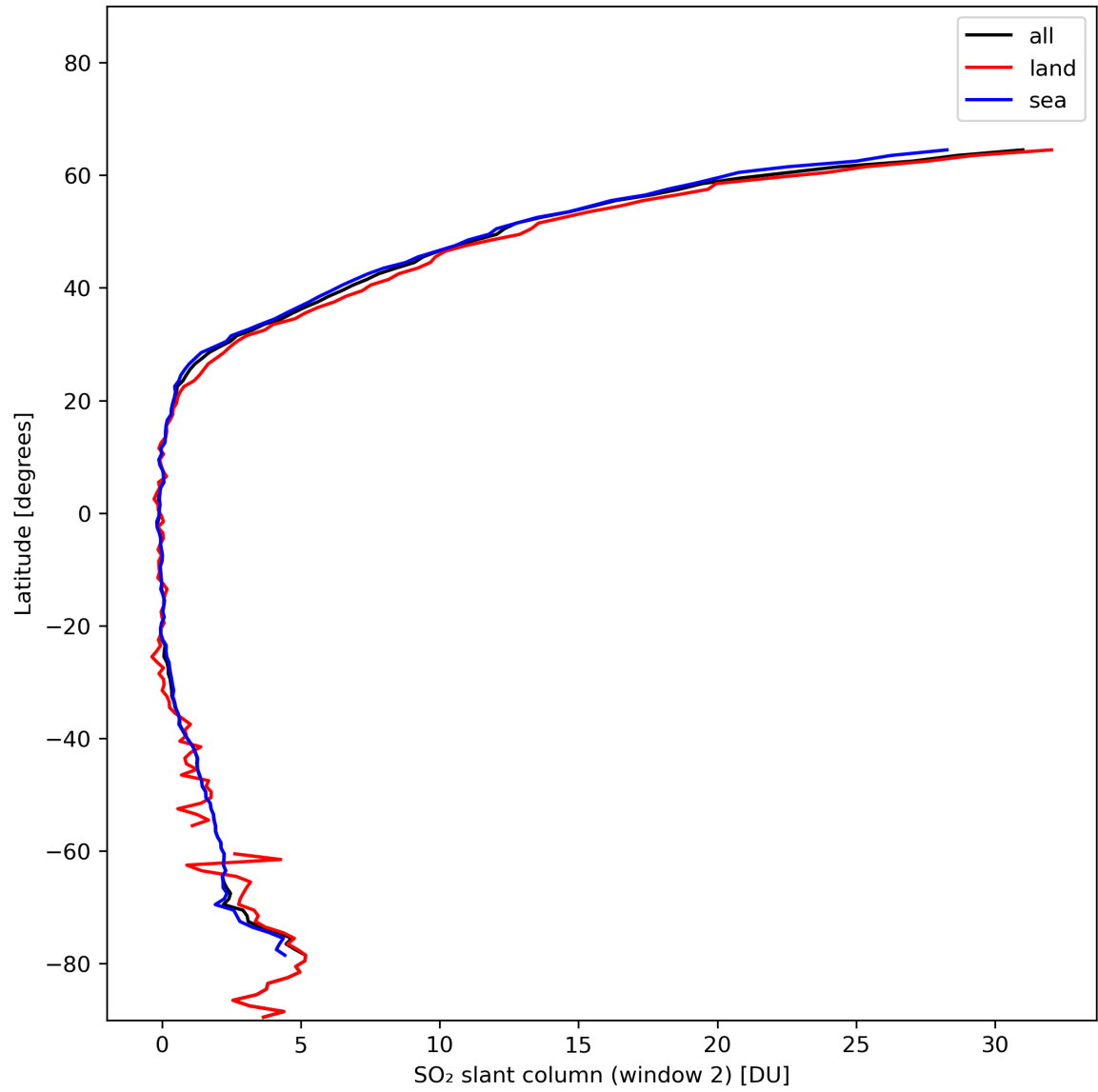
Figure 37: Zonal average of “SO 2 slant column (window 2)” for 2024-01-19 to 2024-01-21.
