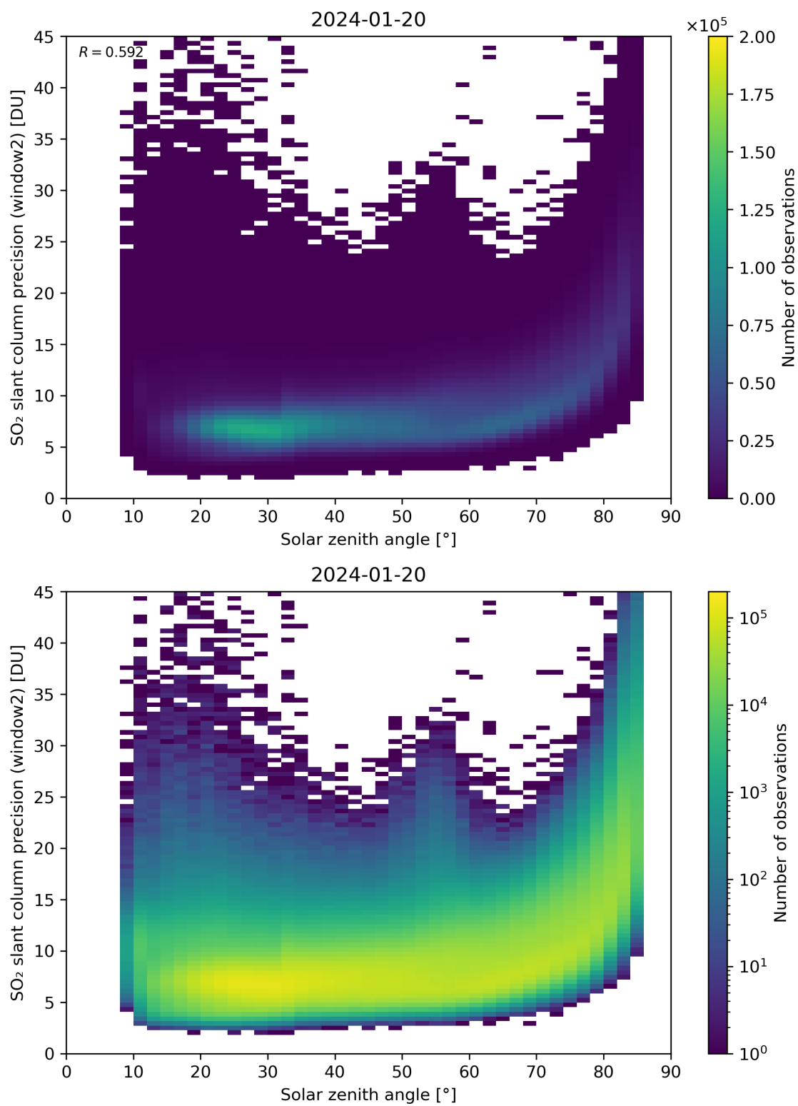
Figure 171: Scatter density plot of “Solar zenith angle” against “SO 2 slant column precision (window2)” for 2024-01-19 to 2024-01-21.
