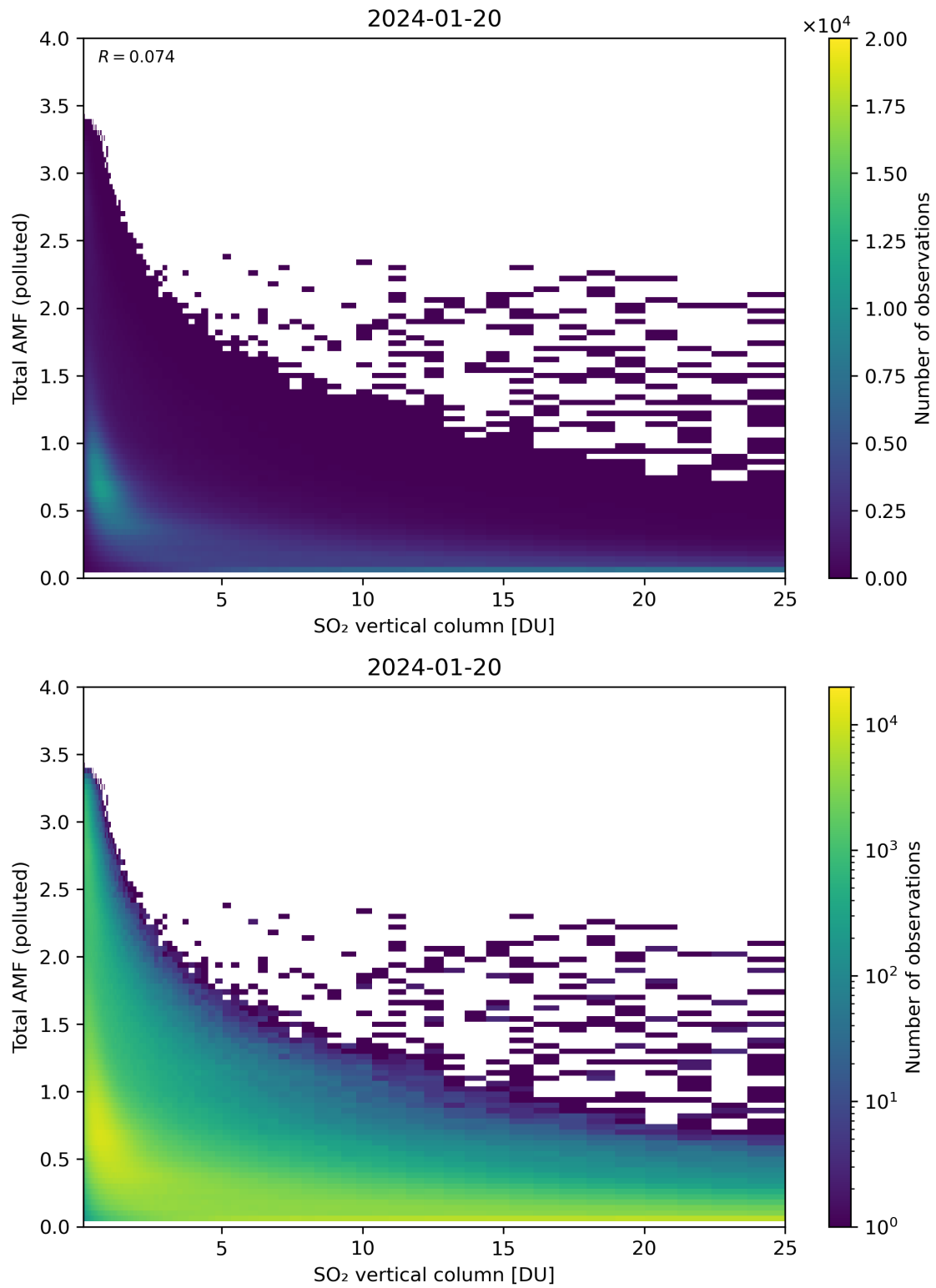
Figure 305: Scatter density plot of “SO 2 vertical column” against “Total AMF (polluted)” for 2024-01-19 to 2024-01-21.
