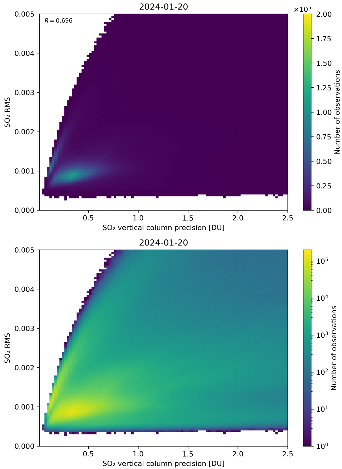
Figure 284: Scatter density plot of “SO 2 vertical column precision” against “SO 2 RMS” for 2024-01-19 to 2024-01-21.
