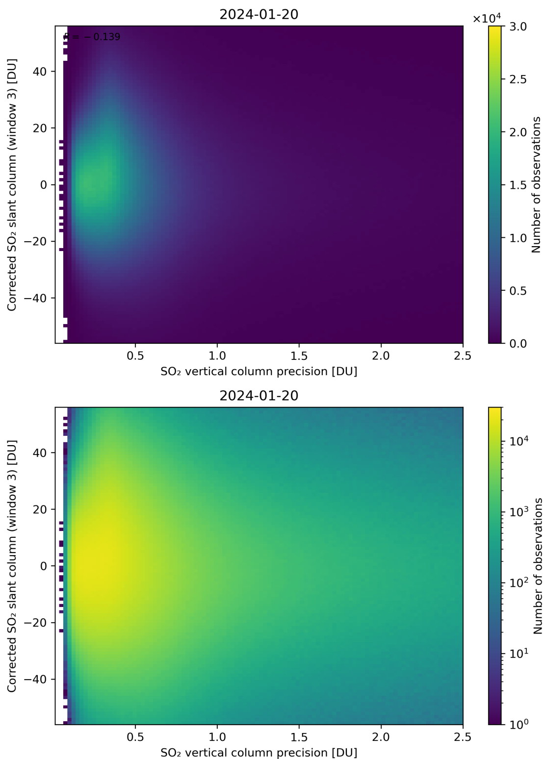
Figure 288: Scatter density plot of “SO 2 vertical column precision” against “Corrected SO 2 slant column (window 3)” for 2024-01-19 to 2024-01-21.
