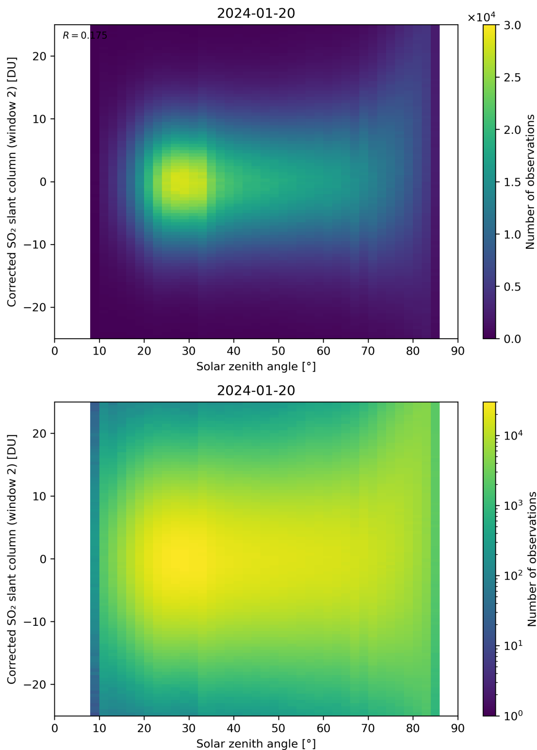
Figure 167: Scatter density plot of “Solar zenith angle” against “Corrected SO 2 slant column (window 2)” for 2024-01-19 to 2024-01-21.
