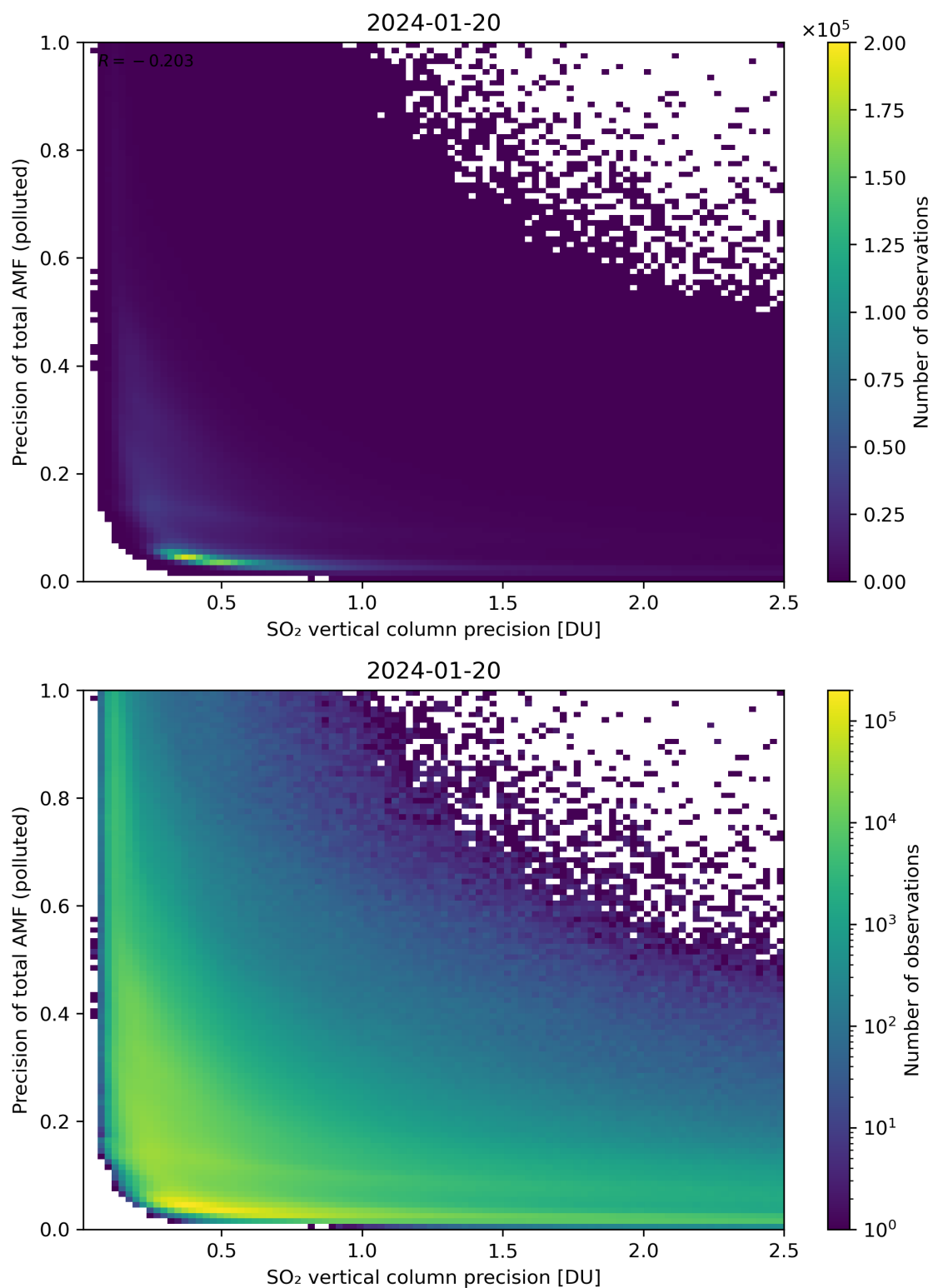
Figure 295: Scatter density plot of “SO 2 vertical column precision” against “Precision of total AMF (polluted)” for 2024-01-19 to 2024-01-21.
