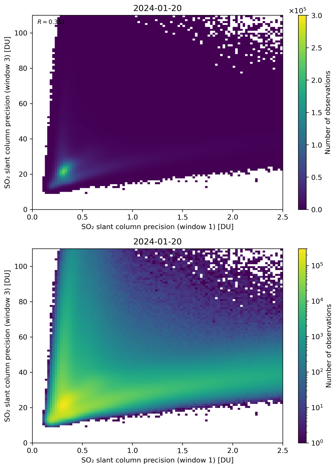
Figure 229: Scatter density plot of “SO 2 slant column precision (window 1)” against “SO 2 slant column precision (window 3)” for 2024-01-19 to 2024-01-21.
