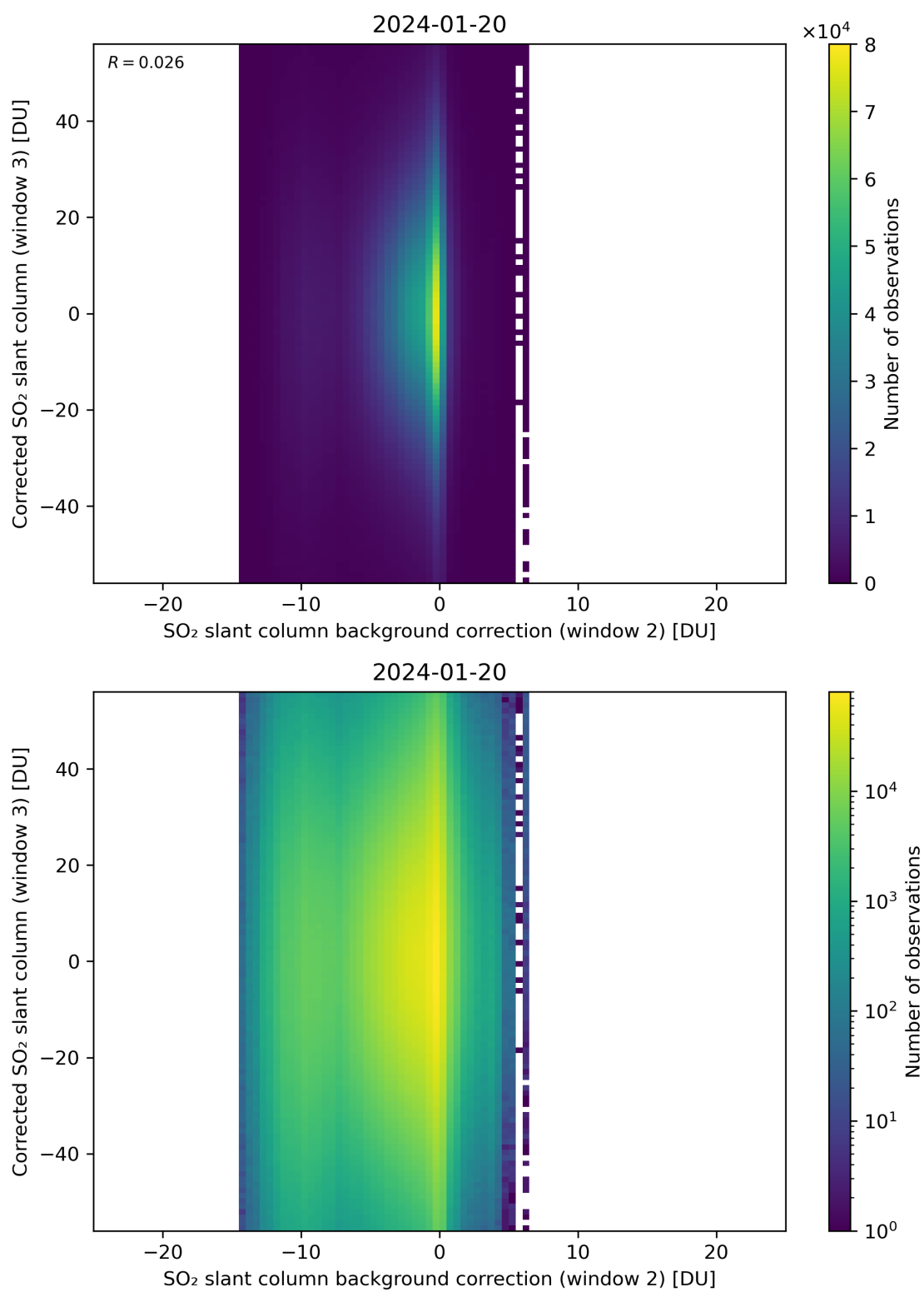
Figure 116: Scatter density plot of “SO 2 slant column background correction (window 2)” against “Corrected SO 2 slant column (window 3)” for 2024-01-19 to 2024-01-21.
