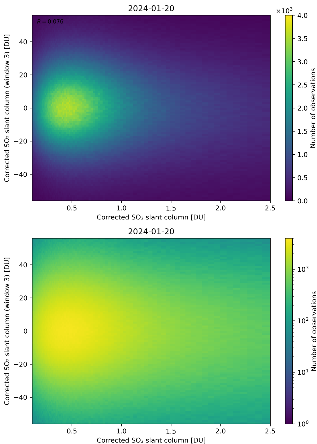
Figure 186: Scatter density plot of “Corrected SO 2 slant column” against “Corrected SO 2 slant column (window 3)” for 2024-01-19 to 2024-01-21.
