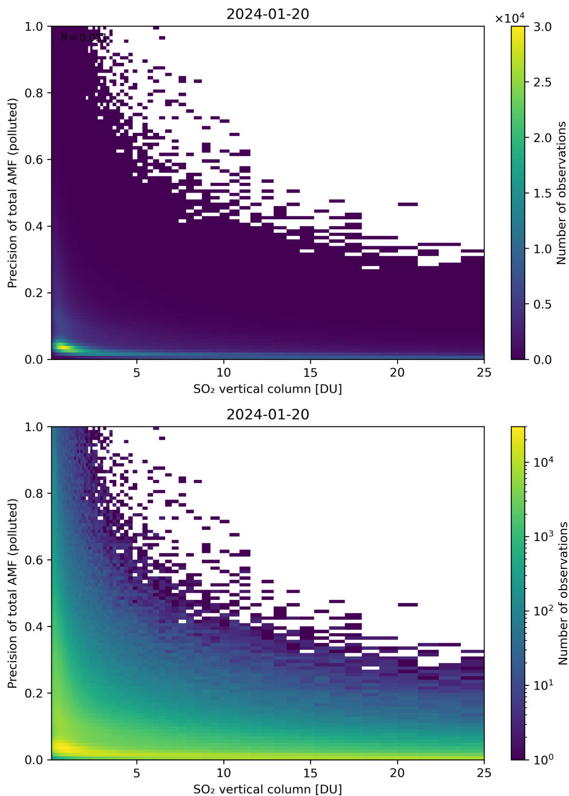
Figure 306: Scatter density plot of “SO 2 vertical column” against “Precision of total AMF (polluted)” for 2024-01-19 to 2024-01-21.
