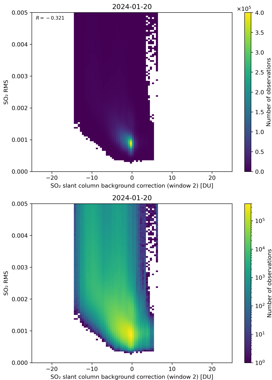
Figure 114: Scatter density plot of “SO 2 slant column background correction (window 2)” against “SO 2 RMS” for 2024-01-19 to 2024-01-21.
