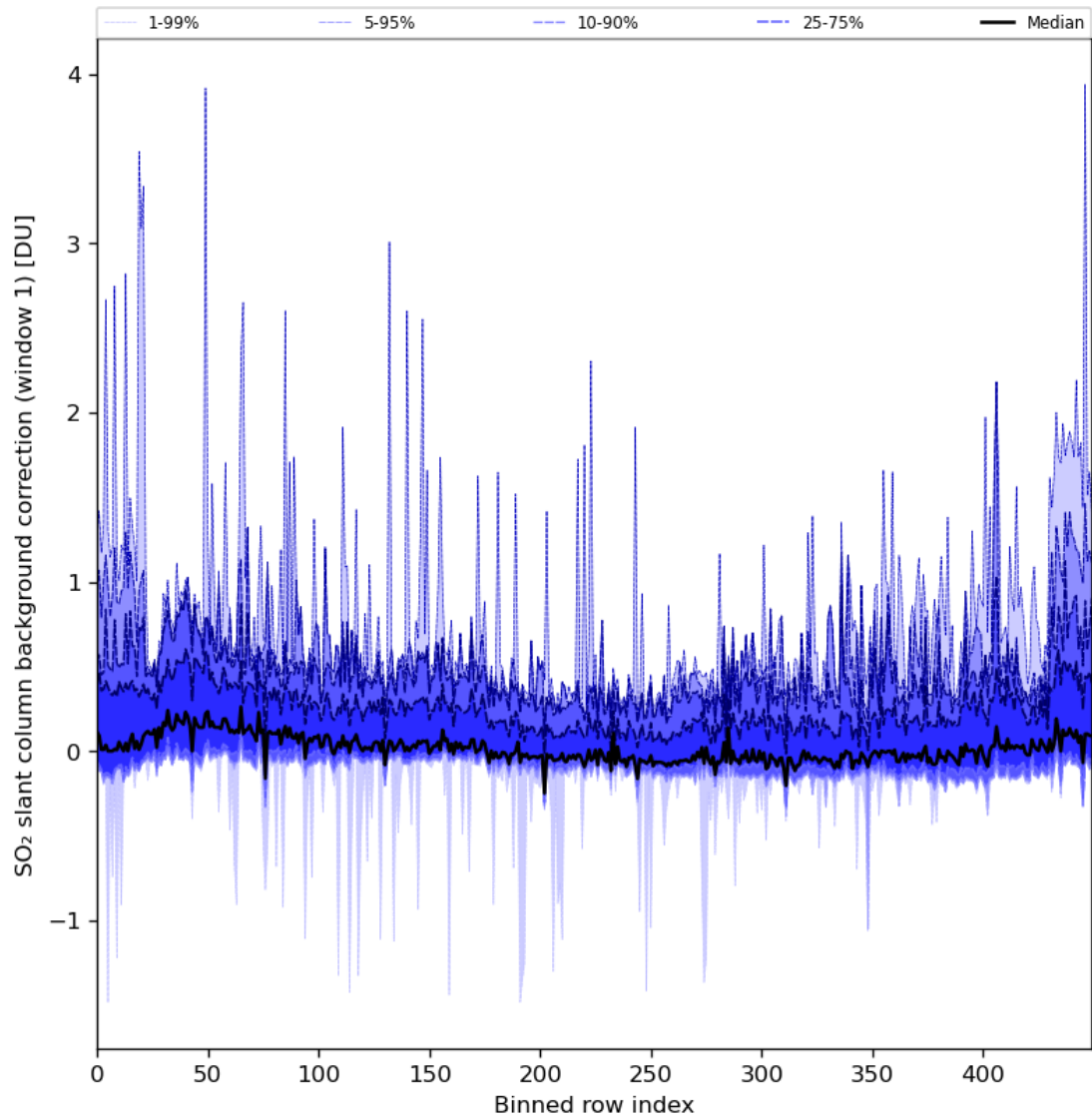
Figure 82: Along track statistics of “SO 2 slant column background correction (window 1)” for 2024-01-19 to 2024-01-21
