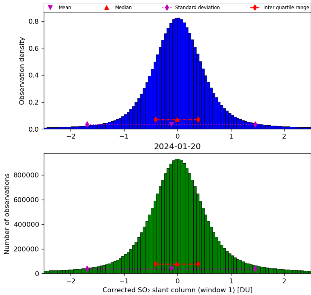
Figure 58: Histogram of “Corrected SO 2 slant column (window 1)” for 2024-01-19 to 2024-01-21
