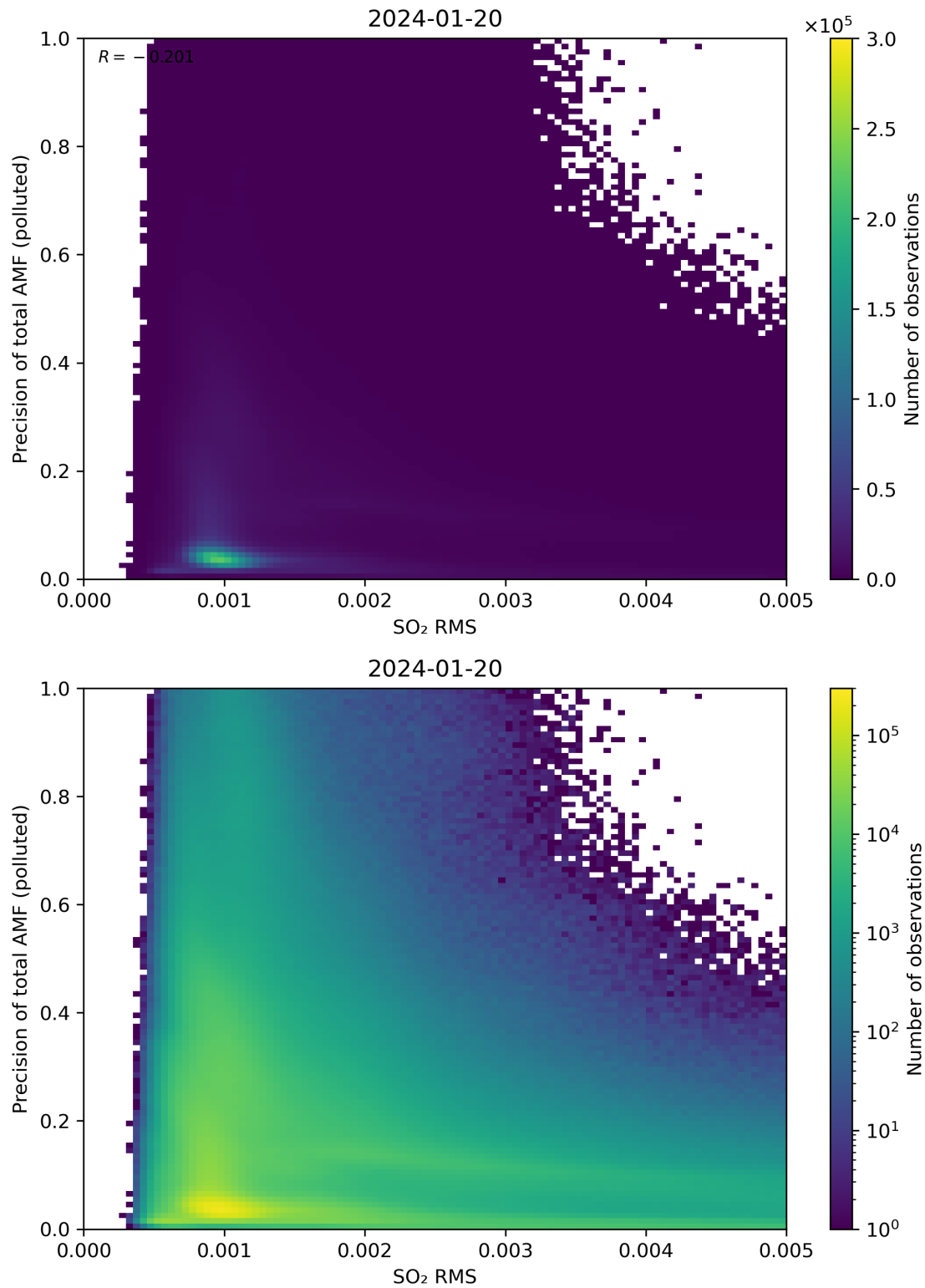
Figure 138: Scatter density plot of “SO 2 RMS” against “Precision of total AMF (polluted)” for 2024-01-19 to 2024-01-21.
