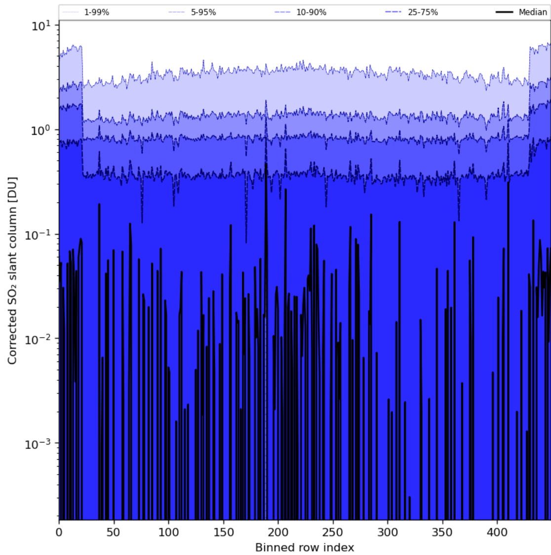
Figure 78: Along track statistics of “Corrected SO 2 slant column” for 2024-01-19 to 2024-01-21
