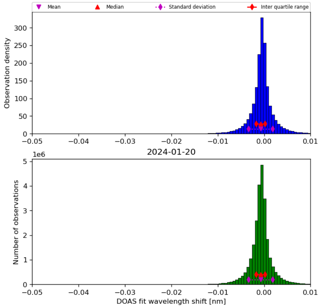
Figure 68: Histogram of “DOAS fit wavelength shift” for 2024-01-19 to 2024-01-21
