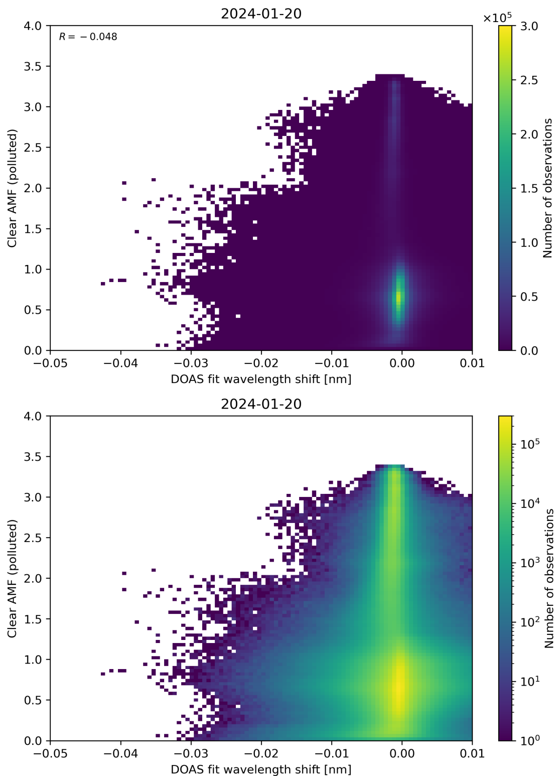
Figure 129: Scatter density plot of “DOAS fit wavelength shift” against “Clear AMF (polluted)” for 2024-01-19 to 2024-01-21.
