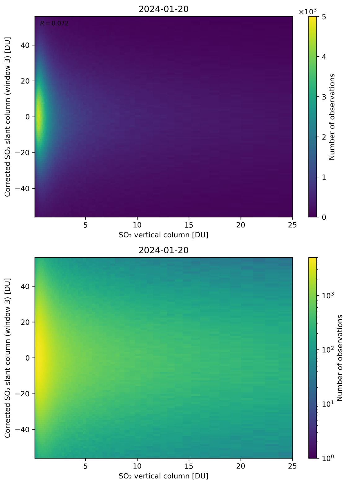
Figure 299: Scatter density plot of “SO 2 vertical column” against “Corrected SO 2 slant column (window 3)” for 2024-01-19 to 2024-01-21.
