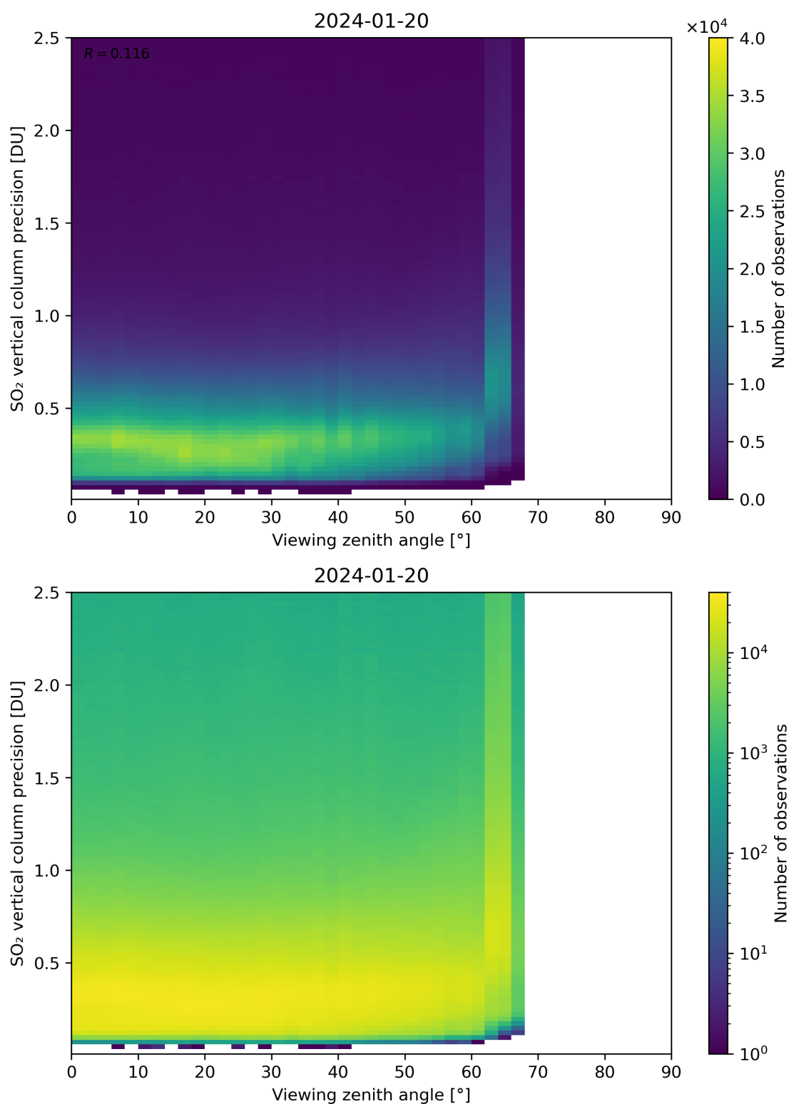
Figure 328: Scatter density plot of “Viewing zenith angle” against “SO 2 vertical column precision” for 2024-01-19 to 2024-01-21.
