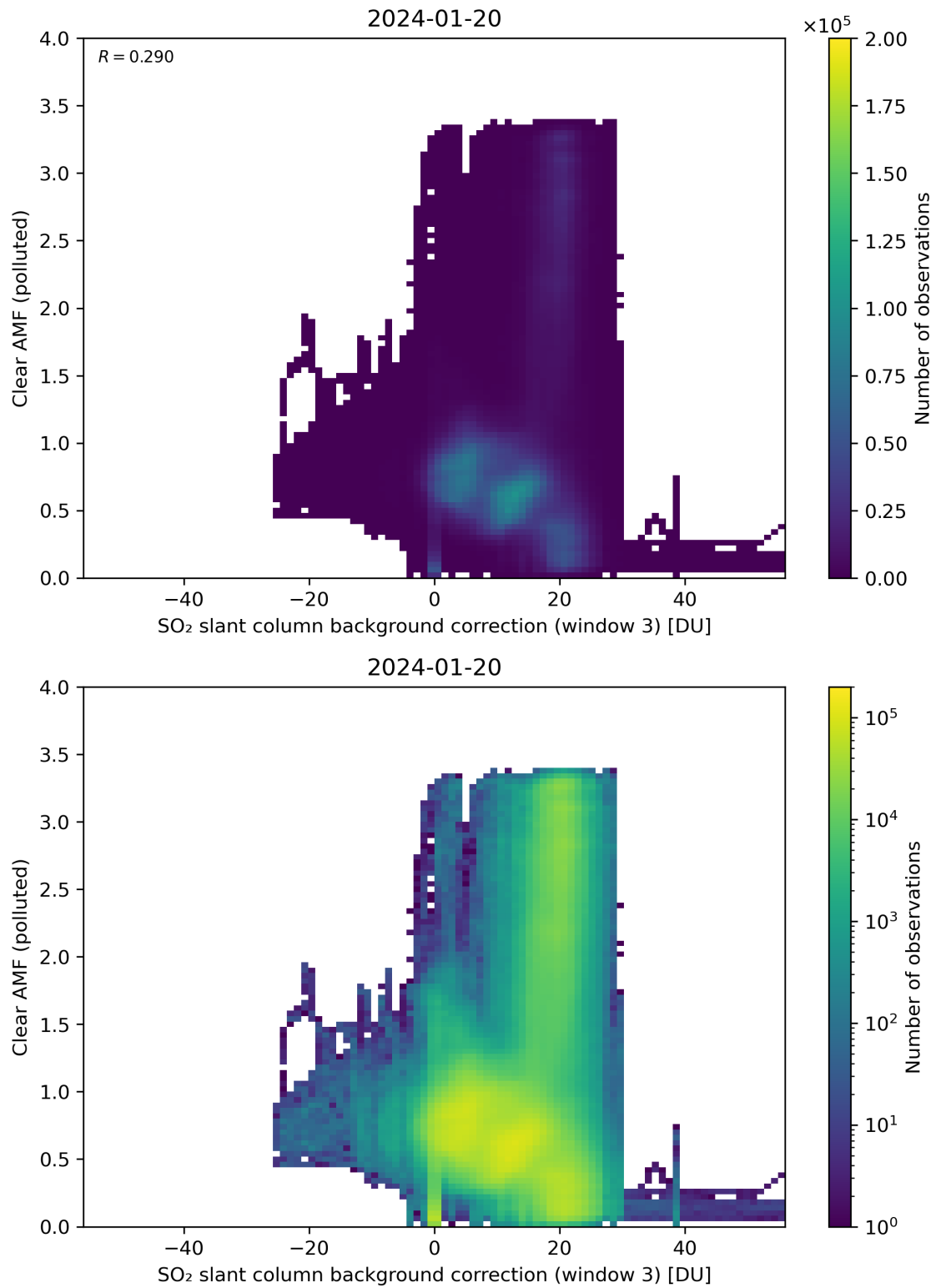
Figure 124: Scatter density plot of “SO 2 slant column background correction (window 3)” against “Clear AMF (polluted)” for 2024-01-19 to 2024-01-21.
