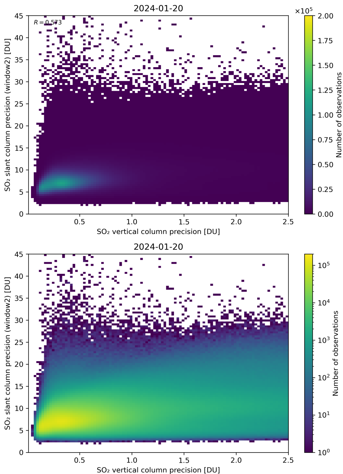
Figure 291: Scatter density plot of “SO 2 vertical column precision” against “SO 2 slant column precision (window2)” for 2024-01-19 to 2024-01-21.
