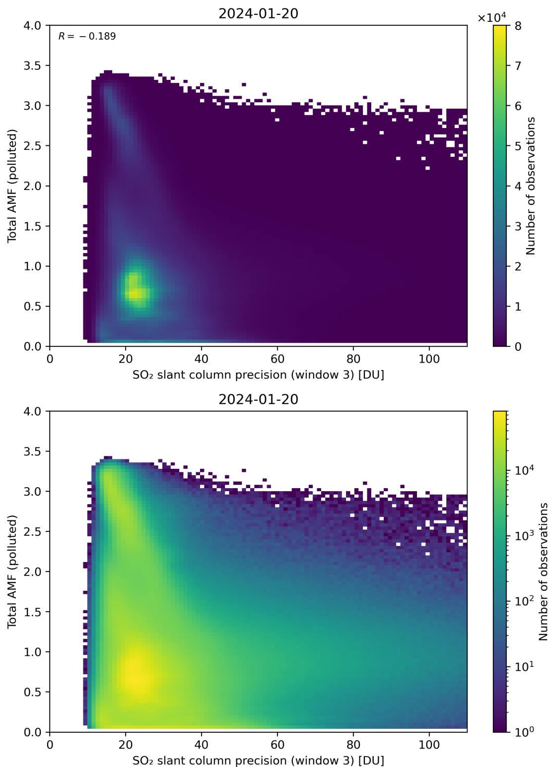
Figure 263: Scatter density plot of “SO 2 slant column precision (window 3)” against “Total AMF (polluted)” for 2024-01-19 to 2024-01-21.
