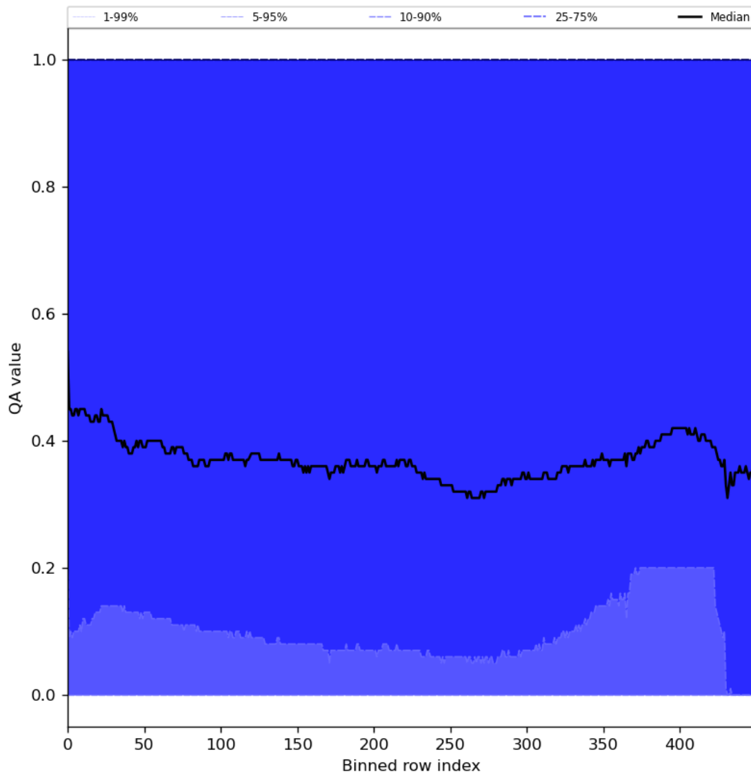
Figure 75: Along track statistics of “QA value” for 2024-01-19 to 2024-01-21
