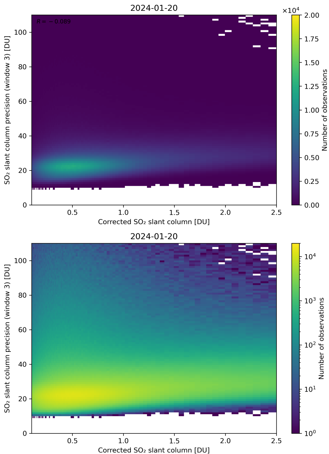
Figure 191: Scatter density plot of “Corrected SO 2 slant column” against “SO 2 slant column precision (window 3)” for 2024-01-19 to 2024-01-21.
