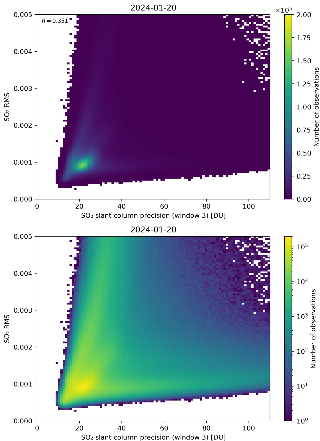
Figure 260: Scatter density plot of “SO 2 slant column precision (window 3)” against “SO 2 RMS” for 2024-01-19 to 2024-01-21.
