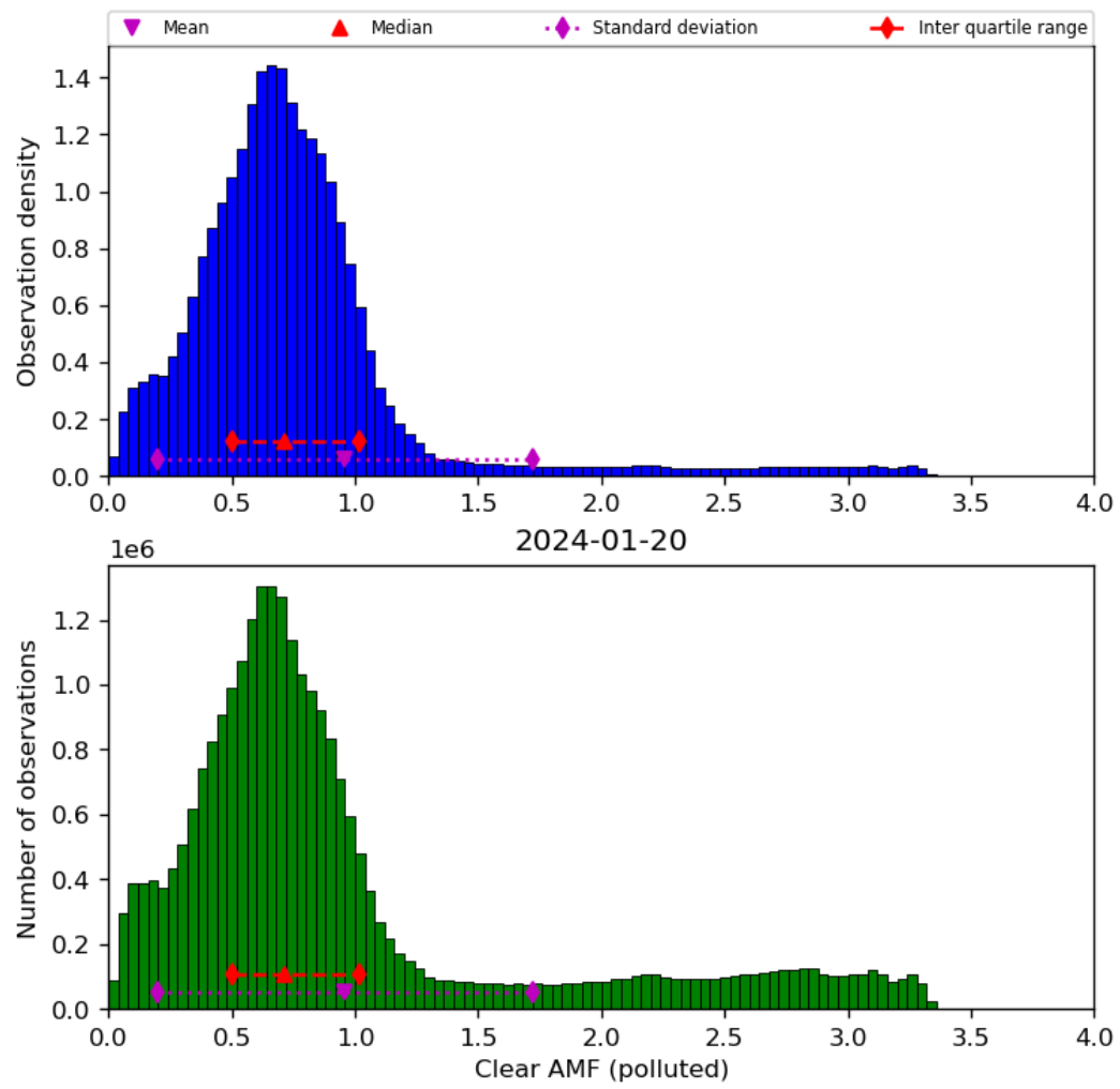
Figure 73: Histogram of “Clear AMF (polluted)” for 2024-01-19 to 2024-01-21
