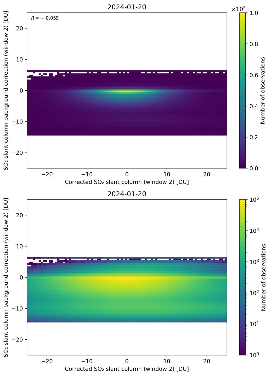
Figure 194: Scatter density plot of “Corrected SO 2 slant column (window 2)” against “SO 2 slant column background correction (window 2)” for 2024-01-19 to 2024-01-21.
