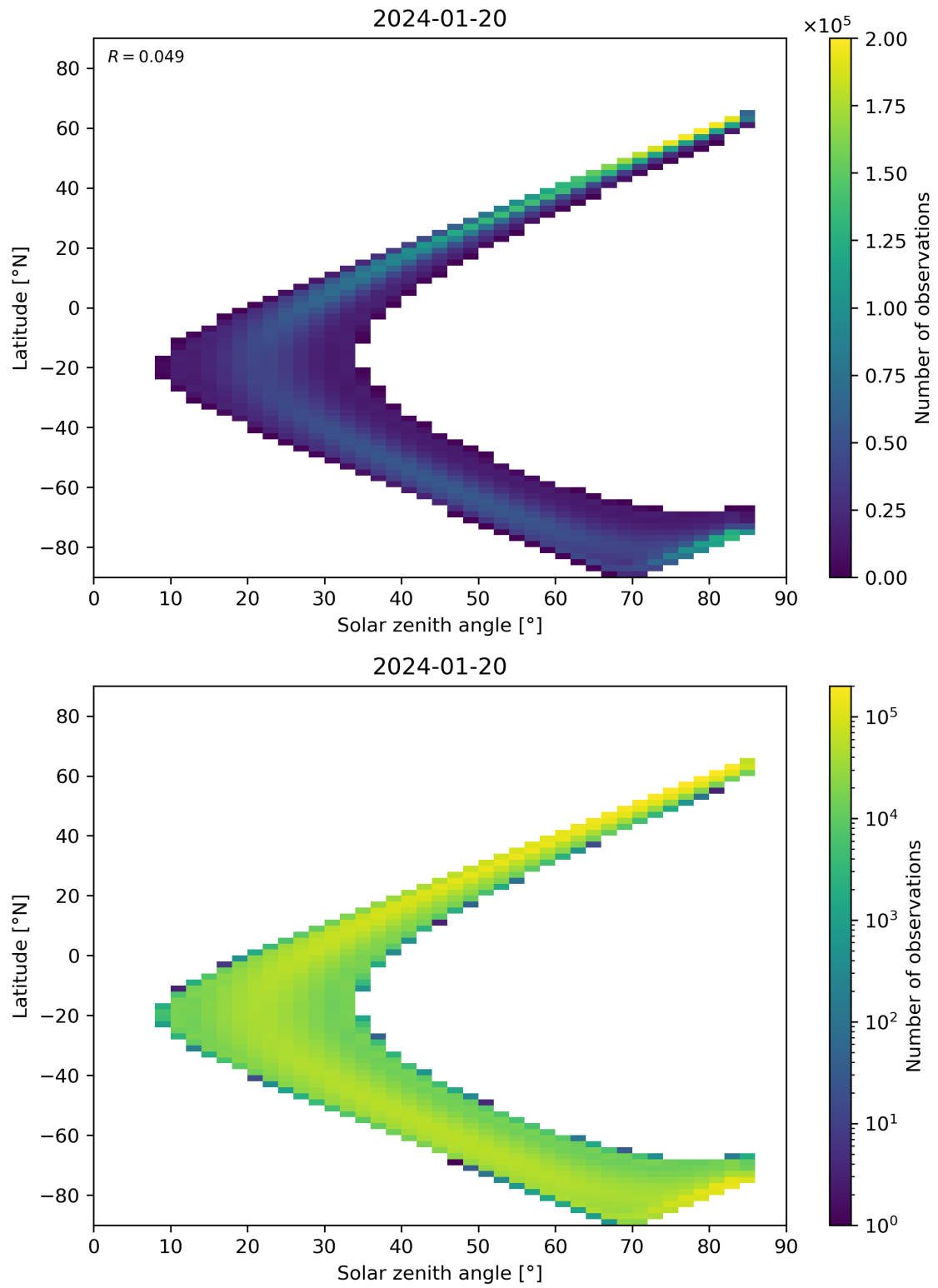
Figure 164: Scatter density plot of “Solar zenith angle” against “Latitude” for 2024-01-19 to 2024-01-21.
