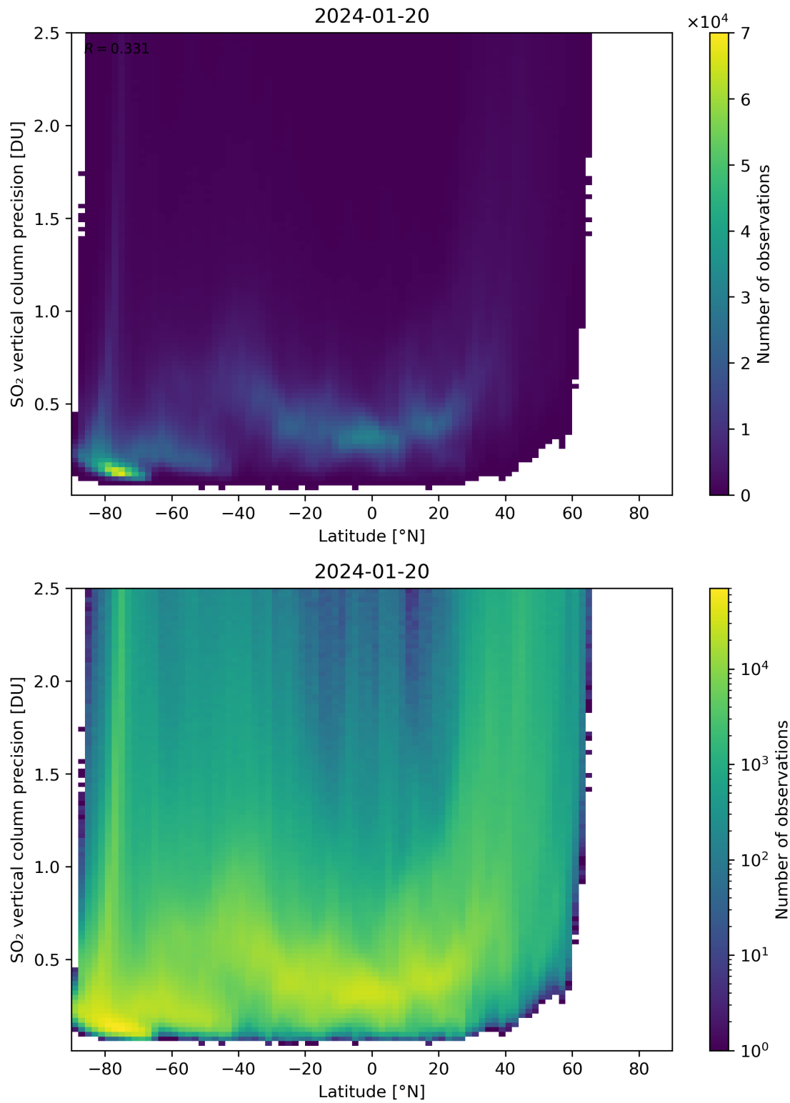
Figure 157: Scatter density plot of “Latitude” against “SO 2 vertical column precision” for 2024-01-19 to 2024-01-21.
