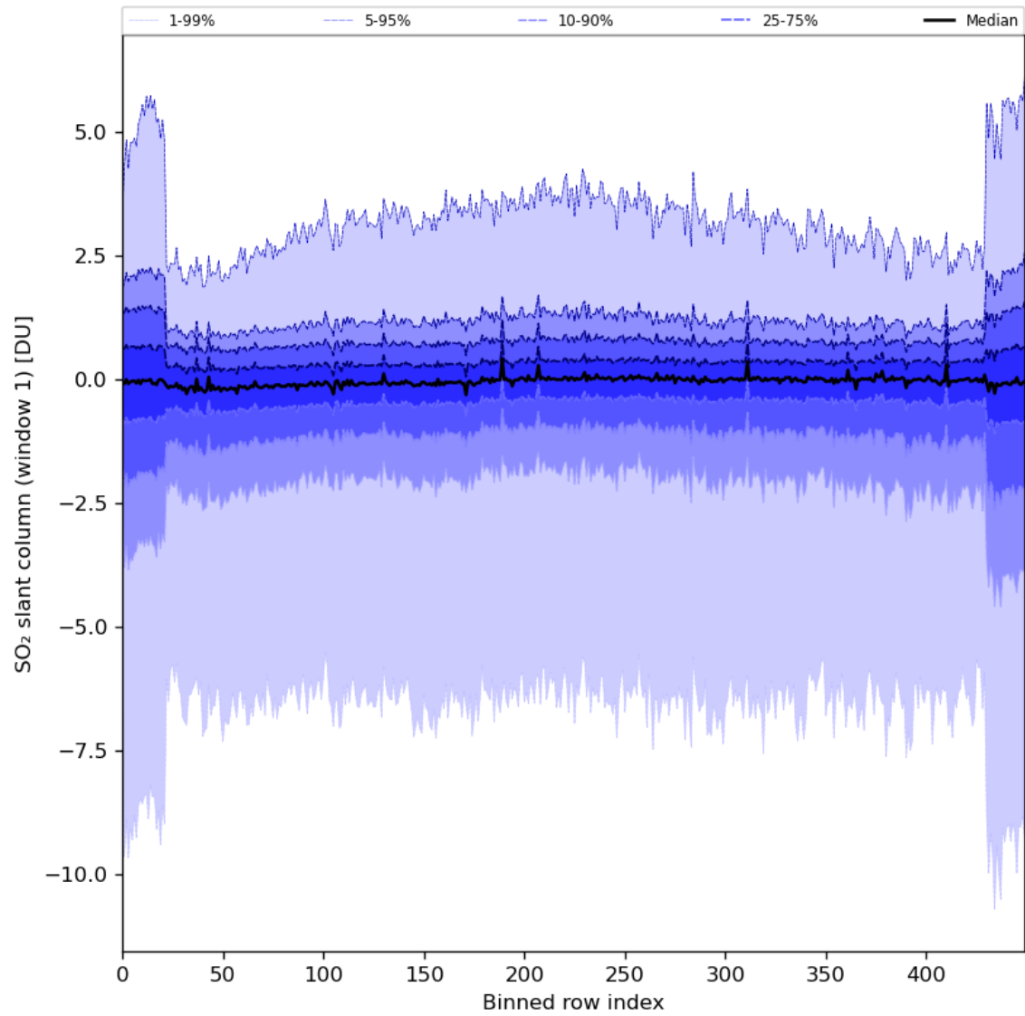
Figure 79: Along track statistics of “SO 2 slant column (window 1)” for 2024-01-19 to 2024-01-21
