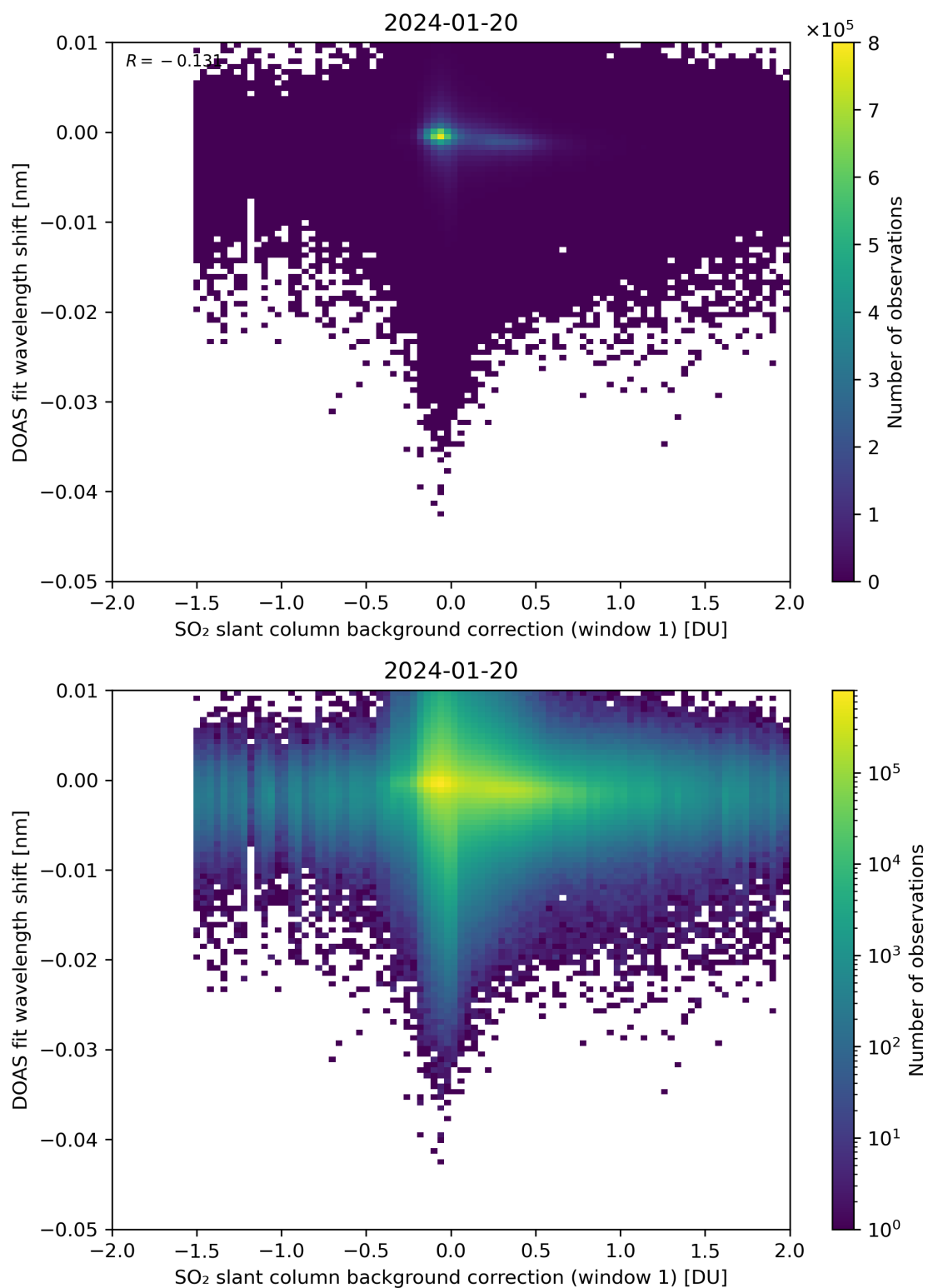
Figure 100: Scatter density plot of “SO 2 slant column background correction (window 1)” against “DOAS fit wavelength shift” for 2024-01-19 to 2024-01-21.
