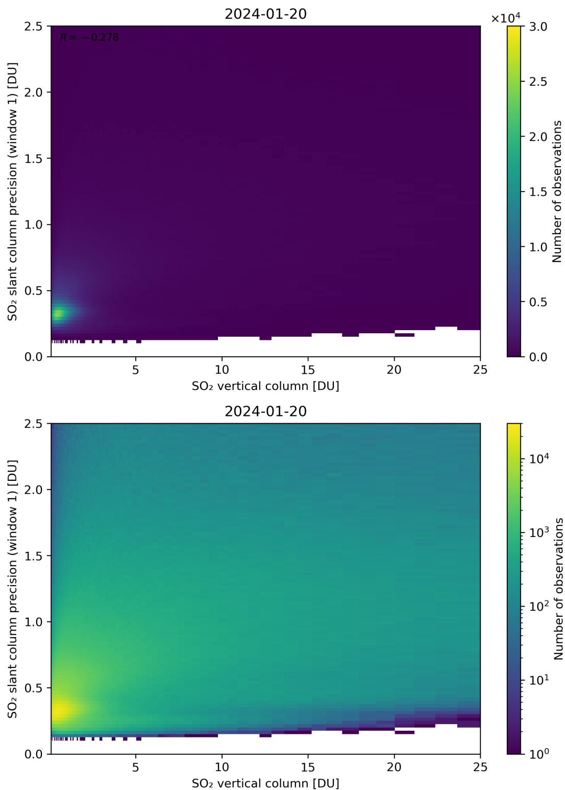
Figure 301: Scatter density plot of “SO 2 vertical column” against “SO 2 slant column precision (window 1)” for 2024-01-19 to 2024-01-21.
