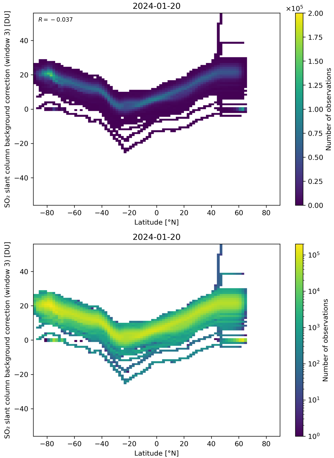
Figure 141: Scatter density plot of “Latitude” against “SO 2 slant column background correction (window 3)” for 2024-01-19 to 2024-01-21.
