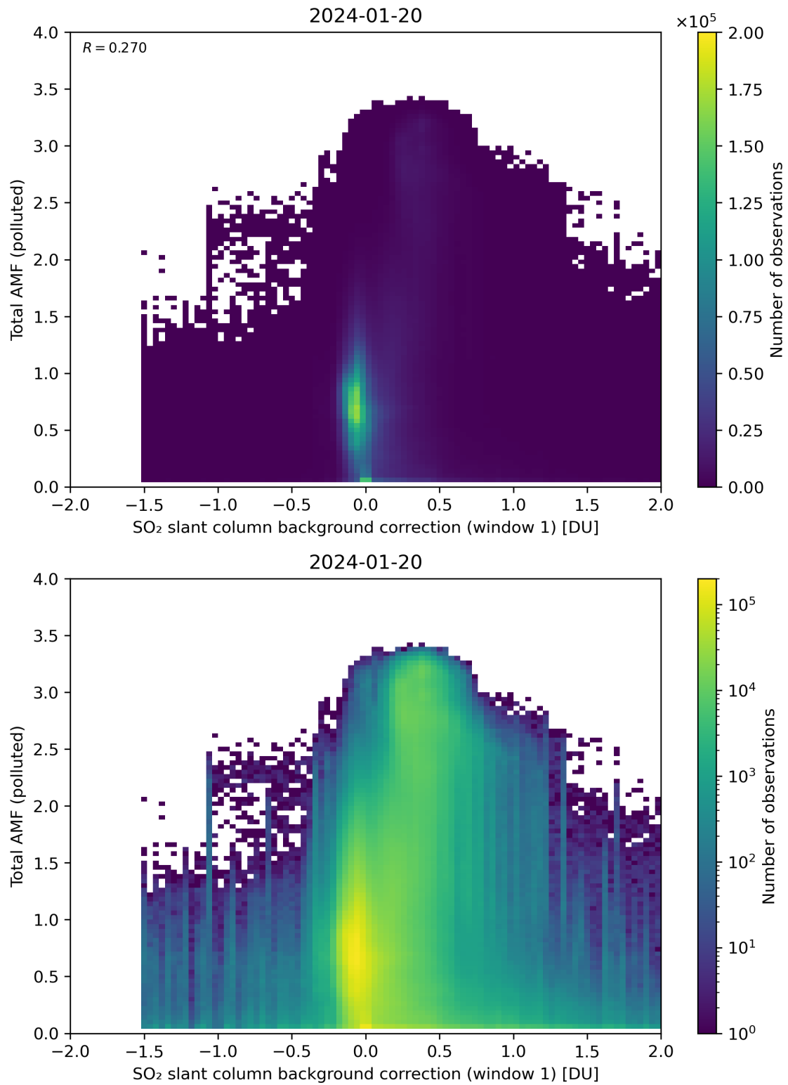
Figure 109: Scatter density plot of “SO 2 slant column background correction (window 1)” against “Total AMF (polluted)” for 2024-01-19 to 2024-01-21.
