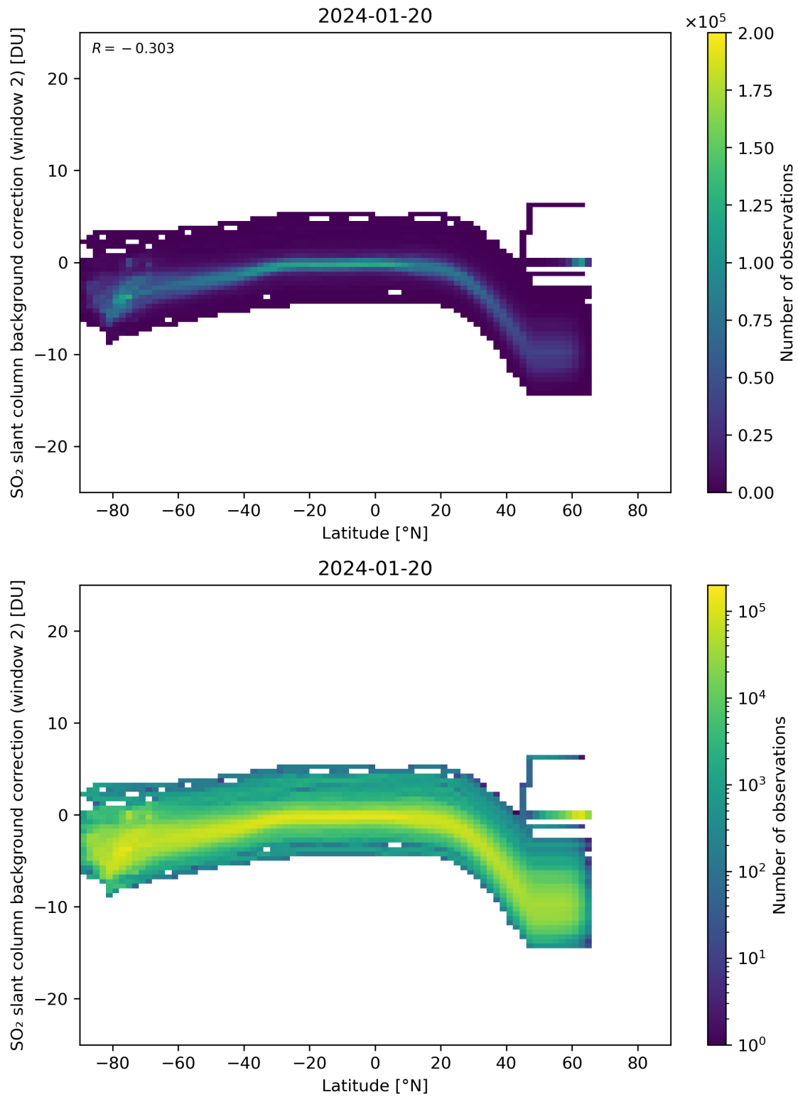
Figure 140: Scatter density plot of “Latitude” against “SO 2 slant column background correction (window 2)” for 2024-01-19 to 2024-01-21.
