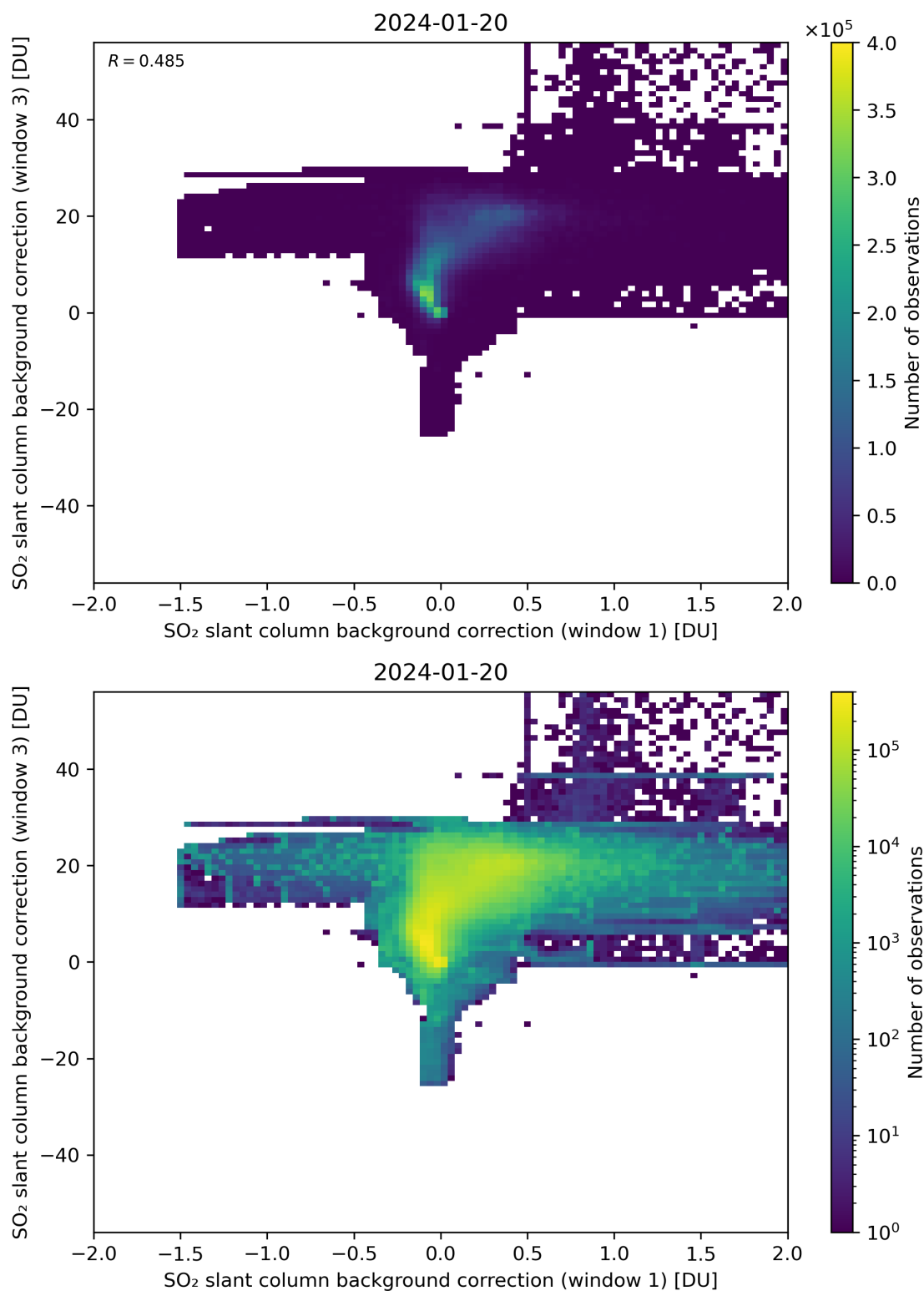
Figure 99: Scatter density plot of “SO 2 slant column background correction (window 1)” against “SO 2 slant column background correction (window 3)” for 2024-01-19 to 2024-01-21.
