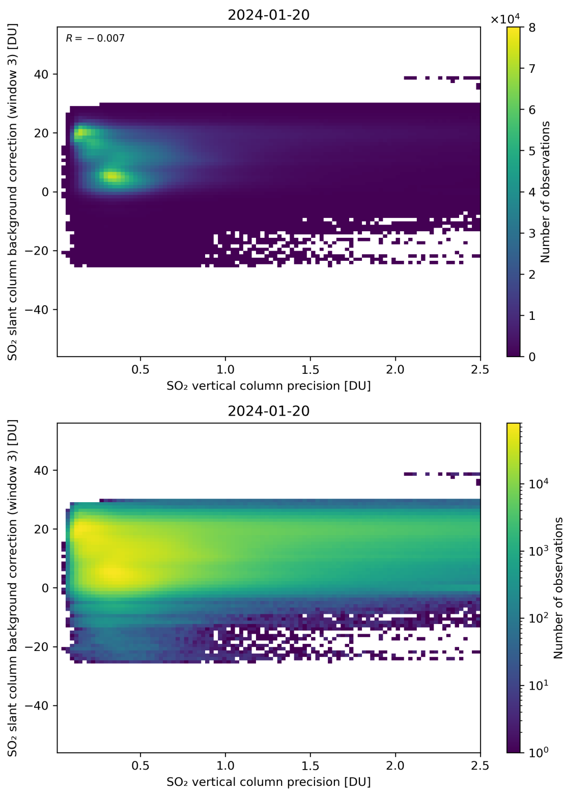
Figure 281: Scatter density plot of “SO 2 vertical column precision” against “SO 2 slant column background correction (window 3)” for 2024-01-19 to 2024-01-21.
