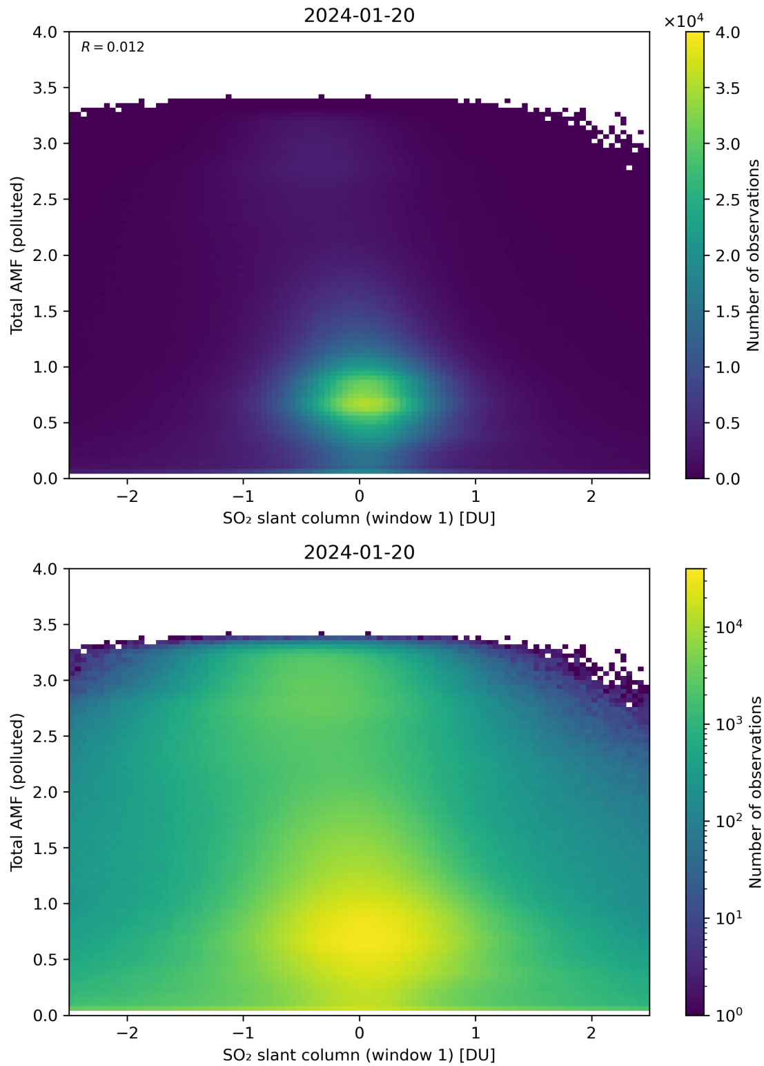
Figure 239: Scatter density plot of “SO 2 slant column (window 1)” against “Total AMF (polluted)” for 2024-01-19 to 2024-01-21.
