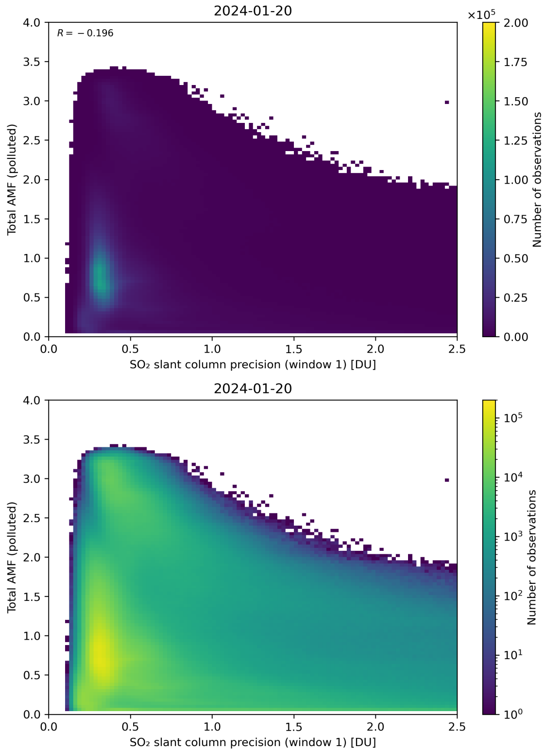
Figure 230: Scatter density plot of “SO 2 slant column precision (window 1)” against “Total AMF (polluted)” for 2024-01-19 to 2024-01-21.
