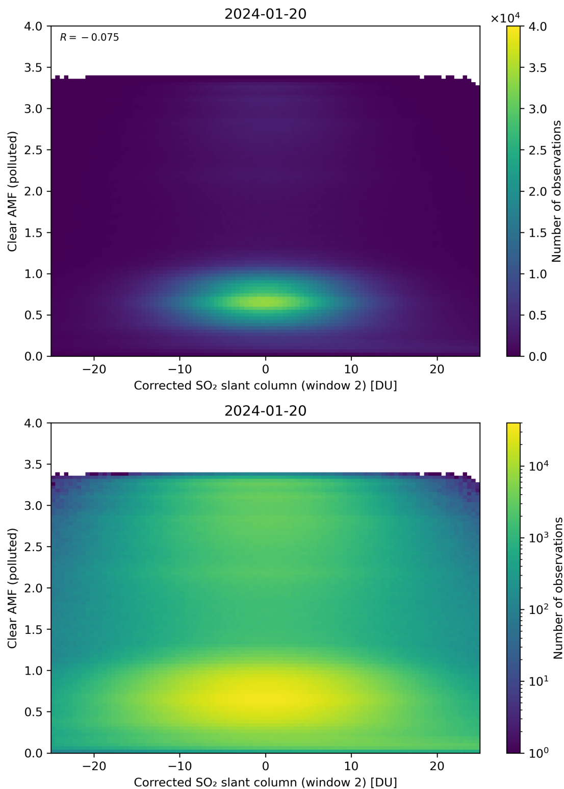
Figure 199: Scatter density plot of “Corrected SO 2 slant column (window 2)” against “Clear AMF (polluted)” for 2024-01-19 to 2024-01-21.
