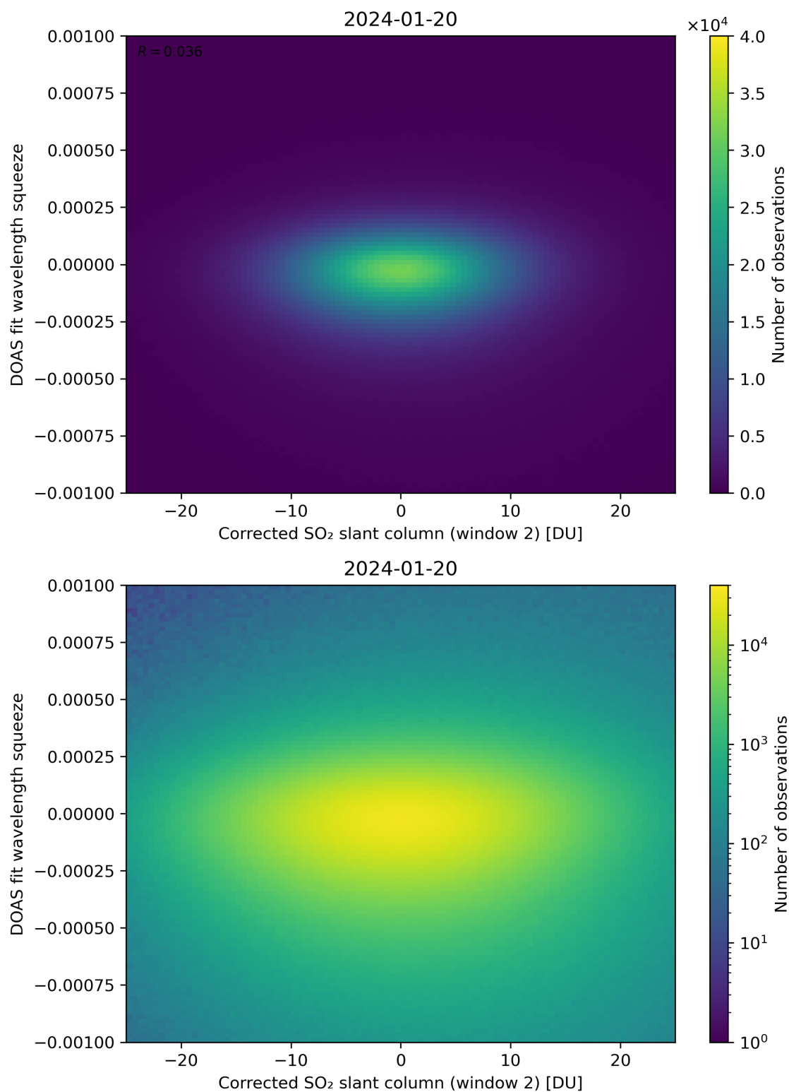
Figure 197: Scatter density plot of “Corrected SO 2 slant column (window 2)” against “DOAS fit wavelength squeeze” for 2024-01-19 to 2024-01-21.
