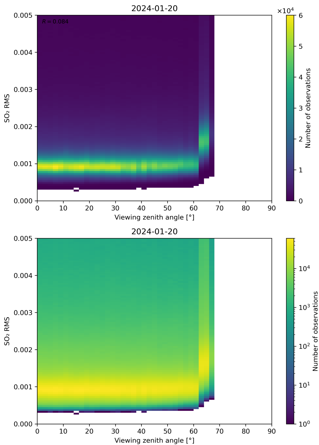
Figure 313: Scatter density plot of “Viewing zenith angle” against “SO 2 RMS” for 2024-01-19 to 2024-01-21.
