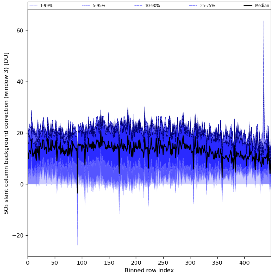
Figure 90: Along track statistics of “SO 2 slant column background correction (window 3)” for 2024-01-19 to 2024-01-21
