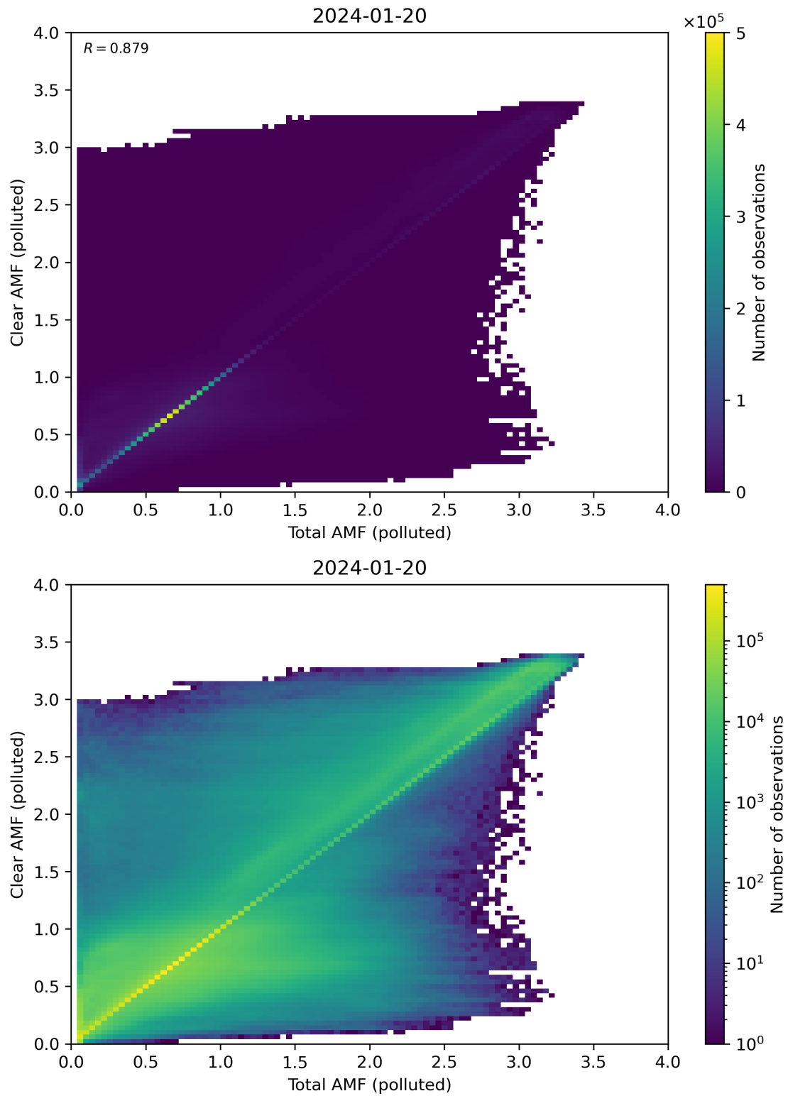
Figure 271: Scatter density plot of “Total AMF (polluted)” against “Clear AMF (polluted)” for 2024-01-19 to 2024-01-21.
