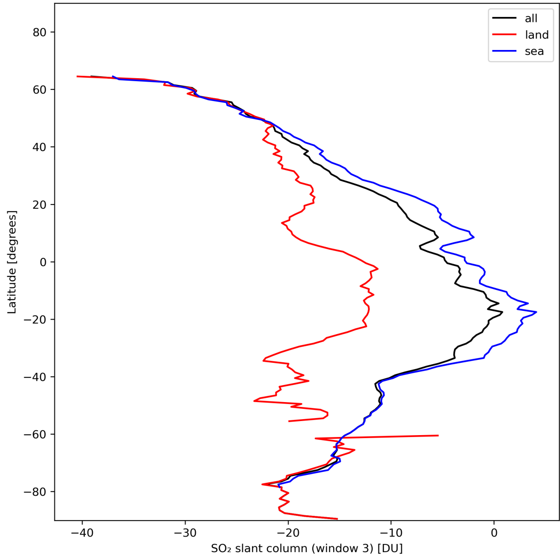
Figure 41: Zonal average of “SO 2 slant column (window 3)” for 2024-01-19 to 2024-01-21.
