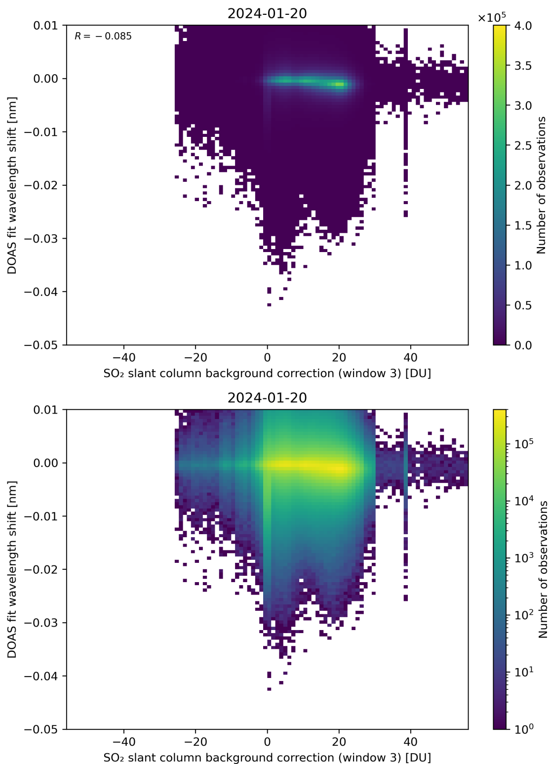
Figure 121: Scatter density plot of “SO 2 slant column background correction (window 3)” against “DOAS fit wavelength shift” for 2024-01-19 to 2024-01-21.
