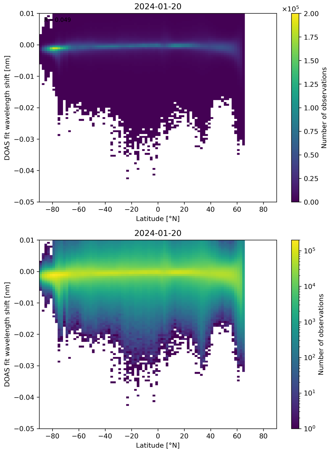
Figure 142: Scatter density plot of “Latitude” against “DOAS fit wavelength shift” for 2024-01-19 to 2024-01-21.
