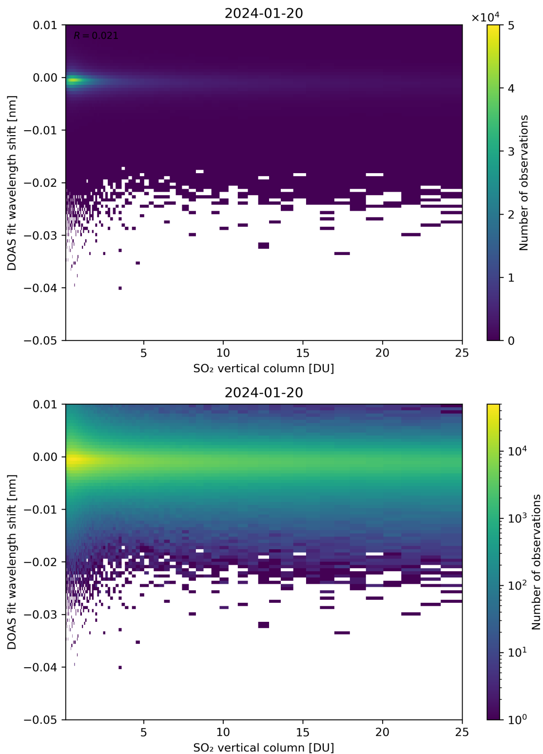
Figure 276: Scatter density plot of “SO 2 vertical column” against “DOAS fit wavelength shift” for 2024-01-19 to 2024-01-21.
