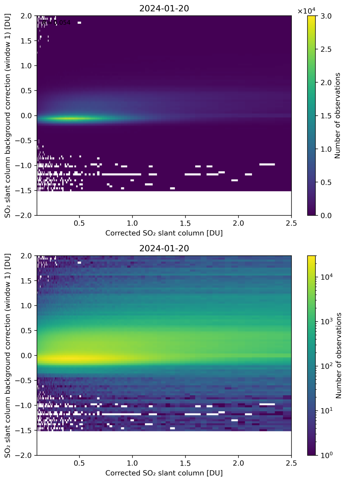
Figure 178: Scatter density plot of “Corrected SO 2 slant column” against “SO 2 slant column background correction (window 1)” for 2024-01-19 to 2024-01-21.
