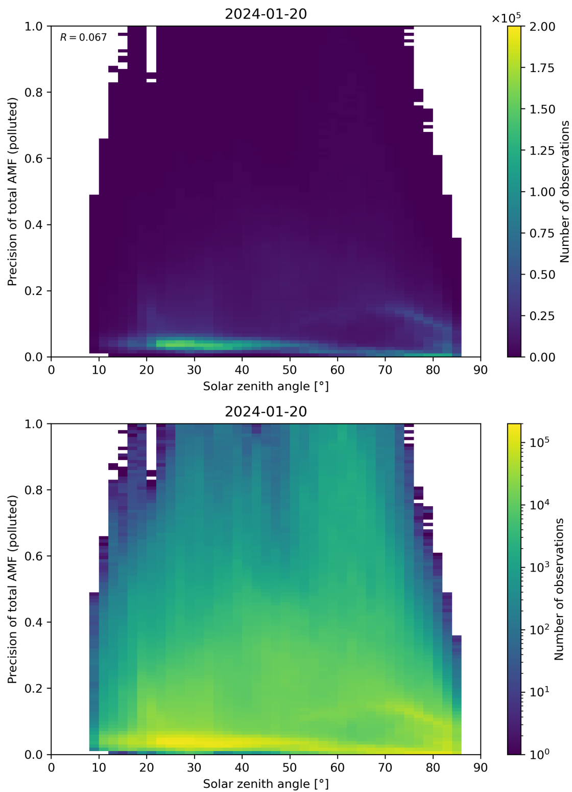
Figure 175: Scatter density plot of “Solar zenith angle” against “Precision of total AMF (polluted)” for 2024-01-19 to 2024-01-21.
