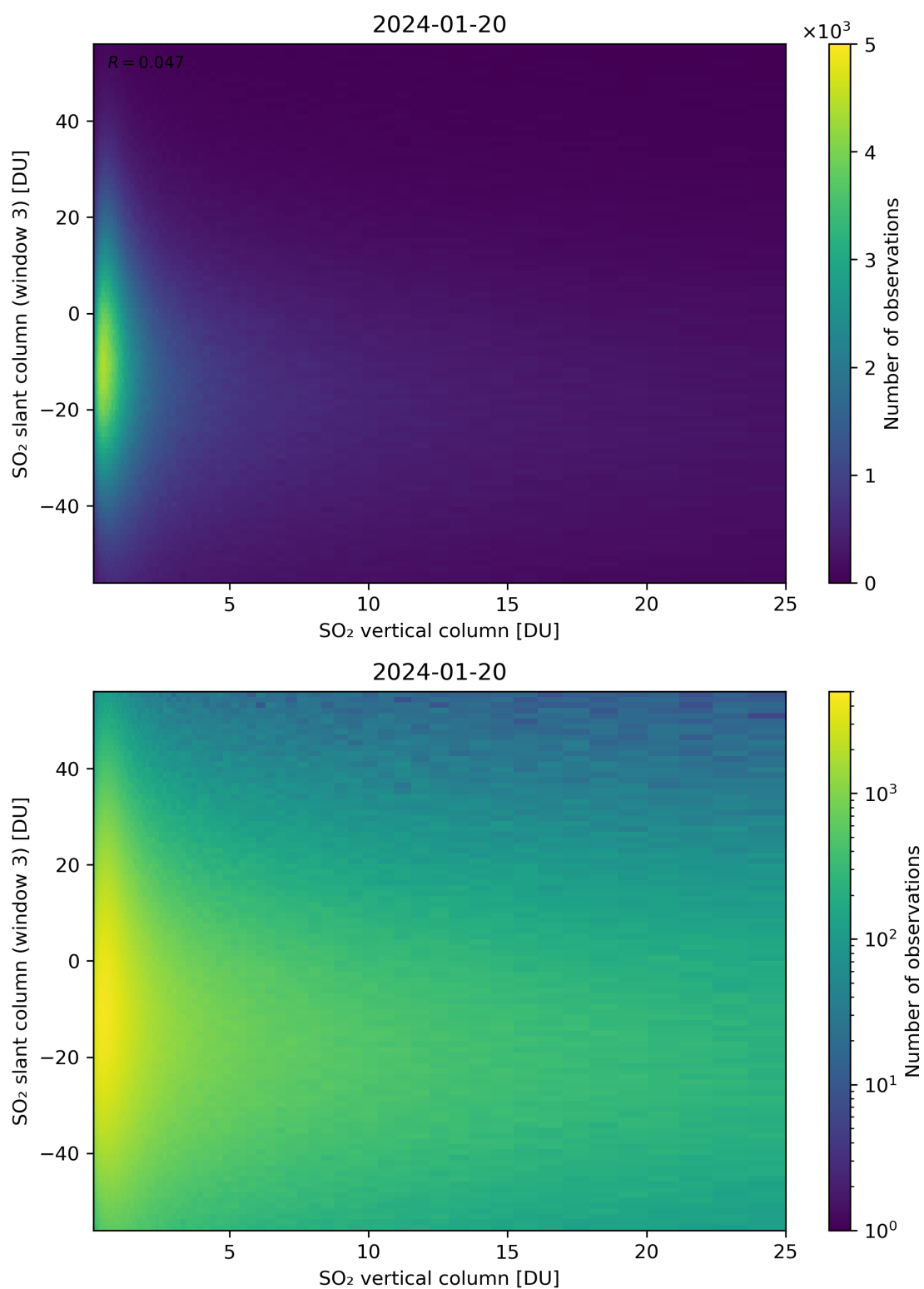
Figure 303: Scatter density plot of “SO 2 vertical column” against “SO 2 slant column (window 3)” for 2024-01-19 to 2024-01-21.
