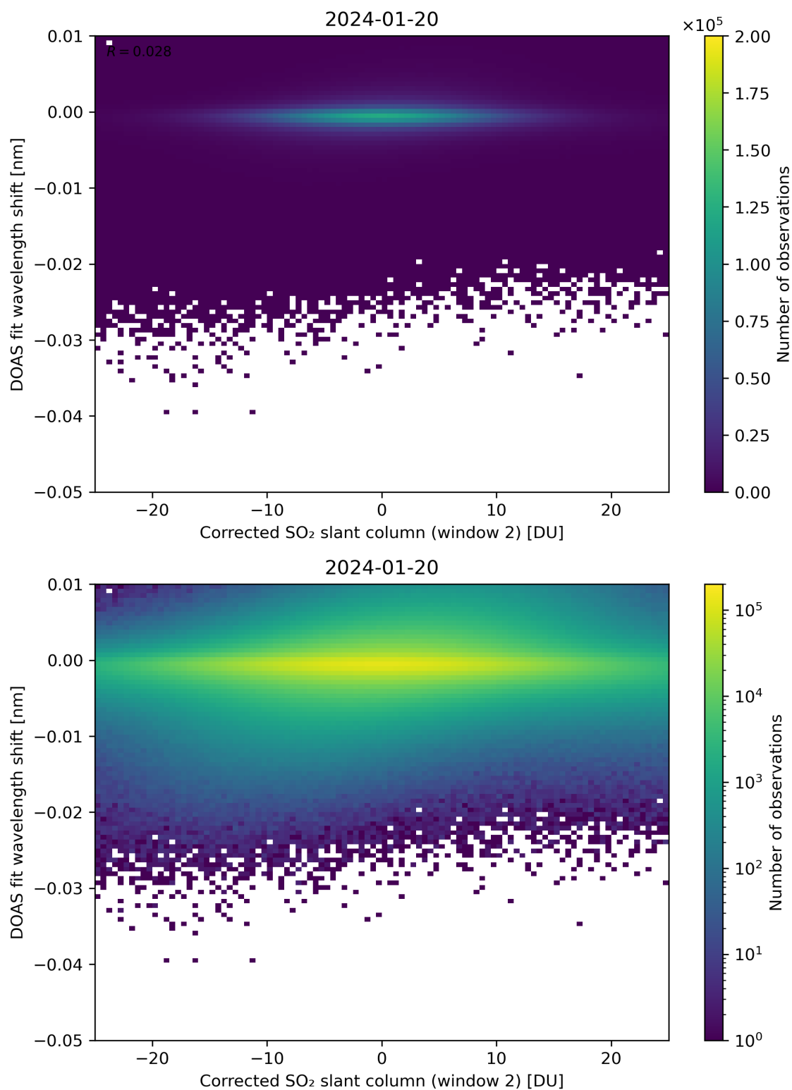
Figure 196: Scatter density plot of “Corrected SO 2 slant column (window 2)” against “DOAS fit wavelength shift” for 2024-01-19 to 2024-01-21.
