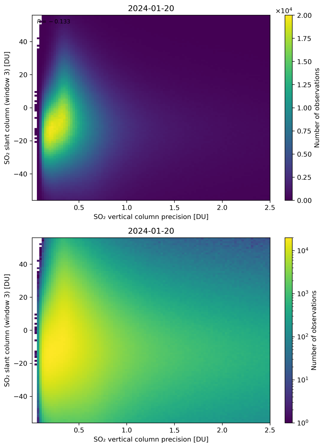
Figure 292: Scatter density plot of “SO 2 vertical column precision” against “SO 2 slant column (window 3)” for 2024-01-19 to 2024-01-21.
