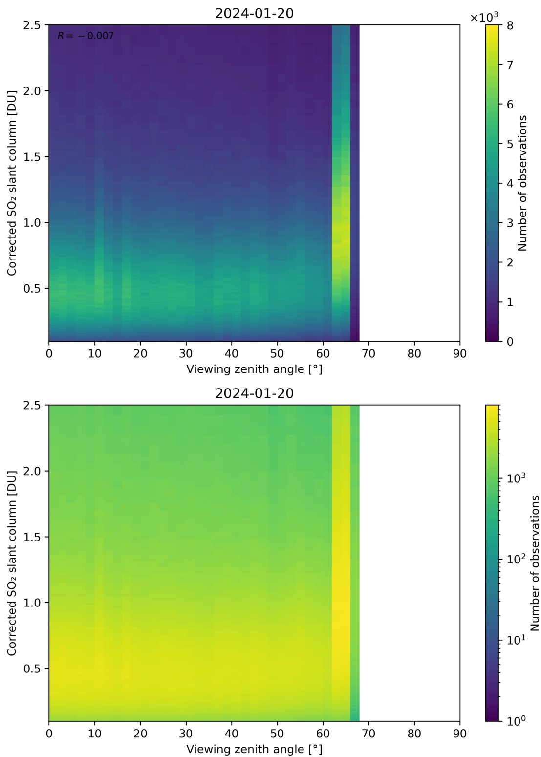
Figure 317: Scatter density plot of “Viewing zenith angle” against “Corrected SO 2 slant column” for 2024-01-19 to 2024-01-21.
