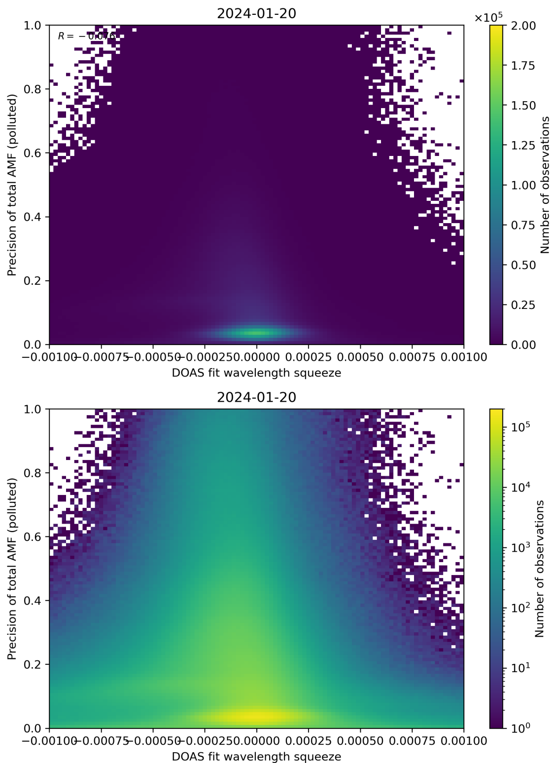
Figure 135: Scatter density plot of “DOAS fit wavelength squeeze” against “Precision of total AMF (polluted)” for 2024-01-19 to 2024-01-21.
