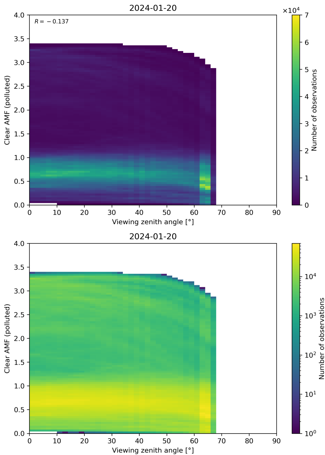
Figure 316: Scatter density plot of “Viewing zenith angle” against “Clear AMF (polluted)” for 2024-01-19 to 2024-01-21.
