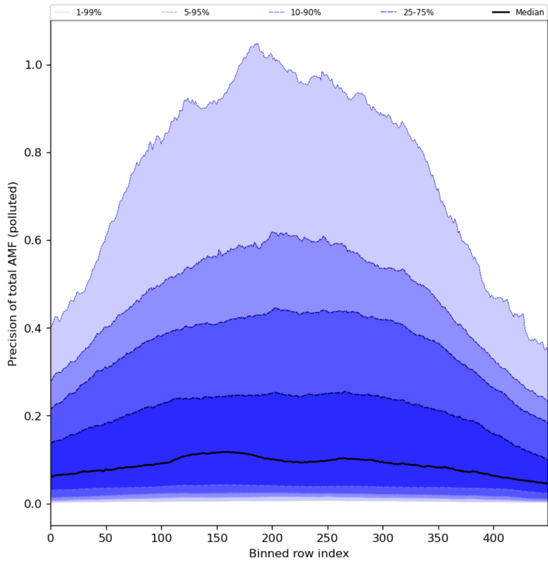
Figure 95: Along track statistics of “Precision of total AMF (polluted)” for 2024-01-19 to 2024-01-21
