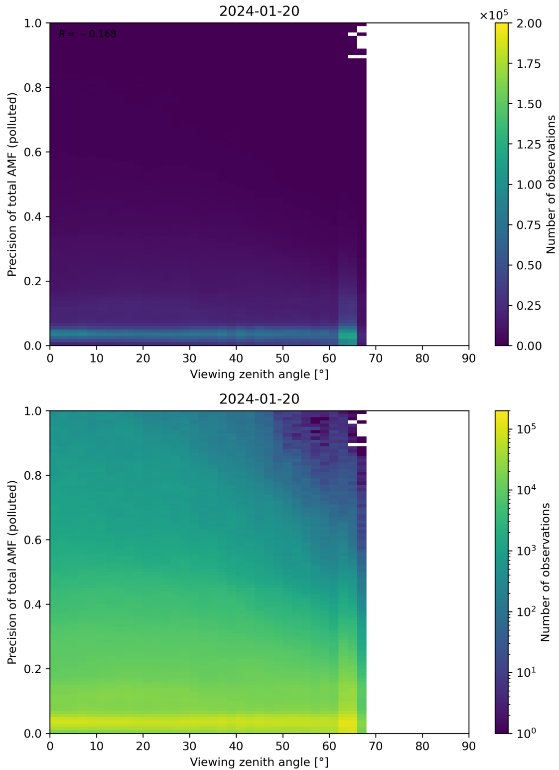
Figure 326: Scatter density plot of “Viewing zenith angle” against “Precision of total AMF (polluted)” for 2024-01-19 to 2024-01-21.
