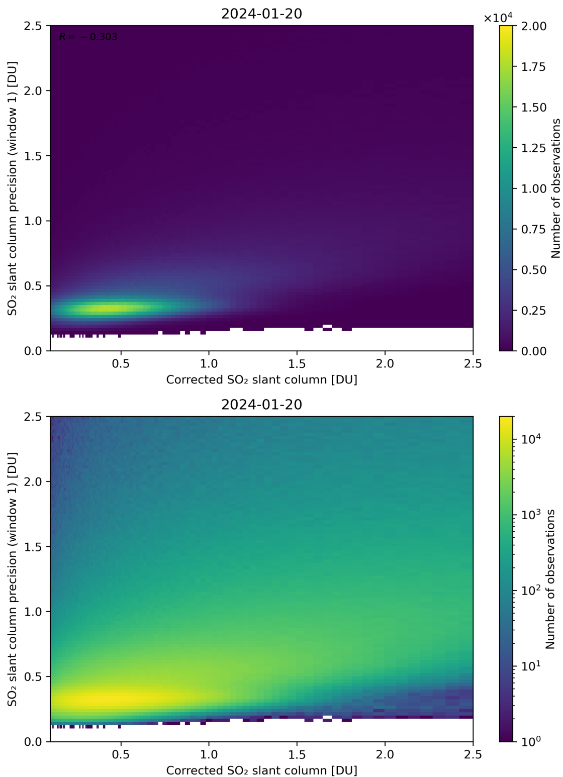
Figure 188: Scatter density plot of “Corrected SO 2 slant column” against “SO 2 slant column precision (window 1)” for 2024-01-19 to 2024-01-21.
