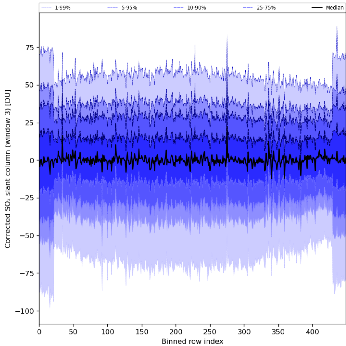
Figure 89: Along track statistics of “Corrected SO 2 slant column (window 3)” for 2024-01-19 to 2024-01-21
