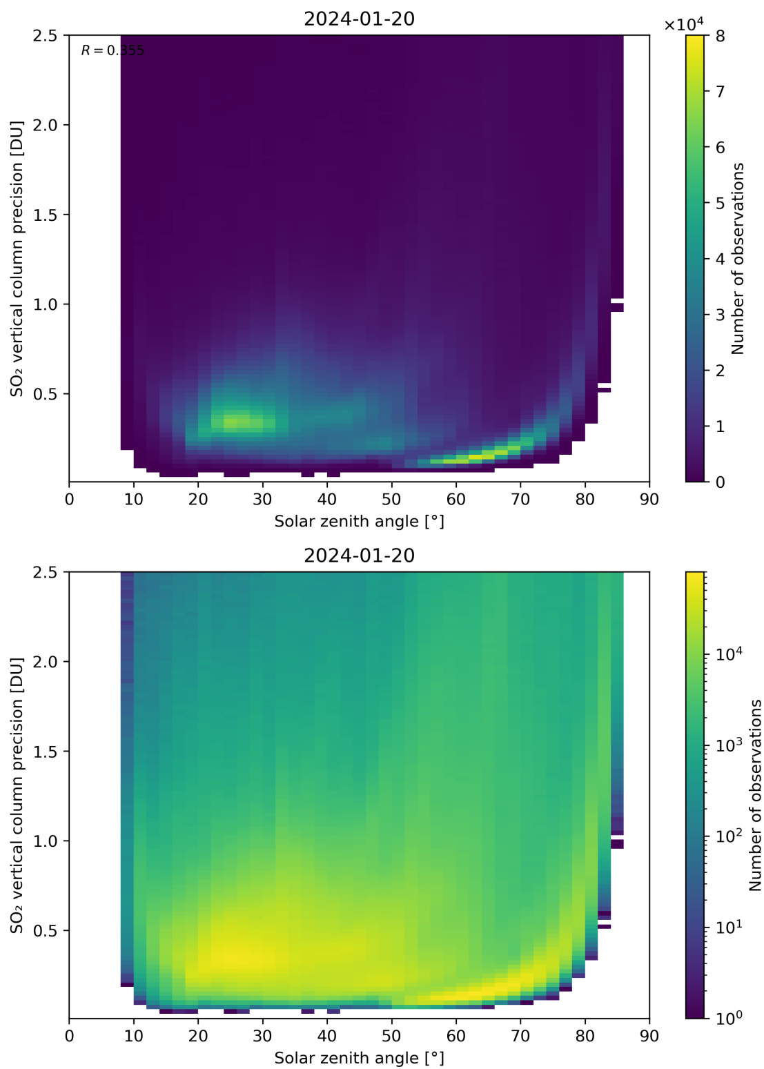
Figure 177: Scatter density plot of “Solar zenith angle” against “SO 2 vertical column precision” for 2024-01-19 to 2024-01-21.
