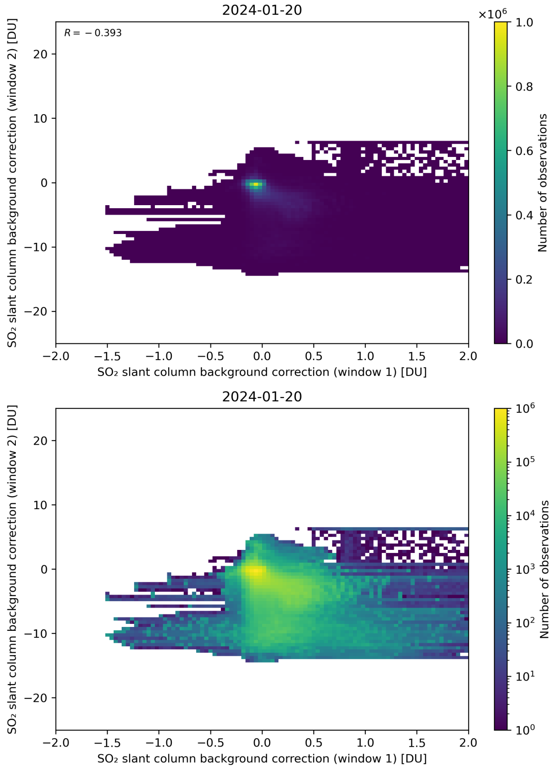
Figure 98: Scatter density plot of “SO 2 slant column background correction (window 1)” against “SO 2 slant column background correction (window 2)” for 2024-01-19 to 2024-01-21.
