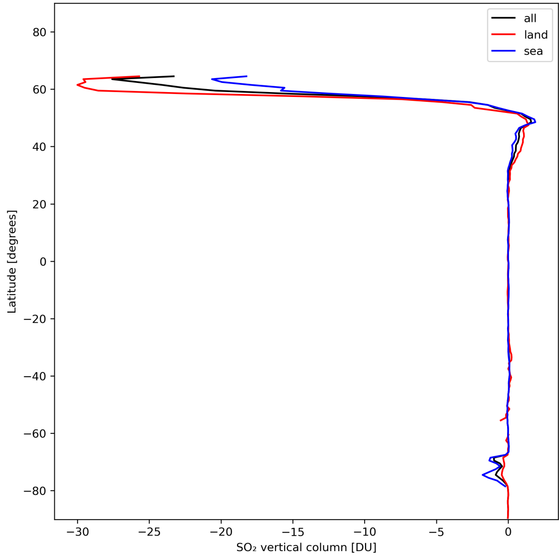
Figure 30: Zonal average of “SO 2 vertical column” for 2024-01-19 to 2024-01-21.
