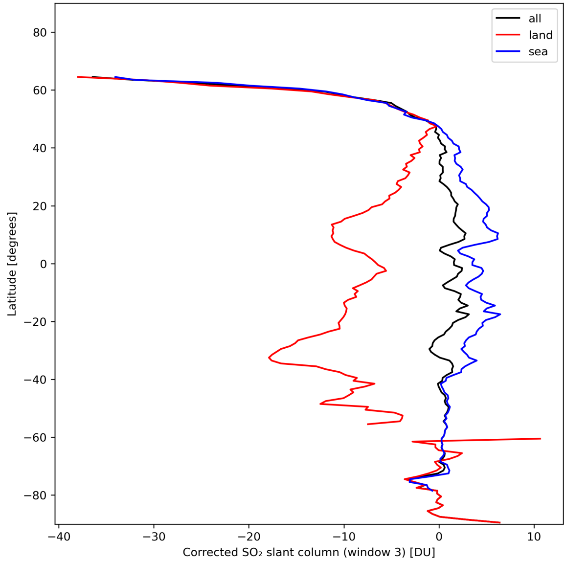
Figure 43: Zonal average of “Corrected SO 2 slant column (window 3)” for 2024-01-19 to 2024-01-21.
