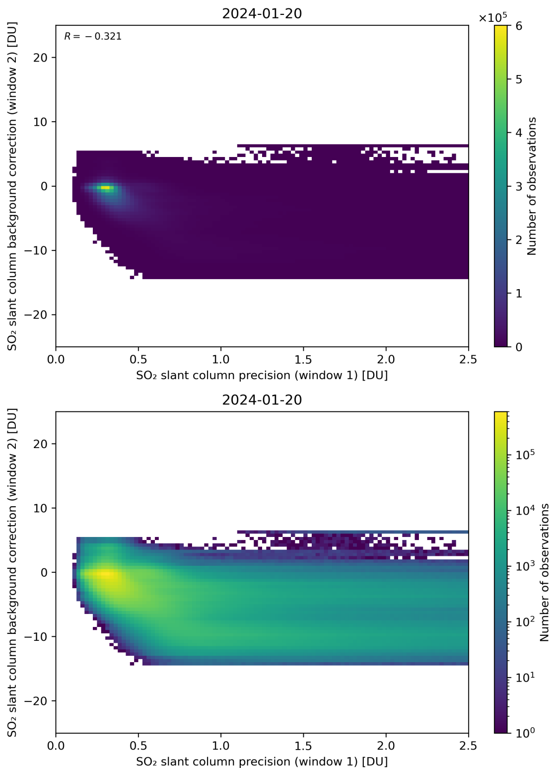
Figure 219: Scatter density plot of “SO 2 slant column precision (window 1)” against “SO 2 slant column background correction (window 2)” for 2024-01-19 to 2024-01-21.
