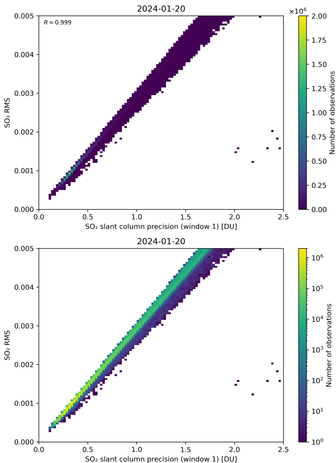
Figure 223: Scatter density plot of “SO 2 slant column precision (window 1)” against “SO 2 RMS” for 2024-01-19 to 2024-01-21.
