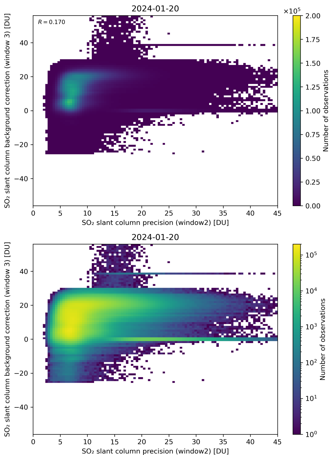
Figure 242: Scatter density plot of “SO 2 slant column precision (window2)” against “SO 2 slant column background correction (window 3)” for 2024-01-19 to 2024-01-21.
