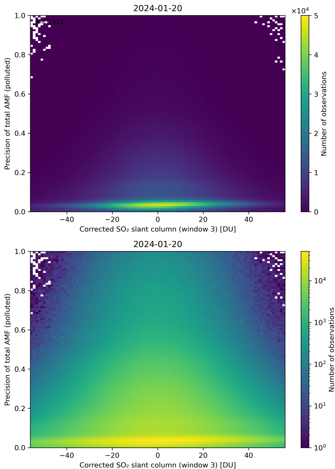
Figure 211: Scatter density plot of “Corrected SO 2 slant column (window 3)” against “Precision of total AMF (polluted)” for 2024-01-19 to 2024-01-21.
