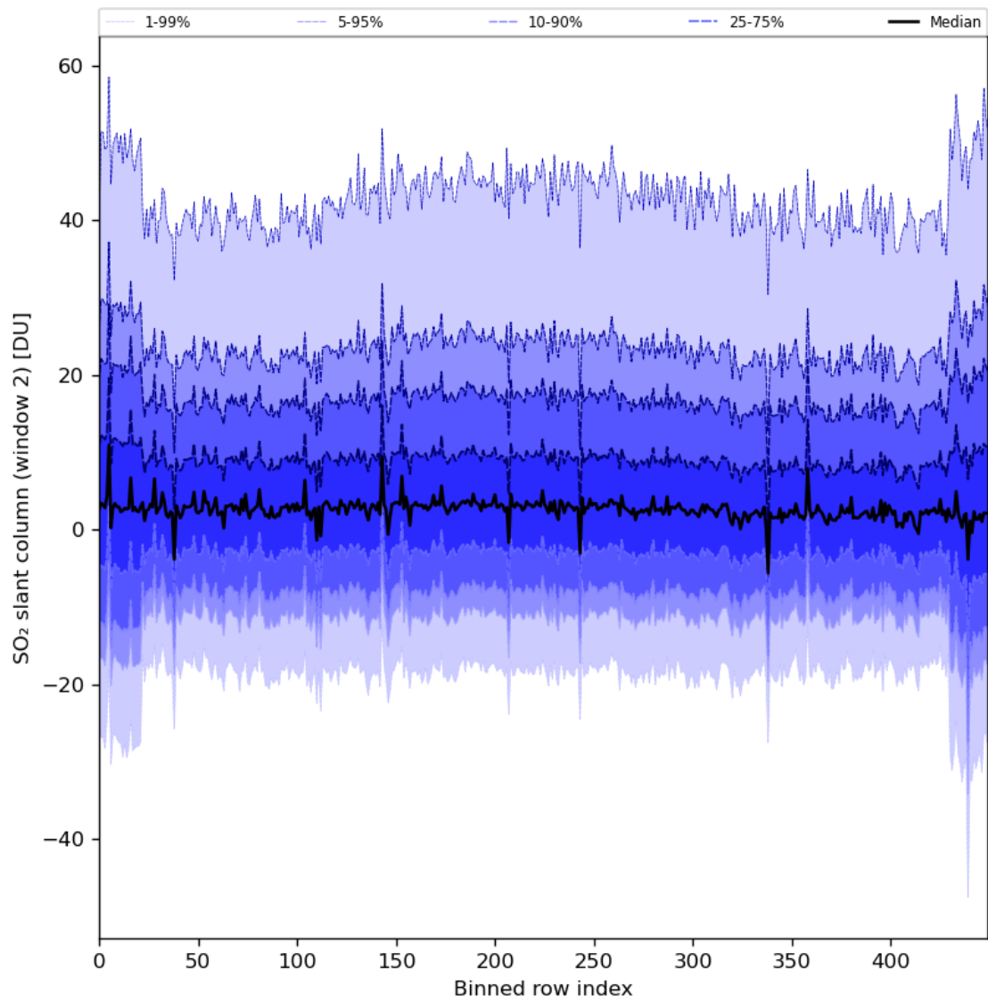
Figure 83: Along track statistics of “SO 2 slant column (window 2)” for 2024-01-19 to 2024-01-21
