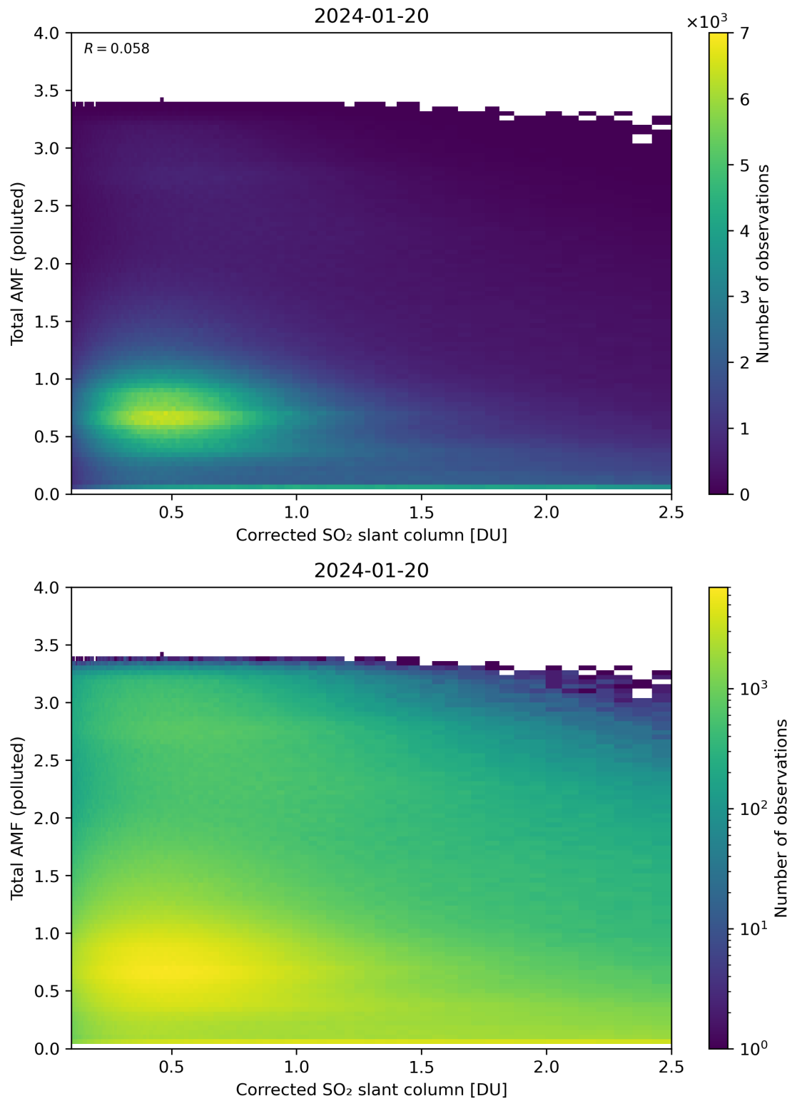
Figure 192: Scatter density plot of “Corrected SO 2 slant column” against “Total AMF (polluted)” for 2024-01-19 to 2024-01-21.
