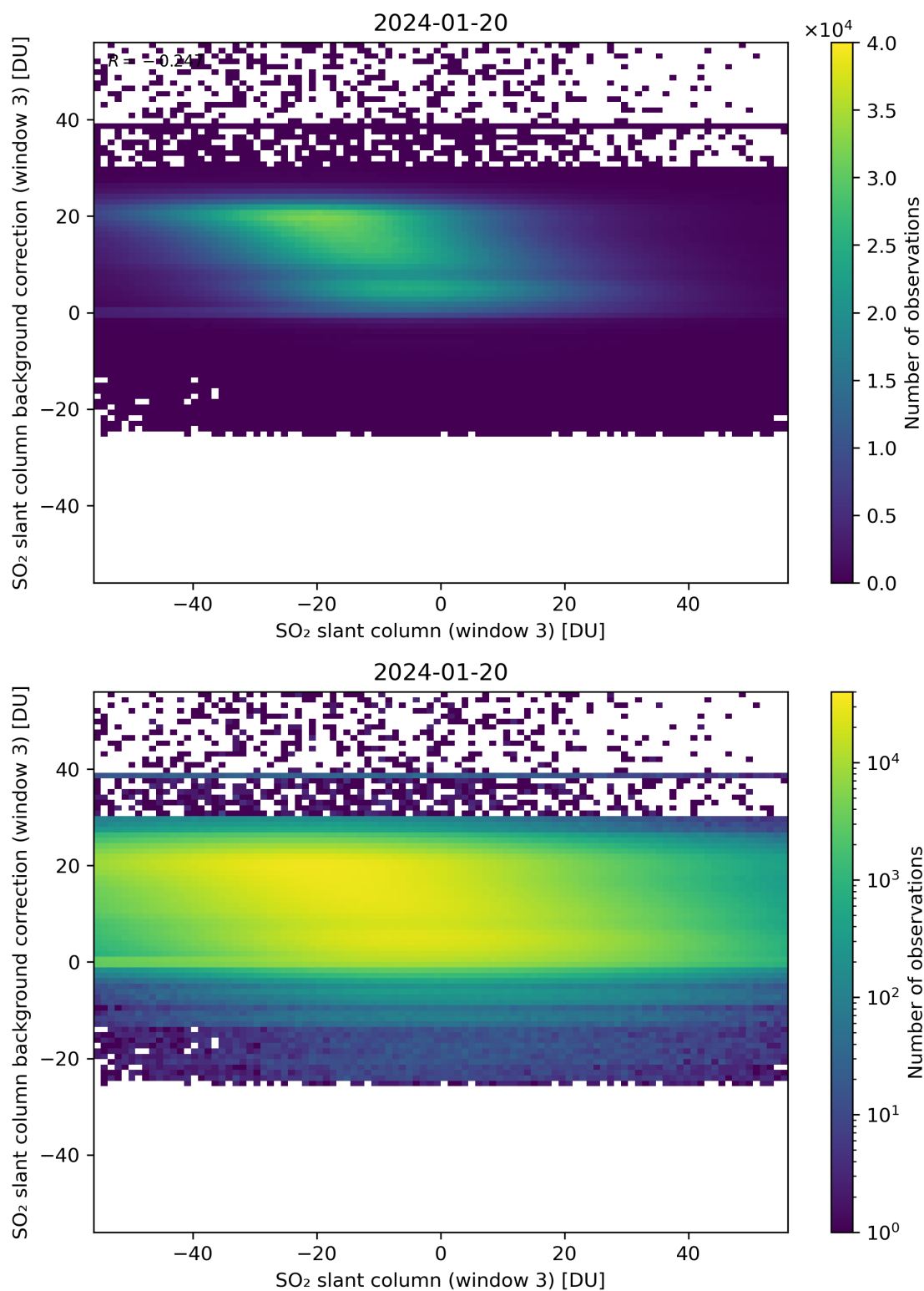
Figure 253: Scatter density plot of “SO 2 slant column (window 3)” against “SO 2 slant column background correction (window 3)” for 2024-01-19 to 2024-01-21.
