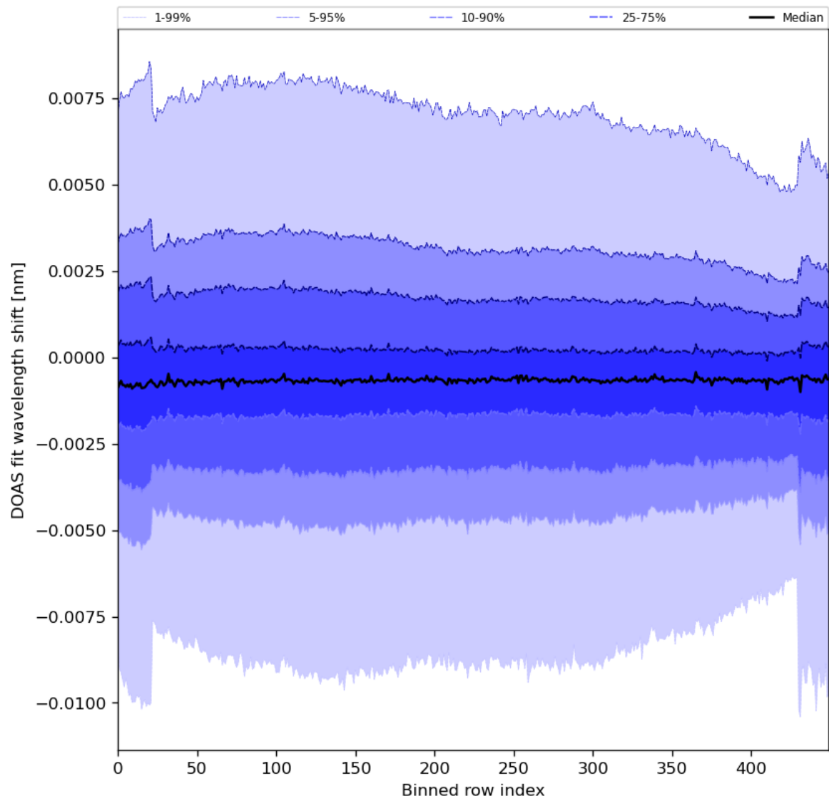
Figure 91: Along track statistics of “DOAS fit wavelength shift” for 2024-01-19 to 2024-01-21
