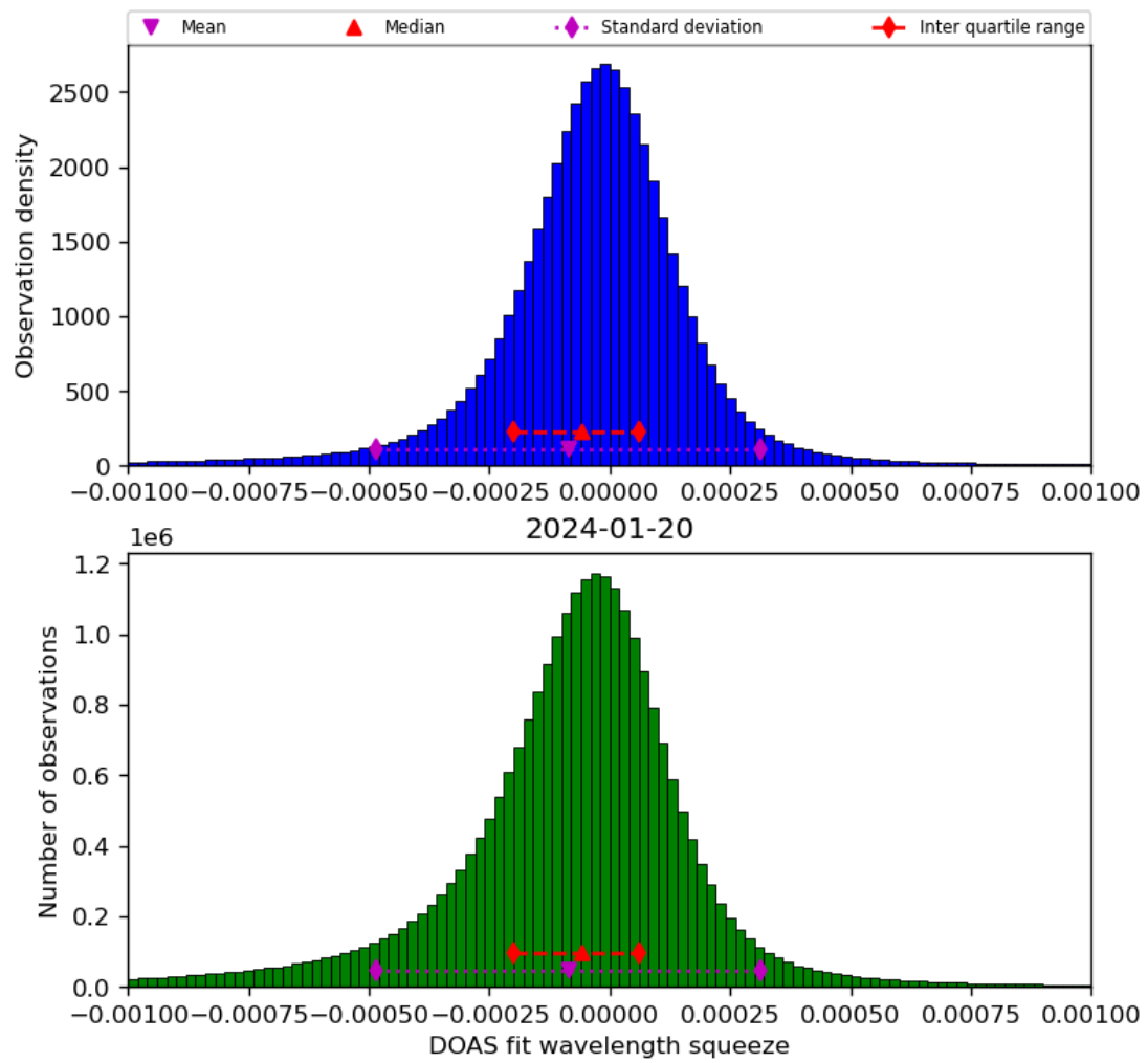
Figure 69: Histogram of “DOAS fit wavelength squeeze” for 2024-01-19 to 2024-01-21
