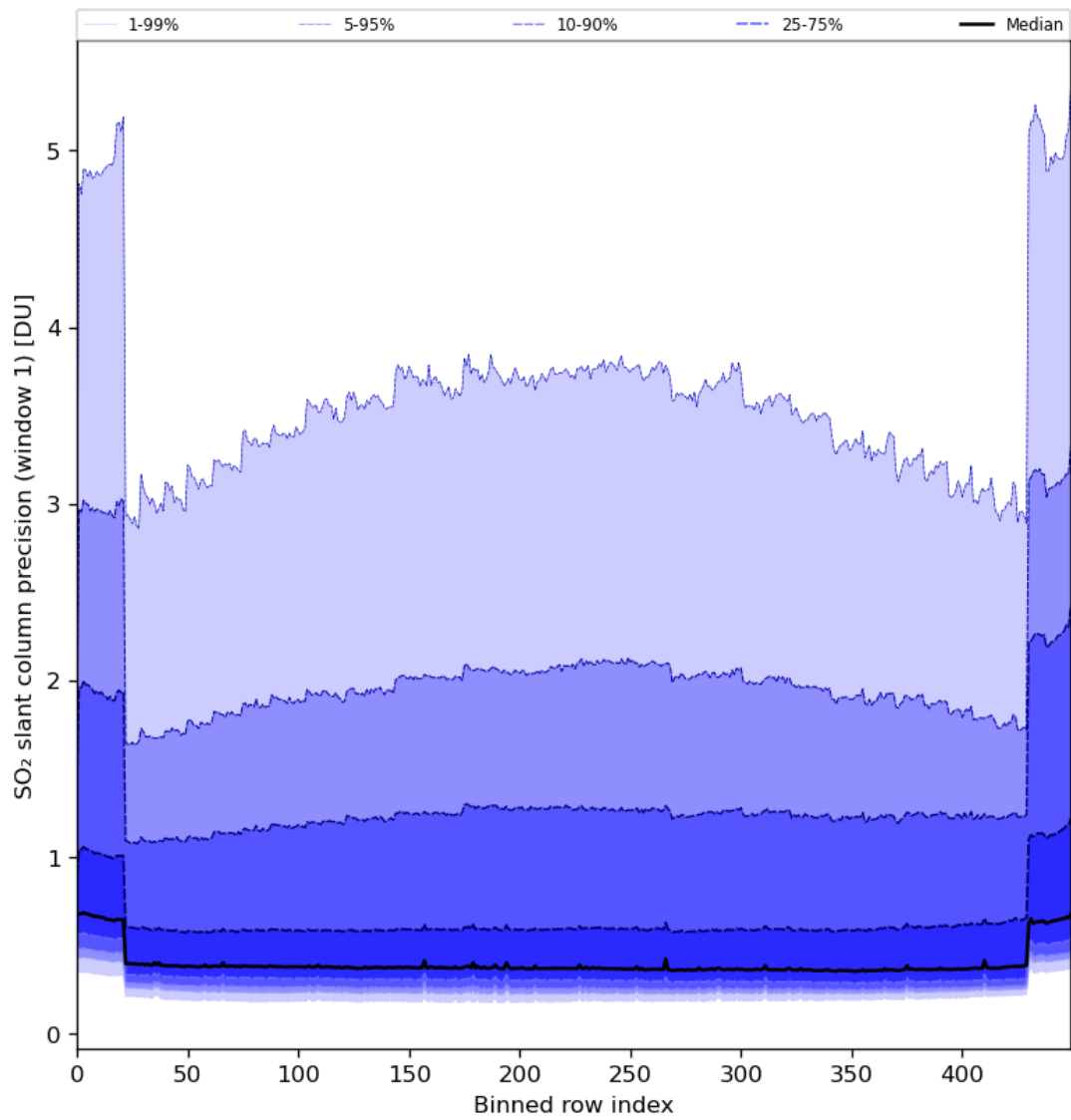
Figure 80: Along track statistics of “SO 2 slant column precision (window 1)” for 2024-01-19 to 2024-01-21
