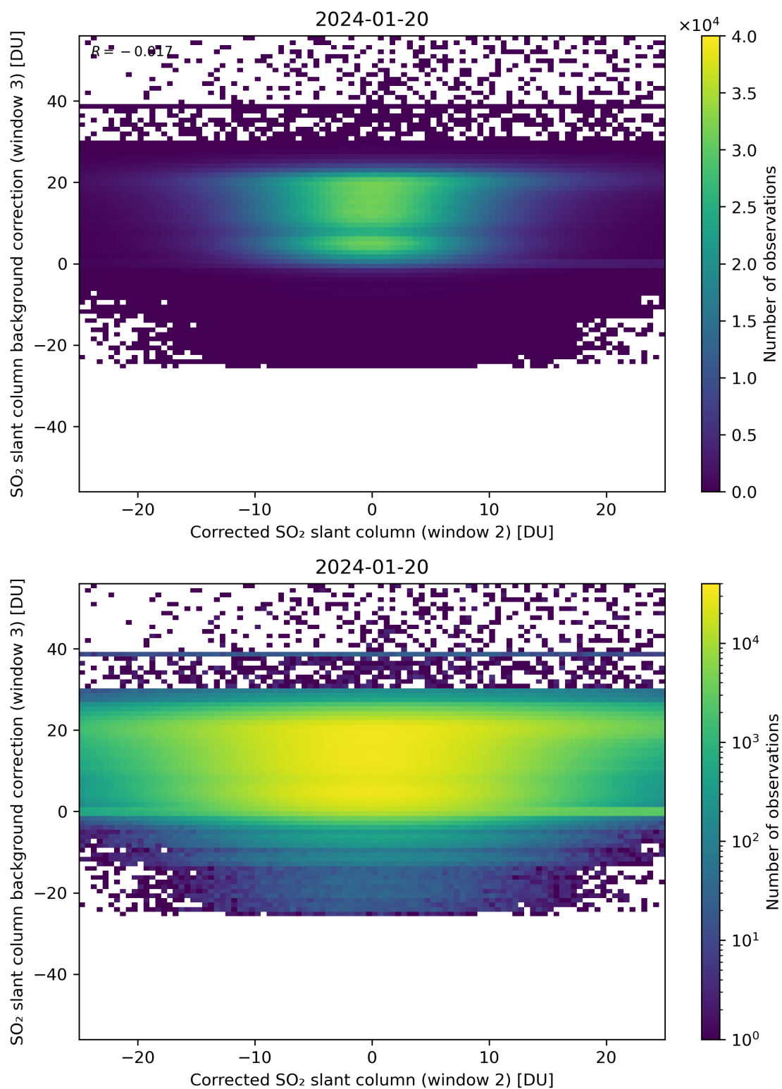
Figure 195: Scatter density plot of “Corrected SO 2 slant column (window 2)” against “SO 2 slant column background correction (window 3)” for 2024-01-19 to 2024-01-21.
