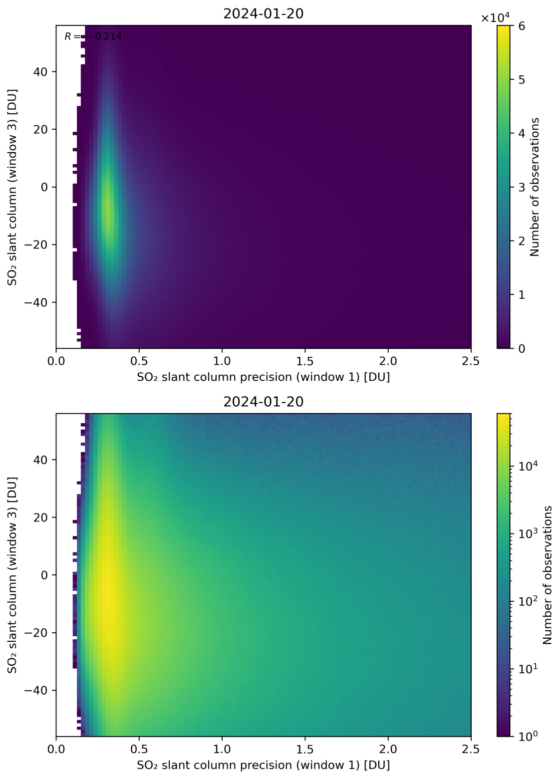
Figure 228: Scatter density plot of “SO 2 slant column precision (window 1)” against “SO 2 slant column (window 3)” for 2024-01-19 to 2024-01-21.
