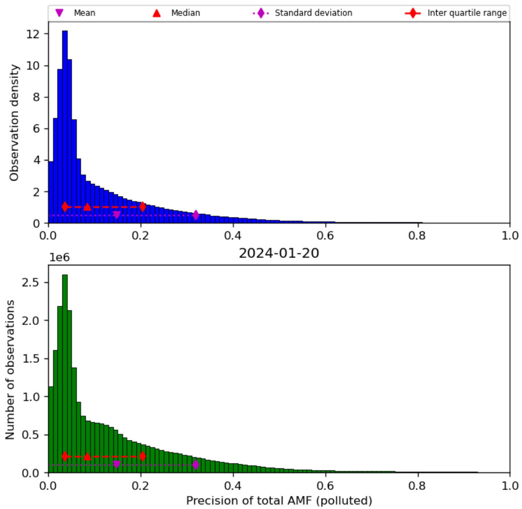
Figure 72: Histogram of “Precision of total AMF (polluted)” for 2024-01-19 to 2024-01-21
