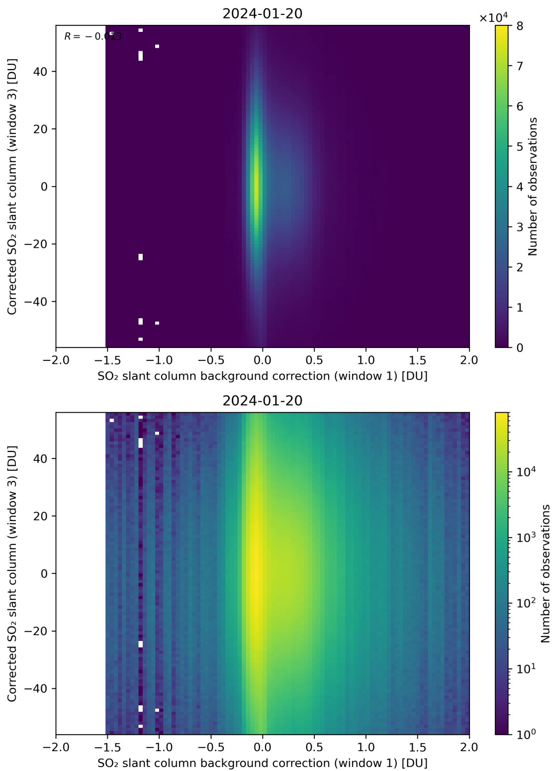
Figure 105: Scatter density plot of “SO 2 slant column background correction (window 1)” against “Corrected SO 2 slant column (window 3)” for 2024-01-19 to 2024-01-21.
