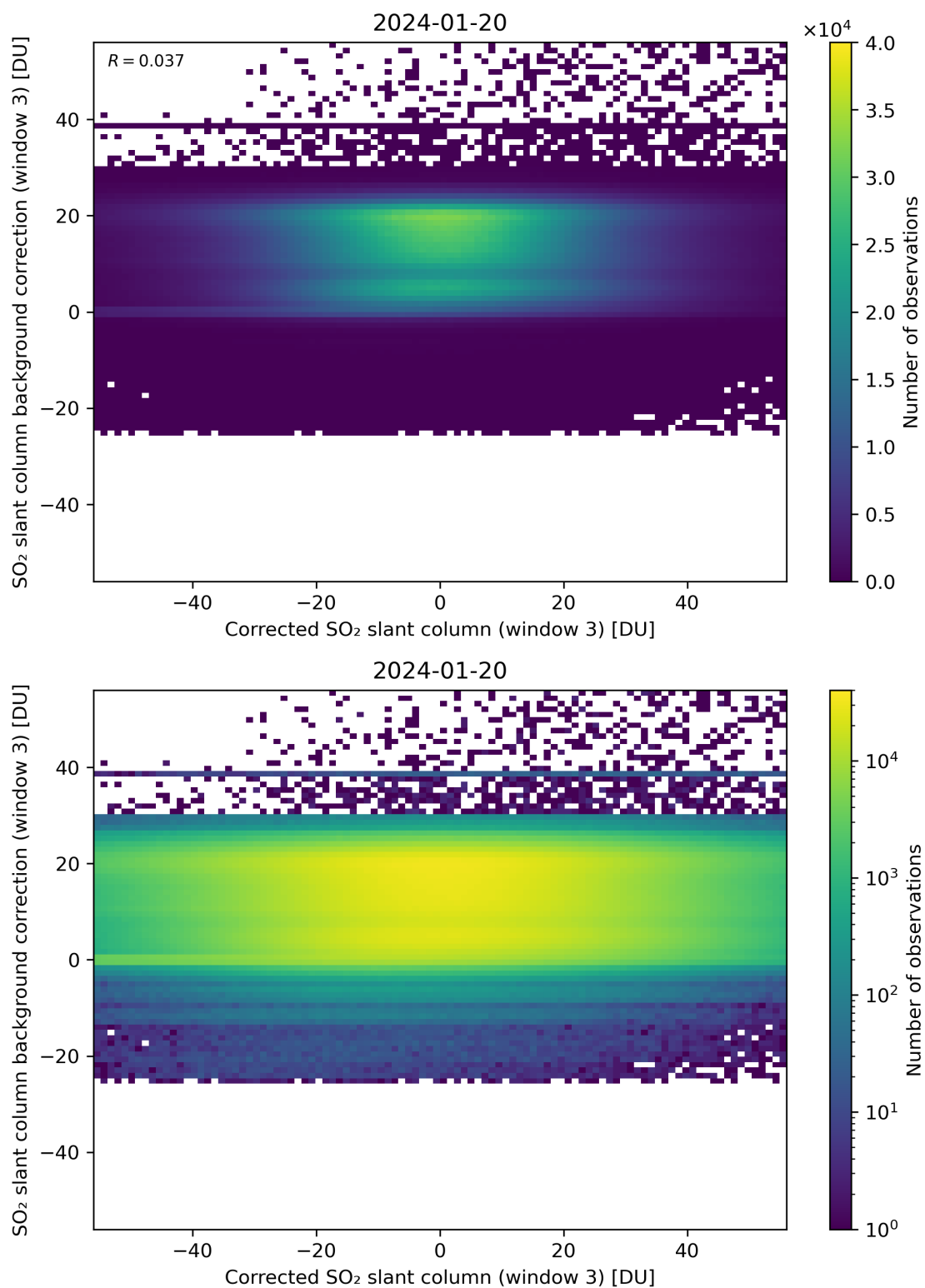
Figure 205: Scatter density plot of “Corrected SO 2 slant column (window 3)” against “SO 2 slant column background correction (window 3)” for 2024-01-19 to 2024-01-21.
