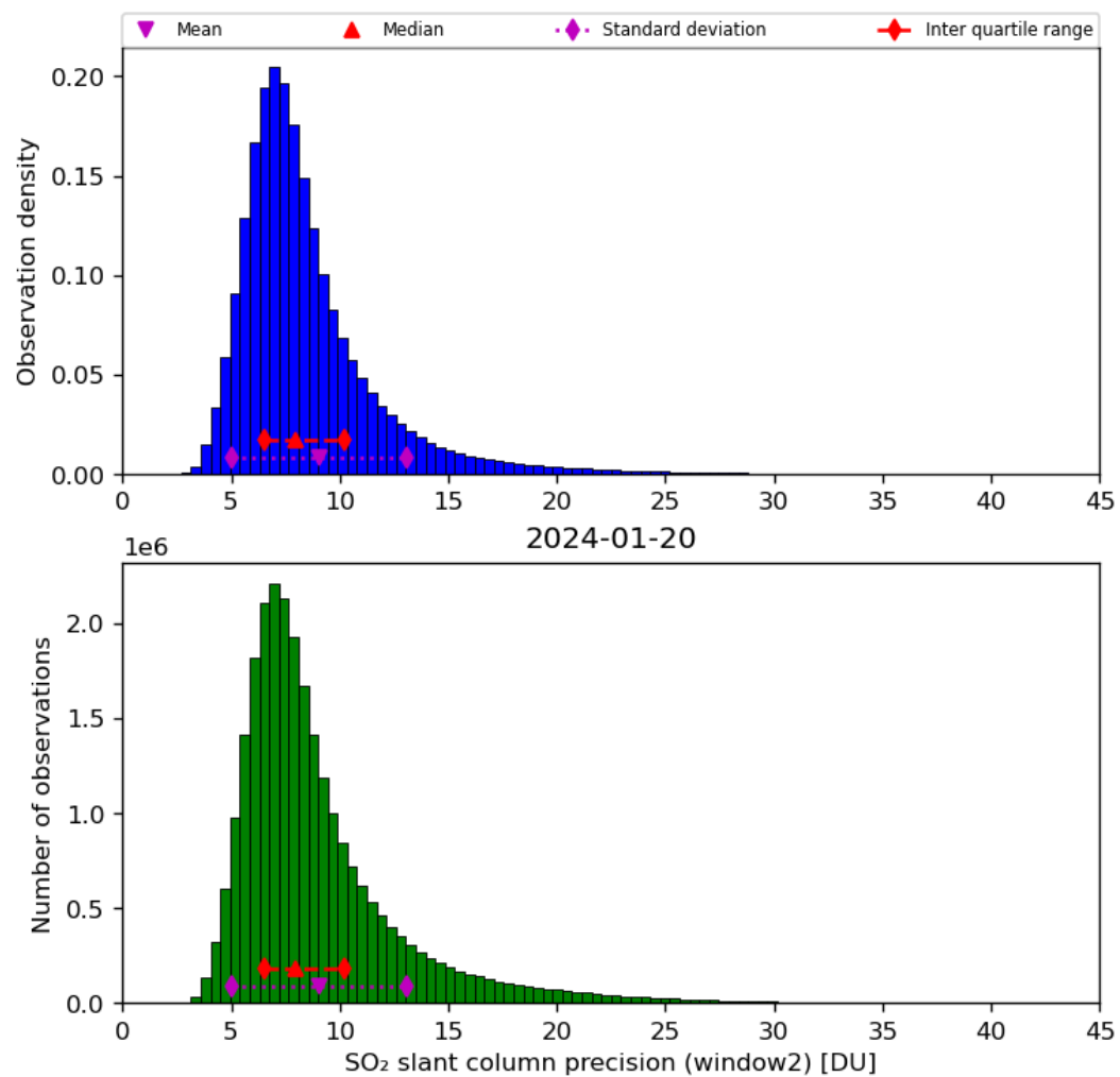
Figure 61: Histogram of “SO 2 slant column precision (window2)” for 2024-01-19 to 2024-01-21
