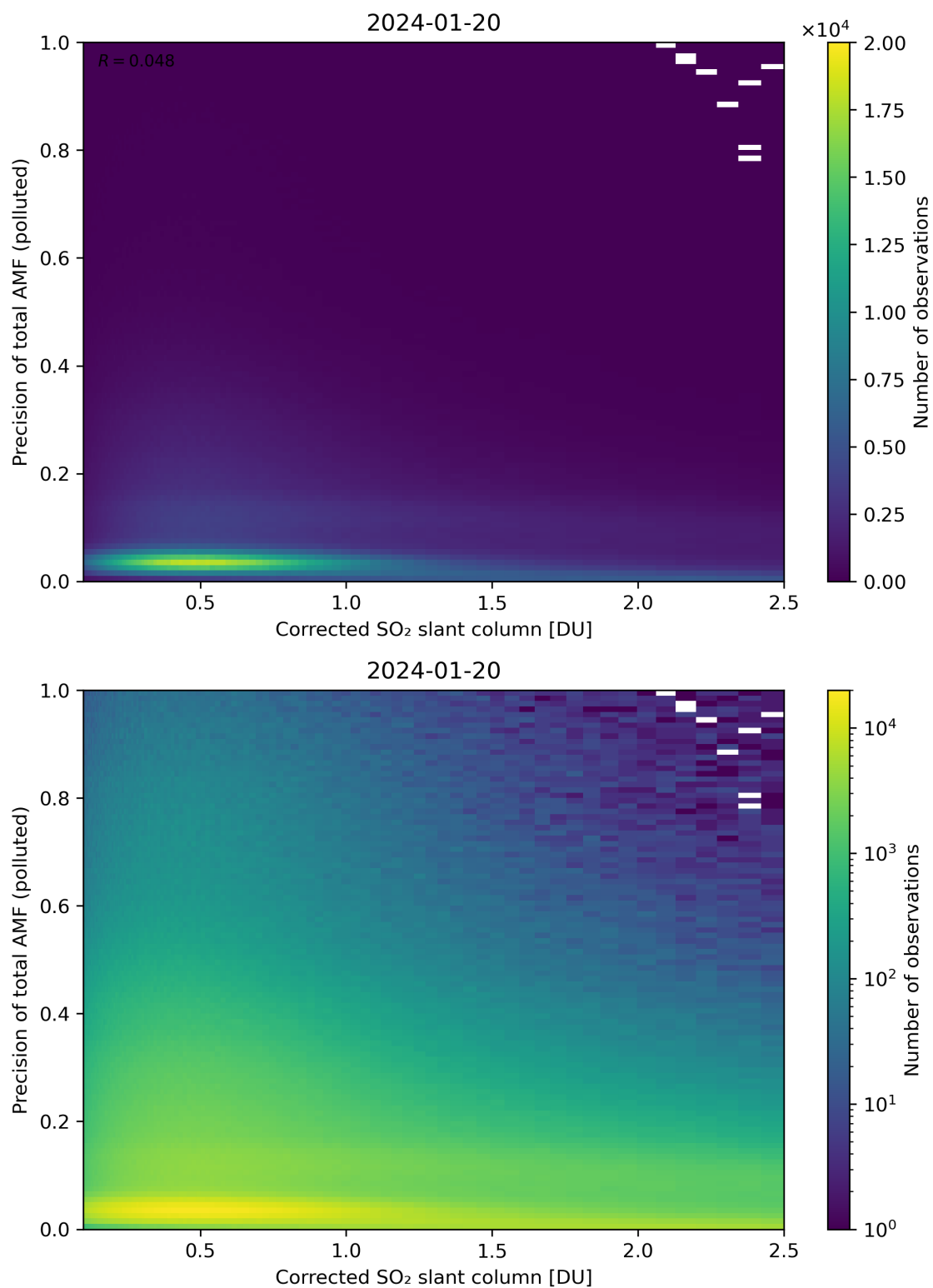
Figure 193: Scatter density plot of “Corrected SO 2 slant column” against “Precision of total AMF (polluted)” for 2024-01-19 to 2024-01-21.
