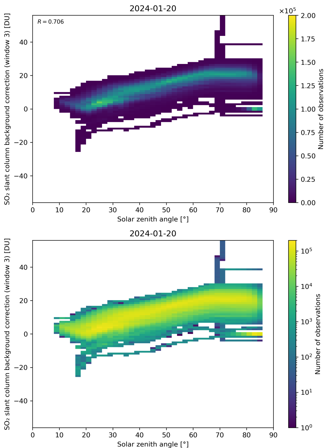
Figure 160: Scatter density plot of “Solar zenith angle” against “SO 2 slant column background correction (window 3)” for 2024-01-19 to 2024-01-21.
