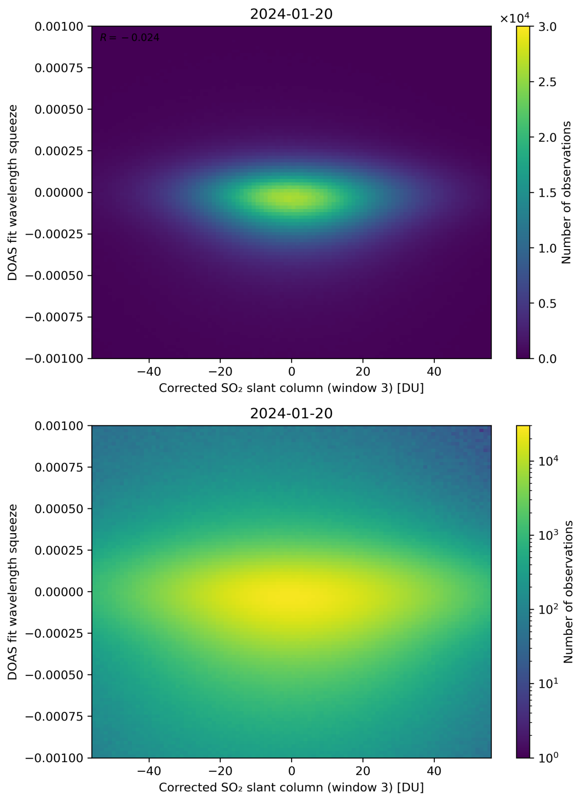
Figure 207: Scatter density plot of “Corrected SO 2 slant column (window 3)” against “DOAS fit wavelength squeeze” for 2024-01-19 to 2024-01-21.
