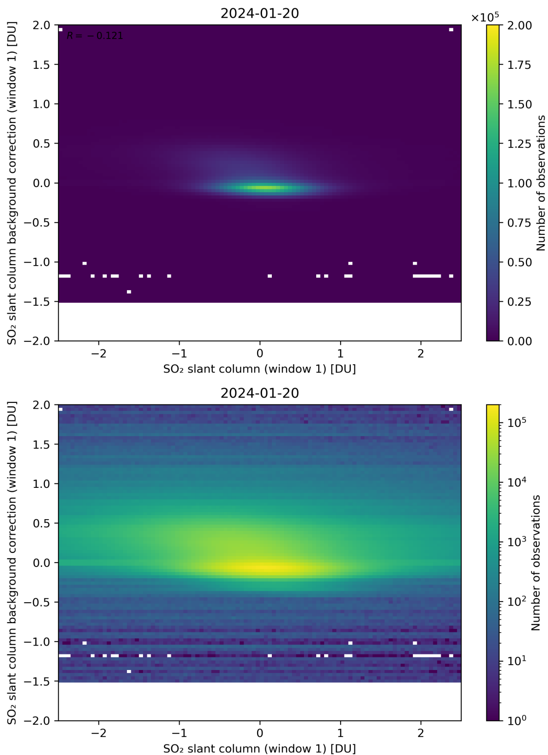
Figure 212: Scatter density plot of “SO 2 slant column (window 1)” against “SO 2 slant column background correction (window 1)” for 2024-01-19 to 2024-01-21.
