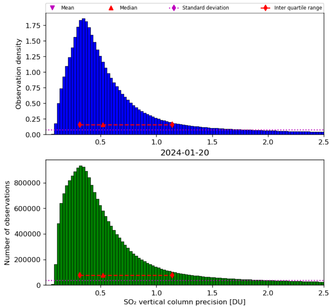
Figure 54: Histogram of “SO 2 vertical column precision” for 2024-01-19 to 2024-01-21
