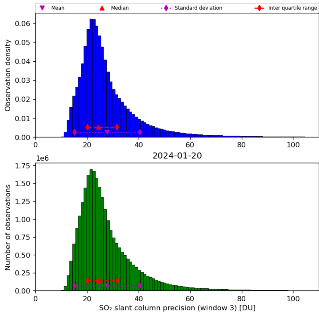
Figure 65: Histogram of “SO 2 slant column precision (window 3)” for 2024-01-19 to 2024-01-21
