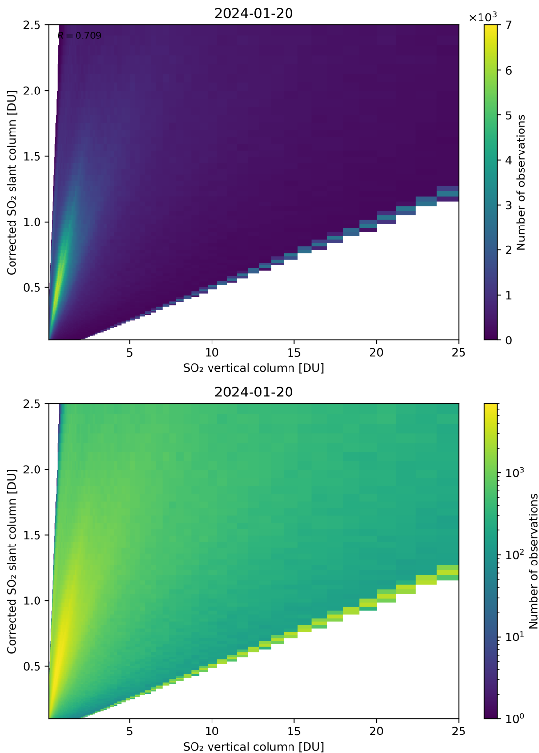
Figure 297: Scatter density plot of “SO 2 vertical column” against “Corrected SO 2 slant column” for 2024-01-19 to 2024-01-21.
