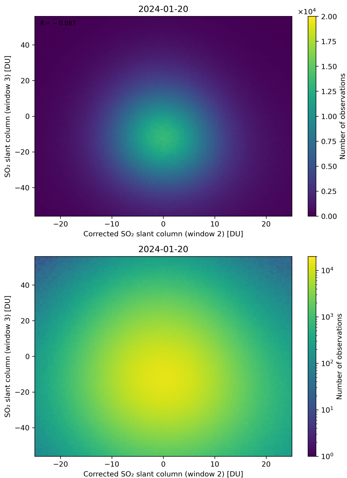
Figure 201: Scatter density plot of “Corrected SO 2 slant column (window 2)” against “SO 2 slant column (window 3)” for 2024-01-19 to 2024-01-21.
