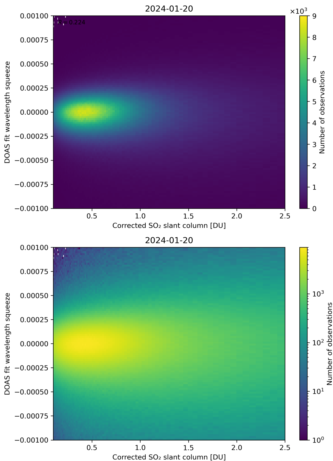
Figure 182: Scatter density plot of “Corrected SO 2 slant column” against “DOAS fit wavelength squeeze” for 2024-01-19 to 2024-01-21.
