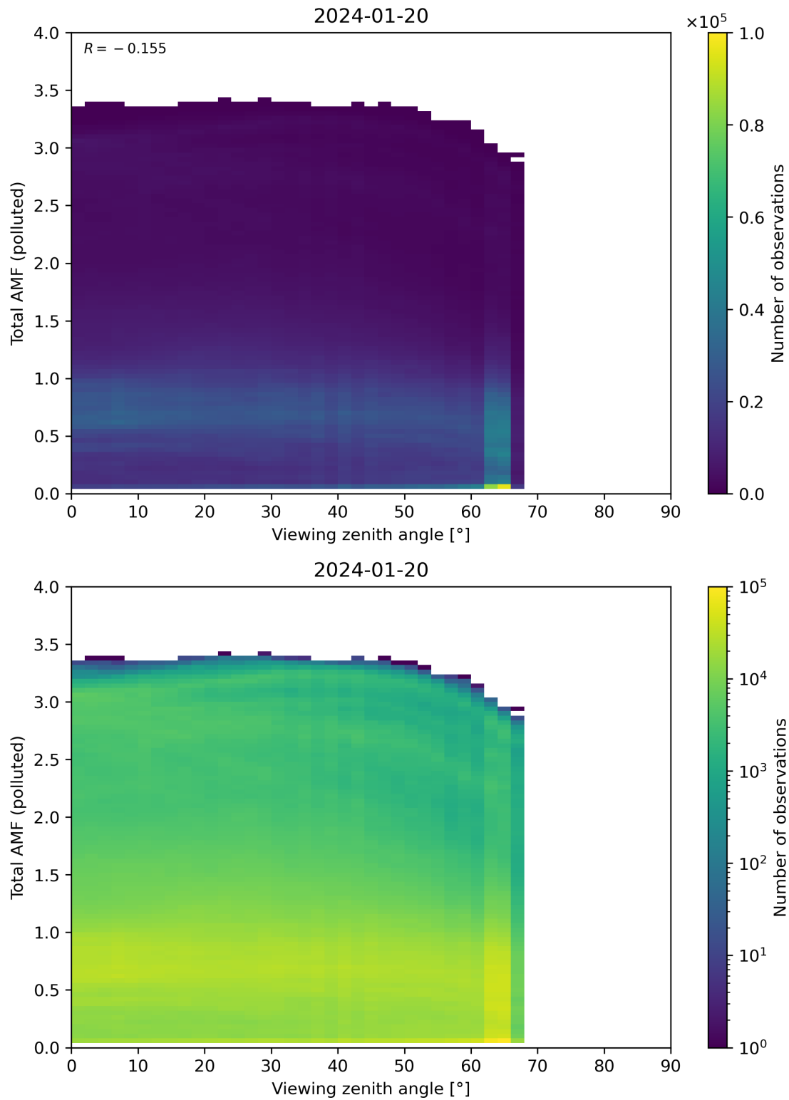
Figure 325: Scatter density plot of “Viewing zenith angle” against “Total AMF (polluted)” for 2024-01-19 to 2024-01-21.
