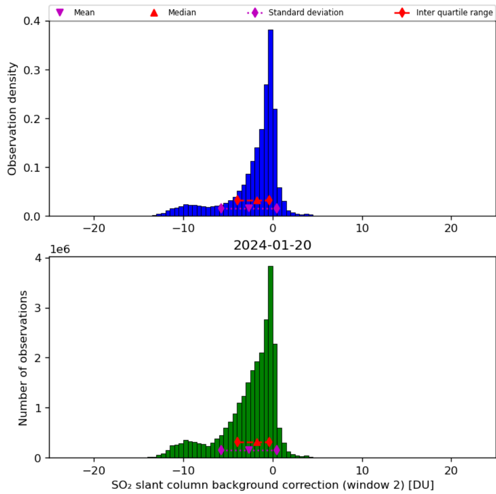
Figure 63: Histogram of “SO 2 slant column background correction (window 2)” for 2024-01-19 to 2024-01-21
