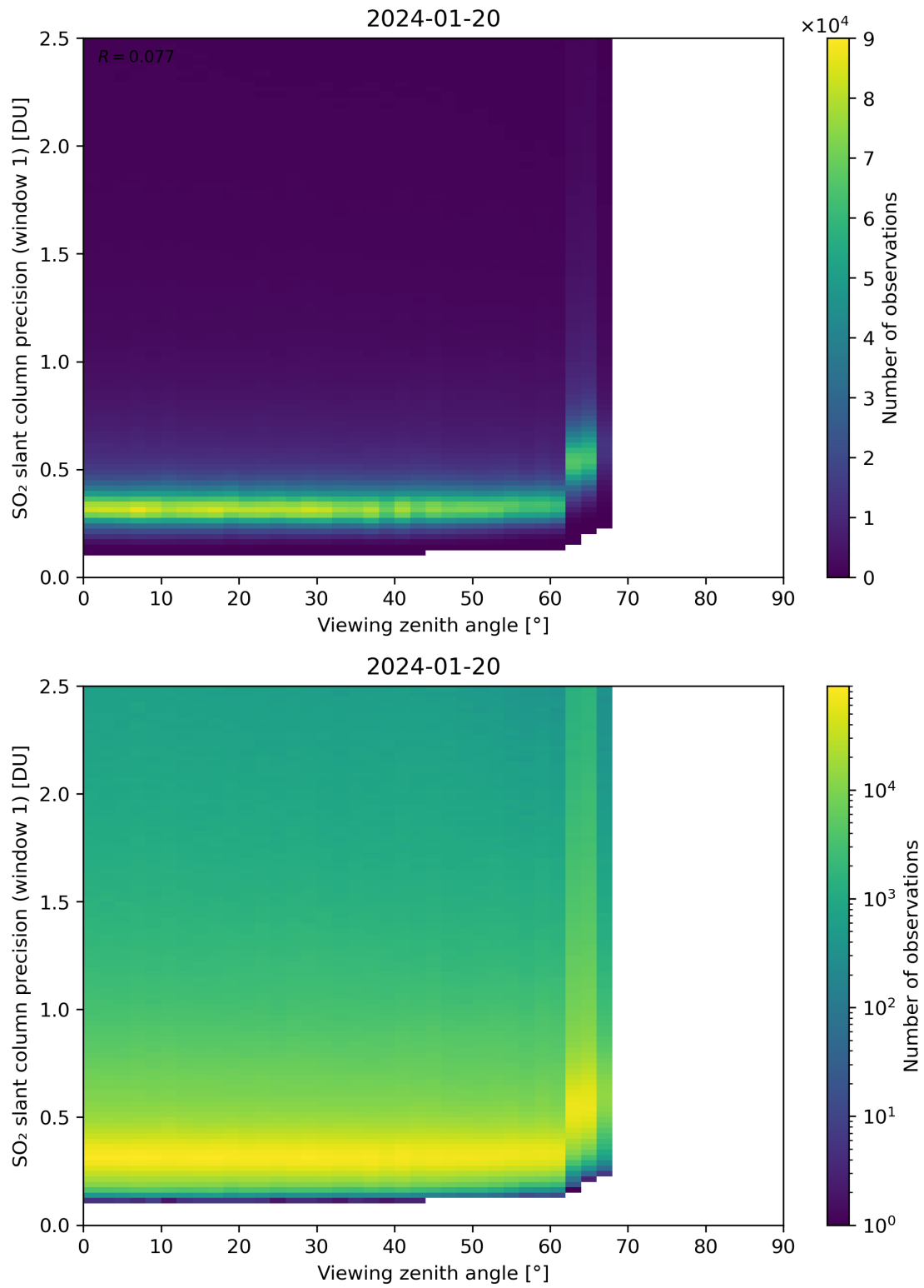
Figure 321: Scatter density plot of “Viewing zenith angle” against “SO 2 slant column precision (window 1)” for 2024-01-19 to 2024-01-21.
