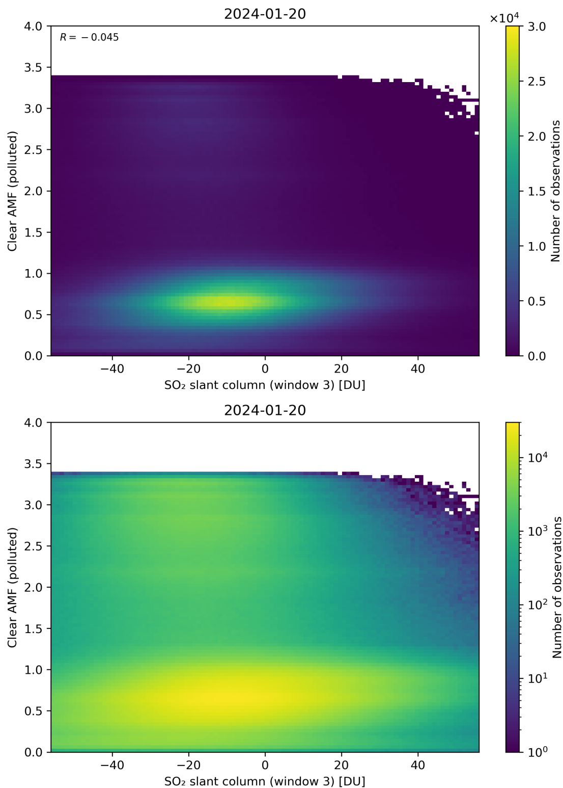
Figure 265: Scatter density plot of “SO 2 slant column (window 3)” against “Clear AMF (polluted)” for 2024-01-19 to 2024-01-21.
