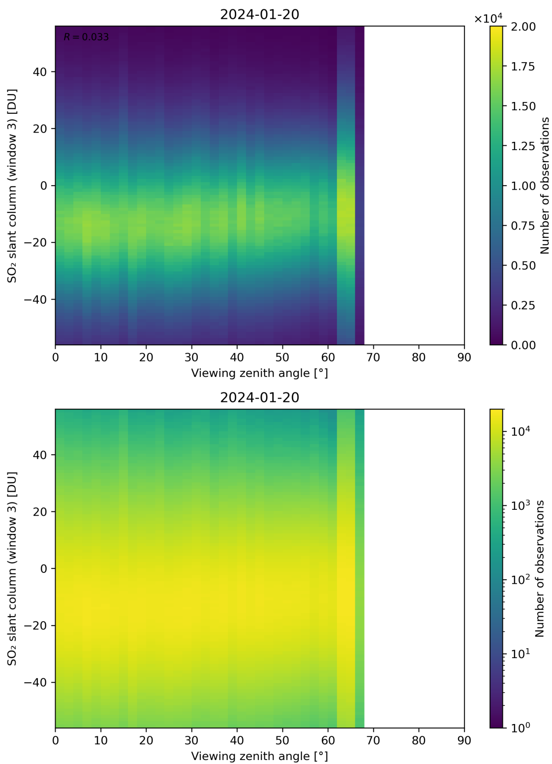
Figure 323: Scatter density plot of “Viewing zenith angle” against “SO 2 slant column (window 3)” for 2024-01-19 to 2024-01-21.
