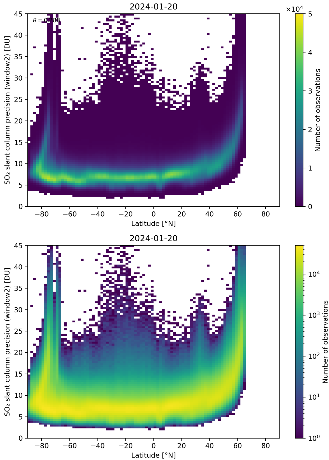
Figure 151: Scatter density plot of “Latitude” against “SO 2 slant column precision (window2)” for 2024-01-19 to 2024-01-21.
