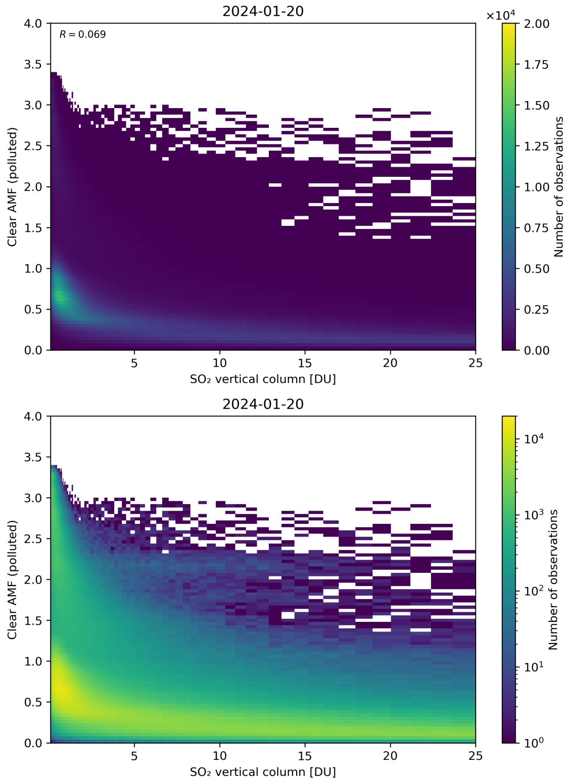
Figure 296: Scatter density plot of “SO 2 vertical column” against “Clear AMF (polluted)” for 2024-01-19 to 2024-01-21.
