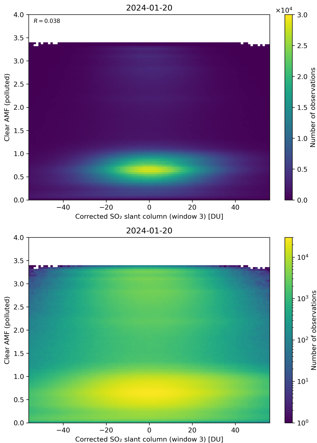
Figure 209: Scatter density plot of “Corrected SO 2 slant column (window 3)” against “Clear AMF (polluted)” for 2024-01-19 to 2024-01-21.
