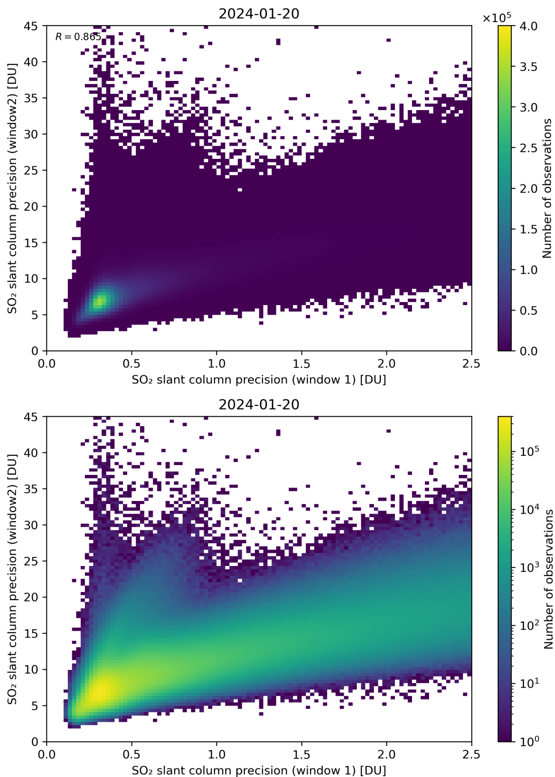
Figure 227: Scatter density plot of “SO 2 slant column precision (window 1)” against “SO 2 slant column precision (window2)” for 2024-01-19 to 2024-01-21.
