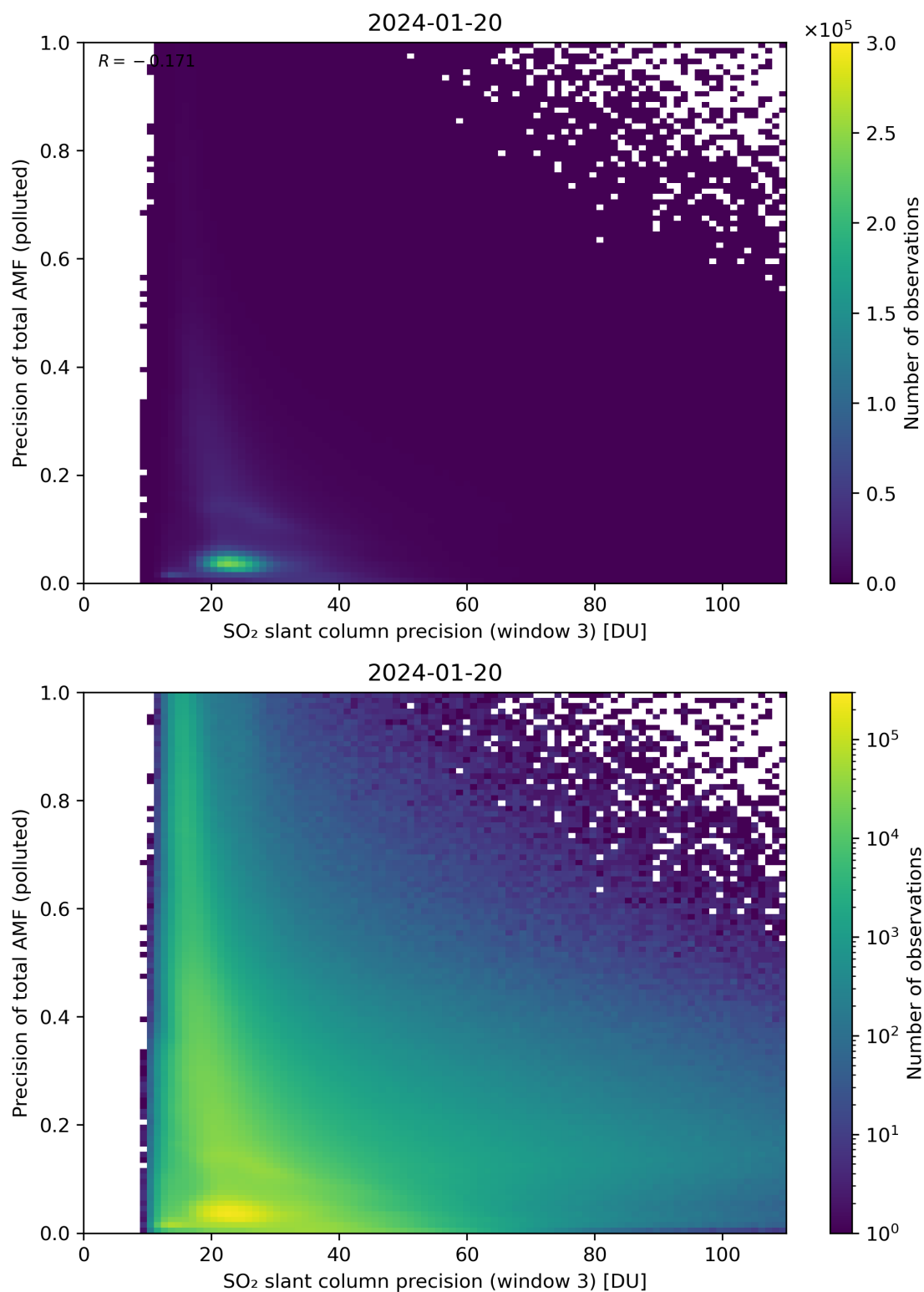
Figure 264: Scatter density plot of “SO 2 slant column precision (window 3)” against “Precision of total AMF (polluted)” for 2024-01-19 to 2024-01-21.
