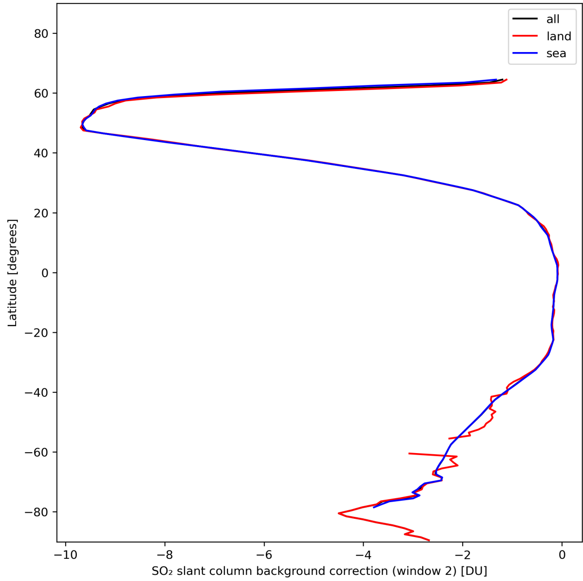
Figure 40: Zonal average of “SO 2 slant column background correction (window 2)” for 2024-01-19 to 2024-01-21.
