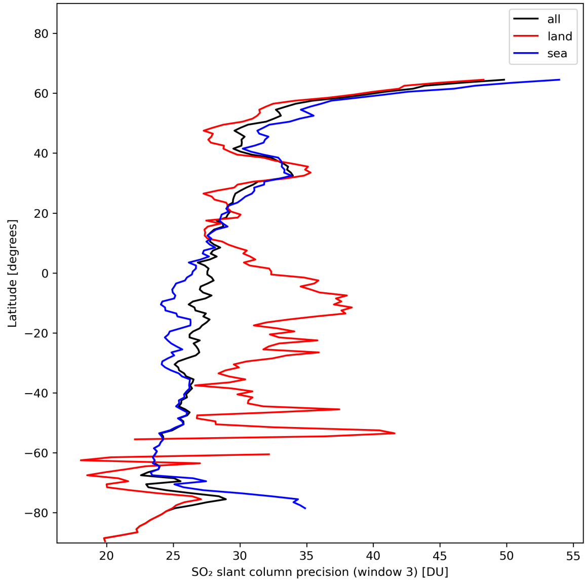
Figure 42: Zonal average of “SO 2 slant column precision (window 3)” for 2024-01-19 to 2024-01-21.
