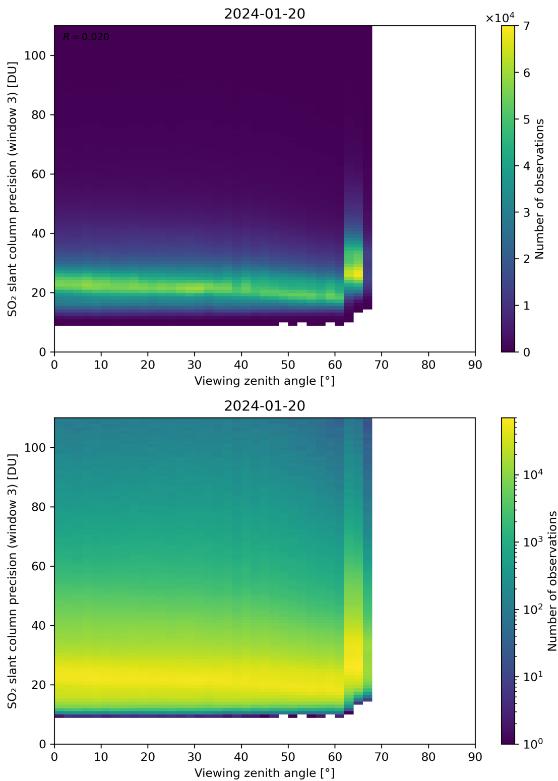
Figure 324: Scatter density plot of “Viewing zenith angle” against “SO 2 slant column precision (window 3)” for 2024-01-19 to 2024-01-21.
