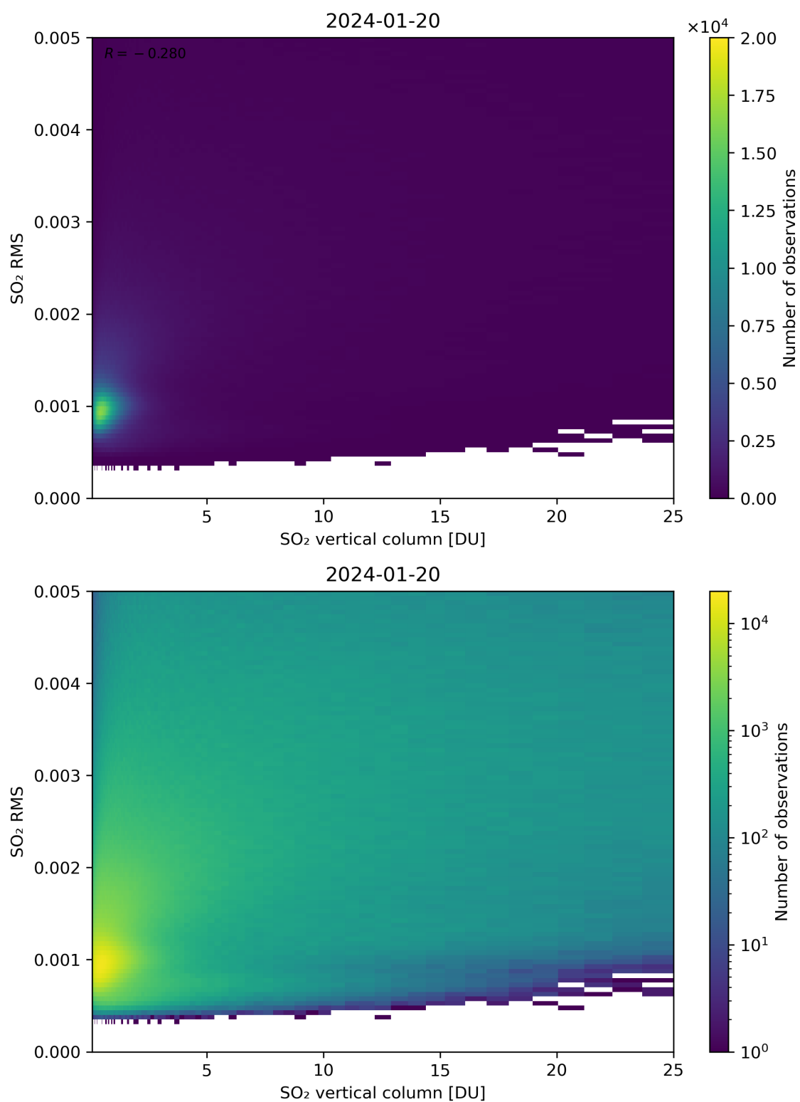
Figure 278: Scatter density plot of “SO 2 vertical column” against “SO 2 RMS” for 2024-01-19 to 2024-01-21.
