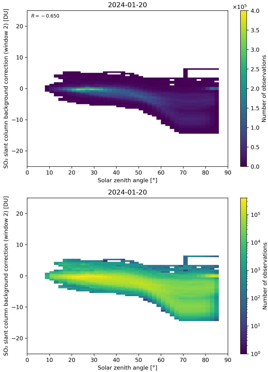
Figure 159: Scatter density plot of “Solar zenith angle” against “SO 2 slant column background correction (window 2)” for 2024-01-19 to 2024-01-21.
