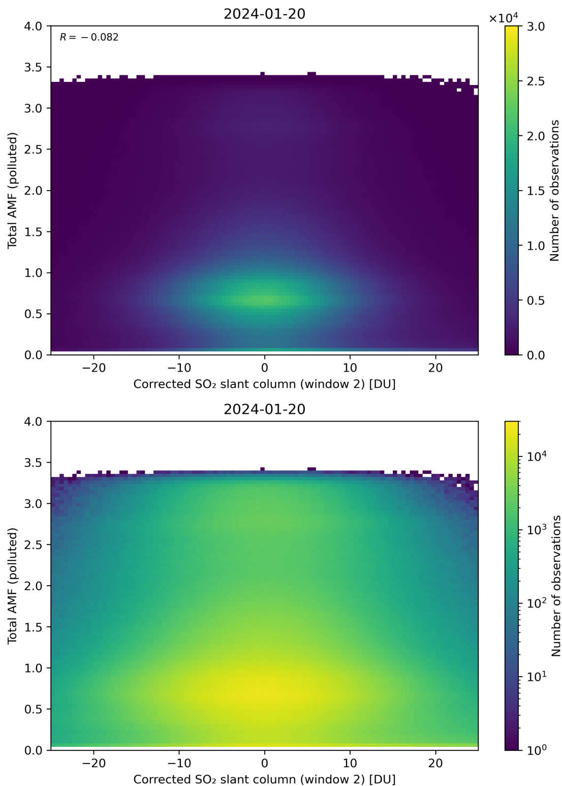
Figure 203: Scatter density plot of “Corrected SO 2 slant column (window 2)” against “Total AMF (polluted)” for 2024-01-19 to 2024-01-21.
