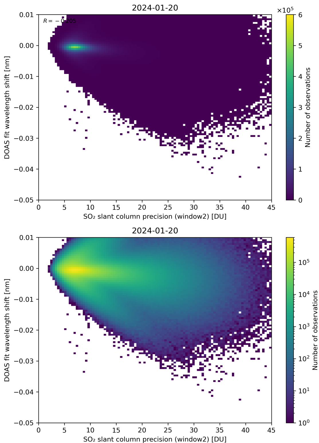
Figure 243: Scatter density plot of “SO 2 slant column precision (window2)” against “DOAS fit wavelength shift” for 2024-01-19 to 2024-01-21.
