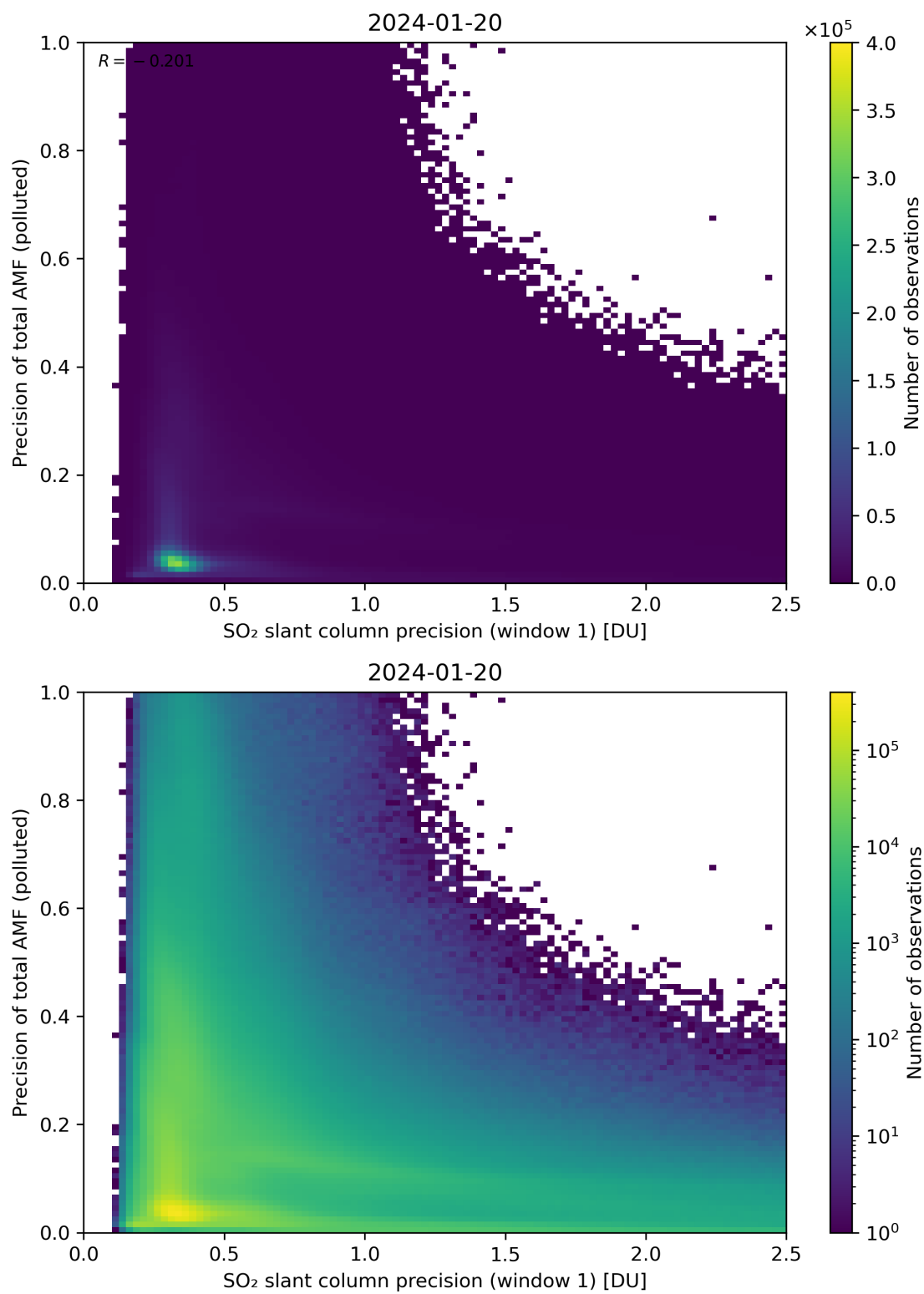
Figure 231: Scatter density plot of “SO 2 slant column precision (window 1)” against “Precision of total AMF (polluted)” for 2024-01-19 to 2024-01-21.
