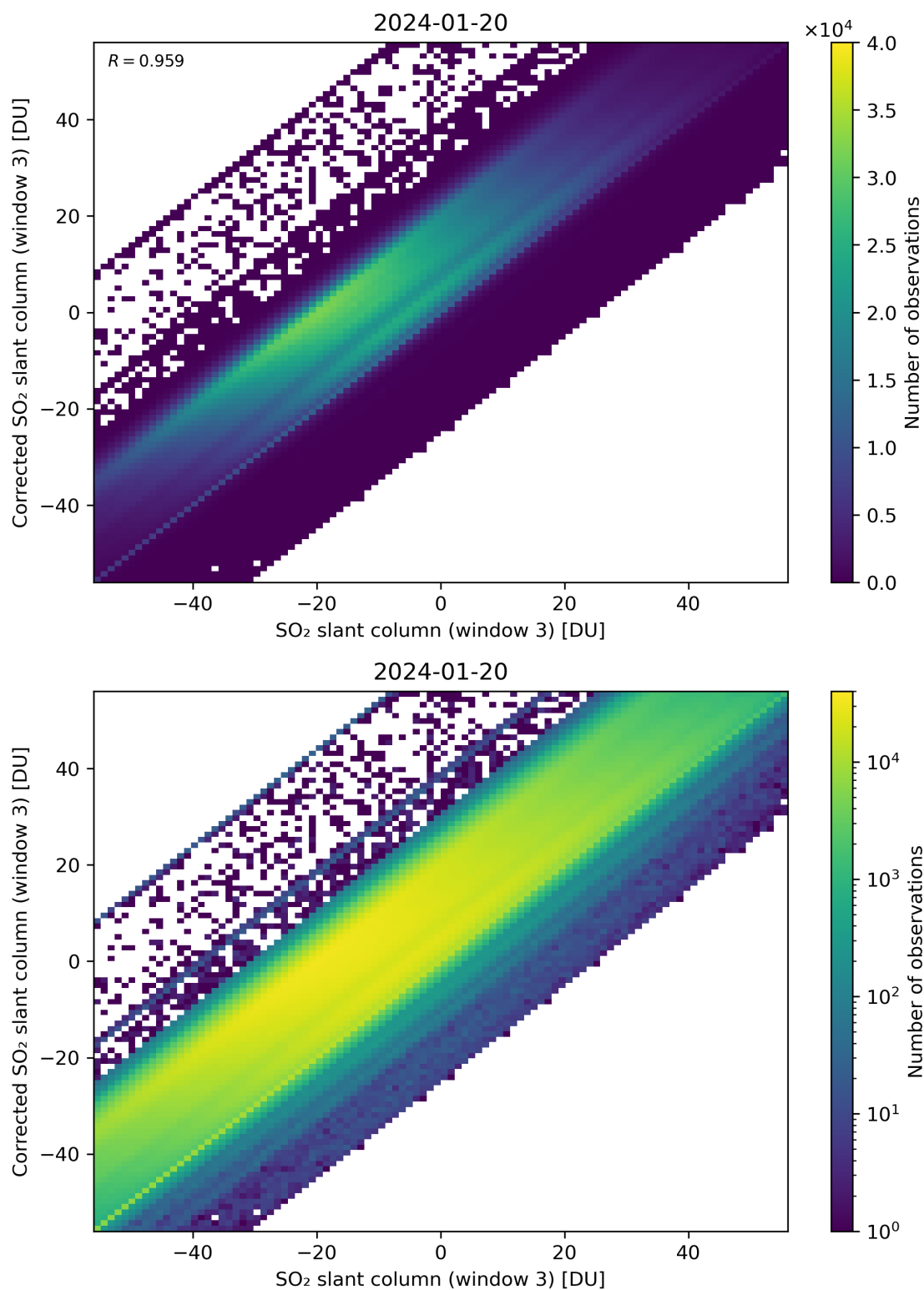
Figure 266: Scatter density plot of “SO 2 slant column (window 3)” against “Corrected SO 2 slant column (window 3)” for 2024-01-19 to 2024-01-21.
