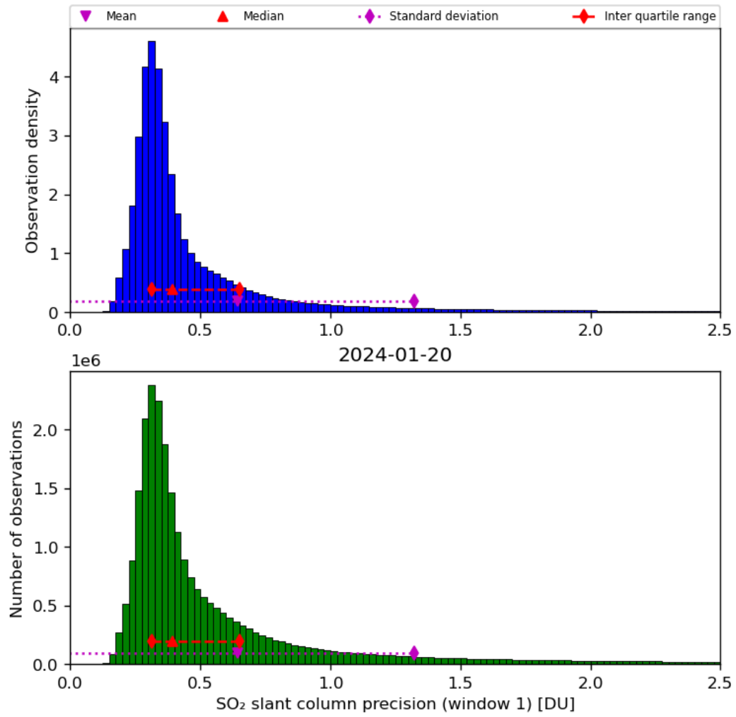
Figure 57: Histogram of “SO 2 slant column precision (window 1)” for 2024-01-19 to 2024-01-21
