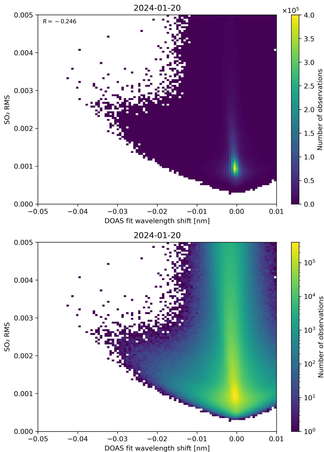
Figure 128: Scatter density plot of “DOAS fit wavelength shift” against “SO 2 RMS” for 2024-01-19 to 2024-01-21.
