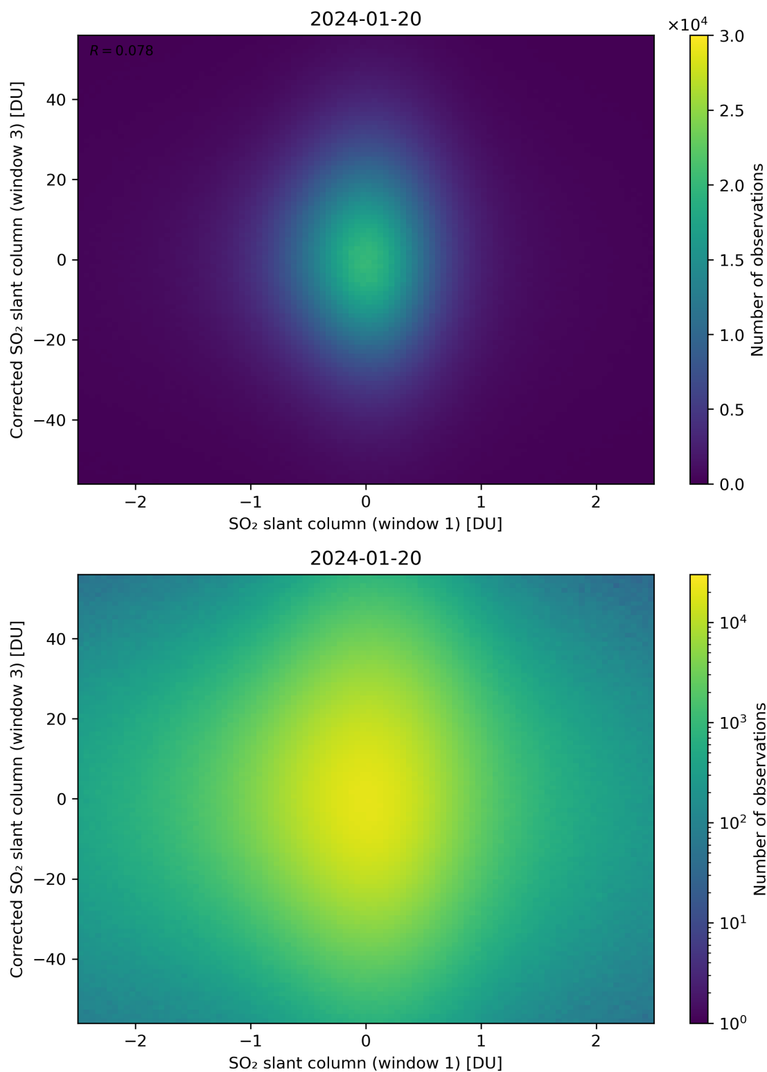
Figure 234: Scatter density plot of “SO 2 slant column (window 1)” against “Corrected SO 2 slant column (window 3)” for 2024-01-19 to 2024-01-21.
