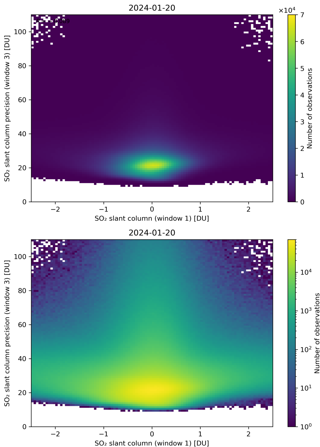
Figure 238: Scatter density plot of “SO 2 slant column (window 1)” against “SO 2 slant column precision (window 3)” for 2024-01-19 to 2024-01-21.
