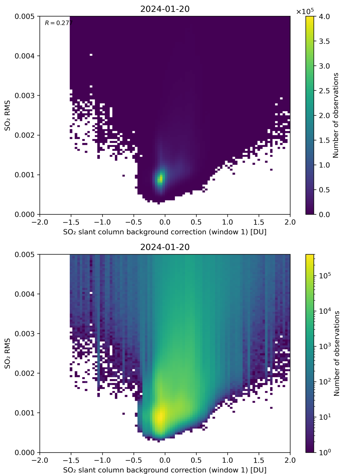
Figure 102: Scatter density plot of “SO 2 slant column background correction (window 1)” against “SO 2 RMS” for 2024-01-19 to 2024-01-21.
