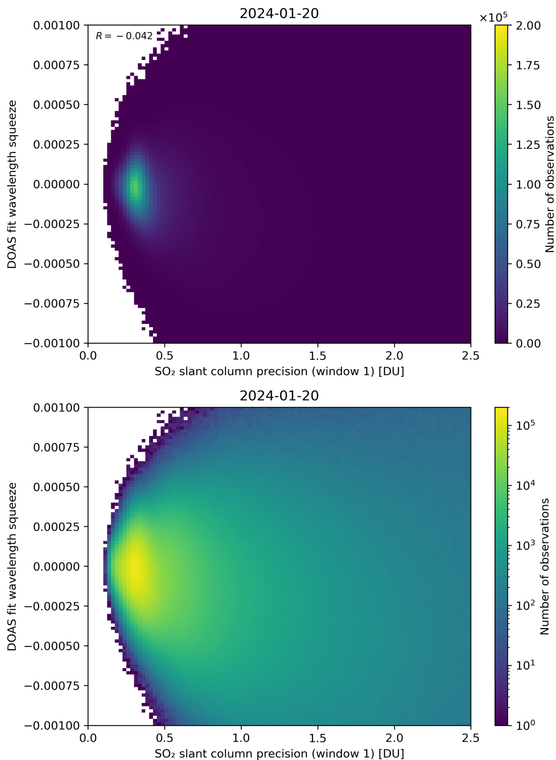
Figure 222: Scatter density plot of “SO 2 slant column precision (window 1)” against “DOAS fit wavelength squeeze” for 2024-01-19 to 2024-01-21.
