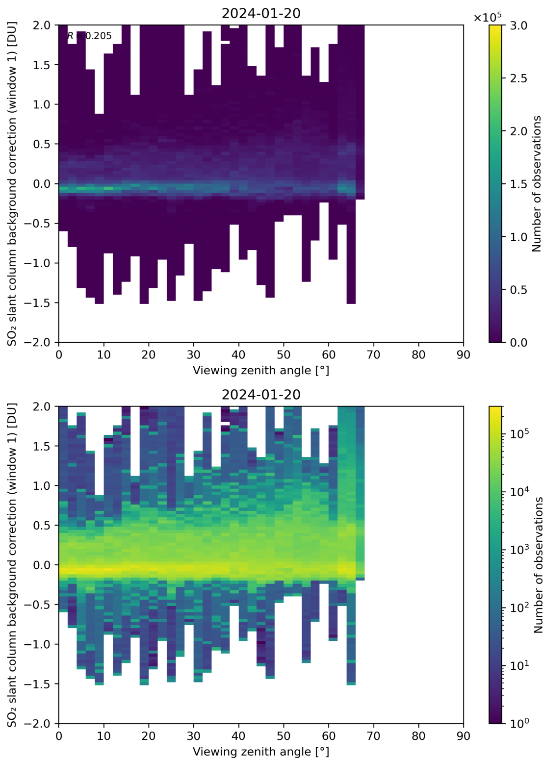
Figure 308: Scatter density plot of “Viewing zenith angle” against “SO 2 slant column background correction (window 1)” for 2024-01-19 to 2024-01-21.
