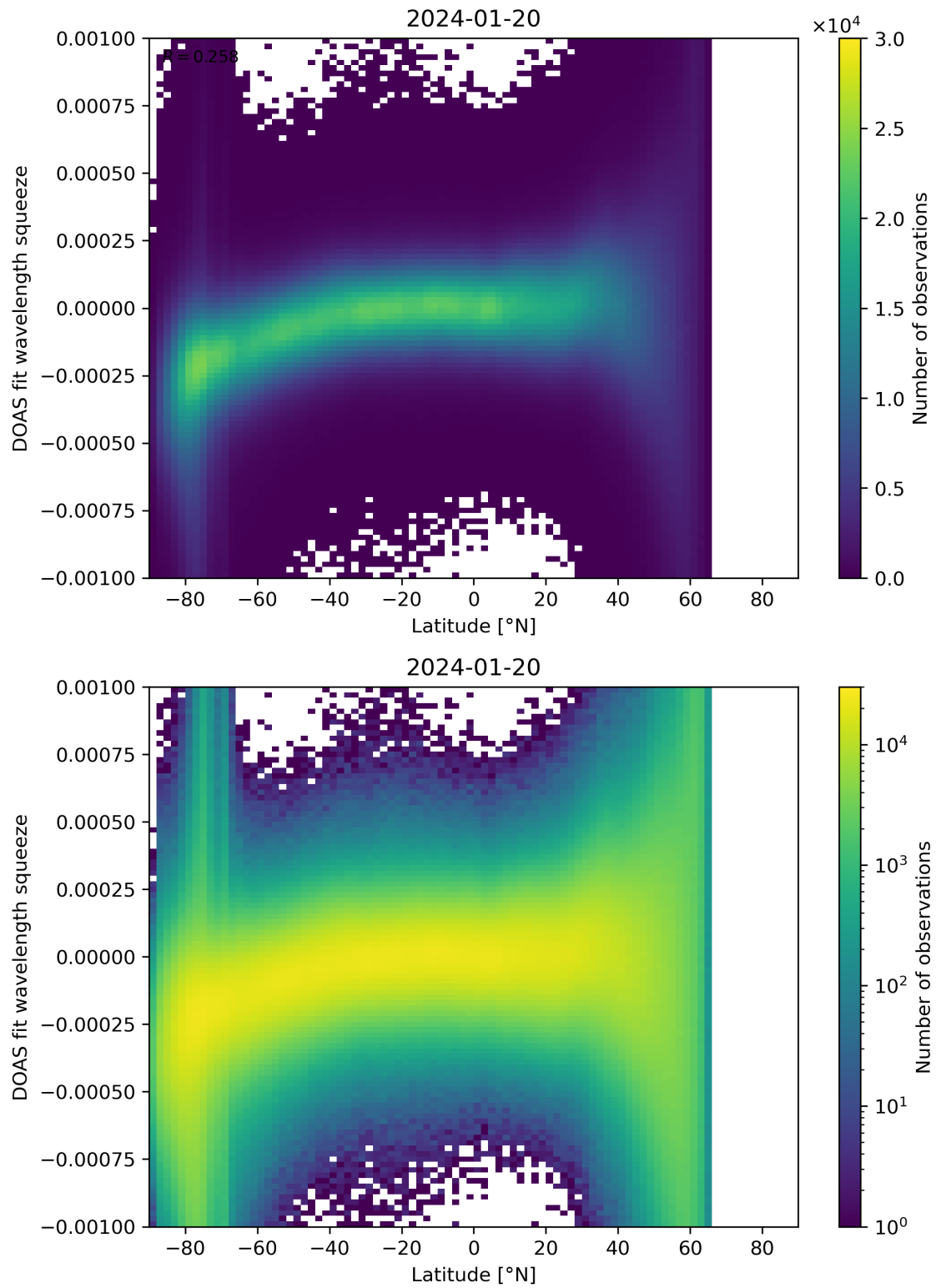
Figure 143: Scatter density plot of “Latitude” against “DOAS fit wavelength squeeze” for 2024-01-19 to 2024-01-21.
