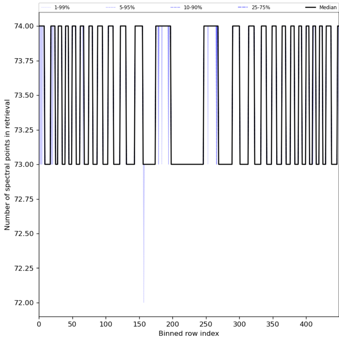
Figure 97: Along track statistics of “Number of spectral points in retrieval” for 2024-01-19 to 2024-01-21
