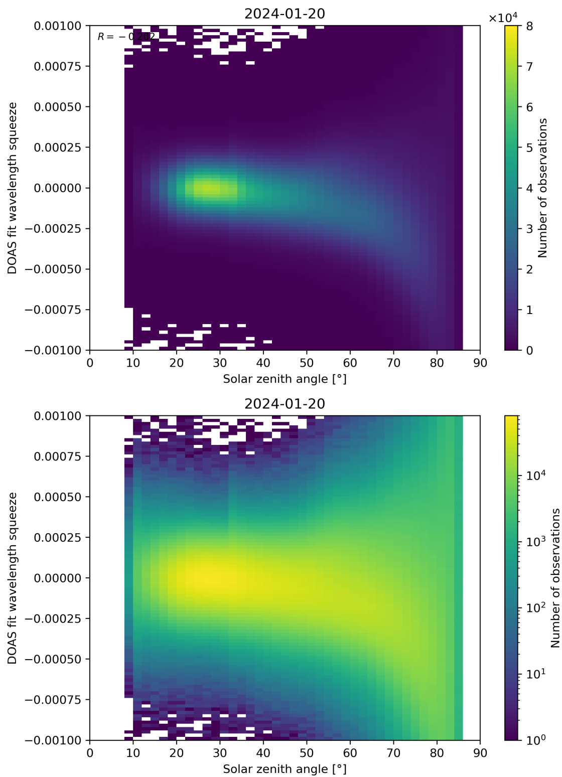
Figure 162: Scatter density plot of “Solar zenith angle” against “DOAS fit wavelength squeeze” for 2024-01-19 to 2024-01-21.
