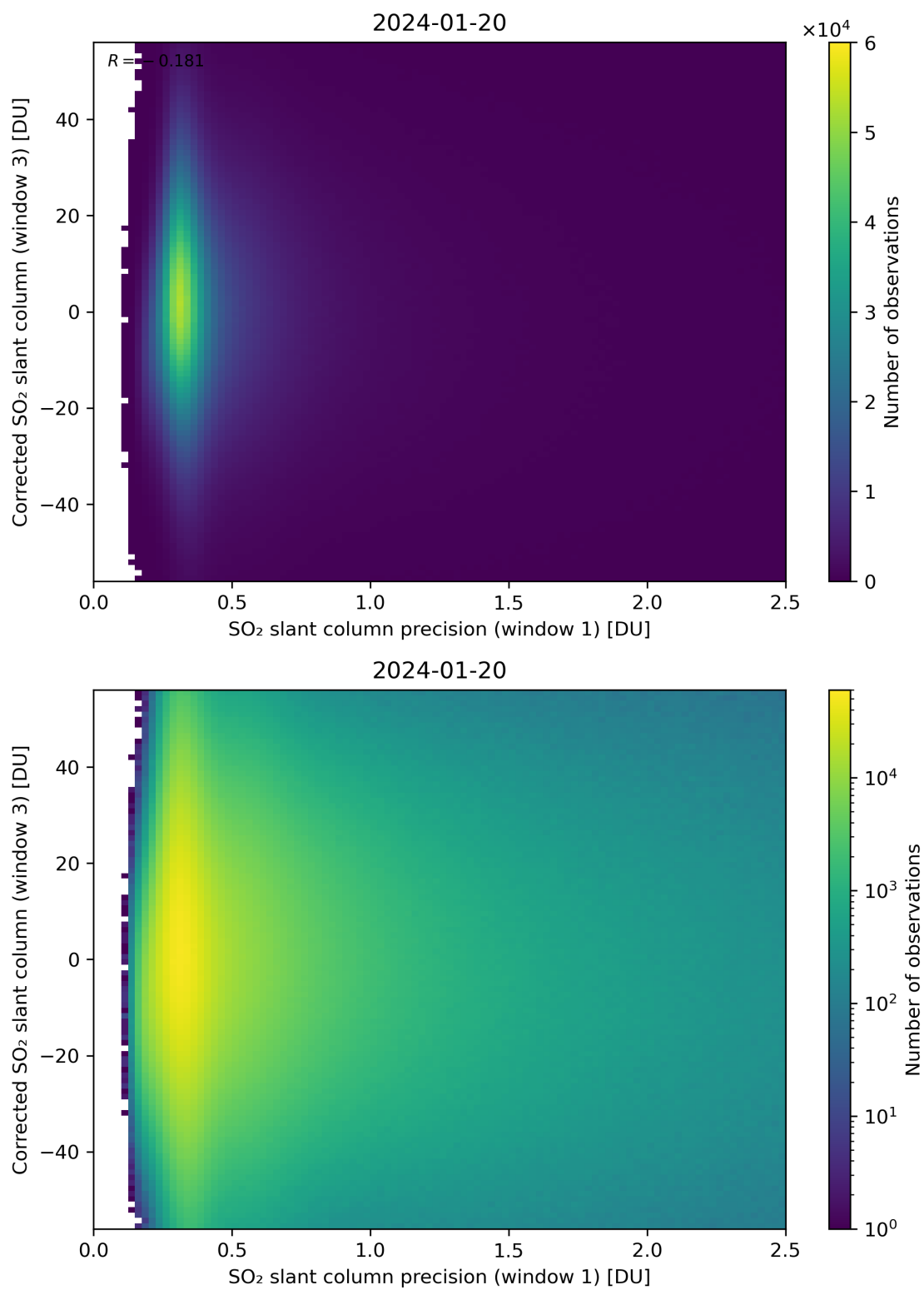
Figure 226: Scatter density plot of “SO 2 slant column precision (window 1)” against “Corrected SO 2 slant column (window 3)” for 2024-01-19 to 2024-01-21.
