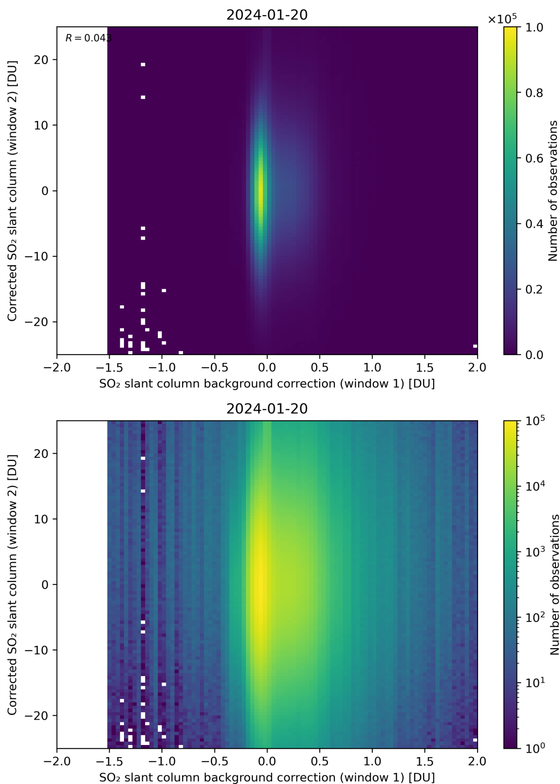
Figure 104: Scatter density plot of “SO 2 slant column background correction (window 1)” against “Corrected SO 2 slant column (window 2)” for 2024-01-19 to 2024-01-21.
