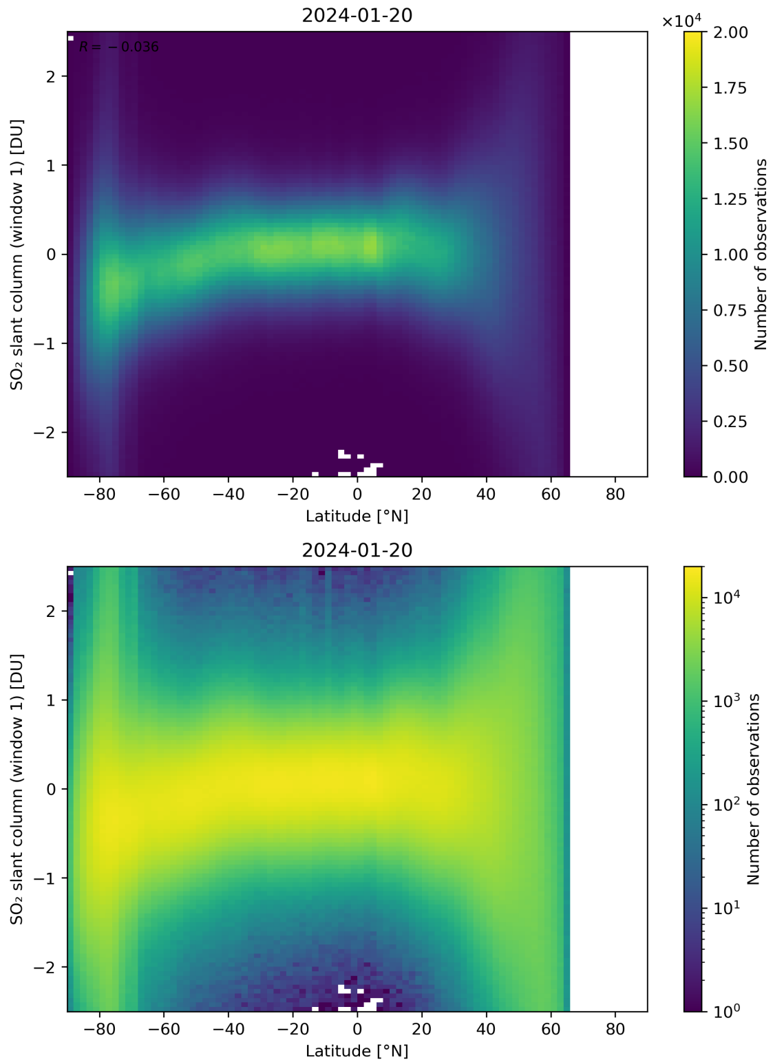
Figure 149: Scatter density plot of “Latitude” against “SO 2 slant column (window 1)” for 2024-01-19 to 2024-01-21.
