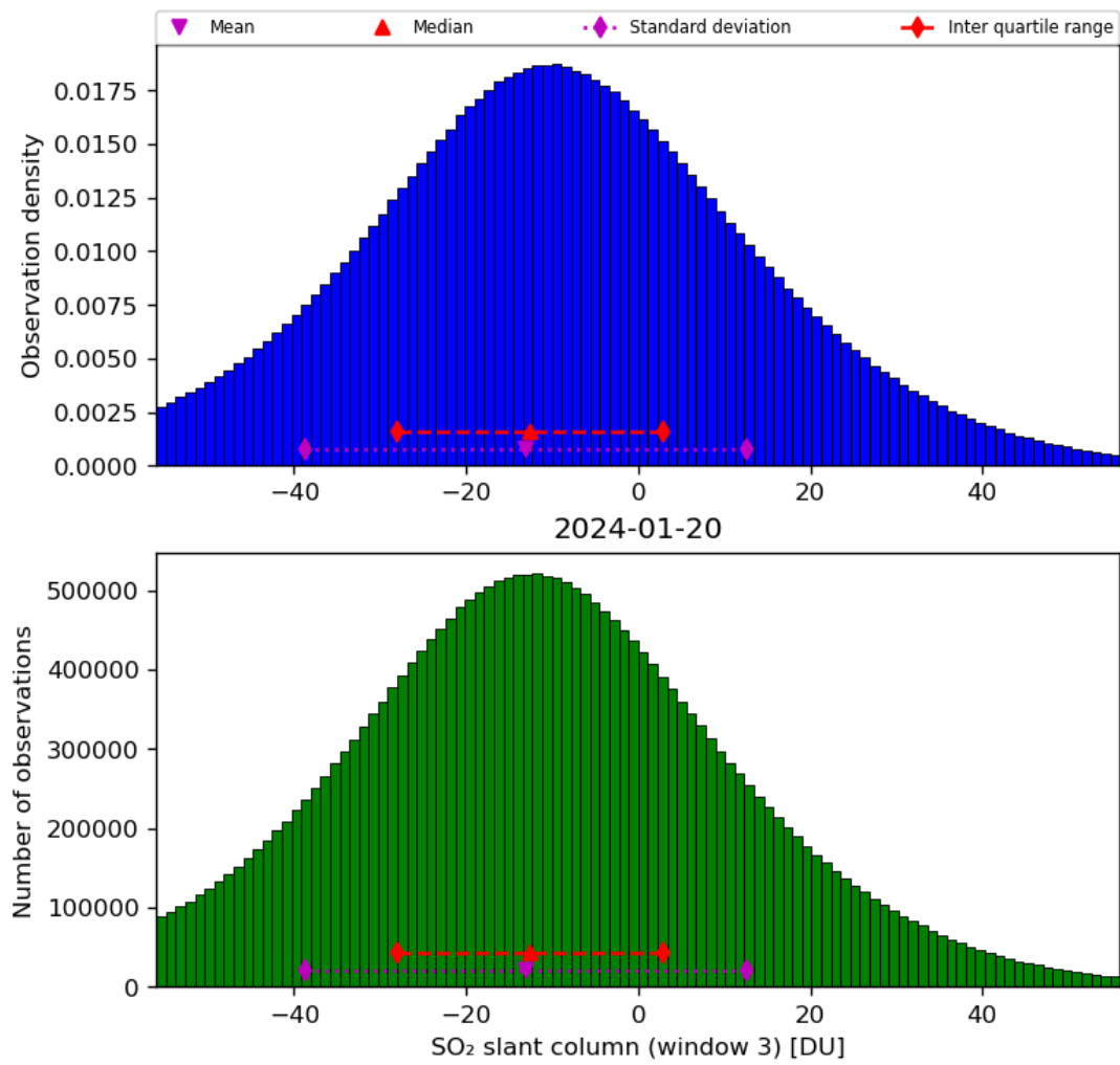
Figure 64: Histogram of “SO 2 slant column (window 3)” for 2024-01-19 to 2024-01-21
