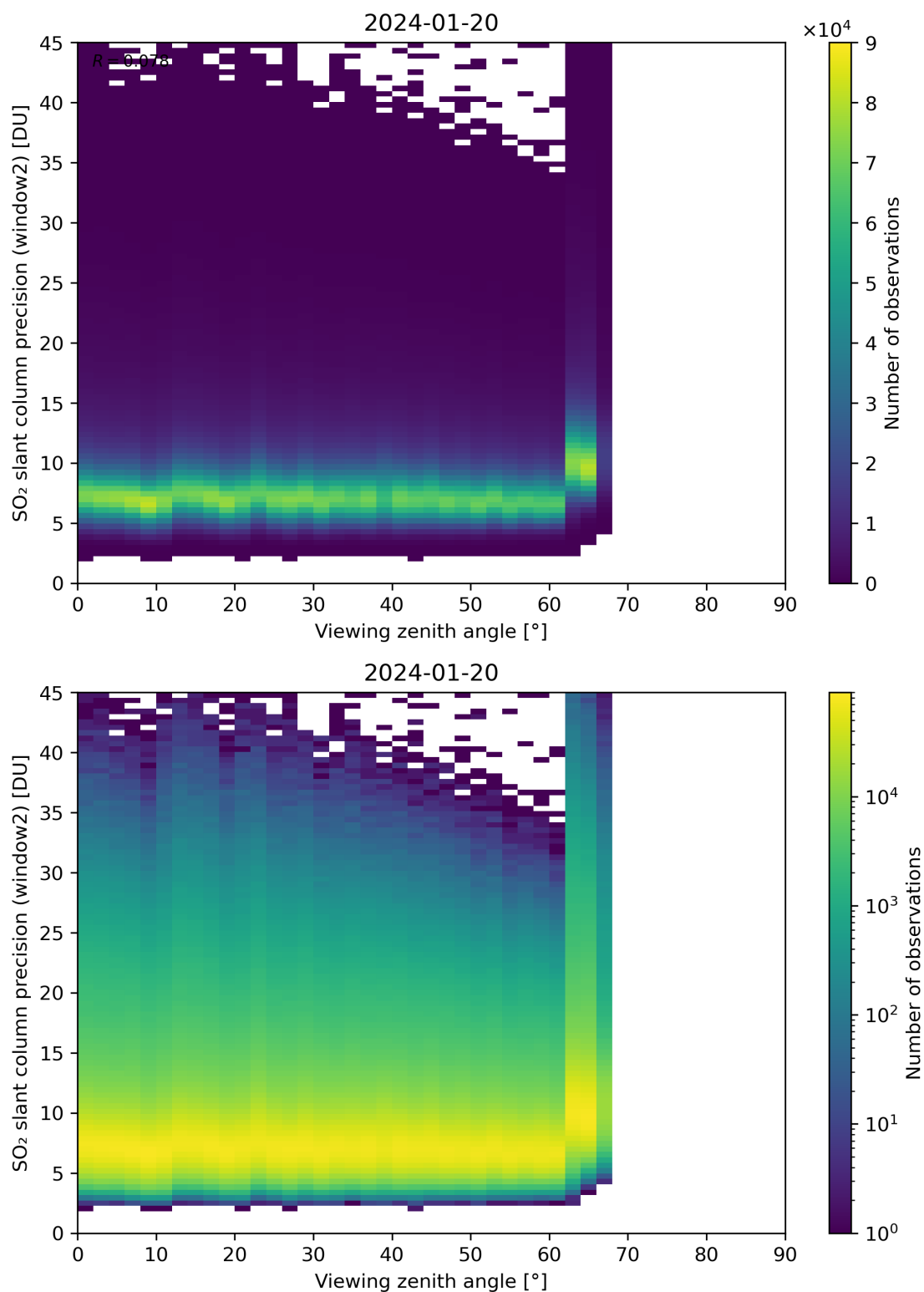
Figure 322: Scatter density plot of “Viewing zenith angle” against “SO 2 slant column precision (window2)” for 2024-01-19 to 2024-01-21.
