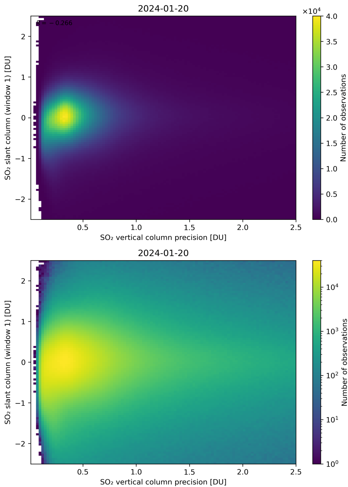
Figure 289: Scatter density plot of “SO 2 vertical column precision” against “SO 2 slant column (window 1)” for 2024-01-19 to 2024-01-21.
