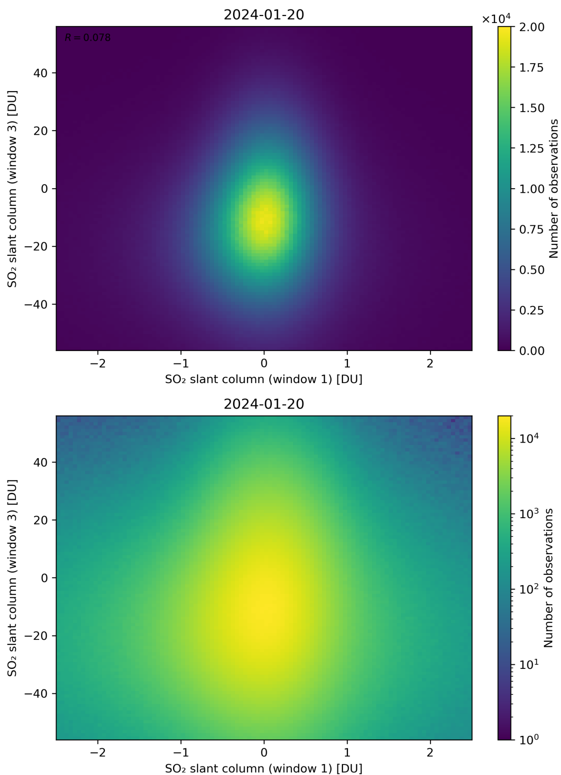
Figure 237: Scatter density plot of “SO 2 slant column (window 1)” against “SO 2 slant column (window 3)” for 2024-01-19 to 2024-01-21.
