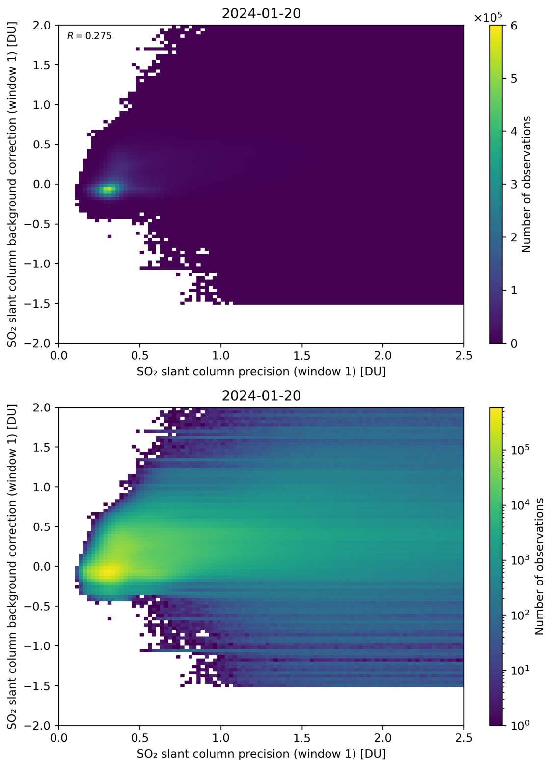
Figure 218: Scatter density plot of “SO 2 slant column precision (window 1)” against “SO 2 slant column background correction (window 1)” for 2024-01-19 to 2024-01-21.
