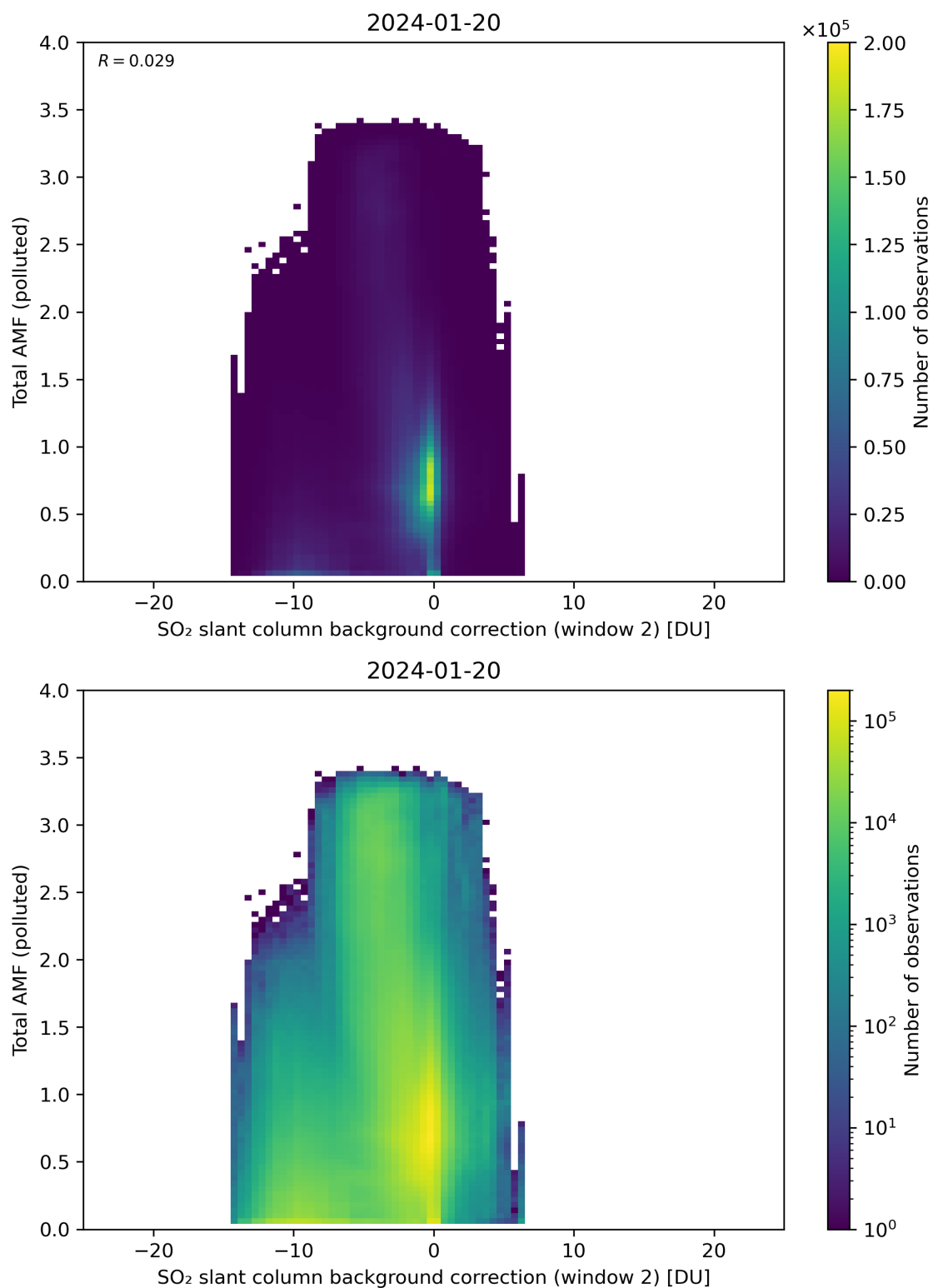
Figure 119: Scatter density plot of “SO 2 slant column background correction (window 2)” against “Total AMF (polluted)” for 2024-01-19 to 2024-01-21.
