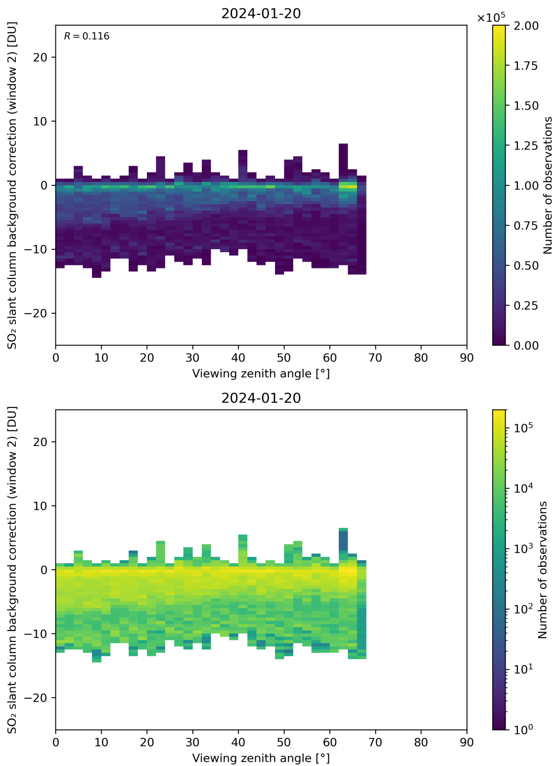
Figure 309: Scatter density plot of “Viewing zenith angle” against “SO 2 slant column background correction (window 2)” for 2024-01-19 to 2024-01-21.
