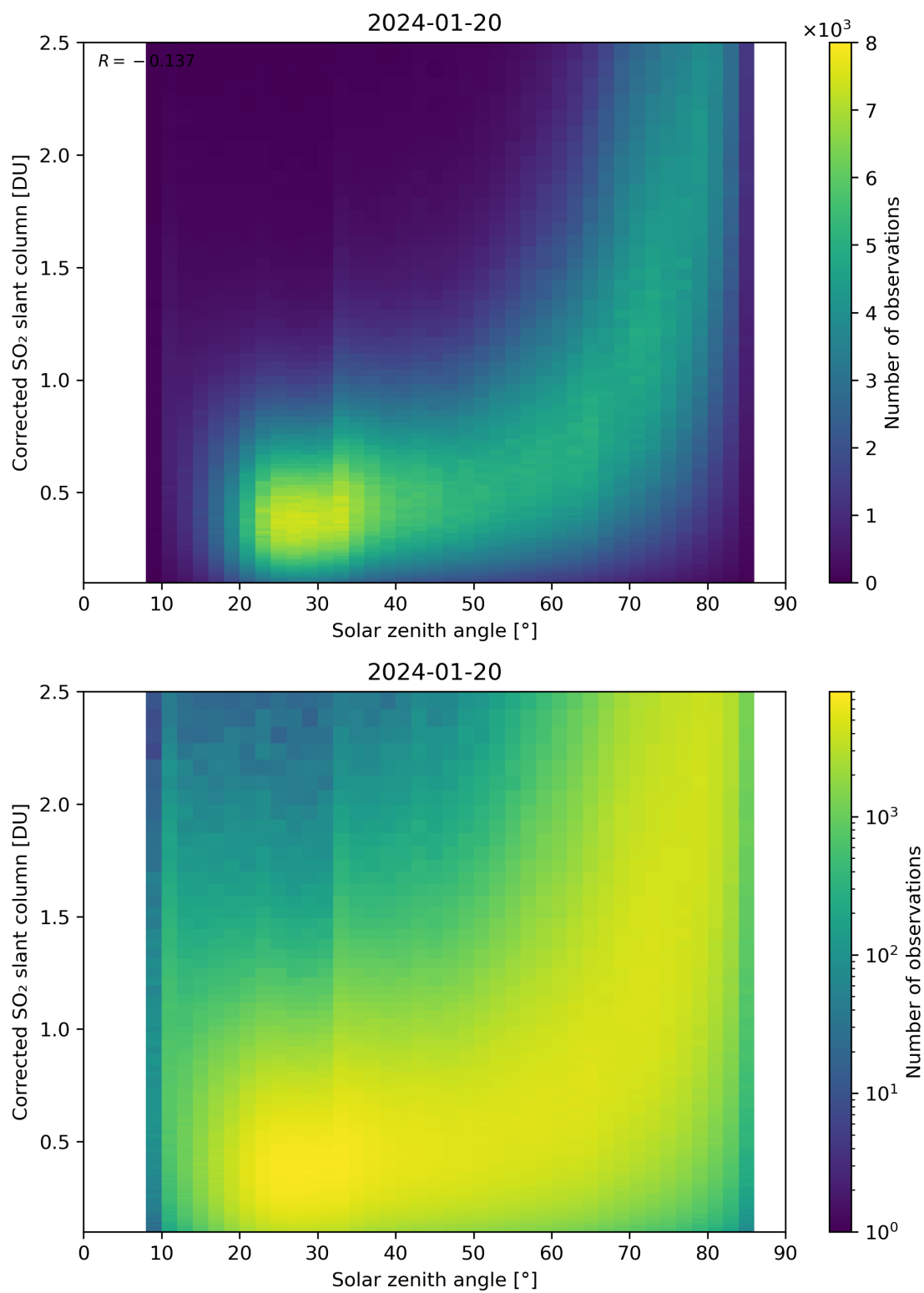
Figure 166: Scatter density plot of “Solar zenith angle” against “Corrected SO 2 slant column” for 2024-01-19 to 2024-01-21.
