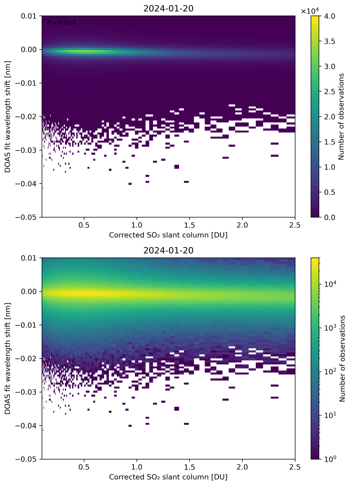
Figure 181: Scatter density plot of “Corrected SO 2 slant column” against “DOAS fit wavelength shift” for 2024-01-19 to 2024-01-21.
