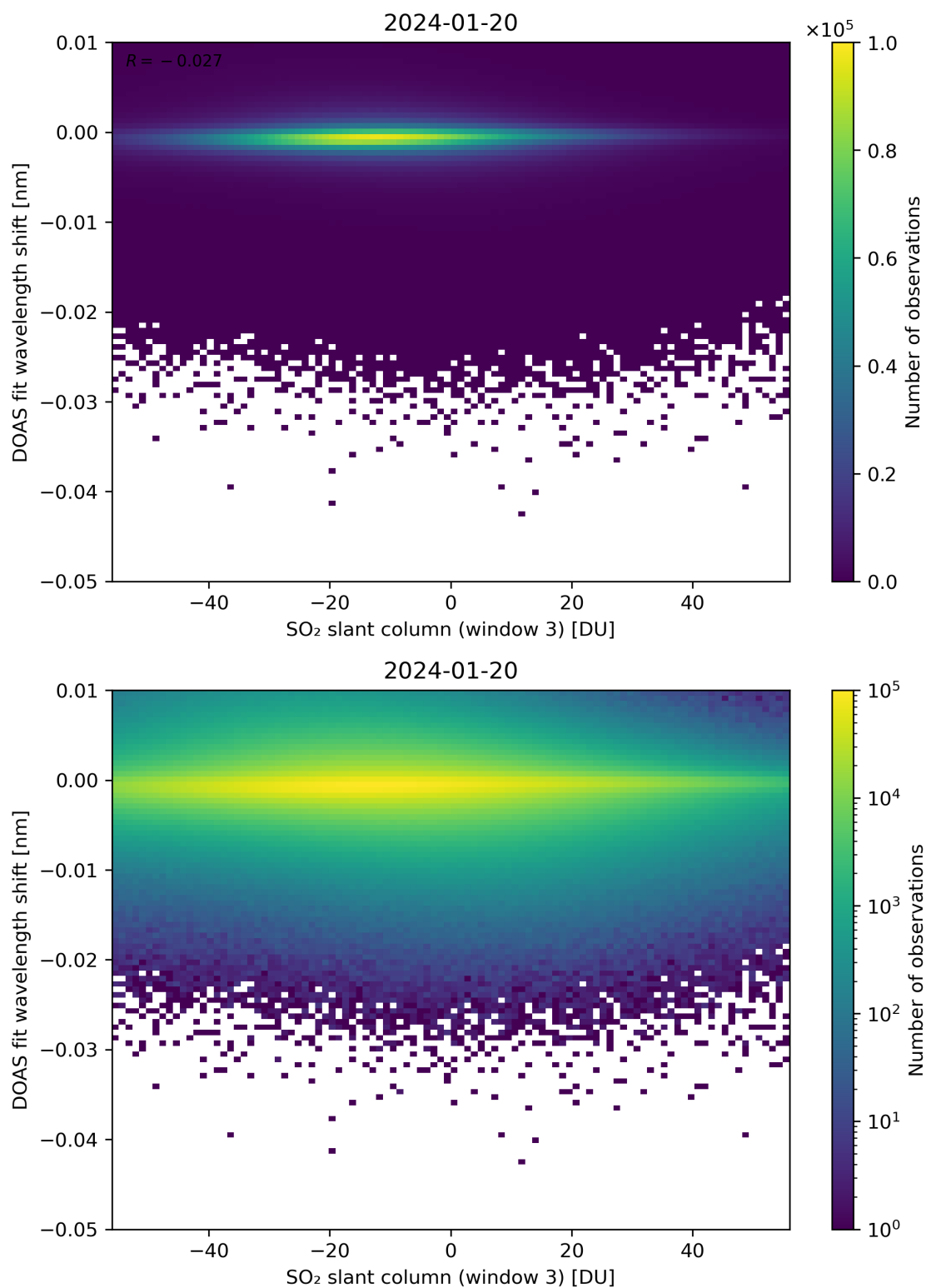
Figure 254: Scatter density plot of “SO 2 slant column (window 3)” against “DOAS fit wavelength shift” for 2024-01-19 to 2024-01-21.
