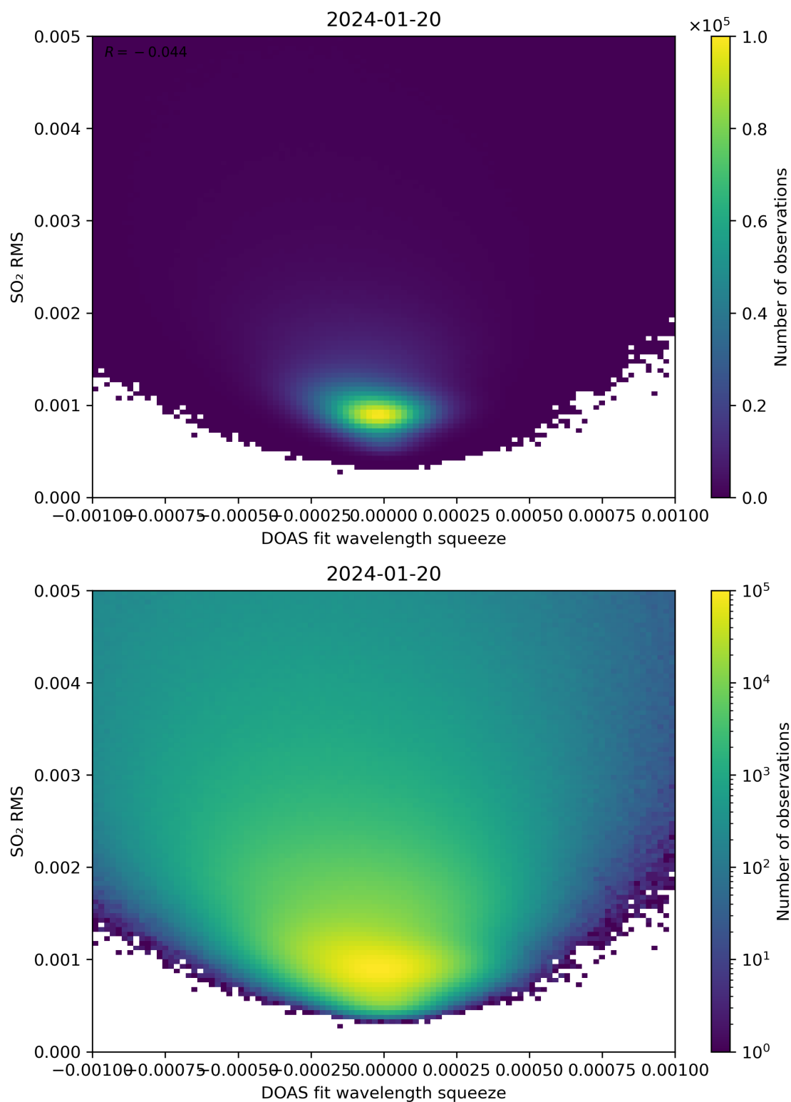
Figure 132: Scatter density plot of “DOAS fit wavelength squeeze” against “SO 2 RMS” for 2024-01-19 to 2024-01-21.
