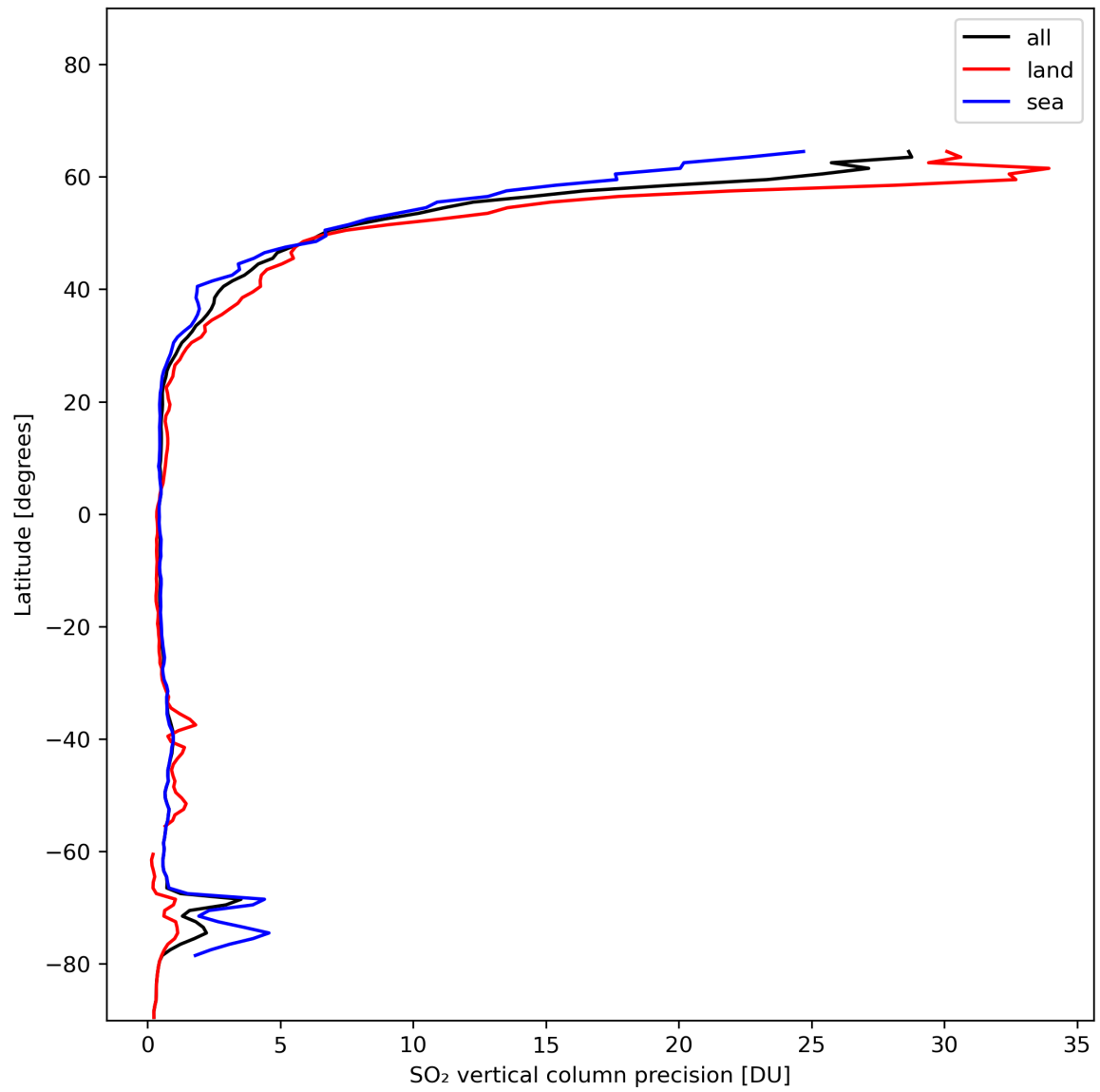
Figure 31: Zonal average of “SO 2 vertical column precision” for 2024-01-19 to 2024-01-21.
