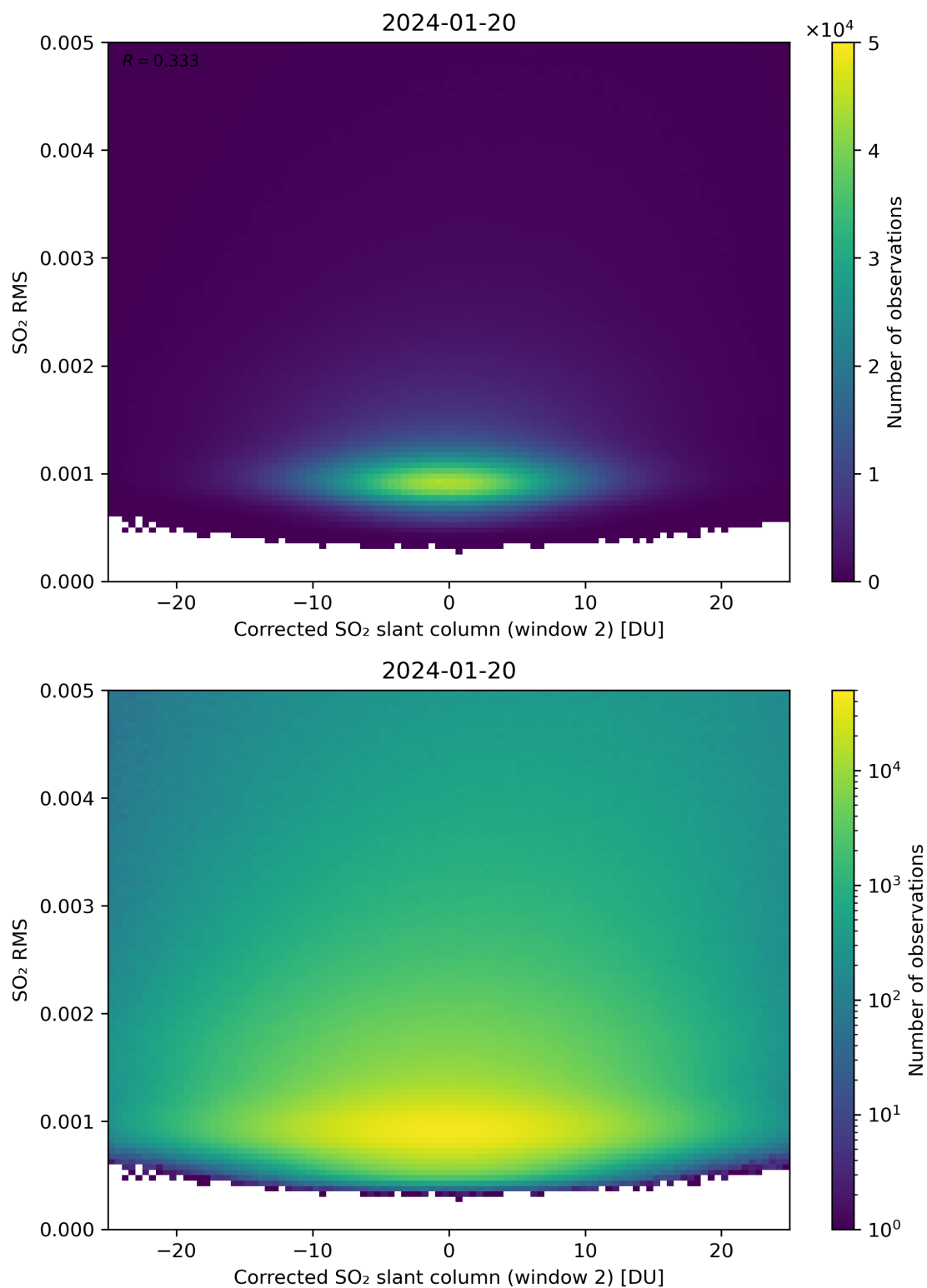
Figure 198: Scatter density plot of “Corrected SO 2 slant column (window 2)” against “SO 2 RMS” for 2024-01-19 to 2024-01-21.
