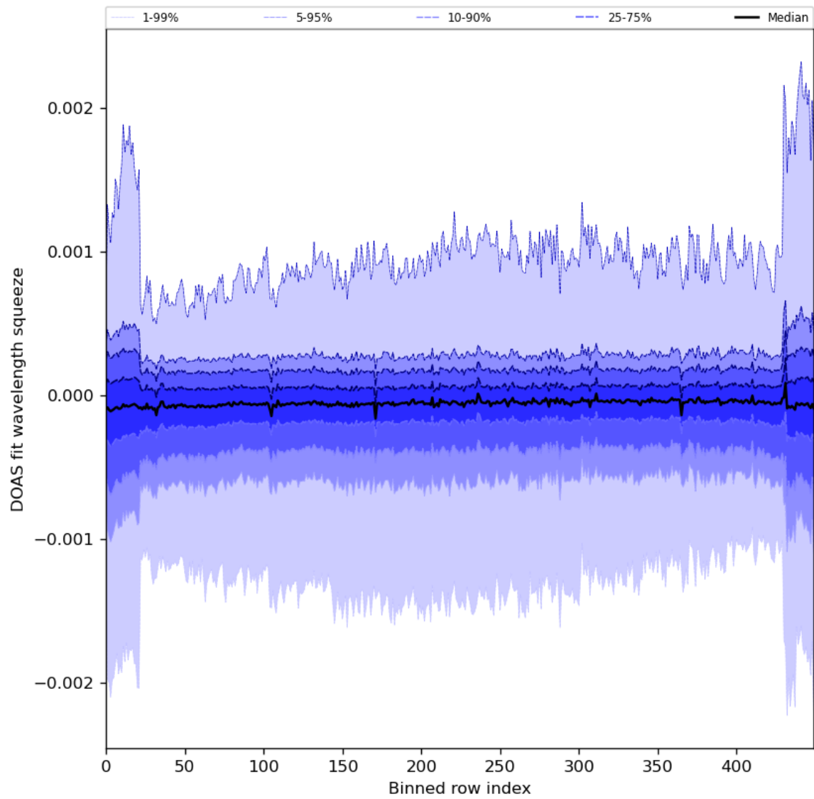
Figure 92: Along track statistics of “DOAS fit wavelength squeeze” for 2024-01-19 to 2024-01-21
