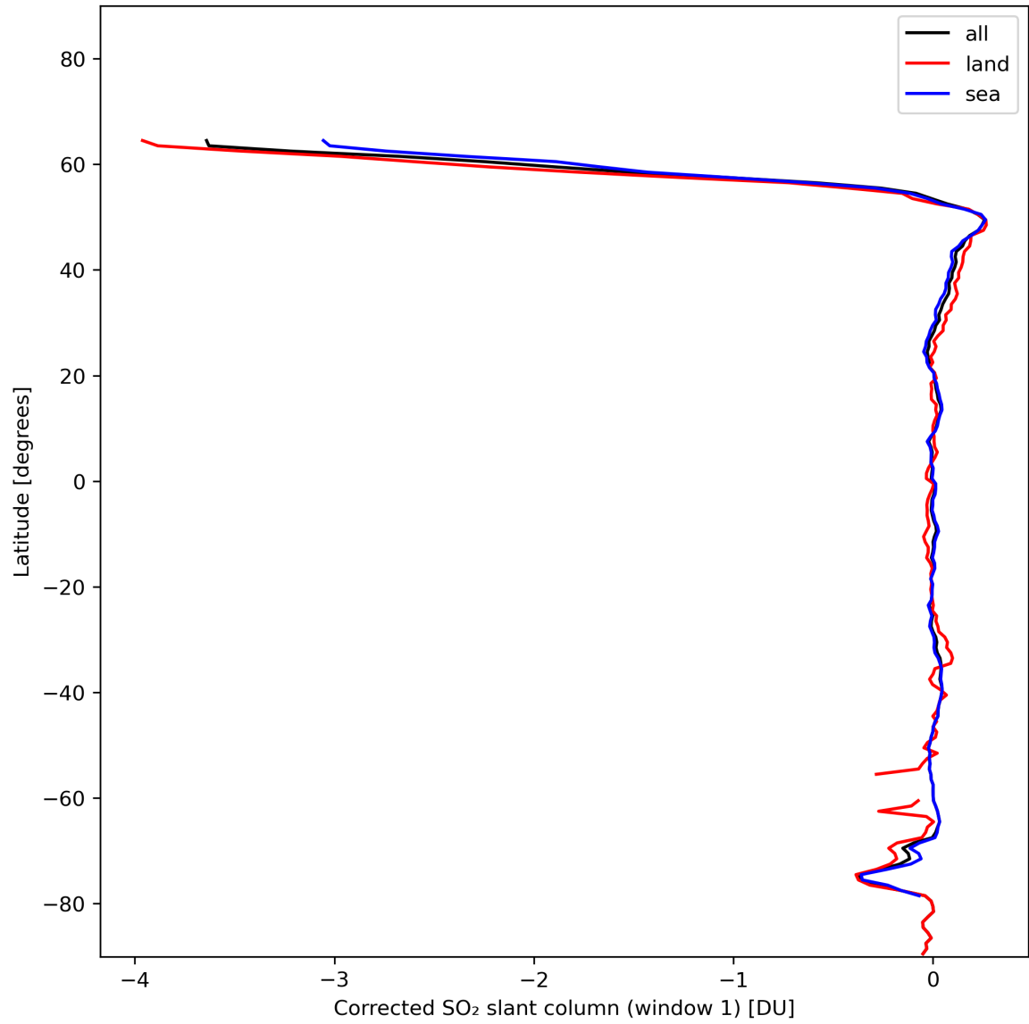
Figure 35: Zonal average of “Corrected SO 2 slant column (window 1)” for 2024-01-19 to 2024-01-21.
