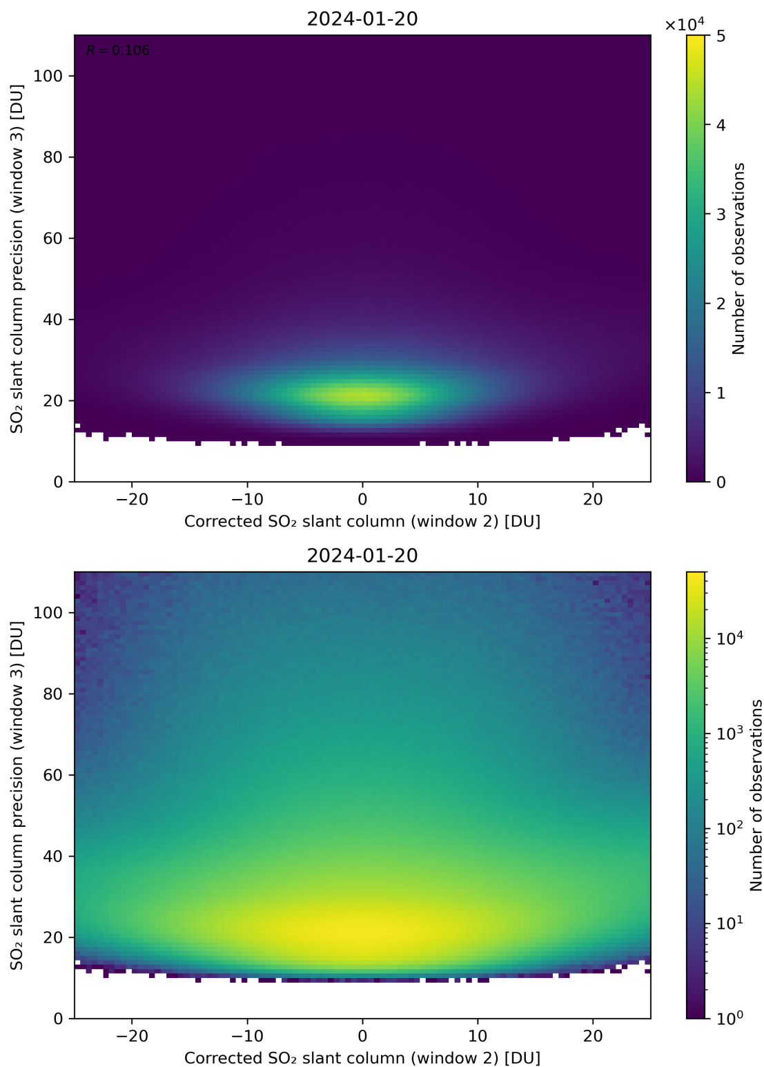
Figure 202: Scatter density plot of “Corrected SO 2 slant column (window 2)” against “SO 2 slant column precision (window 3)” for 2024-01-19 to 2024-01-21.
