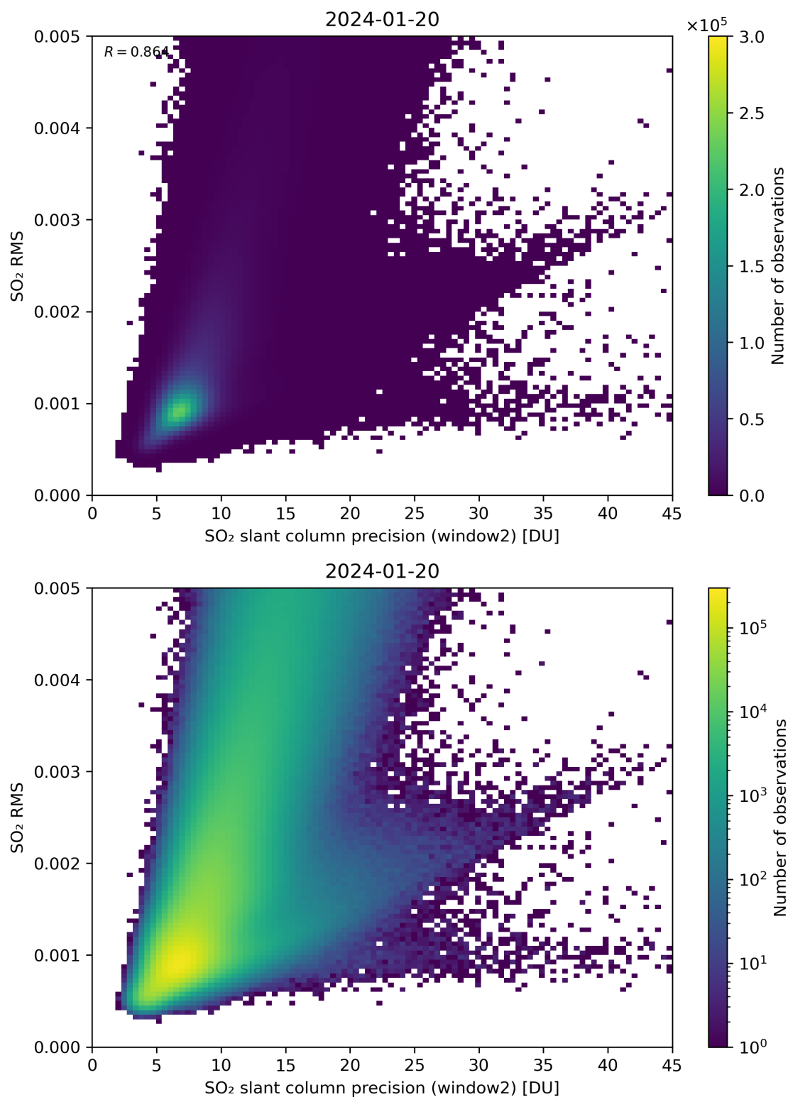
Figure 245: Scatter density plot of “SO 2 slant column precision (window2)” against “SO 2 RMS” for 2024-01-19 to 2024-01-21.
