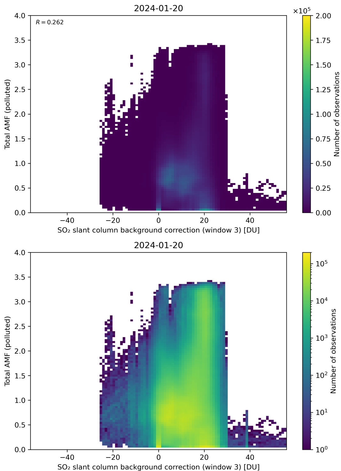
Figure 125: Scatter density plot of “SO 2 slant column background correction (window 3)” against “Total AMF (polluted)” for 2024-01-19 to 2024-01-21.
