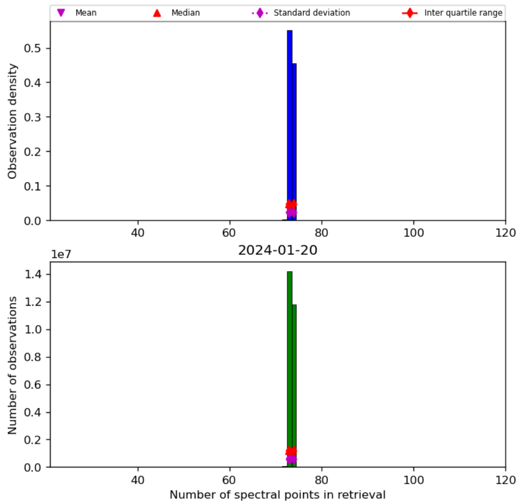
Figure 74: Histogram of “Number of spectral points in retrieval” for 2024-01-19 to 2024-01-21
