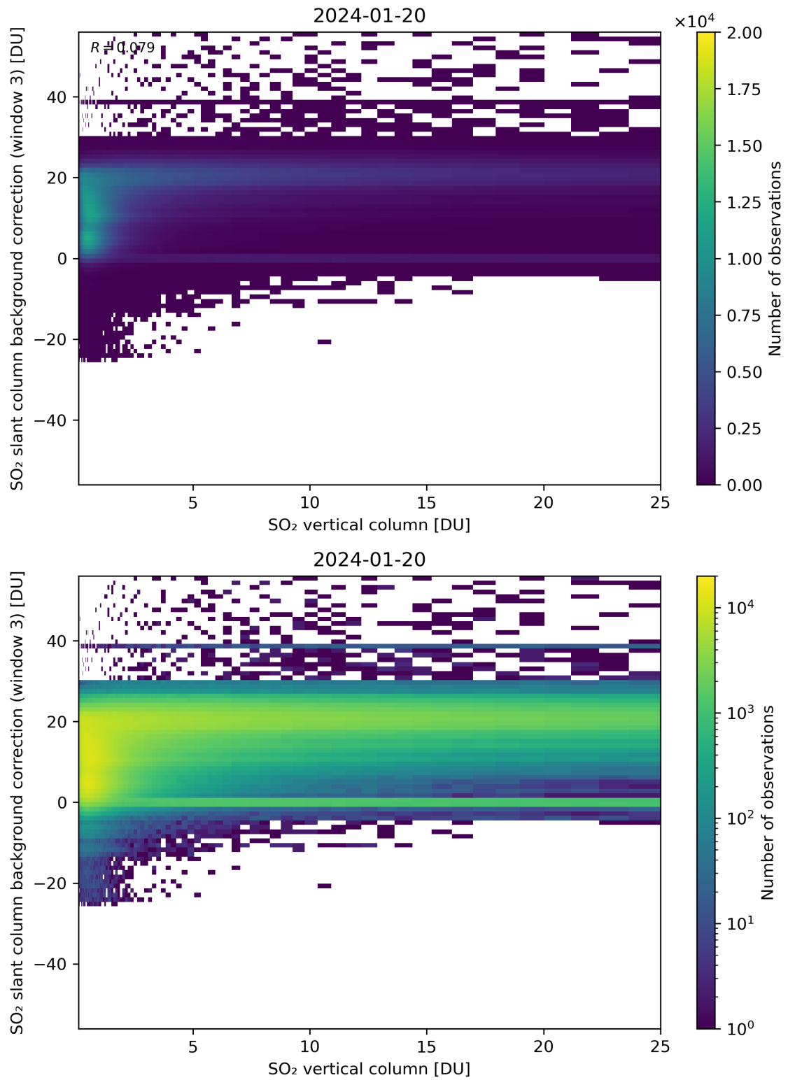
Figure 275: Scatter density plot of “SO 2 vertical column” against “SO 2 slant column background correction (window 3)” for 2024-01-19 to 2024-01-21.
