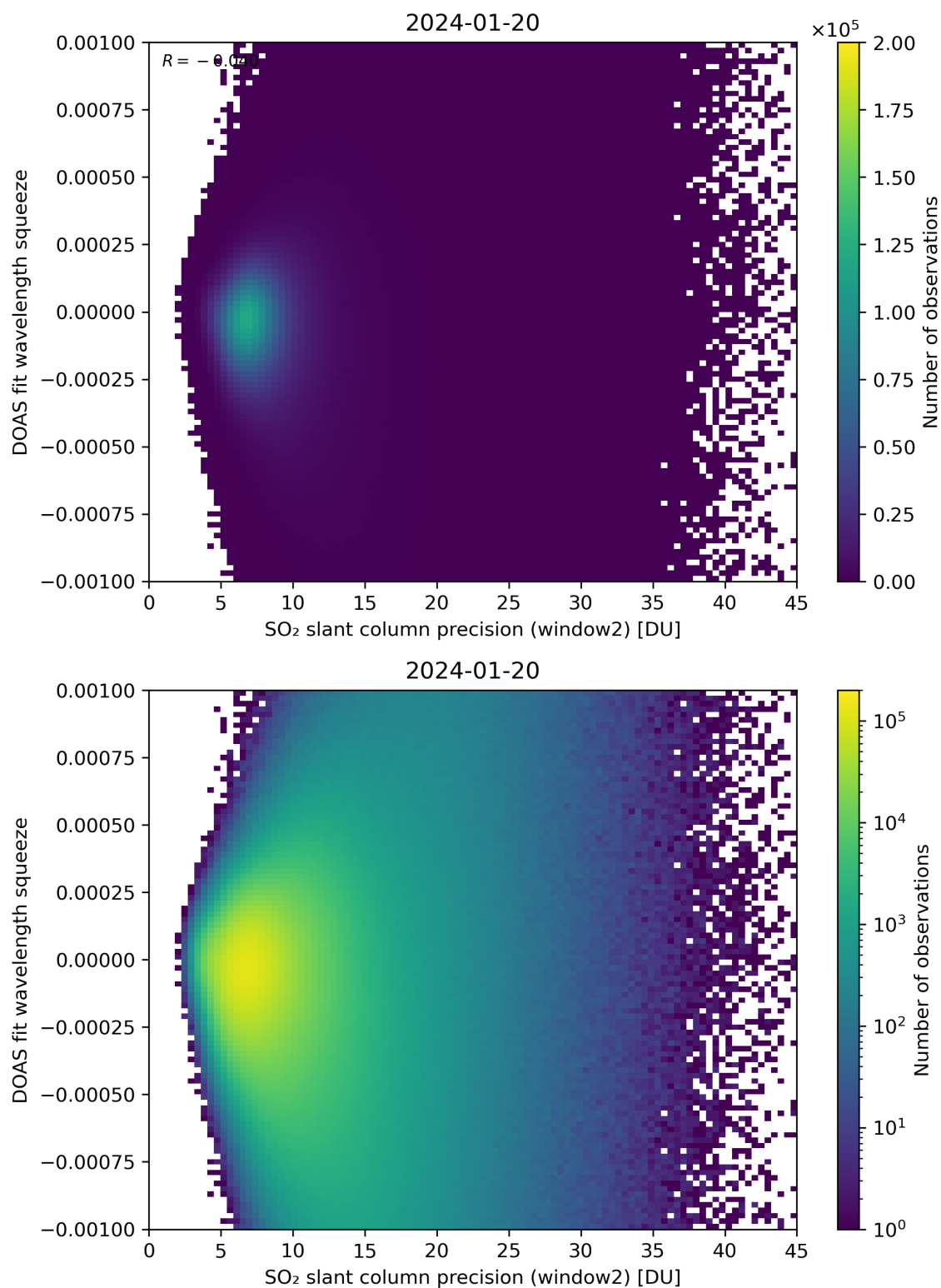
Figure 244: Scatter density plot of “SO 2 slant column precision (window2)” against “DOAS fit wavelength squeeze” for 2024-01-19 to 2024-01-21.
