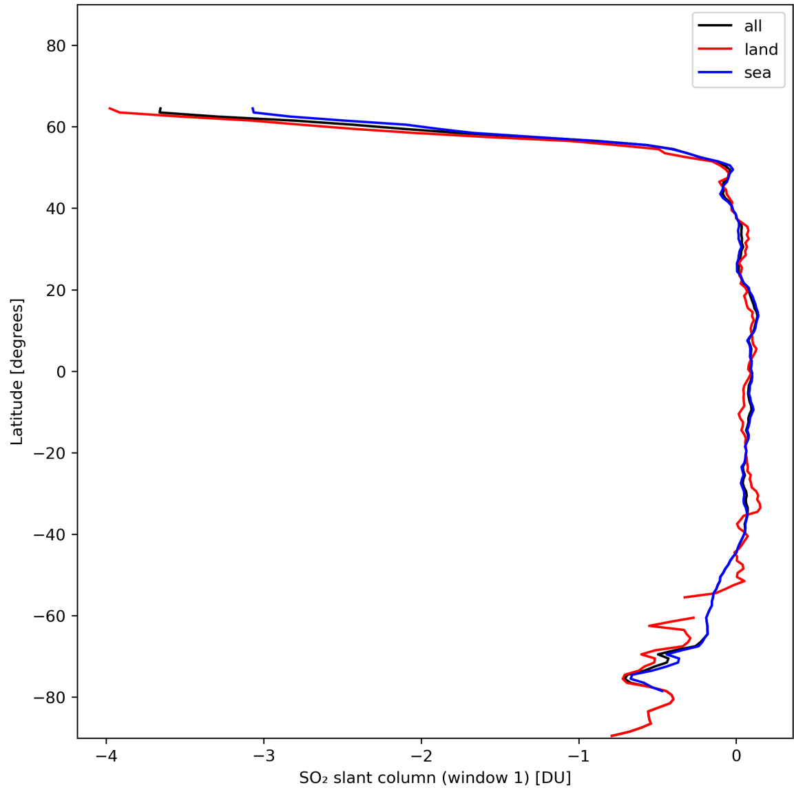
Figure 33: Zonal average of “SO 2 slant column (window 1)” for 2024-01-19 to 2024-01-21.
