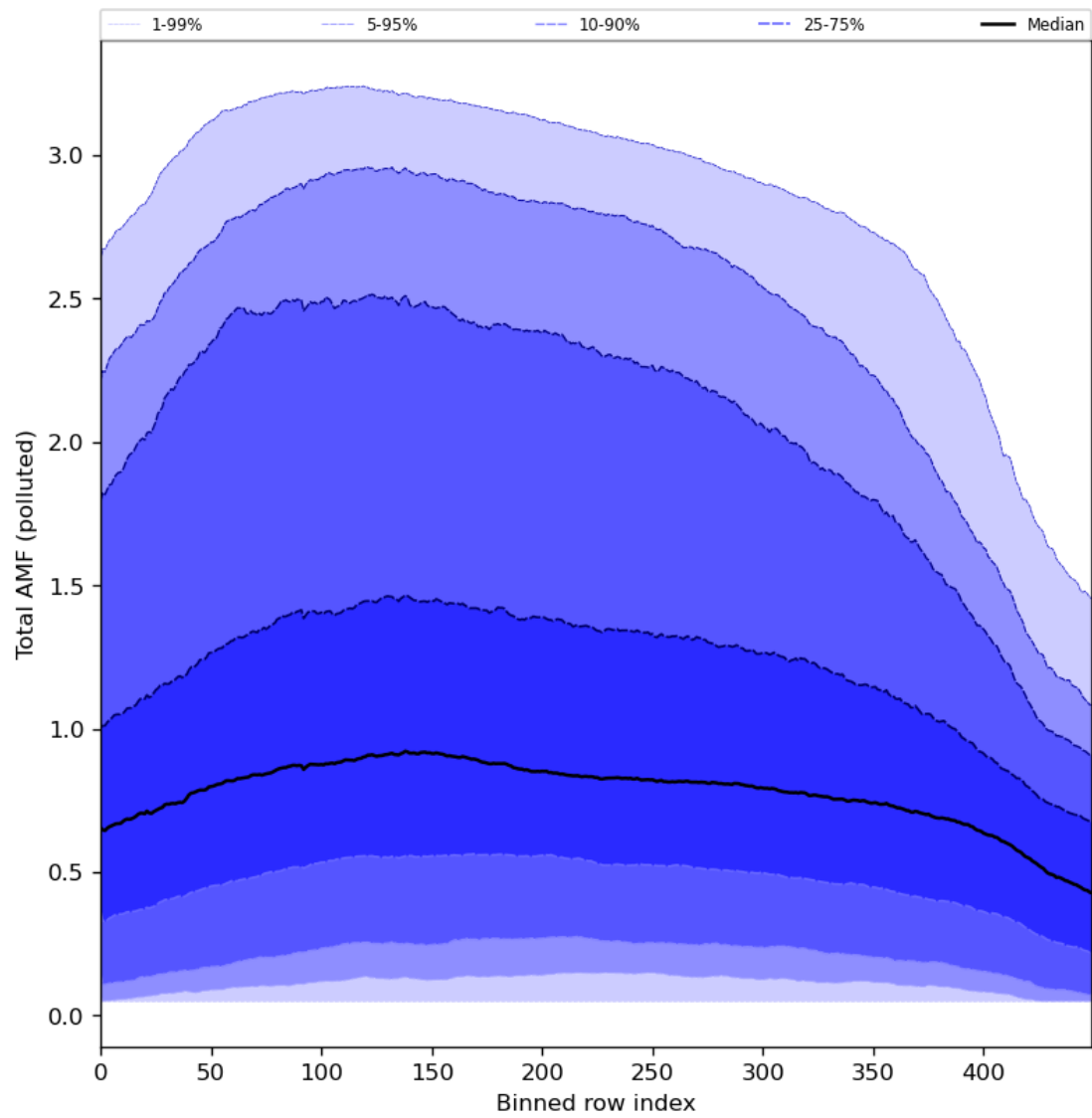
Figure 94: Along track statistics of “Total AMF (polluted)” for 2024-01-19 to 2024-01-21
