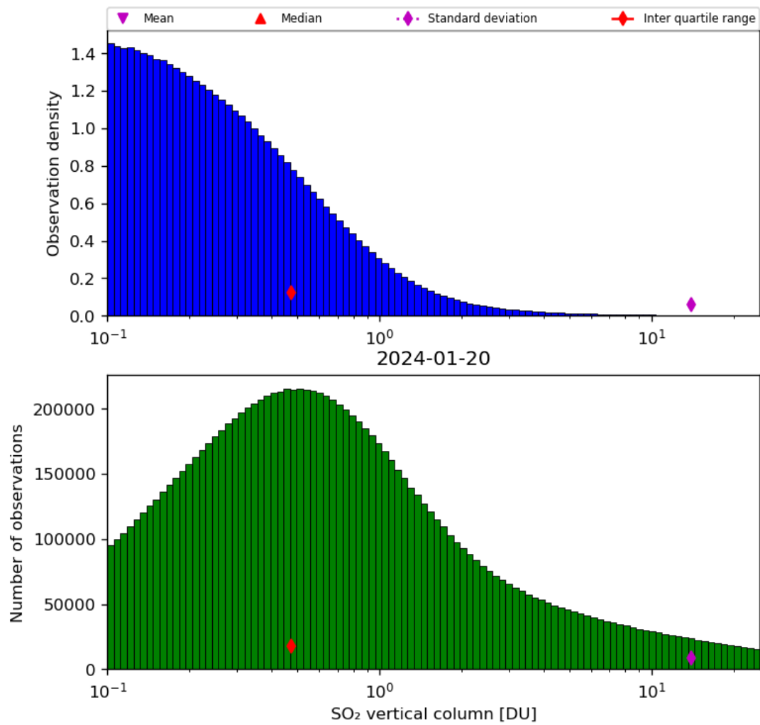
Figure 53: Histogram of “SO 2 vertical column” for 2024-01-19 to 2024-01-21
