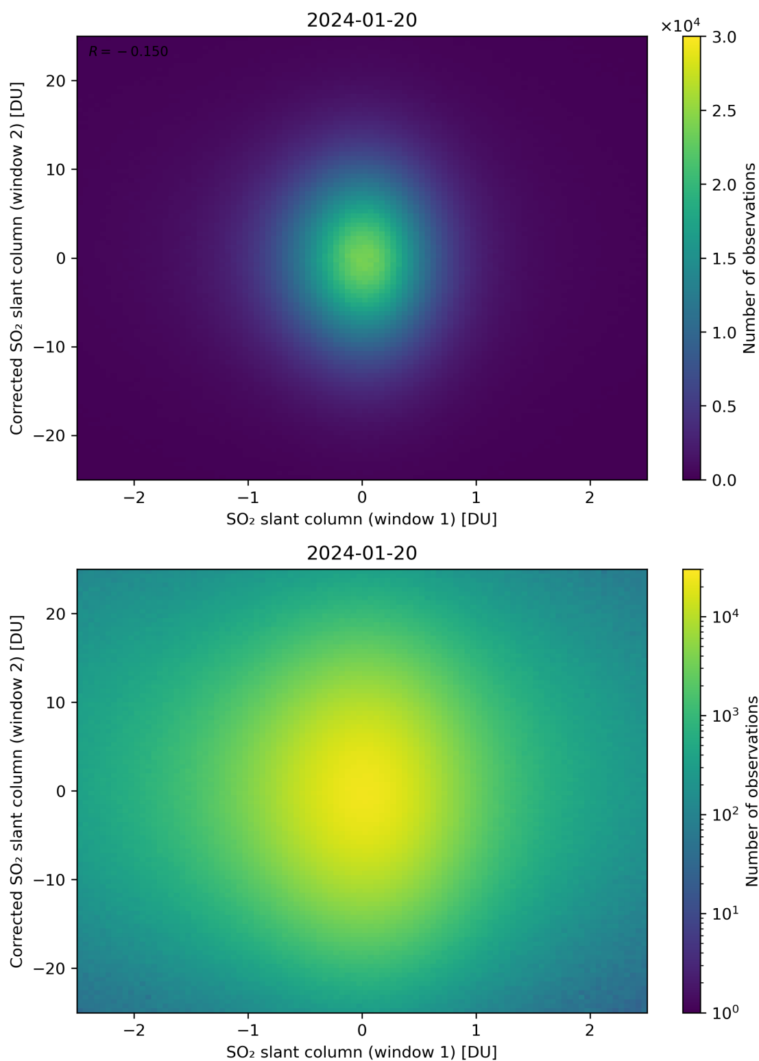
Figure 233: Scatter density plot of “SO 2 slant column (window 1)” against “Corrected SO 2 slant column (window 2)” for 2024-01-19 to 2024-01-21.
