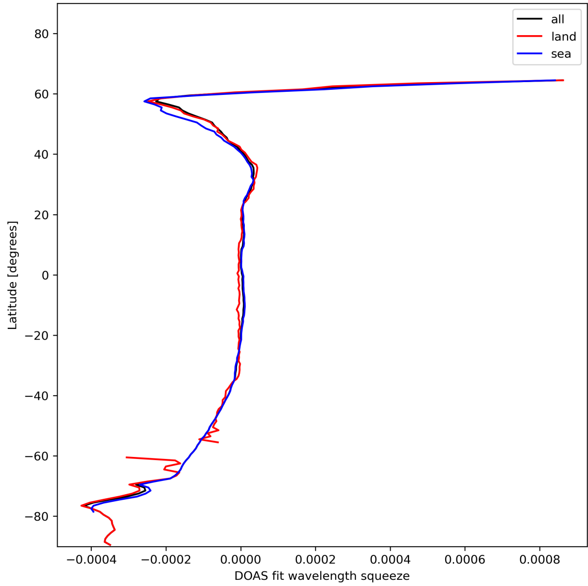
Figure 46: Zonal average of “DOAS fit wavelength squeeze” for 2024-01-19 to 2024-01-21.
