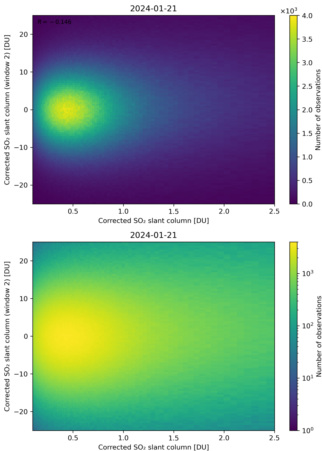
Figure 185: Scatter density plot of “Corrected SO 2 slant column” against “Corrected SO 2 slant column (window 2)” for 2024-01-21 to 2024-01-22.
