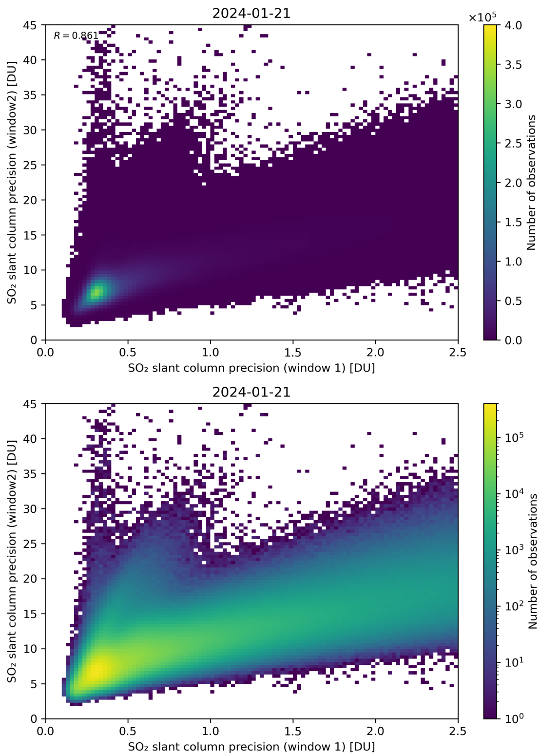
Figure 227: Scatter density plot of “SO 2 slant column precision (window 1)” against “SO 2 slant column precision (window2)” for 2024-01-21 to 2024-01-22.
