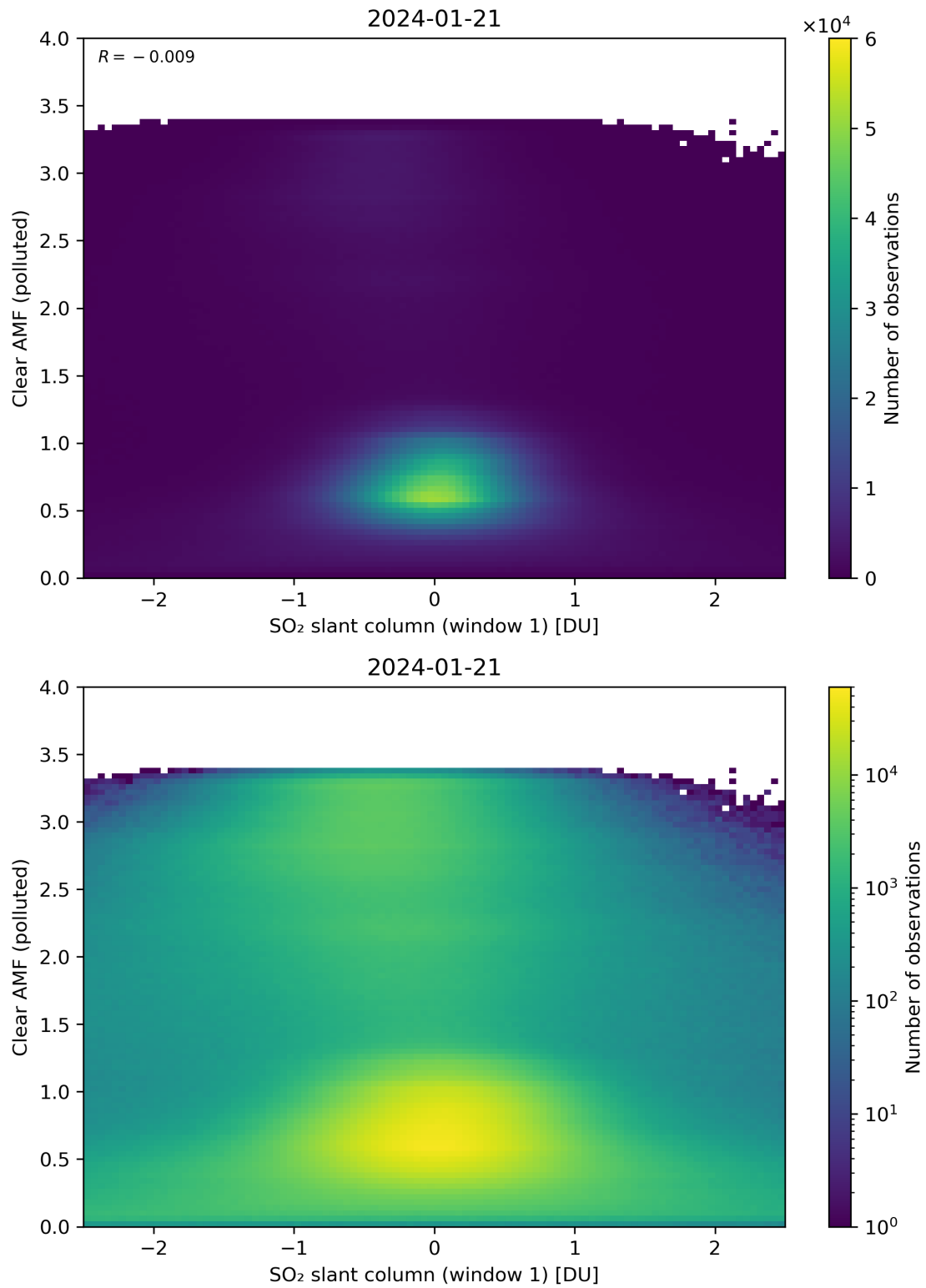
Figure 232: Scatter density plot of “SO 2 slant column (window 1)” against “Clear AMF (polluted)” for 2024-01-21 to 2024-01-22.
