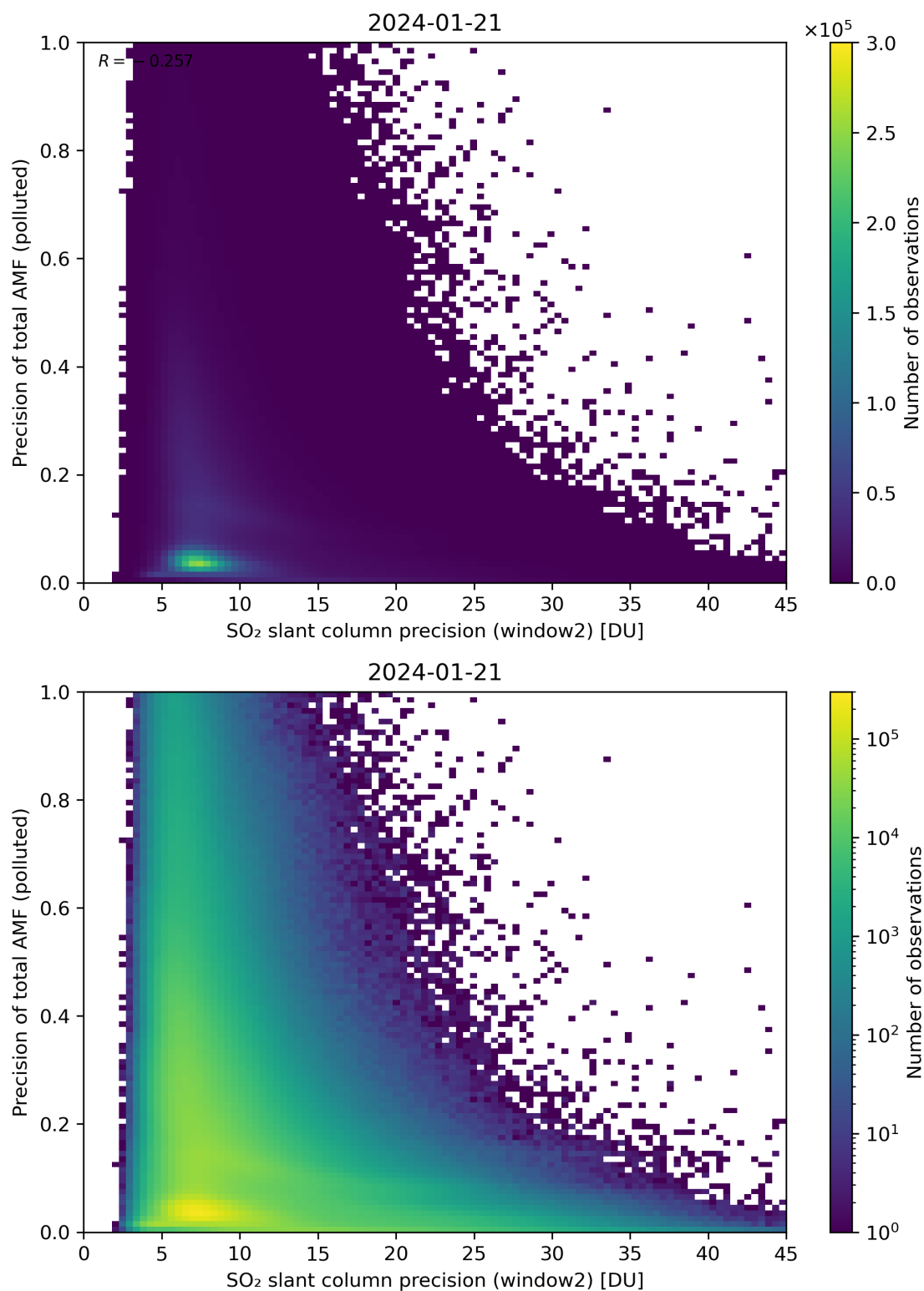
Figure 252: Scatter density plot of “SO 2 slant column precision (window2)” against “Precision of total AMF (polluted)” for 2024-01-21 to 2024-01-22.
