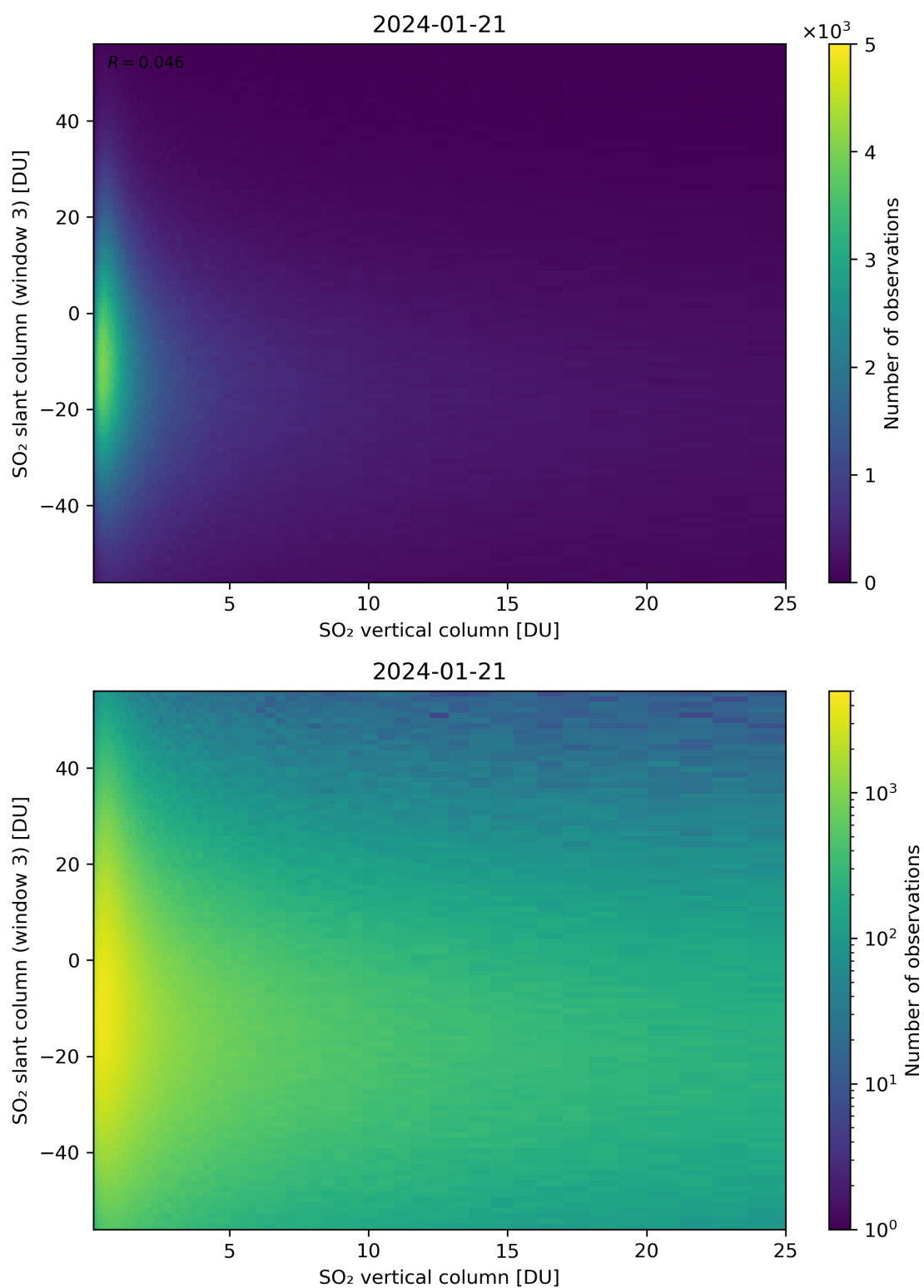
Figure 303: Scatter density plot of “SO 2 vertical column” against “SO 2 slant column (window 3)” for 2024-01-21 to 2024-01-22.
