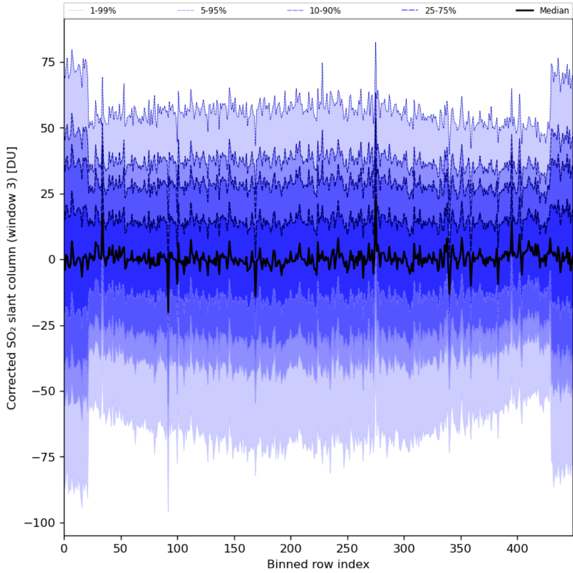
Figure 89: Along track statistics of “Corrected SO 2 slant column (window 3)” for 2024-01-21 to 2024-01-22
