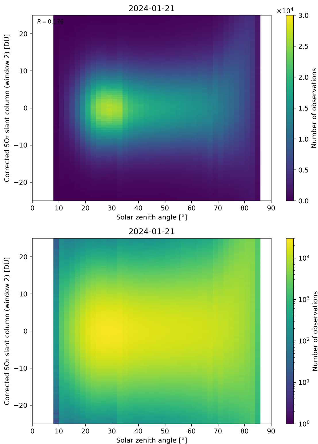
Figure 167: Scatter density plot of “Solar zenith angle” against “Corrected SO 2 slant column (window 2)” for 2024-01-21 to 2024-01-22.
