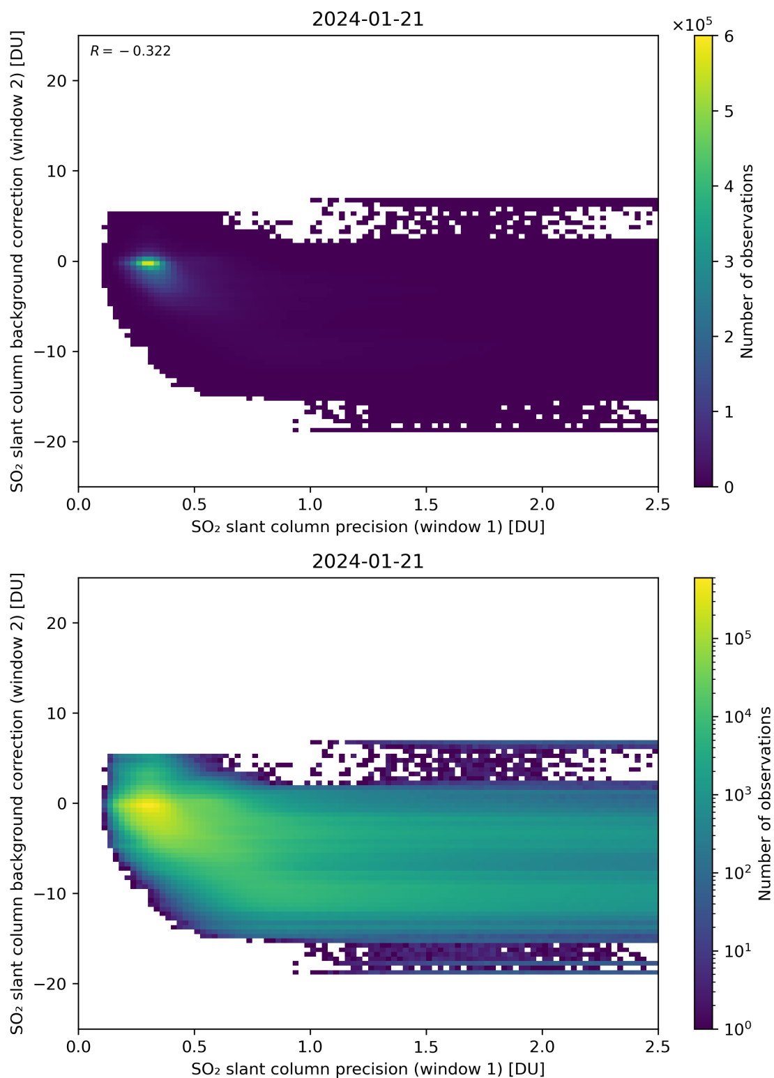
Figure 219: Scatter density plot of “SO 2 slant column precision (window 1)” against “SO 2 slant column background correction (window 2)” for 2024-01-21 to 2024-01-22.
