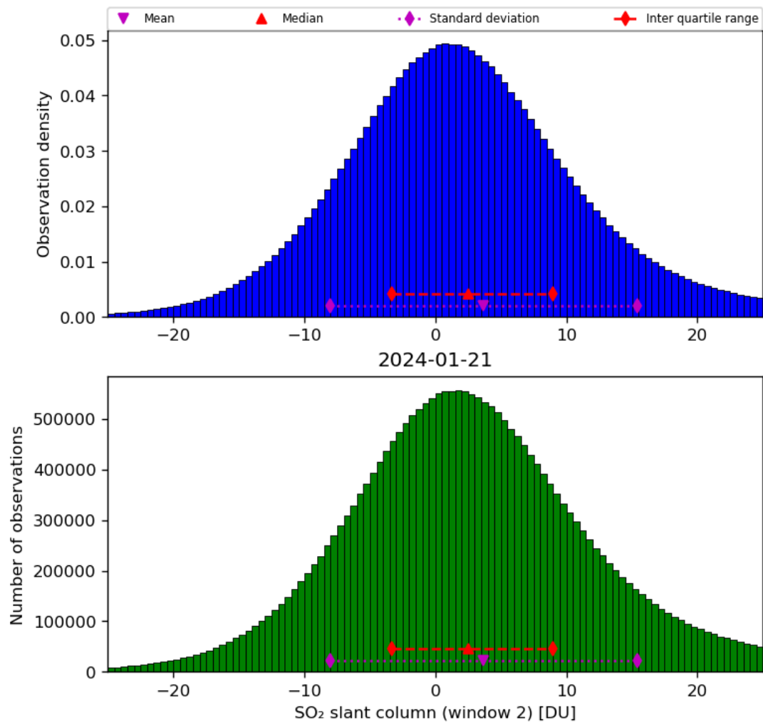
Figure 60: Histogram of “SO 2 slant column (window 2)” for 2024-01-21 to 2024-01-22
