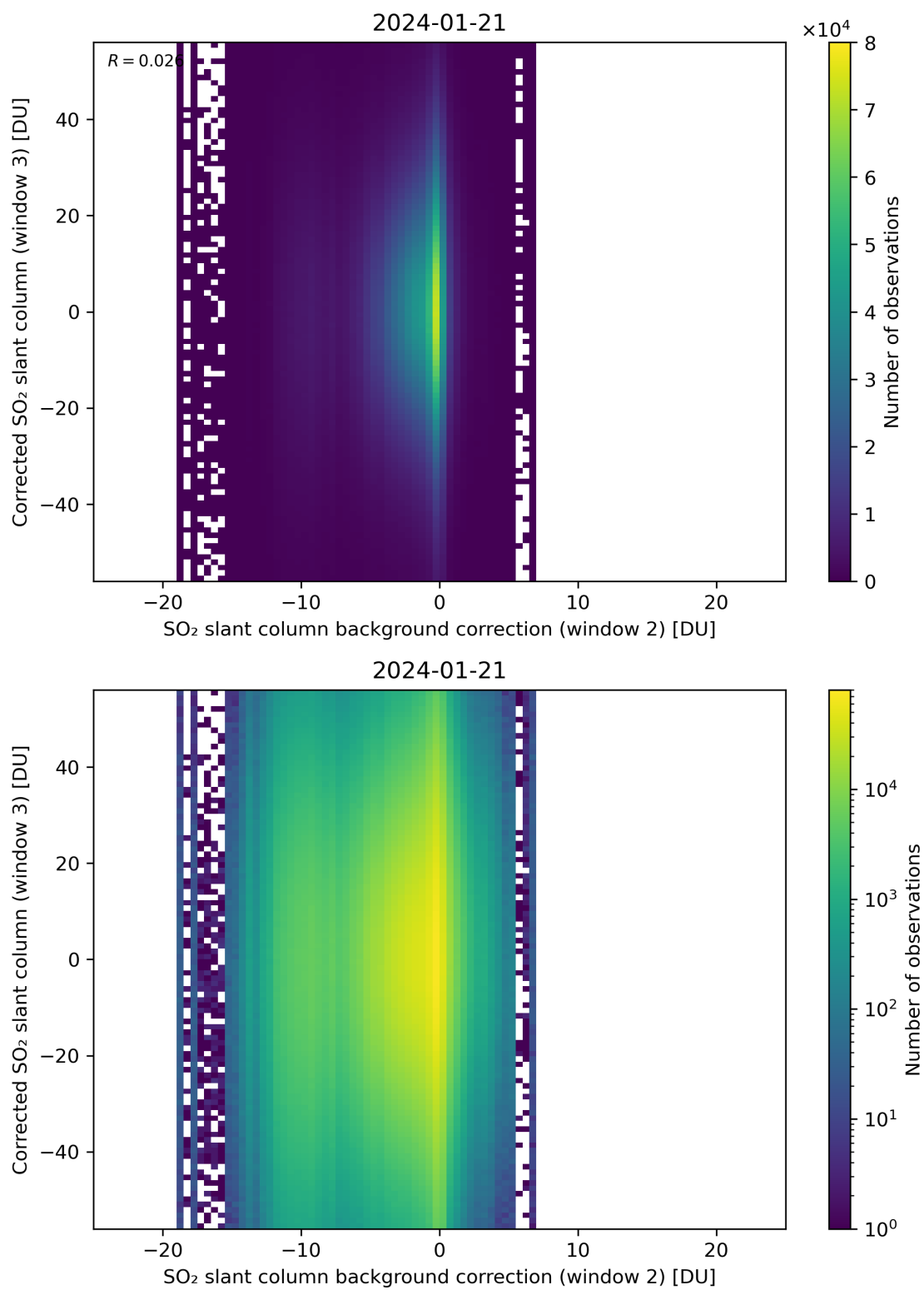
Figure 116: Scatter density plot of “SO 2 slant column background correction (window 2)” against “Corrected SO 2 slant column (window 3)” for 2024-01-21 to 2024-01-22.
