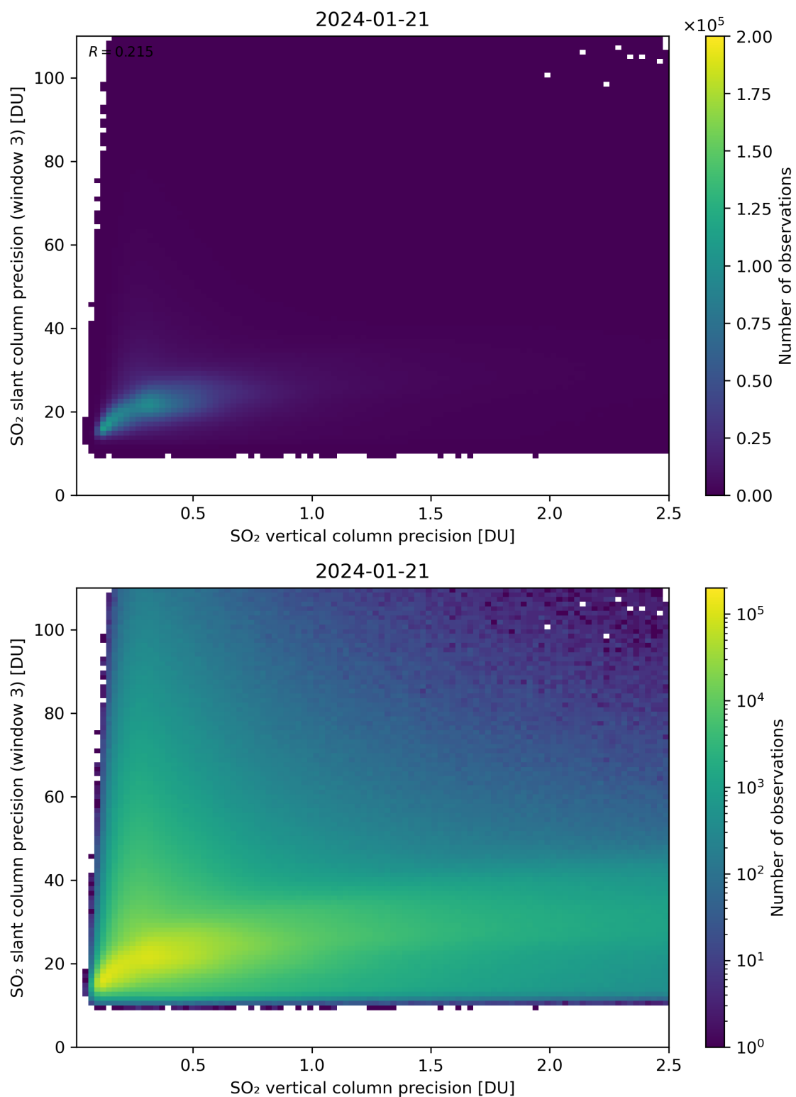
Figure 293: Scatter density plot of “SO 2 vertical column precision” against “SO 2 slant column precision (window 3)” for 2024-01-21 to 2024-01-22.
