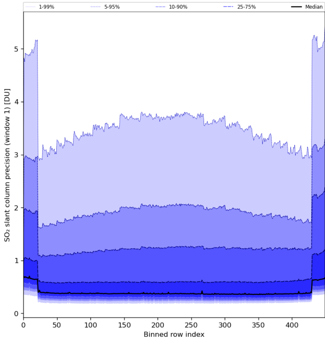
Figure 80: Along track statistics of "SO 2 slant column precision (window 1)" for 2024-01-21 to 2024-01-22
