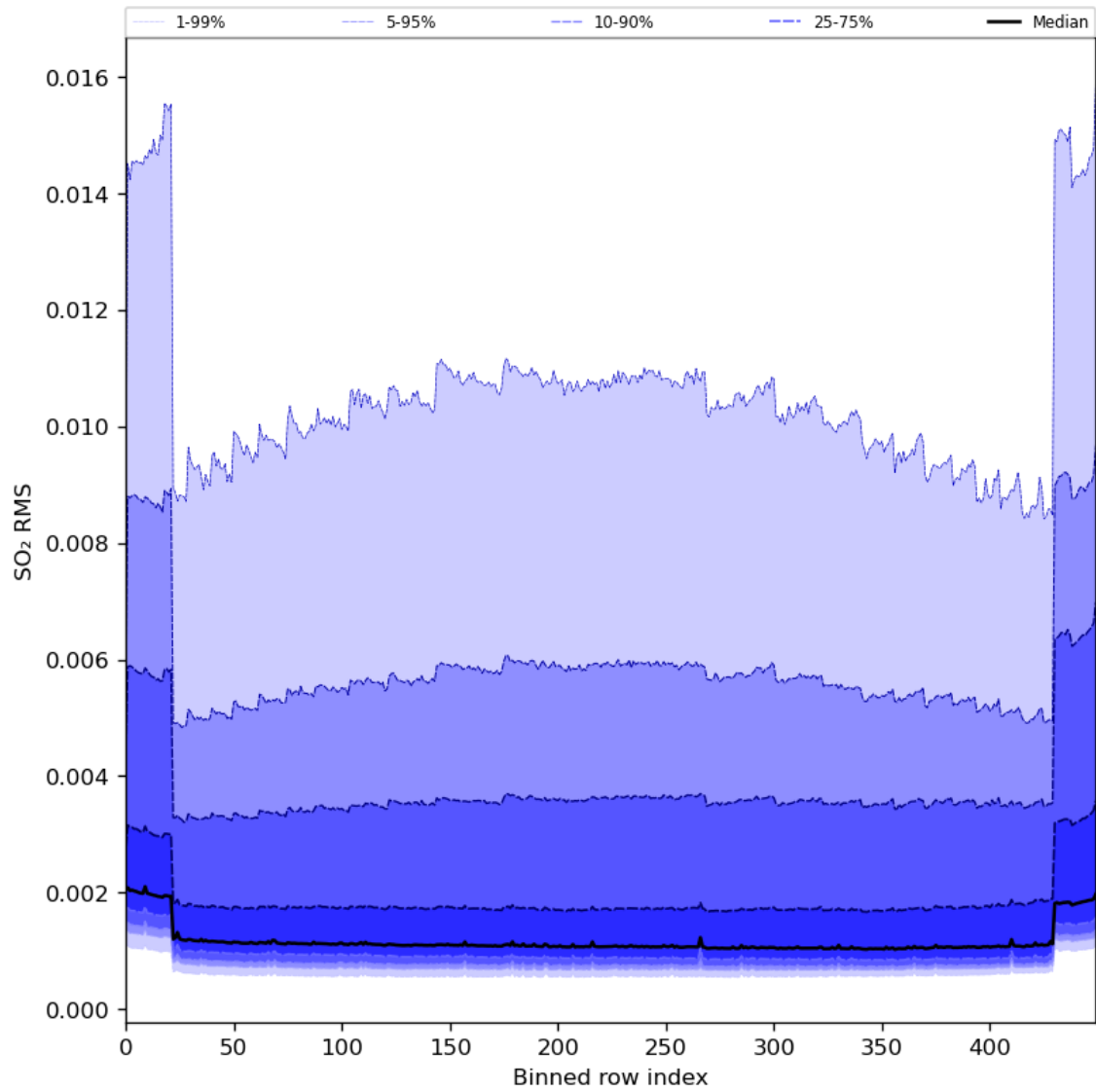
Figure 93: Along track statistics of “SO 2 RMS” for 2024-01-21 to 2024-01-22
