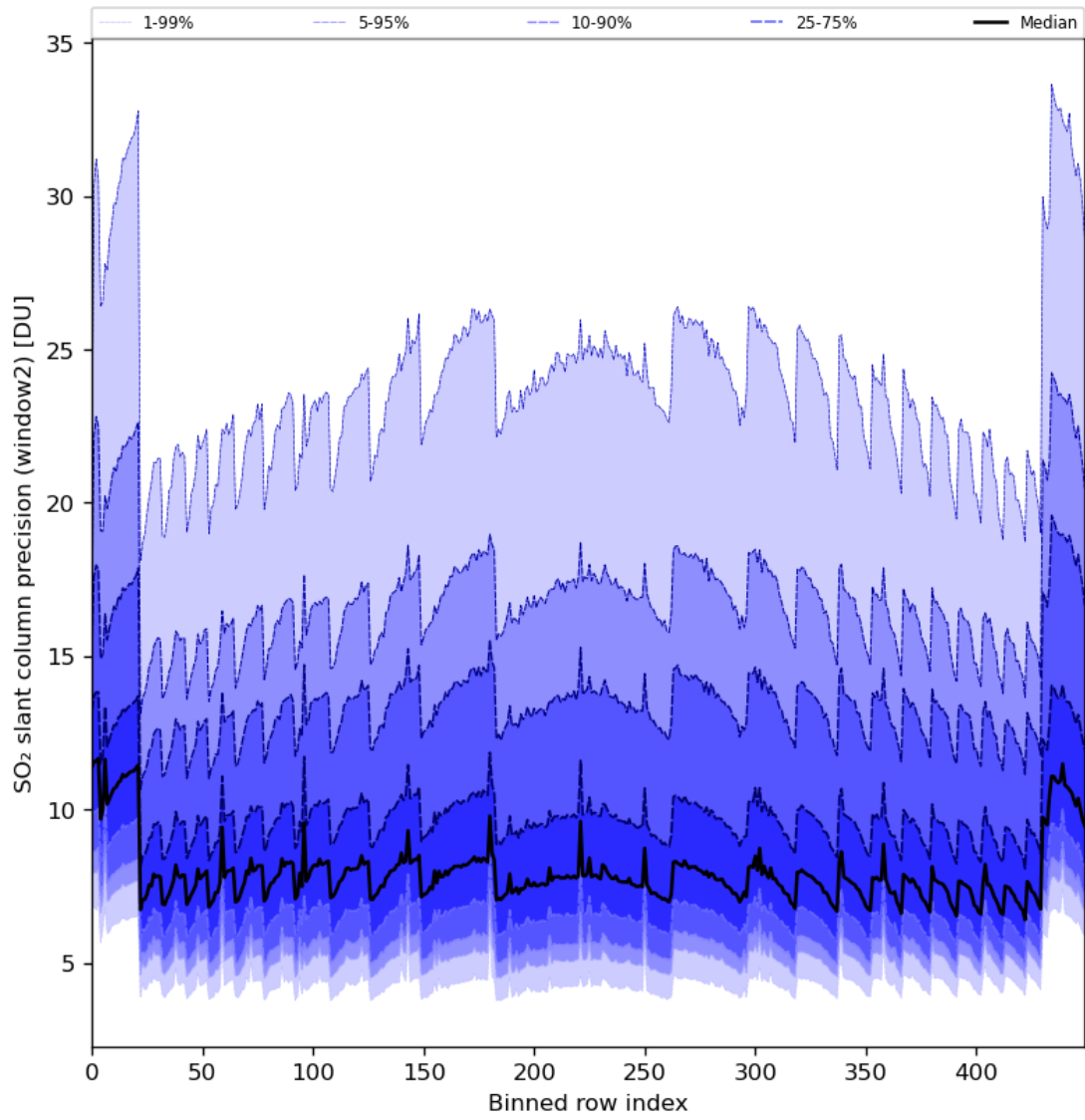
Figure 84: Along track statistics of “SO 2 slant column precision (window2)” for 2024-01-21 to 2024-01-22
