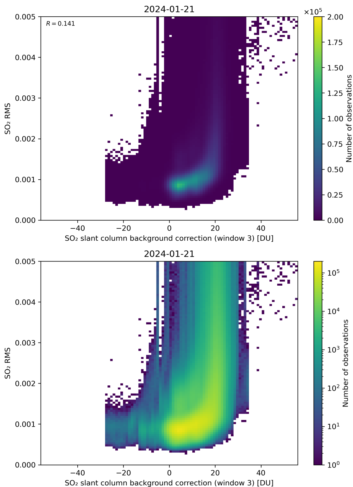
Figure 123: Scatter density plot of “SO 2 slant column background correction (window 3)” against “SO 2 RMS” for 2024-01-21 to 2024-01-22.
