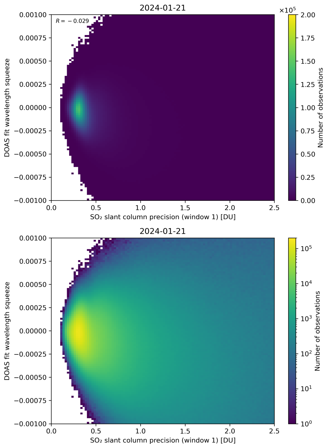
Figure 222: Scatter density plot of “SO 2 slant column precision (window 1)” against “DOAS fit wavelength squeeze” for 2024-01-21 to 2024-01-22.
