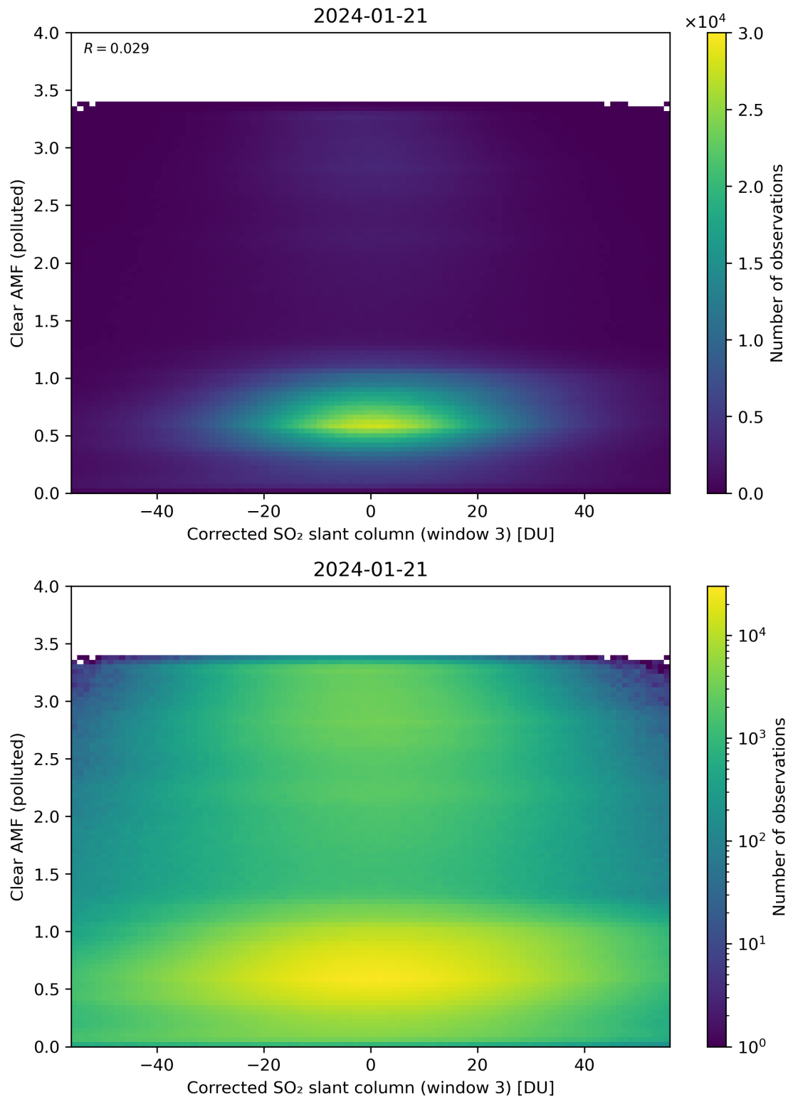
Figure 209: Scatter density plot of “Corrected SO 2 slant column (window 3)” against “Clear AMF (polluted)” for 2024-01-21 to 2024-01-22.
