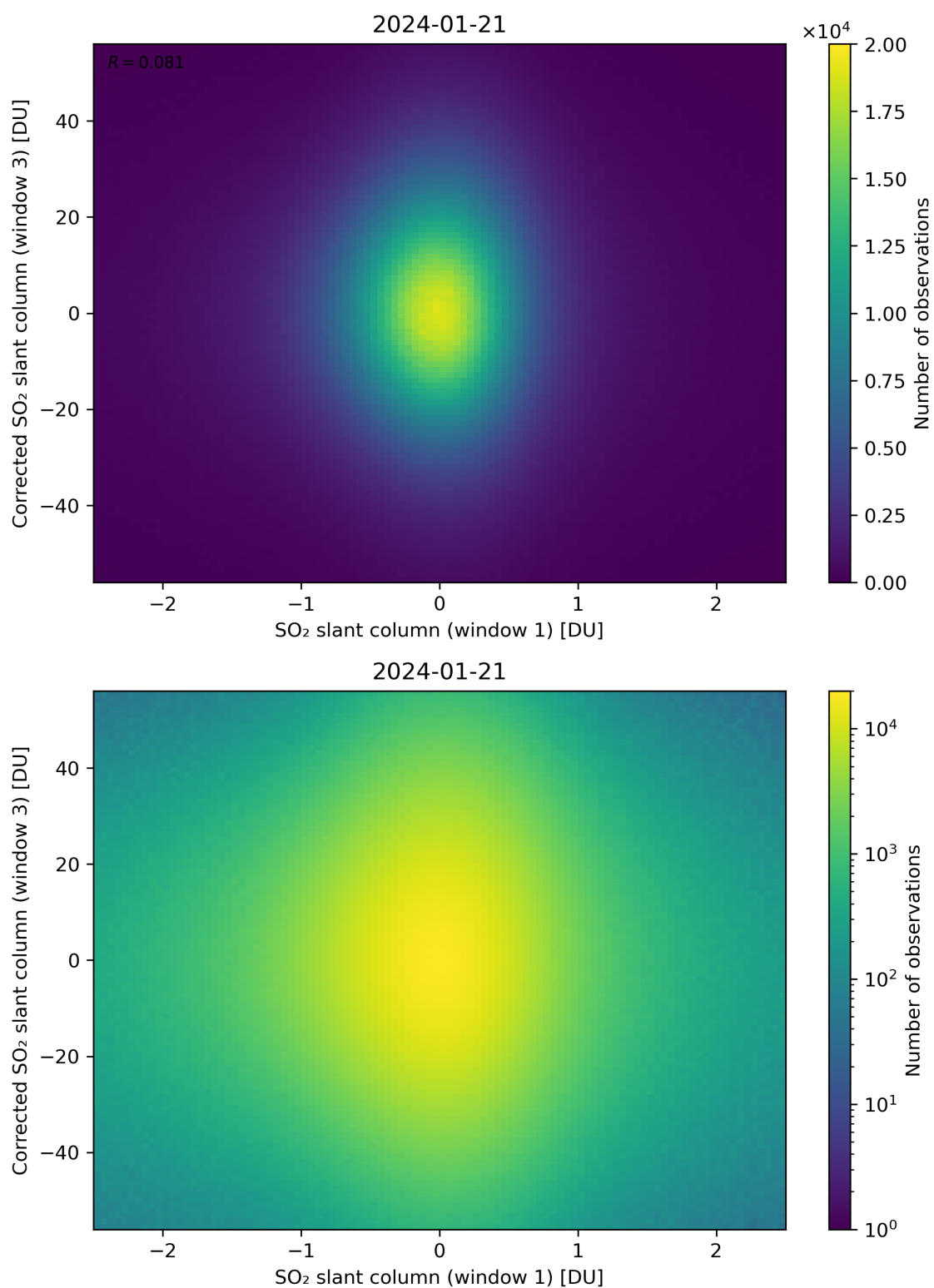
Figure 234: Scatter density plot of “SO 2 slant column (window 1)” against “Corrected SO 2 slant column (window 3)” for 2024-01-21 to 2024-01-22.
