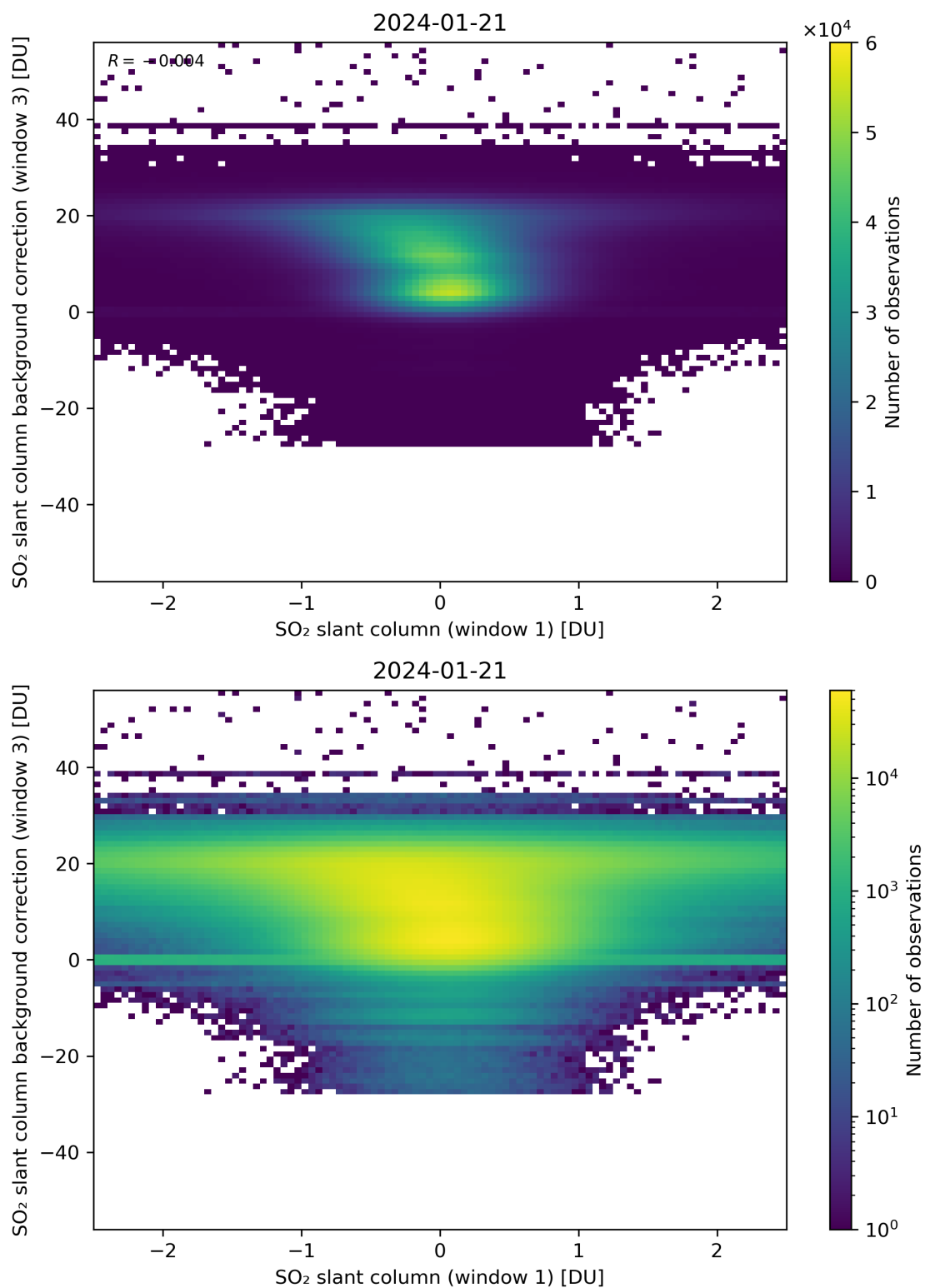
Figure 214: Scatter density plot of “SO 2 slant column (window 1)” against “SO 2 slant column background correction (window 3)” for 2024-01-21 to 2024-01-22.
