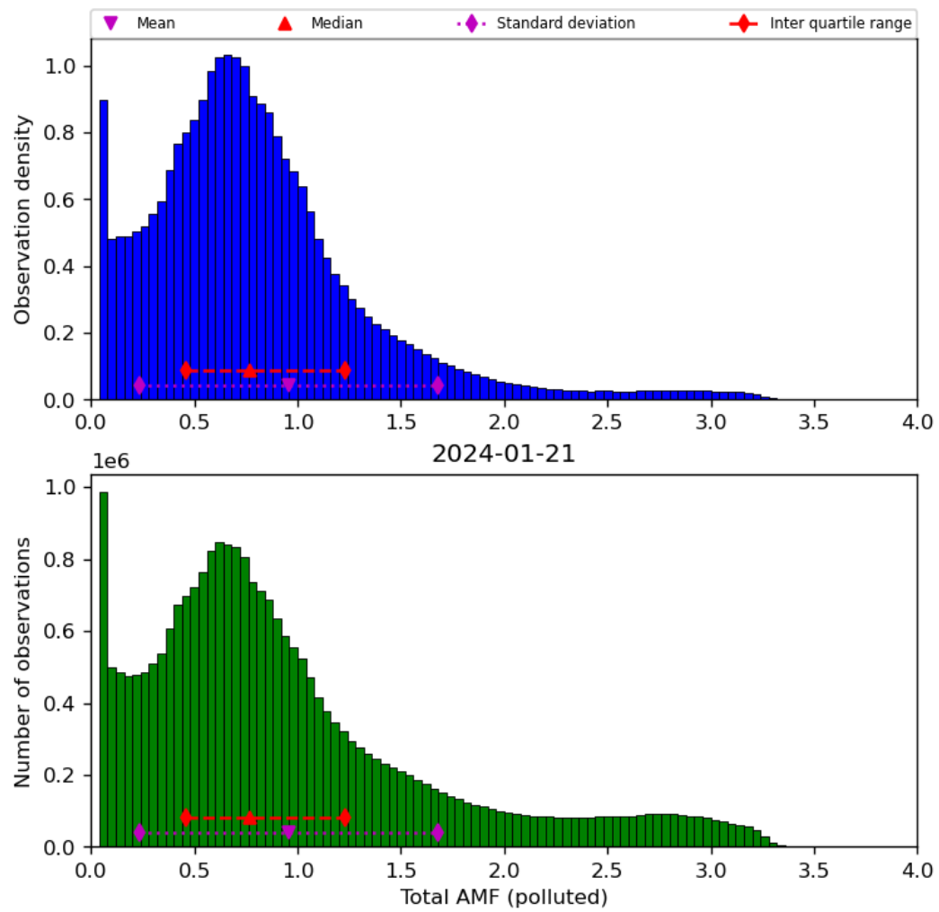
Figure 71: Histogram of “Total AMF (polluted)” for 2024-01-21 to 2024-01-22
