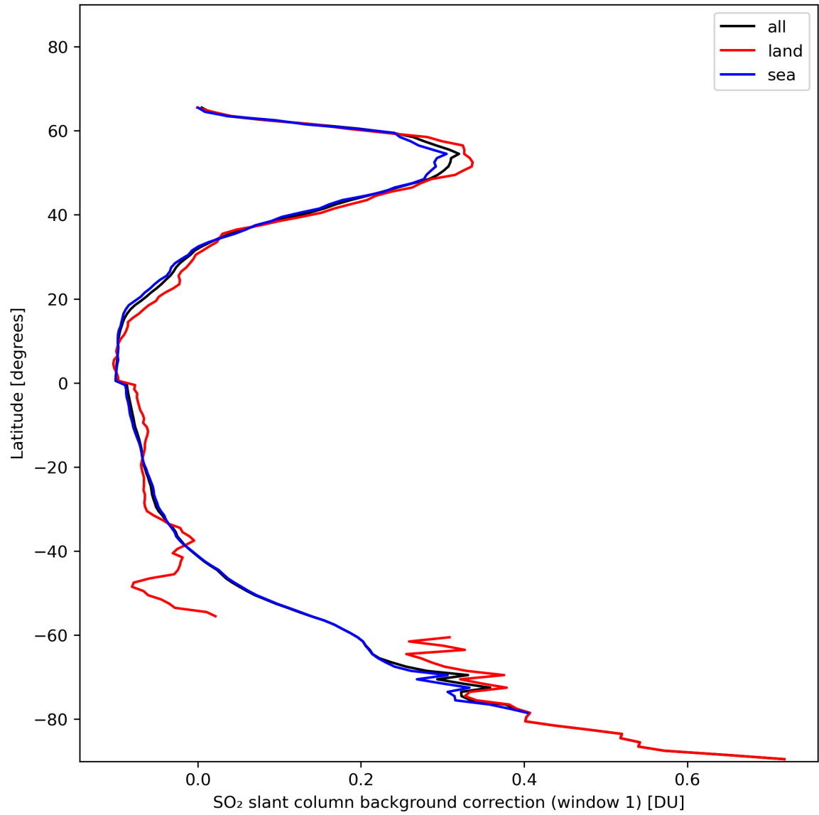
Figure 36: Zonal average of “SO 2 slant column background correction (window 1)” for 2024-01-21 to 2024-01-22.
