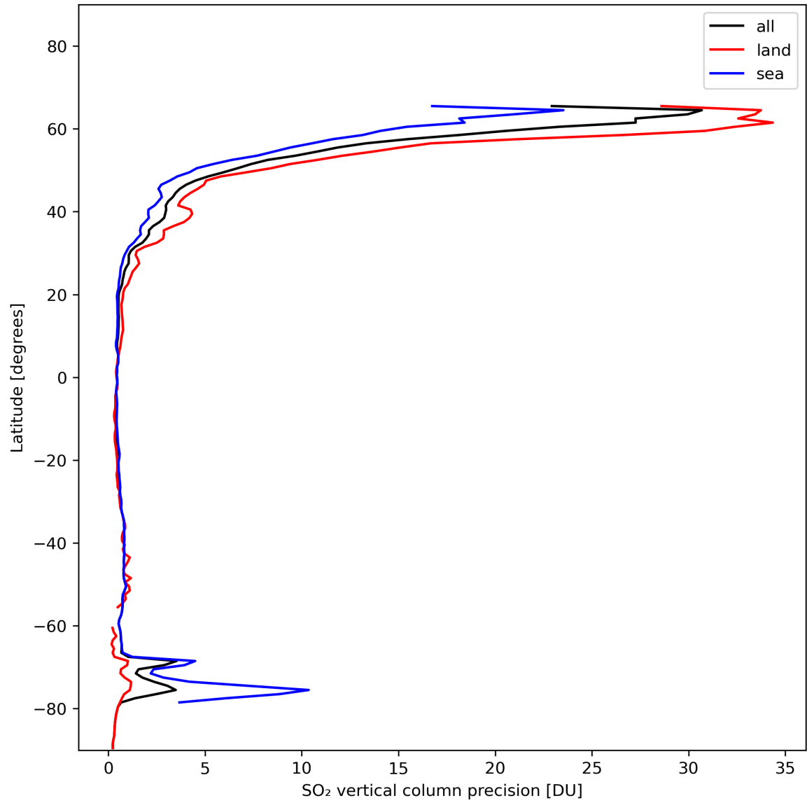
Figure 31: Zonal average of “SO 2 vertical column precision” for 2024-01-21 to 2024-01-22.
