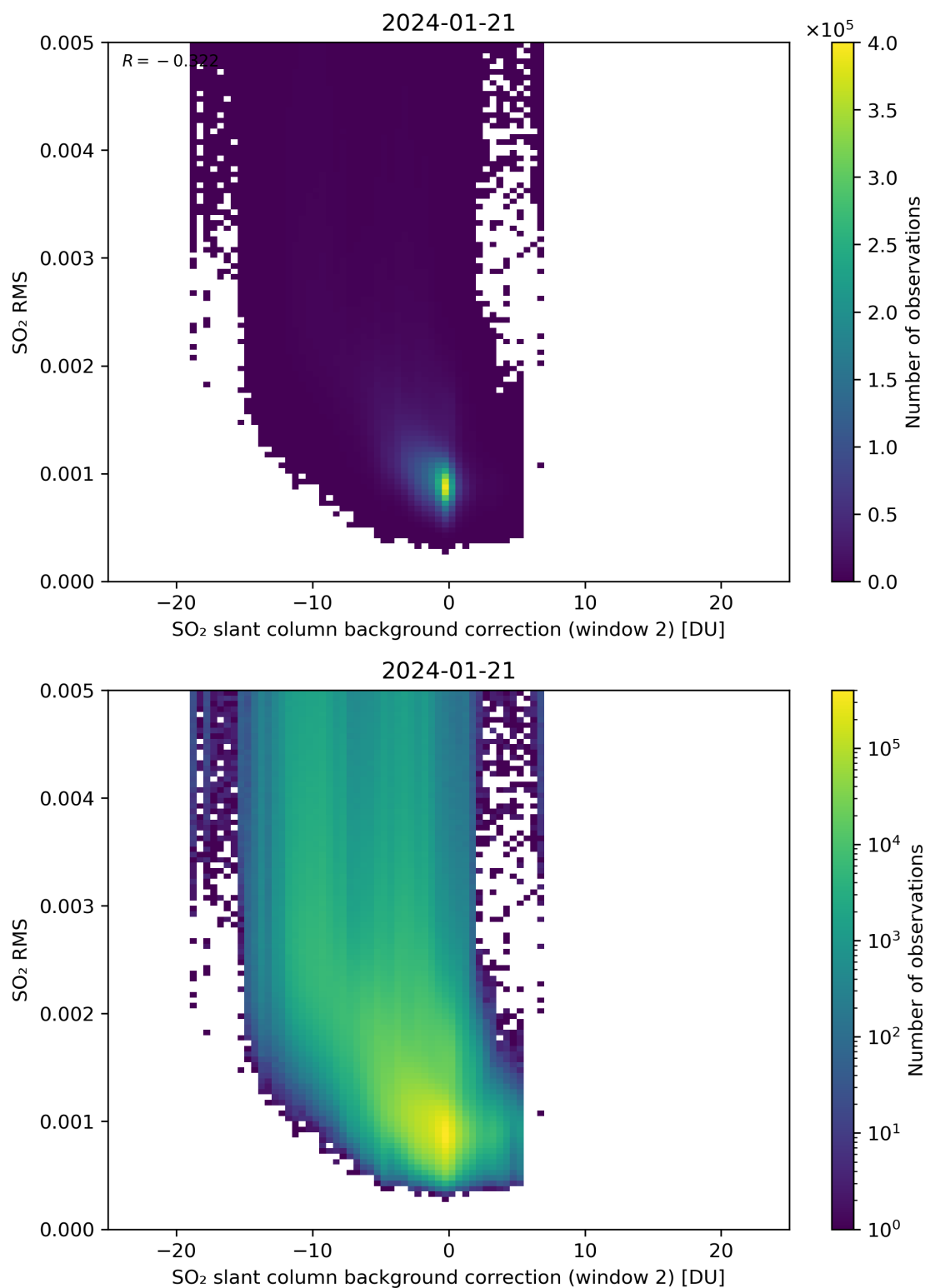
Figure 114: Scatter density plot of “SO 2 slant column background correction (window 2)” against “SO 2 RMS” for 2024-01-21 to 2024-01-22.
