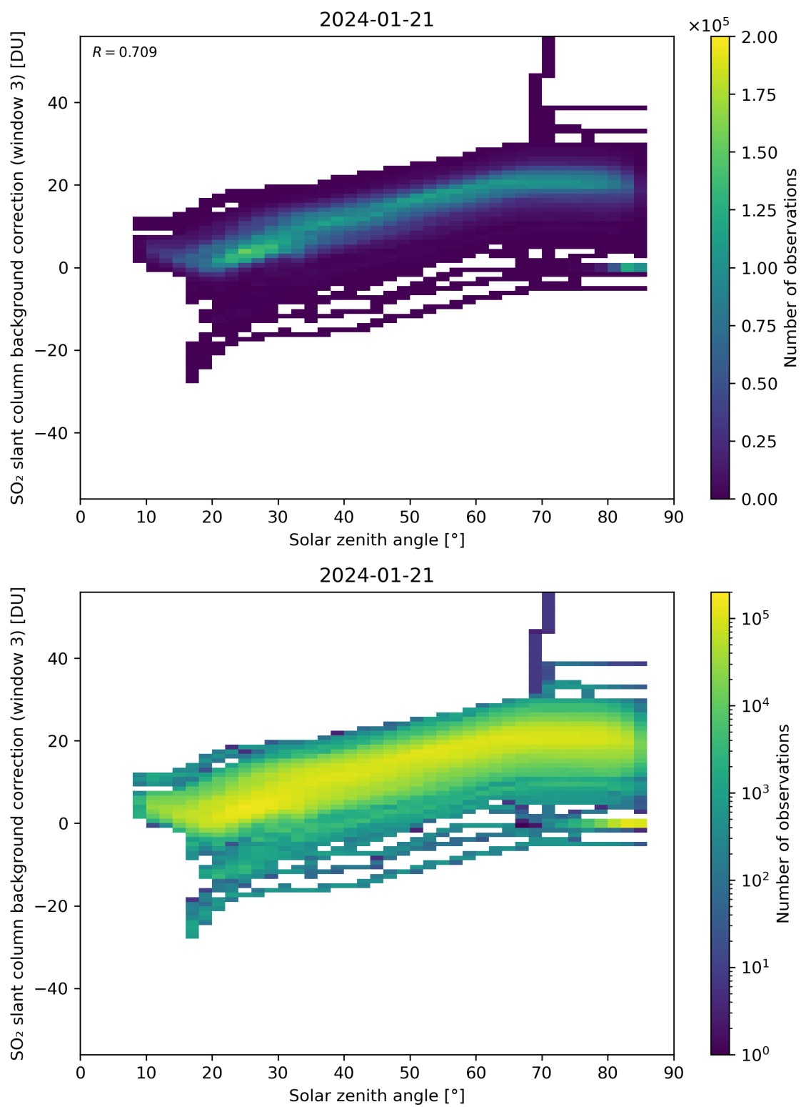
Figure 160: Scatter density plot of “Solar zenith angle” against “SO 2 slant column background correction (window 3)” for 2024-01-21 to 2024-01-22.
