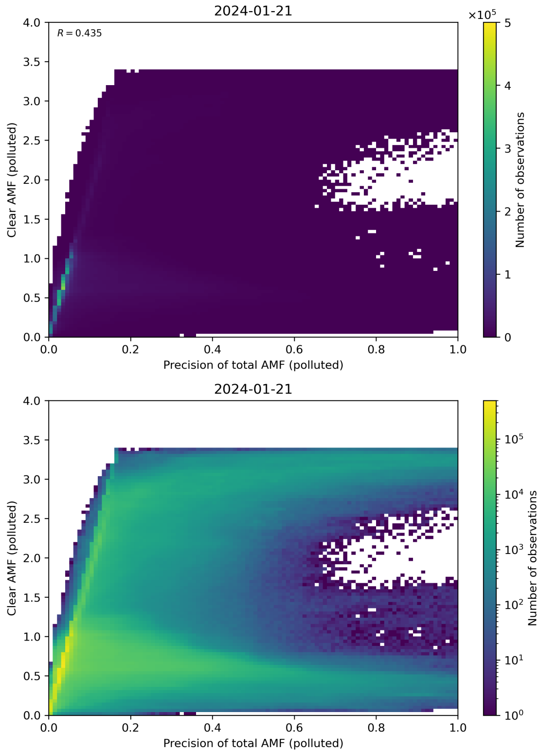
Figure 270: Scatter density plot of “Precision of total AMF (polluted)” against “Clear AMF (polluted)” for 2024-01-21 to 2024-01-22.
