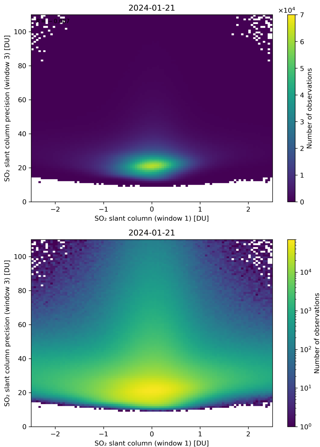
Figure 238: Scatter density plot of “SO 2 slant column (window 1)” against “SO 2 slant column precision (window 3)” for 2024-01-21 to 2024-01-22.
