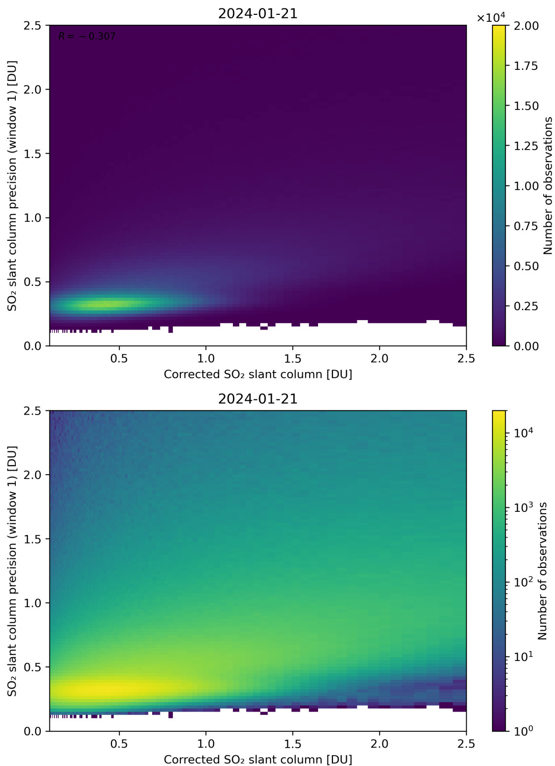
Figure 188: Scatter density plot of “Corrected SO 2 slant column” against “SO 2 slant column precision (window 1)” for 2024-01-21 to 2024-01-22.
