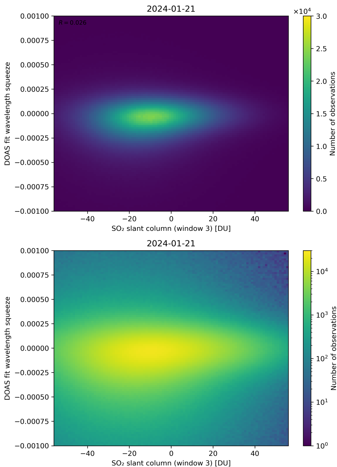
Figure 255: Scatter density plot of “SO 2 slant column (window 3)” against “DOAS fit wavelength squeeze” for 2024-01-21 to 2024-01-22.
