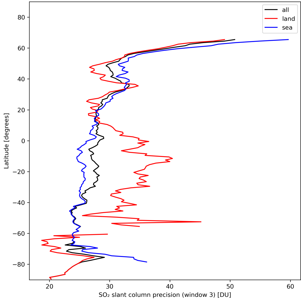
Figure 42: Zonal average of “SO 2 slant column precision (window 3)” for 2024-01-21 to 2024-01-22.
