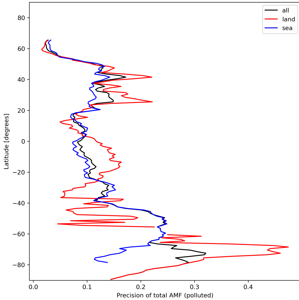
Figure 49: Zonal average of “Precision of total AMF (polluted)” for 2024-01-21 to 2024-01-22.
