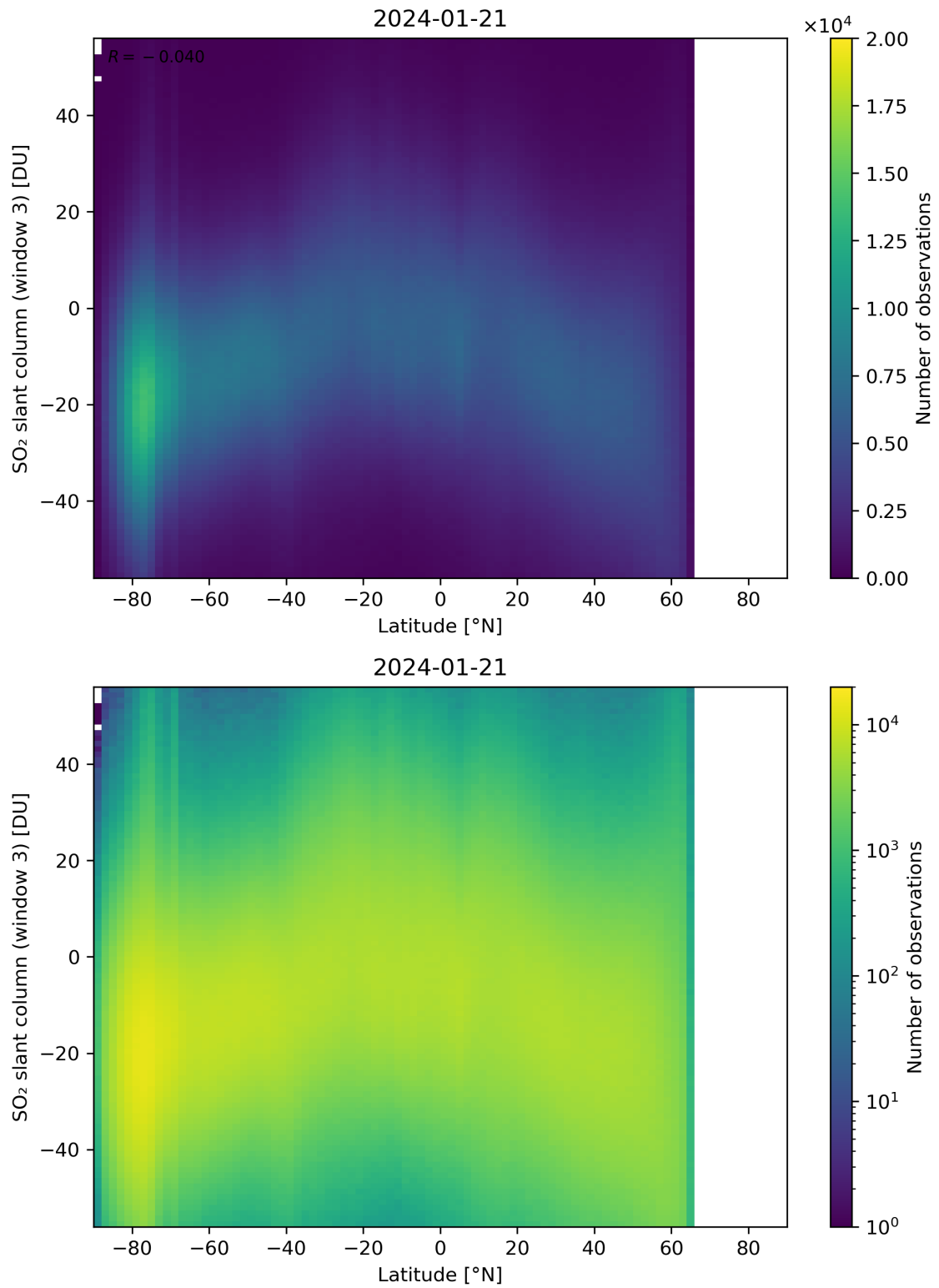
Figure 152: Scatter density plot of “Latitude” against “SO 2 slant column (window 3)” for 2024-01-21 to 2024-01-22.
