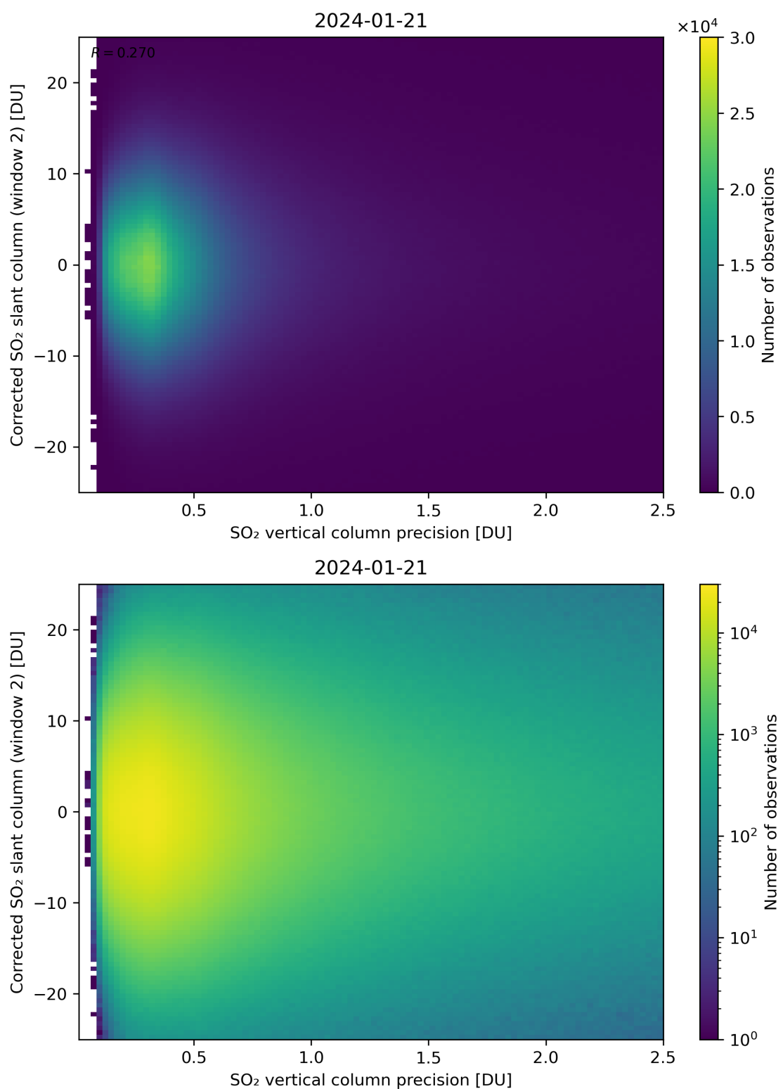
Figure 287: Scatter density plot of “SO 2 vertical column precision” against “Corrected SO 2 slant column (window 2)” for 2024-01-21 to 2024-01-22.
