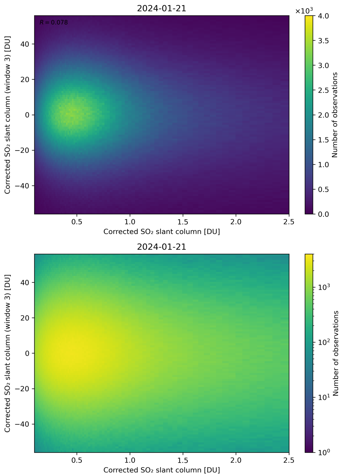
Figure 186: Scatter density plot of “Corrected SO 2 slant column” against “Corrected SO 2 slant column (window 3)” for 2024-01-21 to 2024-01-22.
