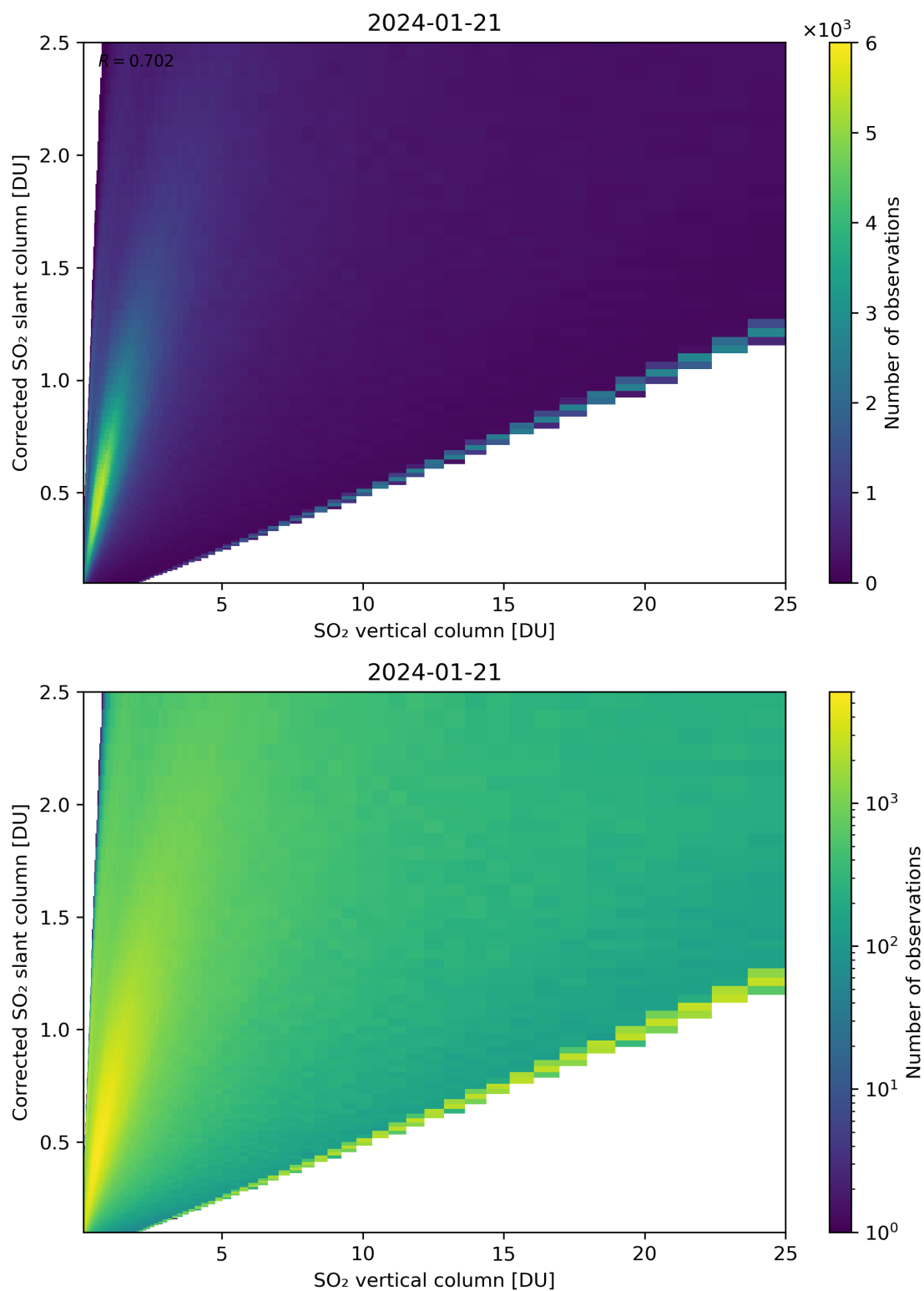
Figure 297: Scatter density plot of “SO 2 vertical column” against “Corrected SO 2 slant column” for 2024-01-21 to 2024-01-22.
