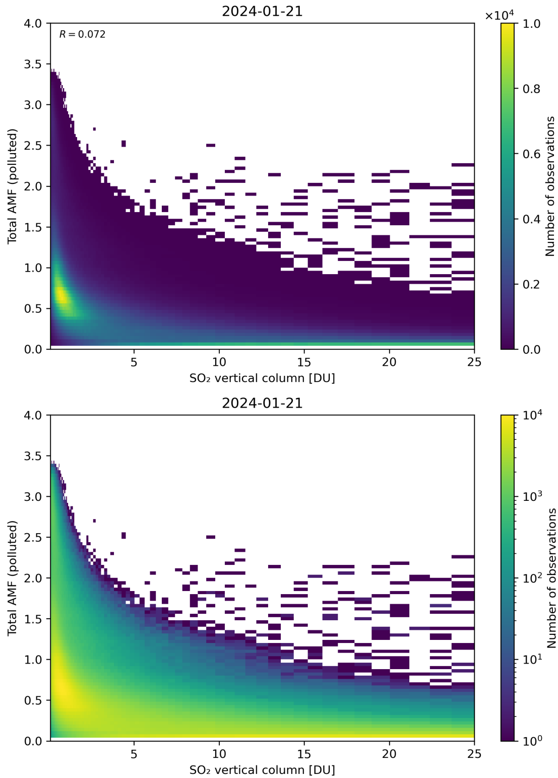
Figure 305: Scatter density plot of “SO 2 vertical column” against “Total AMF (polluted)” for 2024-01-21 to 2024-01-22.
