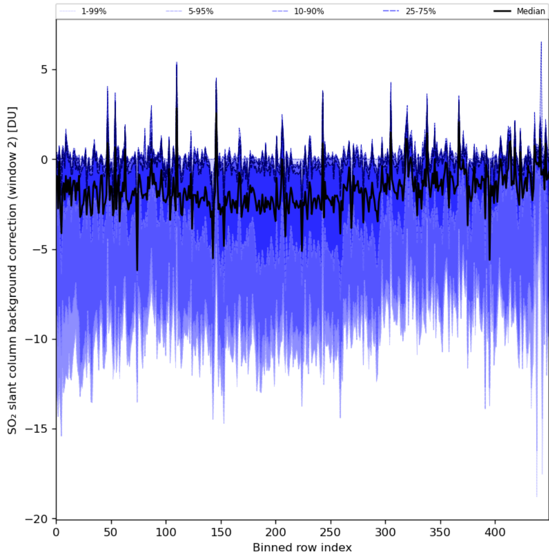
Figure 86: Along track statistics of “SO 2 slant column background correction (window 2)” for 2024-01-21 to 2024-01-22
