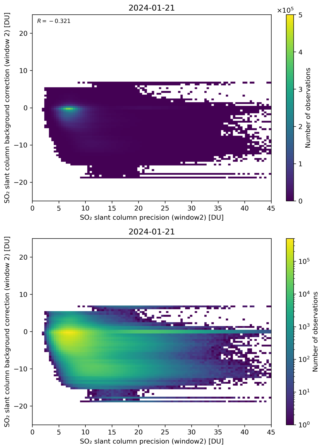
Figure 241: Scatter density plot of “SO 2 slant column precision (window2)” against “SO 2 slant column background correction (window 2)” for 2024-01-21 to 2024-01-22.
