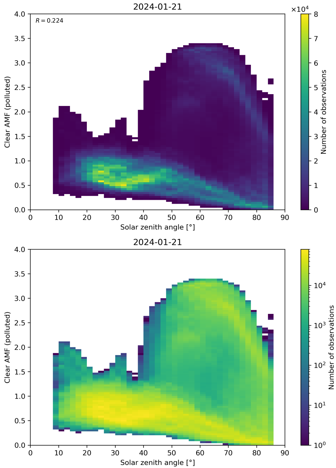
Figure 165: Scatter density plot of “Solar zenith angle” against “Clear AMF (polluted)” for 2024-01-21 to 2024-01-22.
