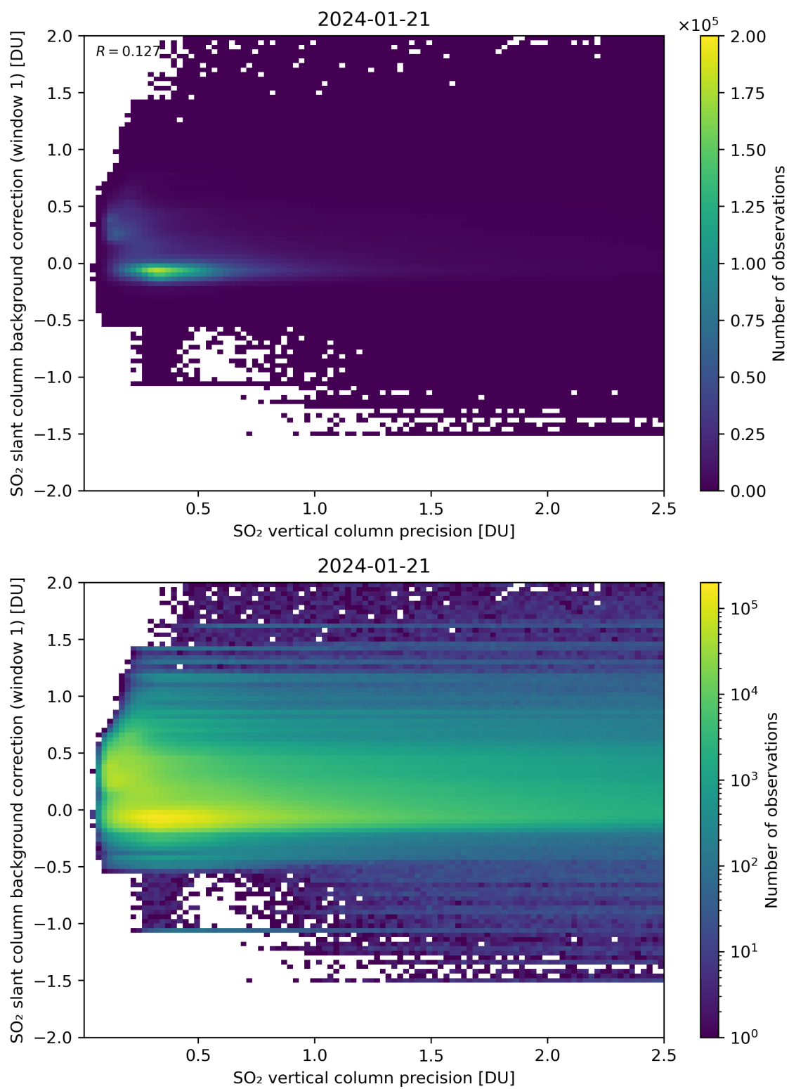
Figure 279: Scatter density plot of “SO 2 vertical column precision” against “SO 2 slant column background correction (window 1)” for 2024-01-21 to 2024-01-22.
