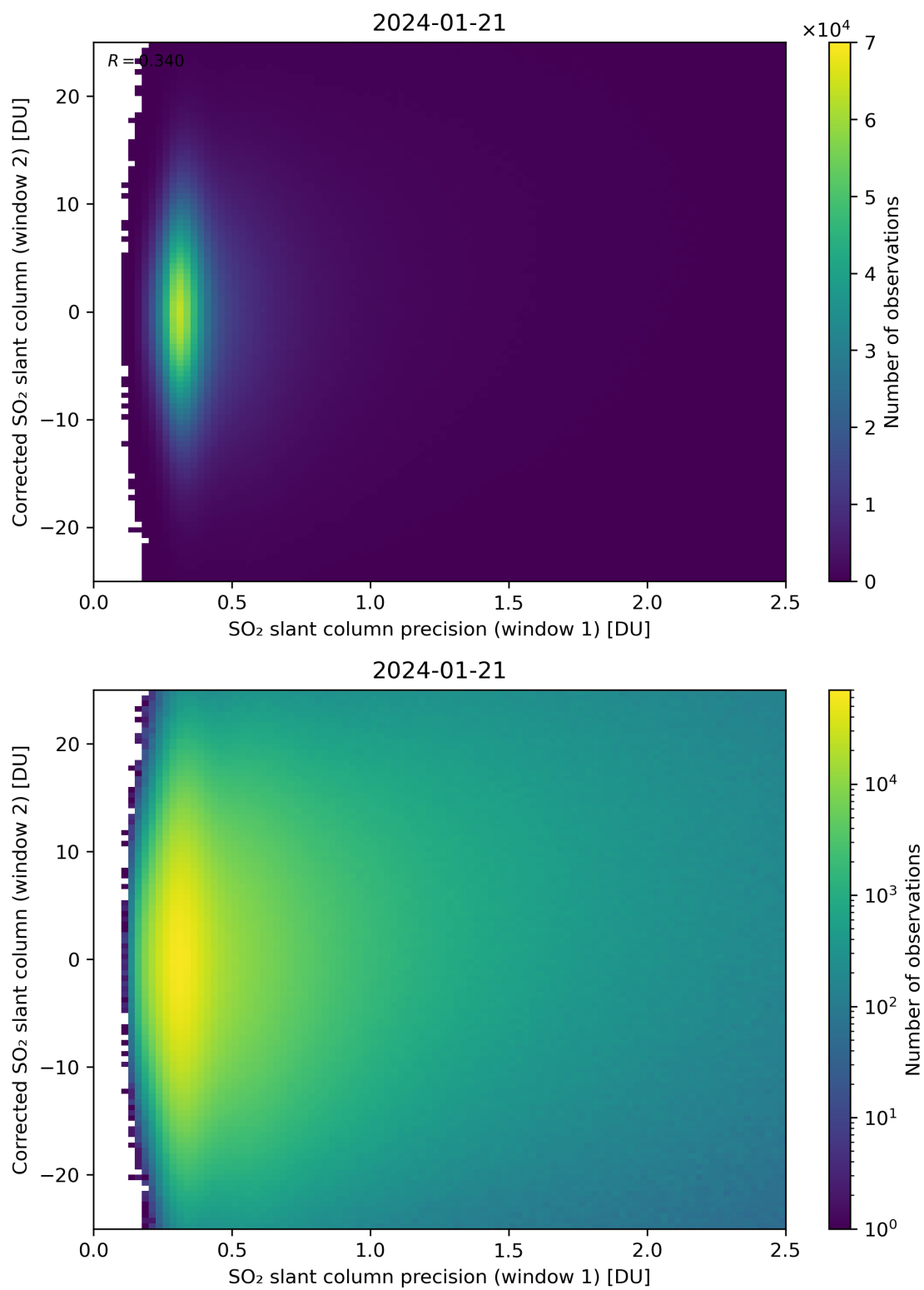
Figure 225: Scatter density plot of “SO 2 slant column precision (window 1)” against “Corrected SO 2 slant column (window 2)” for 2024-01-21 to 2024-01-22.
