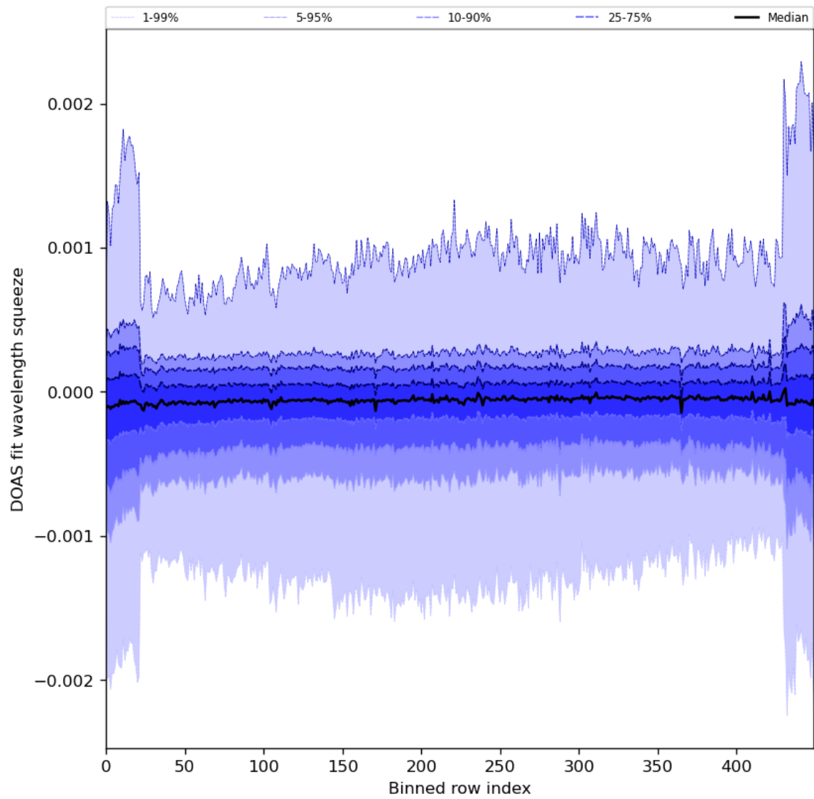
Figure 92: Along track statistics of “DOAS fit wavelength squeeze” for 2024-01-21 to 2024-01-22
