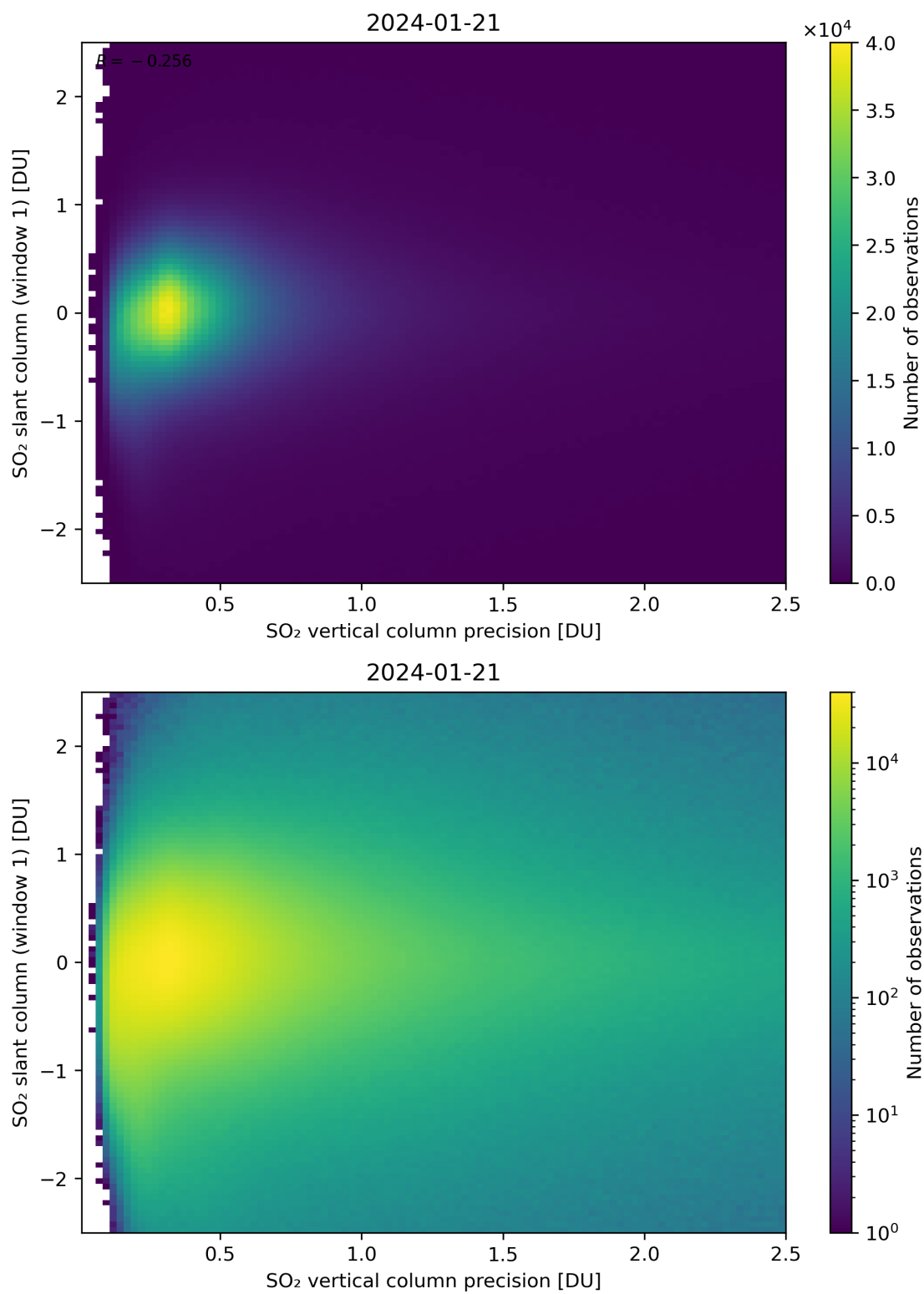
Figure 289: Scatter density plot of “SO 2 vertical column precision” against “SO 2 slant column (window 1)” for 2024-01-21 to 2024-01-22.
