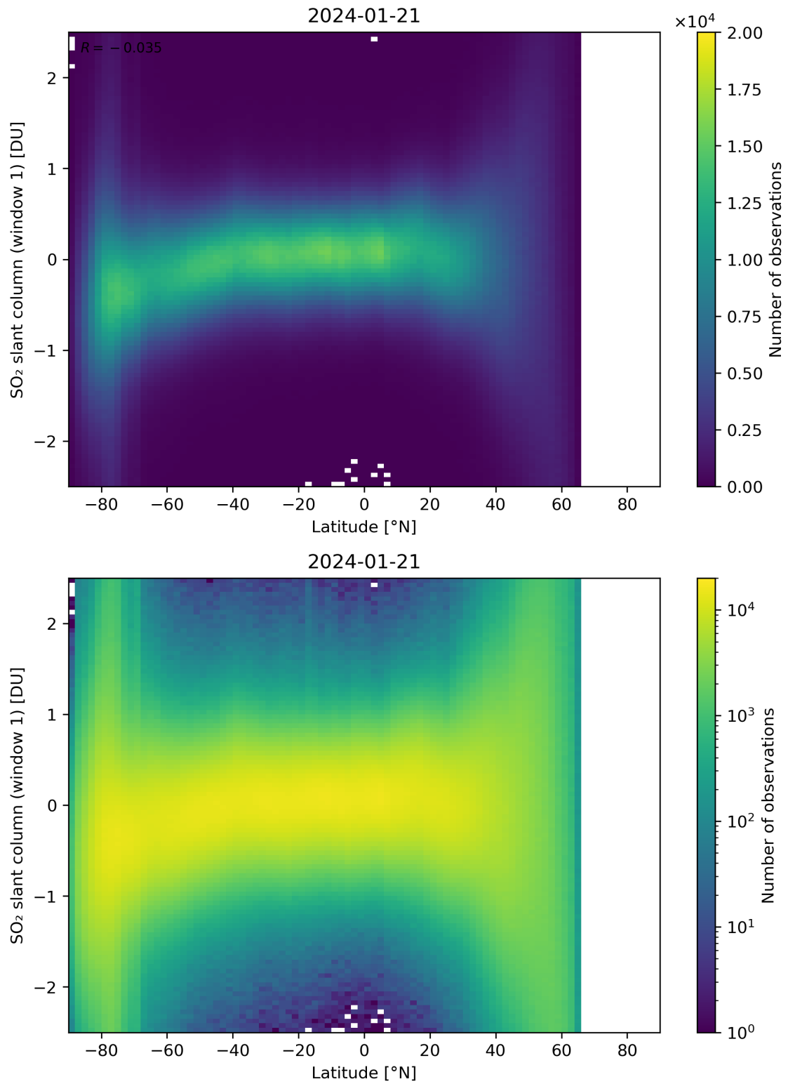
Figure 149: Scatter density plot of “Latitude” against “SO 2 slant column (window 1)” for 2024-01-21 to 2024-01-22.
