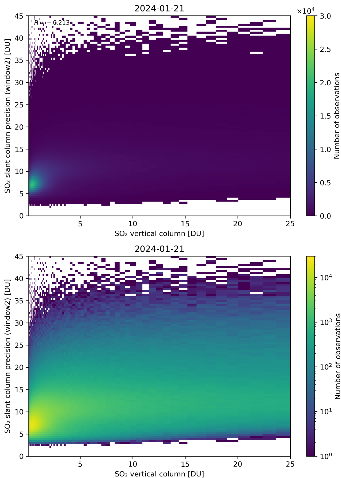
Figure 302: Scatter density plot of “SO 2 vertical column” against “SO 2 slant column precision (window2)” for 2024-01-21 to 2024-01-22.
