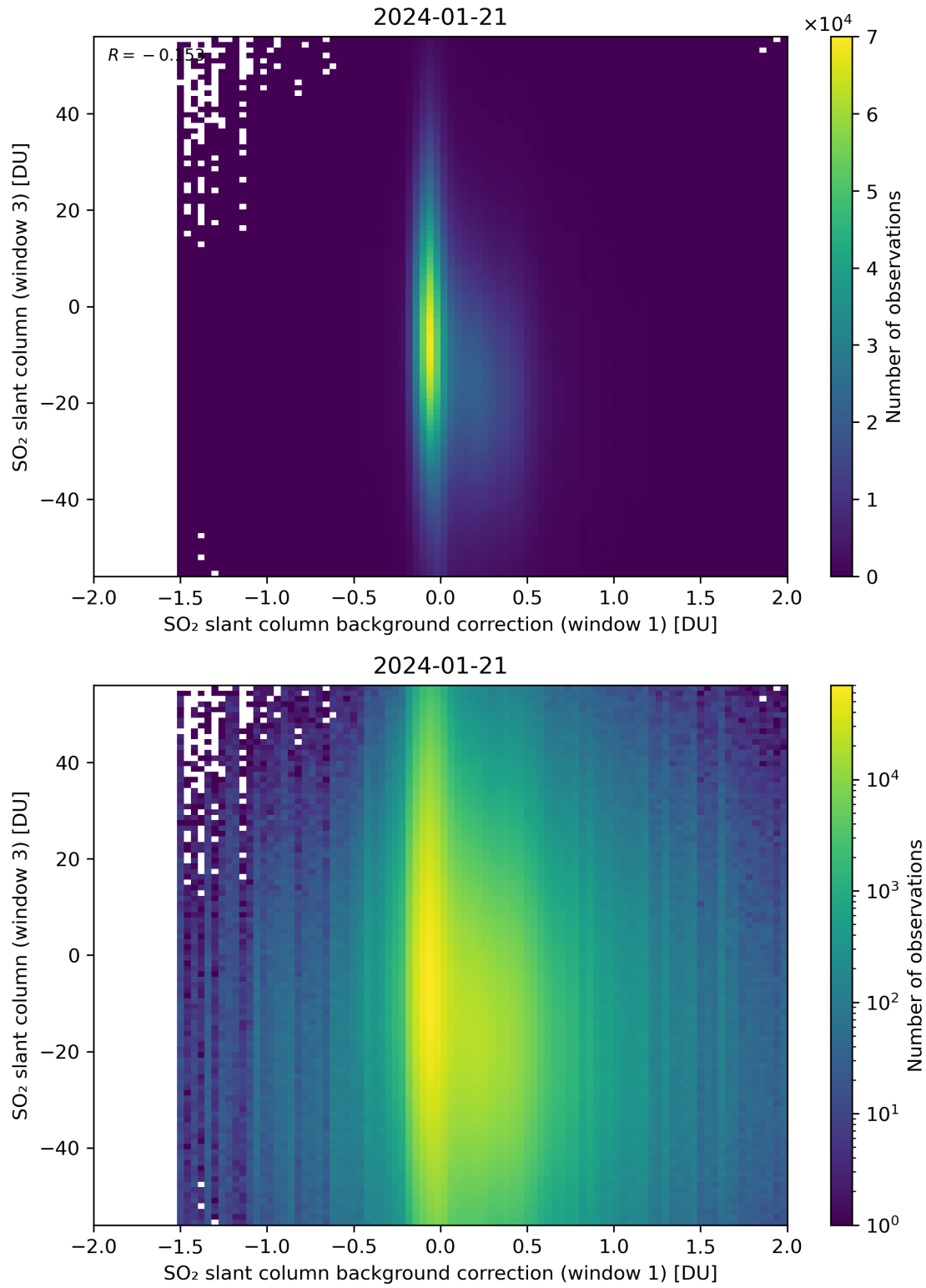
Figure 107: Scatter density plot of “SO 2 slant column background correction (window 1)” against “SO 2 slant column (window 3)” for 2024-01-21 to 2024-01-22.
