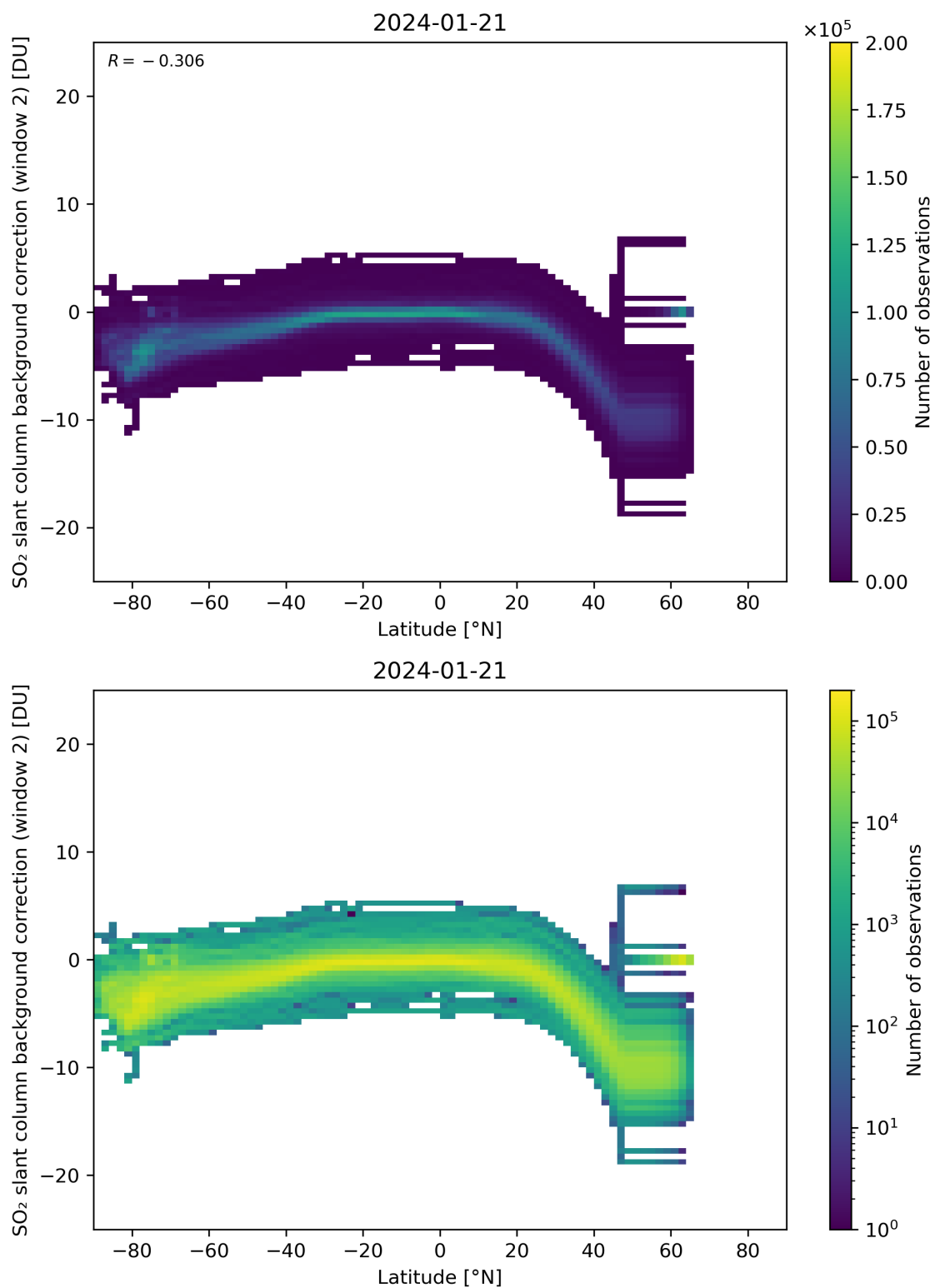
Figure 140: Scatter density plot of “Latitude” against “SO 2 slant column background correction (window 2)” for 2024-01-21 to 2024-01-22.
