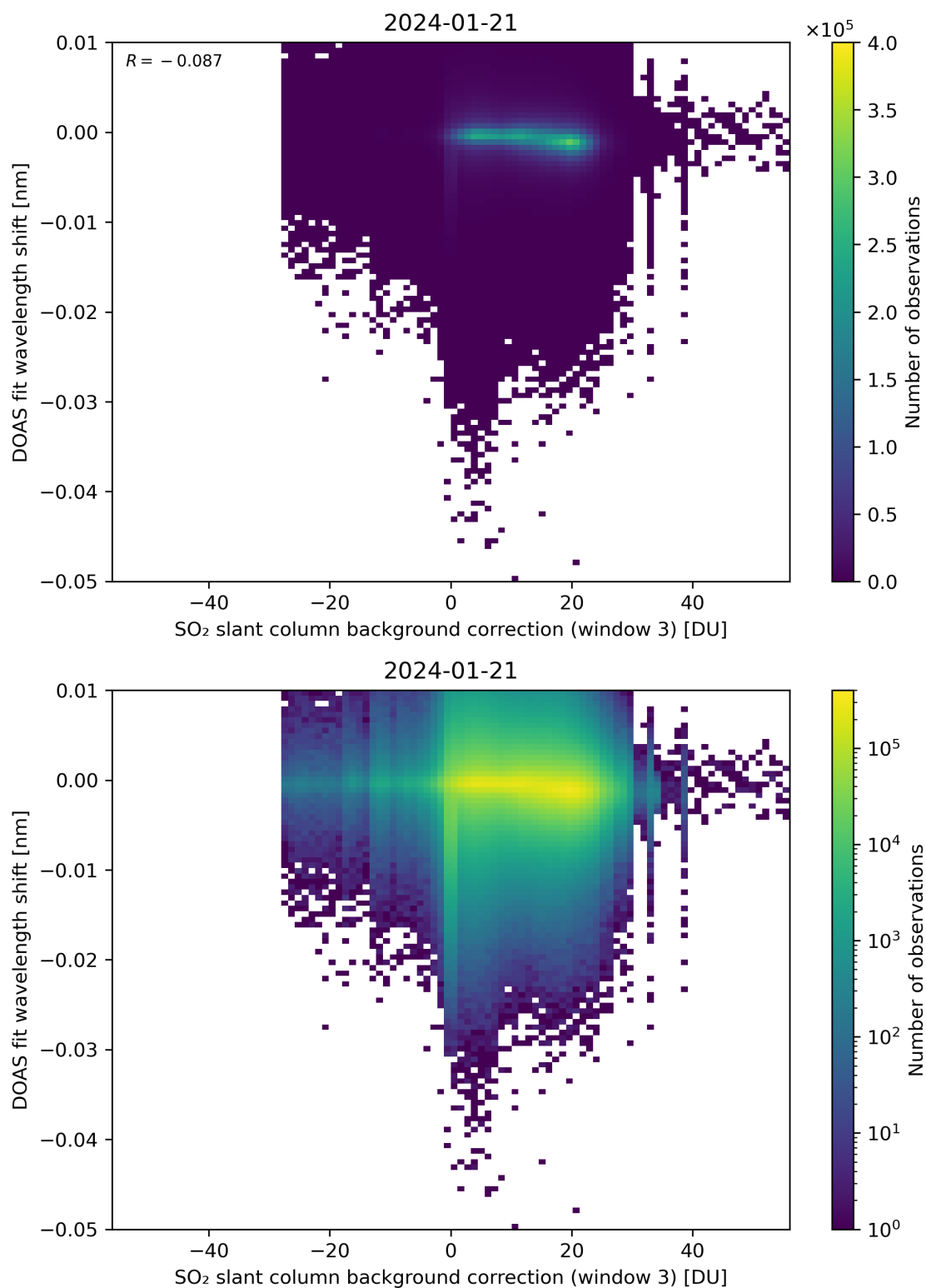
Figure 121: Scatter density plot of “SO 2 slant column background correction (window 3)” against “DOAS fit wavelength shift” for 2024-01-21 to 2024-01-22.
