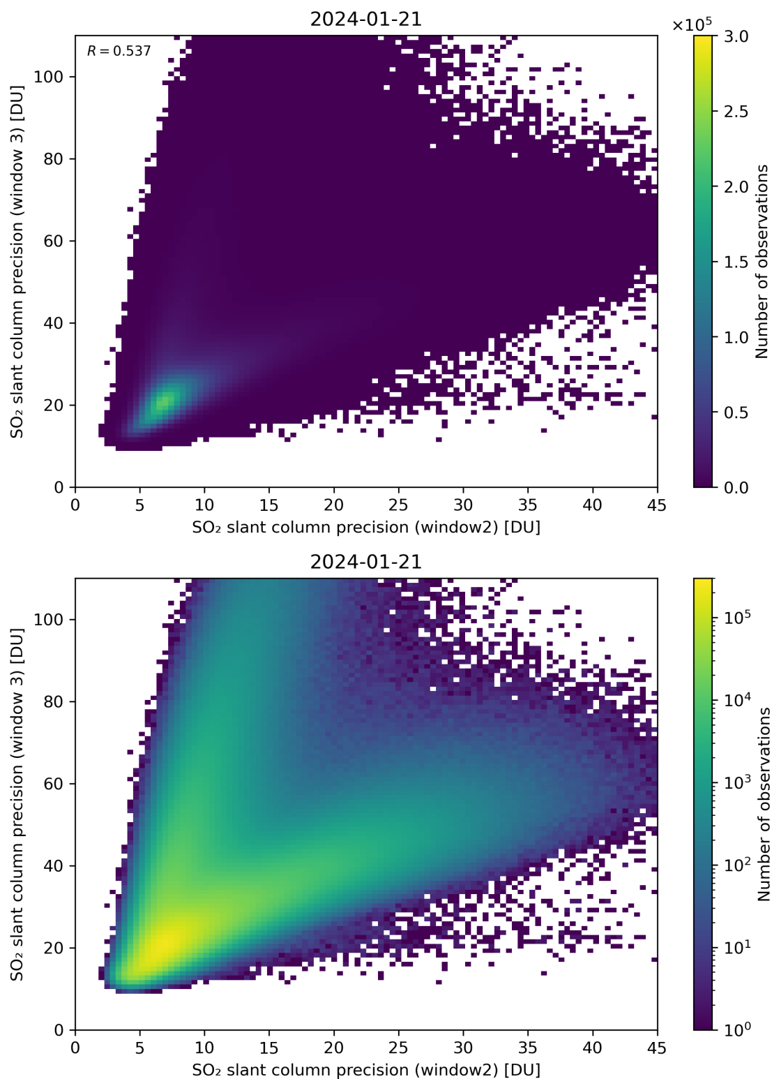
Figure 250: Scatter density plot of “SO 2 slant column precision (window2)” against “SO 2 slant column precision (window 3)” for 2024-01-21 to 2024-01-22.
