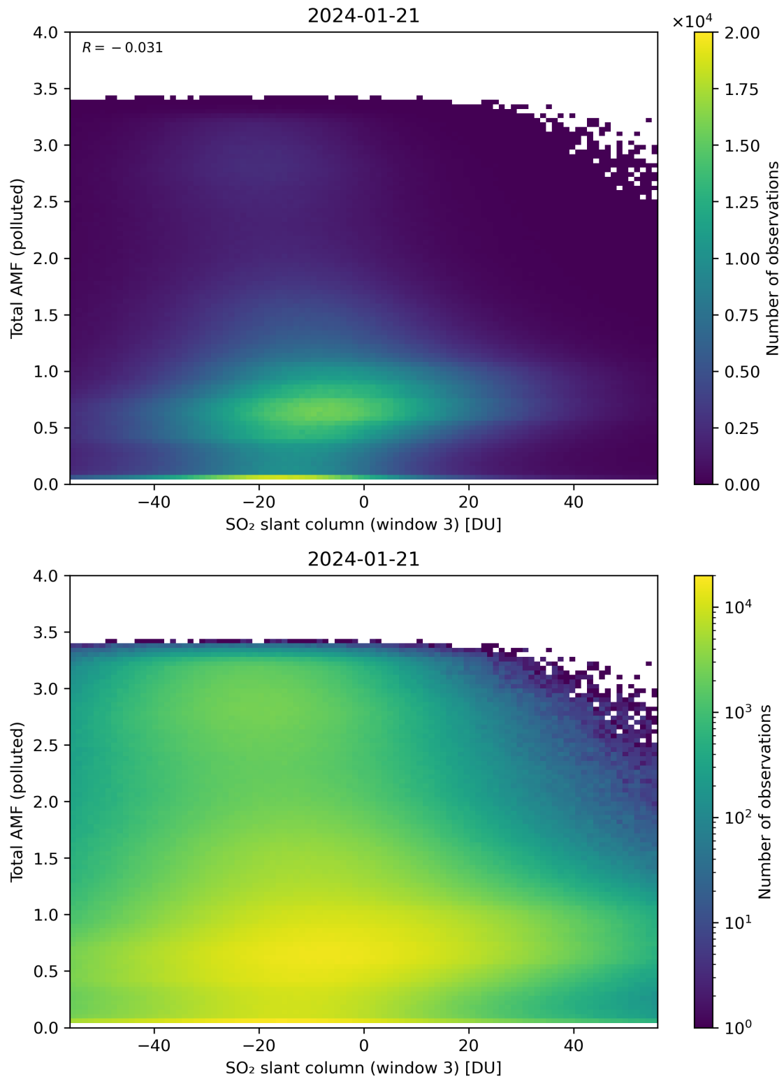
Figure 268: Scatter density plot of “SO 2 slant column (window 3)” against “Total AMF (polluted)” for 2024-01-21 to 2024-01-22.
