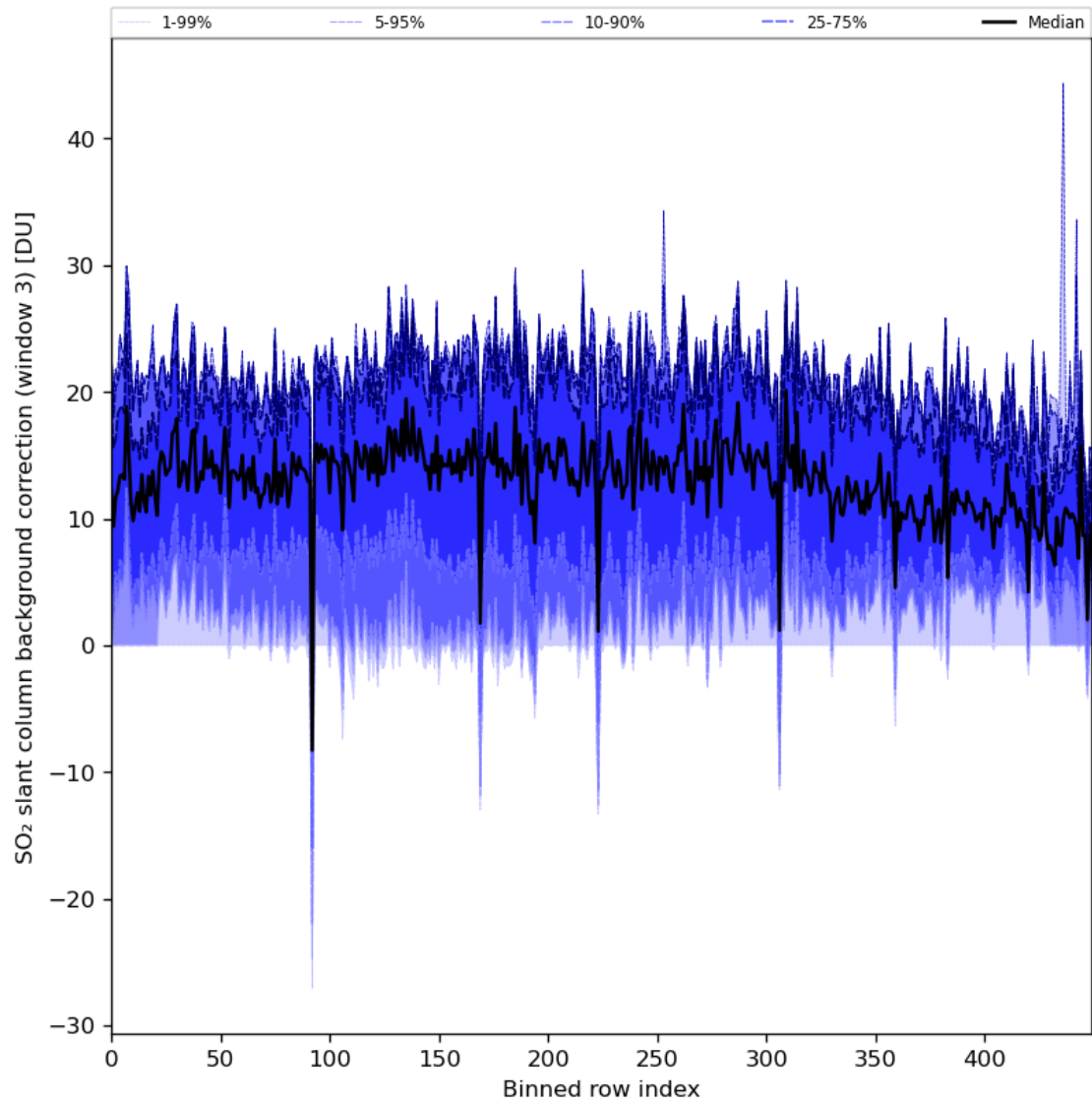
Figure 90: Along track statistics of “SO 2 slant column background correction (window 3)” for 2024-01-21 to 2024-01-22
