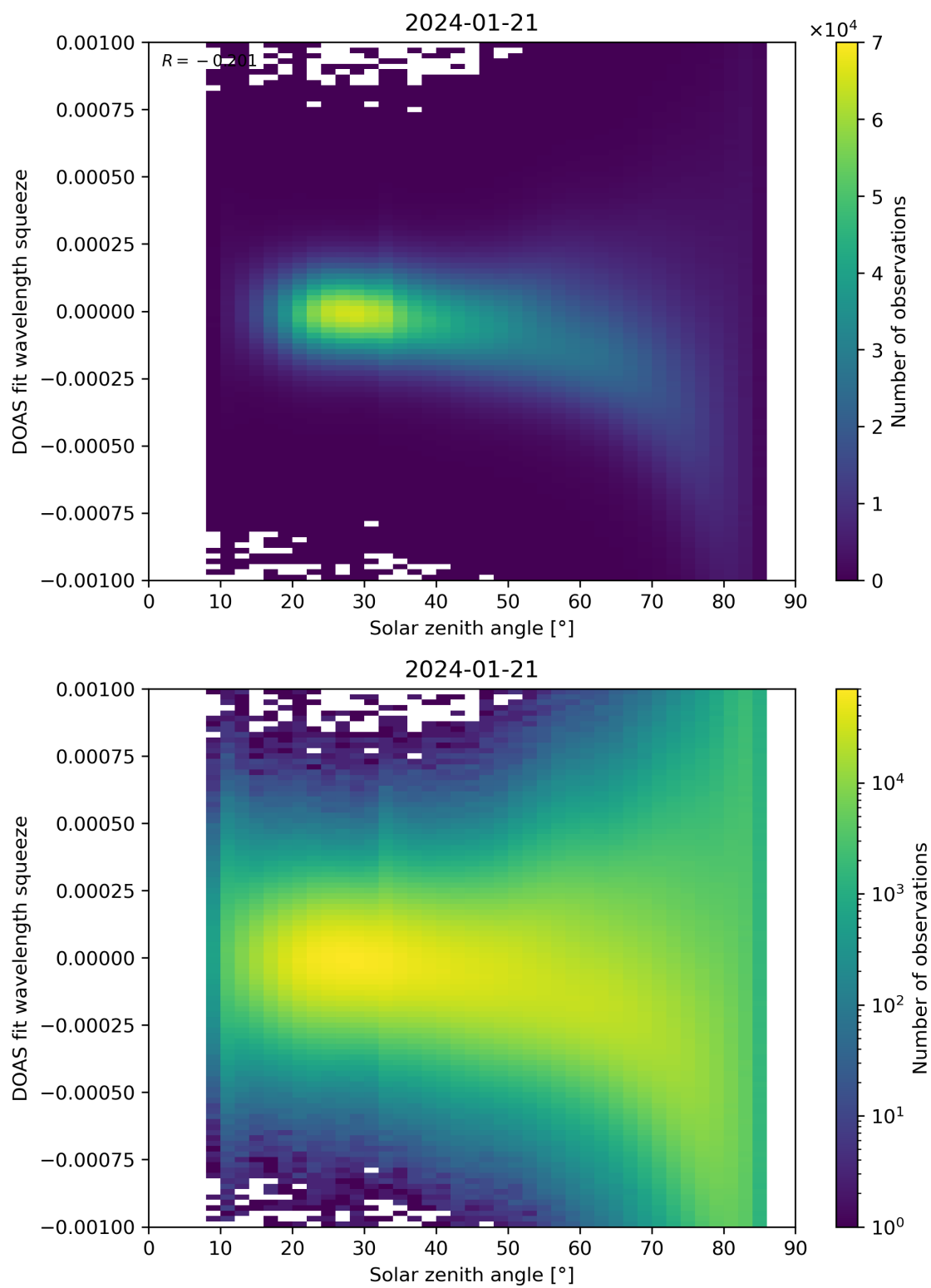
Figure 162: Scatter density plot of “Solar zenith angle” against “DOAS fit wavelength squeeze” for 2024-01-21 to 2024-01-22.
