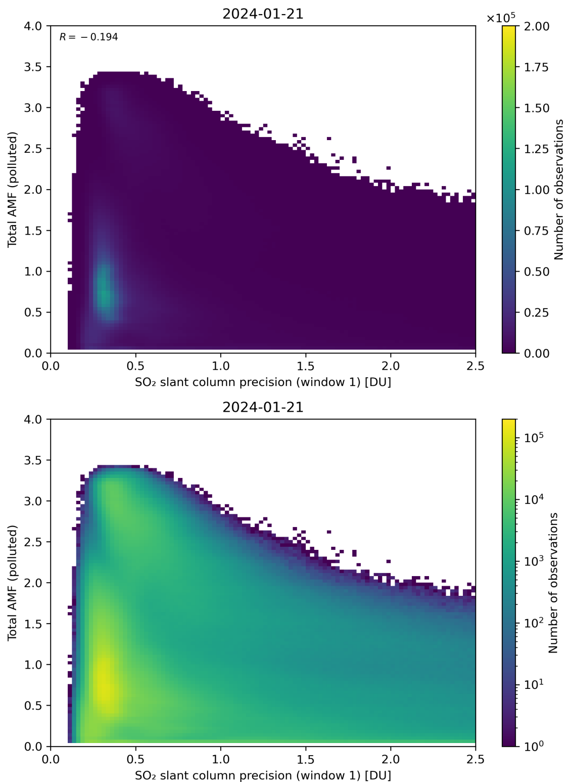
Figure 230: Scatter density plot of “SO 2 slant column precision (window 1)” against “Total AMF (polluted)” for 2024-01-21 to 2024-01-22.
