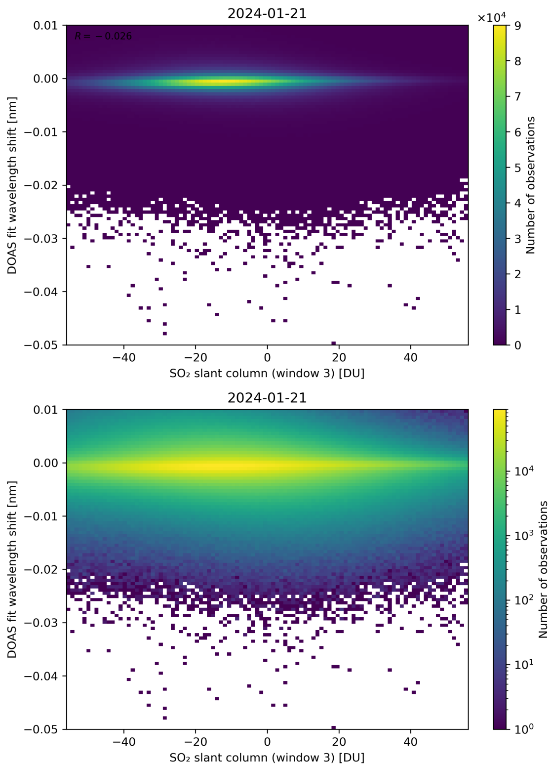
Figure 254: Scatter density plot of “SO 2 slant column (window 3)” against “DOAS fit wavelength shift” for 2024-01-21 to 2024-01-22.
