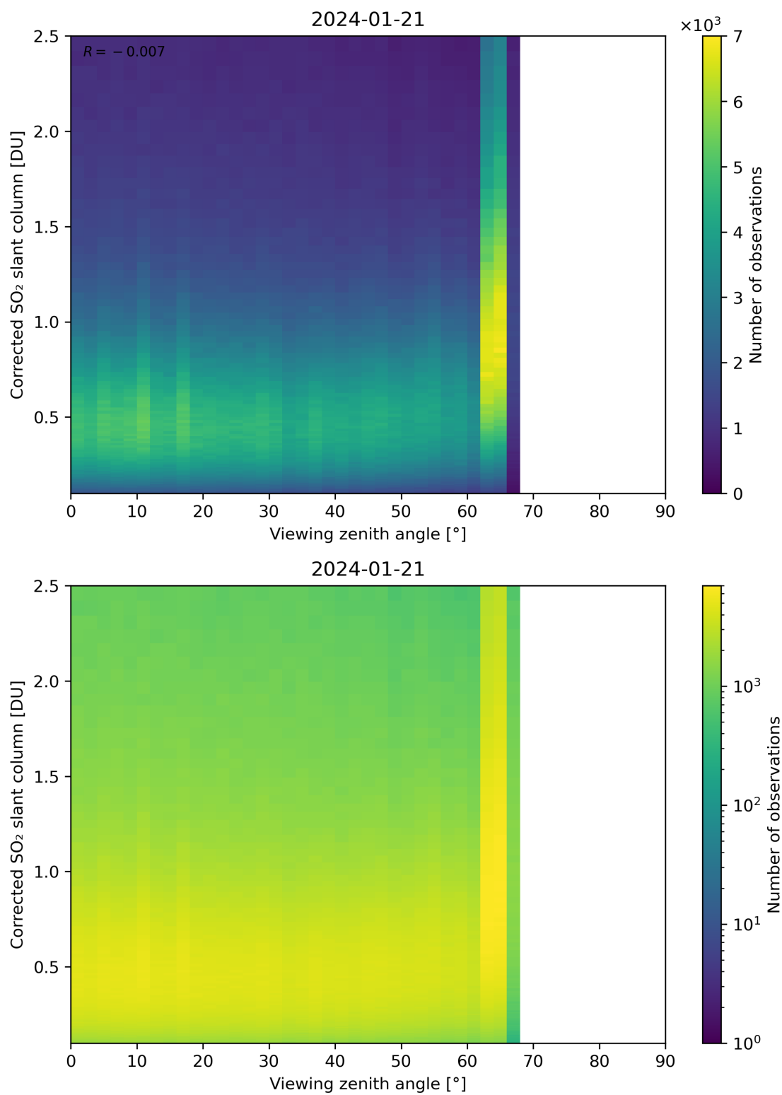
Figure 317: Scatter density plot of “Viewing zenith angle” against “Corrected SO 2 slant column” for 2024-01-21 to 2024-01-22.
