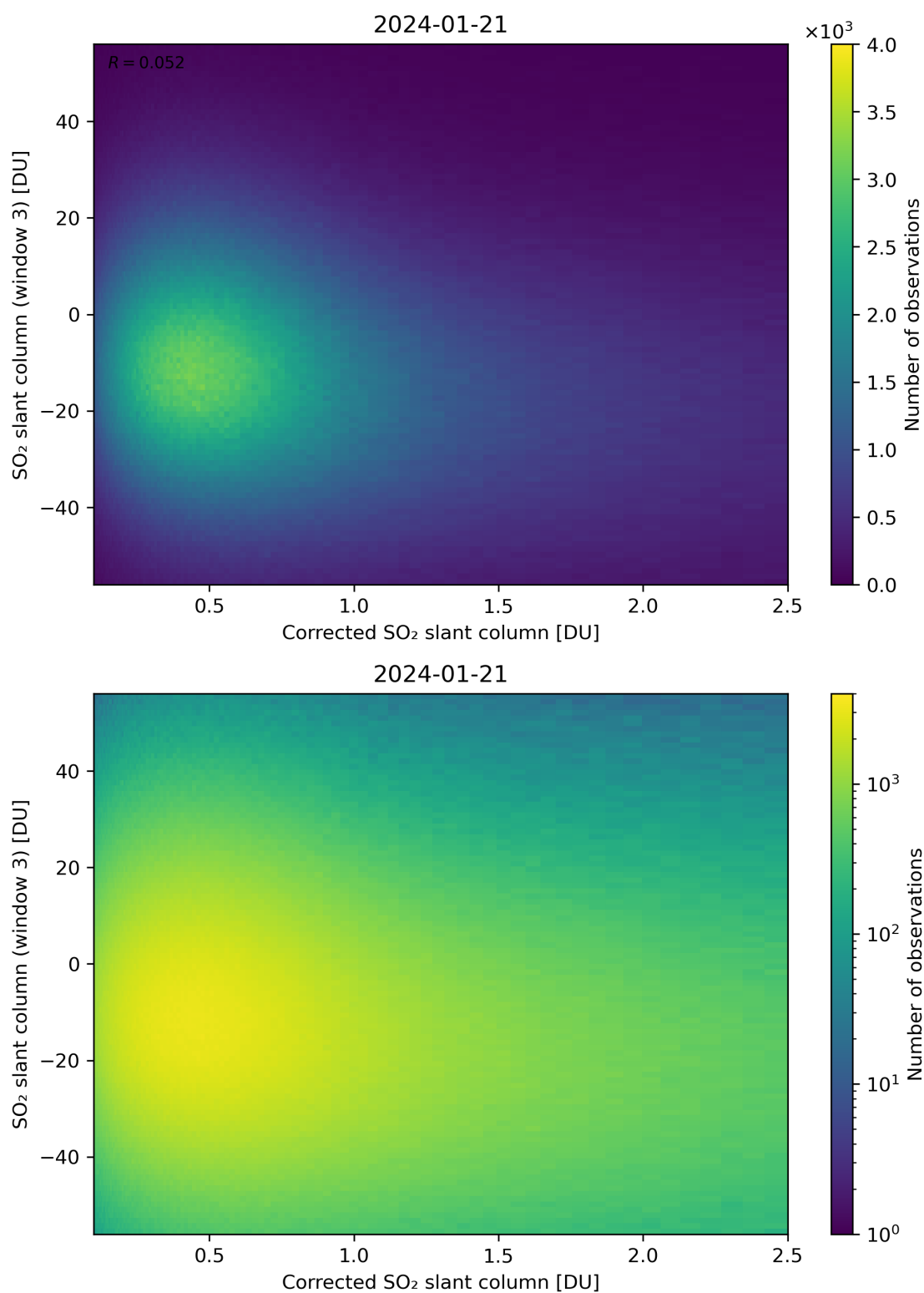
Figure 190: Scatter density plot of “Corrected SO 2 slant column” against “SO 2 slant column (window 3)” for 2024-01-21 to 2024-01-22.
