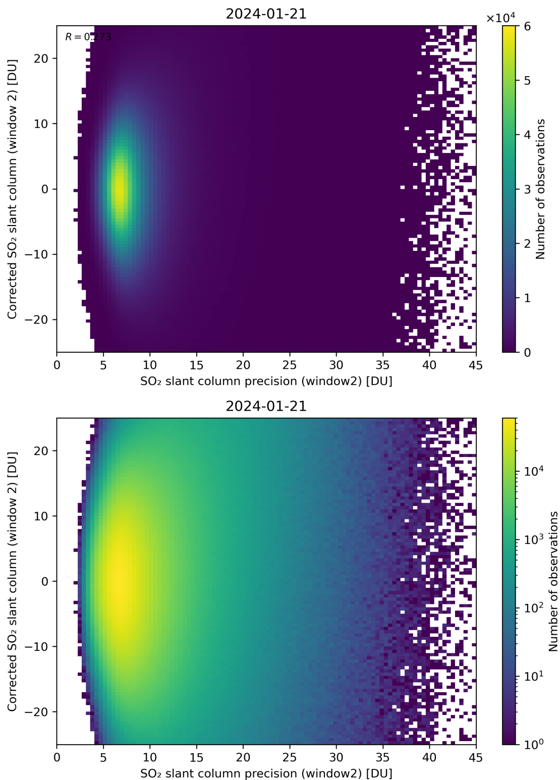
Figure 247: Scatter density plot of “SO 2 slant column precision (window2)” against “Corrected SO 2 slant column (window 2)” for 2024-01-21 to 2024-01-22.
