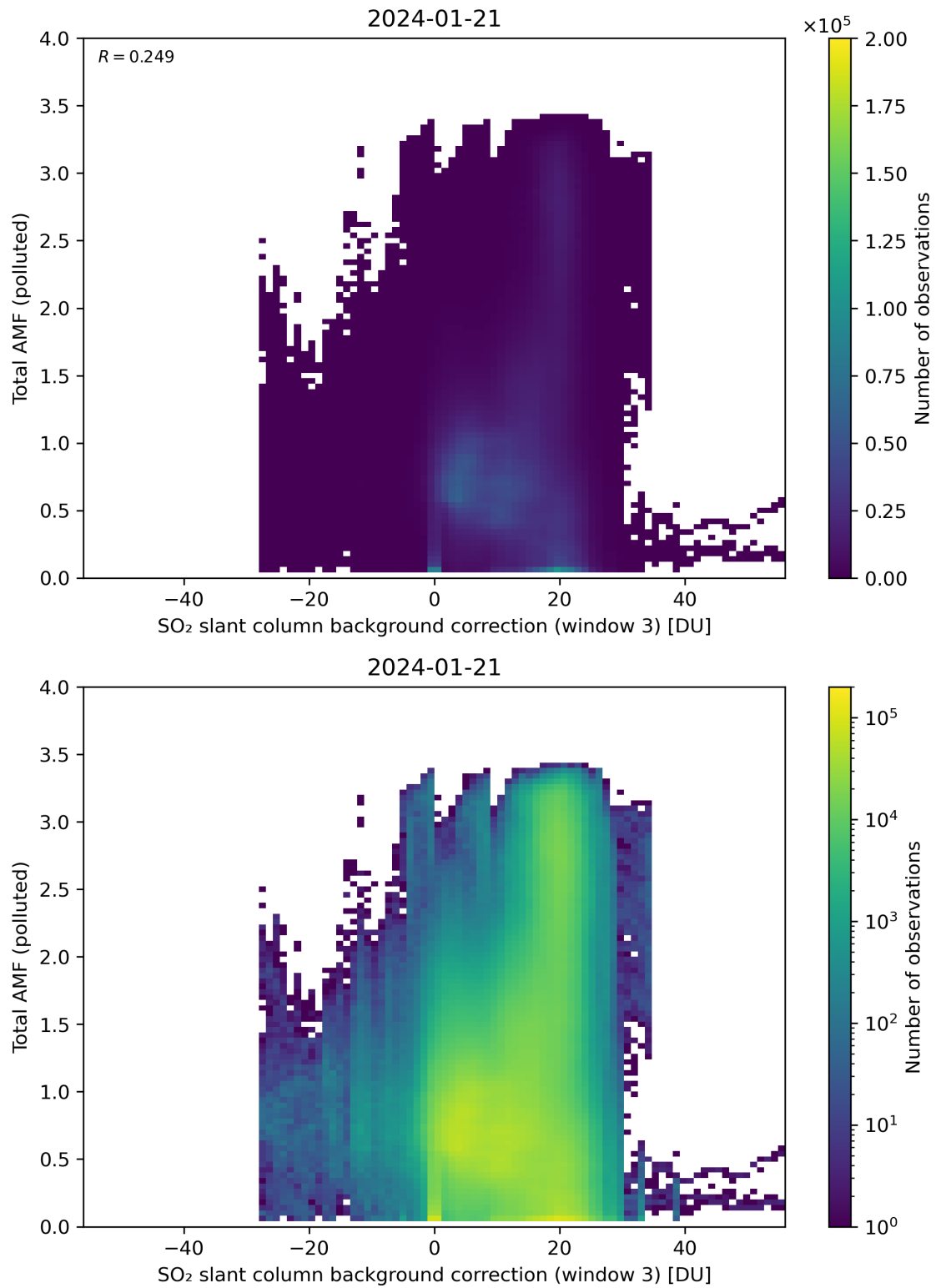
Figure 125: Scatter density plot of “SO 2 slant column background correction (window 3)” against “Total AMF (polluted)” for 2024-01-21 to 2024-01-22.
