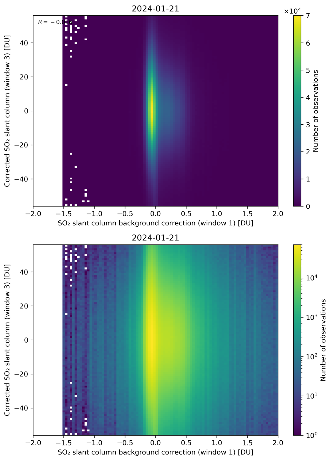
Figure 105: Scatter density plot of “SO 2 slant column background correction (window 1)” against “Corrected SO 2 slant column (window 3)” for 2024-01-21 to 2024-01-22.
