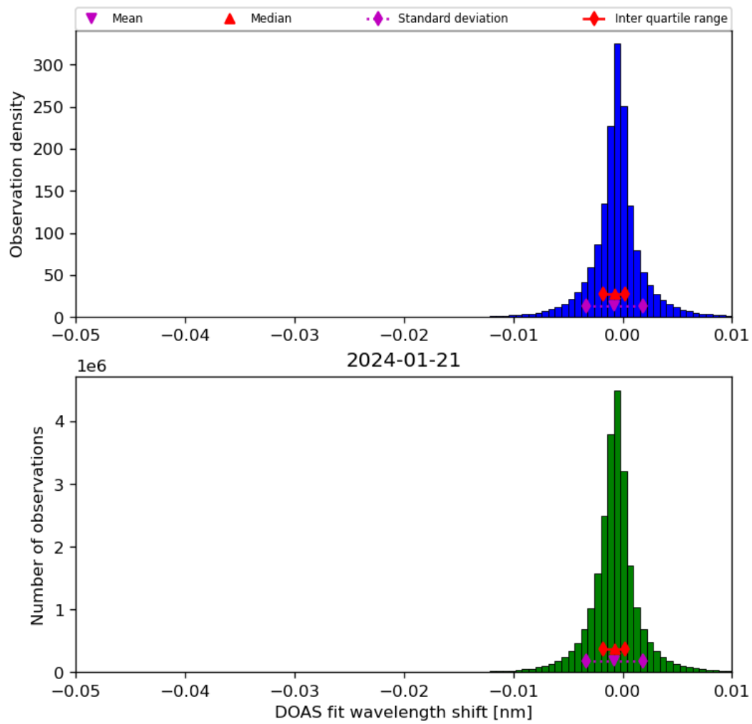
Figure 68: Histogram of “DOAS fit wavelength shift” for 2024-01-21 to 2024-01-22
