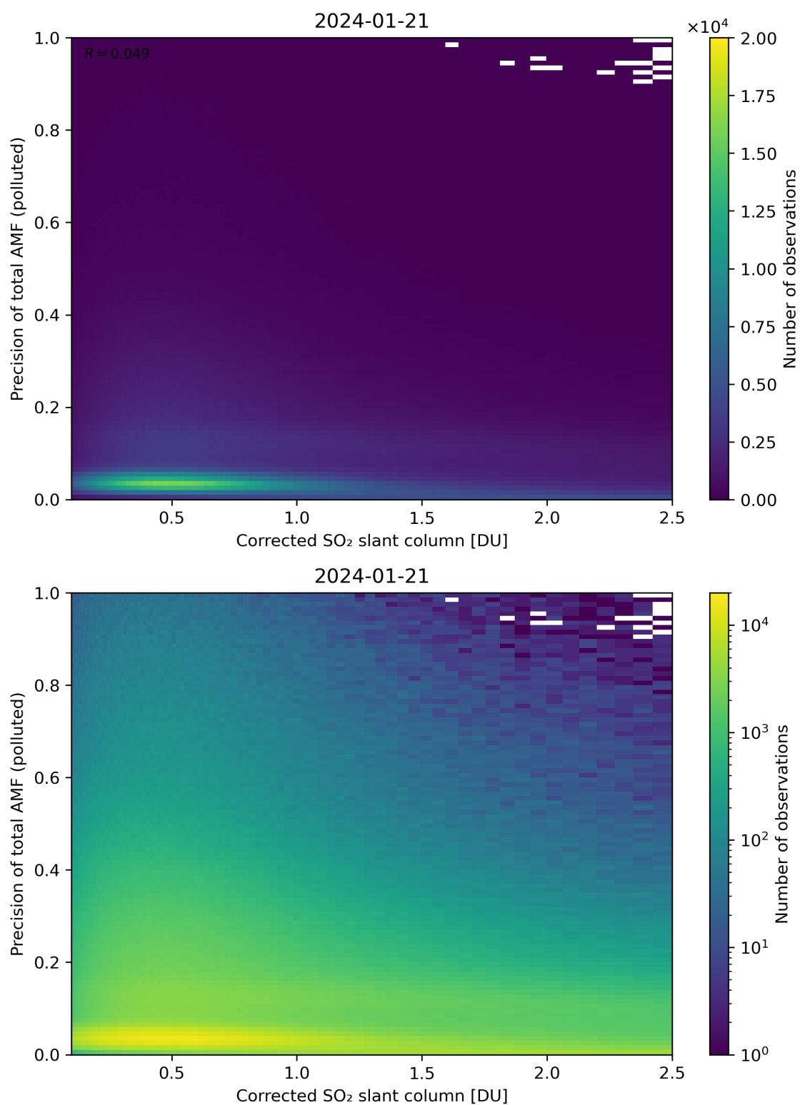
Figure 193: Scatter density plot of “Corrected SO 2 slant column” against “Precision of total AMF (polluted)” for 2024-01-21 to 2024-01-22.
