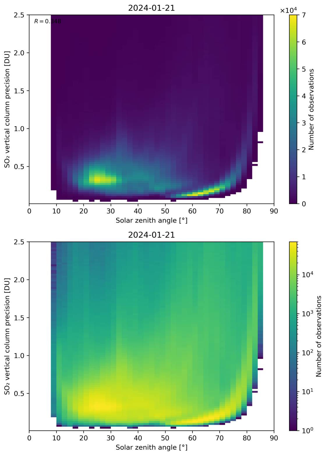
Figure 177: Scatter density plot of “Solar zenith angle” against “SO 2 vertical column precision” for 2024-01-21 to 2024-01-22.
