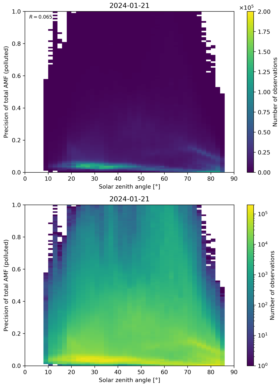
Figure 175: Scatter density plot of “Solar zenith angle” against “Precision of total AMF (polluted)” for 2024-01-21 to 2024-01-22.
