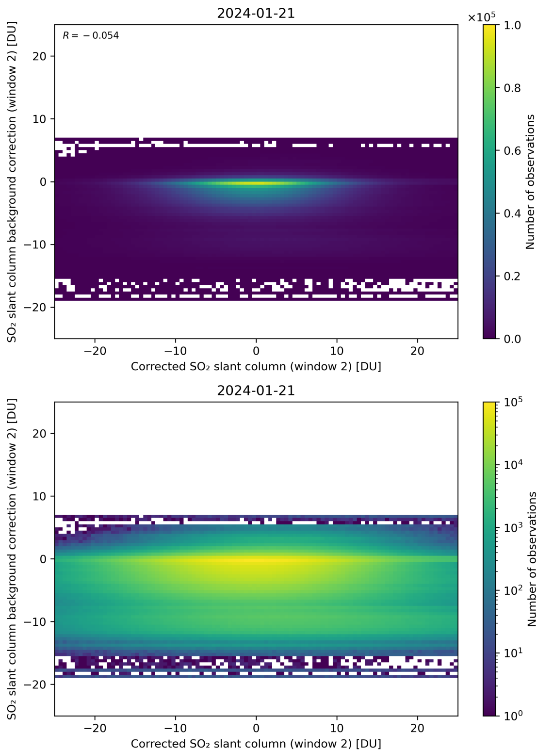
Figure 194: Scatter density plot of “Corrected SO 2 slant column (window 2)” against “SO 2 slant column background correction (window 2)” for 2024-01-21 to 2024-01-22.
