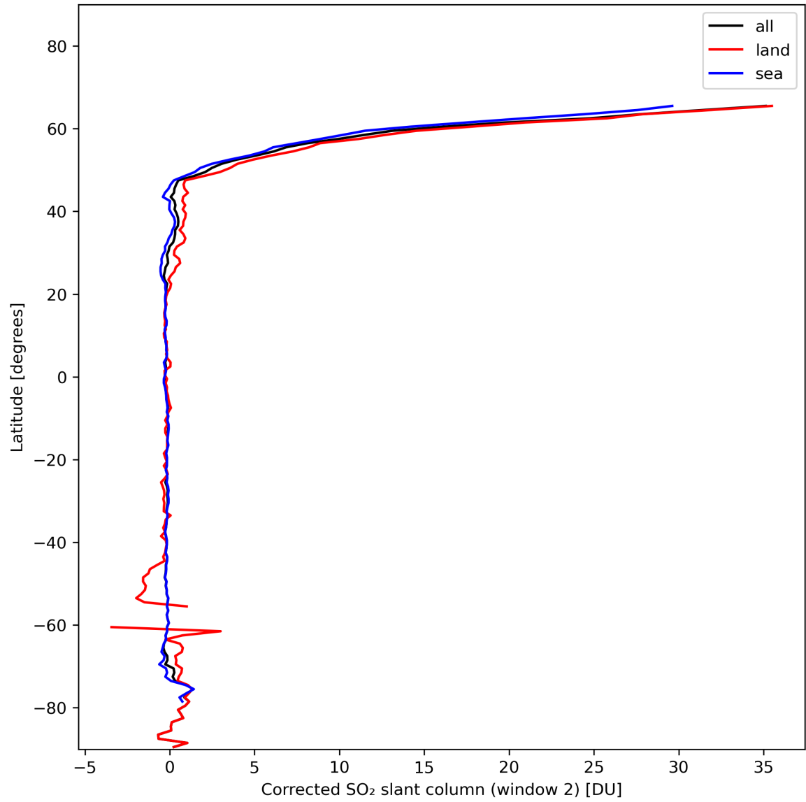
Figure 39: Zonal average of “Corrected SO 2 slant column (window 2)” for 2024-01-21 to 2024-01-22.
