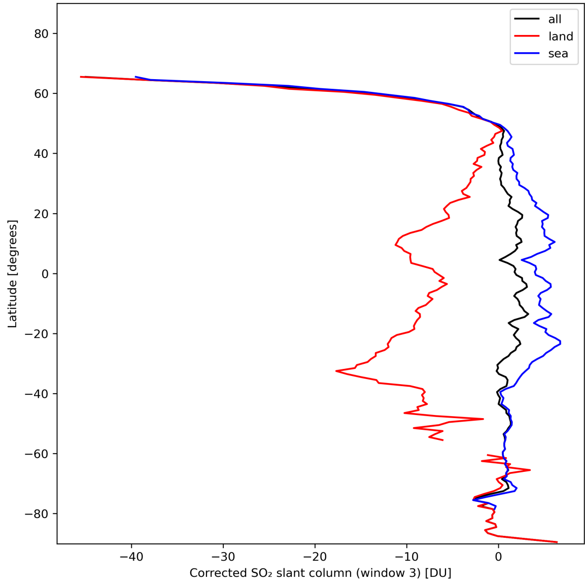
Figure 43: Zonal average of “Corrected SO 2 slant column (window 3)” for 2024-01-21 to 2024-01-22.
