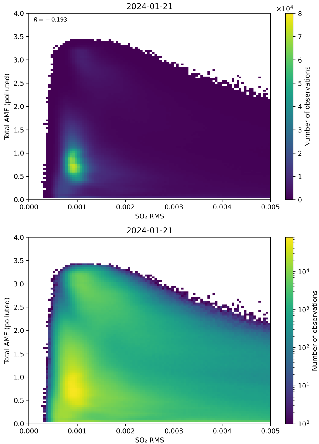
Figure 137: Scatter density plot of “SO 2 RMS” against “Total AMF (polluted)” for 2024-01-21 to 2024-01-22.
