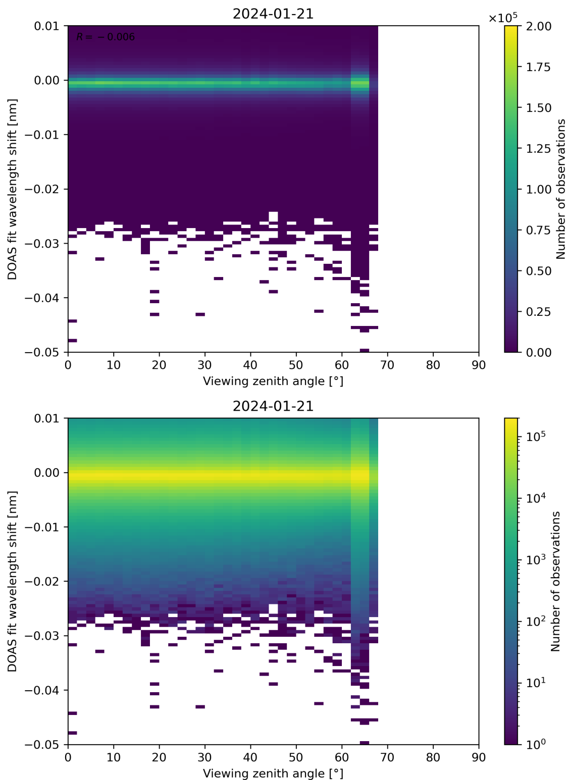
Figure 311: Scatter density plot of “Viewing zenith angle” against “DOAS fit wavelength shift” for 2024-01-21 to 2024-01-22.
