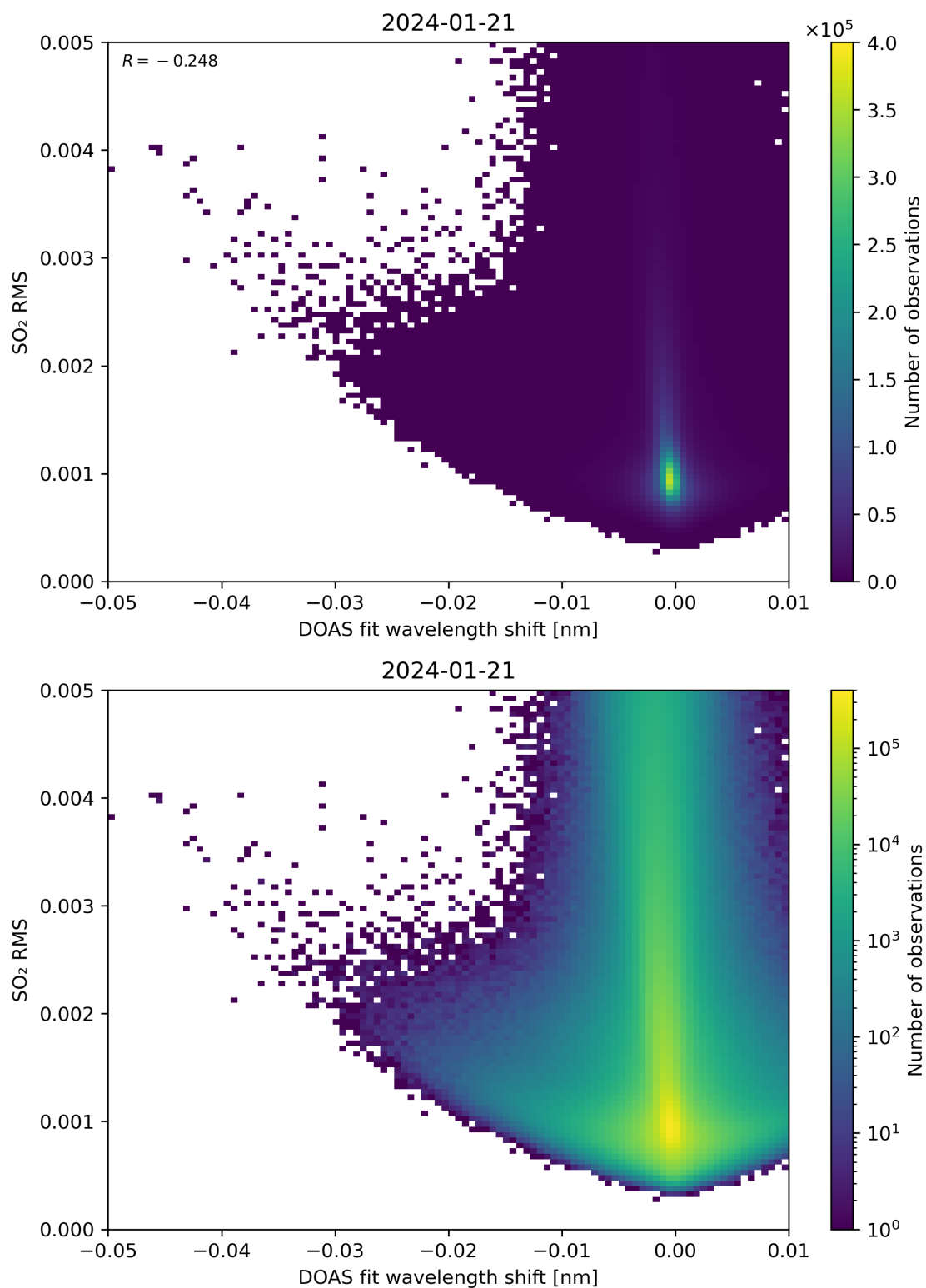
Figure 128: Scatter density plot of “DOAS fit wavelength shift” against “SO 2 RMS” for 2024-01-21 to 2024-01-22.
