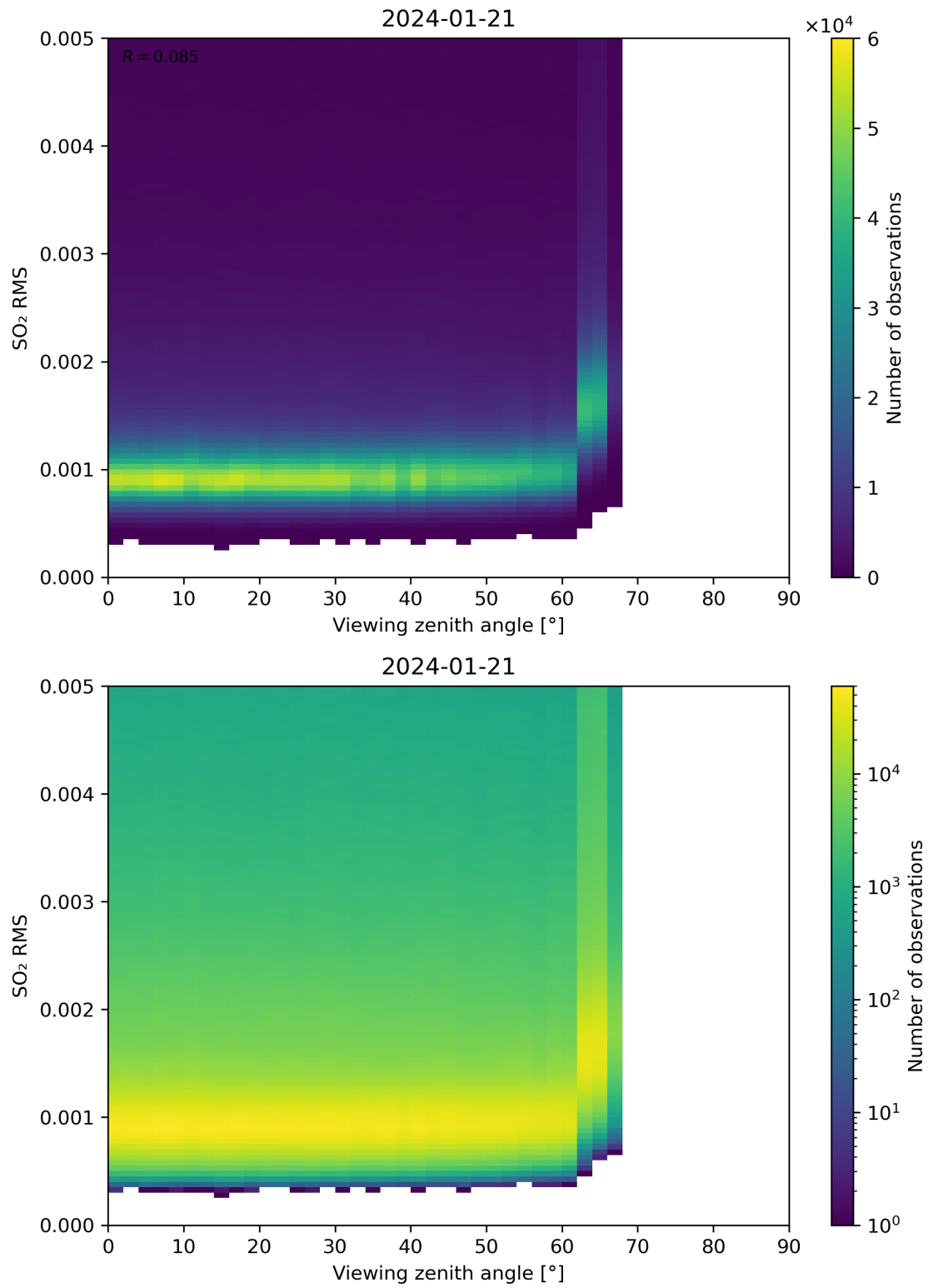
Figure 313: Scatter density plot of “Viewing zenith angle” against “SO 2 RMS” for 2024-01-21 to 2024-01-22.
