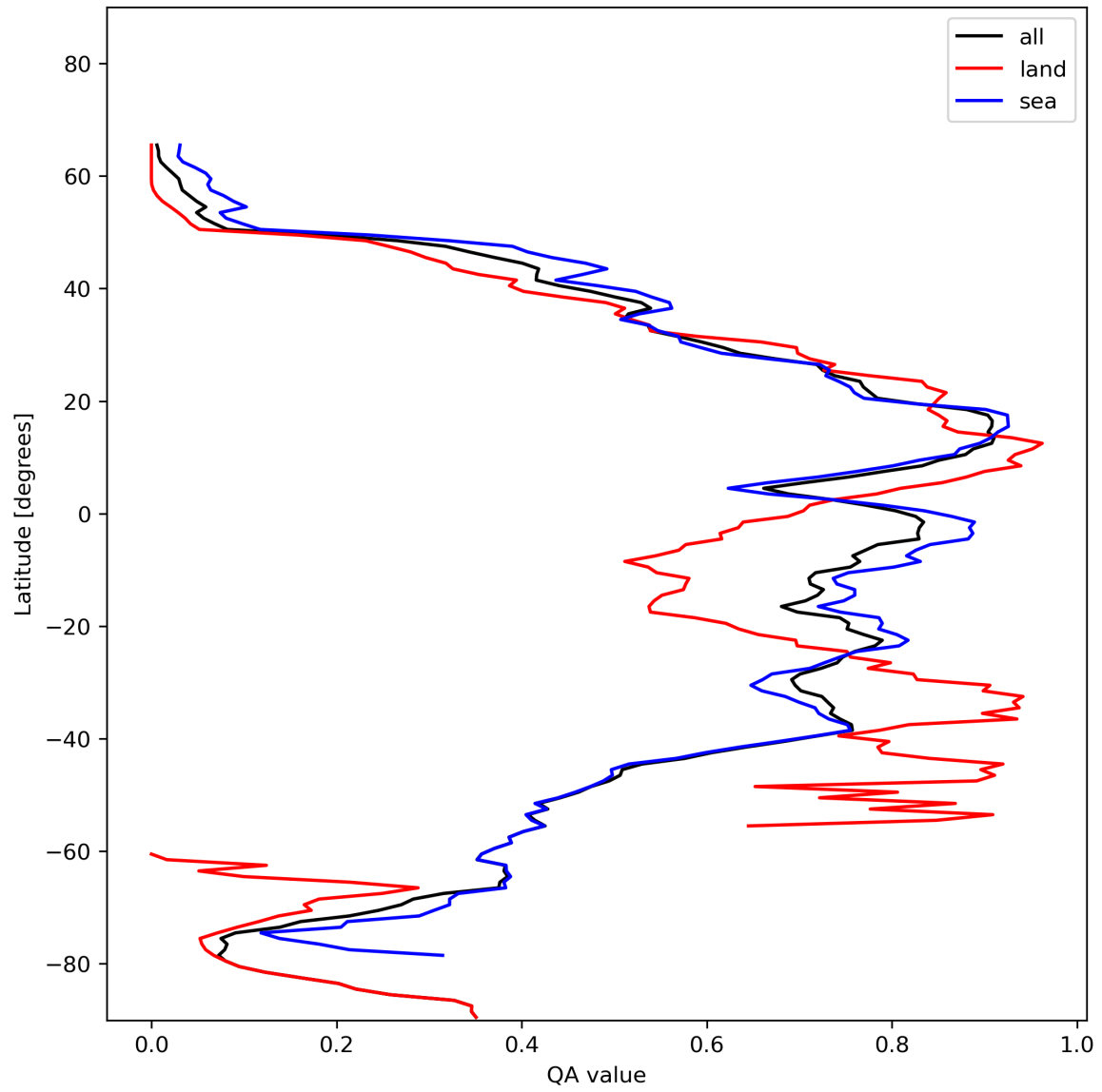
Figure 29: Zonal average of “QA value” for 2024-01-21 to 2024-01-22.
