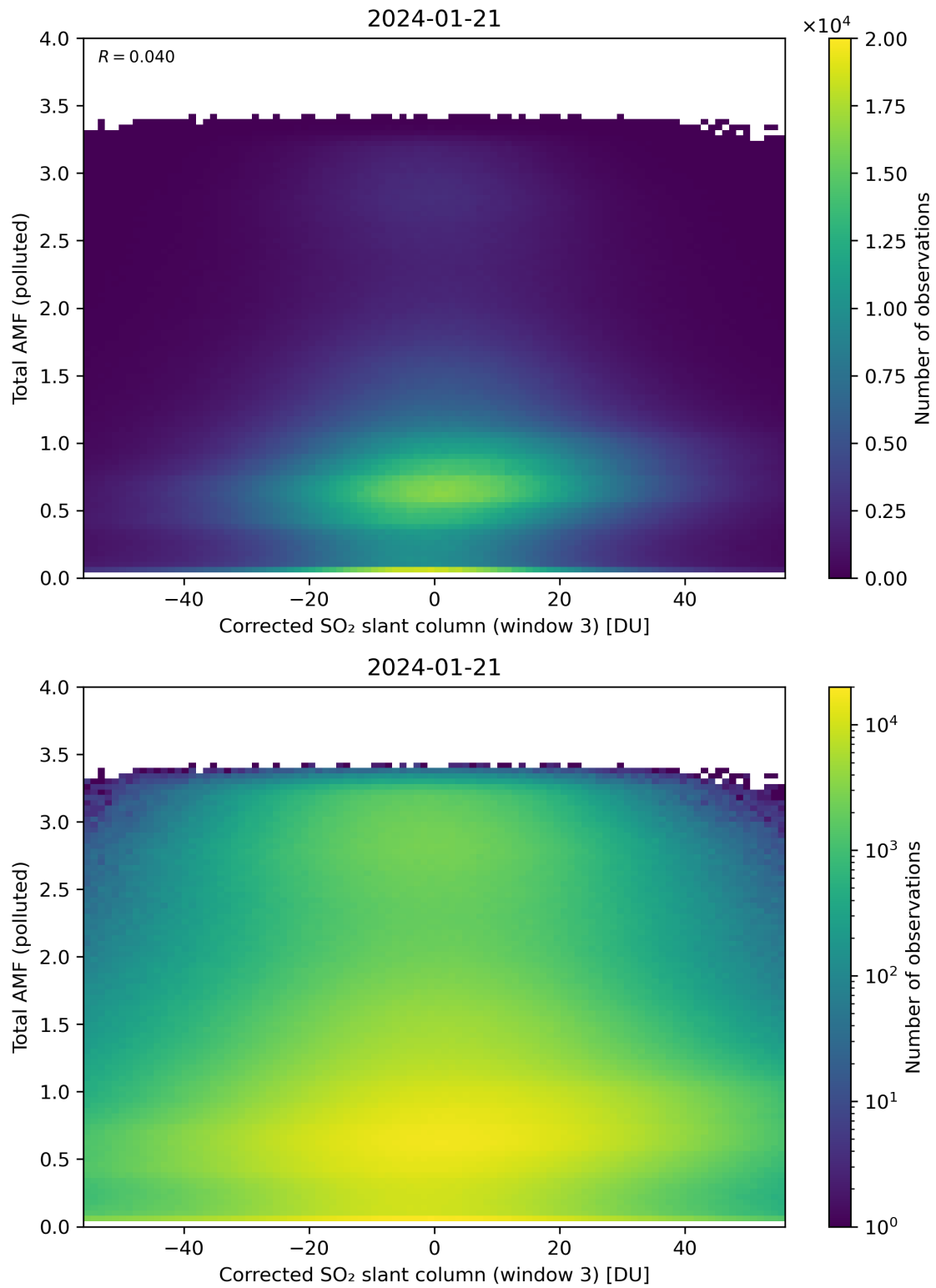
Figure 210: Scatter density plot of “Corrected SO 2 slant column (window 3)” against “Total AMF (polluted)” for 2024-01-21 to 2024-01-22.
