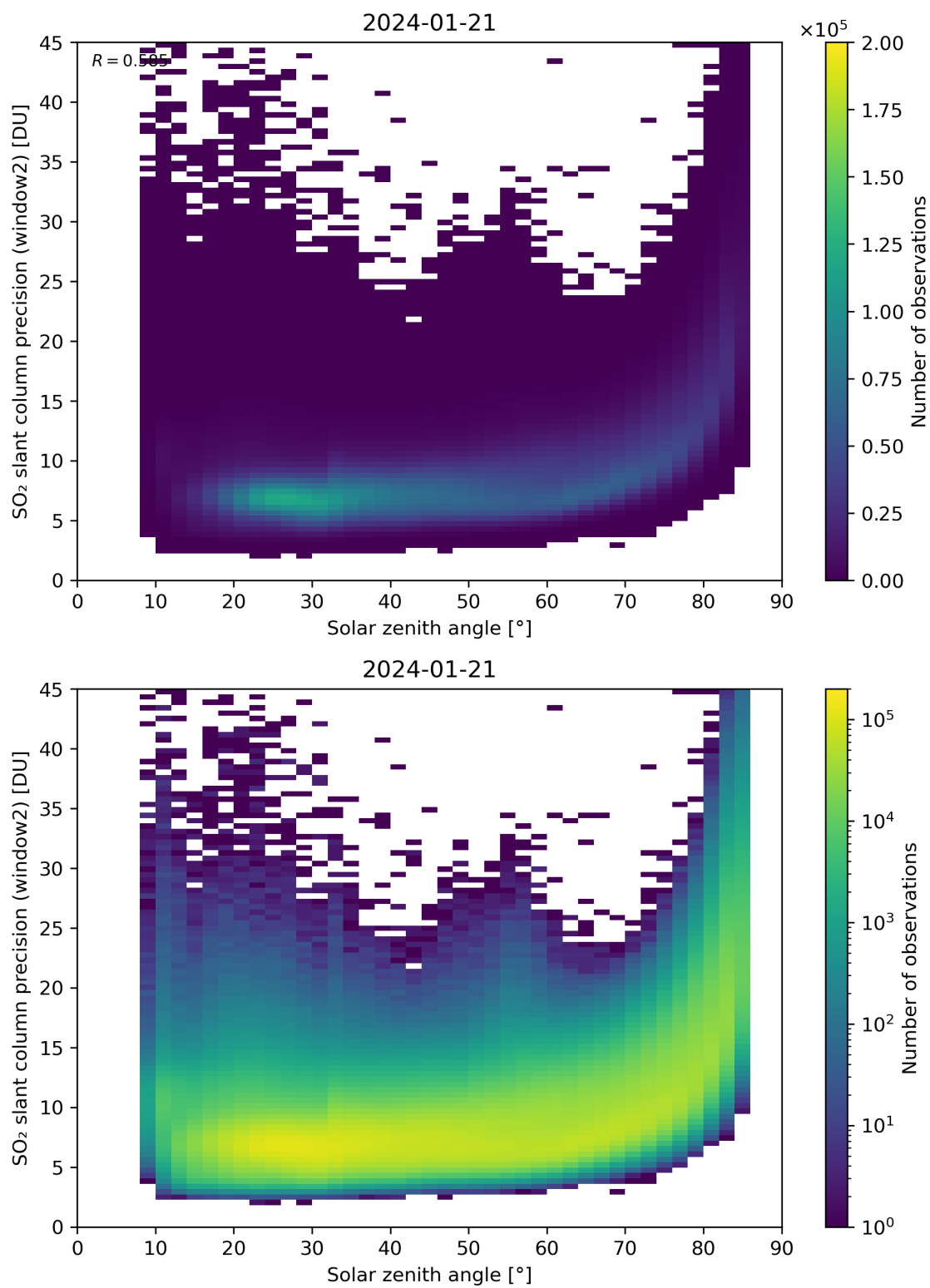
Figure 171: Scatter density plot of “Solar zenith angle” against “SO 2 slant column precision (window2)” for 2024-01-21 to 2024-01-22.
