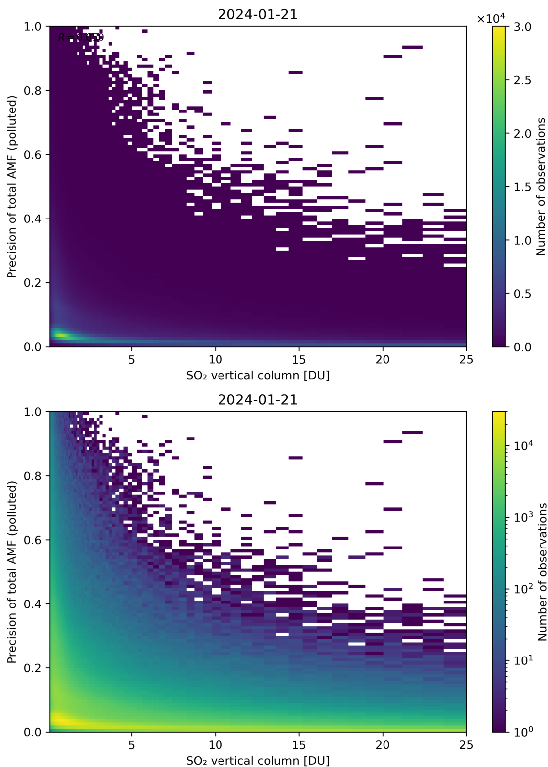
Figure 306: Scatter density plot of “SO 2 vertical column” against “Precision of total AMF (polluted)” for 2024-01-21 to 2024-01-22.
