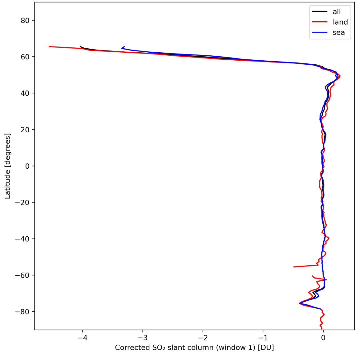
Figure 35: Zonal average of “Corrected SO 2 slant column (window 1)” for 2024-01-21 to 2024-01-22.
