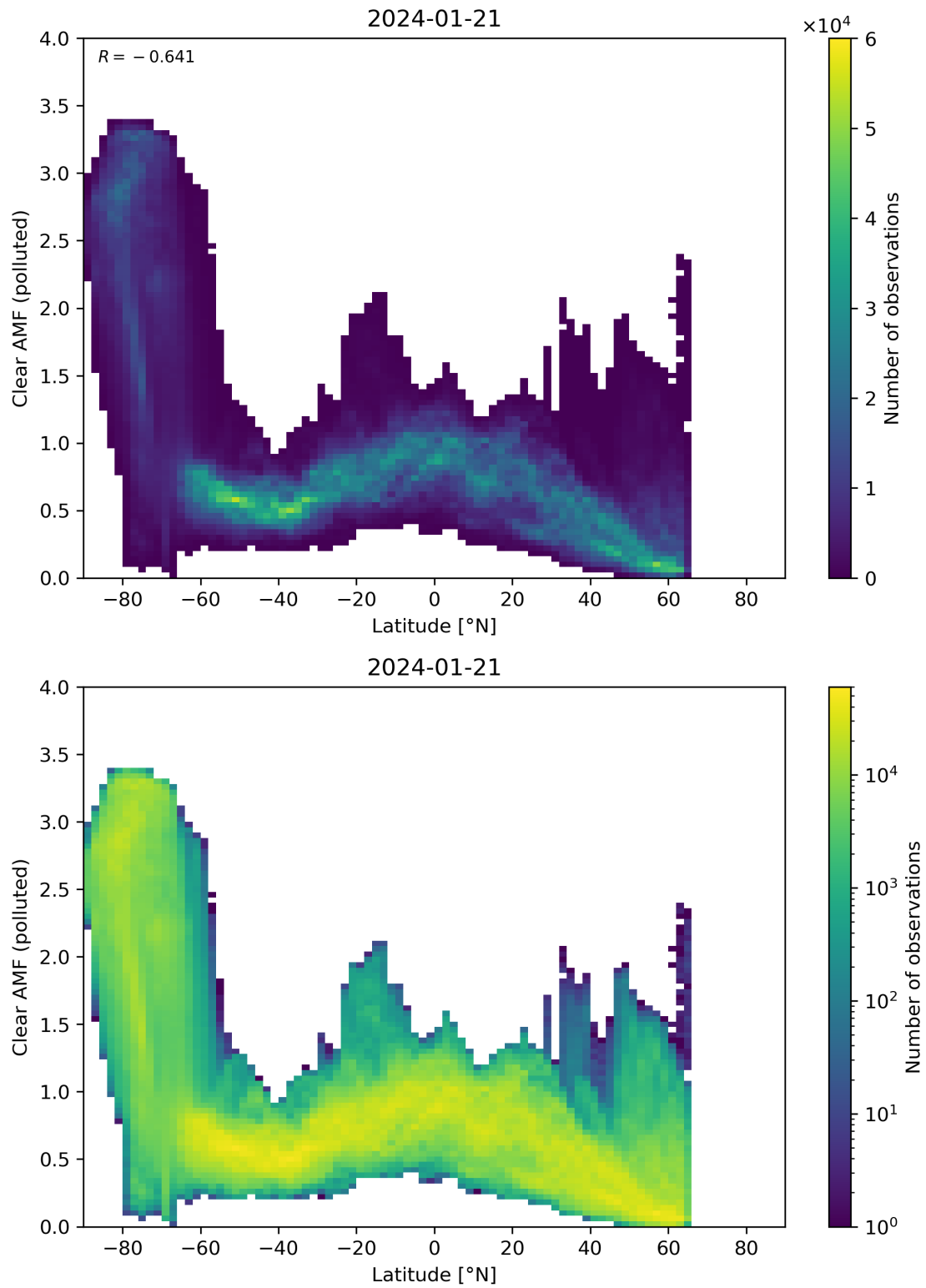
Figure 145: Scatter density plot of “Latitude” against “Clear AMF (polluted)” for 2024-01-21 to 2024-01-22.
