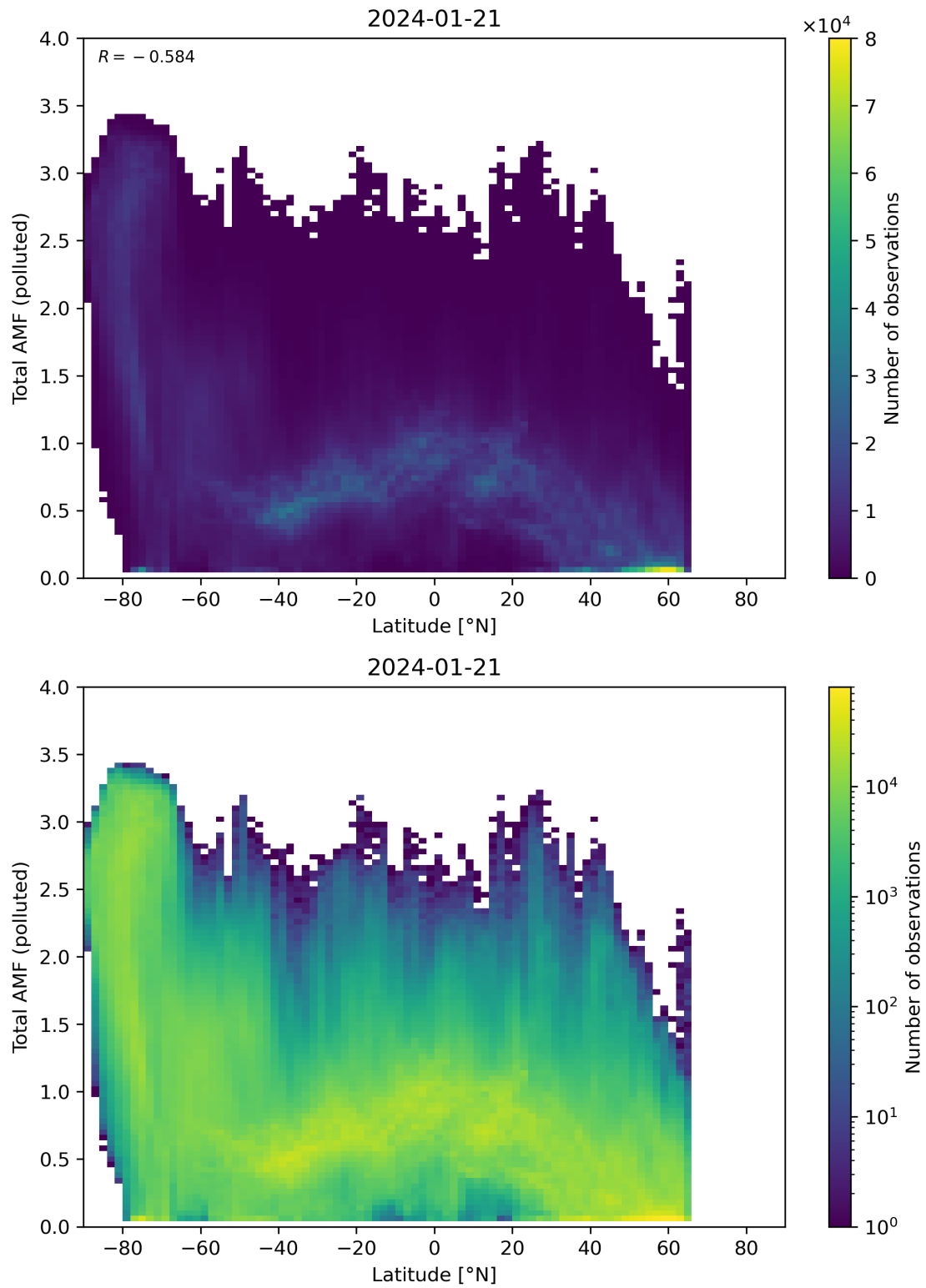
Figure 154: Scatter density plot of “Latitude” against “Total AMF (polluted)” for 2024-01-21 to 2024-01-22.
