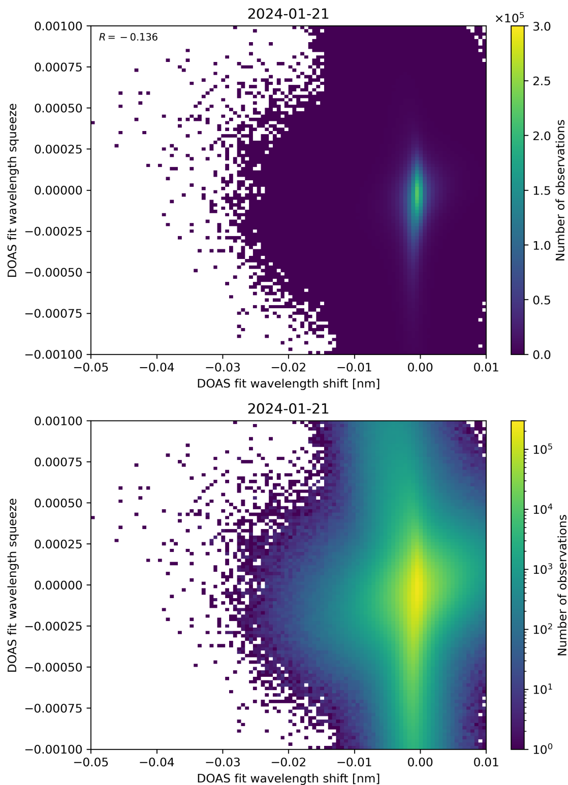
Figure 127: Scatter density plot of “DOAS fit wavelength shift” against “DOAS fit wavelength squeeze” for 2024-01-21 to 2024-01-22.
