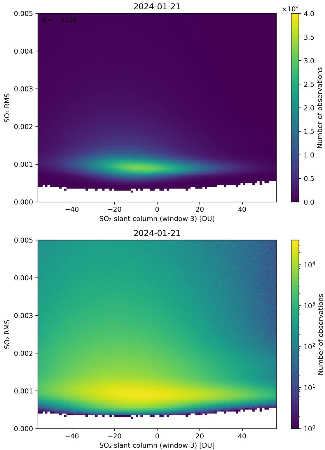
Figure 256: Scatter density plot of “SO 2 slant column (window 3)” against “SO 2 RMS” for 2024-01-21 to 2024-01-22.
