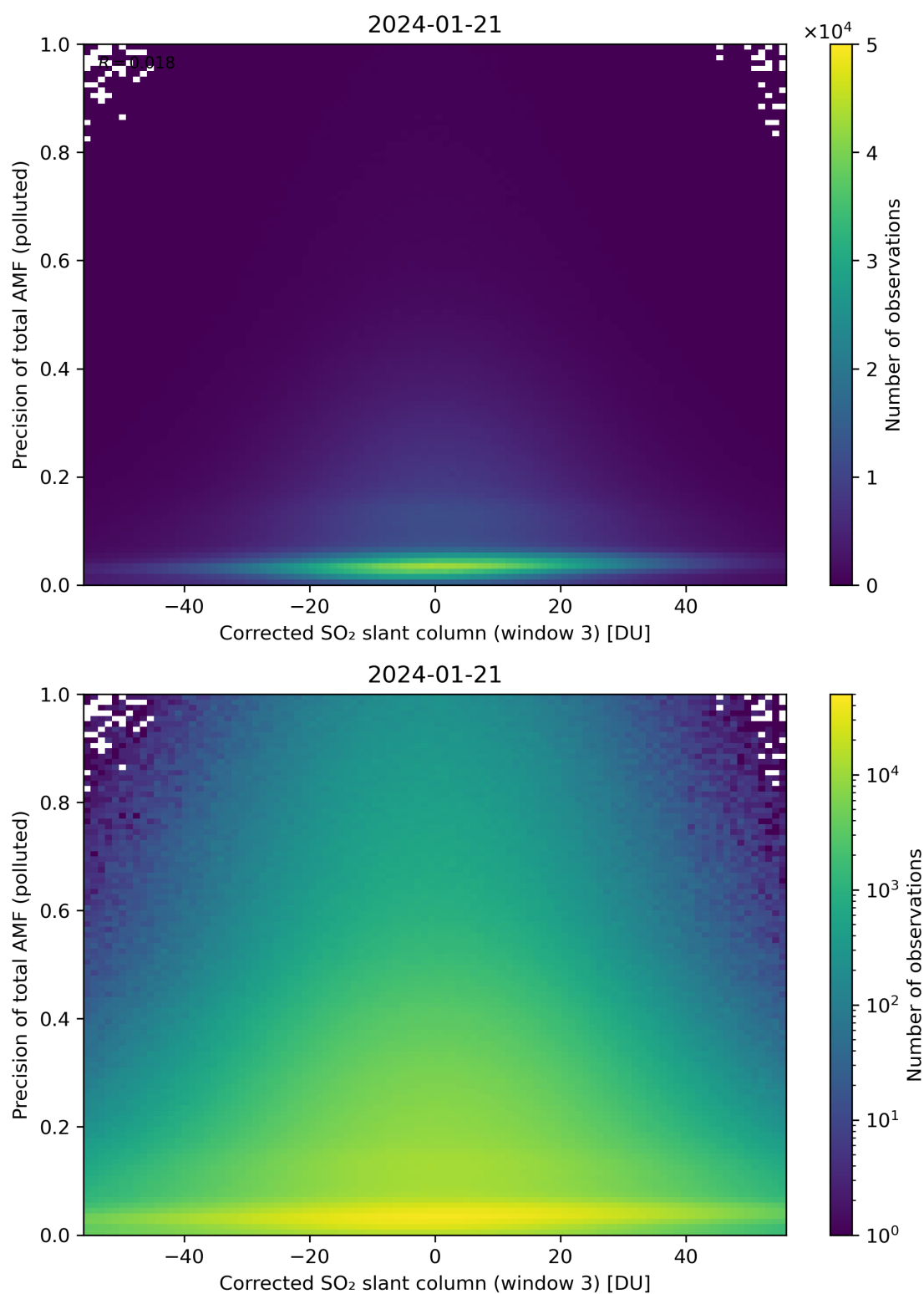
Figure 211: Scatter density plot of “Corrected SO 2 slant column (window 3)” against “Precision of total AMF (polluted)” for 2024-01-21 to 2024-01-22.
