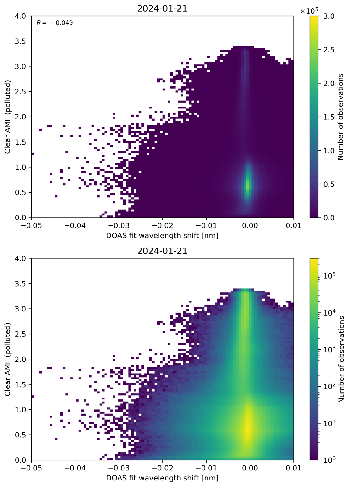
Figure 129: Scatter density plot of “DOAS fit wavelength shift” against “Clear AMF (polluted)” for 2024-01-21 to 2024-01-22.
