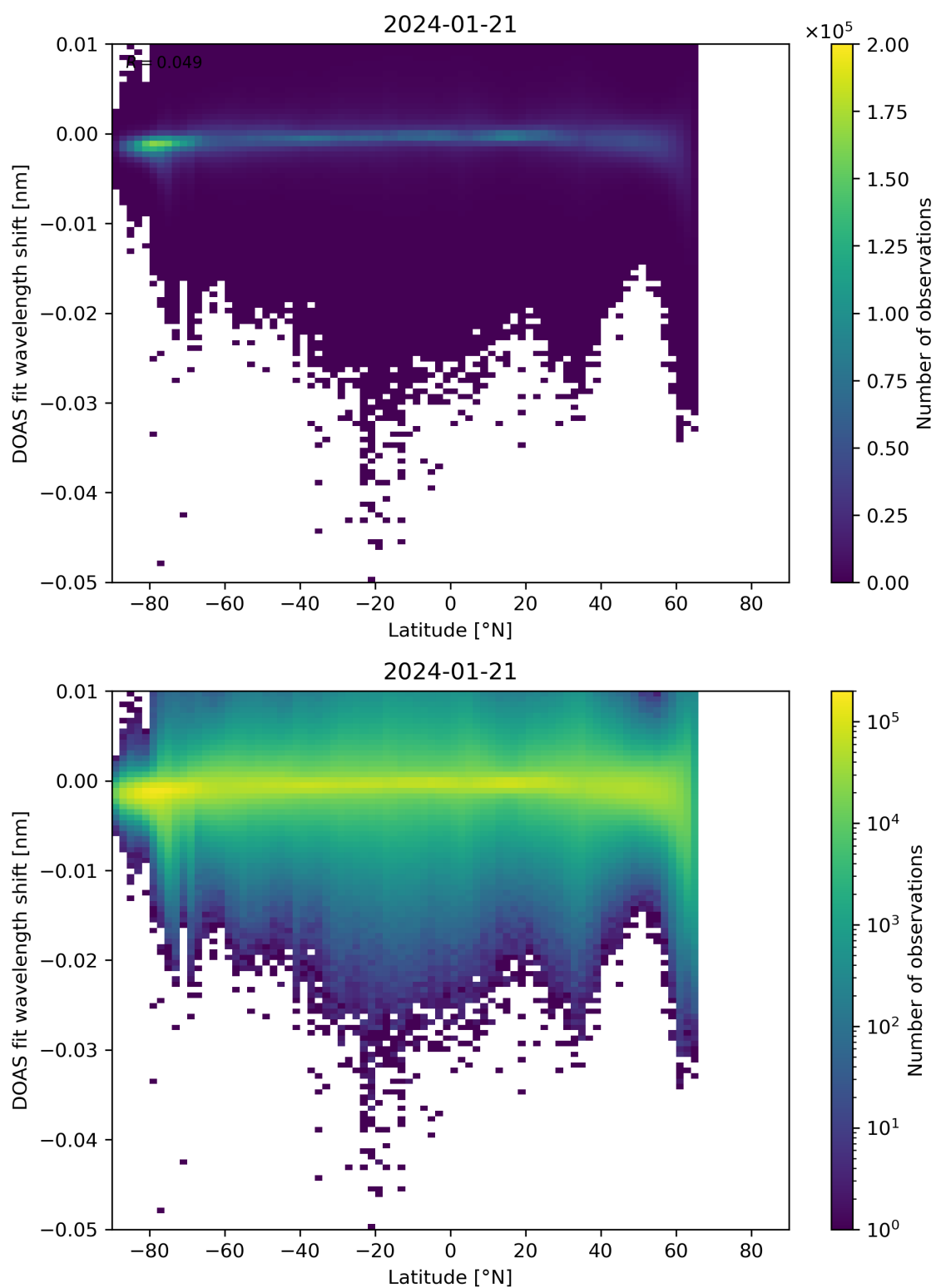
Figure 142: Scatter density plot of “Latitude” against “DOAS fit wavelength shift” for 2024-01-21 to 2024-01-22.
