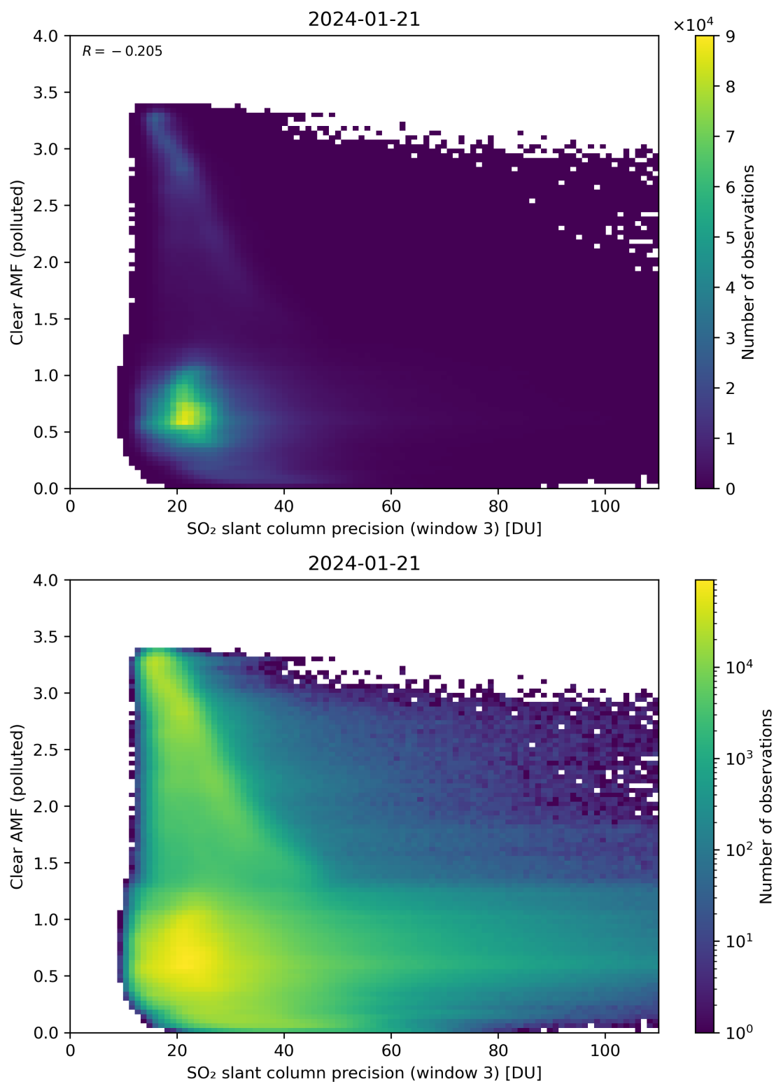
Figure 261: Scatter density plot of “SO 2 slant column precision (window 3)” against “Clear AMF (polluted)” for 2024-01-21 to 2024-01-22.
