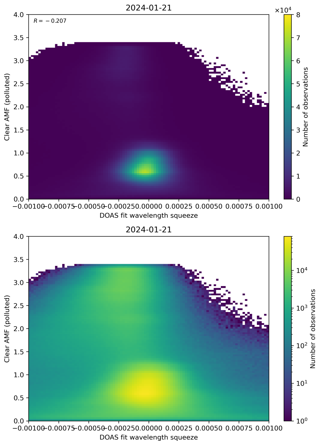
Figure 133: Scatter density plot of “DOAS fit wavelength squeeze” against “Clear AMF (polluted)” for 2024-01-21 to 2024-01-22.
