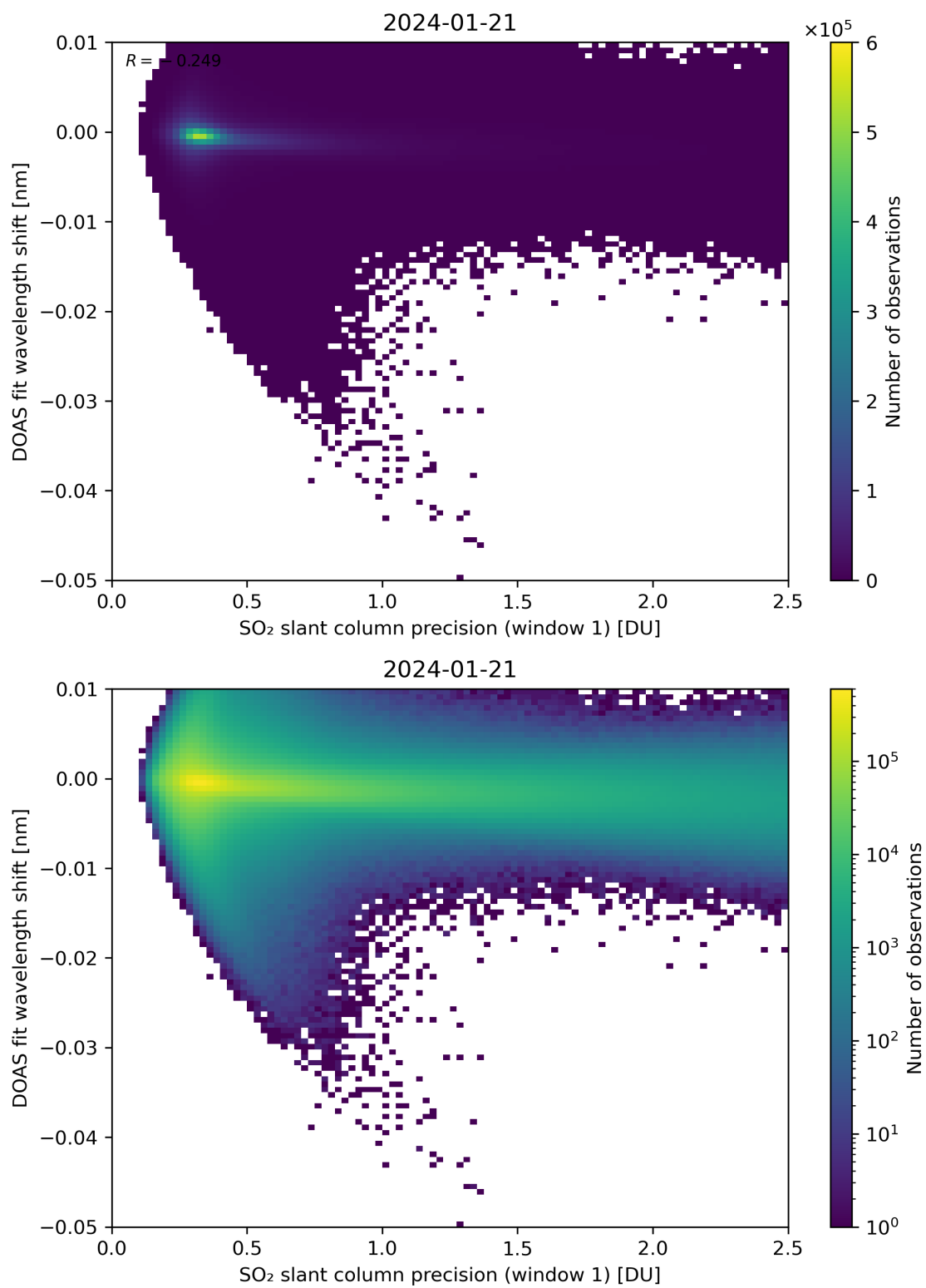
Figure 221: Scatter density plot of “SO 2 slant column precision (window 1)” against “DOAS fit wavelength shift” for 2024-01-21 to 2024-01-22.
