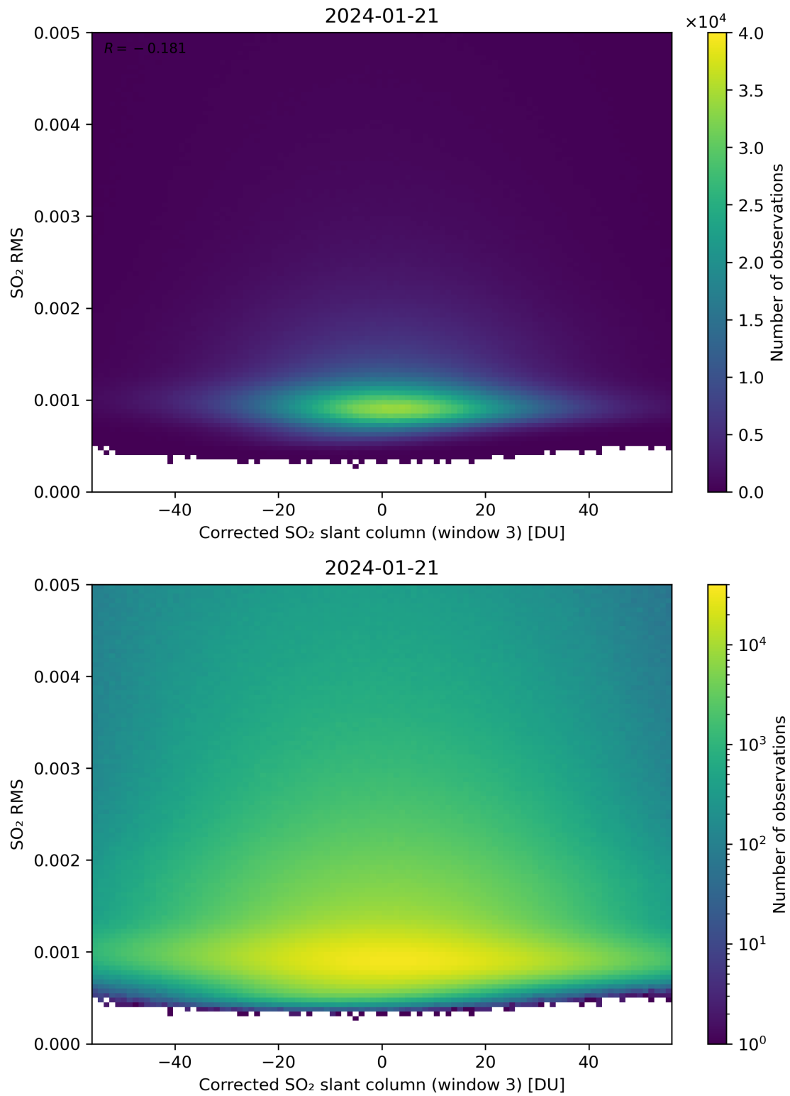
Figure 208: Scatter density plot of “Corrected SO 2 slant column (window 3)” against “SO 2 RMS” for 2024-01-21 to 2024-01-22.
