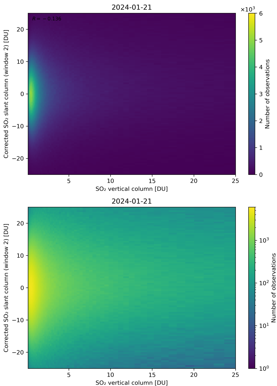
Figure 298: Scatter density plot of “SO 2 vertical column” against “Corrected SO 2 slant column (window 2)” for 2024-01-21 to 2024-01-22.
