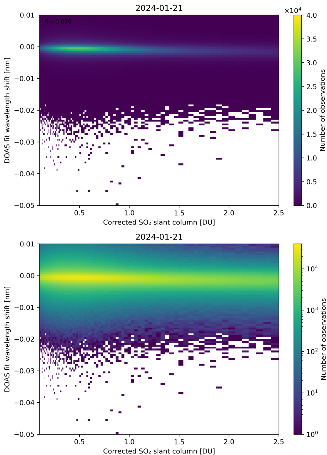
Figure 181: Scatter density plot of “Corrected SO 2 slant column” against “DOAS fit wavelength shift” for 2024-01-21 to 2024-01-22.
