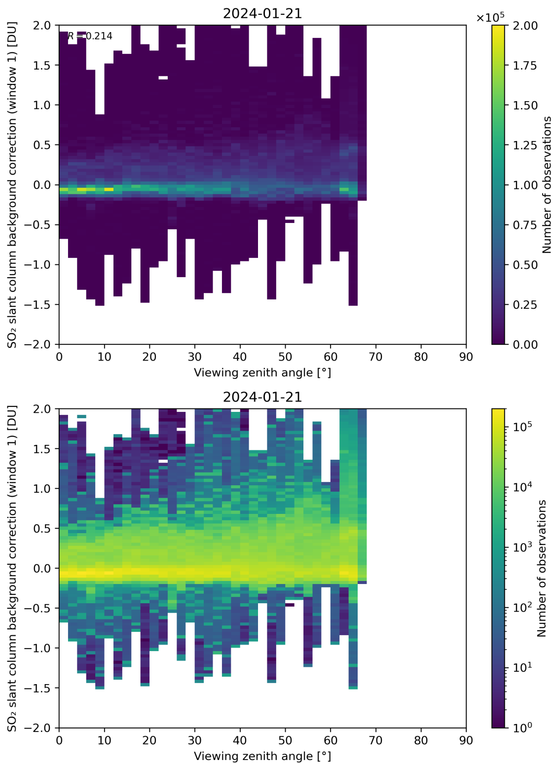
Figure 308: Scatter density plot of “Viewing zenith angle” against “SO 2 slant column background correction (window 1)” for 2024-01-21 to 2024-01-22.
