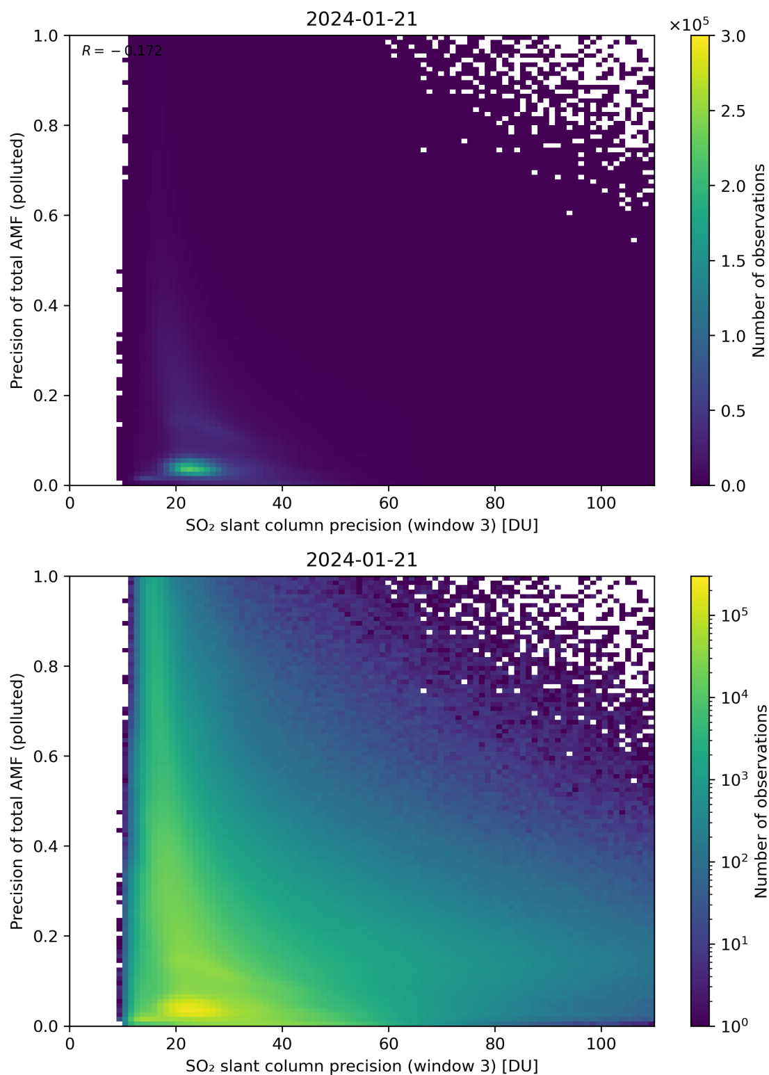
Figure 264: Scatter density plot of “SO 2 slant column precision (window 3)” against “Precision of total AMF (polluted)” for 2024-01-21 to 2024-01-22.
