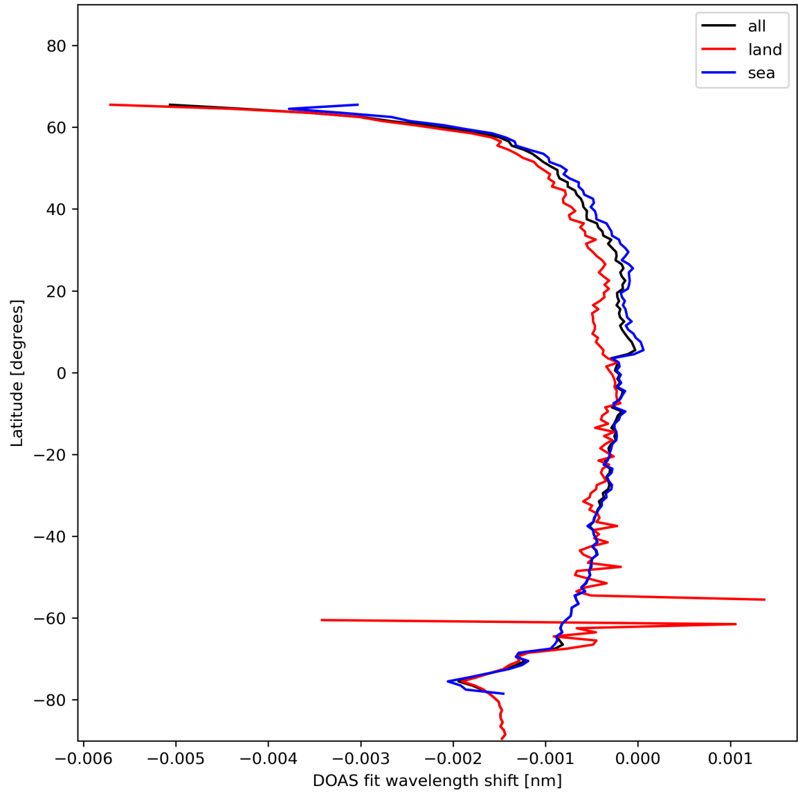
Figure 45: Zonal average of “DOAS fit wavelength shift” for 2024-01-21 to 2024-01-22.
