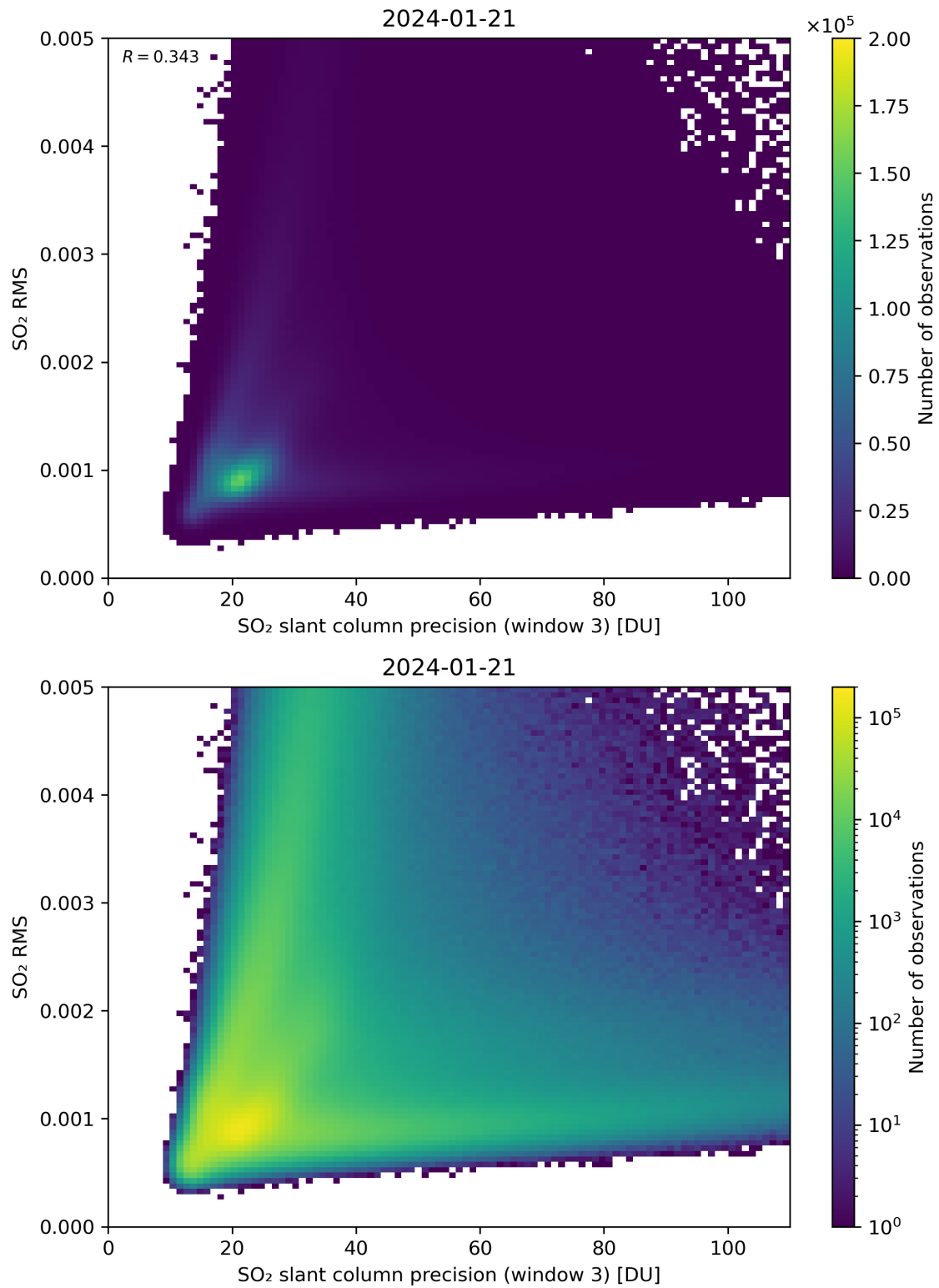
Figure 260: Scatter density plot of “SO 2 slant column precision (window 3)” against “SO 2 RMS” for 2024-01-21 to 2024-01-22.
