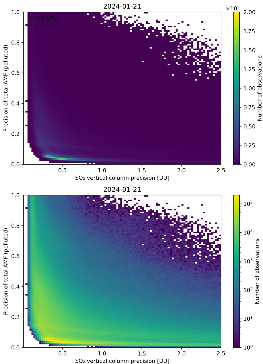
Figure 295: Scatter density plot of “SO 2 vertical column precision” against “Precision of total AMF (polluted)” for 2024-01-21 to 2024-01-22.
