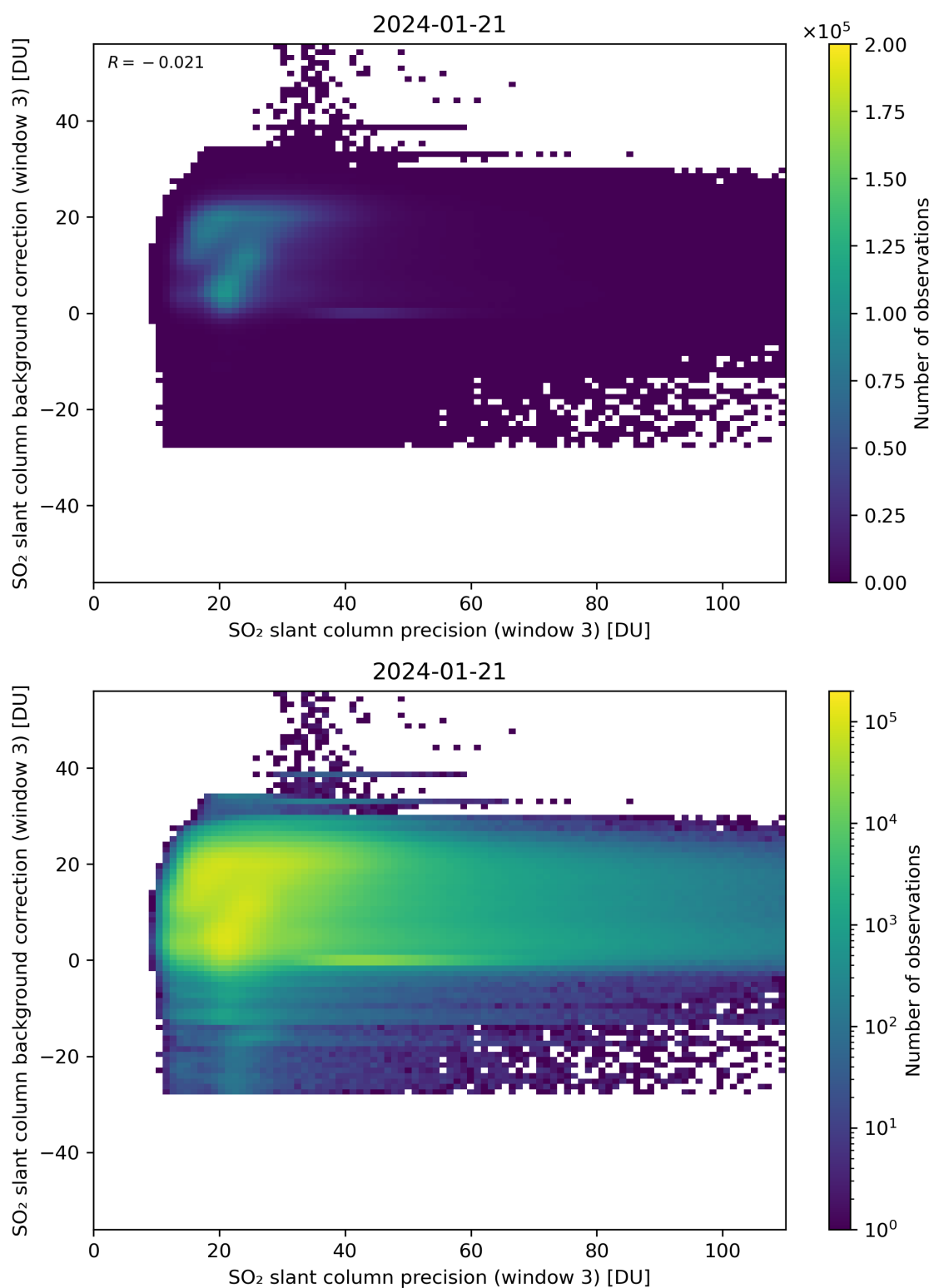
Figure 257: Scatter density plot of “SO 2 slant column precision (window 3)” against “SO 2 slant column background correction (window 3)” for 2024-01-21 to 2024-01-22.
