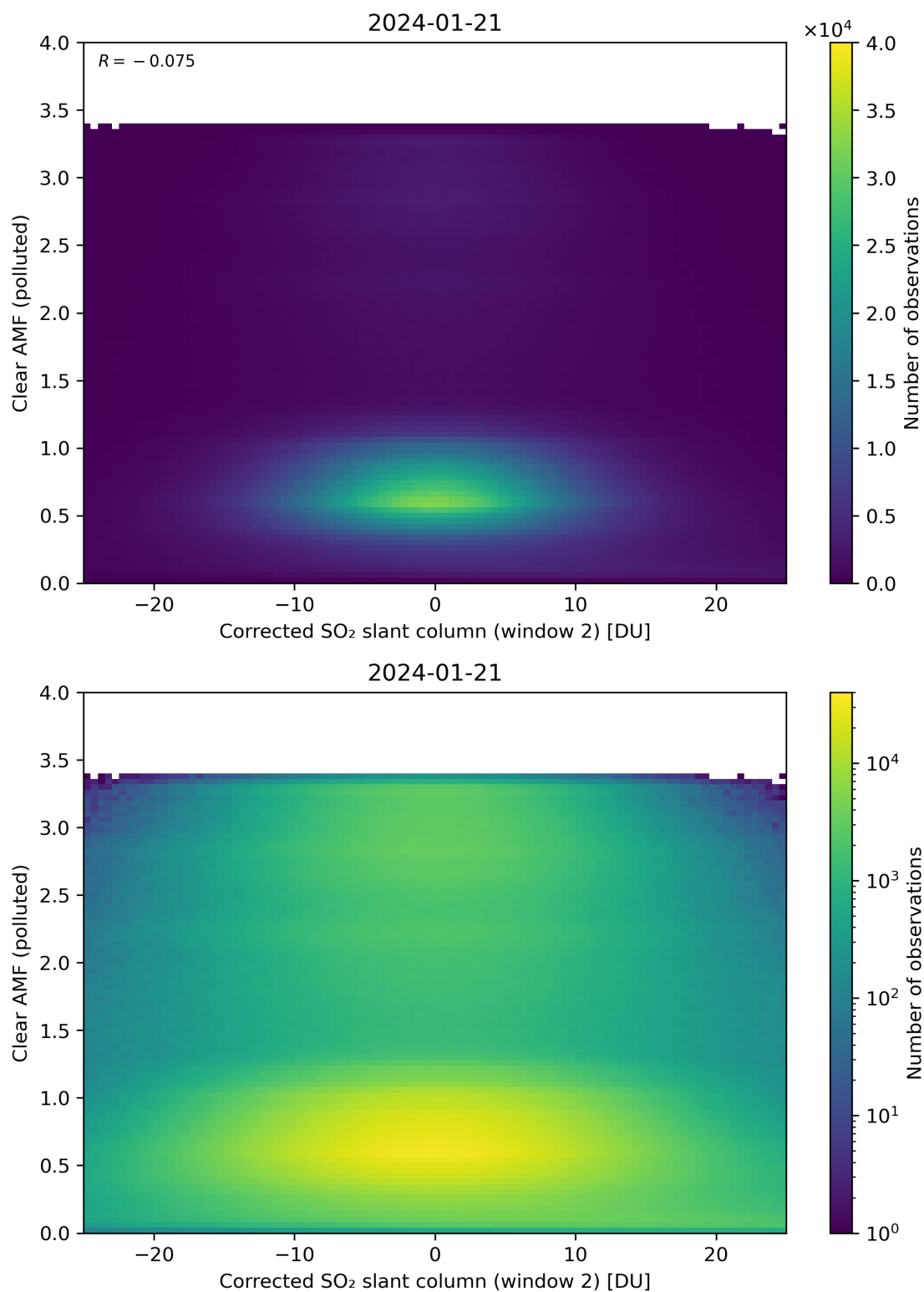
Figure 199: Scatter density plot of “Corrected SO 2 slant column (window 2)” against “Clear AMF (polluted)” for 2024-01-21 to 2024-01-22.
