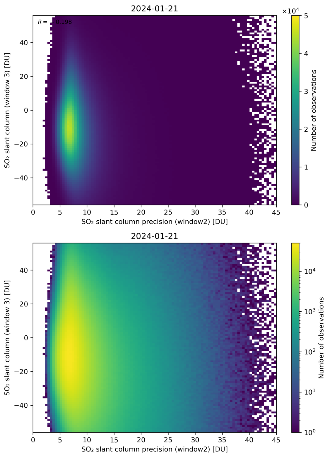
Figure 249: Scatter density plot of “SO 2 slant column precision (window2)” against “SO 2 slant column (window 3)” for 2024-01-21 to 2024-01-22.
