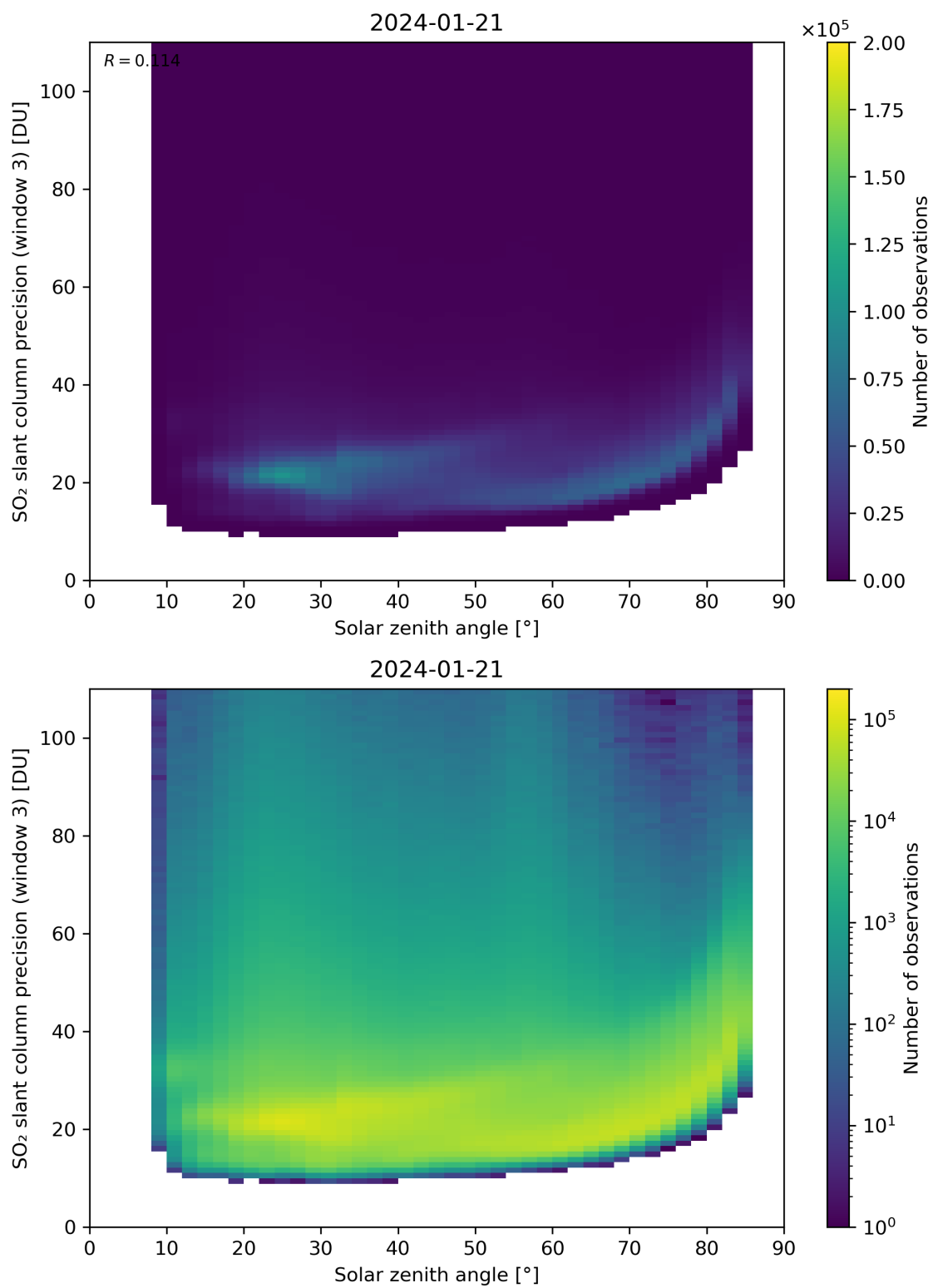
Figure 173: Scatter density plot of “Solar zenith angle” against “SO 2 slant column precision (window 3)” for 2024-01-21 to 2024-01-22.
