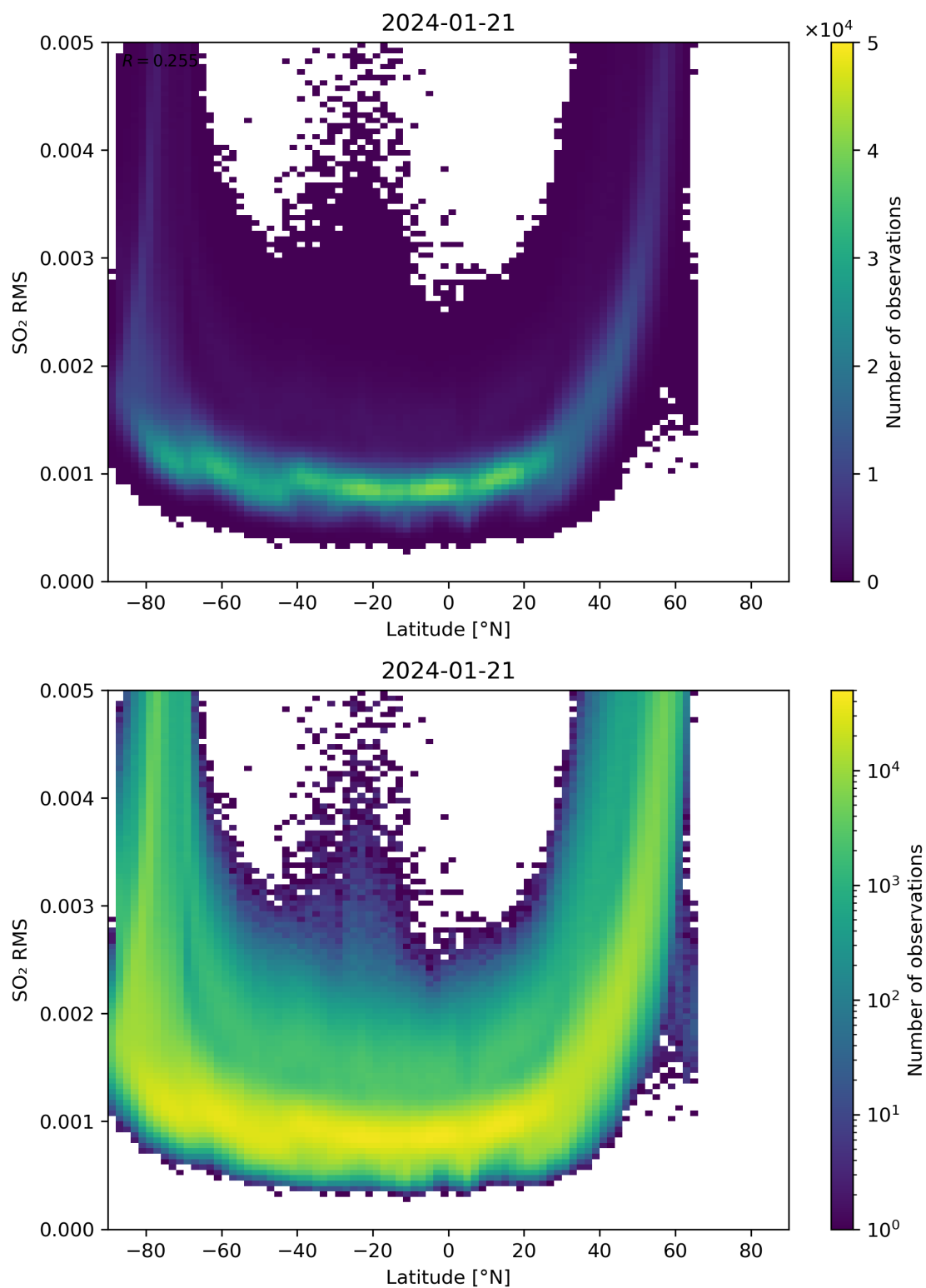
Figure 144: Scatter density plot of “Latitude” against “SO 2 RMS” for 2024-01-21 to 2024-01-22.
