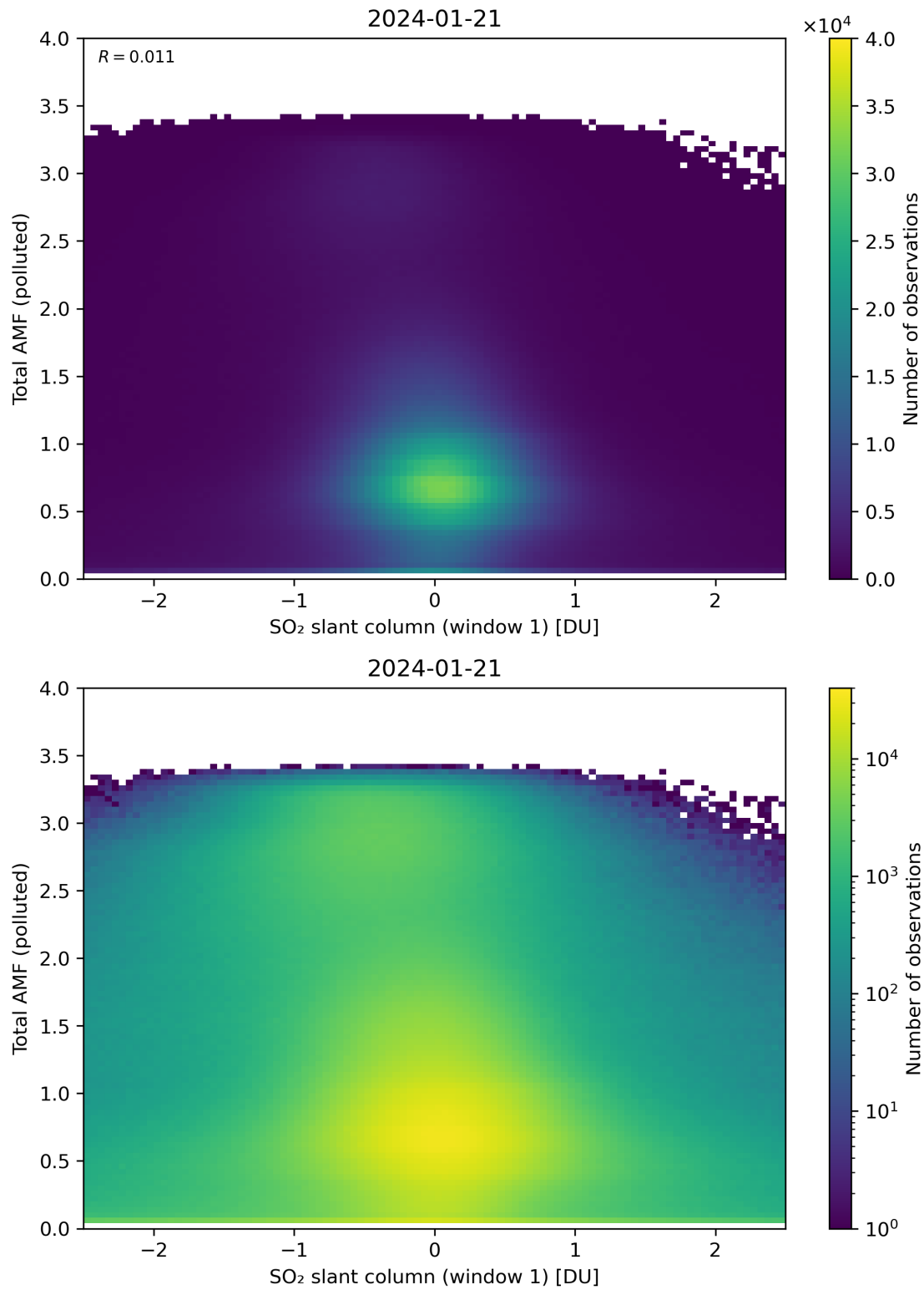
Figure 239: Scatter density plot of “SO 2 slant column (window 1)” against “Total AMF (polluted)” for 2024-01-21 to 2024-01-22.
