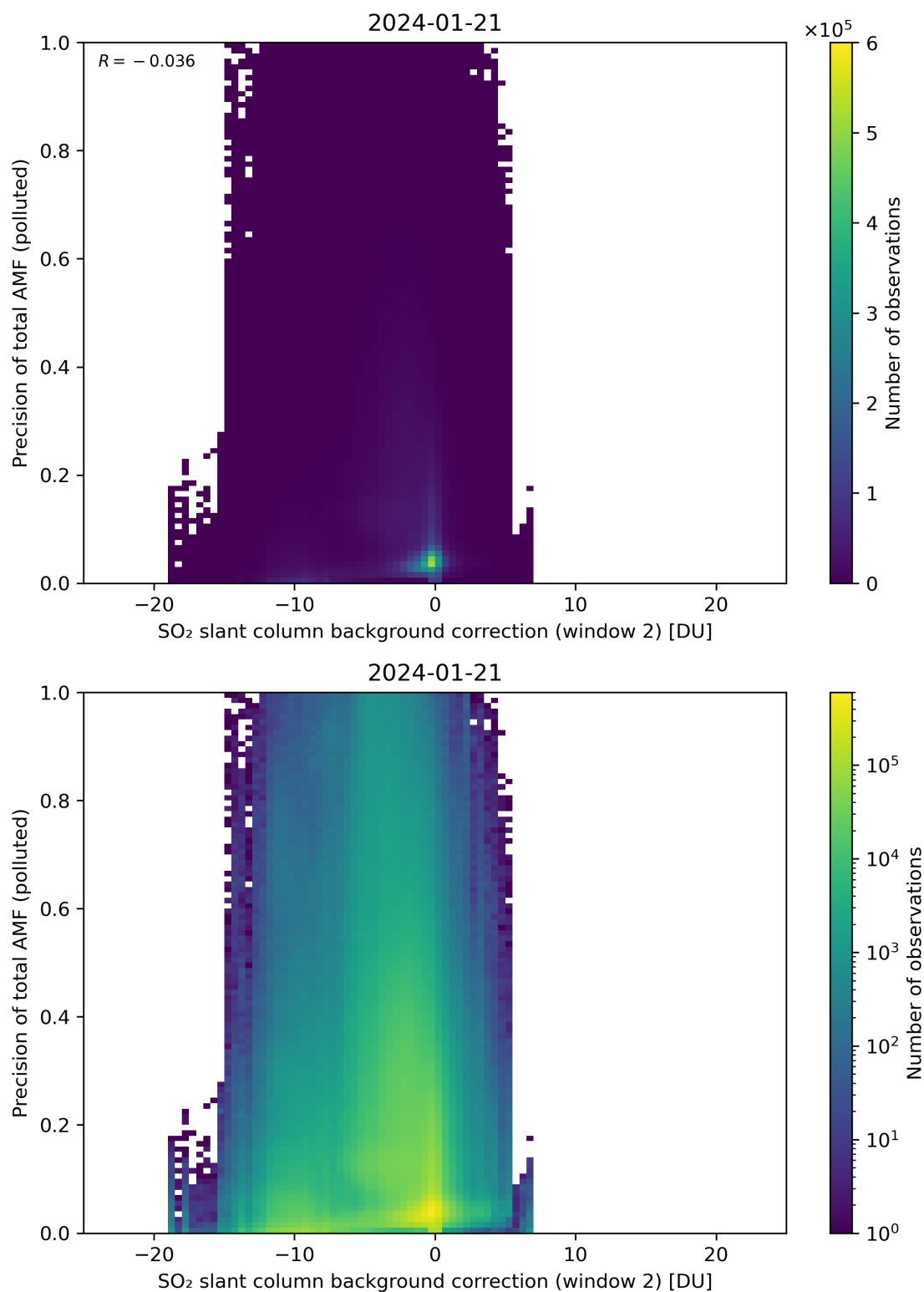
Figure 120: Scatter density plot of “SO 2 slant column background correction (window 2)” against “Precision of total AMF (polluted)” for 2024-01-21 to 2024-01-22.
