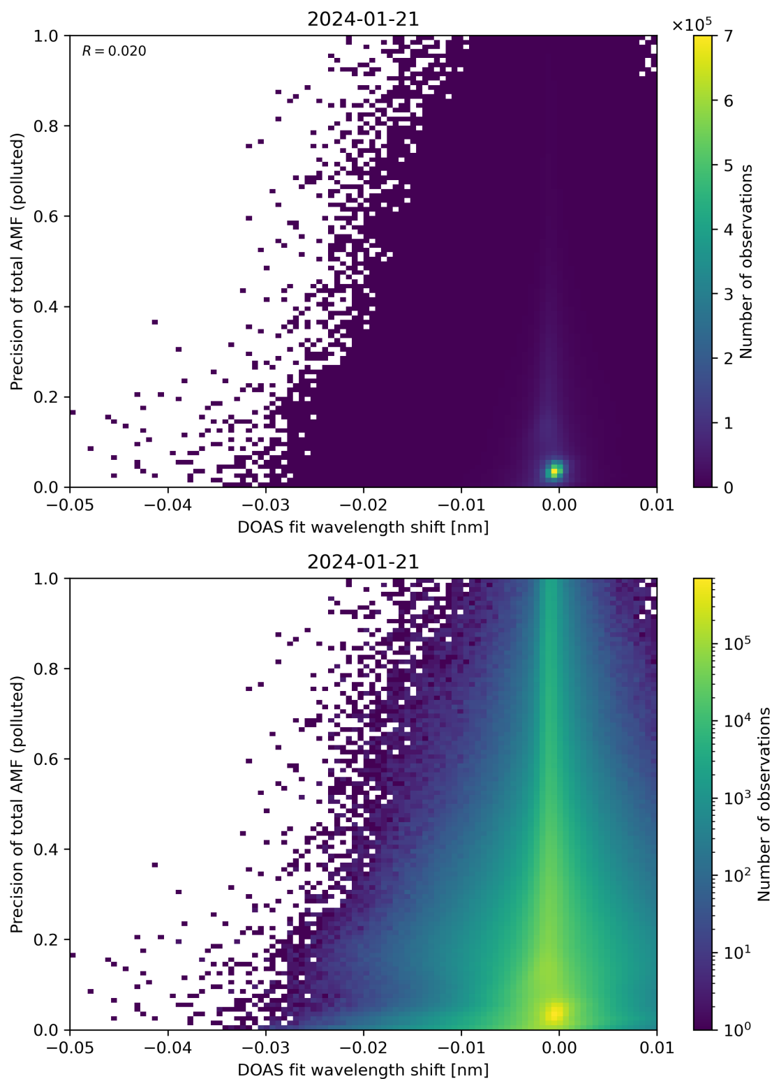
Figure 131: Scatter density plot of “DOAS fit wavelength shift” against “Precision of total AMF (polluted)” for 2024-01-21 to 2024-01-22.
