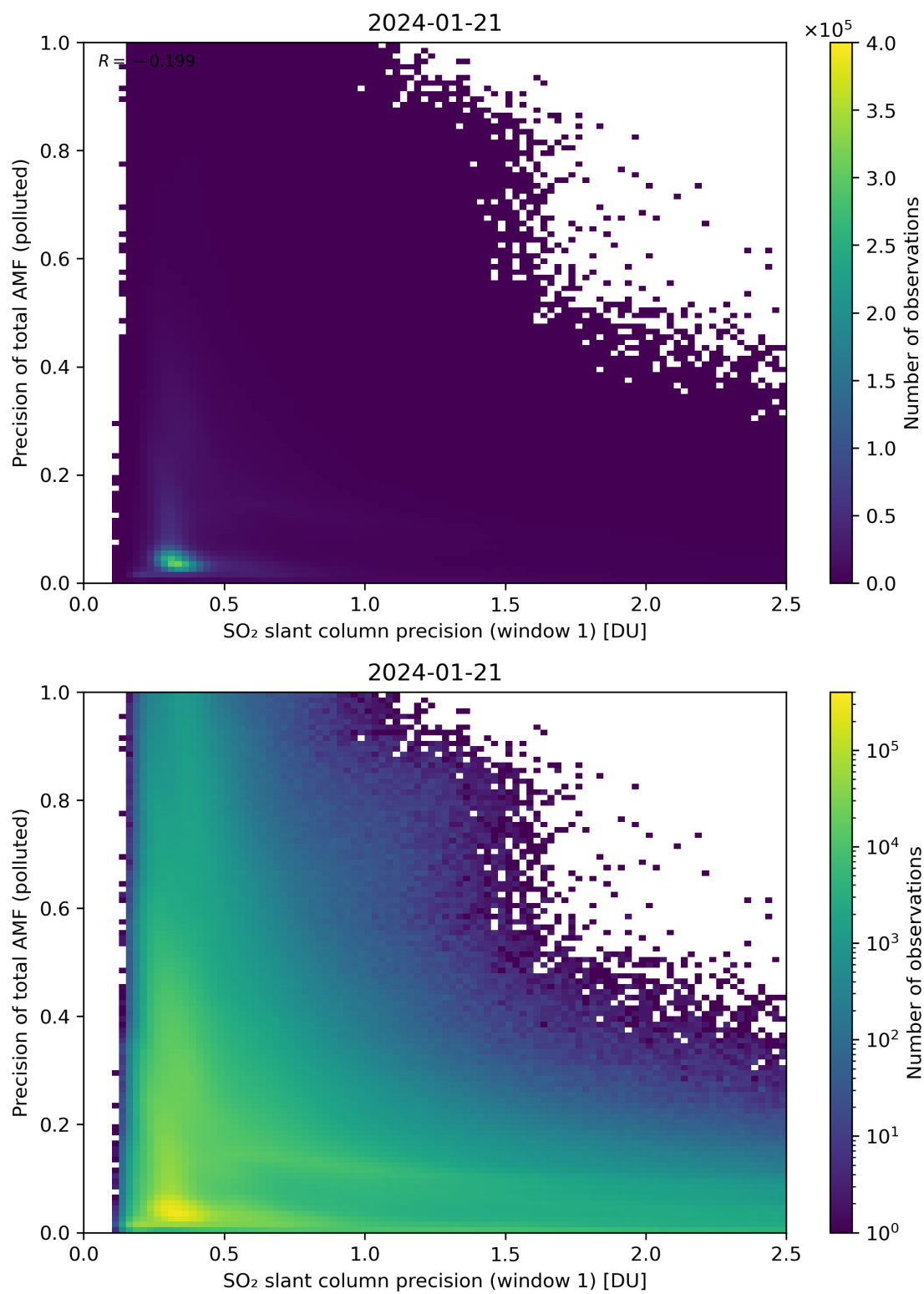
Figure 231: Scatter density plot of “SO 2 slant column precision (window 1)” against “Precision of total AMF (polluted)” for 2024-01-21 to 2024-01-22.
