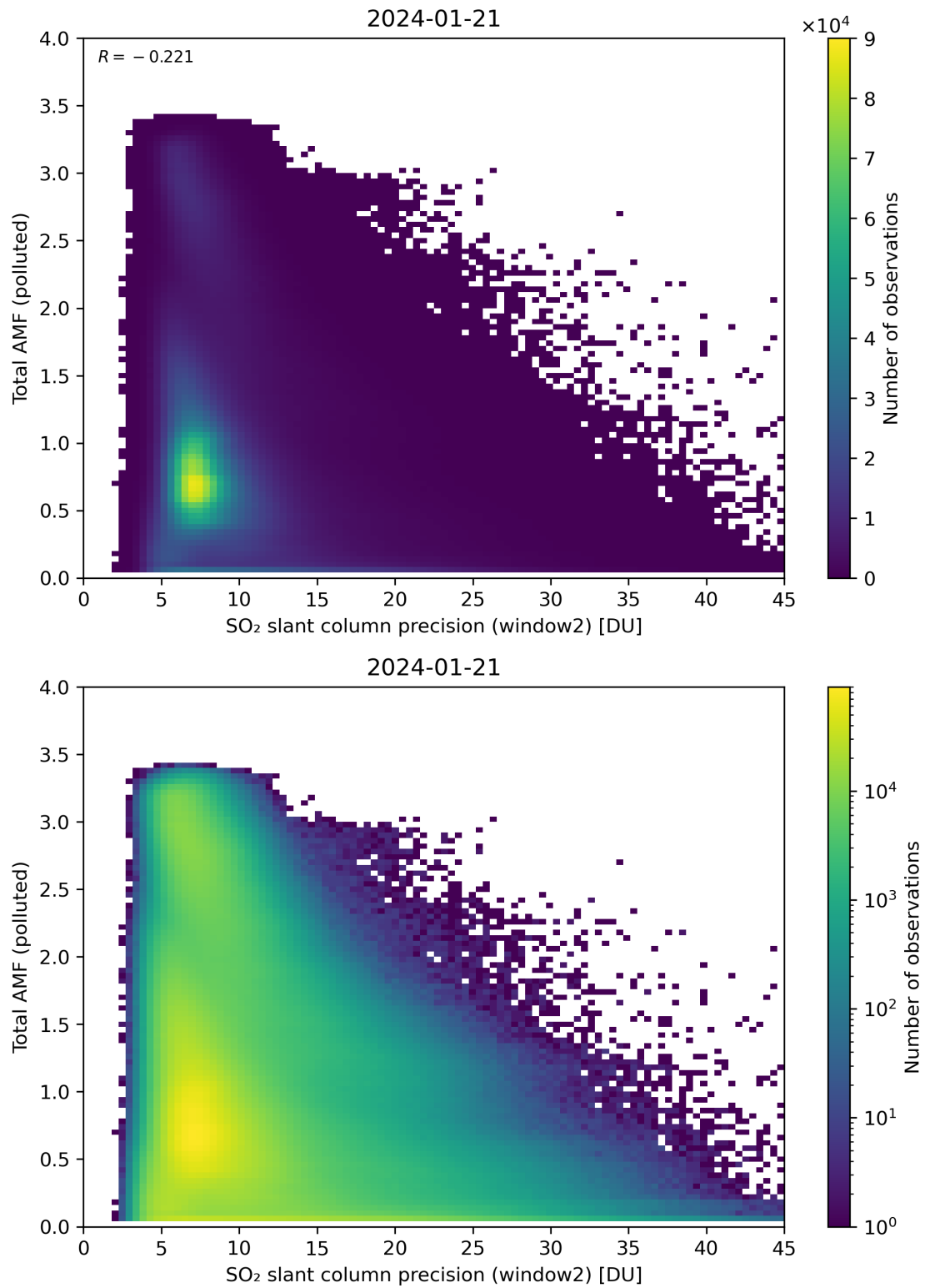
Figure 251: Scatter density plot of “SO 2 slant column precision (window2)” against “Total AMF (polluted)” for 2024-01-21 to 2024-01-22.
