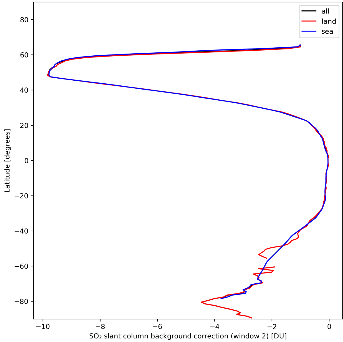
Figure 40: Zonal average of “SO 2 slant column background correction (window 2)” for 2024-01-21 to 2024-01-22.
