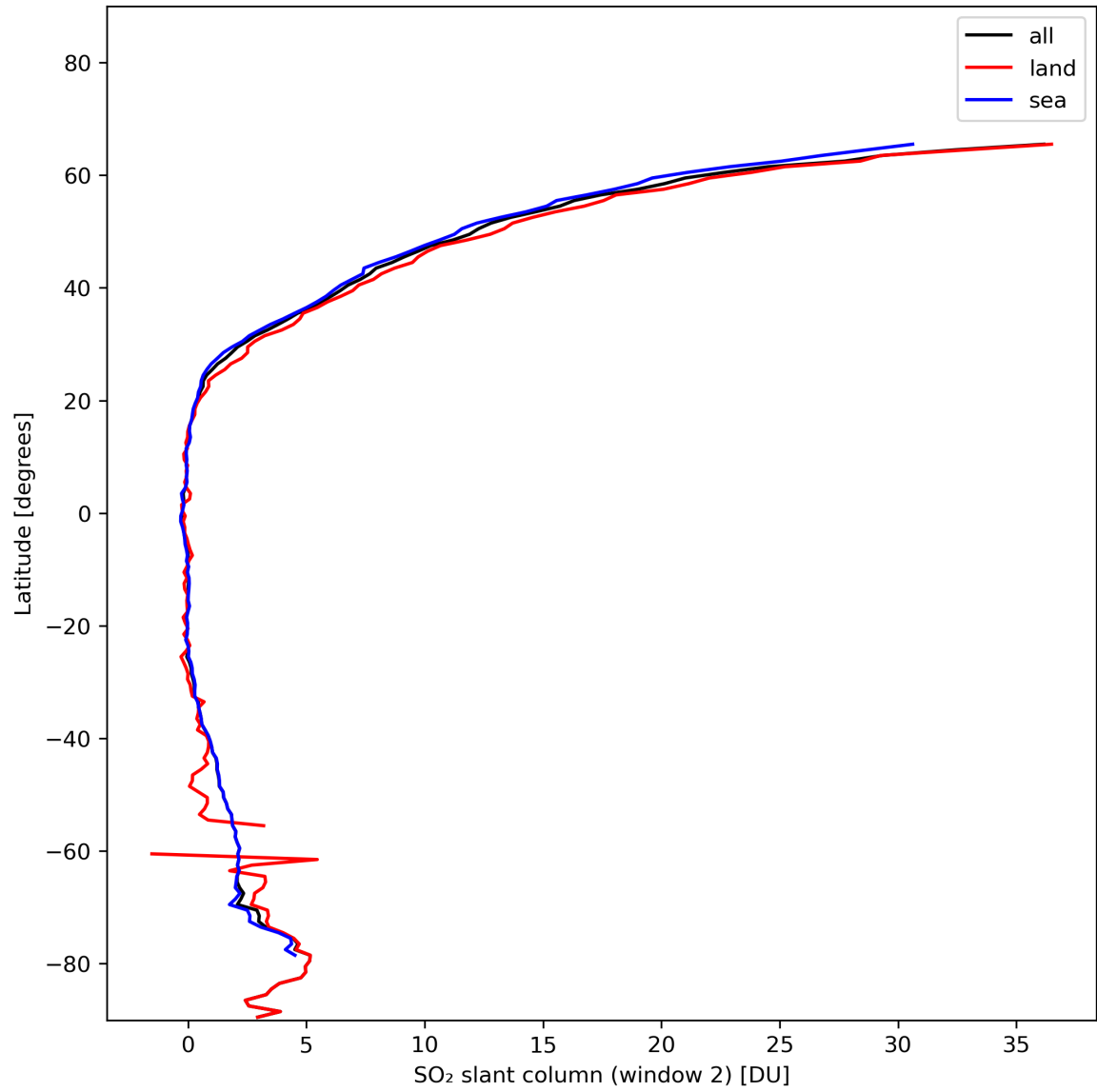
Figure 37: Zonal average of “SO 2 slant column (window 2)” for 2024-01-21 to 2024-01-22.
