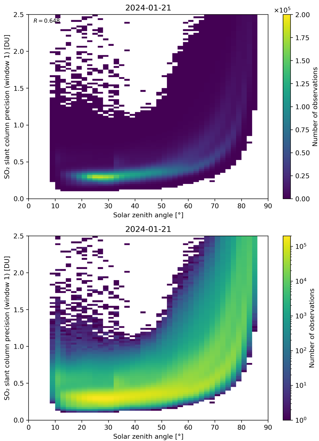
Figure 170: Scatter density plot of “Solar zenith angle” against “SO 2 slant column precision (window 1)” for 2024-01-21 to 2024-01-22.
