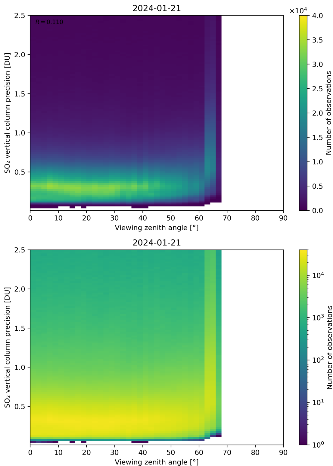
Figure 328: Scatter density plot of “Viewing zenith angle” against “SO 2 vertical column precision” for 2024-01-21 to 2024-01-22.
