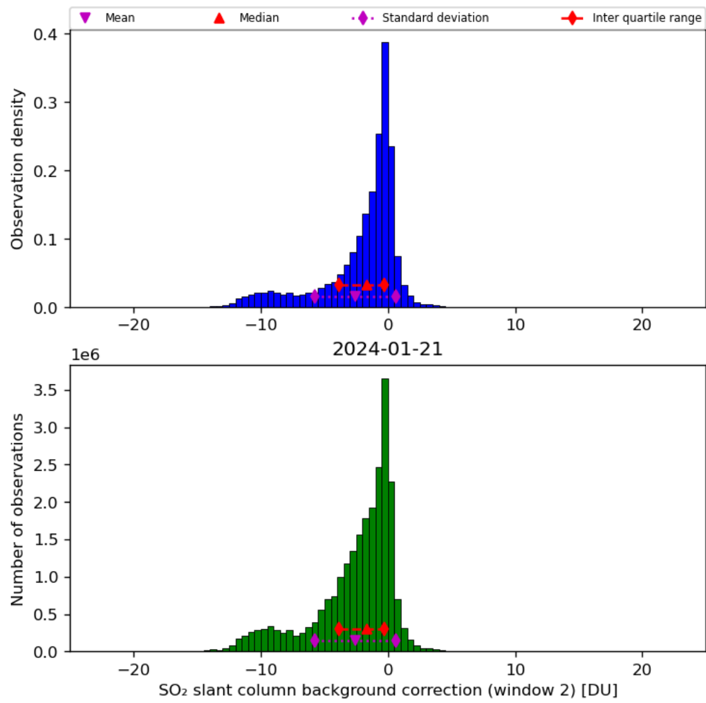
Figure 63: Histogram of “SO 2 slant column background correction (window 2)” for 2024-01-21 to 2024-01-22
