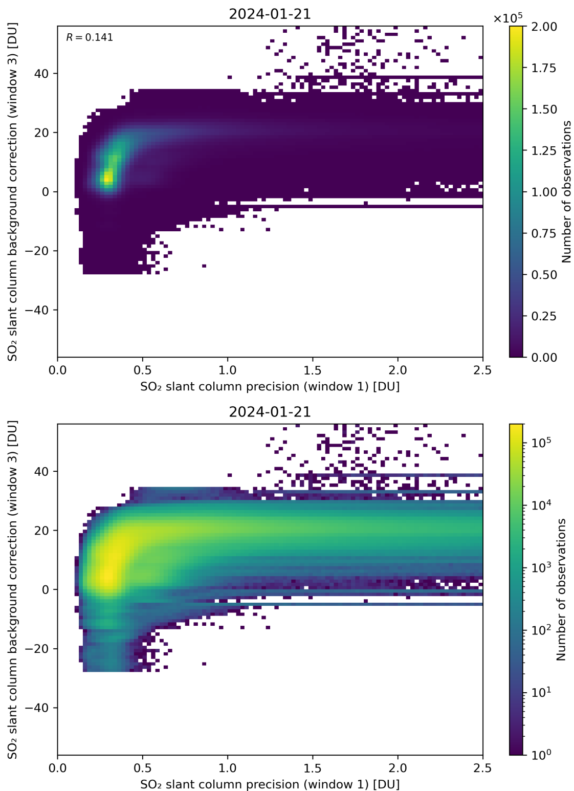
Figure 220: Scatter density plot of “SO 2 slant column precision (window 1)” against “SO 2 slant column background correction (window 3)” for 2024-01-21 to 2024-01-22.
