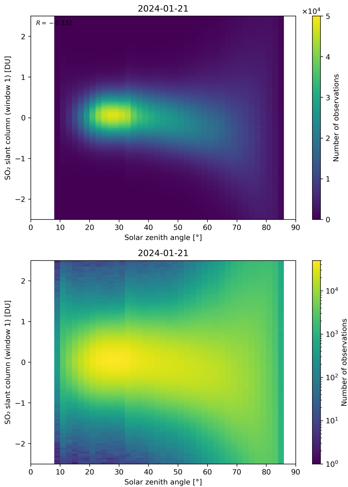
Figure 169: Scatter density plot of “Solar zenith angle” against “SO 2 slant column (window 1)” for 2024-01-21 to 2024-01-22.
