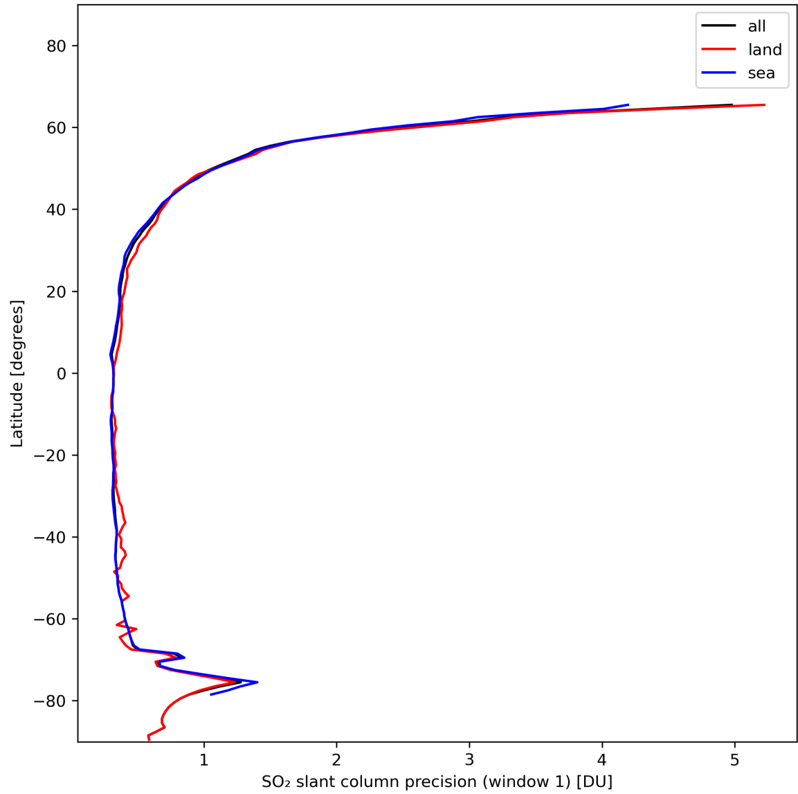
Figure 34: Zonal average of “SO 2 slant column precision (window 1)” for 2024-01-21 to 2024-01-22.
