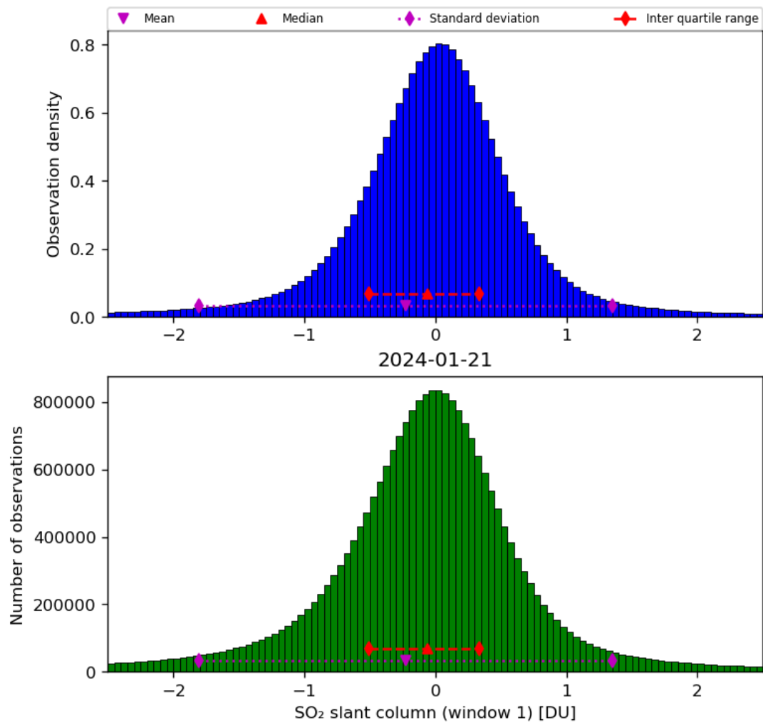
Figure 56: Histogram of “SO 2 slant column (window 1)” for 2024-01-21 to 2024-01-22
