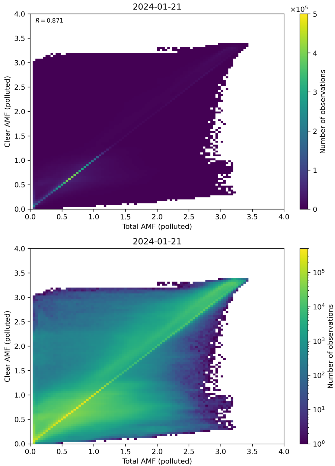
Figure 271: Scatter density plot of “Total AMF (polluted)” against “Clear AMF (polluted)” for 2024-01-21 to 2024-01-22.
