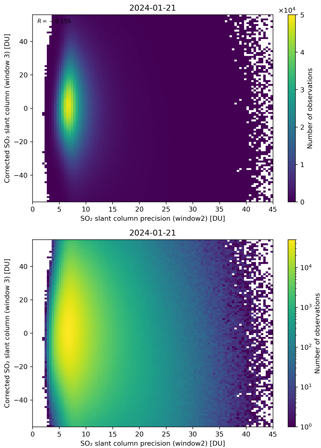
Figure 248: Scatter density plot of “SO 2 slant column precision (window2)” against “Corrected SO 2 slant column (window 3)” for 2024-01-21 to 2024-01-22.
