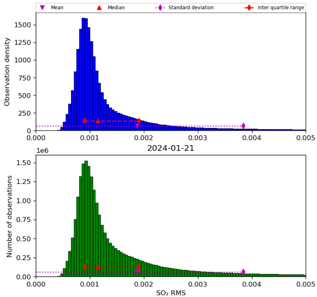
Figure 70: Histogram of “SO 2 RMS” for 2024-01-21 to 2024-01-22
