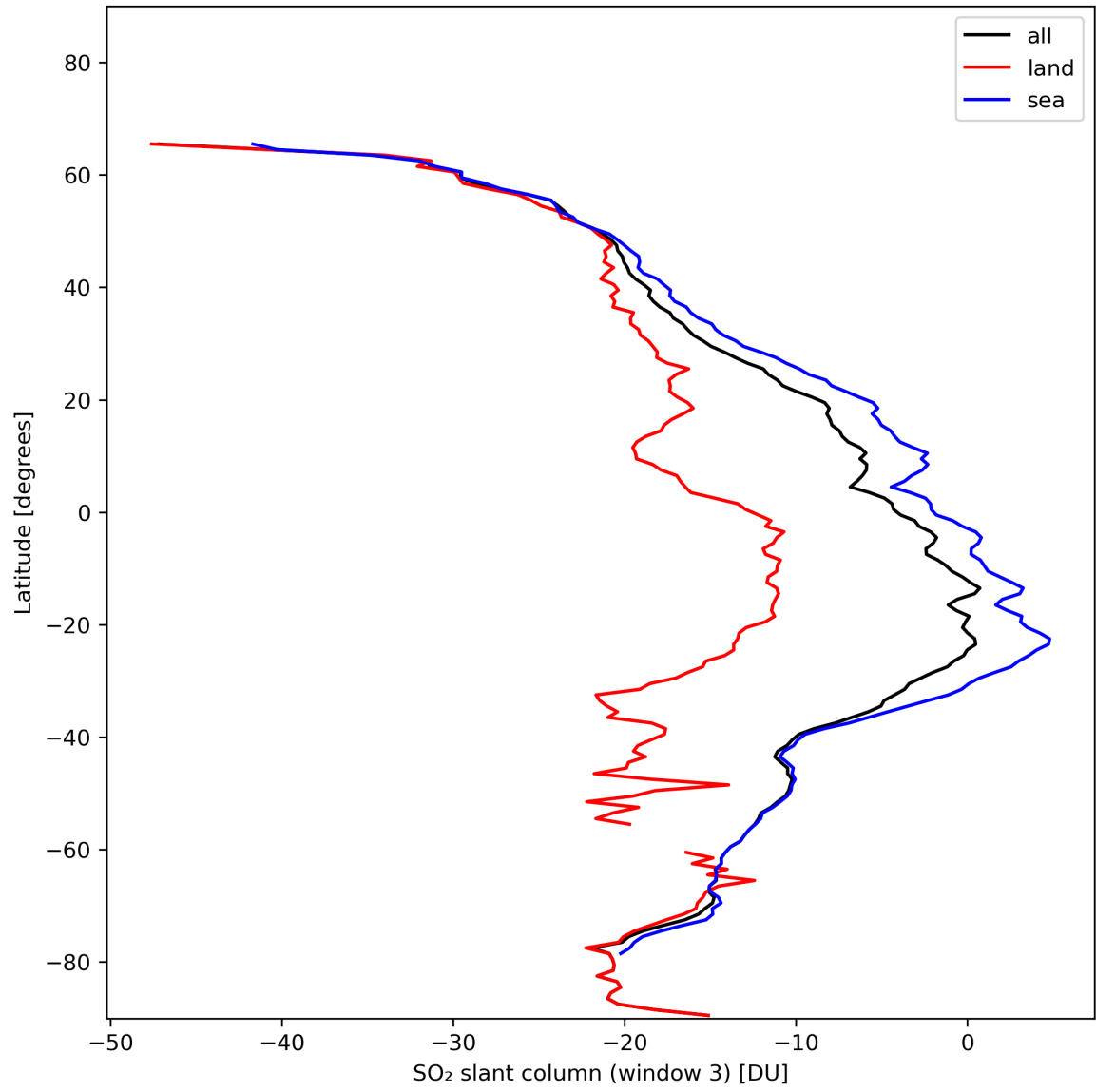
Figure 41: Zonal average of “SO 2 slant column (window 3)” for 2024-01-21 to 2024-01-22.
