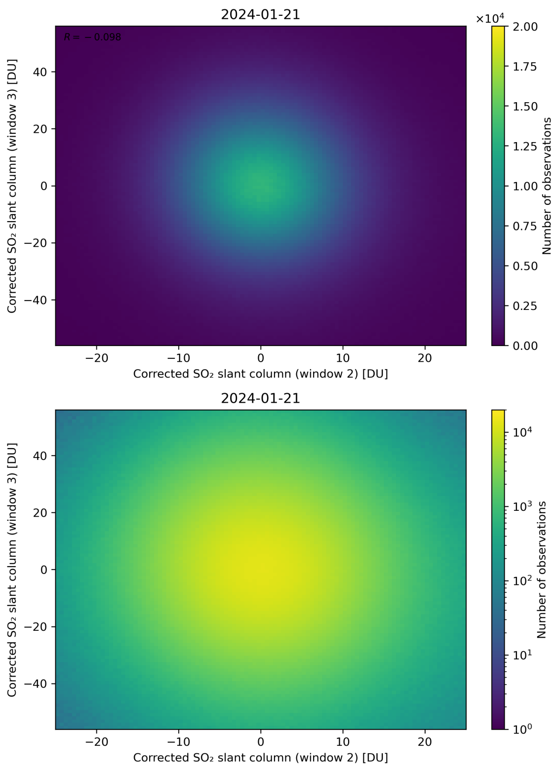
Figure 200: Scatter density plot of “Corrected SO 2 slant column (window 2)” against “Corrected SO 2 slant column (window 3)” for 2024-01-21 to 2024-01-22.
