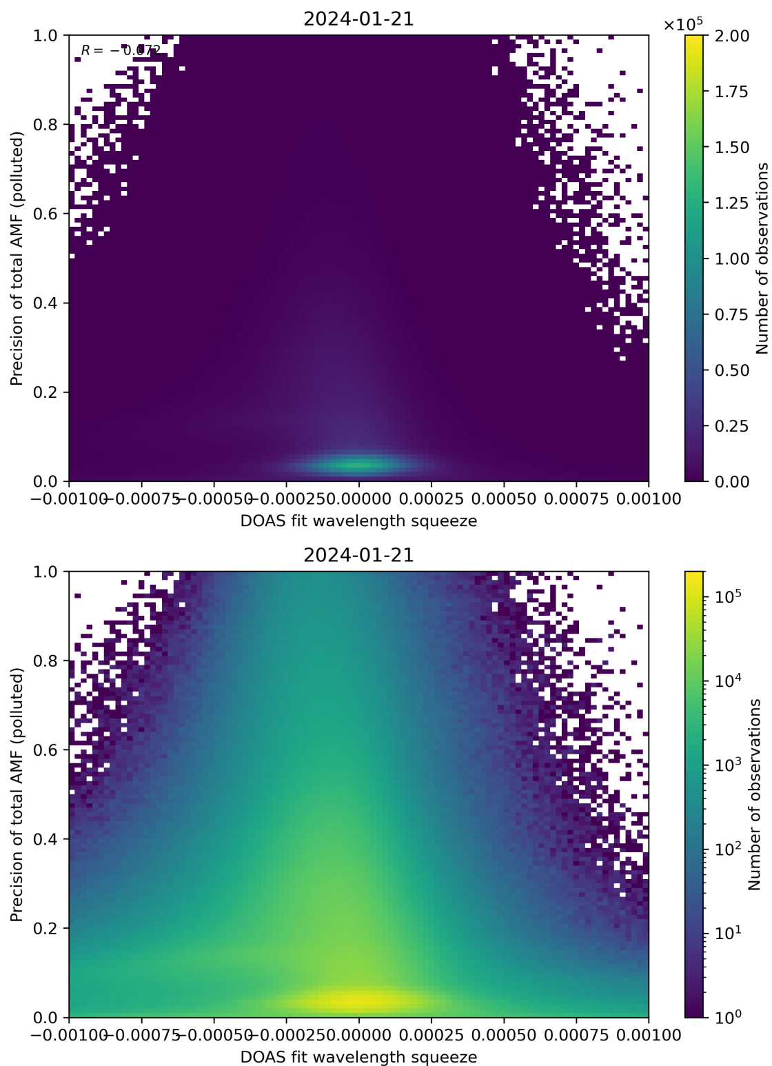
Figure 135: Scatter density plot of “DOAS fit wavelength squeeze” against “Precision of total AMF (polluted)” for 2024-01-21 to 2024-01-22.
