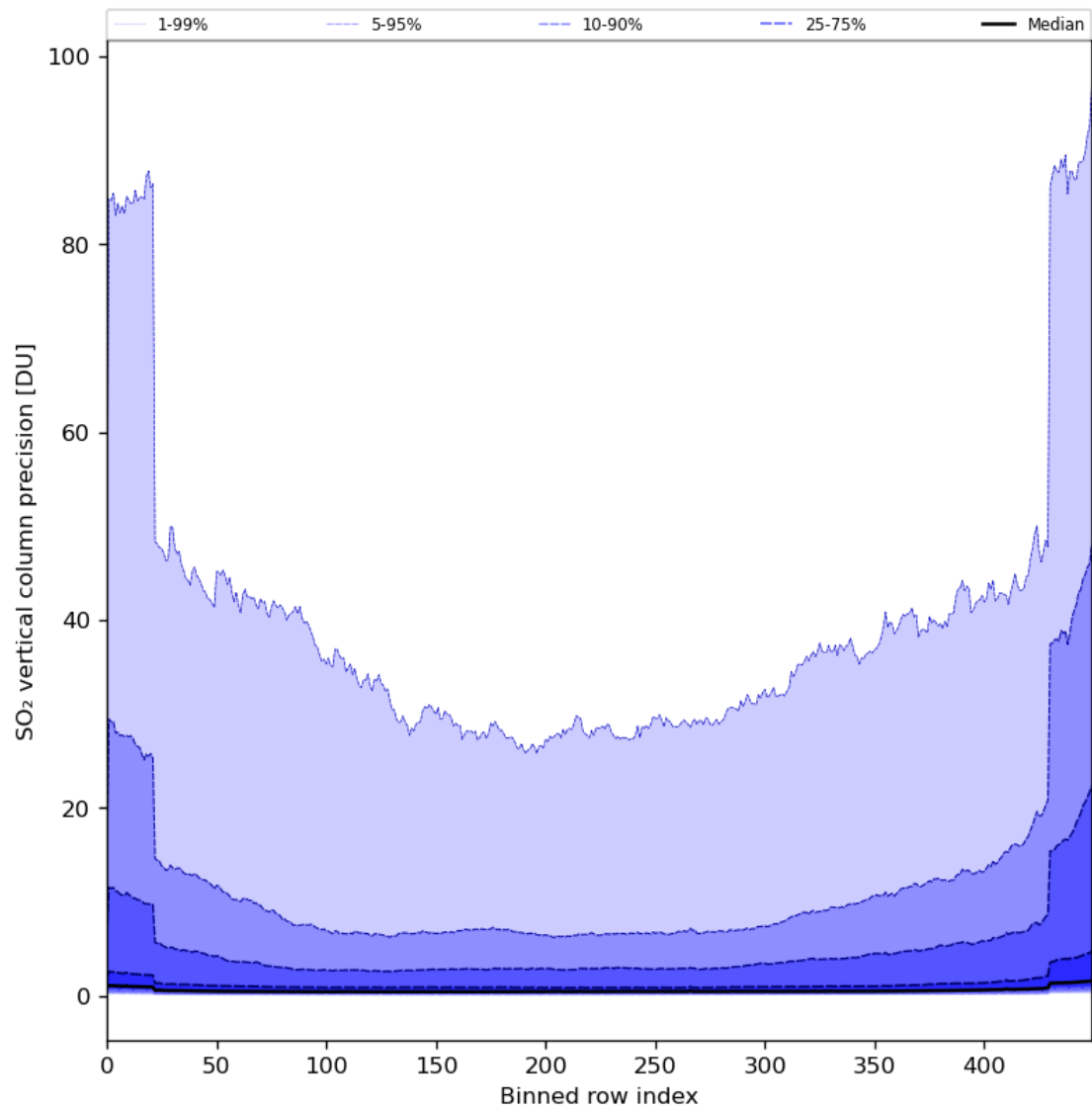
Figure 77: Along track statistics of “SO 2 vertical column precision” for 2024-01-21 to 2024-01-22
