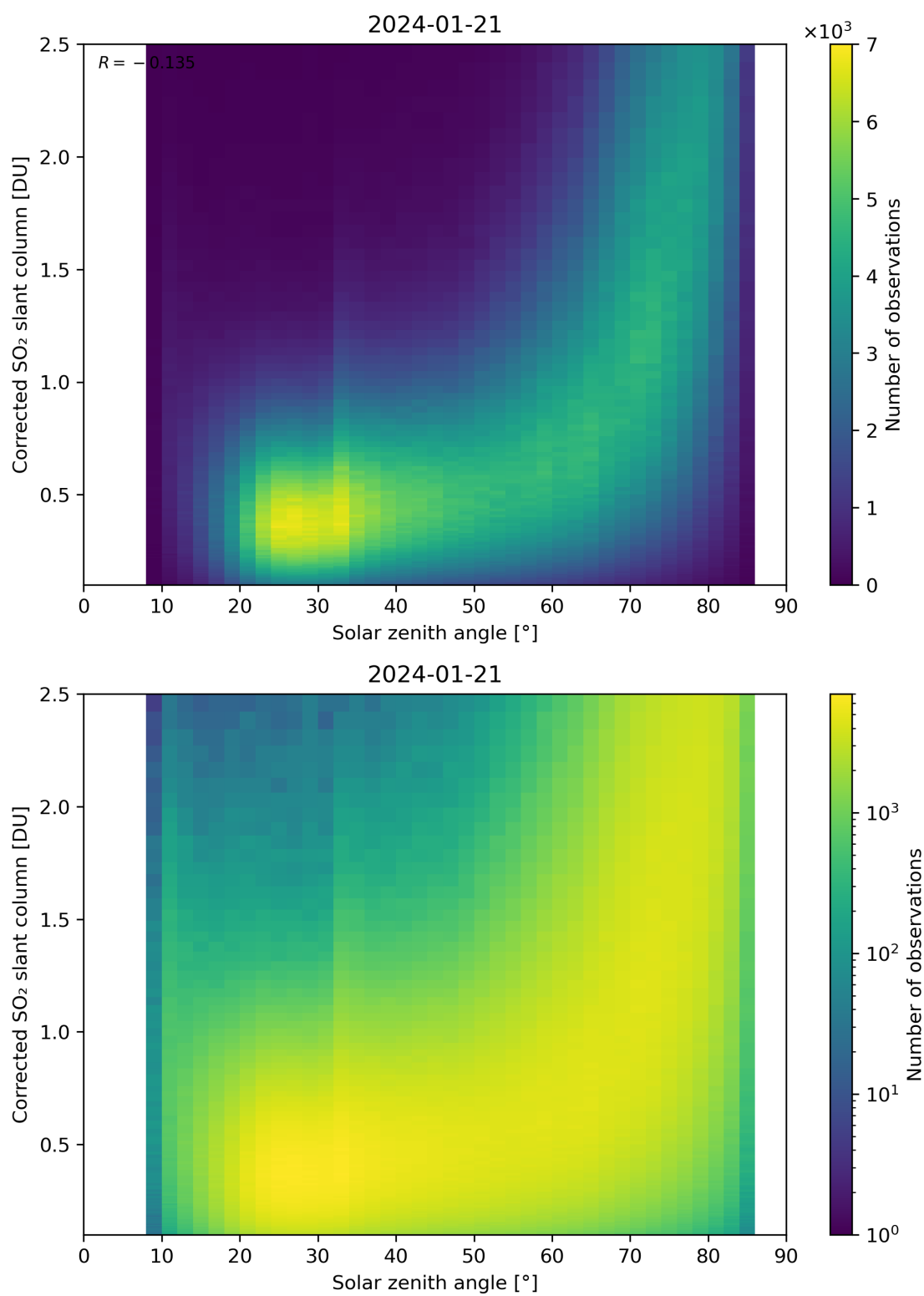
Figure 166: Scatter density plot of “Solar zenith angle” against “Corrected SO 2 slant column” for 2024-01-21 to 2024-01-22.
