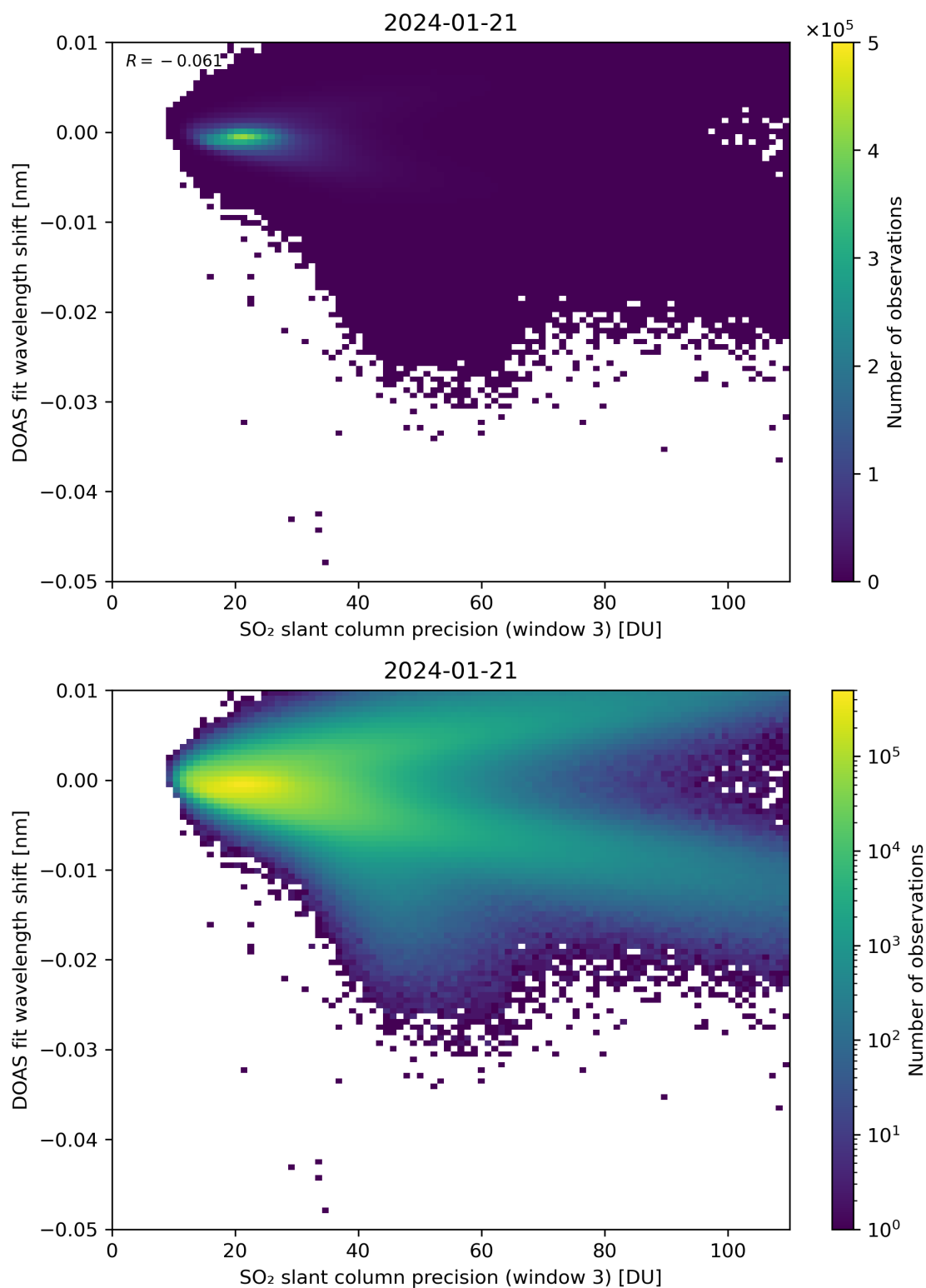
Figure 258: Scatter density plot of “SO 2 slant column precision (window 3)” against “DOAS fit wavelength shift” for 2024-01-21 to 2024-01-22.
