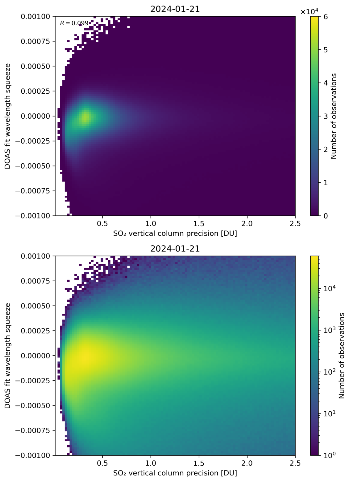
Figure 283: Scatter density plot of “SO 2 vertical column precision” against “DOAS fit wavelength squeeze” for 2024-01-21 to 2024-01-22.
