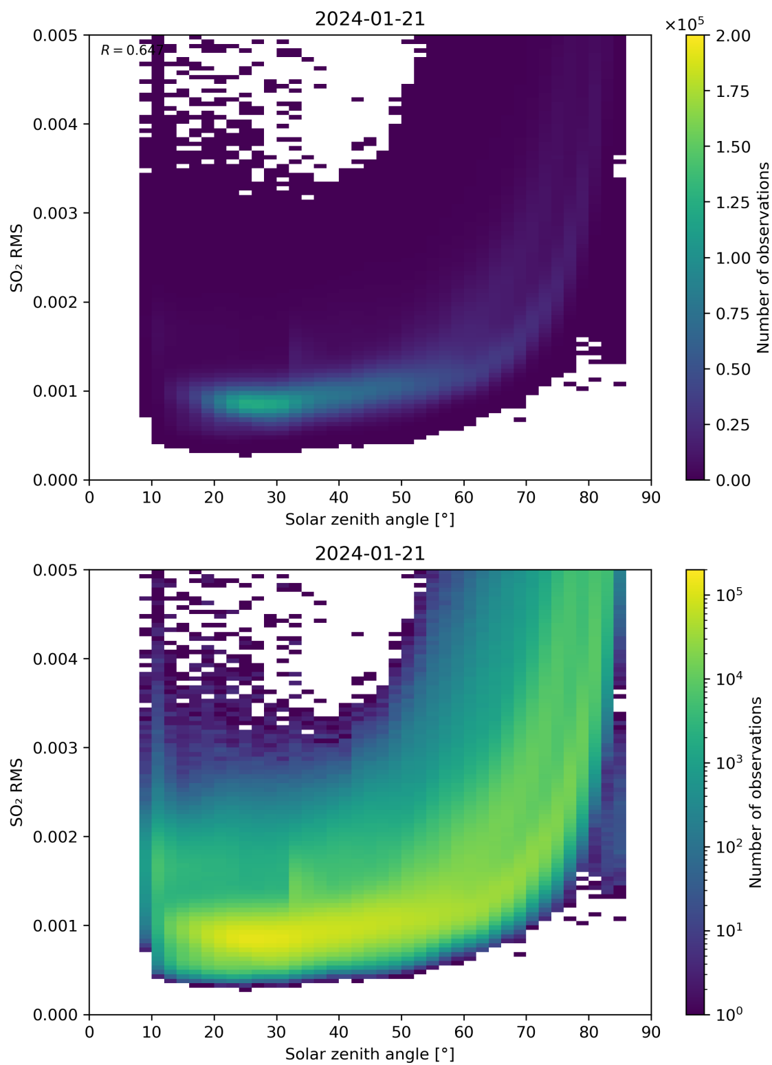
Figure 163: Scatter density plot of “Solar zenith angle” against “SO 2 RMS” for 2024-01-21 to 2024-01-22.
