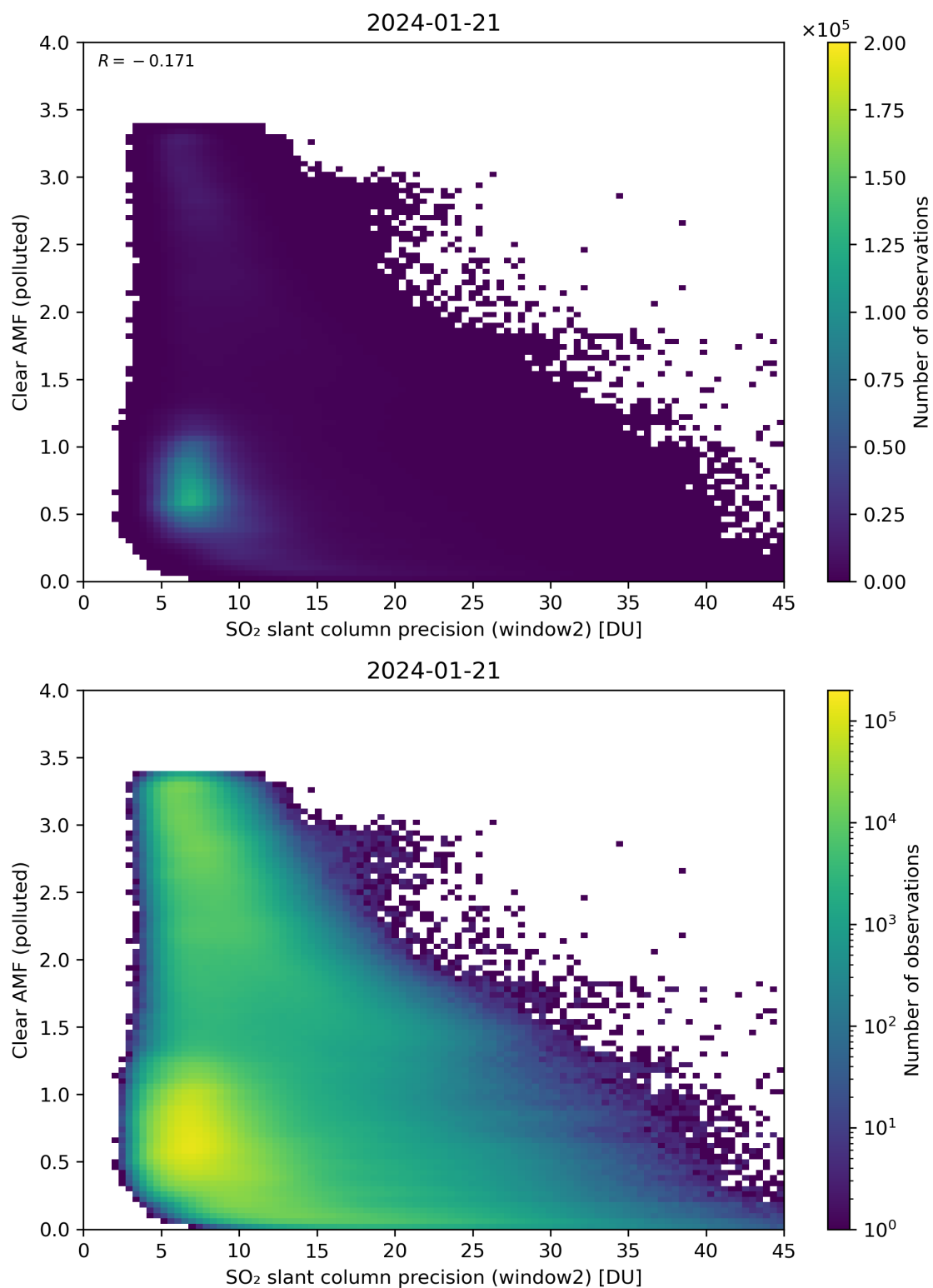
Figure 246: Scatter density plot of “SO 2 slant column precision (window2)” against “Clear AMF (polluted)” for 2024-01-21 to 2024-01-22.
