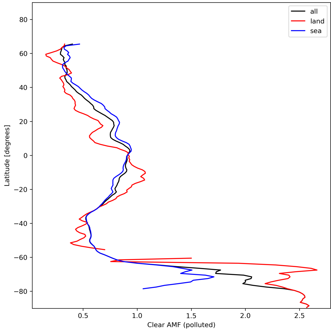
Figure 50: Zonal average of “Clear AMF (polluted)” for 2024-01-21 to 2024-01-22.
