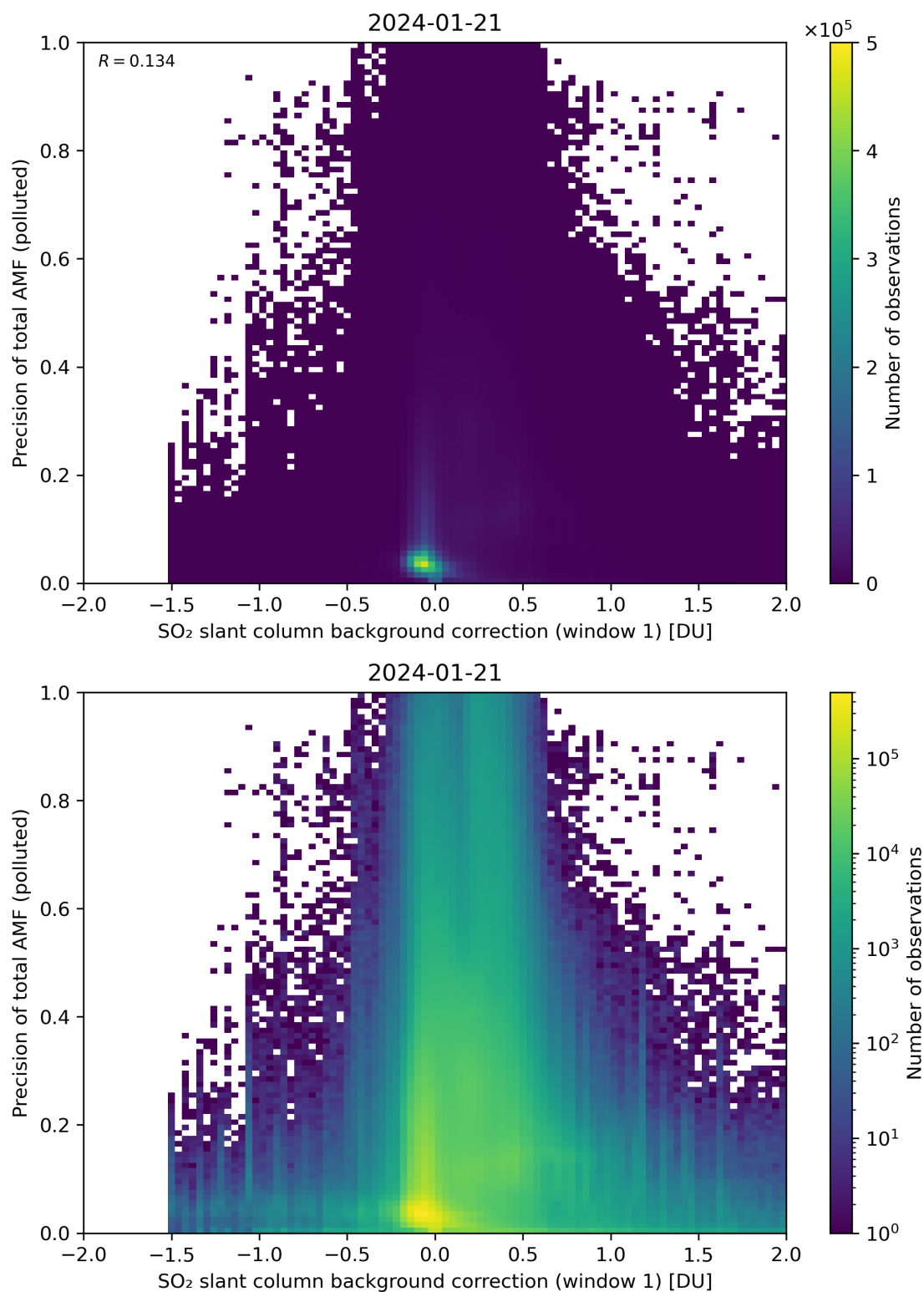
Figure 110: Scatter density plot of “SO 2 slant column background correction (window 1)” against “Precision of total AMF (polluted)” for 2024-01-21 to 2024-01-22.
