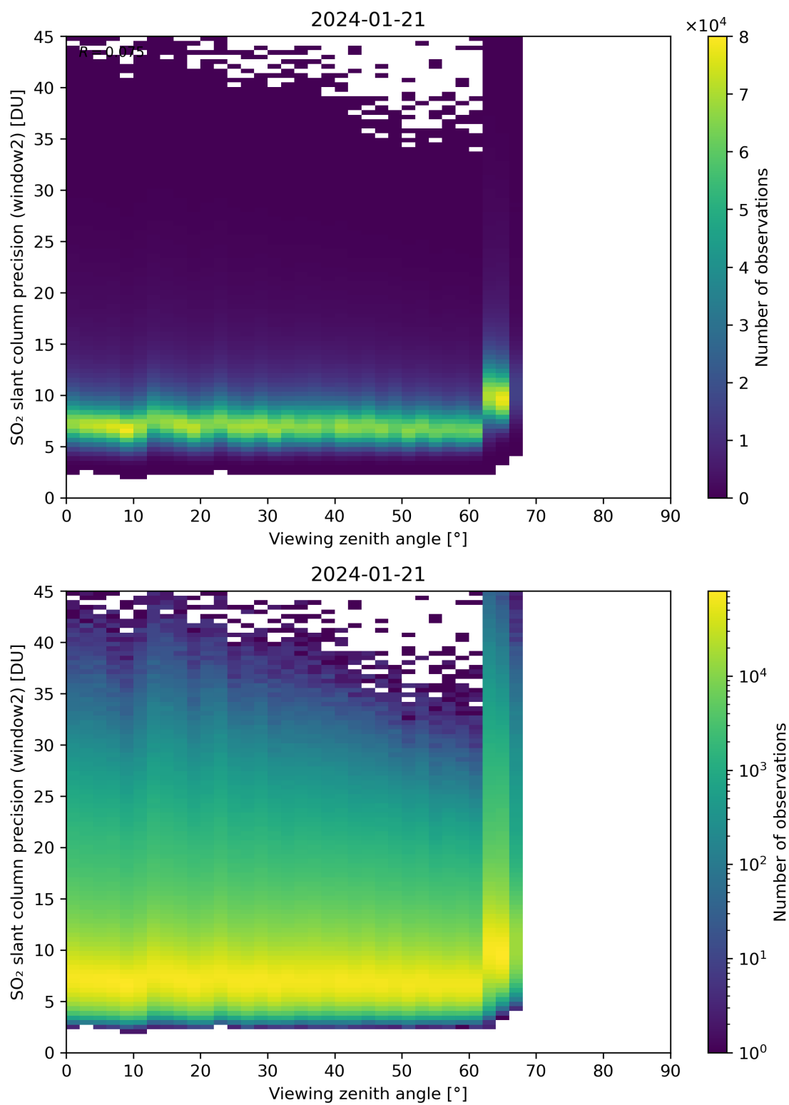
Figure 322: Scatter density plot of “Viewing zenith angle” against “SO 2 slant column precision (window2)” for 2024-01-21 to 2024-01-22.
