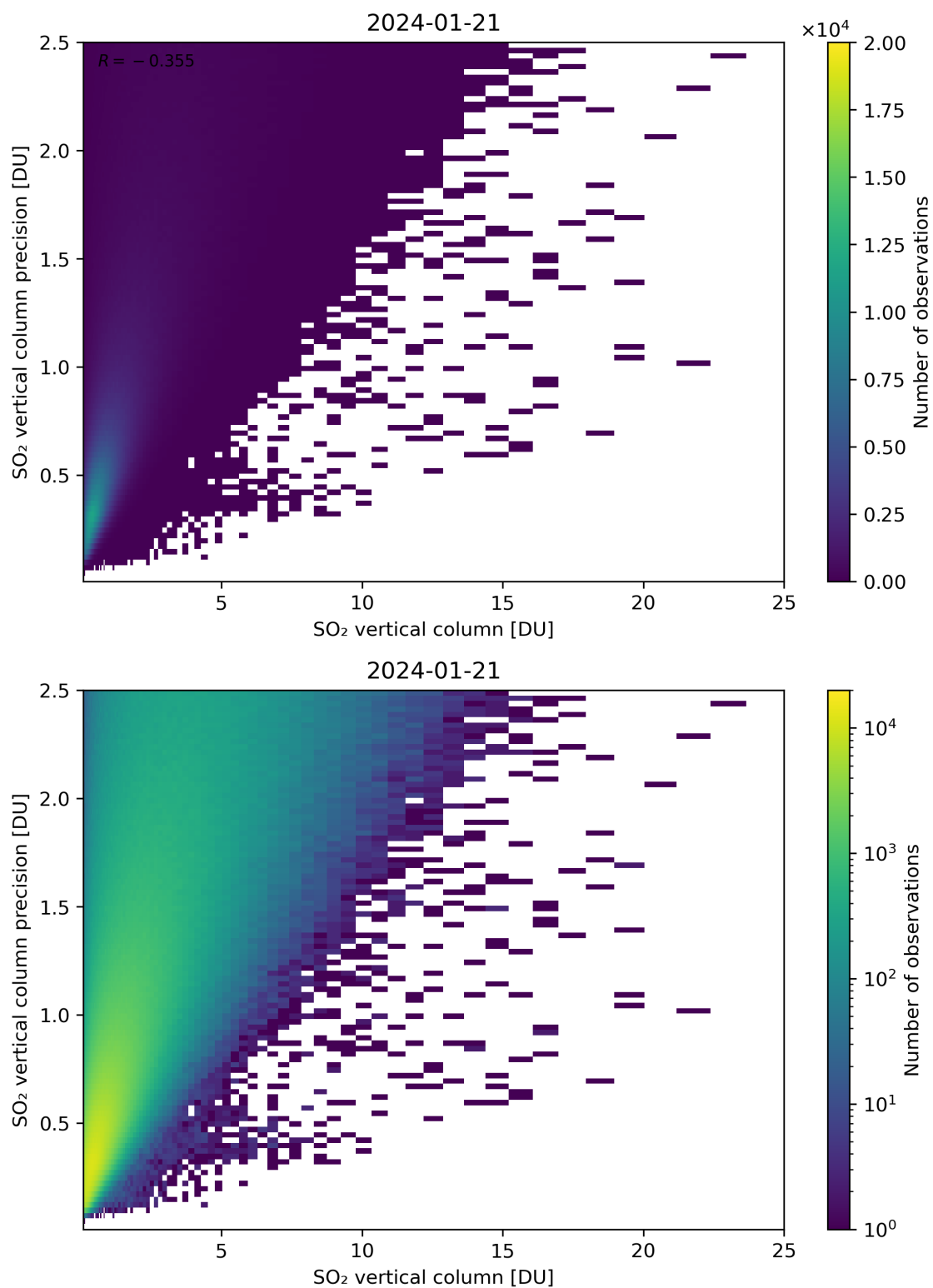
Figure 307: Scatter density plot of “SO 2 vertical column” against “SO 2 vertical column precision” for 2024-01-21 to 2024-01-22.
