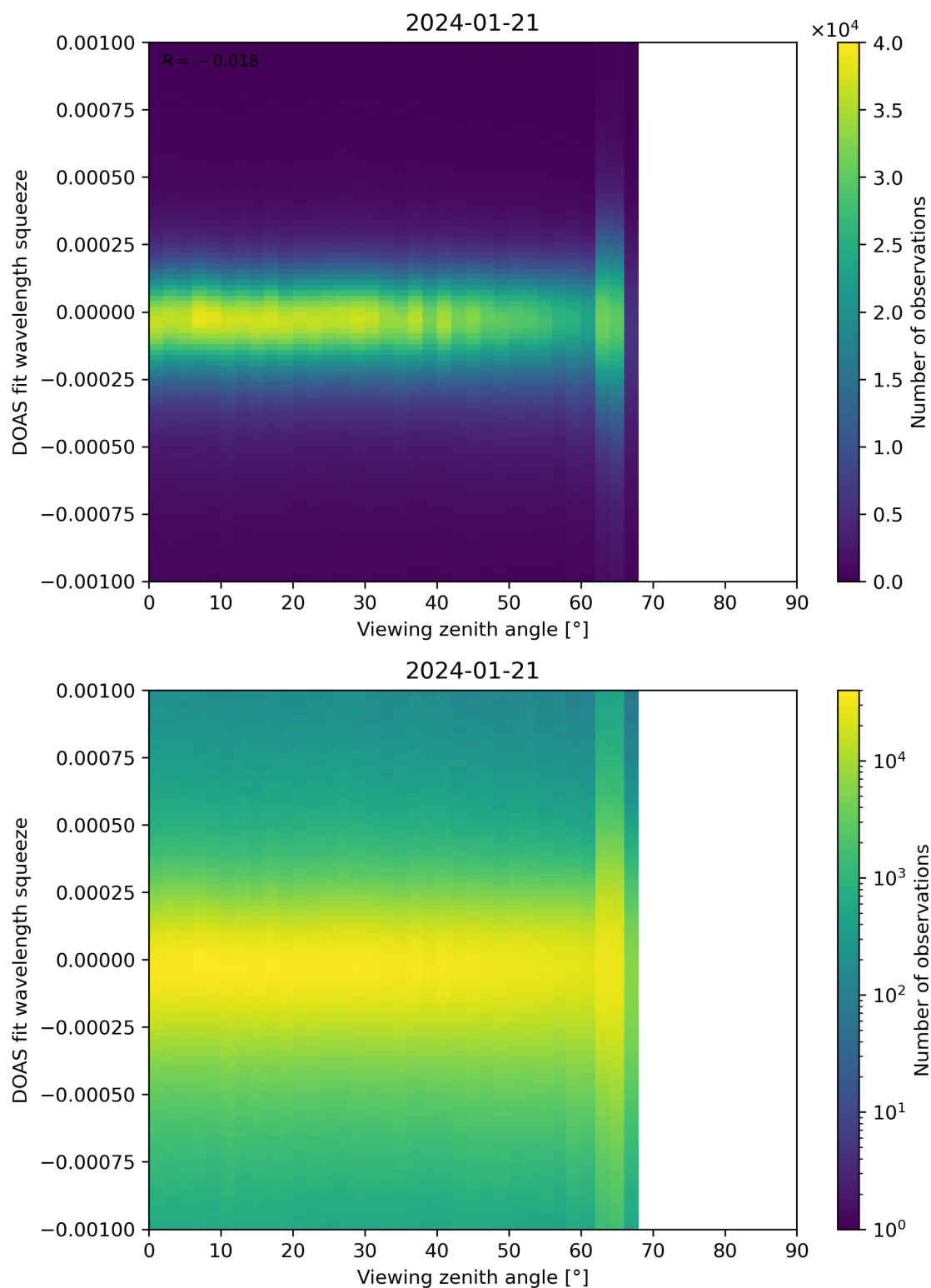
Figure 312: Scatter density plot of “Viewing zenith angle” against “DOAS fit wavelength squeeze” for 2024-01-21 to 2024-01-22.
