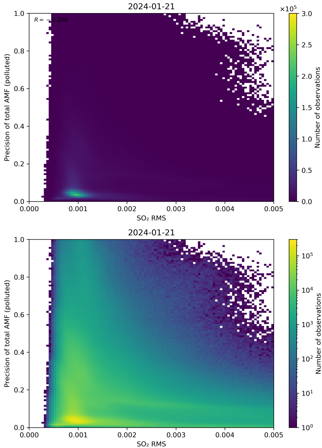
Figure 138: Scatter density plot of “SO 2 RMS” against “Precision of total AMF (polluted)” for 2024-01-21 to 2024-01-22.
