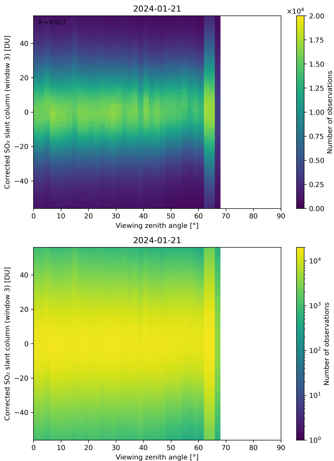
Figure 319: Scatter density plot of “Viewing zenith angle” against “Corrected SO 2 slant column (window 3)” for 2024-01-21 to 2024-01-22.
