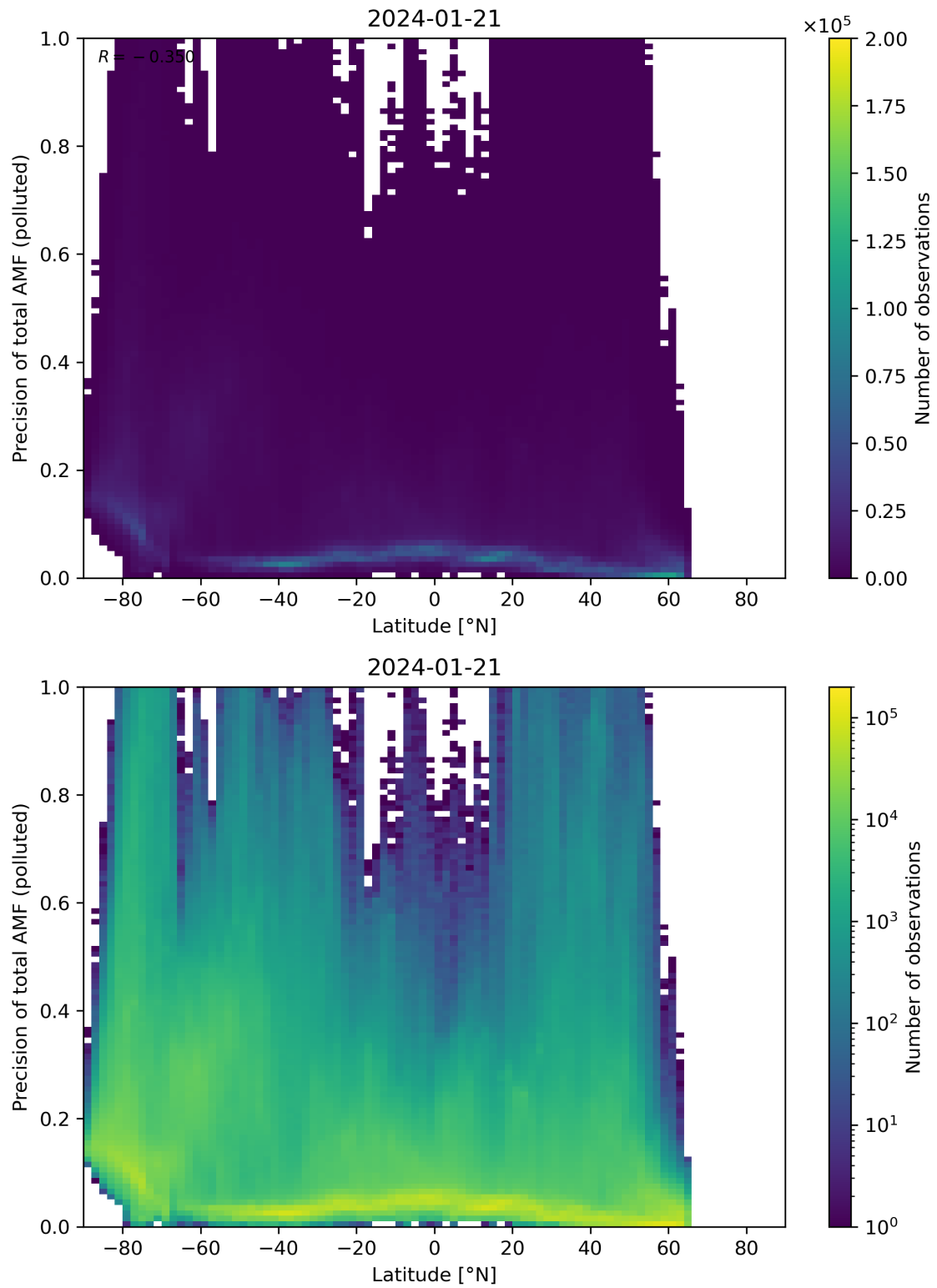
Figure 155: Scatter density plot of “Latitude” against “Precision of total AMF (polluted)” for 2024-01-21 to 2024-01-22.
