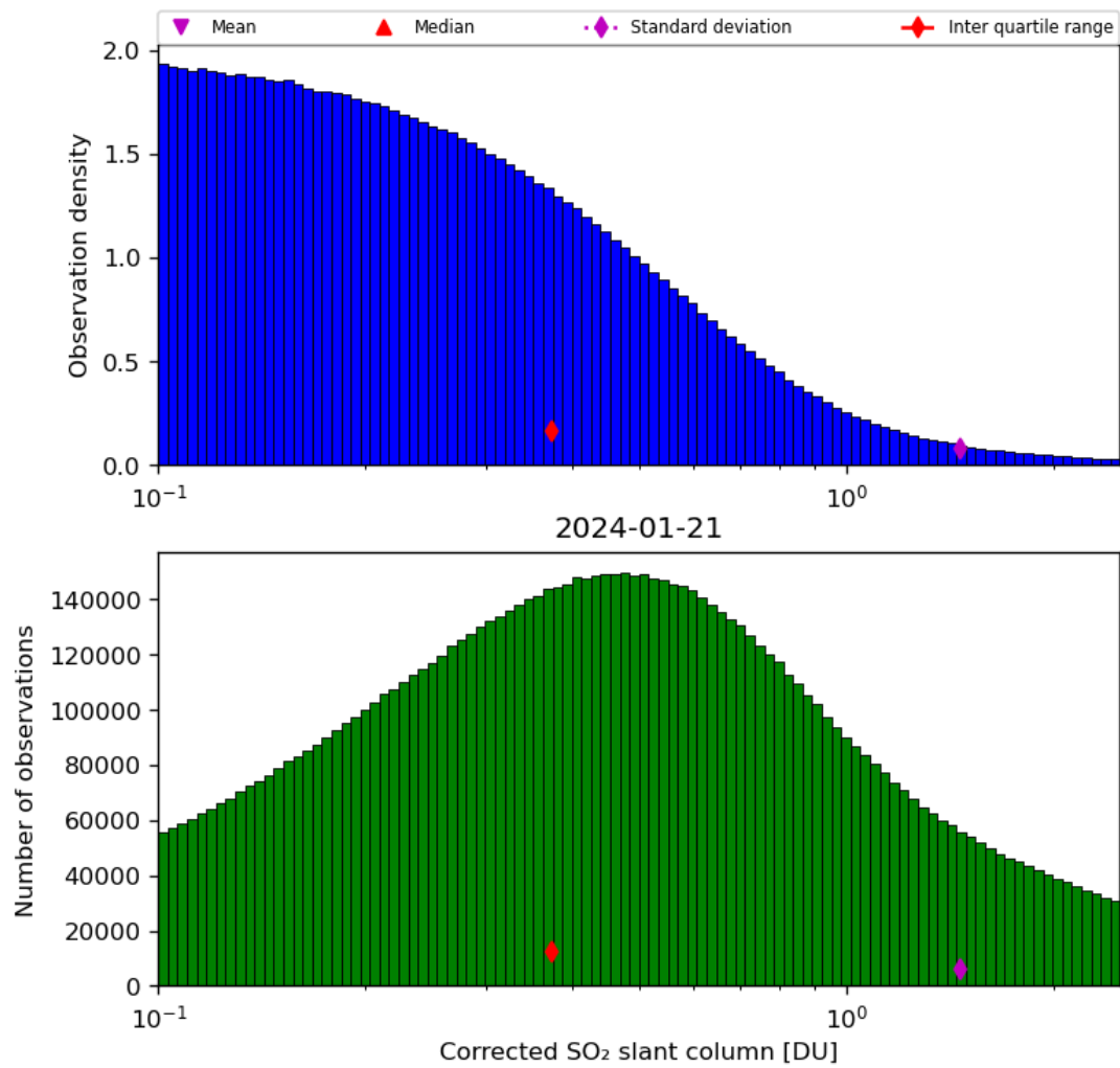
Figure 55: Histogram of “Corrected SO 2 slant column” for 2024-01-21 to 2024-01-22
