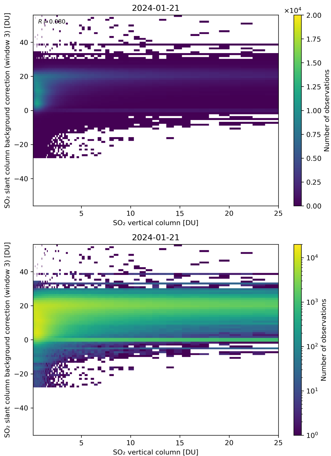
Figure 275: Scatter density plot of “SO 2 vertical column” against “SO 2 slant column background correction (window 3)” for 2024-01-21 to 2024-01-22.
