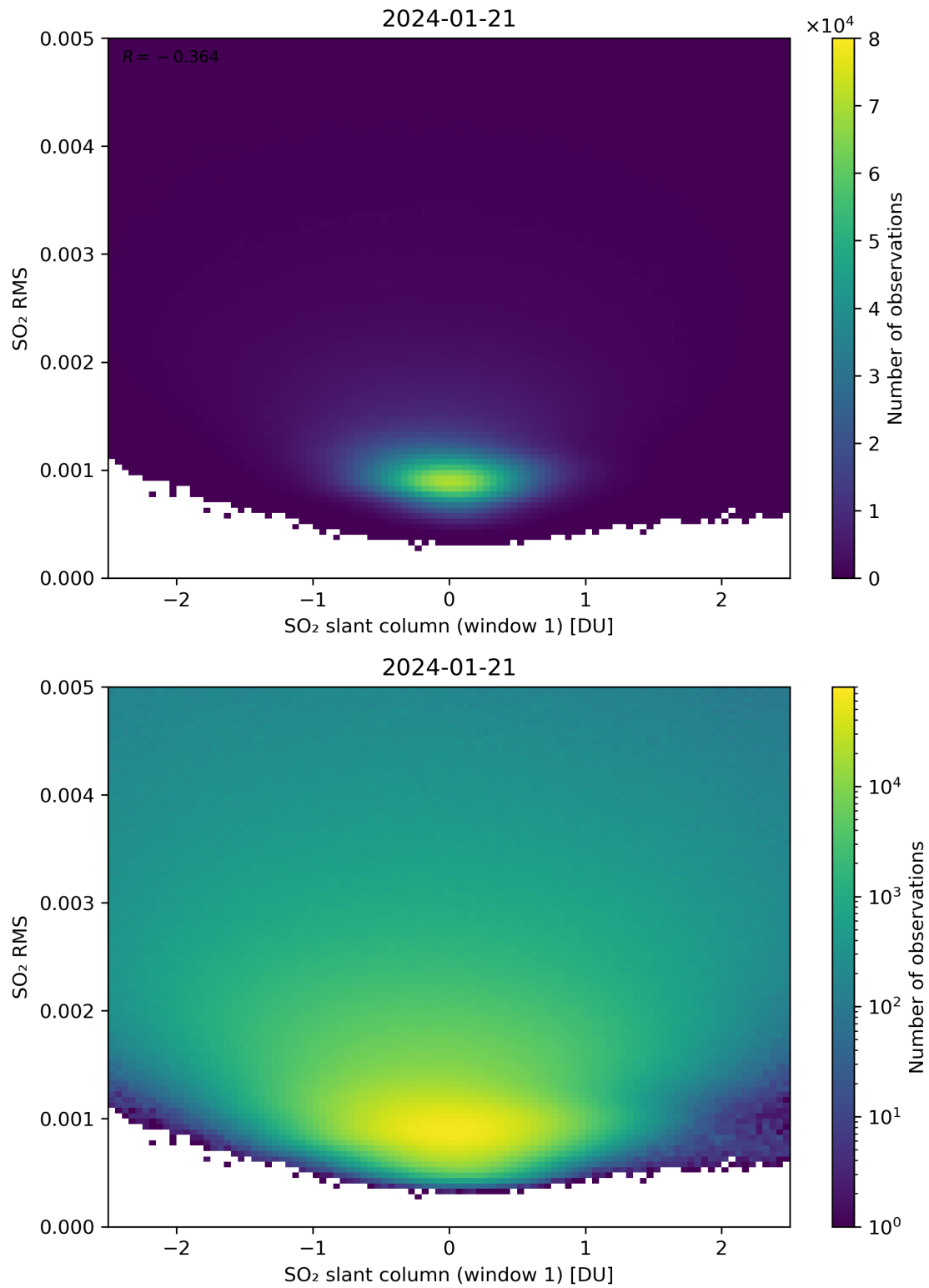
Figure 217: Scatter density plot of “SO 2 slant column (window 1)” against “SO 2 RMS” for 2024-01-21 to 2024-01-22.
