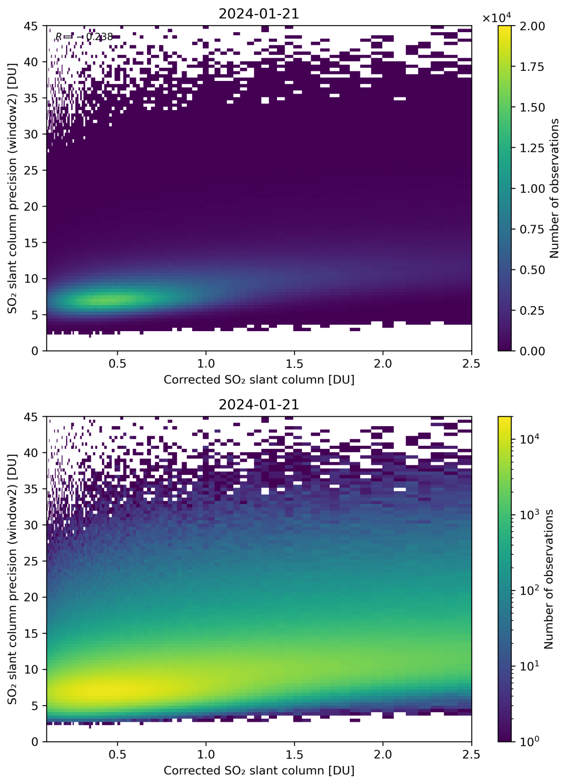
Figure 189: Scatter density plot of “Corrected SO 2 slant column” against “SO 2 slant column precision (window2)” for 2024-01-21 to 2024-01-22.
