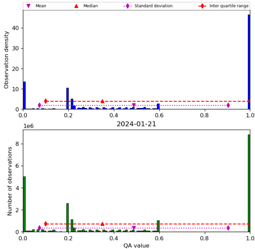
Figure 52: Histogram of “QA value” for 2024-01-21 to 2024-01-22
