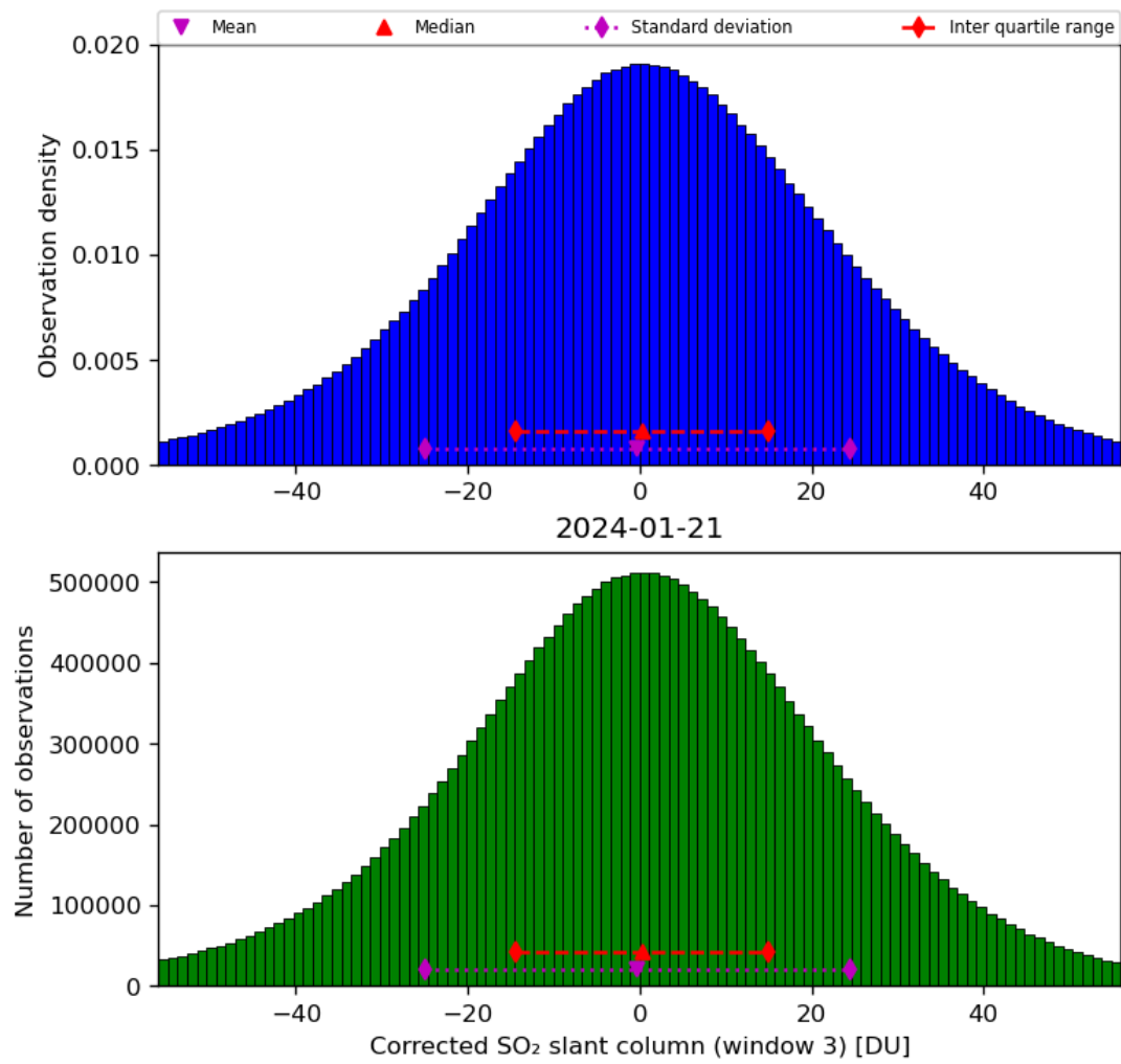
Figure 66: Histogram of “Corrected SO 2 slant column (window 3)” for 2024-01-21 to 2024-01-22
