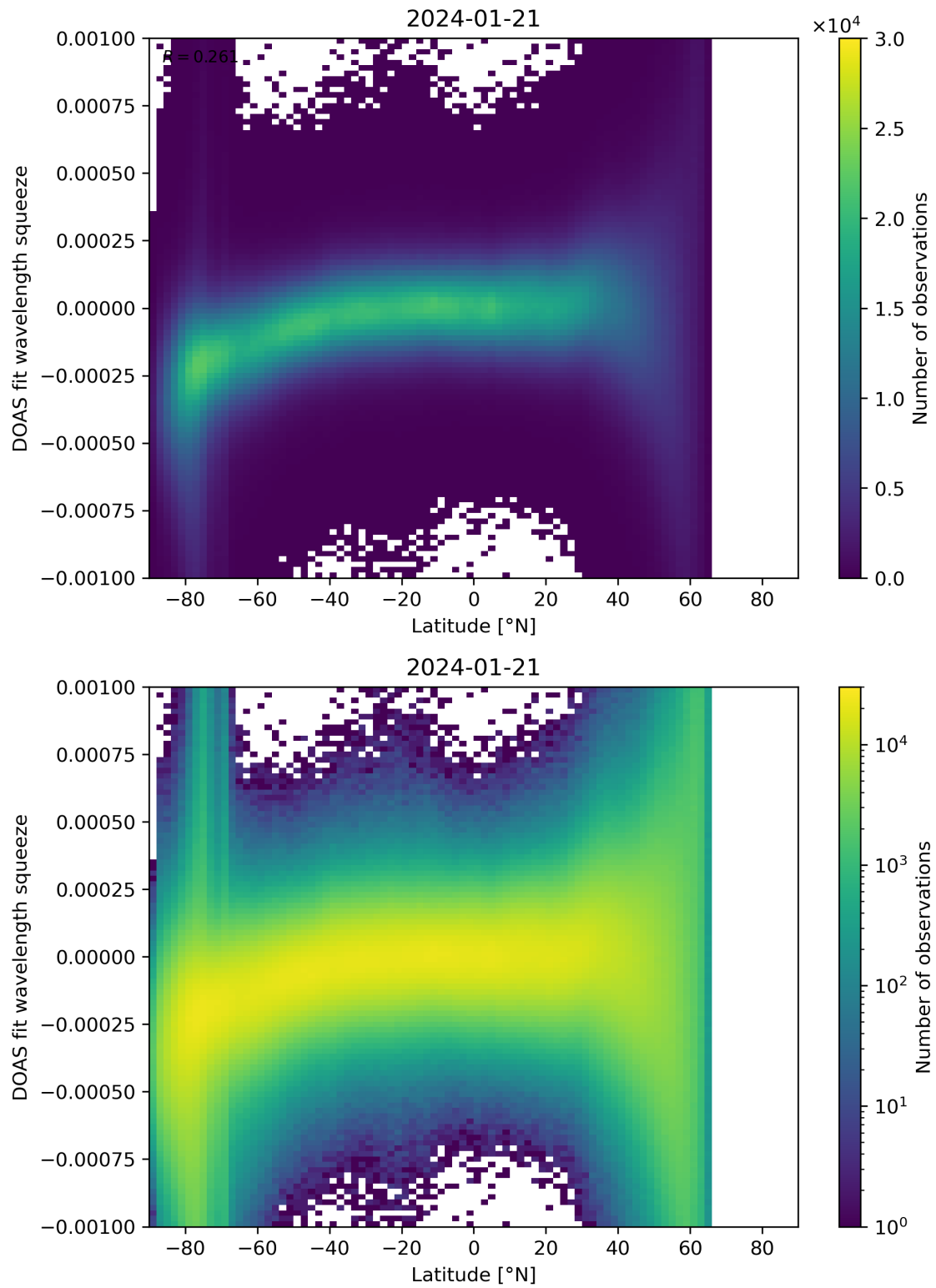
Figure 143: Scatter density plot of “Latitude” against “DOAS fit wavelength squeeze” for 2024-01-21 to 2024-01-22.
