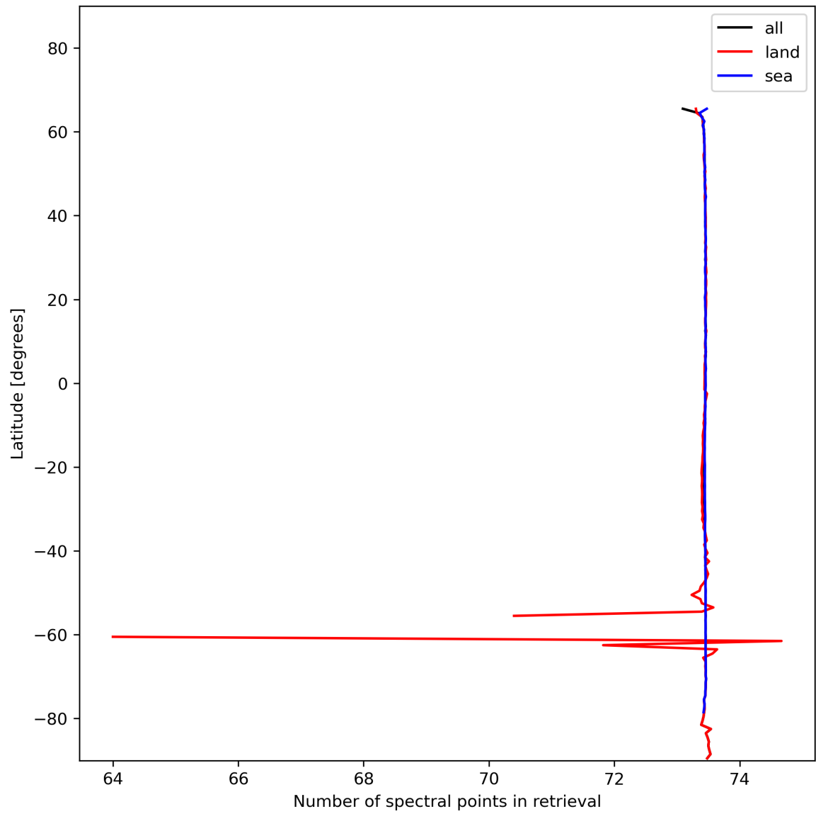
Figure 51: Zonal average of “Number of spectral points in retrieval” for 2024-01-21 to 2024-01-22.
