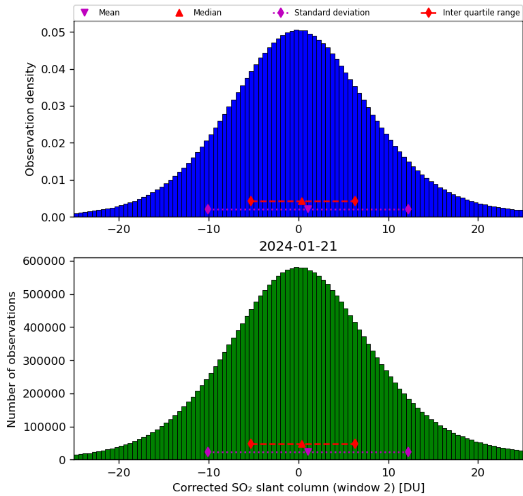
Figure 62: Histogram of “Corrected SO 2 slant column (window 2)” for 2024-01-21 to 2024-01-22
