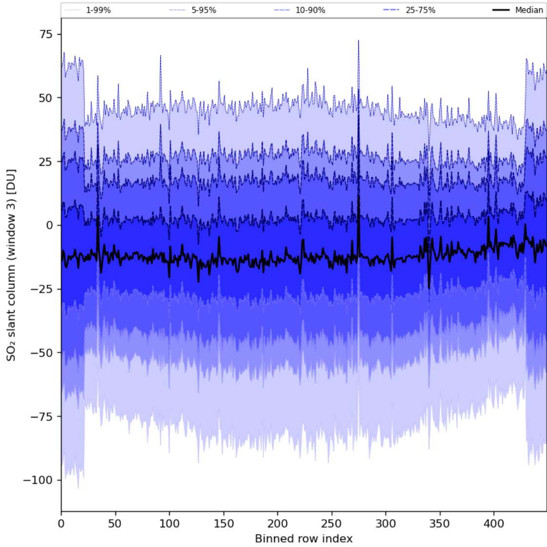
Figure 87: Along track statistics of "SO 2 slant column (window 3)" for 2024-01-21 to 2024-01-22
