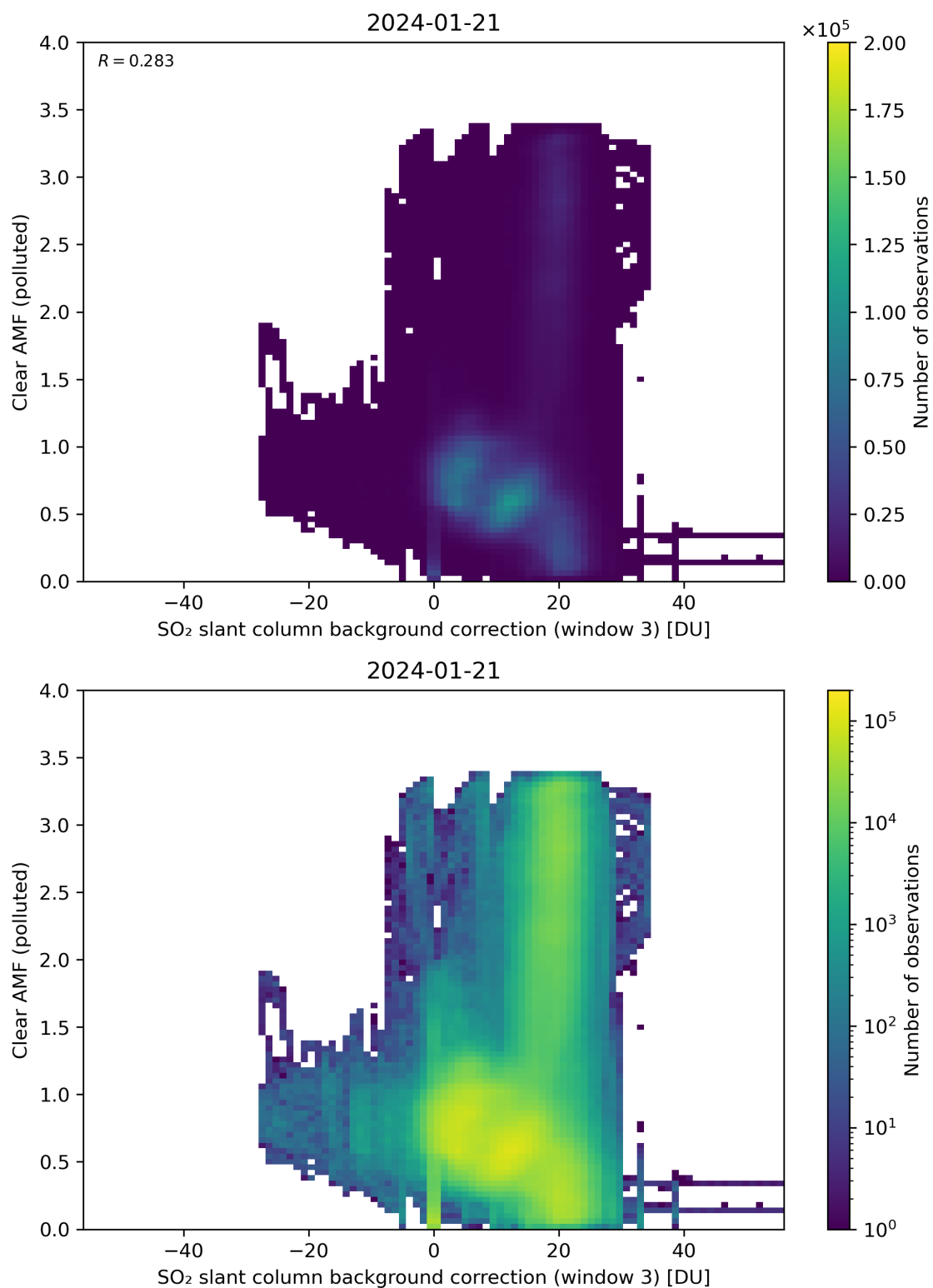
Figure 124: Scatter density plot of “SO 2 slant column background correction (window 3)” against “Clear AMF (polluted)” for 2024-01-21 to 2024-01-22.
