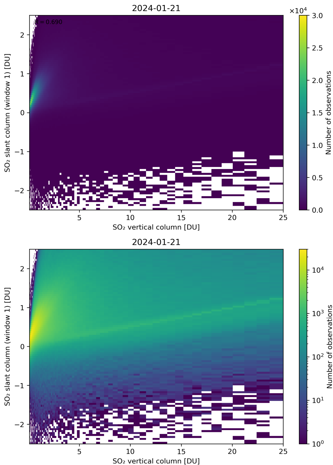
Figure 300: Scatter density plot of “SO 2 vertical column” against “SO 2 slant column (window 1)” for 2024-01-21 to 2024-01-22.
