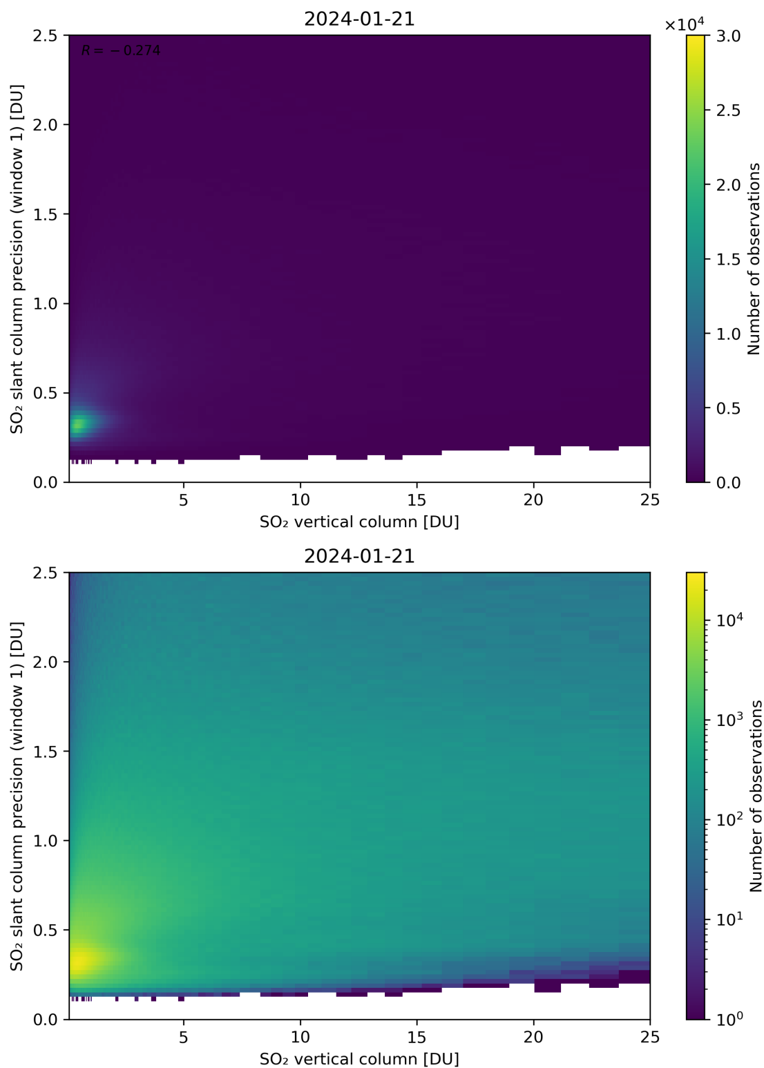
Figure 301: Scatter density plot of “SO 2 vertical column” against “SO 2 slant column precision (window 1)” for 2024-01-21 to 2024-01-22.
