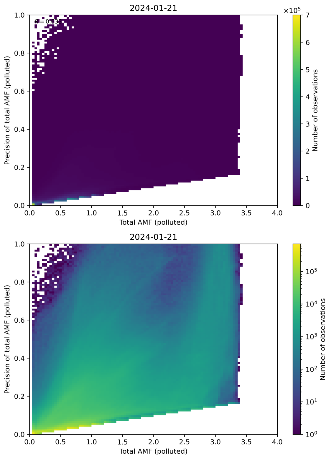
Figure 272: Scatter density plot of “Total AMF (polluted)” against “Precision of total AMF (polluted)” for 2024-01-21 to 2024-01-22.
