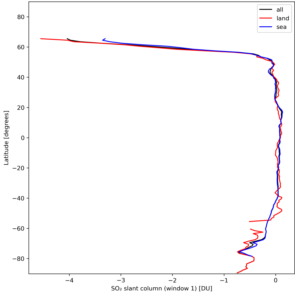
Figure 33: Zonal average of “SO 2 slant column (window 1)” for 2024-01-21 to 2024-01-22.
