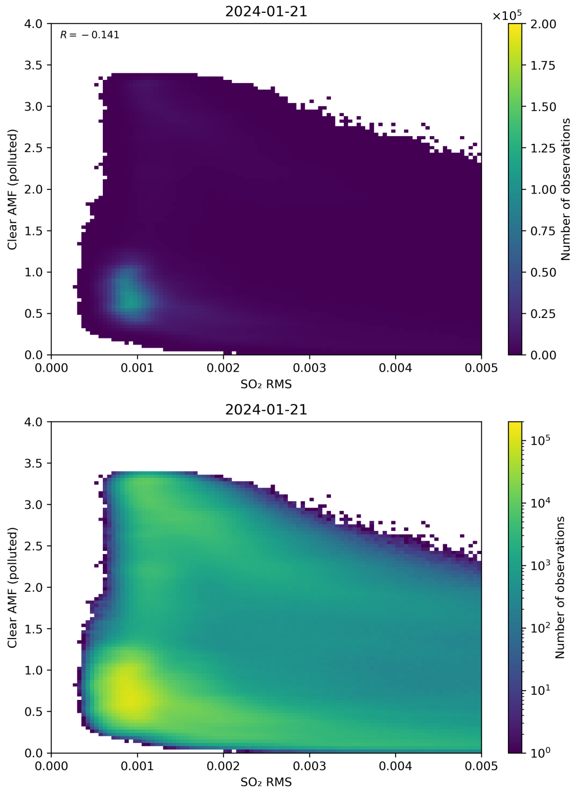
Figure 136: Scatter density plot of “SO 2 RMS” against “Clear AMF (polluted)” for 2024-01-21 to 2024-01-22.
