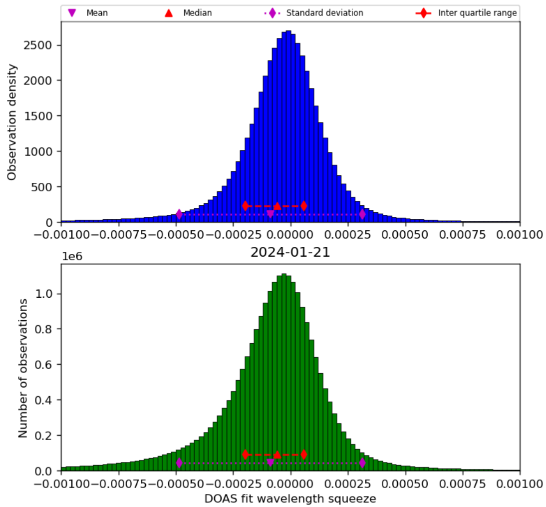
Figure 69: Histogram of “DOAS fit wavelength squeeze” for 2024-01-21 to 2024-01-22
