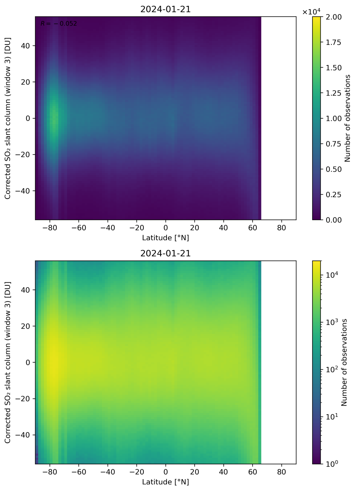
Figure 148: Scatter density plot of “Latitude” against “Corrected SO 2 slant column (window 3)” for 2024-01-21 to 2024-01-22.
