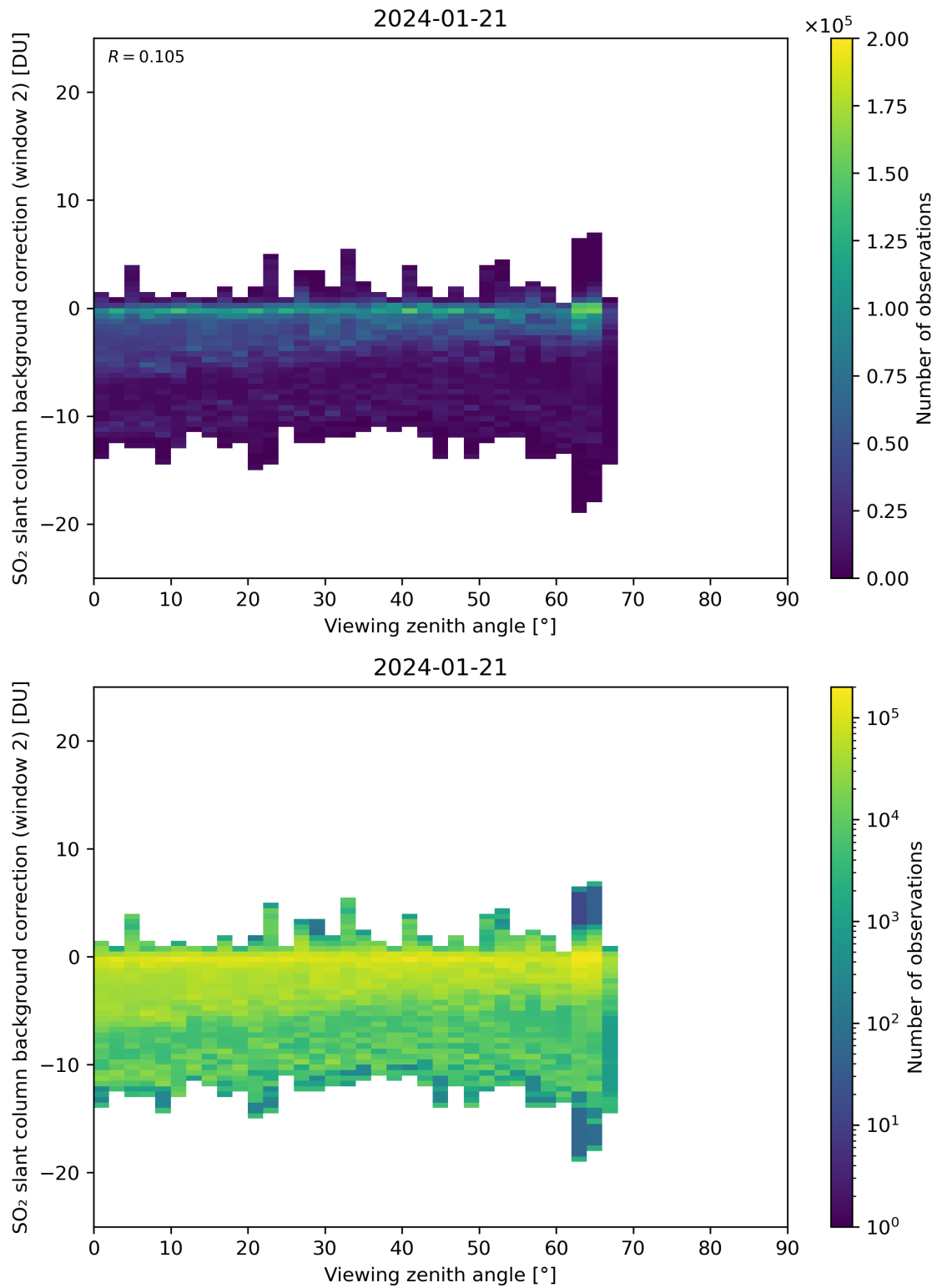
Figure 309: Scatter density plot of “Viewing zenith angle” against “SO 2 slant column background correction (window 2)” for 2024-01-21 to 2024-01-22.
