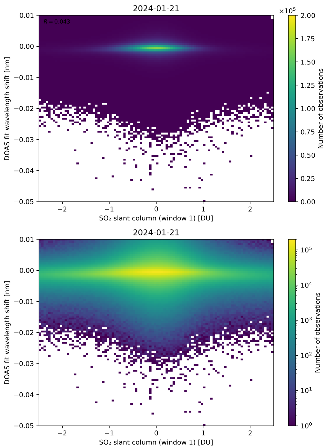
Figure 215: Scatter density plot of “SO 2 slant column (window 1)” against “DOAS fit wavelength shift” for 2024-01-21 to 2024-01-22.
