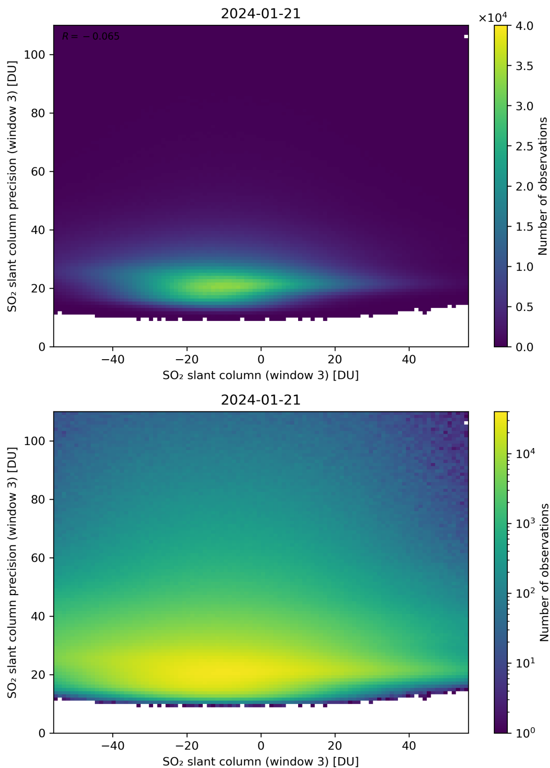
Figure 267: Scatter density plot of “SO 2 slant column (window 3)” against “SO 2 slant column precision (window 3)” for 2024-01-21 to 2024-01-22.
