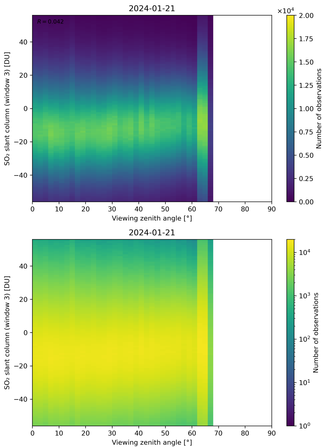
Figure 323: Scatter density plot of “Viewing zenith angle” against “SO 2 slant column (window 3)” for 2024-01-21 to 2024-01-22.
