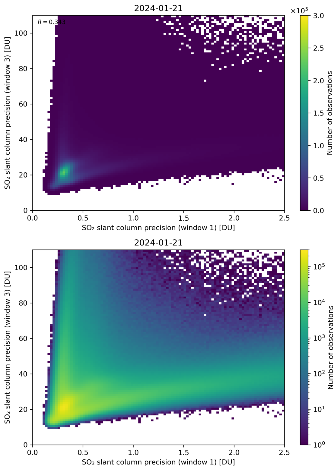
Figure 229: Scatter density plot of “SO 2 slant column precision (window 1)” against “SO 2 slant column precision (window 3)” for 2024-01-21 to 2024-01-22.
