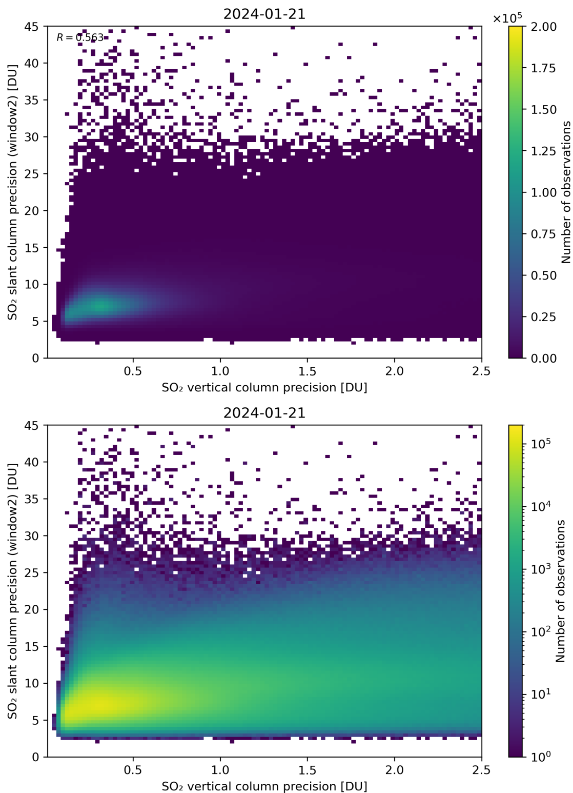
Figure 291: Scatter density plot of “SO 2 vertical column precision” against “SO 2 slant column precision (window2)” for 2024-01-21 to 2024-01-22.
