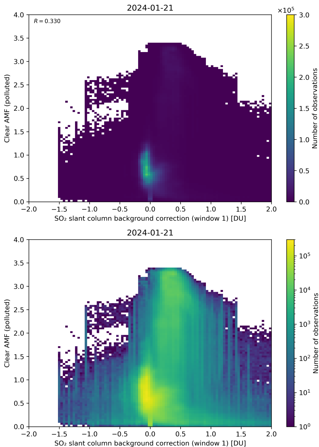
Figure 103: Scatter density plot of “SO 2 slant column background correction (window 1)” against “Clear AMF (polluted)” for 2024-01-21 to 2024-01-22.
