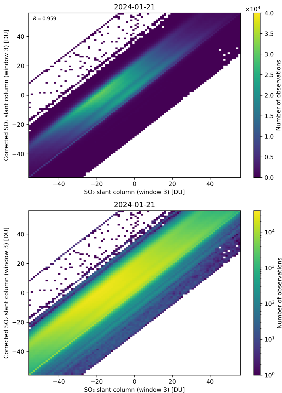
Figure 266: Scatter density plot of “SO 2 slant column (window 3)” against “Corrected SO 2 slant column (window 3)” for 2024-01-21 to 2024-01-22.
