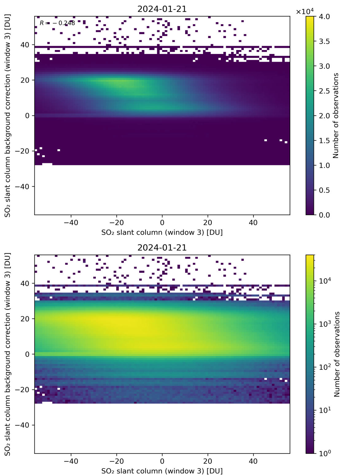
Figure 253: Scatter density plot of “SO 2 slant column (window 3)” against “SO 2 slant column background correction (window 3)” for 2024-01-21 to 2024-01-22.
