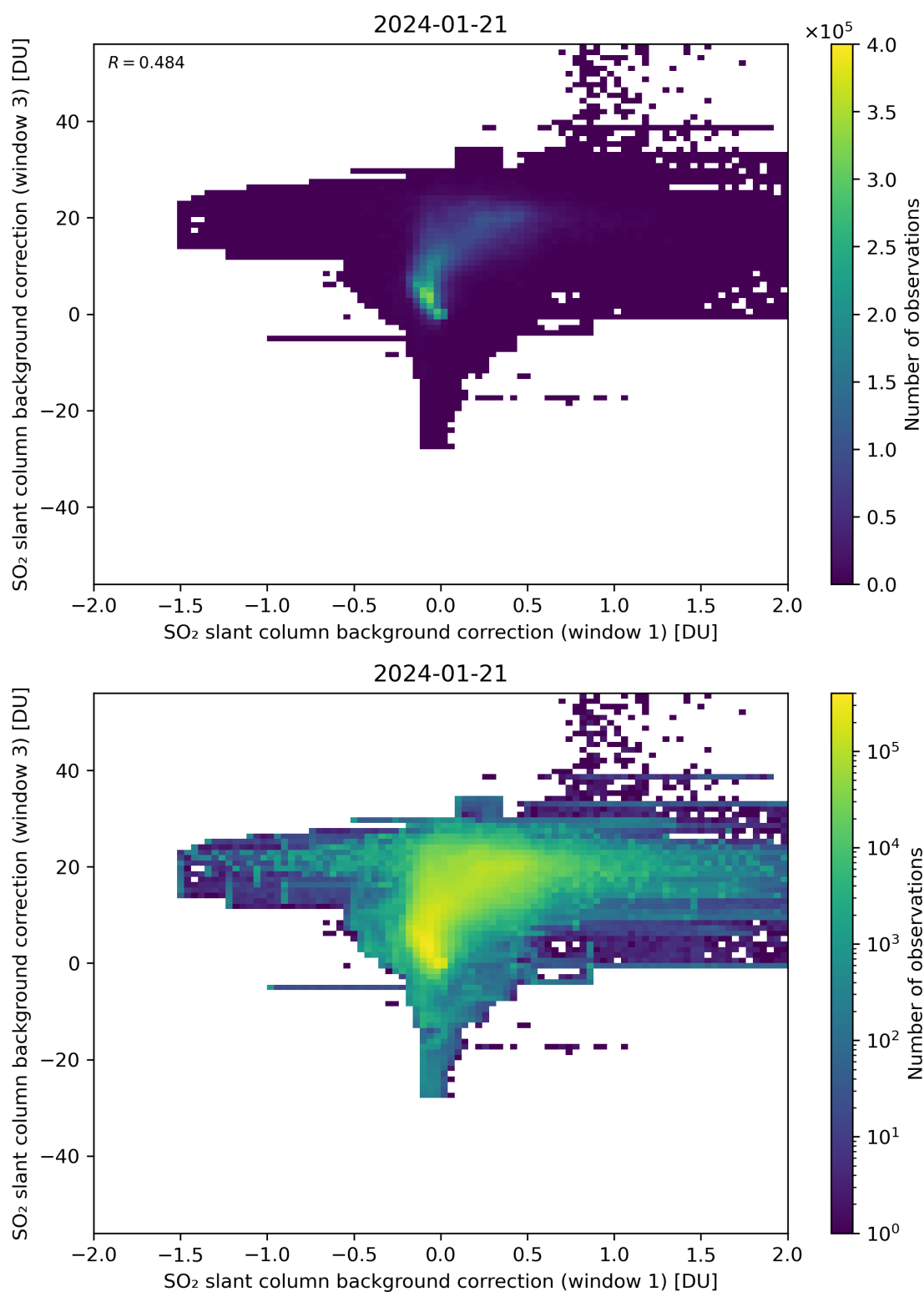
Figure 99: Scatter density plot of “SO 2 slant column background correction (window 1)” against “SO 2 slant column background correction (window 3)” for 2024-01-21 to 2024-01-22.
