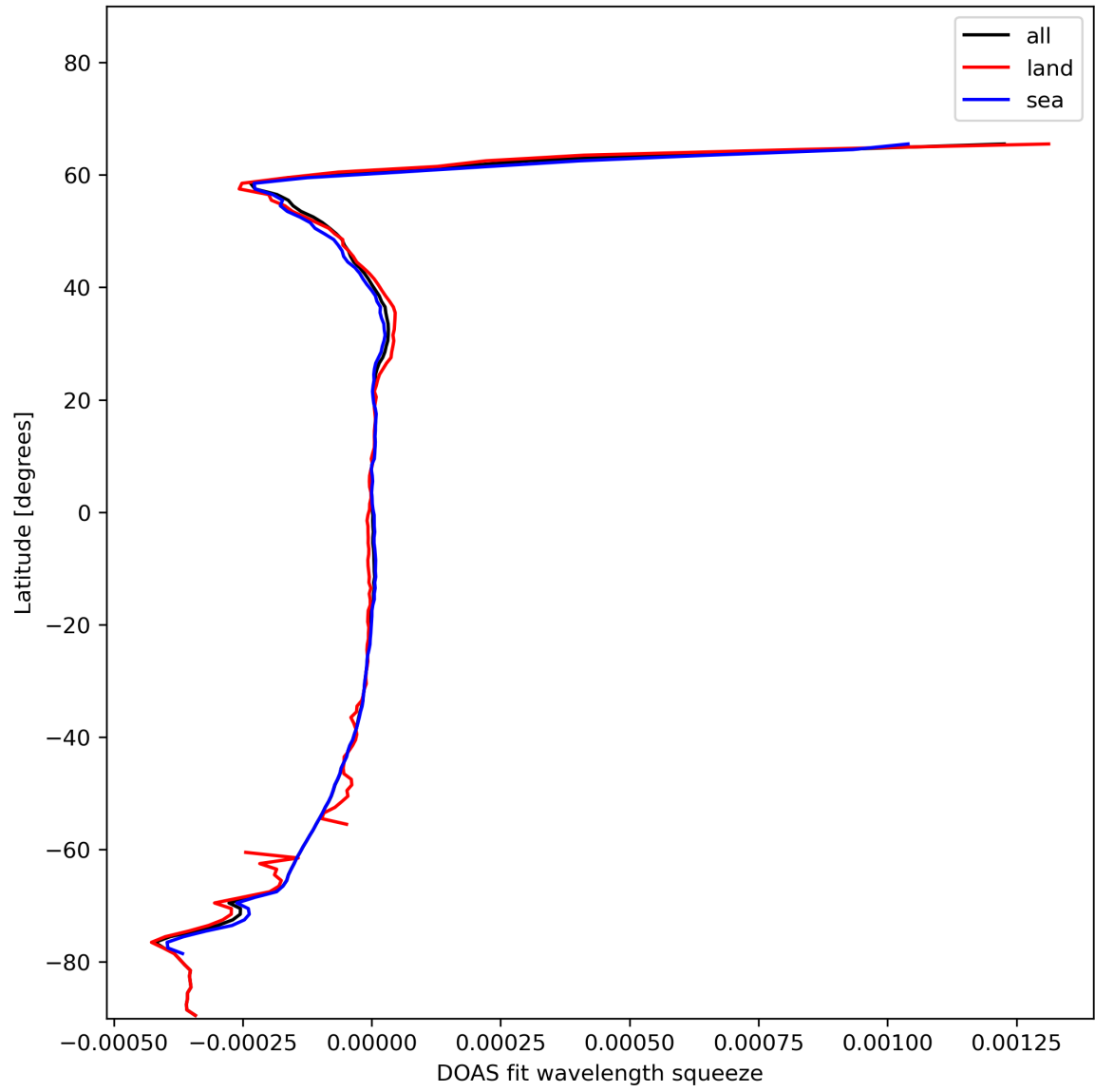
Figure 46: Zonal average of “DOAS fit wavelength squeeze” for 2024-01-21 to 2024-01-22.
