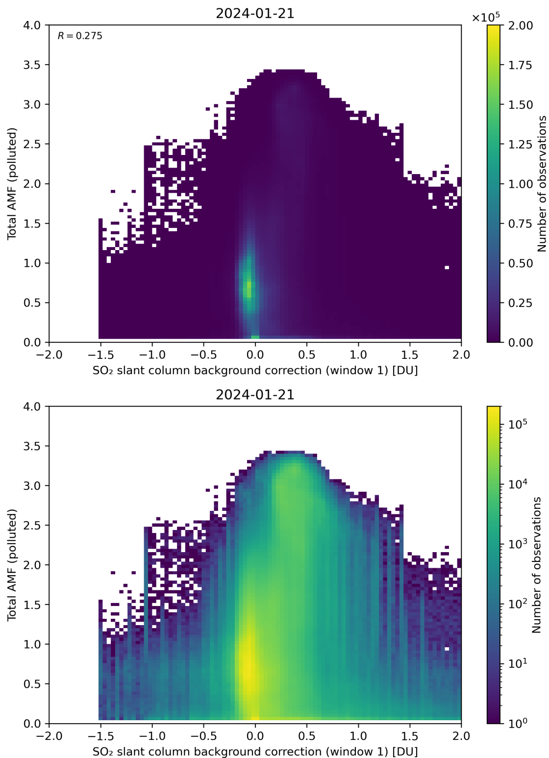
Figure 109: Scatter density plot of “SO 2 slant column background correction (window 1)” against “Total AMF (polluted)” for 2024-01-21 to 2024-01-22.
