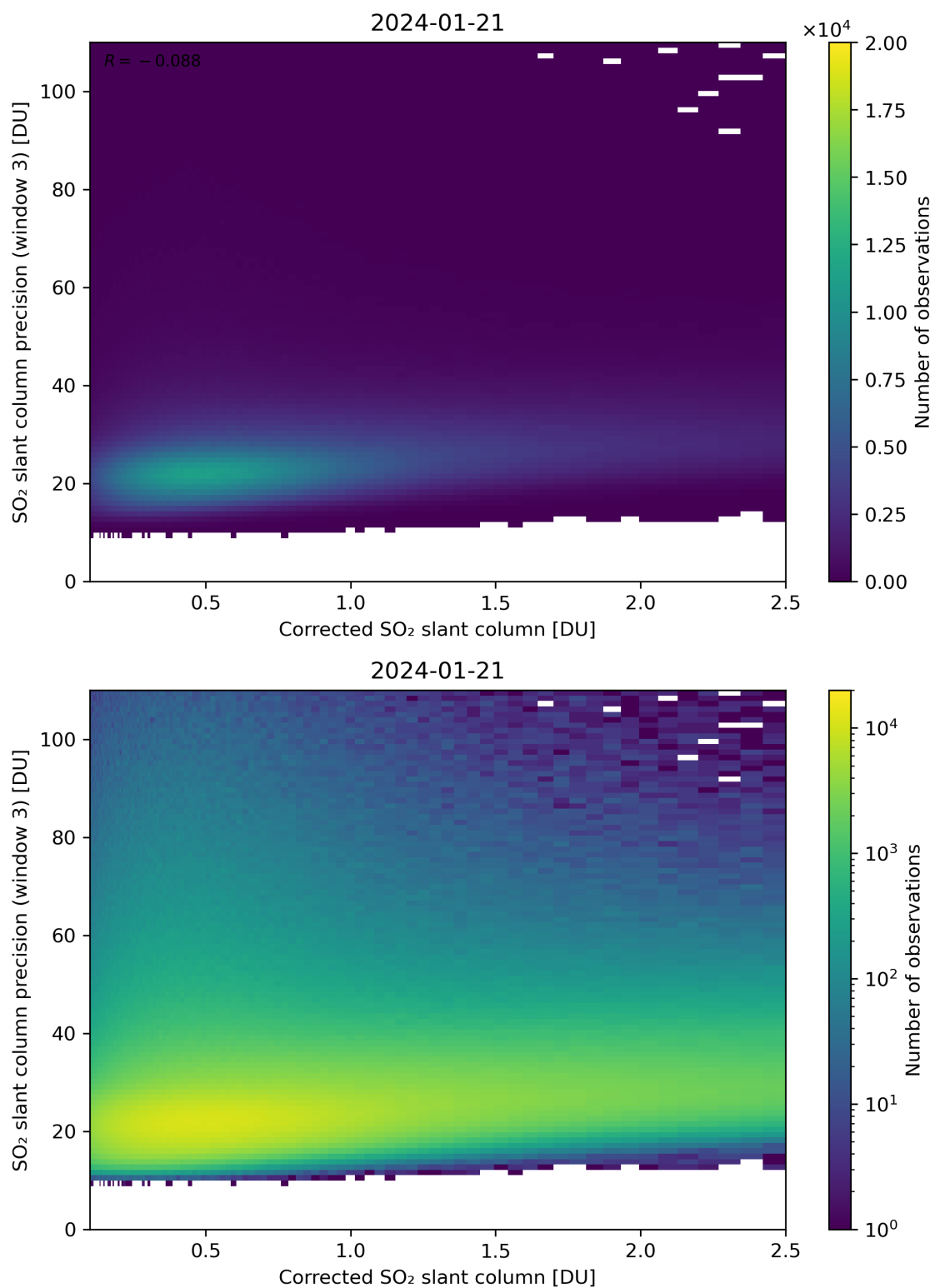
Figure 191: Scatter density plot of “Corrected SO 2 slant column” against “SO 2 slant column precision (window 3)” for 2024-01-21 to 2024-01-22.
