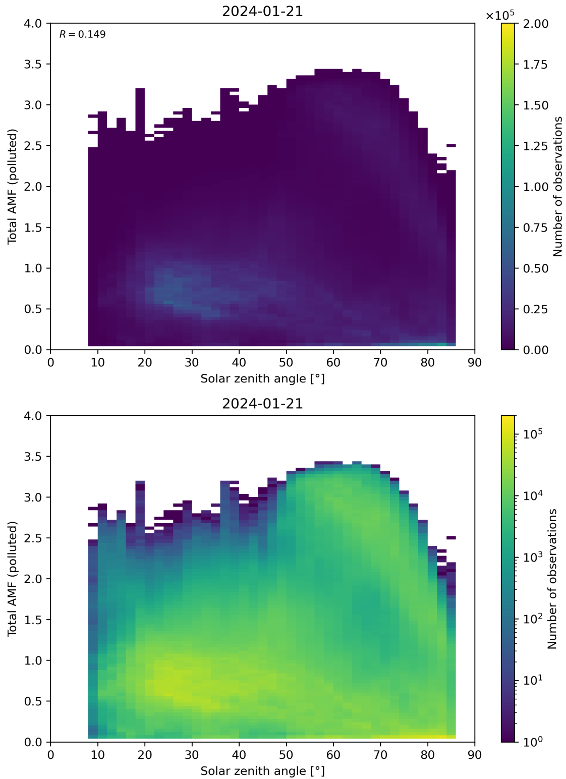
Figure 174: Scatter density plot of “Solar zenith angle” against “Total AMF (polluted)” for 2024-01-21 to 2024-01-22.
