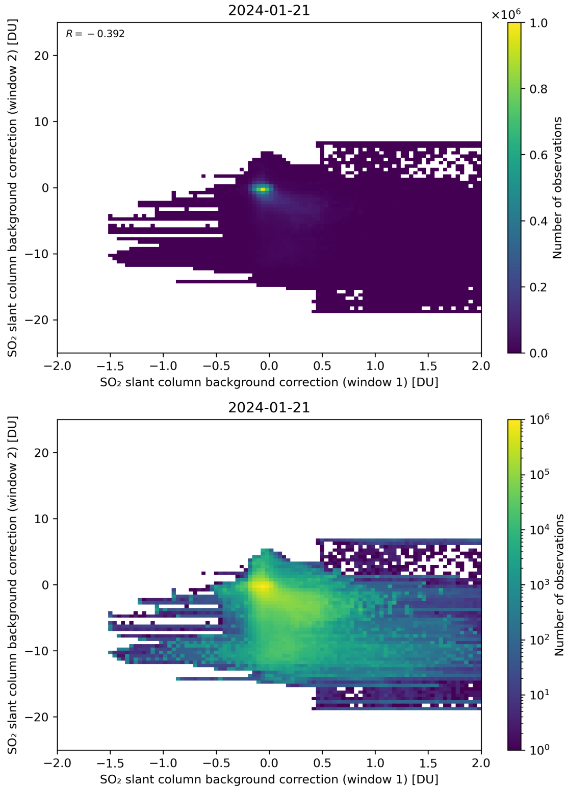
Figure 98: Scatter density plot of “SO 2 slant column background correction (window 1)” against “SO 2 slant column background correction (window 2)” for 2024-01-21 to 2024-01-22.
