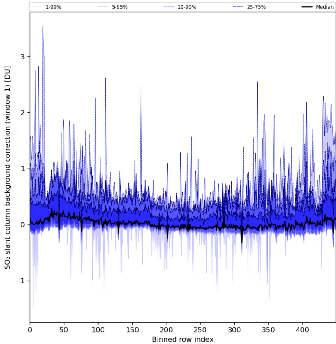
Figure 82: Along track statistics of “SO 2 slant column background correction (window 1)” for 2024-01-21 to 2024-01-22
