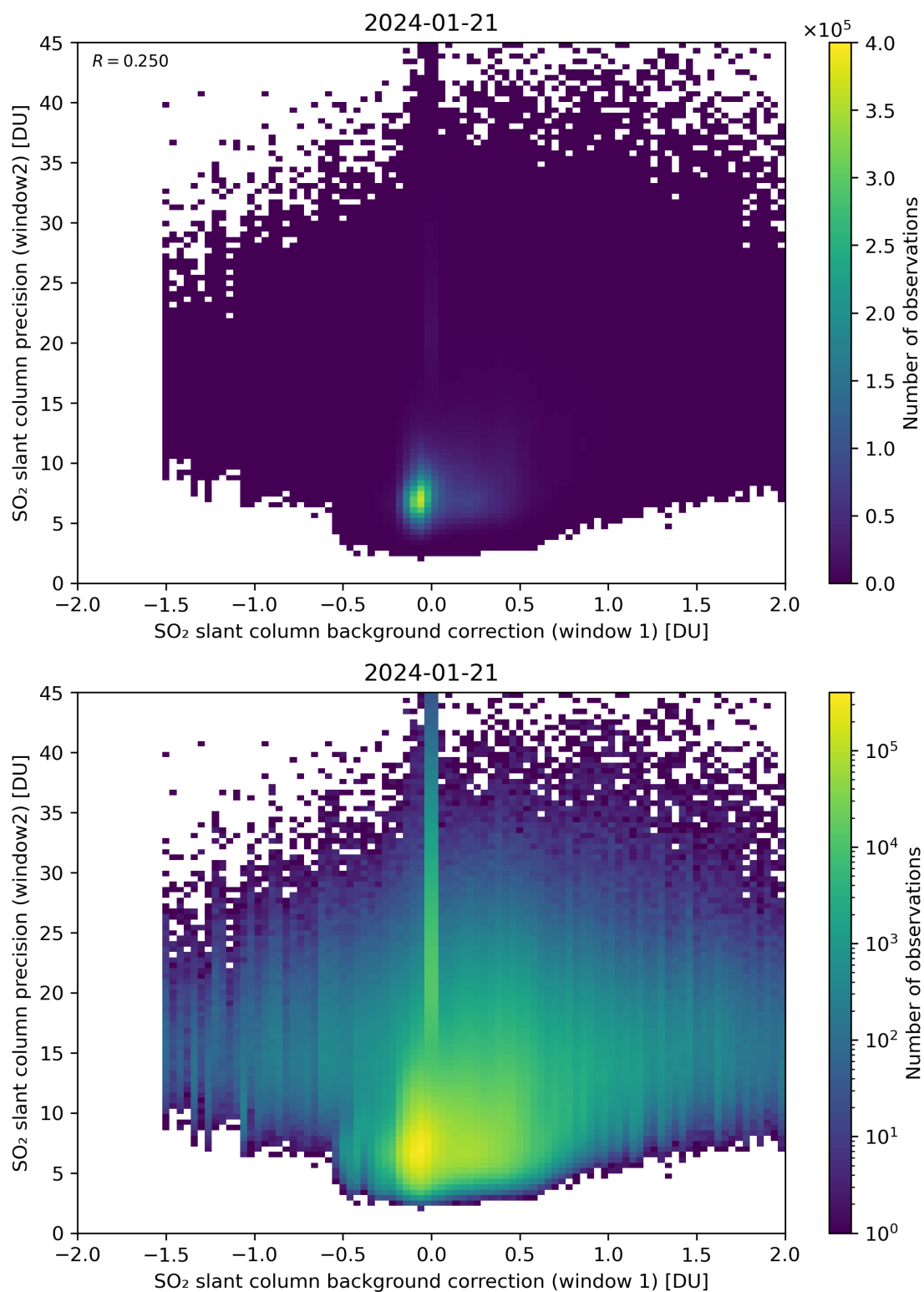
Figure 106: Scatter density plot of “SO 2 slant column background correction (window 1)” against “SO 2 slant column precision (window2)” for 2024-01-21 to 2024-01-22.
