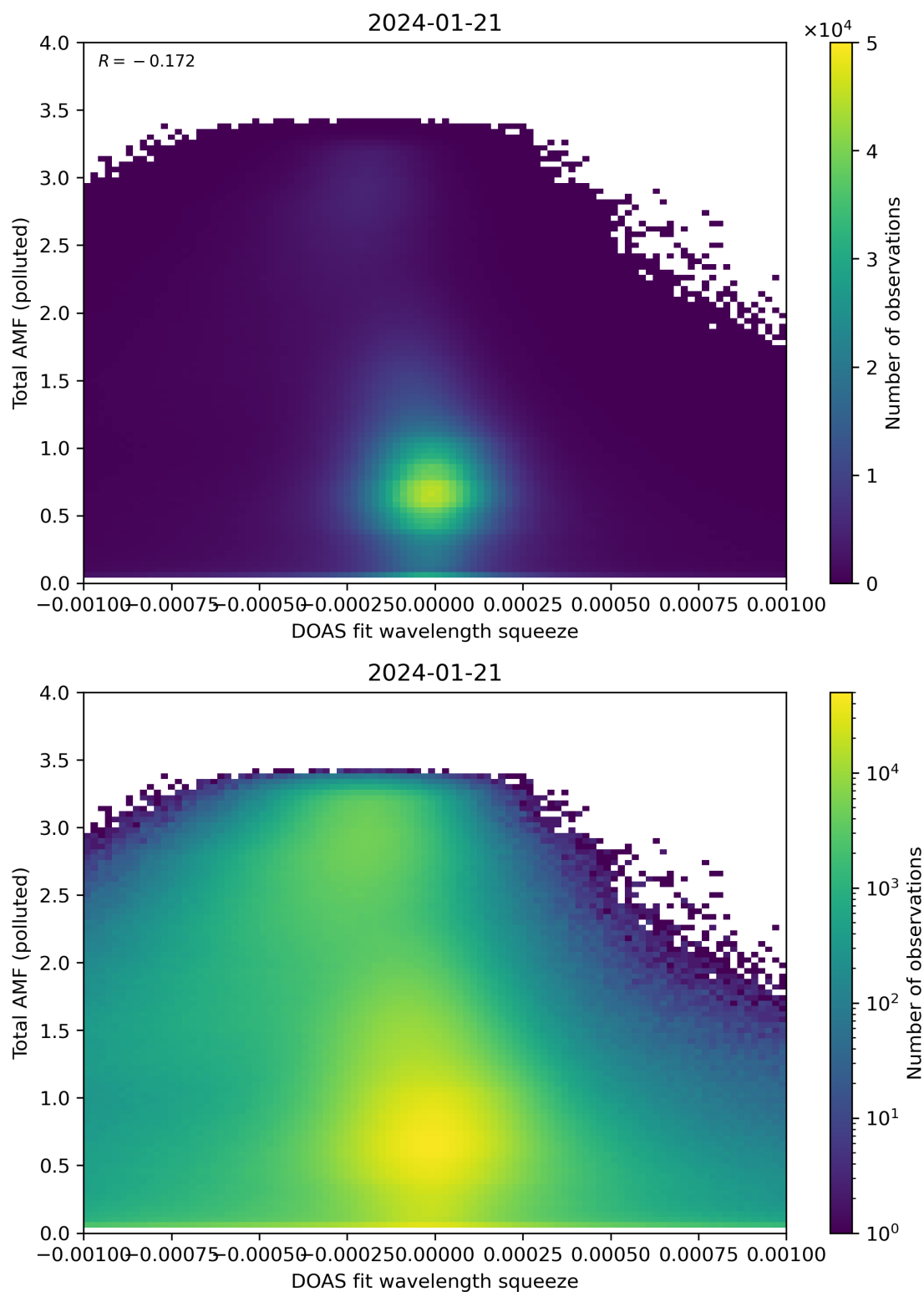
Figure 134: Scatter density plot of “DOAS fit wavelength squeeze” against “Total AMF (polluted)” for 2024-01-21 to 2024-01-22.
