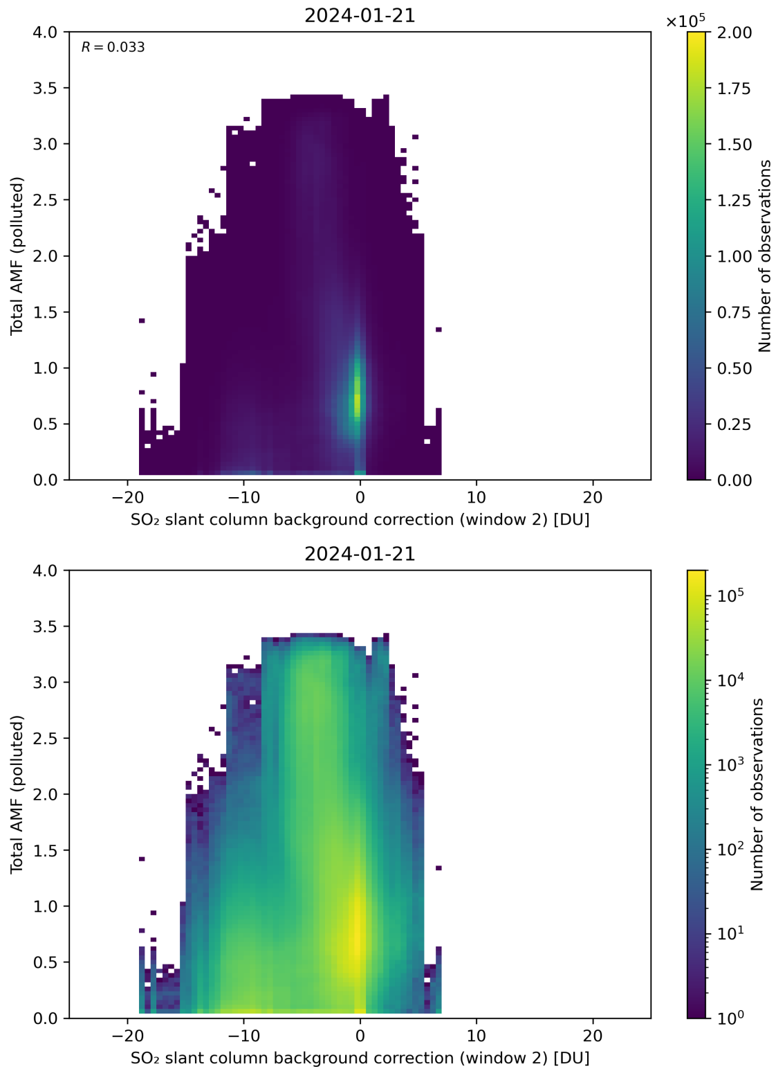
Figure 119: Scatter density plot of “SO 2 slant column background correction (window 2)” against “Total AMF (polluted)” for 2024-01-21 to 2024-01-22.
