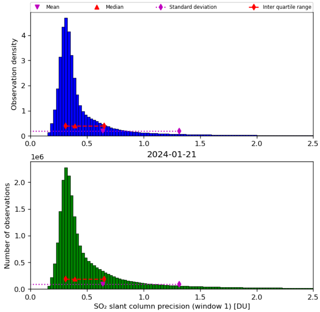
Figure 57: Histogram of “SO 2 slant column precision (window 1)” for 2024-01-21 to 2024-01-22
