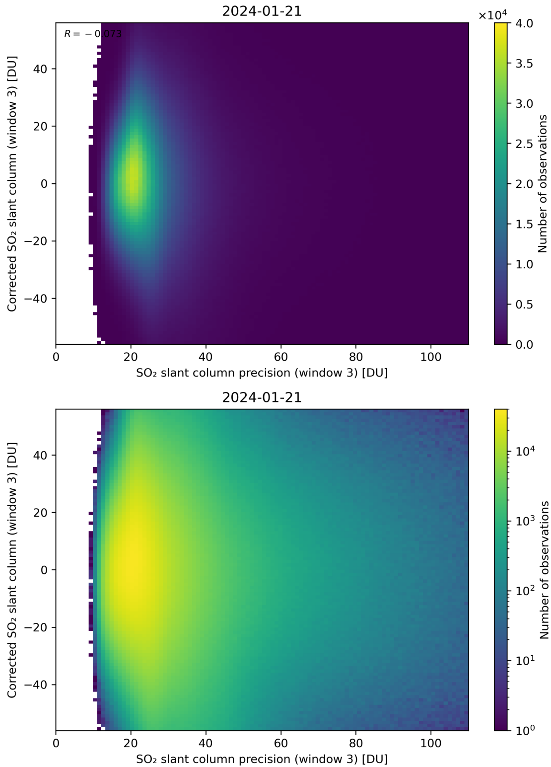
Figure 262: Scatter density plot of “SO 2 slant column precision (window 3)” against “Corrected SO 2 slant column (window 3)” for 2024-01-21 to 2024-01-22.
