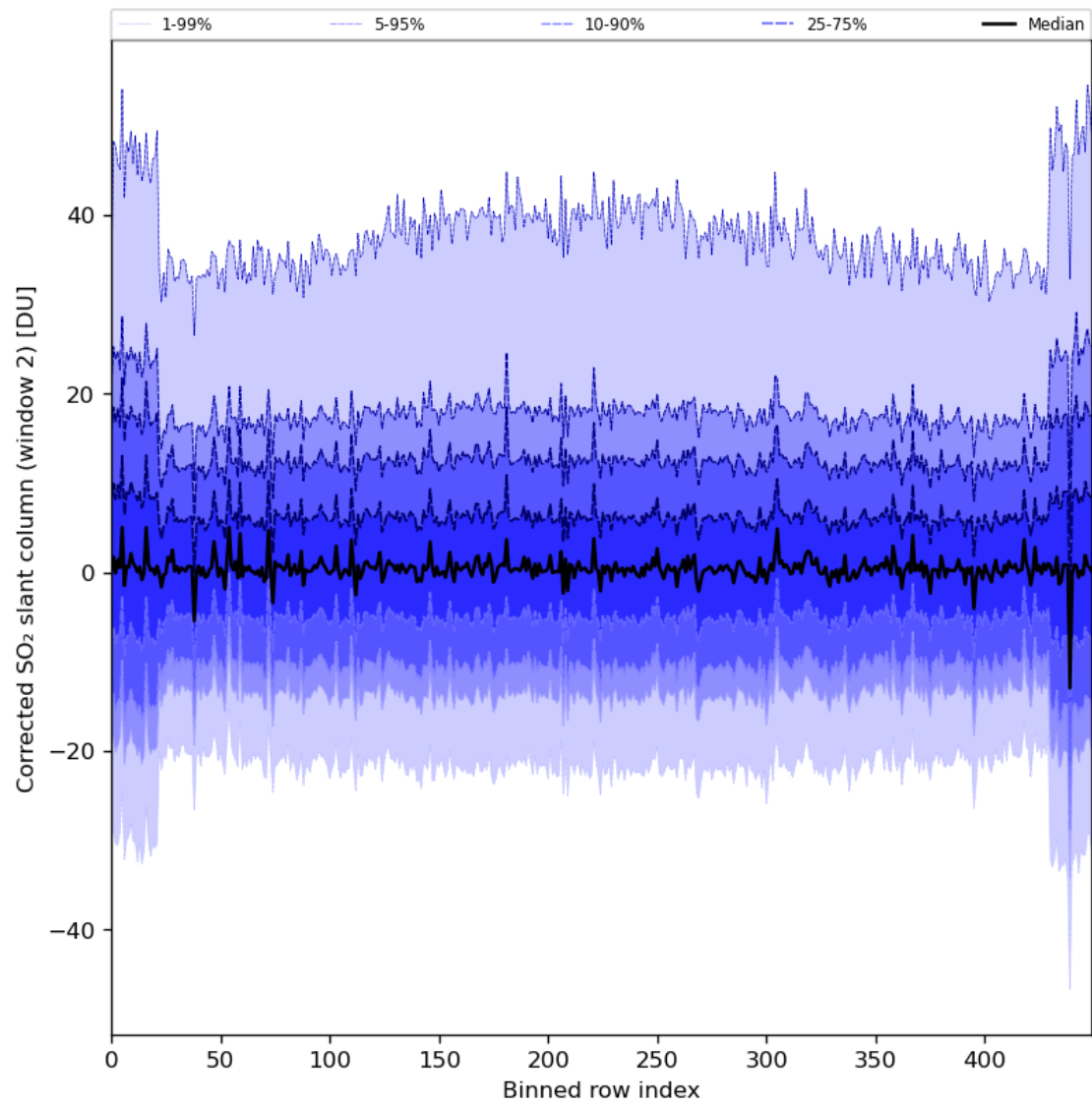
Figure 85: Along track statistics of “Corrected SO 2 slant column (window 2)” for 2024-01-21 to 2024-01-22
