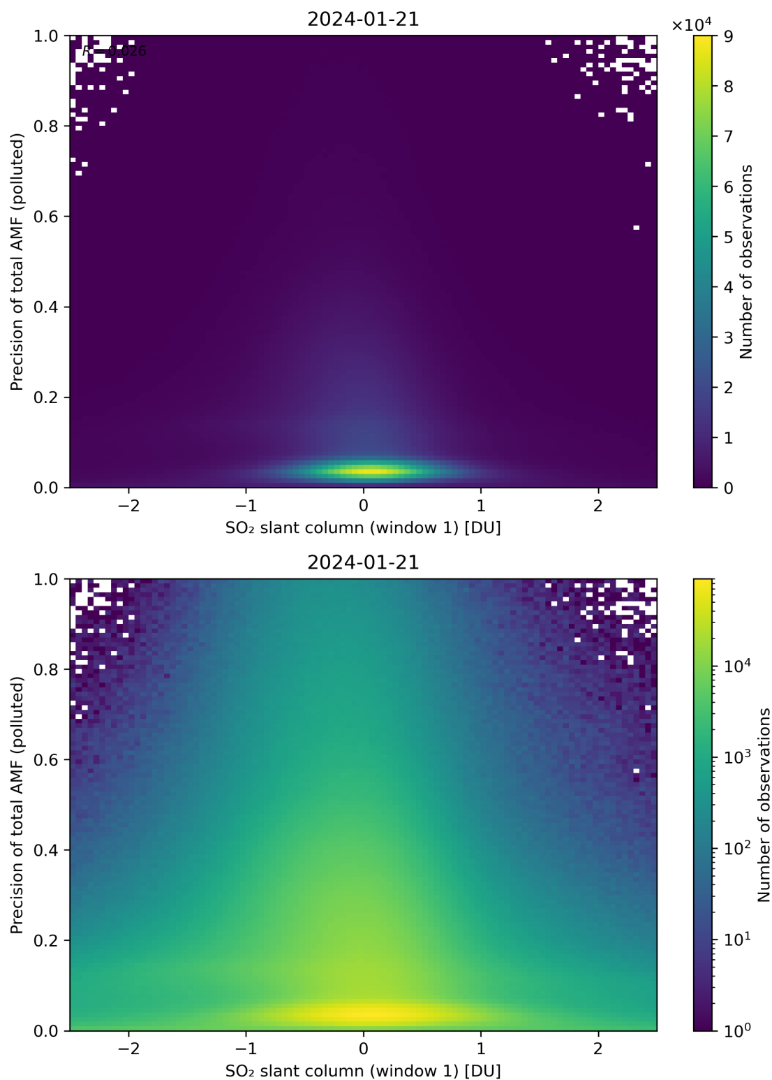
Figure 240: Scatter density plot of “SO 2 slant column (window 1)” against “Precision of total AMF (polluted)” for 2024-01-21 to 2024-01-22.
