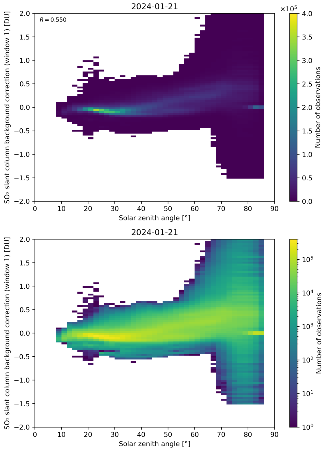
Figure 158: Scatter density plot of “Solar zenith angle” against “SO 2 slant column background correction (window 1)” for 2024-01-21 to 2024-01-22.
