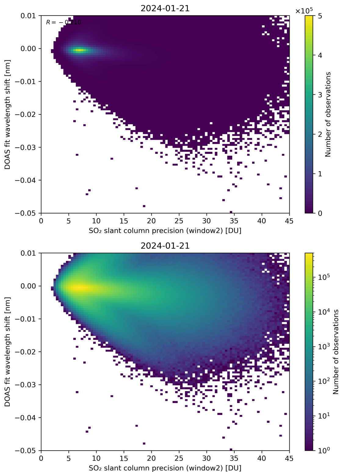
Figure 243: Scatter density plot of “SO 2 slant column precision (window2)” against “DOAS fit wavelength shift” for 2024-01-21 to 2024-01-22.
