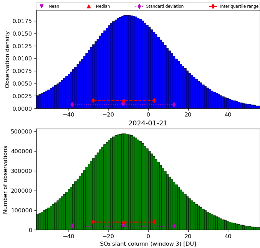
Figure 64: Histogram of “SO 2 slant column (window 3)” for 2024-01-21 to 2024-01-22
