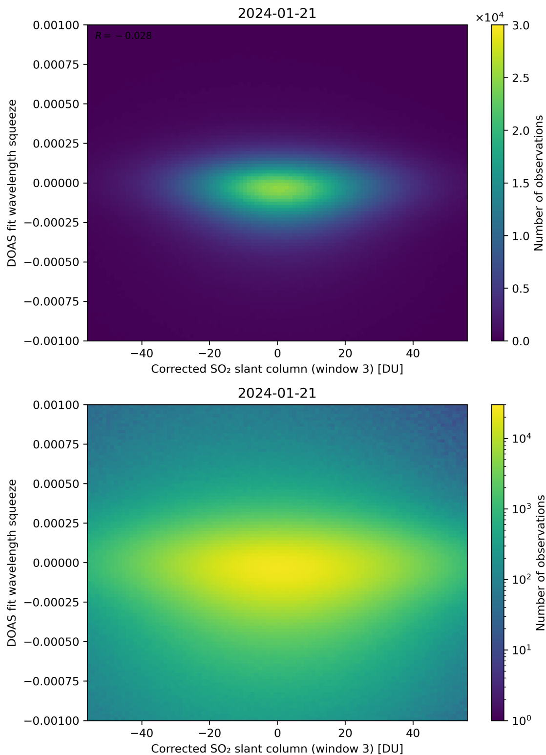
Figure 207: Scatter density plot of “Corrected SO 2 slant column (window 3)” against “DOAS fit wavelength squeeze” for 2024-01-21 to 2024-01-22.
