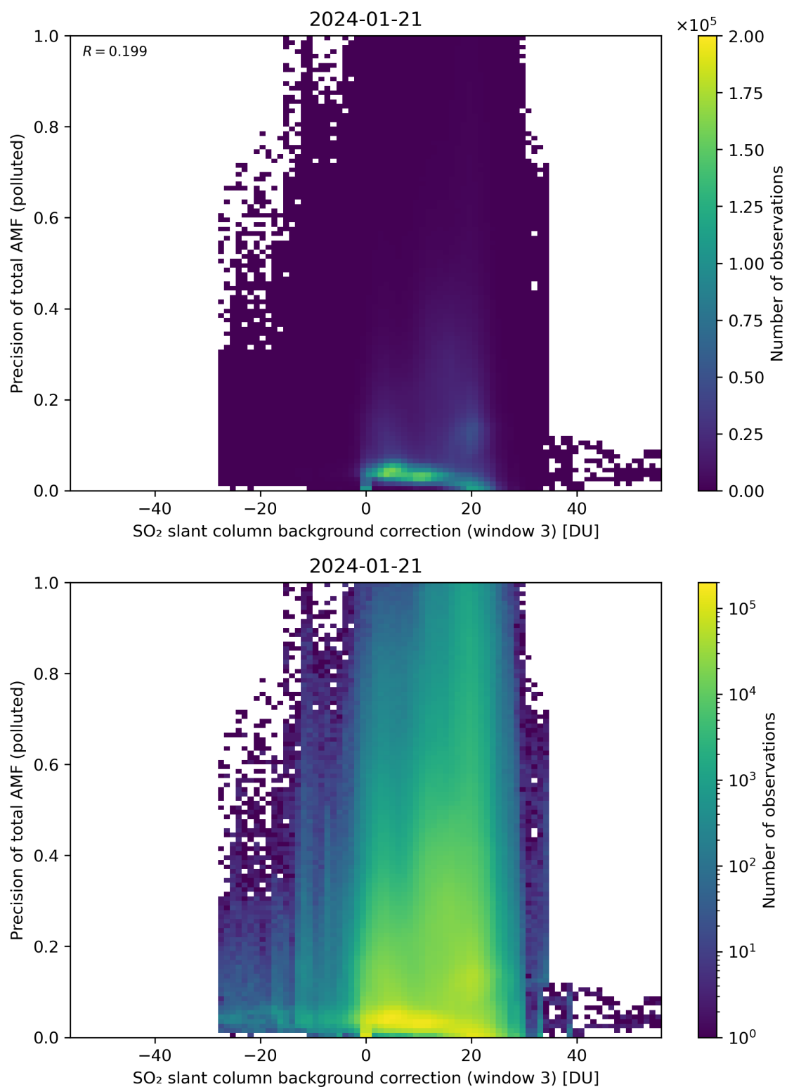
Figure 126: Scatter density plot of “SO 2 slant column background correction (window 3)” against “Precision of total AMF (polluted)” for 2024-01-21 to 2024-01-22.
