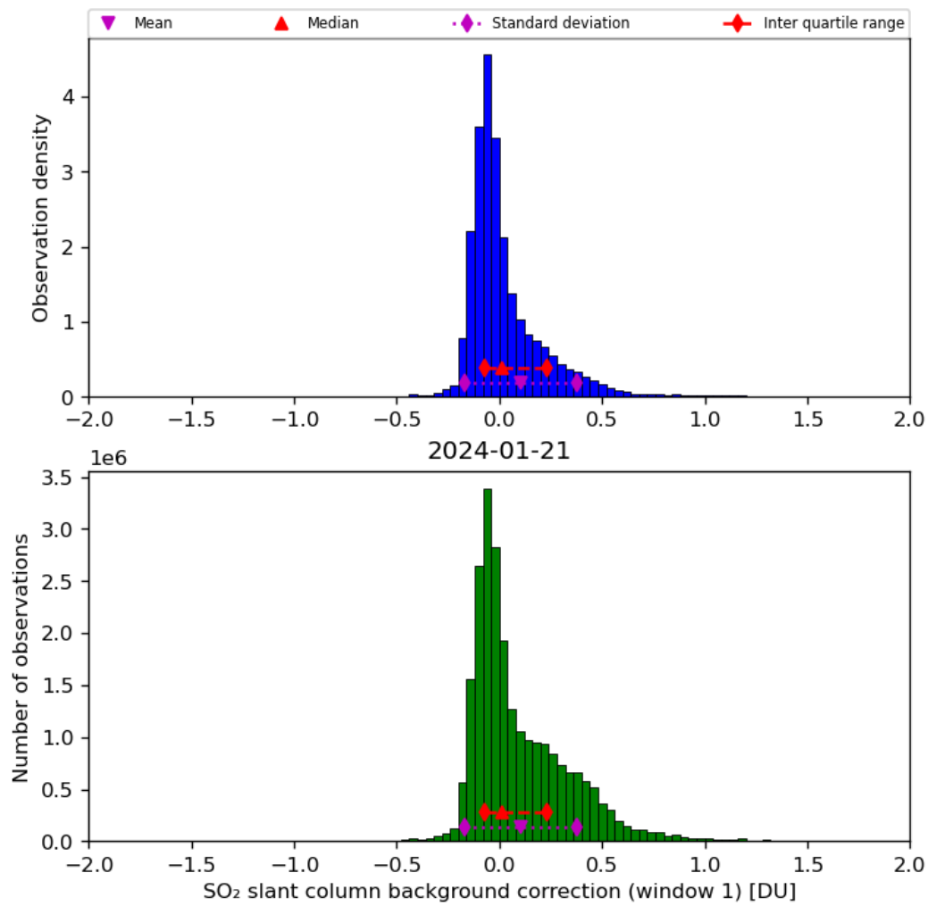
Figure 59: Histogram of “SO 2 slant column background correction (window 1)” for 2024-01-21 to 2024-01-22
