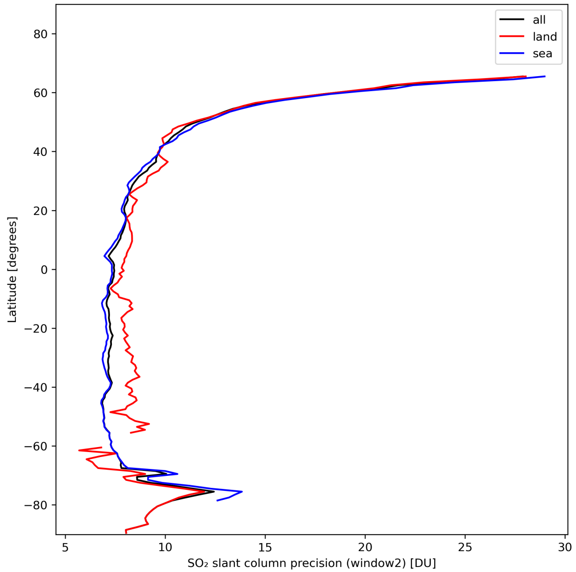
Figure 38: Zonal average of “SO 2 slant column precision (window2)” for 2024-01-21 to 2024-01-22.
