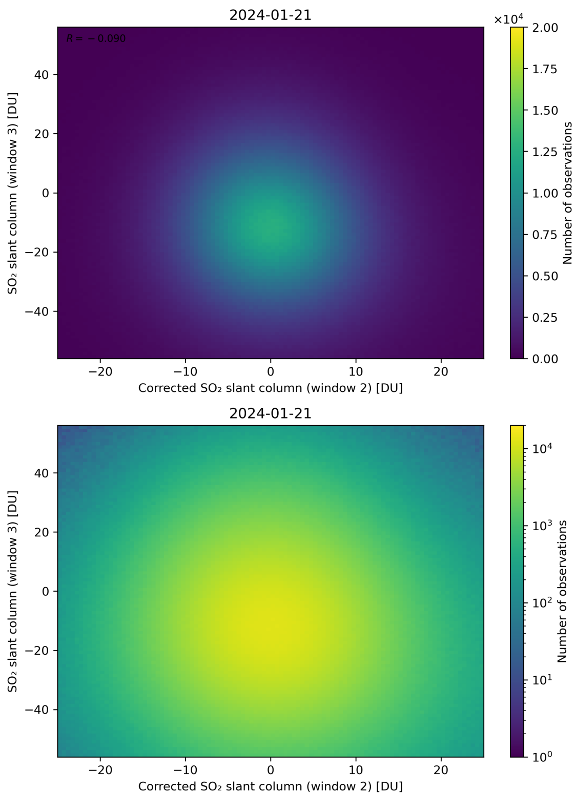
Figure 201: Scatter density plot of “Corrected SO 2 slant column (window 2)” against “SO 2 slant column (window 3)” for 2024-01-21 to 2024-01-22.
