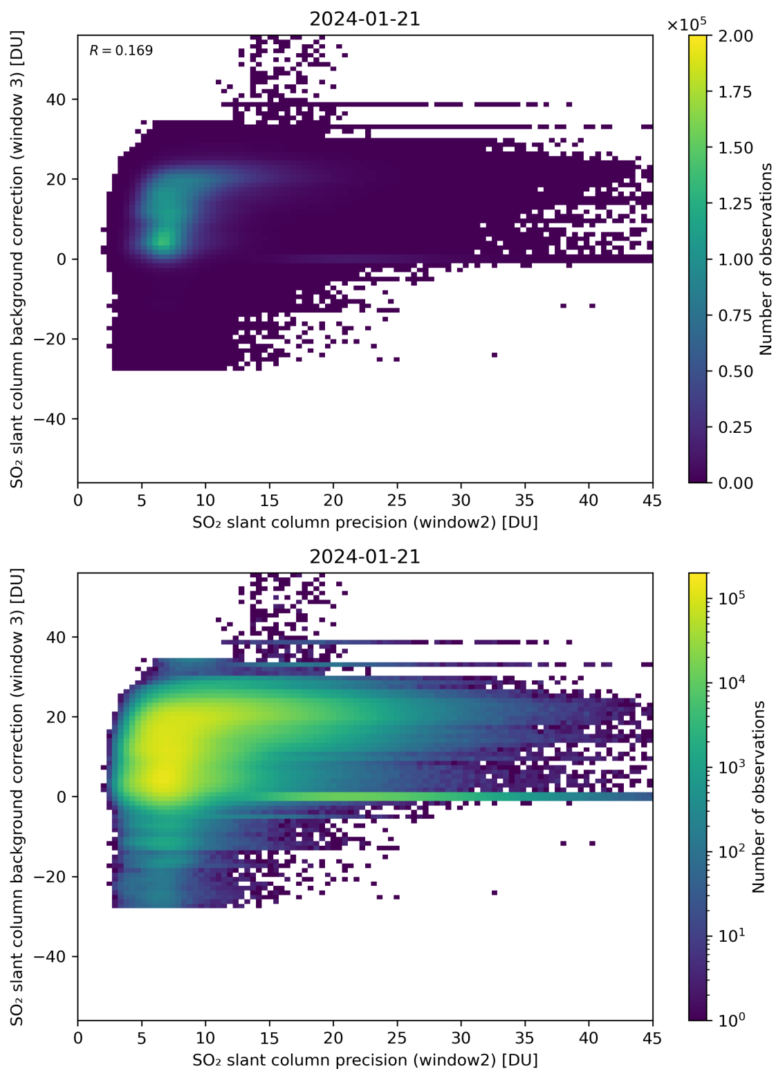
Figure 242: Scatter density plot of “SO 2 slant column precision (window2)” against “SO 2 slant column background correction (window 3)” for 2024-01-21 to 2024-01-22.
