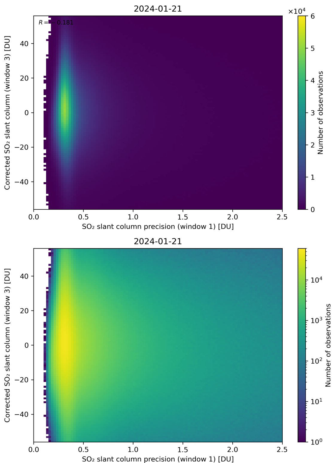
Figure 226: Scatter density plot of “SO 2 slant column precision (window 1)” against “Corrected SO 2 slant column (window 3)” for 2024-01-21 to 2024-01-22.
