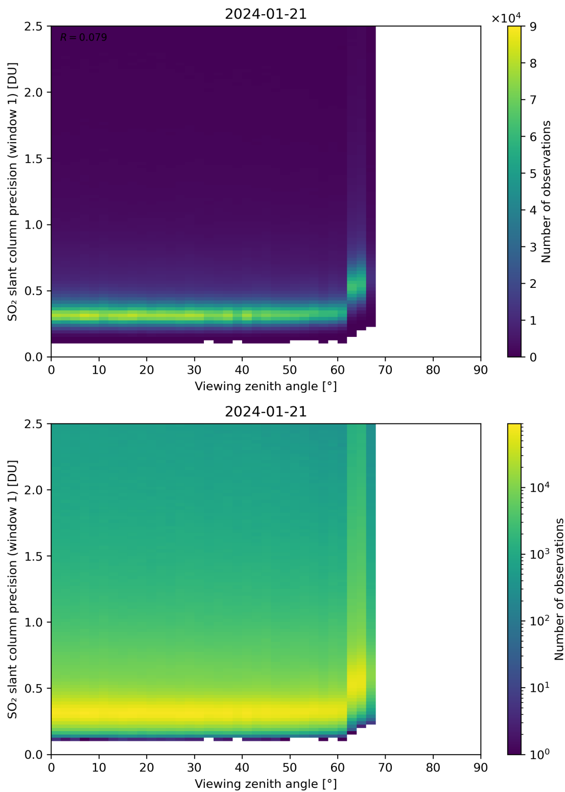
Figure 321: Scatter density plot of “Viewing zenith angle” against “SO 2 slant column precision (window 1)” for 2024-01-21 to 2024-01-22.
