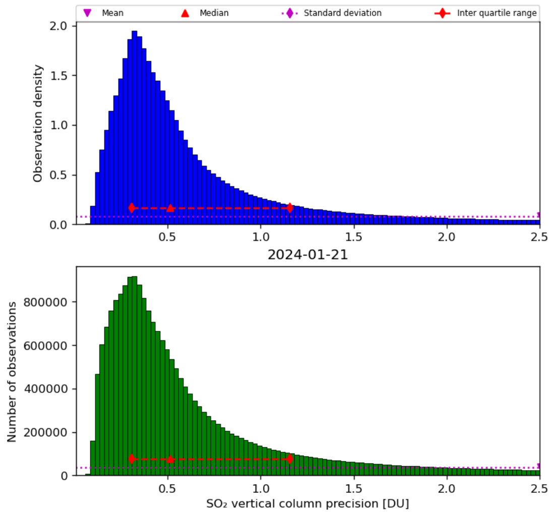
Figure 54: Histogram of “SO 2 vertical column precision” for 2024-01-21 to 2024-01-22
