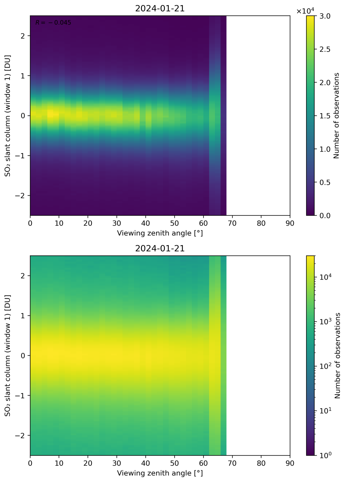
Figure 320: Scatter density plot of “Viewing zenith angle” against “SO 2 slant column (window 1)” for 2024-01-21 to 2024-01-22.
