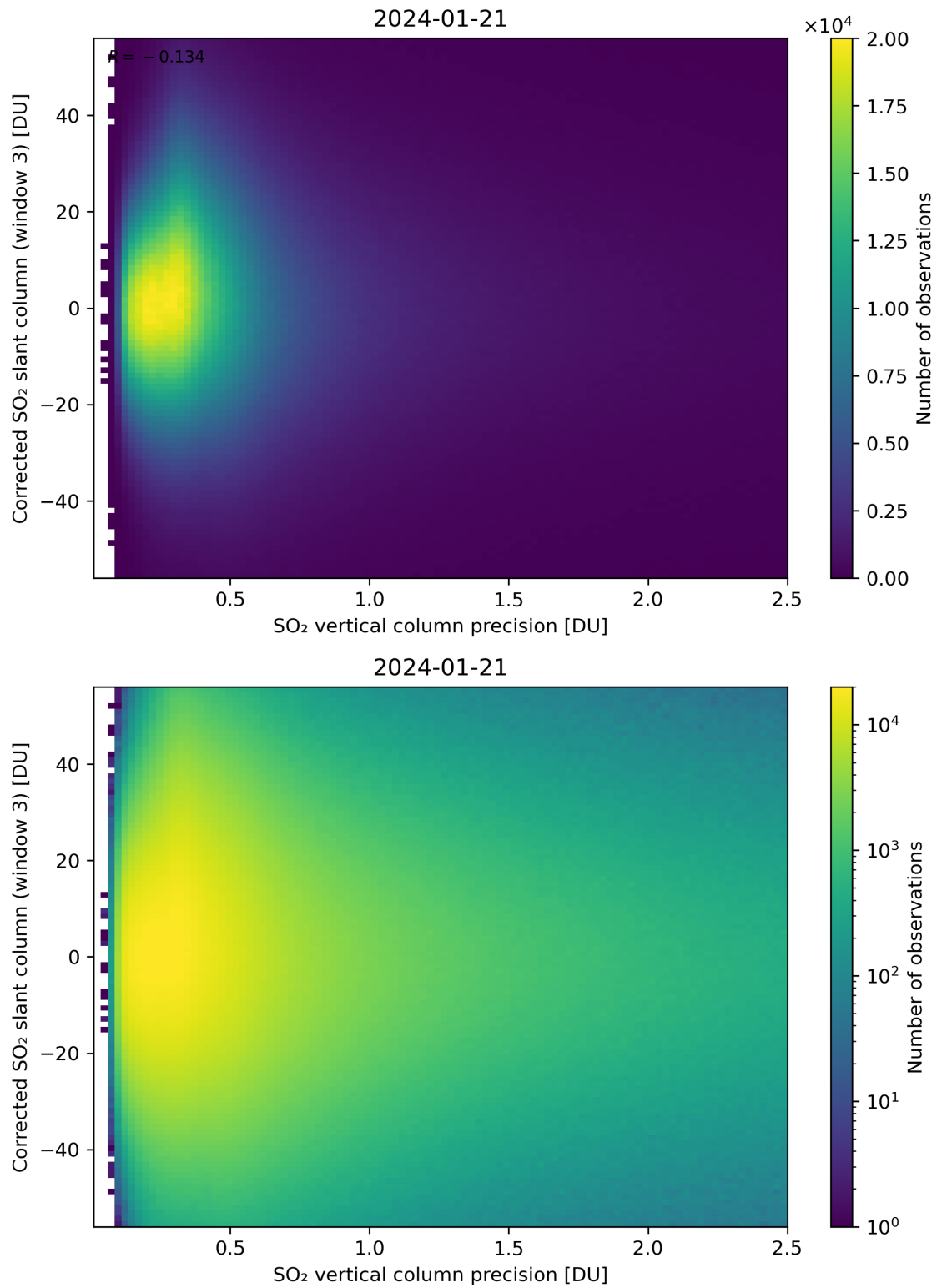
Figure 288: Scatter density plot of “SO 2 vertical column precision” against “Corrected SO 2 slant column (window 3)” for 2024-01-21 to 2024-01-22.
