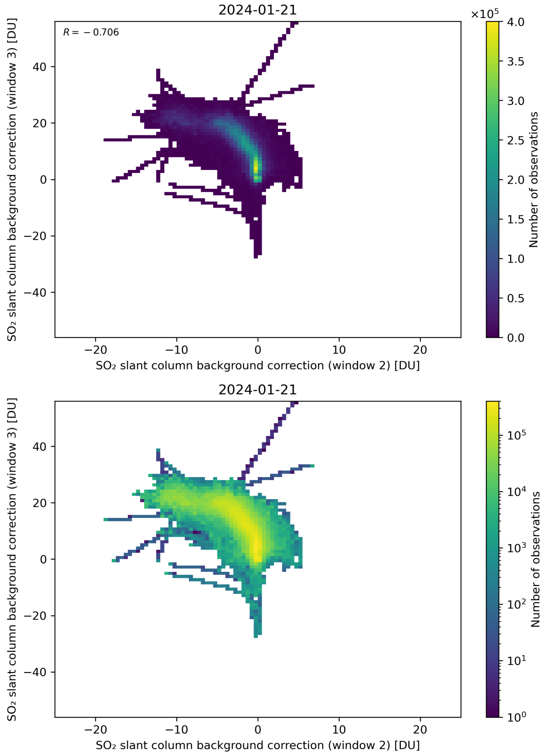
Figure 111: Scatter density plot of “SO 2 slant column background correction (window 2)” against “SO 2 slant column background correction (window 3)” for 2024-01-21 to 2024-01-22.
