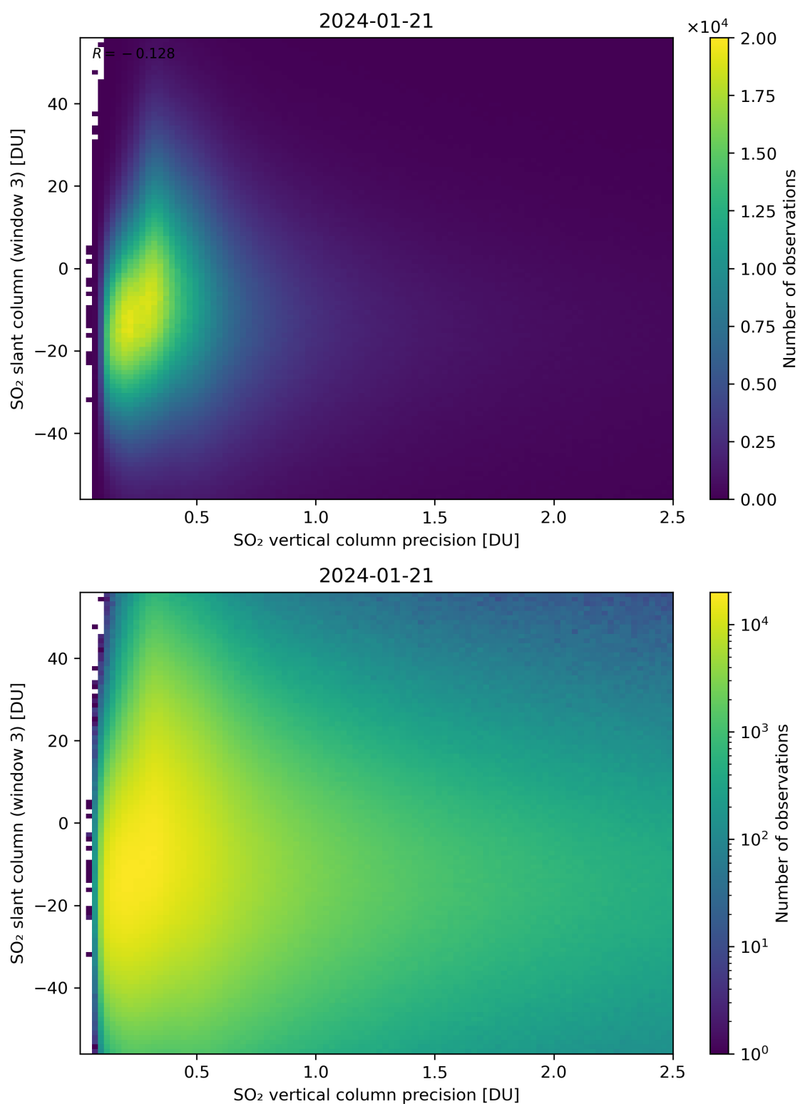
Figure 292: Scatter density plot of “SO 2 vertical column precision” against “SO 2 slant column (window 3)” for 2024-01-21 to 2024-01-22.
