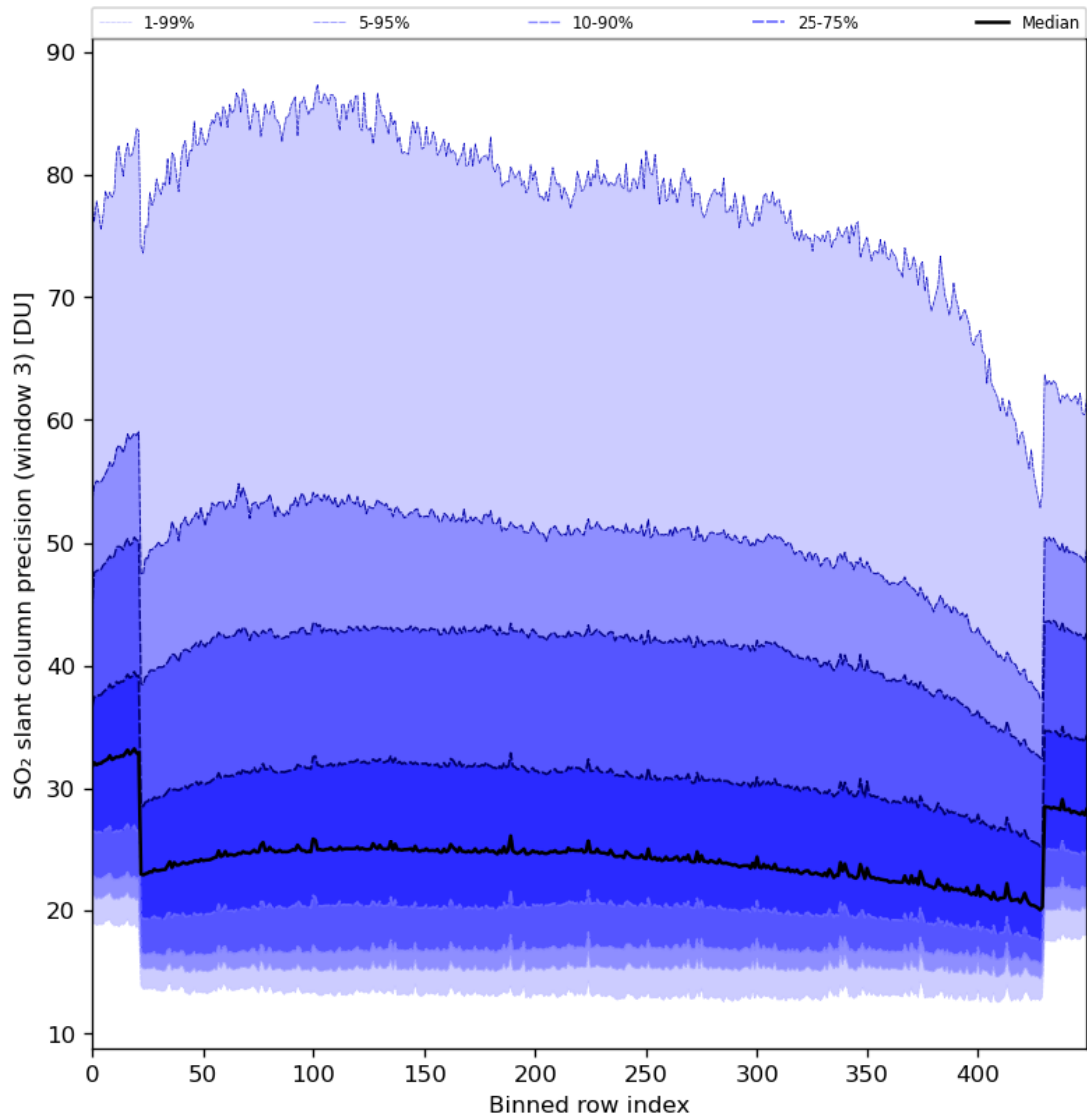
Figure 88: Along track statistics of “SO 2 slant column precision (window 3)” for 2024-01-21 to 2024-01-22
