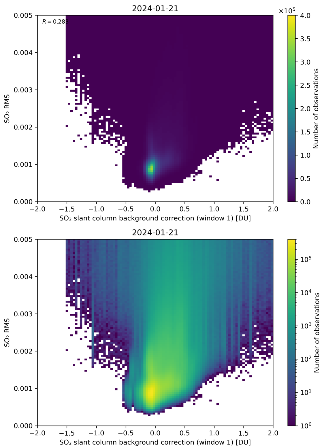
Figure 102: Scatter density plot of “SO 2 slant column background correction (window 1)” against “SO 2 RMS” for 2024-01-21 to 2024-01-22.
