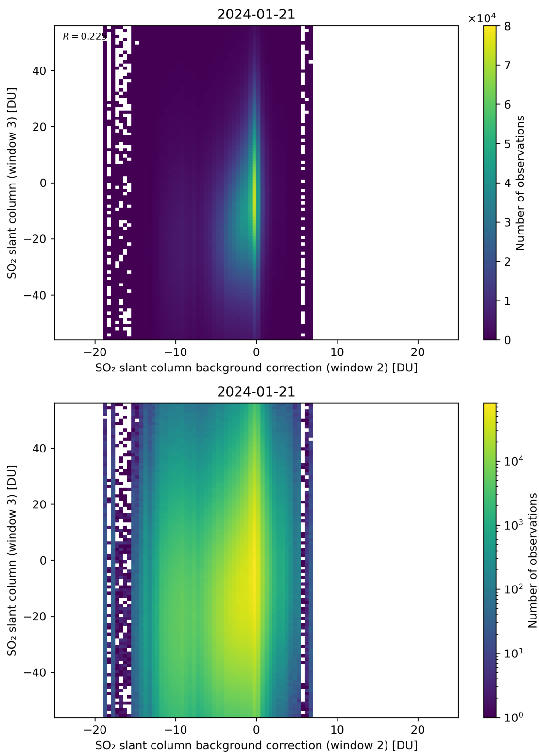
Figure 117: Scatter density plot of “SO 2 slant column background correction (window 2)” against “SO 2 slant column (window 3)” for 2024-01-21 to 2024-01-22.
