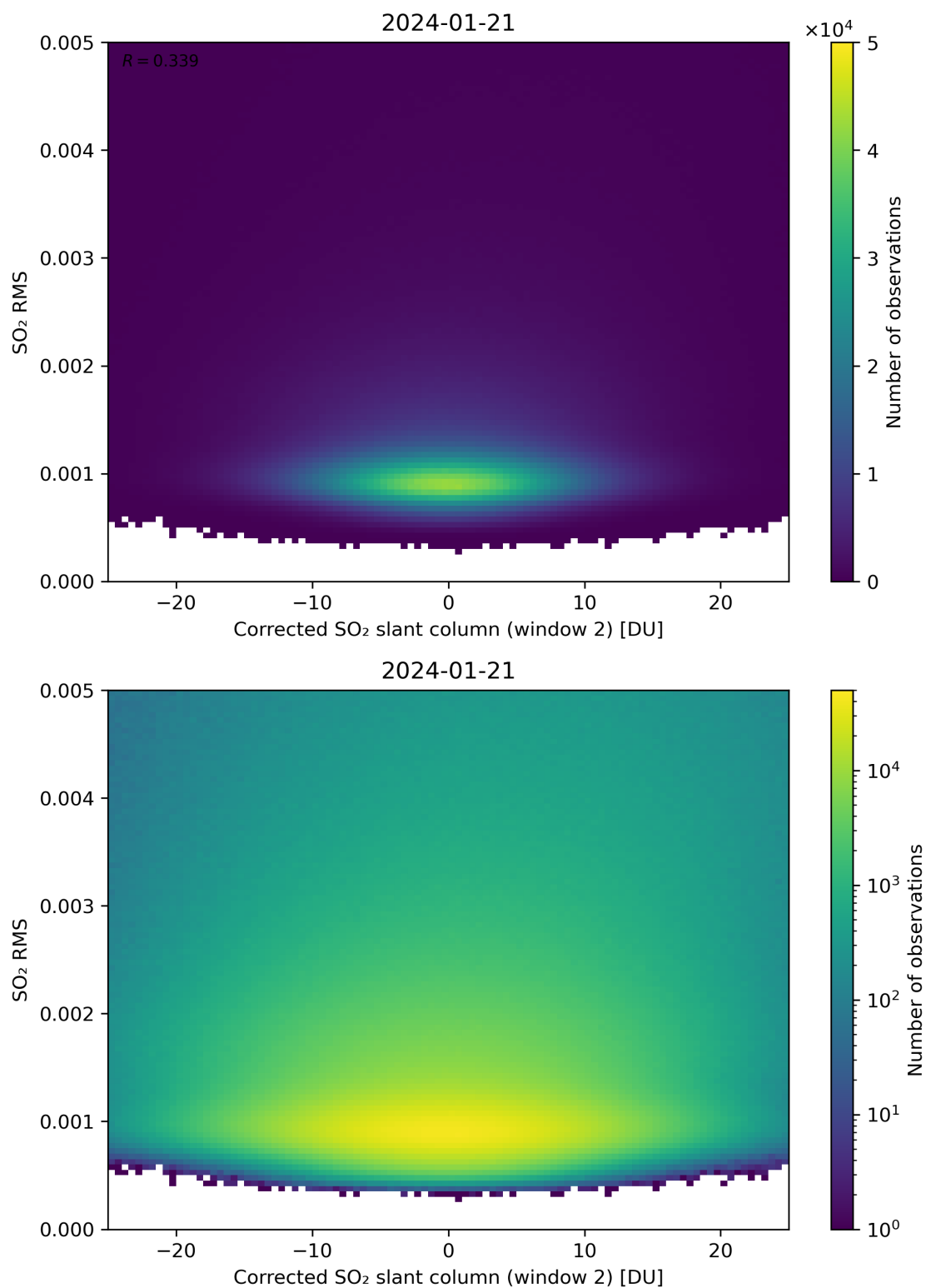
Figure 198: Scatter density plot of “Corrected SO 2 slant column (window 2)” against “SO 2 RMS” for 2024-01-21 to 2024-01-22.
