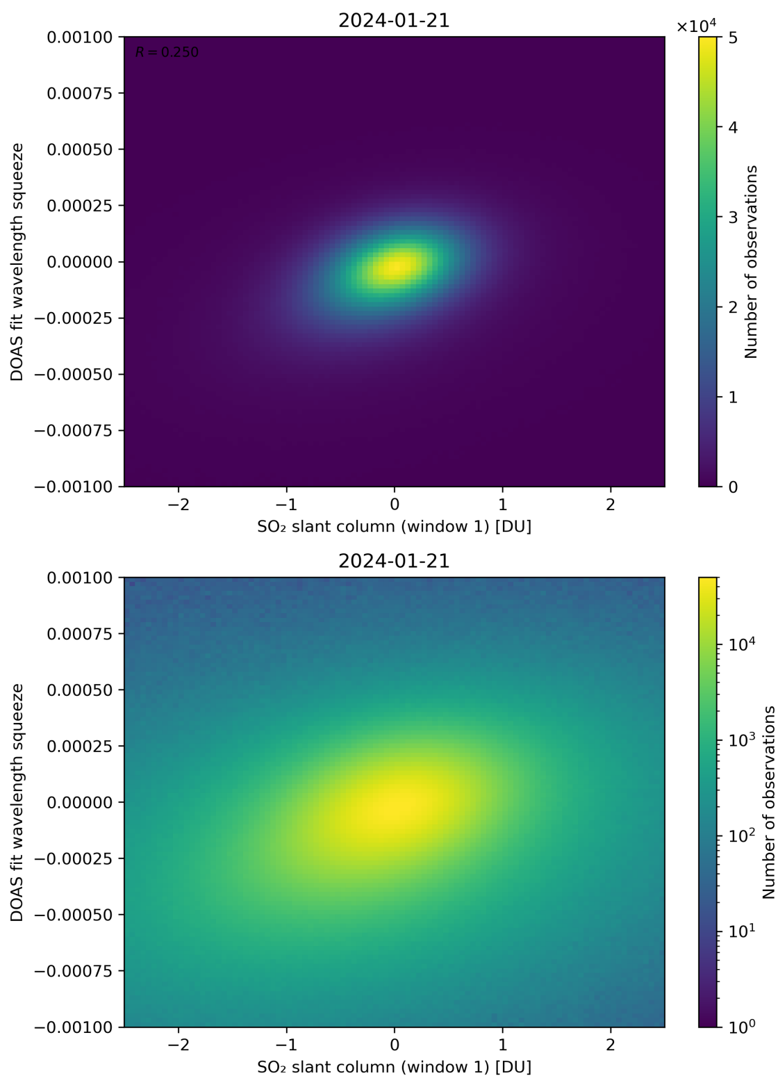
Figure 216: Scatter density plot of “SO 2 slant column (window 1)” against “DOAS fit wavelength squeeze” for 2024-01-21 to 2024-01-22.
