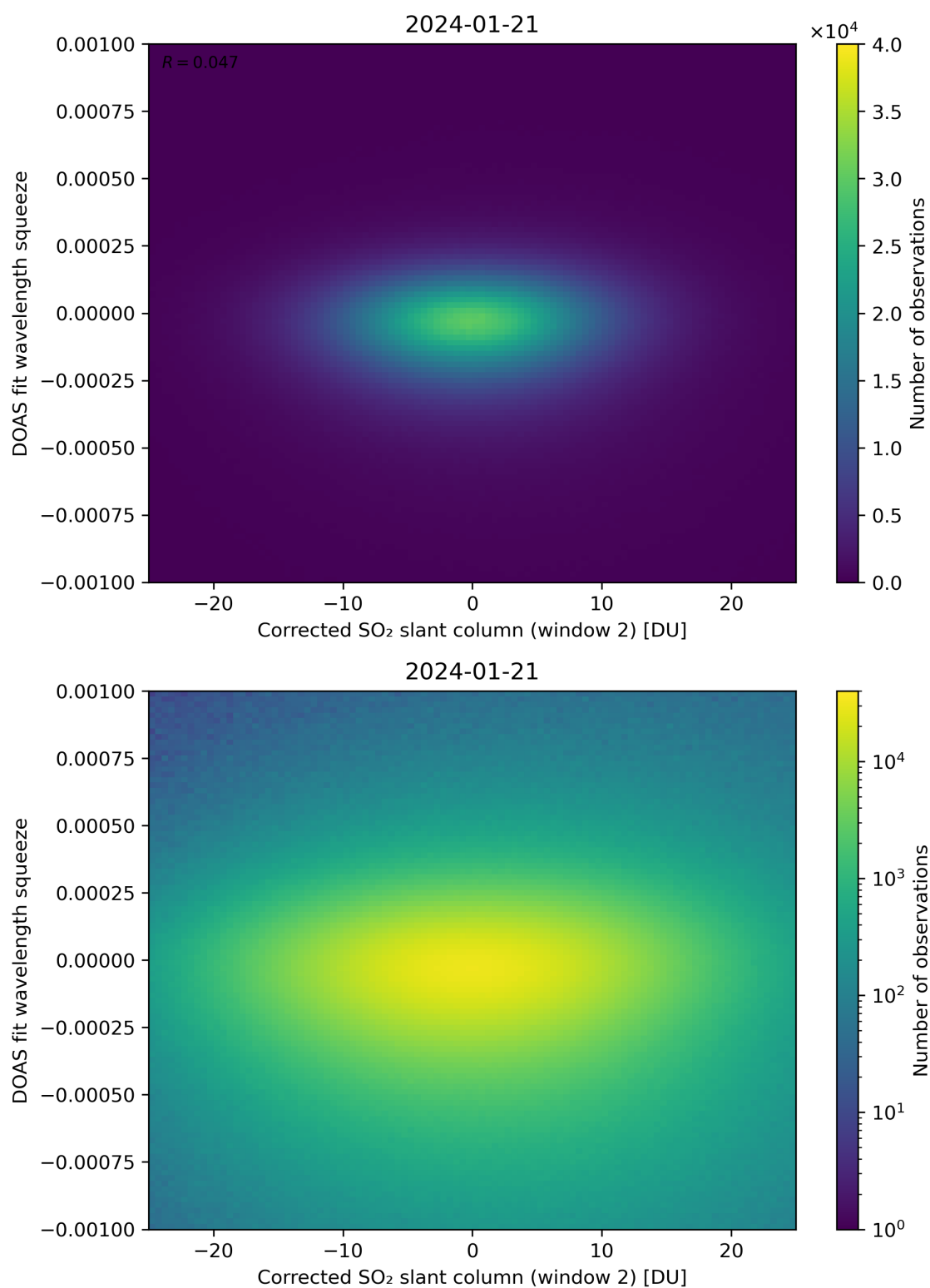
Figure 197: Scatter density plot of “Corrected SO 2 slant column (window 2)” against “DOAS fit wavelength squeeze” for 2024-01-21 to 2024-01-22.
