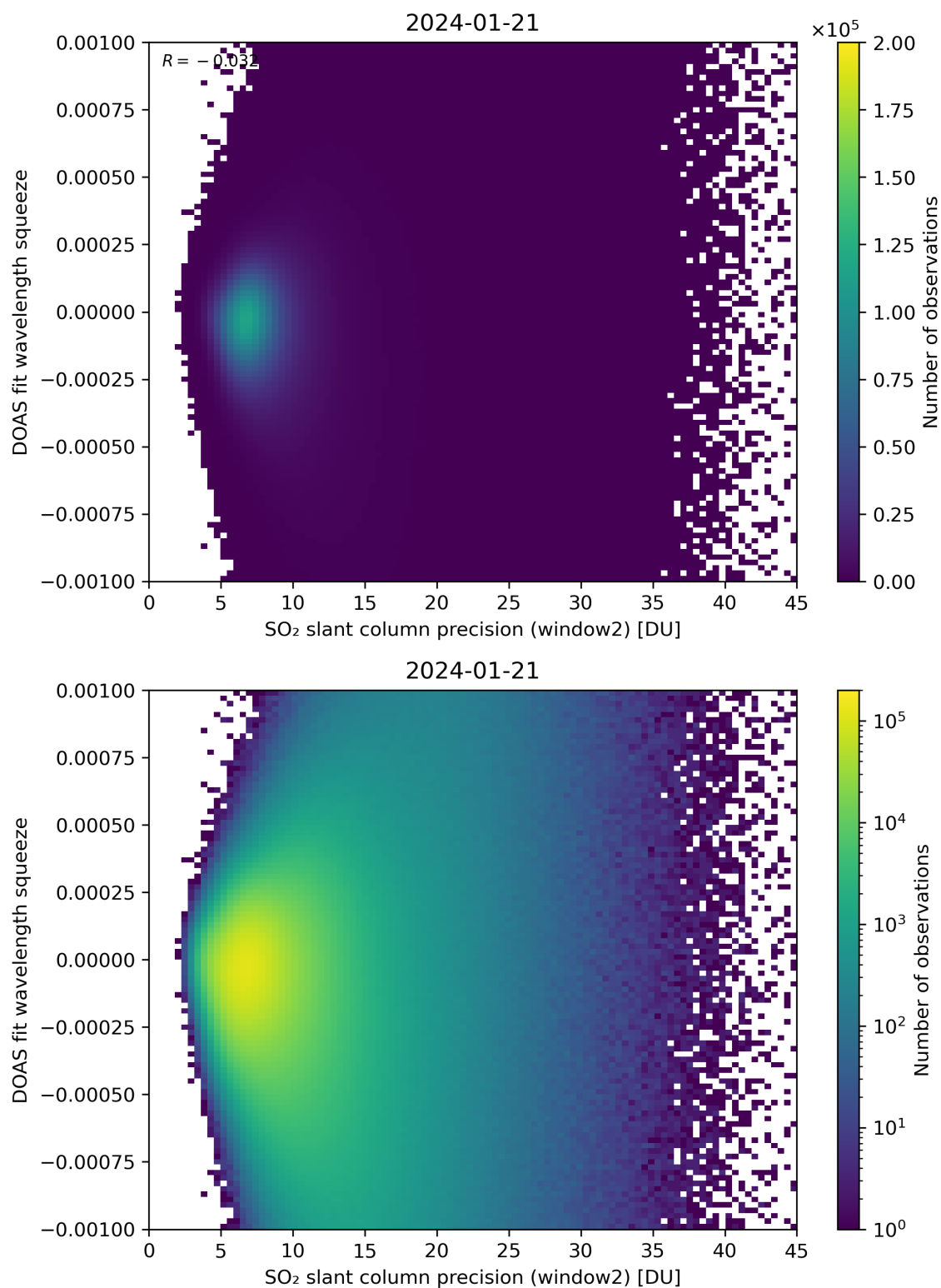
Figure 244: Scatter density plot of “SO 2 slant column precision (window2)” against “DOAS fit wavelength squeeze” for 2024-01-21 to 2024-01-22.
