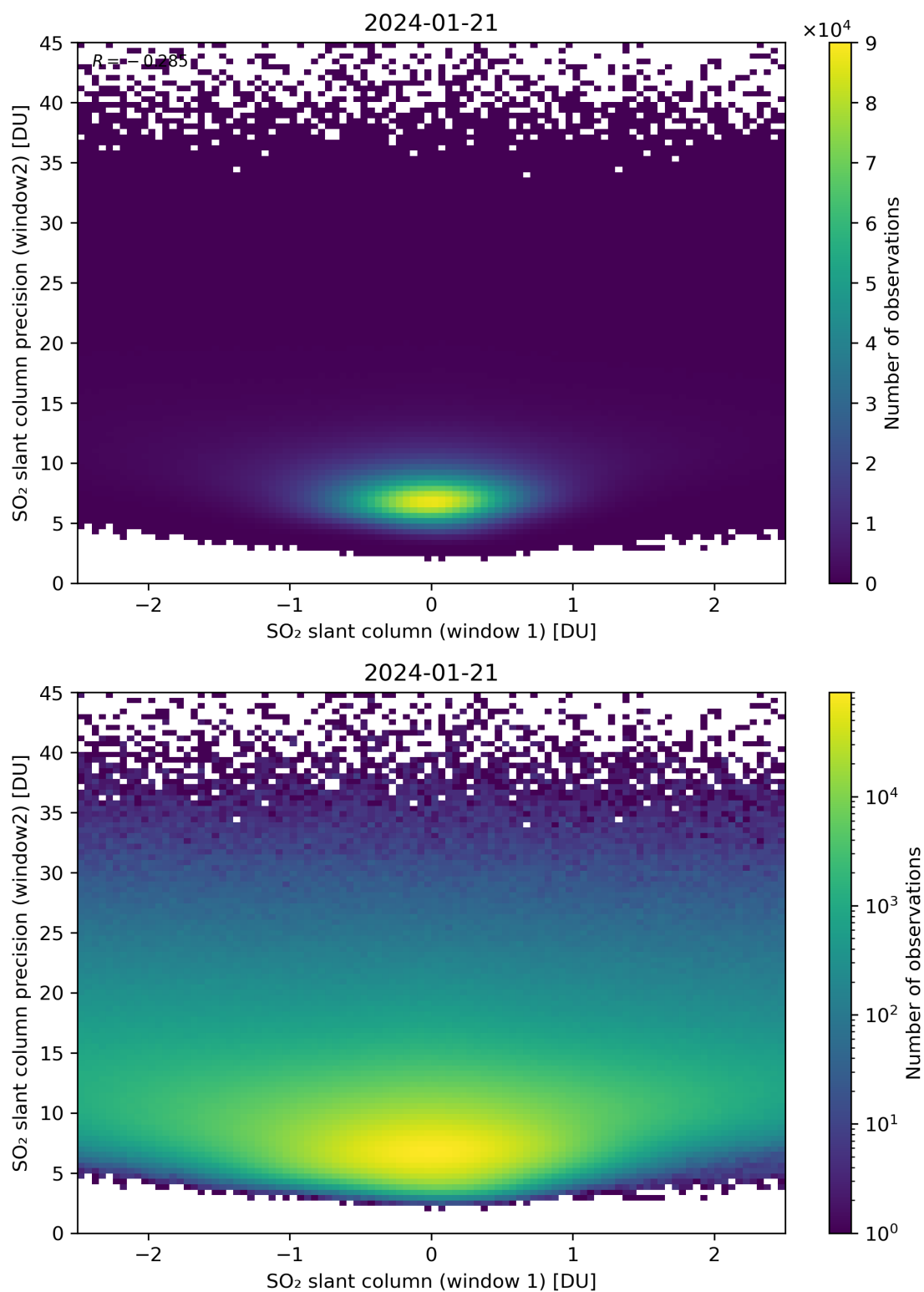
Figure 236: Scatter density plot of “SO 2 slant column (window 1)” against “SO 2 slant column precision (window2)” for 2024-01-21 to 2024-01-22.
