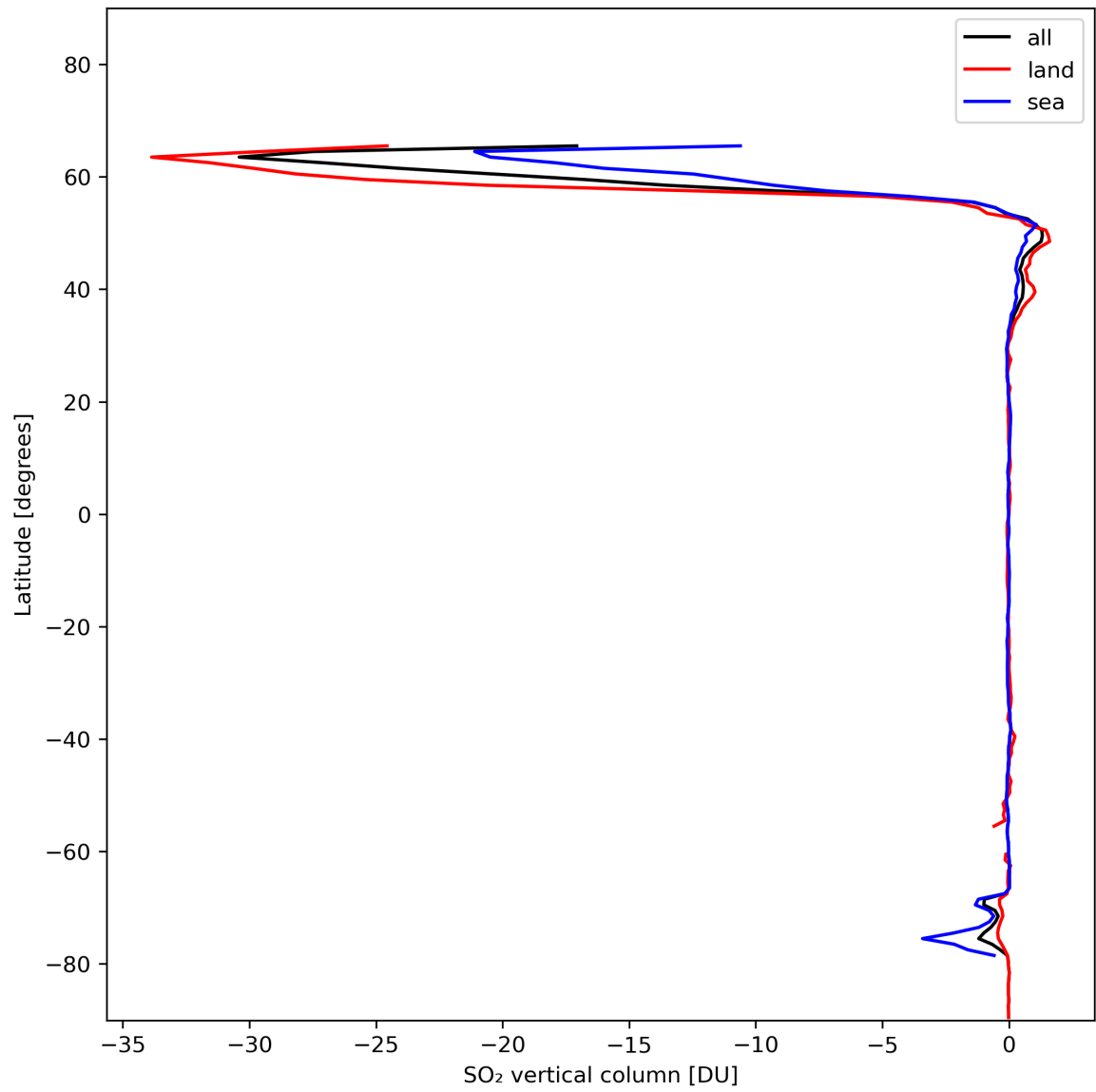
Figure 30: Zonal average of “SO 2 vertical column” for 2024-01-21 to 2024-01-22.
