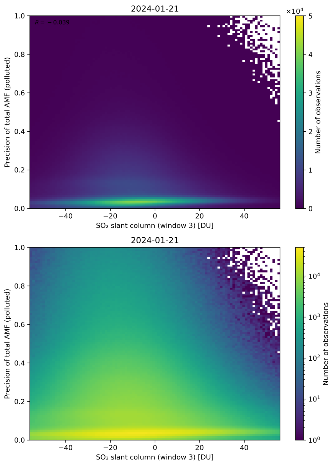
Figure 269: Scatter density plot of “SO 2 slant column (window 3)” against “Precision of total AMF (polluted)” for 2024-01-21 to 2024-01-22.
