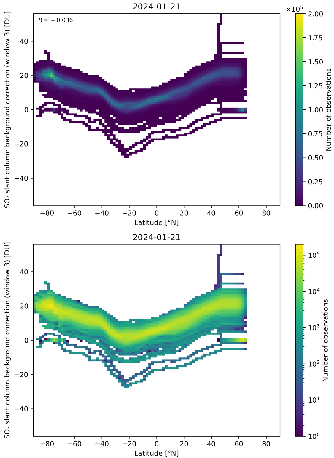
Figure 141: Scatter density plot of “Latitude” against “SO 2 slant column background correction (window 3)” for 2024-01-21 to 2024-01-22.
