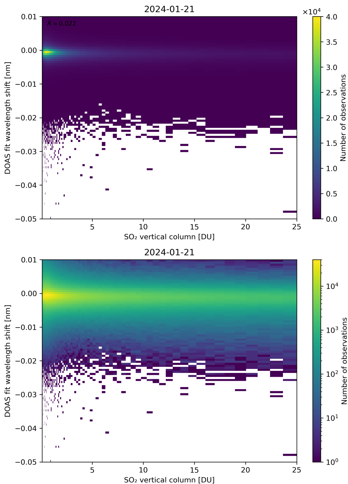
Figure 276: Scatter density plot of “SO 2 vertical column” against “DOAS fit wavelength shift” for 2024-01-21 to 2024-01-22.
