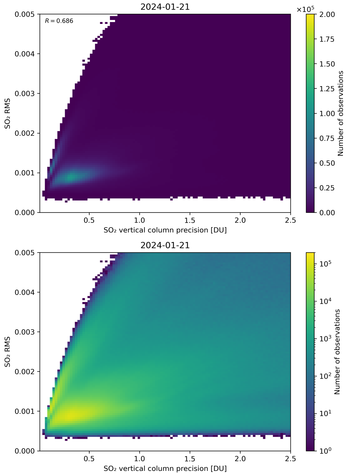
Figure 284: Scatter density plot of “SO 2 vertical column precision” against “SO 2 RMS” for 2024-01-21 to 2024-01-22.
