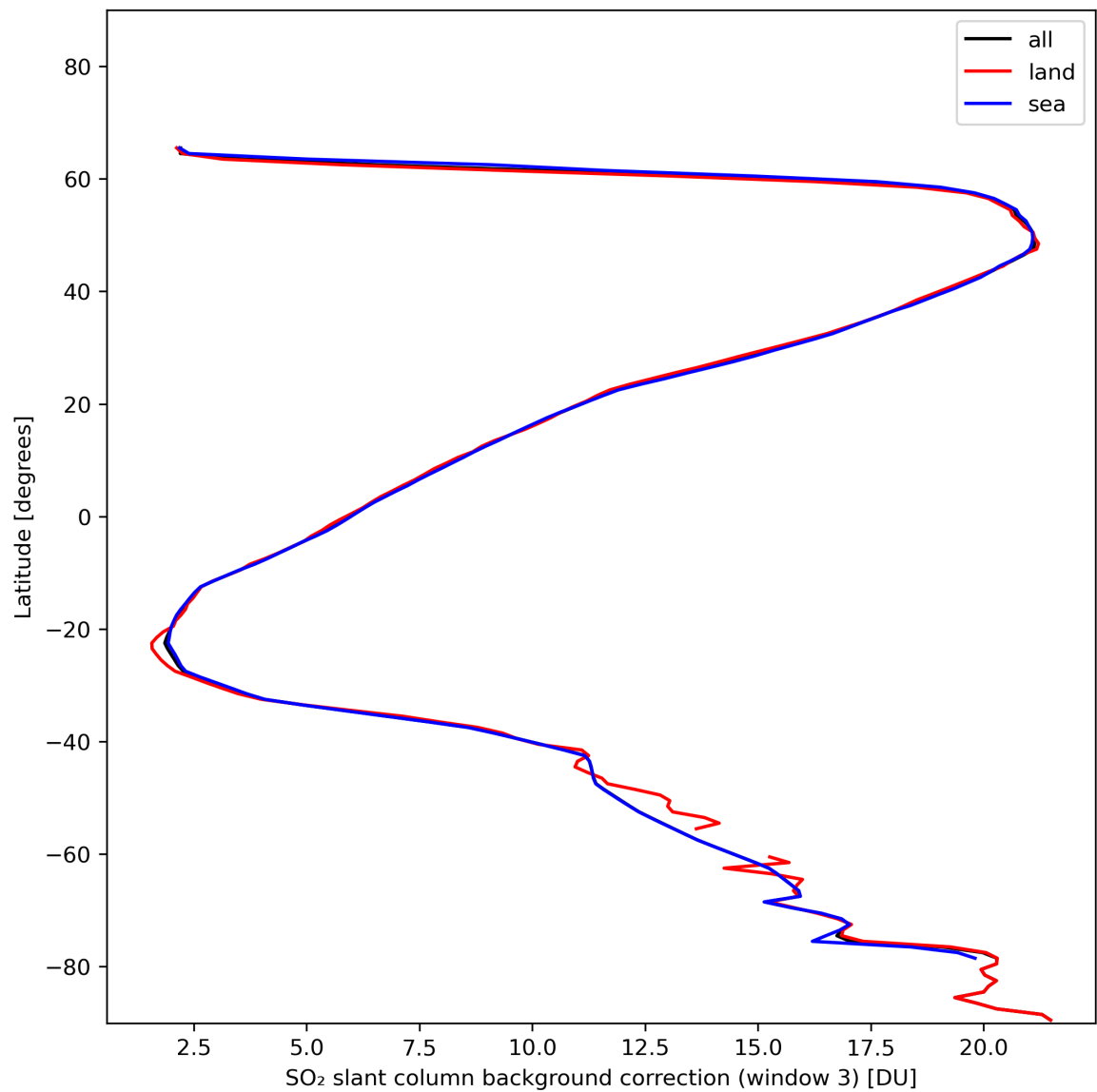
Figure 44: Zonal average of “SO 2 slant column background correction (window 3)” for 2024-01-21 to 2024-01-22.
