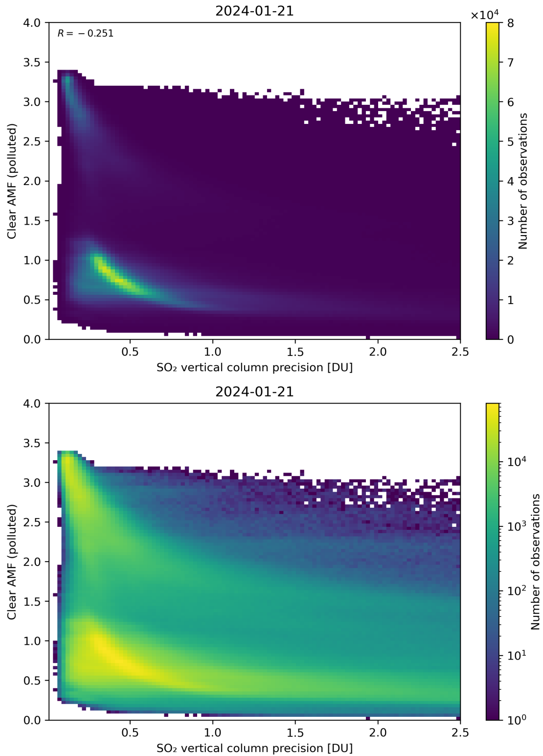
Figure 285: Scatter density plot of “SO 2 vertical column precision” against “Clear AMF (polluted)” for 2024-01-21 to 2024-01-22.
