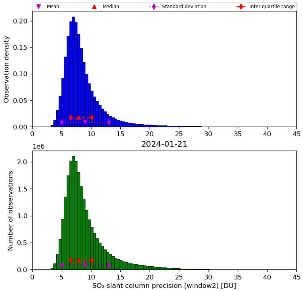
Figure 61: Histogram of “SO 2 slant column precision (window2)” for 2024-01-21 to 2024-01-22
