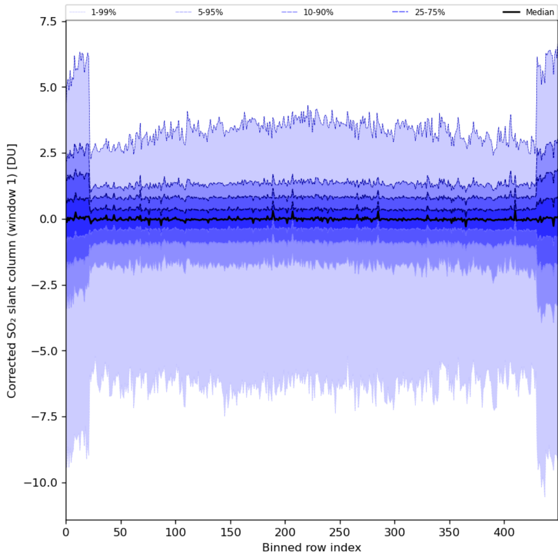
Figure 81: Along track statistics of “Corrected SO 2 slant column (window 1)” for 2024-01-21 to 2024-01-22
