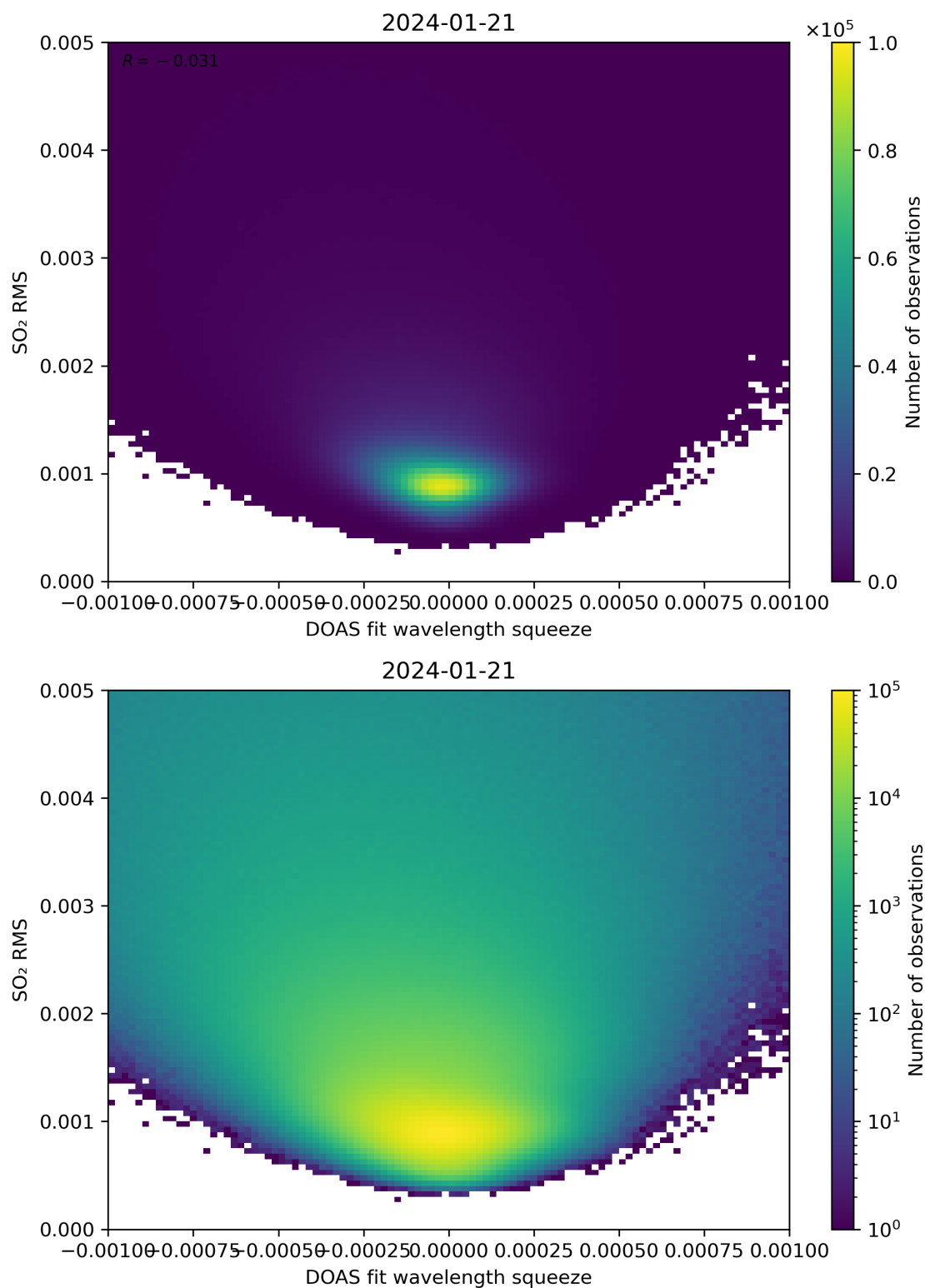
Figure 132: Scatter density plot of “DOAS fit wavelength squeeze” against “SO 2 RMS” for 2024-01-21 to 2024-01-22.
