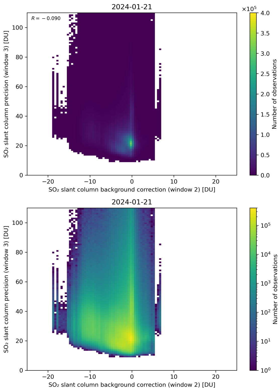
Figure 118: Scatter density plot of “SO 2 slant column background correction (window 2)” against “SO 2 slant column precision (window 3)” for 2024-01-21 to 2024-01-22.
