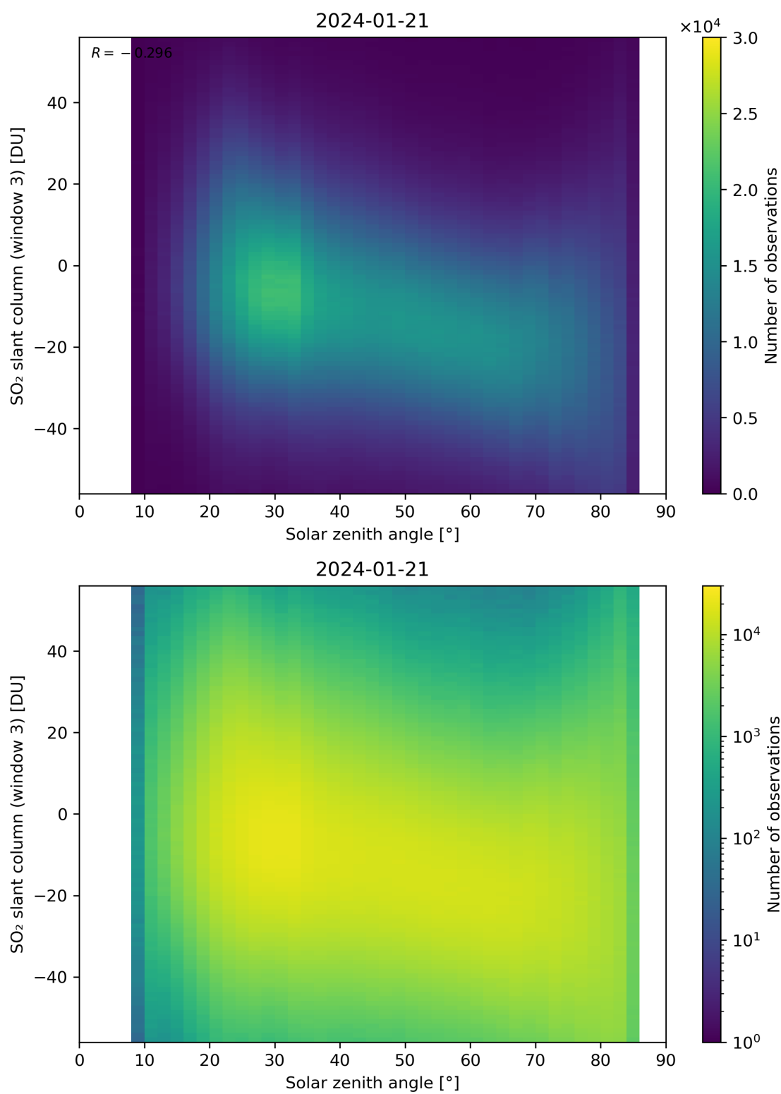
Figure 172: Scatter density plot of “Solar zenith angle” against “SO 2 slant column (window 3)” for 2024-01-21 to 2024-01-22.
