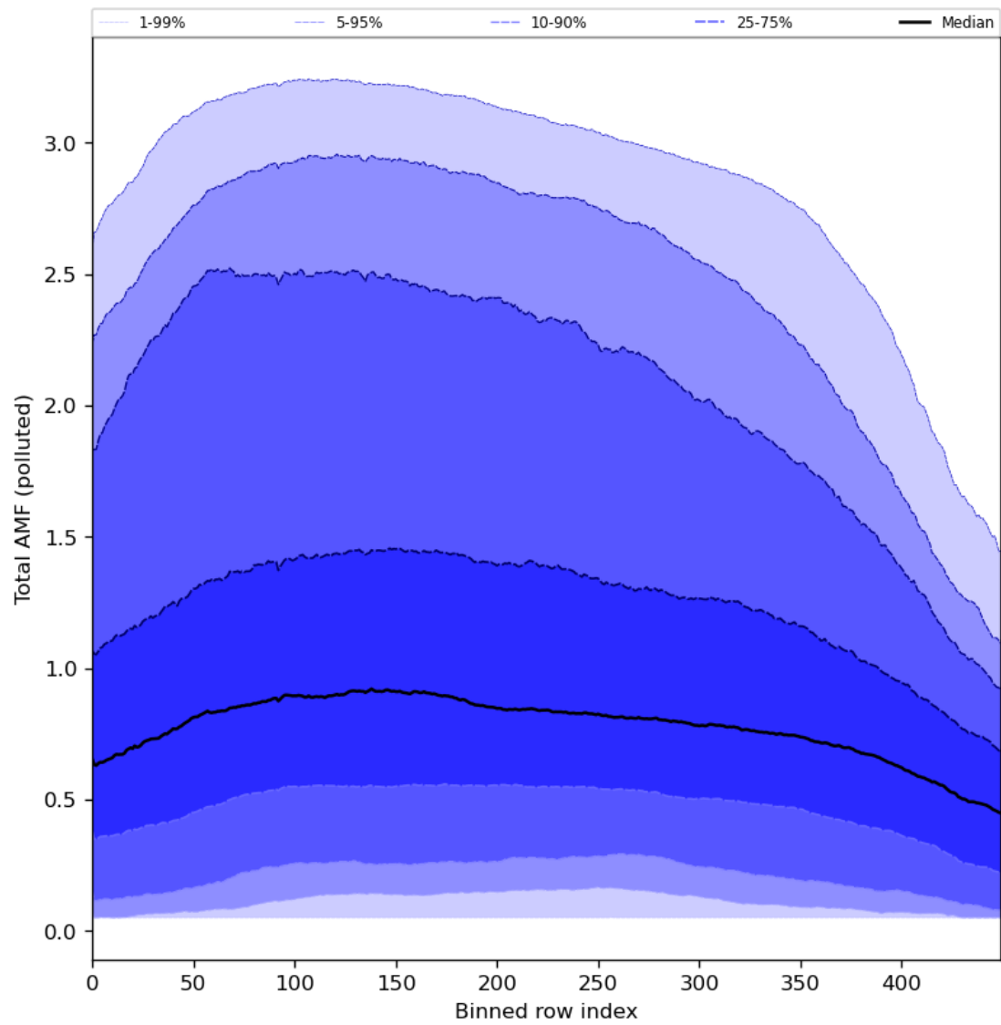
Figure 94: Along track statistics of “Total AMF (polluted)” for 2024-01-21 to 2024-01-22
