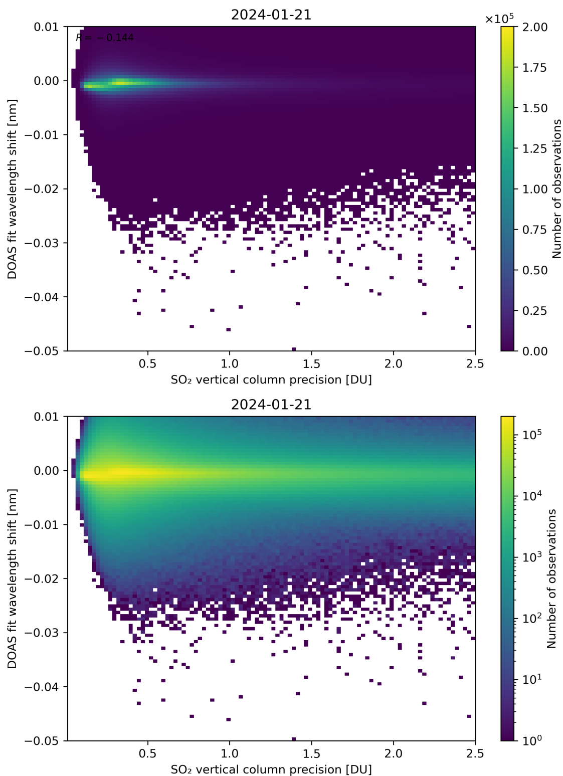
Figure 282: Scatter density plot of “SO 2 vertical column precision” against “DOAS fit wavelength shift” for 2024-01-21 to 2024-01-22.
