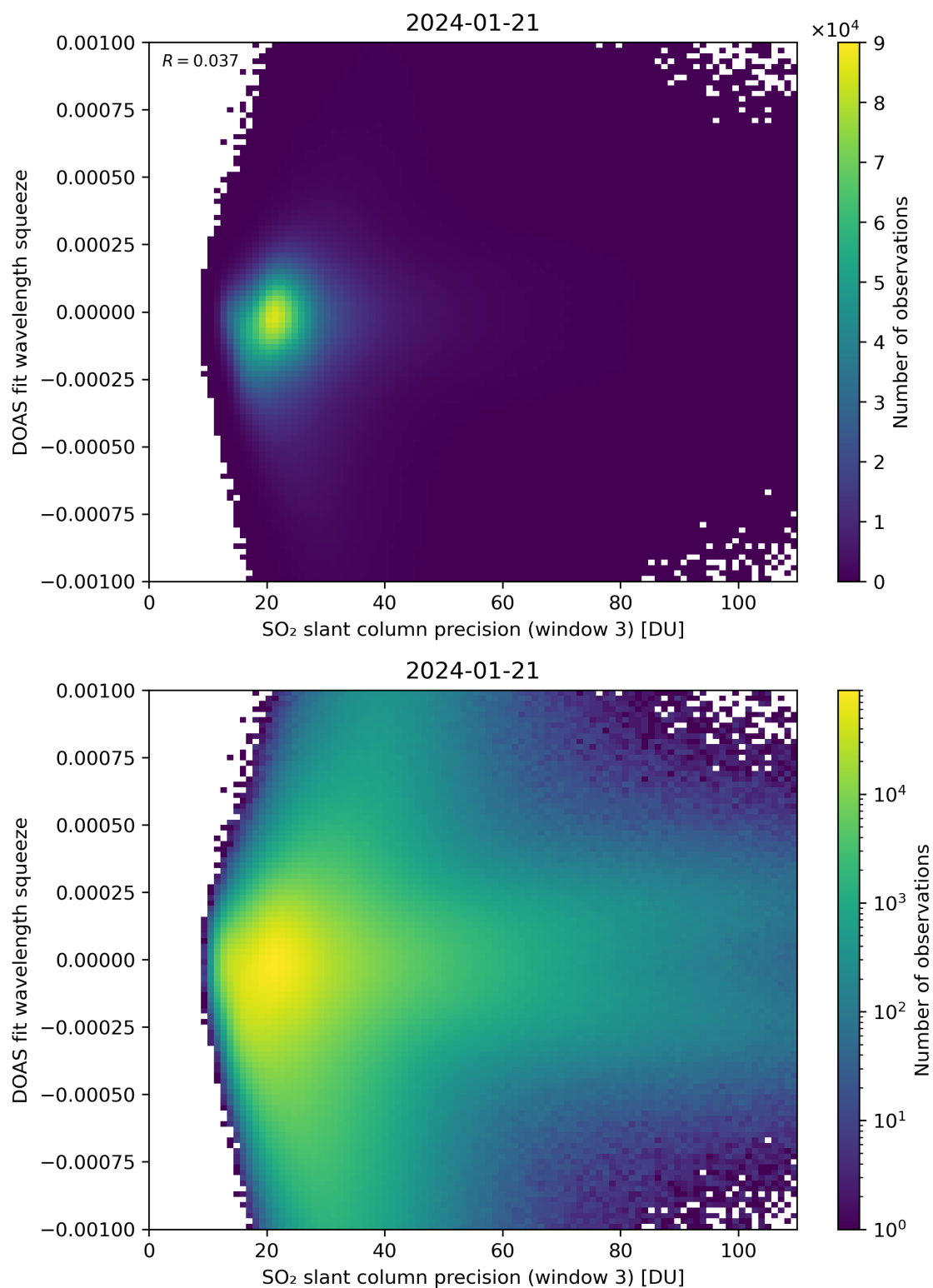
Figure 259: Scatter density plot of “SO 2 slant column precision (window 3)” against “DOAS fit wavelength squeeze” for 2024-01-21 to 2024-01-22.
