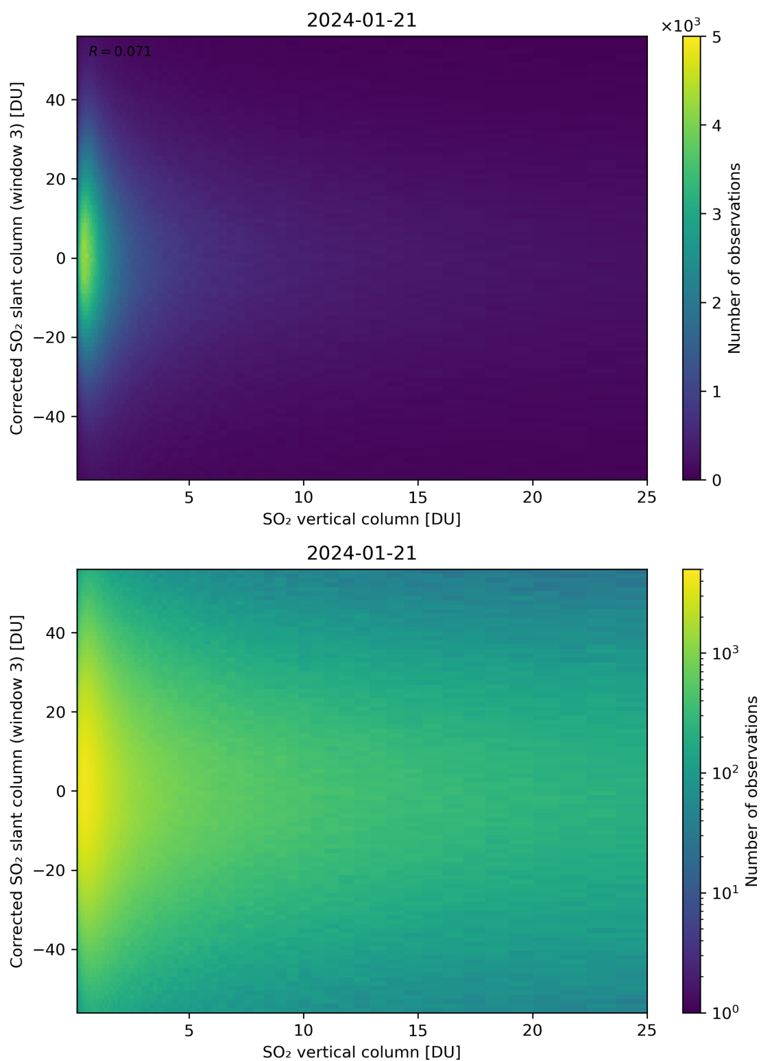
Figure 299: Scatter density plot of “SO 2 vertical column” against “Corrected SO 2 slant column (window 3)” for 2024-01-21 to 2024-01-22.
