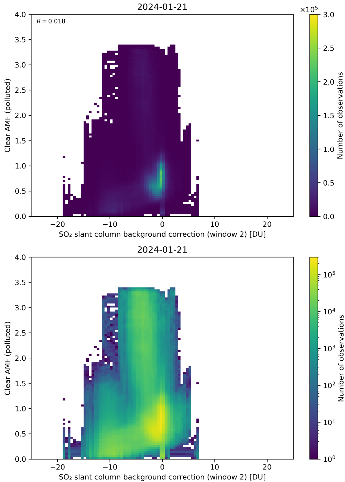
Figure 115: Scatter density plot of “SO 2 slant column background correction (window 2)” against “Clear AMF (polluted)” for 2024-01-21 to 2024-01-22.
