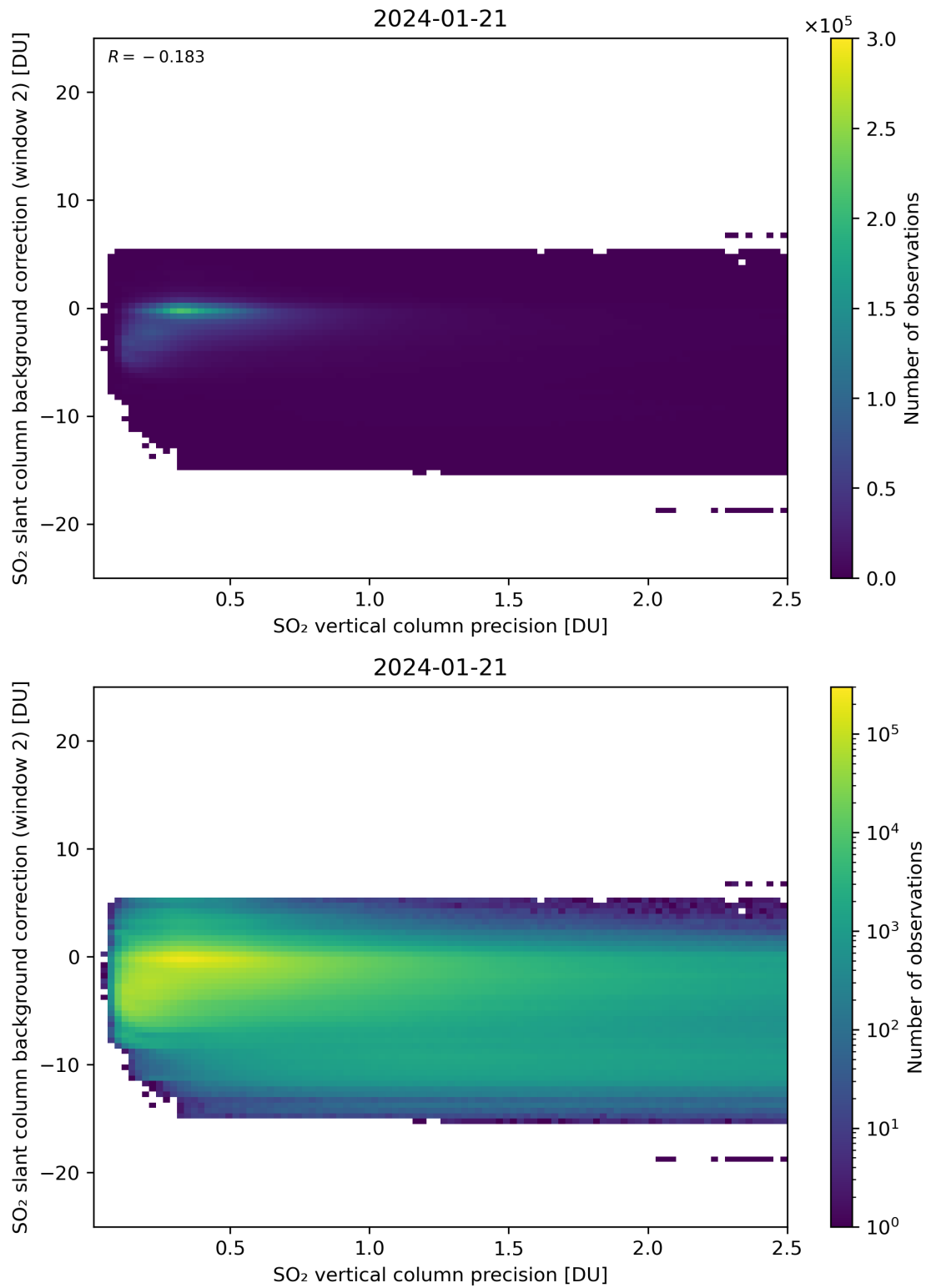
Figure 280: Scatter density plot of “SO 2 vertical column precision” against “SO 2 slant column background correction (window 2)” for 2024-01-21 to 2024-01-22.
