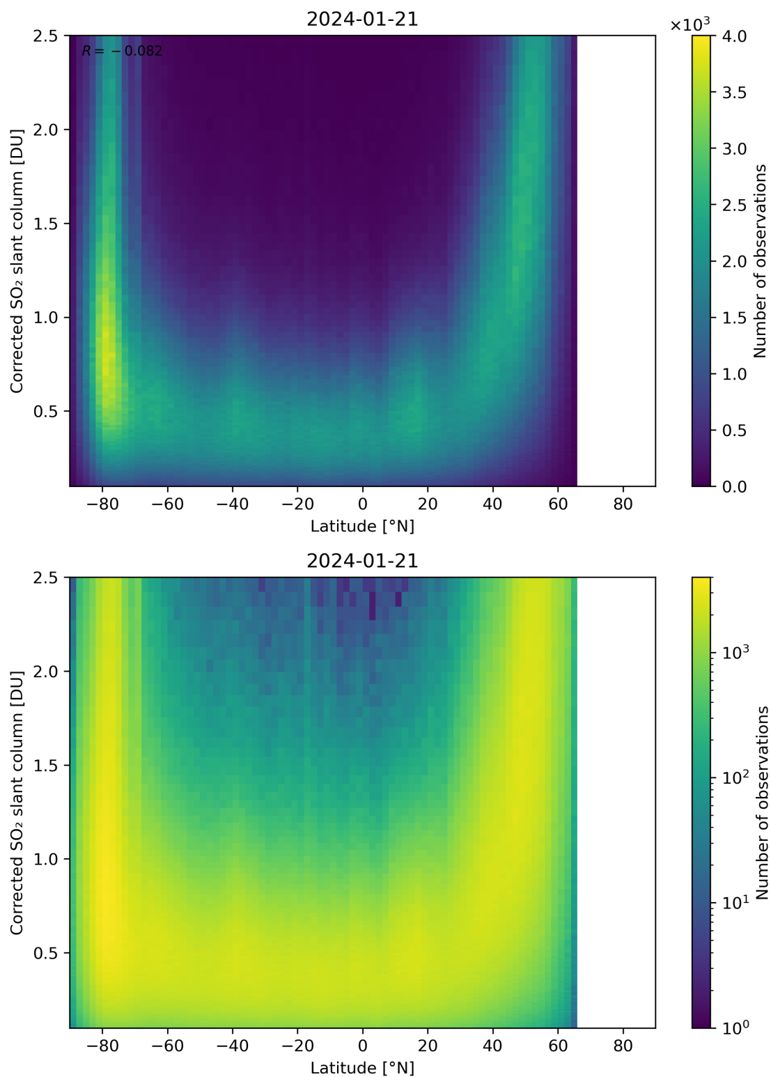
Figure 146: Scatter density plot of “Latitude” against “Corrected SO 2 slant column” for 2024-01-21 to 2024-01-22.
