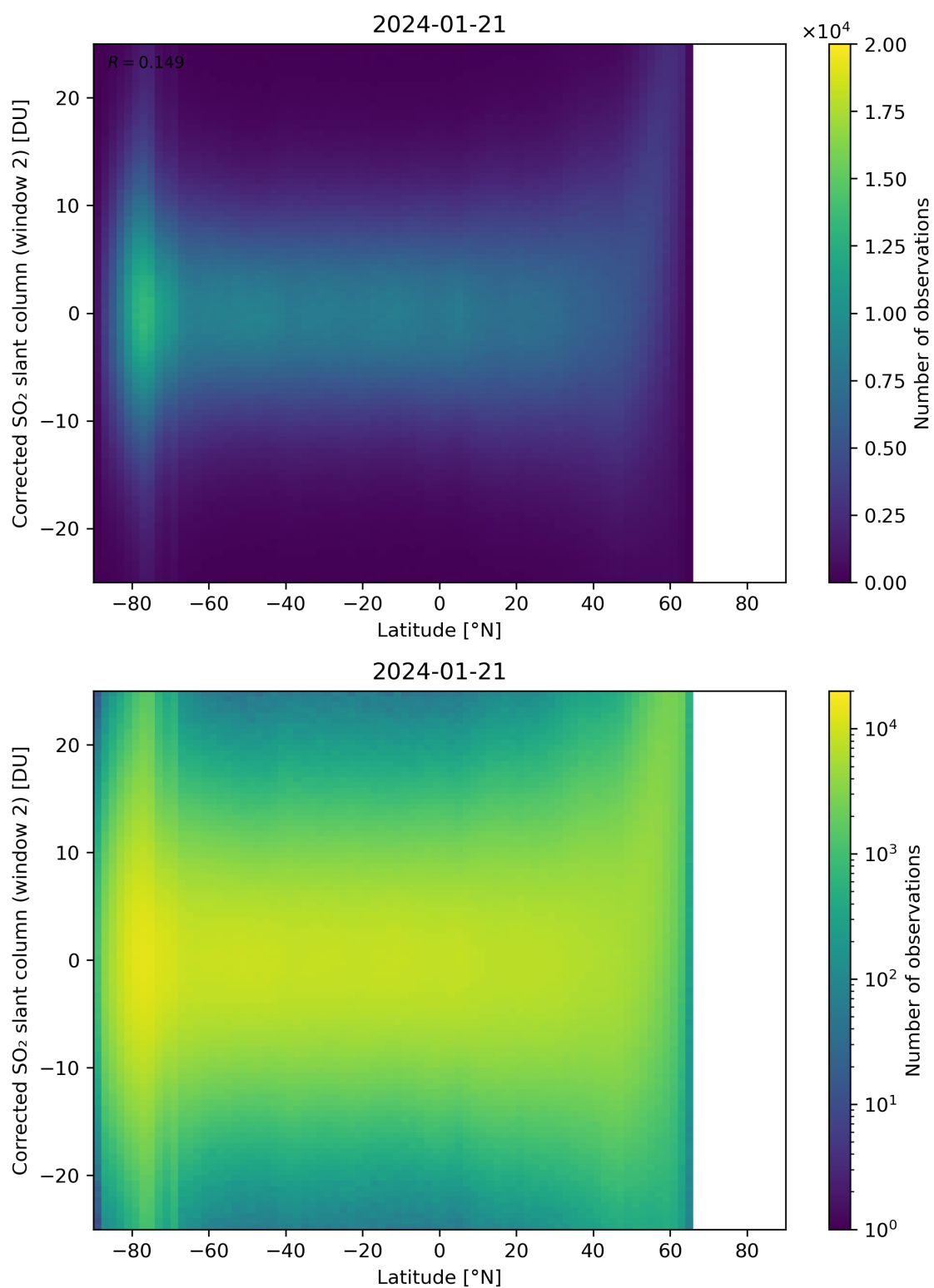
Figure 147: Scatter density plot of “Latitude” against “Corrected SO 2 slant column (window 2)” for 2024-01-21 to 2024-01-22.
