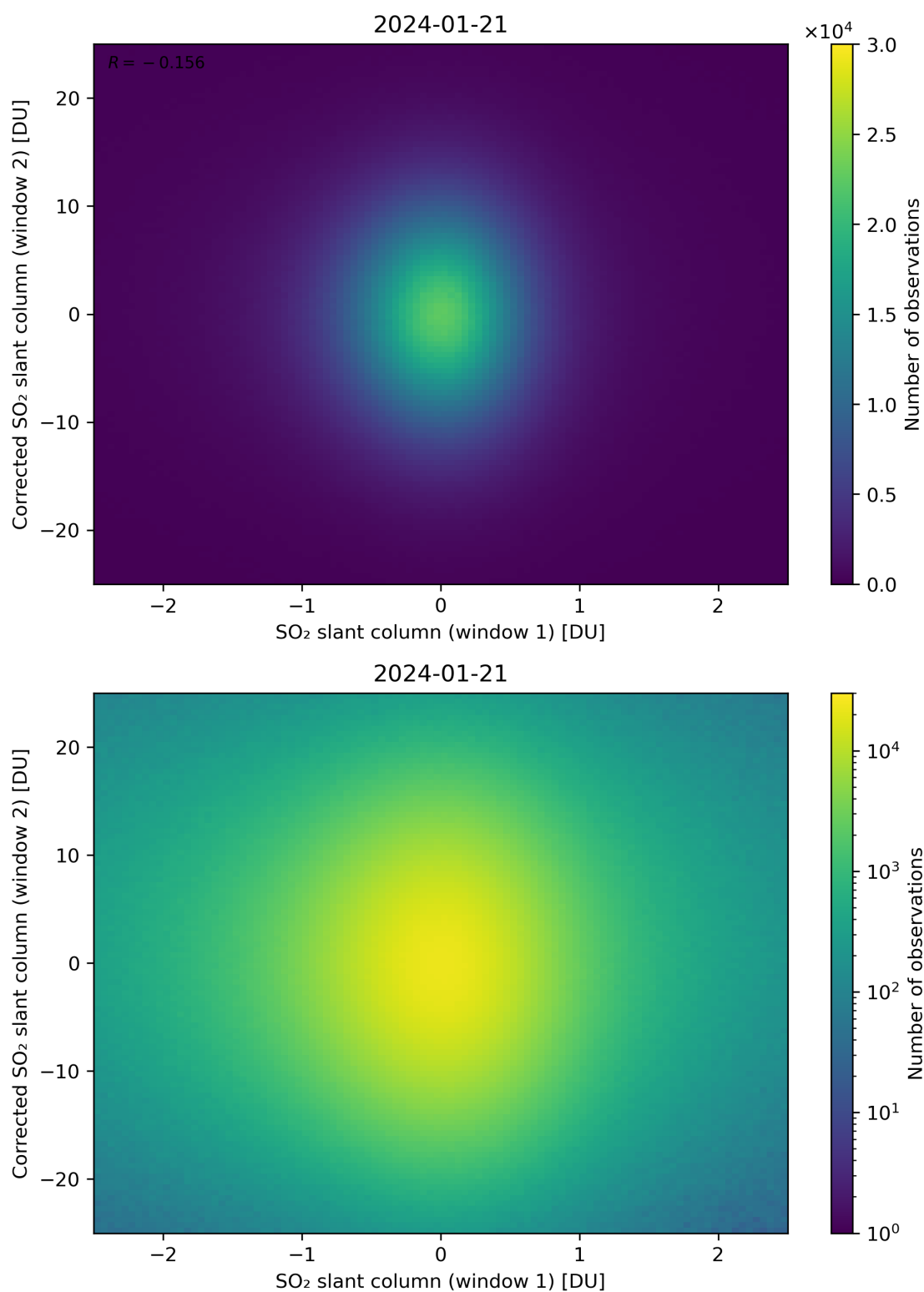
Figure 233: Scatter density plot of “SO 2 slant column (window 1)” against “Corrected SO 2 slant column (window 2)” for 2024-01-21 to 2024-01-22.
