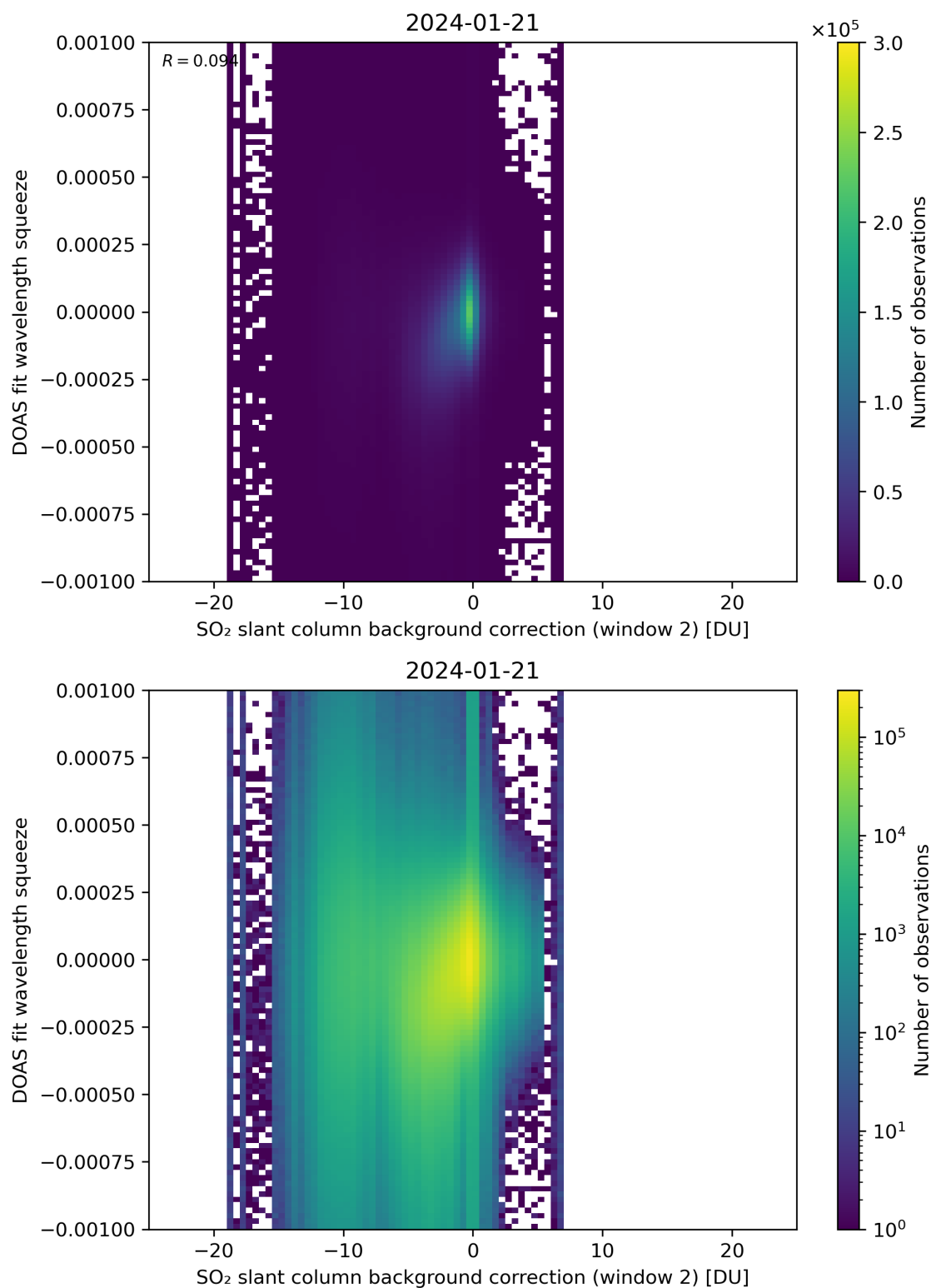
Figure 113: Scatter density plot of “SO 2 slant column background correction (window 2)” against “DOAS fit wavelength squeeze” for 2024-01-21 to 2024-01-22.
