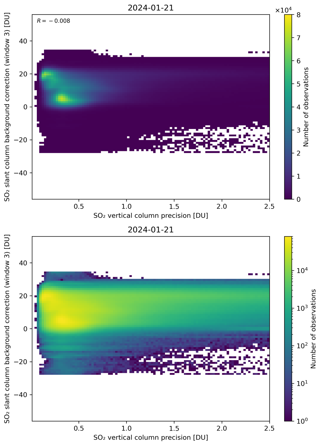
Figure 281: Scatter density plot of “SO 2 vertical column precision” against “SO 2 slant column background correction (window 3)” for 2024-01-21 to 2024-01-22.
