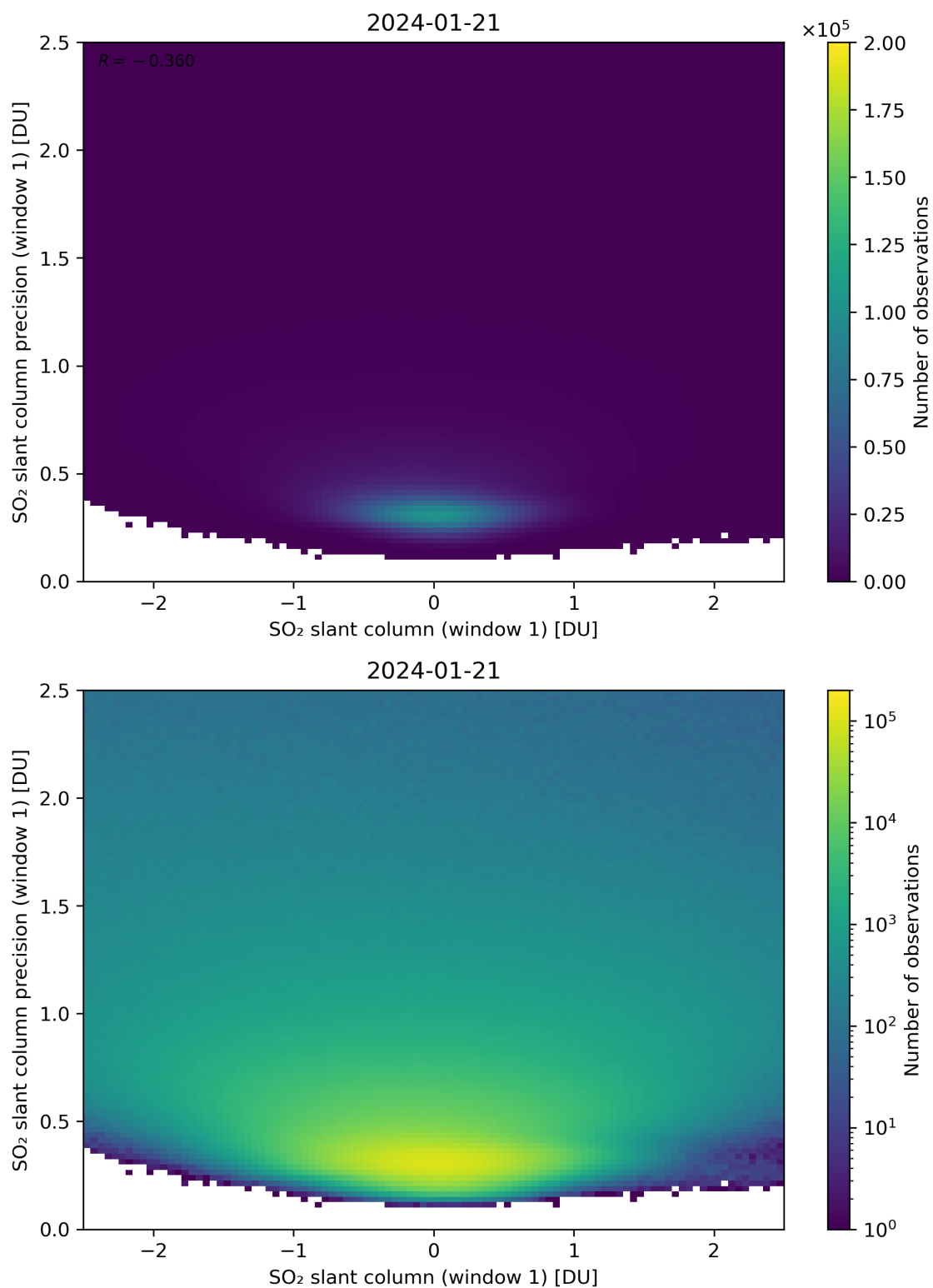
Figure 235: Scatter density plot of “SO 2 slant column (window 1)” against “SO 2 slant column precision (window 1)” for 2024-01-21 to 2024-01-22.
