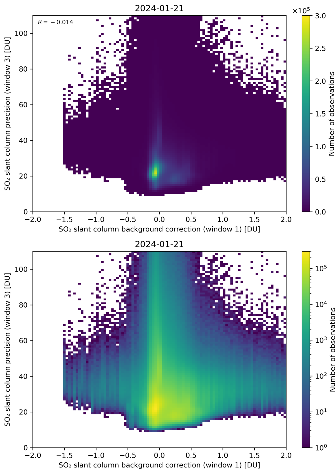
Figure 108: Scatter density plot of “SO 2 slant column background correction (window 1)” against “SO 2 slant column precision (window 3)” for 2024-01-21 to 2024-01-22.
