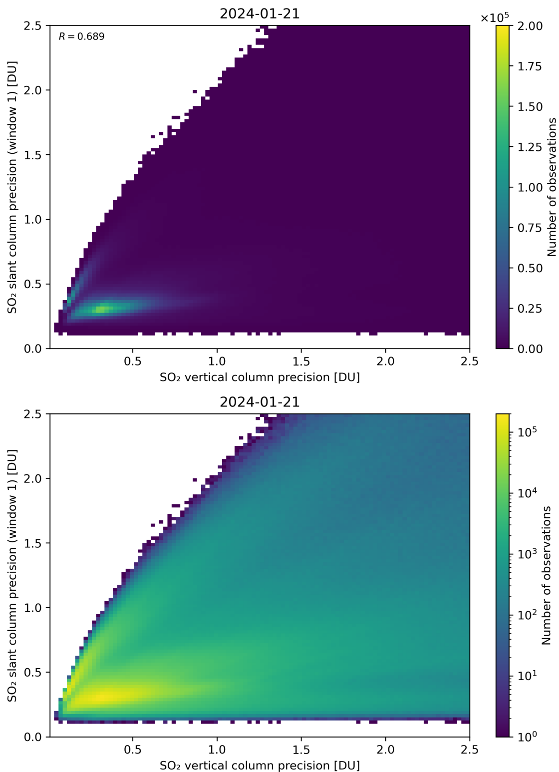
Figure 290: Scatter density plot of “SO 2 vertical column precision” against “SO 2 slant column precision (window 1)” for 2024-01-21 to 2024-01-22.
