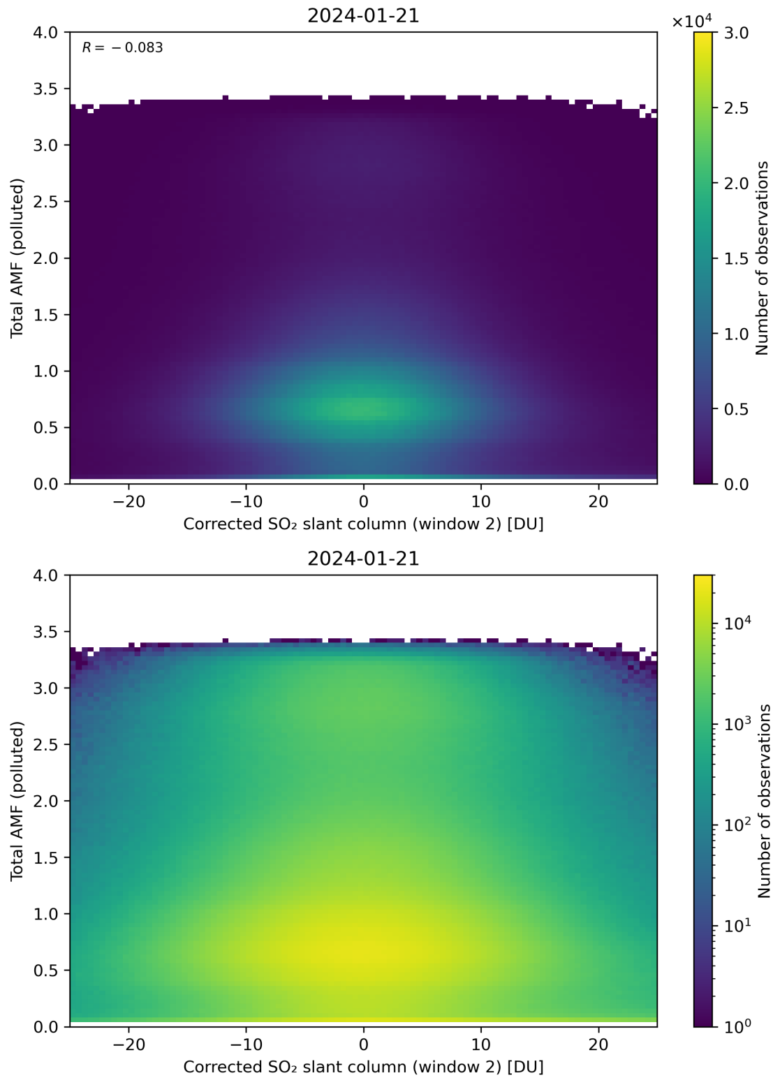
Figure 203: Scatter density plot of “Corrected SO 2 slant column (window 2)” against “Total AMF (polluted)” for 2024-01-21 to 2024-01-22.
