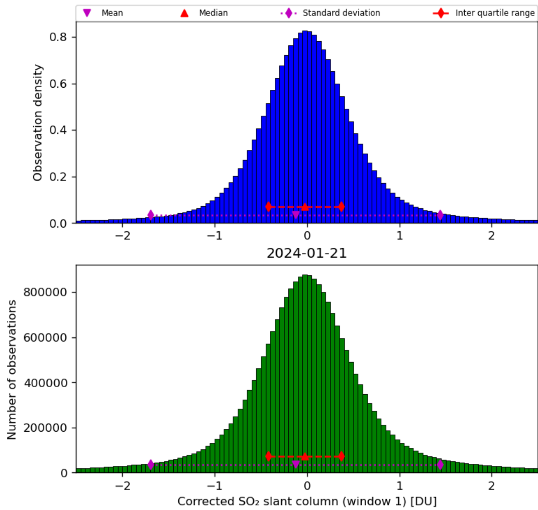
Figure 58: Histogram of “Corrected SO 2 slant column (window 1)” for 2024-01-21 to 2024-01-22
