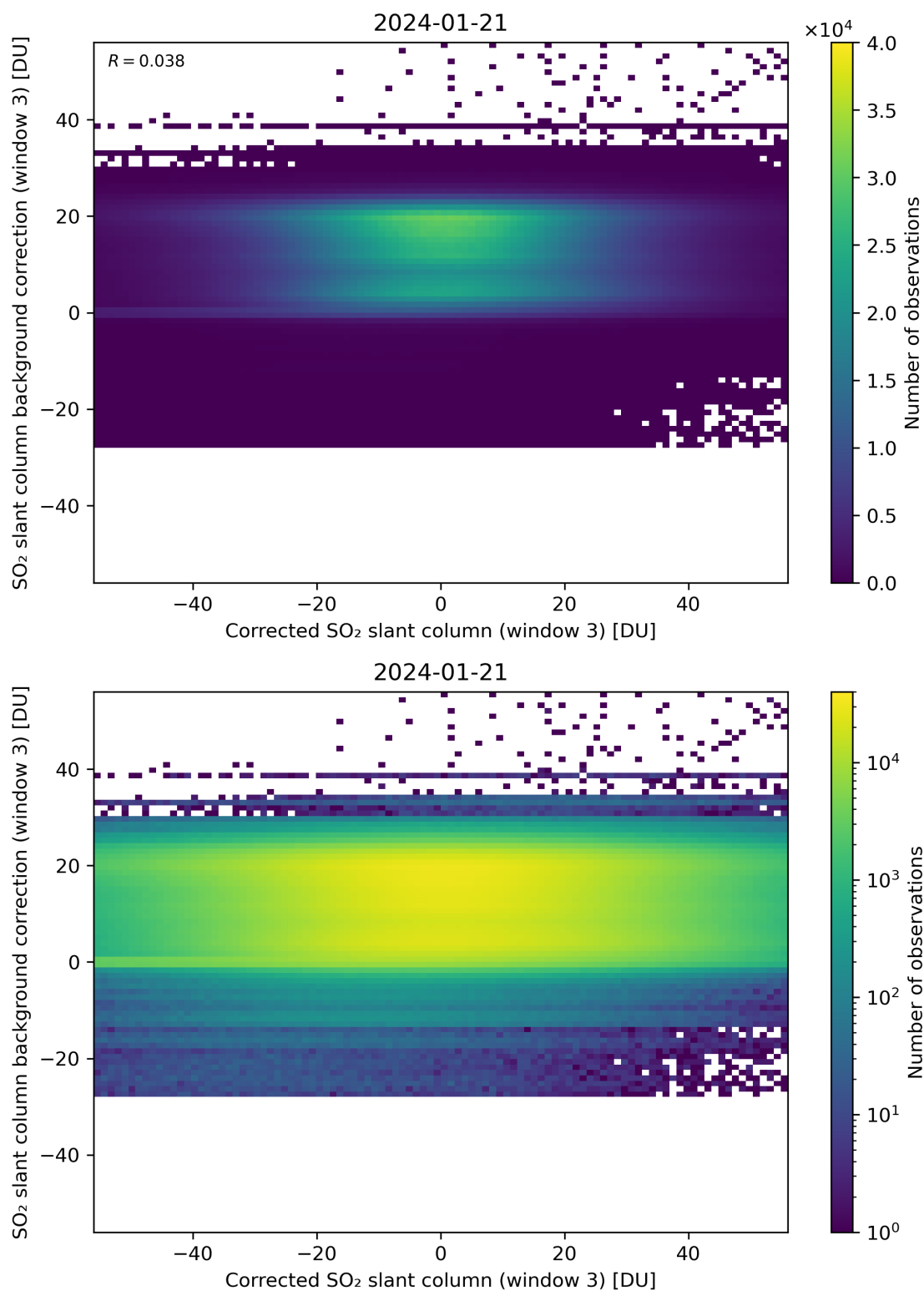
Figure 205: Scatter density plot of “Corrected SO 2 slant column (window 3)” against “SO 2 slant column background correction (window 3)” for 2024-01-21 to 2024-01-22.
