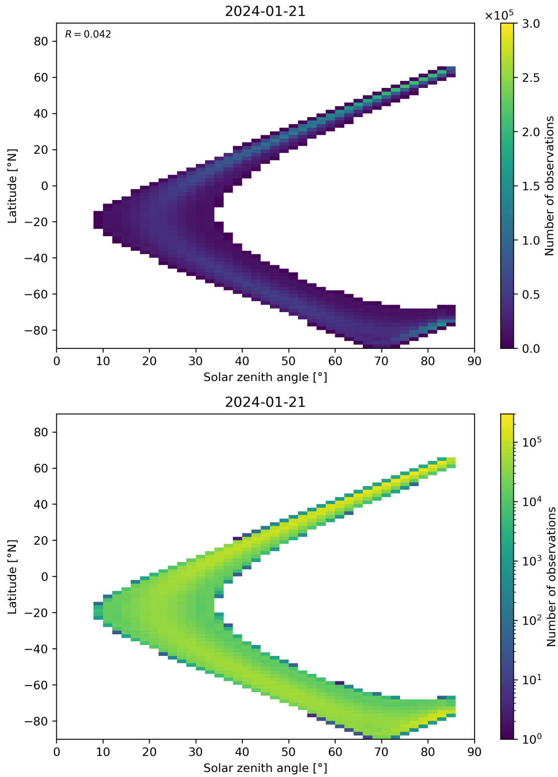
Figure 164: Scatter density plot of “Solar zenith angle” against “Latitude” for 2024-01-21 to 2024-01-22.
