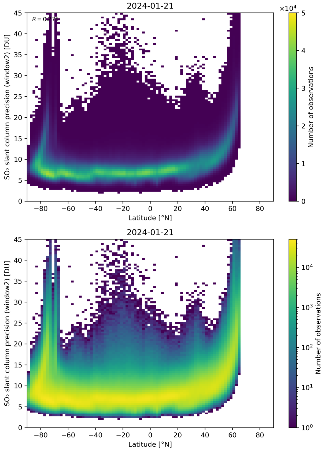
Figure 151: Scatter density plot of “Latitude” against “SO 2 slant column precision (window2)” for 2024-01-21 to 2024-01-22.
