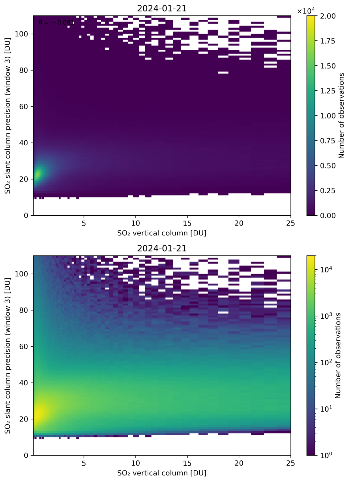
Figure 304: Scatter density plot of “SO 2 vertical column” against “SO 2 slant column precision (window 3)” for 2024-01-21 to 2024-01-22.
