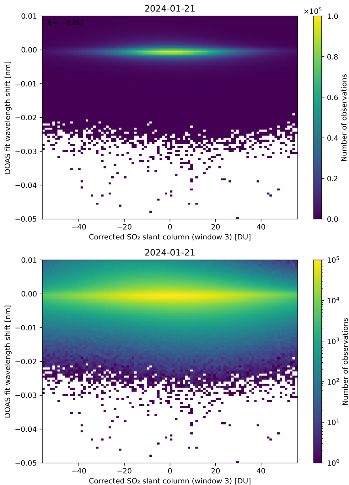
Figure 206: Scatter density plot of “Corrected SO 2 slant column (window 3)” against “DOAS fit wavelength shift” for 2024-01-21 to 2024-01-22.
