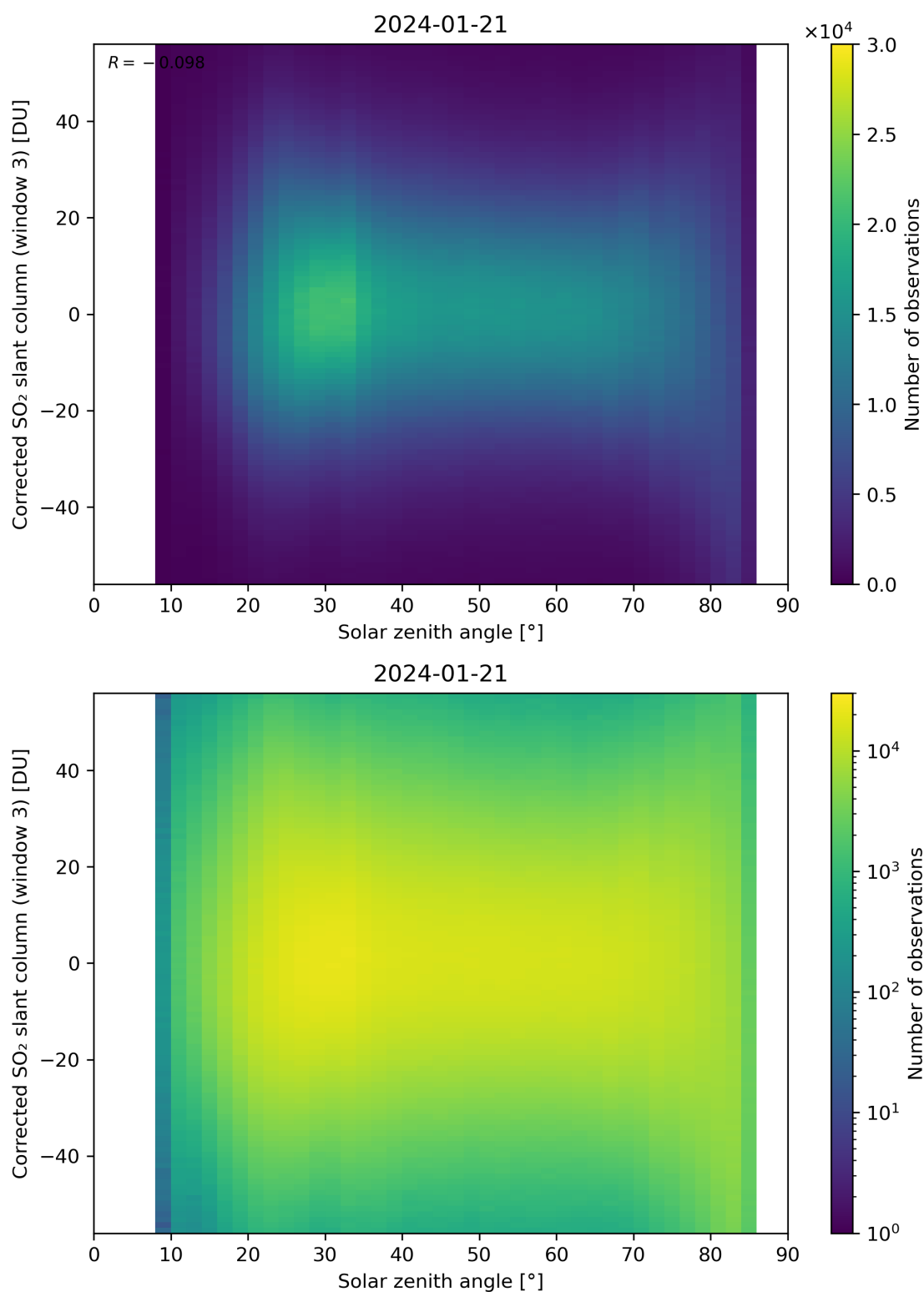
Figure 168: Scatter density plot of “Solar zenith angle” against “Corrected SO 2 slant column (window 3)” for 2024-01-21 to 2024-01-22.
