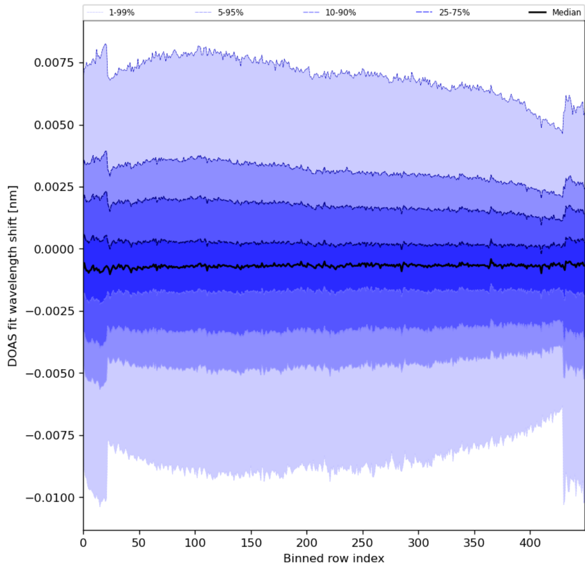
Figure 91: Along track statistics of “DOAS fit wavelength shift” for 2024-01-21 to 2024-01-22
