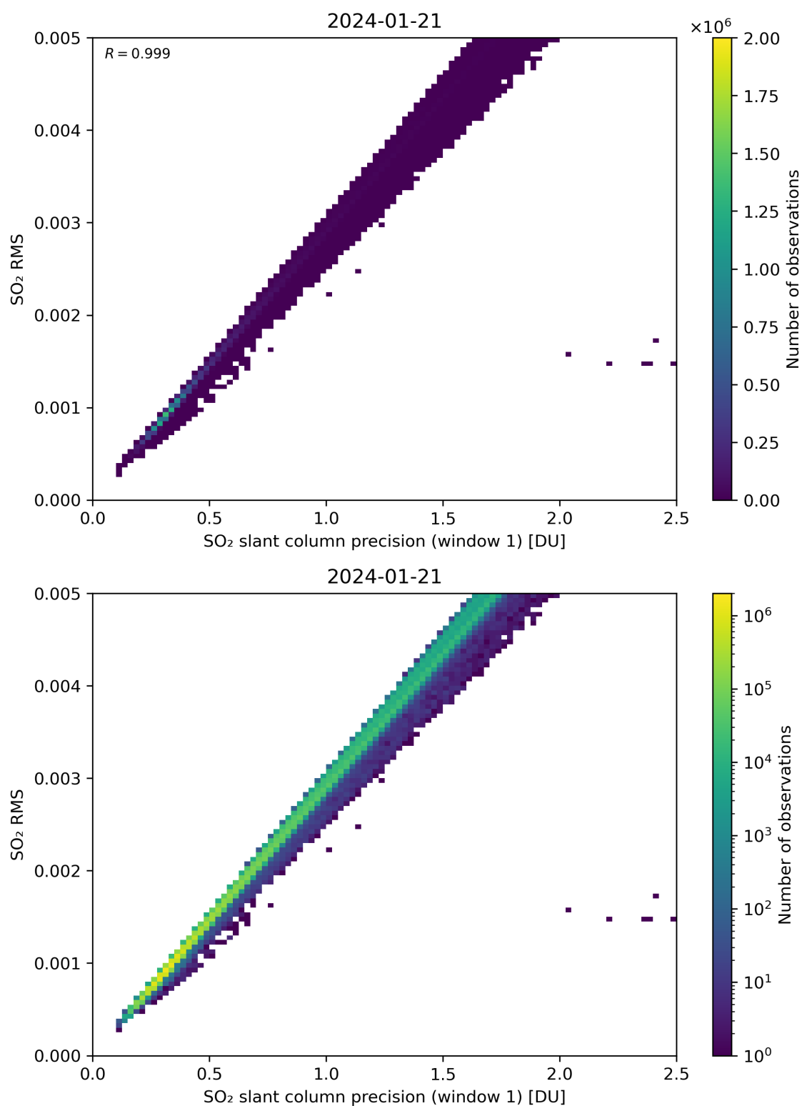
Figure 223: Scatter density plot of “SO 2 slant column precision (window 1)” against “SO 2 RMS” for 2024-01-21 to 2024-01-22.
