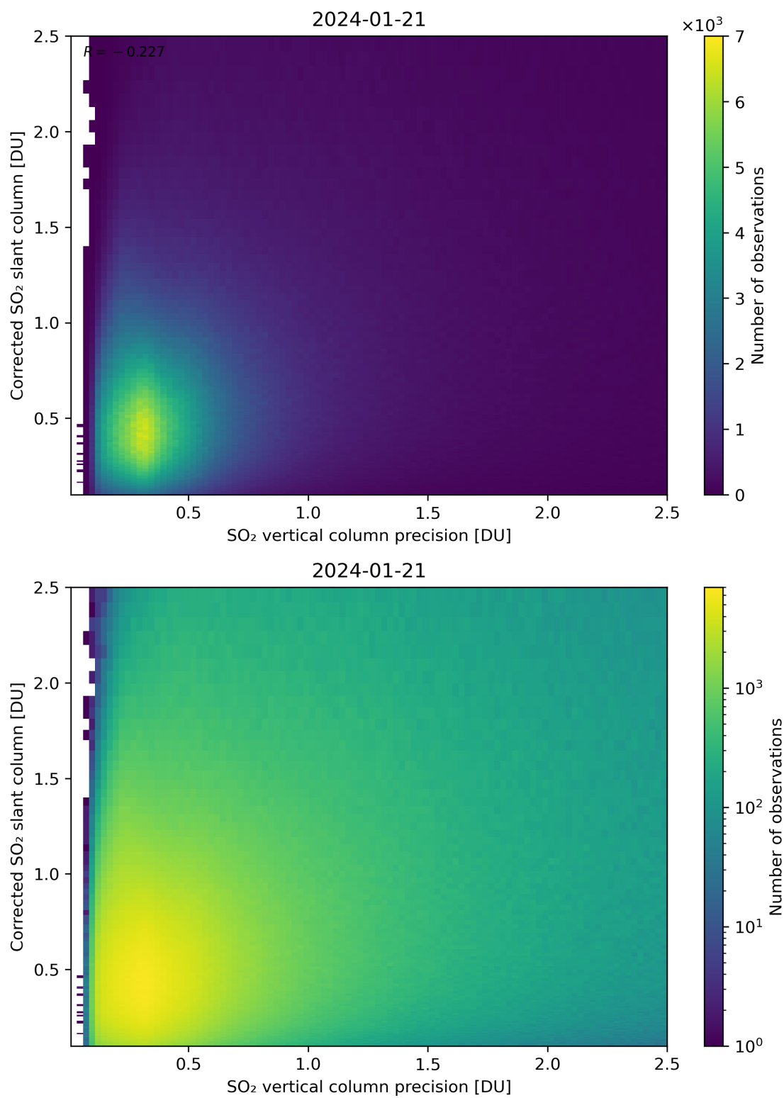
Figure 286: Scatter density plot of “SO 2 vertical column precision” against “Corrected SO 2 slant column” for 2024-01-21 to 2024-01-22.
