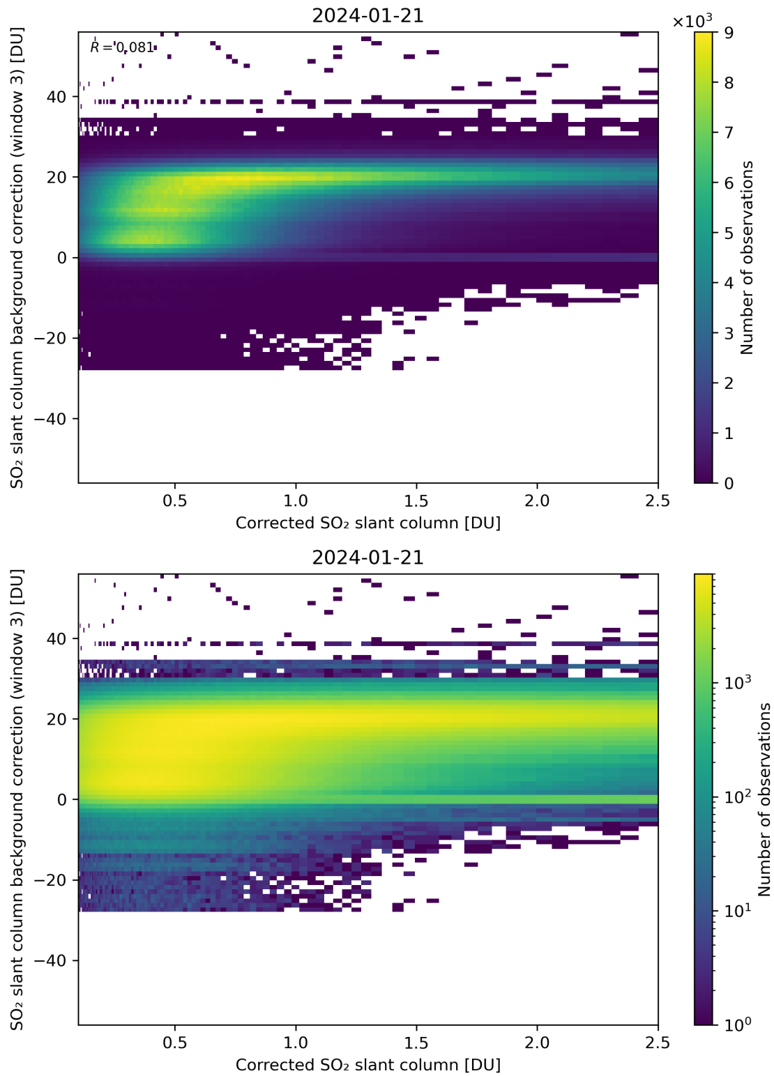
Figure 180: Scatter density plot of “Corrected SO 2 slant column” against “SO 2 slant column background correction (window 3)” for 2024-01-21 to 2024-01-22.
