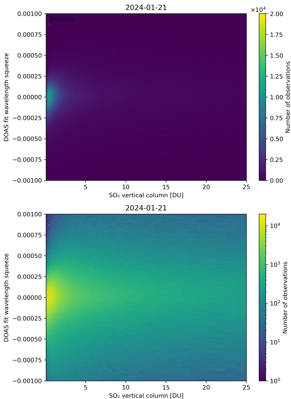
Figure 277: Scatter density plot of “SO 2 vertical column” against “DOAS fit wavelength squeeze” for 2024-01-21 to 2024-01-22.
