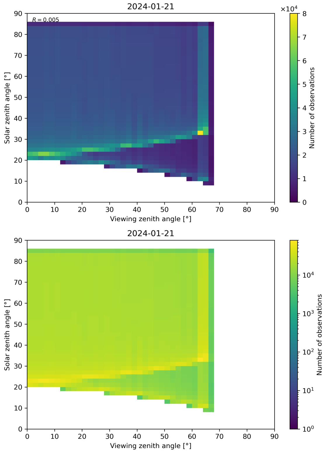
Figure 315: Scatter density plot of “Viewing zenith angle” against “Solar zenith angle” for 2024-01-21 to 2024-01-22.
