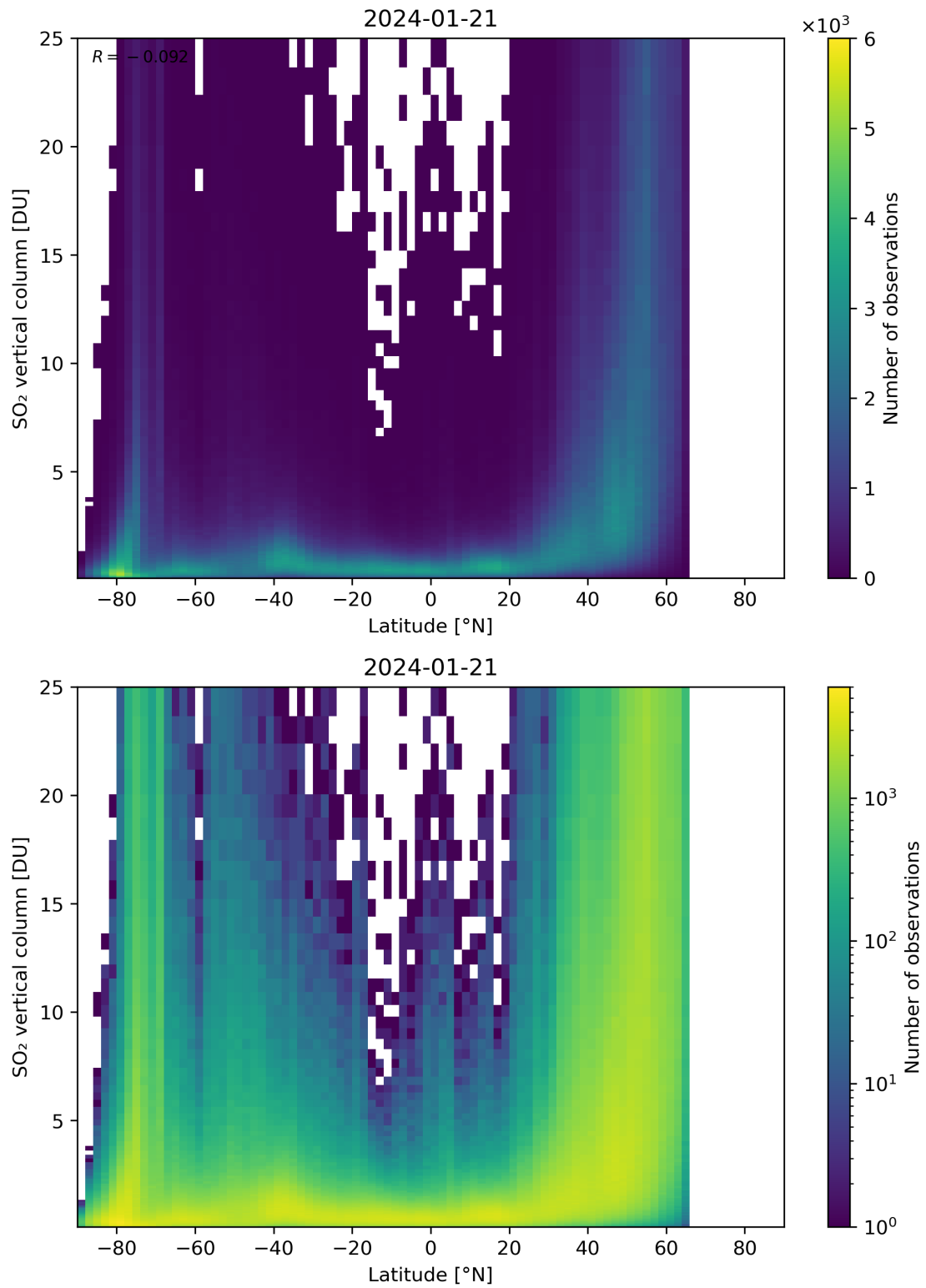
Figure 156: Scatter density plot of “Latitude” against “SO 2 vertical column” for 2024-01-21 to 2024-01-22.
