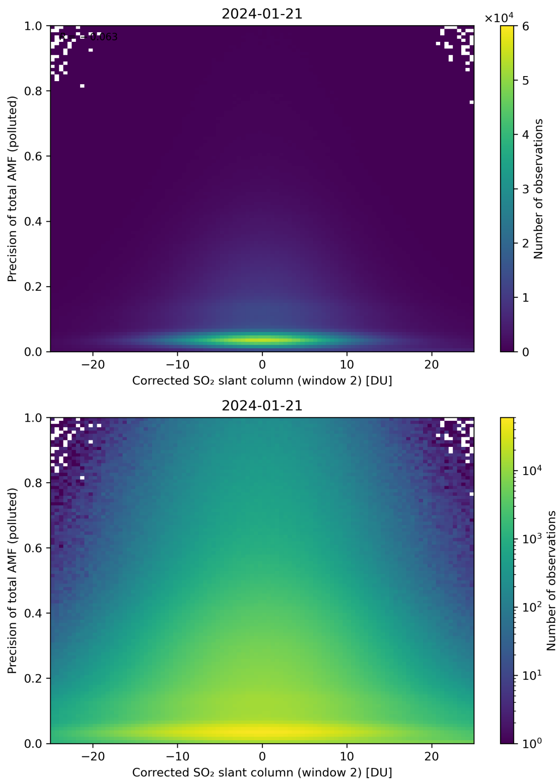
Figure 204: Scatter density plot of “Corrected SO 2 slant column (window 2)” against “Precision of total AMF (polluted)” for 2024-01-21 to 2024-01-22.
