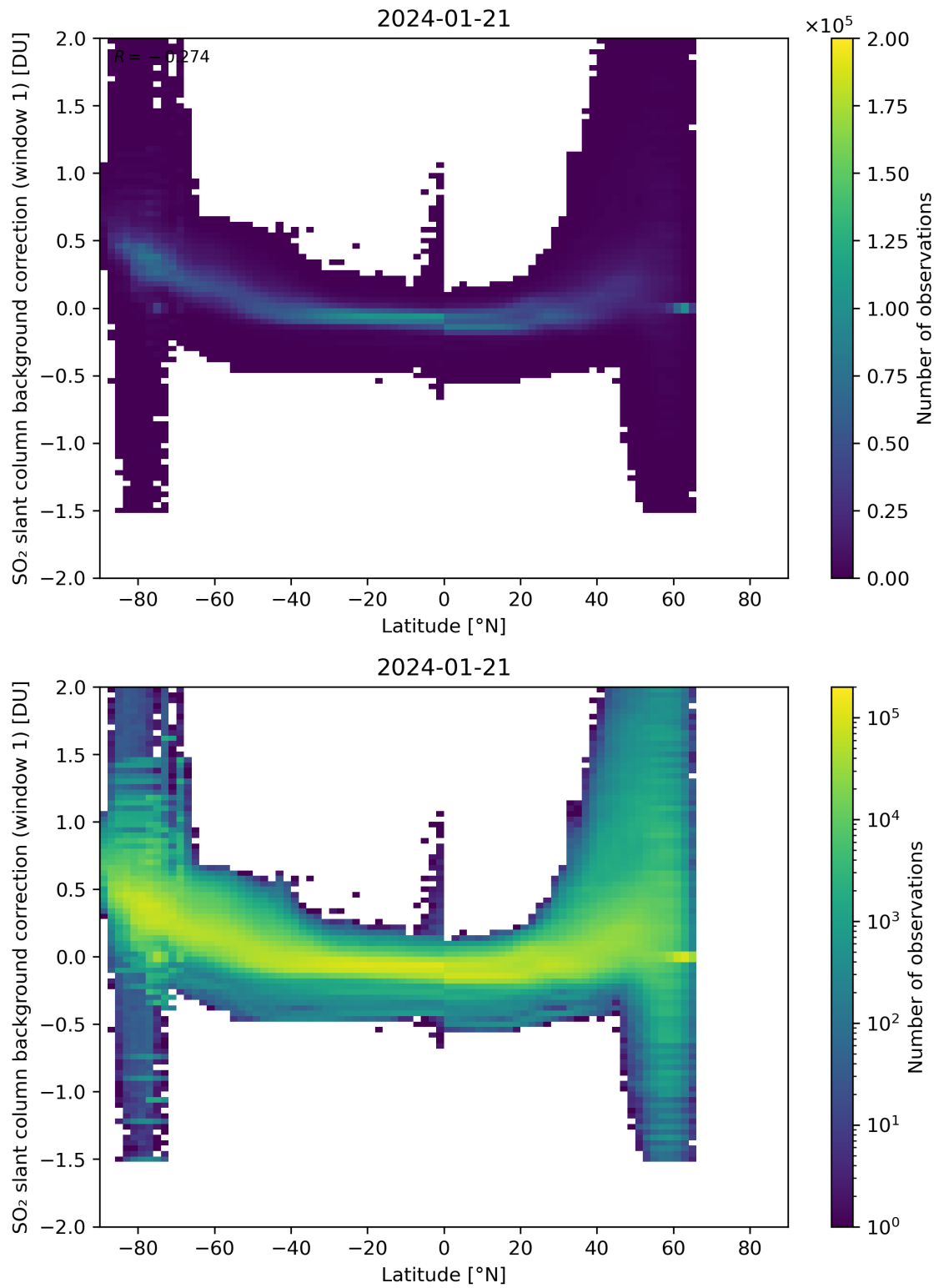
Figure 139: Scatter density plot of “Latitude” against “SO 2 slant column background correction (window 1)” for 2024-01-21 to 2024-01-22.
