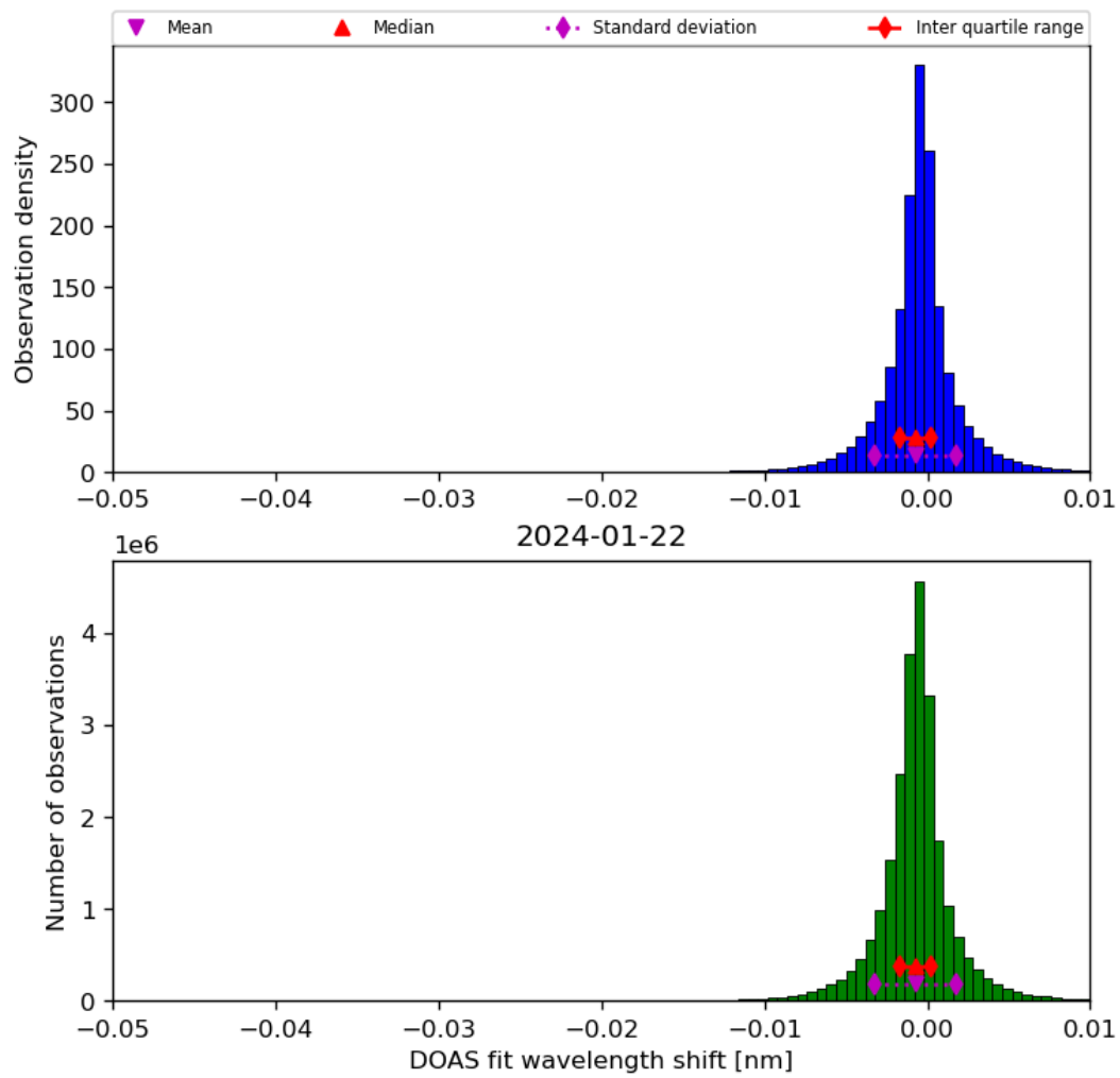
Figure 68: Histogram of “DOAS fit wavelength shift” for 2024-01-21 to 2024-01-23
