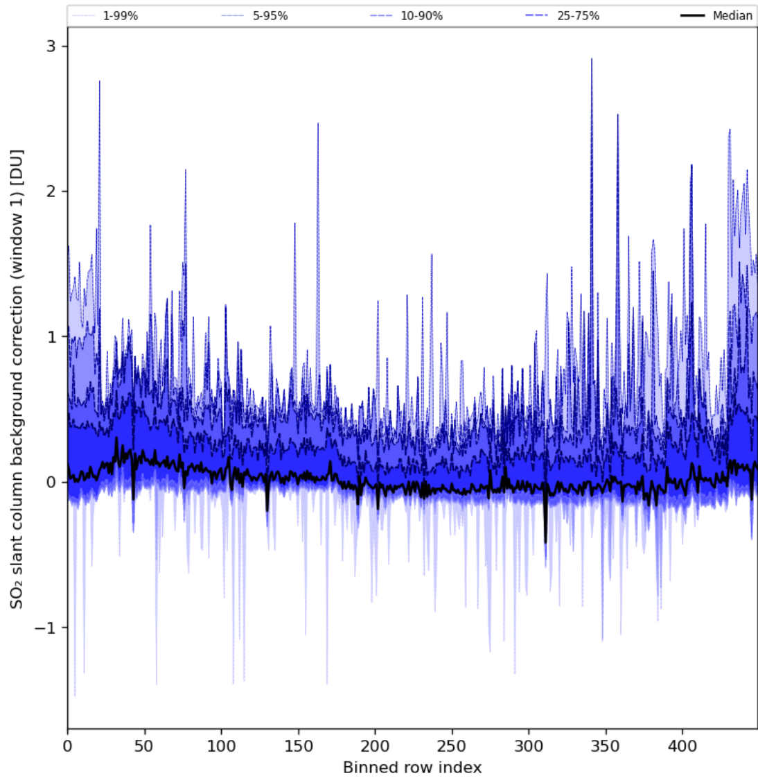
Figure 82: Along track statistics of “SO 2 slant column background correction (window 1)” for 2024-01-21 to 2024-01-23
