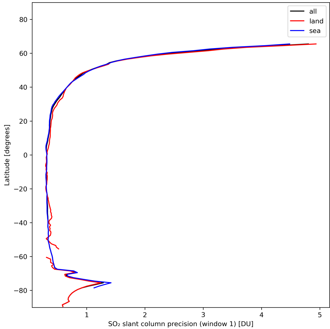
Figure 34: Zonal average of “SO 2 slant column precision (window 1)” for 2024-01-21 to 2024-01-23.
