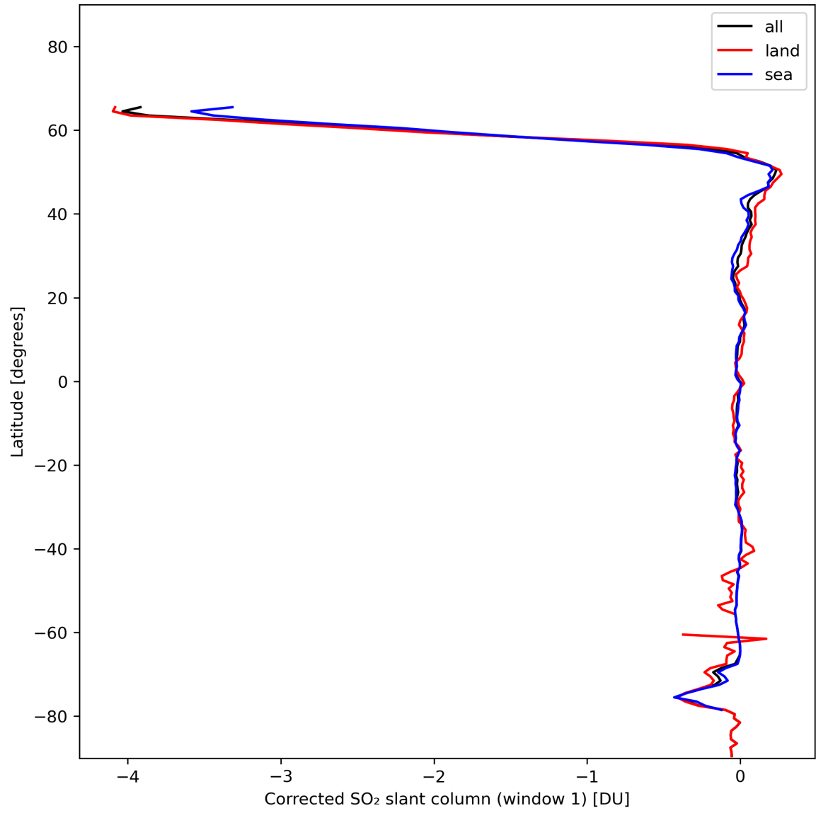
Figure 35: Zonal average of “Corrected SO 2 slant column (window 1)” for 2024-01-21 to 2024-01-23.
