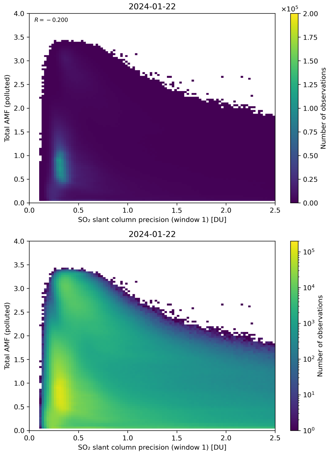
Figure 230: Scatter density plot of “SO 2 slant column precision (window 1)” against “Total AMF (polluted)” for 2024-01-21 to 2024-01-23.
