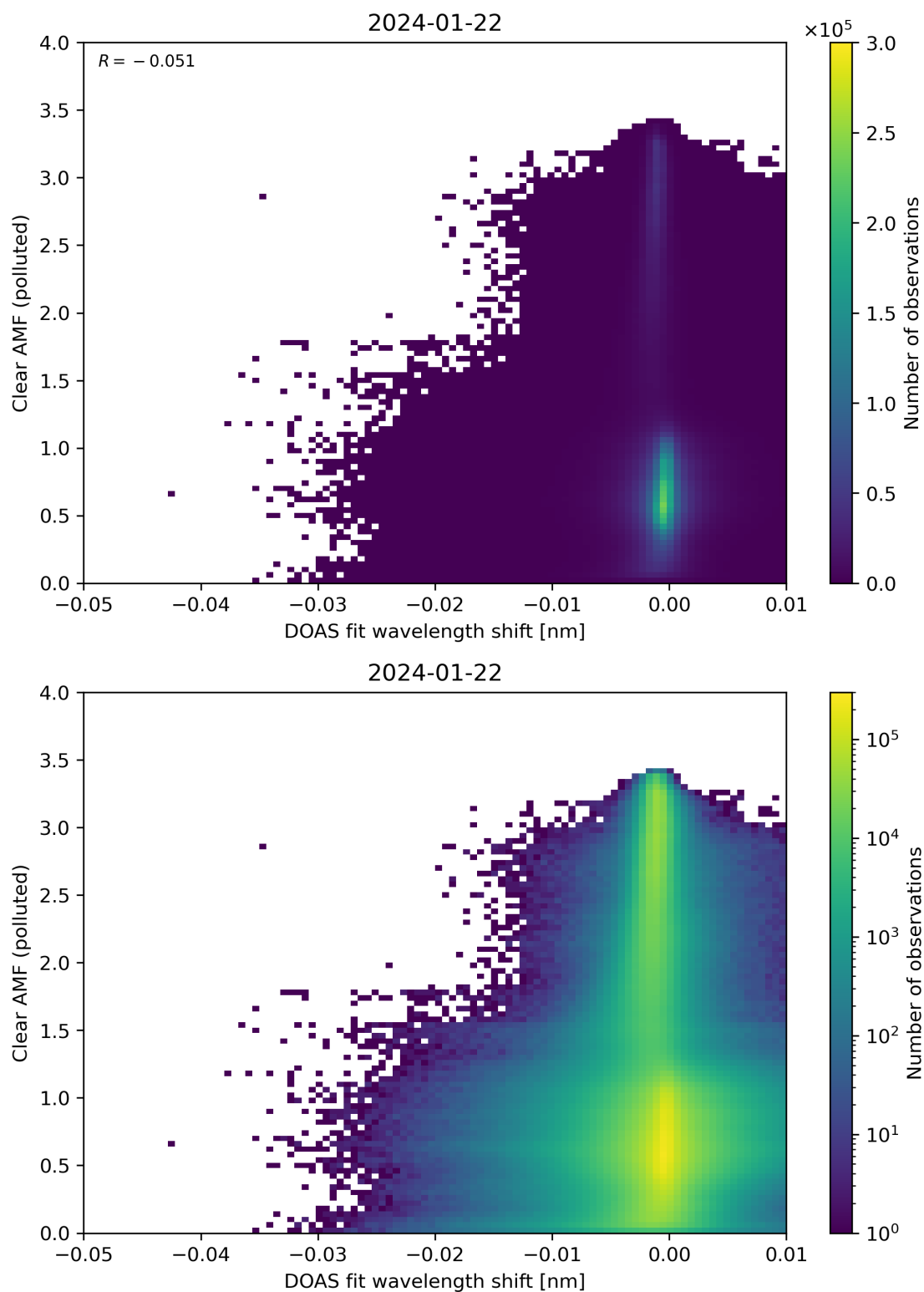
Figure 129: Scatter density plot of “DOAS fit wavelength shift” against “Clear AMF (polluted)” for 2024-01-21 to 2024-01-23.
