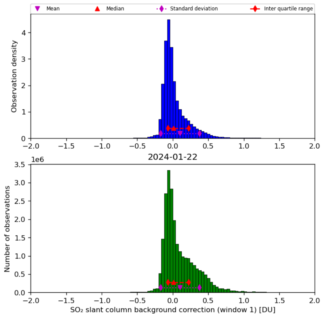
Figure 59: Histogram of “SO 2 slant column background correction (window 1)” for 2024-01-21 to 2024-01-23
