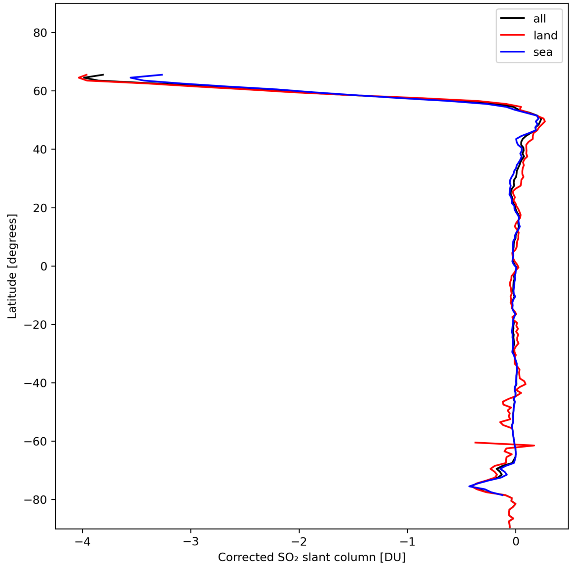
Figure 32: Zonal average of “Corrected SO 2 slant column” for 2024-01-21 to 2024-01-23.
