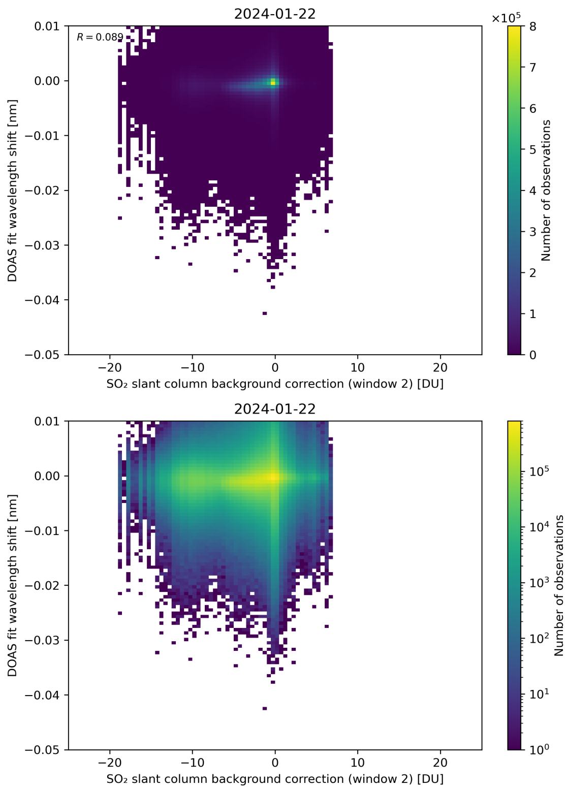
Figure 112: Scatter density plot of “SO 2 slant column background correction (window 2)” against “DOAS fit wavelength shift” for 2024-01-21 to 2024-01-23.
