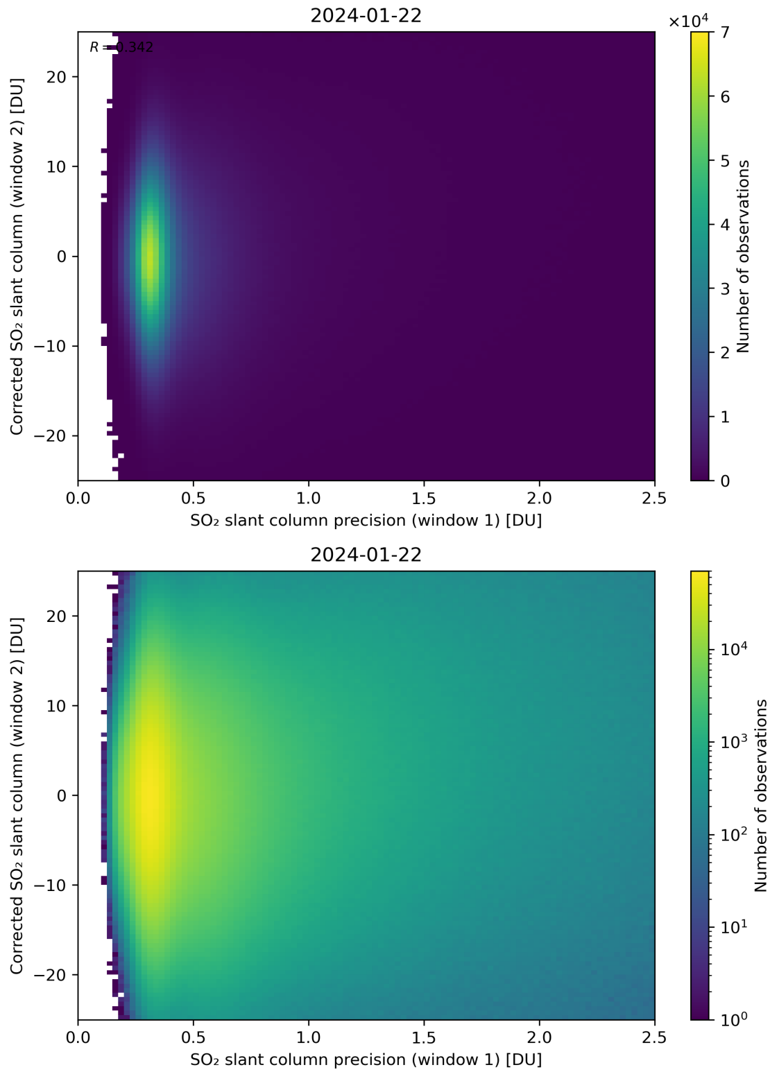
Figure 225: Scatter density plot of “SO 2 slant column precision (window 1)” against “Corrected SO 2 slant column (window 2)” for 2024-01-21 to 2024-01-23.
