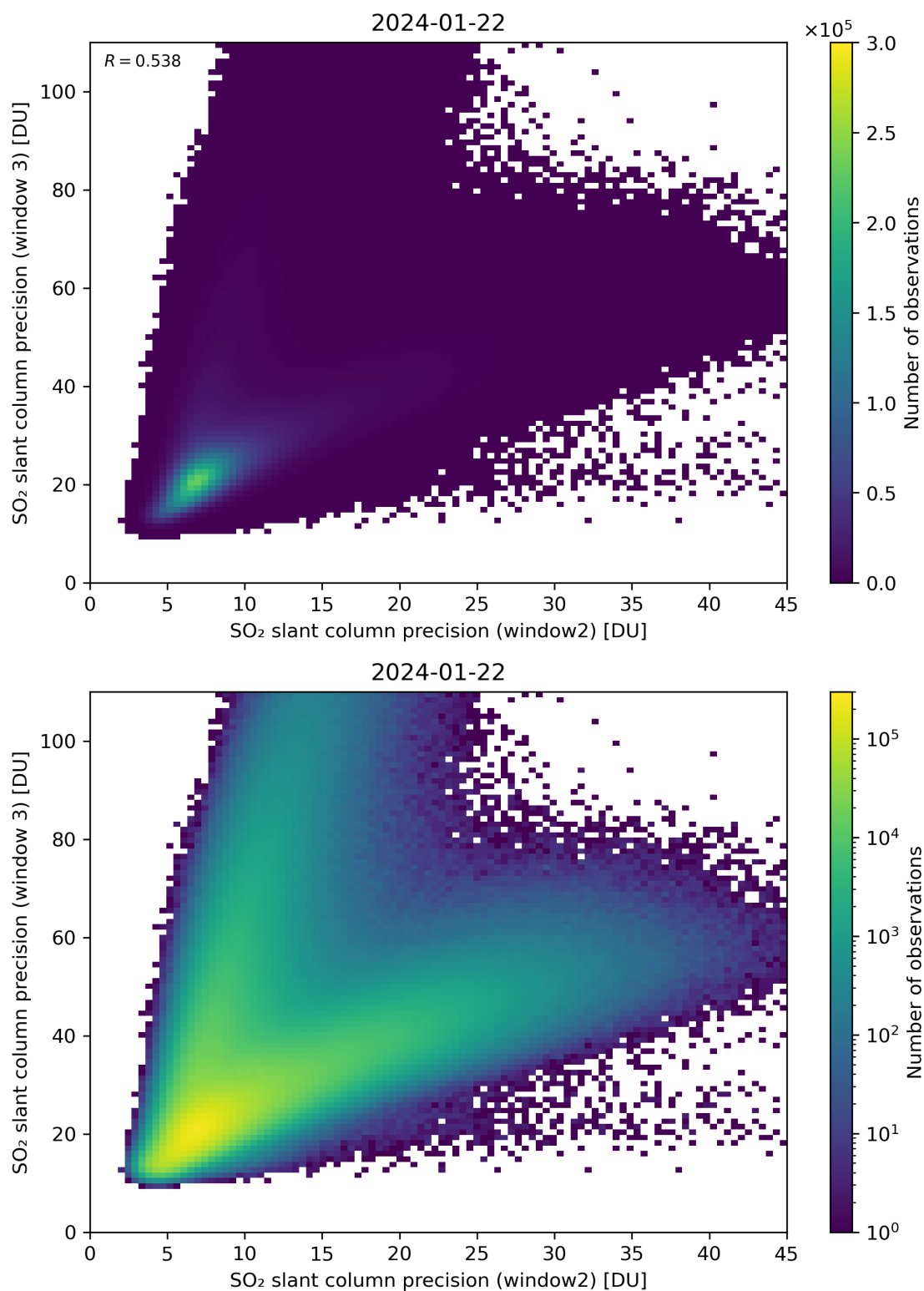
Figure 250: Scatter density plot of “SO 2 slant column precision (window2)” against “SO 2 slant column precision (window 3)” for 2024-01-21 to 2024-01-23.
