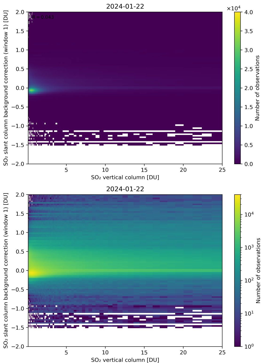
Figure 273: Scatter density plot of “SO 2 vertical column” against “SO 2 slant column background correction (window 1)” for 2024-01-21 to 2024-01-23.
