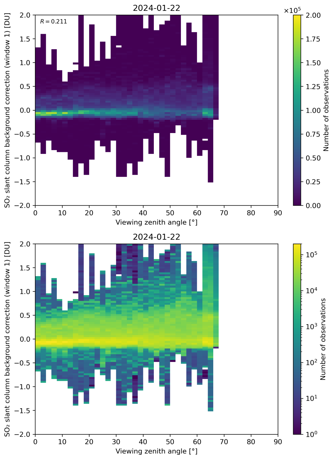
Figure 308: Scatter density plot of “Viewing zenith angle” against “SO 2 slant column background correction (window 1)” for 2024-01-21 to 2024-01-23.
