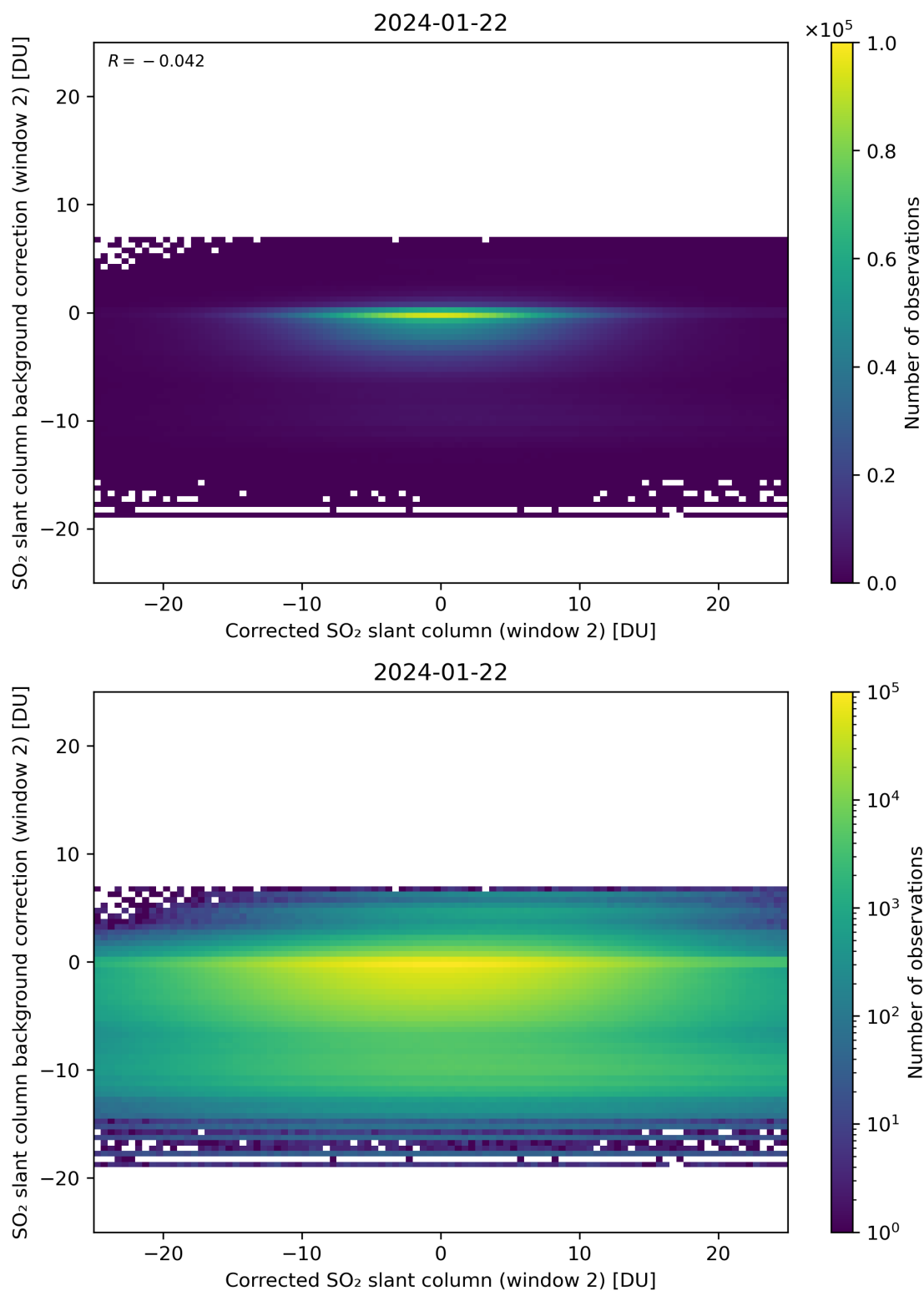
Figure 194: Scatter density plot of “Corrected SO 2 slant column (window 2)” against “SO 2 slant column background correction (window 2)” for 2024-01-21 to 2024-01-23.
