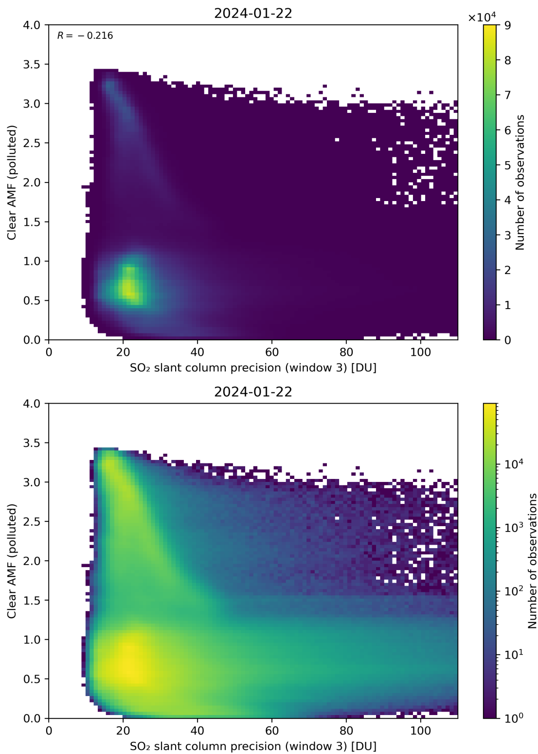
Figure 261: Scatter density plot of “SO 2 slant column precision (window 3)” against “Clear AMF (polluted)” for 2024-01-21 to 2024-01-23.
