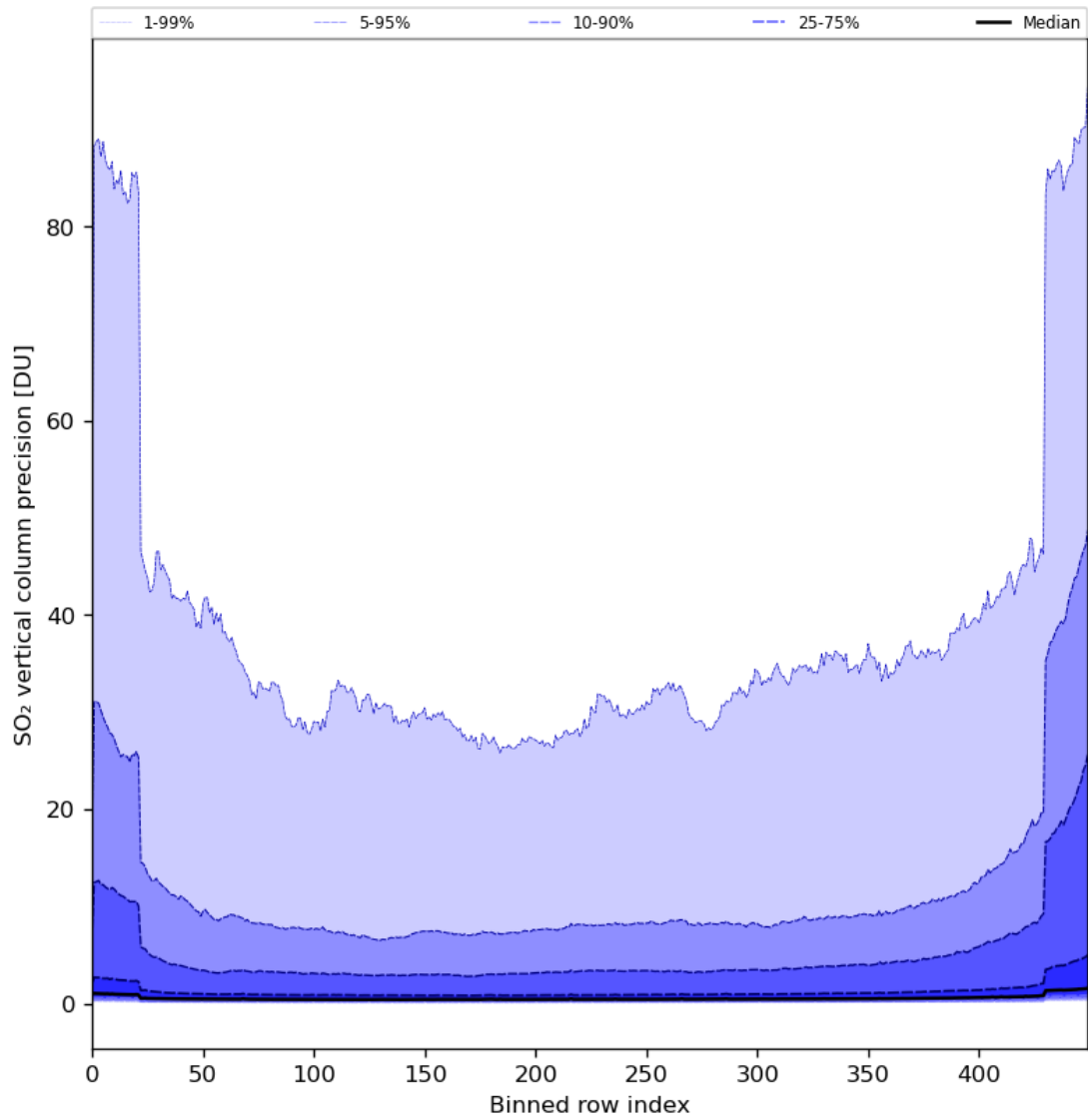
Figure 77: Along track statistics of “SO 2 vertical column precision” for 2024-01-21 to 2024-01-23
