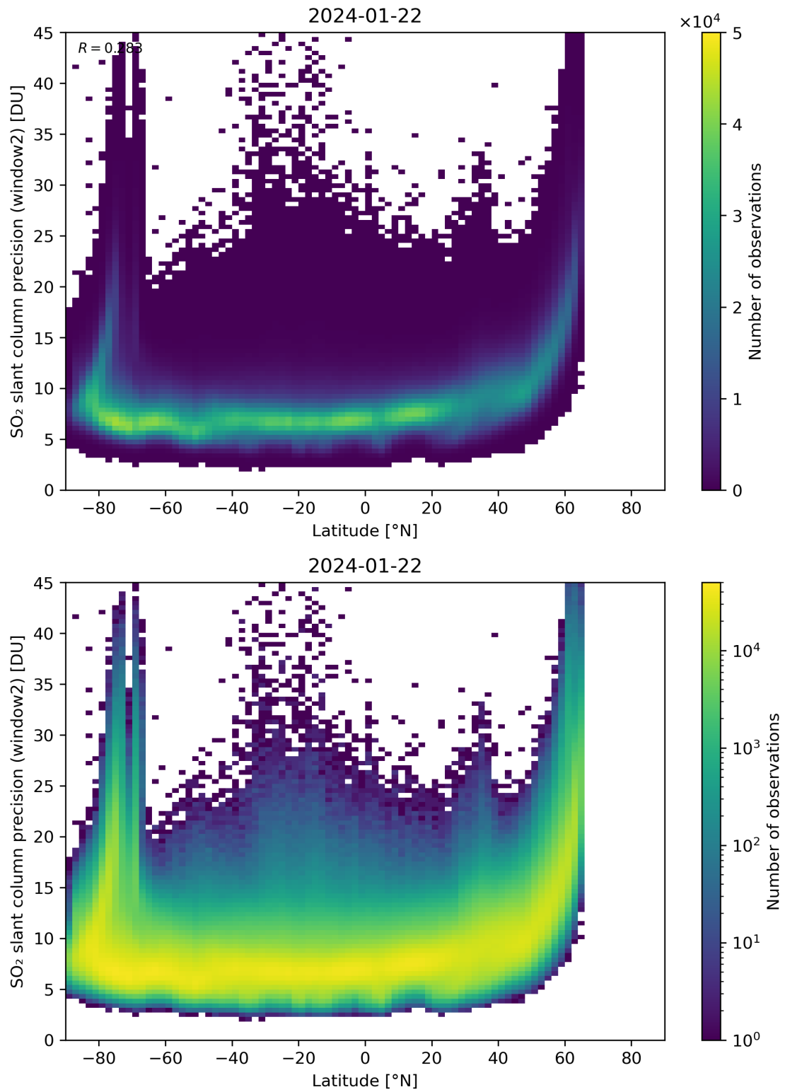
Figure 151: Scatter density plot of “Latitude” against “SO 2 slant column precision (window2)” for 2024-01-21 to 2024-01-23.
