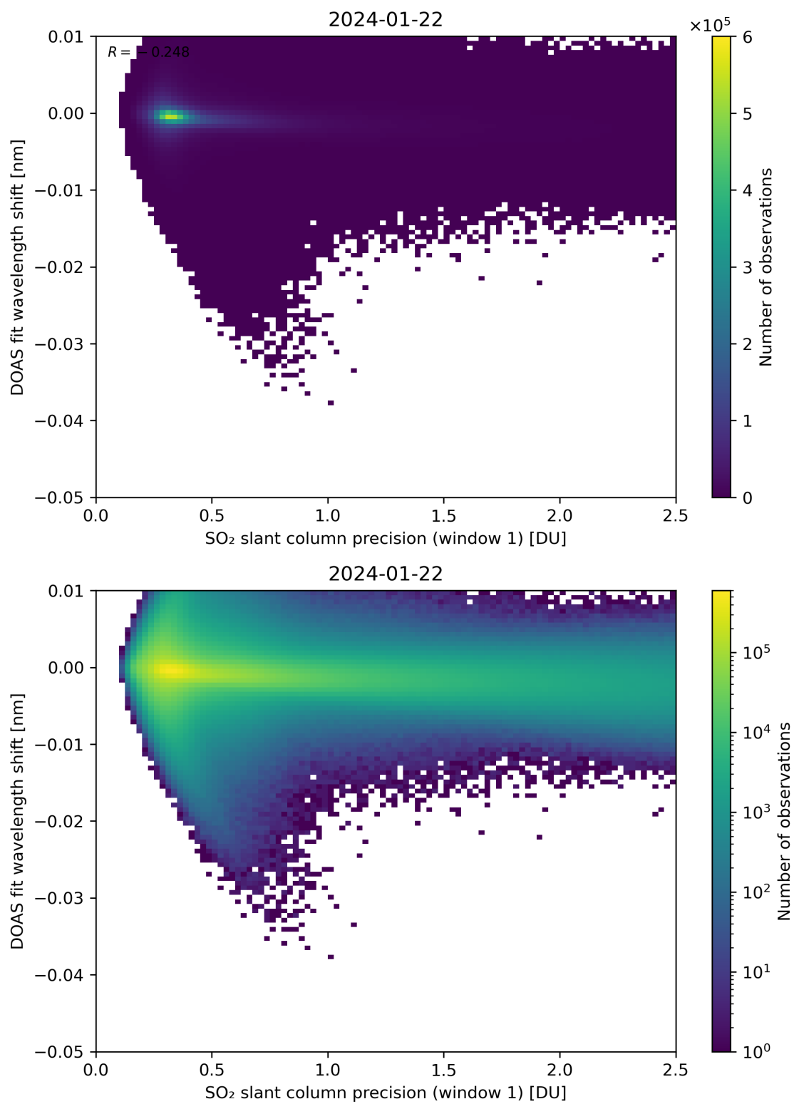
Figure 221: Scatter density plot of “SO 2 slant column precision (window 1)” against “DOAS fit wavelength shift” for 2024-01-21 to 2024-01-23.
