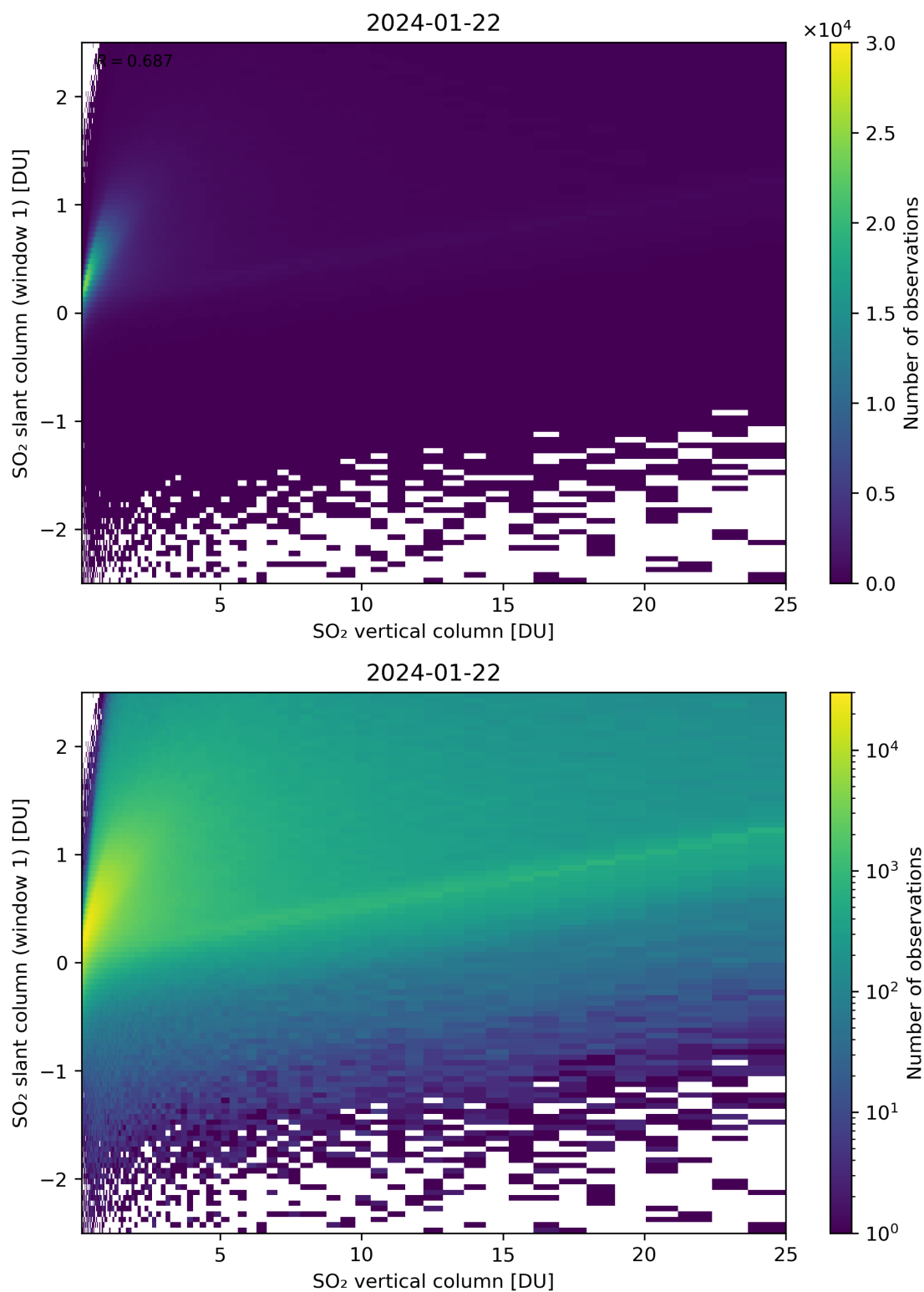
Figure 300: Scatter density plot of “SO 2 vertical column” against “SO 2 slant column (window 1)” for 2024-01-21 to 2024-01-23.
