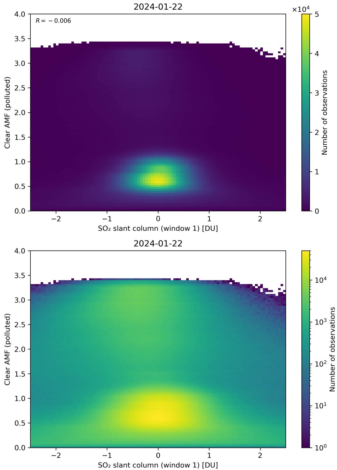
Figure 232: Scatter density plot of “SO 2 slant column (window 1)” against “Clear AMF (polluted)” for 2024-01-21 to 2024-01-23.
