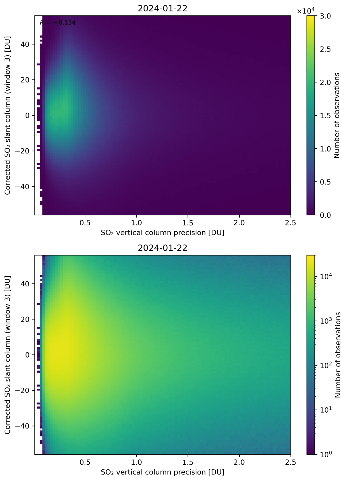
Figure 288: Scatter density plot of “SO 2 vertical column precision” against “Corrected SO 2 slant column (window 3)” for 2024-01-21 to 2024-01-23.
