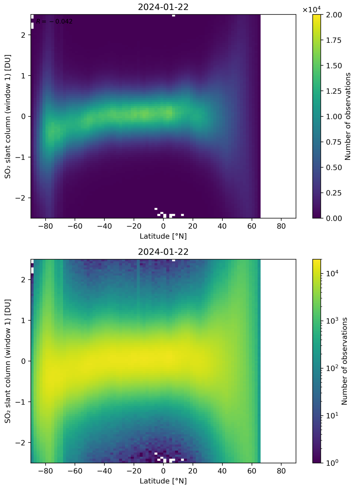
Figure 149: Scatter density plot of “Latitude” against “SO 2 slant column (window 1)” for 2024-01-21 to 2024-01-23.
