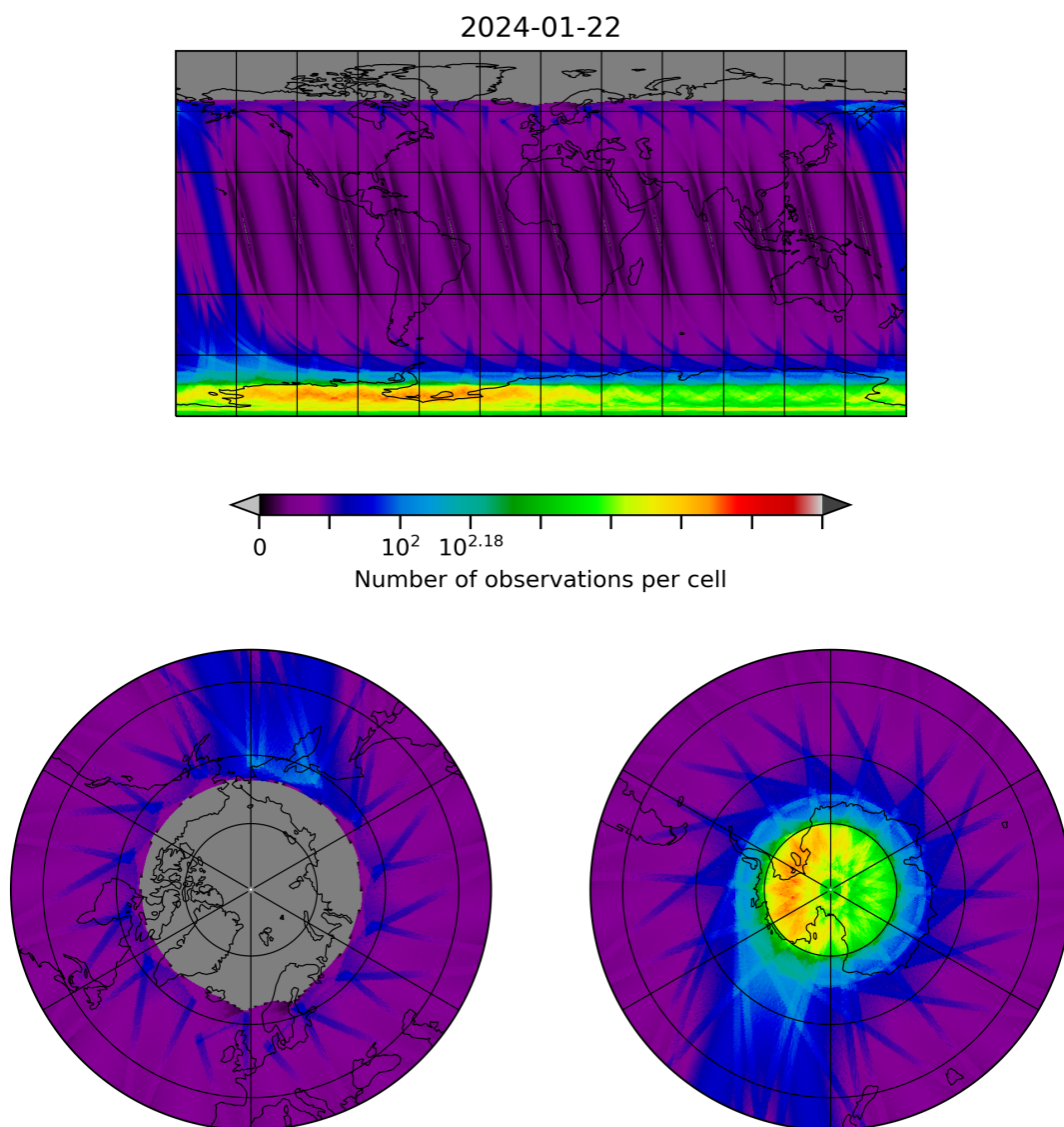
Figure 28: Map of the number of observations for 2024-01-21 to 2024-01-23
