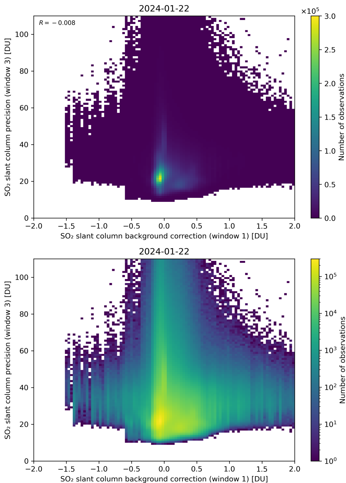
Figure 108: Scatter density plot of “SO 2 slant column background correction (window 1)” against “SO 2 slant column precision (window 3)” for 2024-01-21 to 2024-01-23.
