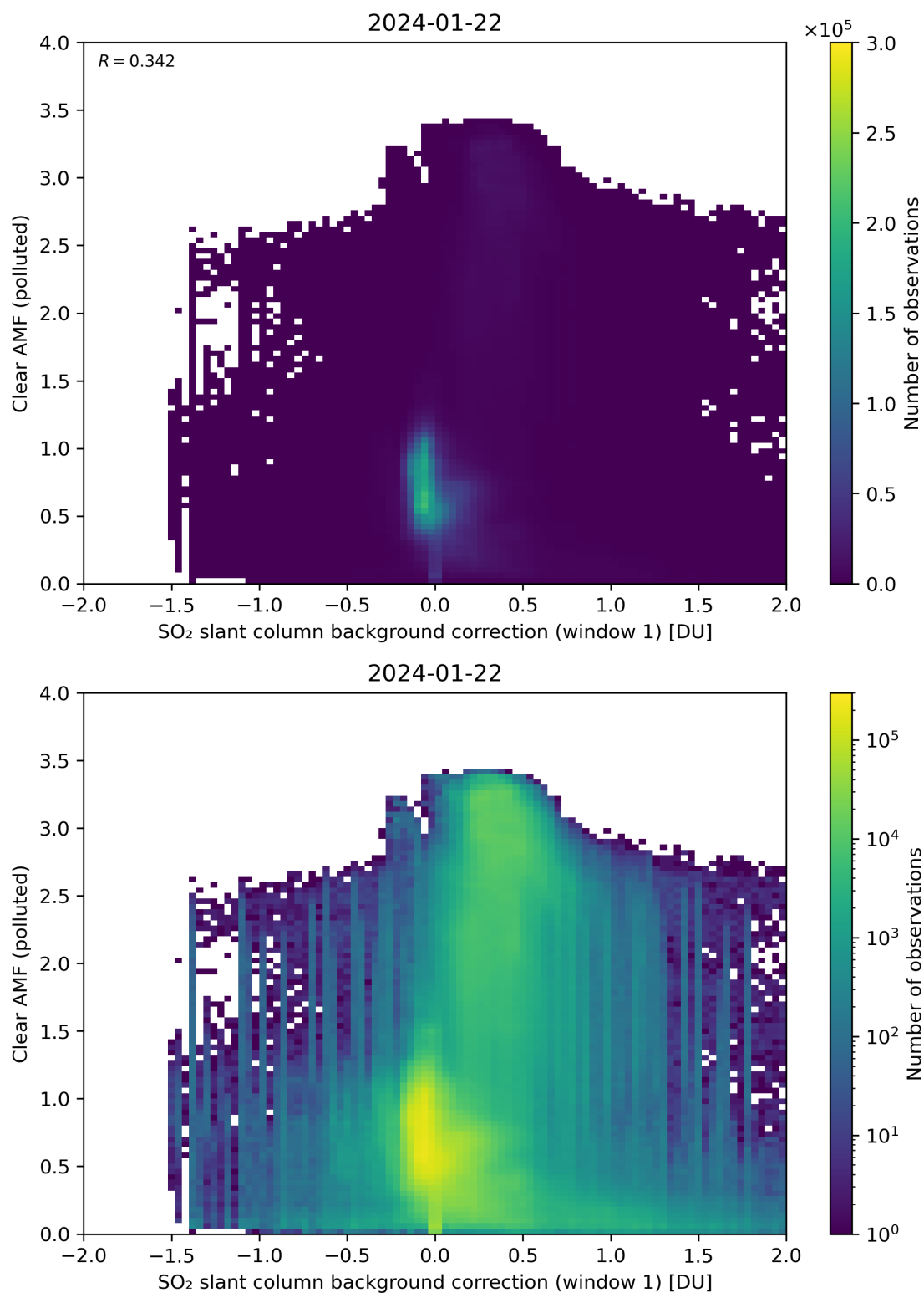
Figure 103: Scatter density plot of “SO 2 slant column background correction (window 1)” against “Clear AMF (polluted)” for 2024-01-21 to 2024-01-23.
