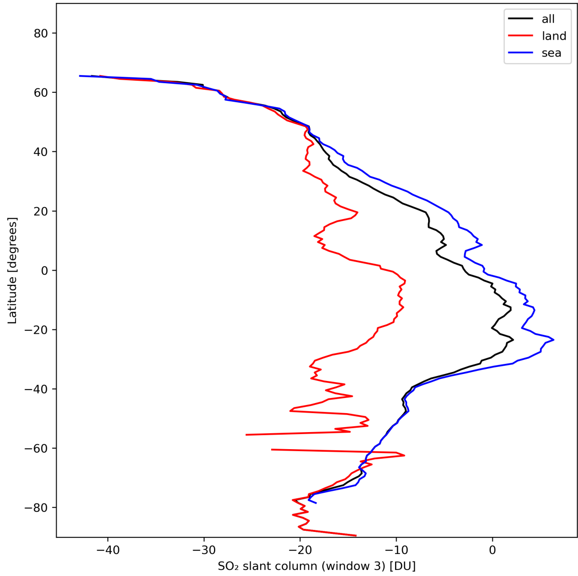
Figure 41: Zonal average of “SO 2 slant column (window 3)” for 2024-01-21 to 2024-01-23.
