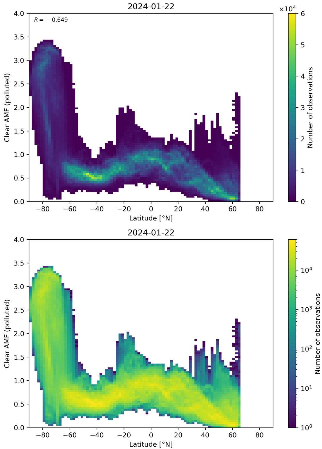
Figure 145: Scatter density plot of “Latitude” against “Clear AMF (polluted)” for 2024-01-21 to 2024-01-23.
