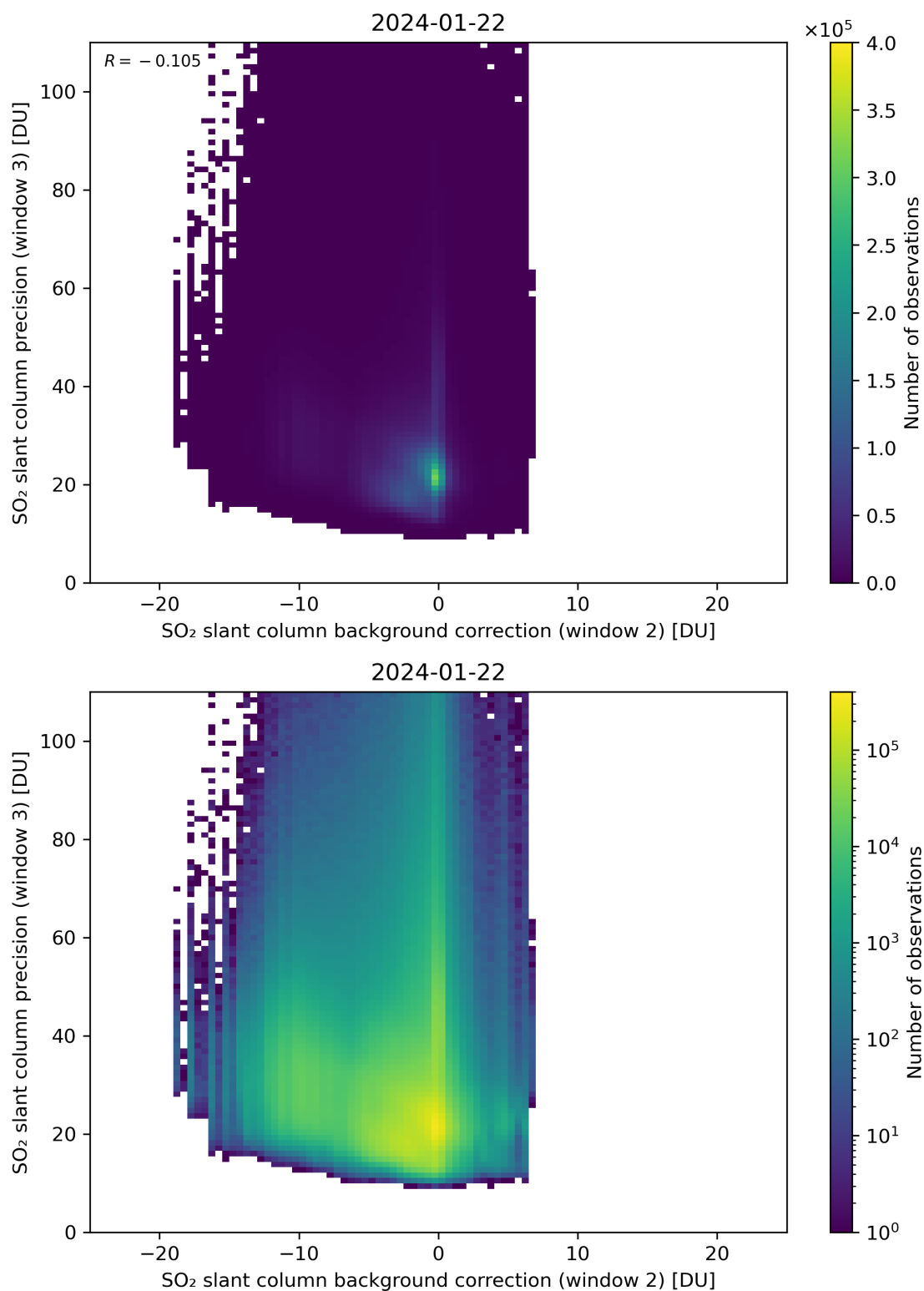
Figure 118: Scatter density plot of “SO 2 slant column background correction (window 2)” against “SO 2 slant column precision (window 3)” for 2024-01-21 to 2024-01-23.
