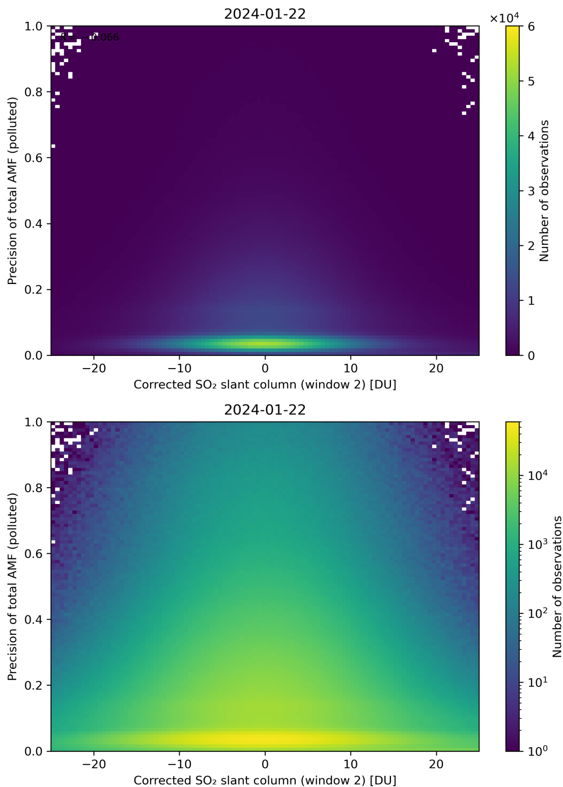
Figure 204: Scatter density plot of “Corrected SO 2 slant column (window 2)” against “Precision of total AMF (polluted)” for 2024-01-21 to 2024-01-23.
