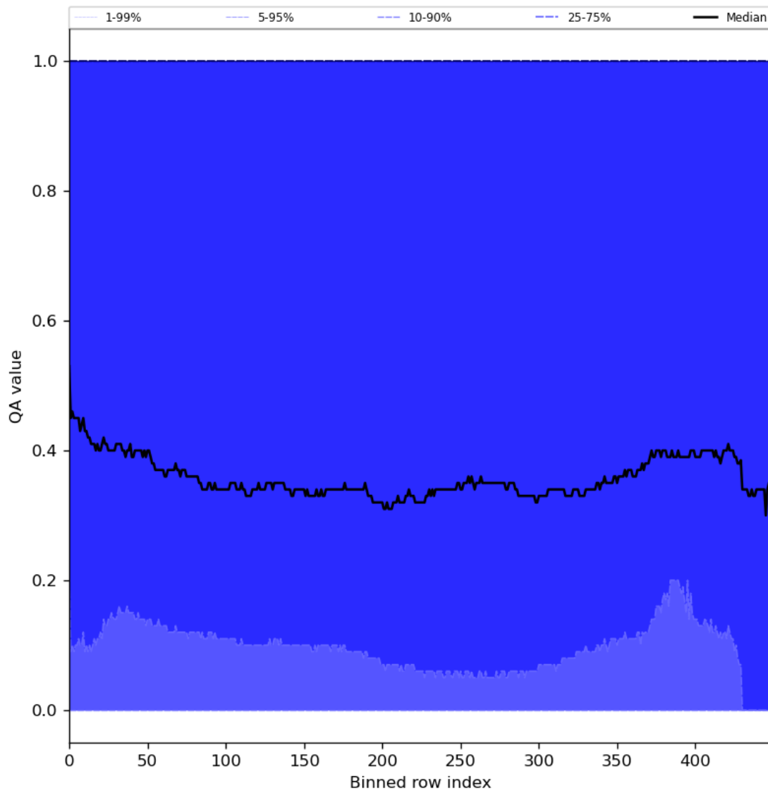
Figure 75: Along track statistics of “QA value” for 2024-01-21 to 2024-01-23
