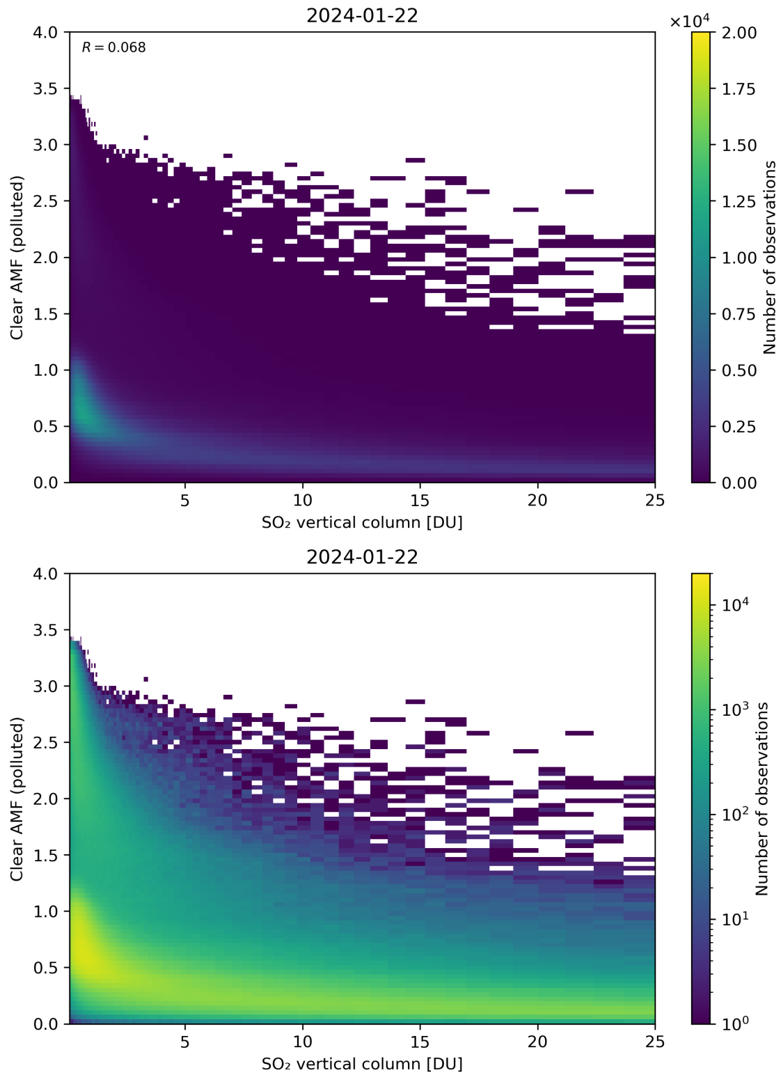
Figure 296: Scatter density plot of “SO 2 vertical column” against “Clear AMF (polluted)” for 2024-01-21 to 2024-01-23.
