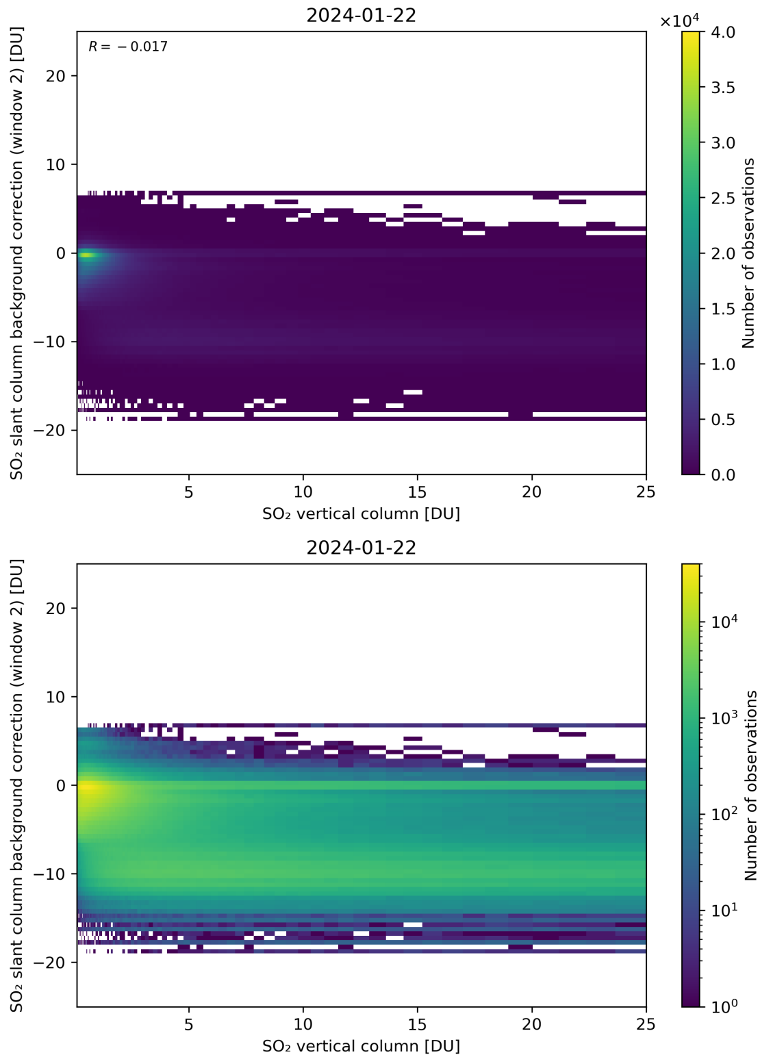
Figure 274: Scatter density plot of “SO 2 vertical column” against “SO 2 slant column background correction (window 2)” for 2024-01-21 to 2024-01-23.
