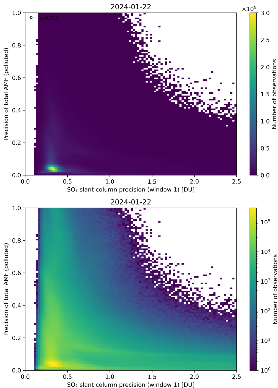
Figure 231: Scatter density plot of “SO 2 slant column precision (window 1)” against “Precision of total AMF (polluted)” for 2024-01-21 to 2024-01-23.
