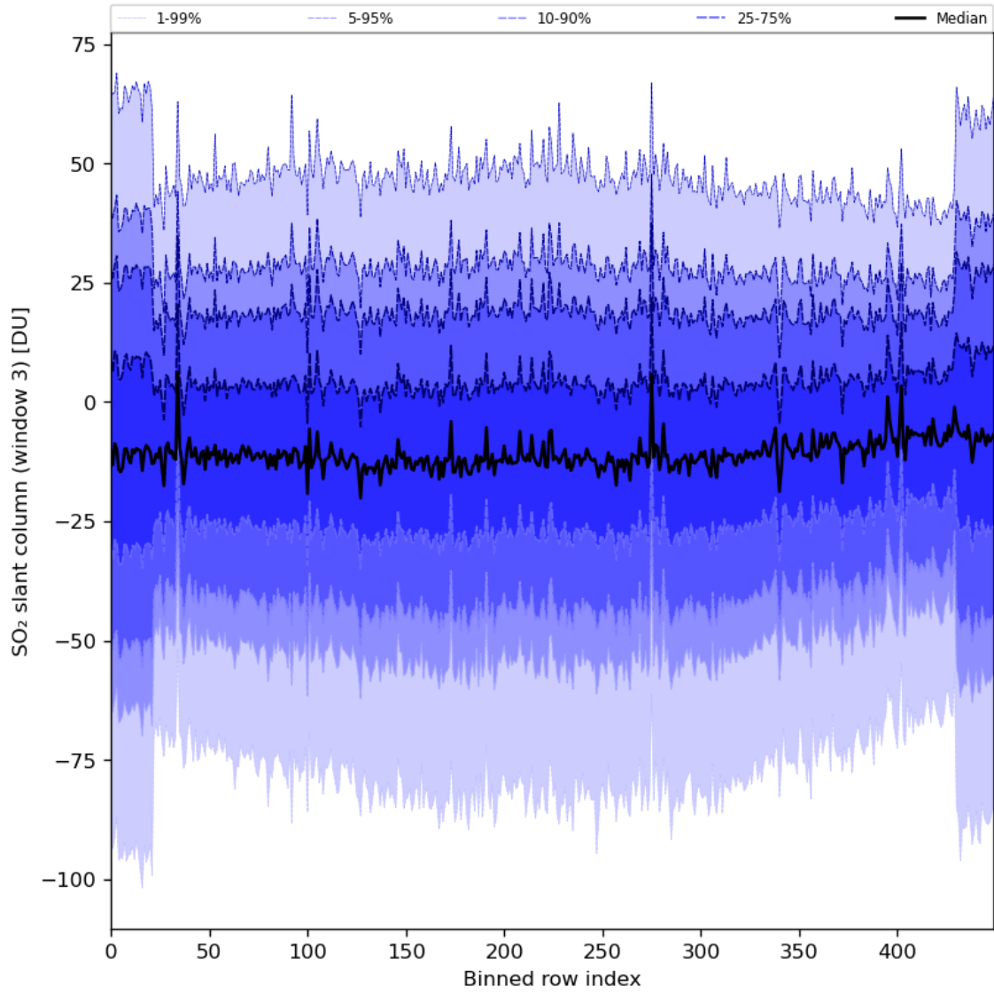
Figure 87: Along track statistics of “SO 2 slant column (window 3)” for 2024-01-21 to 2024-01-23
