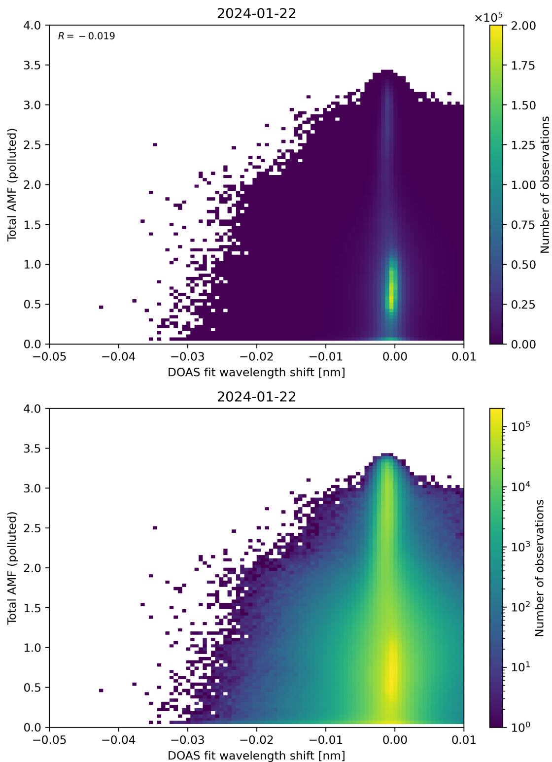
Figure 130: Scatter density plot of “DOAS fit wavelength shift” against “Total AMF (polluted)” for 2024-01-21 to 2024-01-23.
