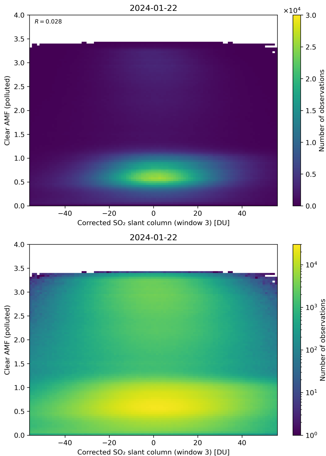
Figure 209: Scatter density plot of “Corrected SO 2 slant column (window 3)” against “Clear AMF (polluted)” for 2024-01-21 to 2024-01-23.
