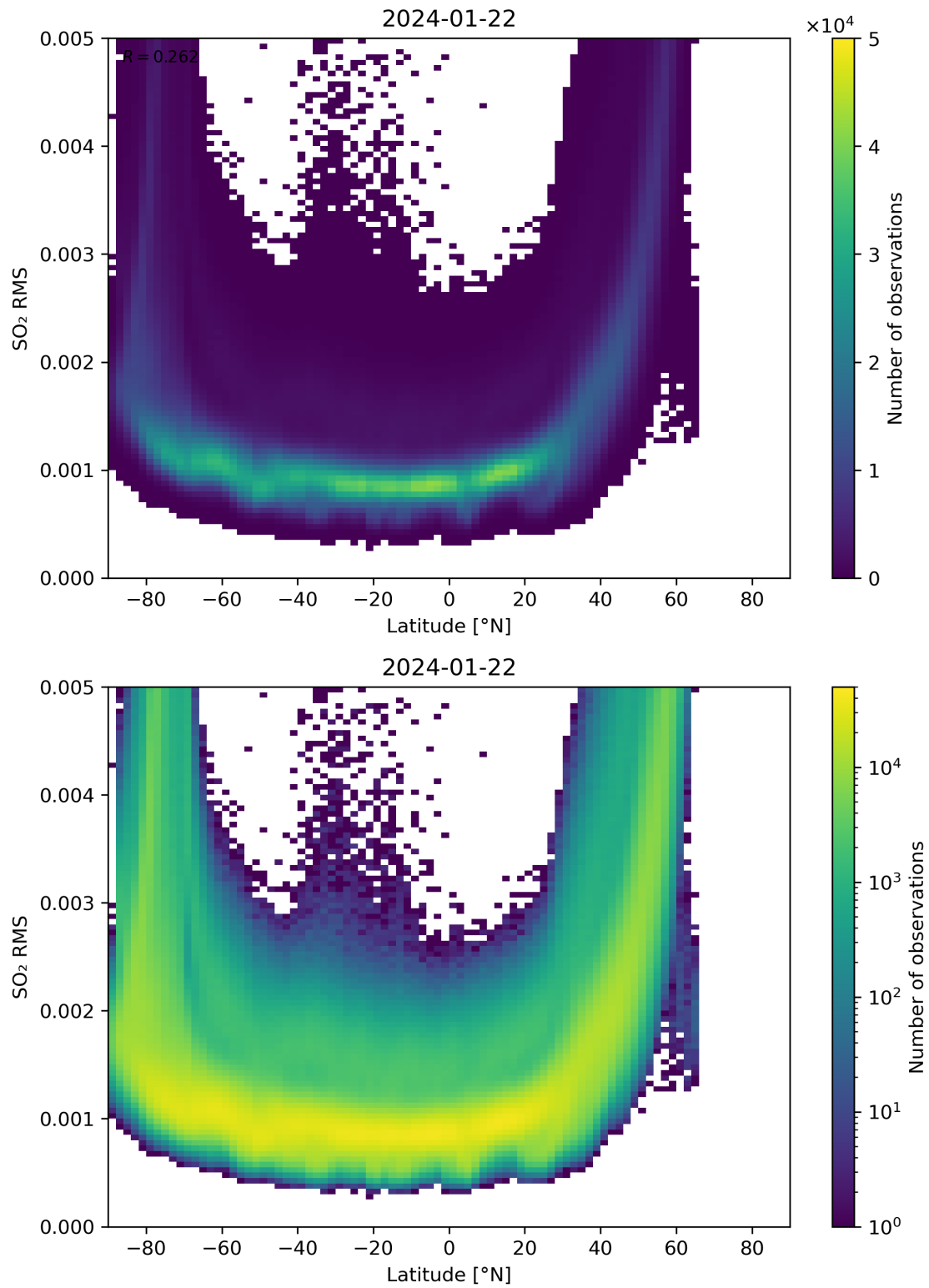
Figure 144: Scatter density plot of “Latitude” against “SO 2 RMS” for 2024-01-21 to 2024-01-23.
