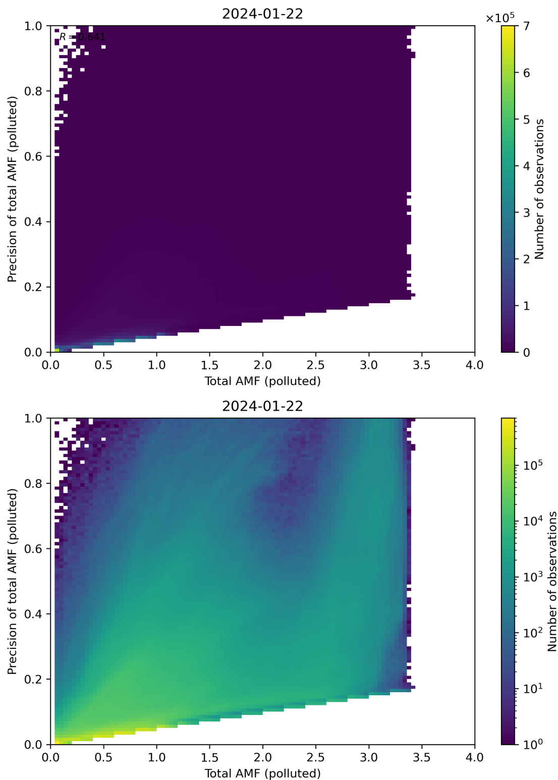
Figure 272: Scatter density plot of “Total AMF (polluted)” against “Precision of total AMF (polluted)” for 2024-01-21 to 2024-01-23.
