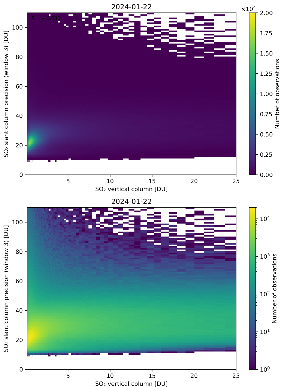
Figure 304: Scatter density plot of “SO 2 vertical column” against “SO 2 slant column precision (window 3)” for 2024-01-21 to 2024-01-23.
