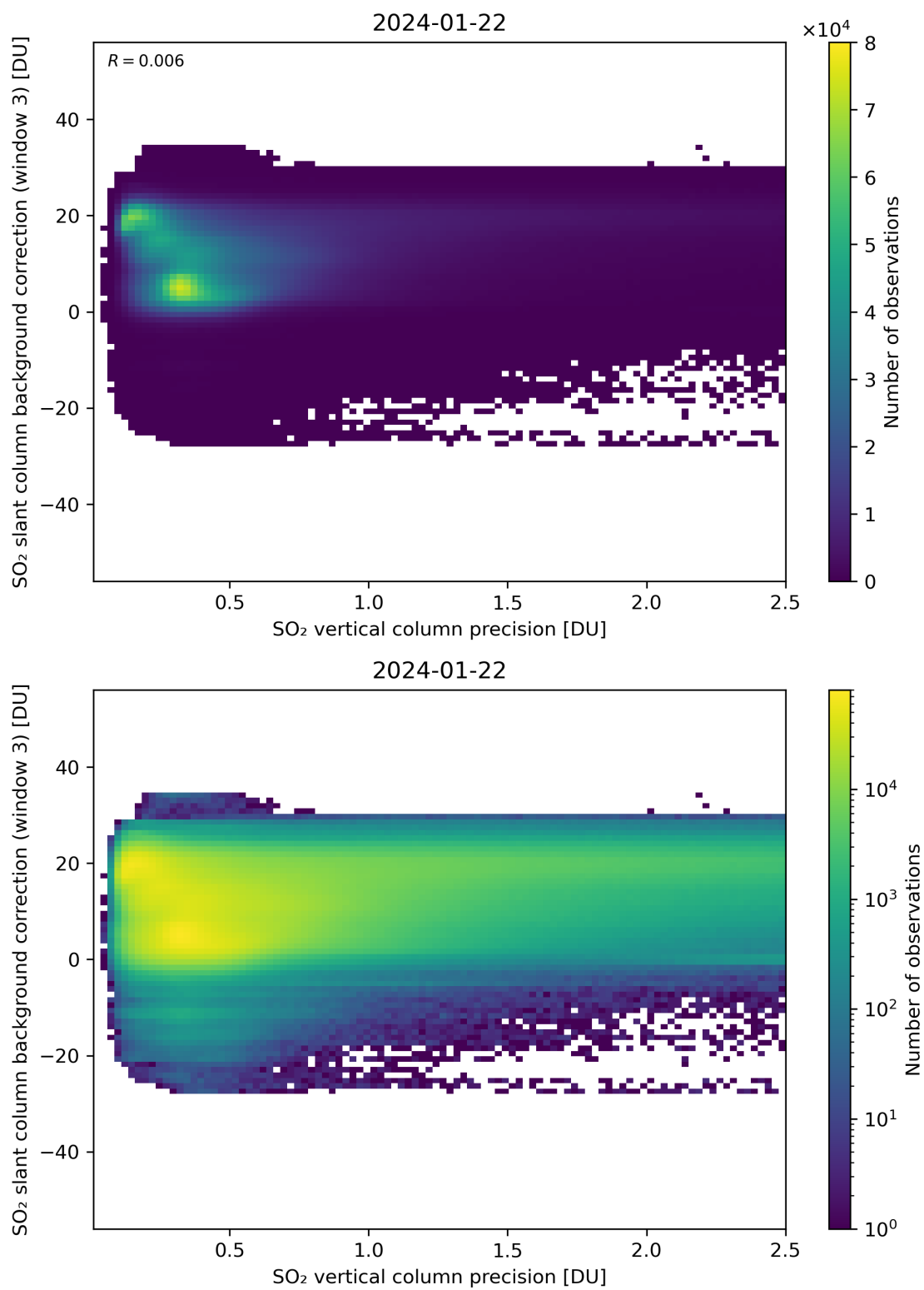
Figure 281: Scatter density plot of “SO 2 vertical column precision” against “SO 2 slant column background correction (window 3)” for 2024-01-21 to 2024-01-23.
