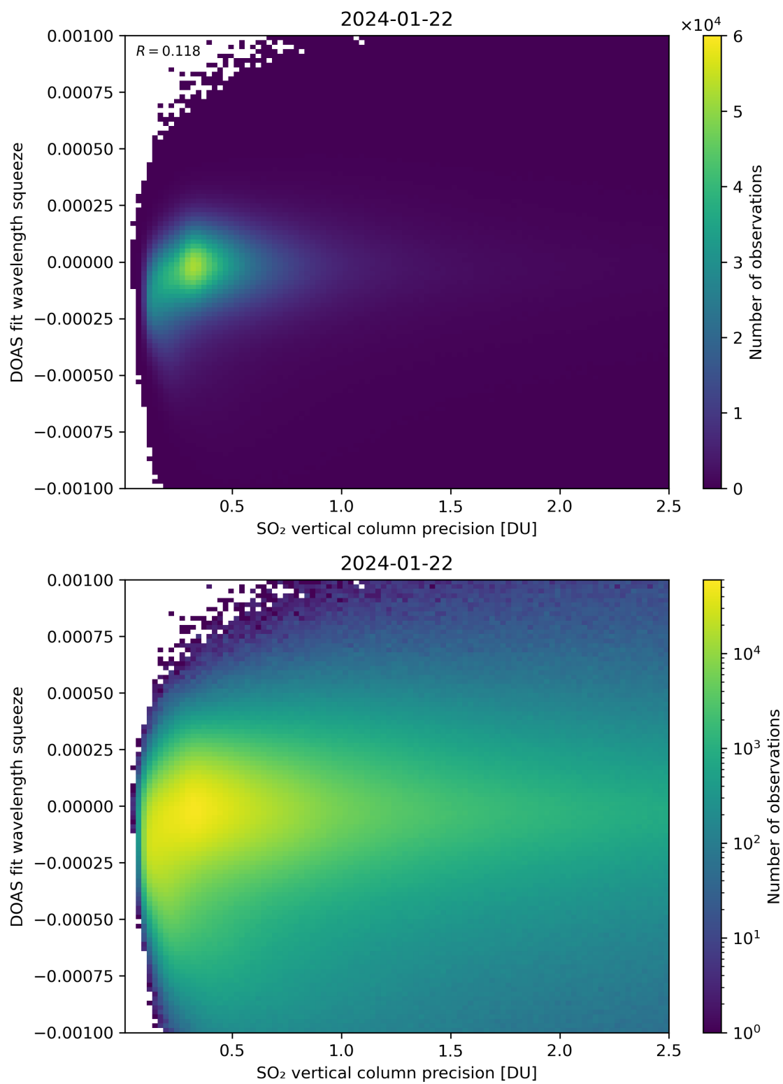
Figure 283: Scatter density plot of “SO 2 vertical column precision” against “DOAS fit wavelength squeeze” for 2024-01-21 to 2024-01-23.
