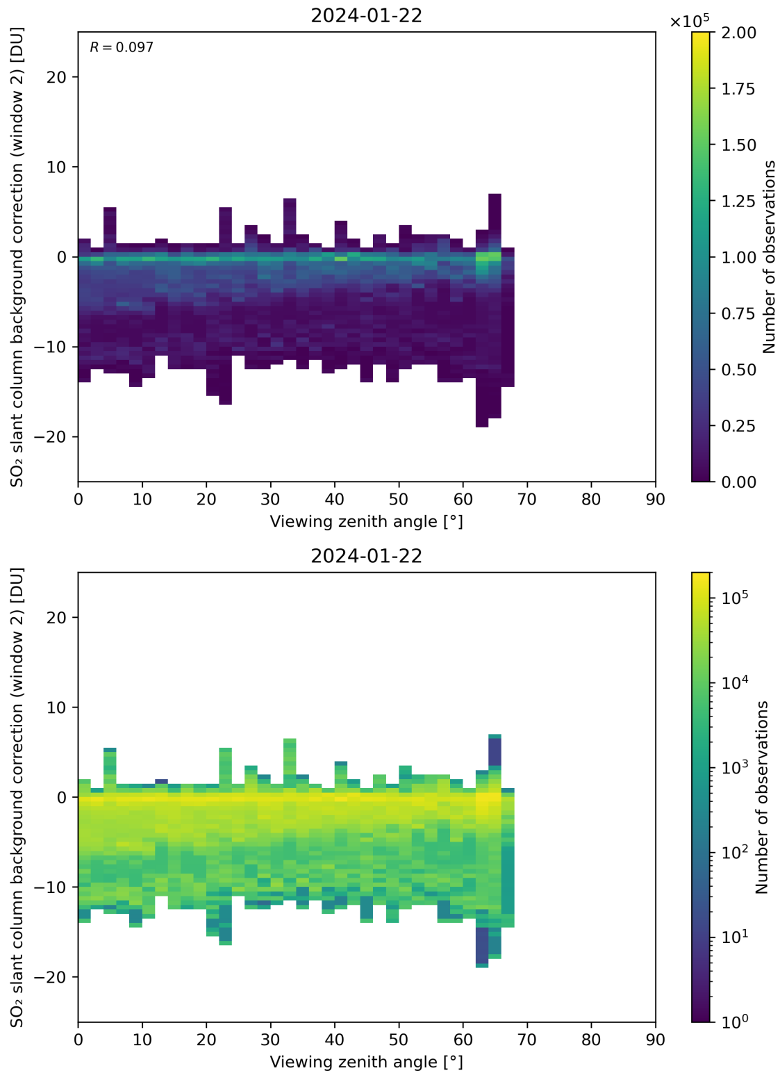
Figure 309: Scatter density plot of “Viewing zenith angle” against “SO 2 slant column background correction (window 2)” for 2024-01-21 to 2024-01-23.
