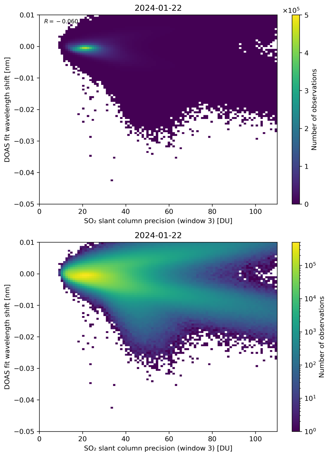
Figure 258: Scatter density plot of “SO 2 slant column precision (window 3)” against “DOAS fit wavelength shift” for 2024-01-21 to 2024-01-23.
