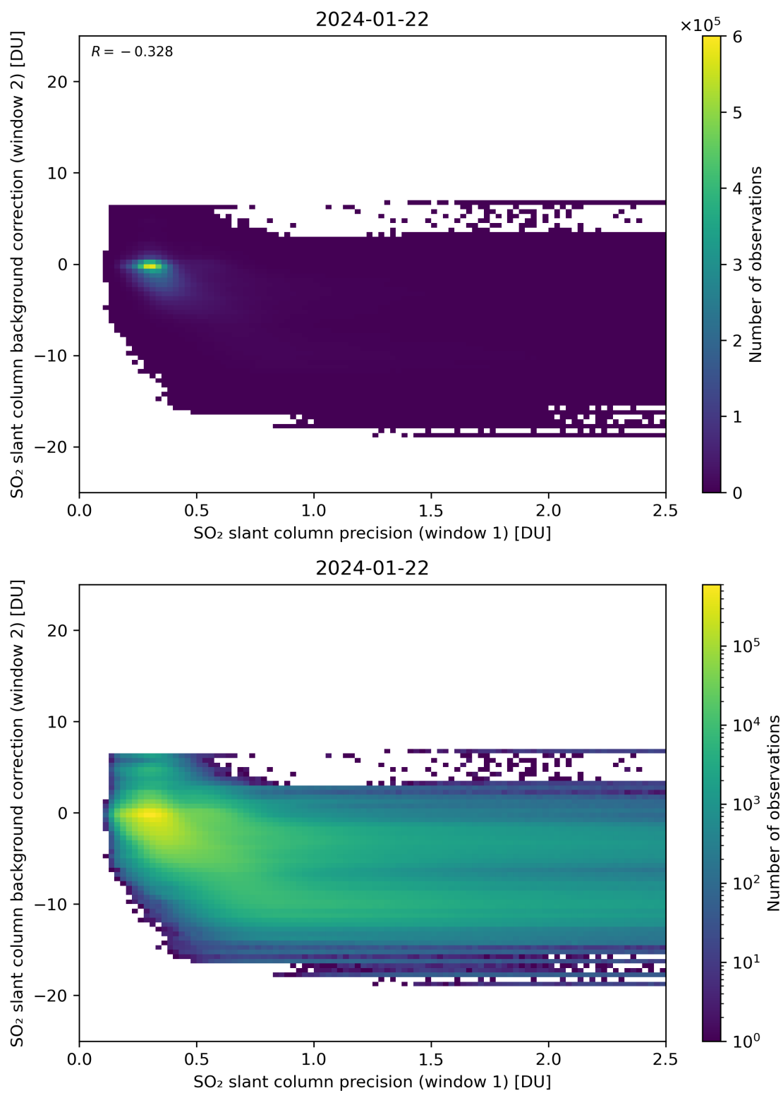
Figure 219: Scatter density plot of “SO 2 slant column precision (window 1)” against “SO 2 slant column background correction (window 2)” for 2024-01-21 to 2024-01-23.
