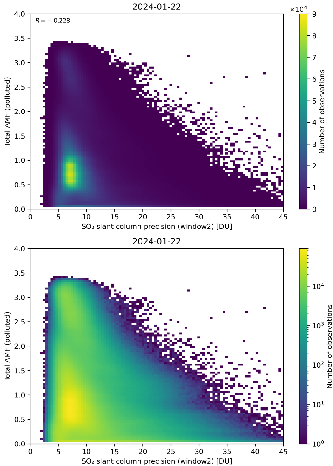
Figure 251: Scatter density plot of “SO 2 slant column precision (window2)” against “Total AMF (polluted)” for 2024-01-21 to 2024-01-23.
