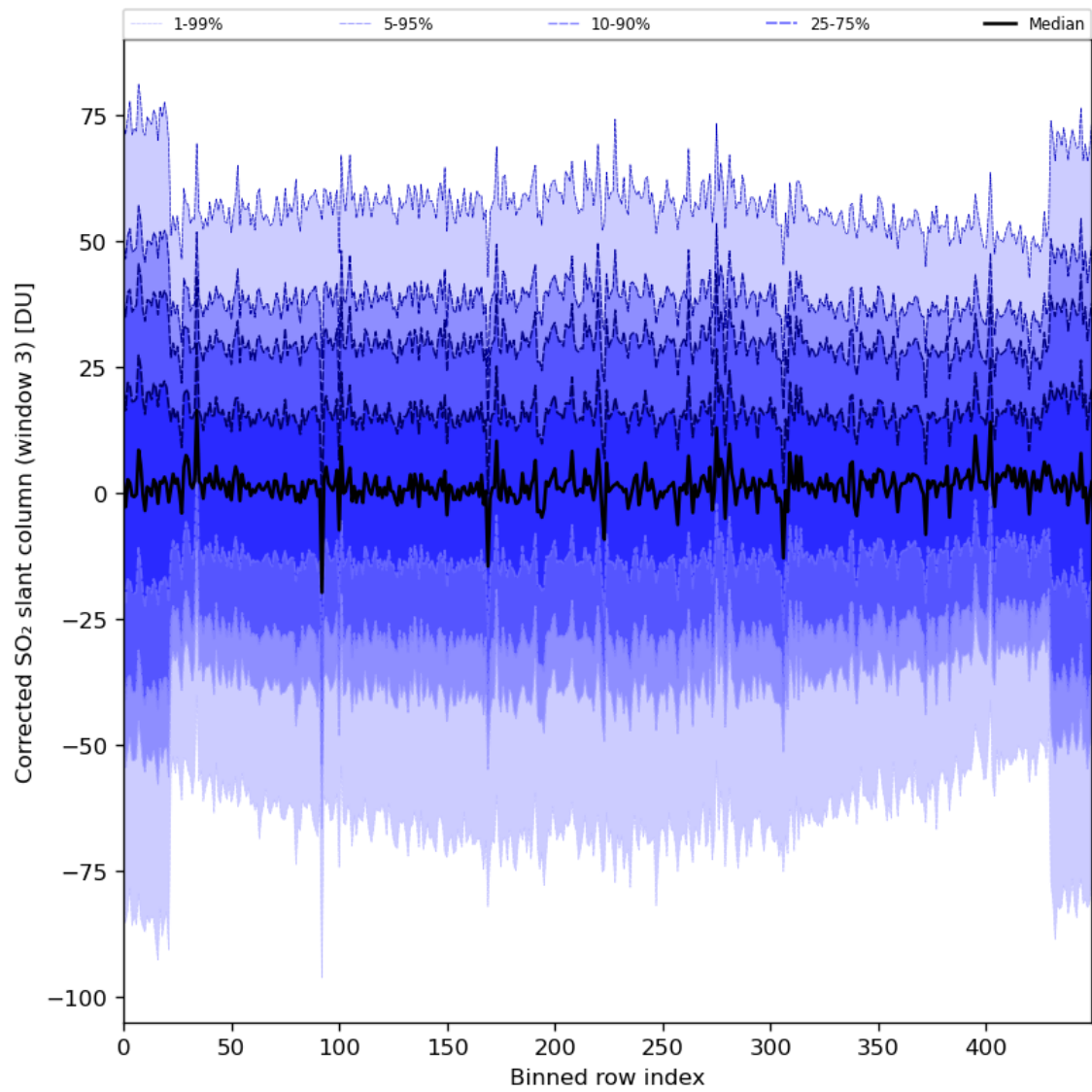
Figure 89: Along track statistics of “Corrected SO 2 slant column (window 3)” for 2024-01-21 to 2024-01-23
