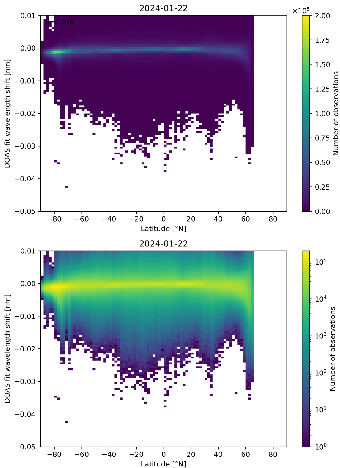
Figure 142: Scatter density plot of “Latitude” against “DOAS fit wavelength shift” for 2024-01-21 to 2024-01-23.
