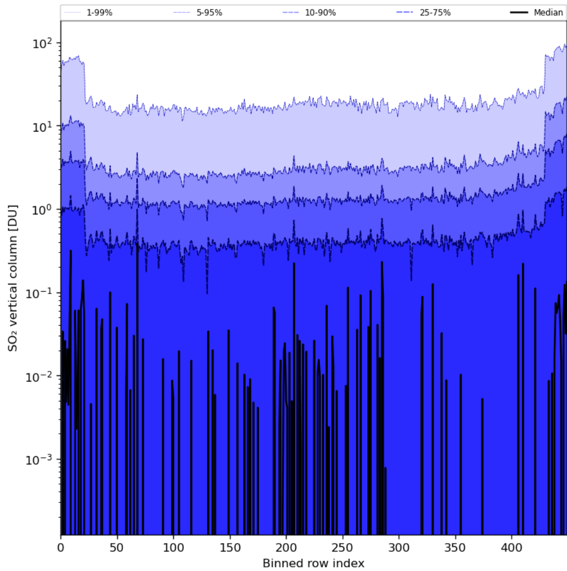
Figure 76: Along track statistics of “SO 2 vertical column” for 2024-01-21 to 2024-01-23
