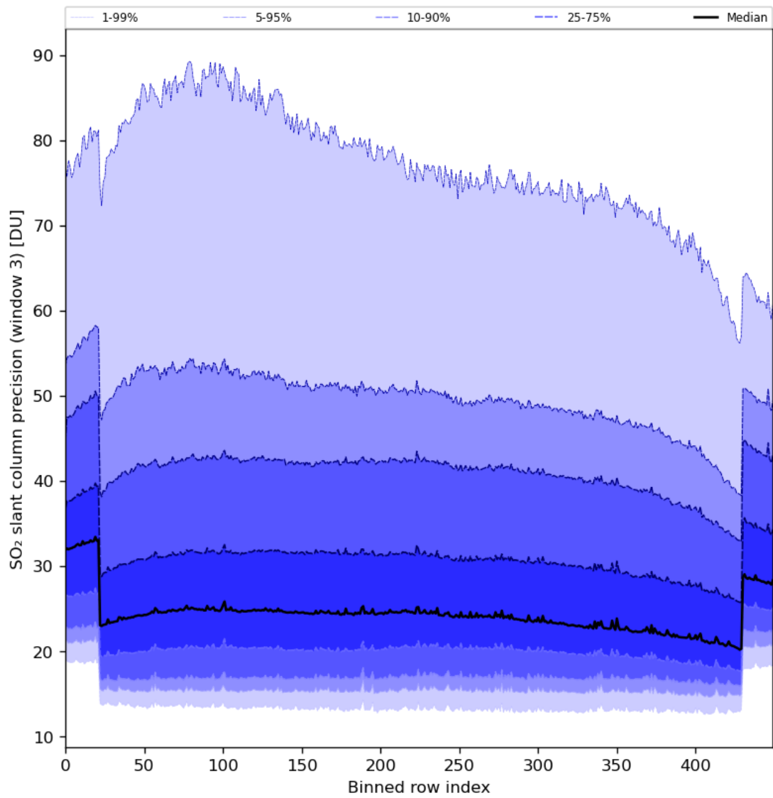
Figure 88: Along track statistics of “SO 2 slant column precision (window 3)” for 2024-01-21 to 2024-01-23
