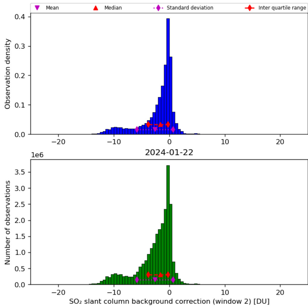
Figure 63: Histogram of “SO 2 slant column background correction (window 2)” for 2024-01-21 to 2024-01-23
