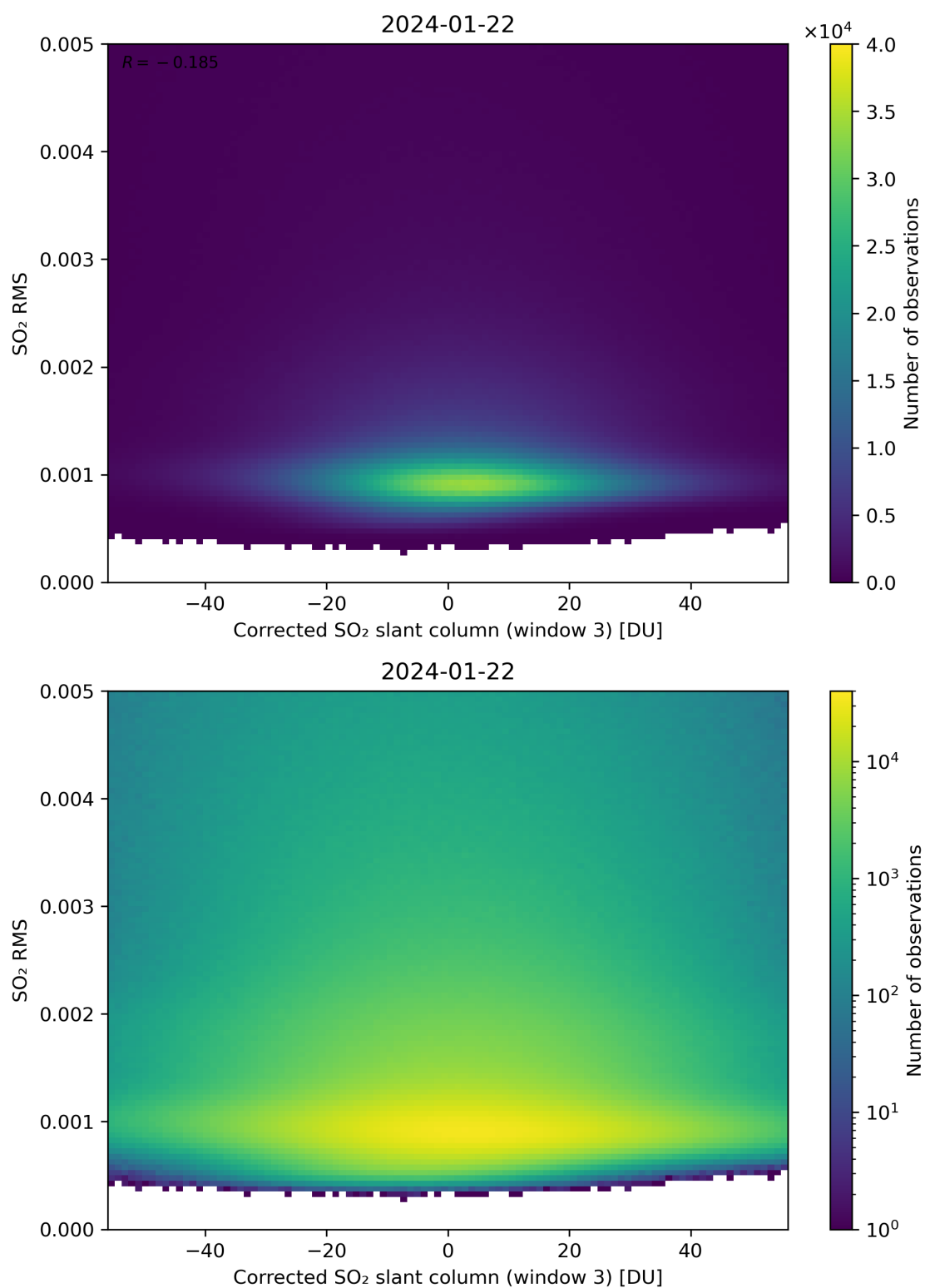
Figure 208: Scatter density plot of “Corrected SO 2 slant column (window 3)” against “SO 2 RMS” for 2024-01-21 to 2024-01-23.
