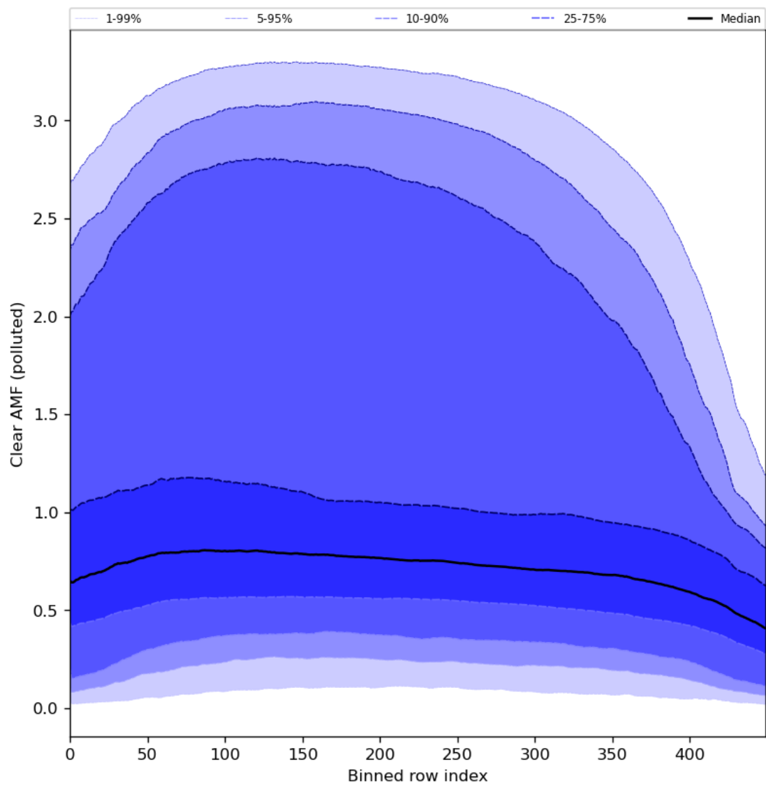
Figure 96: Along track statistics of “Clear AMF (polluted)” for 2024-01-21 to 2024-01-23
