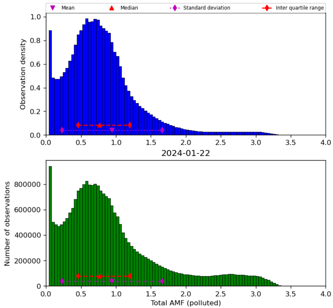
Figure 71: Histogram of “Total AMF (polluted)” for 2024-01-21 to 2024-01-23
