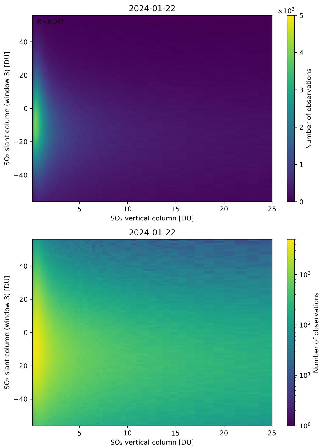
Figure 303: Scatter density plot of “SO 2 vertical column” against “SO 2 slant column (window 3)” for 2024-01-21 to 2024-01-23.
