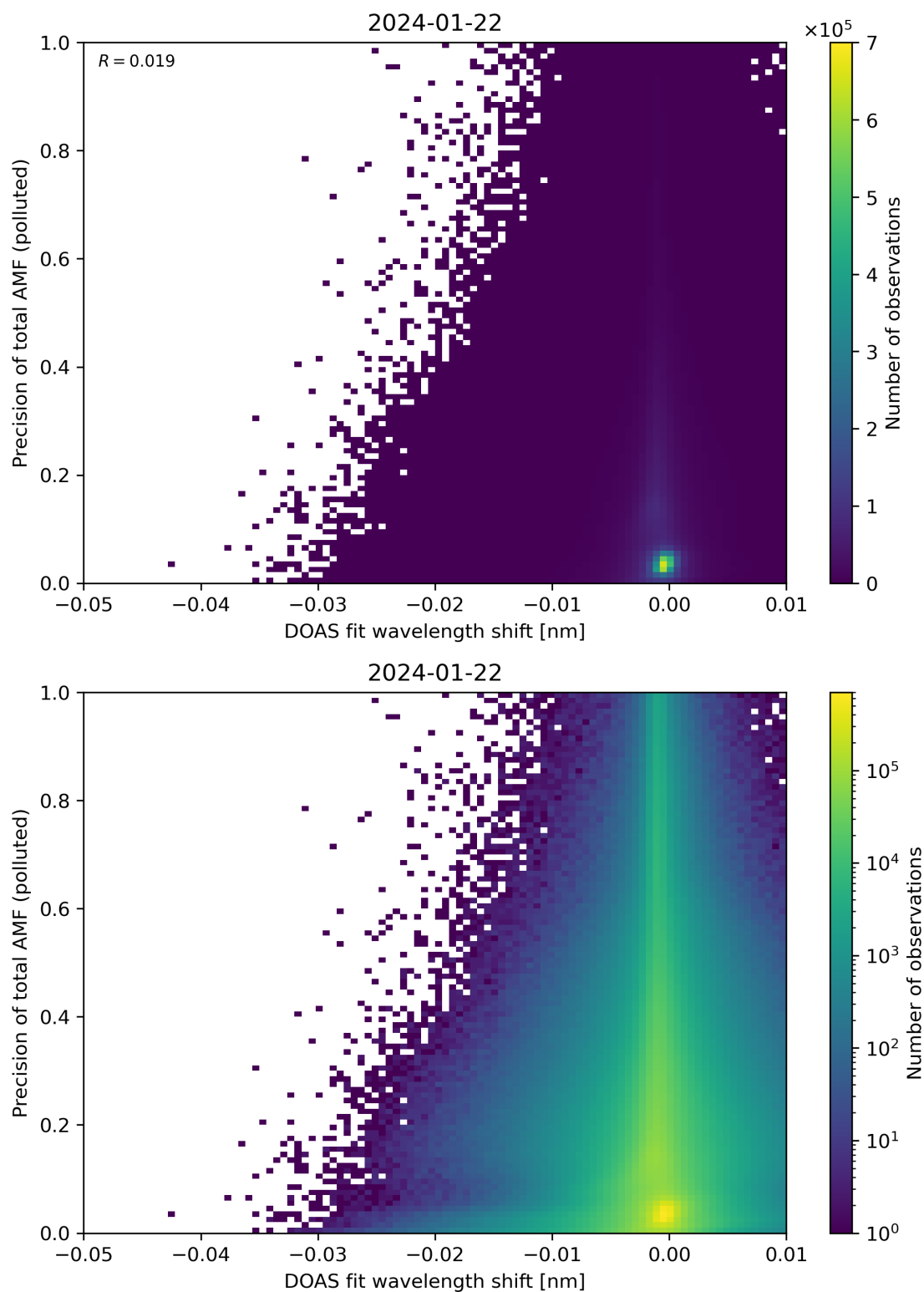
Figure 131: Scatter density plot of “DOAS fit wavelength shift” against “Precision of total AMF (polluted)” for 2024-01-21 to 2024-01-23.
