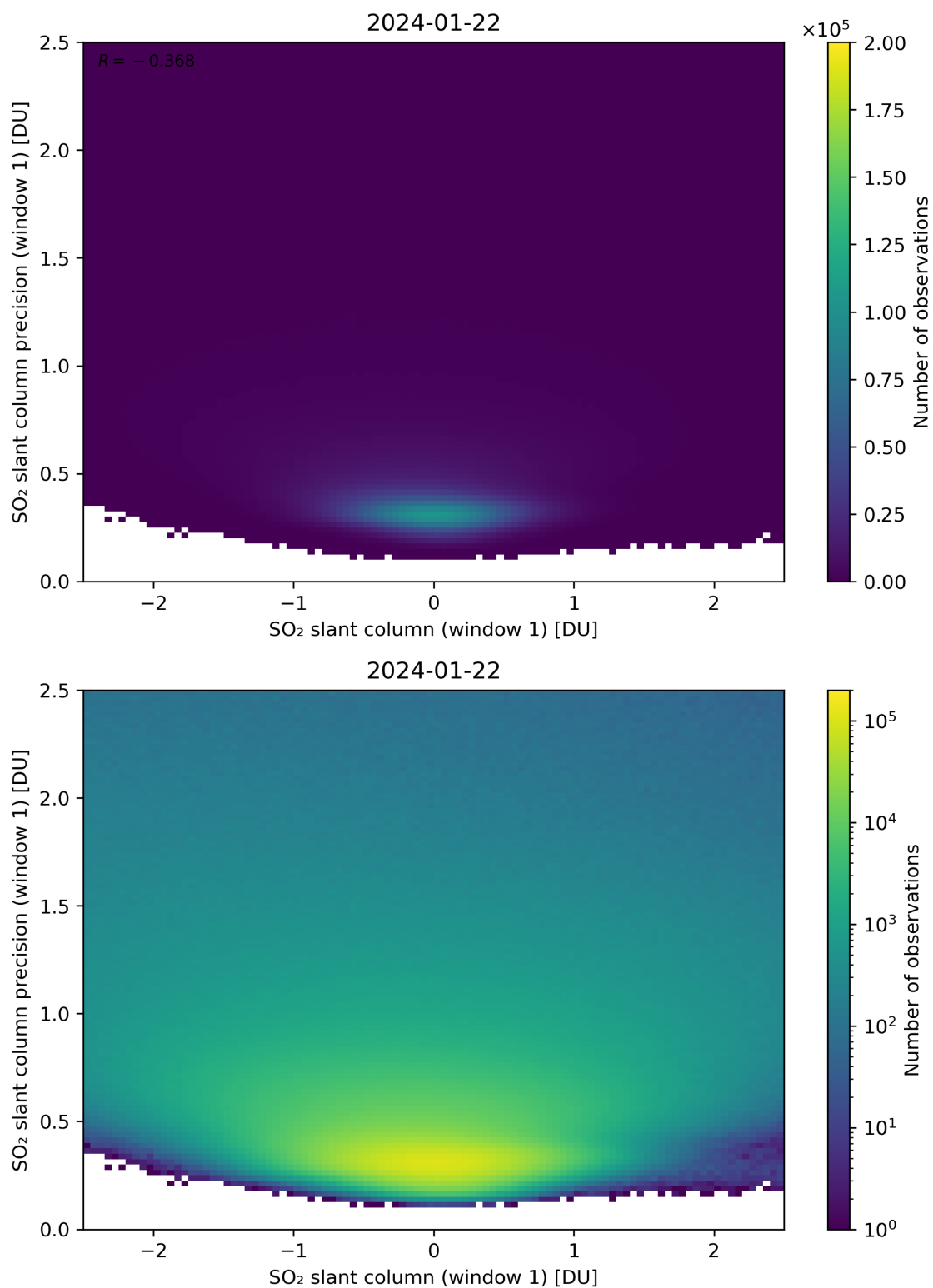
Figure 235: Scatter density plot of “SO 2 slant column (window 1)” against “SO 2 slant column precision (window 1)” for 2024-01-21 to 2024-01-23.
