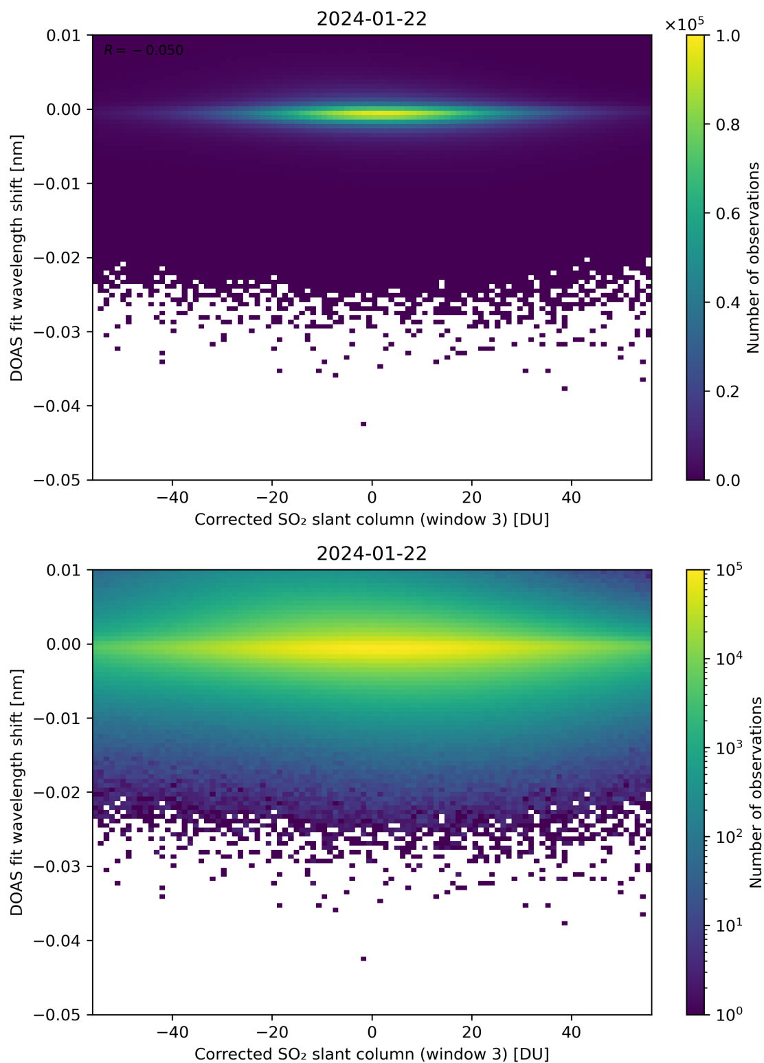
Figure 206: Scatter density plot of “Corrected SO 2 slant column (window 3)” against “DOAS fit wavelength shift” for 2024-01-21 to 2024-01-23.
