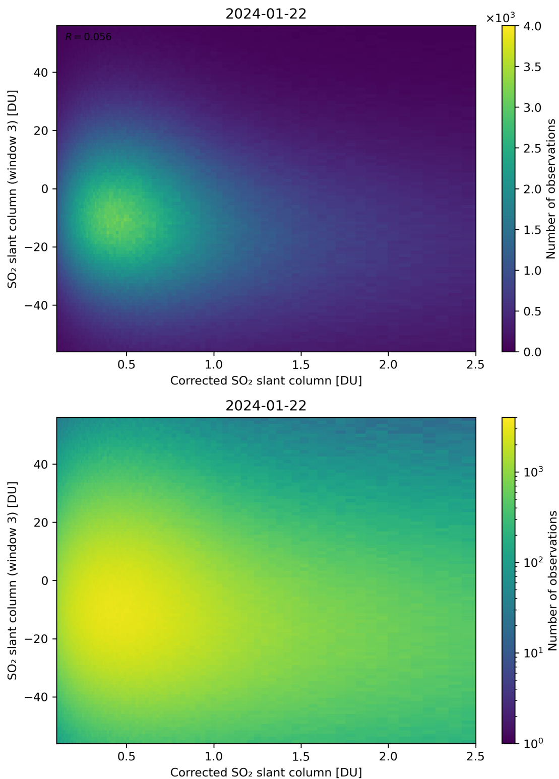
Figure 190: Scatter density plot of “Corrected SO 2 slant column” against “SO 2 slant column (window 3)” for 2024-01-21 to 2024-01-23.
