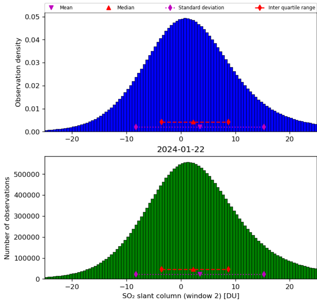
Figure 60: Histogram of “SO 2 slant column (window 2)” for 2024-01-21 to 2024-01-23
