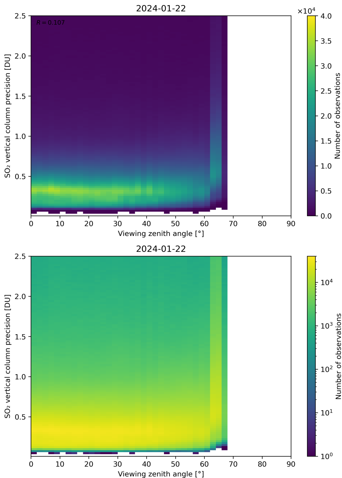
Figure 328: Scatter density plot of “Viewing zenith angle” against “SO 2 vertical column precision” for 2024-01-21 to 2024-01-23.
