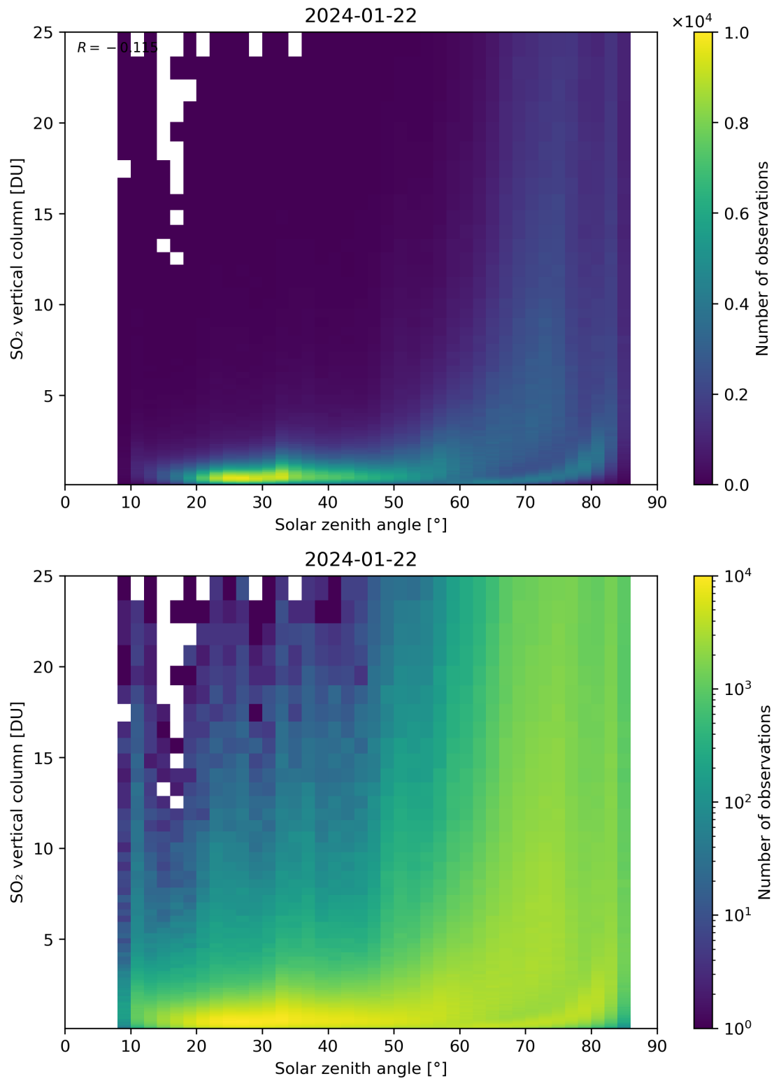
Figure 176: Scatter density plot of “Solar zenith angle” against “SO 2 vertical column” for 2024-01-21 to 2024-01-23.
