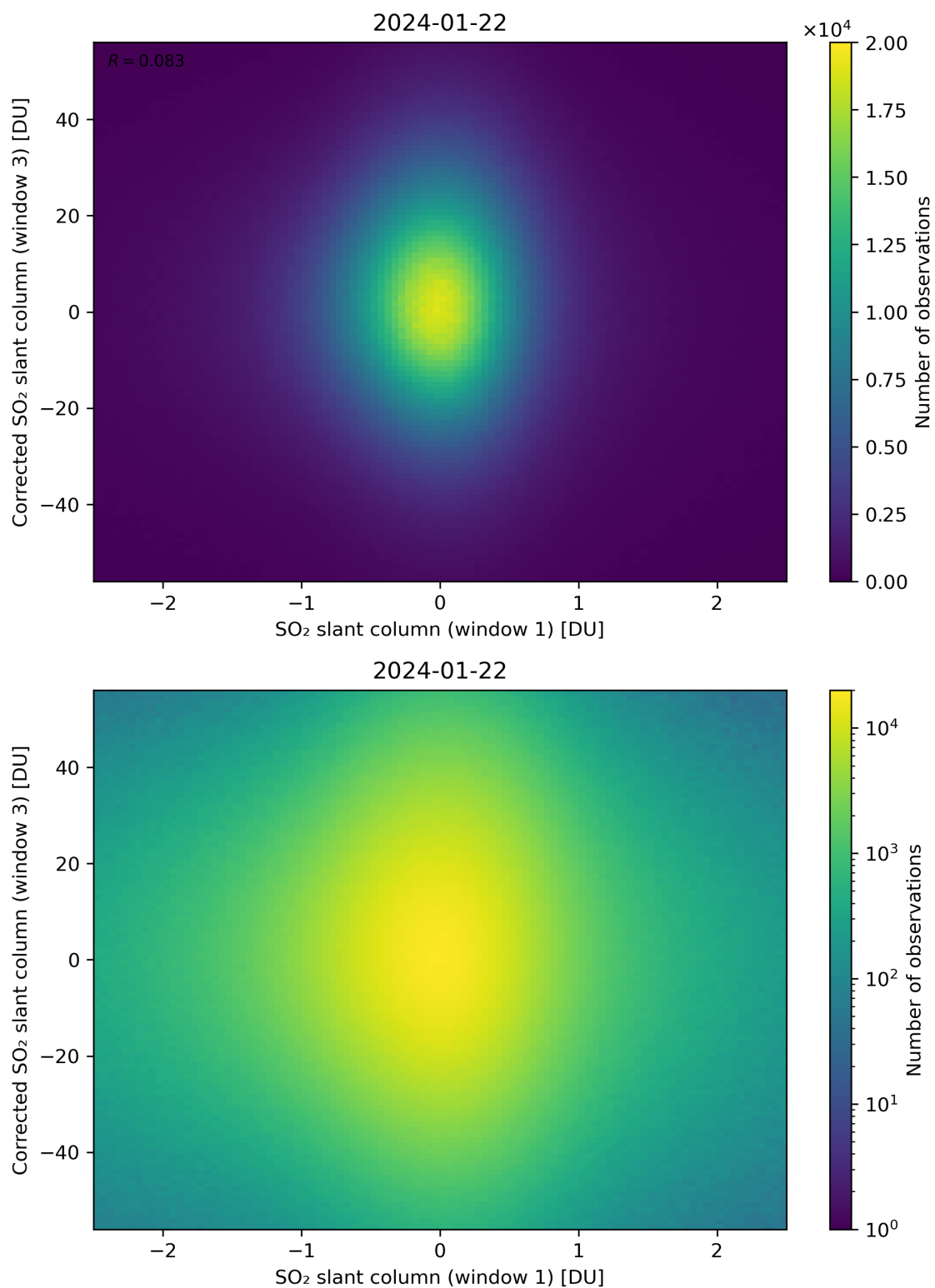
Figure 234: Scatter density plot of “SO 2 slant column (window 1)” against “Corrected SO 2 slant column (window 3)” for 2024-01-21 to 2024-01-23.
