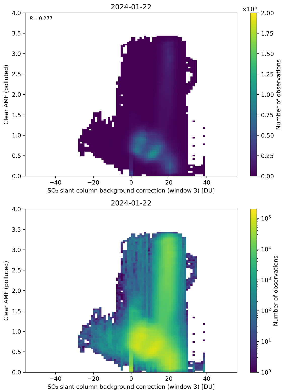
Figure 124: Scatter density plot of “SO 2 slant column background correction (window 3)” against “Clear AMF (polluted)” for 2024-01-21 to 2024-01-23.
