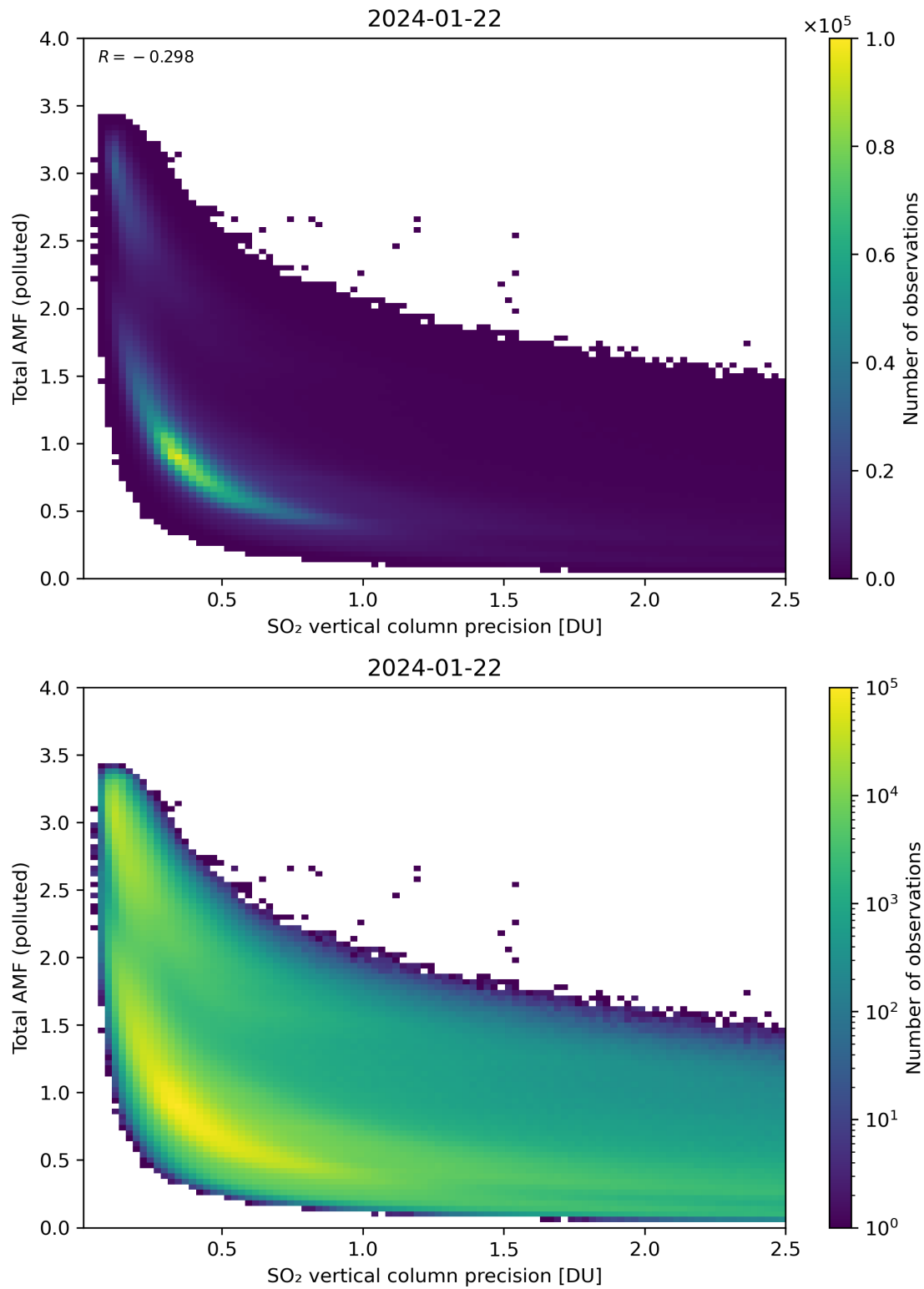
Figure 294: Scatter density plot of “SO 2 vertical column precision” against “Total AMF (polluted)” for 2024-01-21 to 2024-01-23.
