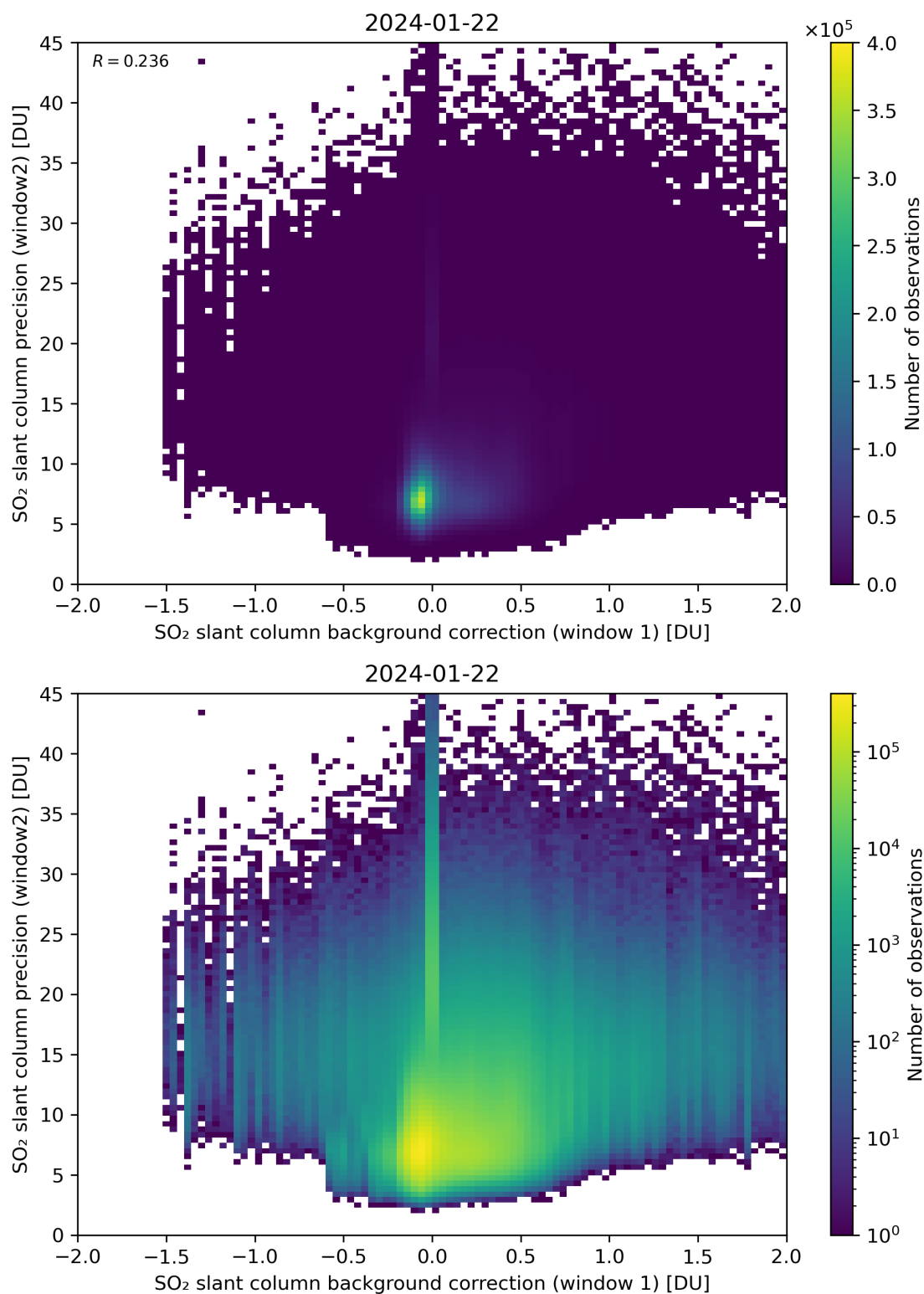
Figure 106: Scatter density plot of “SO 2 slant column background correction (window 1)” against “SO 2 slant column precision (window2)” for 2024-01-21 to 2024-01-23.
