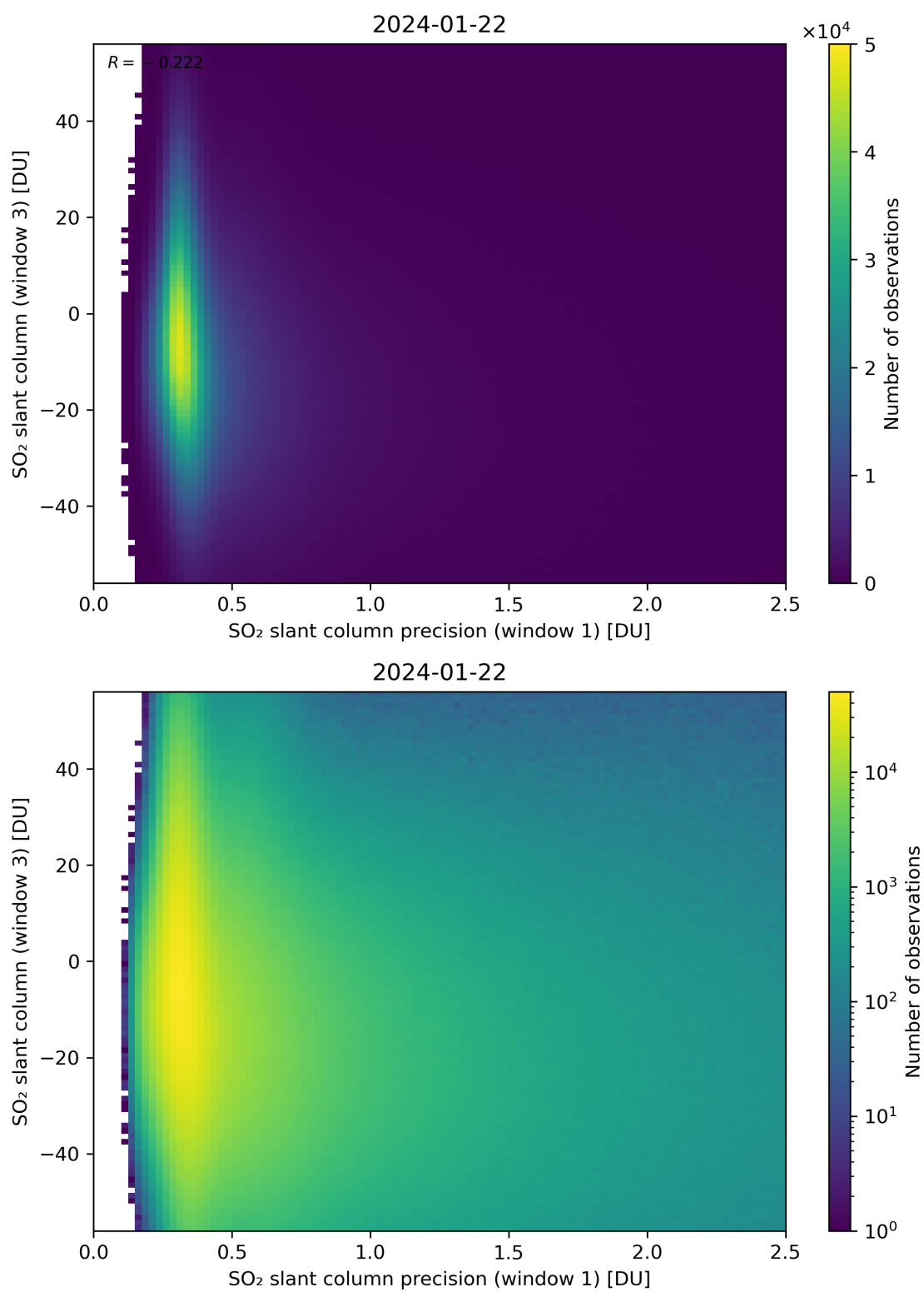
Figure 228: Scatter density plot of “SO 2 slant column precision (window 1)” against “SO 2 slant column (window 3)” for 2024-01-21 to 2024-01-23.
