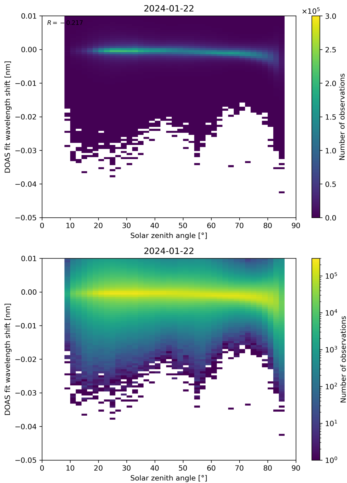
Figure 161: Scatter density plot of “Solar zenith angle” against “DOAS fit wavelength shift” for 2024-01-21 to 2024-01-23.
