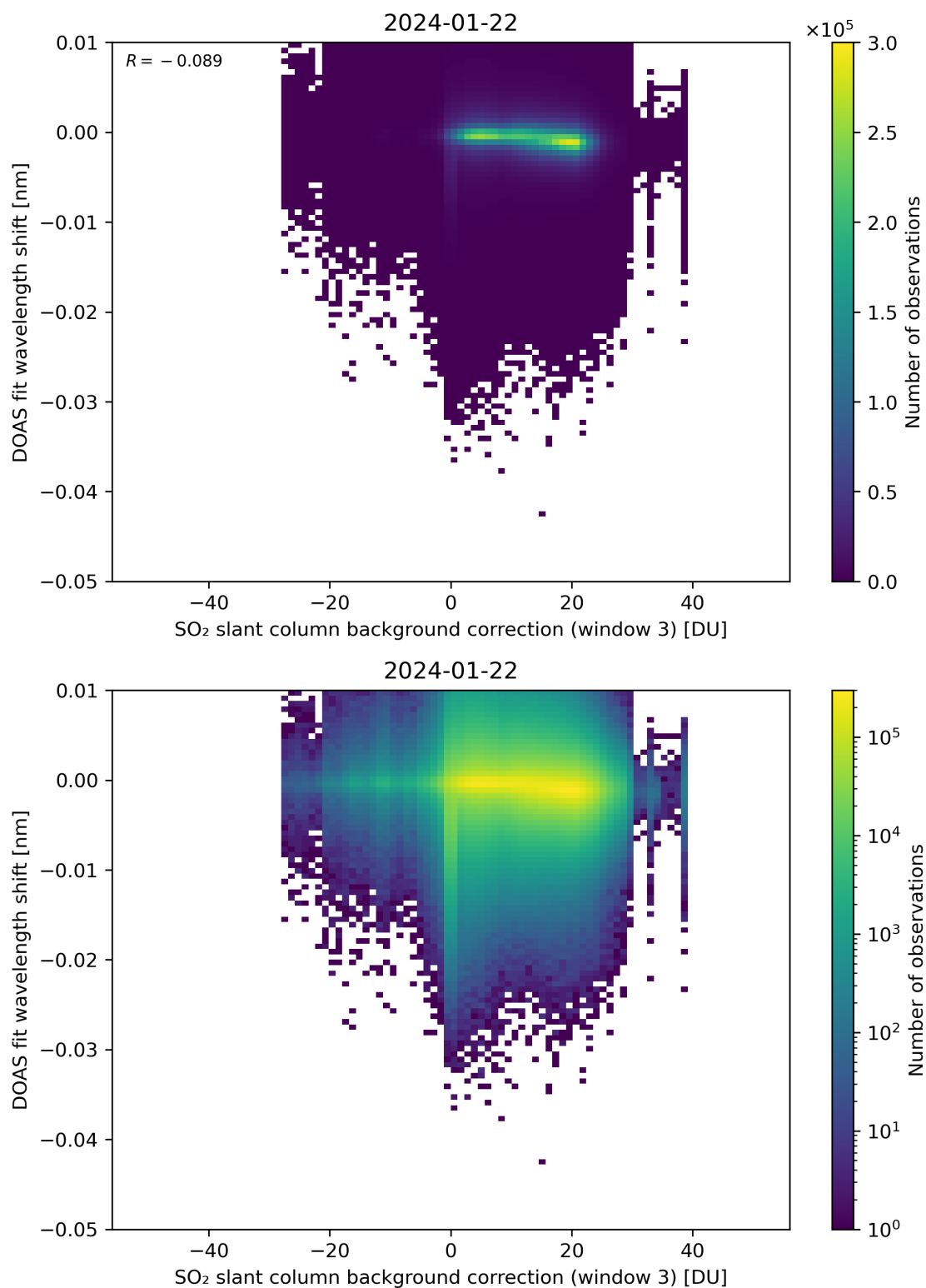
Figure 121: Scatter density plot of “SO 2 slant column background correction (window 3)” against “DOAS fit wavelength shift” for 2024-01-21 to 2024-01-23.
