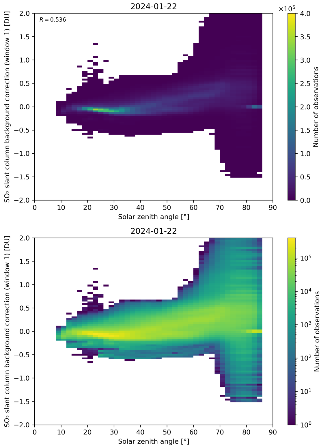
Figure 158: Scatter density plot of “Solar zenith angle” against “SO 2 slant column background correction (window 1)” for 2024-01-21 to 2024-01-23.
