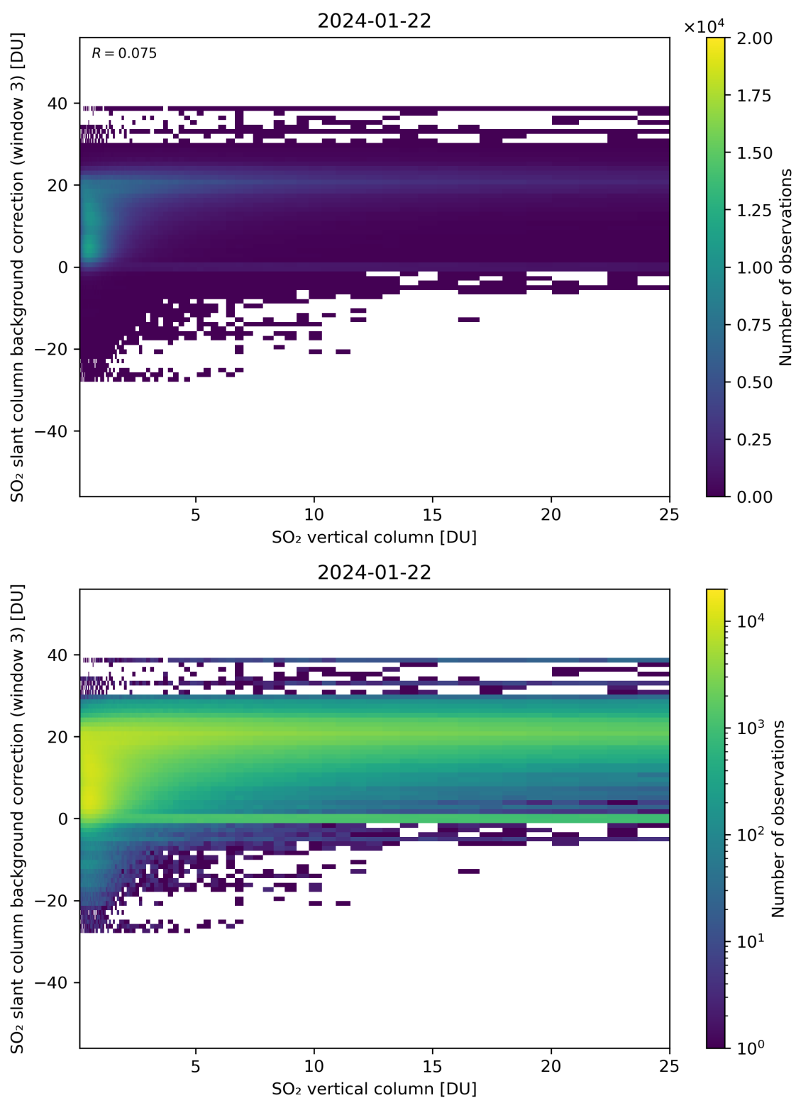
Figure 275: Scatter density plot of “SO 2 vertical column” against “SO 2 slant column background correction (window 3)” for 2024-01-21 to 2024-01-23.
