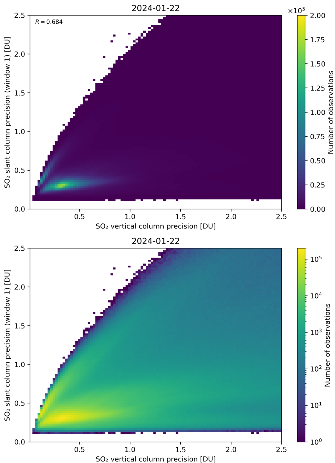
Figure 290: Scatter density plot of “SO 2 vertical column precision” against “SO 2 slant column precision (window 1)” for 2024-01-21 to 2024-01-23.
