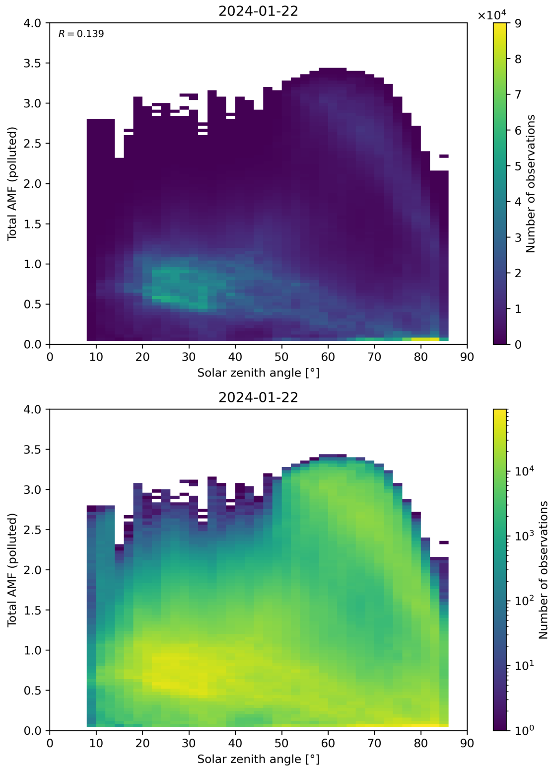
Figure 174: Scatter density plot of “Solar zenith angle” against “Total AMF (polluted)” for 2024-01-21 to 2024-01-23.
