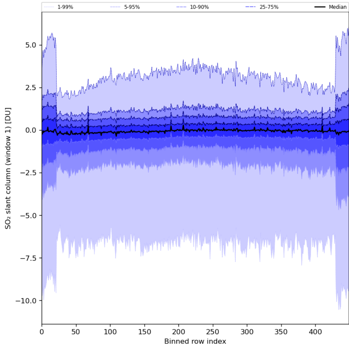
Figure 79: Along track statistics of “SO 2 slant column (window 1)” for 2024-01-21 to 2024-01-23
