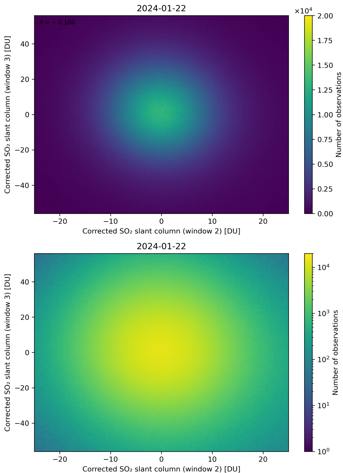
Figure 200: Scatter density plot of “Corrected SO 2 slant column (window 2)” against “Corrected SO 2 slant column (window 3)” for 2024-01-21 to 2024-01-23.
