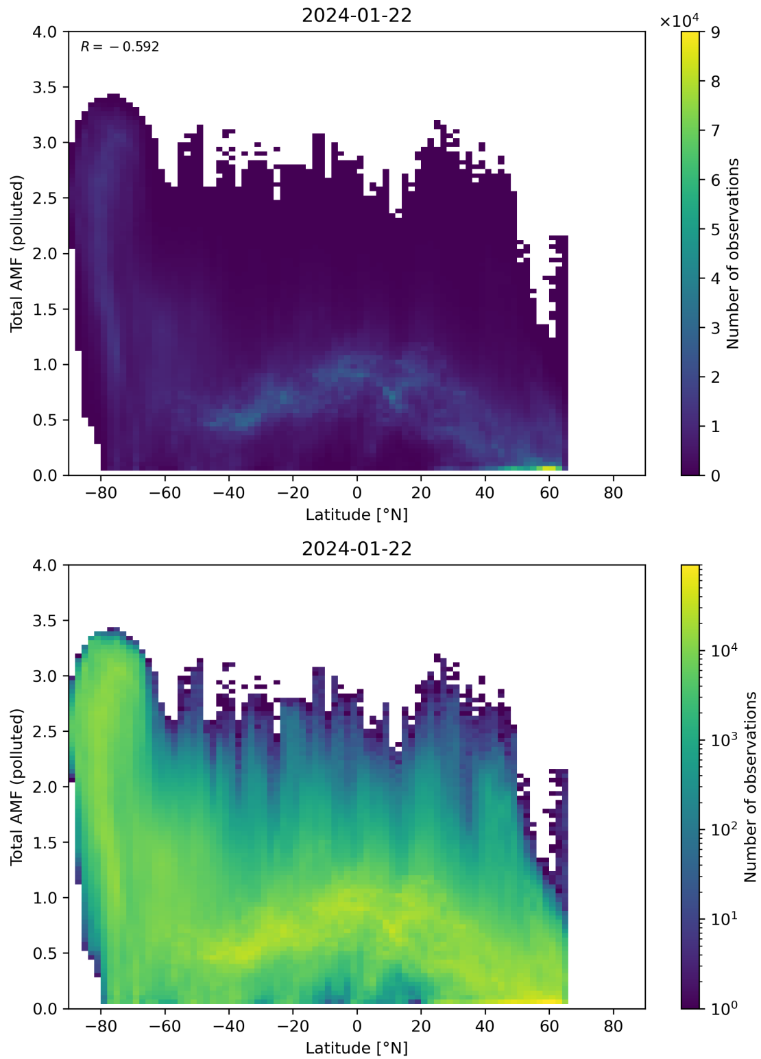
Figure 154: Scatter density plot of “Latitude” against “Total AMF (polluted)” for 2024-01-21 to 2024-01-23.
