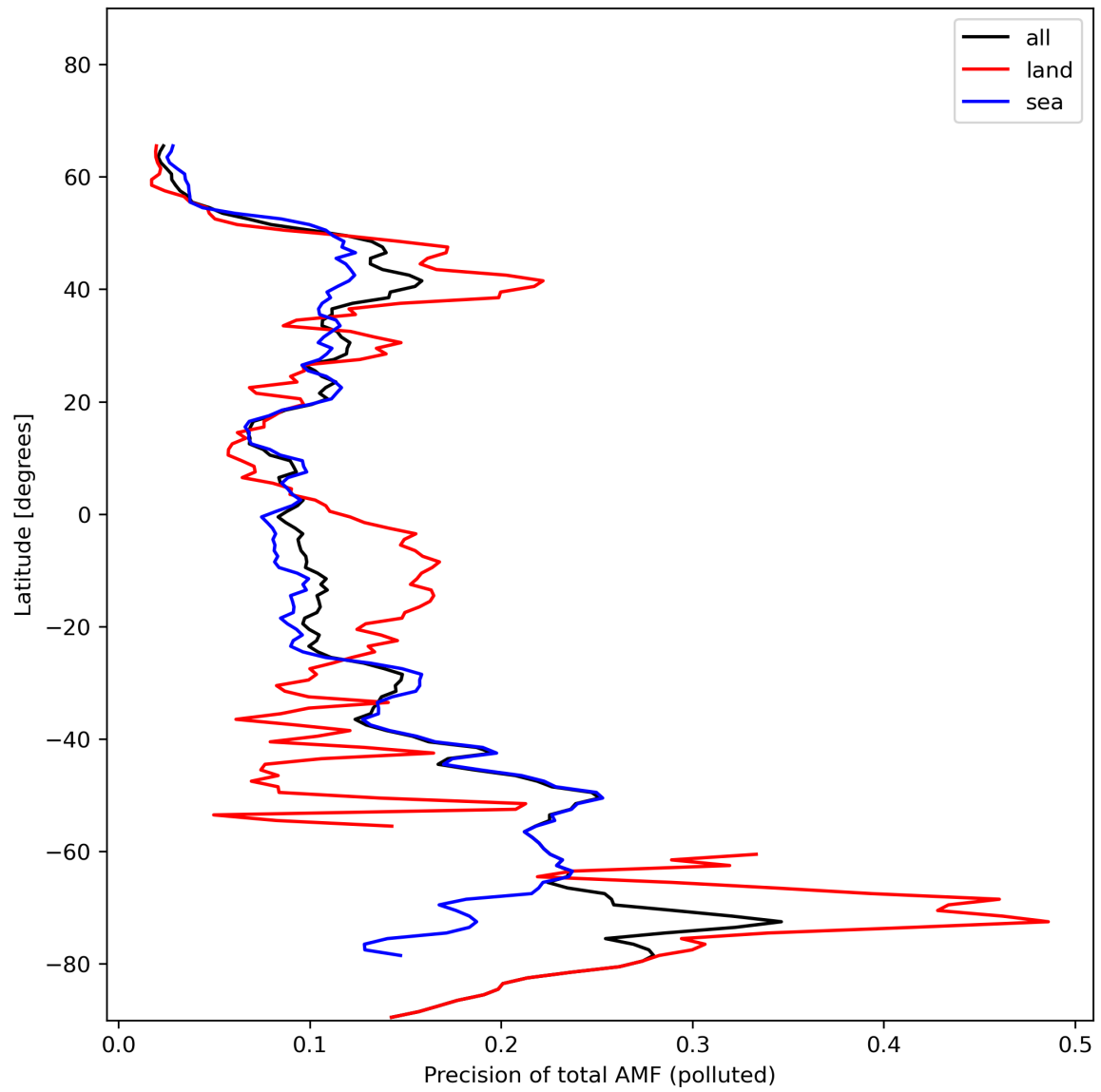
Figure 49: Zonal average of “Precision of total AMF (polluted)” for 2024-01-21 to 2024-01-23.
