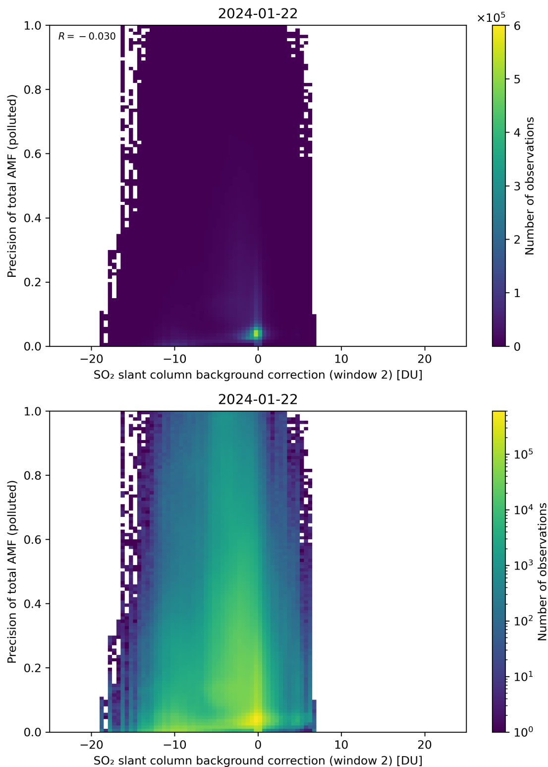
Figure 120: Scatter density plot of “SO 2 slant column background correction (window 2)” against “Precision of total AMF (polluted)” for 2024-01-21 to 2024-01-23.
