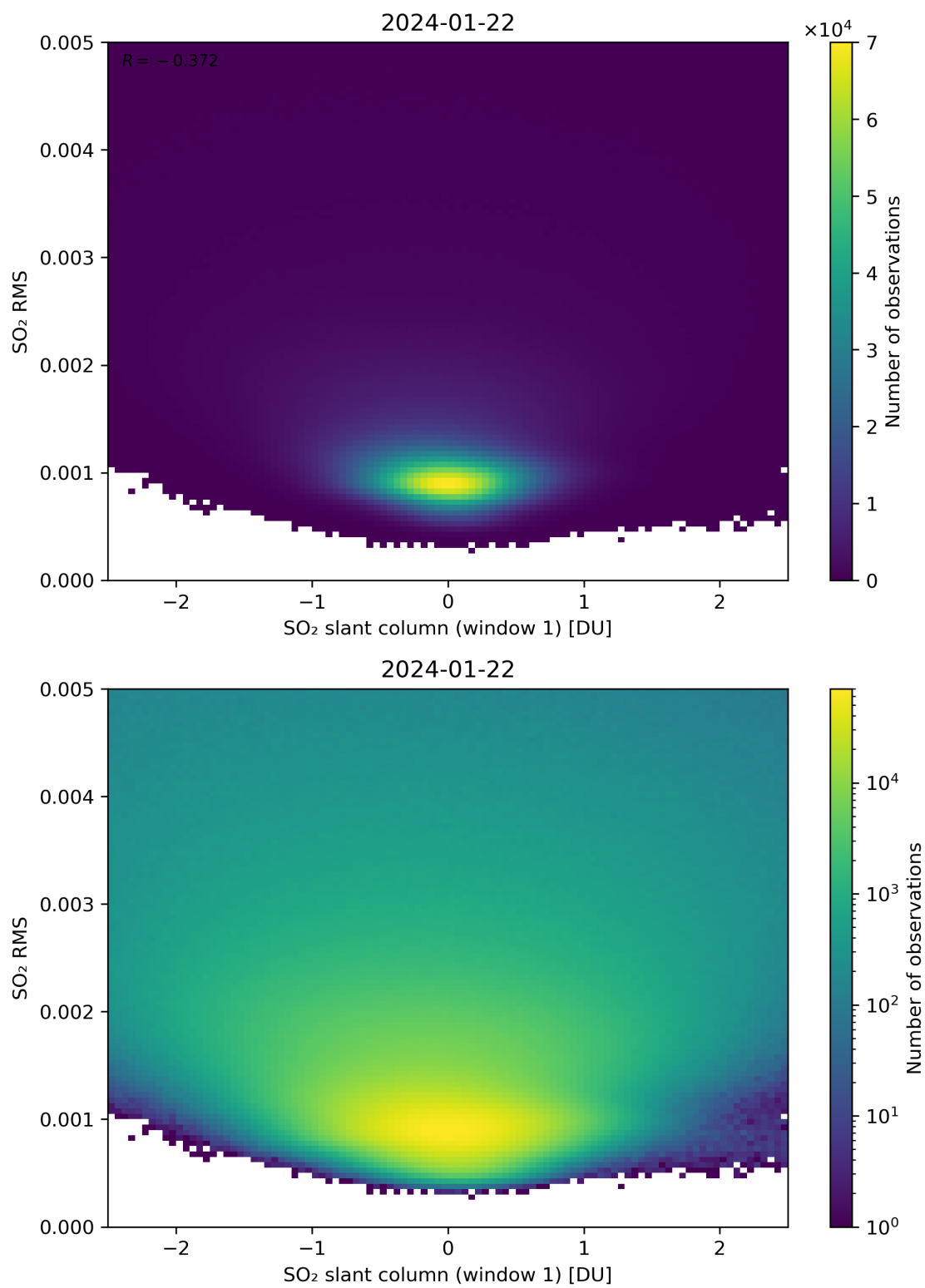
Figure 217: Scatter density plot of “SO 2 slant column (window 1)” against “SO 2 RMS” for 2024-01-21 to 2024-01-23.
