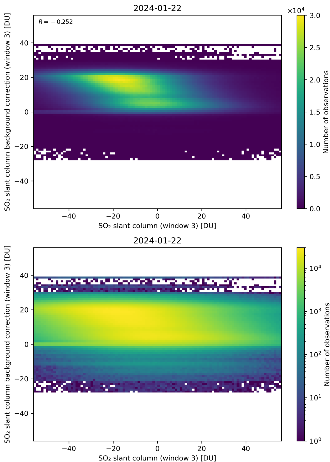
Figure 253: Scatter density plot of “SO 2 slant column (window 3)” against “SO 2 slant column background correction (window 3)” for 2024-01-21 to 2024-01-23.
