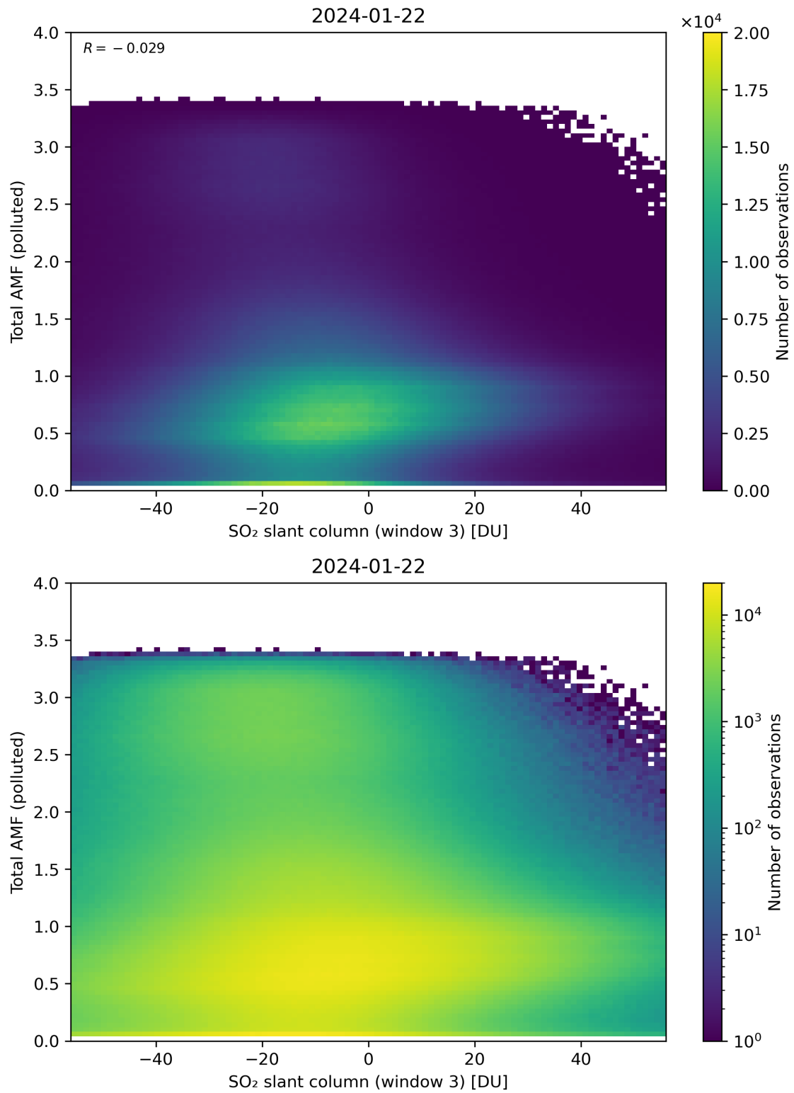
Figure 268: Scatter density plot of “SO 2 slant column (window 3)” against “Total AMF (polluted)” for 2024-01-21 to 2024-01-23.
