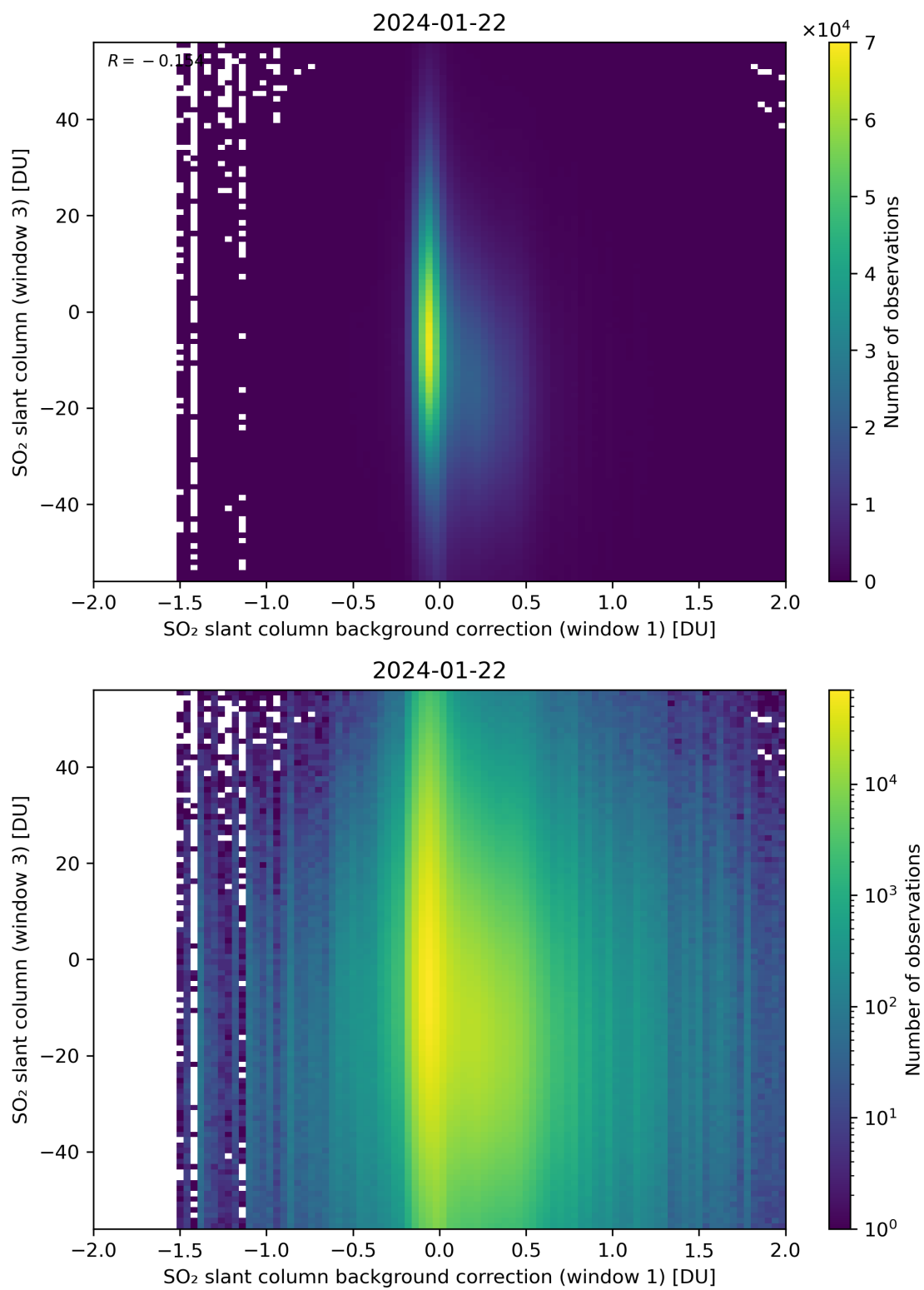
Figure 107: Scatter density plot of “SO 2 slant column background correction (window 1)” against “SO 2 slant column (window 3)” for 2024-01-21 to 2024-01-23.
