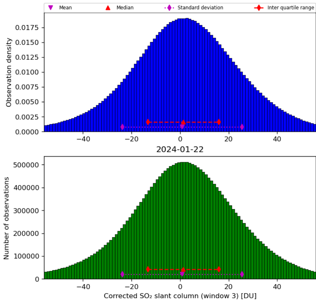
Figure 66: Histogram of “Corrected SO 2 slant column (window 3)” for 2024-01-21 to 2024-01-23
