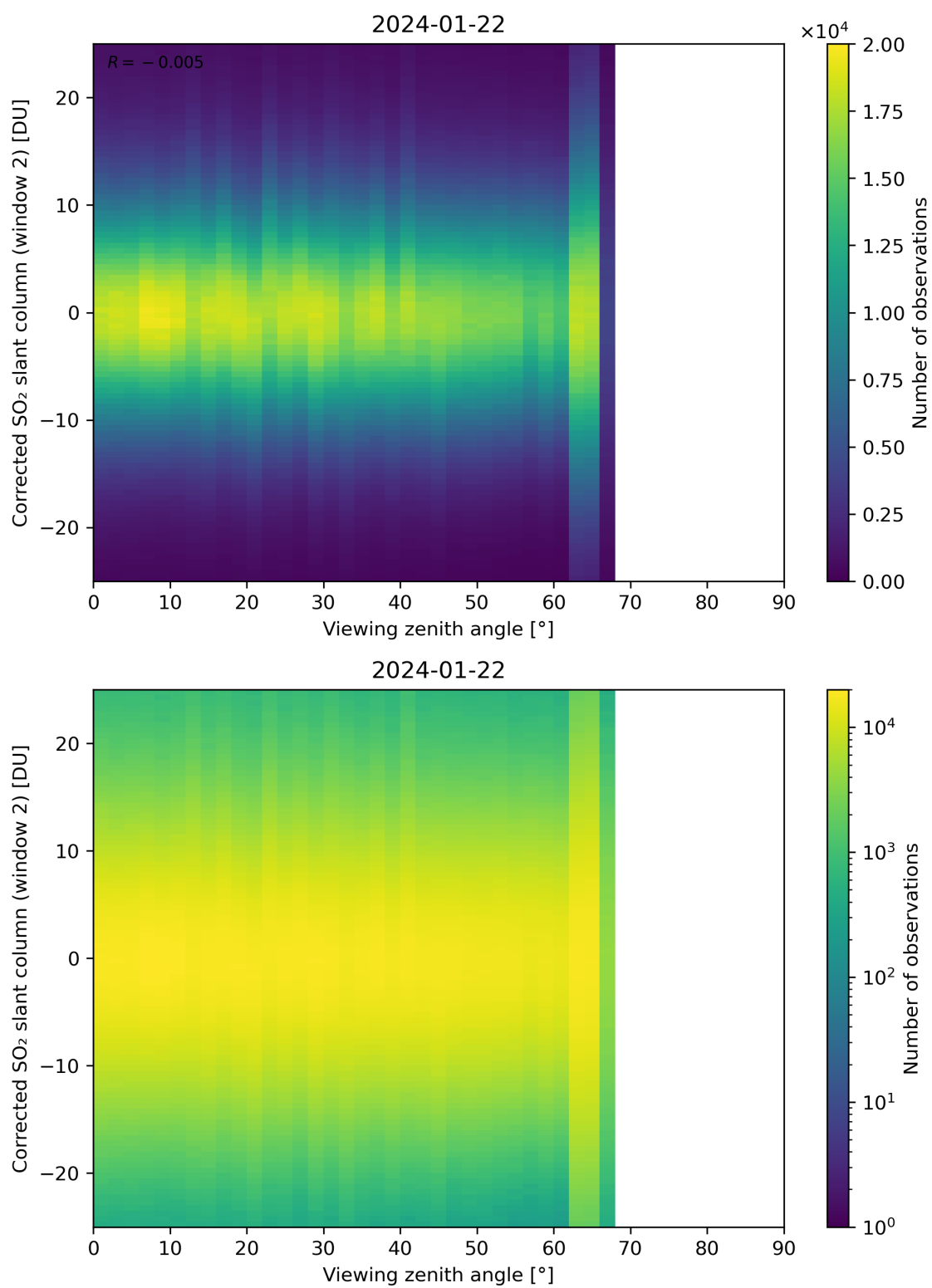
Figure 318: Scatter density plot of “Viewing zenith angle” against “Corrected SO 2 slant column (window 2)” for 2024-01-21 to 2024-01-23.
