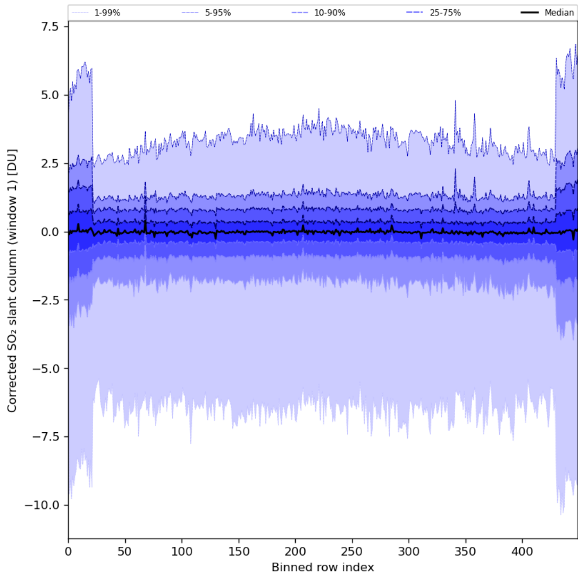
Figure 81: Along track statistics of “Corrected SO 2 slant column (window 1)” for 2024-01-21 to 2024-01-23
