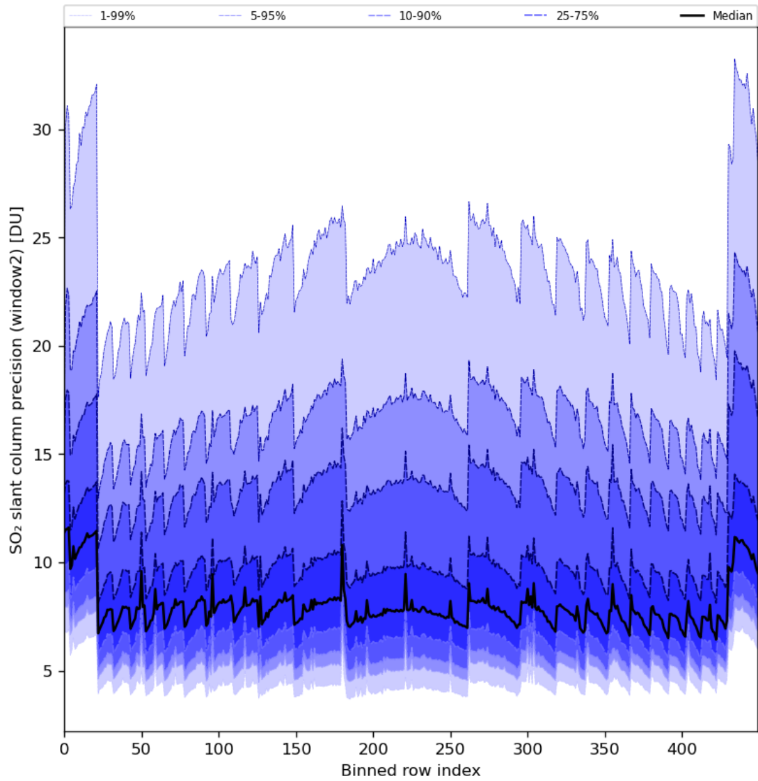
Figure 84: Along track statistics of “SO 2 slant column precision (window2)” for 2024-01-21 to 2024-01-23
