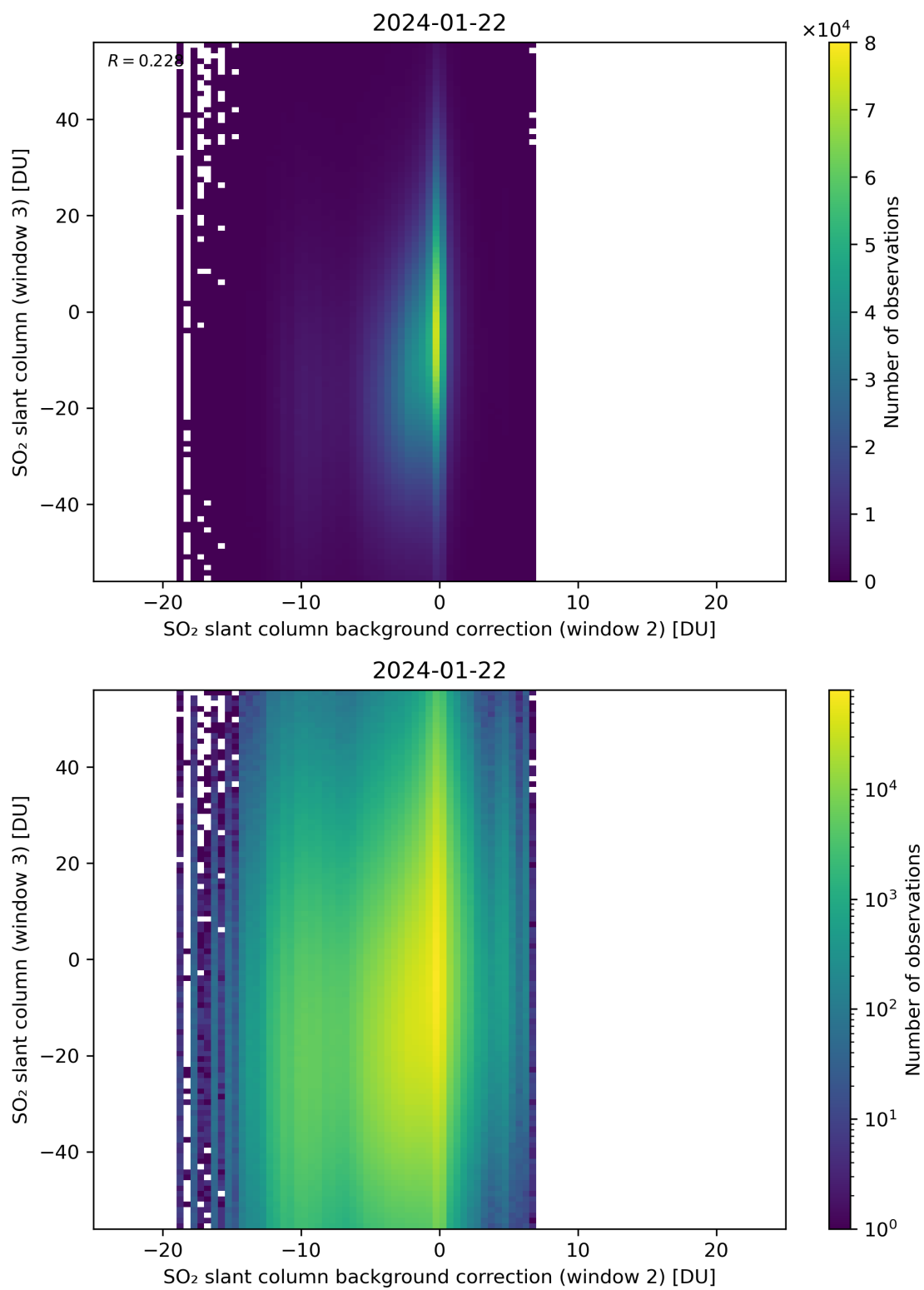
Figure 117: Scatter density plot of “SO 2 slant column background correction (window 2)” against “SO 2 slant column (window 3)” for 2024-01-21 to 2024-01-23.
