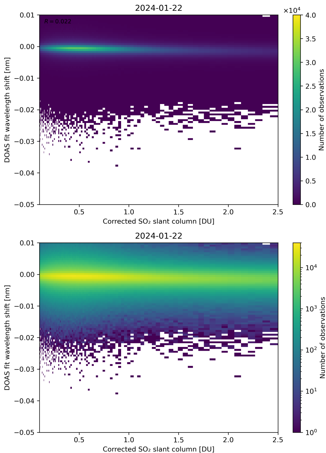
Figure 181: Scatter density plot of “Corrected SO 2 slant column” against “DOAS fit wavelength shift” for 2024-01-21 to 2024-01-23.
