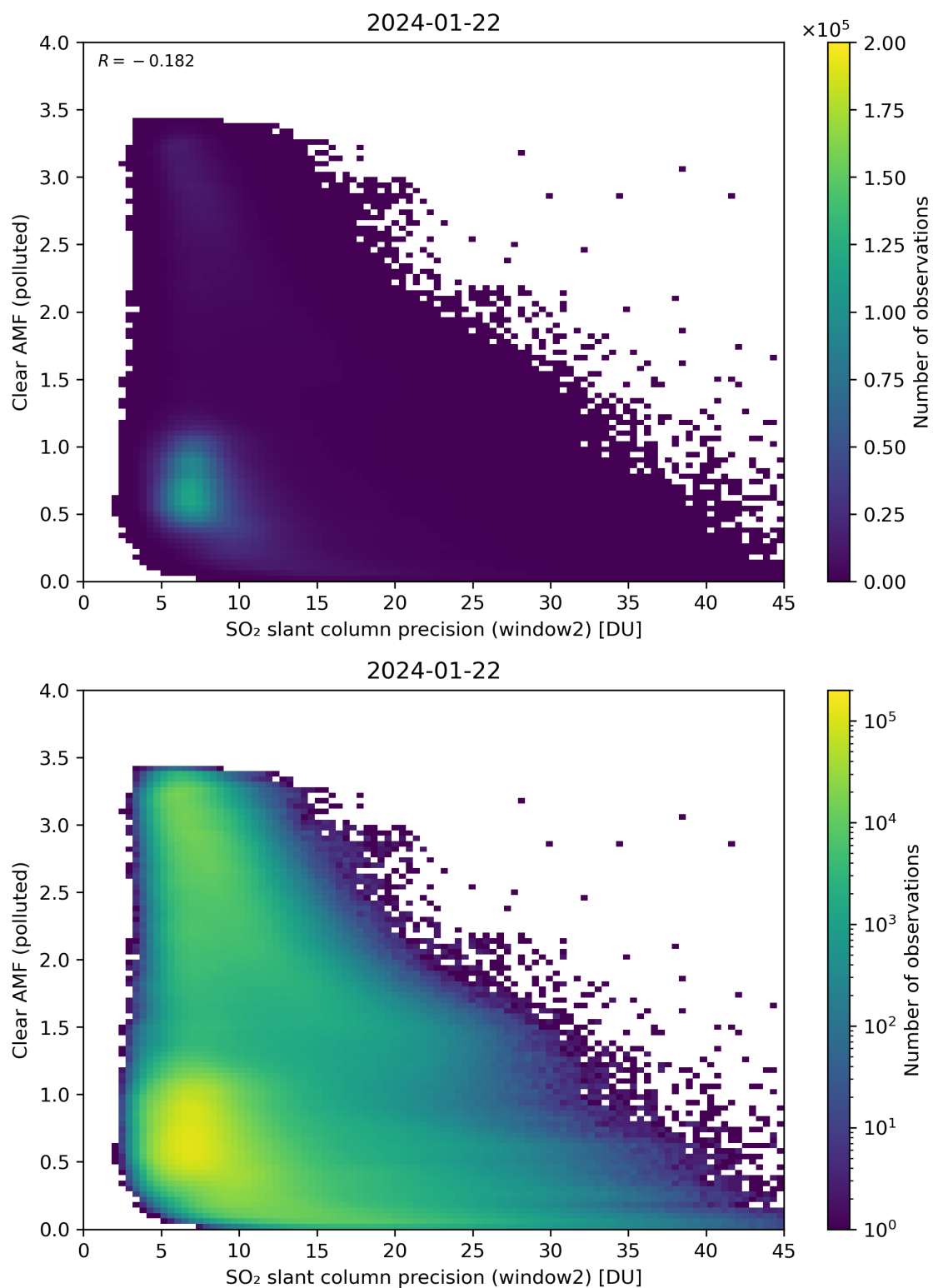
Figure 246: Scatter density plot of “SO 2 slant column precision (window2)” against “Clear AMF (polluted)” for 2024-01-21 to 2024-01-23.
