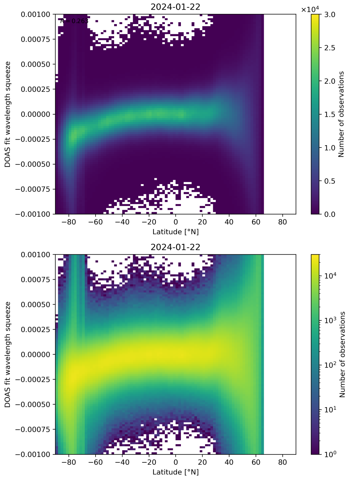
Figure 143: Scatter density plot of “Latitude” against “DOAS fit wavelength squeeze” for 2024-01-21 to 2024-01-23.
