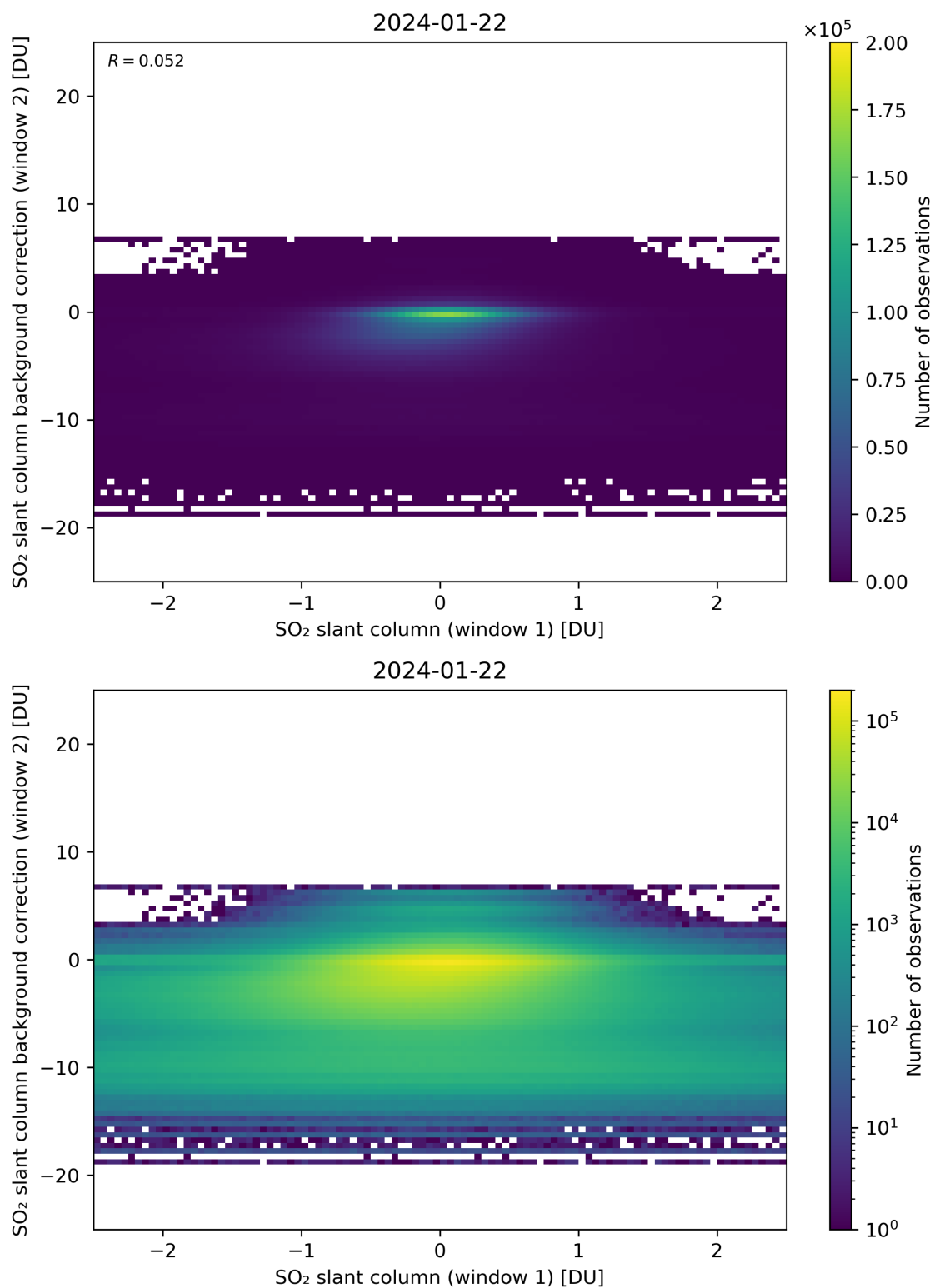
Figure 213: Scatter density plot of “SO 2 slant column (window 1)” against “SO 2 slant column background correction (window 2)” for 2024-01-21 to 2024-01-23.
