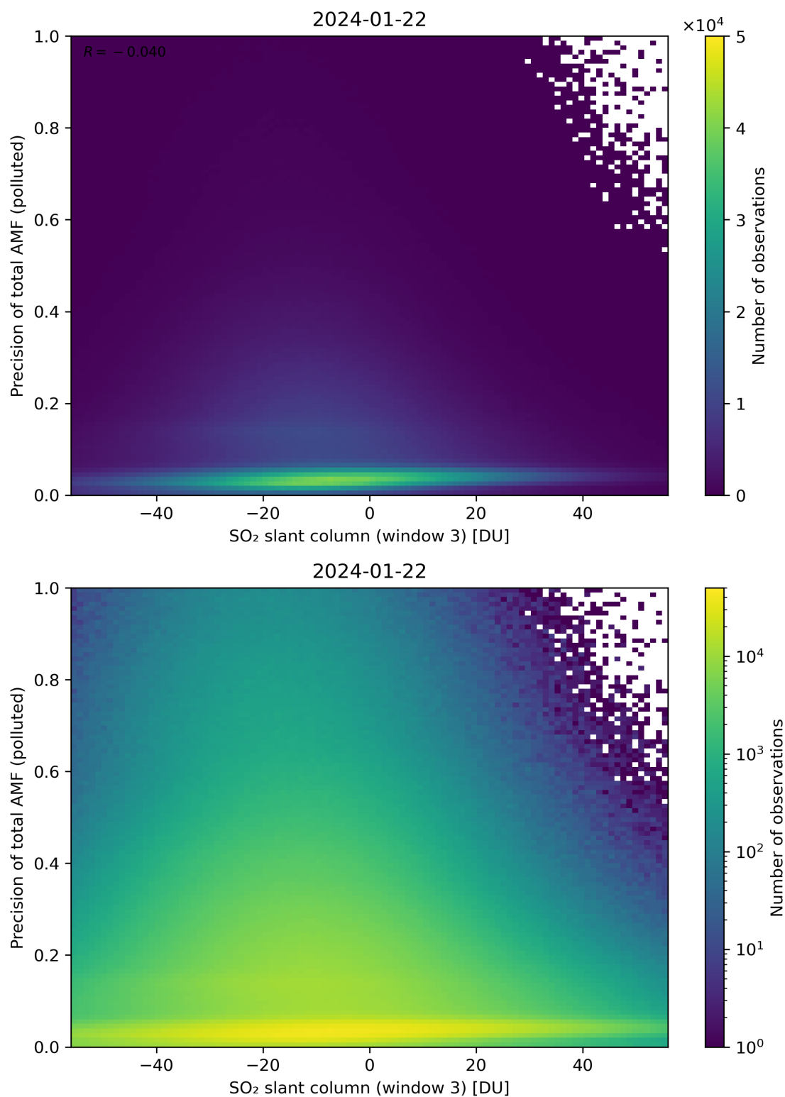
Figure 269: Scatter density plot of “SO 2 slant column (window 3)” against “Precision of total AMF (polluted)” for 2024-01-21 to 2024-01-23.
