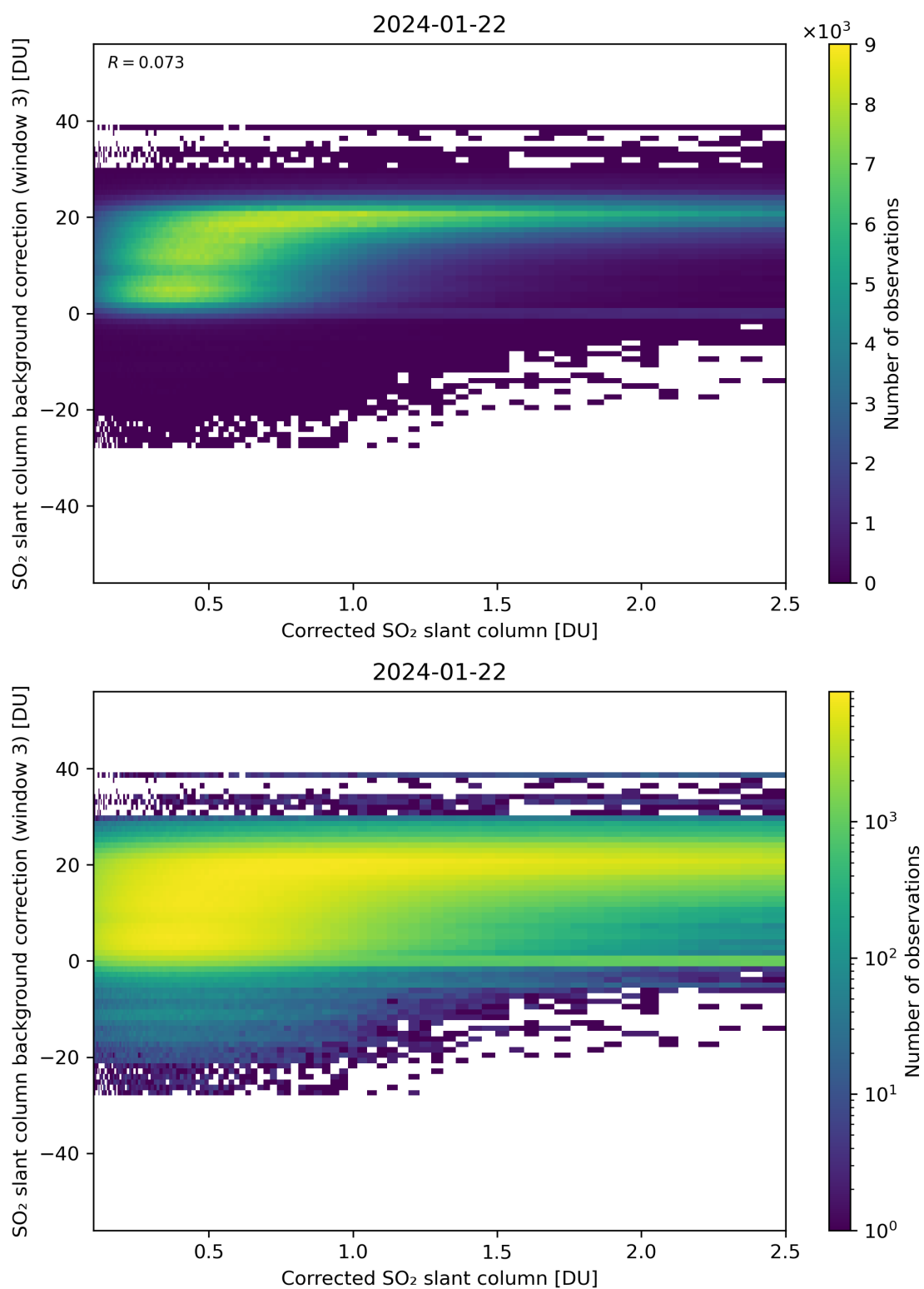
Figure 180: Scatter density plot of “Corrected SO 2 slant column” against “SO 2 slant column background correction (window 3)” for 2024-01-21 to 2024-01-23.
