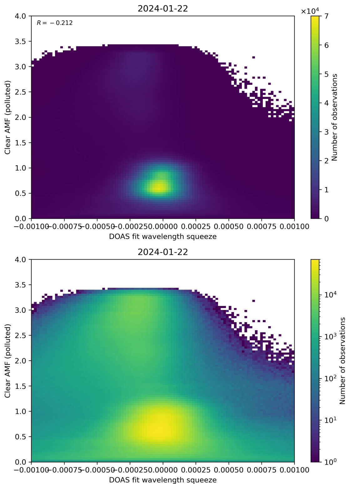
Figure 133: Scatter density plot of “DOAS fit wavelength squeeze” against “Clear AMF (polluted)” for 2024-01-21 to 2024-01-23.
