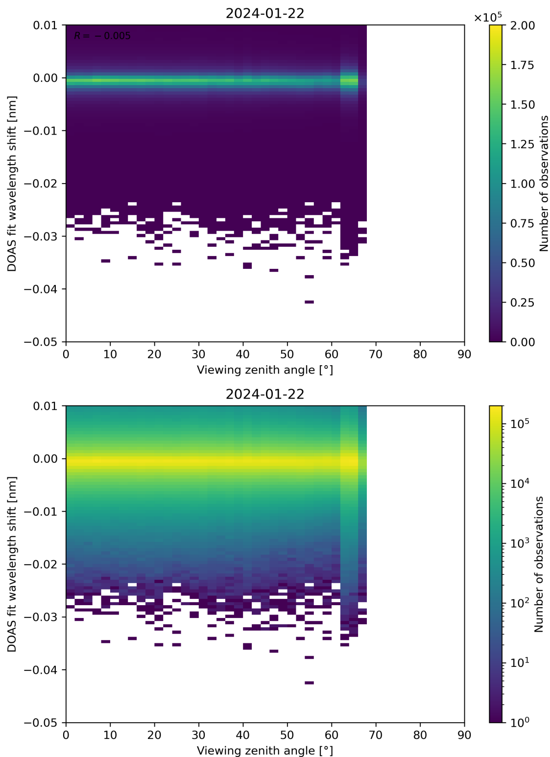
Figure 311: Scatter density plot of “Viewing zenith angle” against “DOAS fit wavelength shift” for 2024-01-21 to 2024-01-23.
