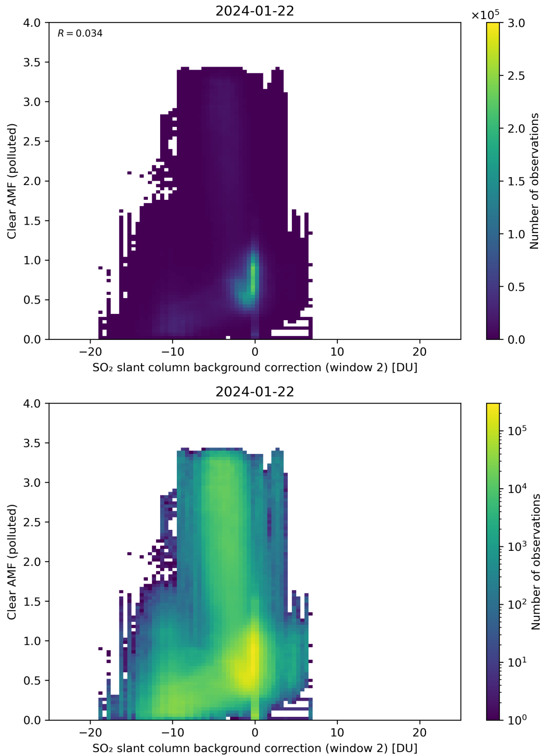
Figure 115: Scatter density plot of “SO 2 slant column background correction (window 2)” against “Clear AMF (polluted)” for 2024-01-21 to 2024-01-23.
