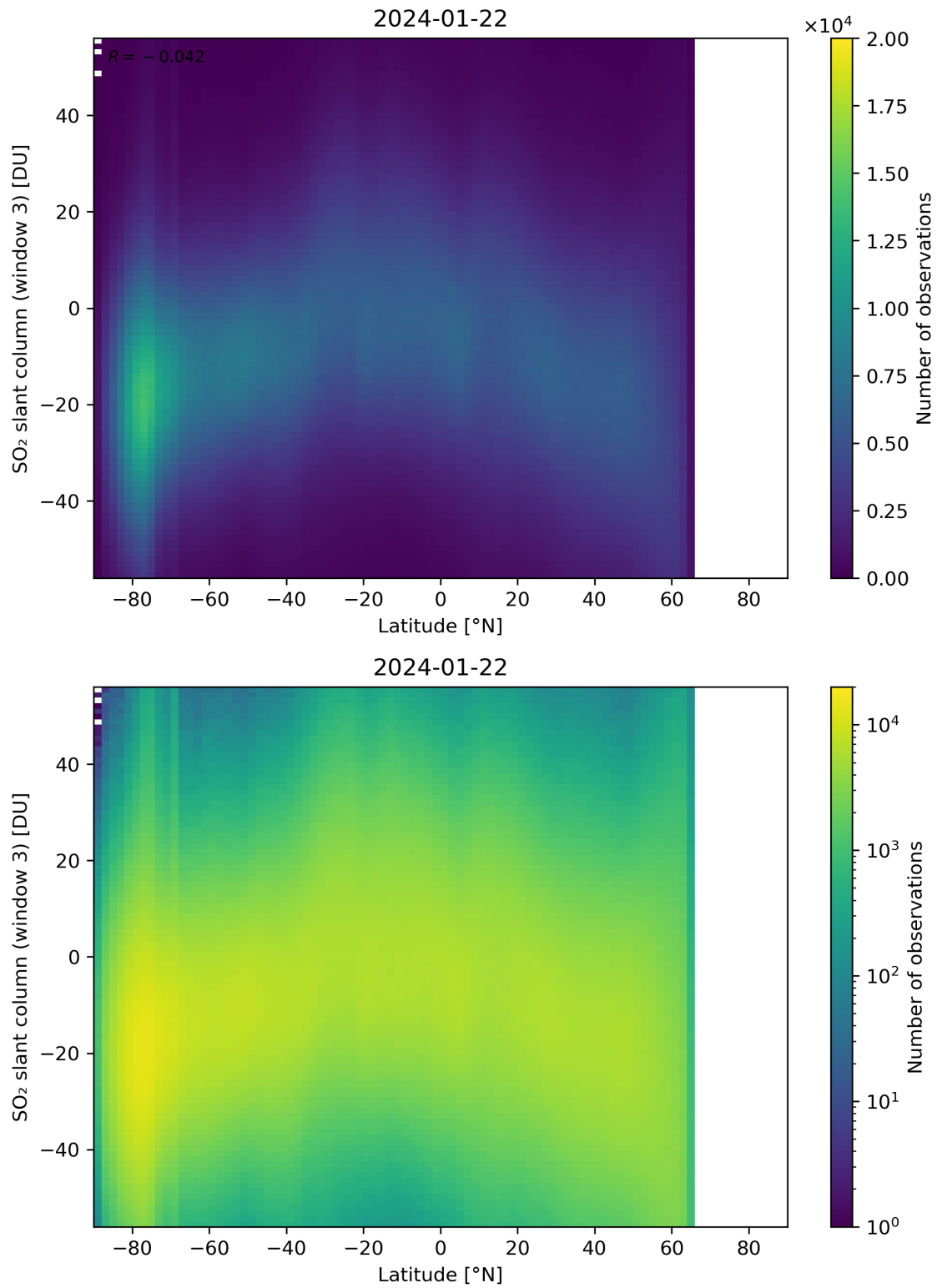
Figure 152: Scatter density plot of “Latitude” against “SO 2 slant column (window 3)” for 2024-01-21 to 2024-01-23.
