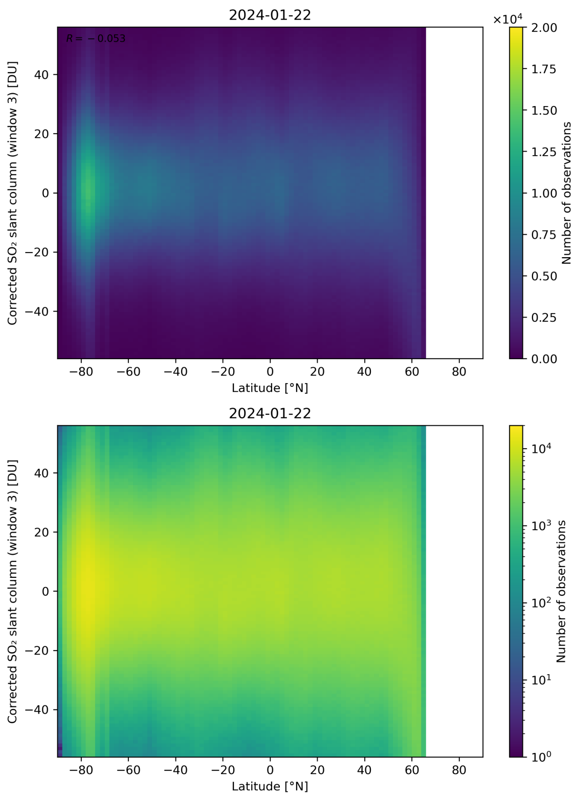
Figure 148: Scatter density plot of “Latitude” against “Corrected SO 2 slant column (window 3)” for 2024-01-21 to 2024-01-23.
