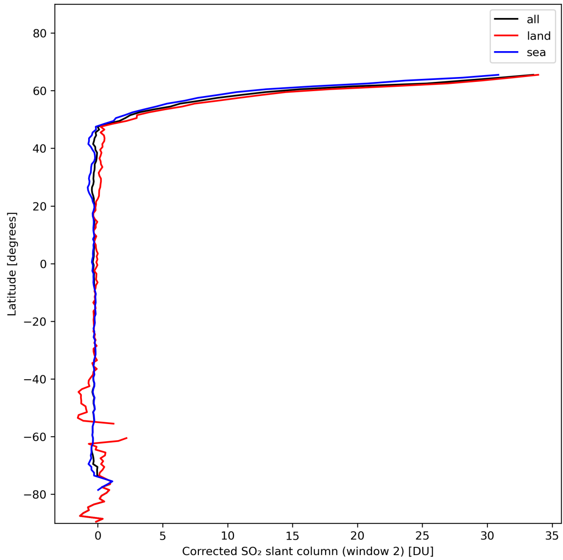
Figure 39: Zonal average of “Corrected SO 2 slant column (window 2)” for 2024-01-21 to 2024-01-23.
