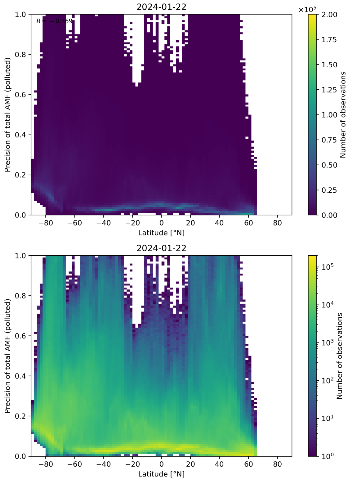
Figure 155: Scatter density plot of “Latitude” against “Precision of total AMF (polluted)” for 2024-01-21 to 2024-01-23.
