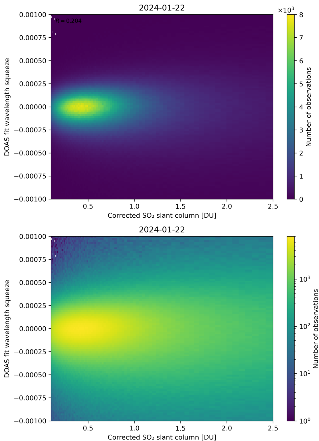
Figure 182: Scatter density plot of “Corrected SO 2 slant column” against “DOAS fit wavelength squeeze” for 2024-01-21 to 2024-01-23.
