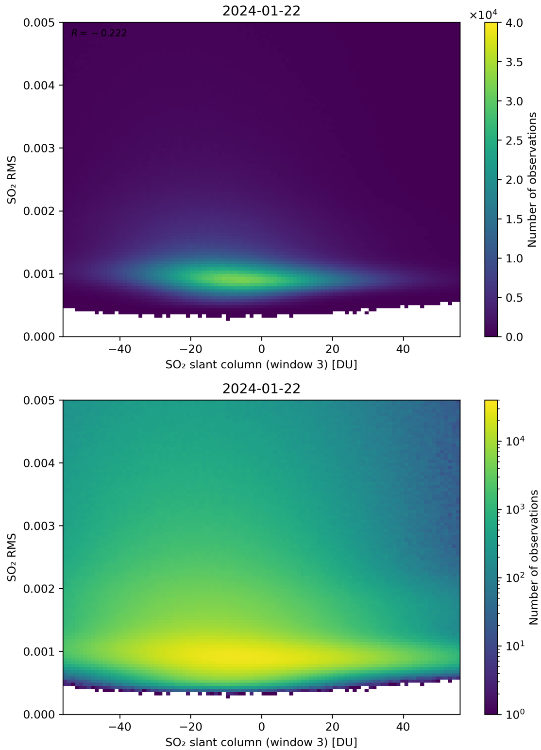
Figure 256: Scatter density plot of “SO 2 slant column (window 3)” against “SO 2 RMS” for 2024-01-21 to 2024-01-23.
