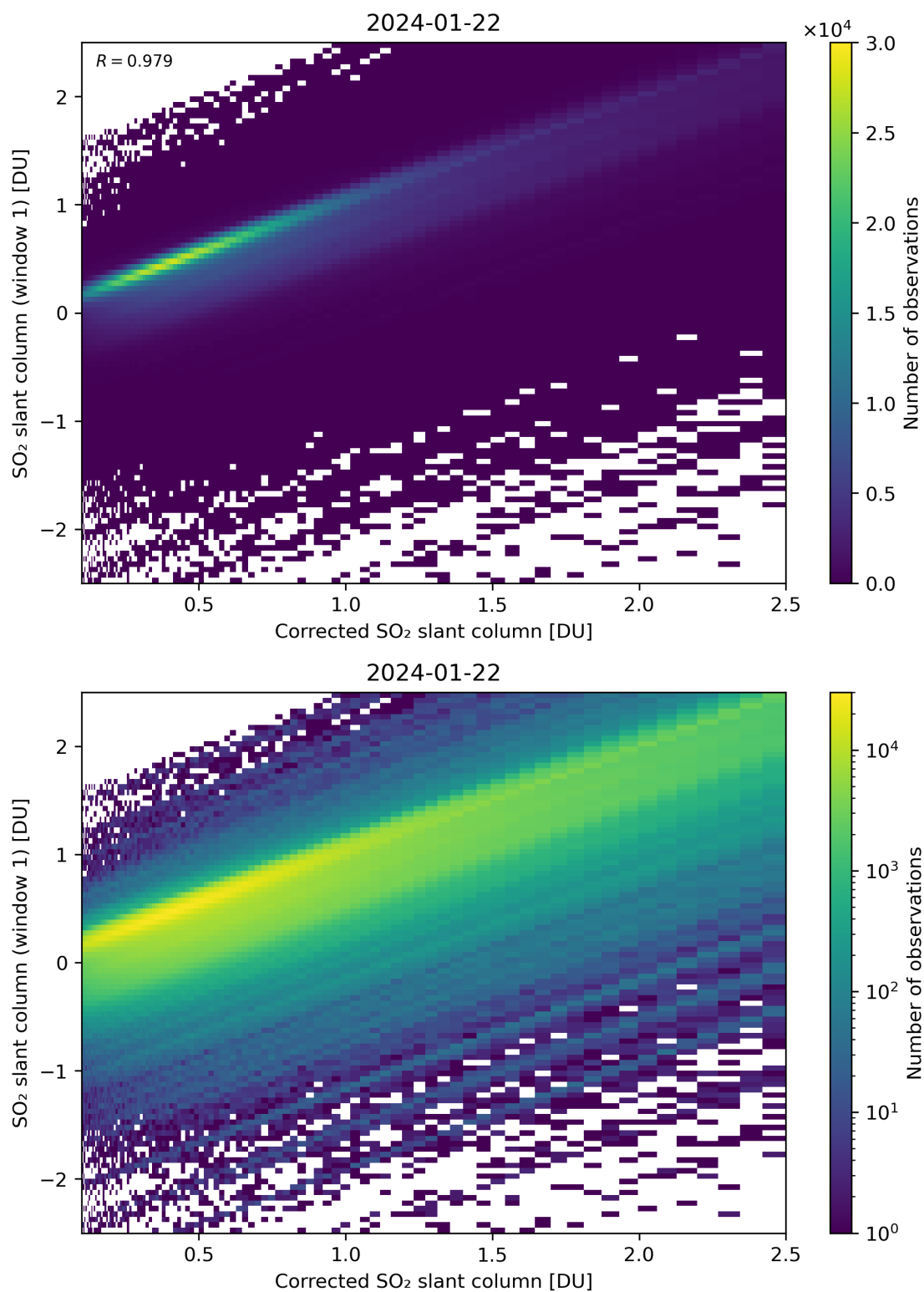
Figure 187: Scatter density plot of “Corrected SO 2 slant column” against “SO 2 slant column (window 1)” for 2024-01-21 to 2024-01-23.
