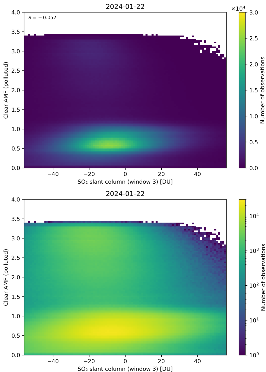
Figure 265: Scatter density plot of “SO 2 slant column (window 3)” against “Clear AMF (polluted)” for 2024-01-21 to 2024-01-23.
