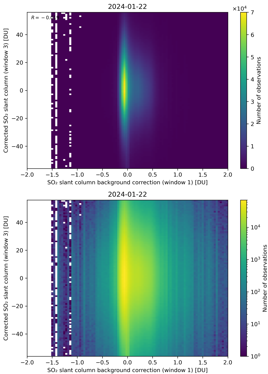
Figure 105: Scatter density plot of “SO 2 slant column background correction (window 1)” against “Corrected SO 2 slant column (window 3)” for 2024-01-21 to 2024-01-23.
