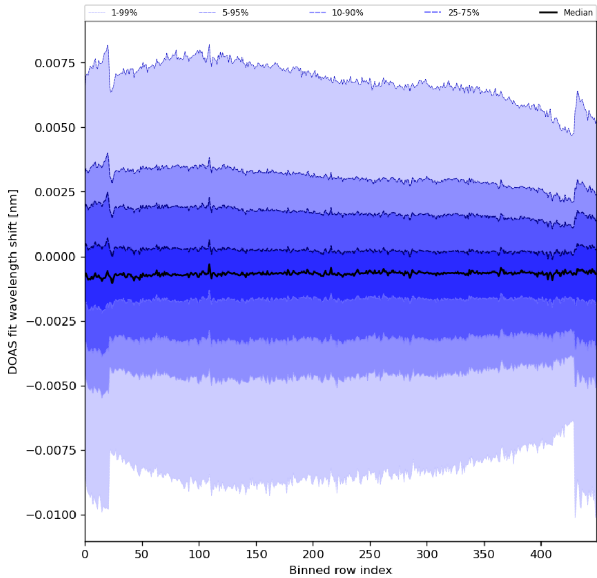
Figure 91: Along track statistics of “DOAS fit wavelength shift” for 2024-01-21 to 2024-01-23
