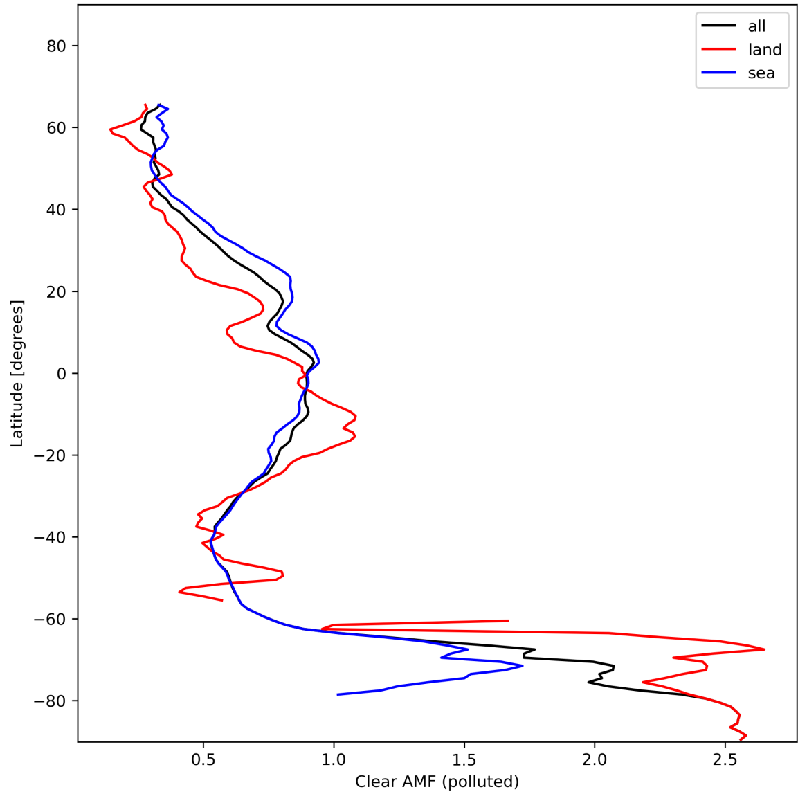
Figure 50: Zonal average of “Clear AMF (polluted)” for 2024-01-21 to 2024-01-23.
