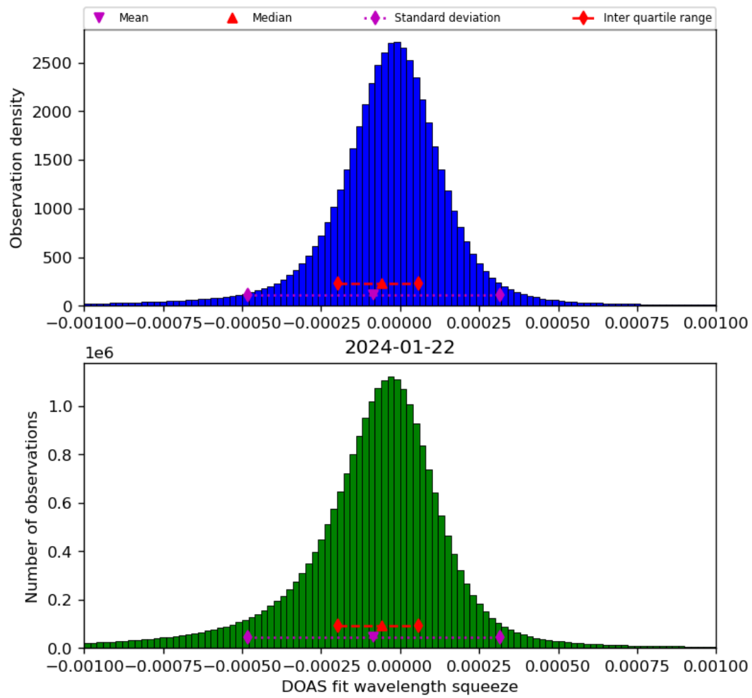
Figure 69: Histogram of “DOAS fit wavelength squeeze” for 2024-01-21 to 2024-01-23
