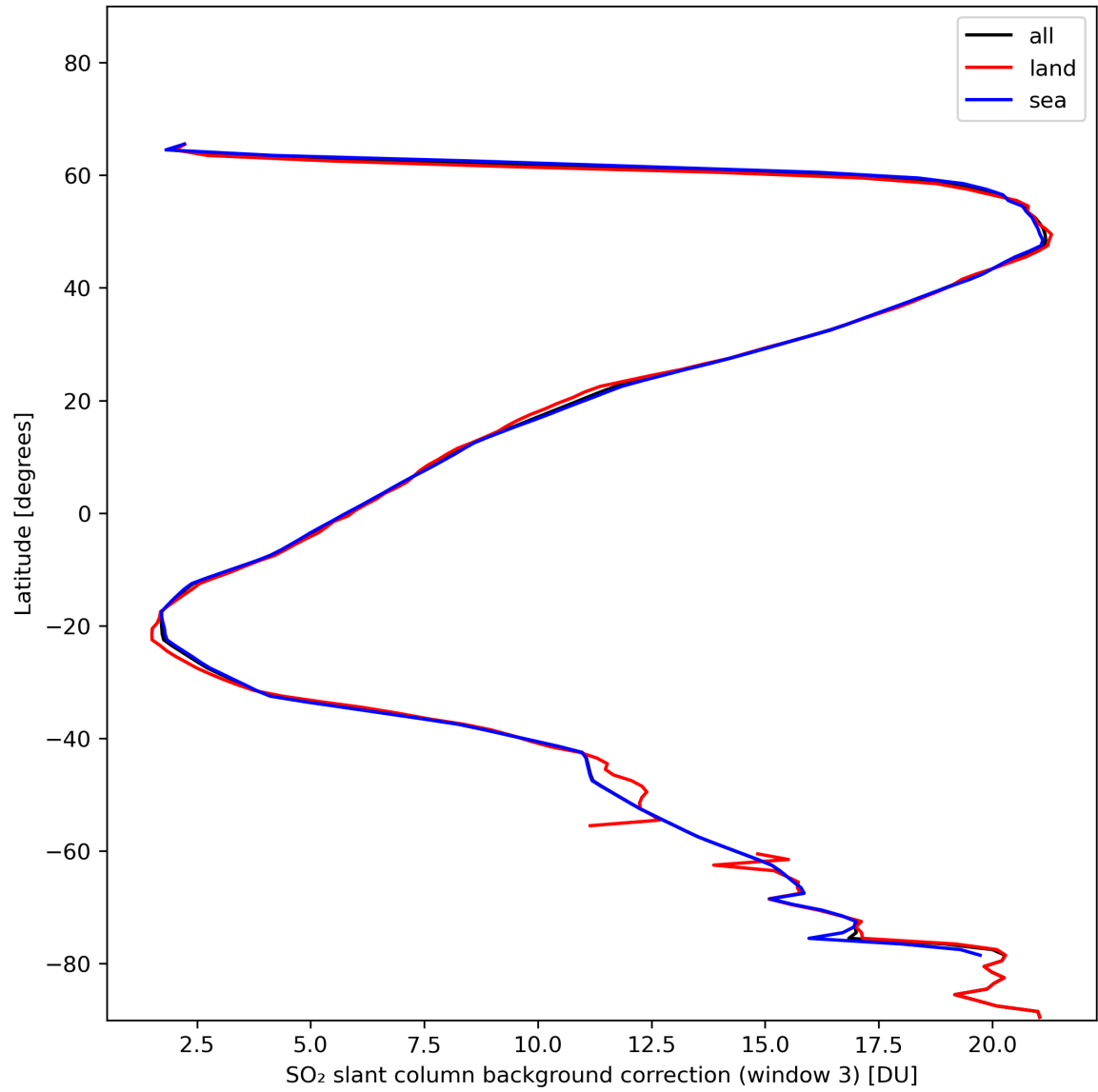
Figure 44: Zonal average of “SO 2 slant column background correction (window 3)” for 2024-01-21 to 2024-01-23.
