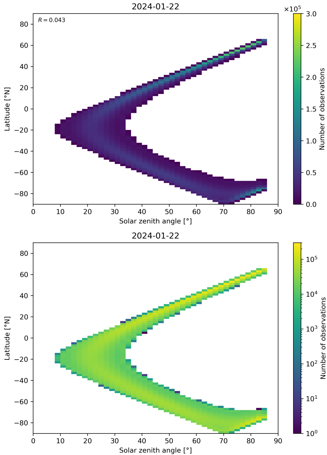
Figure 164: Scatter density plot of “Solar zenith angle” against “Latitude” for 2024-01-21 to 2024-01-23.
