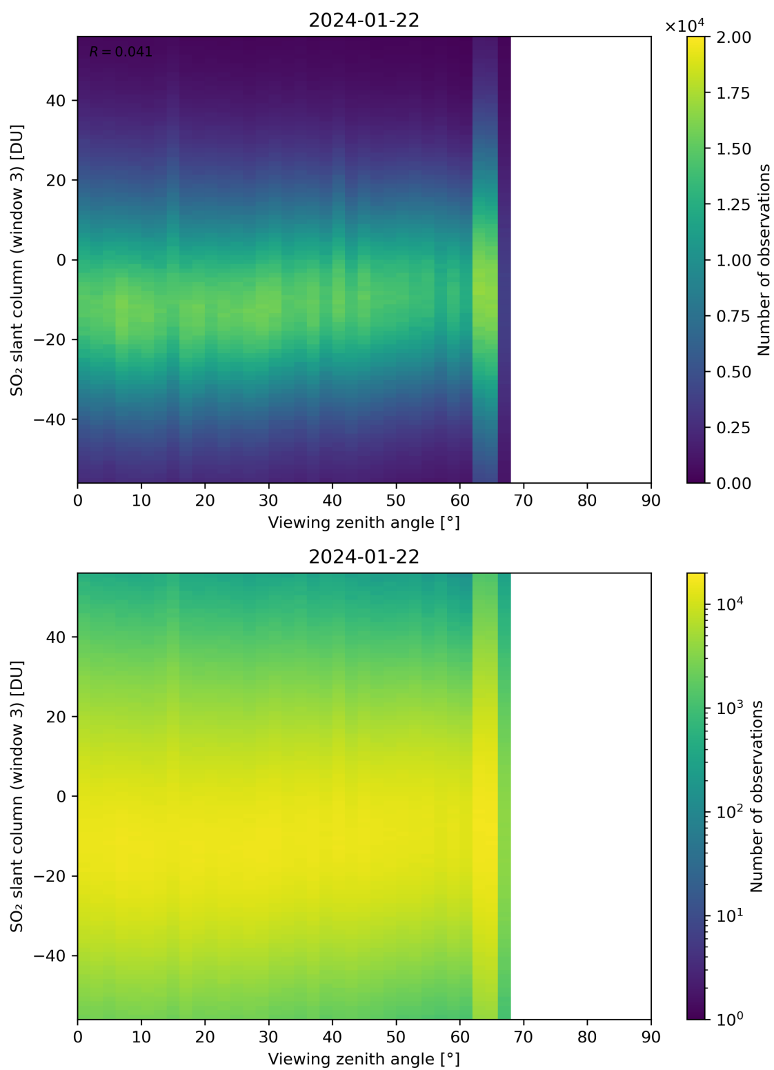
Figure 323: Scatter density plot of “Viewing zenith angle” against “SO 2 slant column (window 3)” for 2024-01-21 to 2024-01-23.
