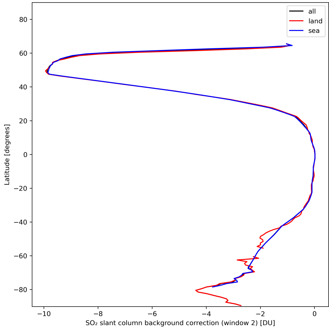
Figure 40: Zonal average of “SO 2 slant column background correction (window 2)” for 2024-01-21 to 2024-01-23.
