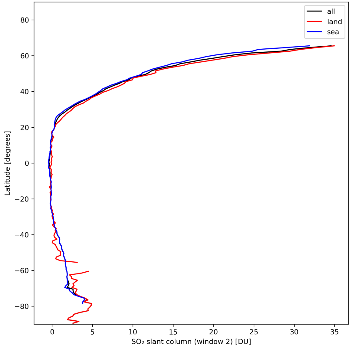
Figure 37: Zonal average of “SO 2 slant column (window 2)” for 2024-01-21 to 2024-01-23.
