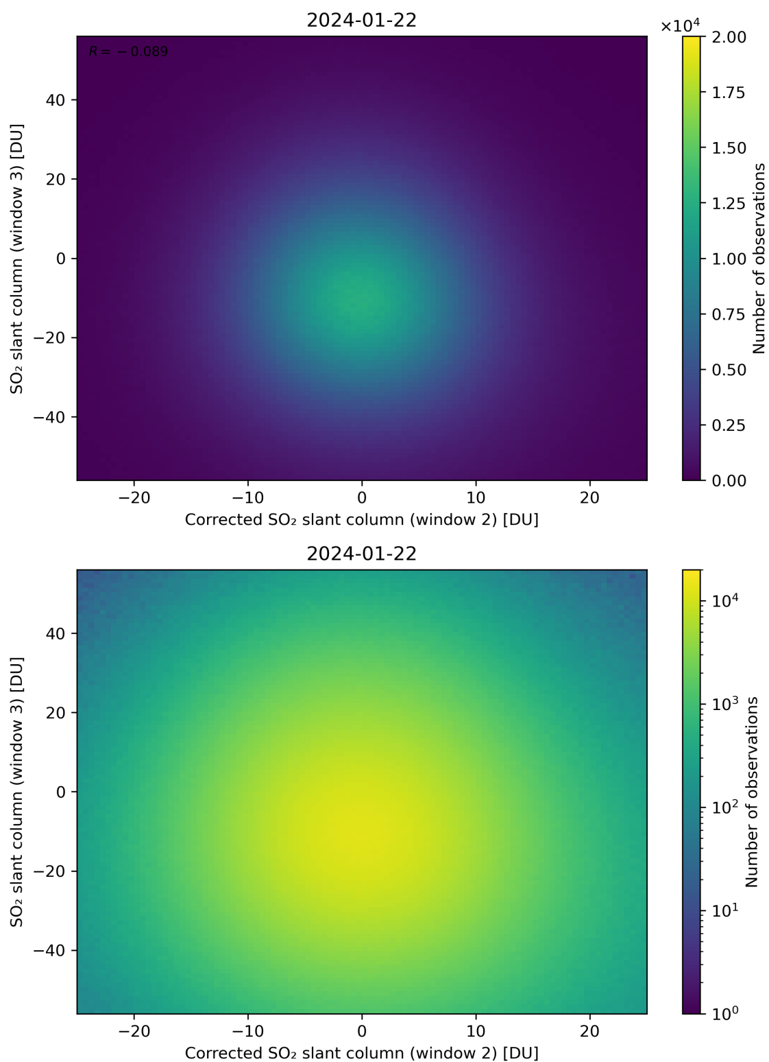
Figure 201: Scatter density plot of “Corrected SO 2 slant column (window 2)” against “SO 2 slant column (window 3)” for 2024-01-21 to 2024-01-23.
