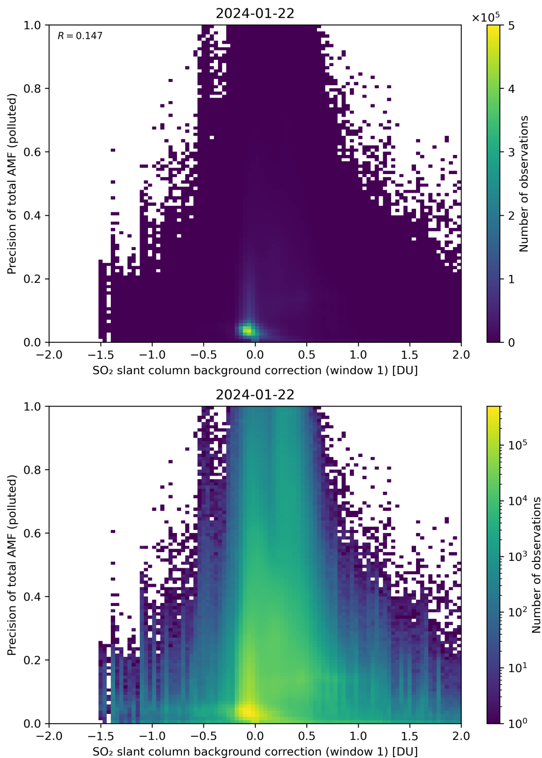
Figure 110: Scatter density plot of “SO 2 slant column background correction (window 1)” against “Precision of total AMF (polluted)” for 2024-01-21 to 2024-01-23.
