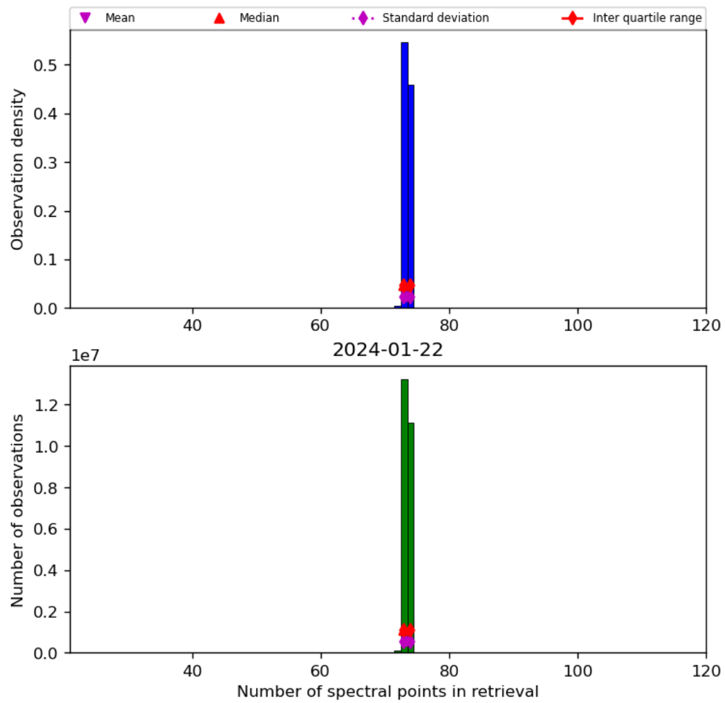
Figure 74: Histogram of “Number of spectral points in retrieval” for 2024-01-21 to 2024-01-23
