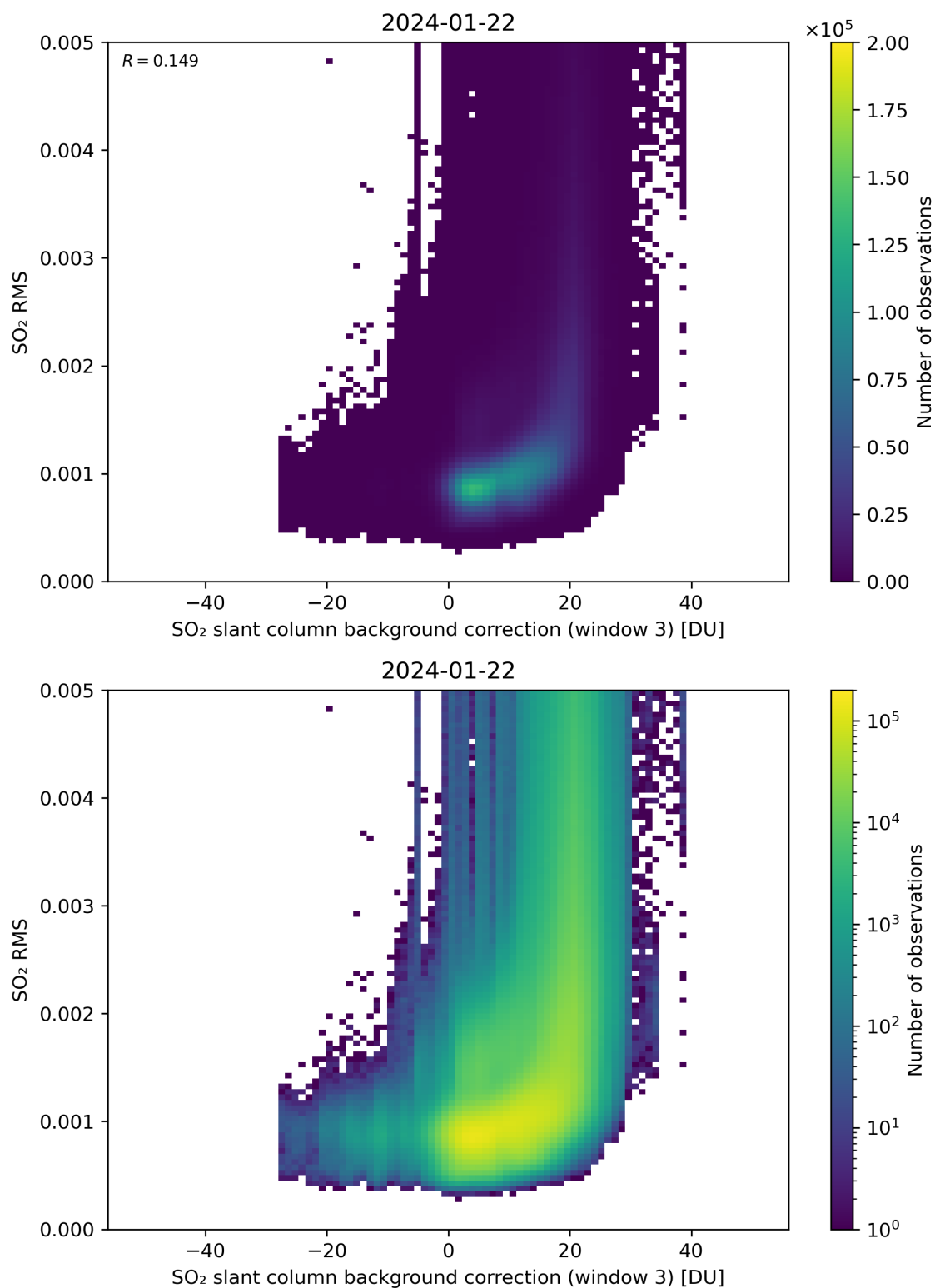
Figure 123: Scatter density plot of “SO 2 slant column background correction (window 3)” against “SO 2 RMS” for 2024-01-21 to 2024-01-23.
