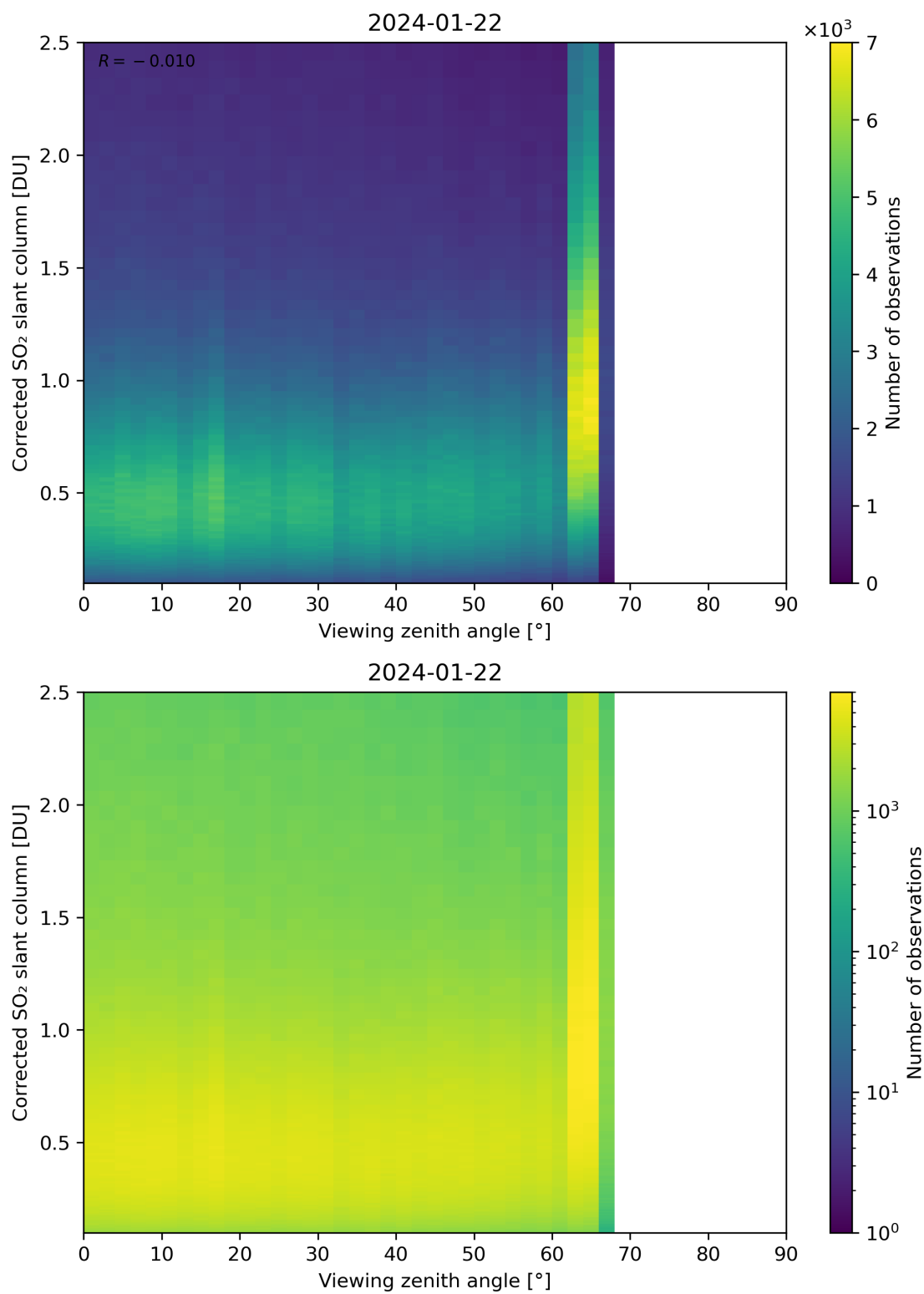
Figure 317: Scatter density plot of “Viewing zenith angle” against “Corrected SO 2 slant column” for 2024-01-21 to 2024-01-23.
