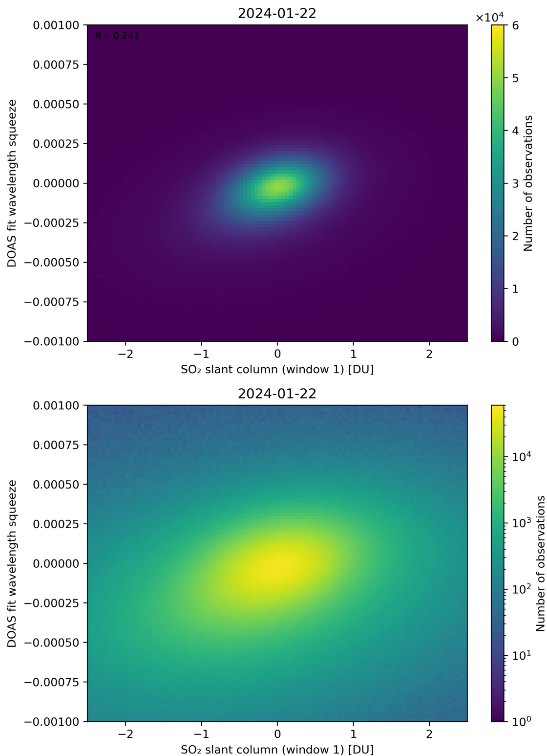
Figure 216: Scatter density plot of “SO 2 slant column (window 1)” against “DOAS fit wavelength squeeze” for 2024-01-21 to 2024-01-23.
