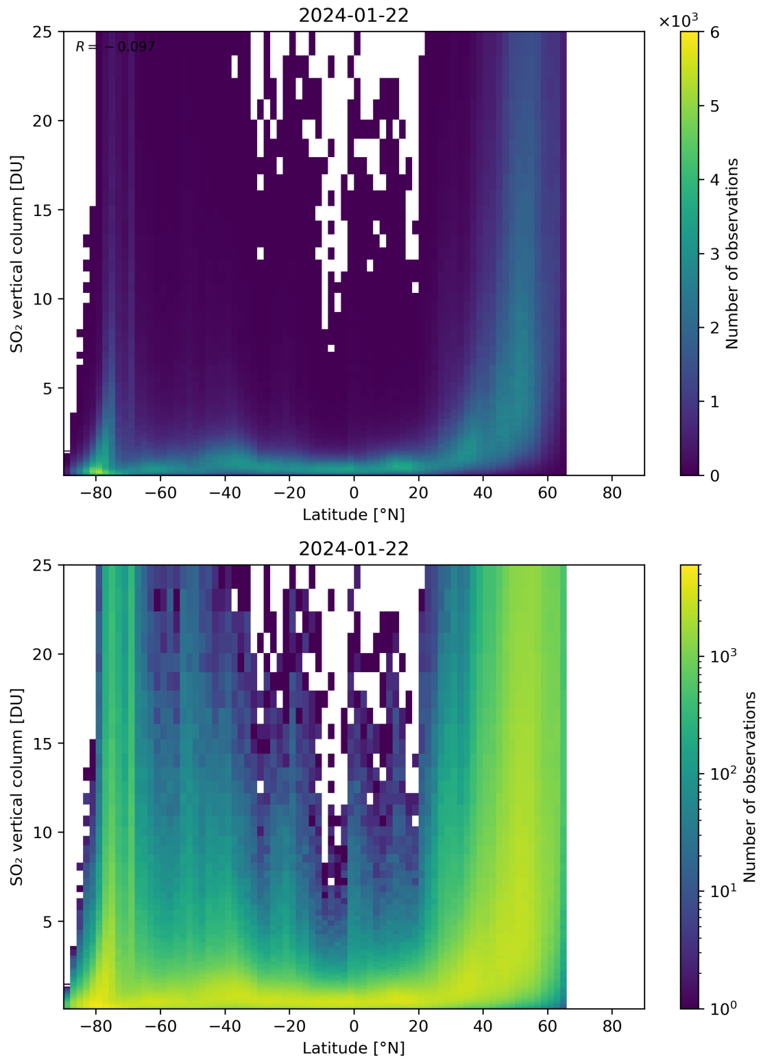
Figure 156: Scatter density plot of “Latitude” against “SO 2 vertical column” for 2024-01-21 to 2024-01-23.
