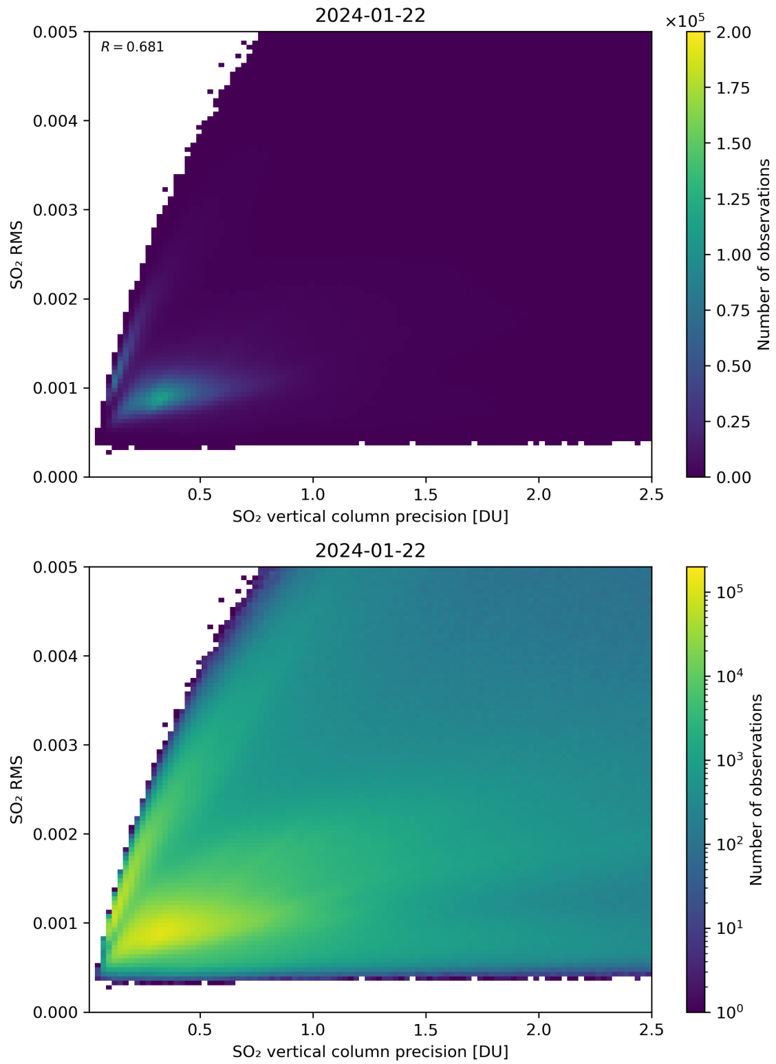
Figure 284: Scatter density plot of “SO 2 vertical column precision” against “SO 2 RMS” for 2024-01-21 to 2024-01-23.
