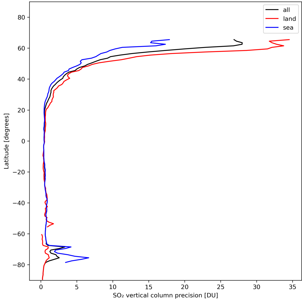
Figure 31: Zonal average of “SO 2 vertical column precision” for 2024-01-21 to 2024-01-23.
