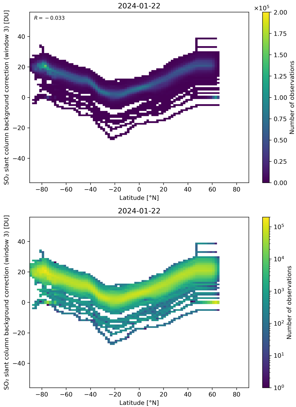
Figure 141: Scatter density plot of “Latitude” against “SO 2 slant column background correction (window 3)” for 2024-01-21 to 2024-01-23.
