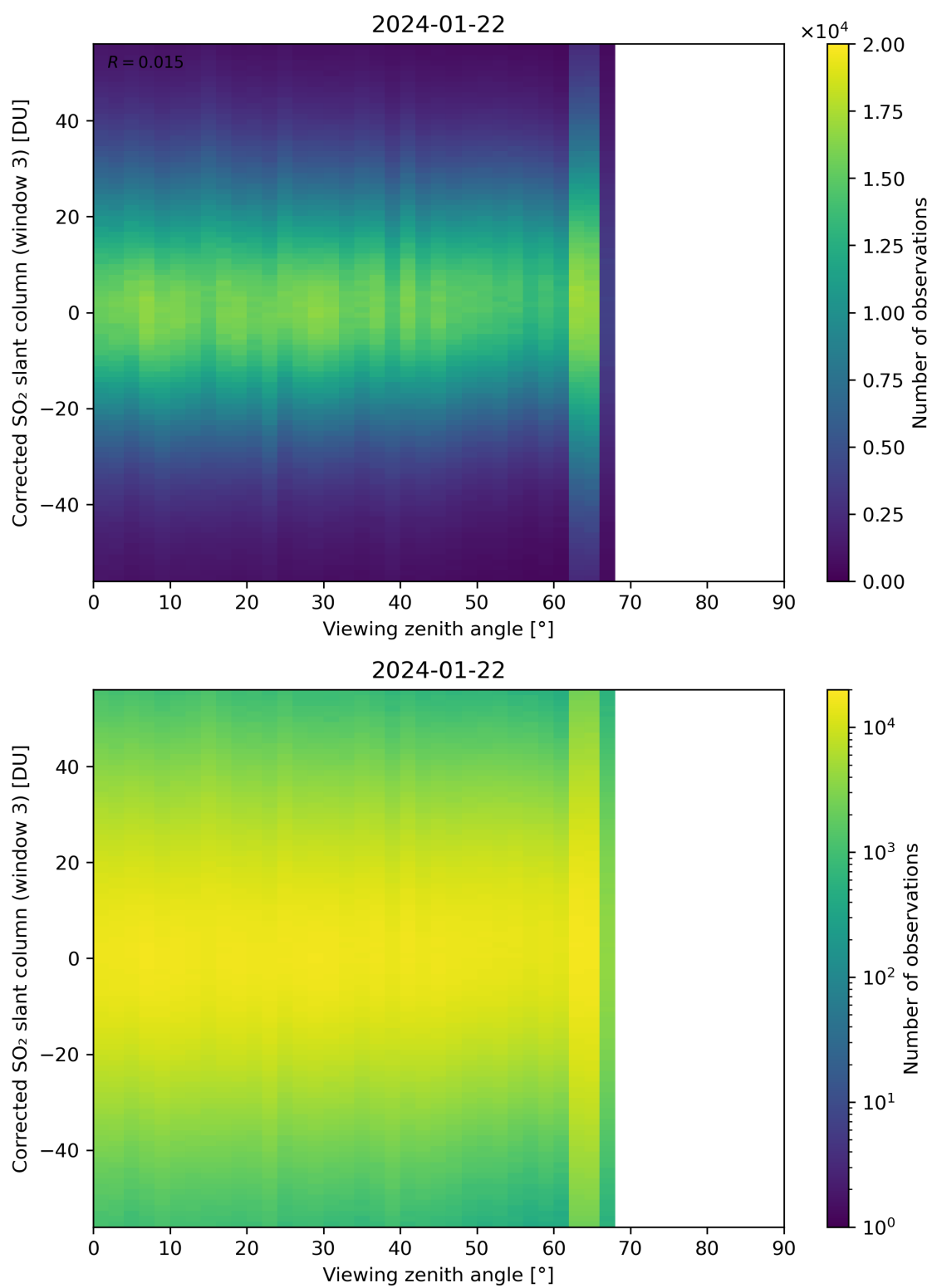
Figure 319: Scatter density plot of “Viewing zenith angle” against “Corrected SO 2 slant column (window 3)” for 2024-01-21 to 2024-01-23.
