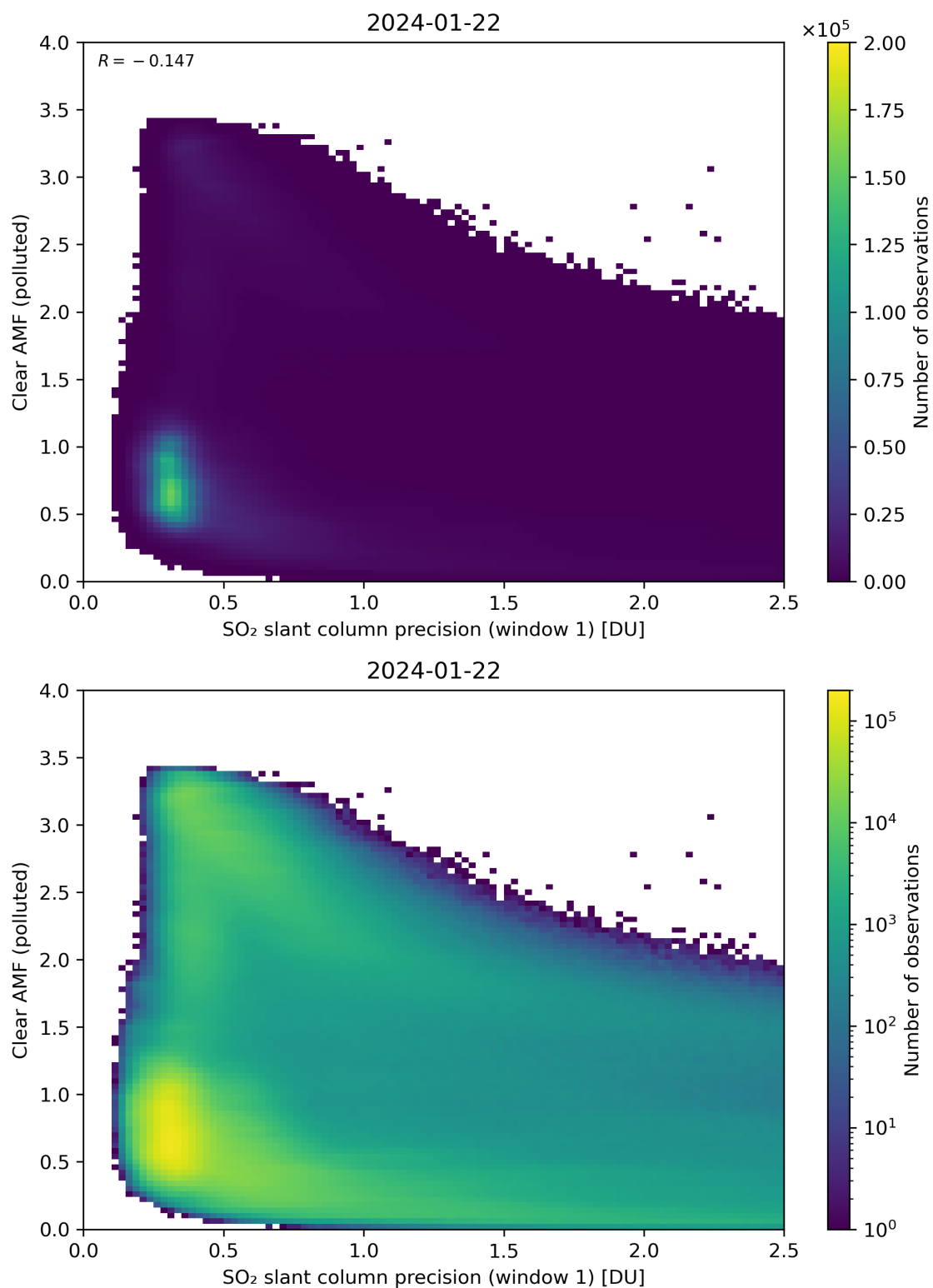
Figure 224: Scatter density plot of “SO 2 slant column precision (window 1)” against “Clear AMF (polluted)” for 2024-01-21 to 2024-01-23.
