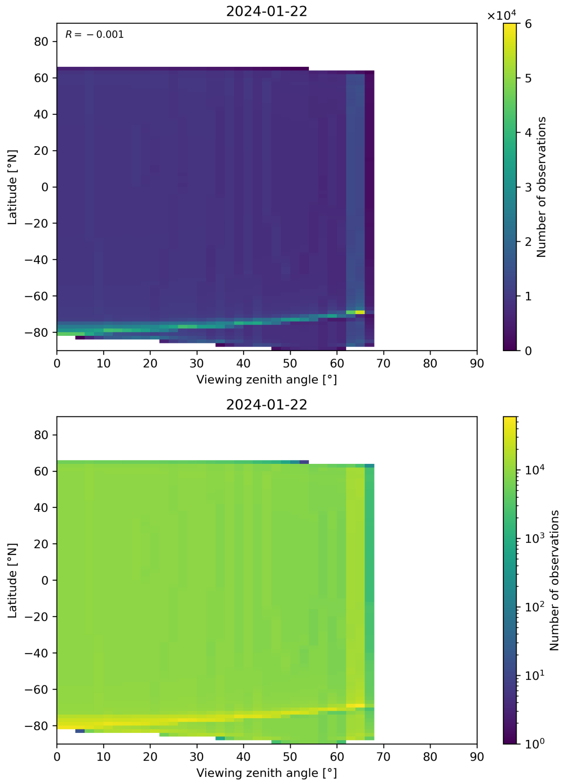
Figure 314: Scatter density plot of “Viewing zenith angle” against “Latitude” for 2024-01-21 to 2024-01-23.
