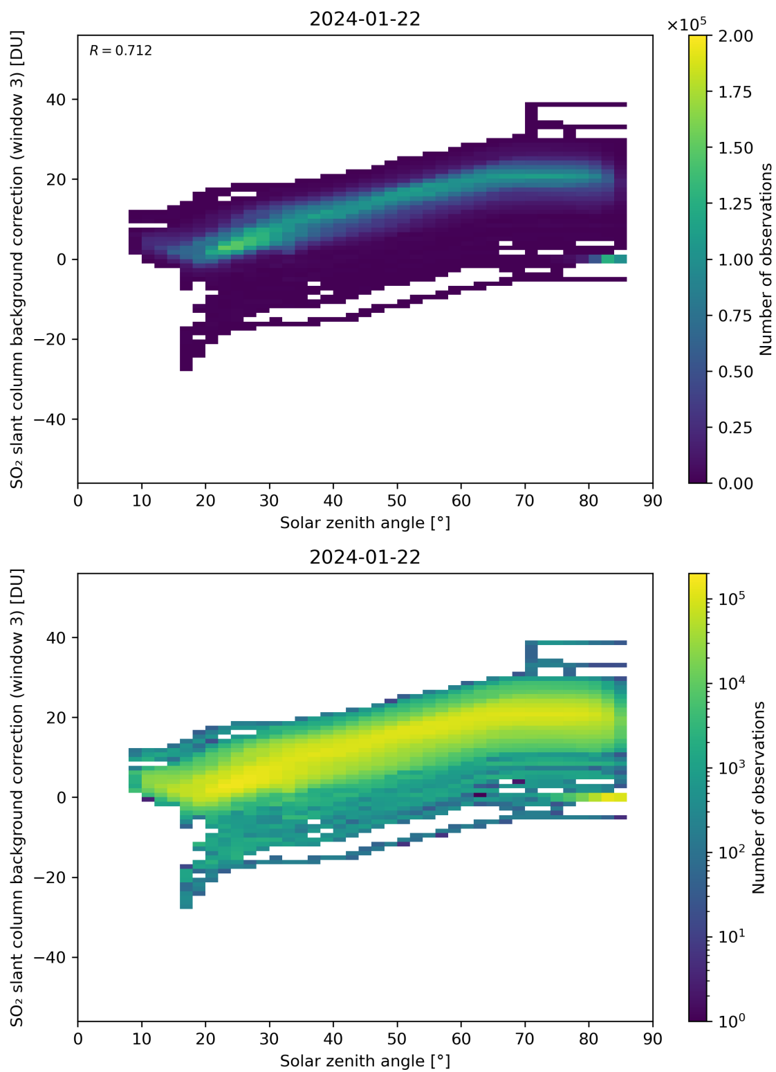
Figure 160: Scatter density plot of “Solar zenith angle” against “SO 2 slant column background correction (window 3)” for 2024-01-21 to 2024-01-23.
