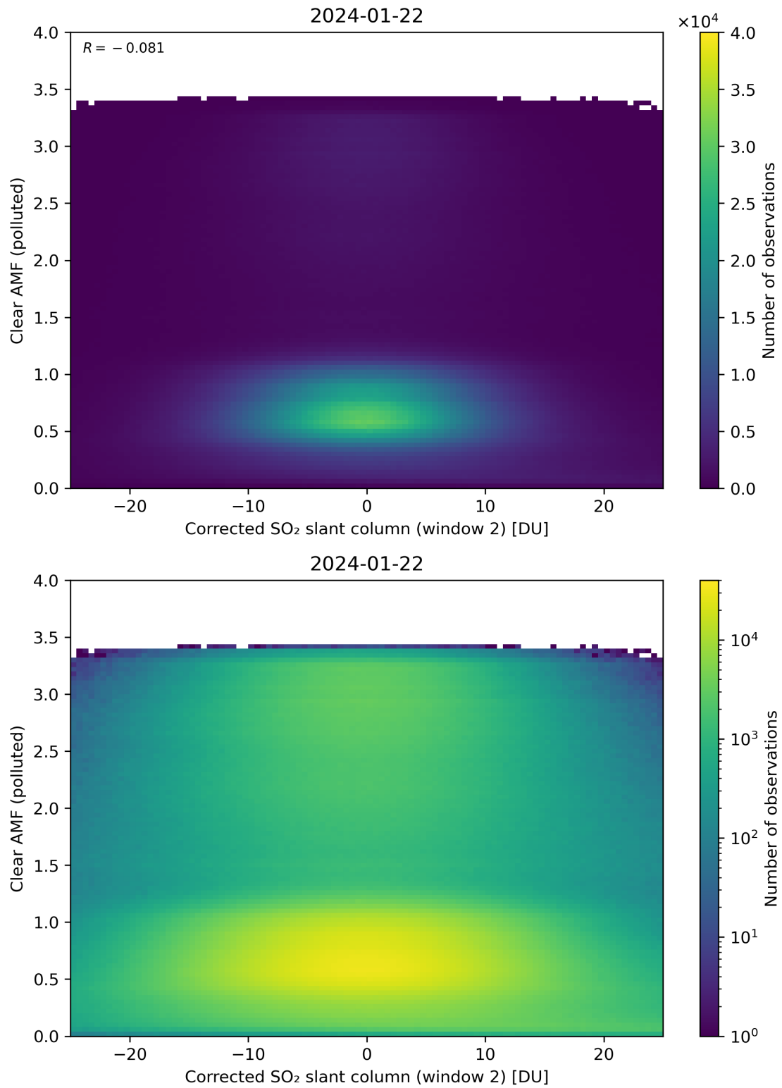
Figure 199: Scatter density plot of “Corrected SO 2 slant column (window 2)” against “Clear AMF (polluted)” for 2024-01-21 to 2024-01-23.
