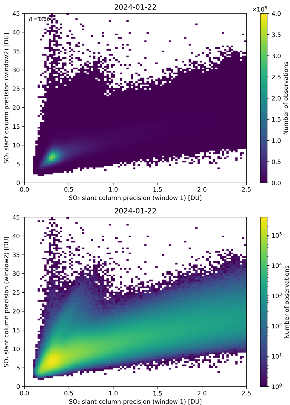
Figure 227: Scatter density plot of “SO 2 slant column precision (window 1)” against “SO 2 slant column precision (window2)” for 2024-01-21 to 2024-01-23.
