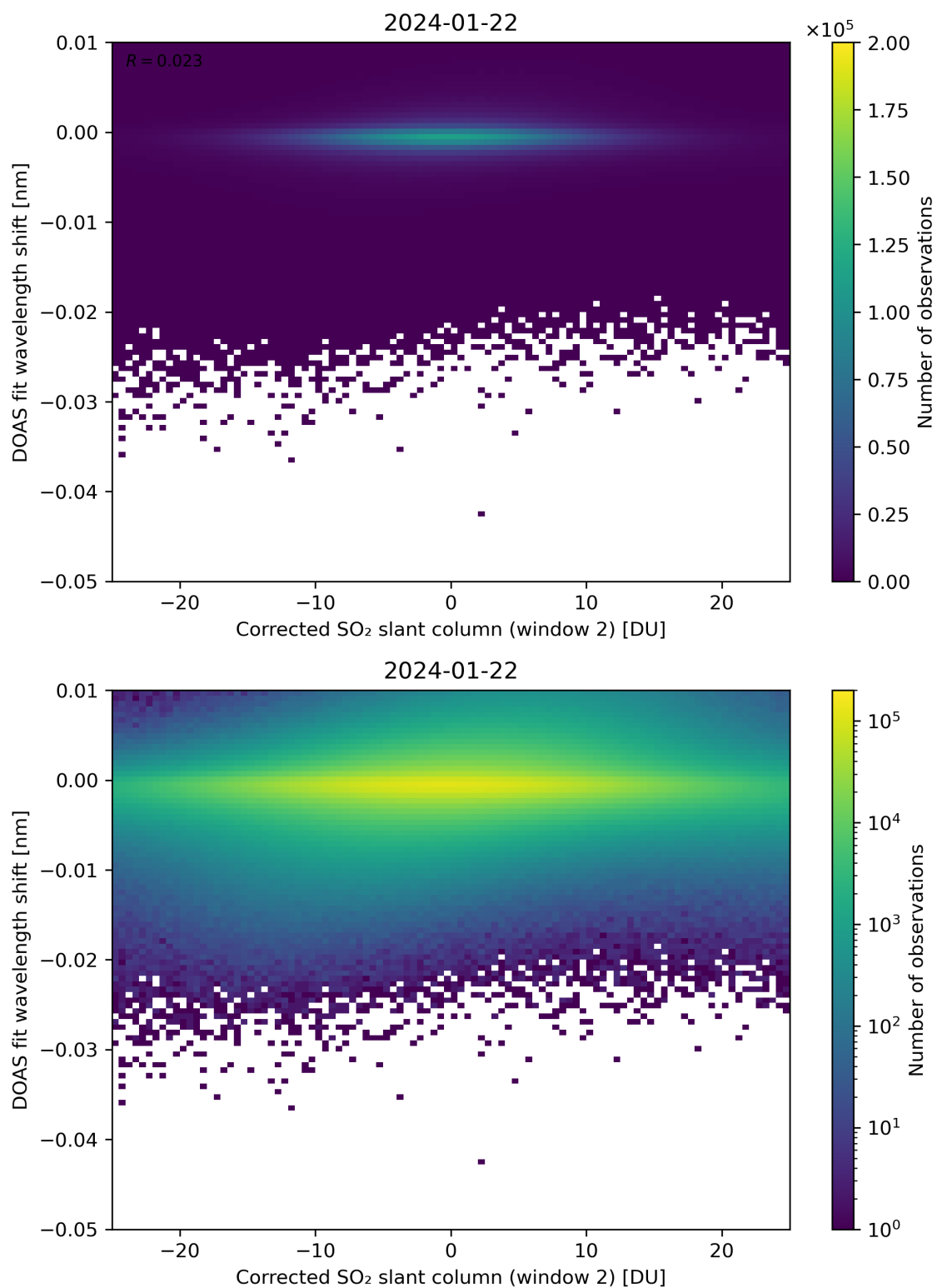
Figure 196: Scatter density plot of “Corrected SO 2 slant column (window 2)” against “DOAS fit wavelength shift” for 2024-01-21 to 2024-01-23.
