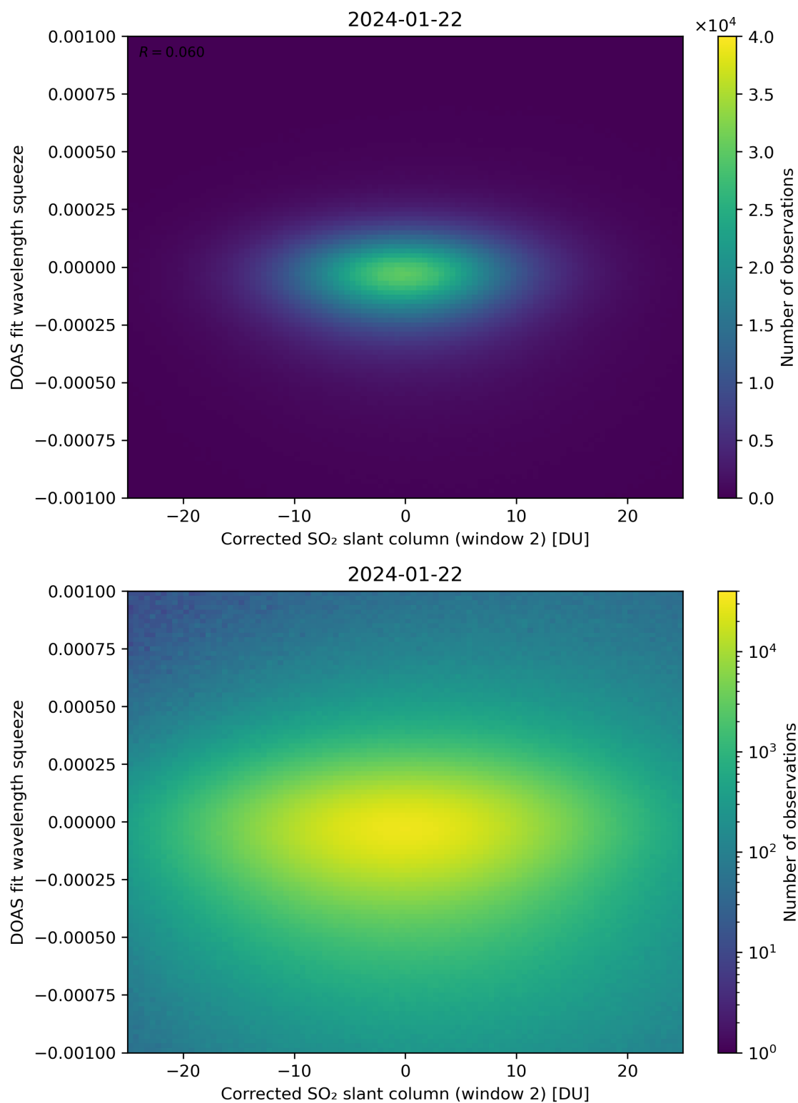
Figure 197: Scatter density plot of “Corrected SO 2 slant column (window 2)” against “DOAS fit wavelength squeeze” for 2024-01-21 to 2024-01-23.
