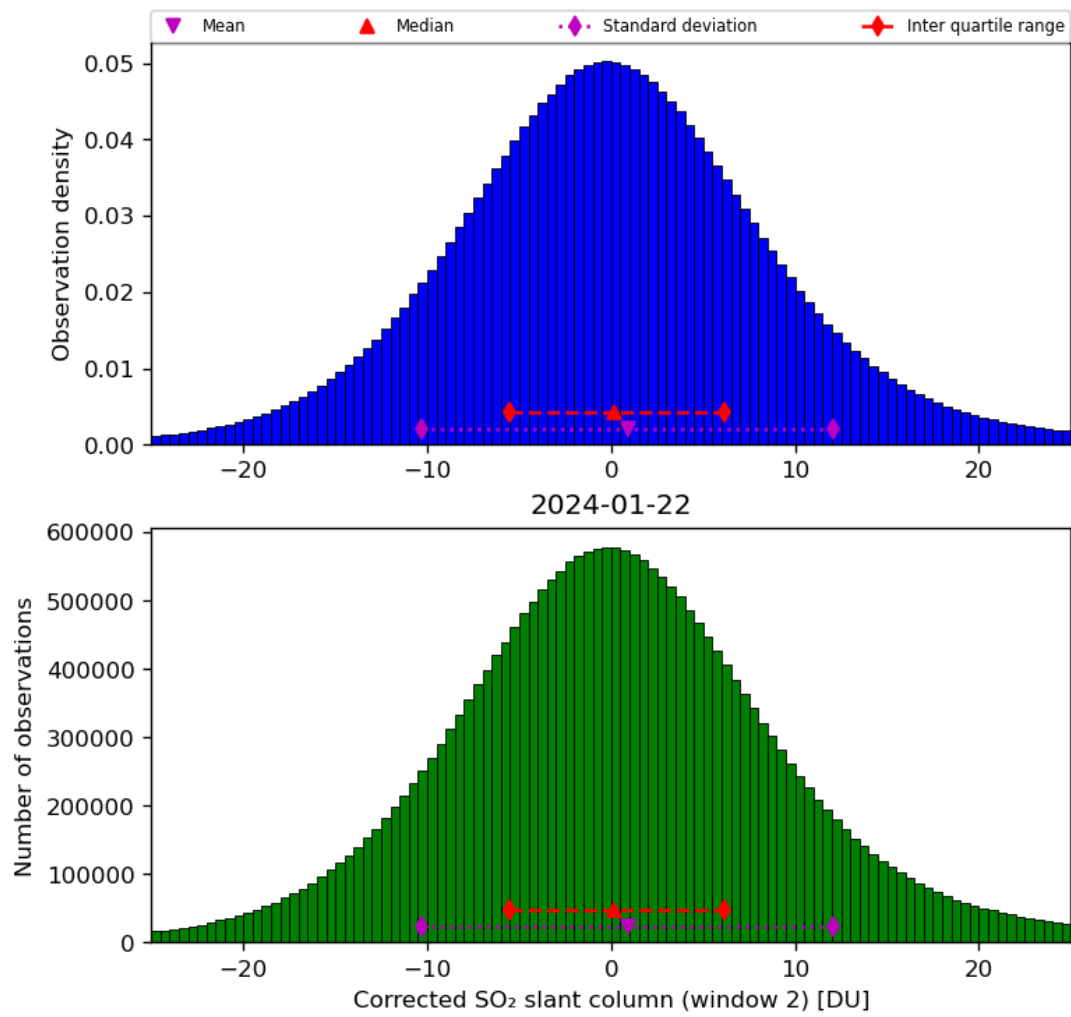
Figure 62: Histogram of “Corrected SO 2 slant column (window 2)” for 2024-01-21 to 2024-01-23
