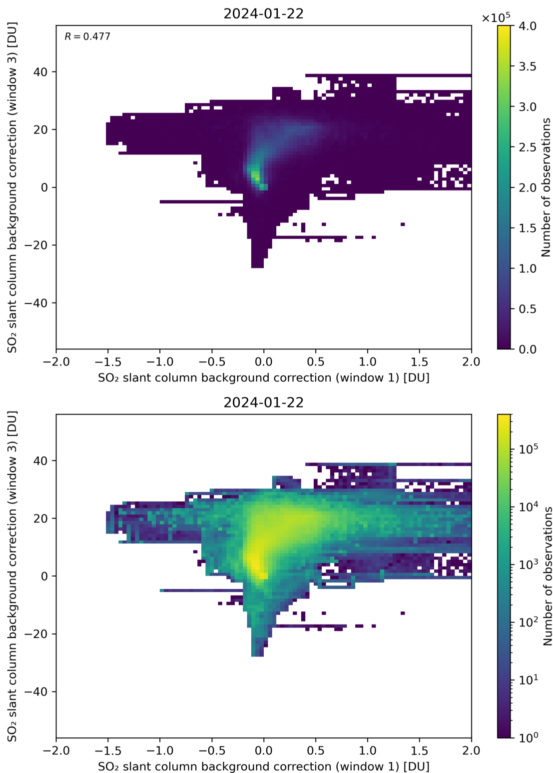
Figure 99: Scatter density plot of “SO 2 slant column background correction (window 1)” against “SO 2 slant column background correction (window 3)” for 2024-01-21 to 2024-01-23.
