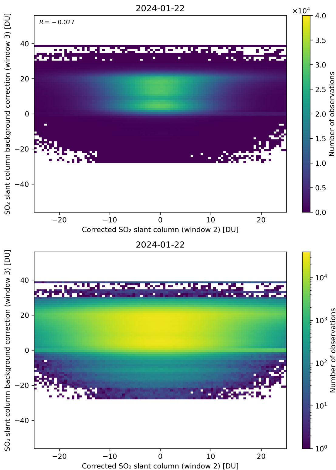
Figure 195: Scatter density plot of “Corrected SO 2 slant column (window 2)” against “SO 2 slant column background correction (window 3)” for 2024-01-21 to 2024-01-23.
