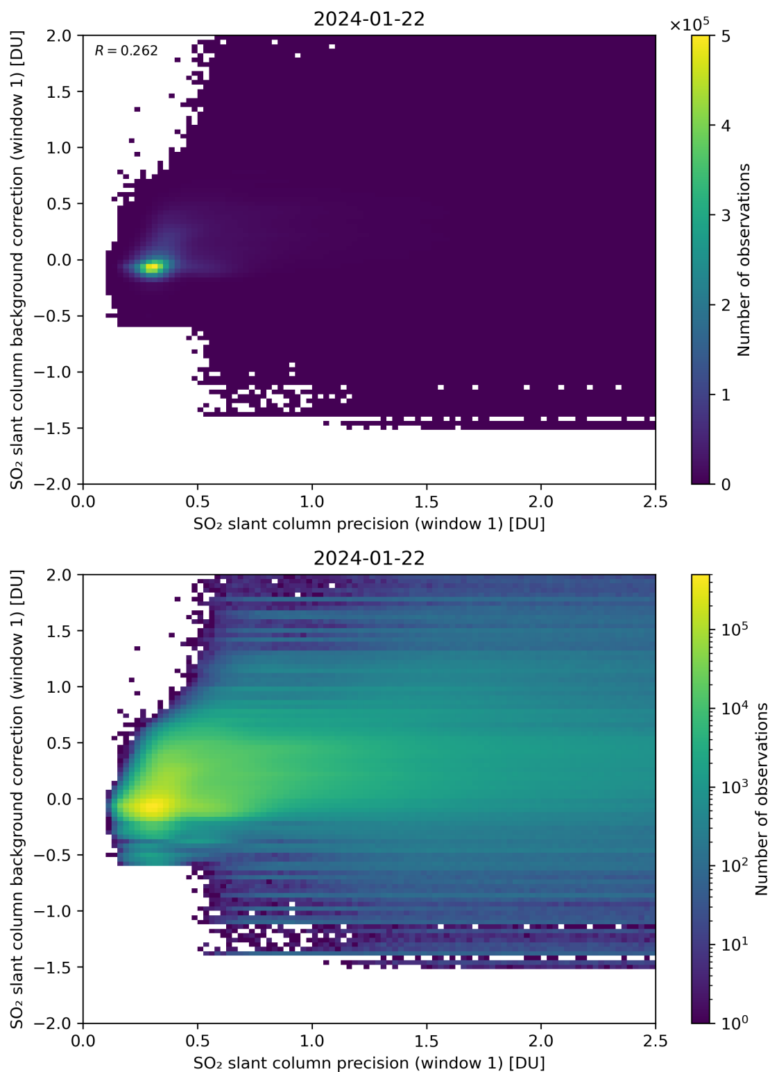
Figure 218: Scatter density plot of “SO 2 slant column precision (window 1)” against “SO 2 slant column background correction (window 1)” for 2024-01-21 to 2024-01-23.
