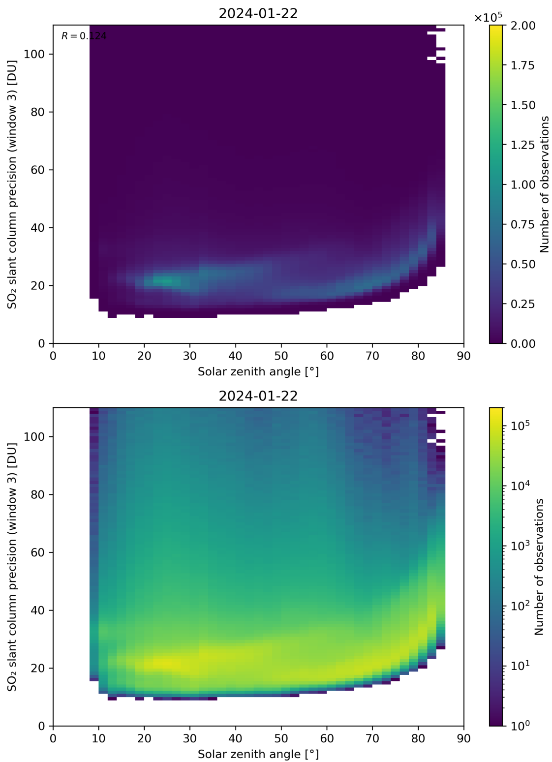
Figure 173: Scatter density plot of “Solar zenith angle” against “SO 2 slant column precision (window 3)” for 2024-01-21 to 2024-01-23.
