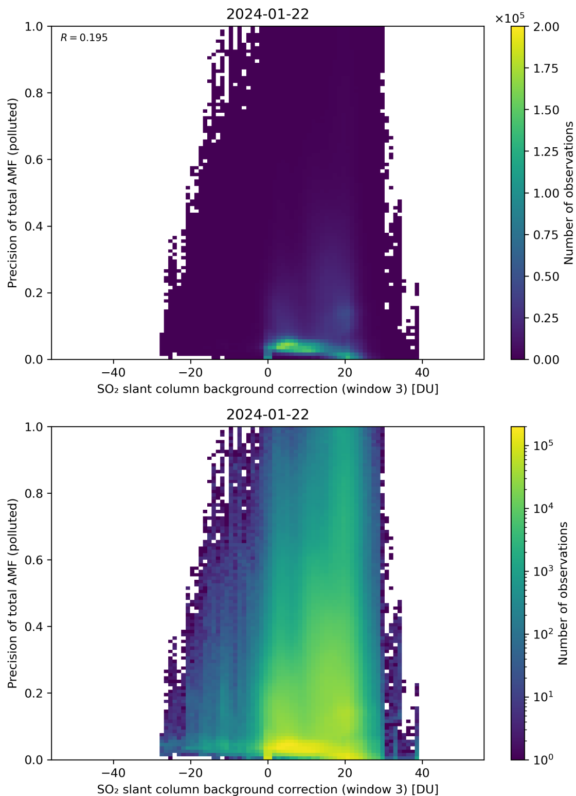
Figure 126: Scatter density plot of “SO 2 slant column background correction (window 3)” against “Precision of total AMF (polluted)” for 2024-01-21 to 2024-01-23.
