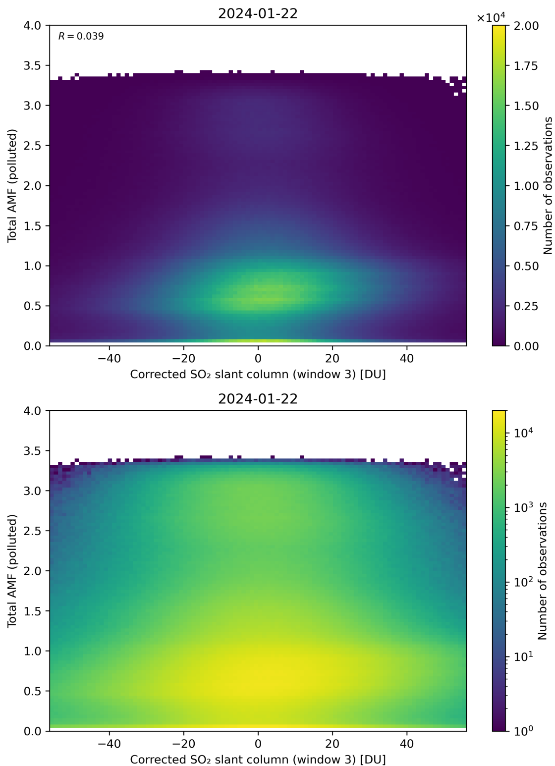
Figure 210: Scatter density plot of “Corrected SO 2 slant column (window 3)” against “Total AMF (polluted)” for 2024-01-21 to 2024-01-23.
