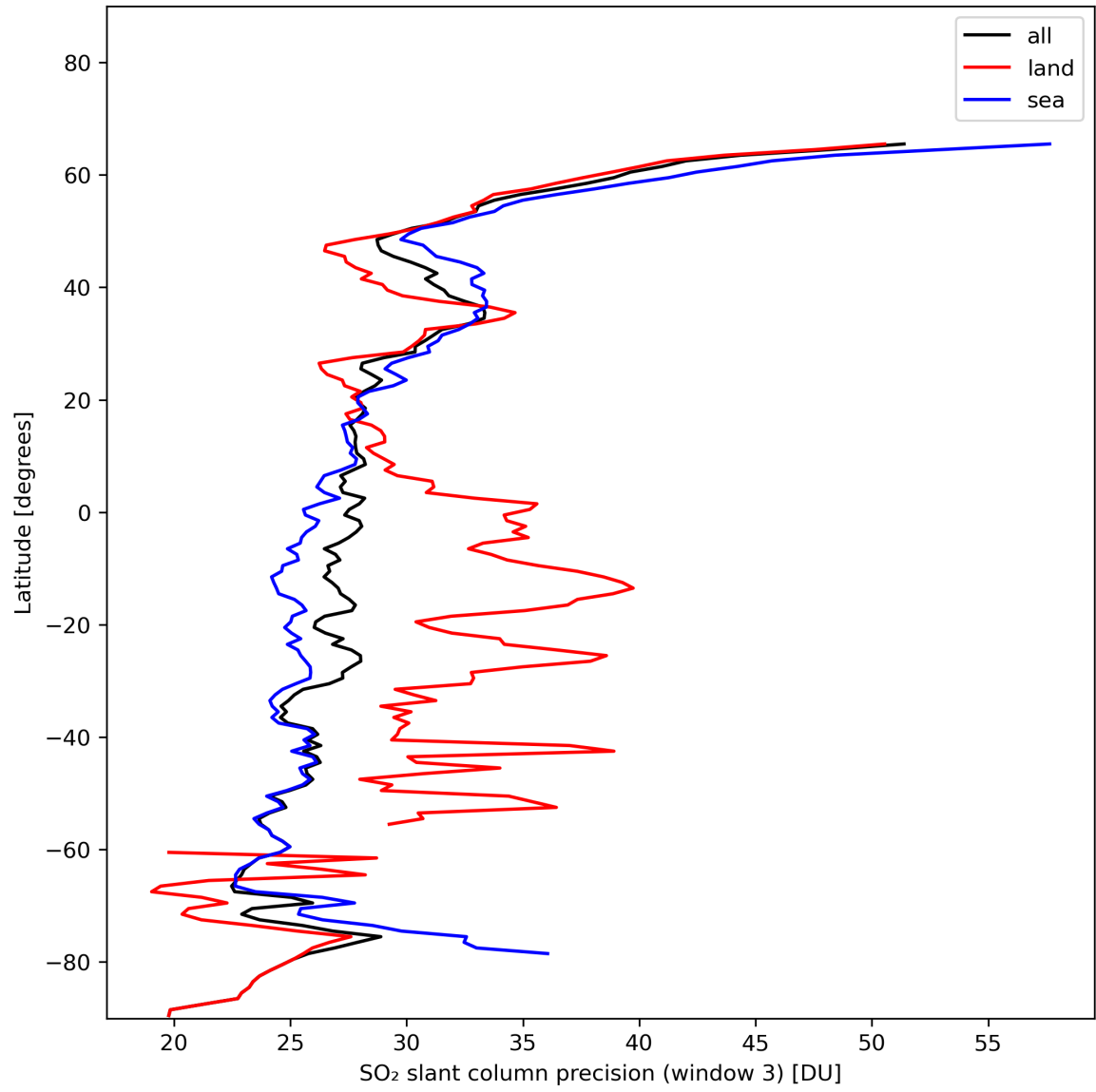
Figure 42: Zonal average of “SO 2 slant column precision (window 3)” for 2024-01-21 to 2024-01-23.
