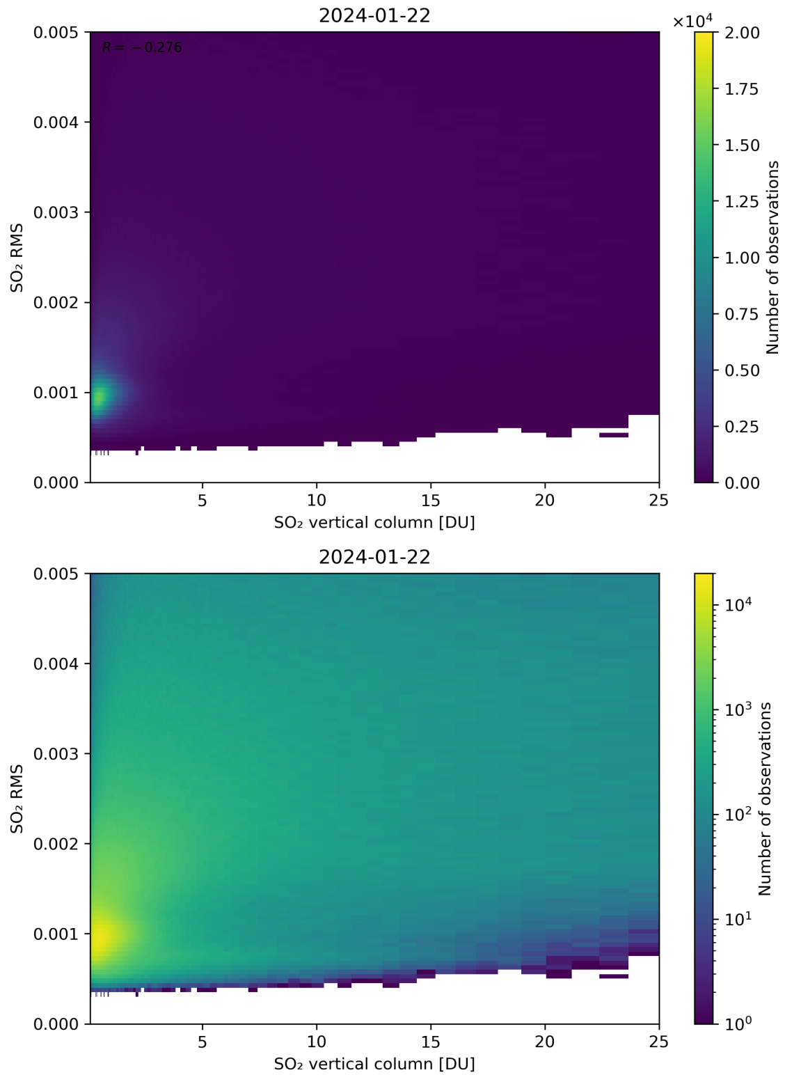
Figure 278: Scatter density plot of “SO 2 vertical column” against “SO 2 RMS” for 2024-01-21 to 2024-01-23.
