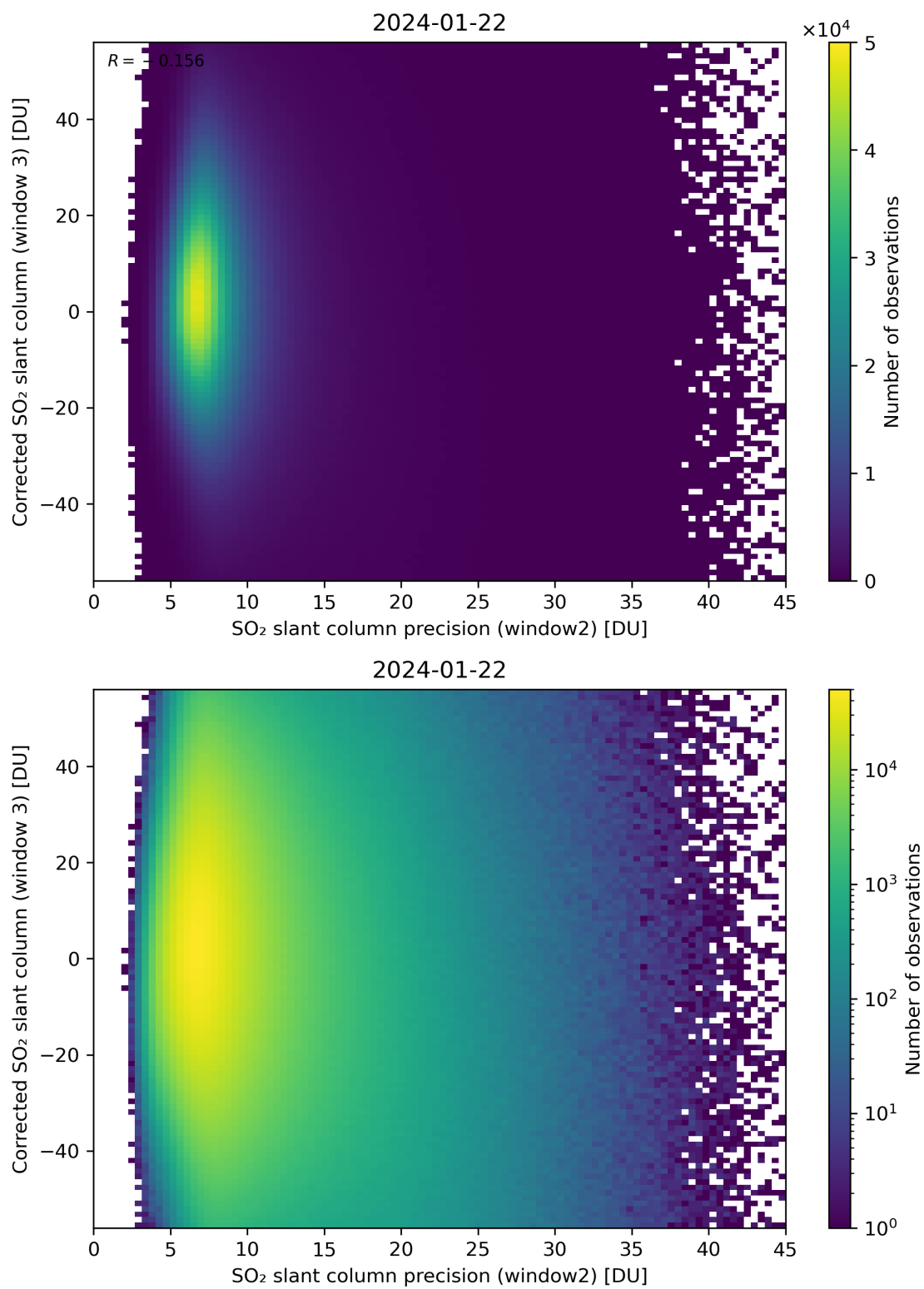
Figure 248: Scatter density plot of “SO 2 slant column precision (window2)” against “Corrected SO 2 slant column (window 3)” for 2024-01-21 to 2024-01-23.
