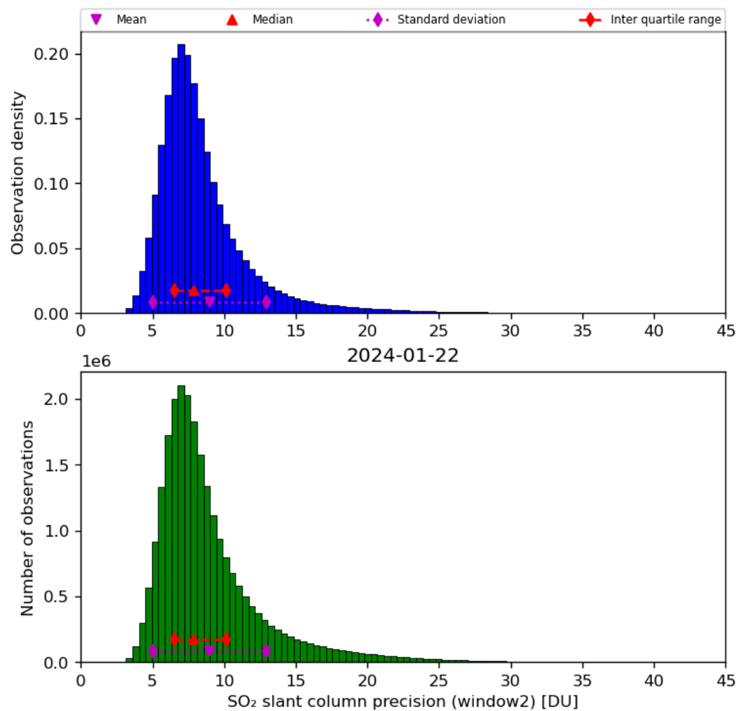
Figure 61: Histogram of “SO 2 slant column precision (window2)” for 2024-01-21 to 2024-01-23
