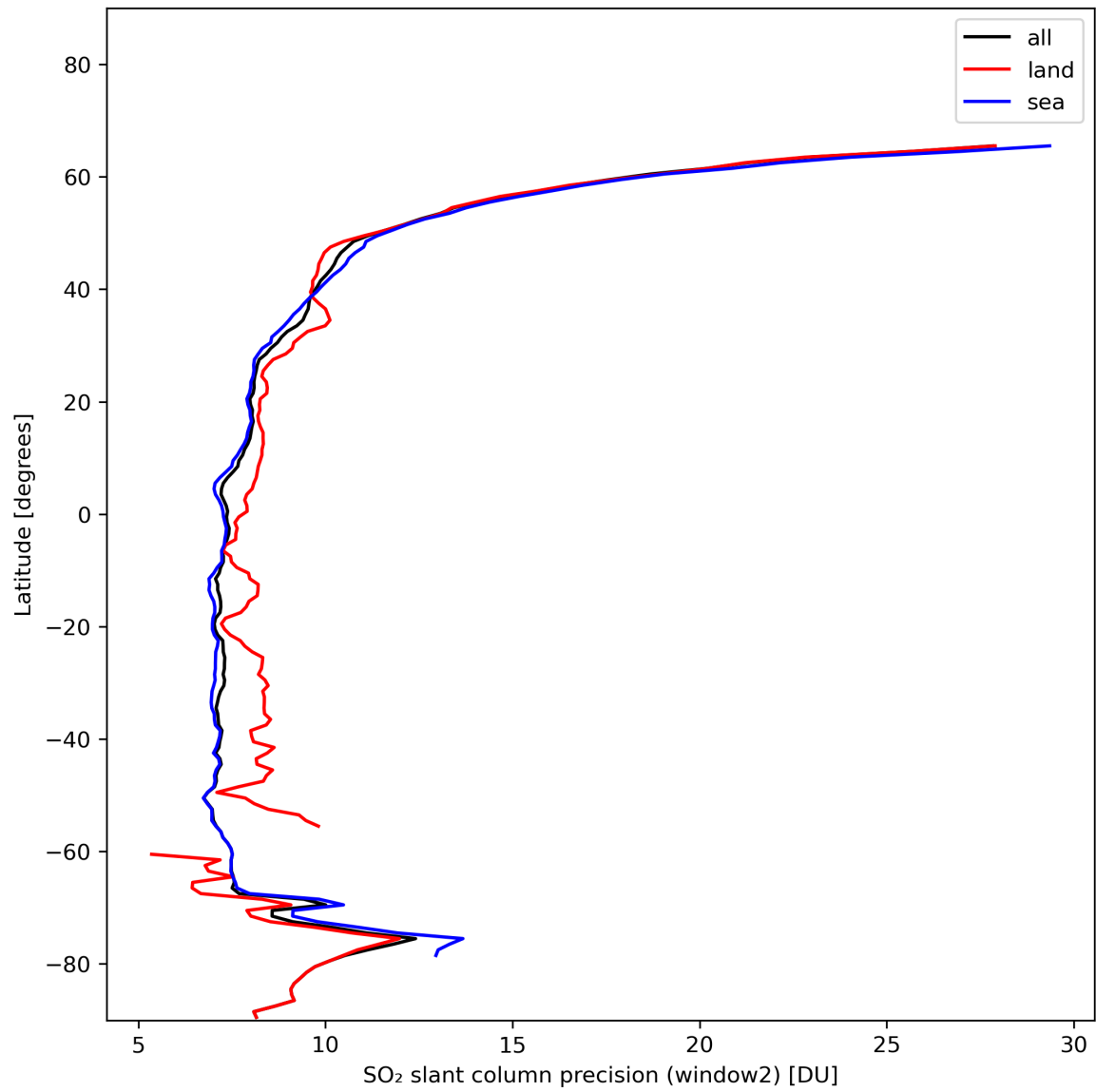
Figure 38: Zonal average of “SO 2 slant column precision (window2)” for 2024-01-21 to 2024-01-23.
