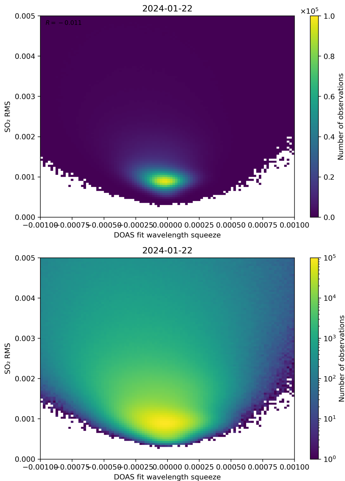
Figure 132: Scatter density plot of “DOAS fit wavelength squeeze” against “SO 2 RMS” for 2024-01-21 to 2024-01-23.
