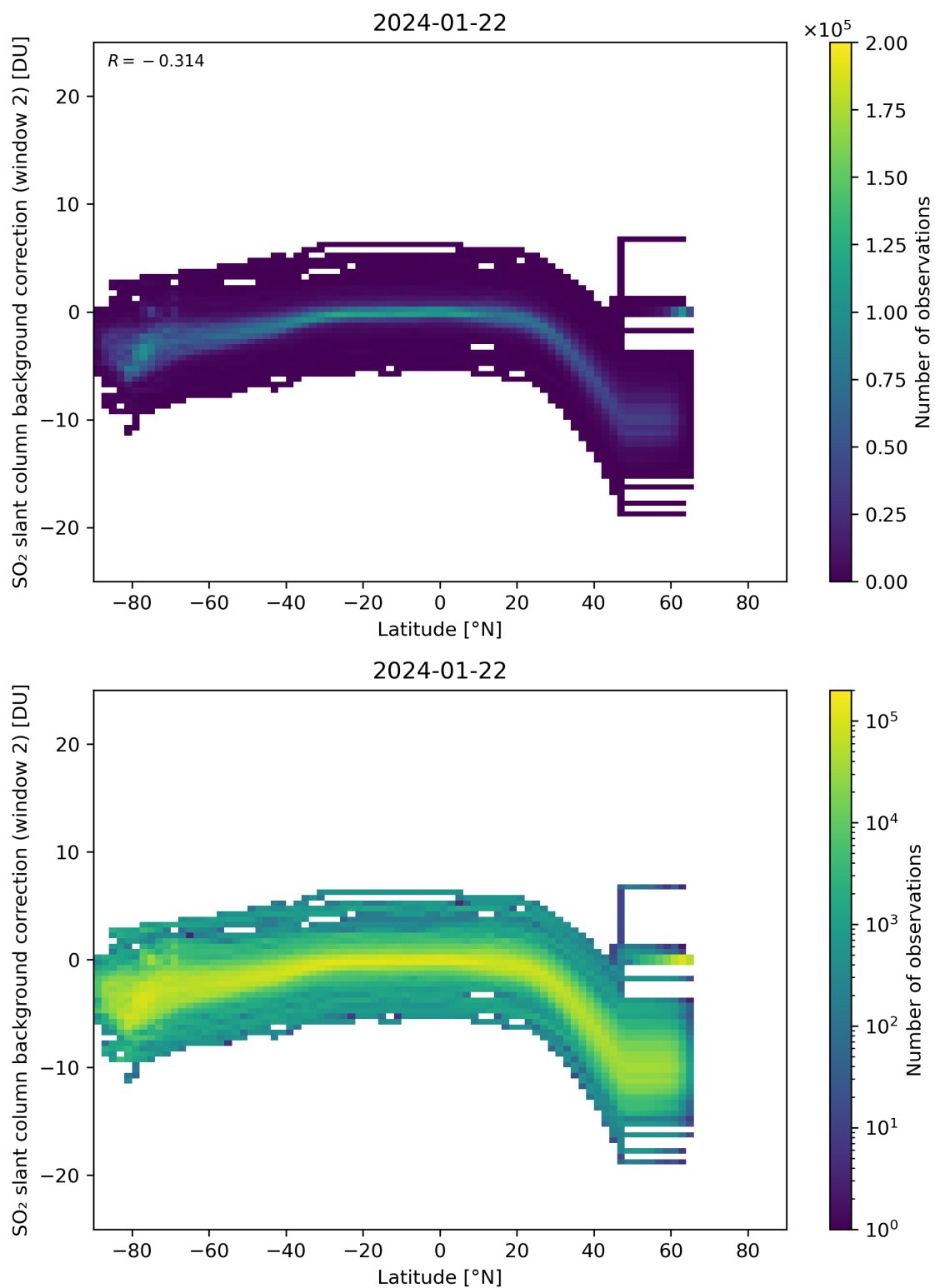
Figure 140: Scatter density plot of “Latitude” against “SO 2 slant column background correction (window 2)” for 2024-01-21 to 2024-01-23.
