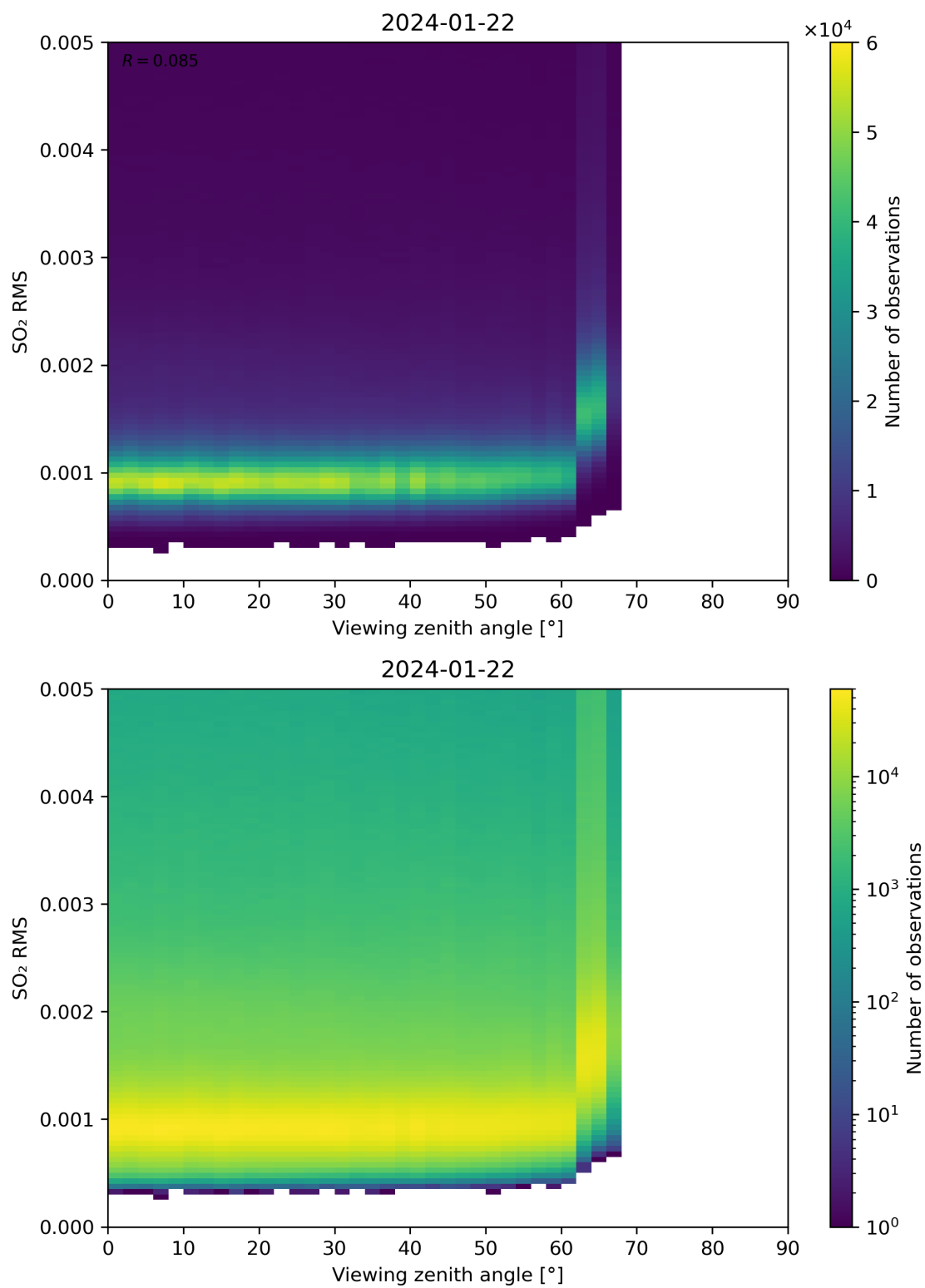
Figure 313: Scatter density plot of “Viewing zenith angle” against “SO 2 RMS” for 2024-01-21 to 2024-01-23.
