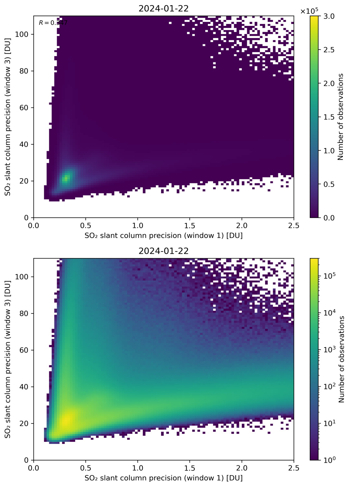
Figure 229: Scatter density plot of “SO 2 slant column precision (window 1)” against “SO 2 slant column precision (window 3)” for 2024-01-21 to 2024-01-23.
