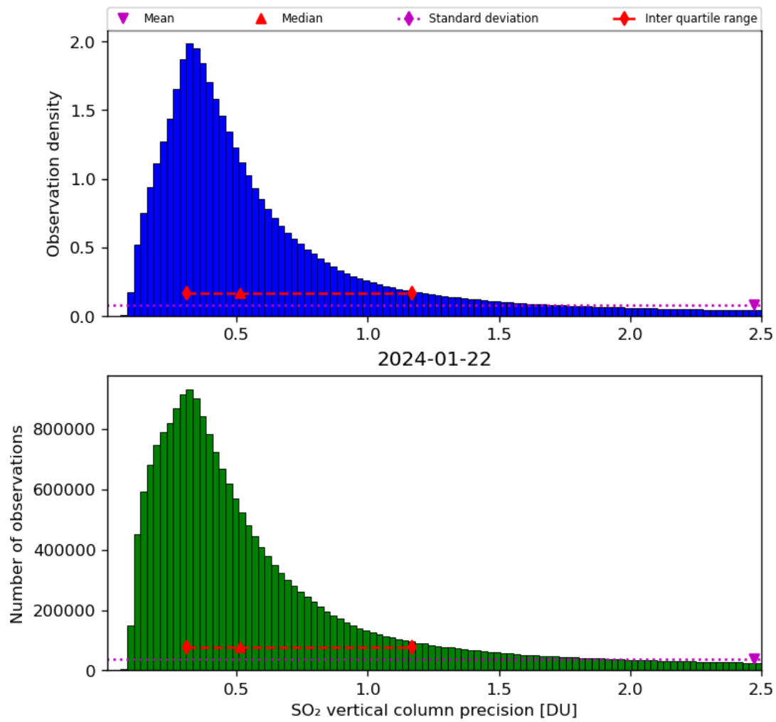
Figure 54: Histogram of “SO 2 vertical column precision” for 2024-01-21 to 2024-01-23
