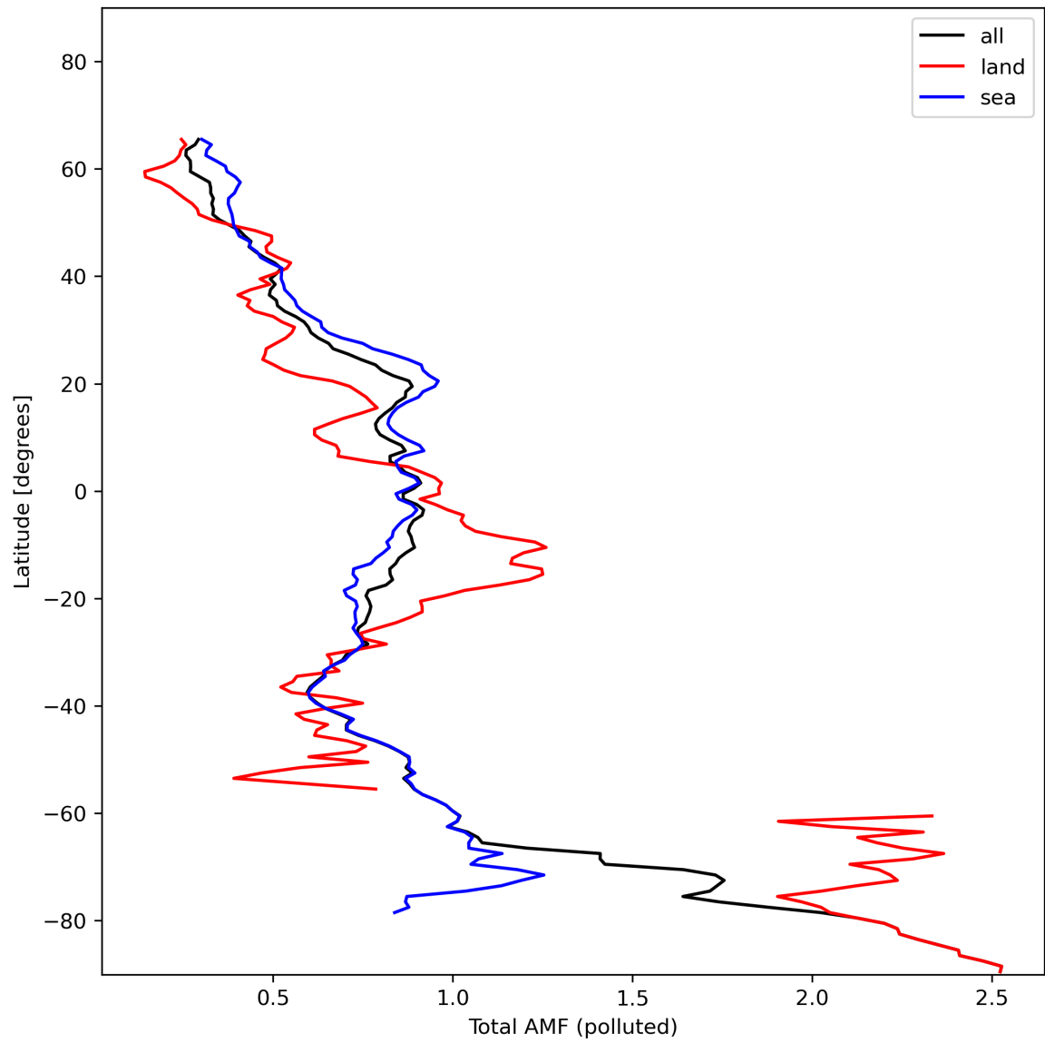
Figure 48: Zonal average of “Total AMF (polluted)” for 2024-01-21 to 2024-01-23.
