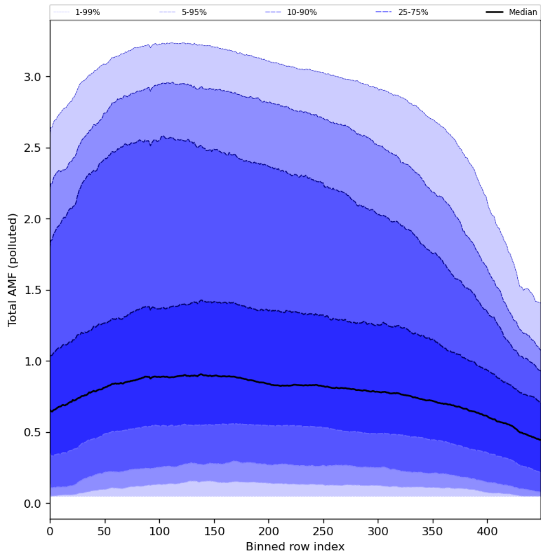
Figure 94: Along track statistics of “Total AMF (polluted)” for 2024-01-21 to 2024-01-23
