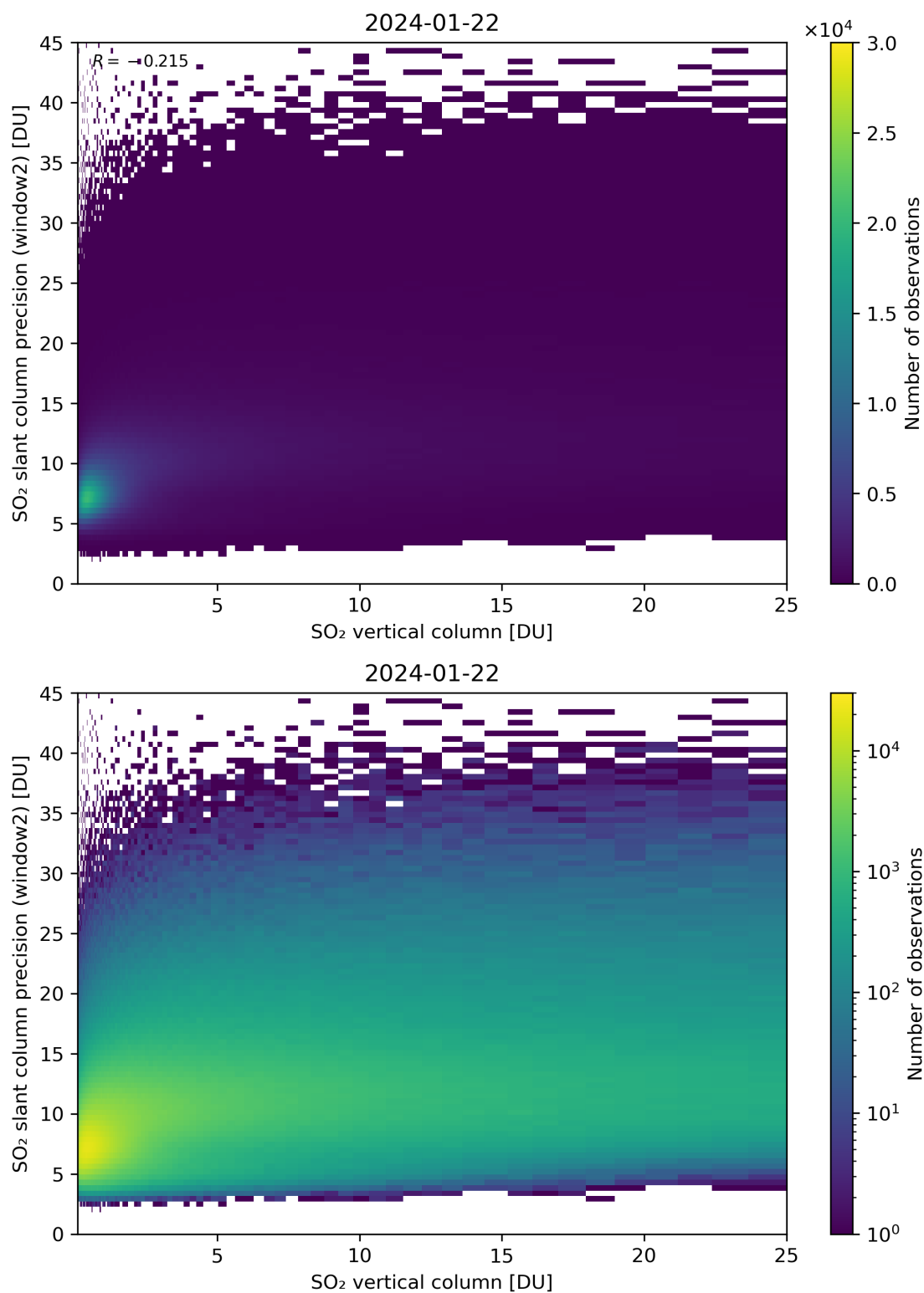
Figure 302: Scatter density plot of “SO 2 vertical column” against “SO 2 slant column precision (window2)” for 2024-01-21 to 2024-01-23.
