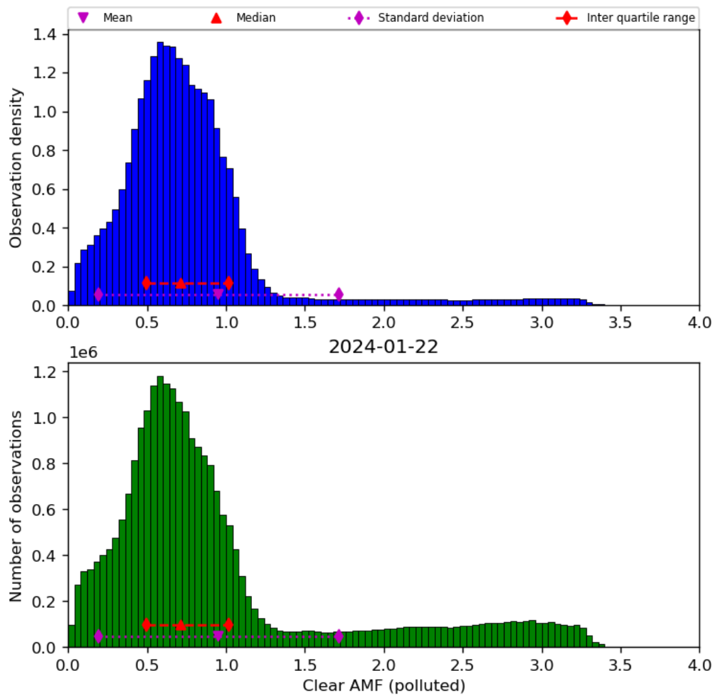
Figure 73: Histogram of “Clear AMF (polluted)” for 2024-01-21 to 2024-01-23
