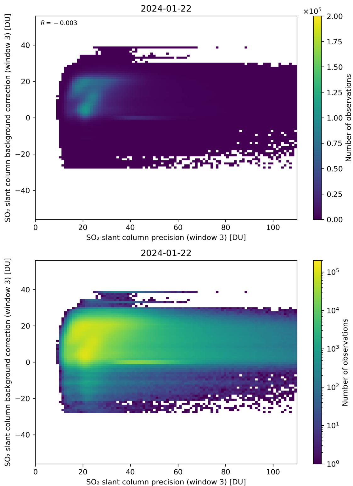
Figure 257: Scatter density plot of “SO 2 slant column precision (window 3)” against “SO 2 slant column background correction (window 3)” for 2024-01-21 to 2024-01-23.
