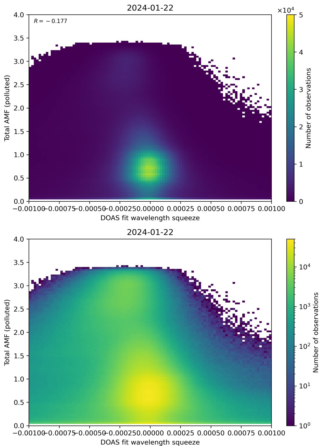
Figure 134: Scatter density plot of “DOAS fit wavelength squeeze” against “Total AMF (polluted)” for 2024-01-21 to 2024-01-23.
