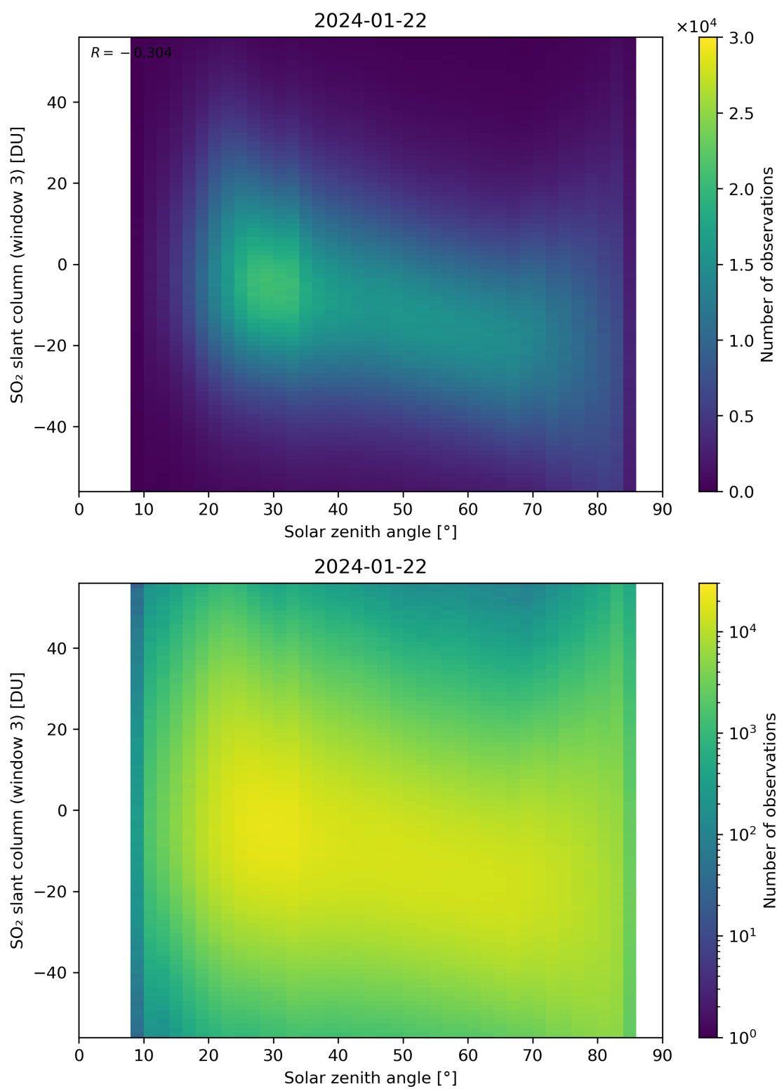
Figure 172: Scatter density plot of “Solar zenith angle” against “SO 2 slant column (window 3)” for 2024-01-21 to 2024-01-23.
