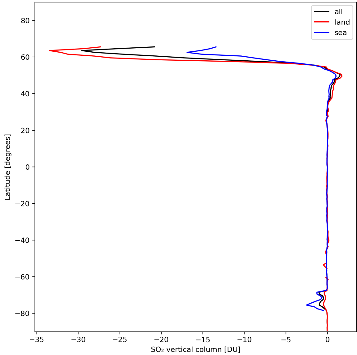
Figure 30: Zonal average of “SO 2 vertical column” for 2024-01-21 to 2024-01-23.
