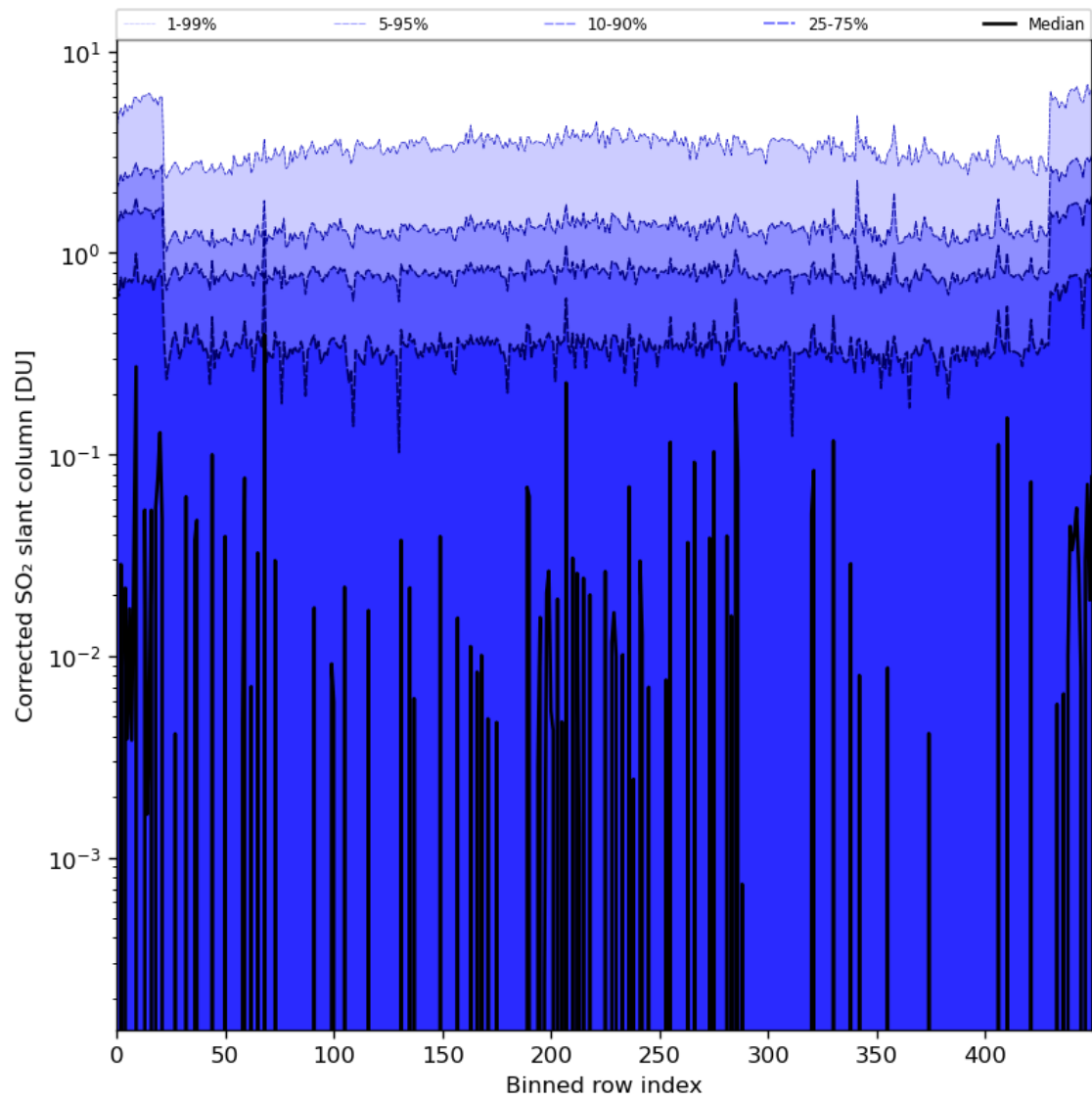
Figure 78: Along track statistics of “Corrected SO 2 slant column” for 2024-01-21 to 2024-01-23
