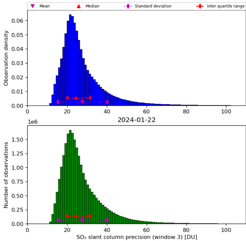
Figure 65: Histogram of “SO 2 slant column precision (window 3)” for 2024-01-21 to 2024-01-23
