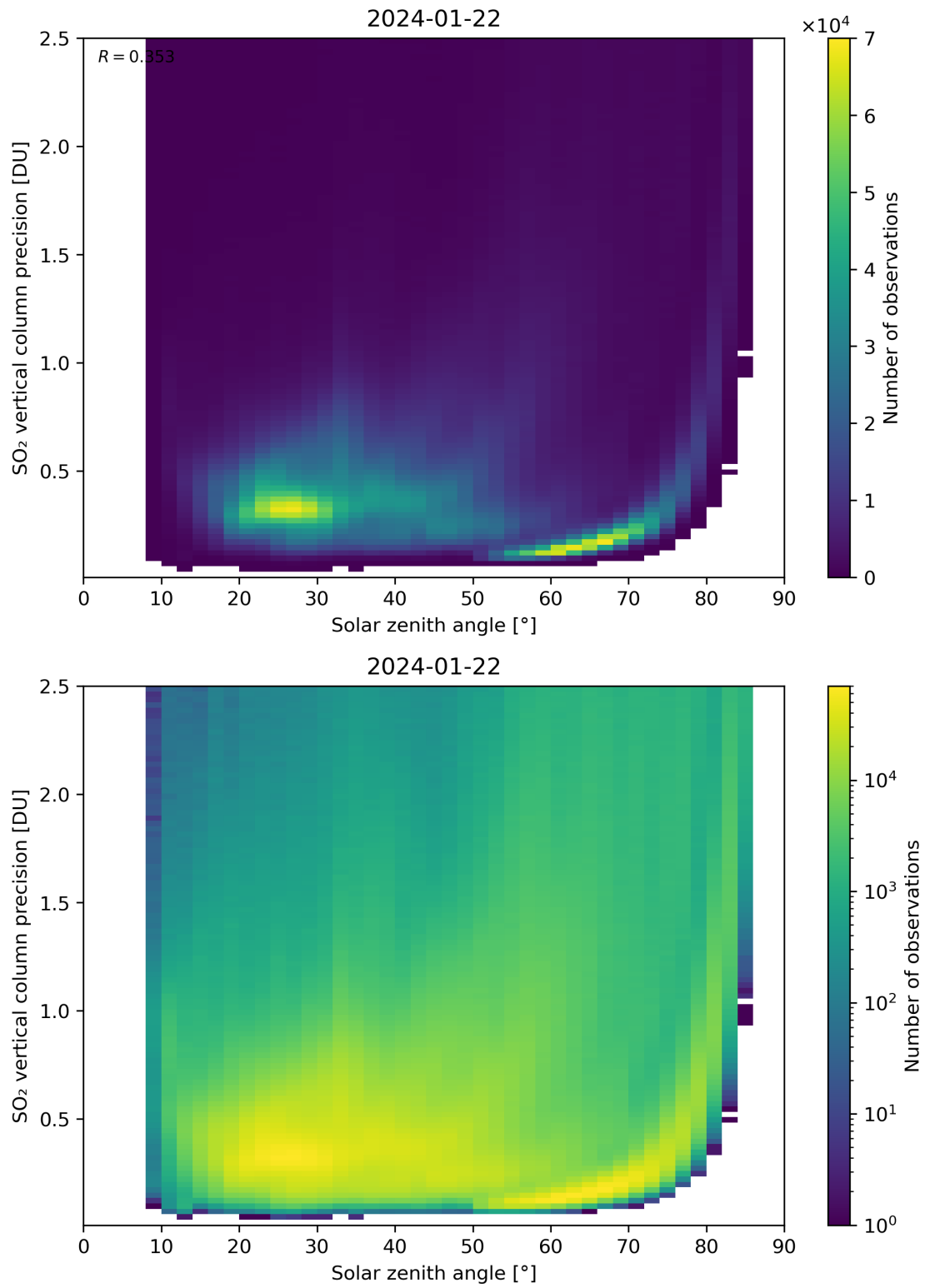
Figure 177: Scatter density plot of “Solar zenith angle” against “SO 2 vertical column precision” for 2024-01-21 to 2024-01-23.
