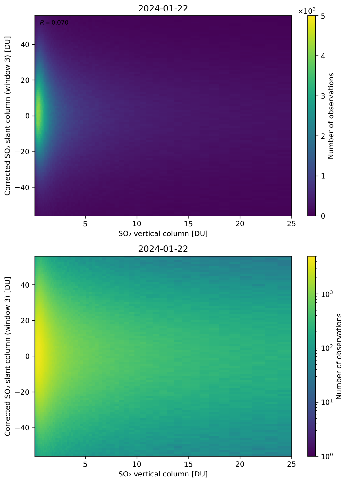
Figure 299: Scatter density plot of “SO 2 vertical column” against “Corrected SO 2 slant column (window 3)” for 2024-01-21 to 2024-01-23.
