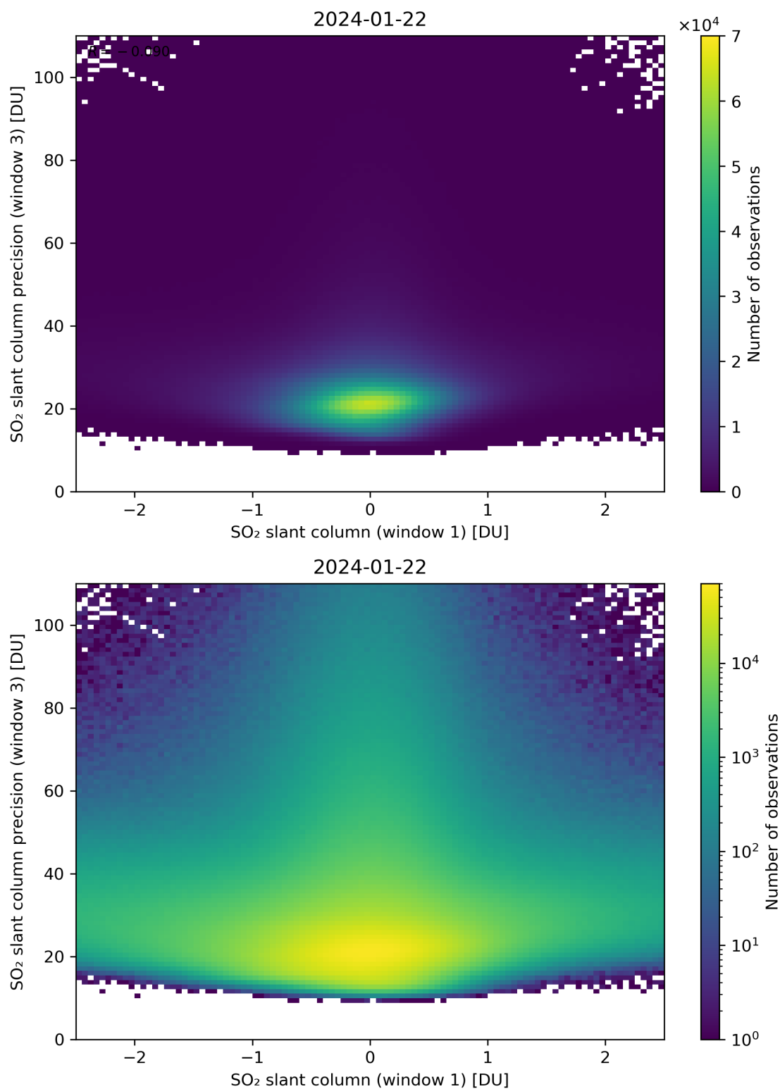
Figure 238: Scatter density plot of “SO 2 slant column (window 1)” against “SO 2 slant column precision (window 3)” for 2024-01-21 to 2024-01-23.
