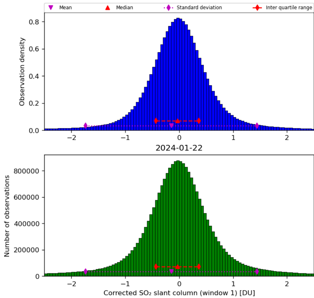
Figure 58: Histogram of “Corrected SO 2 slant column (window 1)” for 2024-01-21 to 2024-01-23
