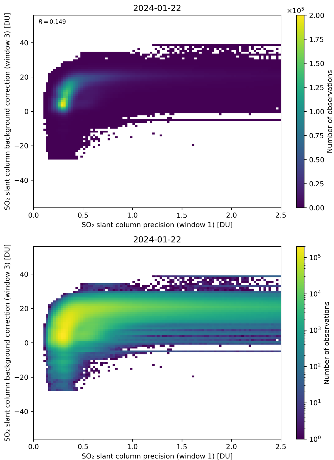
Figure 220: Scatter density plot of “SO 2 slant column precision (window 1)” against “SO 2 slant column background correction (window 3)” for 2024-01-21 to 2024-01-23.
