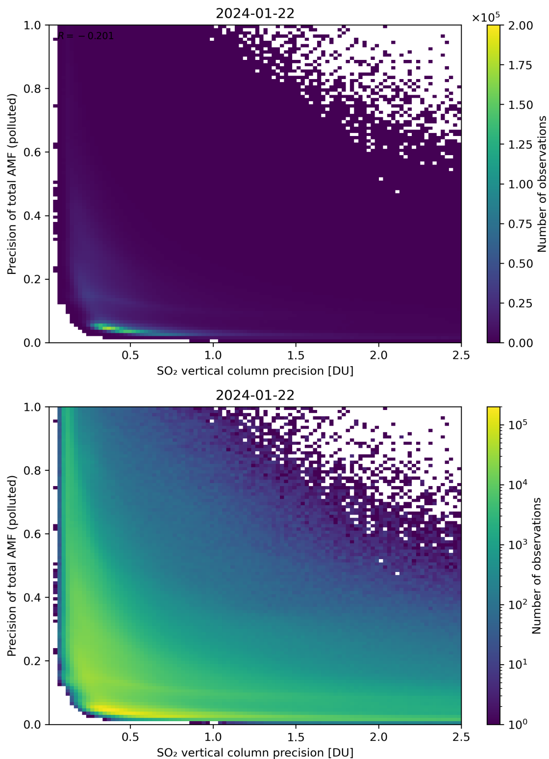
Figure 295: Scatter density plot of “SO 2 vertical column precision” against “Precision of total AMF (polluted)” for 2024-01-21 to 2024-01-23.
