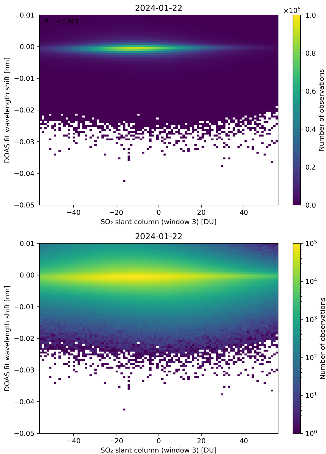
Figure 254: Scatter density plot of “SO 2 slant column (window 3)” against “DOAS fit wavelength shift” for 2024-01-21 to 2024-01-23.
