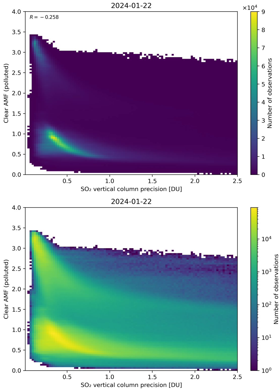
Figure 285: Scatter density plot of “SO 2 vertical column precision” against “Clear AMF (polluted)” for 2024-01-21 to 2024-01-23.
