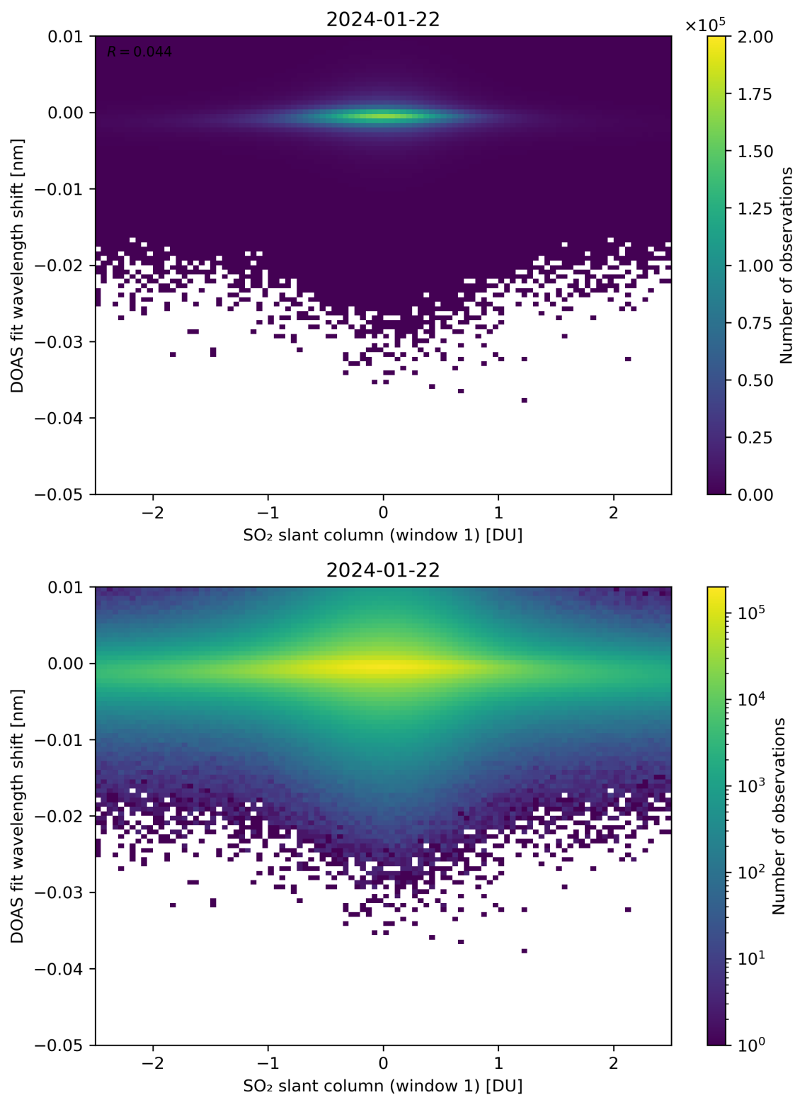
Figure 215: Scatter density plot of “SO 2 slant column (window 1)” against “DOAS fit wavelength shift” for 2024-01-21 to 2024-01-23.
