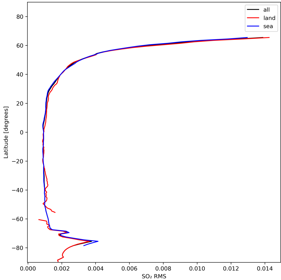
Figure 47: Zonal average of “SO 2 RMS” for 2024-01-21 to 2024-01-23.
