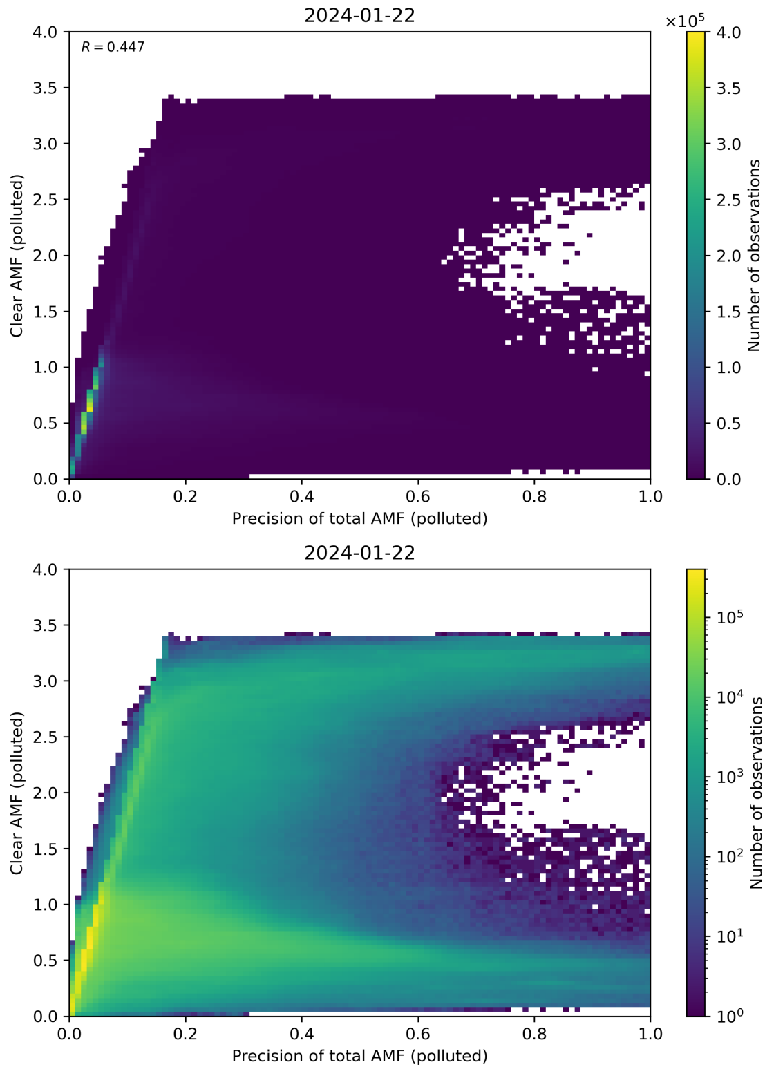
Figure 270: Scatter density plot of “Precision of total AMF (polluted)” against “Clear AMF (polluted)” for 2024-01-21 to 2024-01-23.
