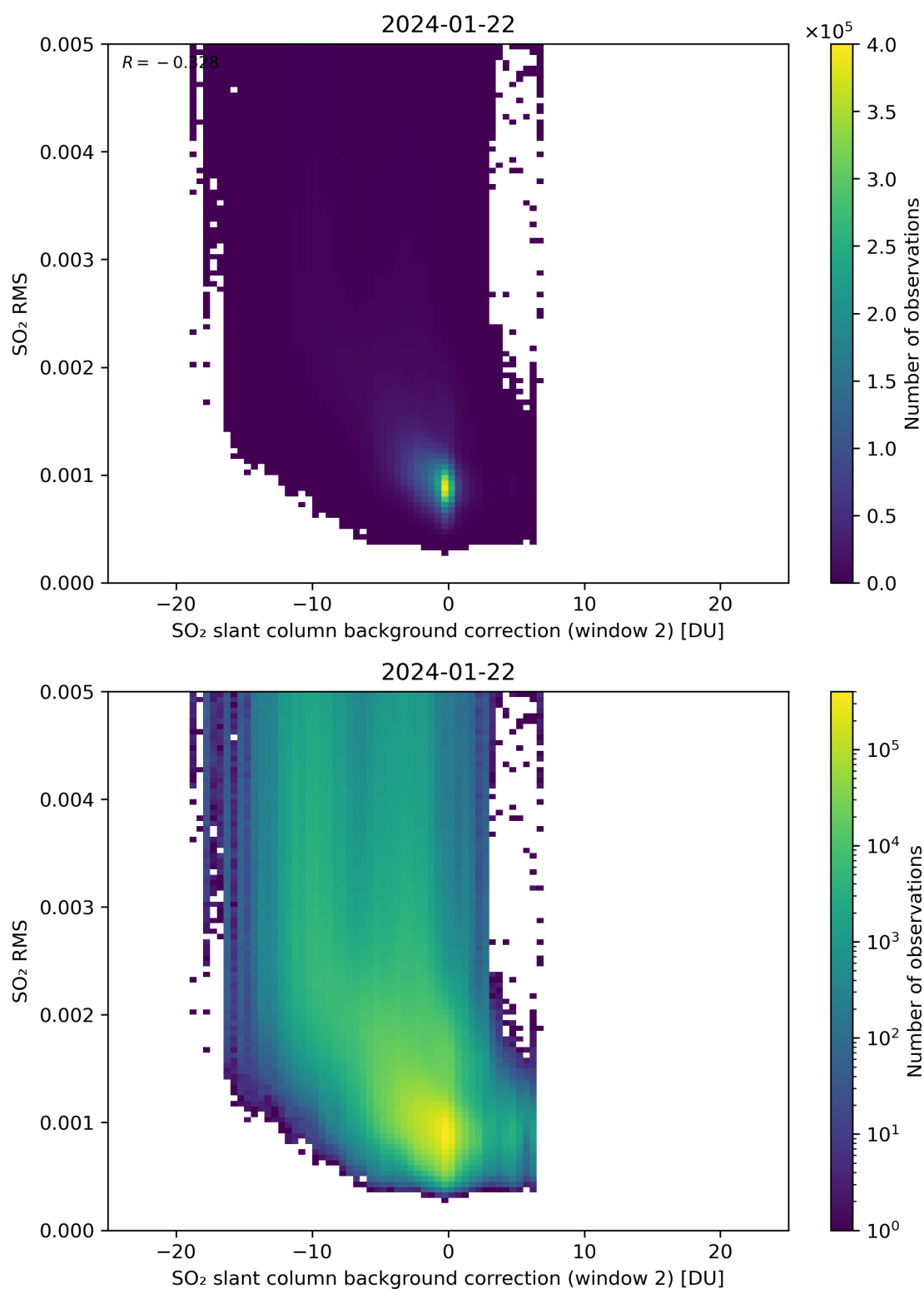
Figure 114: Scatter density plot of “SO 2 slant column background correction (window 2)” against “SO 2 RMS” for 2024-01-21 to 2024-01-23.
