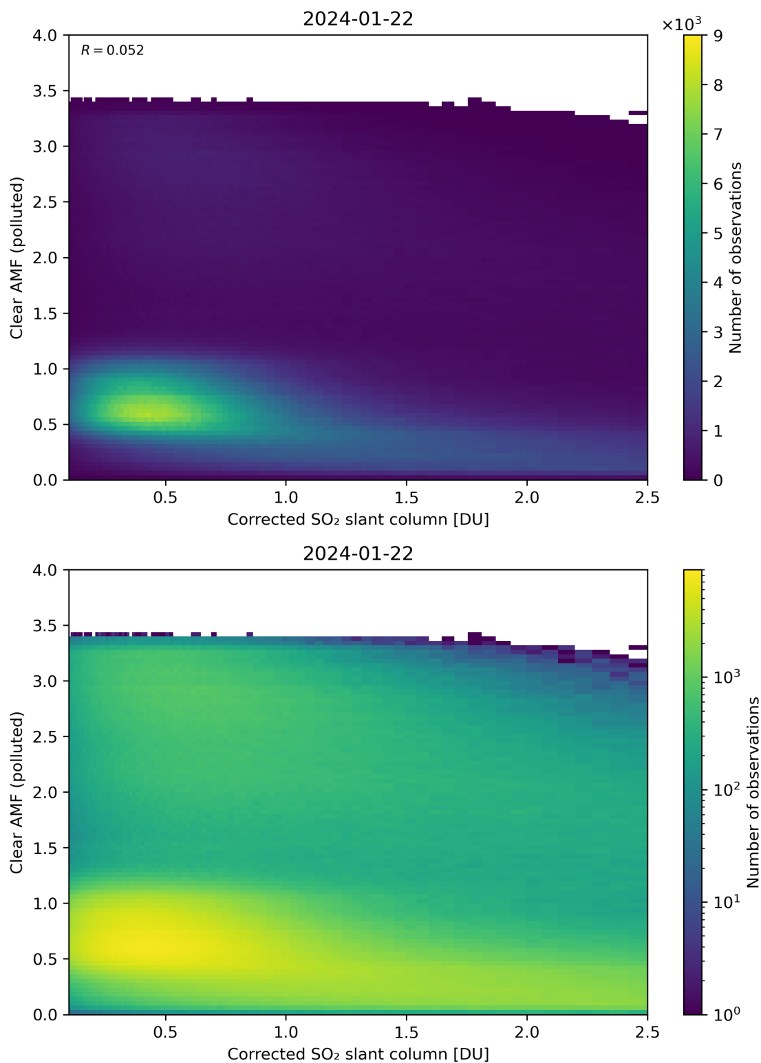
Figure 184: Scatter density plot of “Corrected SO 2 slant column” against “Clear AMF (polluted)” for 2024-01-21 to 2024-01-23.
