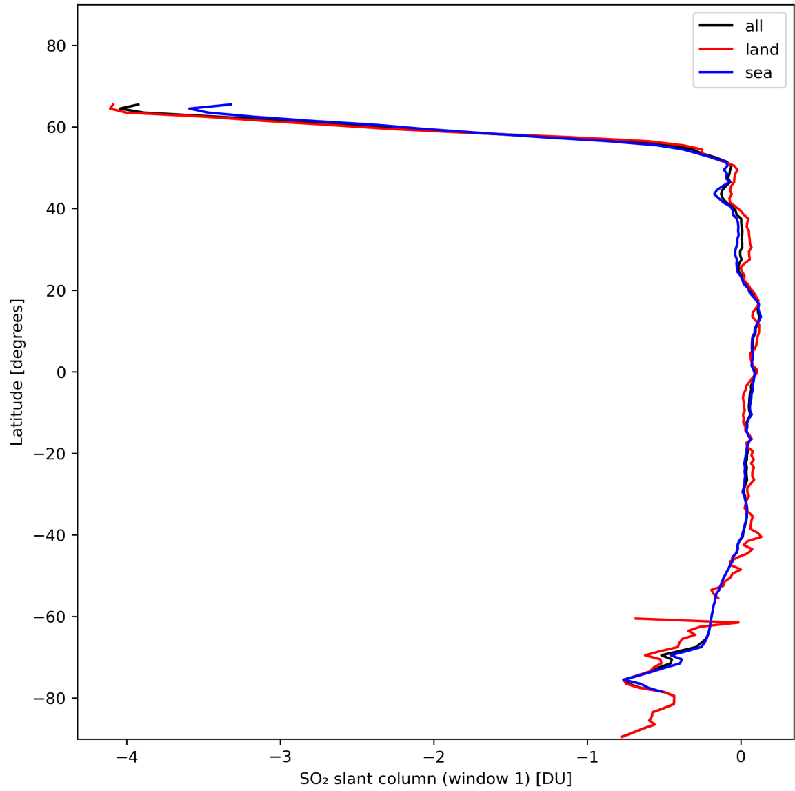
Figure 33: Zonal average of “SO 2 slant column (window 1)” for 2024-01-21 to 2024-01-23.
