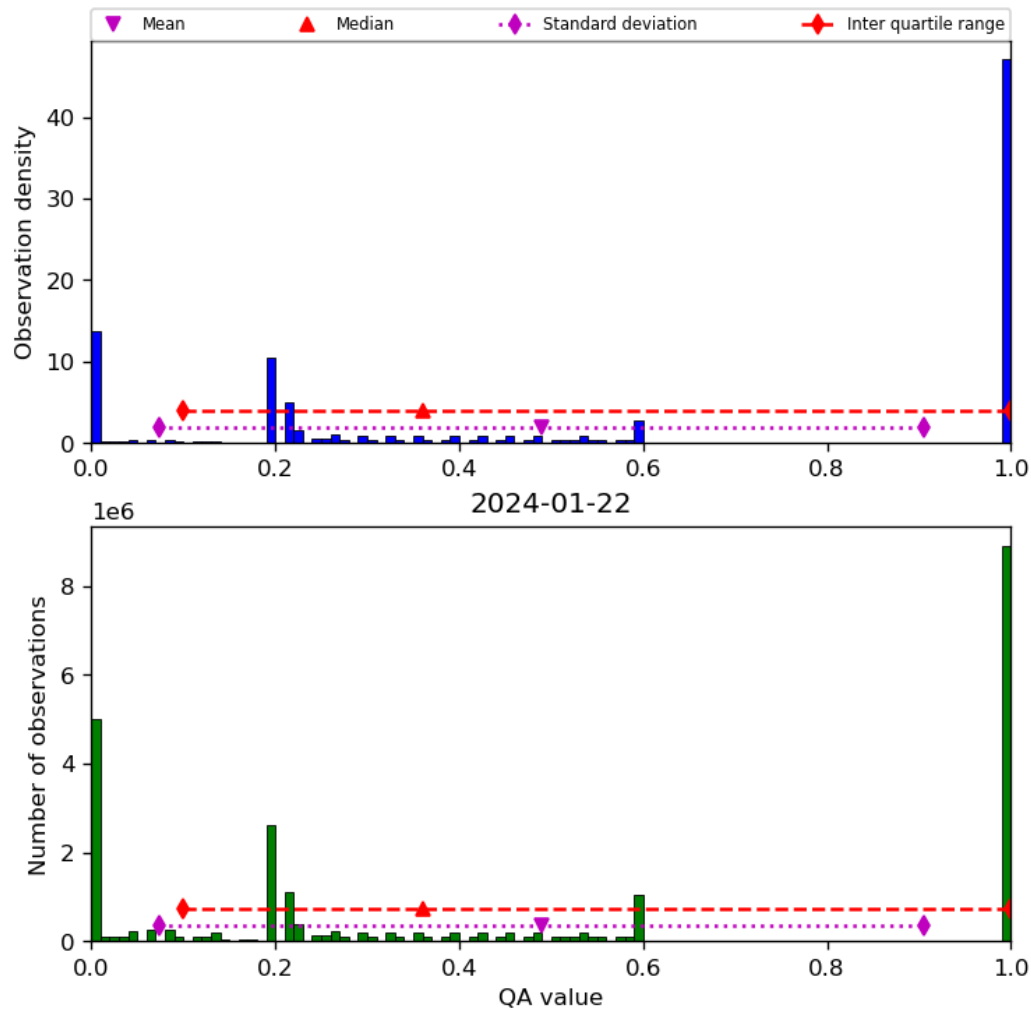
Figure 52: Histogram of “QA value” for 2024-01-21 to 2024-01-23
