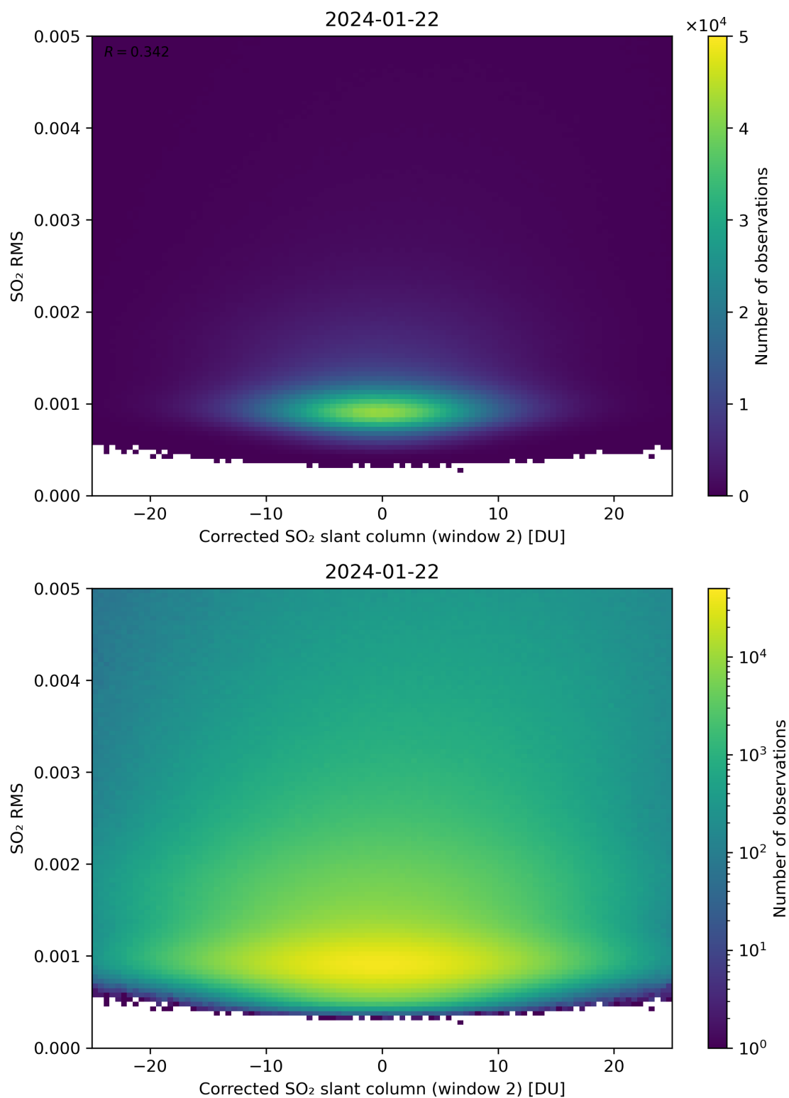
Figure 198: Scatter density plot of “Corrected SO 2 slant column (window 2)” against “SO 2 RMS” for 2024-01-21 to 2024-01-23.
