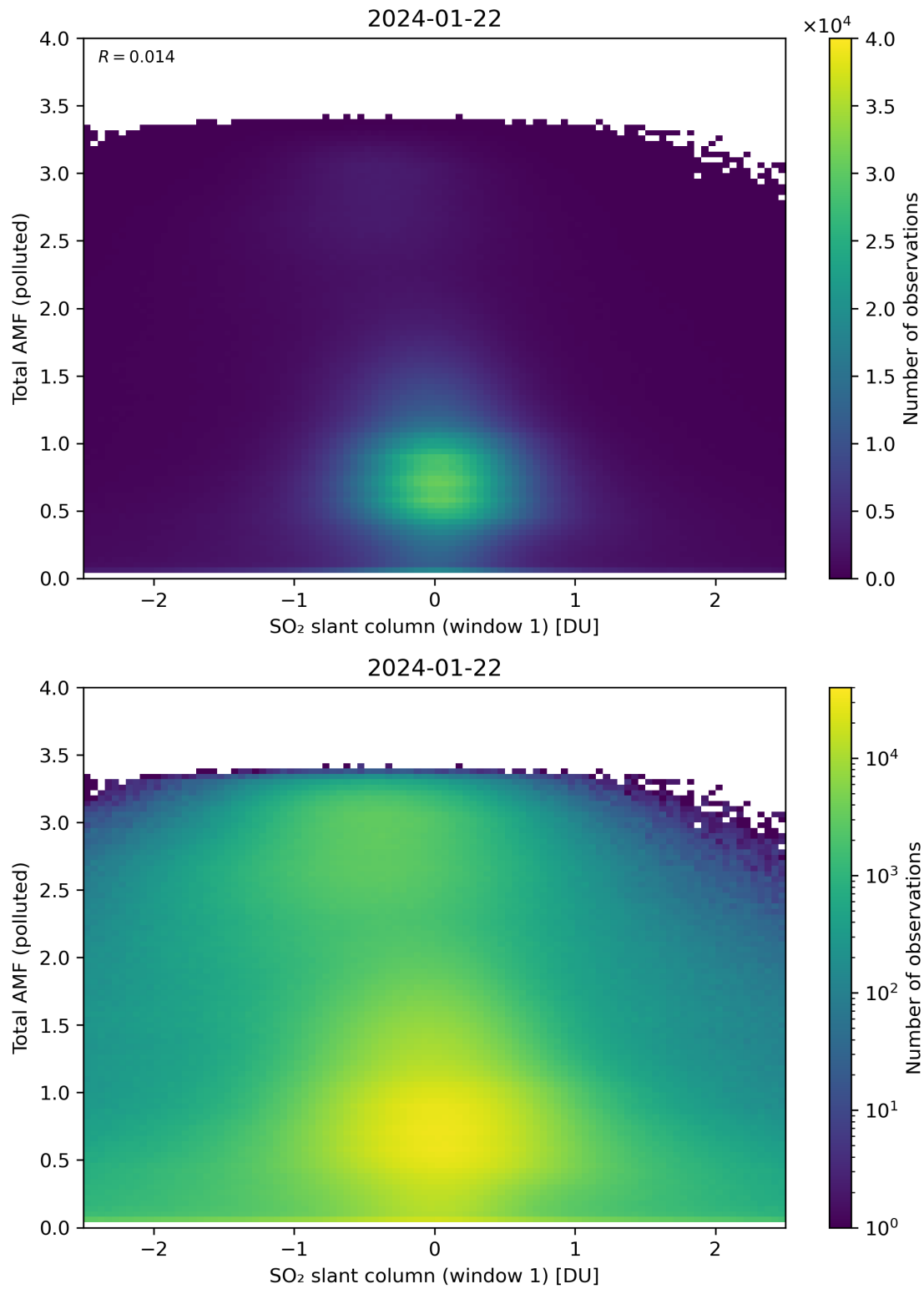
Figure 239: Scatter density plot of “SO 2 slant column (window 1)” against “Total AMF (polluted)” for 2024-01-21 to 2024-01-23.
