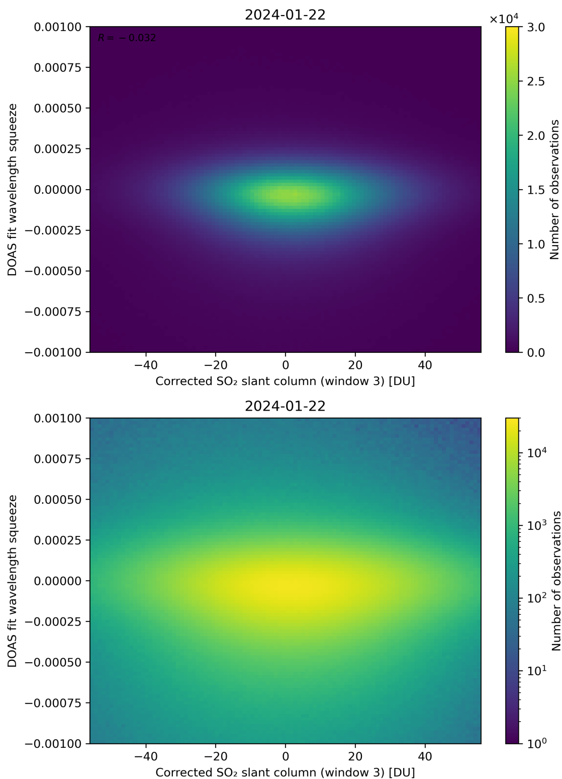
Figure 207: Scatter density plot of “Corrected SO 2 slant column (window 3)” against “DOAS fit wavelength squeeze” for 2024-01-21 to 2024-01-23.
