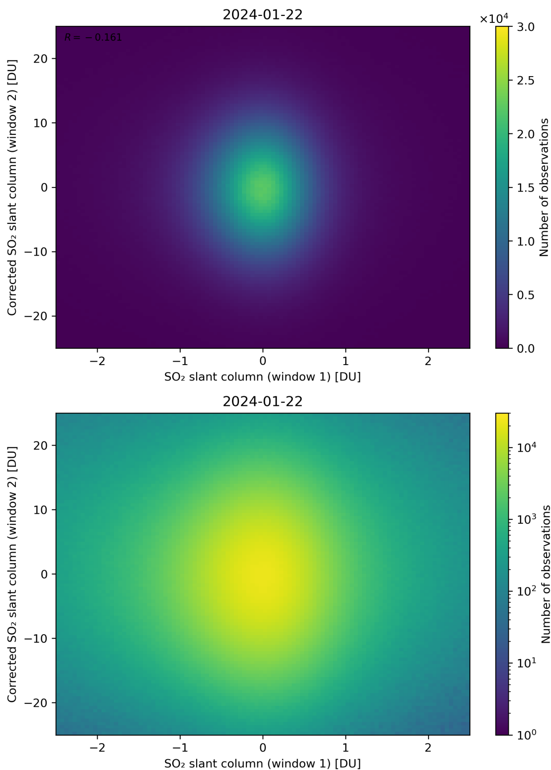
Figure 233: Scatter density plot of “SO 2 slant column (window 1)” against “Corrected SO 2 slant column (window 2)” for 2024-01-21 to 2024-01-23.
