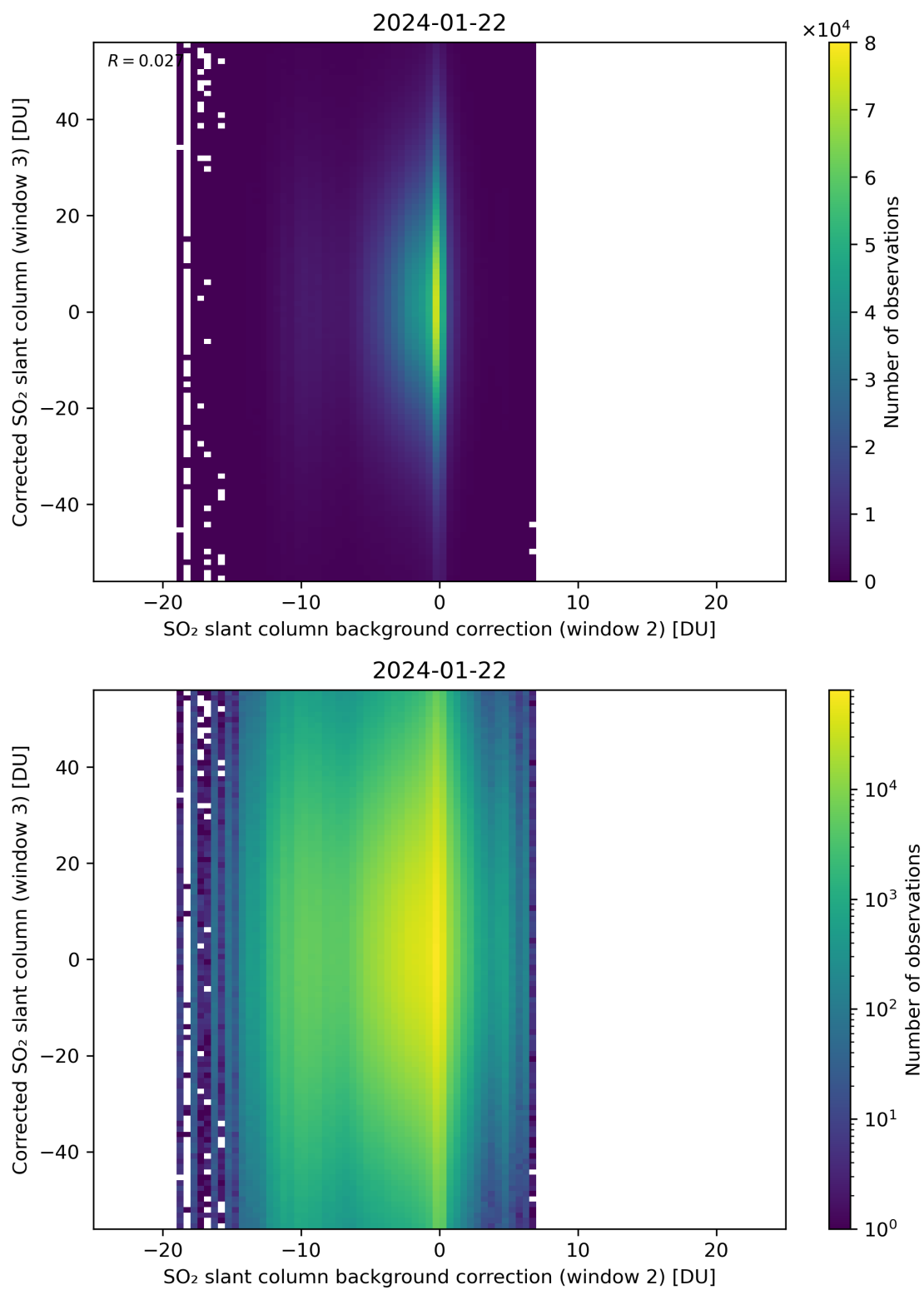
Figure 116: Scatter density plot of “SO 2 slant column background correction (window 2)” against “Corrected SO 2 slant column (window 3)” for 2024-01-21 to 2024-01-23.
