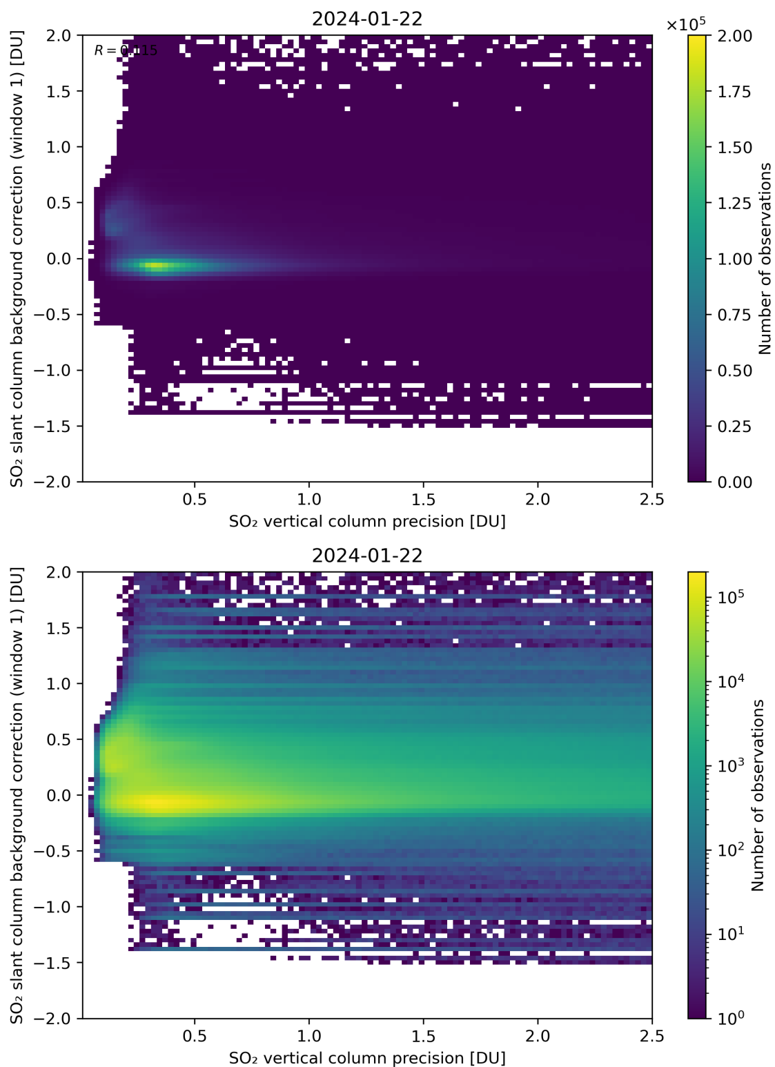
Figure 279: Scatter density plot of “SO 2 vertical column precision” against “SO 2 slant column background correction (window 1)” for 2024-01-21 to 2024-01-23.
