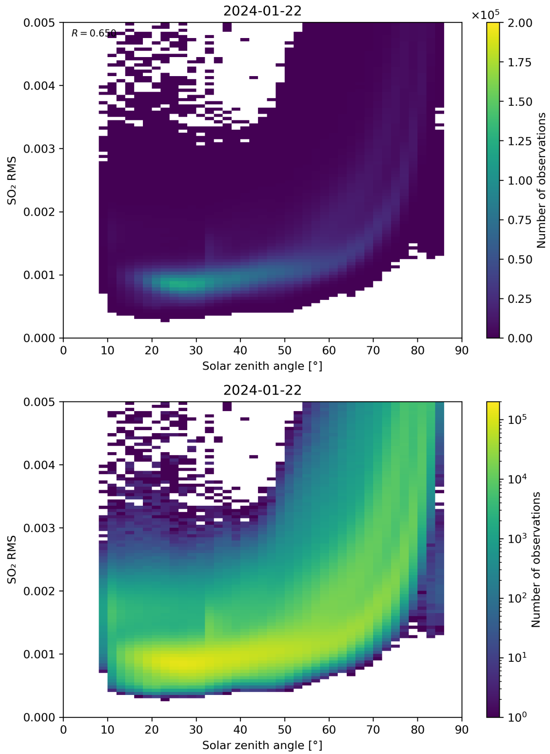
Figure 163: Scatter density plot of “Solar zenith angle” against “SO 2 RMS” for 2024-01-21 to 2024-01-23.
