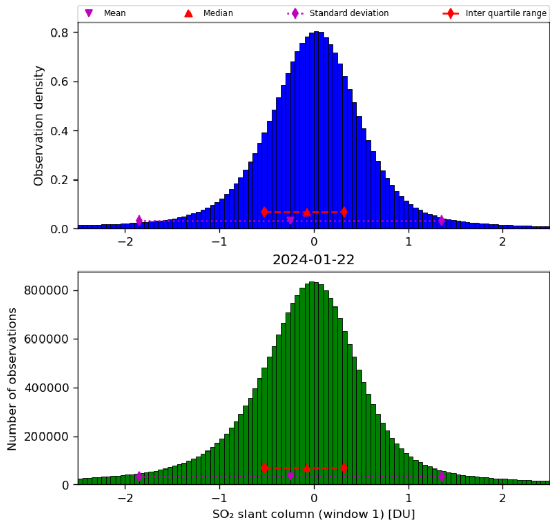
Figure 56: Histogram of “SO 2 slant column (window 1)” for 2024-01-21 to 2024-01-23
