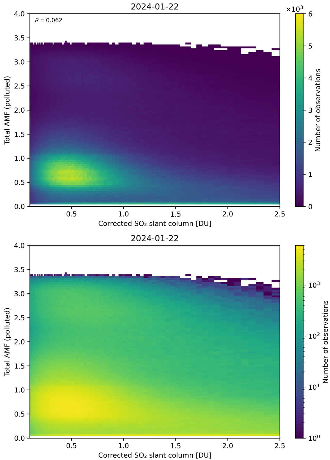
Figure 192: Scatter density plot of “Corrected SO 2 slant column” against “Total AMF (polluted)” for 2024-01-21 to 2024-01-23.
