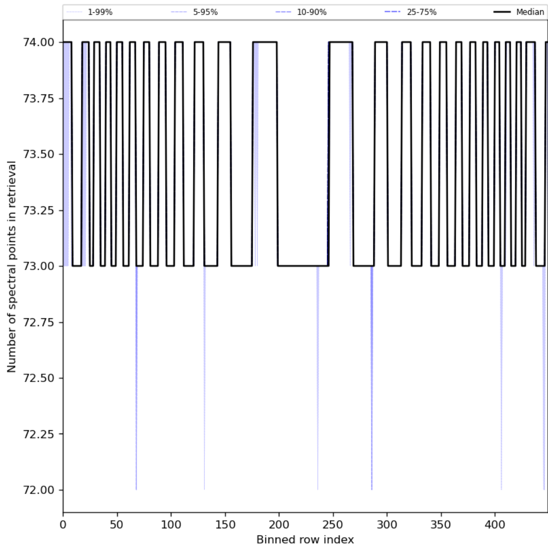
Figure 97: Along track statistics of “Number of spectral points in retrieval” for 2024-01-21 to 2024-01-23
