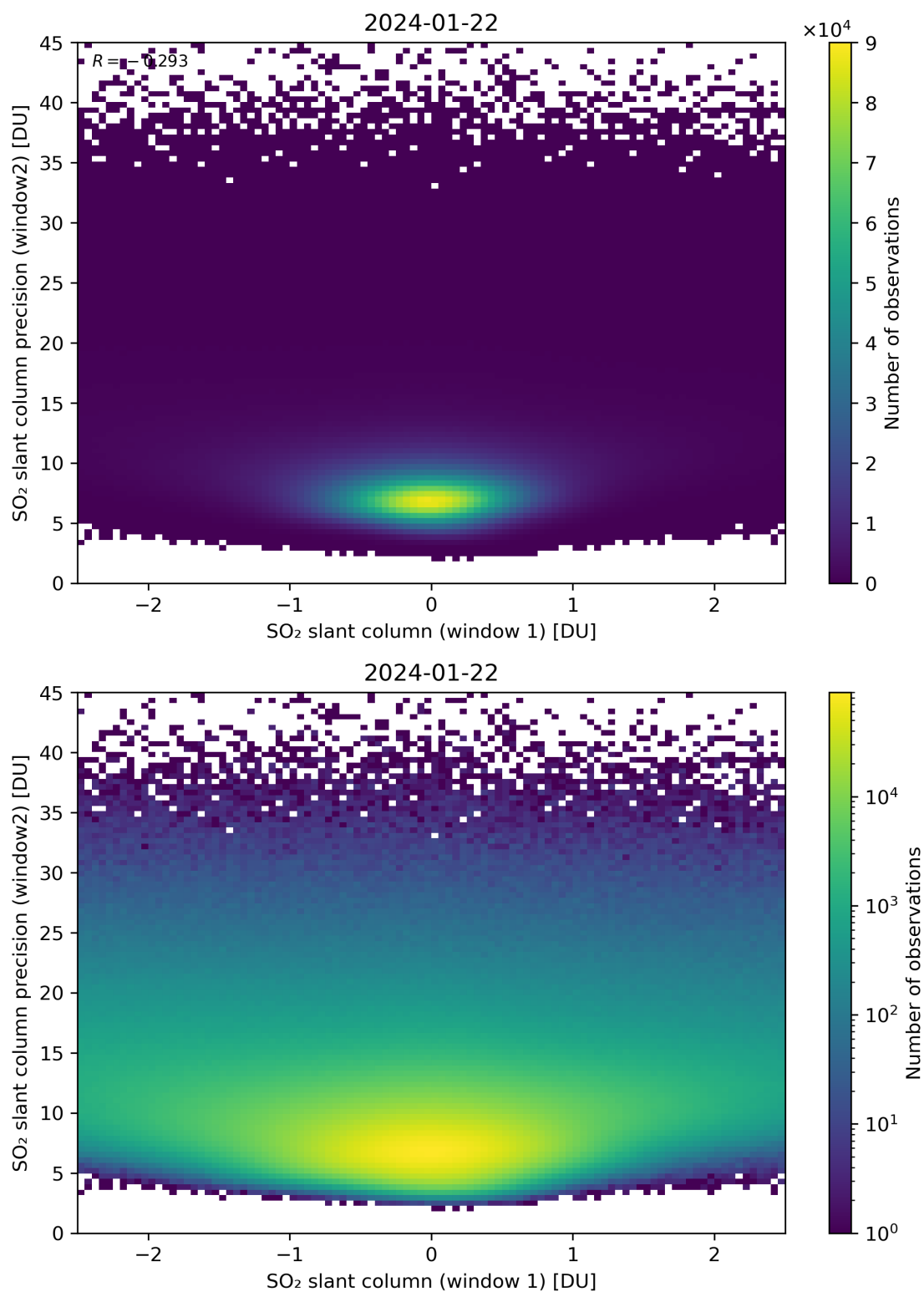
Figure 236: Scatter density plot of “SO 2 slant column (window 1)” against “SO 2 slant column precision (window2)” for 2024-01-21 to 2024-01-23.
