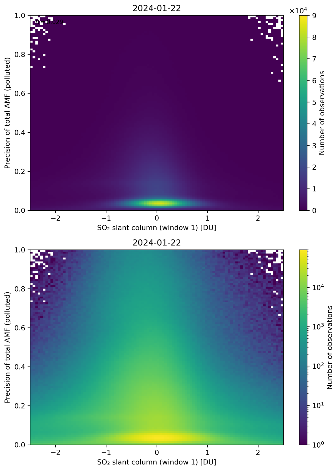
Figure 240: Scatter density plot of “SO 2 slant column (window 1)” against “Precision of total AMF (polluted)” for 2024-01-21 to 2024-01-23.
