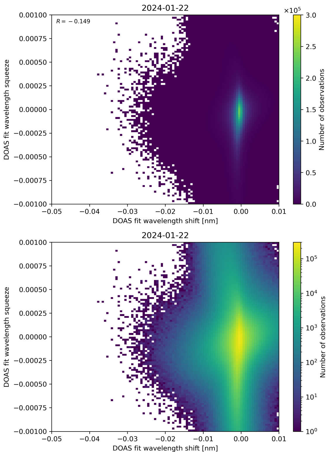
Figure 127: Scatter density plot of “DOAS fit wavelength shift” against “DOAS fit wavelength squeeze” for 2024-01-21 to 2024-01-23.
