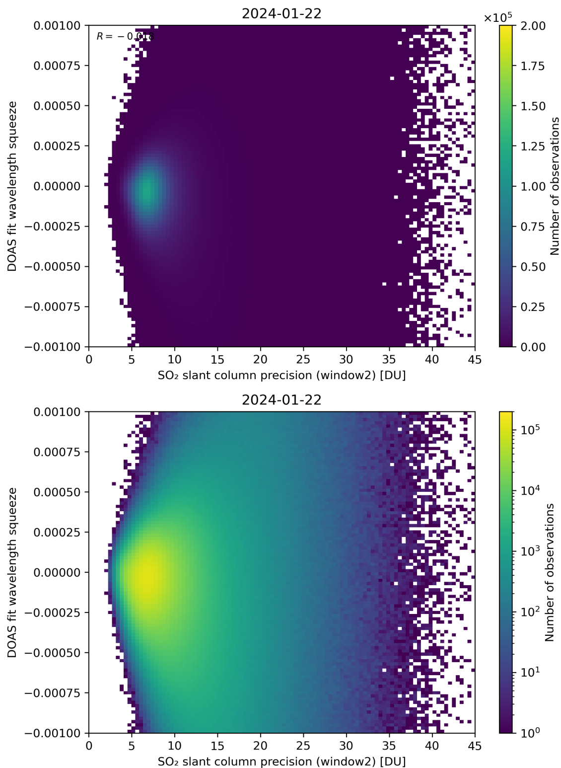
Figure 244: Scatter density plot of “SO 2 slant column precision (window2)” against “DOAS fit wavelength squeeze” for 2024-01-21 to 2024-01-23.
