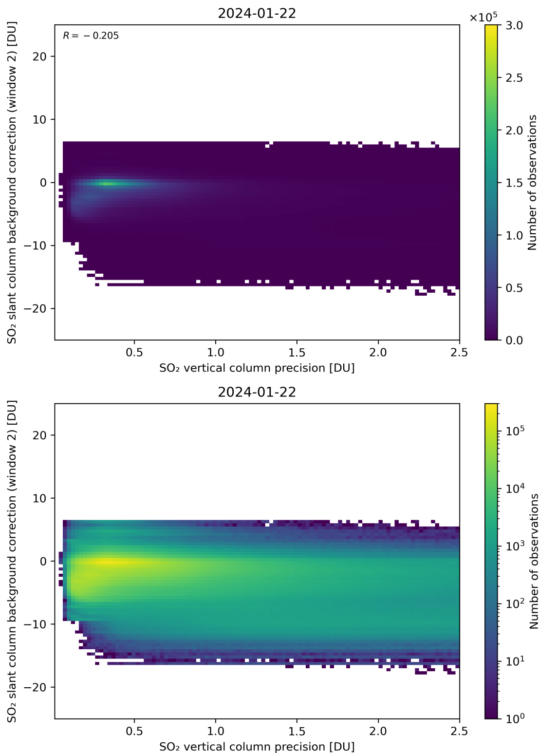
Figure 280: Scatter density plot of “SO 2 vertical column precision” against “SO 2 slant column background correction (window 2)” for 2024-01-21 to 2024-01-23.
