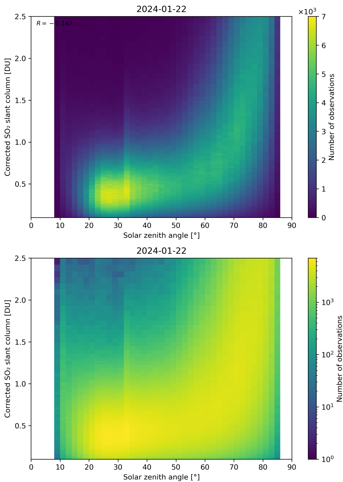
Figure 166: Scatter density plot of “Solar zenith angle” against “Corrected SO 2 slant column” for 2024-01-21 to 2024-01-23.
