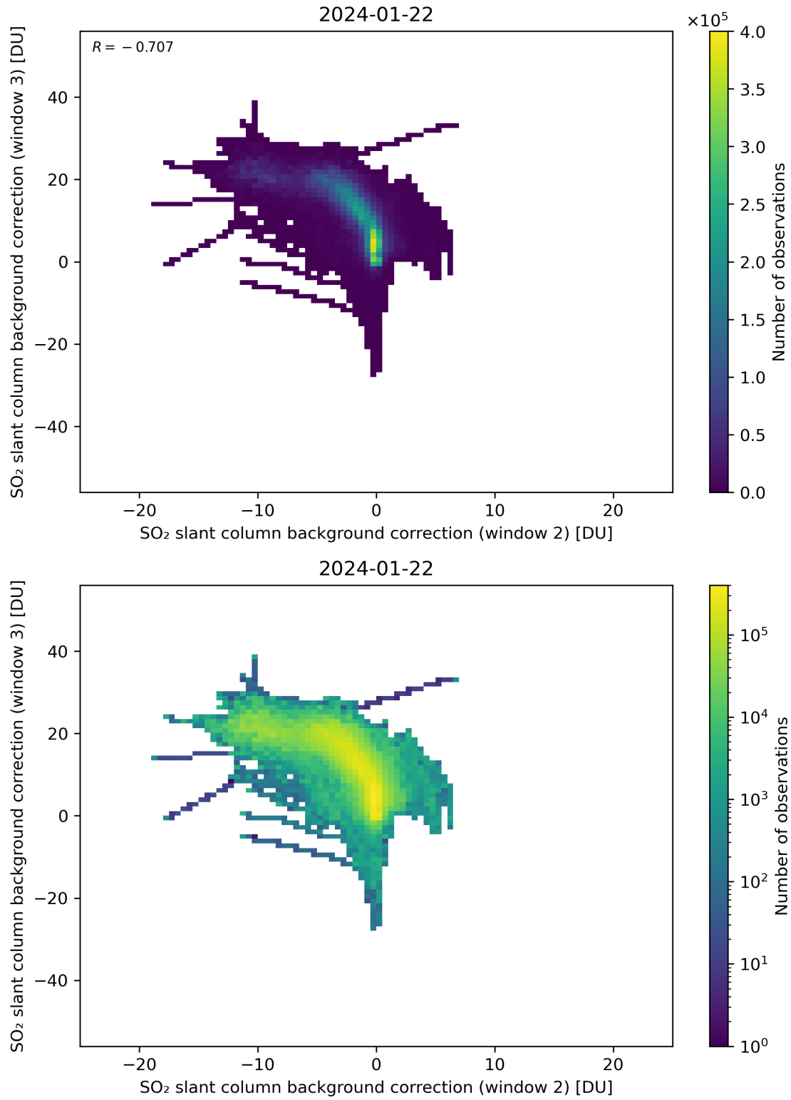
Figure 111: Scatter density plot of “SO 2 slant column background correction (window 2)” against “SO 2 slant column background correction (window 3)” for 2024-01-21 to 2024-01-23.
