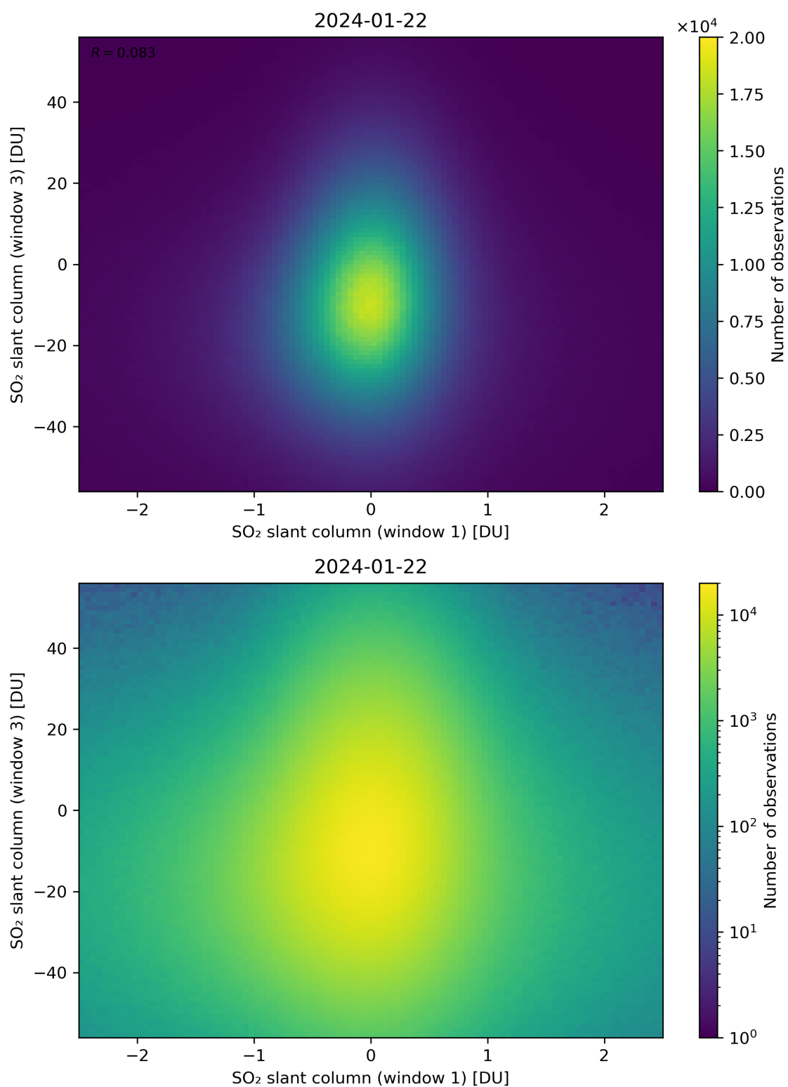
Figure 237: Scatter density plot of “SO 2 slant column (window 1)” against “SO 2 slant column (window 3)” for 2024-01-21 to 2024-01-23.
