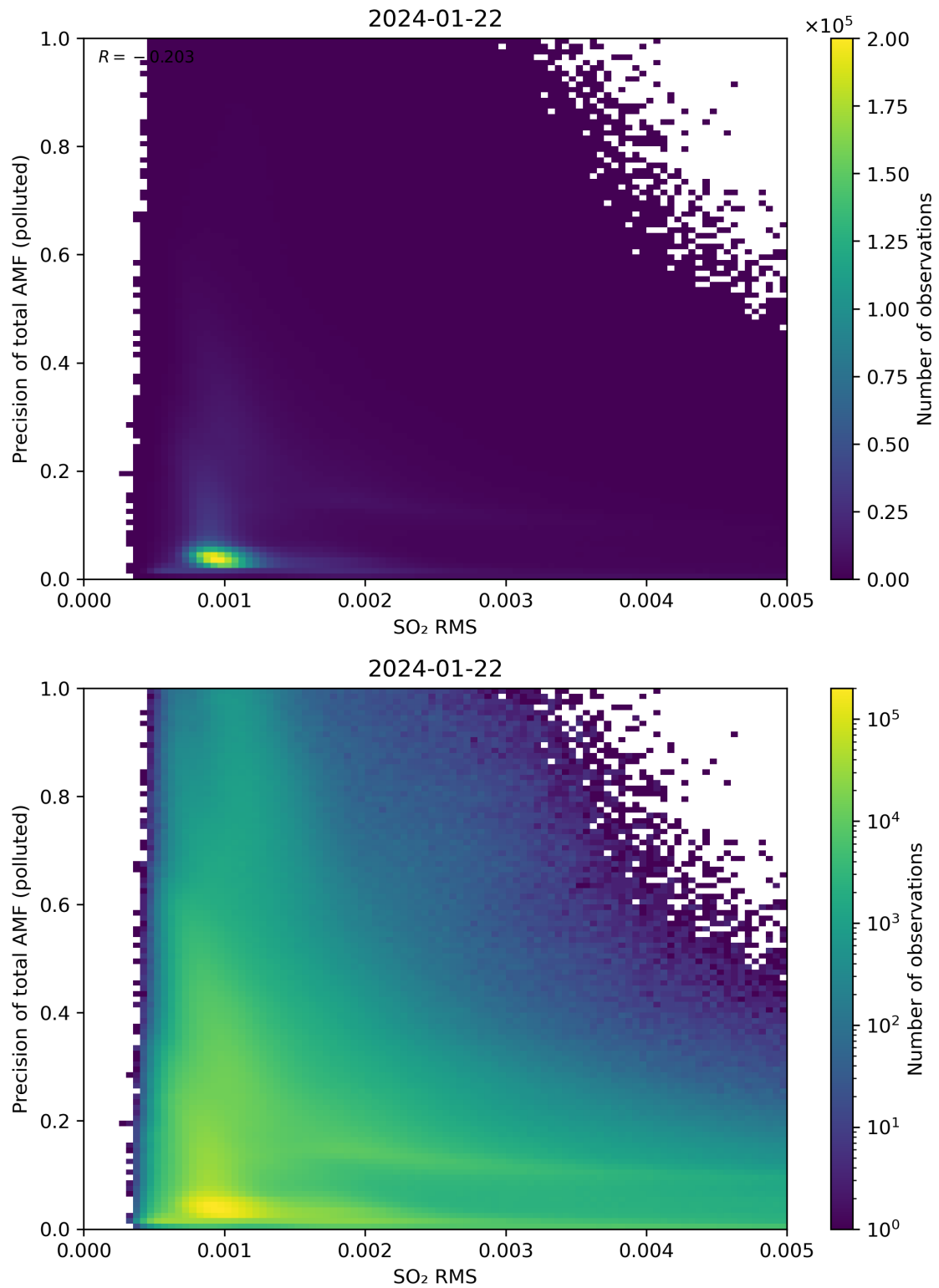
Figure 138: Scatter density plot of “SO 2 RMS” against “Precision of total AMF (polluted)” for 2024-01-21 to 2024-01-23.
