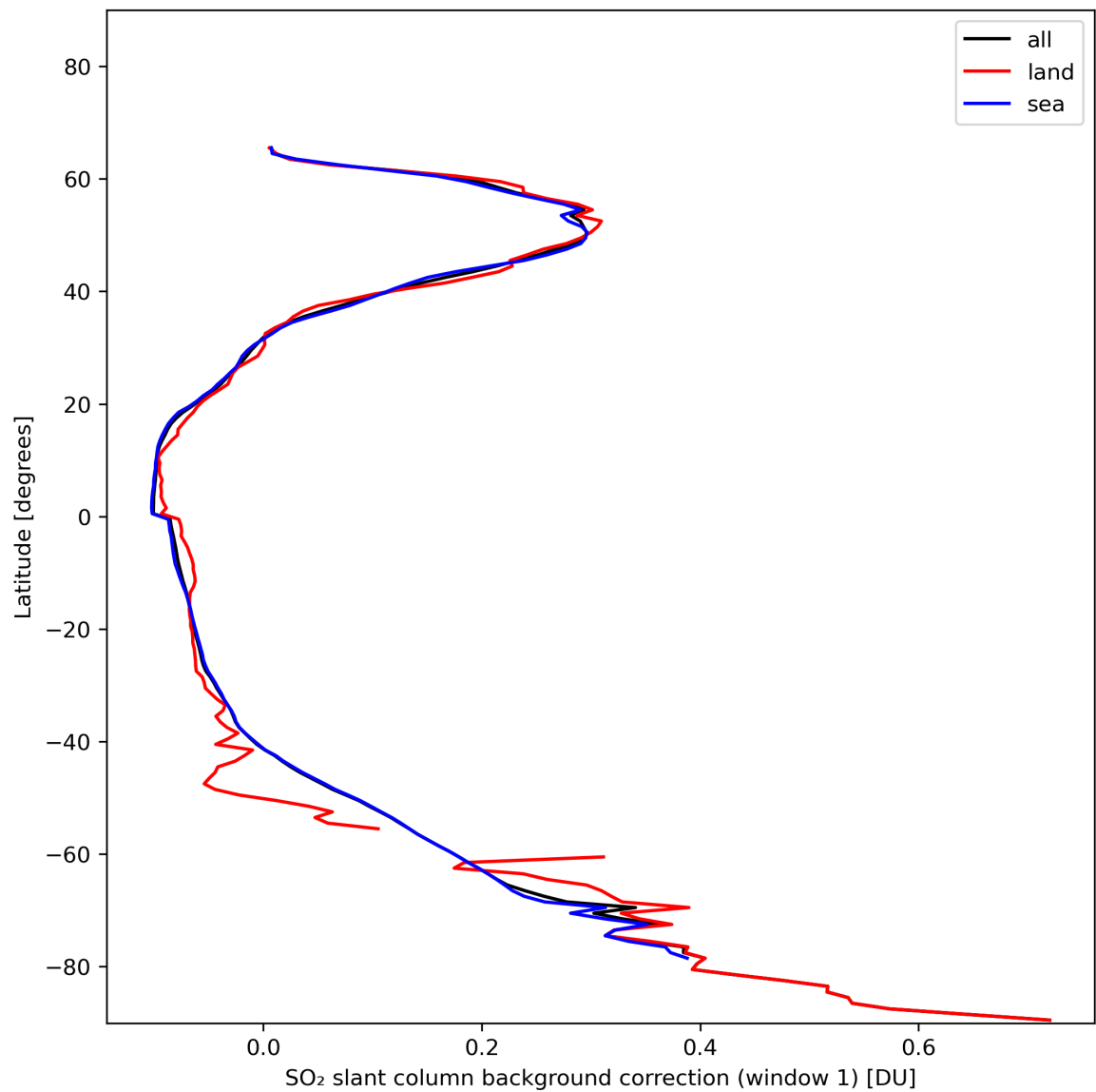
Figure 36: Zonal average of “SO 2 slant column background correction (window 1)” for 2024-01-21 to 2024-01-23.
