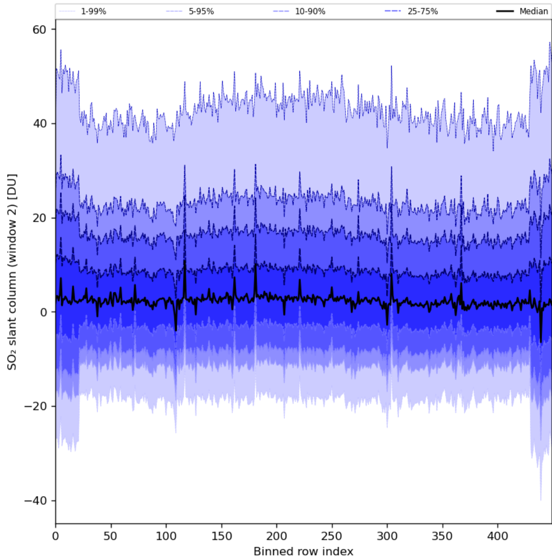
Figure 83: Along track statistics of “SO 2 slant column (window 2)” for 2024-01-21 to 2024-01-23
