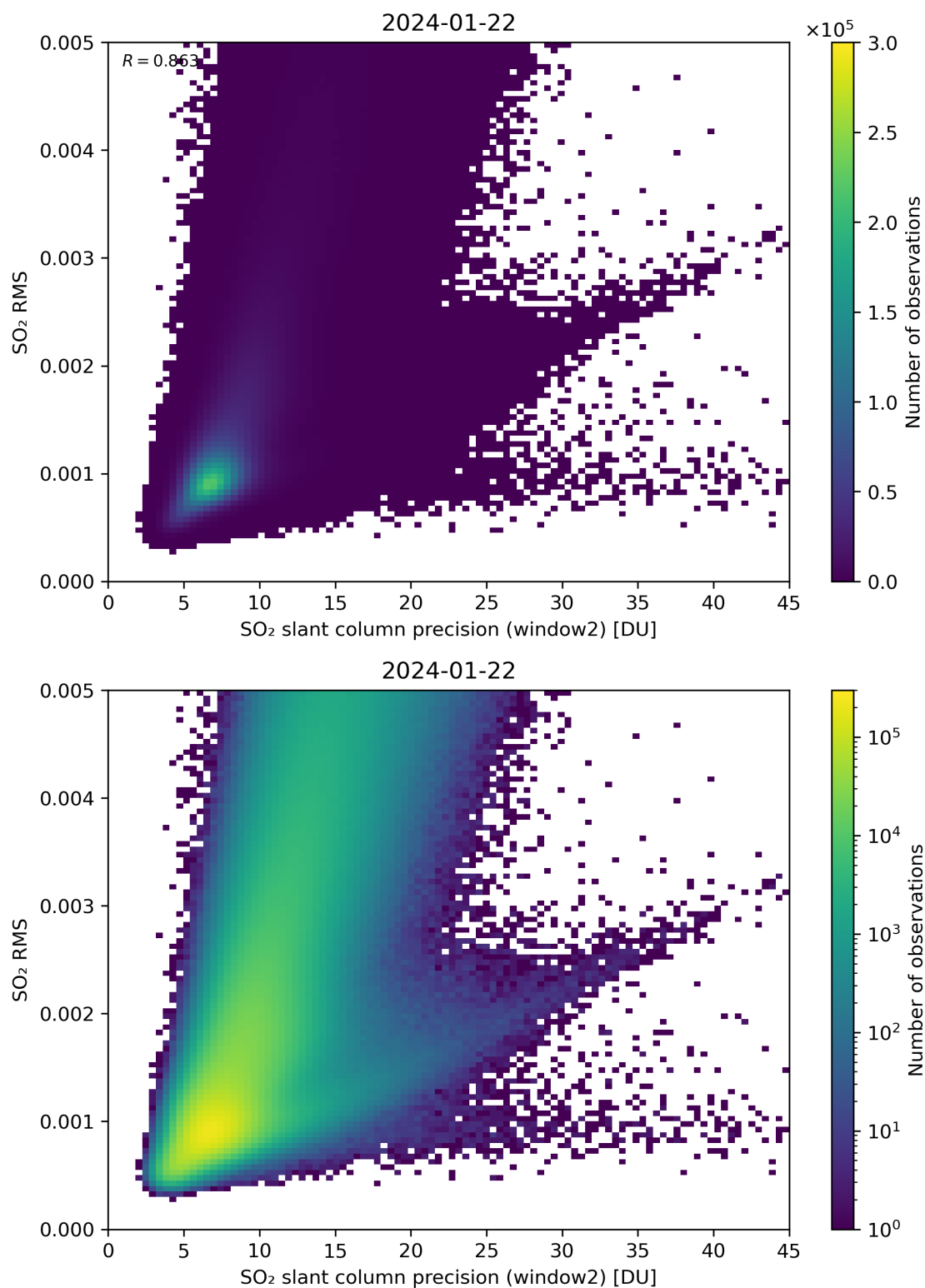
Figure 245: Scatter density plot of “SO 2 slant column precision (window2)” against “SO 2 RMS” for 2024-01-21 to 2024-01-23.
