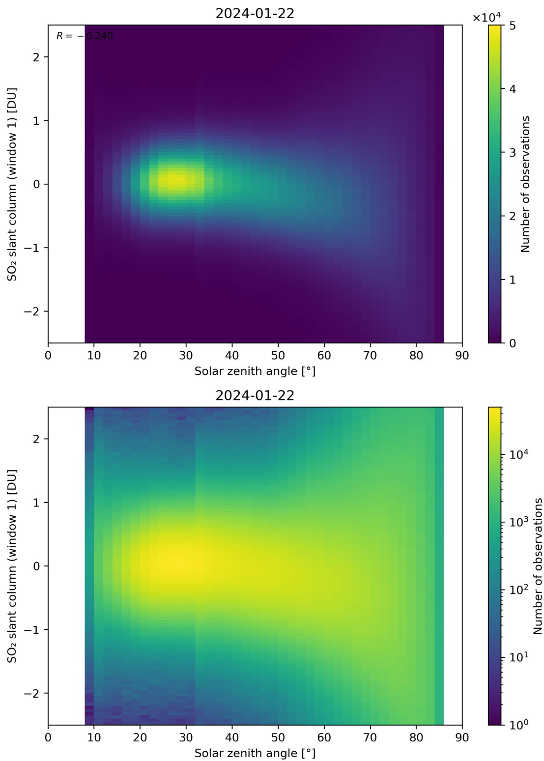
Figure 169: Scatter density plot of “Solar zenith angle” against “SO 2 slant column (window 1)” for 2024-01-21 to 2024-01-23.
