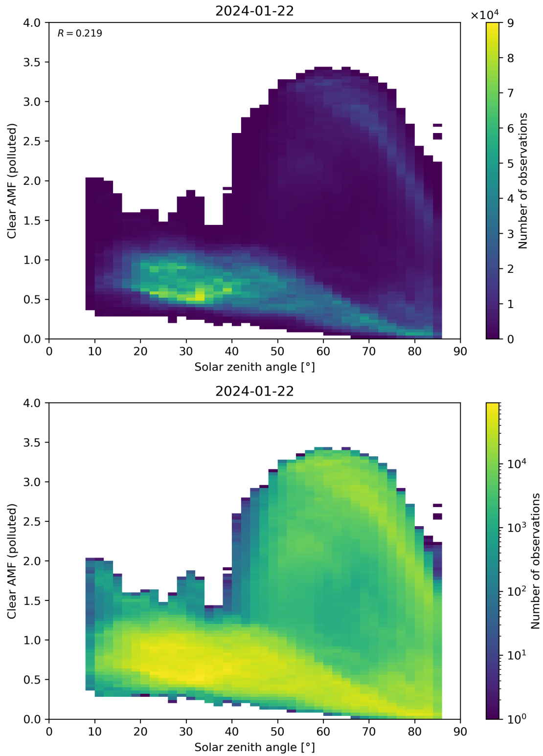
Figure 165: Scatter density plot of “Solar zenith angle” against “Clear AMF (polluted)” for 2024-01-21 to 2024-01-23.
