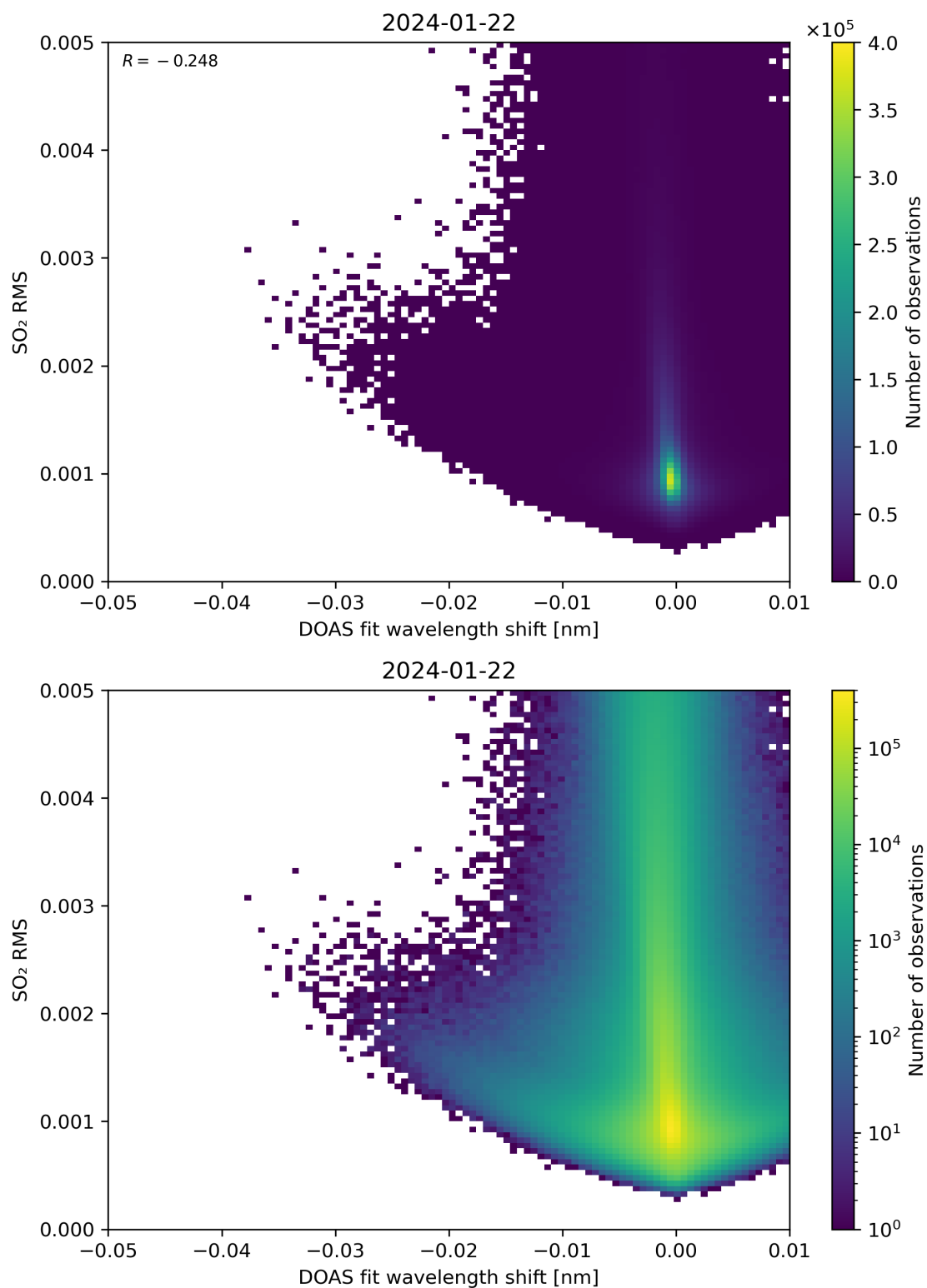
Figure 128: Scatter density plot of “DOAS fit wavelength shift” against “SO 2 RMS” for 2024-01-21 to 2024-01-23.
