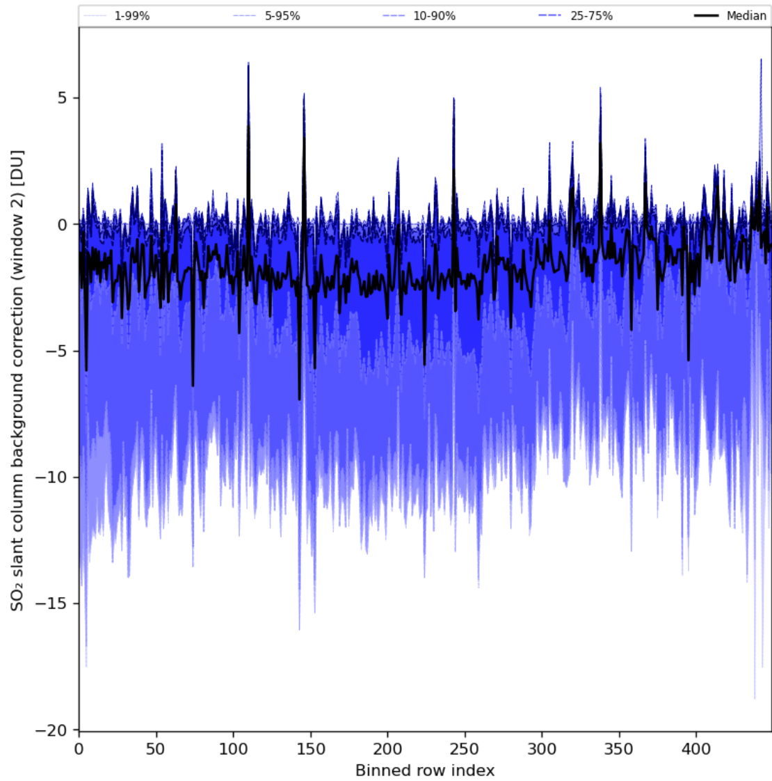
Figure 86: Along track statistics of “SO 2 slant column background correction (window 2)” for 2024-01-21 to 2024-01-23
