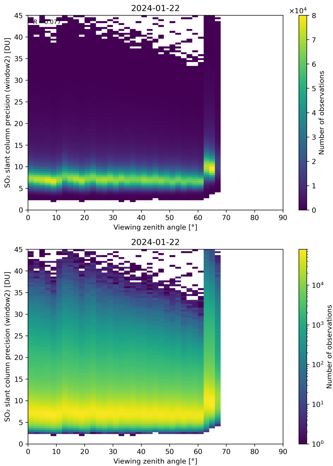
Figure 322: Scatter density plot of “Viewing zenith angle” against “SO 2 slant column precision (window2)” for 2024-01-21 to 2024-01-23.
