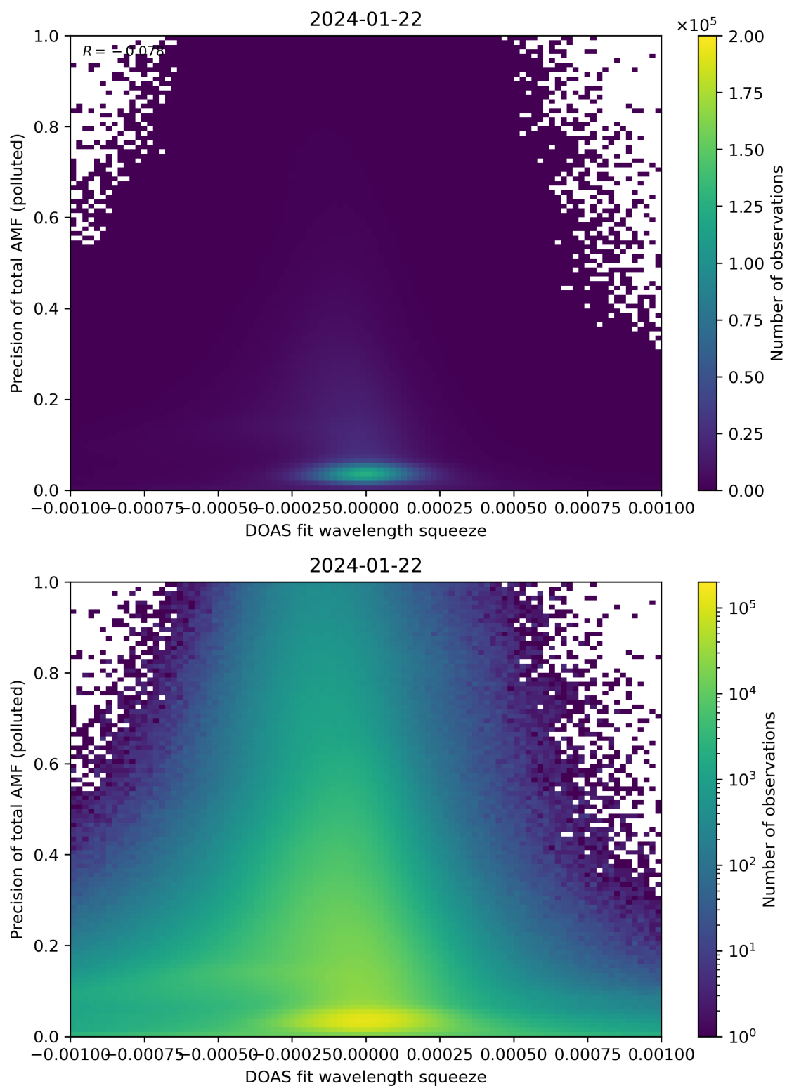
Figure 135: Scatter density plot of “DOAS fit wavelength squeeze” against “Precision of total AMF (polluted)” for 2024-01-21 to 2024-01-23.
