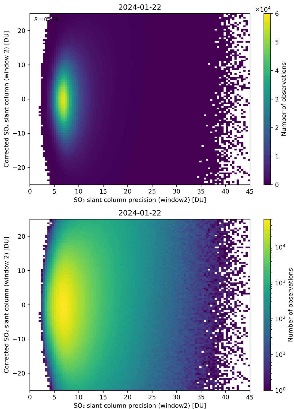
Figure 247: Scatter density plot of “SO 2 slant column precision (window2)” against “Corrected SO 2 slant column (window 2)” for 2024-01-21 to 2024-01-23.
