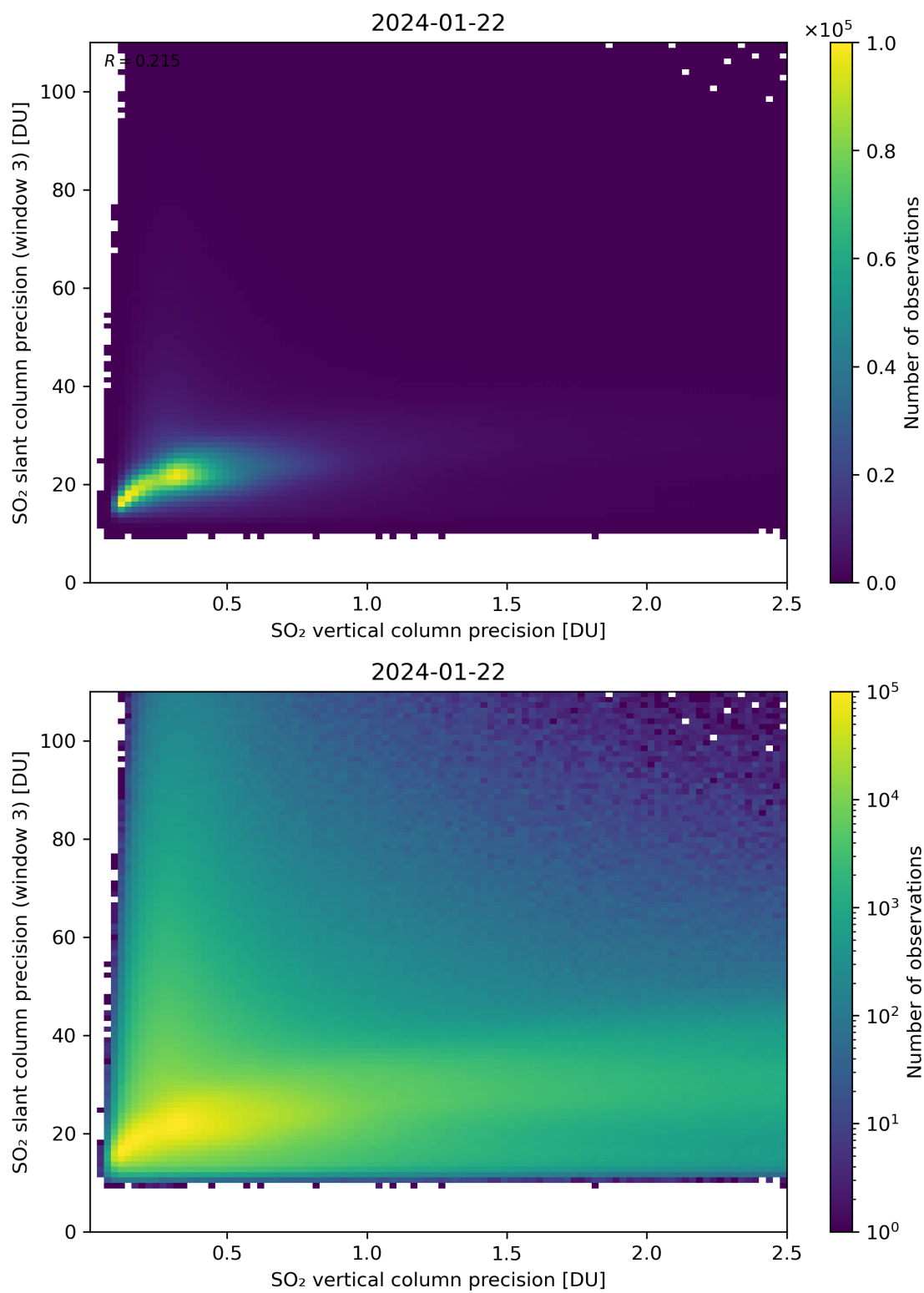
Figure 293: Scatter density plot of “SO 2 vertical column precision” against “SO 2 slant column precision (window 3)” for 2024-01-21 to 2024-01-23.
