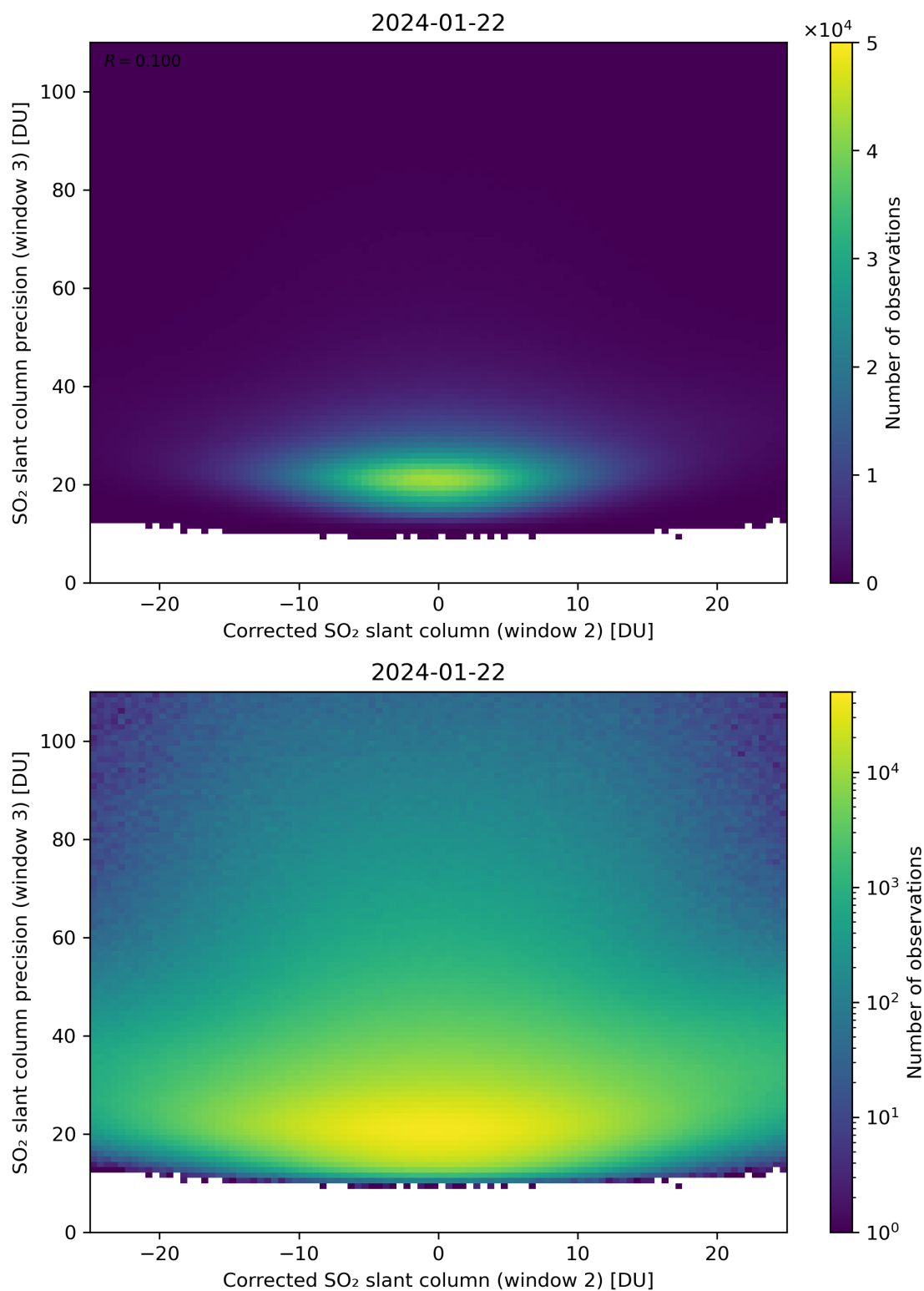
Figure 202: Scatter density plot of “Corrected SO 2 slant column (window 2)” against “SO 2 slant column precision (window 3)” for 2024-01-21 to 2024-01-23.
