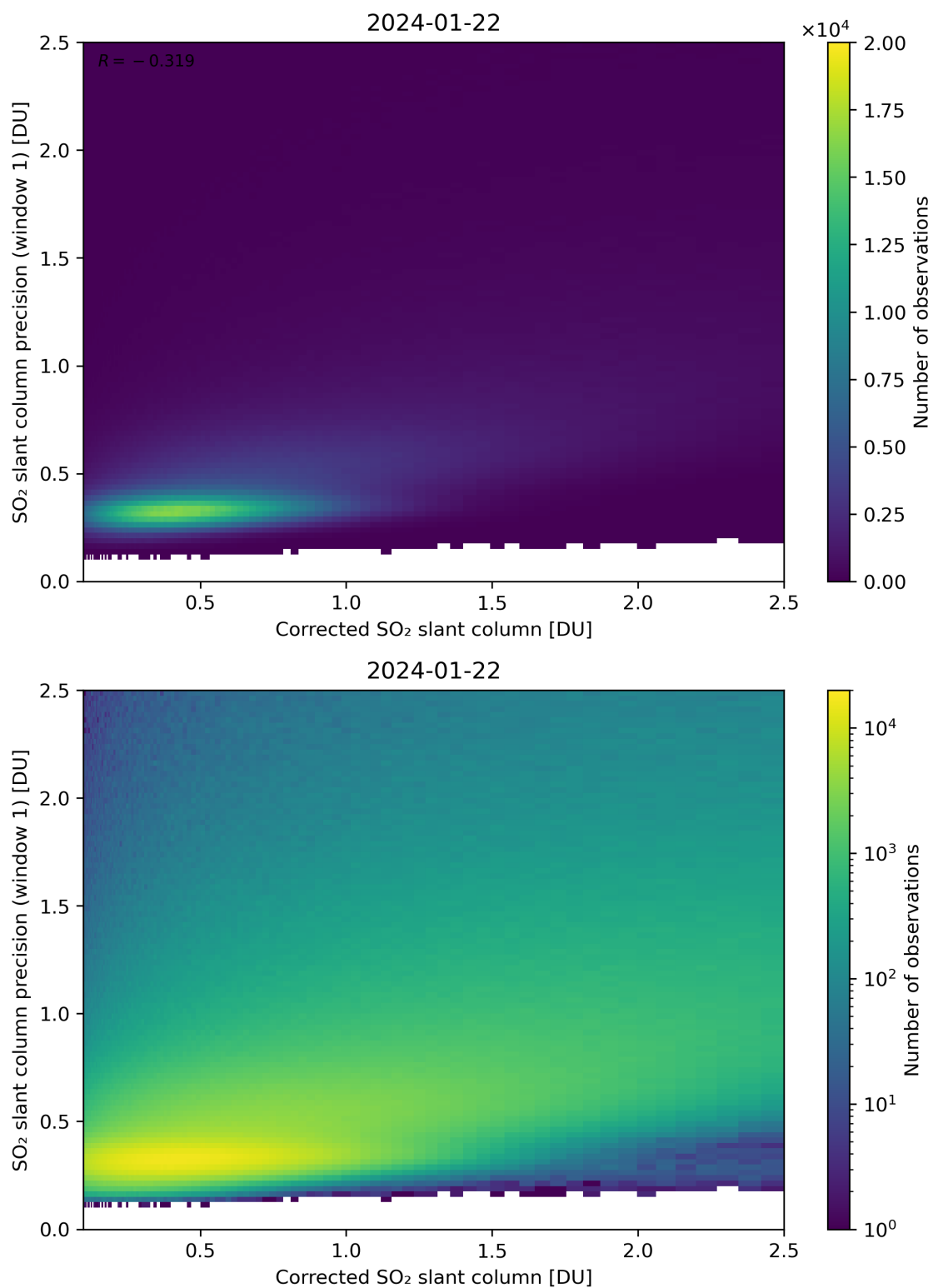
Figure 188: Scatter density plot of “Corrected SO 2 slant column” against “SO 2 slant column precision (window 1)” for 2024-01-21 to 2024-01-23.
