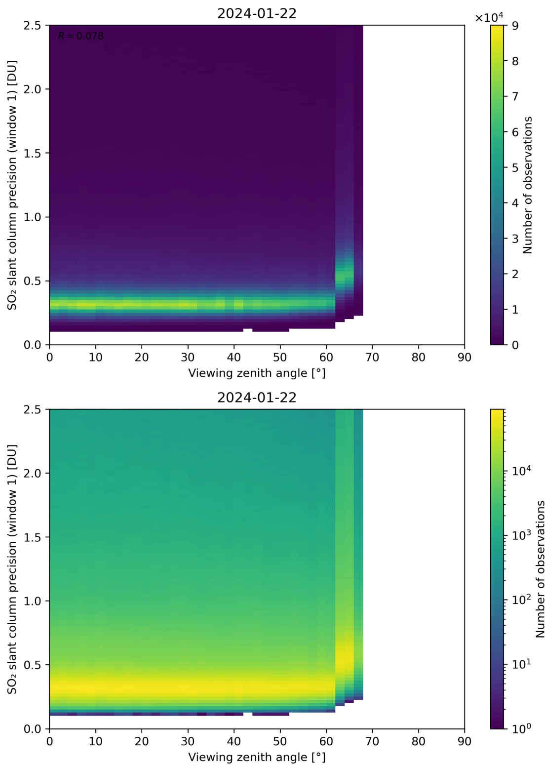
Figure 321: Scatter density plot of “Viewing zenith angle” against “SO 2 slant column precision (window 1)” for 2024-01-21 to 2024-01-23.
