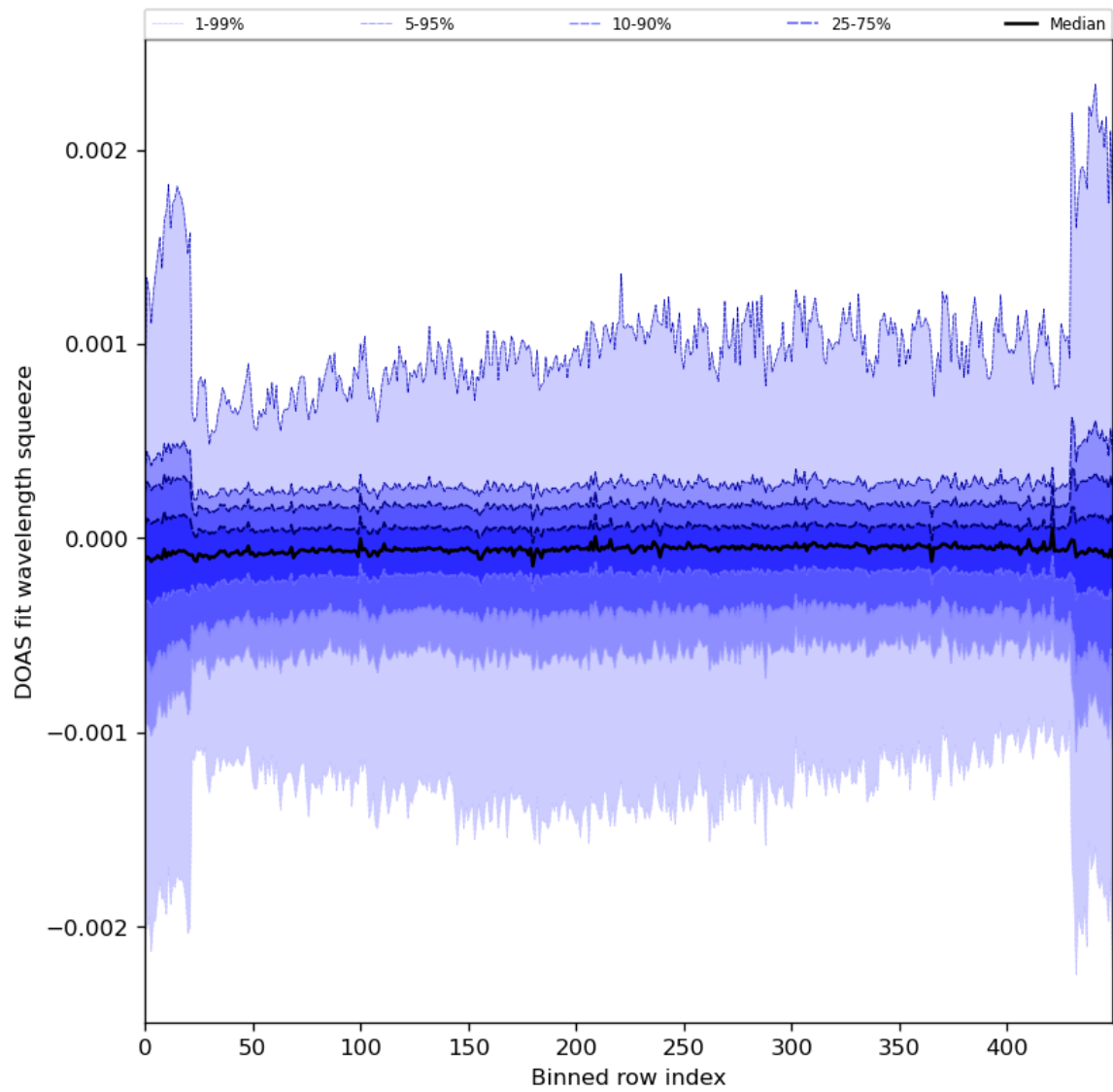
Figure 92: Along track statistics of “DOAS fit wavelength squeeze” for 2024-01-21 to 2024-01-23
