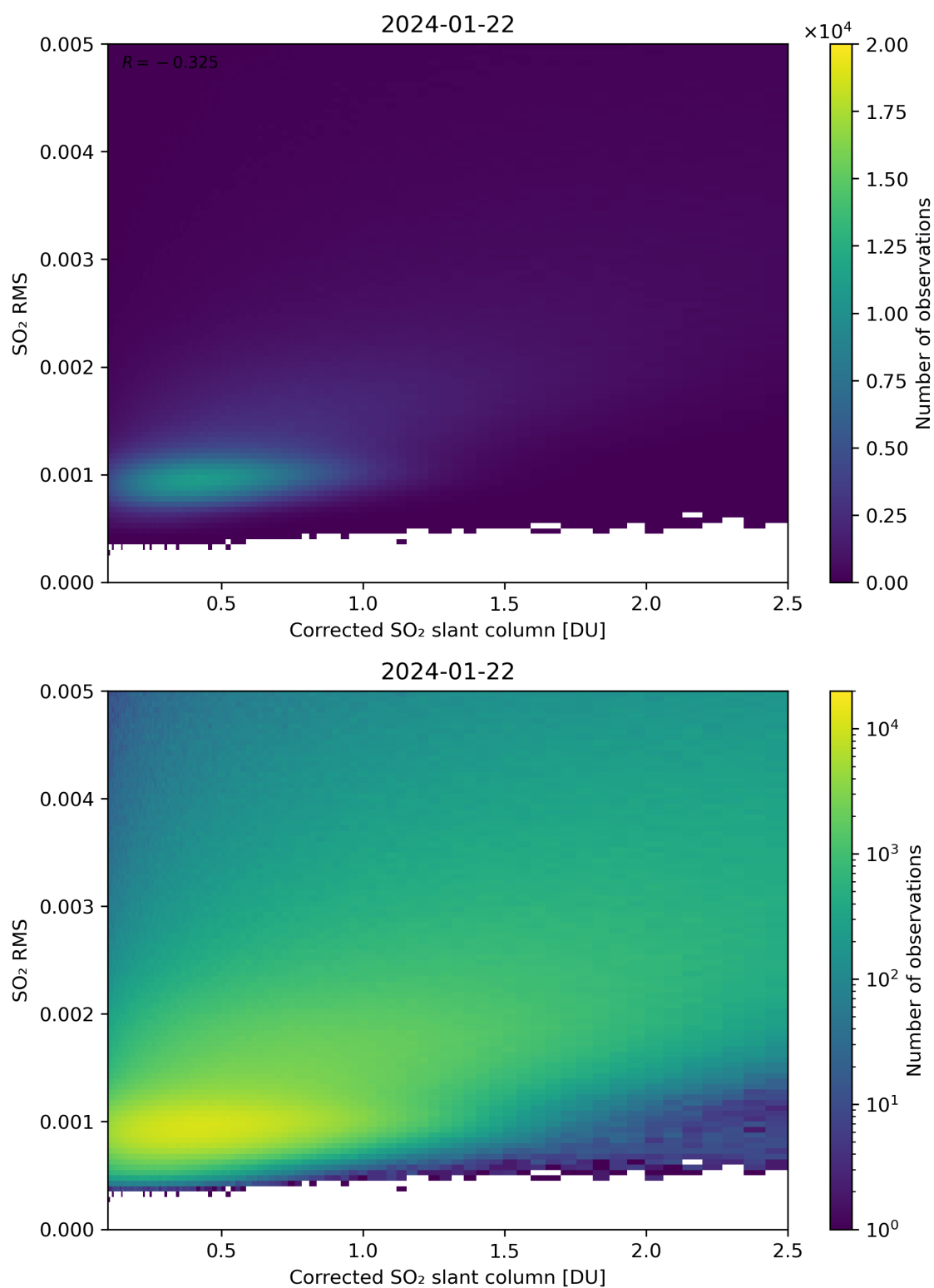
Figure 183: Scatter density plot of “Corrected SO 2 slant column” against “SO 2 RMS” for 2024-01-21 to 2024-01-23.
