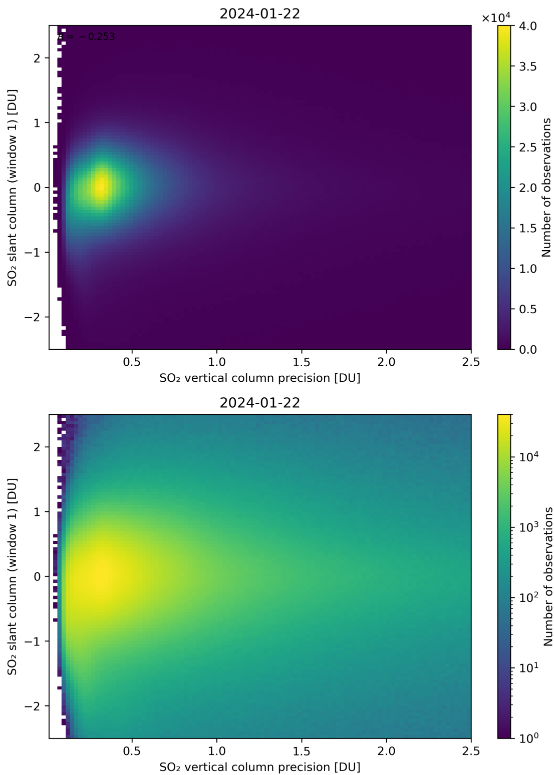
Figure 289: Scatter density plot of “SO 2 vertical column precision” against “SO 2 slant column (window 1)” for 2024-01-21 to 2024-01-23.
