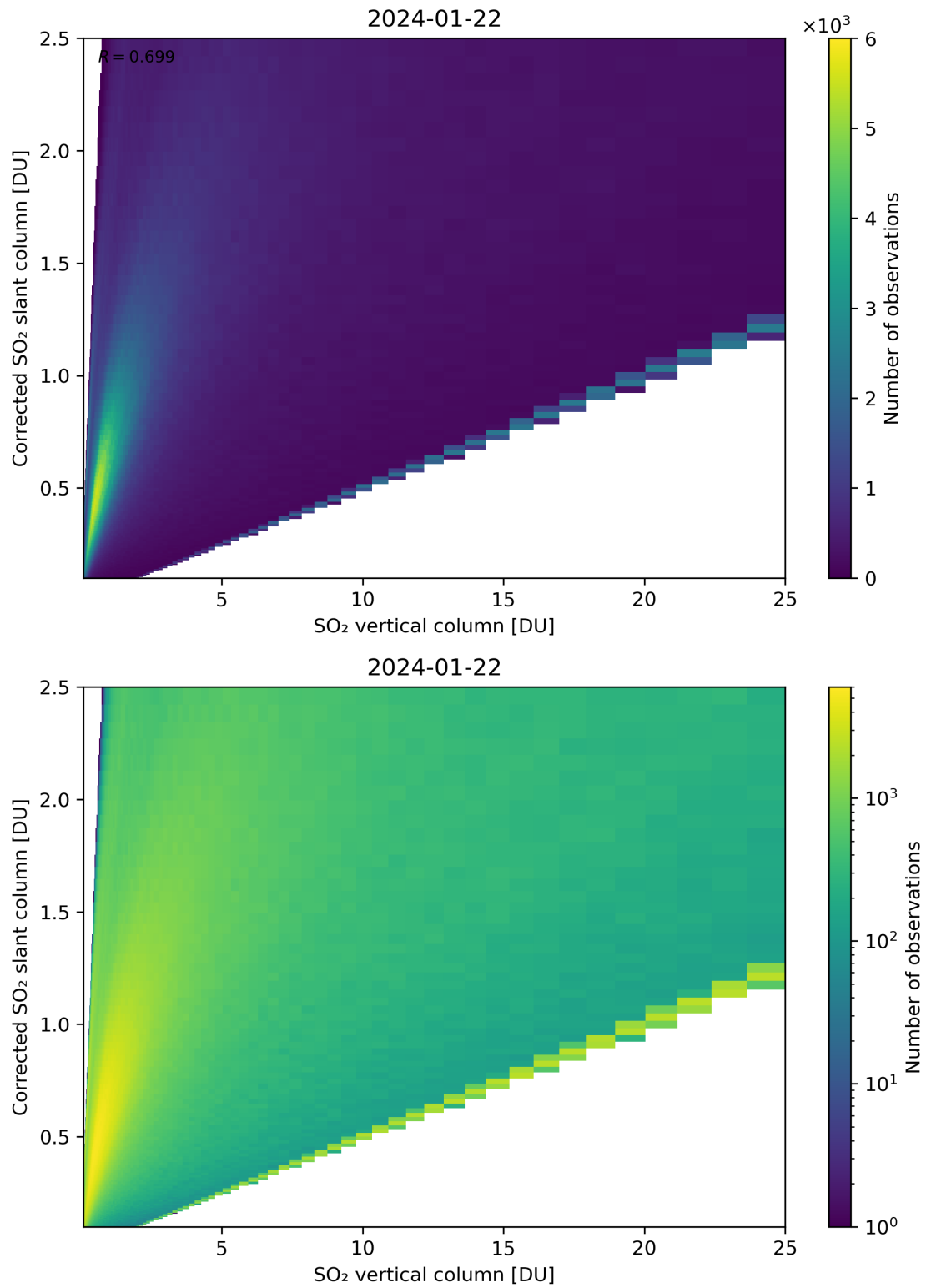
Figure 297: Scatter density plot of “SO 2 vertical column” against “Corrected SO 2 slant column” for 2024-01-21 to 2024-01-23.
