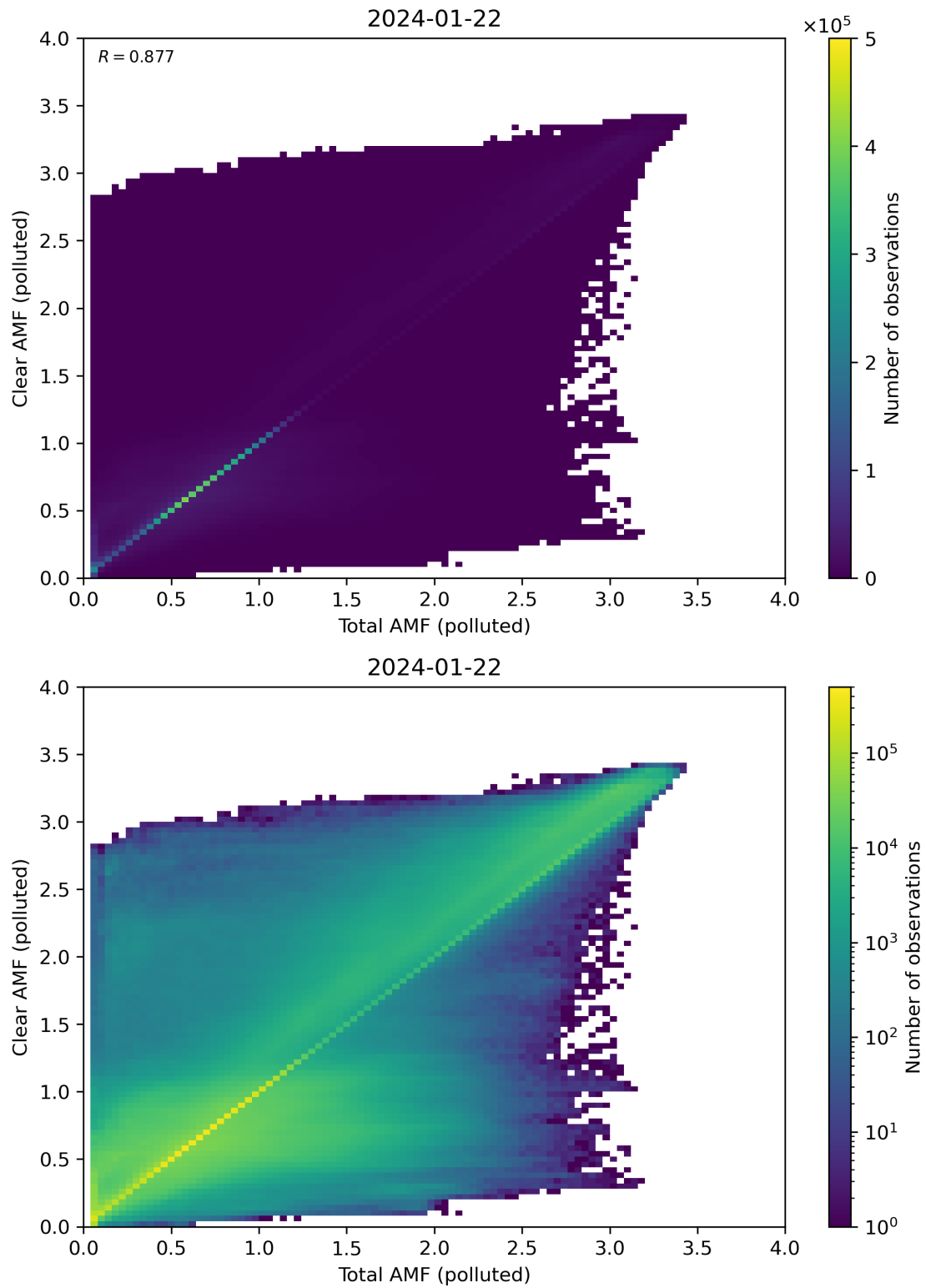
Figure 271: Scatter density plot of “Total AMF (polluted)” against “Clear AMF (polluted)” for 2024-01-21 to 2024-01-23.
