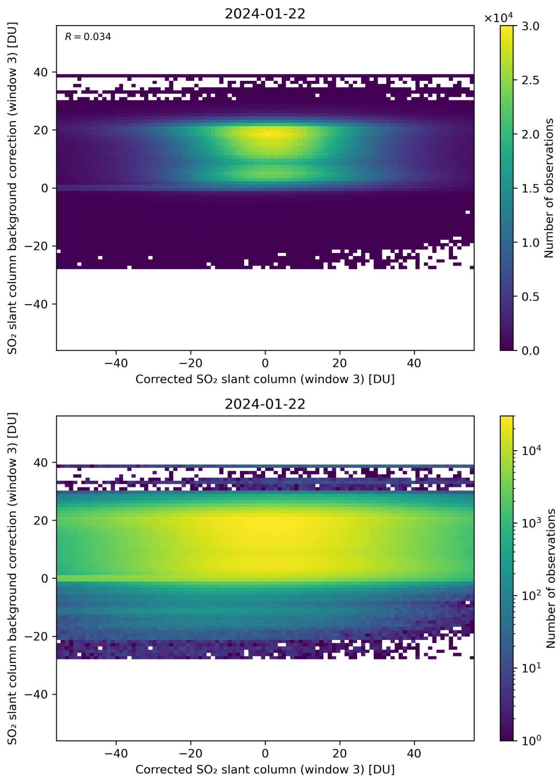
Figure 205: Scatter density plot of “Corrected SO 2 slant column (window 3)” against “SO 2 slant column background correction (window 3)” for 2024-01-21 to 2024-01-23.
