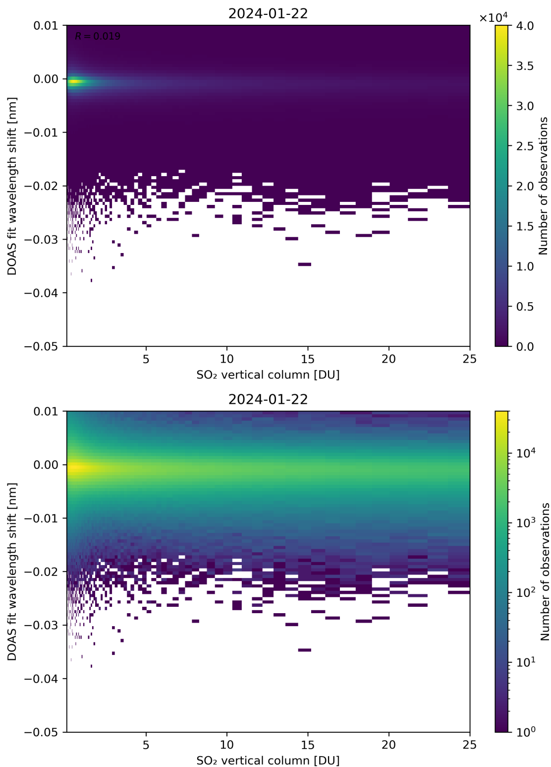
Figure 276: Scatter density plot of “SO 2 vertical column” against “DOAS fit wavelength shift” for 2024-01-21 to 2024-01-23.
