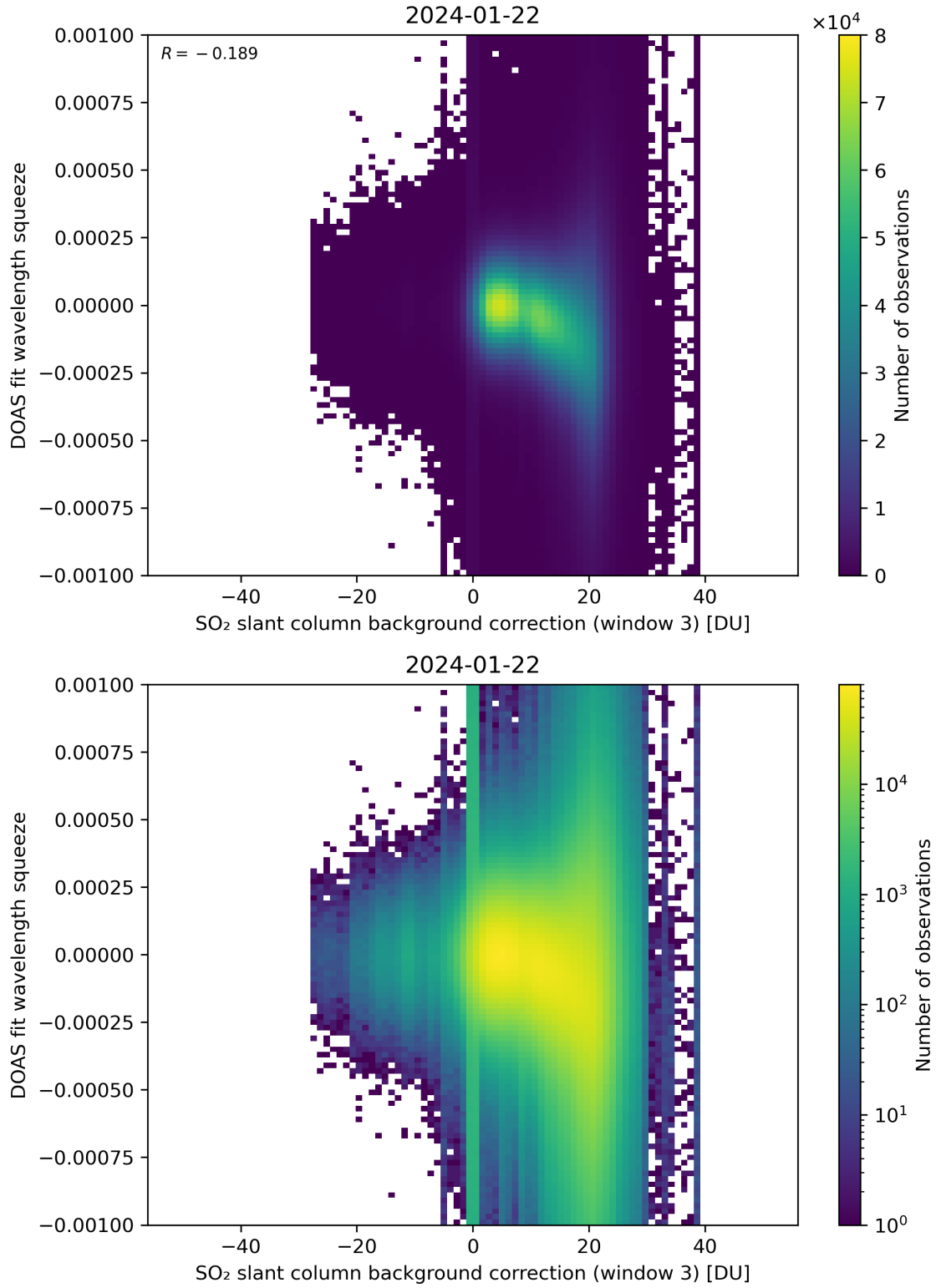
Figure 122: Scatter density plot of “SO 2 slant column background correction (window 3)” against “DOAS fit wavelength squeeze” for 2024-01-21 to 2024-01-23.
