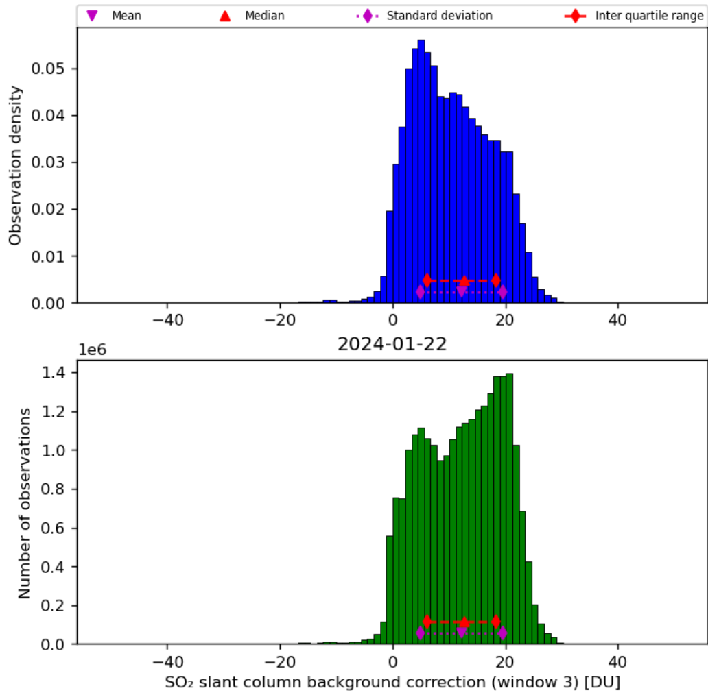
Figure 67: Histogram of “SO 2 slant column background correction (window 3)” for 2024-01-21 to 2024-01-23
