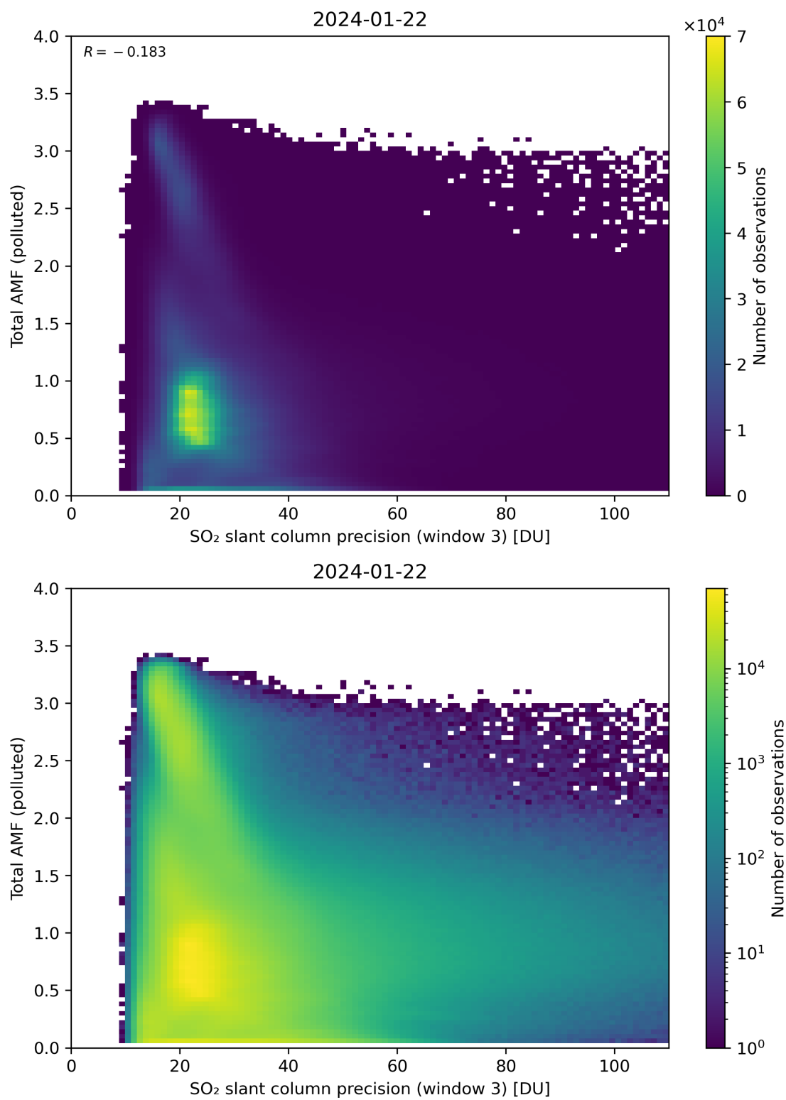
Figure 263: Scatter density plot of “SO 2 slant column precision (window 3)” against “Total AMF (polluted)” for 2024-01-21 to 2024-01-23.
