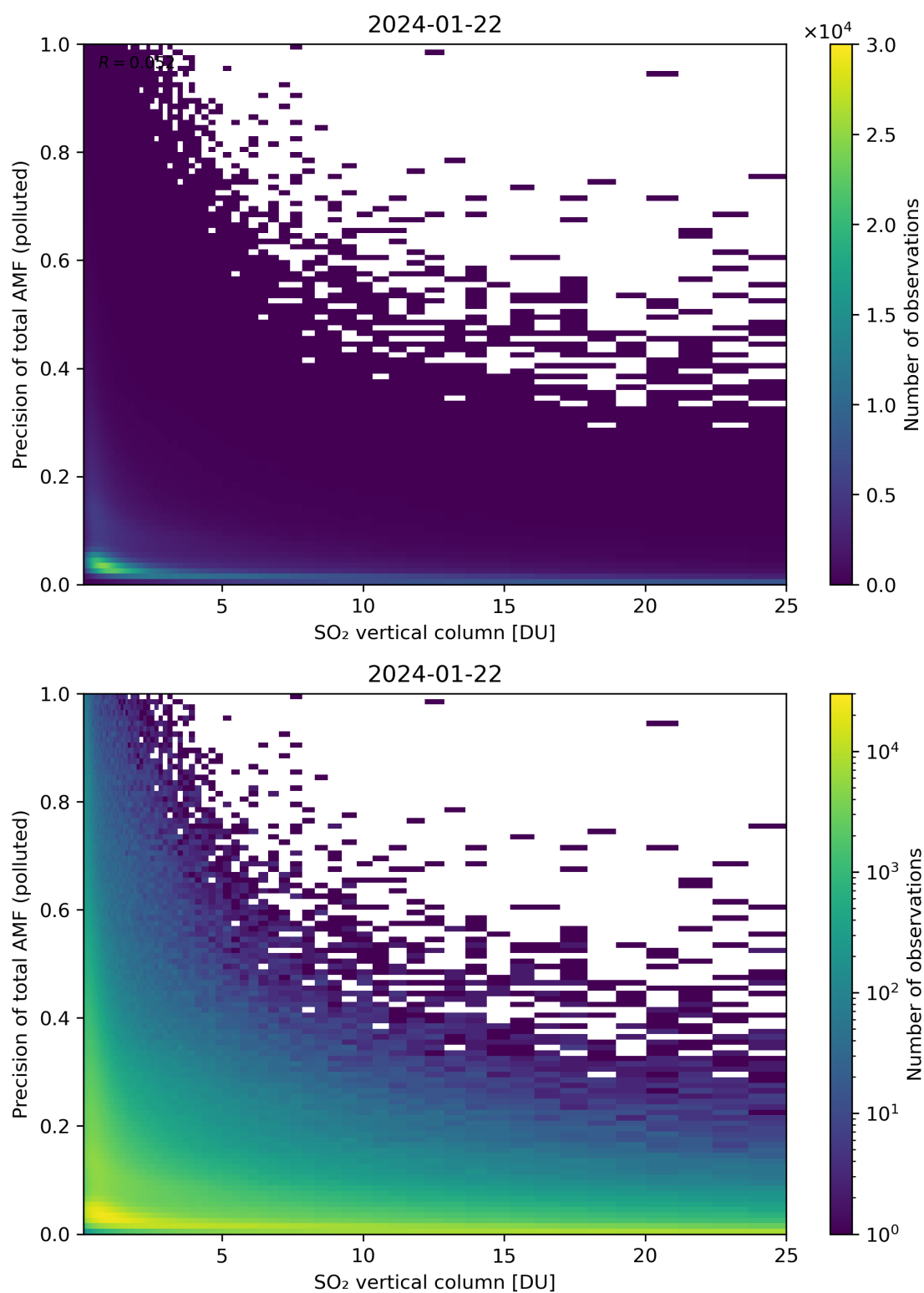
Figure 306: Scatter density plot of “SO 2 vertical column” against “Precision of total AMF (polluted)” for 2024-01-21 to 2024-01-23.
