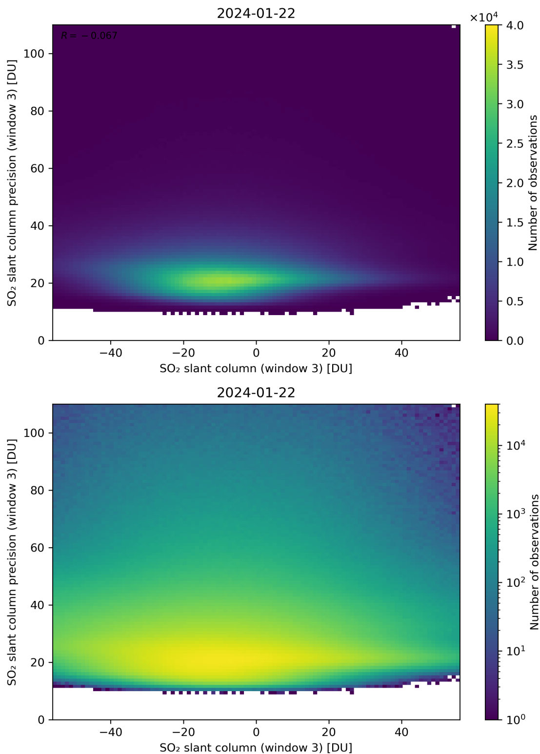
Figure 267: Scatter density plot of “SO 2 slant column (window 3)” against “SO 2 slant column precision (window 3)” for 2024-01-21 to 2024-01-23.
