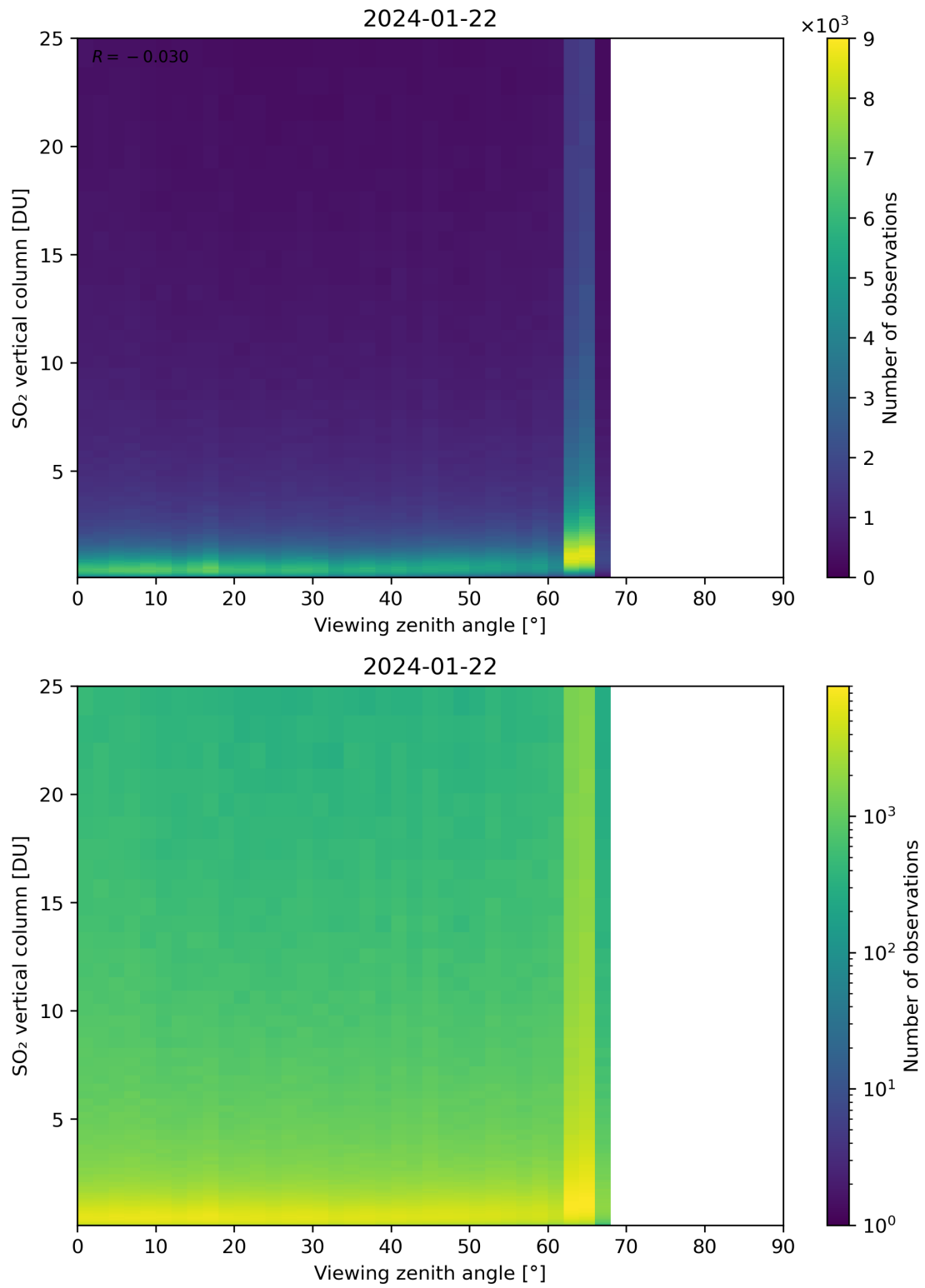
Figure 327: Scatter density plot of “Viewing zenith angle” against “SO 2 vertical column” for 2024-01-21 to 2024-01-23.
