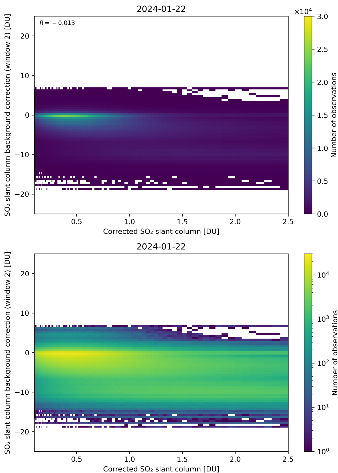
Figure 179: Scatter density plot of “Corrected SO 2 slant column” against “SO 2 slant column background correction (window 2)” for 2024-01-21 to 2024-01-23.
