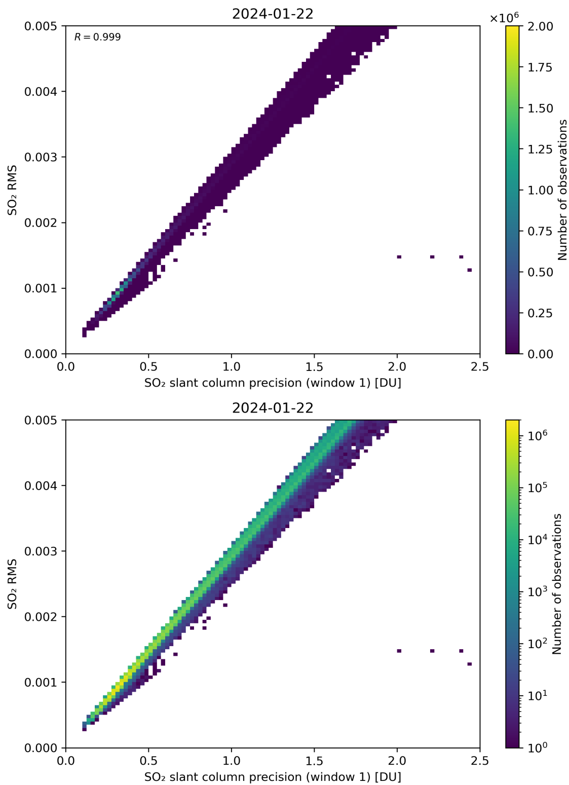
Figure 223: Scatter density plot of “SO 2 slant column precision (window 1)” against “SO 2 RMS” for 2024-01-21 to 2024-01-23.
