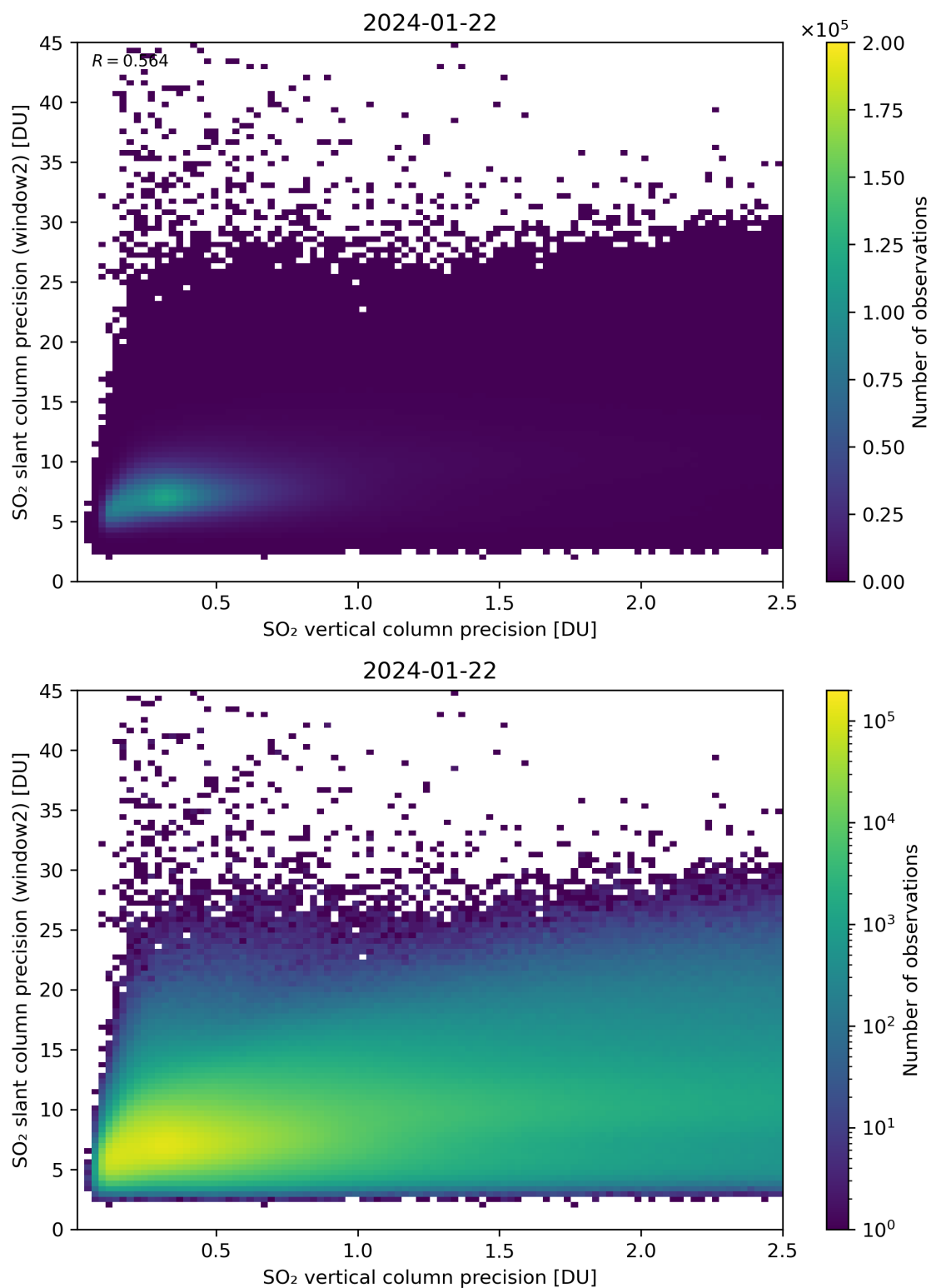
Figure 291: Scatter density plot of “SO 2 vertical column precision” against “SO 2 slant column precision (window2)” for 2024-01-21 to 2024-01-23.
