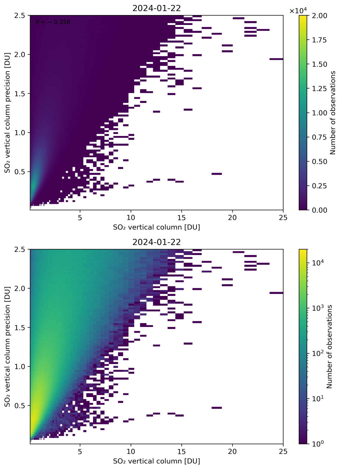
Figure 307: Scatter density plot of “SO 2 vertical column” against “SO 2 vertical column precision” for 2024-01-21 to 2024-01-23.
