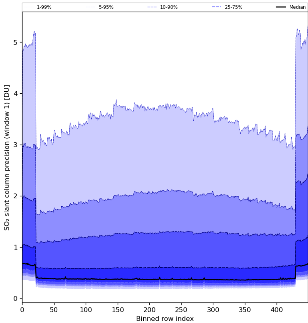
Figure 80: Along track statistics of “SO 2 slant column precision (window 1)” for 2024-01-21 to 2024-01-23
