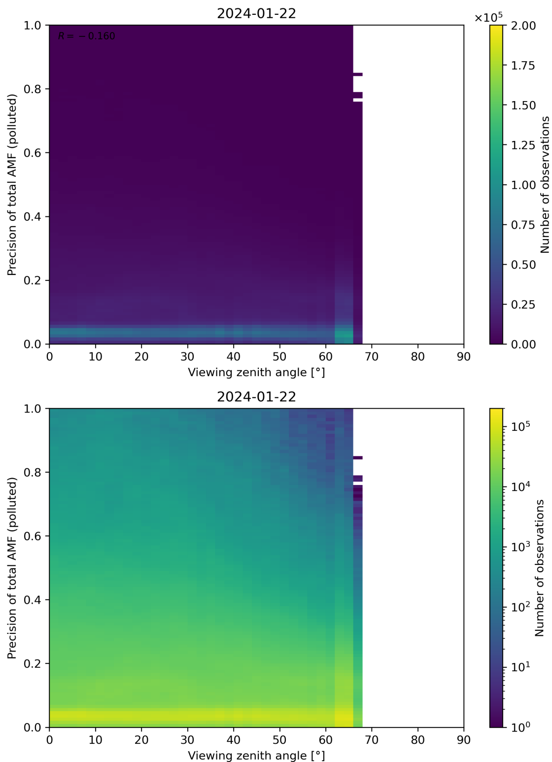
Figure 326: Scatter density plot of “Viewing zenith angle” against “Precision of total AMF (polluted)” for 2024-01-21 to 2024-01-23.
