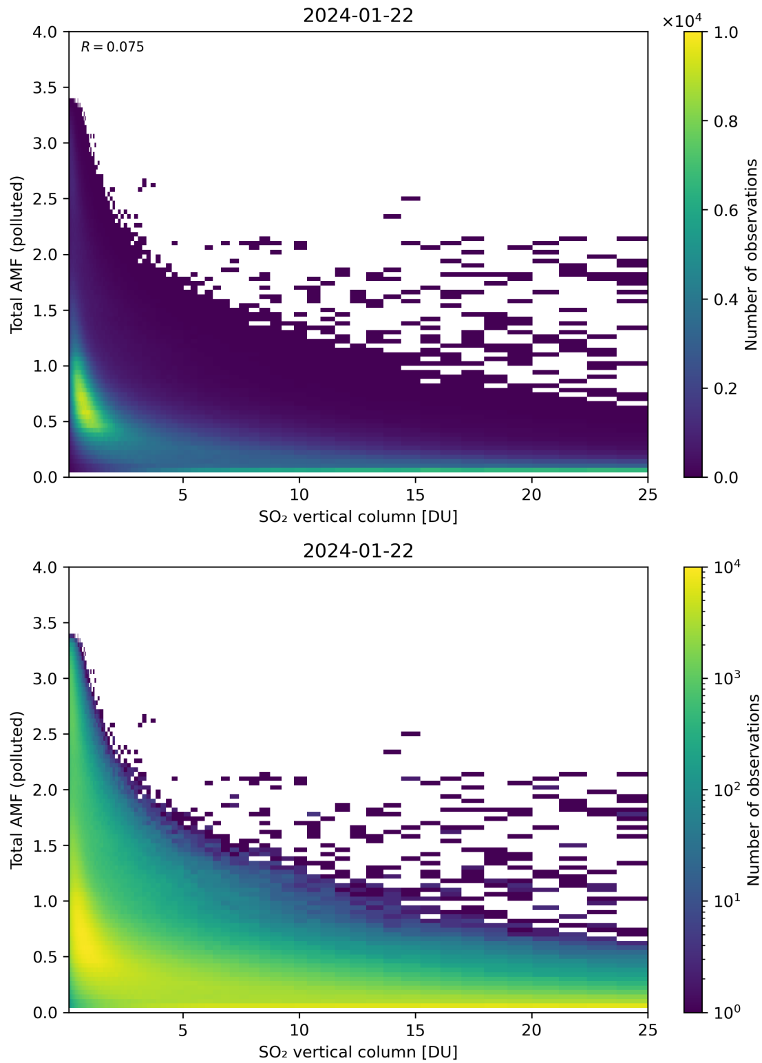
Figure 305: Scatter density plot of “SO 2 vertical column” against “Total AMF (polluted)” for 2024-01-21 to 2024-01-23.
