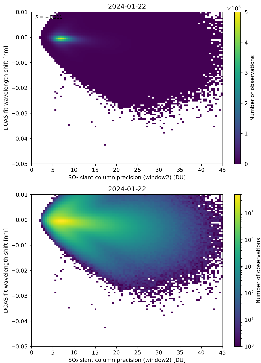
Figure 243: Scatter density plot of “SO 2 slant column precision (window2)” against “DOAS fit wavelength shift” for 2024-01-21 to 2024-01-23.
