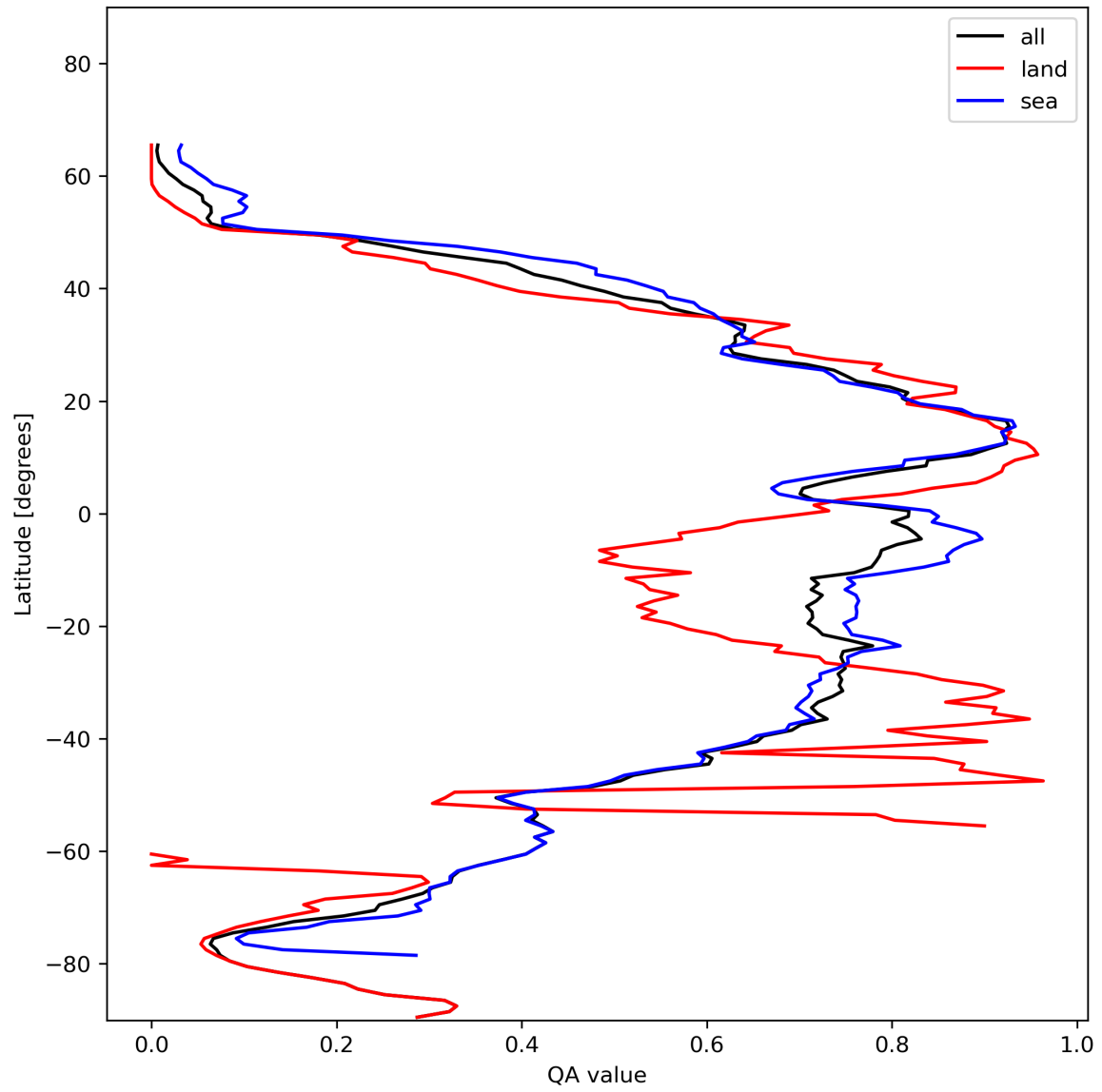
Figure 29: Zonal average of “QA value” for 2024-01-21 to 2024-01-23.
