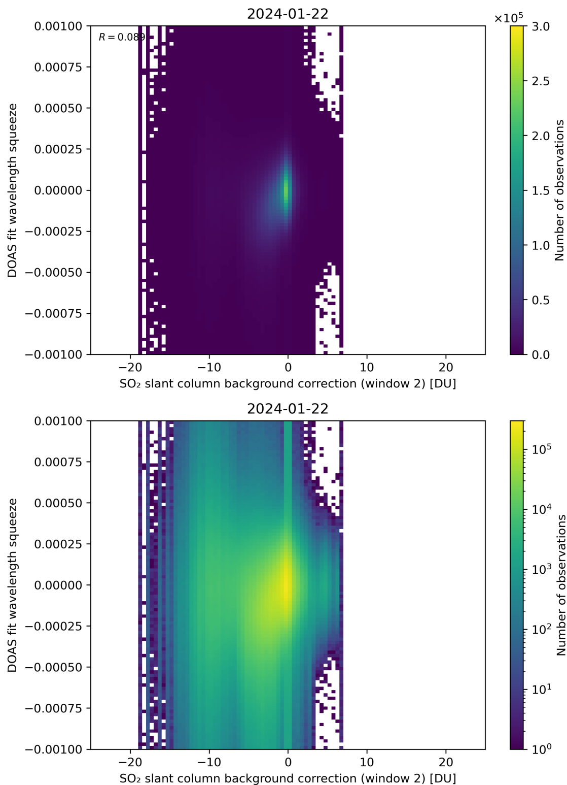
Figure 113: Scatter density plot of “SO 2 slant column background correction (window 2)” against “DOAS fit wavelength squeeze” for 2024-01-21 to 2024-01-23.
