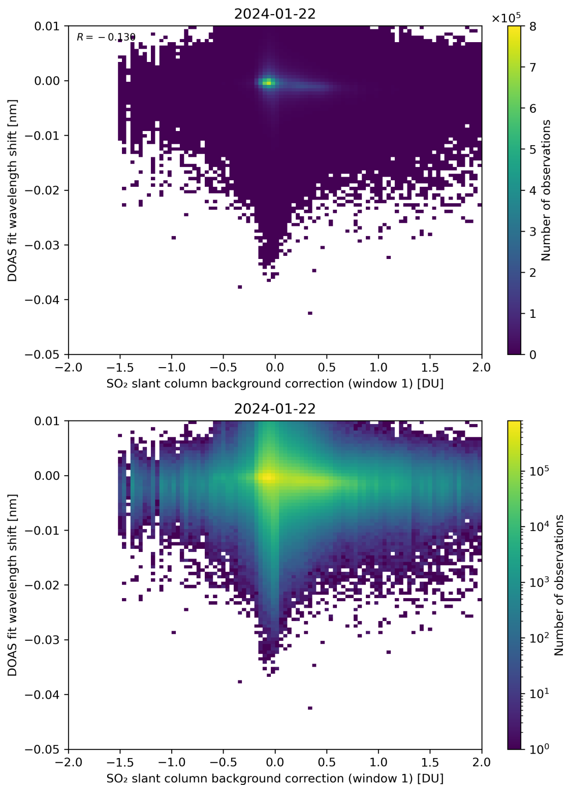
Figure 100: Scatter density plot of “SO 2 slant column background correction (window 1)” against “DOAS fit wavelength shift” for 2024-01-21 to 2024-01-23.
