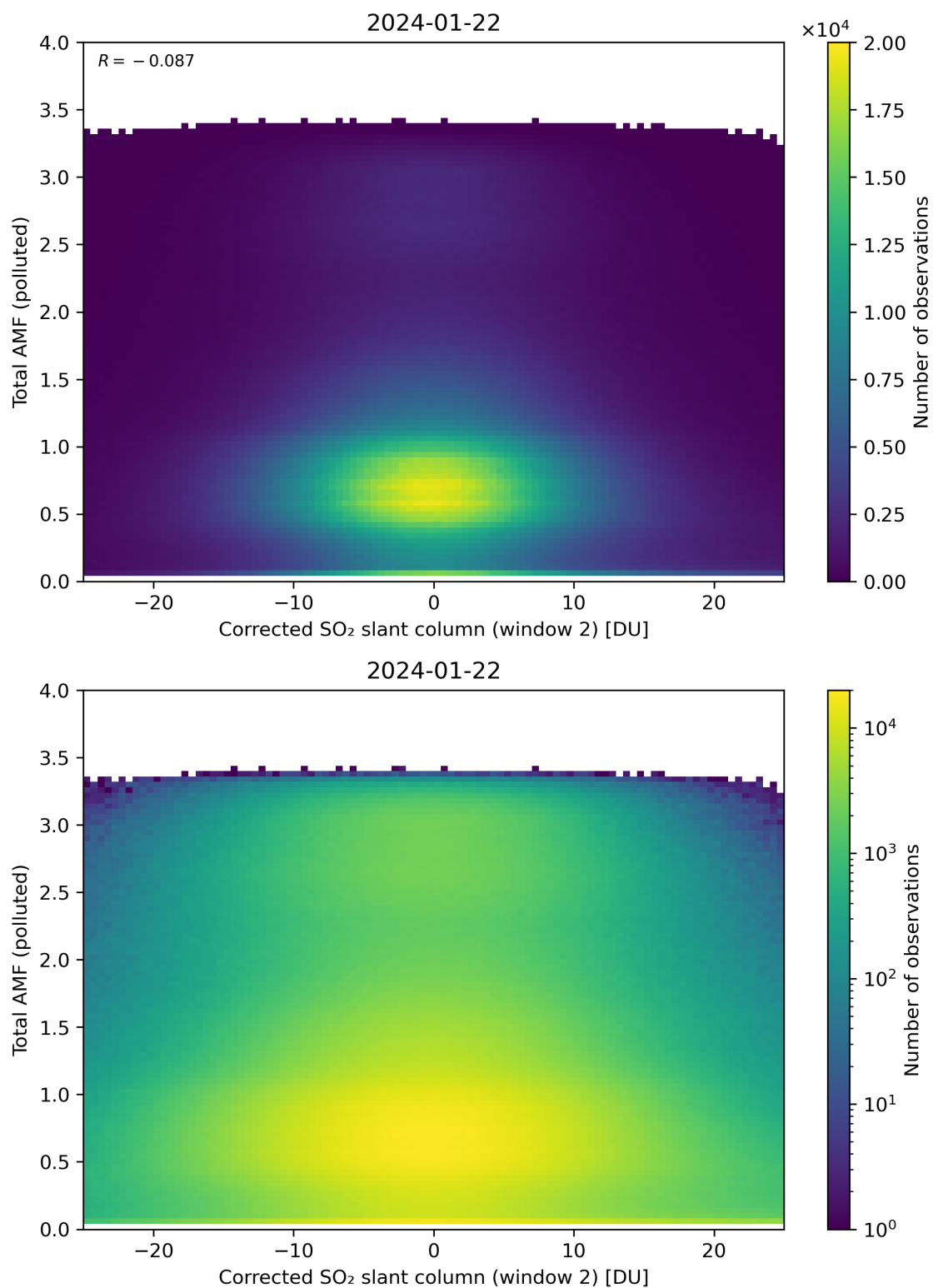
Figure 203: Scatter density plot of “Corrected SO 2 slant column (window 2)” against “Total AMF (polluted)” for 2024-01-21 to 2024-01-23.
