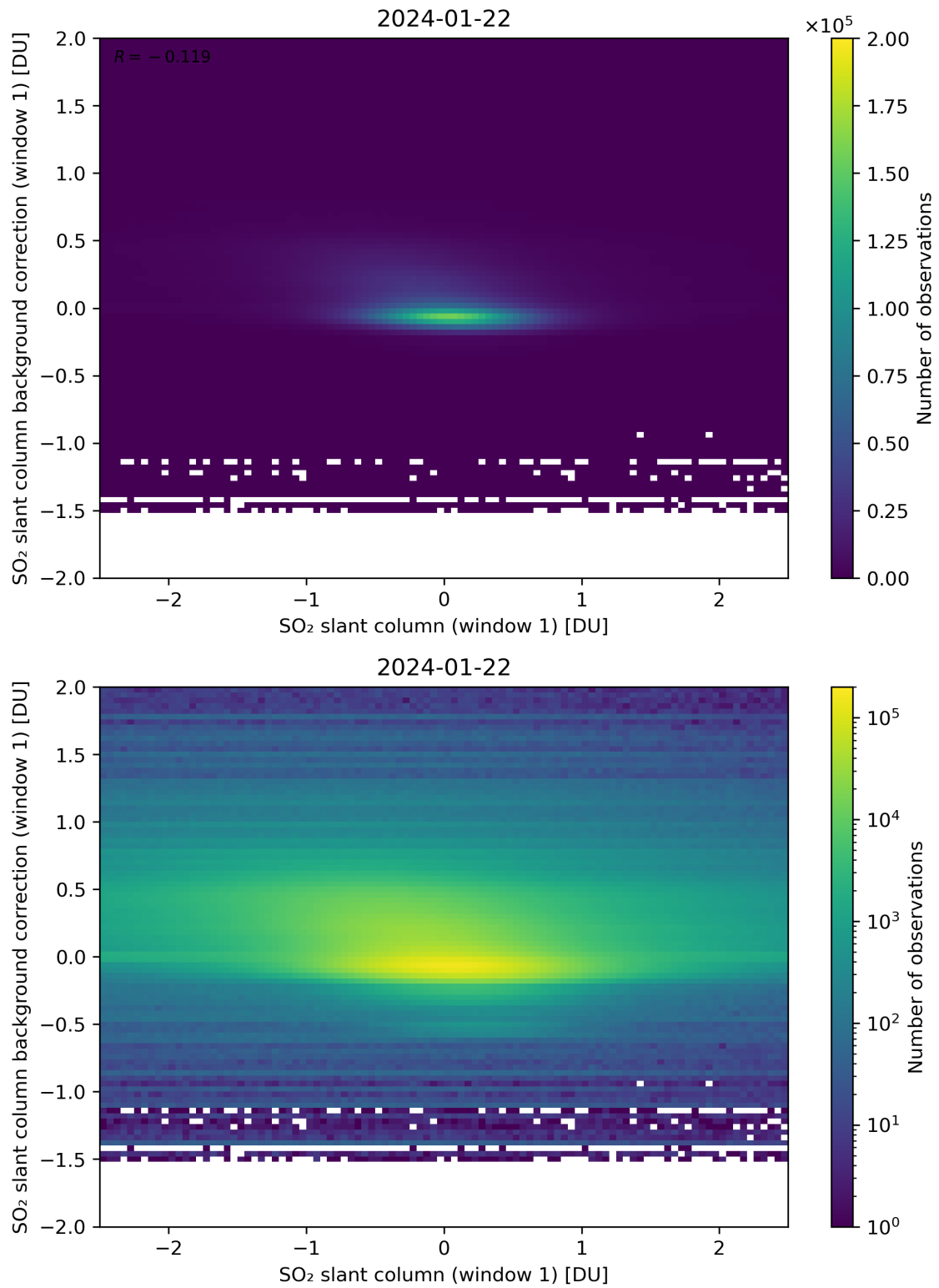
Figure 212: Scatter density plot of “SO 2 slant column (window 1)” against “SO 2 slant column background correction (window 1)” for 2024-01-21 to 2024-01-23.
