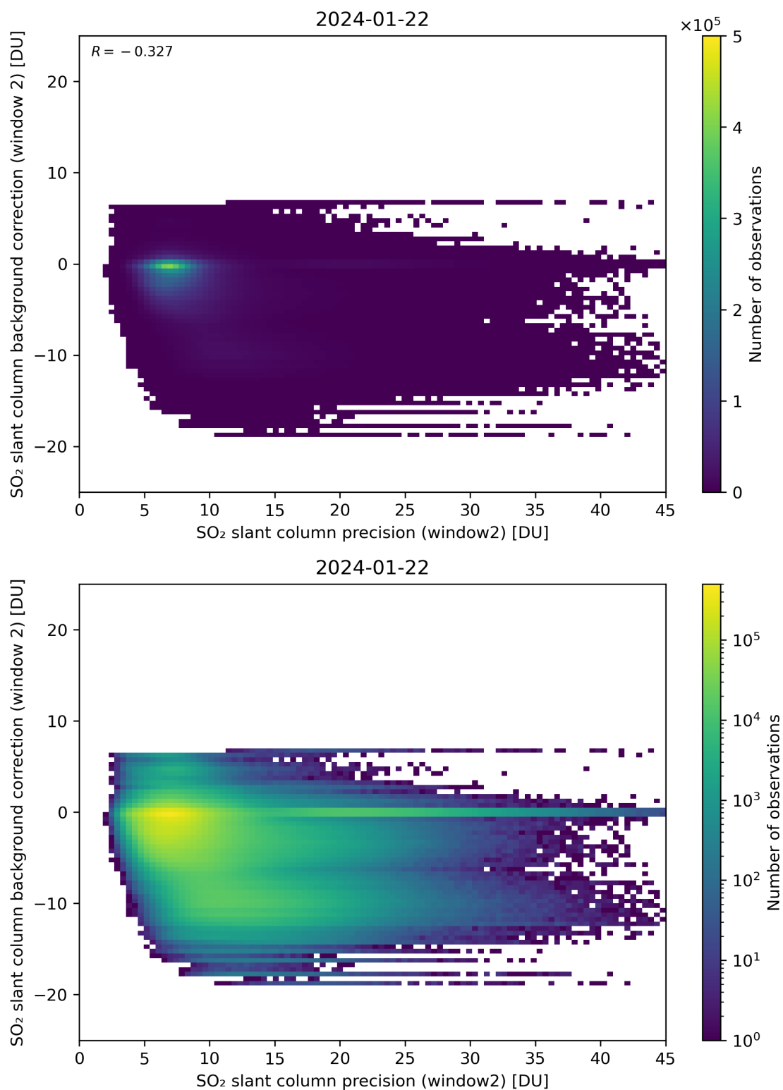
Figure 241: Scatter density plot of “SO 2 slant column precision (window2)” against “SO 2 slant column background correction (window 2)” for 2024-01-21 to 2024-01-23.
