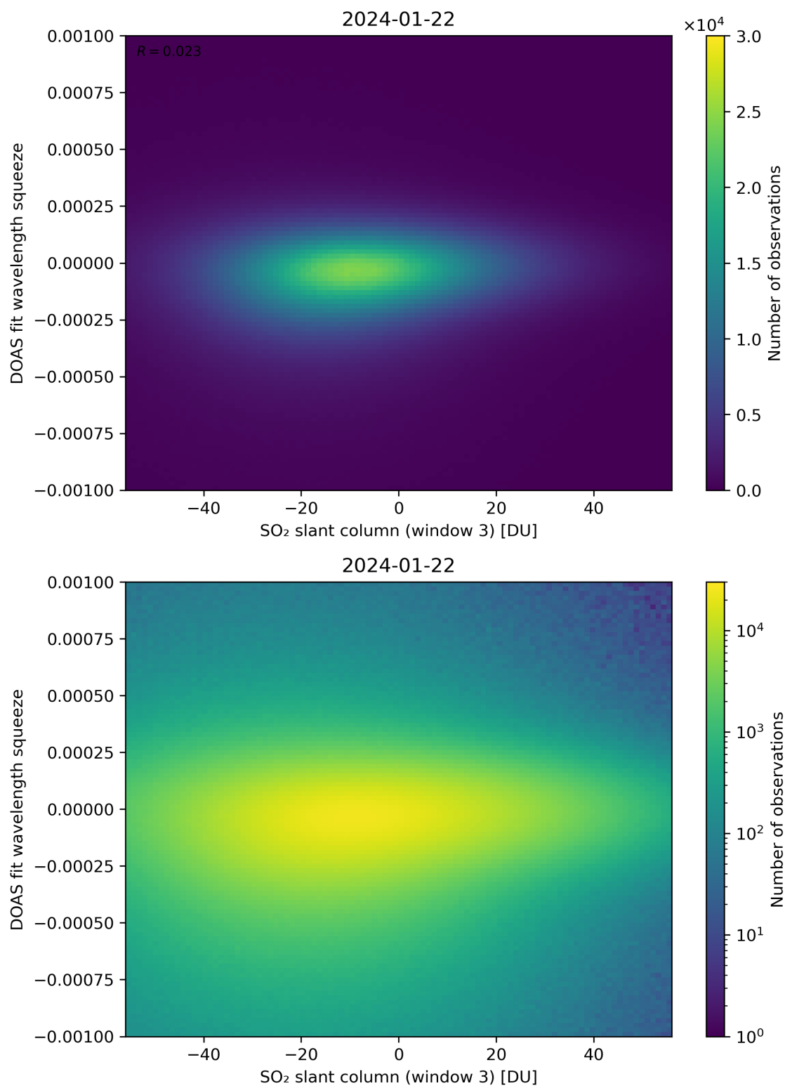
Figure 255: Scatter density plot of “SO 2 slant column (window 3)” against “DOAS fit wavelength squeeze” for 2024-01-21 to 2024-01-23.
