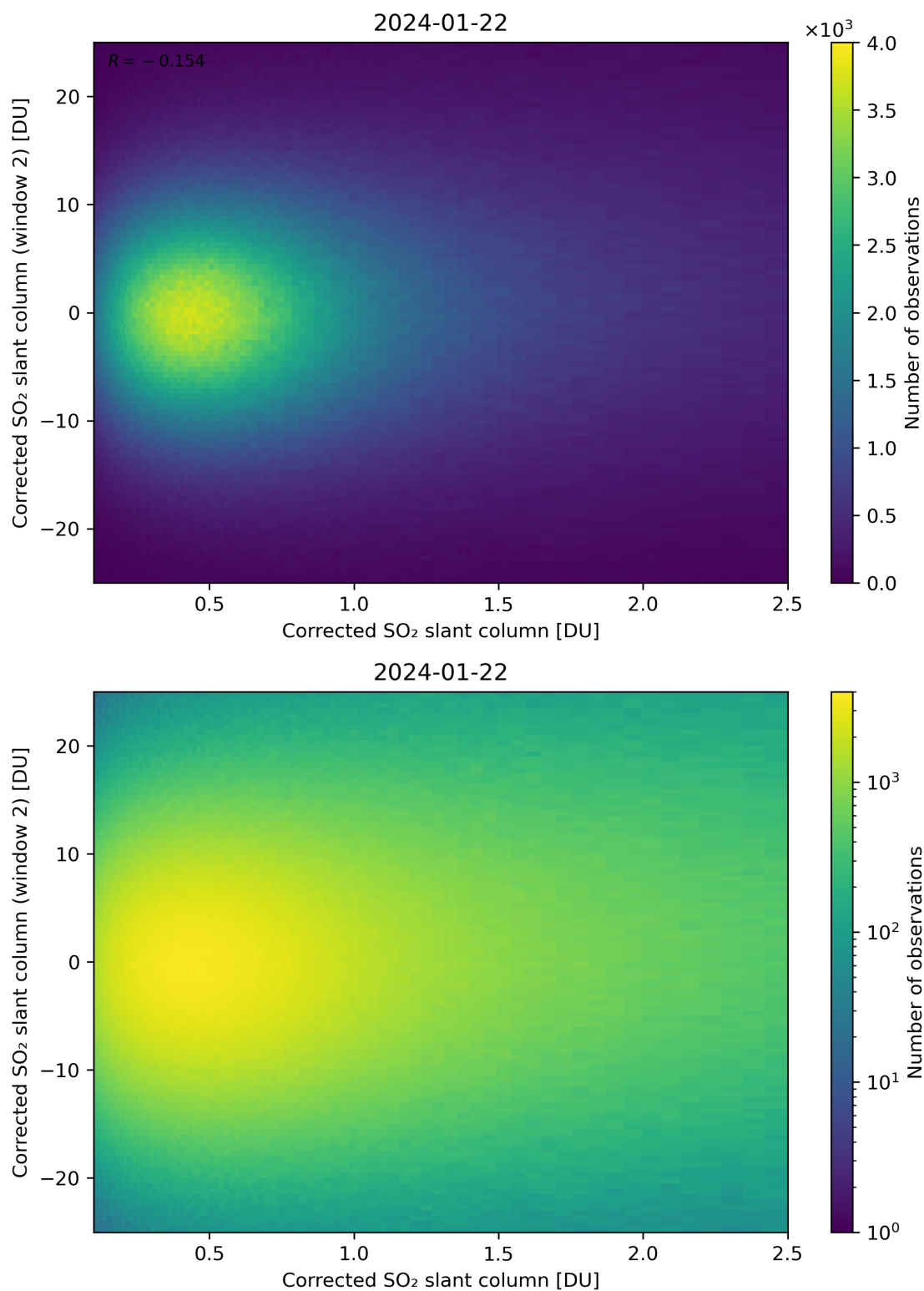
Figure 185: Scatter density plot of “Corrected SO 2 slant column” against “Corrected SO 2 slant column (window 2)” for 2024-01-21 to 2024-01-23.
