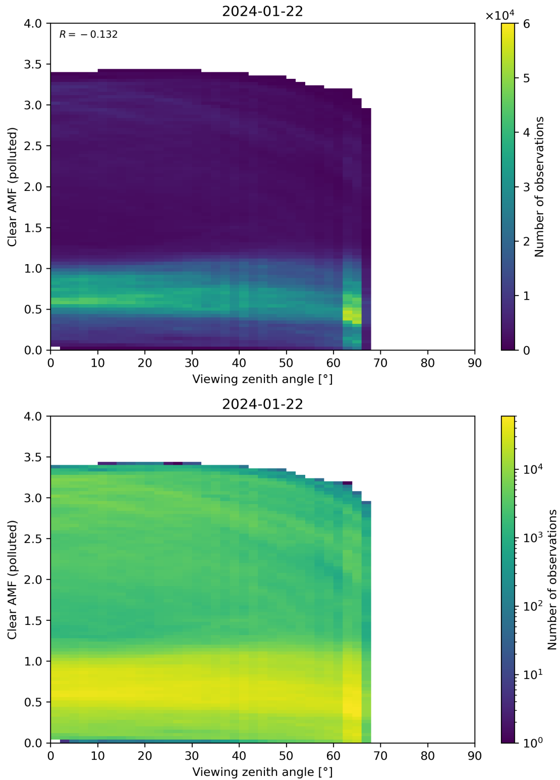
Figure 316: Scatter density plot of “Viewing zenith angle” against “Clear AMF (polluted)” for 2024-01-21 to 2024-01-23.
