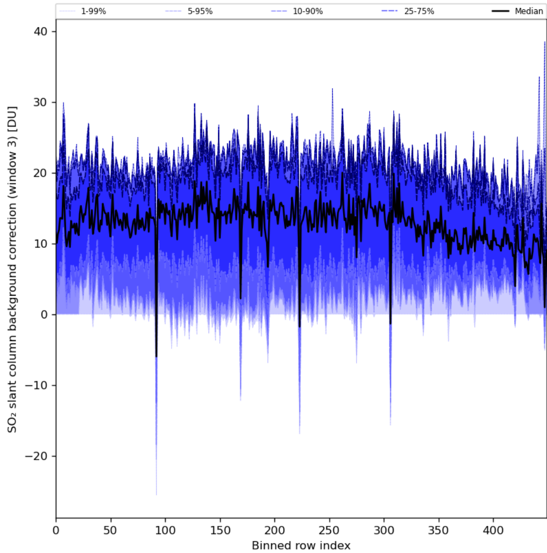
Figure 90: Along track statistics of “SO 2 slant column background correction (window 3)” for 2024-01-21 to 2024-01-23
