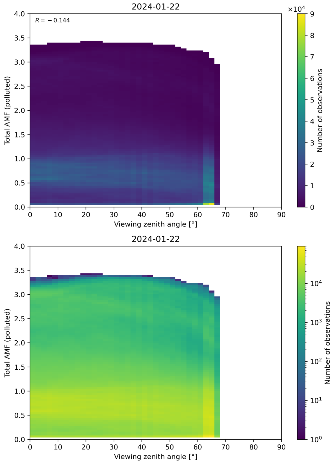
Figure 325: Scatter density plot of “Viewing zenith angle” against “Total AMF (polluted)” for 2024-01-21 to 2024-01-23.
