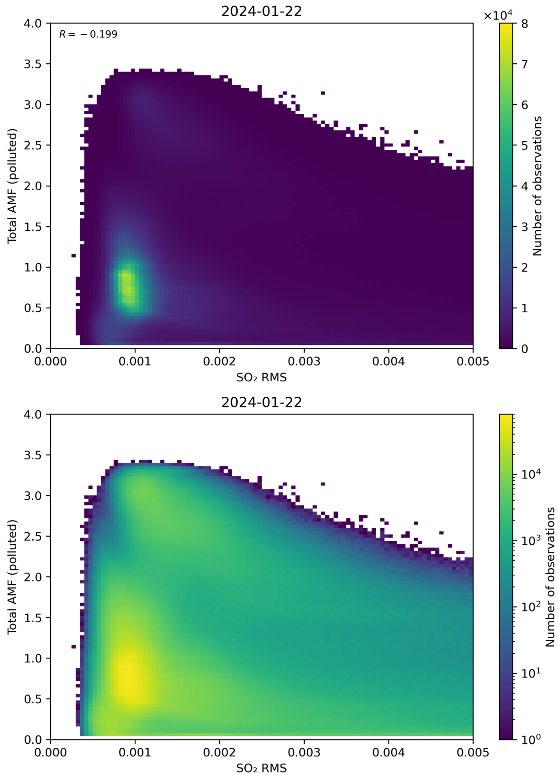
Figure 137: Scatter density plot of “SO 2 RMS” against “Total AMF (polluted)” for 2024-01-21 to 2024-01-23.
