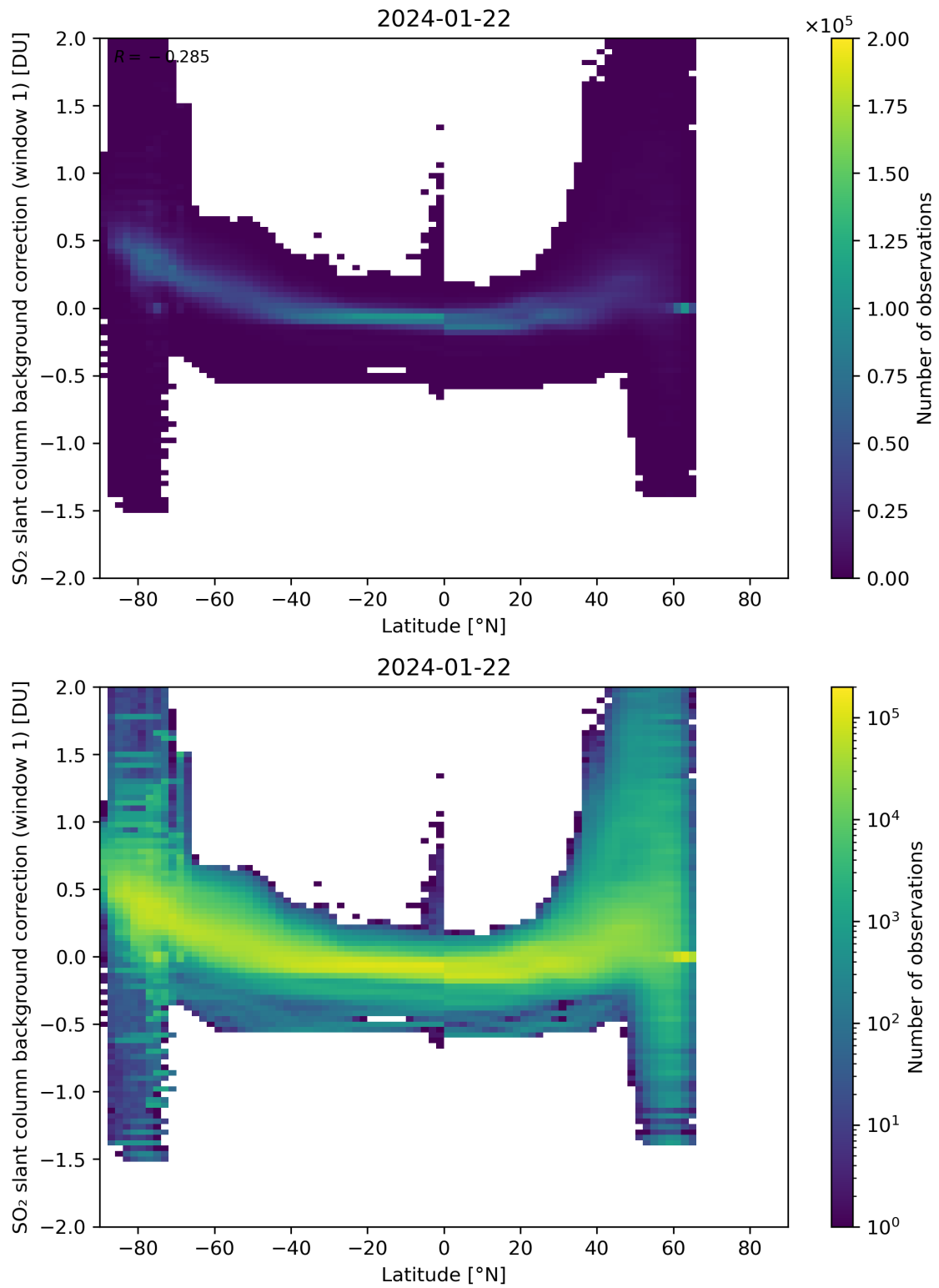
Figure 139: Scatter density plot of “Latitude” against “SO 2 slant column background correction (window 1)” for 2024-01-21 to 2024-01-23.
