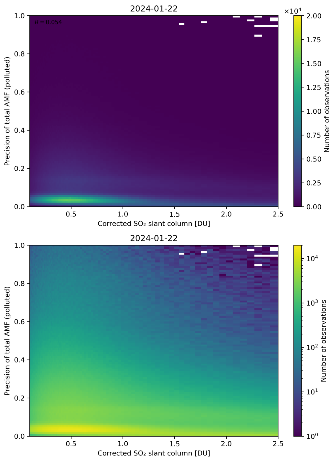
Figure 193: Scatter density plot of “Corrected SO 2 slant column” against “Precision of total AMF (polluted)” for 2024-01-21 to 2024-01-23.
