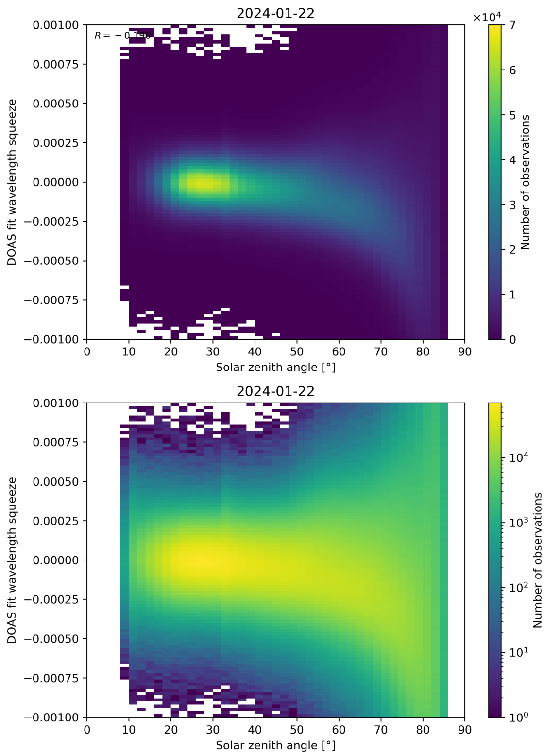
Figure 162: Scatter density plot of “Solar zenith angle” against “DOAS fit wavelength squeeze” for 2024-01-21 to 2024-01-23.
