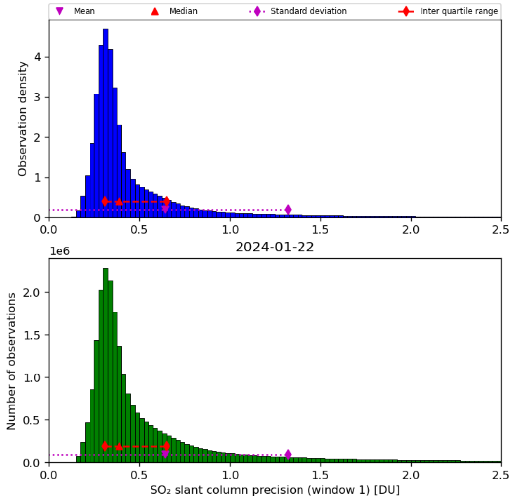
Figure 57: Histogram of “SO 2 slant column precision (window 1)” for 2024-01-21 to 2024-01-23
