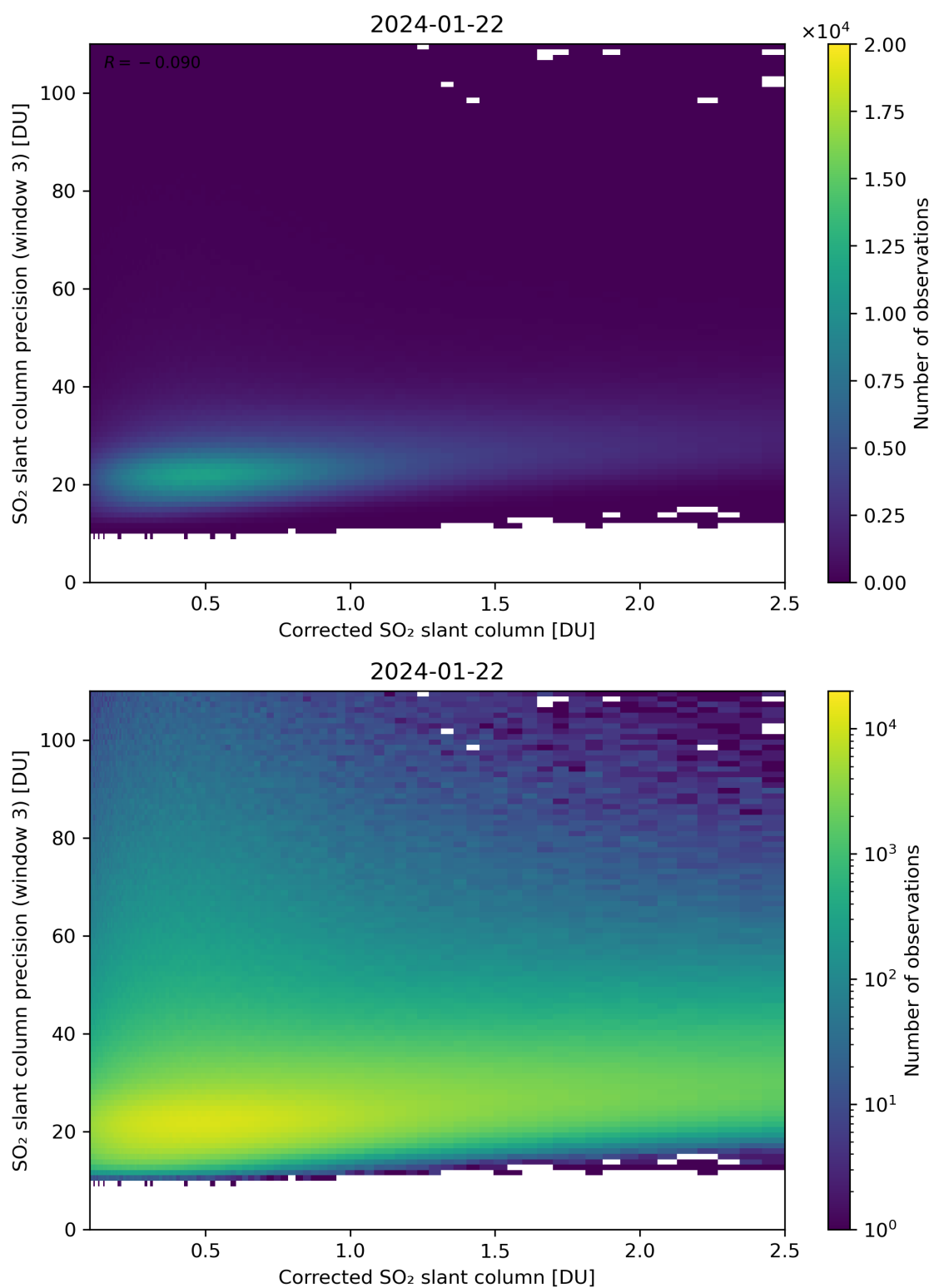
Figure 191: Scatter density plot of “Corrected SO 2 slant column” against “SO 2 slant column precision (window 3)” for 2024-01-21 to 2024-01-23.
