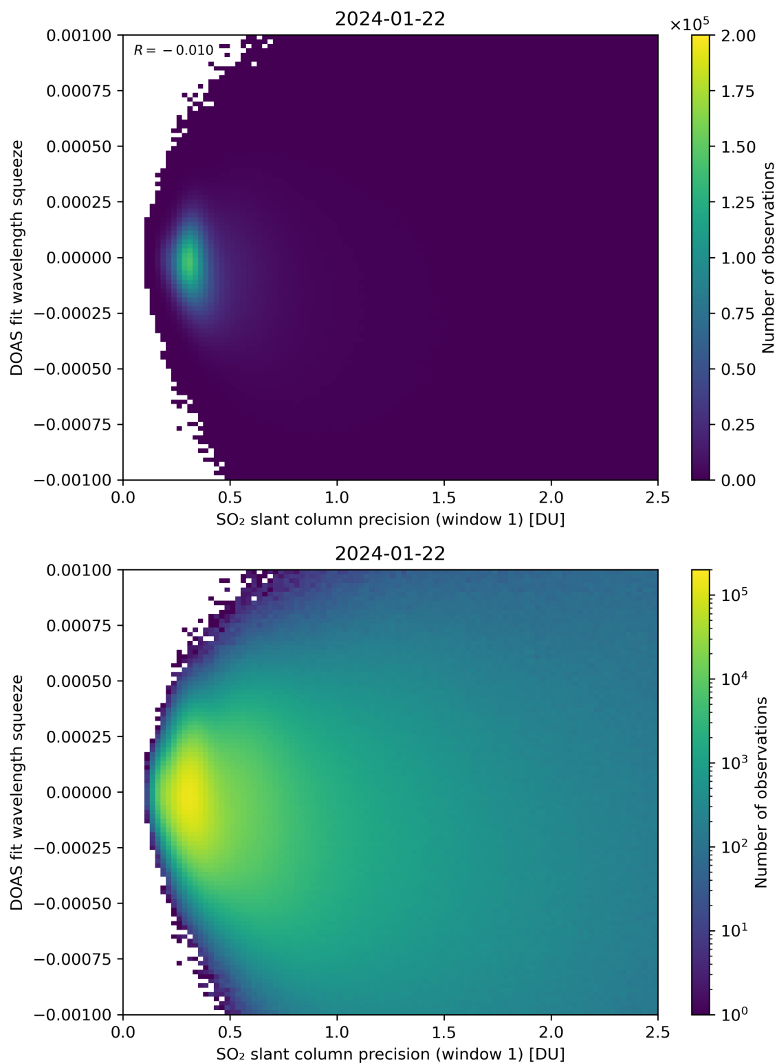
Figure 222: Scatter density plot of “SO 2 slant column precision (window 1)” against “DOAS fit wavelength squeeze” for 2024-01-21 to 2024-01-23.
