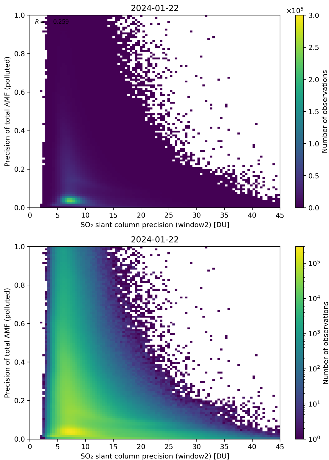
Figure 252: Scatter density plot of “SO 2 slant column precision (window2)” against “Precision of total AMF (polluted)” for 2024-01-21 to 2024-01-23.
