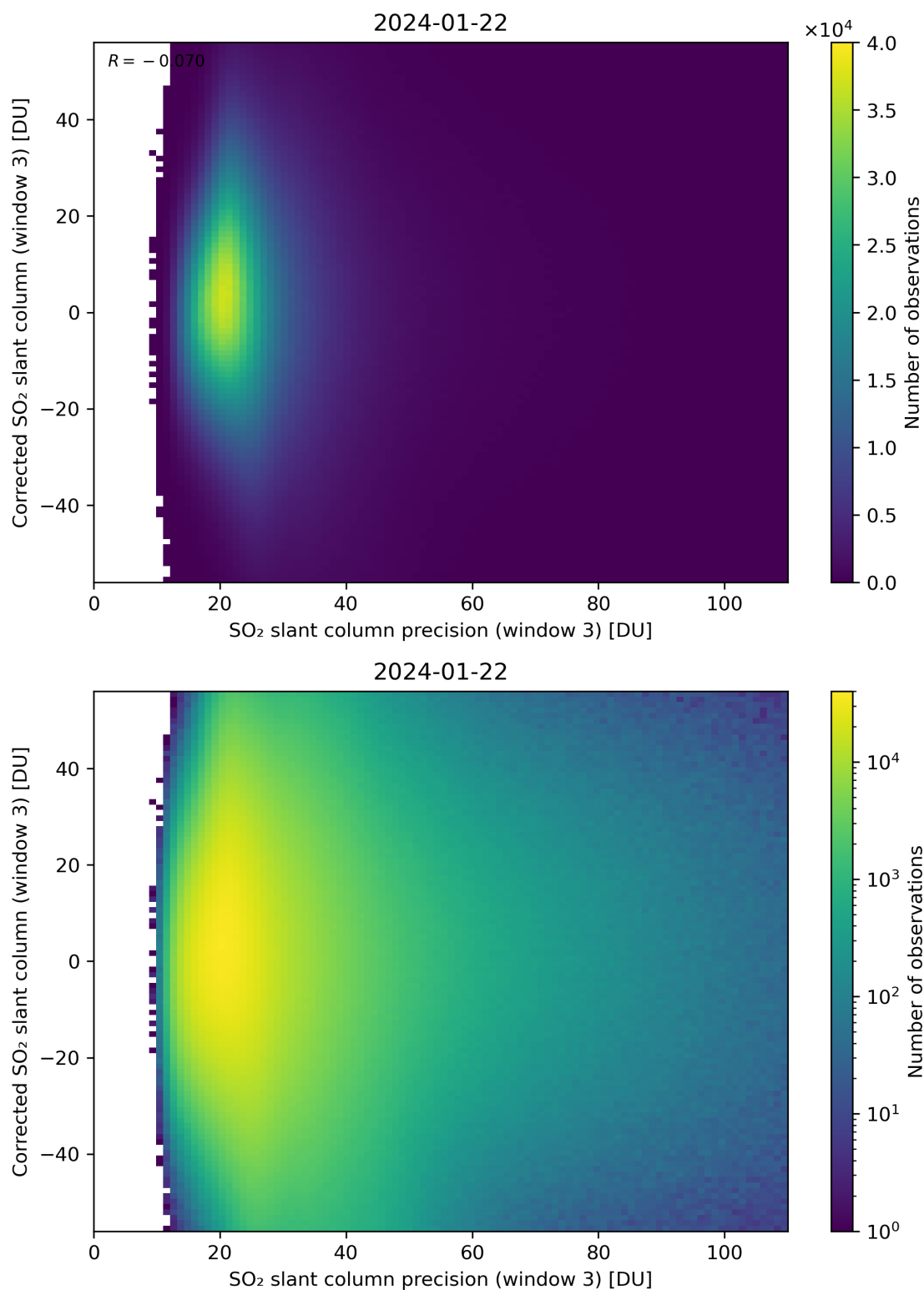
Figure 262: Scatter density plot of “SO 2 slant column precision (window 3)” against “Corrected SO 2 slant column (window 3)” for 2024-01-21 to 2024-01-23.
