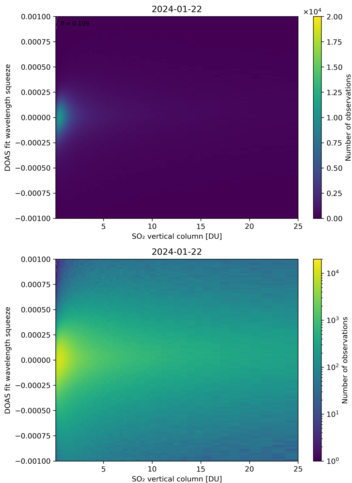
Figure 277: Scatter density plot of “SO 2 vertical column” against “DOAS fit wavelength squeeze” for 2024-01-21 to 2024-01-23.
