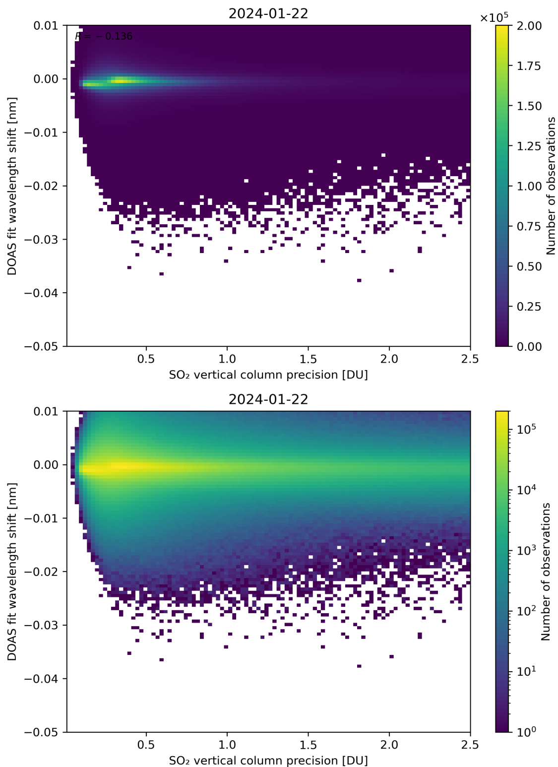
Figure 282: Scatter density plot of “SO 2 vertical column precision” against “DOAS fit wavelength shift” for 2024-01-21 to 2024-01-23.
