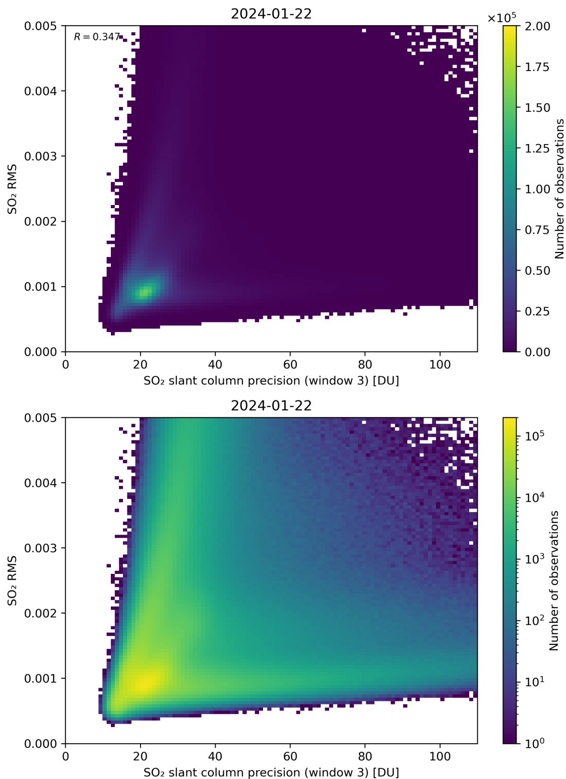
Figure 260: Scatter density plot of “SO 2 slant column precision (window 3)” against “SO 2 RMS” for 2024-01-21 to 2024-01-23.
