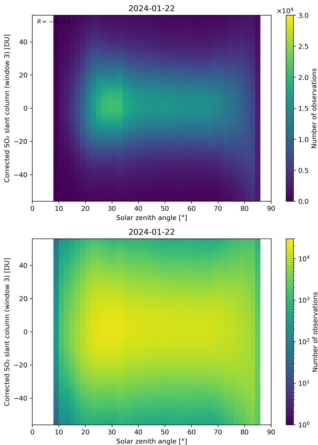
Figure 168: Scatter density plot of “Solar zenith angle” against “Corrected SO 2 slant column (window 3)” for 2024-01-21 to 2024-01-23.
