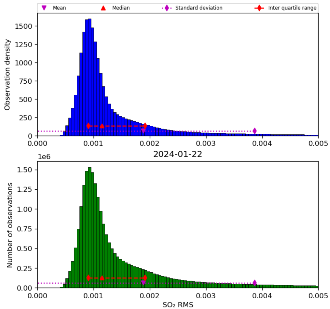
Figure 70: Histogram of “SO 2 RMS” for 2024-01-21 to 2024-01-23
