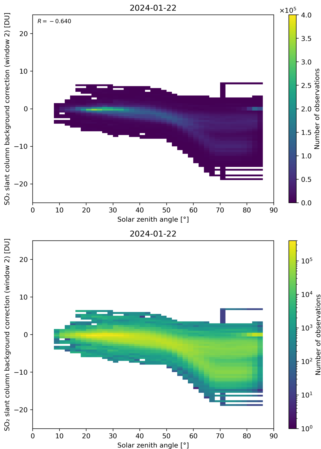
Figure 159: Scatter density plot of “Solar zenith angle” against “SO 2 slant column background correction (window 2)” for 2024-01-21 to 2024-01-23.
