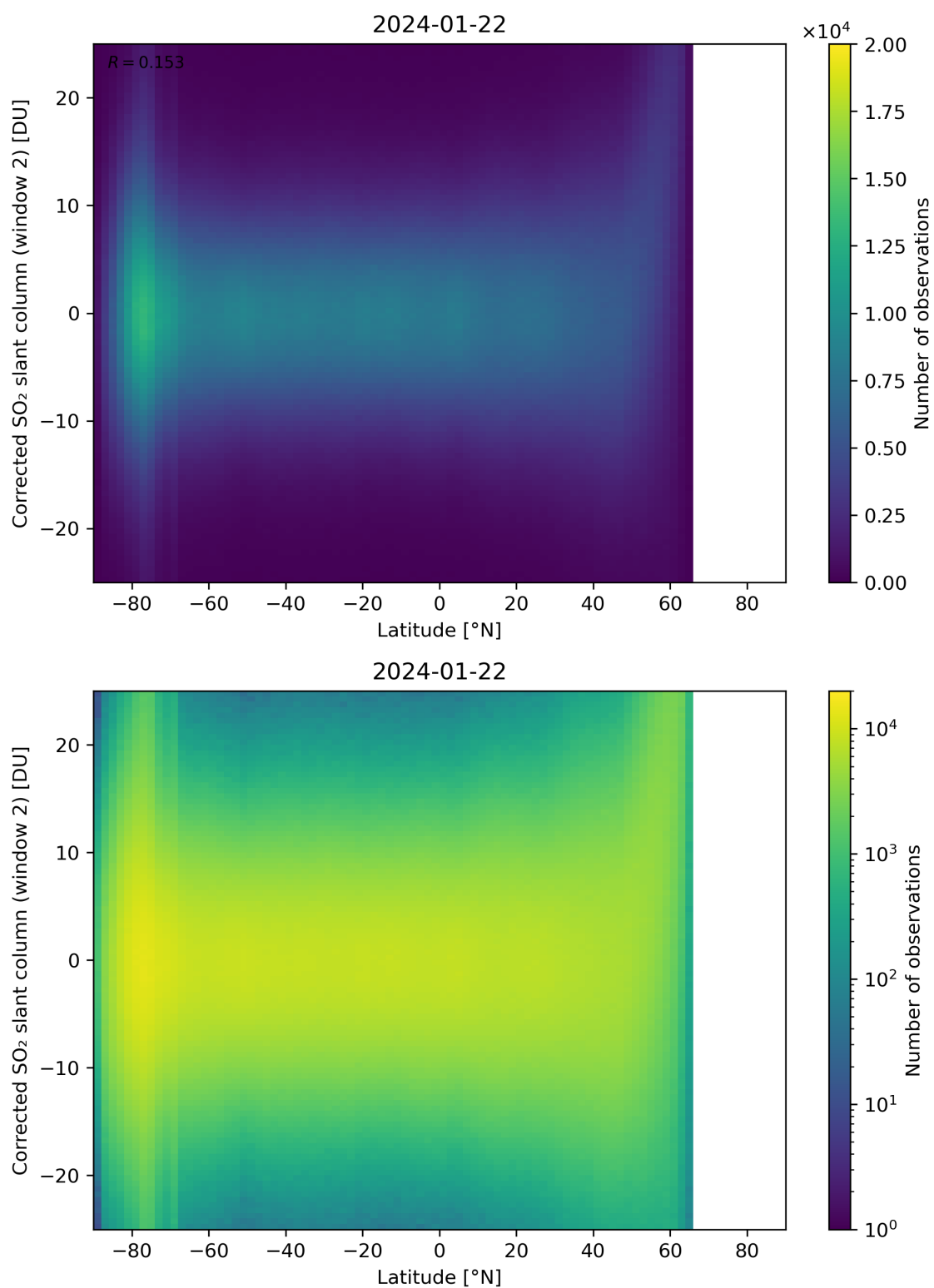
Figure 147: Scatter density plot of “Latitude” against “Corrected SO 2 slant column (window 2)” for 2024-01-21 to 2024-01-23.
