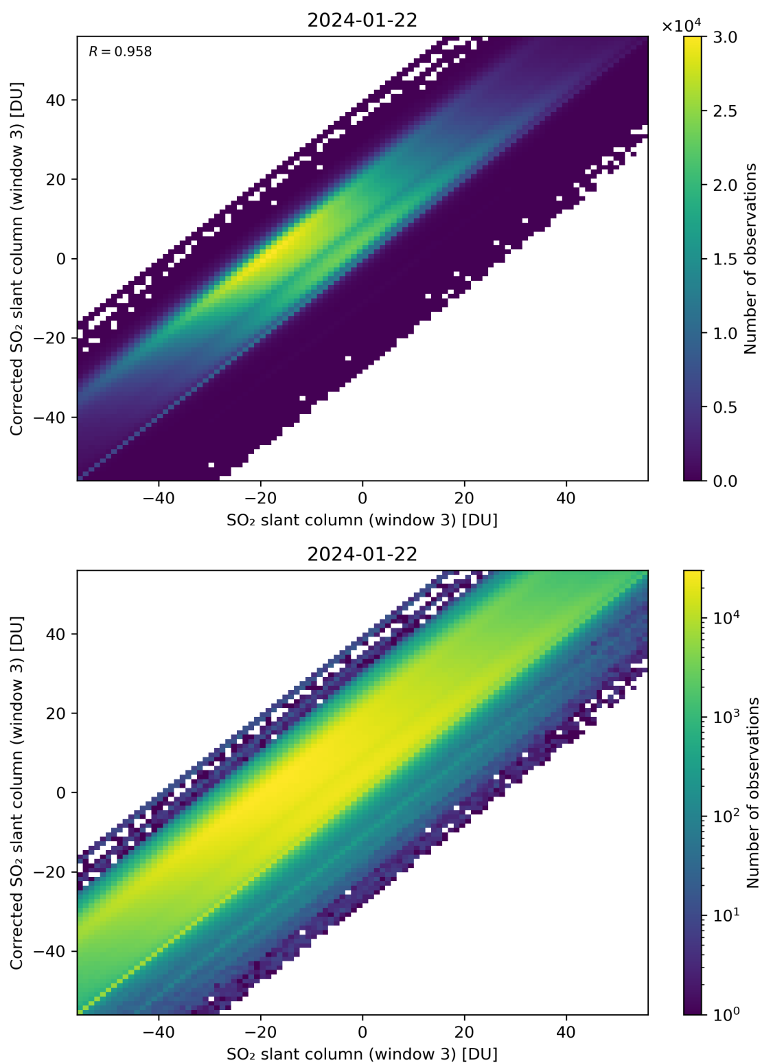
Figure 266: Scatter density plot of “SO 2 slant column (window 3)” against “Corrected SO 2 slant column (window 3)” for 2024-01-21 to 2024-01-23.
