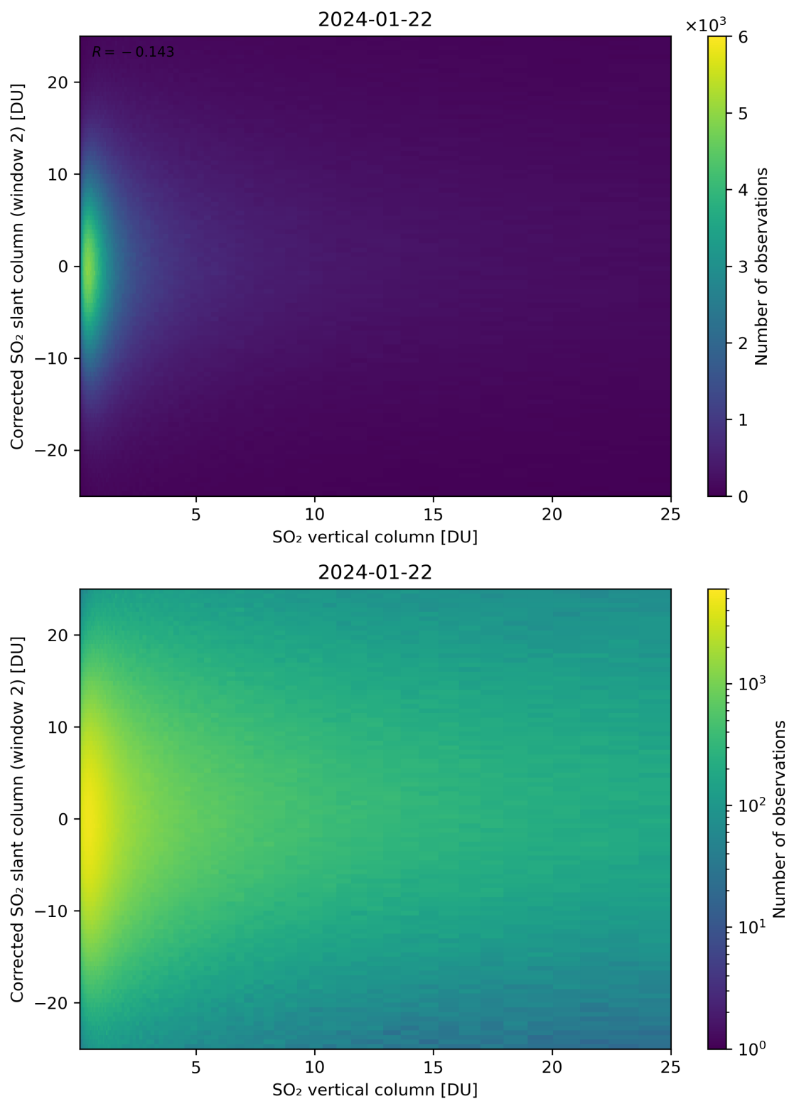
Figure 298: Scatter density plot of “SO 2 vertical column” against “Corrected SO 2 slant column (window 2)” for 2024-01-21 to 2024-01-23.
