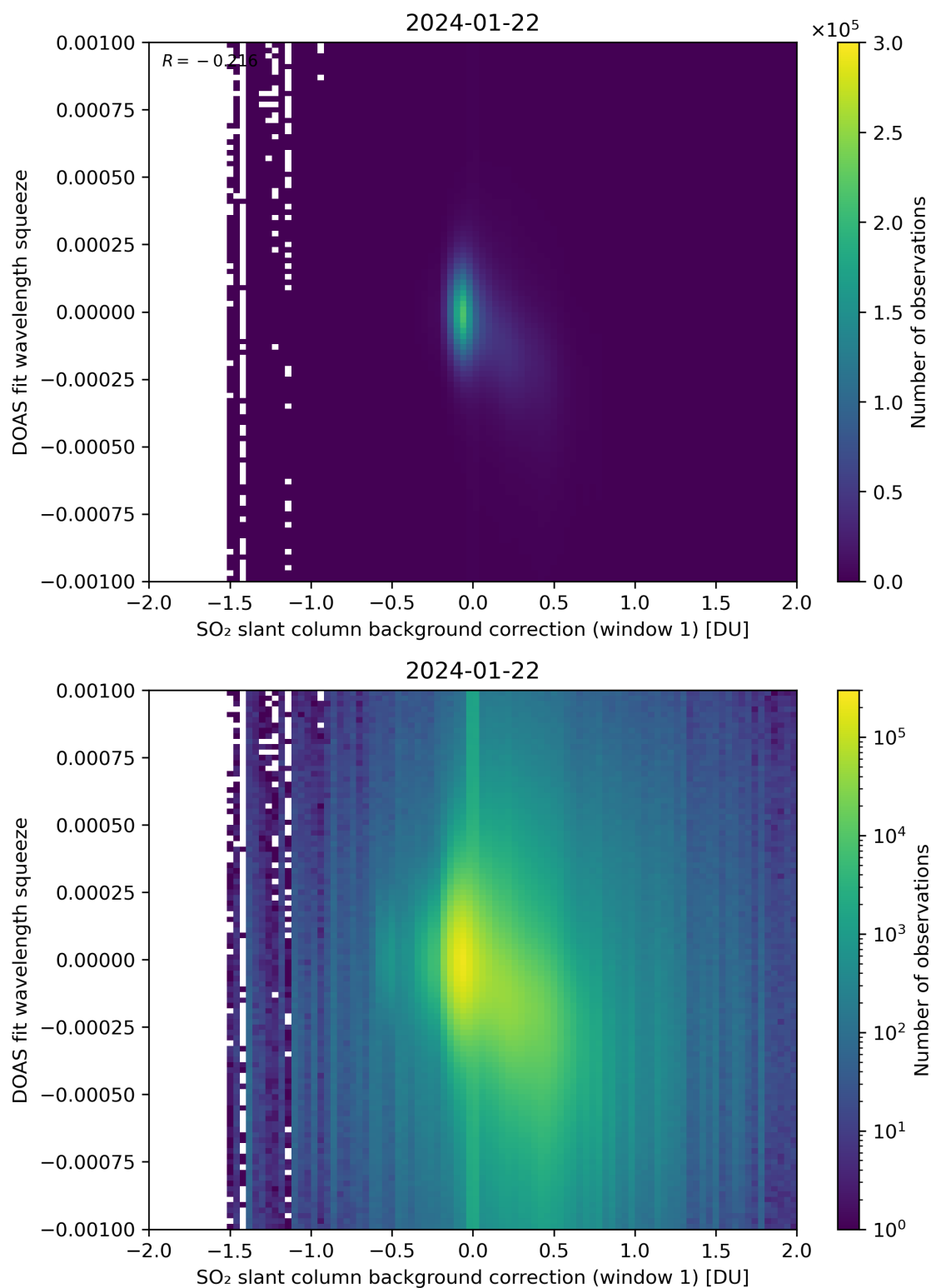
Figure 101: Scatter density plot of “SO 2 slant column background correction (window 1)” against “DOAS fit wavelength squeeze” for 2024-01-21 to 2024-01-23.
