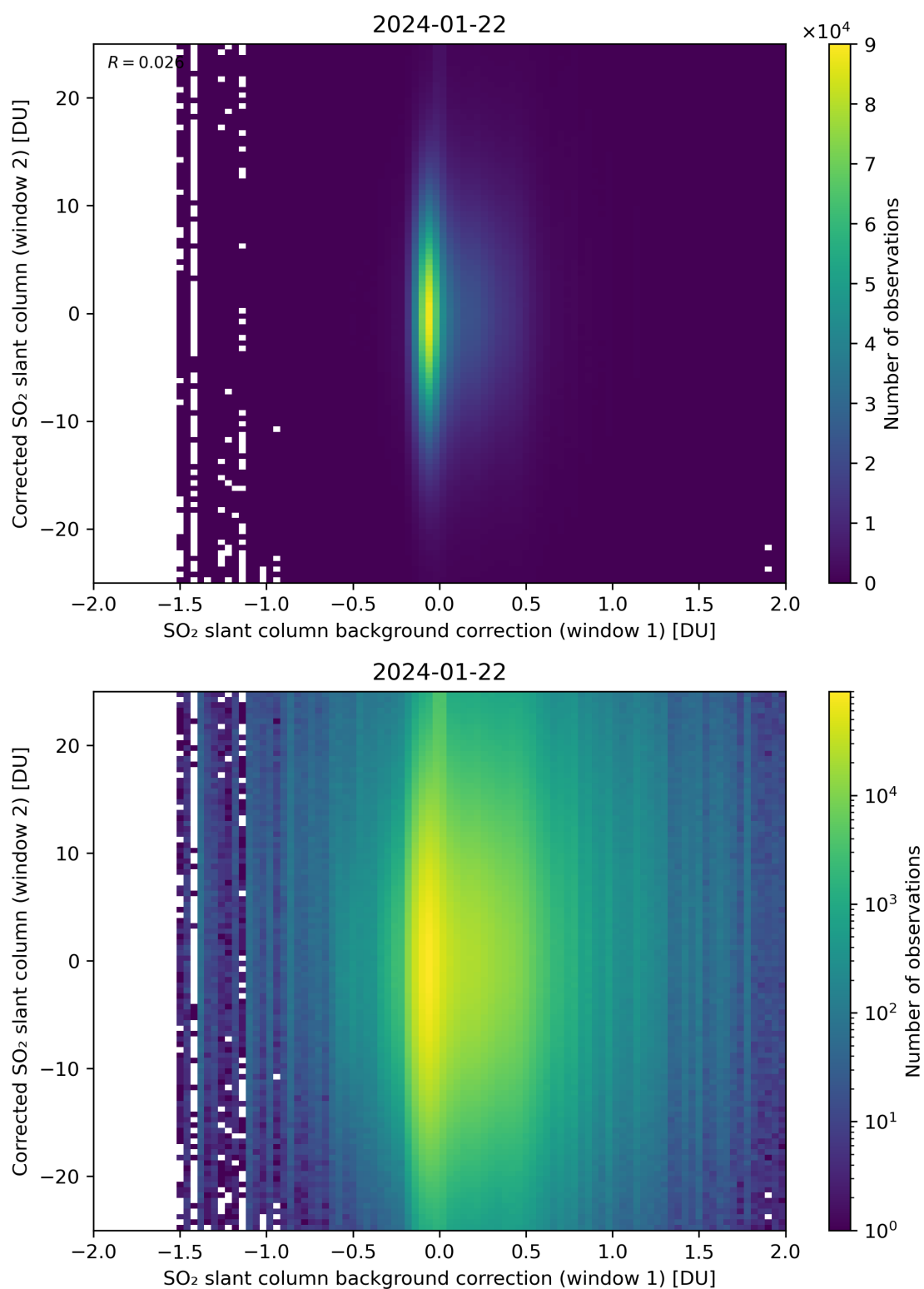
Figure 104: Scatter density plot of “SO 2 slant column background correction (window 1)” against “Corrected SO 2 slant column (window 2)” for 2024-01-21 to 2024-01-23.
