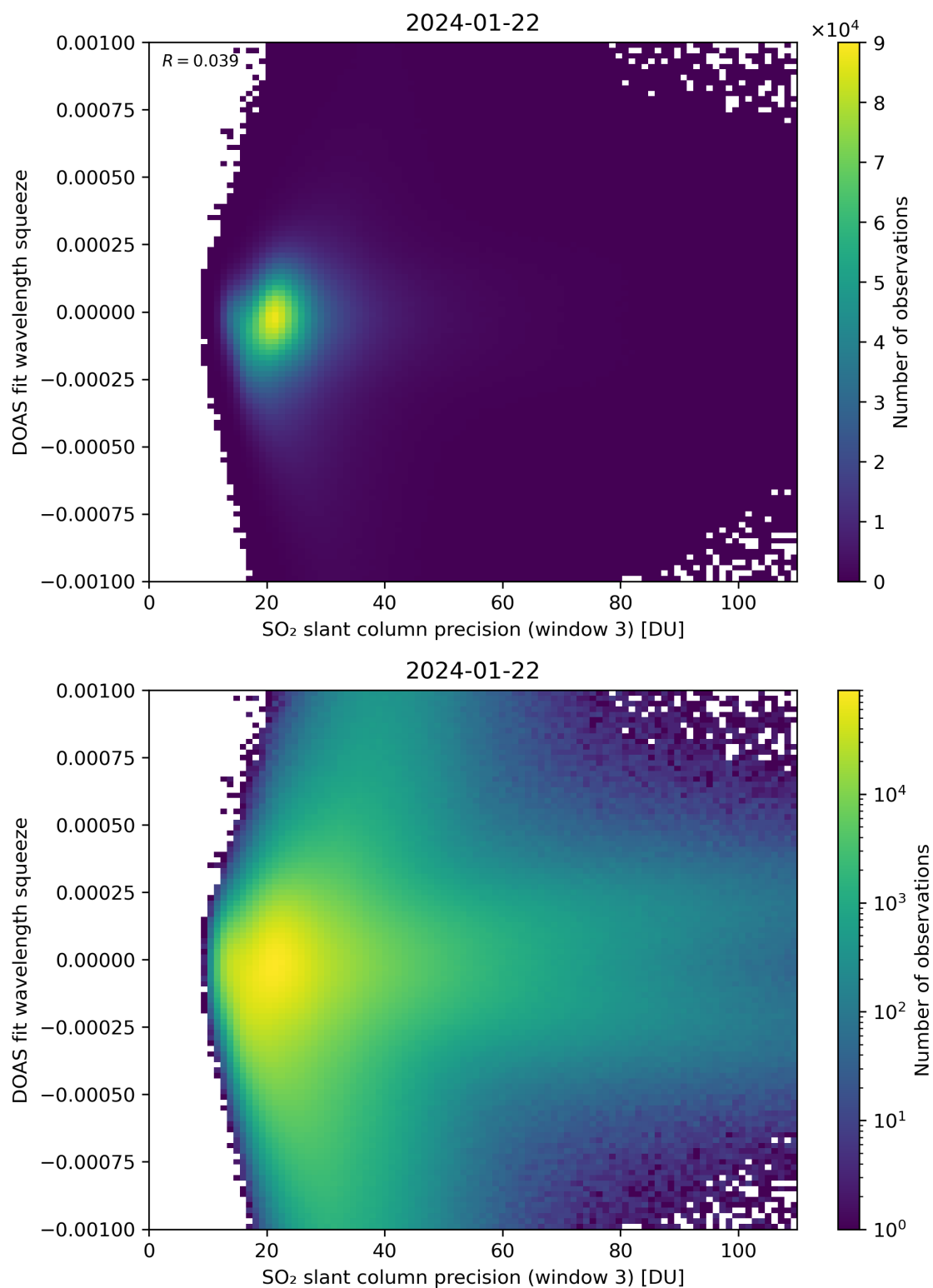
Figure 259: Scatter density plot of “SO 2 slant column precision (window 3)” against “DOAS fit wavelength squeeze” for 2024-01-21 to 2024-01-23.
