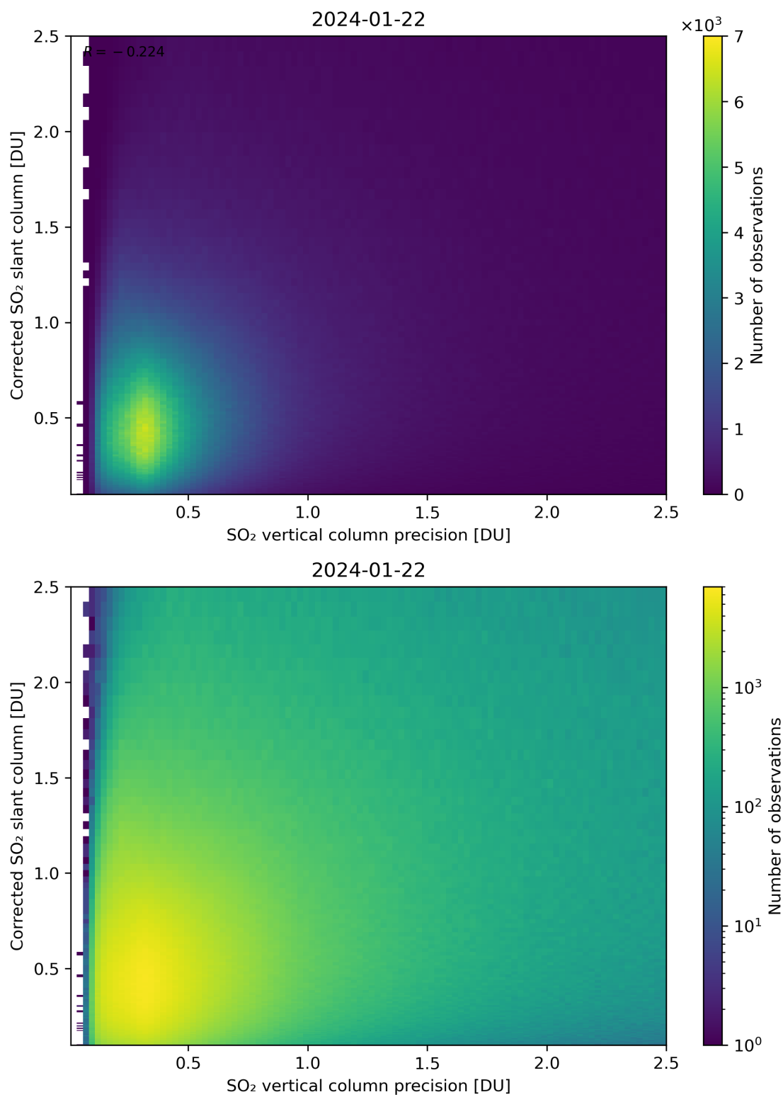
Figure 286: Scatter density plot of “SO 2 vertical column precision” against “Corrected SO 2 slant column” for 2024-01-21 to 2024-01-23.
