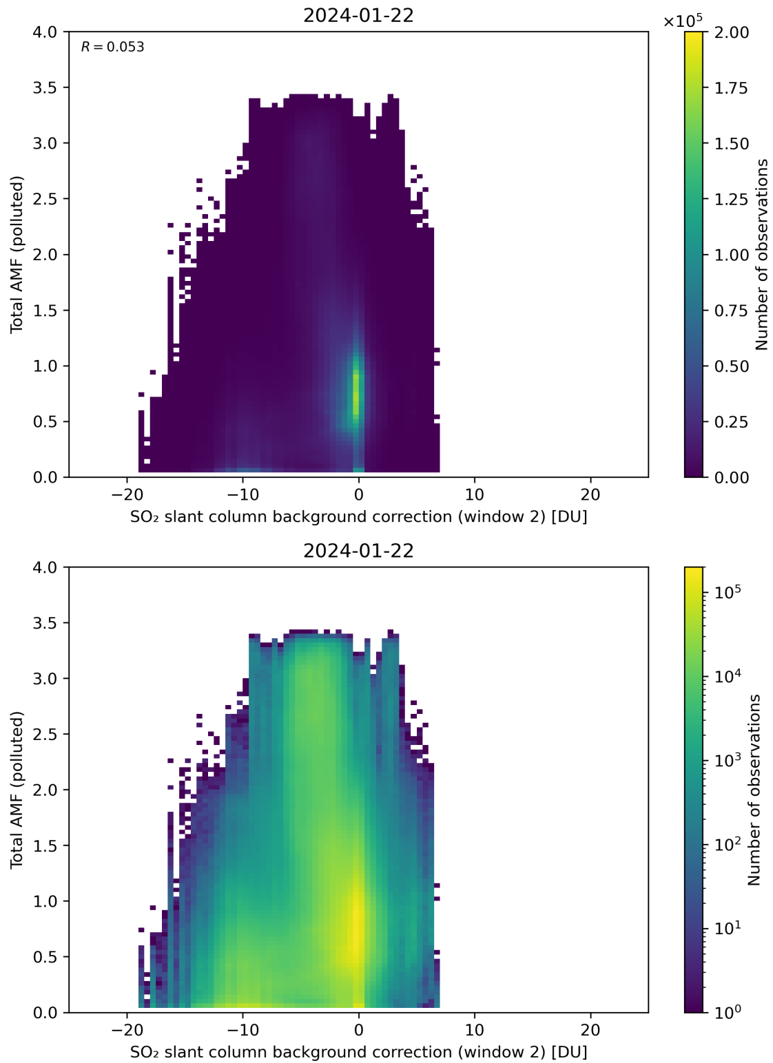
Figure 119: Scatter density plot of “SO 2 slant column background correction (window 2)” against “Total AMF (polluted)” for 2024-01-21 to 2024-01-23.
