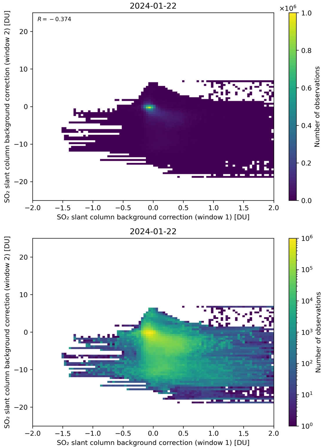
Figure 98: Scatter density plot of “SO 2 slant column background correction (window 1)” against “SO 2 slant column background correction (window 2)” for 2024-01-21 to 2024-01-23.
