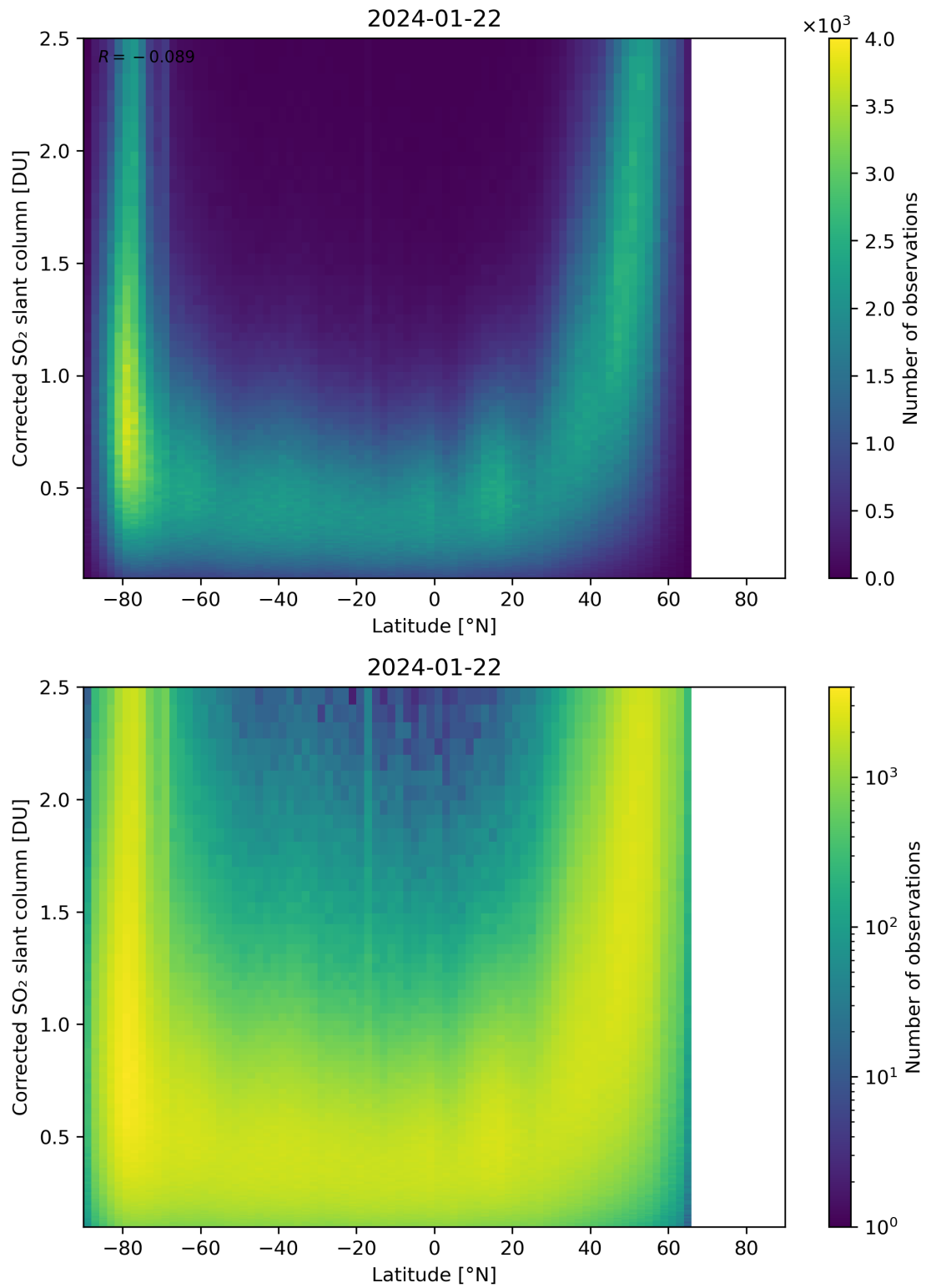
Figure 146: Scatter density plot of “Latitude” against “Corrected SO 2 slant column” for 2024-01-21 to 2024-01-23.
