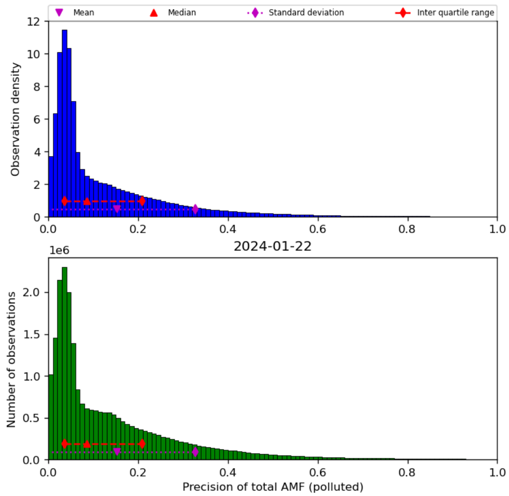
Figure 72: Histogram of “Precision of total AMF (polluted)” for 2024-01-21 to 2024-01-23
