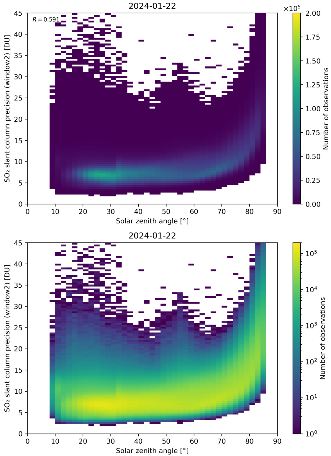
Figure 171: Scatter density plot of “Solar zenith angle” against “SO 2 slant column precision (window2)” for 2024-01-21 to 2024-01-23.
