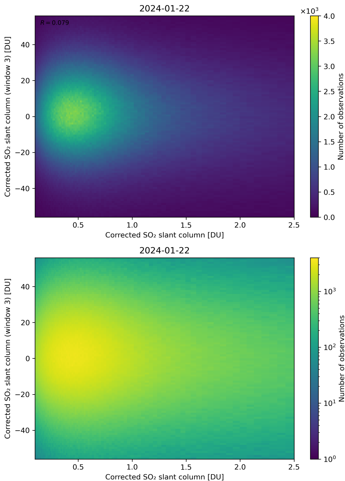
Figure 186: Scatter density plot of “Corrected SO 2 slant column” against “Corrected SO 2 slant column (window 3)” for 2024-01-21 to 2024-01-23.
