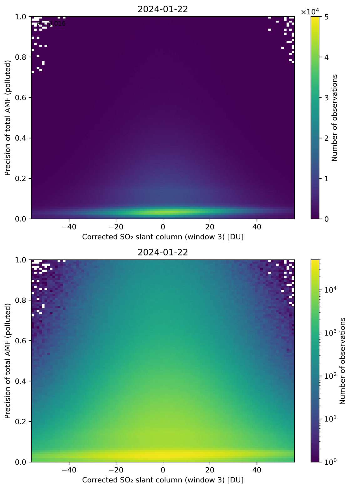
Figure 211: Scatter density plot of “Corrected SO 2 slant column (window 3)” against “Precision of total AMF (polluted)” for 2024-01-21 to 2024-01-23.
