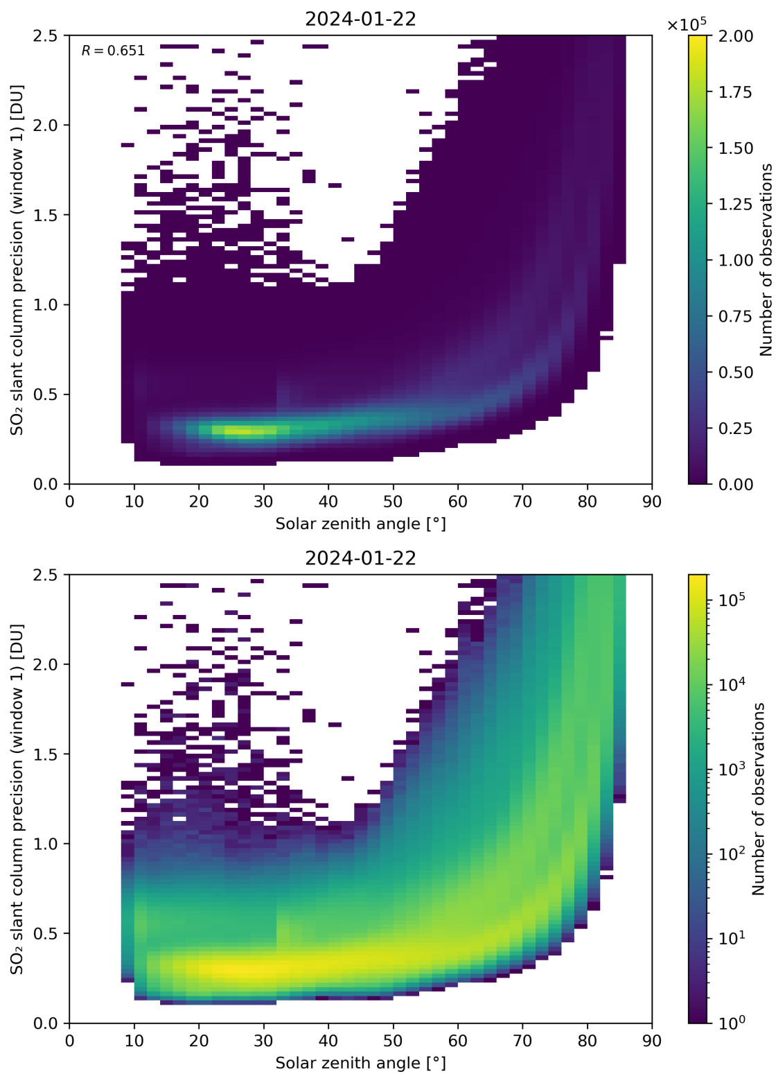
Figure 170: Scatter density plot of “Solar zenith angle” against “SO 2 slant column precision (window 1)” for 2024-01-21 to 2024-01-23.
