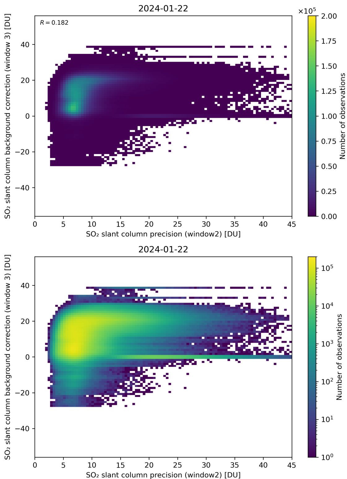
Figure 242: Scatter density plot of “SO 2 slant column precision (window2)” against “SO 2 slant column background correction (window 3)” for 2024-01-21 to 2024-01-23.
