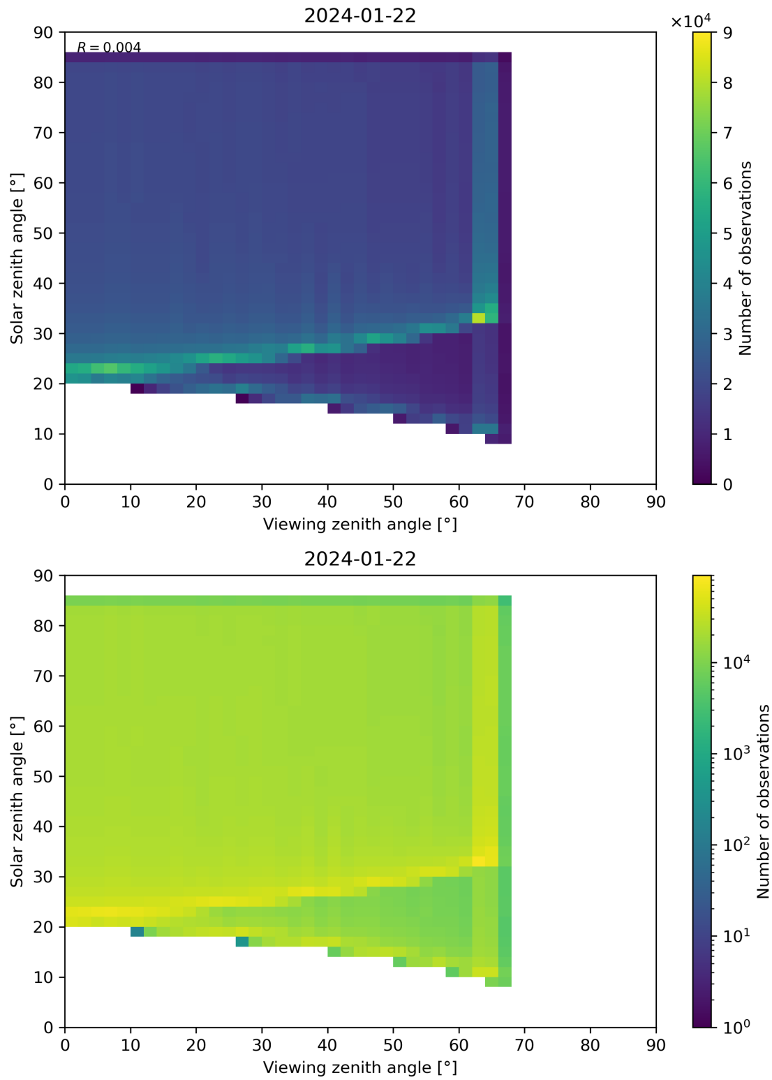
Figure 315: Scatter density plot of “Viewing zenith angle” against “Solar zenith angle” for 2024-01-21 to 2024-01-23.
