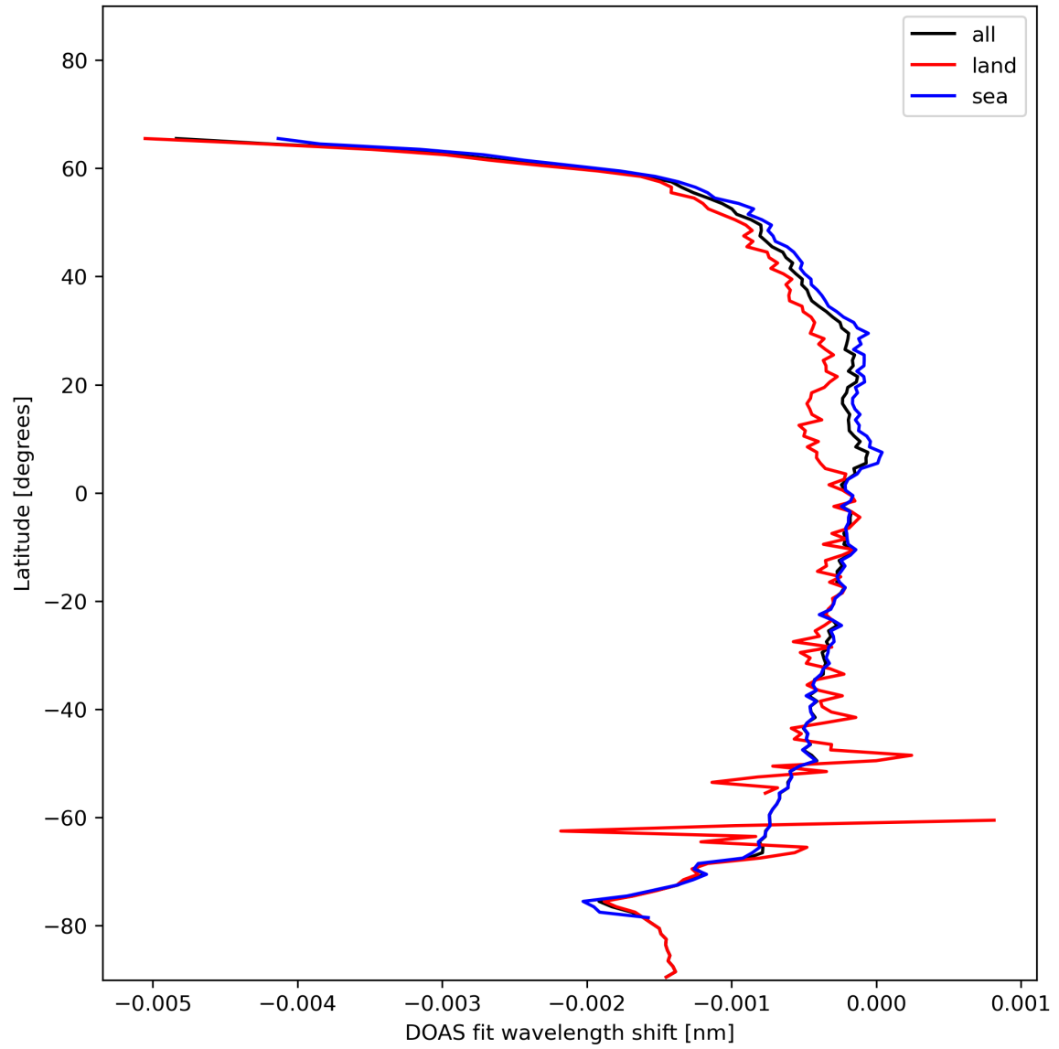
Figure 45: Zonal average of “DOAS fit wavelength shift” for 2024-01-21 to 2024-01-23.
