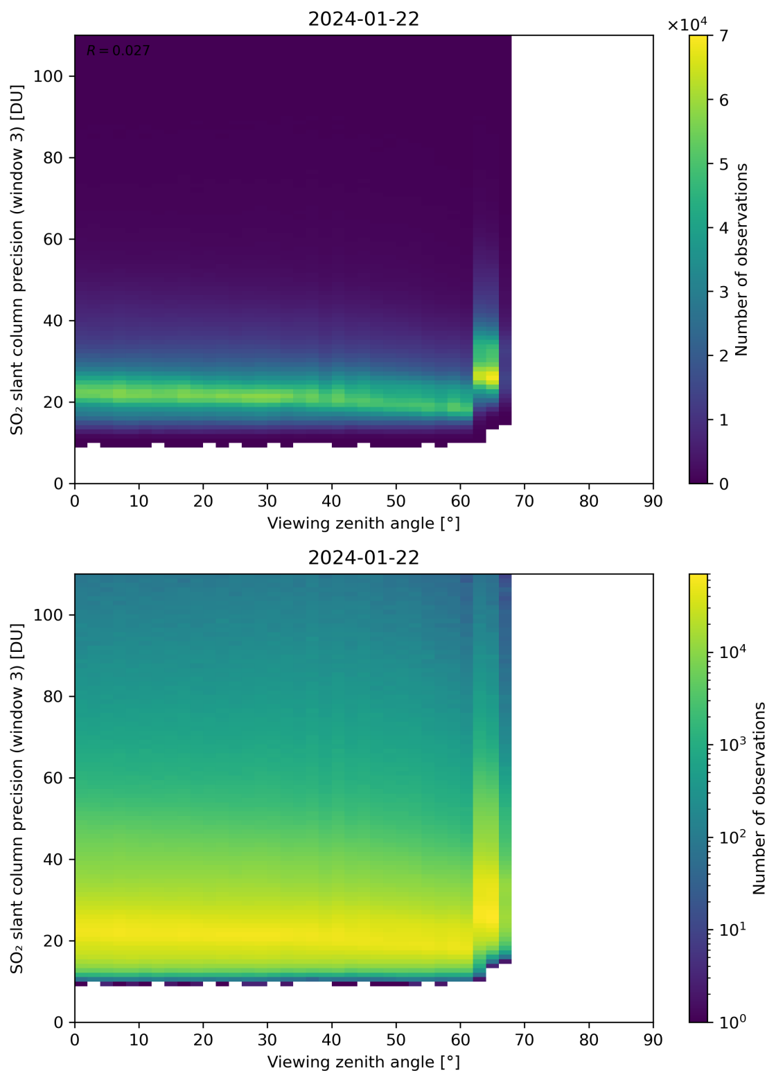
Figure 324: Scatter density plot of “Viewing zenith angle” against “SO 2 slant column precision (window 3)” for 2024-01-21 to 2024-01-23.
