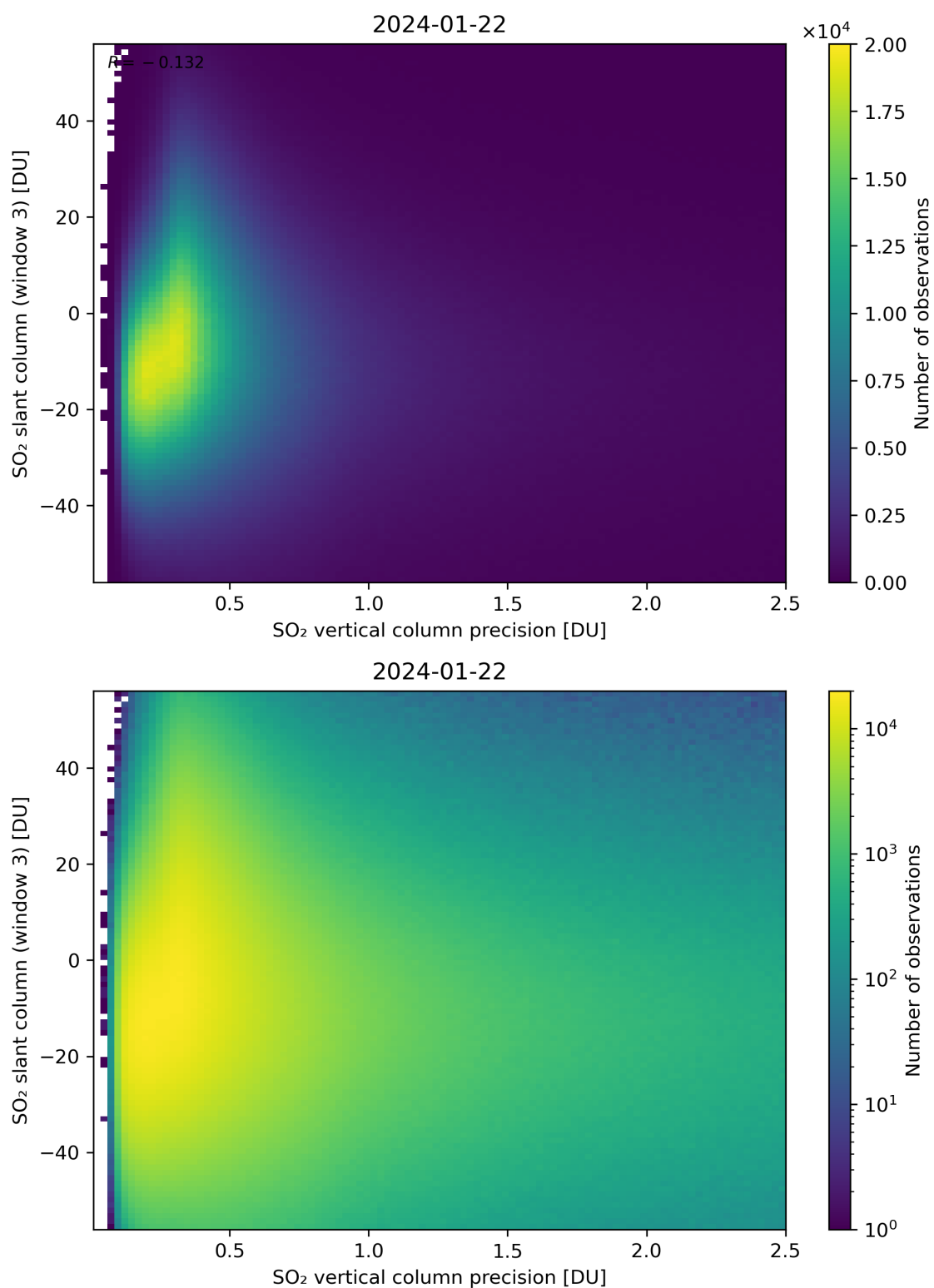
Figure 292: Scatter density plot of “SO 2 vertical column precision” against “SO 2 slant column (window 3)” for 2024-01-21 to 2024-01-23.
