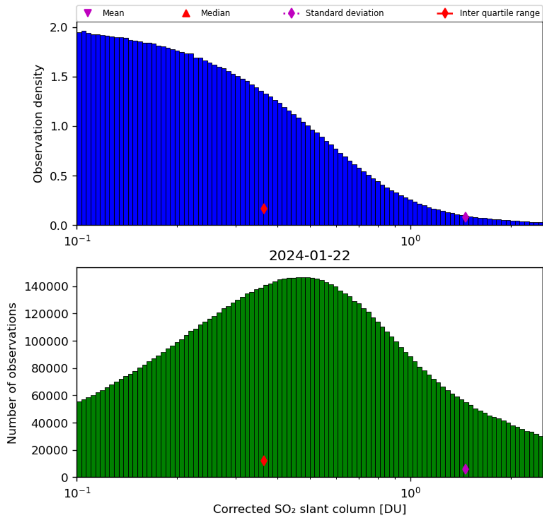
Figure 55: Histogram of “Corrected SO 2 slant column” for 2024-01-21 to 2024-01-23
