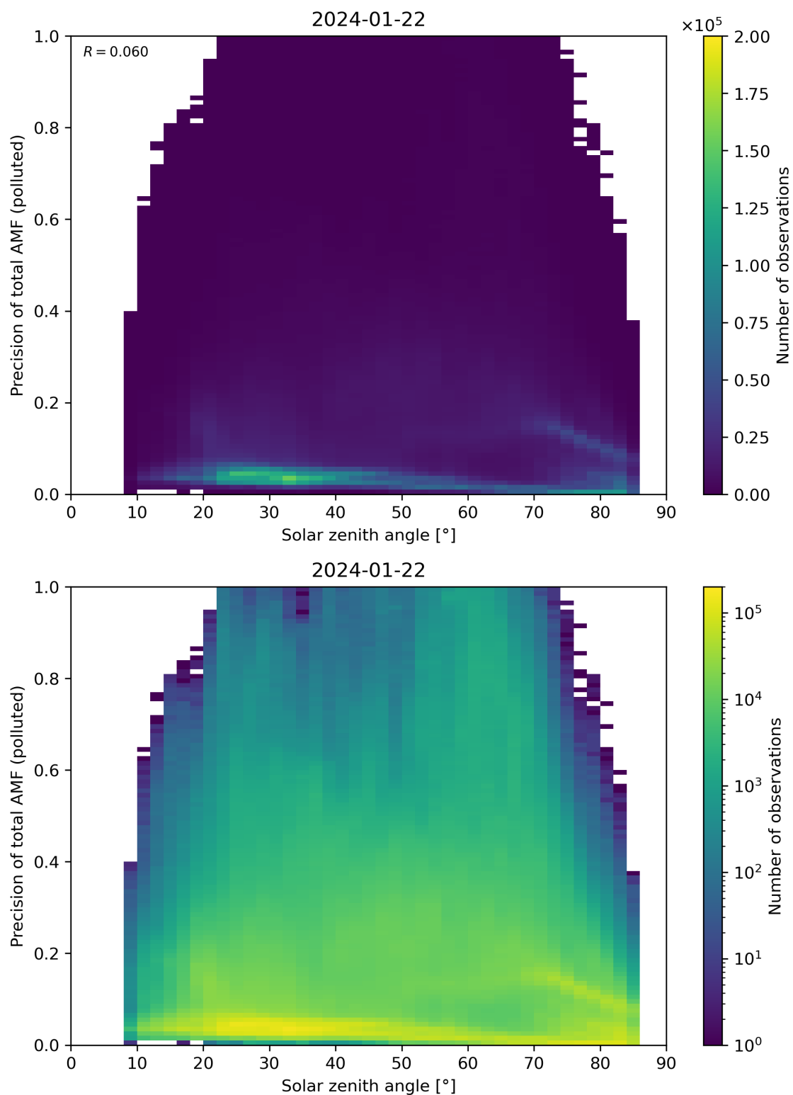
Figure 175: Scatter density plot of “Solar zenith angle” against “Precision of total AMF (polluted)” for 2024-01-21 to 2024-01-23.
