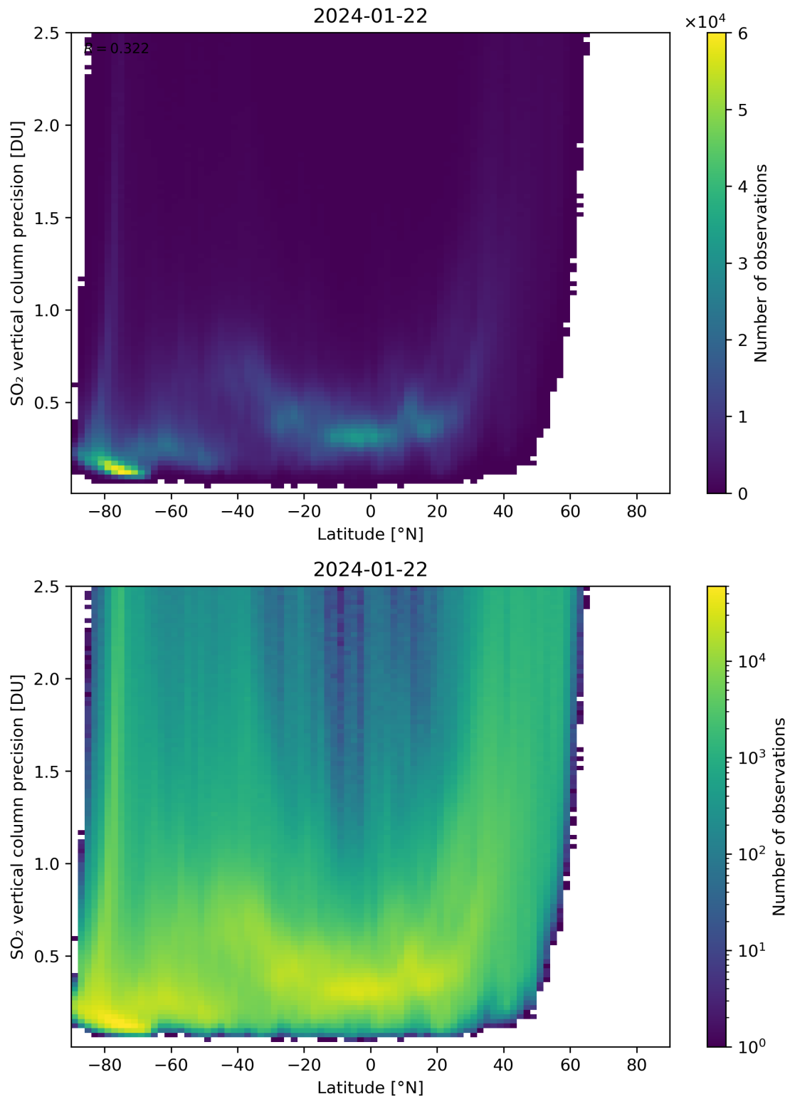
Figure 157: Scatter density plot of “Latitude” against “SO 2 vertical column precision” for 2024-01-21 to 2024-01-23.
