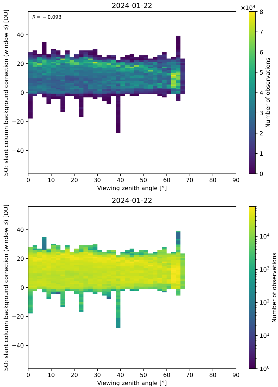
Figure 310: Scatter density plot of “Viewing zenith angle” against “SO 2 slant column background correction (window 3)” for 2024-01-21 to 2024-01-23.
