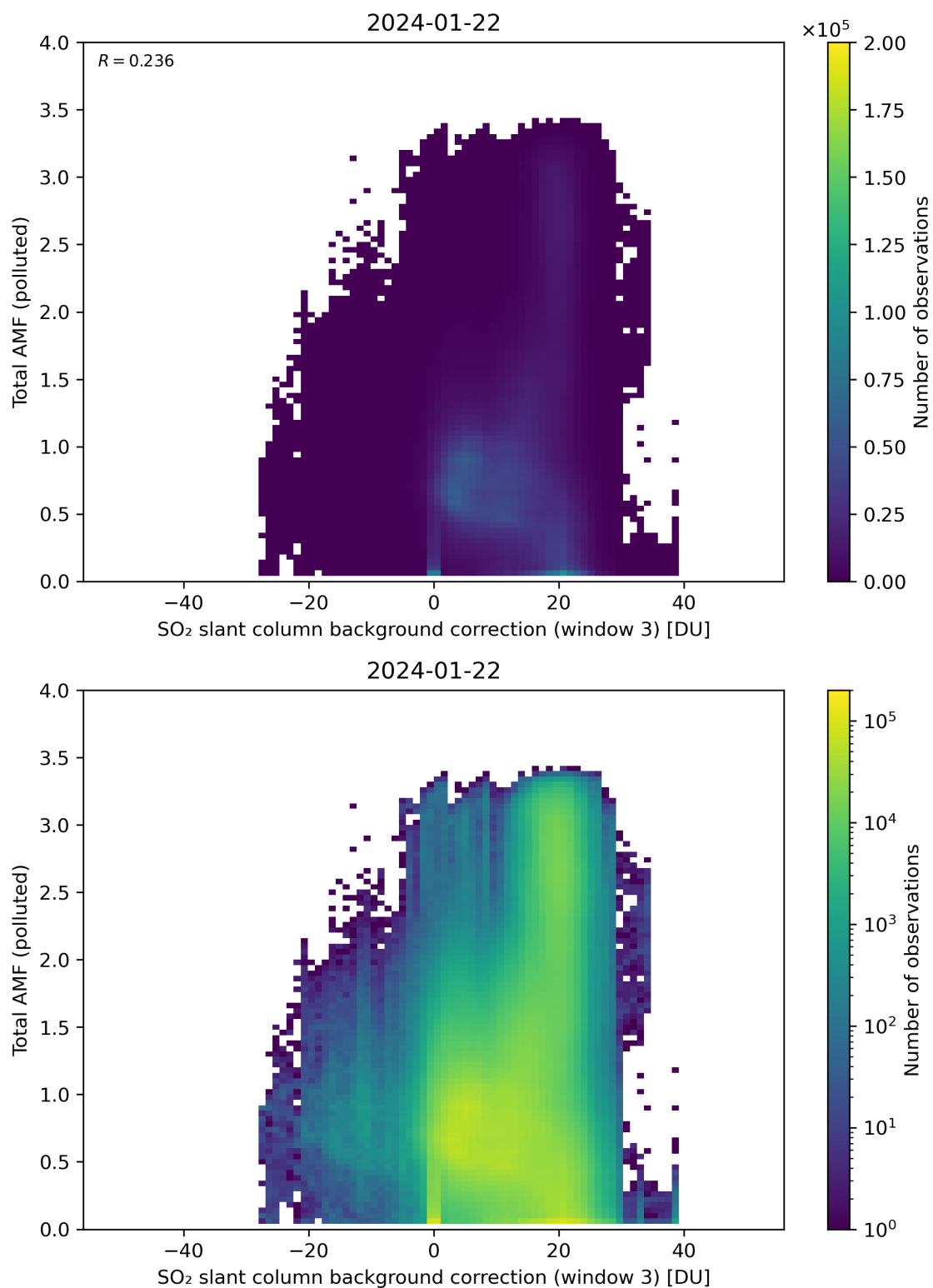
Figure 125: Scatter density plot of “SO 2 slant column background correction (window 3)” against “Total AMF (polluted)” for 2024-01-21 to 2024-01-23.
