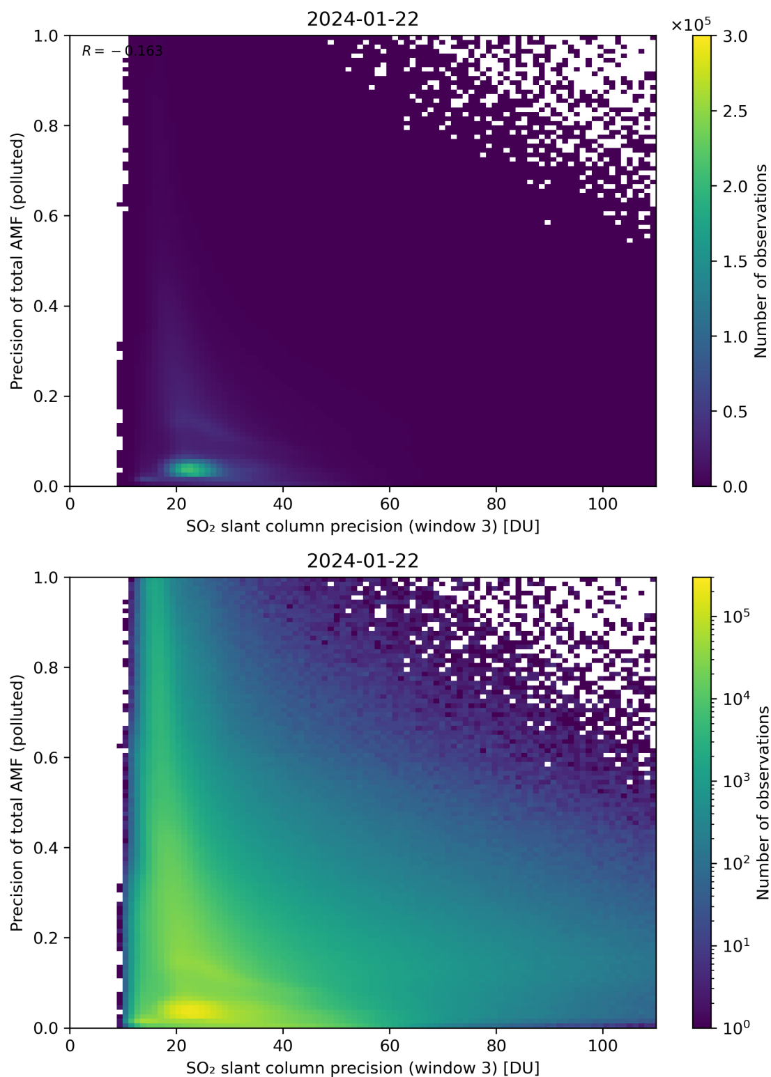
Figure 264: Scatter density plot of “SO 2 slant column precision (window 3)” against “Precision of total AMF (polluted)” for 2024-01-21 to 2024-01-23.
