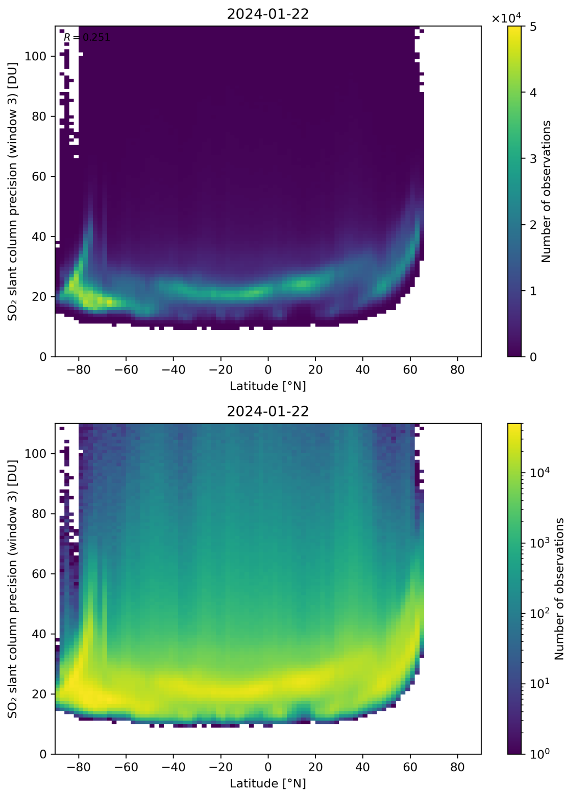
Figure 153: Scatter density plot of “Latitude” against “SO 2 slant column precision (window 3)” for 2024-01-21 to 2024-01-23.
