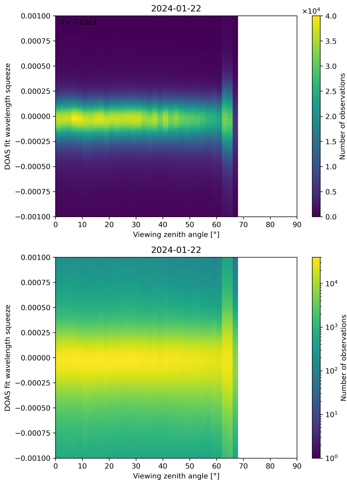
Figure 312: Scatter density plot of “Viewing zenith angle” against “DOAS fit wavelength squeeze” for 2024-01-21 to 2024-01-23.
