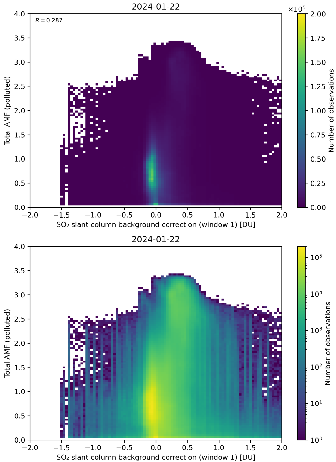
Figure 109: Scatter density plot of “SO 2 slant column background correction (window 1)” against “Total AMF (polluted)” for 2024-01-21 to 2024-01-23.
