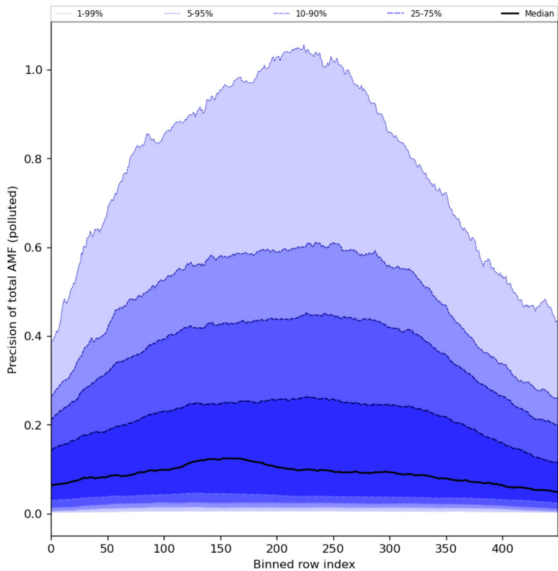
Figure 95: Along track statistics of “Precision of total AMF (polluted)” for 2024-01-21 to 2024-01-23
