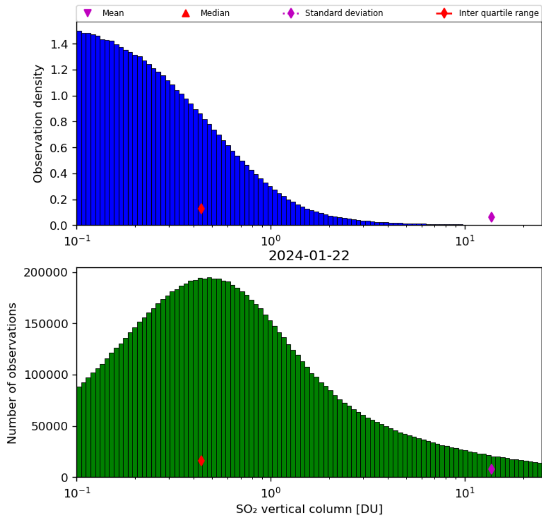
Figure 53: Histogram of “SO 2 vertical column” for 2024-01-21 to 2024-01-23
