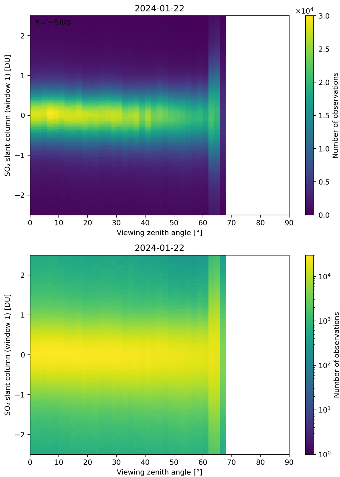
Figure 320: Scatter density plot of “Viewing zenith angle” against “SO 2 slant column (window 1)” for 2024-01-21 to 2024-01-23.
