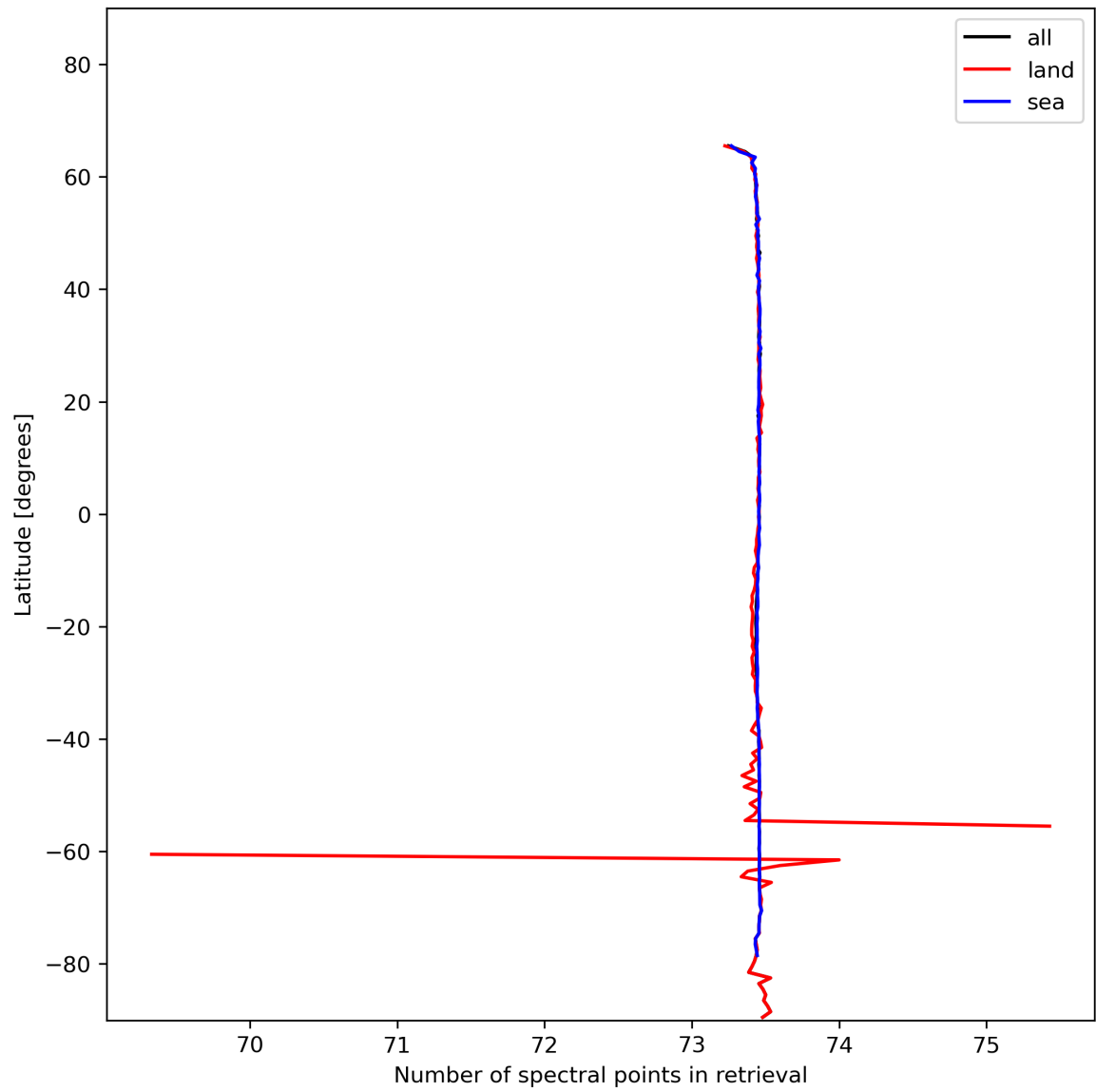
Figure 51: Zonal average of “Number of spectral points in retrieval” for 2024-01-21 to 2024-01-23.
