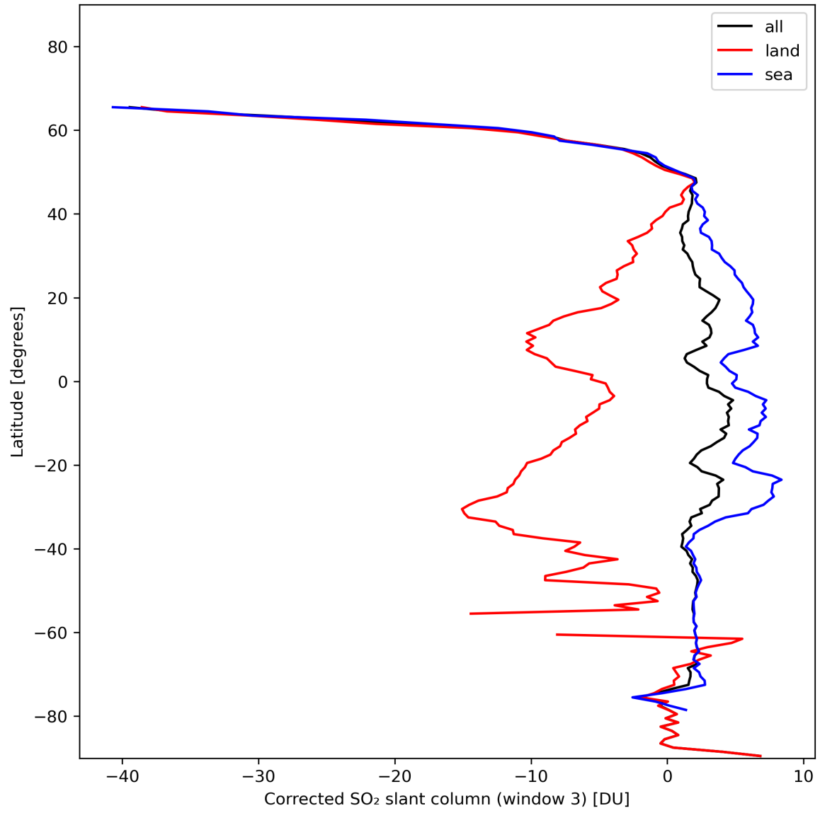
Figure 43: Zonal average of “Corrected SO 2 slant column (window 3)” for 2024-01-21 to 2024-01-23.
