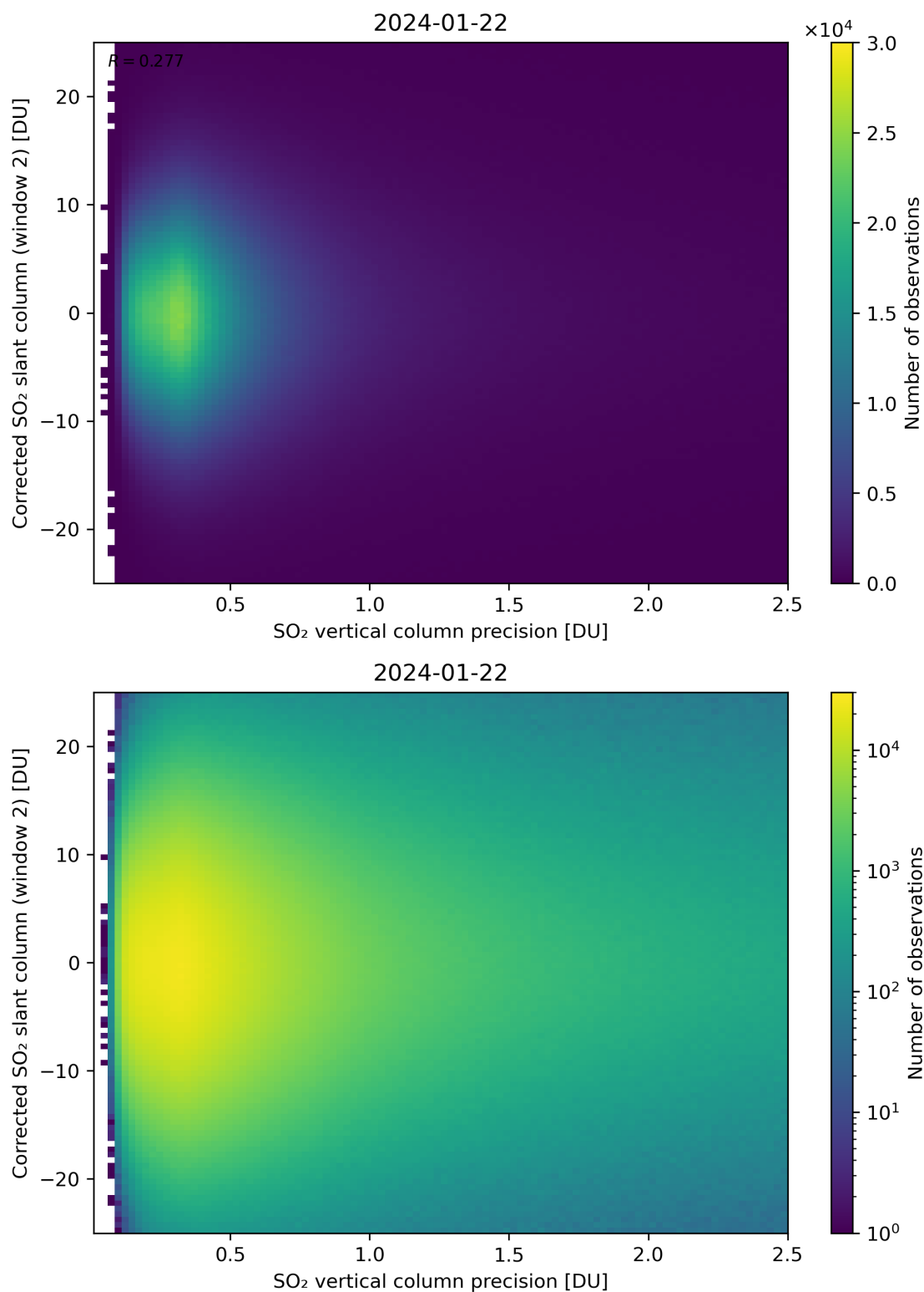
Figure 287: Scatter density plot of “SO 2 vertical column precision” against “Corrected SO 2 slant column (window 2)” for 2024-01-21 to 2024-01-23.
