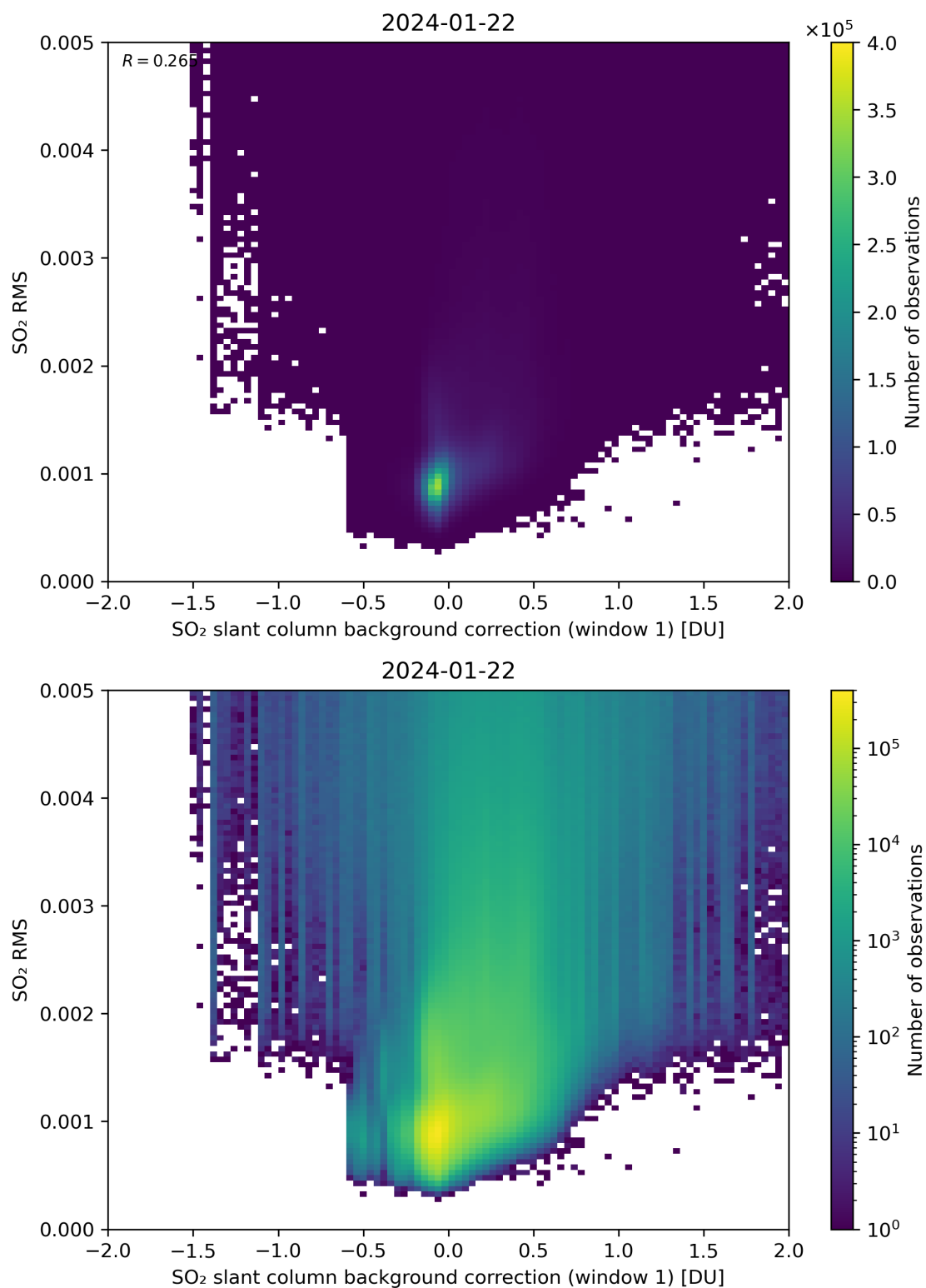
Figure 102: Scatter density plot of “SO 2 slant column background correction (window 1)” against “SO 2 RMS” for 2024-01-21 to 2024-01-23.
