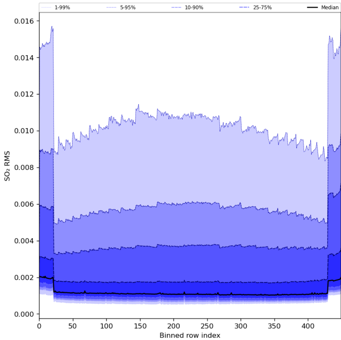
Figure 93: Along track statistics of “SO 2 RMS” for 2024-01-21 to 2024-01-23
