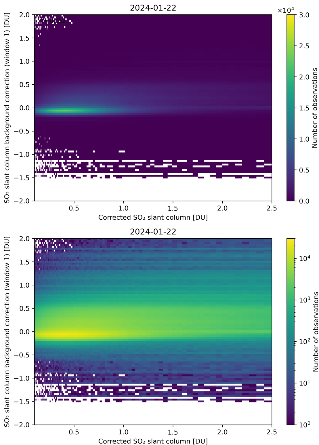
Figure 178: Scatter density plot of “Corrected SO 2 slant column” against “SO 2 slant column background correction (window 1)” for 2024-01-21 to 2024-01-23.
