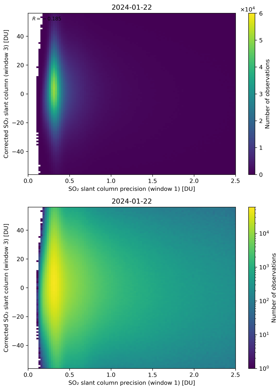
Figure 226: Scatter density plot of “SO 2 slant column precision (window 1)” against “Corrected SO 2 slant column (window 3)” for 2024-01-21 to 2024-01-23.
