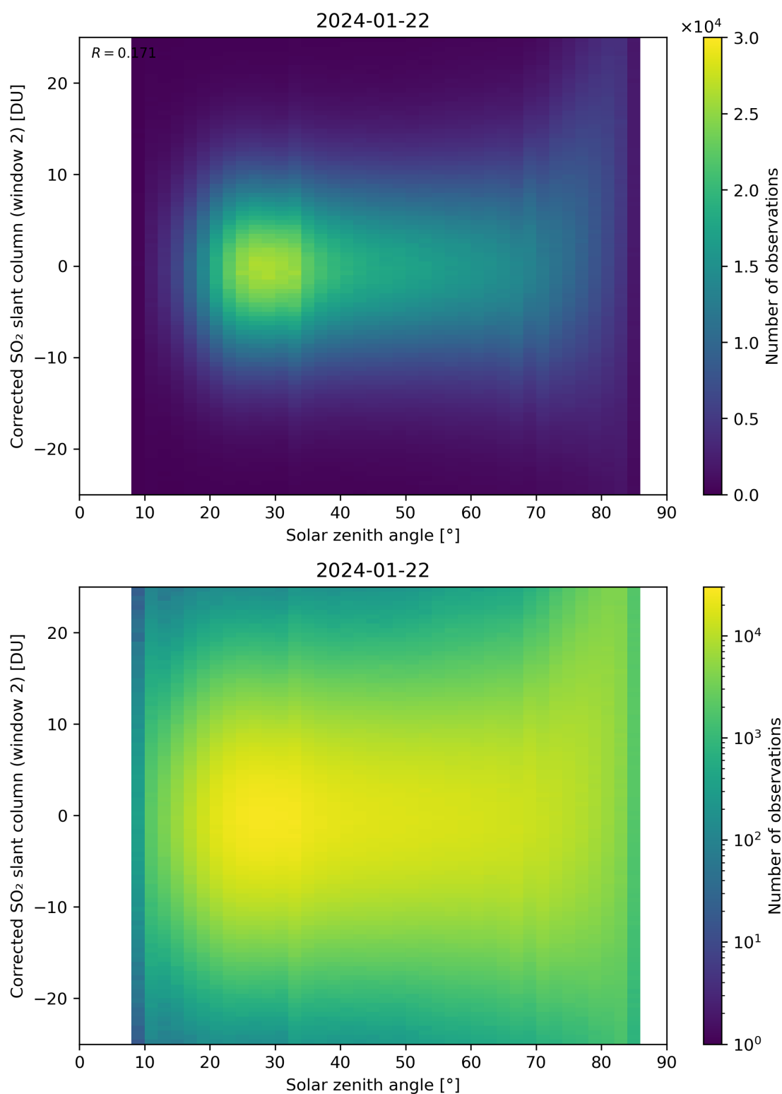
Figure 167: Scatter density plot of “Solar zenith angle” against “Corrected SO 2 slant column (window 2)” for 2024-01-21 to 2024-01-23.
