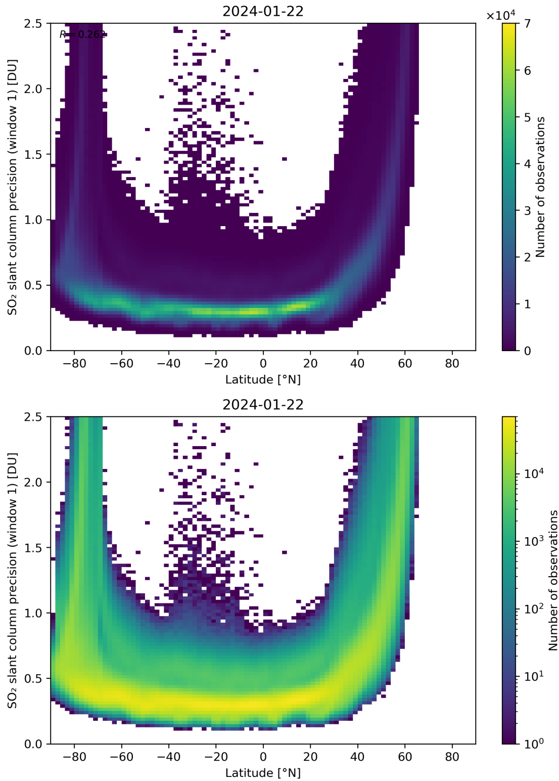
Figure 150: Scatter density plot of “Latitude” against “SO 2 slant column precision (window 1)” for 2024-01-21 to 2024-01-23.
