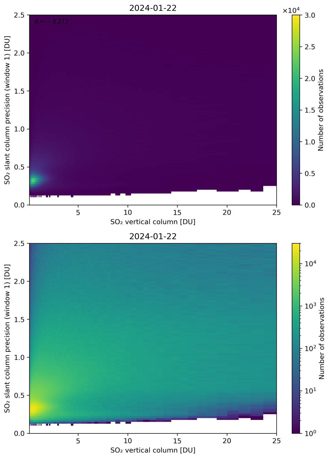
Figure 301: Scatter density plot of “SO 2 vertical column” against “SO 2 slant column precision (window 1)” for 2024-01-21 to 2024-01-23.
