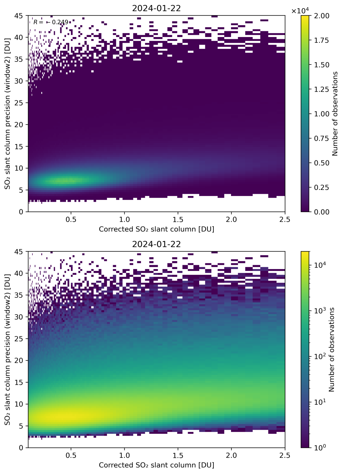
Figure 189: Scatter density plot of “Corrected SO 2 slant column” against “SO 2 slant column precision (window2)” for 2024-01-21 to 2024-01-23.
