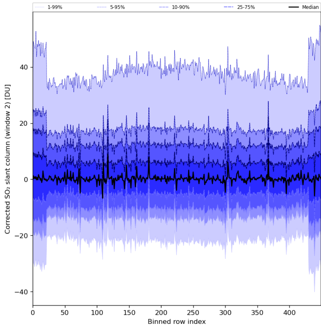
Figure 85: Along track statistics of “Corrected SO 2 slant column (window 2)” for 2024-01-21 to 2024-01-23
