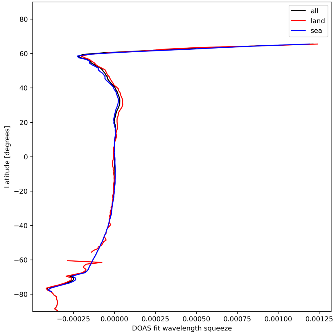
Figure 46: Zonal average of “DOAS fit wavelength squeeze” for 2024-01-21 to 2024-01-23.
