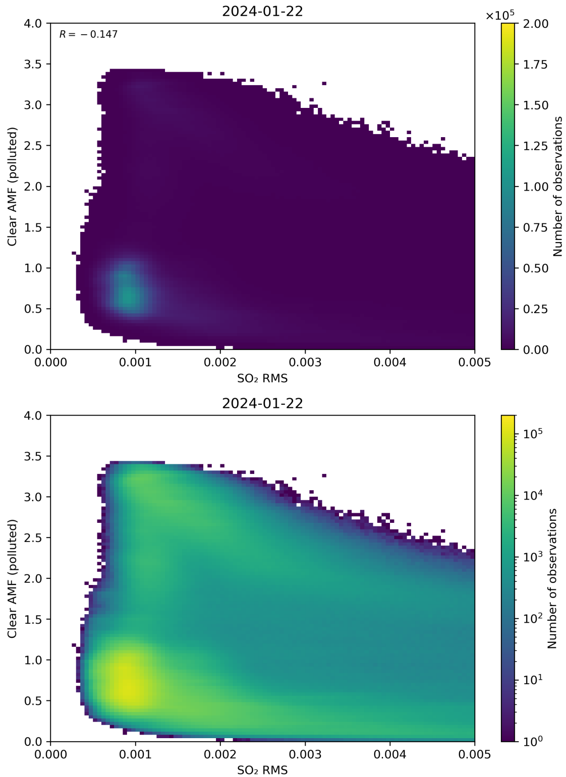
Figure 136: Scatter density plot of “SO 2 RMS” against “Clear AMF (polluted)” for 2024-01-21 to 2024-01-23.
