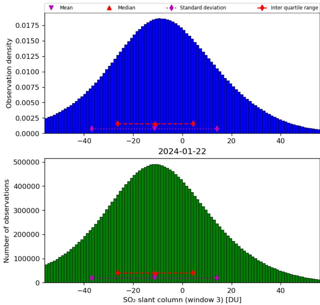
Figure 64: Histogram of “SO 2 slant column (window 3)” for 2024-01-21 to 2024-01-23
