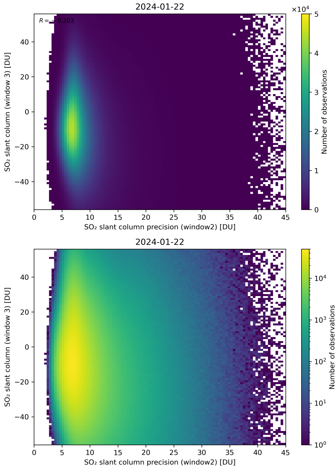
Figure 249: Scatter density plot of “SO 2 slant column precision (window2)” against “SO 2 slant column (window 3)” for 2024-01-21 to 2024-01-23.
