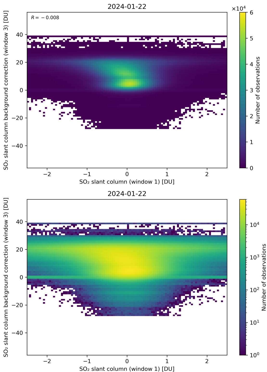
Figure 214: Scatter density plot of “SO 2 slant column (window 1)” against “SO 2 slant column background correction (window 3)” for 2024-01-21 to 2024-01-23.
