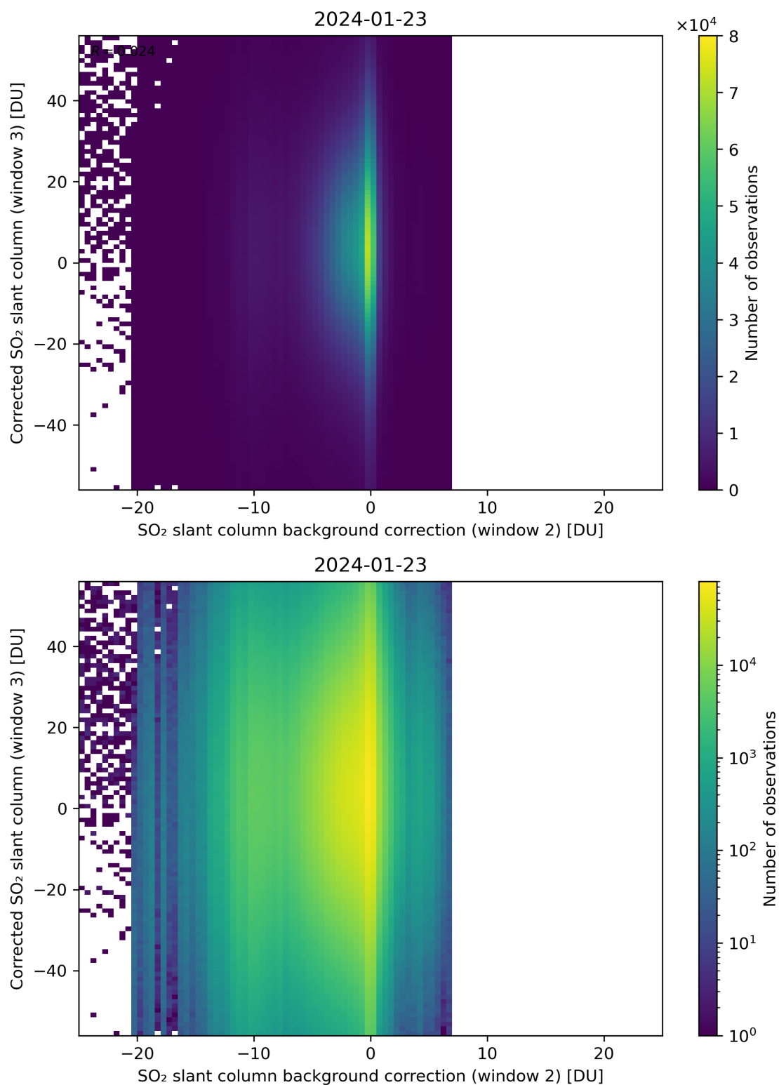
Figure 116: Scatter density plot of “SO 2 slant column background correction (window 2)” against “Corrected SO 2 slant column (window 3)” for 2024-01-22 to 2024-01-24.
