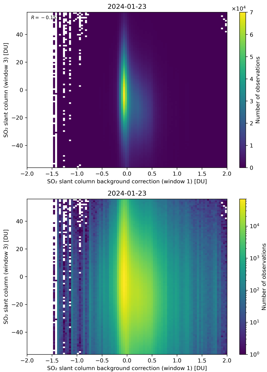
Figure 107: Scatter density plot of “SO 2 slant column background correction (window 1)” against “SO 2 slant column (window 3)” for 2024-01-22 to 2024-01-24.
