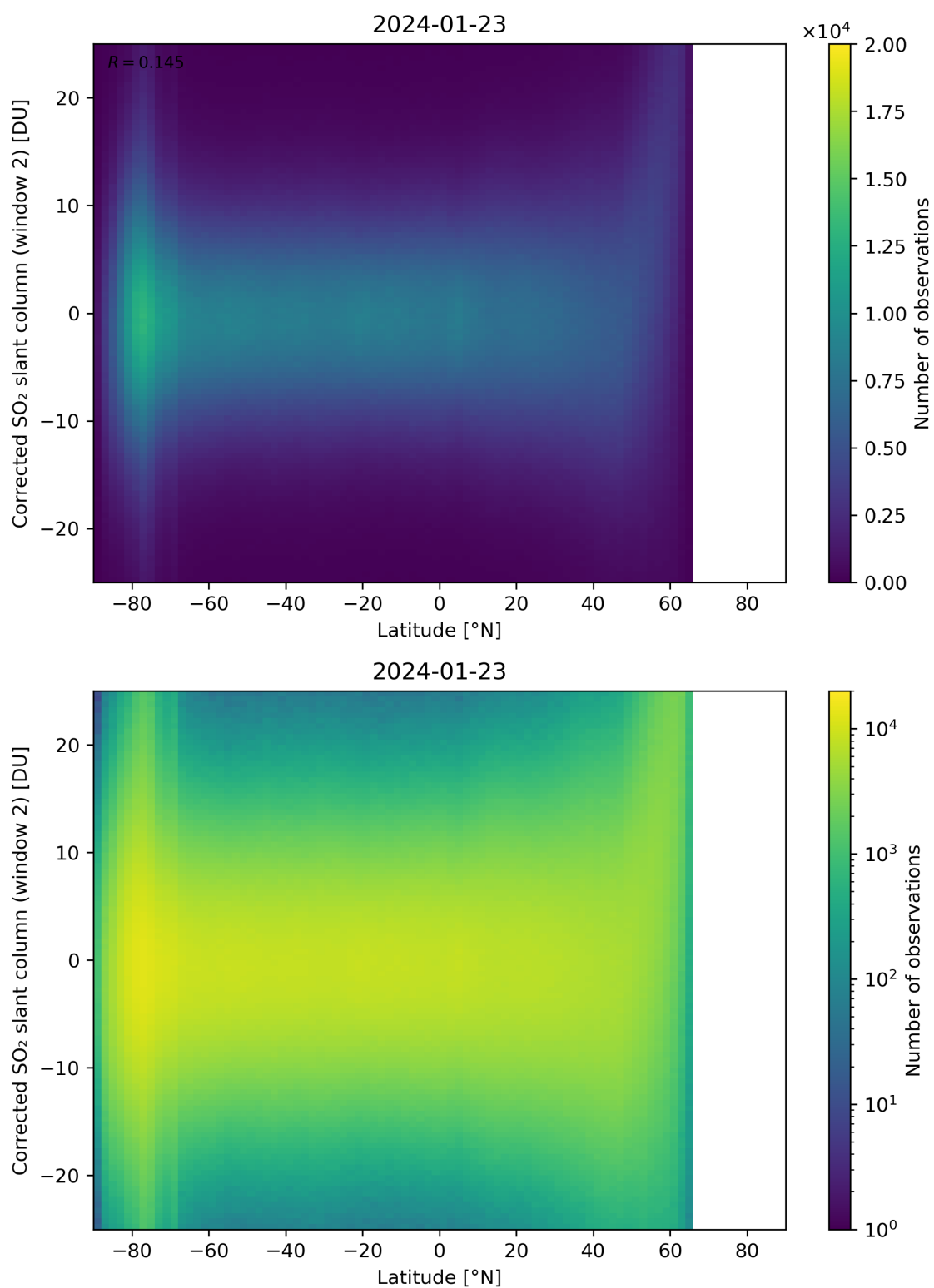
Figure 147: Scatter density plot of “Latitude” against “Corrected SO 2 slant column (window 2)” for 2024-01-22 to 2024-01-24.
