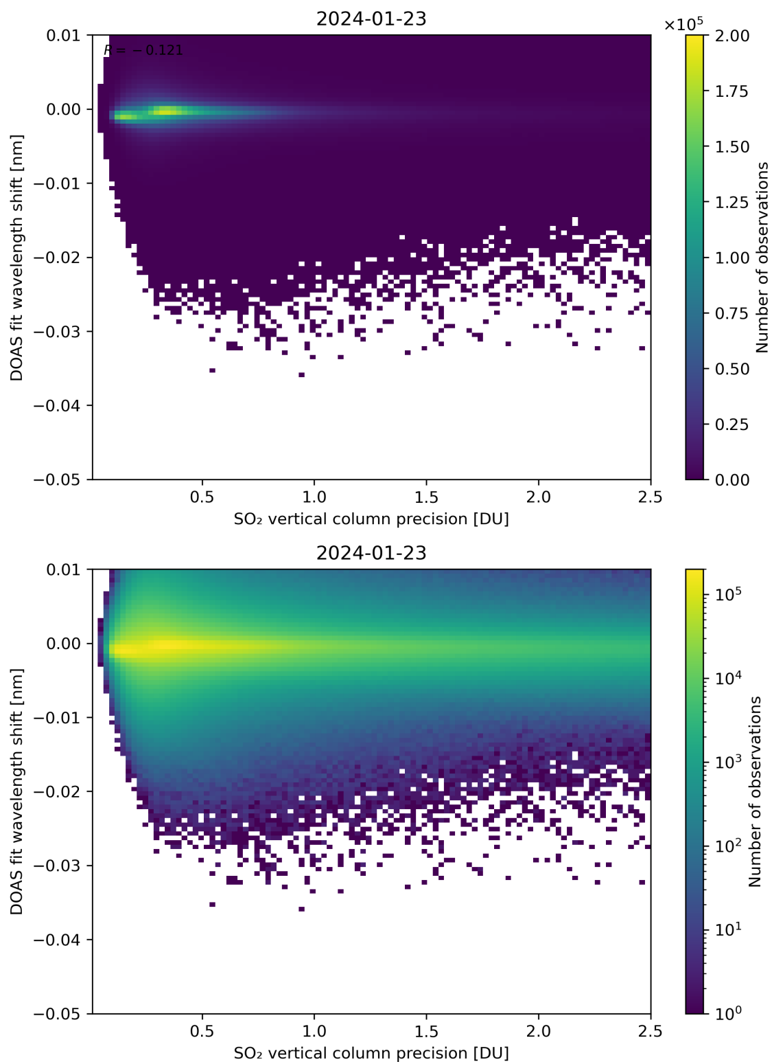
Figure 282: Scatter density plot of “SO 2 vertical column precision” against “DOAS fit wavelength shift” for 2024-01-22 to 2024-01-24.
