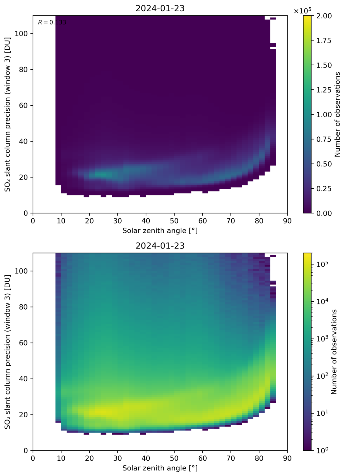
Figure 173: Scatter density plot of “Solar zenith angle” against “SO 2 slant column precision (window 3)” for 2024-01-22 to 2024-01-24.
