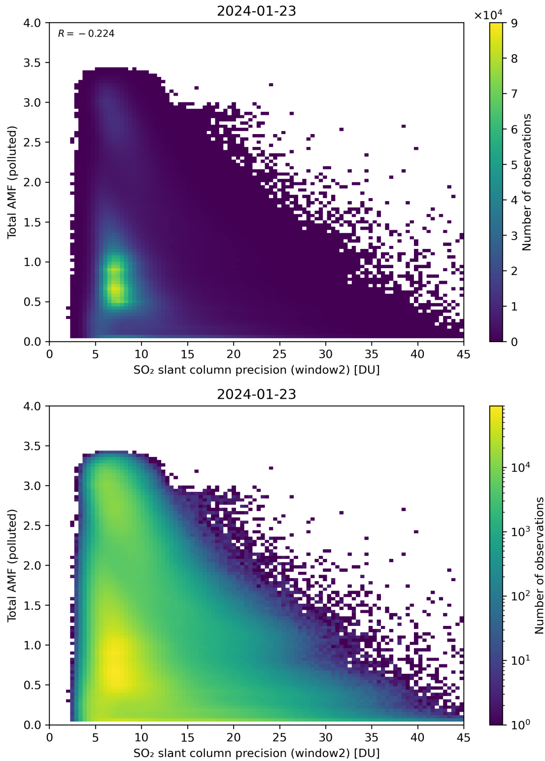
Figure 251: Scatter density plot of “SO 2 slant column precision (window2)” against “Total AMF (polluted)” for 2024-01-22 to 2024-01-24.
