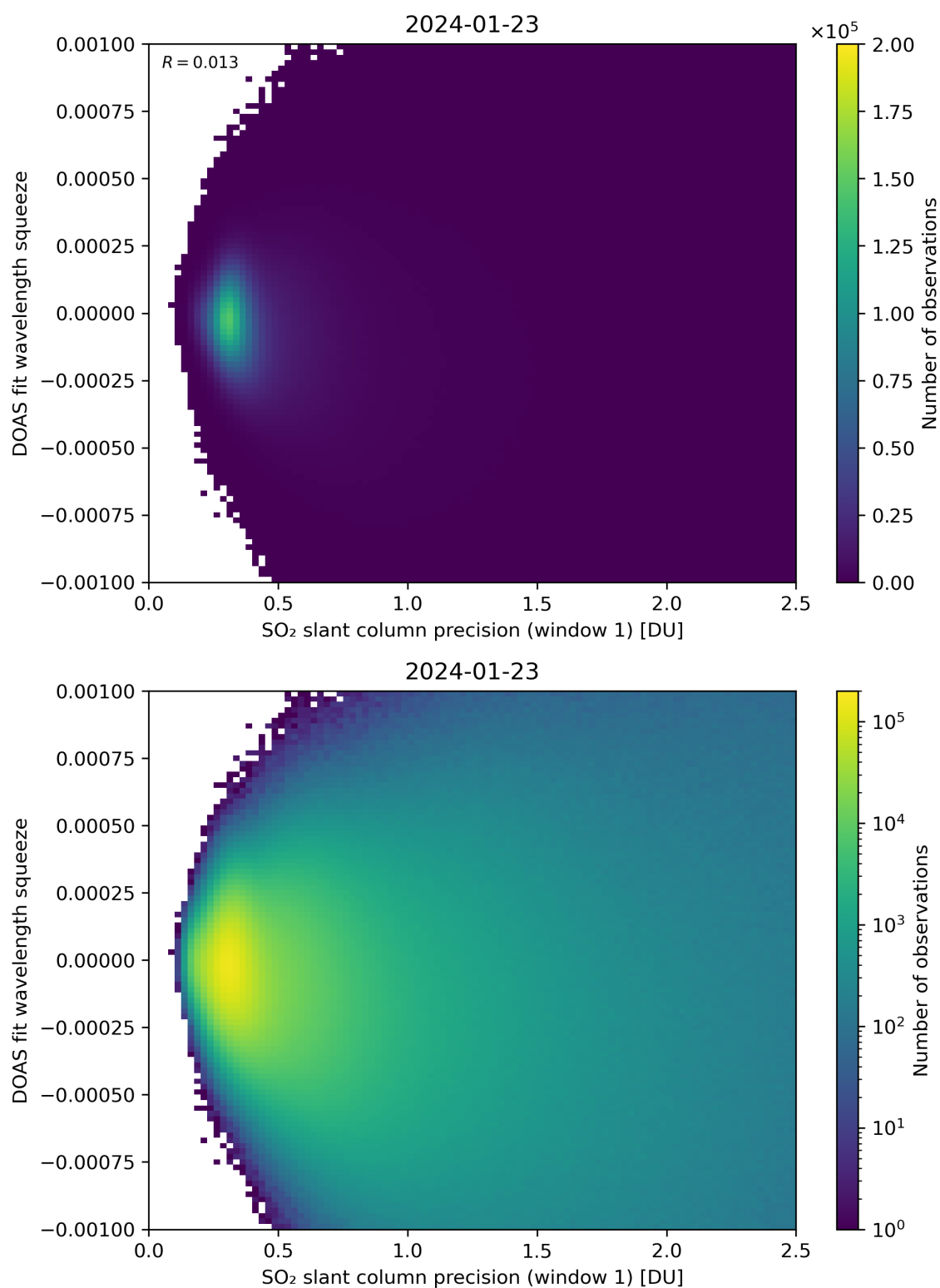
Figure 222: Scatter density plot of “SO 2 slant column precision (window 1)” against “DOAS fit wavelength squeeze” for 2024-01-22 to 2024-01-24.
