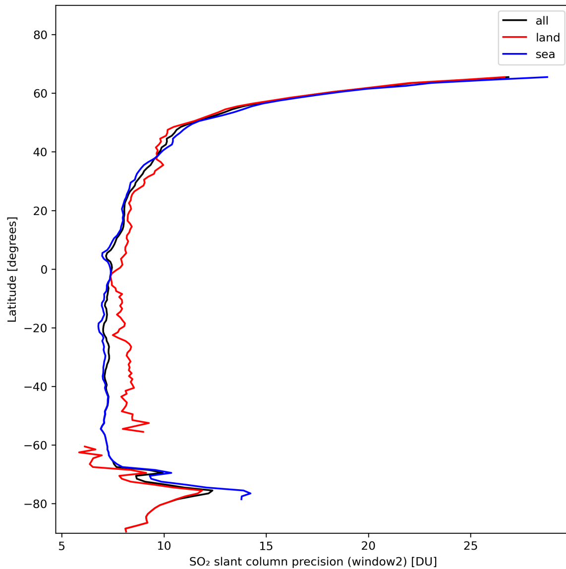
Figure 38: Zonal average of “SO 2 slant column precision (window2)” for 2024-01-22 to 2024-01-24.
