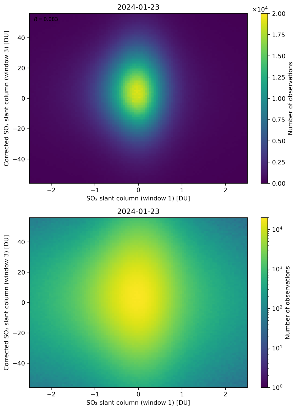
Figure 234: Scatter density plot of “SO 2 slant column (window 1)” against “Corrected SO 2 slant column (window 3)” for 2024-01-22 to 2024-01-24.
