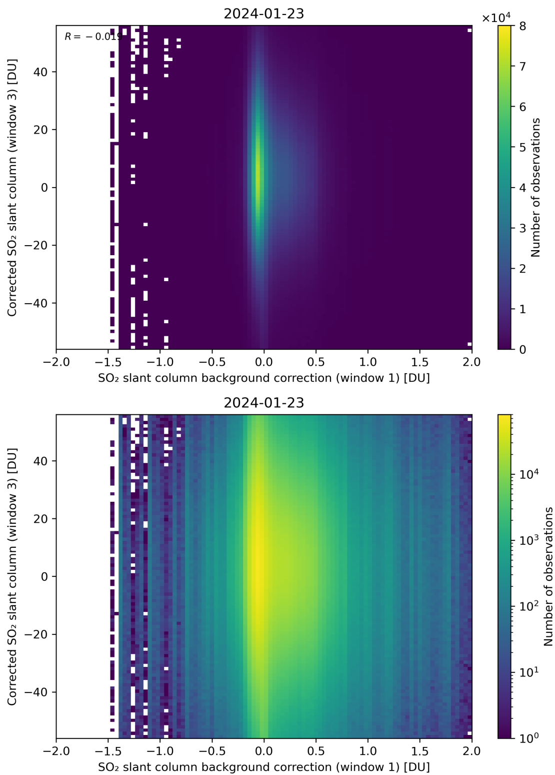
Figure 105: Scatter density plot of “SO 2 slant column background correction (window 1)” against “Corrected SO 2 slant column (window 3)” for 2024-01-22 to 2024-01-24.
