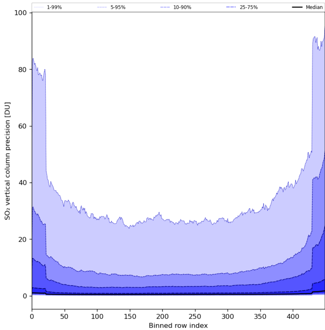
Figure 77: Along track statistics of “SO 2 vertical column precision” for 2024-01-22 to 2024-01-24
