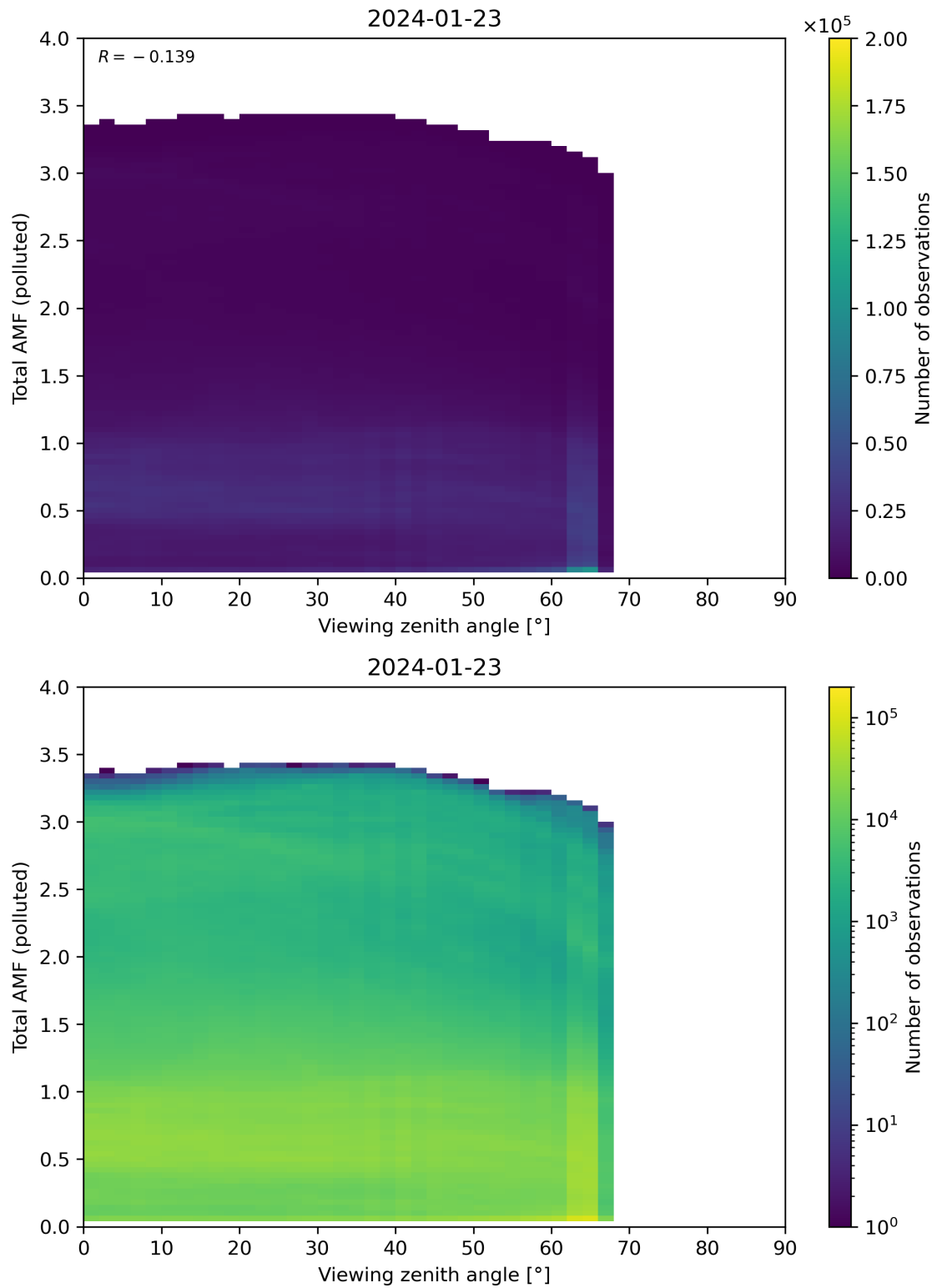
Figure 325: Scatter density plot of “Viewing zenith angle” against “Total AMF (polluted)” for 2024-01-22 to 2024-01-24.
