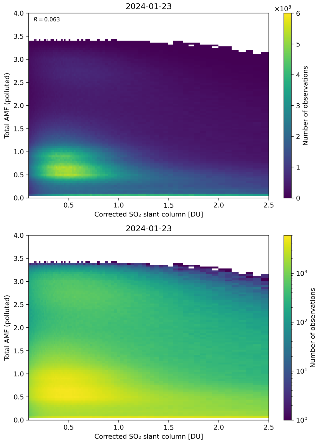
Figure 192: Scatter density plot of “Corrected SO 2 slant column” against “Total AMF (polluted)” for 2024-01-22 to 2024-01-24.
