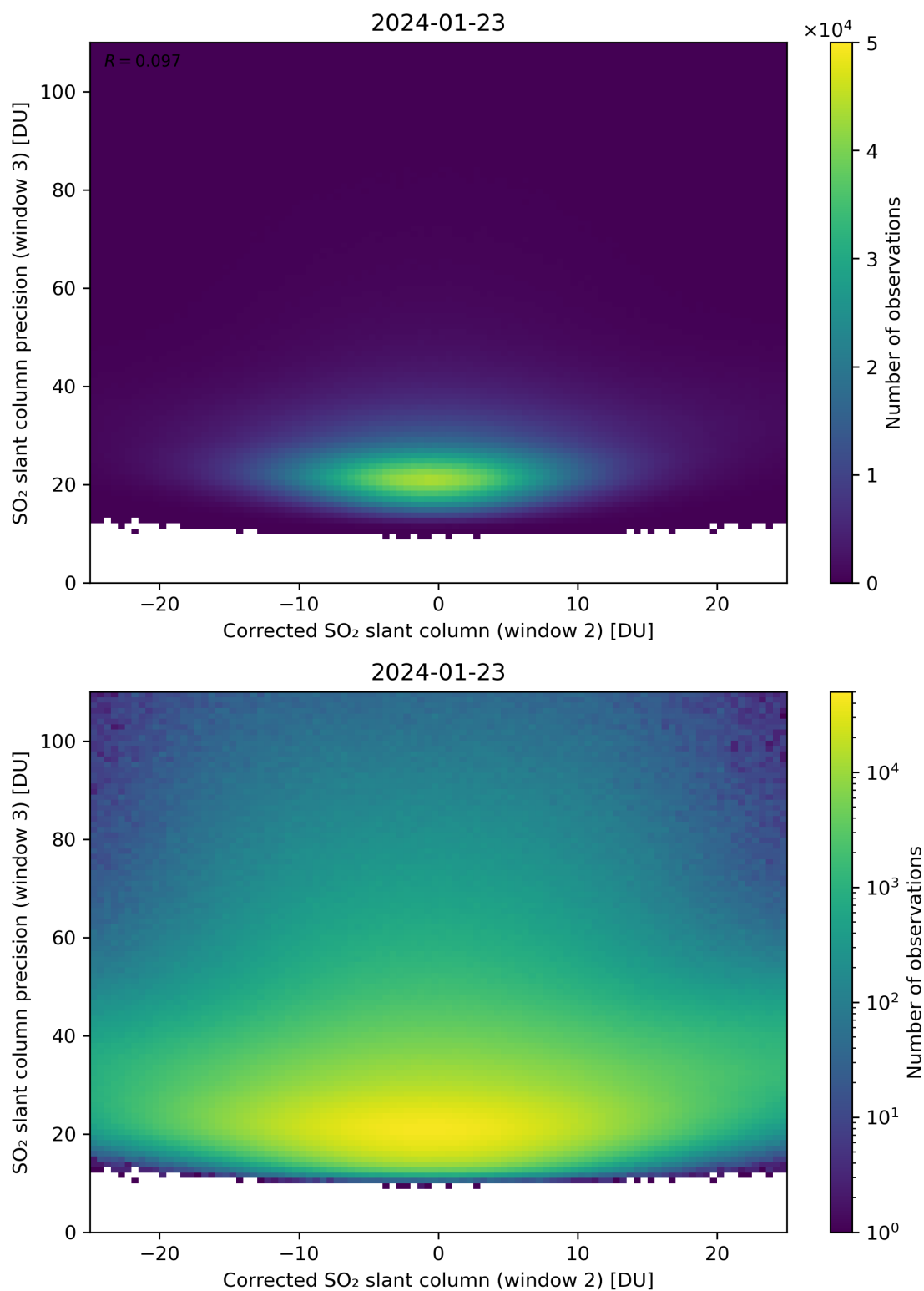
Figure 202: Scatter density plot of “Corrected SO 2 slant column (window 2)” against “SO 2 slant column precision (window 3)” for 2024-01-22 to 2024-01-24.
