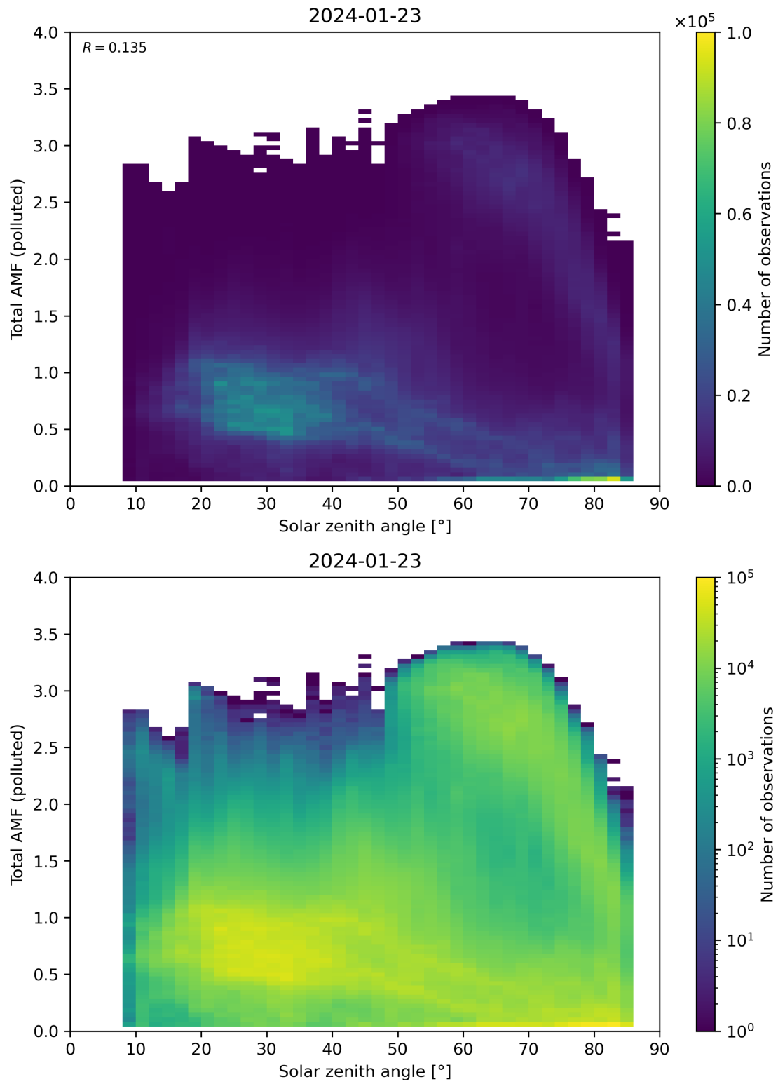
Figure 174: Scatter density plot of “Solar zenith angle” against “Total AMF (polluted)” for 2024-01-22 to 2024-01-24.
