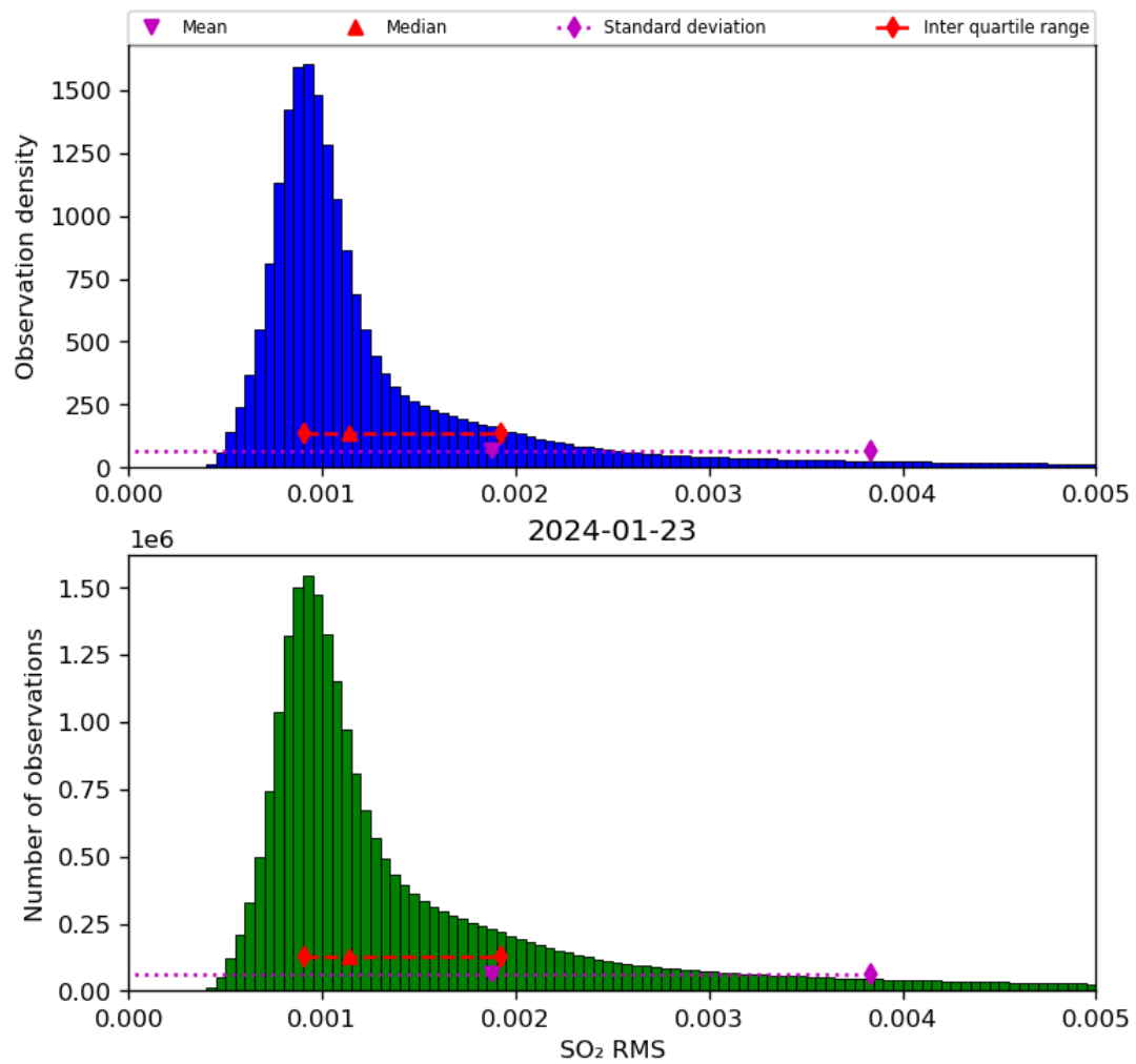
Figure 70: Histogram of “SO 2 RMS” for 2024-01-22 to 2024-01-24
