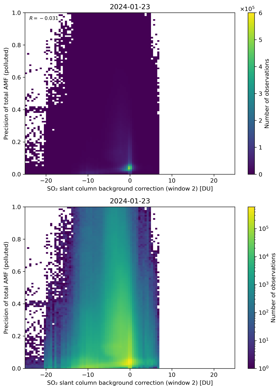
Figure 120: Scatter density plot of “SO 2 slant column background correction (window 2)” against “Precision of total AMF (polluted)” for 2024-01-22 to 2024-01-24.
