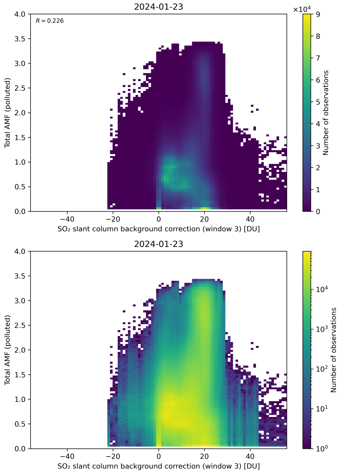
Figure 125: Scatter density plot of “SO 2 slant column background correction (window 3)” against “Total AMF (polluted)” for 2024-01-22 to 2024-01-24.
