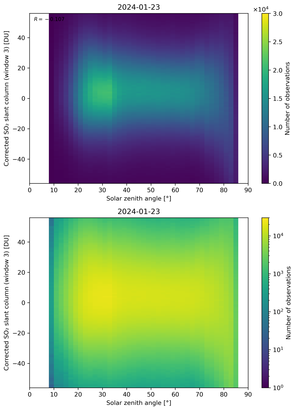
Figure 168: Scatter density plot of “Solar zenith angle” against “Corrected SO 2 slant column (window 3)” for 2024-01-22 to 2024-01-24.
