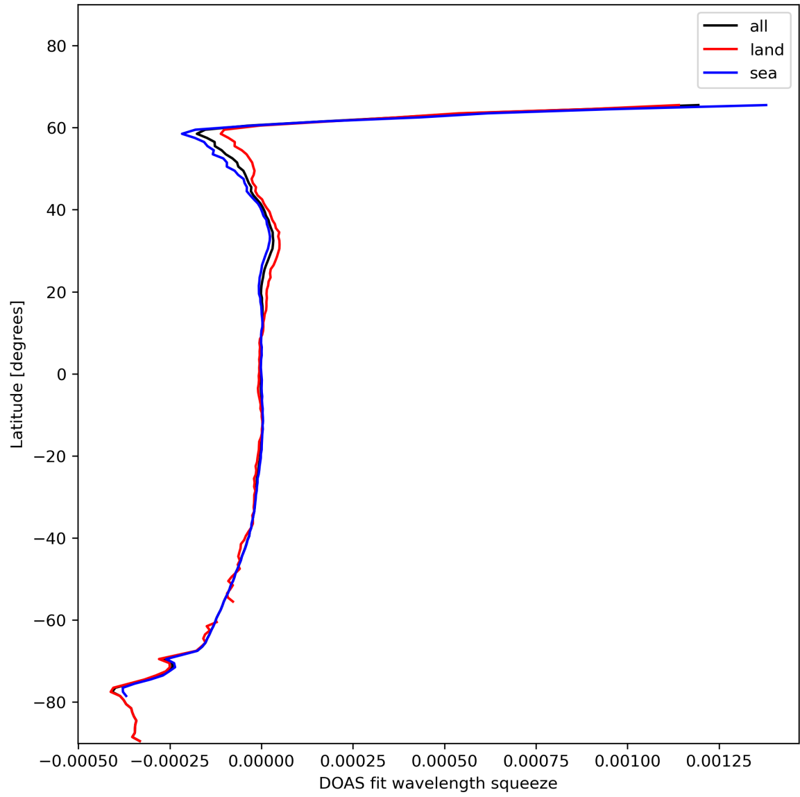
Figure 46: Zonal average of “DOAS fit wavelength squeeze” for 2024-01-22 to 2024-01-24.
