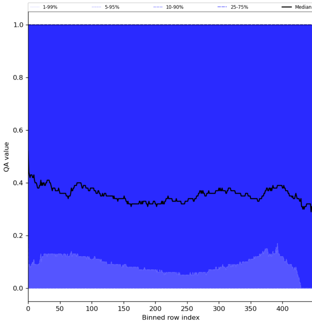
Figure 75: Along track statistics of “QA value” for 2024-01-22 to 2024-01-24
