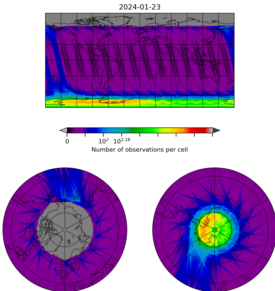
Figure 28: Map of the number of observations for 2024-01-22 to 2024-01-24
