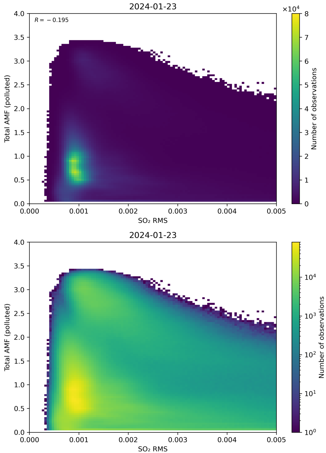
Figure 137: Scatter density plot of “SO 2 RMS” against “Total AMF (polluted)” for 2024-01-22 to 2024-01-24.
