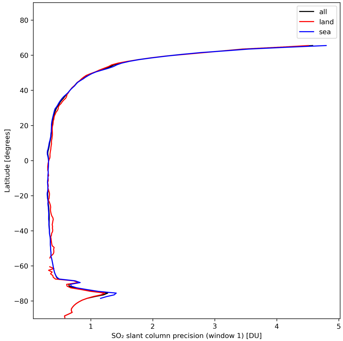
Figure 34: Zonal average of “SO 2 slant column precision (window 1)” for 2024-01-22 to 2024-01-24.
