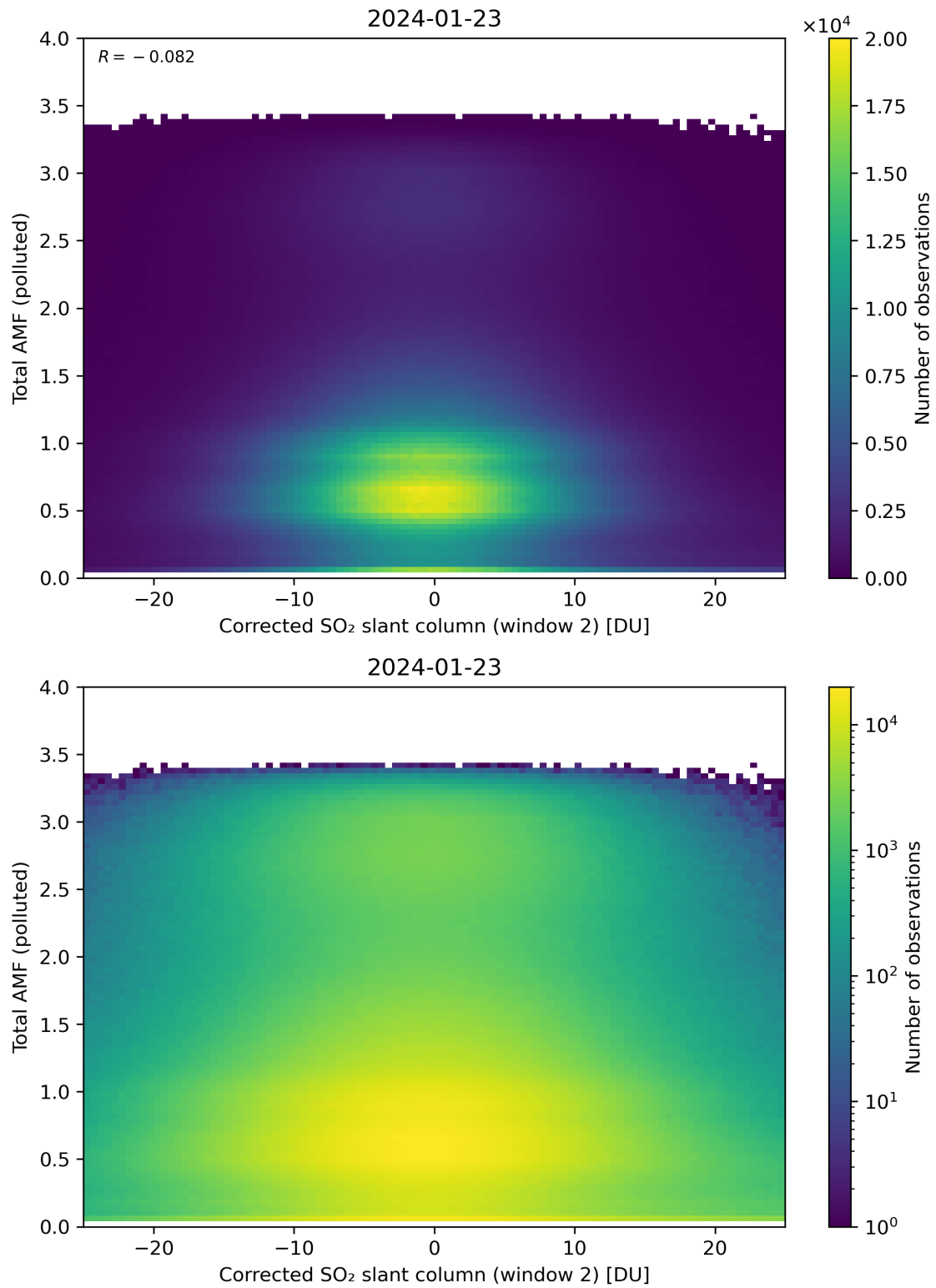
Figure 203: Scatter density plot of “Corrected SO 2 slant column (window 2)” against “Total AMF (polluted)” for 2024-01-22 to 2024-01-24.
