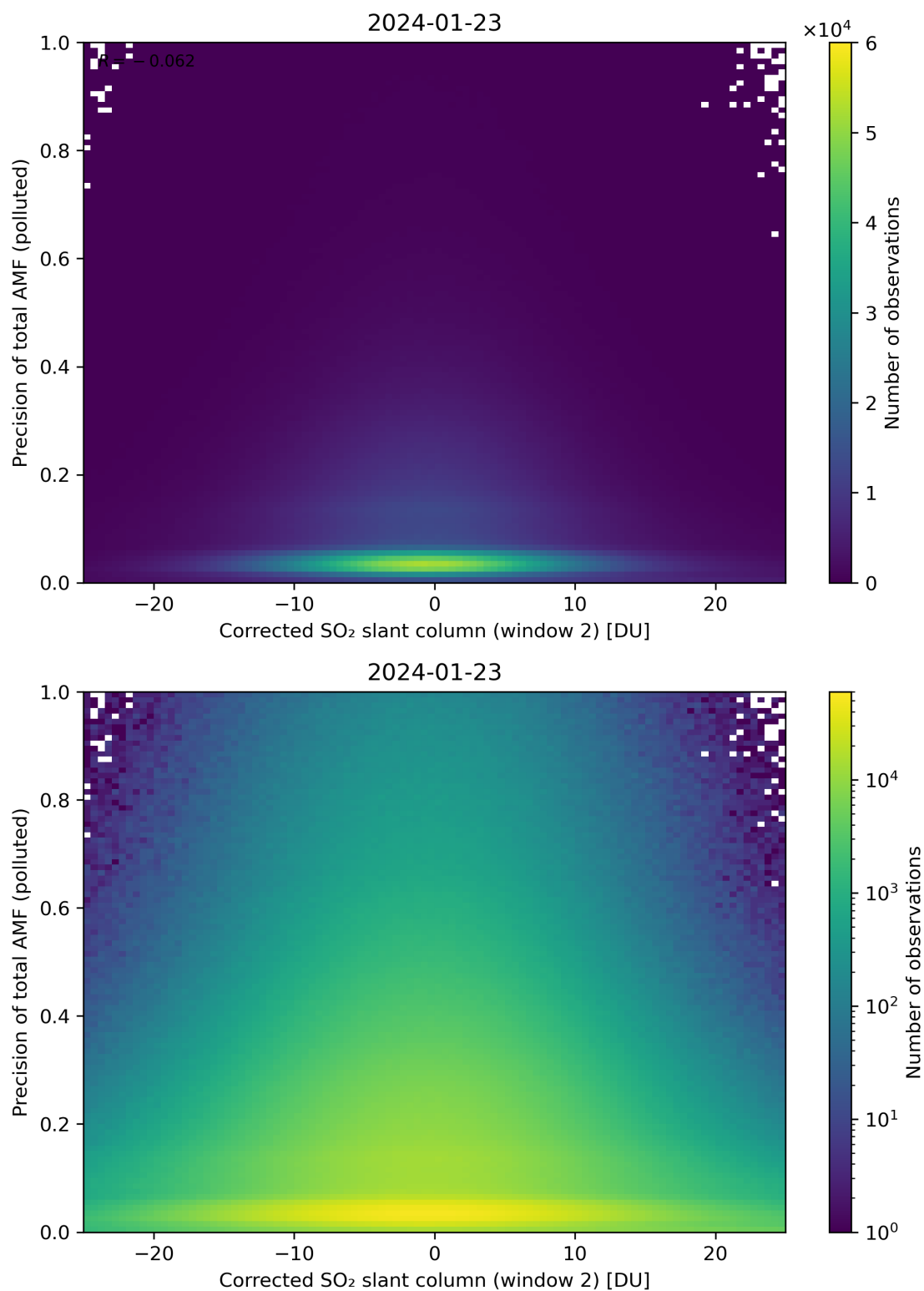
Figure 204: Scatter density plot of “Corrected SO 2 slant column (window 2)” against “Precision of total AMF (polluted)” for 2024-01-22 to 2024-01-24.
