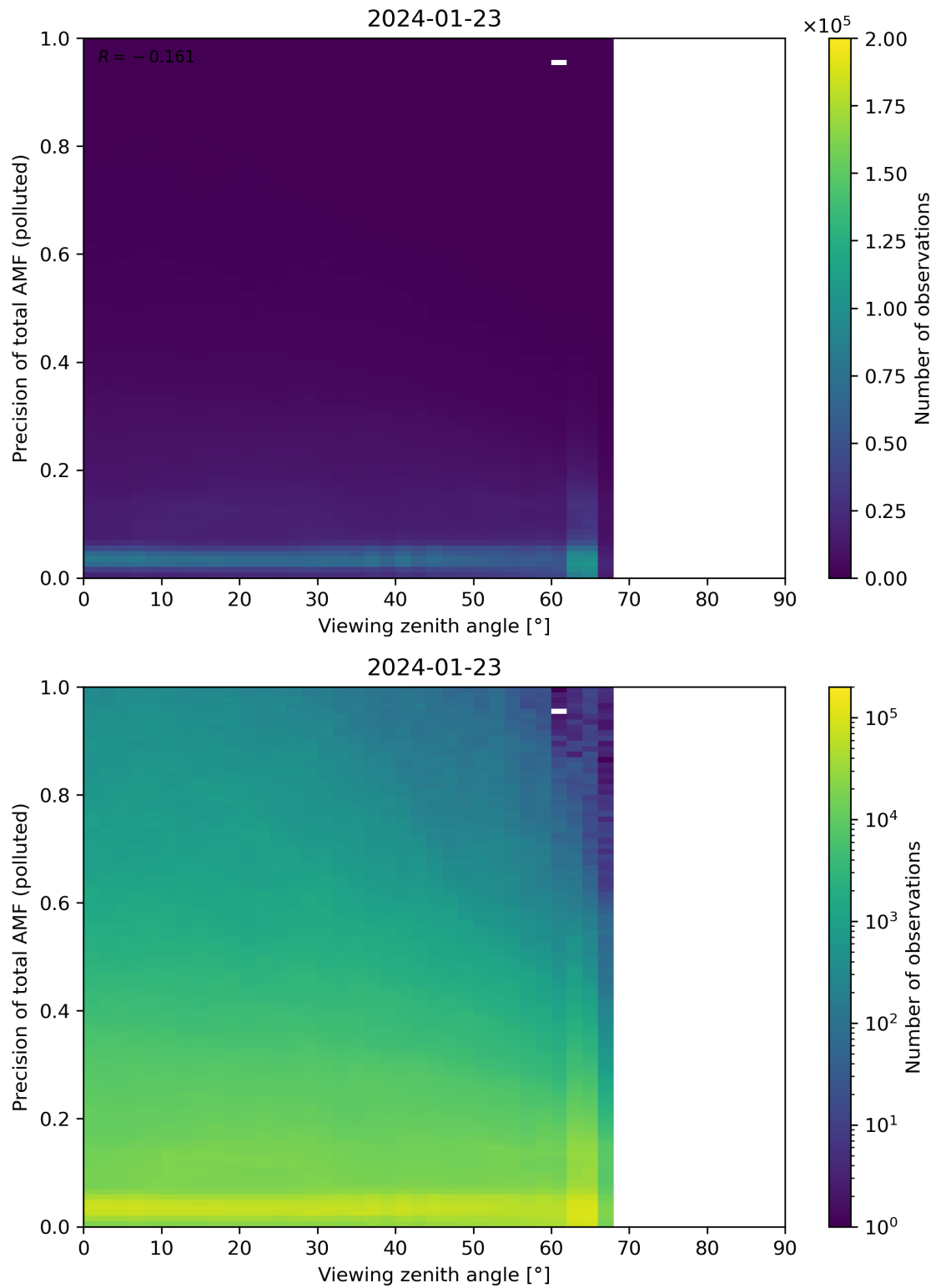
Figure 326: Scatter density plot of “Viewing zenith angle” against “Precision of total AMF (polluted)” for 2024-01-22 to 2024-01-24.
