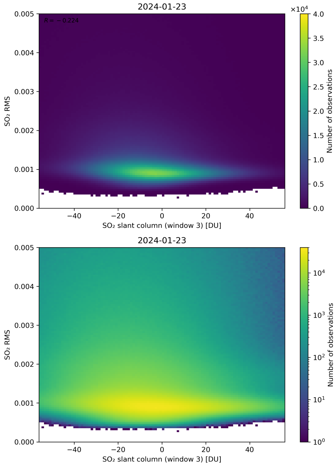
Figure 256: Scatter density plot of “SO 2 slant column (window 3)” against “SO 2 RMS” for 2024-01-22 to 2024-01-24.
