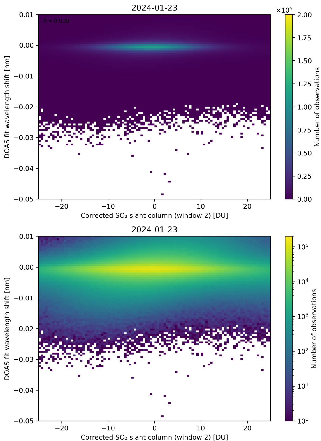
Figure 196: Scatter density plot of “Corrected SO 2 slant column (window 2)” against “DOAS fit wavelength shift” for 2024-01-22 to 2024-01-24.
