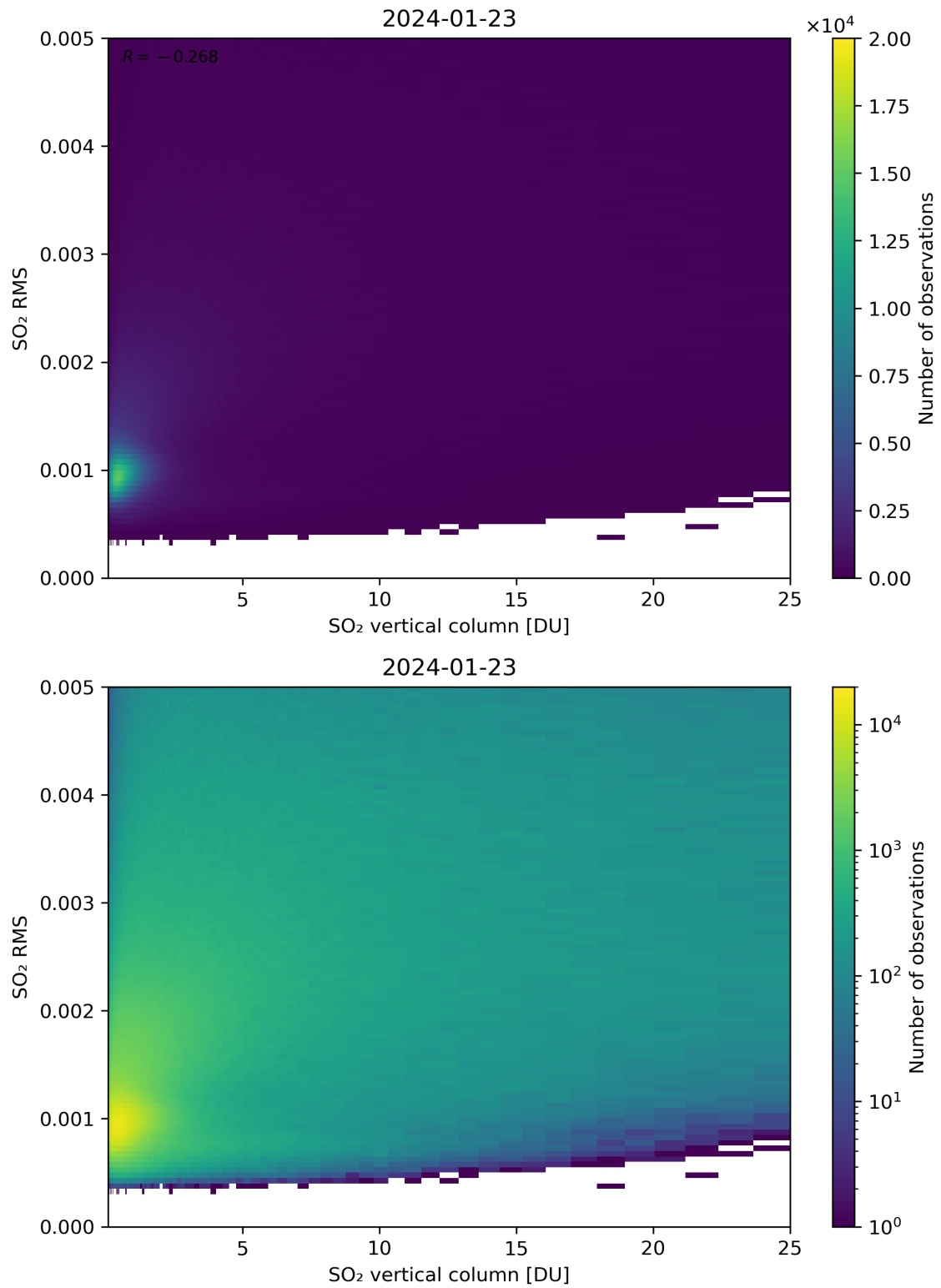
Figure 278: Scatter density plot of “SO 2 vertical column” against “SO 2 RMS” for 2024-01-22 to 2024-01-24.
