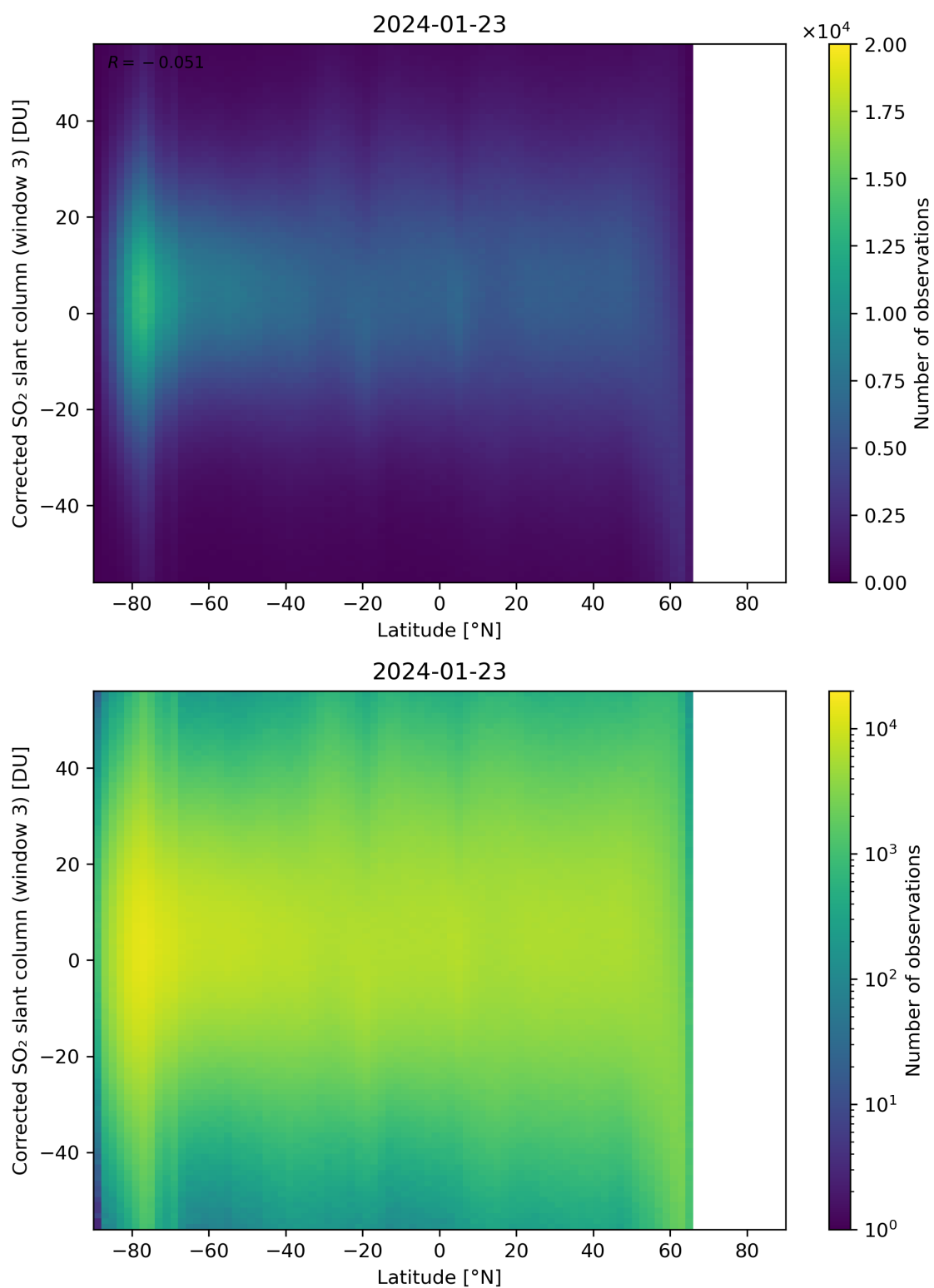
Figure 148: Scatter density plot of “Latitude” against “Corrected SO 2 slant column (window 3)” for 2024-01-22 to 2024-01-24.
