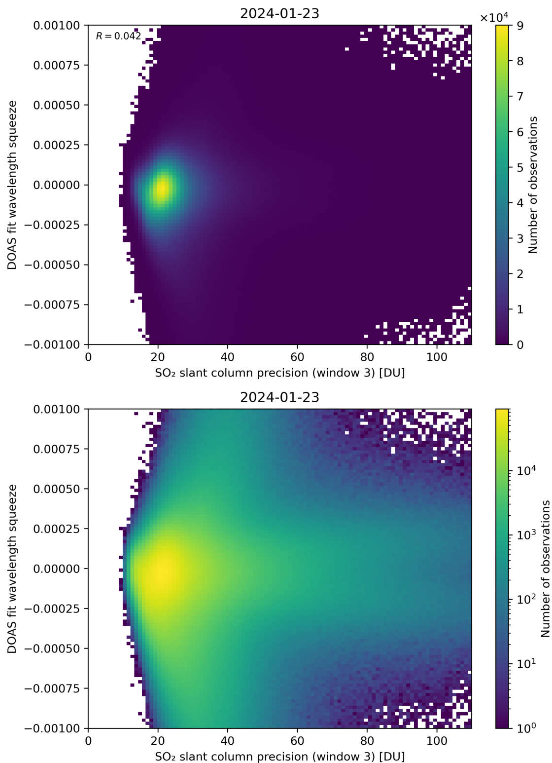
Figure 259: Scatter density plot of “SO 2 slant column precision (window 3)” against “DOAS fit wavelength squeeze” for 2024-01-22 to 2024-01-24.
