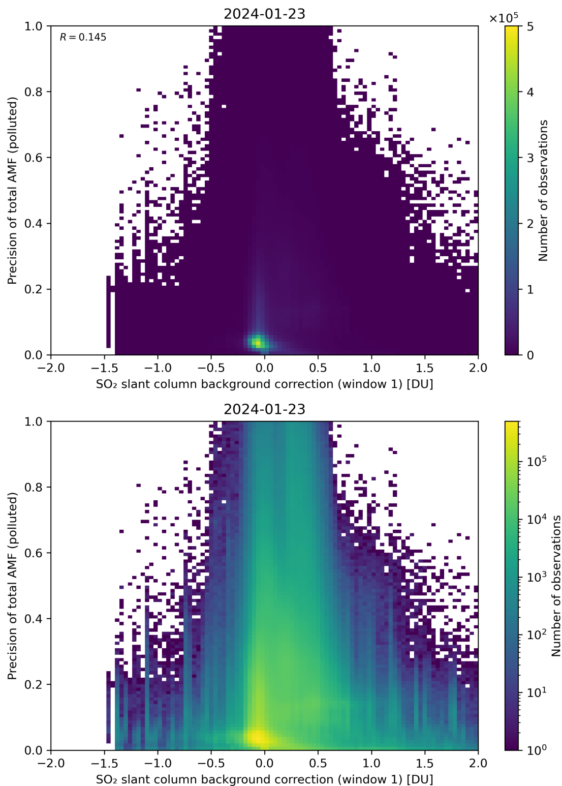
Figure 110: Scatter density plot of “SO 2 slant column background correction (window 1)” against “Precision of total AMF (polluted)” for 2024-01-22 to 2024-01-24.
