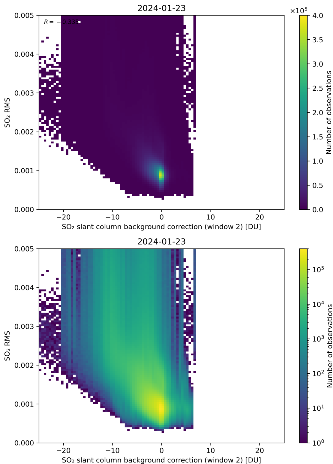
Figure 114: Scatter density plot of “SO 2 slant column background correction (window 2)” against “SO 2 RMS” for 2024-01-22 to 2024-01-24.
