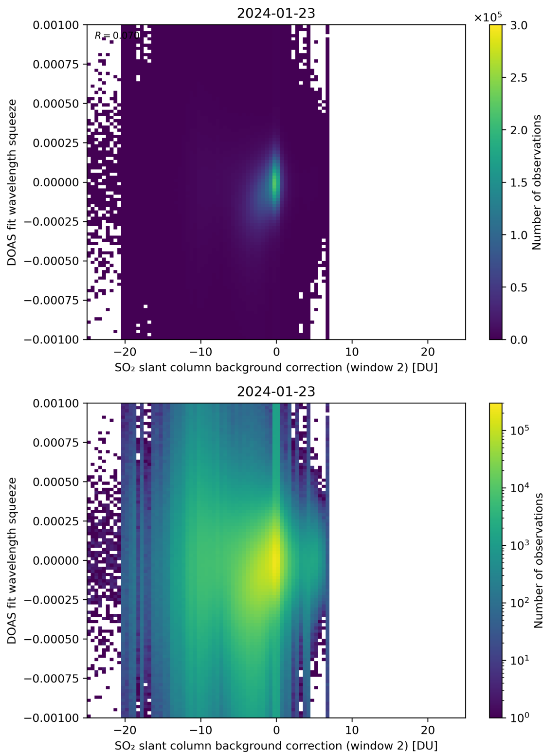
Figure 113: Scatter density plot of “SO 2 slant column background correction (window 2)” against “DOAS fit wavelength squeeze” for 2024-01-22 to 2024-01-24.
