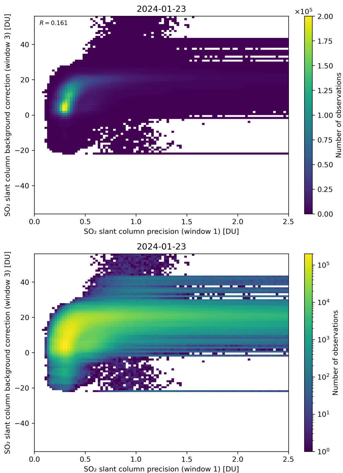
Figure 220: Scatter density plot of “SO 2 slant column precision (window 1)” against “SO 2 slant column background correction (window 3)” for 2024-01-22 to 2024-01-24.
