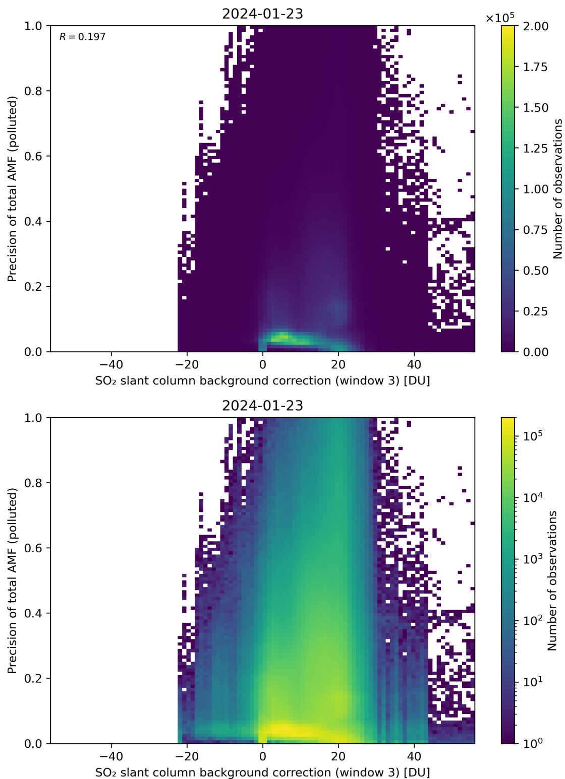
Figure 126: Scatter density plot of “SO 2 slant column background correction (window 3)” against “Precision of total AMF (polluted)” for 2024-01-22 to 2024-01-24.
