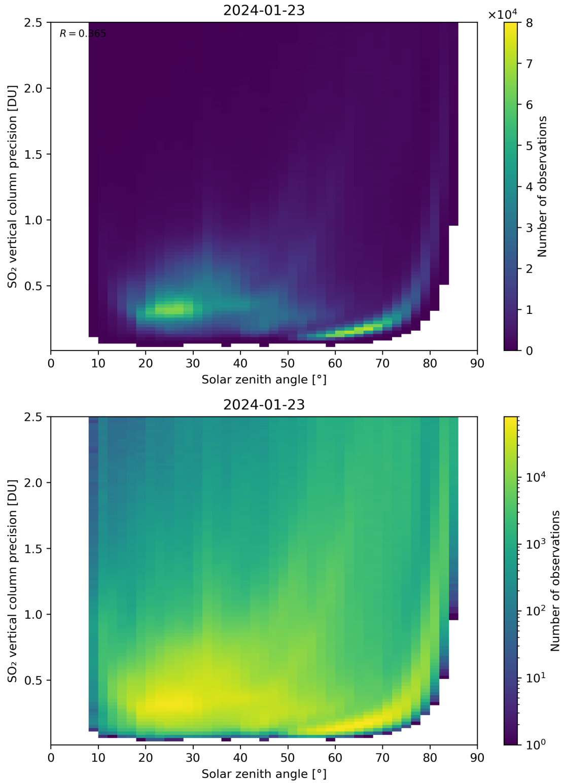
Figure 177: Scatter density plot of “Solar zenith angle” against “SO 2 vertical column precision” for 2024-01-22 to 2024-01-24.
