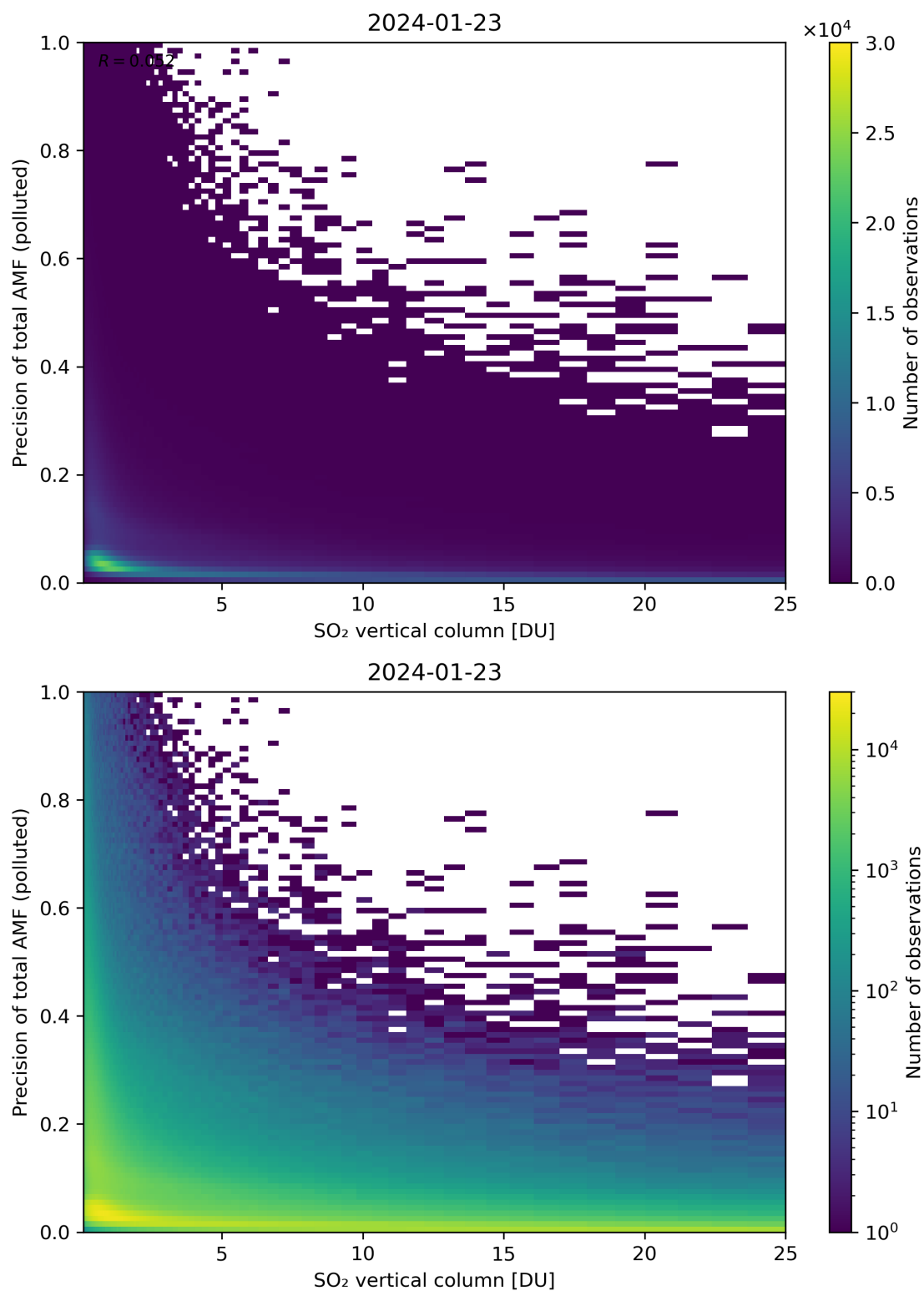
Figure 306: Scatter density plot of “SO 2 vertical column” against “Precision of total AMF (polluted)” for 2024-01-22 to 2024-01-24.
