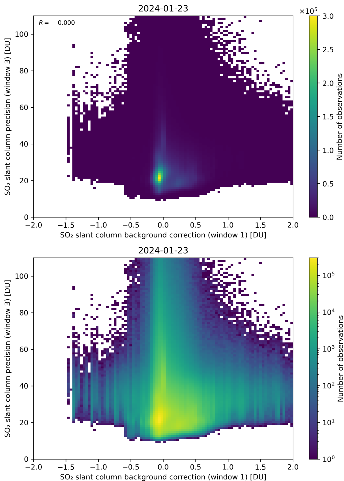
Figure 108: Scatter density plot of “SO 2 slant column background correction (window 1)” against “SO 2 slant column precision (window 3)” for 2024-01-22 to 2024-01-24.
