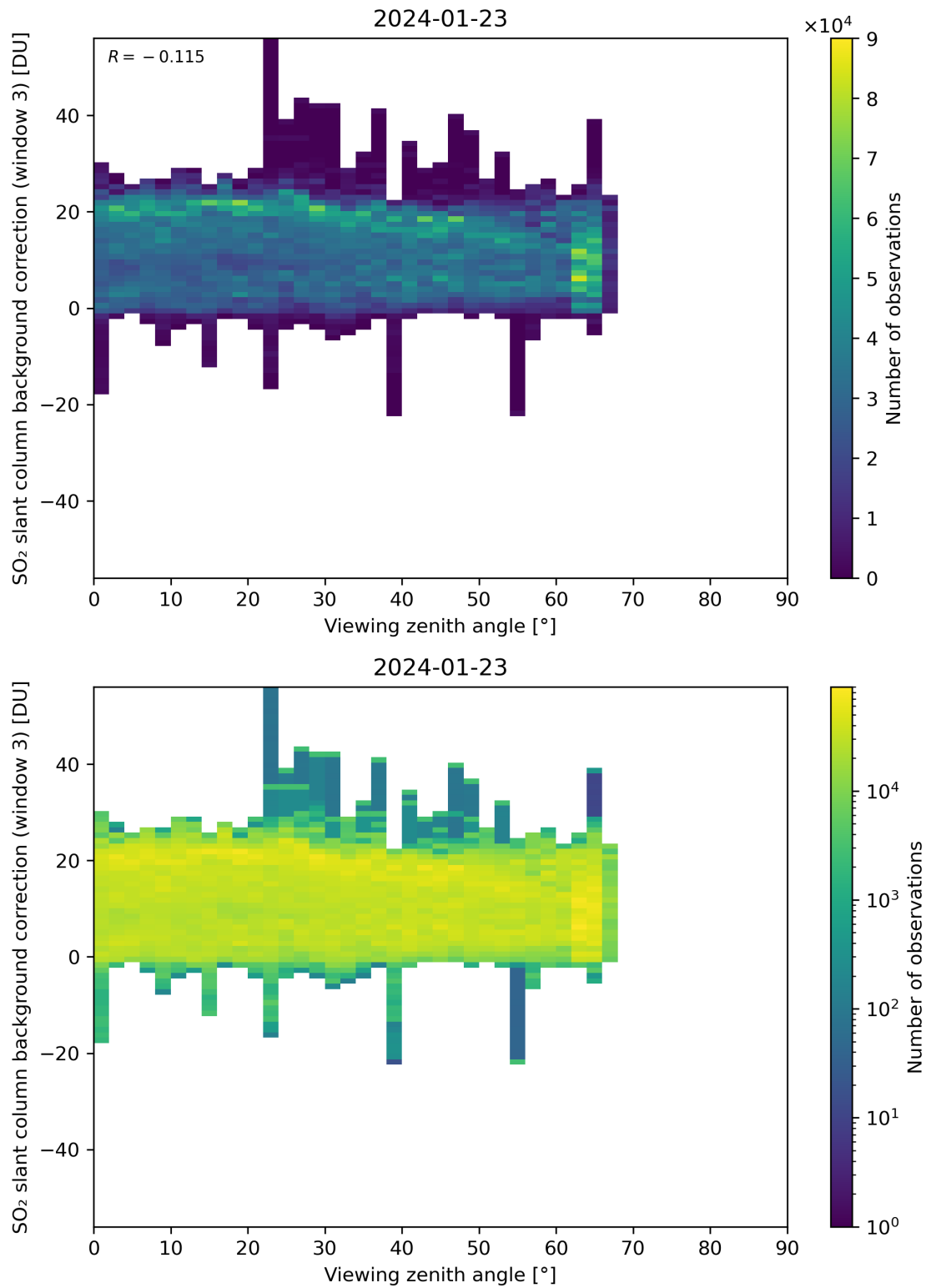
Figure 310: Scatter density plot of “Viewing zenith angle” against “SO 2 slant column background correction (window 3)” for 2024-01-22 to 2024-01-24.
