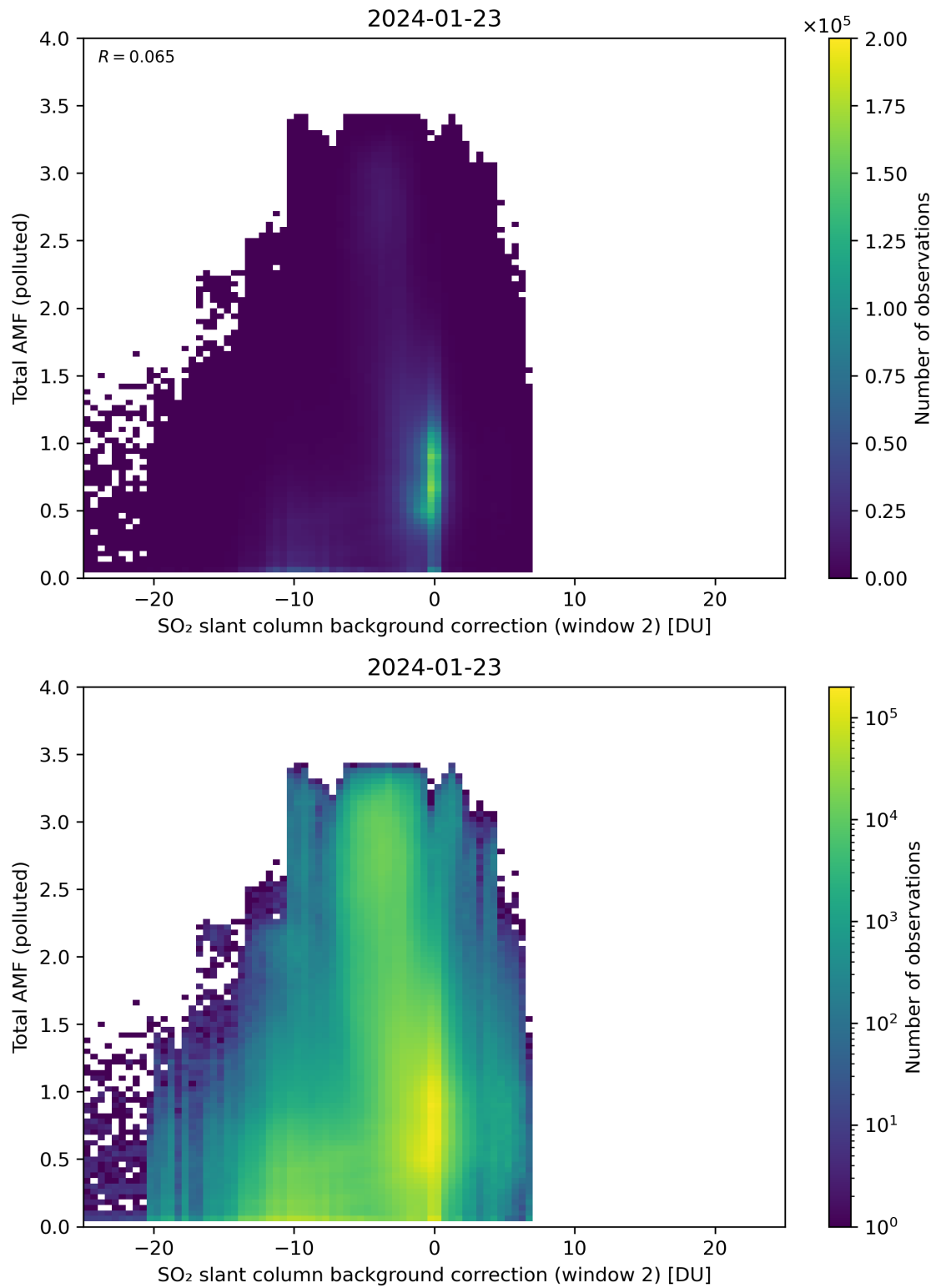
Figure 119: Scatter density plot of “SO 2 slant column background correction (window 2)” against “Total AMF (polluted)” for 2024-01-22 to 2024-01-24.
