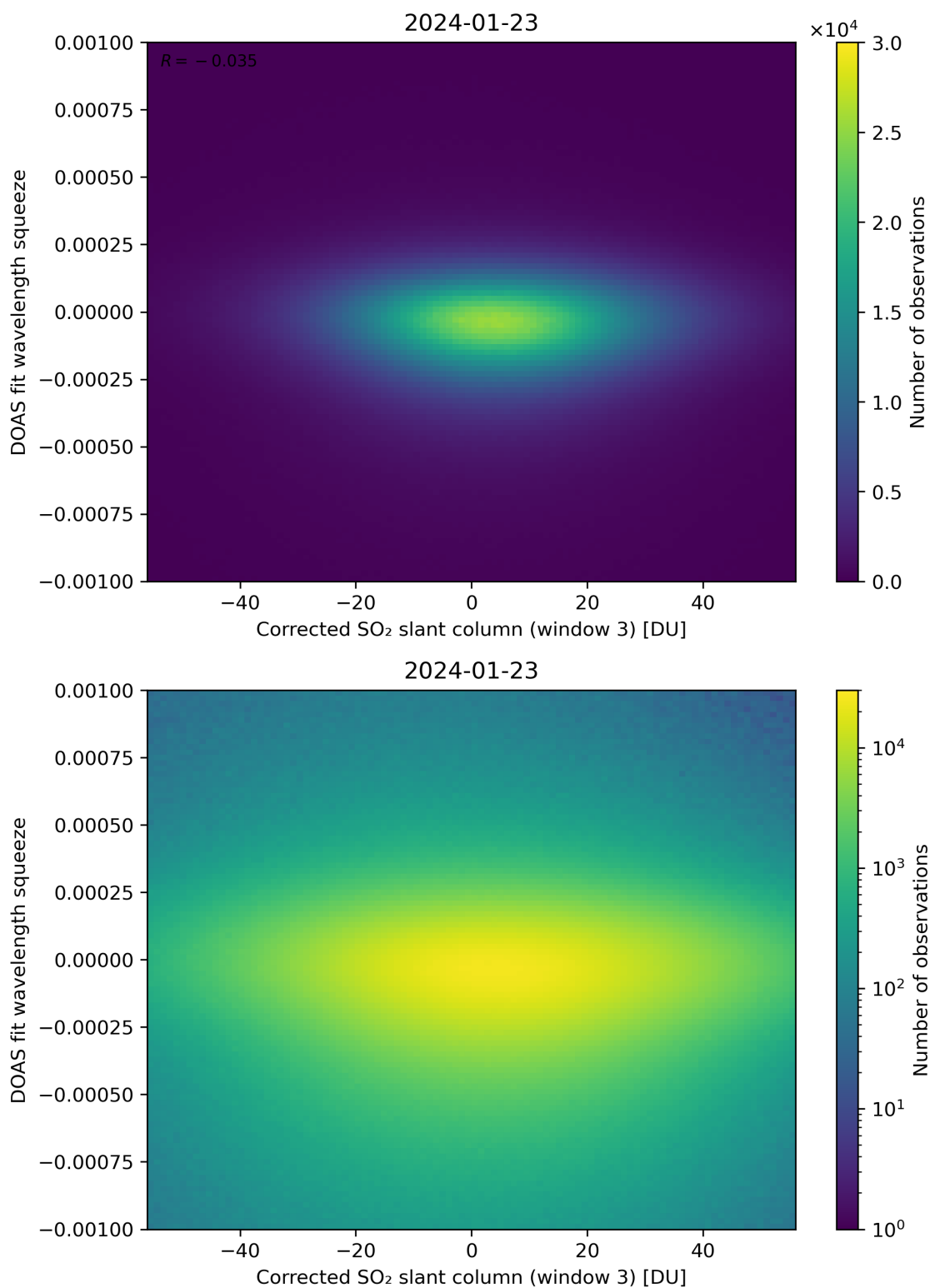
Figure 207: Scatter density plot of “Corrected SO 2 slant column (window 3)” against “DOAS fit wavelength squeeze” for 2024-01-22 to 2024-01-24.
