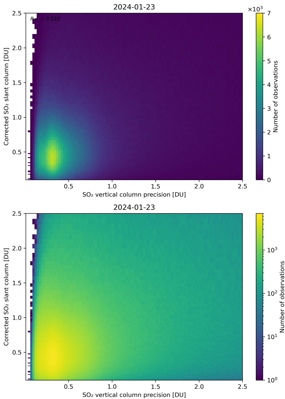
Figure 286: Scatter density plot of “SO 2 vertical column precision” against “Corrected SO 2 slant column” for 2024-01-22 to 2024-01-24.
