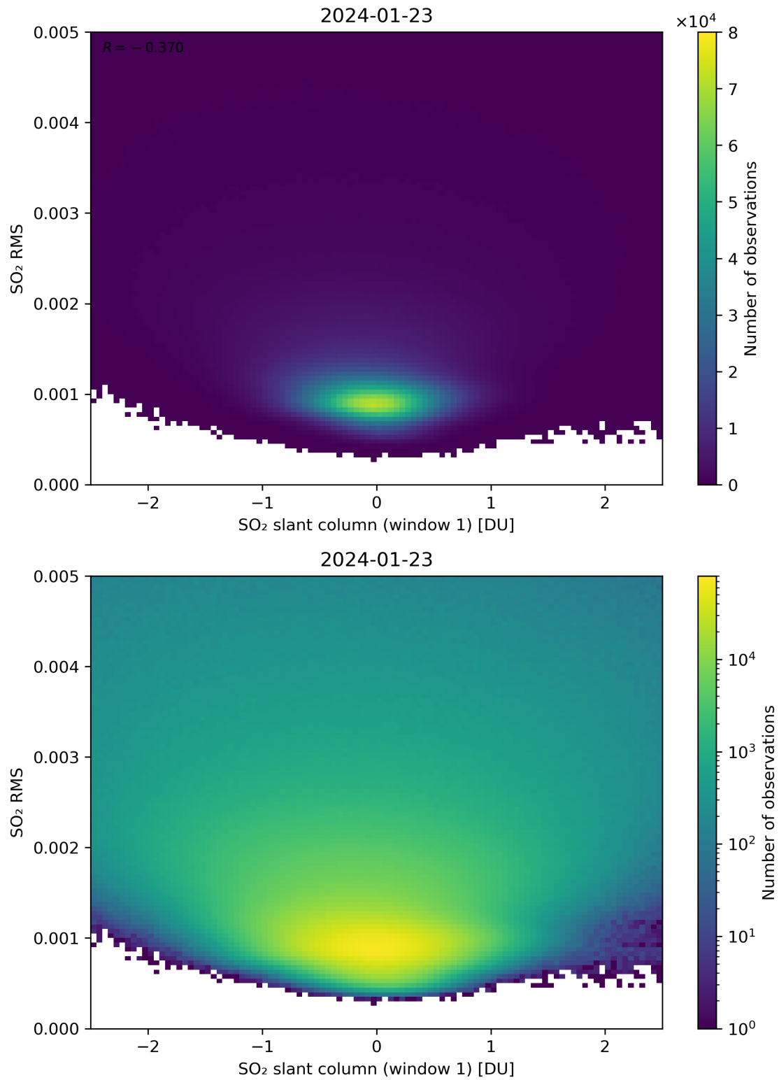
Figure 217: Scatter density plot of “SO 2 slant column (window 1)” against “SO 2 RMS” for 2024-01-22 to 2024-01-24.
