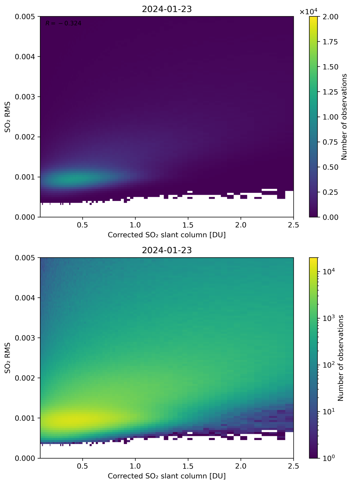
Figure 183: Scatter density plot of “Corrected SO 2 slant column” against “SO 2 RMS” for 2024-01-22 to 2024-01-24.
