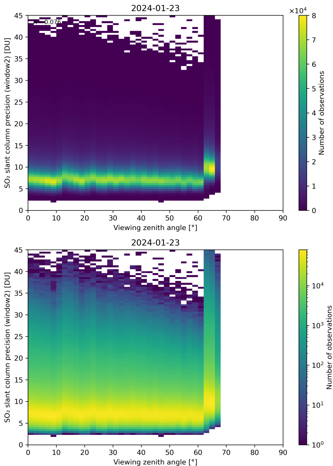
Figure 322: Scatter density plot of “Viewing zenith angle” against “SO 2 slant column precision (window2)” for 2024-01-22 to 2024-01-24.
