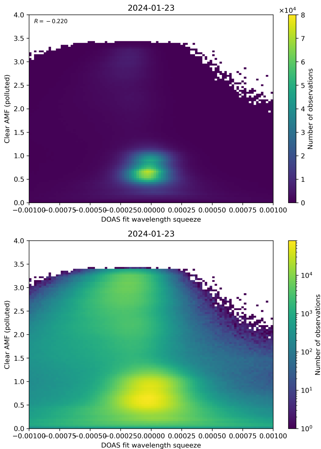
Figure 133: Scatter density plot of “DOAS fit wavelength squeeze” against “Clear AMF (polluted)” for 2024-01-22 to 2024-01-24.
