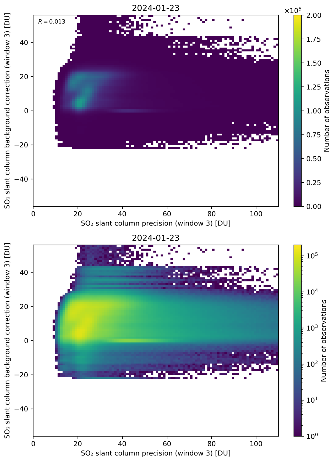
Figure 257: Scatter density plot of “SO 2 slant column precision (window 3)” against “SO 2 slant column background correction (window 3)” for 2024-01-22 to 2024-01-24.
