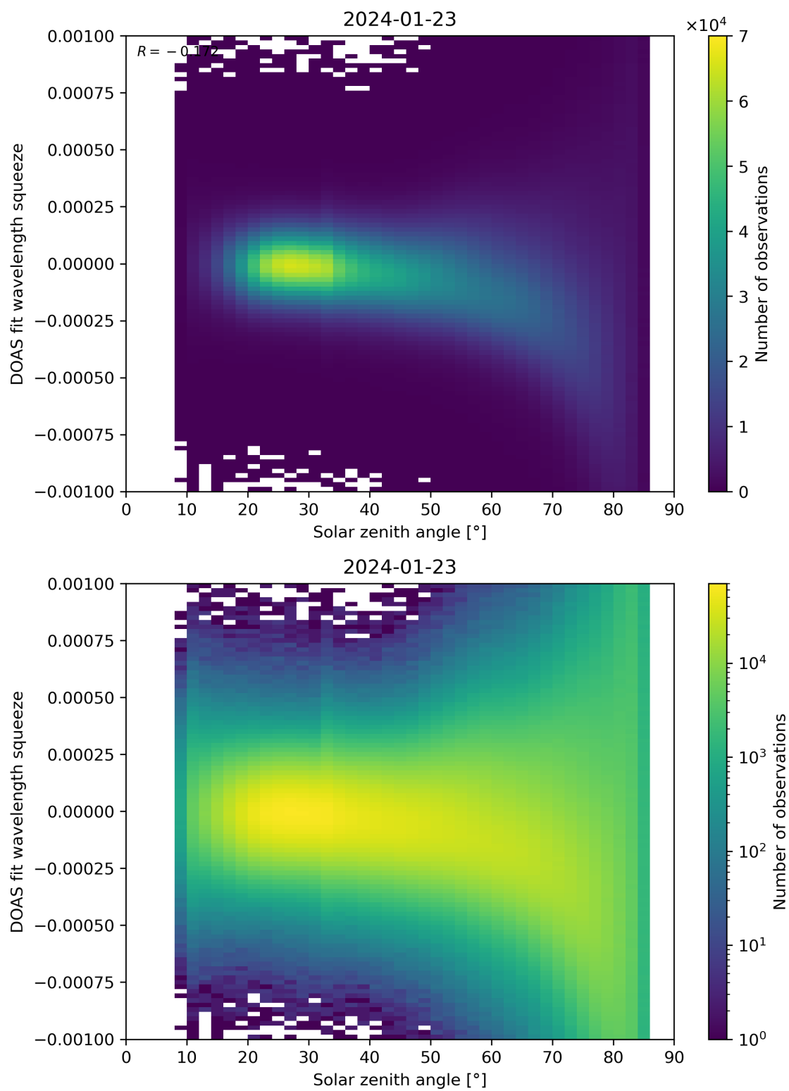
Figure 162: Scatter density plot of “Solar zenith angle” against “DOAS fit wavelength squeeze” for 2024-01-22 to 2024-01-24.
