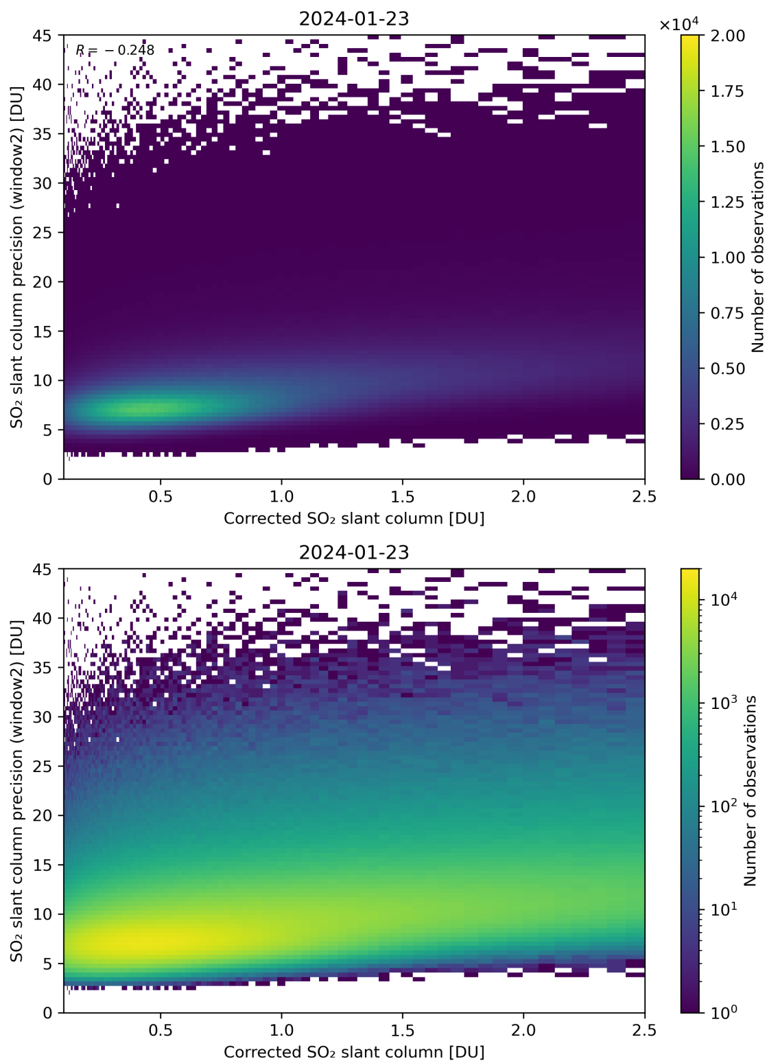
Figure 189: Scatter density plot of “Corrected SO 2 slant column” against “SO 2 slant column precision (window2)” for 2024-01-22 to 2024-01-24.
