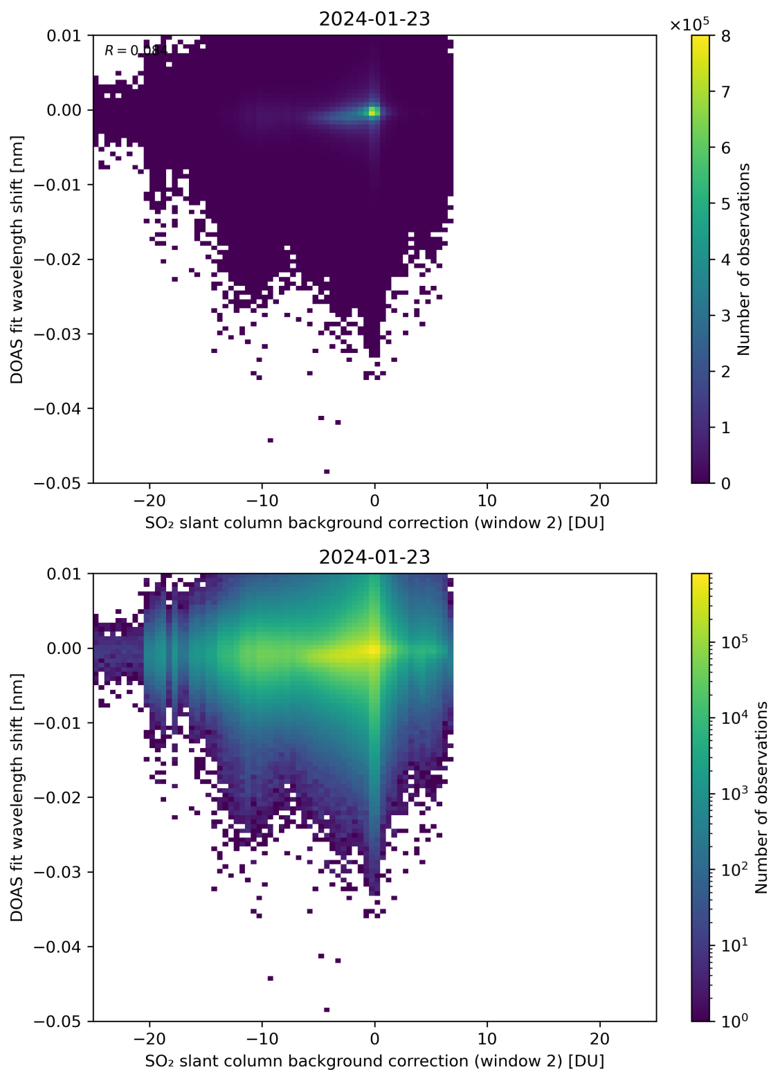
Figure 112: Scatter density plot of “SO 2 slant column background correction (window 2)” against “DOAS fit wavelength shift” for 2024-01-22 to 2024-01-24.
