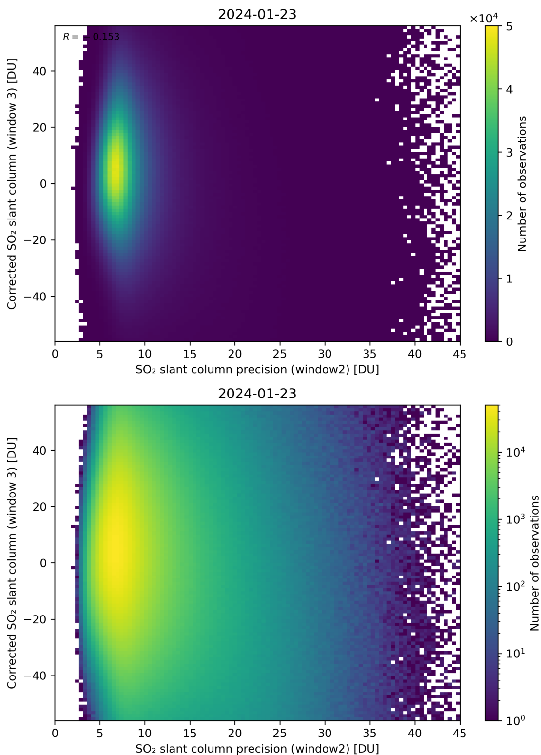
Figure 248: Scatter density plot of “SO 2 slant column precision (window2)” against “Corrected SO 2 slant column (window 3)” for 2024-01-22 to 2024-01-24.
