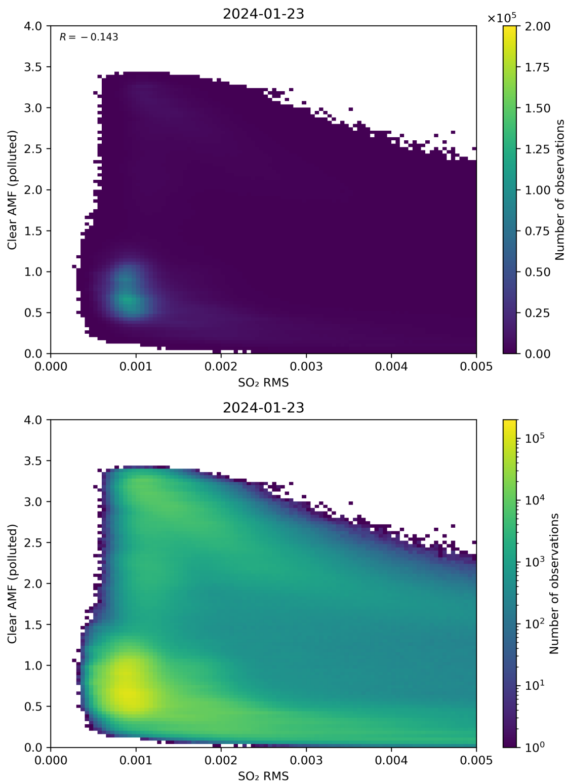
Figure 136: Scatter density plot of “SO 2 RMS” against “Clear AMF (polluted)” for 2024-01-22 to 2024-01-24.
