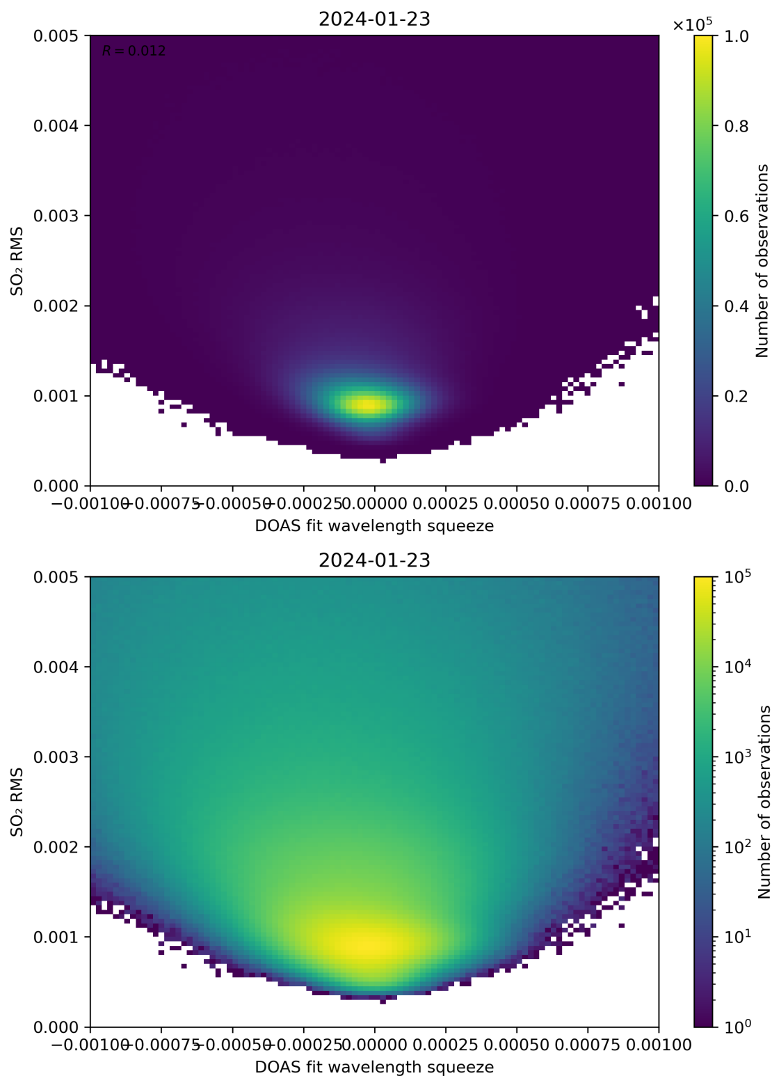
Figure 132: Scatter density plot of “DOAS fit wavelength squeeze” against “SO 2 RMS” for 2024-01-22 to 2024-01-24.
