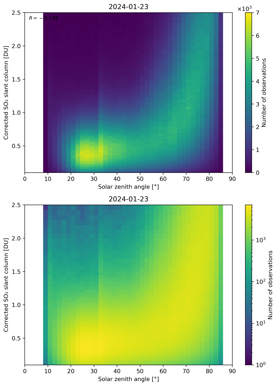
Figure 166: Scatter density plot of “Solar zenith angle” against “Corrected SO 2 slant column” for 2024-01-22 to 2024-01-24.
