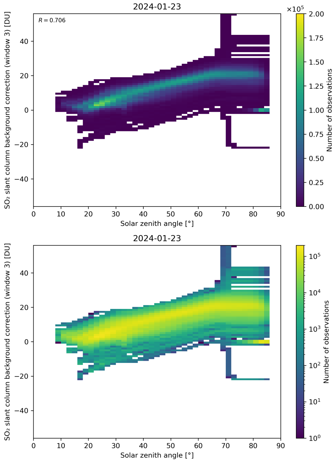
Figure 160: Scatter density plot of “Solar zenith angle” against “SO 2 slant column background correction (window 3)” for 2024-01-22 to 2024-01-24.
