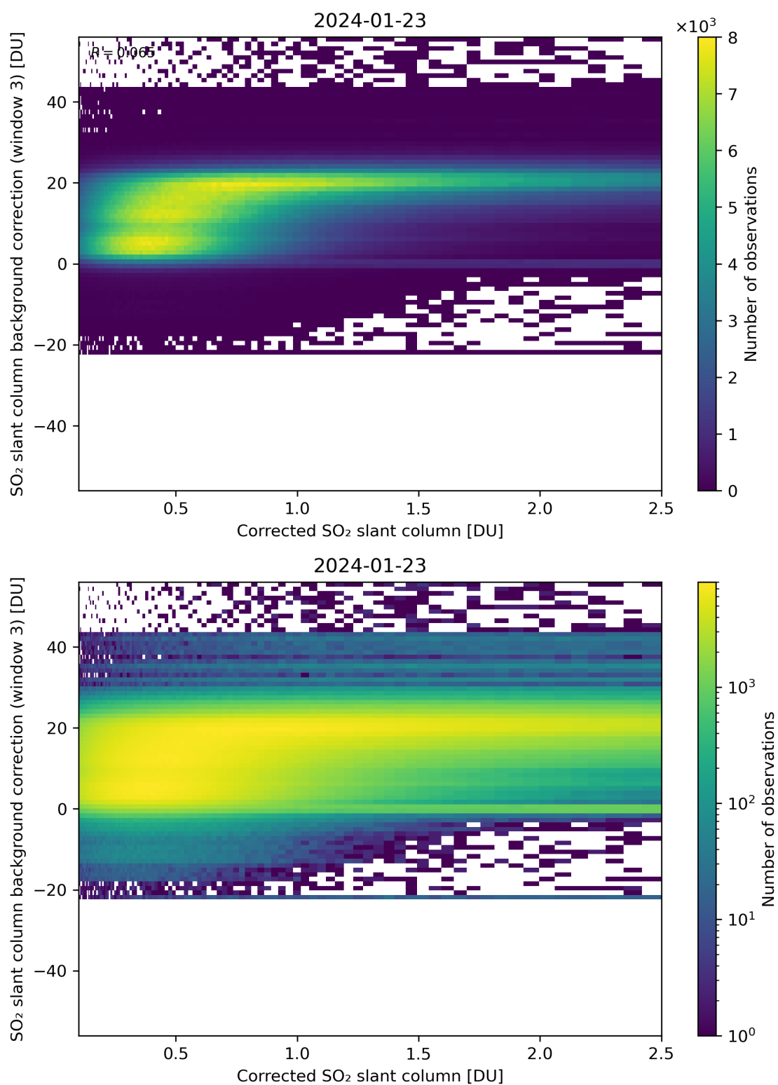
Figure 180: Scatter density plot of “Corrected SO 2 slant column” against “SO 2 slant column background correction (window 3)” for 2024-01-22 to 2024-01-24.
