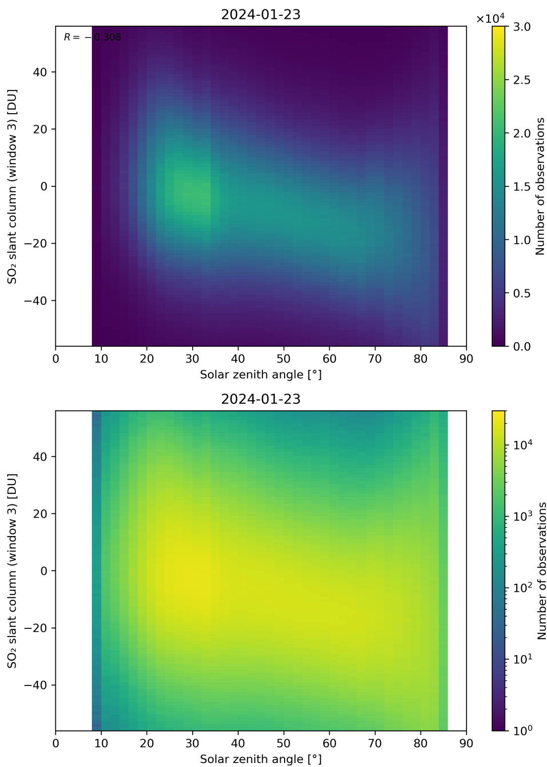
Figure 172: Scatter density plot of “Solar zenith angle” against “SO 2 slant column (window 3)” for 2024-01-22 to 2024-01-24.
