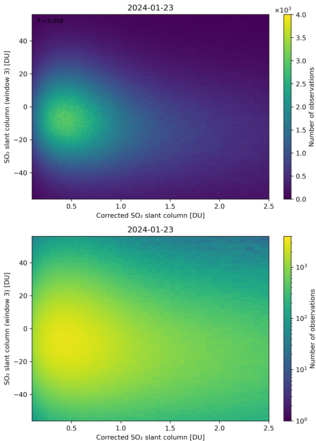
Figure 190: Scatter density plot of “Corrected SO 2 slant column” against “SO 2 slant column (window 3)” for 2024-01-22 to 2024-01-24.
