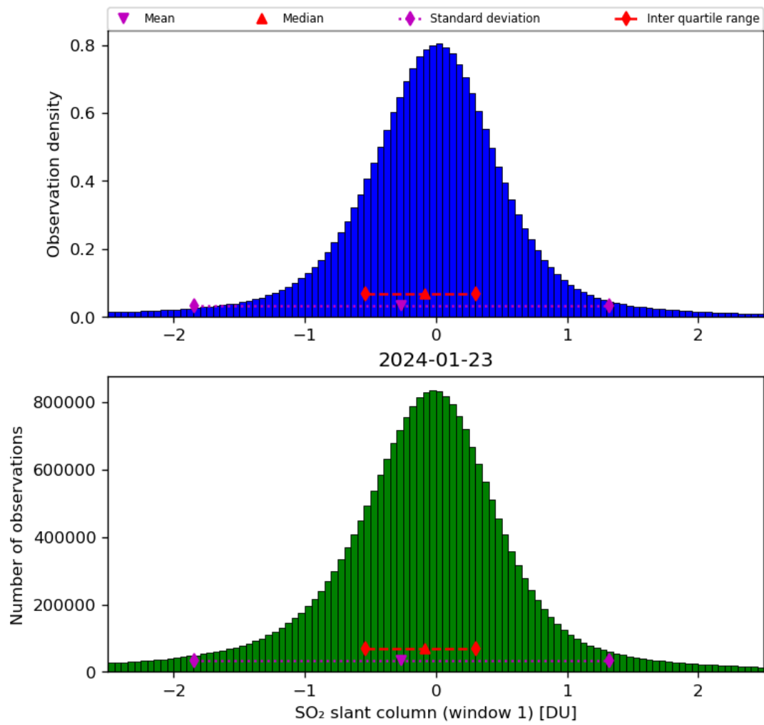
Figure 56: Histogram of “SO 2 slant column (window 1)” for 2024-01-22 to 2024-01-24
