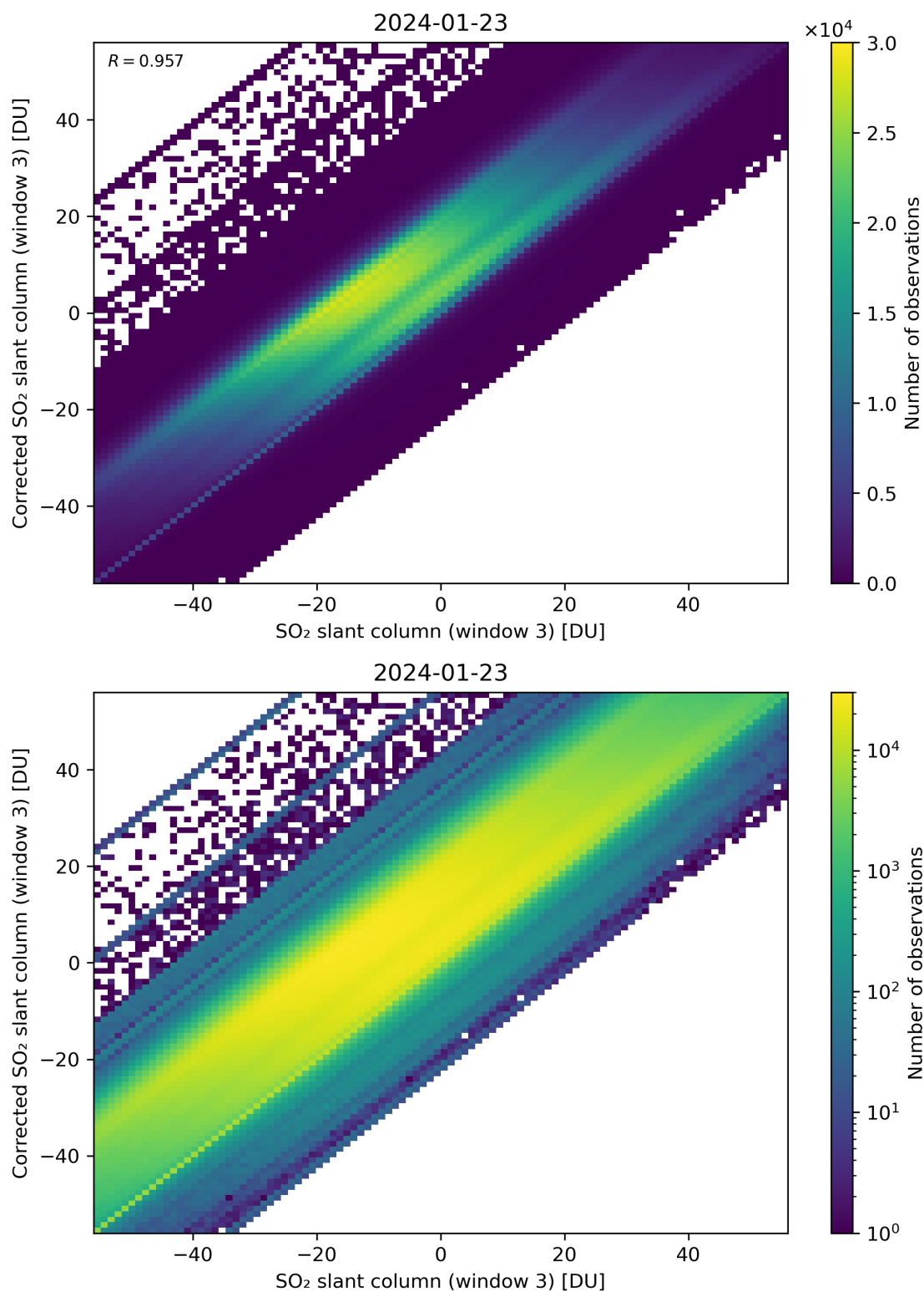
Figure 266: Scatter density plot of “SO 2 slant column (window 3)” against “Corrected SO 2 slant column (window 3)” for 2024-01-22 to 2024-01-24.
