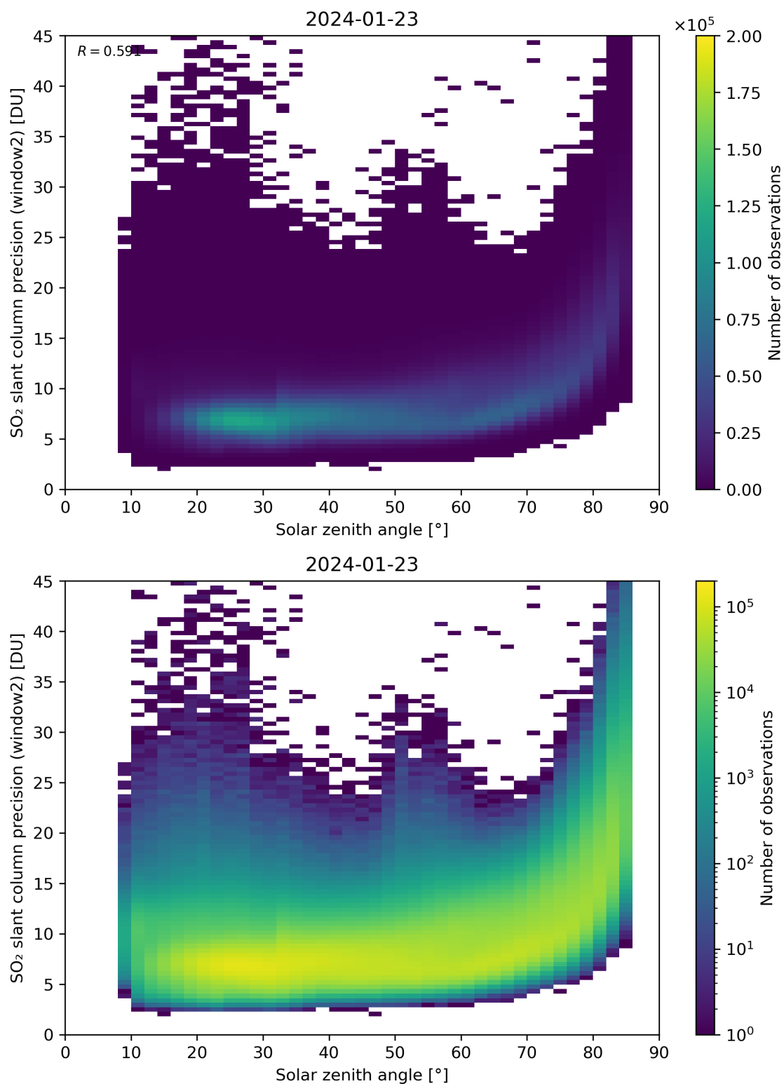
Figure 171: Scatter density plot of “Solar zenith angle” against “SO 2 slant column precision (window2)” for 2024-01-22 to 2024-01-24.
