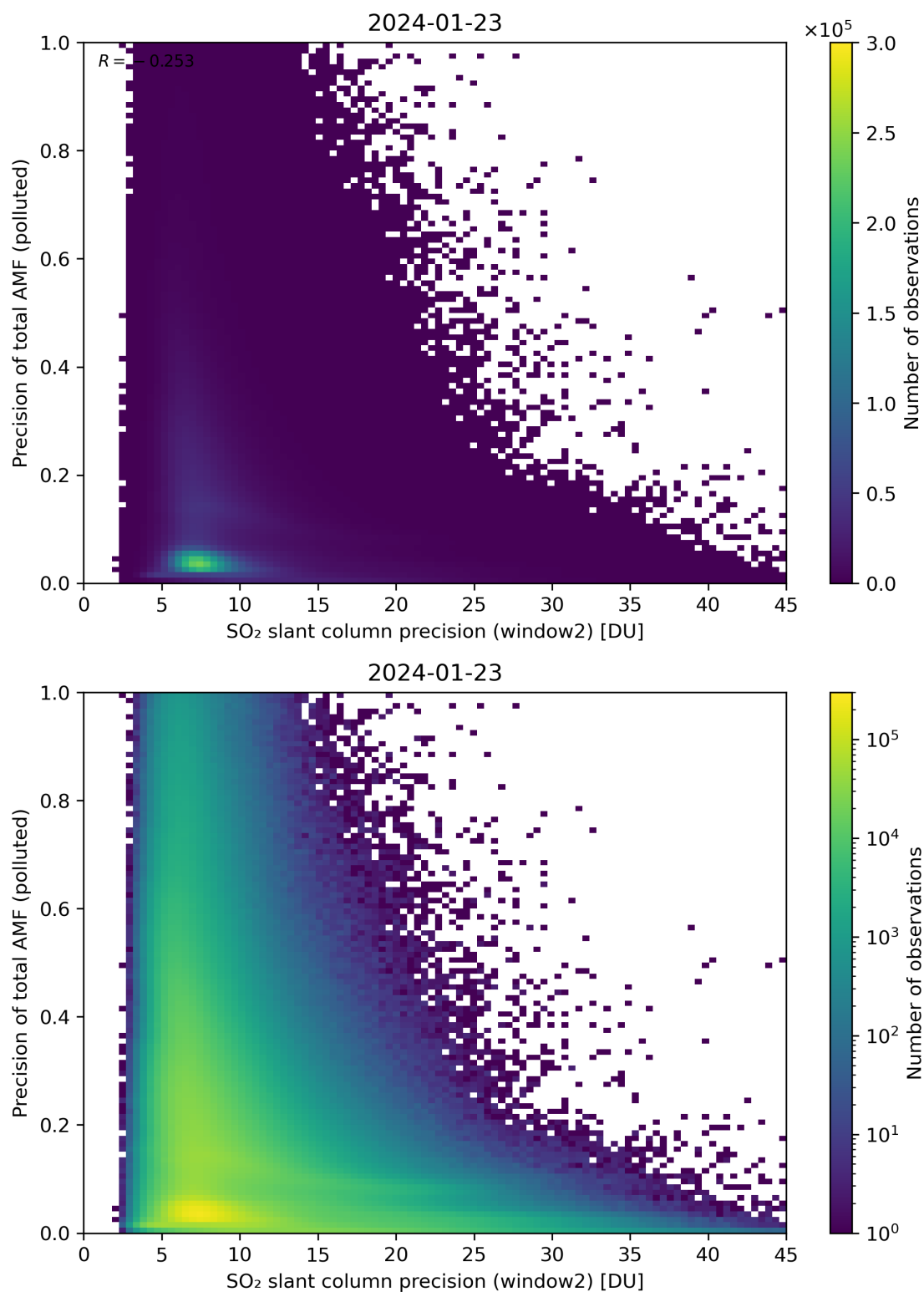
Figure 252: Scatter density plot of “SO 2 slant column precision (window2)” against “Precision of total AMF (polluted)” for 2024-01-22 to 2024-01-24.
