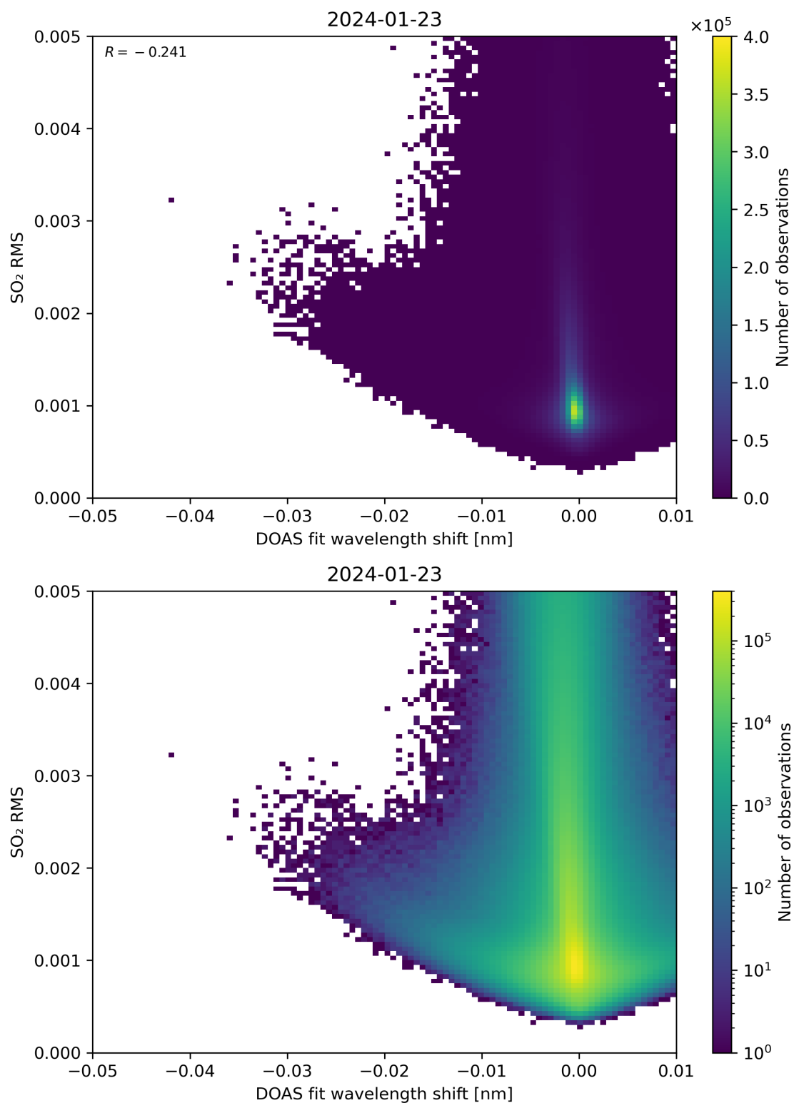
Figure 128: Scatter density plot of “DOAS fit wavelength shift” against “SO 2 RMS” for 2024-01-22 to 2024-01-24.
