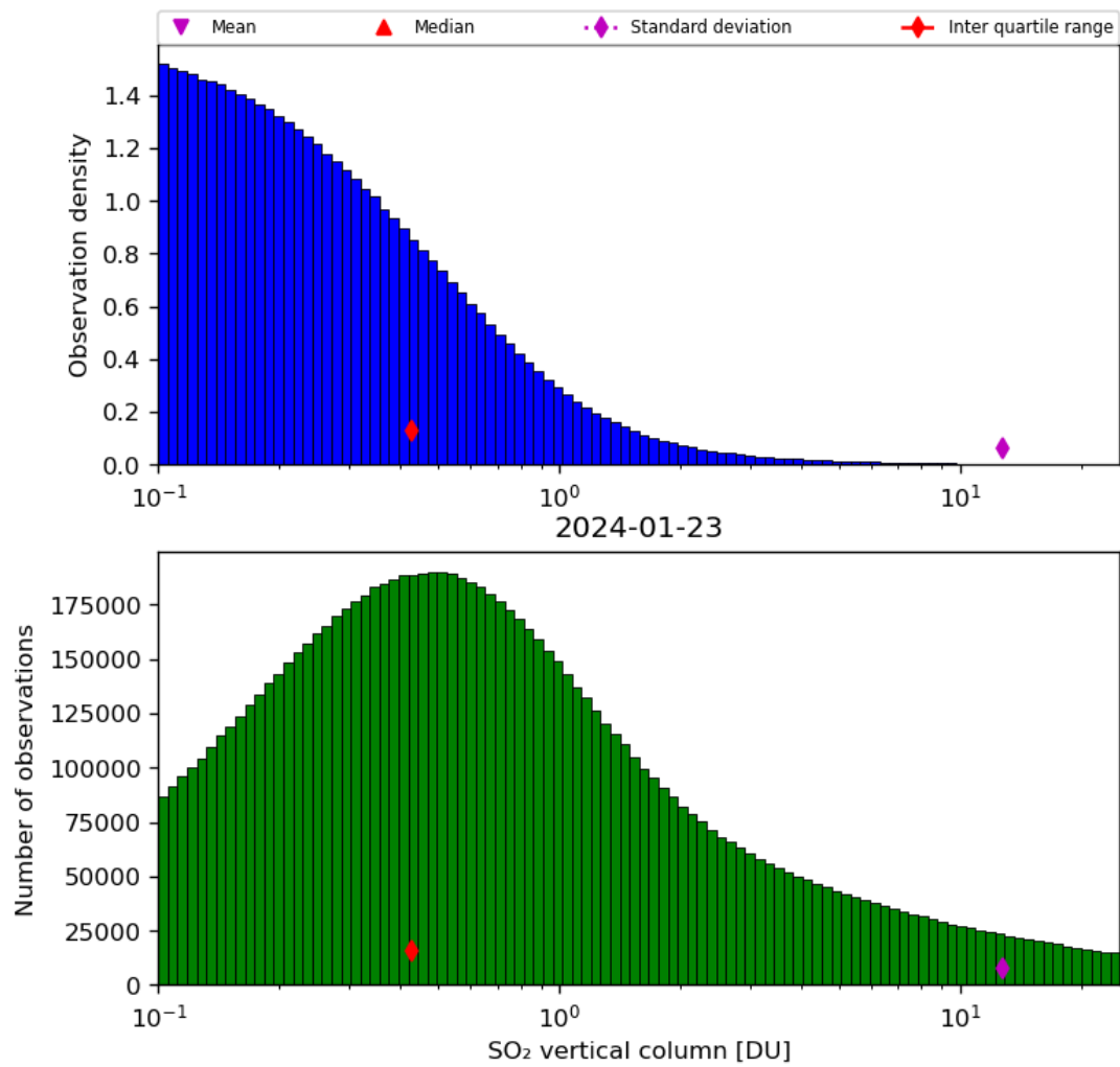
Figure 53: Histogram of “SO 2 vertical column” for 2024-01-22 to 2024-01-24
