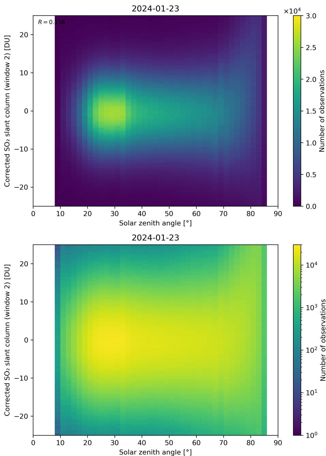
Figure 167: Scatter density plot of “Solar zenith angle” against “Corrected SO 2 slant column (window 2)” for 2024-01-22 to 2024-01-24.
