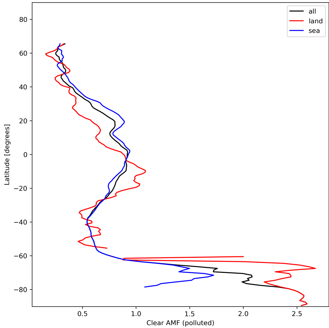
Figure 50: Zonal average of “Clear AMF (polluted)” for 2024-01-22 to 2024-01-24.
