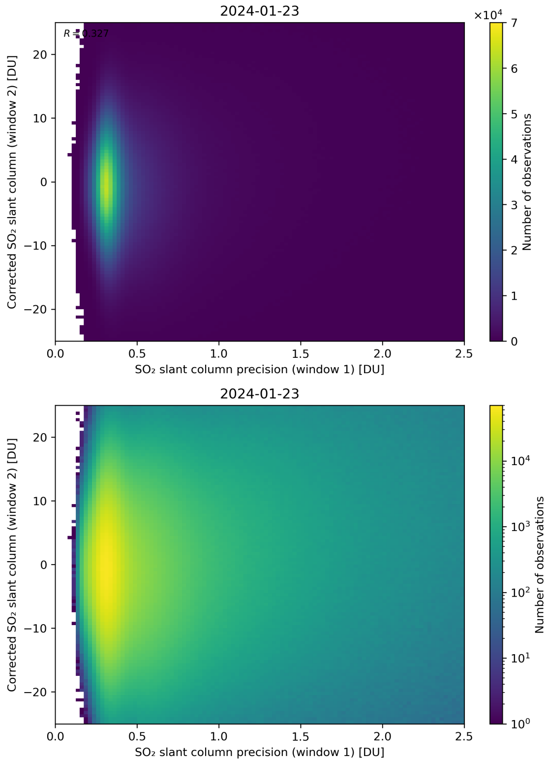
Figure 225: Scatter density plot of “SO 2 slant column precision (window 1)” against “Corrected SO 2 slant column (window 2)” for 2024-01-22 to 2024-01-24.
