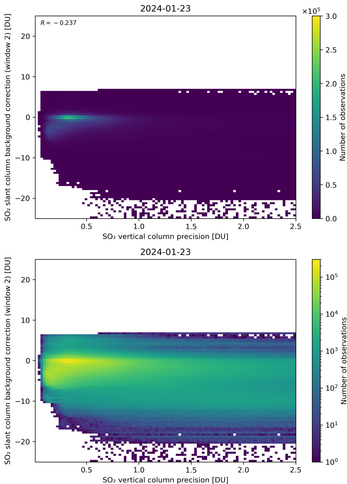
Figure 280: Scatter density plot of “SO 2 vertical column precision” against “SO 2 slant column background correction (window 2)” for 2024-01-22 to 2024-01-24.
