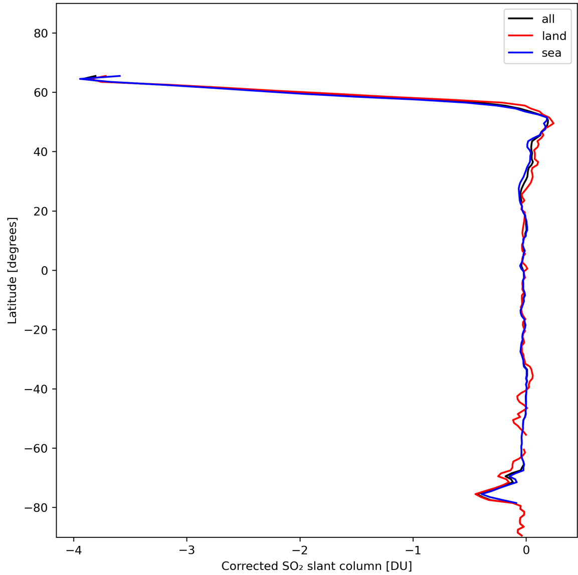
Figure 32: Zonal average of “Corrected SO 2 slant column” for 2024-01-22 to 2024-01-24.
