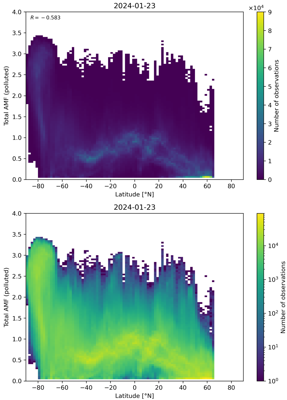
Figure 154: Scatter density plot of “Latitude” against “Total AMF (polluted)” for 2024-01-22 to 2024-01-24.
