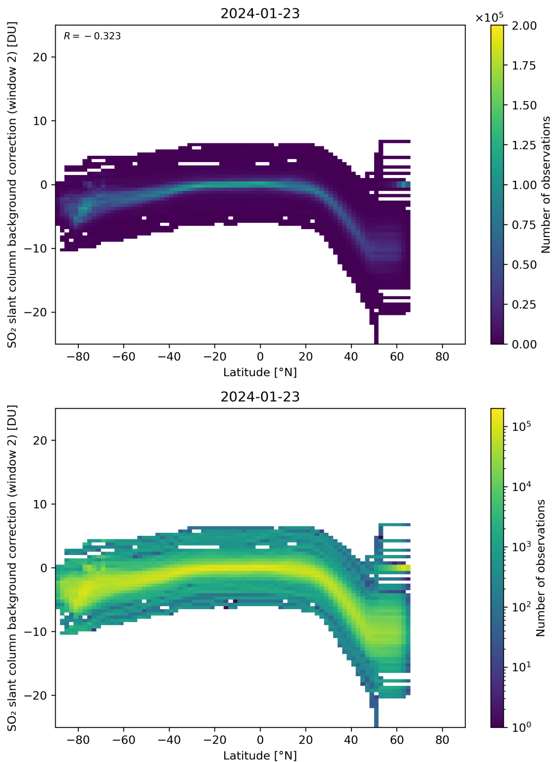
Figure 140: Scatter density plot of “Latitude” against “SO 2 slant column background correction (window 2)” for 2024-01-22 to 2024-01-24.
