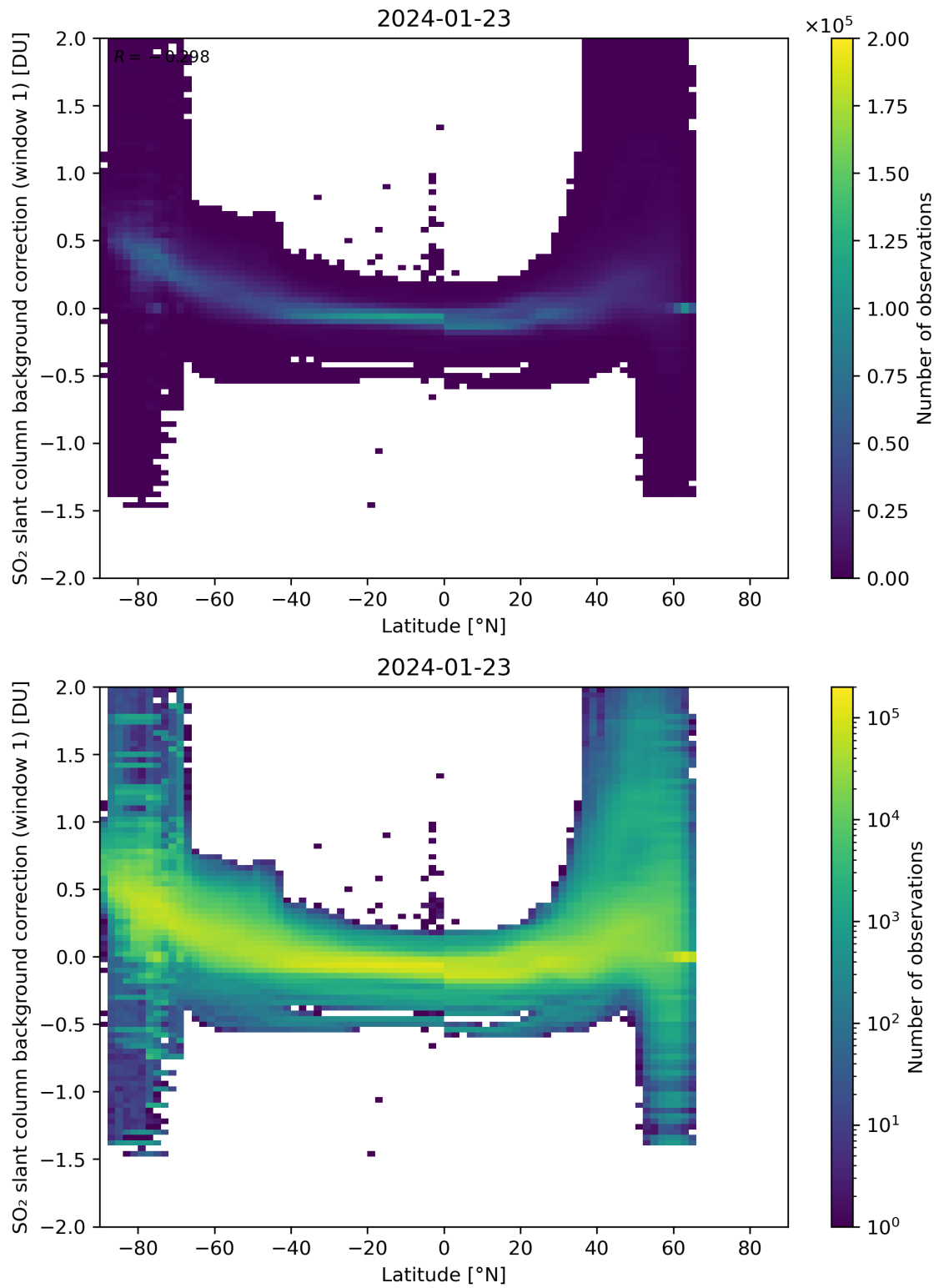
Figure 139: Scatter density plot of “Latitude” against “SO 2 slant column background correction (window 1)” for 2024-01-22 to 2024-01-24.
