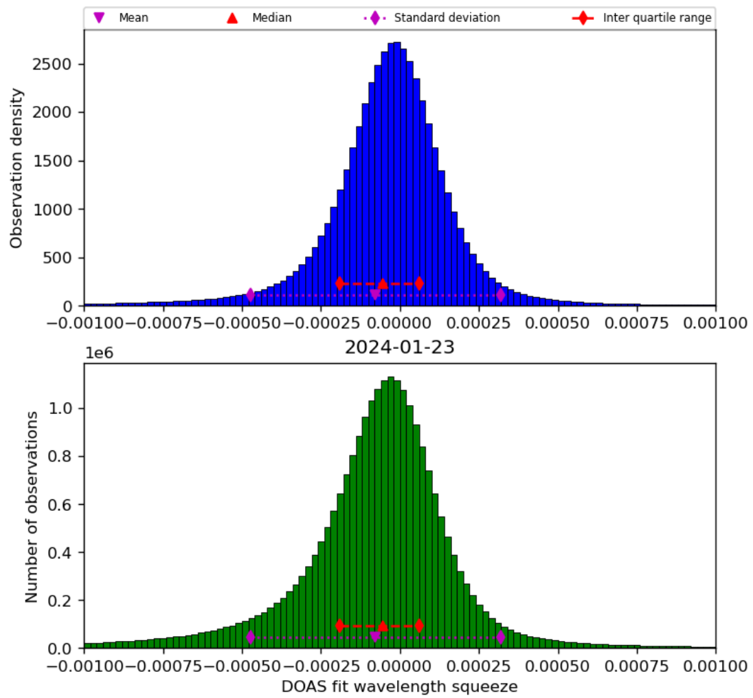
Figure 69: Histogram of “DOAS fit wavelength squeeze” for 2024-01-22 to 2024-01-24
