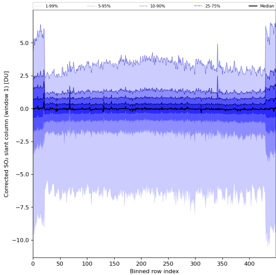
Figure 81: Along track statistics of “Corrected SO 2 slant column (window 1)” for 2024-01-22 to 2024-01-24
