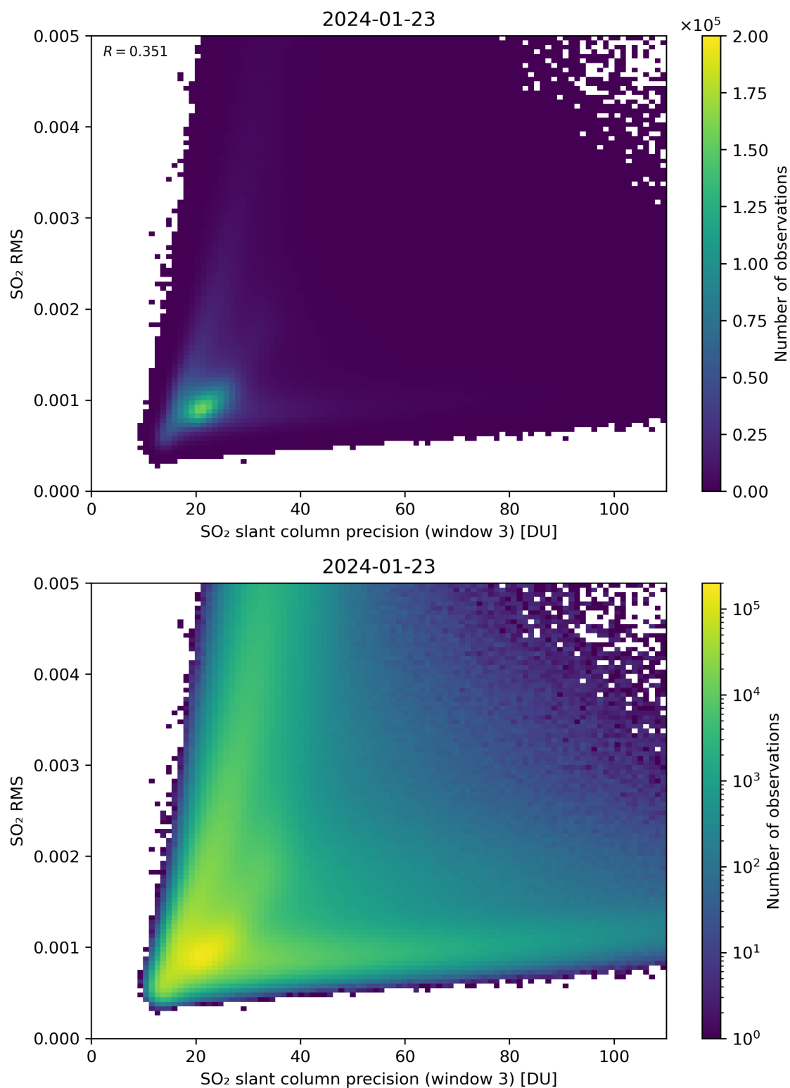
Figure 260: Scatter density plot of “SO 2 slant column precision (window 3)” against “SO 2 RMS” for 2024-01-22 to 2024-01-24.
