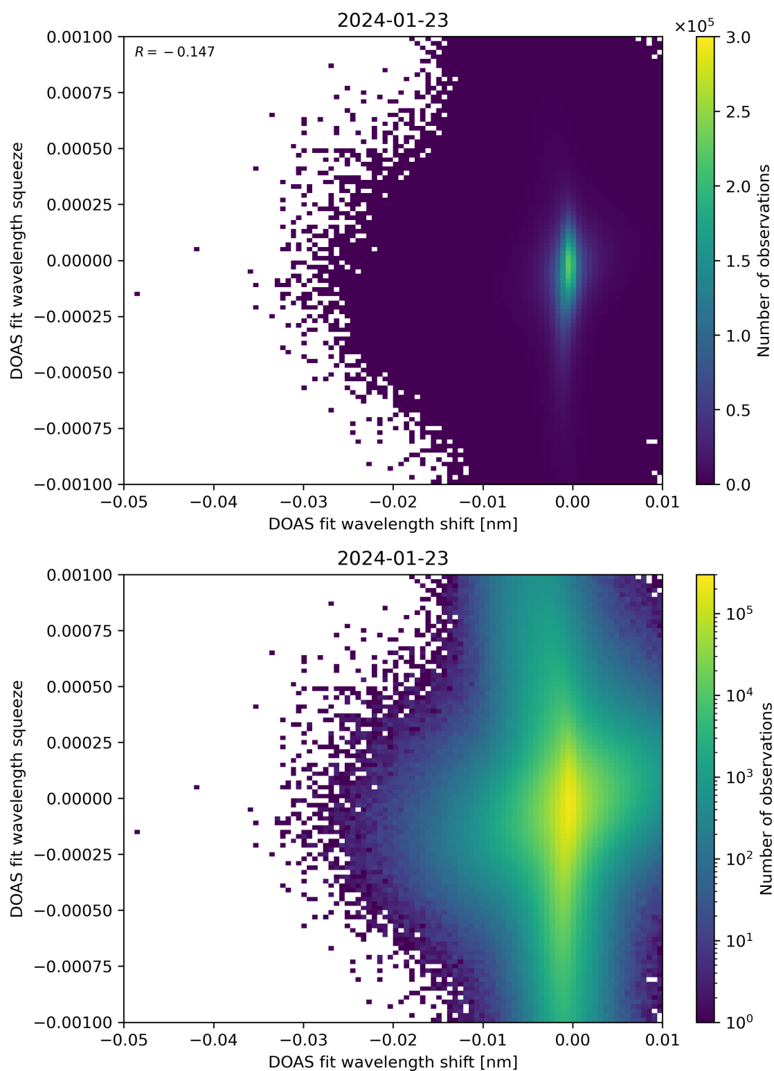
Figure 127: Scatter density plot of “DOAS fit wavelength shift” against “DOAS fit wavelength squeeze” for 2024-01-22 to 2024-01-24.
