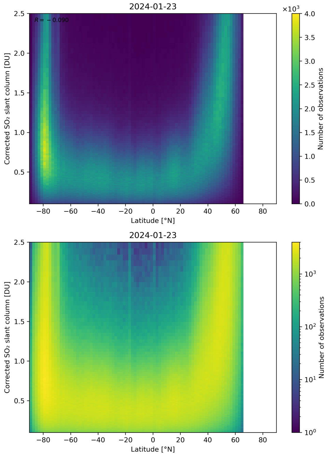
Figure 146: Scatter density plot of “Latitude” against “Corrected SO 2 slant column” for 2024-01-22 to 2024-01-24.
