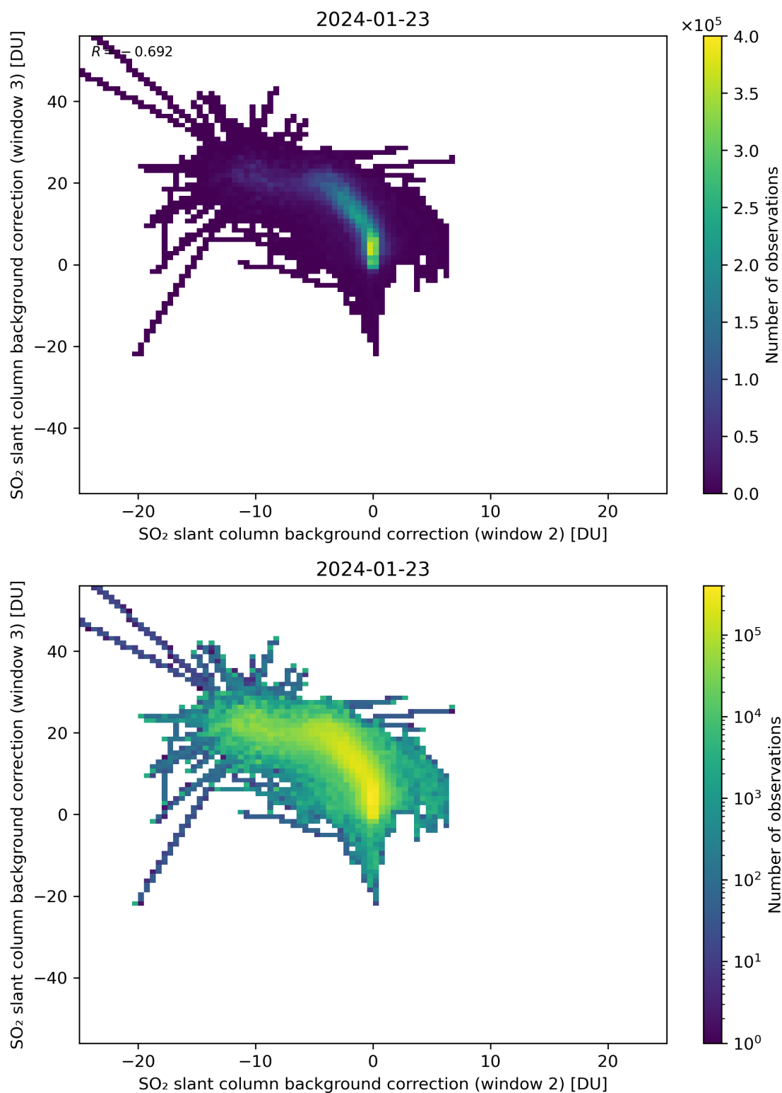
Figure 111: Scatter density plot of “SO 2 slant column background correction (window 2)” against “SO 2 slant column background correction (window 3)” for 2024-01-22 to 2024-01-24.
