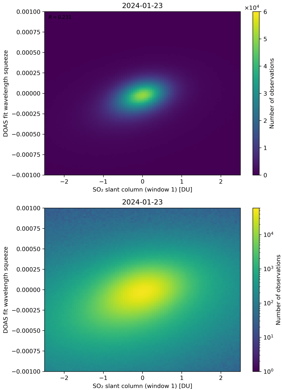
Figure 216: Scatter density plot of “SO 2 slant column (window 1)” against “DOAS fit wavelength squeeze” for 2024-01-22 to 2024-01-24.
