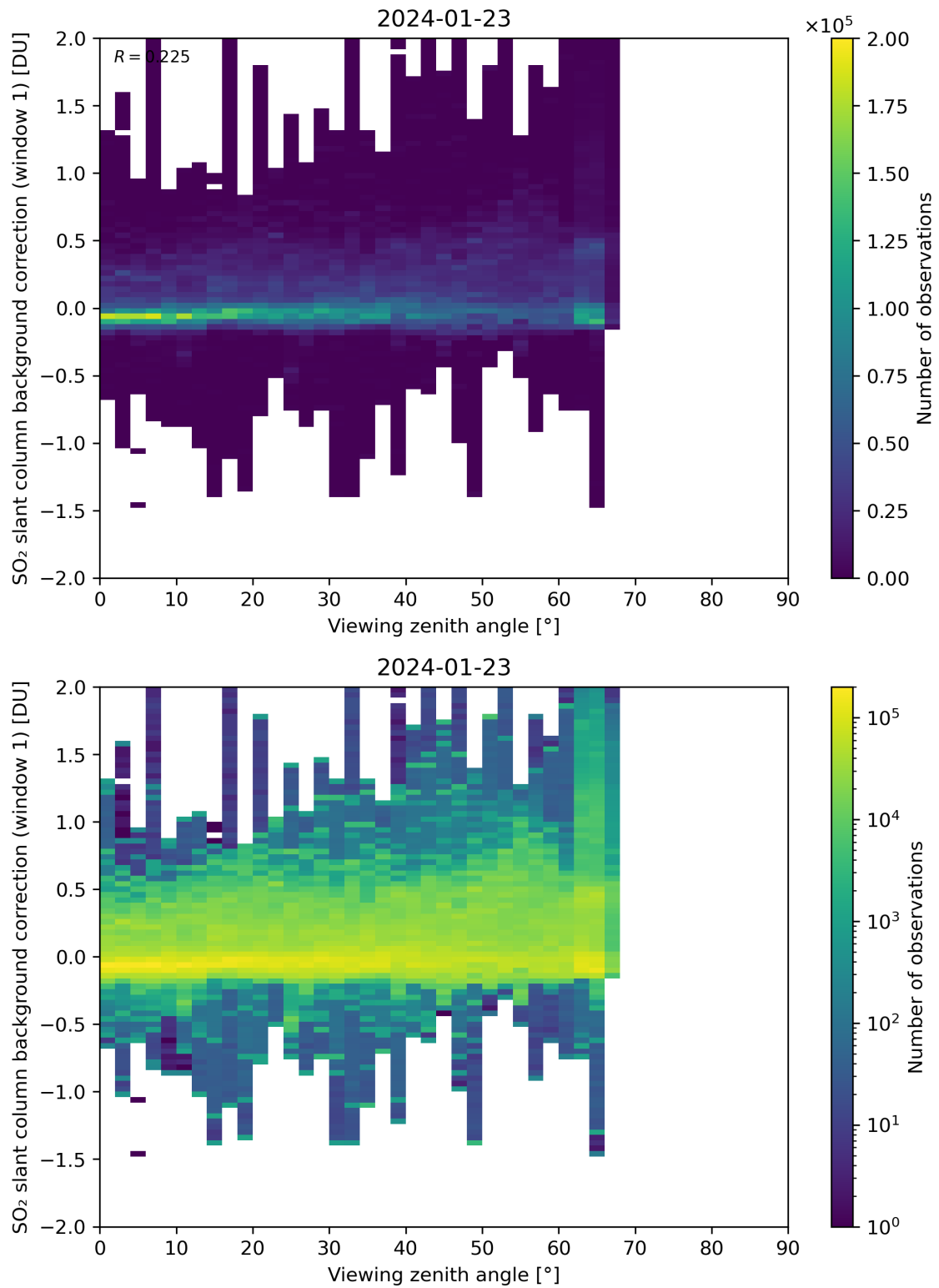
Figure 308: Scatter density plot of “Viewing zenith angle” against “SO 2 slant column background correction (window 1)” for 2024-01-22 to 2024-01-24.
