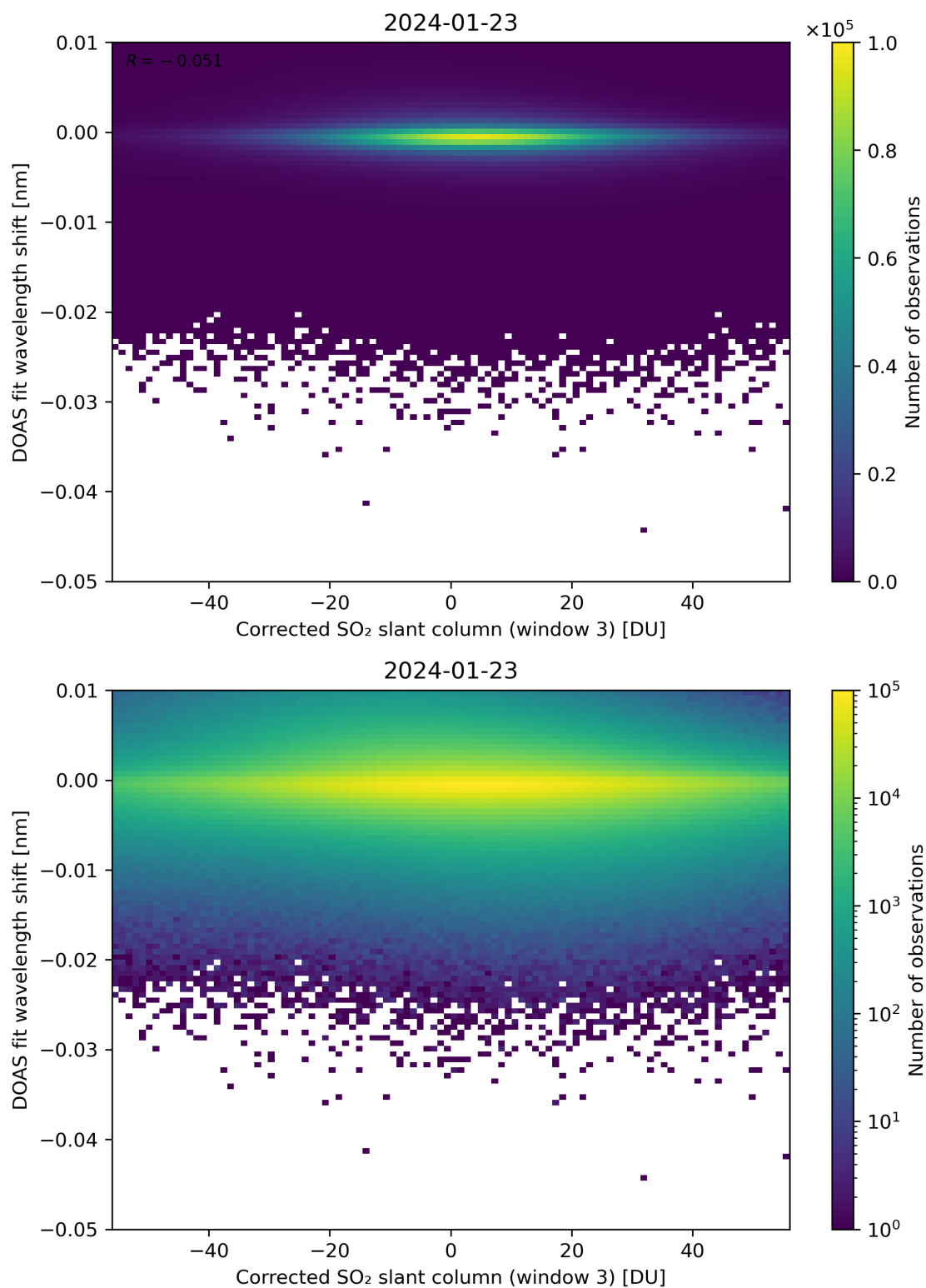
Figure 206: Scatter density plot of “Corrected SO 2 slant column (window 3)” against “DOAS fit wavelength shift” for 2024-01-22 to 2024-01-24.
