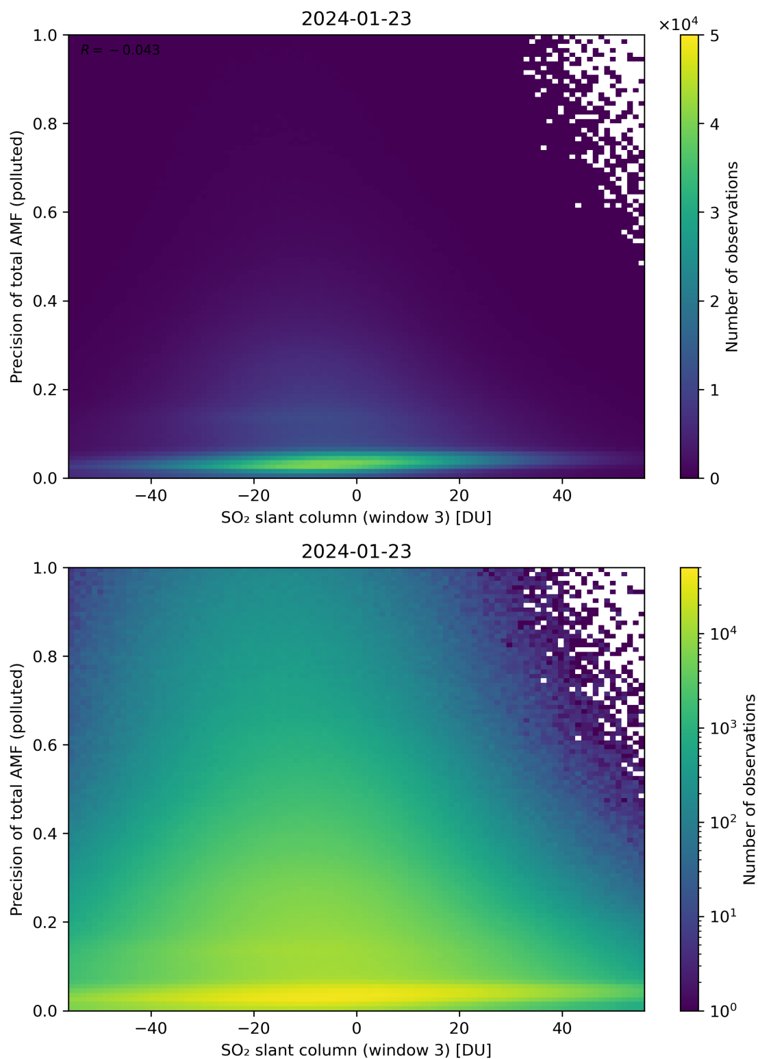
Figure 269: Scatter density plot of “SO 2 slant column (window 3)” against “Precision of total AMF (polluted)” for 2024-01-22 to 2024-01-24.
