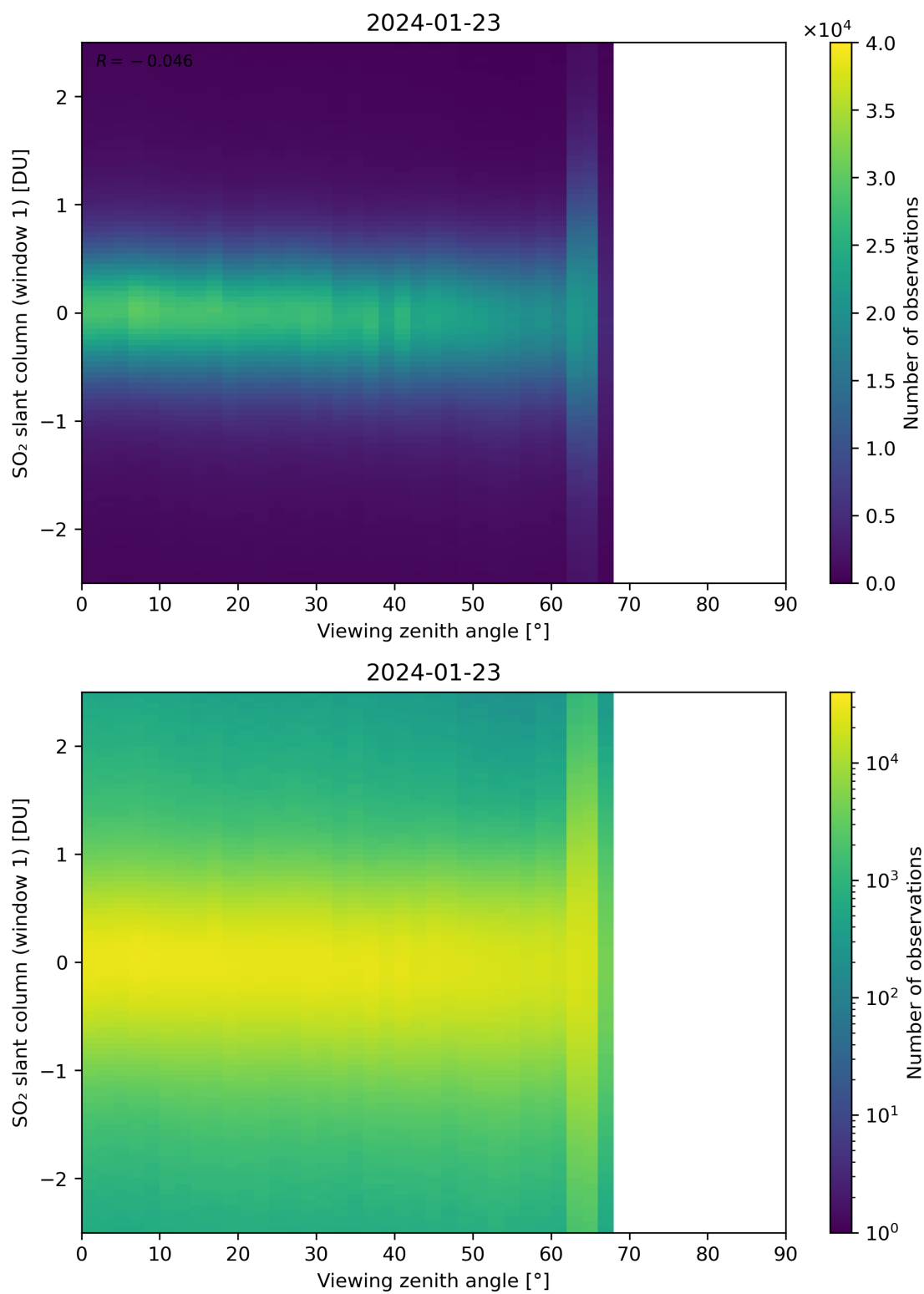
Figure 320: Scatter density plot of “Viewing zenith angle” against “SO 2 slant column (window 1)” for 2024-01-22 to 2024-01-24.
