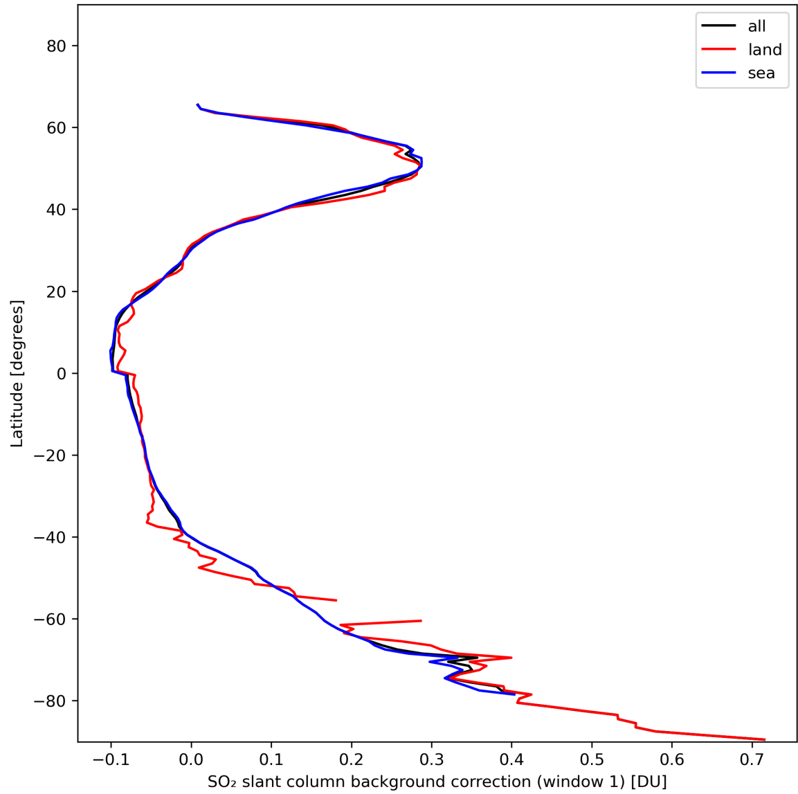
Figure 36: Zonal average of "SO 2 slant column background correction (window 1)" for 2024-01-22 to 2024-01-24.
