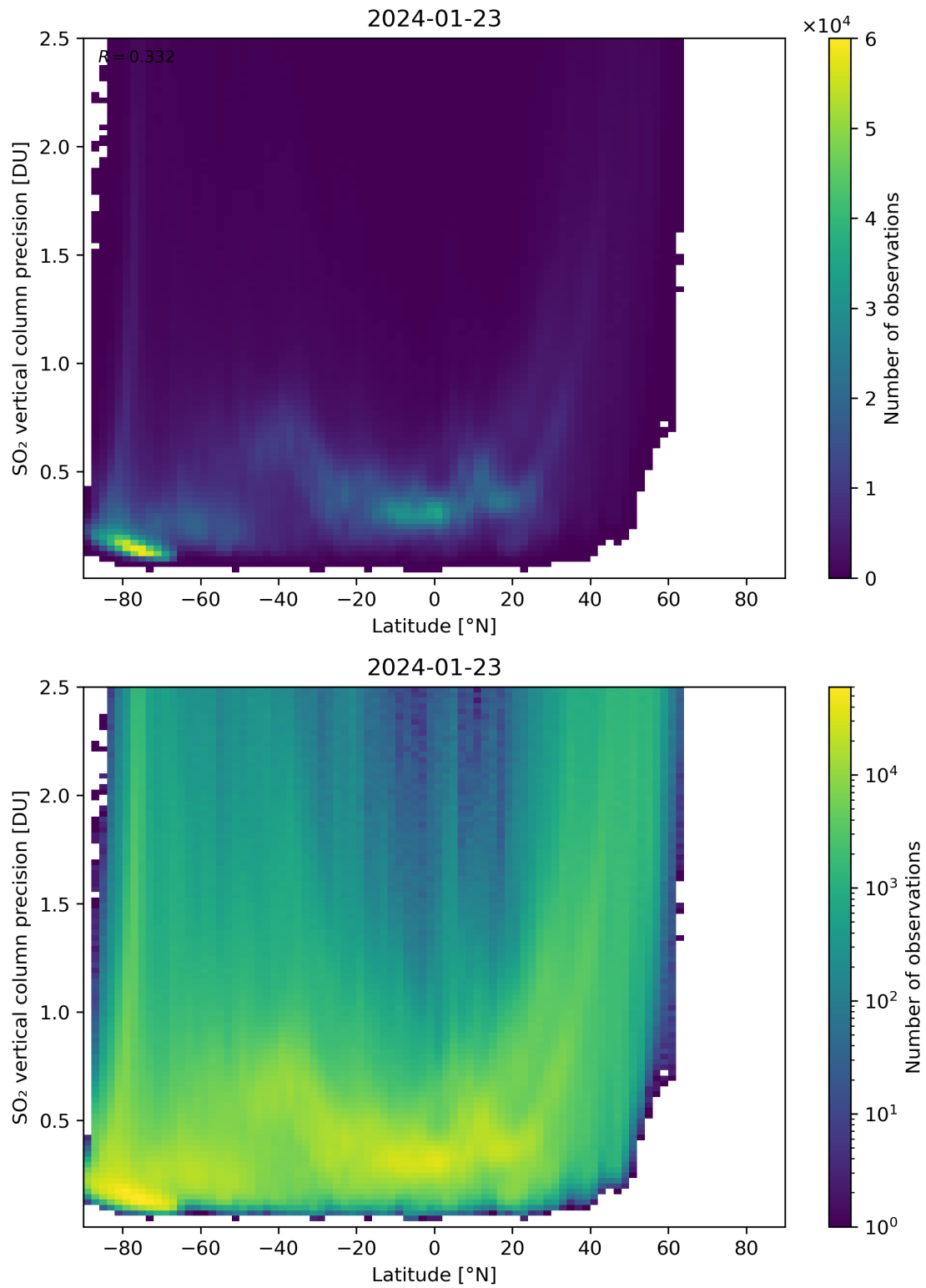
Figure 157: Scatter density plot of “Latitude” against “SO 2 vertical column precision” for 2024-01-22 to 2024-01-24.
