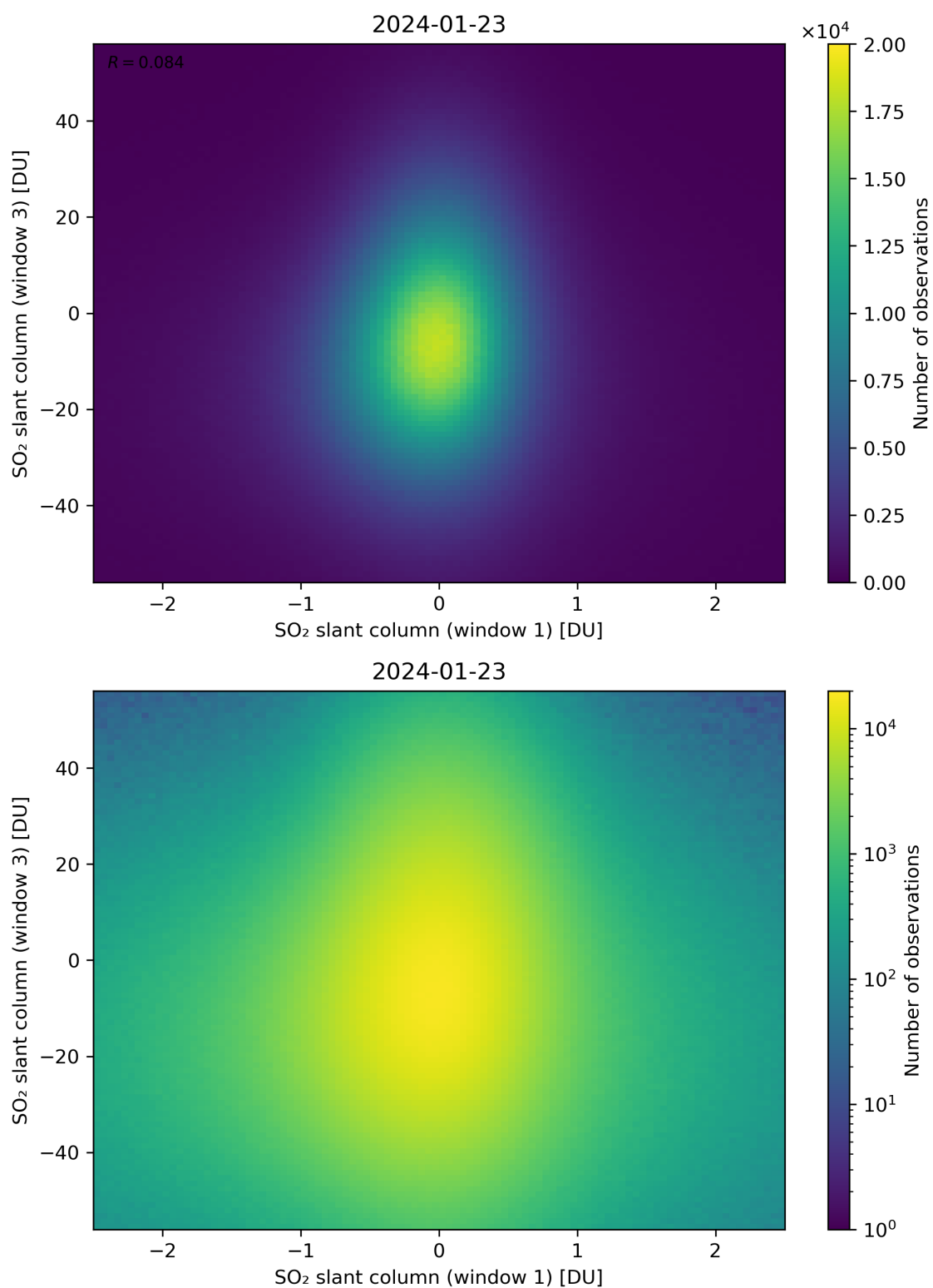
Figure 237: Scatter density plot of “SO 2 slant column (window 1)” against “SO 2 slant column (window 3)” for 2024-01-22 to 2024-01-24.
