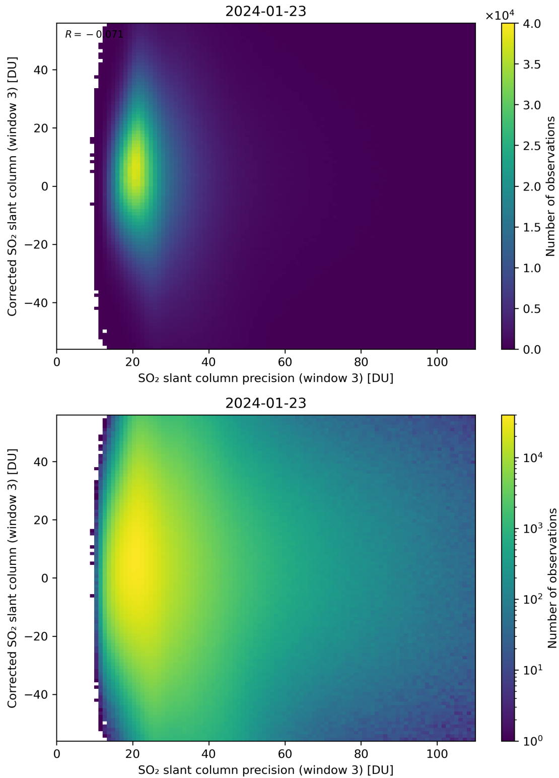
Figure 262: Scatter density plot of “SO 2 slant column precision (window 3)” against “Corrected SO 2 slant column (window 3)” for 2024-01-22 to 2024-01-24.
