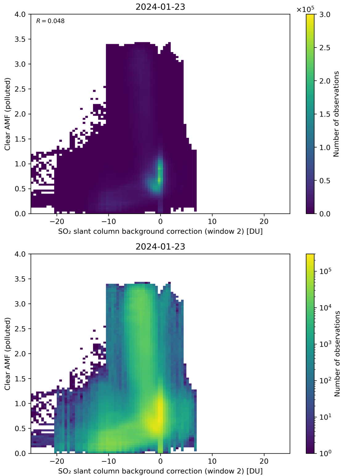
Figure 115: Scatter density plot of “SO 2 slant column background correction (window 2)” against “Clear AMF (polluted)” for 2024-01-22 to 2024-01-24.
