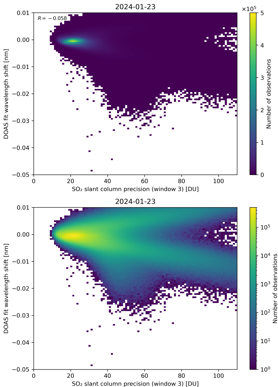
Figure 258: Scatter density plot of “SO 2 slant column precision (window 3)” against “DOAS fit wavelength shift” for 2024-01-22 to 2024-01-24.
