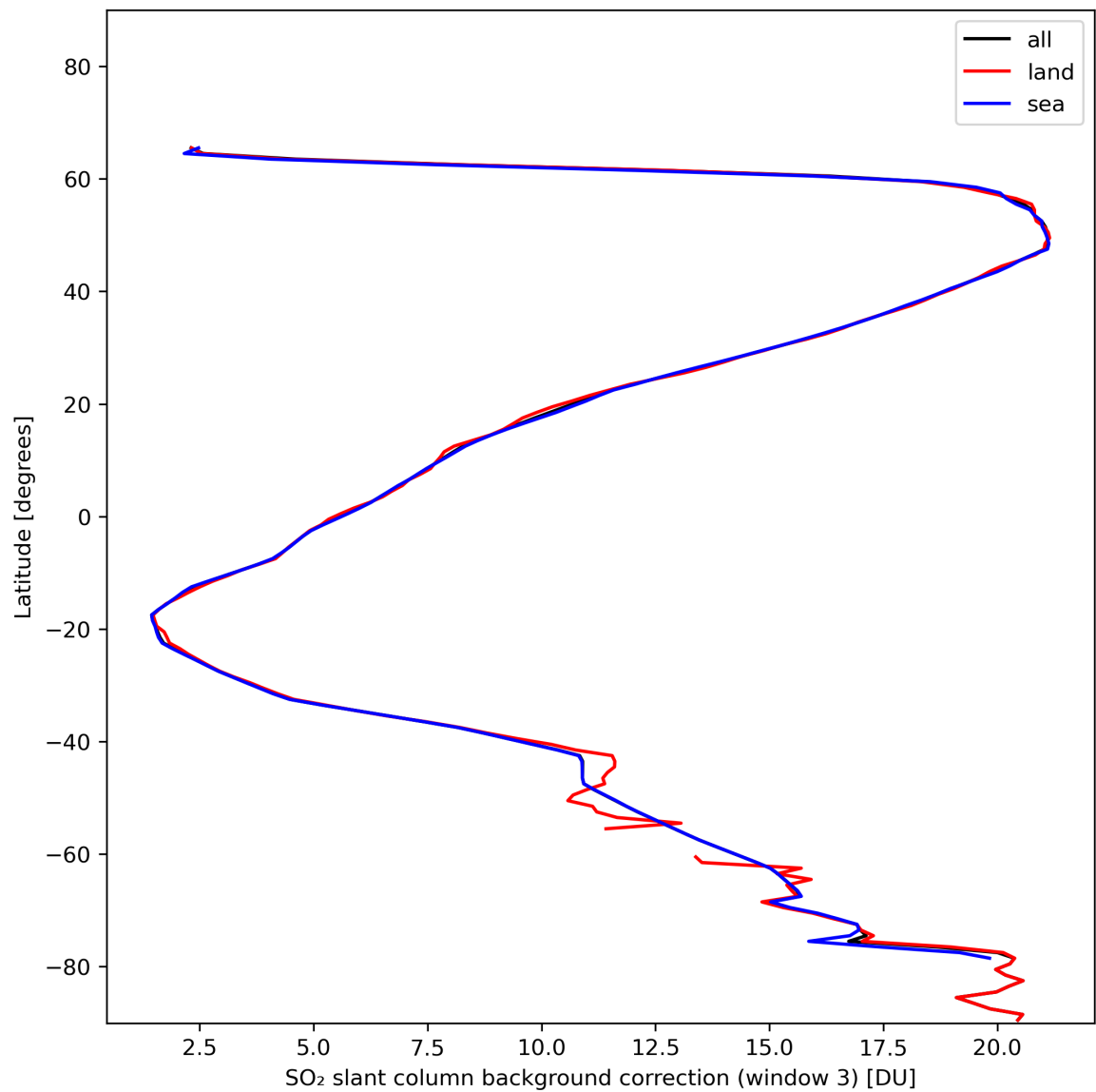
Figure 44: Zonal average of “SO 2 slant column background correction (window 3)” for 2024-01-22 to 2024-01-24.
