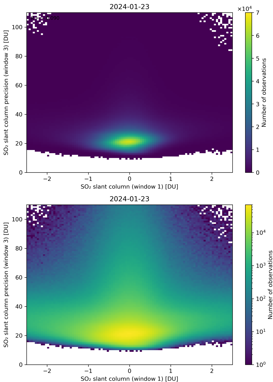
Figure 238: Scatter density plot of “SO 2 slant column (window 1)” against “SO 2 slant column precision (window 3)” for 2024-01-22 to 2024-01-24.
