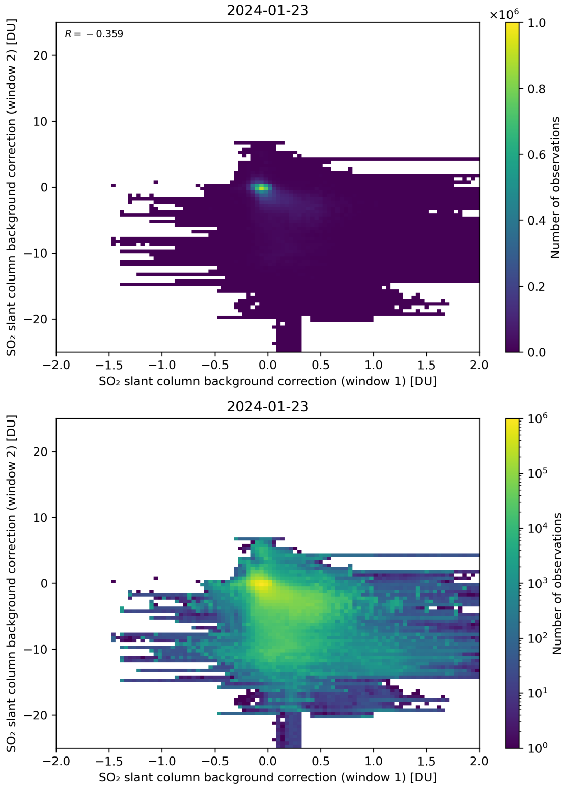
Figure 98: Scatter density plot of “SO 2 slant column background correction (window 1)” against “SO 2 slant column background correction (window 2)” for 2024-01-22 to 2024-01-24.
