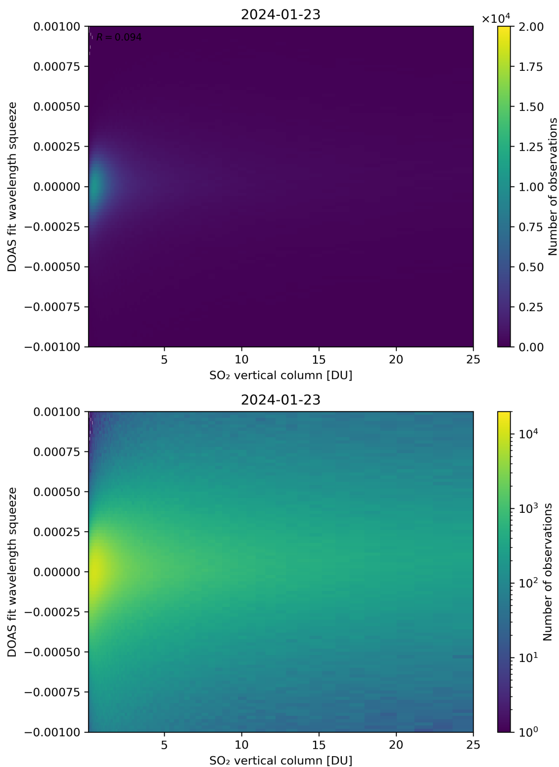
Figure 277: Scatter density plot of “SO 2 vertical column” against “DOAS fit wavelength squeeze” for 2024-01-22 to 2024-01-24.
