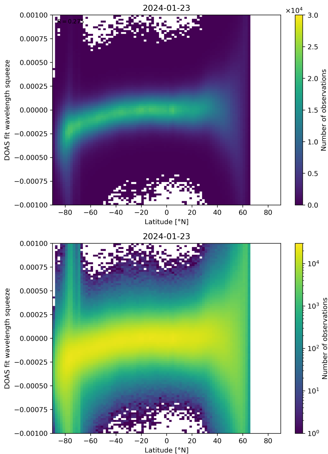
Figure 143: Scatter density plot of “Latitude” against “DOAS fit wavelength squeeze” for 2024-01-22 to 2024-01-24.
