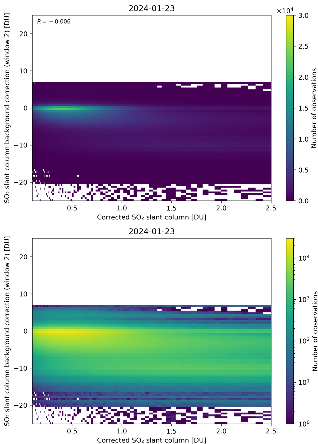
Figure 179: Scatter density plot of “Corrected SO 2 slant column” against “SO 2 slant column background correction (window 2)” for 2024-01-22 to 2024-01-24.
