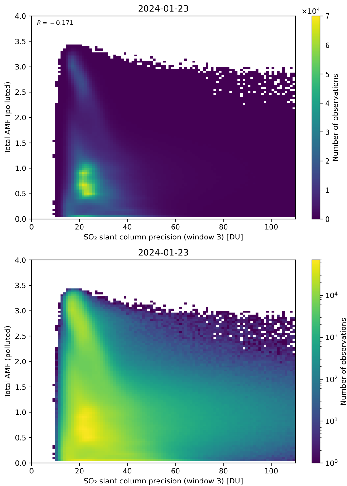
Figure 263: Scatter density plot of “SO 2 slant column precision (window 3)” against “Total AMF (polluted)” for 2024-01-22 to 2024-01-24.
