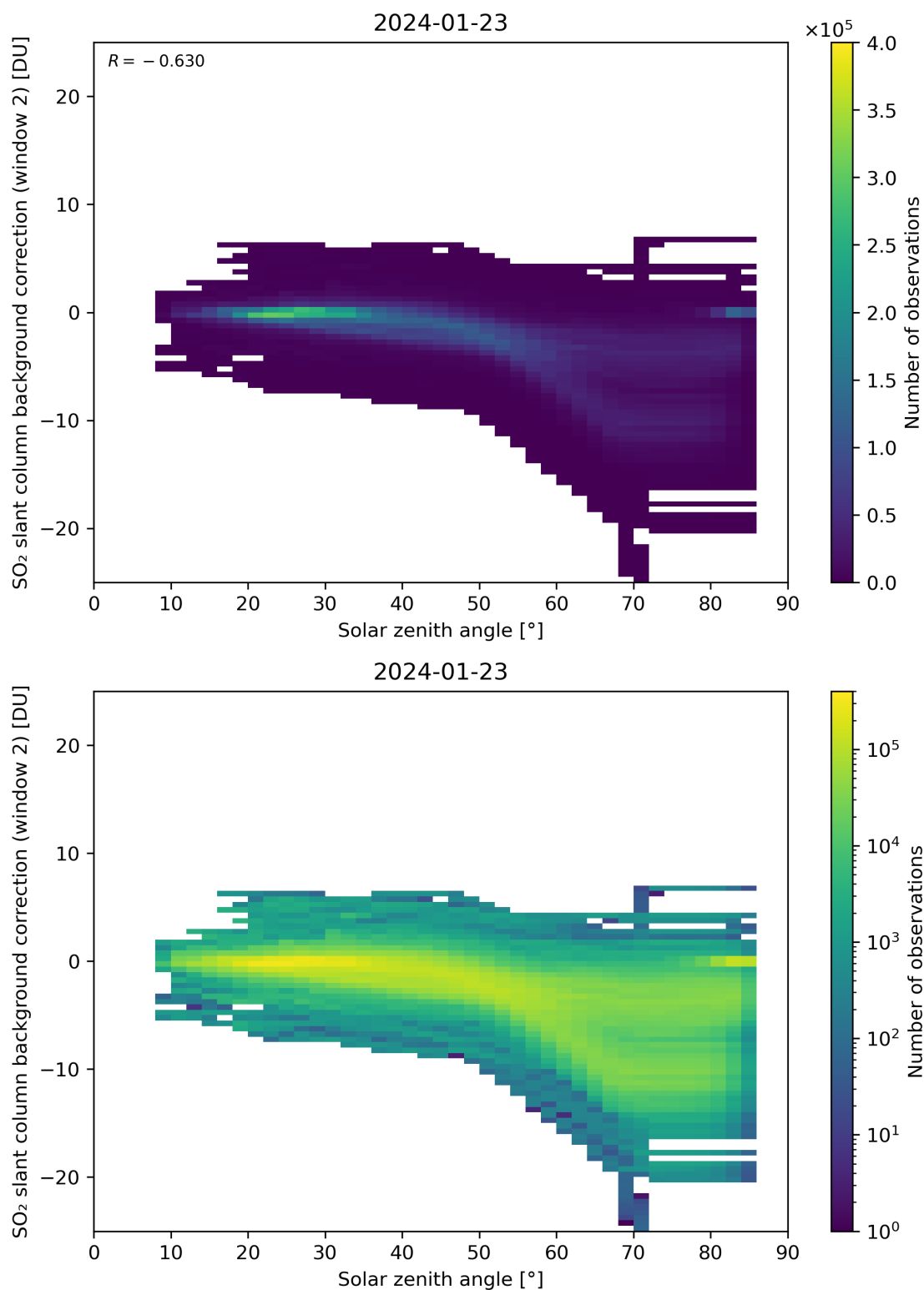
Figure 159: Scatter density plot of “Solar zenith angle” against “SO 2 slant column background correction (window 2)” for 2024-01-22 to 2024-01-24.
