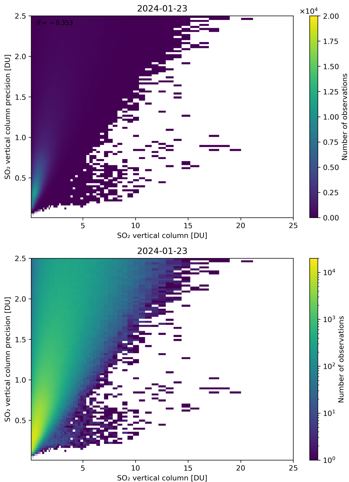
Figure 307: Scatter density plot of “SO 2 vertical column” against “SO 2 vertical column precision” for 2024-01-22 to 2024-01-24.
