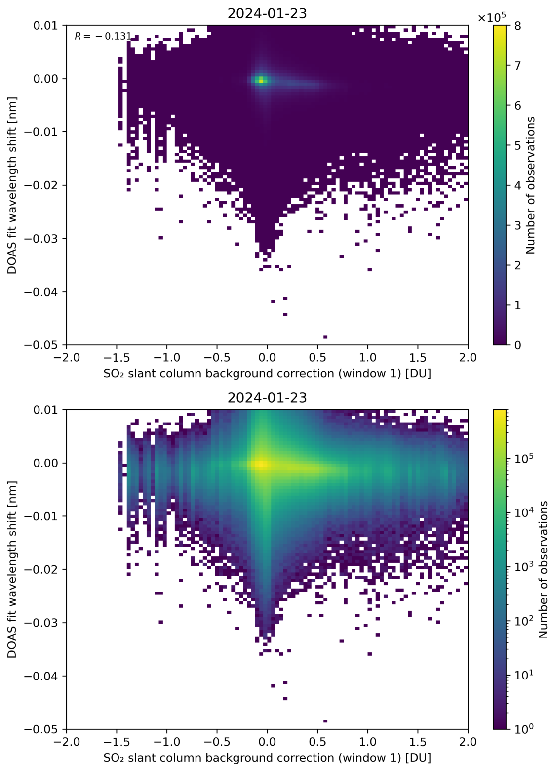
Figure 100: Scatter density plot of “SO 2 slant column background correction (window 1)” against “DOAS fit wavelength shift” for 2024-01-22 to 2024-01-24.
