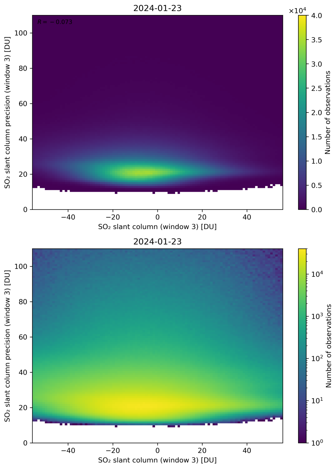
Figure 267: Scatter density plot of “SO 2 slant column (window 3)” against “SO 2 slant column precision (window 3)” for 2024-01-22 to 2024-01-24.
