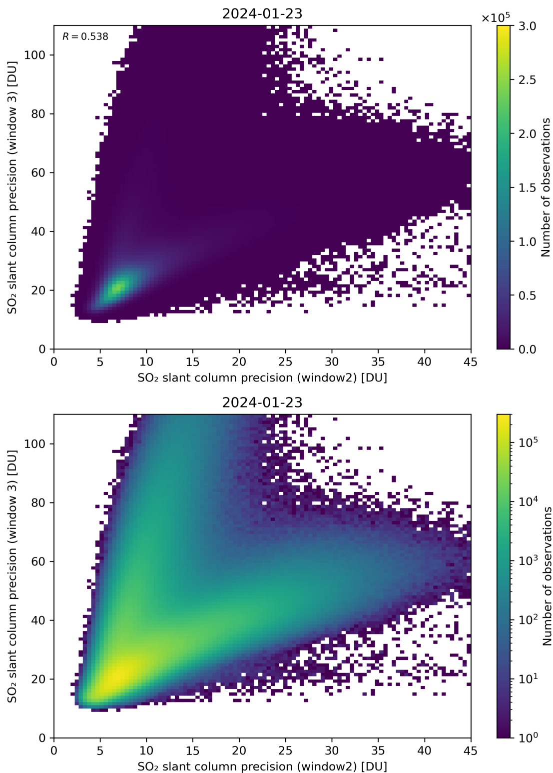
Figure 250: Scatter density plot of “SO 2 slant column precision (window2)” against “SO 2 slant column precision (window 3)” for 2024-01-22 to 2024-01-24.
