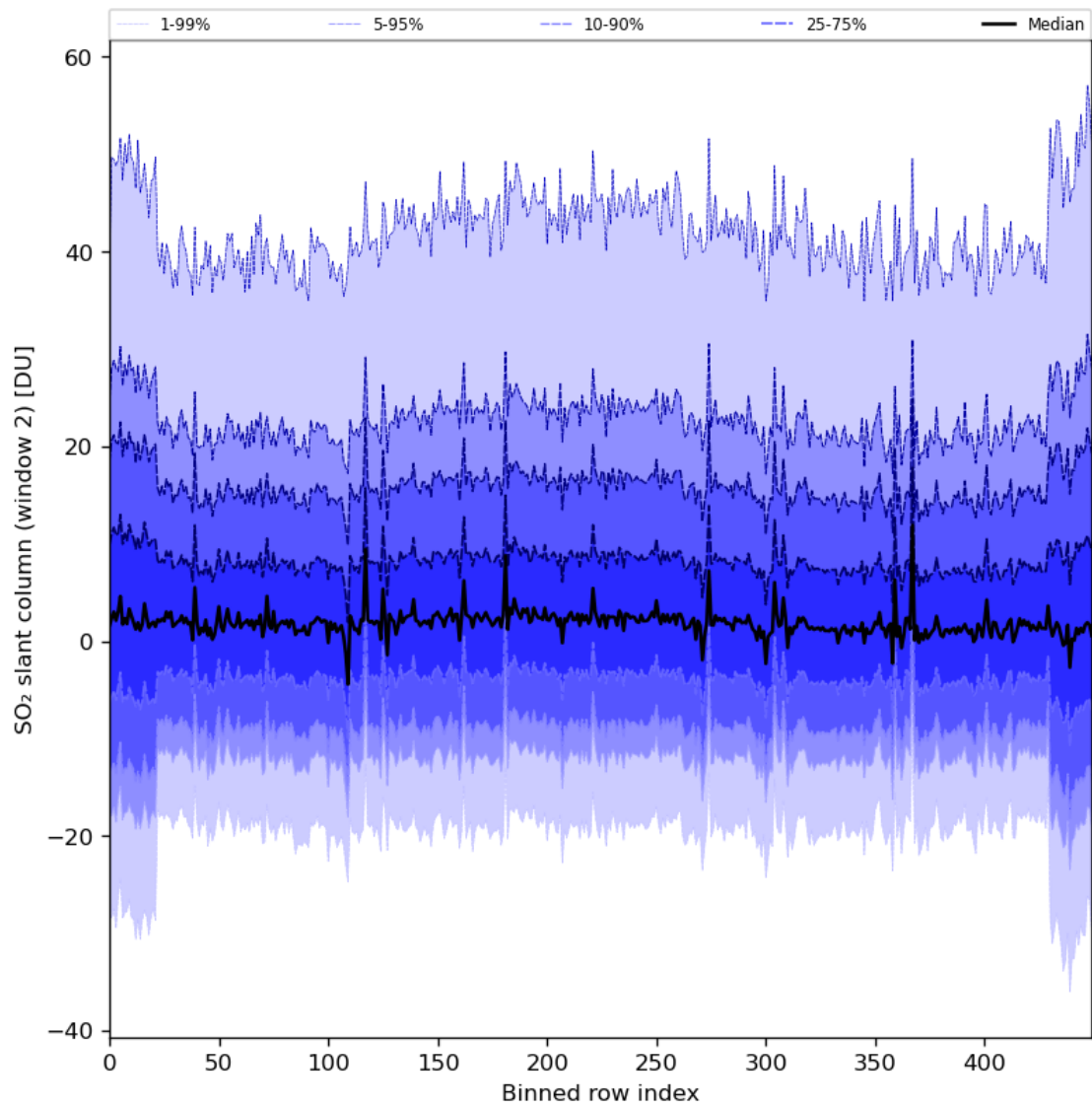
Figure 83: Along track statistics of “SO 2 slant column (window 2)” for 2024-01-22 to 2024-01-24
