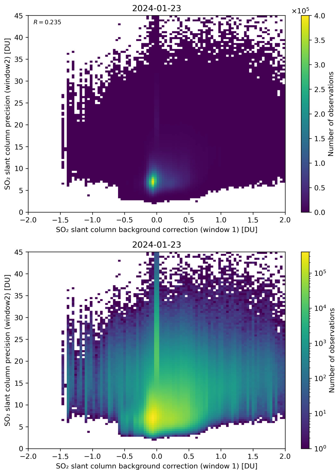
Figure 106: Scatter density plot of “SO 2 slant column background correction (window 1)” against “SO 2 slant column precision (window2)” for 2024-01-22 to 2024-01-24.
