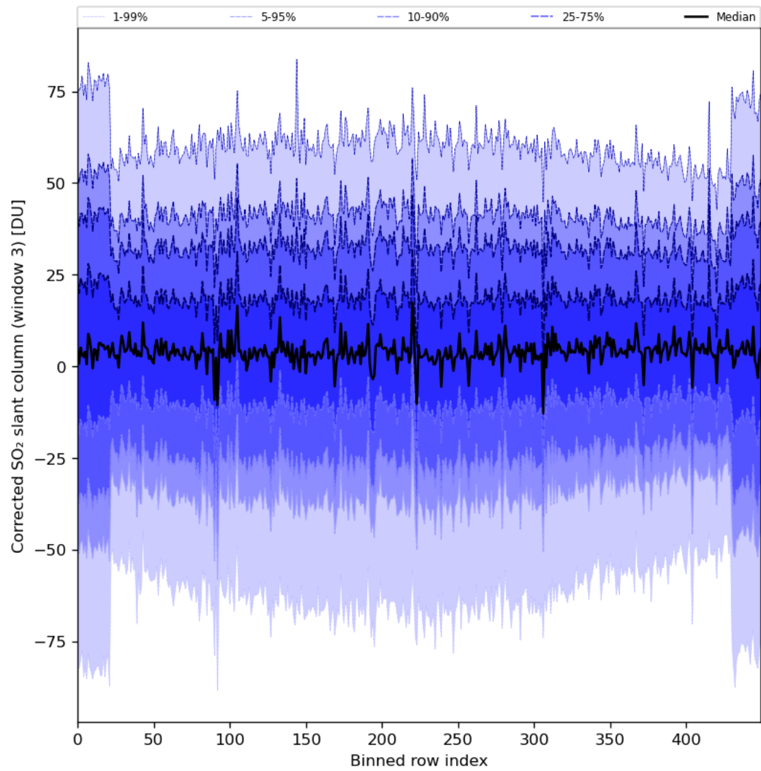
Figure 89: Along track statistics of “Corrected SO 2 slant column (window 3)” for 2024-01-22 to 2024-01-24
