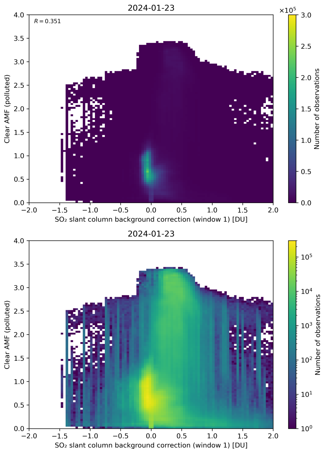
Figure 103: Scatter density plot of “SO 2 slant column background correction (window 1)” against “Clear AMF (polluted)” for 2024-01-22 to 2024-01-24.
