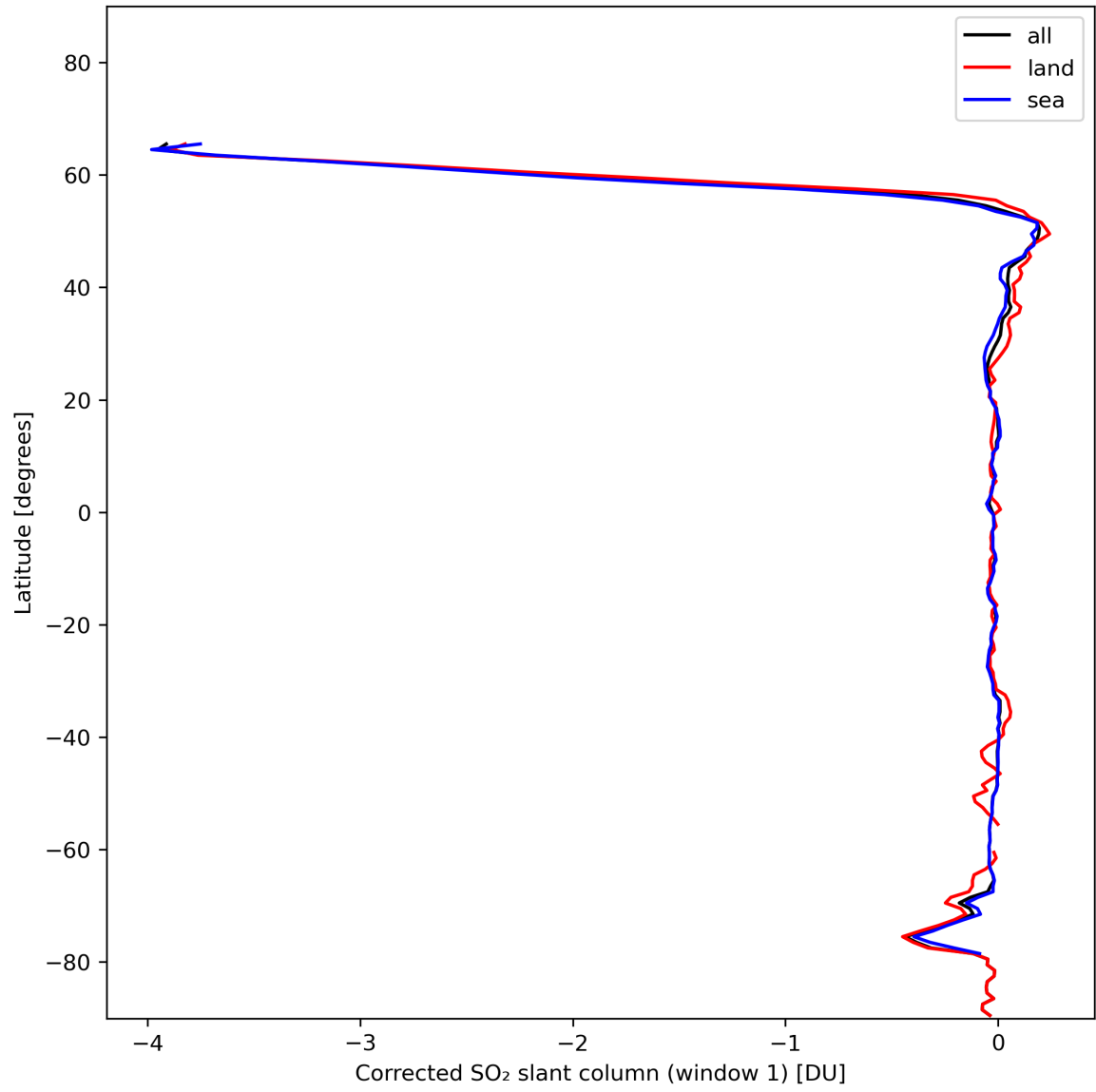
Figure 35: Zonal average of “Corrected SO 2 slant column (window 1)” for 2024-01-22 to 2024-01-24.
