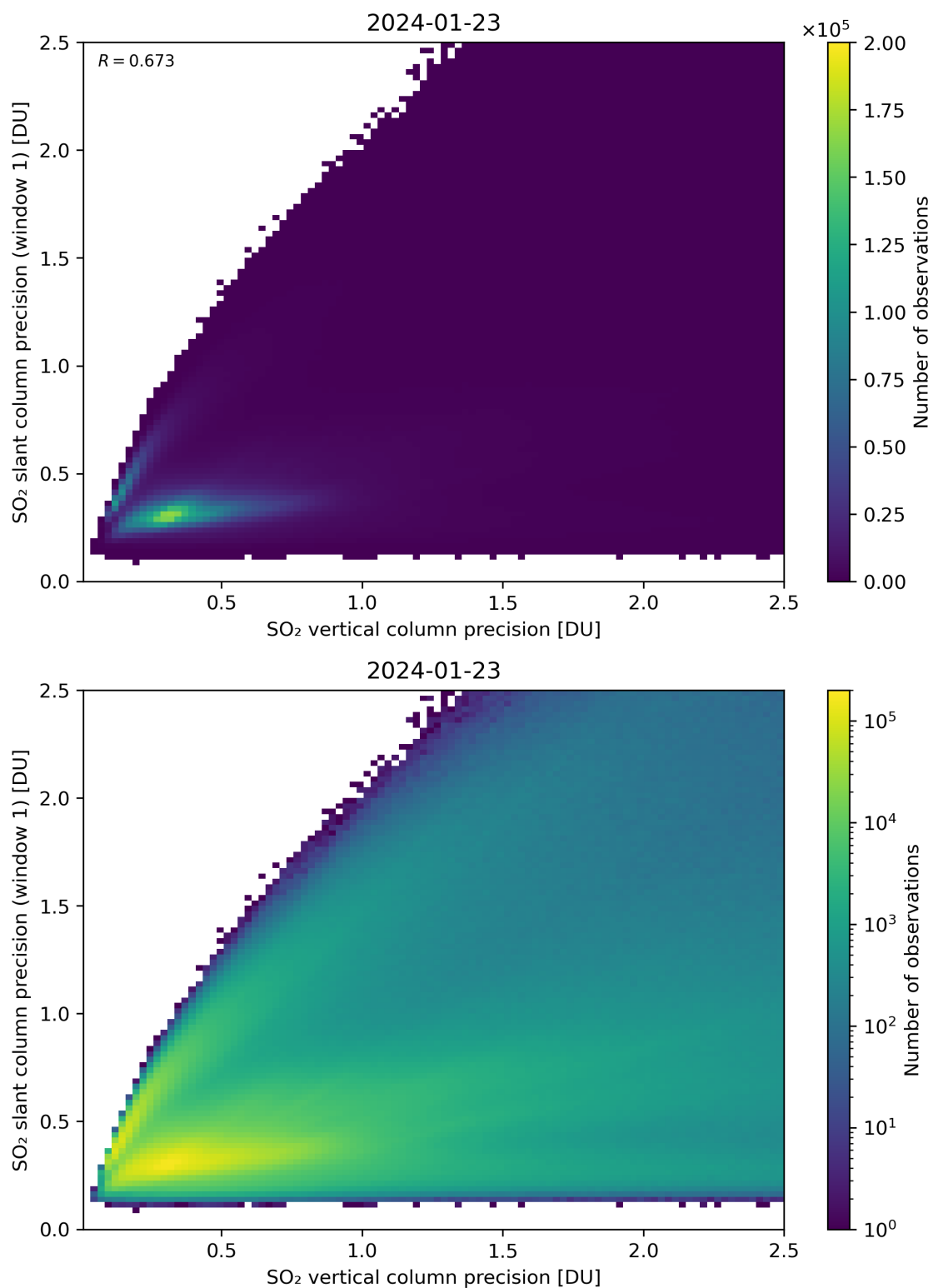
Figure 290: Scatter density plot of “SO 2 vertical column precision” against “SO 2 slant column precision (window 1)” for 2024-01-22 to 2024-01-24.
