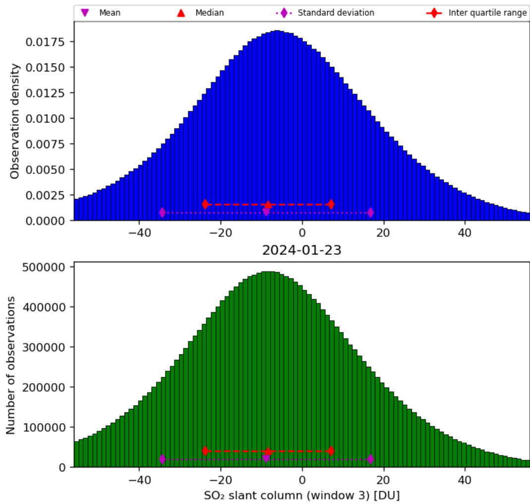
Figure 64: Histogram of “SO 2 slant column (window 3)” for 2024-01-22 to 2024-01-24
