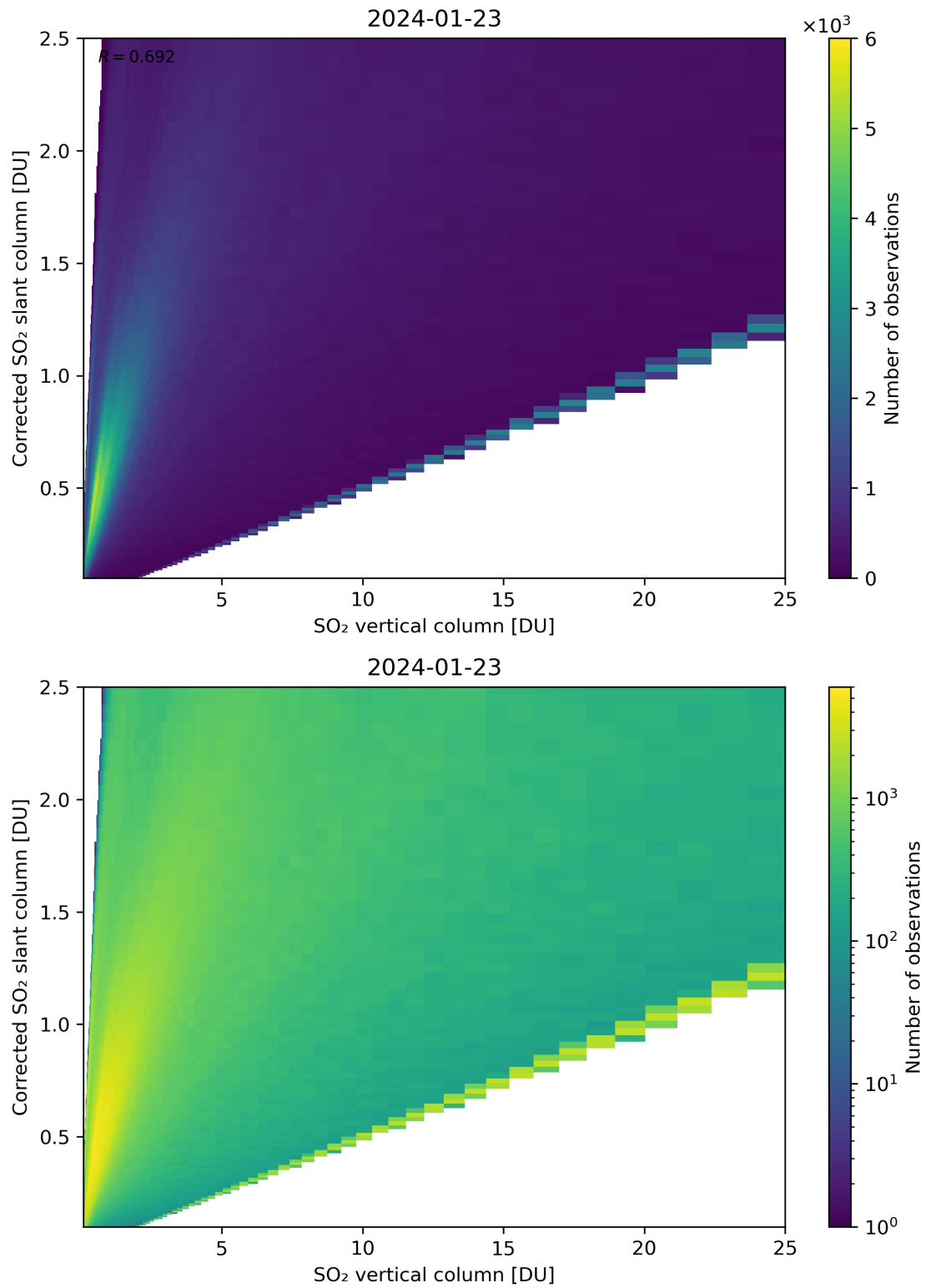
Figure 297: Scatter density plot of “SO 2 vertical column” against “Corrected SO 2 slant column” for 2024-01-22 to 2024-01-24.
