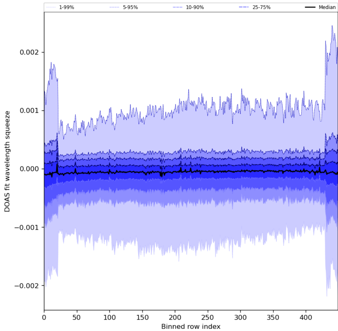
Figure 92: Along track statistics of “DOAS fit wavelength squeeze” for 2024-01-22 to 2024-01-24
