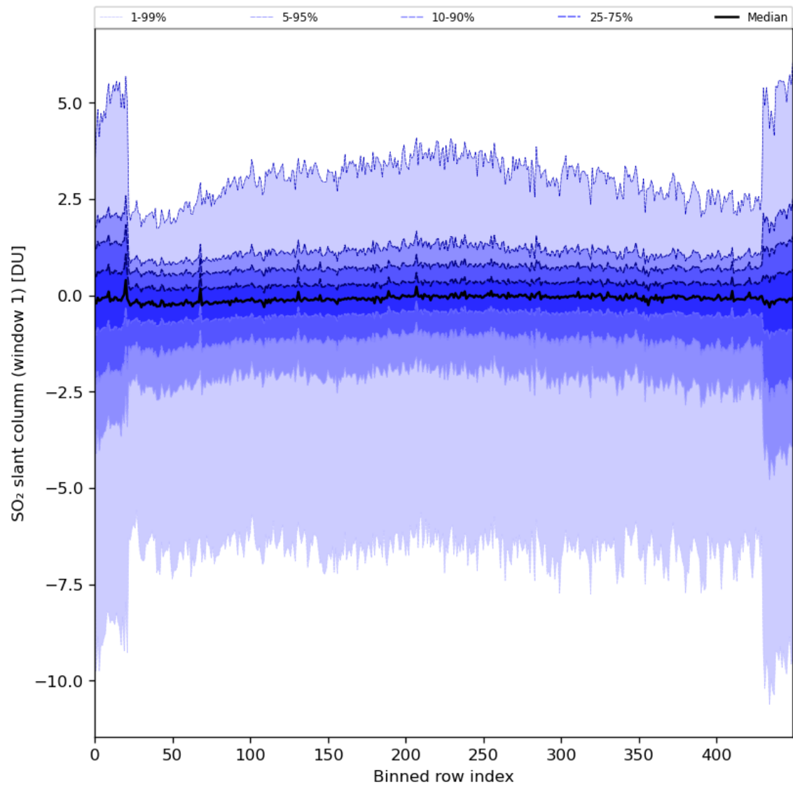
Figure 79: Along track statistics of “SO 2 slant column (window 1)” for 2024-01-22 to 2024-01-24
