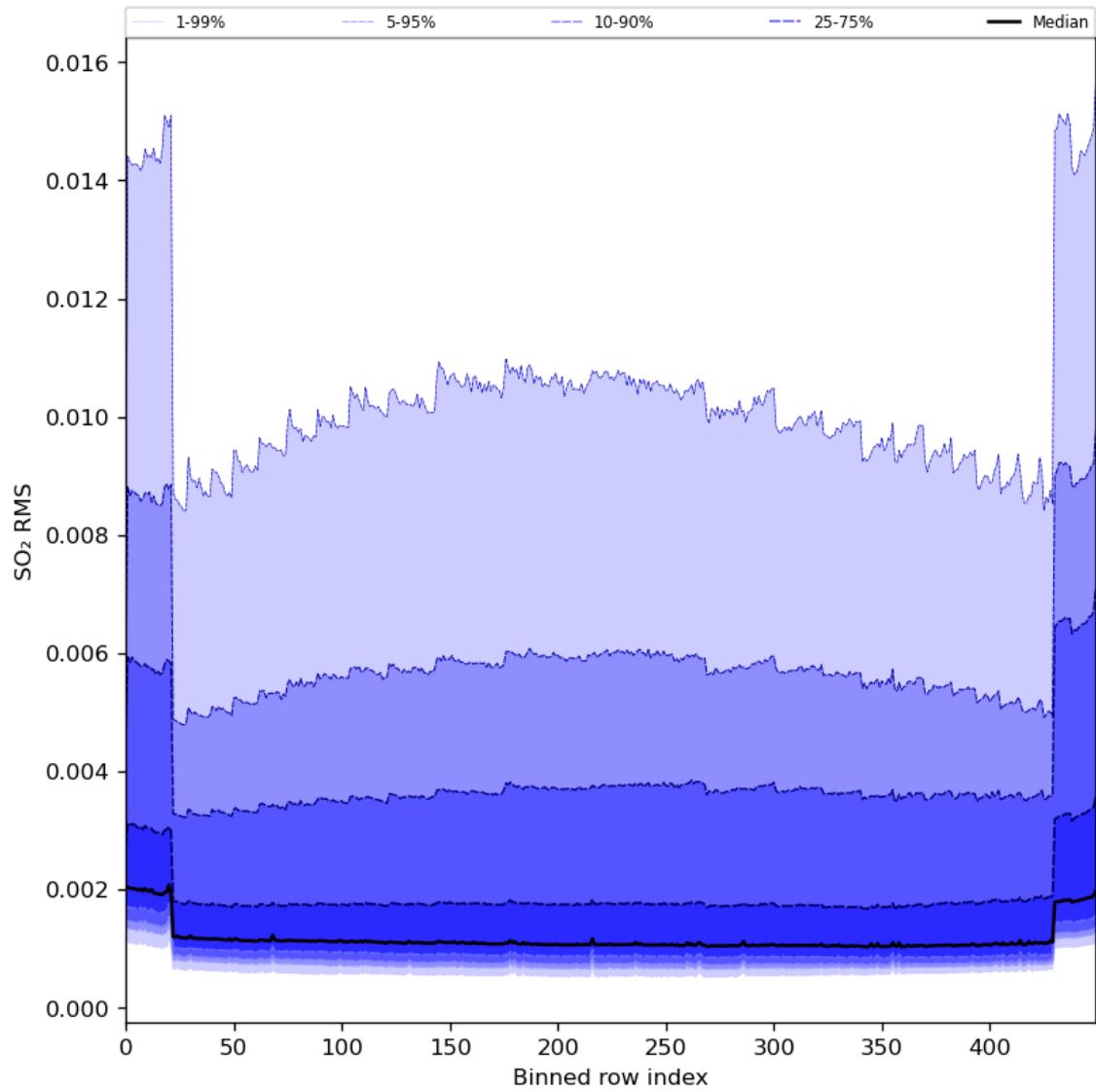
Figure 93: Along track statistics of “SO 2 RMS” for 2024-01-22 to 2024-01-24
