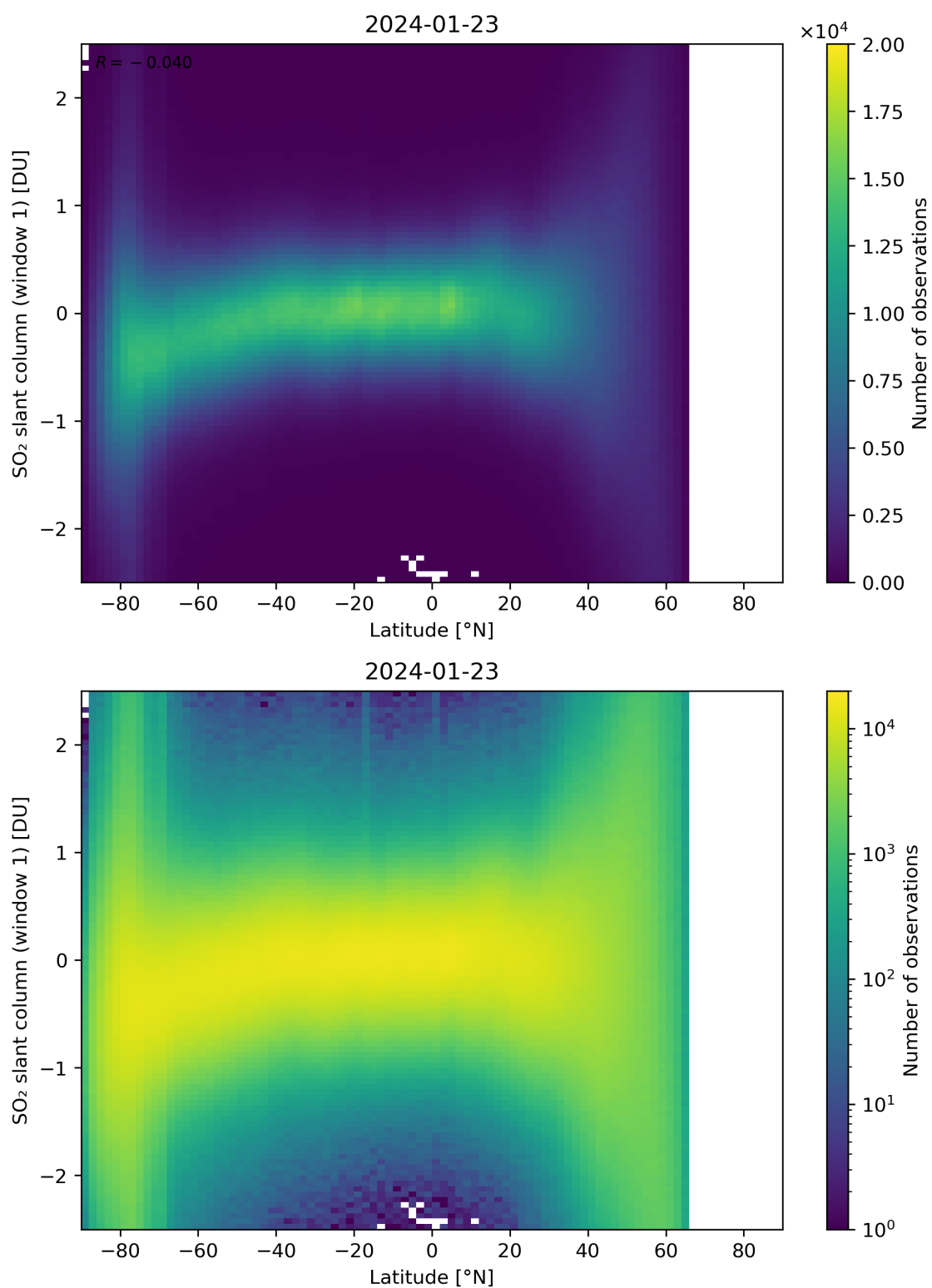
Figure 149: Scatter density plot of “Latitude” against “SO 2 slant column (window 1)” for 2024-01-22 to 2024-01-24.
