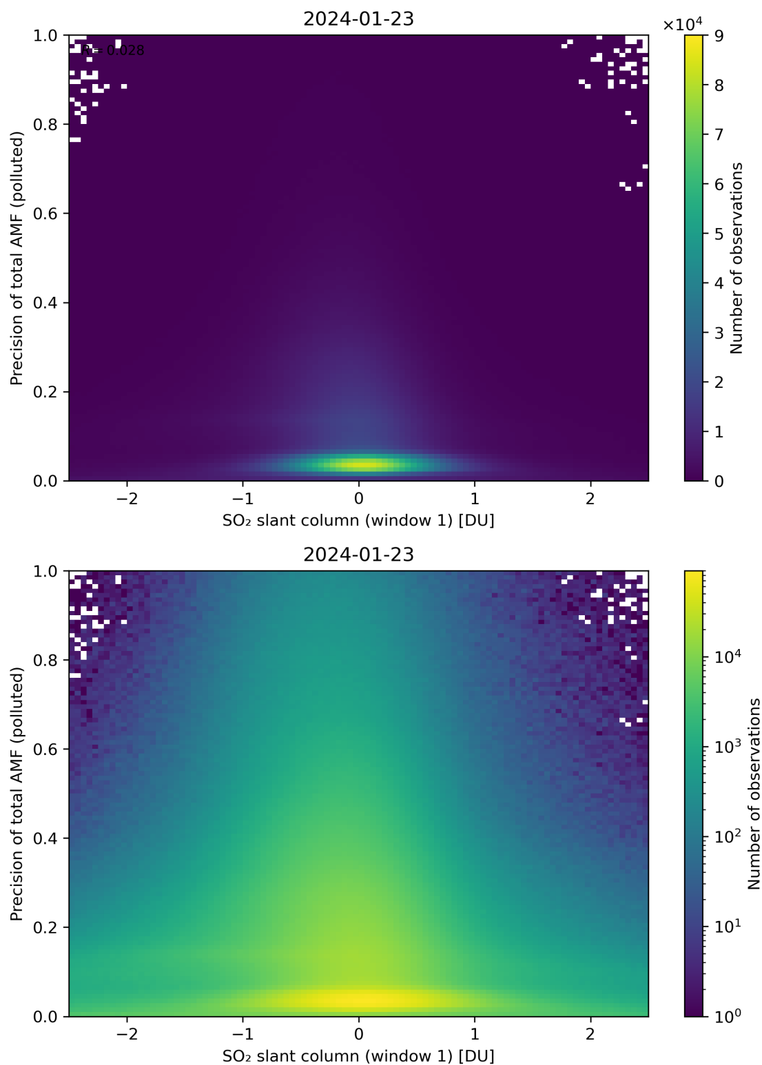
Figure 240: Scatter density plot of “SO 2 slant column (window 1)” against “Precision of total AMF (polluted)” for 2024-01-22 to 2024-01-24.
