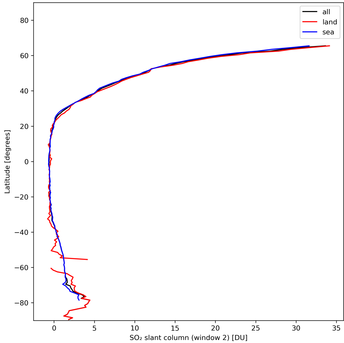
Figure 37: Zonal average of “SO 2 slant column (window 2)” for 2024-01-22 to 2024-01-24.
