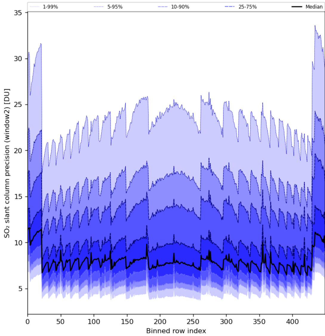
Figure 84: Along track statistics of “SO 2 slant column precision (window2)” for 2024-01-22 to 2024-01-24
