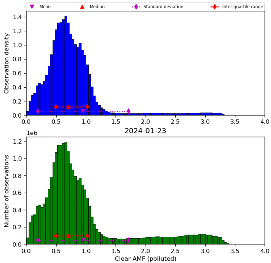
Figure 73: Histogram of “Clear AMF (polluted)” for 2024-01-22 to 2024-01-24
