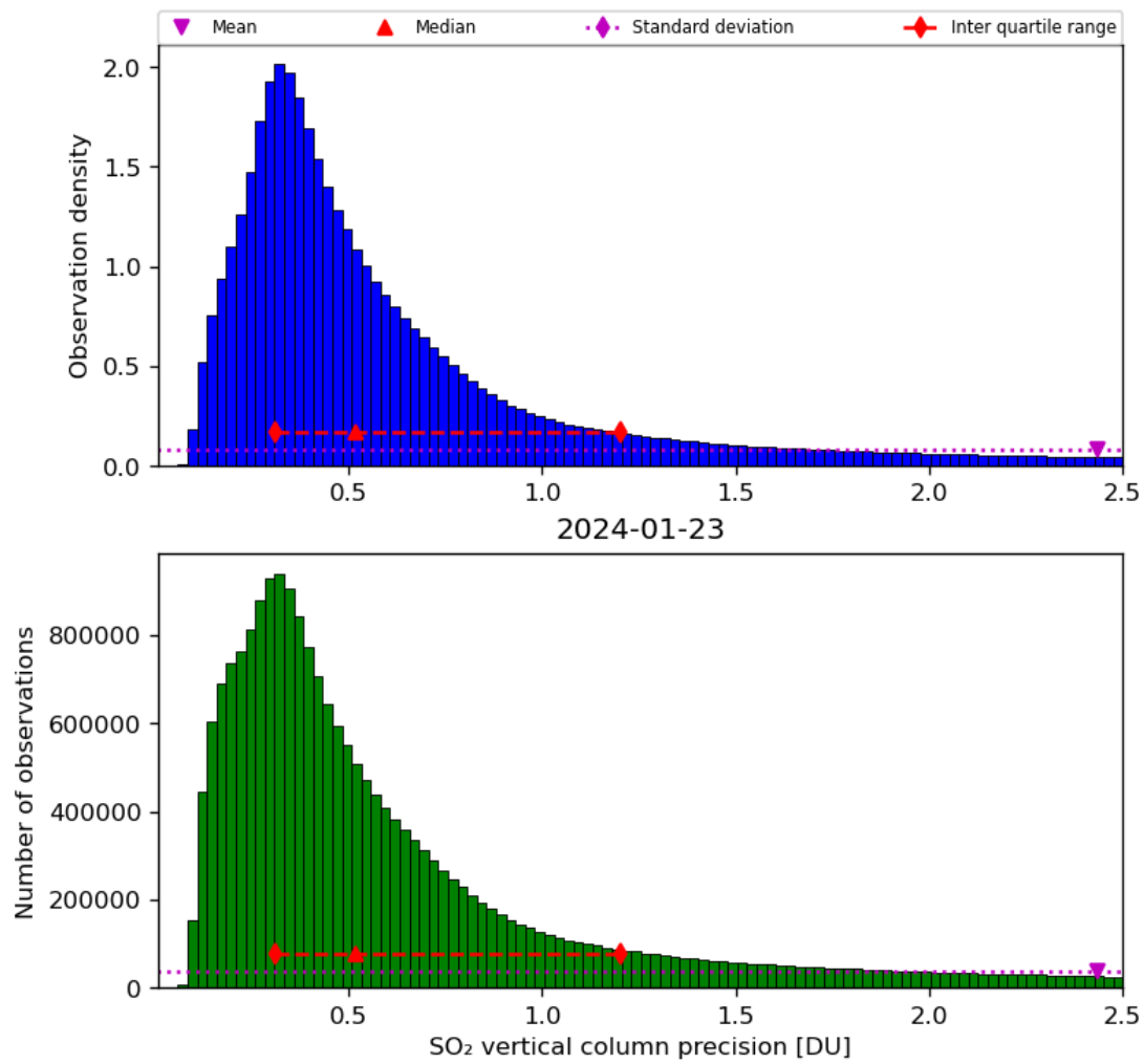
Figure 54: Histogram of “SO 2 vertical column precision” for 2024-01-22 to 2024-01-24
