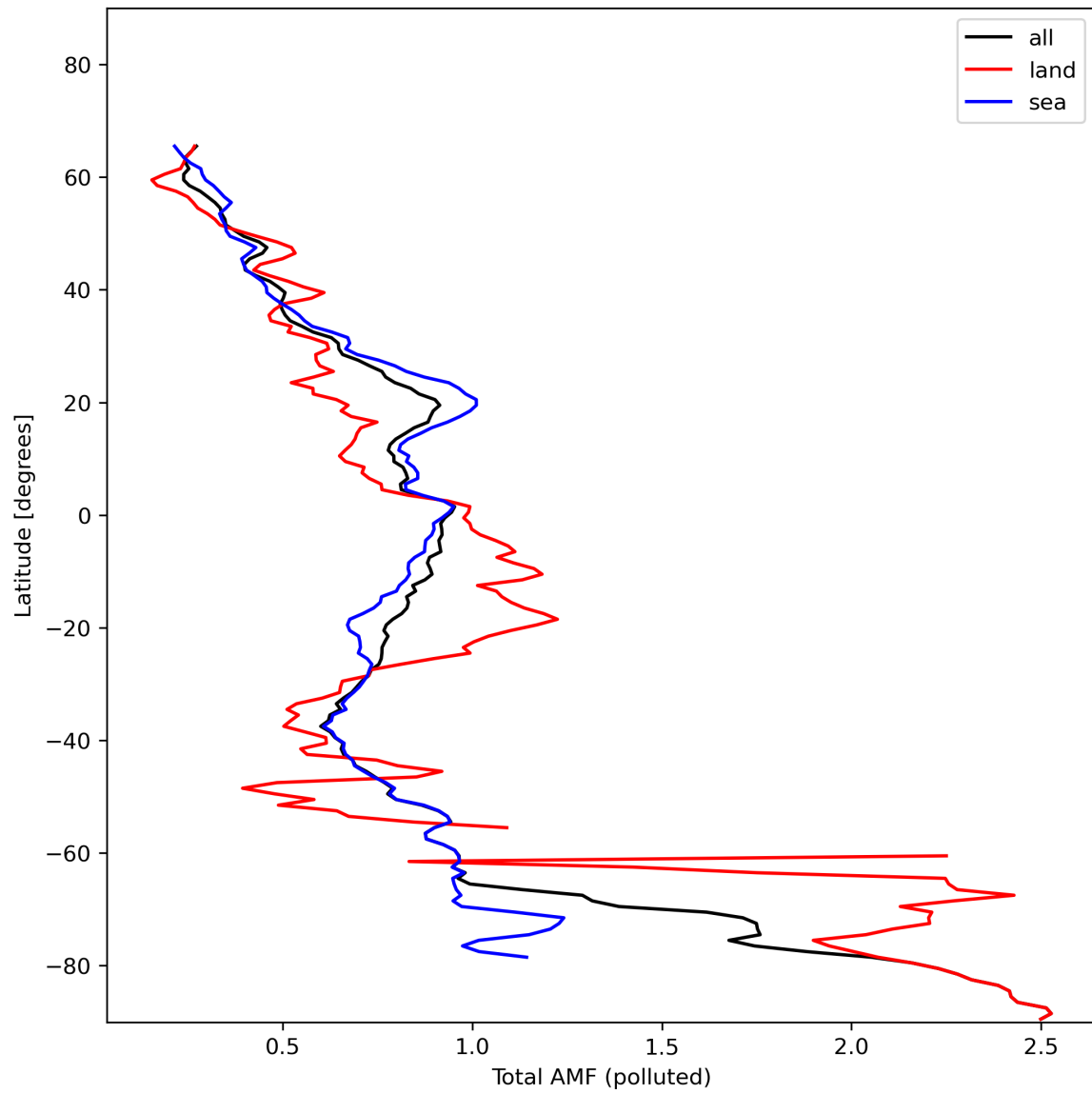
Figure 48: Zonal average of “Total AMF (polluted)” for 2024-01-22 to 2024-01-24.
