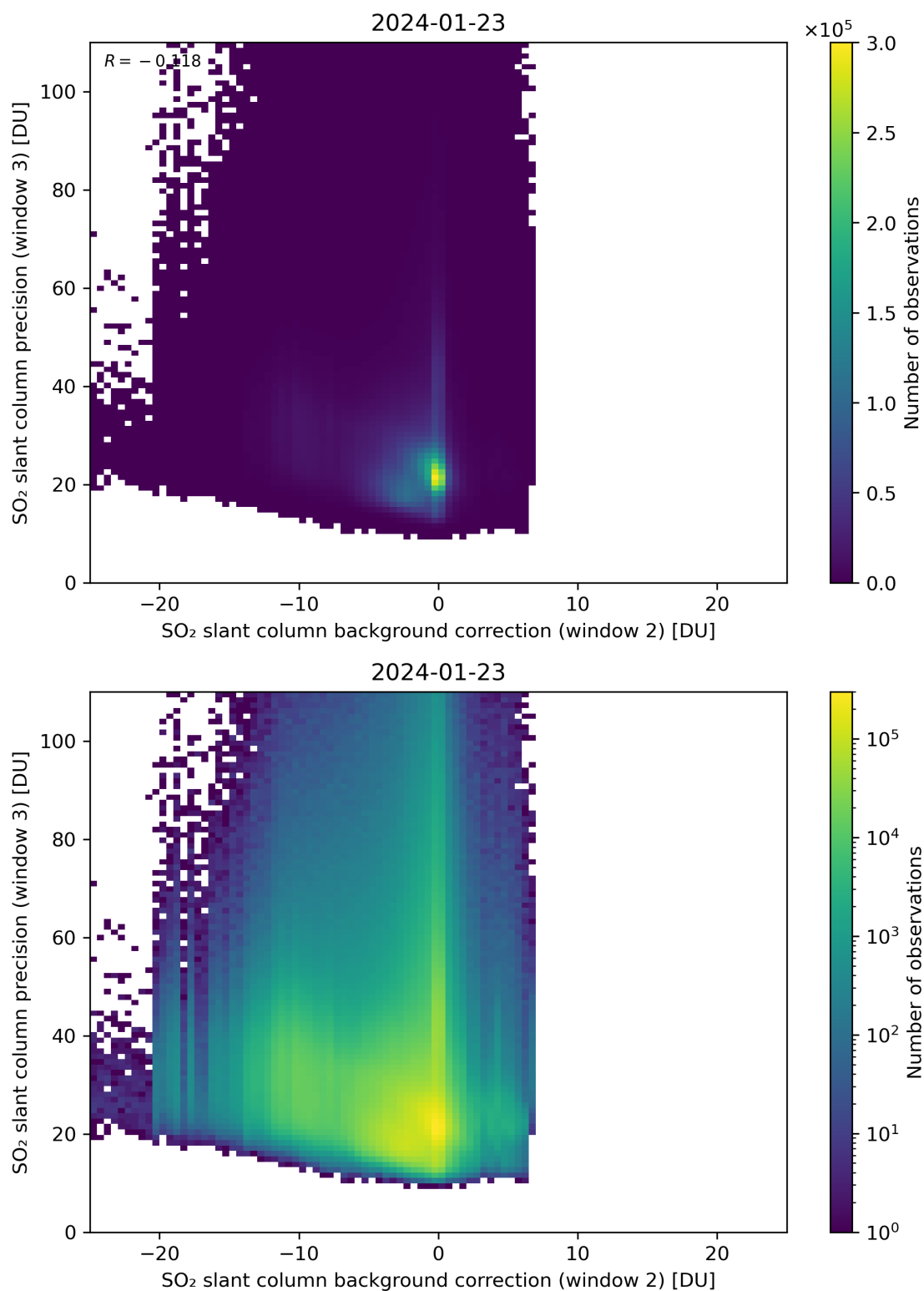
Figure 118: Scatter density plot of “SO 2 slant column background correction (window 2)” against “SO 2 slant column precision (window 3)” for 2024-01-22 to 2024-01-24.
