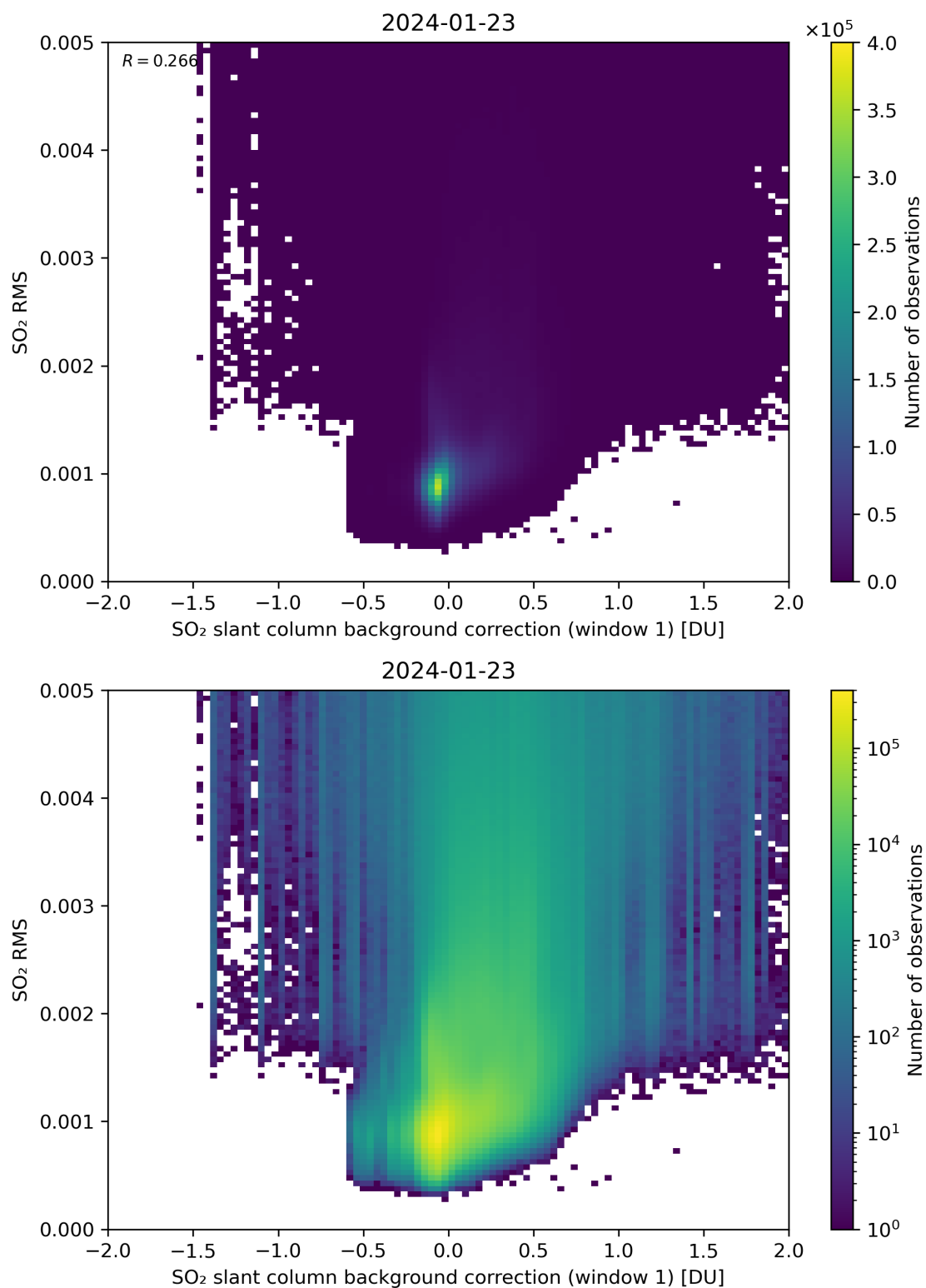
Figure 102: Scatter density plot of “SO 2 slant column background correction (window 1)” against “SO 2 RMS” for 2024-01-22 to 2024-01-24.
