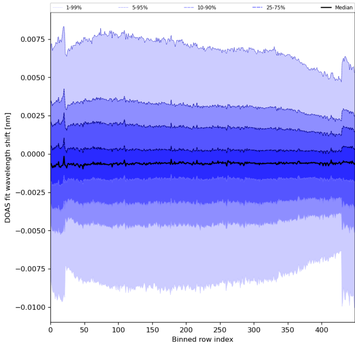
Figure 91: Along track statistics of “DOAS fit wavelength shift” for 2024-01-22 to 2024-01-24
