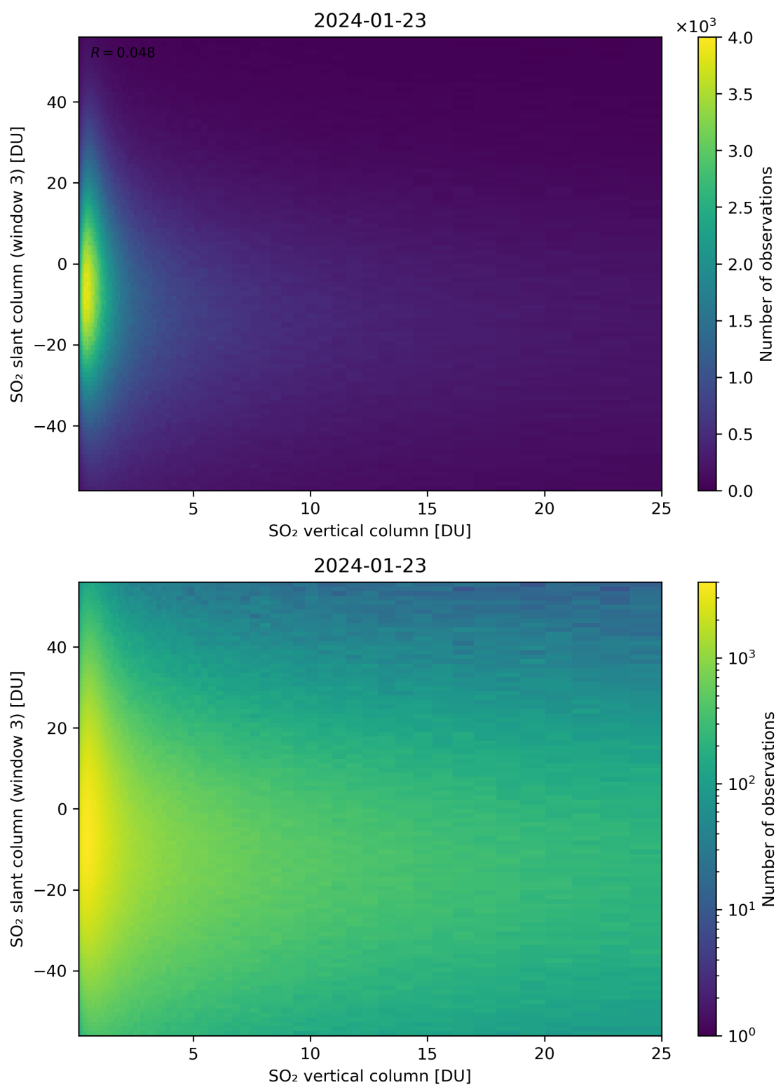
Figure 303: Scatter density plot of “SO 2 vertical column” against “SO 2 slant column (window 3)” for 2024-01-22 to 2024-01-24.
