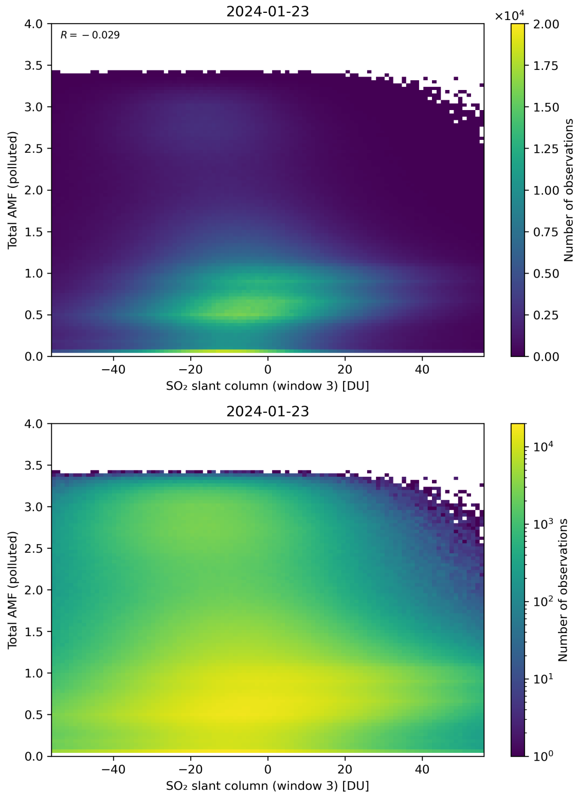
Figure 268: Scatter density plot of “SO 2 slant column (window 3)” against “Total AMF (polluted)” for 2024-01-22 to 2024-01-24.
