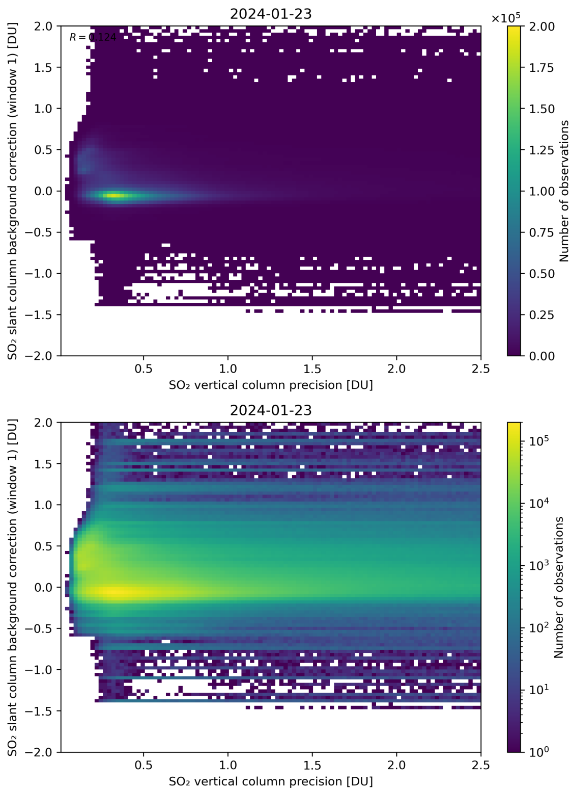
Figure 279: Scatter density plot of “SO 2 vertical column precision” against “SO 2 slant column background correction (window 1)” for 2024-01-22 to 2024-01-24.
