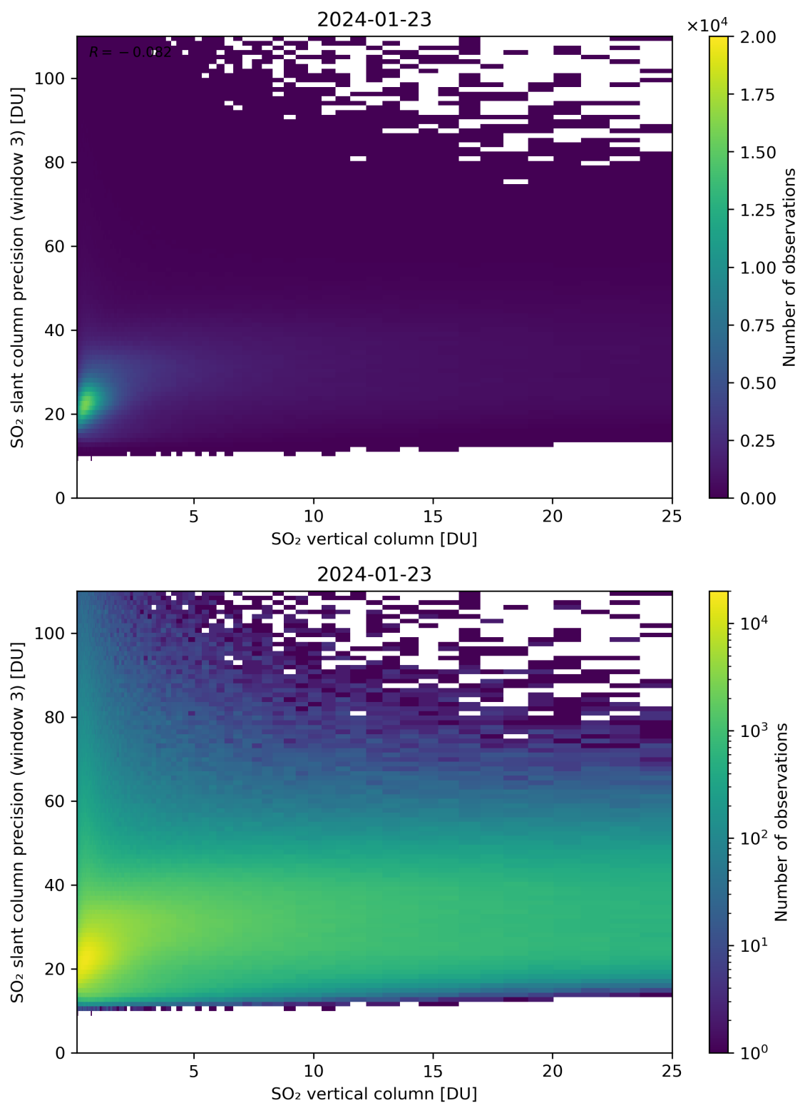
Figure 304: Scatter density plot of “SO 2 vertical column” against “SO 2 slant column precision (window 3)” for 2024-01-22 to 2024-01-24.
