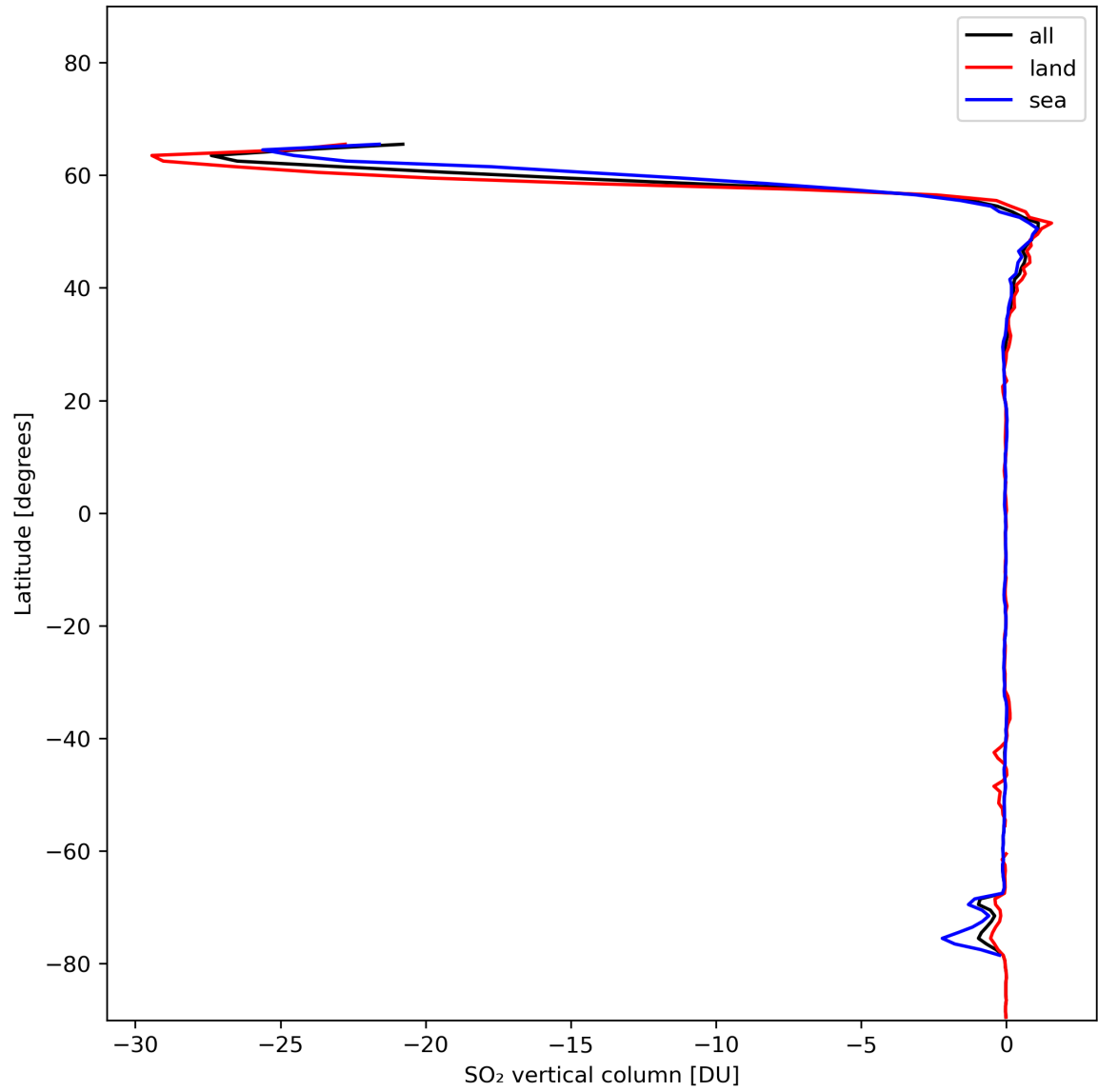
Figure 30: Zonal average of “SO 2 vertical column” for 2024-01-22 to 2024-01-24.
