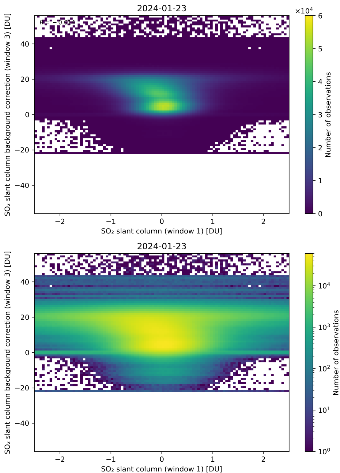
Figure 214: Scatter density plot of “SO 2 slant column (window 1)” against “SO 2 slant column background correction (window 3)” for 2024-01-22 to 2024-01-24.
