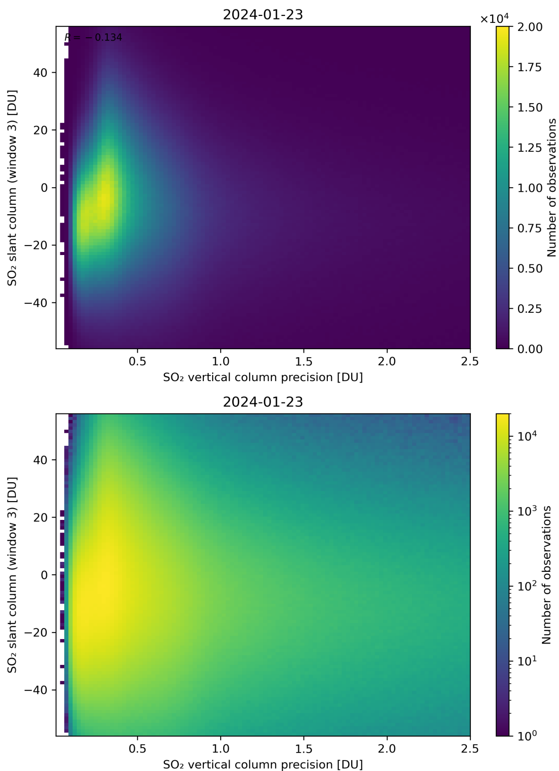
Figure 292: Scatter density plot of “SO 2 vertical column precision” against “SO 2 slant column (window 3)” for 2024-01-22 to 2024-01-24.
