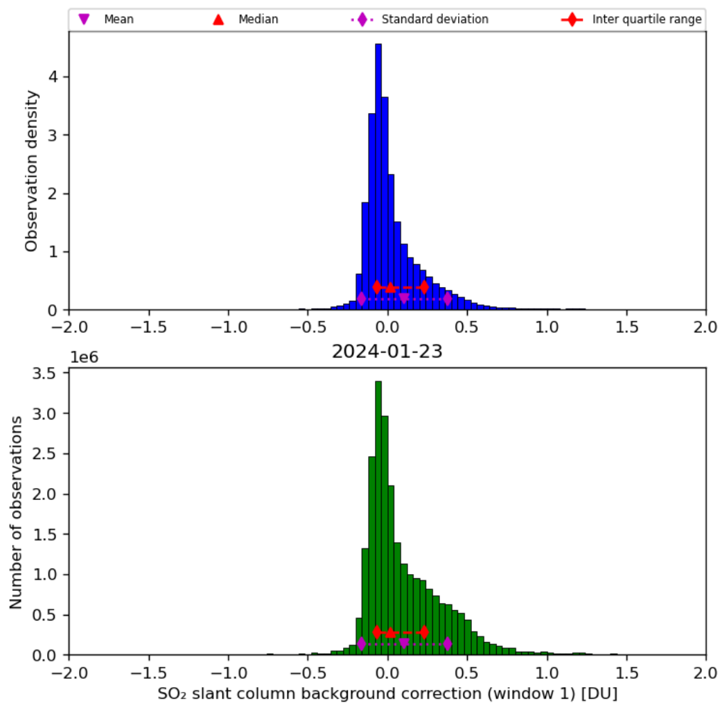
Figure 59: Histogram of “SO 2 slant column background correction (window 1)” for 2024-01-22 to 2024-01-24
