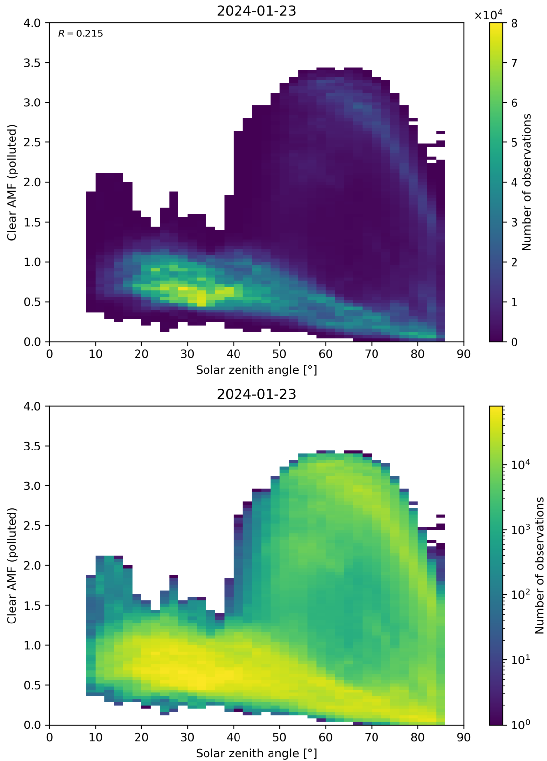
Figure 165: Scatter density plot of “Solar zenith angle” against “Clear AMF (polluted)” for 2024-01-22 to 2024-01-24.
