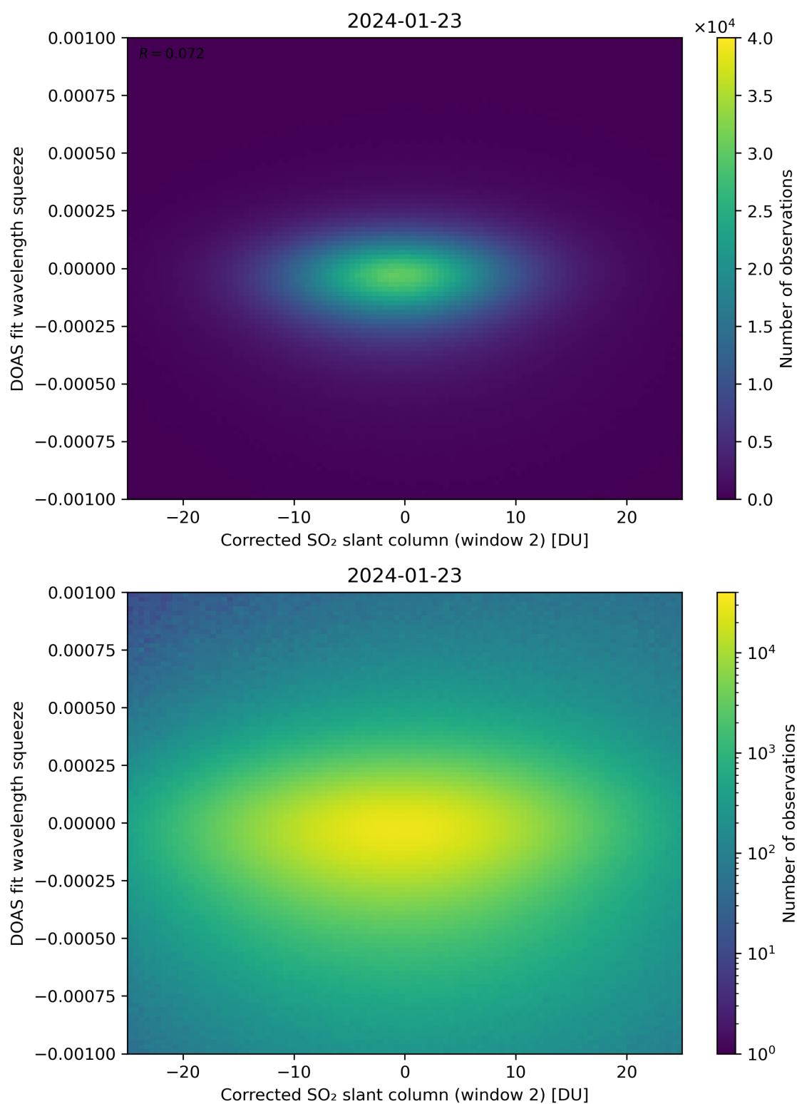
Figure 197: Scatter density plot of “Corrected SO 2 slant column (window 2)” against “DOAS fit wavelength squeeze” for 2024-01-22 to 2024-01-24.
