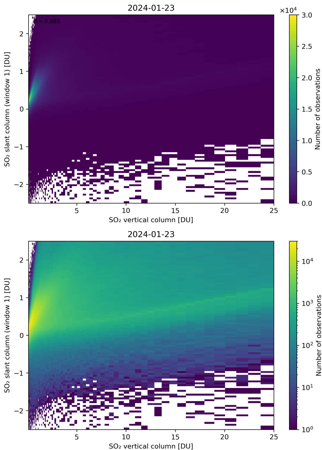
Figure 300: Scatter density plot of “SO 2 vertical column” against “SO 2 slant column (window 1)” for 2024-01-22 to 2024-01-24.
