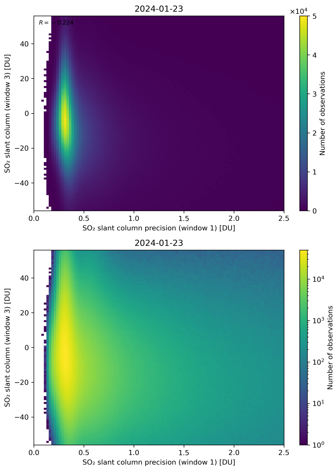
Figure 228: Scatter density plot of “SO 2 slant column precision (window 1)” against “SO 2 slant column (window 3)” for 2024-01-22 to 2024-01-24.
