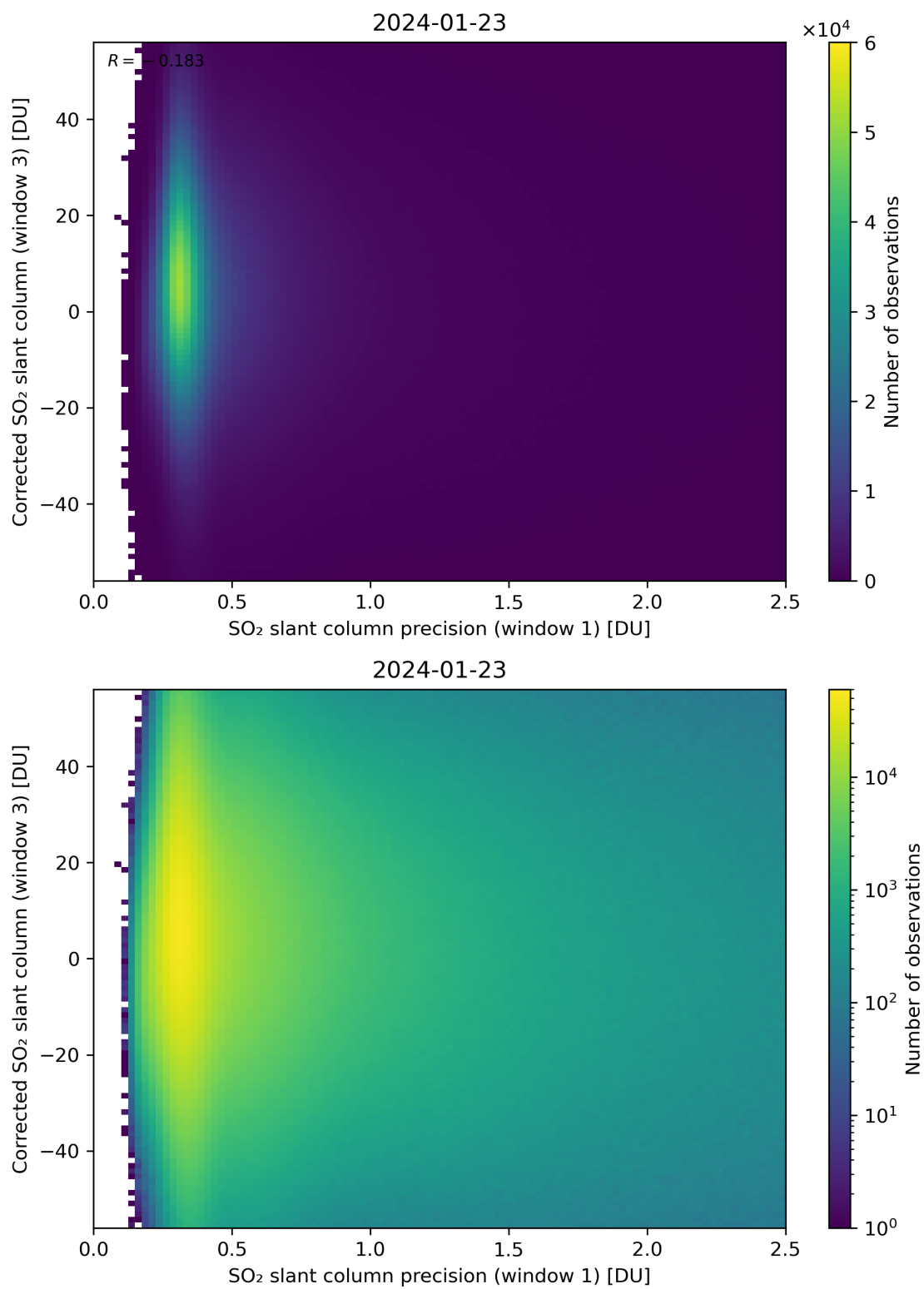
Figure 226: Scatter density plot of “SO 2 slant column precision (window 1)” against “Corrected SO 2 slant column (window 3)” for 2024-01-22 to 2024-01-24.
