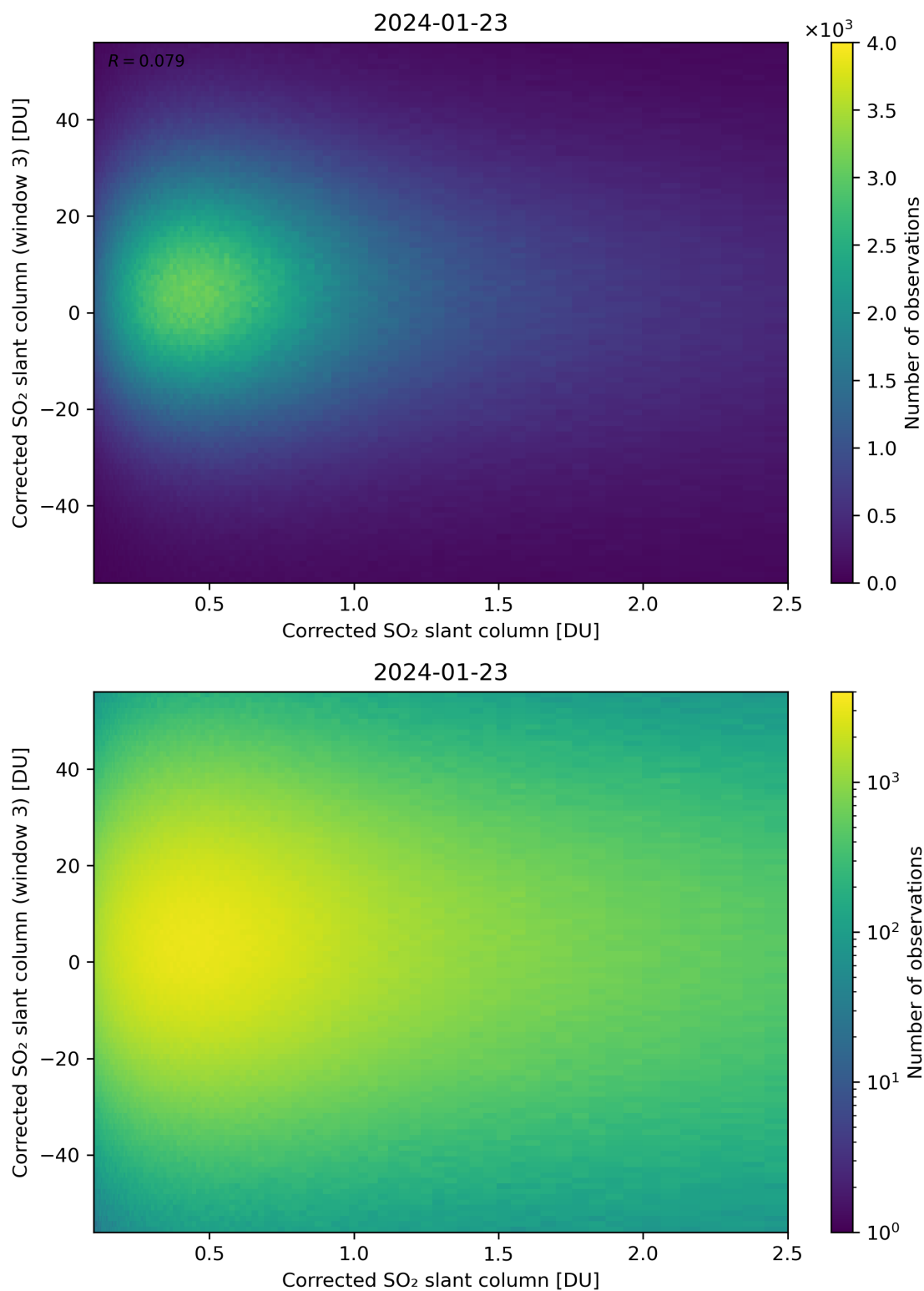
Figure 186: Scatter density plot of “Corrected SO 2 slant column” against “Corrected SO 2 slant column (window 3)” for 2024-01-22 to 2024-01-24.
