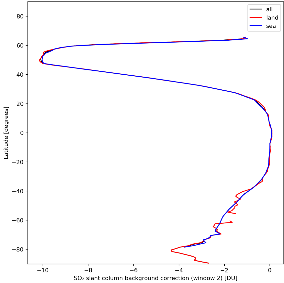
Figure 40: Zonal average of “SO 2 slant column background correction (window 2)” for 2024-01-22 to 2024-01-24.
