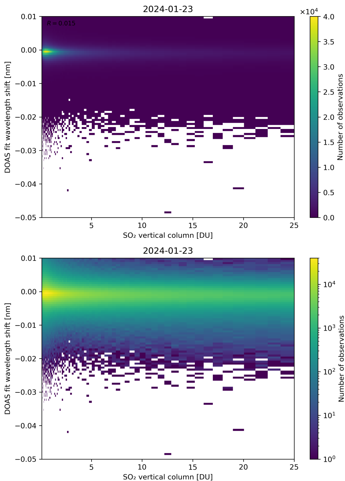
Figure 276: Scatter density plot of “SO 2 vertical column” against “DOAS fit wavelength shift” for 2024-01-22 to 2024-01-24.
