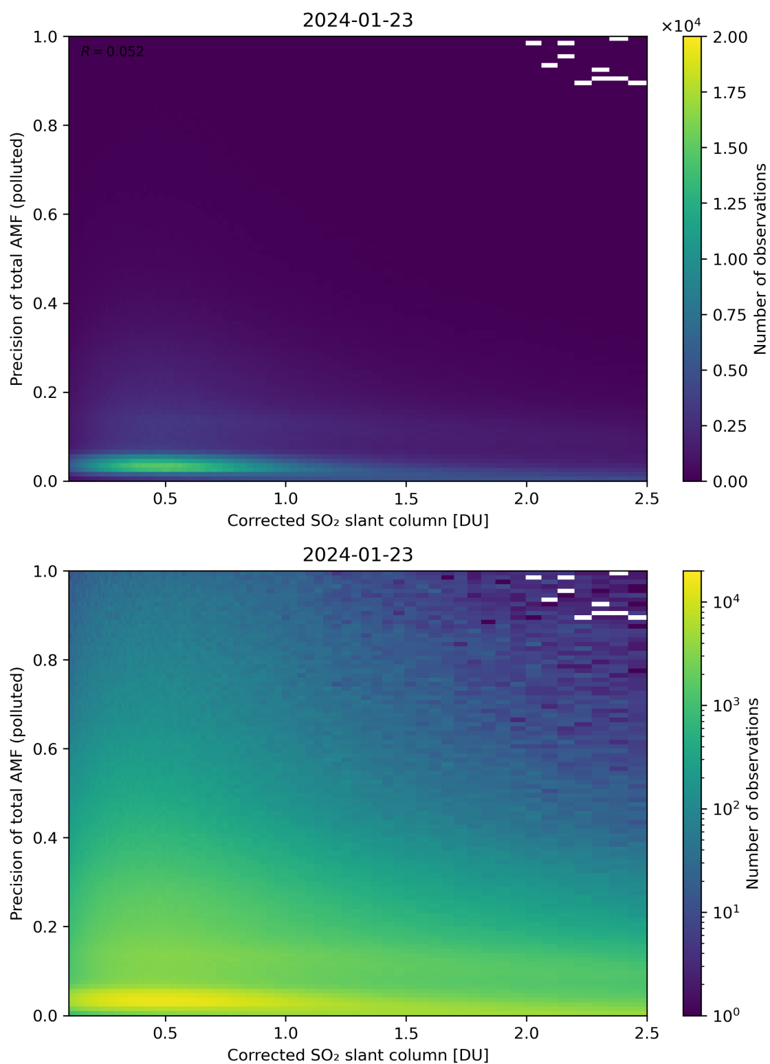
Figure 193: Scatter density plot of “Corrected SO 2 slant column” against “Precision of total AMF (polluted)” for 2024-01-22 to 2024-01-24.
