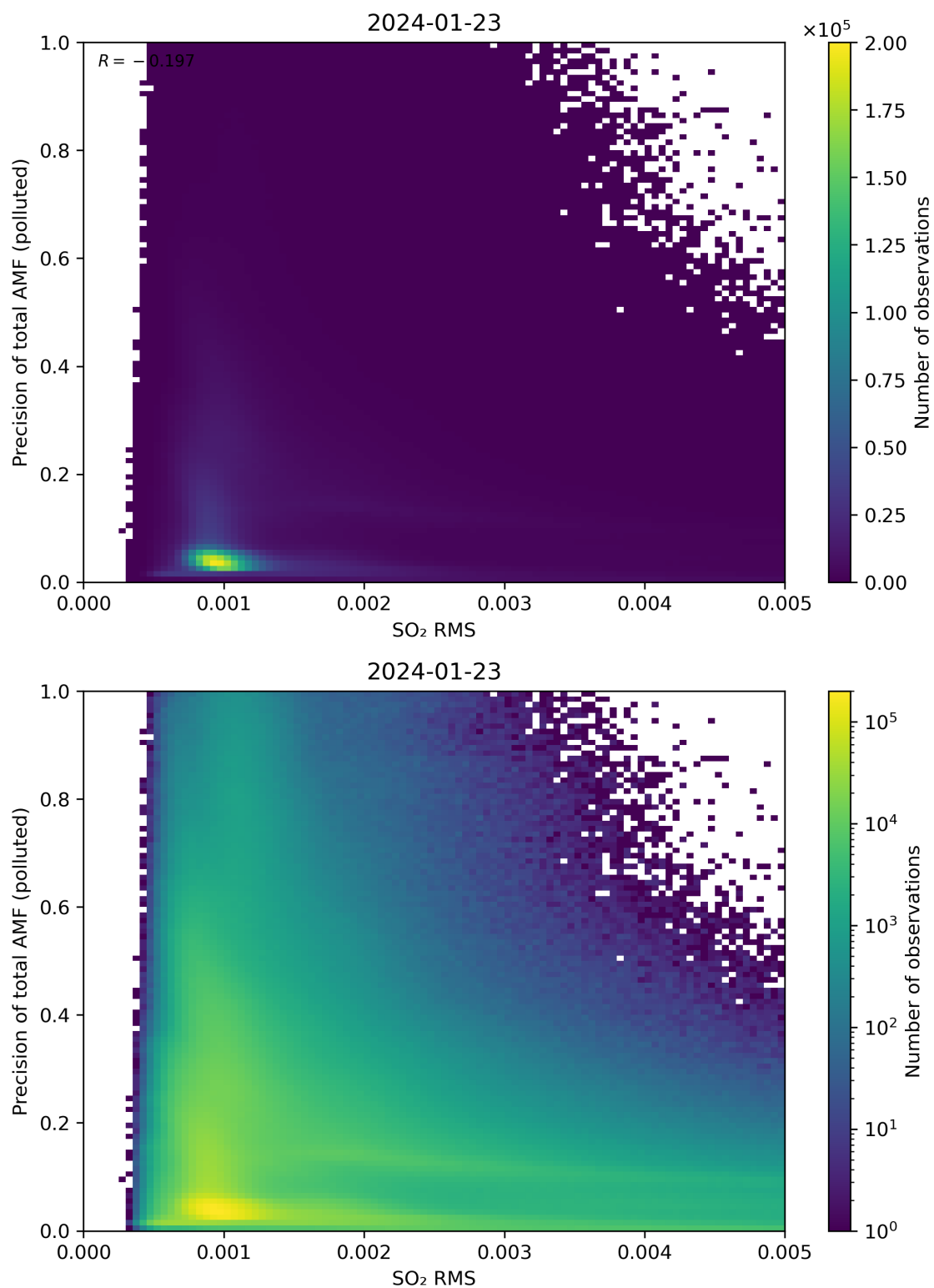
Figure 138: Scatter density plot of “SO 2 RMS” against “Precision of total AMF (polluted)” for 2024-01-22 to 2024-01-24.
