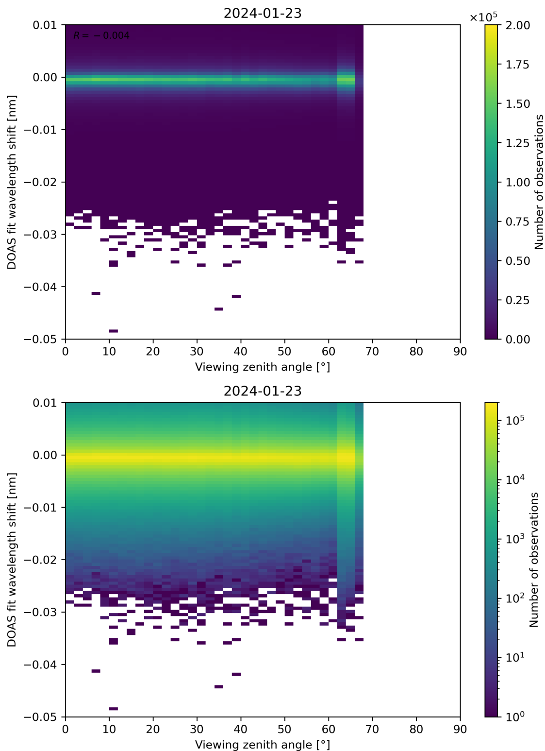
Figure 311: Scatter density plot of “Viewing zenith angle” against “DOAS fit wavelength shift” for 2024-01-22 to 2024-01-24.
