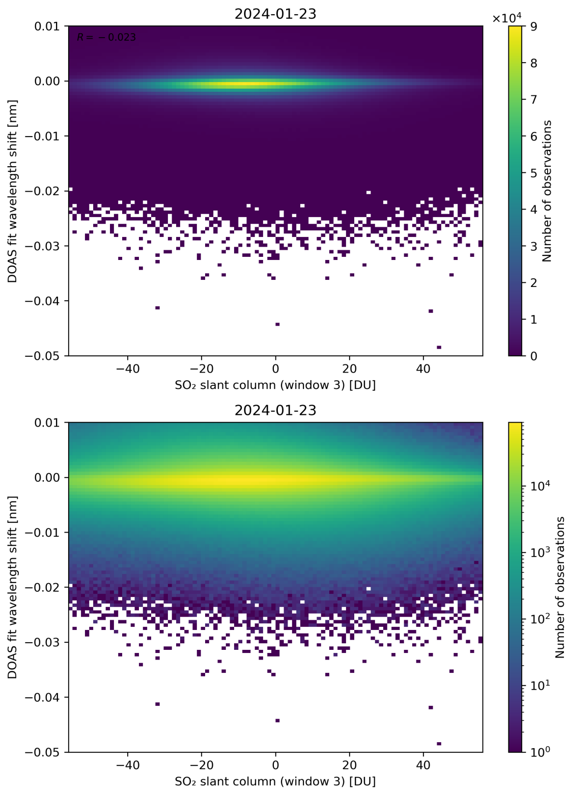
Figure 254: Scatter density plot of “SO 2 slant column (window 3)” against “DOAS fit wavelength shift” for 2024-01-22 to 2024-01-24.
