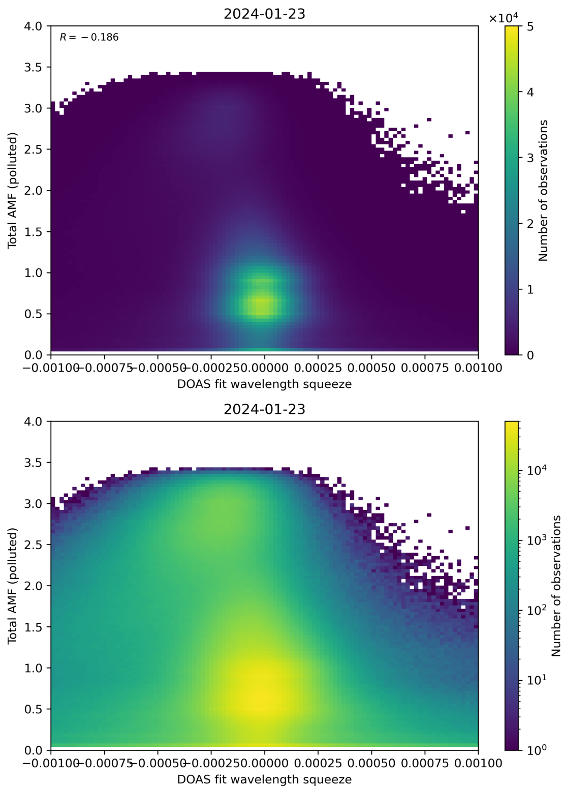
Figure 134: Scatter density plot of “DOAS fit wavelength squeeze” against “Total AMF (polluted)” for 2024-01-22 to 2024-01-24.
