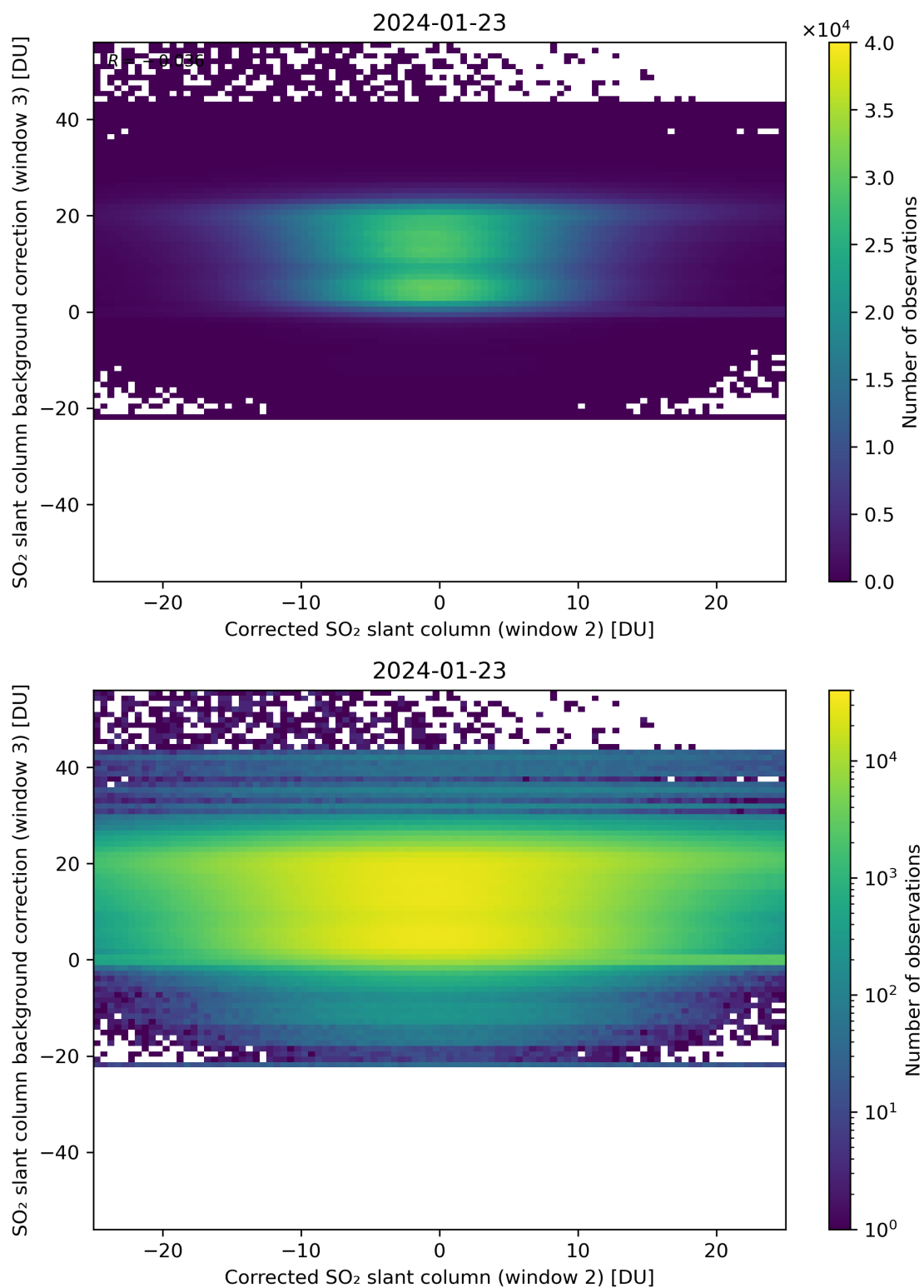
Figure 195: Scatter density plot of “Corrected SO 2 slant column (window 2)” against “SO 2 slant column background correction (window 3)” for 2024-01-22 to 2024-01-24.
