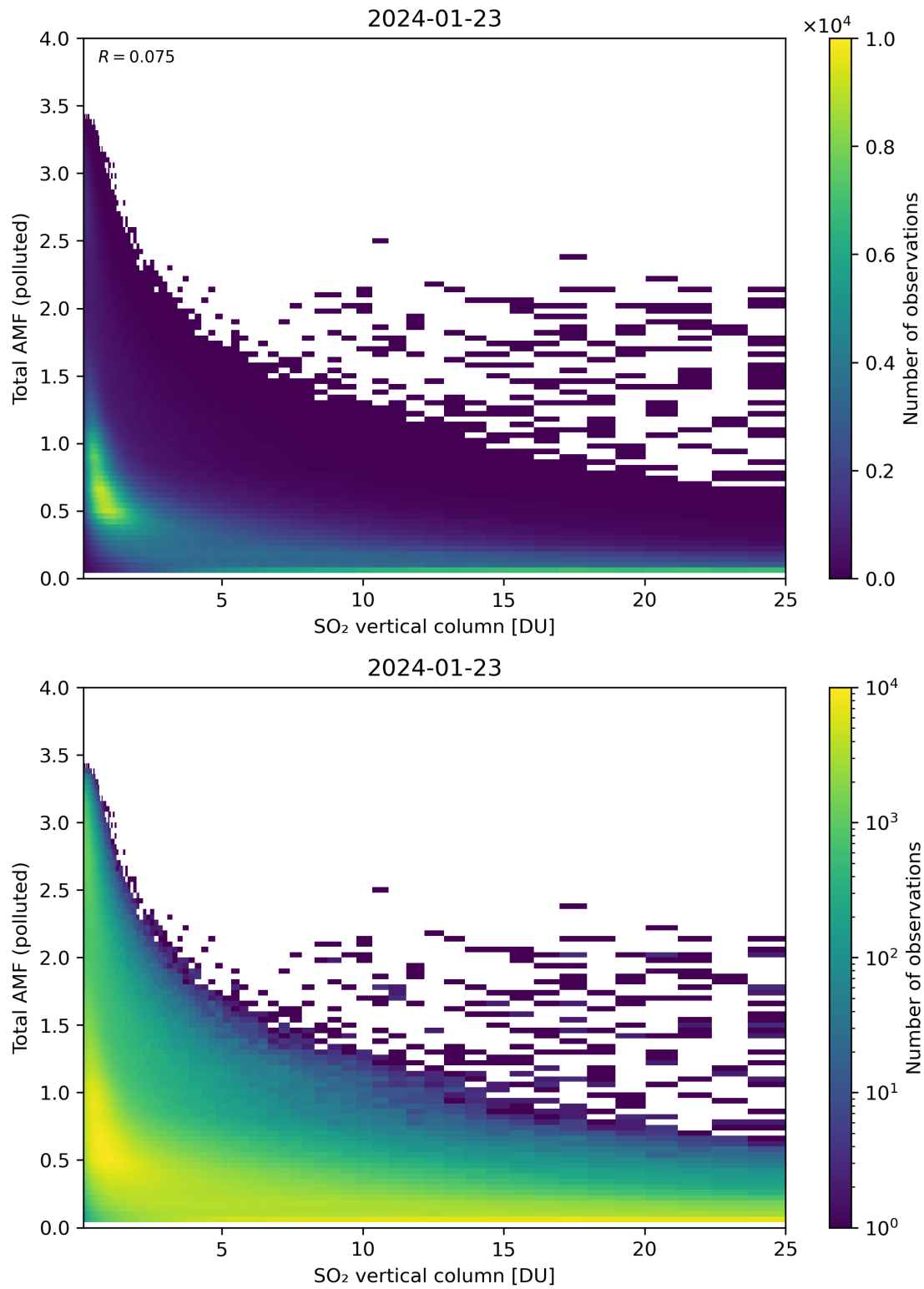
Figure 305: Scatter density plot of “SO 2 vertical column” against “Total AMF (polluted)” for 2024-01-22 to 2024-01-24.
