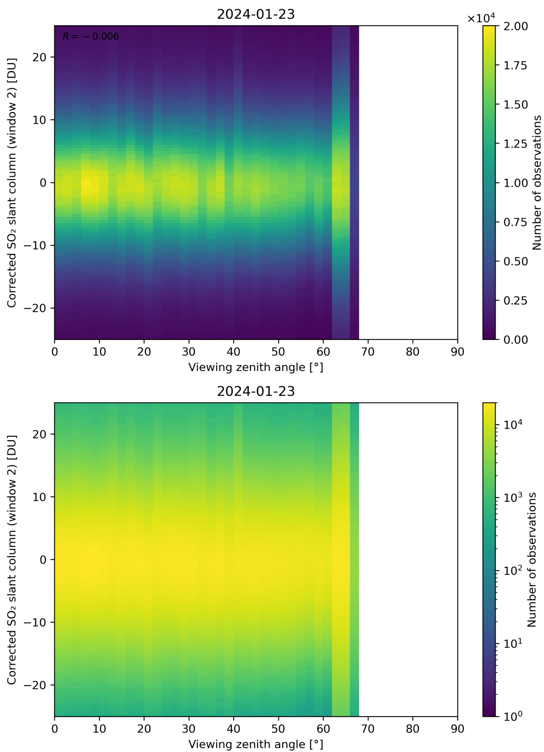
Figure 318: Scatter density plot of “Viewing zenith angle” against “Corrected SO 2 slant column (window 2)” for 2024-01-22 to 2024-01-24.
