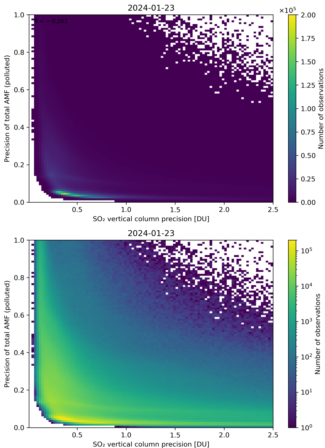
Figure 295: Scatter density plot of “SO 2 vertical column precision” against “Precision of total AMF (polluted)” for 2024-01-22 to 2024-01-24.
