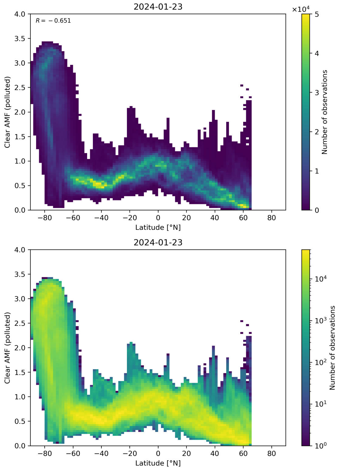
Figure 145: Scatter density plot of “Latitude” against “Clear AMF (polluted)” for 2024-01-22 to 2024-01-24.
