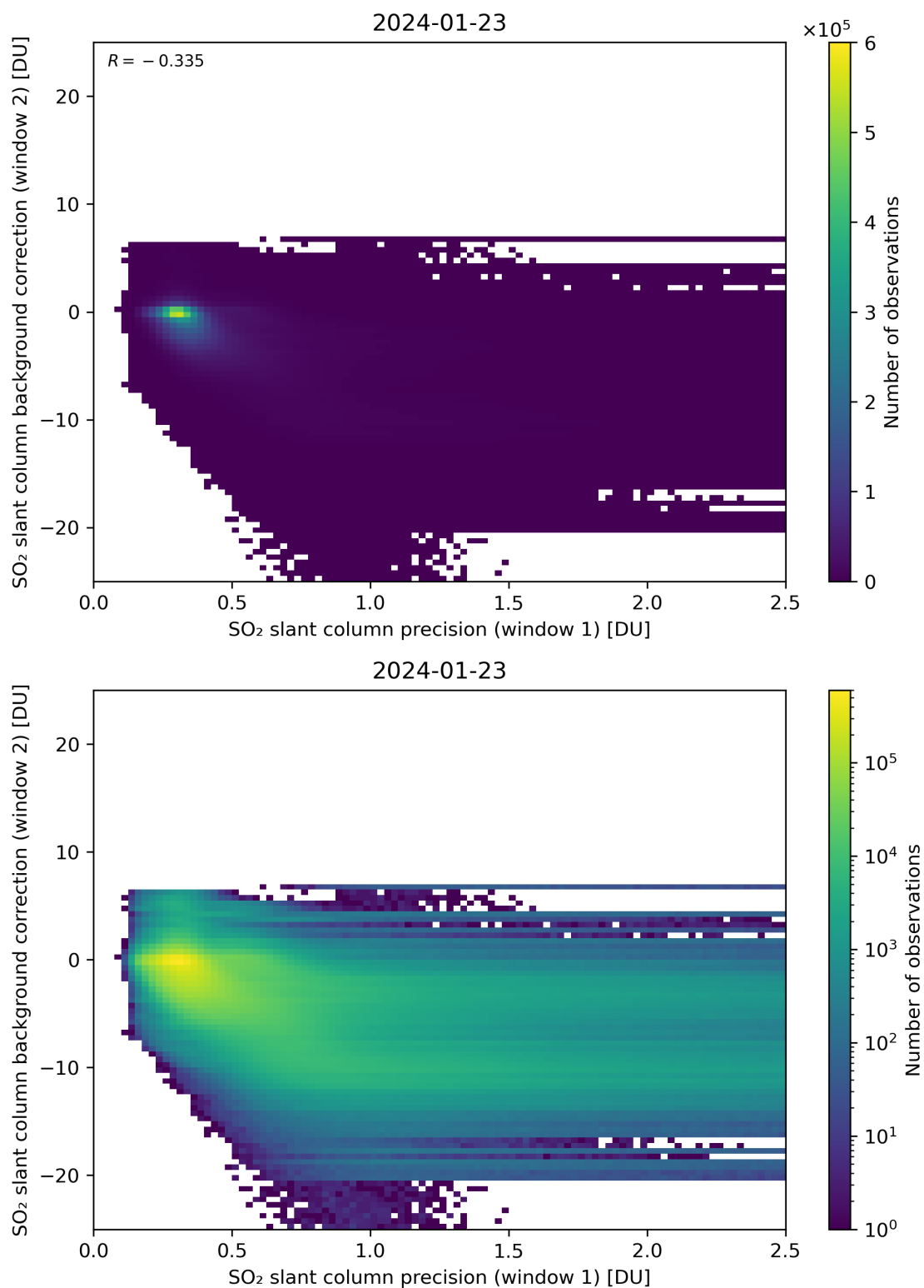
Figure 219: Scatter density plot of “SO 2 slant column precision (window 1)” against “SO 2 slant column background correction (window 2)” for 2024-01-22 to 2024-01-24.
