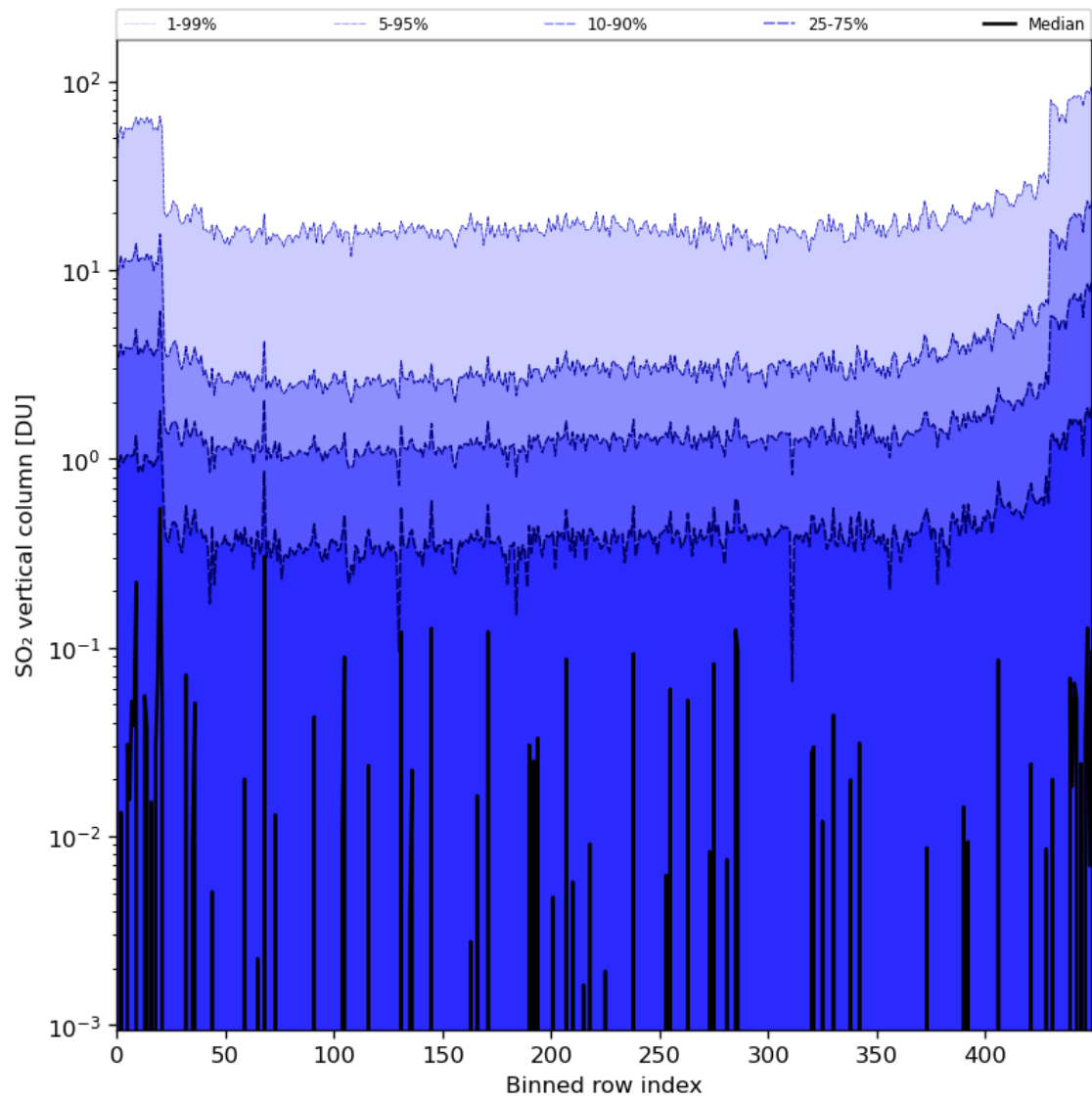
Figure 76: Along track statistics of “SO 2 vertical column” for 2024-01-22 to 2024-01-24
