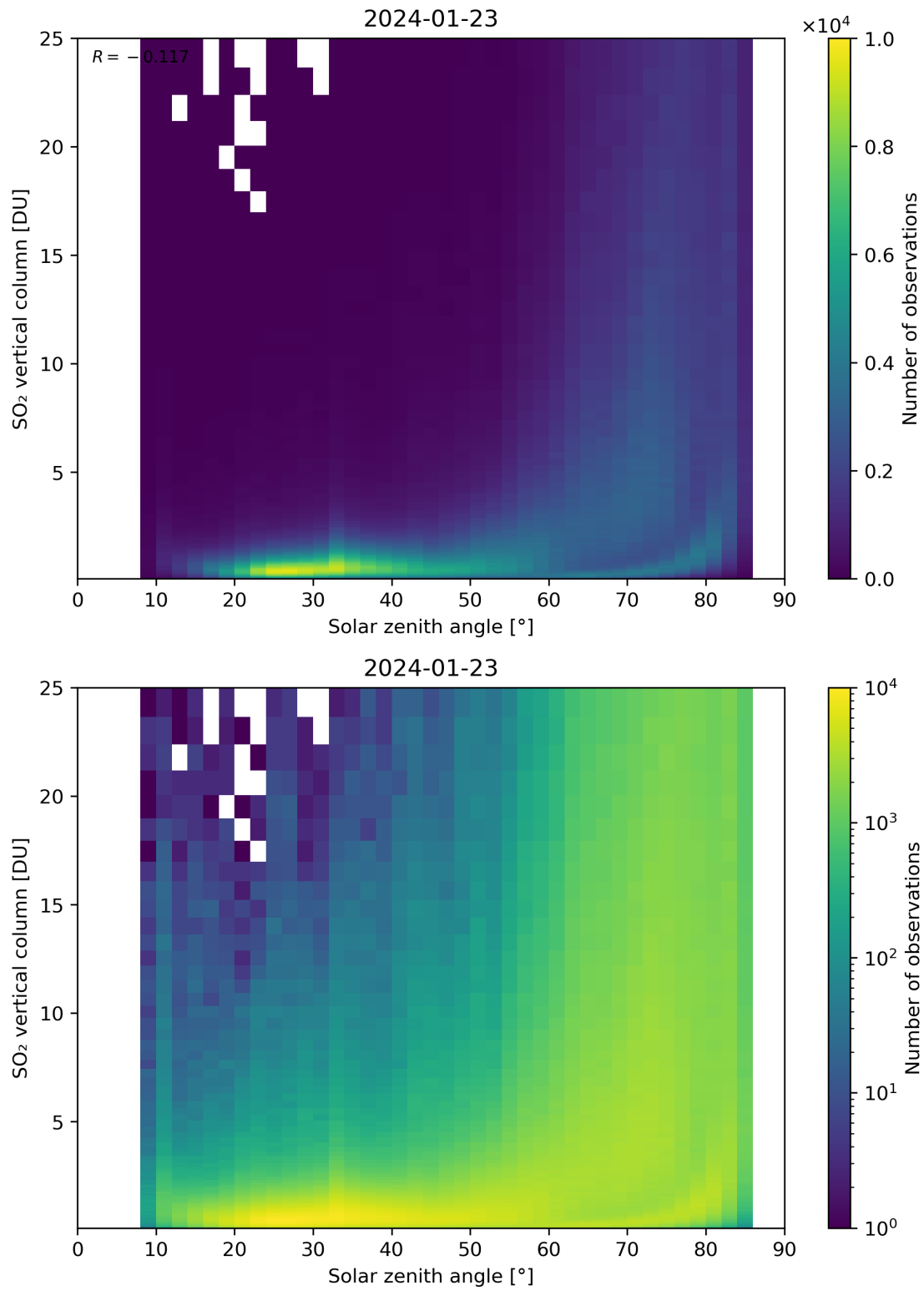
Figure 176: Scatter density plot of “Solar zenith angle” against “SO 2 vertical column” for 2024-01-22 to 2024-01-24.
