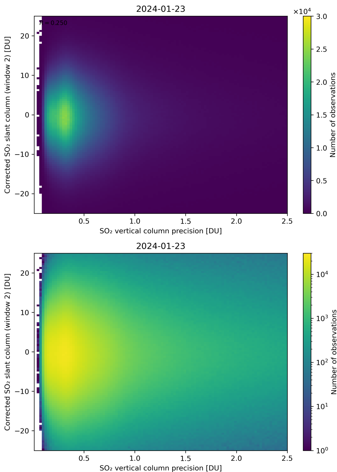
Figure 287: Scatter density plot of “SO 2 vertical column precision” against “Corrected SO 2 slant column (window 2)” for 2024-01-22 to 2024-01-24.
