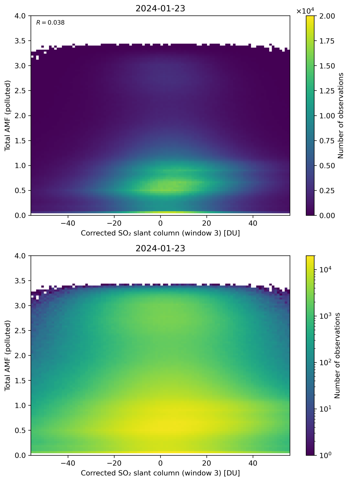
Figure 210: Scatter density plot of “Corrected SO 2 slant column (window 3)” against “Total AMF (polluted)” for 2024-01-22 to 2024-01-24.
