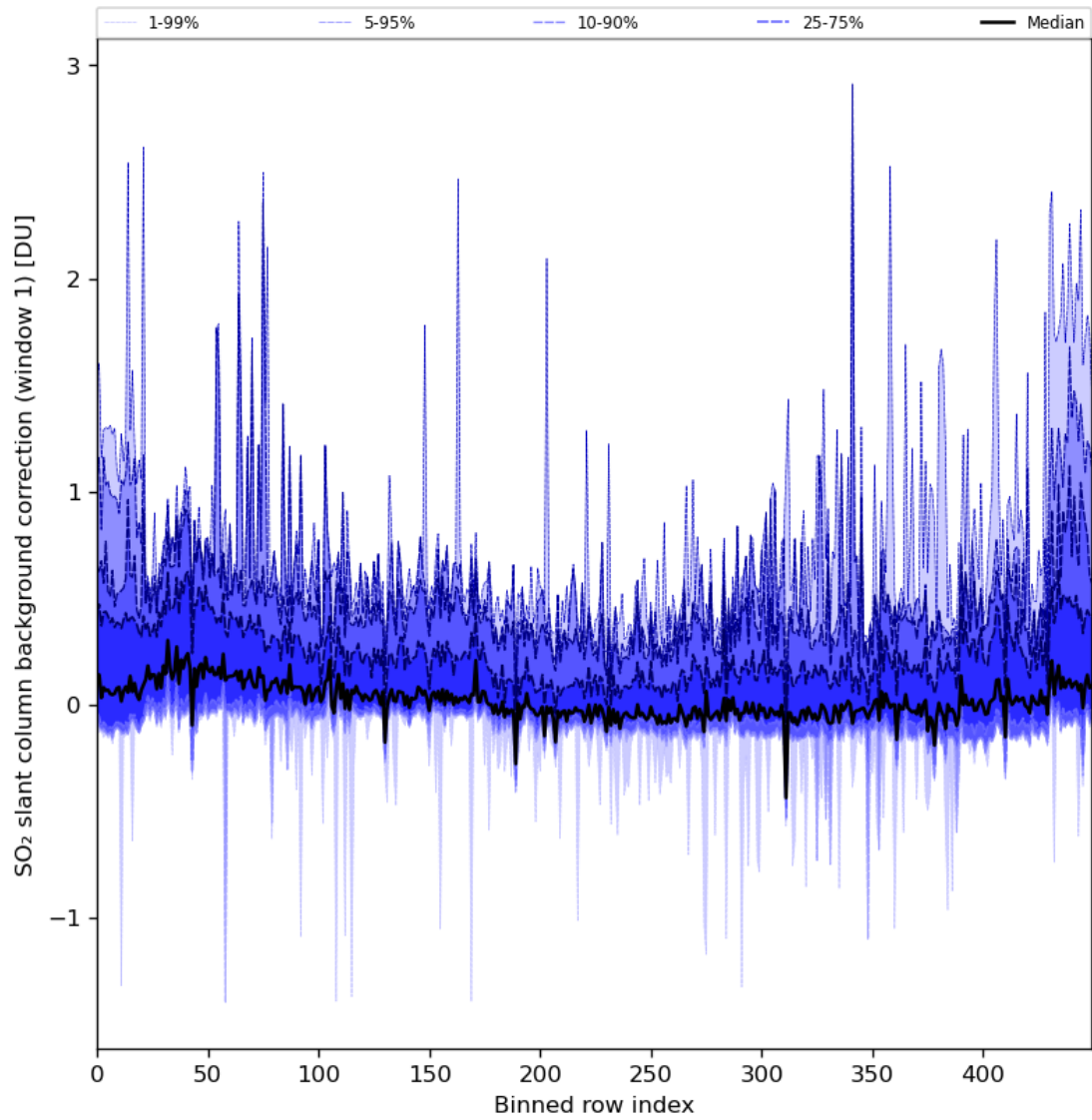
Figure 82: Along track statistics of “SO 2 slant column background correction (window 1)” for 2024-01-22 to 2024-01-24
