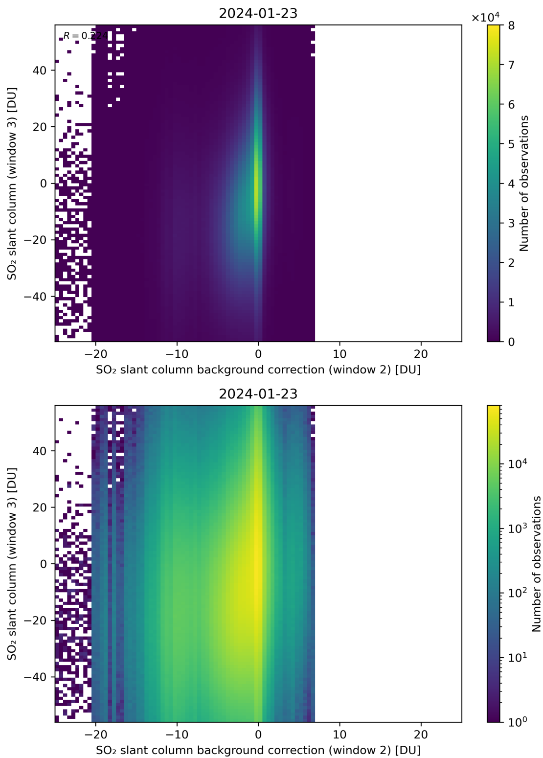
Figure 117: Scatter density plot of “SO 2 slant column background correction (window 2)” against “SO 2 slant column (window 3)” for 2024-01-22 to 2024-01-24.
