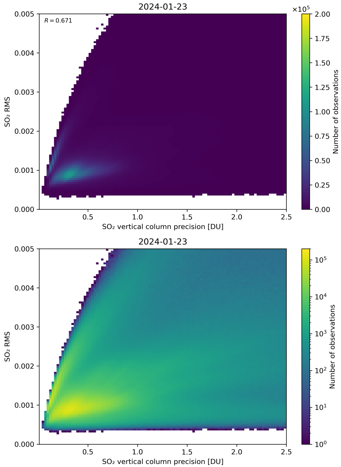
Figure 284: Scatter density plot of “SO 2 vertical column precision” against “SO 2 RMS” for 2024-01-22 to 2024-01-24.
