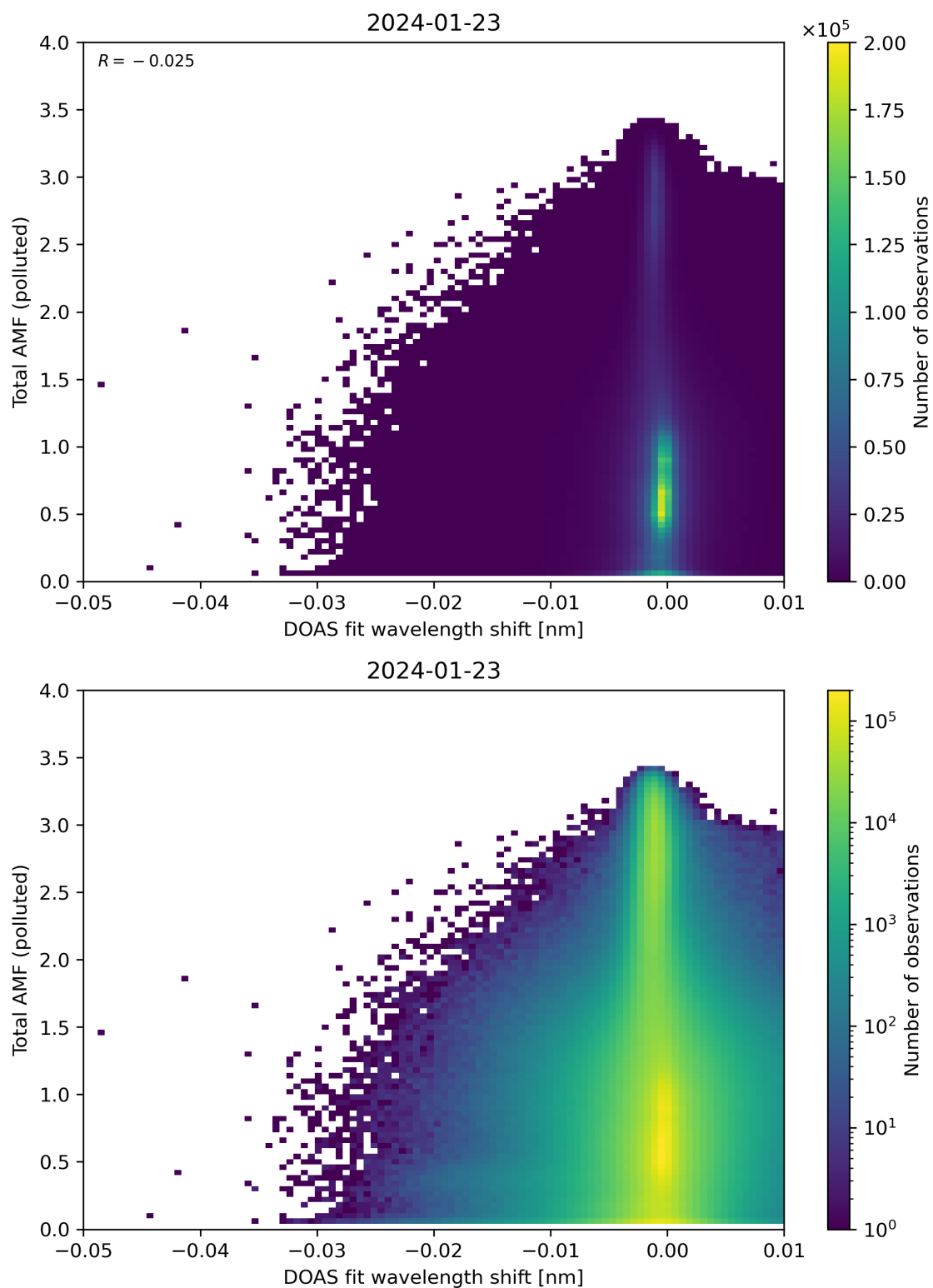
Figure 130: Scatter density plot of “DOAS fit wavelength shift” against “Total AMF (polluted)” for 2024-01-22 to 2024-01-24.
