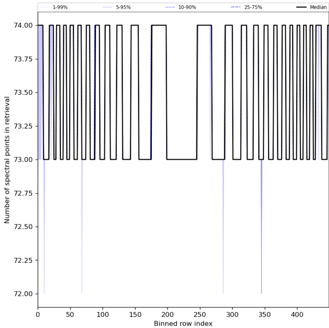
Figure 97: Along track statistics of “Number of spectral points in retrieval” for 2024-01-22 to 2024-01-24
