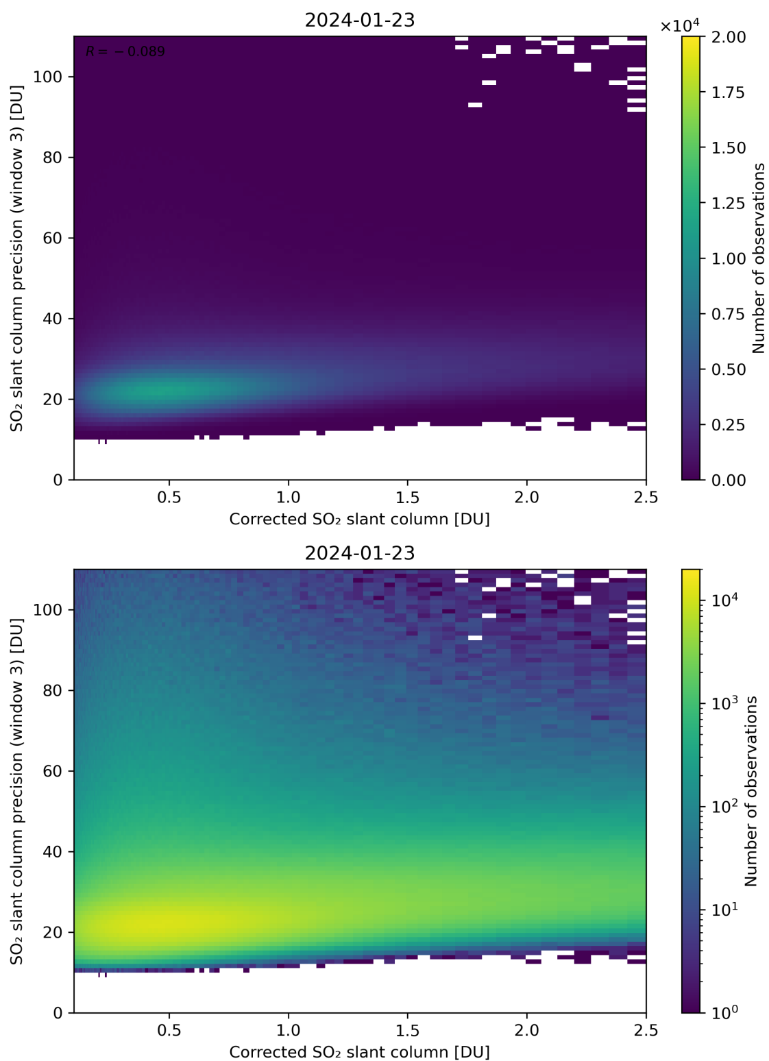
Figure 191: Scatter density plot of “Corrected SO 2 slant column” against “SO 2 slant column precision (window 3)” for 2024-01-22 to 2024-01-24.
