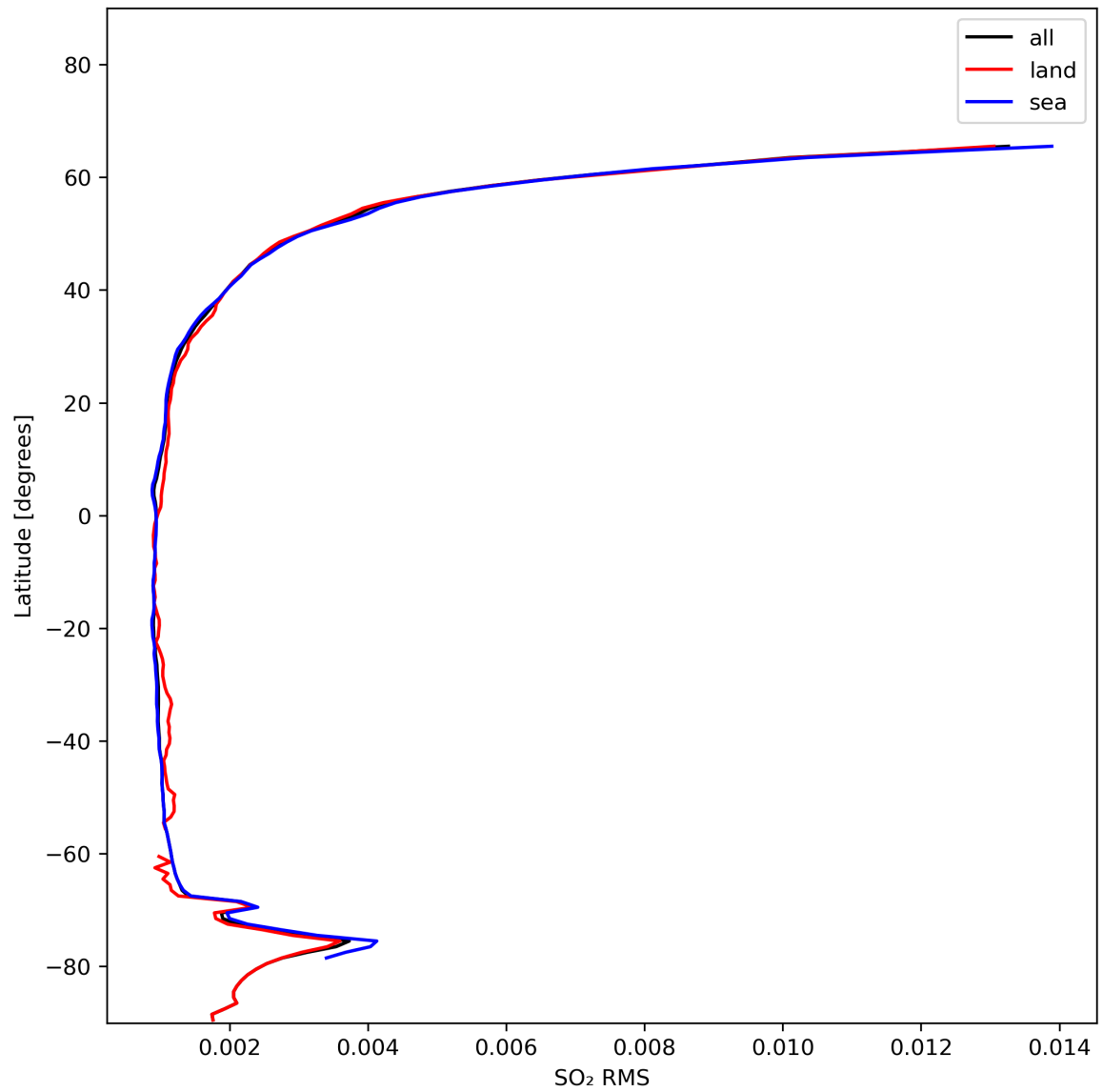
Figure 47: Zonal average of “SO 2 RMS” for 2024-01-22 to 2024-01-24.
