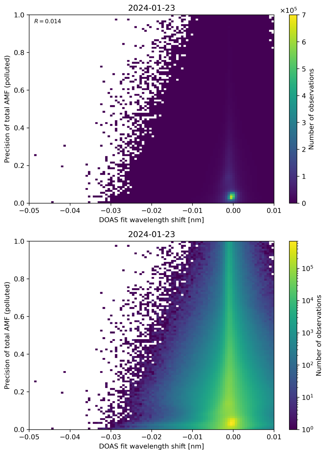
Figure 131: Scatter density plot of “DOAS fit wavelength shift” against “Precision of total AMF (polluted)” for 2024-01-22 to 2024-01-24.
