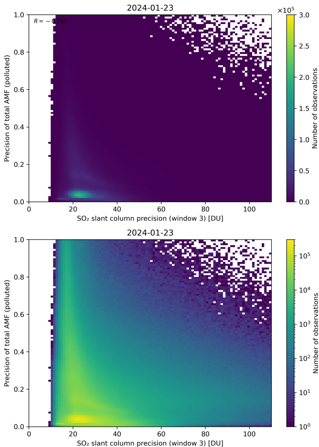
Figure 264: Scatter density plot of “SO 2 slant column precision (window 3)” against “Precision of total AMF (polluted)” for 2024-01-22 to 2024-01-24.
