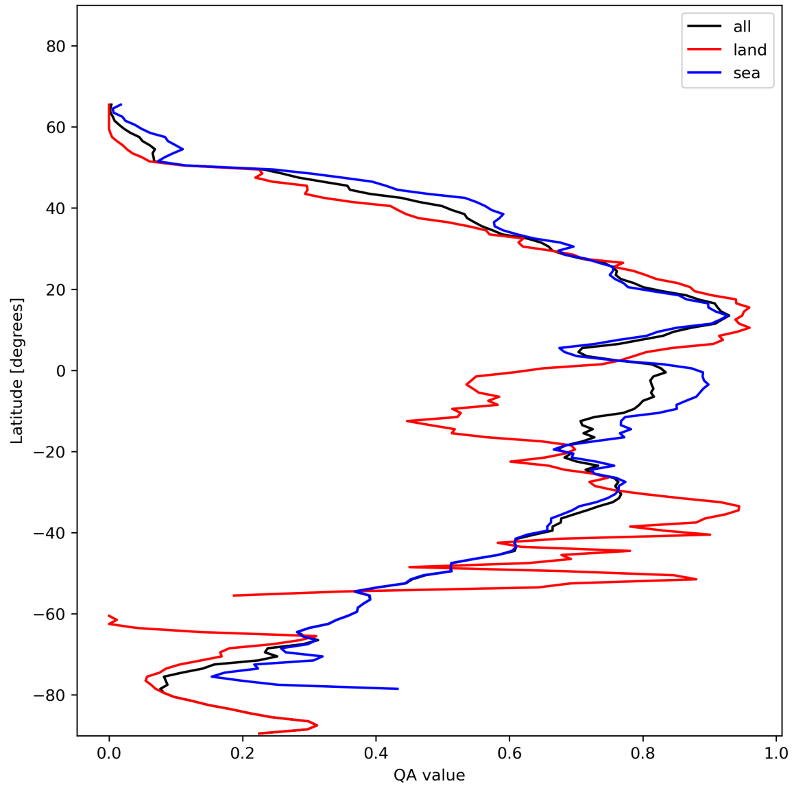
Figure 29: Zonal average of “QA value” for 2024-01-22 to 2024-01-24.
