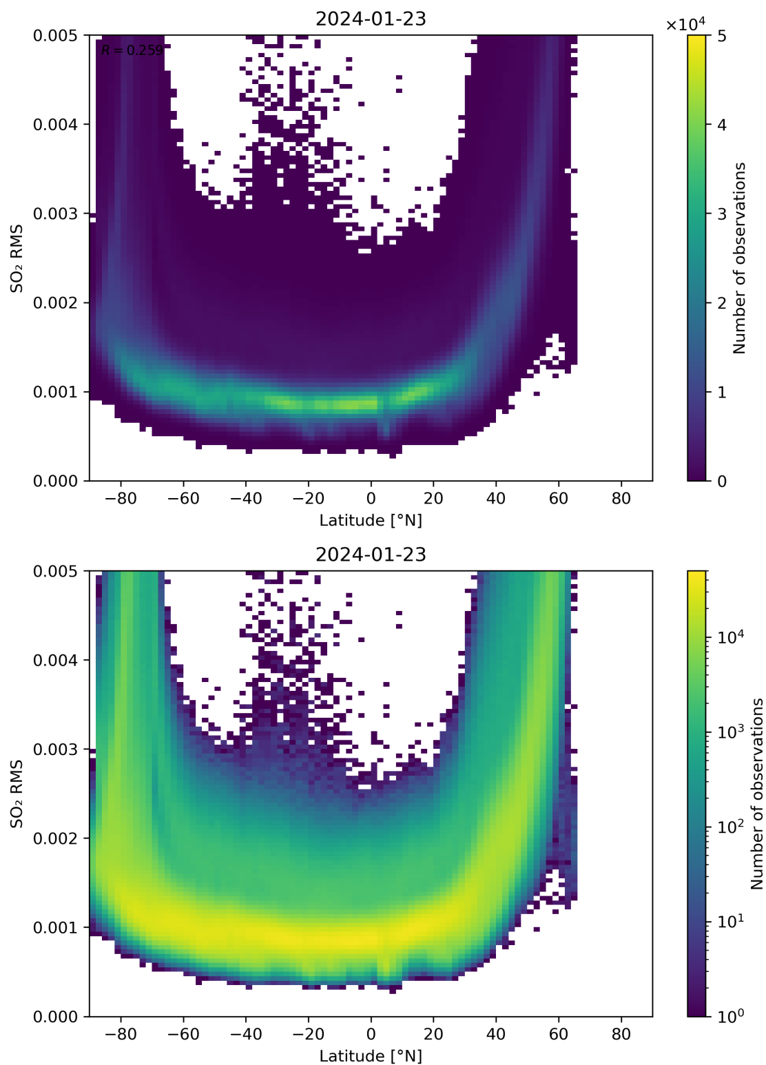
Figure 144: Scatter density plot of “Latitude” against “SO 2 RMS” for 2024-01-22 to 2024-01-24.
