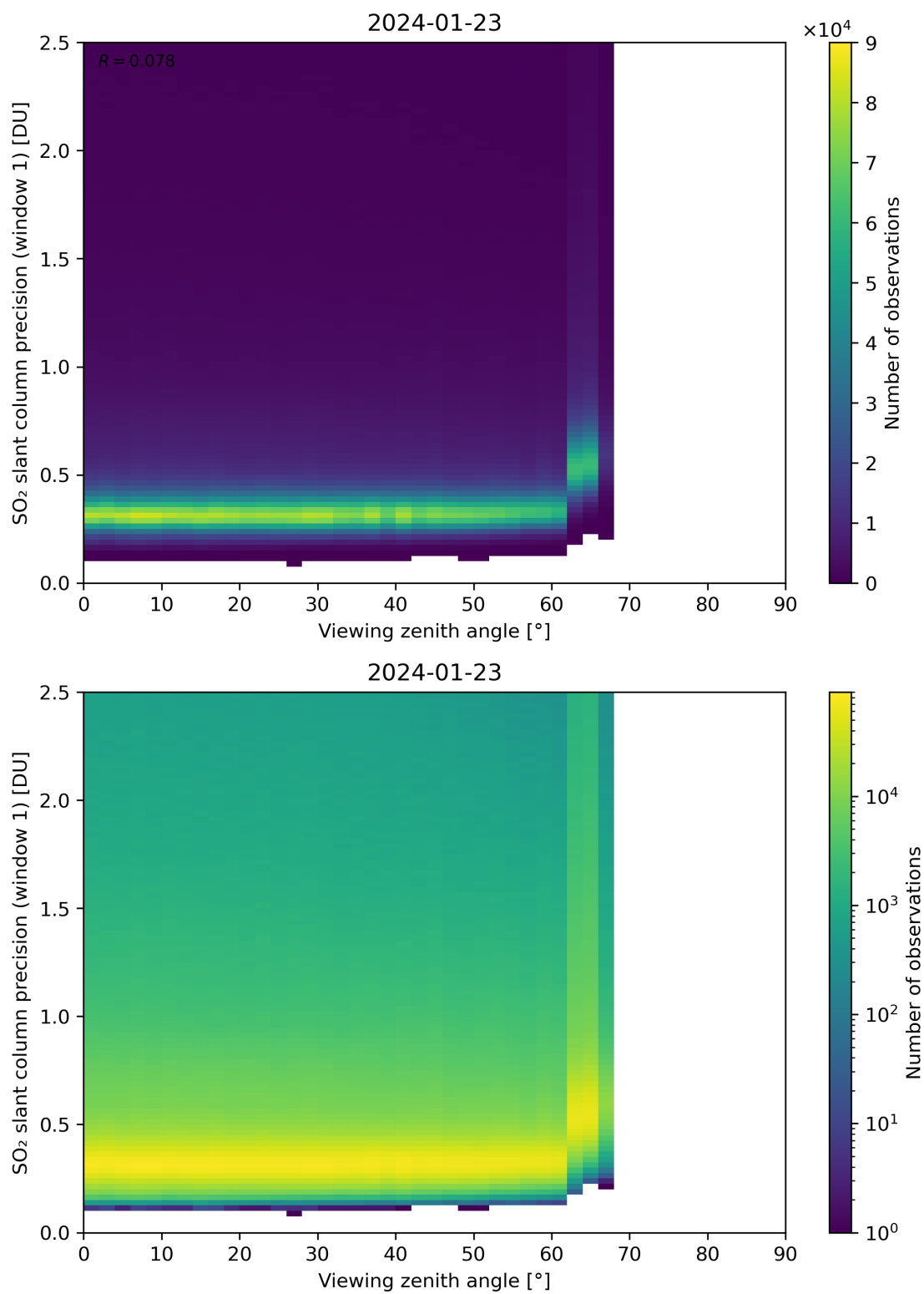
Figure 321: Scatter density plot of “Viewing zenith angle” against “SO 2 slant column precision (window 1)” for 2024-01-22 to 2024-01-24.
