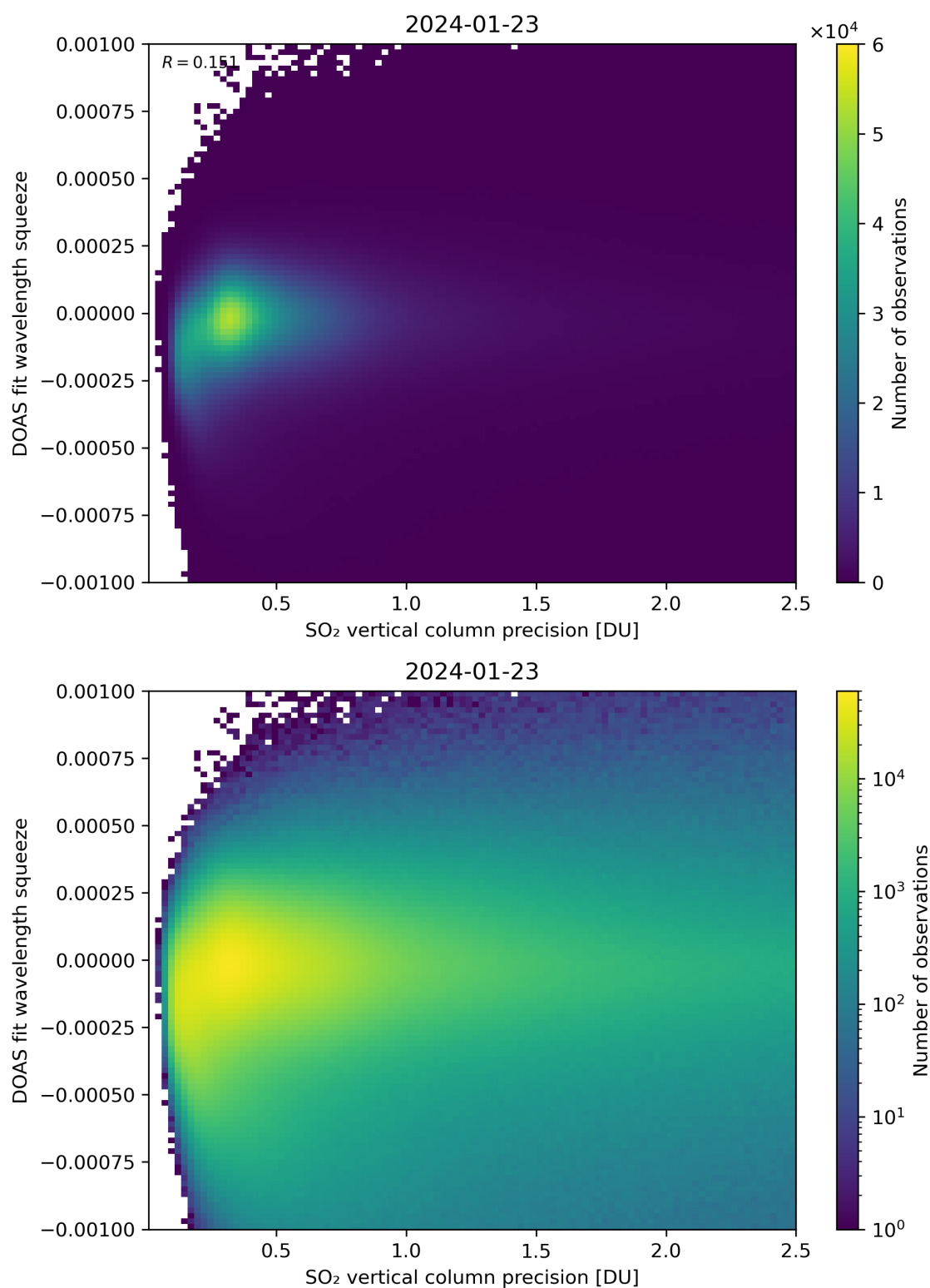
Figure 283: Scatter density plot of “SO 2 vertical column precision” against “DOAS fit wavelength squeeze” for 2024-01-22 to 2024-01-24.
