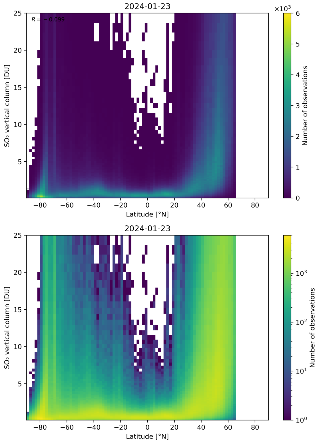
Figure 156: Scatter density plot of “Latitude” against “SO 2 vertical column” for 2024-01-22 to 2024-01-24.
