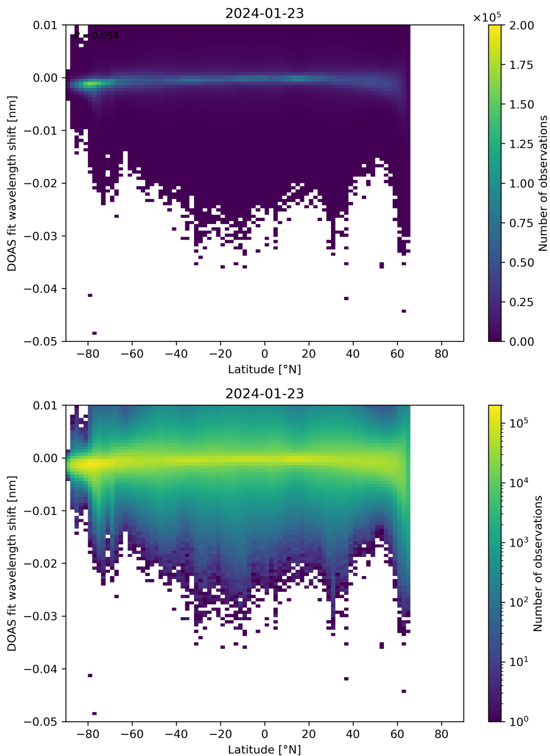
Figure 142: Scatter density plot of “Latitude” against “DOAS fit wavelength shift” for 2024-01-22 to 2024-01-24.
