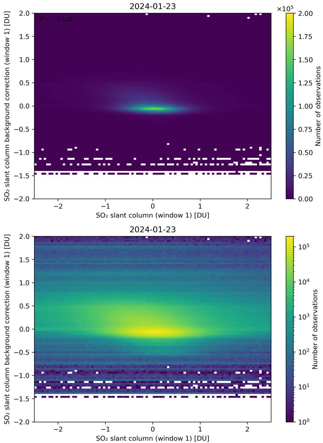
Figure 212: Scatter density plot of “SO 2 slant column (window 1)” against “SO 2 slant column background correction (window 1)” for 2024-01-22 to 2024-01-24.
