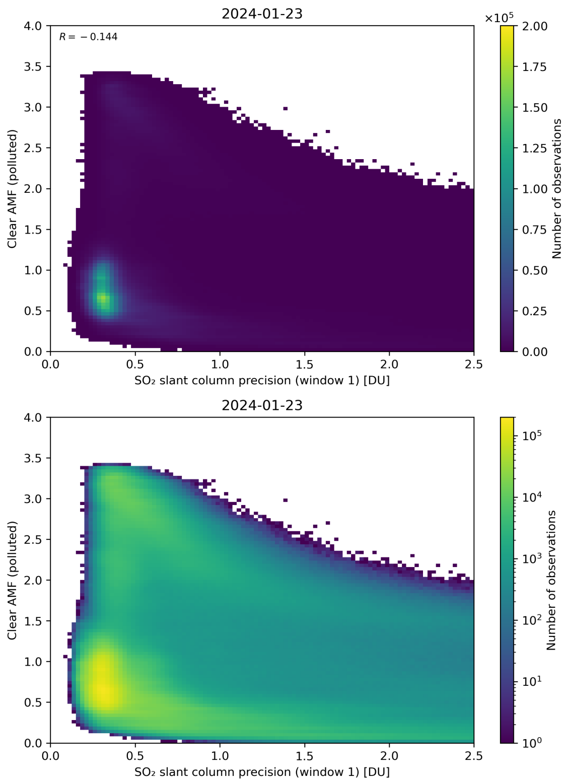
Figure 224: Scatter density plot of “SO 2 slant column precision (window 1)” against “Clear AMF (polluted)” for 2024-01-22 to 2024-01-24.
