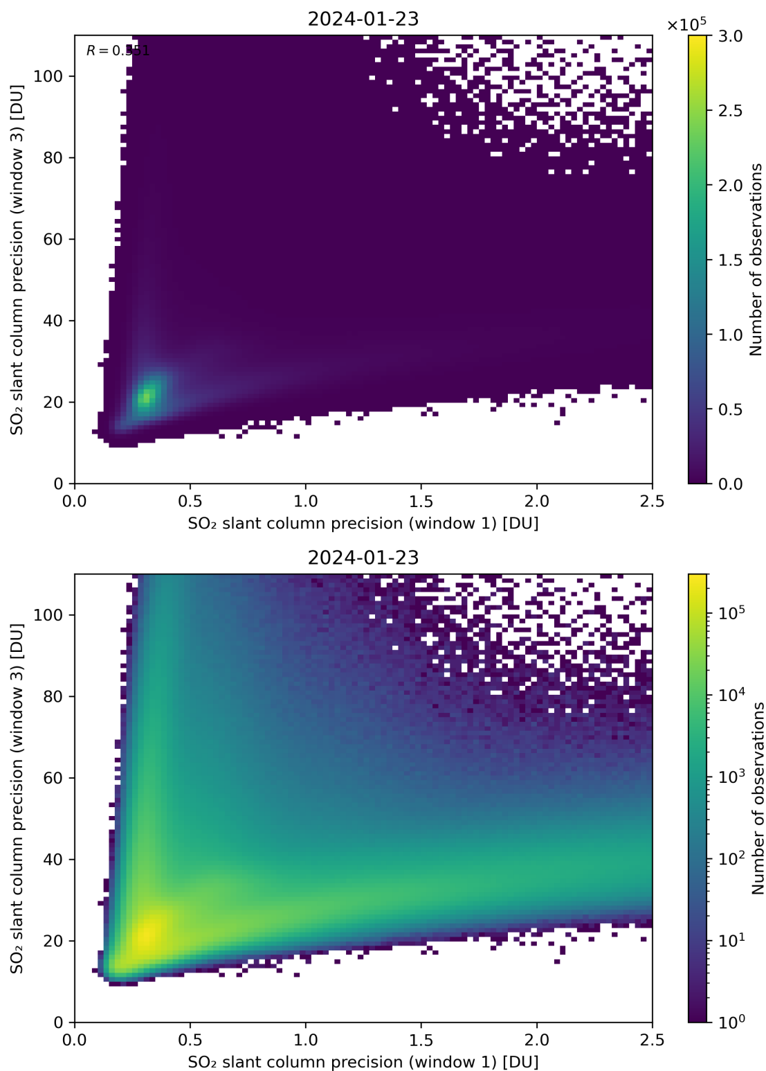
Figure 229: Scatter density plot of “SO 2 slant column precision (window 1)” against “SO 2 slant column precision (window 3)” for 2024-01-22 to 2024-01-24.
