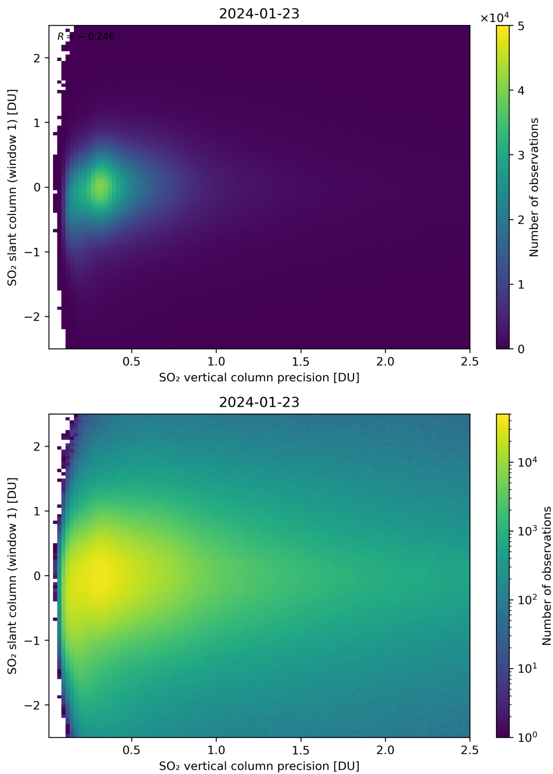
Figure 289: Scatter density plot of “SO 2 vertical column precision” against “SO 2 slant column (window 1)” for 2024-01-22 to 2024-01-24.
