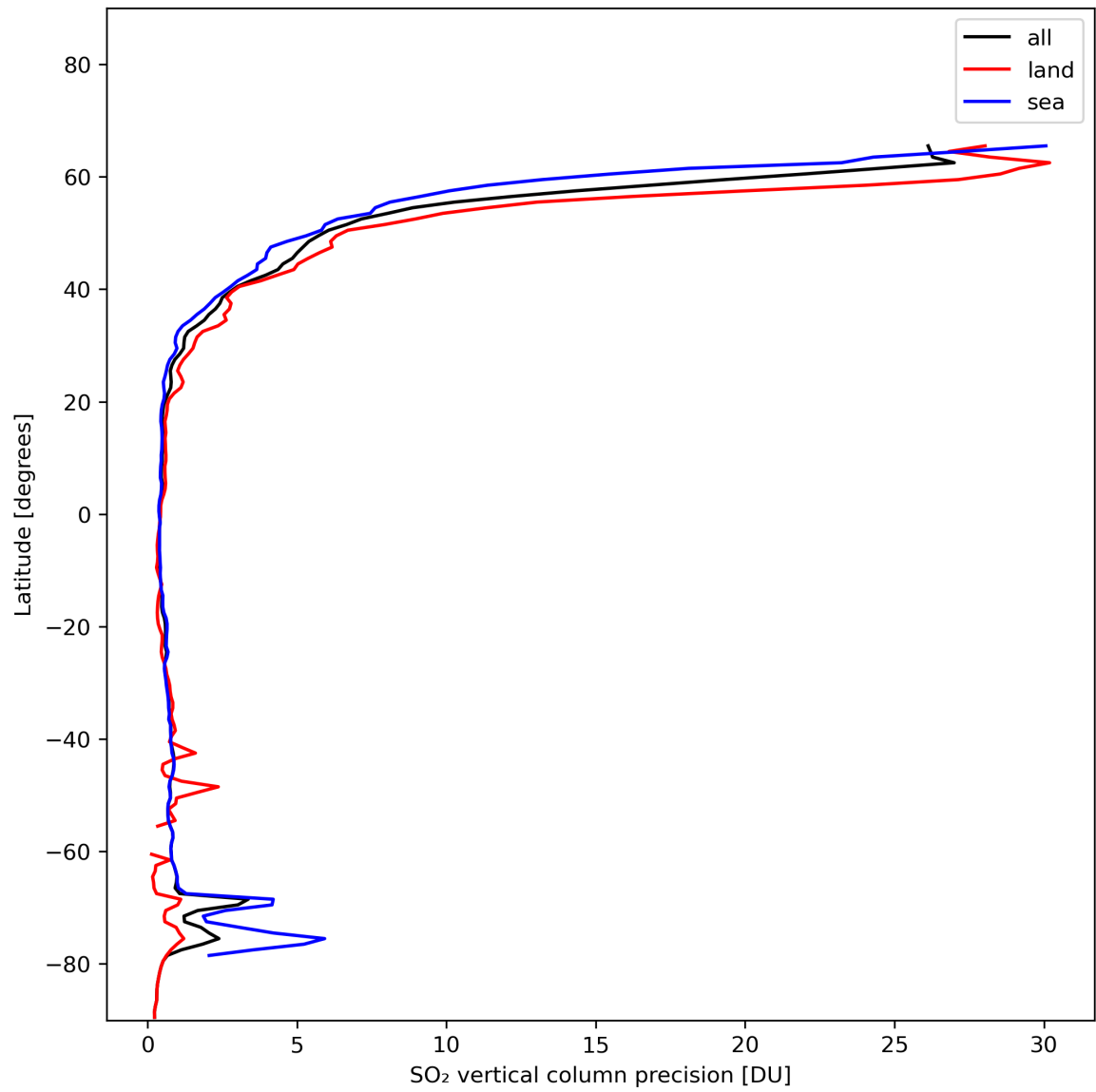
Figure 31: Zonal average of “SO 2 vertical column precision” for 2024-01-22 to 2024-01-24.
