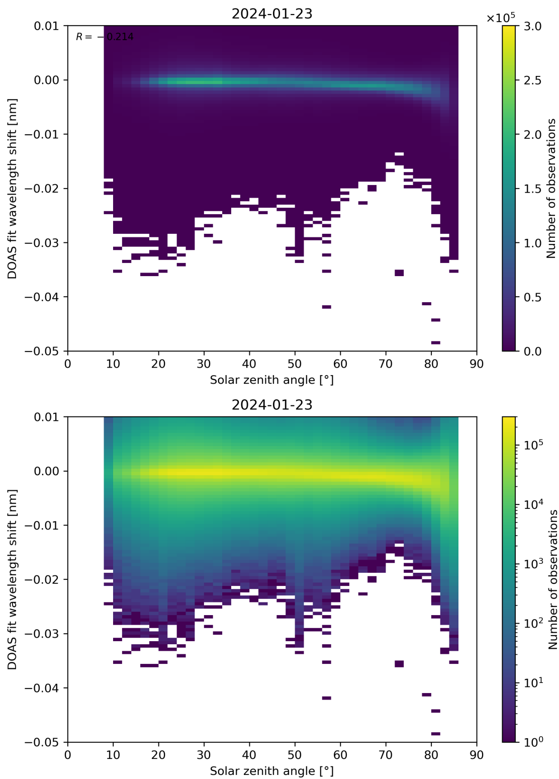
Figure 161: Scatter density plot of “Solar zenith angle” against “DOAS fit wavelength shift” for 2024-01-22 to 2024-01-24.
