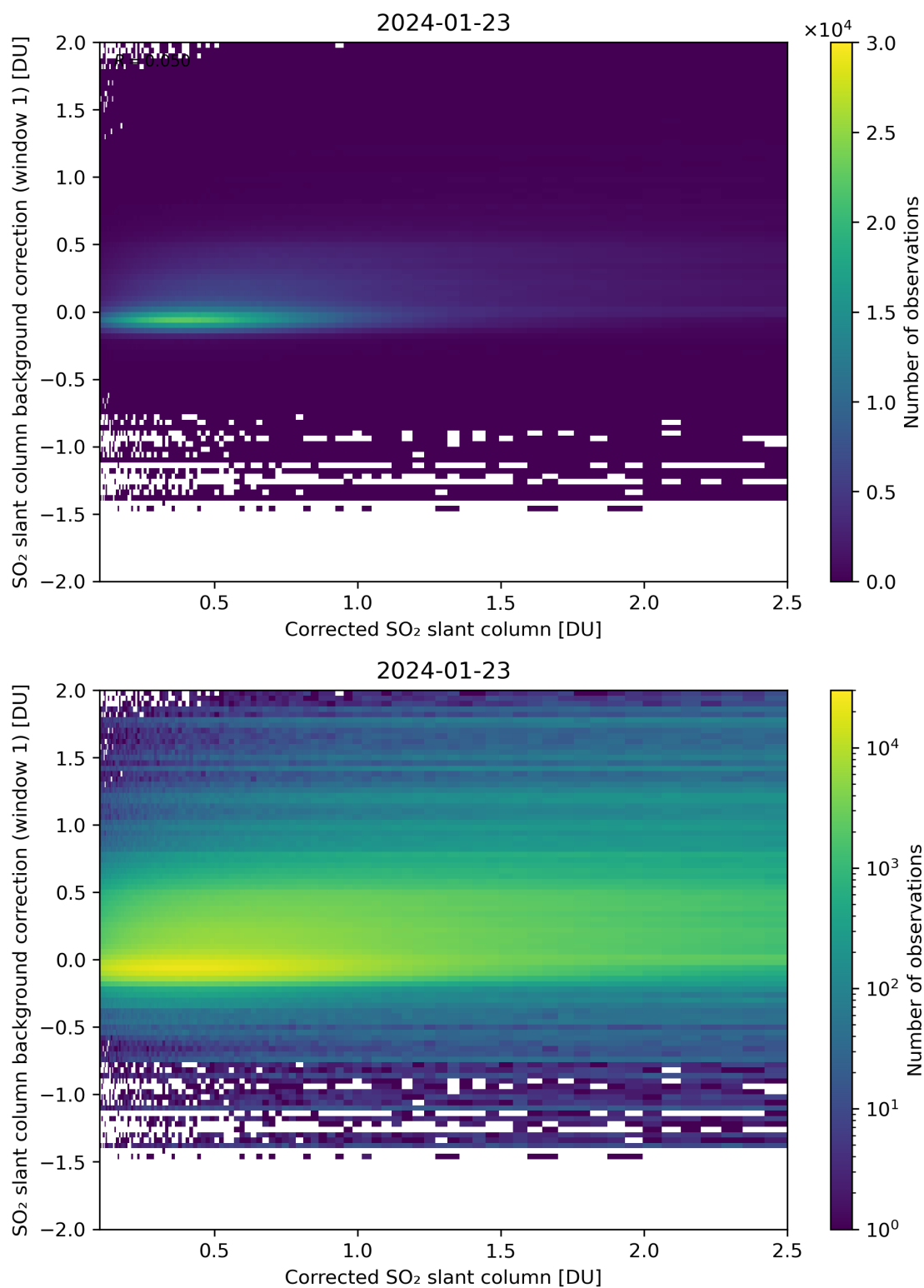
Figure 178: Scatter density plot of “Corrected SO 2 slant column” against “SO 2 slant column background correction (window 1)” for 2024-01-22 to 2024-01-24.
