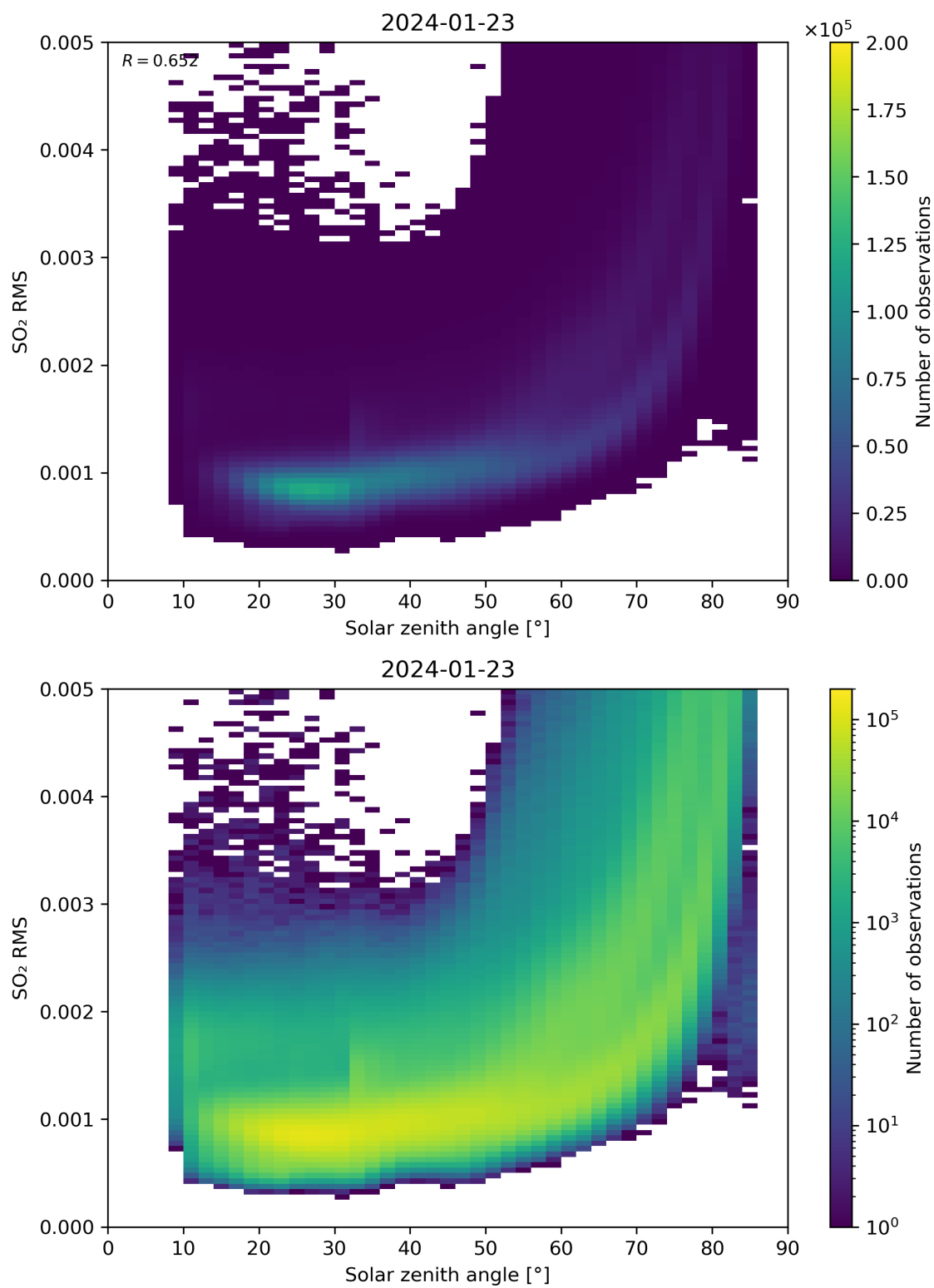
Figure 163: Scatter density plot of “Solar zenith angle” against “SO 2 RMS” for 2024-01-22 to 2024-01-24.
