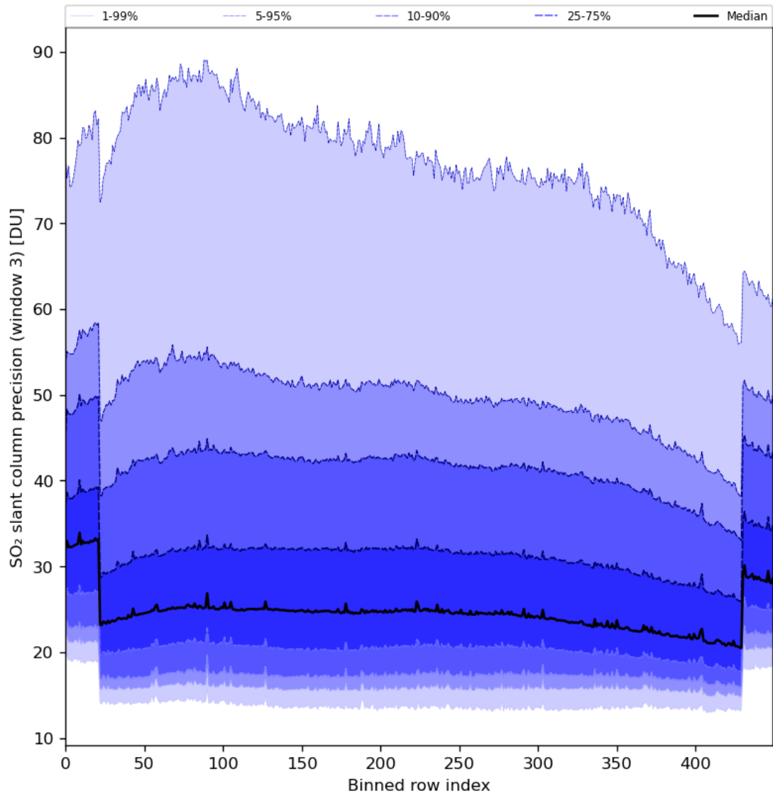
Figure 88: Along track statistics of “SO 2 slant column precision (window 3)” for 2024-01-22 to 2024-01-24
