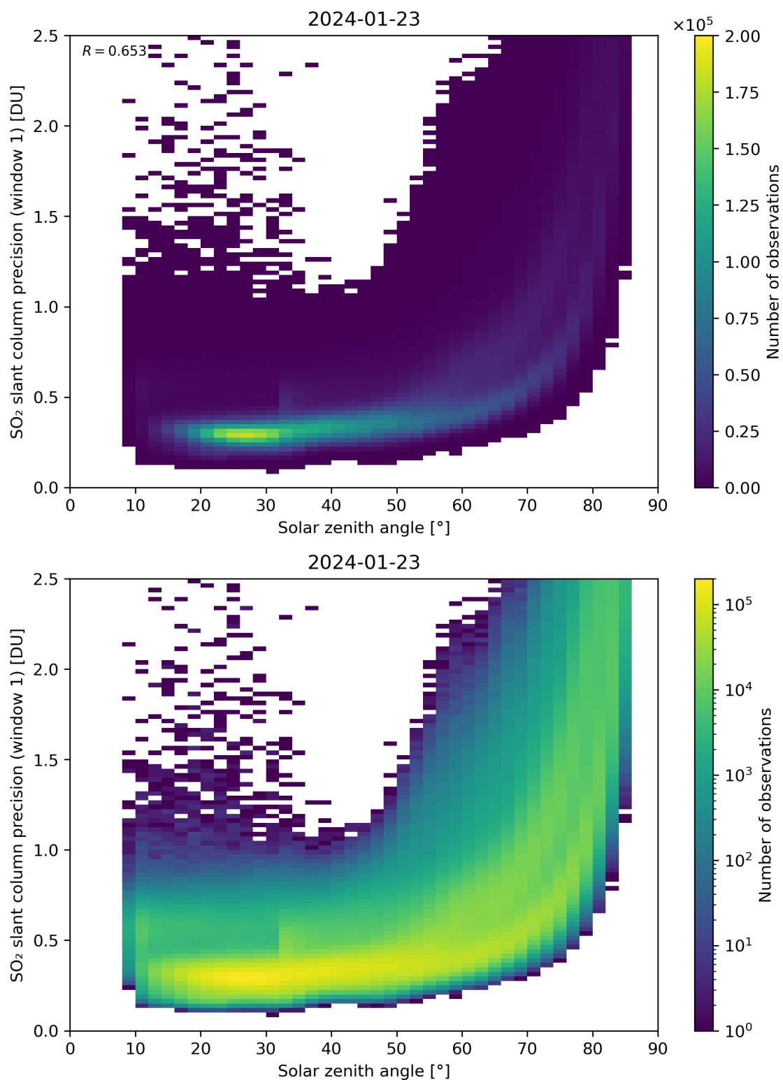
Figure 170: Scatter density plot of “Solar zenith angle” against “SO 2 slant column precision (window 1)” for 2024-01-22 to 2024-01-24.
