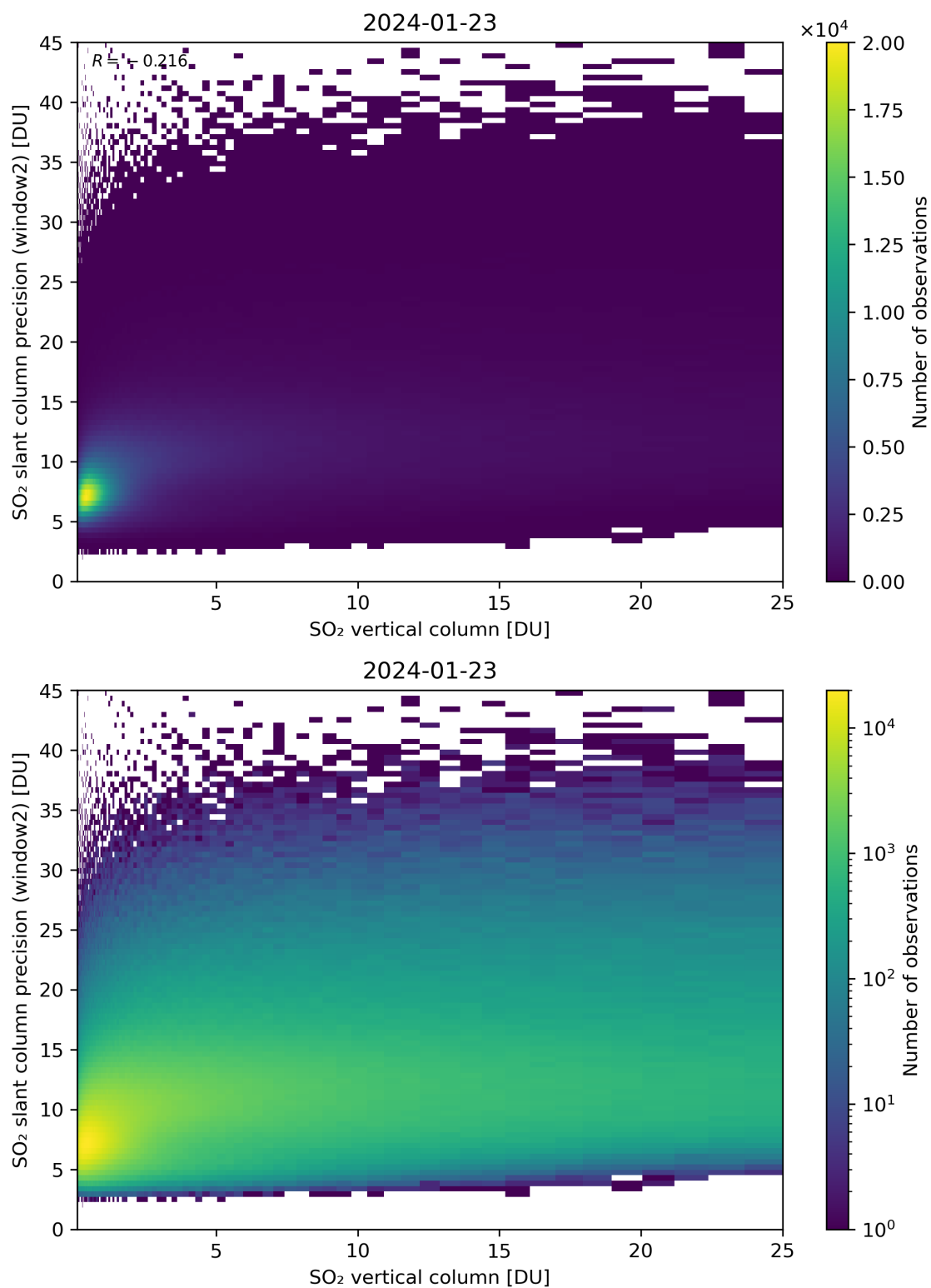
Figure 302: Scatter density plot of “SO 2 vertical column” against “SO 2 slant column precision (window2)” for 2024-01-22 to 2024-01-24.
