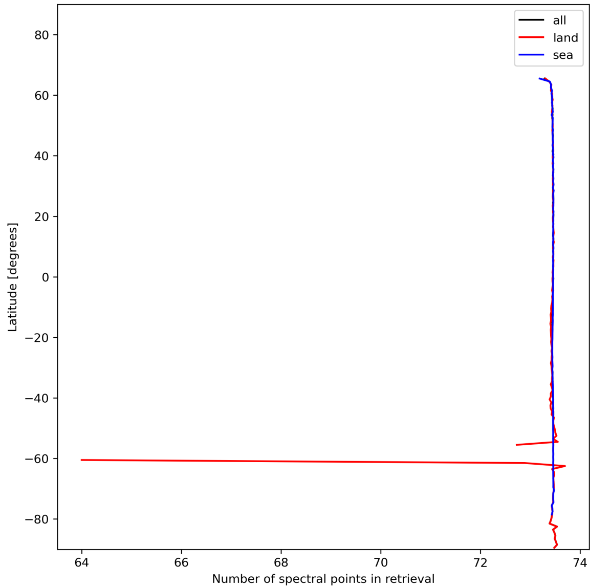
Figure 51: Zonal average of “Number of spectral points in retrieval” for 2024-01-22 to 2024-01-24.
