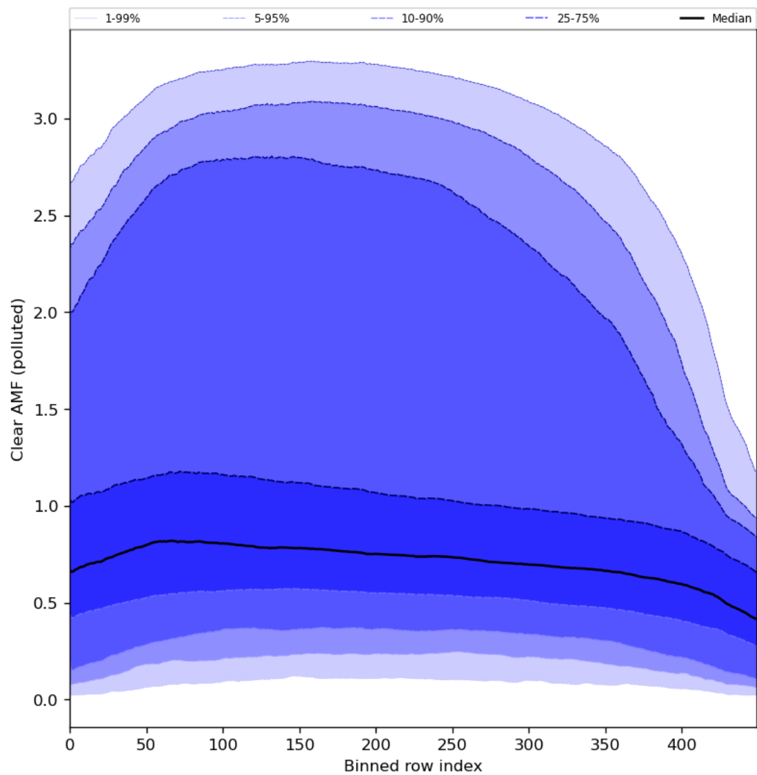
Figure 96: Along track statistics of “Clear AMF (polluted)” for 2024-01-22 to 2024-01-24
