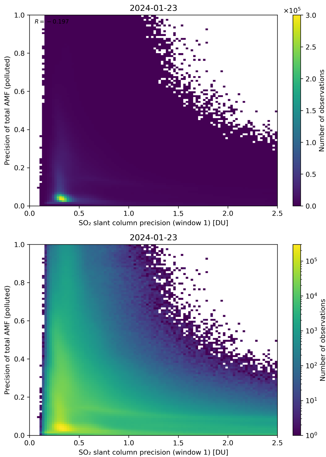
Figure 231: Scatter density plot of “SO 2 slant column precision (window 1)” against “Precision of total AMF (polluted)” for 2024-01-22 to 2024-01-24.
