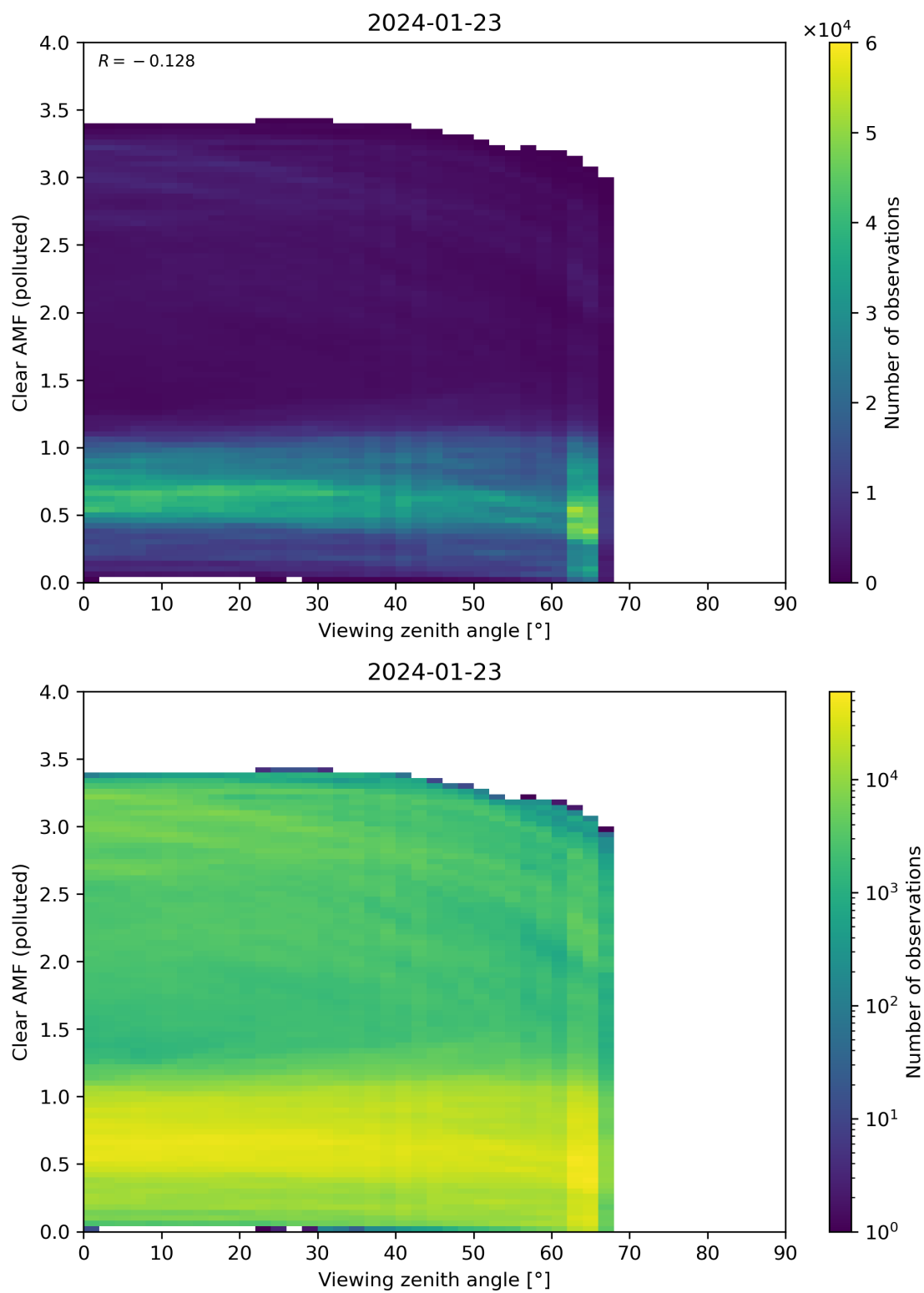
Figure 316: Scatter density plot of “Viewing zenith angle” against “Clear AMF (polluted)” for 2024-01-22 to 2024-01-24.
