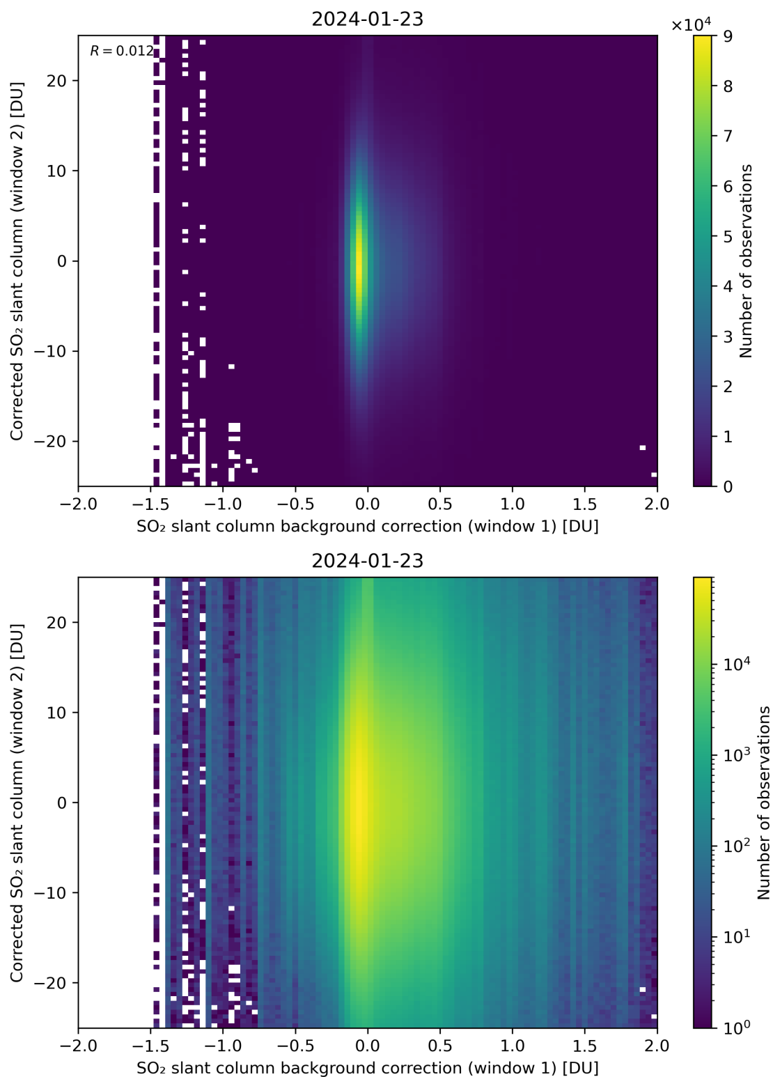
Figure 104: Scatter density plot of “SO 2 slant column background correction (window 1)” against “Corrected SO 2 slant column (window 2)” for 2024-01-22 to 2024-01-24.
