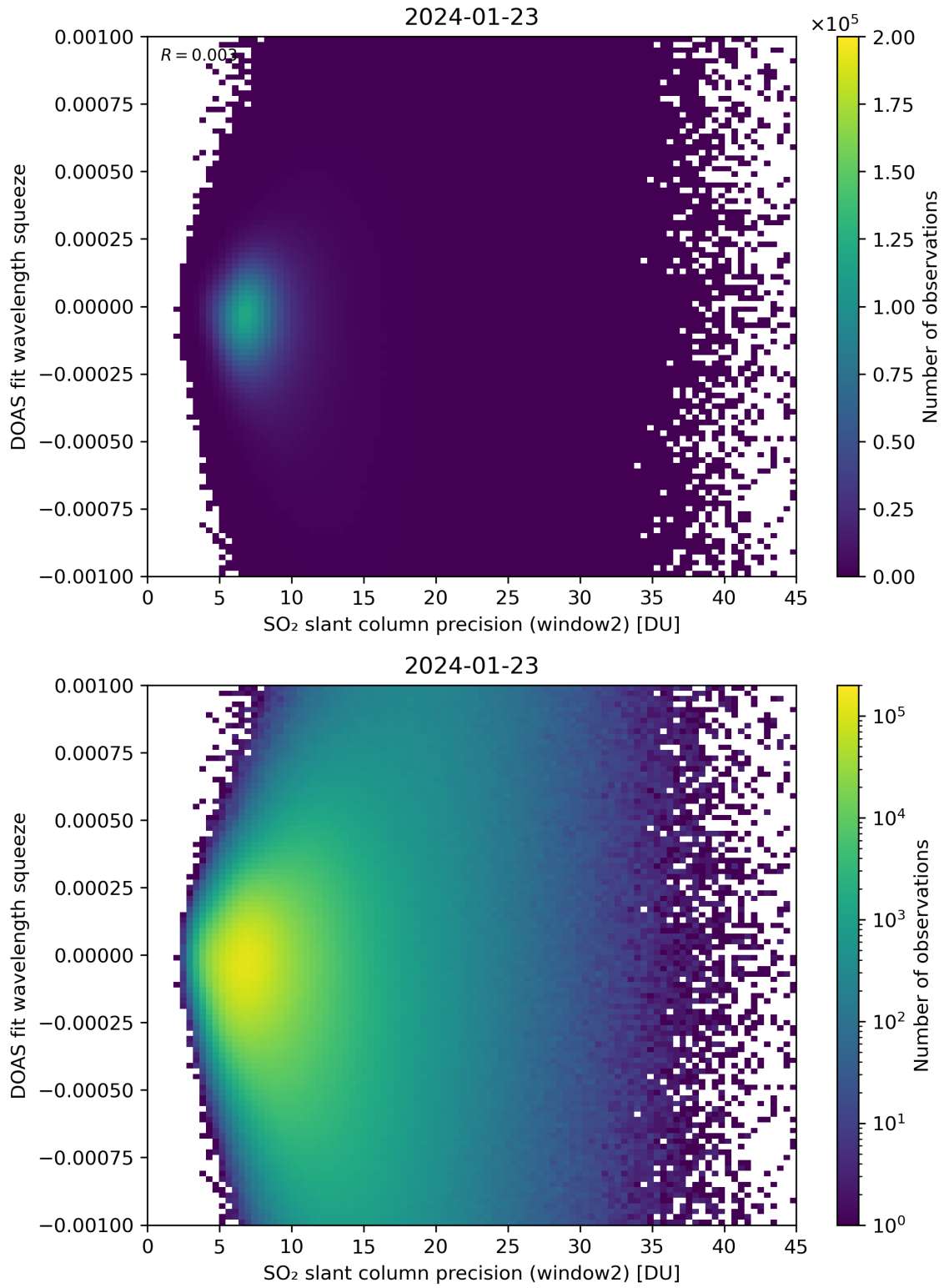
Figure 244: Scatter density plot of “SO 2 slant column precision (window2)” against “DOAS fit wavelength squeeze” for 2024-01-22 to 2024-01-24.
