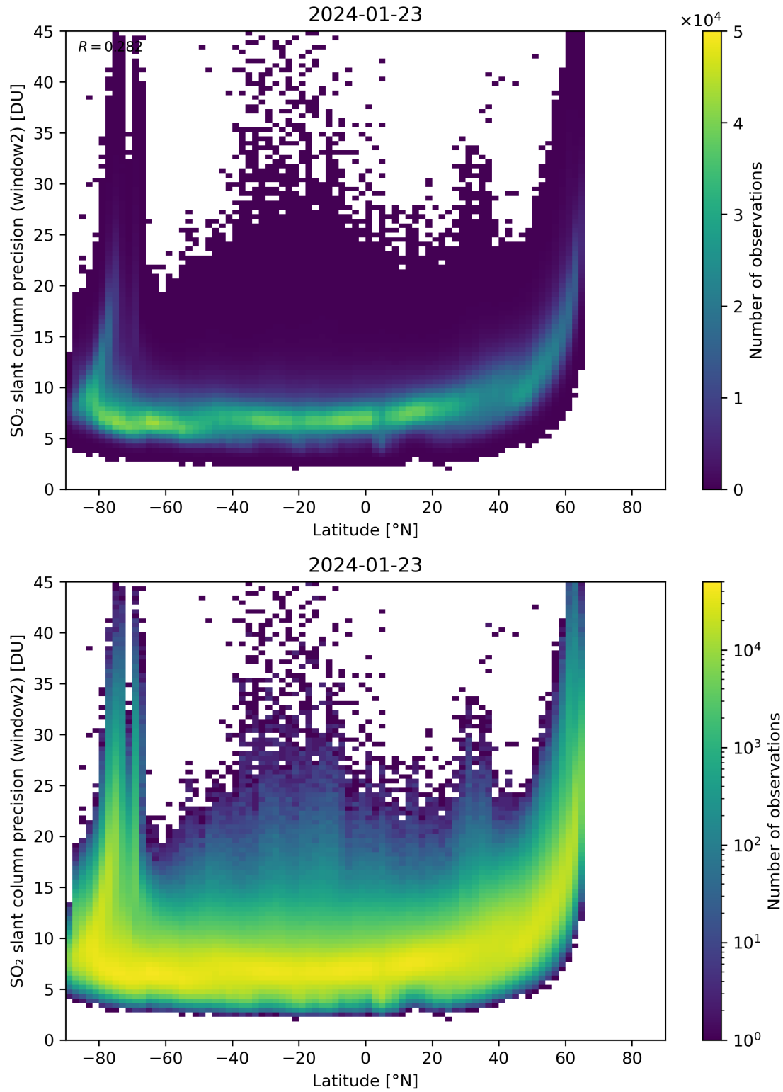
Figure 151: Scatter density plot of “Latitude” against “SO 2 slant column precision (window2)” for 2024-01-22 to 2024-01-24.
