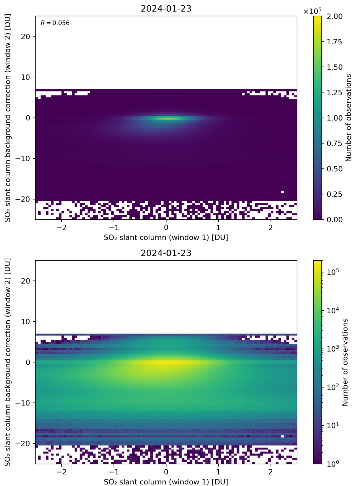
Figure 213: Scatter density plot of “SO 2 slant column (window 1)” against “SO 2 slant column background correction (window 2)” for 2024-01-22 to 2024-01-24.
