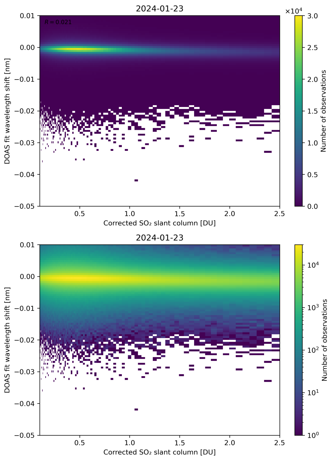
Figure 181: Scatter density plot of “Corrected SO 2 slant column” against “DOAS fit wavelength shift” for 2024-01-22 to 2024-01-24.
