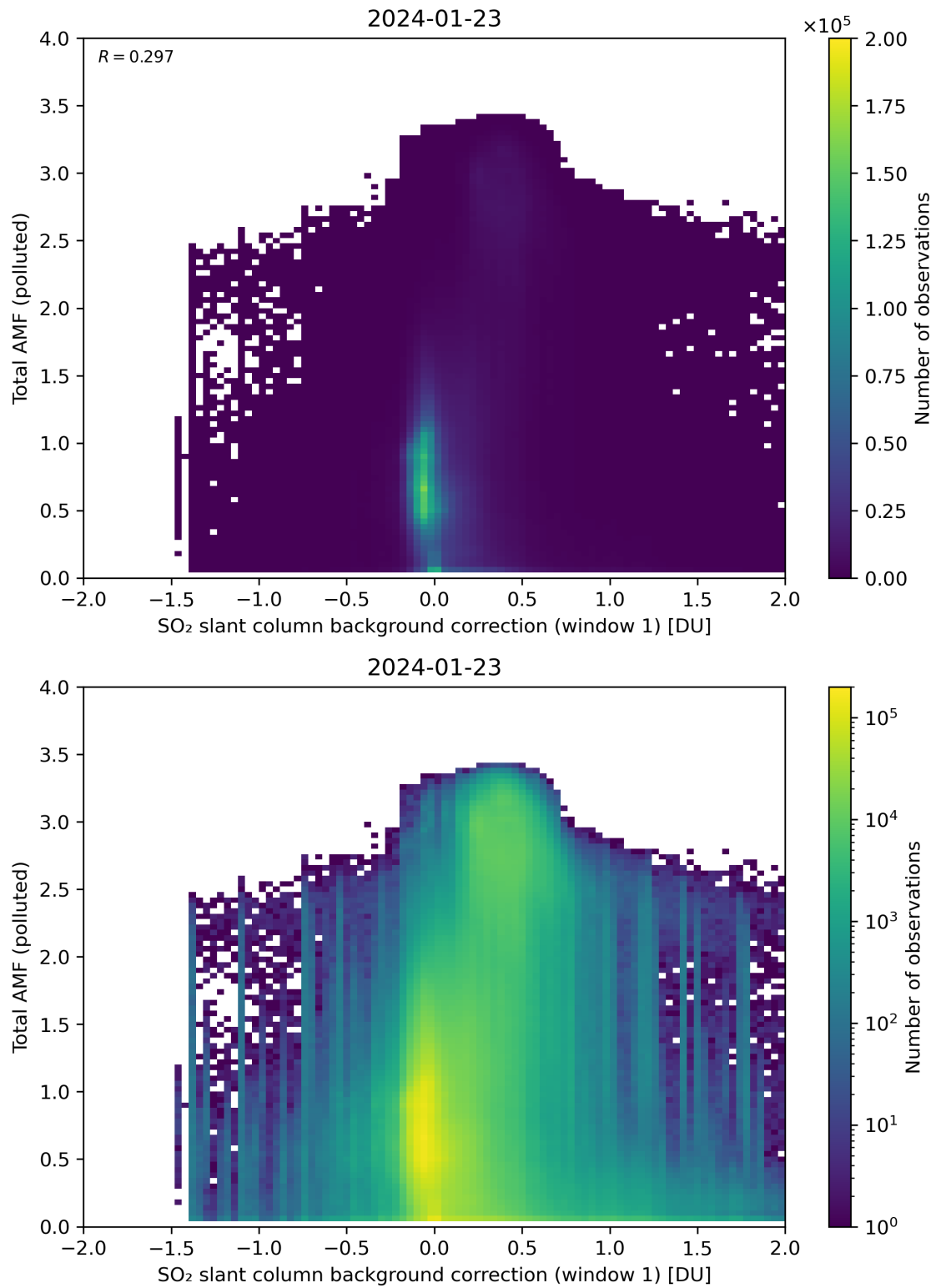
Figure 109: Scatter density plot of “SO 2 slant column background correction (window 1)” against “Total AMF (polluted)” for 2024-01-22 to 2024-01-24.
