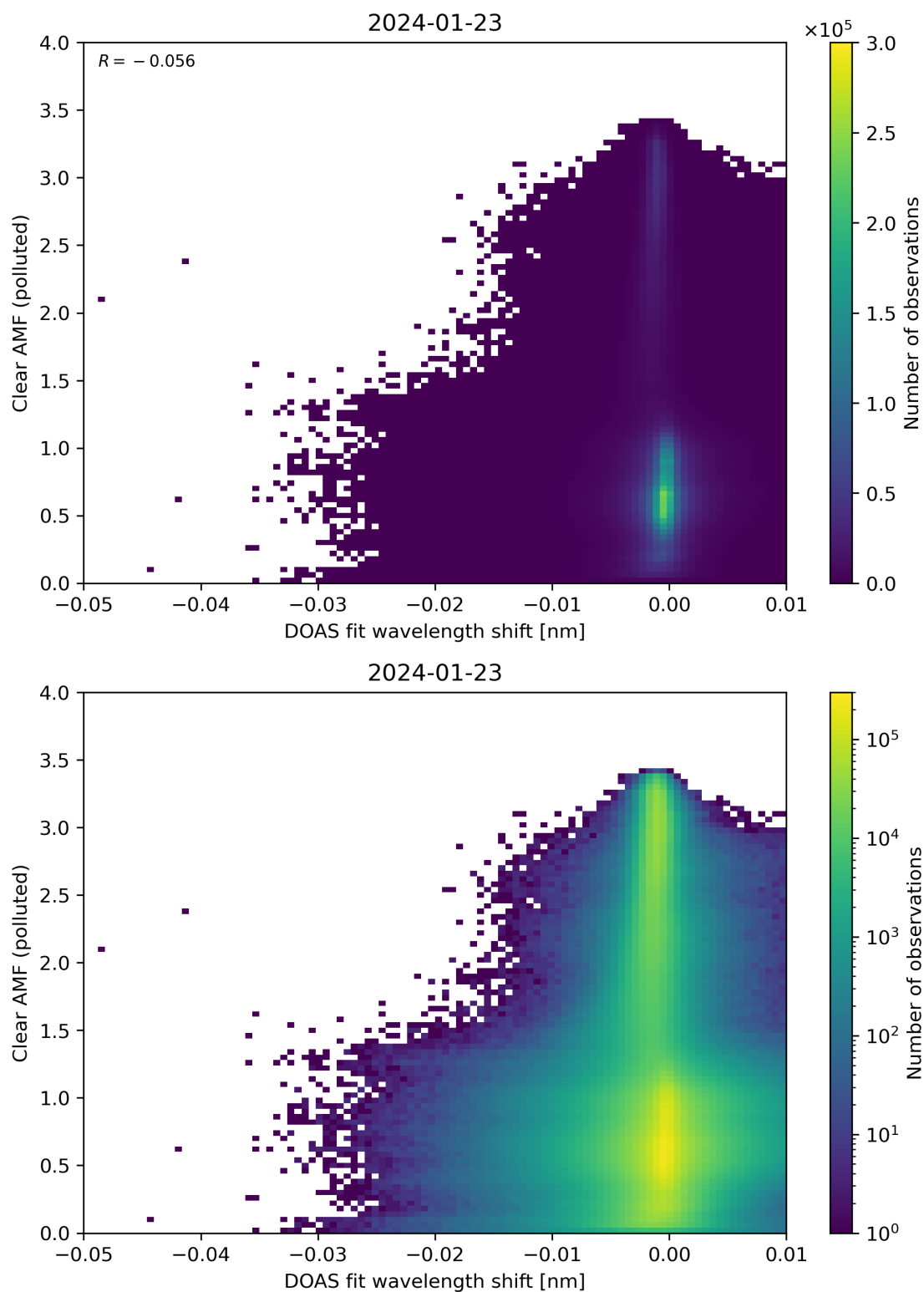
Figure 129: Scatter density plot of “DOAS fit wavelength shift” against “Clear AMF (polluted)” for 2024-01-22 to 2024-01-24.
