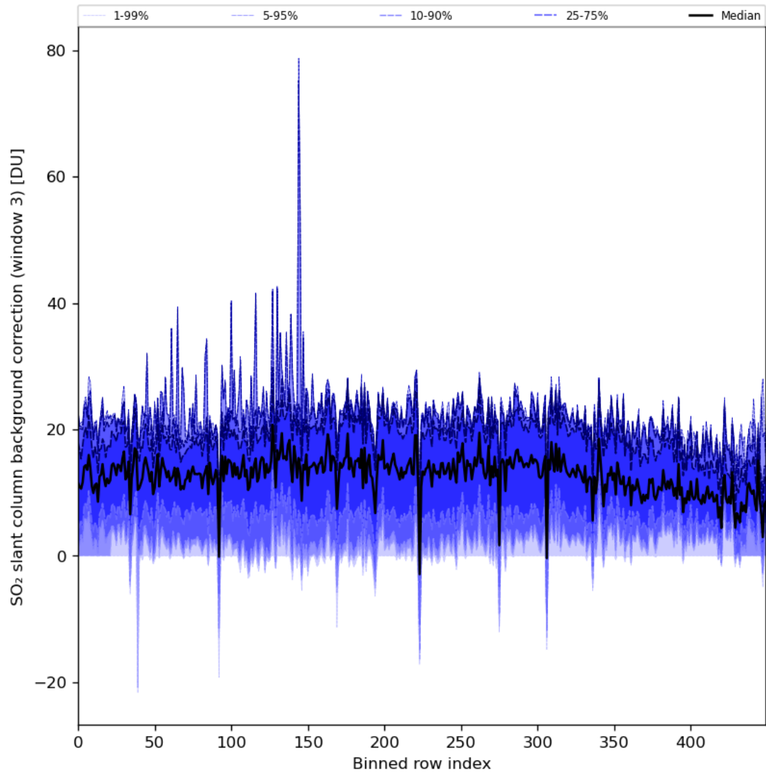
Figure 90: Along track statistics of “SO 2 slant column background correction (window 3)” for 2024-01-22 to 2024-01-24
