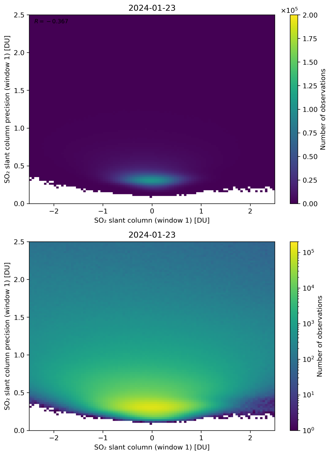
Figure 235: Scatter density plot of “SO 2 slant column (window 1)” against “SO 2 slant column precision (window 1)” for 2024-01-22 to 2024-01-24.
