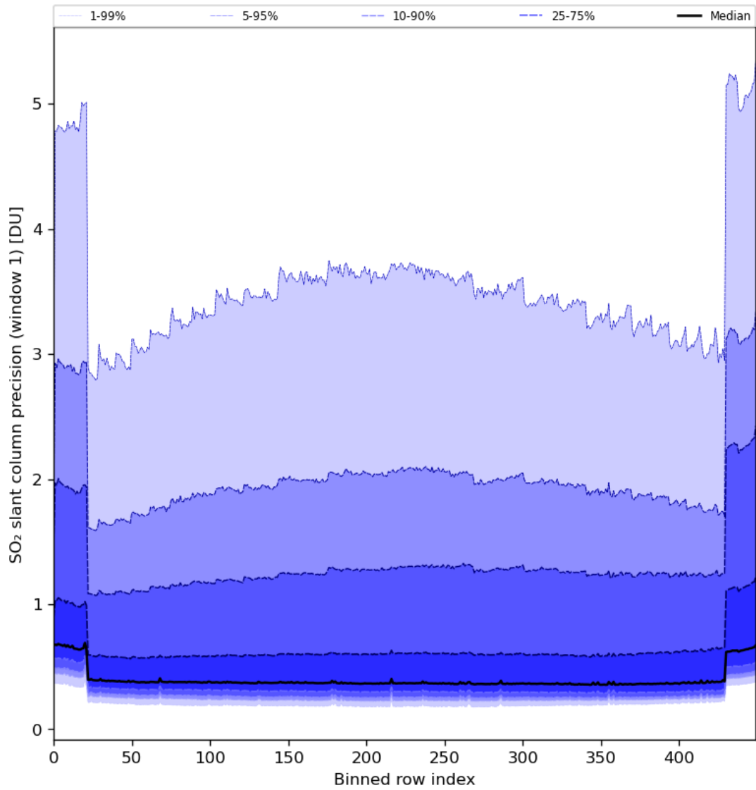
Figure 80: Along track statistics of “SO 2 slant column precision (window 1)” for 2024-01-22 to 2024-01-24
