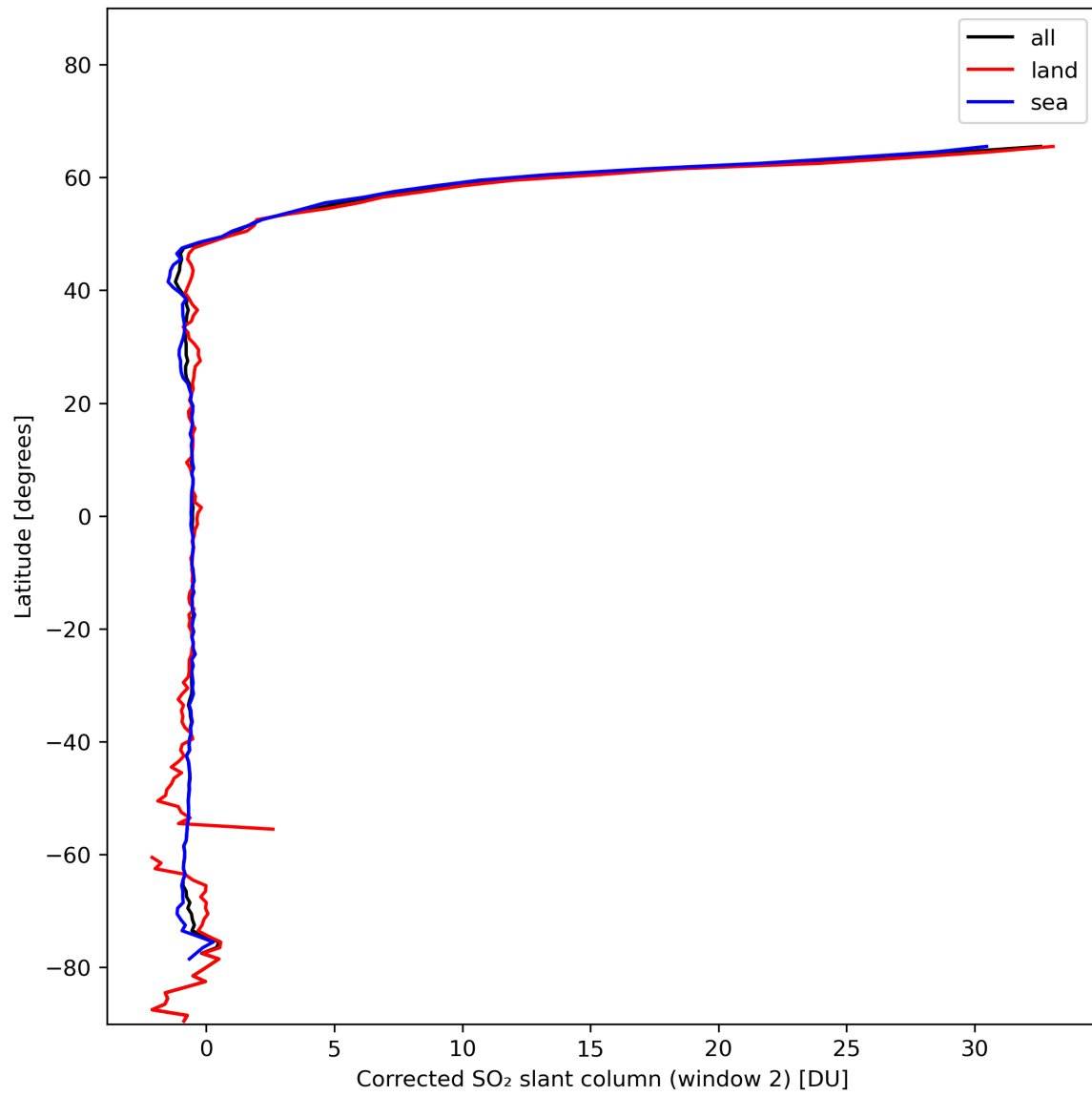
Figure 39: Zonal average of “Corrected SO 2 slant column (window 2)” for 2024-01-22 to 2024-01-24.
