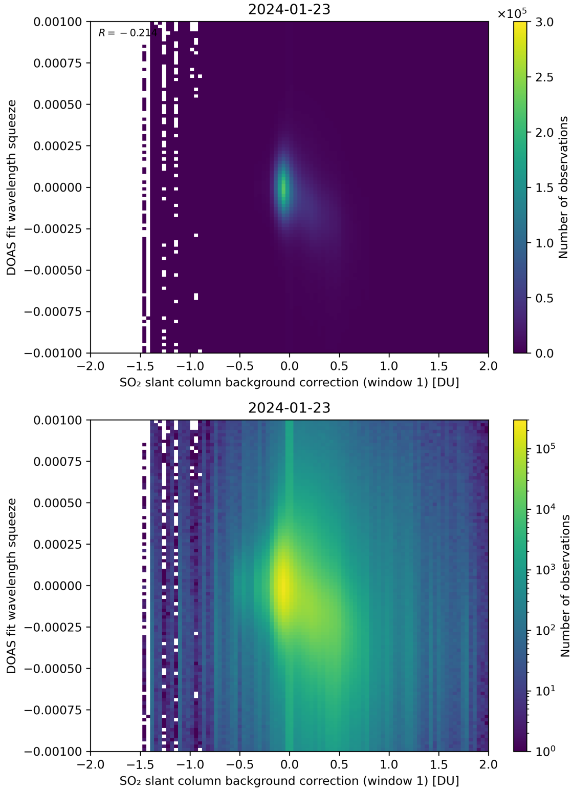
Figure 101: Scatter density plot of “SO 2 slant column background correction (window 1)” against “DOAS fit wavelength squeeze” for 2024-01-22 to 2024-01-24.
