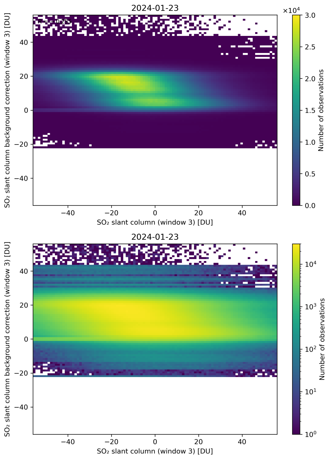
Figure 253: Scatter density plot of “SO 2 slant column (window 3)” against “SO 2 slant column background correction (window 3)” for 2024-01-22 to 2024-01-24.
