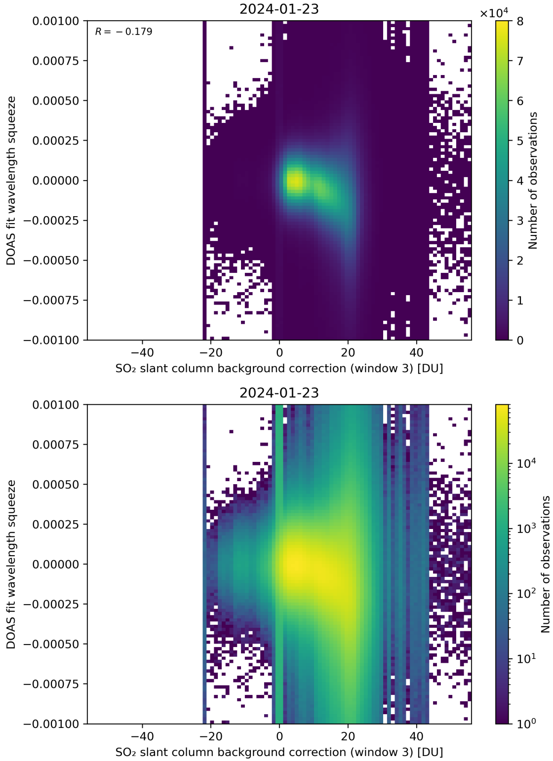
Figure 122: Scatter density plot of “SO 2 slant column background correction (window 3)” against “DOAS fit wavelength squeeze” for 2024-01-22 to 2024-01-24.
