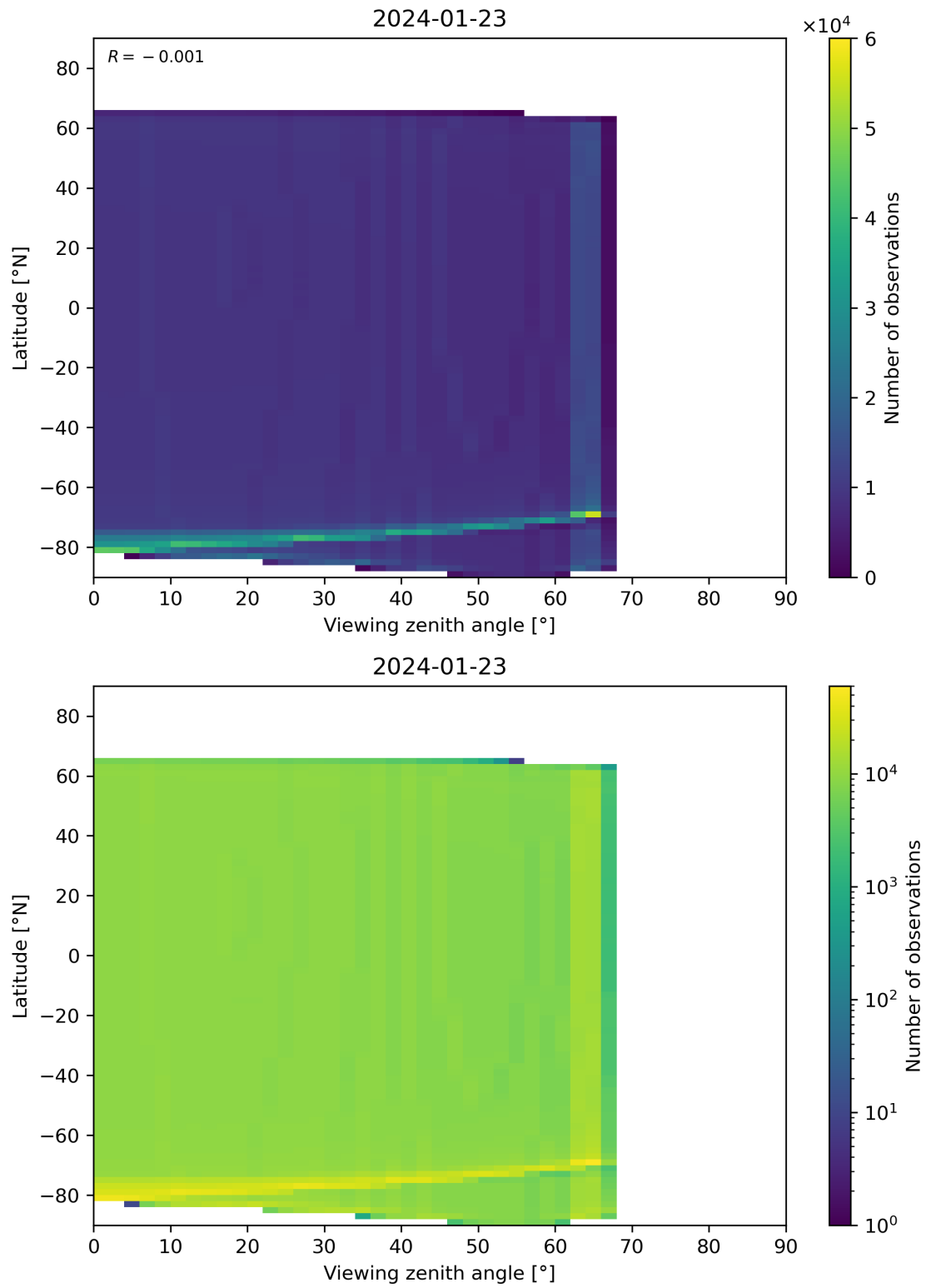
Figure 314: Scatter density plot of “Viewing zenith angle” against “Latitude” for 2024-01-22 to 2024-01-24.
