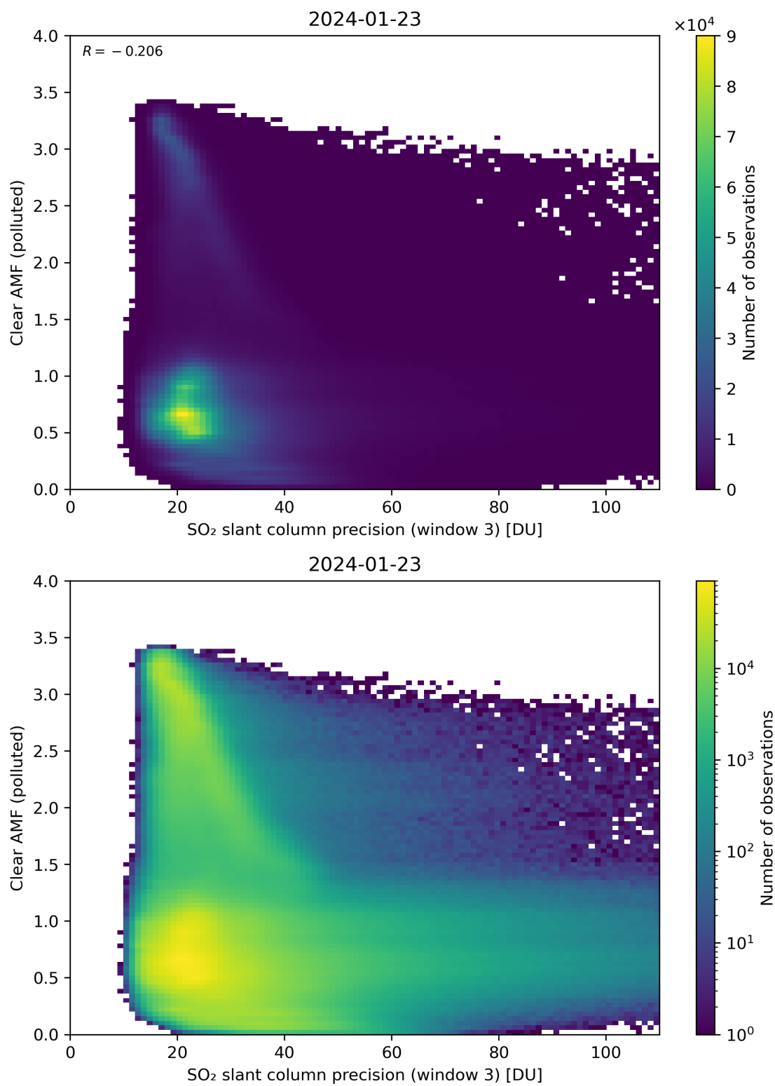
Figure 261: Scatter density plot of “SO 2 slant column precision (window 3)” against “Clear AMF (polluted)” for 2024-01-22 to 2024-01-24.
