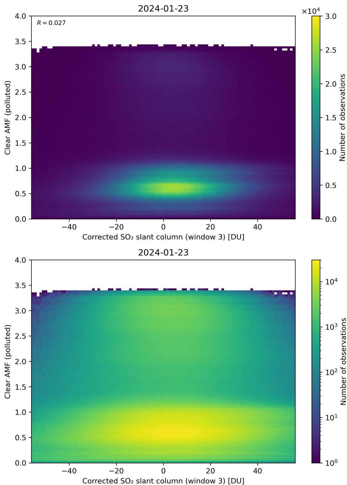
Figure 209: Scatter density plot of “Corrected SO 2 slant column (window 3)” against “Clear AMF (polluted)” for 2024-01-22 to 2024-01-24.
