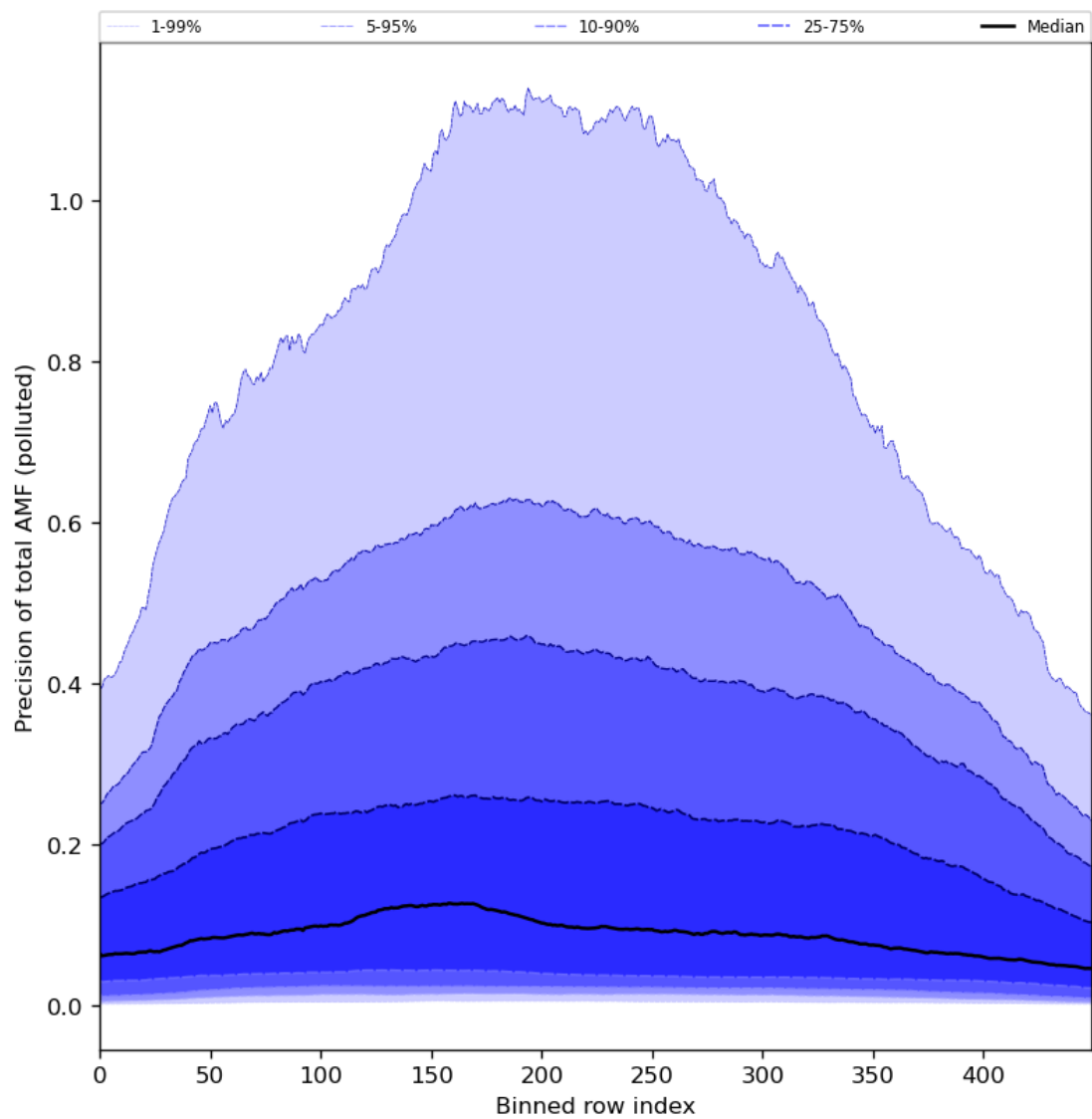
Figure 95: Along track statistics of “Precision of total AMF (polluted)” for 2024-01-22 to 2024-01-24
