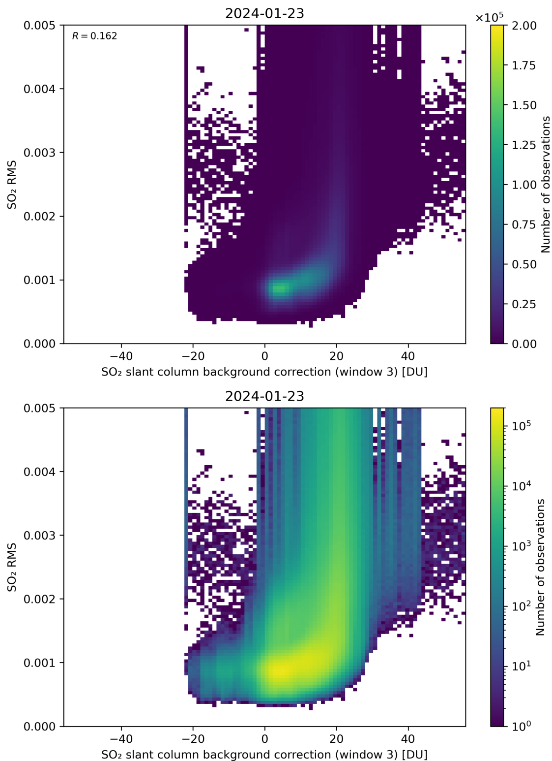
Figure 123: Scatter density plot of “SO 2 slant column background correction (window 3)” against “SO 2 RMS” for 2024-01-22 to 2024-01-24.
