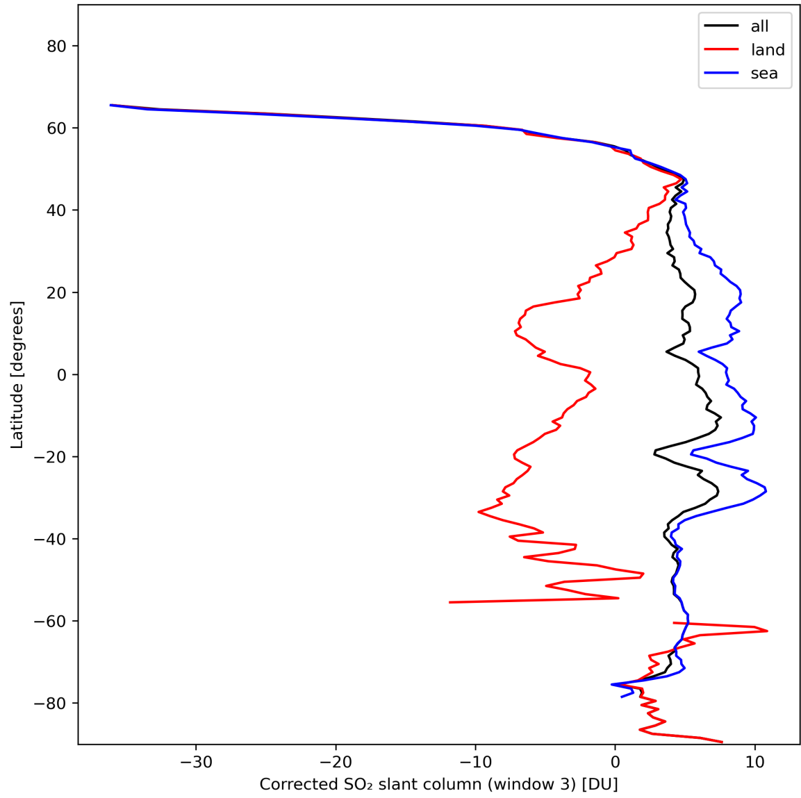
Figure 43: Zonal average of “Corrected SO 2 slant column (window 3)” for 2024-01-22 to 2024-01-24.
