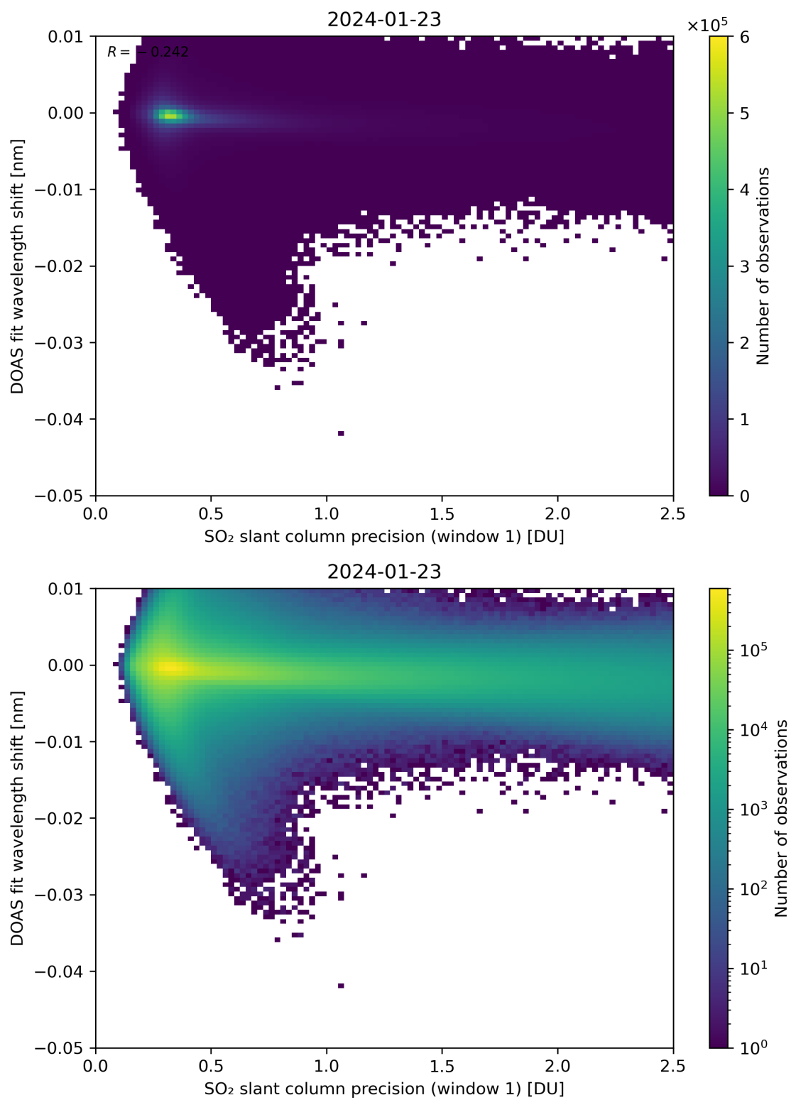
Figure 221: Scatter density plot of “SO 2 slant column precision (window 1)” against “DOAS fit wavelength shift” for 2024-01-22 to 2024-01-24.
