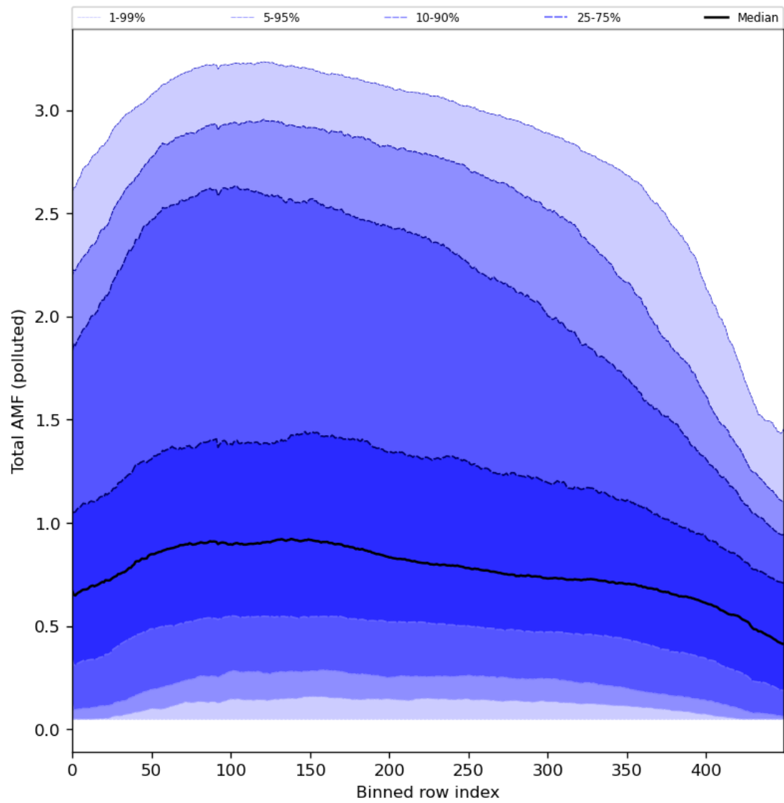
Figure 94: Along track statistics of “Total AMF (polluted)” for 2024-01-22 to 2024-01-24
