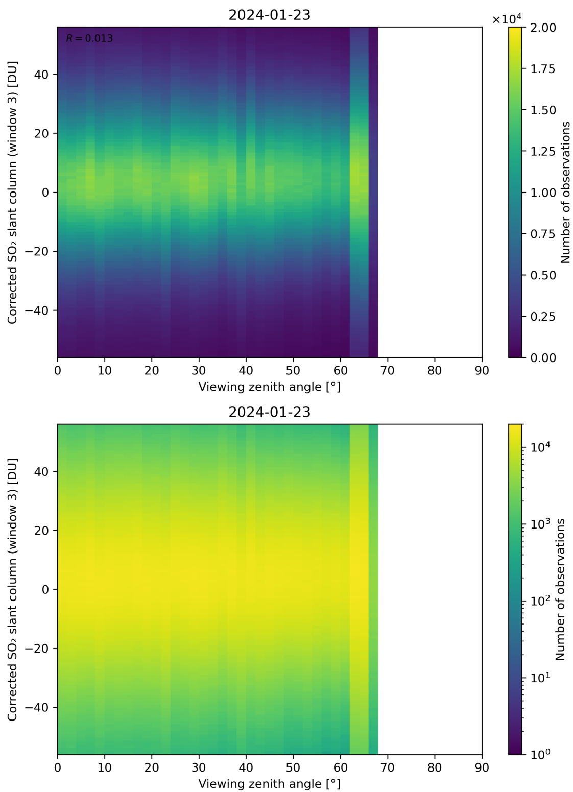
Figure 319: Scatter density plot of “Viewing zenith angle” against “Corrected SO 2 slant column (window 3)” for 2024-01-22 to 2024-01-24.
