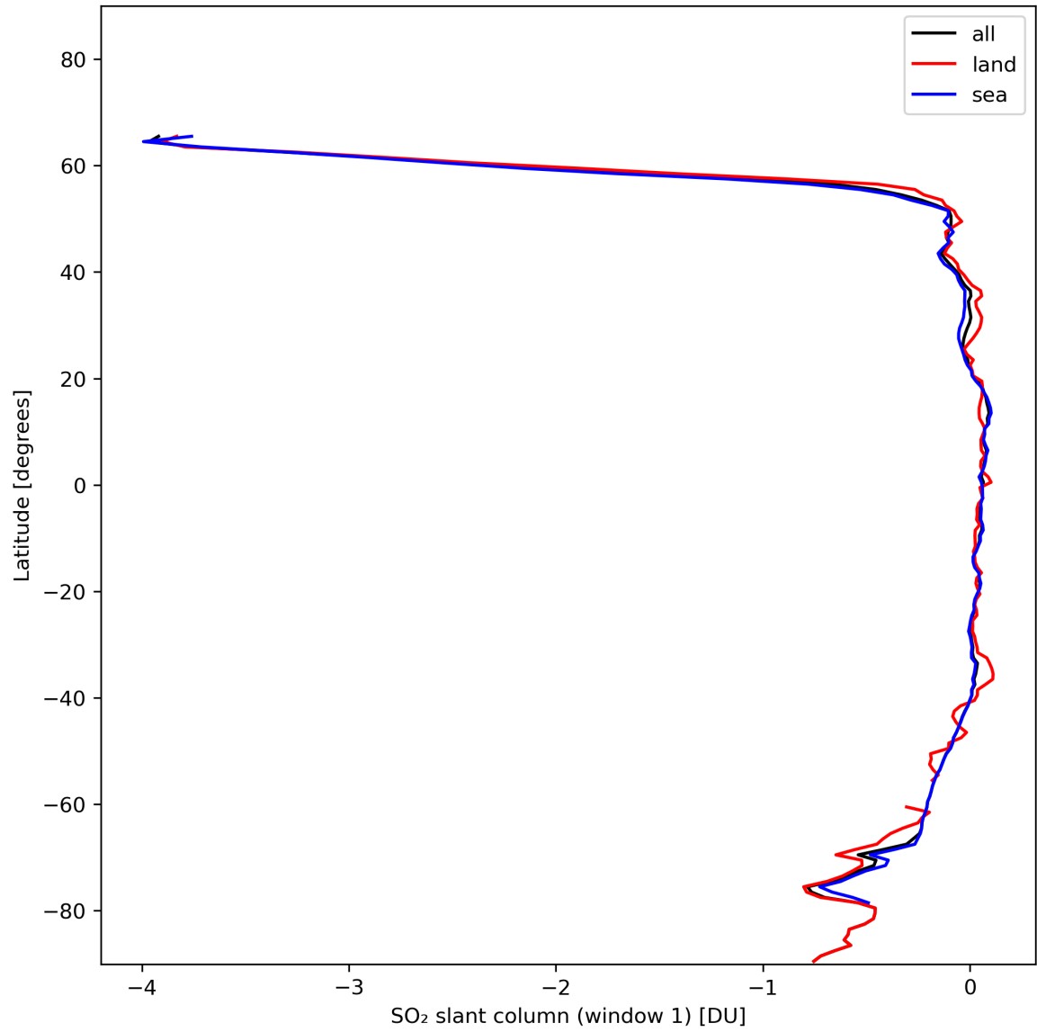
Figure 33: Zonal average of “SO 2 slant column (window 1)” for 2024-01-22 to 2024-01-24.
