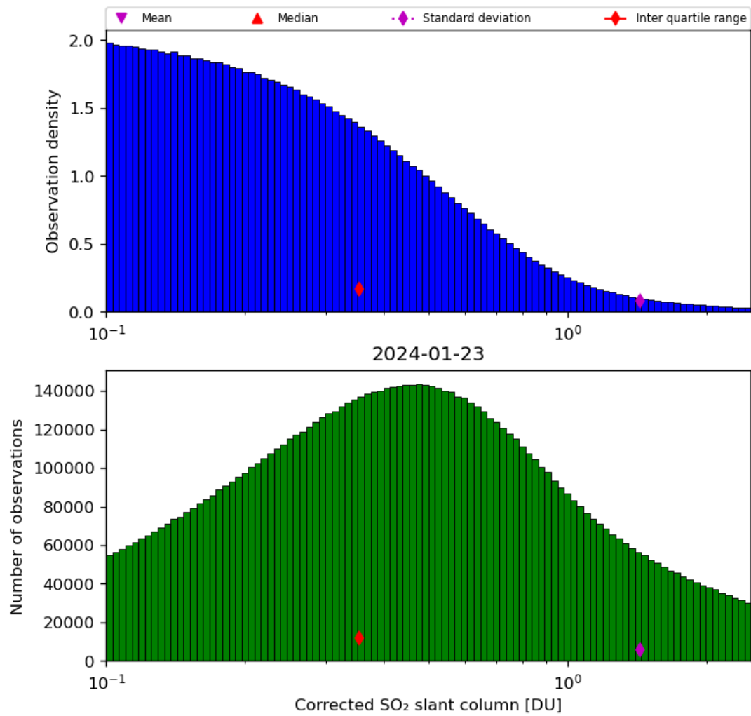
Figure 55: Histogram of “Corrected SO 2 slant column” for 2024-01-22 to 2024-01-24
