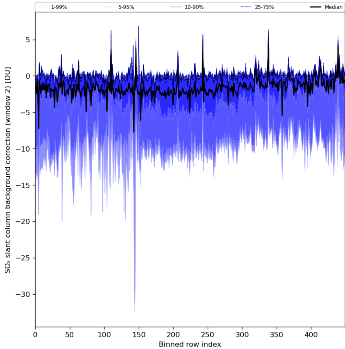
Figure 86: Along track statistics of “SO 2 slant column background correction (window 2)” for 2024-01-22 to 2024-01-24
