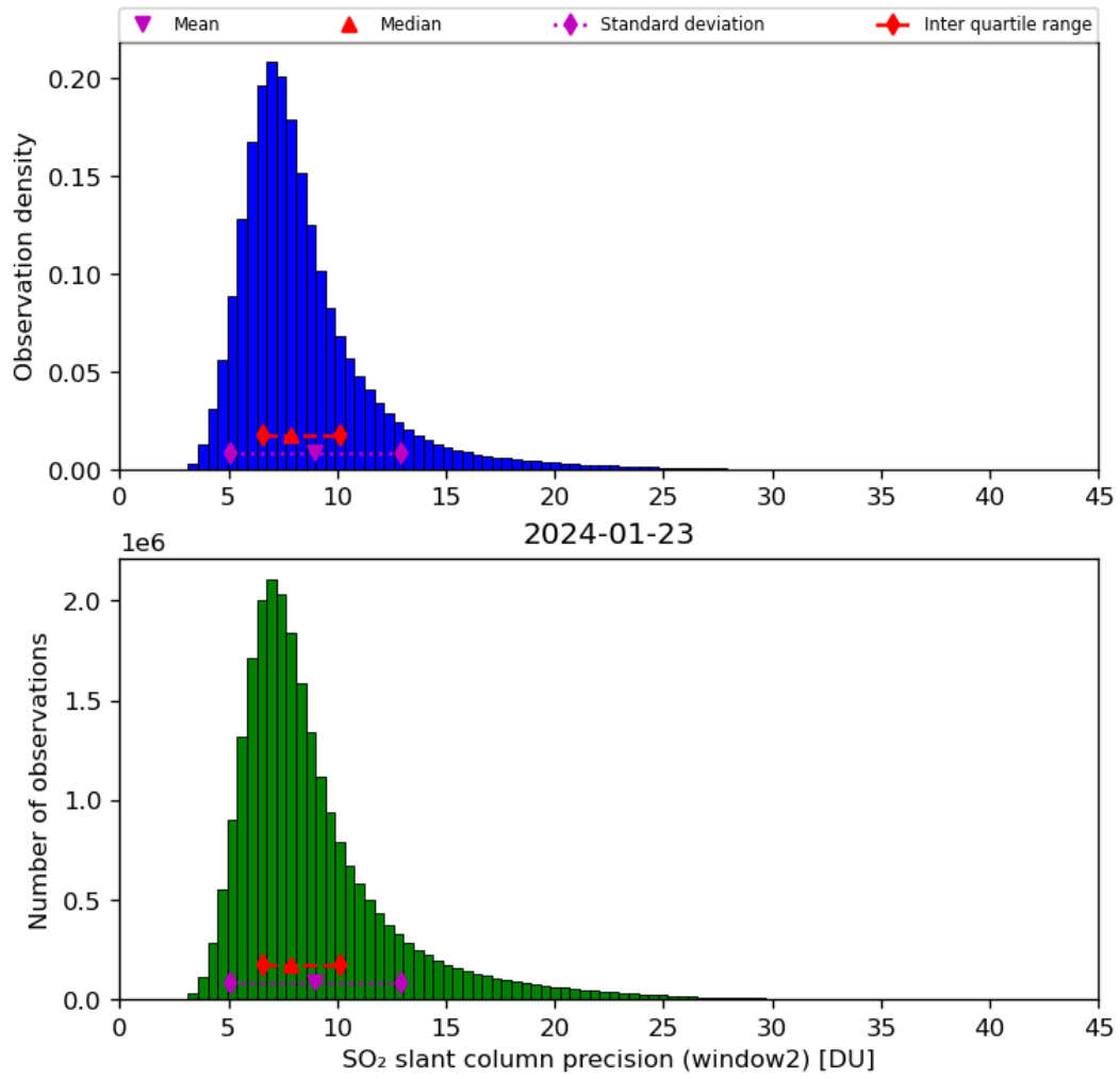
Figure 61: Histogram of “SO 2 slant column precision (window2)” for 2024-01-22 to 2024-01-24
