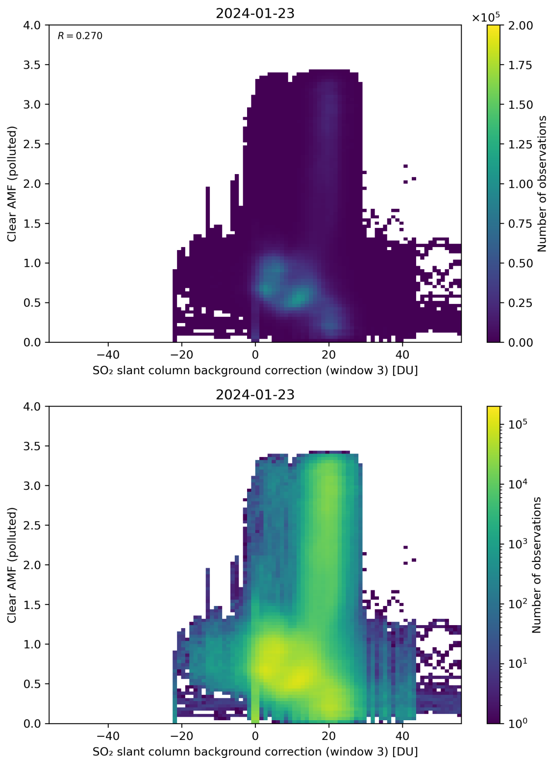
Figure 124: Scatter density plot of “SO 2 slant column background correction (window 3)” against “Clear AMF (polluted)” for 2024-01-22 to 2024-01-24.
