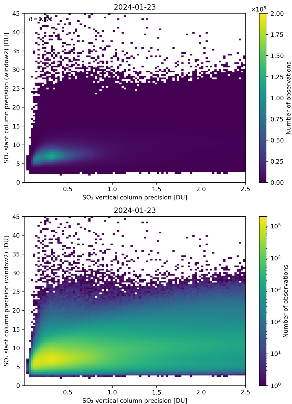
Figure 291: Scatter density plot of “SO 2 vertical column precision” against “SO 2 slant column precision (window2)” for 2024-01-22 to 2024-01-24.
