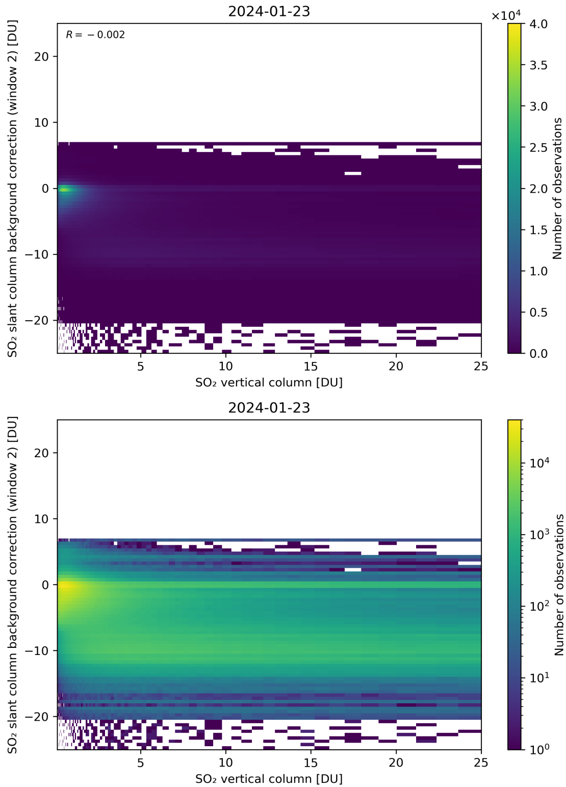
Figure 274: Scatter density plot of “SO 2 vertical column” against “SO 2 slant column background correction (window 2)” for 2024-01-22 to 2024-01-24.
