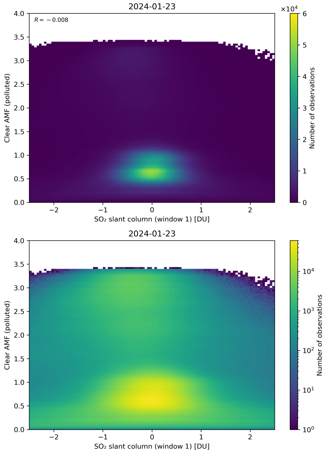
Figure 232: Scatter density plot of “SO 2 slant column (window 1)” against “Clear AMF (polluted)” for 2024-01-22 to 2024-01-24.
