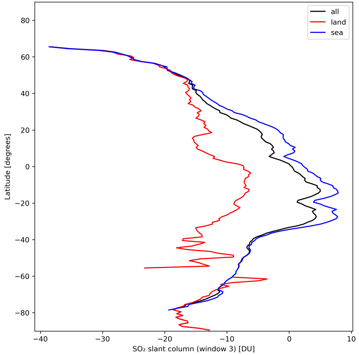
Figure 41: Zonal average of “SO 2 slant column (window 3)” for 2024-01-22 to 2024-01-24.
