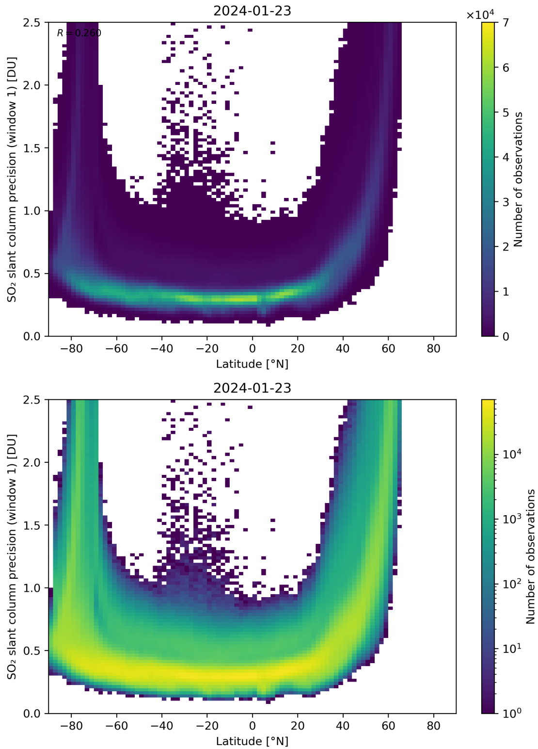
Figure 150: Scatter density plot of “Latitude” against “SO 2 slant column precision (window 1)” for 2024-01-22 to 2024-01-24.
