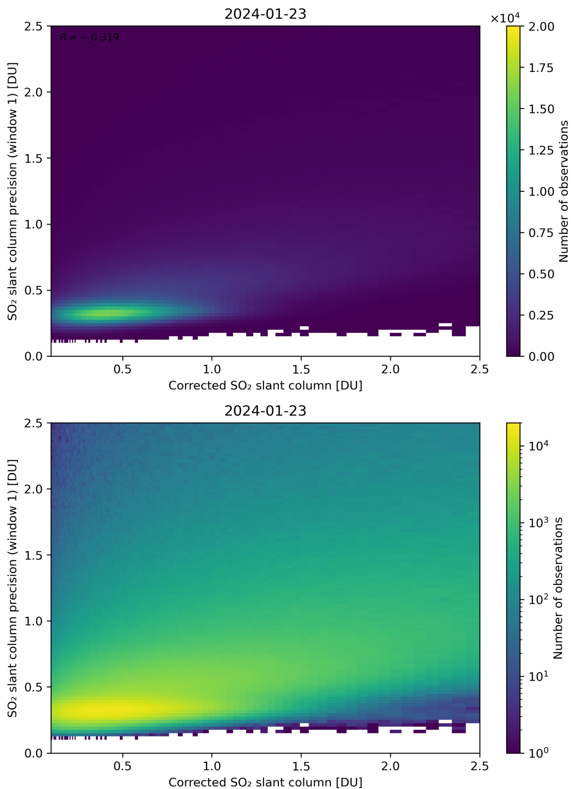
Figure 188: Scatter density plot of “Corrected SO 2 slant column” against “SO 2 slant column precision (window 1)” for 2024-01-22 to 2024-01-24.
