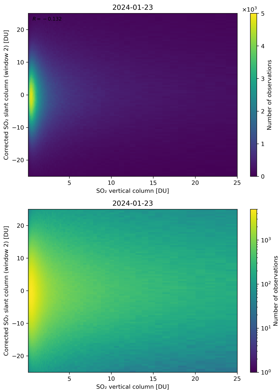
Figure 298: Scatter density plot of “SO 2 vertical column” against “Corrected SO 2 slant column (window 2)” for 2024-01-22 to 2024-01-24.
