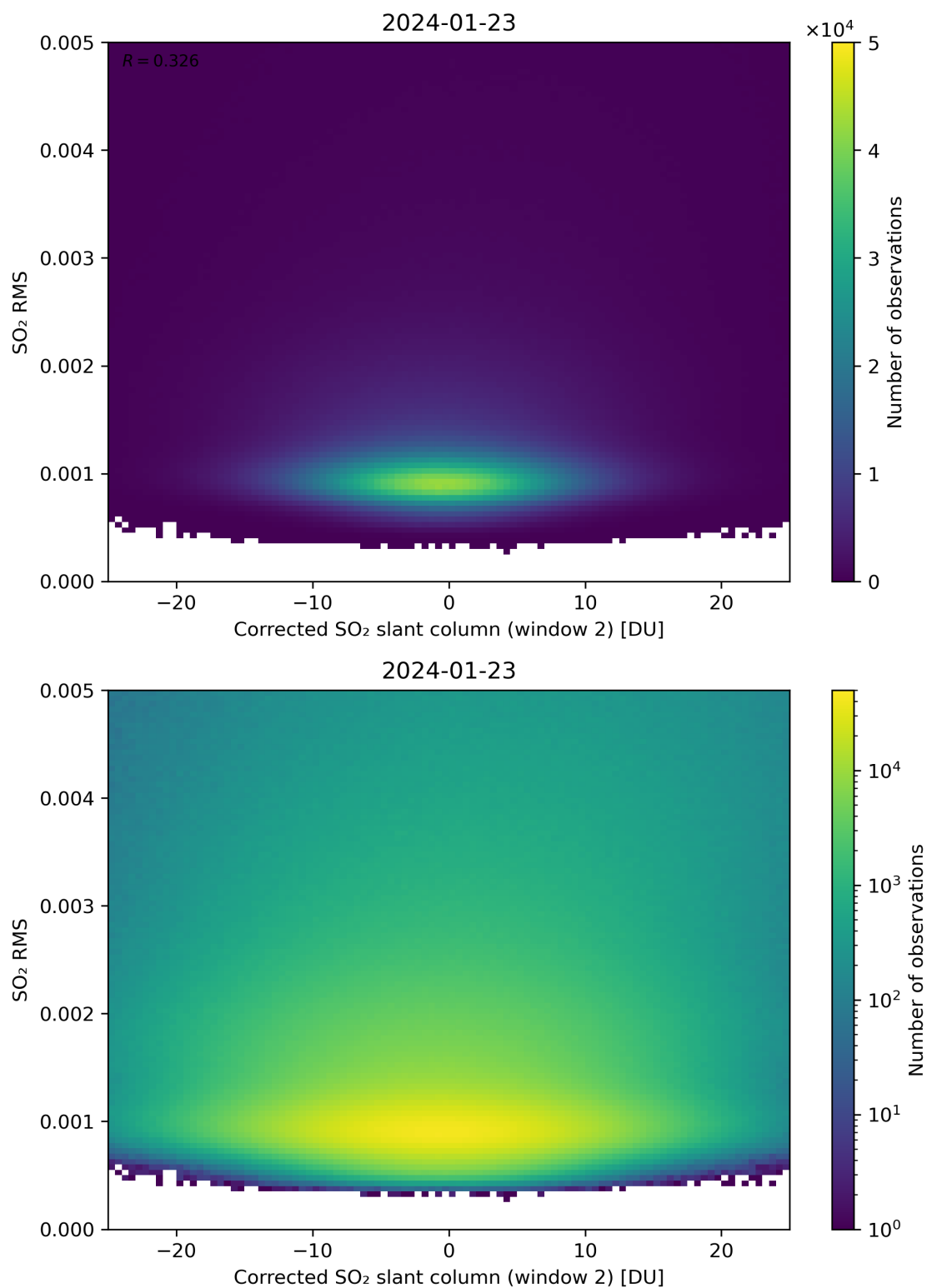
Figure 198: Scatter density plot of “Corrected SO 2 slant column (window 2)” against “SO 2 RMS” for 2024-01-22 to 2024-01-24.
