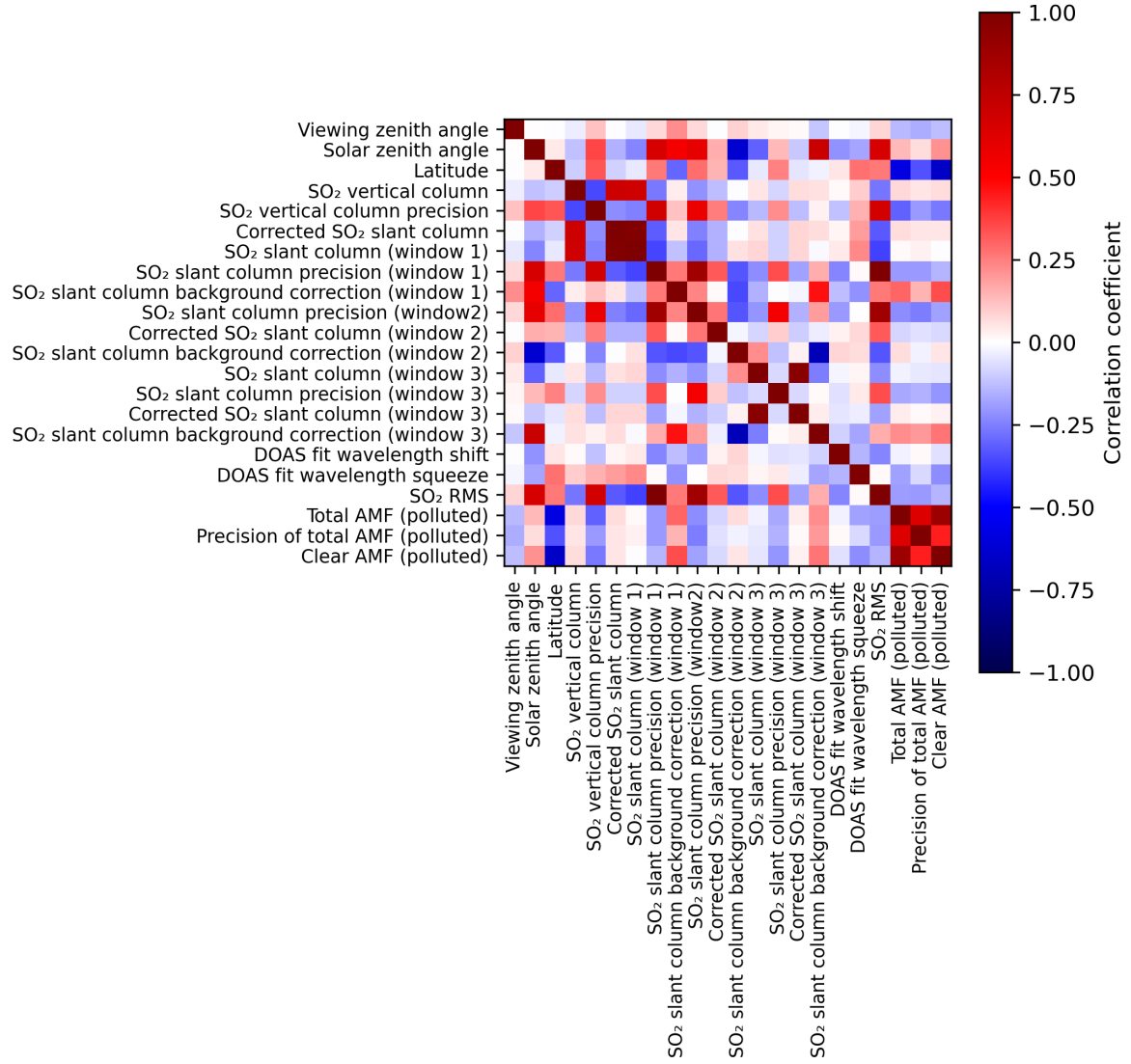
Figure 2: Map of correlation matrix for 2024-01-22 to 2024-01-24.
