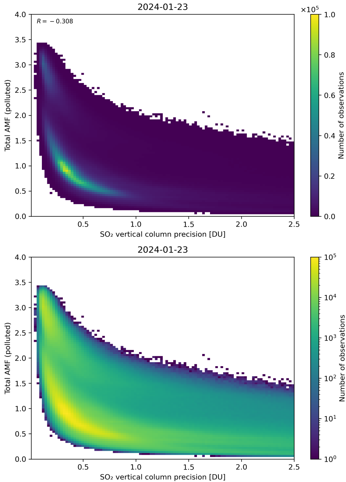
Figure 294: Scatter density plot of “SO 2 vertical column precision” against “Total AMF (polluted)” for 2024-01-22 to 2024-01-24.
