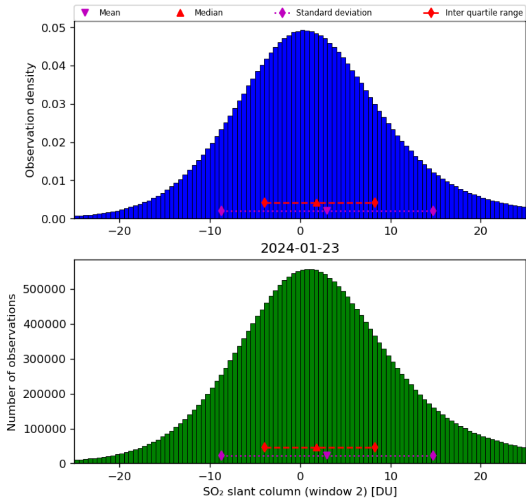
Figure 60: Histogram of “SO 2 slant column (window 2)” for 2024-01-22 to 2024-01-24
