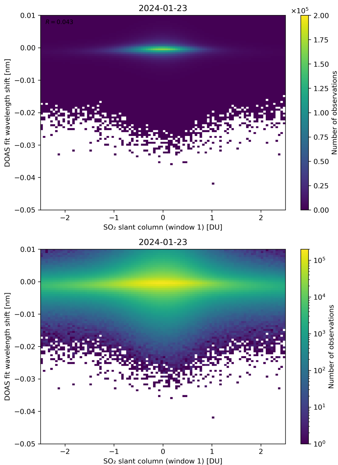
Figure 215: Scatter density plot of “SO 2 slant column (window 1)” against “DOAS fit wavelength shift” for 2024-01-22 to 2024-01-24.
