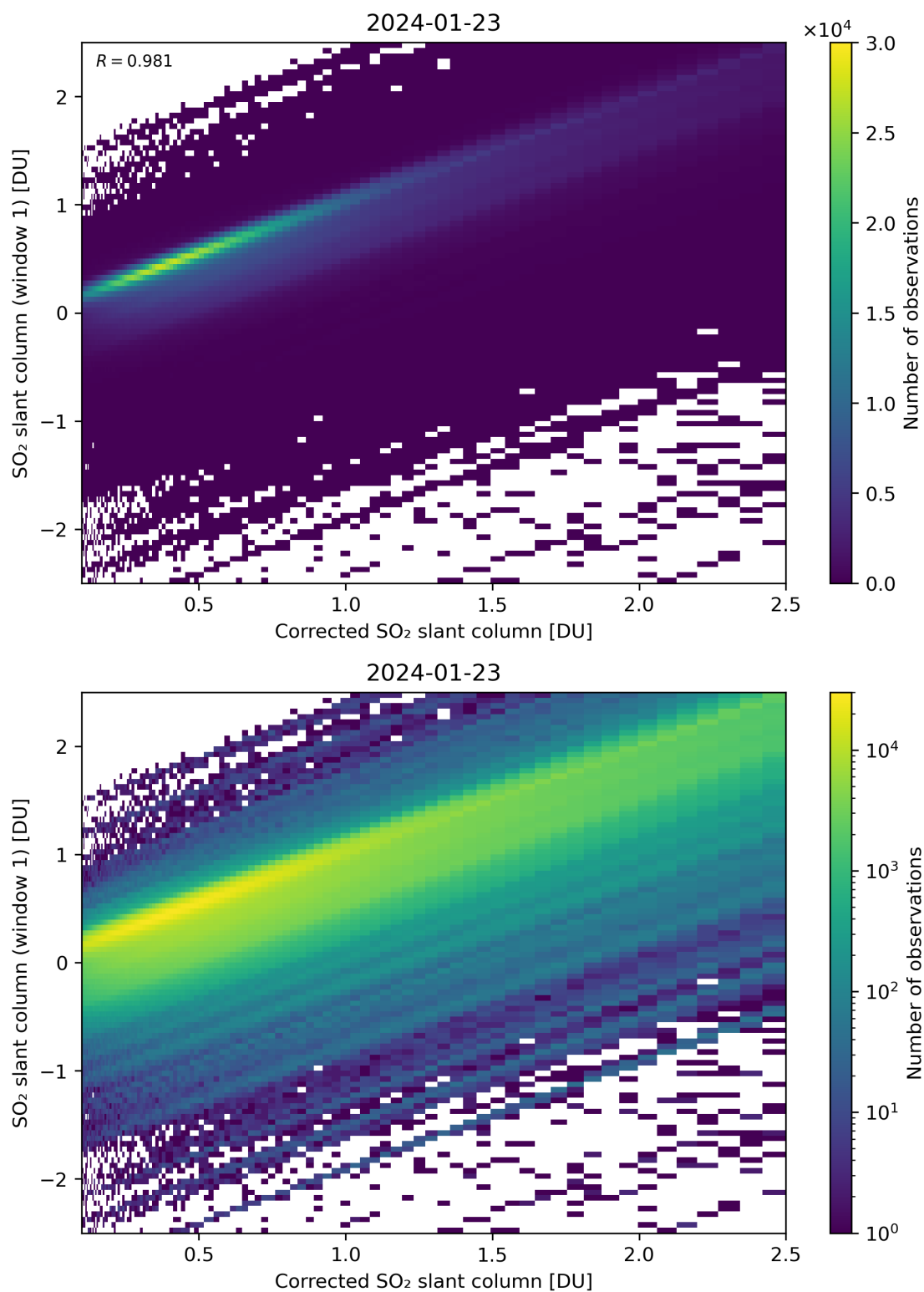
Figure 187: Scatter density plot of “Corrected SO 2 slant column” against “SO 2 slant column (window 1)” for 2024-01-22 to 2024-01-24.
