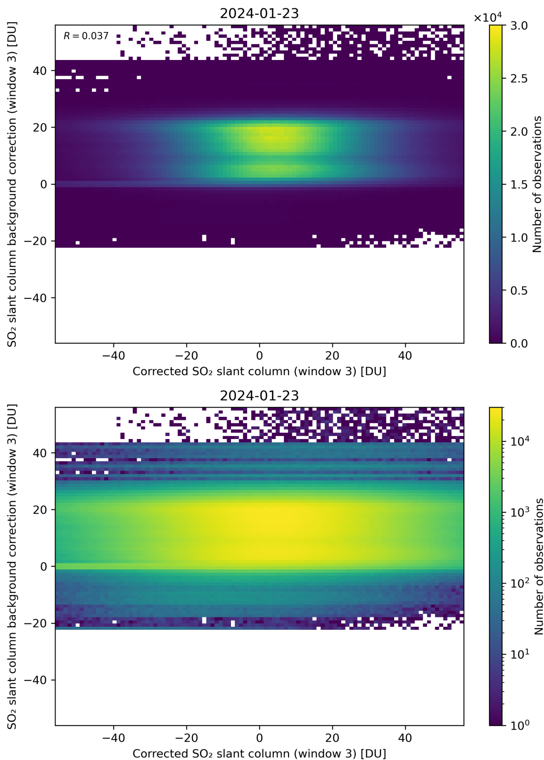
Figure 205: Scatter density plot of “Corrected SO 2 slant column (window 3)” against “SO 2 slant column background correction (window 3)” for 2024-01-22 to 2024-01-24.
