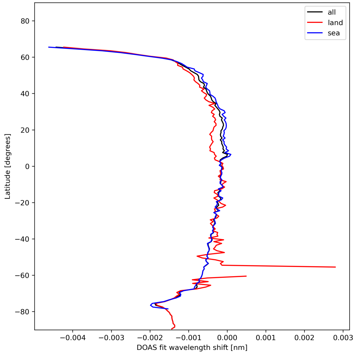
Figure 45: Zonal average of “DOAS fit wavelength shift” for 2024-01-22 to 2024-01-24.
