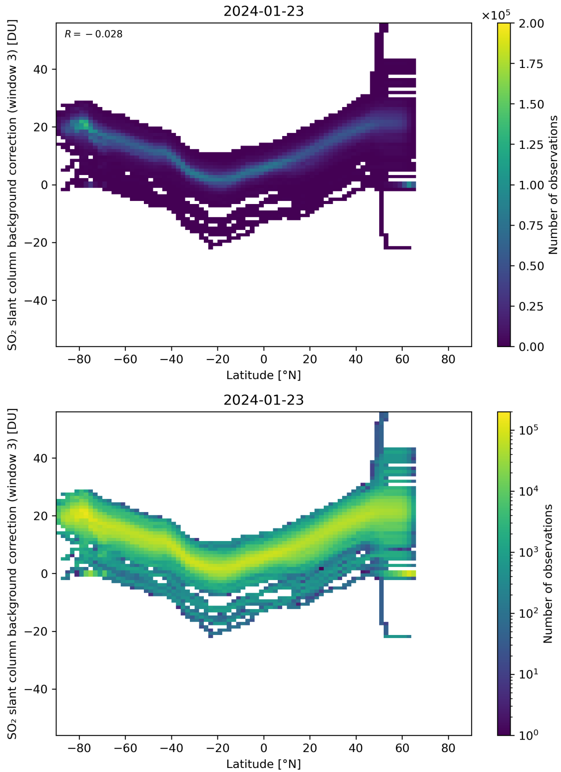
Figure 141: Scatter density plot of “Latitude” against “SO 2 slant column background correction (window 3)” for 2024-01-22 to 2024-01-24.
