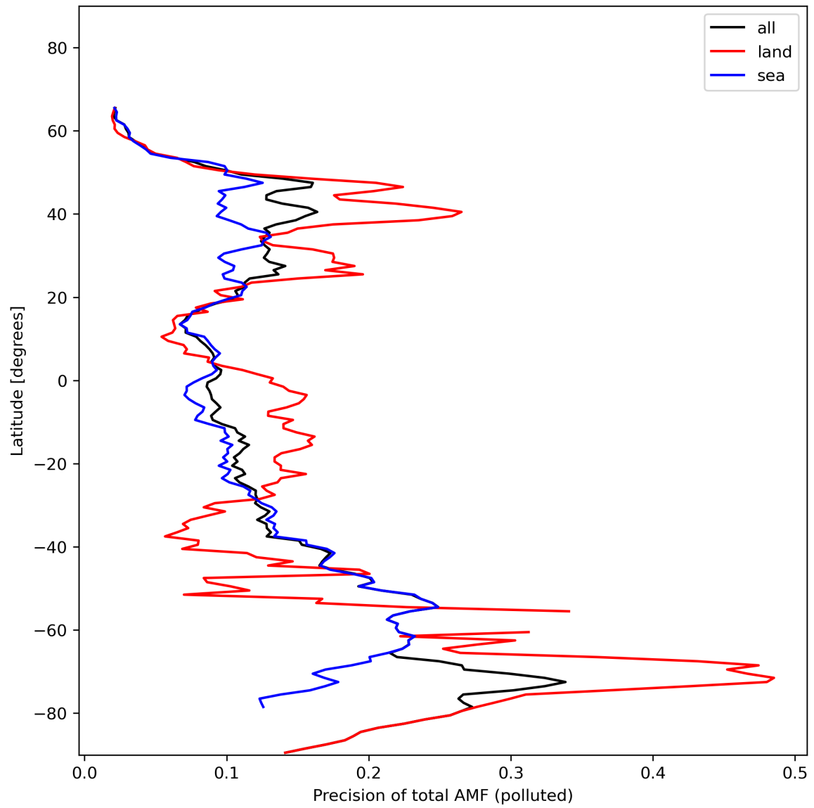
Figure 49: Zonal average of “Precision of total AMF (polluted)” for 2024-01-22 to 2024-01-24.
