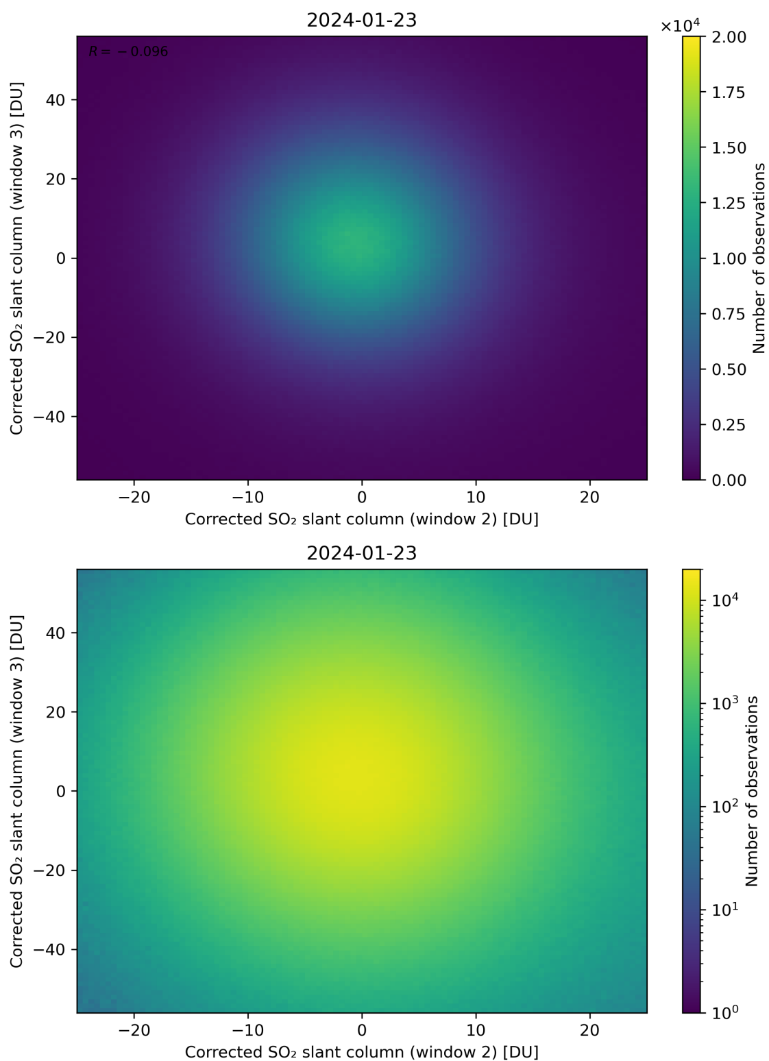
Figure 200: Scatter density plot of “Corrected SO 2 slant column (window 2)” against “Corrected SO 2 slant column (window 3)” for 2024-01-22 to 2024-01-24.
