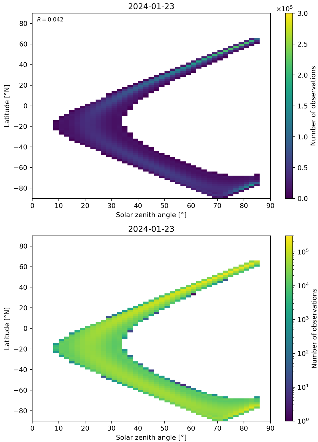
Figure 164: Scatter density plot of “Solar zenith angle” against “Latitude” for 2024-01-22 to 2024-01-24.
