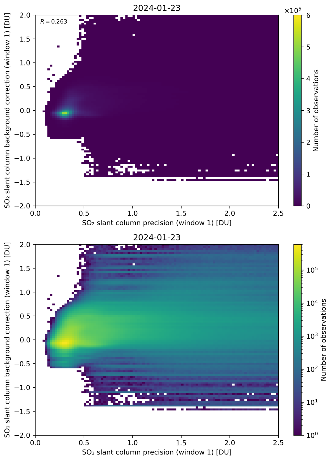
Figure 218: Scatter density plot of “SO 2 slant column precision (window 1)” against “SO 2 slant column background correction (window 1)” for 2024-01-22 to 2024-01-24.
