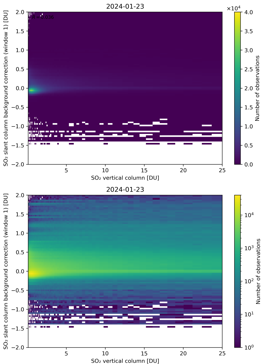
Figure 273: Scatter density plot of “SO 2 vertical column” against “SO 2 slant column background correction (window 1)” for 2024-01-22 to 2024-01-24.
