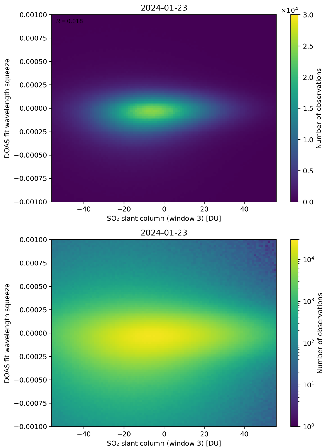
Figure 255: Scatter density plot of “SO 2 slant column (window 3)” against “DOAS fit wavelength squeeze” for 2024-01-22 to 2024-01-24.
