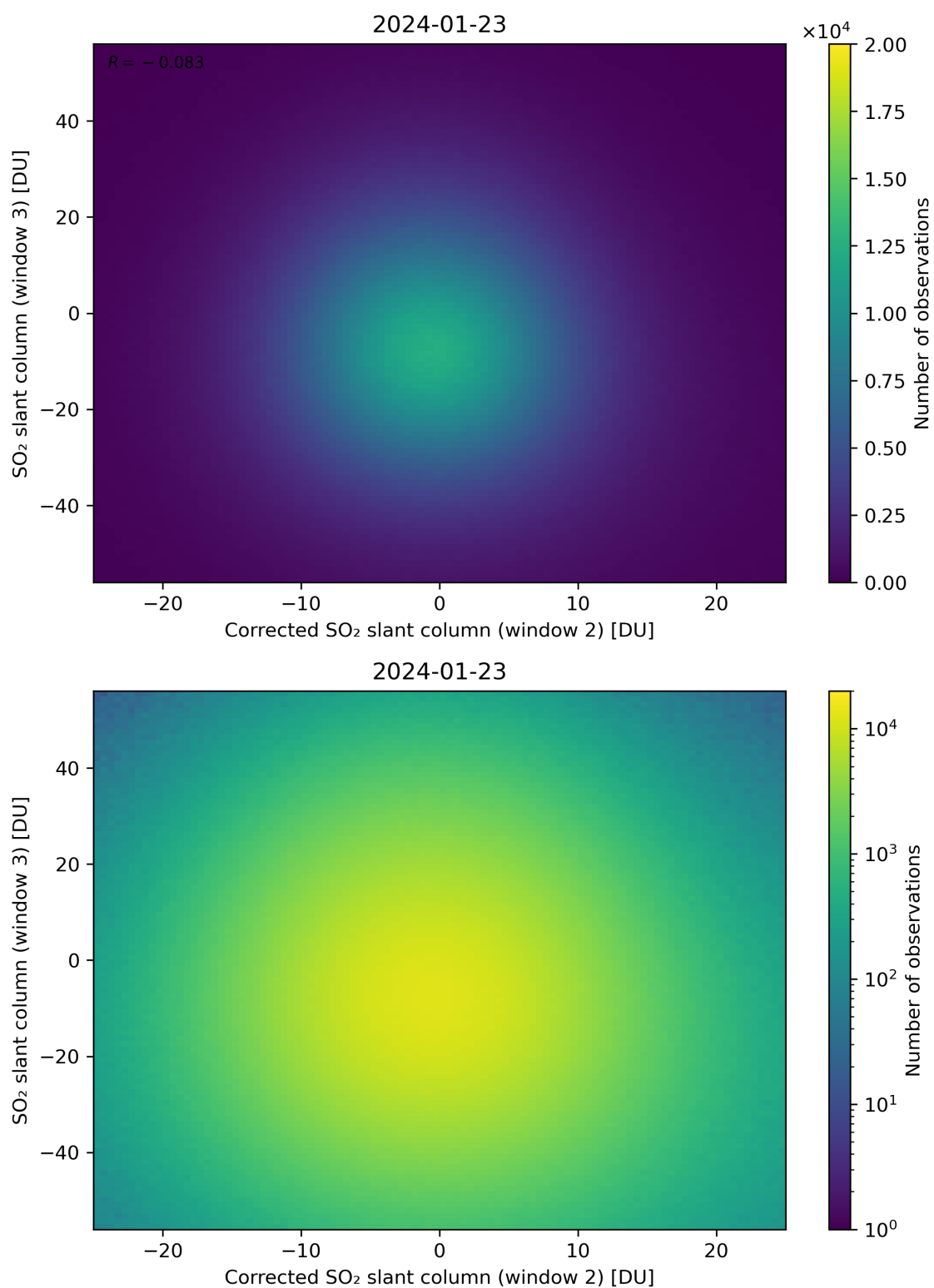
Figure 201: Scatter density plot of “Corrected SO 2 slant column (window 2)” against “SO 2 slant column (window 3)” for 2024-01-22 to 2024-01-24.
