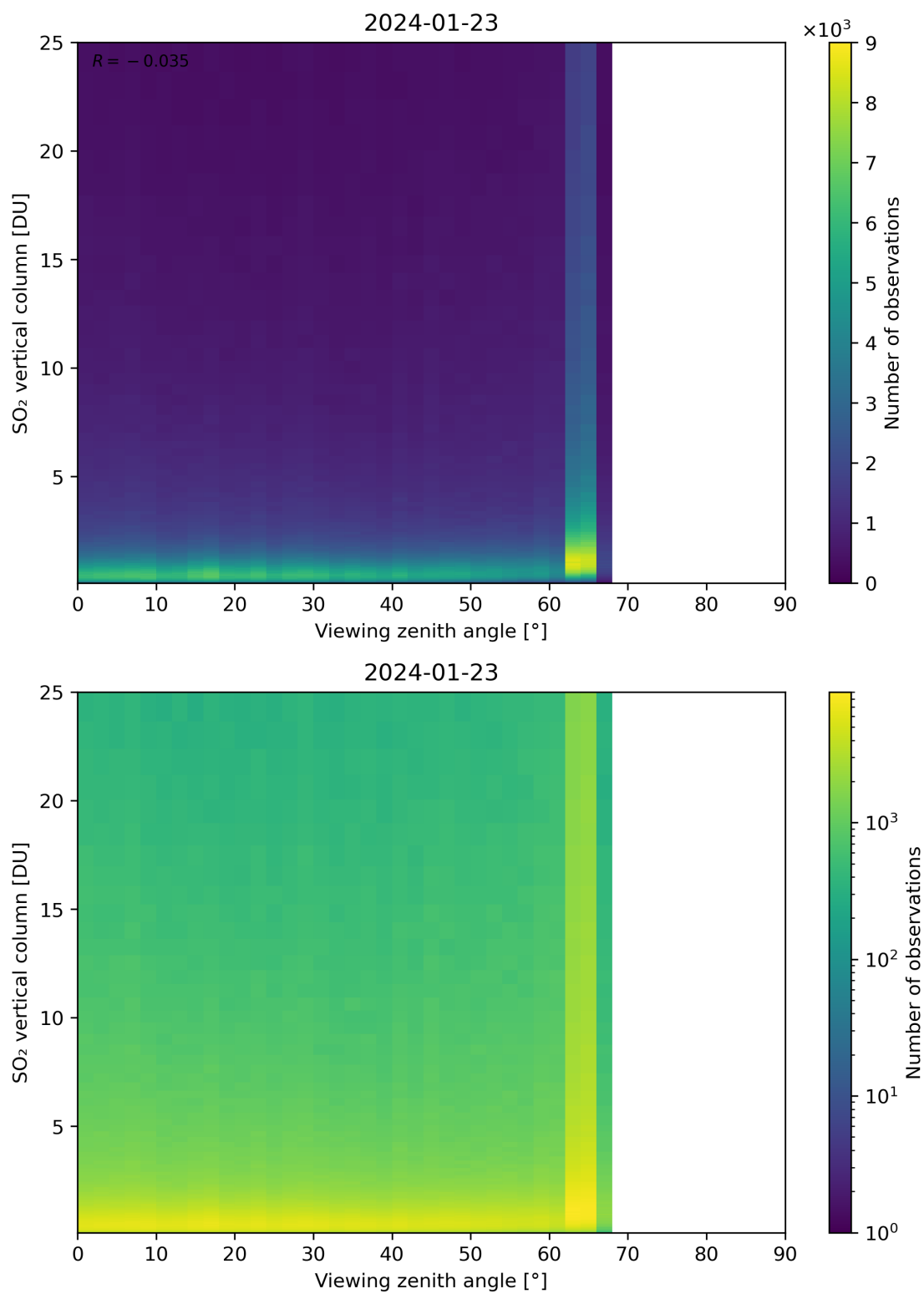
Figure 327: Scatter density plot of “Viewing zenith angle” against “SO 2 vertical column” for 2024-01-22 to 2024-01-24.
