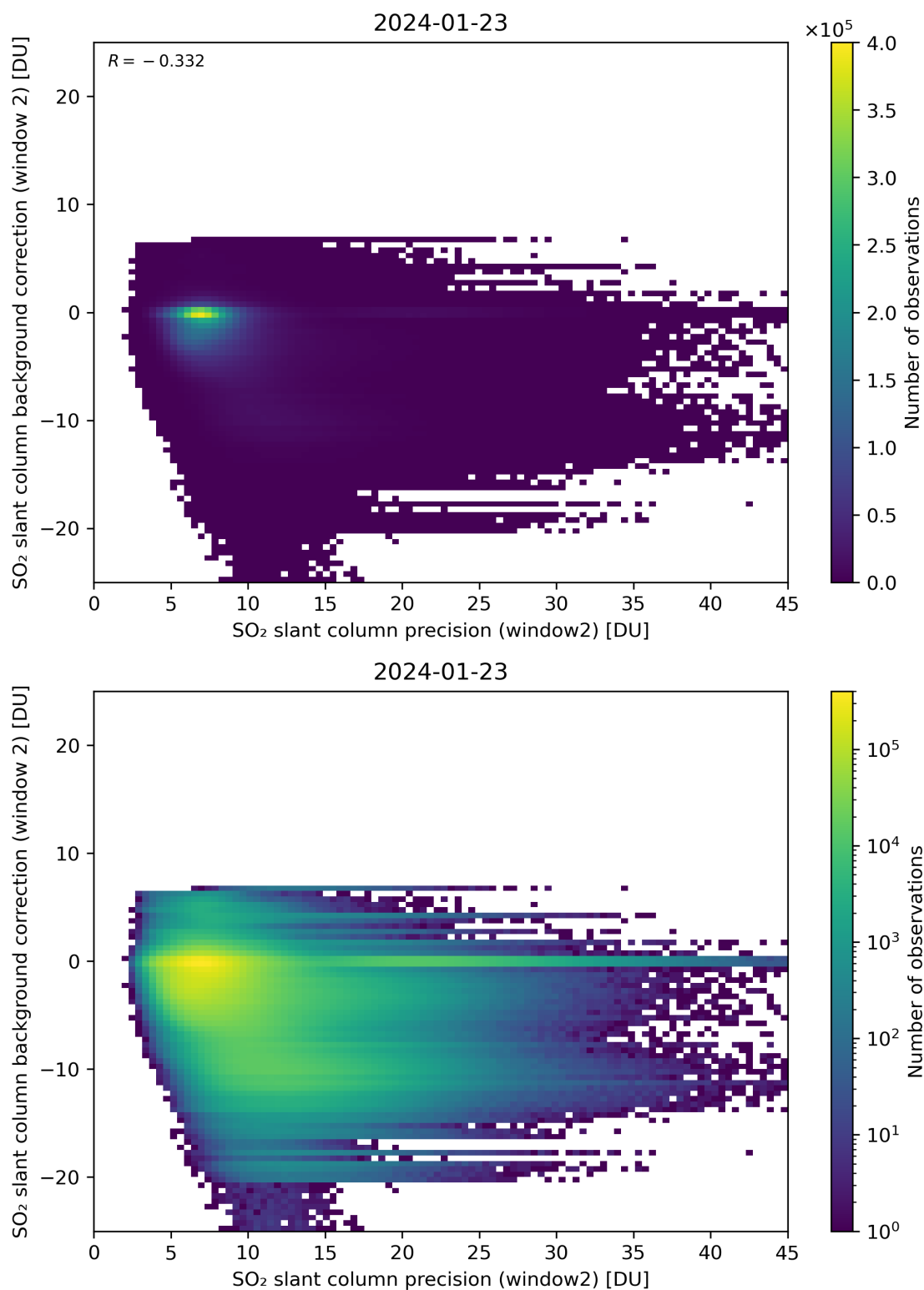
Figure 241: Scatter density plot of “SO 2 slant column precision (window2)” against “SO 2 slant column background correction (window 2)” for 2024-01-22 to 2024-01-24.
