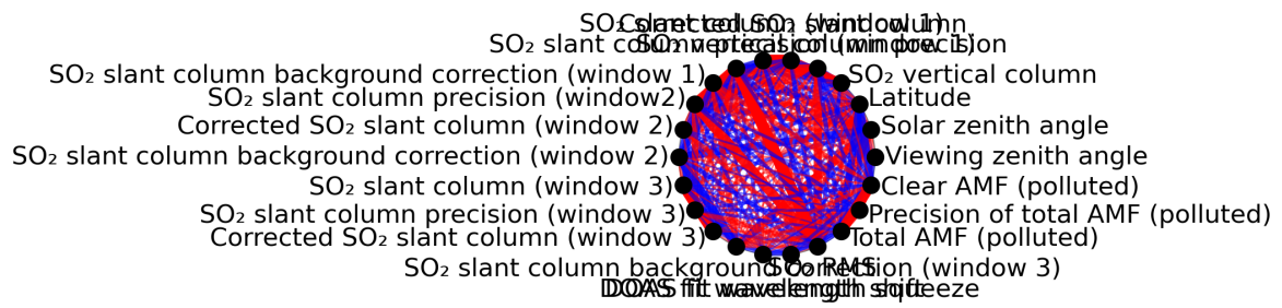
Figure 1: Map of correlation graph for 2024-01-22 to 2024-01-24.
