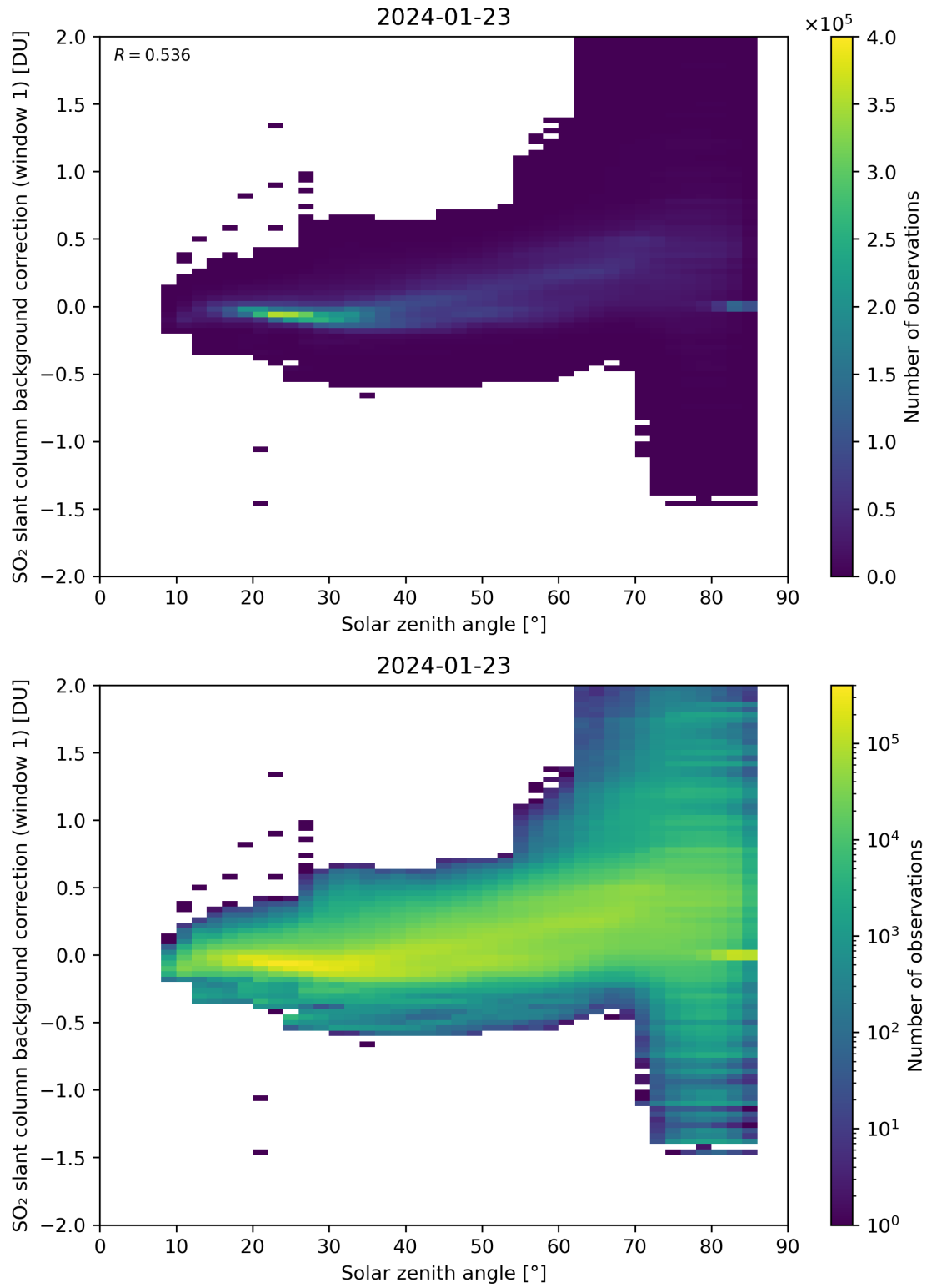
Figure 158: Scatter density plot of “Solar zenith angle” against “SO 2 slant column background correction (window 1)” for 2024-01-22 to 2024-01-24.
