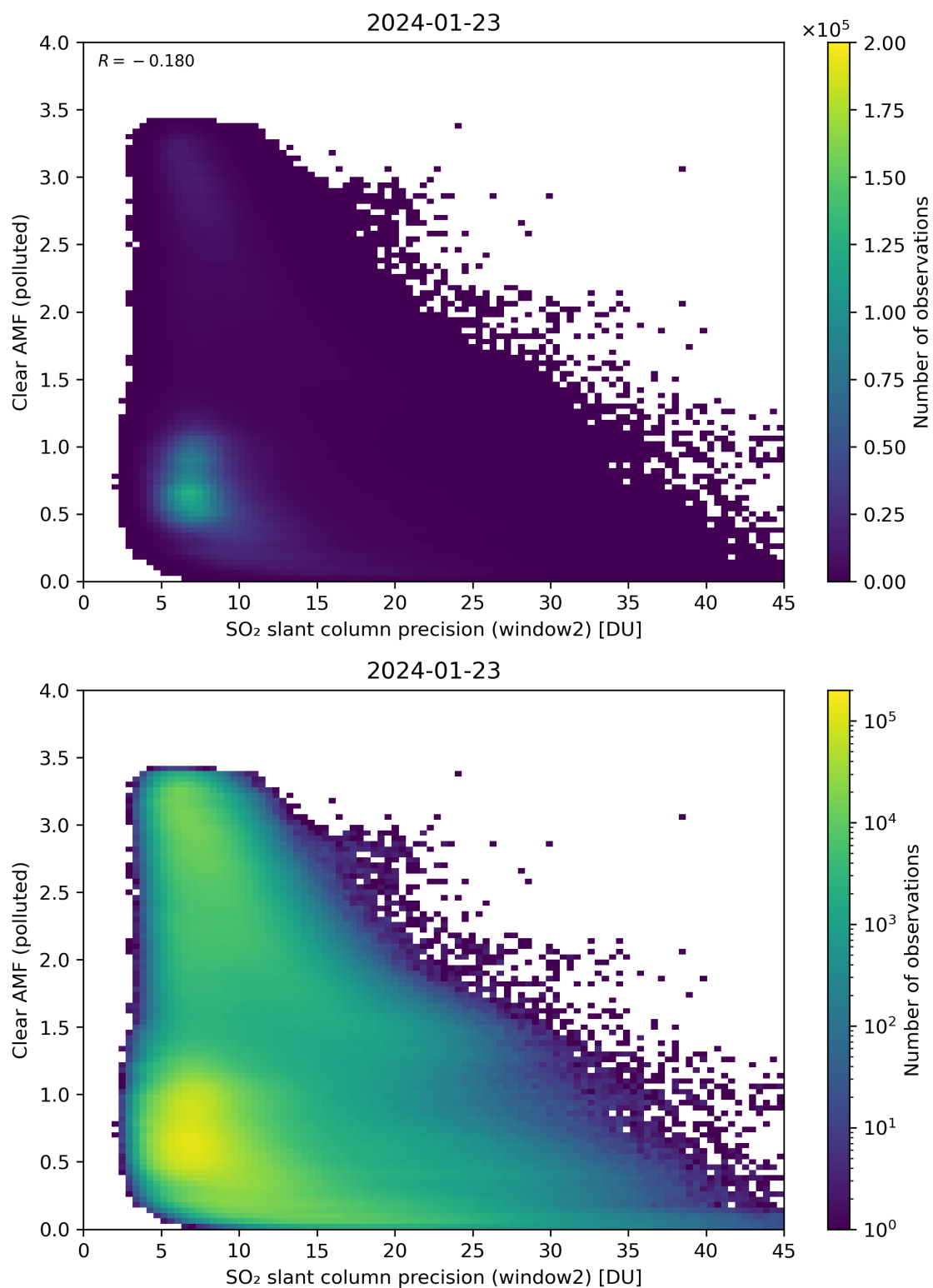
Figure 246: Scatter density plot of “SO 2 slant column precision (window2)” against “Clear AMF (polluted)” for 2024-01-22 to 2024-01-24.
