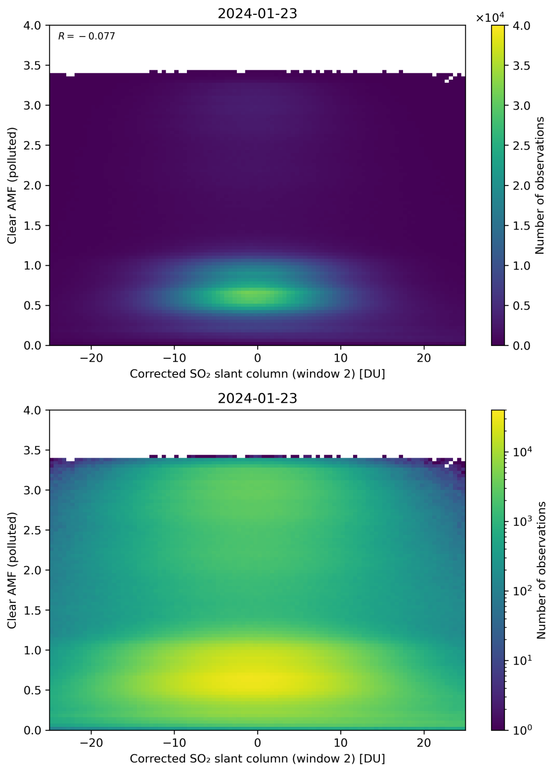
Figure 199: Scatter density plot of “Corrected SO 2 slant column (window 2)” against “Clear AMF (polluted)” for 2024-01-22 to 2024-01-24.
