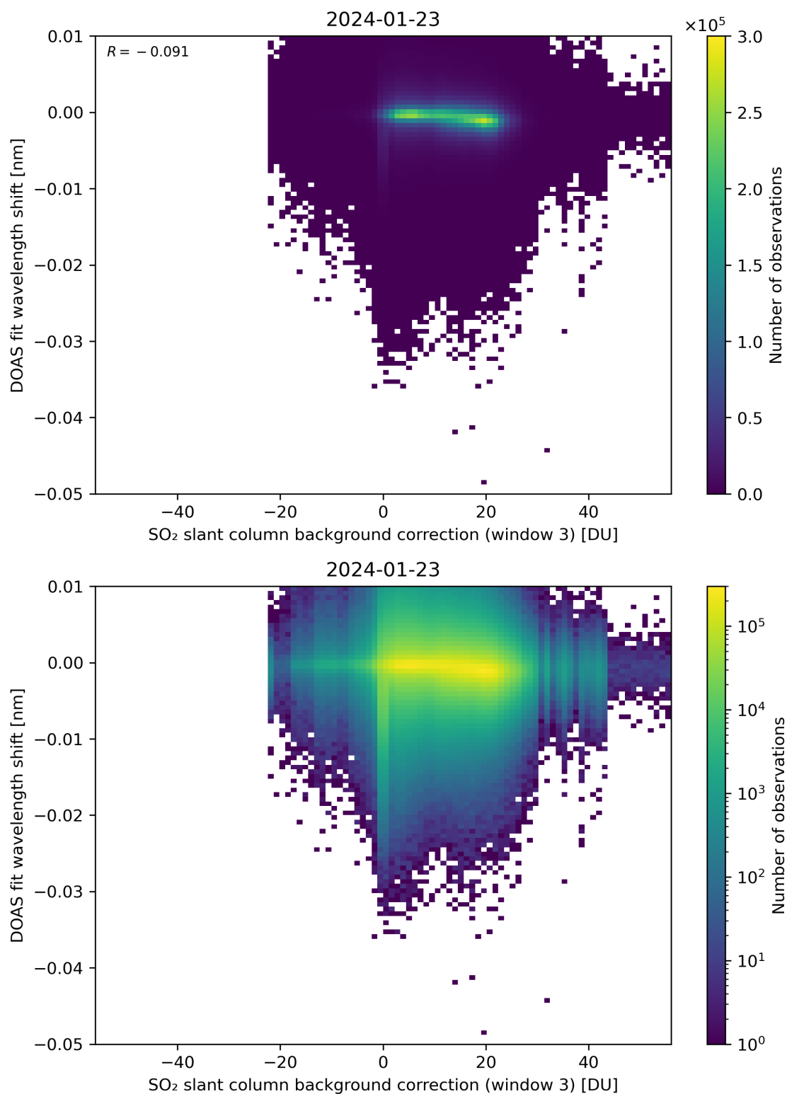
Figure 121: Scatter density plot of “SO 2 slant column background correction (window 3)” against “DOAS fit wavelength shift” for 2024-01-22 to 2024-01-24.
