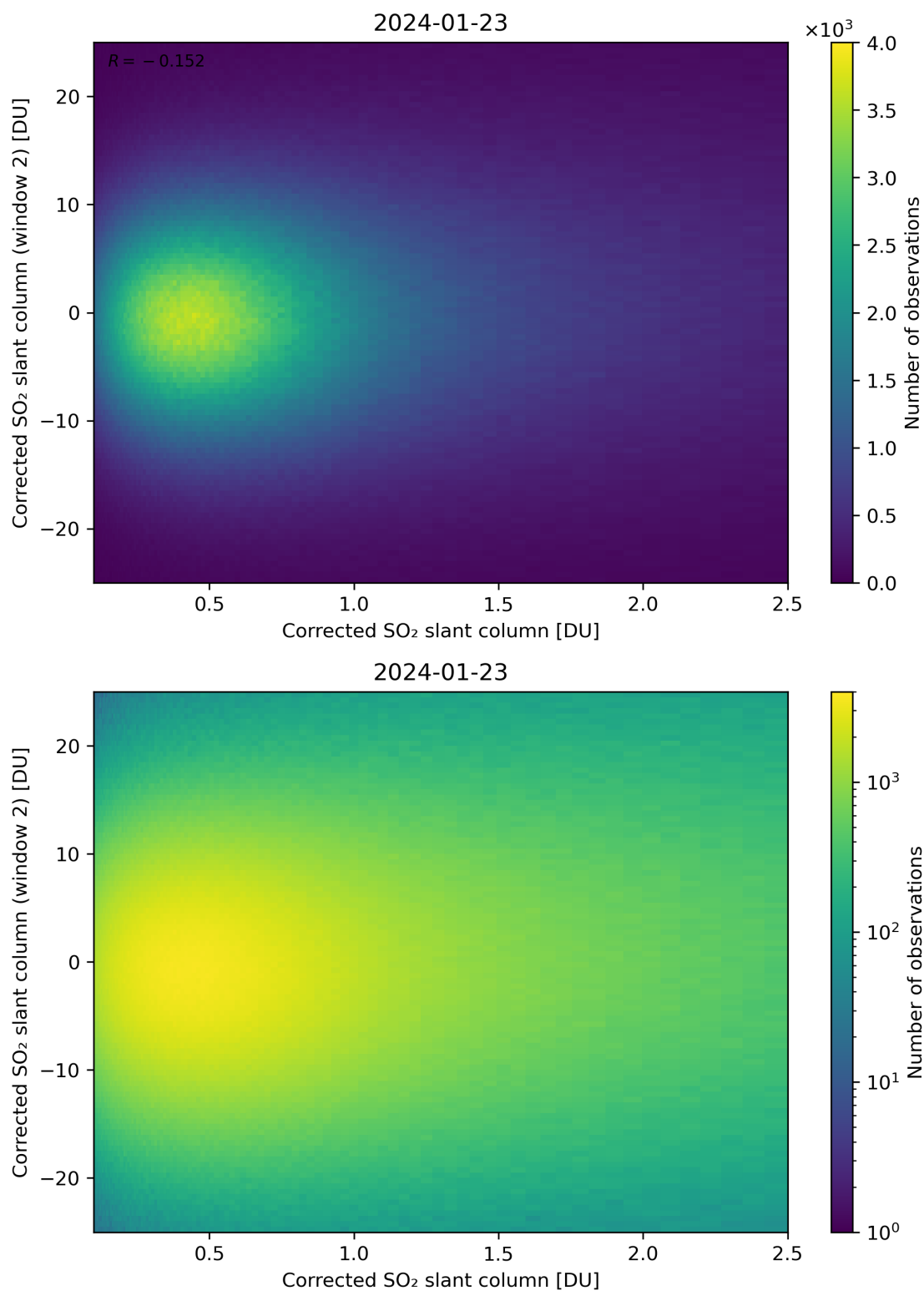
Figure 185: Scatter density plot of “Corrected SO 2 slant column” against “Corrected SO 2 slant column (window 2)” for 2024-01-22 to 2024-01-24.
