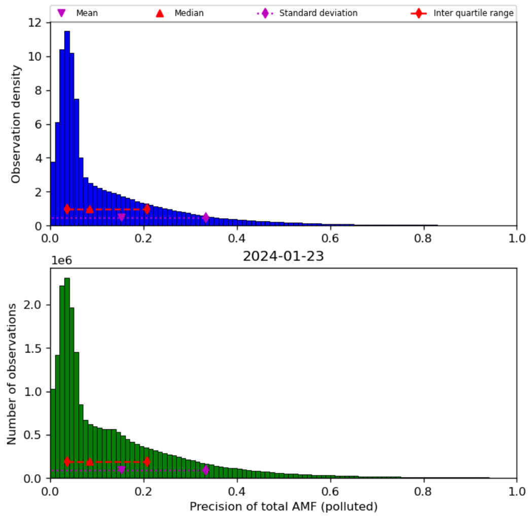
Figure 72: Histogram of “Precision of total AMF (polluted)” for 2024-01-22 to 2024-01-24
