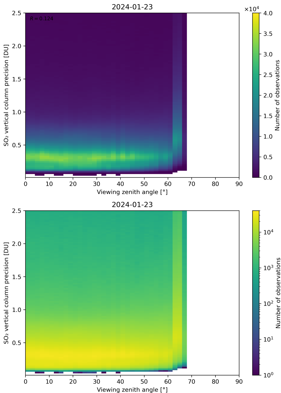
Figure 328: Scatter density plot of “Viewing zenith angle” against “SO 2 vertical column precision” for 2024-01-22 to 2024-01-24.
