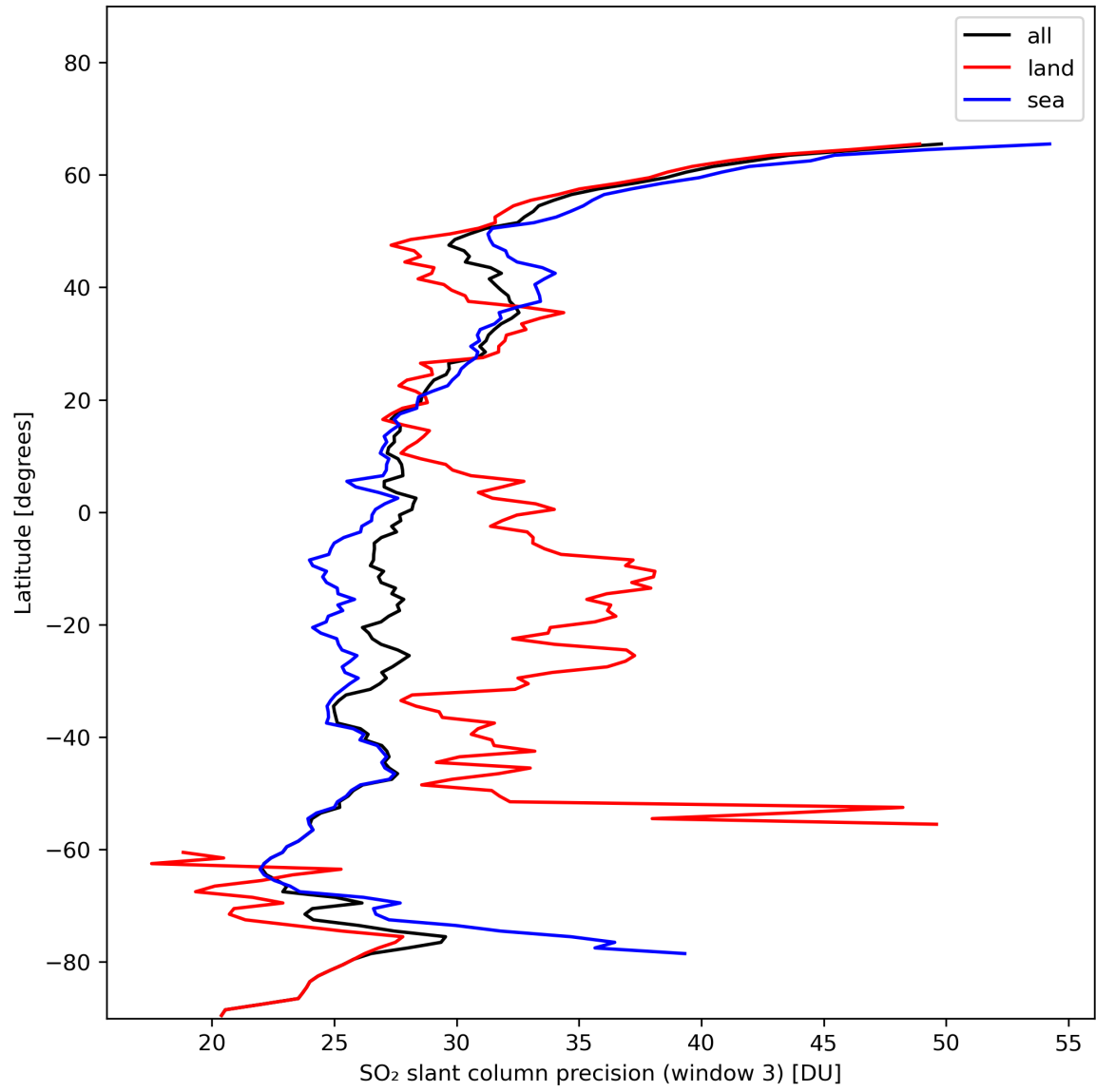
Figure 42: Zonal average of “SO 2 slant column precision (window 3)” for 2024-01-22 to 2024-01-24.
