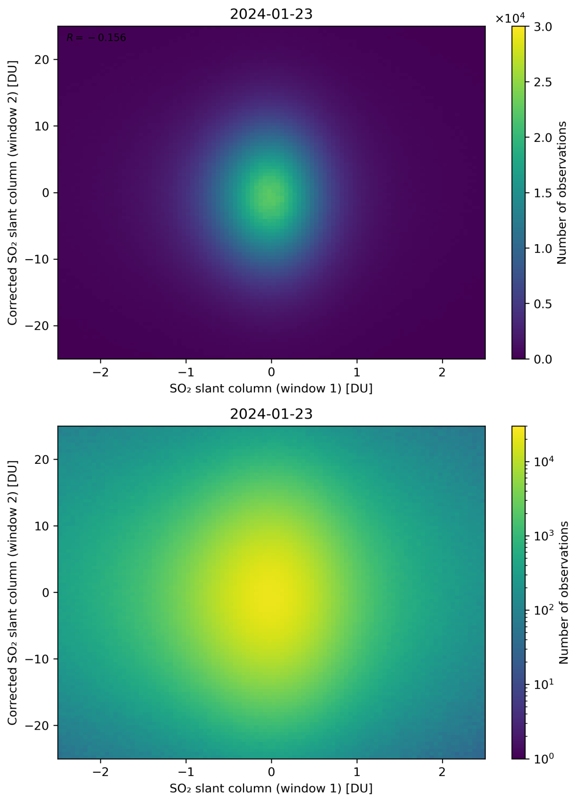
Figure 233: Scatter density plot of “SO 2 slant column (window 1)” against “Corrected SO 2 slant column (window 2)” for 2024-01-22 to 2024-01-24.
