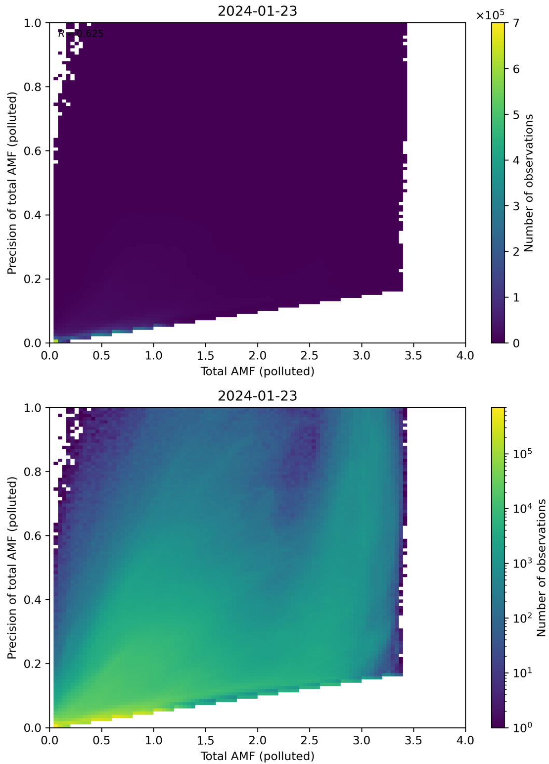
Figure 272: Scatter density plot of “Total AMF (polluted)” against “Precision of total AMF (polluted)” for 2024-01-22 to 2024-01-24.
