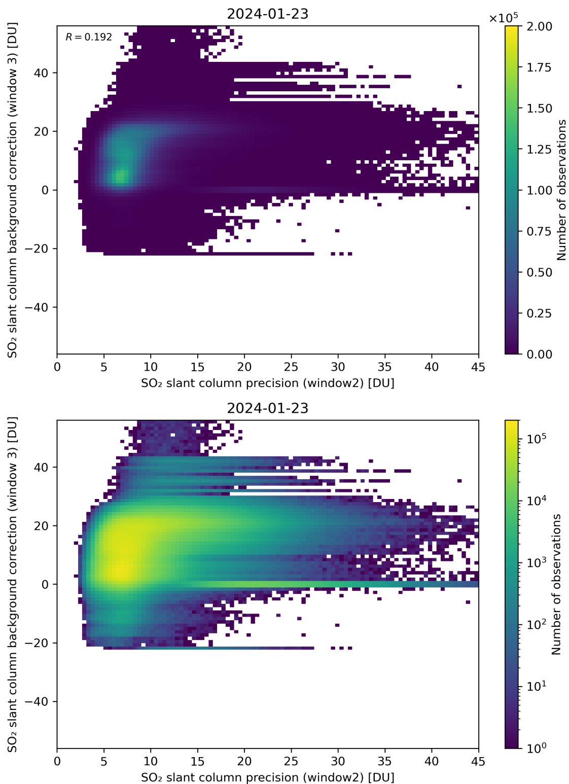
Figure 242: Scatter density plot of “SO 2 slant column precision (window2)” against “SO 2 slant column background correction (window 3)” for 2024-01-22 to 2024-01-24.
