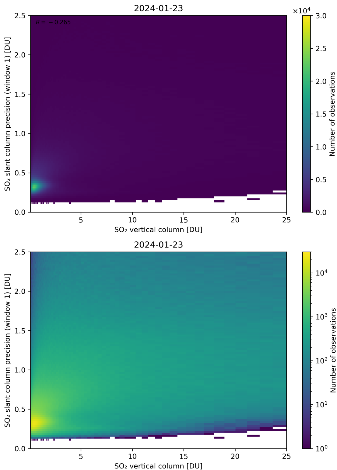
Figure 301: Scatter density plot of “SO 2 vertical column” against “SO 2 slant column precision (window 1)” for 2024-01-22 to 2024-01-24.
