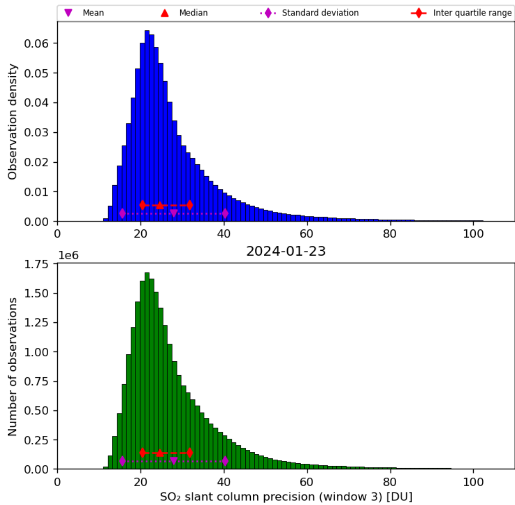
Figure 65: Histogram of “SO 2 slant column precision (window 3)” for 2024-01-22 to 2024-01-24
