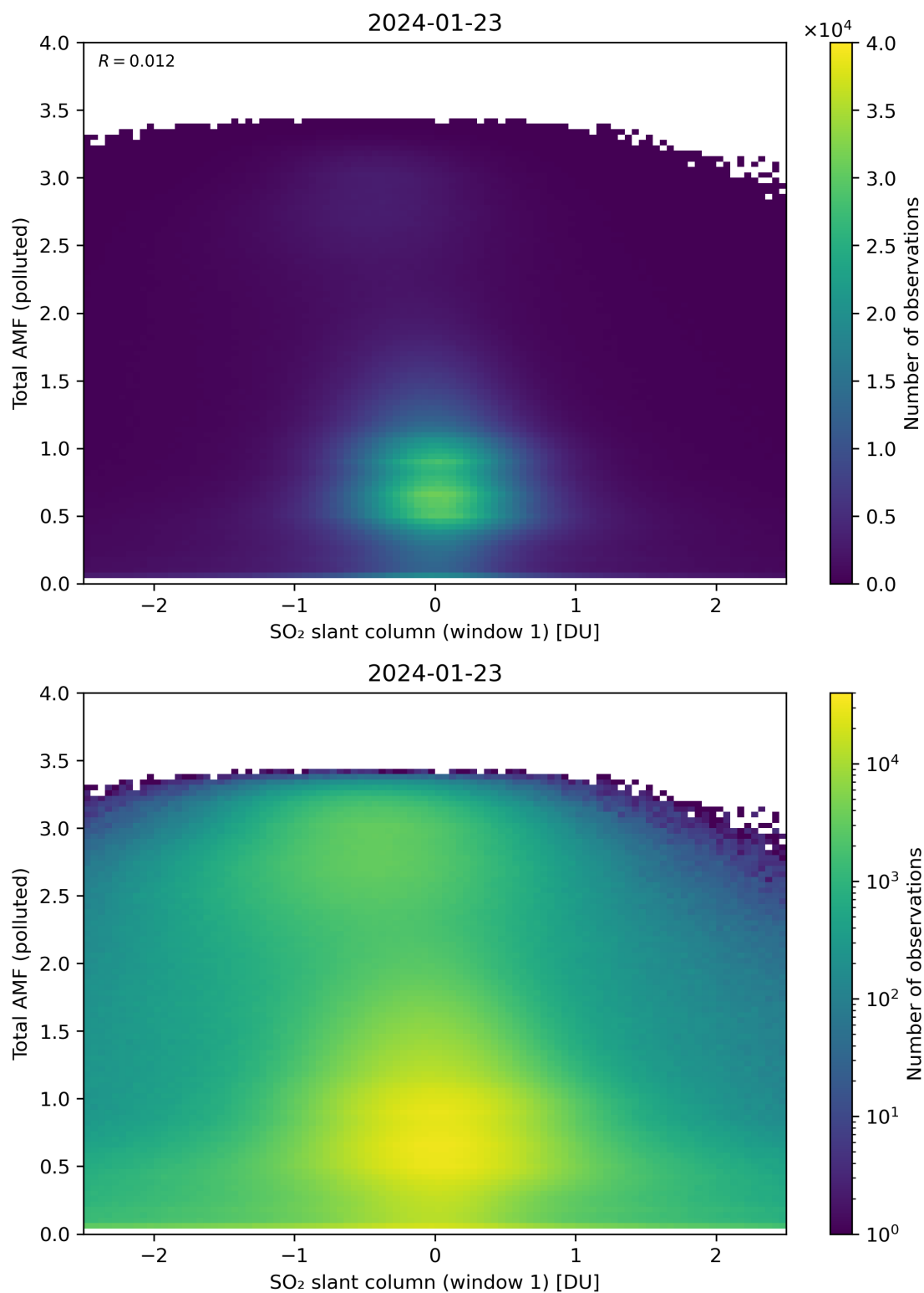
Figure 239: Scatter density plot of “SO 2 slant column (window 1)” against “Total AMF (polluted)” for 2024-01-22 to 2024-01-24.
