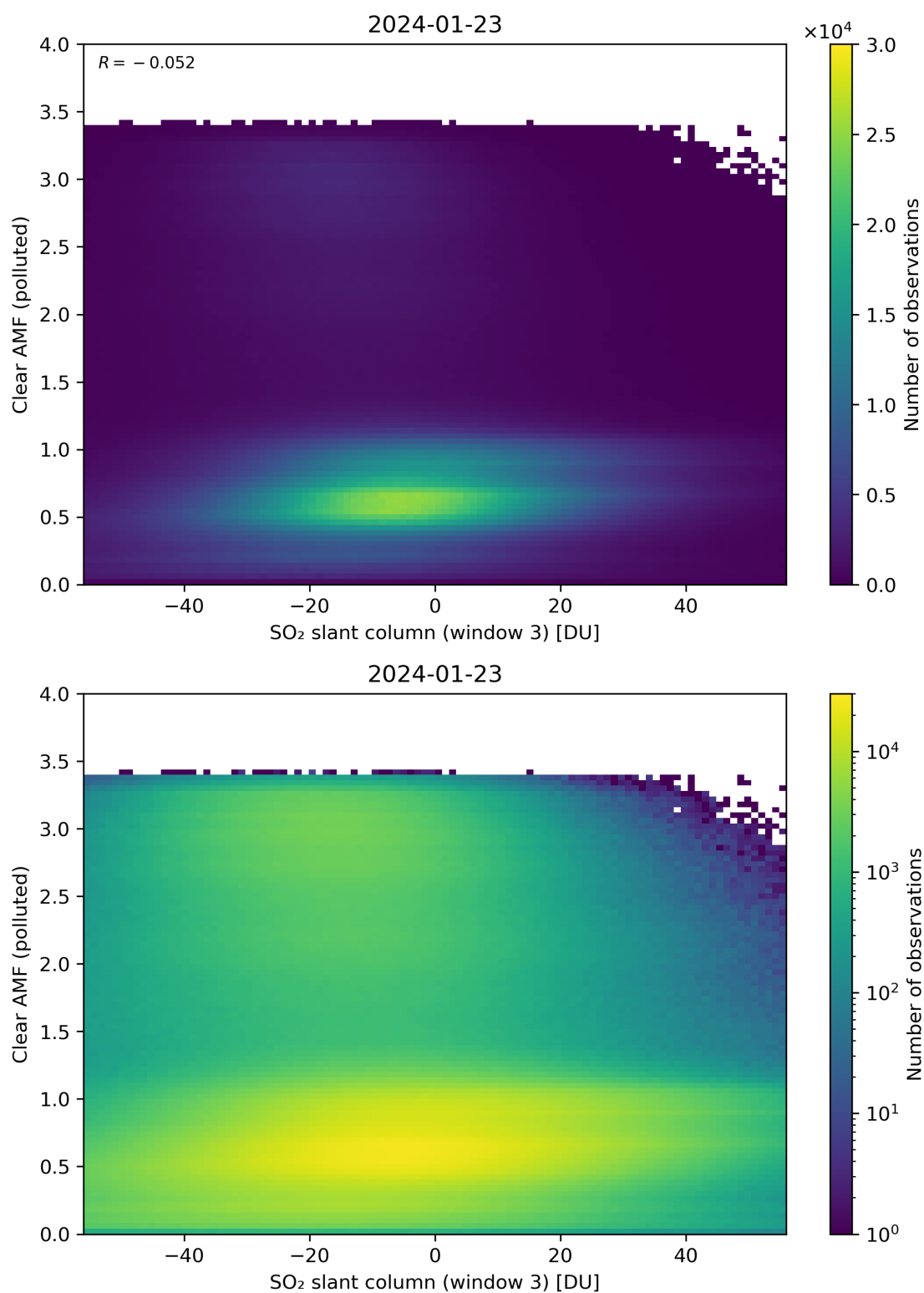
Figure 265: Scatter density plot of “SO 2 slant column (window 3)” against “Clear AMF (polluted)” for 2024-01-22 to 2024-01-24.
