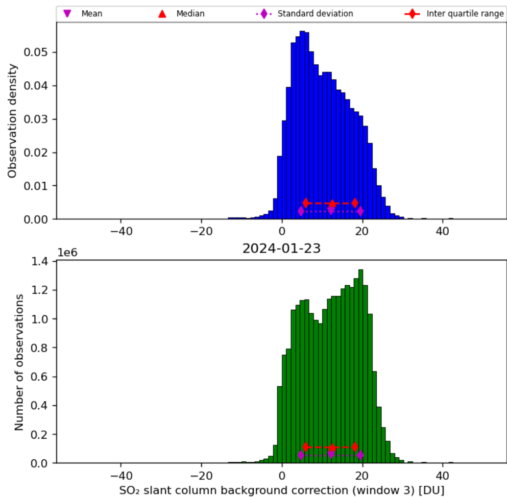
Figure 67: Histogram of “SO 2 slant column background correction (window 3)” for 2024-01-22 to 2024-01-24
