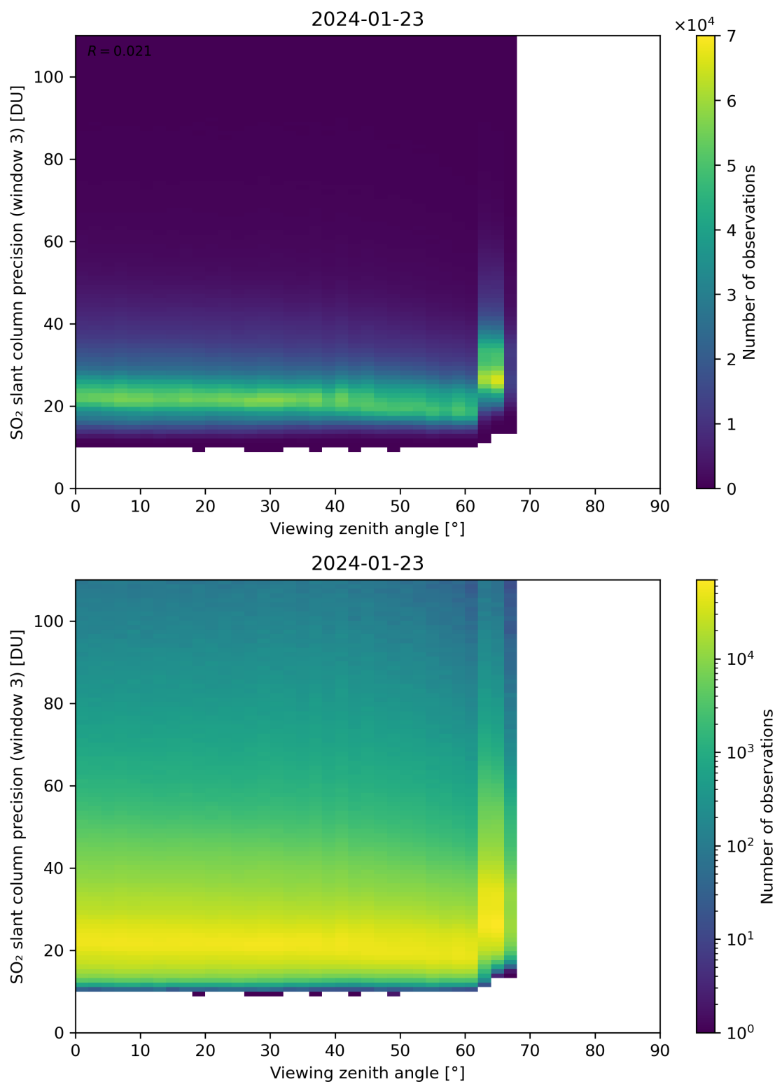
Figure 324: Scatter density plot of “Viewing zenith angle” against “SO 2 slant column precision (window 3)” for 2024-01-22 to 2024-01-24.
