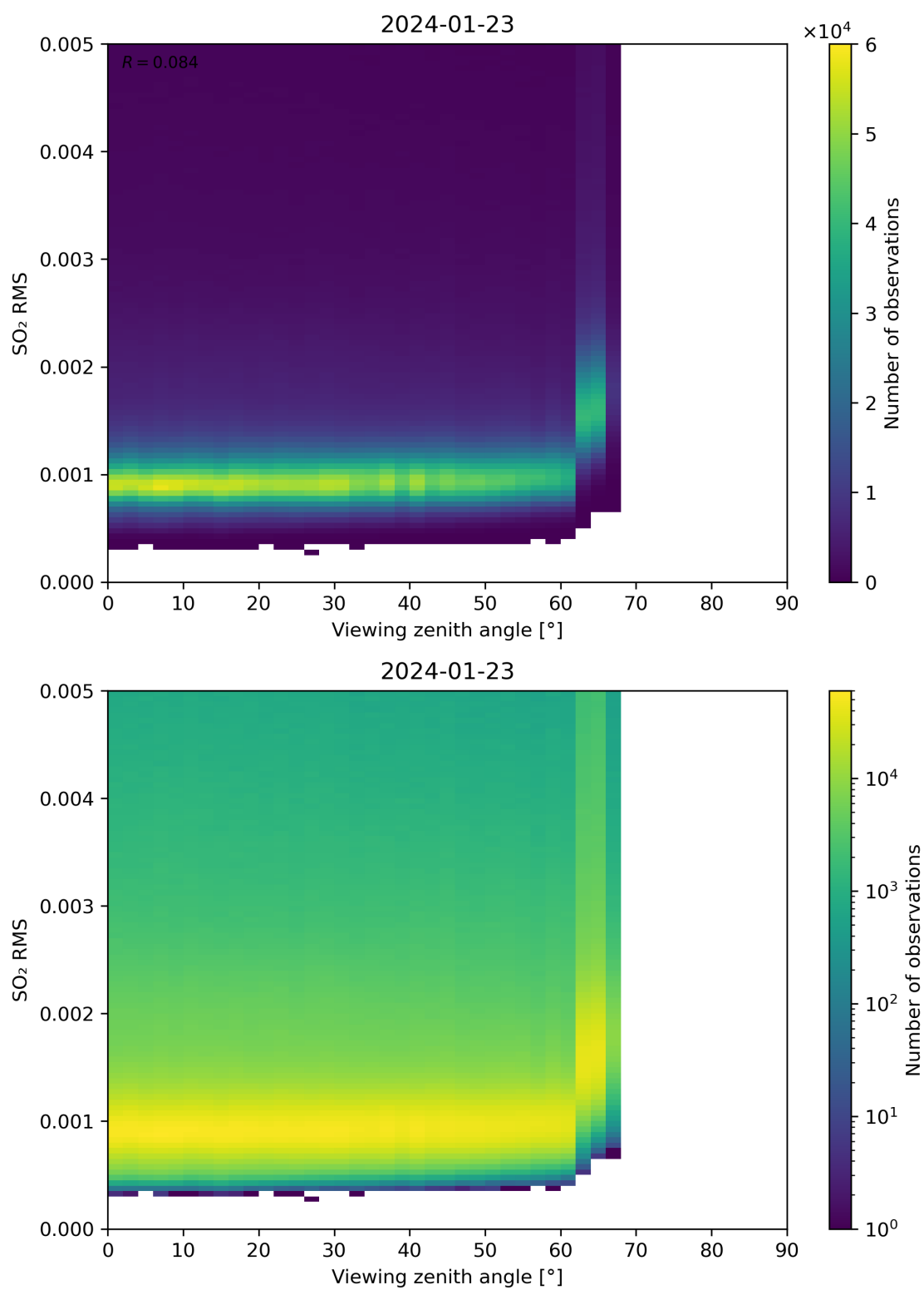
Figure 313: Scatter density plot of “Viewing zenith angle” against “SO 2 RMS” for 2024-01-22 to 2024-01-24.
