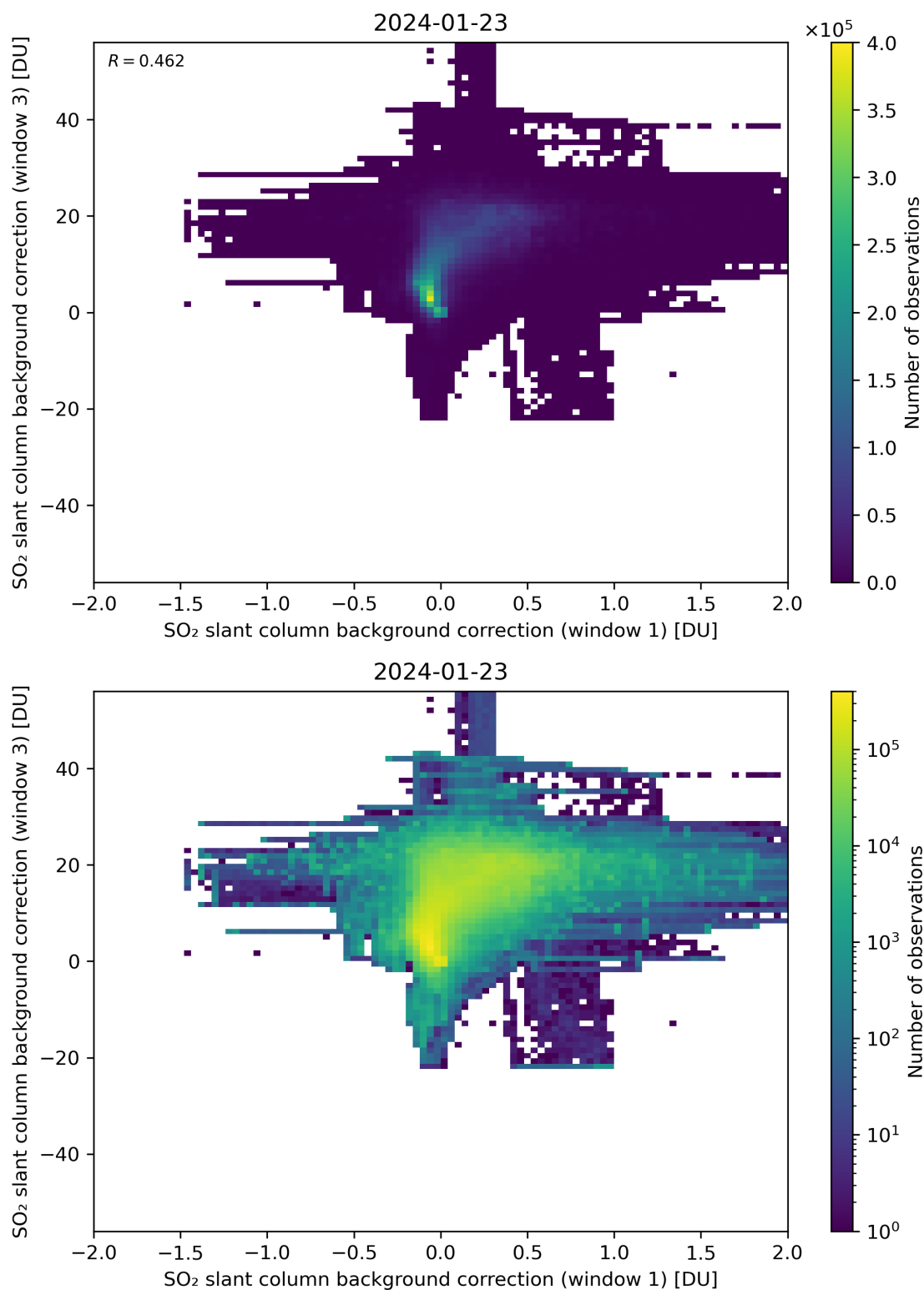
Figure 99: Scatter density plot of “SO 2 slant column background correction (window 1)” against “SO 2 slant column background correction (window 3)” for 2024-01-22 to 2024-01-24.
