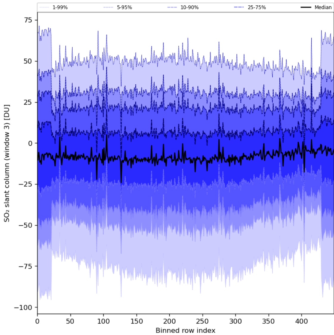
Figure 87: Along track statistics of “SO 2 slant column (window 3)” for 2024-01-22 to 2024-01-24
