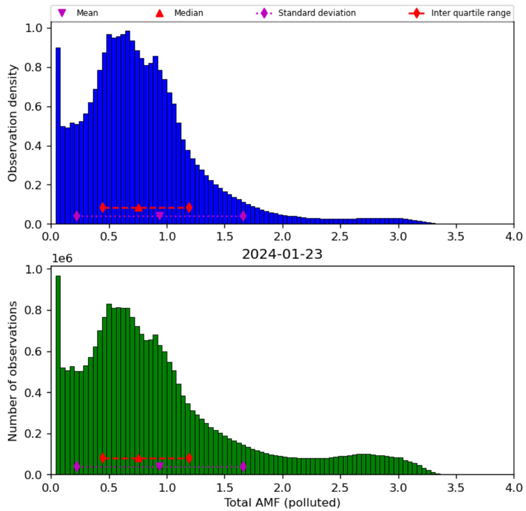
Figure 71: Histogram of “Total AMF (polluted)” for 2024-01-22 to 2024-01-24
