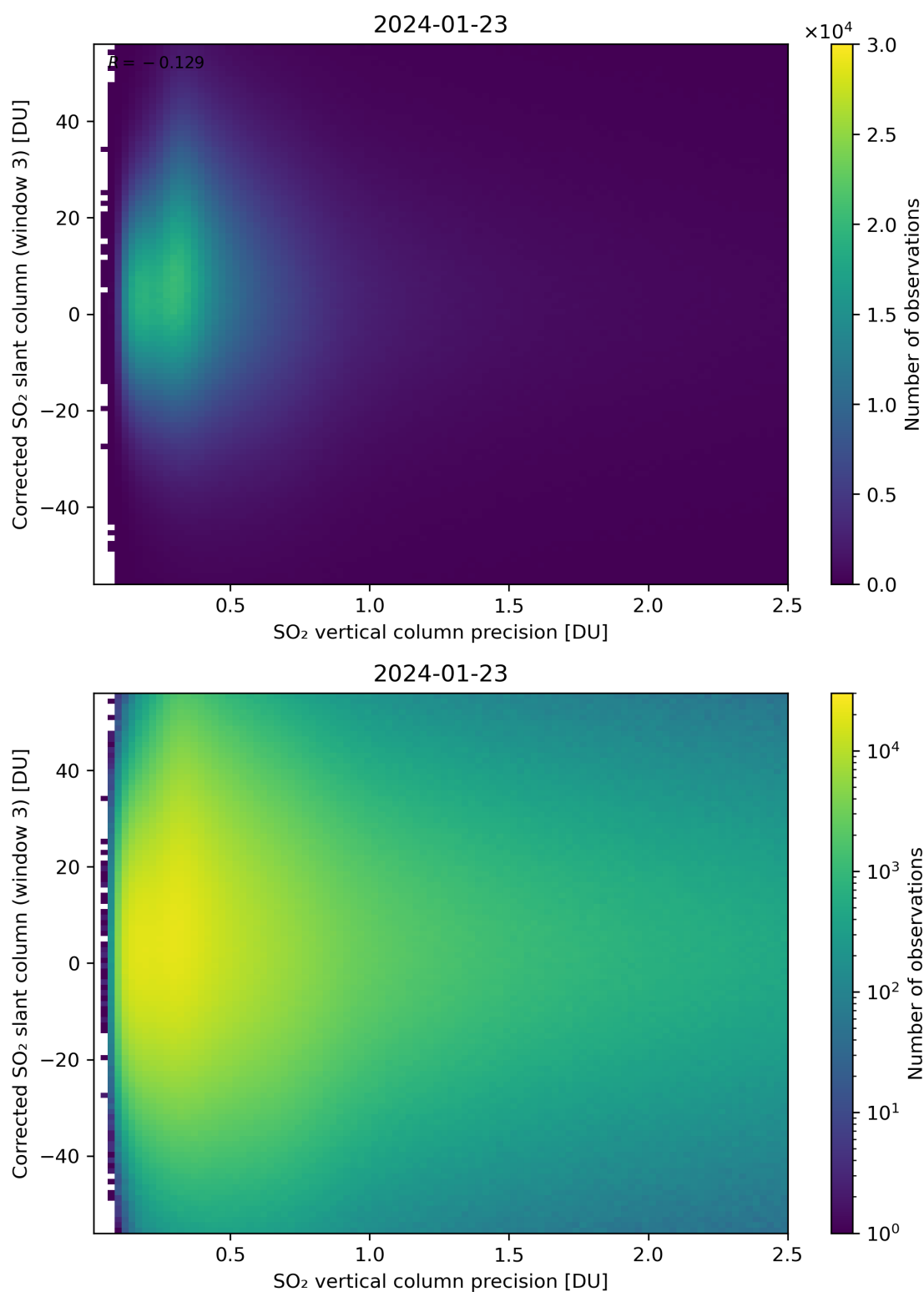
Figure 288: Scatter density plot of “SO 2 vertical column precision” against “Corrected SO 2 slant column (window 3)” for 2024-01-22 to 2024-01-24.
