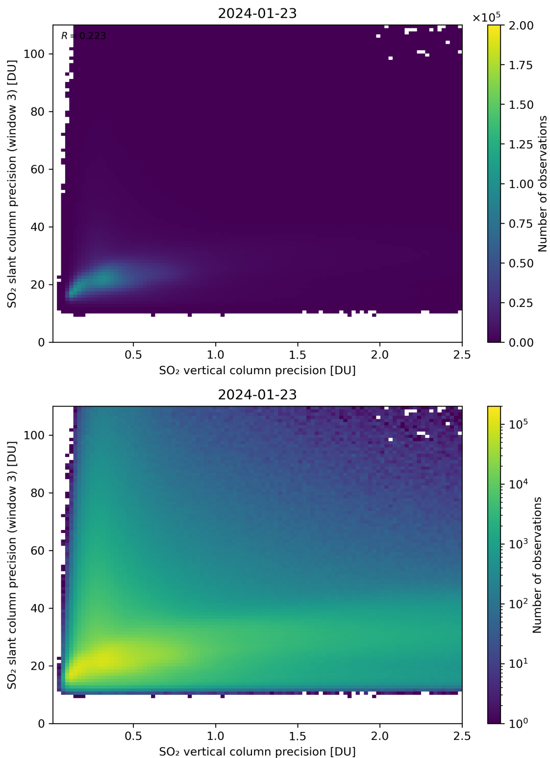
Figure 293: Scatter density plot of “SO 2 vertical column precision” against “SO 2 slant column precision (window 3)” for 2024-01-22 to 2024-01-24.
