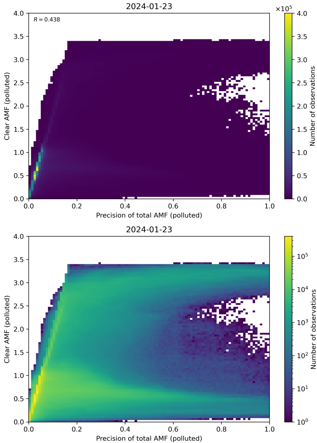
Figure 270: Scatter density plot of “Precision of total AMF (polluted)” against “Clear AMF (polluted)” for 2024-01-22 to 2024-01-24.
