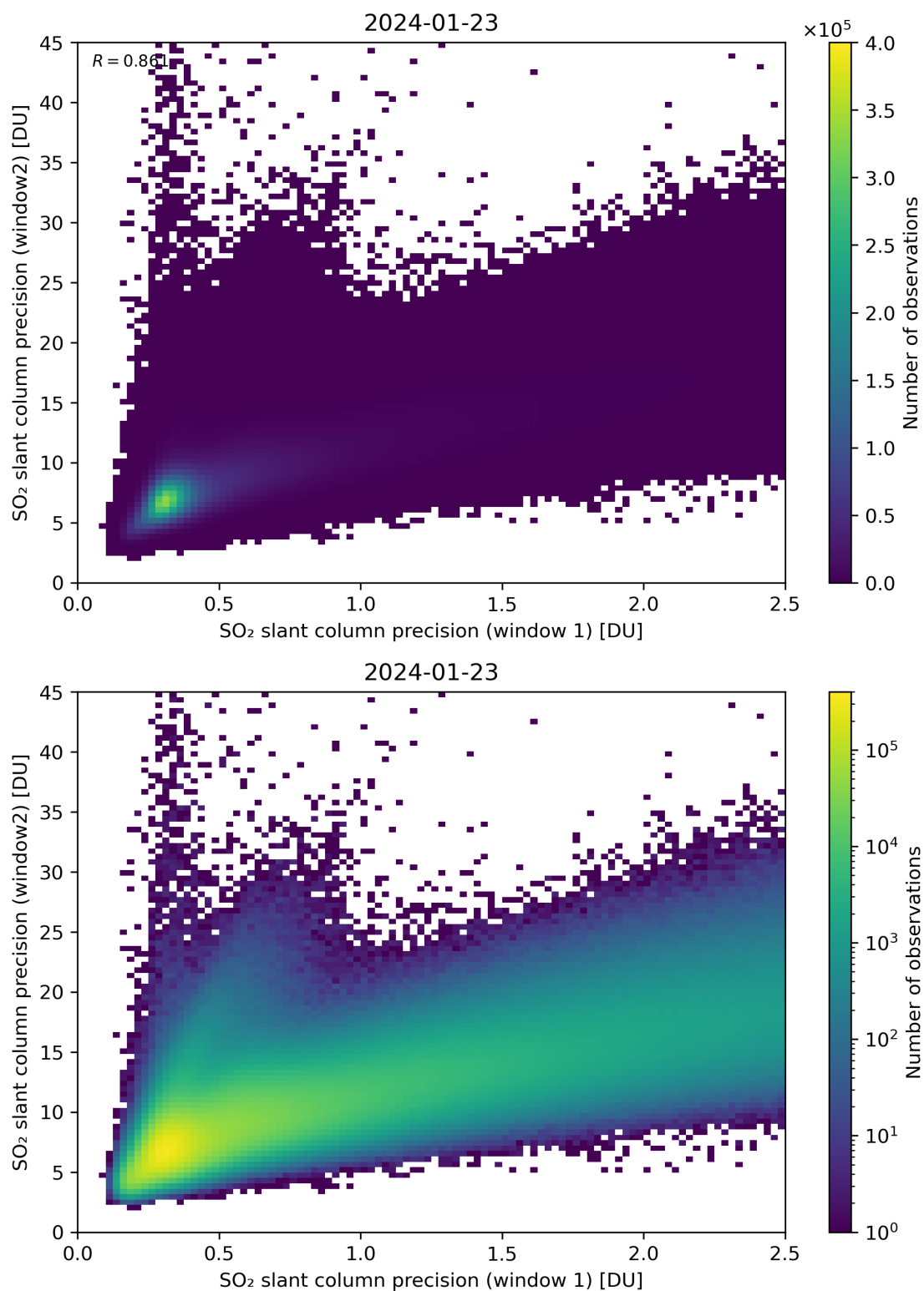
Figure 227: Scatter density plot of “SO 2 slant column precision (window 1)” against “SO 2 slant column precision (window2)” for 2024-01-22 to 2024-01-24.
