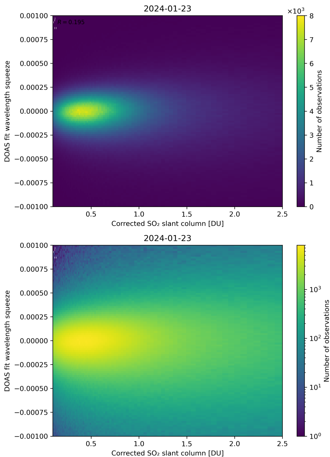
Figure 182: Scatter density plot of “Corrected SO 2 slant column” against “DOAS fit wavelength squeeze” for 2024-01-22 to 2024-01-24.
