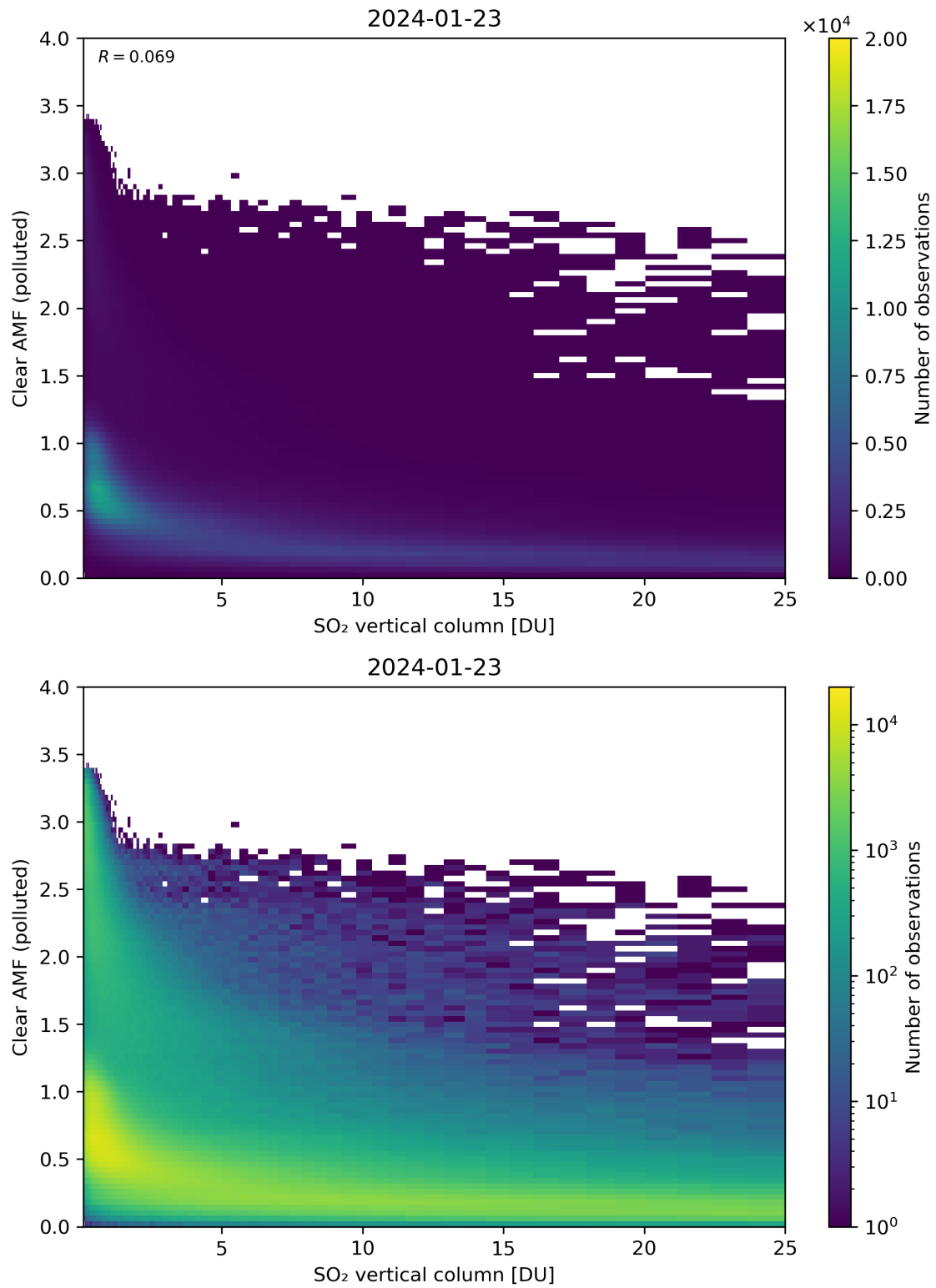
Figure 296: Scatter density plot of “SO 2 vertical column” against “Clear AMF (polluted)” for 2024-01-22 to 2024-01-24.
