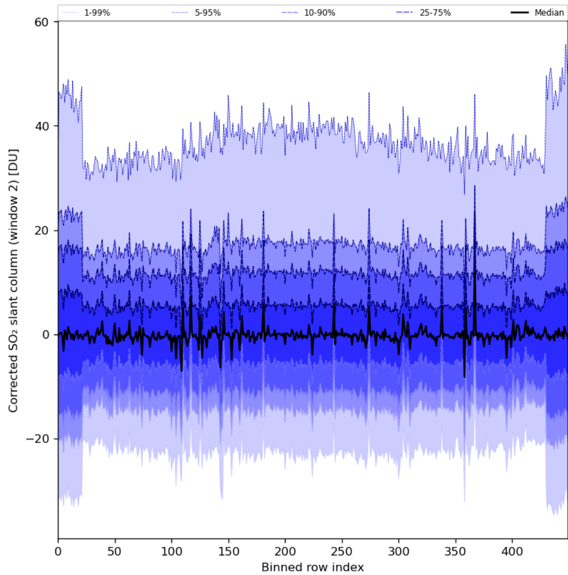
Figure 85: Along track statistics of “Corrected SO 2 slant column (window 2)” for 2024-01-22 to 2024-01-24
