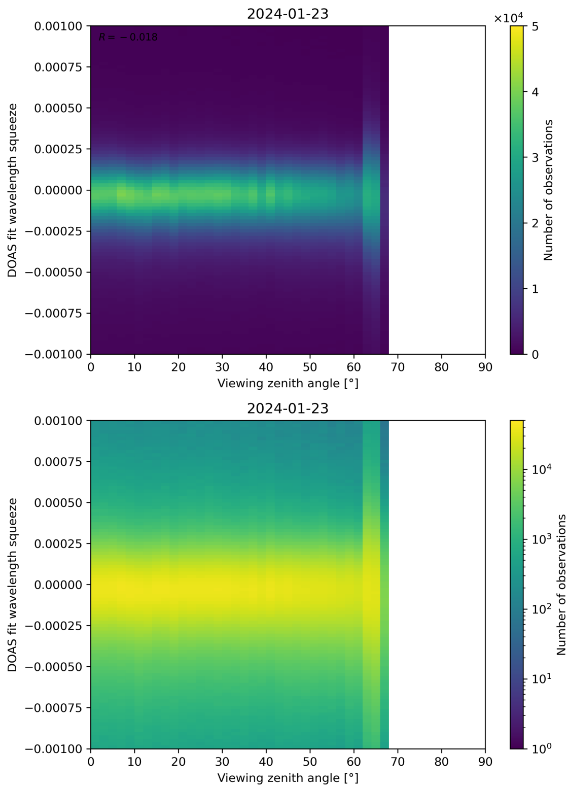
Figure 312: Scatter density plot of “Viewing zenith angle” against “DOAS fit wavelength squeeze” for 2024-01-22 to 2024-01-24.
