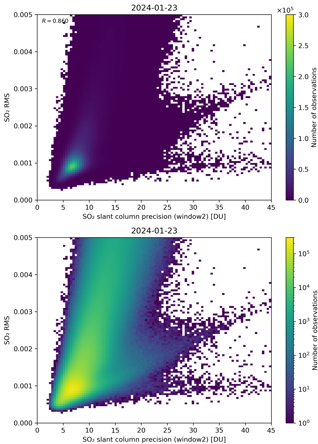
Figure 245: Scatter density plot of “SO 2 slant column precision (window2)” against “SO 2 RMS” for 2024-01-22 to 2024-01-24.
