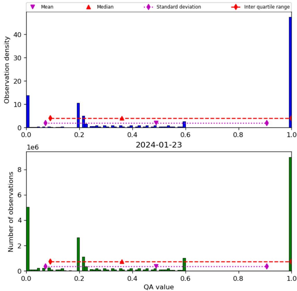
Figure 52: Histogram of “QA value” for 2024-01-22 to 2024-01-24
