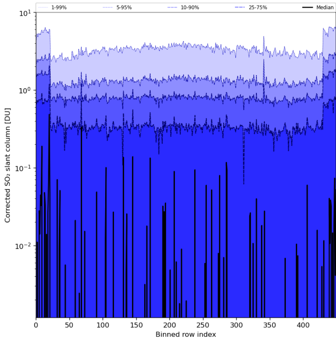
Figure 78: Along track statistics of “Corrected SO 2 slant column” for 2024-01-22 to 2024-01-24
