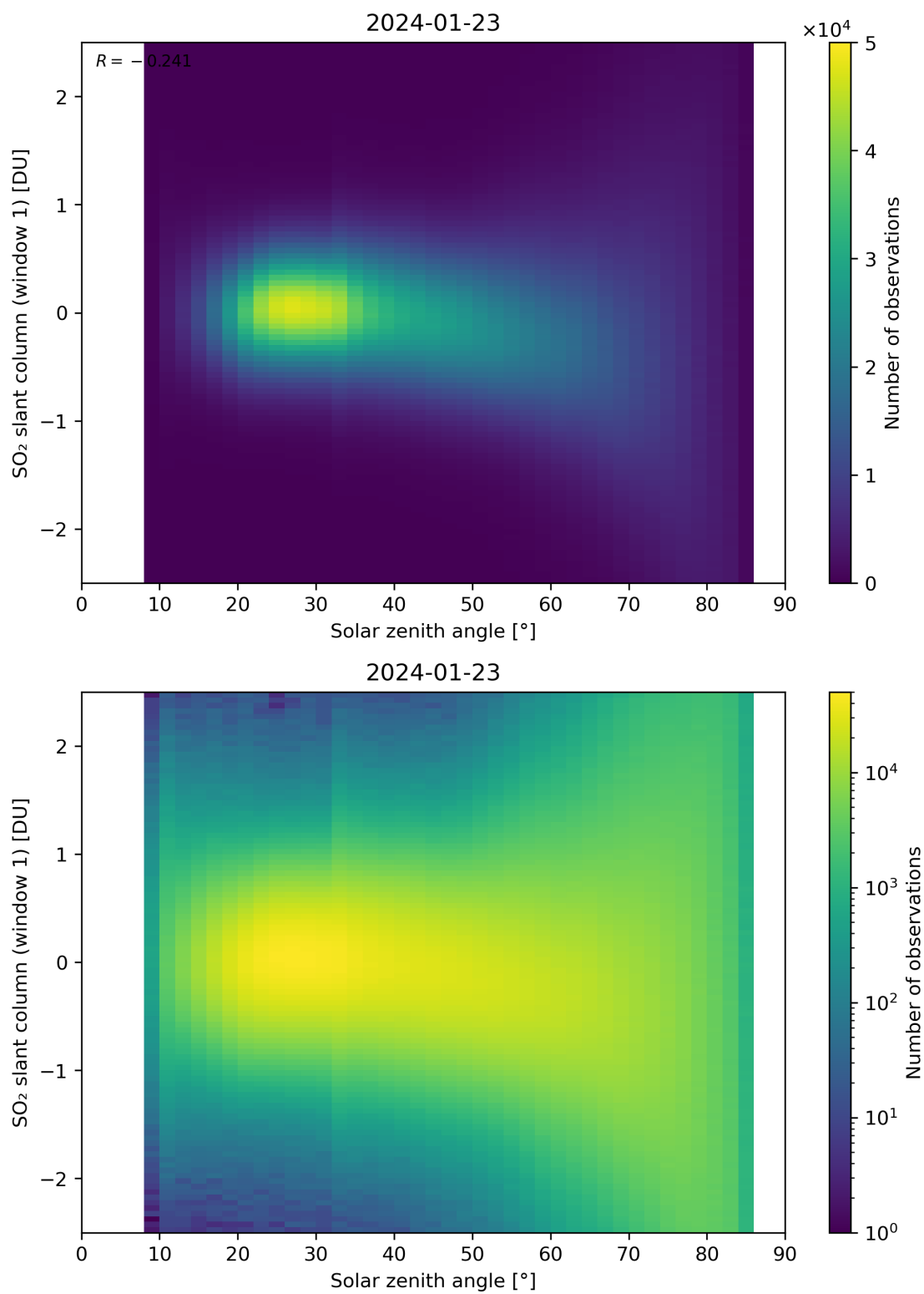
Figure 169: Scatter density plot of “Solar zenith angle” against “SO 2 slant column (window 1)” for 2024-01-22 to 2024-01-24.
