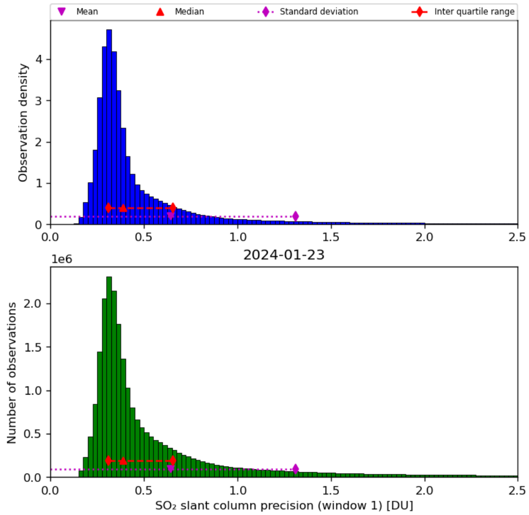
Figure 57: Histogram of “SO 2 slant column precision (window 1)” for 2024-01-22 to 2024-01-24
