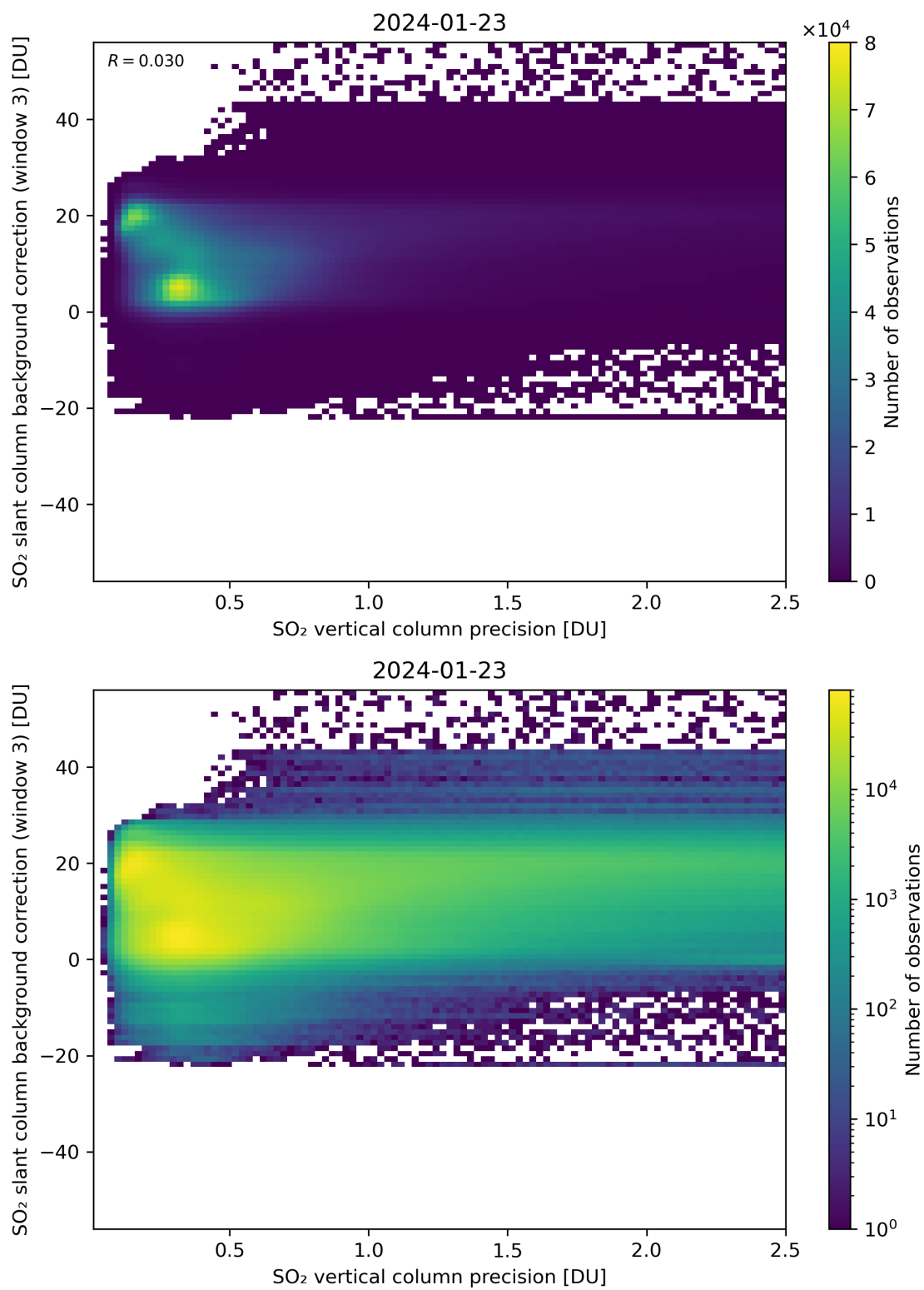
Figure 281: Scatter density plot of “SO 2 vertical column precision” against “SO 2 slant column background correction (window 3)” for 2024-01-22 to 2024-01-24.
