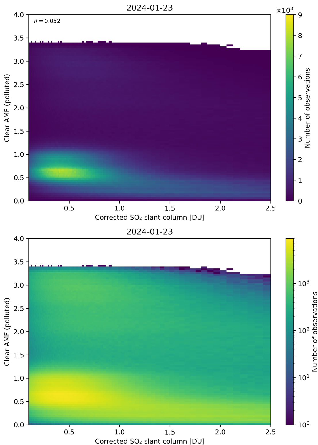
Figure 184: Scatter density plot of “Corrected SO 2 slant column” against “Clear AMF (polluted)” for 2024-01-22 to 2024-01-24.
