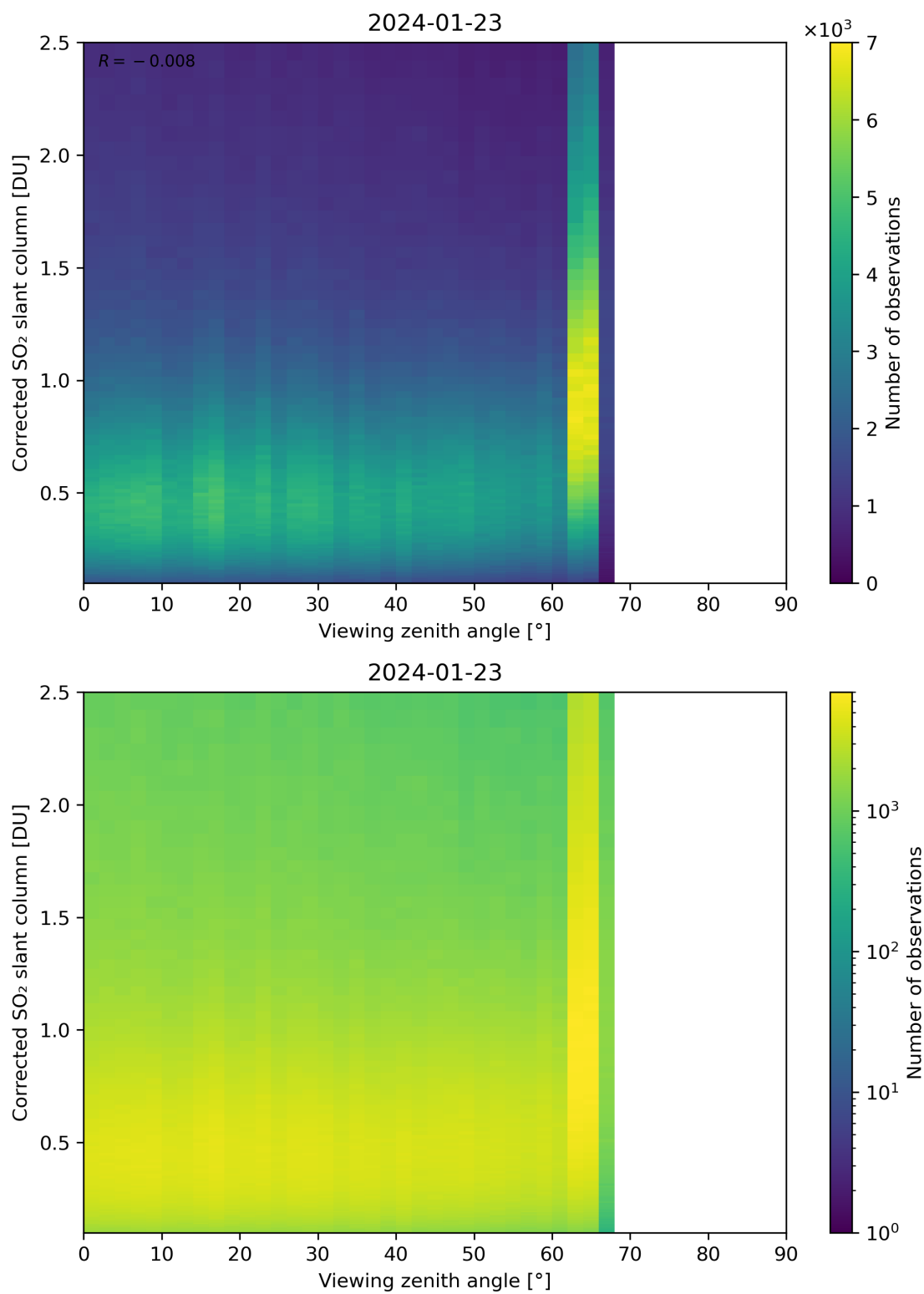
Figure 317: Scatter density plot of “Viewing zenith angle” against “Corrected SO 2 slant column” for 2024-01-22 to 2024-01-24.
