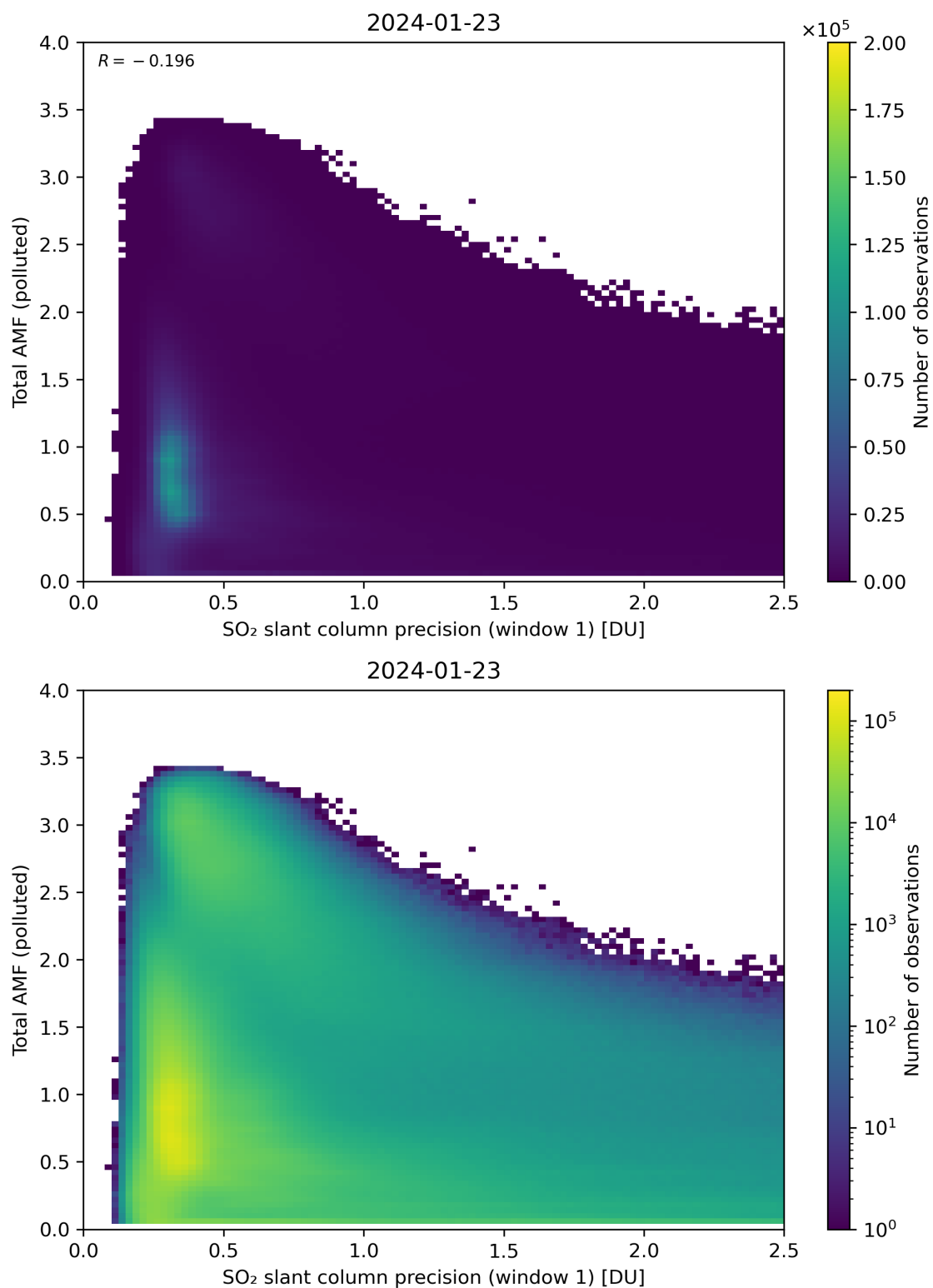
Figure 230: Scatter density plot of “SO 2 slant column precision (window 1)” against “Total AMF (polluted)” for 2024-01-22 to 2024-01-24.
