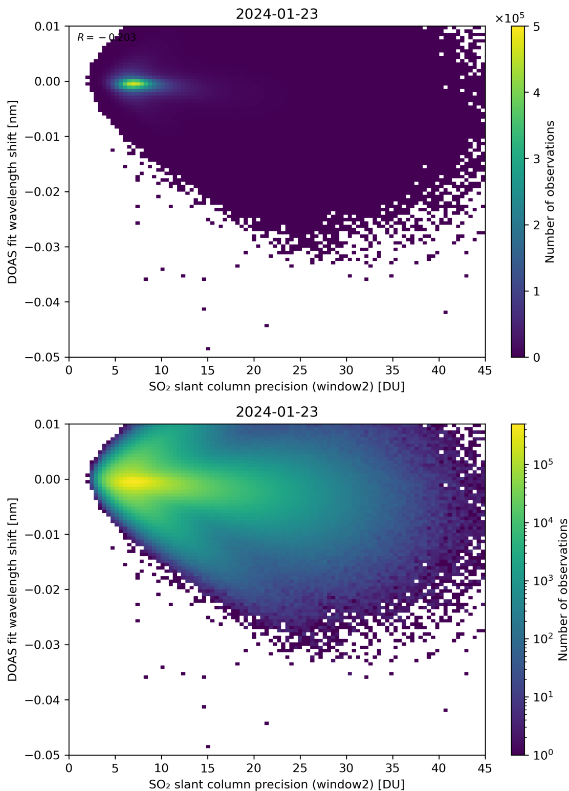
Figure 243: Scatter density plot of “SO 2 slant column precision (window2)” against “DOAS fit wavelength shift” for 2024-01-22 to 2024-01-24.
