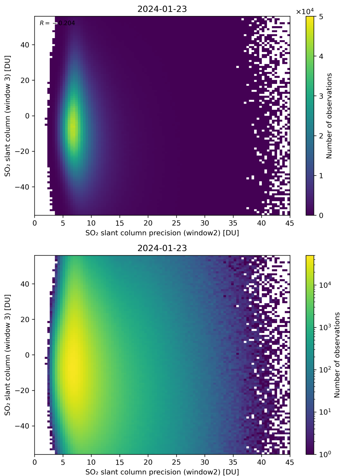
Figure 249: Scatter density plot of “SO 2 slant column precision (window2)” against “SO 2 slant column (window 3)” for 2024-01-22 to 2024-01-24.
