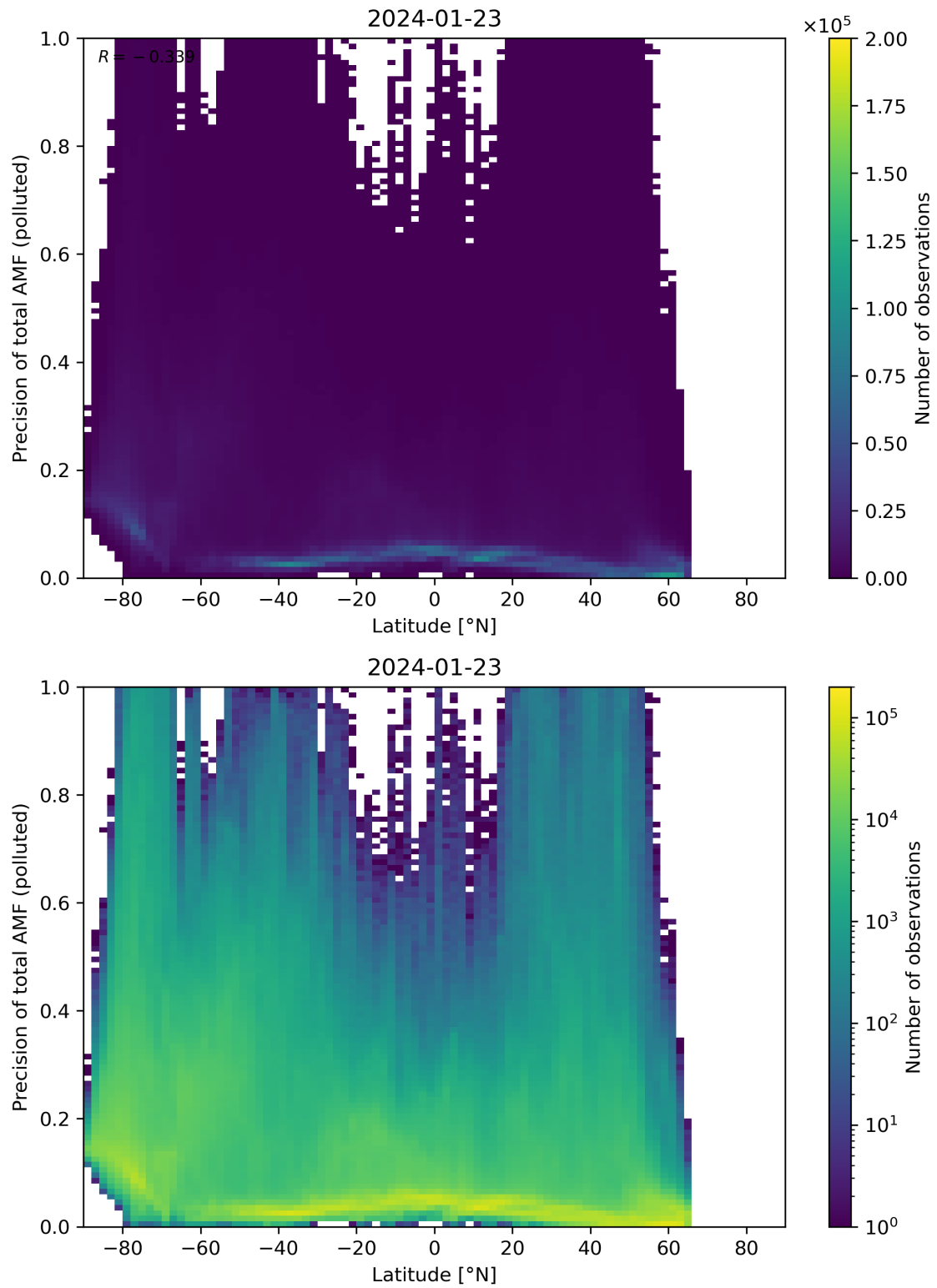
Figure 155: Scatter density plot of “Latitude” against “Precision of total AMF (polluted)” for 2024-01-22 to 2024-01-24.
