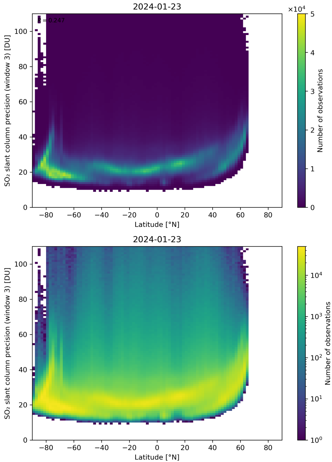
Figure 153: Scatter density plot of “Latitude” against “SO 2 slant column precision (window 3)” for 2024-01-22 to 2024-01-24.
