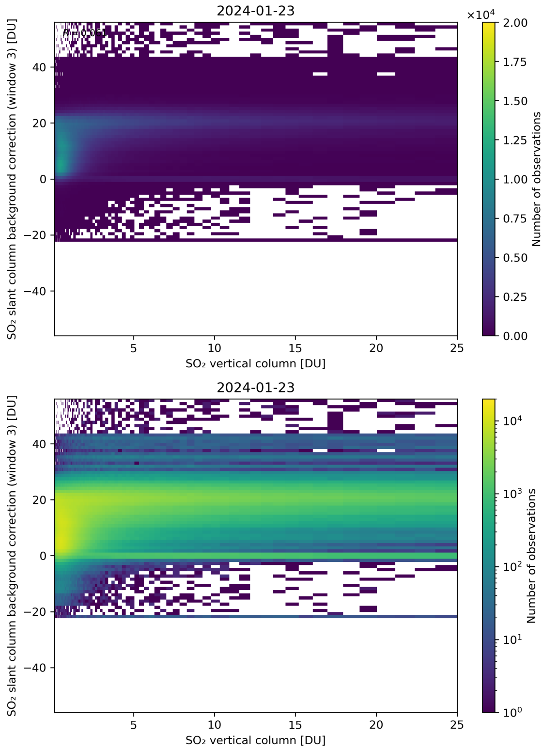
Figure 275: Scatter density plot of “SO 2 vertical column” against “SO 2 slant column background correction (window 3)” for 2024-01-22 to 2024-01-24.
