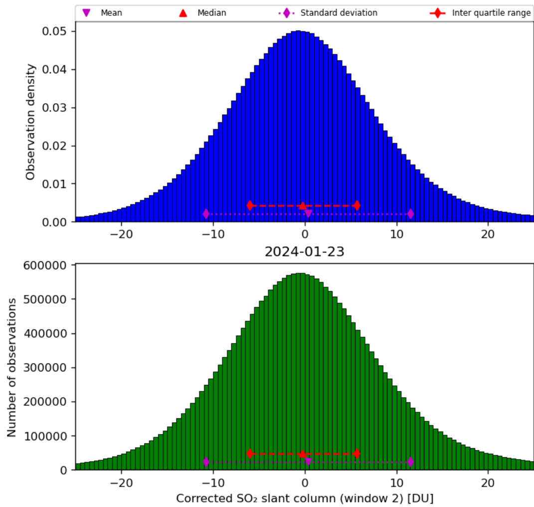
Figure 62: Histogram of “Corrected SO 2 slant column (window 2)” for 2024-01-22 to 2024-01-24
