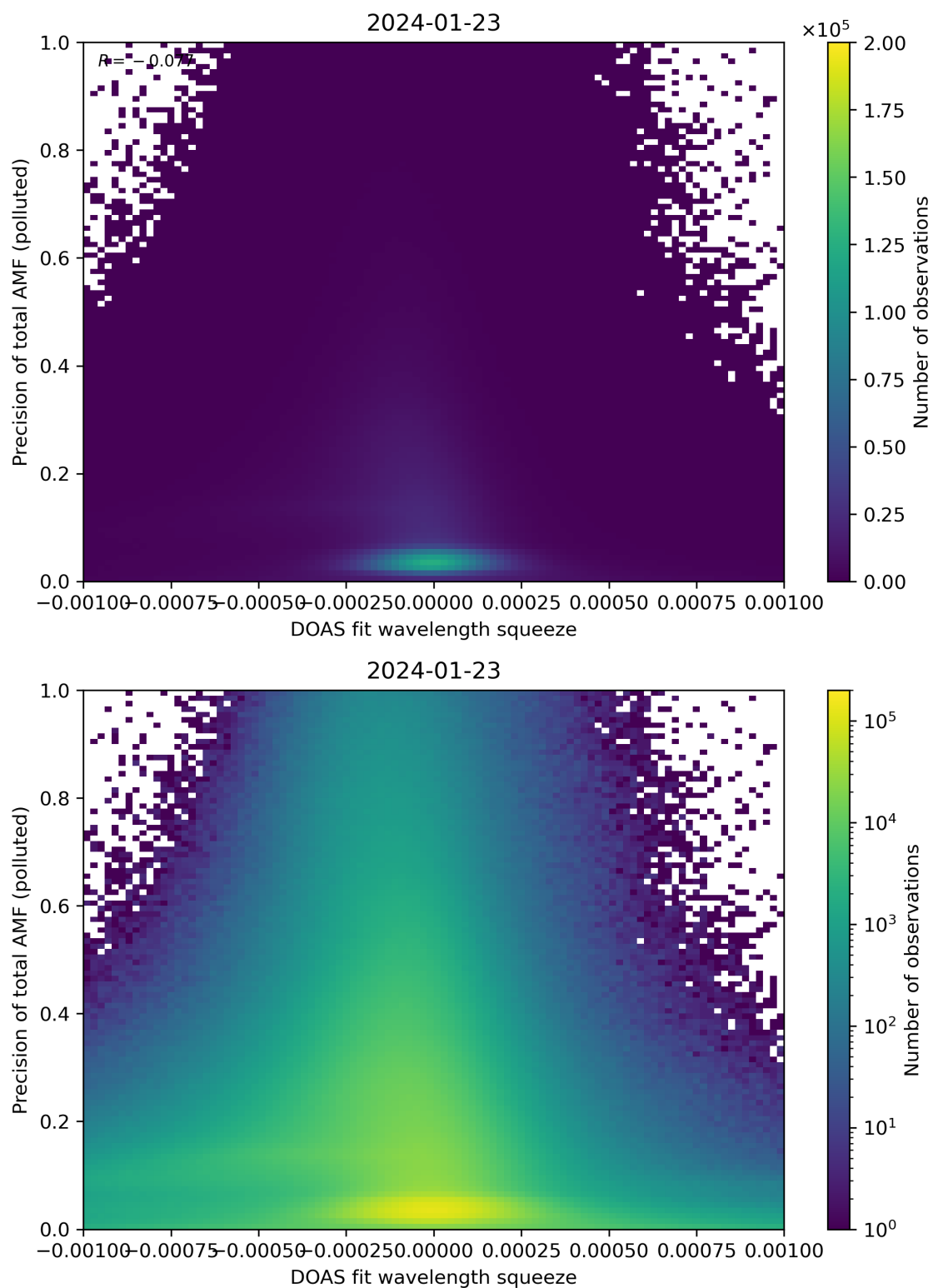
Figure 135: Scatter density plot of “DOAS fit wavelength squeeze” against “Precision of total AMF (polluted)” for 2024-01-22 to 2024-01-24.
