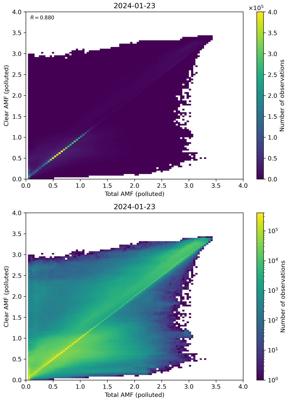
Figure 271: Scatter density plot of “Total AMF (polluted)” against “Clear AMF (polluted)” for 2024-01-22 to 2024-01-24.
