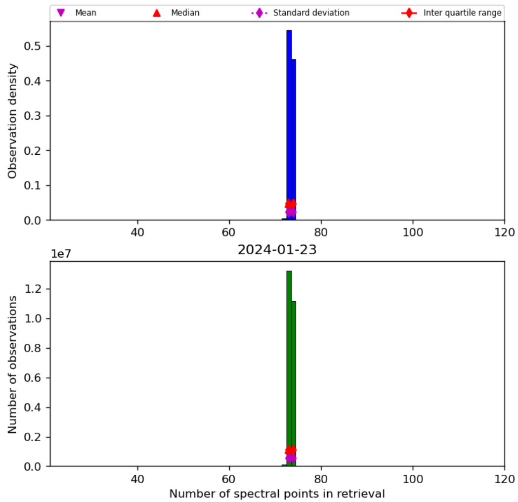
Figure 74: Histogram of “Number of spectral points in retrieval” for 2024-01-22 to 2024-01-24
