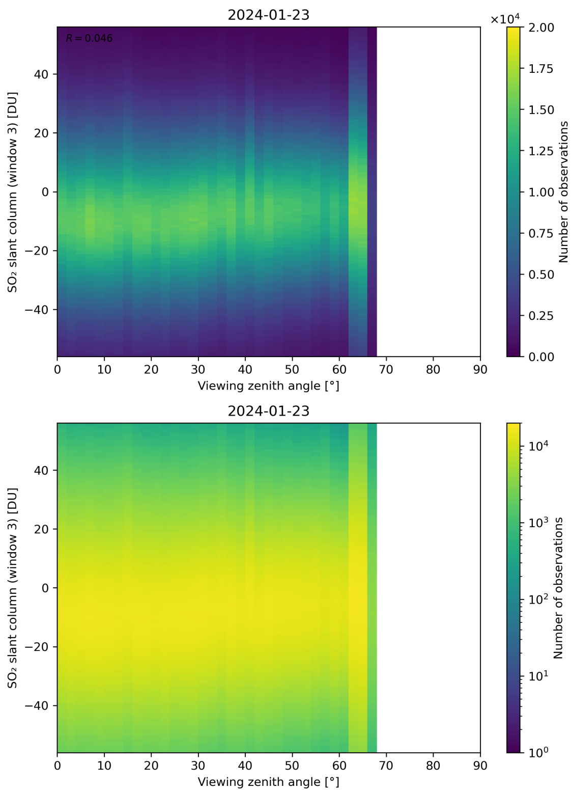
Figure 323: Scatter density plot of “Viewing zenith angle” against “SO 2 slant column (window 3)” for 2024-01-22 to 2024-01-24.
