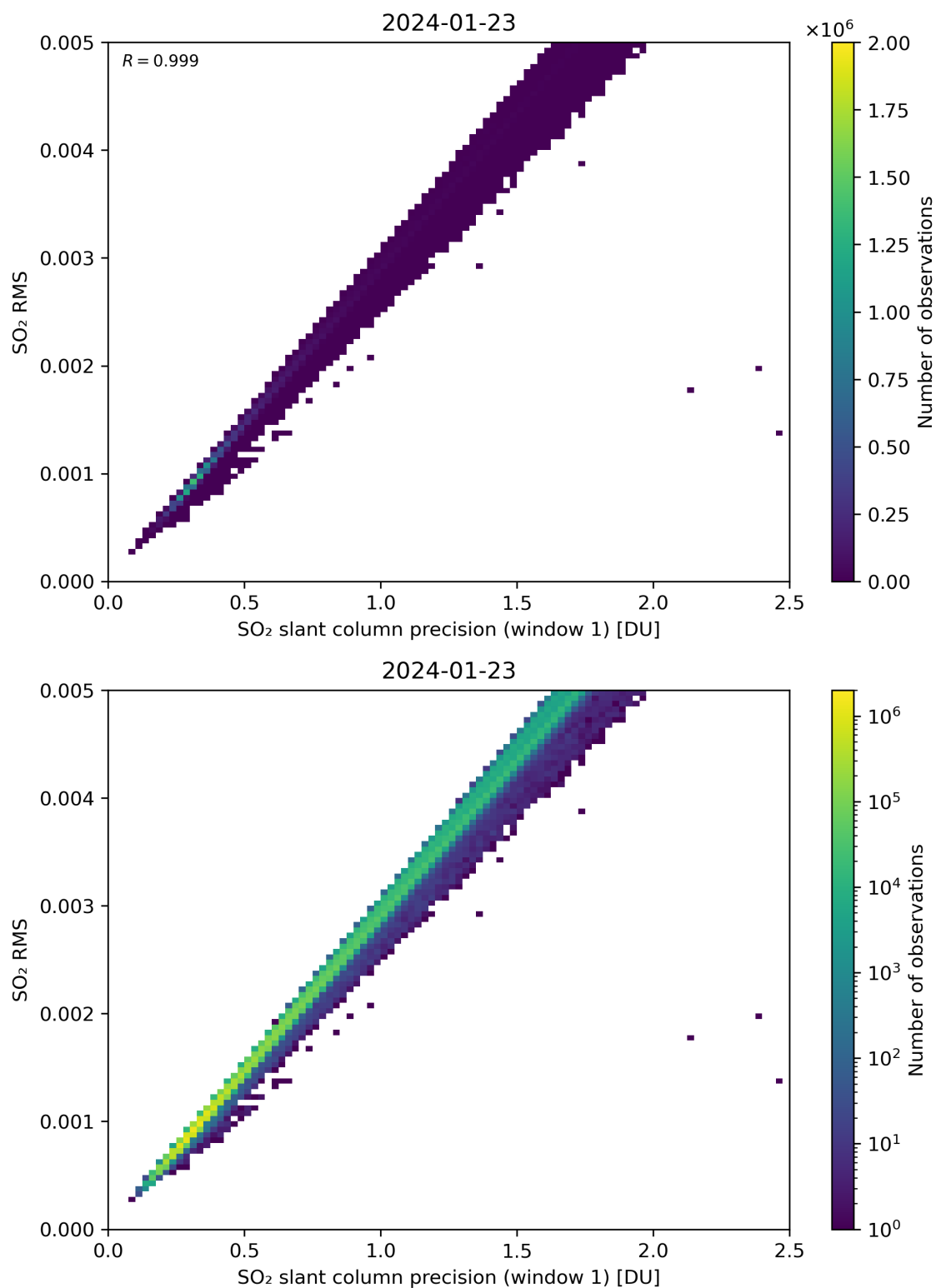
Figure 223: Scatter density plot of “SO 2 slant column precision (window 1)” against “SO 2 RMS” for 2024-01-22 to 2024-01-24.
