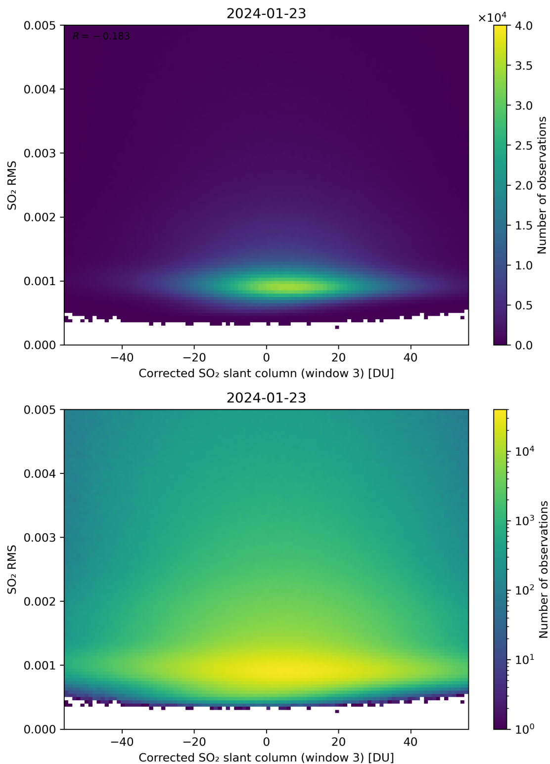
Figure 208: Scatter density plot of “Corrected SO 2 slant column (window 3)” against “SO 2 RMS” for 2024-01-22 to 2024-01-24.
