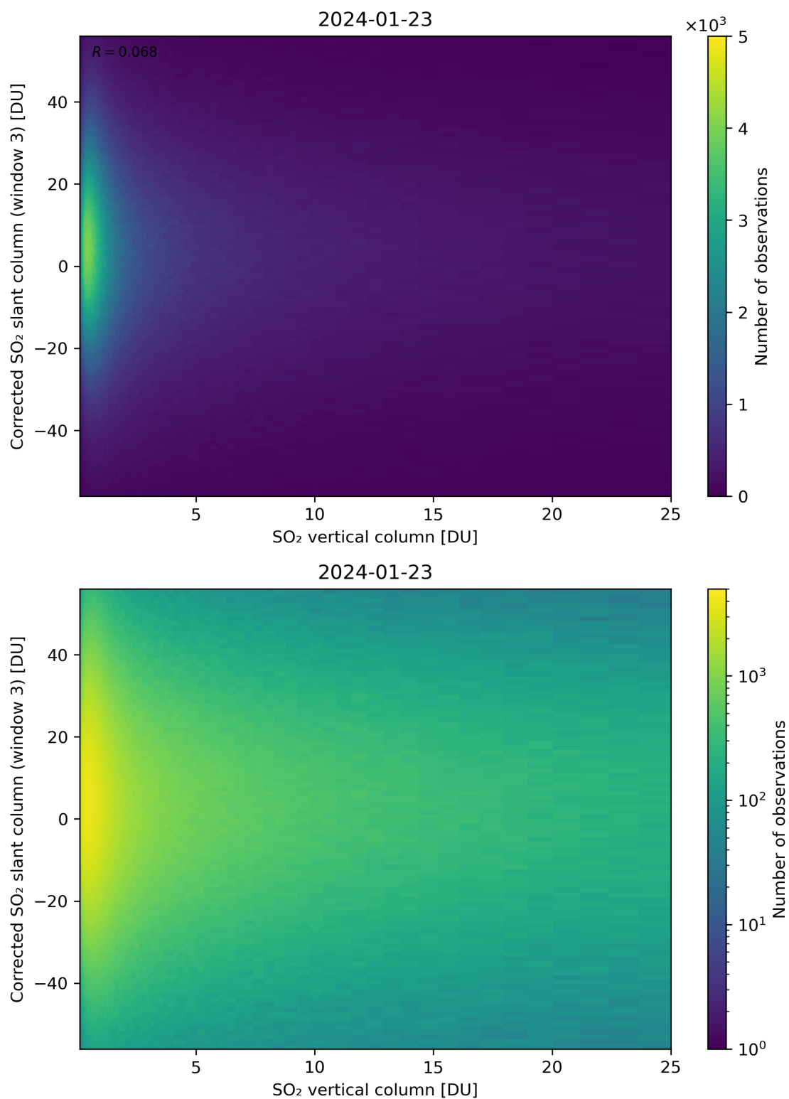
Figure 299: Scatter density plot of “SO 2 vertical column” against “Corrected SO 2 slant column (window 3)” for 2024-01-22 to 2024-01-24.
