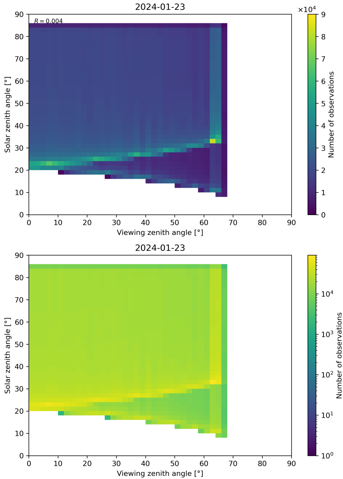
Figure 315: Scatter density plot of “Viewing zenith angle” against “Solar zenith angle” for 2024-01-22 to 2024-01-24.
