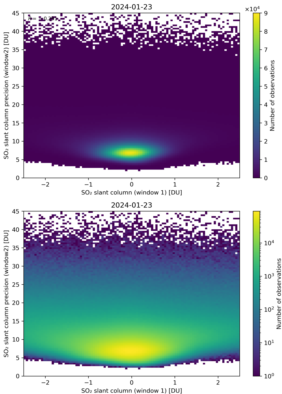
Figure 236: Scatter density plot of “SO 2 slant column (window 1)” against “SO 2 slant column precision (window2)” for 2024-01-22 to 2024-01-24.
