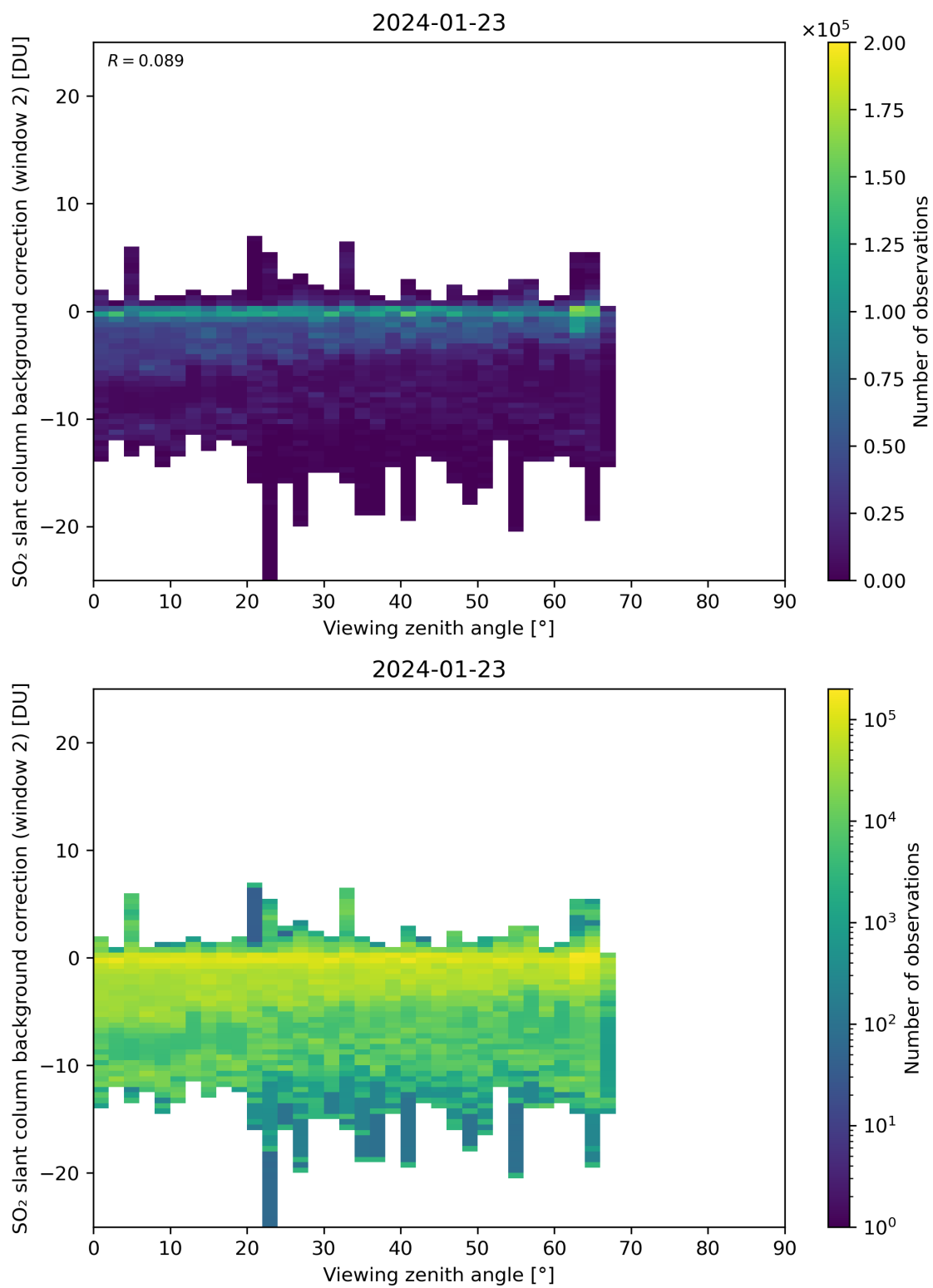
Figure 309: Scatter density plot of “Viewing zenith angle” against “SO 2 slant column background correction (window 2)” for 2024-01-22 to 2024-01-24.
