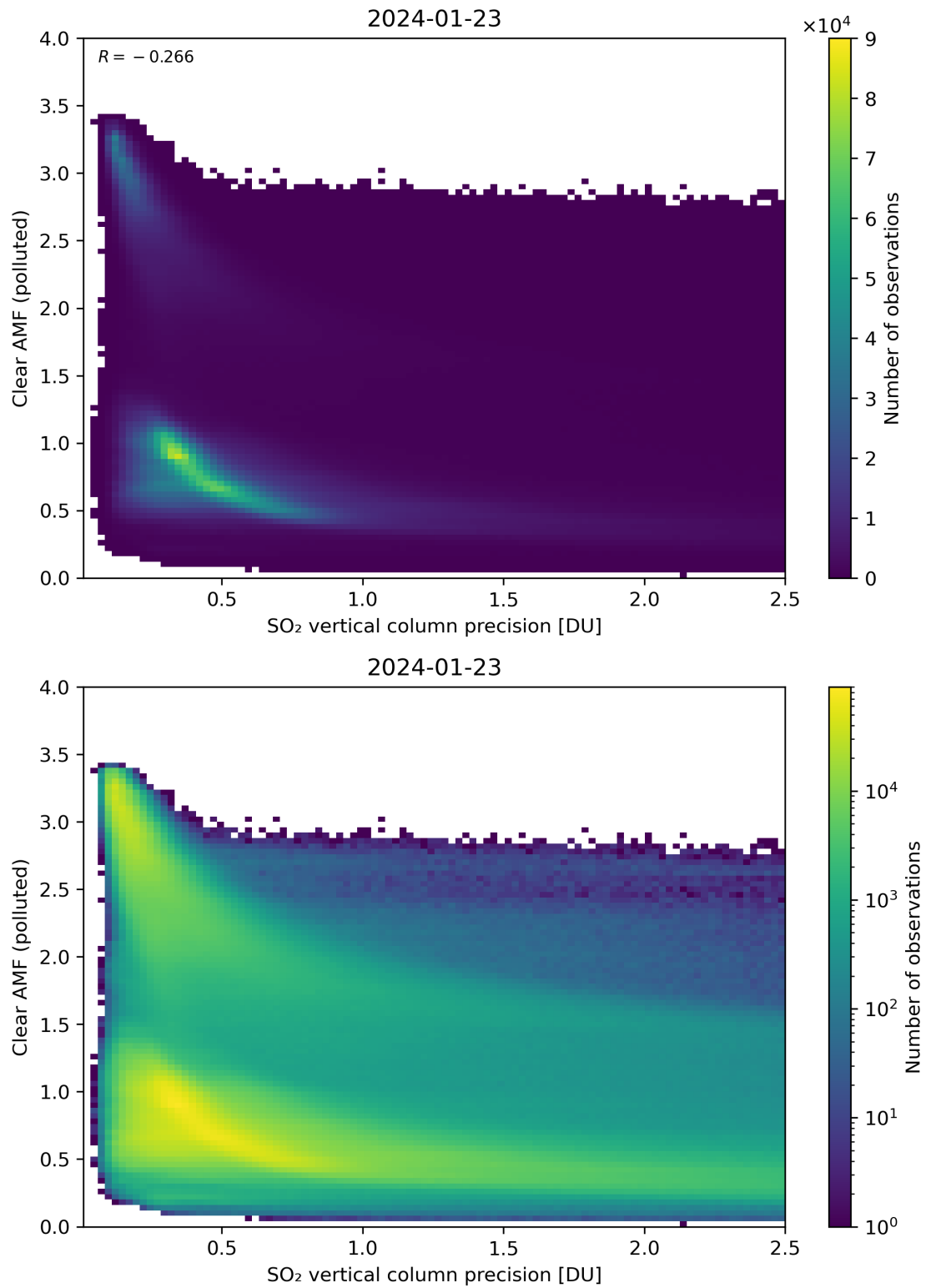
Figure 285: Scatter density plot of “SO 2 vertical column precision” against “Clear AMF (polluted)” for 2024-01-22 to 2024-01-24.
