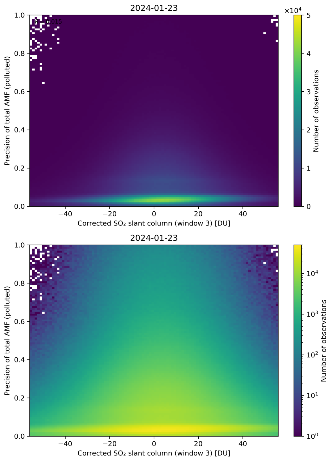
Figure 211: Scatter density plot of “Corrected SO 2 slant column (window 3)” against “Precision of total AMF (polluted)” for 2024-01-22 to 2024-01-24.
