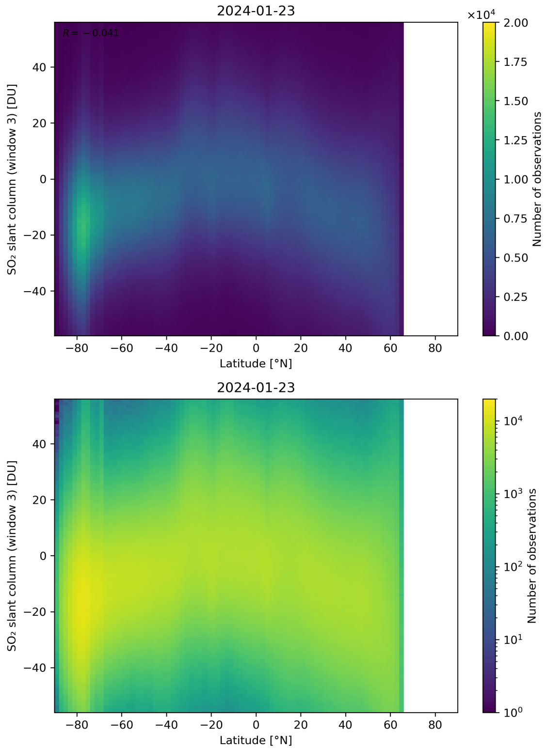
Figure 152: Scatter density plot of “Latitude” against “SO 2 slant column (window 3)” for 2024-01-22 to 2024-01-24.
