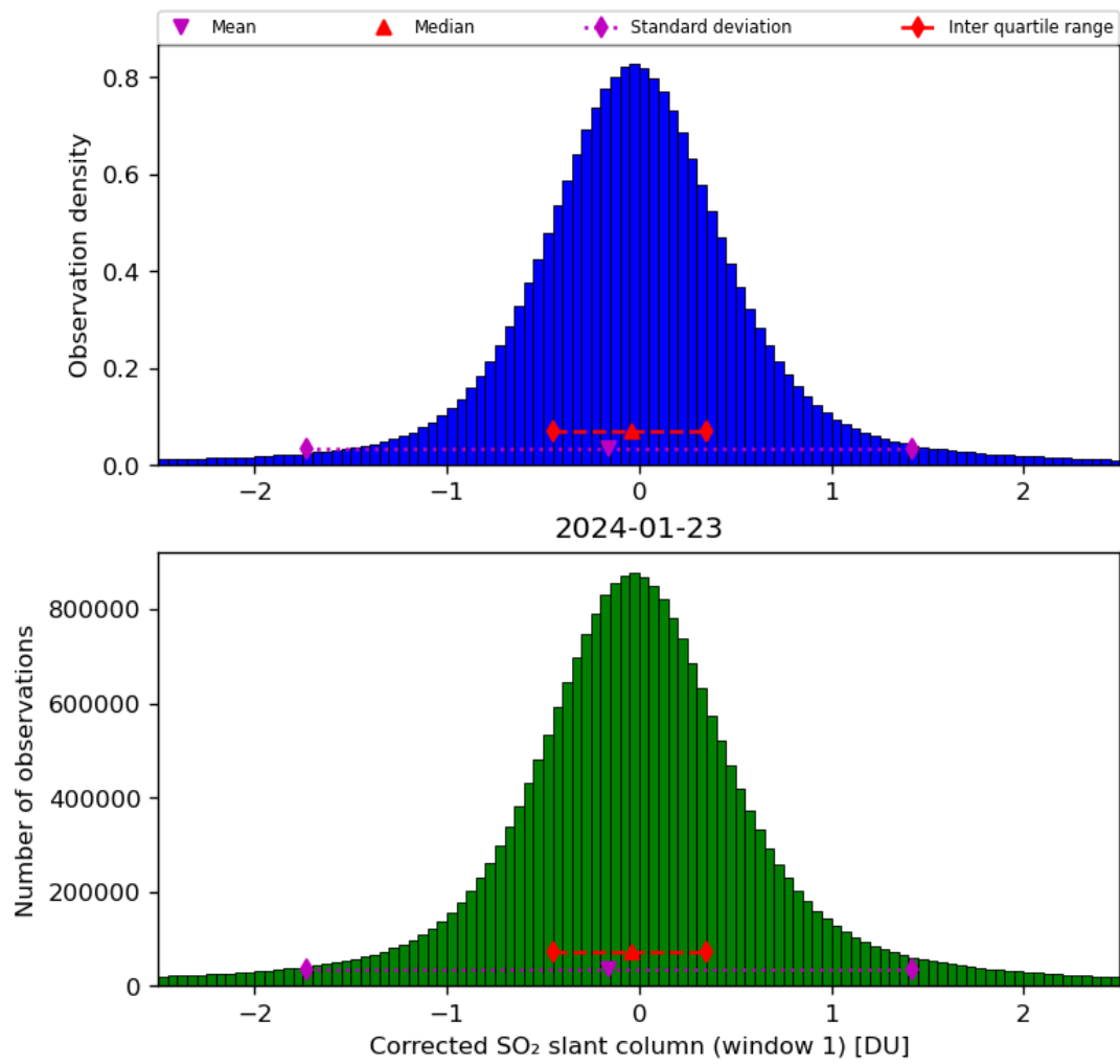
Figure 58: Histogram of “Corrected SO 2 slant column (window 1)” for 2024-01-22 to 2024-01-24
