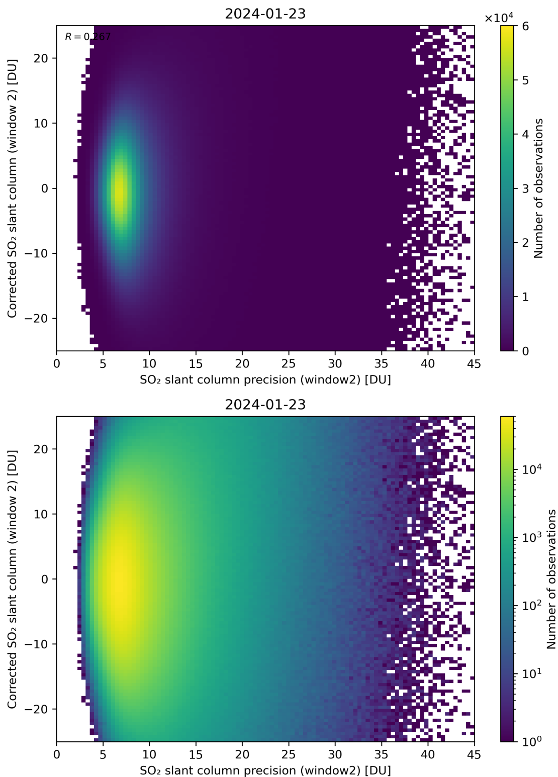
Figure 247: Scatter density plot of “SO 2 slant column precision (window2)” against “Corrected SO 2 slant column (window 2)” for 2024-01-22 to 2024-01-24.
