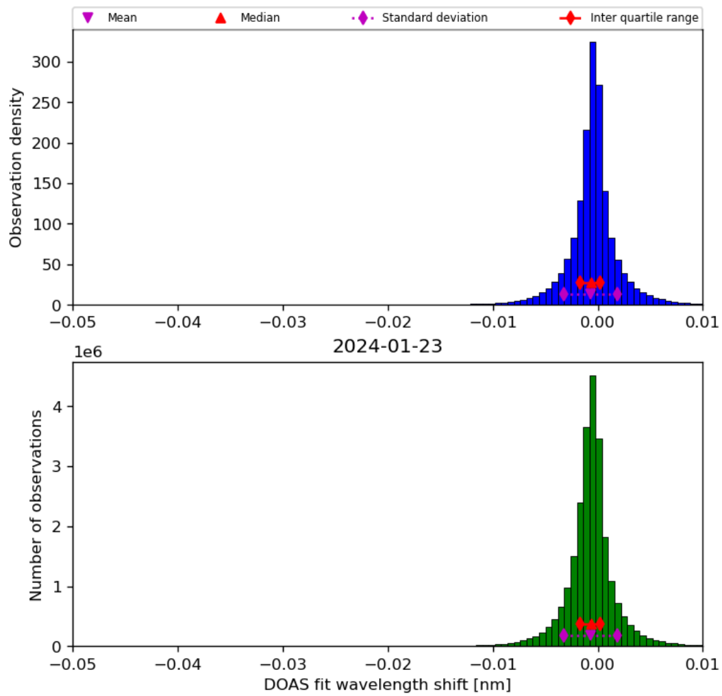
Figure 68: Histogram of “DOAS fit wavelength shift” for 2024-01-22 to 2024-01-24
