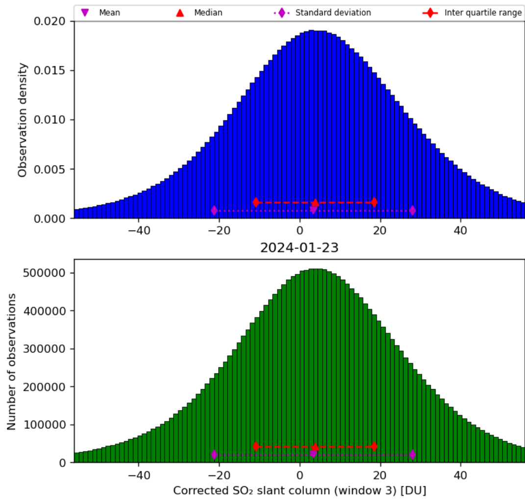
Figure 66: Histogram of "Corrected SO 2 slant column (window 3)" for 2024-01-22 to 2024-01-24
