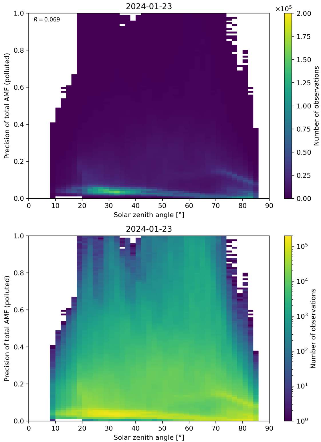
Figure 175: Scatter density plot of “Solar zenith angle” against “Precision of total AMF (polluted)” for 2024-01-22 to 2024-01-24.
