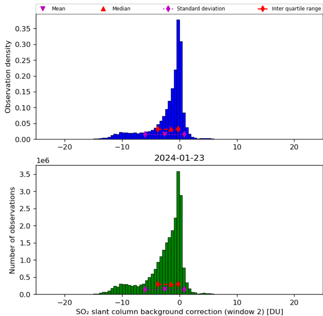
Figure 63: Histogram of “SO 2 slant column background correction (window 2)” for 2024-01-22 to 2024-01-24
