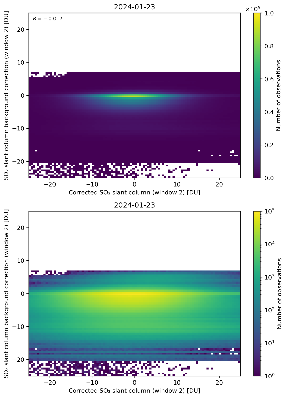
Figure 194: Scatter density plot of “Corrected SO 2 slant column (window 2)” against “SO 2 slant column background correction (window 2)” for 2024-01-22 to 2024-01-24.
