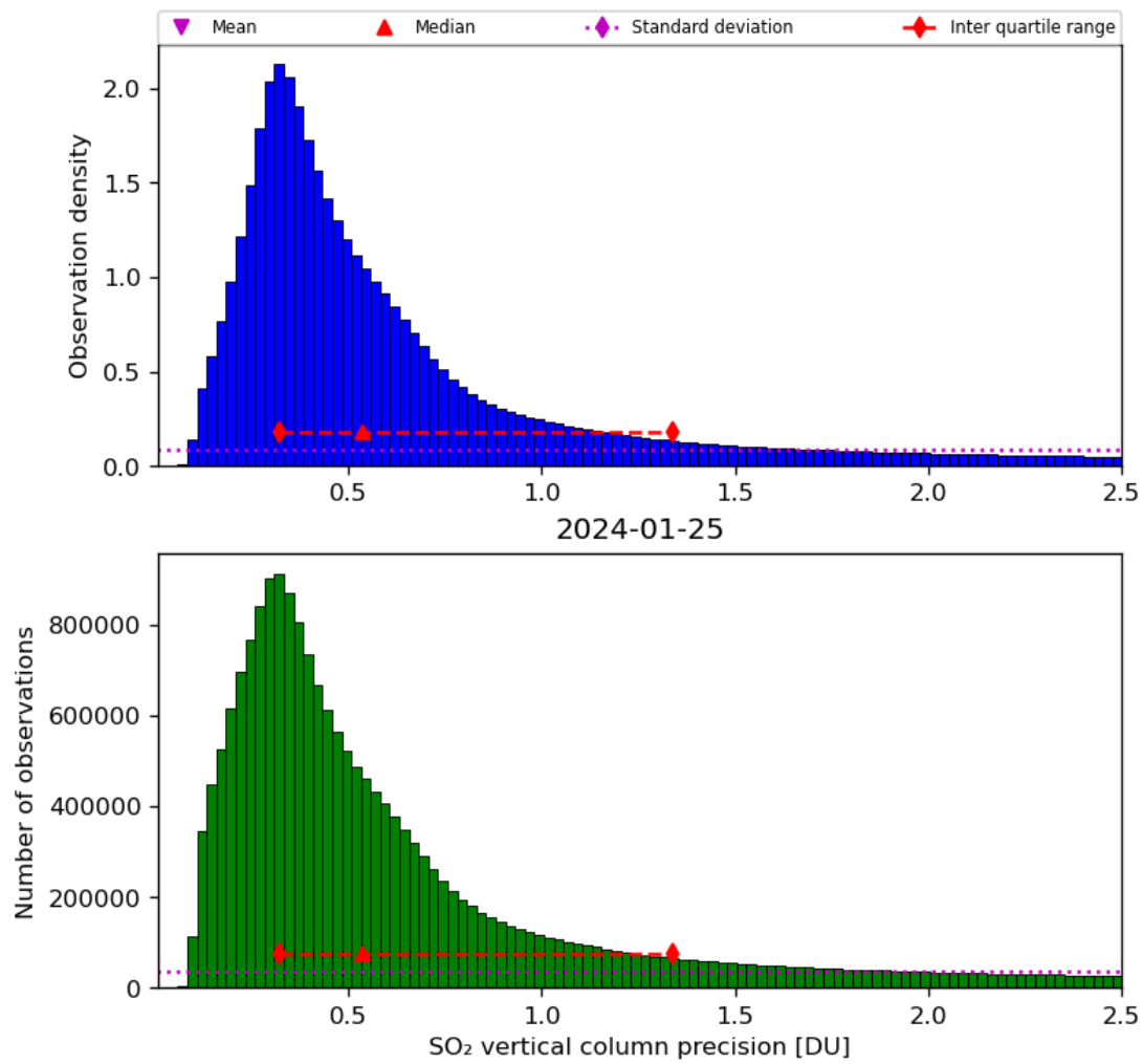
Figure 54: Histogram of “SO 2 vertical column precision” for 2024-01-24 to 2024-01-26
