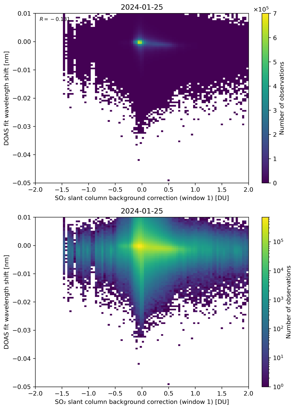
Figure 100: Scatter density plot of “SO 2 slant column background correction (window 1)” against “DOAS fit wavelength shift” for 2024-01-24 to 2024-01-26.
