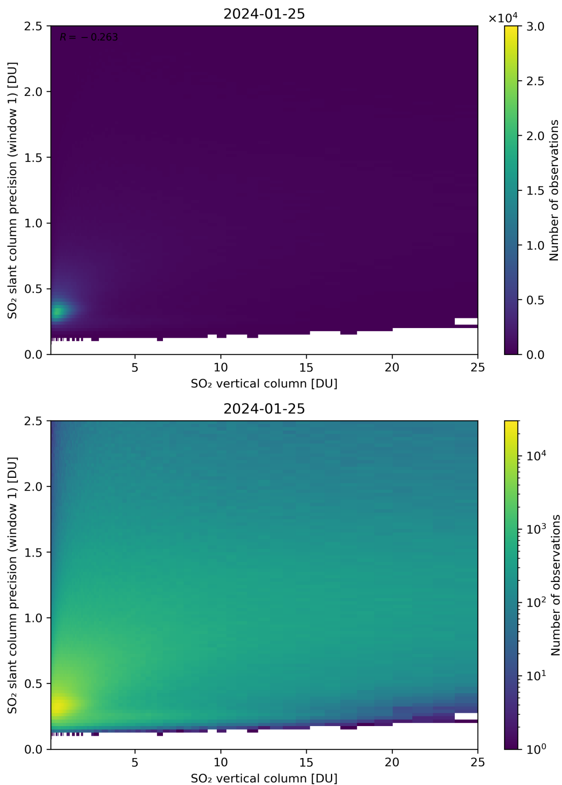
Figure 301: Scatter density plot of “SO 2 vertical column” against “SO 2 slant column precision (window 1)” for 2024-01-24 to 2024-01-26.
