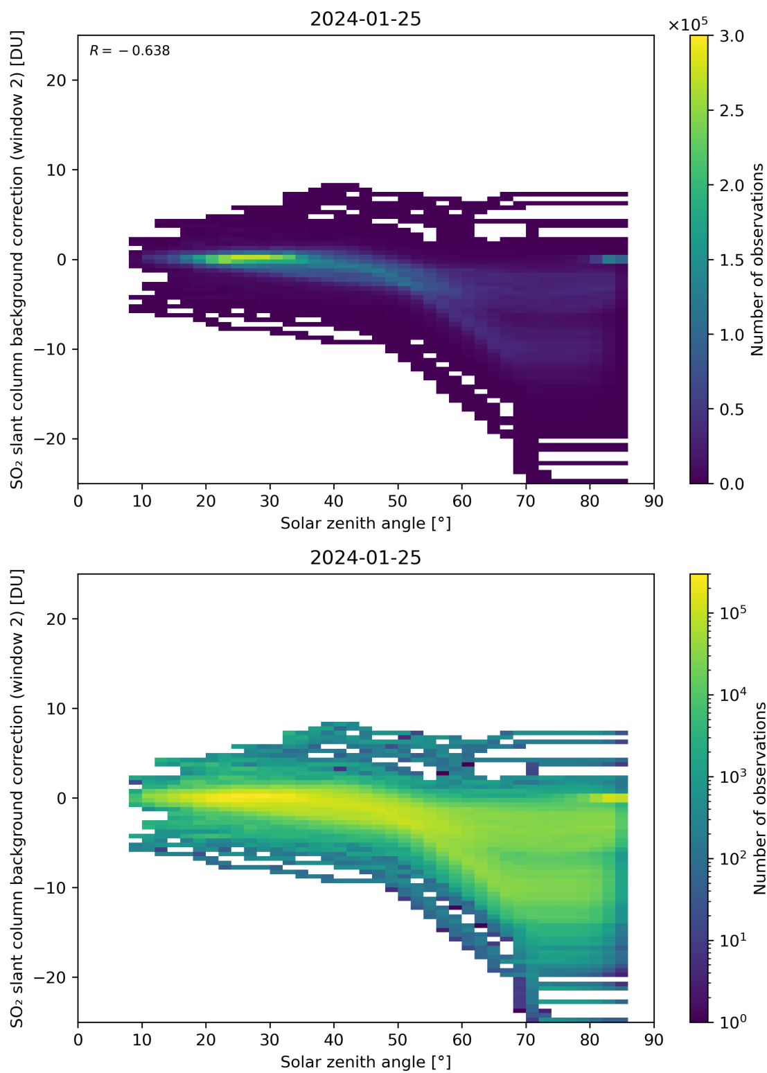
Figure 159: Scatter density plot of “Solar zenith angle” against “SO 2 slant column background correction (window 2)” for 2024-01-24 to 2024-01-26.
