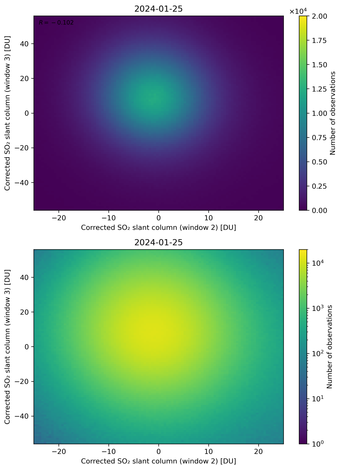
Figure 200: Scatter density plot of “Corrected SO 2 slant column (window 2)” against “Corrected SO 2 slant column (window 3)” for 2024-01-24 to 2024-01-26.
