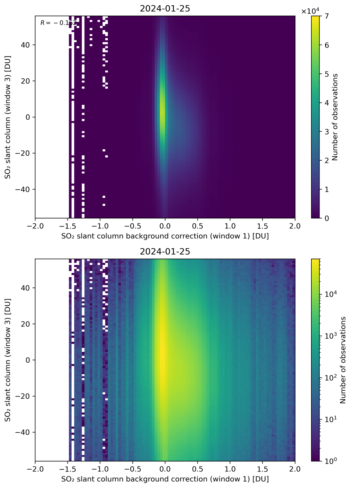
Figure 107: Scatter density plot of “SO 2 slant column background correction (window 1)” against “SO 2 slant column (window 3)” for 2024-01-24 to 2024-01-26.
