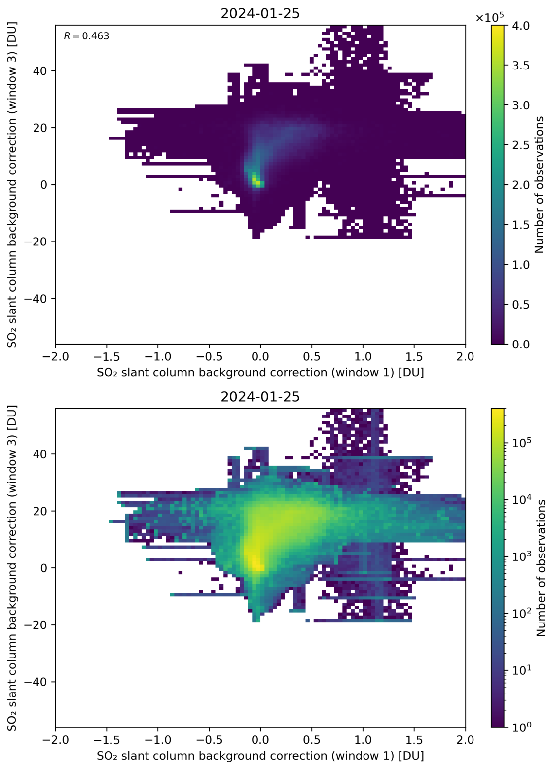
Figure 99: Scatter density plot of “SO 2 slant column background correction (window 1)” against “SO 2 slant column background correction (window 3)” for 2024-01-24 to 2024-01-26.
