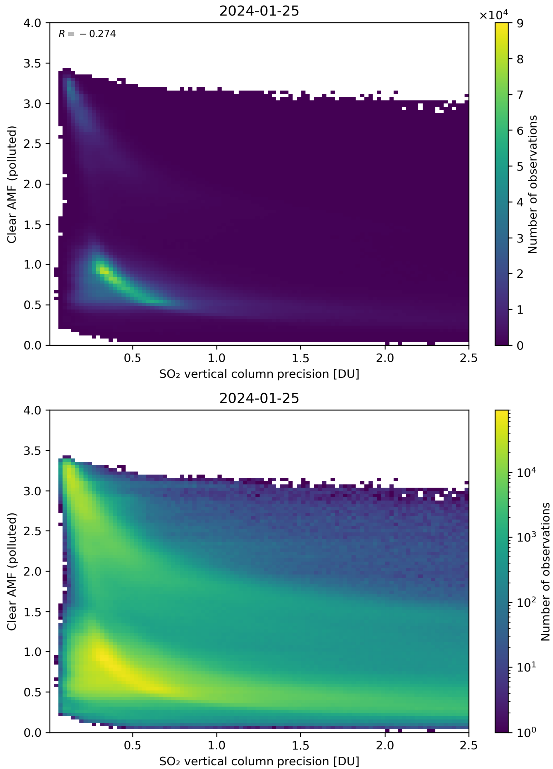
Figure 285: Scatter density plot of “SO 2 vertical column precision” against “Clear AMF (polluted)” for 2024-01-24 to 2024-01-26.
