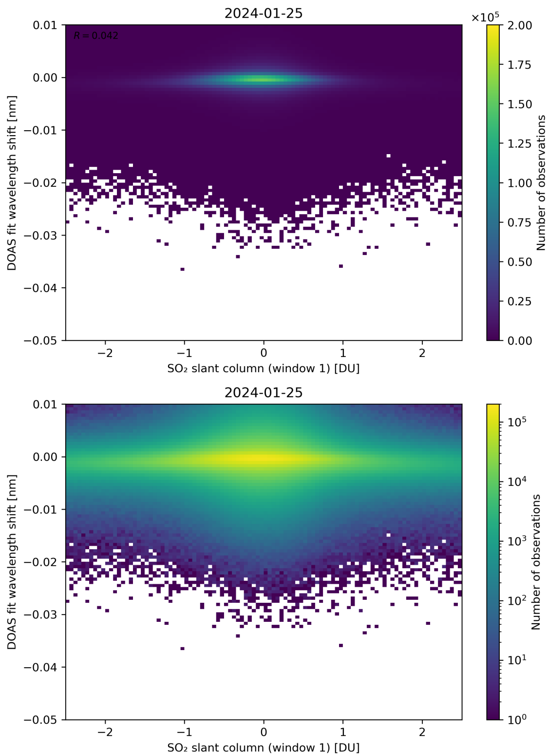
Figure 215: Scatter density plot of “SO 2 slant column (window 1)” against “DOAS fit wavelength shift” for 2024-01-24 to 2024-01-26.
