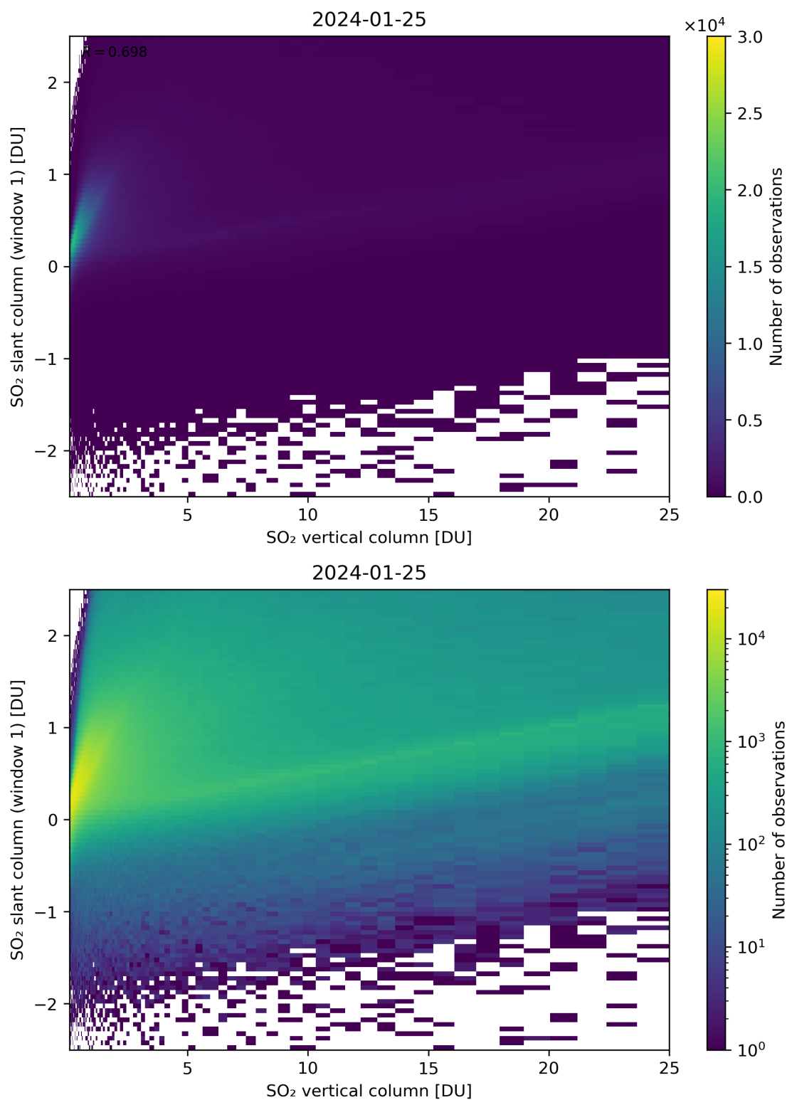
Figure 300: Scatter density plot of “SO 2 vertical column” against “SO 2 slant column (window 1)” for 2024-01-24 to 2024-01-26.
