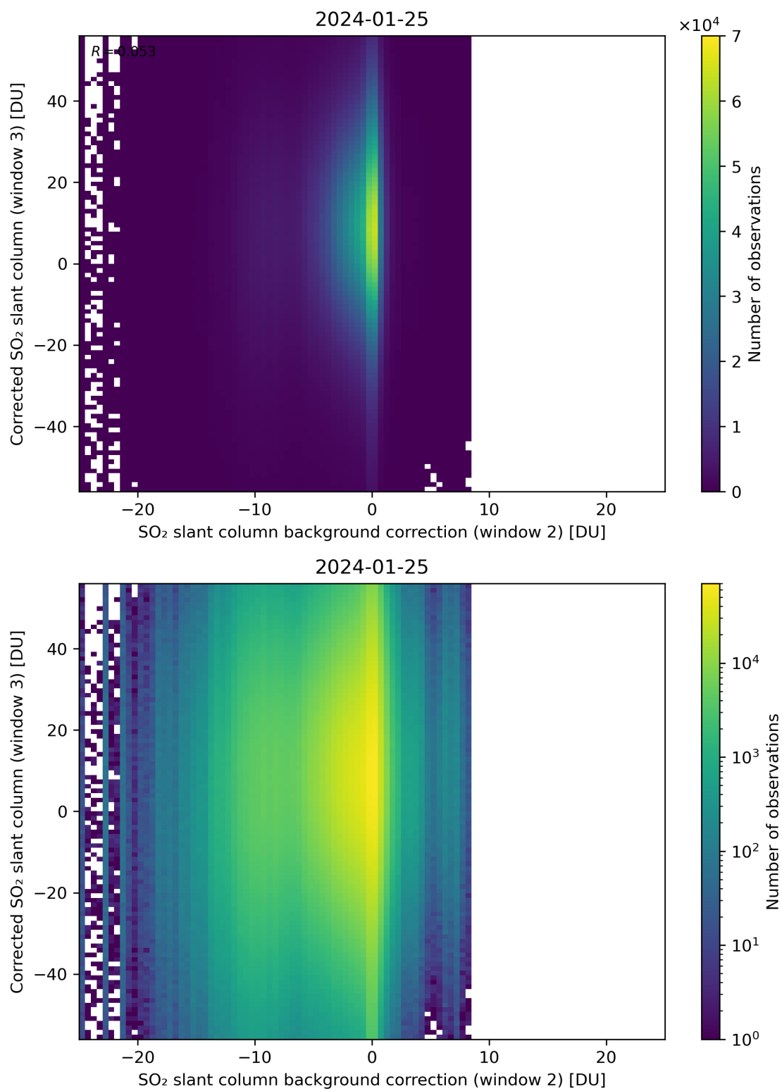
Figure 116: Scatter density plot of “SO 2 slant column background correction (window 2)” against “Corrected SO 2 slant column (window 3)” for 2024-01-24 to 2024-01-26.
