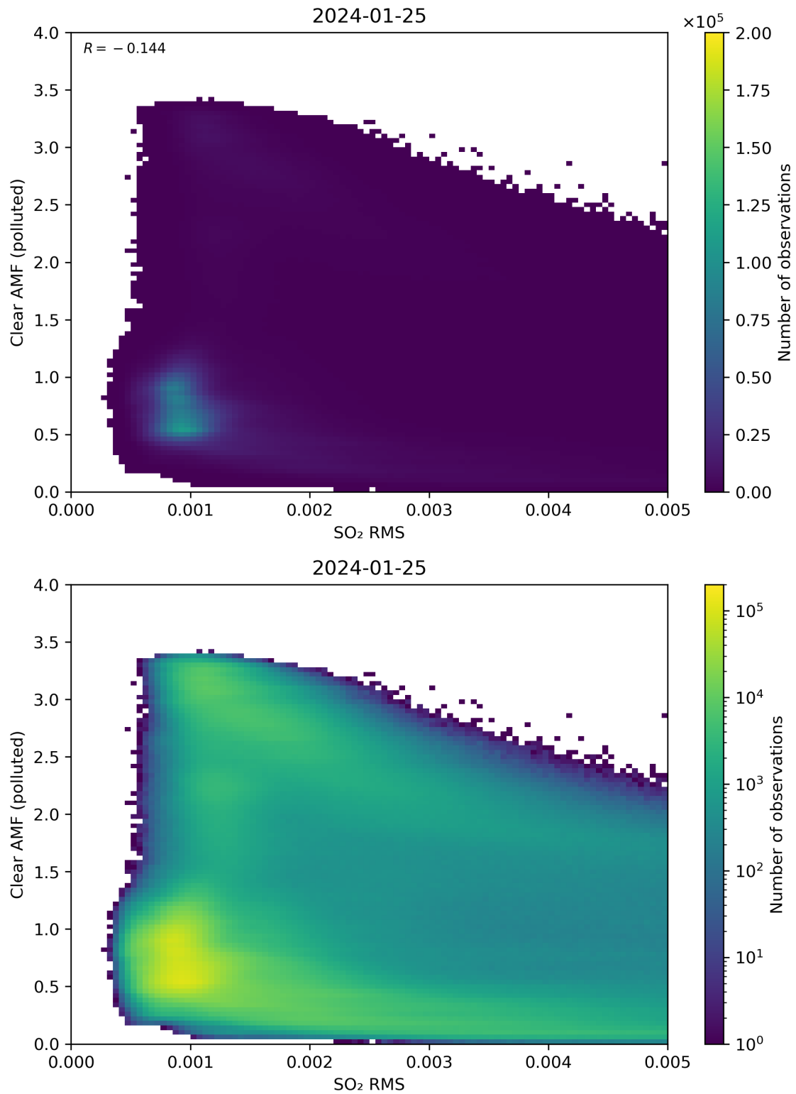
Figure 136: Scatter density plot of “SO 2 RMS” against “Clear AMF (polluted)” for 2024-01-24 to 2024-01-26.
