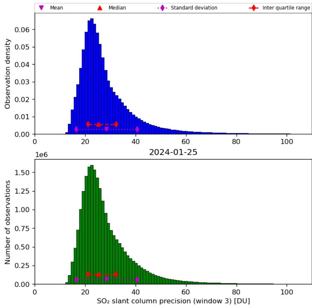
Figure 65: Histogram of “SO 2 slant column precision (window 3)” for 2024-01-24 to 2024-01-26
