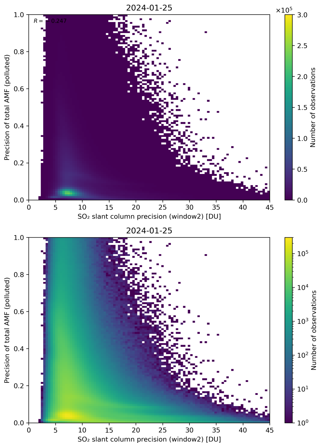
Figure 252: Scatter density plot of “SO 2 slant column precision (window2)” against “Precision of total AMF (polluted)” for 2024-01-24 to 2024-01-26.
