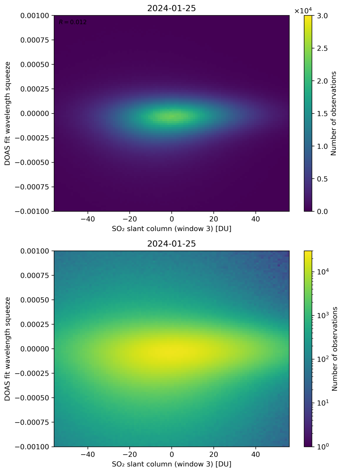
Figure 255: Scatter density plot of “SO 2 slant column (window 3)” against “DOAS fit wavelength squeeze” for 2024-01-24 to 2024-01-26.
