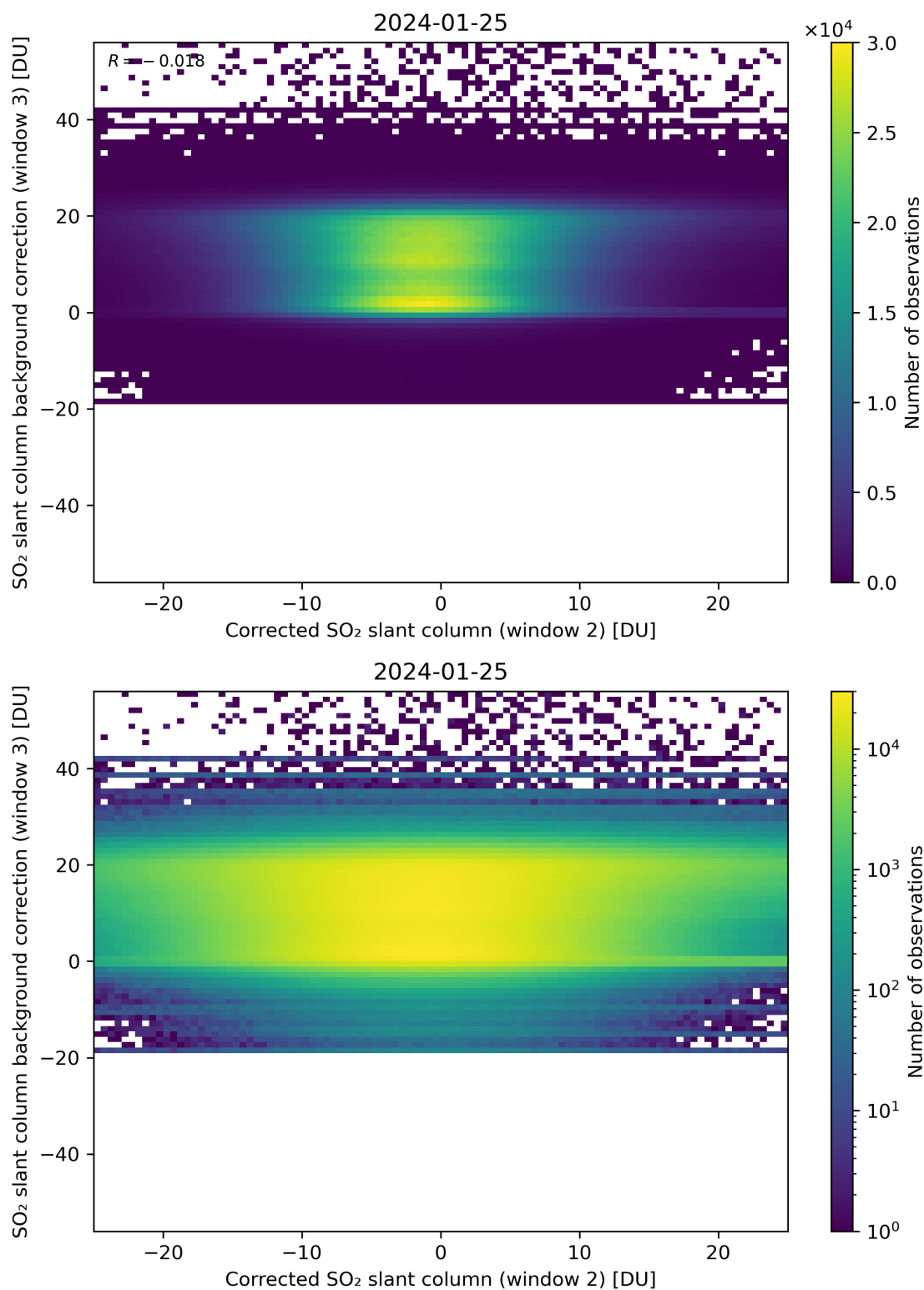
Figure 195: Scatter density plot of “Corrected SO 2 slant column (window 2)” against “SO 2 slant column background correction (window 3)” for 2024-01-24 to 2024-01-26.
