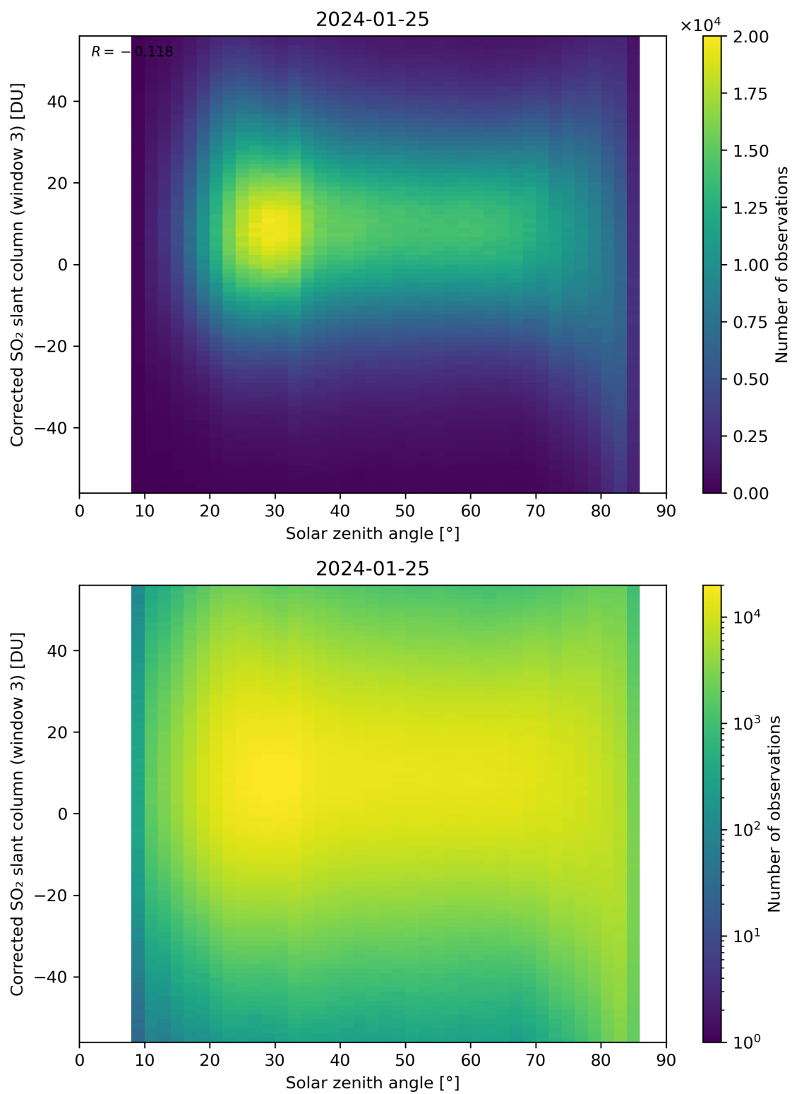
Figure 168: Scatter density plot of “Solar zenith angle” against “Corrected SO 2 slant column (window 3)” for 2024-01-24 to 2024-01-26.
