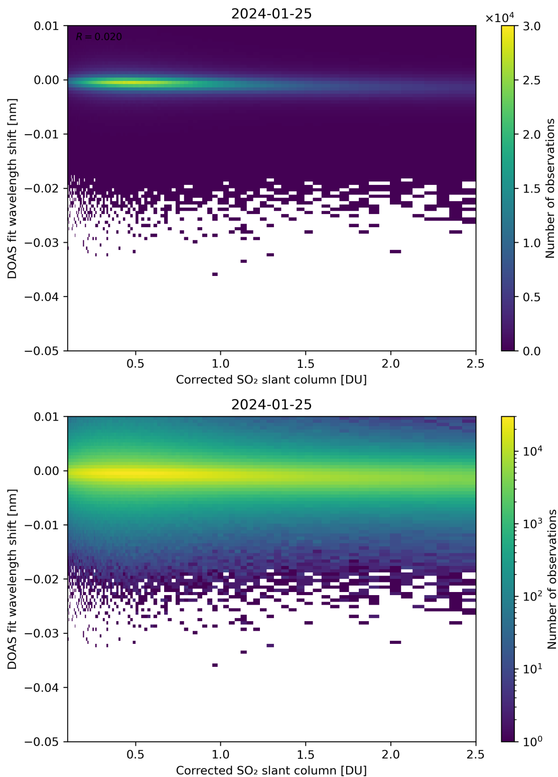
Figure 181: Scatter density plot of “Corrected SO 2 slant column” against “DOAS fit wavelength shift” for 2024-01-24 to 2024-01-26.
