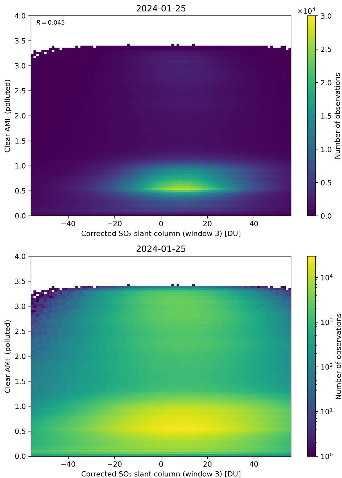
Figure 209: Scatter density plot of “Corrected SO 2 slant column (window 3)” against “Clear AMF (polluted)” for 2024-01-24 to 2024-01-26.
