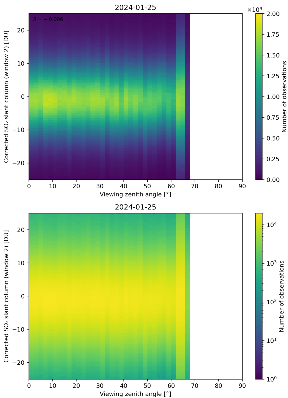
Figure 318: Scatter density plot of “Viewing zenith angle” against “Corrected SO 2 slant column (window 2)” for 2024-01-24 to 2024-01-26.
