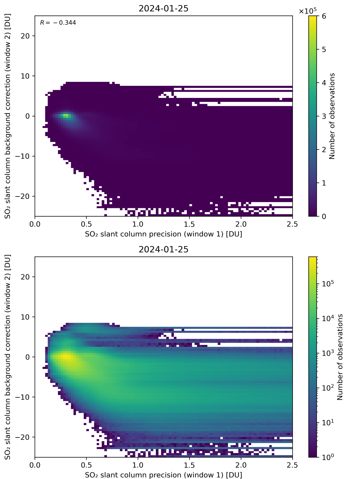
Figure 219: Scatter density plot of “SO 2 slant column precision (window 1)” against “SO 2 slant column background correction (window 2)” for 2024-01-24 to 2024-01-26.
