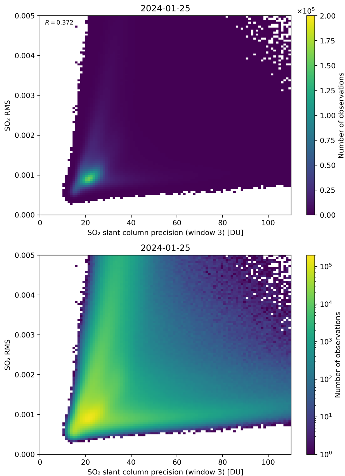
Figure 260: Scatter density plot of “SO 2 slant column precision (window 3)” against “SO 2 RMS” for 2024-01-24 to 2024-01-26.
