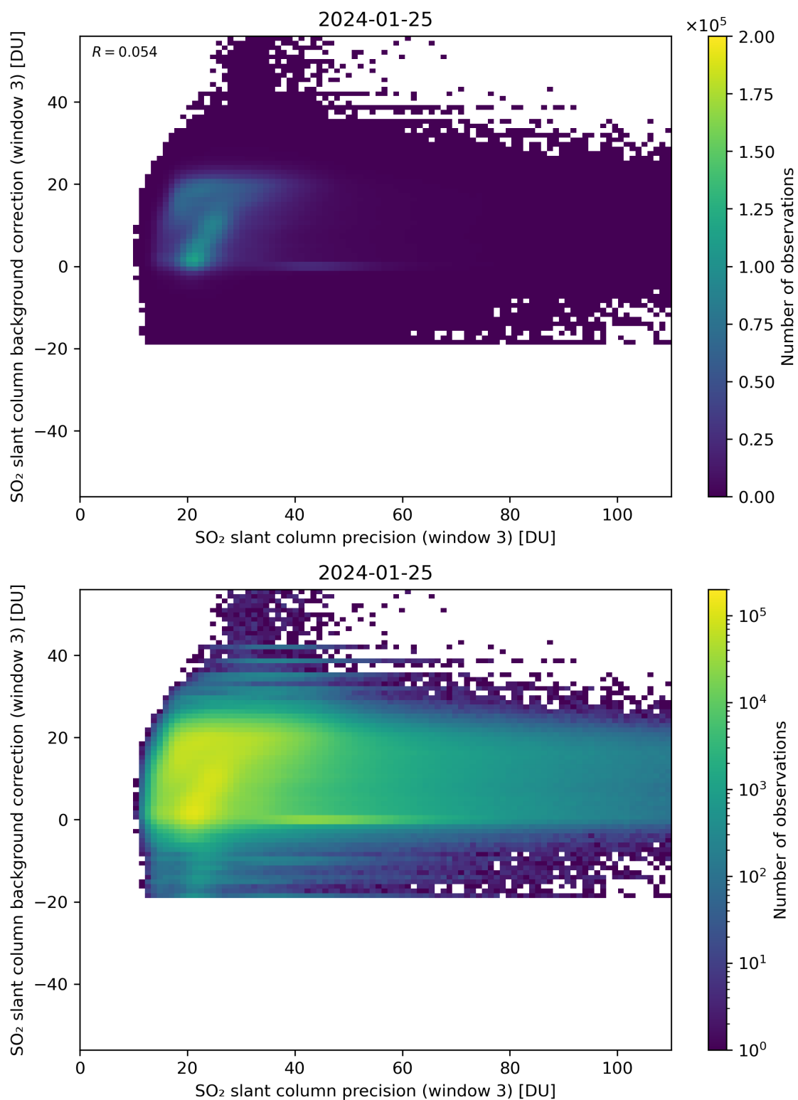
Figure 257: Scatter density plot of “SO 2 slant column precision (window 3)” against “SO 2 slant column background correction (window 3)” for 2024-01-24 to 2024-01-26.
