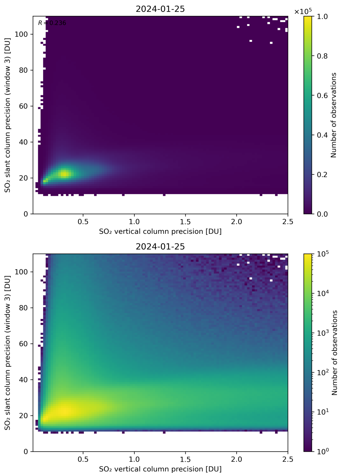
Figure 293: Scatter density plot of “SO 2 vertical column precision” against “SO 2 slant column precision (window 3)” for 2024-01-24 to 2024-01-26.
