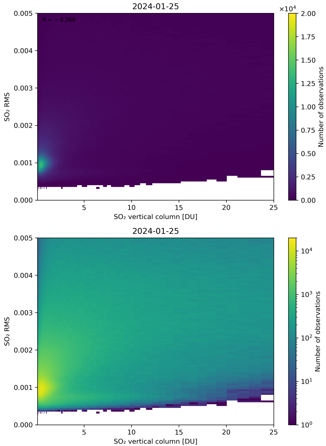
Figure 278: Scatter density plot of “SO 2 vertical column” against “SO 2 RMS” for 2024-01-24 to 2024-01-26.
