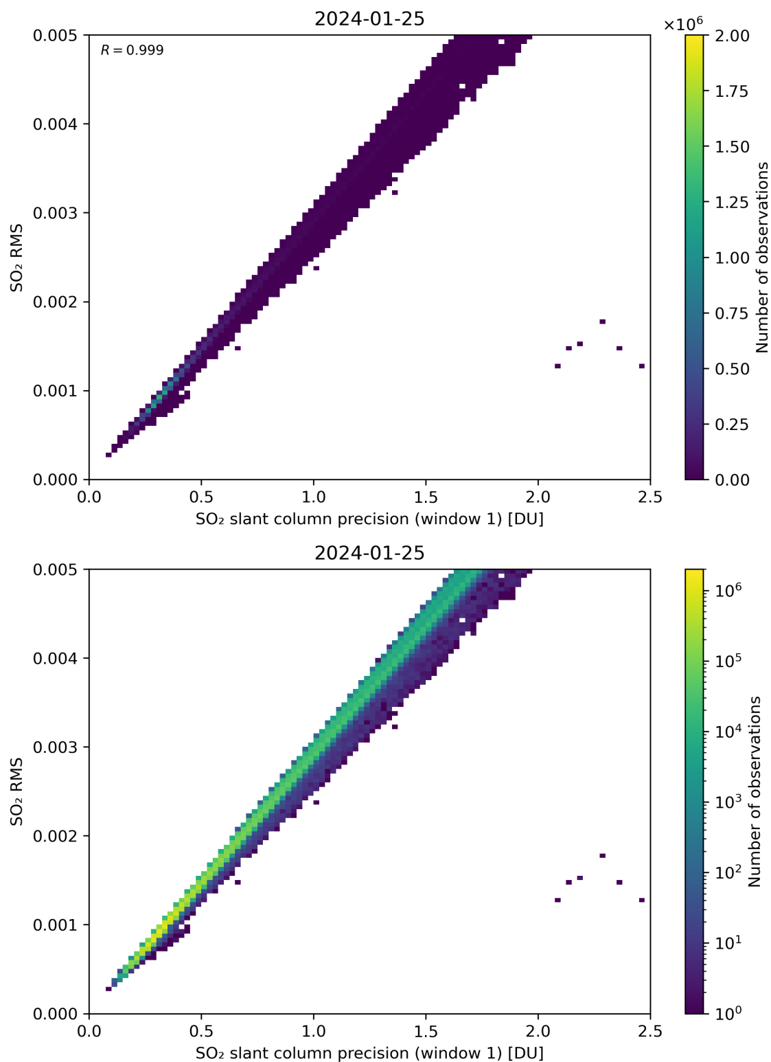
Figure 223: Scatter density plot of “SO 2 slant column precision (window 1)” against “SO 2 RMS” for 2024-01-24 to 2024-01-26.
