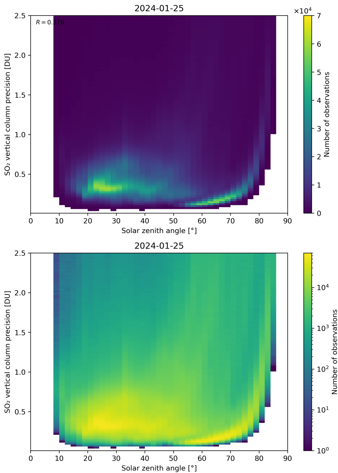
Figure 177: Scatter density plot of “Solar zenith angle” against “SO 2 vertical column precision” for 2024-01-24 to 2024-01-26.
