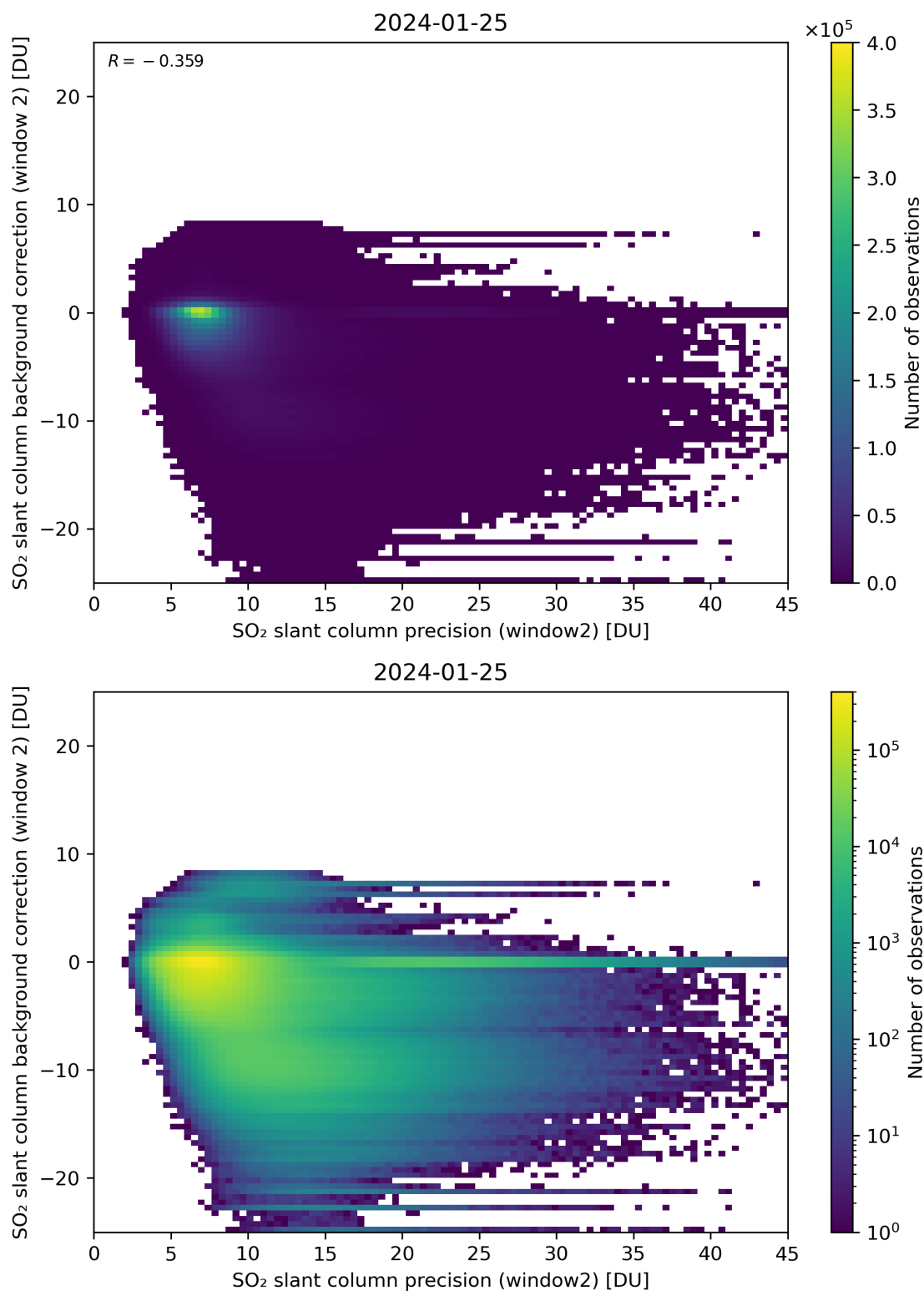
Figure 241: Scatter density plot of “SO 2 slant column precision (window2)” against “SO 2 slant column background correction (window 2)” for 2024-01-24 to 2024-01-26.
