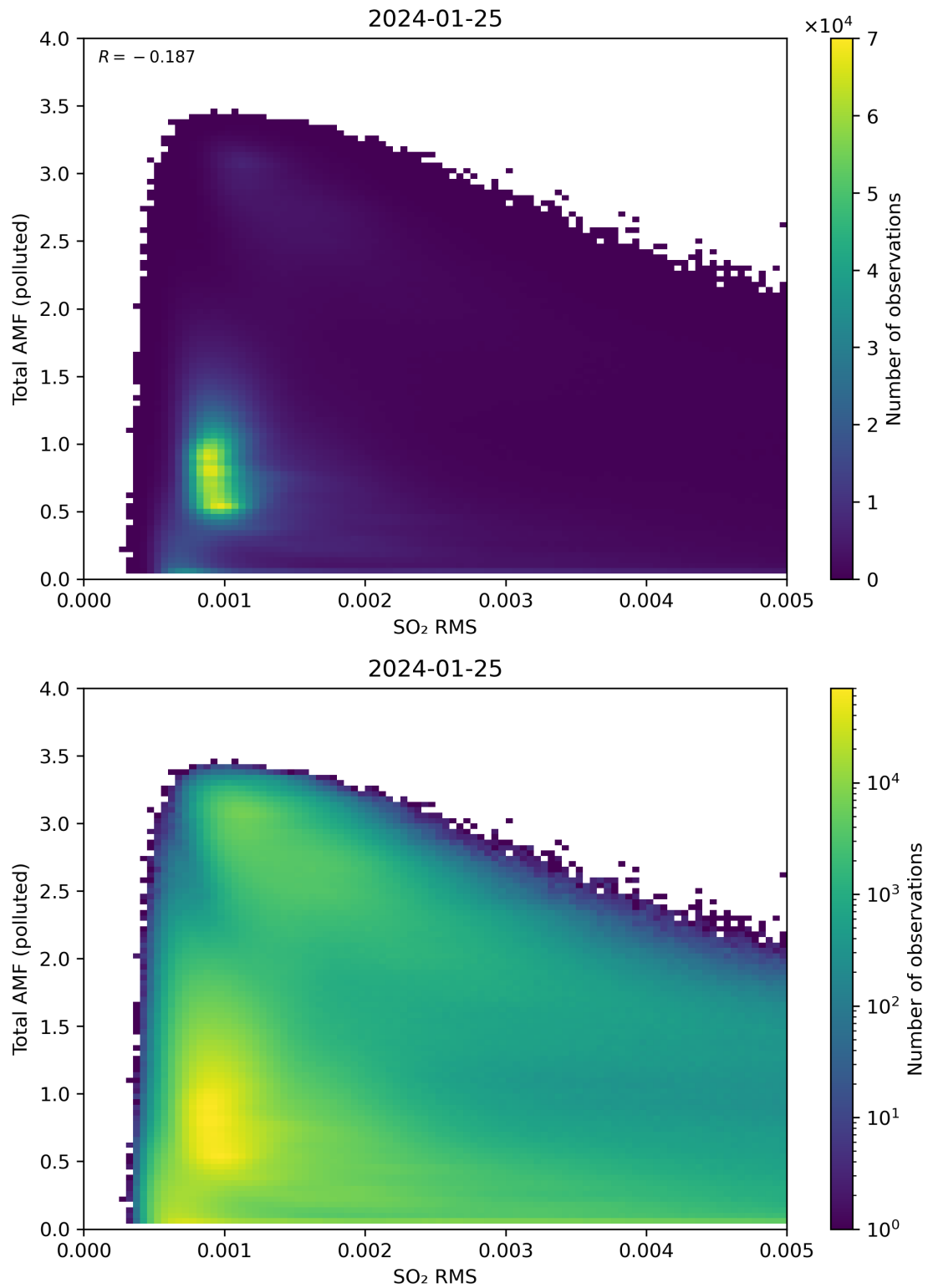
Figure 137: Scatter density plot of “SO 2 RMS” against “Total AMF (polluted)” for 2024-01-24 to 2024-01-26.
