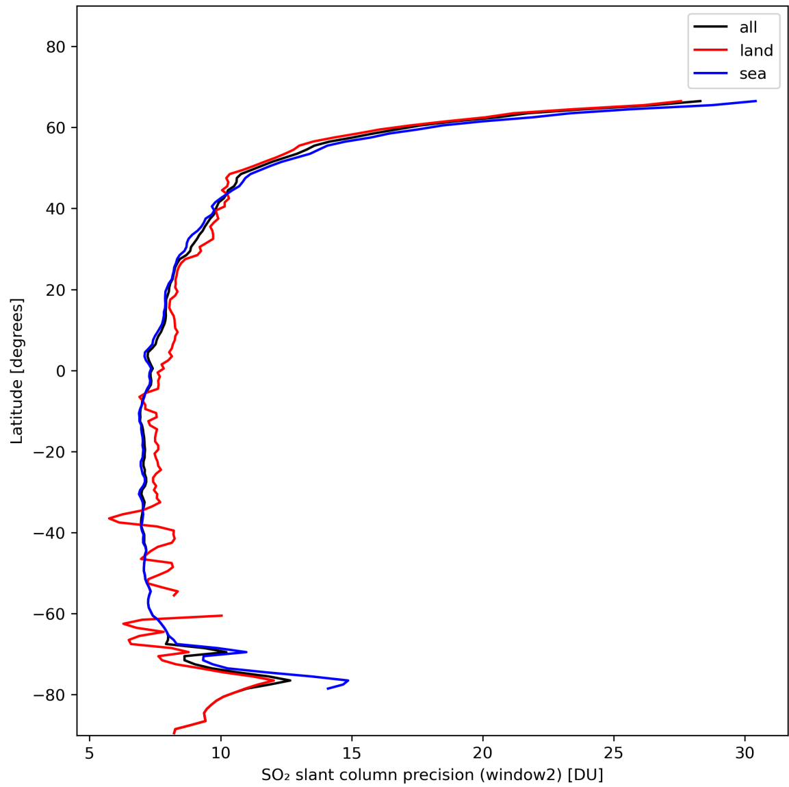
Figure 38: Zonal average of “SO 2 slant column precision (window2)” for 2024-01-24 to 2024-01-26.
