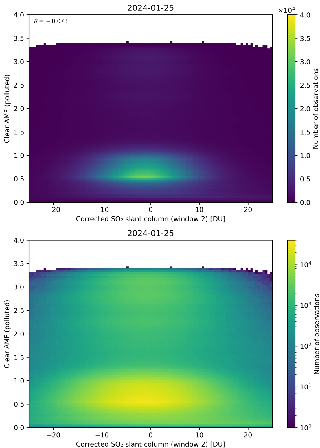
Figure 199: Scatter density plot of “Corrected SO 2 slant column (window 2)” against “Clear AMF (polluted)” for 2024-01-24 to 2024-01-26.
