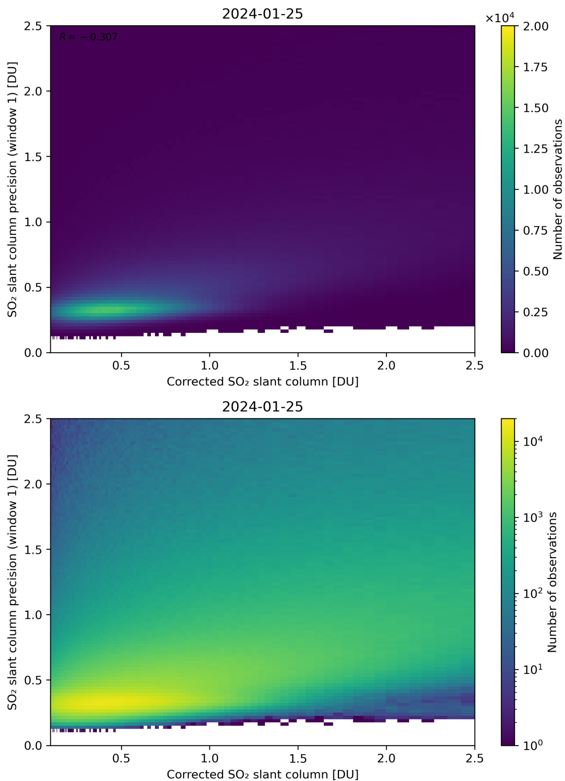
Figure 188: Scatter density plot of “Corrected SO 2 slant column” against “SO 2 slant column precision (window 1)” for 2024-01-24 to 2024-01-26.
