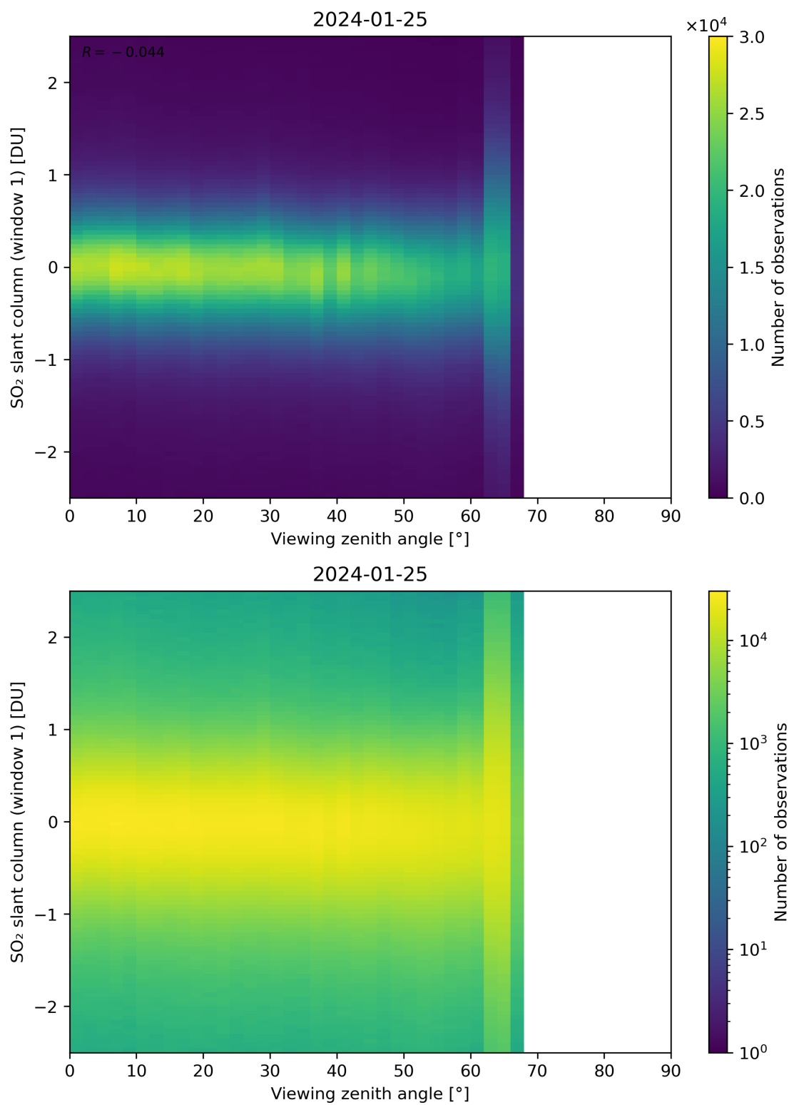
Figure 320: Scatter density plot of “Viewing zenith angle” against “SO 2 slant column (window 1)” for 2024-01-24 to 2024-01-26.
