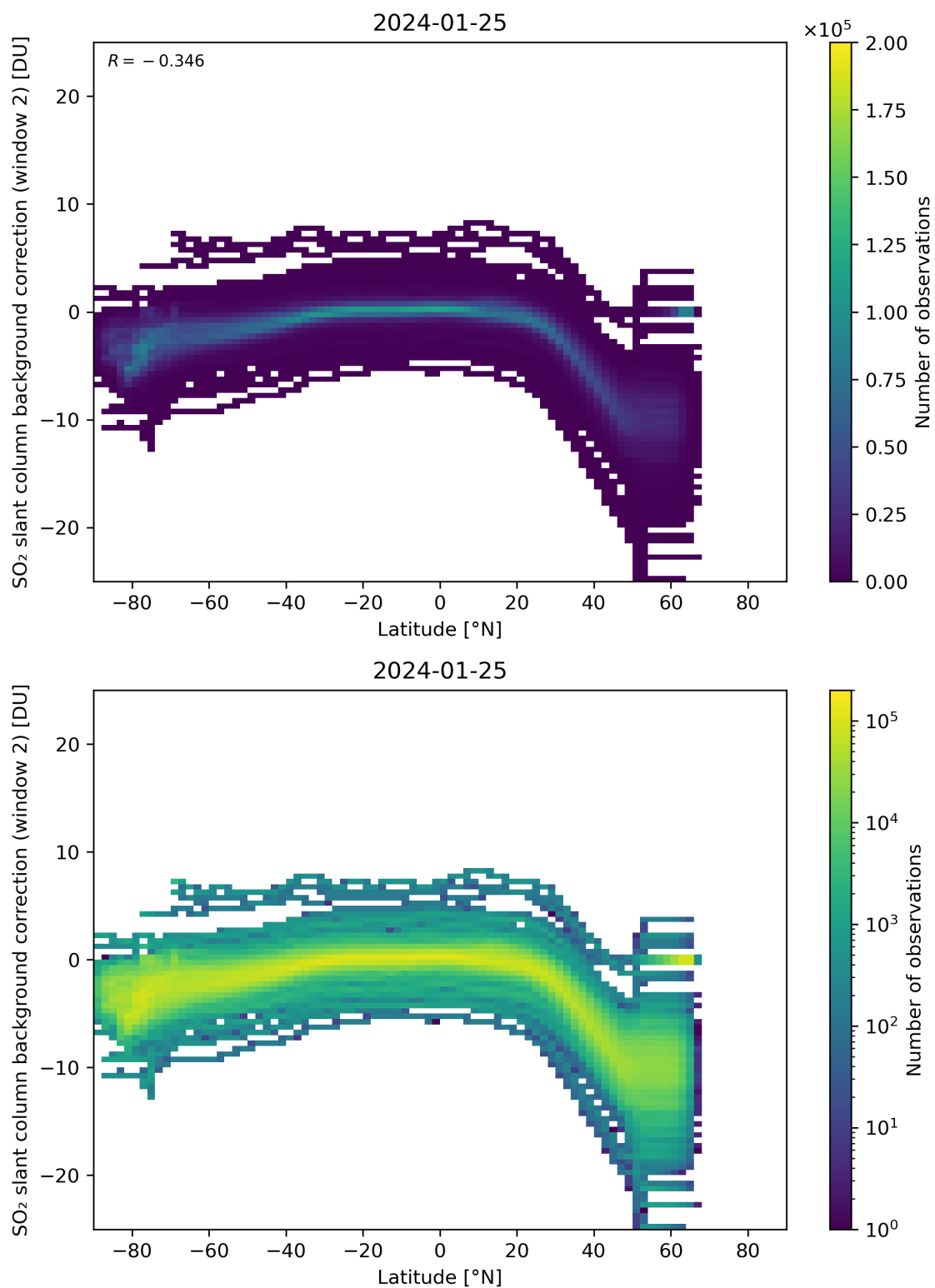
Figure 140: Scatter density plot of “Latitude” against “SO 2 slant column background correction (window 2)” for 2024-01-24 to 2024-01-26.
