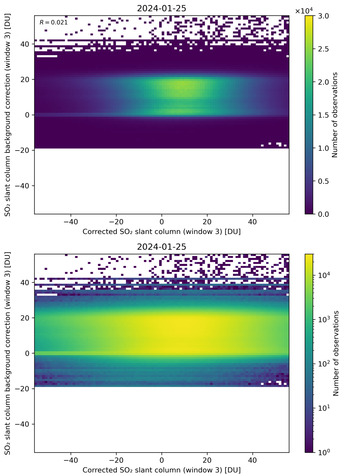
Figure 205: Scatter density plot of “Corrected SO 2 slant column (window 3)” against “SO 2 slant column background correction (window 3)” for 2024-01-24 to 2024-01-26.
