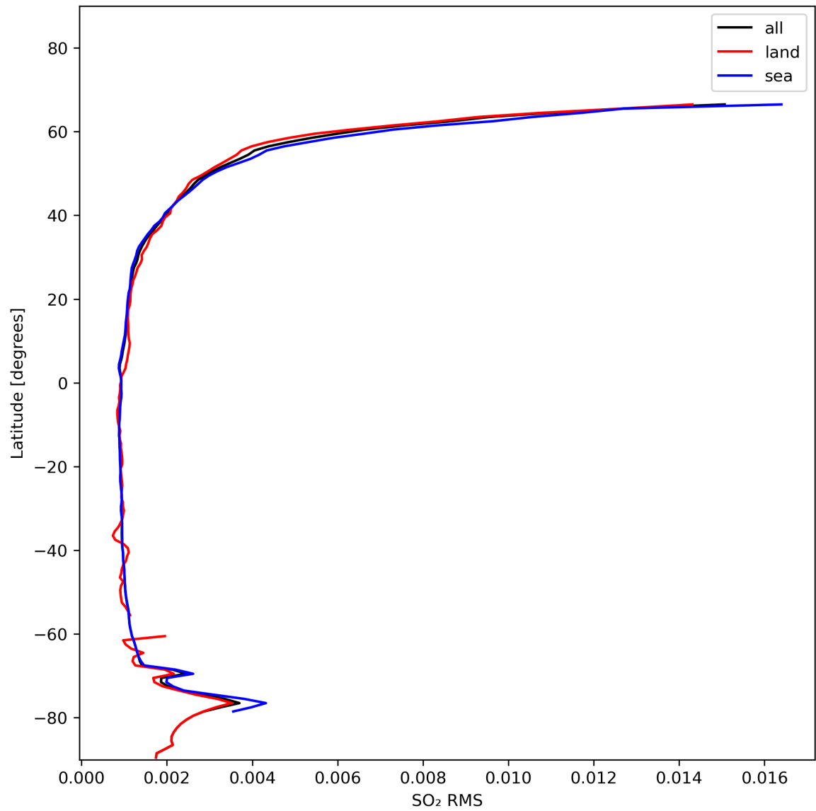
Figure 47: Zonal average of “SO 2 RMS” for 2024-01-24 to 2024-01-26.
