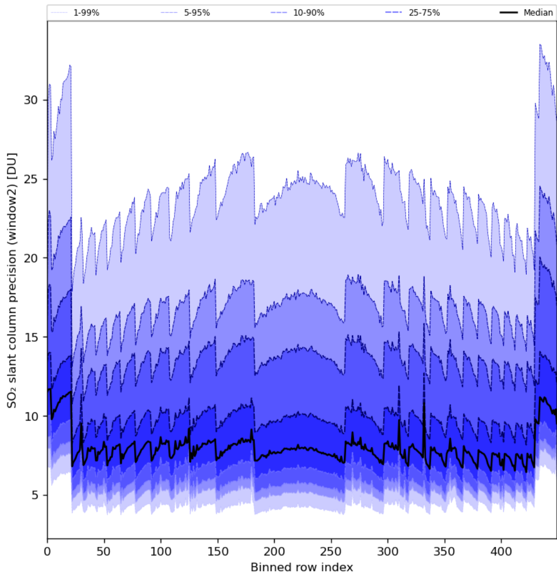
Figure 84: Along track statistics of “SO 2 slant column precision (window2)” for 2024-01-24 to 2024-01-26
