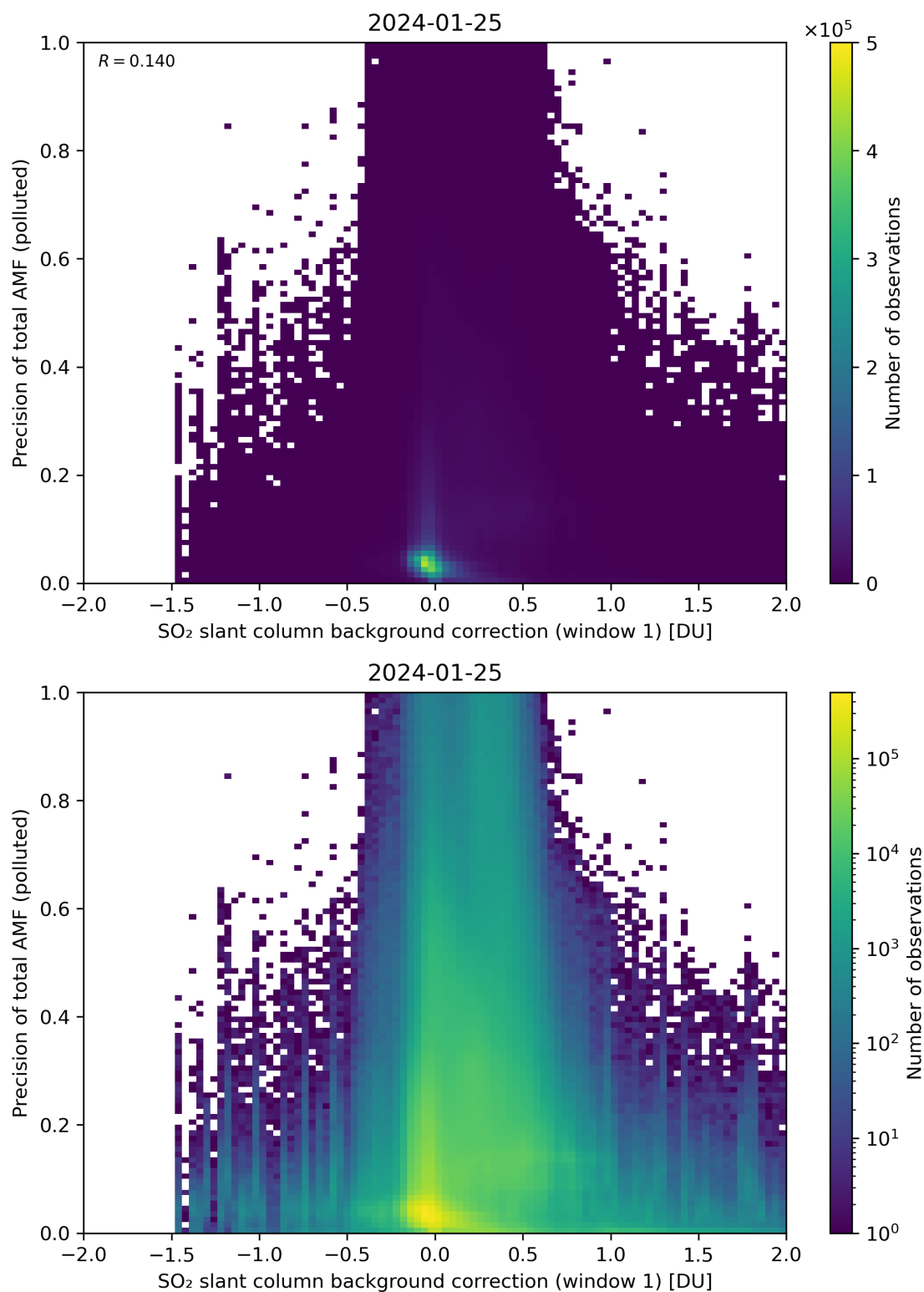
Figure 110: Scatter density plot of “SO 2 slant column background correction (window 1)” against “Precision of total AMF (polluted)” for 2024-01-24 to 2024-01-26.
