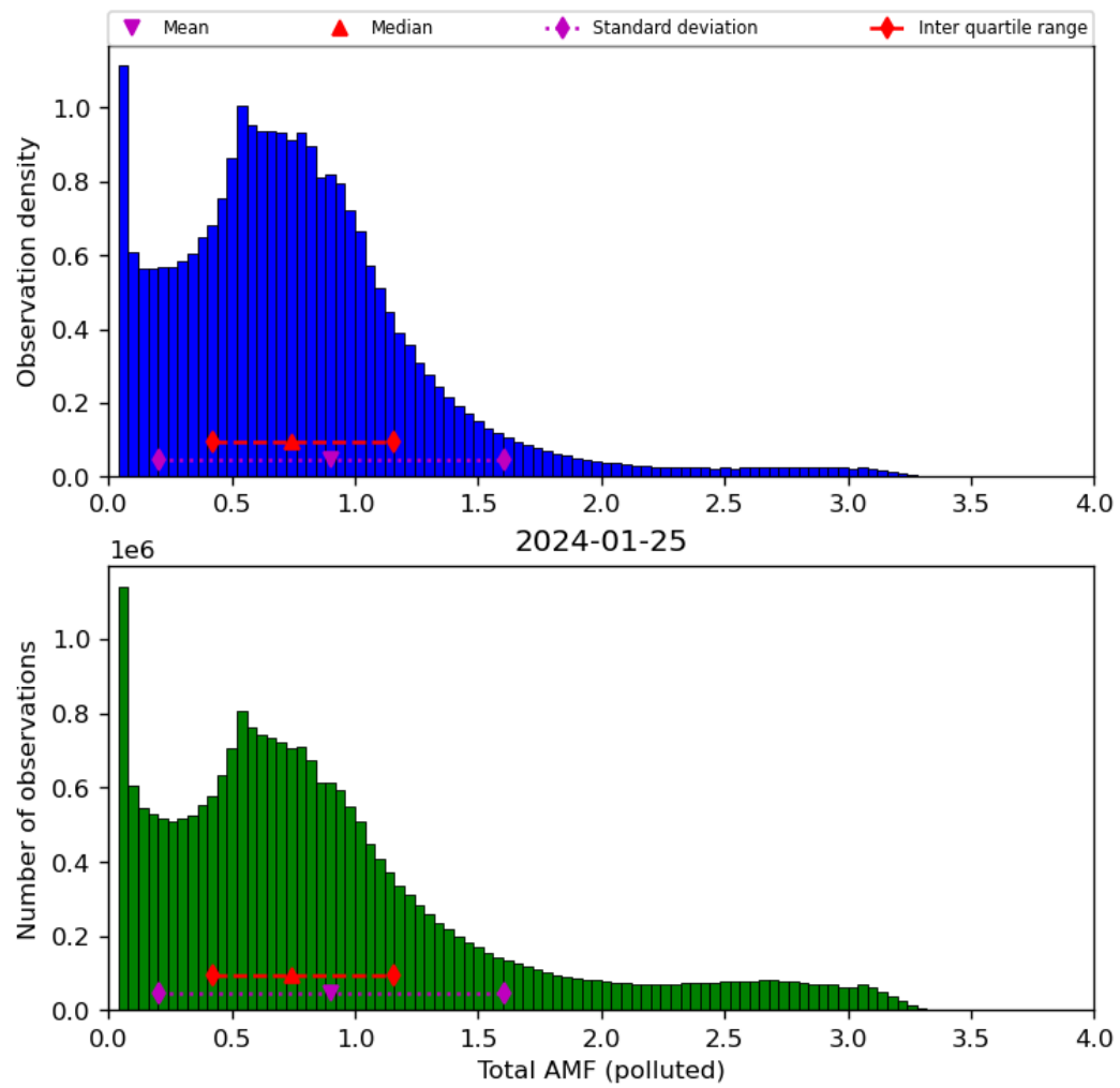
Figure 71: Histogram of “Total AMF (polluted)” for 2024-01-24 to 2024-01-26
