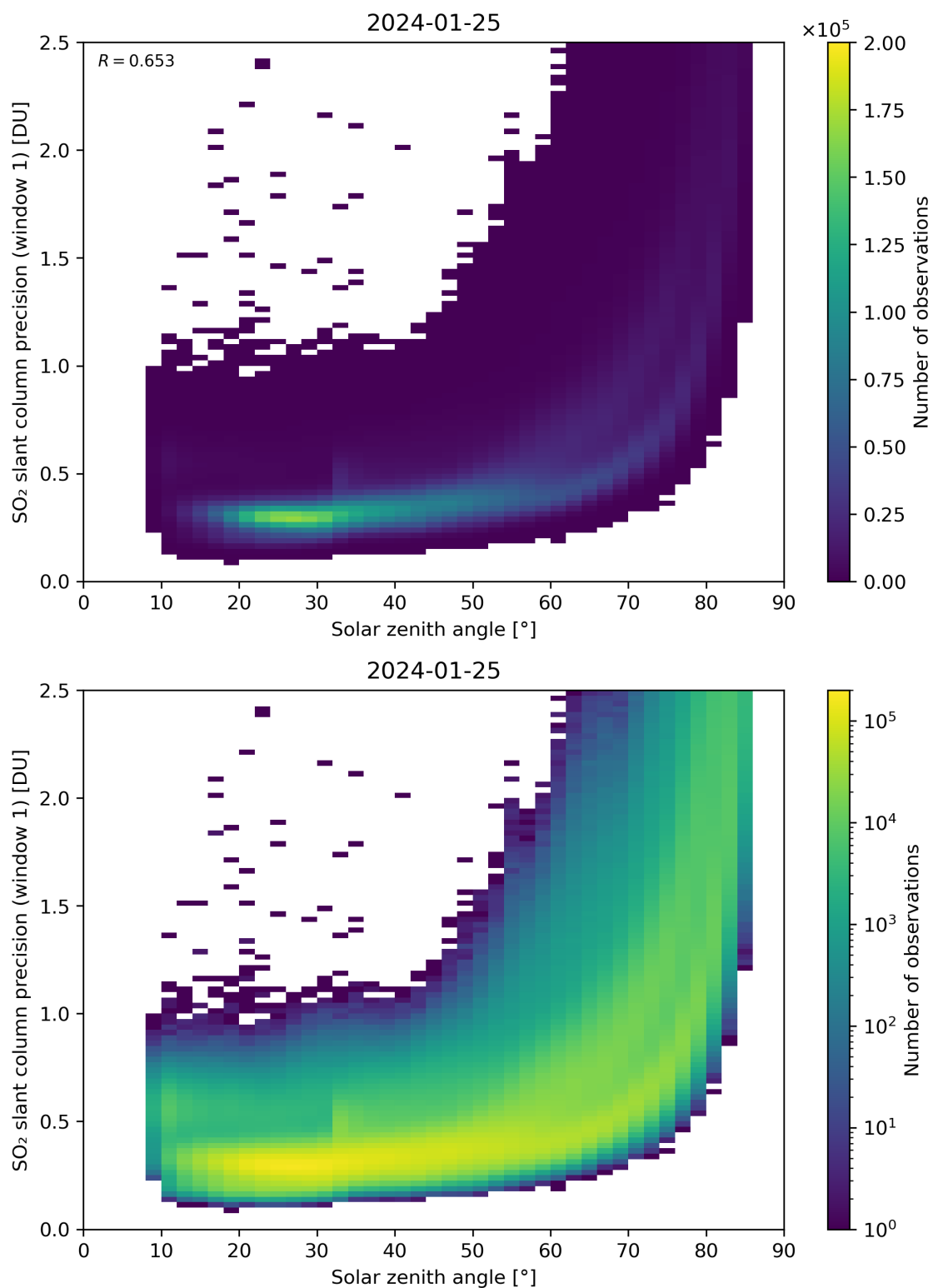
Figure 170: Scatter density plot of “Solar zenith angle” against “SO 2 slant column precision (window 1)” for 2024-01-24 to 2024-01-26.
