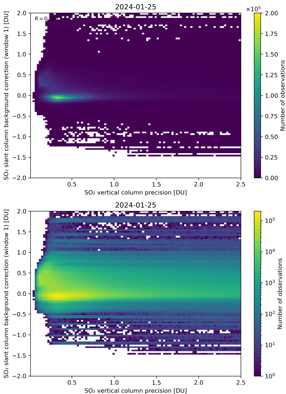
Figure 279: Scatter density plot of “SO 2 vertical column precision” against “SO 2 slant column background correction (window 1)” for 2024-01-24 to 2024-01-26.
