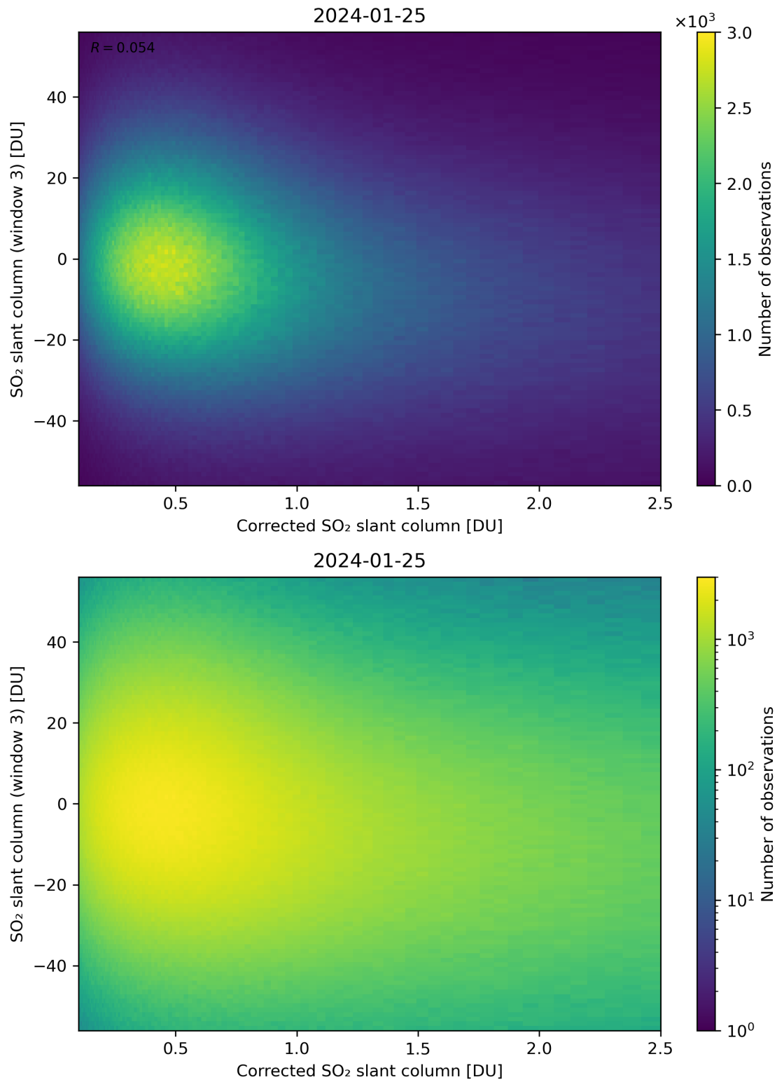
Figure 190: Scatter density plot of “Corrected SO 2 slant column” against “SO 2 slant column (window 3)” for 2024-01-24 to 2024-01-26.
