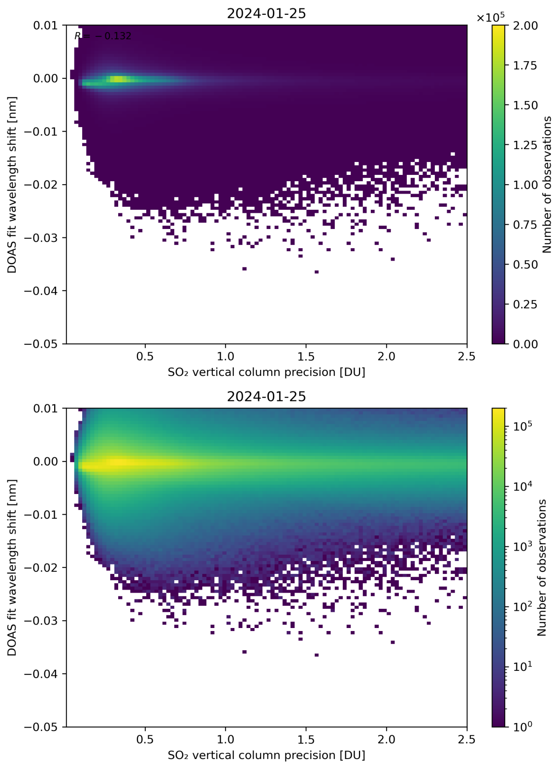
Figure 282: Scatter density plot of “SO 2 vertical column precision” against “DOAS fit wavelength shift” for 2024-01-24 to 2024-01-26.
