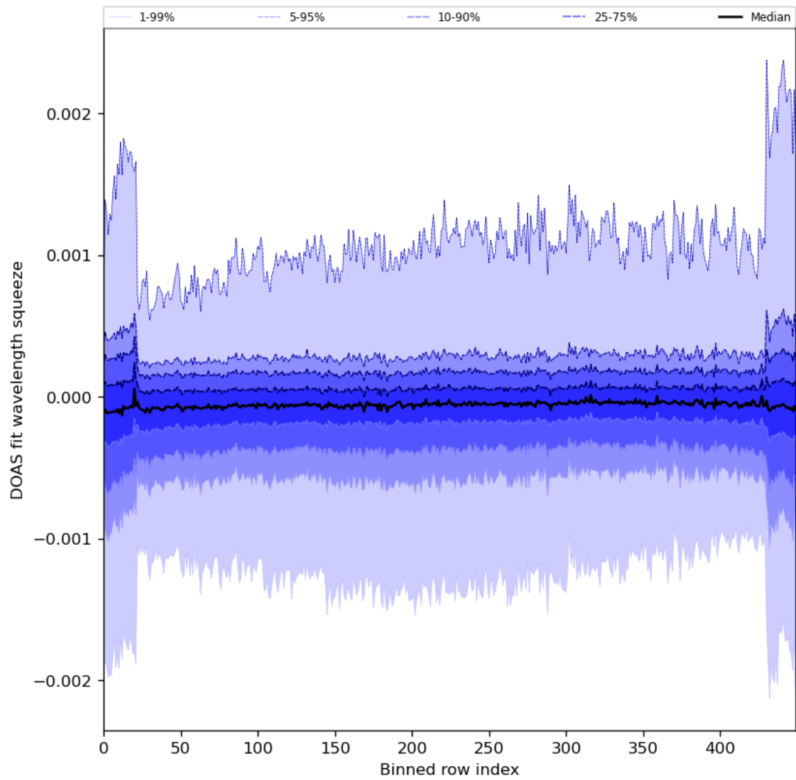
Figure 92: Along track statistics of “DOAS fit wavelength squeeze” for 2024-01-24 to 2024-01-26
