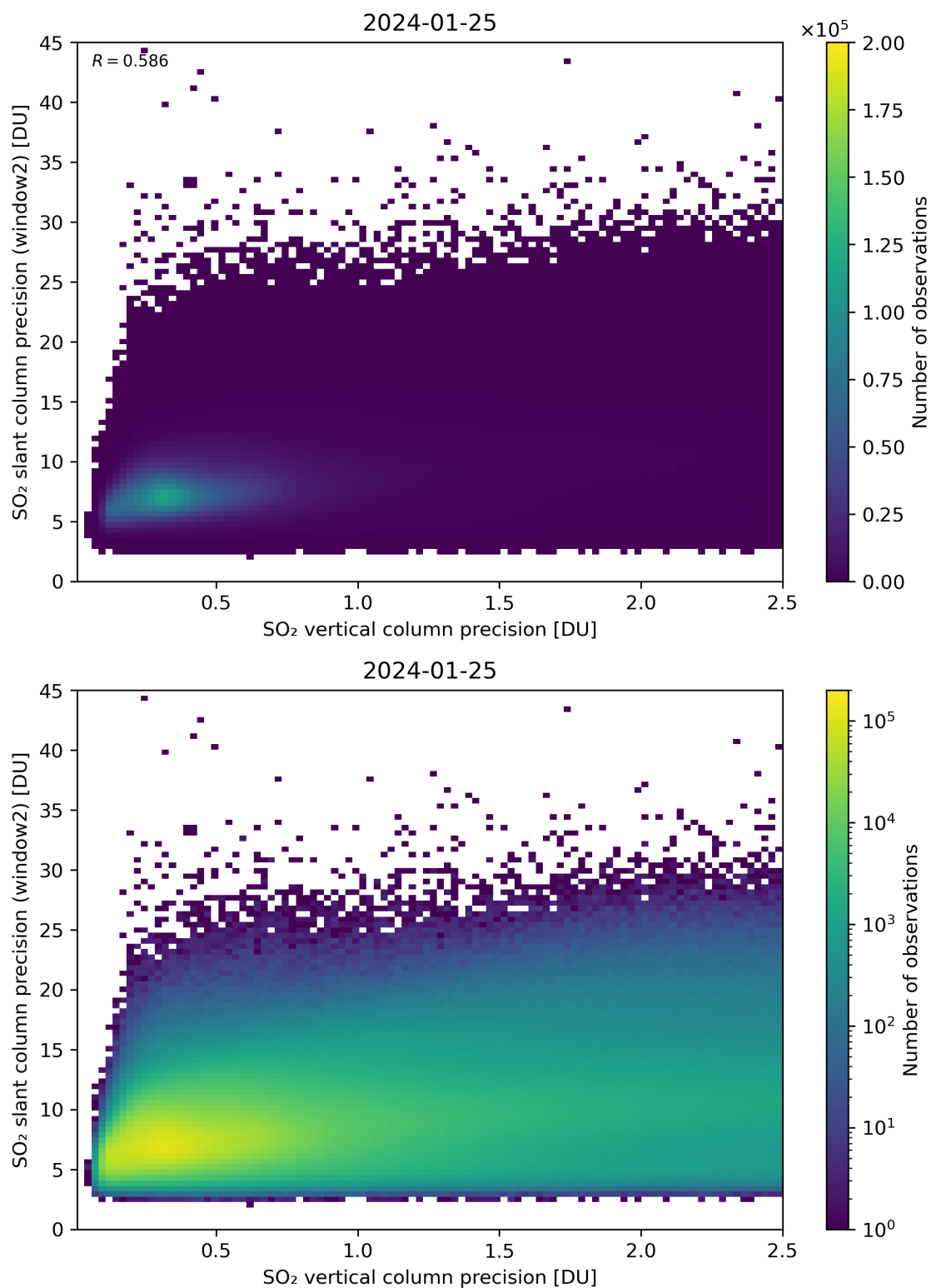
Figure 291: Scatter density plot of “SO 2 vertical column precision” against “SO 2 slant column precision (window2)” for 2024-01-24 to 2024-01-26.
