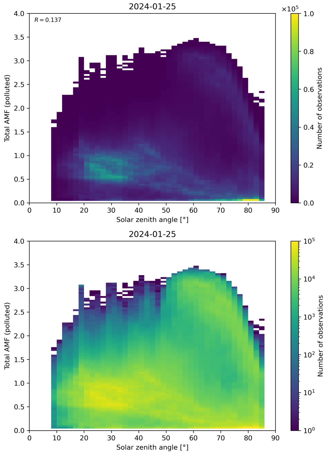
Figure 174: Scatter density plot of “Solar zenith angle” against “Total AMF (polluted)” for 2024-01-24 to 2024-01-26.
