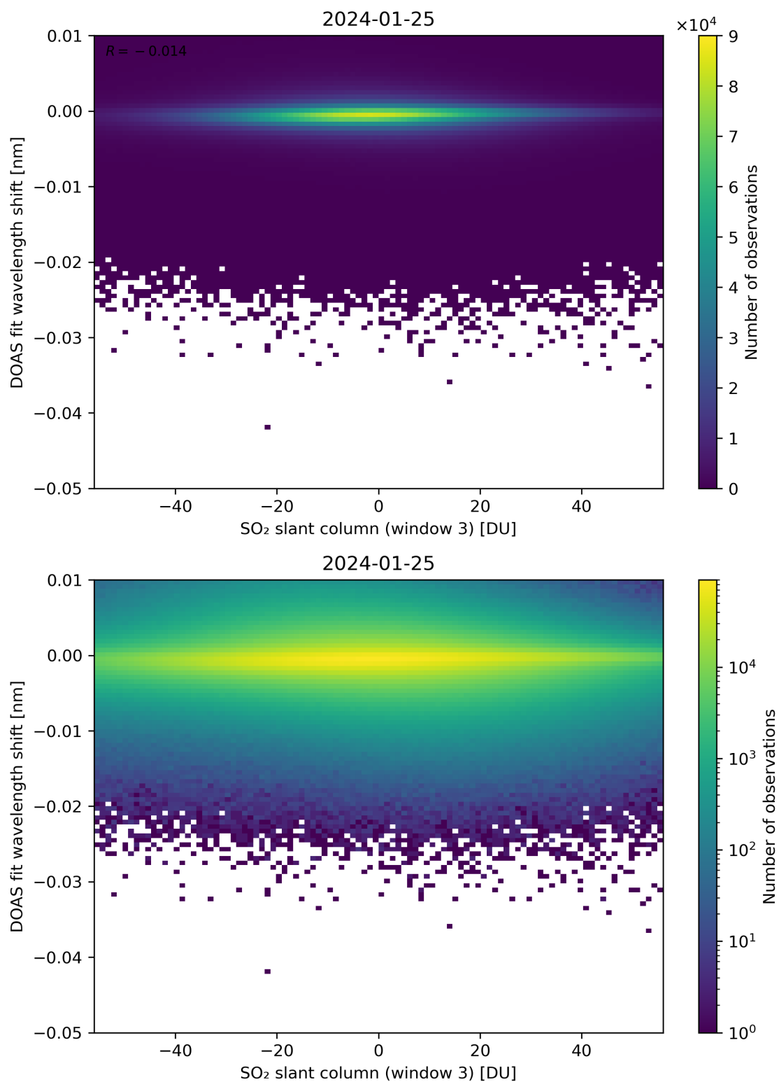
Figure 254: Scatter density plot of “SO 2 slant column (window 3)” against “DOAS fit wavelength shift” for 2024-01-24 to 2024-01-26.
