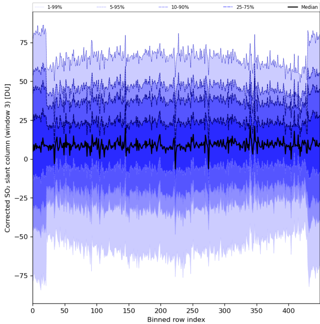
Figure 89: Along track statistics of “Corrected SO 2 slant column (window 3)” for 2024-01-24 to 2024-01-26
