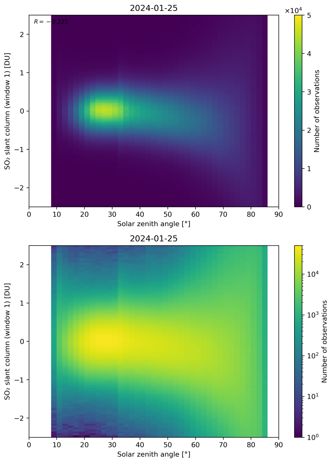
Figure 169: Scatter density plot of “Solar zenith angle” against “SO 2 slant column (window 1)” for 2024-01-24 to 2024-01-26.
