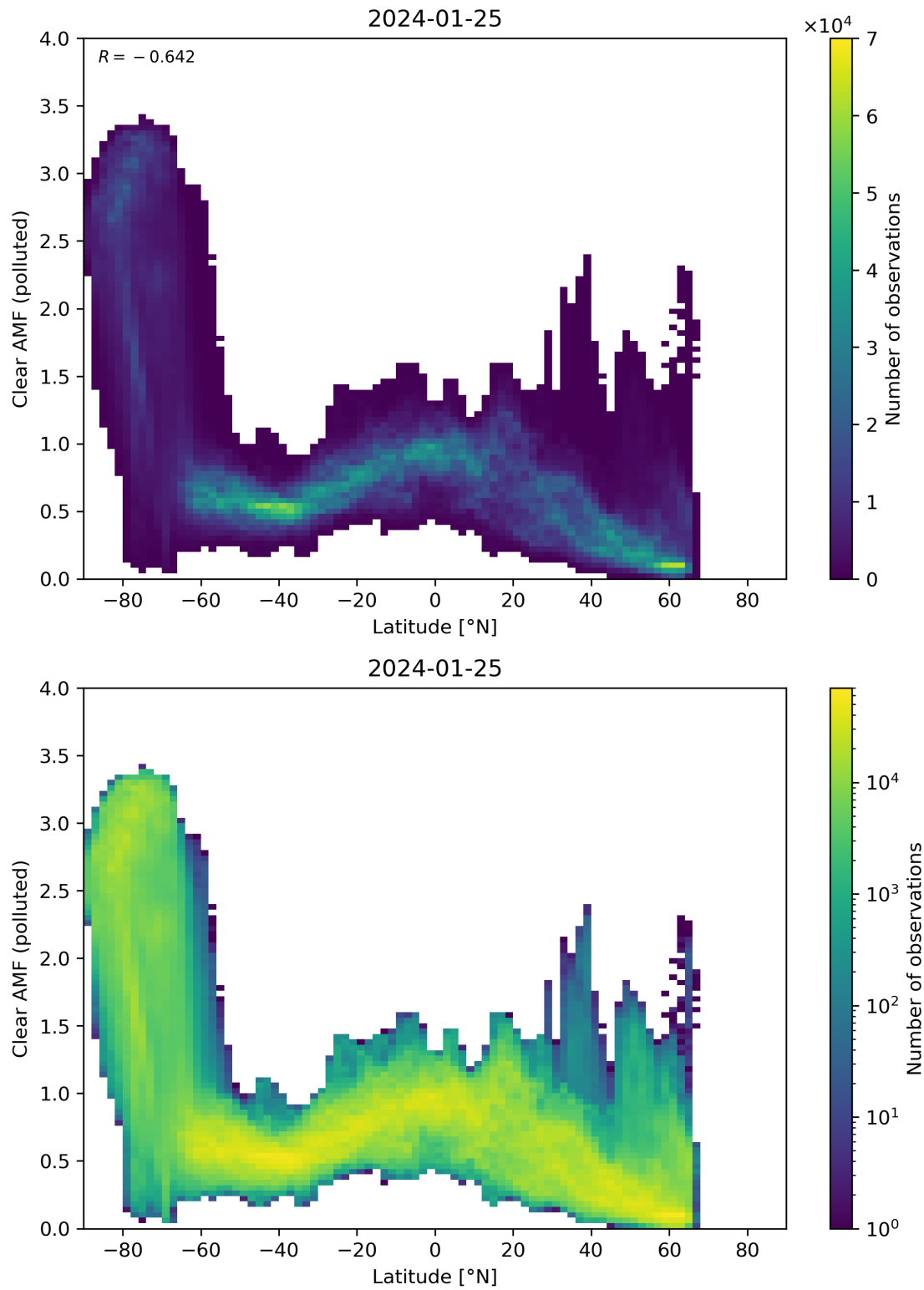
Figure 145: Scatter density plot of “Latitude” against “Clear AMF (polluted)” for 2024-01-24 to 2024-01-26.
