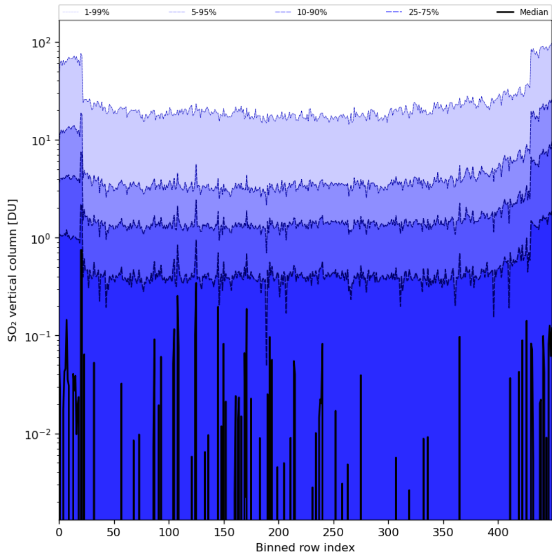
Figure 76: Along track statistics of “SO 2 vertical column” for 2024-01-24 to 2024-01-26
