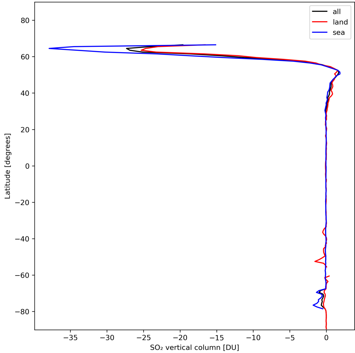
Figure 30: Zonal average of “SO 2 vertical column” for 2024-01-24 to 2024-01-26.
