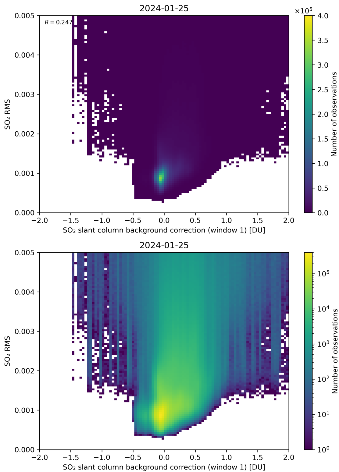
Figure 102: Scatter density plot of “SO 2 slant column background correction (window 1)” against “SO 2 RMS” for 2024-01-24 to 2024-01-26.
