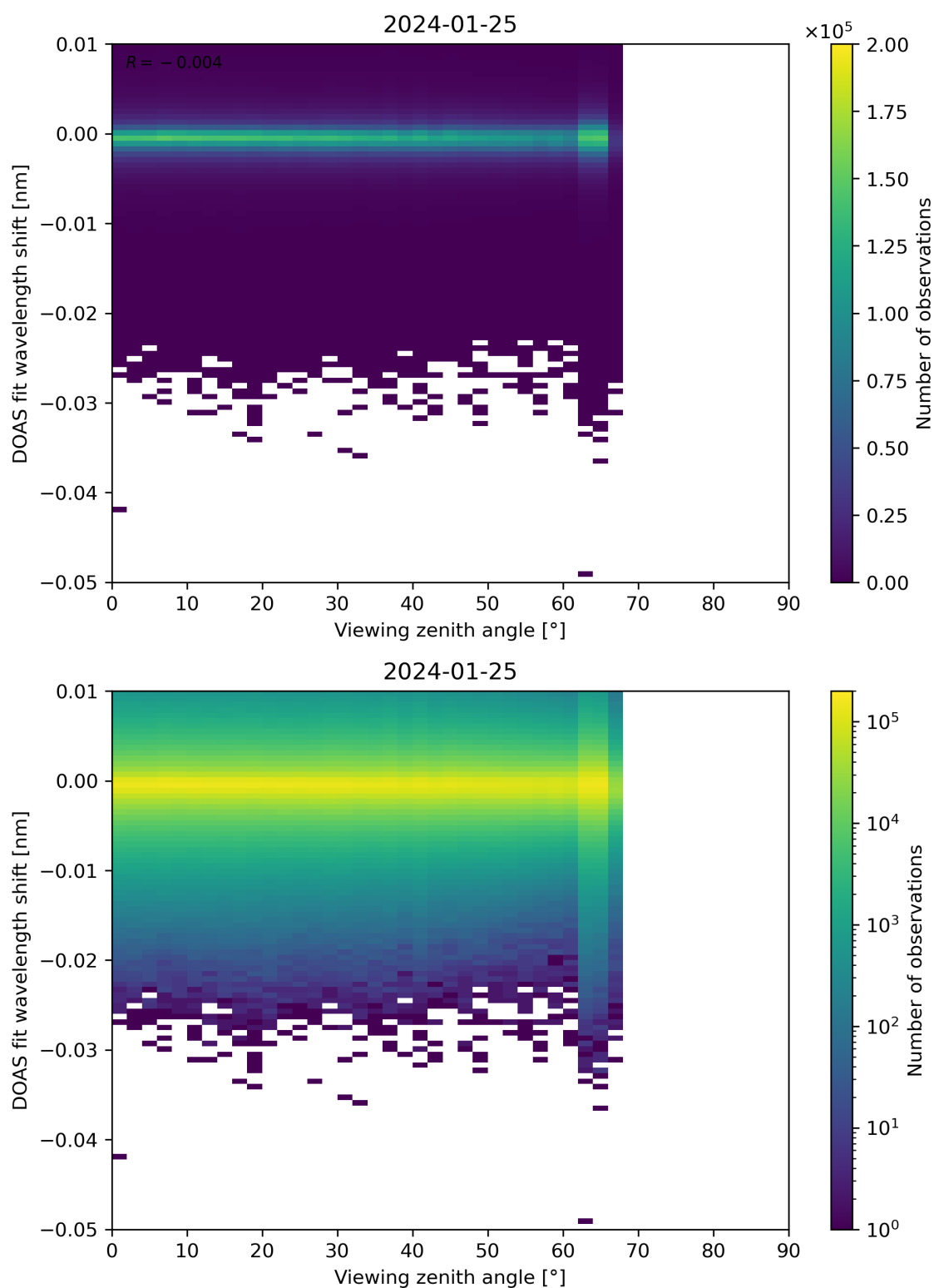
Figure 311: Scatter density plot of “Viewing zenith angle” against “DOAS fit wavelength shift” for 2024-01-24 to 2024-01-26.
