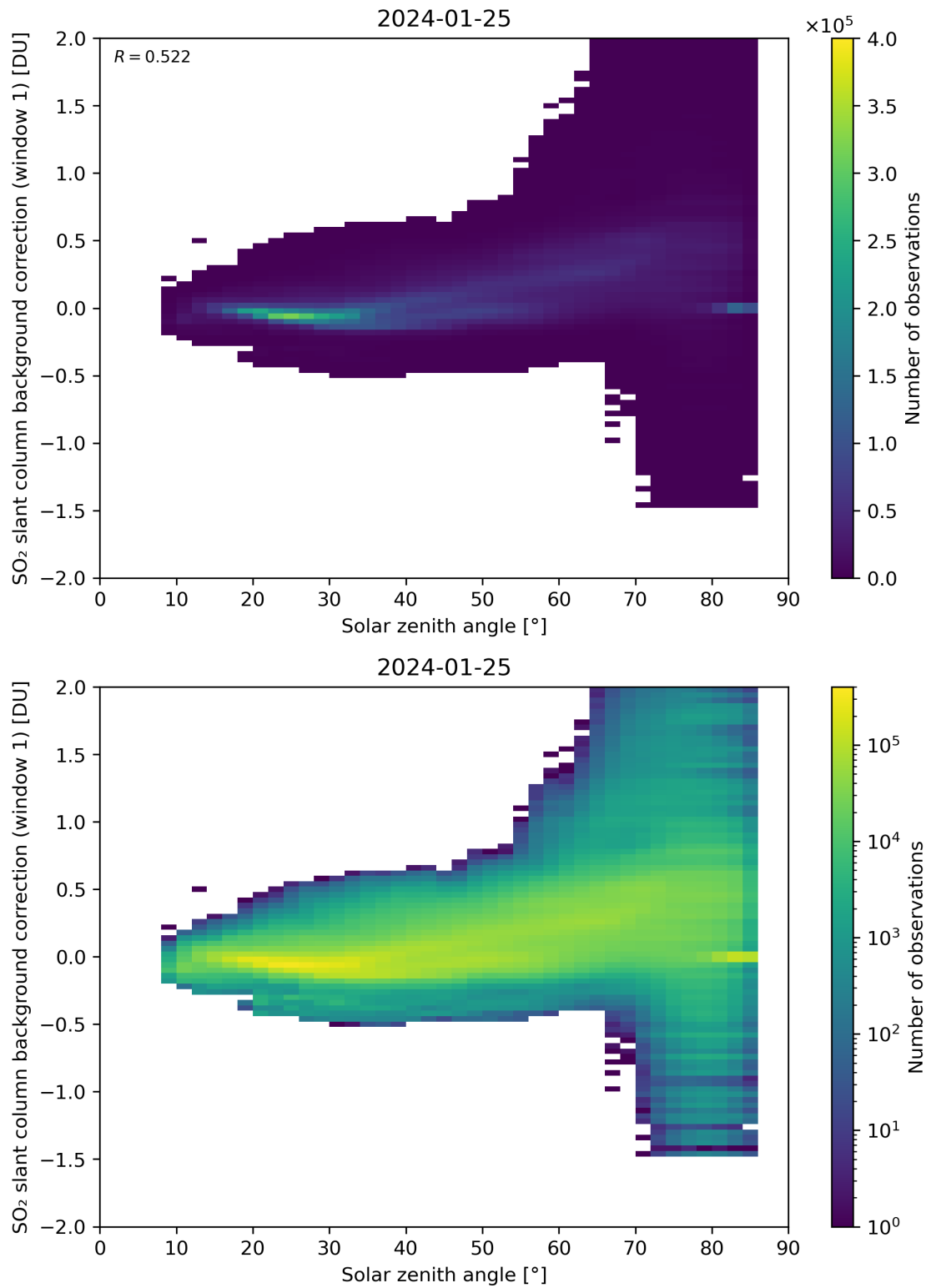
Figure 158: Scatter density plot of “Solar zenith angle” against “SO 2 slant column background correction (window 1)” for 2024-01-24 to 2024-01-26.
