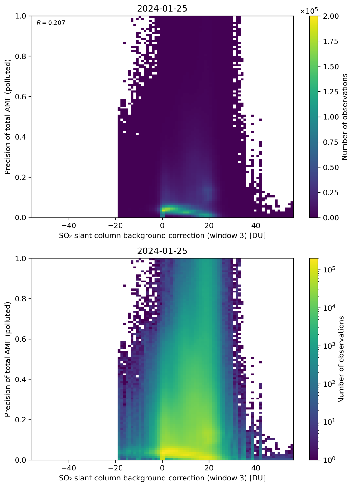
Figure 126: Scatter density plot of “SO 2 slant column background correction (window 3)” against “Precision of total AMF (polluted)” for 2024-01-24 to 2024-01-26.
