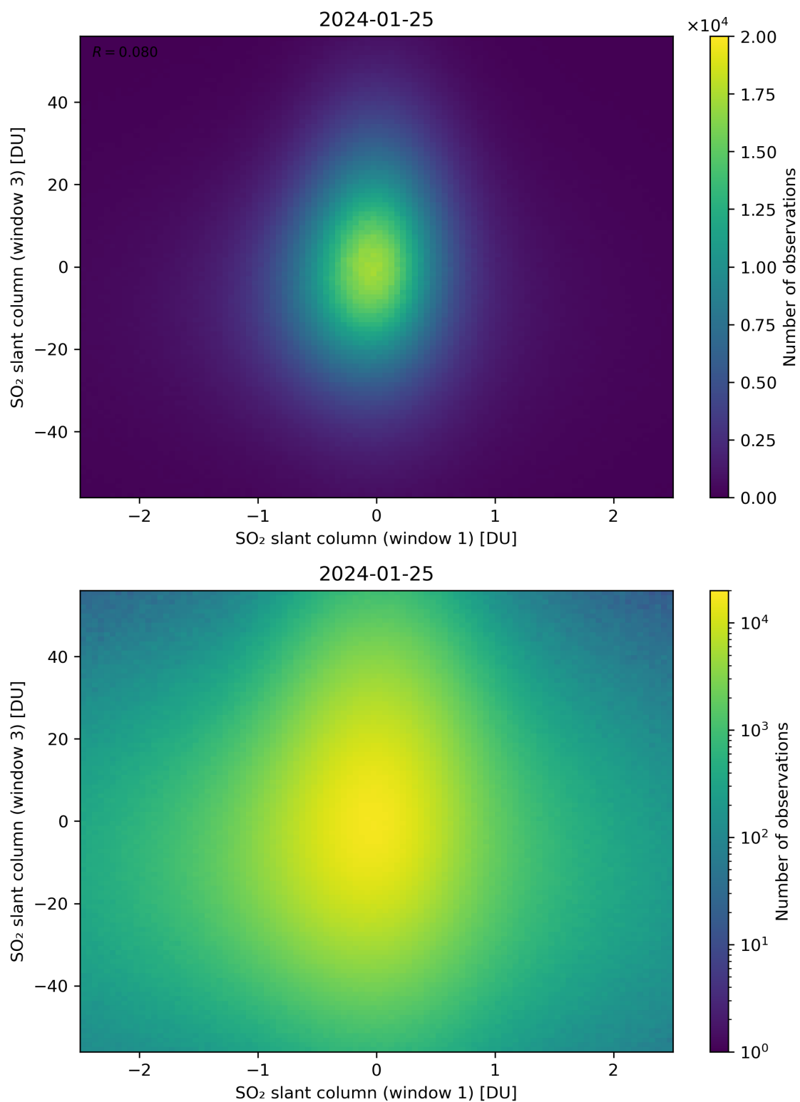
Figure 237: Scatter density plot of “SO 2 slant column (window 1)” against “SO 2 slant column (window 3)” for 2024-01-24 to 2024-01-26.
