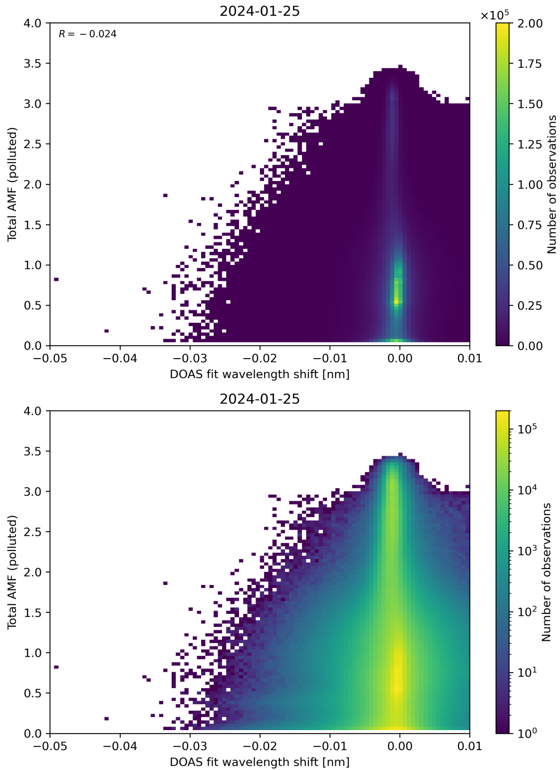
Figure 130: Scatter density plot of “DOAS fit wavelength shift” against “Total AMF (polluted)” for 2024-01-24 to 2024-01-26.
