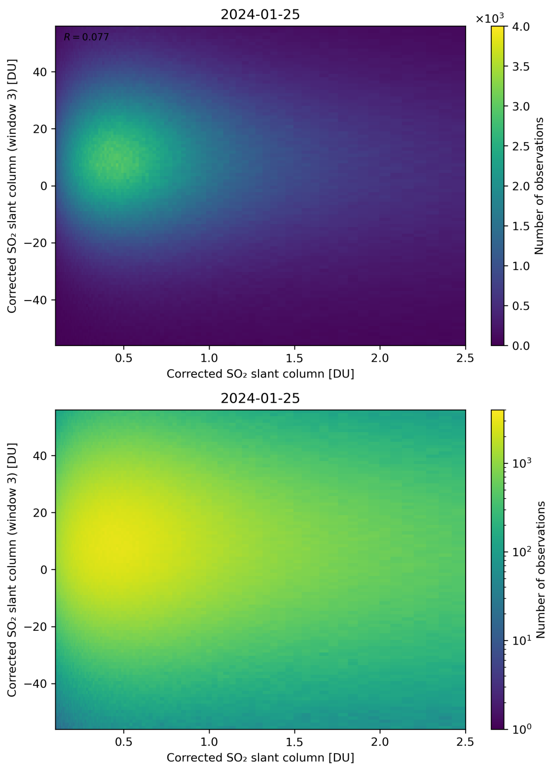
Figure 186: Scatter density plot of “Corrected SO 2 slant column” against “Corrected SO 2 slant column (window 3)” for 2024-01-24 to 2024-01-26.
