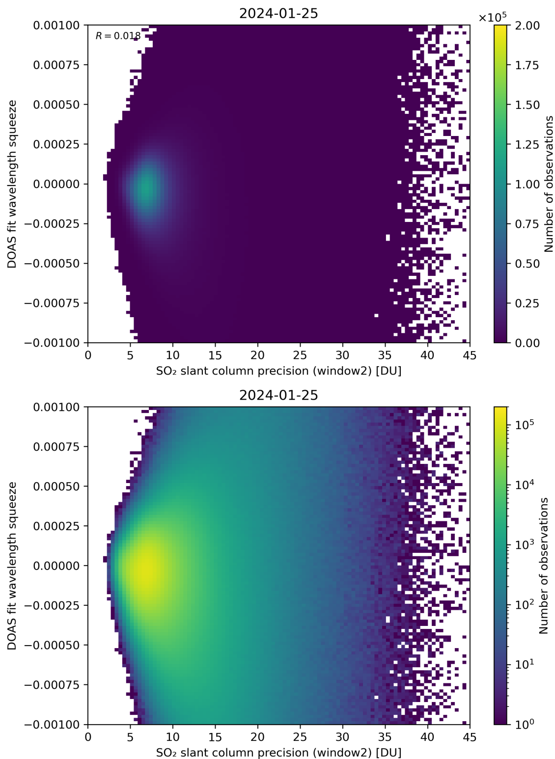
Figure 244: Scatter density plot of “SO 2 slant column precision (window2)” against “DOAS fit wavelength squeeze” for 2024-01-24 to 2024-01-26.
