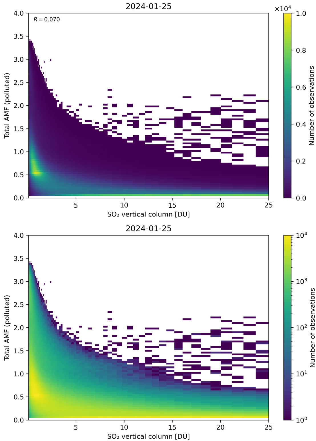
Figure 305: Scatter density plot of “SO 2 vertical column” against “Total AMF (polluted)” for 2024-01-24 to 2024-01-26.
