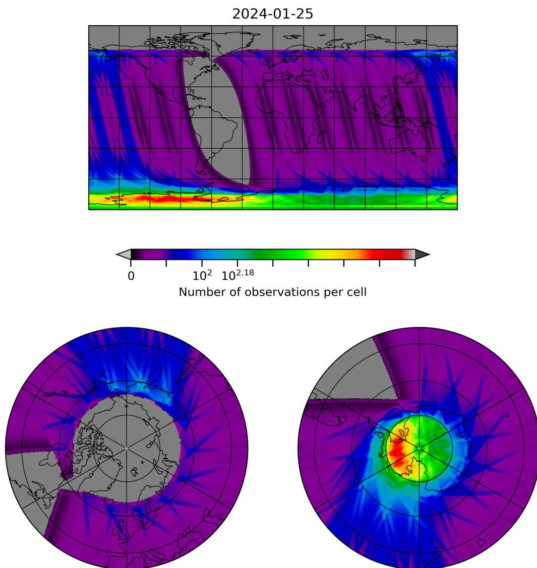
Figure 28: Map of the number of observations for 2024-01-24 to 2024-01-26
