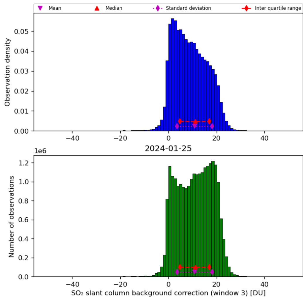
Figure 67: Histogram of “SO 2 slant column background correction (window 3)” for 2024-01-24 to 2024-01-26
