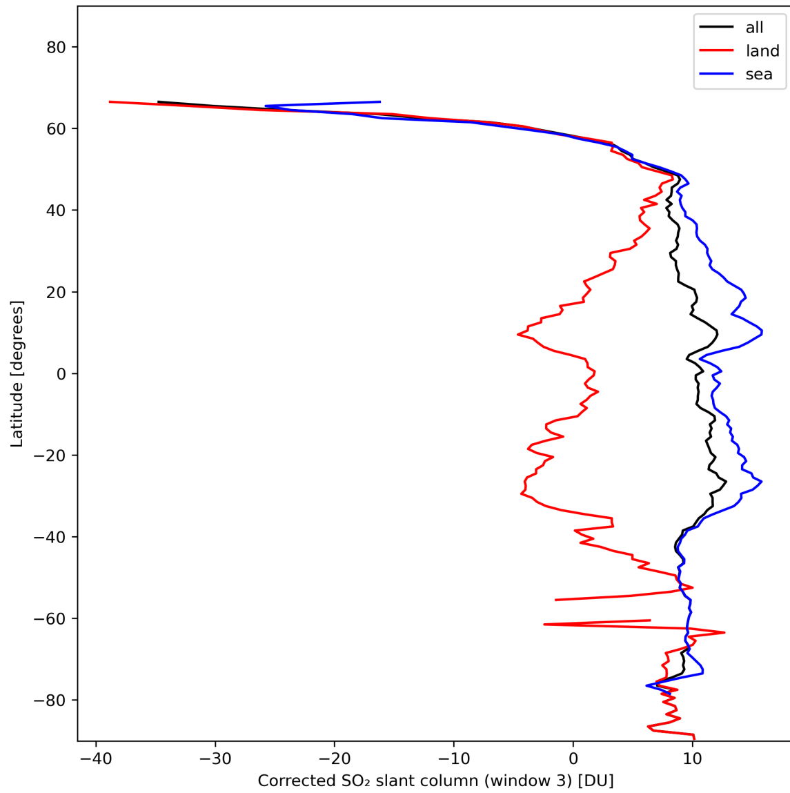
Figure 43: Zonal average of “Corrected SO 2 slant column (window 3)” for 2024-01-24 to 2024-01-26.
