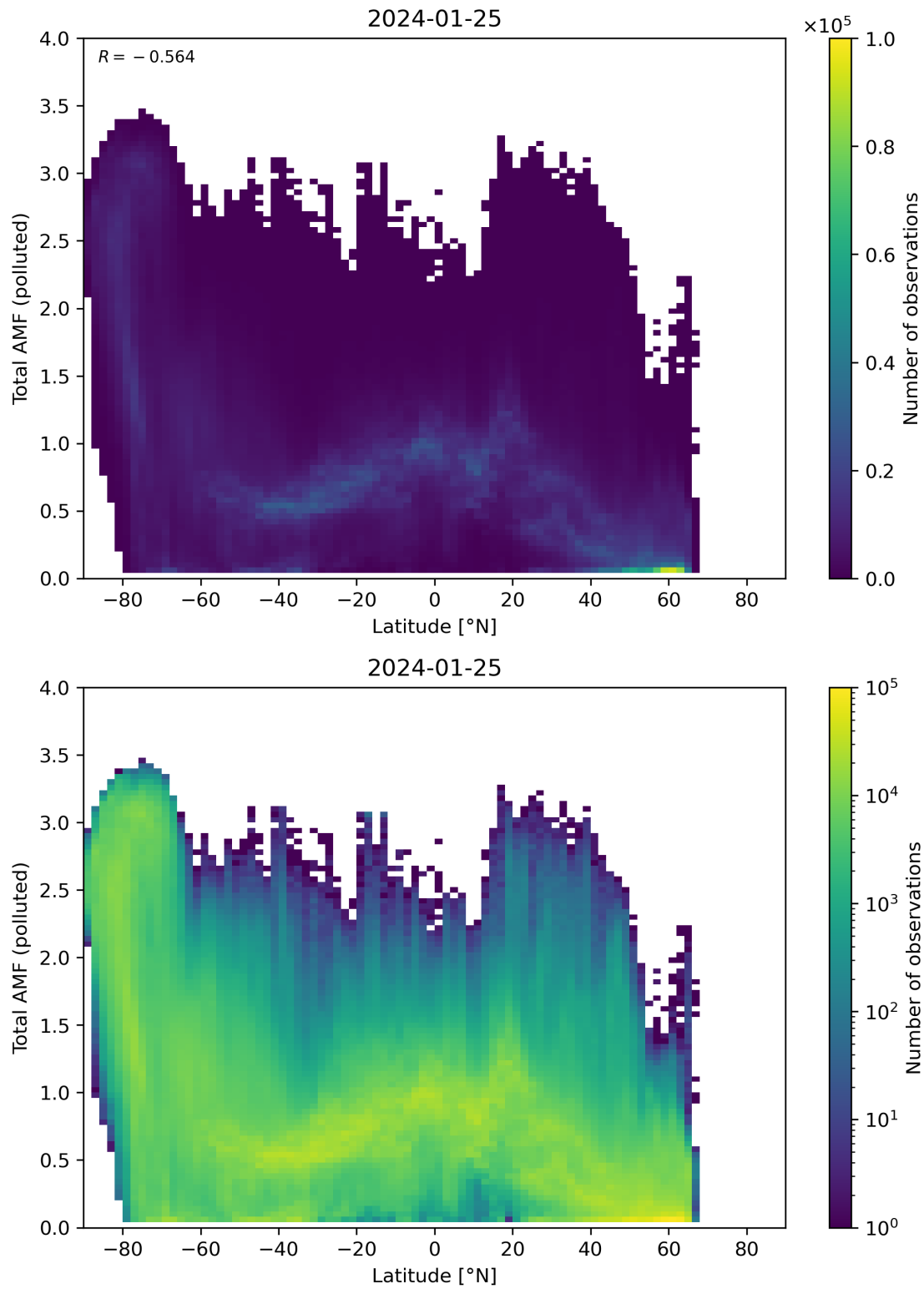
Figure 154: Scatter density plot of “Latitude” against “Total AMF (polluted)” for 2024-01-24 to 2024-01-26.
