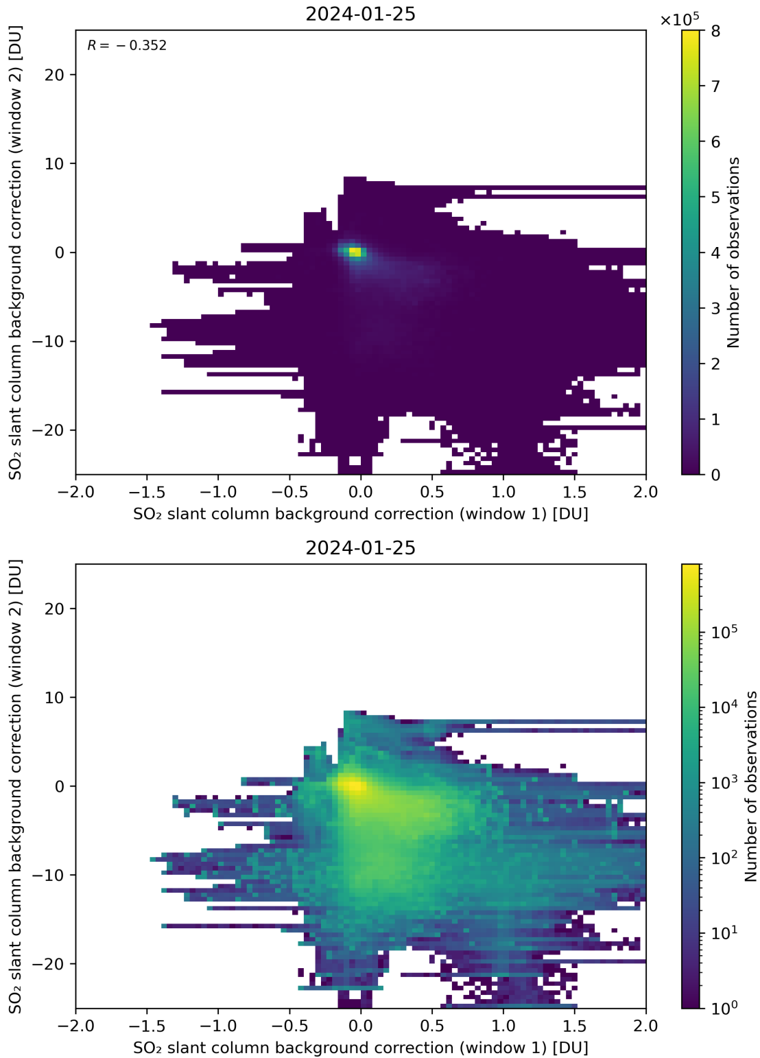
Figure 98: Scatter density plot of “SO 2 slant column background correction (window 1)” against “SO 2 slant column background correction (window 2)” for 2024-01-24 to 2024-01-26.
