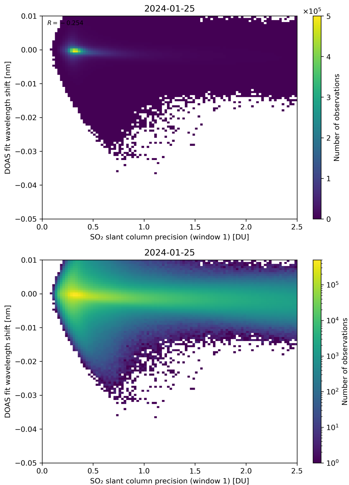
Figure 221: Scatter density plot of “SO 2 slant column precision (window 1)” against “DOAS fit wavelength shift” for 2024-01-24 to 2024-01-26.
