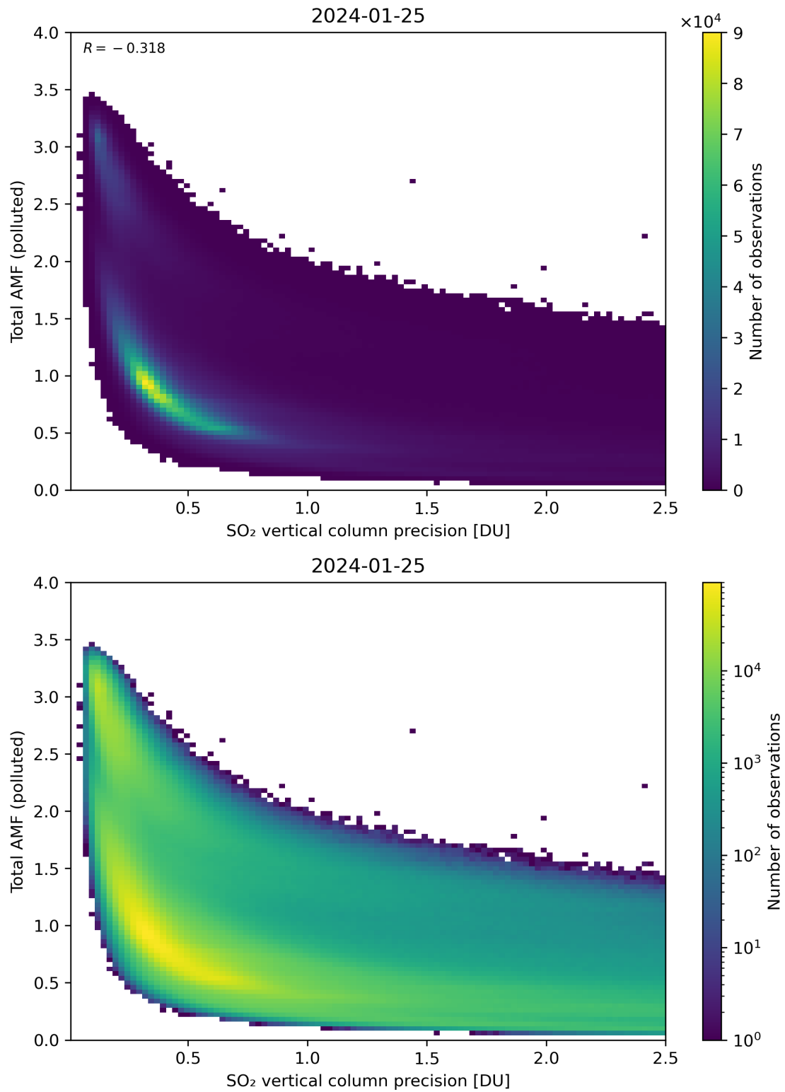
Figure 294: Scatter density plot of “SO 2 vertical column precision” against “Total AMF (polluted)” for 2024-01-24 to 2024-01-26.
