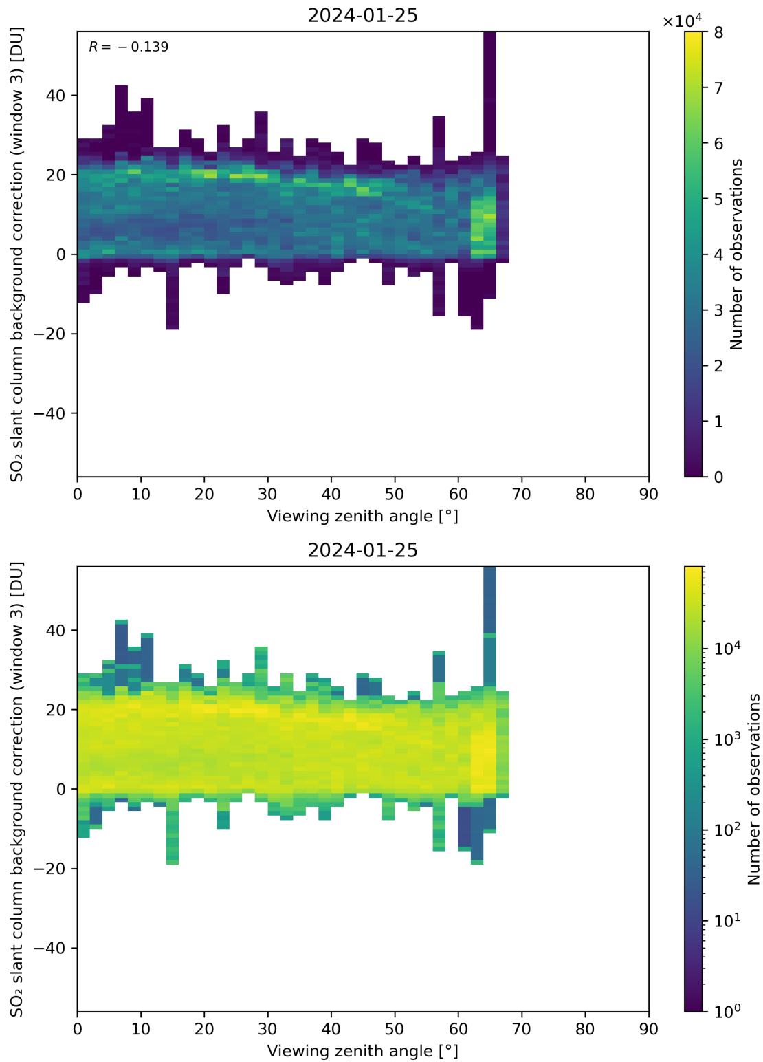
Figure 310: Scatter density plot of “Viewing zenith angle” against “SO 2 slant column background correction (window 3)” for 2024-01-24 to 2024-01-26.
