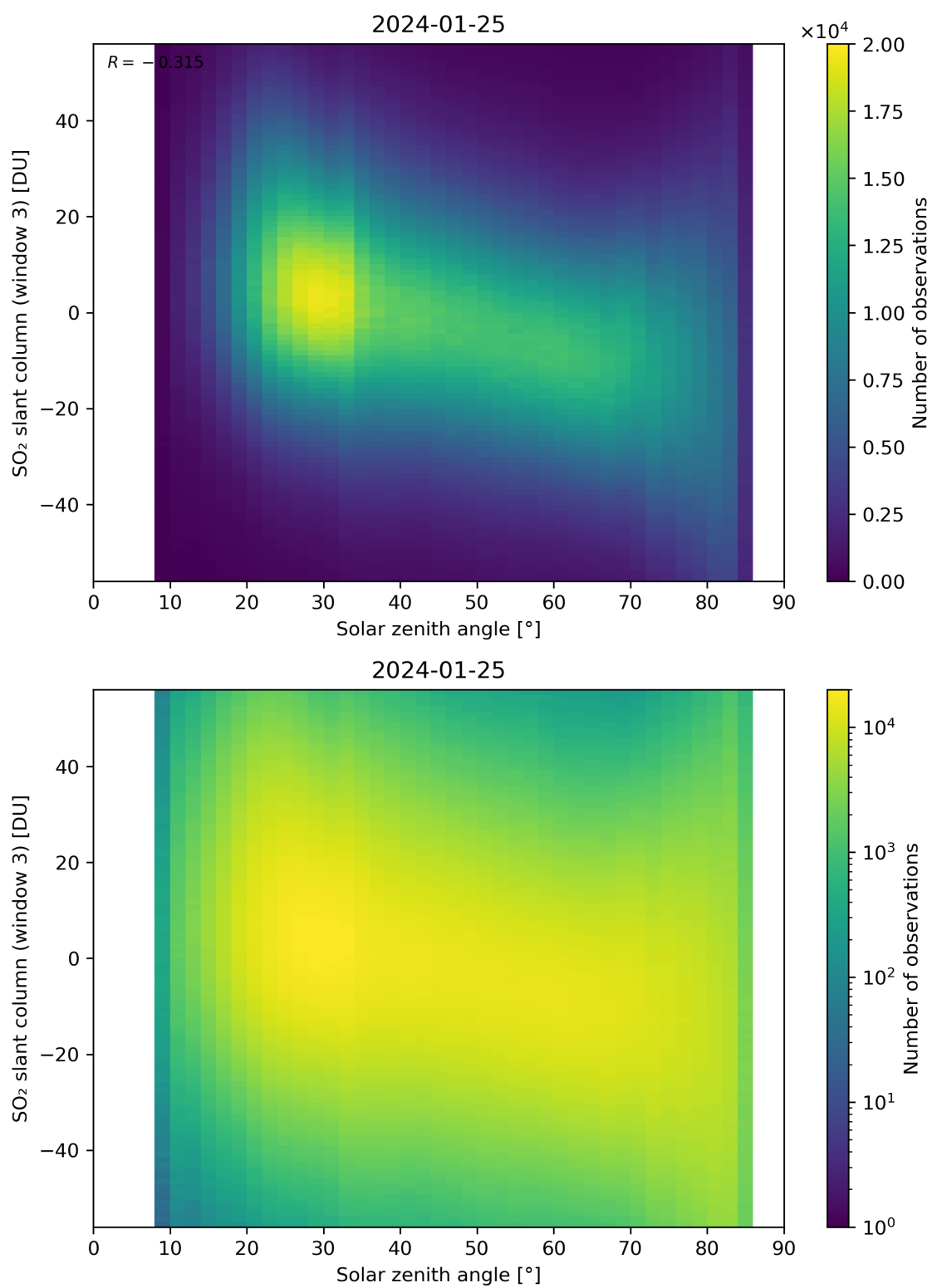
Figure 172: Scatter density plot of “Solar zenith angle” against “SO 2 slant column (window 3)” for 2024-01-24 to 2024-01-26.
