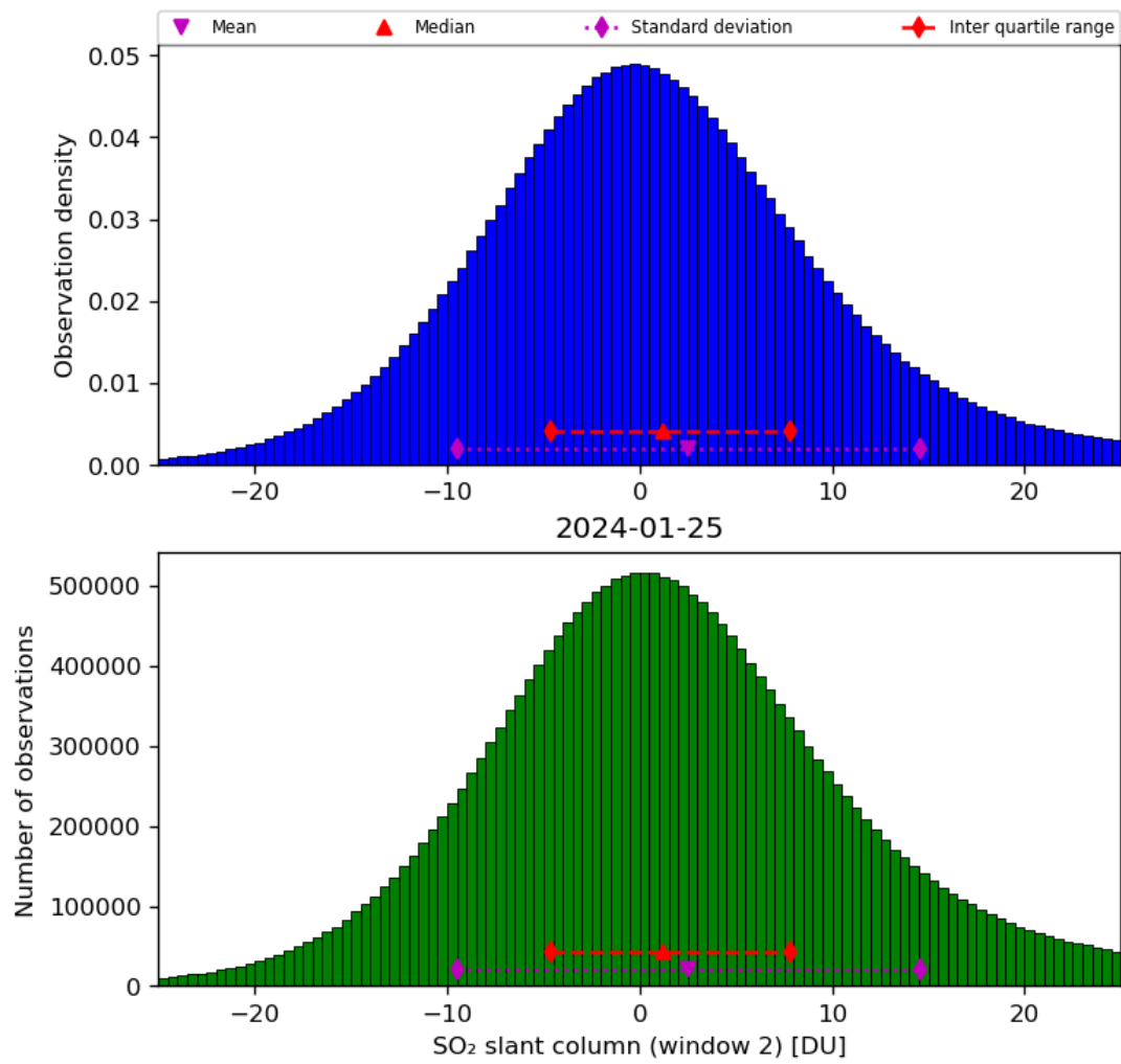
Figure 60: Histogram of “SO 2 slant column (window 2)” for 2024-01-24 to 2024-01-26
