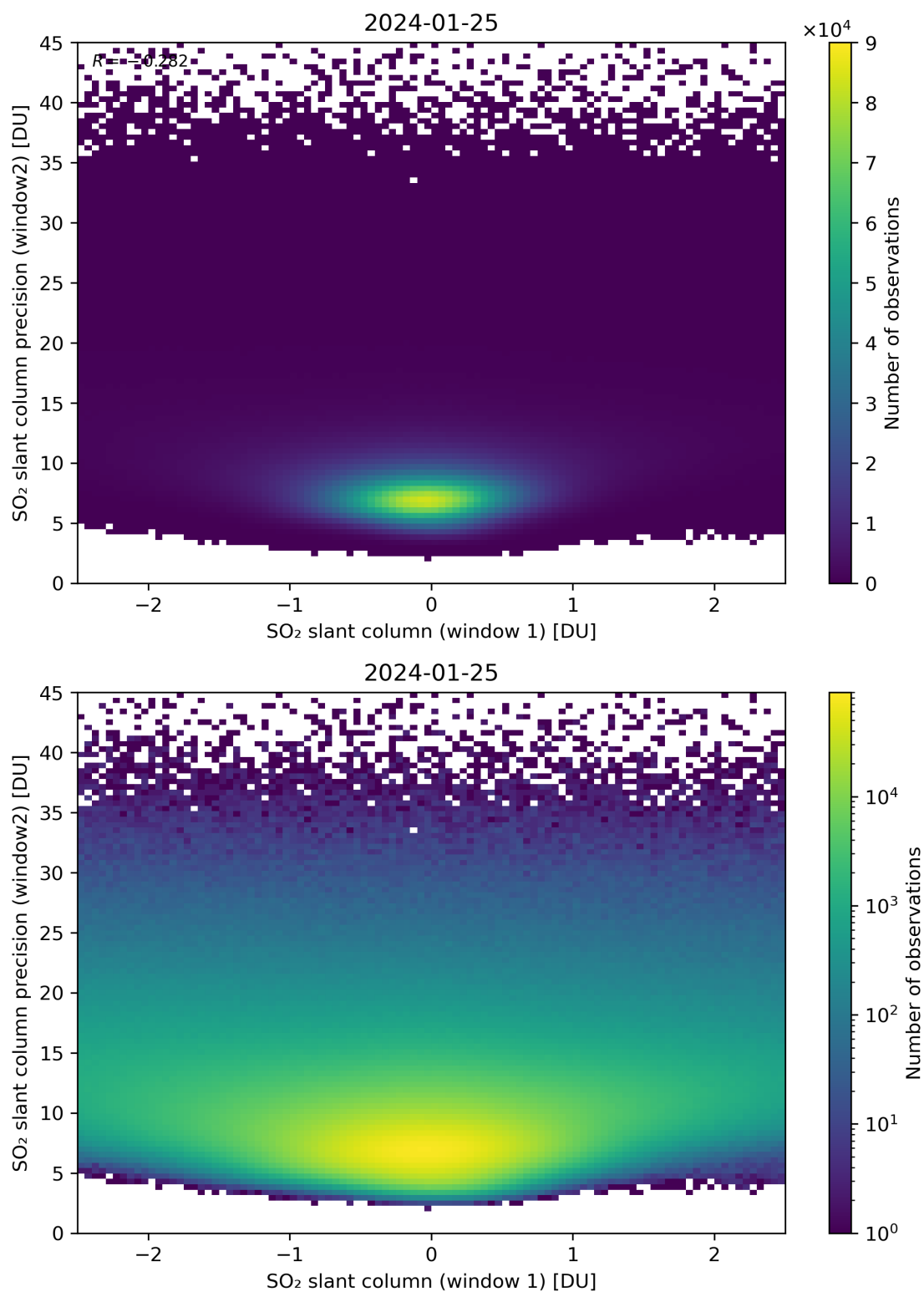
Figure 236: Scatter density plot of “SO 2 slant column (window 1)” against “SO 2 slant column precision (window2)” for 2024-01-24 to 2024-01-26.
