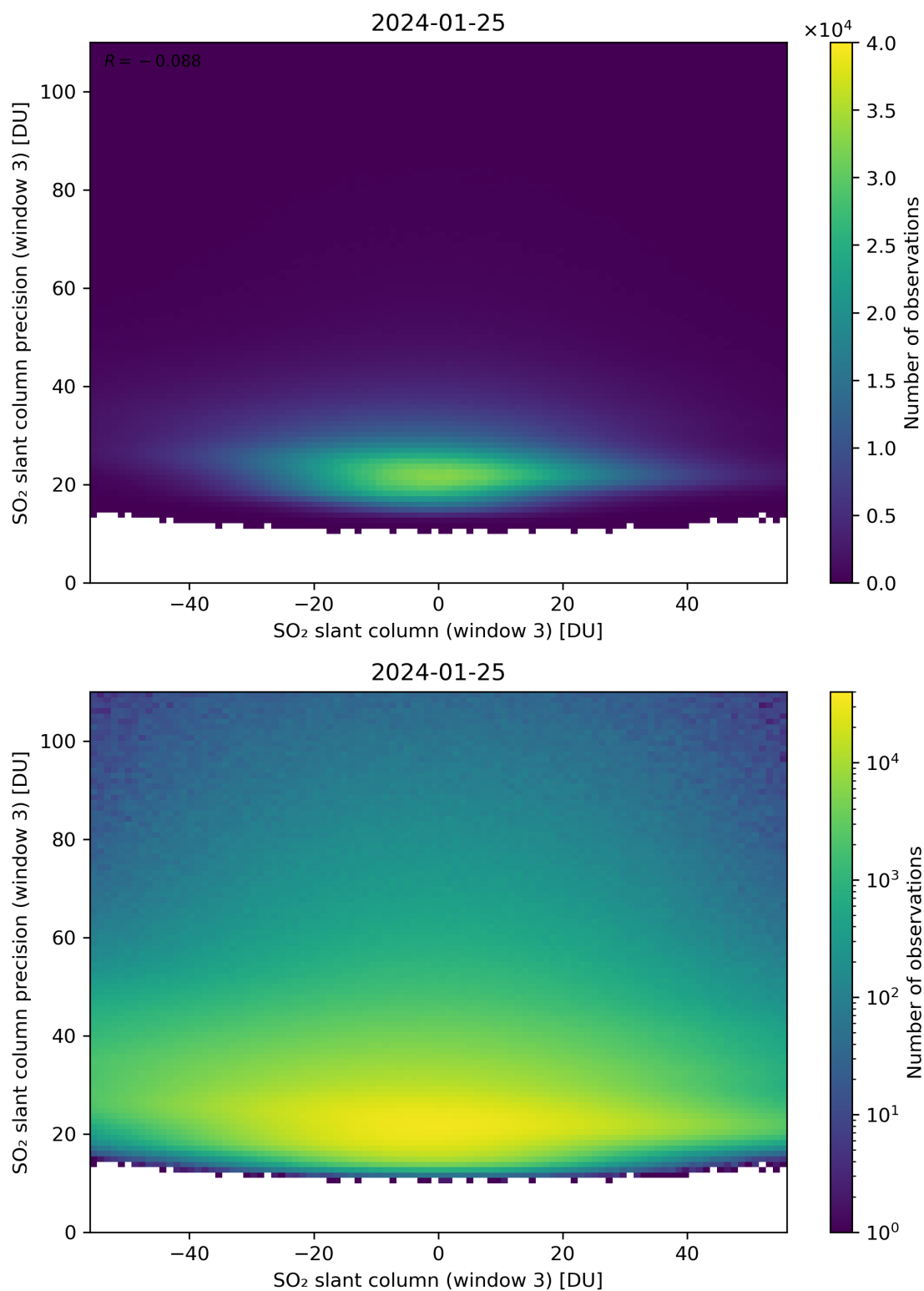
Figure 267: Scatter density plot of “SO 2 slant column (window 3)” against “SO 2 slant column precision (window 3)” for 2024-01-24 to 2024-01-26.
