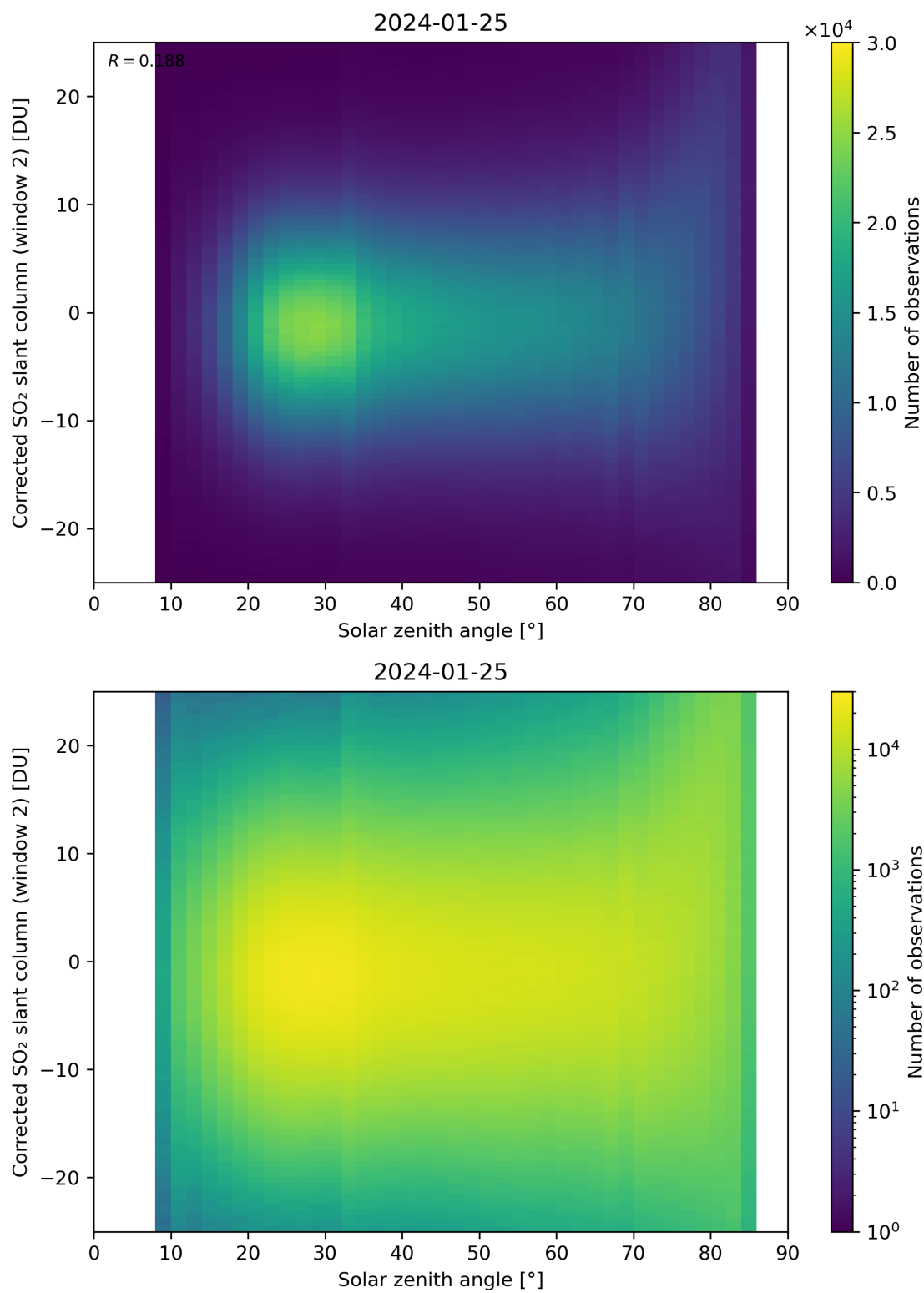
Figure 167: Scatter density plot of “Solar zenith angle” against “Corrected SO 2 slant column (window 2)” for 2024-01-24 to 2024-01-26.
