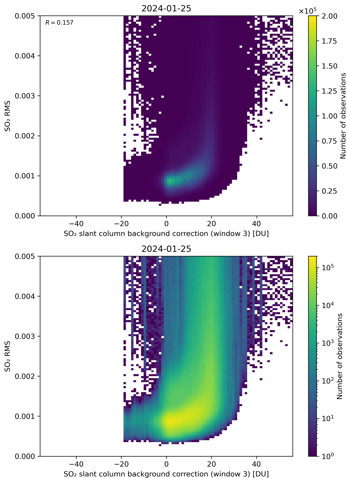
Figure 123: Scatter density plot of “SO 2 slant column background correction (window 3)” against “SO 2 RMS” for 2024-01-24 to 2024-01-26.
