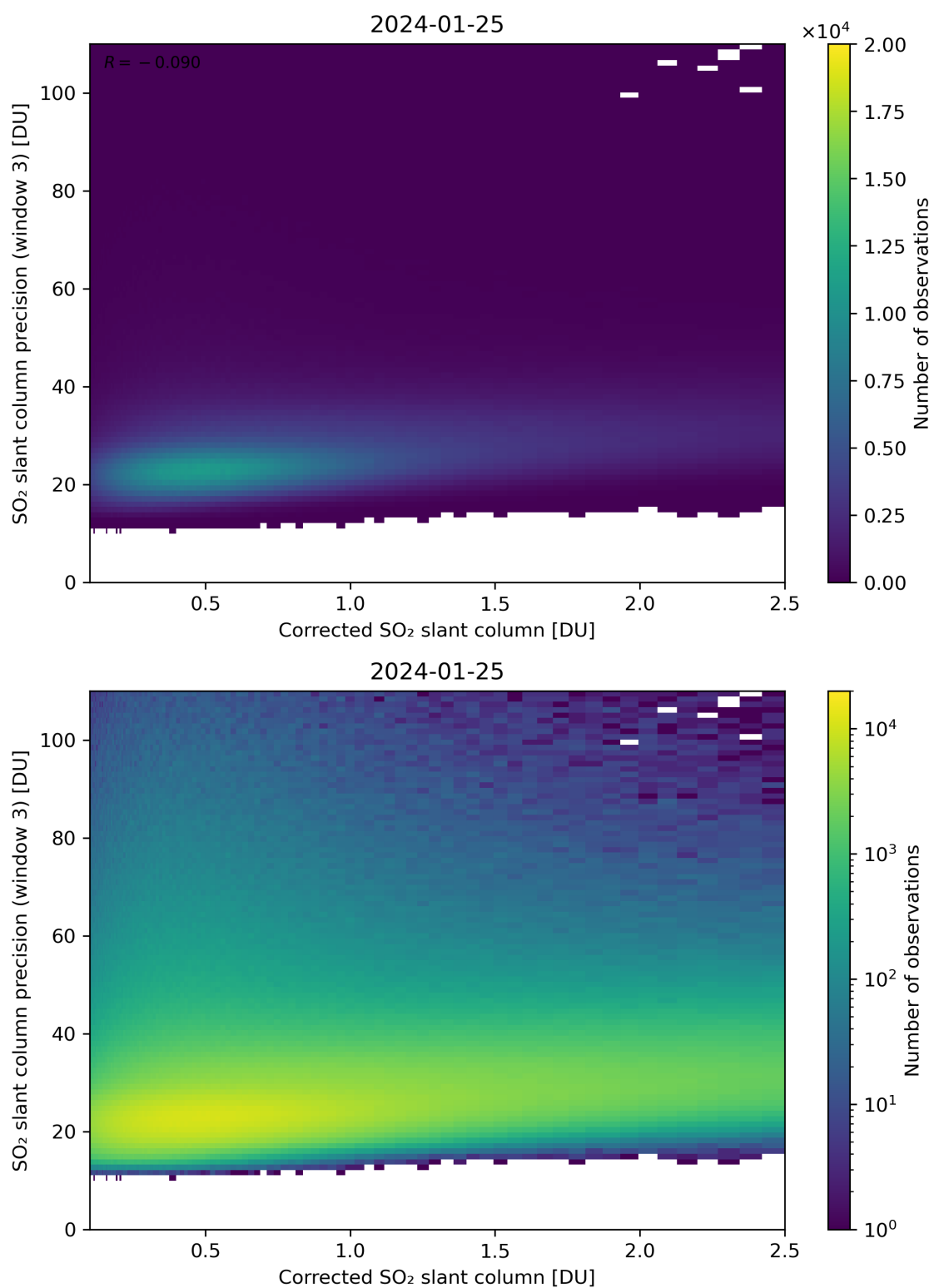
Figure 191: Scatter density plot of “Corrected SO 2 slant column” against “SO 2 slant column precision (window 3)” for 2024-01-24 to 2024-01-26.
