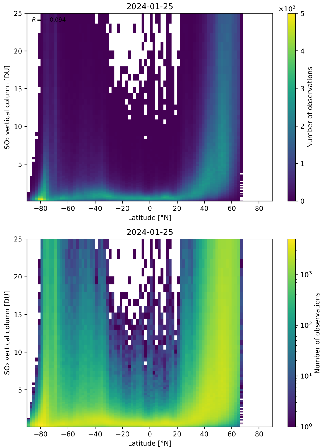
Figure 156: Scatter density plot of “Latitude” against “SO 2 vertical column” for 2024-01-24 to 2024-01-26.
