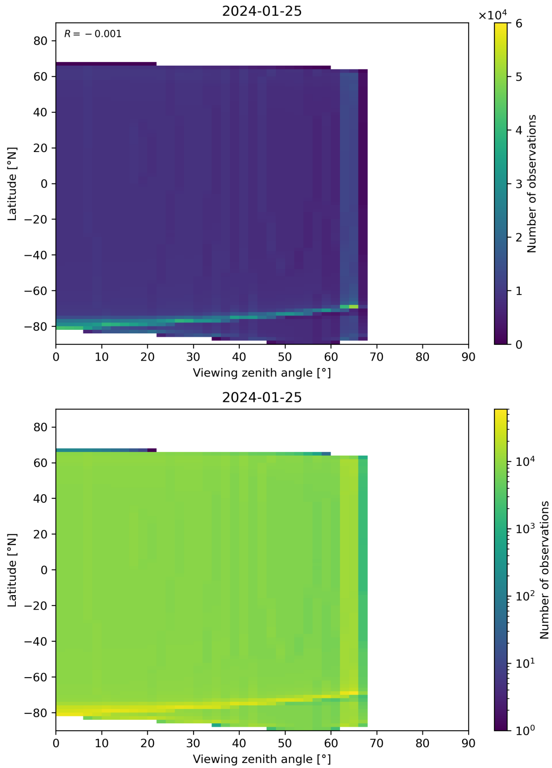
Figure 314: Scatter density plot of “Viewing zenith angle” against “Latitude” for 2024-01-24 to 2024-01-26.
