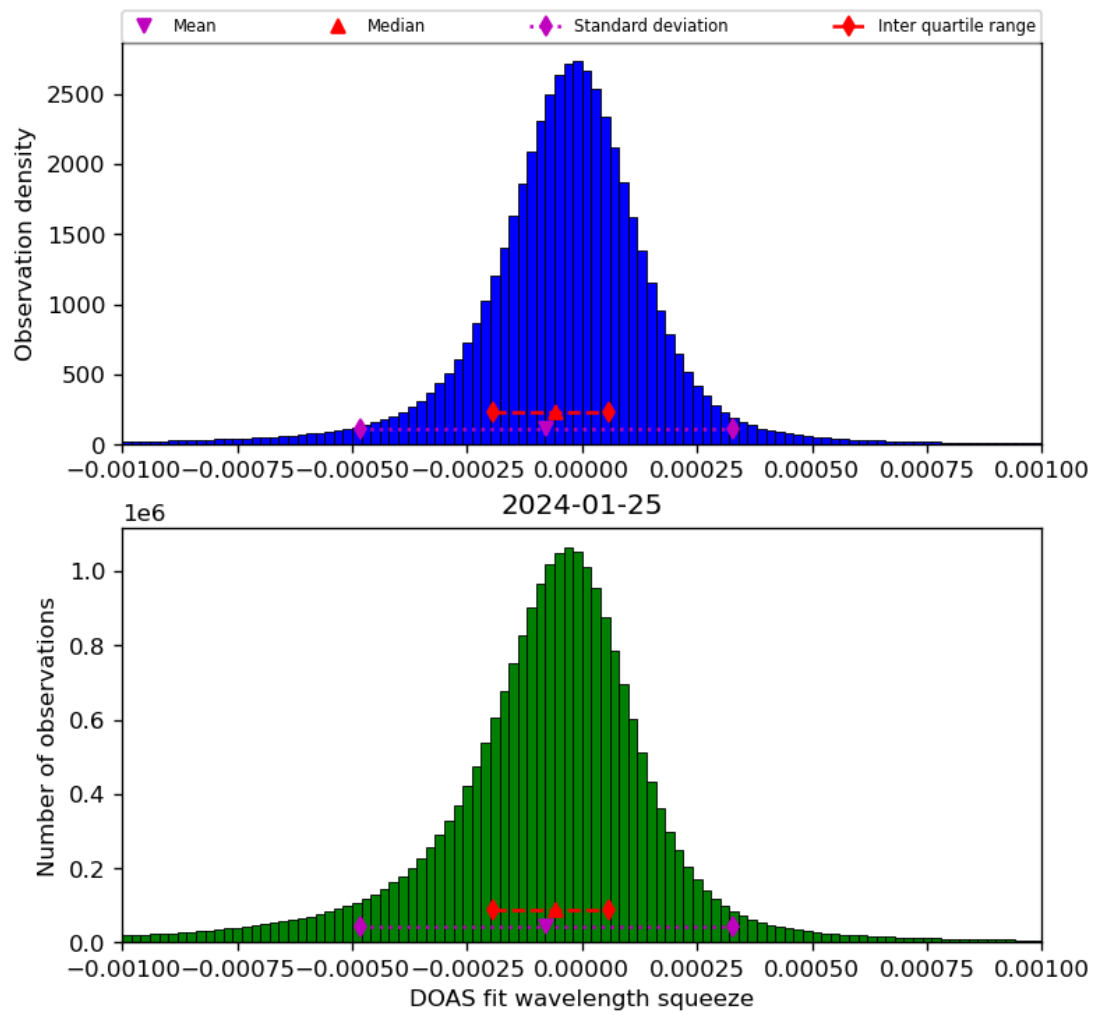
Figure 69: Histogram of “DOAS fit wavelength squeeze” for 2024-01-24 to 2024-01-26
