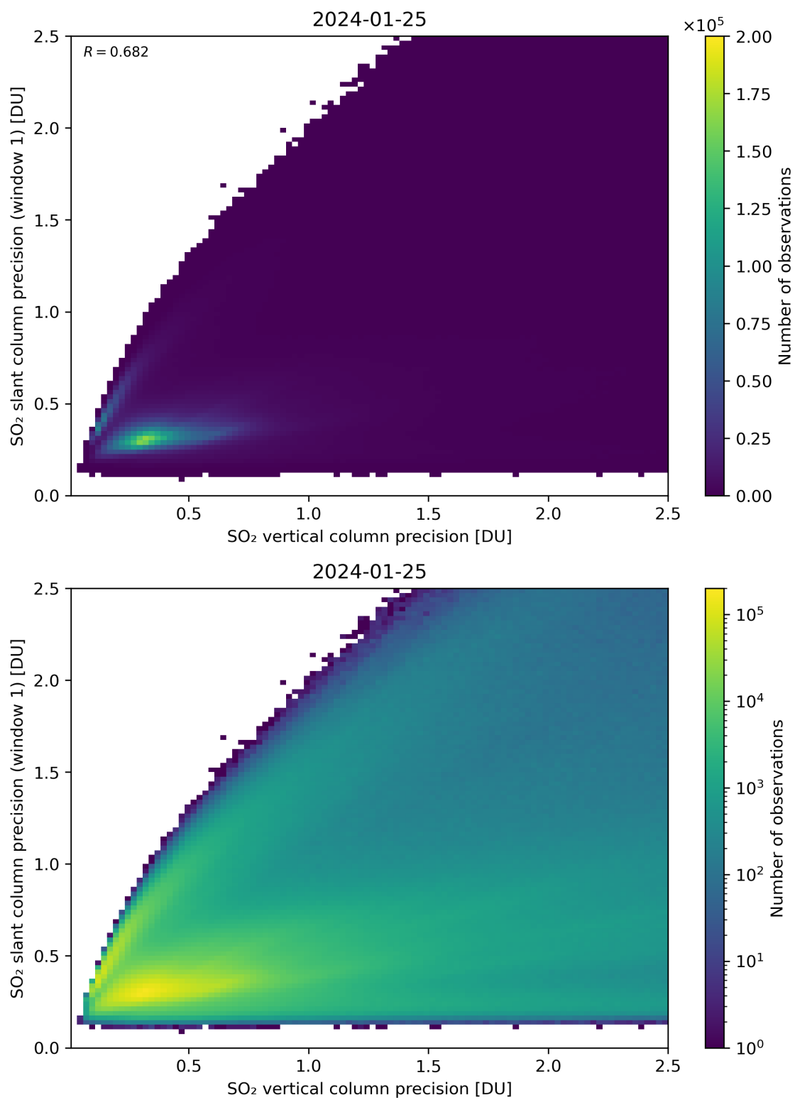
Figure 290: Scatter density plot of “SO 2 vertical column precision” against “SO 2 slant column precision (window 1)” for 2024-01-24 to 2024-01-26.
