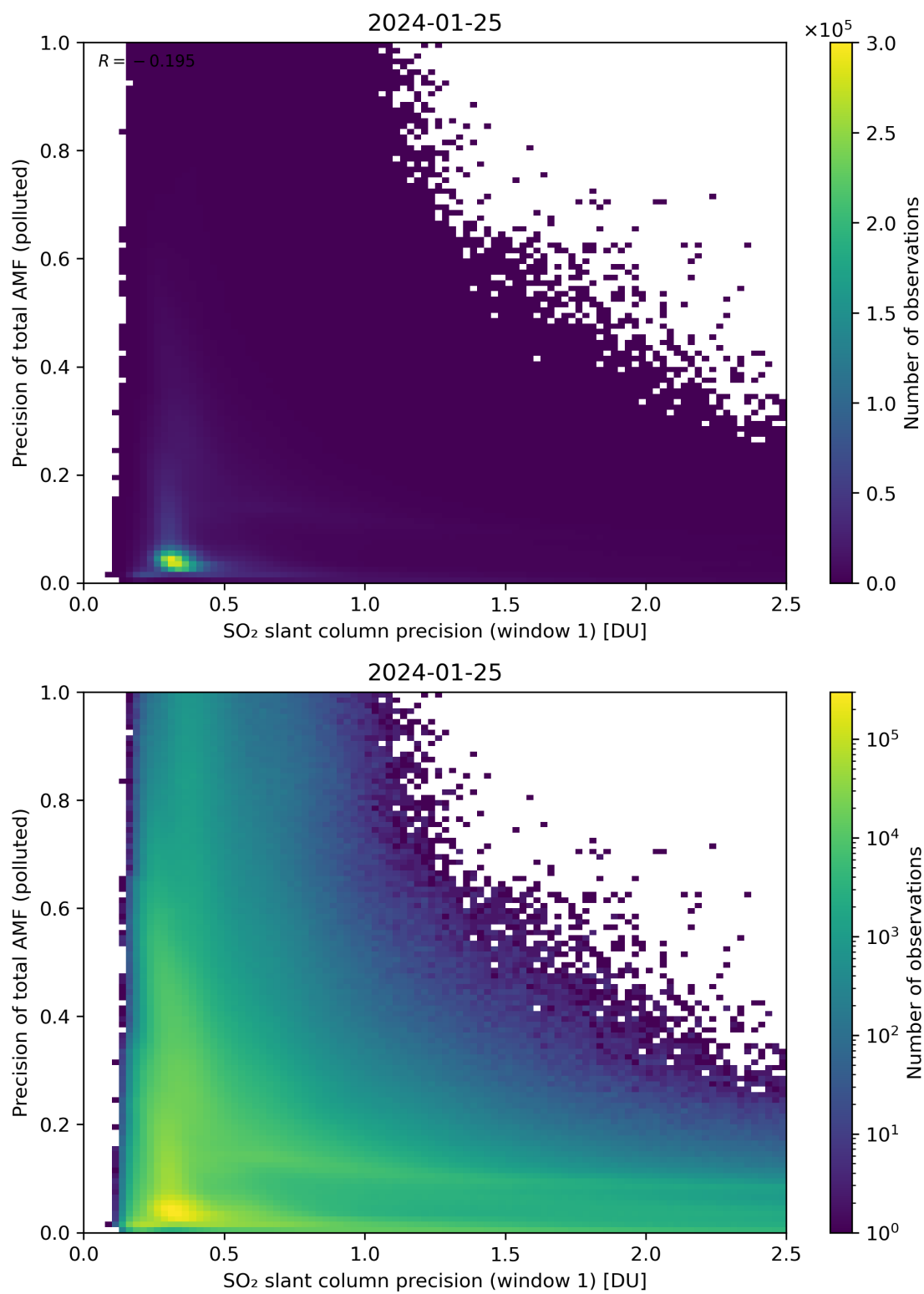
Figure 231: Scatter density plot of “SO 2 slant column precision (window 1)” against “Precision of total AMF (polluted)” for 2024-01-24 to 2024-01-26.
