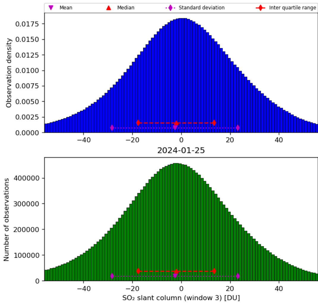
Figure 64: Histogram of “SO 2 slant column (window 3)” for 2024-01-24 to 2024-01-26
