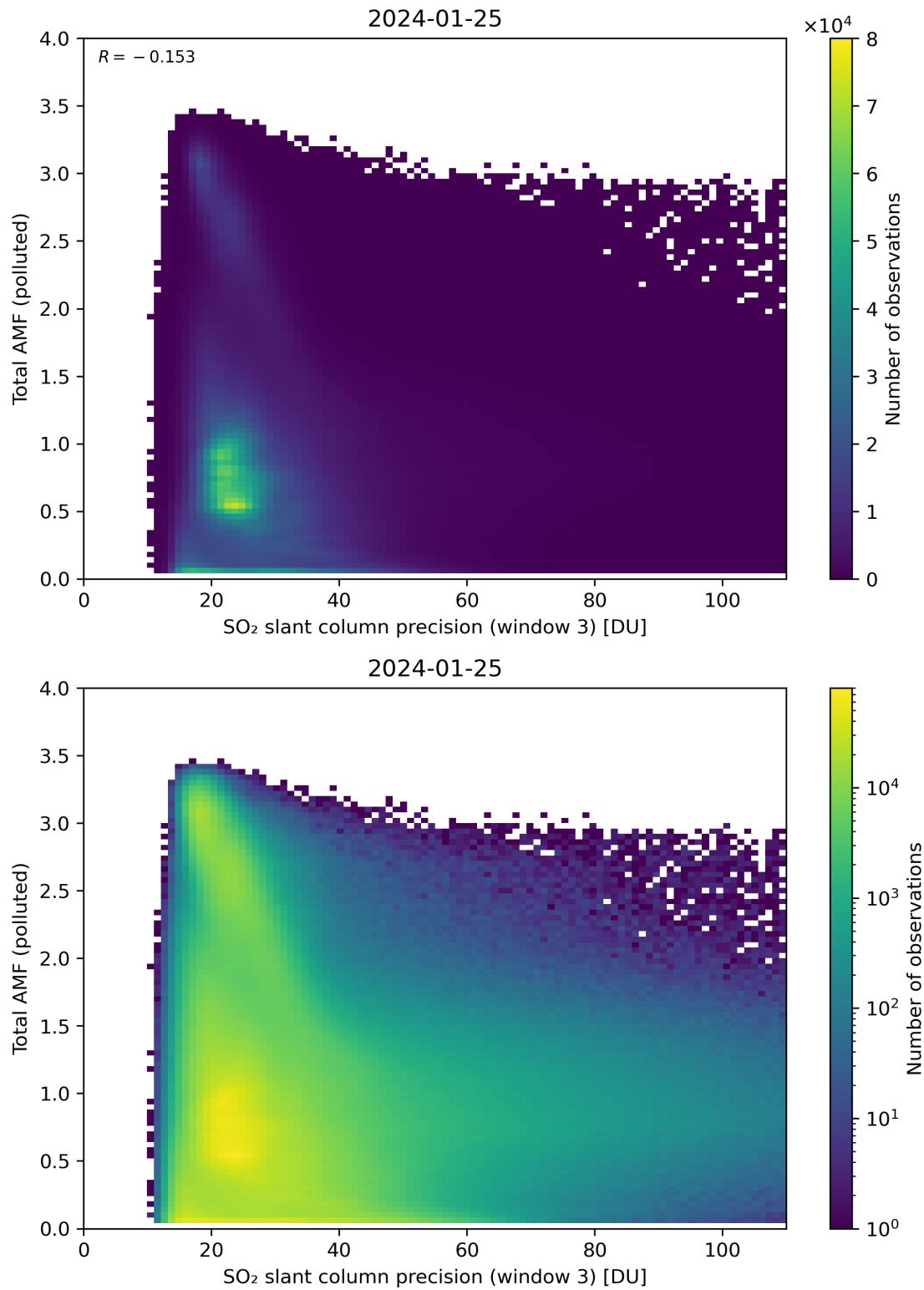
Figure 263: Scatter density plot of “SO 2 slant column precision (window 3)” against “Total AMF (polluted)” for 2024-01-24 to 2024-01-26.
