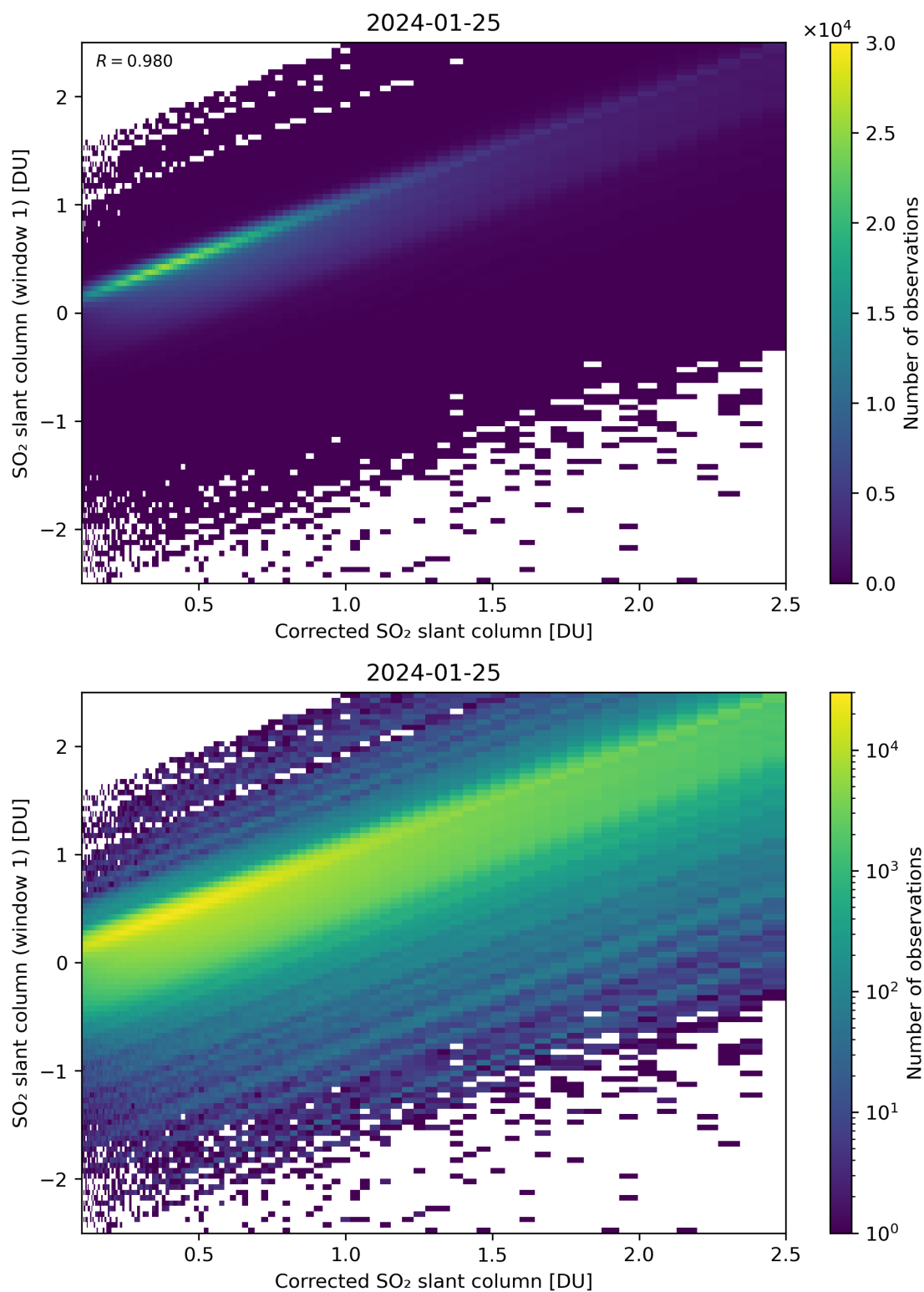
Figure 187: Scatter density plot of “Corrected SO 2 slant column” against “SO 2 slant column (window 1)” for 2024-01-24 to 2024-01-26.
