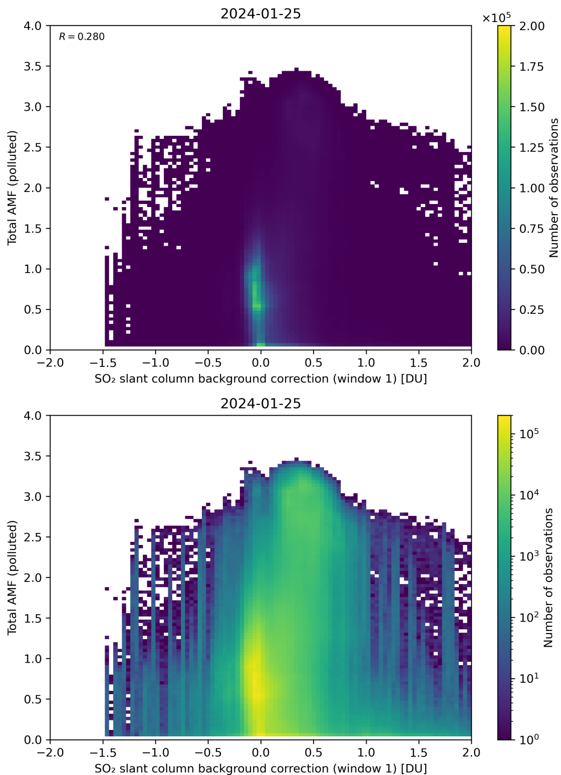
Figure 109: Scatter density plot of “SO 2 slant column background correction (window 1)” against “Total AMF (polluted)” for 2024-01-24 to 2024-01-26.
