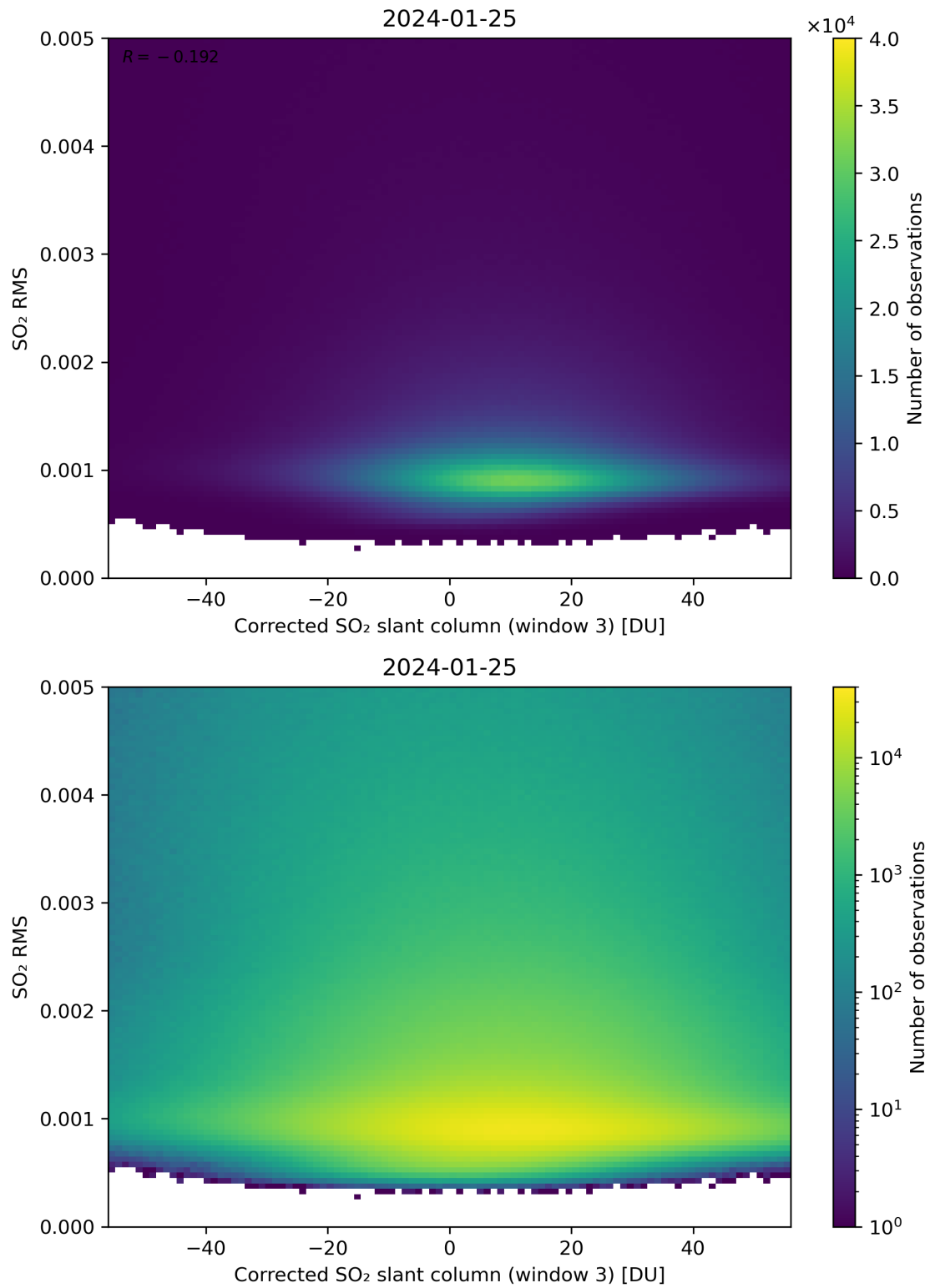
Figure 208: Scatter density plot of “Corrected SO 2 slant column (window 3)” against “SO 2 RMS” for 2024-01-24 to 2024-01-26.
