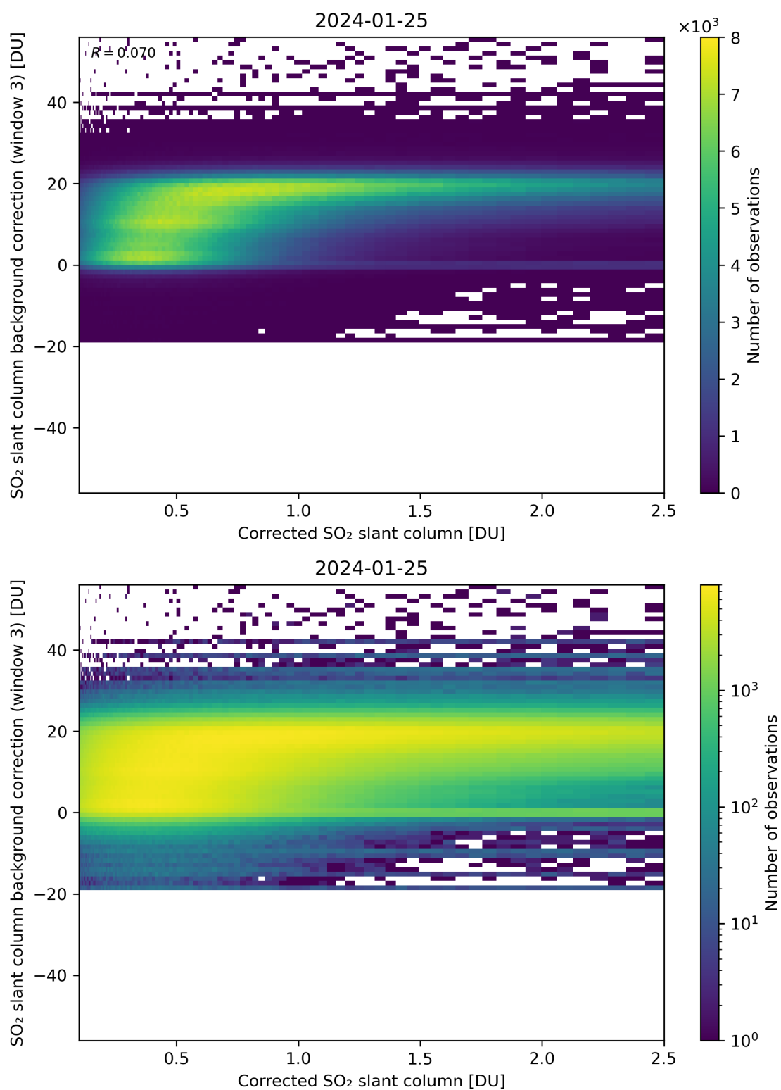
Figure 180: Scatter density plot of “Corrected SO 2 slant column” against “SO 2 slant column background correction (window 3)” for 2024-01-24 to 2024-01-26.
