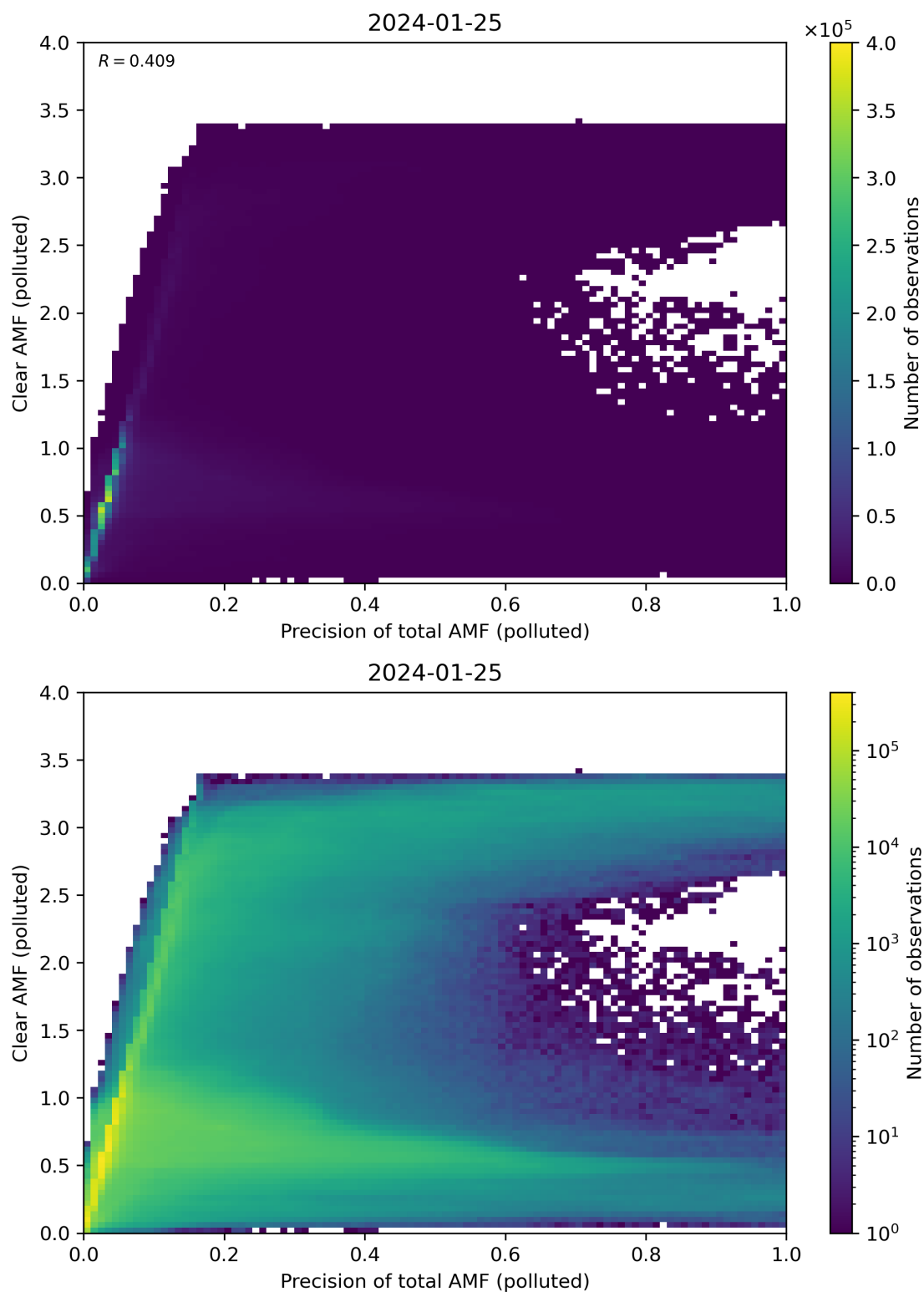
Figure 270: Scatter density plot of “Precision of total AMF (polluted)” against “Clear AMF (polluted)” for 2024-01-24 to 2024-01-26.
