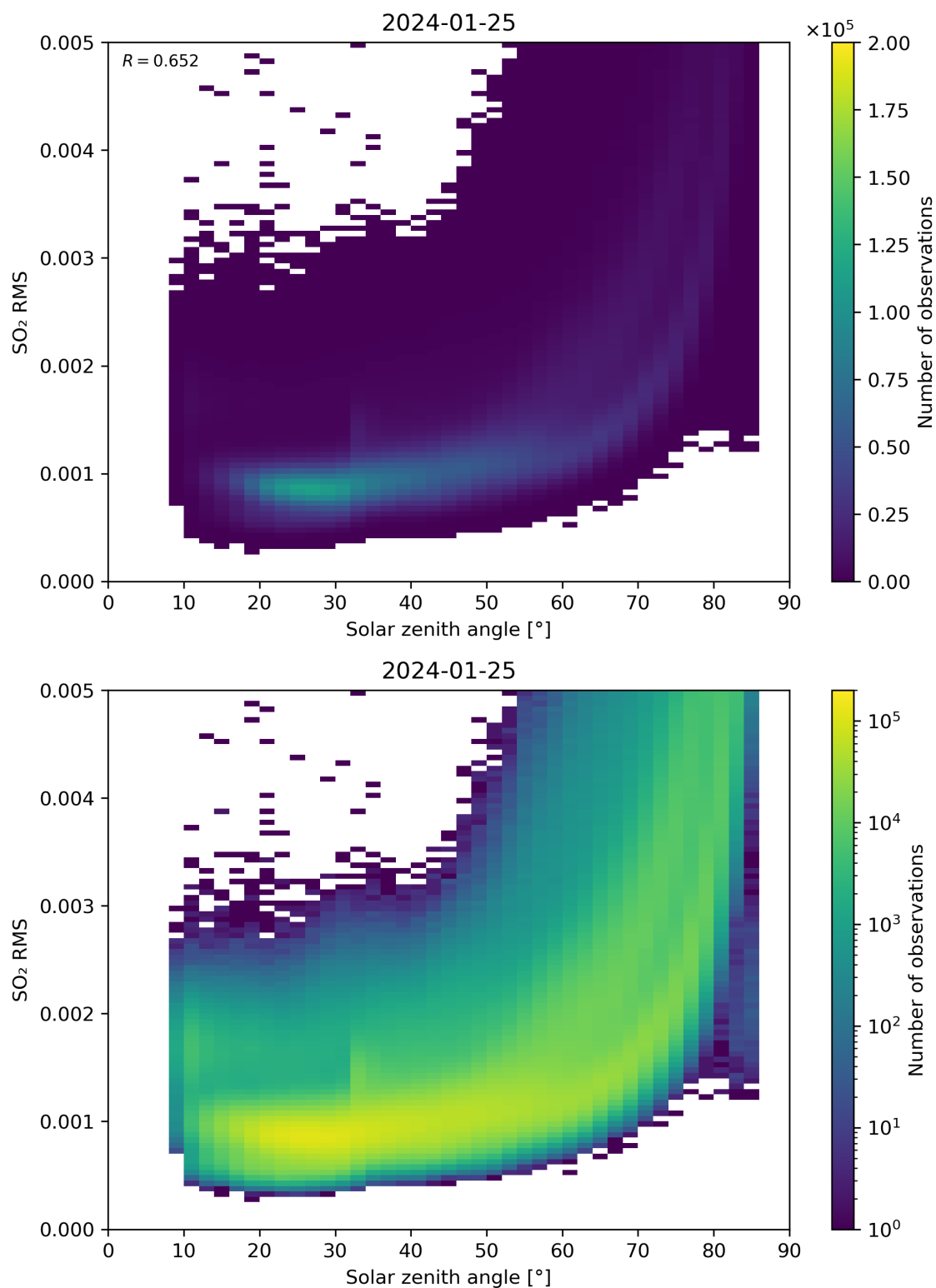
Figure 163: Scatter density plot of “Solar zenith angle” against “SO 2 RMS” for 2024-01-24 to 2024-01-26.
