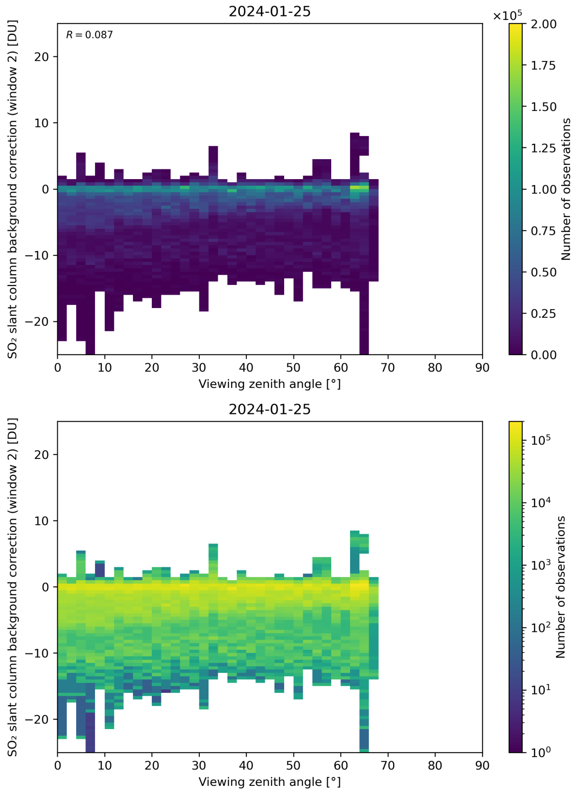
Figure 309: Scatter density plot of “Viewing zenith angle” against “SO 2 slant column background correction (window 2)” for 2024-01-24 to 2024-01-26.
