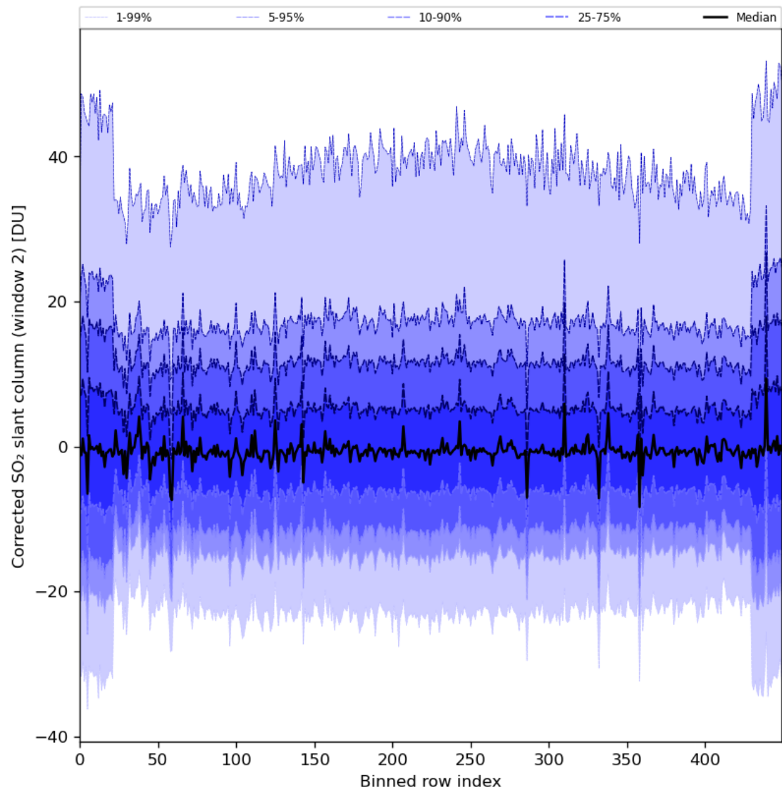
Figure 85: Along track statistics of “Corrected SO 2 slant column (window 2)” for 2024-01-24 to 2024-01-26
