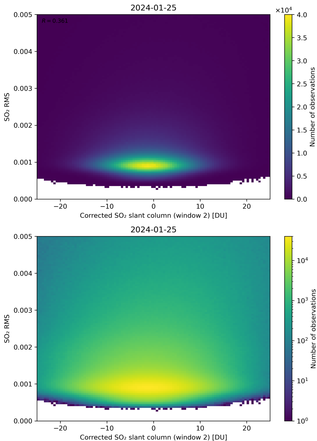
Figure 198: Scatter density plot of “Corrected SO 2 slant column (window 2)” against “SO 2 RMS” for 2024-01-24 to 2024-01-26.
