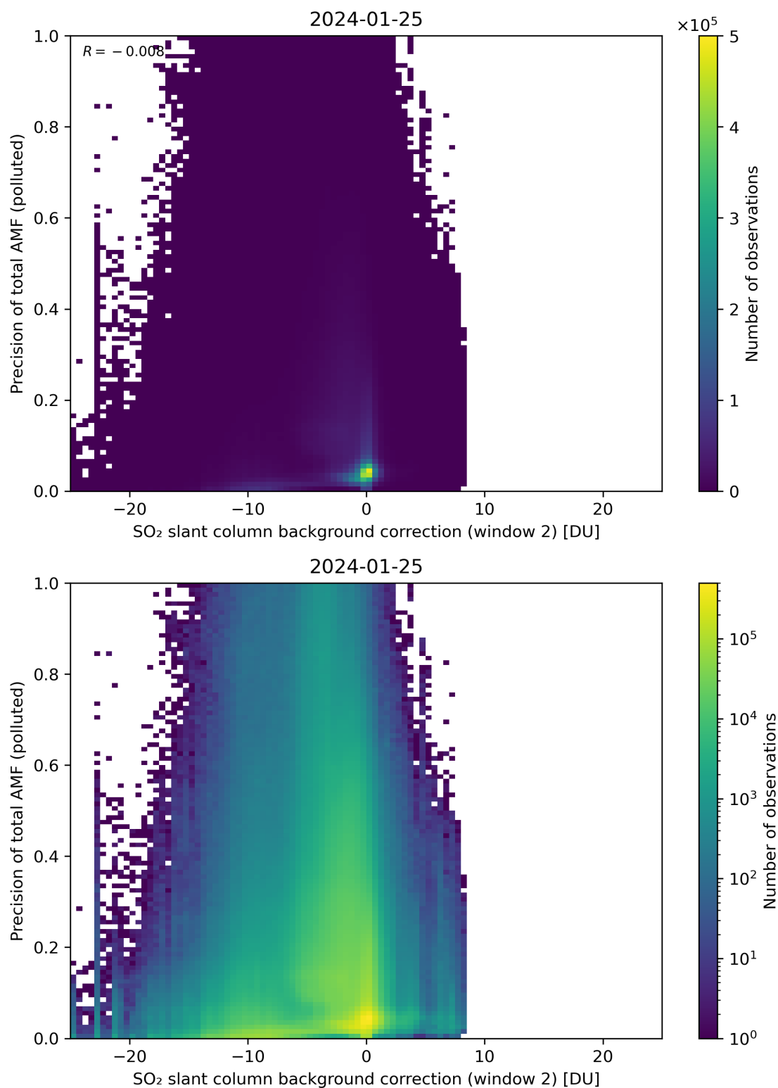
Figure 120: Scatter density plot of “SO 2 slant column background correction (window 2)” against “Precision of total AMF (polluted)” for 2024-01-24 to 2024-01-26.
