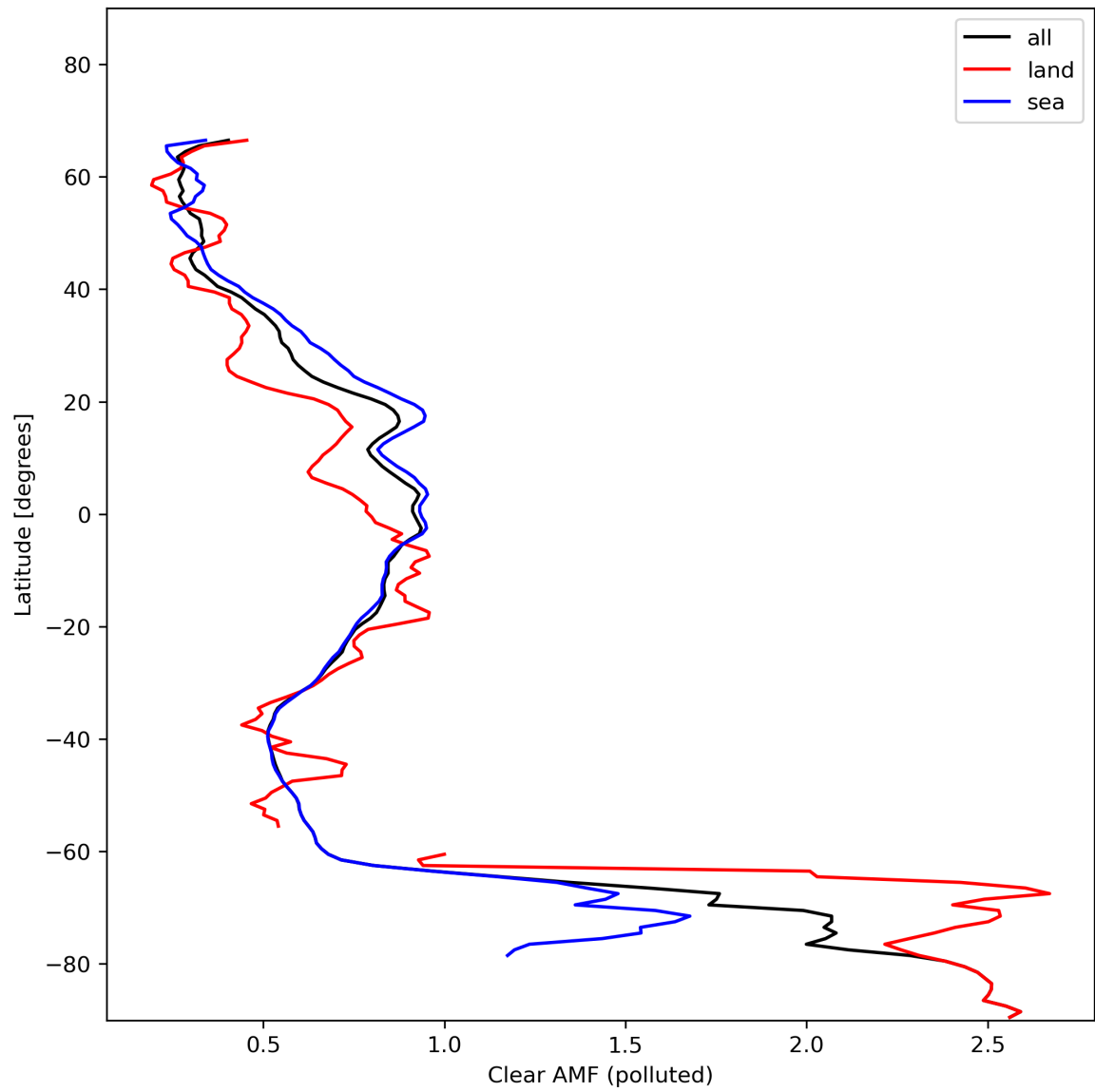
Figure 50: Zonal average of “Clear AMF (polluted)” for 2024-01-24 to 2024-01-26.
