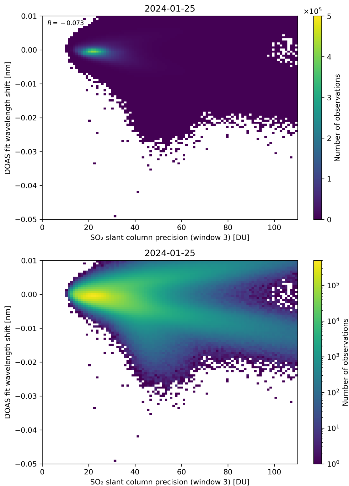
Figure 258: Scatter density plot of “SO 2 slant column precision (window 3)” against “DOAS fit wavelength shift” for 2024-01-24 to 2024-01-26.
