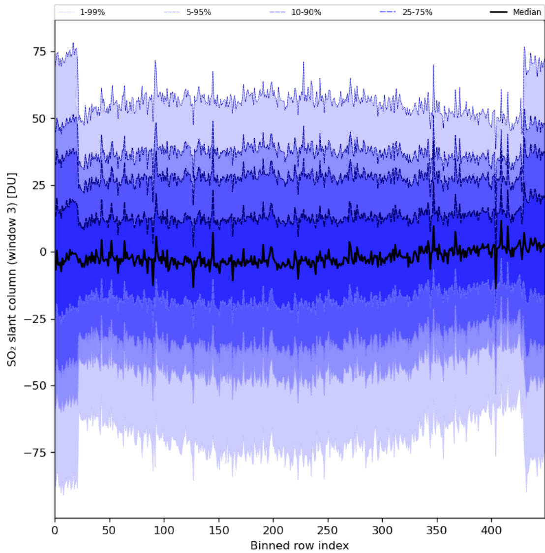
Figure 87: Along track statistics of “SO 2 slant column (window 3)” for 2024-01-24 to 2024-01-26
