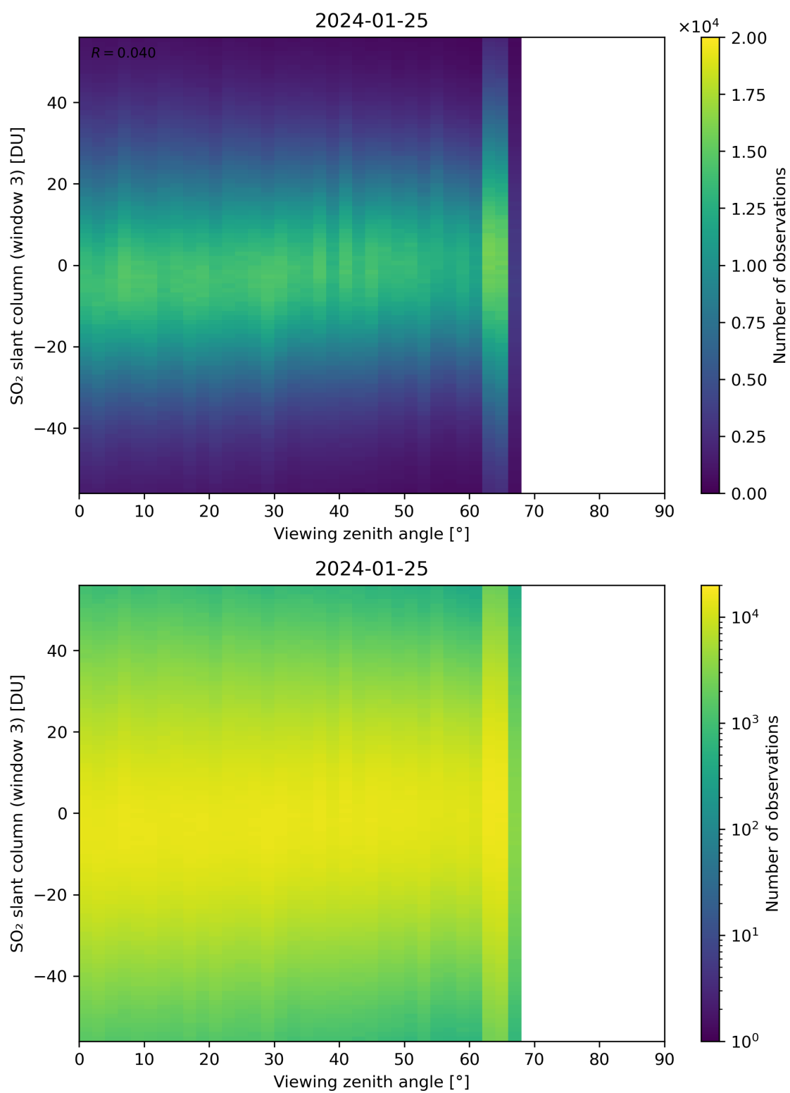
Figure 323: Scatter density plot of “Viewing zenith angle” against “SO 2 slant column (window 3)” for 2024-01-24 to 2024-01-26.
