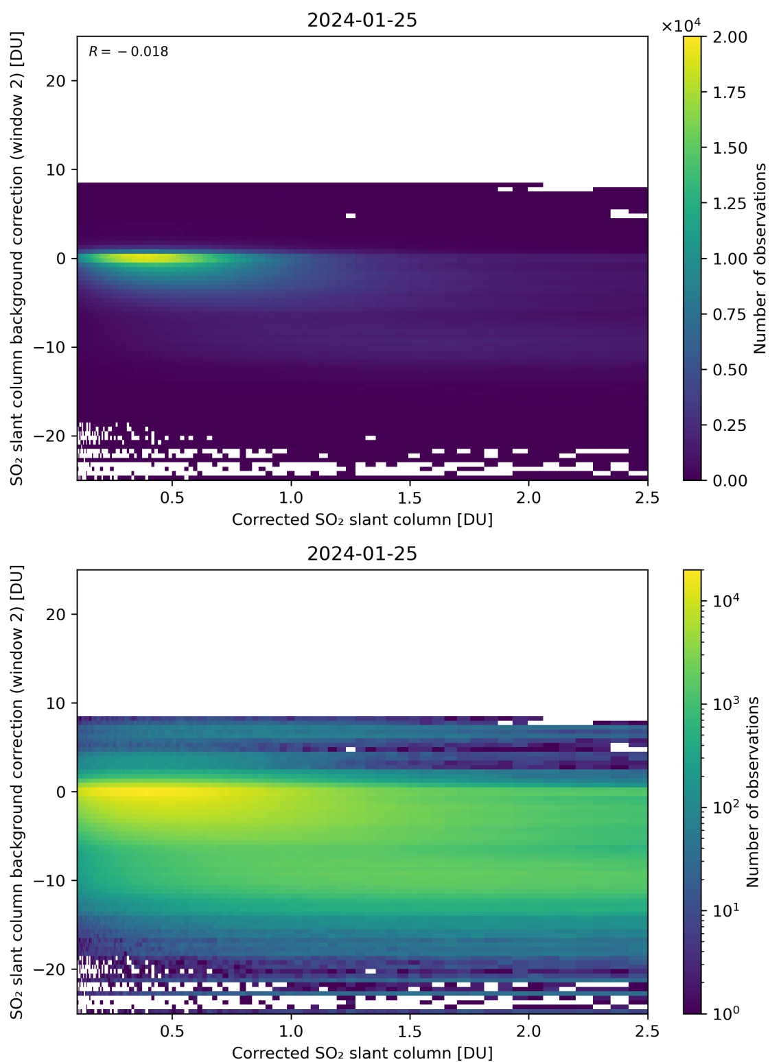
Figure 179: Scatter density plot of “Corrected SO 2 slant column” against “SO 2 slant column background correction (window 2)” for 2024-01-24 to 2024-01-26.
