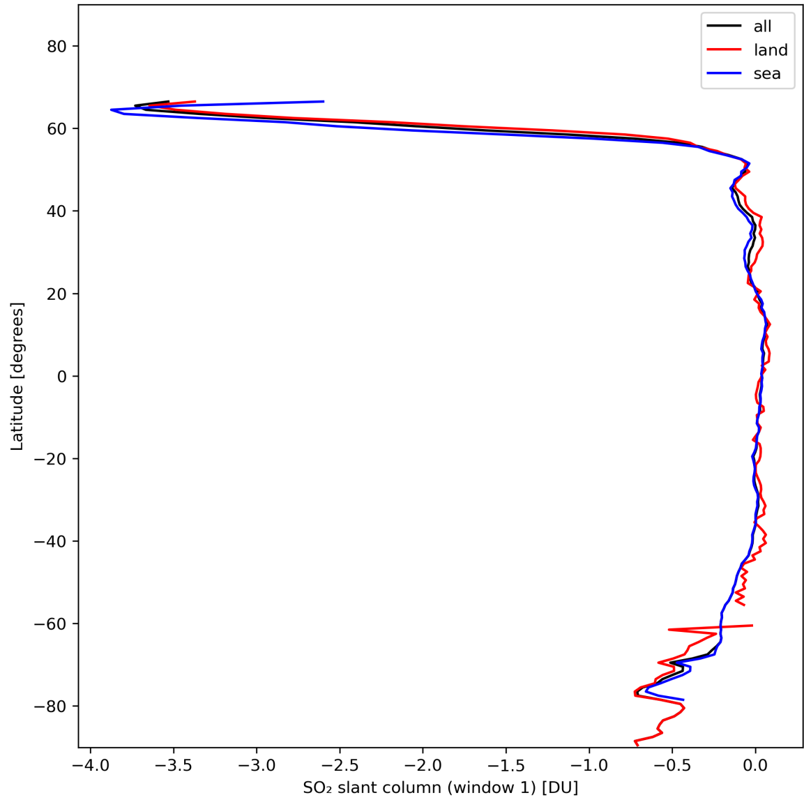
Figure 33: Zonal average of “SO 2 slant column (window 1)” for 2024-01-24 to 2024-01-26.
