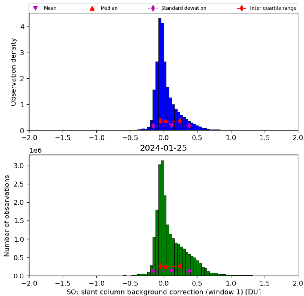
Figure 59: Histogram of “SO 2 slant column background correction (window 1)” for 2024-01-24 to 2024-01-26
