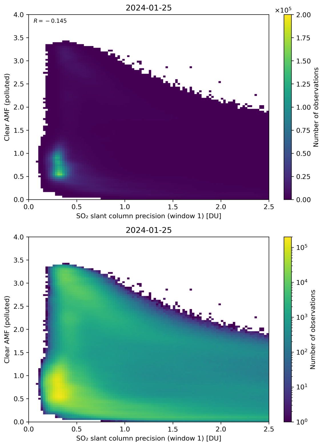
Figure 224: Scatter density plot of “SO 2 slant column precision (window 1)” against “Clear AMF (polluted)” for 2024-01-24 to 2024-01-26.
