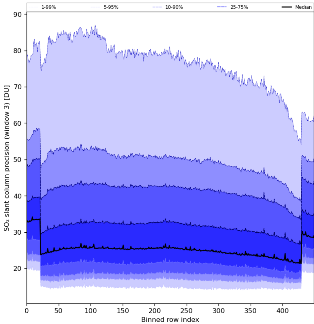
Figure 88: Along track statistics of “SO 2 slant column precision (window 3)” for 2024-01-24 to 2024-01-26
