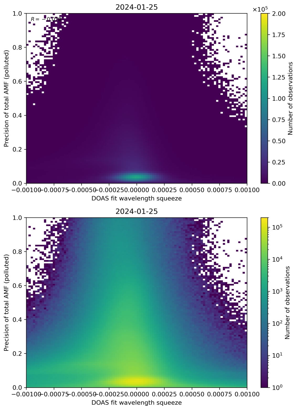
Figure 135: Scatter density plot of “DOAS fit wavelength squeeze” against “Precision of total AMF (polluted)” for 2024-01-24 to 2024-01-26.
