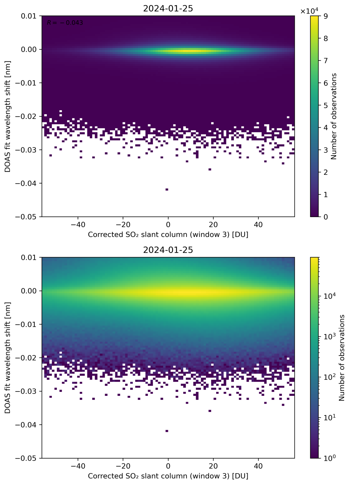
Figure 206: Scatter density plot of “Corrected SO 2 slant column (window 3)” against “DOAS fit wavelength shift” for 2024-01-24 to 2024-01-26.
