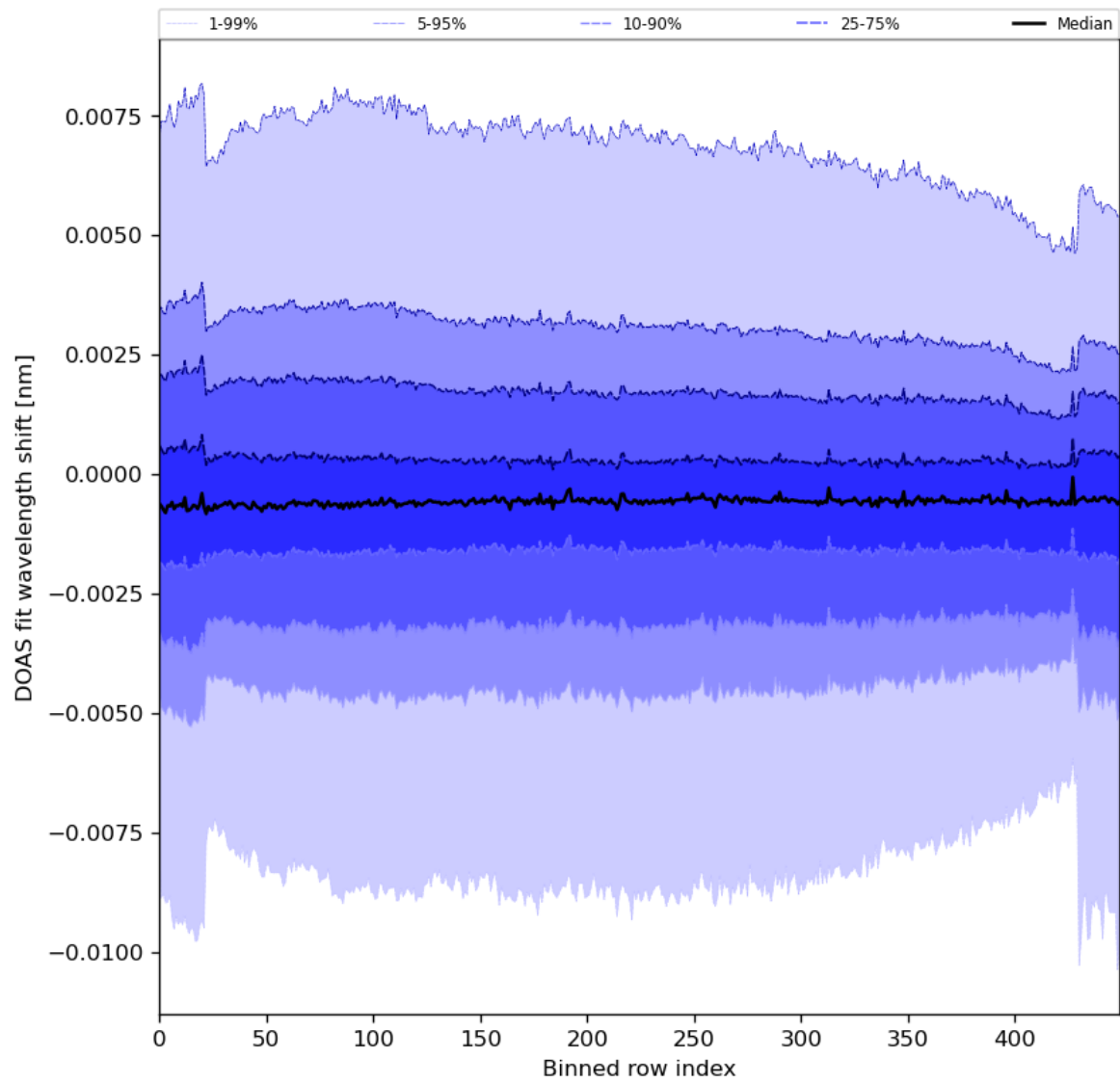
Figure 91: Along track statistics of “DOAS fit wavelength shift” for 2024-01-24 to 2024-01-26
