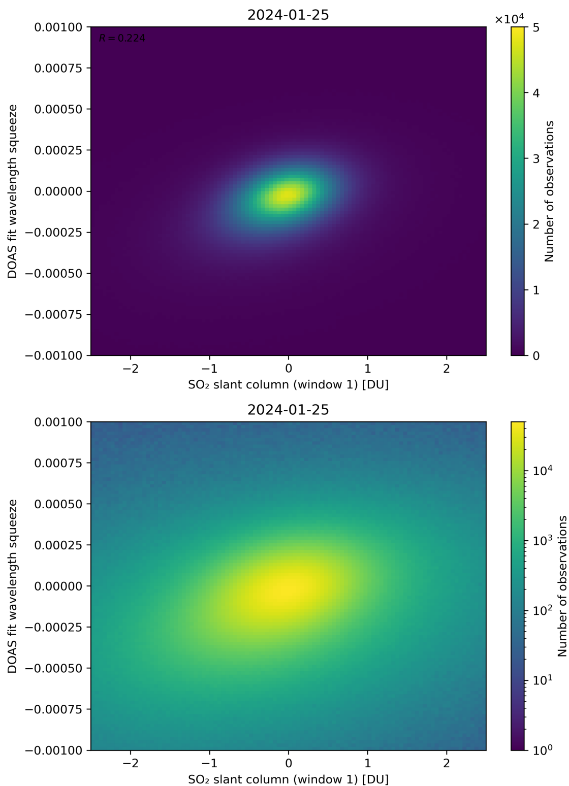
Figure 216: Scatter density plot of “SO 2 slant column (window 1)” against “DOAS fit wavelength squeeze” for 2024-01-24 to 2024-01-26.
