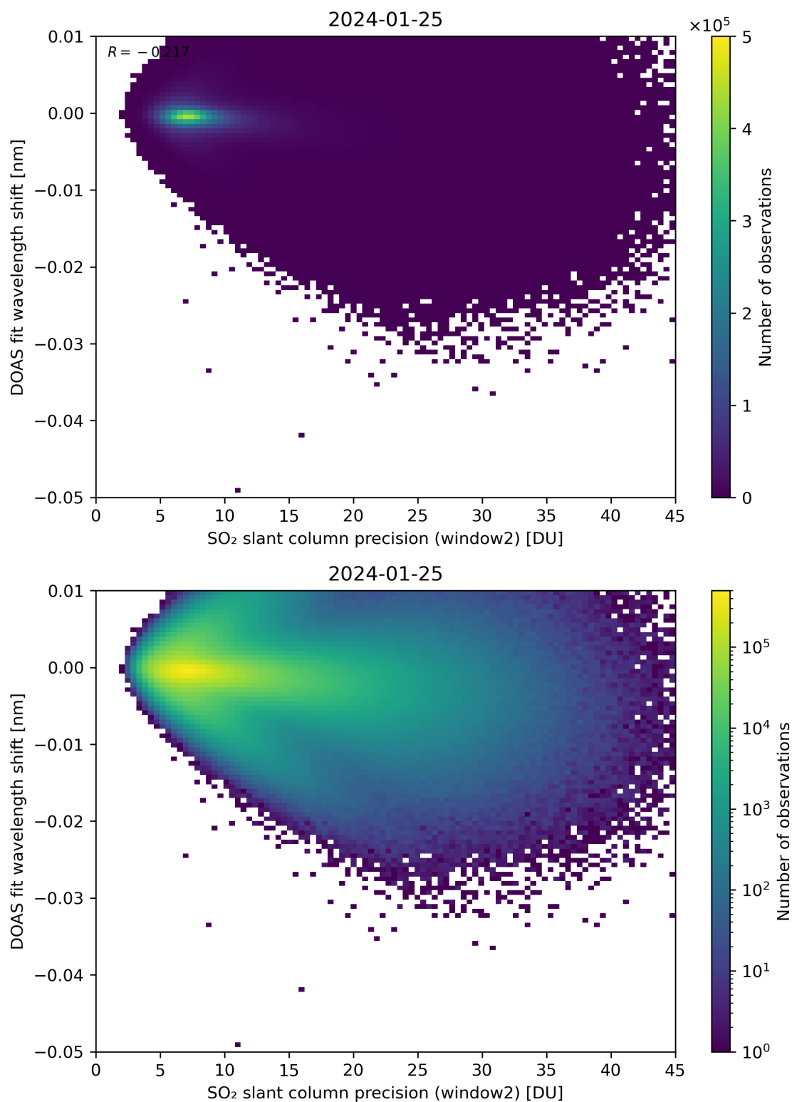
Figure 243: Scatter density plot of “SO 2 slant column precision (window2)” against “DOAS fit wavelength shift” for 2024-01-24 to 2024-01-26.
