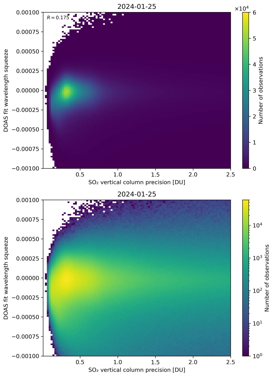
Figure 283: Scatter density plot of “SO 2 vertical column precision” against “DOAS fit wavelength squeeze” for 2024-01-24 to 2024-01-26.
