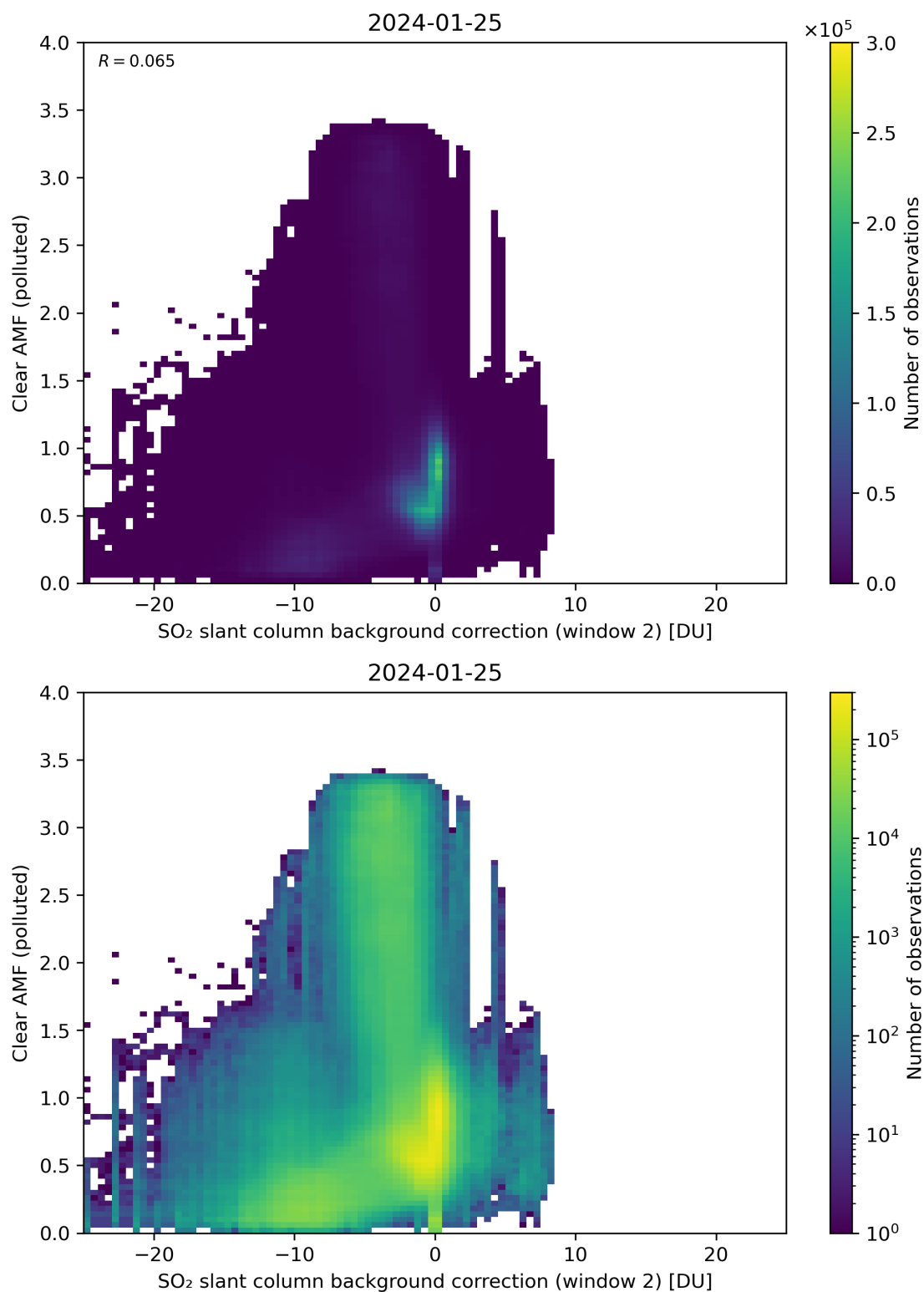
Figure 115: Scatter density plot of “SO 2 slant column background correction (window 2)” against “Clear AMF (polluted)” for 2024-01-24 to 2024-01-26.
