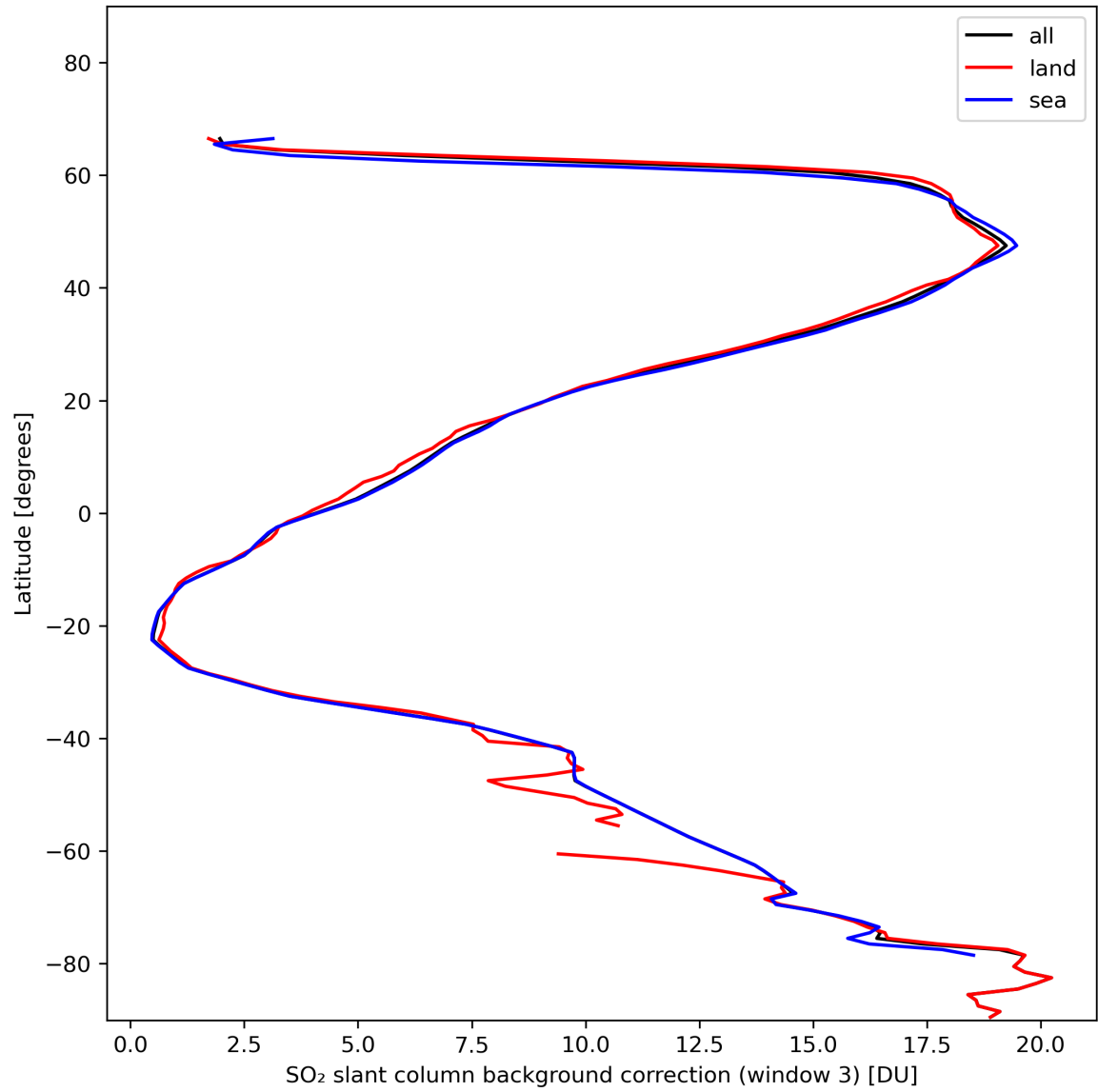
Figure 44: Zonal average of “SO 2 slant column background correction (window 3)” for 2024-01-24 to 2024-01-26.
