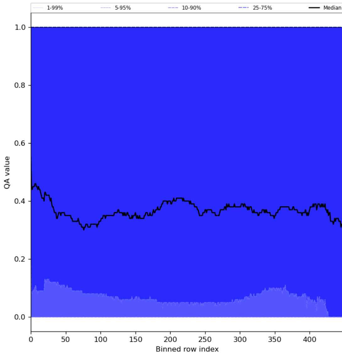
Figure 75: Along track statistics of “QA value” for 2024-01-24 to 2024-01-26
