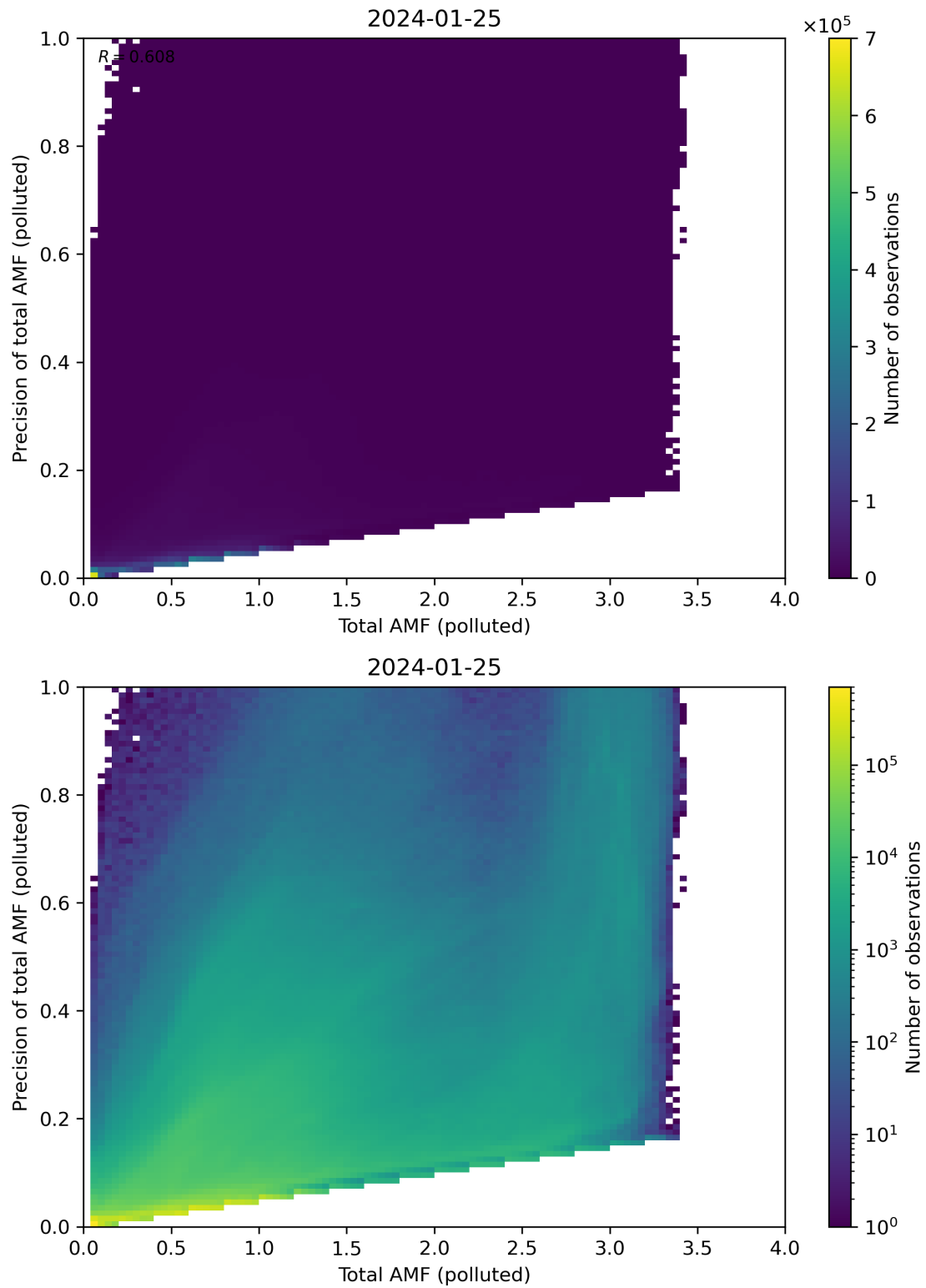
Figure 272: Scatter density plot of “Total AMF (polluted)” against “Precision of total AMF (polluted)” for 2024-01-24 to 2024-01-26.
