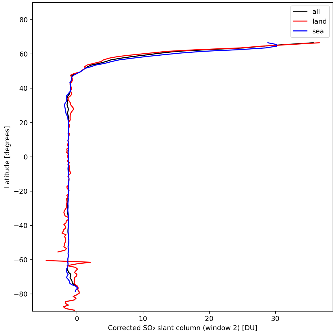
Figure 39: Zonal average of “Corrected SO 2 slant column (window 2)” for 2024-01-24 to 2024-01-26.
