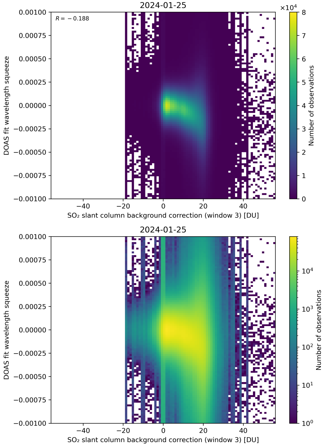
Figure 122: Scatter density plot of “SO 2 slant column background correction (window 3)” against “DOAS fit wavelength squeeze” for 2024-01-24 to 2024-01-26.
