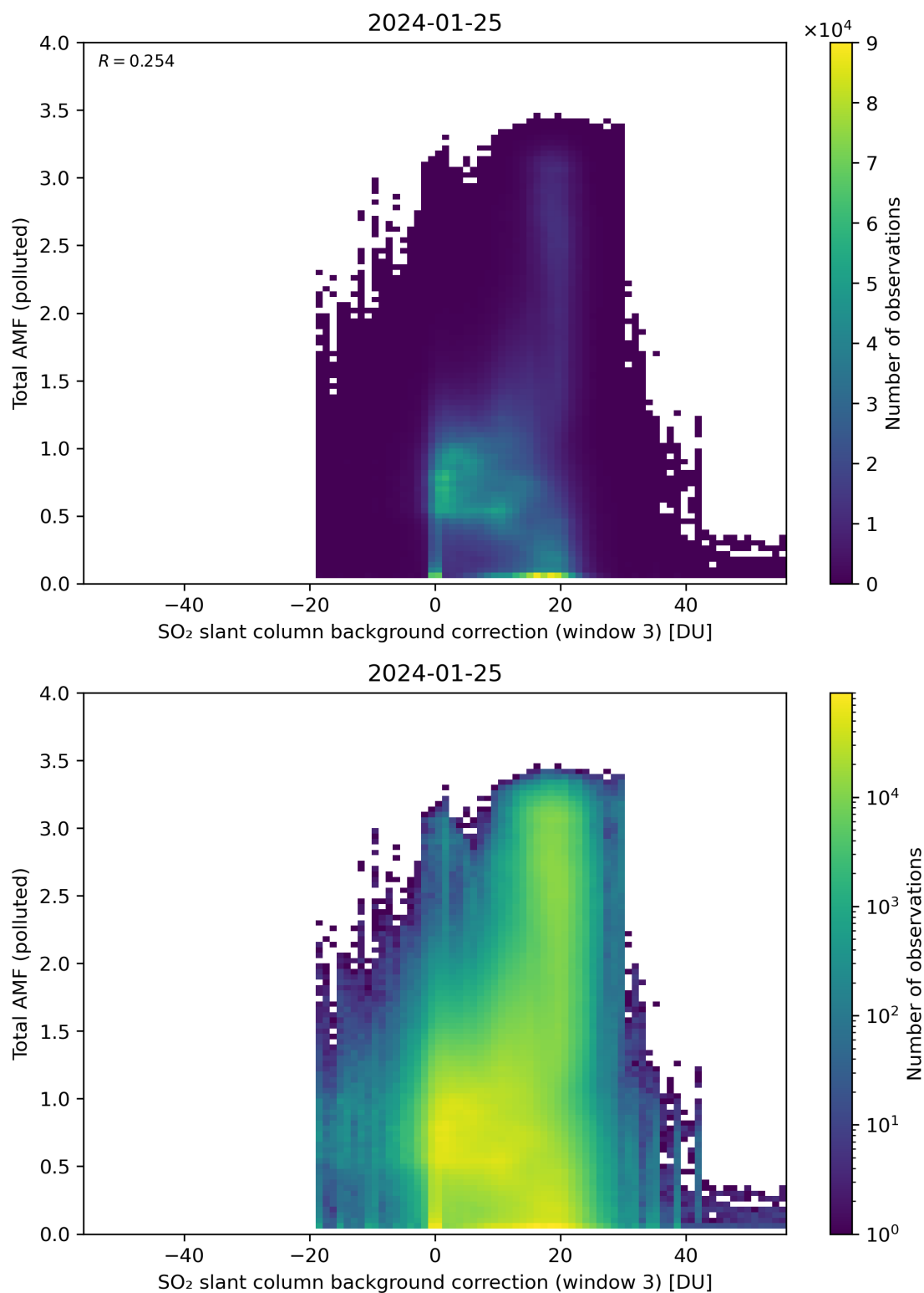
Figure 125: Scatter density plot of “SO 2 slant column background correction (window 3)” against “Total AMF (polluted)” for 2024-01-24 to 2024-01-26.
