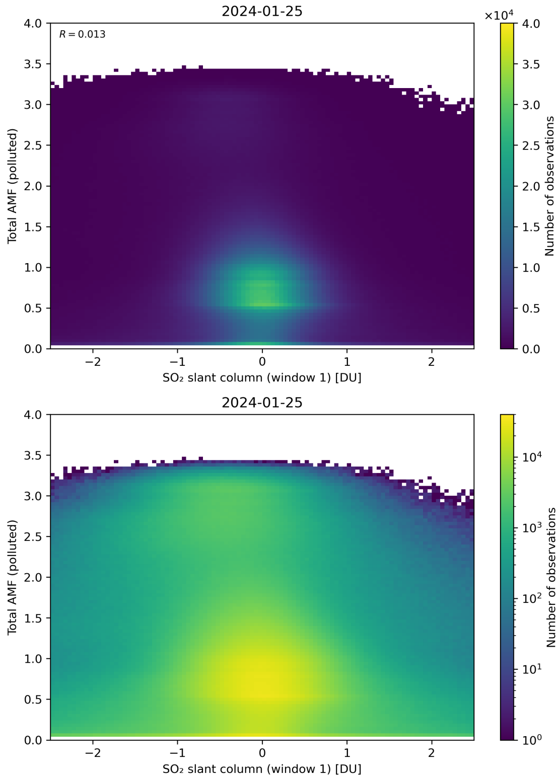
Figure 239: Scatter density plot of “SO 2 slant column (window 1)” against “Total AMF (polluted)” for 2024-01-24 to 2024-01-26.
