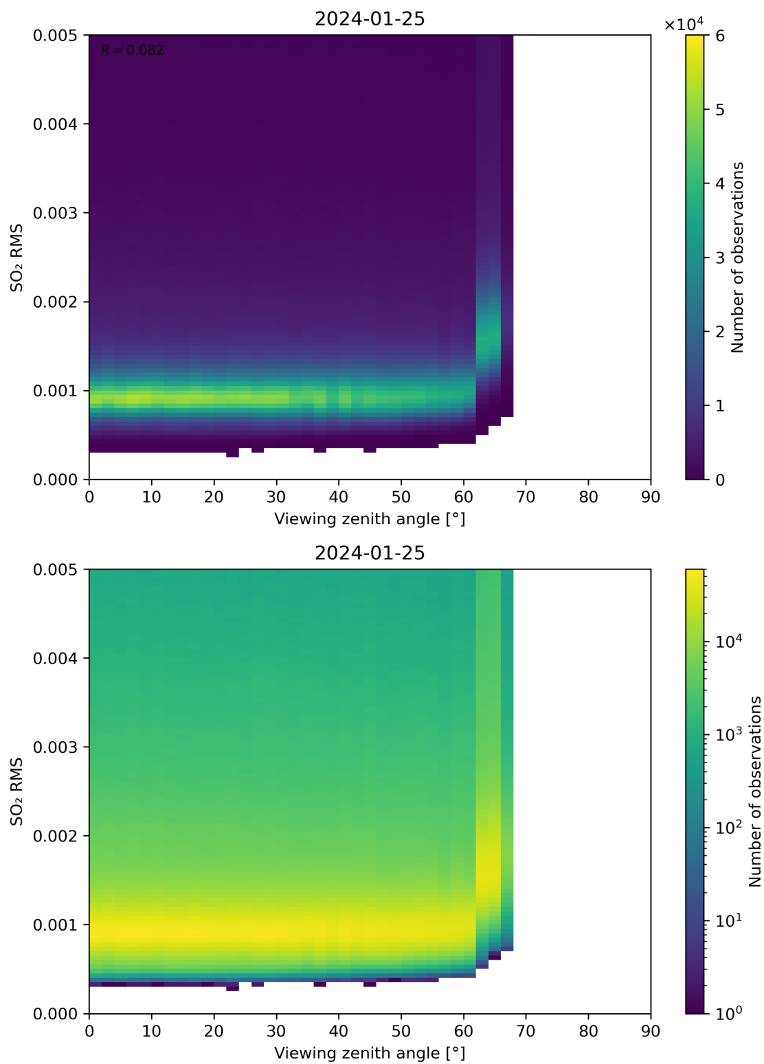
Figure 313: Scatter density plot of “Viewing zenith angle” against “SO 2 RMS” for 2024-01-24 to 2024-01-26.
