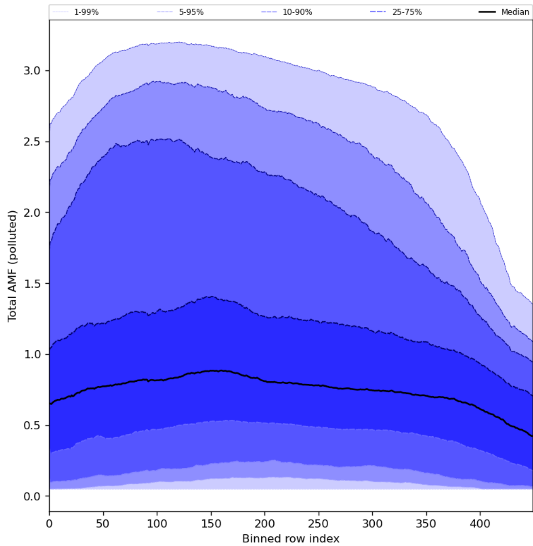
Figure 94: Along track statistics of “Total AMF (polluted)” for 2024-01-24 to 2024-01-26
