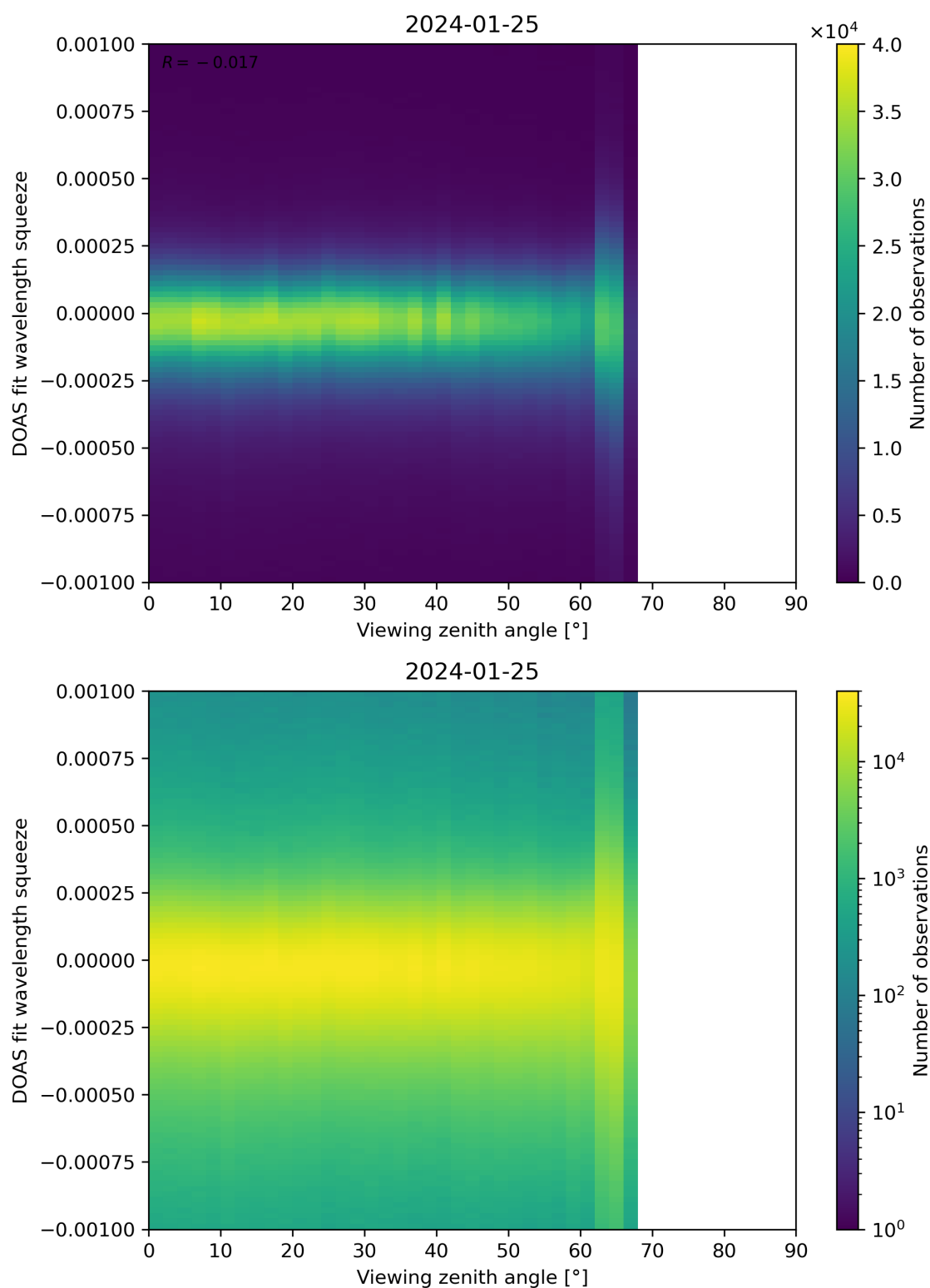
Figure 312: Scatter density plot of “Viewing zenith angle” against “DOAS fit wavelength squeeze” for 2024-01-24 to 2024-01-26.
