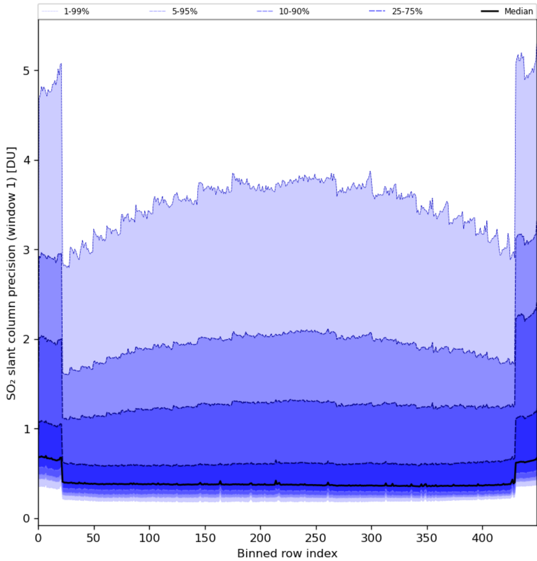
Figure 80: Along track statistics of “SO 2 slant column precision (window 1)” for 2024-01-24 to 2024-01-26
