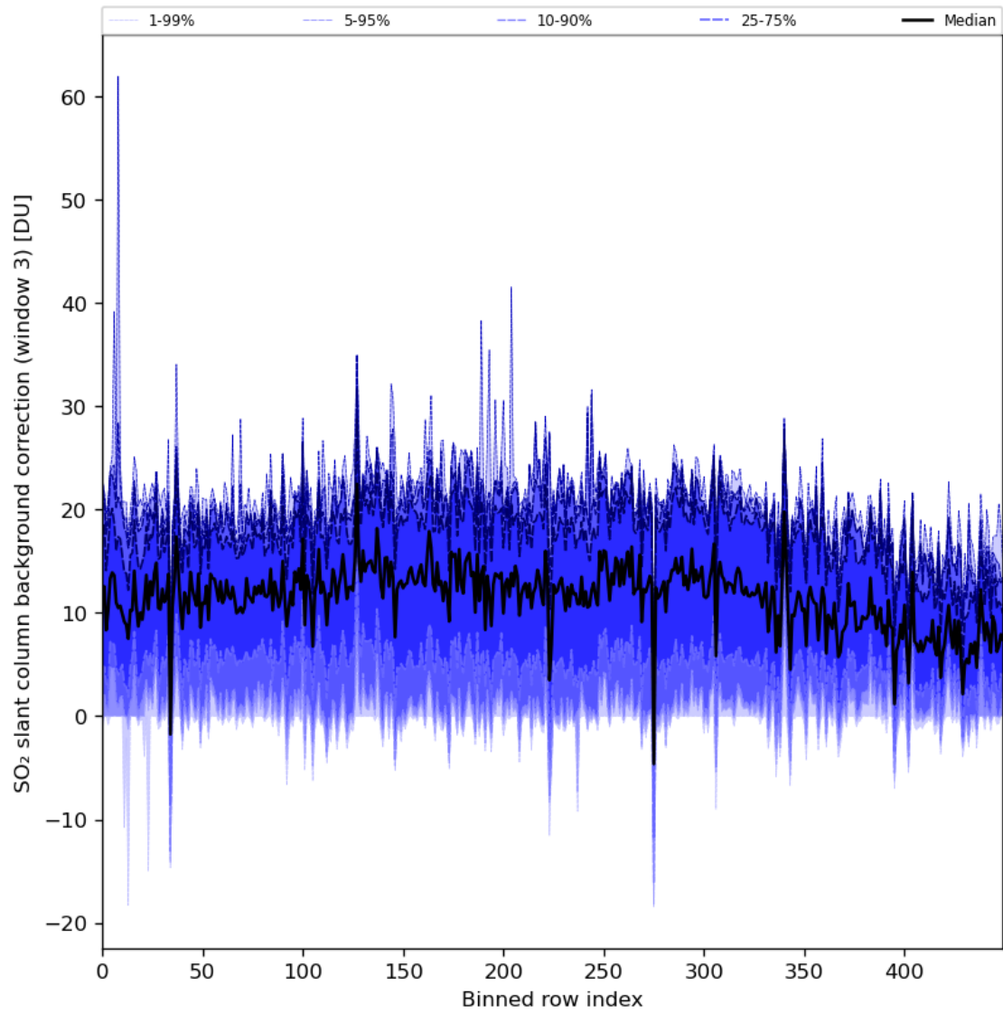
Figure 90: Along track statistics of “SO 2 slant column background correction (window 3)” for 2024-01-24 to 2024-01-26
