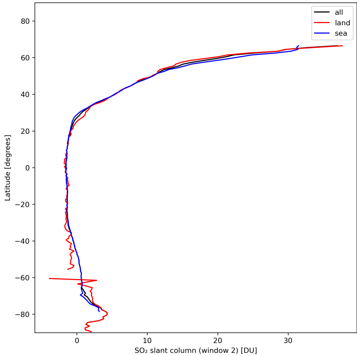
Figure 37: Zonal average of “SO 2 slant column (window 2)” for 2024-01-24 to 2024-01-26.
