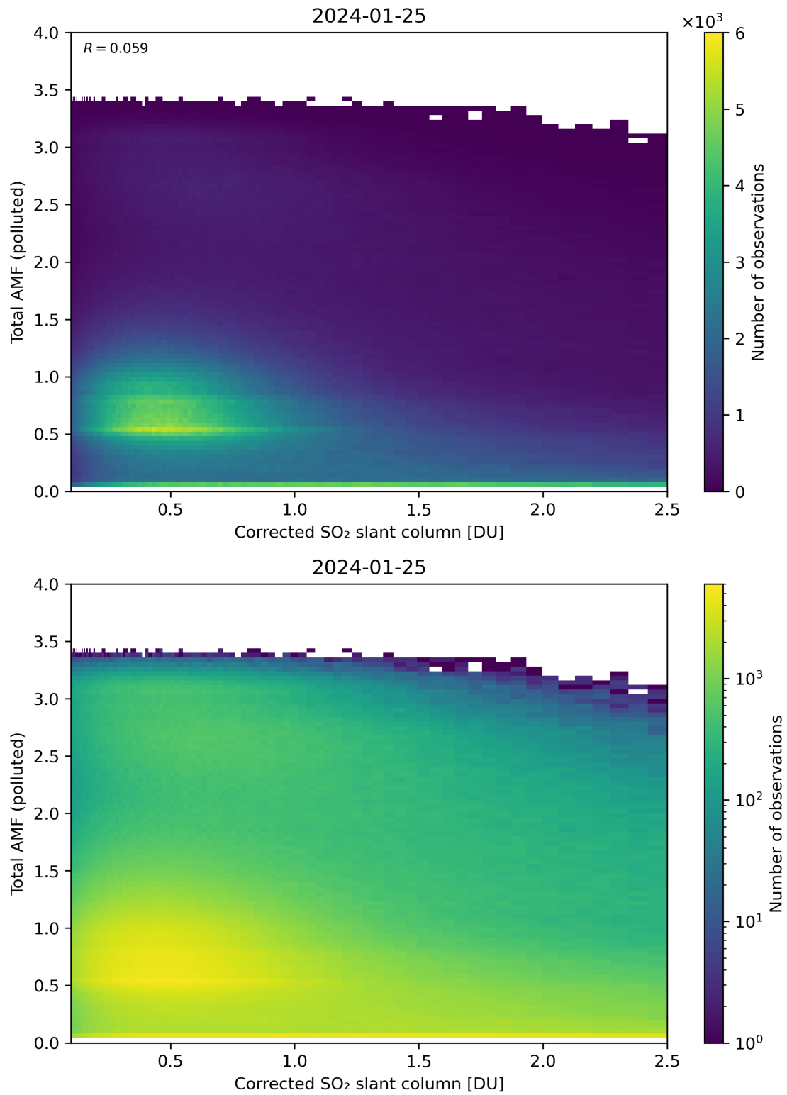
Figure 192: Scatter density plot of “Corrected SO 2 slant column” against “Total AMF (polluted)” for 2024-01-24 to 2024-01-26.
