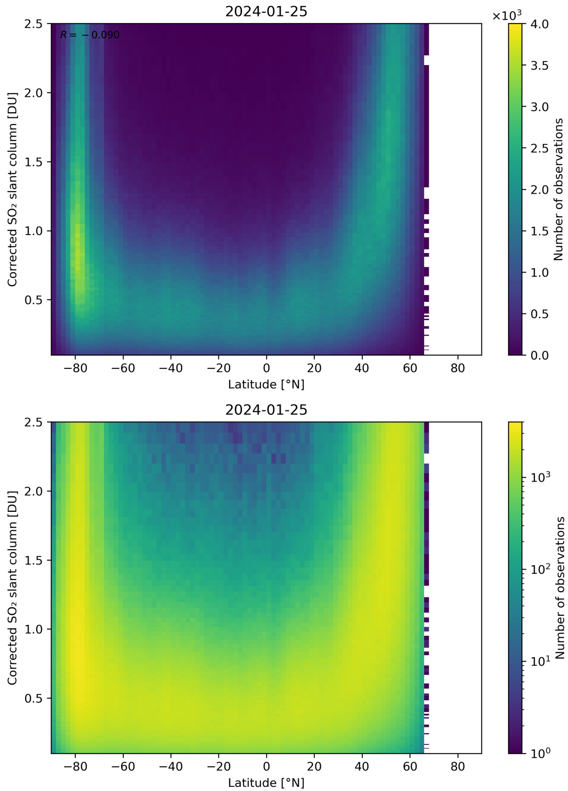
Figure 146: Scatter density plot of “Latitude” against “Corrected SO 2 slant column” for 2024-01-24 to 2024-01-26.
