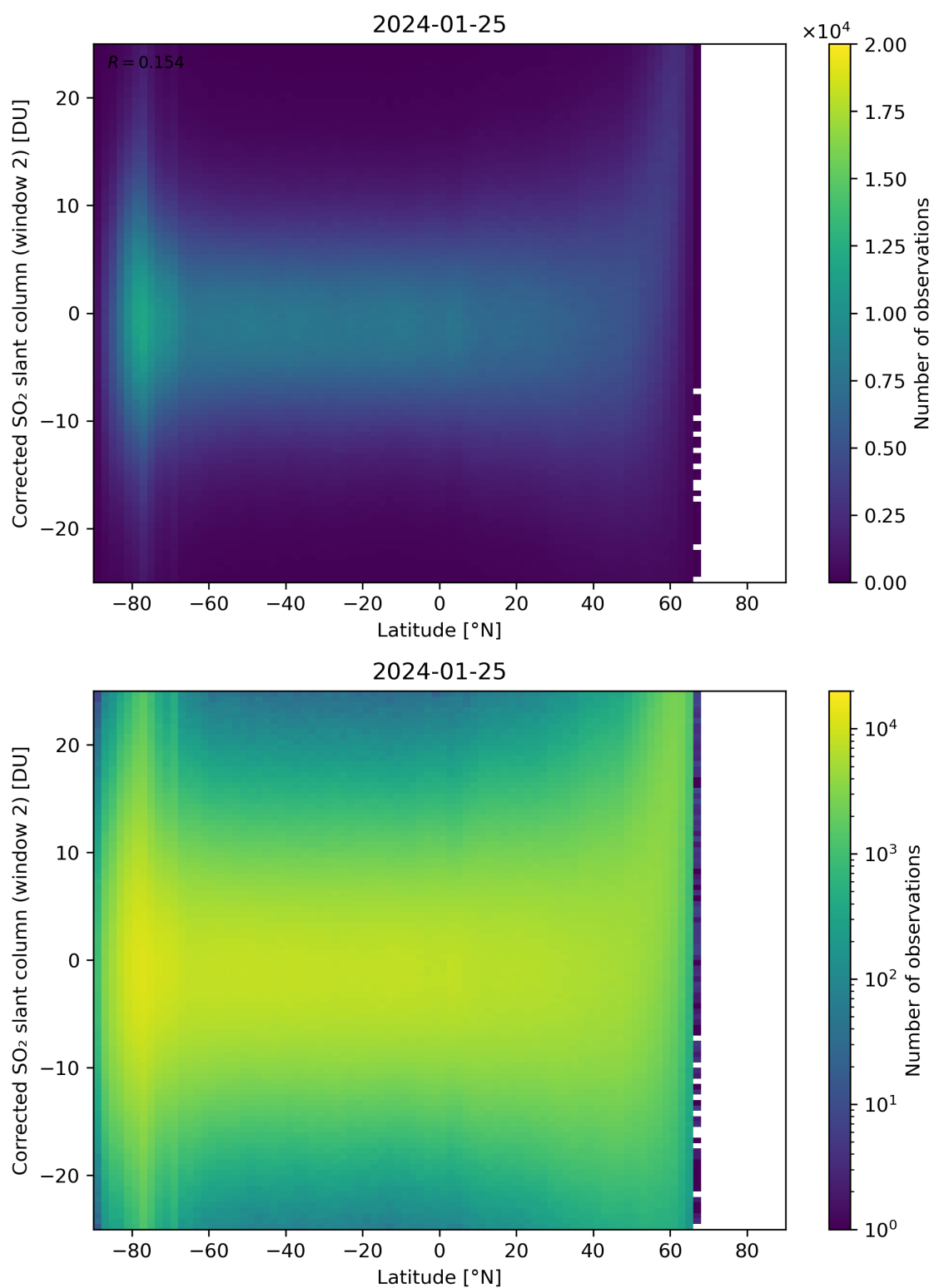
Figure 147: Scatter density plot of “Latitude” against “Corrected SO 2 slant column (window 2)” for 2024-01-24 to 2024-01-26.
