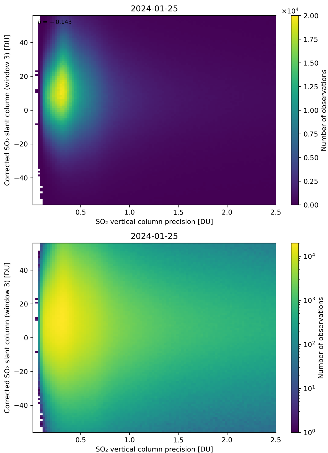
Figure 288: Scatter density plot of “SO 2 vertical column precision” against “Corrected SO 2 slant column (window 3)” for 2024-01-24 to 2024-01-26.
