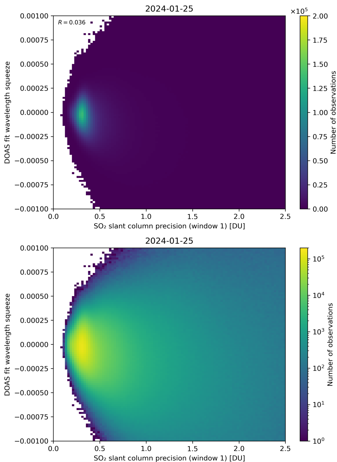
Figure 222: Scatter density plot of “SO 2 slant column precision (window 1)” against “DOAS fit wavelength squeeze” for 2024-01-24 to 2024-01-26.
