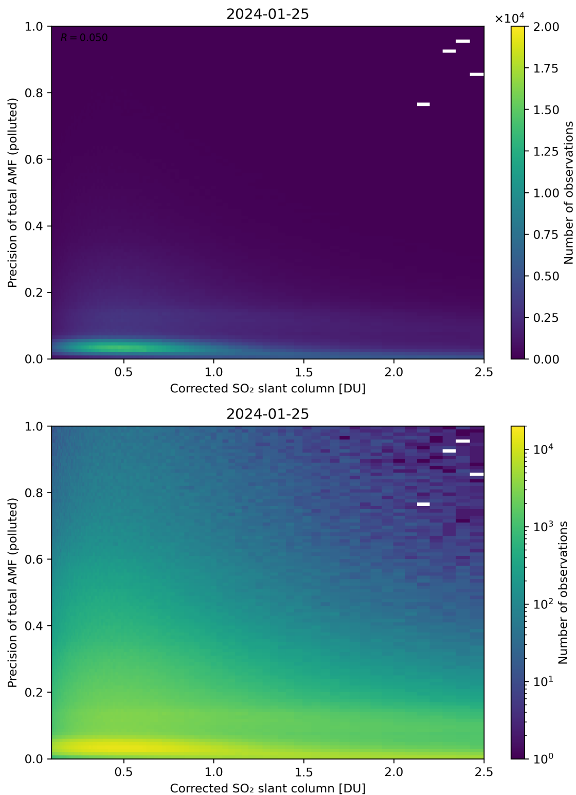
Figure 193: Scatter density plot of “Corrected SO 2 slant column” against “Precision of total AMF (polluted)” for 2024-01-24 to 2024-01-26.
