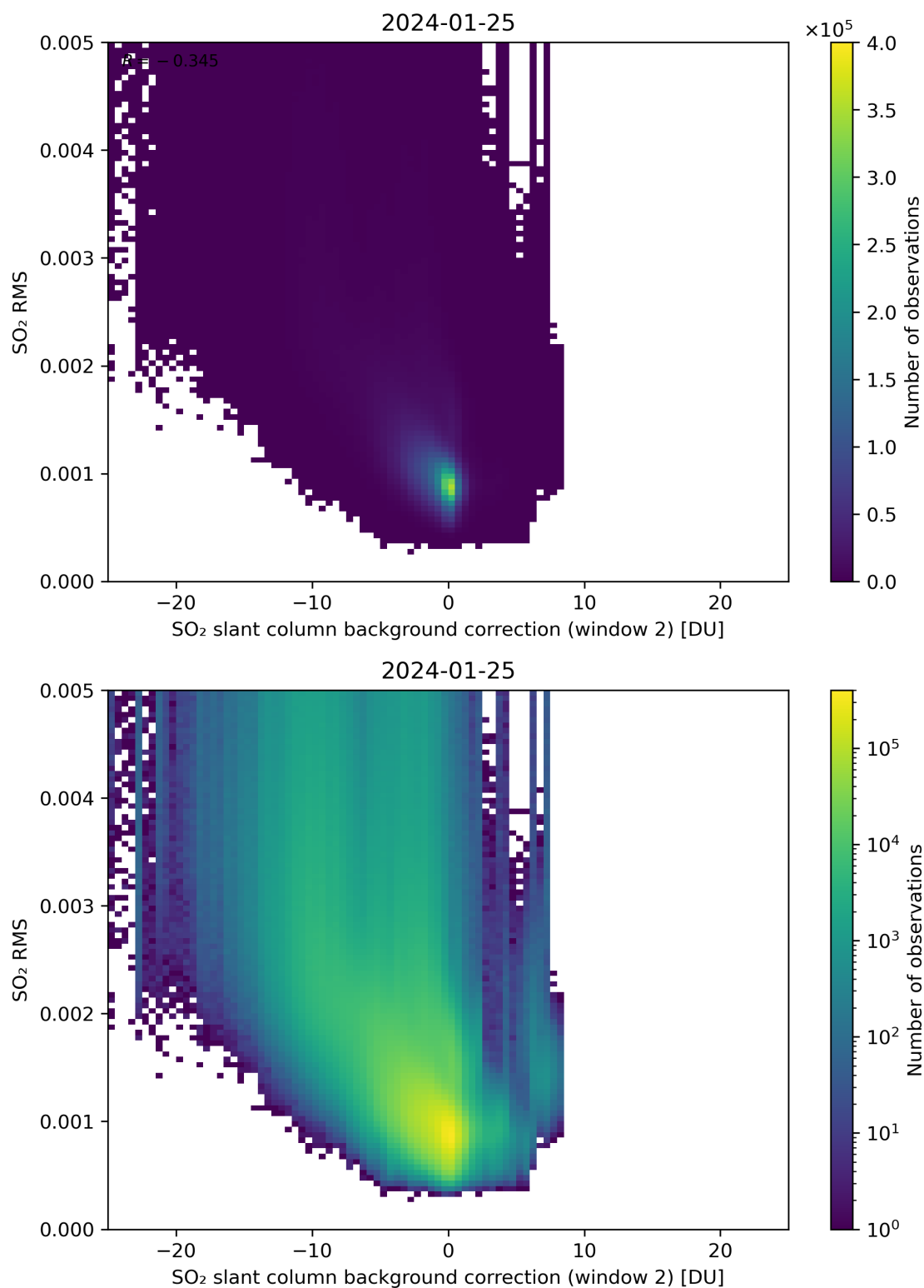
Figure 114: Scatter density plot of “SO 2 slant column background correction (window 2)” against “SO 2 RMS” for 2024-01-24 to 2024-01-26.
