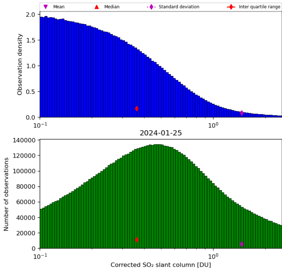
Figure 55: Histogram of “Corrected SO 2 slant column” for 2024-01-24 to 2024-01-26
