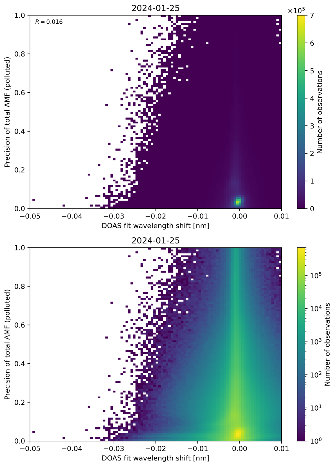
Figure 131: Scatter density plot of “DOAS fit wavelength shift” against “Precision of total AMF (polluted)” for 2024-01-24 to 2024-01-26.
