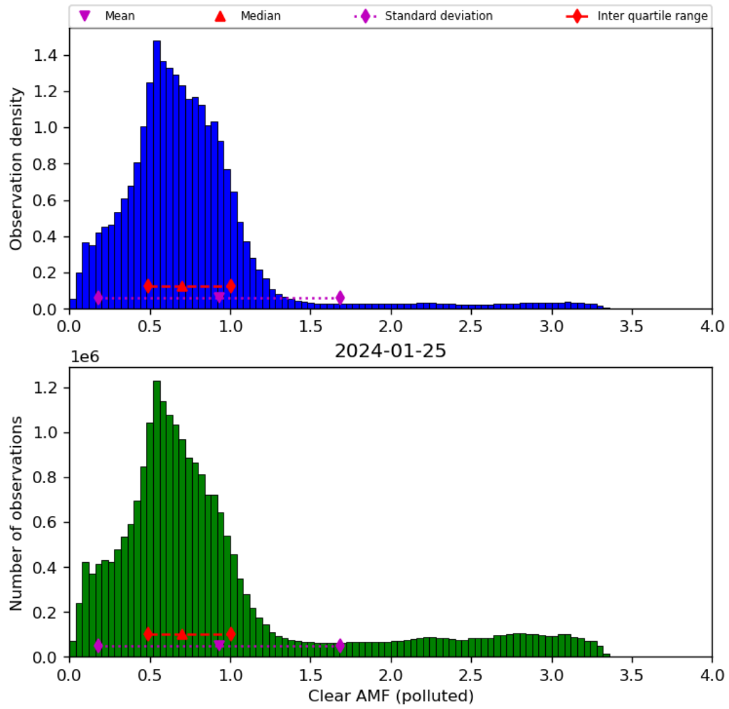
Figure 73: Histogram of “Clear AMF (polluted)” for 2024-01-24 to 2024-01-26
