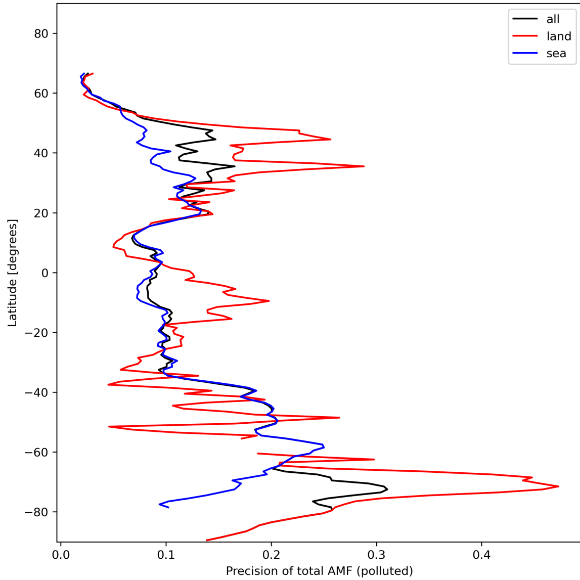
Figure 49: Zonal average of “Precision of total AMF (polluted)” for 2024-01-24 to 2024-01-26.
