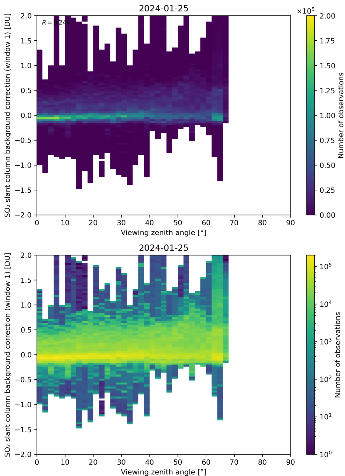
Figure 308: Scatter density plot of “Viewing zenith angle” against “SO 2 slant column background correction (window 1)” for 2024-01-24 to 2024-01-26.
