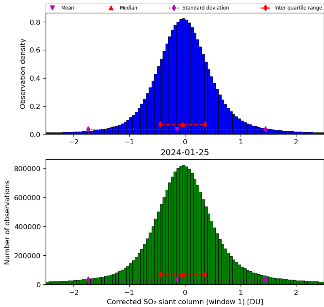
Figure 58: Histogram of “Corrected SO 2 slant column (window 1)” for 2024-01-24 to 2024-01-26
