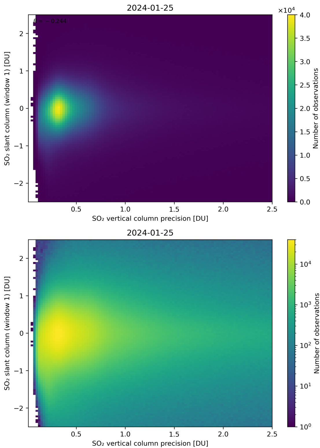
Figure 289: Scatter density plot of “SO 2 vertical column precision” against “SO 2 slant column (window 1)” for 2024-01-24 to 2024-01-26.
