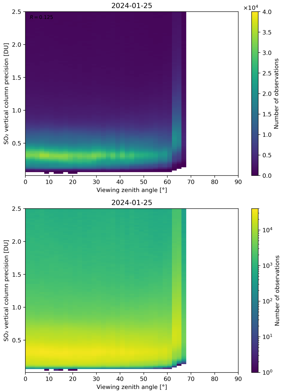
Figure 328: Scatter density plot of “Viewing zenith angle” against “SO 2 vertical column precision” for 2024-01-24 to 2024-01-26.
