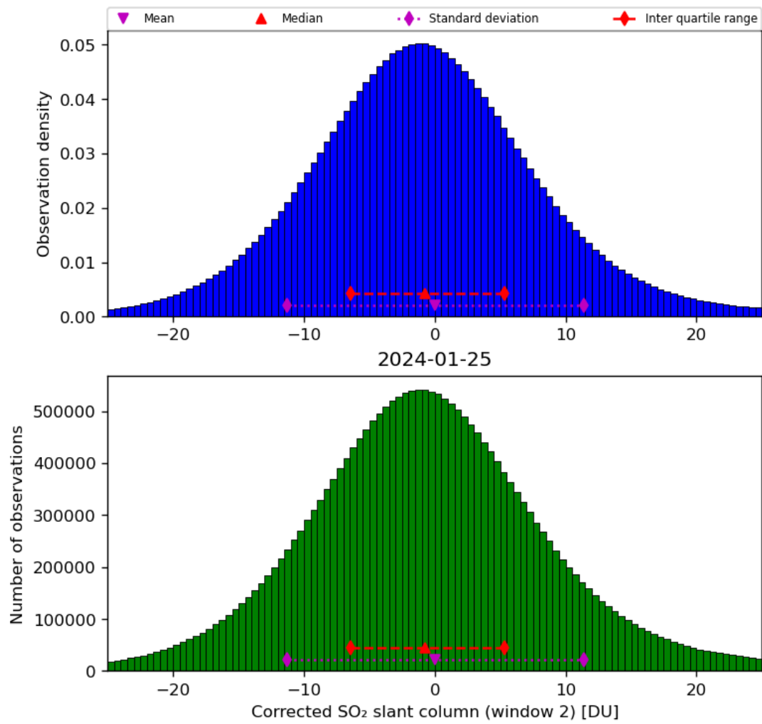
Figure 62: Histogram of “Corrected SO 2 slant column (window 2)” for 2024-01-24 to 2024-01-26
