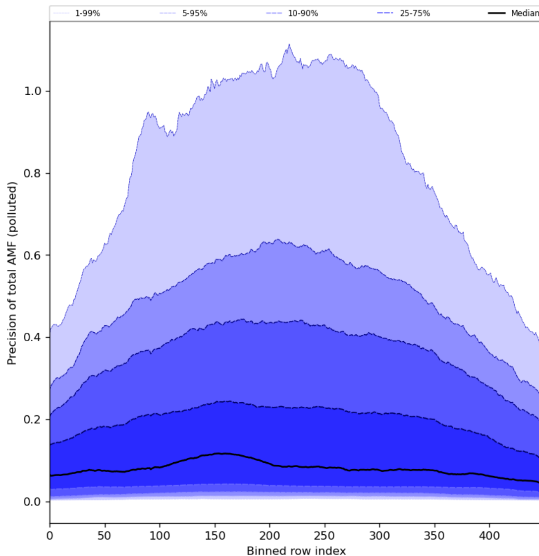
Figure 95: Along track statistics of “Precision of total AMF (polluted)” for 2024-01-24 to 2024-01-26
