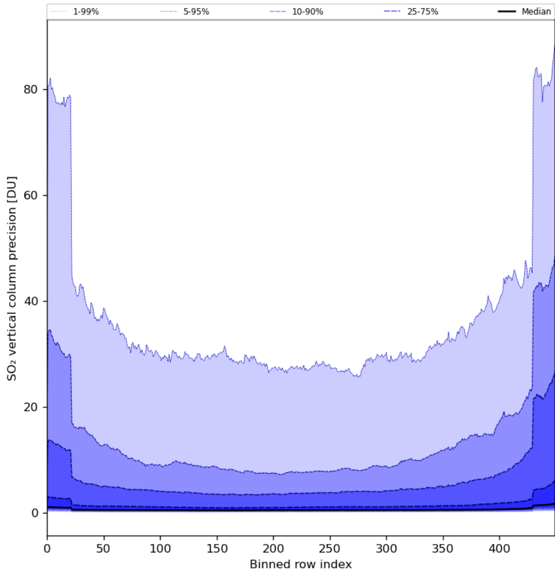
Figure 77: Along track statistics of “SO 2 vertical column precision” for 2024-01-24 to 2024-01-26
