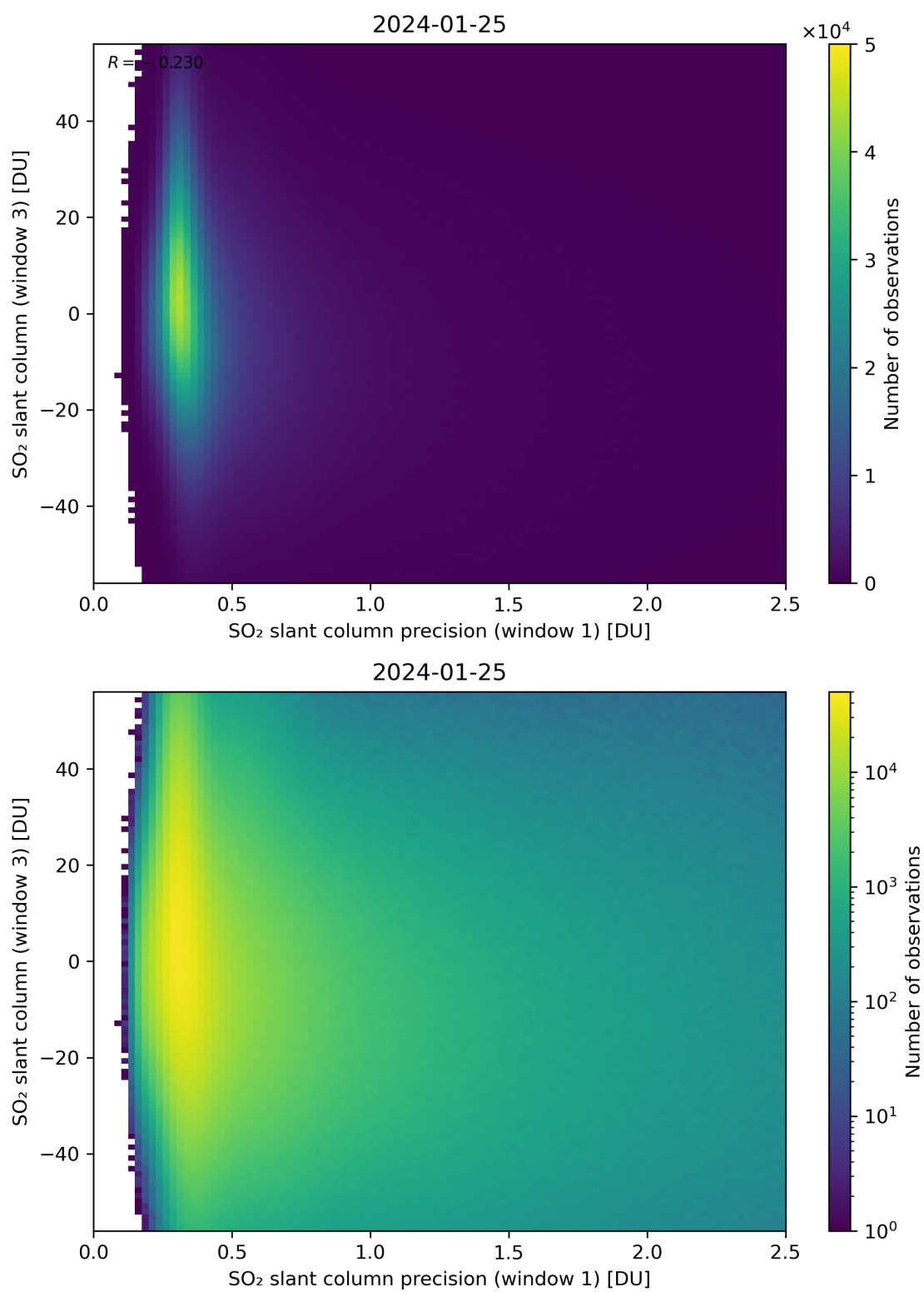
Figure 228: Scatter density plot of “SO 2 slant column precision (window 1)” against “SO 2 slant column (window 3)” for 2024-01-24 to 2024-01-26.
