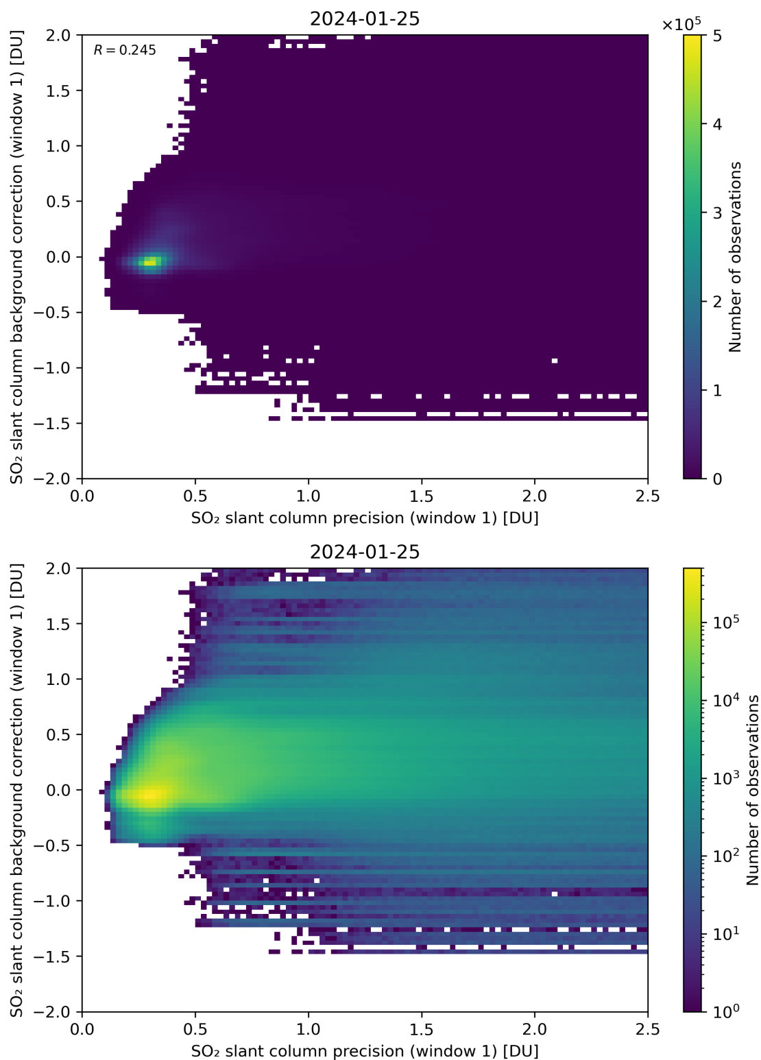
Figure 218: Scatter density plot of “SO 2 slant column precision (window 1)” against “SO 2 slant column background correction (window 1)” for 2024-01-24 to 2024-01-26.
