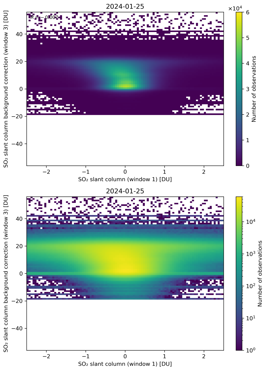
Figure 214: Scatter density plot of “SO 2 slant column (window 1)” against “SO 2 slant column background correction (window 3)” for 2024-01-24 to 2024-01-26.
