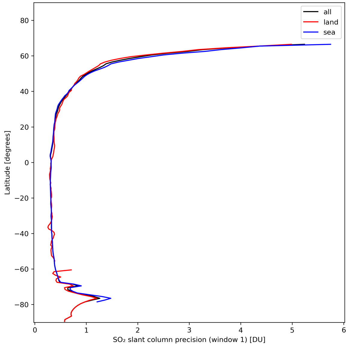
Figure 34: Zonal average of “SO 2 slant column precision (window 1)” for 2024-01-24 to 2024-01-26.
