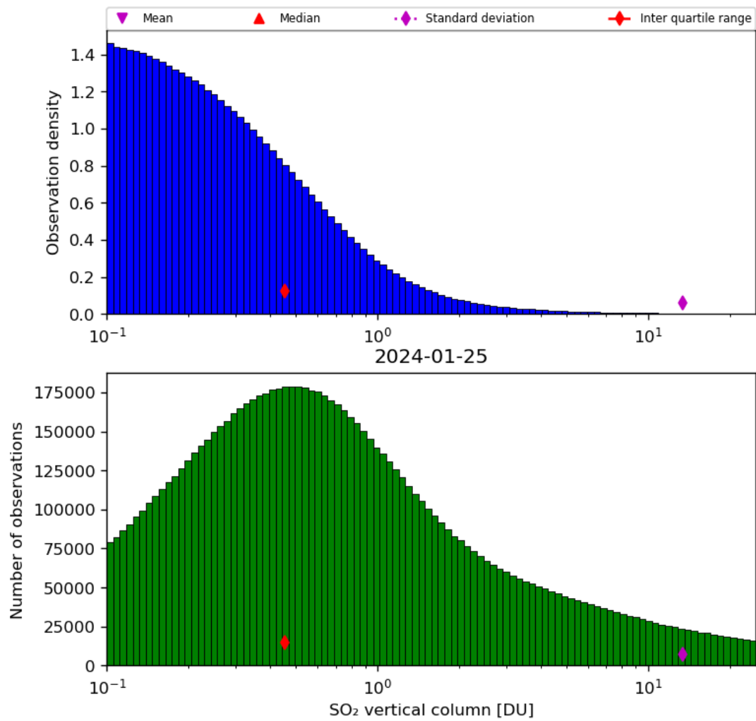
Figure 53: Histogram of “SO 2 vertical column” for 2024-01-24 to 2024-01-26
