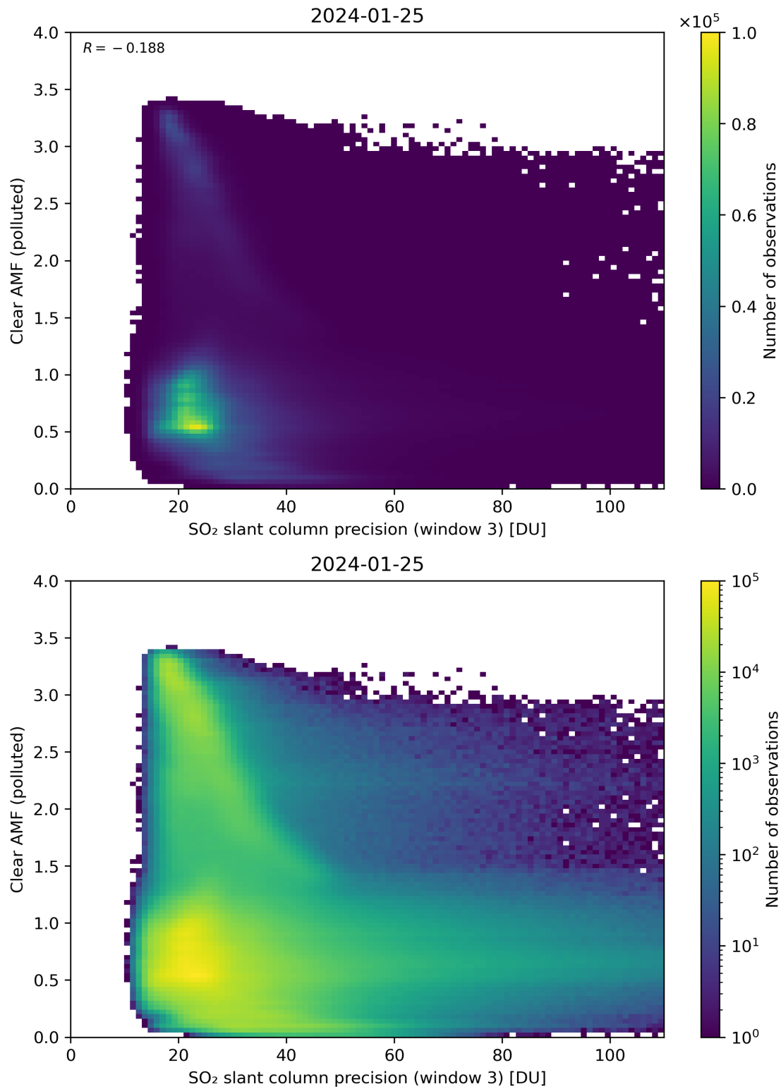
Figure 261: Scatter density plot of “SO 2 slant column precision (window 3)” against “Clear AMF (polluted)” for 2024-01-24 to 2024-01-26.
