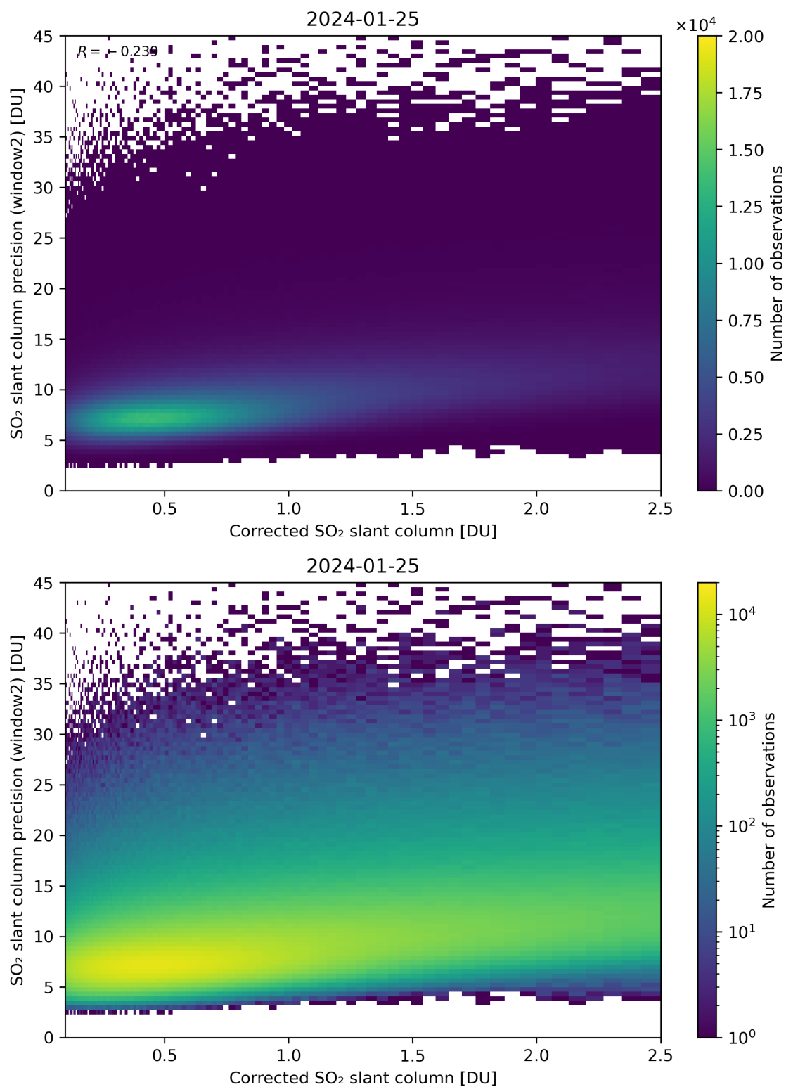
Figure 189: Scatter density plot of “Corrected SO 2 slant column” against “SO 2 slant column precision (window2)” for 2024-01-24 to 2024-01-26.
