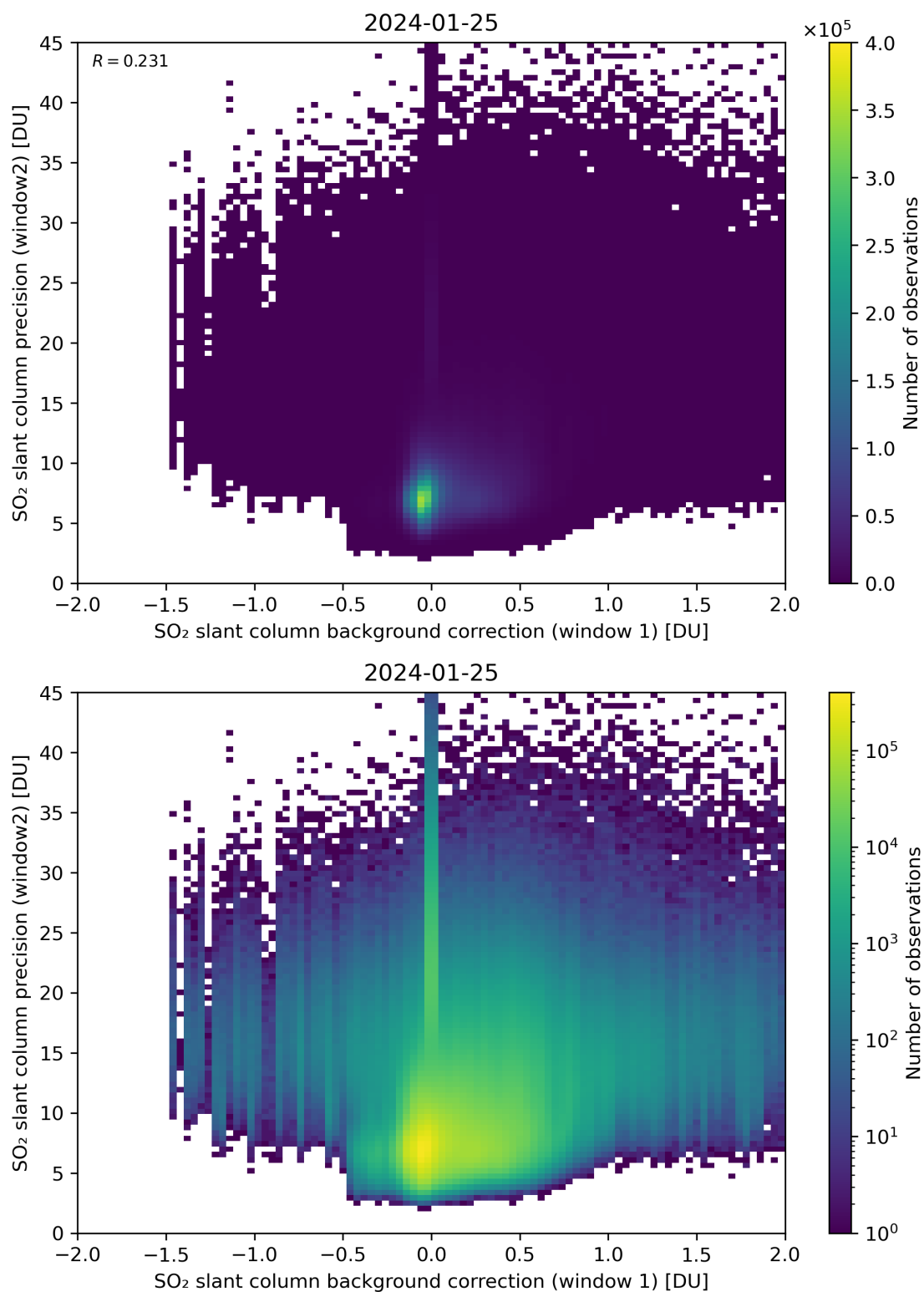
Figure 106: Scatter density plot of “SO 2 slant column background correction (window 1)” against “SO 2 slant column precision (window2)” for 2024-01-24 to 2024-01-26.
