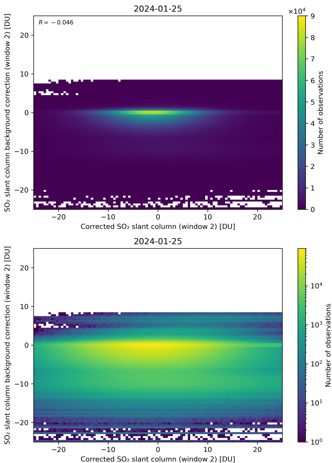
Figure 194: Scatter density plot of “Corrected SO 2 slant column (window 2)” against “SO 2 slant column background correction (window 2)” for 2024-01-24 to 2024-01-26.
