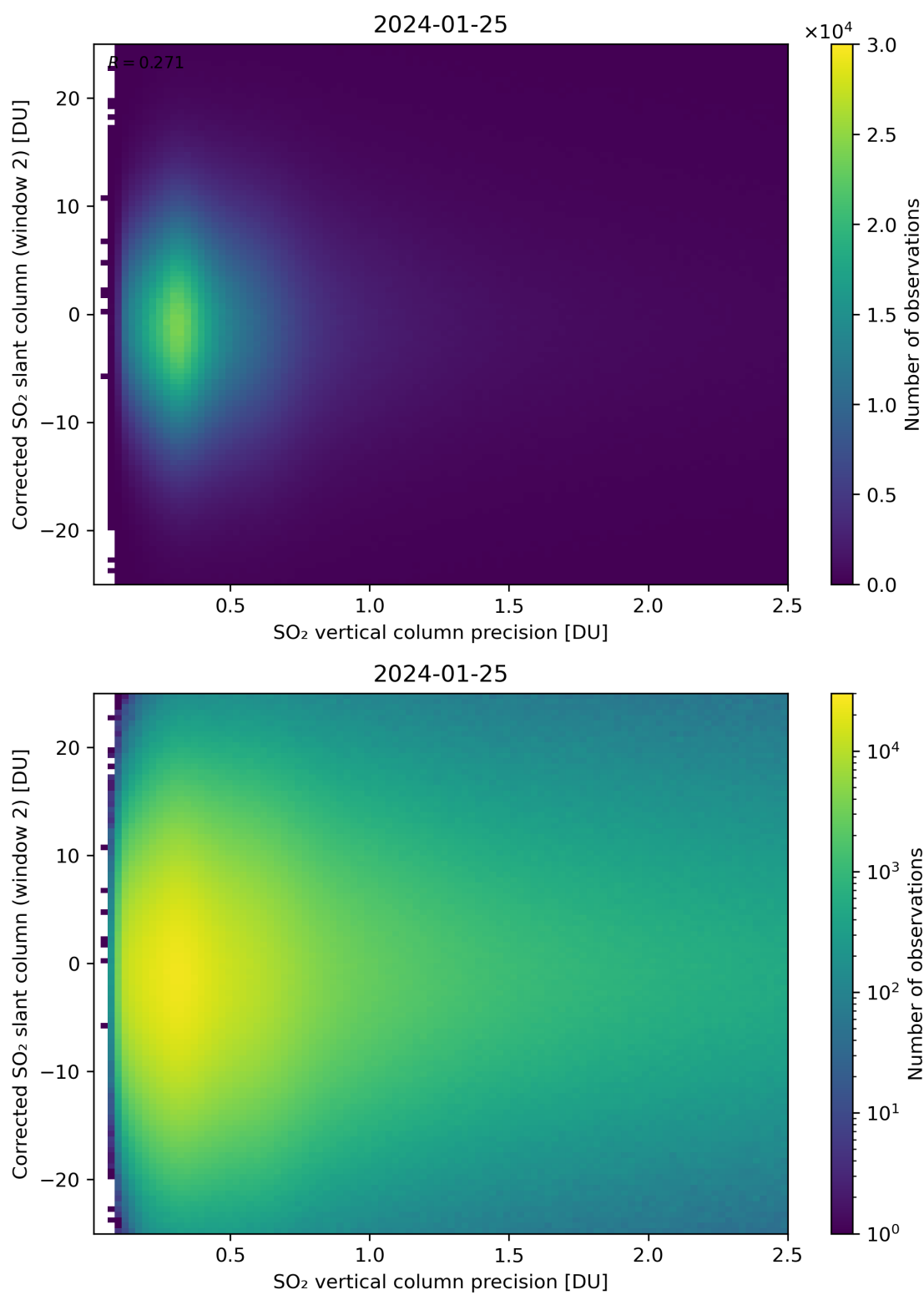
Figure 287: Scatter density plot of “SO 2 vertical column precision” against “Corrected SO 2 slant column (window 2)” for 2024-01-24 to 2024-01-26.
