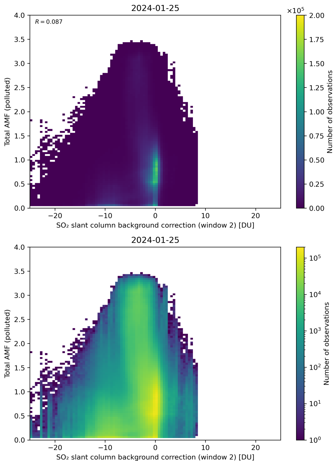
Figure 119: Scatter density plot of “SO 2 slant column background correction (window 2)” against “Total AMF (polluted)” for 2024-01-24 to 2024-01-26.
