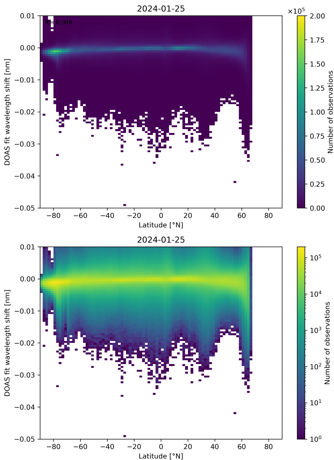
Figure 142: Scatter density plot of “Latitude” against “DOAS fit wavelength shift” for 2024-01-24 to 2024-01-26.
