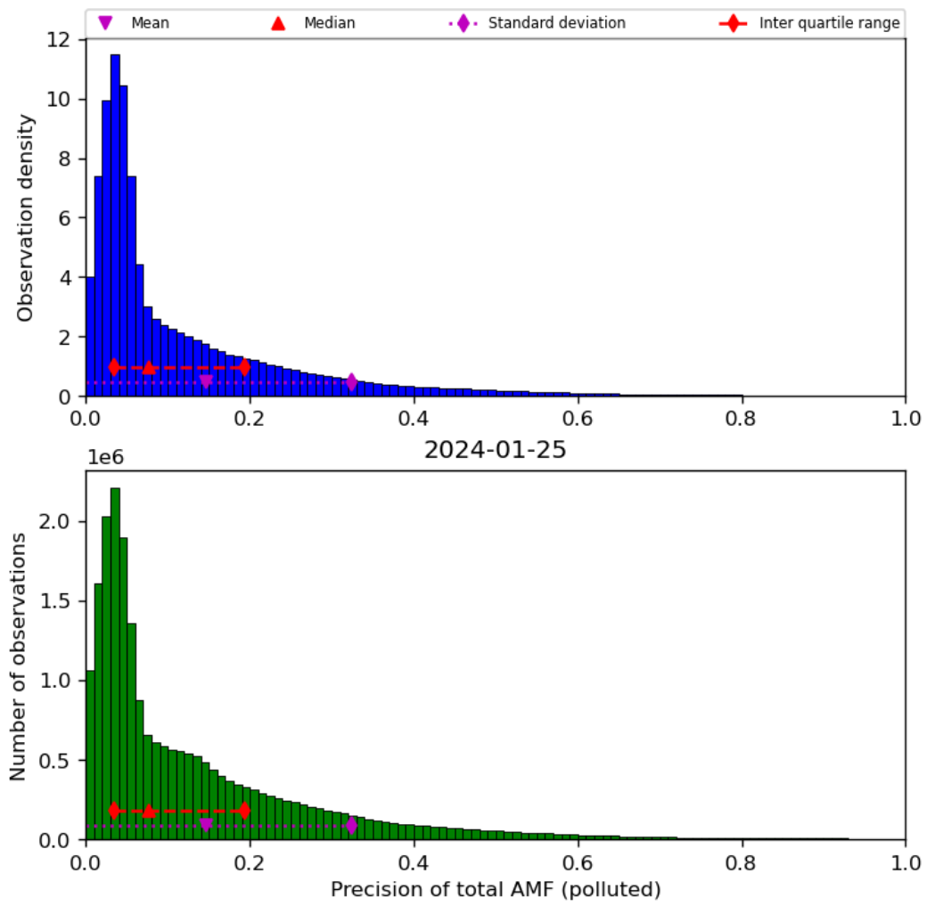
Figure 72: Histogram of “Precision of total AMF (polluted)” for 2024-01-24 to 2024-01-26
