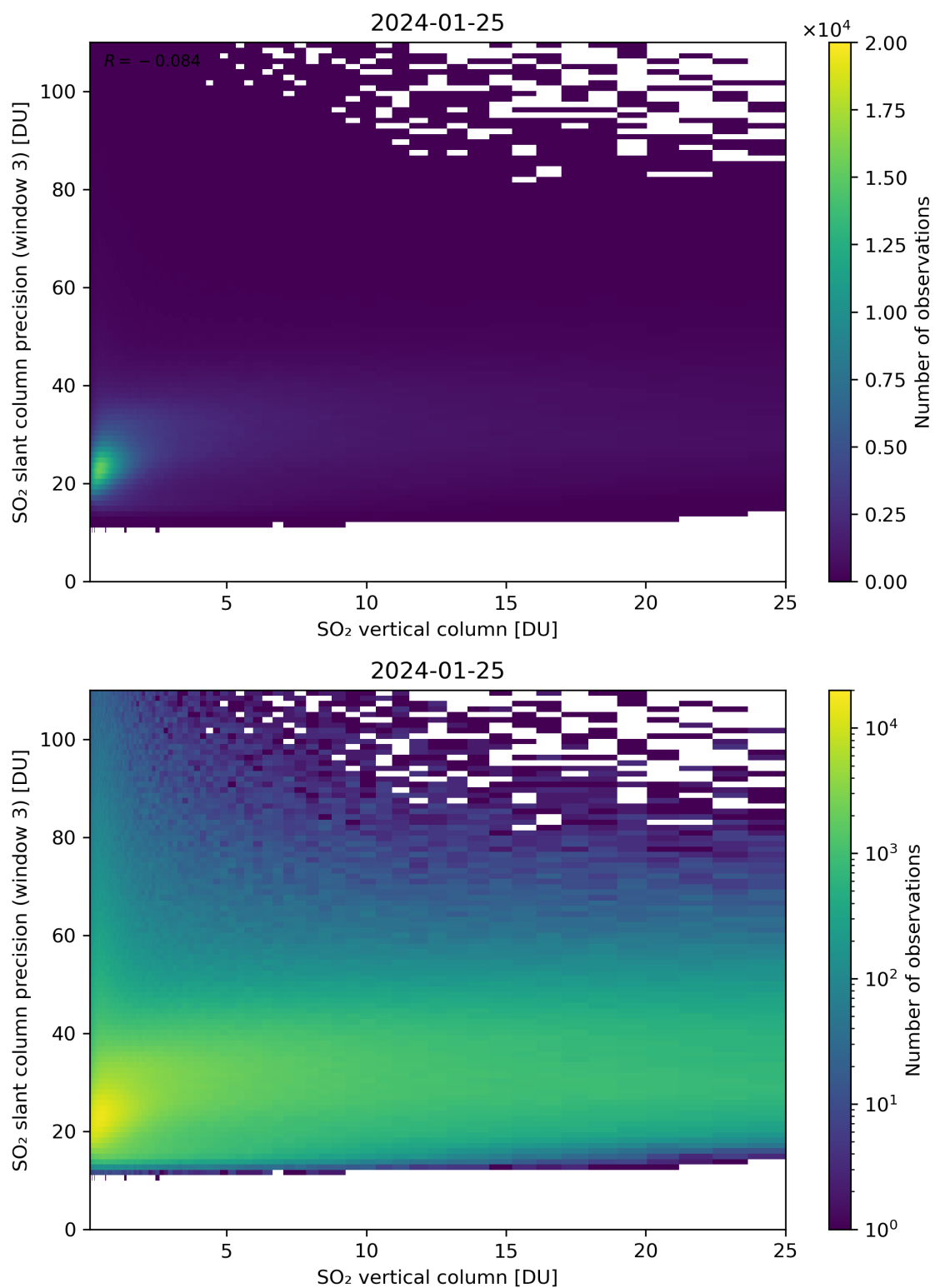
Figure 304: Scatter density plot of “SO 2 vertical column” against “SO 2 slant column precision (window 3)” for 2024-01-24 to 2024-01-26.
