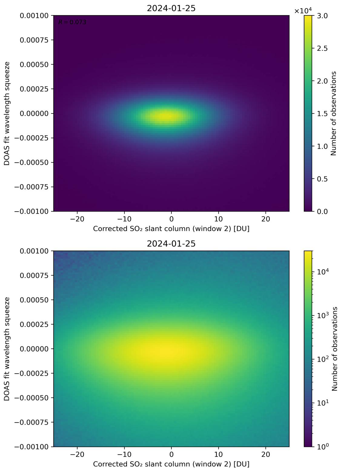
Figure 197: Scatter density plot of “Corrected SO 2 slant column (window 2)” against “DOAS fit wavelength squeeze” for 2024-01-24 to 2024-01-26.
