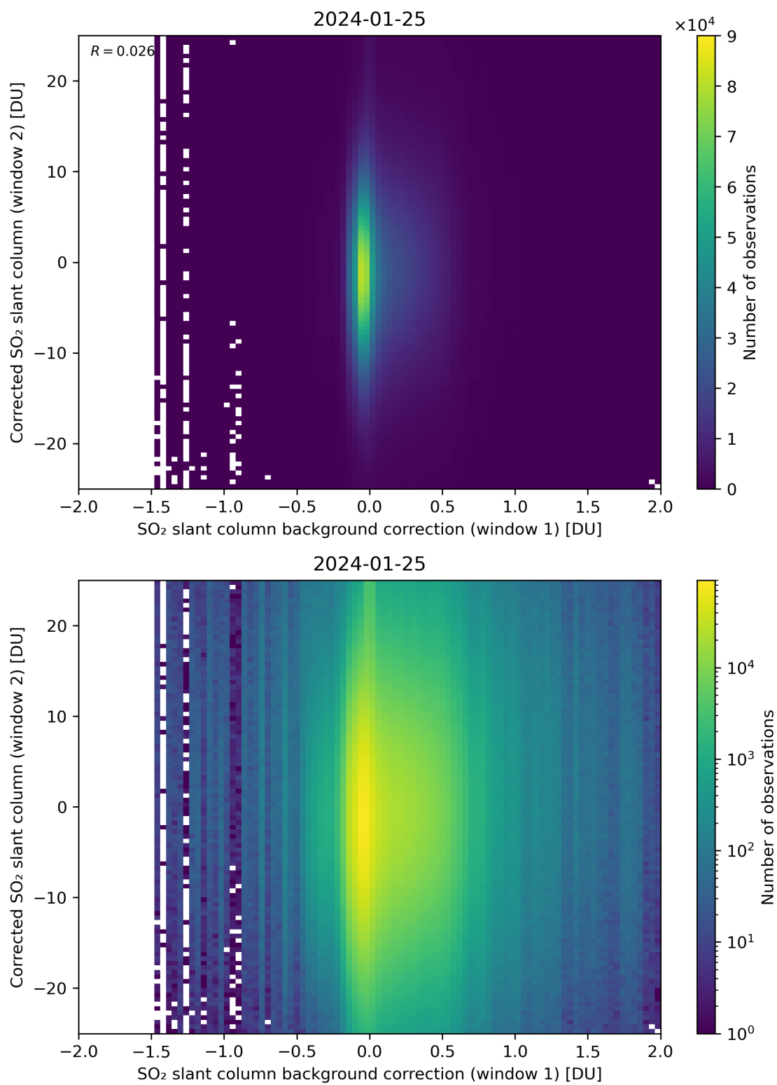
Figure 104: Scatter density plot of “SO 2 slant column background correction (window 1)” against “Corrected SO 2 slant column (window 2)” for 2024-01-24 to 2024-01-26.
