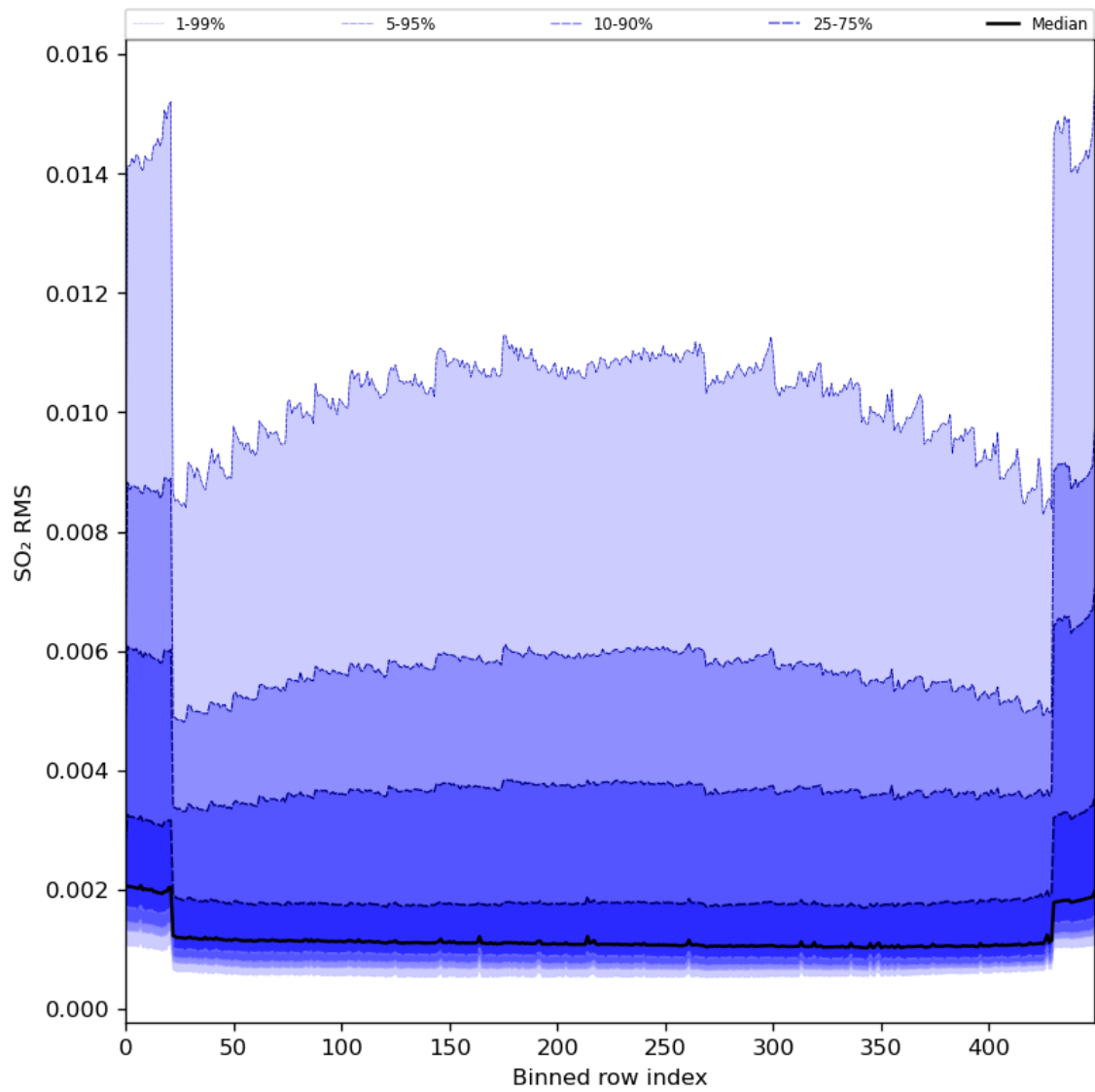
Figure 93: Along track statistics of “SO 2 RMS” for 2024-01-24 to 2024-01-26
