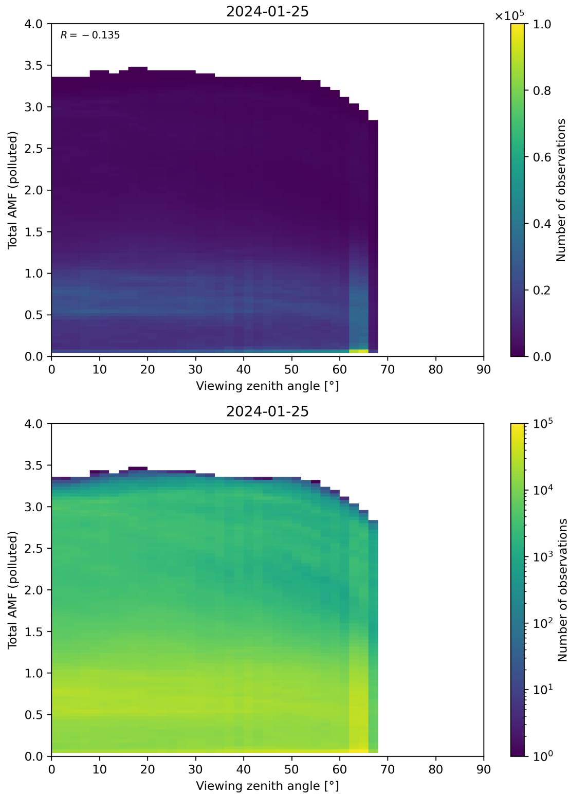
Figure 325: Scatter density plot of “Viewing zenith angle” against “Total AMF (polluted)” for 2024-01-24 to 2024-01-26.
