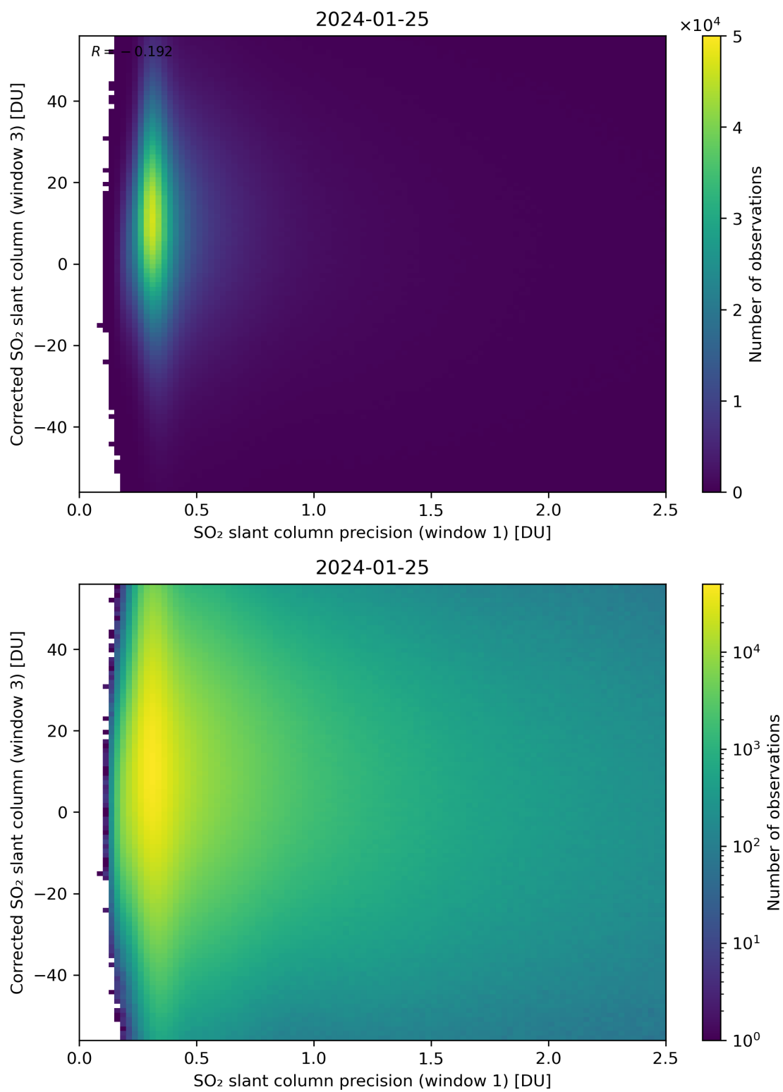
Figure 226: Scatter density plot of “SO 2 slant column precision (window 1)” against “Corrected SO 2 slant column (window 3)” for 2024-01-24 to 2024-01-26.
