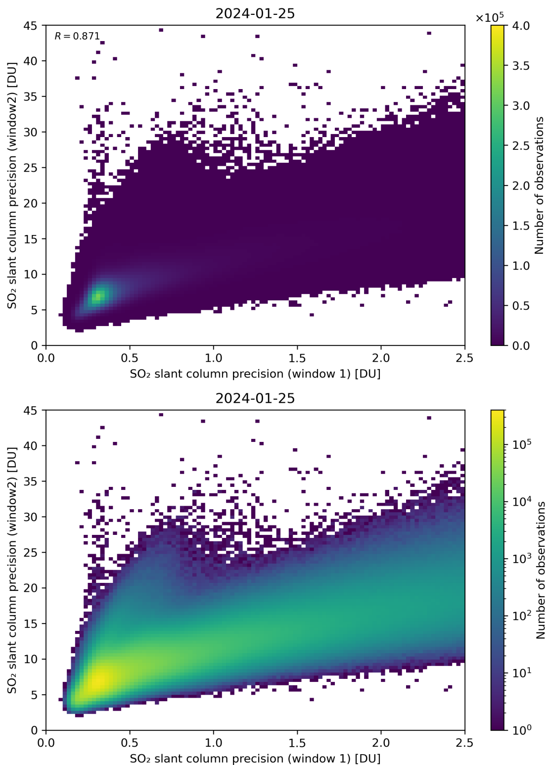
Figure 227: Scatter density plot of “SO 2 slant column precision (window 1)” against “SO 2 slant column precision (window2)” for 2024-01-24 to 2024-01-26.
