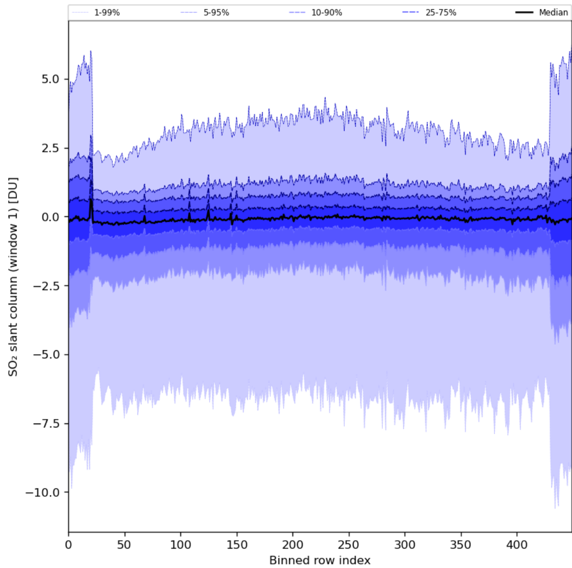
Figure 79: Along track statistics of “SO 2 slant column (window 1)” for 2024-01-24 to 2024-01-26
