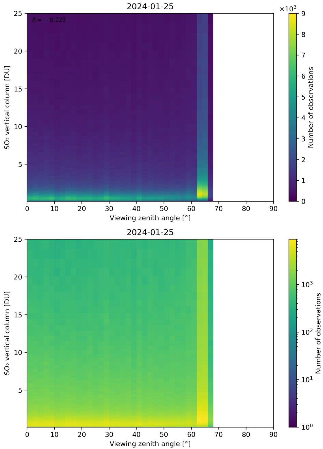
Figure 327: Scatter density plot of “Viewing zenith angle” against “SO 2 vertical column” for 2024-01-24 to 2024-01-26.
