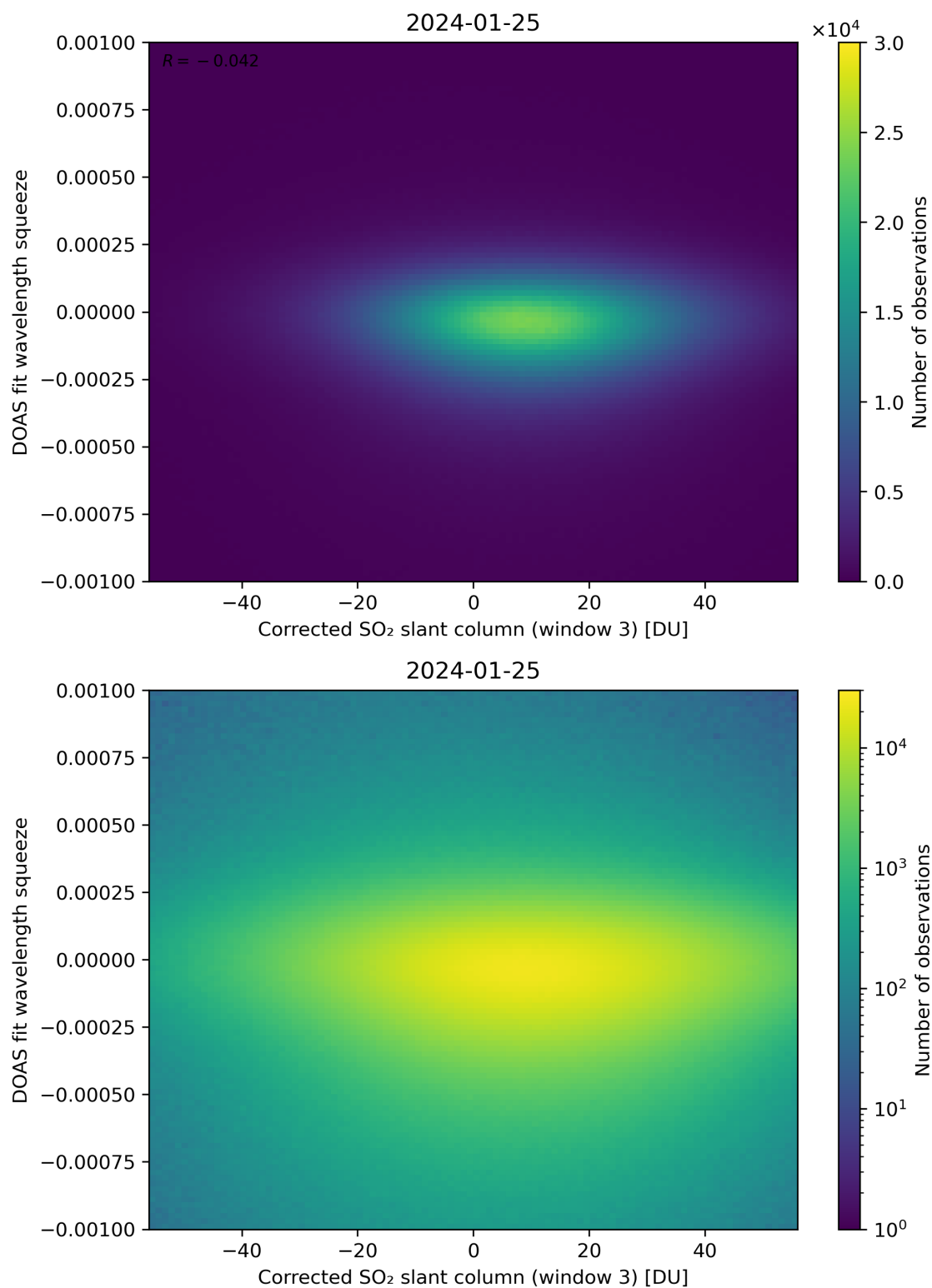
Figure 207: Scatter density plot of “Corrected SO 2 slant column (window 3)” against “DOAS fit wavelength squeeze” for 2024-01-24 to 2024-01-26.
