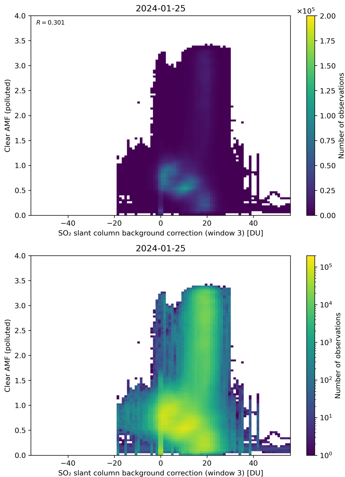
Figure 124: Scatter density plot of “SO 2 slant column background correction (window 3)” against “Clear AMF (polluted)” for 2024-01-24 to 2024-01-26.
