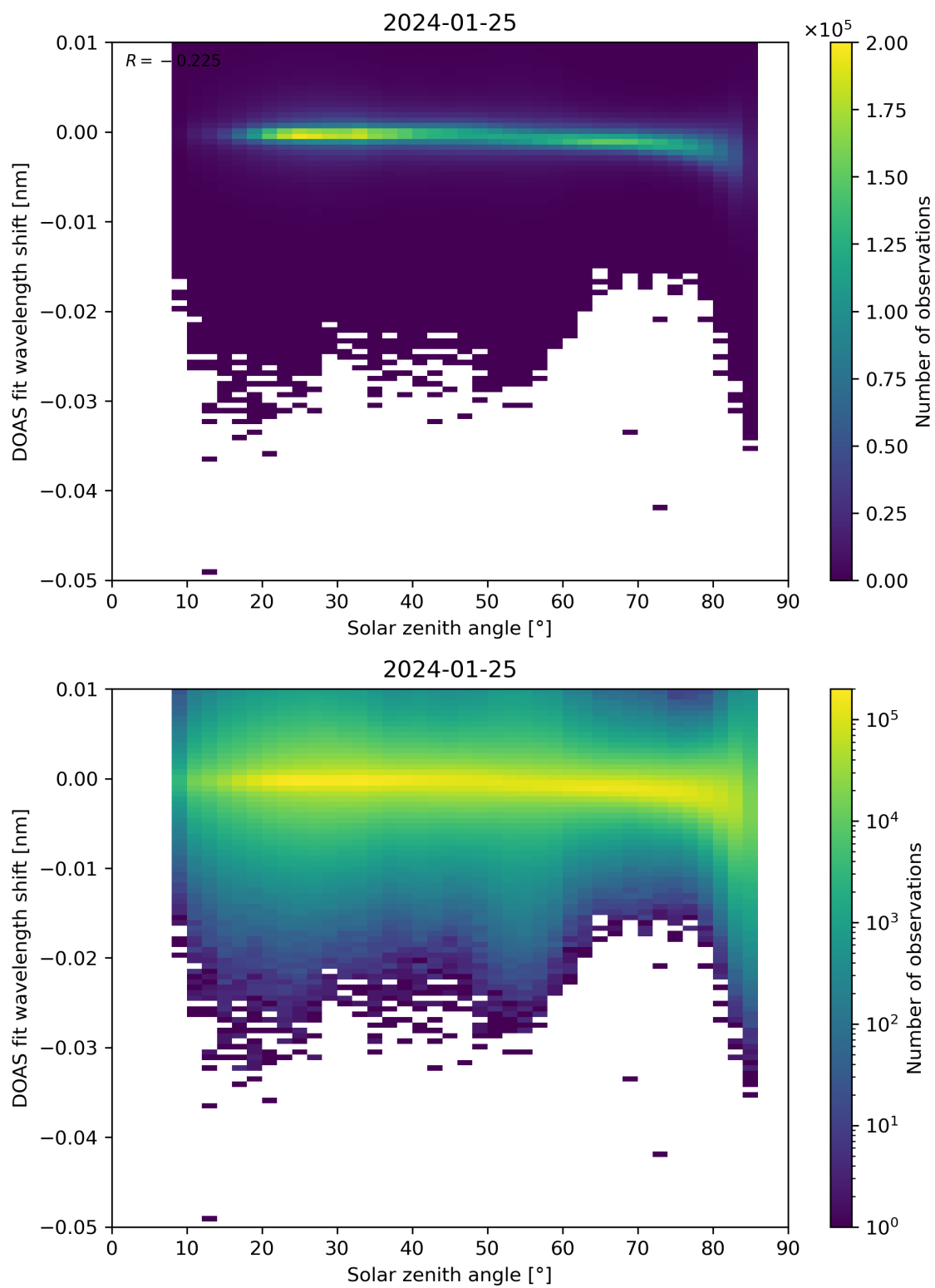
Figure 161: Scatter density plot of “Solar zenith angle” against “DOAS fit wavelength shift” for 2024-01-24 to 2024-01-26.
