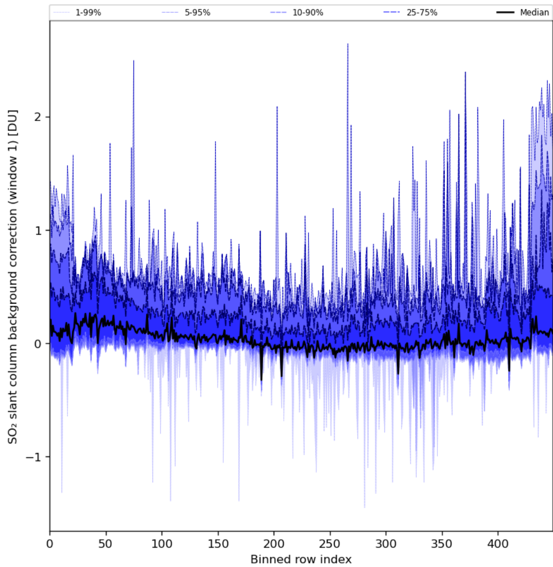
Figure 82: Along track statistics of “SO 2 slant column background correction (window 1)” for 2024-01-24 to 2024-01-26
