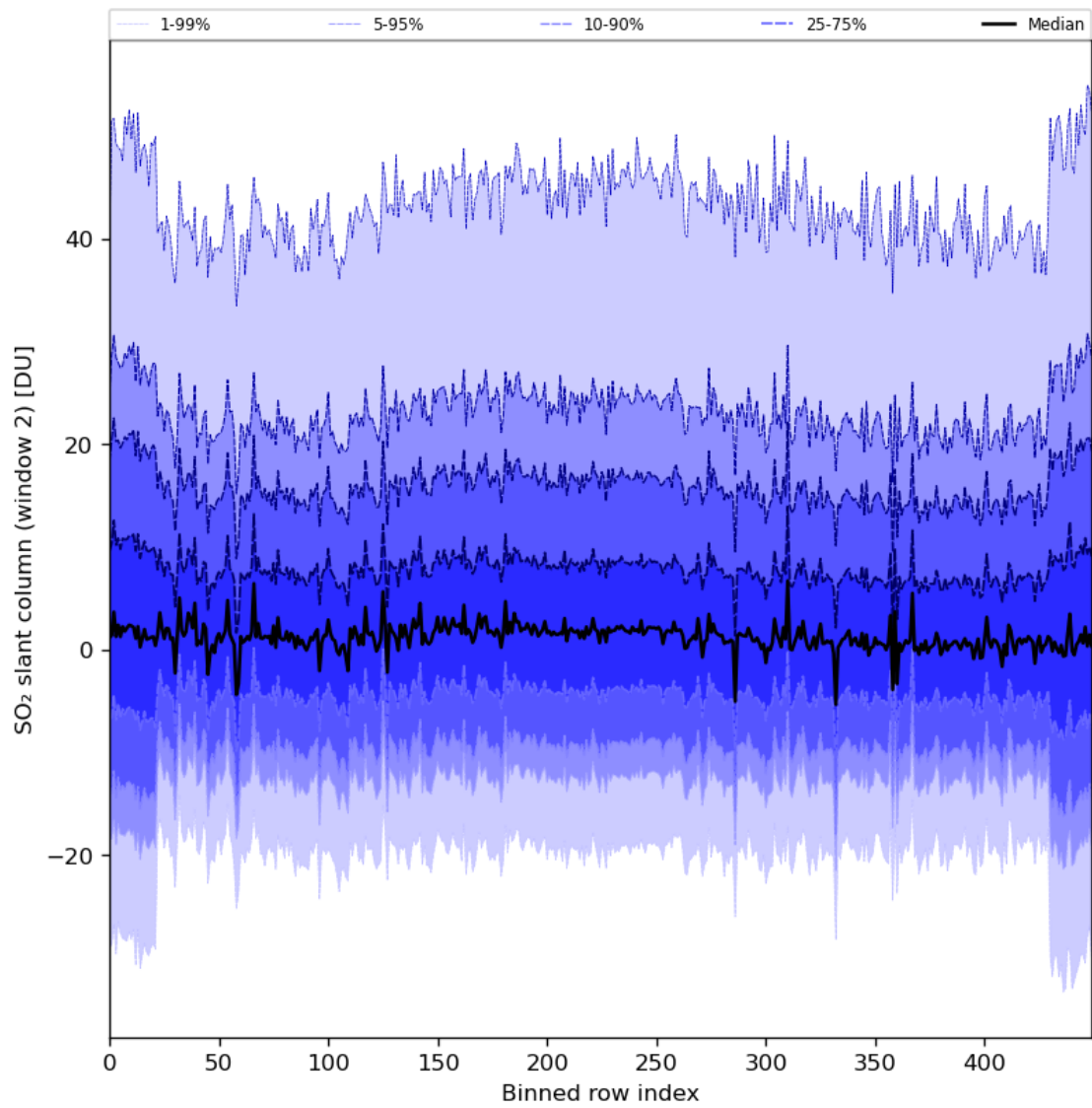
Figure 83: Along track statistics of “SO 2 slant column (window 2)” for 2024-01-24 to 2024-01-26
