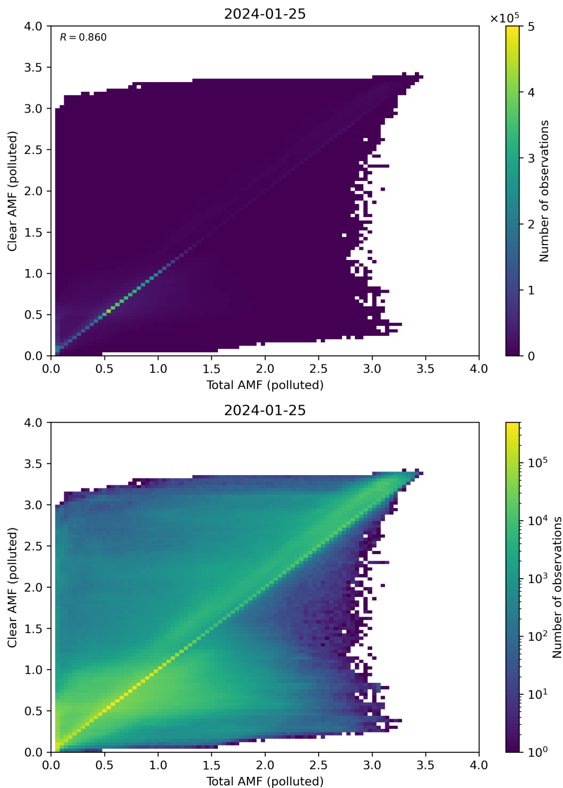
Figure 271: Scatter density plot of “Total AMF (polluted)” against “Clear AMF (polluted)” for 2024-01-24 to 2024-01-26.
