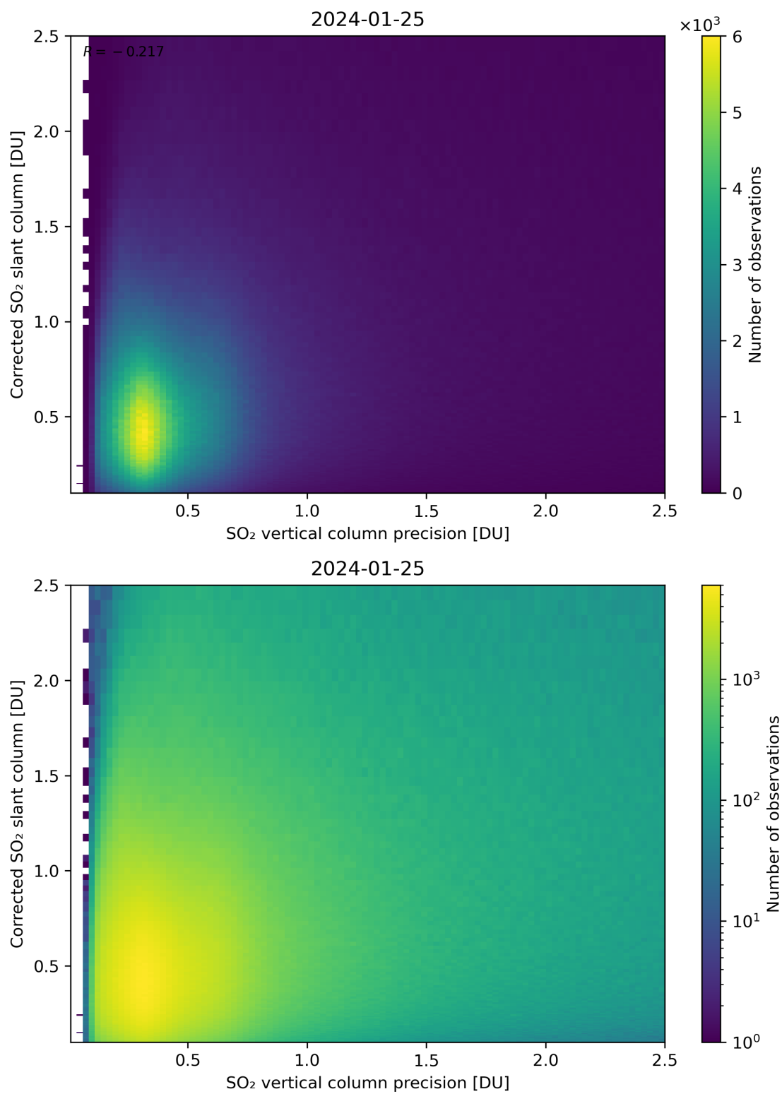
Figure 286: Scatter density plot of “SO 2 vertical column precision” against “Corrected SO 2 slant column” for 2024-01-24 to 2024-01-26.
