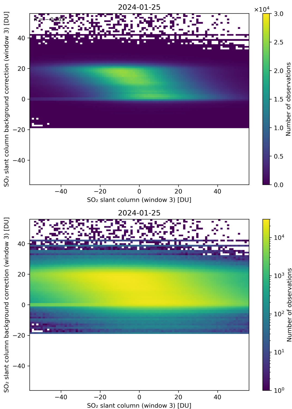
Figure 253: Scatter density plot of “SO 2 slant column (window 3)” against “SO 2 slant column background correction (window 3)” for 2024-01-24 to 2024-01-26.
