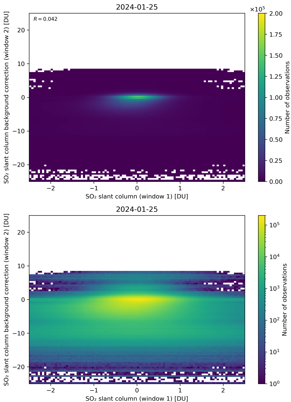
Figure 213: Scatter density plot of “SO 2 slant column (window 1)” against “SO 2 slant column background correction (window 2)” for 2024-01-24 to 2024-01-26.
