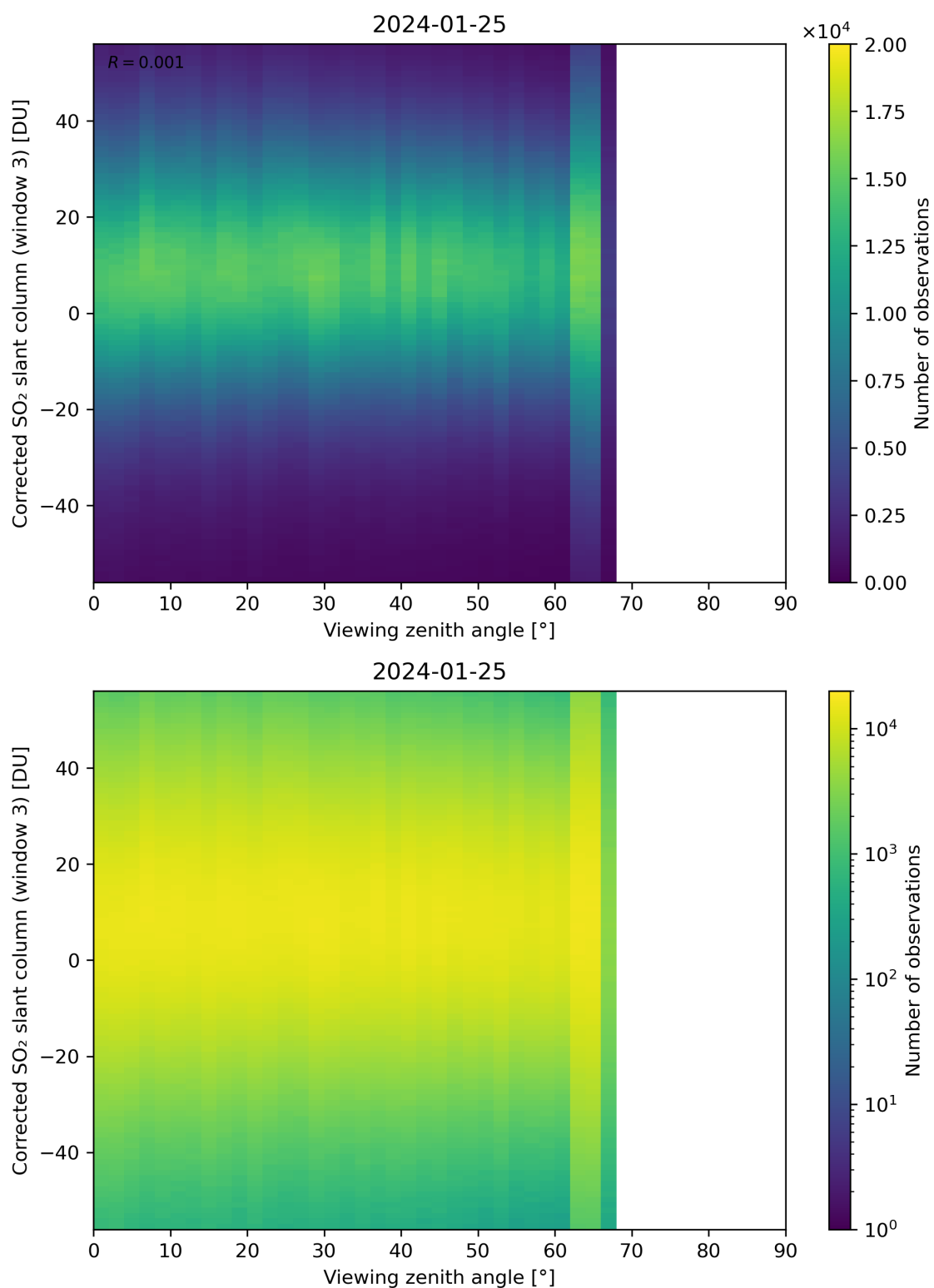
Figure 319: Scatter density plot of “Viewing zenith angle” against “Corrected SO 2 slant column (window 3)” for 2024-01-24 to 2024-01-26.
