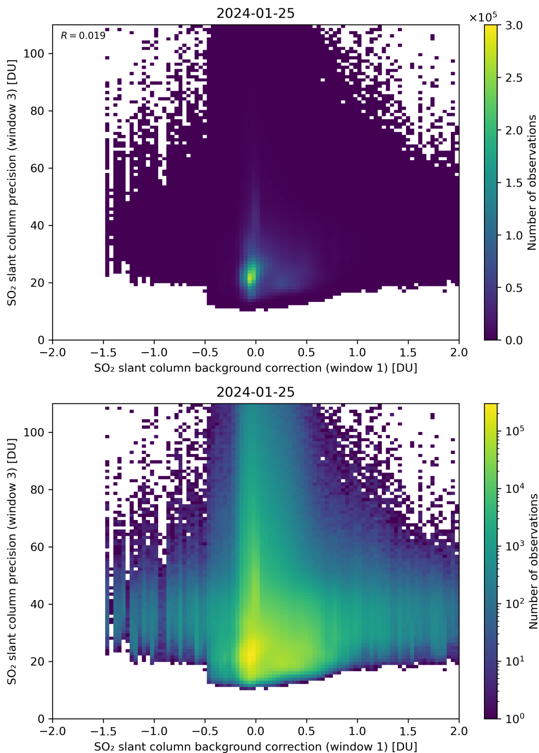
Figure 108: Scatter density plot of “SO 2 slant column background correction (window 1)” against “SO 2 slant column precision (window 3)” for 2024-01-24 to 2024-01-26.
