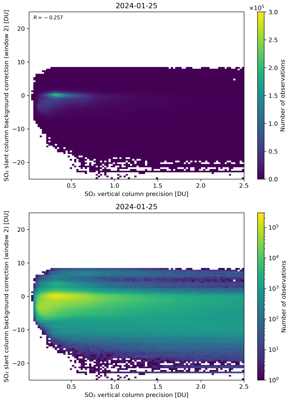
Figure 280: Scatter density plot of “SO 2 vertical column precision” against “SO 2 slant column background correction (window 2)” for 2024-01-24 to 2024-01-26.
