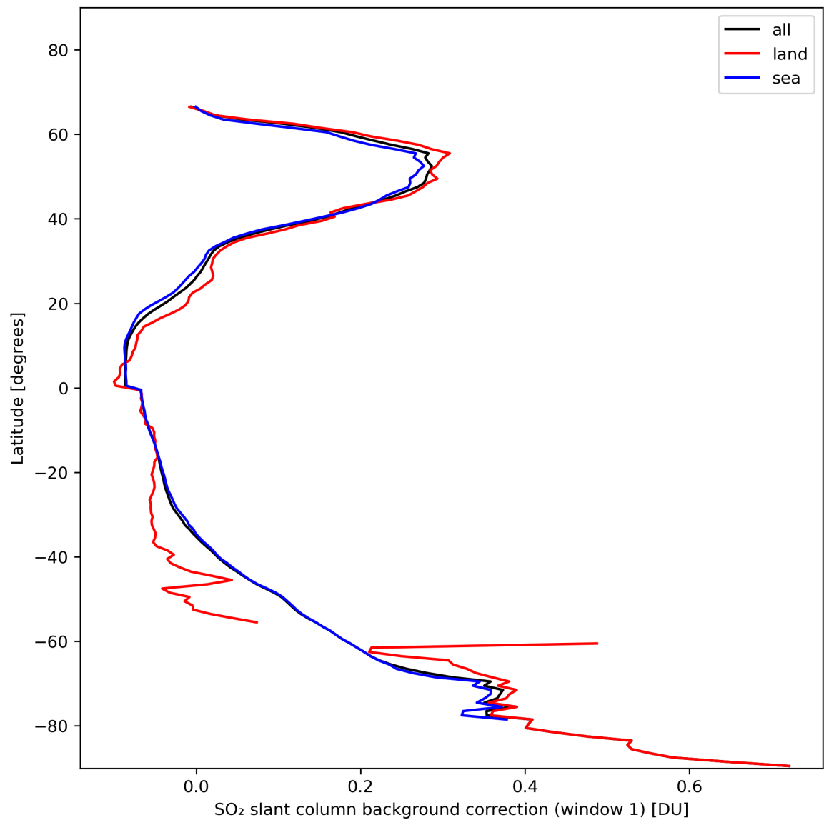
Figure 36: Zonal average of “SO 2 slant column background correction (window 1)” for 2024-01-24 to 2024-01-26.
