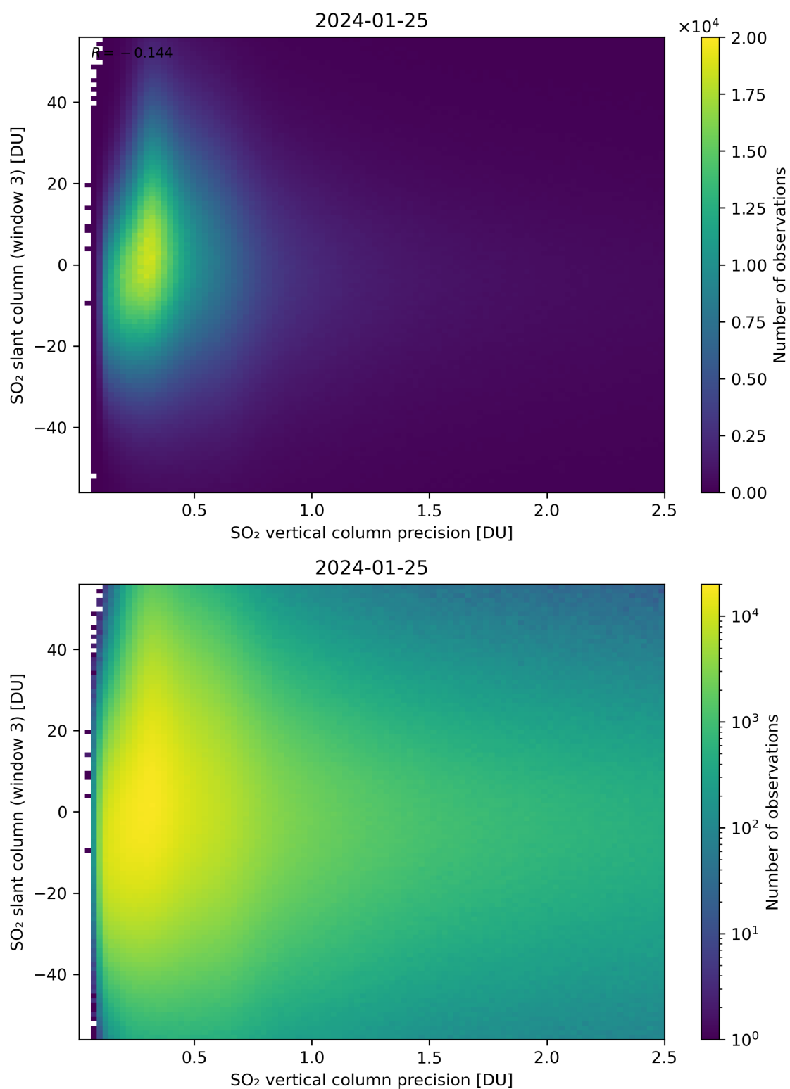
Figure 292: Scatter density plot of “SO 2 vertical column precision” against “SO 2 slant column (window 3)” for 2024-01-24 to 2024-01-26.
