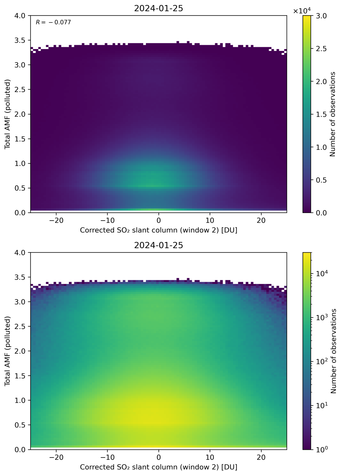
Figure 203: Scatter density plot of “Corrected SO 2 slant column (window 2)” against “Total AMF (polluted)” for 2024-01-24 to 2024-01-26.
