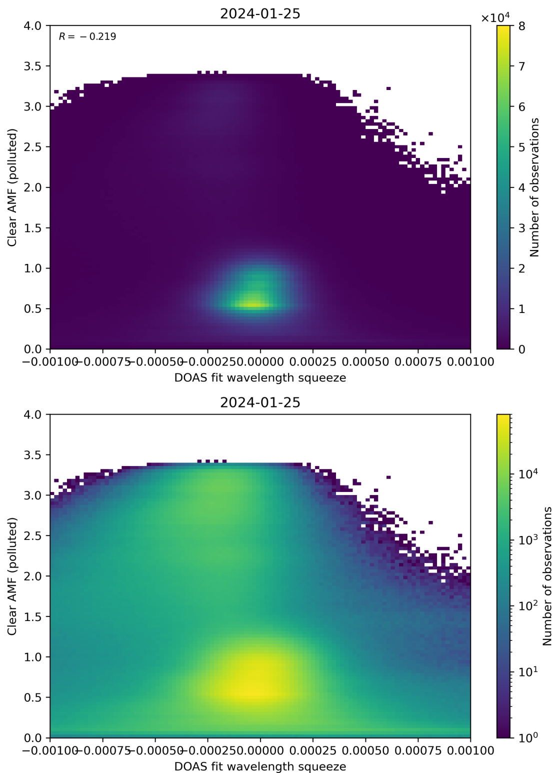
Figure 133: Scatter density plot of “DOAS fit wavelength squeeze” against “Clear AMF (polluted)” for 2024-01-24 to 2024-01-26.
