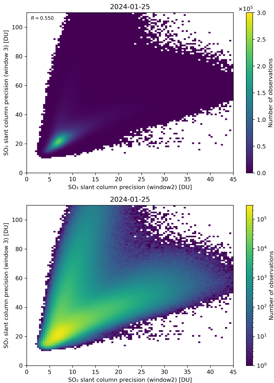
Figure 250: Scatter density plot of “SO 2 slant column precision (window2)” against “SO 2 slant column precision (window 3)” for 2024-01-24 to 2024-01-26.
