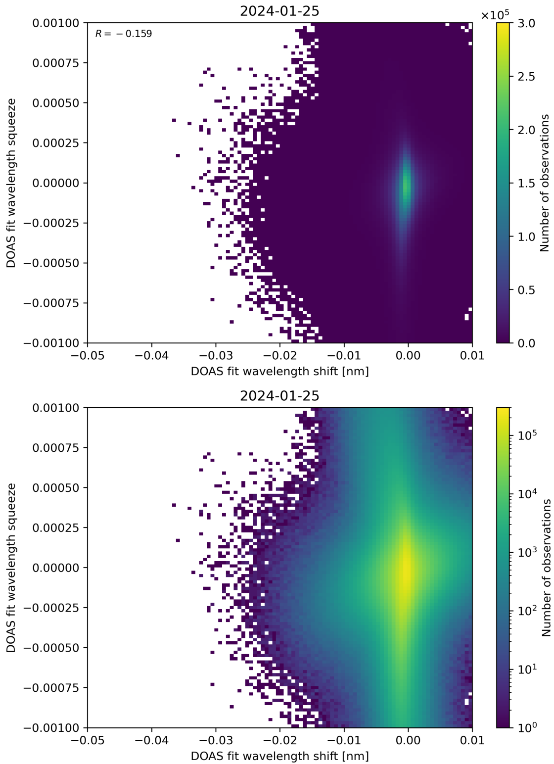
Figure 127: Scatter density plot of “DOAS fit wavelength shift” against “DOAS fit wavelength squeeze” for 2024-01-24 to 2024-01-26.
