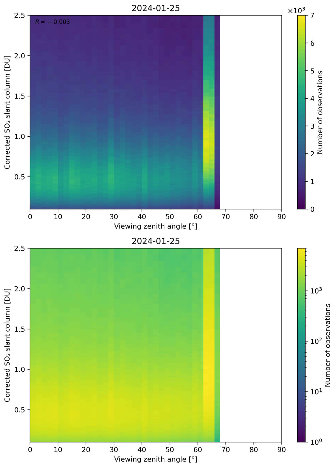
Figure 317: Scatter density plot of “Viewing zenith angle” against “Corrected SO 2 slant column” for 2024-01-24 to 2024-01-26.
