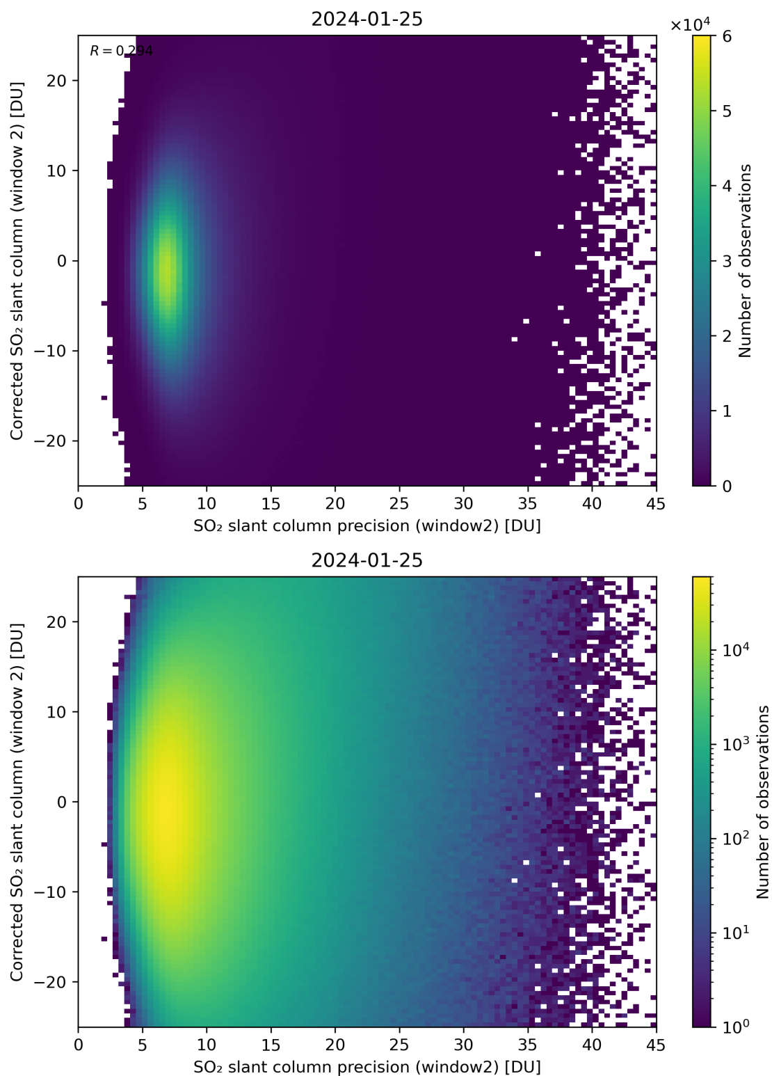
Figure 247: Scatter density plot of “SO 2 slant column precision (window2)” against “Corrected SO 2 slant column (window 2)” for 2024-01-24 to 2024-01-26.
