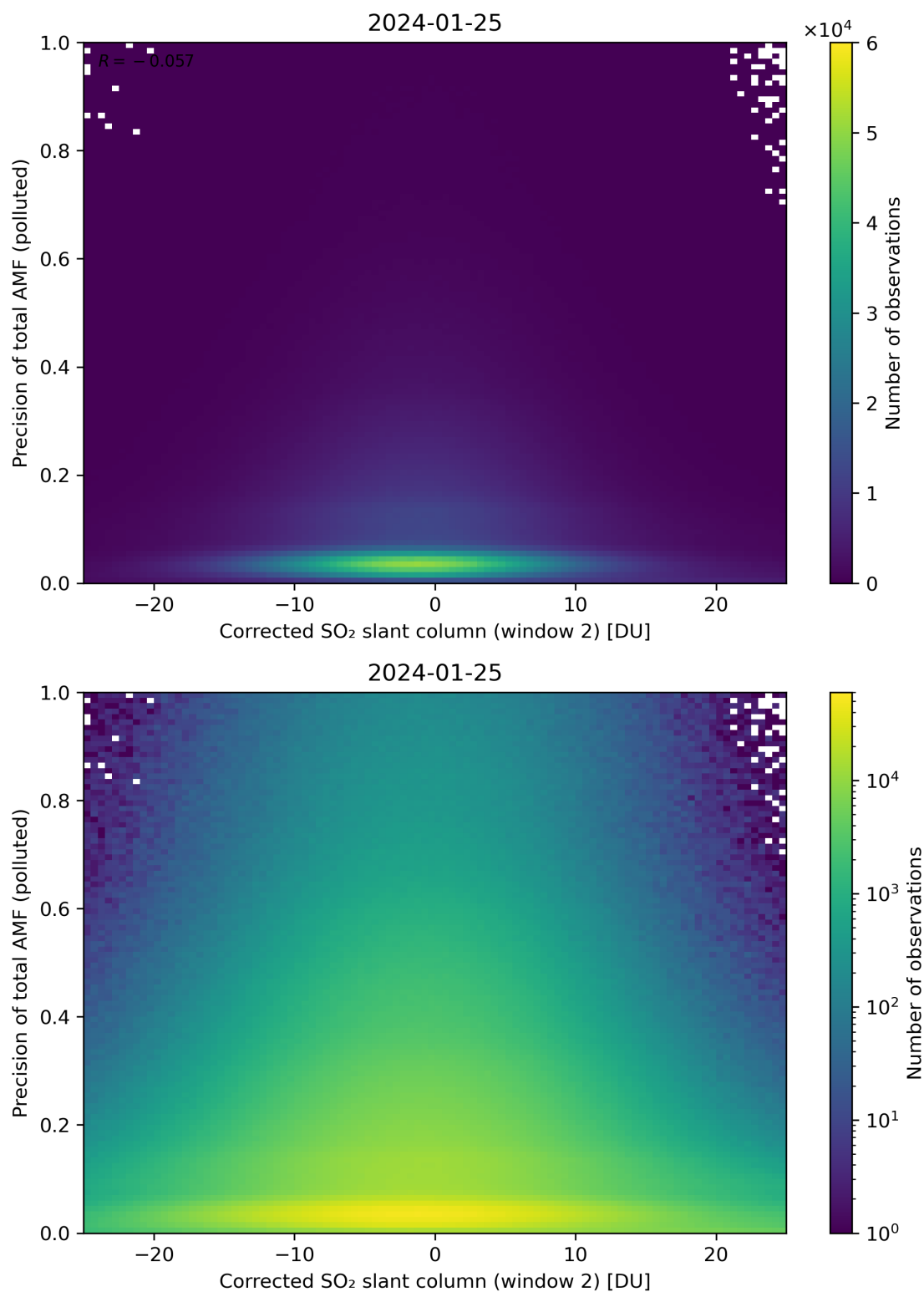
Figure 204: Scatter density plot of “Corrected SO 2 slant column (window 2)” against “Precision of total AMF (polluted)” for 2024-01-24 to 2024-01-26.
