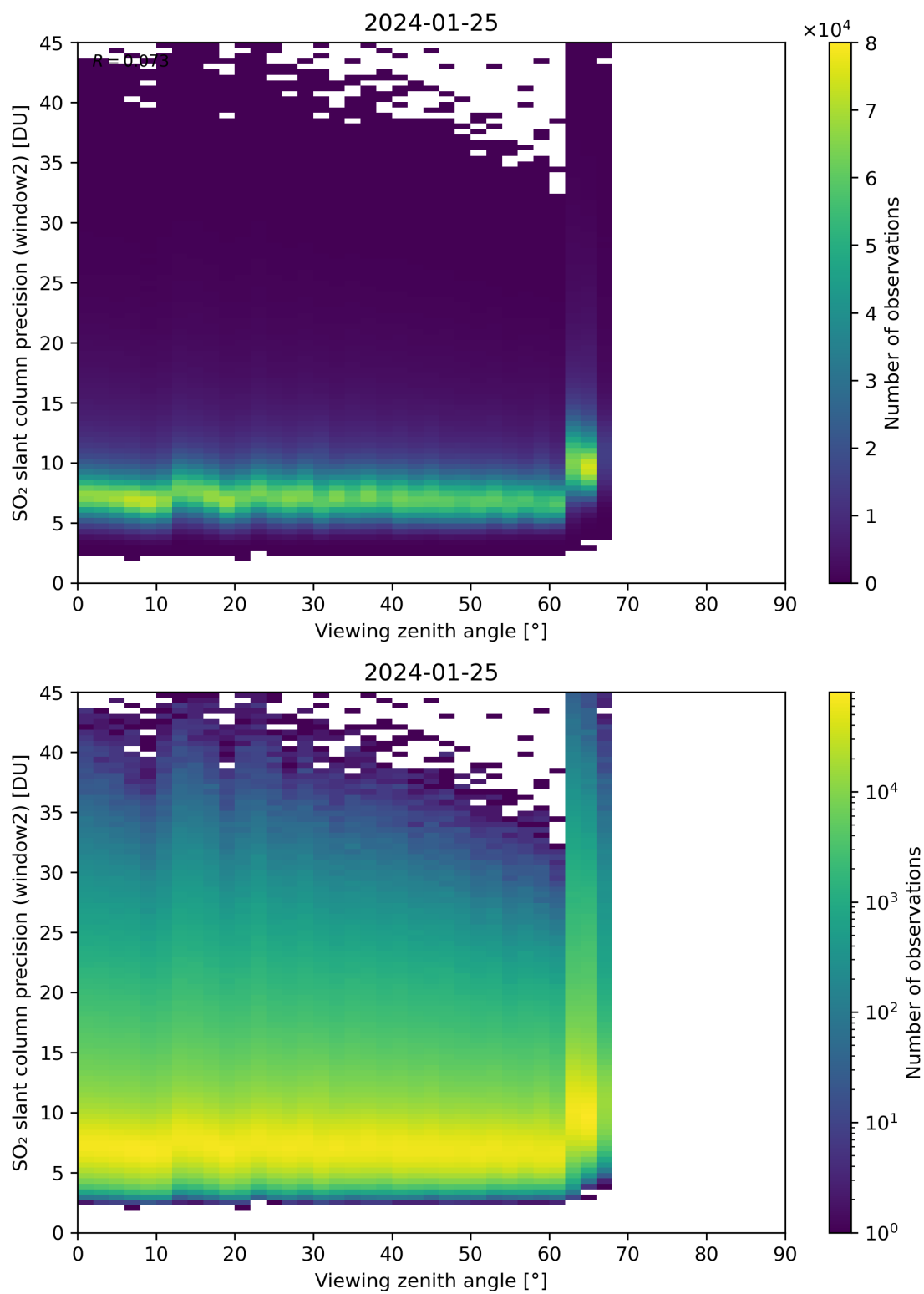
Figure 322: Scatter density plot of “Viewing zenith angle” against “SO 2 slant column precision (window2)” for 2024-01-24 to 2024-01-26.
