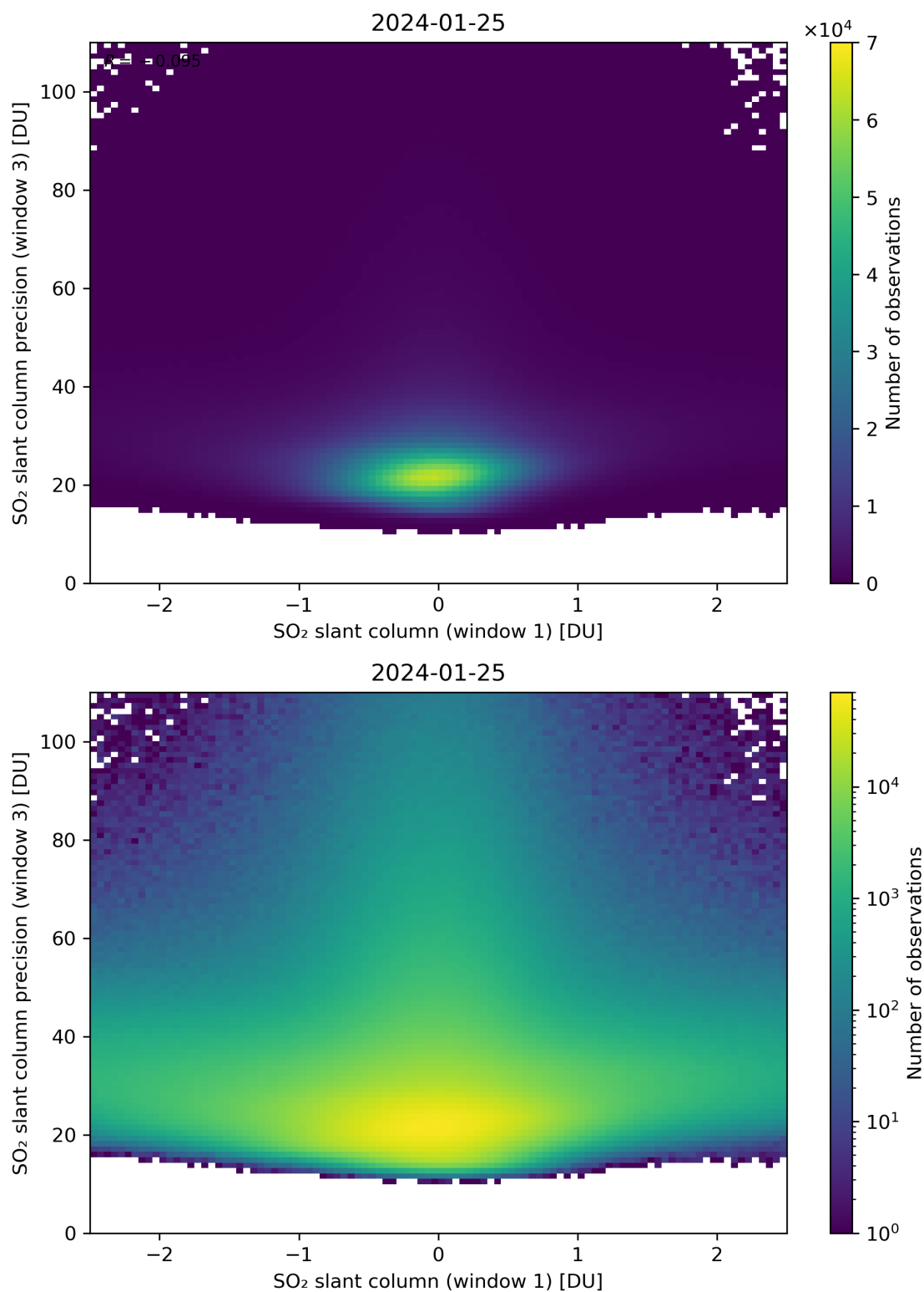
Figure 238: Scatter density plot of “SO 2 slant column (window 1)” against “SO 2 slant column precision (window 3)” for 2024-01-24 to 2024-01-26.
