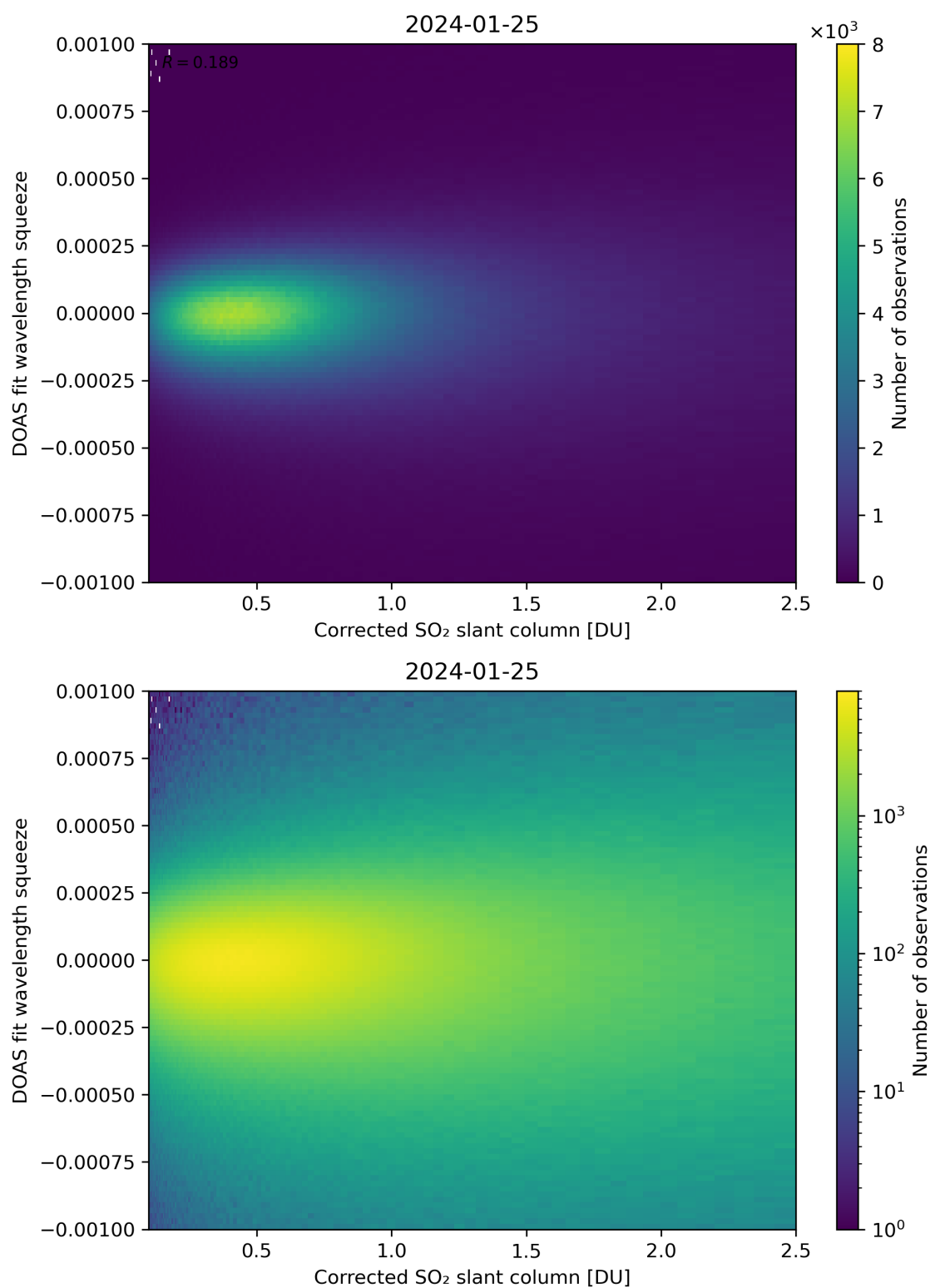
Figure 182: Scatter density plot of “Corrected SO 2 slant column” against “DOAS fit wavelength squeeze” for 2024-01-24 to 2024-01-26.
