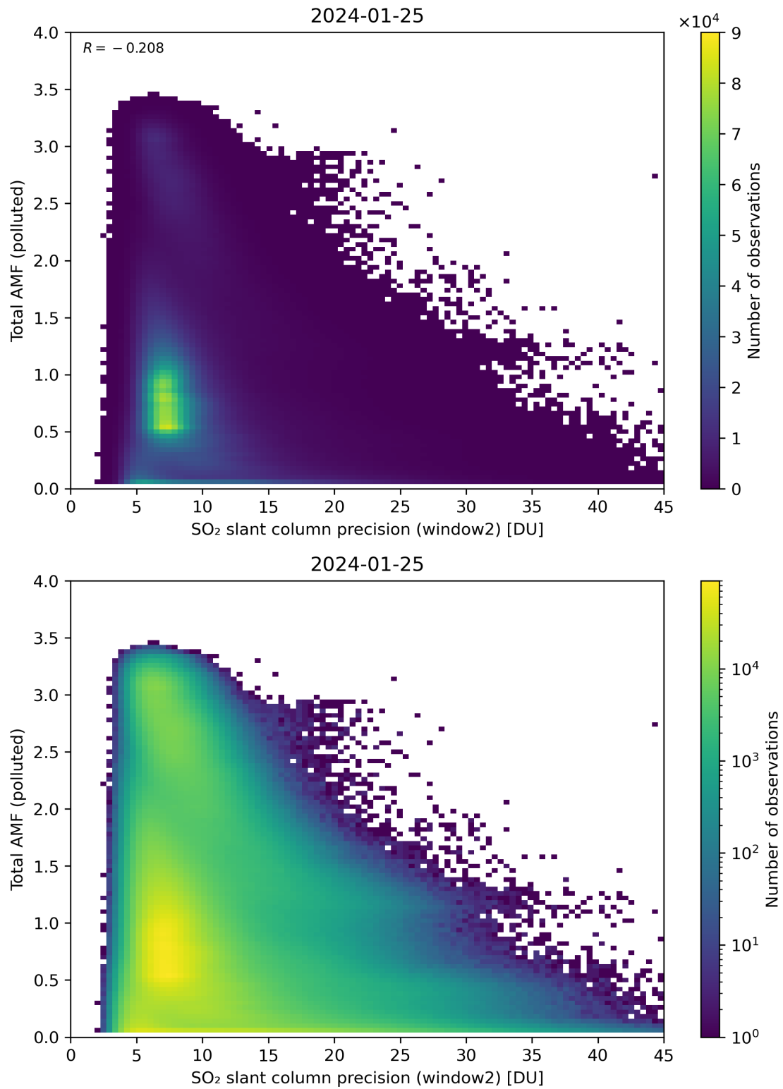
Figure 251: Scatter density plot of “SO 2 slant column precision (window2)” against “Total AMF (polluted)” for 2024-01-24 to 2024-01-26.
