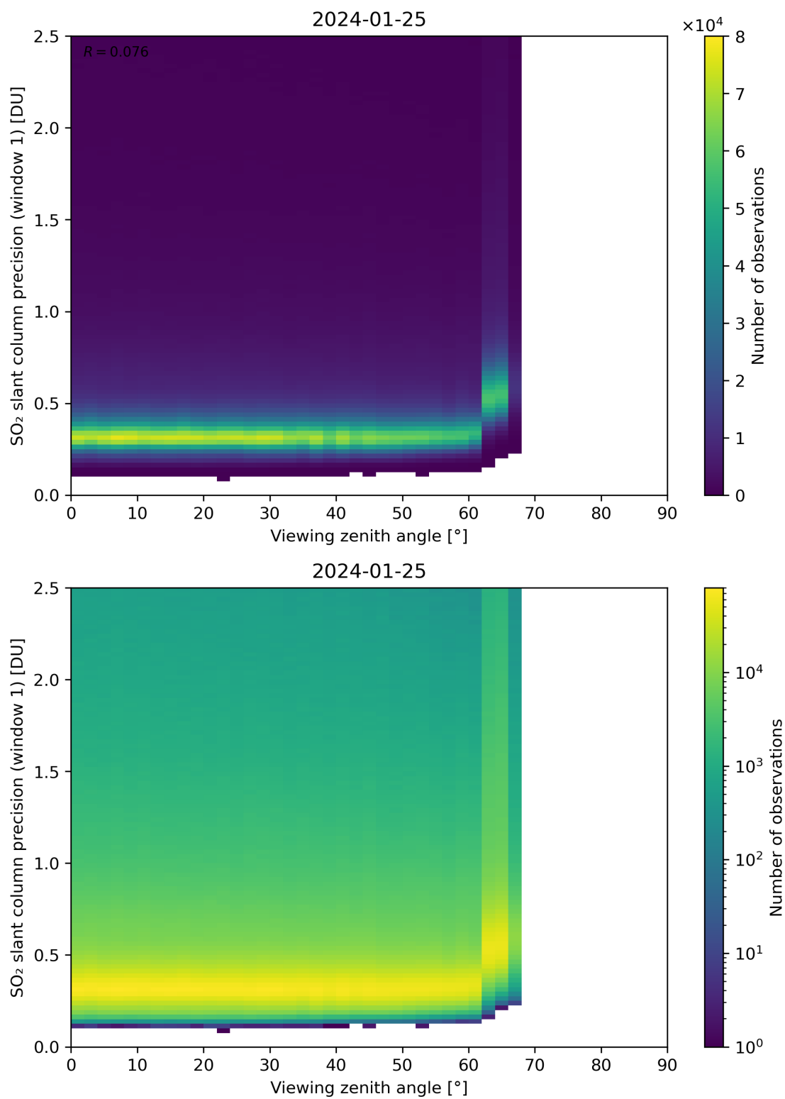
Figure 321: Scatter density plot of “Viewing zenith angle” against “SO 2 slant column precision (window 1)” for 2024-01-24 to 2024-01-26.
