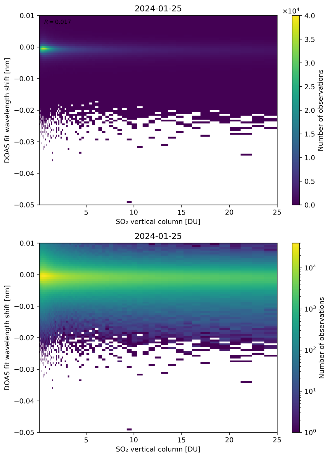
Figure 276: Scatter density plot of “SO 2 vertical column” against “DOAS fit wavelength shift” for 2024-01-24 to 2024-01-26.
