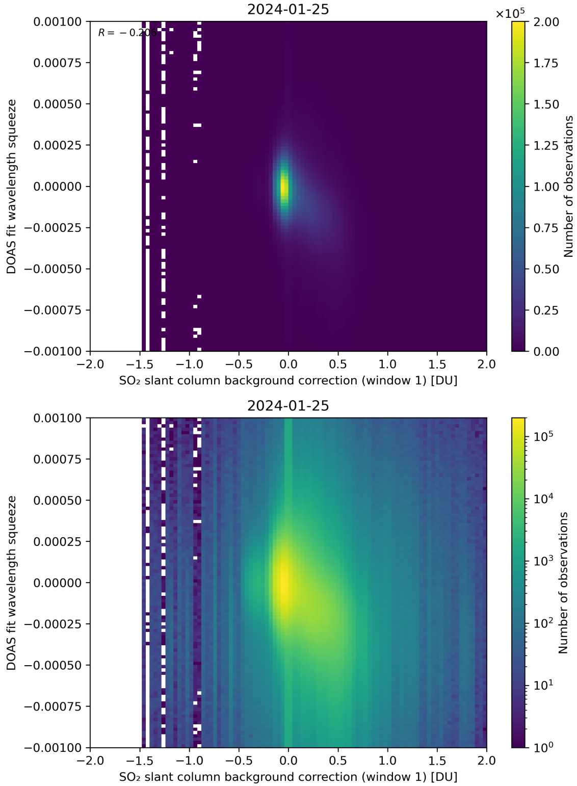
Figure 101: Scatter density plot of “SO 2 slant column background correction (window 1)” against “DOAS fit wavelength squeeze” for 2024-01-24 to 2024-01-26.
