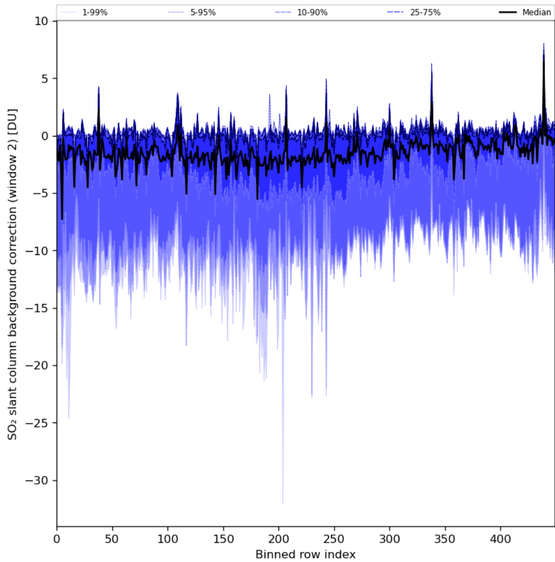
Figure 86: Along track statistics of “SO 2 slant column background correction (window 2)” for 2024-01-24 to 2024-01-26
