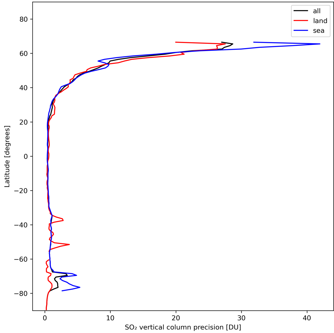
Figure 31: Zonal average of “SO 2 vertical column precision” for 2024-01-24 to 2024-01-26.
