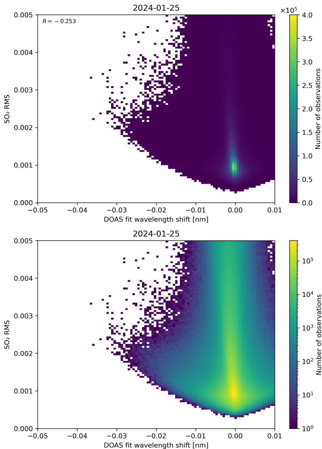
Figure 128: Scatter density plot of “DOAS fit wavelength shift” against “SO 2 RMS” for 2024-01-24 to 2024-01-26.
