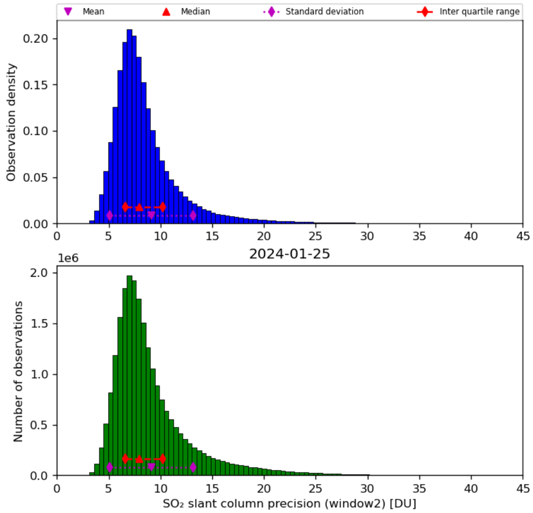
Figure 61: Histogram of “SO 2 slant column precision (window2)” for 2024-01-24 to 2024-01-26
