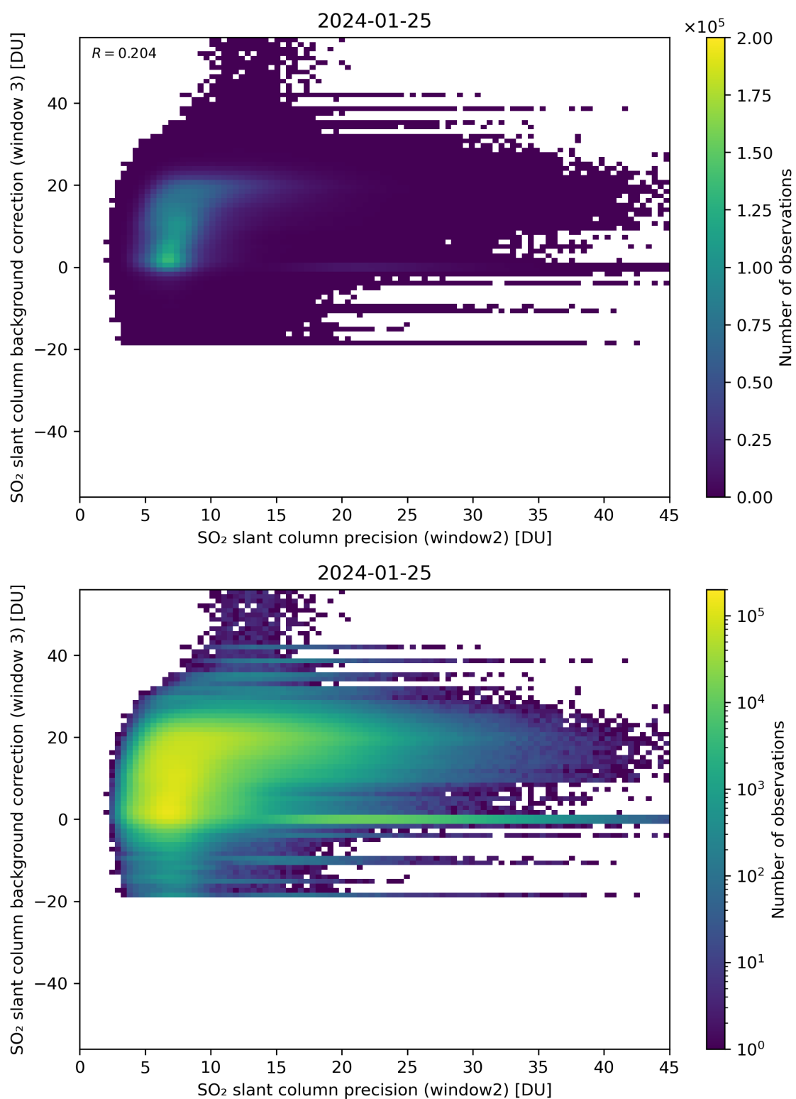
Figure 242: Scatter density plot of “SO 2 slant column precision (window2)” against “SO 2 slant column background correction (window 3)” for 2024-01-24 to 2024-01-26.
