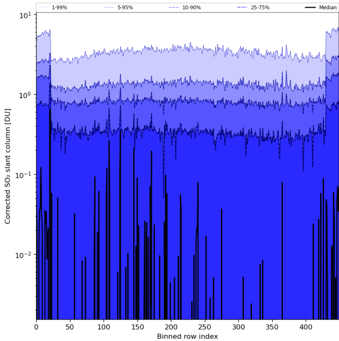
Figure 78: Along track statistics of “Corrected SO 2 slant column” for 2024-01-24 to 2024-01-26
