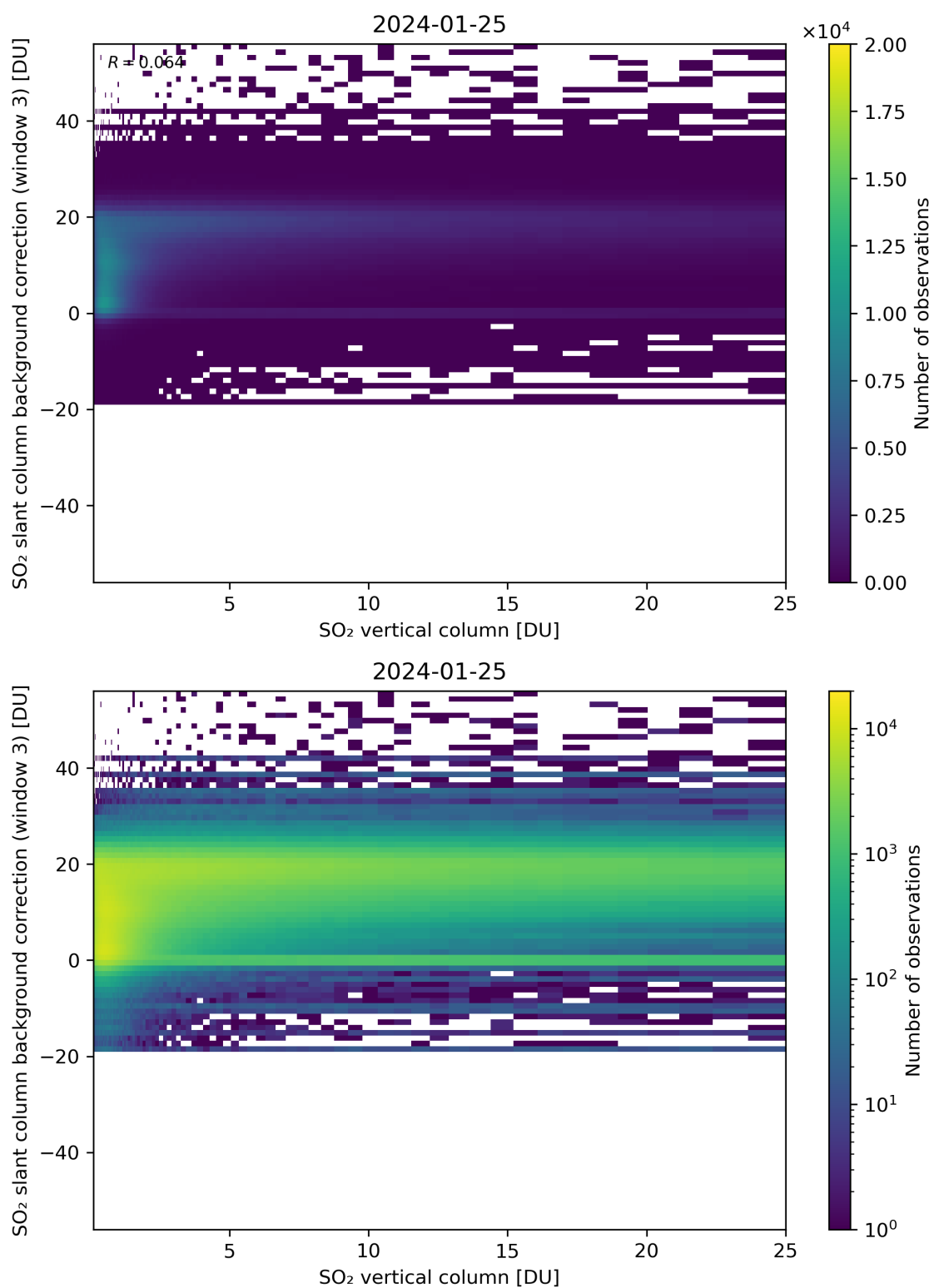
Figure 275: Scatter density plot of “SO 2 vertical column” against “SO 2 slant column background correction (window 3)” for 2024-01-24 to 2024-01-26.
