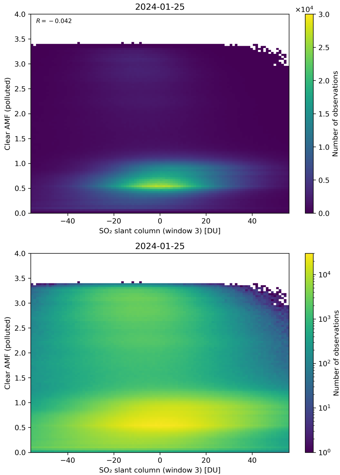
Figure 265: Scatter density plot of “SO 2 slant column (window 3)” against “Clear AMF (polluted)” for 2024-01-24 to 2024-01-26.
