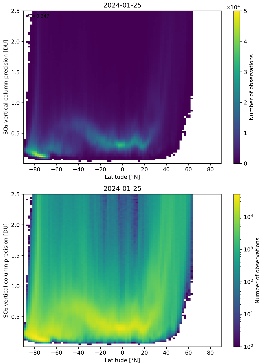
Figure 157: Scatter density plot of “Latitude” against “SO 2 vertical column precision” for 2024-01-24 to 2024-01-26.
