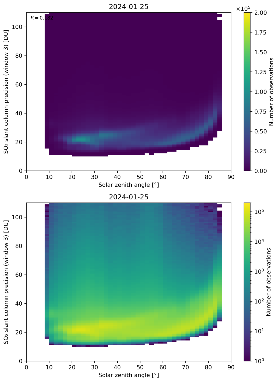
Figure 173: Scatter density plot of “Solar zenith angle” against “SO 2 slant column precision (window 3)” for 2024-01-24 to 2024-01-26.
