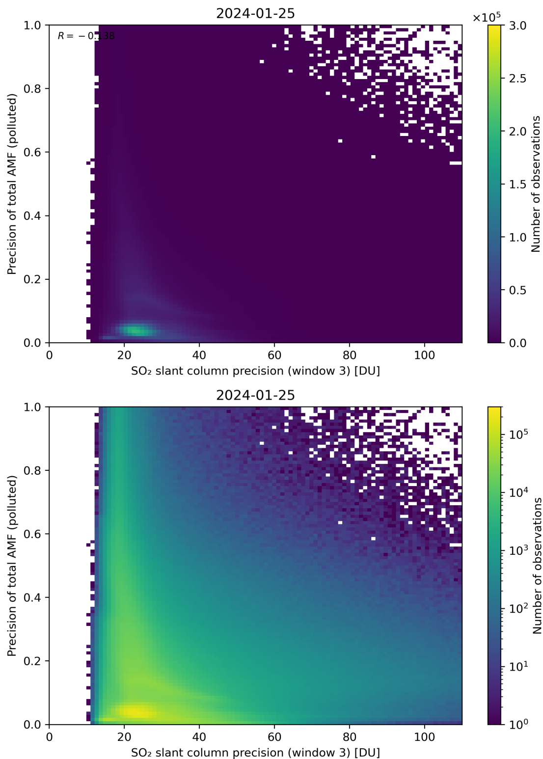
Figure 264: Scatter density plot of “SO 2 slant column precision (window 3)” against “Precision of total AMF (polluted)” for 2024-01-24 to 2024-01-26.
