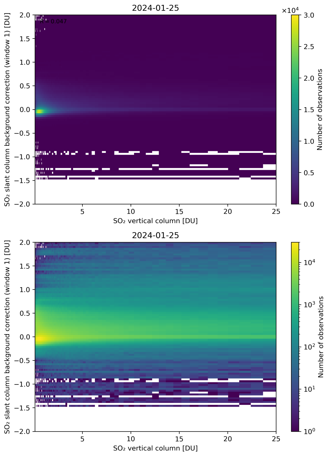
Figure 273: Scatter density plot of “SO 2 vertical column” against “SO 2 slant column background correction (window 1)” for 2024-01-24 to 2024-01-26.
