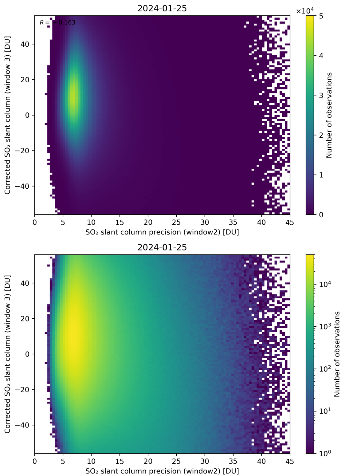
Figure 248: Scatter density plot of “SO 2 slant column precision (window2)” against “Corrected SO 2 slant column (window 3)” for 2024-01-24 to 2024-01-26.
