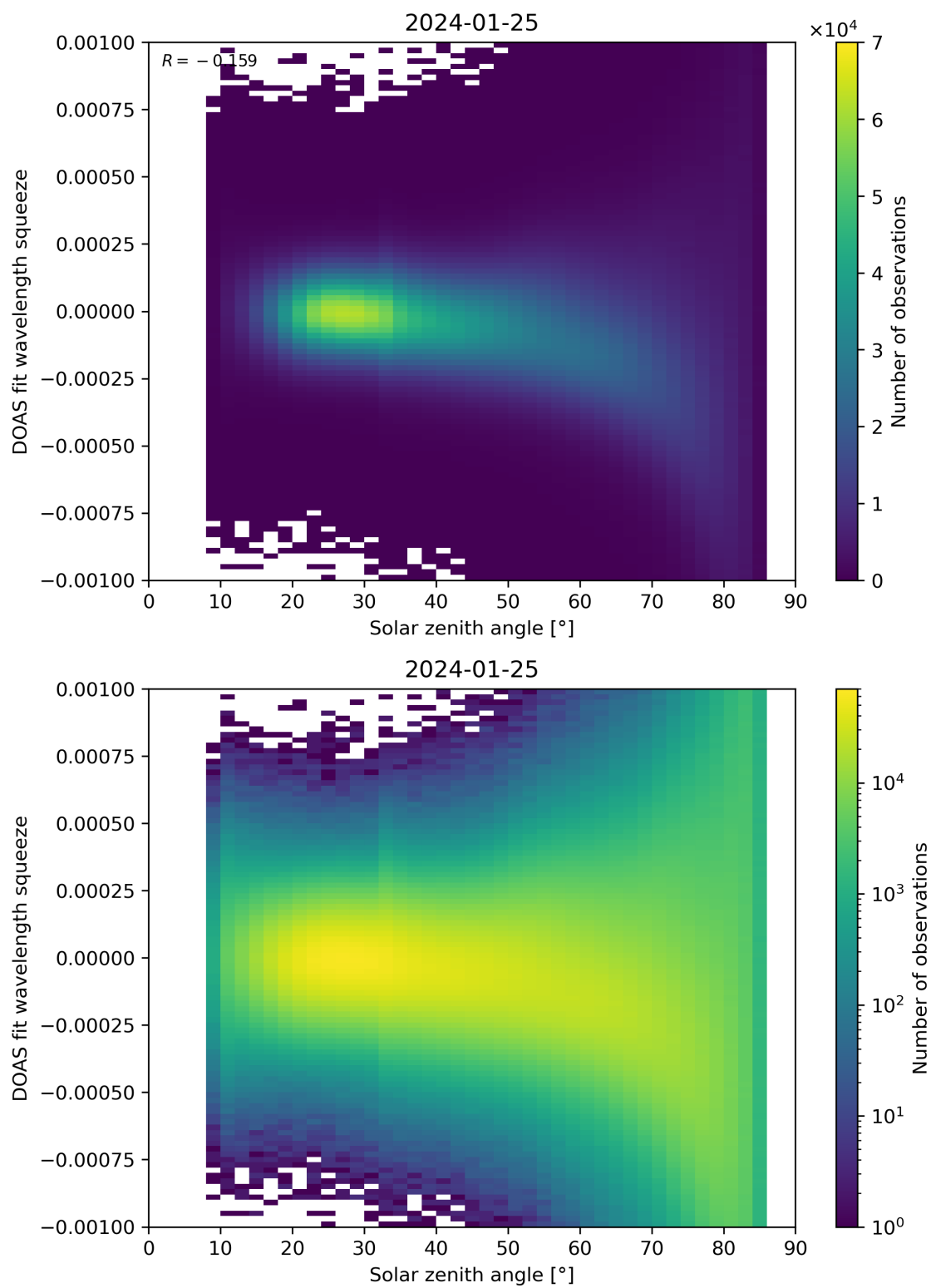
Figure 162: Scatter density plot of “Solar zenith angle” against “DOAS fit wavelength squeeze” for 2024-01-24 to 2024-01-26.
