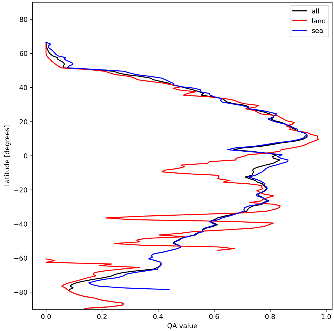
Figure 29: Zonal average of “QA value” for 2024-01-24 to 2024-01-26.
