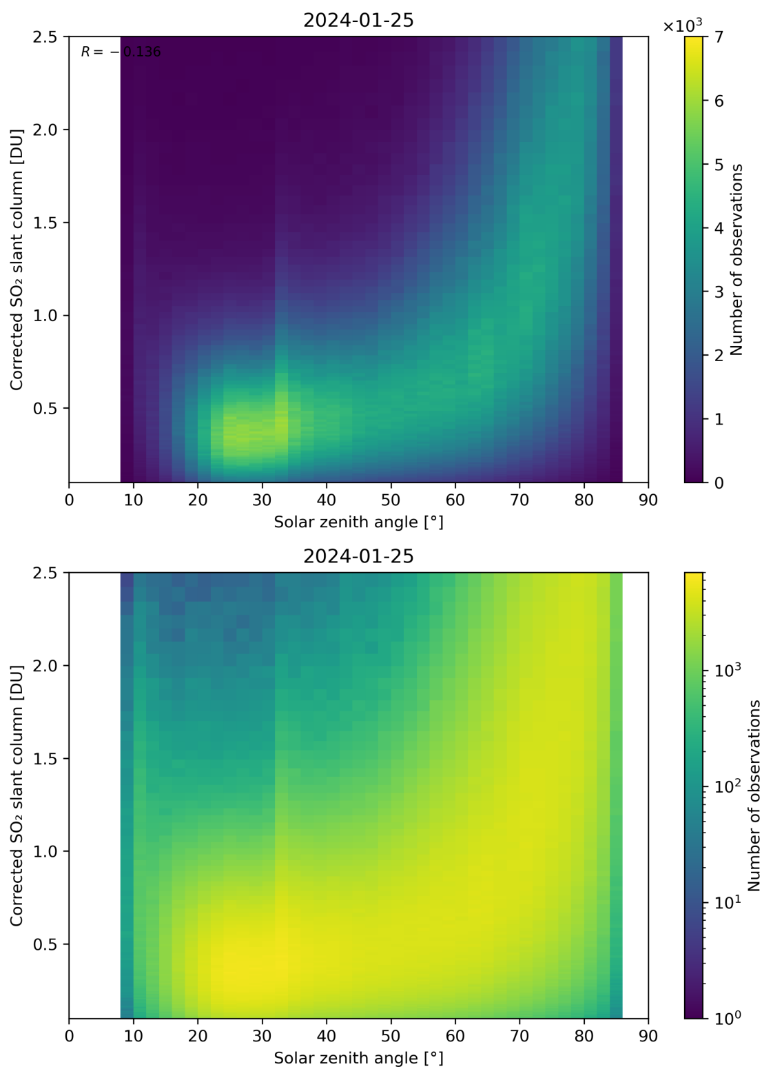
Figure 166: Scatter density plot of “Solar zenith angle” against “Corrected SO 2 slant column” for 2024-01-24 to 2024-01-26.
