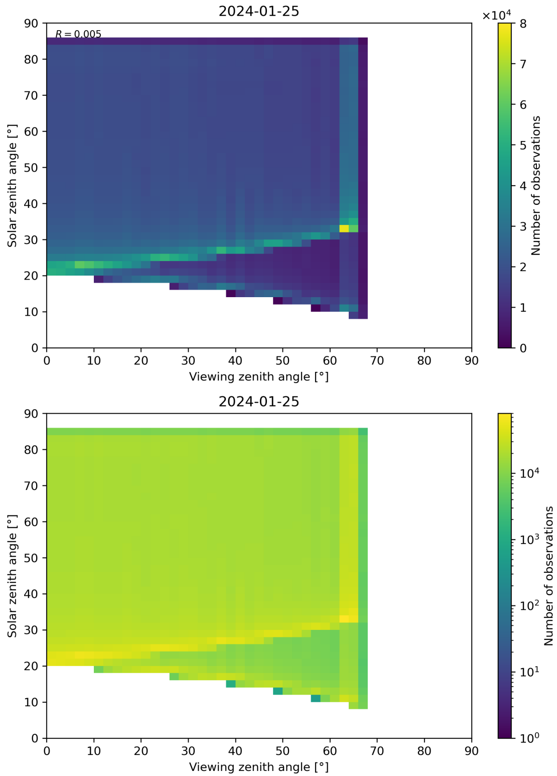
Figure 315: Scatter density plot of “Viewing zenith angle” against “Solar zenith angle” for 2024-01-24 to 2024-01-26.
