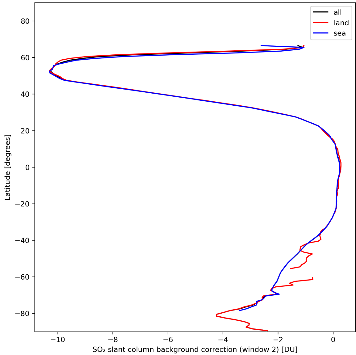
Figure 40: Zonal average of “SO 2 slant column background correction (window 2)” for 2024-01-24 to 2024-01-26.
