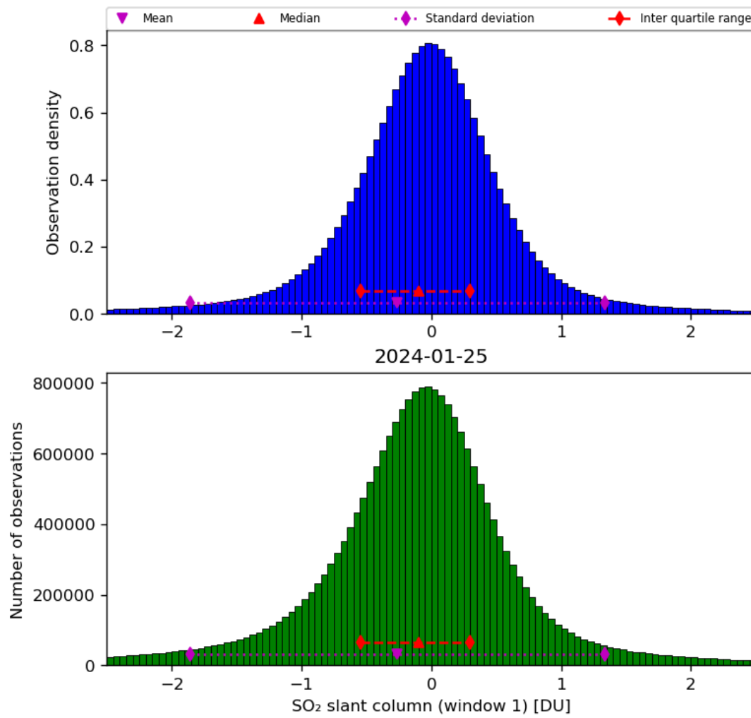
Figure 56: Histogram of “SO 2 slant column (window 1)” for 2024-01-24 to 2024-01-26
