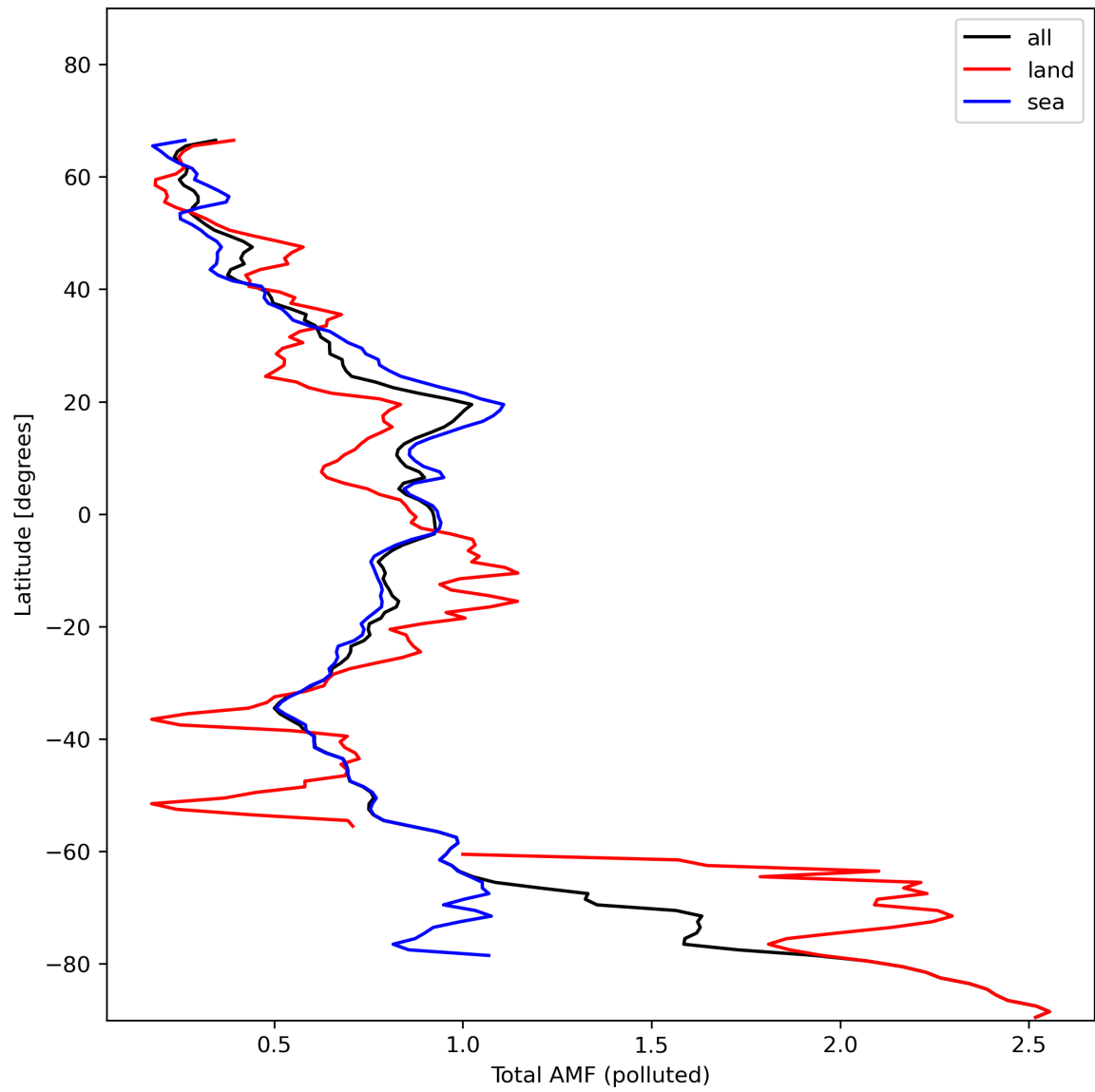
Figure 48: Zonal average of “Total AMF (polluted)” for 2024-01-24 to 2024-01-26.
