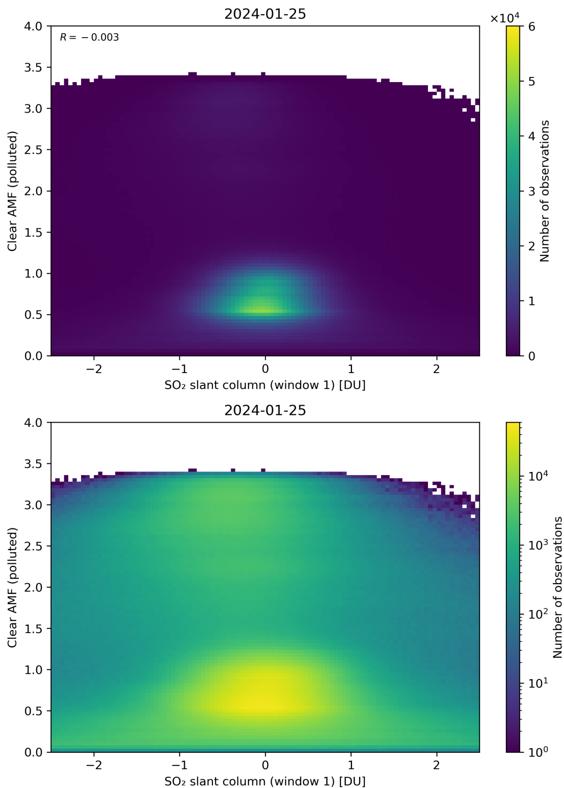
Figure 232: Scatter density plot of “SO 2 slant column (window 1)” against “Clear AMF (polluted)” for 2024-01-24 to 2024-01-26.
