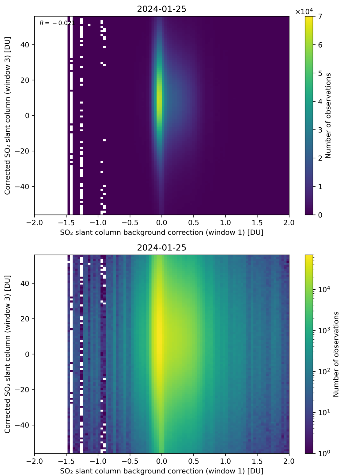
Figure 105: Scatter density plot of “SO 2 slant column background correction (window 1)” against “Corrected SO 2 slant column (window 3)” for 2024-01-24 to 2024-01-26.
