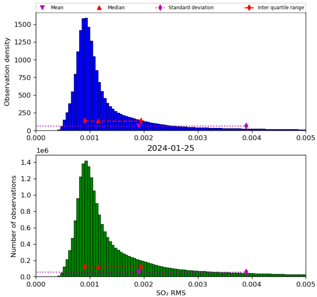
Figure 70: Histogram of “SO 2 RMS” for 2024-01-24 to 2024-01-26
