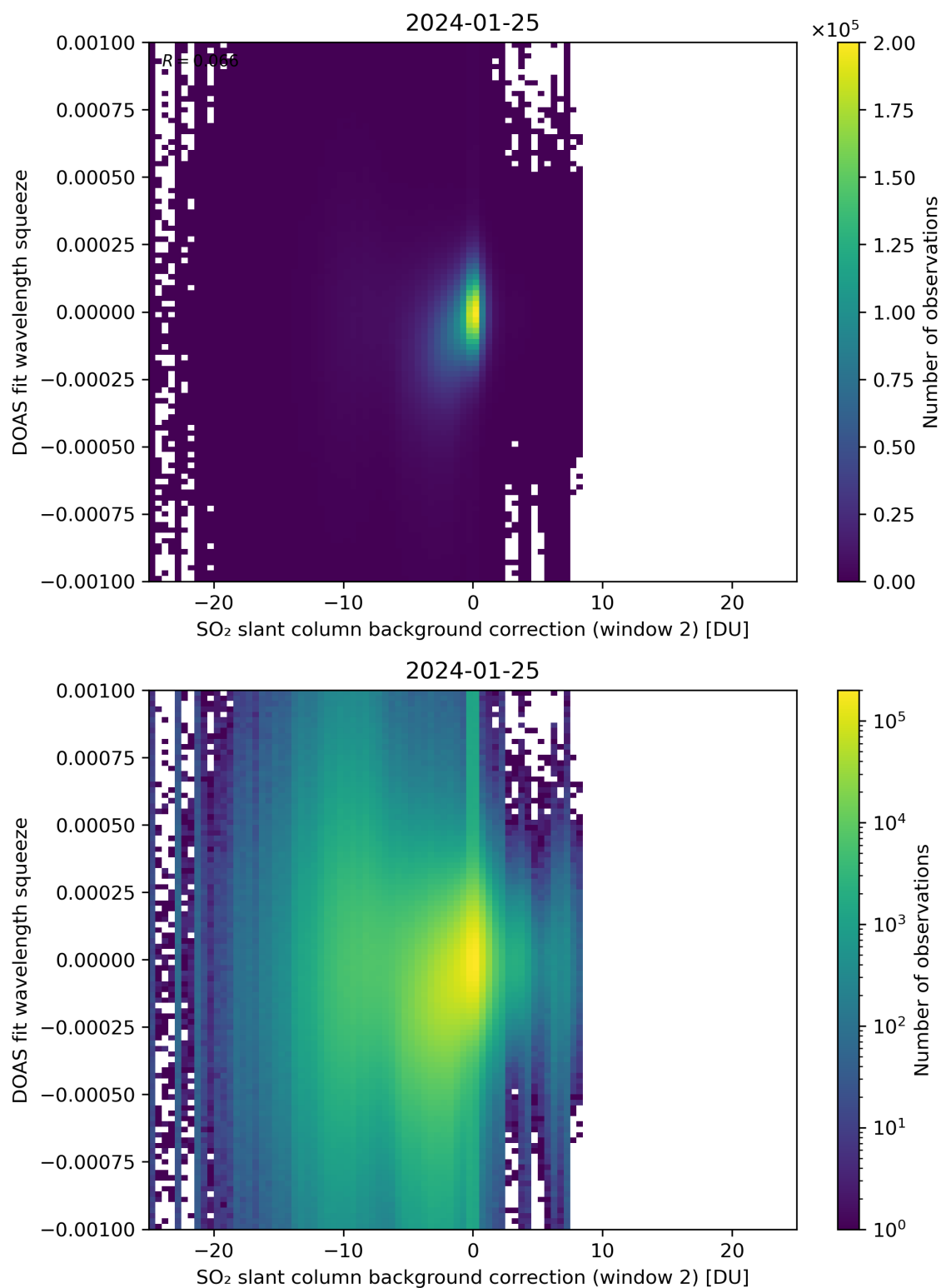
Figure 113: Scatter density plot of “SO 2 slant column background correction (window 2)” against “DOAS fit wavelength squeeze” for 2024-01-24 to 2024-01-26.
