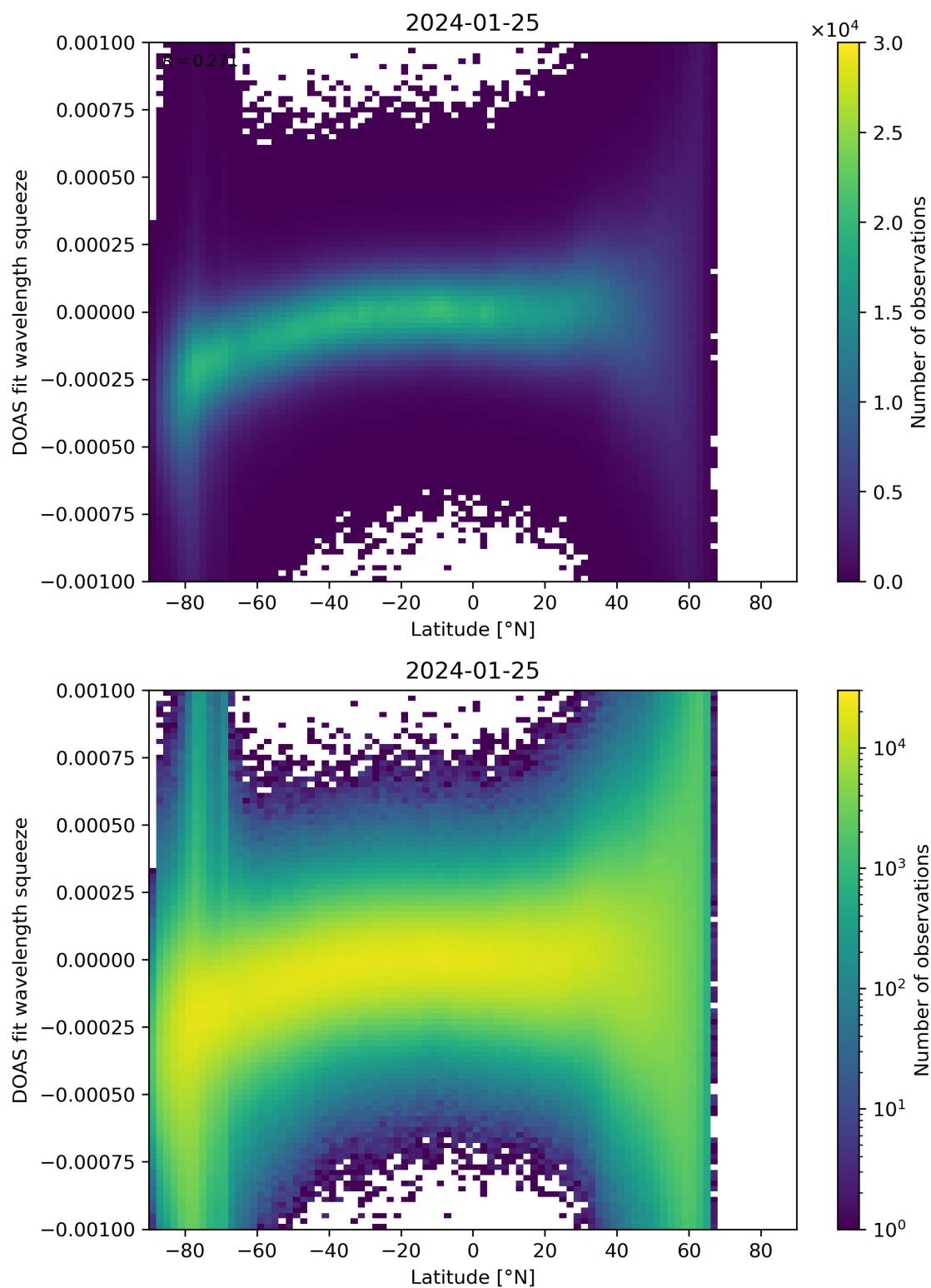
Figure 143: Scatter density plot of “Latitude” against “DOAS fit wavelength squeeze” for 2024-01-24 to 2024-01-26.
