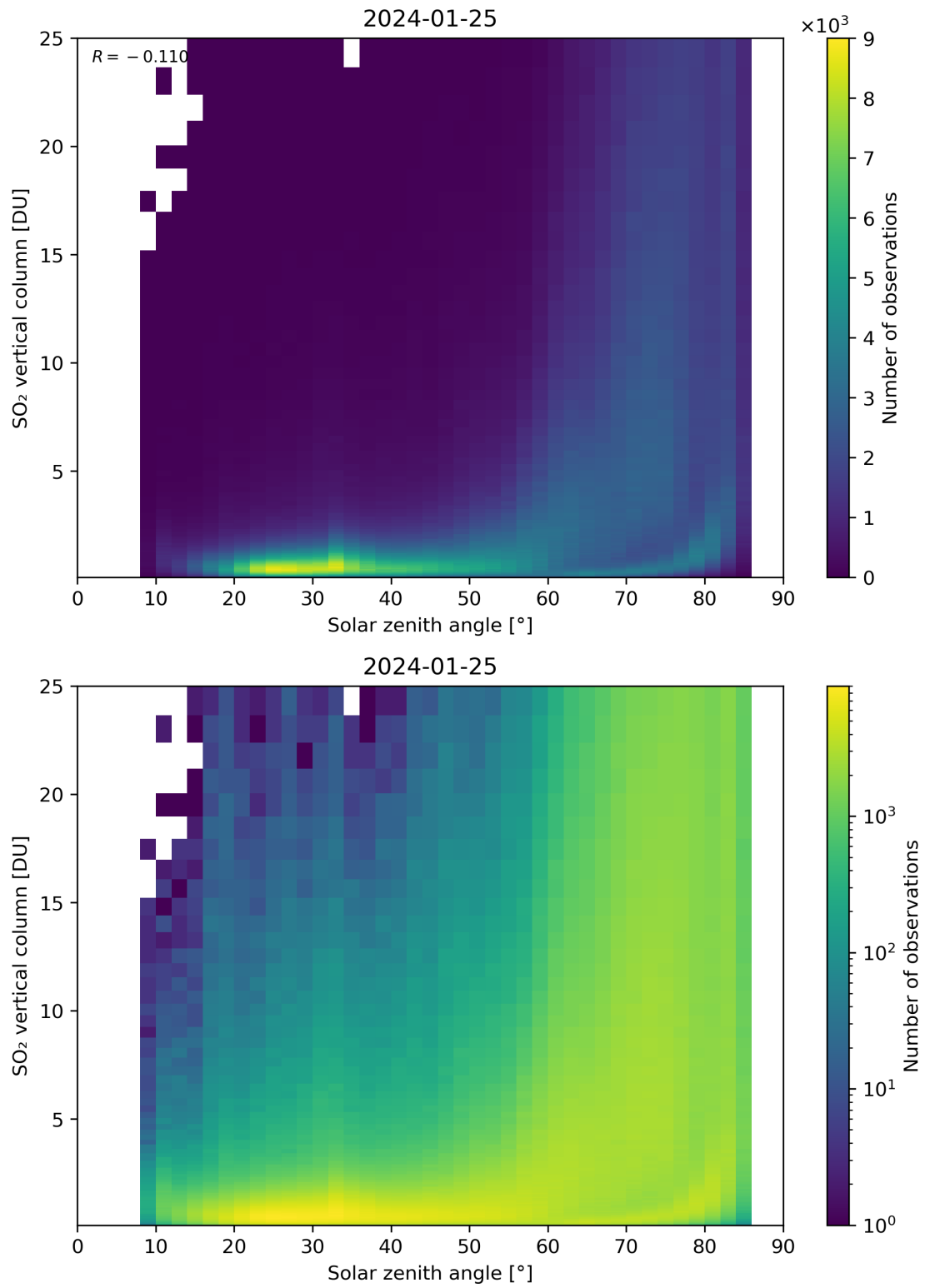
Figure 176: Scatter density plot of “Solar zenith angle” against “SO 2 vertical column” for 2024-01-24 to 2024-01-26.
