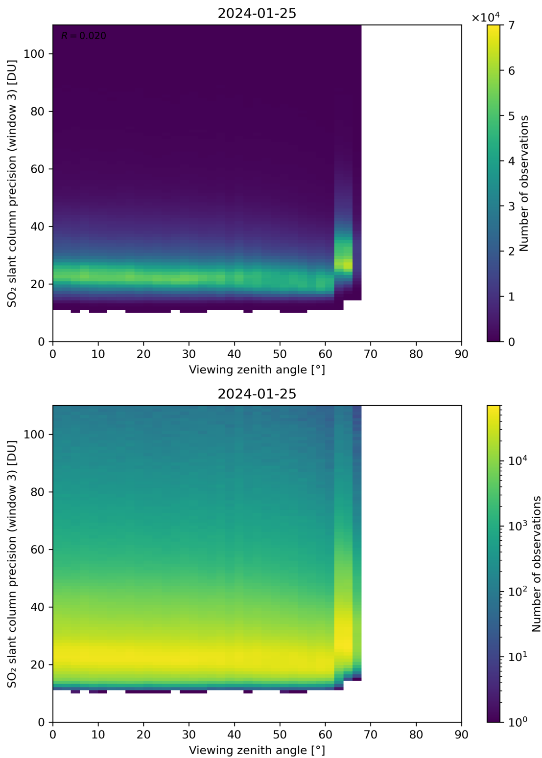
Figure 324: Scatter density plot of “Viewing zenith angle” against “SO 2 slant column precision (window 3)” for 2024-01-24 to 2024-01-26.
