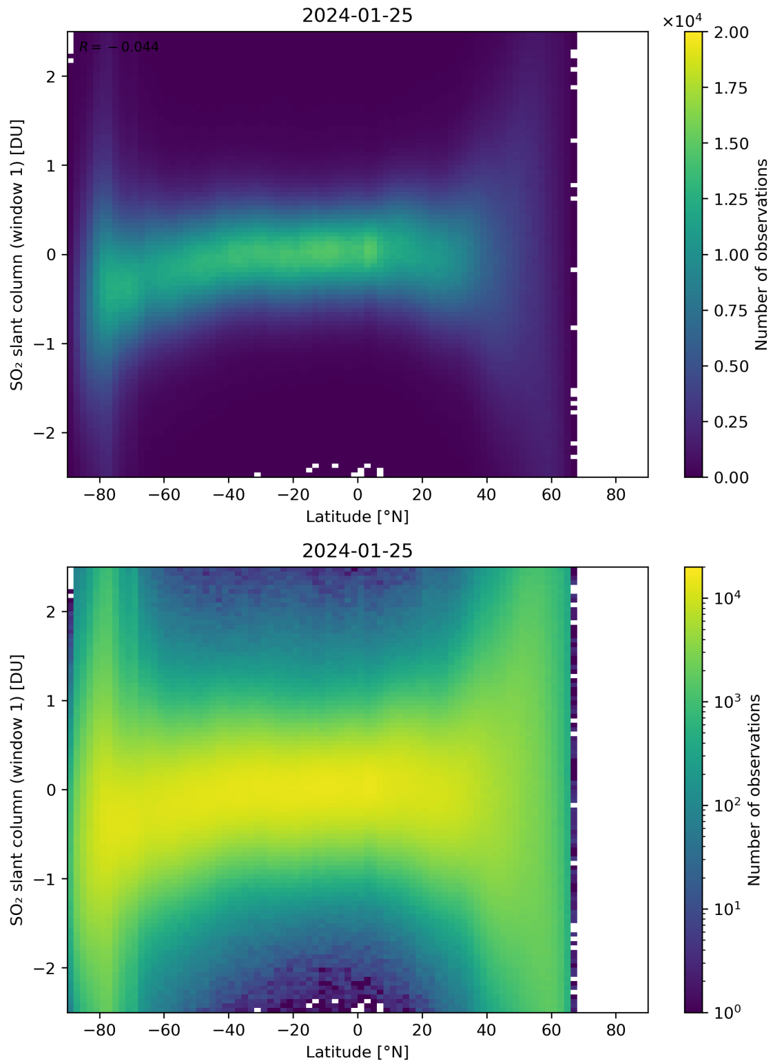
Figure 149: Scatter density plot of “Latitude” against “SO 2 slant column (window 1)” for 2024-01-24 to 2024-01-26.
