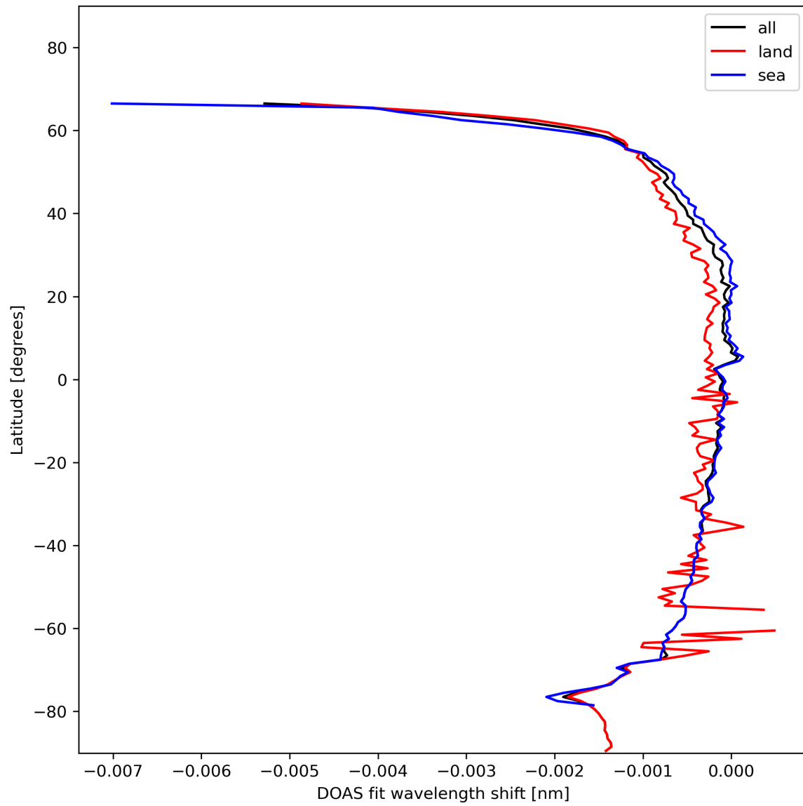
Figure 45: Zonal average of “DOAS fit wavelength shift” for 2024-01-24 to 2024-01-26.
