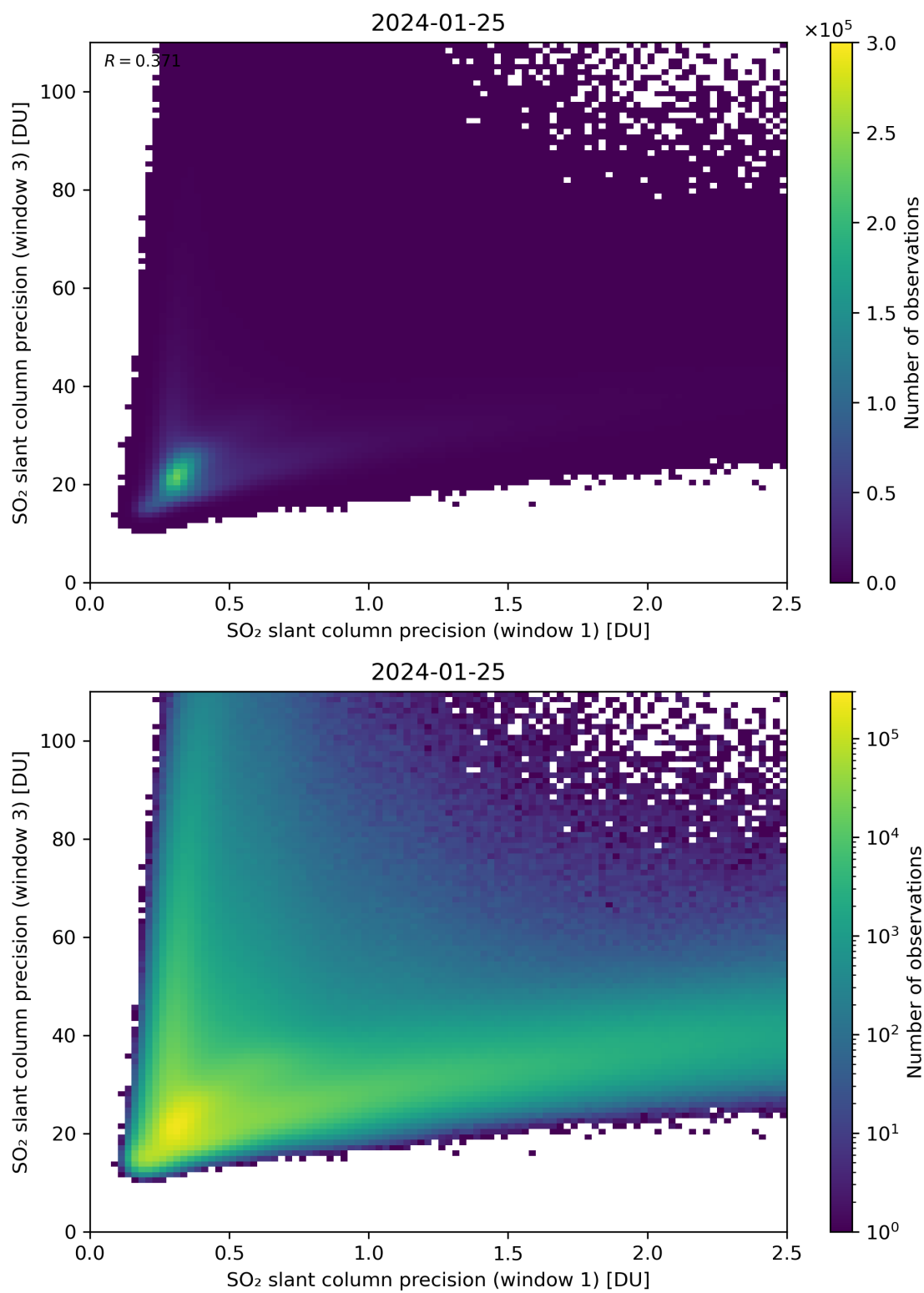
Figure 229: Scatter density plot of “SO 2 slant column precision (window 1)” against “SO 2 slant column precision (window 3)” for 2024-01-24 to 2024-01-26.
