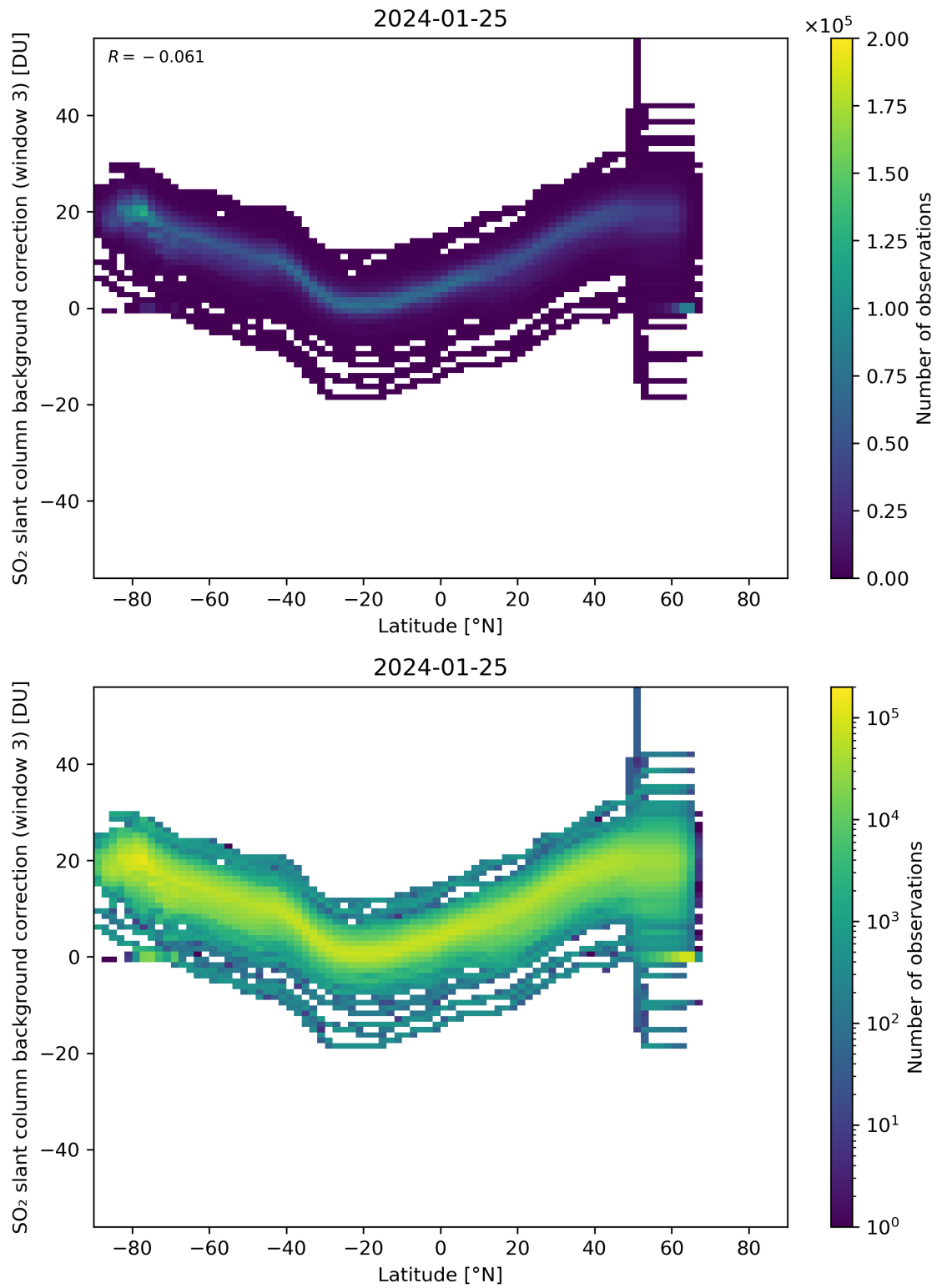
Figure 141: Scatter density plot of “Latitude” against “SO 2 slant column background correction (window 3)” for 2024-01-24 to 2024-01-26.
