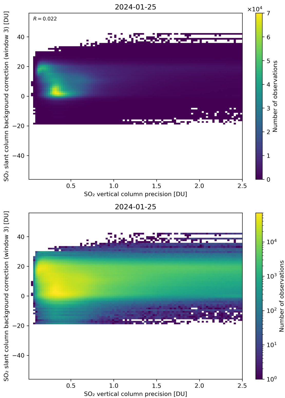
Figure 281: Scatter density plot of “SO 2 vertical column precision” against “SO 2 slant column background correction (window 3)” for 2024-01-24 to 2024-01-26.
