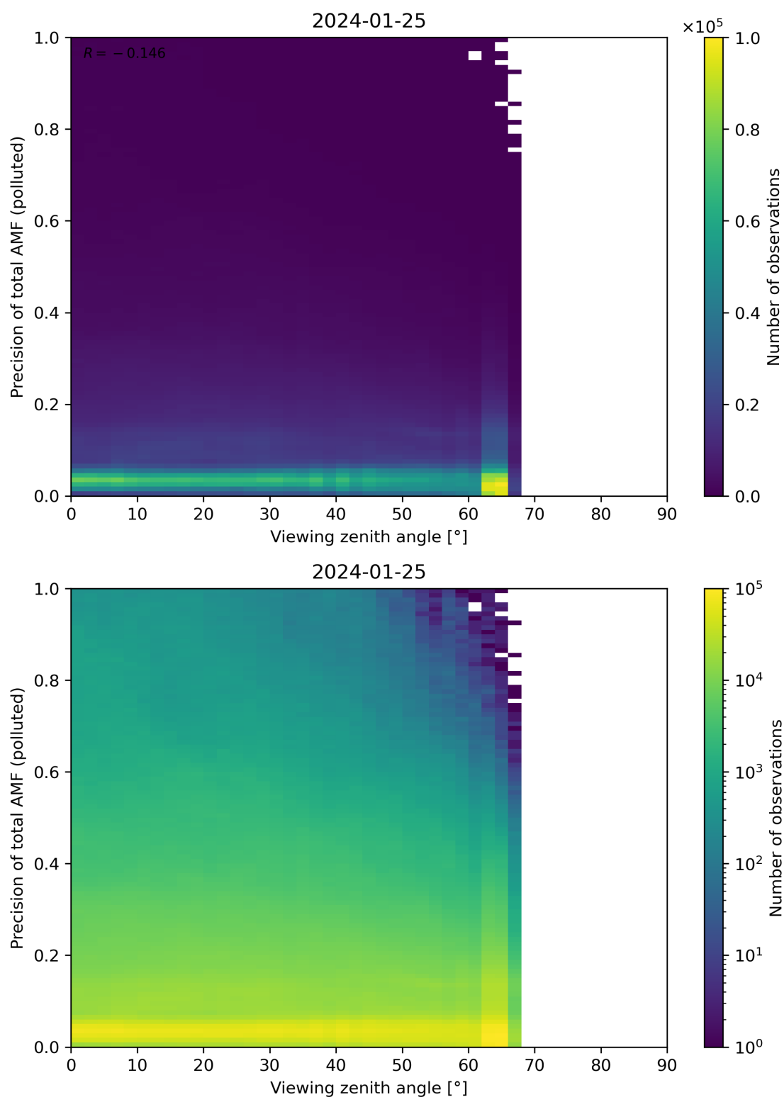
Figure 326: Scatter density plot of “Viewing zenith angle” against “Precision of total AMF (polluted)” for 2024-01-24 to 2024-01-26.
