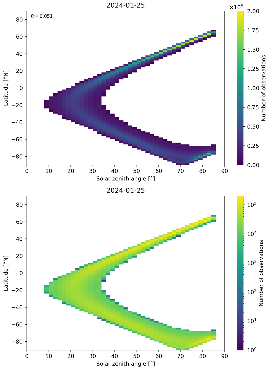
Figure 164: Scatter density plot of “Solar zenith angle” against “Latitude” for 2024-01-24 to 2024-01-26.
