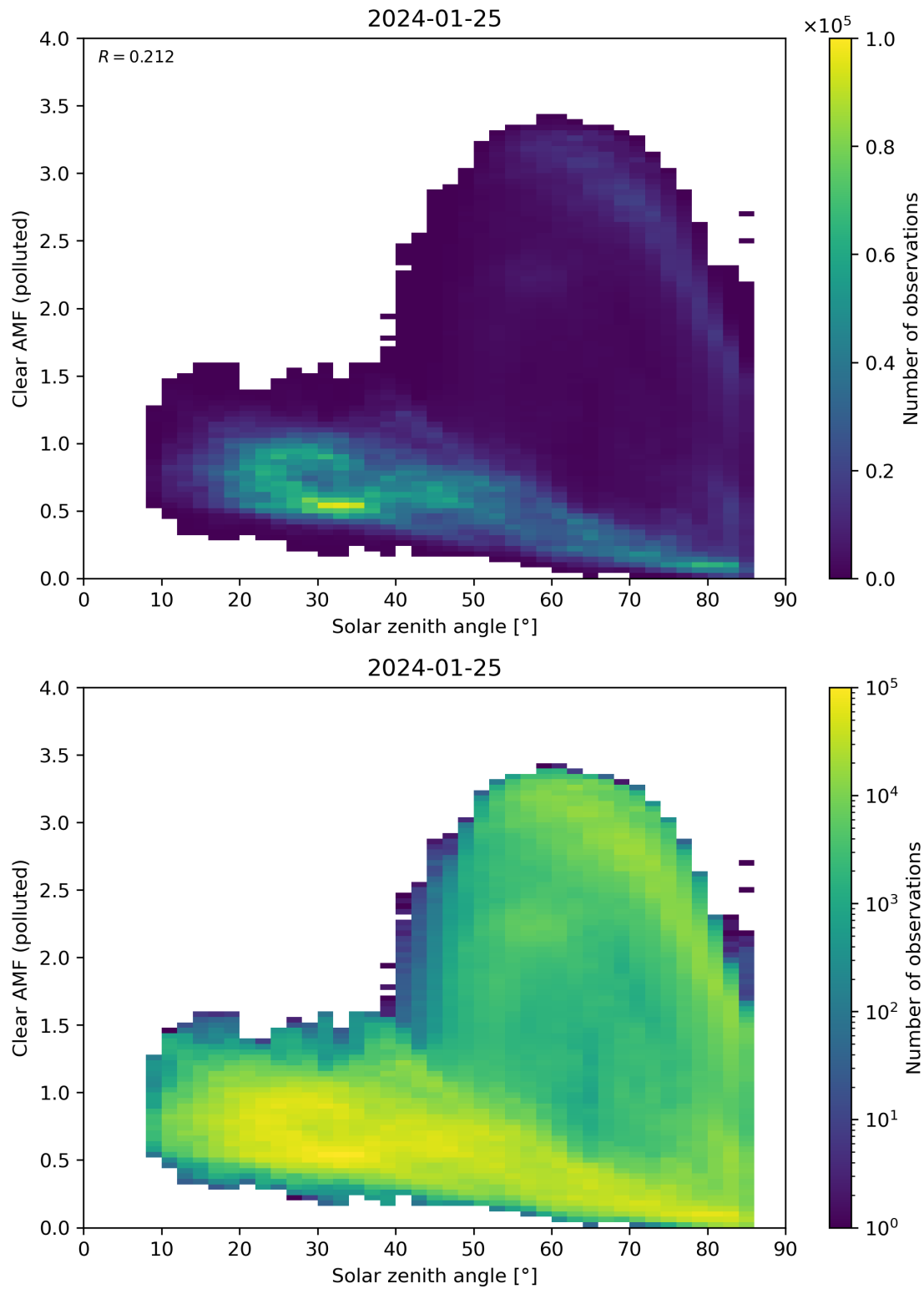
Figure 165: Scatter density plot of “Solar zenith angle” against “Clear AMF (polluted)” for 2024-01-24 to 2024-01-26.
