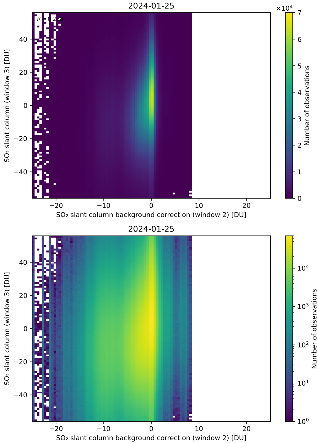
Figure 117: Scatter density plot of “SO 2 slant column background correction (window 2)” against “SO 2 slant column (window 3)” for 2024-01-24 to 2024-01-26.
