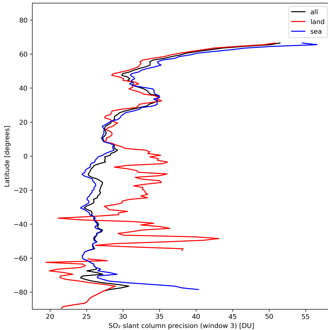
Figure 42: Zonal average of “SO 2 slant column precision (window 3)” for 2024-01-24 to 2024-01-26.
