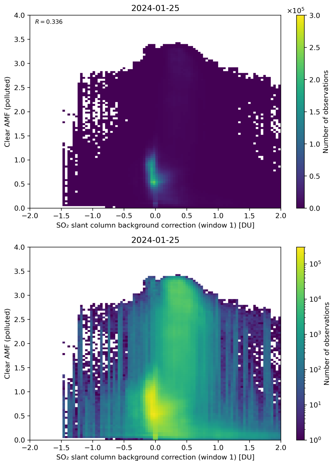
Figure 103: Scatter density plot of “SO 2 slant column background correction (window 1)” against “Clear AMF (polluted)” for 2024-01-24 to 2024-01-26.
