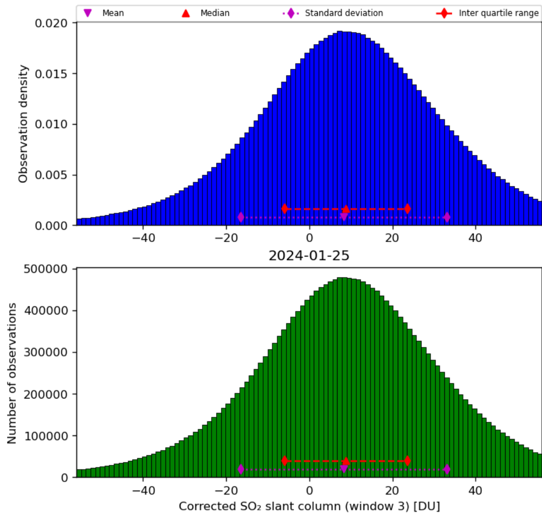
Figure 66: Histogram of “Corrected SO 2 slant column (window 3)” for 2024-01-24 to 2024-01-26
