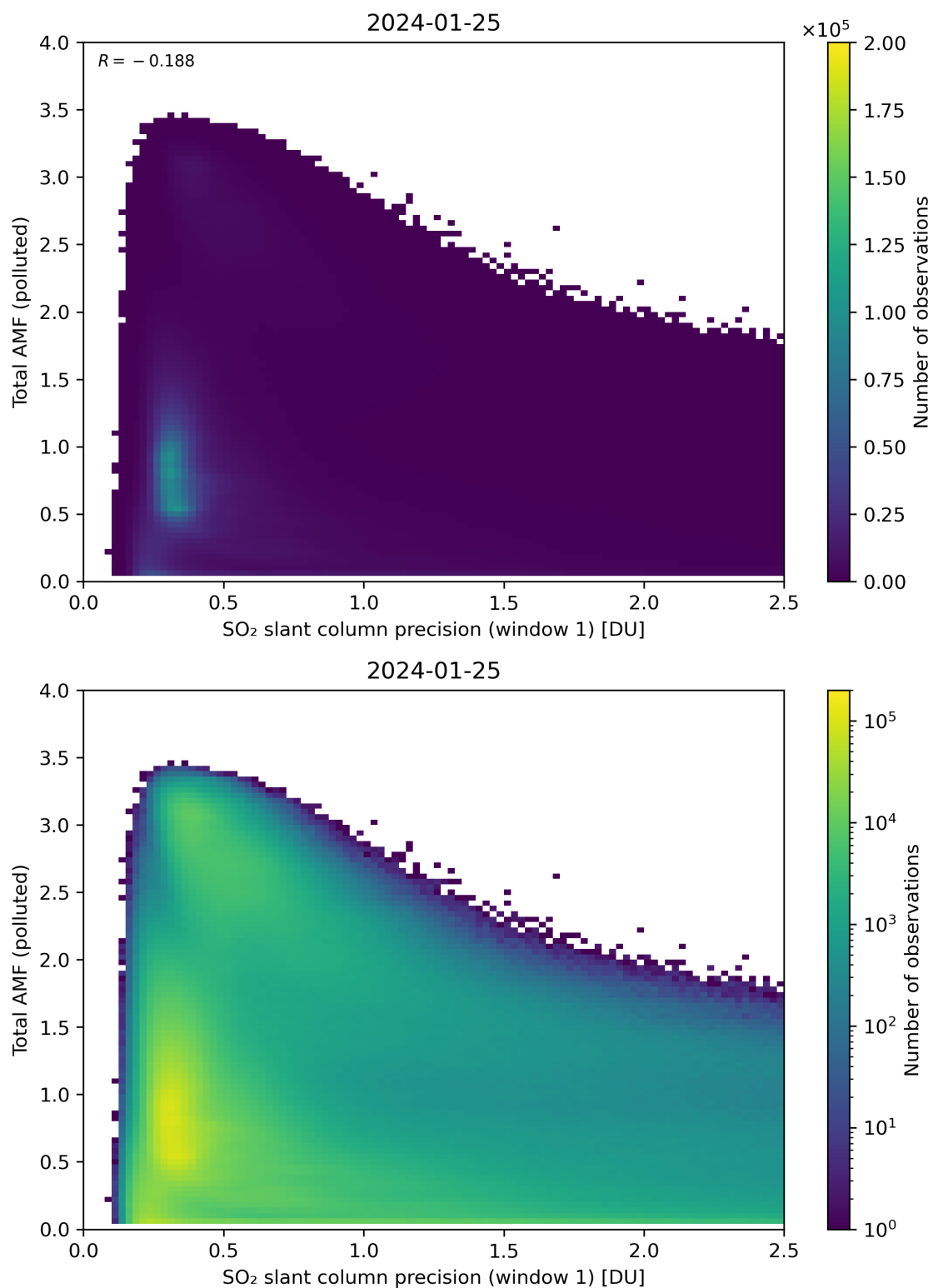
Figure 230: Scatter density plot of “SO 2 slant column precision (window 1)” against “Total AMF (polluted)” for 2024-01-24 to 2024-01-26.
