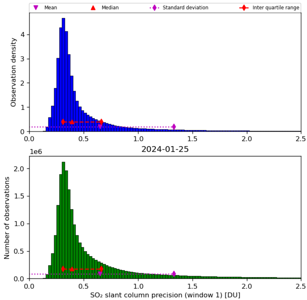
Figure 57: Histogram of “SO 2 slant column precision (window 1)” for 2024-01-24 to 2024-01-26
