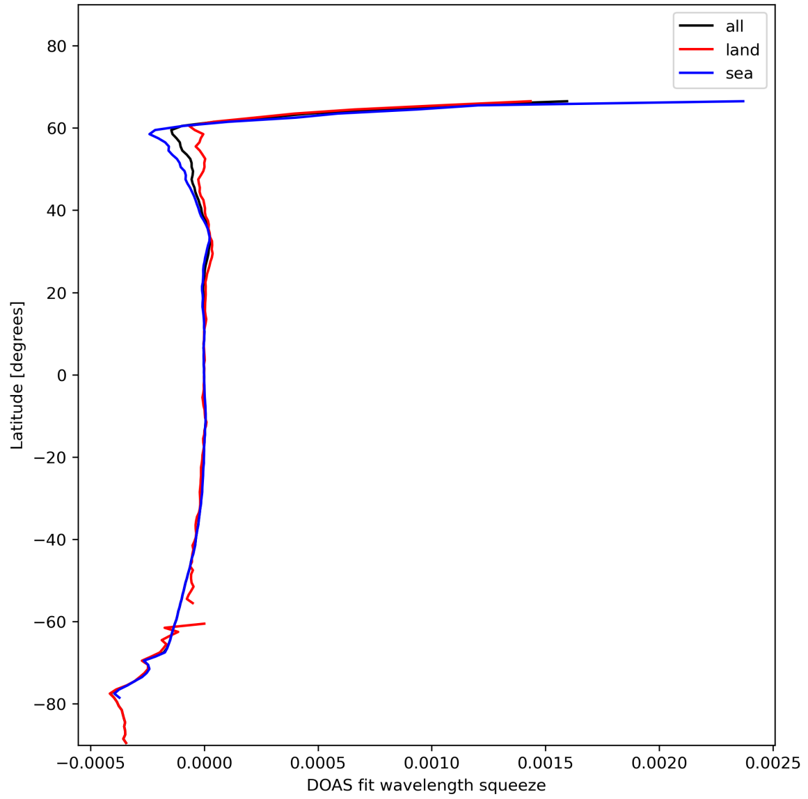
Figure 46: Zonal average of “DOAS fit wavelength squeeze” for 2024-01-24 to 2024-01-26.
