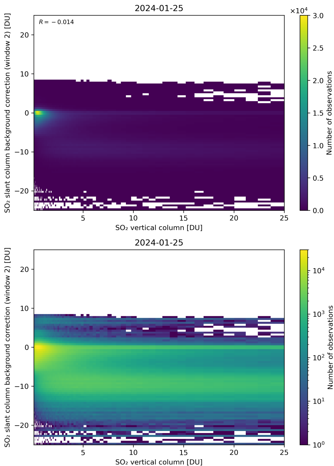
Figure 274: Scatter density plot of “SO 2 vertical column” against “SO 2 slant column background correction (window 2)” for 2024-01-24 to 2024-01-26.
