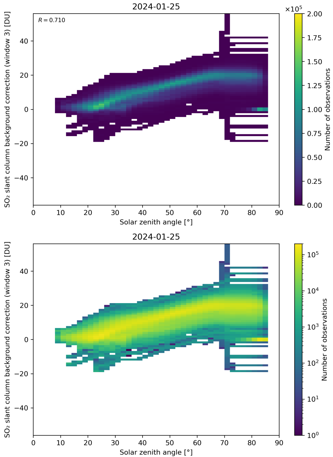
Figure 160: Scatter density plot of “Solar zenith angle” against “SO 2 slant column background correction (window 3)” for 2024-01-24 to 2024-01-26.
