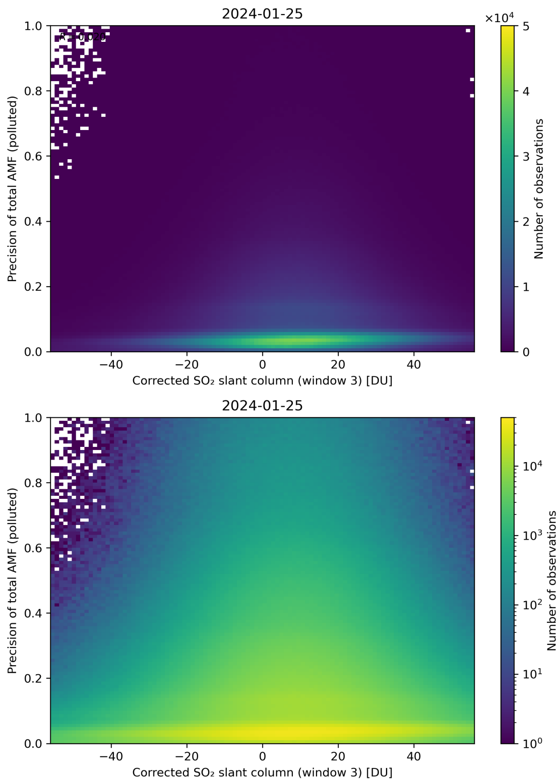
Figure 211: Scatter density plot of “Corrected SO 2 slant column (window 3)” against “Precision of total AMF (polluted)” for 2024-01-24 to 2024-01-26.
