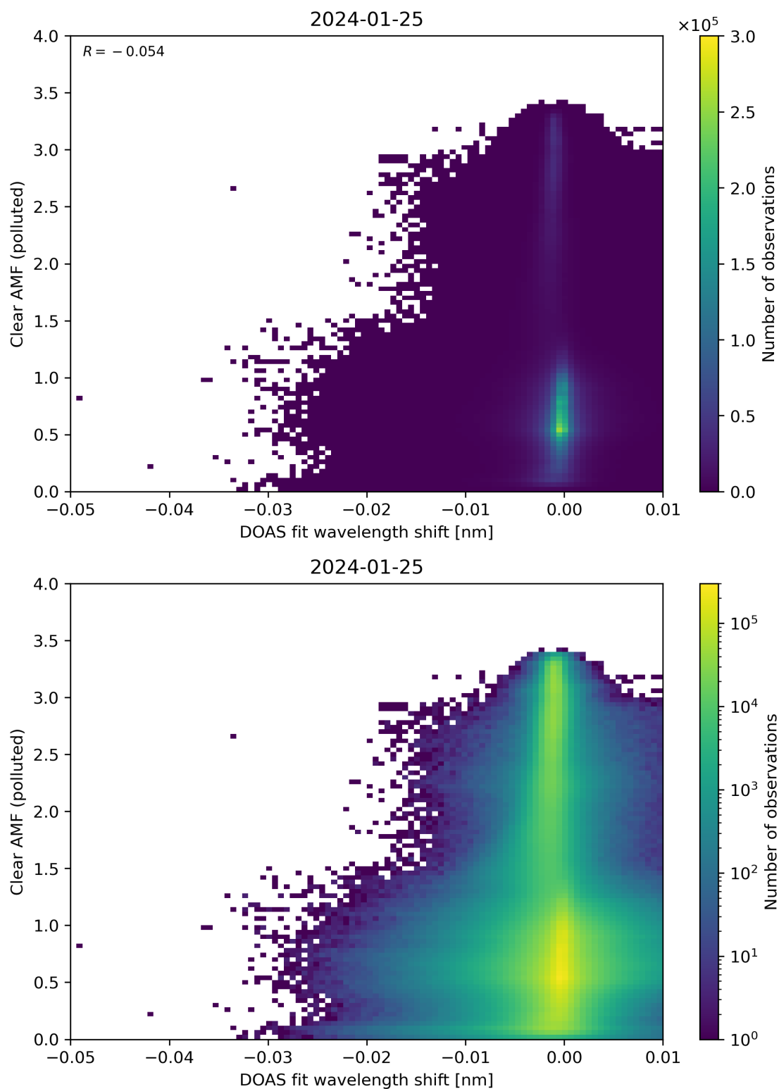
Figure 129: Scatter density plot of “DOAS fit wavelength shift” against “Clear AMF (polluted)” for 2024-01-24 to 2024-01-26.
