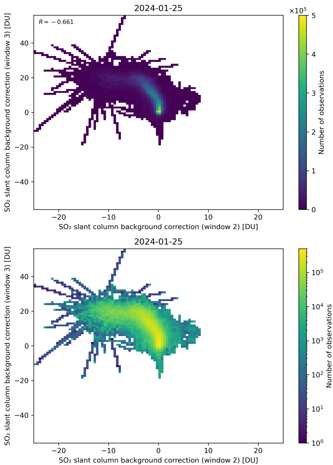
Figure 111: Scatter density plot of “SO 2 slant column background correction (window 2)” against “SO 2 slant column background correction (window 3)” for 2024-01-24 to 2024-01-26.
