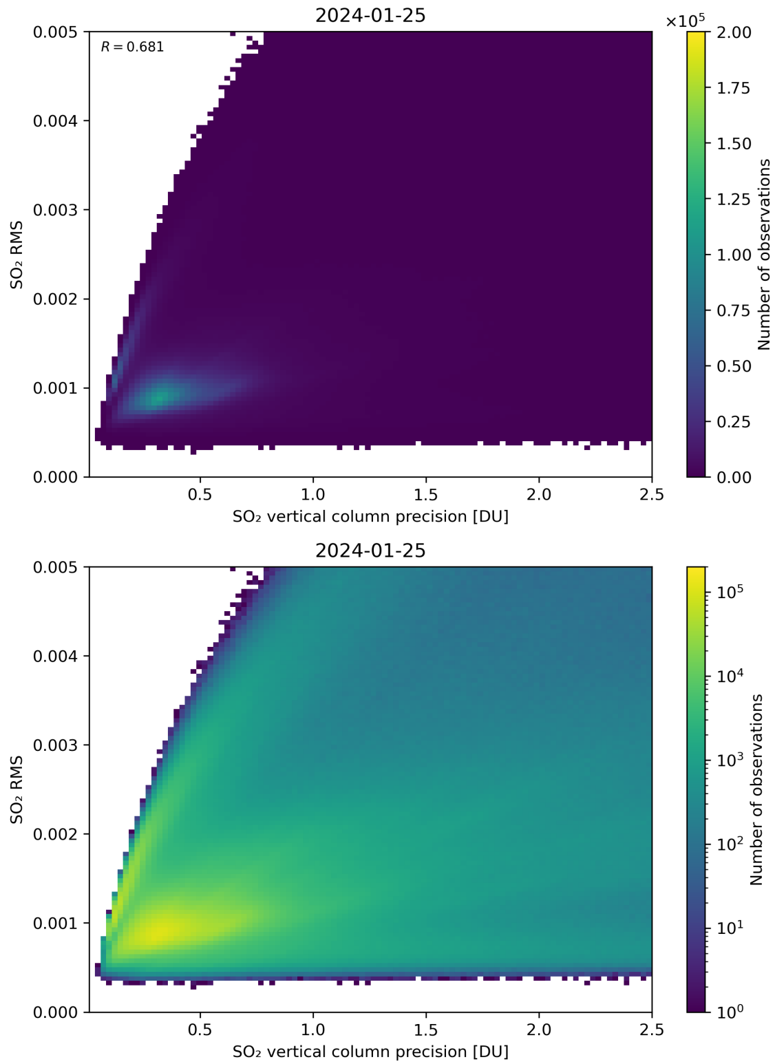
Figure 284: Scatter density plot of “SO 2 vertical column precision” against “SO 2 RMS” for 2024-01-24 to 2024-01-26.
