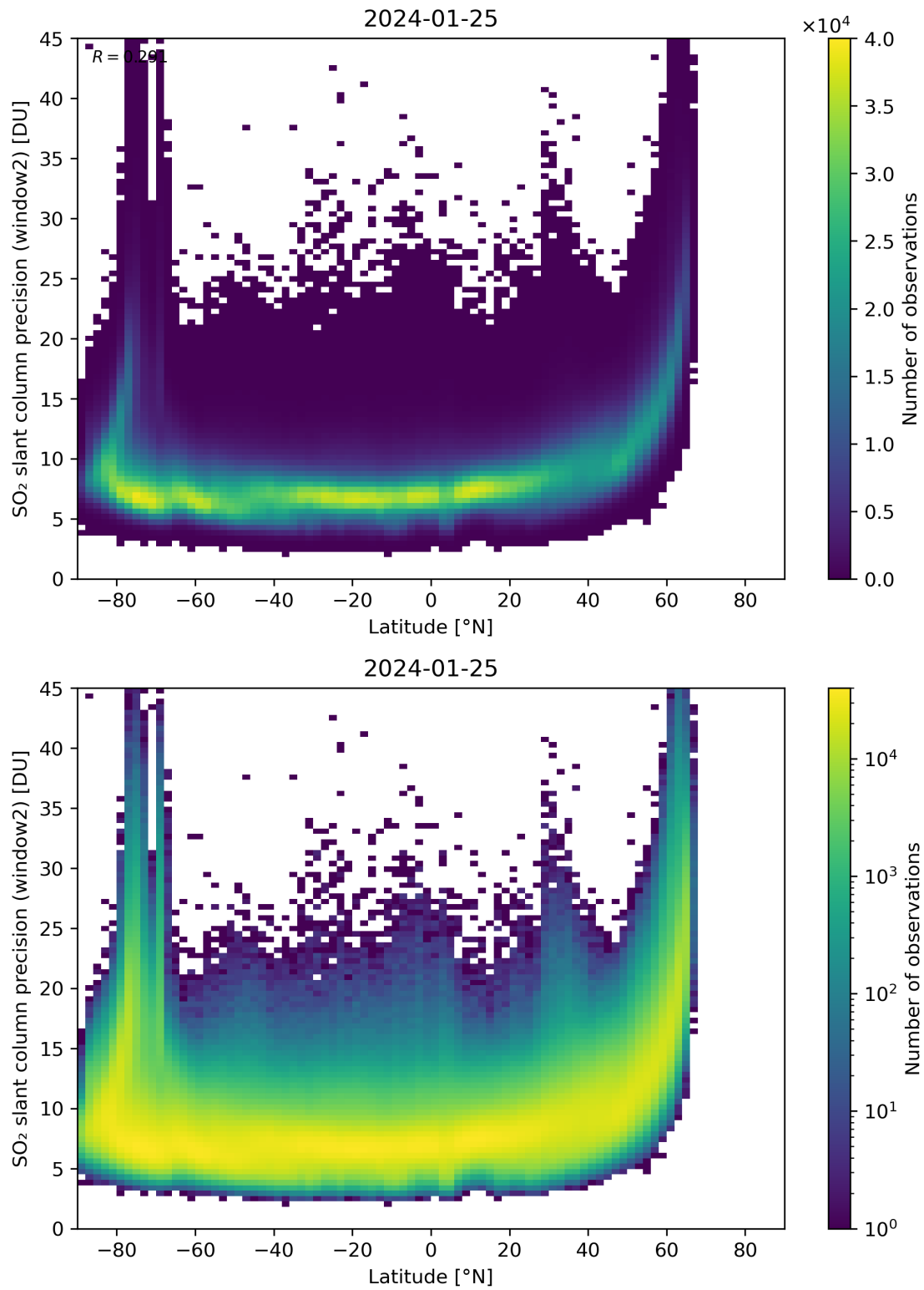
Figure 151: Scatter density plot of “Latitude” against “SO 2 slant column precision (window2)” for 2024-01-24 to 2024-01-26.
