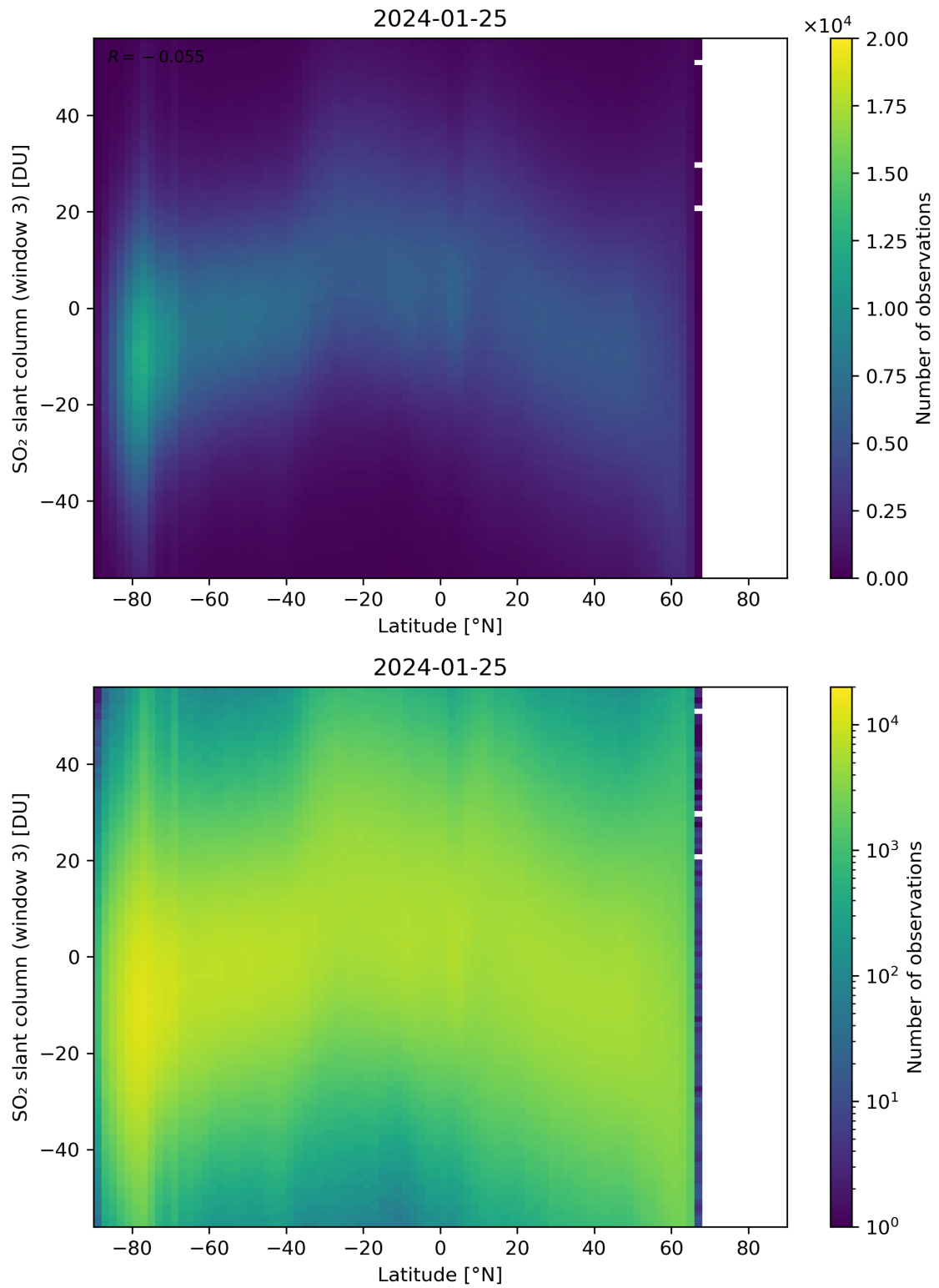
Figure 152: Scatter density plot of “Latitude” against “SO 2 slant column (window 3)” for 2024-01-24 to 2024-01-26.
