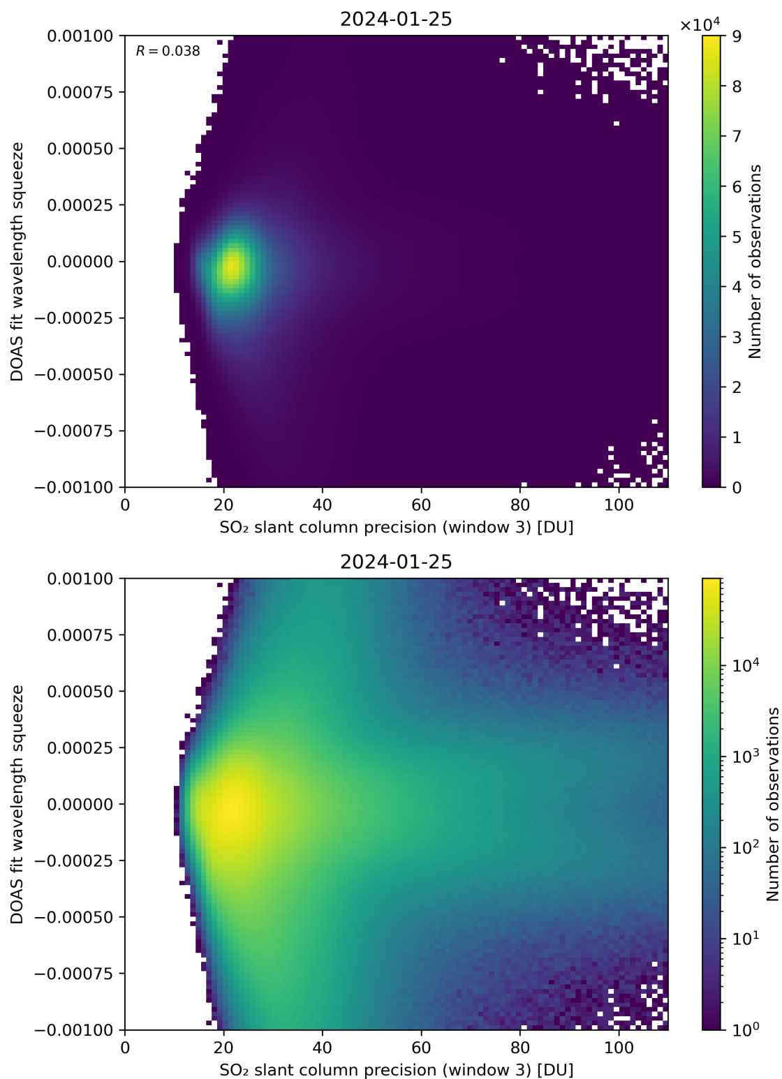
Figure 259: Scatter density plot of “SO 2 slant column precision (window 3)” against “DOAS fit wavelength squeeze” for 2024-01-24 to 2024-01-26.
