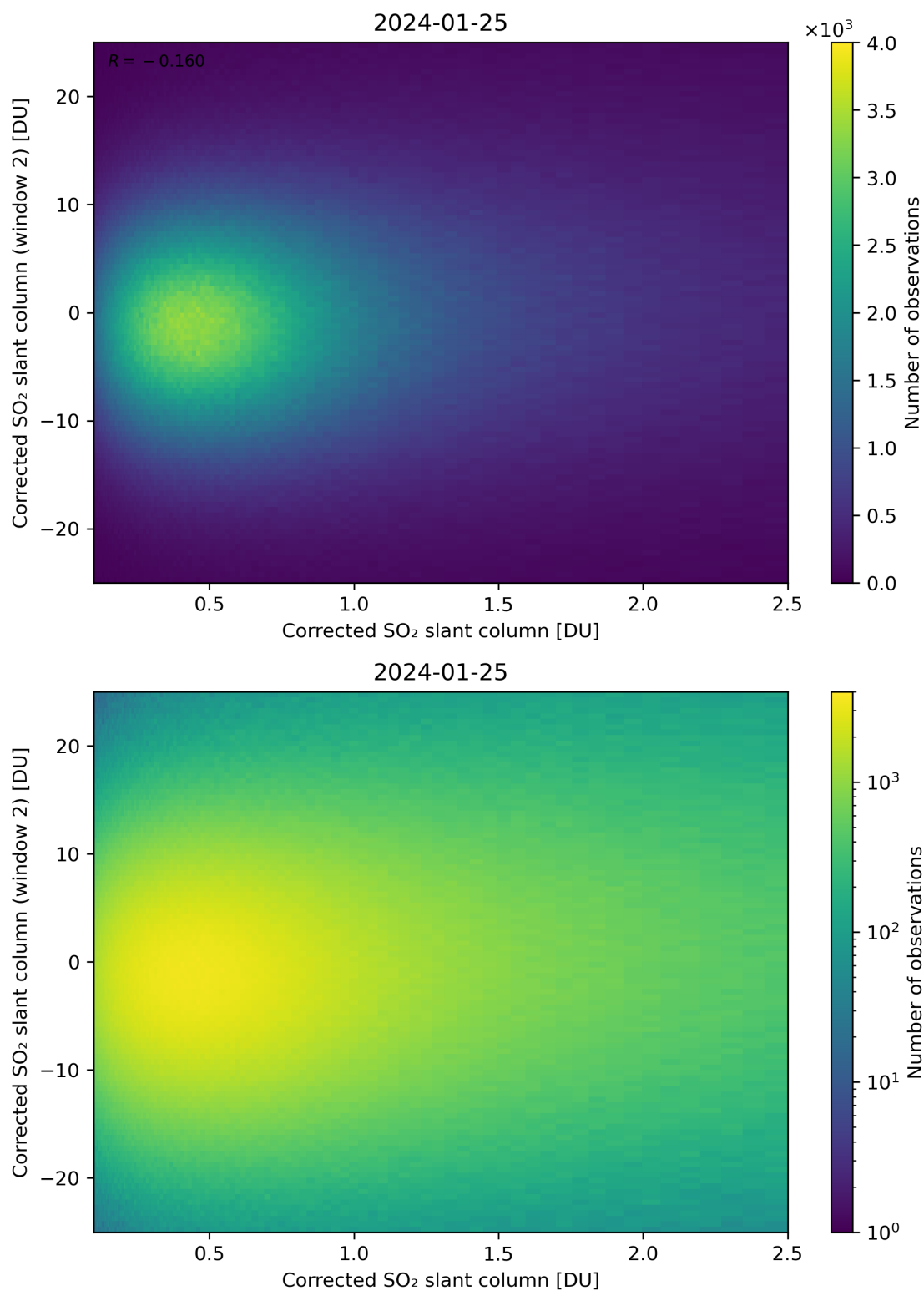
Figure 185: Scatter density plot of “Corrected SO 2 slant column” against “Corrected SO 2 slant column (window 2)” for 2024-01-24 to 2024-01-26.
