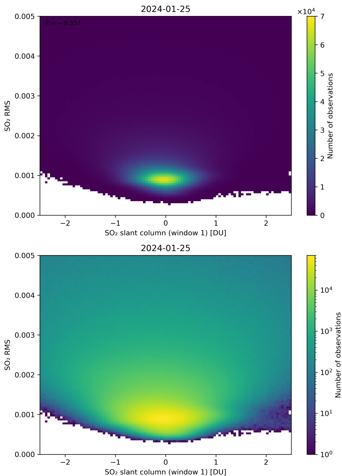
Figure 217: Scatter density plot of “SO 2 slant column (window 1)” against “SO 2 RMS” for 2024-01-24 to 2024-01-26.
