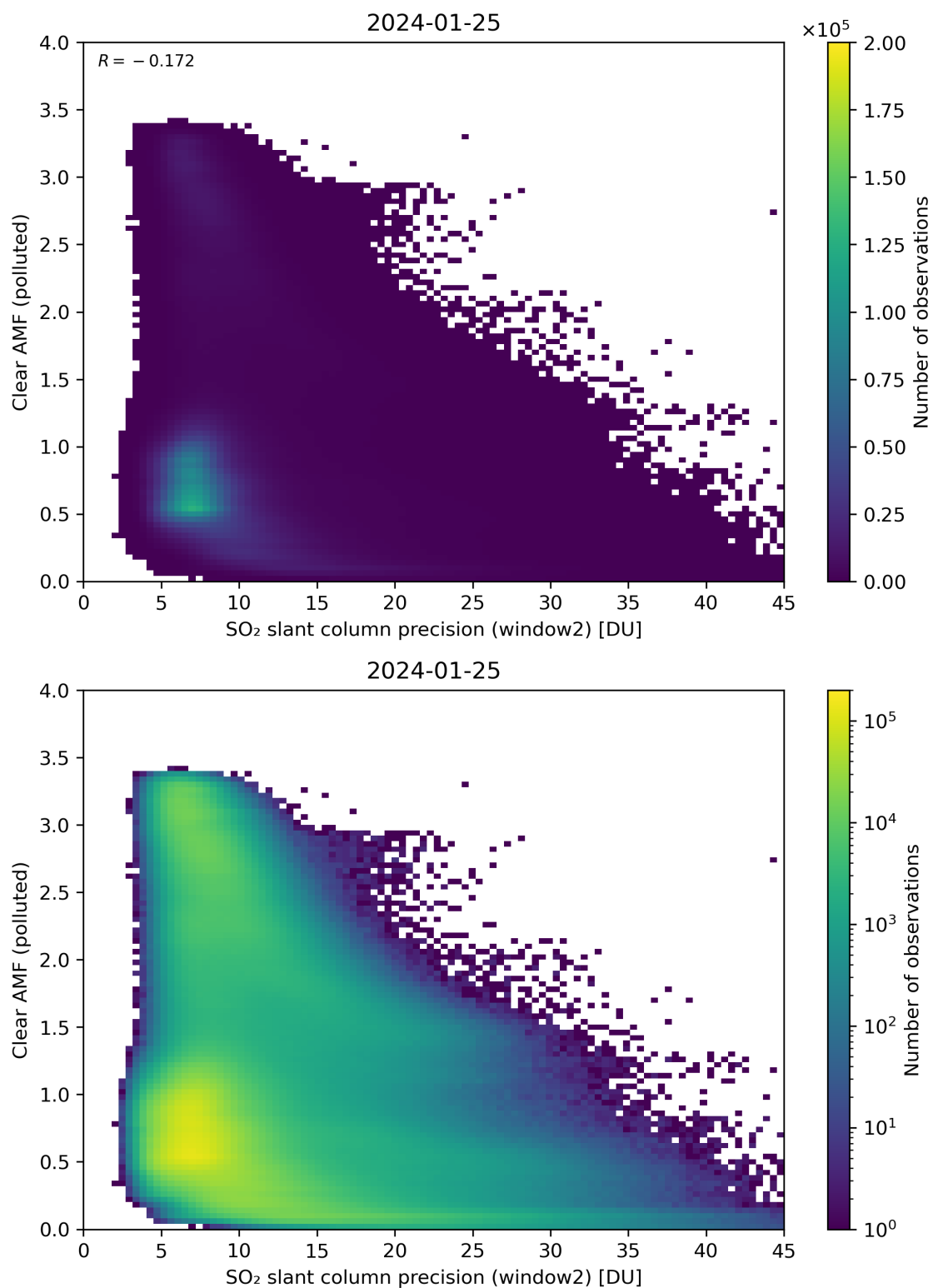
Figure 246: Scatter density plot of “SO 2 slant column precision (window2)” against “Clear AMF (polluted)” for 2024-01-24 to 2024-01-26.
