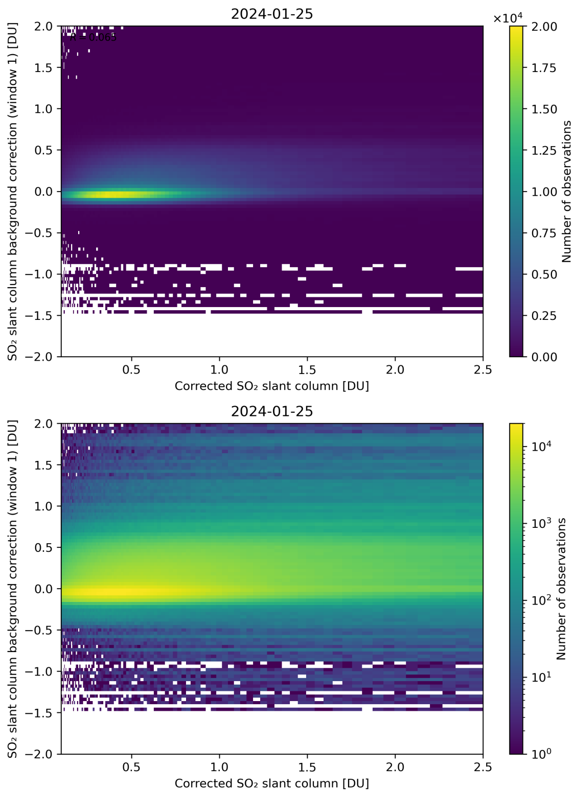
Figure 178: Scatter density plot of “Corrected SO 2 slant column” against “SO 2 slant column background correction (window 1)” for 2024-01-24 to 2024-01-26.
