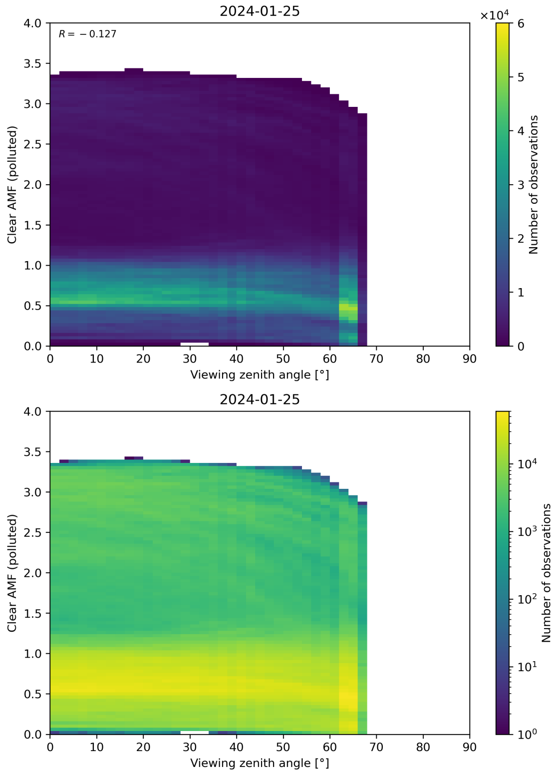
Figure 316: Scatter density plot of “Viewing zenith angle” against “Clear AMF (polluted)” for 2024-01-24 to 2024-01-26.
