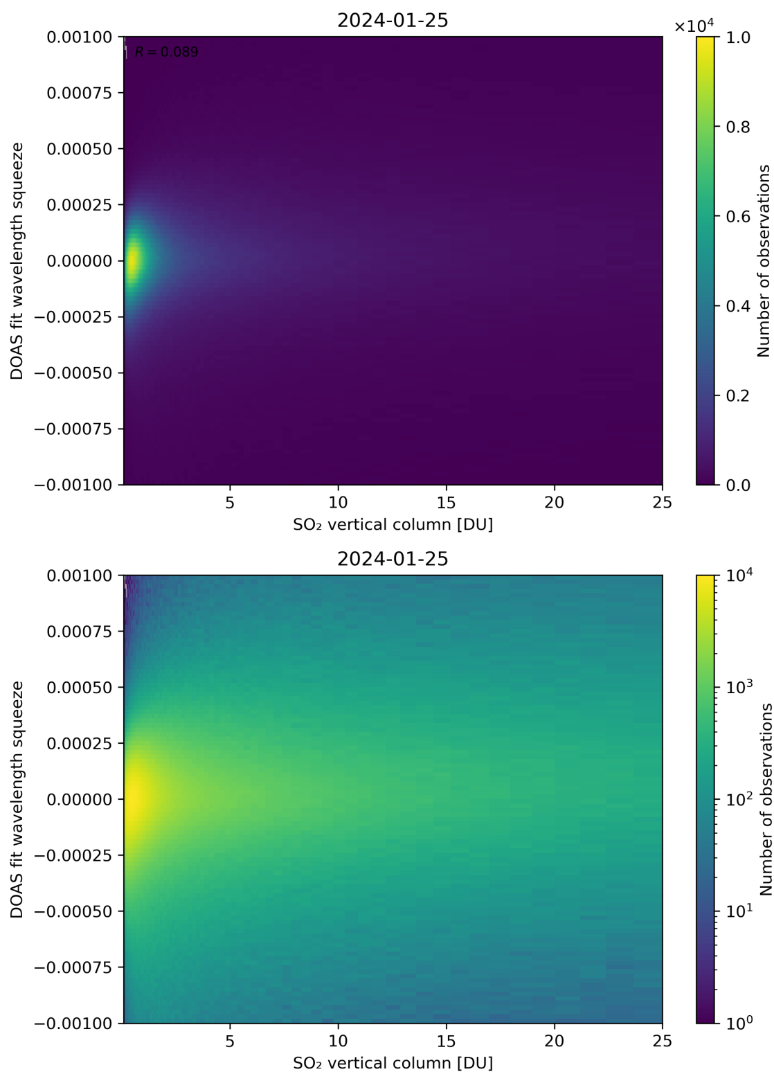
Figure 277: Scatter density plot of “SO 2 vertical column” against “DOAS fit wavelength squeeze” for 2024-01-24 to 2024-01-26.
