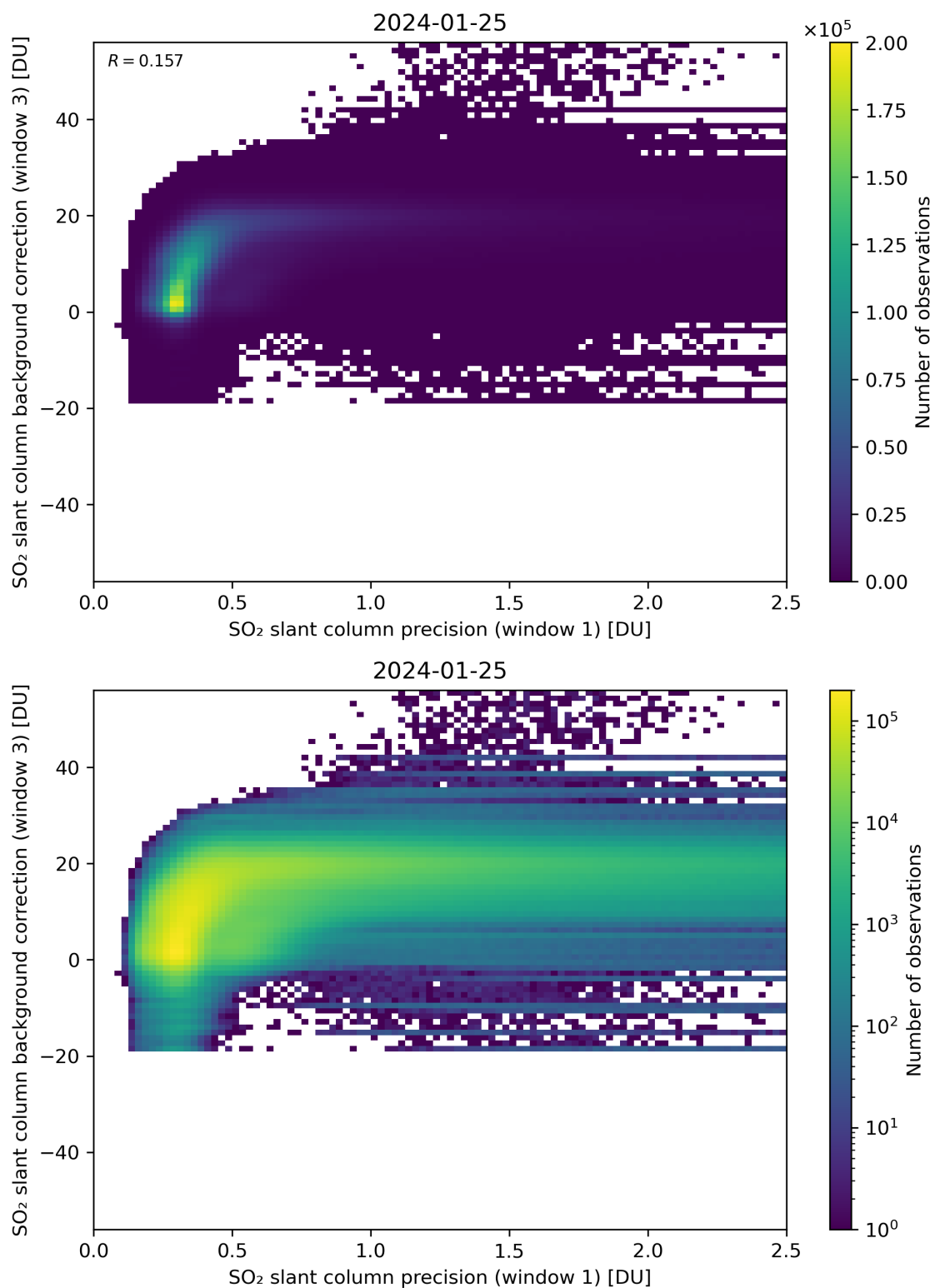
Figure 220: Scatter density plot of “SO 2 slant column precision (window 1)” against “SO 2 slant column background correction (window 3)” for 2024-01-24 to 2024-01-26.
