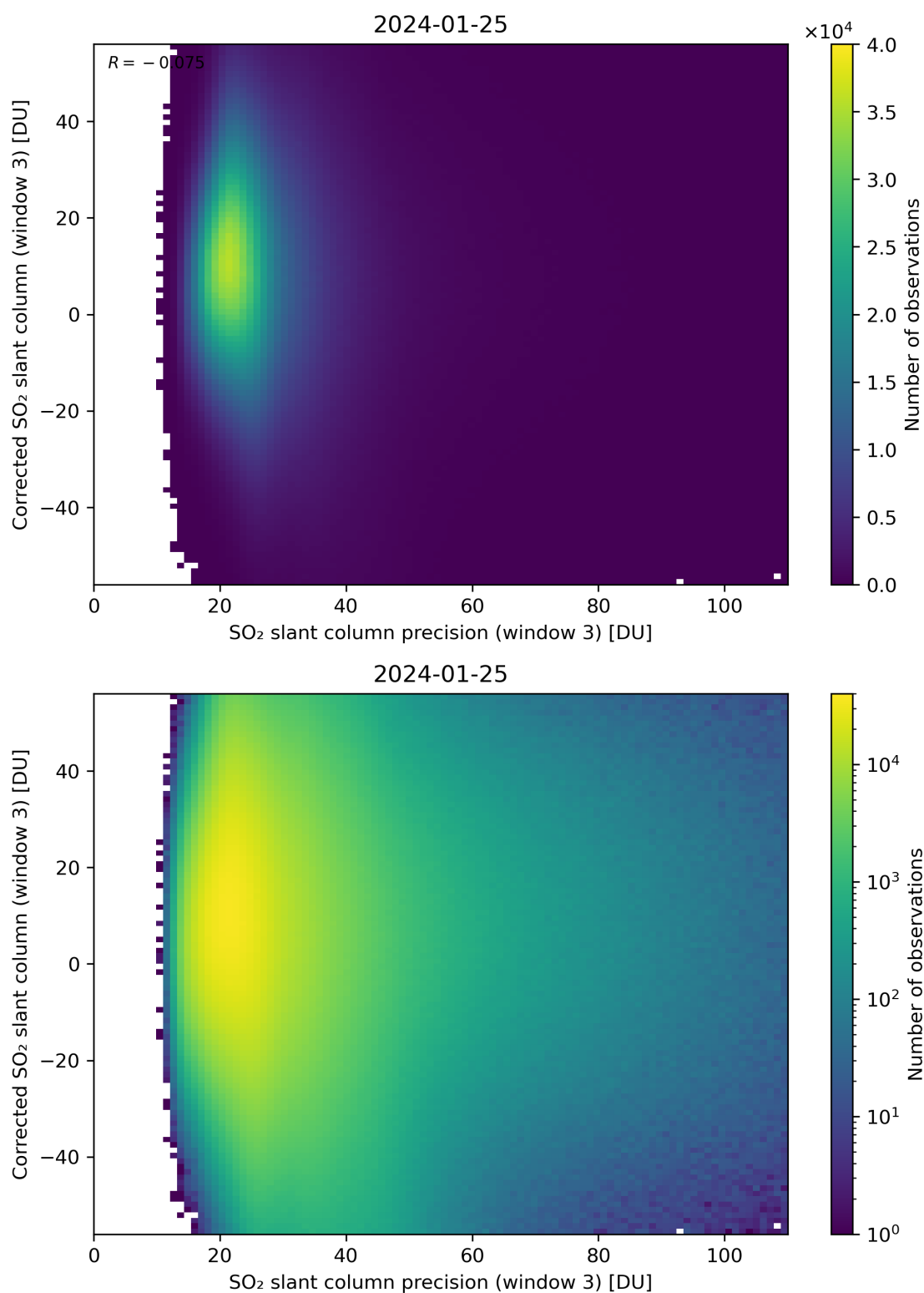
Figure 262: Scatter density plot of “SO 2 slant column precision (window 3)” against “Corrected SO 2 slant column (window 3)” for 2024-01-24 to 2024-01-26.
