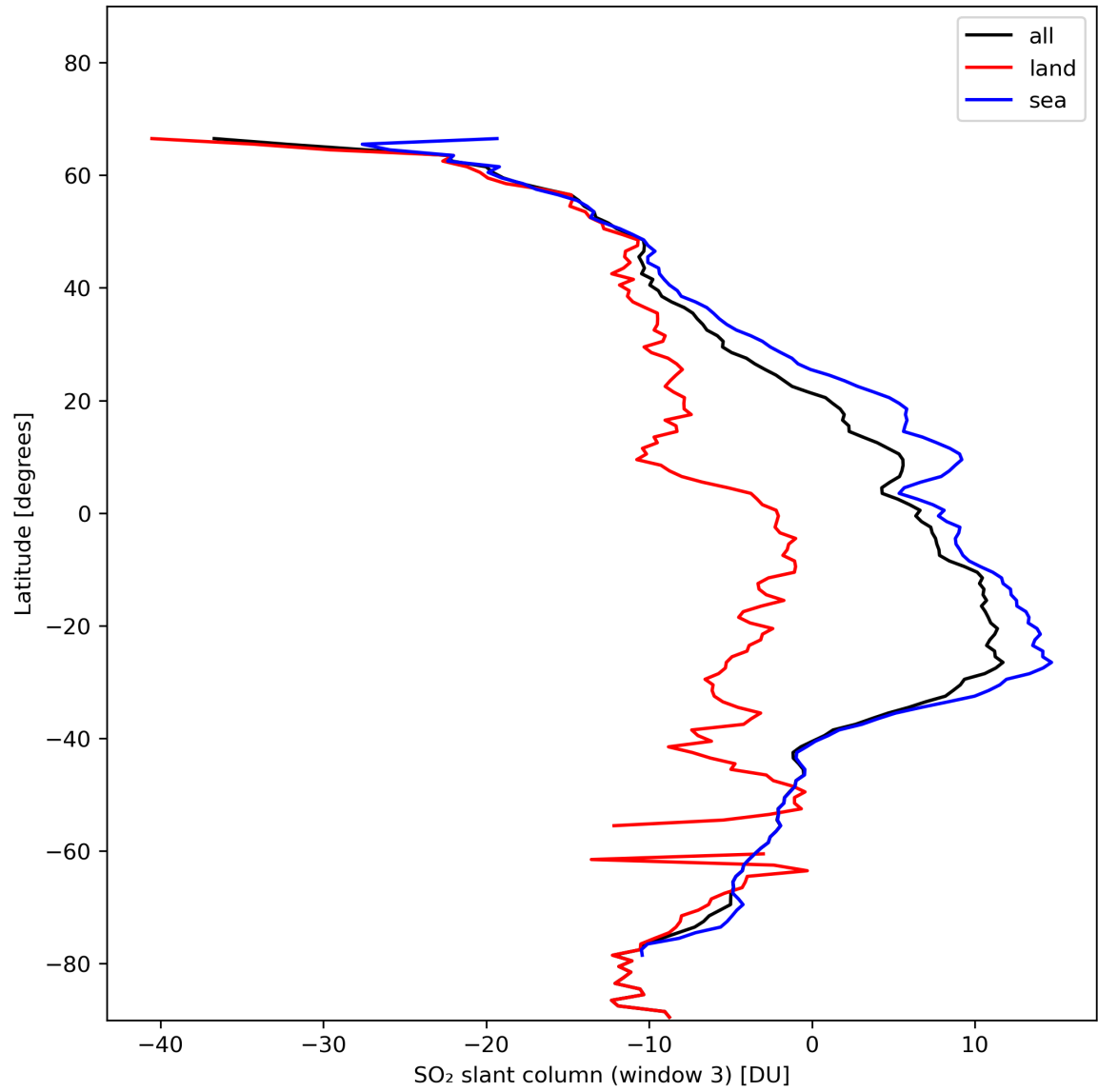
Figure 41: Zonal average of “SO 2 slant column (window 3)” for 2024-01-24 to 2024-01-26.
