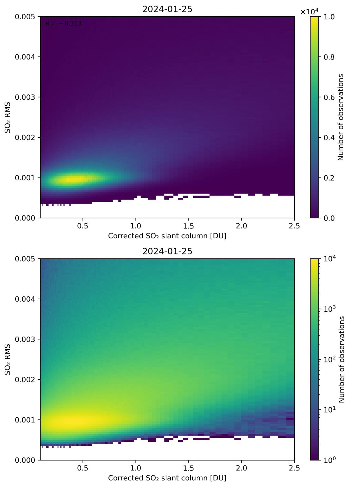
Figure 183: Scatter density plot of “Corrected SO 2 slant column” against “SO 2 RMS” for 2024-01-24 to 2024-01-26.
