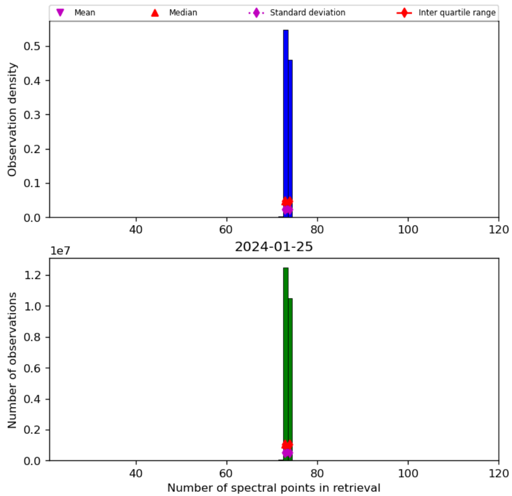
Figure 74: Histogram of “Number of spectral points in retrieval” for 2024-01-24 to 2024-01-26
