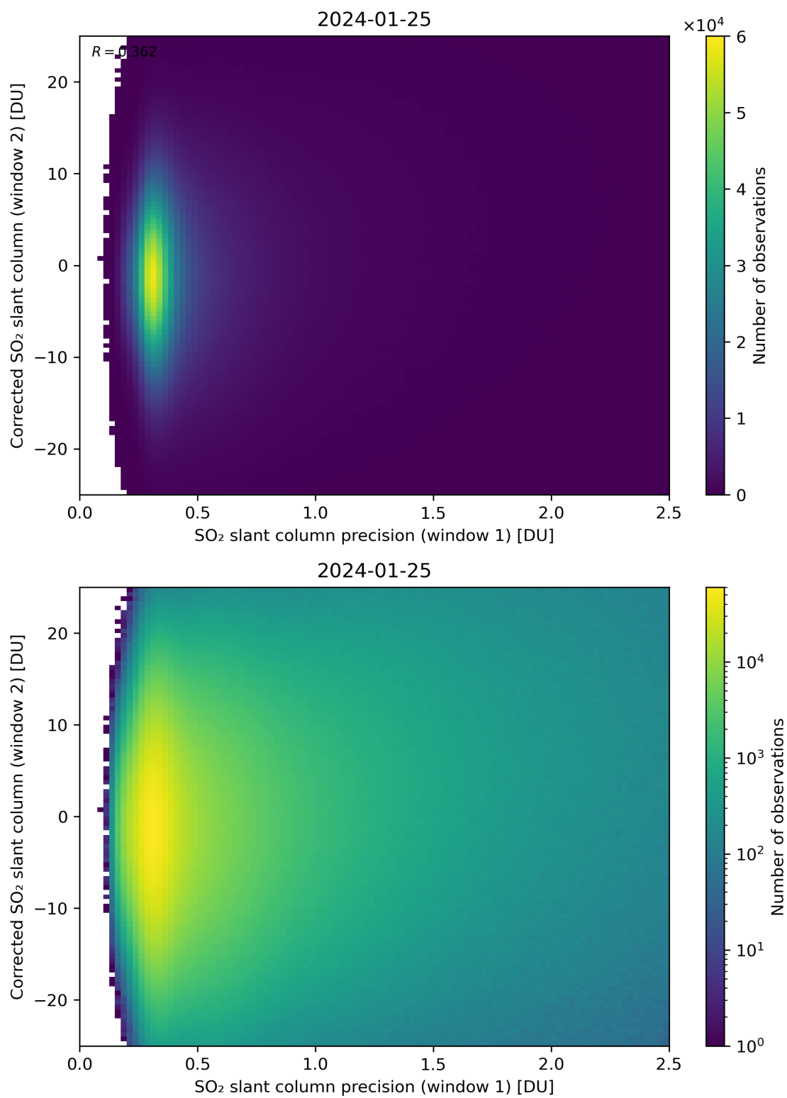
Figure 225: Scatter density plot of “SO 2 slant column precision (window 1)” against “Corrected SO 2 slant column (window 2)” for 2024-01-24 to 2024-01-26.
