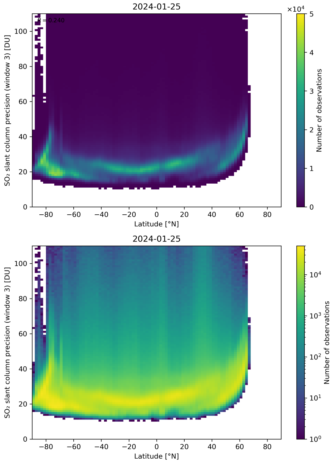
Figure 153: Scatter density plot of “Latitude” against “SO 2 slant column precision (window 3)” for 2024-01-24 to 2024-01-26.
