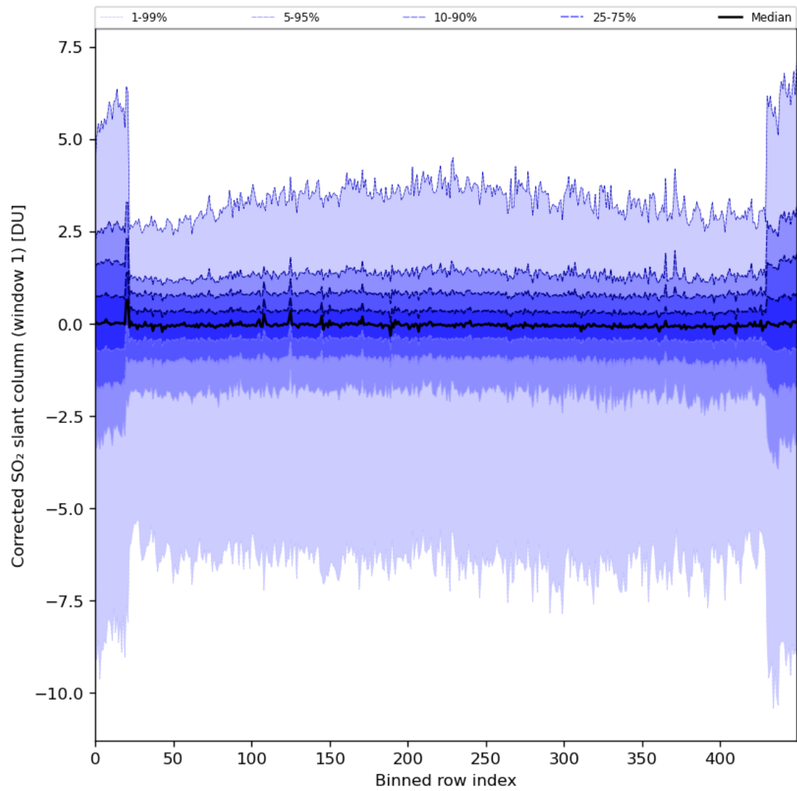
Figure 81: Along track statistics of “Corrected SO 2 slant column (window 1)” for 2024-01-24 to 2024-01-26
