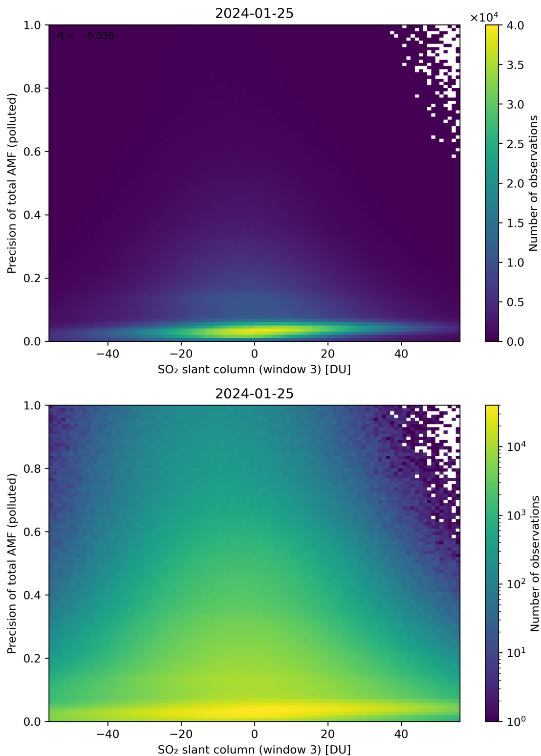
Figure 269: Scatter density plot of “SO 2 slant column (window 3)” against “Precision of total AMF (polluted)” for 2024-01-24 to 2024-01-26.
