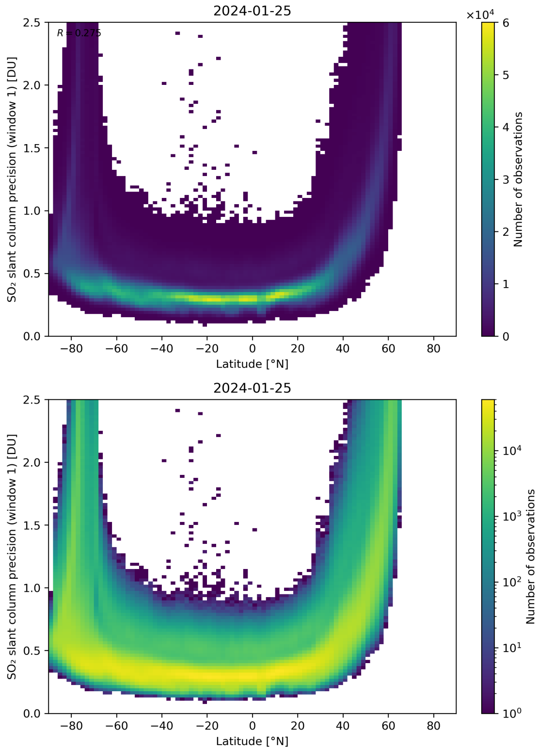
Figure 150: Scatter density plot of “Latitude” against “SO 2 slant column precision (window 1)” for 2024-01-24 to 2024-01-26.
