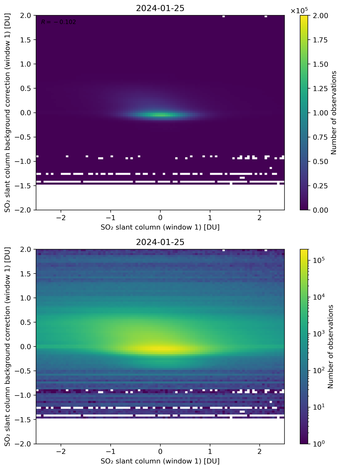
Figure 212: Scatter density plot of “SO 2 slant column (window 1)” against “SO 2 slant column background correction (window 1)” for 2024-01-24 to 2024-01-26.
