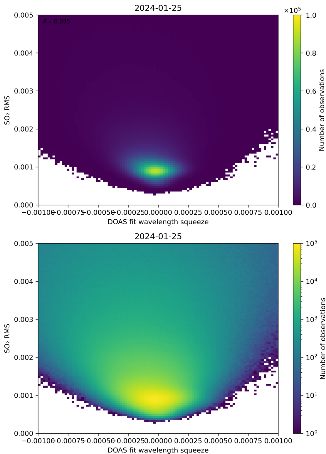
Figure 132: Scatter density plot of “DOAS fit wavelength squeeze” against “SO 2 RMS” for 2024-01-24 to 2024-01-26.
