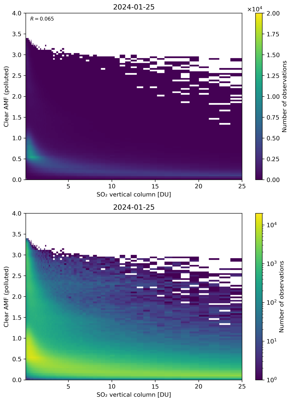
Figure 296: Scatter density plot of “SO 2 vertical column” against “Clear AMF (polluted)” for 2024-01-24 to 2024-01-26.
