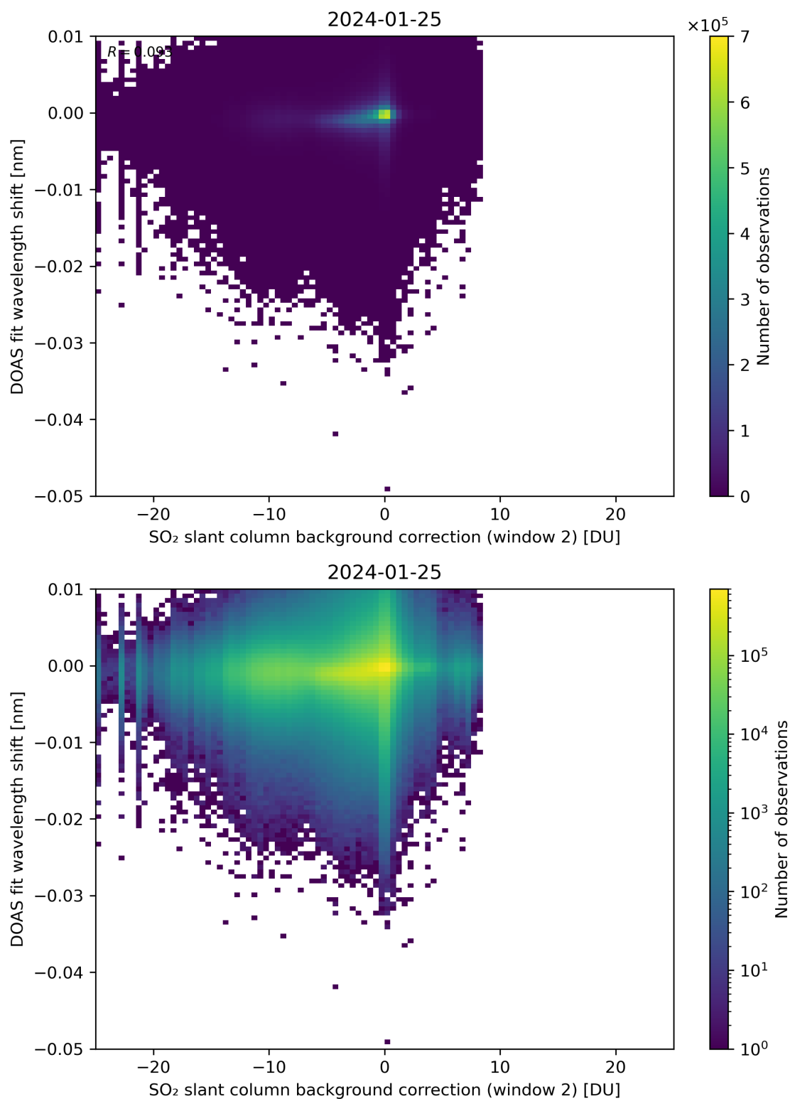
Figure 112: Scatter density plot of “SO 2 slant column background correction (window 2)” against “DOAS fit wavelength shift” for 2024-01-24 to 2024-01-26.
