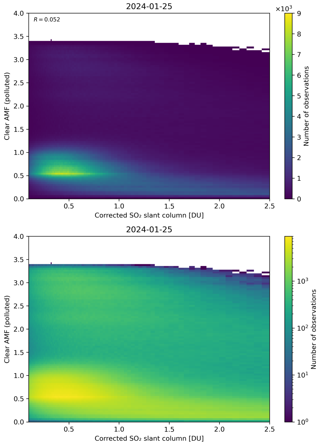
Figure 184: Scatter density plot of “Corrected SO 2 slant column” against “Clear AMF (polluted)” for 2024-01-24 to 2024-01-26.
