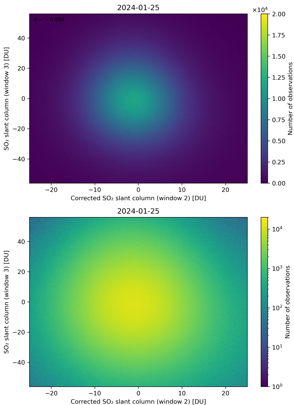
Figure 201: Scatter density plot of “Corrected SO 2 slant column (window 2)” against “SO 2 slant column (window 3)” for 2024-01-24 to 2024-01-26.
