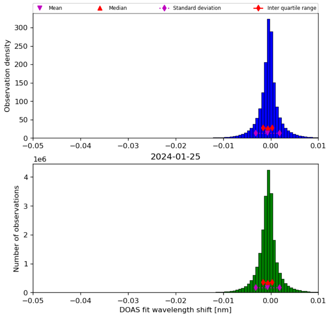
Figure 68: Histogram of “DOAS fit wavelength shift” for 2024-01-24 to 2024-01-26
