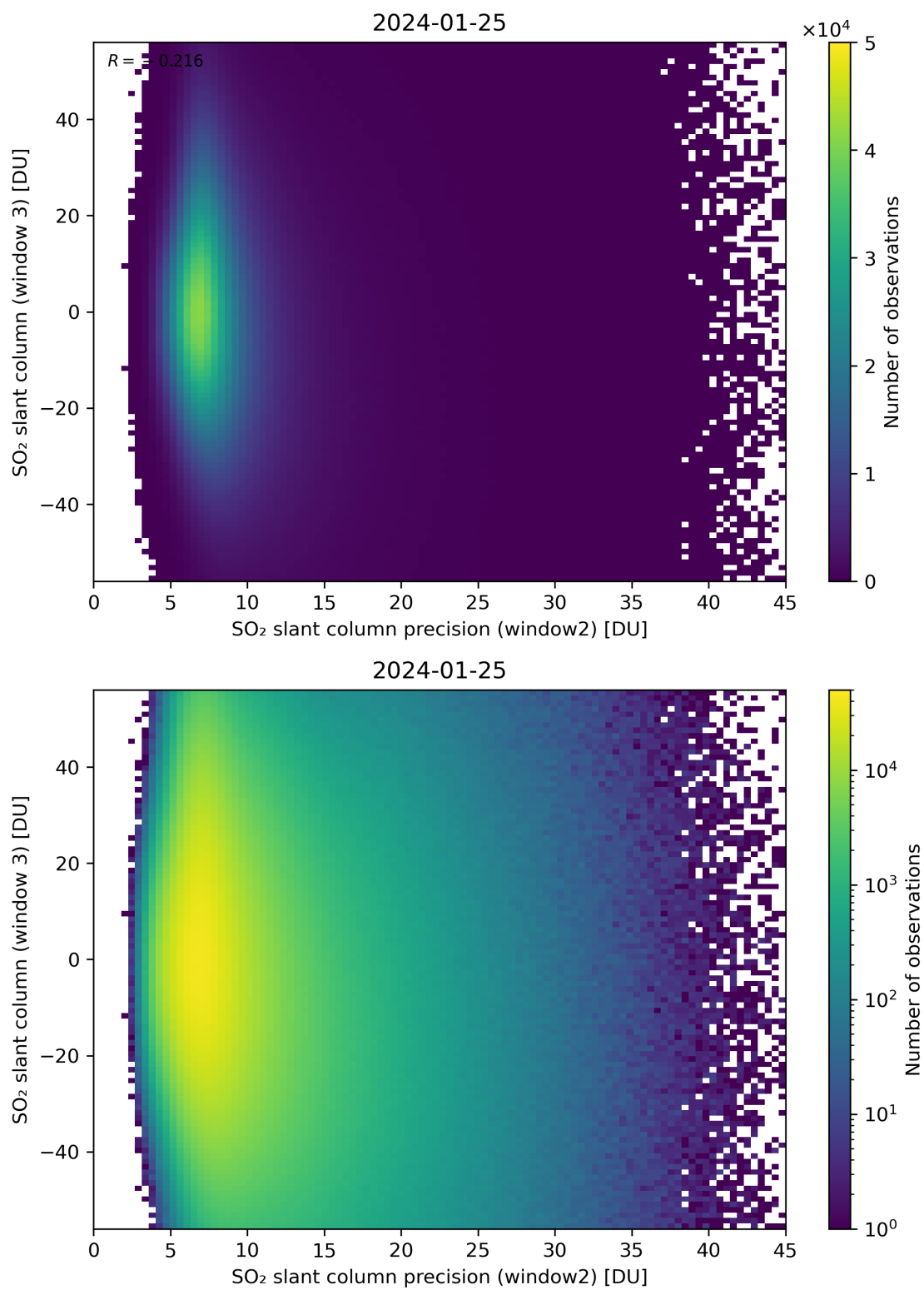
Figure 249: Scatter density plot of “SO 2 slant column precision (window2)” against “SO 2 slant column (window 3)” for 2024-01-24 to 2024-01-26.
