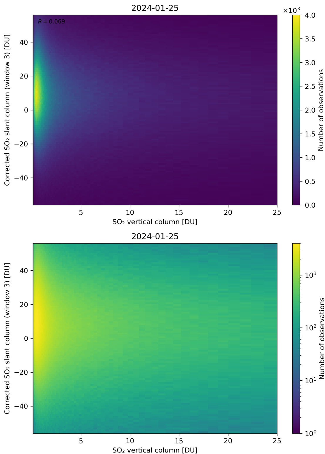
Figure 299: Scatter density plot of “SO 2 vertical column” against “Corrected SO 2 slant column (window 3)” for 2024-01-24 to 2024-01-26.
