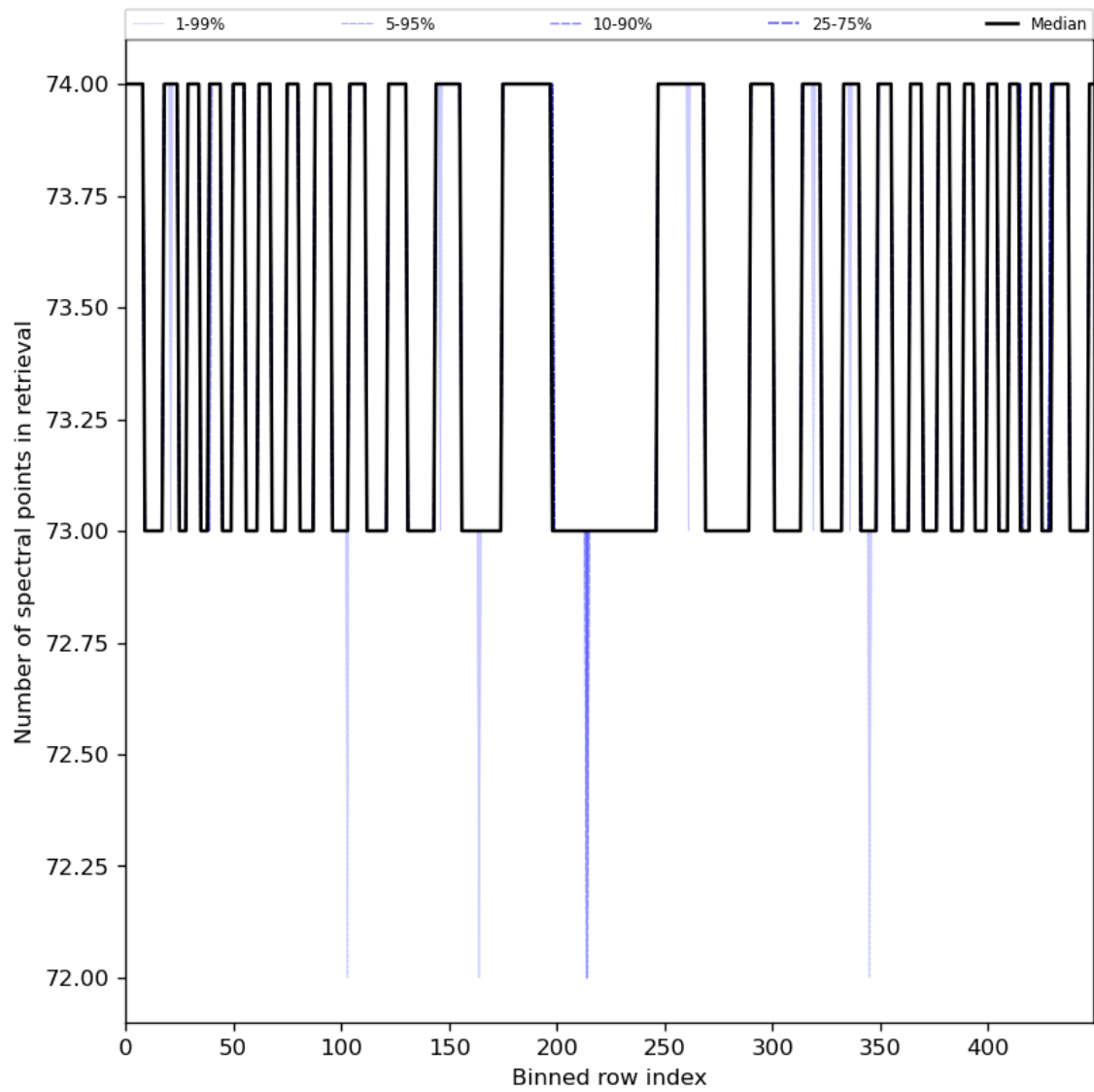
Figure 97: Along track statistics of “Number of spectral points in retrieval” for 2024-01-24 to 2024-01-26
