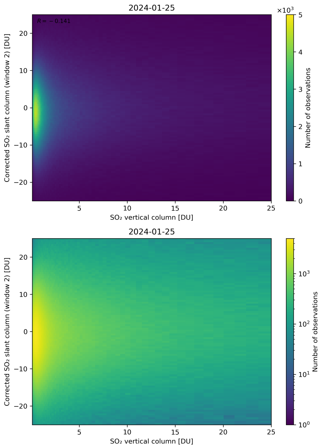
Figure 298: Scatter density plot of “SO 2 vertical column” against “Corrected SO 2 slant column (window 2)” for 2024-01-24 to 2024-01-26.
