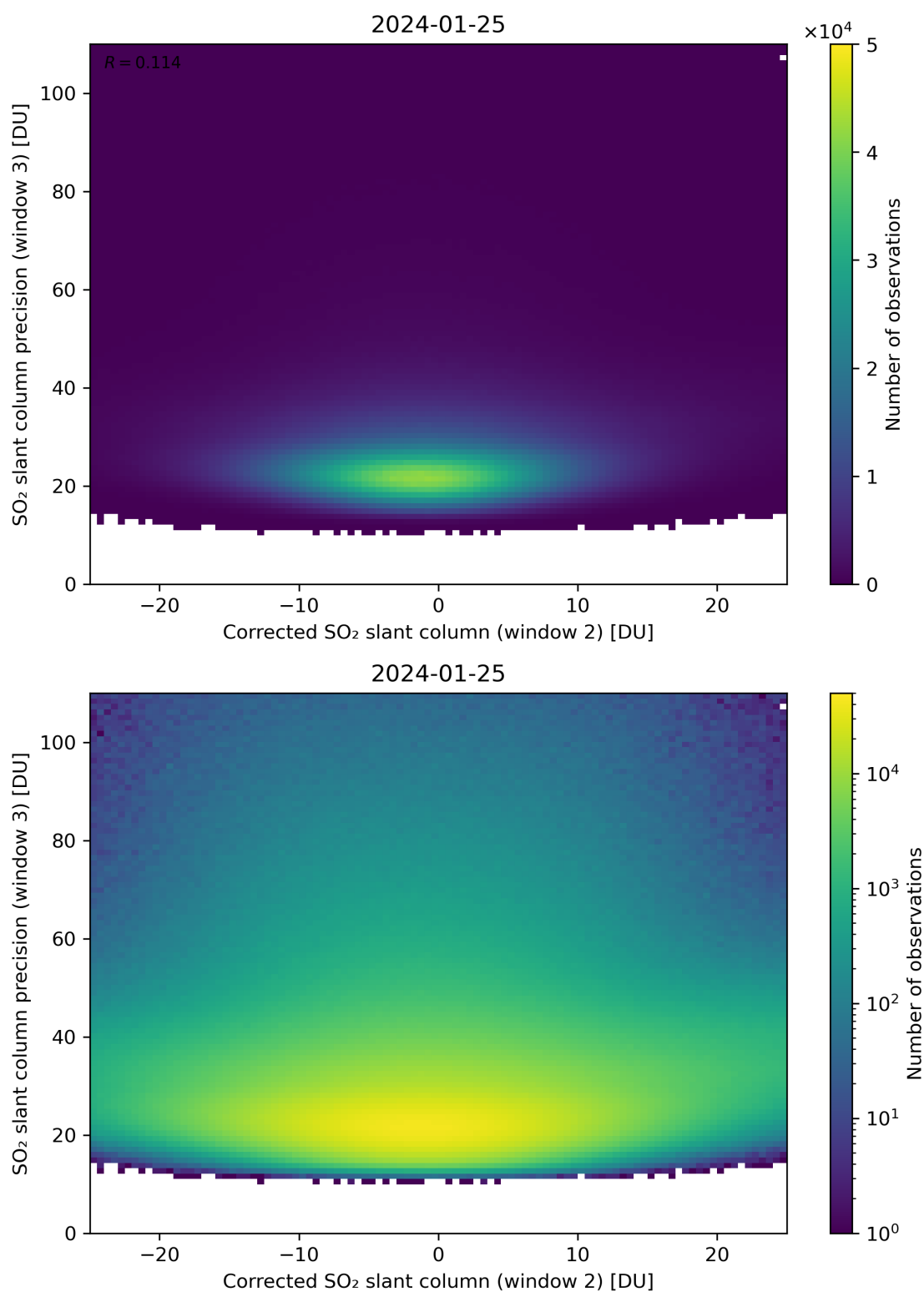
Figure 202: Scatter density plot of “Corrected SO 2 slant column (window 2)” against “SO 2 slant column precision (window 3)” for 2024-01-24 to 2024-01-26.
