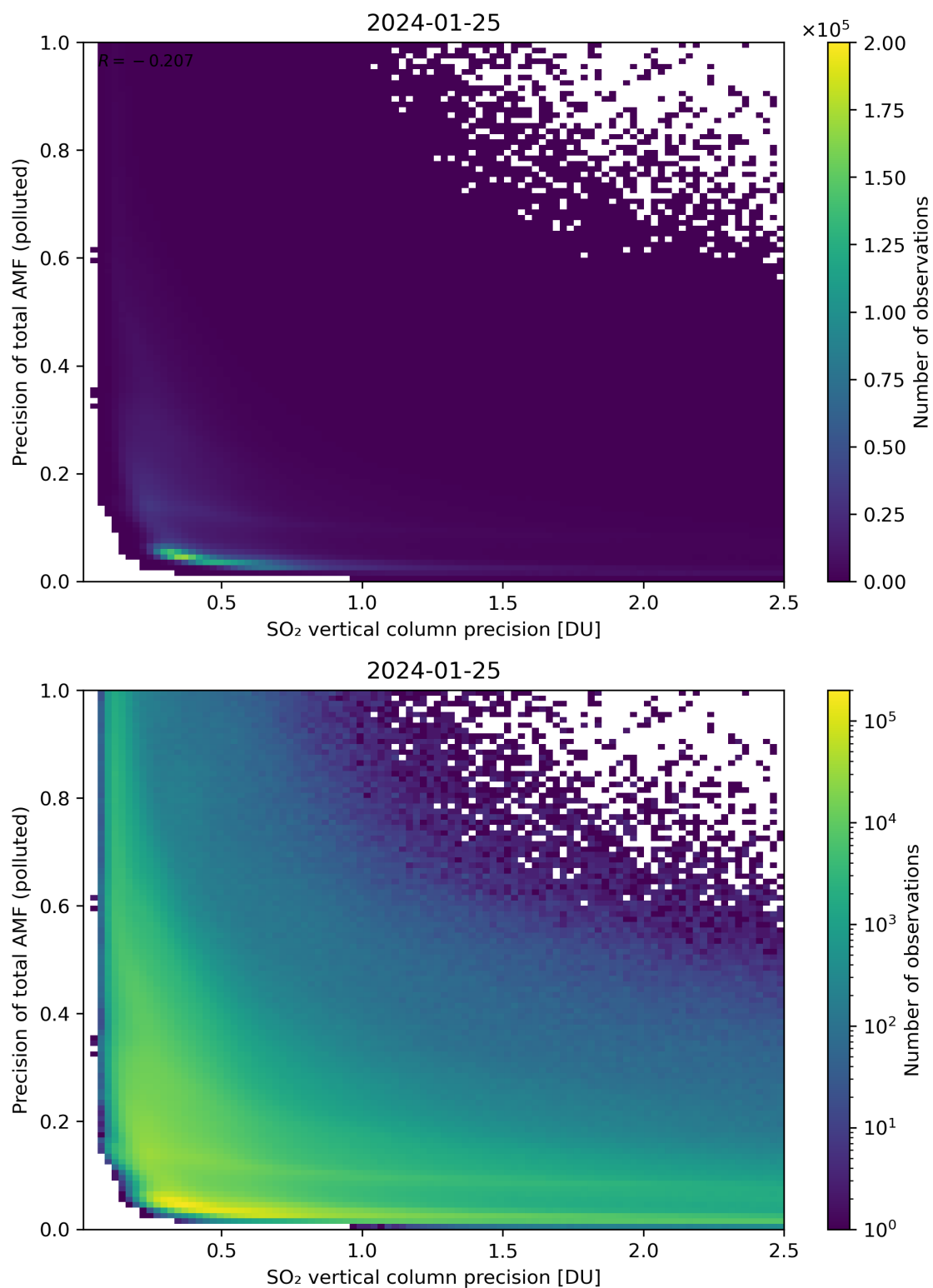
Figure 295: Scatter density plot of “SO 2 vertical column precision” against “Precision of total AMF (polluted)” for 2024-01-24 to 2024-01-26.
