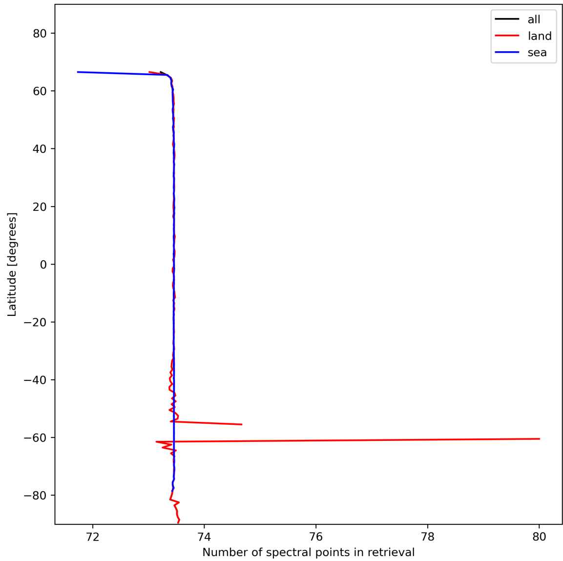
Figure 51: Zonal average of “Number of spectral points in retrieval” for 2024-01-24 to 2024-01-26.
