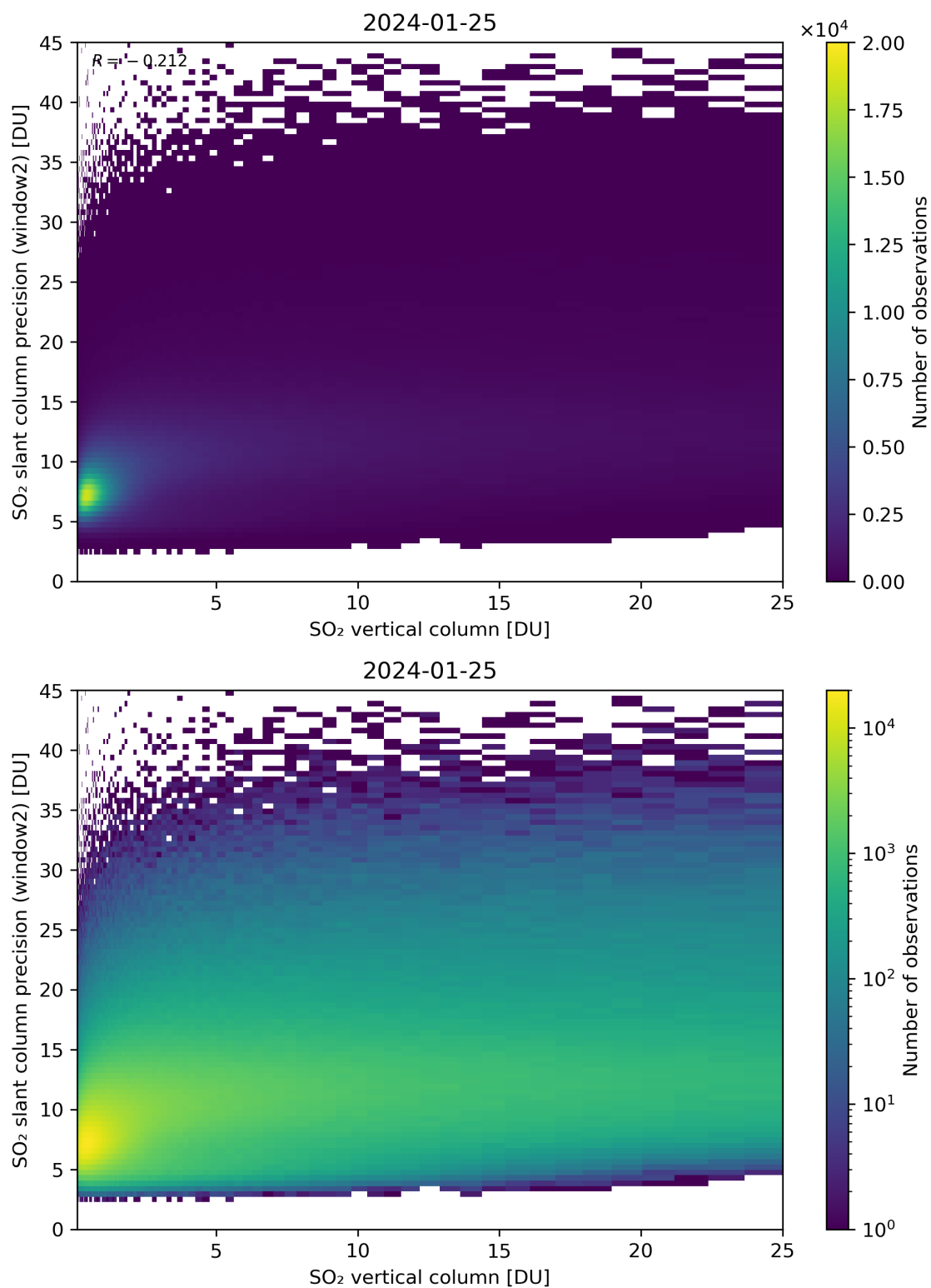
Figure 302: Scatter density plot of “SO 2 vertical column” against “SO 2 slant column precision (window2)” for 2024-01-24 to 2024-01-26.
