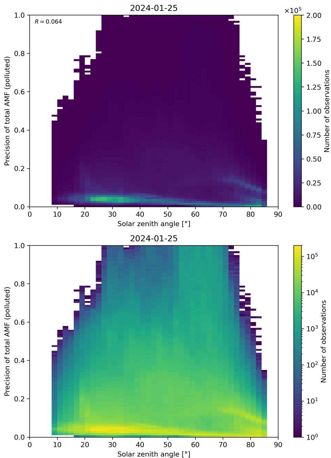
Figure 175: Scatter density plot of “Solar zenith angle” against “Precision of total AMF (polluted)” for 2024-01-24 to 2024-01-26.
