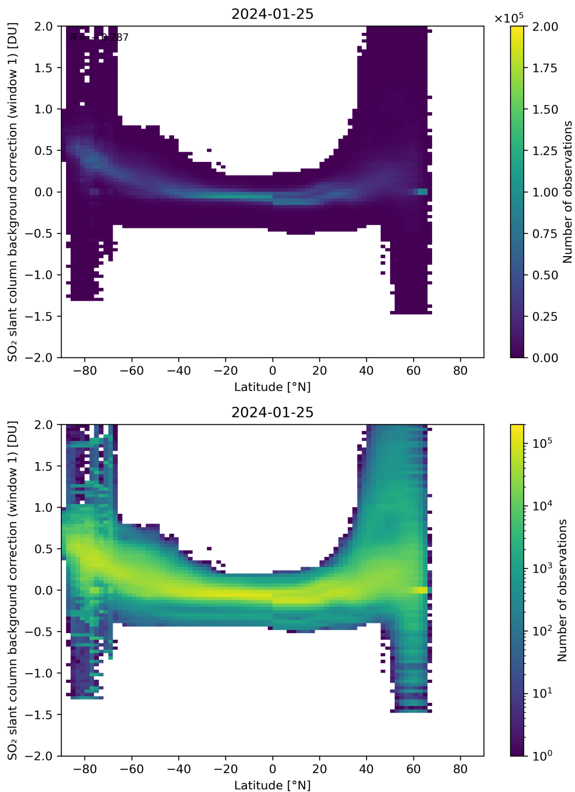
Figure 139: Scatter density plot of “Latitude” against “SO 2 slant column background correction (window 1)” for 2024-01-24 to 2024-01-26.
