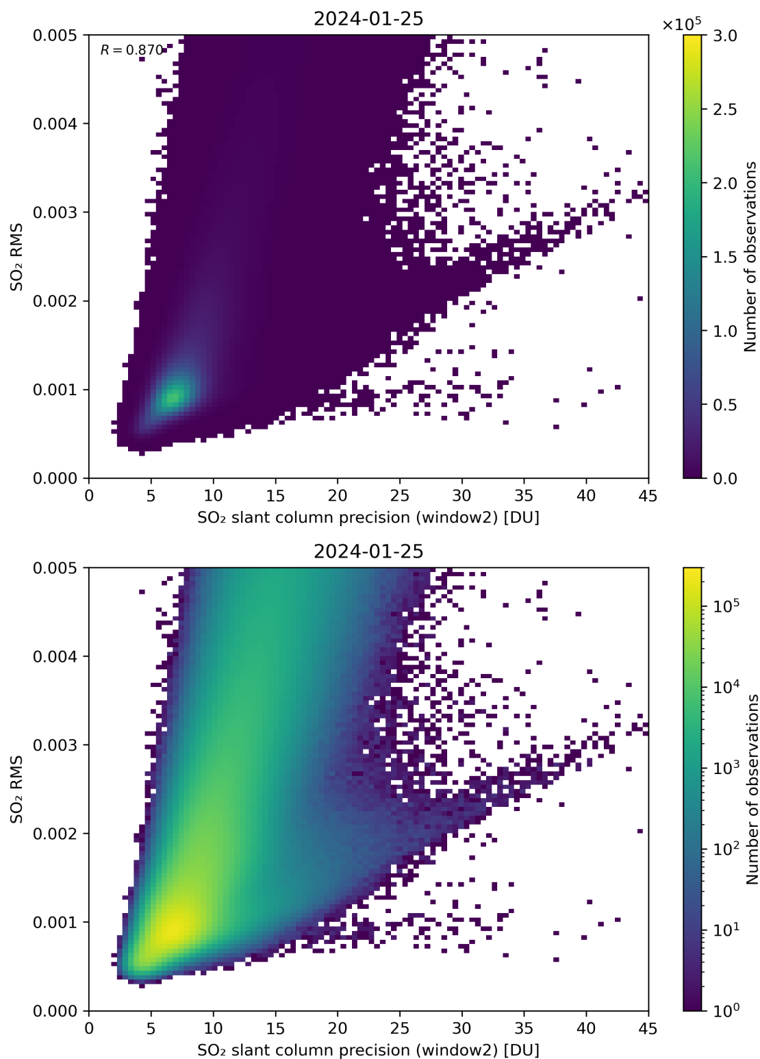
Figure 245: Scatter density plot of “SO 2 slant column precision (window2)” against “SO 2 RMS” for 2024-01-24 to 2024-01-26.
