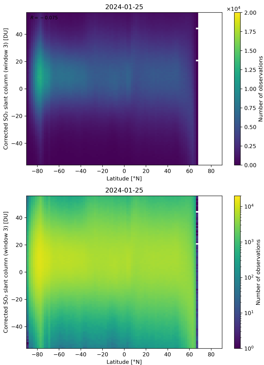
Figure 148: Scatter density plot of “Latitude” against “Corrected SO 2 slant column (window 3)” for 2024-01-24 to 2024-01-26.
