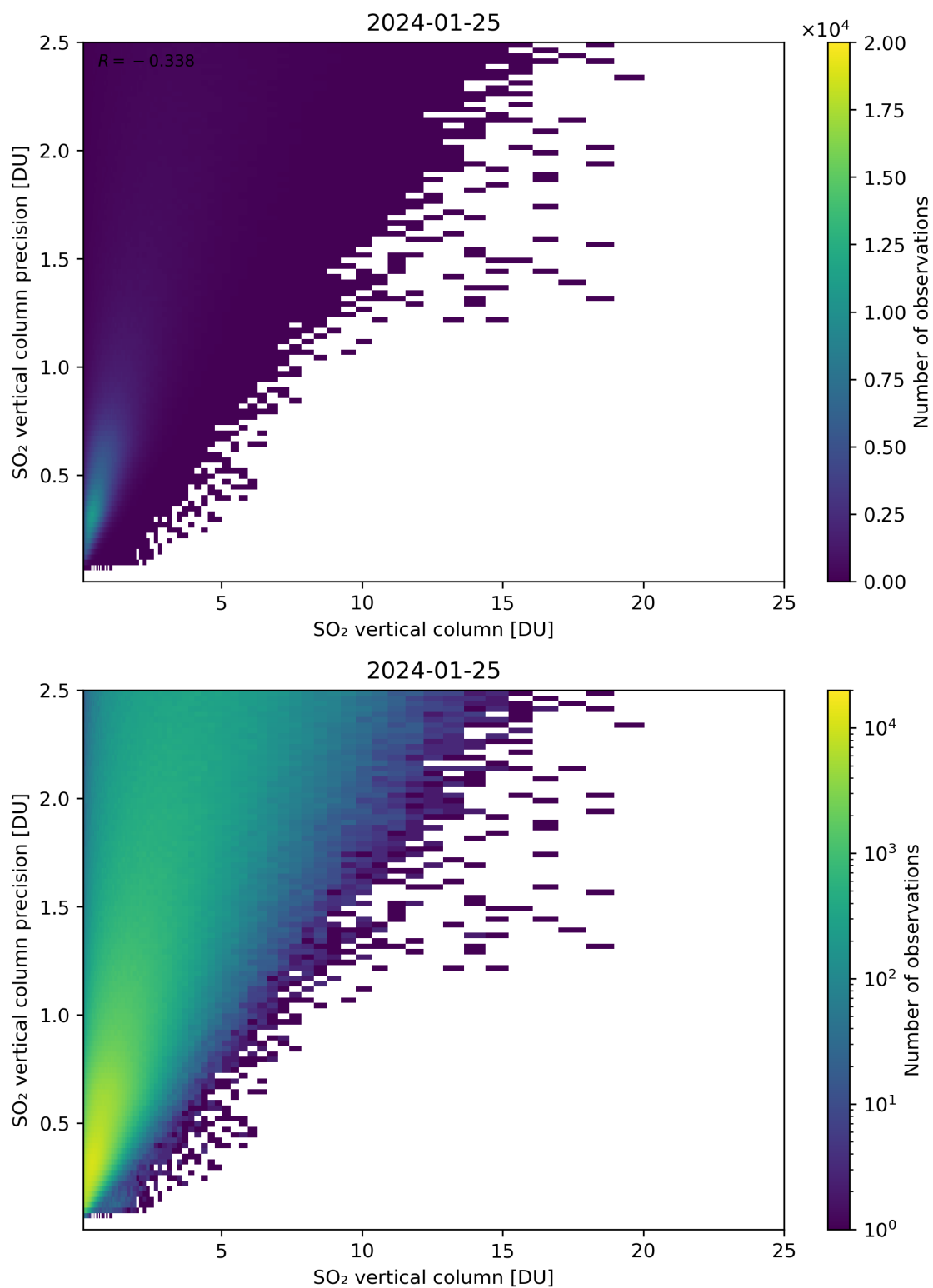
Figure 307: Scatter density plot of “SO 2 vertical column” against “SO 2 vertical column precision” for 2024-01-24 to 2024-01-26.
