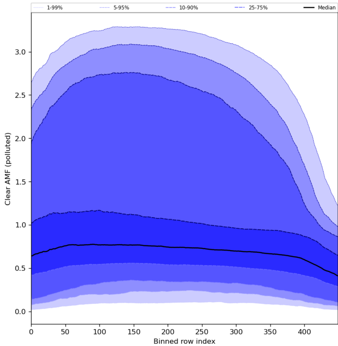
Figure 96: Along track statistics of “Clear AMF (polluted)” for 2024-01-24 to 2024-01-26
