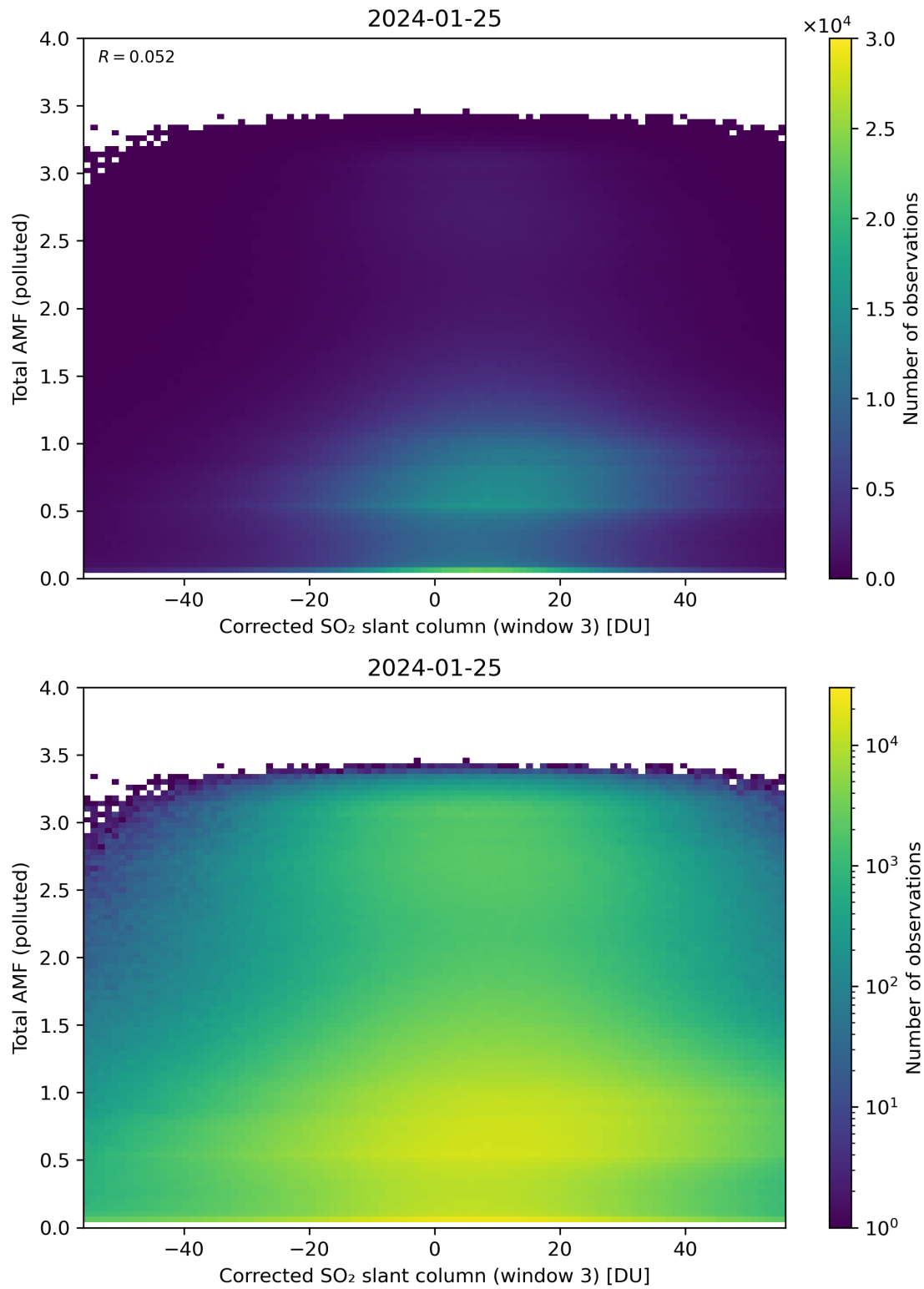
Figure 210: Scatter density plot of “Corrected SO 2 slant column (window 3)” against “Total AMF (polluted)” for 2024-01-24 to 2024-01-26.
