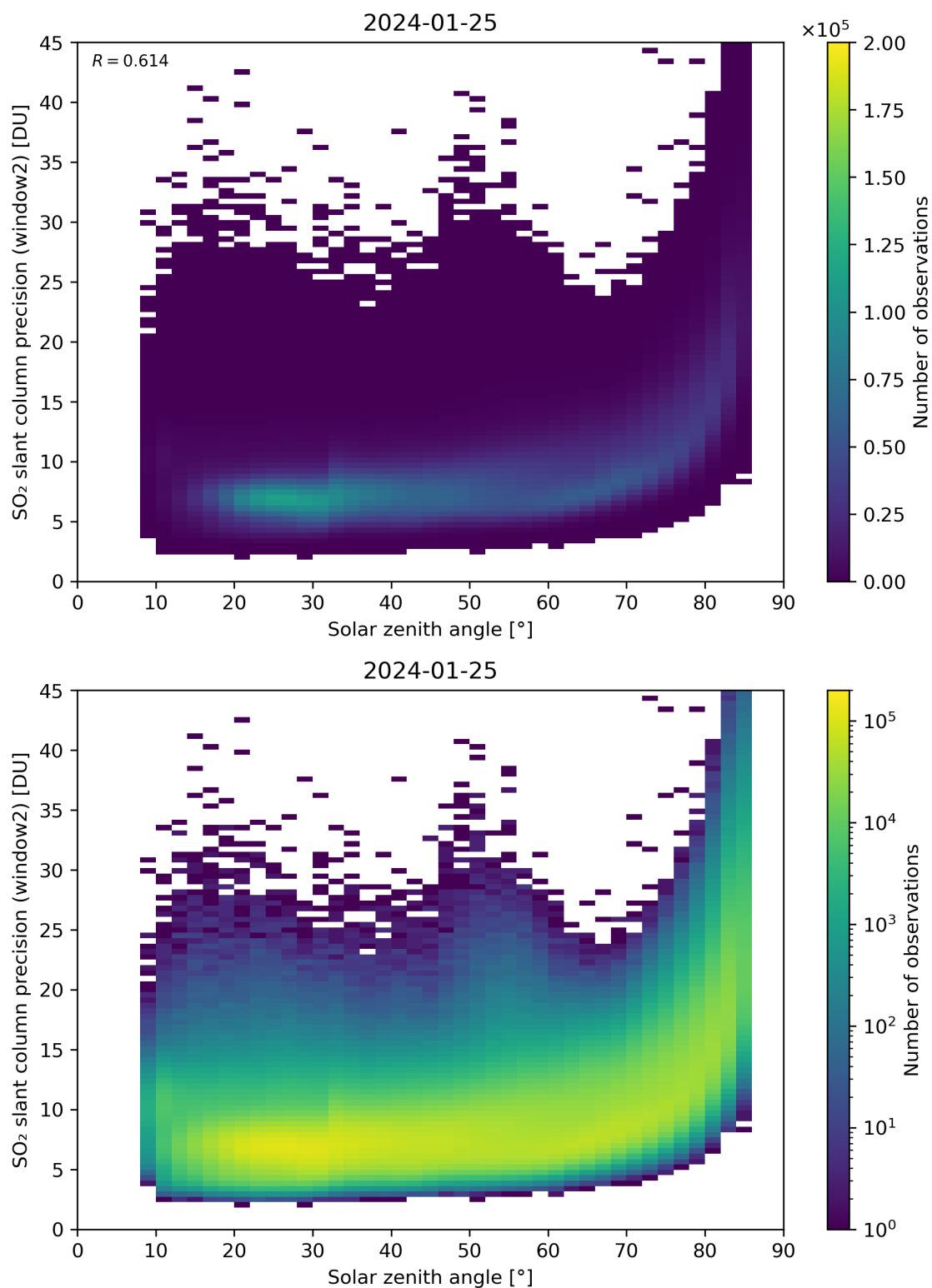
Figure 171: Scatter density plot of “Solar zenith angle” against “SO 2 slant column precision (window2)” for 2024-01-24 to 2024-01-26.
