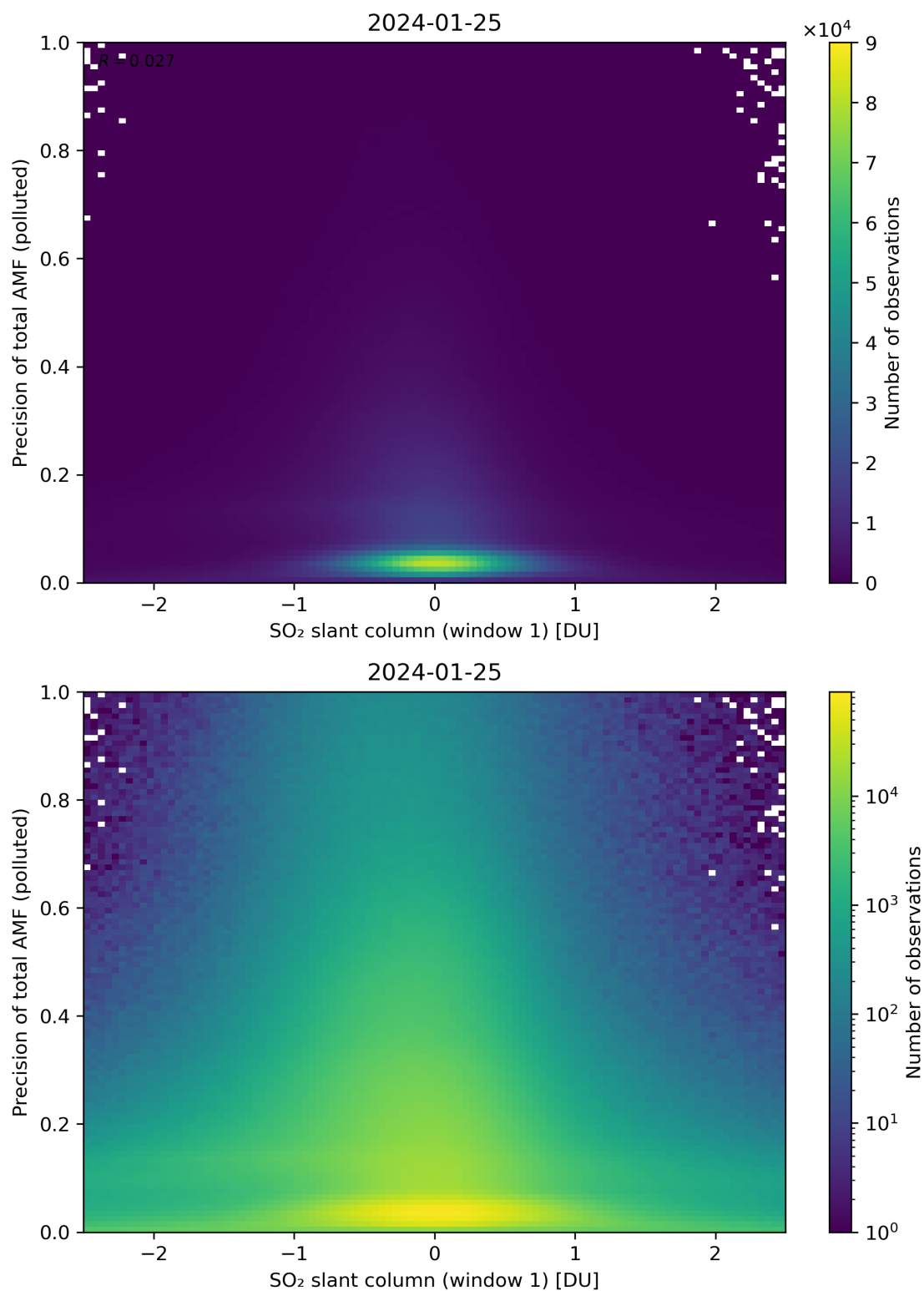
Figure 240: Scatter density plot of “SO 2 slant column (window 1)” against “Precision of total AMF (polluted)” for 2024-01-24 to 2024-01-26.
