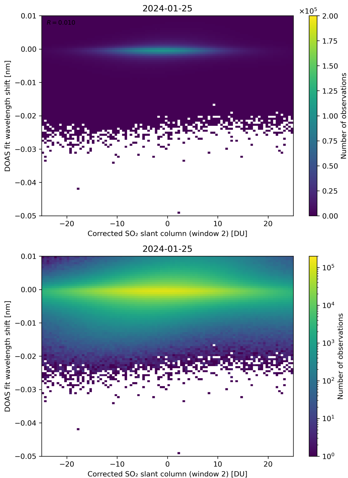
Figure 196: Scatter density plot of “Corrected SO 2 slant column (window 2)” against “DOAS fit wavelength shift” for 2024-01-24 to 2024-01-26.
