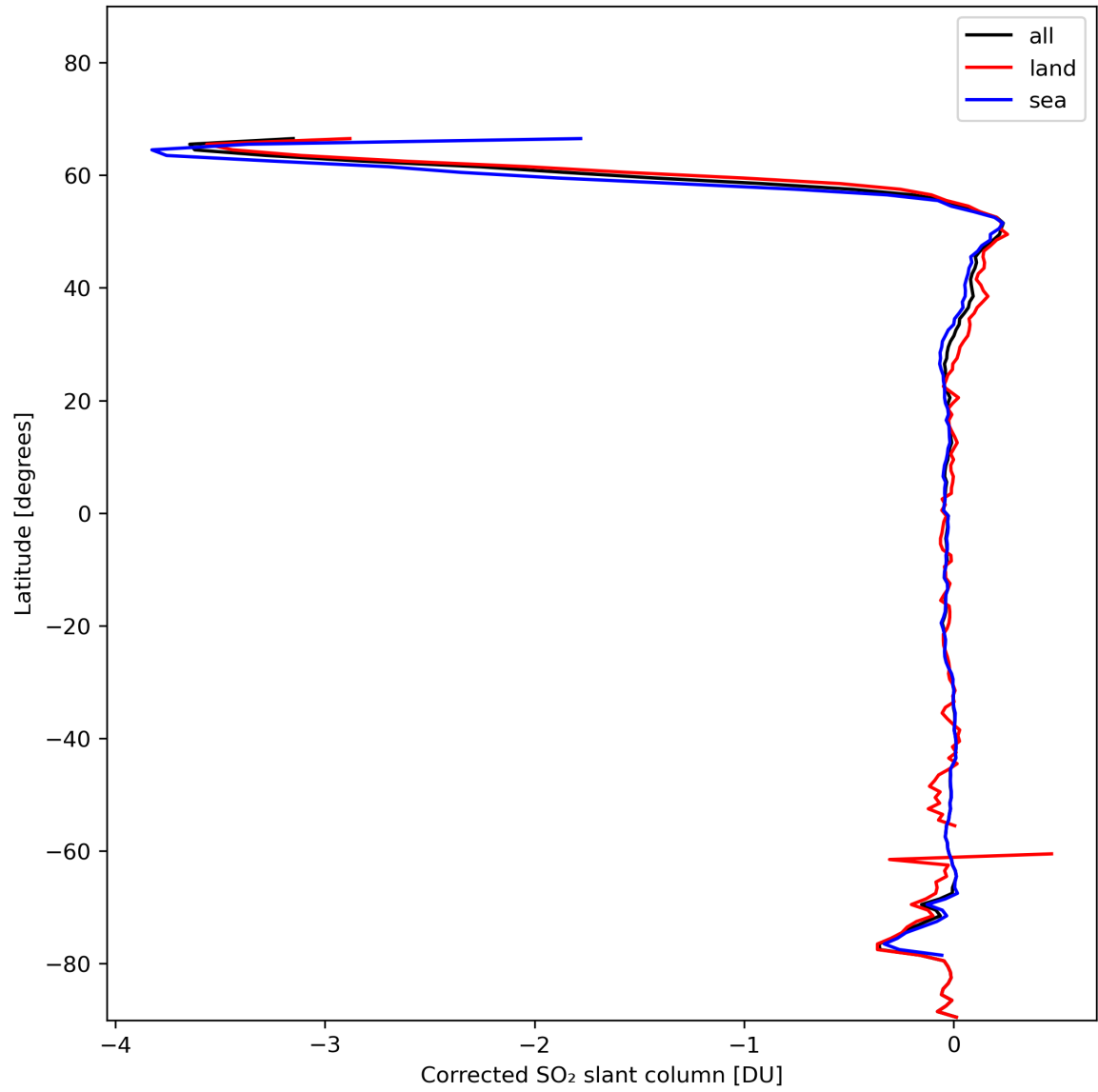
Figure 32: Zonal average of “Corrected SO 2 slant column” for 2024-01-24 to 2024-01-26.
