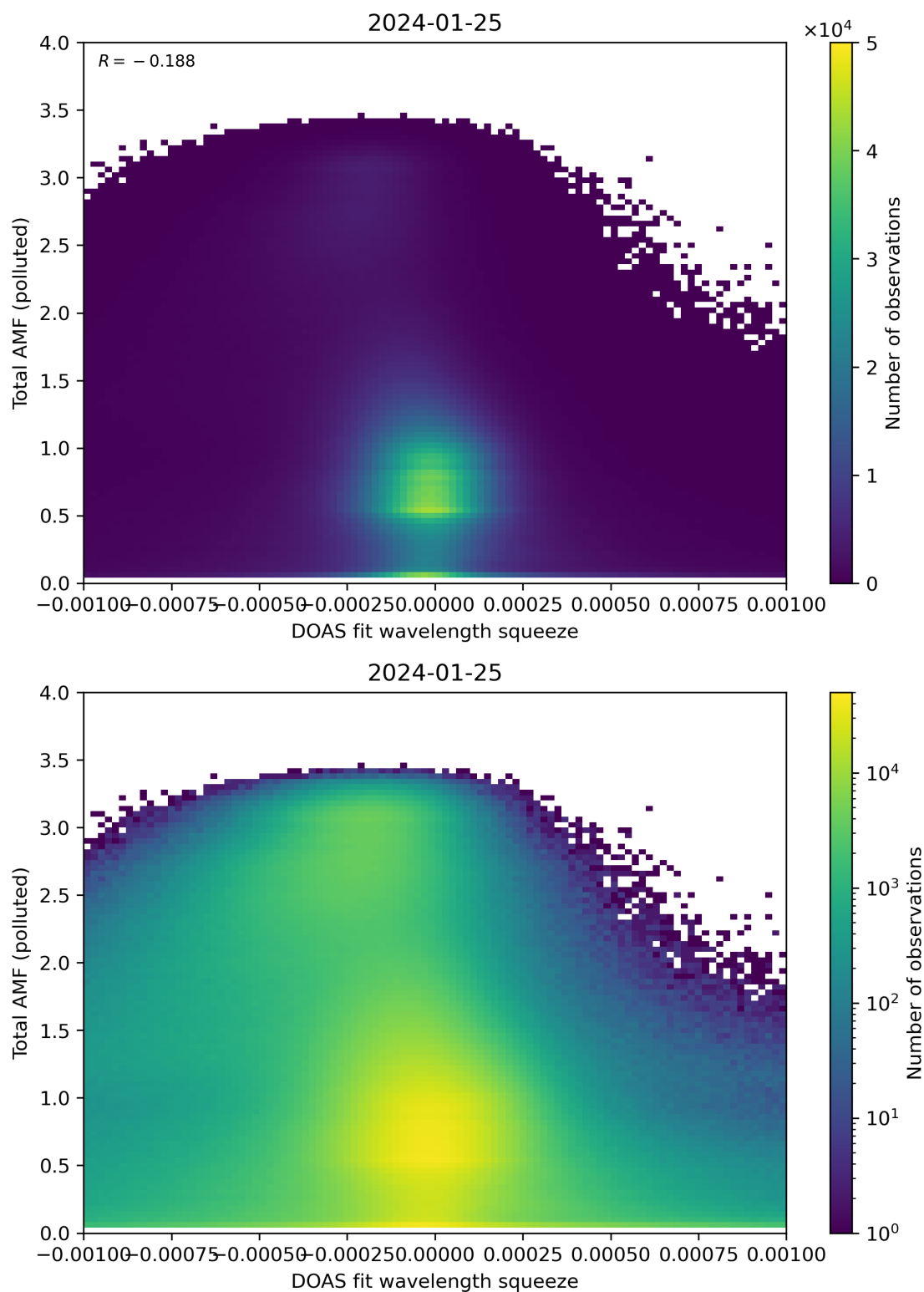
Figure 134: Scatter density plot of “DOAS fit wavelength squeeze” against “Total AMF (polluted)” for 2024-01-24 to 2024-01-26.
