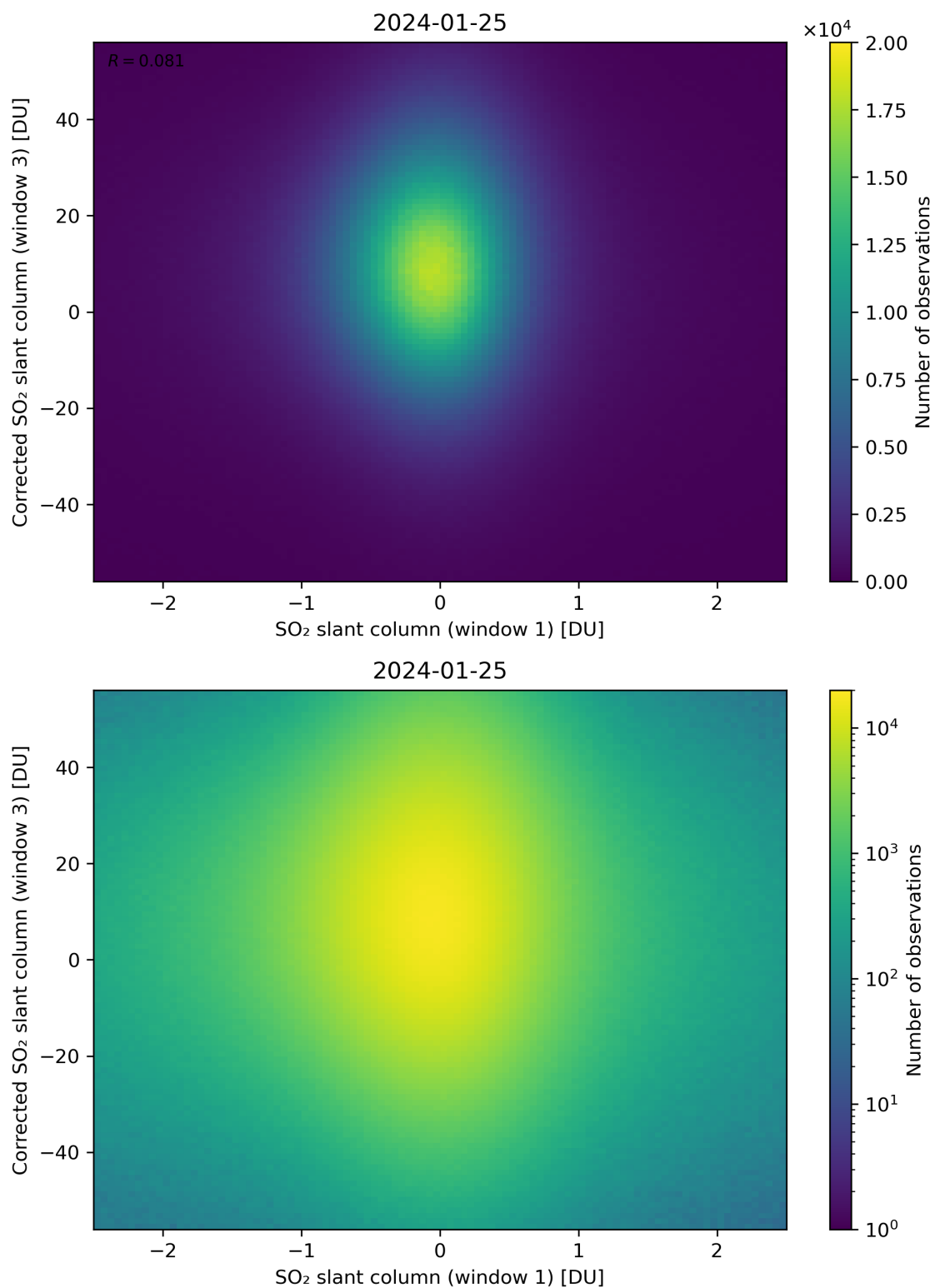
Figure 234: Scatter density plot of “SO 2 slant column (window 1)” against “Corrected SO 2 slant column (window 3)” for 2024-01-24 to 2024-01-26.
