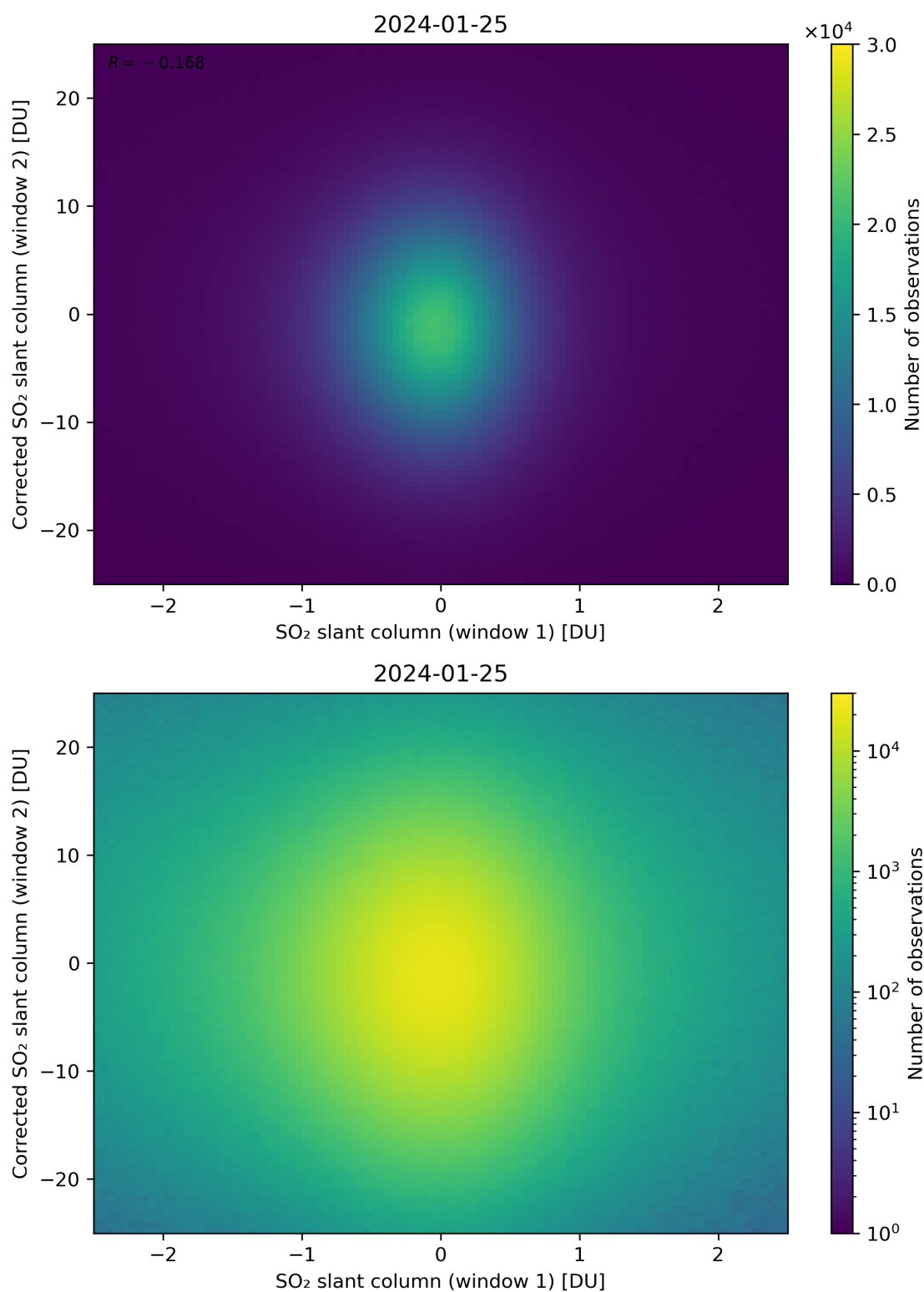
Figure 233: Scatter density plot of “SO 2 slant column (window 1)” against “Corrected SO 2 slant column (window 2)” for 2024-01-24 to 2024-01-26.
