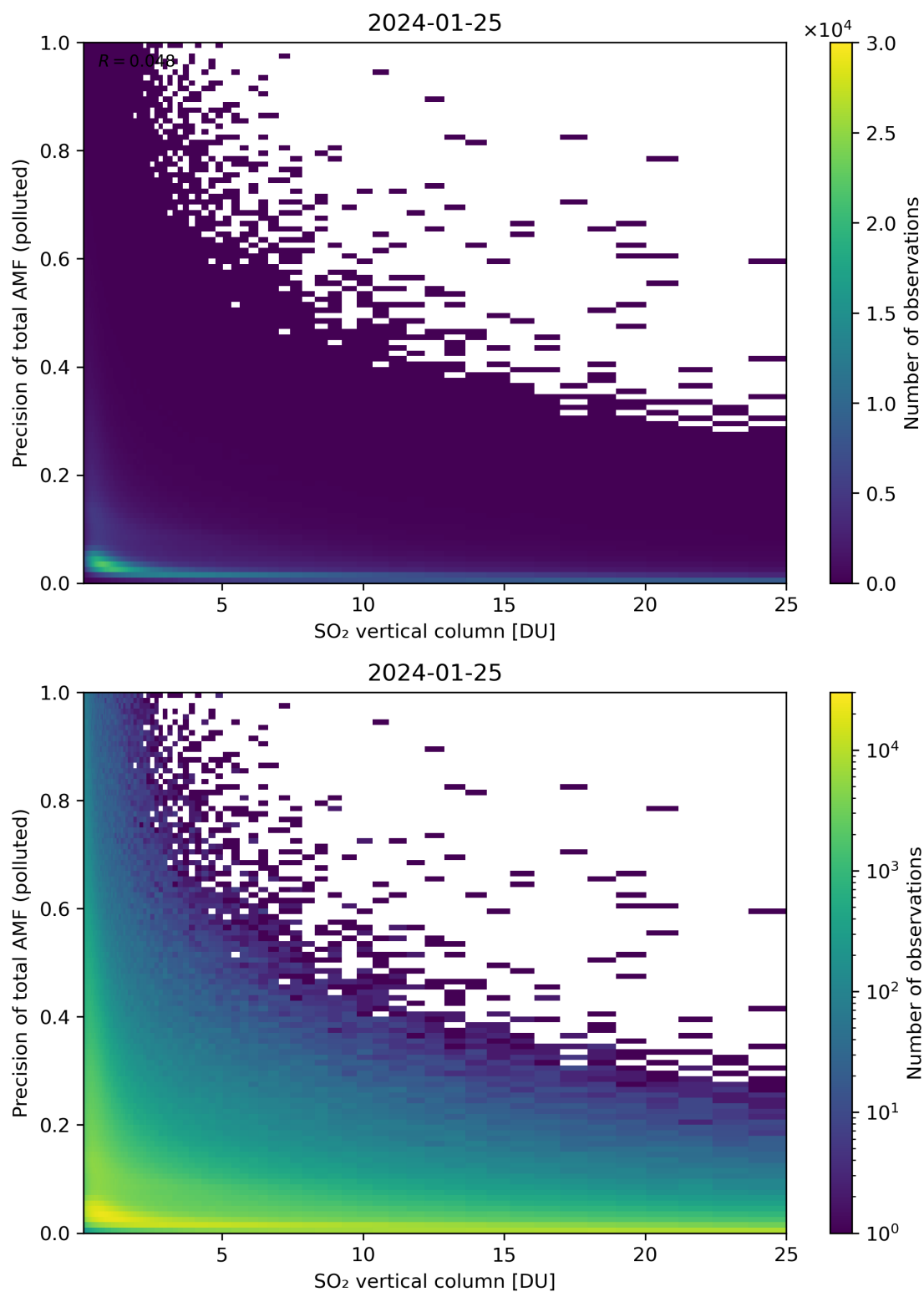
Figure 306: Scatter density plot of “SO 2 vertical column” against “Precision of total AMF (polluted)” for 2024-01-24 to 2024-01-26.
