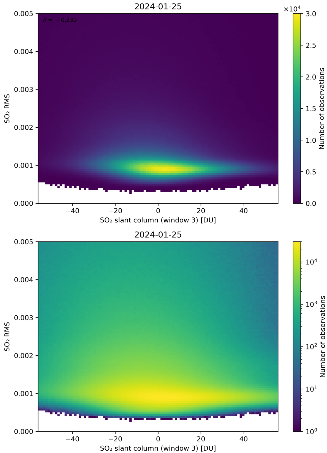
Figure 256: Scatter density plot of “SO 2 slant column (window 3)” against “SO 2 RMS” for 2024-01-24 to 2024-01-26.
