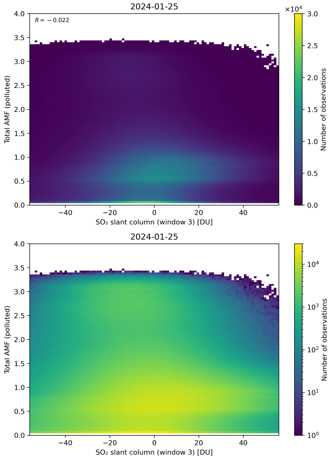
Figure 268: Scatter density plot of “SO 2 slant column (window 3)” against “Total AMF (polluted)” for 2024-01-24 to 2024-01-26.
