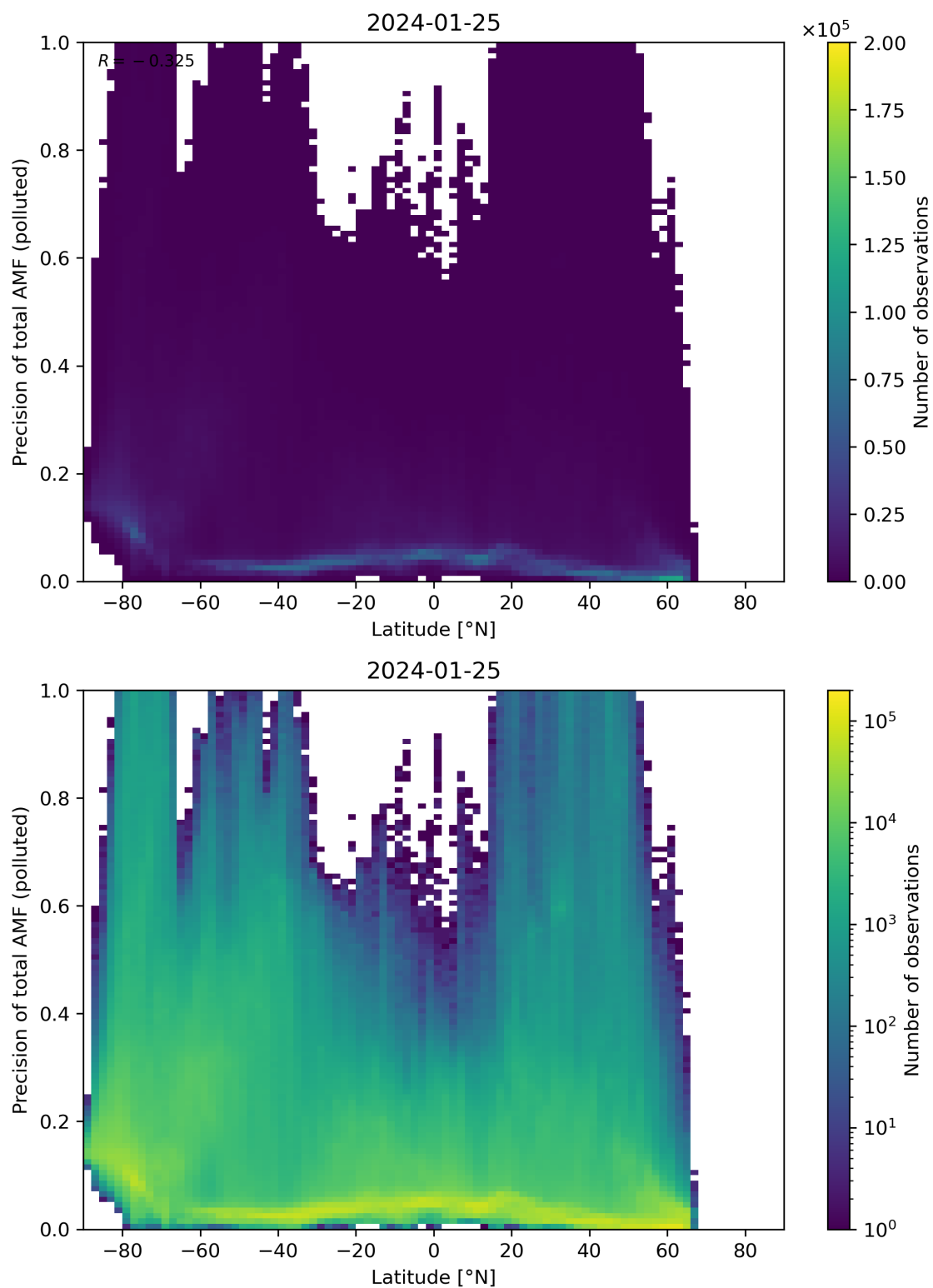
Figure 155: Scatter density plot of “Latitude” against “Precision of total AMF (polluted)” for 2024-01-24 to 2024-01-26.
