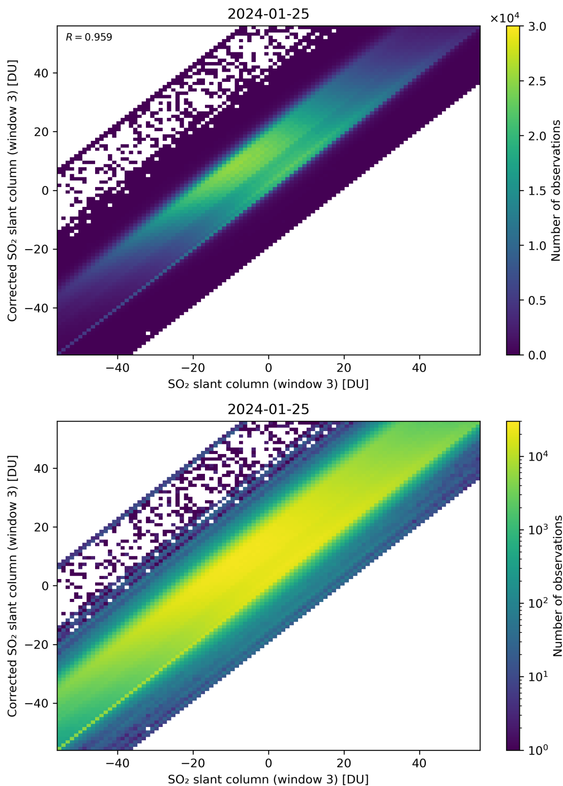
Figure 266: Scatter density plot of “SO 2 slant column (window 3)” against “Corrected SO 2 slant column (window 3)” for 2024-01-24 to 2024-01-26.
