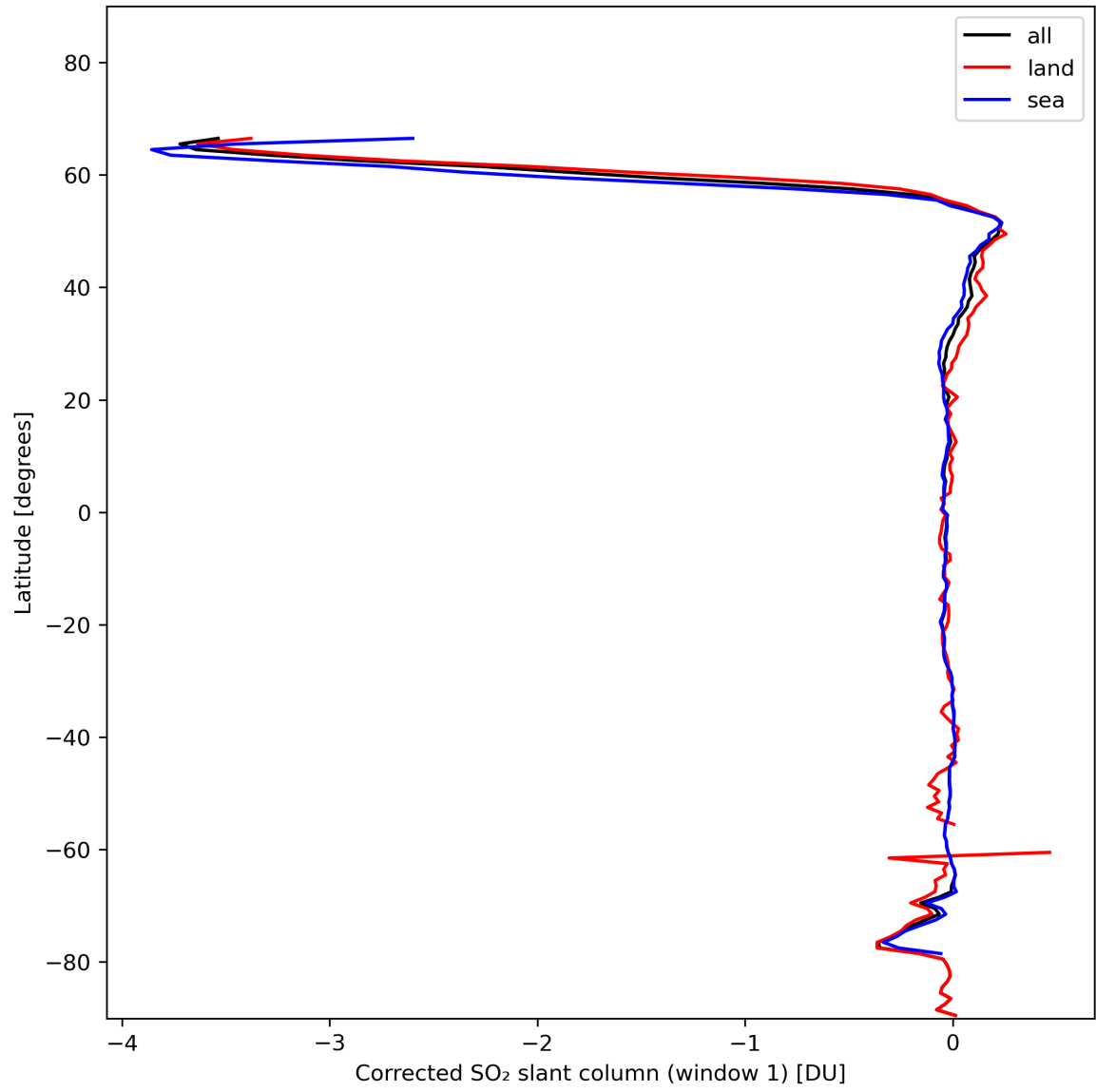
Figure 35: Zonal average of “Corrected SO 2 slant column (window 1)” for 2024-01-24 to 2024-01-26.
