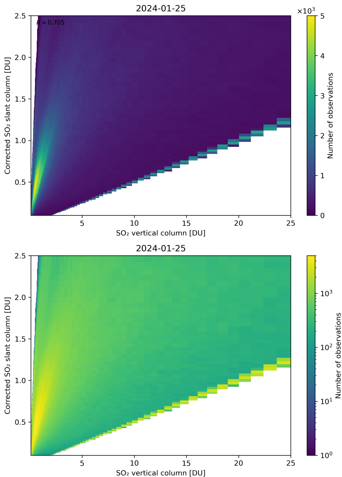
Figure 297: Scatter density plot of “SO 2 vertical column” against “Corrected SO 2 slant column” for 2024-01-24 to 2024-01-26.
