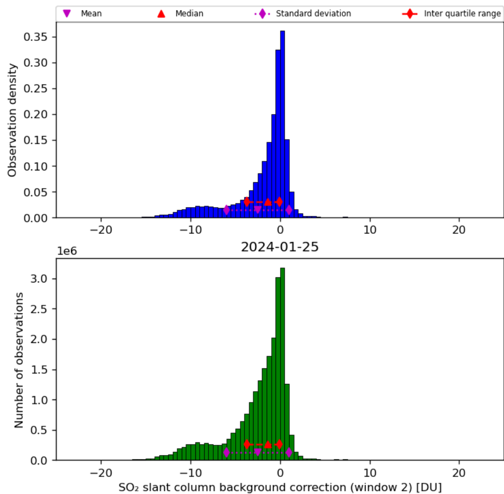
Figure 63: Histogram of “SO 2 slant column background correction (window 2)” for 2024-01-24 to 2024-01-26
