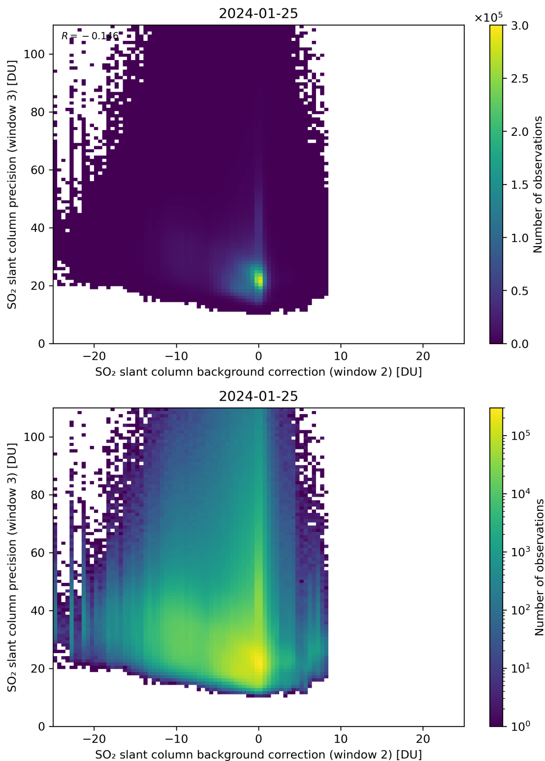
Figure 118: Scatter density plot of “SO 2 slant column background correction (window 2)” against “SO 2 slant column precision (window 3)” for 2024-01-24 to 2024-01-26.
