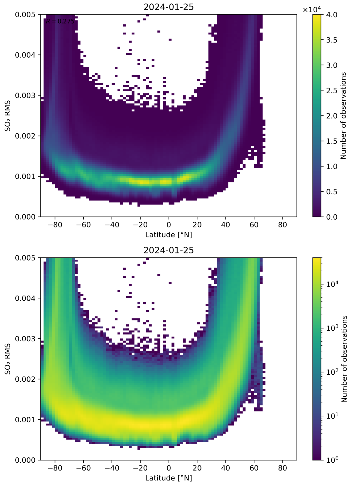
Figure 144: Scatter density plot of “Latitude” against “SO 2 RMS” for 2024-01-24 to 2024-01-26.
