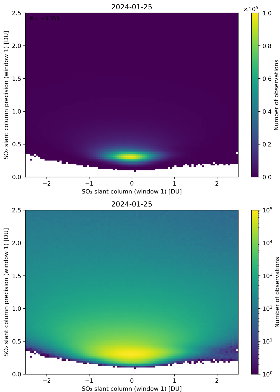
Figure 235: Scatter density plot of “SO 2 slant column (window 1)” against “SO 2 slant column precision (window 1)” for 2024-01-24 to 2024-01-26.
