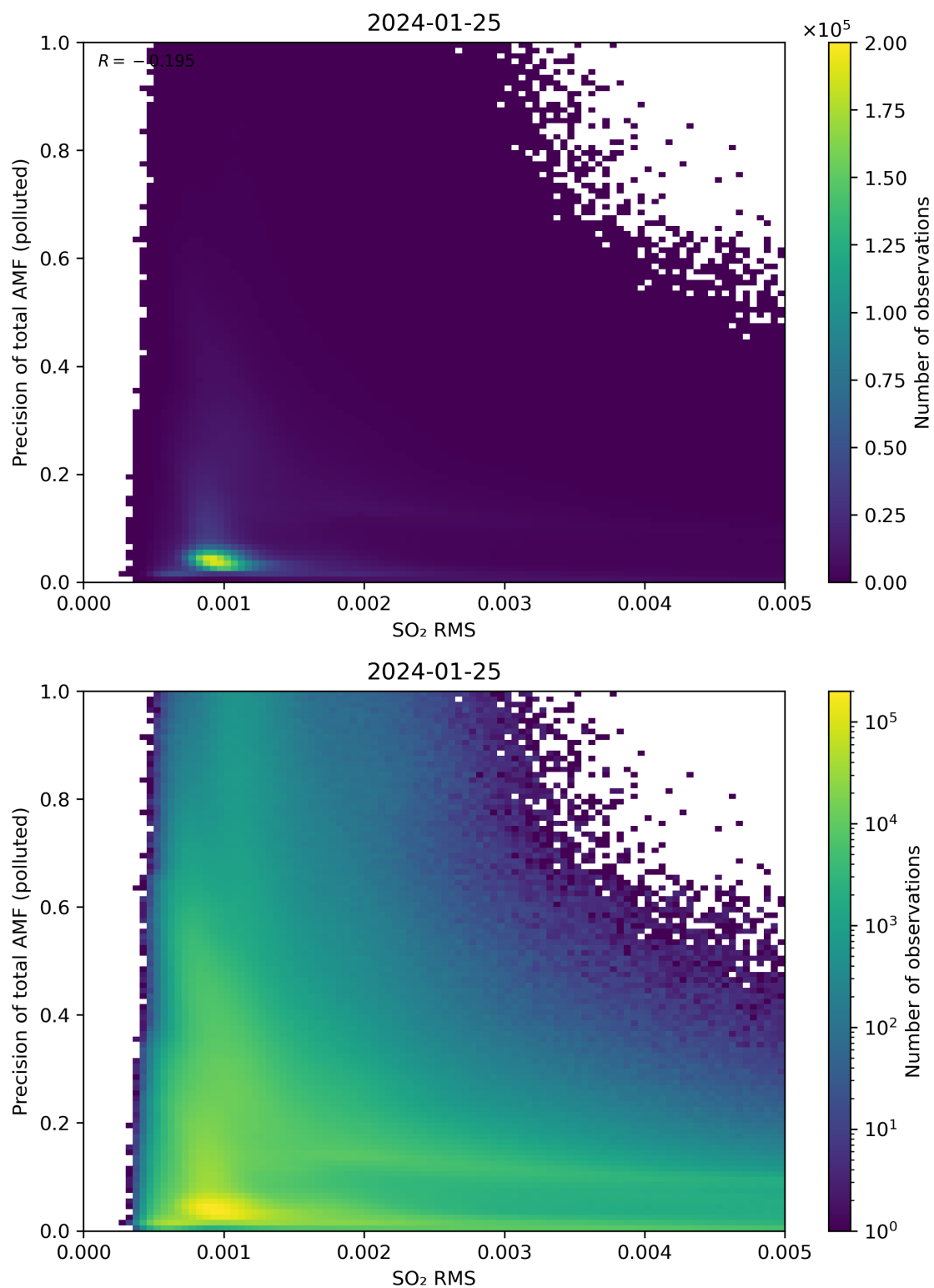
Figure 138: Scatter density plot of “SO 2 RMS” against “Precision of total AMF (polluted)” for 2024-01-24 to 2024-01-26.
