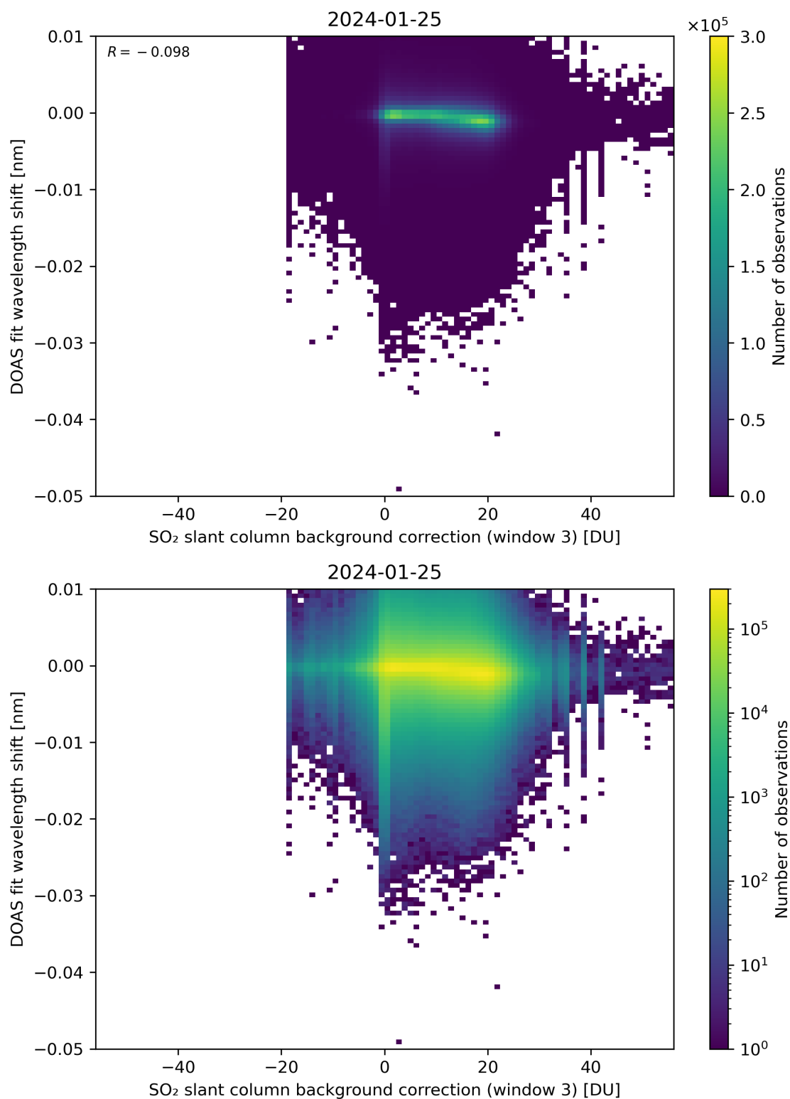
Figure 121: Scatter density plot of “SO 2 slant column background correction (window 3)” against “DOAS fit wavelength shift” for 2024-01-24 to 2024-01-26.
