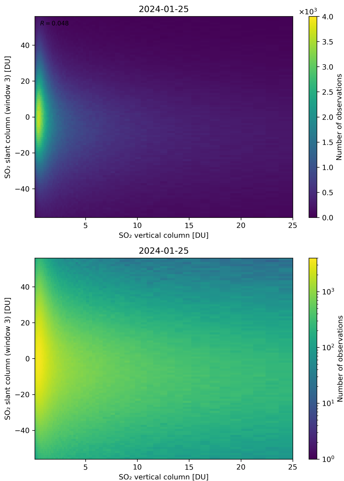
Figure 303: Scatter density plot of “SO 2 vertical column” against “SO 2 slant column (window 3)” for 2024-01-24 to 2024-01-26.
