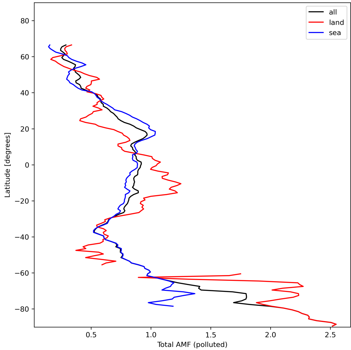
Figure 48: Zonal average of “Total AMF (polluted)” for 2024-01-26 to 2024-01-27.
