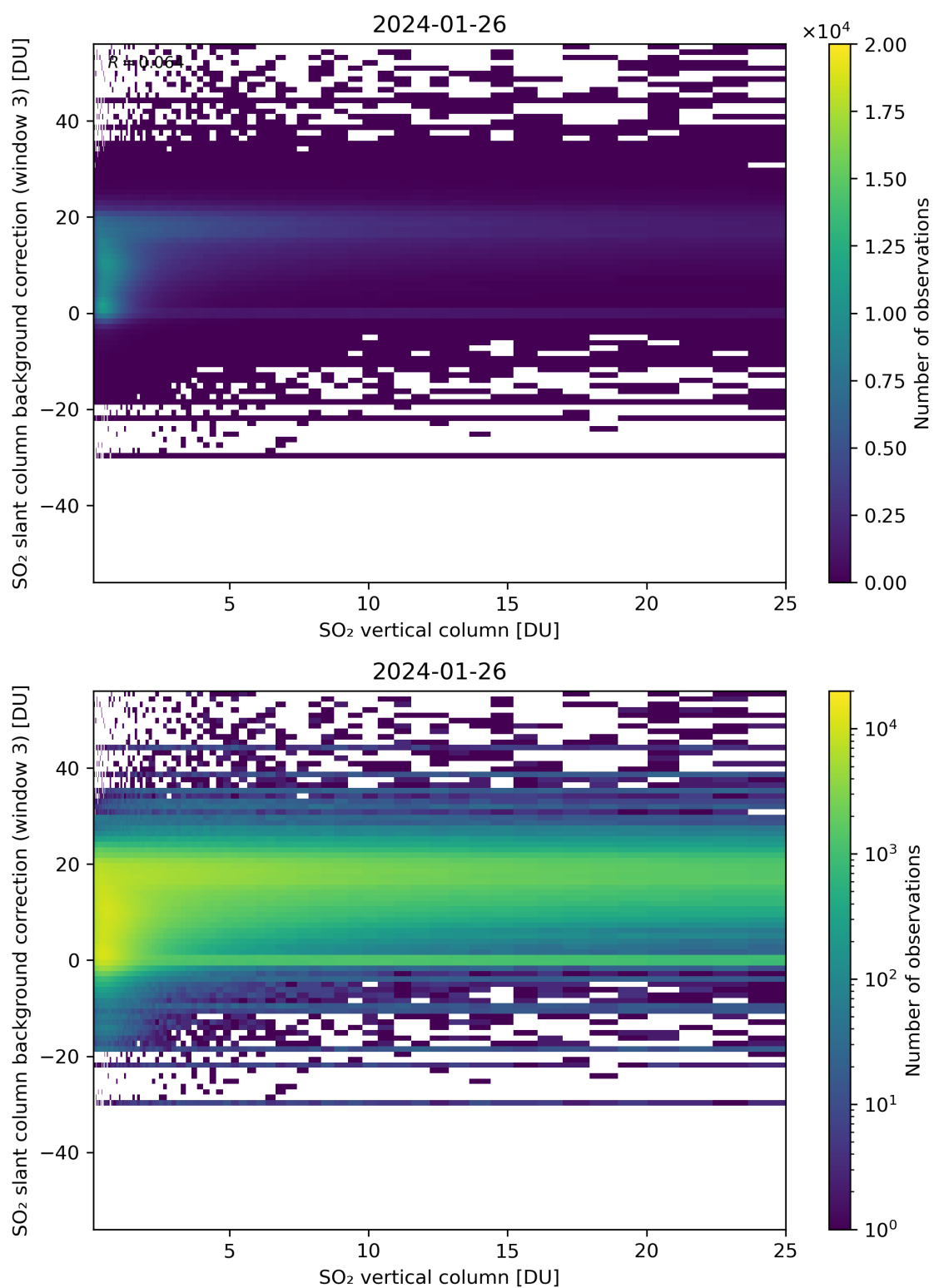
Figure 275: Scatter density plot of “SO 2 vertical column” against “SO 2 slant column background correction (window 3)” for 2024-01-26 to 2024-01-27.
