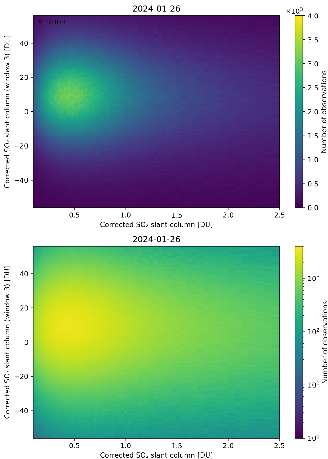
Figure 186: Scatter density plot of “Corrected SO 2 slant column” against “Corrected SO 2 slant column (window 3)” for 2024-01-26 to 2024-01-27.
