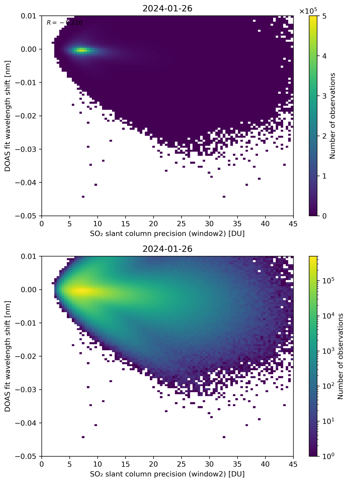
Figure 243: Scatter density plot of “SO 2 slant column precision (window2)” against “DOAS fit wavelength shift” for 2024-01-26 to 2024-01-27.
