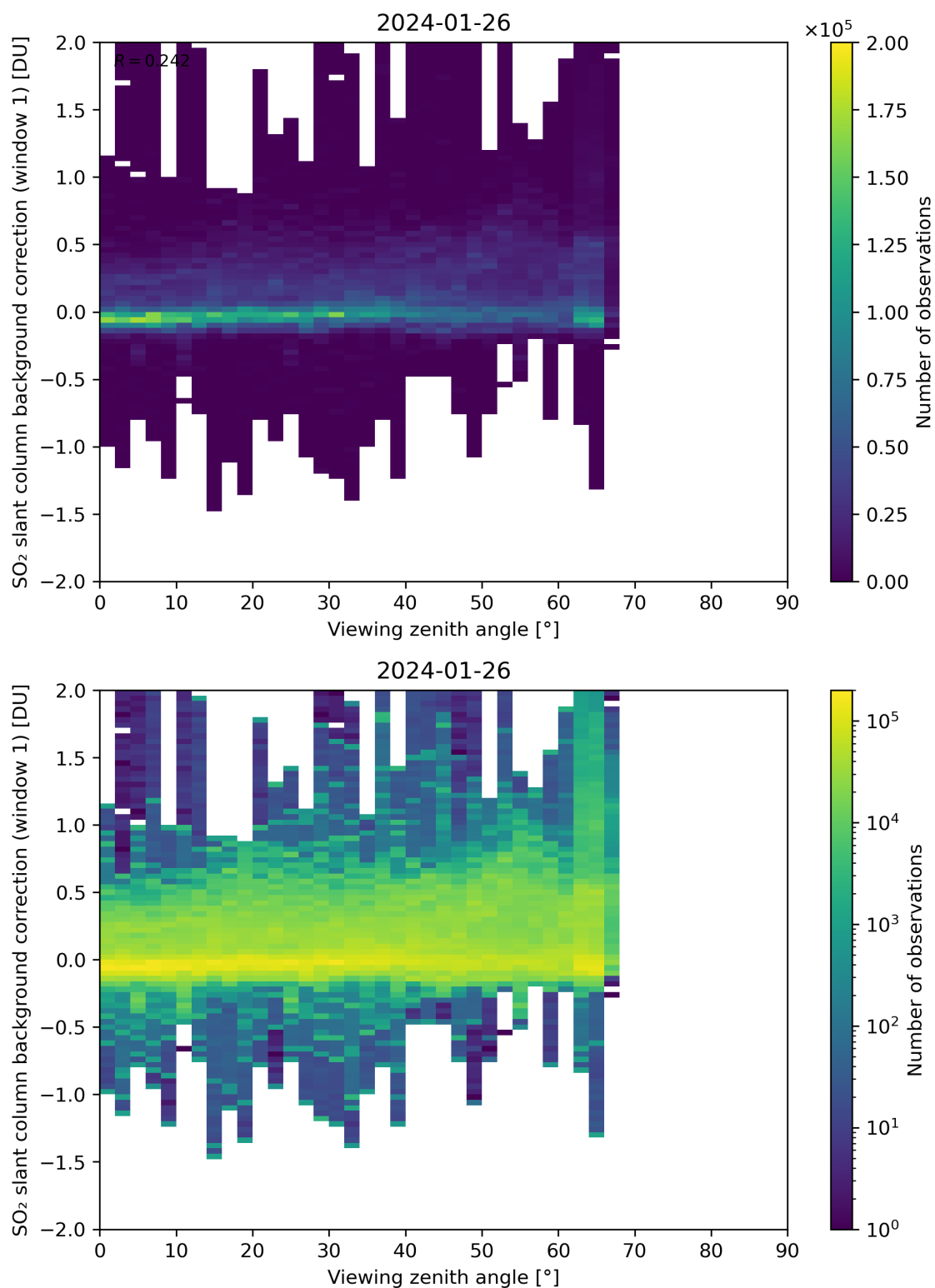
Figure 308: Scatter density plot of “Viewing zenith angle” against “SO 2 slant column background correction (window 1)” for 2024-01-26 to 2024-01-27.
