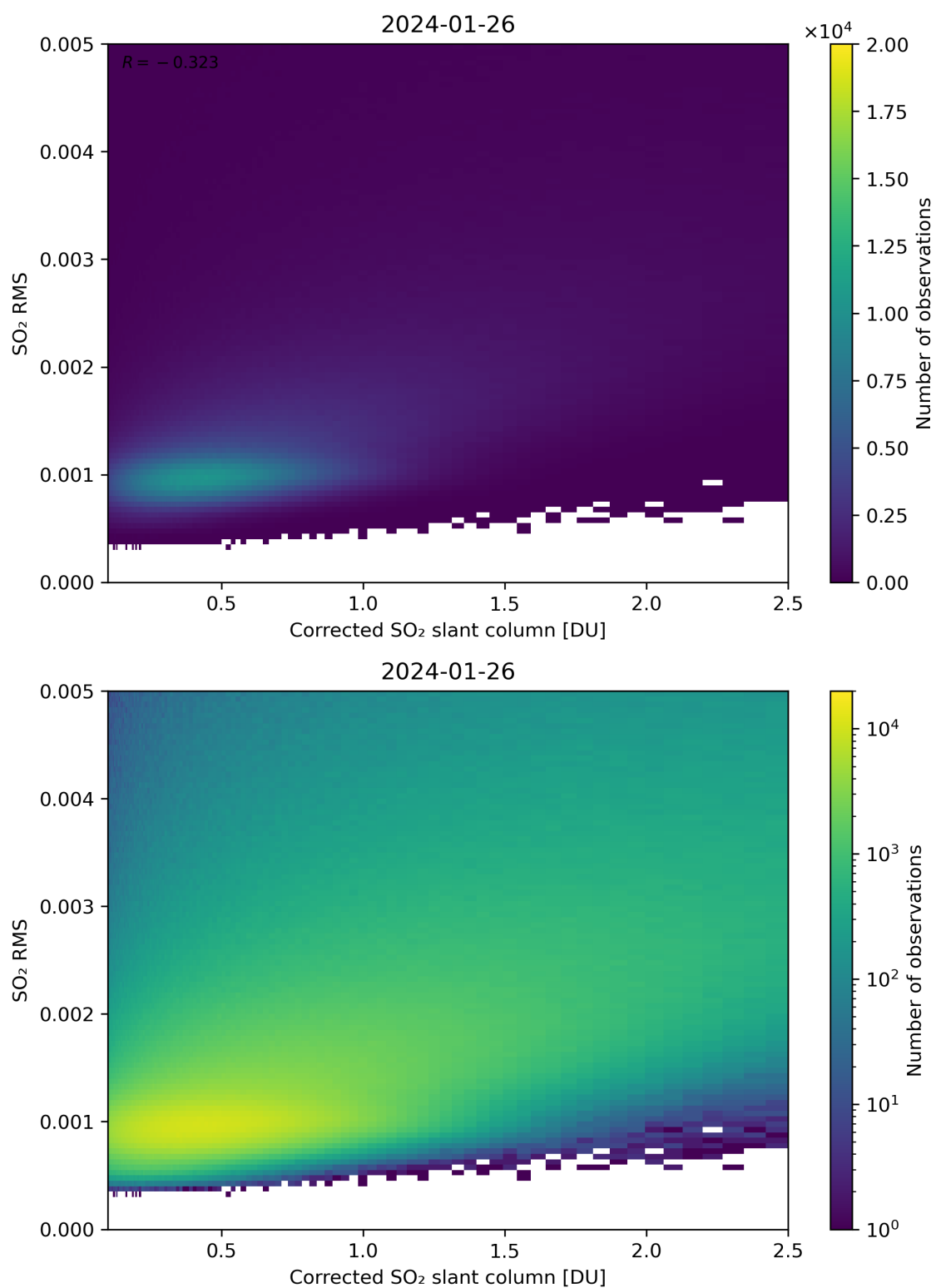
Figure 183: Scatter density plot of “Corrected SO 2 slant column” against “SO 2 RMS” for 2024-01-26 to 2024-01-27.
