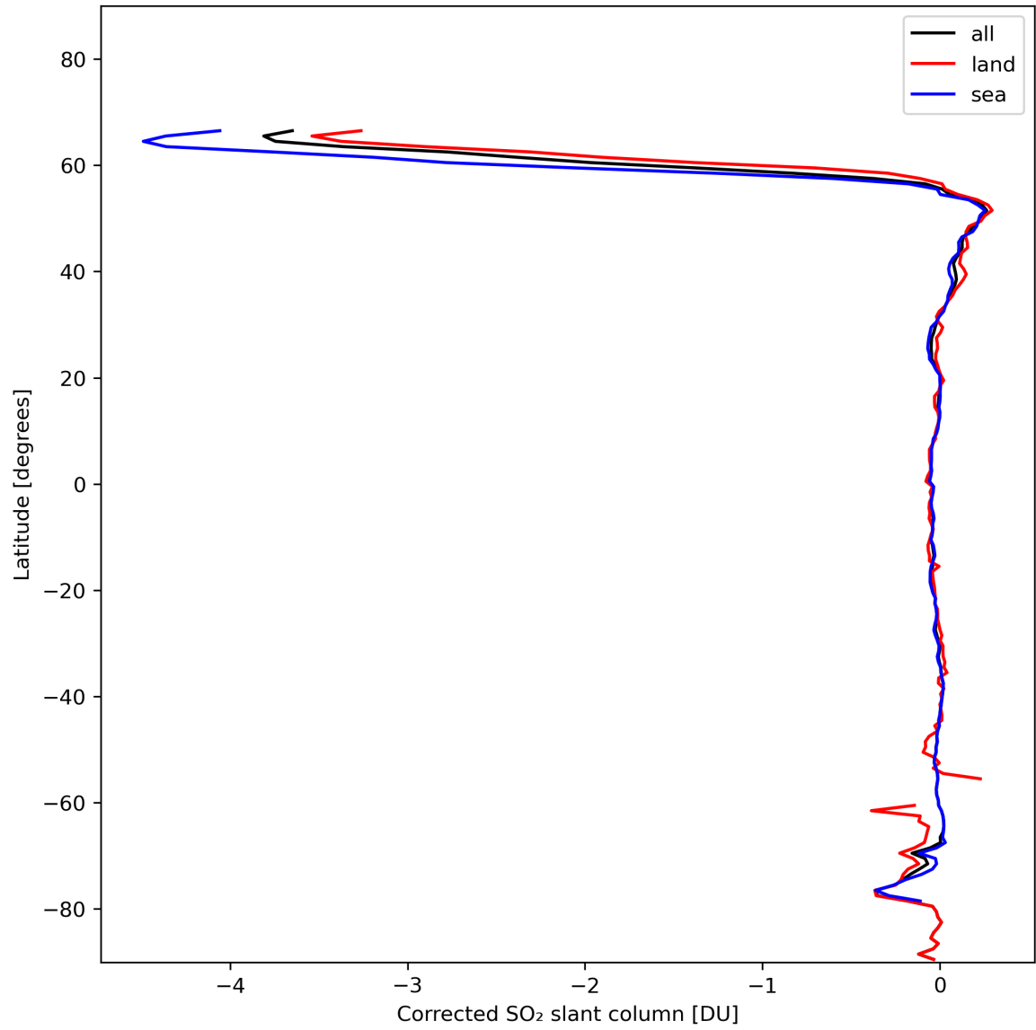
Figure 32: Zonal average of "Corrected SO 2 slant column" for 2024-01-26 to 2024-01-27.
