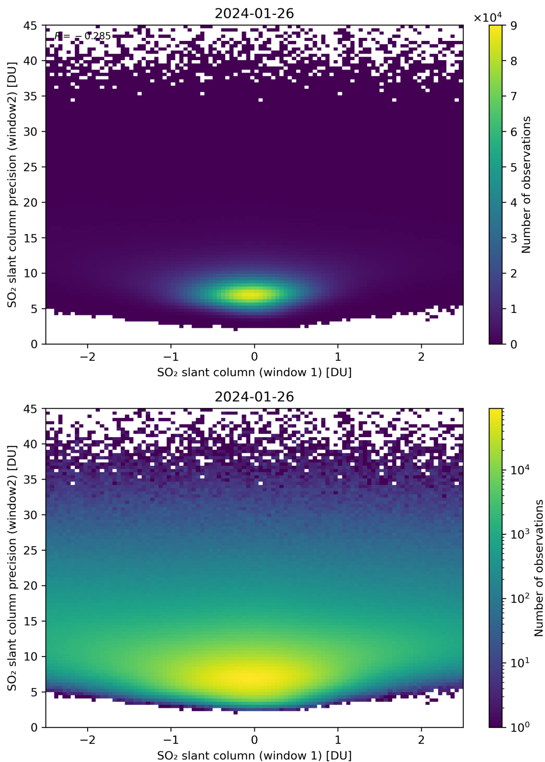
Figure 236: Scatter density plot of “SO 2 slant column (window 1)” against “SO 2 slant column precision (window2)” for 2024-01-26 to 2024-01-27.
