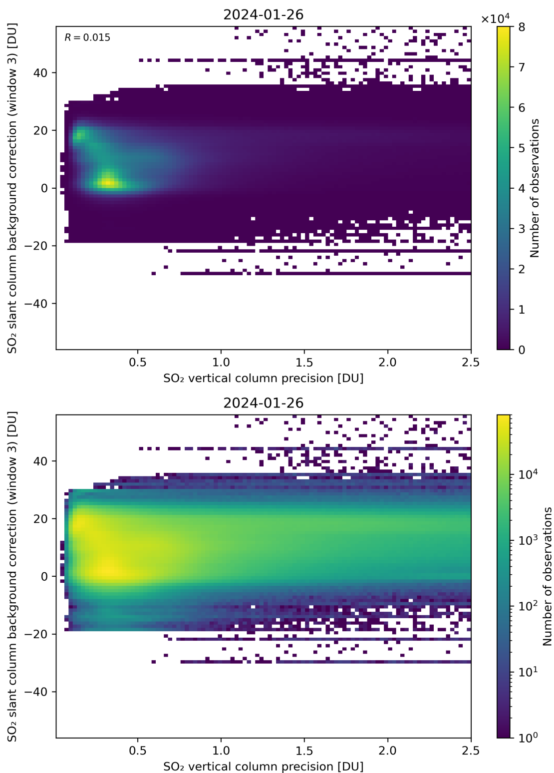
Figure 281: Scatter density plot of “SO 2 vertical column precision” against “SO 2 slant column background correction (window 3)” for 2024-01-26 to 2024-01-27.
