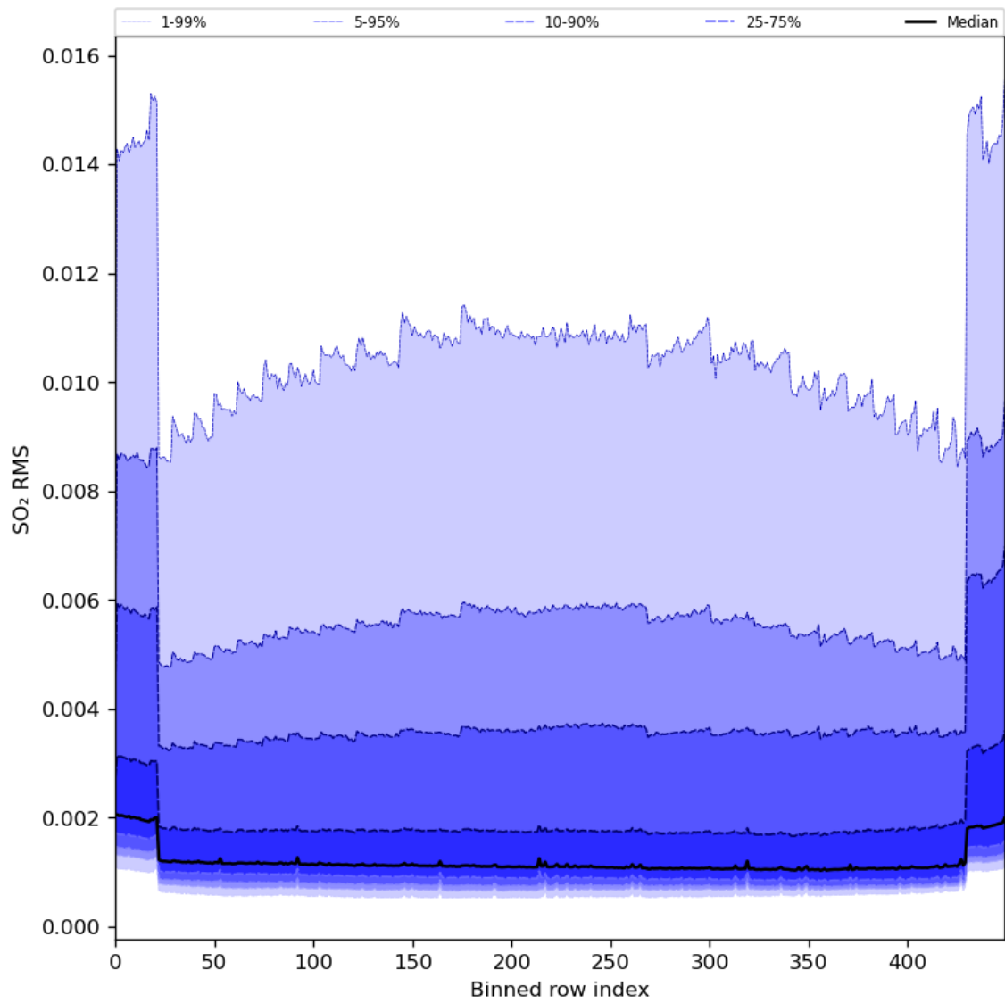
Figure 93: Along track statistics of “SO 2 RMS” for 2024-01-26 to 2024-01-27
