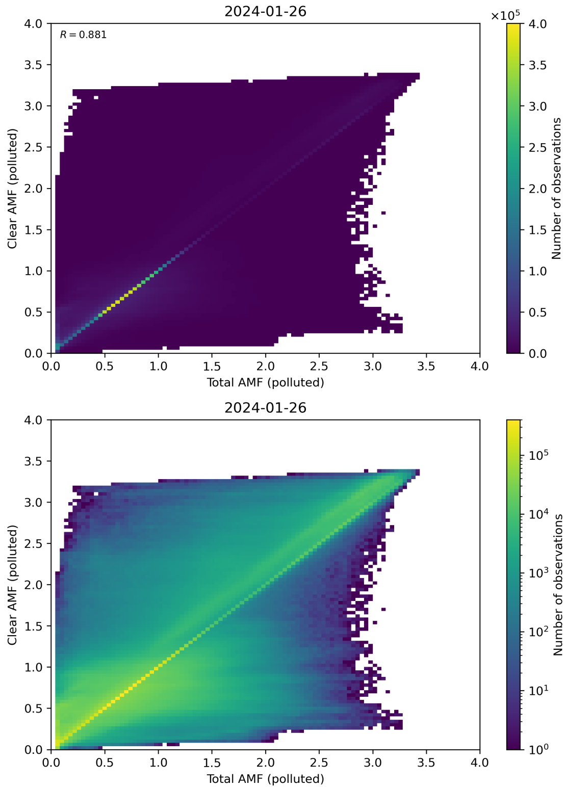
Figure 271: Scatter density plot of “Total AMF (polluted)” against “Clear AMF (polluted)” for 2024-01-26 to 2024-01-27.
