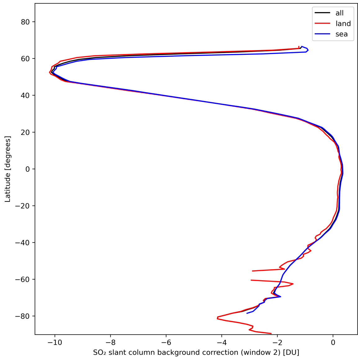
Figure 40: Zonal average of “SO 2 slant column background correction (window 2)” for 2024-01-26 to 2024-01-27.
