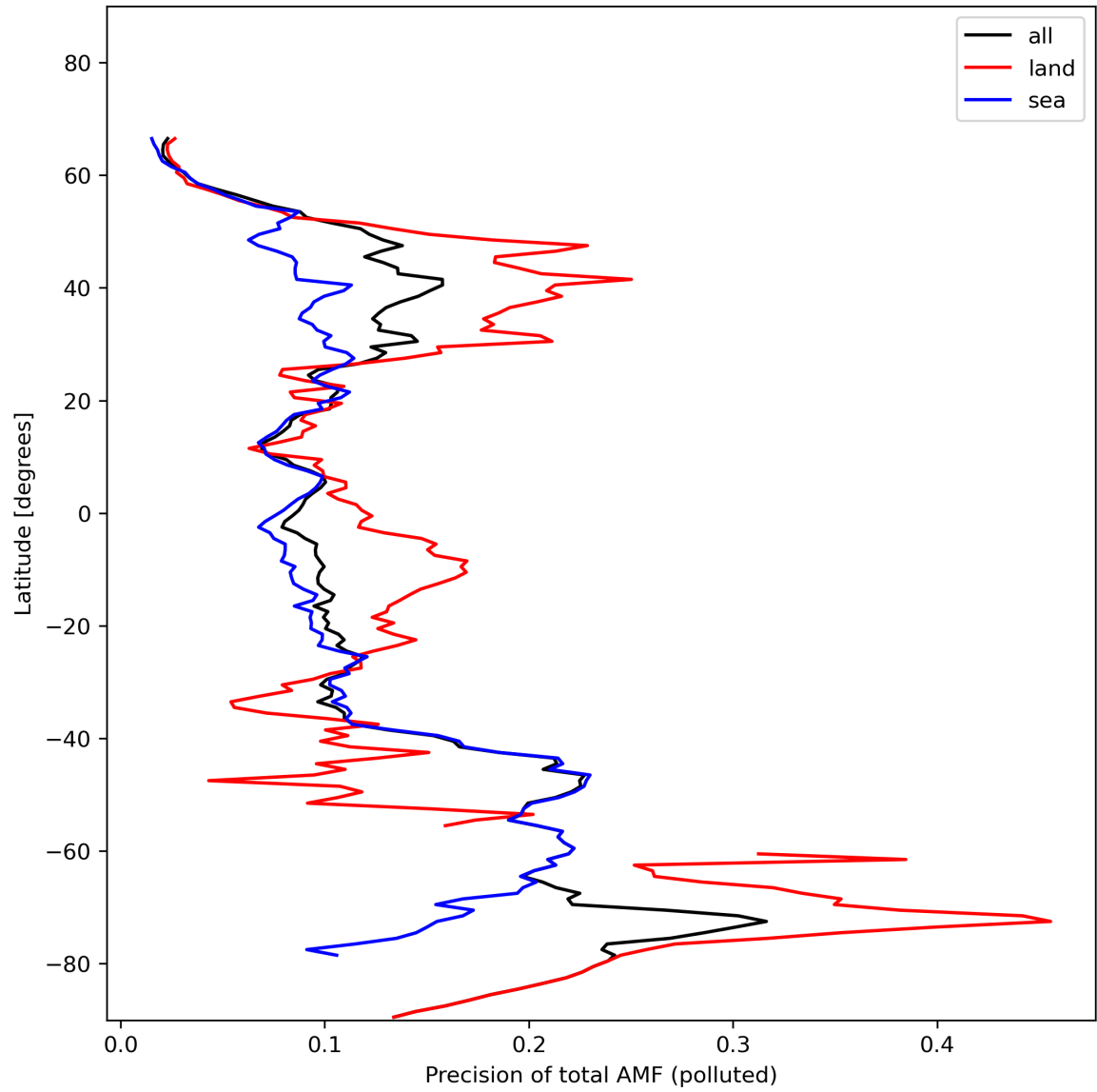
Figure 49: Zonal average of “Precision of total AMF (polluted)” for 2024-01-26 to 2024-01-27.
