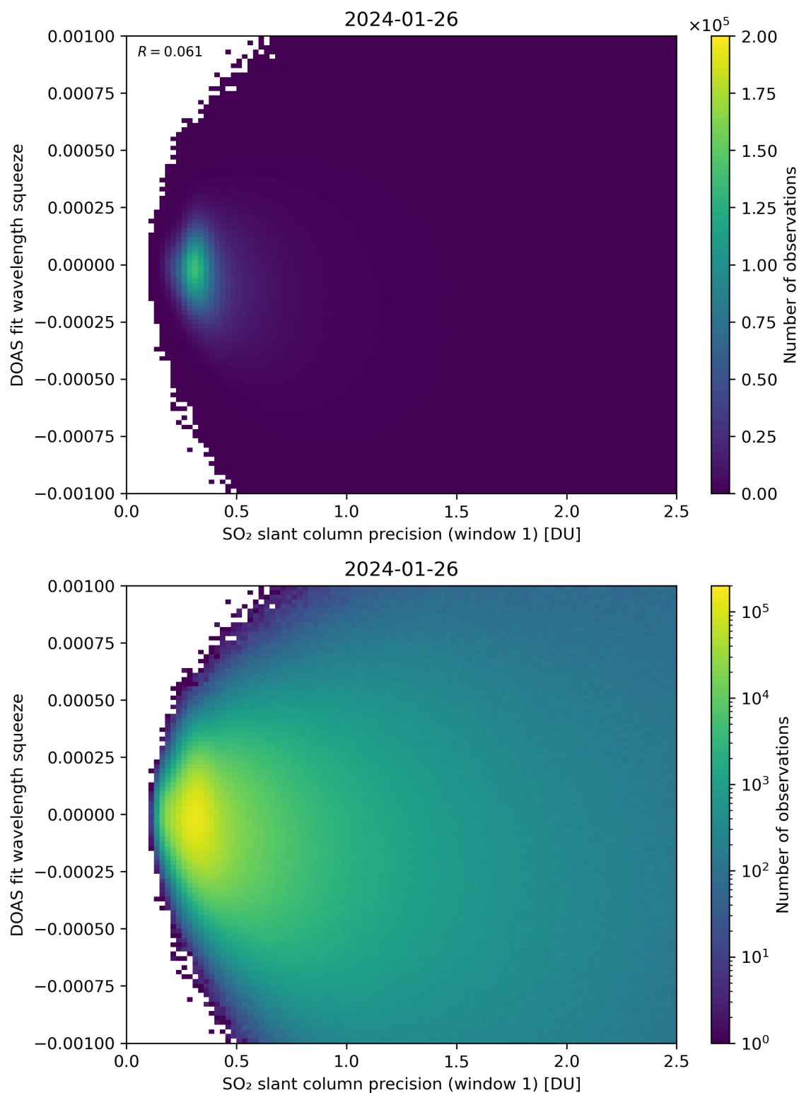
Figure 222: Scatter density plot of “SO 2 slant column precision (window 1)” against “DOAS fit wavelength squeeze” for 2024-01-26 to 2024-01-27.
