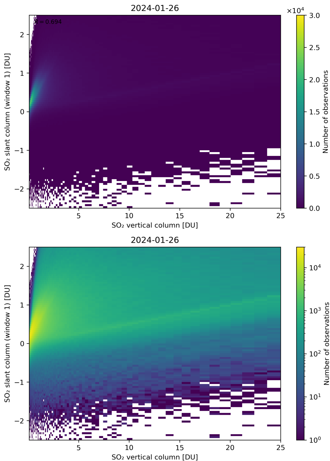
Figure 300: Scatter density plot of “SO 2 vertical column” against “SO 2 slant column (window 1)” for 2024-01-26 to 2024-01-27.
