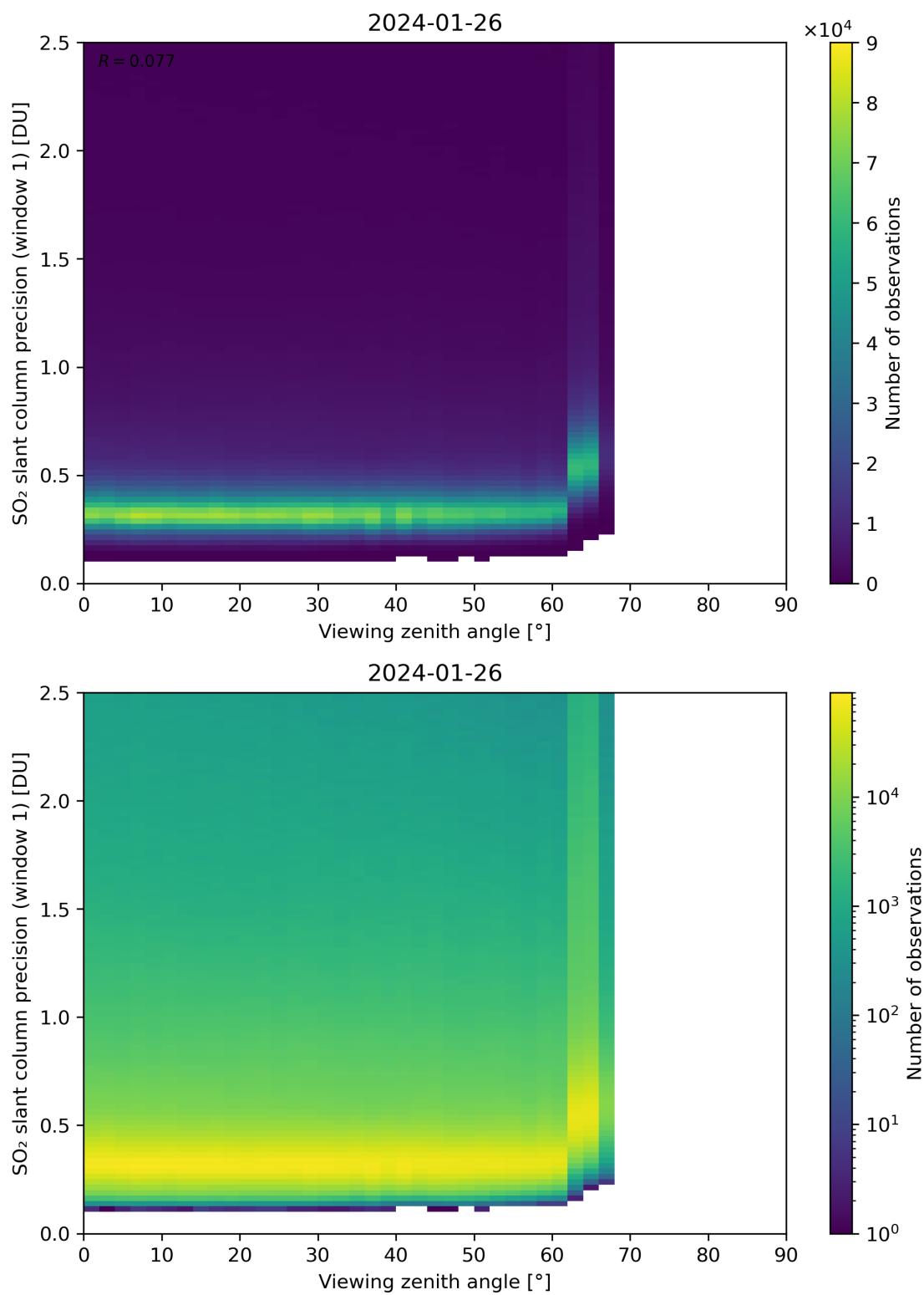
Figure 321: Scatter density plot of “Viewing zenith angle” against “SO 2 slant column precision (window 1)” for 2024-01-26 to 2024-01-27.
