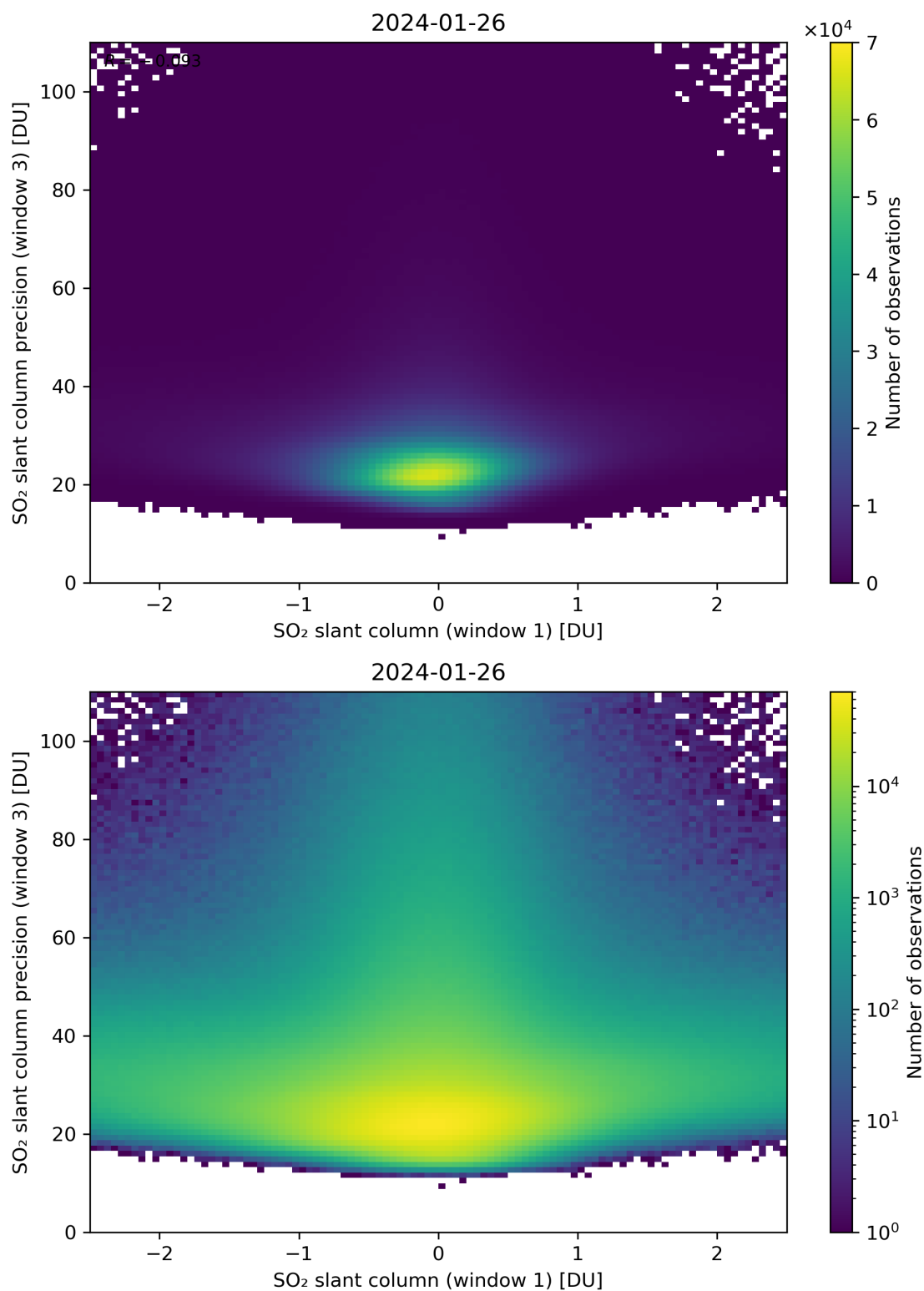
Figure 238: Scatter density plot of “SO 2 slant column (window 1)” against “SO 2 slant column precision (window 3)” for 2024-01-26 to 2024-01-27.
