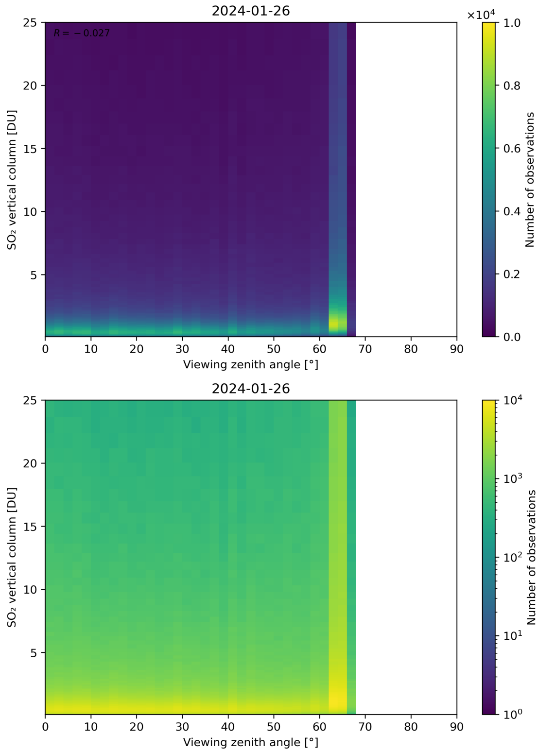
Figure 327: Scatter density plot of “Viewing zenith angle” against “SO 2 vertical column” for 2024-01-26 to 2024-01-27.
