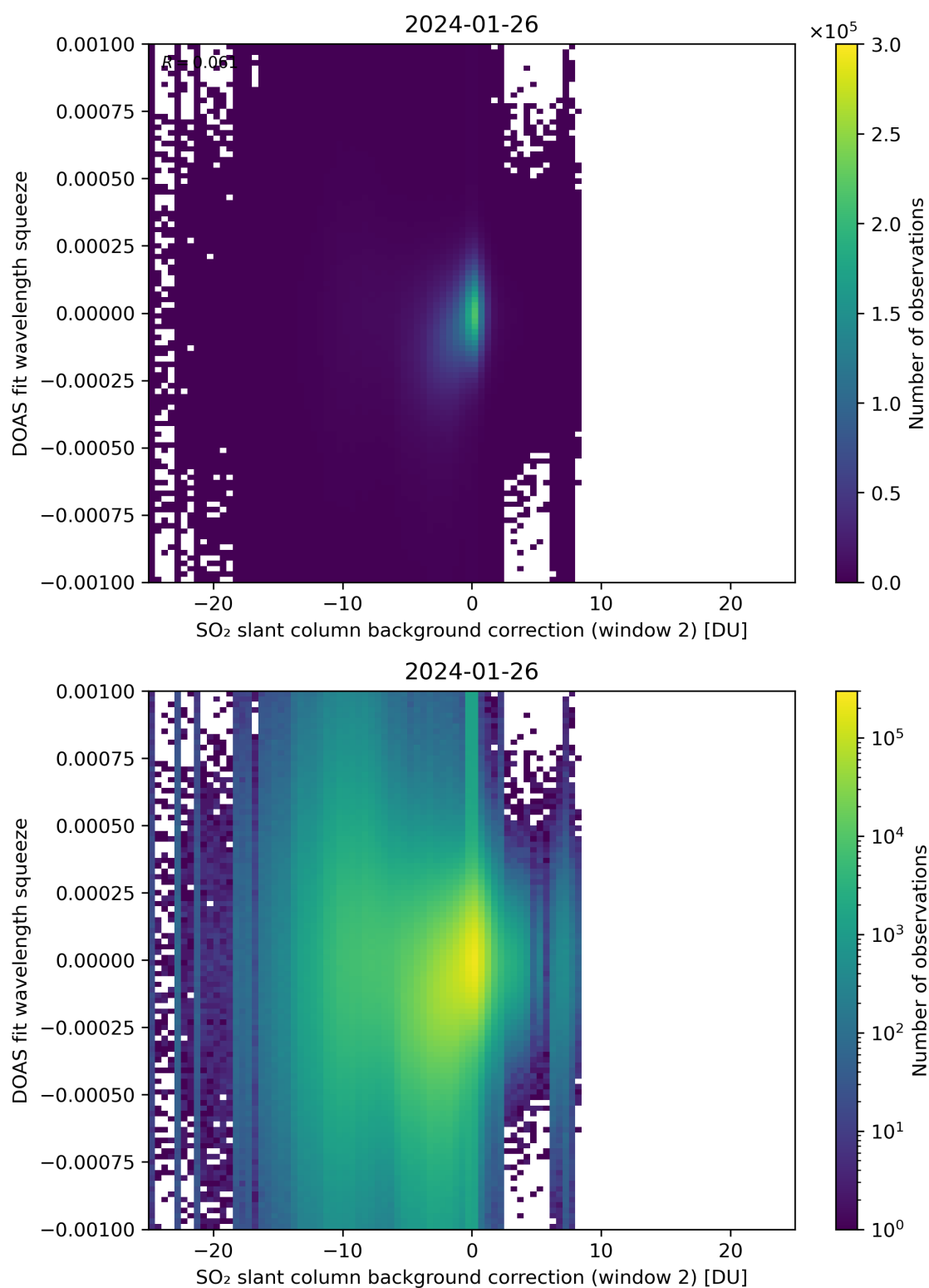
Figure 113: Scatter density plot of “SO 2 slant column background correction (window 2)” against “DOAS fit wavelength squeeze” for 2024-01-26 to 2024-01-27.
