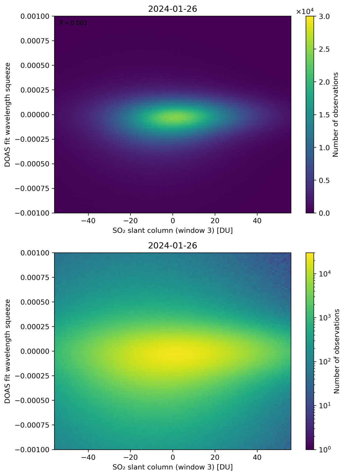
Figure 255: Scatter density plot of “SO 2 slant column (window 3)” against “DOAS fit wavelength squeeze” for 2024-01-26 to 2024-01-27.
