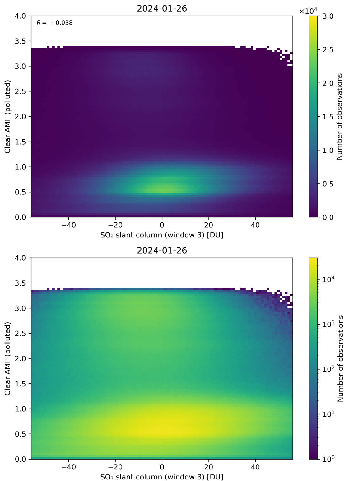
Figure 265: Scatter density plot of “SO 2 slant column (window 3)” against “Clear AMF (polluted)” for 2024-01-26 to 2024-01-27.
