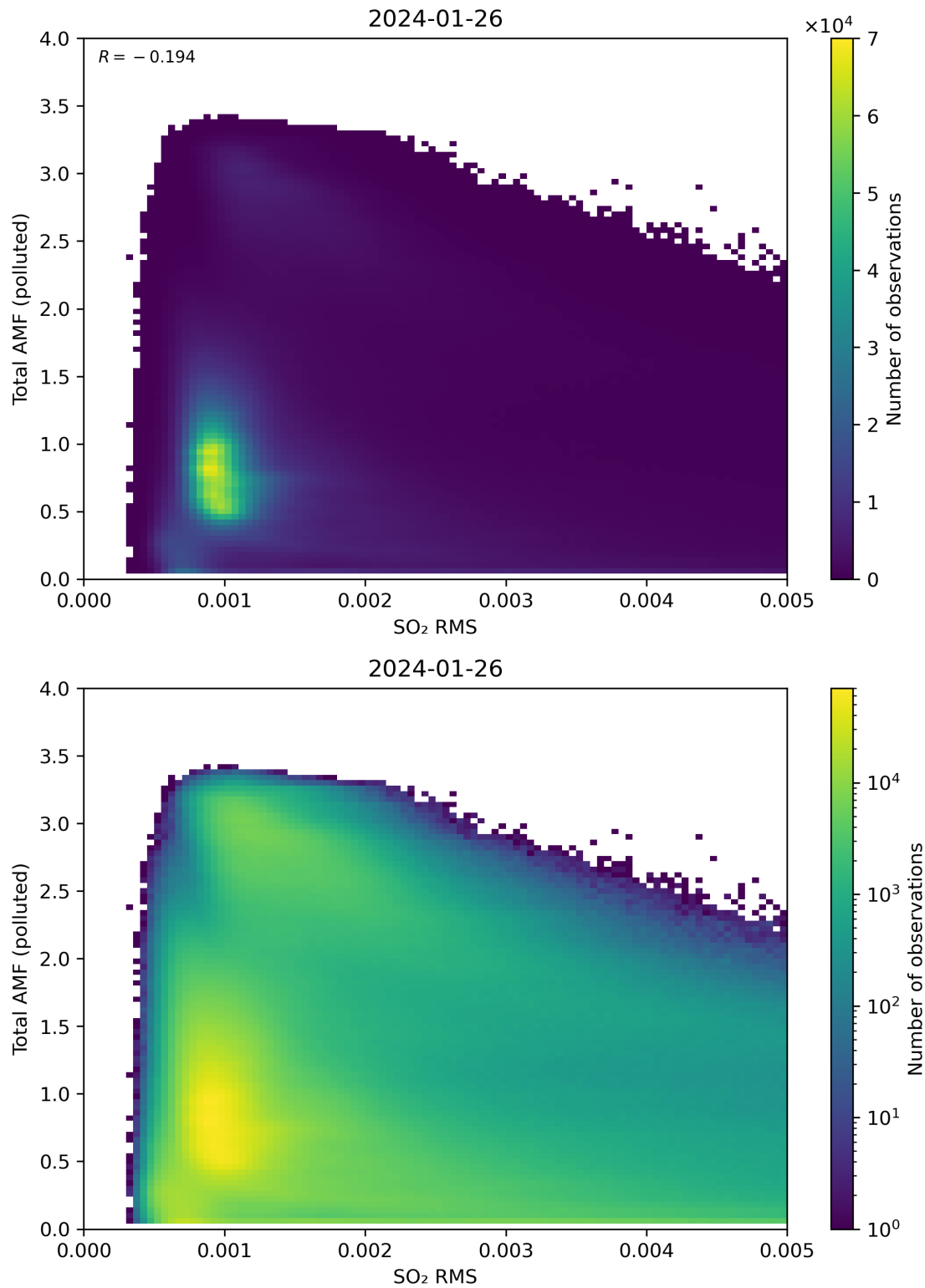
Figure 137: Scatter density plot of “SO 2 RMS” against “Total AMF (polluted)” for 2024-01-26 to 2024-01-27.
