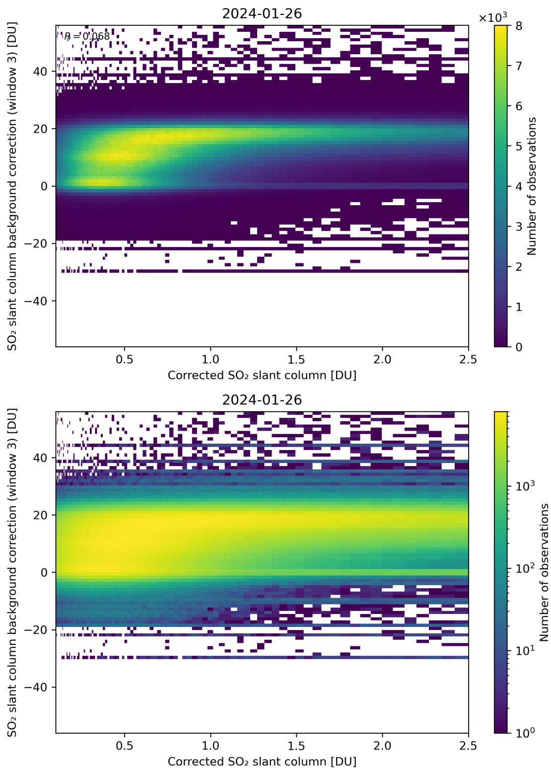
Figure 180: Scatter density plot of “Corrected SO 2 slant column” against “SO 2 slant column background correction (window 3)” for 2024-01-26 to 2024-01-27.
