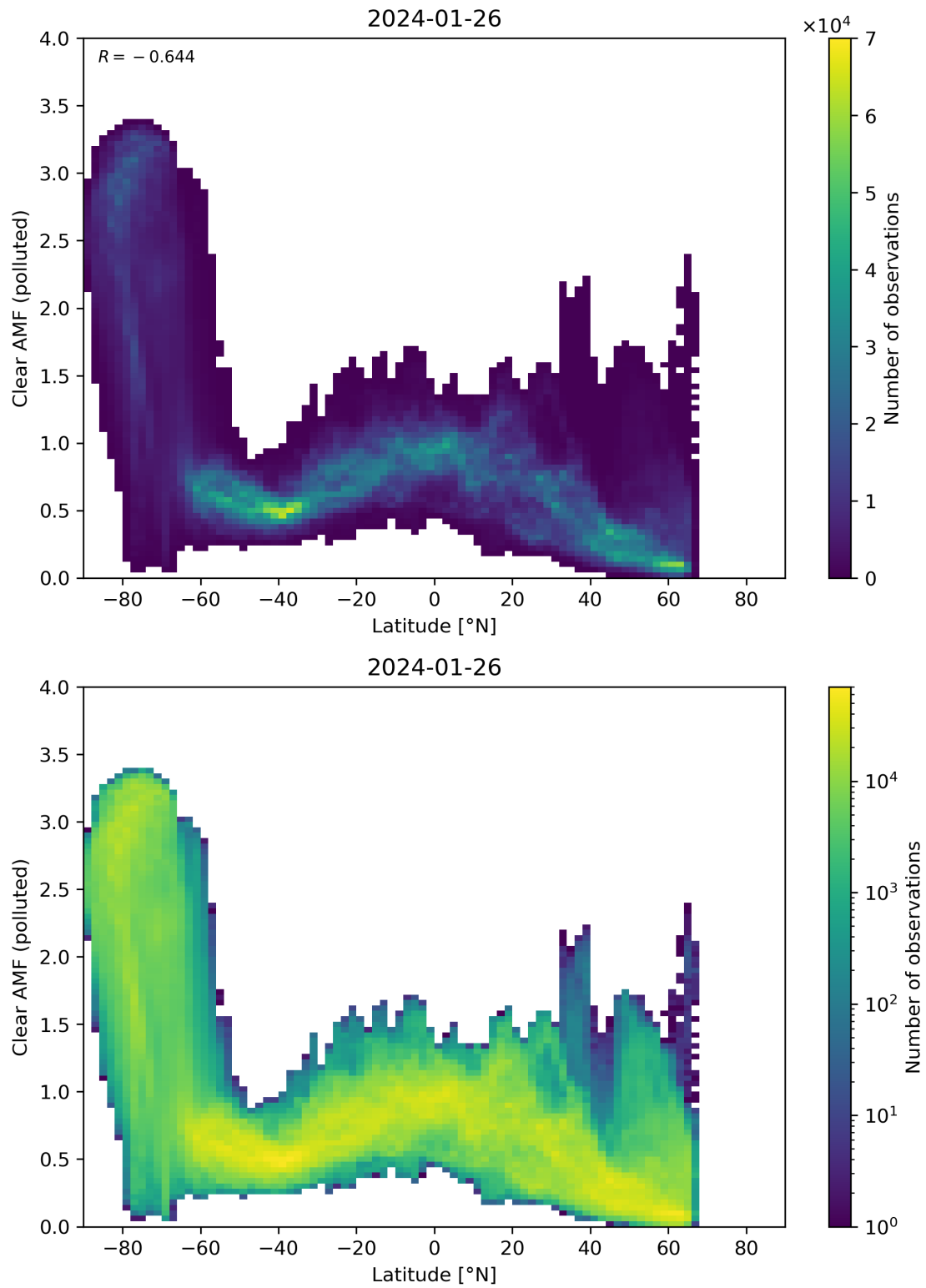
Figure 145: Scatter density plot of “Latitude” against “Clear AMF (polluted)” for 2024-01-26 to 2024-01-27.
