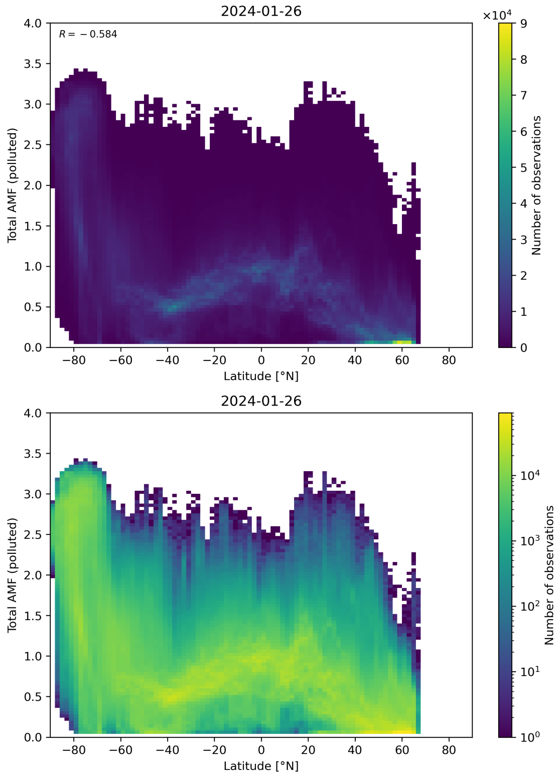
Figure 154: Scatter density plot of “Latitude” against “Total AMF (polluted)” for 2024-01-26 to 2024-01-27.
