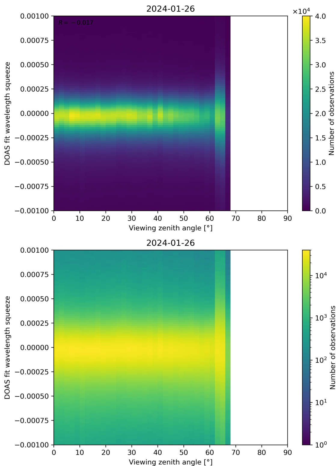
Figure 312: Scatter density plot of “Viewing zenith angle” against “DOAS fit wavelength squeeze” for 2024-01-26 to 2024-01-27.
