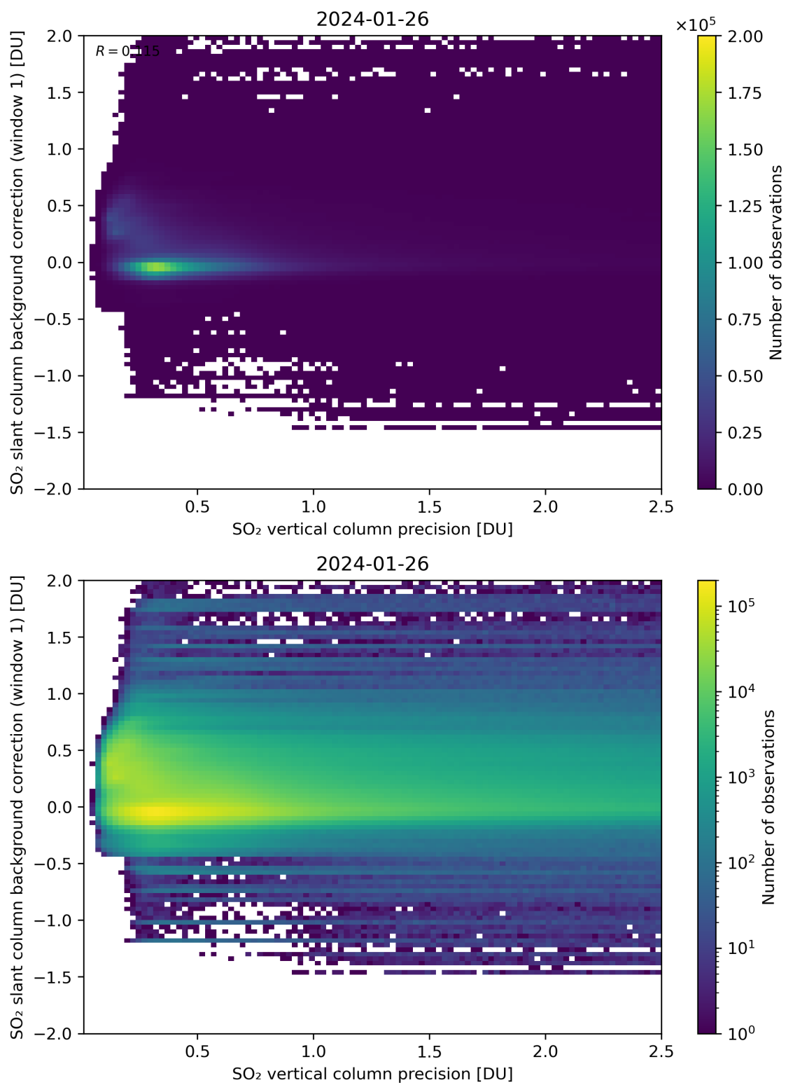
Figure 279: Scatter density plot of “SO 2 vertical column precision” against “SO 2 slant column background correction (window 1)” for 2024-01-26 to 2024-01-27.
