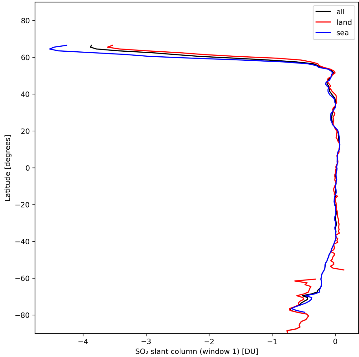
Figure 33: Zonal average of “SO 2 slant column (window 1)” for 2024-01-26 to 2024-01-27.
