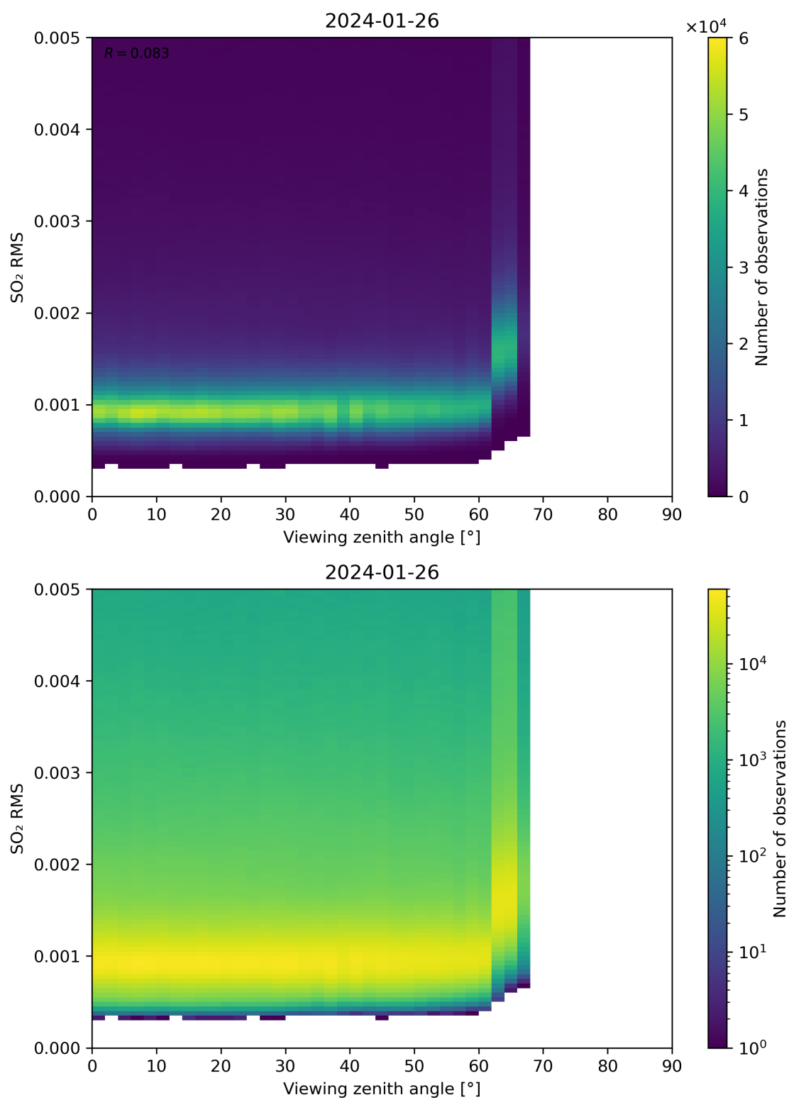
Figure 313: Scatter density plot of “Viewing zenith angle” against “SO 2 RMS” for 2024-01-26 to 2024-01-27.
