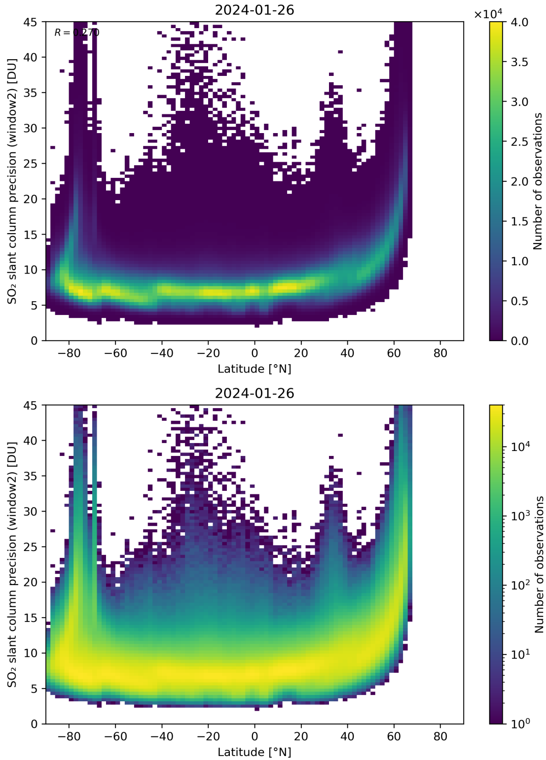
Figure 151: Scatter density plot of “Latitude” against “SO 2 slant column precision (window2)” for 2024-01-26 to 2024-01-27.
