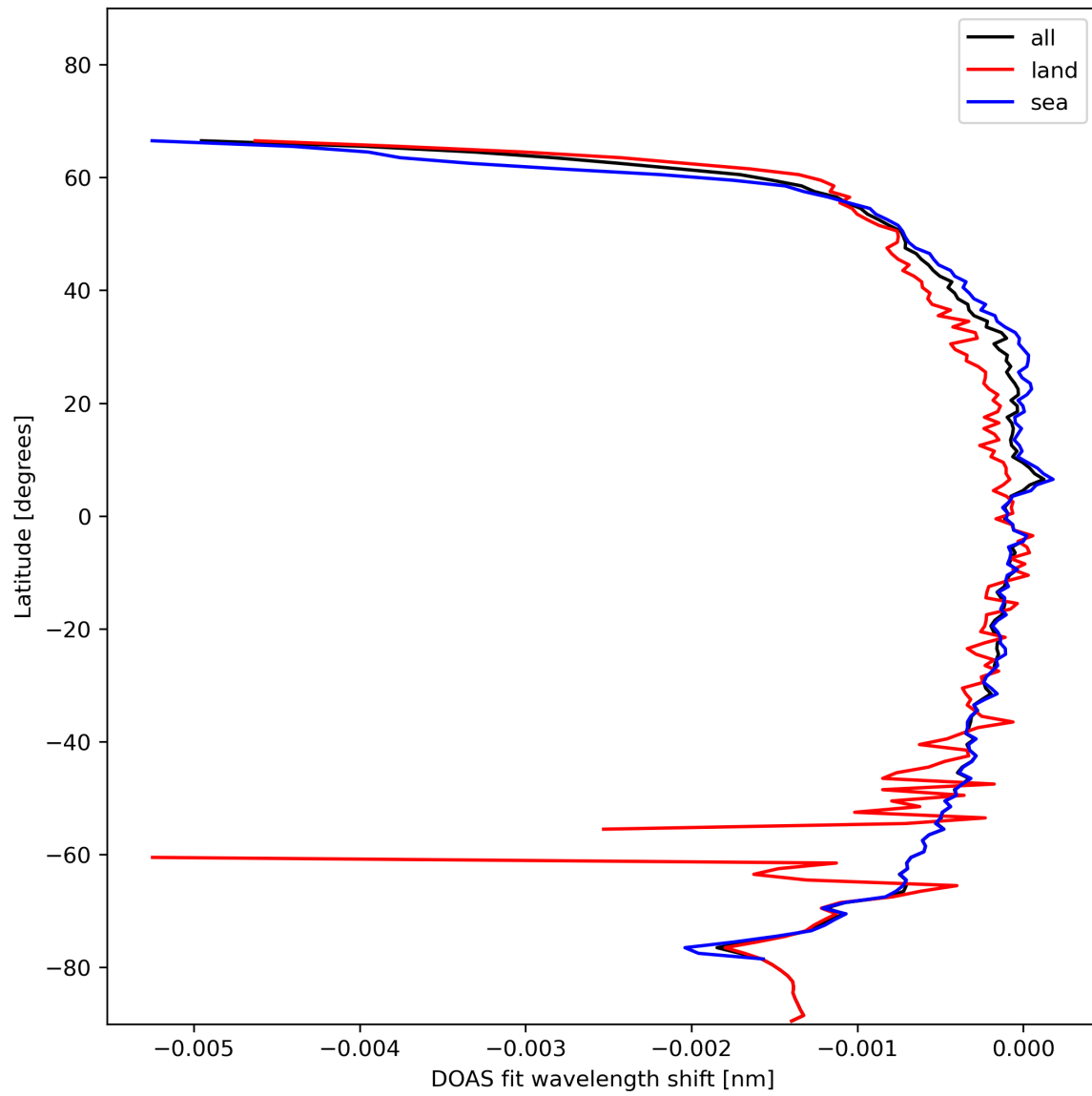
Figure 45: Zonal average of “DOAS fit wavelength shift” for 2024-01-26 to 2024-01-27.
