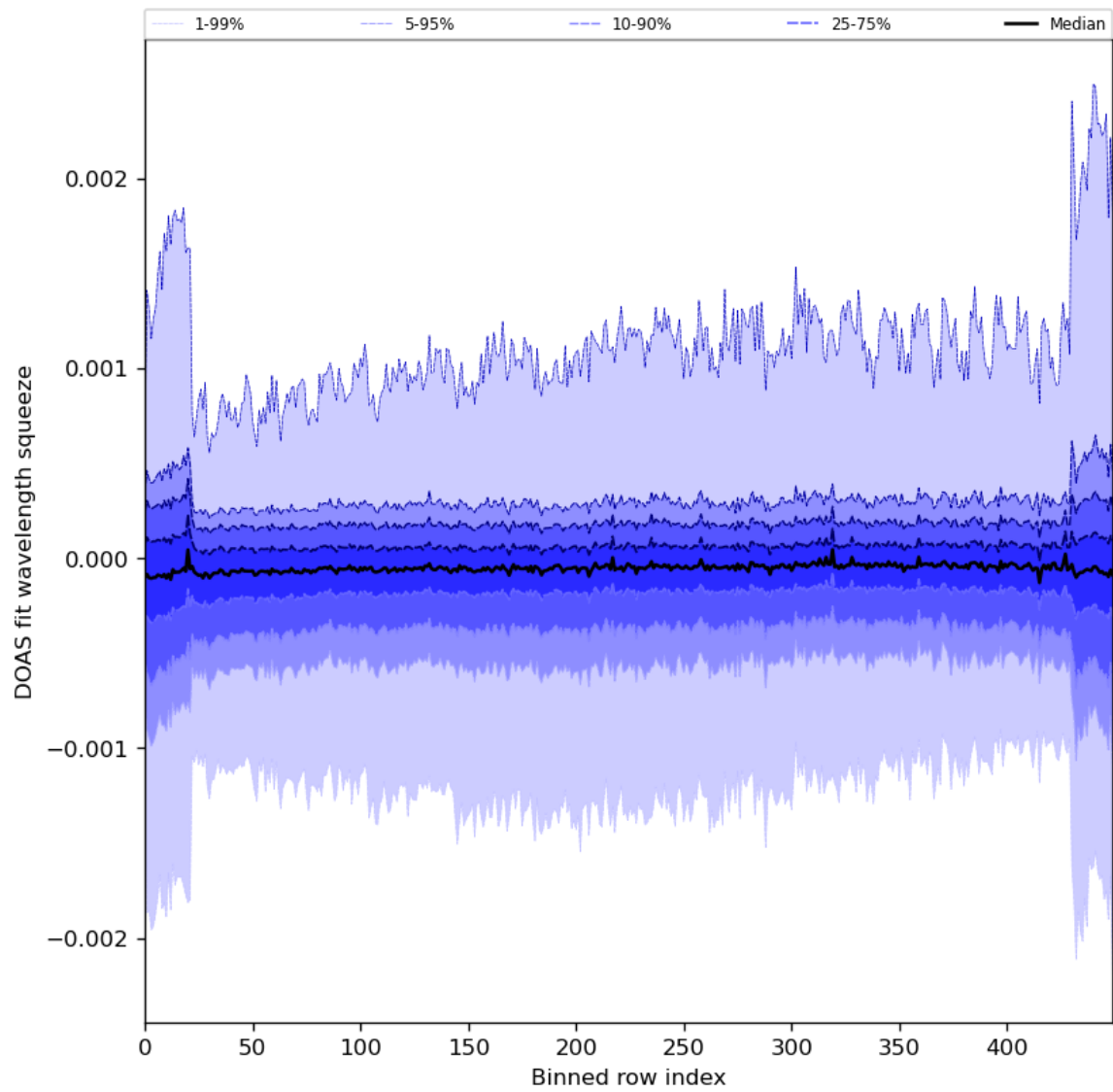
Figure 92: Along track statistics of “DOAS fit wavelength squeeze” for 2024-01-26 to 2024-01-27
