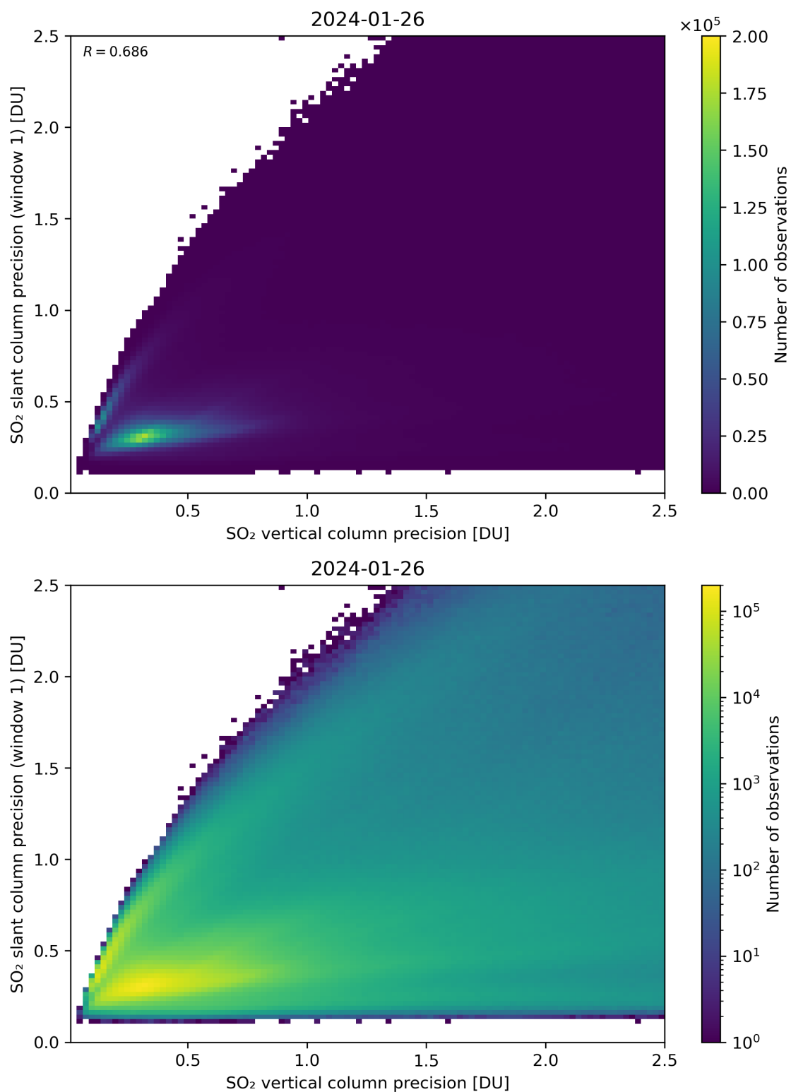
Figure 290: Scatter density plot of “SO 2 vertical column precision” against “SO 2 slant column precision (window 1)” for 2024-01-26 to 2024-01-27.
