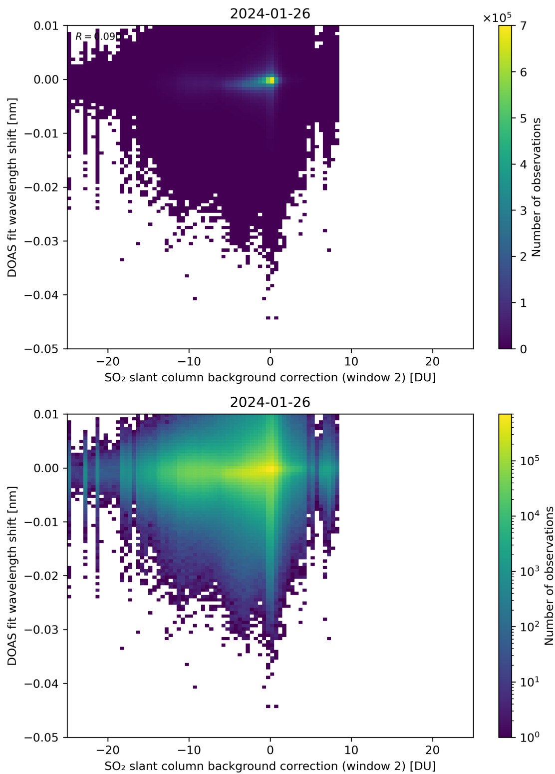
Figure 112: Scatter density plot of “SO 2 slant column background correction (window 2)” against “DOAS fit wavelength shift” for 2024-01-26 to 2024-01-27.
