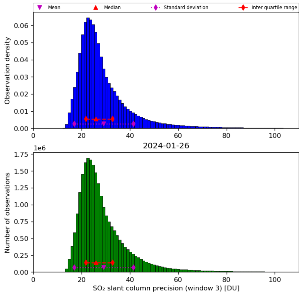
Figure 65: Histogram of “SO 2 slant column precision (window 3)” for 2024-01-26 to 2024-01-27
