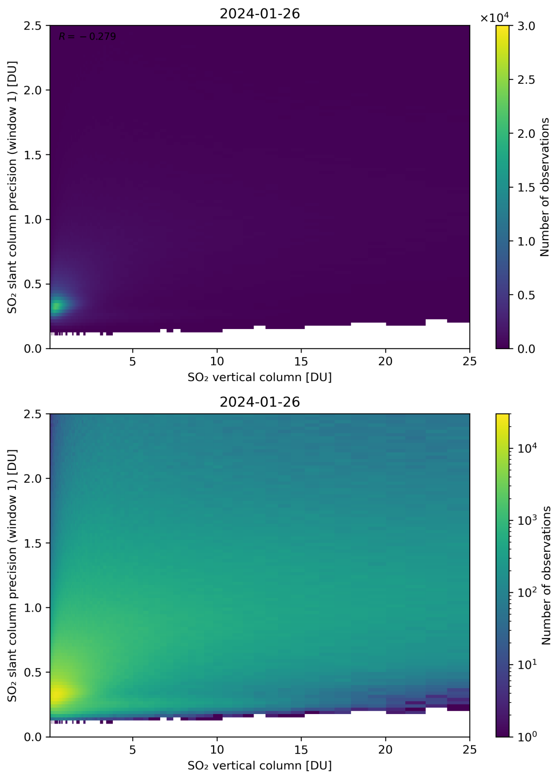
Figure 301: Scatter density plot of “SO 2 vertical column” against “SO 2 slant column precision (window 1)” for 2024-01-26 to 2024-01-27.
