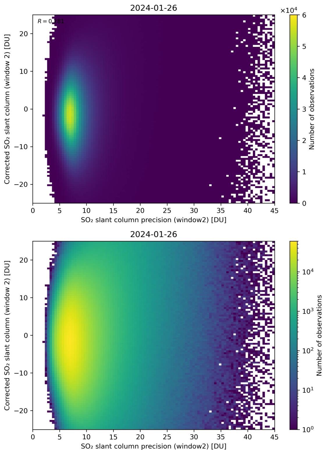
Figure 247: Scatter density plot of “SO 2 slant column precision (window2)” against “Corrected SO 2 slant column (window 2)” for 2024-01-26 to 2024-01-27.
