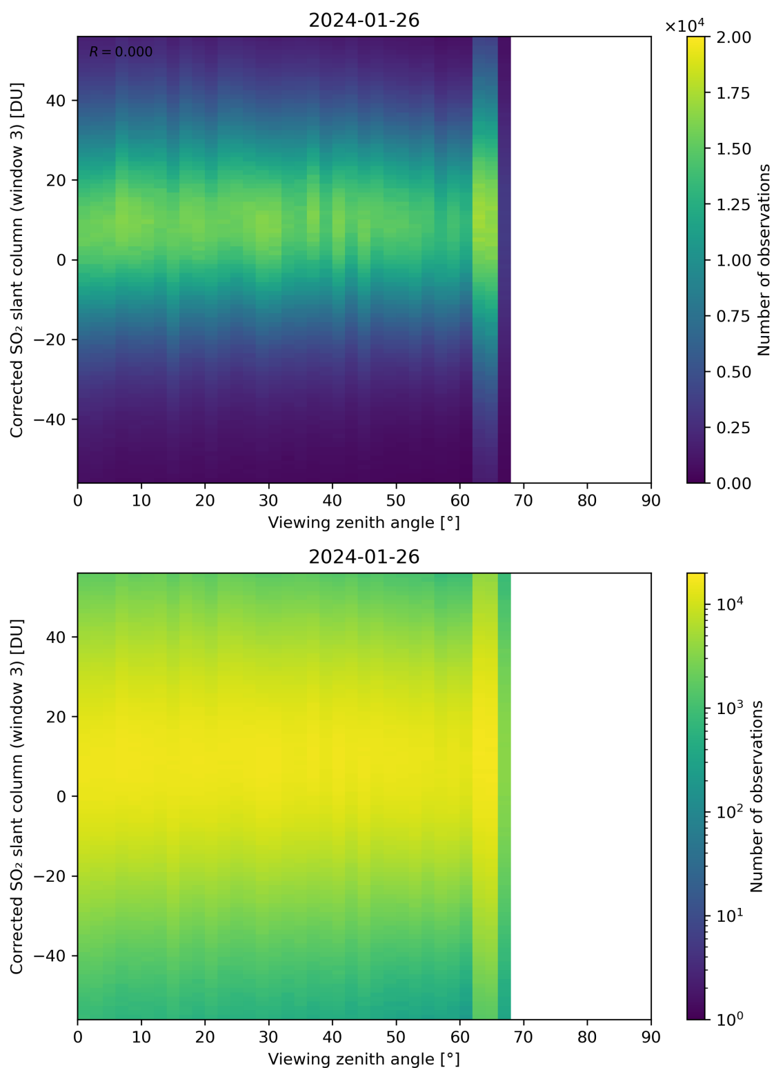
Figure 319: Scatter density plot of “Viewing zenith angle” against “Corrected SO 2 slant column (window 3)” for 2024-01-26 to 2024-01-27.
