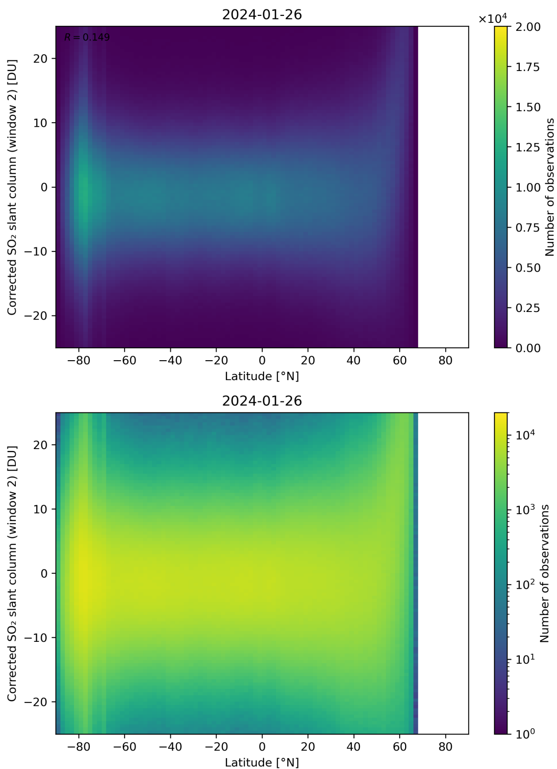
Figure 147: Scatter density plot of “Latitude” against “Corrected SO 2 slant column (window 2)” for 2024-01-26 to 2024-01-27.
