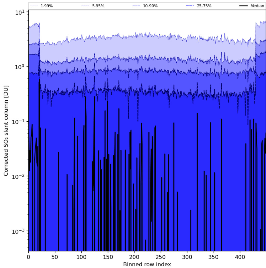
Figure 78: Along track statistics of “Corrected SO 2 slant column” for 2024-01-26 to 2024-01-27
