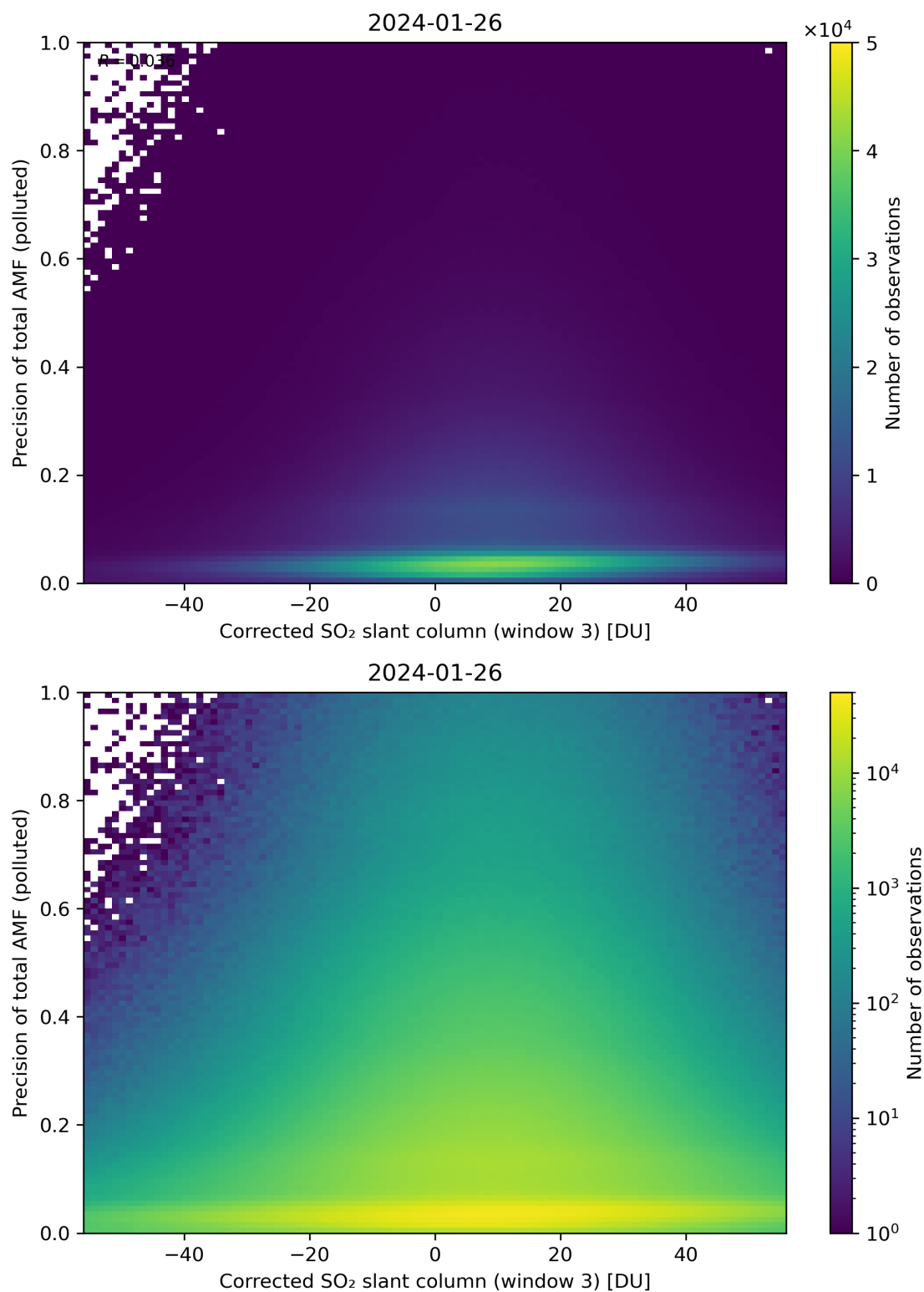
Figure 211: Scatter density plot of “Corrected SO 2 slant column (window 3)” against “Precision of total AMF (polluted)” for 2024-01-26 to 2024-01-27.
