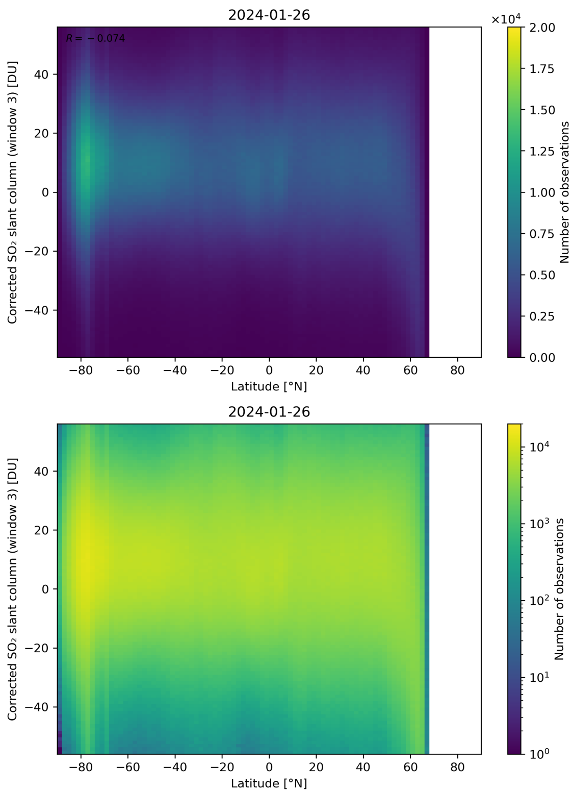
Figure 148: Scatter density plot of “Latitude” against “Corrected SO 2 slant column (window 3)” for 2024-01-26 to 2024-01-27.
