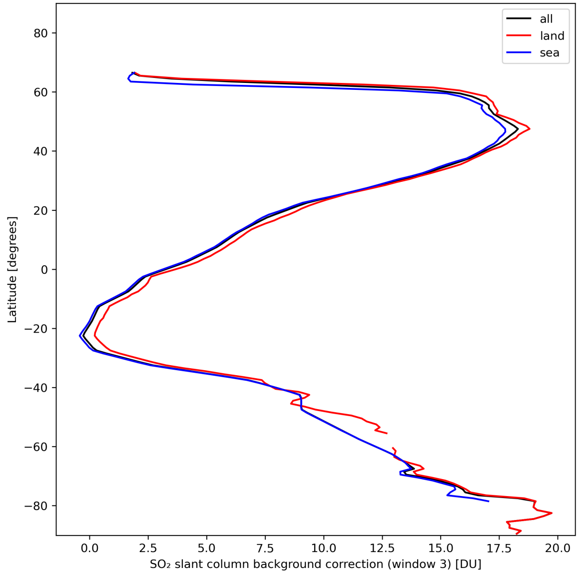
Figure 44: Zonal average of “SO 2 slant column background correction (window 3)” for 2024-01-26 to 2024-01-27.
