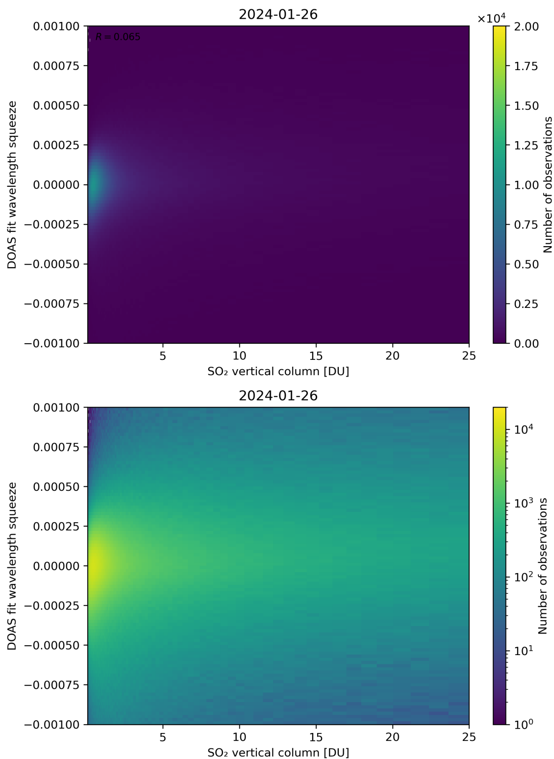
Figure 277: Scatter density plot of “SO 2 vertical column” against “DOAS fit wavelength squeeze” for 2024-01-26 to 2024-01-27.
