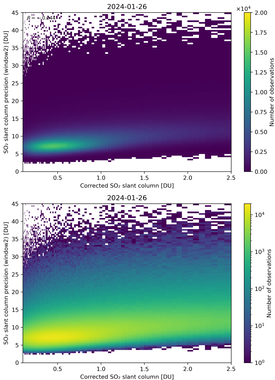
Figure 189: Scatter density plot of “Corrected SO 2 slant column” against “SO 2 slant column precision (window2)” for 2024-01-26 to 2024-01-27.
