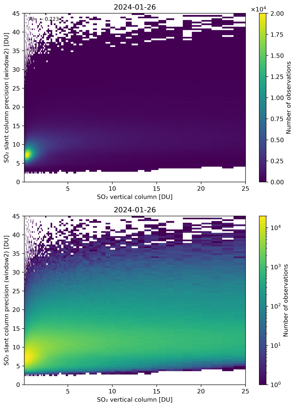
Figure 302: Scatter density plot of “SO 2 vertical column” against “SO 2 slant column precision (window2)” for 2024-01-26 to 2024-01-27.
