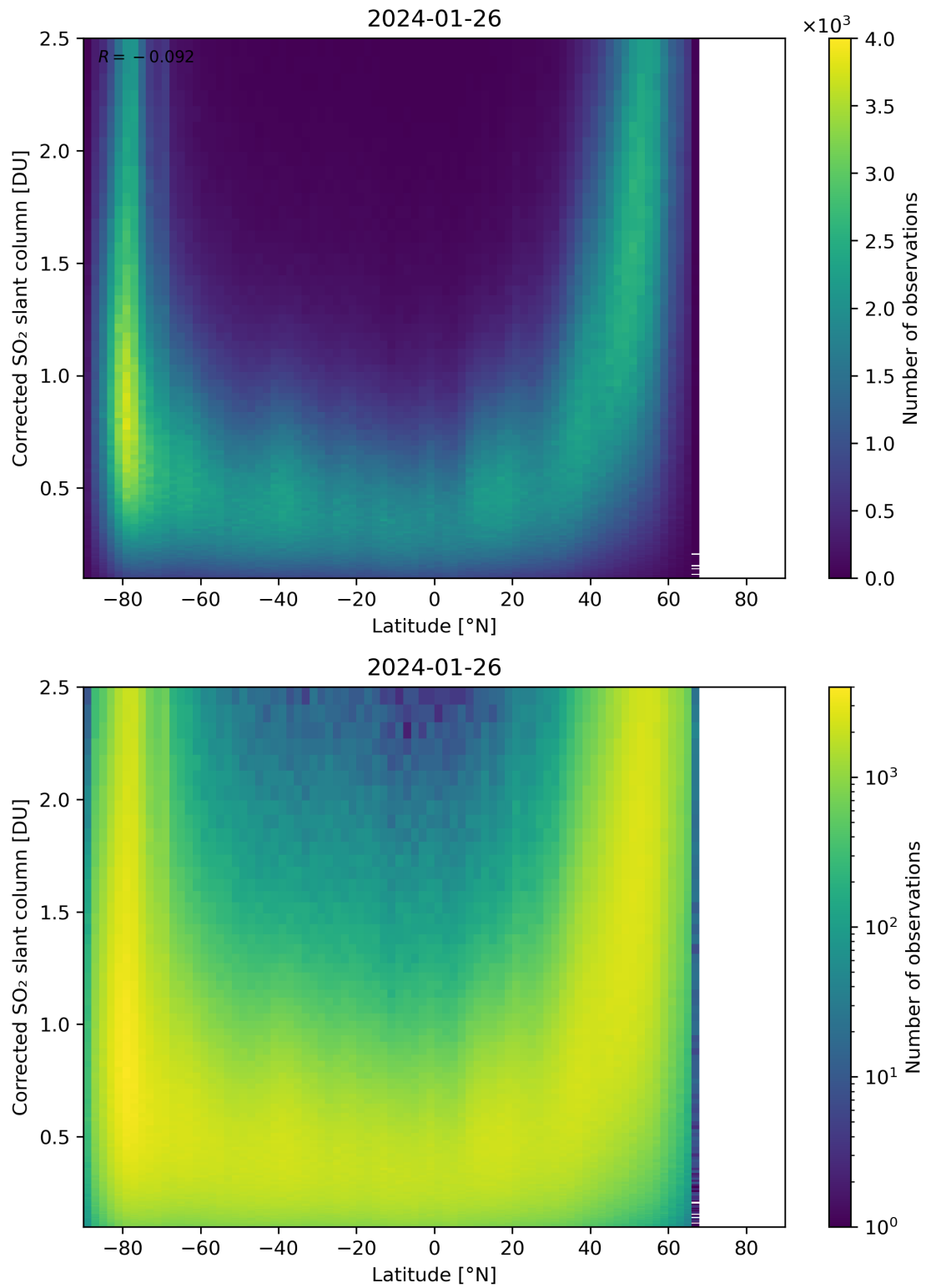
Figure 146: Scatter density plot of “Latitude” against “Corrected SO 2 slant column” for 2024-01-26 to 2024-01-27.
