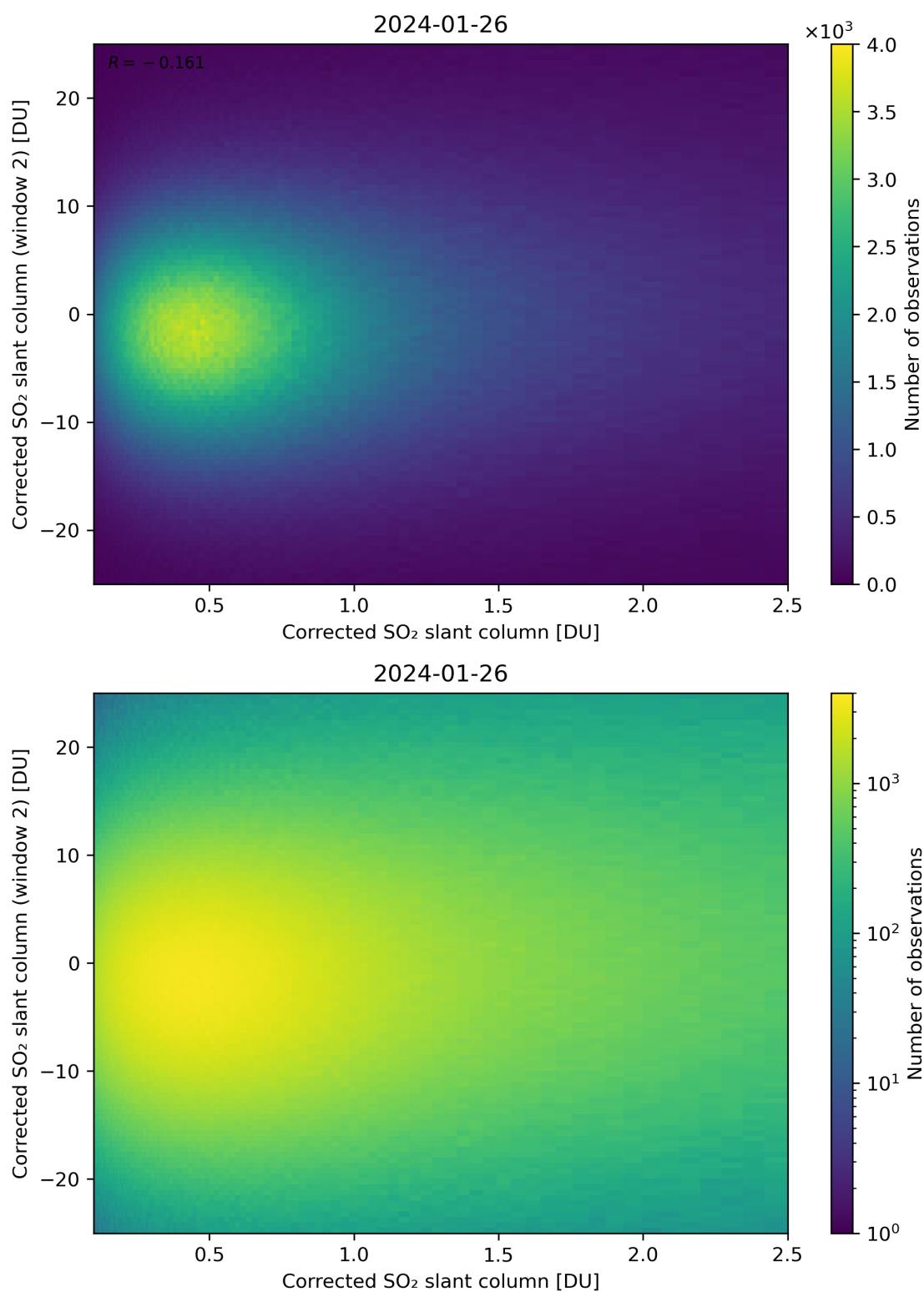
Figure 185: Scatter density plot of “Corrected SO 2 slant column” against “Corrected SO 2 slant column (window 2)” for 2024-01-26 to 2024-01-27.
