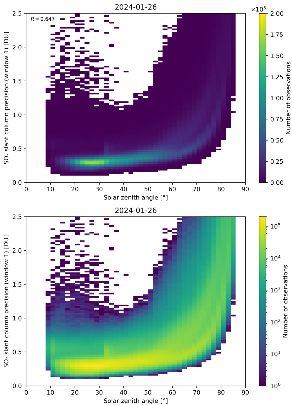
Figure 170: Scatter density plot of “Solar zenith angle” against “SO 2 slant column precision (window 1)” for 2024-01-26 to 2024-01-27.
