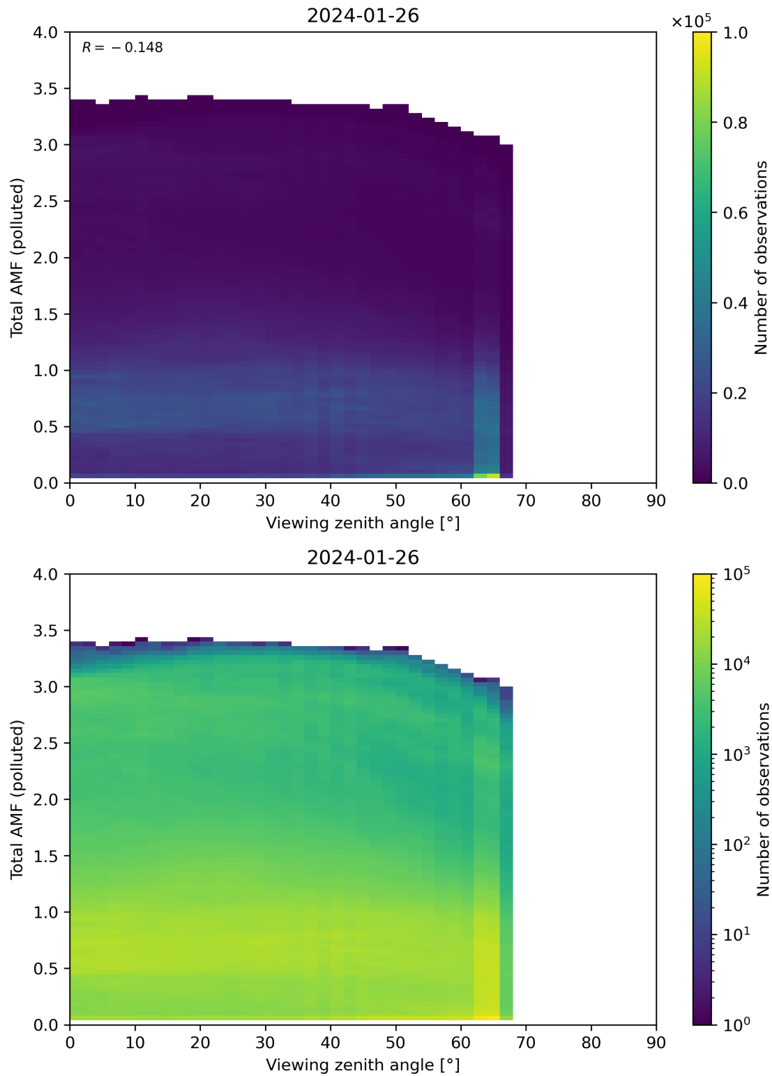
Figure 325: Scatter density plot of “Viewing zenith angle” against “Total AMF (polluted)” for 2024-01-26 to 2024-01-27.
