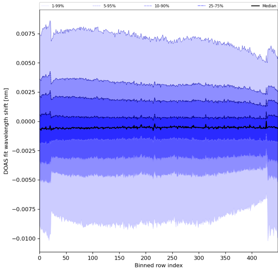
Figure 91: Along track statistics of “DOAS fit wavelength shift” for 2024-01-26 to 2024-01-27
