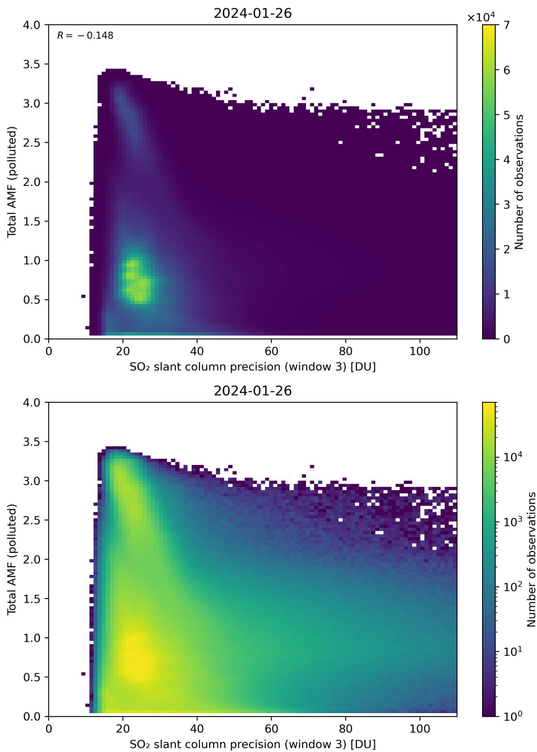
Figure 263: Scatter density plot of “SO 2 slant column precision (window 3)” against “Total AMF (polluted)” for 2024-01-26 to 2024-01-27.
