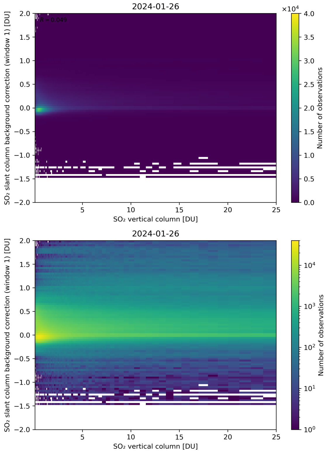
Figure 273: Scatter density plot of “SO 2 vertical column” against “SO 2 slant column background correction (window 1)” for 2024-01-26 to 2024-01-27.
