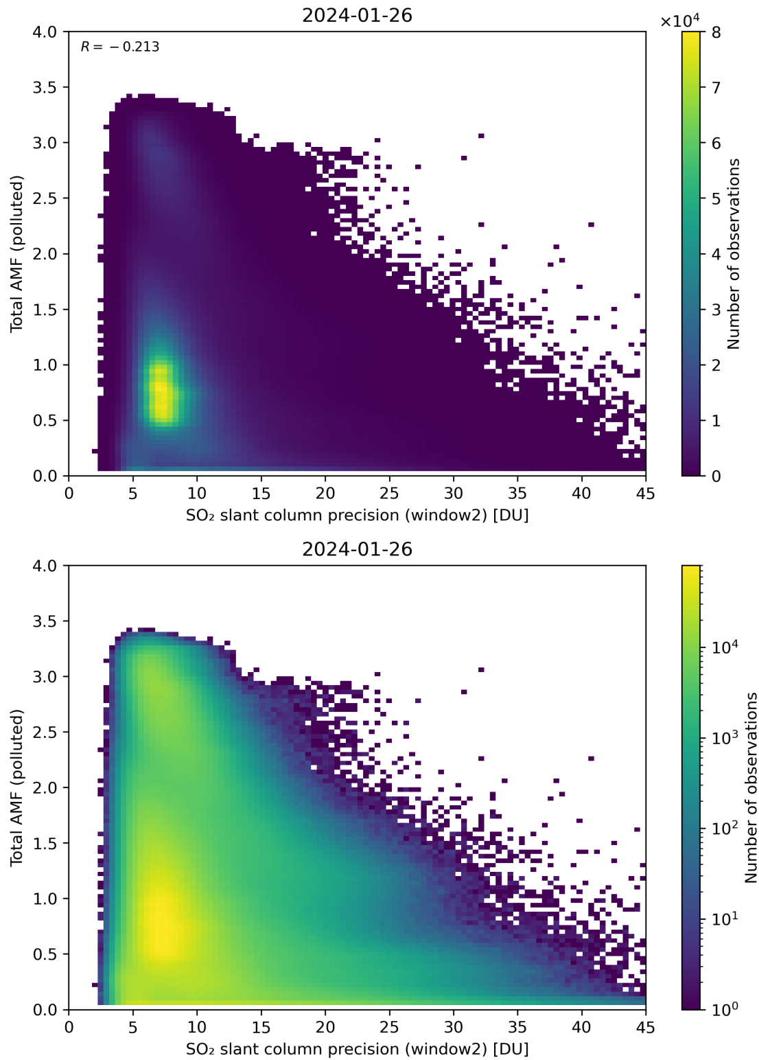
Figure 251: Scatter density plot of “SO 2 slant column precision (window2)” against “Total AMF (polluted)” for 2024-01-26 to 2024-01-27.
