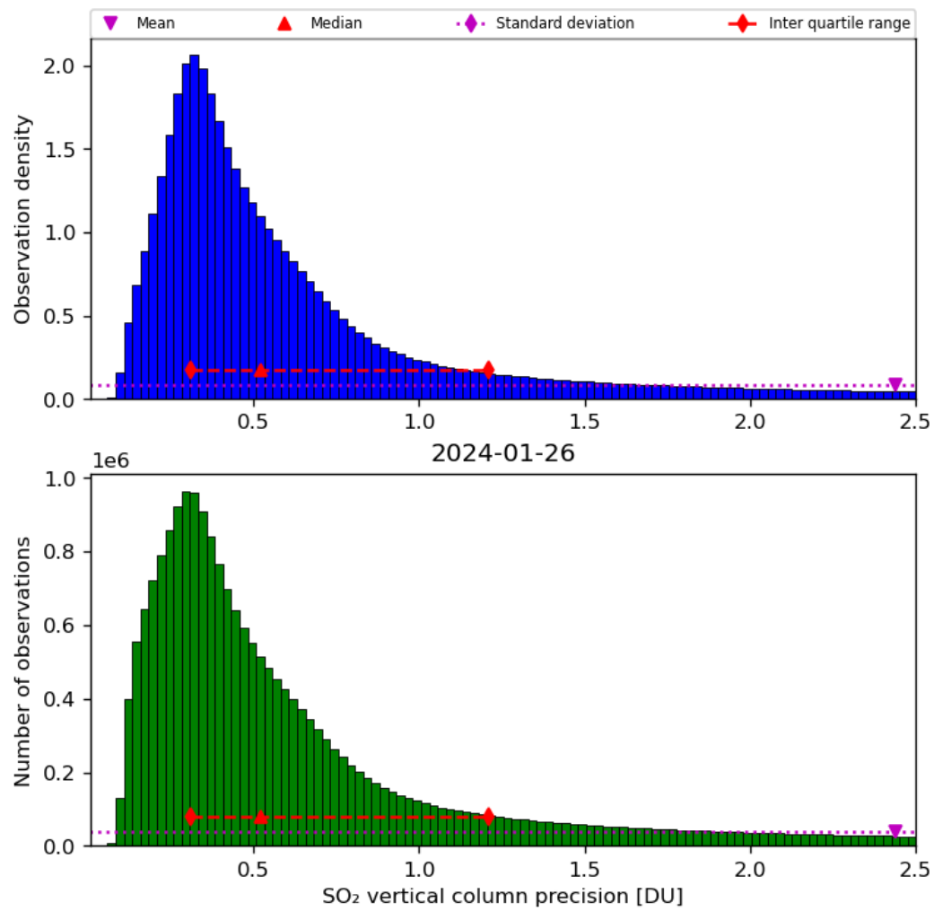
Figure 54: Histogram of “SO 2 vertical column precision” for 2024-01-26 to 2024-01-27
