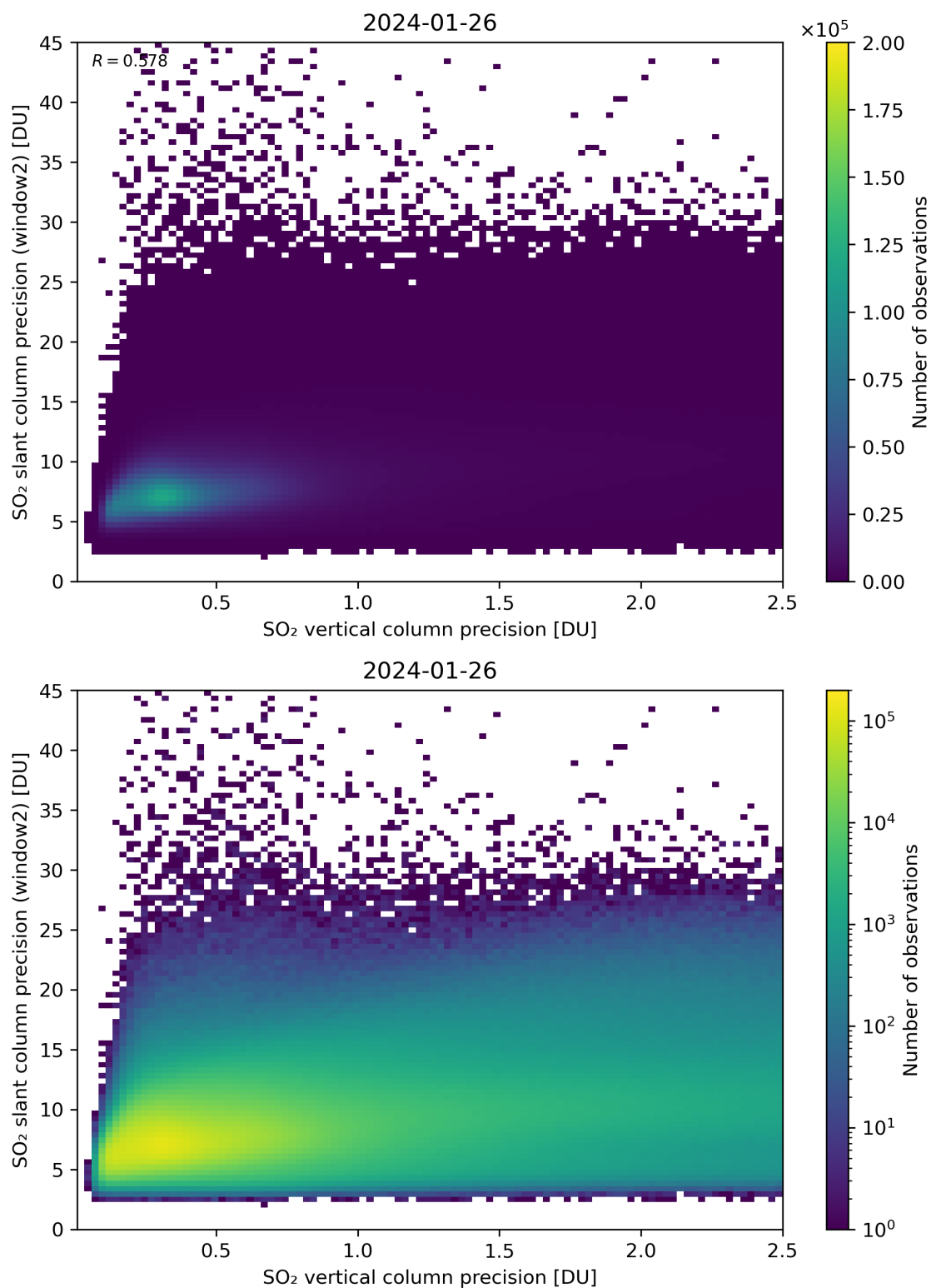
Figure 291: Scatter density plot of “SO 2 vertical column precision” against “SO 2 slant column precision (window2)” for 2024-01-26 to 2024-01-27.
