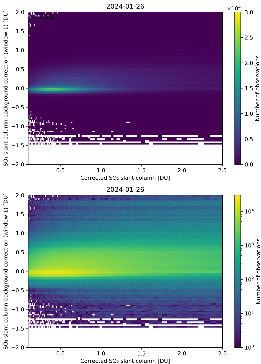
Figure 178: Scatter density plot of “Corrected SO 2 slant column” against “SO 2 slant column background correction (window 1)” for 2024-01-26 to 2024-01-27.
