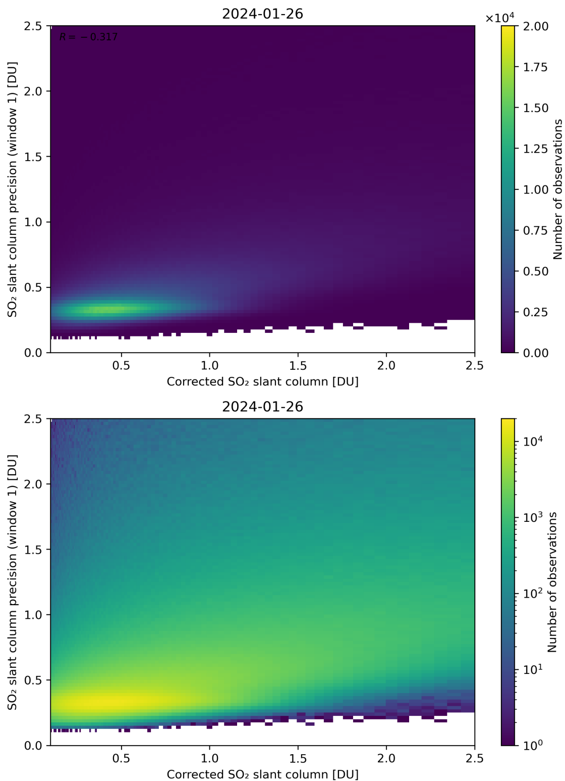
Figure 188: Scatter density plot of “Corrected SO 2 slant column” against “SO 2 slant column precision (window 1)” for 2024-01-26 to 2024-01-27.
