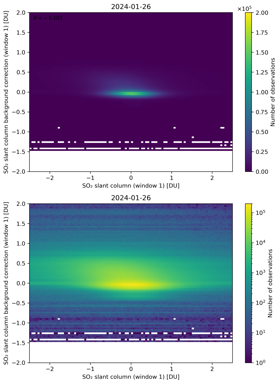
Figure 212: Scatter density plot of “SO 2 slant column (window 1)” against “SO 2 slant column background correction (window 1)” for 2024-01-26 to 2024-01-27.
