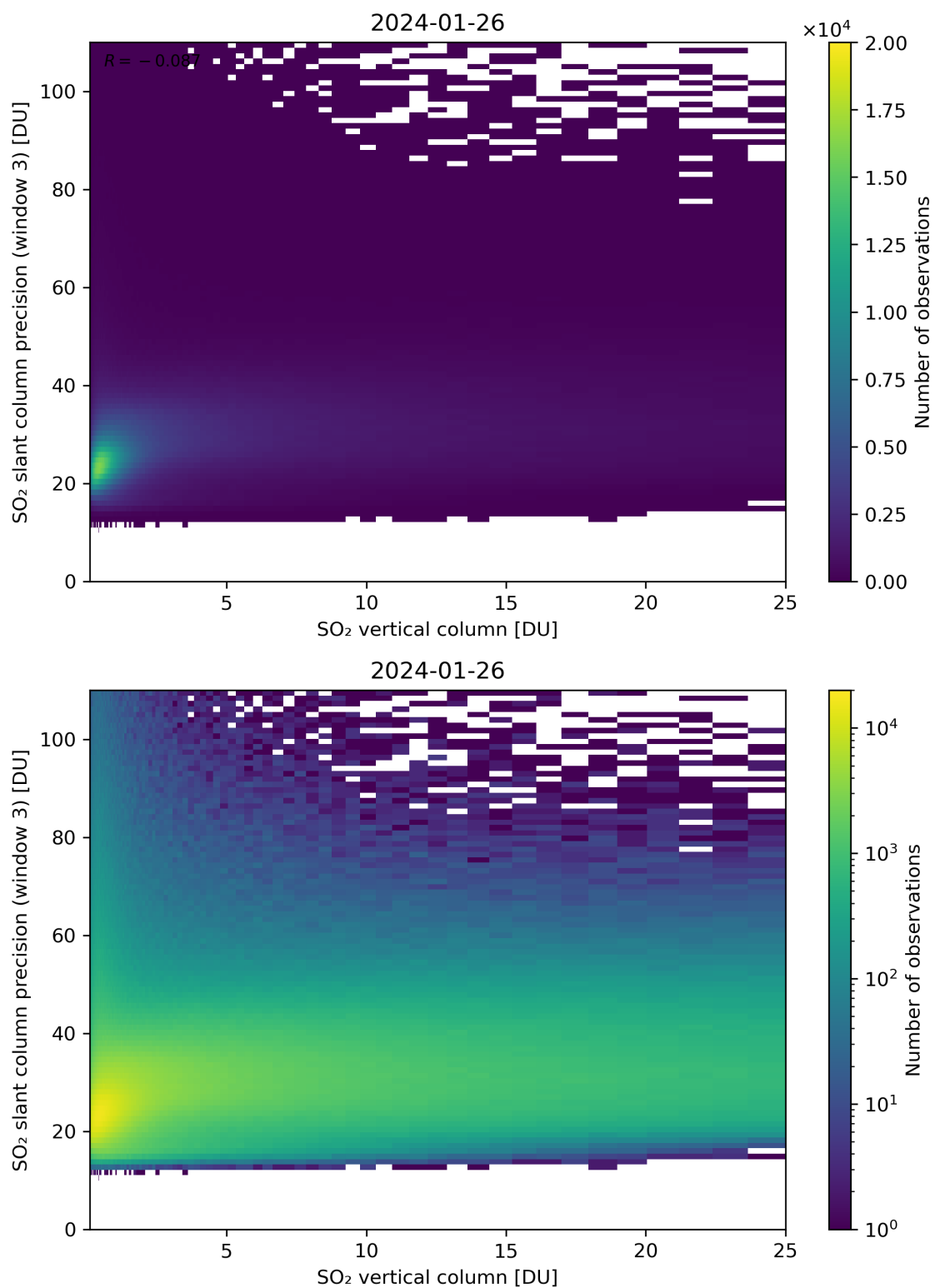
Figure 304: Scatter density plot of “SO 2 vertical column” against “SO 2 slant column precision (window 3)” for 2024-01-26 to 2024-01-27.
