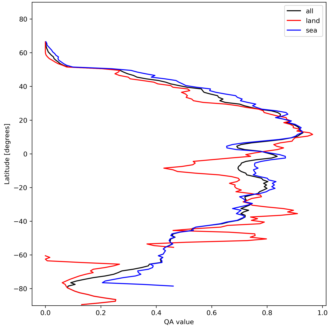
Figure 29: Zonal average of “QA value” for 2024-01-26 to 2024-01-27.
