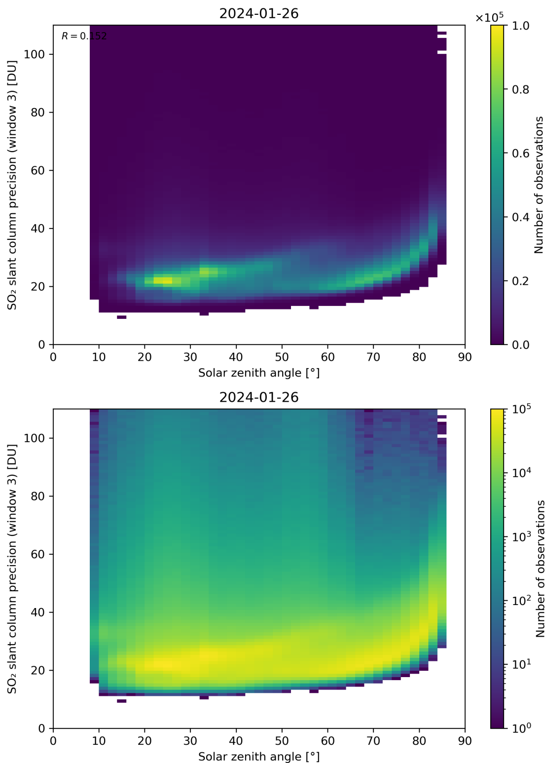
Figure 173: Scatter density plot of “Solar zenith angle” against “SO 2 slant column precision (window 3)” for 2024-01-26 to 2024-01-27.
