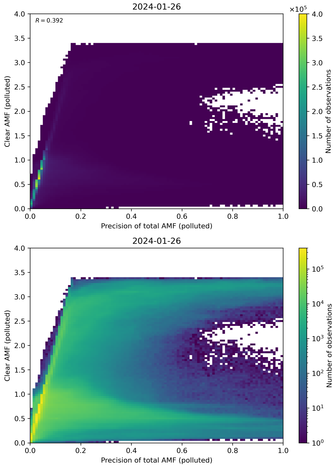
Figure 270: Scatter density plot of “Precision of total AMF (polluted)” against “Clear AMF (polluted)” for 2024-01-26 to 2024-01-27.
