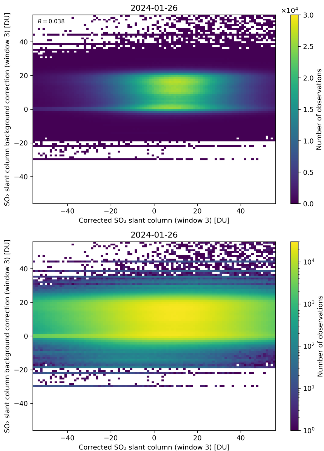
Figure 205: Scatter density plot of “Corrected SO 2 slant column (window 3)” against “SO 2 slant column background correction (window 3)” for 2024-01-26 to 2024-01-27.
