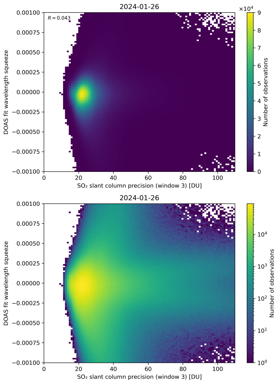
Figure 259: Scatter density plot of “SO 2 slant column precision (window 3)” against “DOAS fit wavelength squeeze” for 2024-01-26 to 2024-01-27.
