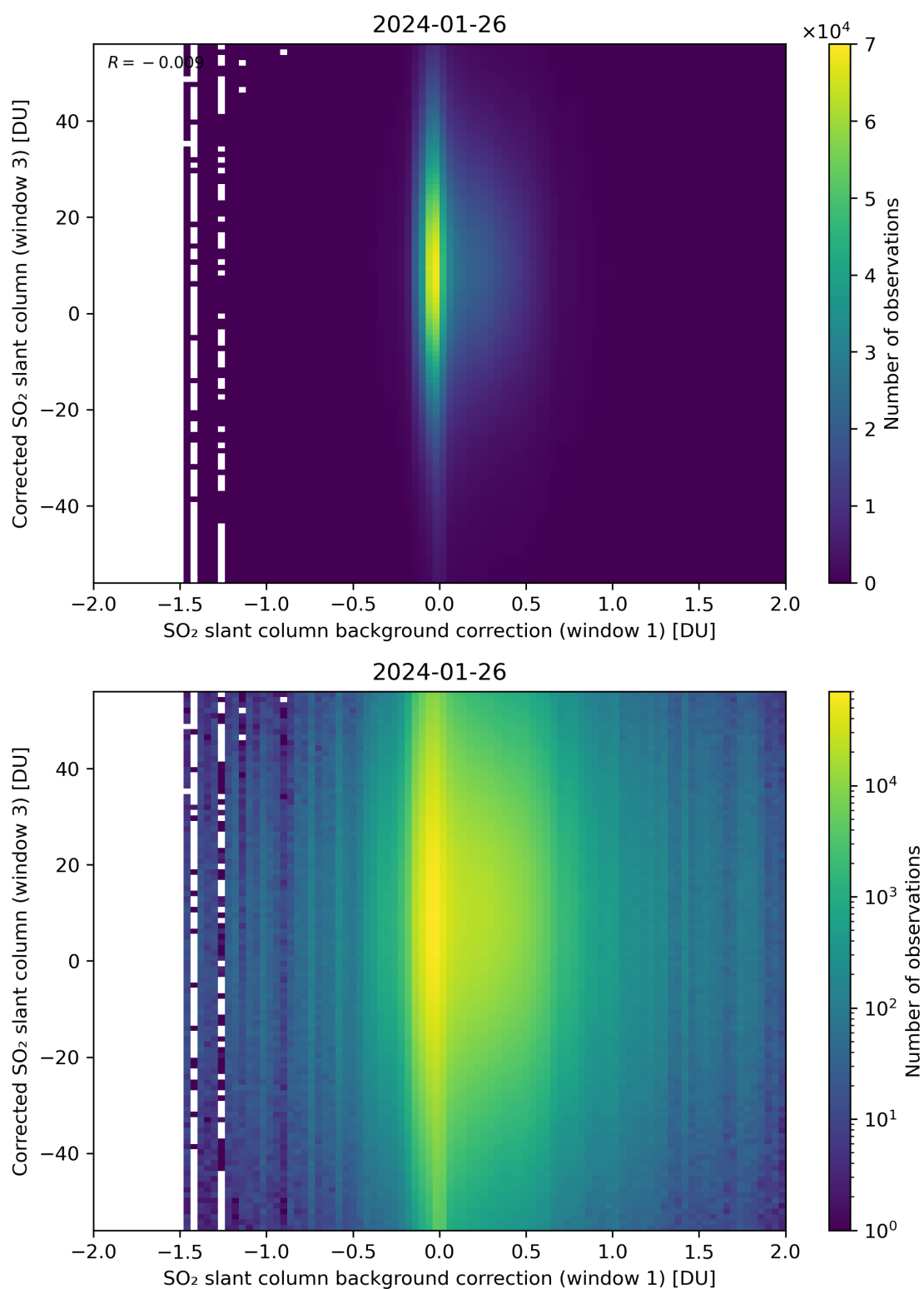
Figure 105: Scatter density plot of “SO 2 slant column background correction (window 1)” against “Corrected SO 2 slant column (window 3)” for 2024-01-26 to 2024-01-27.
