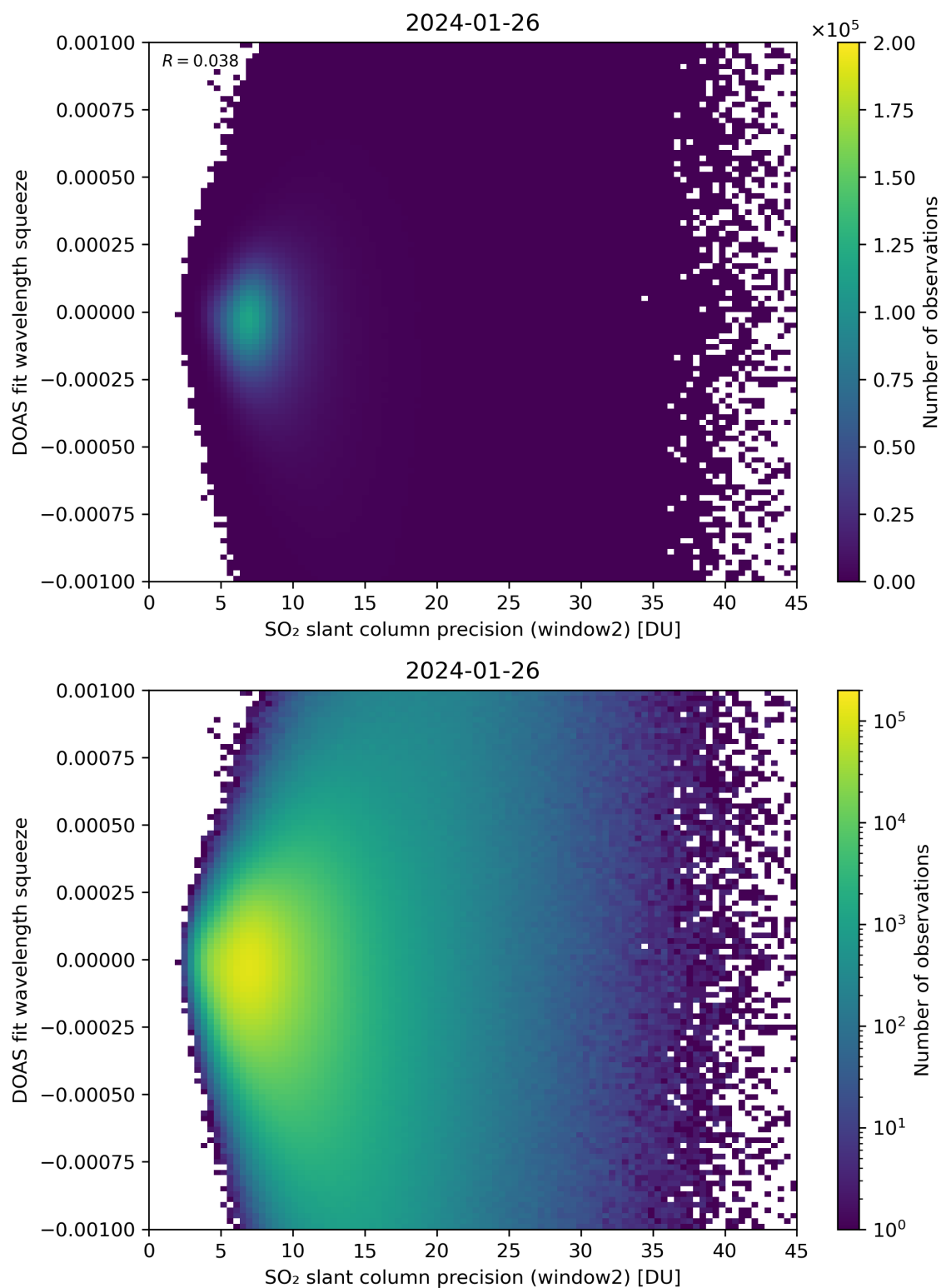
Figure 244: Scatter density plot of “SO 2 slant column precision (window2)” against “DOAS fit wavelength squeeze” for 2024-01-26 to 2024-01-27.
