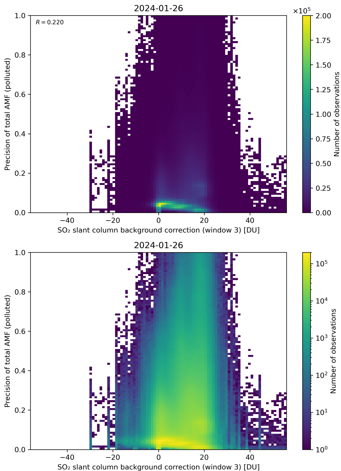
Figure 126: Scatter density plot of “SO 2 slant column background correction (window 3)” against “Precision of total AMF (polluted)” for 2024-01-26 to 2024-01-27.
