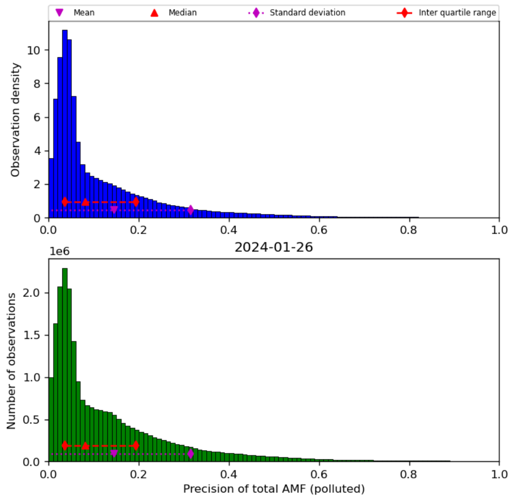
Figure 72: Histogram of “Precision of total AMF (polluted)” for 2024-01-26 to 2024-01-27
