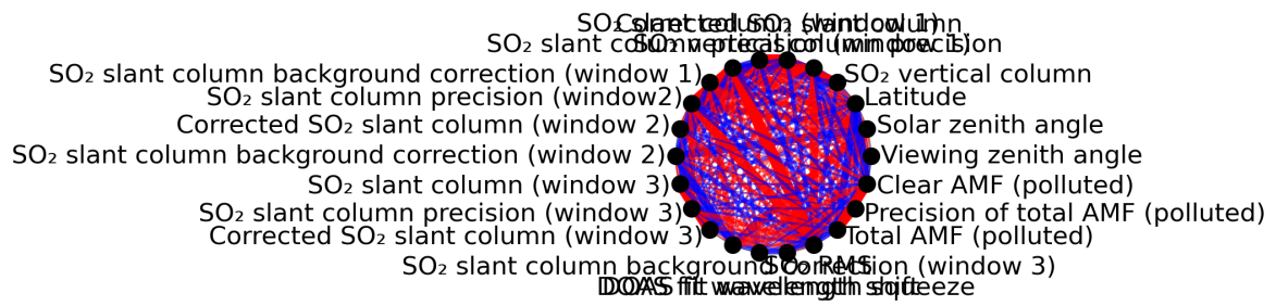
Figure 1: Map of correlation graph for 2024-01-26 to 2024-01-27.
