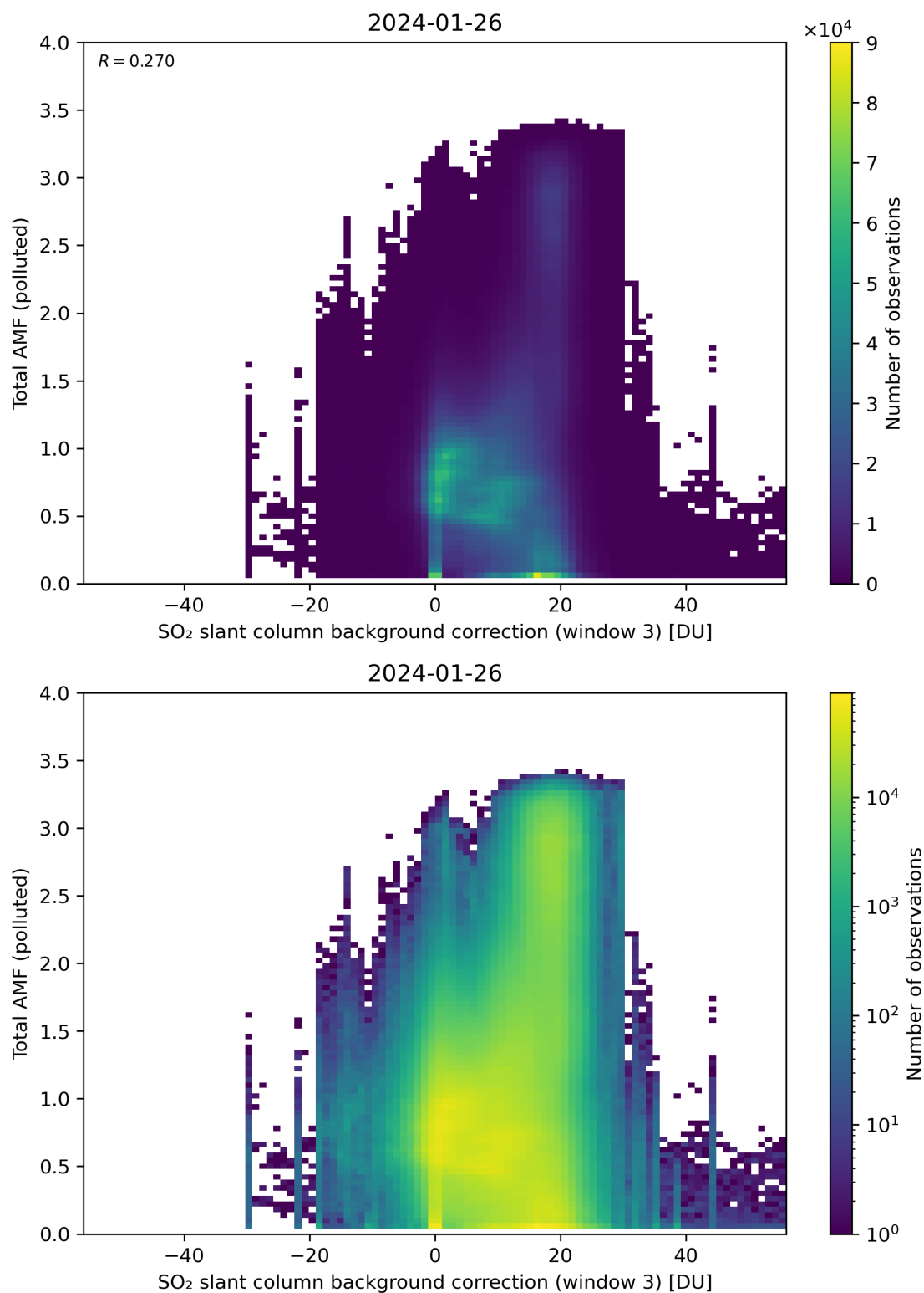
Figure 125: Scatter density plot of “SO 2 slant column background correction (window 3)” against “Total AMF (polluted)” for 2024-01-26 to 2024-01-27.
