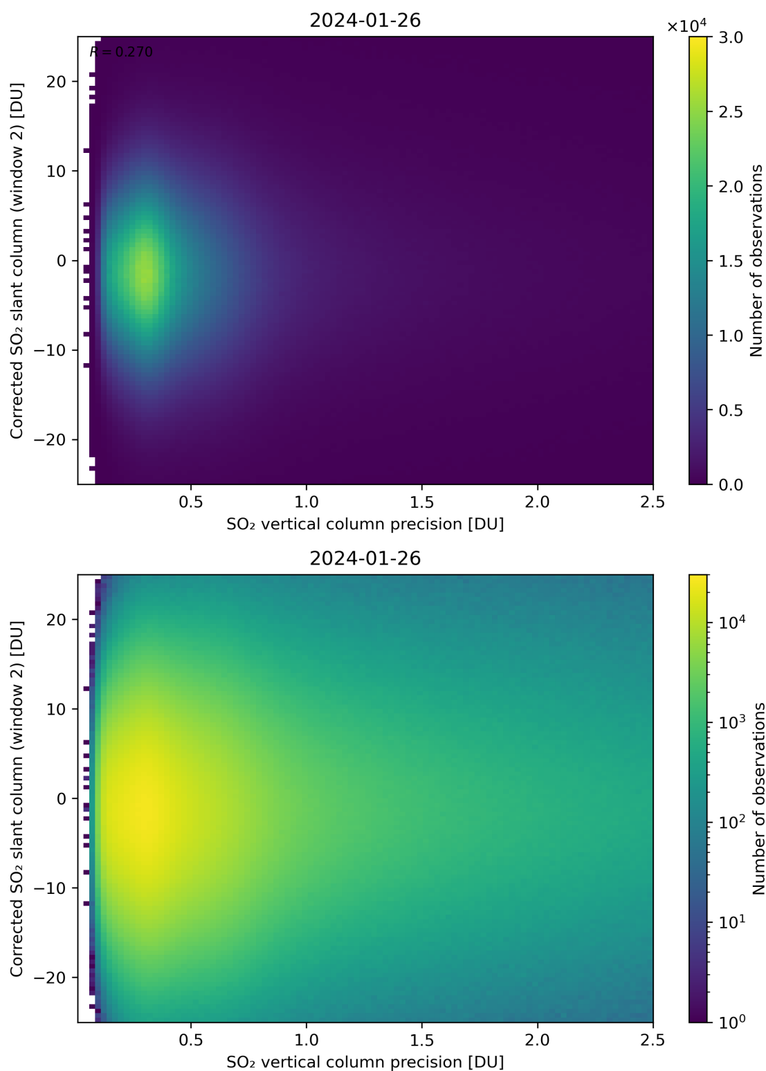
Figure 287: Scatter density plot of “SO 2 vertical column precision” against “Corrected SO 2 slant column (window 2)” for 2024-01-26 to 2024-01-27.
