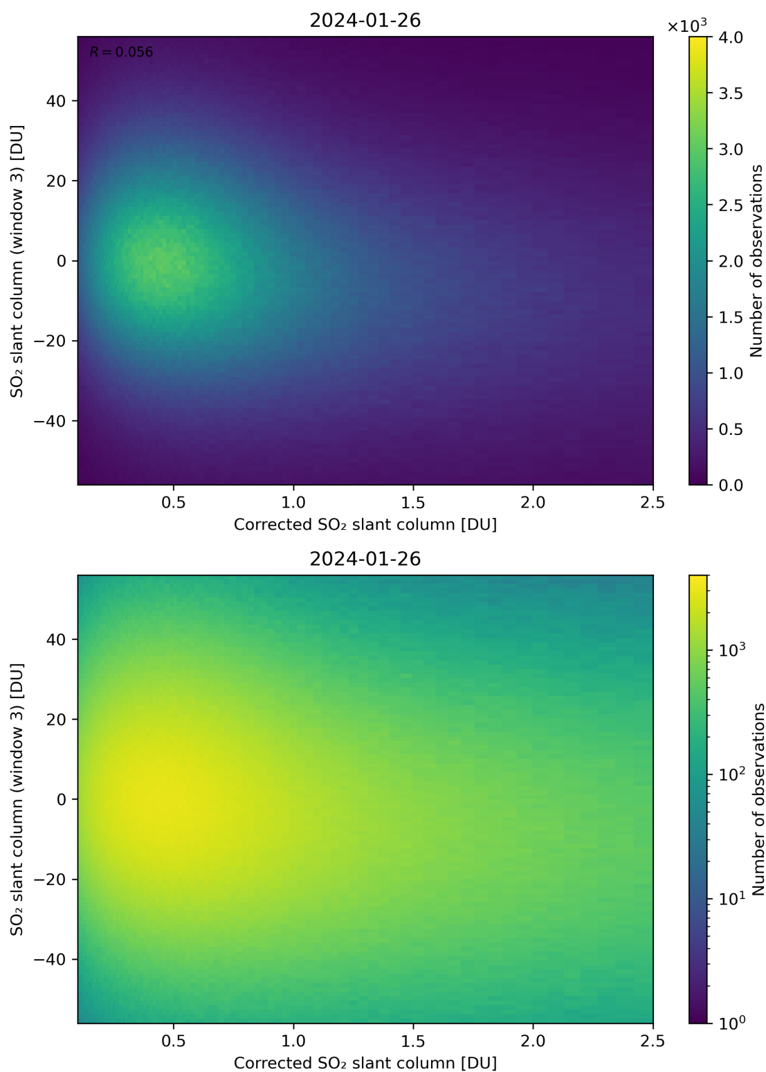
Figure 190: Scatter density plot of “Corrected SO 2 slant column” against “SO 2 slant column (window 3)” for 2024-01-26 to 2024-01-27.
