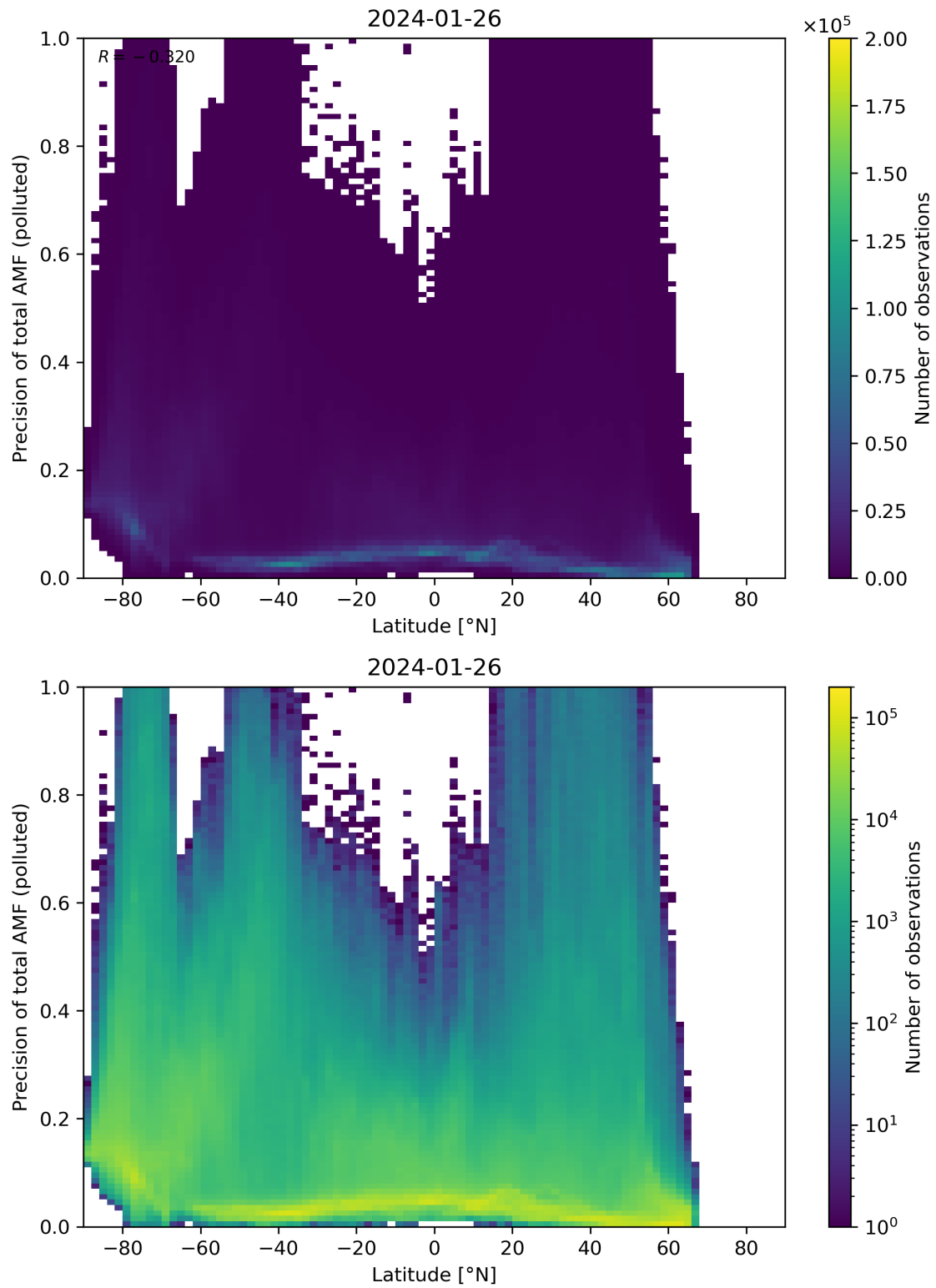
Figure 155: Scatter density plot of “Latitude” against “Precision of total AMF (polluted)” for 2024-01-26 to 2024-01-27.
