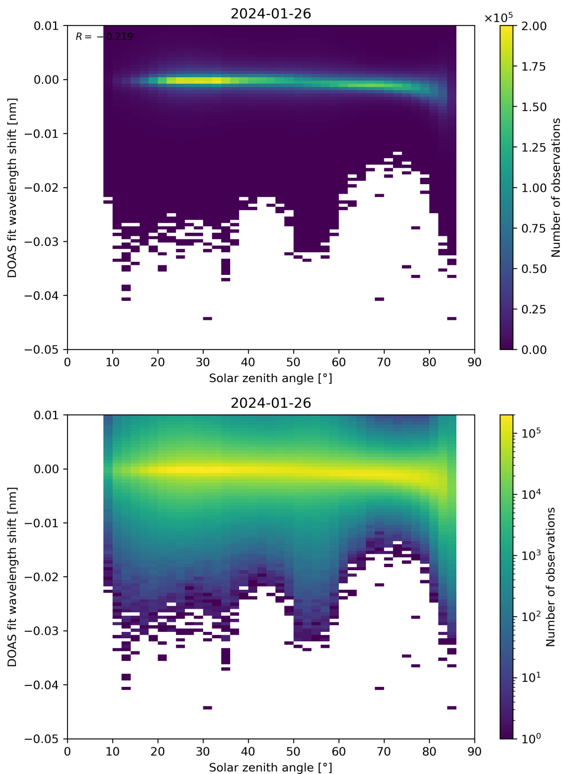
Figure 161: Scatter density plot of “Solar zenith angle” against “DOAS fit wavelength shift” for 2024-01-26 to 2024-01-27.
