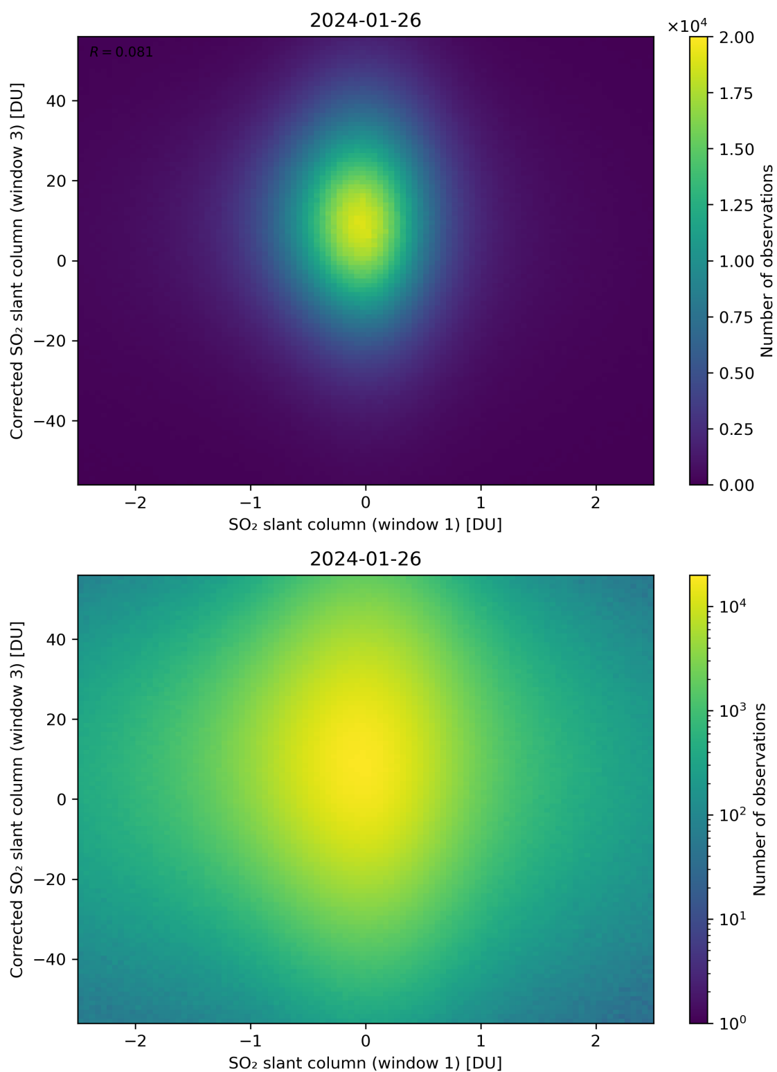
Figure 234: Scatter density plot of “SO 2 slant column (window 1)” against “Corrected SO 2 slant column (window 3)” for 2024-01-26 to 2024-01-27.
