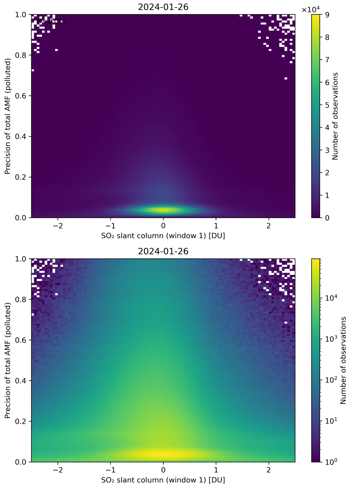
Figure 240: Scatter density plot of “SO 2 slant column (window 1)” against “Precision of total AMF (polluted)” for 2024-01-26 to 2024-01-27.
