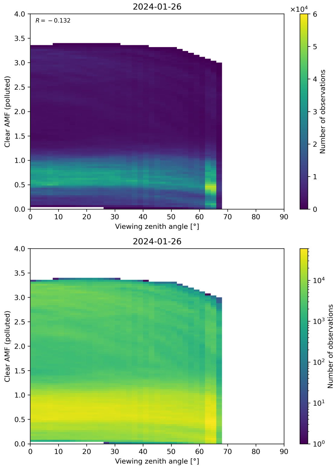
Figure 316: Scatter density plot of “Viewing zenith angle” against “Clear AMF (polluted)” for 2024-01-26 to 2024-01-27.
