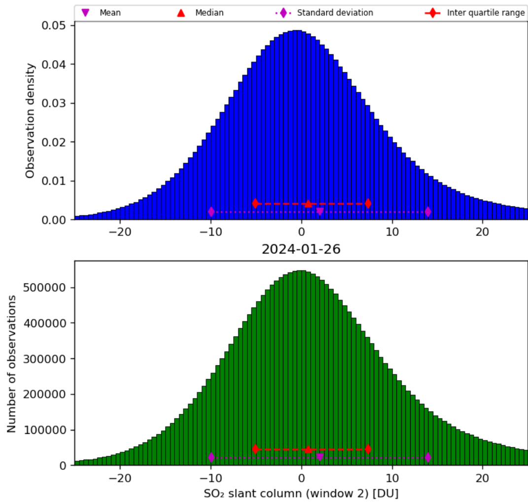
Figure 60: Histogram of “SO 2 slant column (window 2)” for 2024-01-26 to 2024-01-27
