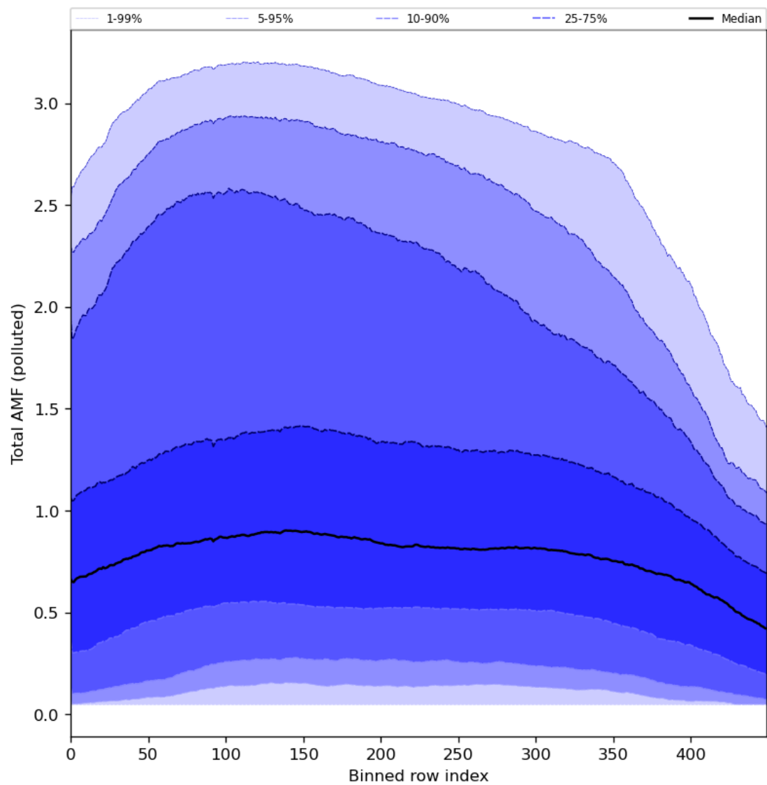
Figure 94: Along track statistics of “Total AMF (polluted)” for 2024-01-26 to 2024-01-27
