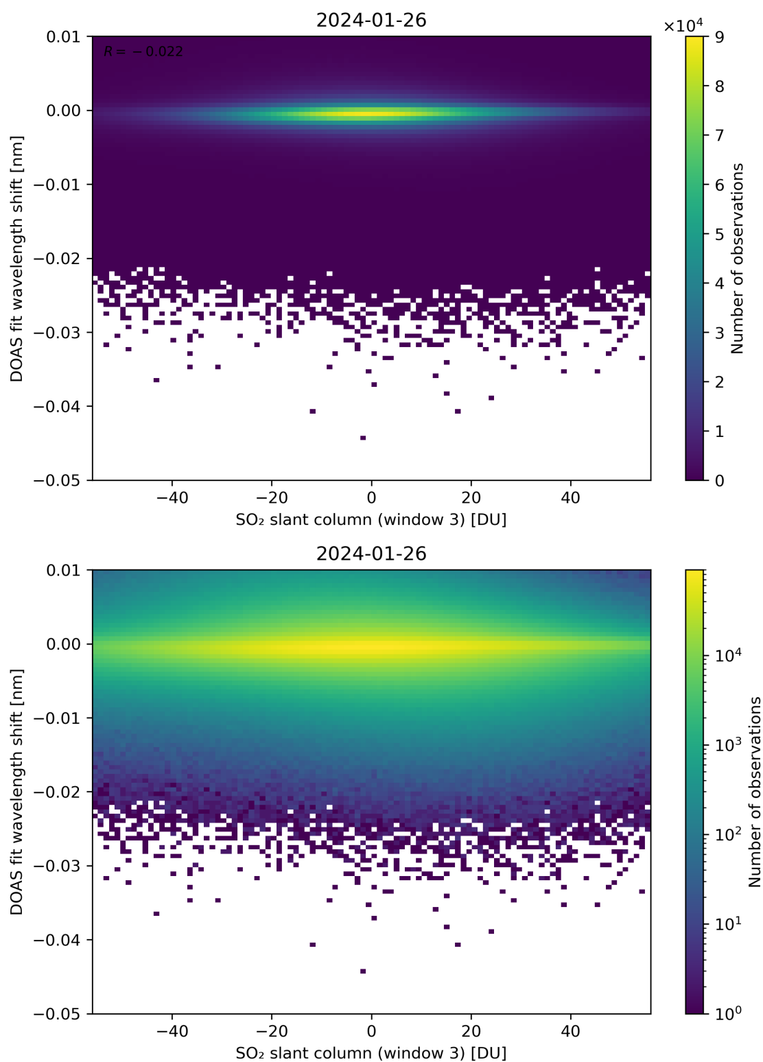
Figure 254: Scatter density plot of “SO 2 slant column (window 3)” against “DOAS fit wavelength shift” for 2024-01-26 to 2024-01-27.
