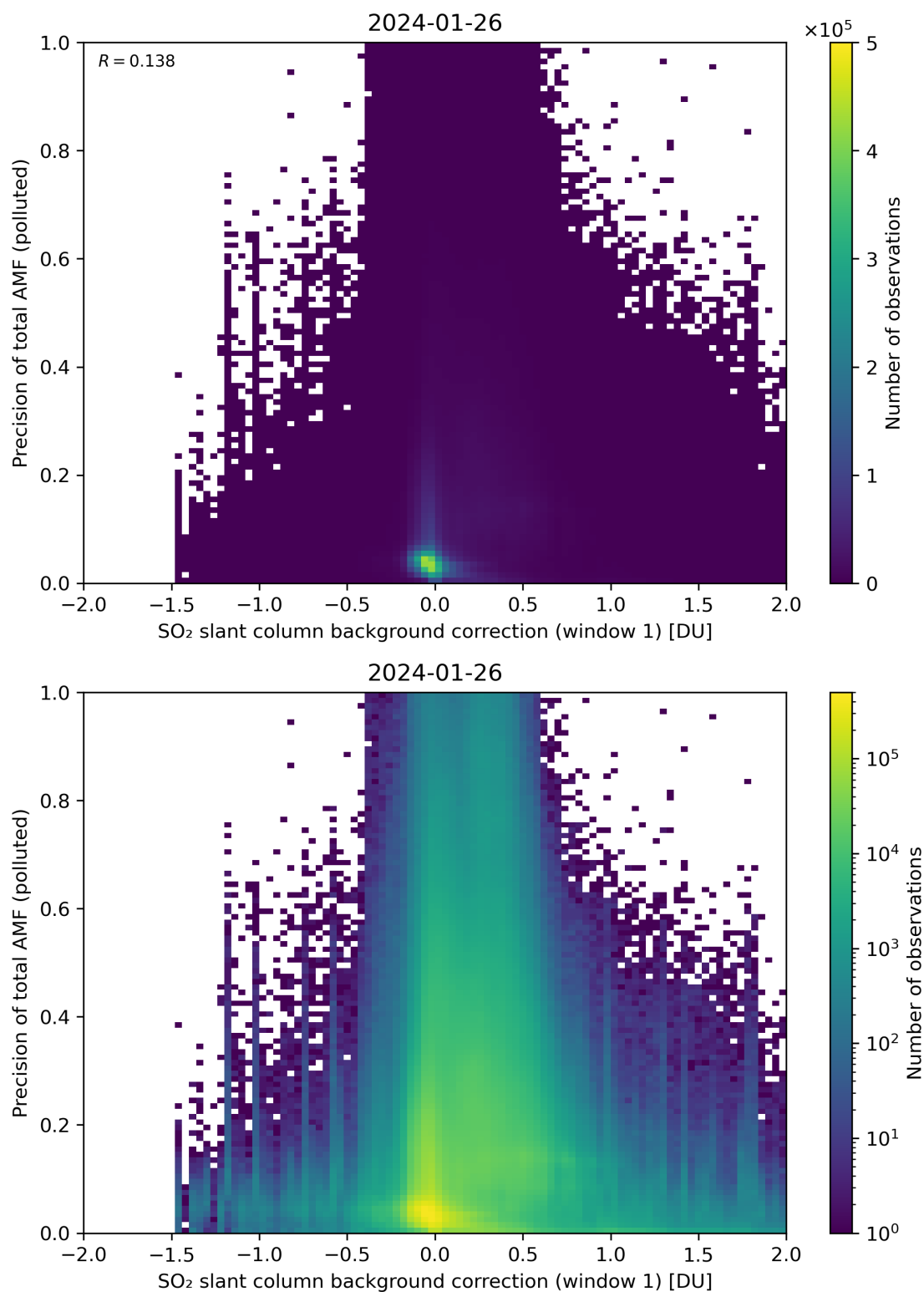
Figure 110: Scatter density plot of “SO 2 slant column background correction (window 1)” against “Precision of total AMF (polluted)” for 2024-01-26 to 2024-01-27.
