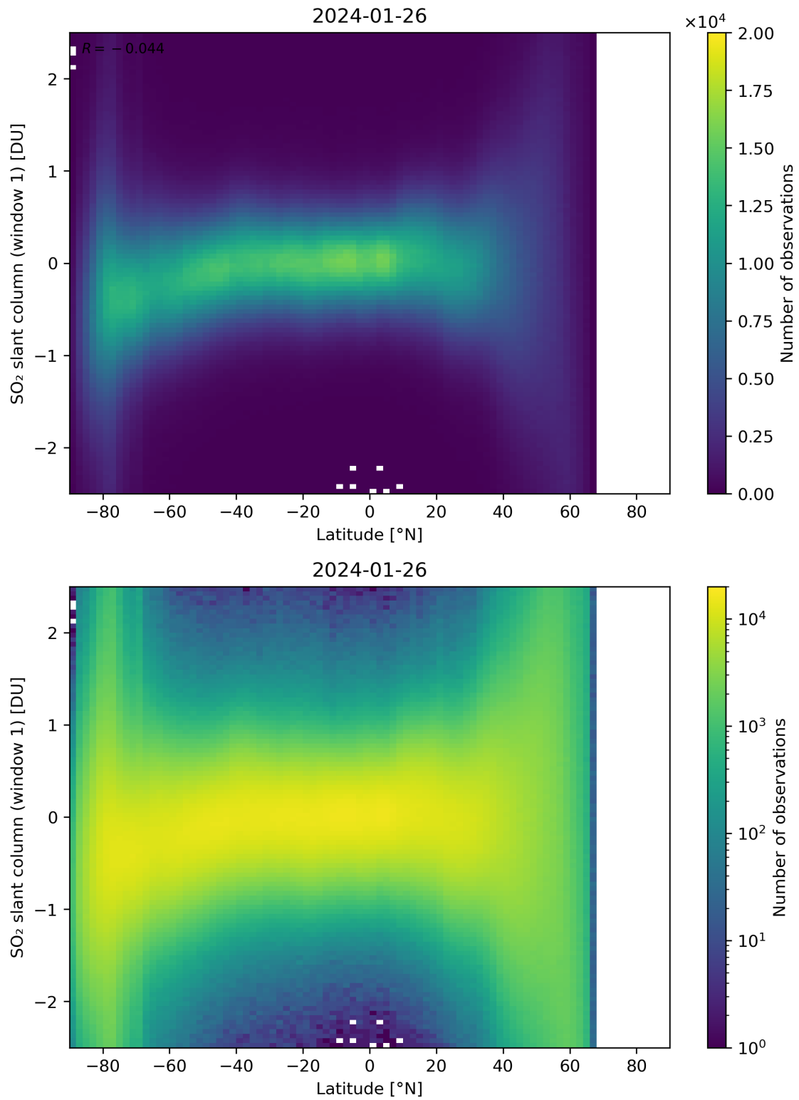
Figure 149: Scatter density plot of “Latitude” against “SO 2 slant column (window 1)” for 2024-01-26 to 2024-01-27.
