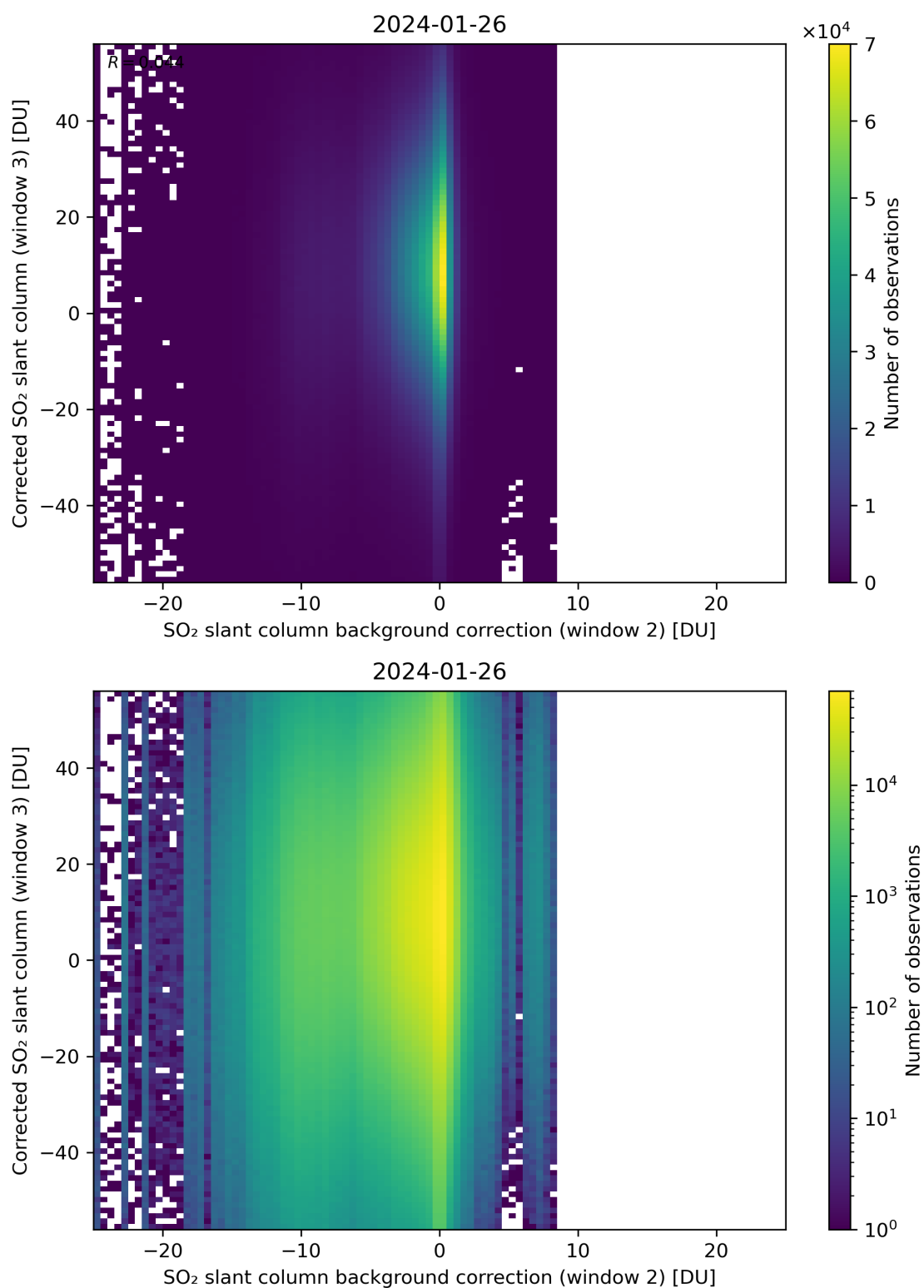
Figure 116: Scatter density plot of “SO 2 slant column background correction (window 2)” against “Corrected SO 2 slant column (window 3)” for 2024-01-26 to 2024-01-27.
