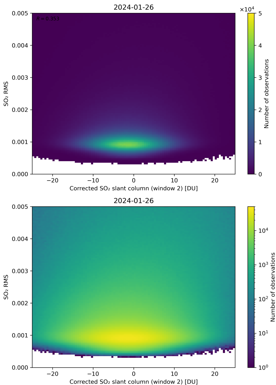
Figure 198: Scatter density plot of “Corrected SO 2 slant column (window 2)” against “SO 2 RMS” for 2024-01-26 to 2024-01-27.
