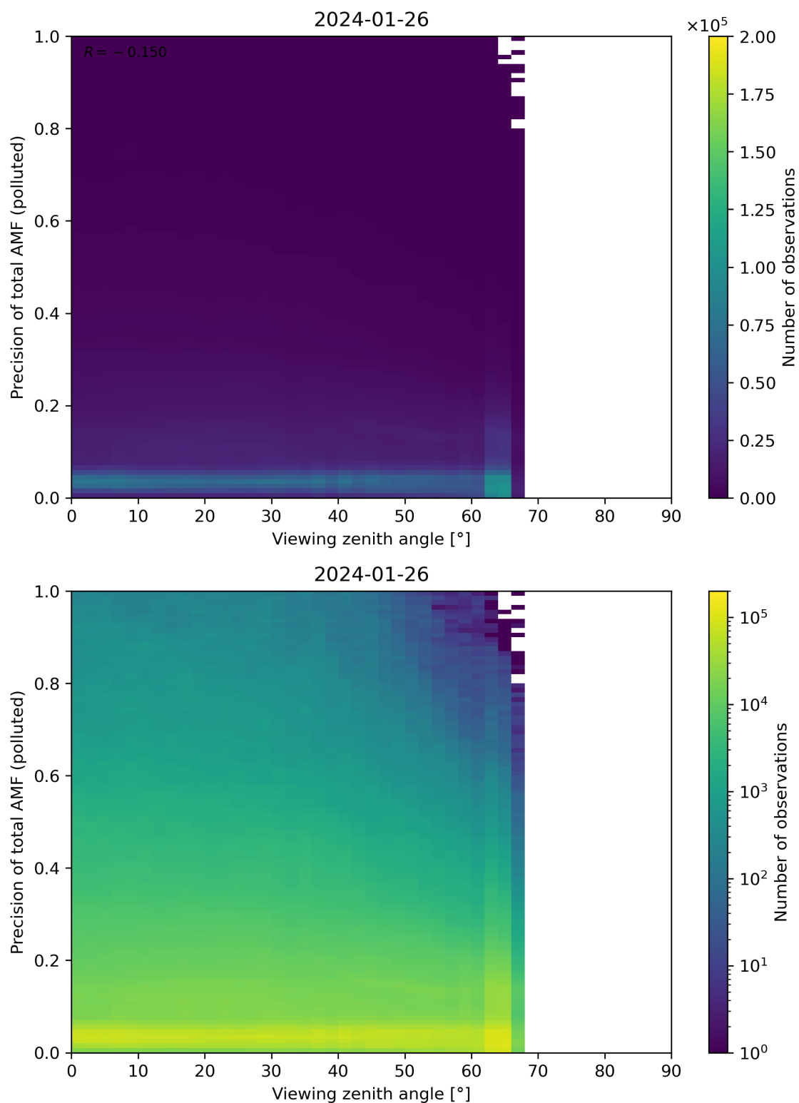
Figure 326: Scatter density plot of “Viewing zenith angle” against “Precision of total AMF (polluted)” for 2024-01-26 to 2024-01-27.
