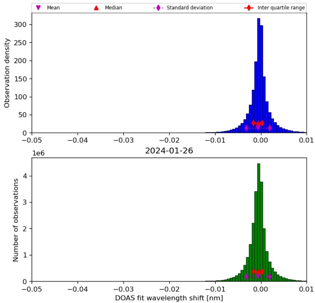
Figure 68: Histogram of “DOAS fit wavelength shift” for 2024-01-26 to 2024-01-27
