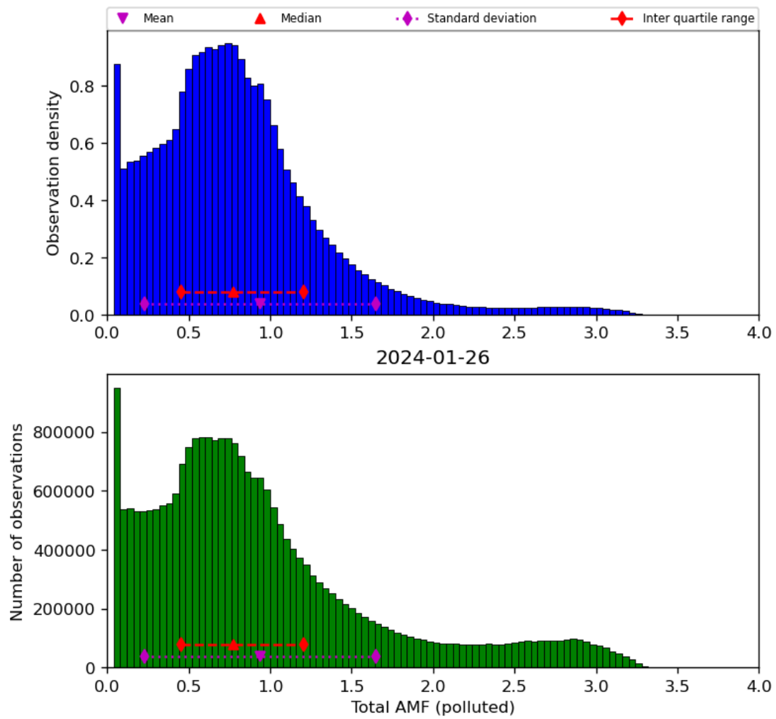
Figure 71: Histogram of “Total AMF (polluted)” for 2024-01-26 to 2024-01-27
