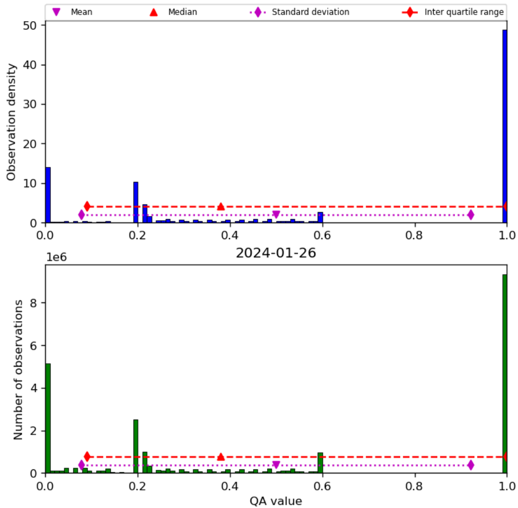
Figure 52: Histogram of “QA value” for 2024-01-26 to 2024-01-27
