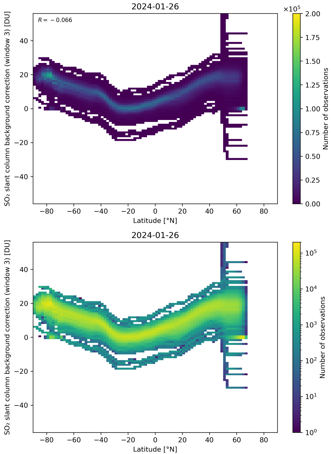
Figure 141: Scatter density plot of “Latitude” against “SO 2 slant column background correction (window 3)” for 2024-01-26 to 2024-01-27.
