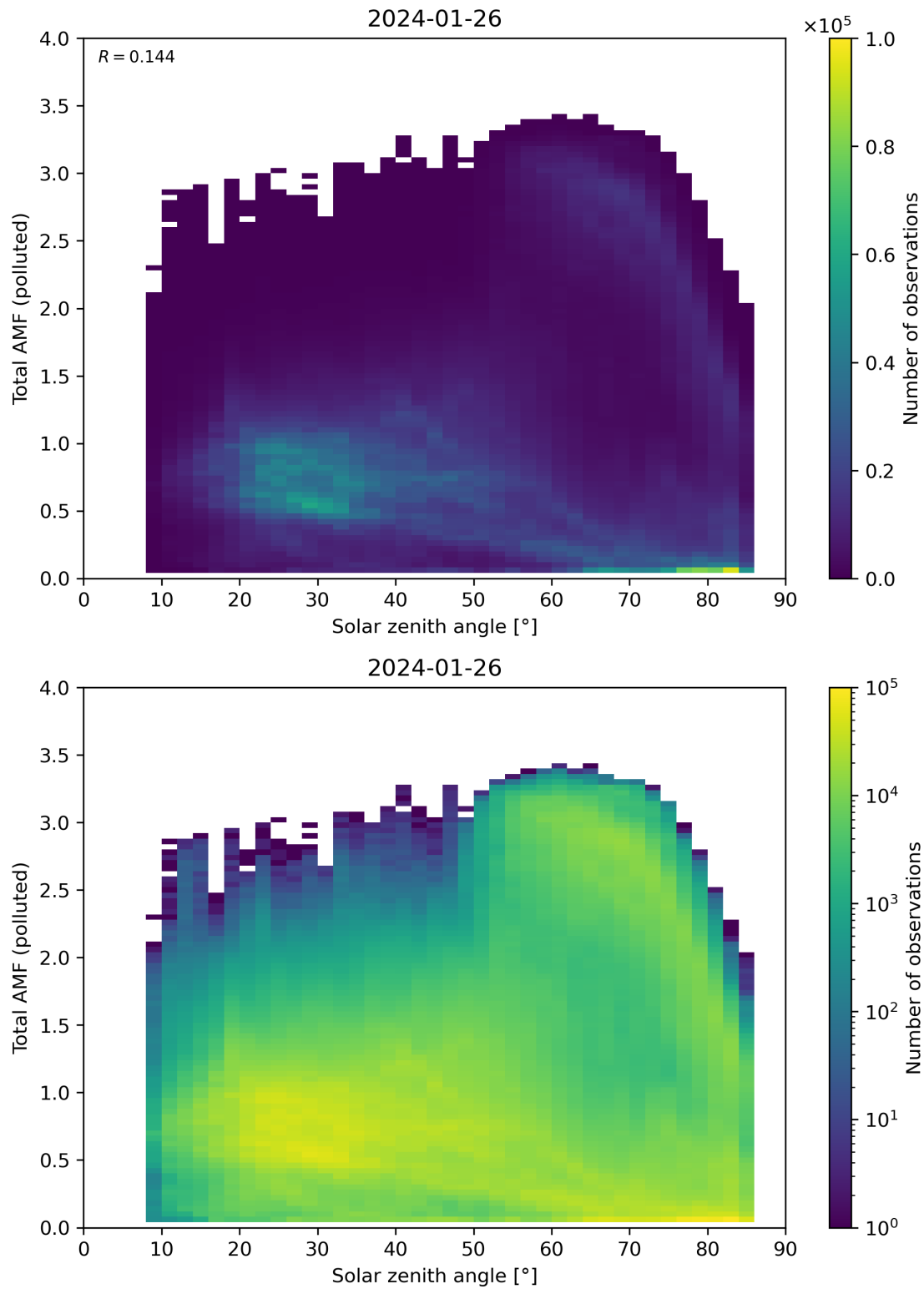
Figure 174: Scatter density plot of “Solar zenith angle” against “Total AMF (polluted)” for 2024-01-26 to 2024-01-27.
