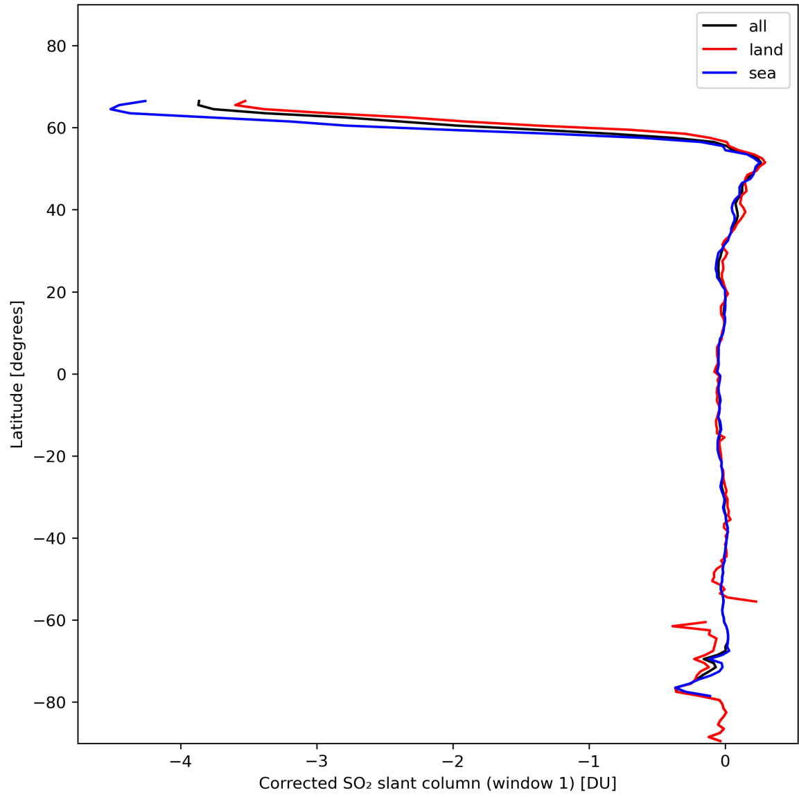
Figure 35: Zonal average of “Corrected SO 2 slant column (window 1)” for 2024-01-26 to 2024-01-27.
