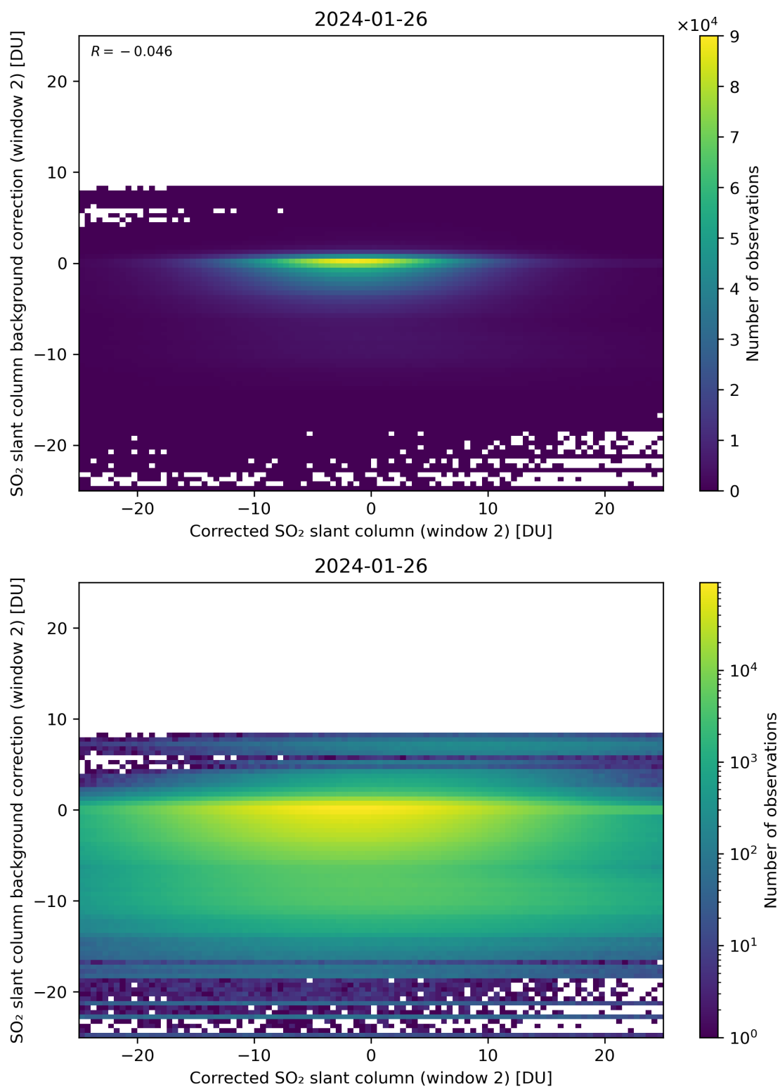
Figure 194: Scatter density plot of “Corrected SO 2 slant column (window 2)” against “SO 2 slant column background correction (window 2)” for 2024-01-26 to 2024-01-27.
