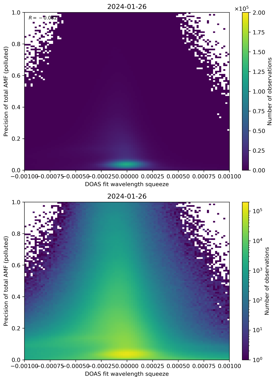
Figure 135: Scatter density plot of “DOAS fit wavelength squeeze” against “Precision of total AMF (polluted)” for 2024-01-26 to 2024-01-27.
