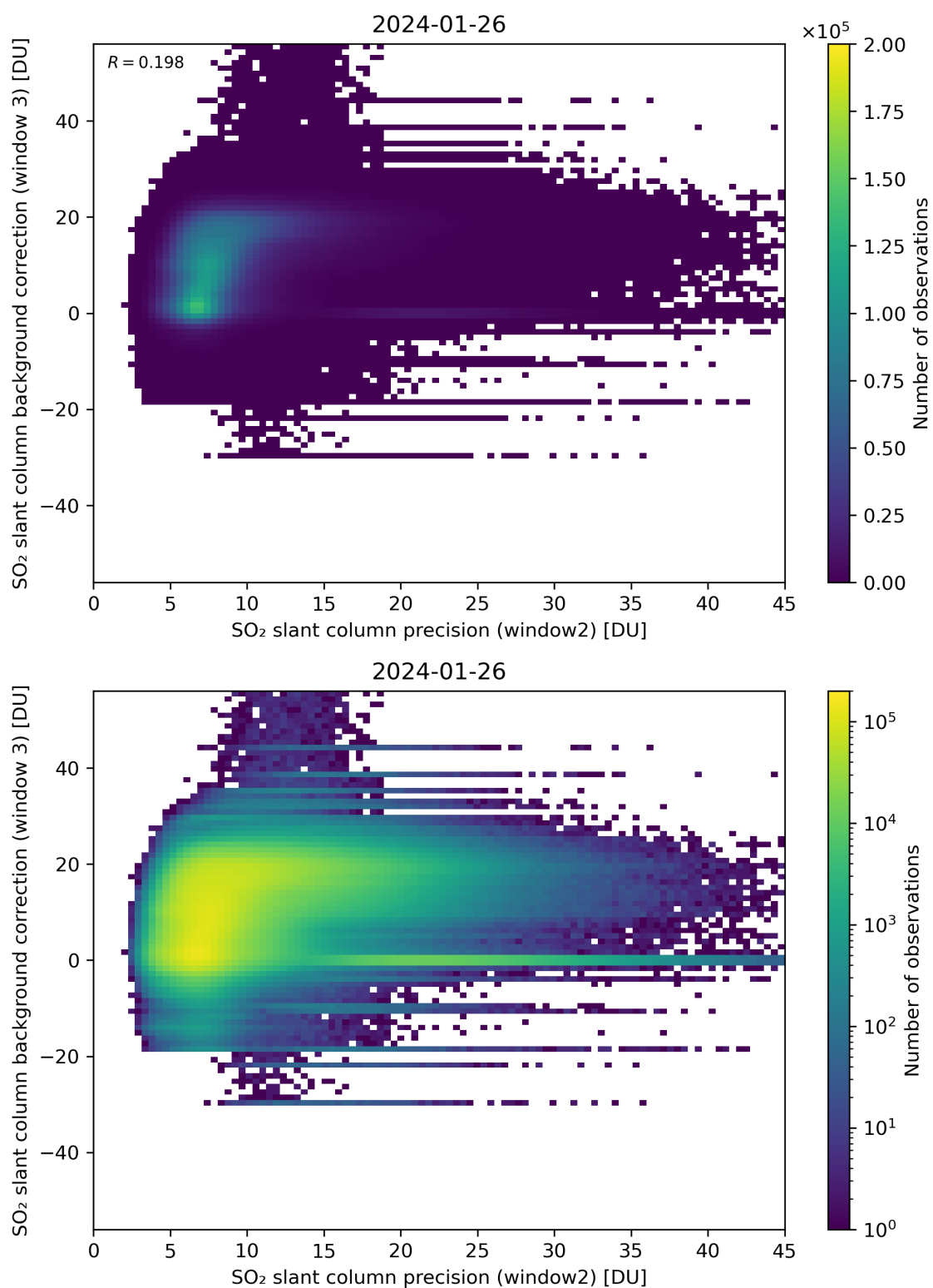
Figure 242: Scatter density plot of “SO 2 slant column precision (window2)” against “SO 2 slant column background correction (window 3)” for 2024-01-26 to 2024-01-27.
