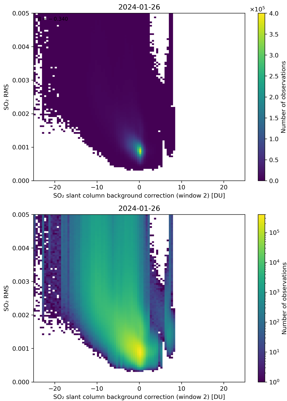
Figure 114: Scatter density plot of “SO 2 slant column background correction (window 2)” against “SO 2 RMS” for 2024-01-26 to 2024-01-27.
