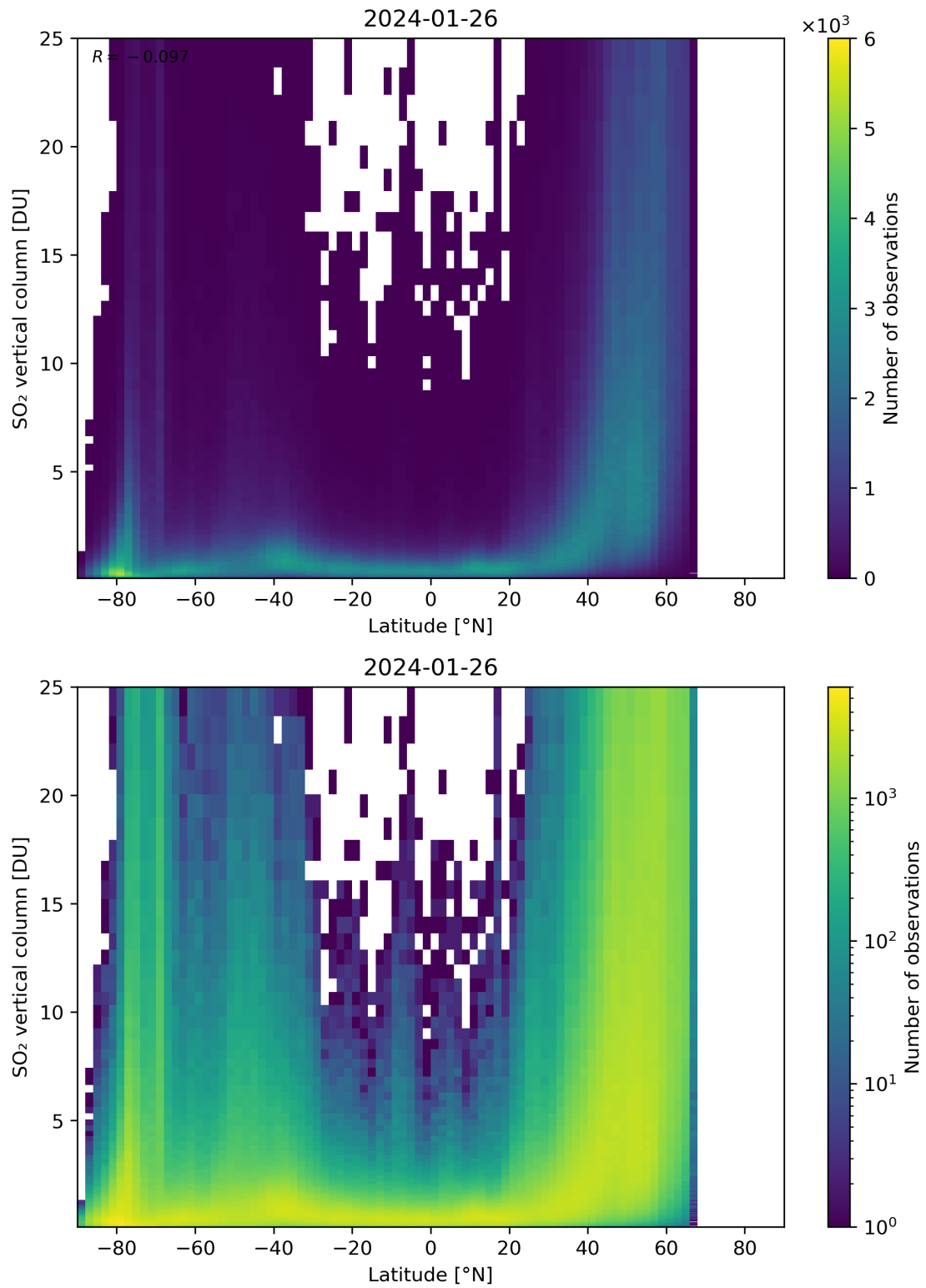
Figure 156: Scatter density plot of “Latitude” against “SO 2 vertical column” for 2024-01-26 to 2024-01-27.
