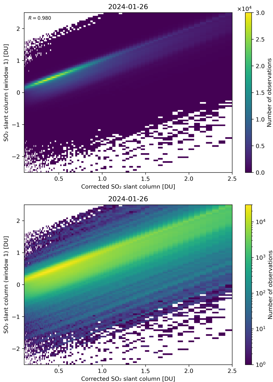
Figure 187: Scatter density plot of “Corrected SO 2 slant column” against “SO 2 slant column (window 1)” for 2024-01-26 to 2024-01-27.
