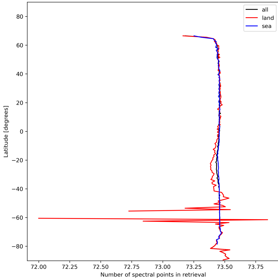
Figure 51: Zonal average of “Number of spectral points in retrieval” for 2024-01-26 to 2024-01-27.
