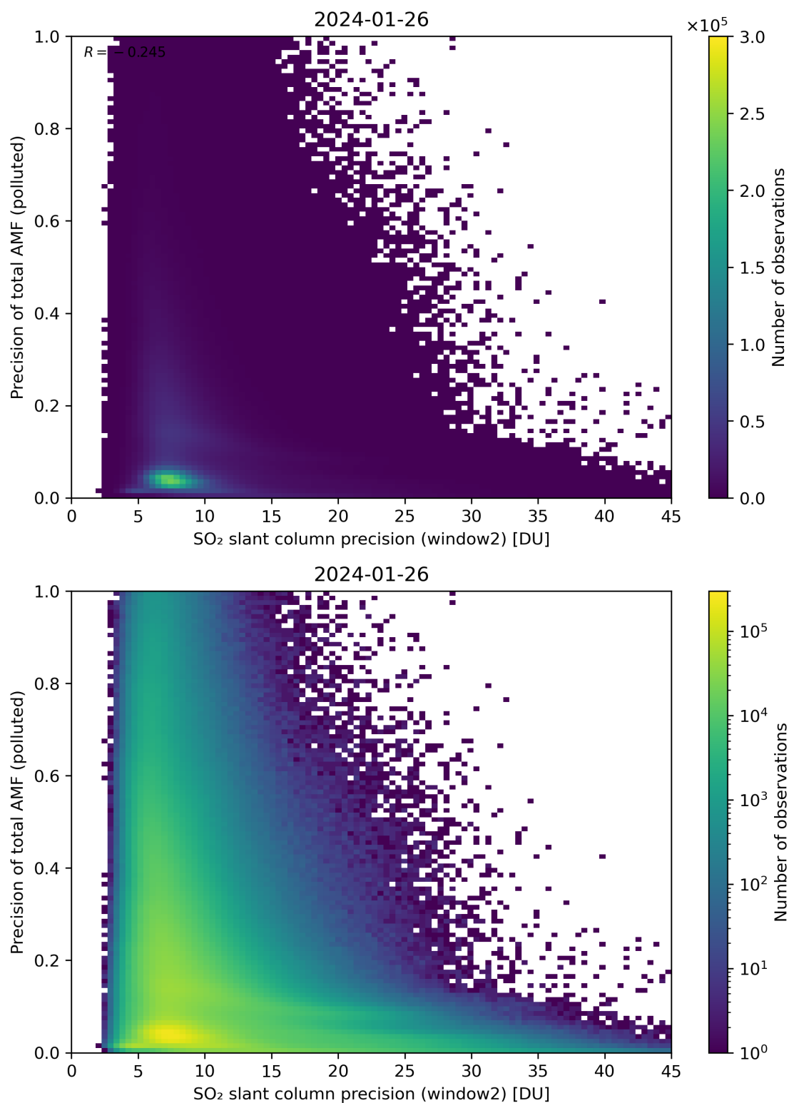
Figure 252: Scatter density plot of “SO 2 slant column precision (window2)” against “Precision of total AMF (polluted)” for 2024-01-26 to 2024-01-27.
