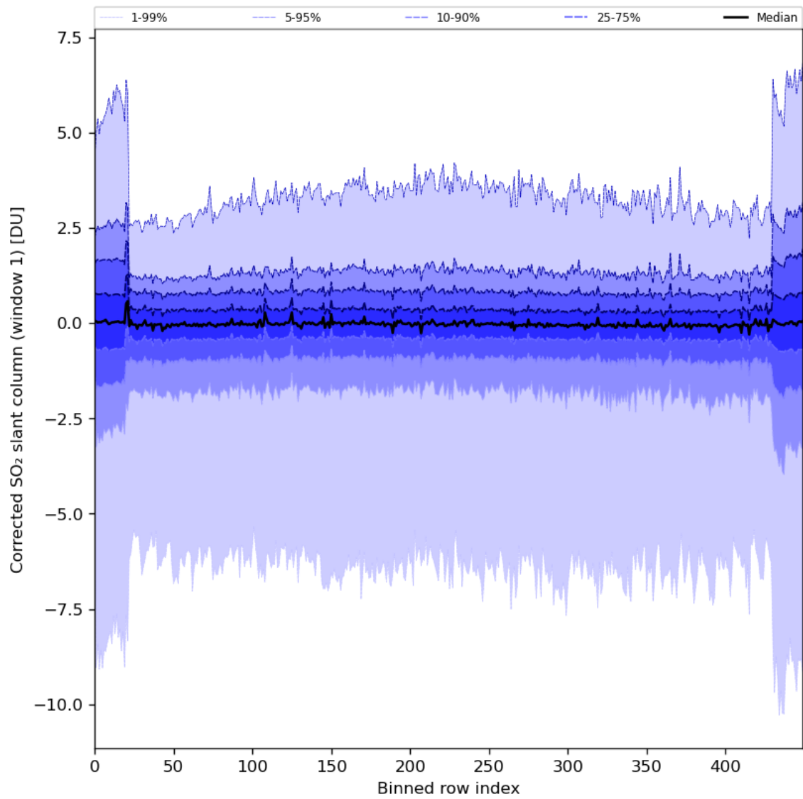
Figure 81: Along track statistics of "Corrected SO 2 slant column (window 1)" for 2024-01-26 to 2024-01-27
