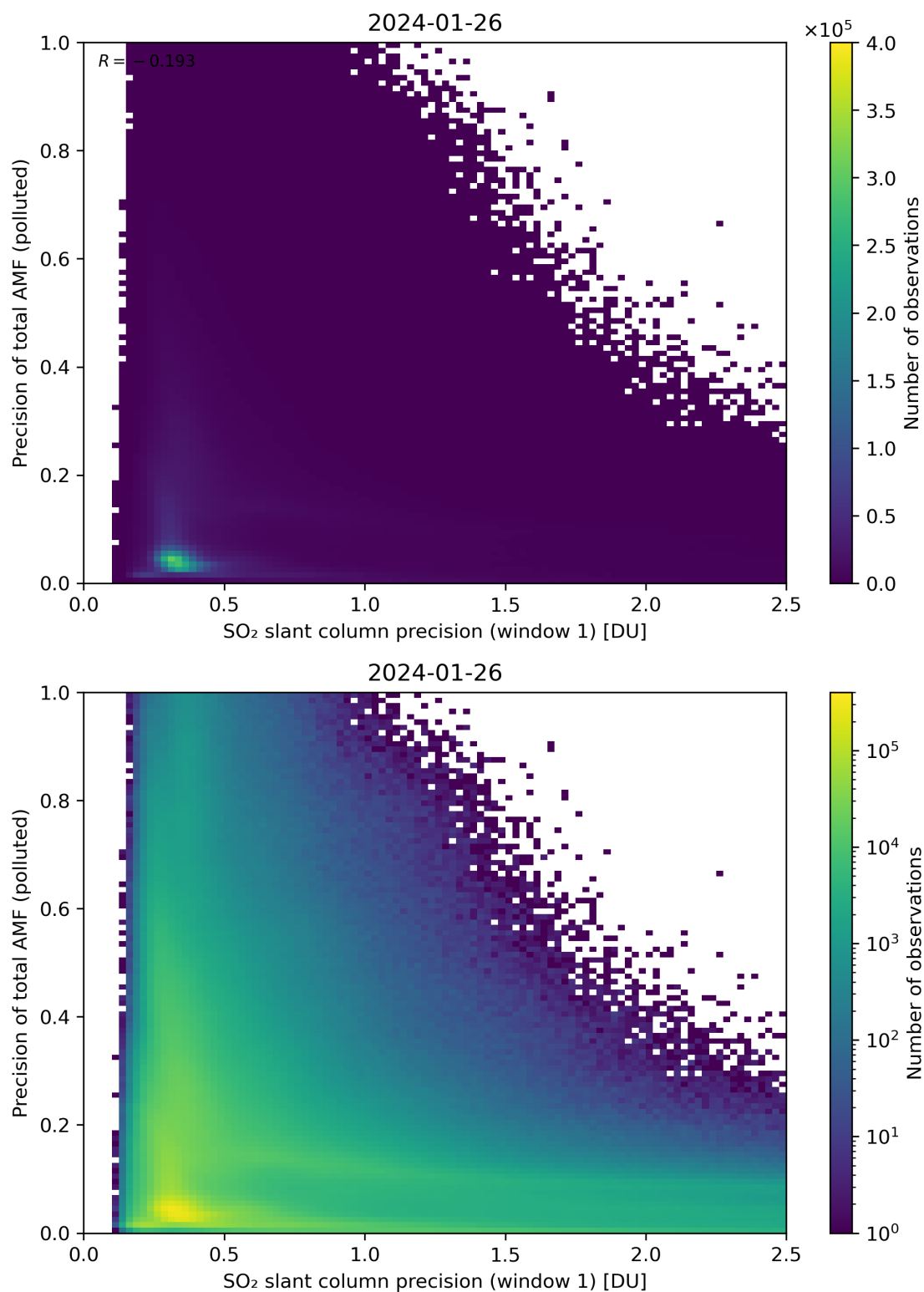
Figure 231: Scatter density plot of “SO 2 slant column precision (window 1)” against “Precision of total AMF (polluted)” for 2024-01-26 to 2024-01-27.
