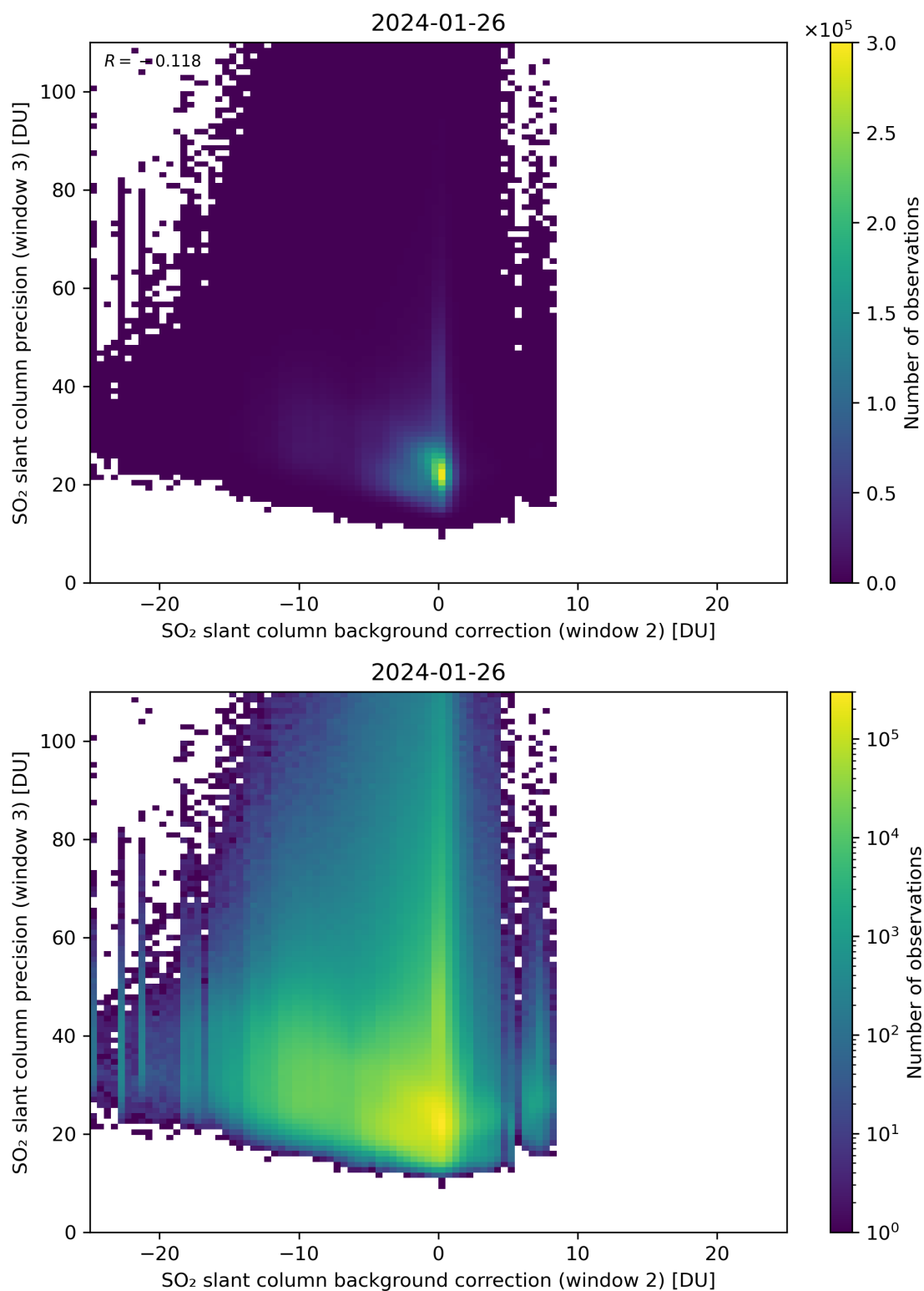
Figure 118: Scatter density plot of “SO 2 slant column background correction (window 2)” against “SO 2 slant column precision (window 3)” for 2024-01-26 to 2024-01-27.
