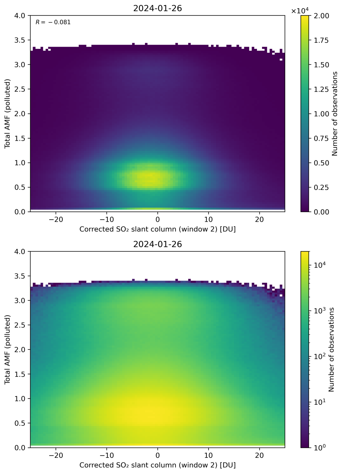
Figure 203: Scatter density plot of “Corrected SO 2 slant column (window 2)” against “Total AMF (polluted)” for 2024-01-26 to 2024-01-27.
