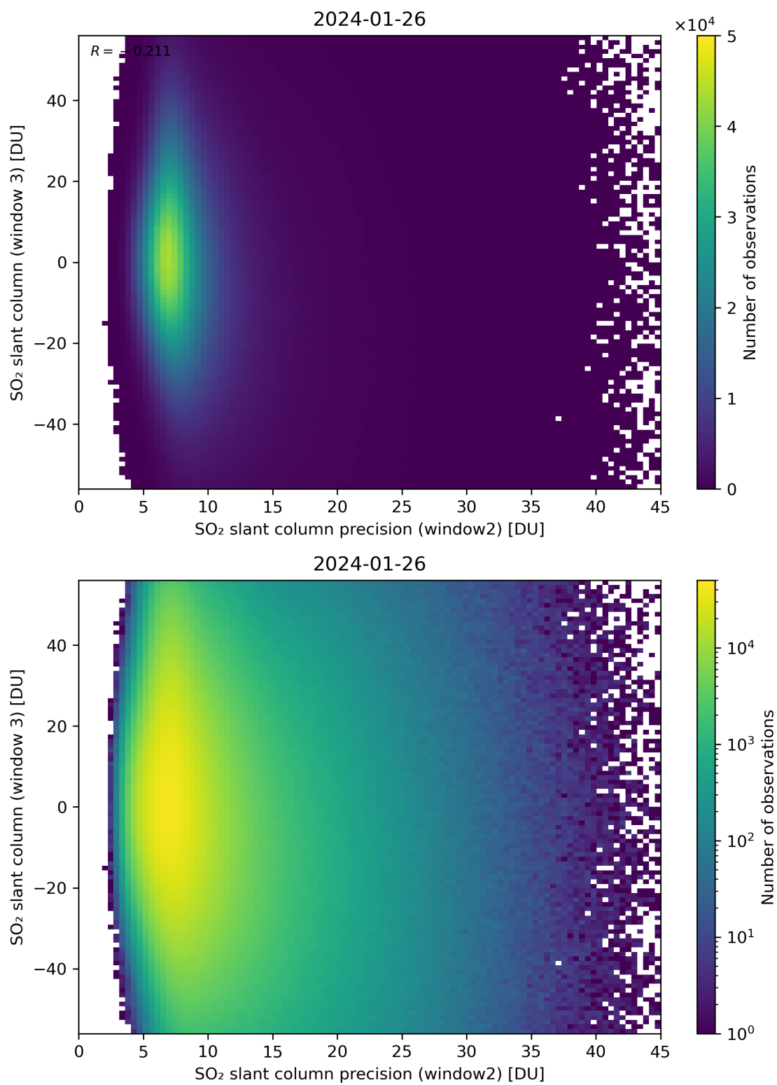
Figure 249: Scatter density plot of “SO 2 slant column precision (window2)” against “SO 2 slant column (window 3)” for 2024-01-26 to 2024-01-27.
