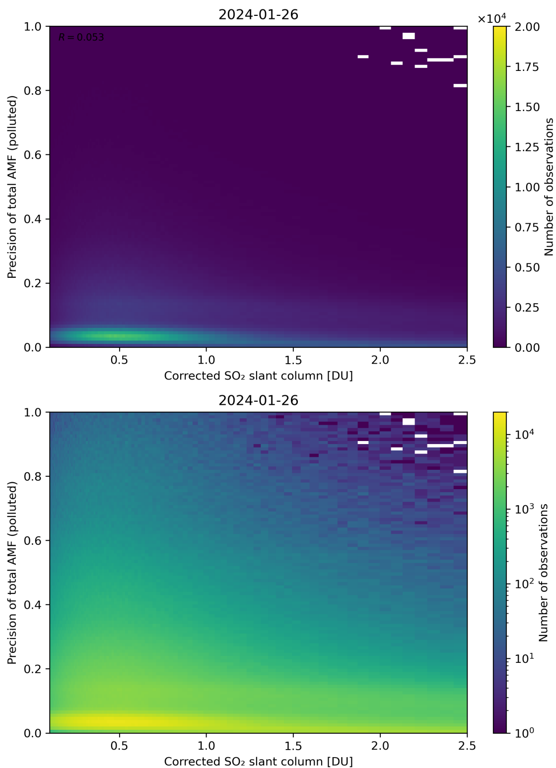
Figure 193: Scatter density plot of “Corrected SO 2 slant column” against “Precision of total AMF (polluted)” for 2024-01-26 to 2024-01-27.
