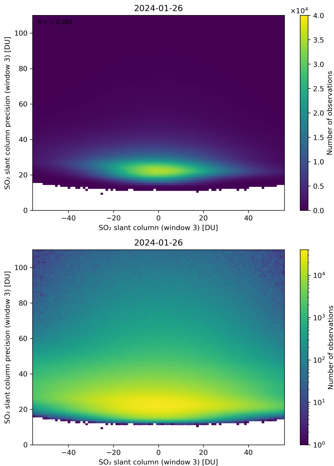
Figure 267: Scatter density plot of “SO 2 slant column (window 3)” against “SO 2 slant column precision (window 3)” for 2024-01-26 to 2024-01-27.
