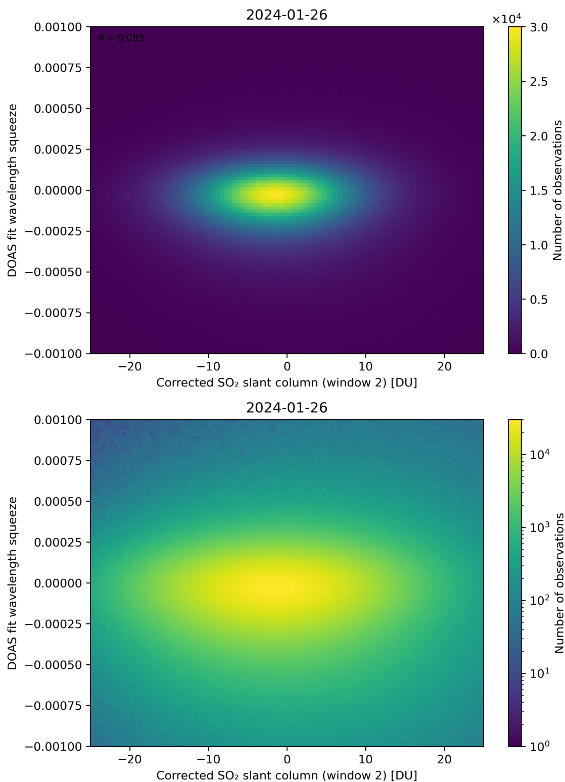
Figure 197: Scatter density plot of “Corrected SO 2 slant column (window 2)” against “DOAS fit wavelength squeeze” for 2024-01-26 to 2024-01-27.
