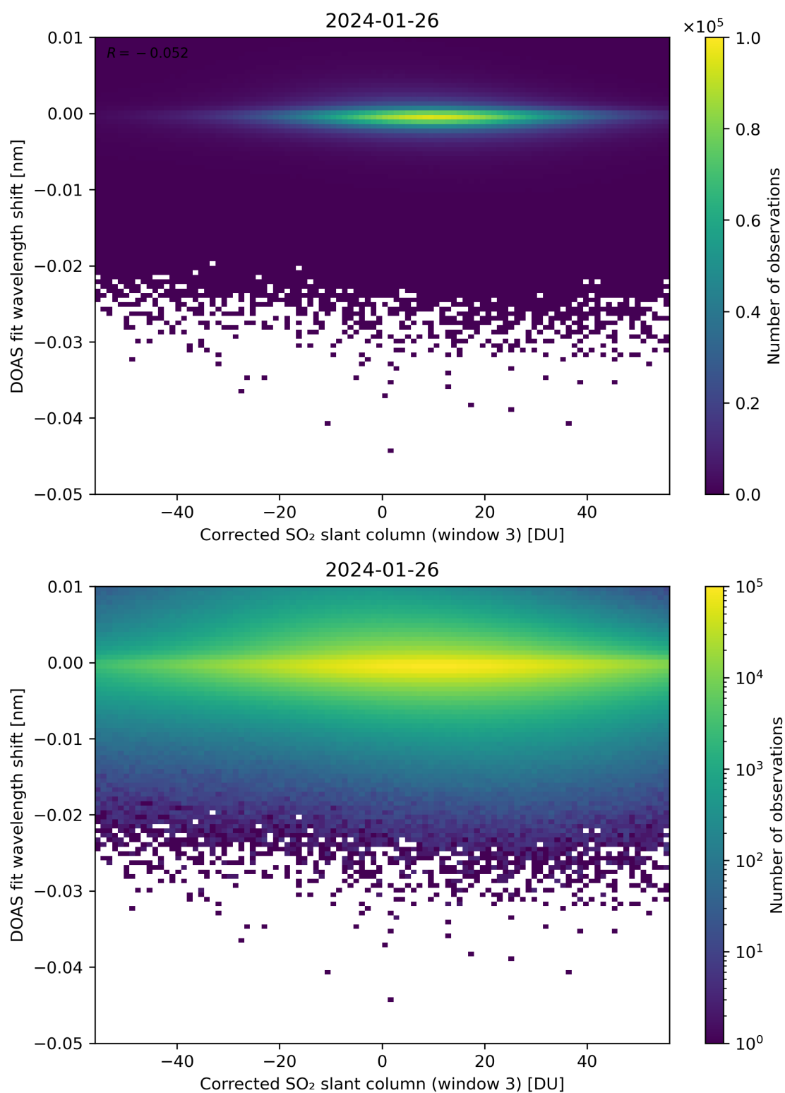
Figure 206: Scatter density plot of “Corrected SO 2 slant column (window 3)” against “DOAS fit wavelength shift” for 2024-01-26 to 2024-01-27.
