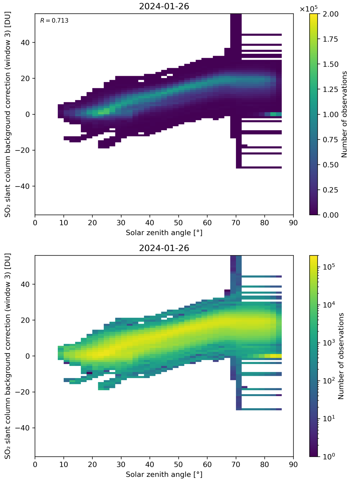
Figure 160: Scatter density plot of “Solar zenith angle” against “SO 2 slant column background correction (window 3)” for 2024-01-26 to 2024-01-27.
