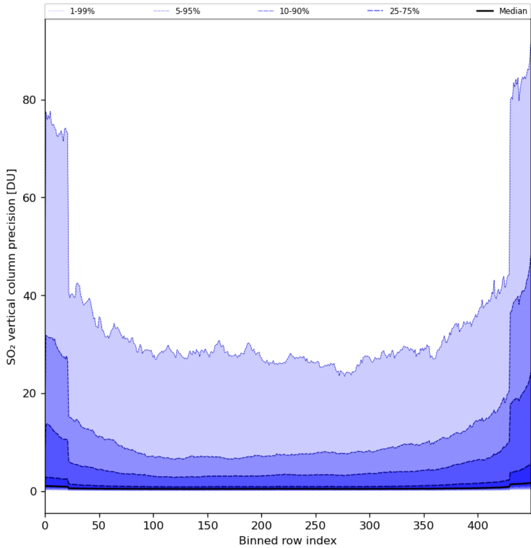
Figure 77: Along track statistics of “SO 2 vertical column precision” for 2024-01-26 to 2024-01-27
