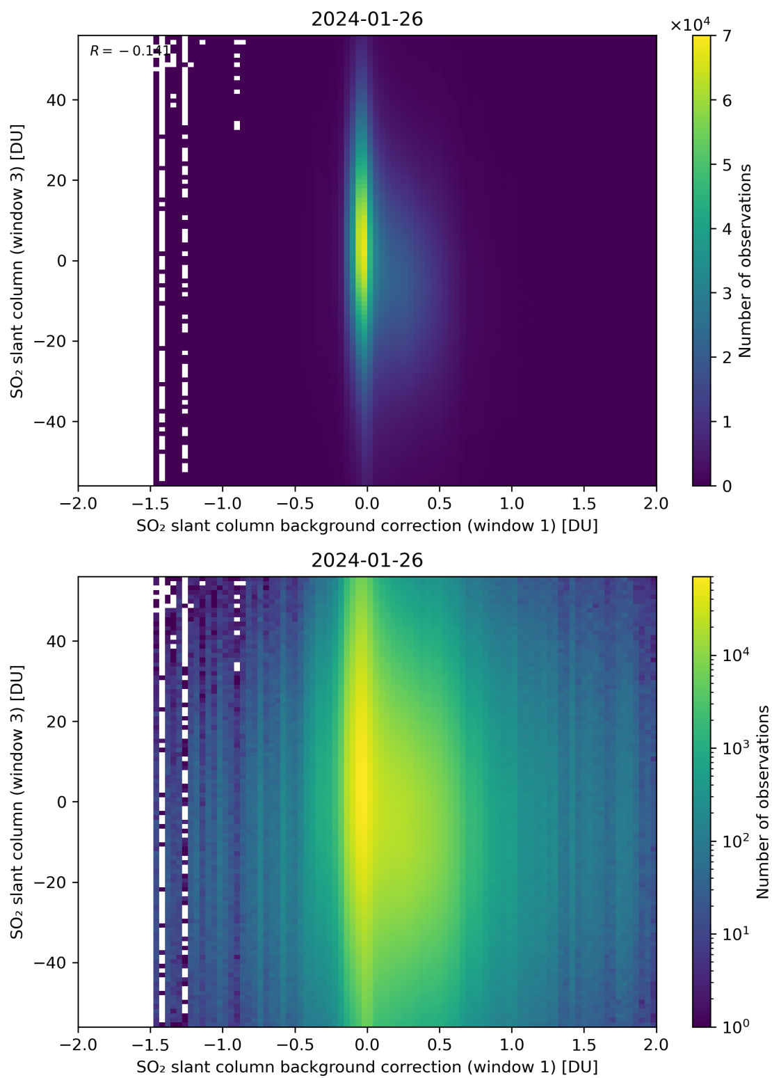
Figure 107: Scatter density plot of “SO 2 slant column background correction (window 1)” against “SO 2 slant column (window 3)” for 2024-01-26 to 2024-01-27.
