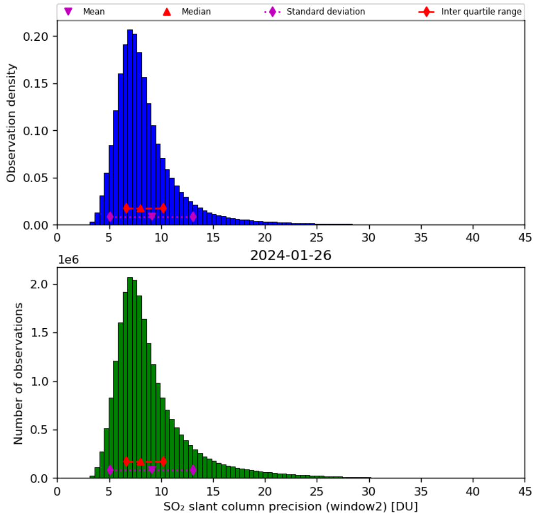
Figure 61: Histogram of “SO 2 slant column precision (window2)” for 2024-01-26 to 2024-01-27
