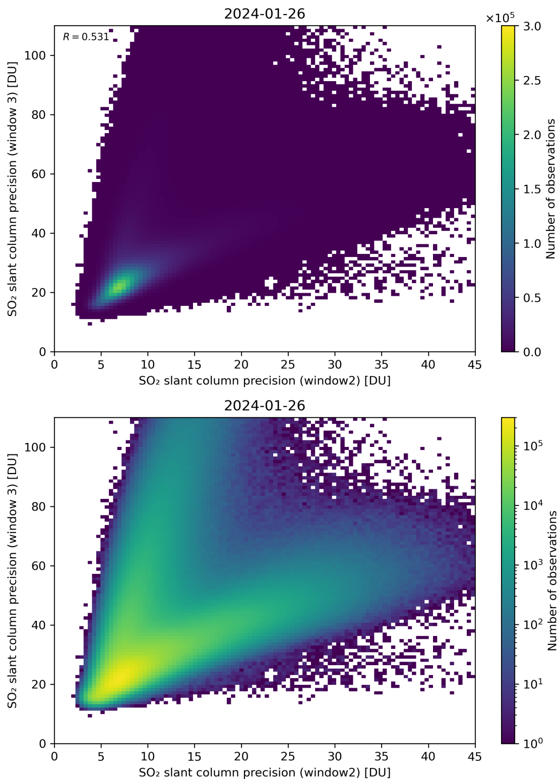
Figure 250: Scatter density plot of “SO 2 slant column precision (window2)” against “SO 2 slant column precision (window 3)” for 2024-01-26 to 2024-01-27.
