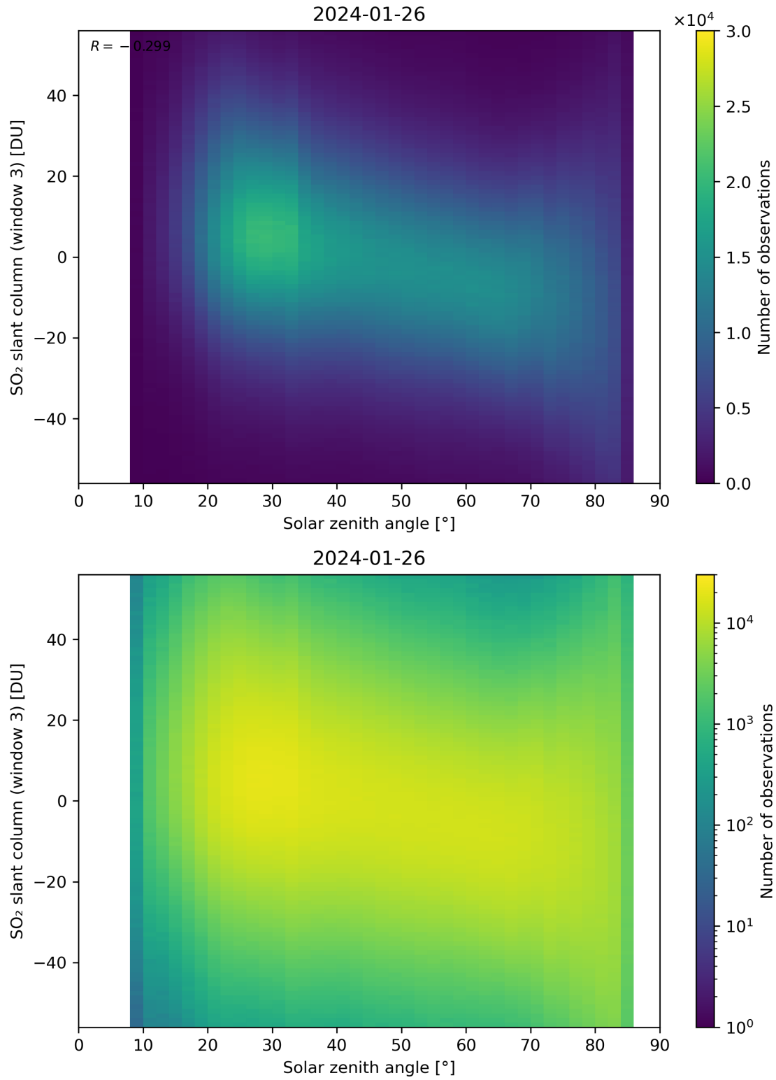
Figure 172: Scatter density plot of “Solar zenith angle” against “SO 2 slant column (window 3)” for 2024-01-26 to 2024-01-27.
