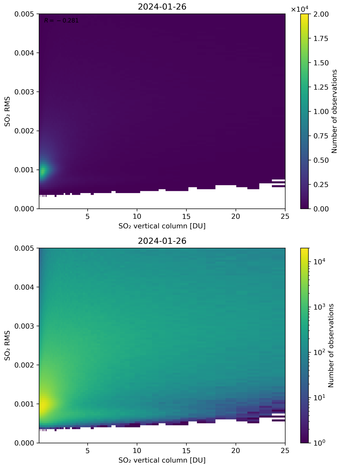
Figure 278: Scatter density plot of “SO 2 vertical column” against “SO 2 RMS” for 2024-01-26 to 2024-01-27.
