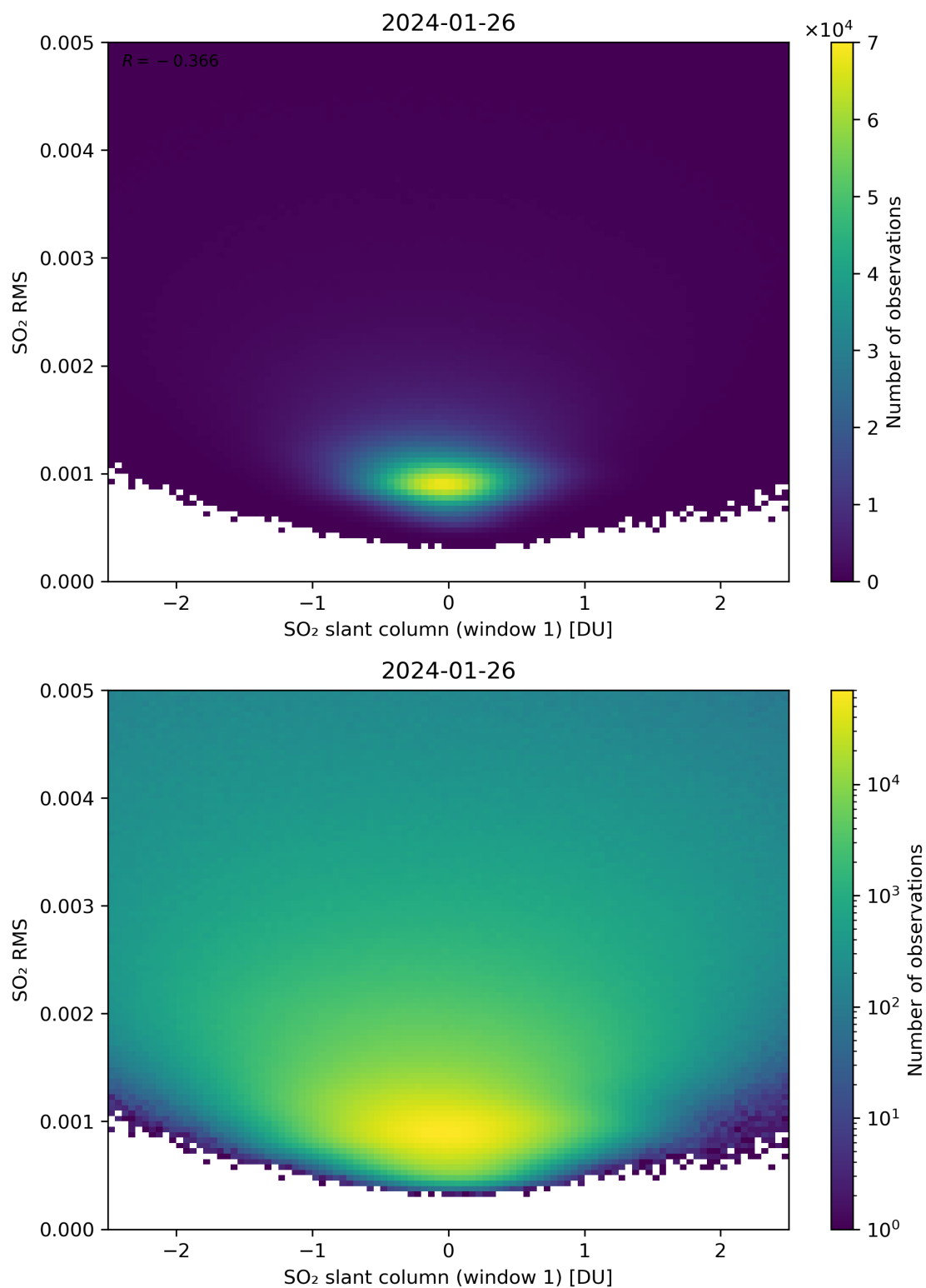
Figure 217: Scatter density plot of “SO 2 slant column (window 1)” against “SO 2 RMS” for 2024-01-26 to 2024-01-27.
