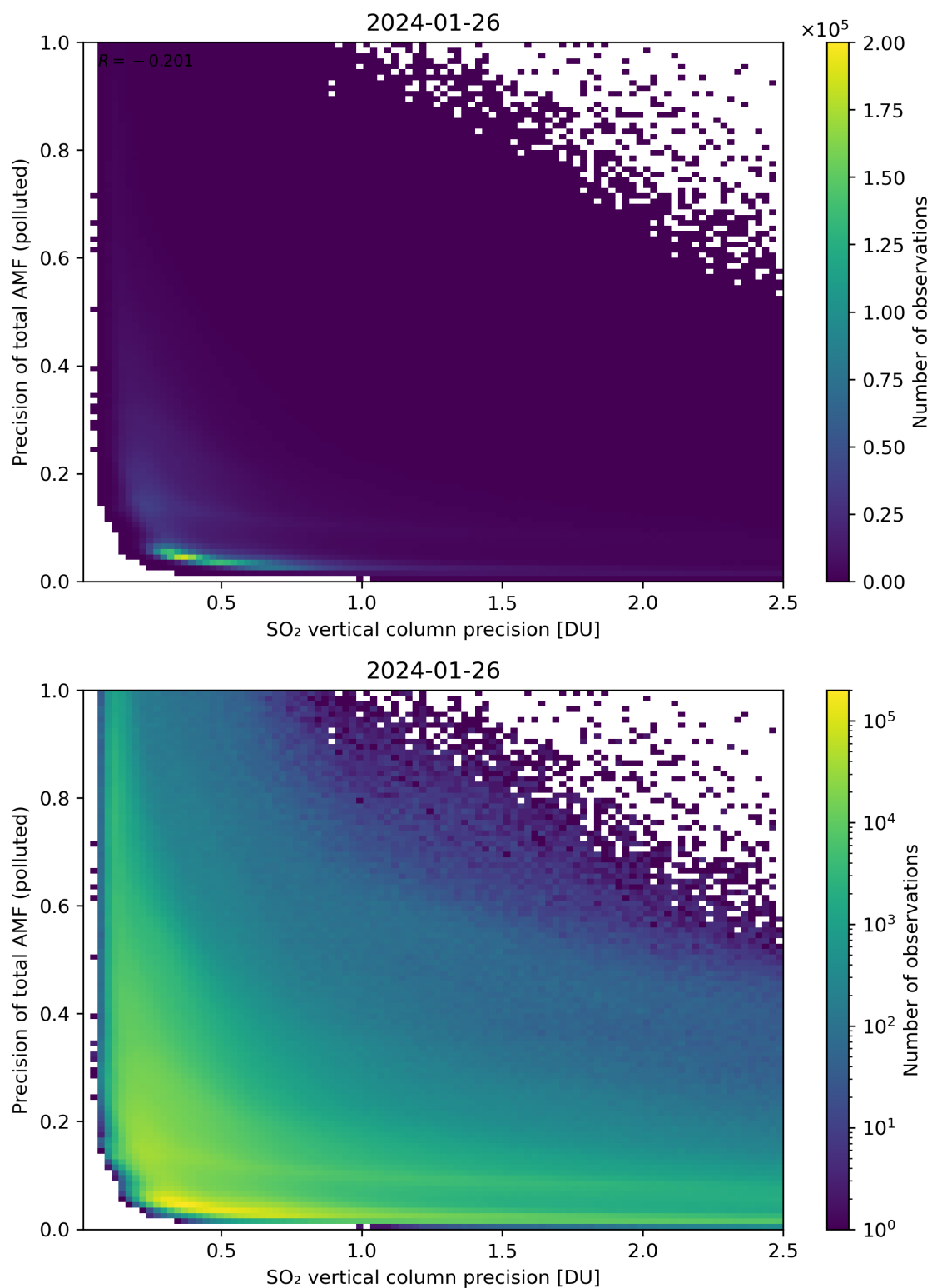
Figure 295: Scatter density plot of “SO 2 vertical column precision” against “Precision of total AMF (polluted)” for 2024-01-26 to 2024-01-27.
