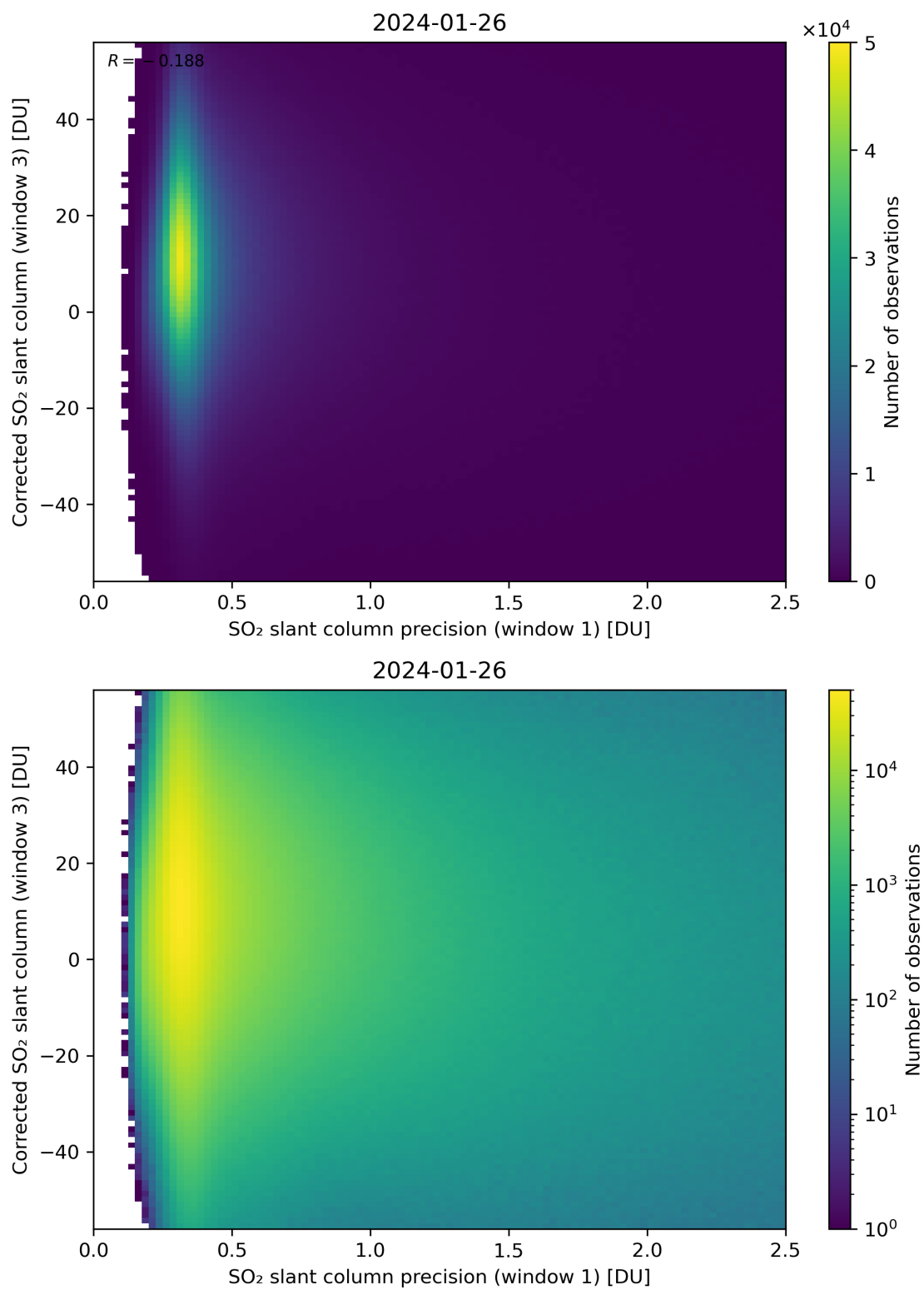
Figure 226: Scatter density plot of “SO 2 slant column precision (window 1)” against “Corrected SO 2 slant column (window 3)” for 2024-01-26 to 2024-01-27.
