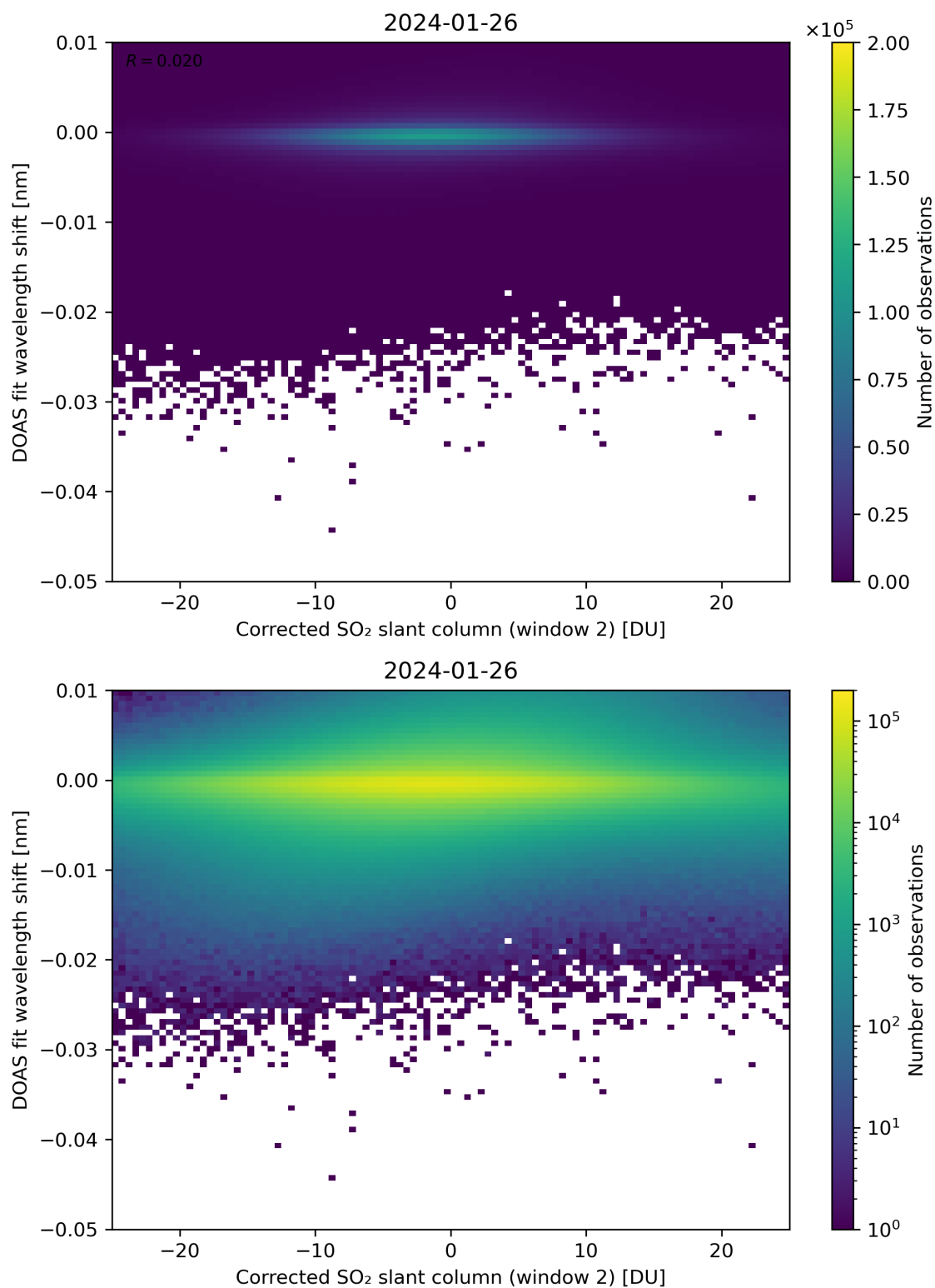
Figure 196: Scatter density plot of “Corrected SO 2 slant column (window 2)” against “DOAS fit wavelength shift” for 2024-01-26 to 2024-01-27.
