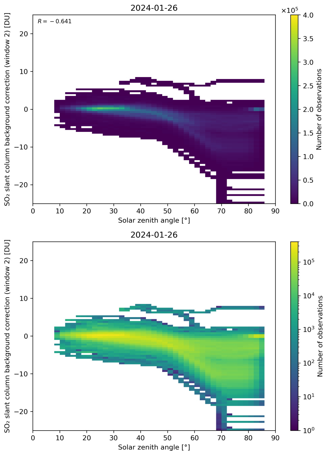
Figure 159: Scatter density plot of “Solar zenith angle” against “SO 2 slant column background correction (window 2)” for 2024-01-26 to 2024-01-27.
