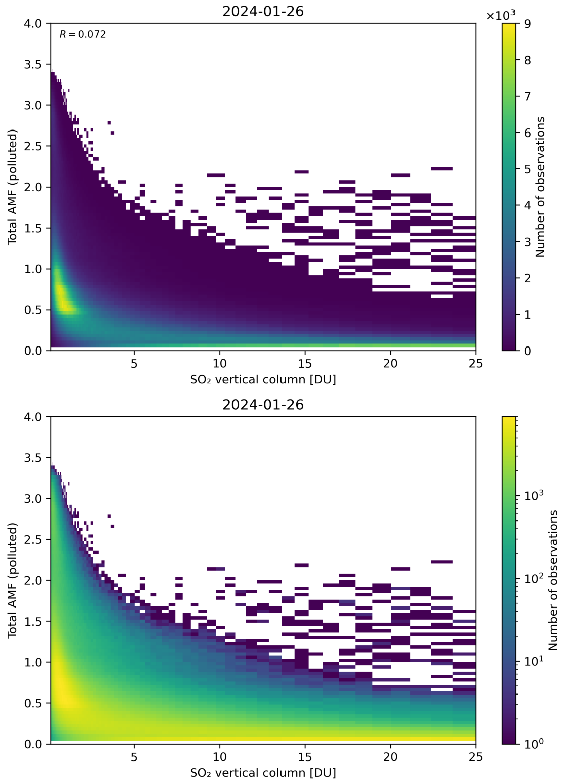
Figure 305: Scatter density plot of “SO 2 vertical column” against “Total AMF (polluted)” for 2024-01-26 to 2024-01-27.
