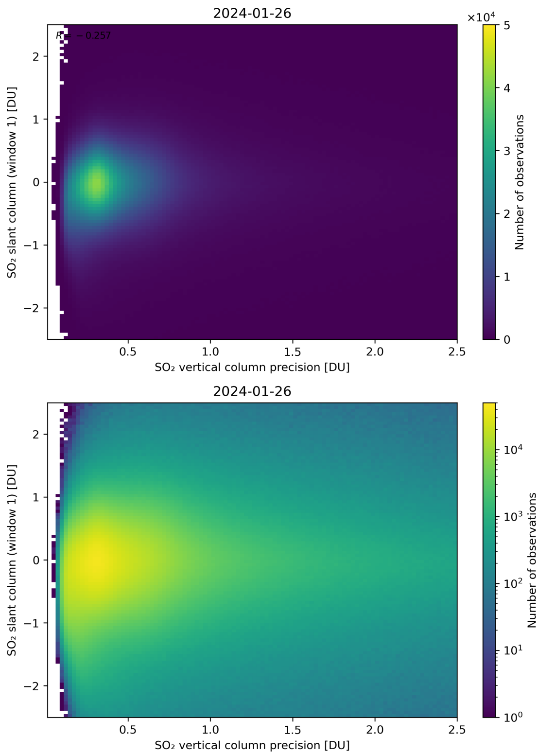
Figure 289: Scatter density plot of “SO 2 vertical column precision” against “SO 2 slant column (window 1)” for 2024-01-26 to 2024-01-27.
