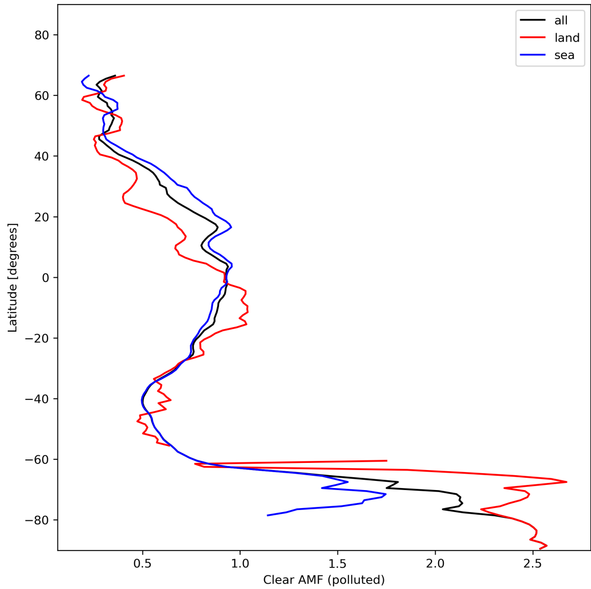
Figure 50: Zonal average of “Clear AMF (polluted)” for 2024-01-26 to 2024-01-27.
