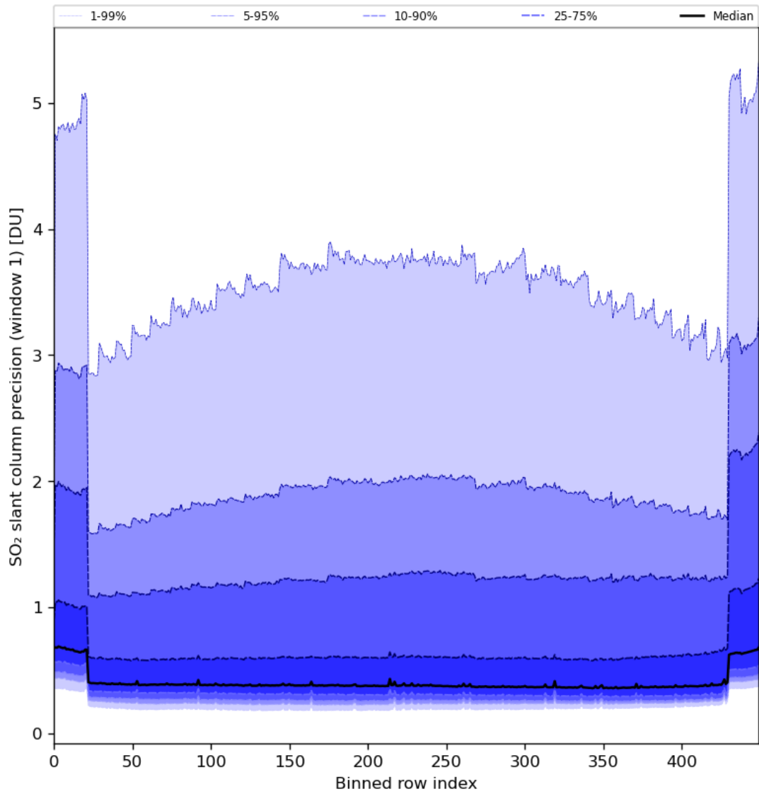
Figure 80: Along track statistics of “SO 2 slant column precision (window 1)” for 2024-01-26 to 2024-01-27
