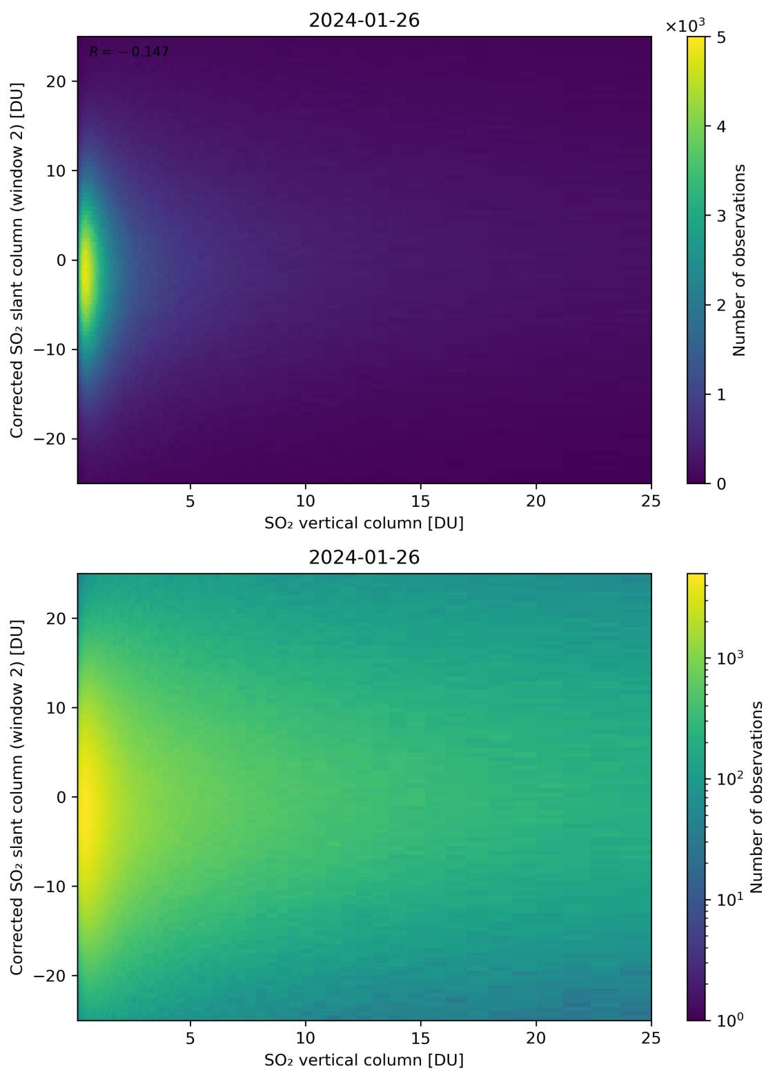
Figure 298: Scatter density plot of “SO 2 vertical column” against “Corrected SO 2 slant column (window 2)” for 2024-01-26 to 2024-01-27.
