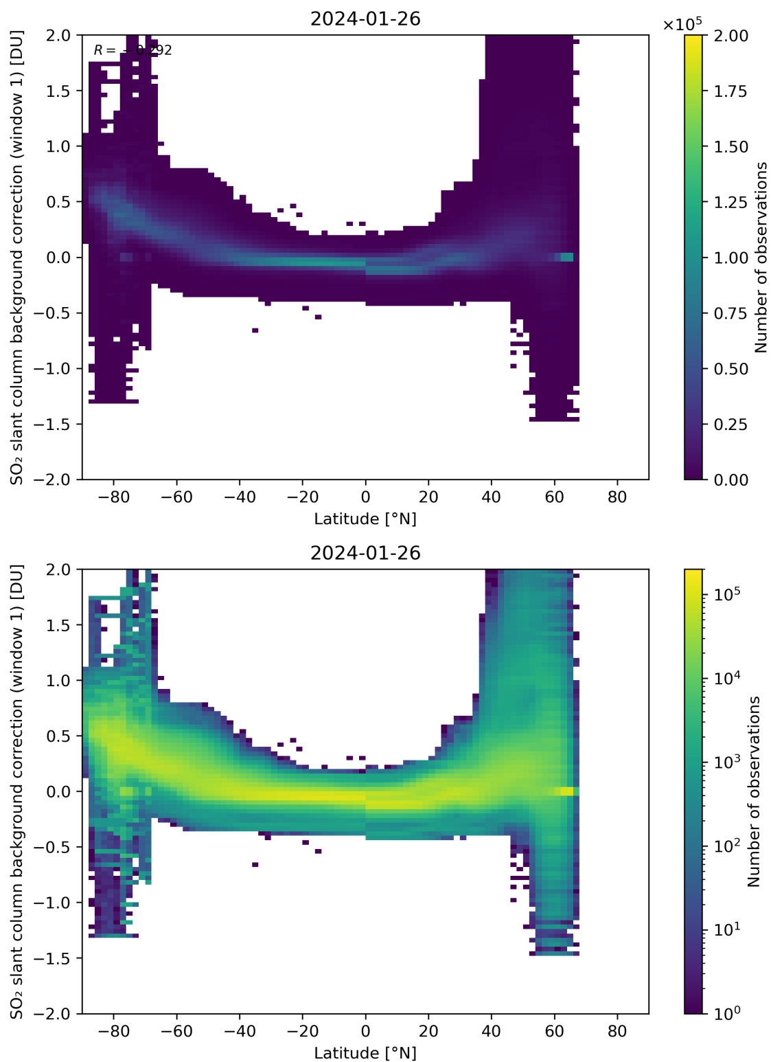
Figure 139: Scatter density plot of “Latitude” against “SO 2 slant column background correction (window 1)” for 2024-01-26 to 2024-01-27.
