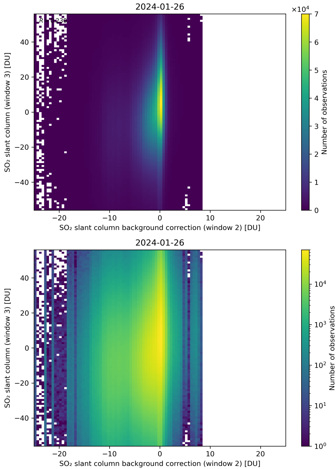
Figure 117: Scatter density plot of “SO 2 slant column background correction (window 2)” against “SO 2 slant column (window 3)” for 2024-01-26 to 2024-01-27.
