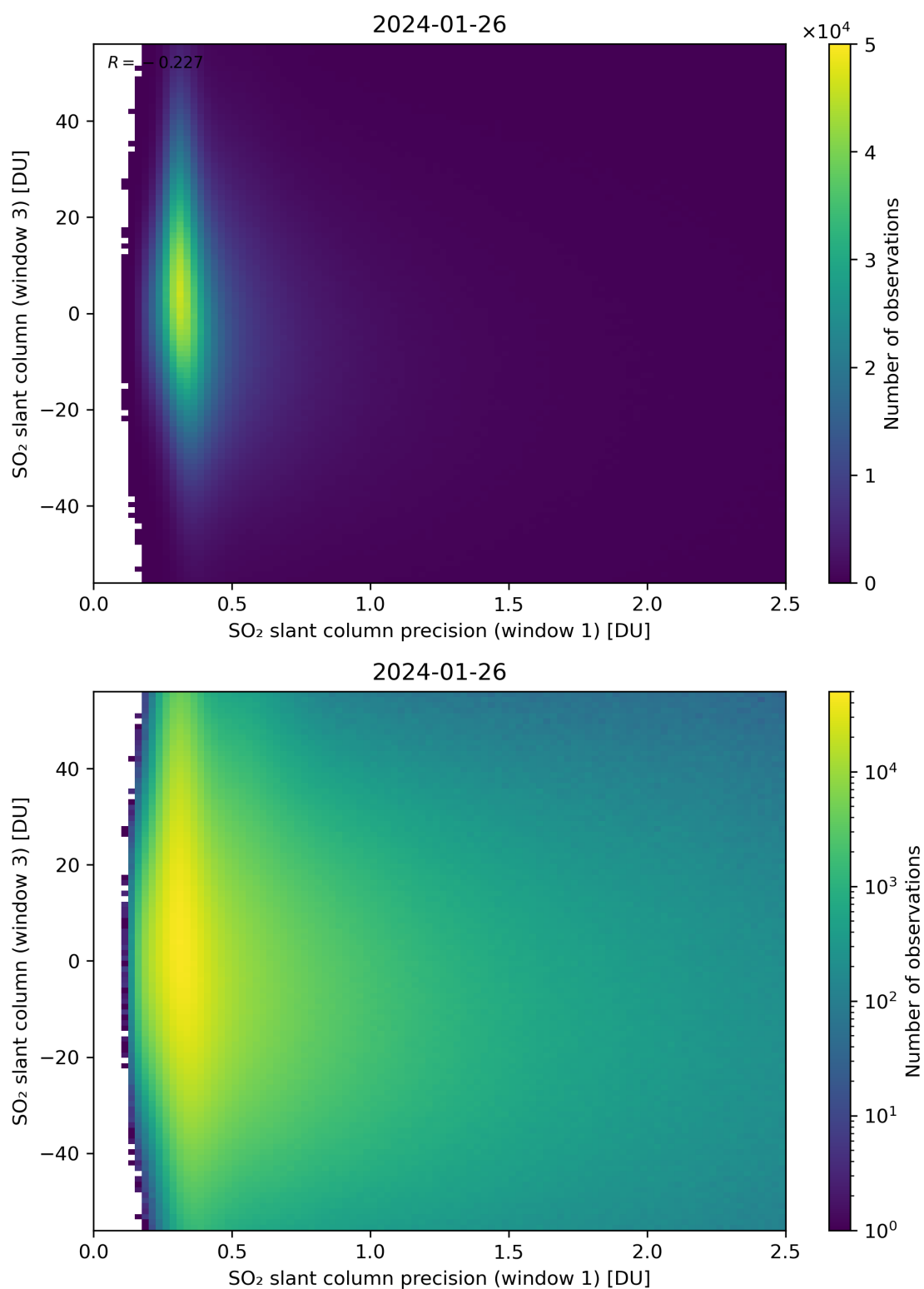
Figure 228: Scatter density plot of “SO 2 slant column precision (window 1)” against “SO 2 slant column (window 3)” for 2024-01-26 to 2024-01-27.
