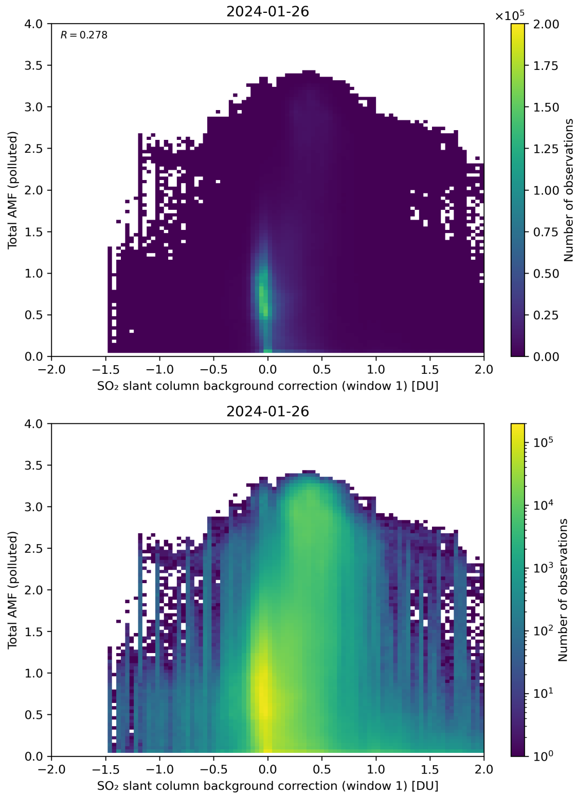
Figure 109: Scatter density plot of “SO 2 slant column background correction (window 1)” against “Total AMF (polluted)” for 2024-01-26 to 2024-01-27.
