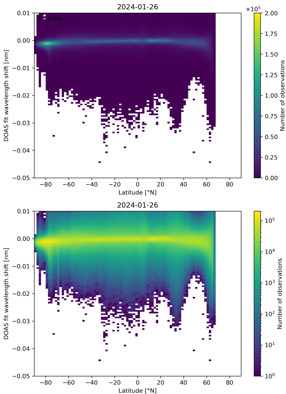
Figure 142: Scatter density plot of “Latitude” against “DOAS fit wavelength shift” for 2024-01-26 to 2024-01-27.
