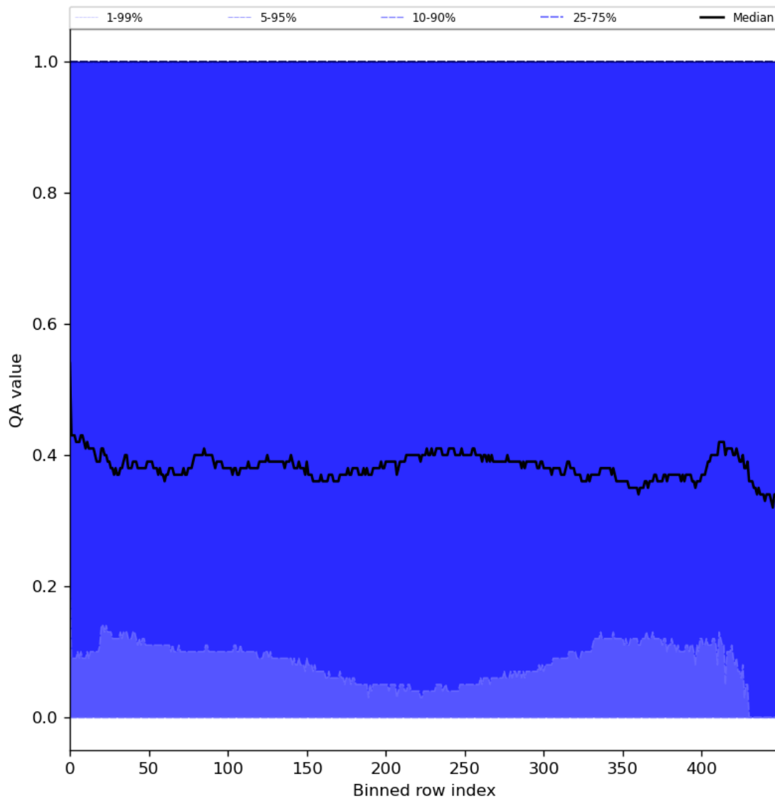
Figure 75: Along track statistics of “QA value” for 2024-01-26 to 2024-01-27
