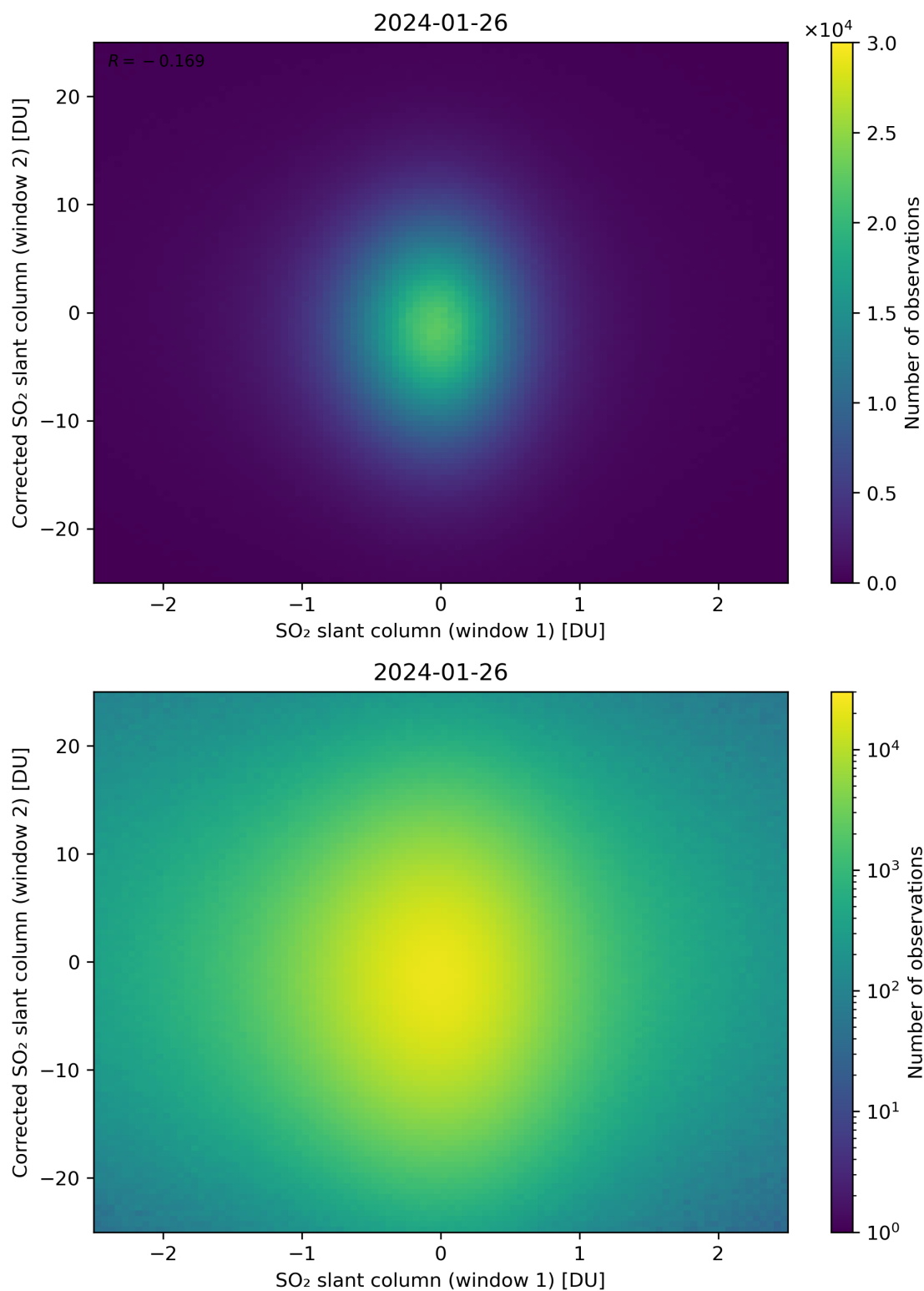
Figure 233: Scatter density plot of “SO 2 slant column (window 1)” against “Corrected SO 2 slant column (window 2)” for 2024-01-26 to 2024-01-27.
