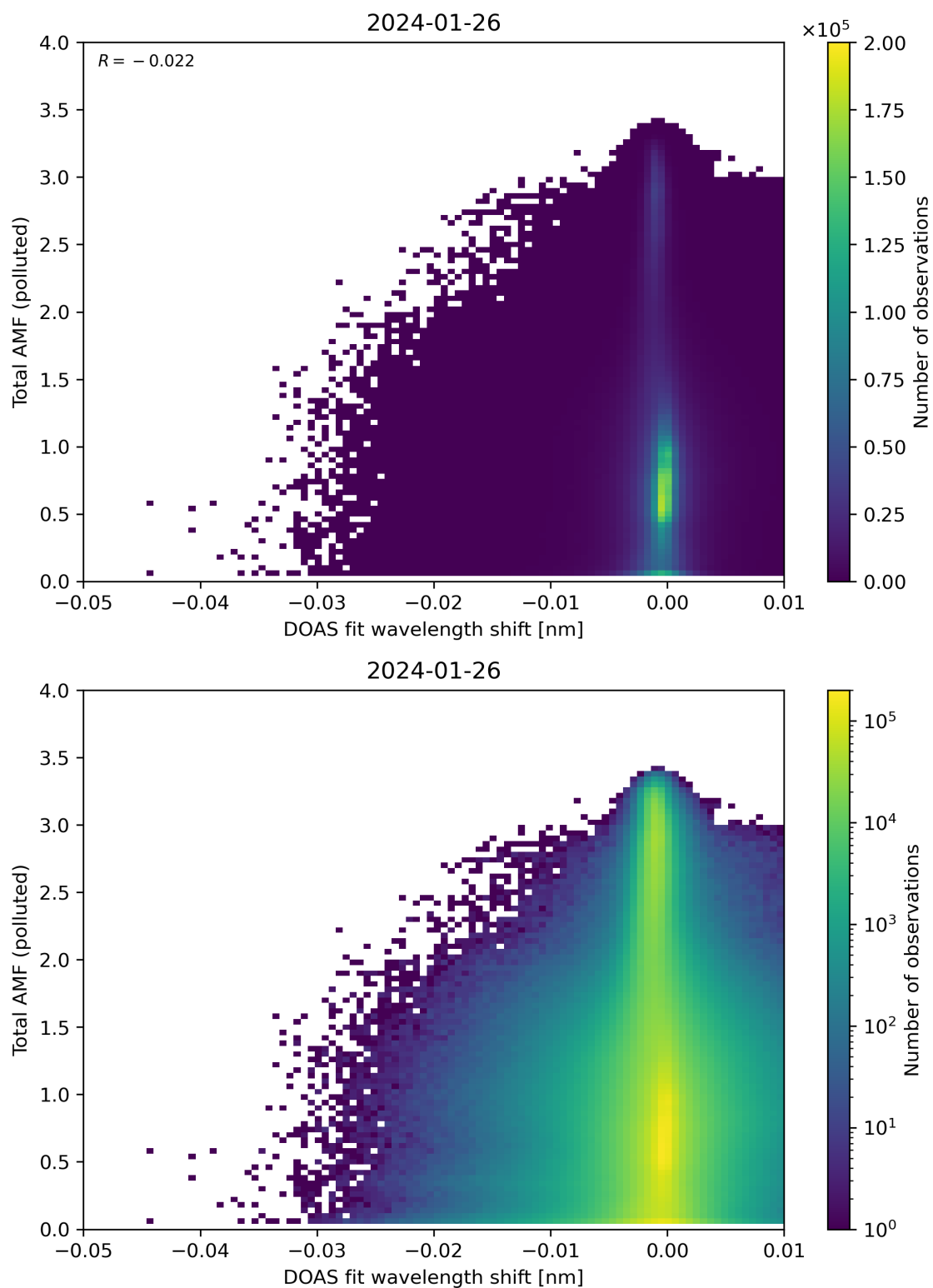
Figure 130: Scatter density plot of “DOAS fit wavelength shift” against “Total AMF (polluted)” for 2024-01-26 to 2024-01-27.
