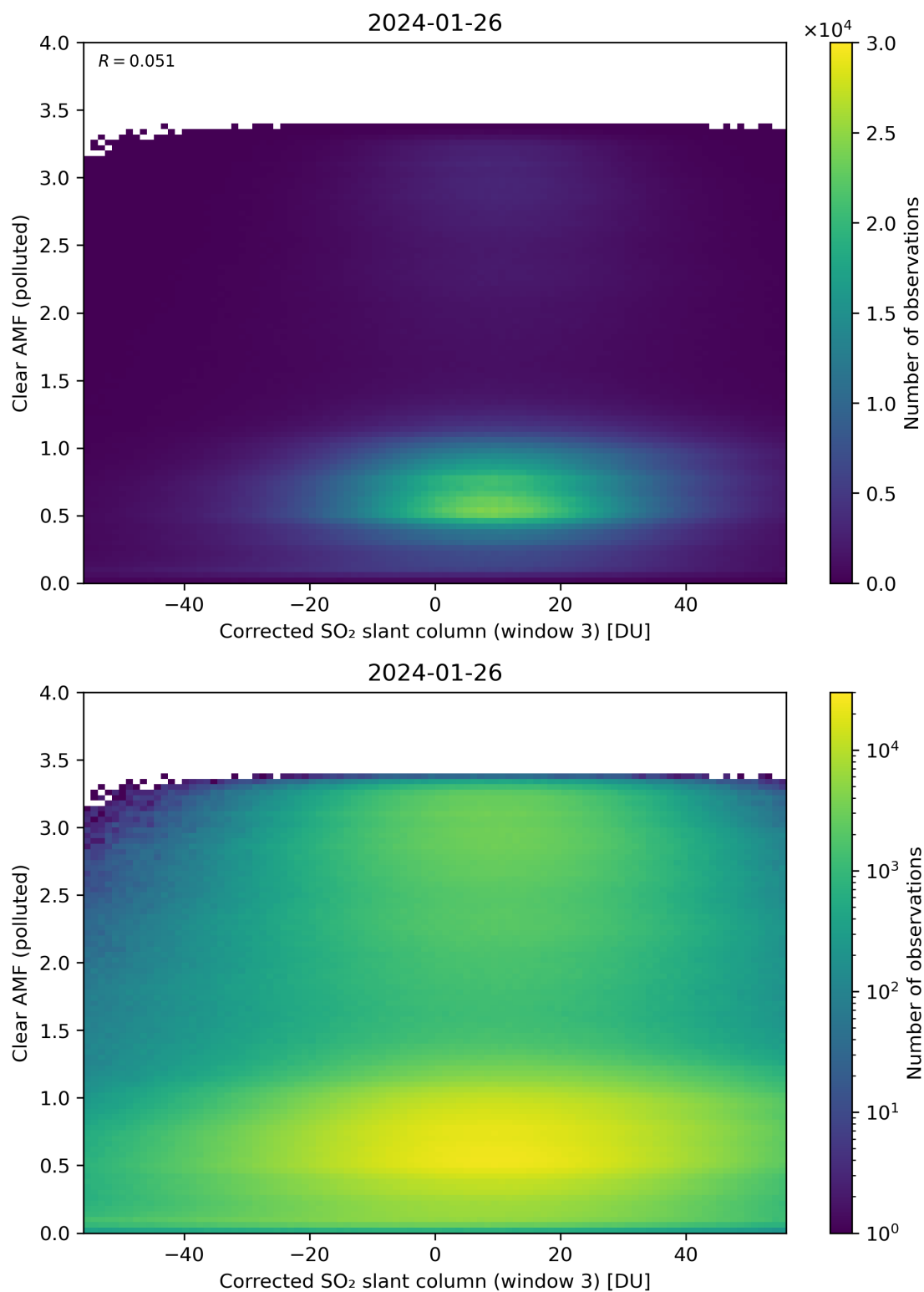
Figure 209: Scatter density plot of “Corrected SO 2 slant column (window 3)” against “Clear AMF (polluted)” for 2024-01-26 to 2024-01-27.
