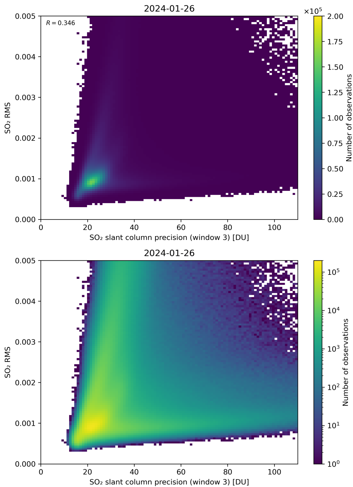
Figure 260: Scatter density plot of “SO 2 slant column precision (window 3)” against “SO 2 RMS” for 2024-01-26 to 2024-01-27.
