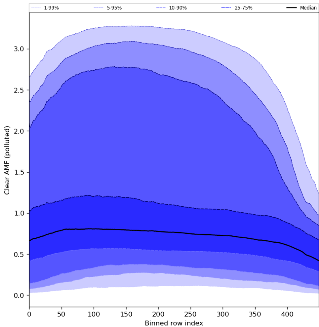
Figure 96: Along track statistics of “Clear AMF (polluted)” for 2024-01-26 to 2024-01-27
