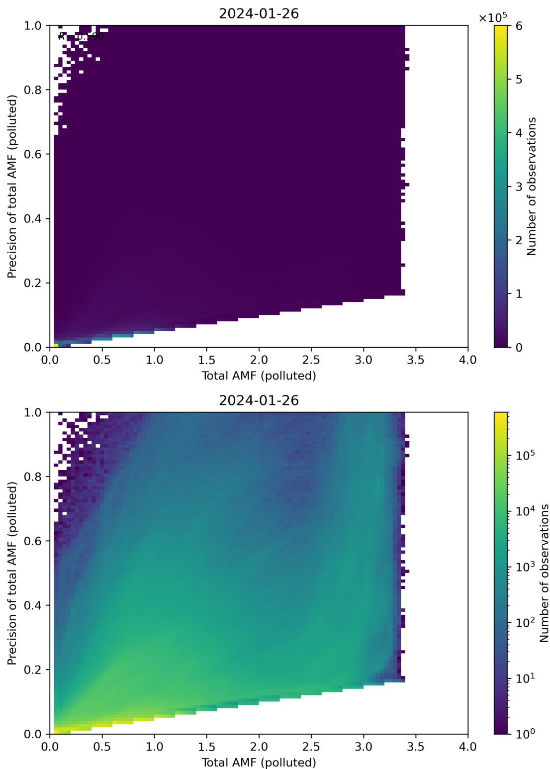
Figure 272: Scatter density plot of “Total AMF (polluted)” against “Precision of total AMF (polluted)” for 2024-01-26 to 2024-01-27.
