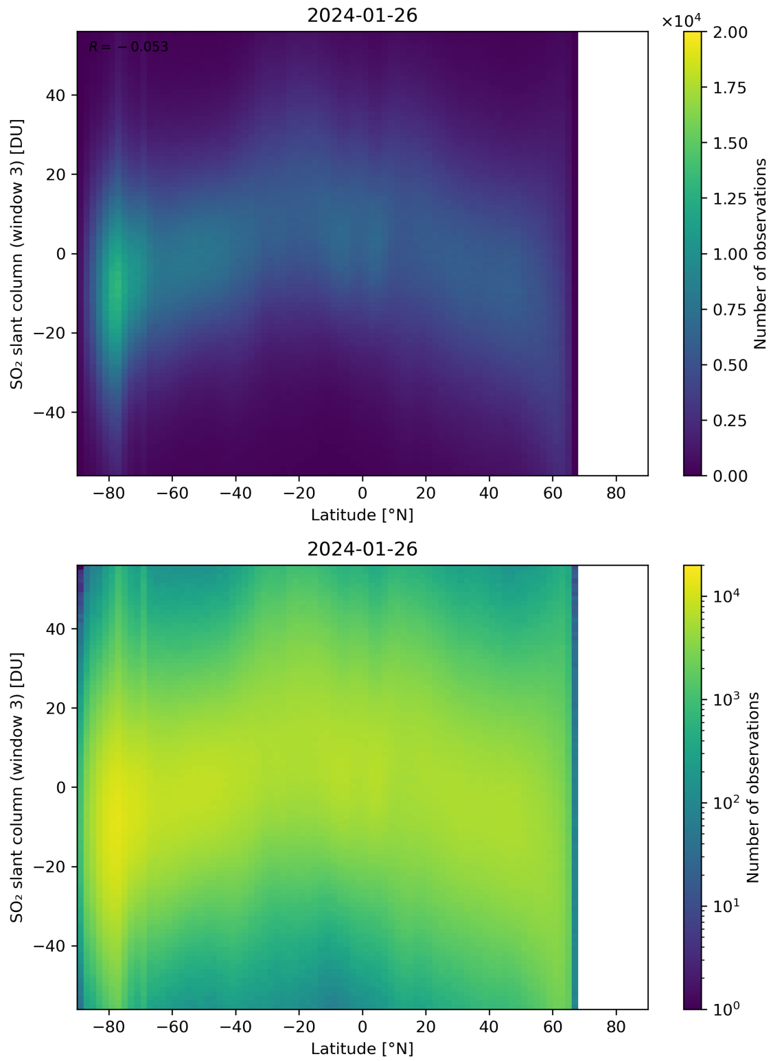
Figure 152: Scatter density plot of “Latitude” against “SO 2 slant column (window 3)” for 2024-01-26 to 2024-01-27.
