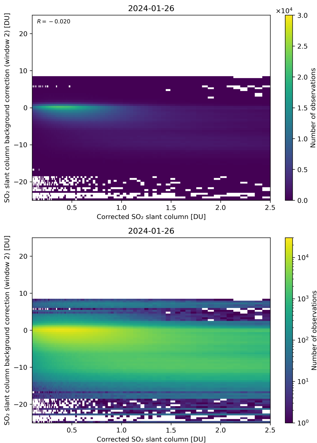
Figure 179: Scatter density plot of “Corrected SO 2 slant column” against “SO 2 slant column background correction (window 2)” for 2024-01-26 to 2024-01-27.
