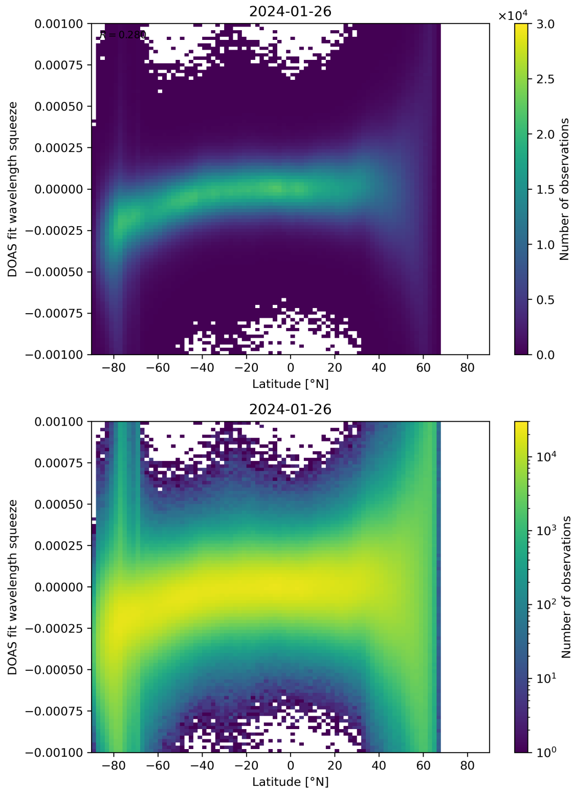
Figure 143: Scatter density plot of “Latitude” against “DOAS fit wavelength squeeze” for 2024-01-26 to 2024-01-27.
