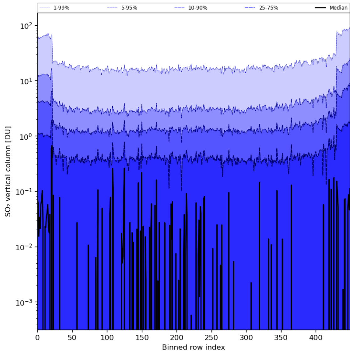
Figure 76: Along track statistics of “SO 2 vertical column” for 2024-01-26 to 2024-01-27
