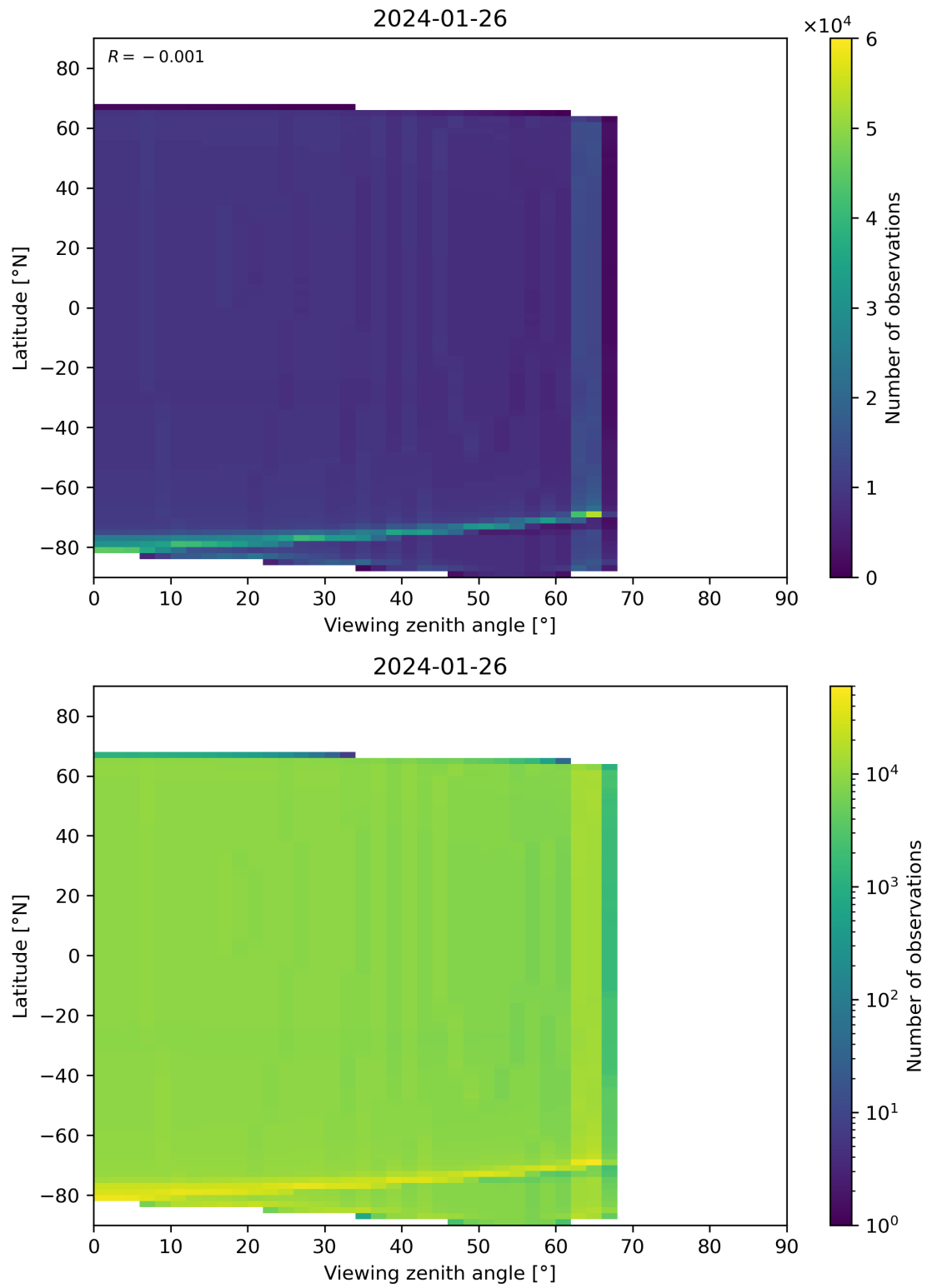
Figure 314: Scatter density plot of “Viewing zenith angle” against “Latitude” for 2024-01-26 to 2024-01-27.
