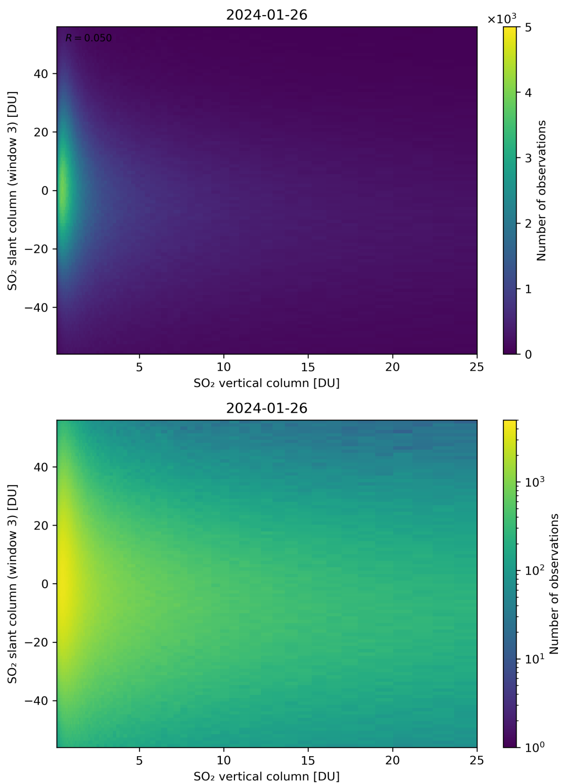
Figure 303: Scatter density plot of “SO 2 vertical column” against “SO 2 slant column (window 3)” for 2024-01-26 to 2024-01-27.
