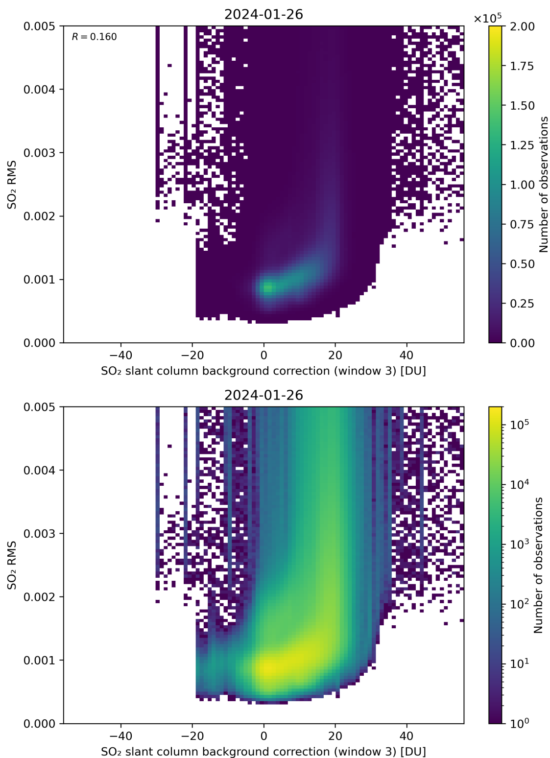
Figure 123: Scatter density plot of “SO 2 slant column background correction (window 3)” against “SO 2 RMS” for 2024-01-26 to 2024-01-27.
