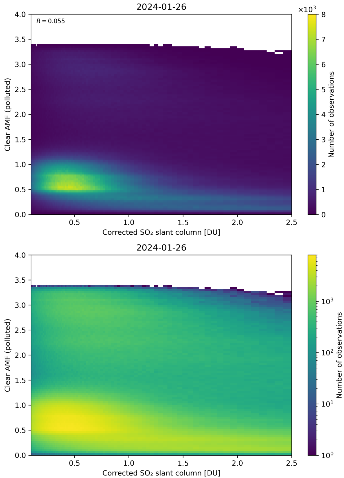
Figure 184: Scatter density plot of “Corrected SO 2 slant column” against “Clear AMF (polluted)” for 2024-01-26 to 2024-01-27.
