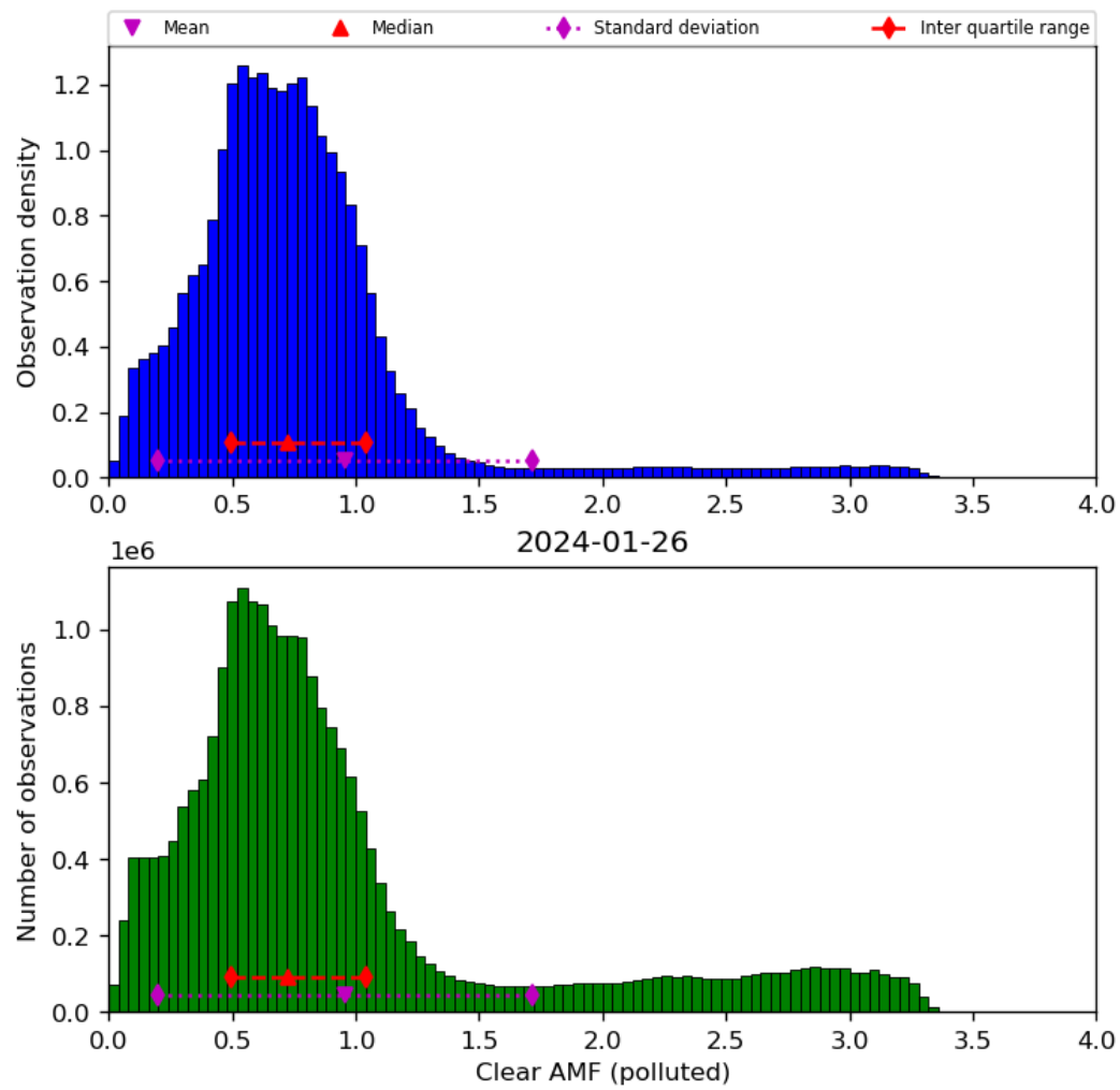
Figure 73: Histogram of “Clear AMF (polluted)” for 2024-01-26 to 2024-01-27
