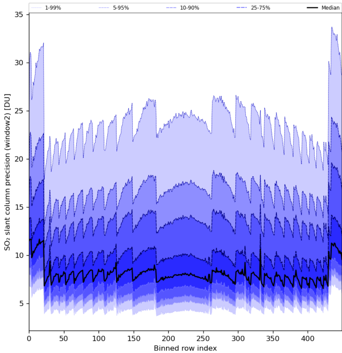
Figure 84: Along track statistics of “SO 2 slant column precision (window2)” for 2024-01-26 to 2024-01-27
