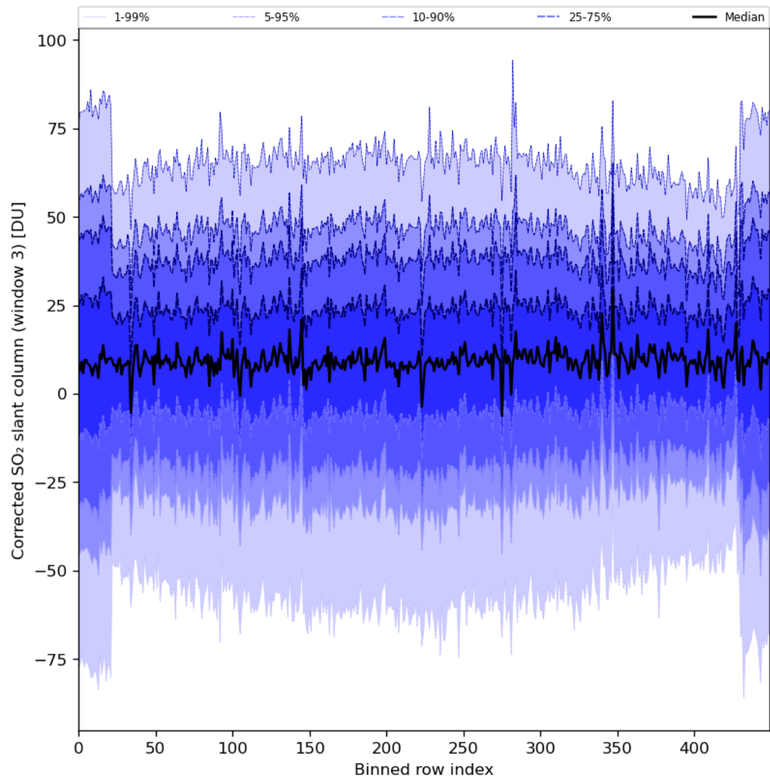
Figure 89: Along track statistics of “Corrected SO 2 slant column (window 3)” for 2024-01-26 to 2024-01-27
