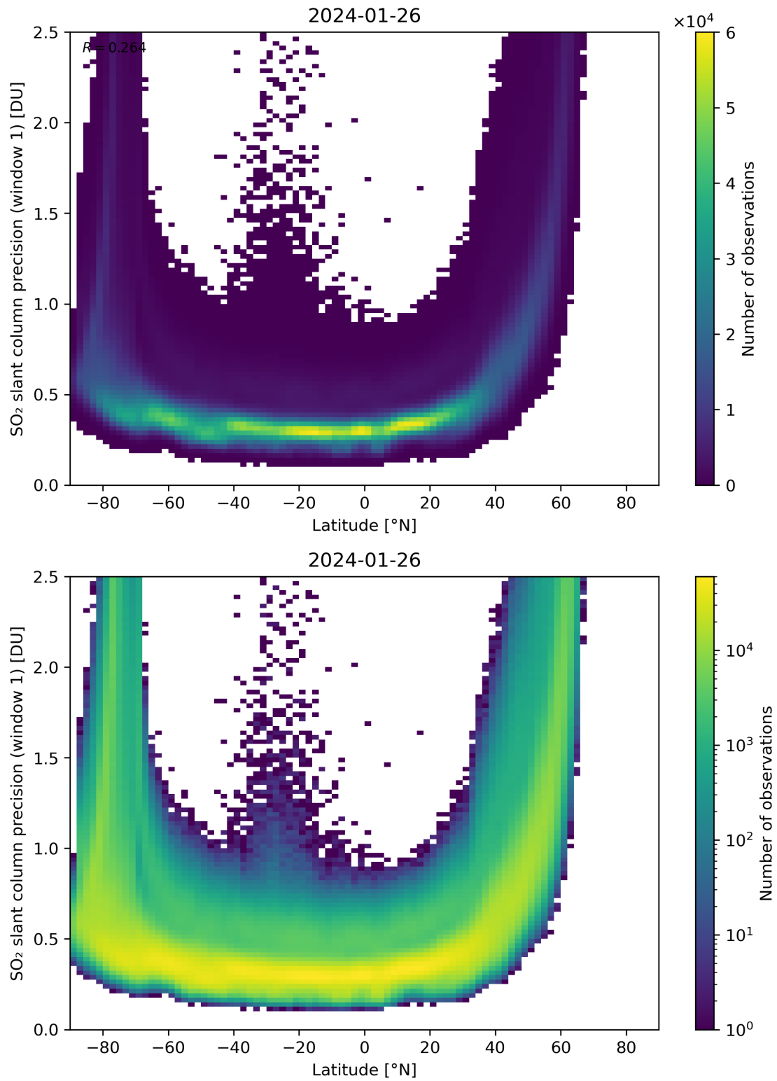
Figure 150: Scatter density plot of “Latitude” against “SO 2 slant column precision (window 1)” for 2024-01-26 to 2024-01-27.
