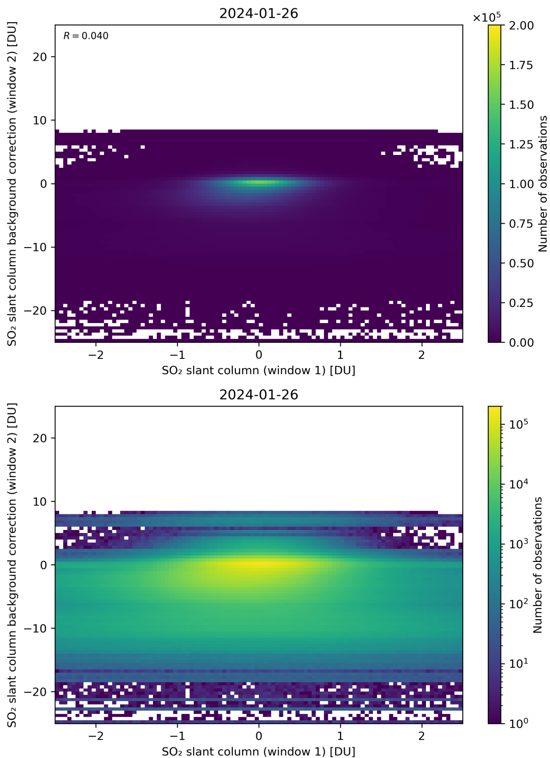
Figure 213: Scatter density plot of “SO 2 slant column (window 1)” against “SO 2 slant column background correction (window 2)” for 2024-01-26 to 2024-01-27.
