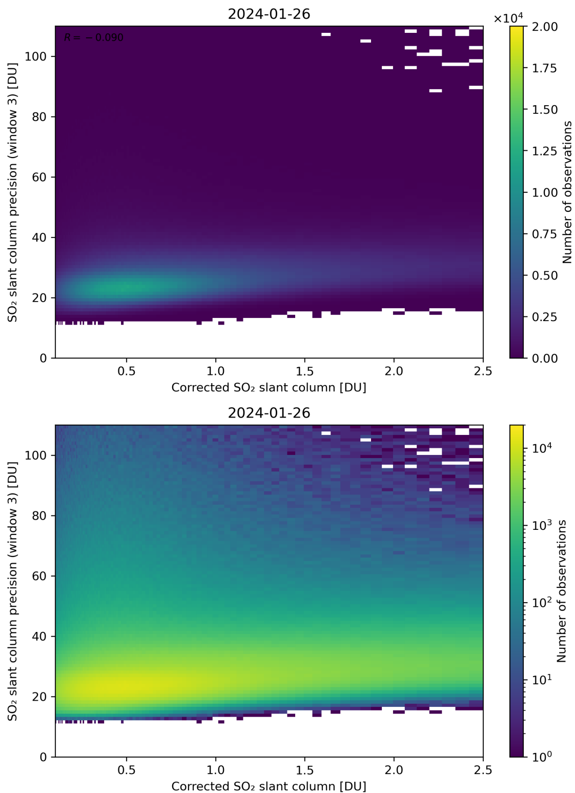
Figure 191: Scatter density plot of “Corrected SO 2 slant column” against “SO 2 slant column precision (window 3)” for 2024-01-26 to 2024-01-27.
