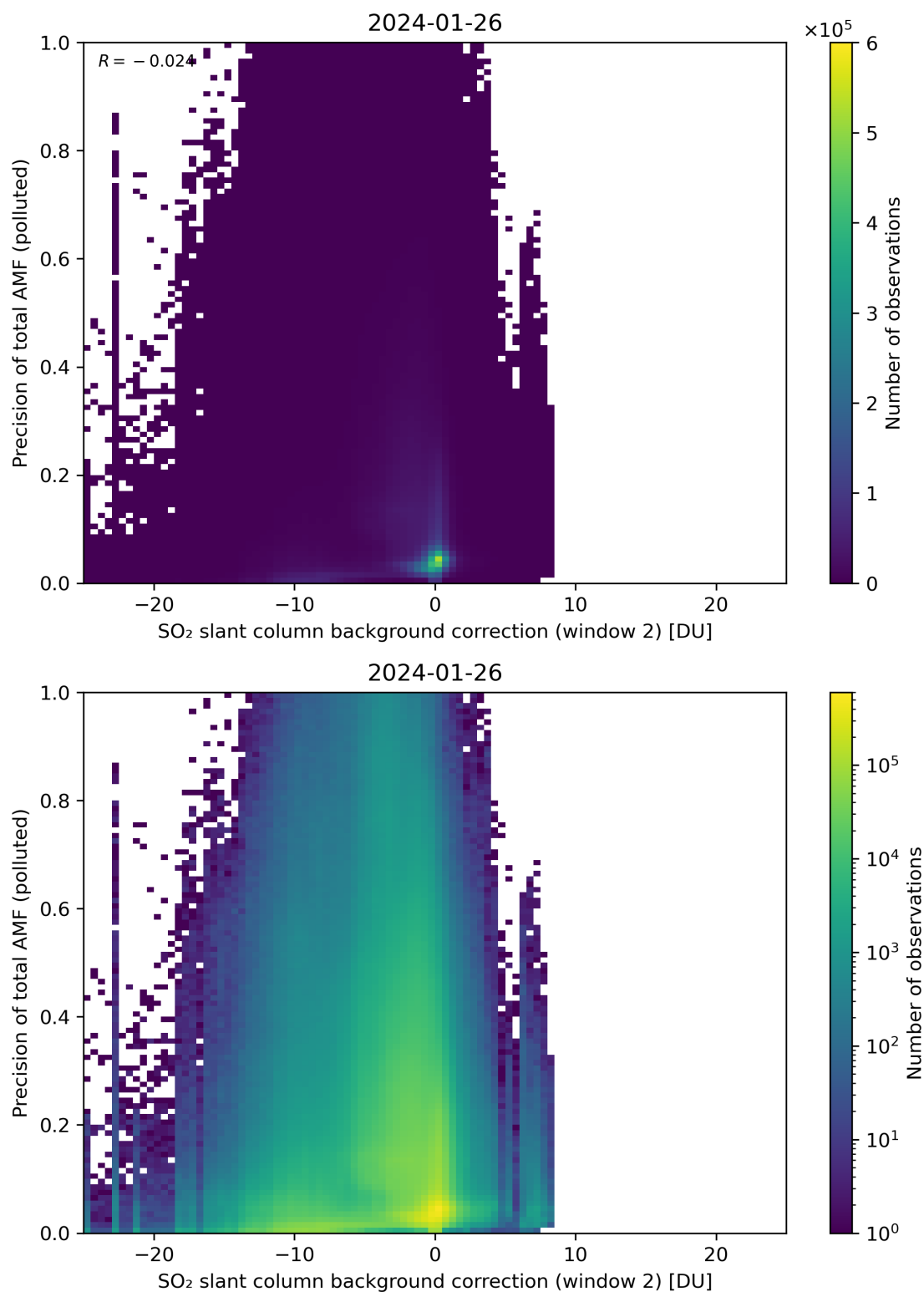
Figure 120: Scatter density plot of “SO 2 slant column background correction (window 2)” against “Precision of total AMF (polluted)” for 2024-01-26 to 2024-01-27.
