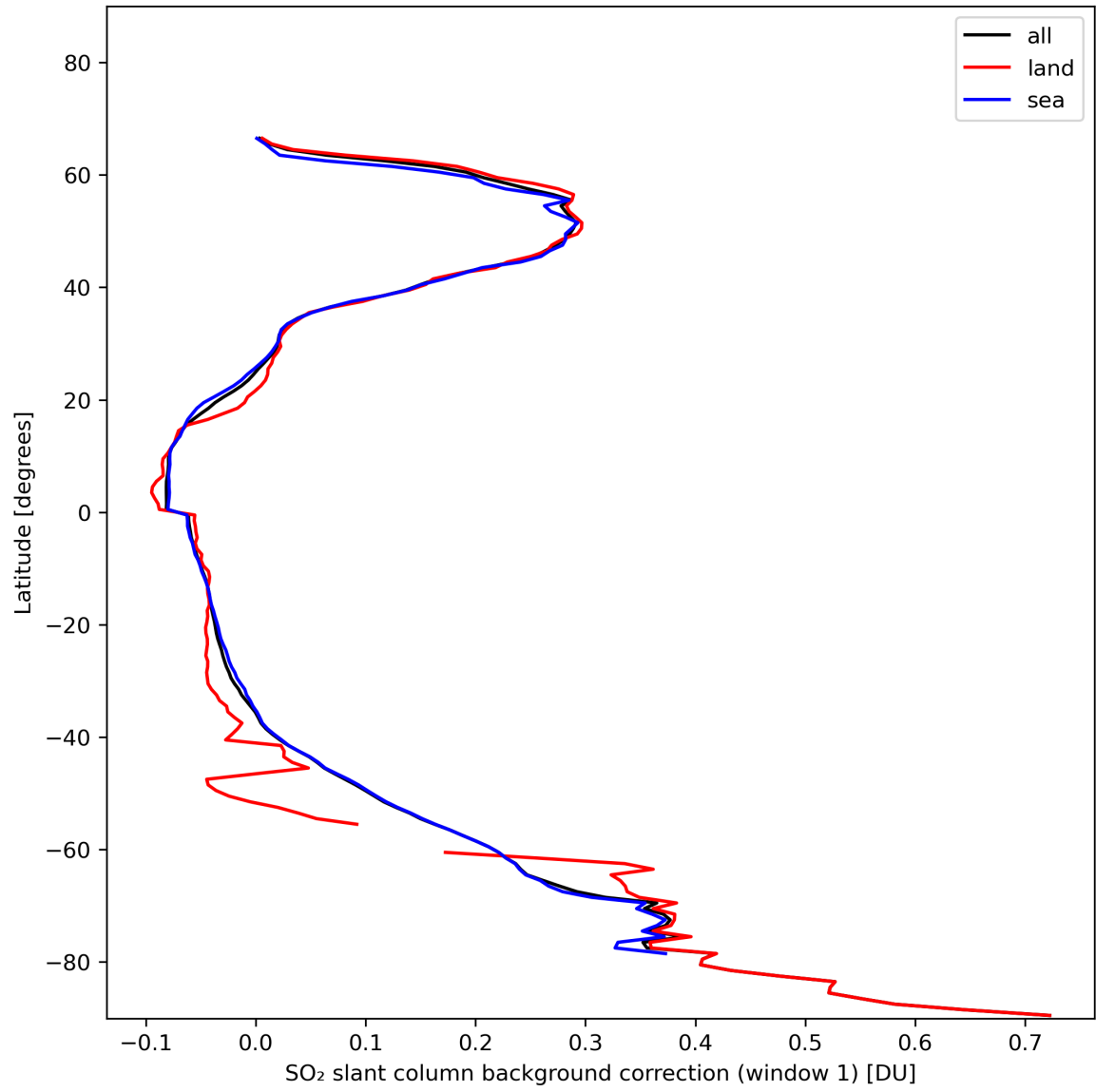
Figure 36: Zonal average of “SO 2 slant column background correction (window 1)” for 2024-01-26 to 2024-01-27.
