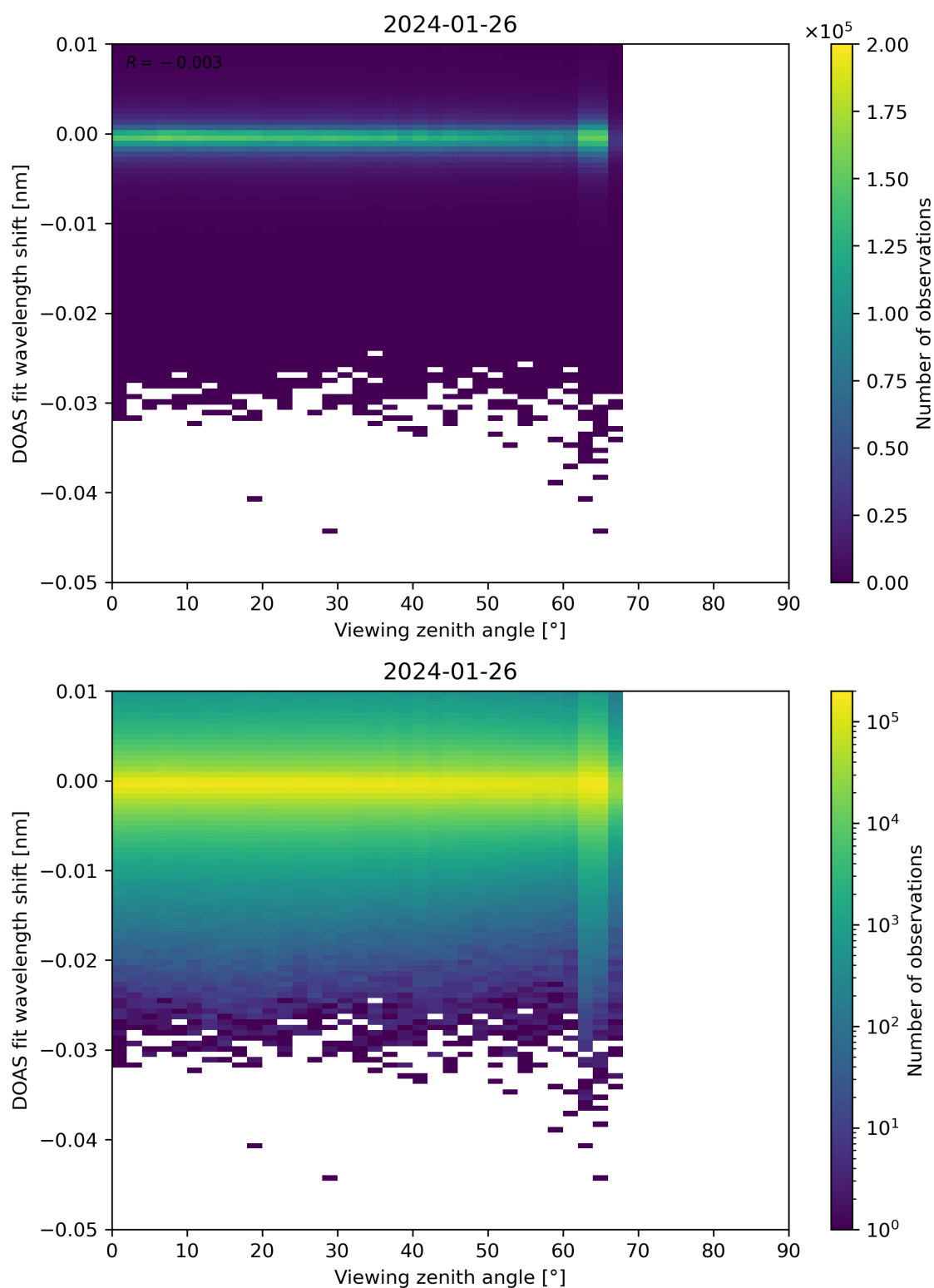
Figure 311: Scatter density plot of “Viewing zenith angle” against “DOAS fit wavelength shift” for 2024-01-26 to 2024-01-27.
