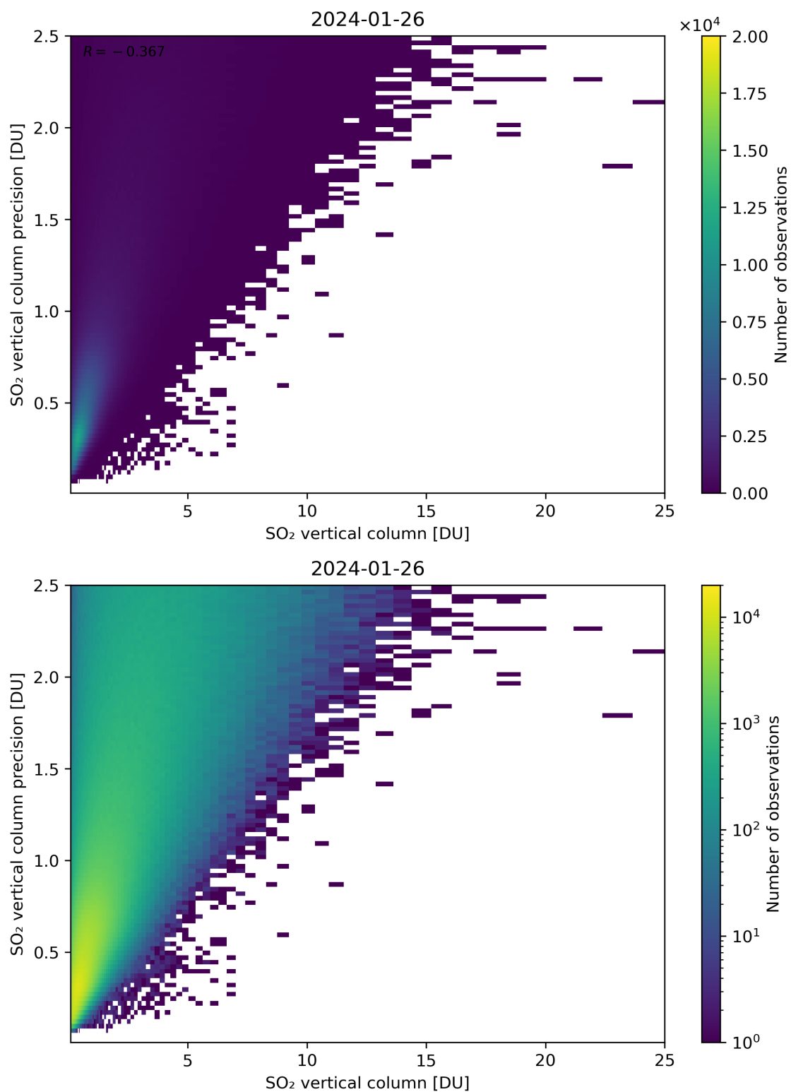
Figure 307: Scatter density plot of “SO 2 vertical column” against “SO 2 vertical column precision” for 2024-01-26 to 2024-01-27.
