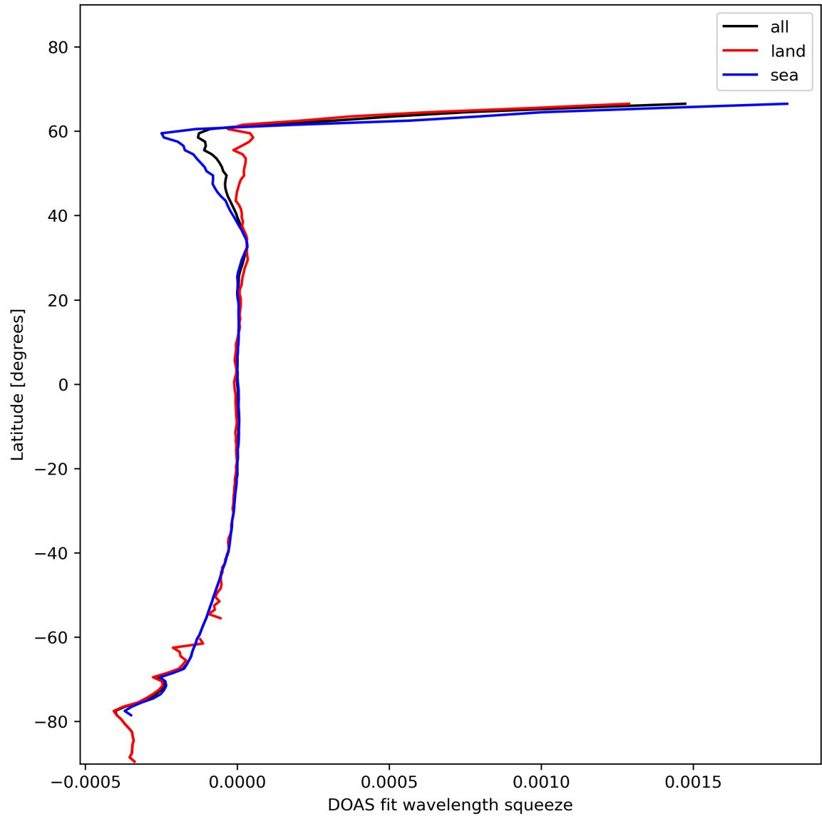
Figure 46: Zonal average of "DOAS fit wavelength squeeze" for 2024-01-26 to 2024-01-27.
