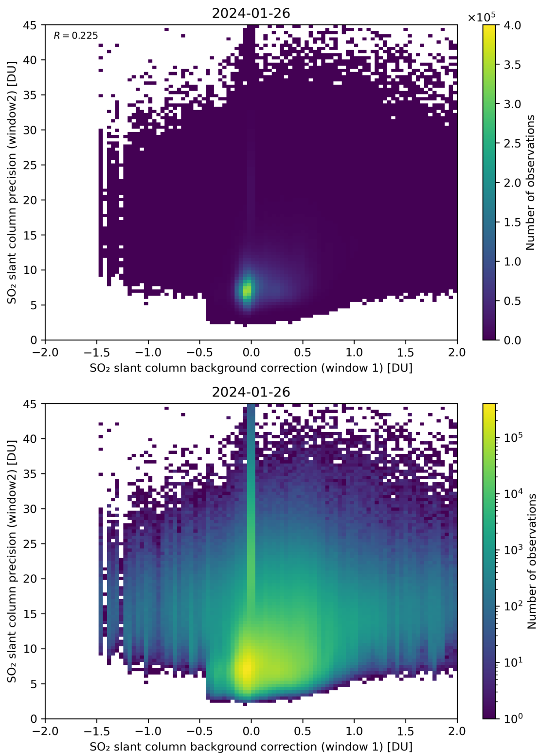
Figure 106: Scatter density plot of “SO 2 slant column background correction (window 1)” against “SO 2 slant column precision (window2)” for 2024-01-26 to 2024-01-27.
