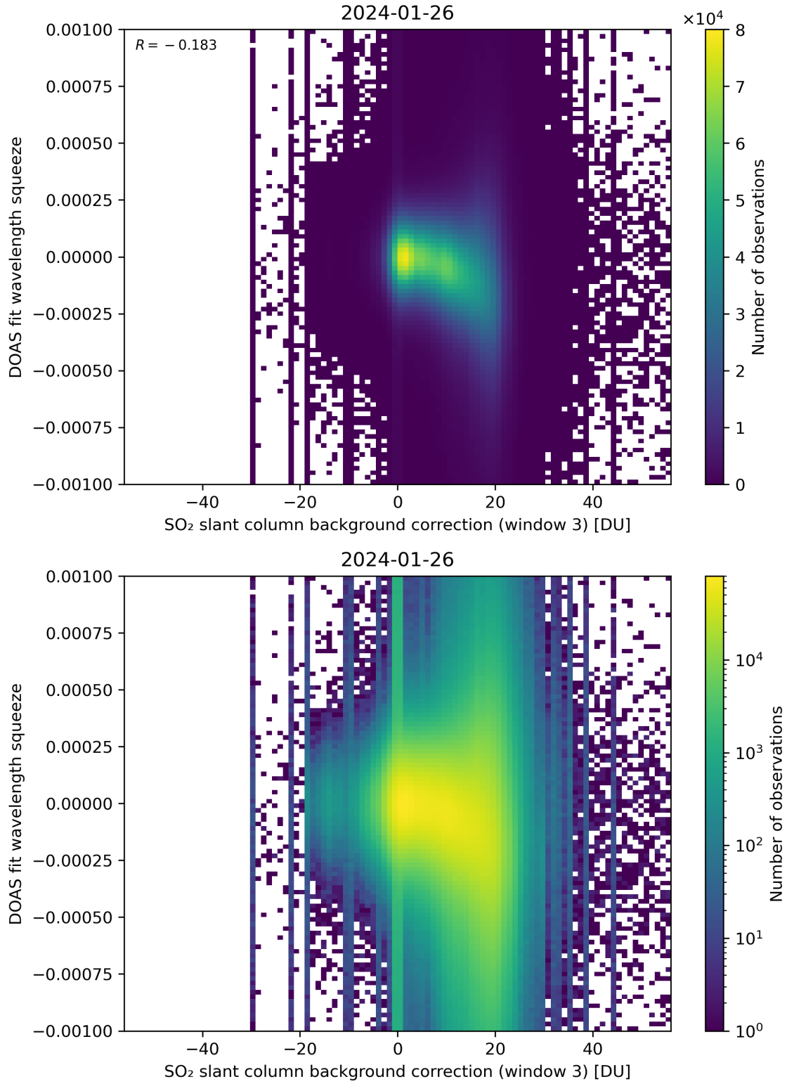
Figure 122: Scatter density plot of “SO 2 slant column background correction (window 3)” against “DOAS fit wavelength squeeze” for 2024-01-26 to 2024-01-27.
