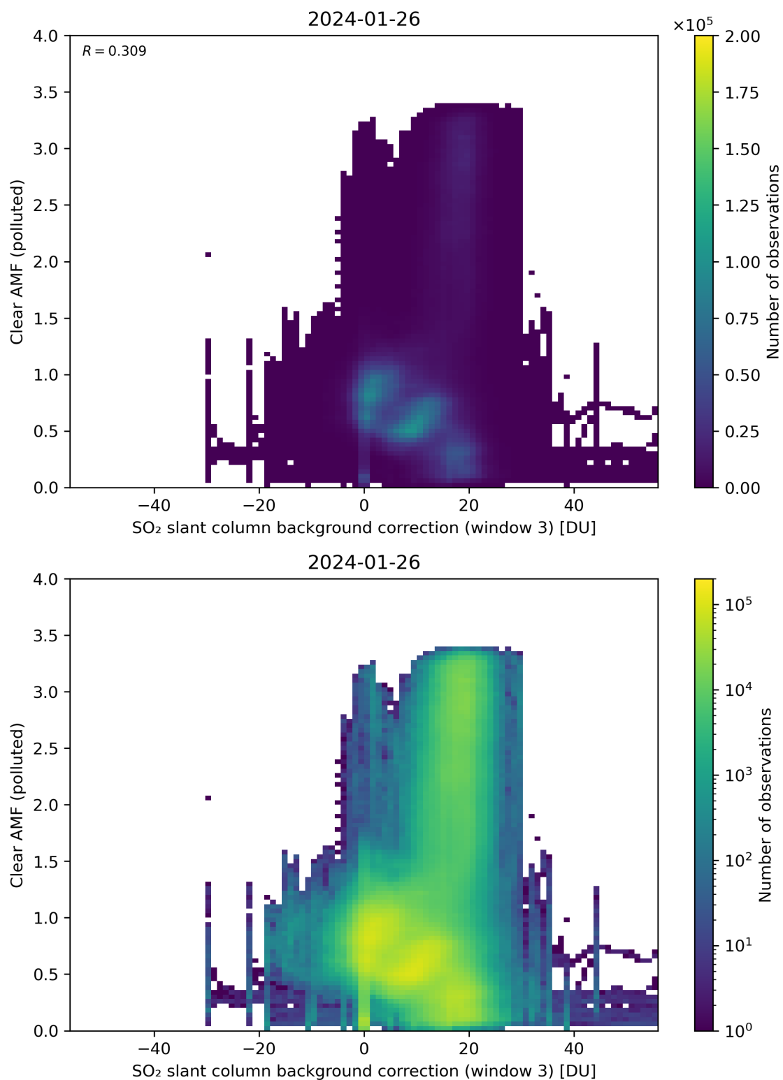
Figure 124: Scatter density plot of “SO 2 slant column background correction (window 3)” against “Clear AMF (polluted)” for 2024-01-26 to 2024-01-27.
