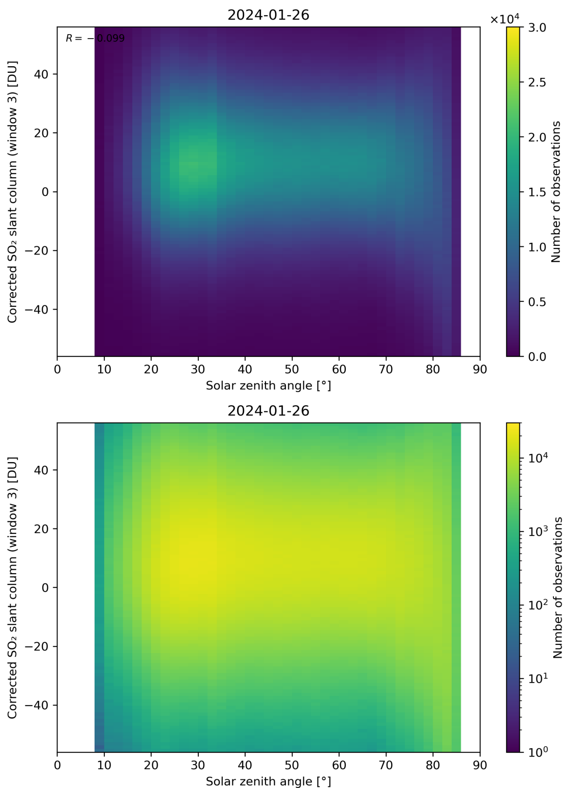
Figure 168: Scatter density plot of “Solar zenith angle” against “Corrected SO 2 slant column (window 3)” for 2024-01-26 to 2024-01-27.
