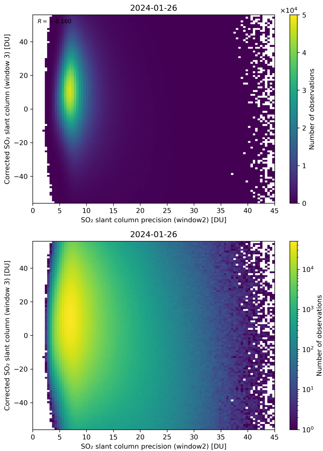
Figure 248: Scatter density plot of “SO 2 slant column precision (window2)” against “Corrected SO 2 slant column (window 3)” for 2024-01-26 to 2024-01-27.
