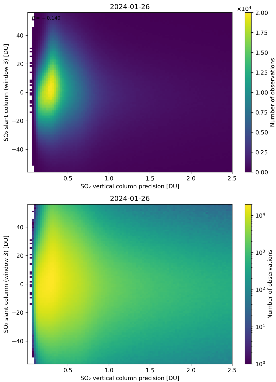
Figure 292: Scatter density plot of “SO 2 vertical column precision” against “SO 2 slant column (window 3)” for 2024-01-26 to 2024-01-27.
