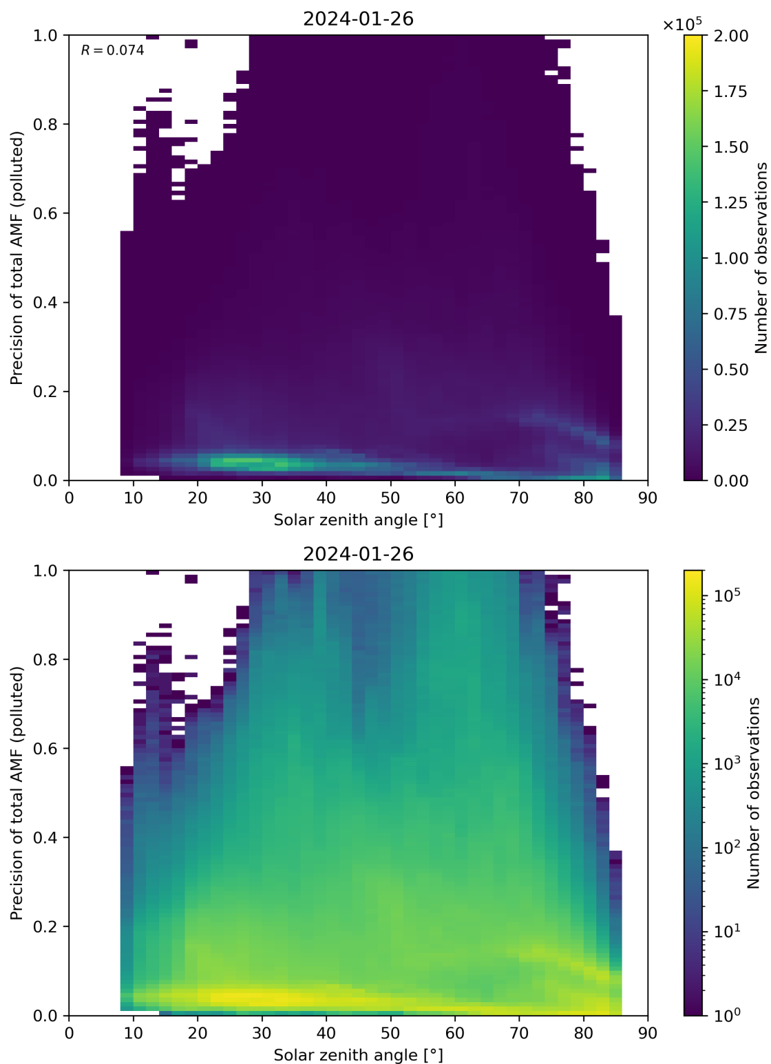
Figure 175: Scatter density plot of “Solar zenith angle” against “Precision of total AMF (polluted)” for 2024-01-26 to 2024-01-27.
