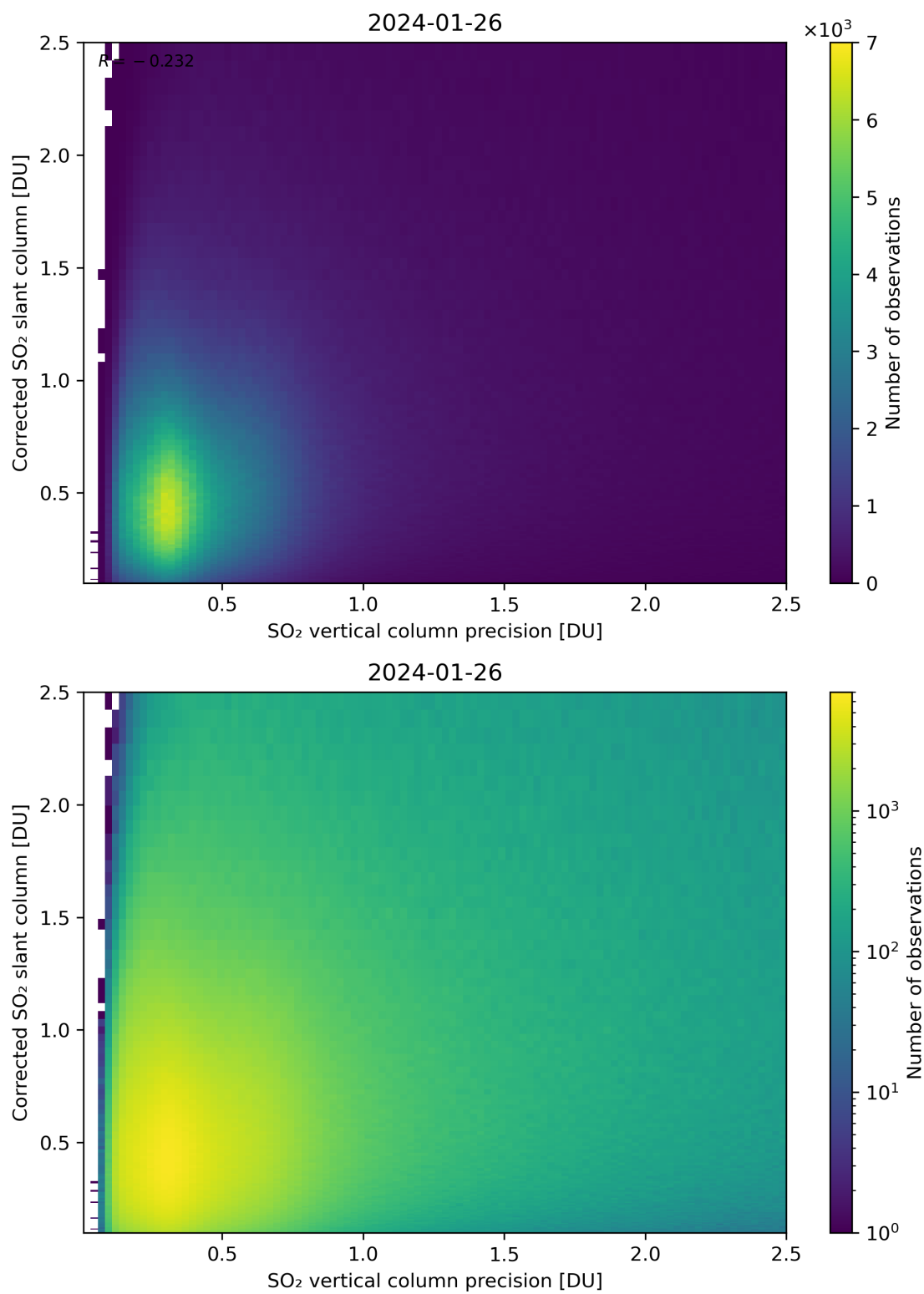
Figure 286: Scatter density plot of “SO 2 vertical column precision” against “Corrected SO 2 slant column” for 2024-01-26 to 2024-01-27.
