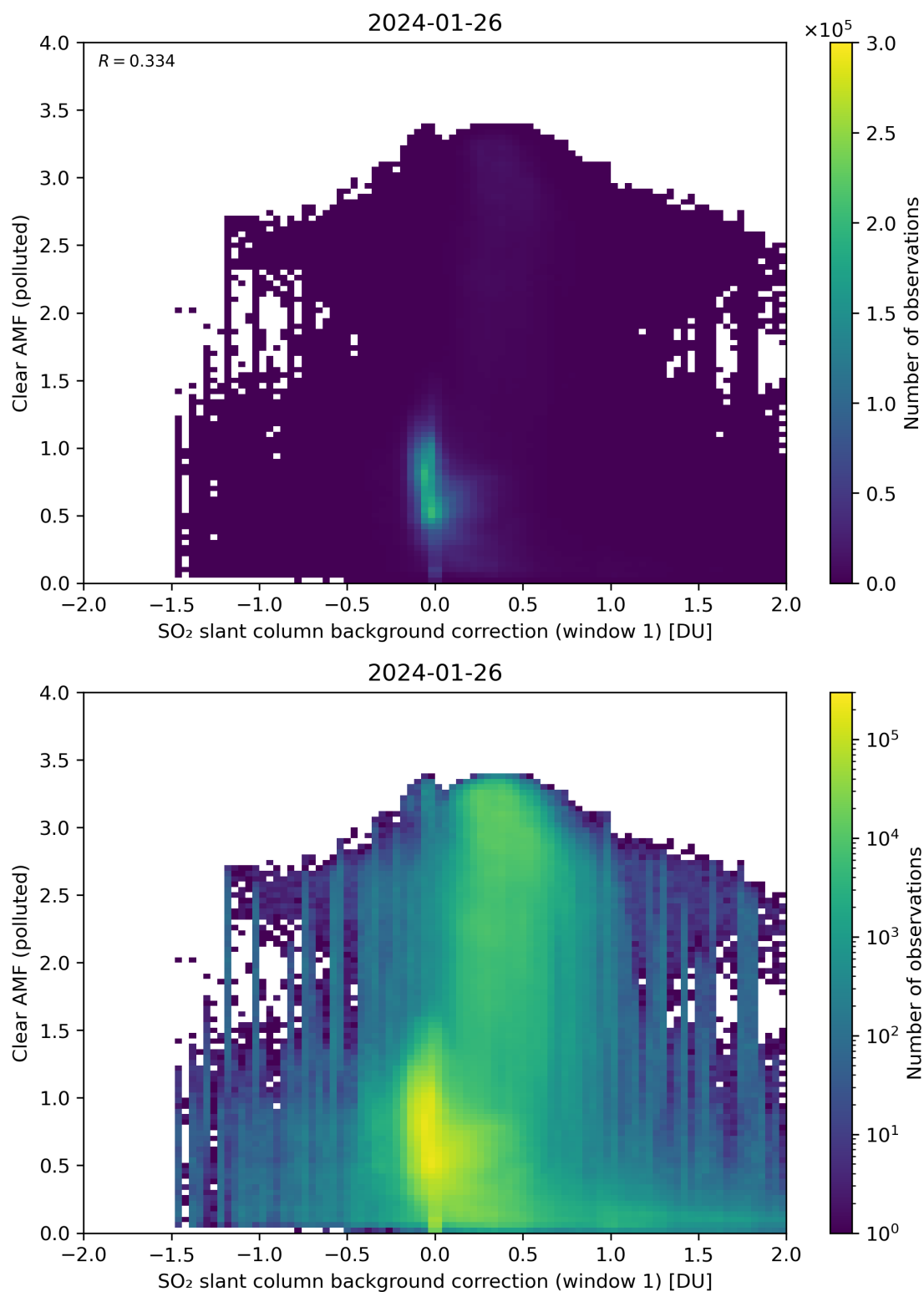
Figure 103: Scatter density plot of “SO 2 slant column background correction (window 1)” against “Clear AMF (polluted)” for 2024-01-26 to 2024-01-27.
