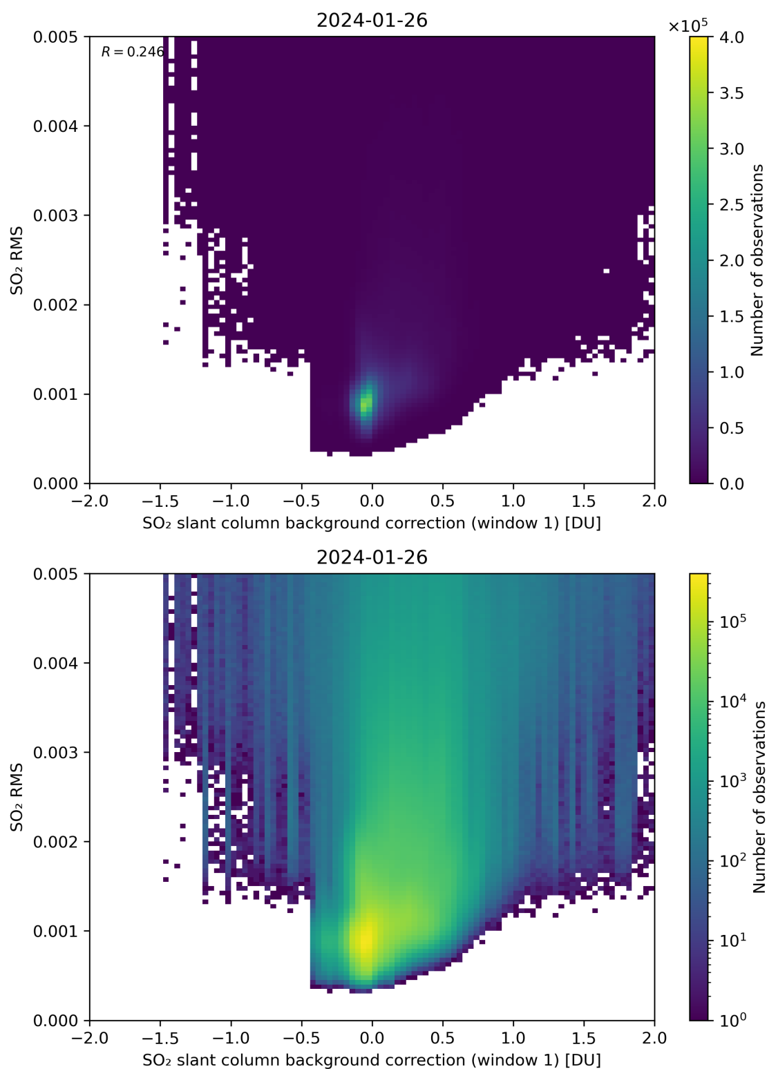
Figure 102: Scatter density plot of “SO 2 slant column background correction (window 1)” against “SO 2 RMS” for 2024-01-26 to 2024-01-27.
