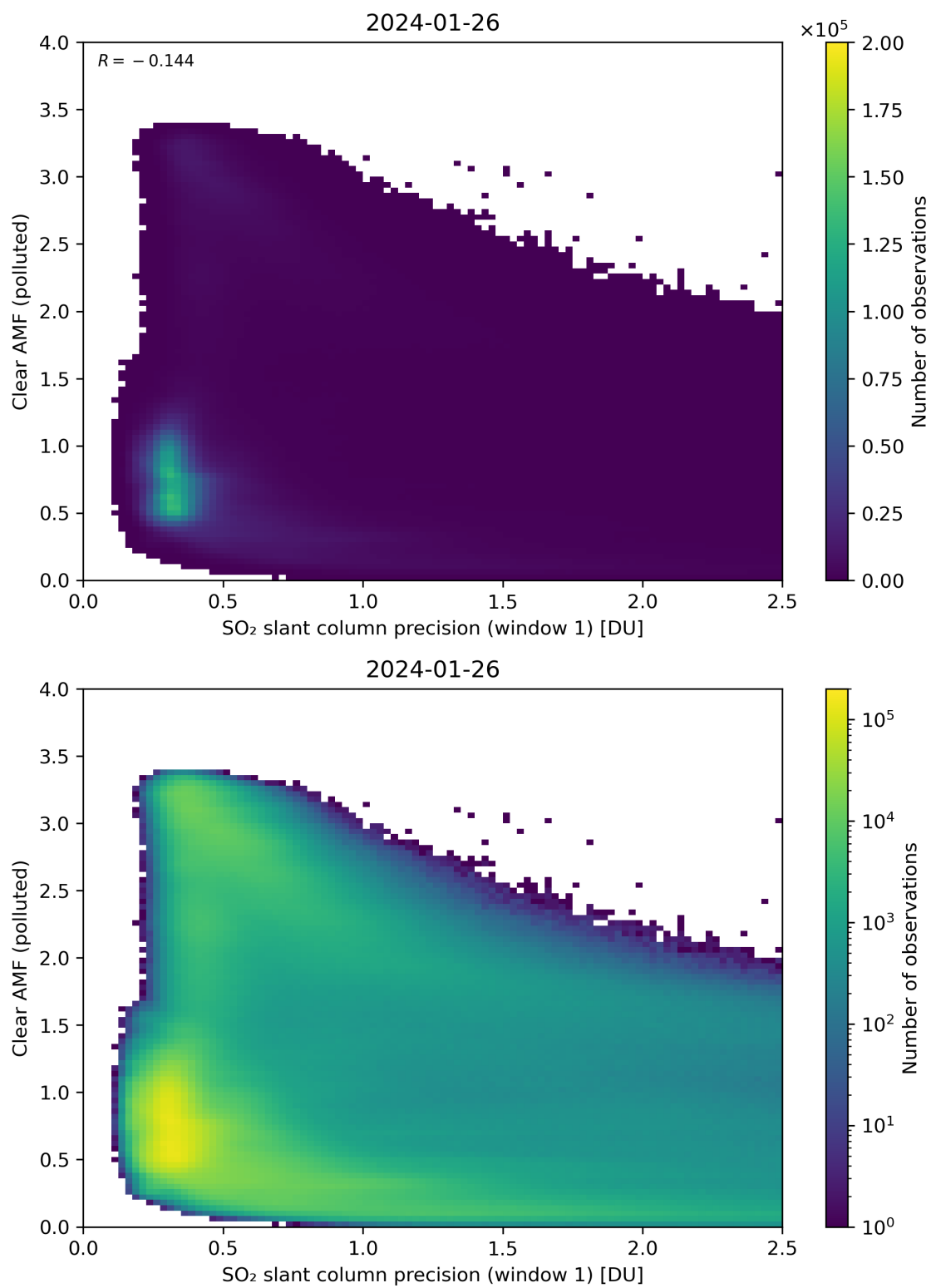
Figure 224: Scatter density plot of “SO 2 slant column precision (window 1)” against “Clear AMF (polluted)” for 2024-01-26 to 2024-01-27.
