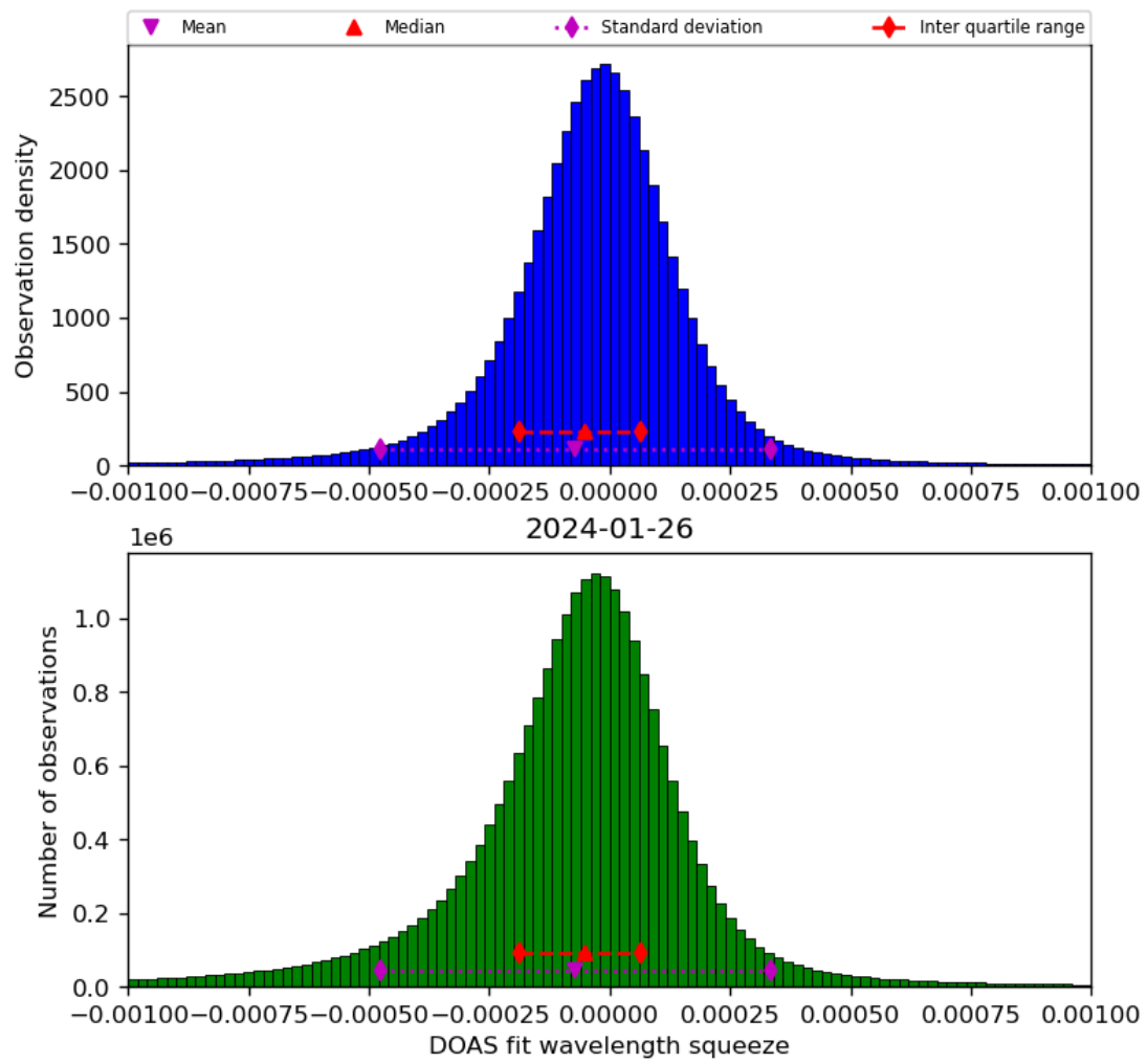
Figure 69: Histogram of “DOAS fit wavelength squeeze” for 2024-01-26 to 2024-01-27
