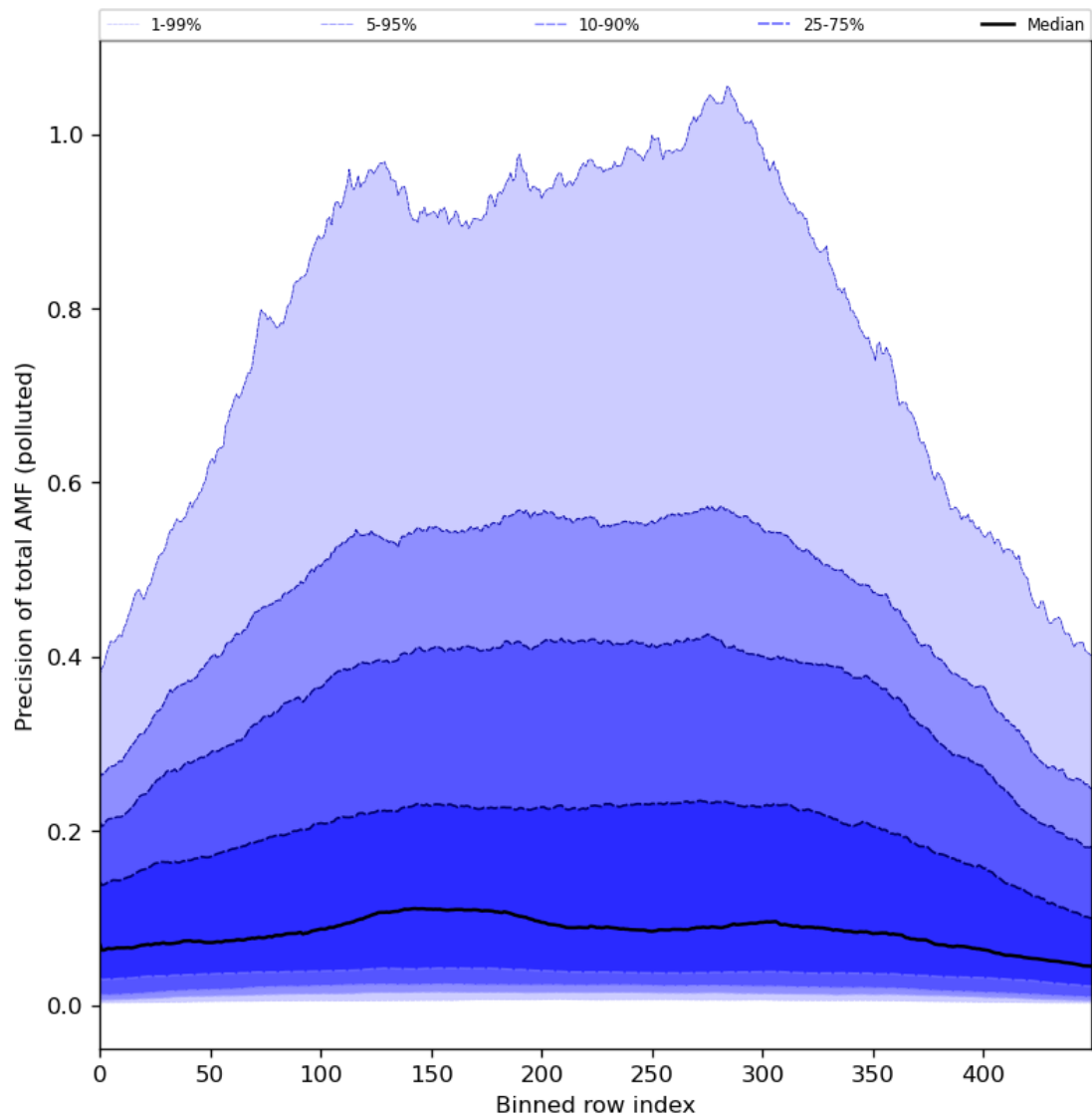
Figure 95: Along track statistics of “Precision of total AMF (polluted)” for 2024-01-26 to 2024-01-27
