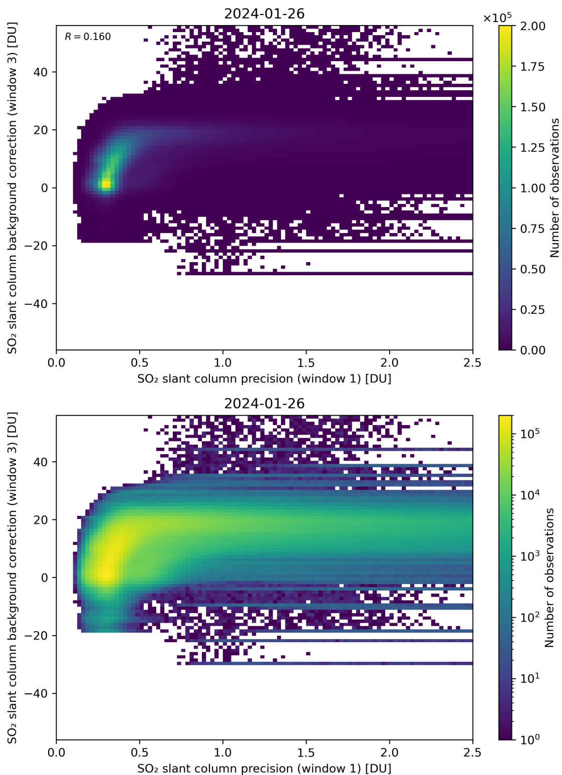
Figure 220: Scatter density plot of “SO 2 slant column precision (window 1)” against “SO 2 slant column background correction (window 3)” for 2024-01-26 to 2024-01-27.
