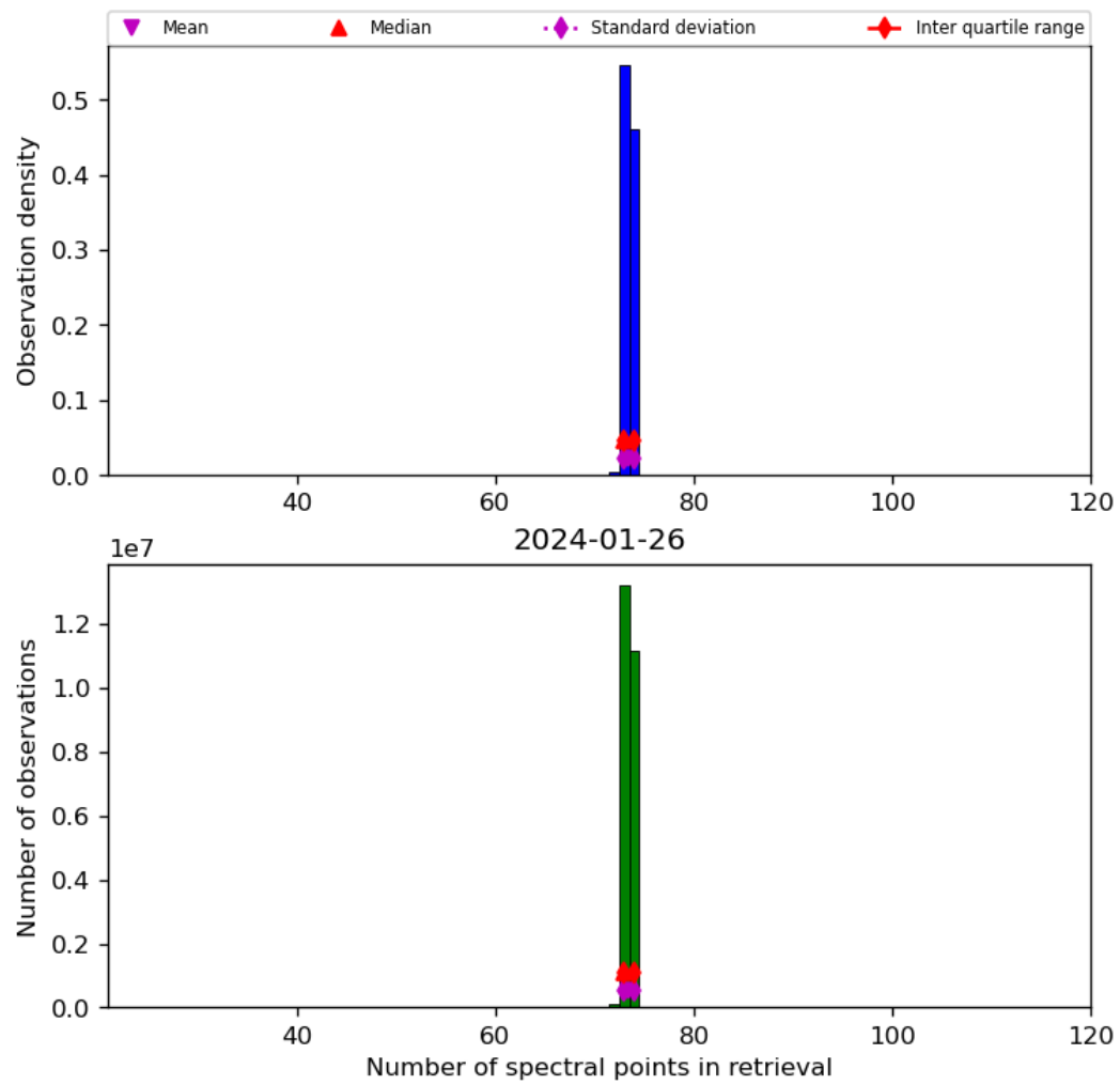
Figure 74: Histogram of “Number of spectral points in retrieval” for 2024-01-26 to 2024-01-27
