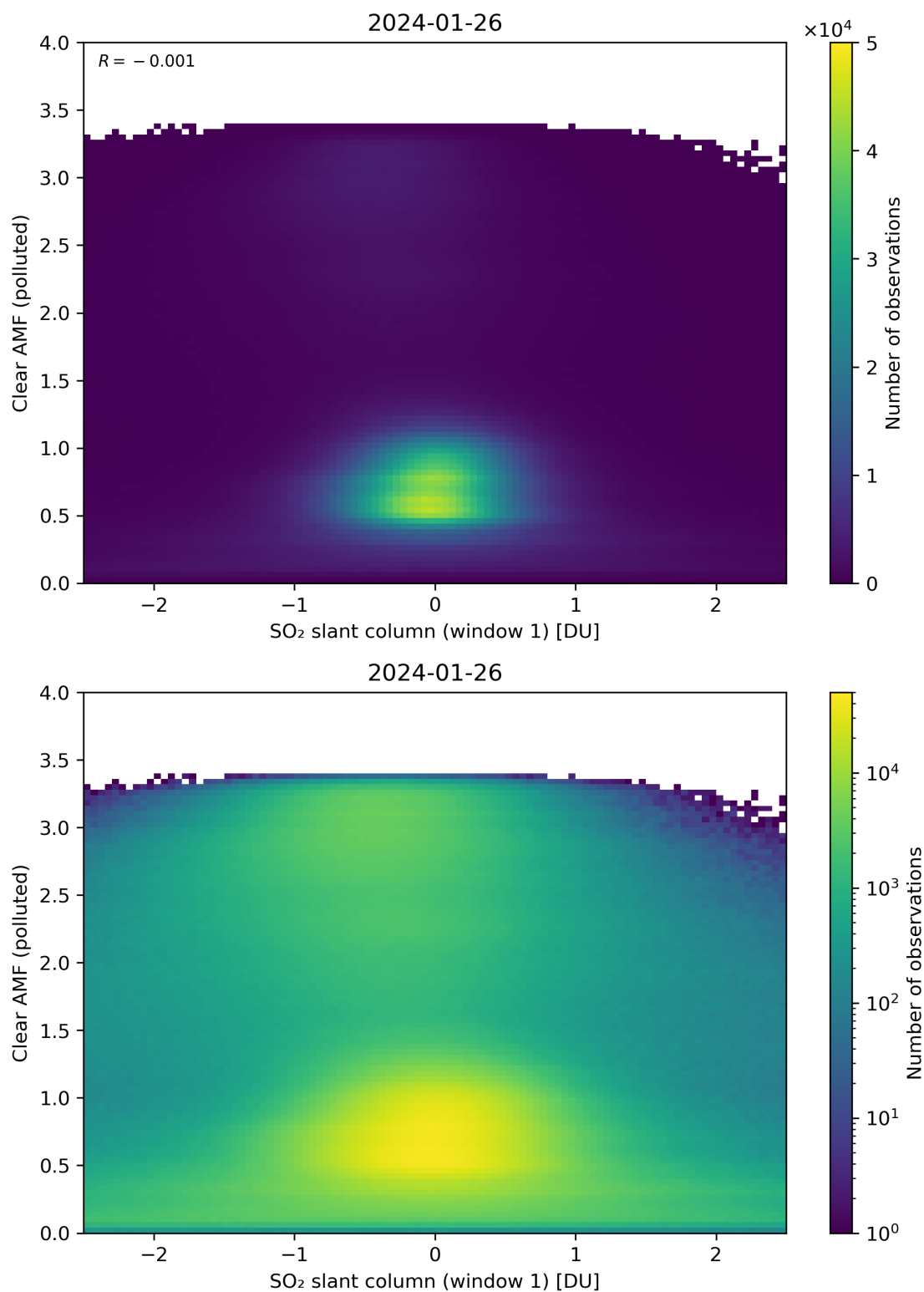
Figure 232: Scatter density plot of “SO 2 slant column (window 1)” against “Clear AMF (polluted)” for 2024-01-26 to 2024-01-27.
