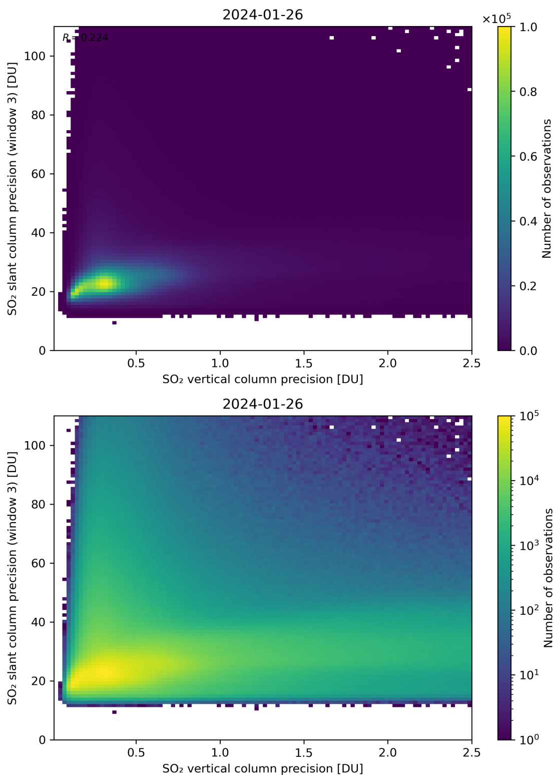
Figure 293: Scatter density plot of “SO 2 vertical column precision” against “SO 2 slant column precision (window 3)” for 2024-01-26 to 2024-01-27.
