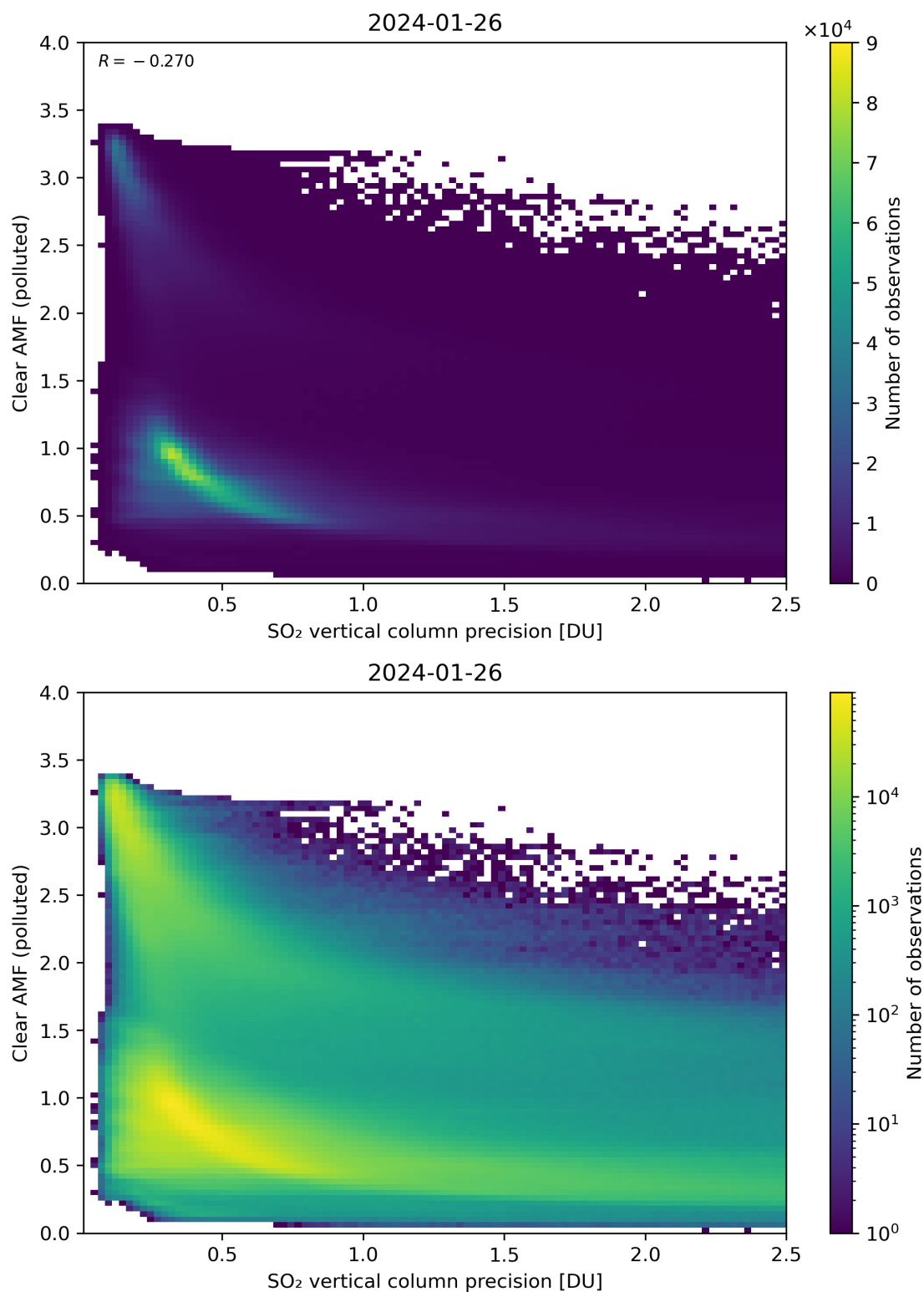
Figure 285: Scatter density plot of “SO 2 vertical column precision” against “Clear AMF (polluted)” for 2024-01-26 to 2024-01-27.
