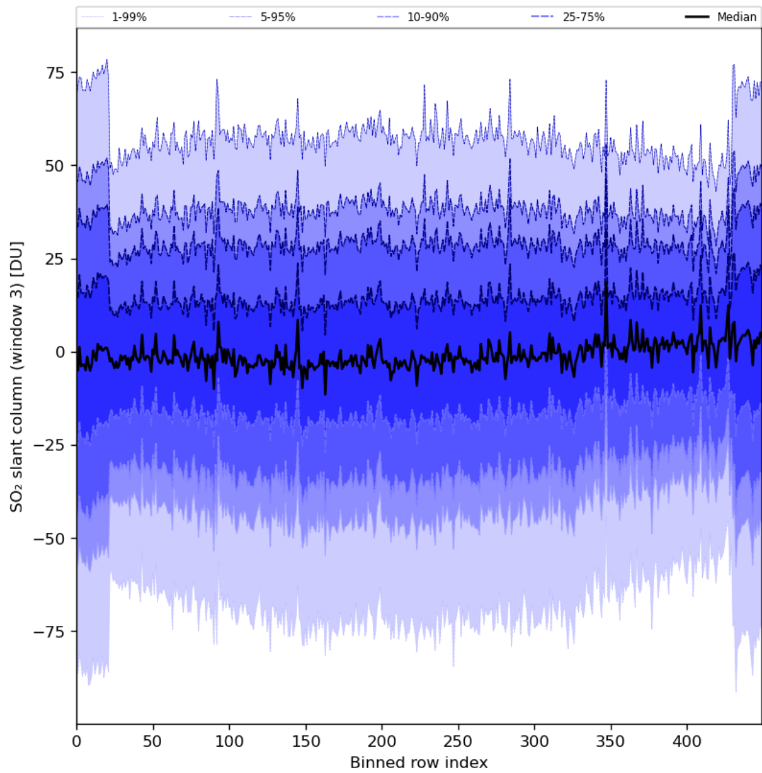
Figure 87: Along track statistics of “SO 2 slant column (window 3)” for 2024-01-26 to 2024-01-27
