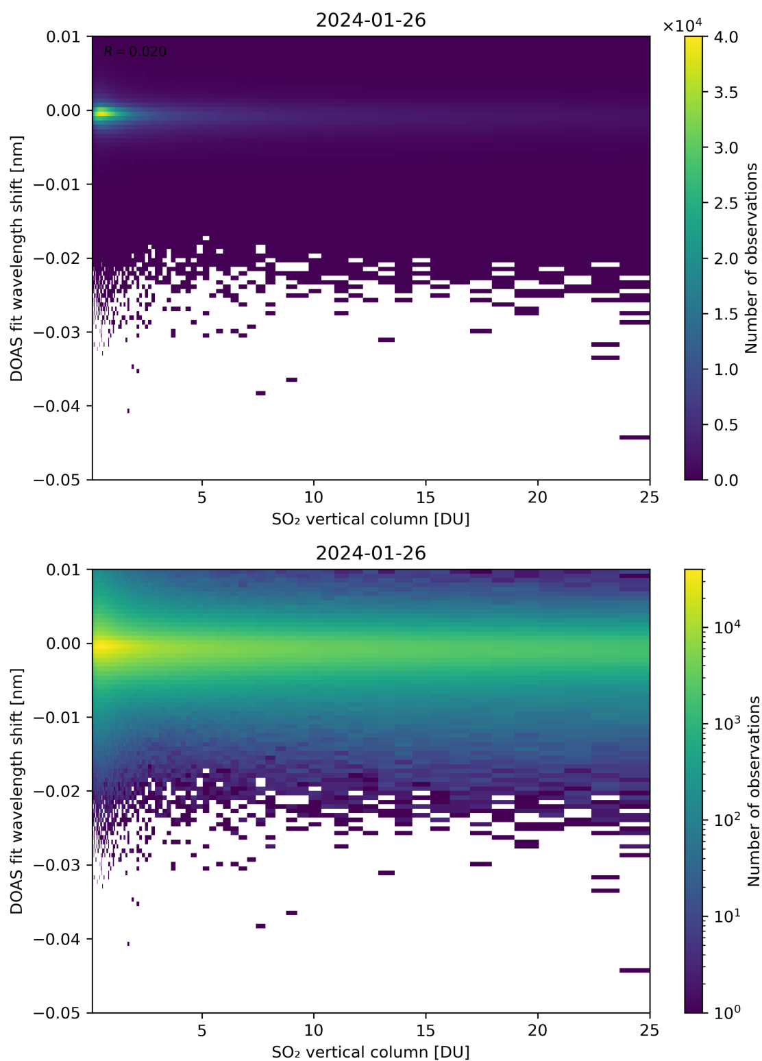
Figure 276: Scatter density plot of “SO 2 vertical column” against “DOAS fit wavelength shift” for 2024-01-26 to 2024-01-27.
