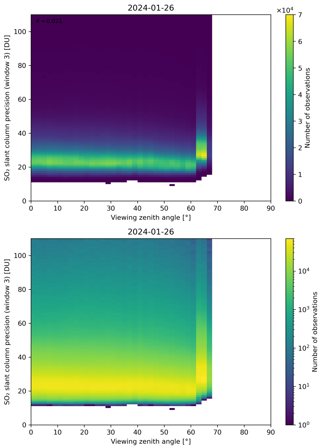
Figure 324: Scatter density plot of “Viewing zenith angle” against “SO 2 slant column precision (window 3)” for 2024-01-26 to 2024-01-27.
