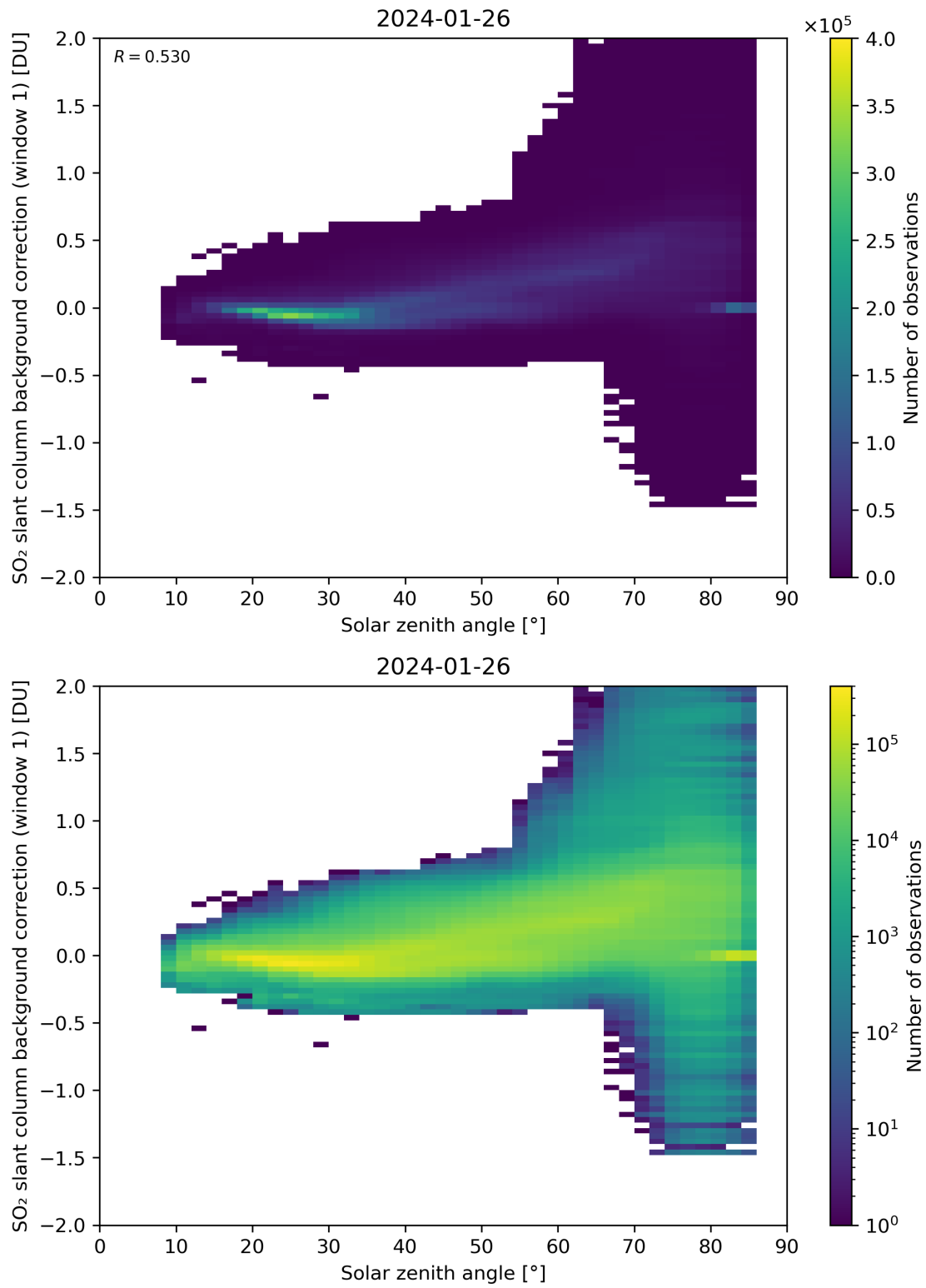
Figure 158: Scatter density plot of “Solar zenith angle” against “SO 2 slant column background correction (window 1)” for 2024-01-26 to 2024-01-27.
