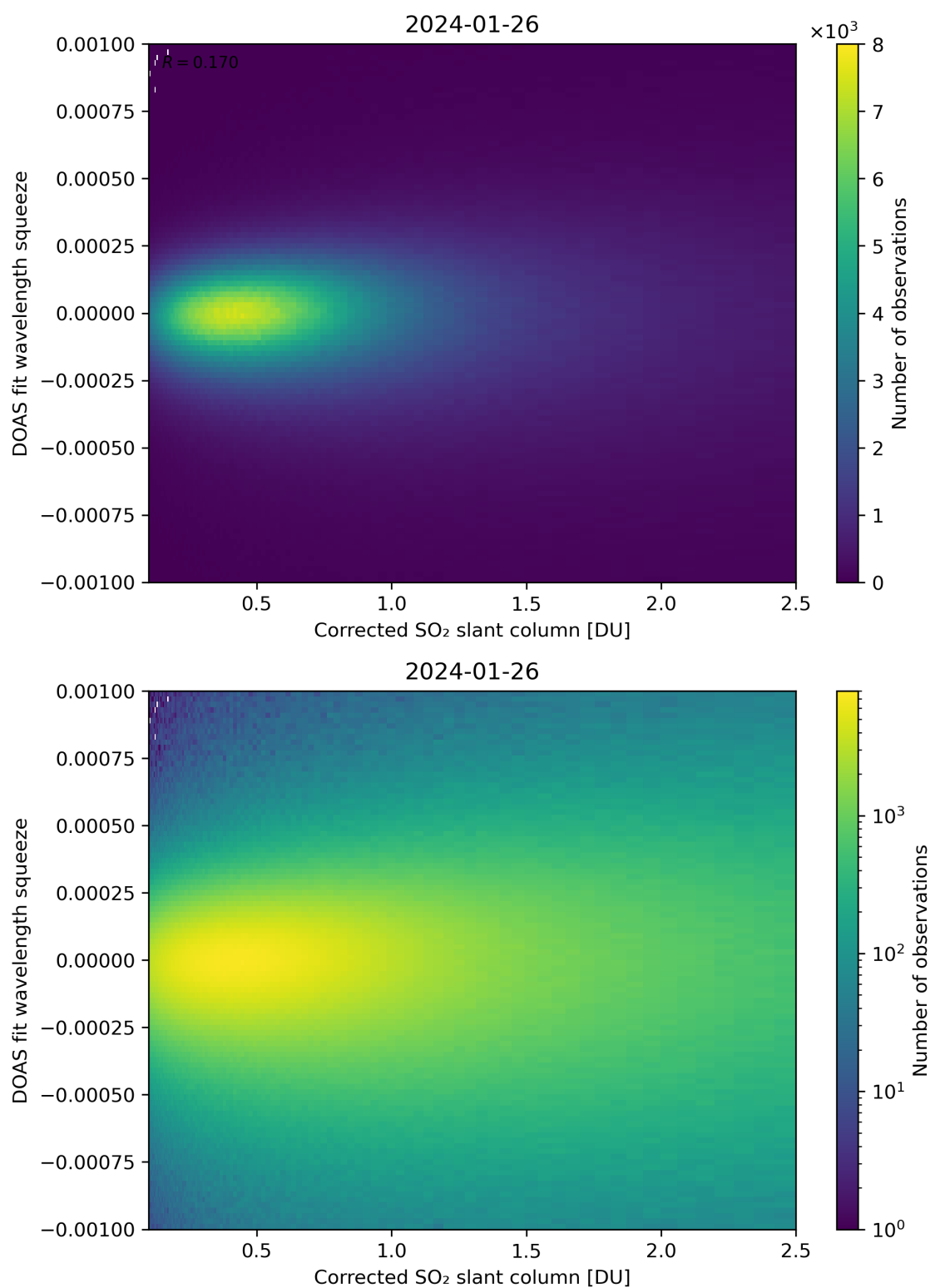
Figure 182: Scatter density plot of “Corrected SO 2 slant column” against “DOAS fit wavelength squeeze” for 2024-01-26 to 2024-01-27.
