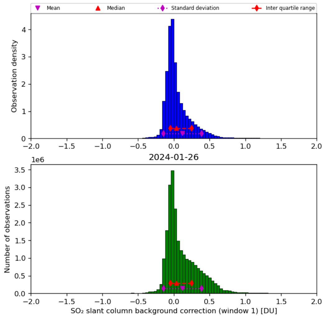
Figure 59: Histogram of “SO 2 slant column background correction (window 1)” for 2024-01-26 to 2024-01-27
