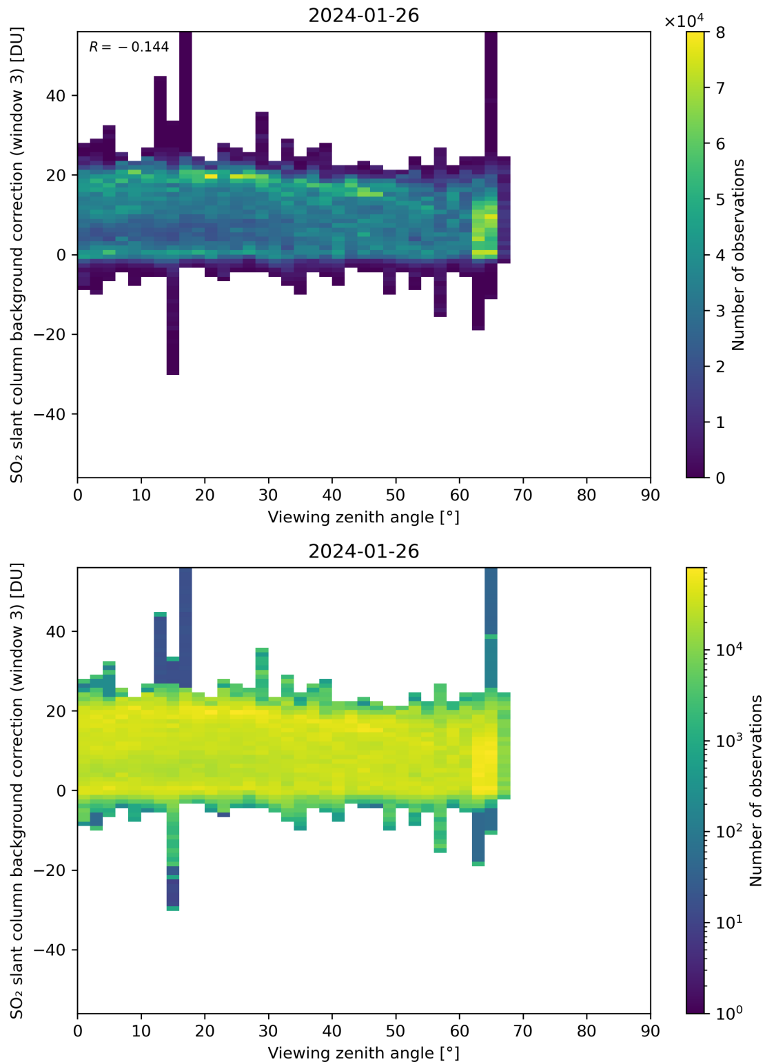
Figure 310: Scatter density plot of “Viewing zenith angle” against “SO 2 slant column background correction (window 3)” for 2024-01-26 to 2024-01-27.
