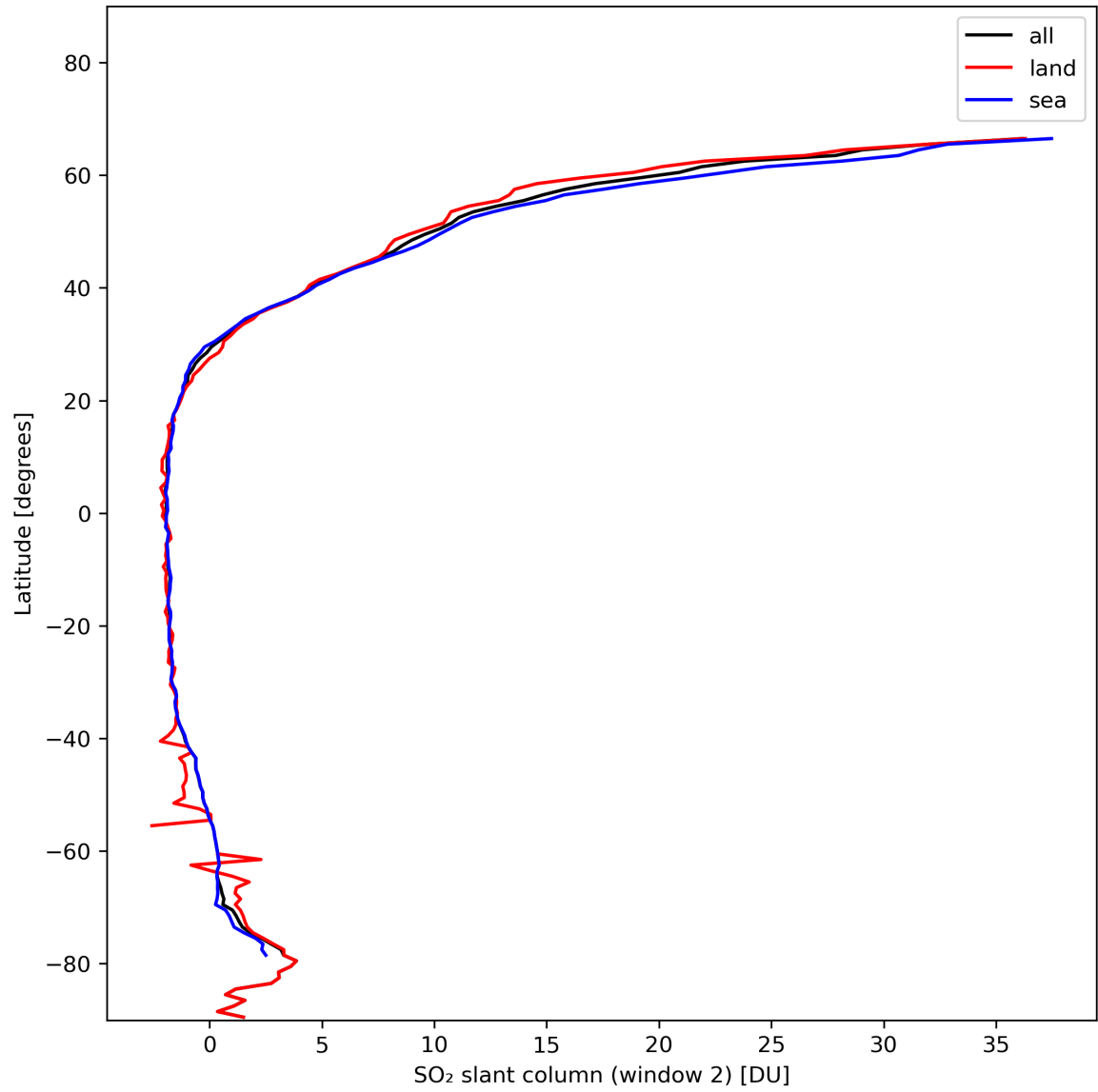
Figure 37: Zonal average of “SO 2 slant column (window 2)” for 2024-01-26 to 2024-01-27.
