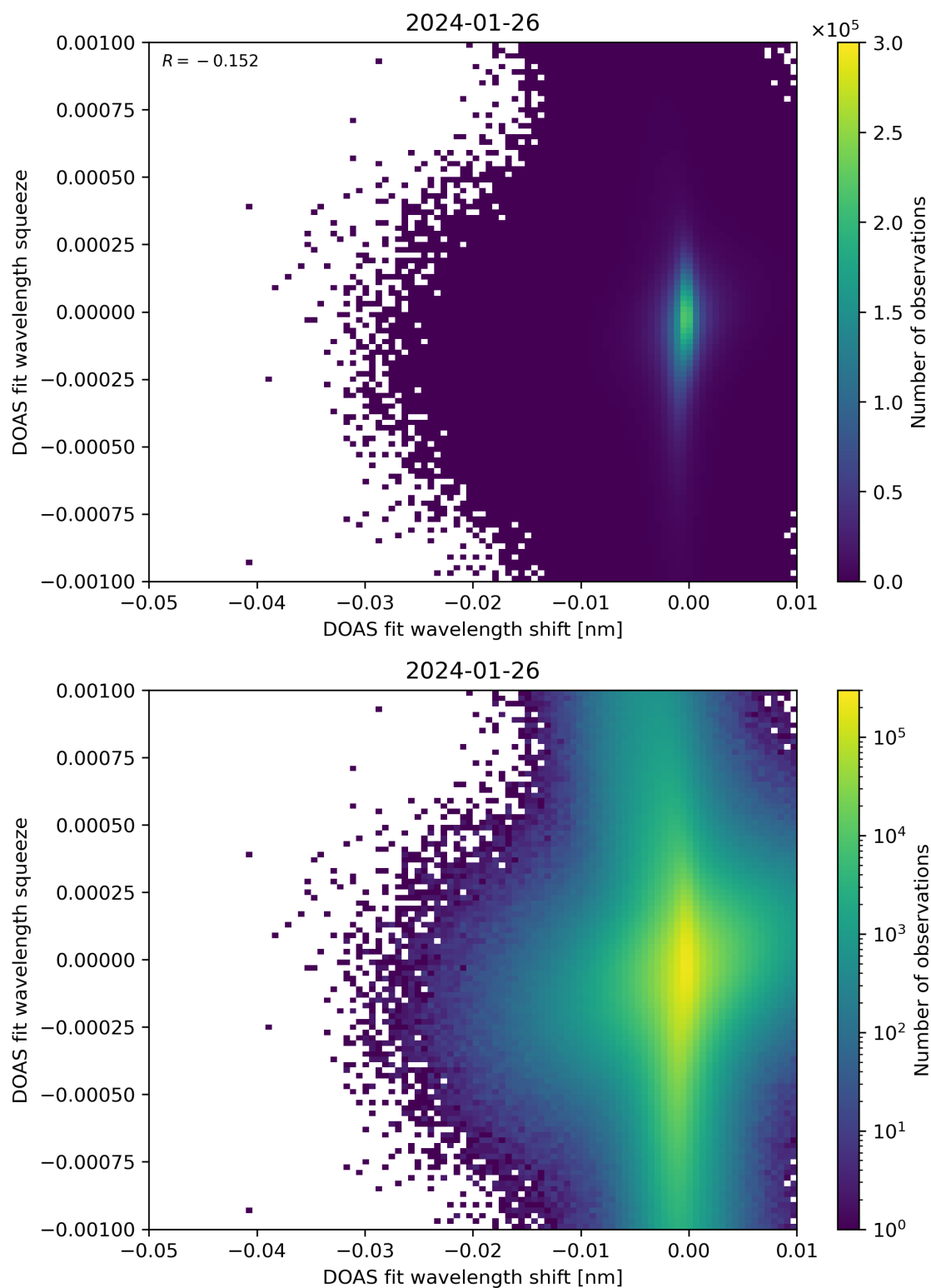
Figure 127: Scatter density plot of “DOAS fit wavelength shift” against “DOAS fit wavelength squeeze” for 2024-01-26 to 2024-01-27.
