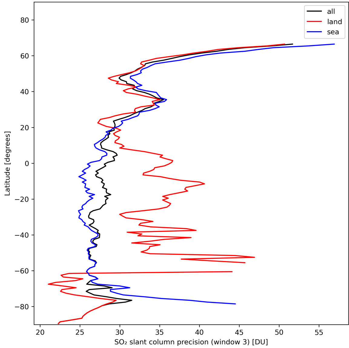
Figure 42: Zonal average of “SO 2 slant column precision (window 3)” for 2024-01-26 to 2024-01-27.
