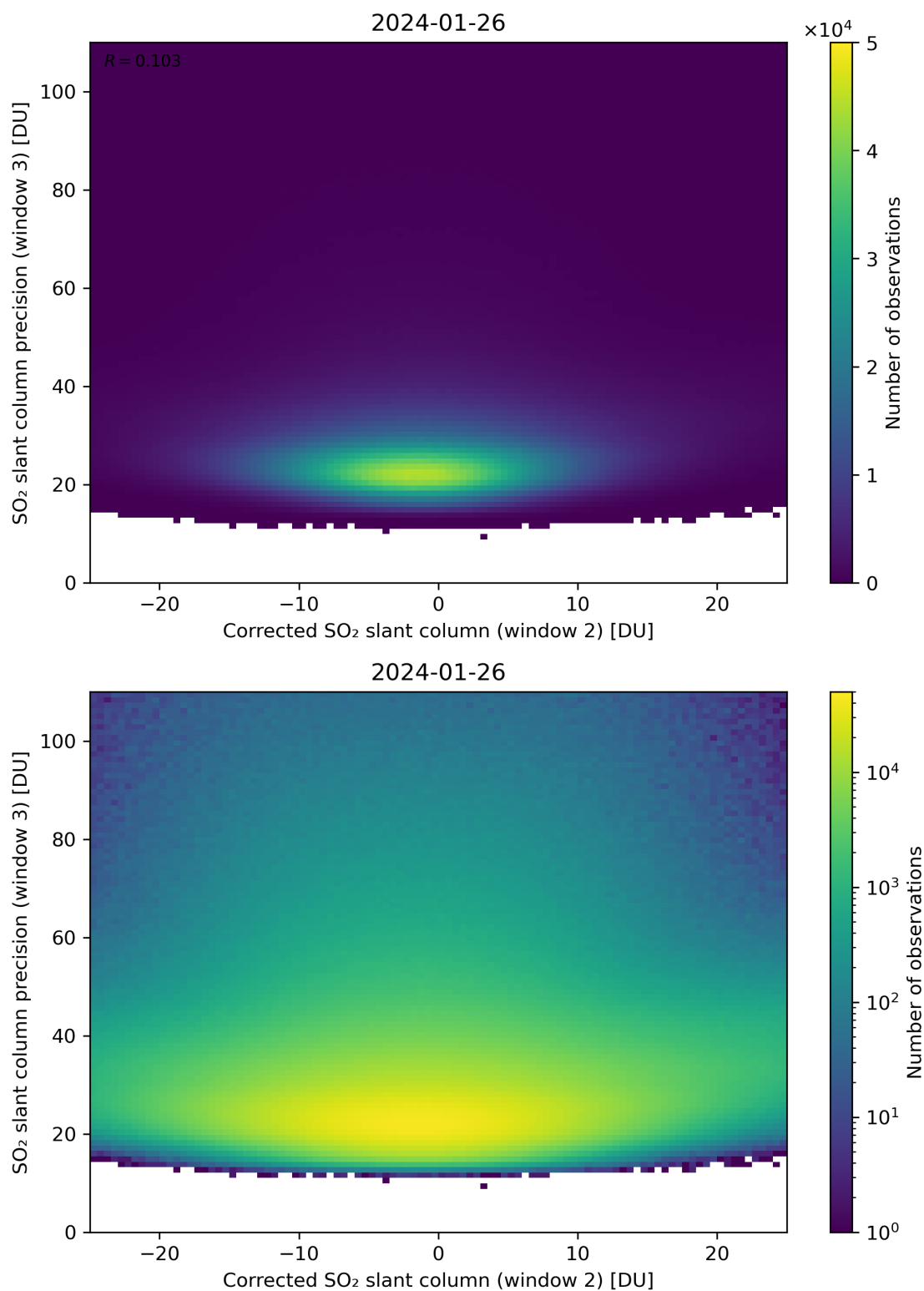
Figure 202: Scatter density plot of “Corrected SO 2 slant column (window 2)” against “SO 2 slant column precision (window 3)” for 2024-01-26 to 2024-01-27.
