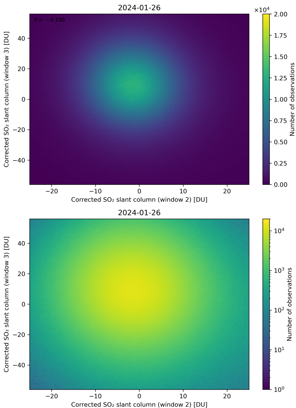
Figure 200: Scatter density plot of “Corrected SO 2 slant column (window 2)” against “Corrected SO 2 slant column (window 3)” for 2024-01-26 to 2024-01-27.
