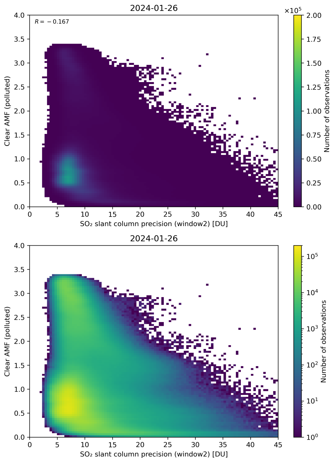
Figure 246: Scatter density plot of “SO 2 slant column precision (window2)” against “Clear AMF (polluted)” for 2024-01-26 to 2024-01-27.
