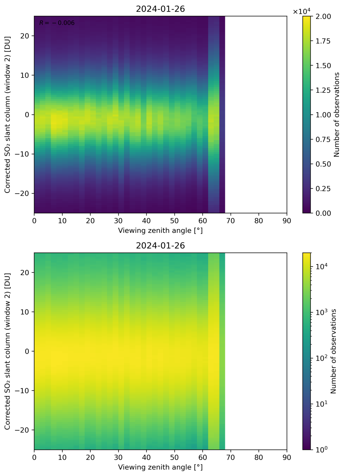
Figure 318: Scatter density plot of “Viewing zenith angle” against “Corrected SO 2 slant column (window 2)” for 2024-01-26 to 2024-01-27.
