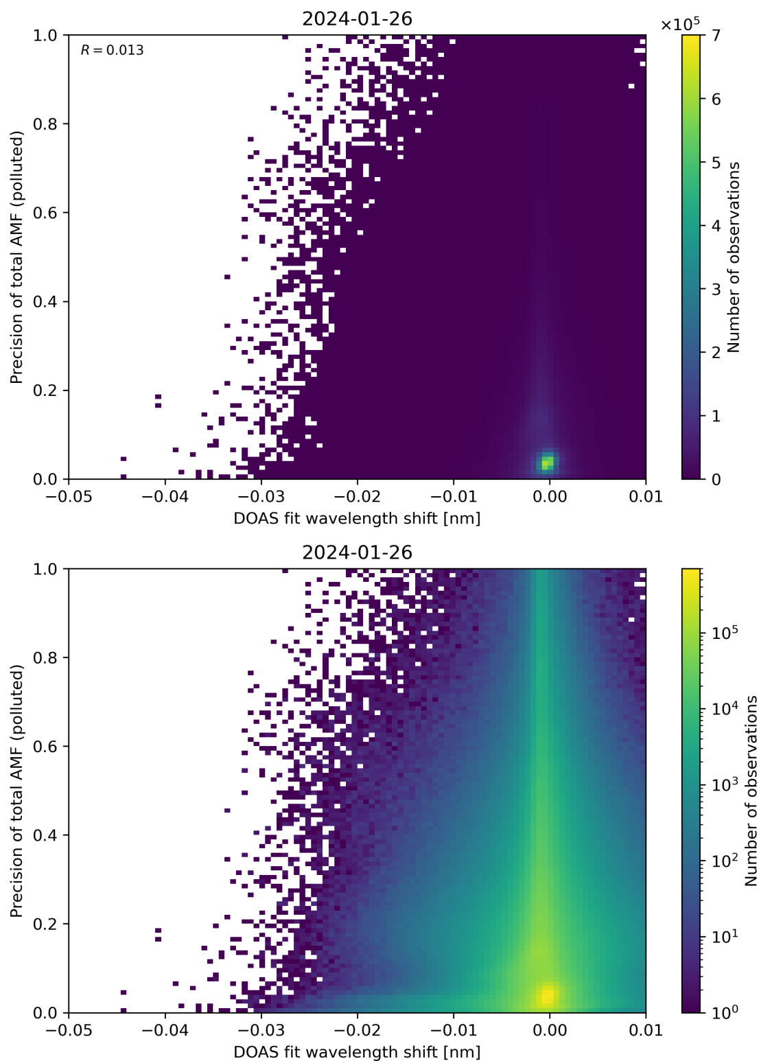
Figure 131: Scatter density plot of “DOAS fit wavelength shift” against “Precision of total AMF (polluted)” for 2024-01-26 to 2024-01-27.
