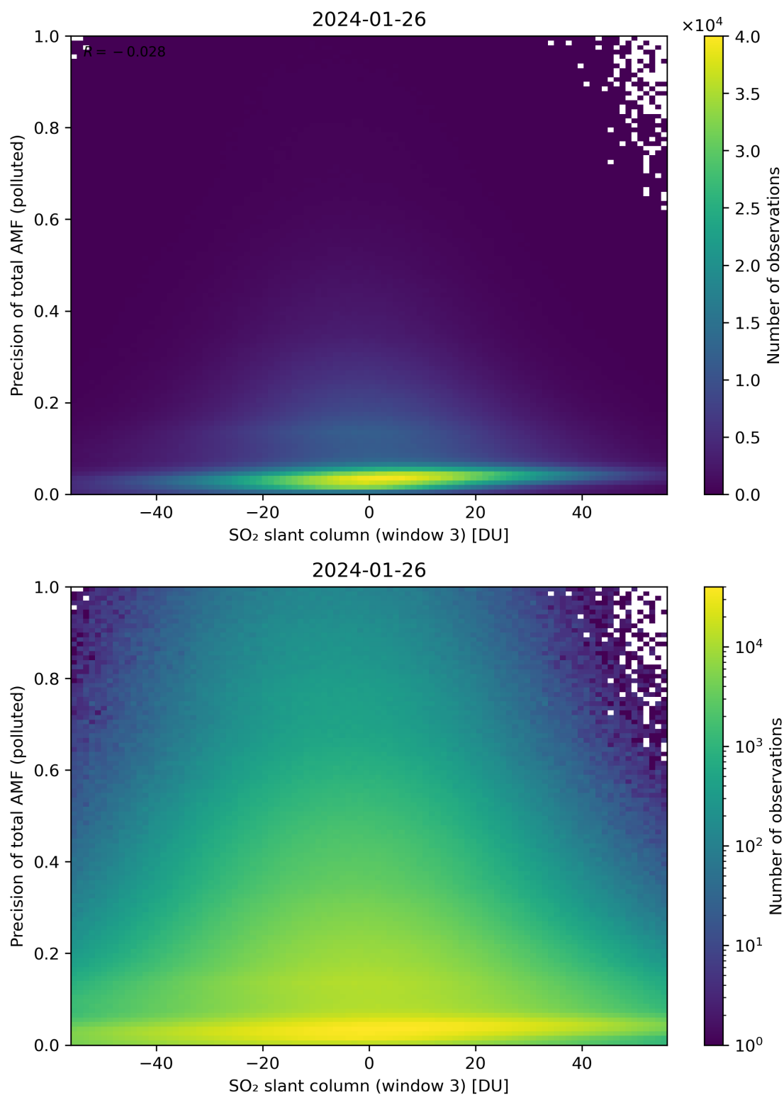
Figure 269: Scatter density plot of “SO 2 slant column (window 3)” against “Precision of total AMF (polluted)” for 2024-01-26 to 2024-01-27.
