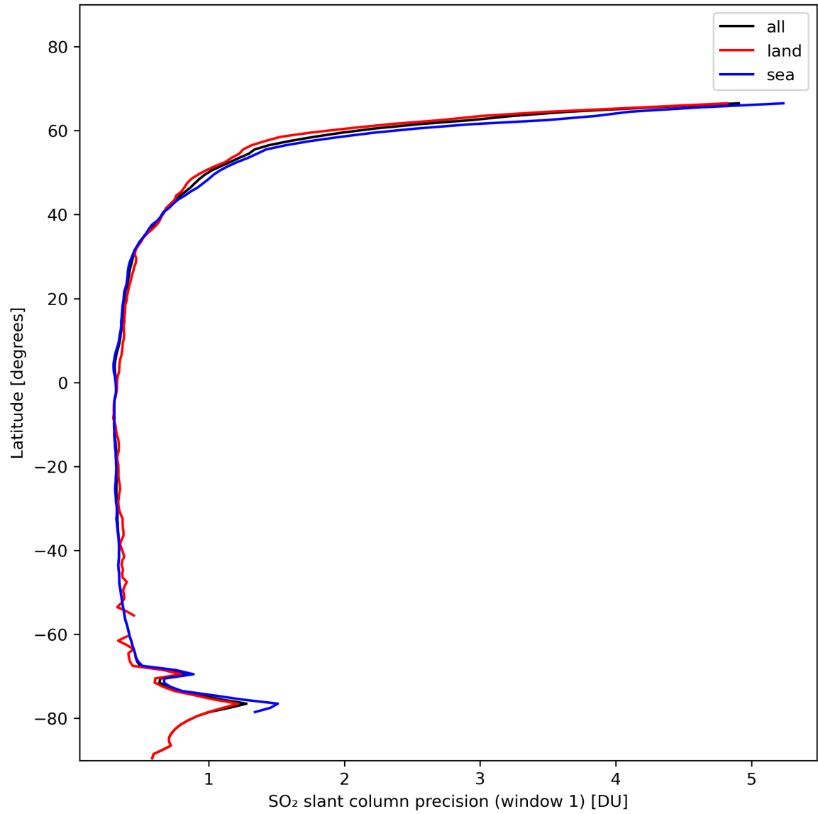
Figure 34: Zonal average of “SO 2 slant column precision (window 1)” for 2024-01-26 to 2024-01-27.
