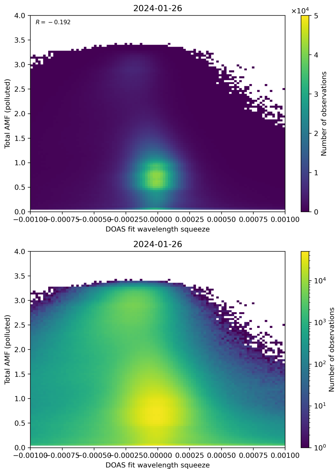
Figure 134: Scatter density plot of “DOAS fit wavelength squeeze” against “Total AMF (polluted)” for 2024-01-26 to 2024-01-27.
