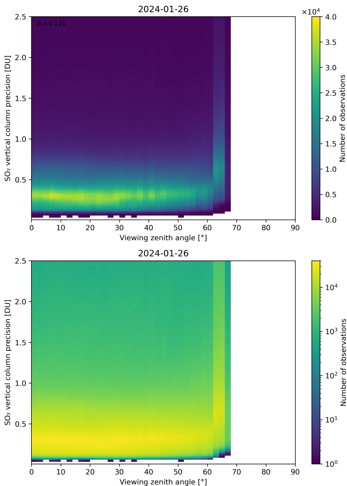
Figure 328: Scatter density plot of “Viewing zenith angle” against “SO 2 vertical column precision” for 2024-01-26 to 2024-01-27.
