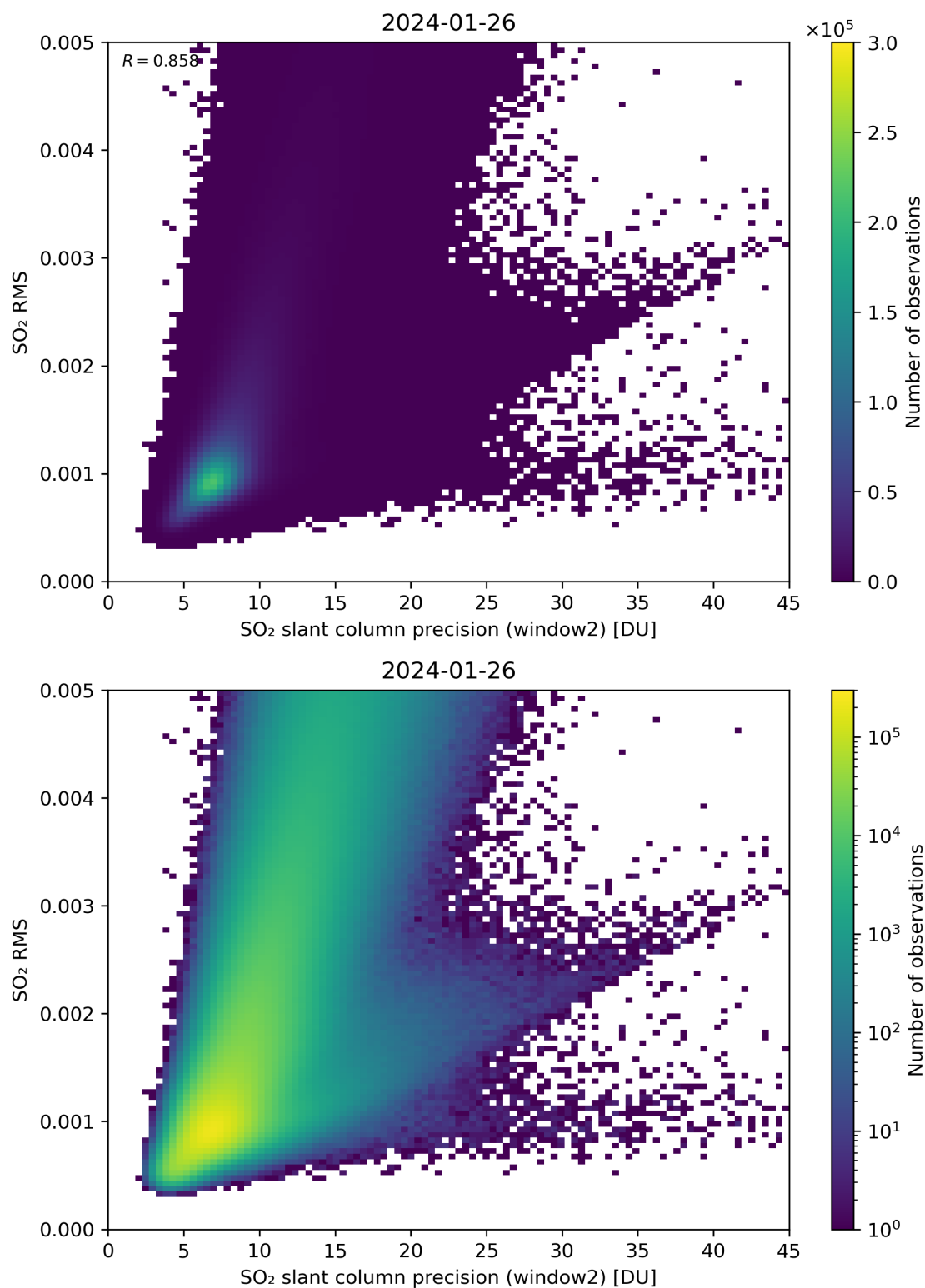
Figure 245: Scatter density plot of “SO 2 slant column precision (window2)” against “SO 2 RMS” for 2024-01-26 to 2024-01-27.
