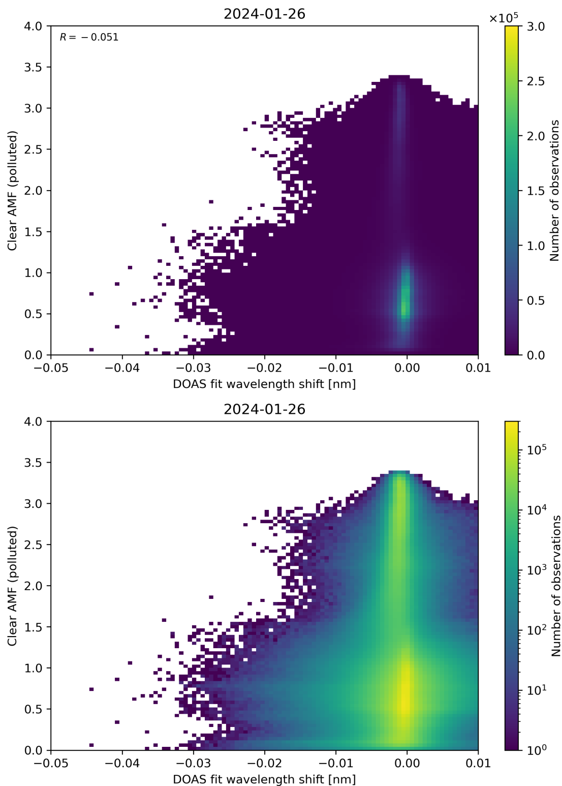
Figure 129: Scatter density plot of “DOAS fit wavelength shift” against “Clear AMF (polluted)” for 2024-01-26 to 2024-01-27.
