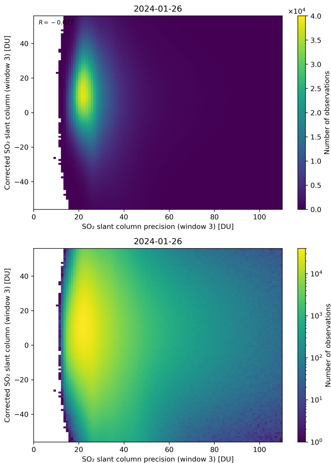
Figure 262: Scatter density plot of “SO 2 slant column precision (window 3)” against “Corrected SO 2 slant column (window 3)” for 2024-01-26 to 2024-01-27.
