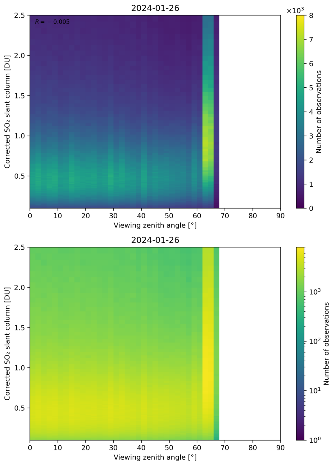
Figure 317: Scatter density plot of “Viewing zenith angle” against “Corrected SO 2 slant column” for 2024-01-26 to 2024-01-27.
