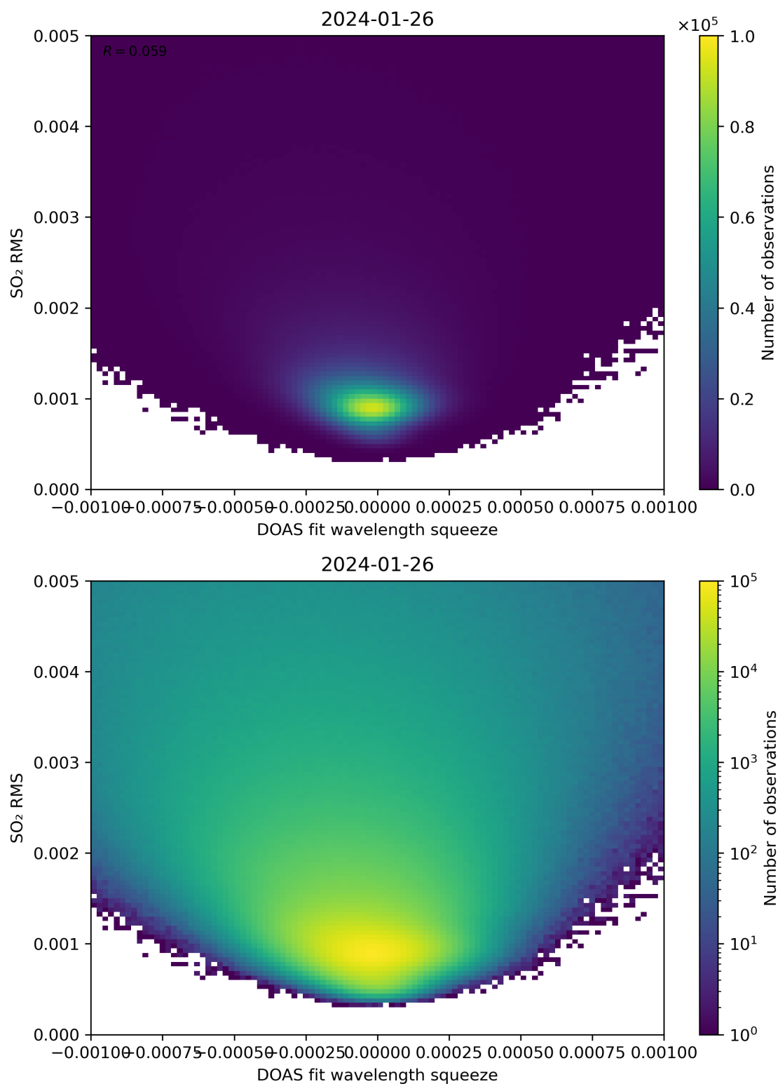
Figure 132: Scatter density plot of “DOAS fit wavelength squeeze” against “SO 2 RMS” for 2024-01-26 to 2024-01-27.
