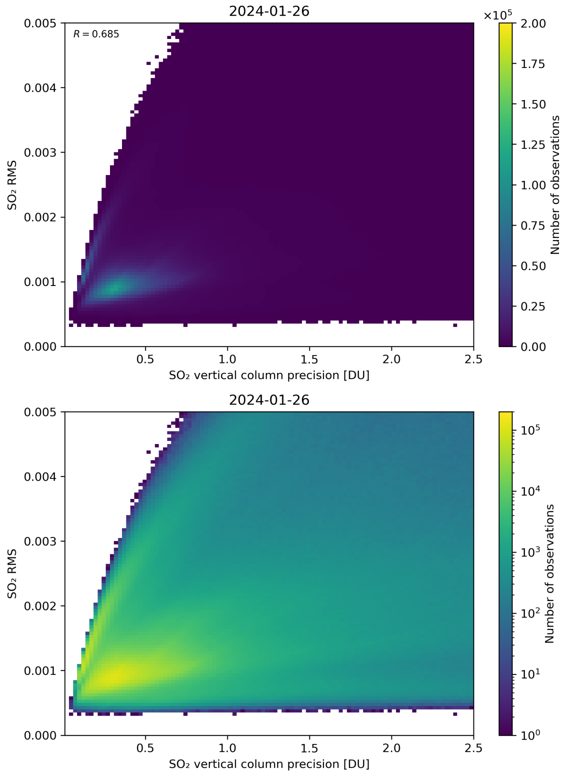
Figure 284: Scatter density plot of “SO 2 vertical column precision” against “SO 2 RMS” for 2024-01-26 to 2024-01-27.
