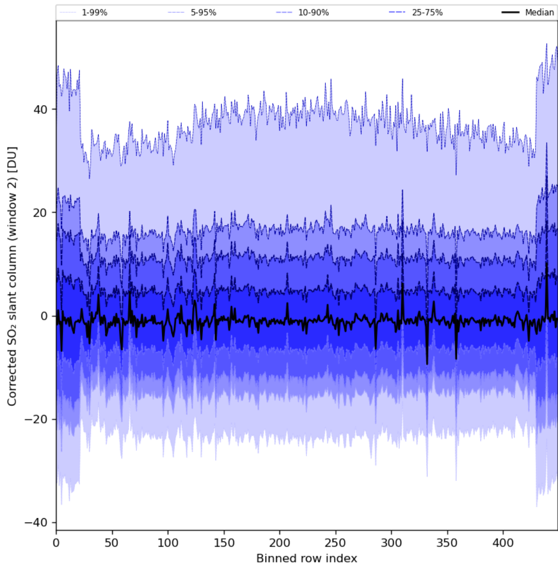
Figure 85: Along track statistics of “Corrected SO 2 slant column (window 2)” for 2024-01-26 to 2024-01-27
