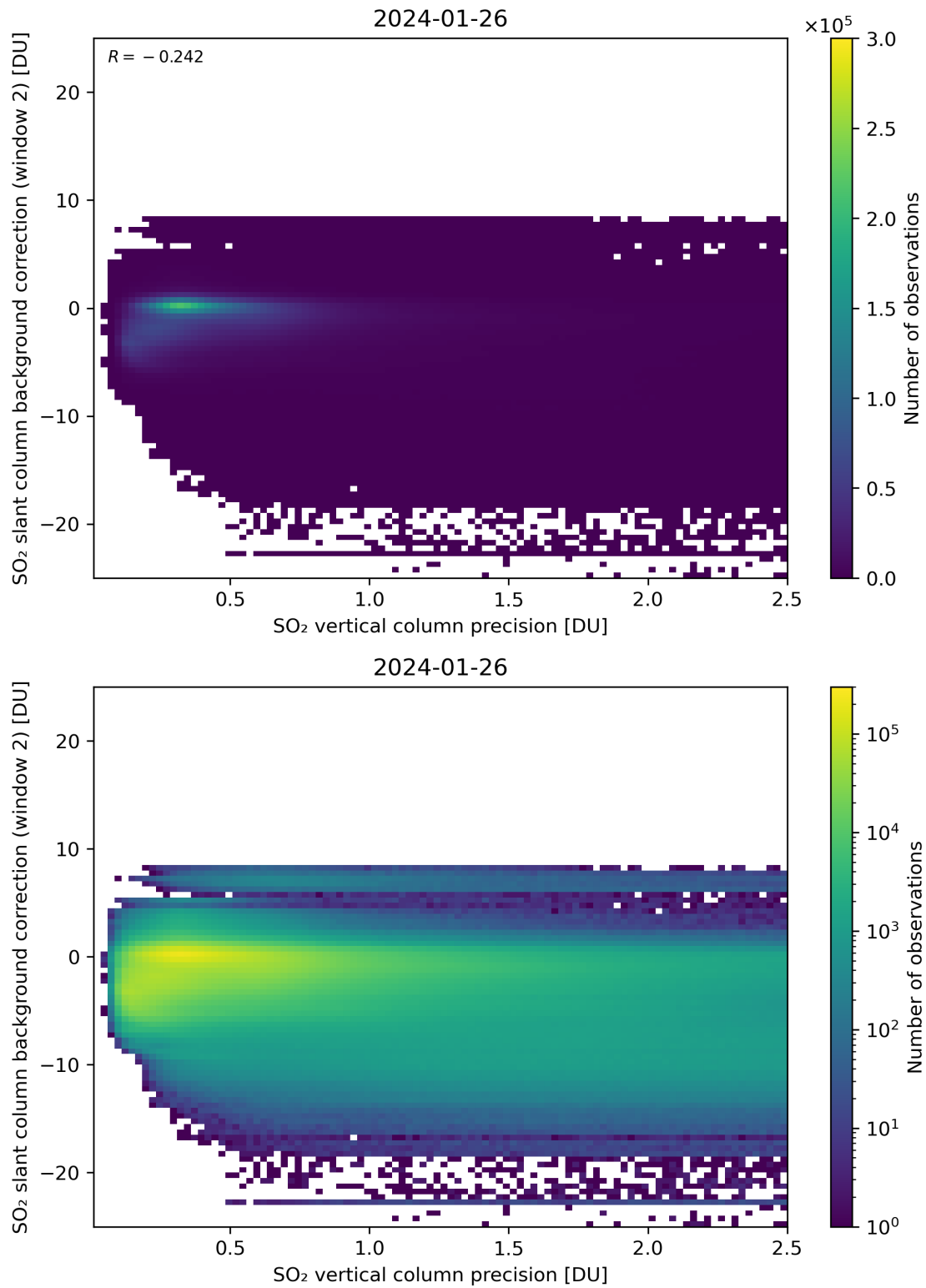
Figure 280: Scatter density plot of “SO 2 vertical column precision” against “SO 2 slant column background correction (window 2)” for 2024-01-26 to 2024-01-27.
