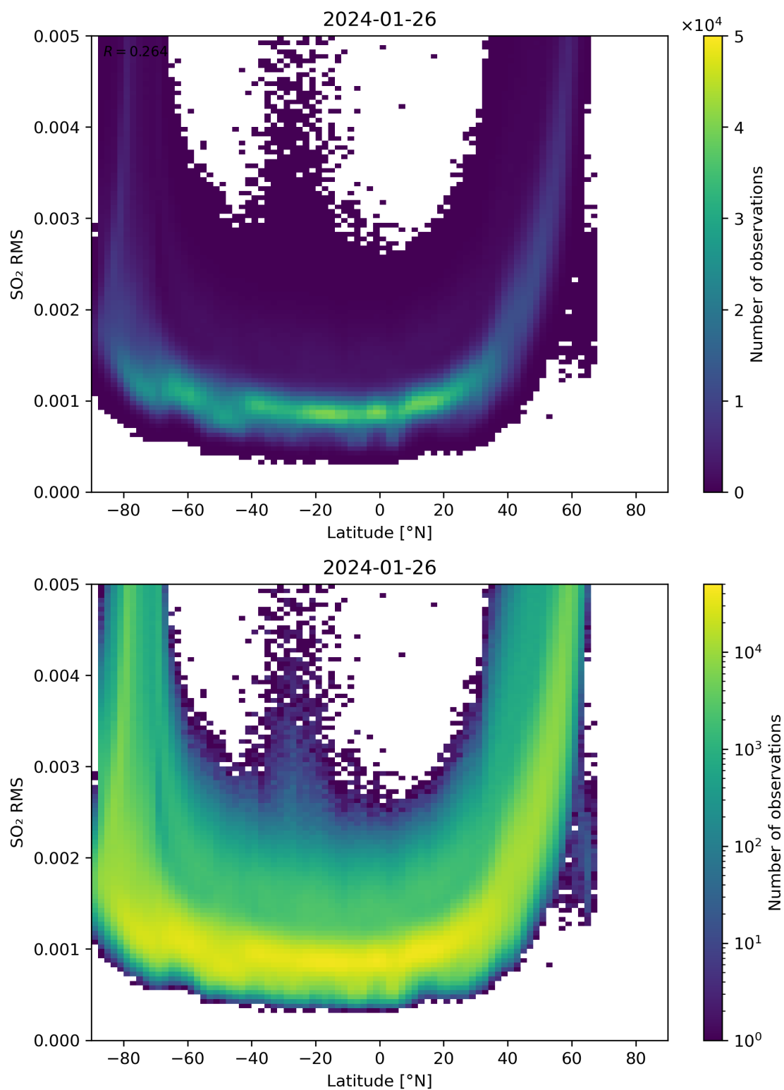
Figure 144: Scatter density plot of “Latitude” against “SO 2 RMS” for 2024-01-26 to 2024-01-27.
