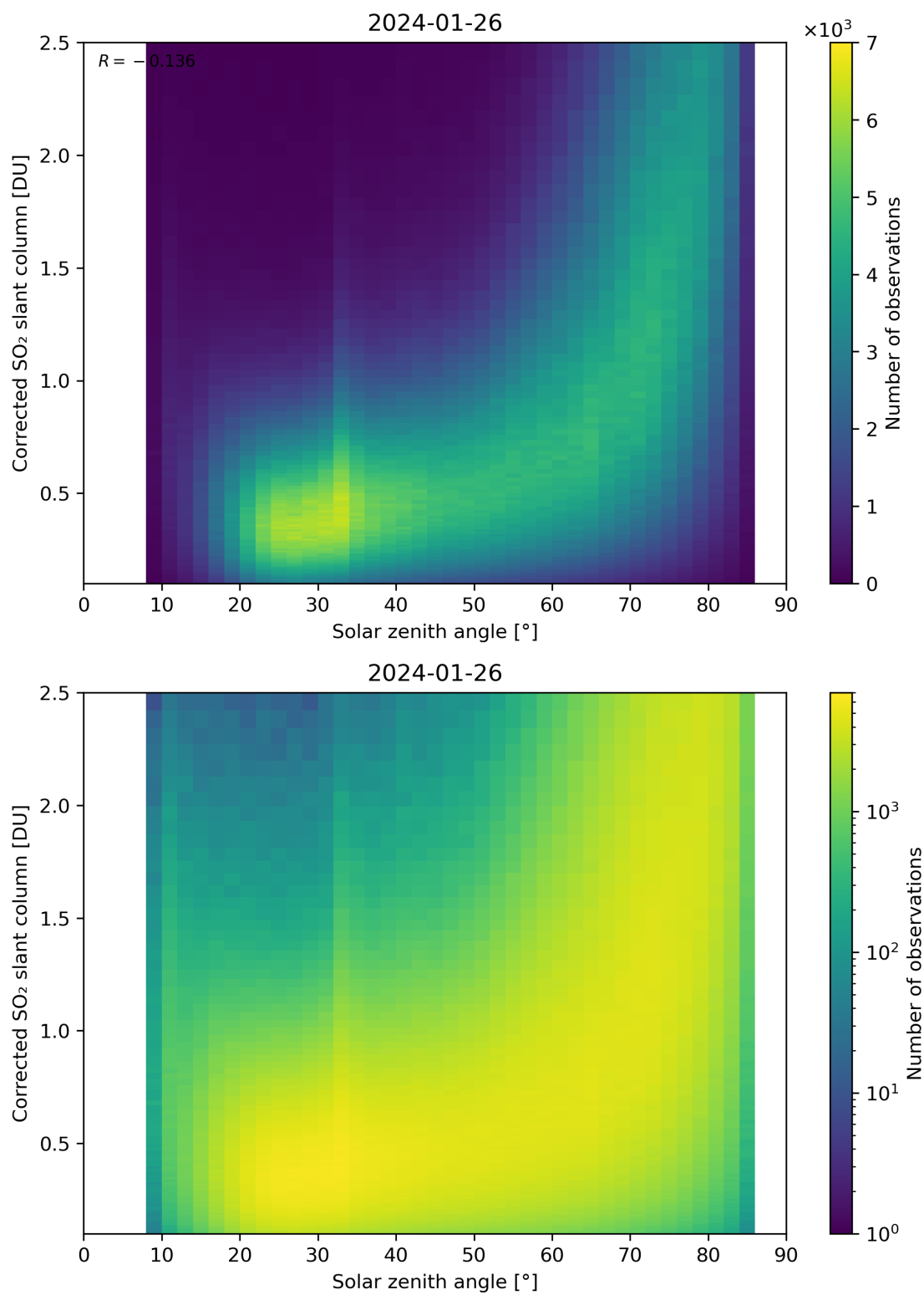
Figure 166: Scatter density plot of “Solar zenith angle” against “Corrected SO 2 slant column” for 2024-01-26 to 2024-01-27.
