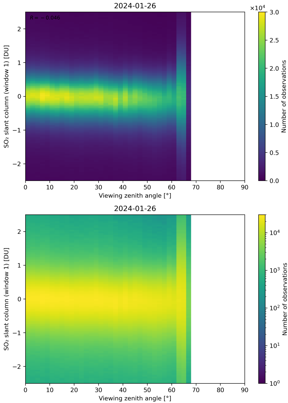
Figure 320: Scatter density plot of “Viewing zenith angle” against “SO 2 slant column (window 1)” for 2024-01-26 to 2024-01-27.
