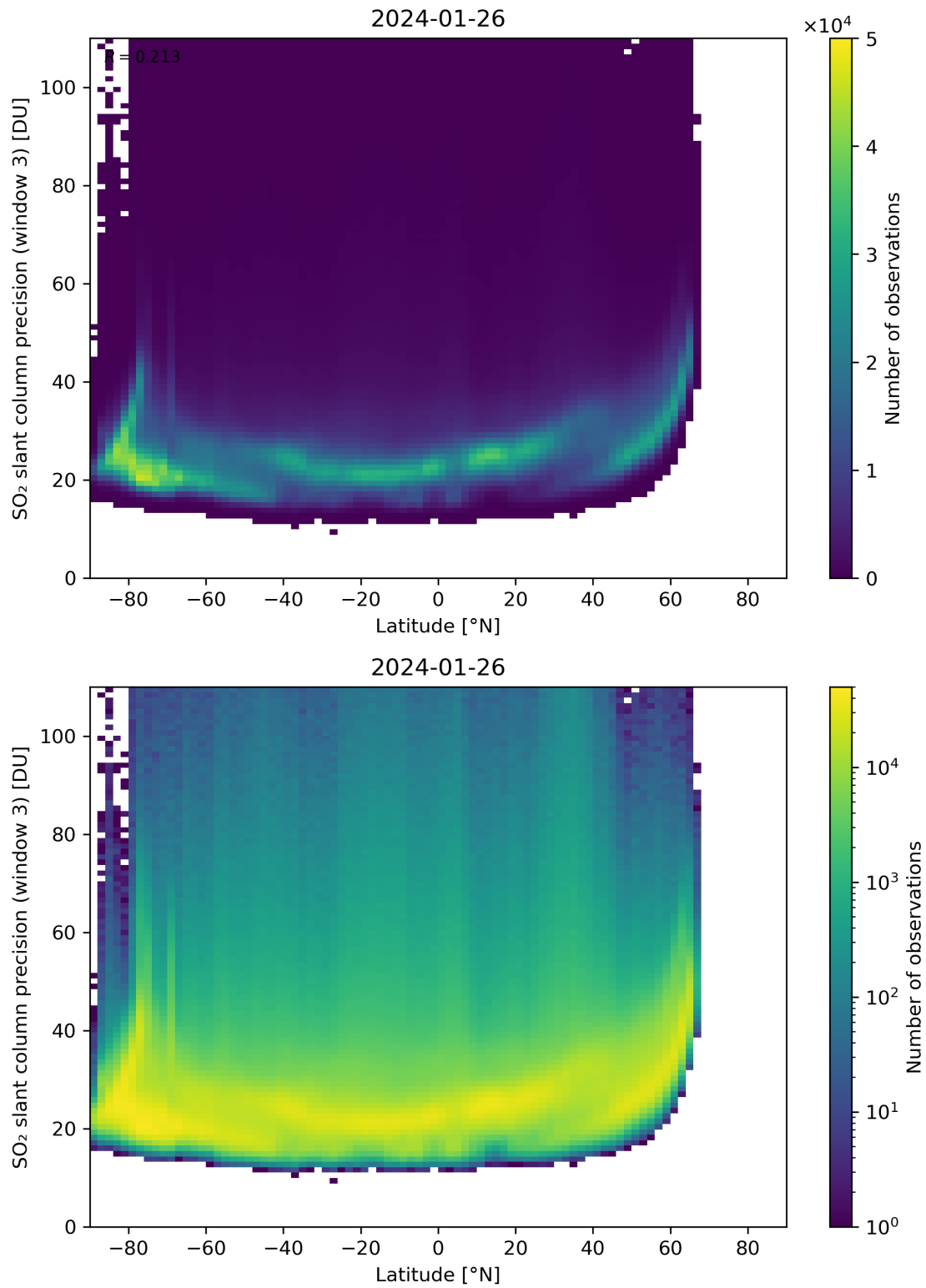
Figure 153: Scatter density plot of “Latitude” against “SO 2 slant column precision (window 3)” for 2024-01-26 to 2024-01-27.
