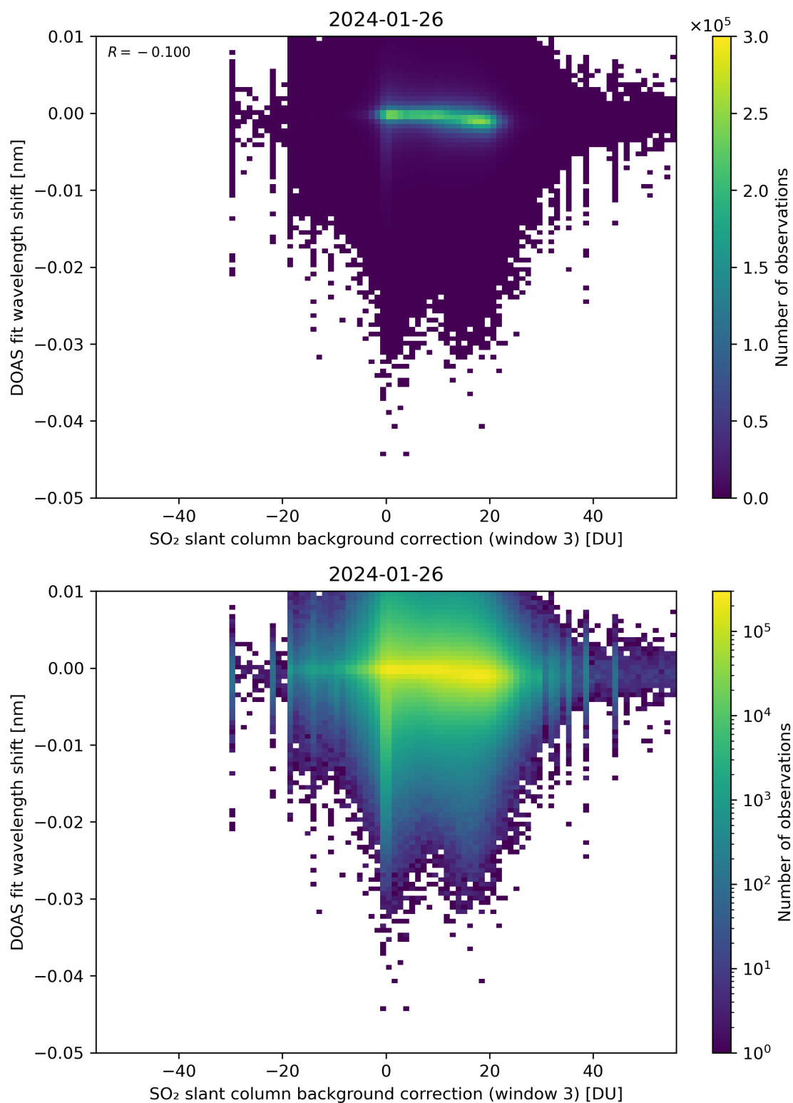
Figure 121: Scatter density plot of “SO 2 slant column background correction (window 3)” against “DOAS fit wavelength shift” for 2024-01-26 to 2024-01-27.
