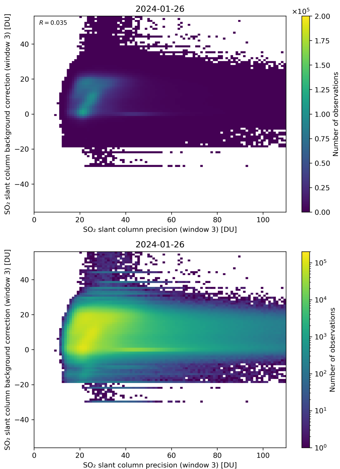
Figure 257: Scatter density plot of “SO 2 slant column precision (window 3)” against “SO 2 slant column background correction (window 3)” for 2024-01-26 to 2024-01-27.
