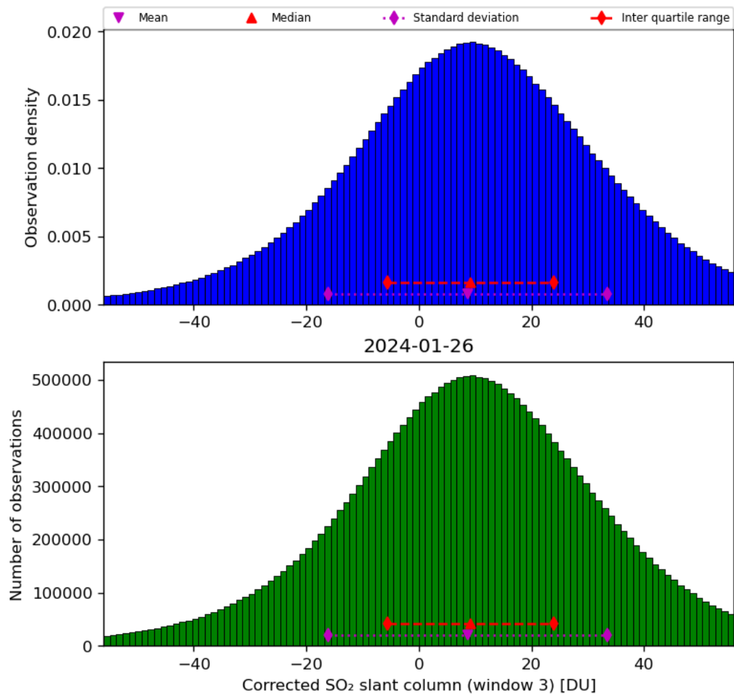
Figure 66: Histogram of “Corrected SO 2 slant column (window 3)” for 2024-01-26 to 2024-01-27
