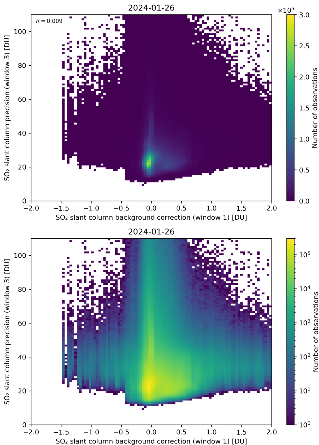
Figure 108: Scatter density plot of “SO 2 slant column background correction (window 1)” against “SO 2 slant column precision (window 3)” for 2024-01-26 to 2024-01-27.
