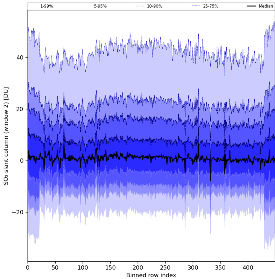
Figure 83: Along track statistics of “SO 2 slant column (window 2)” for 2024-01-26 to 2024-01-27
