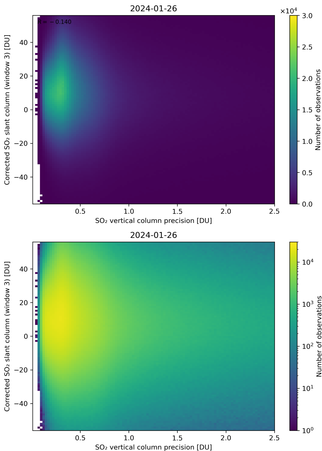
Figure 288: Scatter density plot of “SO 2 vertical column precision” against “Corrected SO 2 slant column (window 3)” for 2024-01-26 to 2024-01-27.
