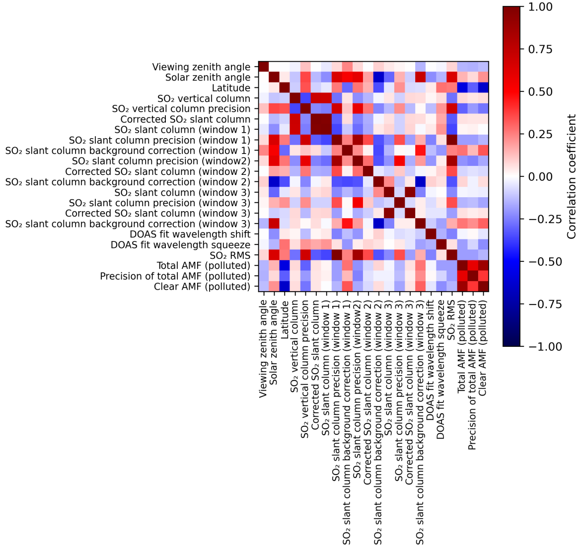
Figure 2: Map of correlation matrix for 2024-01-26 to 2024-01-27.
