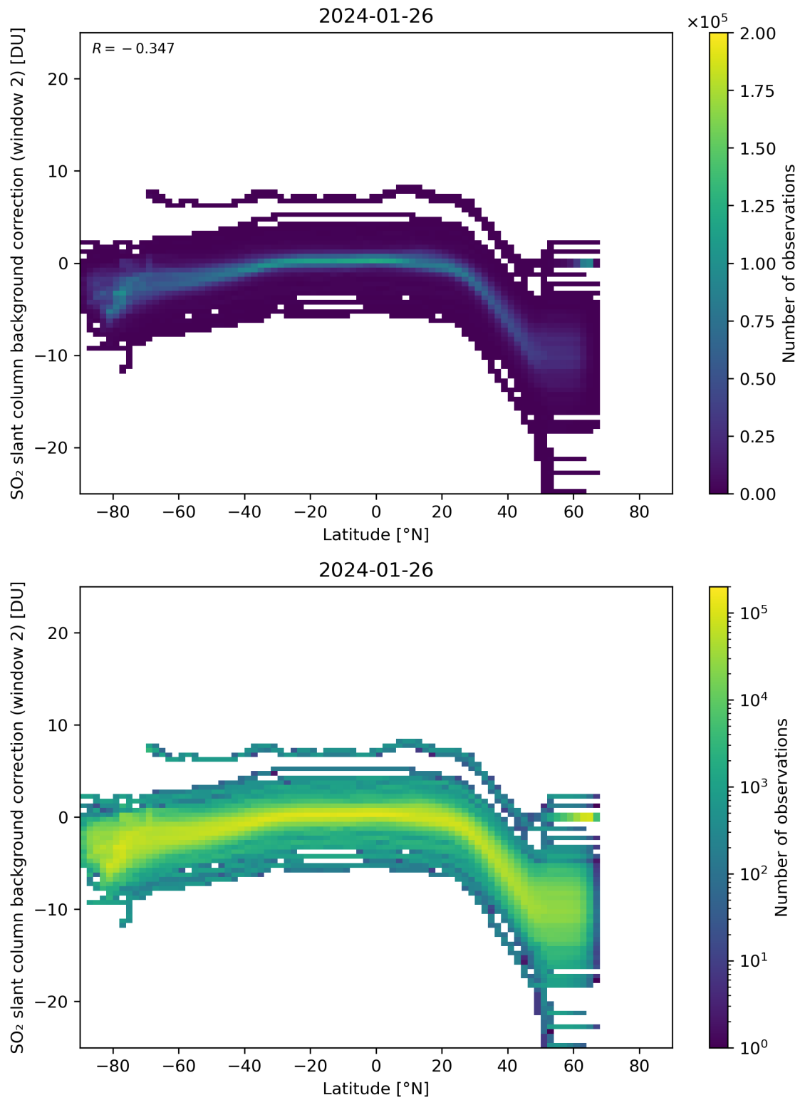
Figure 140: Scatter density plot of “Latitude” against “SO 2 slant column background correction (window 2)” for 2024-01-26 to 2024-01-27.
