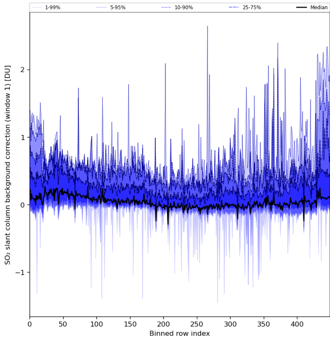
Figure 82: Along track statistics of “SO 2 slant column background correction (window 1)” for 2024-01-26 to 2024-01-27
