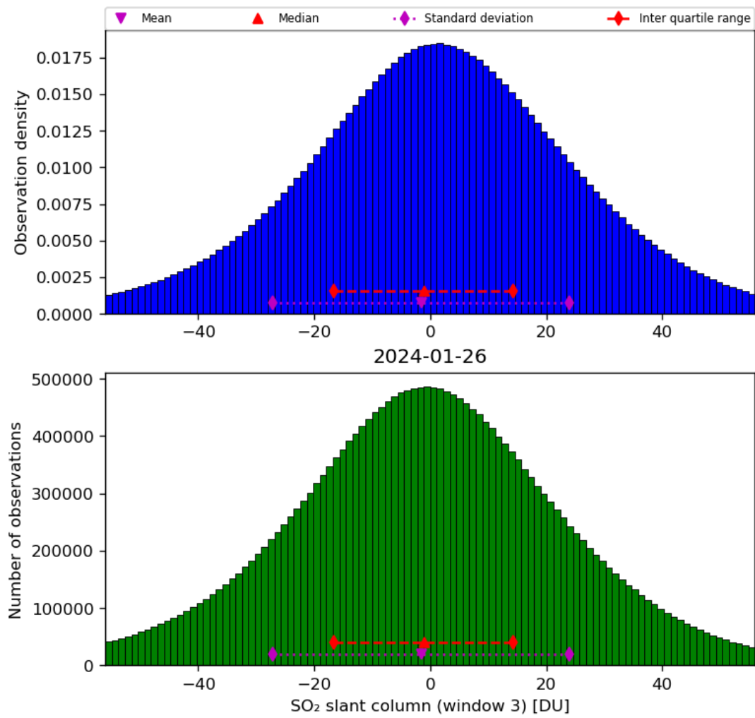
Figure 64: Histogram of “SO 2 slant column (window 3)” for 2024-01-26 to 2024-01-27
