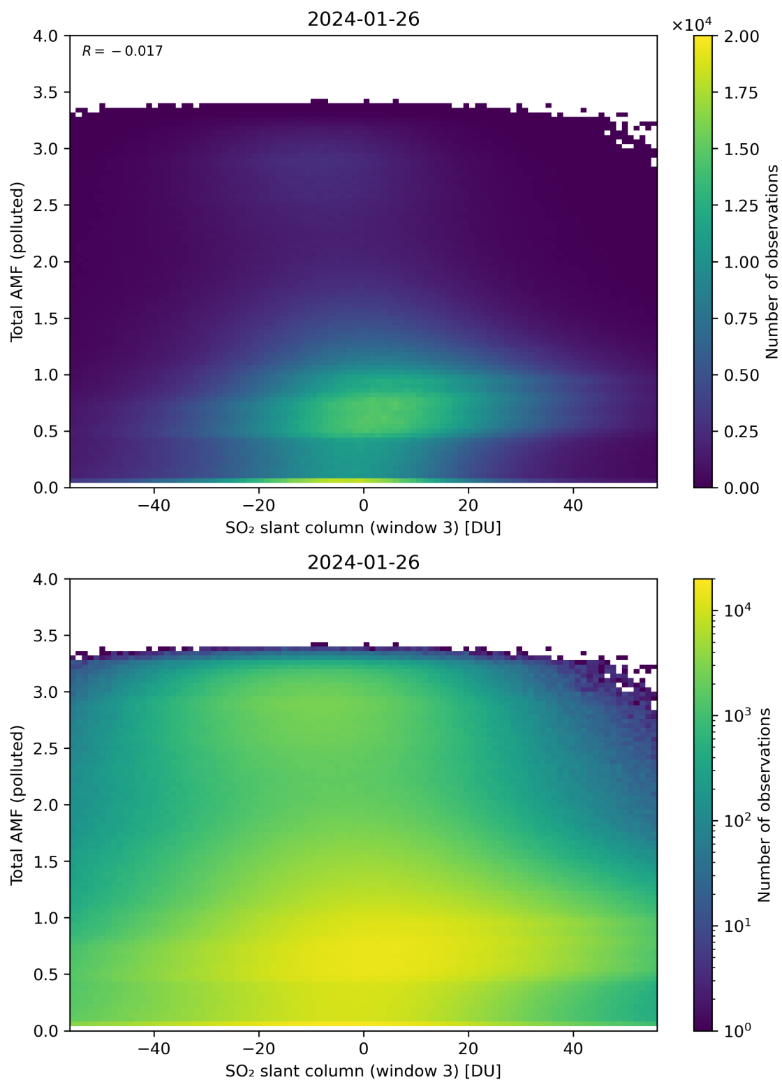
Figure 268: Scatter density plot of “SO 2 slant column (window 3)” against “Total AMF (polluted)” for 2024-01-26 to 2024-01-27.
