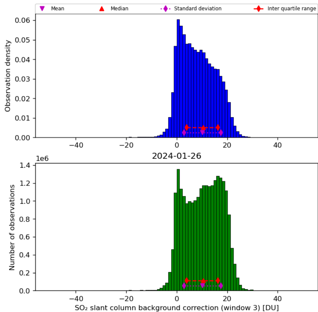
Figure 67: Histogram of “SO 2 slant column background correction (window 3)” for 2024-01-26 to 2024-01-27
