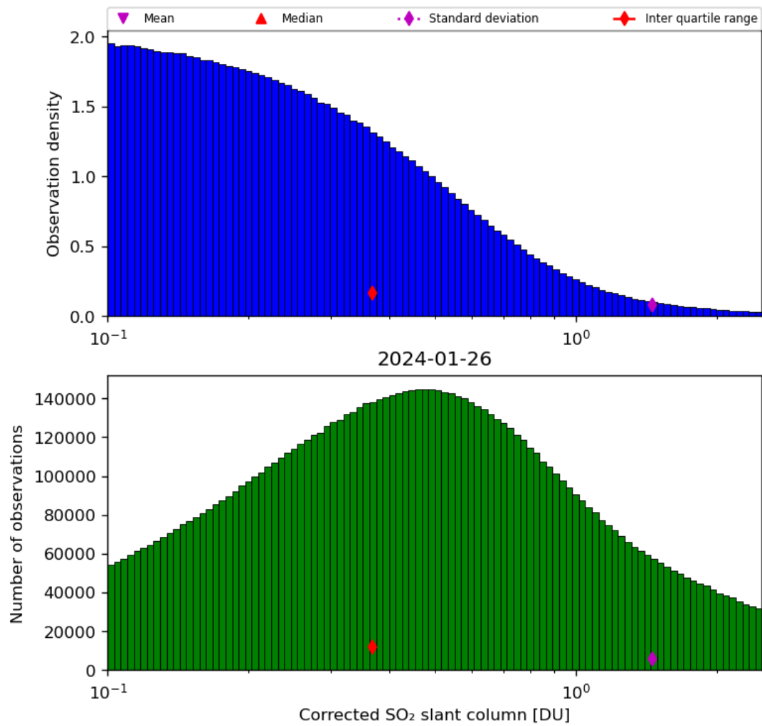
Figure 55: Histogram of “Corrected SO 2 slant column” for 2024-01-26 to 2024-01-27
