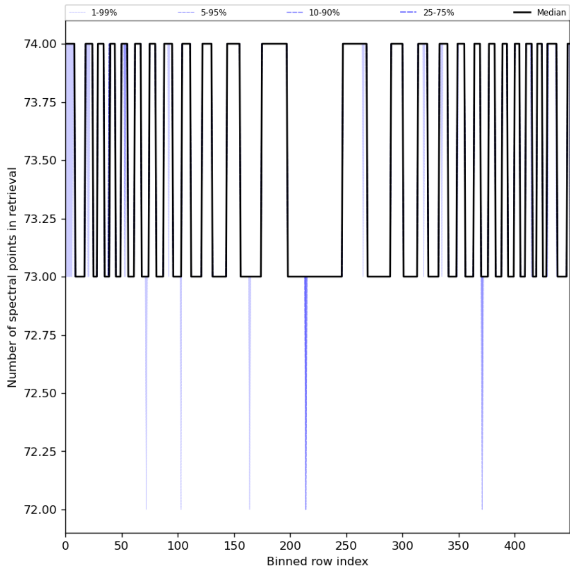
Figure 97: Along track statistics of “Number of spectral points in retrieval” for 2024-01-26 to 2024-01-27
