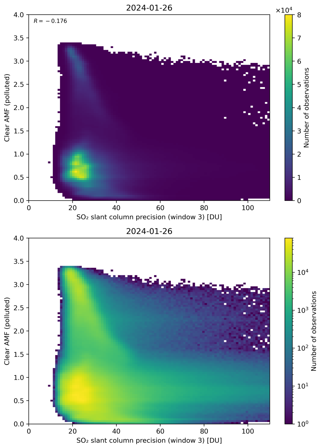
Figure 261: Scatter density plot of “SO 2 slant column precision (window 3)” against “Clear AMF (polluted)” for 2024-01-26 to 2024-01-27.
