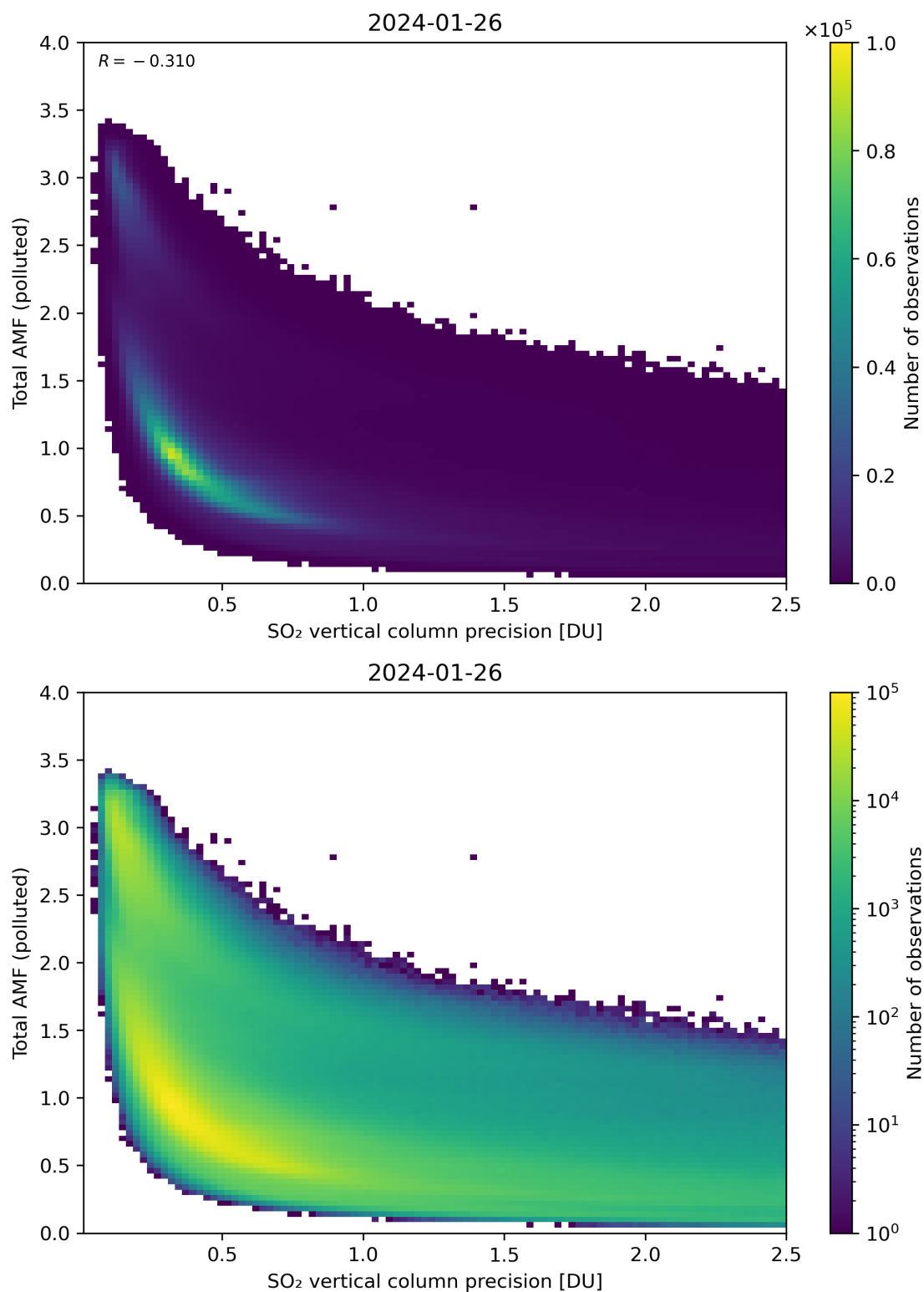
Figure 294: Scatter density plot of “SO 2 vertical column precision” against “Total AMF (polluted)” for 2024-01-26 to 2024-01-27.
