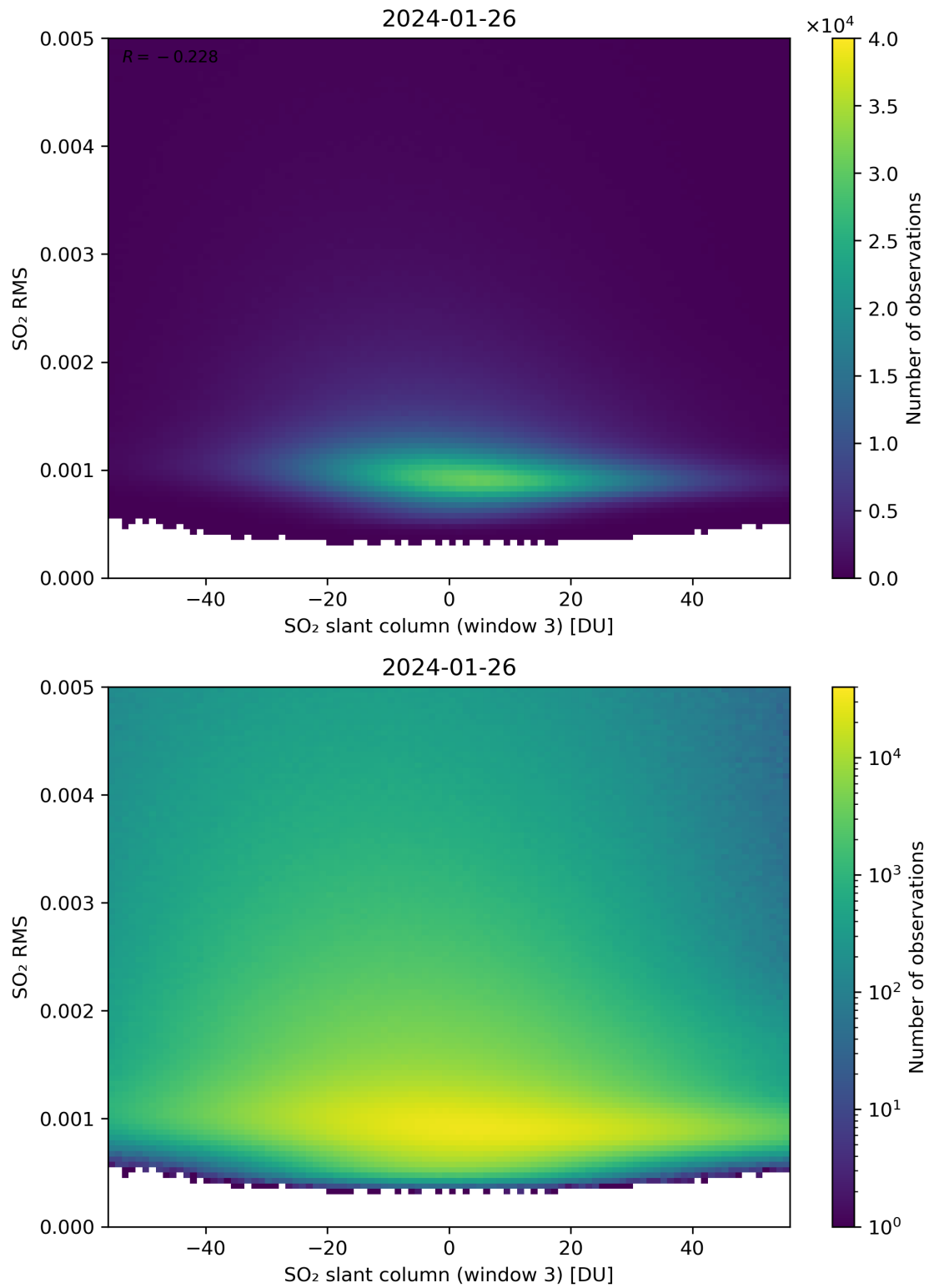
Figure 256: Scatter density plot of “SO 2 slant column (window 3)” against “SO 2 RMS” for 2024-01-26 to 2024-01-27.
