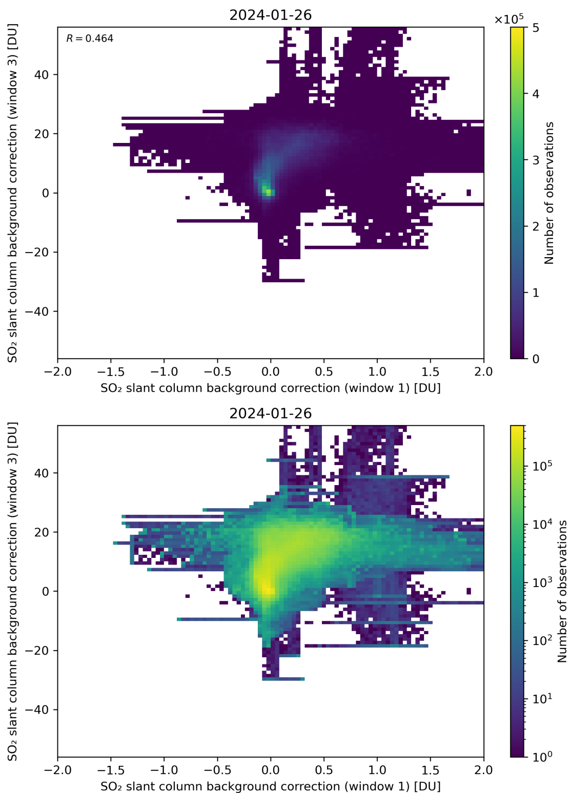
Figure 99: Scatter density plot of “SO 2 slant column background correction (window 1)” against “SO 2 slant column background correction (window 3)” for 2024-01-26 to 2024-01-27.
