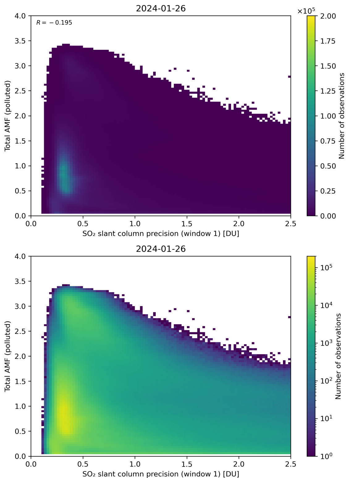
Figure 230: Scatter density plot of “SO 2 slant column precision (window 1)” against “Total AMF (polluted)” for 2024-01-26 to 2024-01-27.
