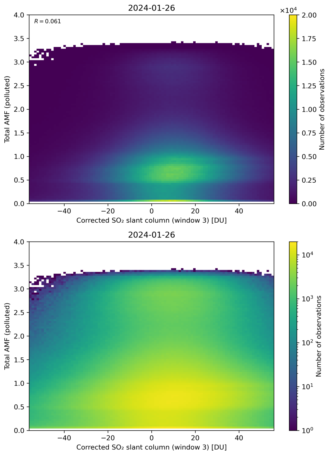
Figure 210: Scatter density plot of “Corrected SO 2 slant column (window 3)” against “Total AMF (polluted)” for 2024-01-26 to 2024-01-27.
