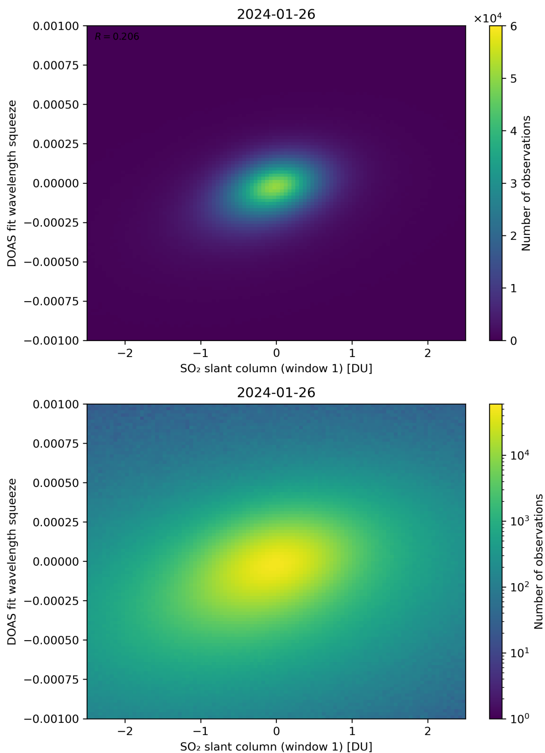
Figure 216: Scatter density plot of “SO 2 slant column (window 1)” against “DOAS fit wavelength squeeze” for 2024-01-26 to 2024-01-27.
