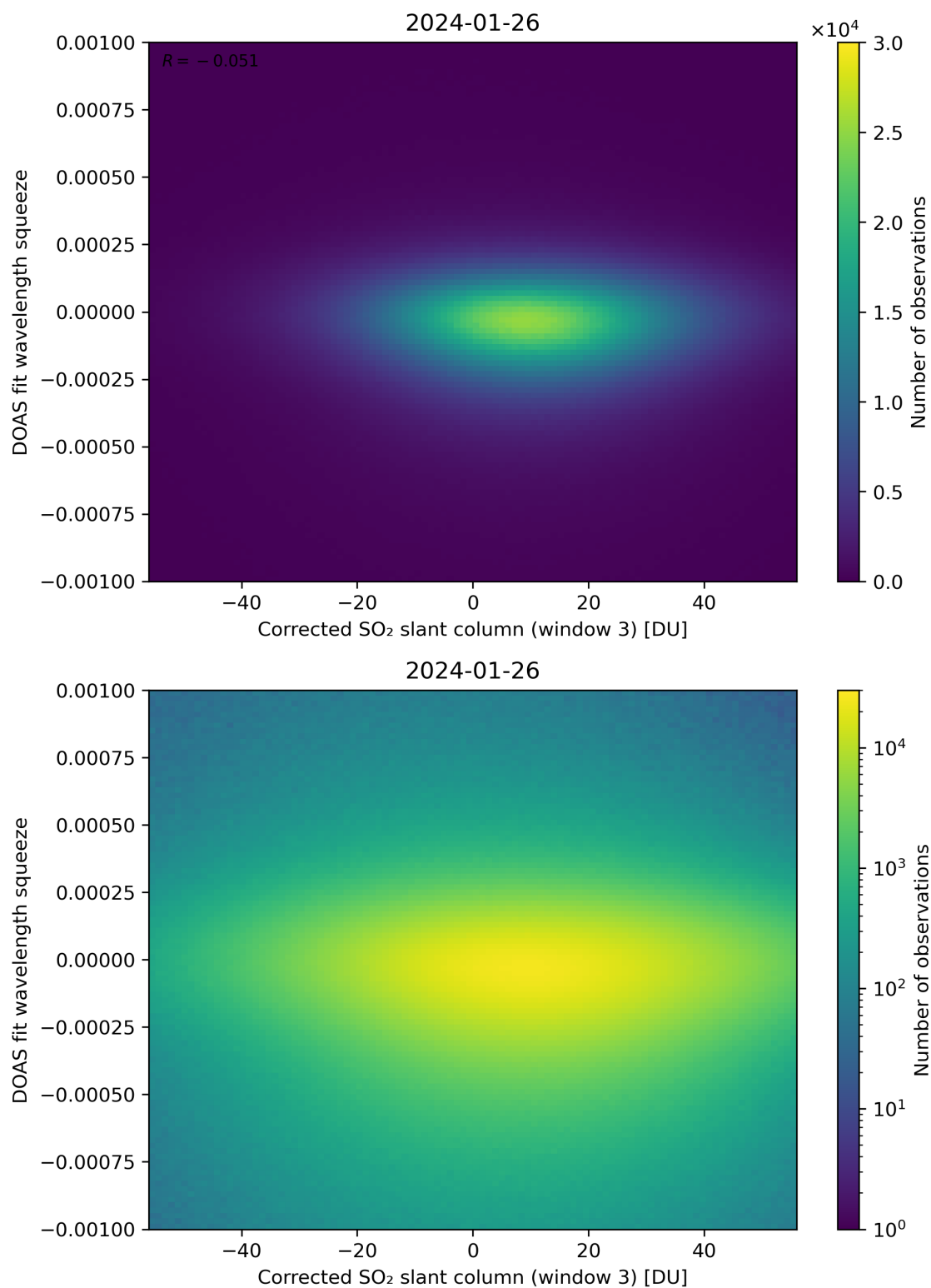
Figure 207: Scatter density plot of “Corrected SO 2 slant column (window 3)” against “DOAS fit wavelength squeeze” for 2024-01-26 to 2024-01-27.
