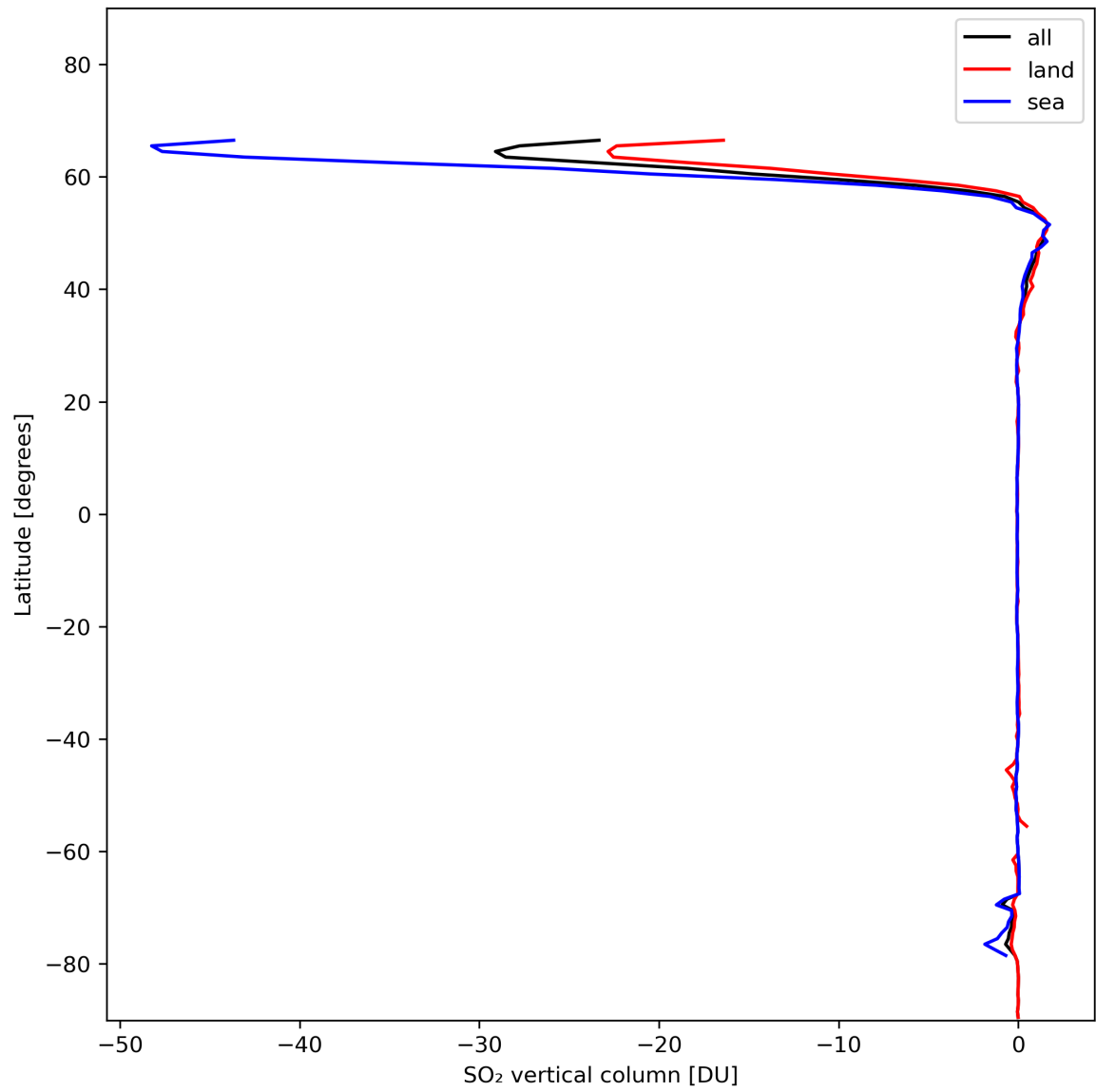
Figure 30: Zonal average of “SO 2 vertical column” for 2024-01-26 to 2024-01-27.
