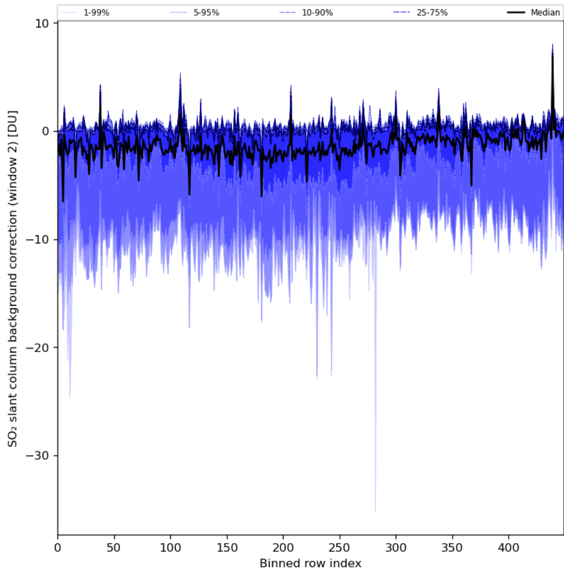
Figure 86: Along track statistics of “SO 2 slant column background correction (window 2)” for 2024-01-26 to 2024-01-27
