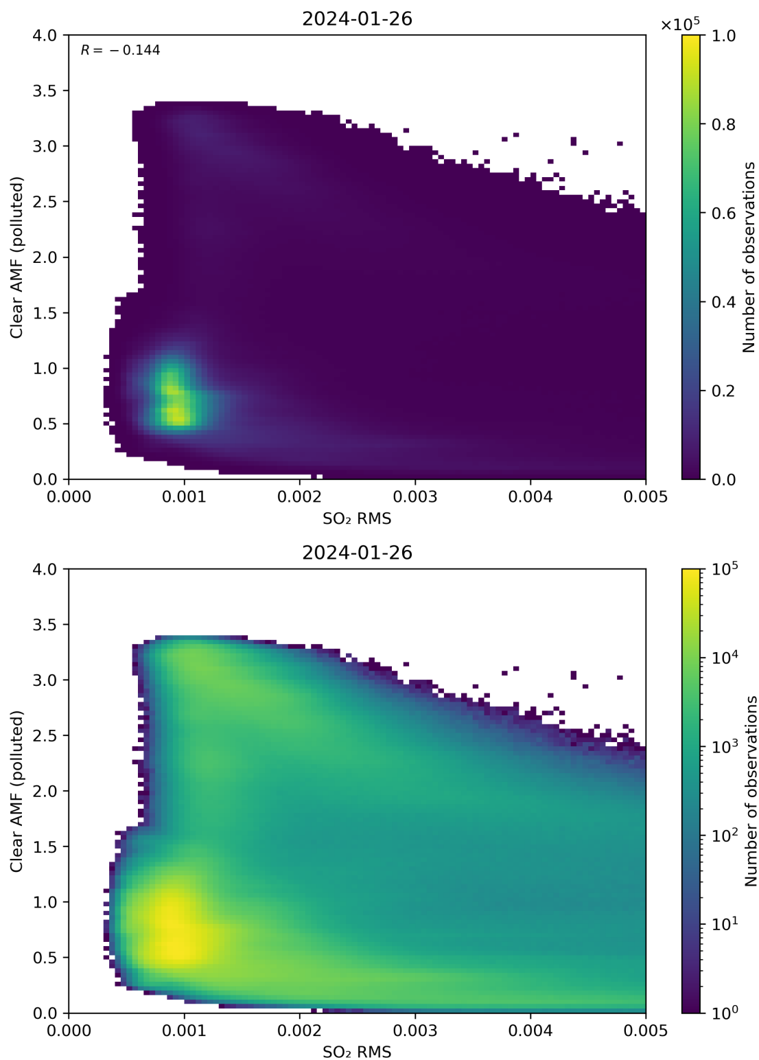
Figure 136: Scatter density plot of “SO 2 RMS” against “Clear AMF (polluted)” for 2024-01-26 to 2024-01-27.
