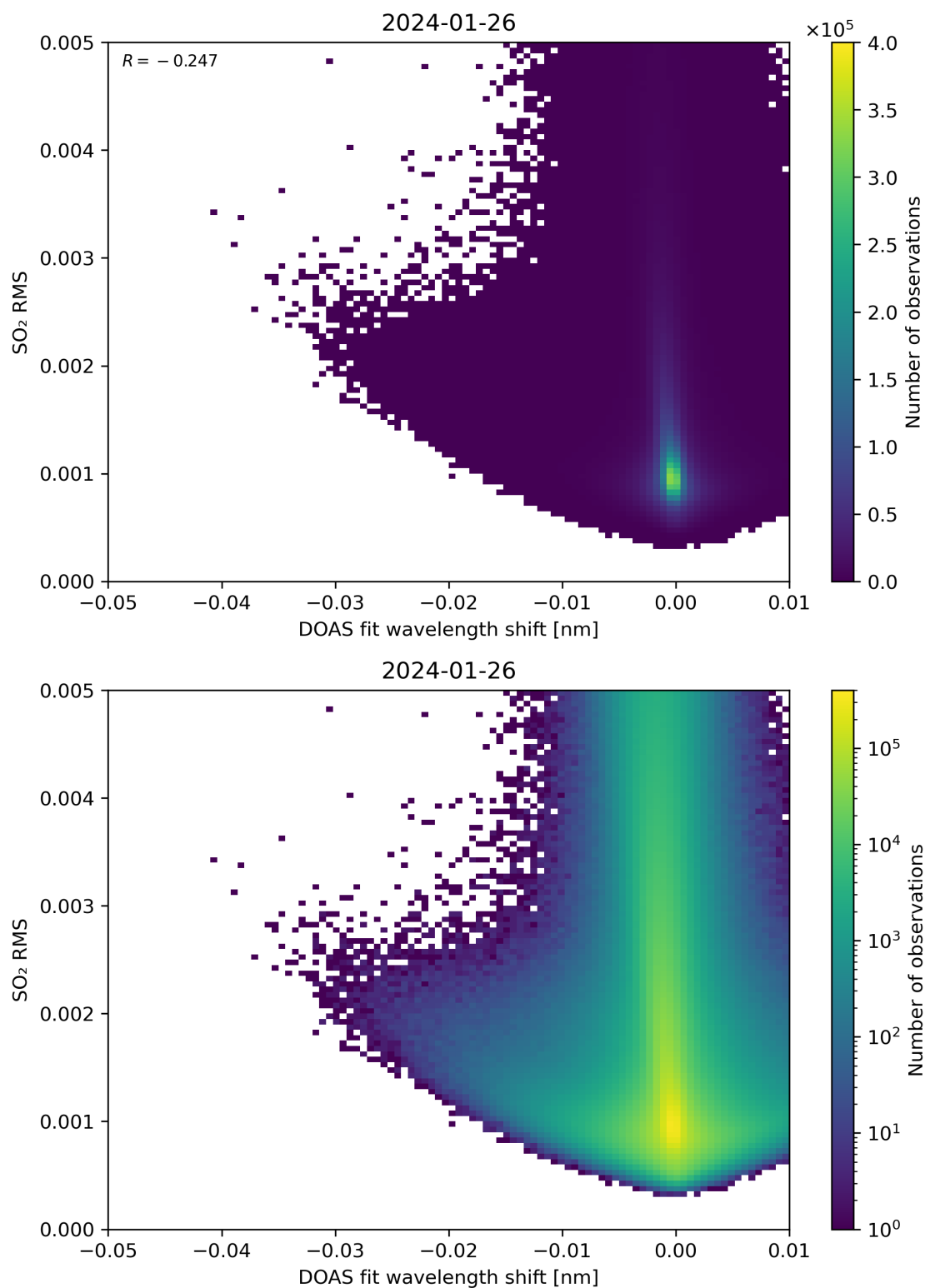
Figure 128: Scatter density plot of “DOAS fit wavelength shift” against “SO 2 RMS” for 2024-01-26 to 2024-01-27.
