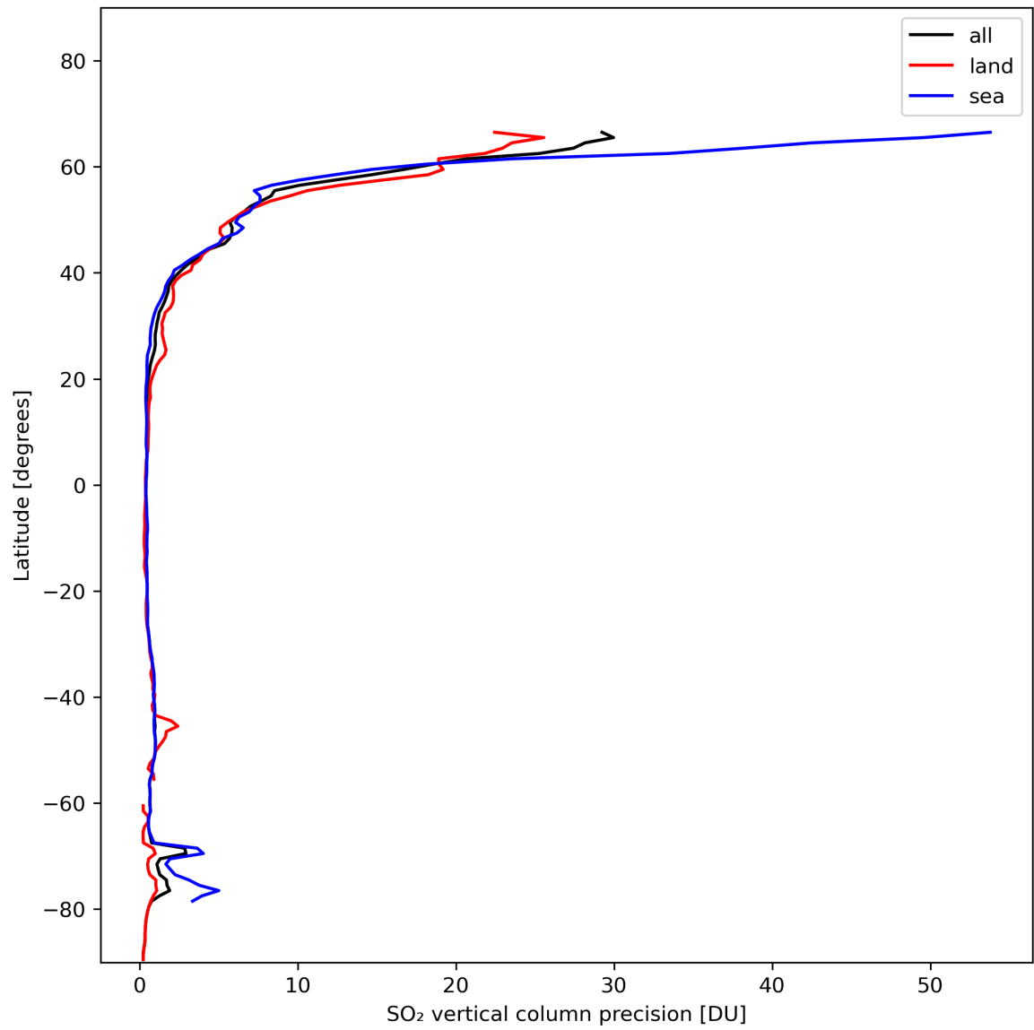
Figure 31: Zonal average of “SO 2 vertical column precision” for 2024-01-26 to 2024-01-27.
