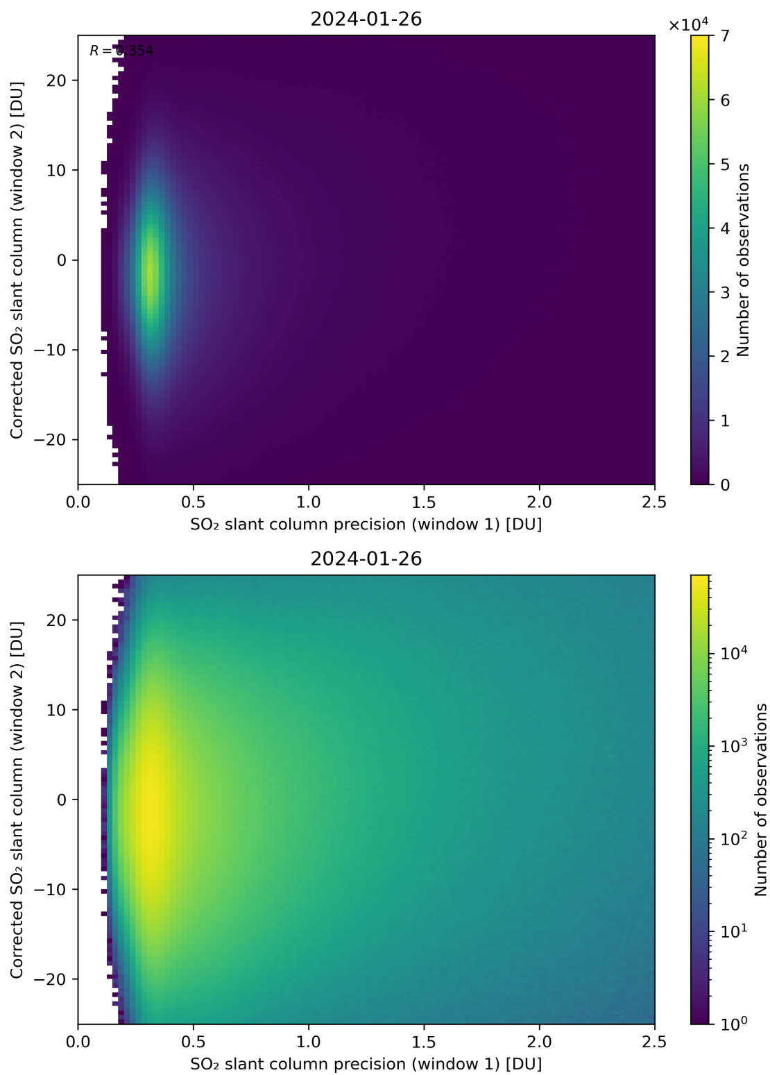
Figure 225: Scatter density plot of “SO 2 slant column precision (window 1)” against “Corrected SO 2 slant column (window 2)” for 2024-01-26 to 2024-01-27.
