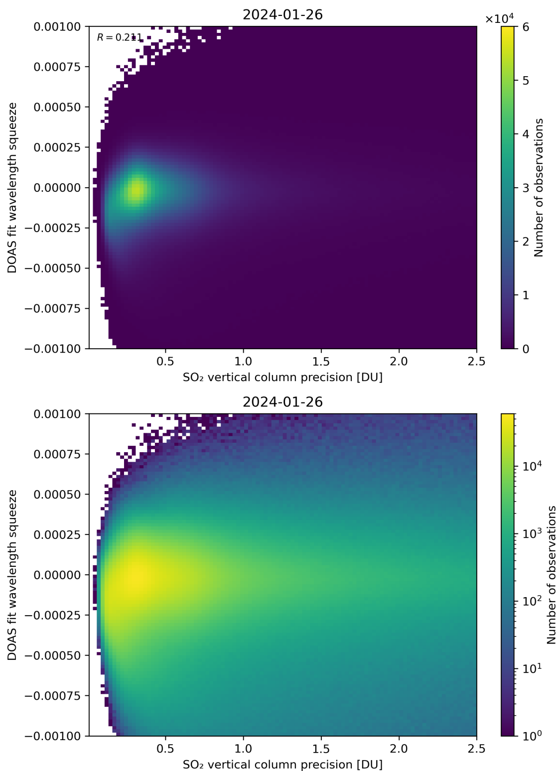
Figure 283: Scatter density plot of “SO 2 vertical column precision” against “DOAS fit wavelength squeeze” for 2024-01-26 to 2024-01-27.
