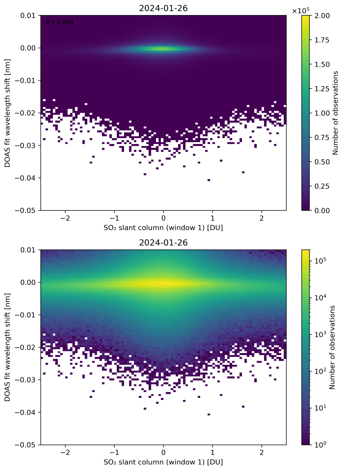
Figure 215: Scatter density plot of “SO 2 slant column (window 1)” against “DOAS fit wavelength shift” for 2024-01-26 to 2024-01-27.
