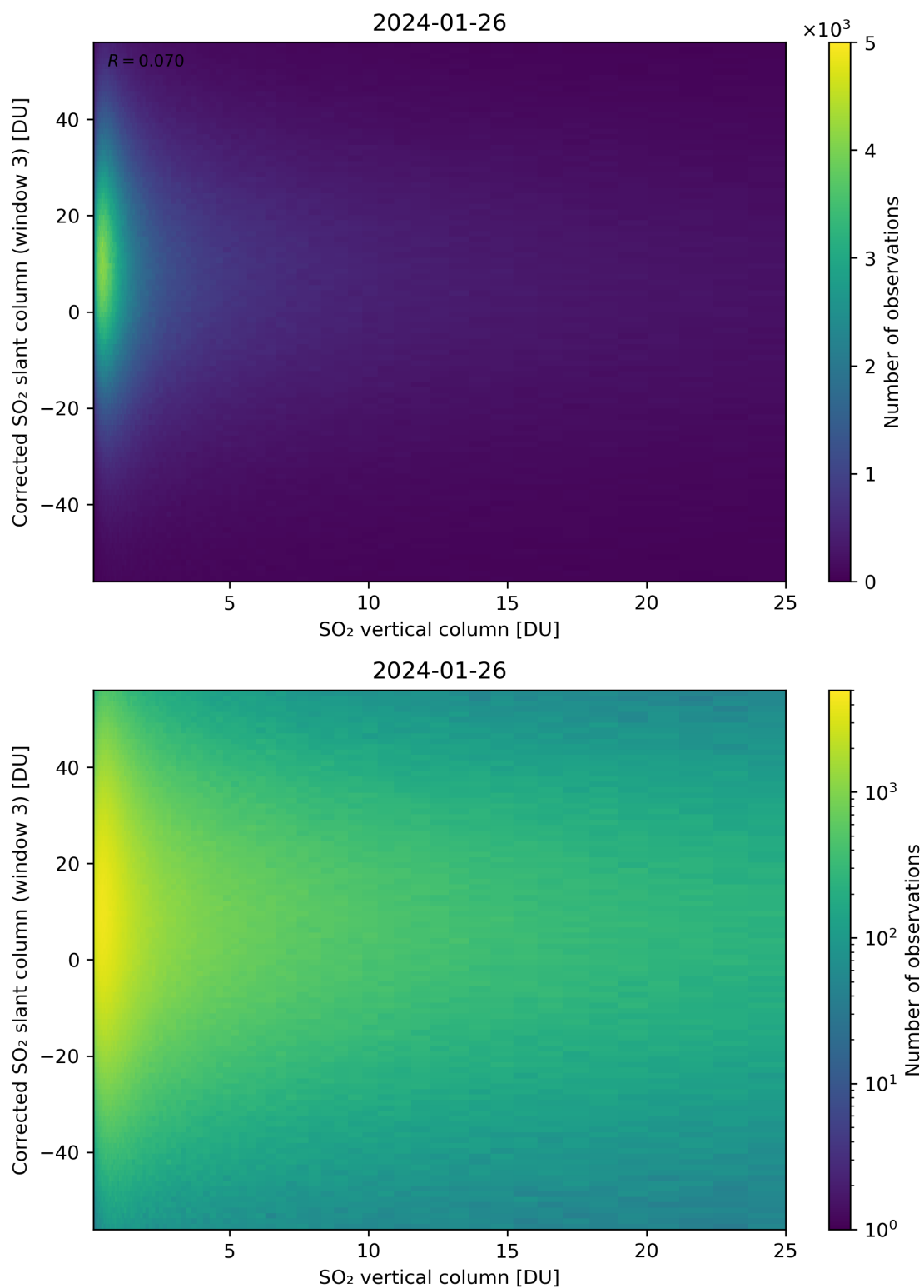
Figure 299: Scatter density plot of “SO 2 vertical column” against “Corrected SO 2 slant column (window 3)” for 2024-01-26 to 2024-01-27.
