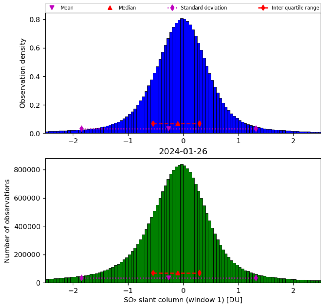
Figure 56: Histogram of “SO 2 slant column (window 1)” for 2024-01-26 to 2024-01-27
