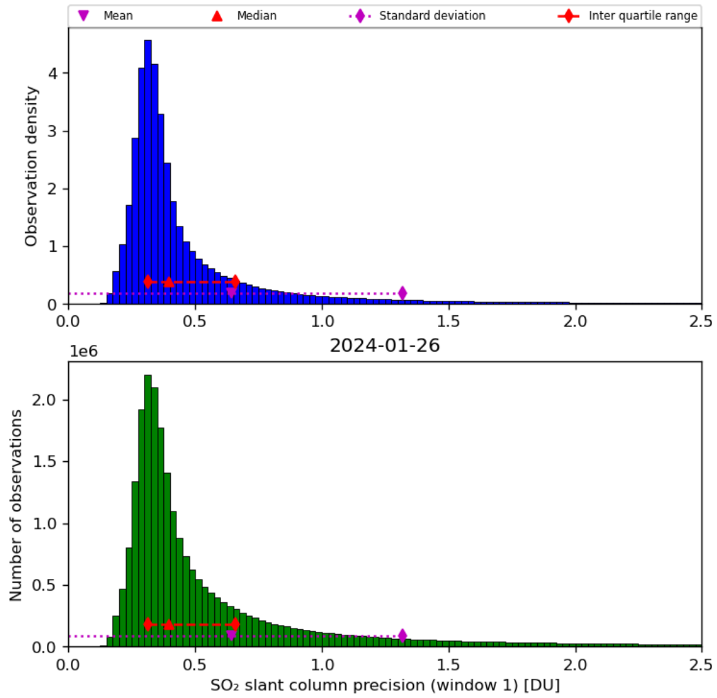
Figure 57: Histogram of “SO 2 slant column precision (window 1)” for 2024-01-26 to 2024-01-27
