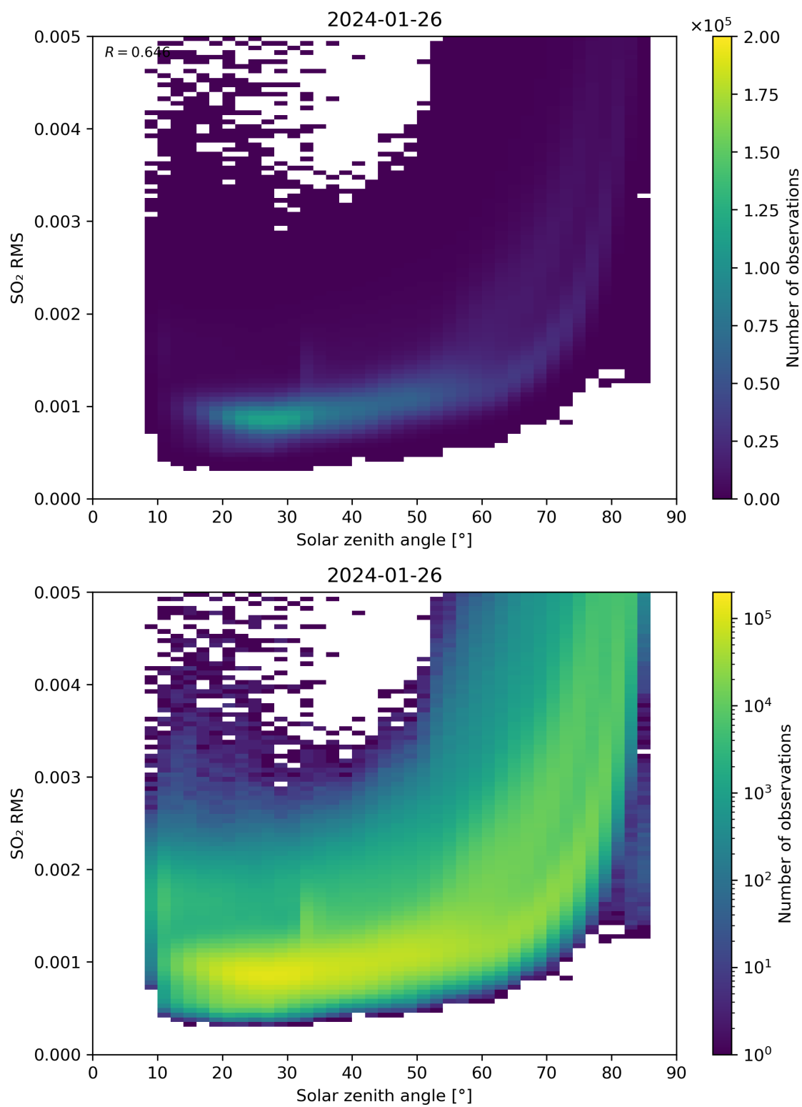
Figure 163: Scatter density plot of “Solar zenith angle” against “SO 2 RMS” for 2024-01-26 to 2024-01-27.
