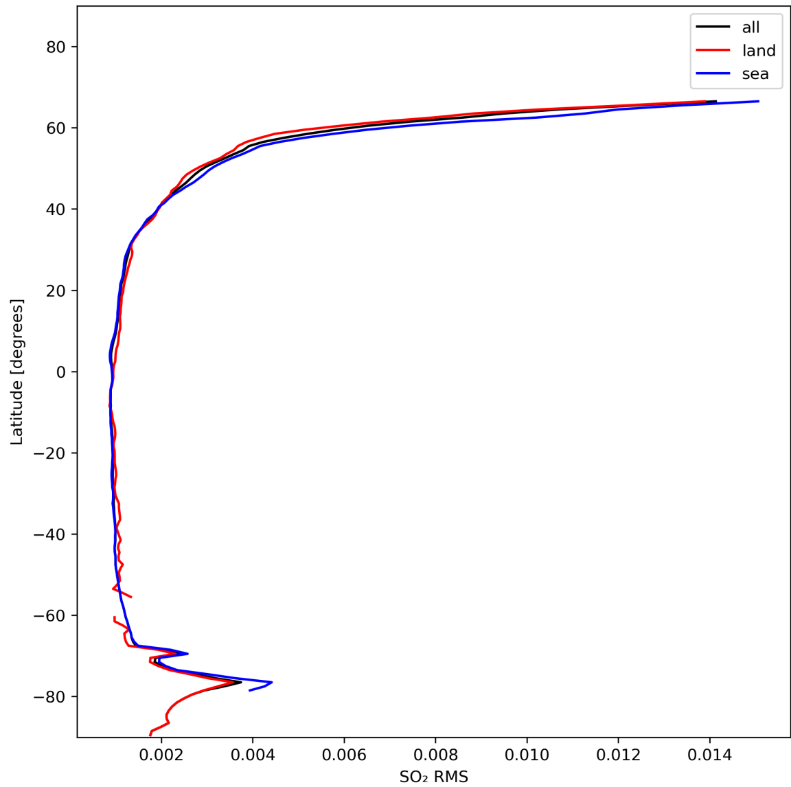
Figure 47: Zonal average of “SO 2 RMS” for 2024-01-26 to 2024-01-27.
