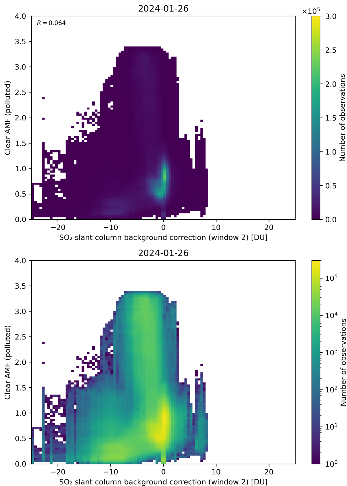
Figure 115: Scatter density plot of “SO 2 slant column background correction (window 2)” against “Clear AMF (polluted)” for 2024-01-26 to 2024-01-27.
