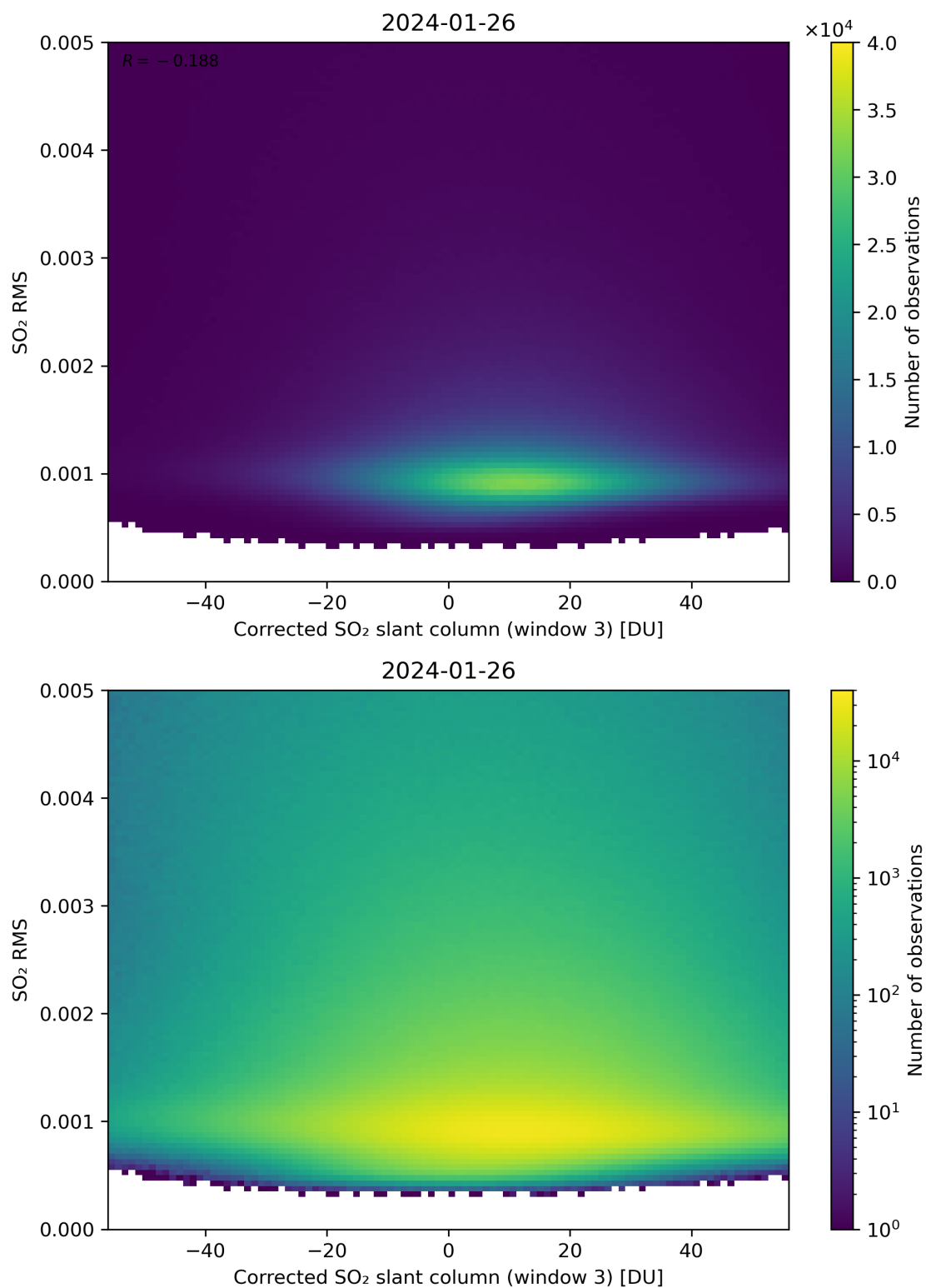
Figure 208: Scatter density plot of “Corrected SO 2 slant column (window 3)” against “SO 2 RMS” for 2024-01-26 to 2024-01-27.
