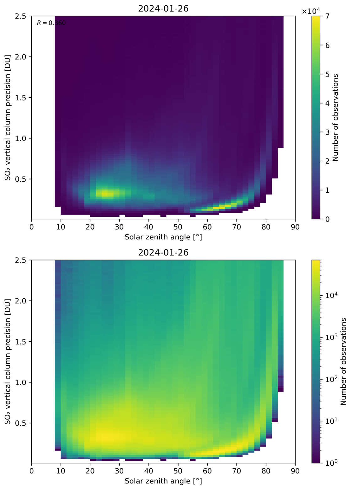
Figure 177: Scatter density plot of “Solar zenith angle” against “SO 2 vertical column precision” for 2024-01-26 to 2024-01-27.
