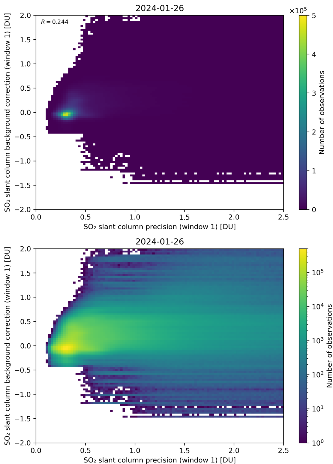
Figure 218: Scatter density plot of “SO 2 slant column precision (window 1)” against “SO 2 slant column background correction (window 1)” for 2024-01-26 to 2024-01-27.
