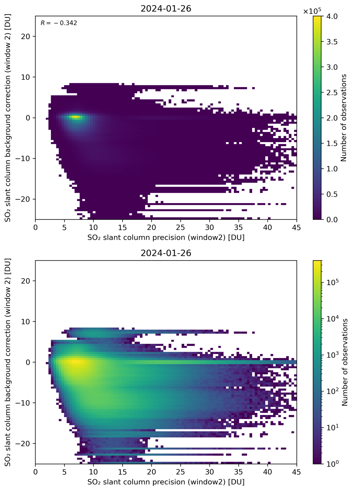
Figure 241: Scatter density plot of “SO 2 slant column precision (window2)” against “SO 2 slant column background correction (window 2)” for 2024-01-26 to 2024-01-27.
