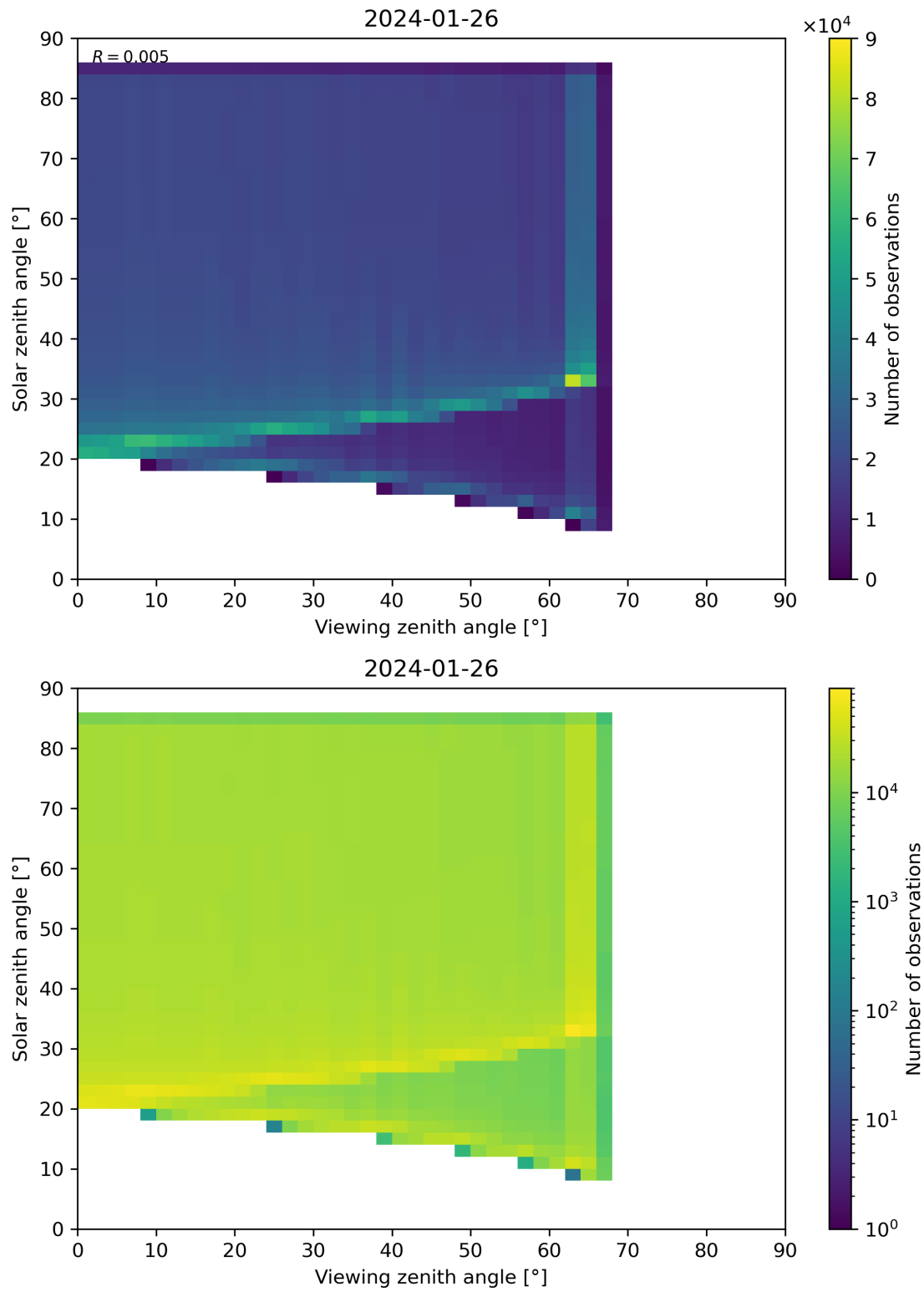
Figure 315: Scatter density plot of “Viewing zenith angle” against “Solar zenith angle” for 2024-01-26 to 2024-01-27.
