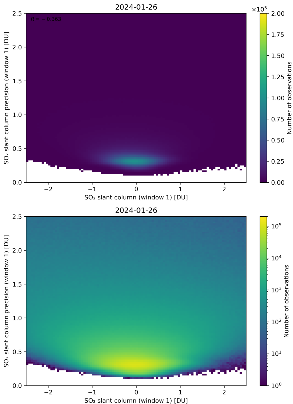
Figure 235: Scatter density plot of “SO 2 slant column (window 1)” against “SO 2 slant column precision (window 1)” for 2024-01-26 to 2024-01-27.
