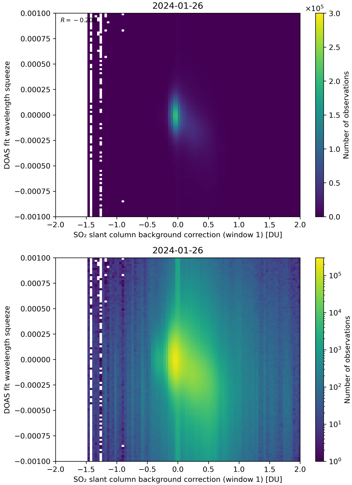
Figure 101: Scatter density plot of “SO 2 slant column background correction (window 1)” against “DOAS fit wavelength squeeze” for 2024-01-26 to 2024-01-27.
