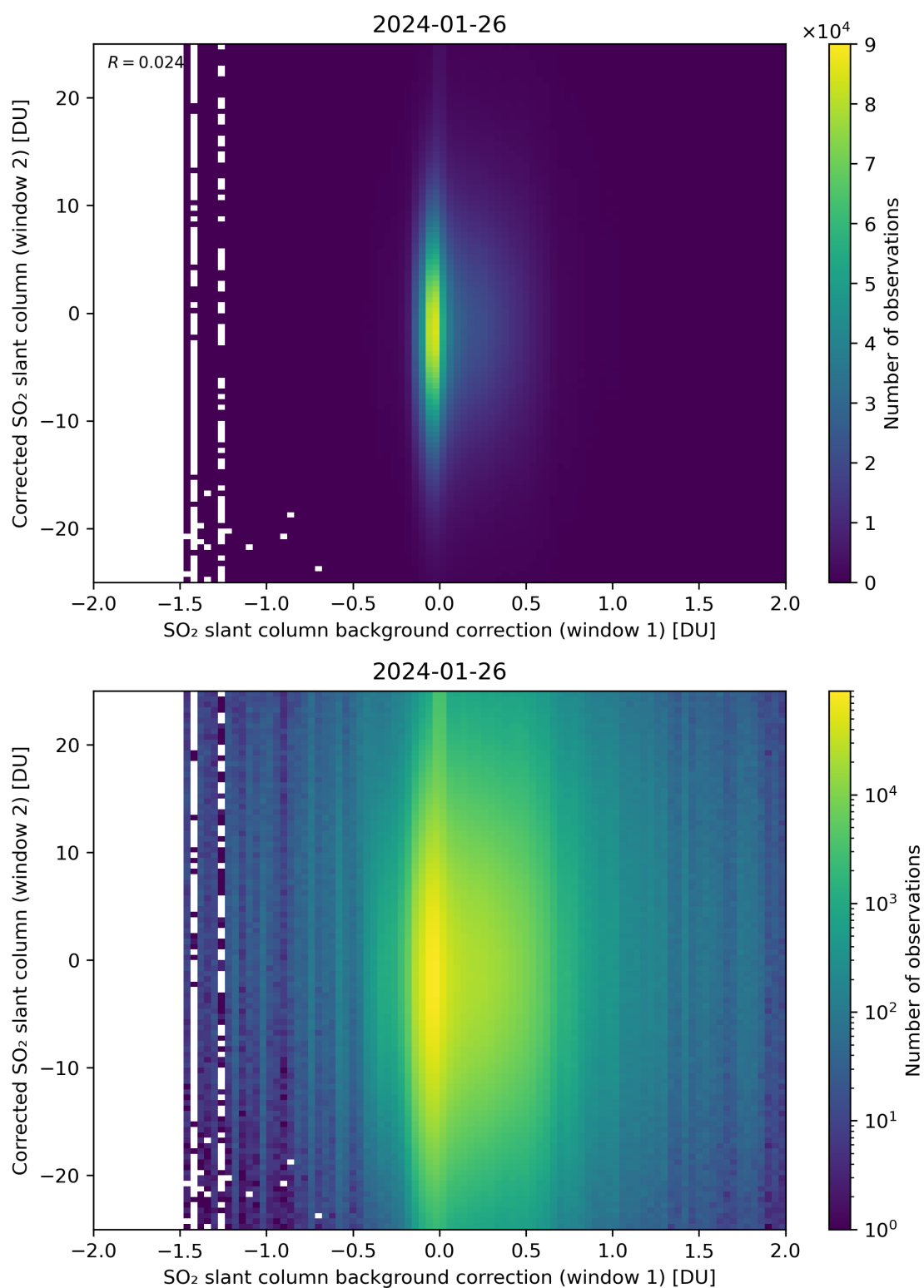
Figure 104: Scatter density plot of “SO 2 slant column background correction (window 1)” against “Corrected SO 2 slant column (window 2)” for 2024-01-26 to 2024-01-27.
