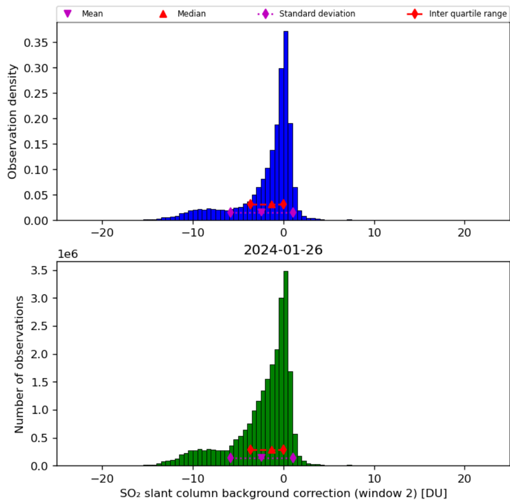
Figure 63: Histogram of “SO 2 slant column background correction (window 2)” for 2024-01-26 to 2024-01-27
