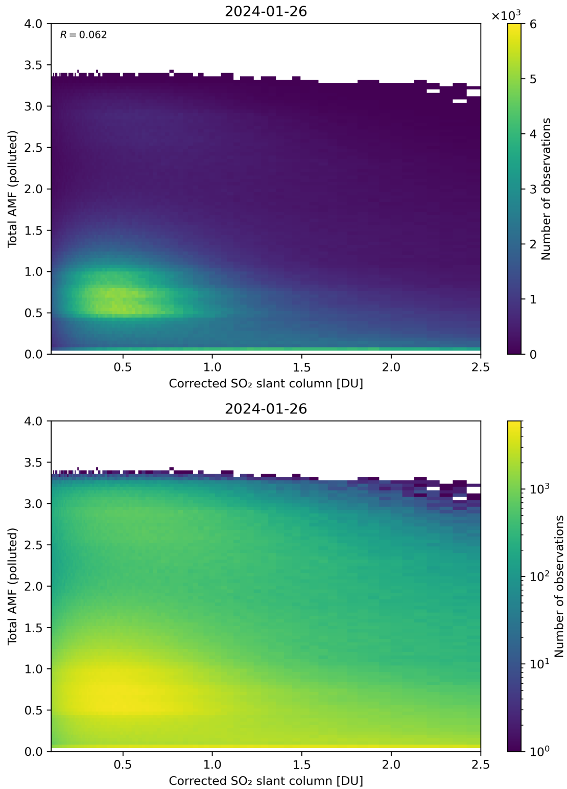
Figure 192: Scatter density plot of “Corrected SO 2 slant column” against “Total AMF (polluted)” for 2024-01-26 to 2024-01-27.
