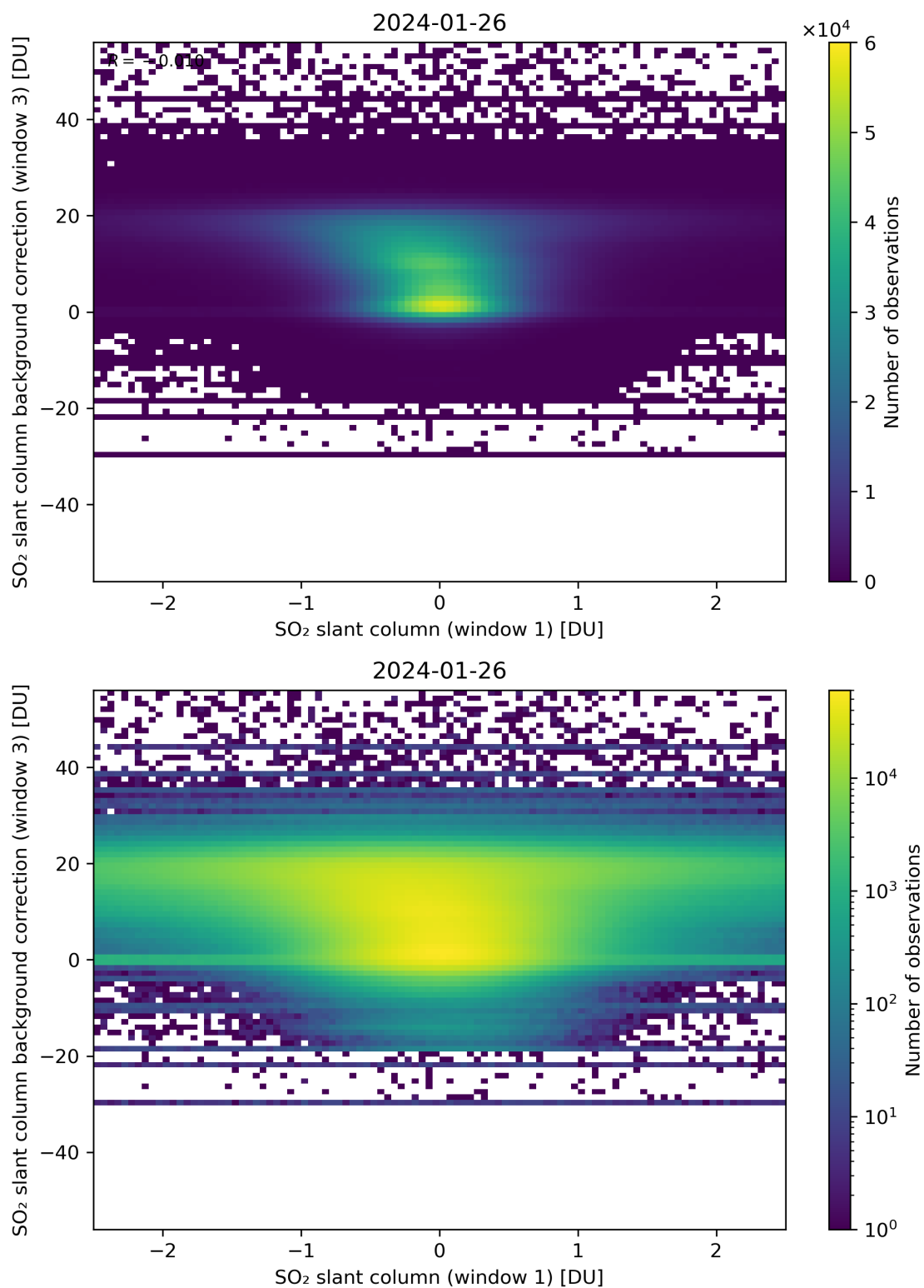
Figure 214: Scatter density plot of “SO 2 slant column (window 1)” against “SO 2 slant column background correction (window 3)” for 2024-01-26 to 2024-01-27.
