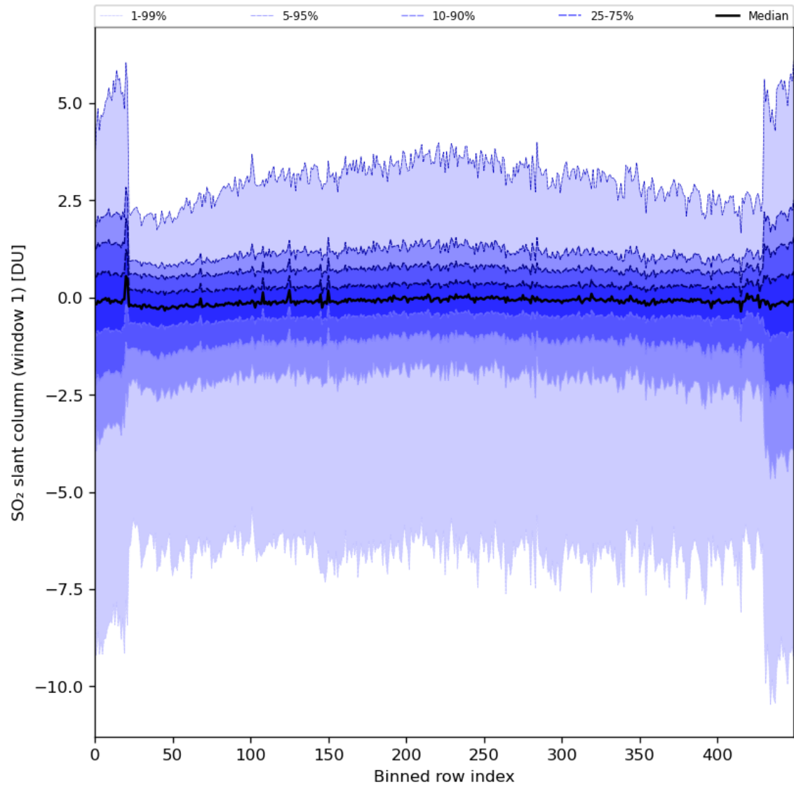
Figure 79: Along track statistics of “SO 2 slant column (window 1)” for 2024-01-26 to 2024-01-27
