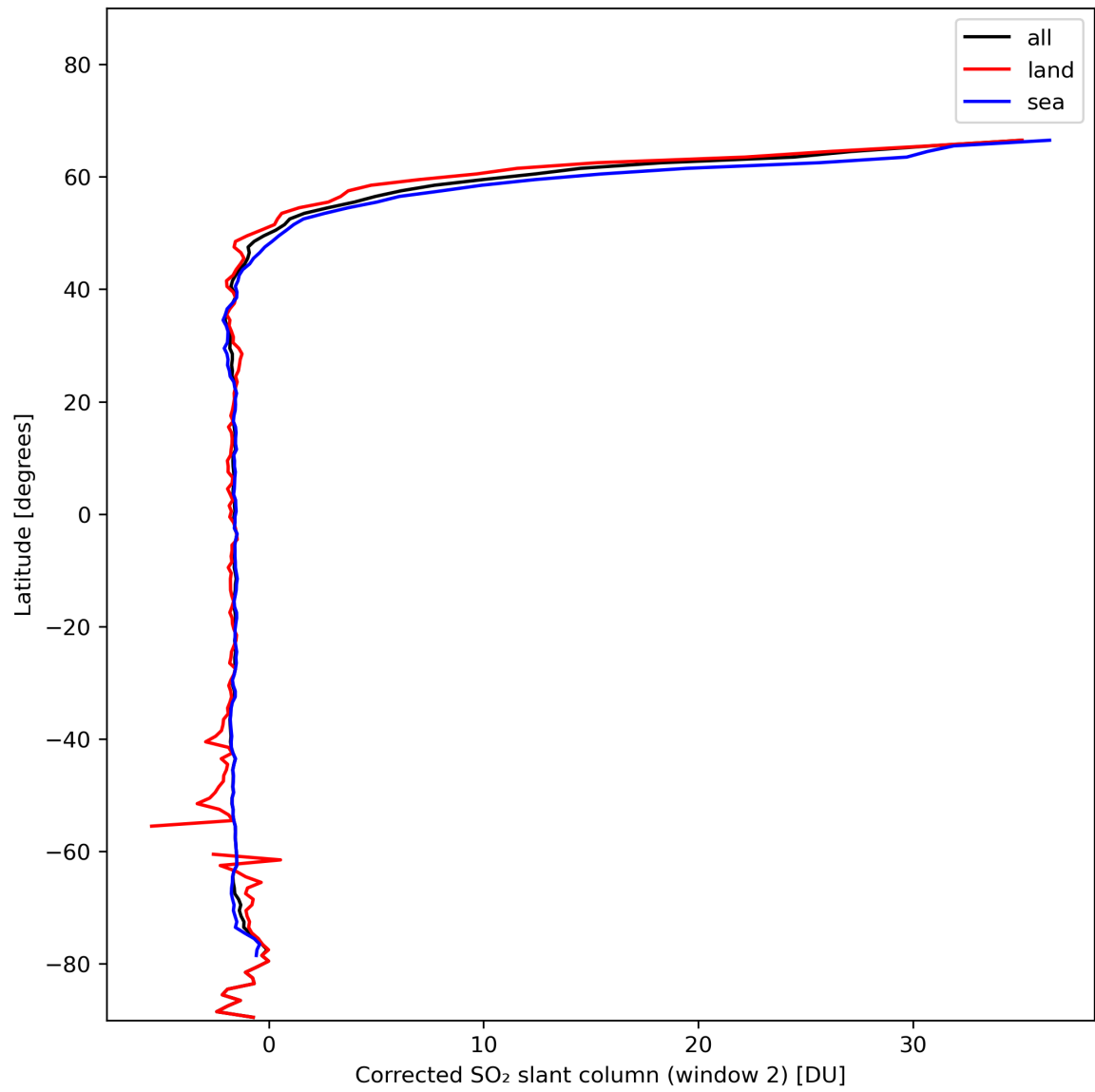
Figure 39: Zonal average of “Corrected SO 2 slant column (window 2)” for 2024-01-26 to 2024-01-27.
