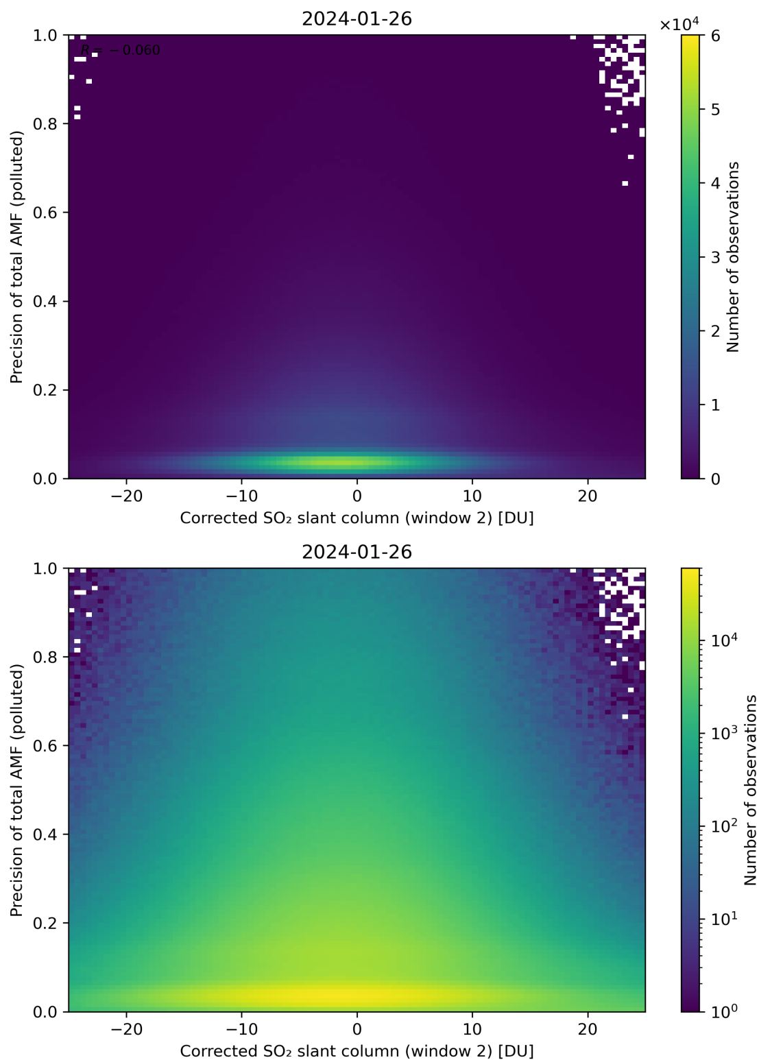
Figure 204: Scatter density plot of “Corrected SO 2 slant column (window 2)” against “Precision of total AMF (polluted)” for 2024-01-26 to 2024-01-27.
