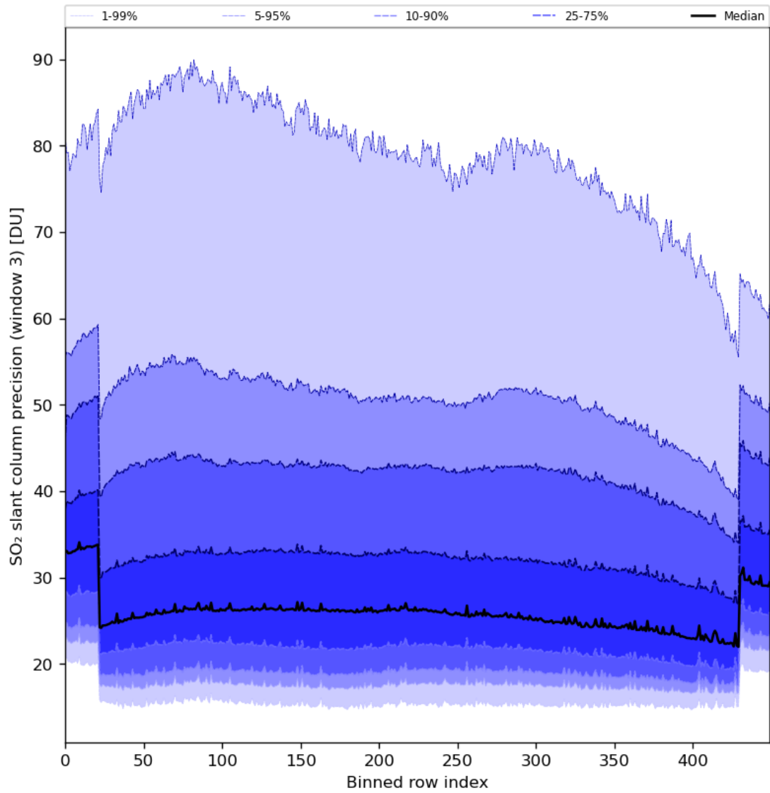
Figure 88: Along track statistics of “SO 2 slant column precision (window 3)” for 2024-01-26 to 2024-01-27
