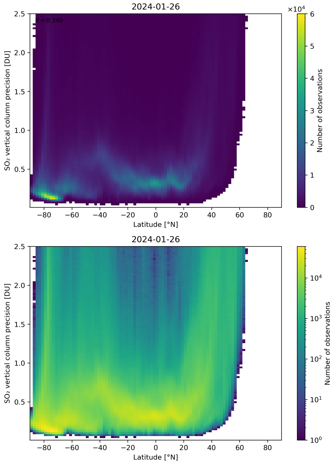
Figure 157: Scatter density plot of “Latitude” against “SO 2 vertical column precision” for 2024-01-26 to 2024-01-27.
