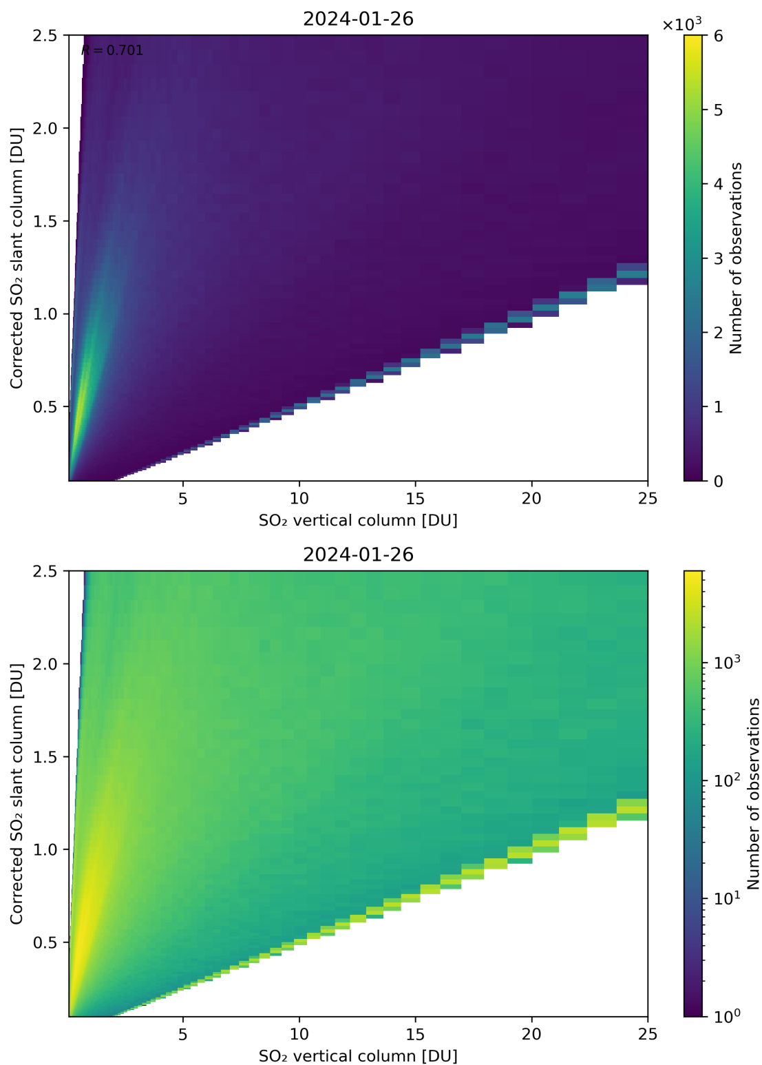
Figure 297: Scatter density plot of “SO 2 vertical column” against “Corrected SO 2 slant column” for 2024-01-26 to 2024-01-27.
