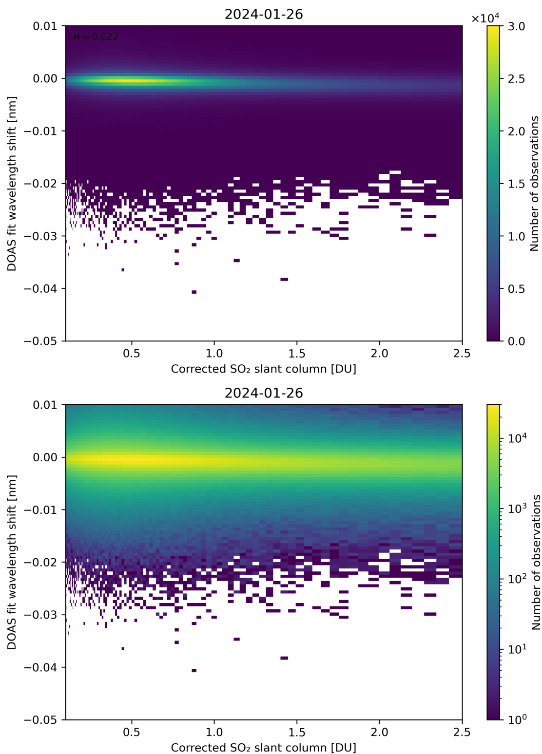
Figure 181: Scatter density plot of “Corrected SO 2 slant column” against “DOAS fit wavelength shift” for 2024-01-26 to 2024-01-27.
