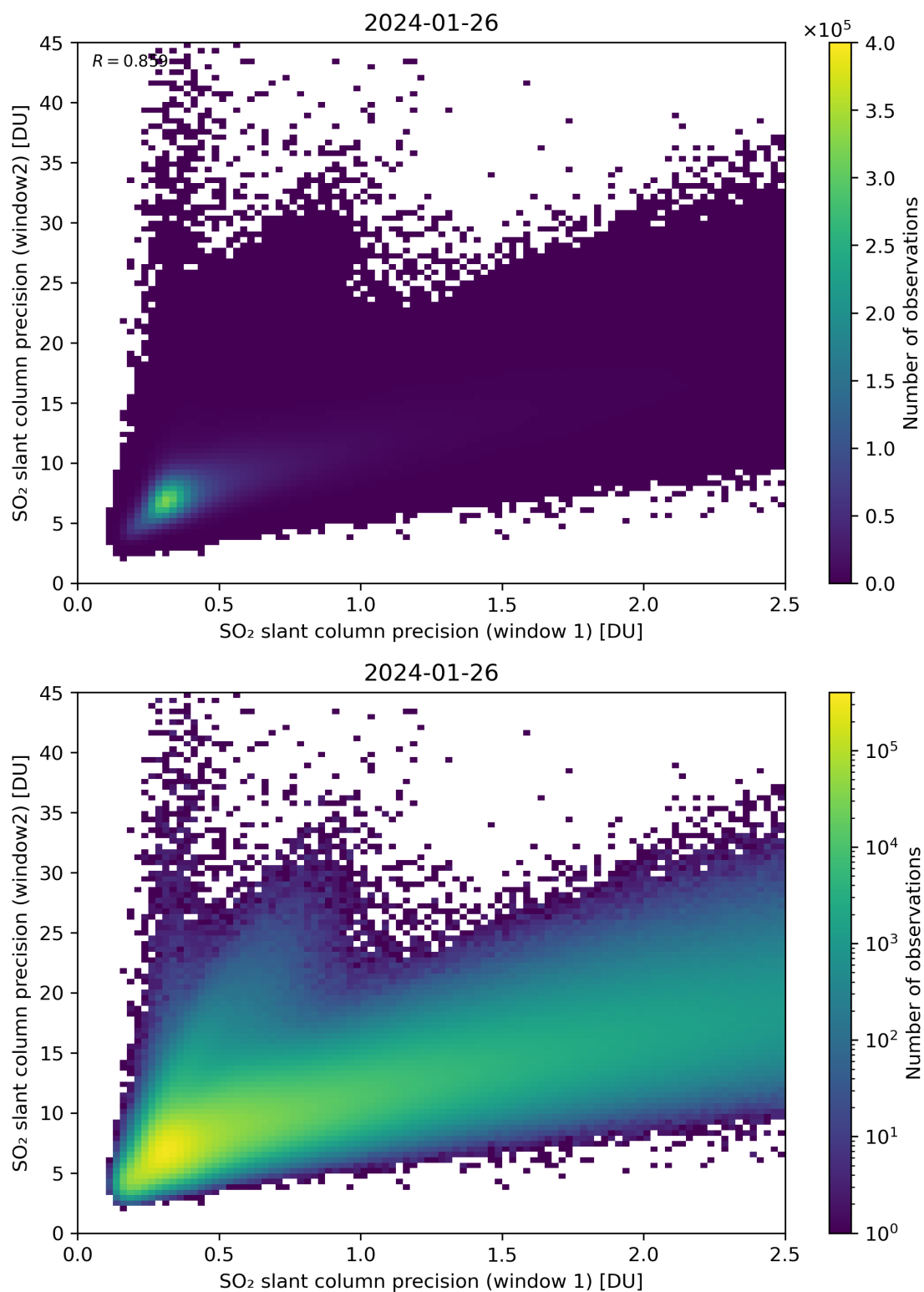
Figure 227: Scatter density plot of “SO 2 slant column precision (window 1)” against “SO 2 slant column precision (window2)” for 2024-01-26 to 2024-01-27.
