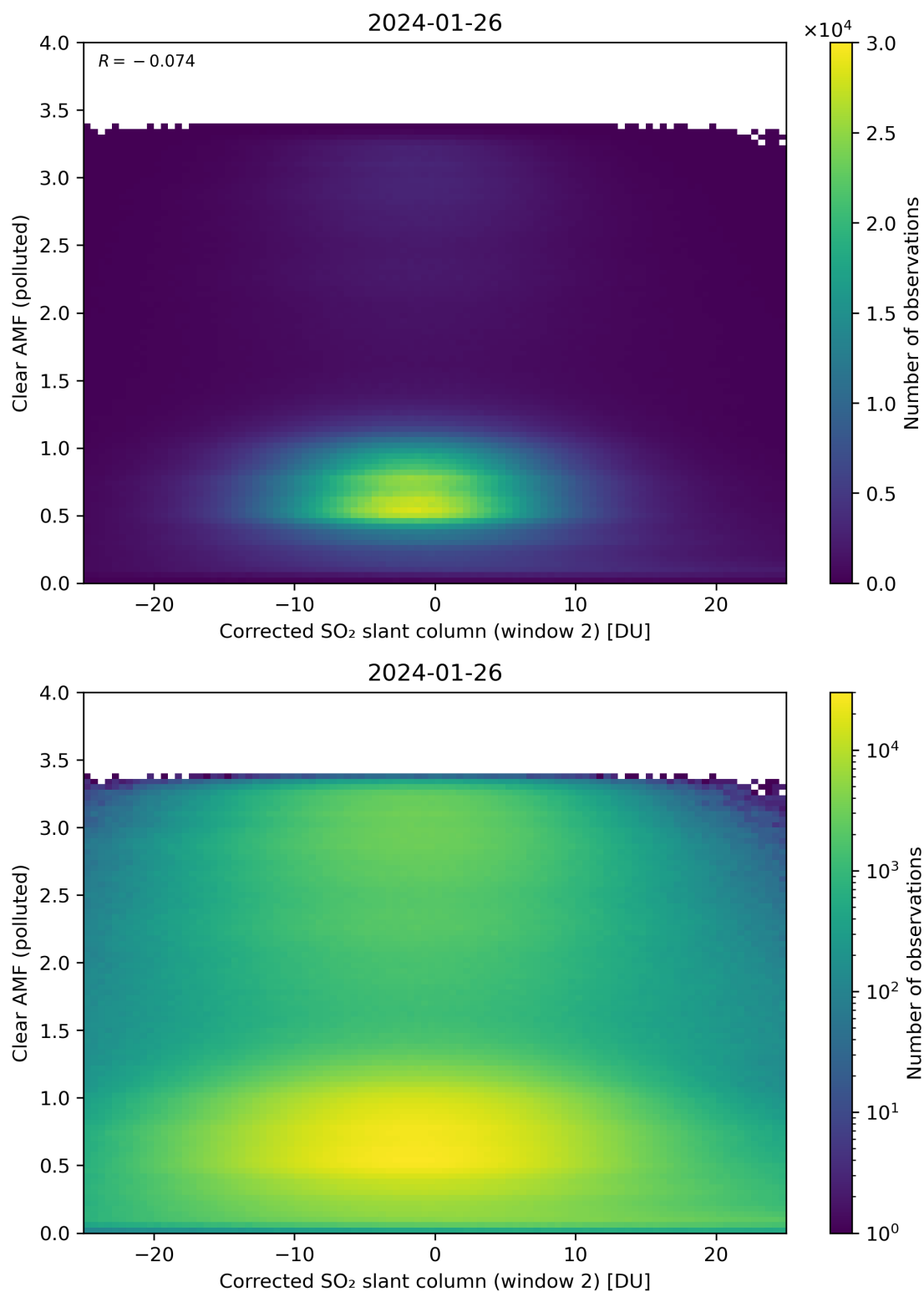
Figure 199: Scatter density plot of “Corrected SO 2 slant column (window 2)” against “Clear AMF (polluted)” for 2024-01-26 to 2024-01-27.
