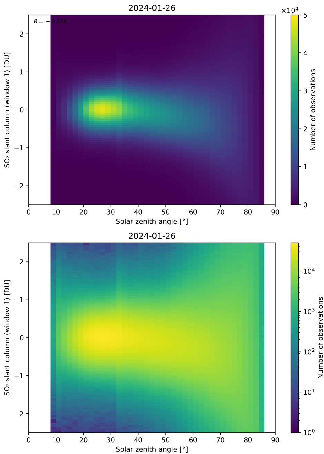
Figure 169: Scatter density plot of “Solar zenith angle” against “SO 2 slant column (window 1)” for 2024-01-26 to 2024-01-27.
