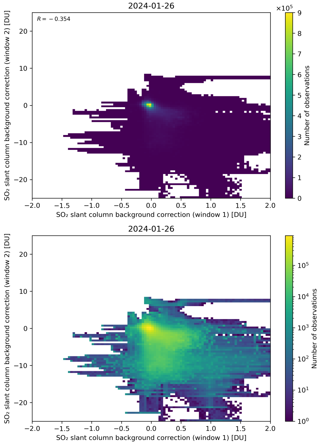
Figure 98: Scatter density plot of “SO 2 slant column background correction (window 1)” against “SO 2 slant column background correction (window 2)” for 2024-01-26 to 2024-01-27.
