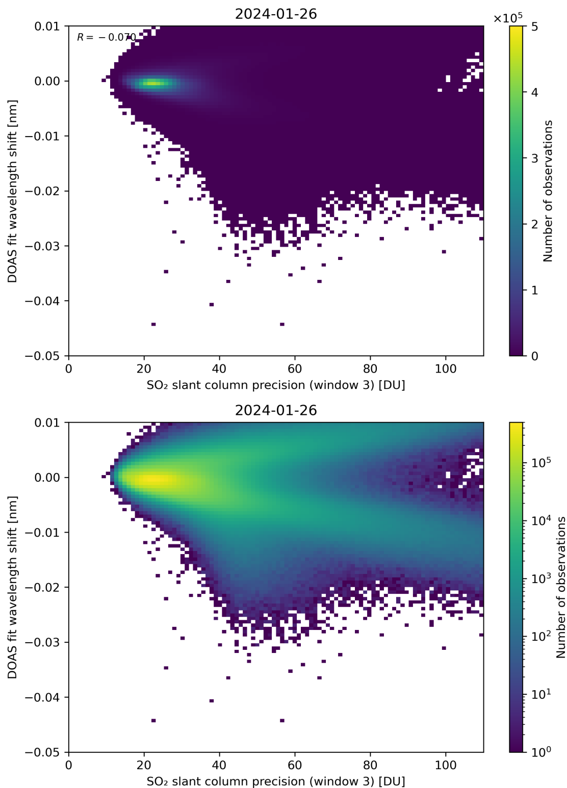
Figure 258: Scatter density plot of “SO 2 slant column precision (window 3)” against “DOAS fit wavelength shift” for 2024-01-26 to 2024-01-27.
