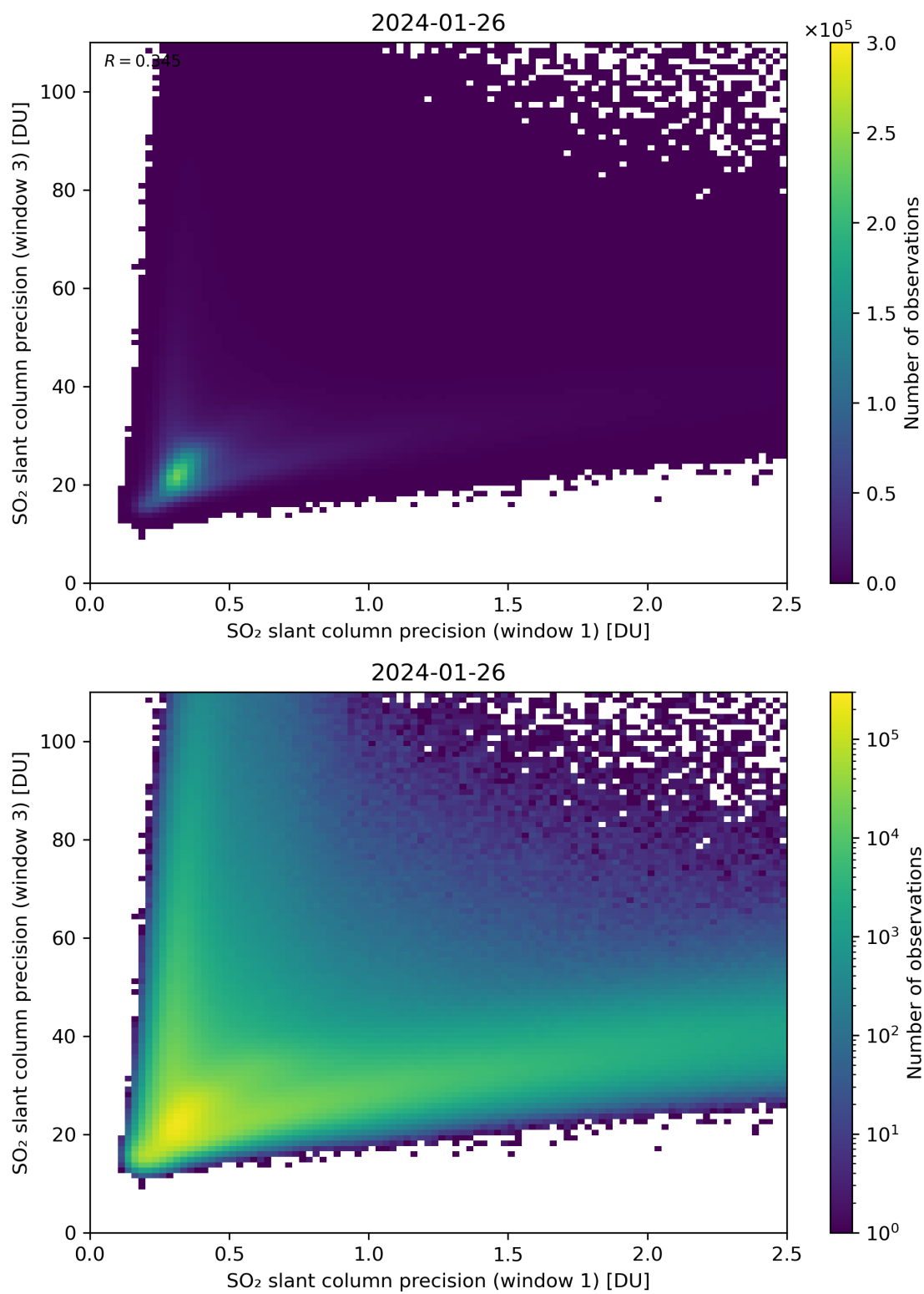
Figure 229: Scatter density plot of “SO 2 slant column precision (window 1)” against “SO 2 slant column precision (window 3)” for 2024-01-26 to 2024-01-27.
