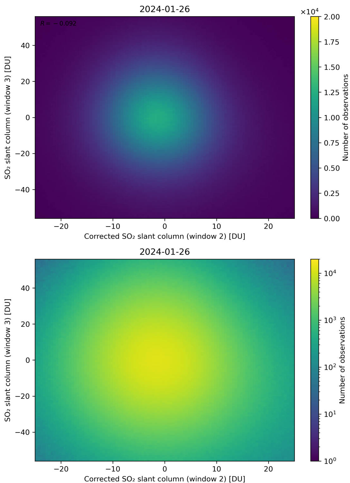
Figure 201: Scatter density plot of “Corrected SO 2 slant column (window 2)” against “SO 2 slant column (window 3)” for 2024-01-26 to 2024-01-27.
