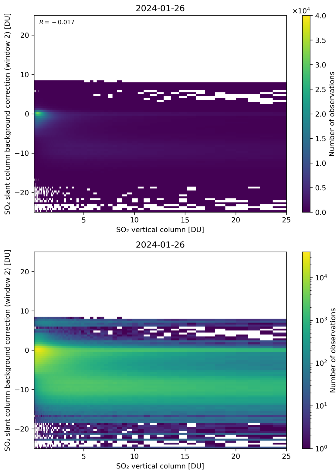
Figure 274: Scatter density plot of “SO 2 vertical column” against “SO 2 slant column background correction (window 2)” for 2024-01-26 to 2024-01-27.
