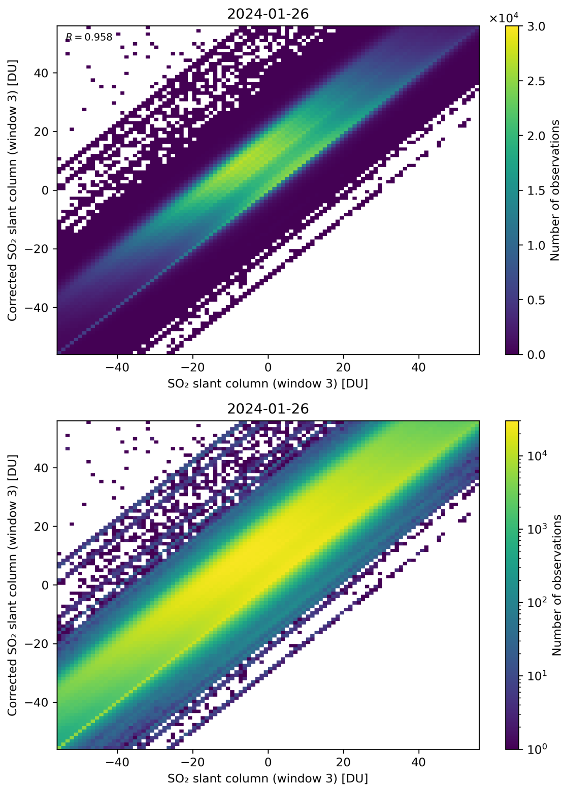
Figure 266: Scatter density plot of “SO 2 slant column (window 3)” against “Corrected SO 2 slant column (window 3)” for 2024-01-26 to 2024-01-27.
