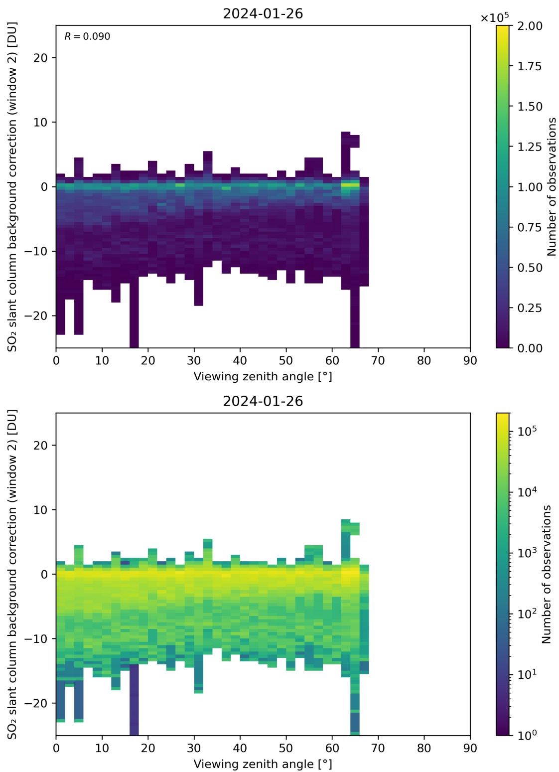
Figure 309: Scatter density plot of “Viewing zenith angle” against “SO 2 slant column background correction (window 2)” for 2024-01-26 to 2024-01-27.
