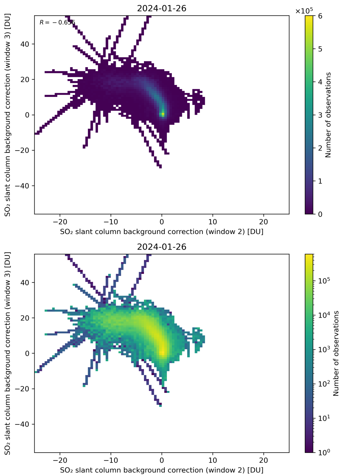
Figure 111: Scatter density plot of “SO 2 slant column background correction (window 2)” against “SO 2 slant column background correction (window 3)” for 2024-01-26 to 2024-01-27.
