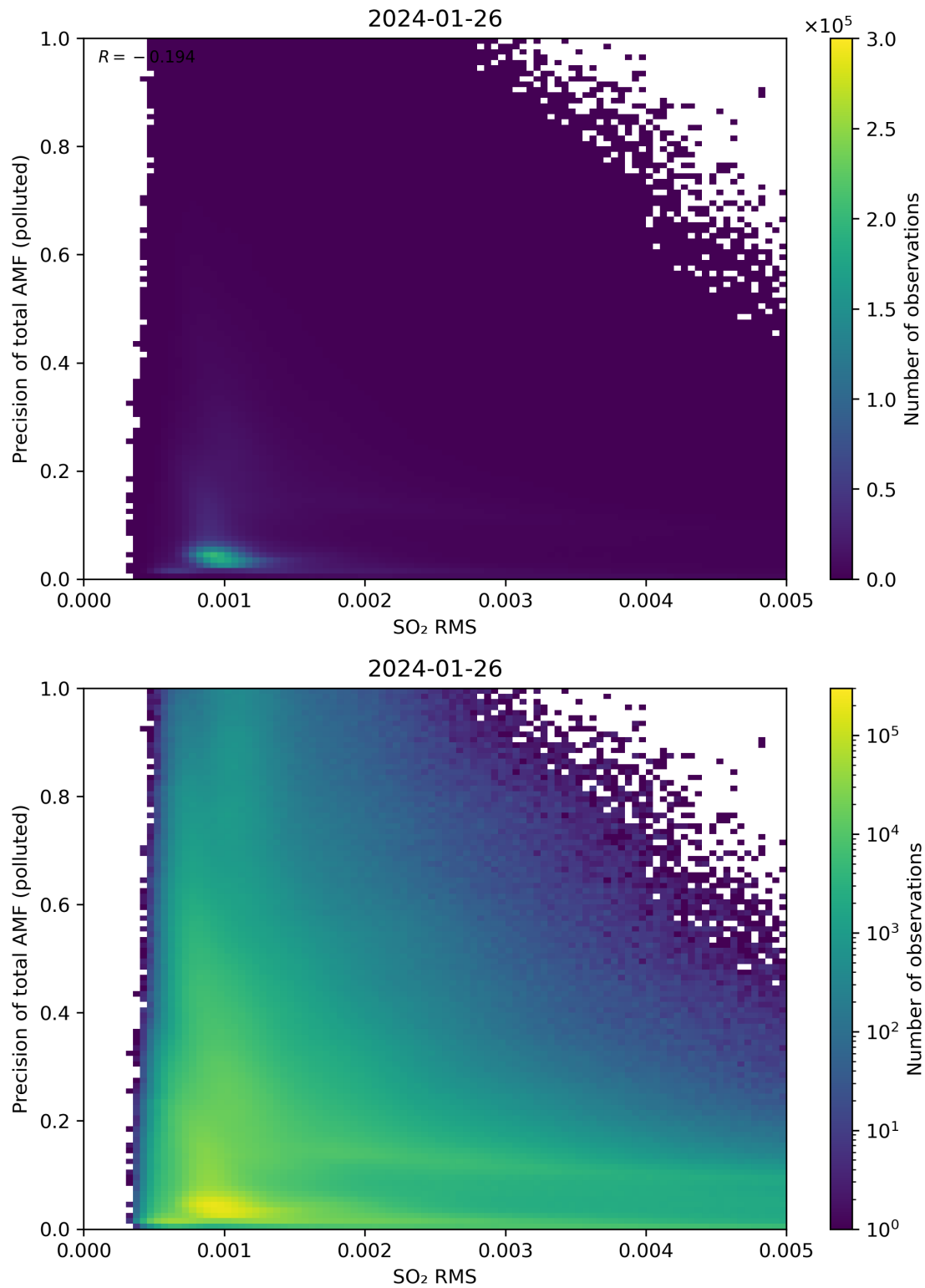
Figure 138: Scatter density plot of “SO 2 RMS” against “Precision of total AMF (polluted)” for 2024-01-26 to 2024-01-27.
