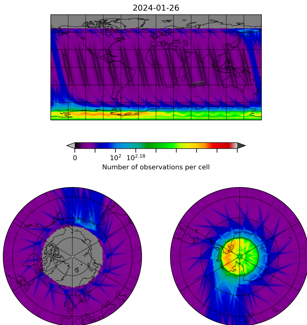
Figure 28: Map of the number of observations for 2024-01-26 to 2024-01-27
