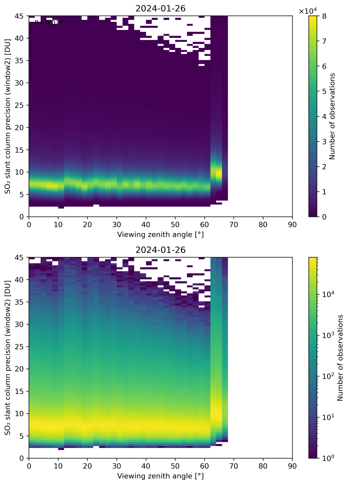
Figure 322: Scatter density plot of “Viewing zenith angle” against “SO 2 slant column precision (window2)” for 2024-01-26 to 2024-01-27.
