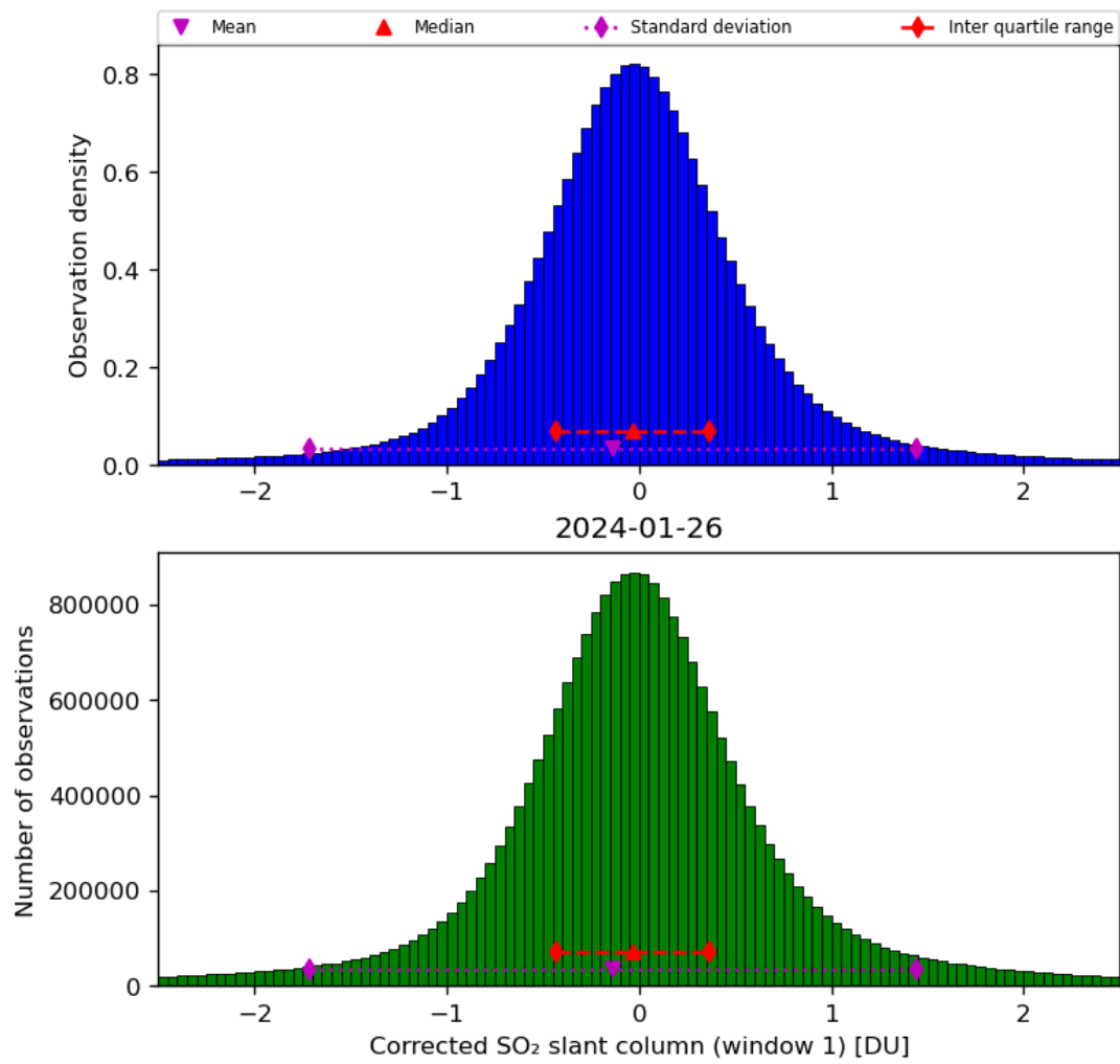
Figure 58: Histogram of “Corrected SO 2 slant column (window 1)” for 2024-01-26 to 2024-01-27
