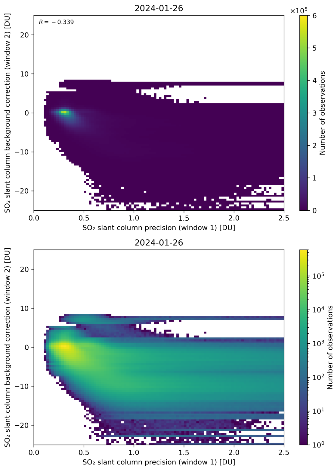
Figure 219: Scatter density plot of “SO 2 slant column precision (window 1)” against “SO 2 slant column background correction (window 2)” for 2024-01-26 to 2024-01-27.
