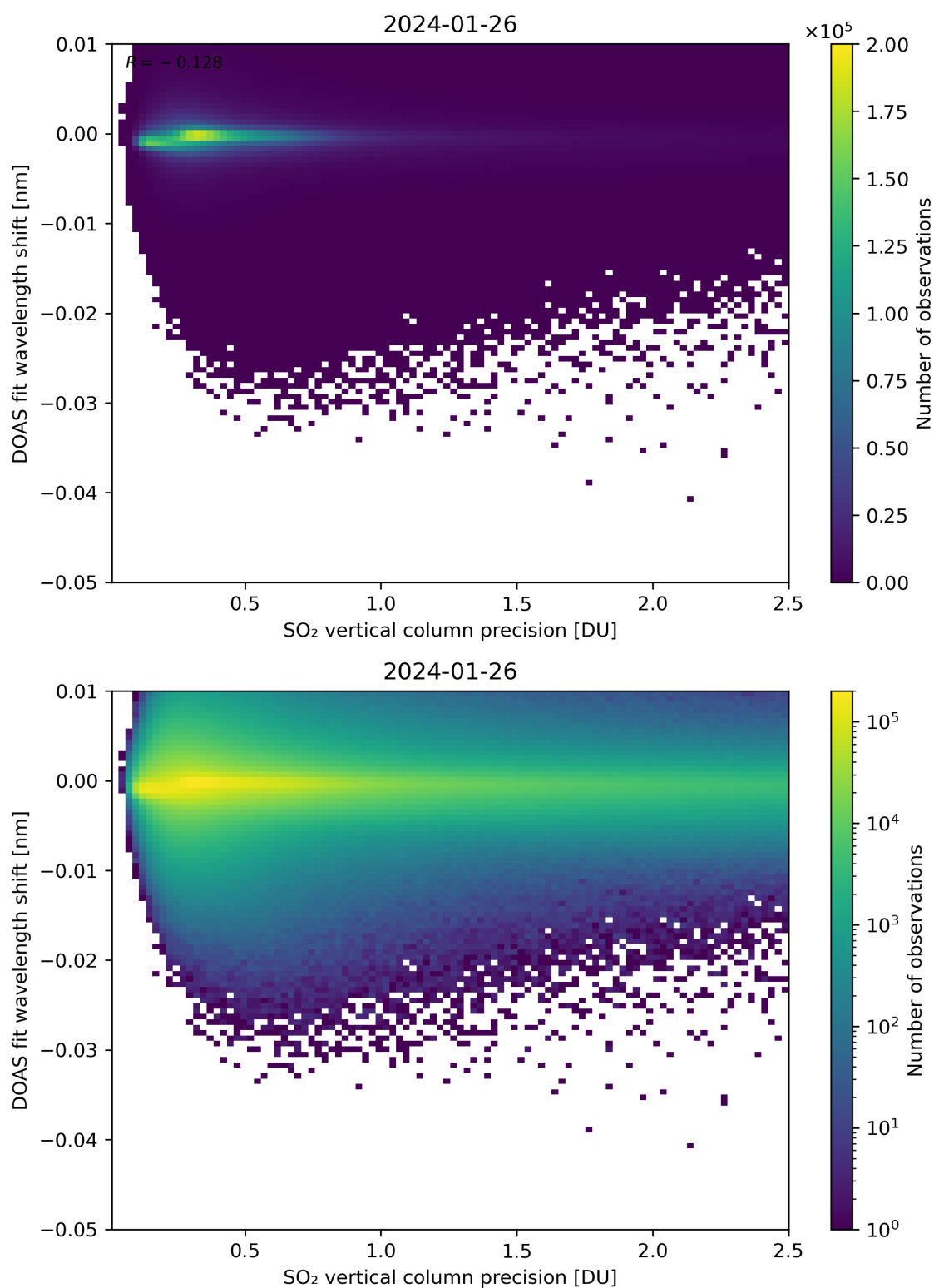
Figure 282: Scatter density plot of “SO 2 vertical column precision” against “DOAS fit wavelength shift” for 2024-01-26 to 2024-01-27.
