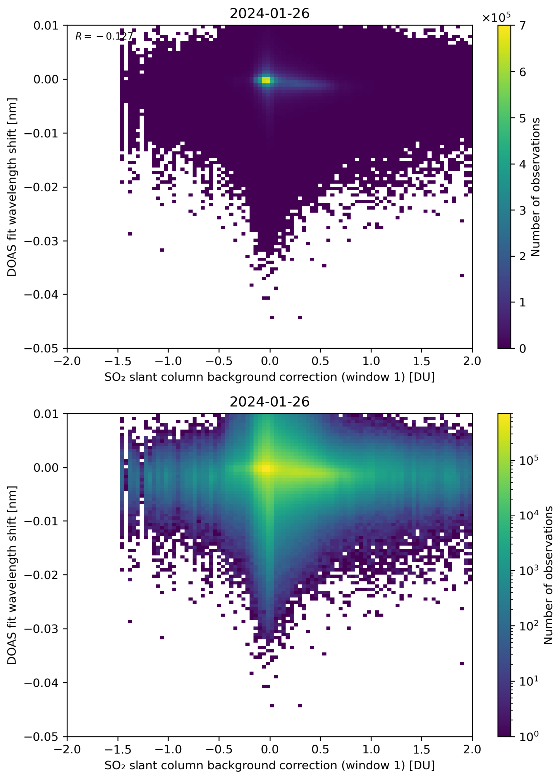
Figure 100: Scatter density plot of “SO 2 slant column background correction (window 1)” against “DOAS fit wavelength shift” for 2024-01-26 to 2024-01-27.
