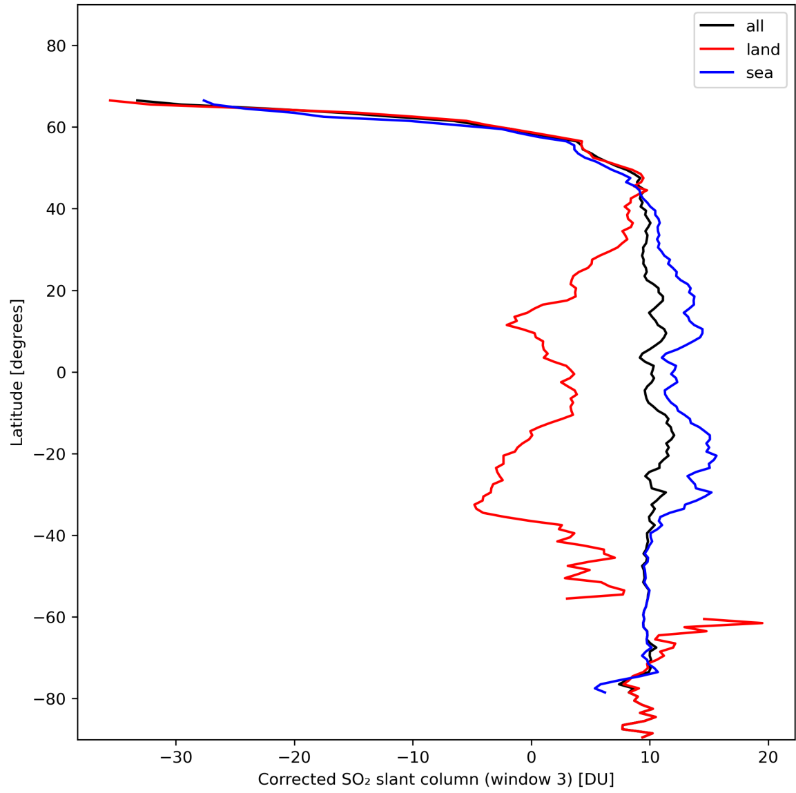
Figure 43: Zonal average of “Corrected SO 2 slant column (window 3)” for 2024-01-26 to 2024-01-27.
