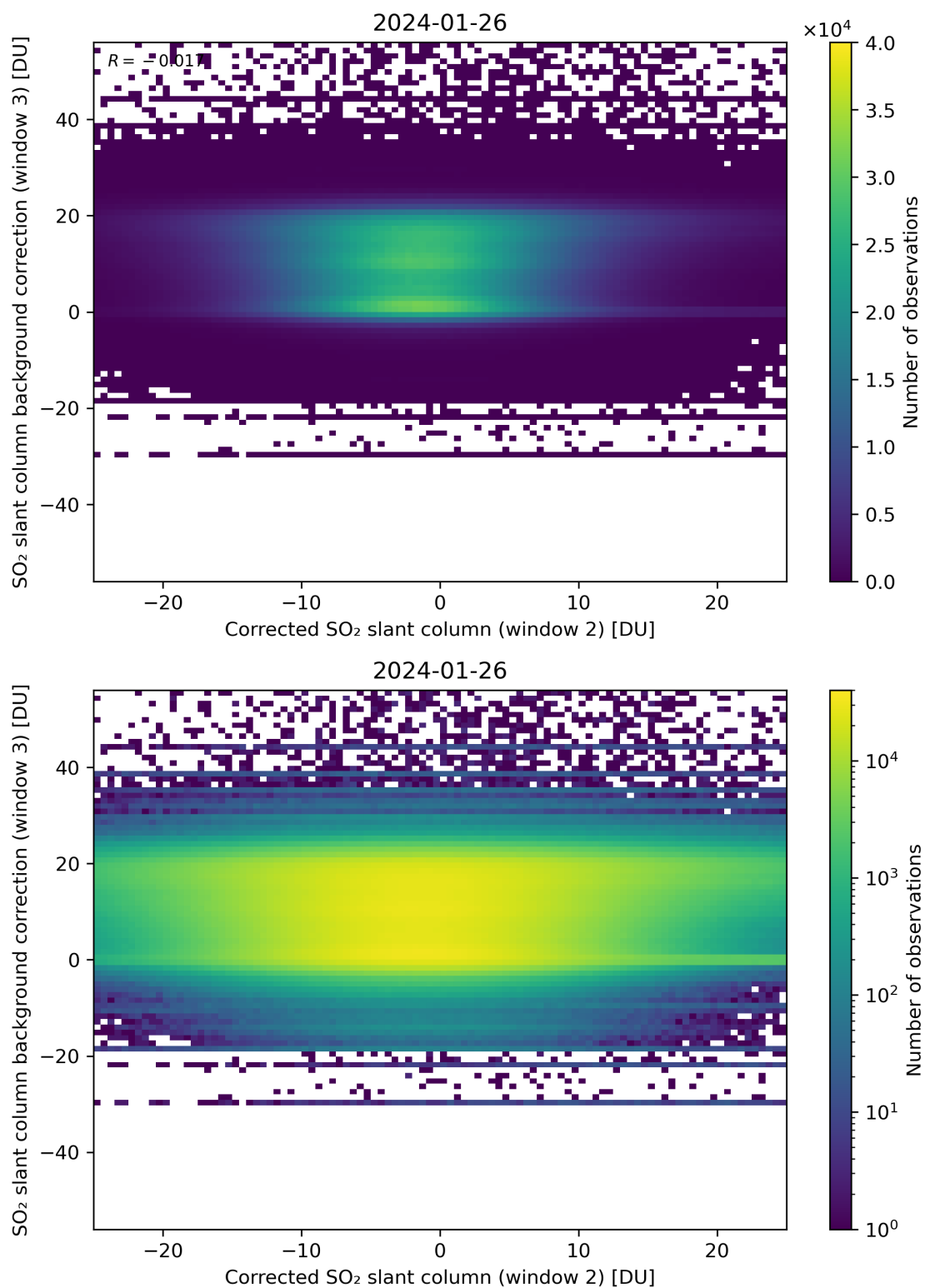
Figure 195: Scatter density plot of “Corrected SO 2 slant column (window 2)” against “SO 2 slant column background correction (window 3)” for 2024-01-26 to 2024-01-27.
