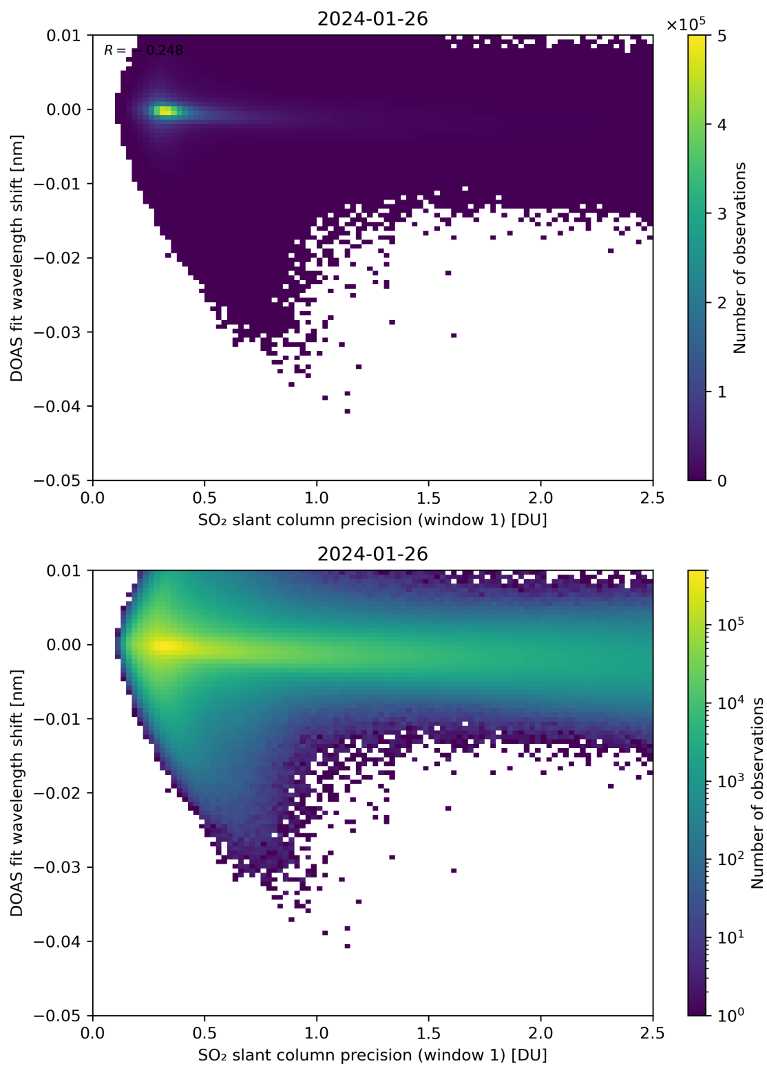
Figure 221: Scatter density plot of “SO 2 slant column precision (window 1)” against “DOAS fit wavelength shift” for 2024-01-26 to 2024-01-27.
