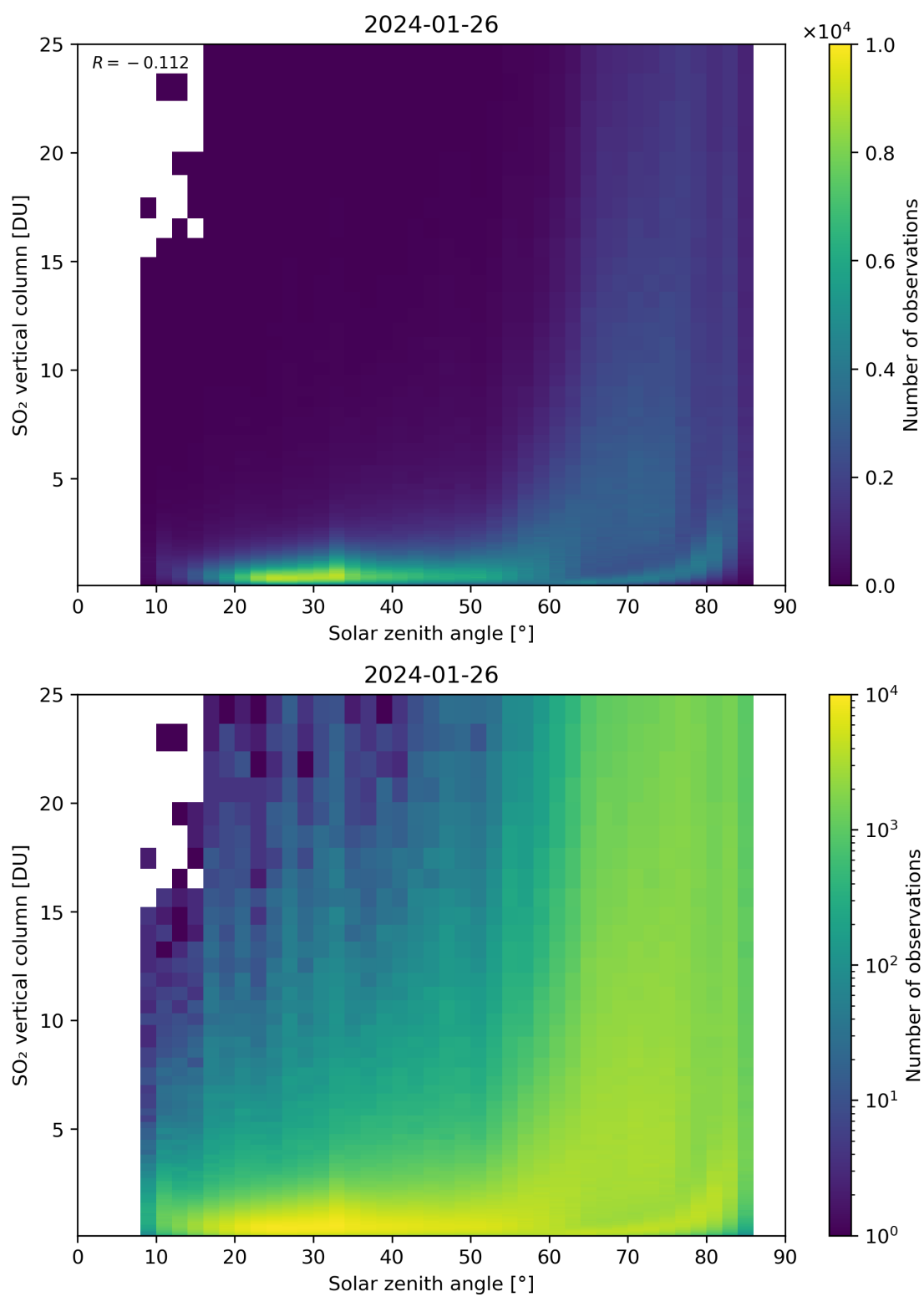
Figure 176: Scatter density plot of “Solar zenith angle” against “SO 2 vertical column” for 2024-01-26 to 2024-01-27.
