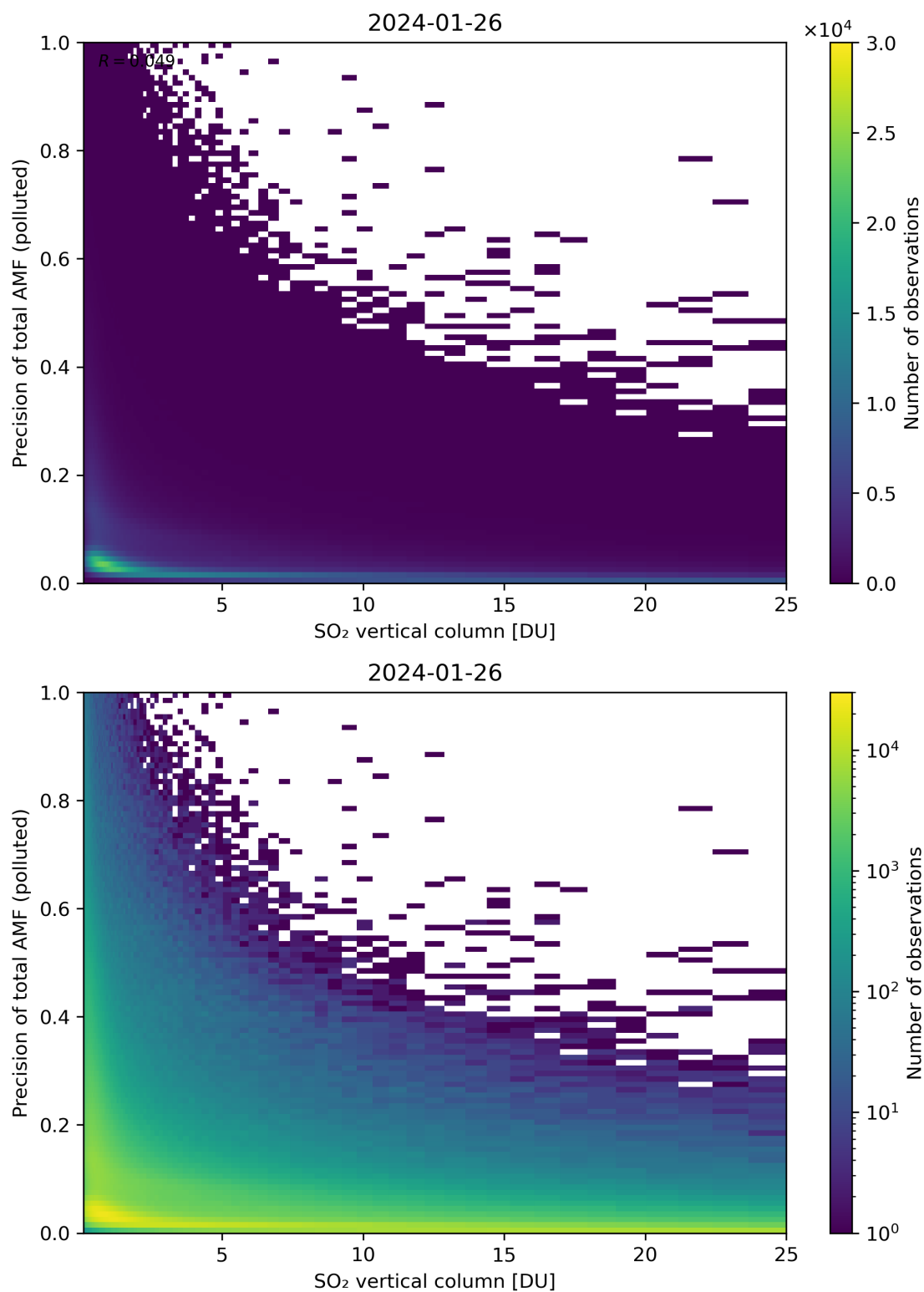
Figure 306: Scatter density plot of “SO 2 vertical column” against “Precision of total AMF (polluted)” for 2024-01-26 to 2024-01-27.
