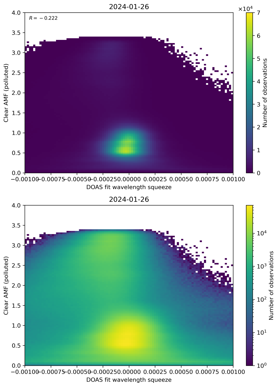
Figure 133: Scatter density plot of “DOAS fit wavelength squeeze” against “Clear AMF (polluted)” for 2024-01-26 to 2024-01-27.
