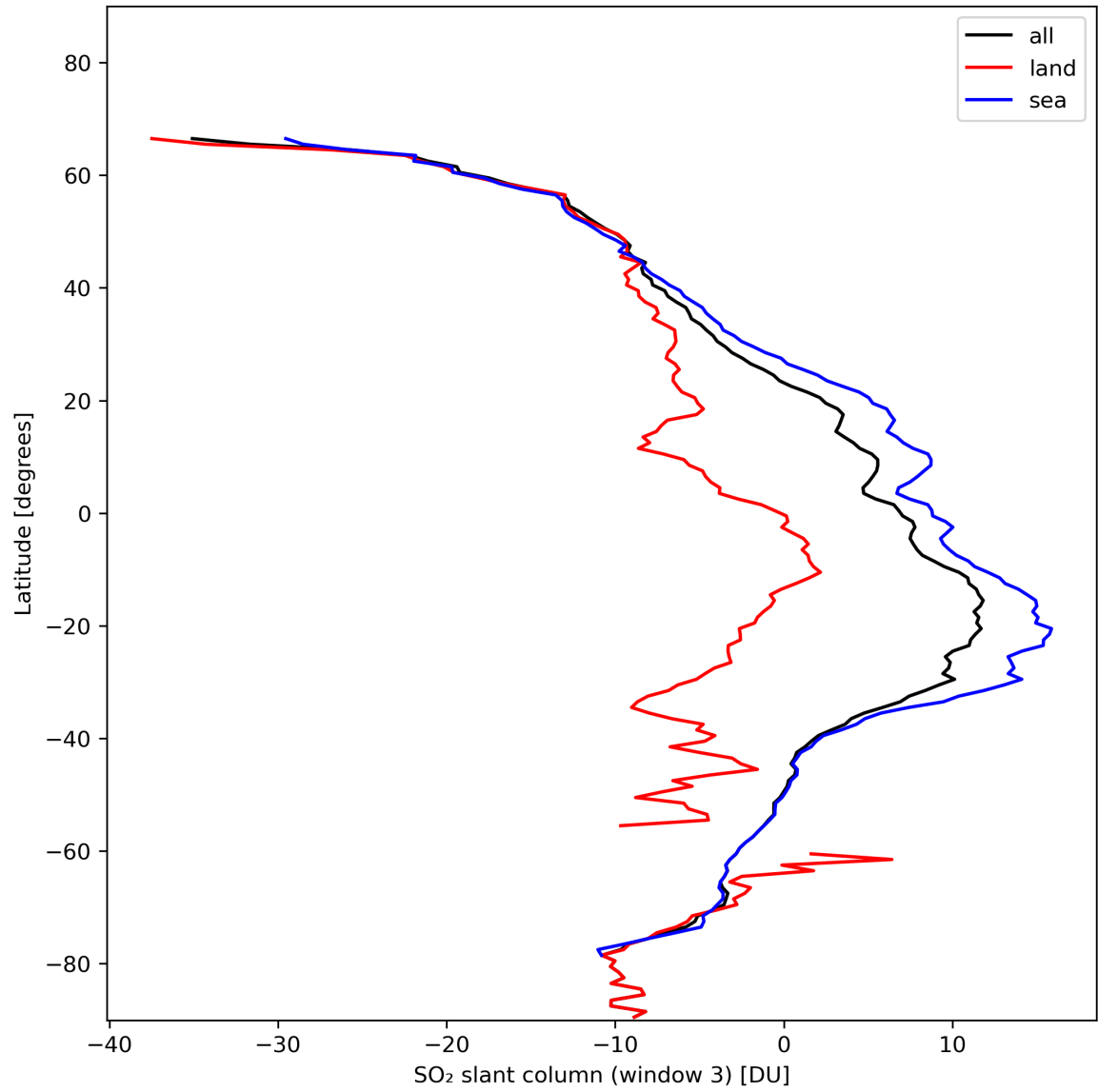
Figure 41: Zonal average of “SO 2 slant column (window 3)” for 2024-01-26 to 2024-01-27.
