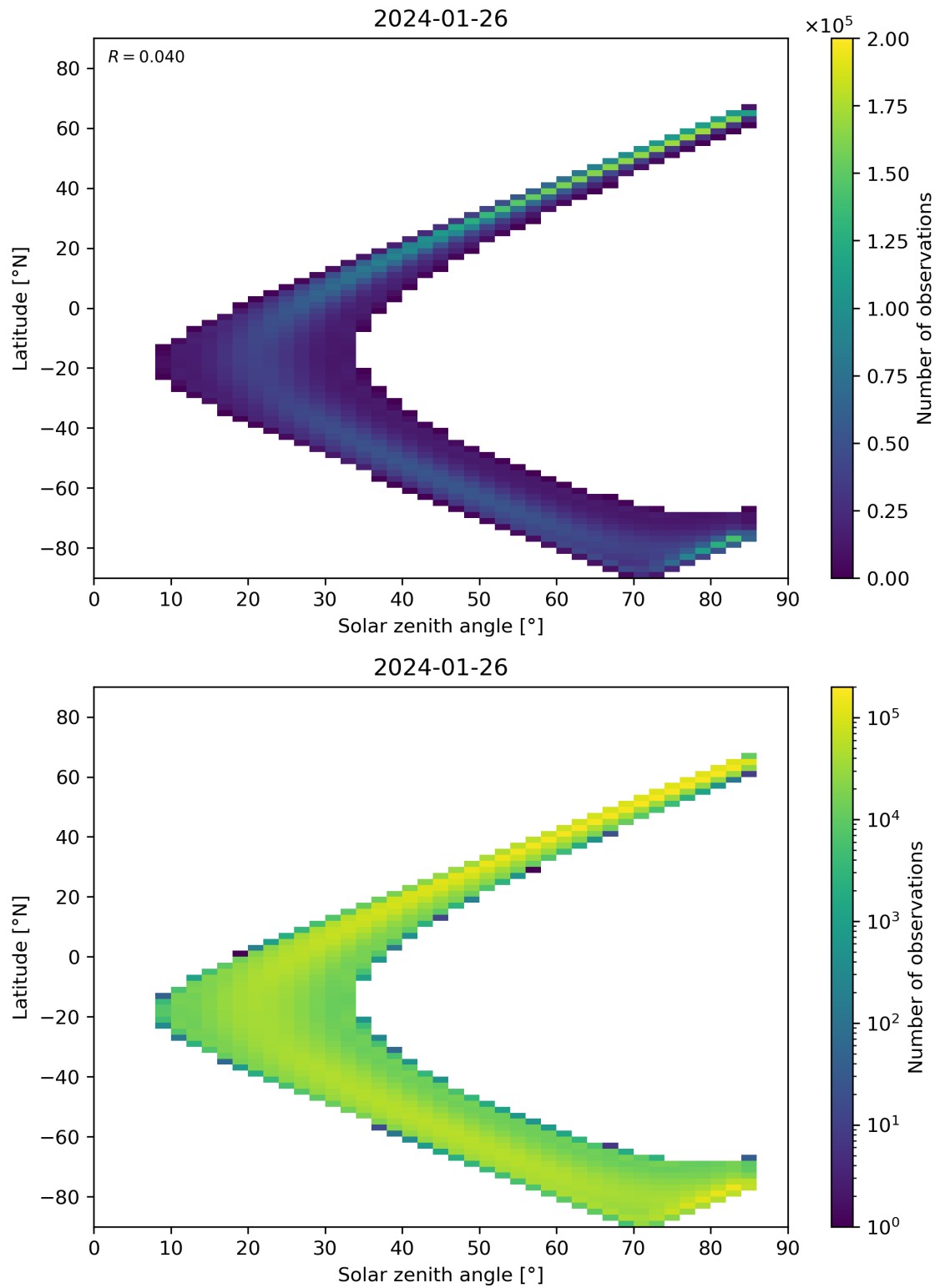
Figure 164: Scatter density plot of “Solar zenith angle” against “Latitude” for 2024-01-26 to 2024-01-27.
