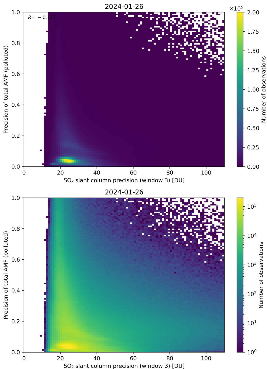
Figure 264: Scatter density plot of “SO 2 slant column precision (window 3)” against “Precision of total AMF (polluted)” for 2024-01-26 to 2024-01-27.
