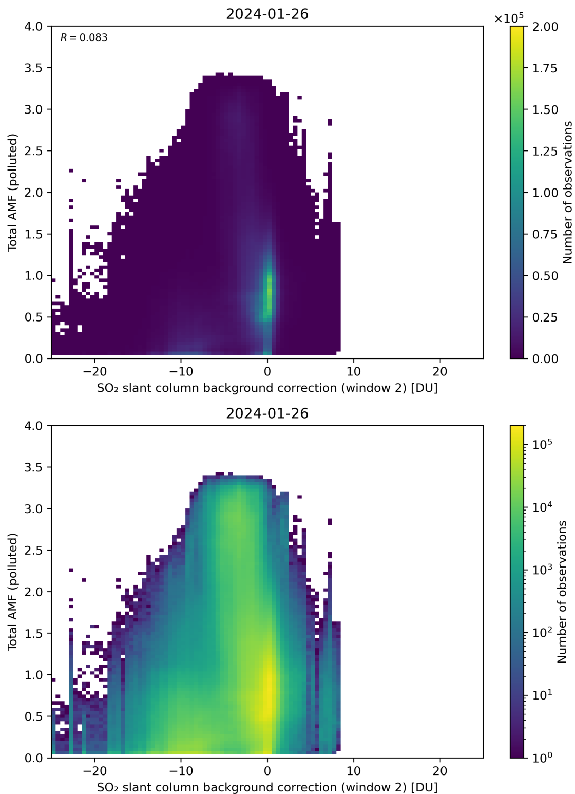
Figure 119: Scatter density plot of “SO 2 slant column background correction (window 2)” against “Total AMF (polluted)” for 2024-01-26 to 2024-01-27.
