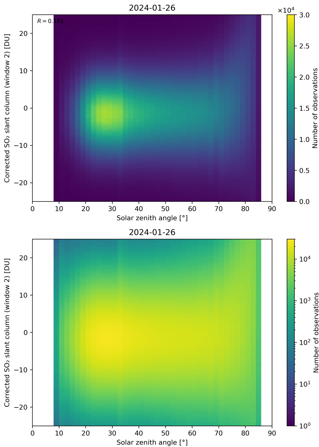
Figure 167: Scatter density plot of “Solar zenith angle” against “Corrected SO 2 slant column (window 2)” for 2024-01-26 to 2024-01-27.
