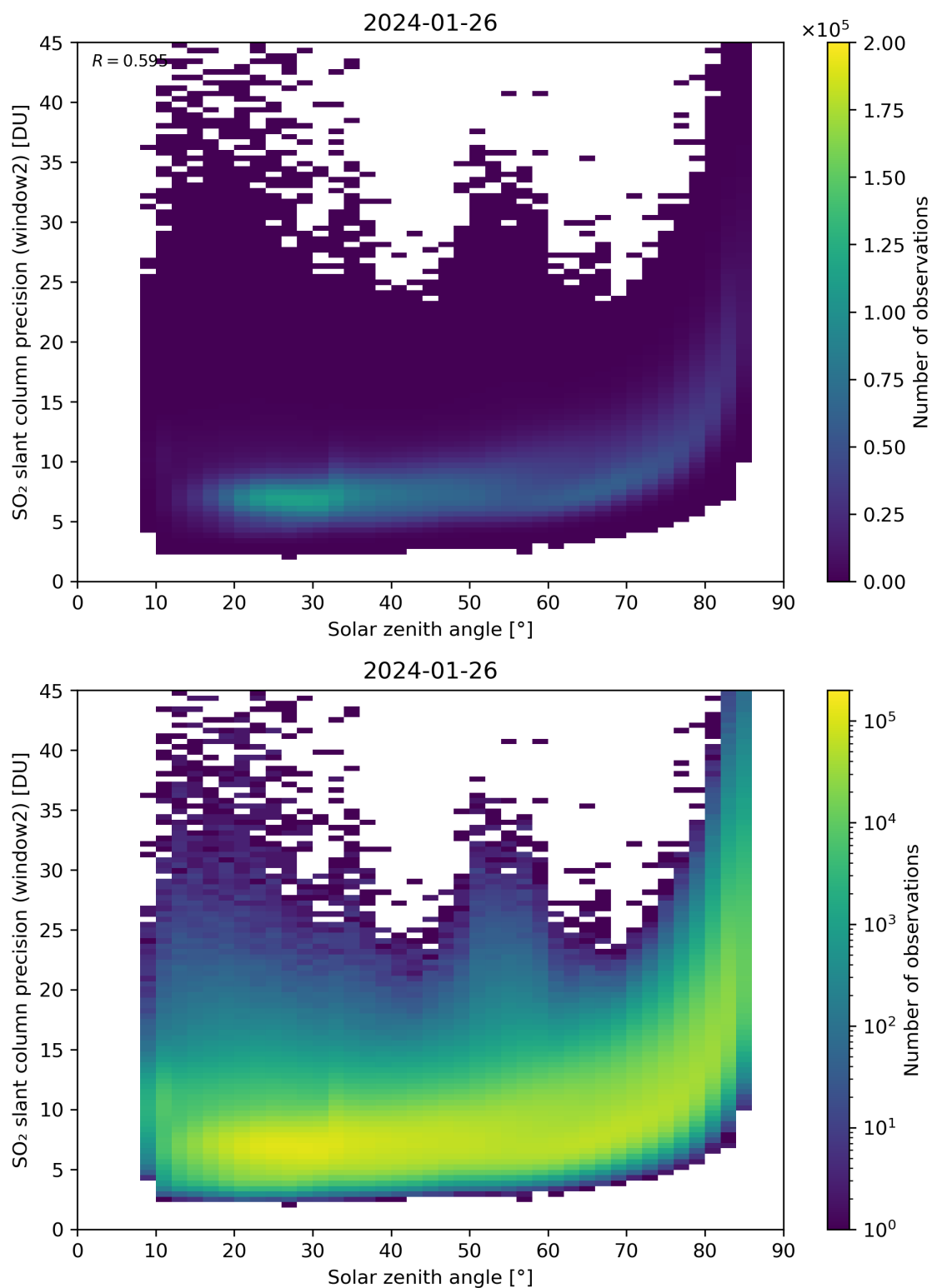
Figure 171: Scatter density plot of “Solar zenith angle” against “SO 2 slant column precision (window2)” for 2024-01-26 to 2024-01-27.
