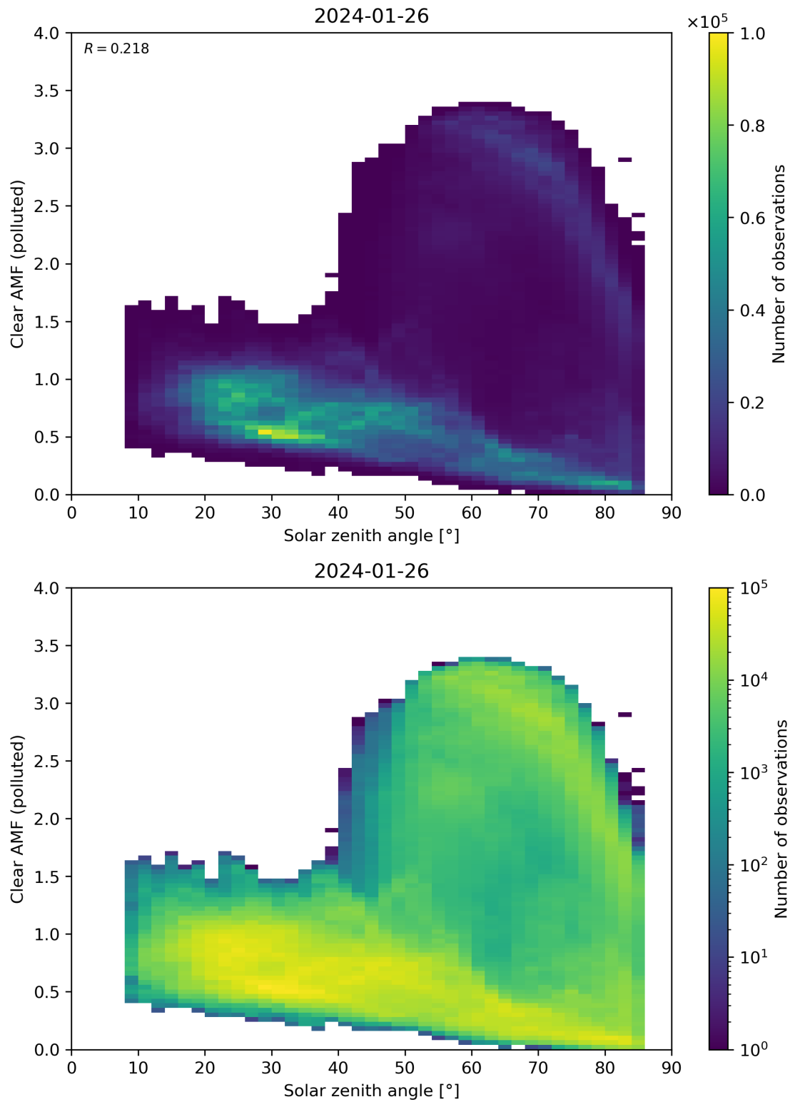
Figure 165: Scatter density plot of “Solar zenith angle” against “Clear AMF (polluted)” for 2024-01-26 to 2024-01-27.
