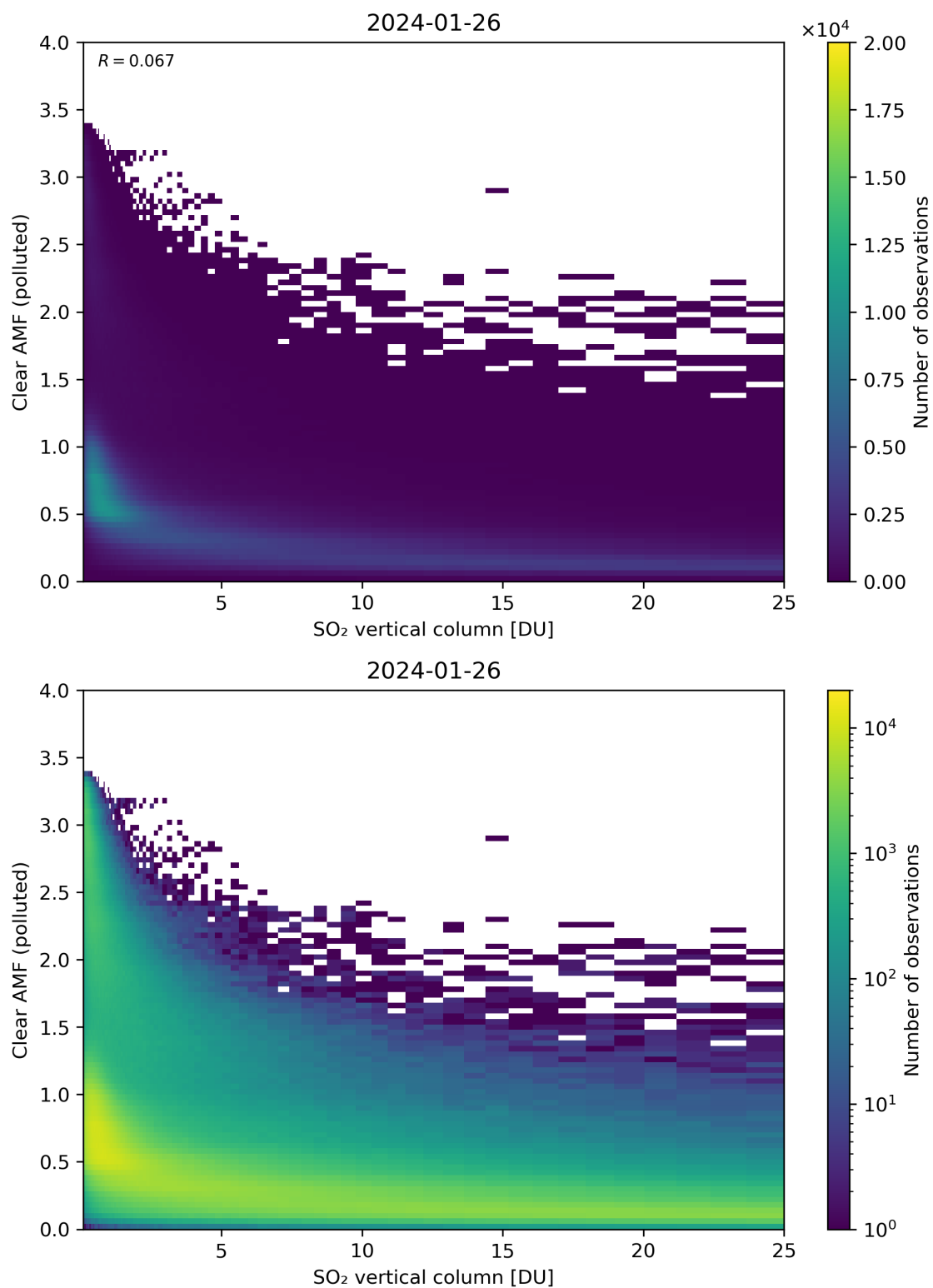
Figure 296: Scatter density plot of “SO 2 vertical column” against “Clear AMF (polluted)” for 2024-01-26 to 2024-01-27.
