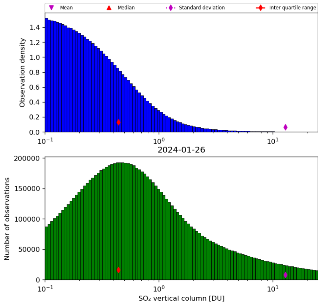
Figure 53: Histogram of “SO 2 vertical column” for 2024-01-26 to 2024-01-27
