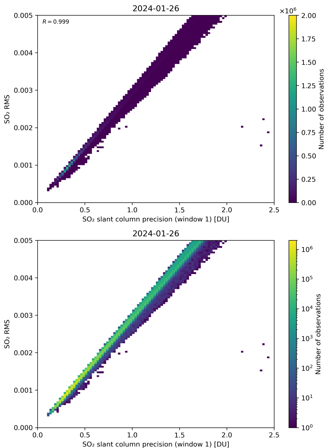
Figure 223: Scatter density plot of “SO 2 slant column precision (window 1)” against “SO 2 RMS” for 2024-01-26 to 2024-01-27.
