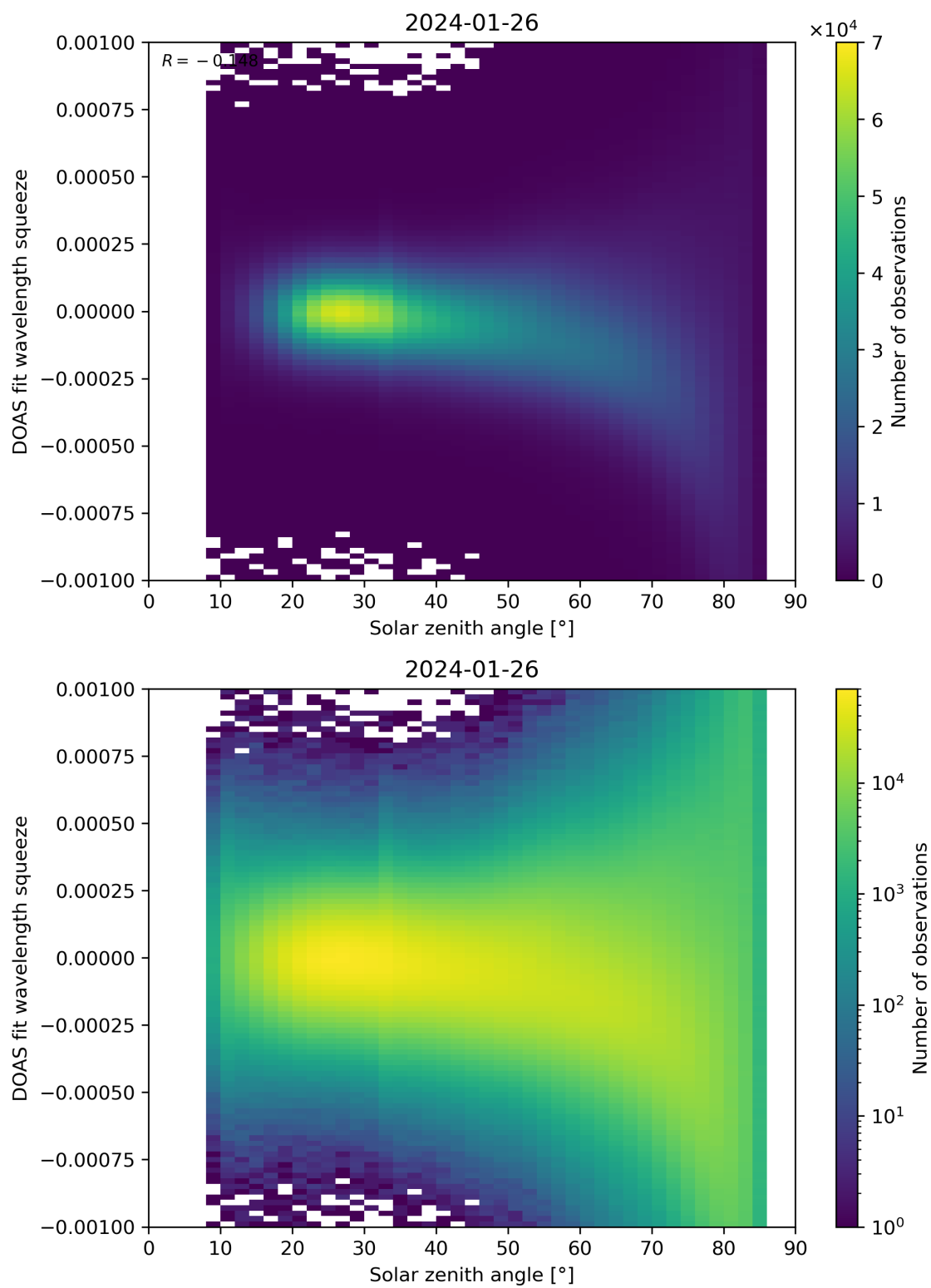
Figure 162: Scatter density plot of “Solar zenith angle” against “DOAS fit wavelength squeeze” for 2024-01-26 to 2024-01-27.
