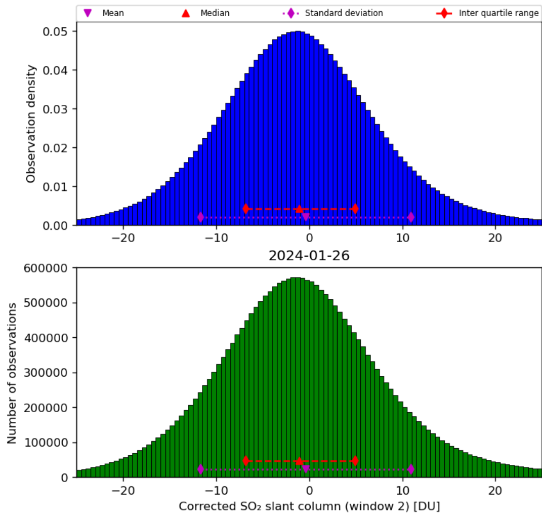
Figure 62: Histogram of “Corrected SO 2 slant column (window 2)” for 2024-01-26 to 2024-01-27
