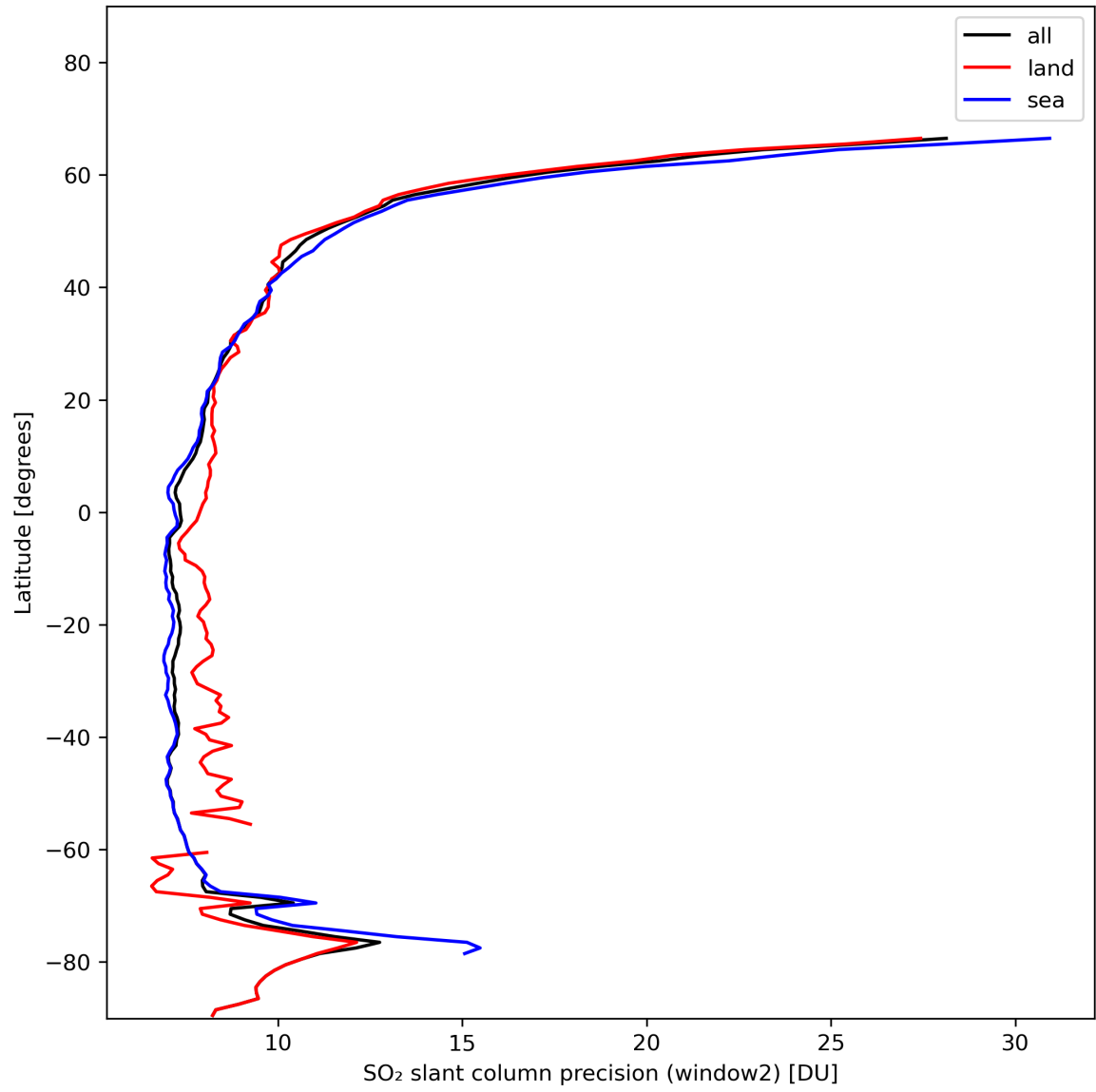
Figure 38: Zonal average of "SO 2 slant column precision (window2)" for 2024-01-26 to 2024-01-27.
