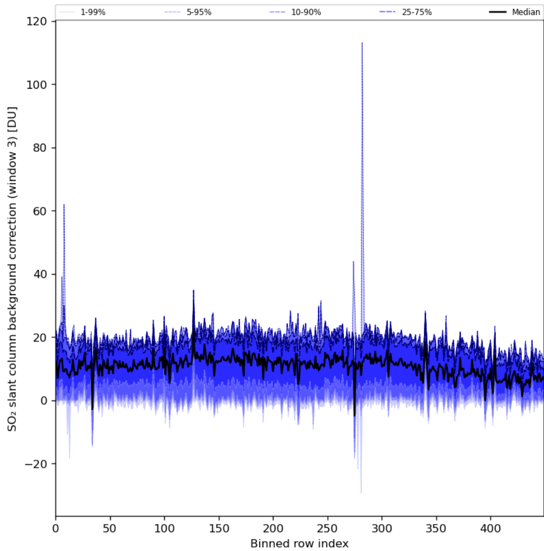
Figure 90: Along track statistics of “SO 2 slant column background correction (window 3)” for 2024-01-26 to 2024-01-27
