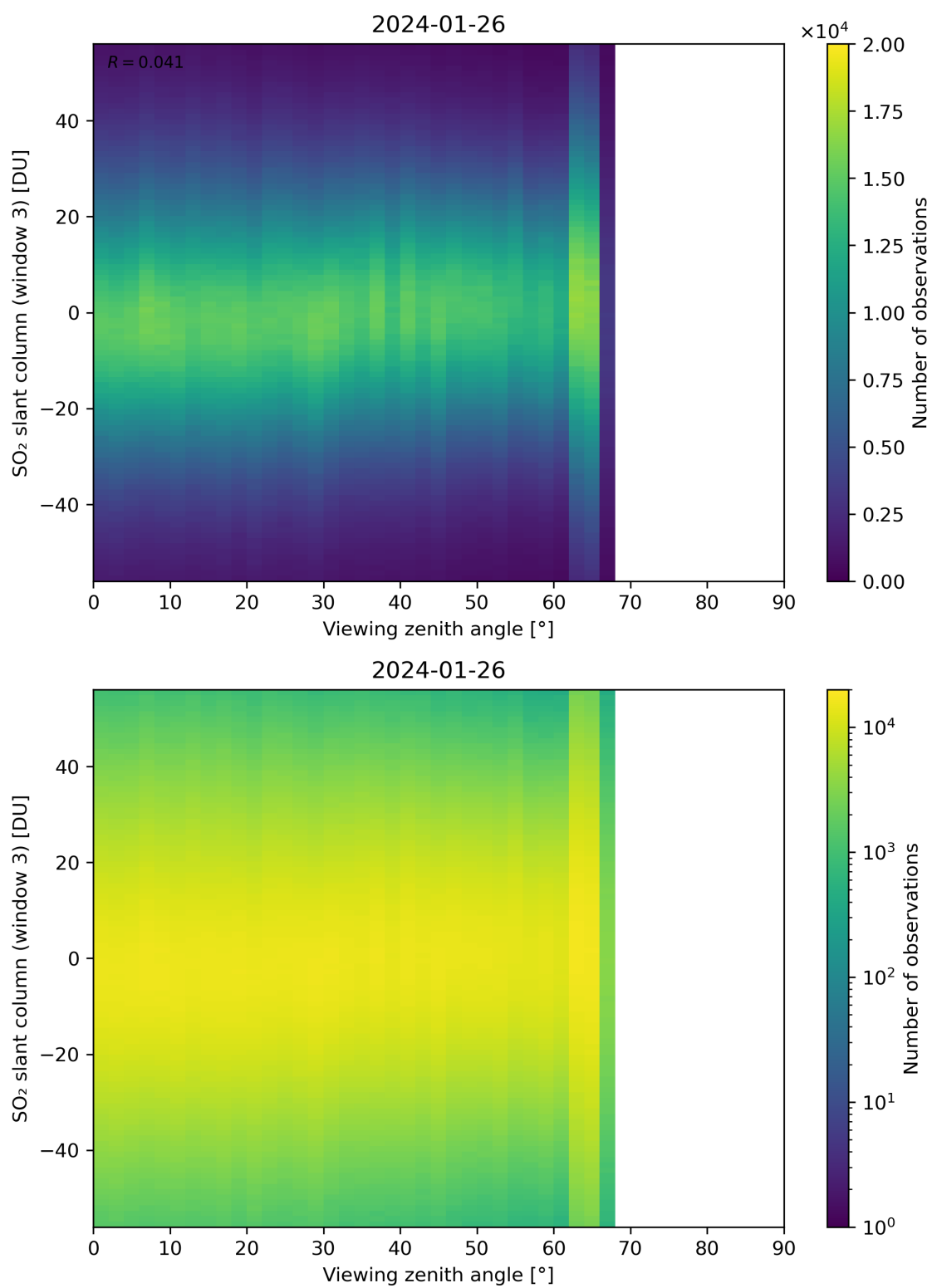
Figure 323: Scatter density plot of “Viewing zenith angle” against “SO 2 slant column (window 3)” for 2024-01-26 to 2024-01-27.
