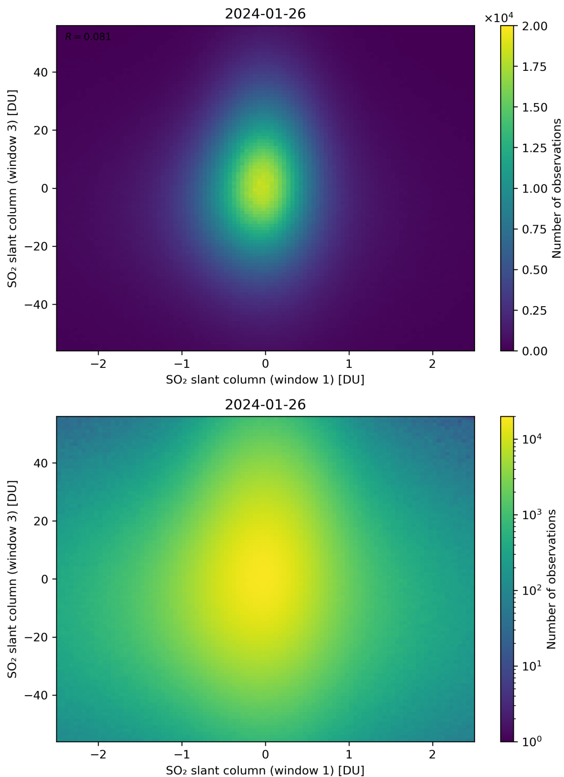
Figure 237: Scatter density plot of “SO 2 slant column (window 1)” against “SO 2 slant column (window 3)” for 2024-01-26 to 2024-01-27.
