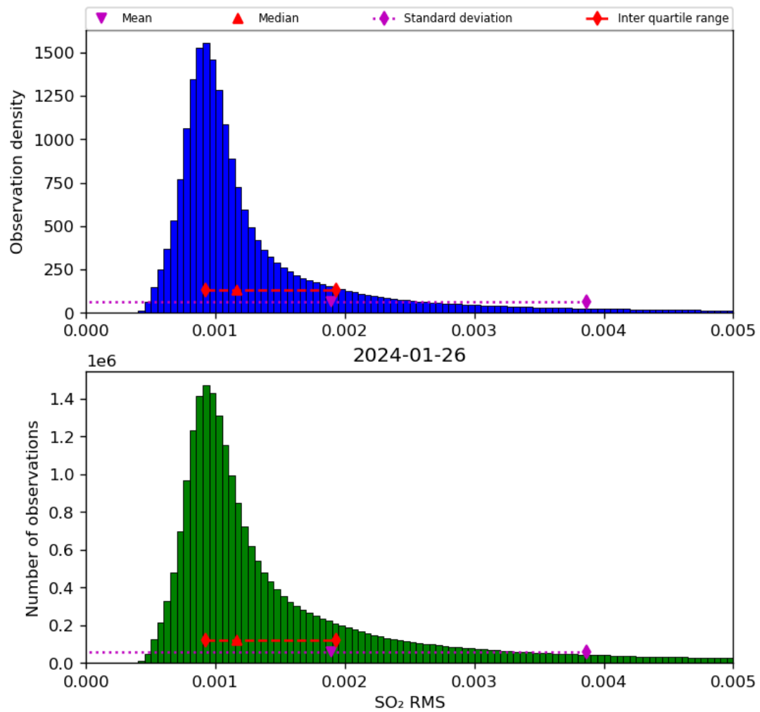
Figure 70: Histogram of “SO 2 RMS” for 2024-01-26 to 2024-01-27
