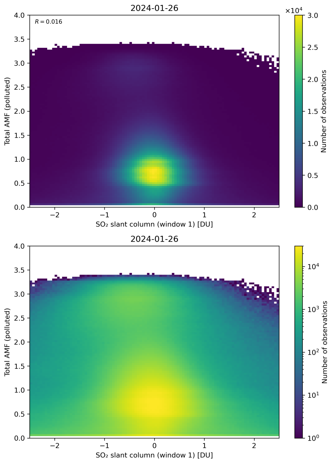
Figure 239: Scatter density plot of “SO 2 slant column (window 1)” against “Total AMF (polluted)” for 2024-01-26 to 2024-01-27.
