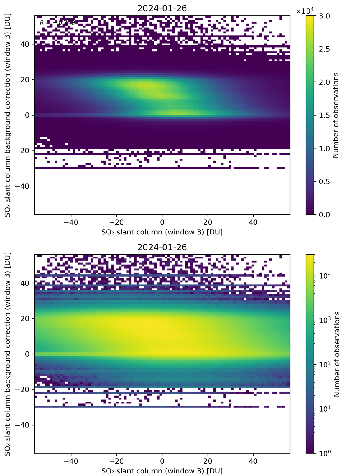
Figure 253: Scatter density plot of “SO 2 slant column (window 3)” against “SO 2 slant column background correction (window 3)” for 2024-01-26 to 2024-01-27.
