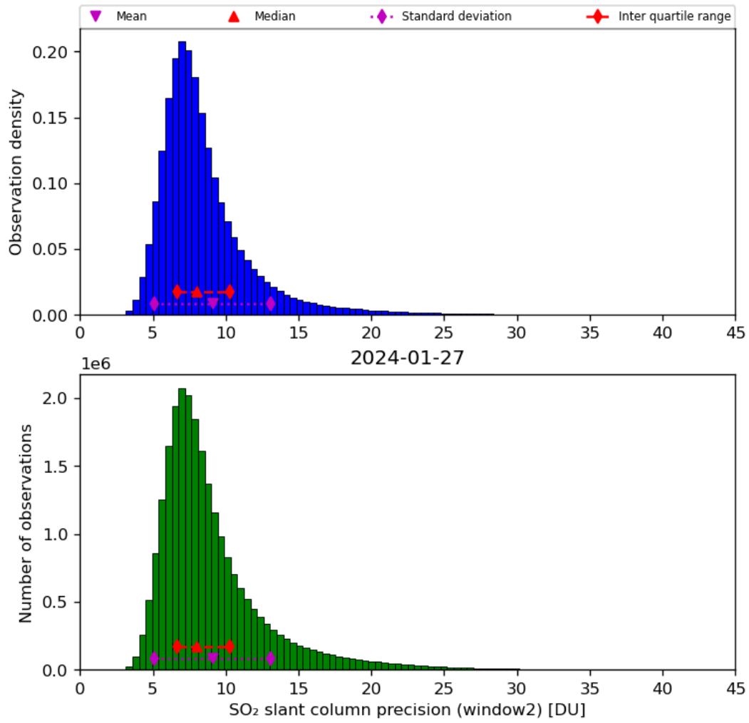
Figure 61: Histogram of “SO 2 slant column precision (window2)” for 2024-01-26 to 2024-01-28
