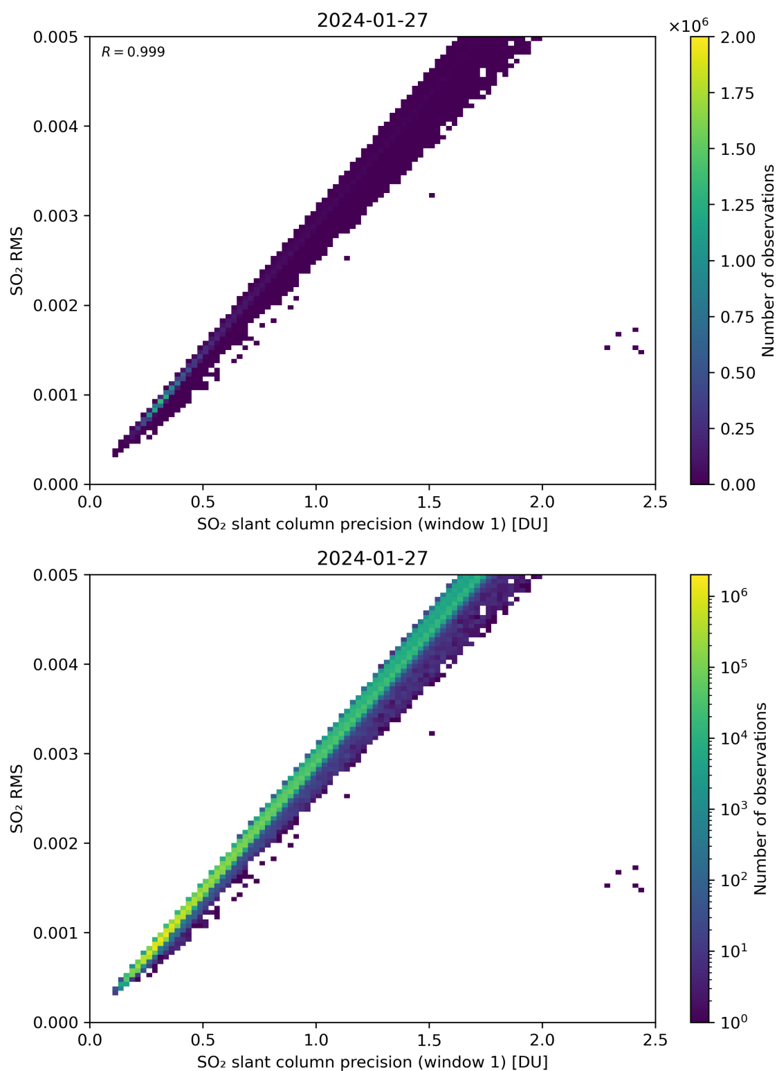
Figure 223: Scatter density plot of “SO 2 slant column precision (window 1)” against “SO 2 RMS” for 2024-01-26 to 2024-01-28.
