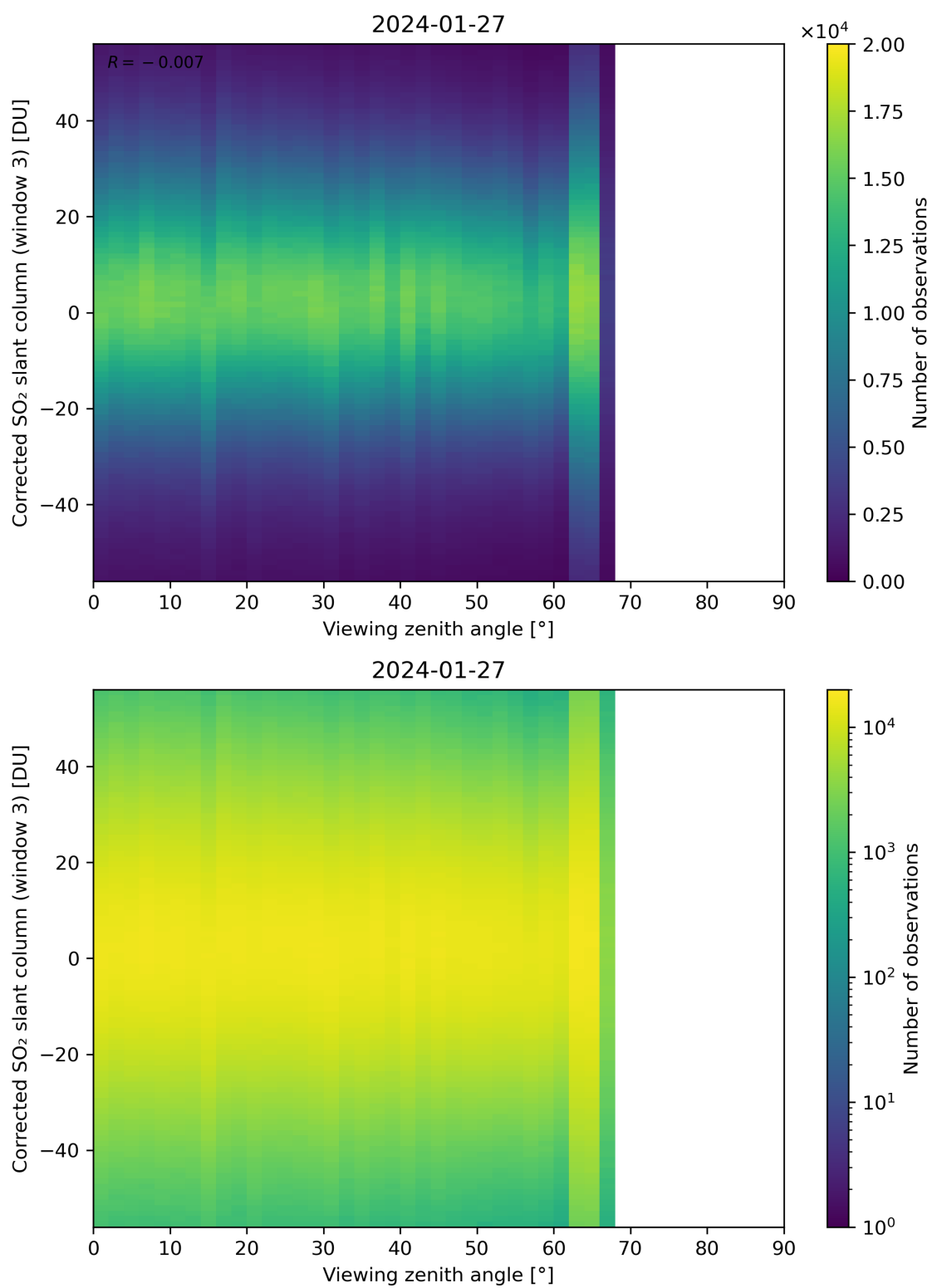
Figure 319: Scatter density plot of “Viewing zenith angle” against “Corrected SO 2 slant column (window 3)” for 2024-01-26 to 2024-01-28.
