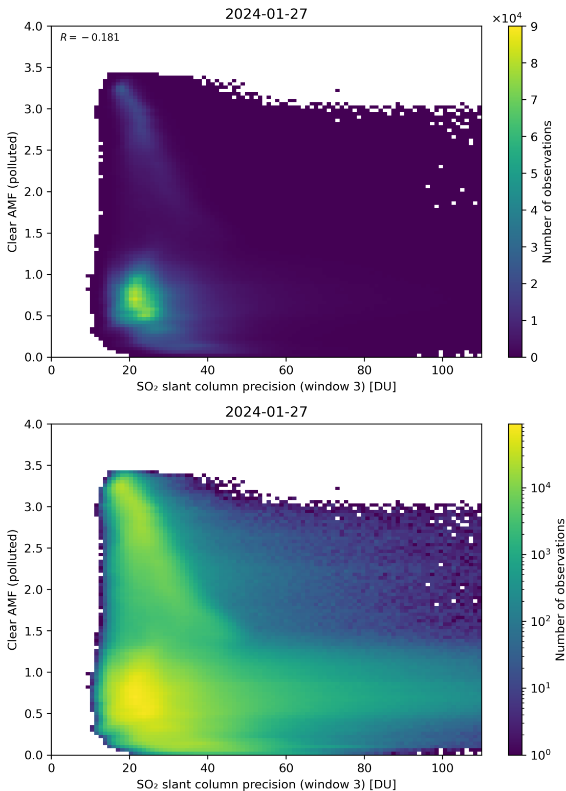
Figure 261: Scatter density plot of “SO 2 slant column precision (window 3)” against “Clear AMF (polluted)” for 2024-01-26 to 2024-01-28.
