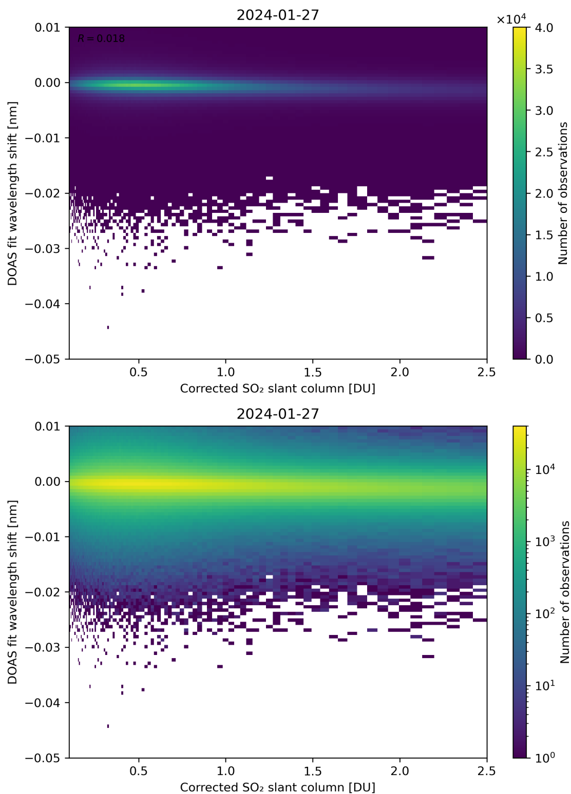
Figure 181: Scatter density plot of “Corrected SO 2 slant column” against “DOAS fit wavelength shift” for 2024-01-26 to 2024-01-28.
