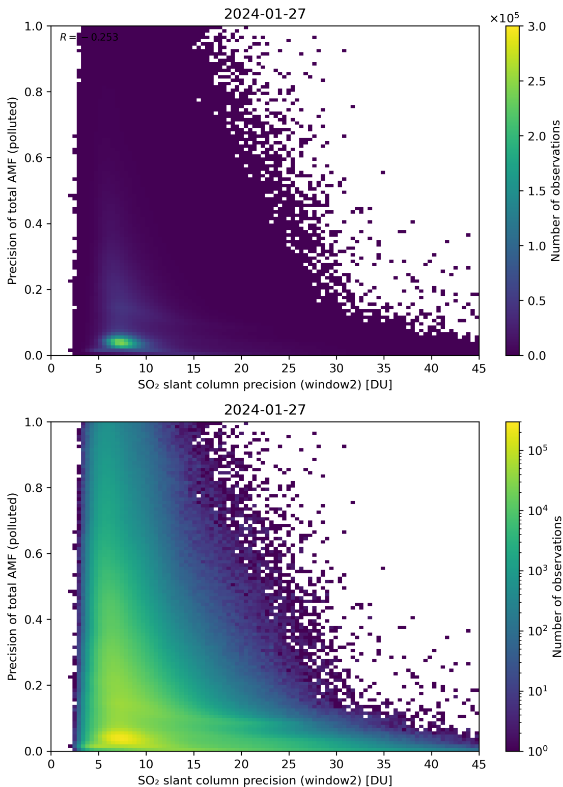
Figure 252: Scatter density plot of “SO 2 slant column precision (window2)” against “Precision of total AMF (polluted)” for 2024-01-26 to 2024-01-28.
