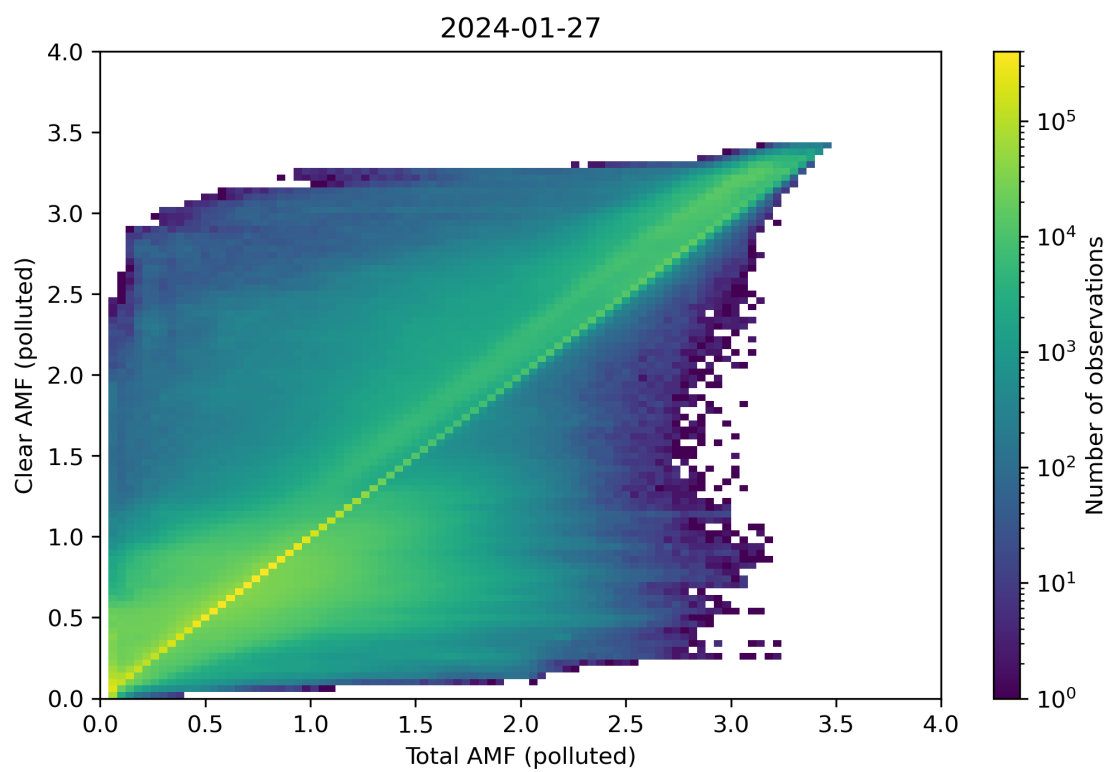
Figure 271: Scatter density plot of “Total AMF (polluted)” against “Clear AMF (polluted)” for 2024-01-26 to 2024-01-28.
