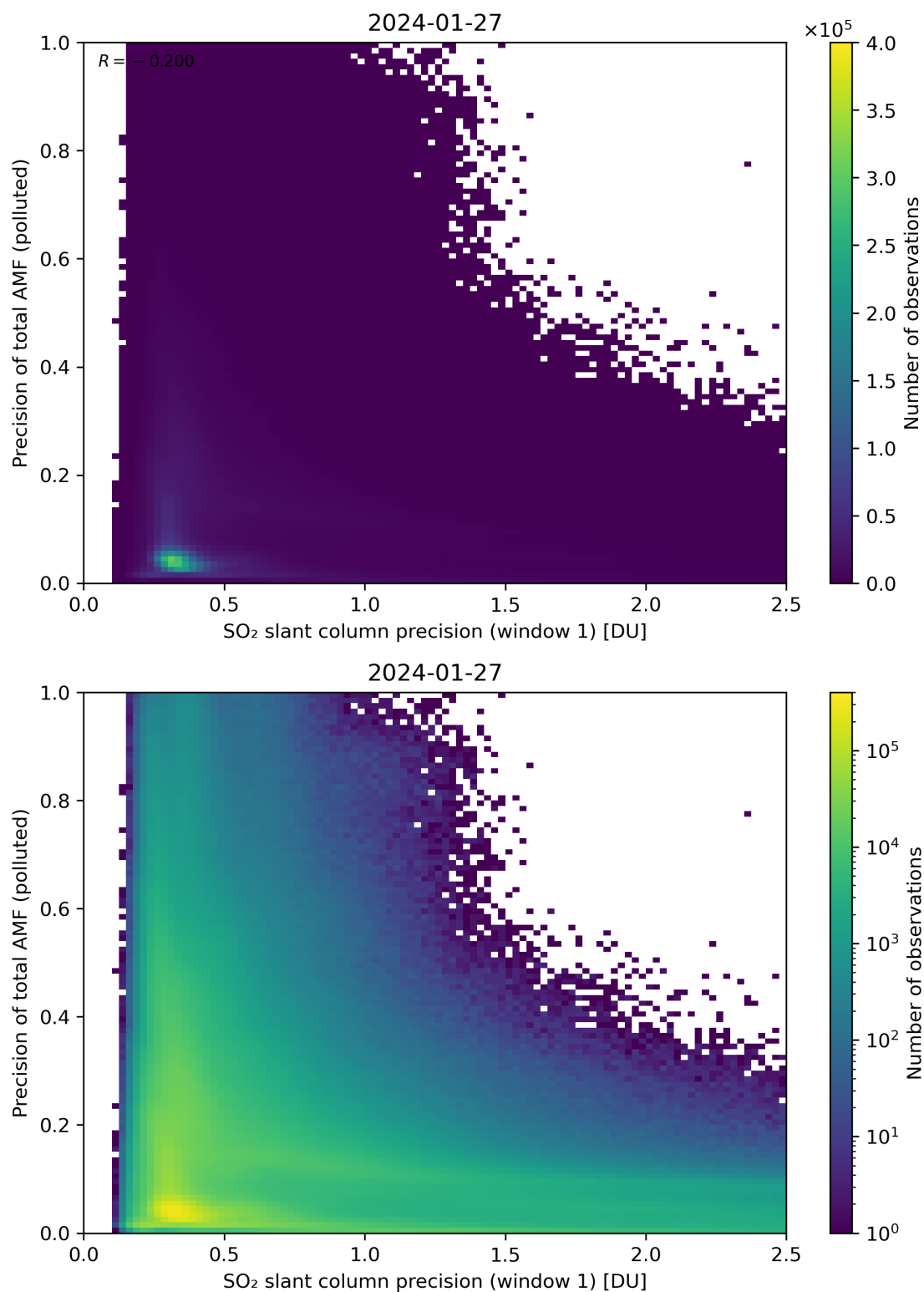
Figure 231: Scatter density plot of “SO 2 slant column precision (window 1)” against “Precision of total AMF (polluted)” for 2024-01-26 to 2024-01-28.
