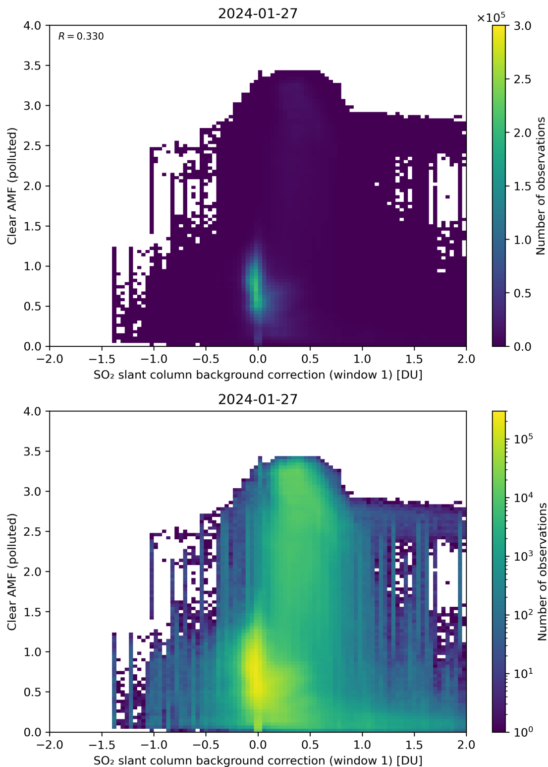
Figure 103: Scatter density plot of “SO 2 slant column background correction (window 1)” against “Clear AMF (polluted)” for 2024-01-26 to 2024-01-28.
