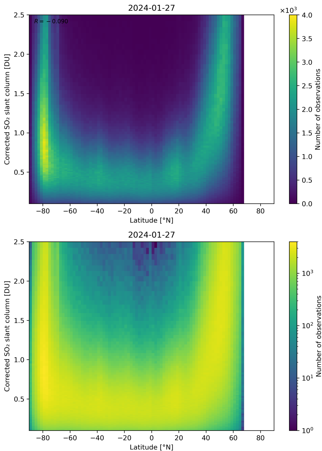
Figure 146: Scatter density plot of “Latitude” against “Corrected SO 2 slant column” for 2024-01-26 to 2024-01-28.
