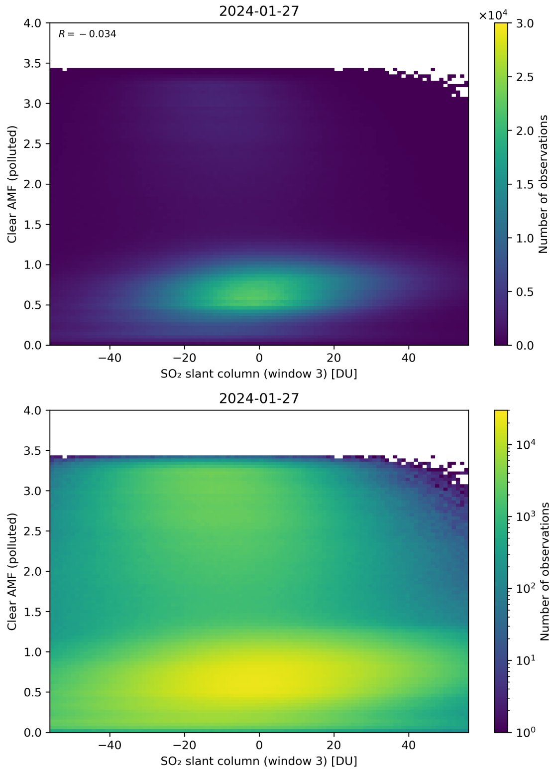
Figure 265: Scatter density plot of “SO 2 slant column (window 3)” against “Clear AMF (polluted)” for 2024-01-26 to 2024-01-28.
