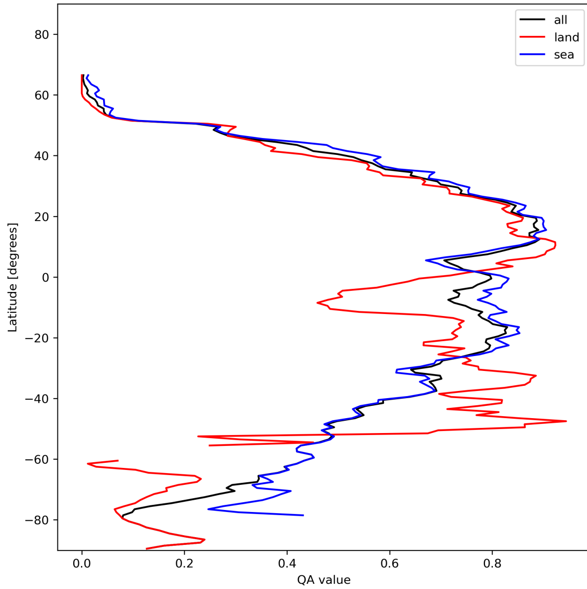
Figure 29: Zonal average of “QA value” for 2024-01-26 to 2024-01-28.
