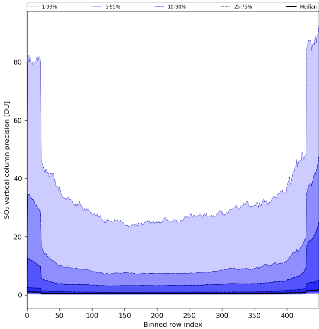
Figure 77: Along track statistics of “SO 2 vertical column precision” for 2024-01-26 to 2024-01-28
