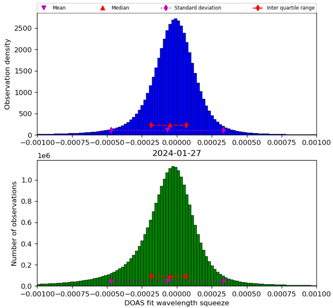
Figure 69: Histogram of “DOAS fit wavelength squeeze” for 2024-01-26 to 2024-01-28
