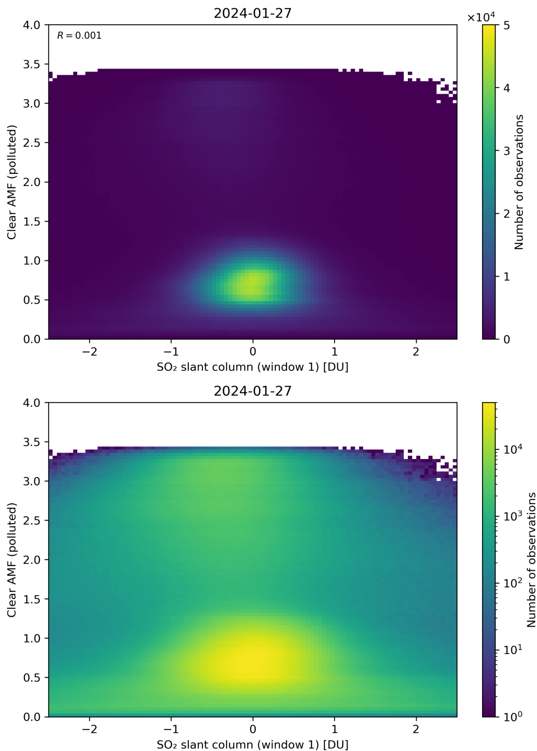
Figure 232: Scatter density plot of “SO 2 slant column (window 1)” against “Clear AMF (polluted)” for 2024-01-26 to 2024-01-28.
