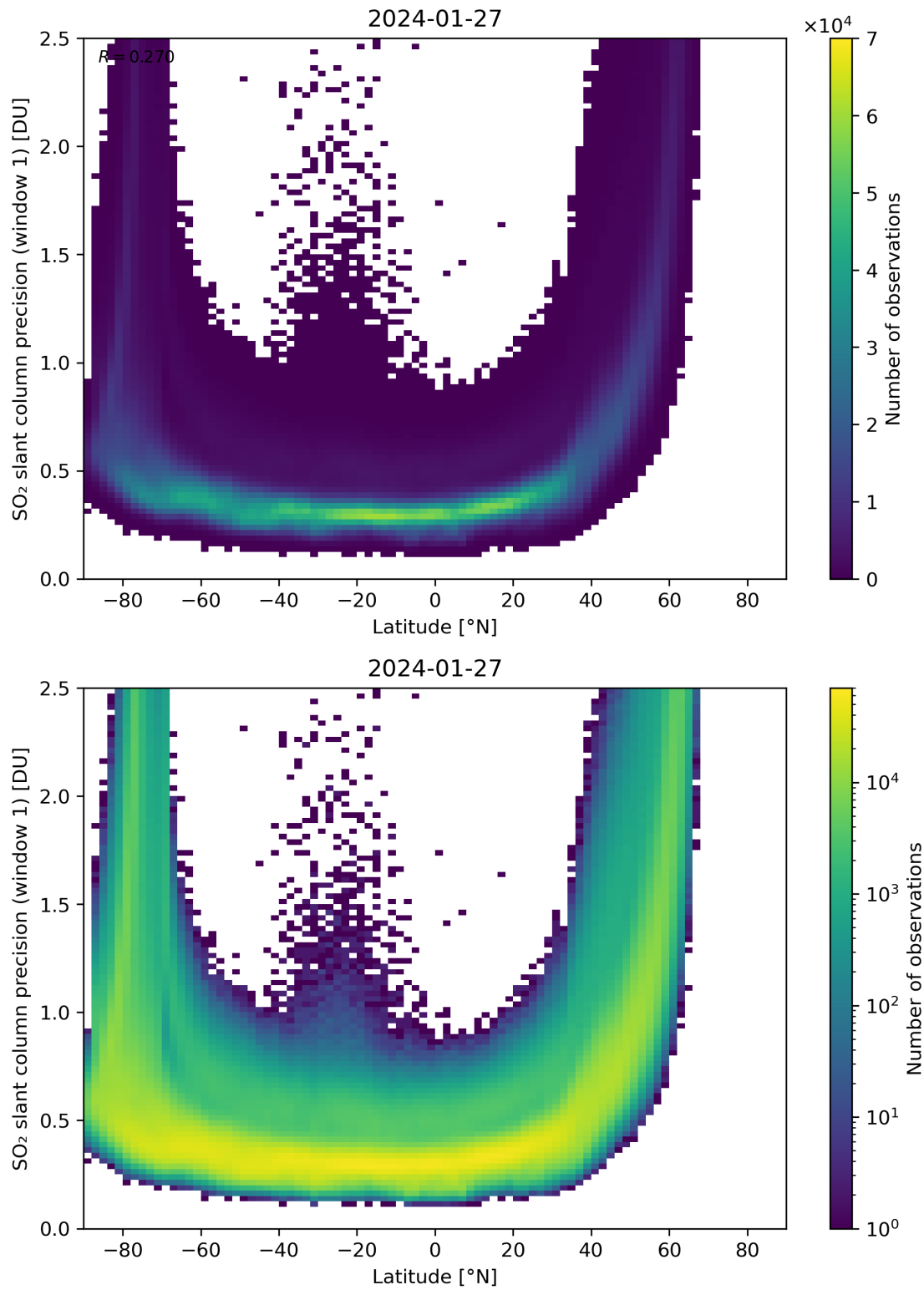
Figure 150: Scatter density plot of “Latitude” against “SO 2 slant column precision (window 1)” for 2024-01-26 to 2024-01-28.
