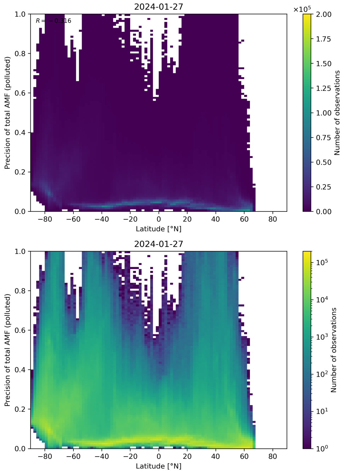
Figure 155: Scatter density plot of “Latitude” against “Precision of total AMF (polluted)” for 2024-01-26 to 2024-01-28.
