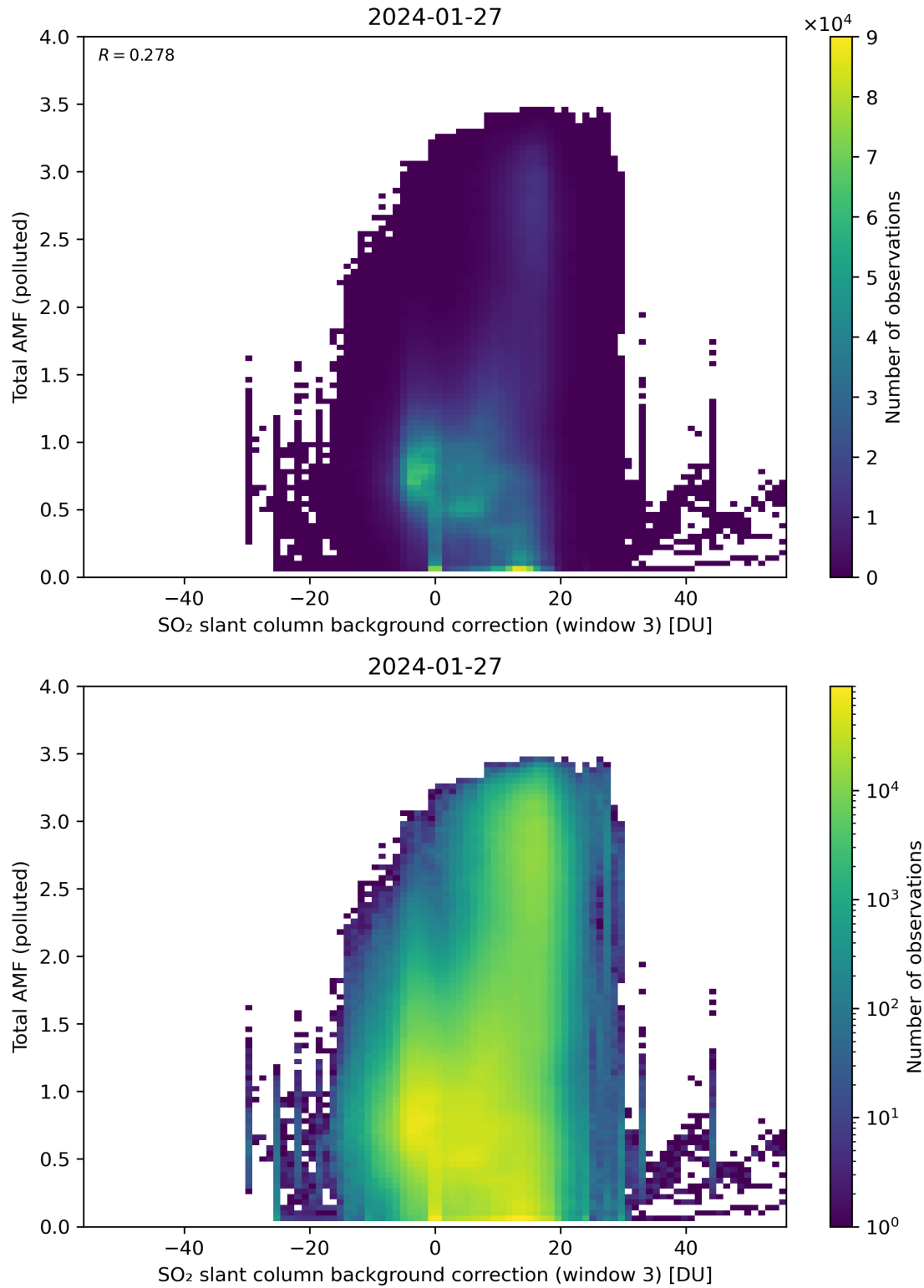
Figure 125: Scatter density plot of “SO 2 slant column background correction (window 3)” against “Total AMF (polluted)” for 2024-01-26 to 2024-01-28.
