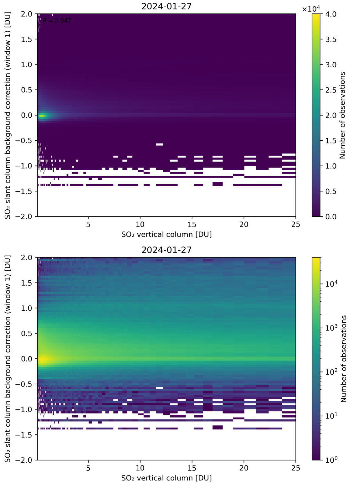
Figure 273: Scatter density plot of “SO 2 vertical column” against “SO 2 slant column background correction (window 1)” for 2024-01-26 to 2024-01-28.
