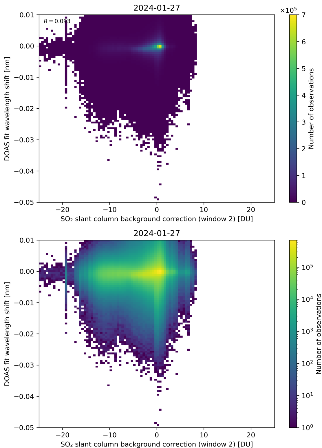
Figure 112: Scatter density plot of “SO 2 slant column background correction (window 2)” against “DOAS fit wavelength shift” for 2024-01-26 to 2024-01-28.
