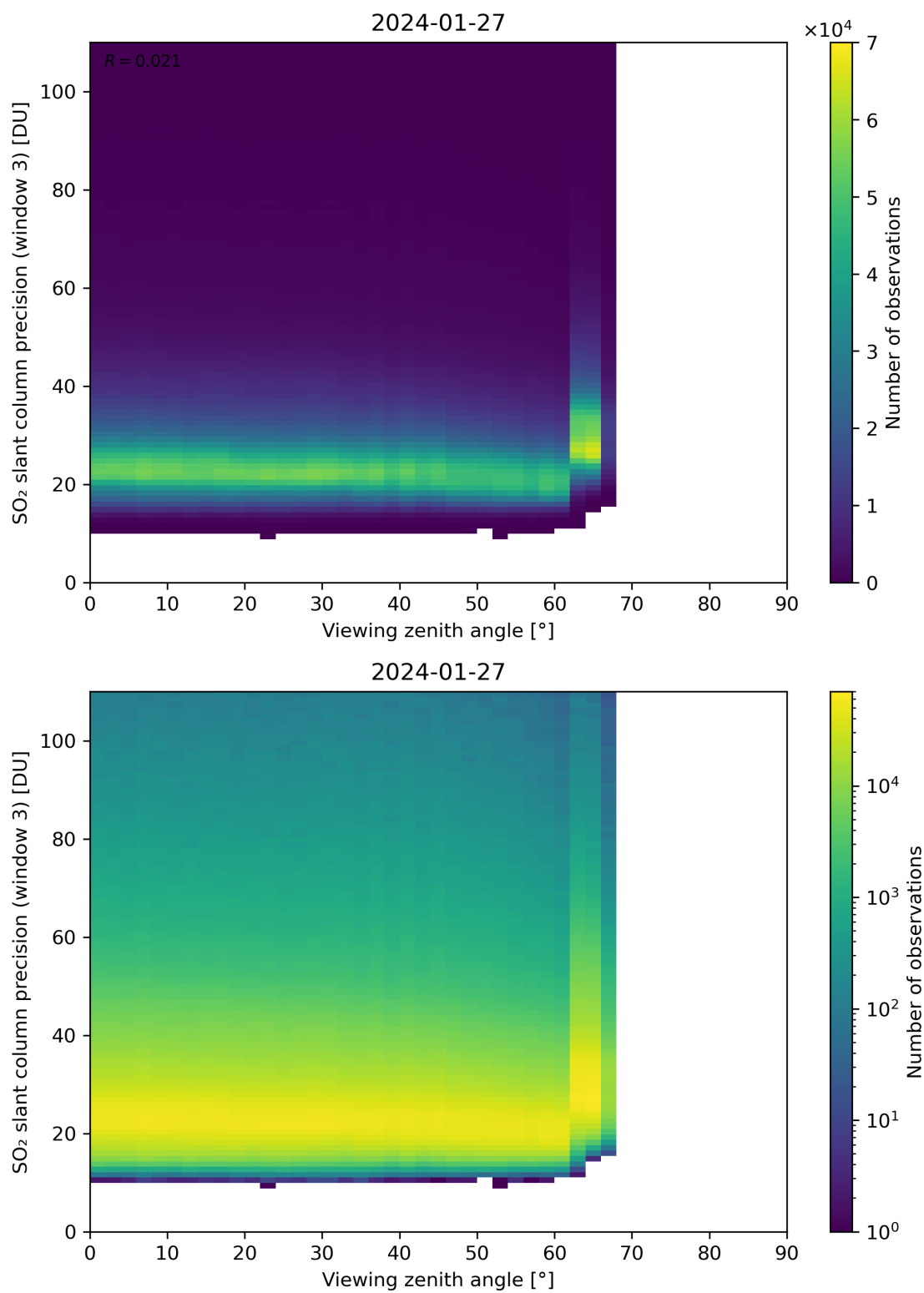
Figure 324: Scatter density plot of “Viewing zenith angle” against “SO 2 slant column precision (window 3)” for 2024-01-26 to 2024-01-28.
