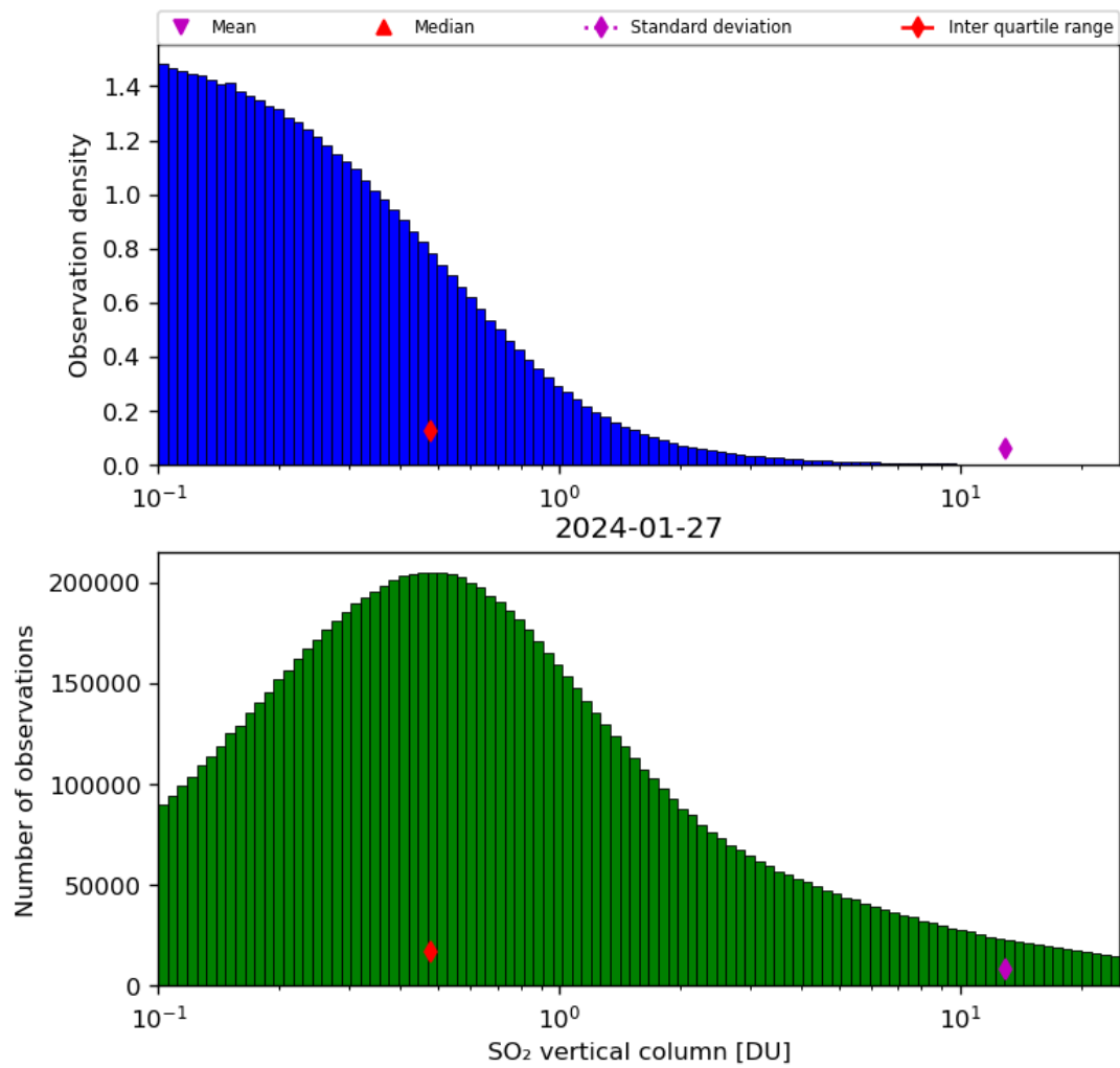
Figure 53: Histogram of “SO 2 vertical column” for 2024-01-26 to 2024-01-28
