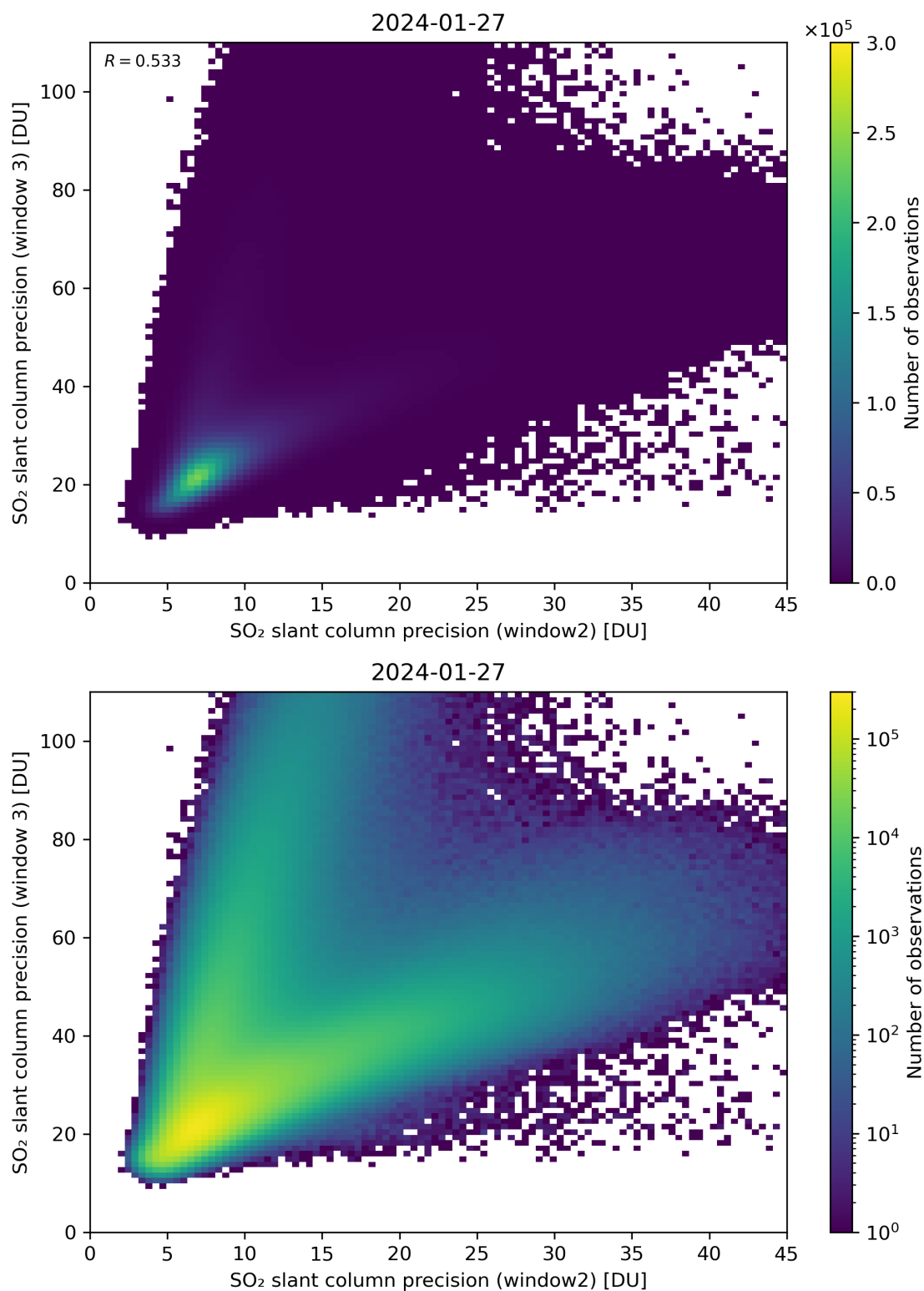
Figure 250: Scatter density plot of “SO 2 slant column precision (window2)” against “SO 2 slant column precision (window 3)” for 2024-01-26 to 2024-01-28.
