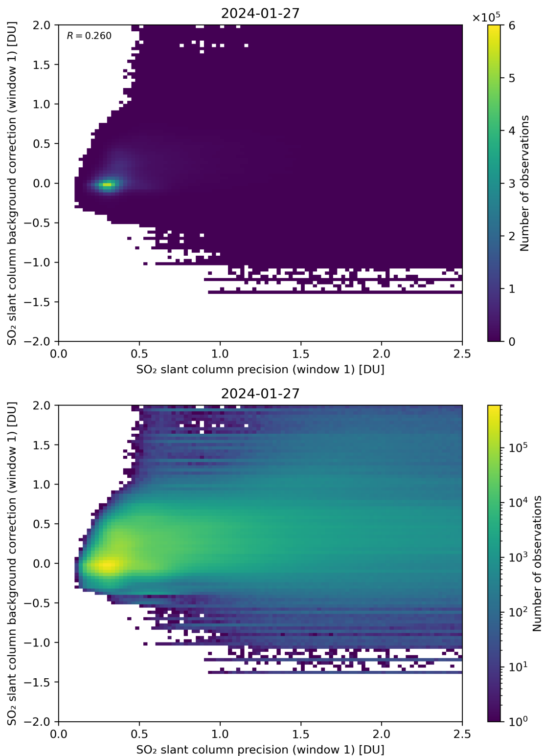
Figure 218: Scatter density plot of “SO 2 slant column precision (window 1)” against “SO 2 slant column background correction (window 1)” for 2024-01-26 to 2024-01-28.
