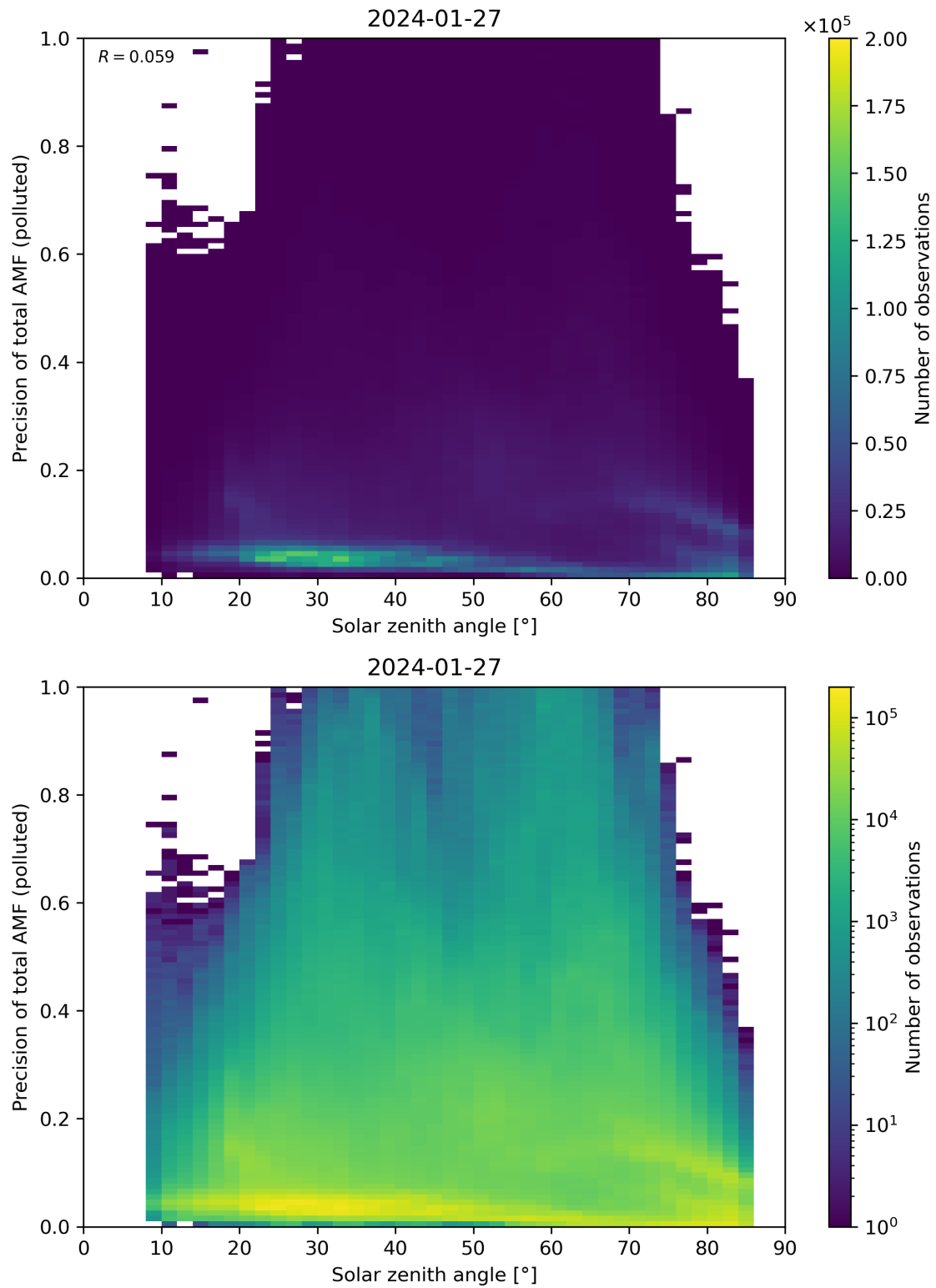
Figure 175: Scatter density plot of “Solar zenith angle” against “Precision of total AMF (polluted)” for 2024-01-26 to 2024-01-28.
