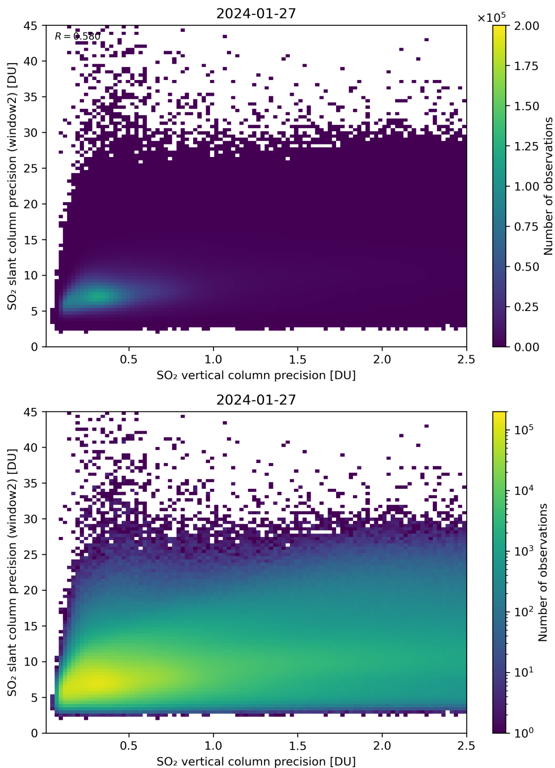
Figure 291: Scatter density plot of “SO 2 vertical column precision” against “SO 2 slant column precision (window2)” for 2024-01-26 to 2024-01-28.
