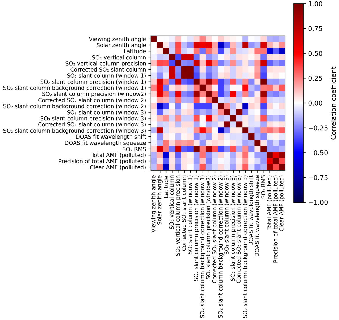
Figure 2: Map of correlation matrix for 2024-01-26 to 2024-01-28.
