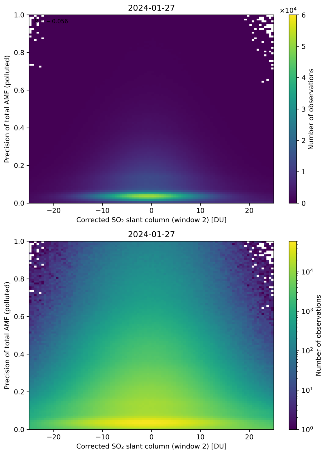
Figure 204: Scatter density plot of “Corrected SO 2 slant column (window 2)” against “Precision of total AMF (polluted)” for 2024-01-26 to 2024-01-28.
