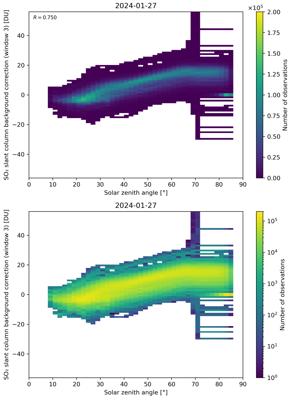
Figure 160: Scatter density plot of “Solar zenith angle” against “SO 2 slant column background correction (window 3)” for 2024-01-26 to 2024-01-28.
