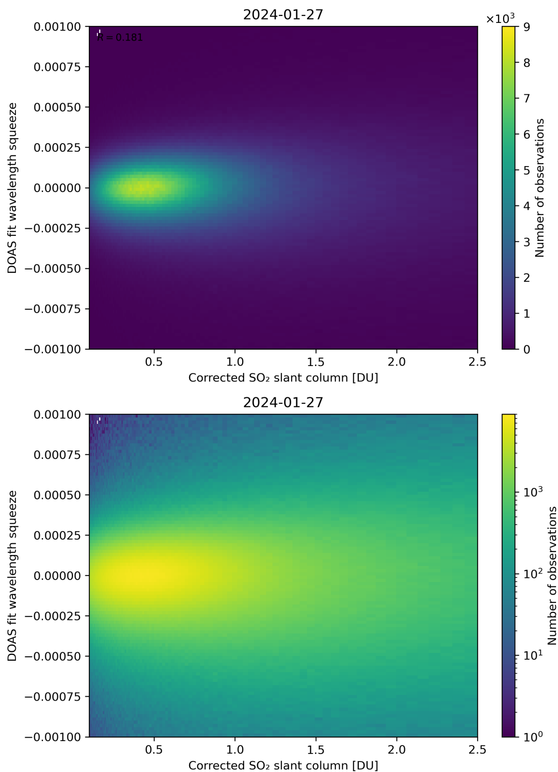
Figure 182: Scatter density plot of “Corrected SO 2 slant column” against “DOAS fit wavelength squeeze” for 2024-01-26 to 2024-01-28.
