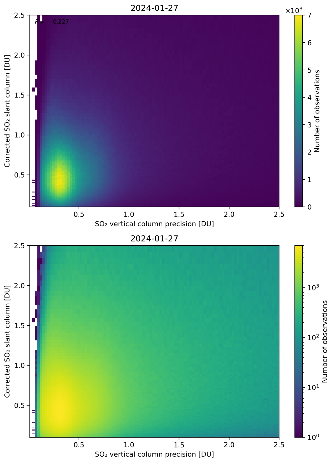
Figure 286: Scatter density plot of “SO 2 vertical column precision” against “Corrected SO 2 slant column” for 2024-01-26 to 2024-01-28.
