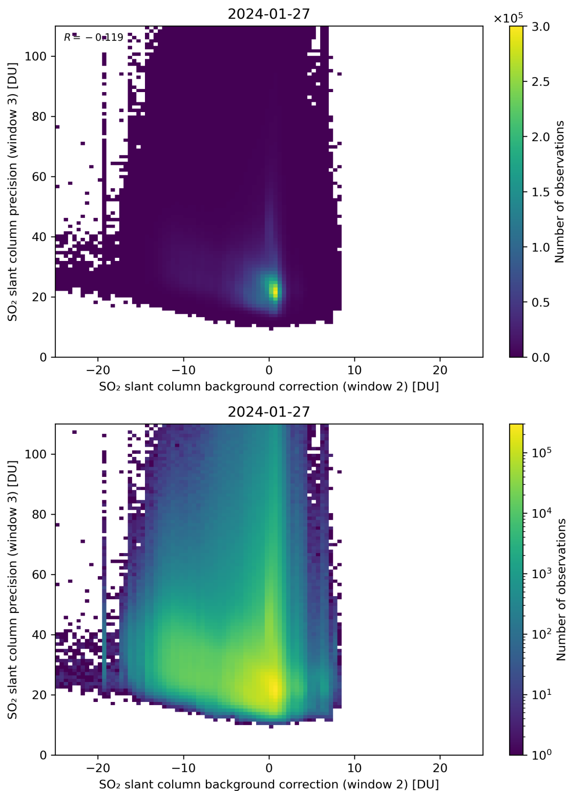
Figure 118: Scatter density plot of “SO 2 slant column background correction (window 2)” against “SO 2 slant column precision (window 3)” for 2024-01-26 to 2024-01-28.
