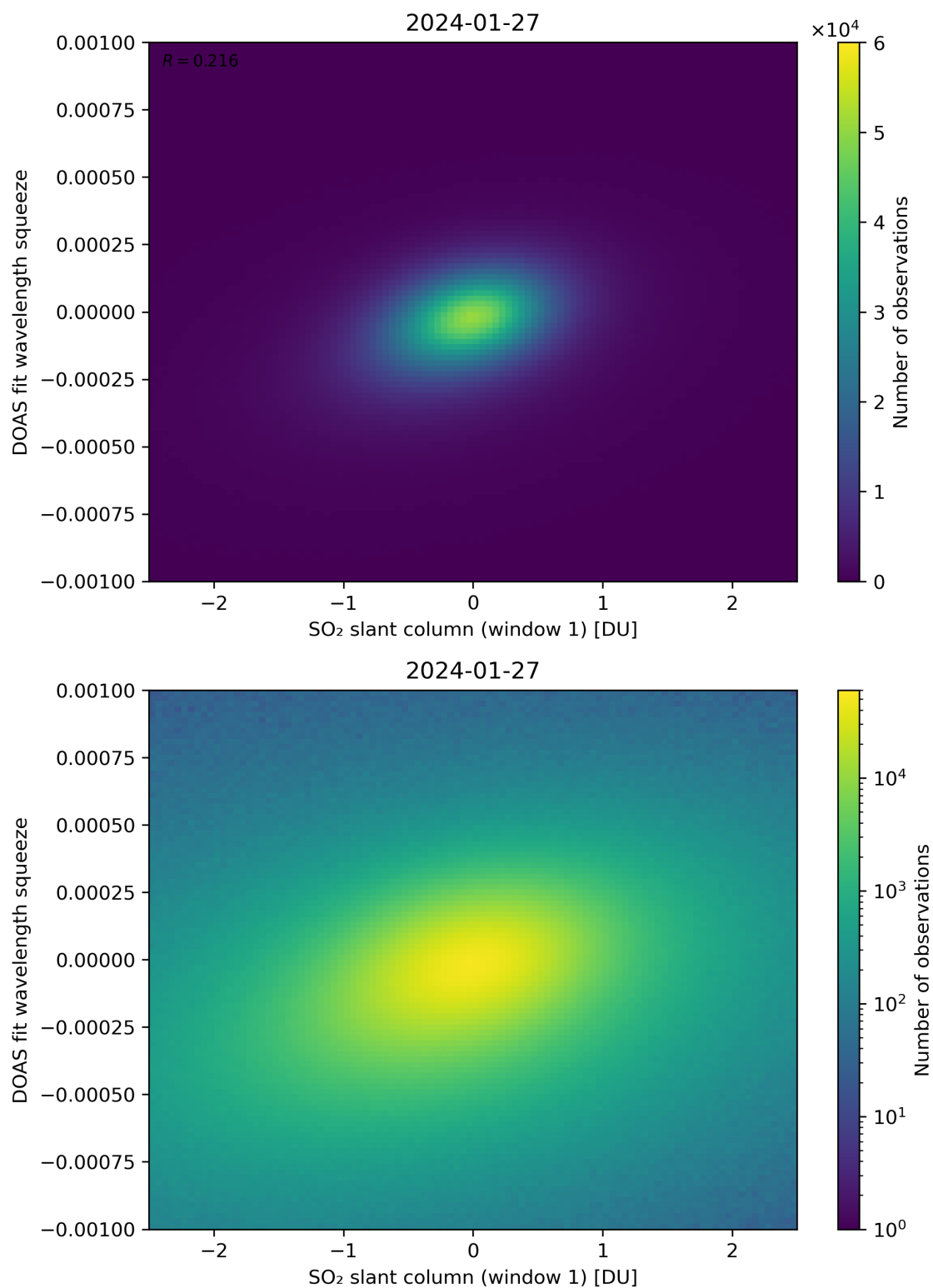
Figure 216: Scatter density plot of “SO 2 slant column (window 1)” against “DOAS fit wavelength squeeze” for 2024-01-26 to 2024-01-28.
