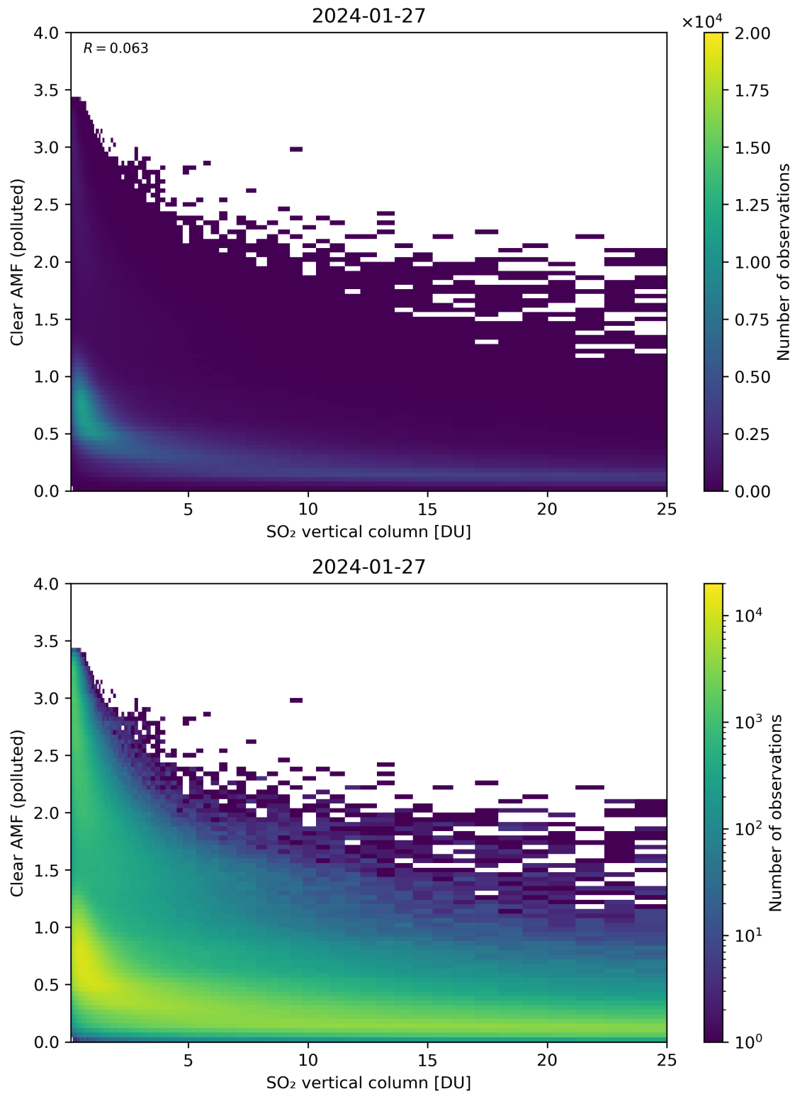
Figure 296: Scatter density plot of “SO 2 vertical column” against “Clear AMF (polluted)” for 2024-01-26 to 2024-01-28.
