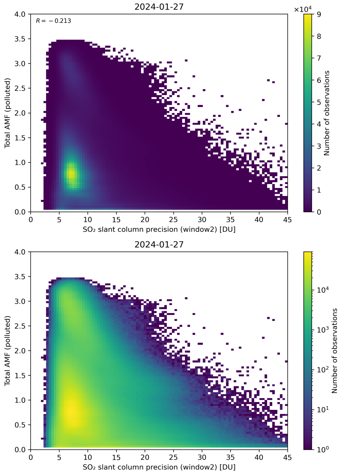
Figure 251: Scatter density plot of “SO 2 slant column precision (window2)” against “Total AMF (polluted)” for 2024-01-26 to 2024-01-28.
