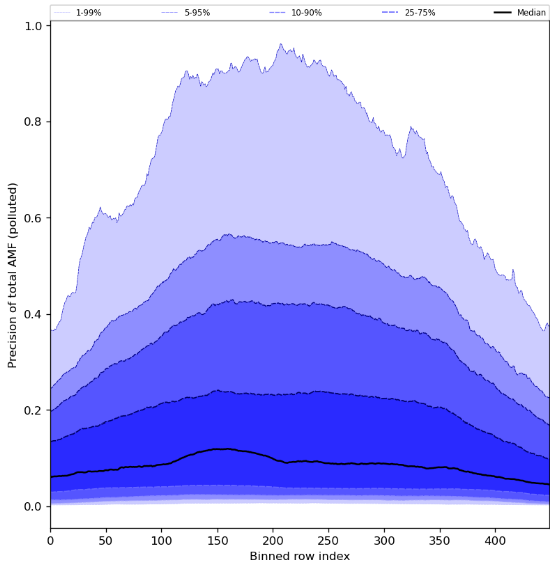
Figure 95: Along track statistics of “Precision of total AMF (polluted)” for 2024-01-26 to 2024-01-28
