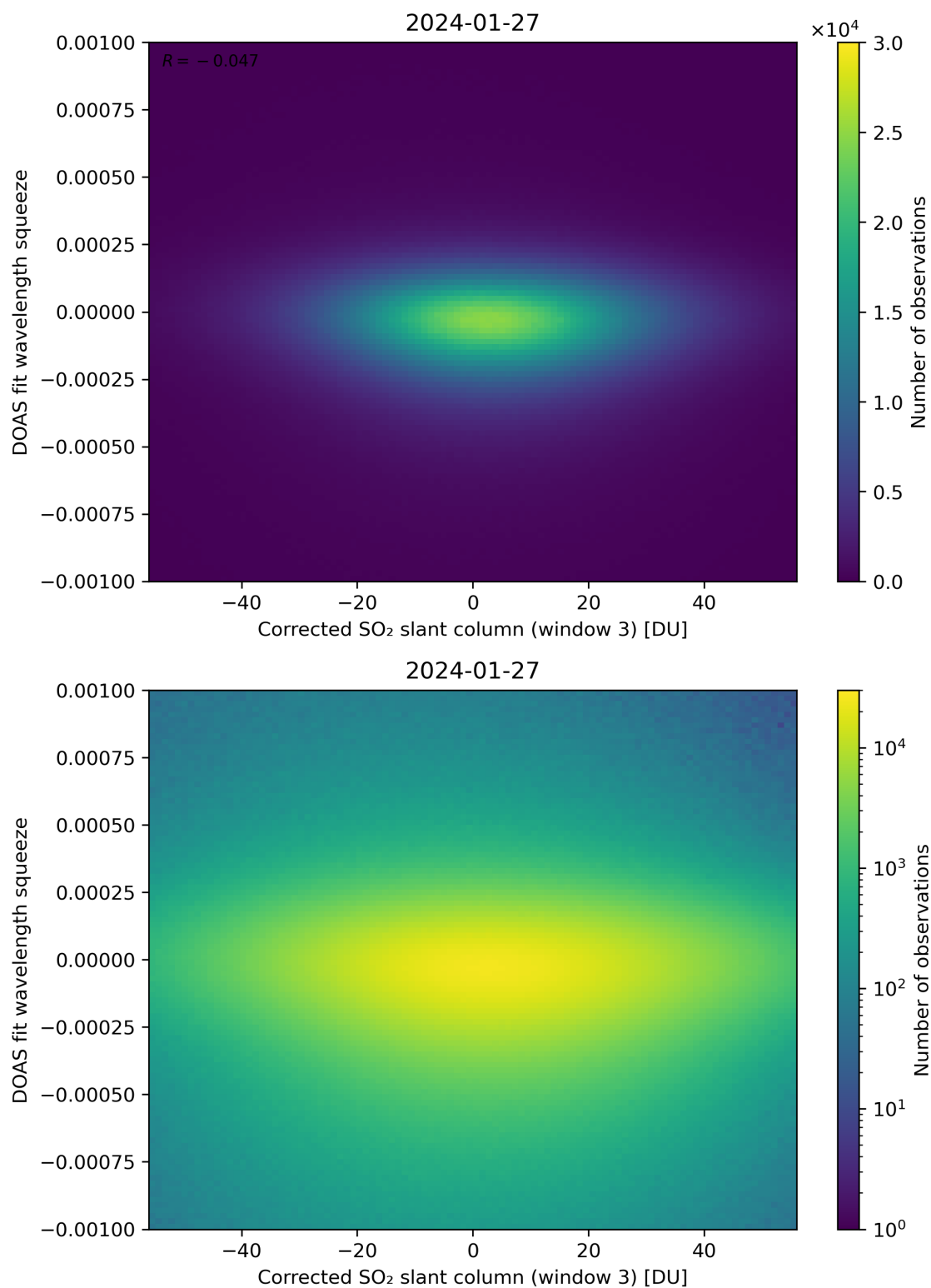
Figure 207: Scatter density plot of “Corrected SO 2 slant column (window 3)” against “DOAS fit wavelength squeeze” for 2024-01-26 to 2024-01-28.
