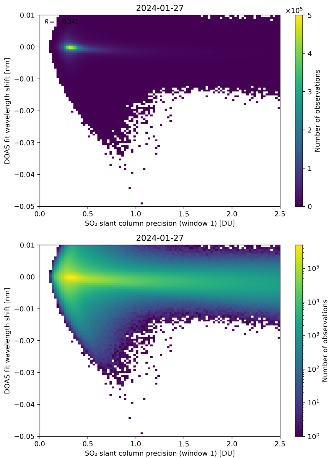
Figure 221: Scatter density plot of “SO 2 slant column precision (window 1)” against “DOAS fit wavelength shift” for 2024-01-26 to 2024-01-28.
