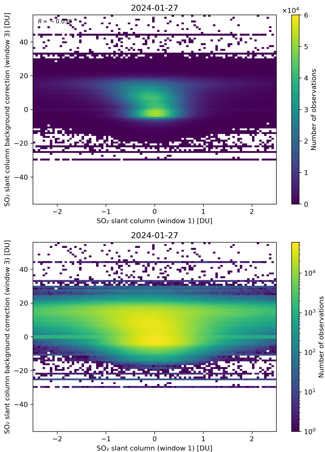
Figure 214: Scatter density plot of “SO 2 slant column (window 1)” against “SO 2 slant column background correction (window 3)” for 2024-01-26 to 2024-01-28.
