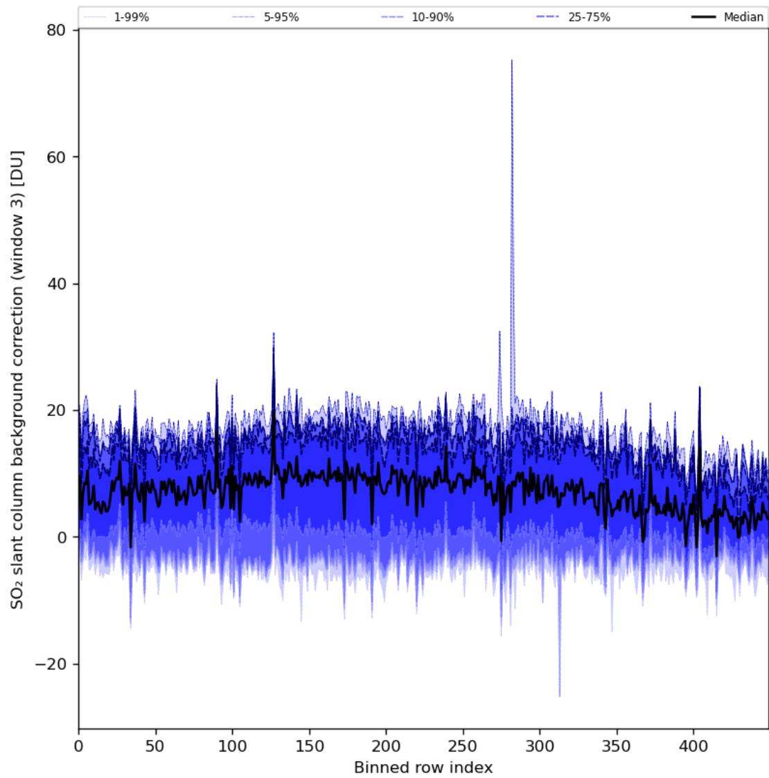
Figure 90: Along track statistics of “SO 2 slant column background correction (window 3)” for 2024-01-26 to 2024-01-28
