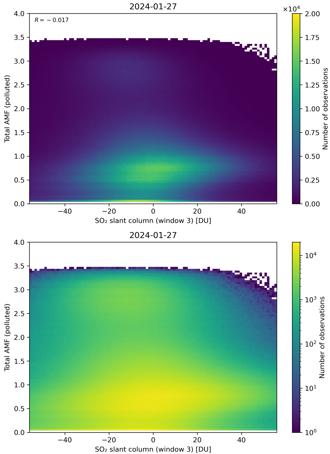
Figure 268: Scatter density plot of “SO 2 slant column (window 3)” against “Total AMF (polluted)” for 2024-01-26 to 2024-01-28.
