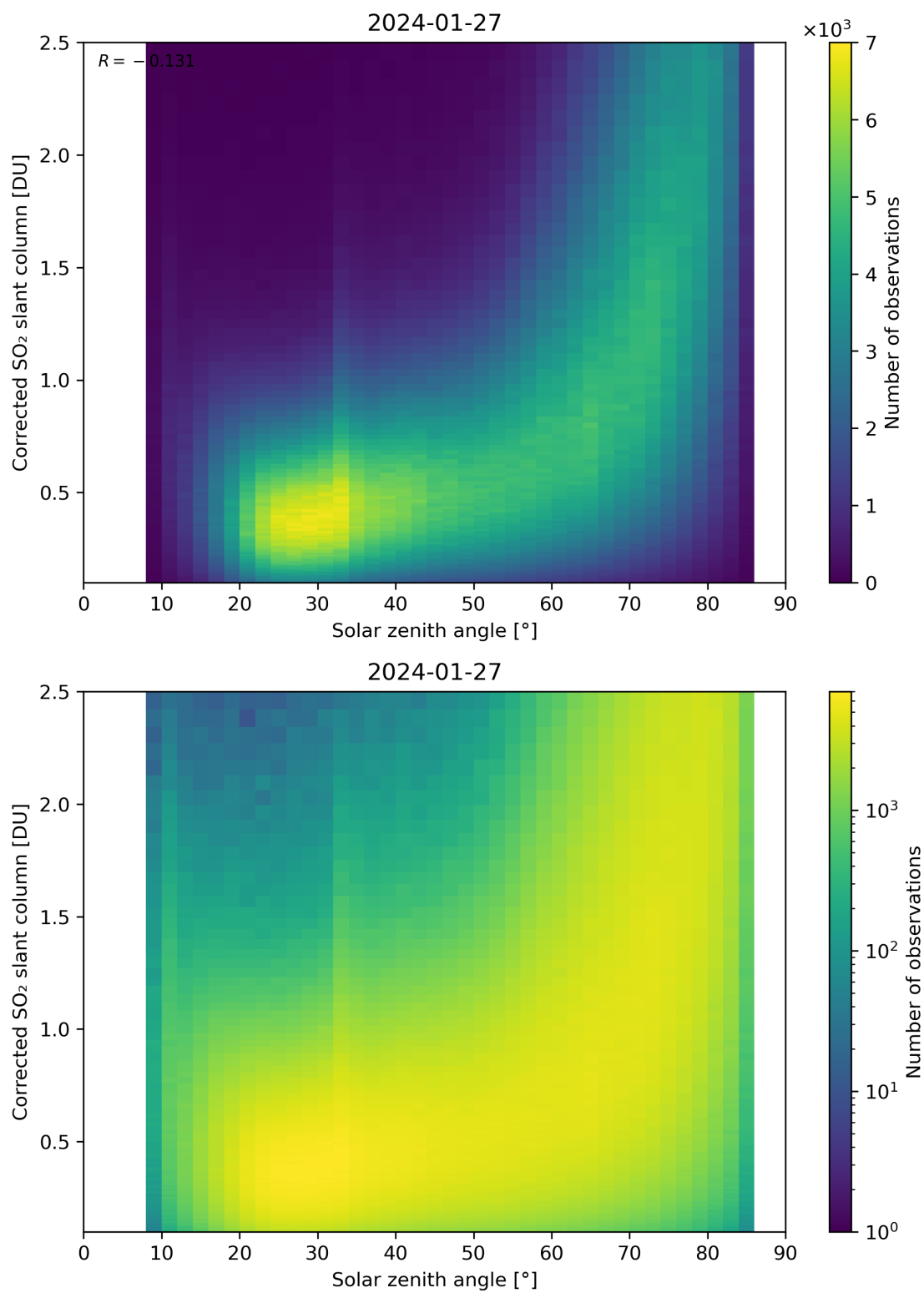
Figure 166: Scatter density plot of “Solar zenith angle” against “Corrected SO 2 slant column” for 2024-01-26 to 2024-01-28.
