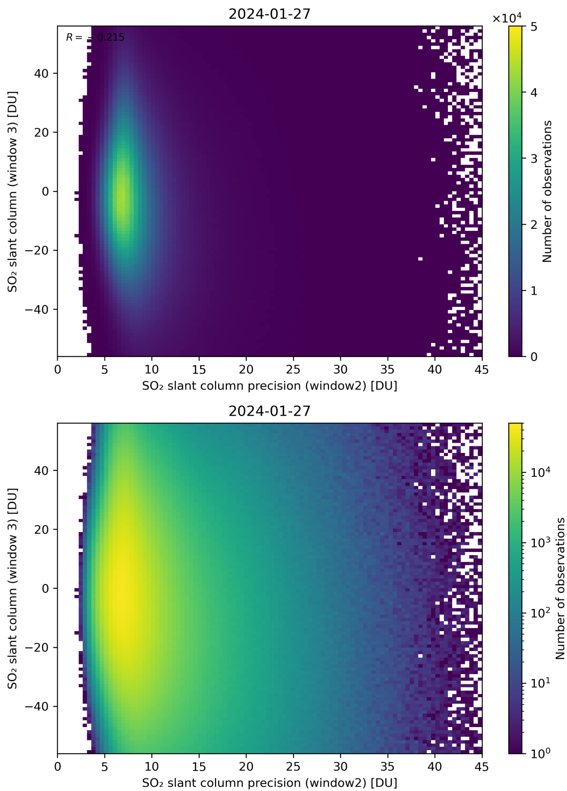
Figure 249: Scatter density plot of “SO 2 slant column precision (window2)” against “SO 2 slant column (window 3)” for 2024-01-26 to 2024-01-28.
