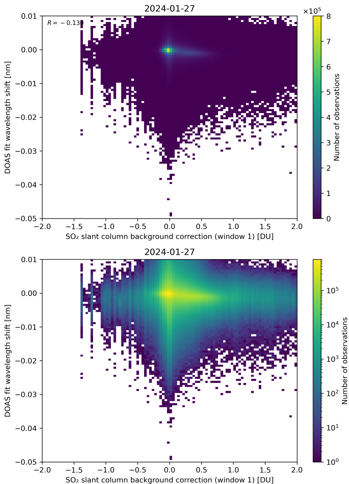
Figure 100: Scatter density plot of “SO 2 slant column background correction (window 1)” against “DOAS fit wavelength shift” for 2024-01-26 to 2024-01-28.
