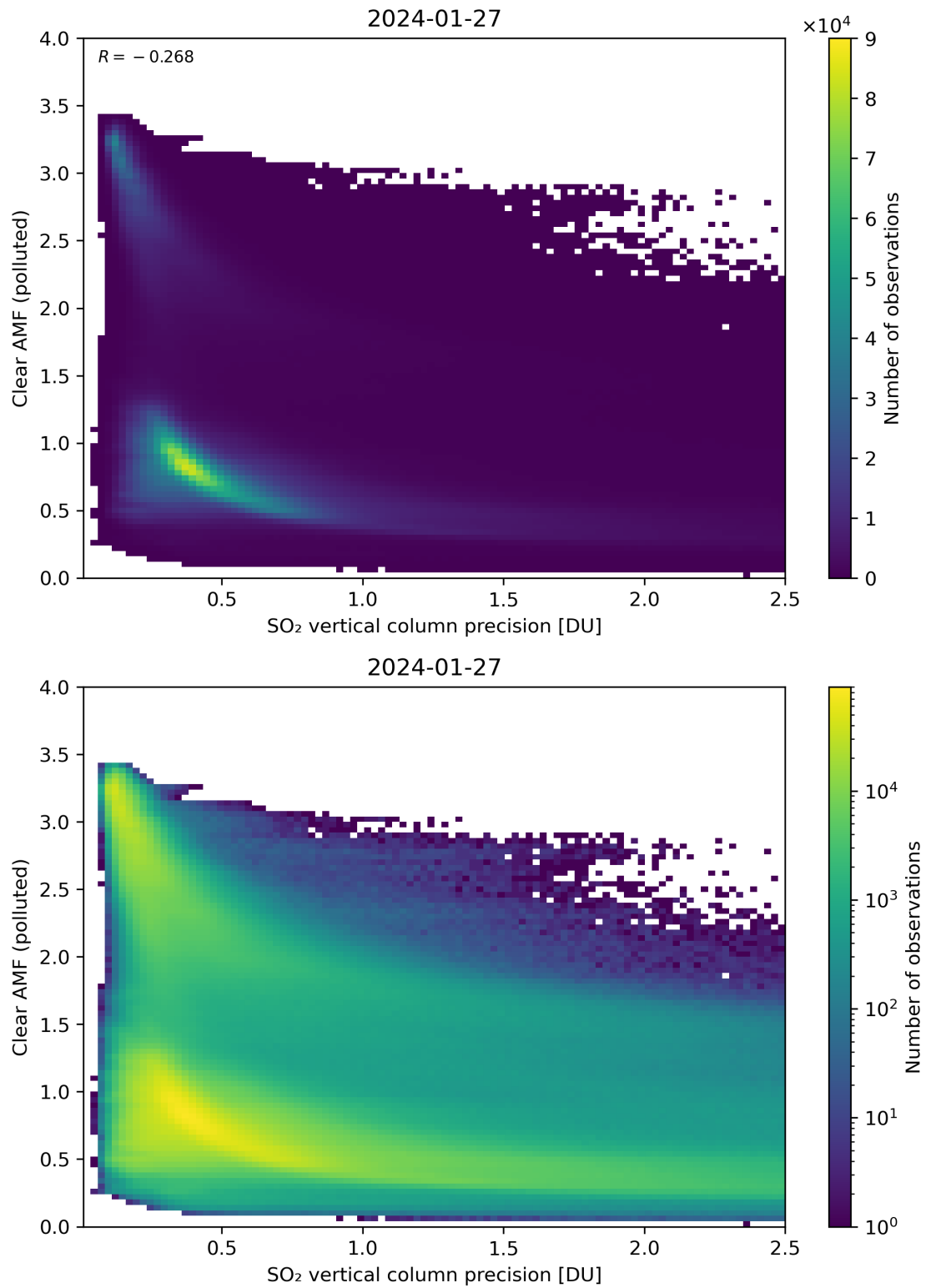
Figure 285: Scatter density plot of “SO 2 vertical column precision” against “Clear AMF (polluted)” for 2024-01-26 to 2024-01-28.
