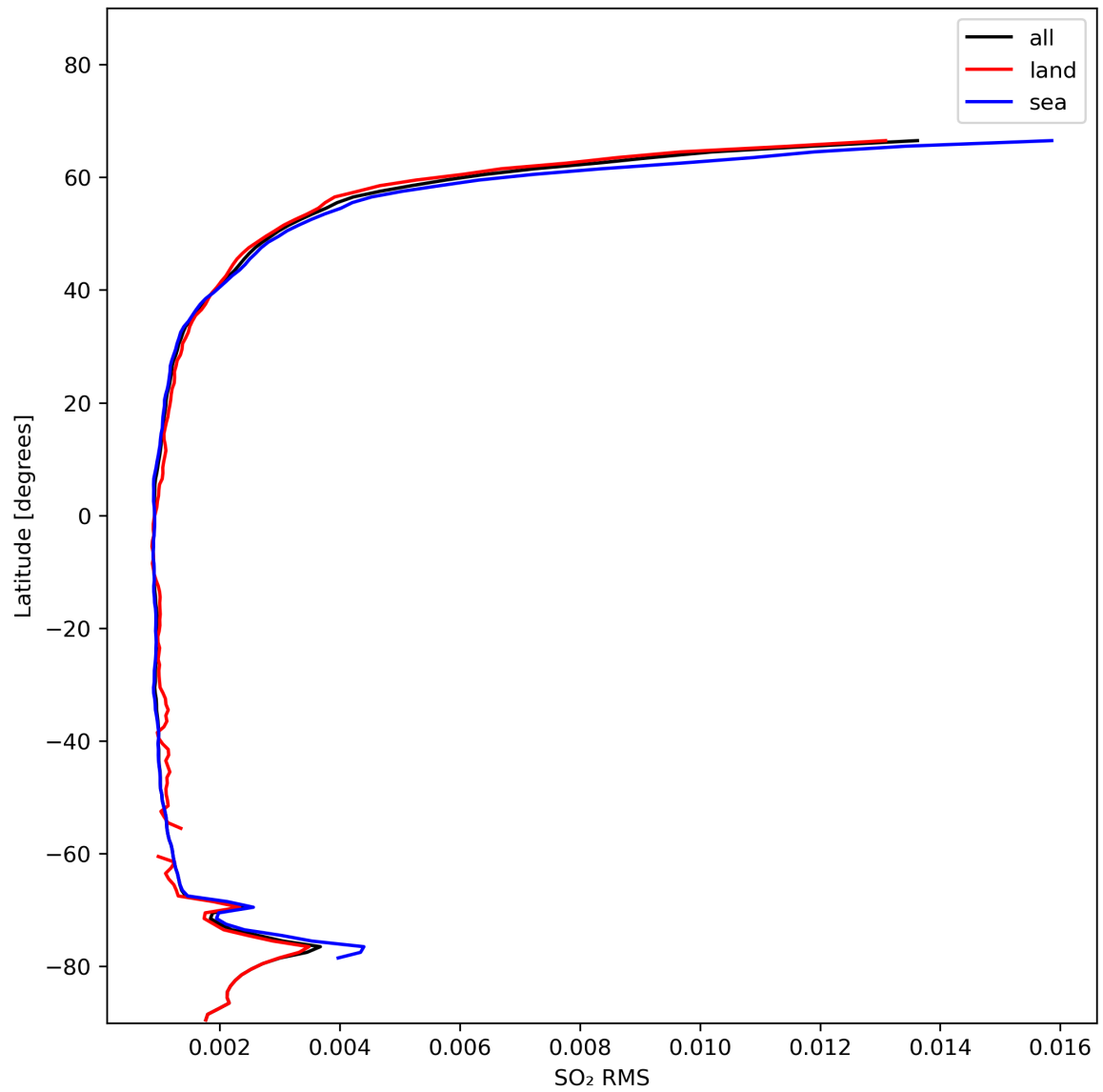
Figure 47: Zonal average of “SO 2 RMS” for 2024-01-26 to 2024-01-28.
