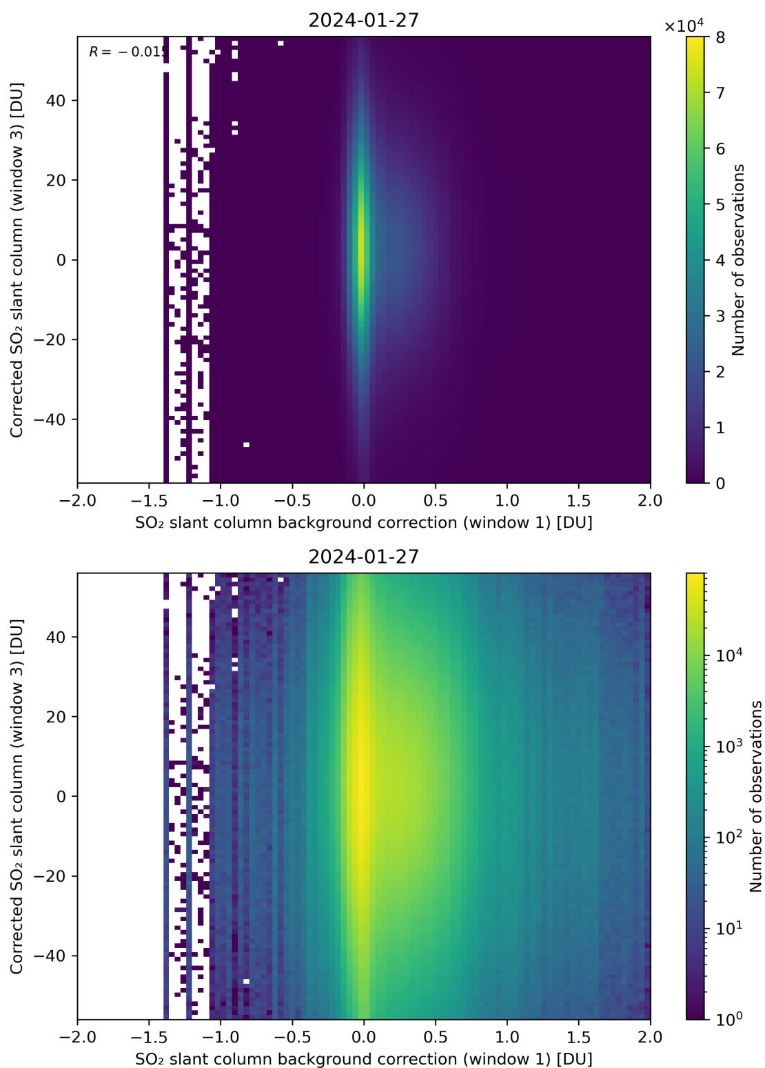
Figure 105: Scatter density plot of “SO 2 slant column background correction (window 1)” against “Corrected SO 2 slant column (window 3)” for 2024-01-26 to 2024-01-28.
