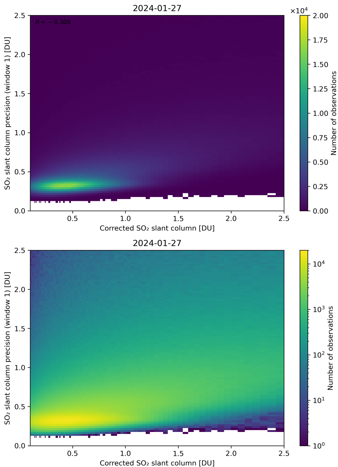
Figure 188: Scatter density plot of “Corrected SO 2 slant column” against “SO 2 slant column precision (window 1)” for 2024-01-26 to 2024-01-28.
