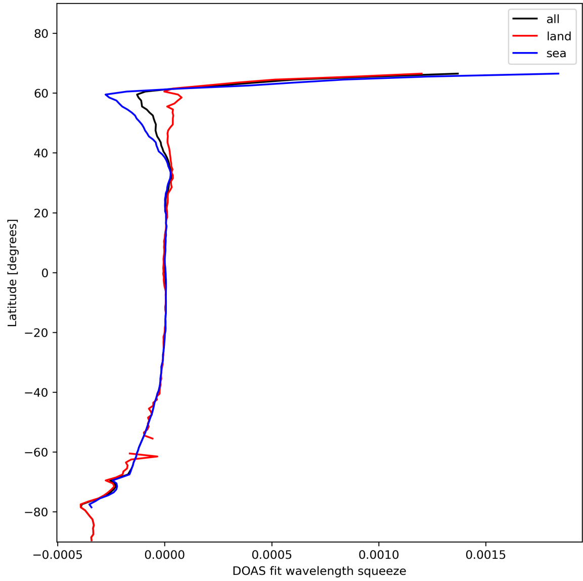
Figure 46: Zonal average of “DOAS fit wavelength squeeze” for 2024-01-26 to 2024-01-28.
