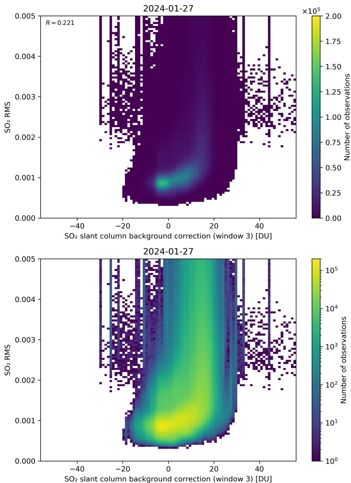
Figure 123: Scatter density plot of “SO 2 slant column background correction (window 3)” against “SO 2 RMS” for 2024-01-26 to 2024-01-28.
