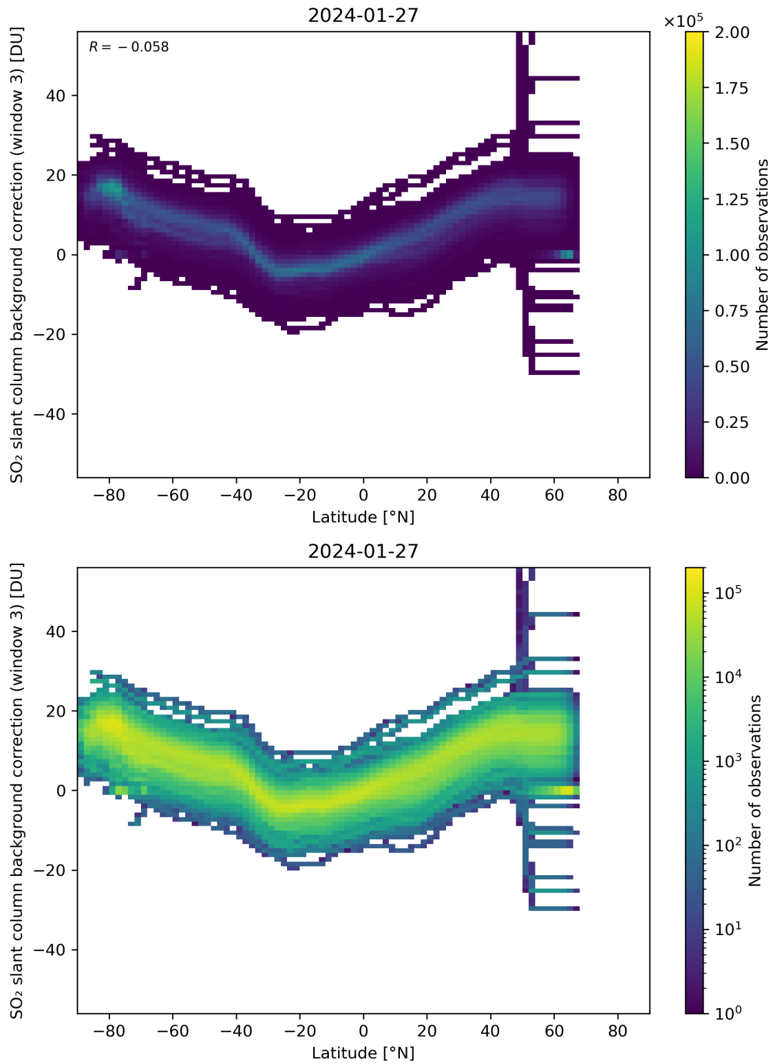
Figure 141: Scatter density plot of “Latitude” against “SO 2 slant column background correction (window 3)” for 2024-01-26 to 2024-01-28.
