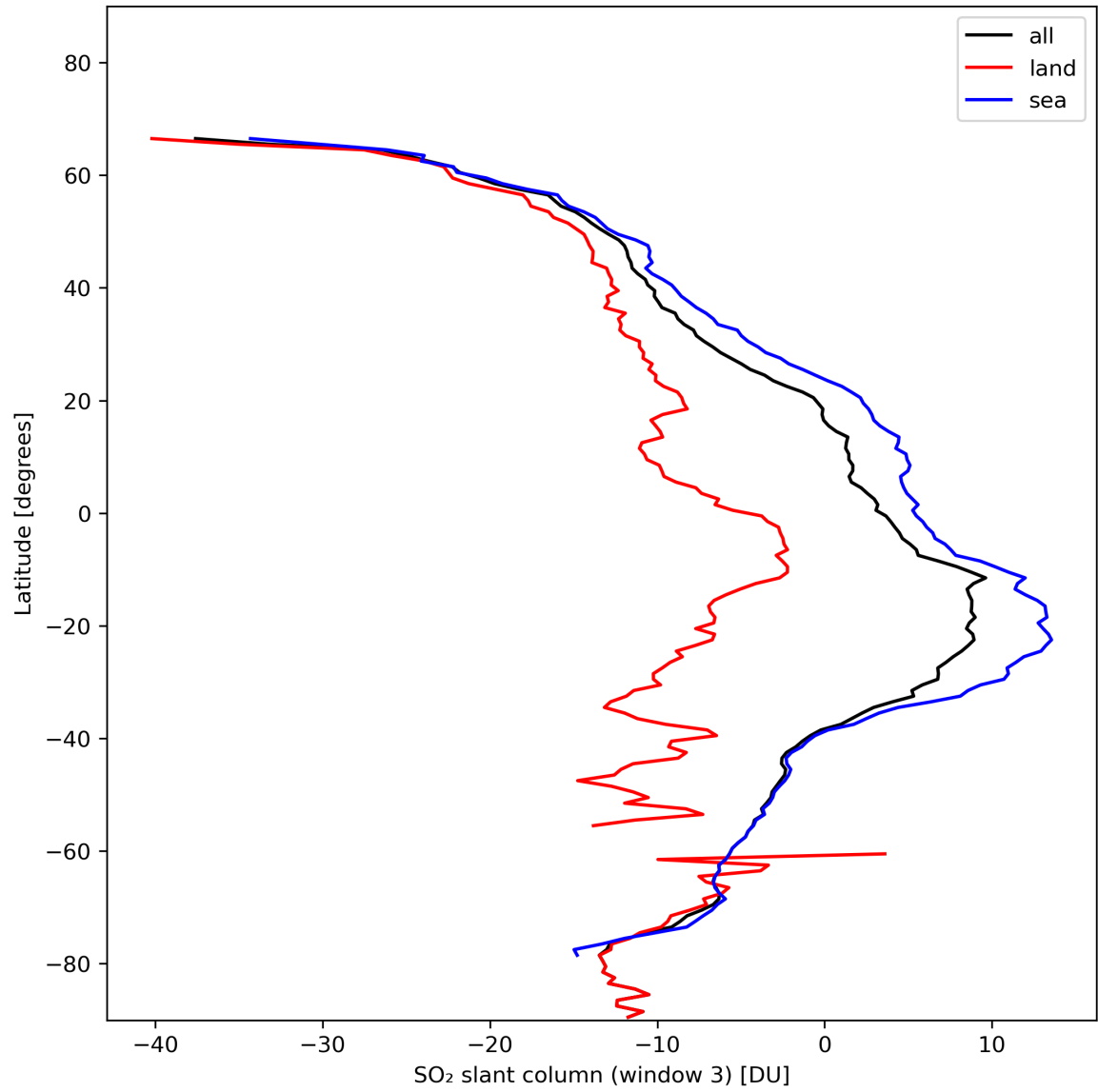
Figure 41: Zonal average of “SO 2 slant column (window 3)” for 2024-01-26 to 2024-01-28.
