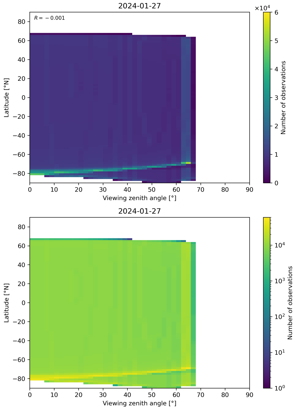
Figure 314: Scatter density plot of “Viewing zenith angle” against “Latitude” for 2024-01-26 to 2024-01-28.
