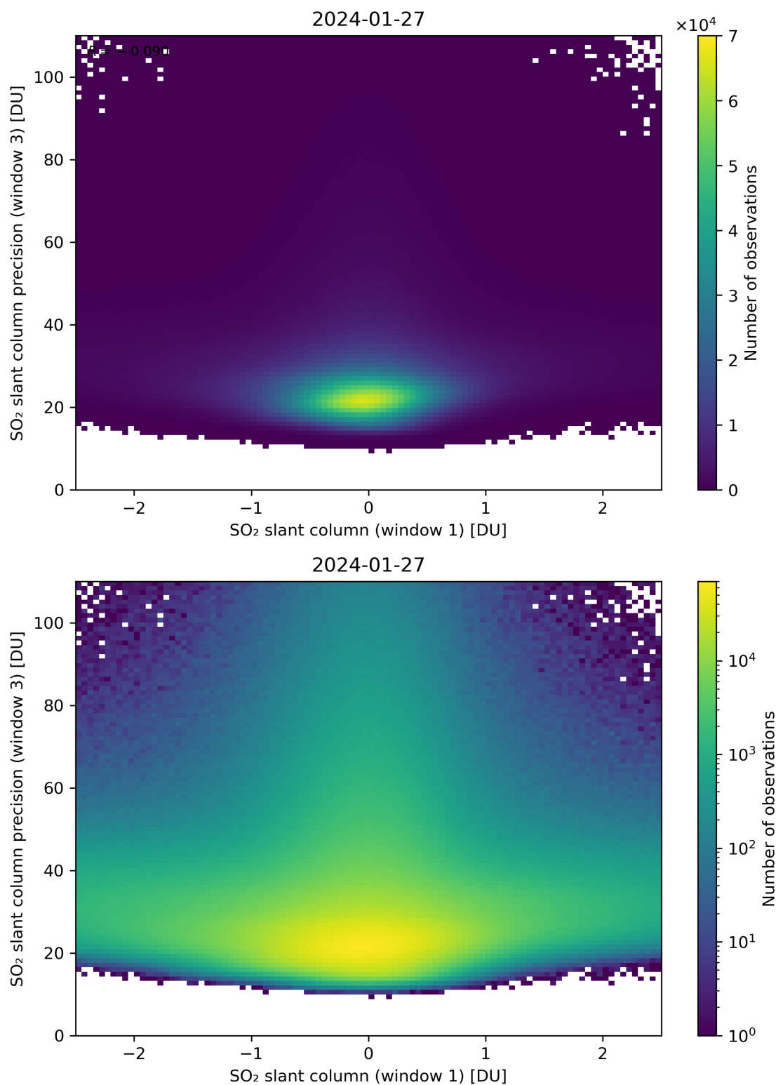
Figure 238: Scatter density plot of “SO 2 slant column (window 1)” against “SO 2 slant column precision (window 3)” for 2024-01-26 to 2024-01-28.
