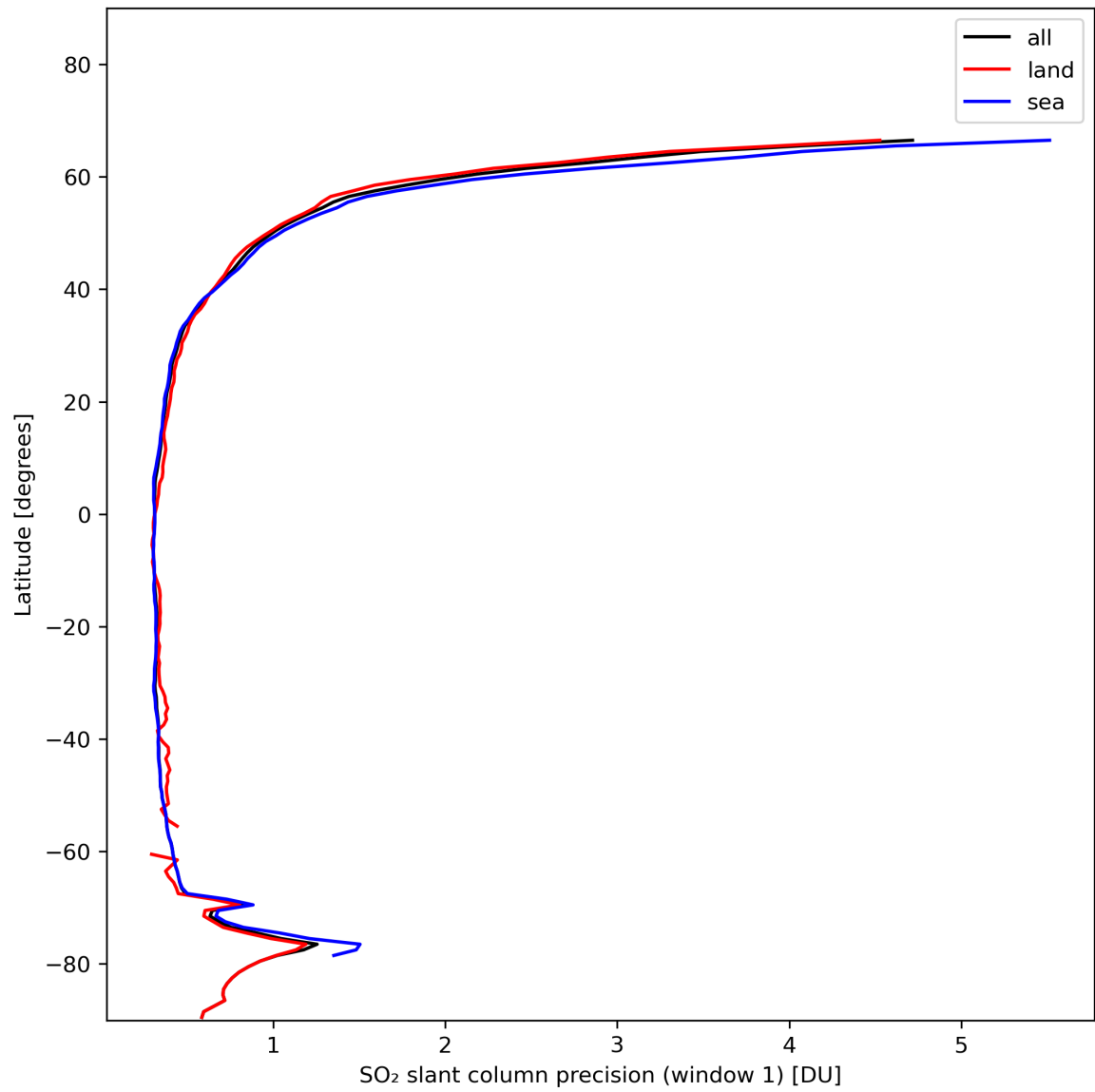
Figure 34: Zonal average of “SO 2 slant column precision (window 1)” for 2024-01-26 to 2024-01-28.
