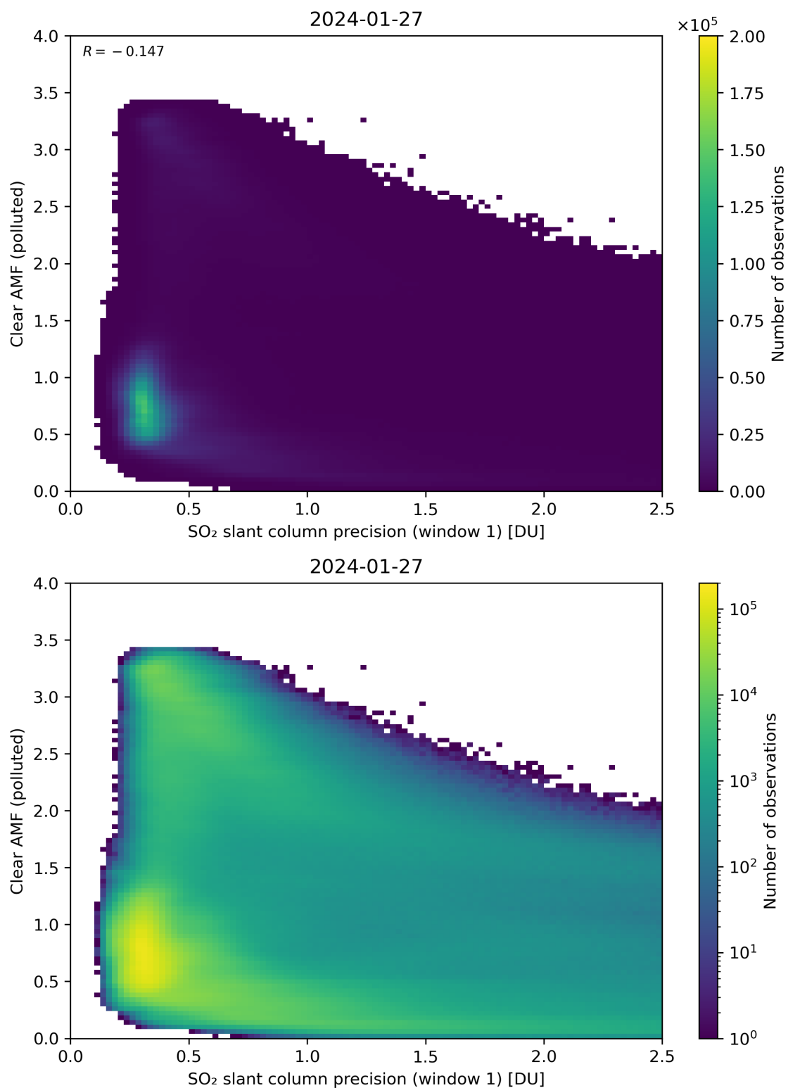
Figure 224: Scatter density plot of “SO 2 slant column precision (window 1)” against “Clear AMF (polluted)” for 2024-01-26 to 2024-01-28.
