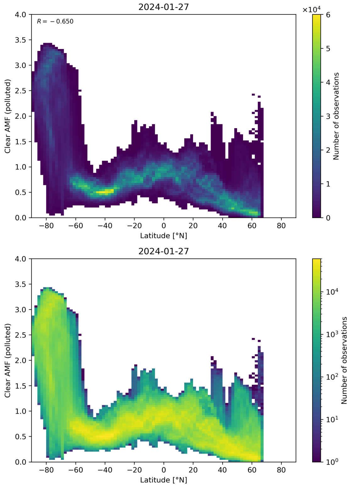
Figure 145: Scatter density plot of “Latitude” against “Clear AMF (polluted)” for 2024-01-26 to 2024-01-28.
