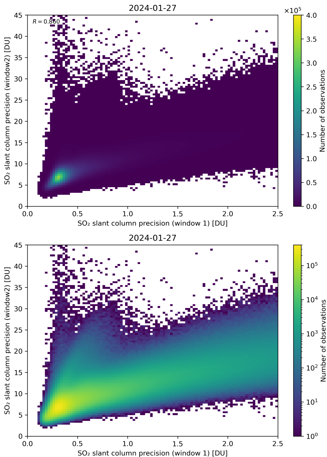
Figure 227: Scatter density plot of “SO 2 slant column precision (window 1)” against “SO 2 slant column precision (window2)” for 2024-01-26 to 2024-01-28.
