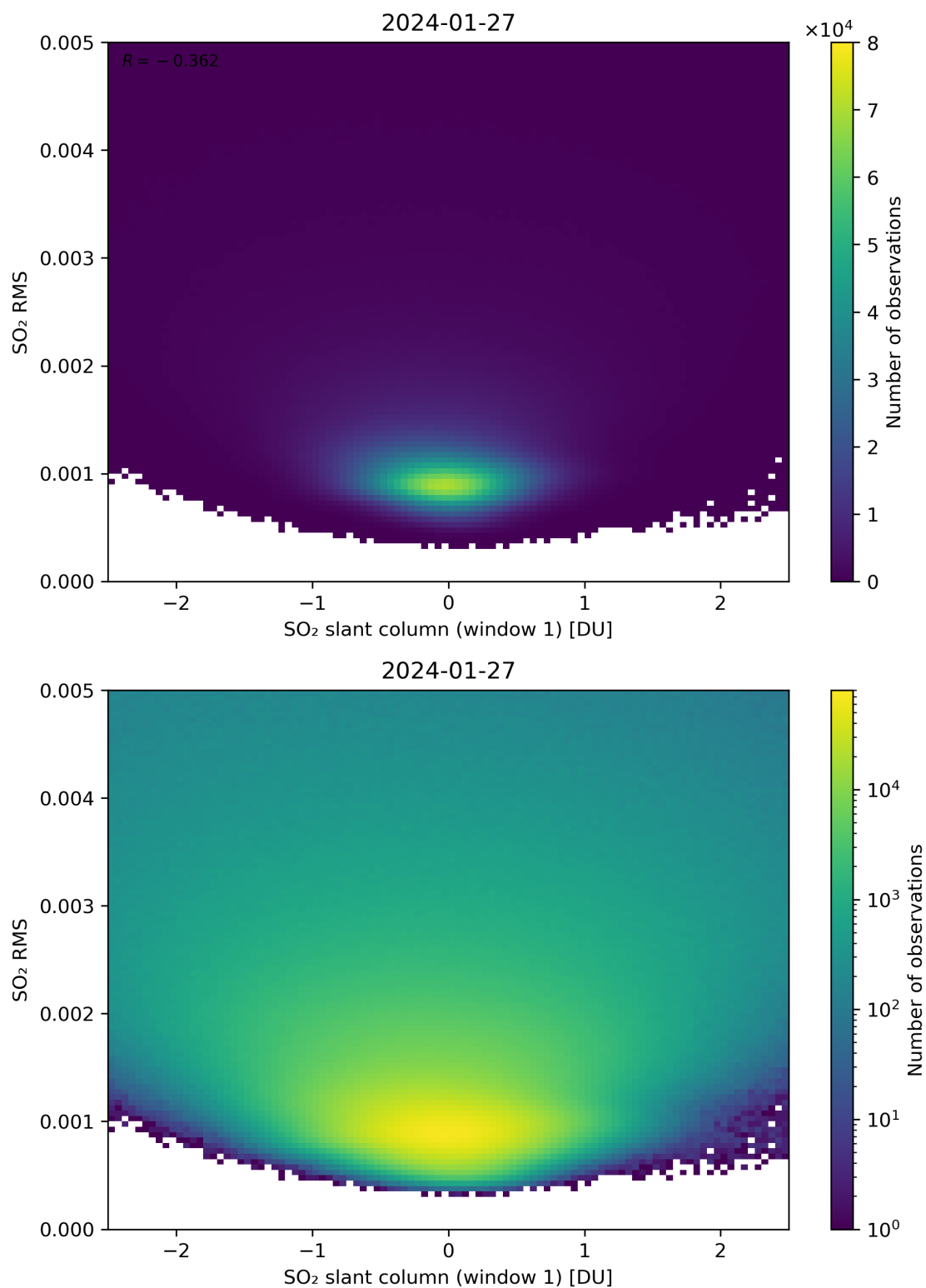
Figure 217: Scatter density plot of “SO 2 slant column (window 1)” against “SO 2 RMS” for 2024-01-26 to 2024-01-28.
