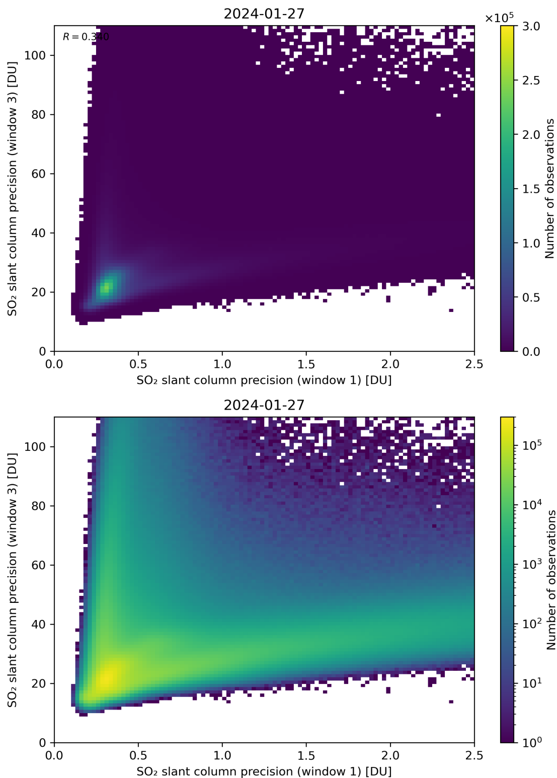
Figure 229: Scatter density plot of “SO 2 slant column precision (window 1)” against “SO 2 slant column precision (window 3)” for 2024-01-26 to 2024-01-28.
