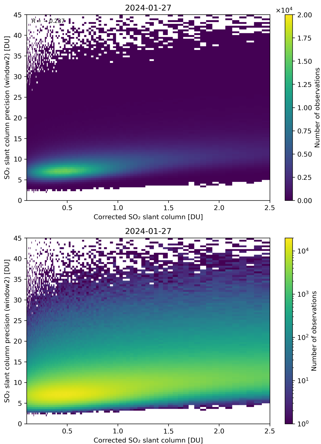
Figure 189: Scatter density plot of “Corrected SO 2 slant column” against “SO 2 slant column precision (window2)” for 2024-01-26 to 2024-01-28.
