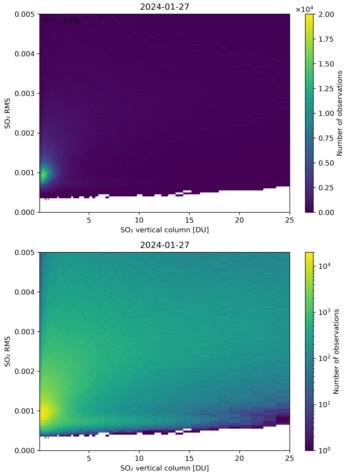
Figure 278: Scatter density plot of “SO 2 vertical column” against “SO 2 RMS” for 2024-01-26 to 2024-01-28.
