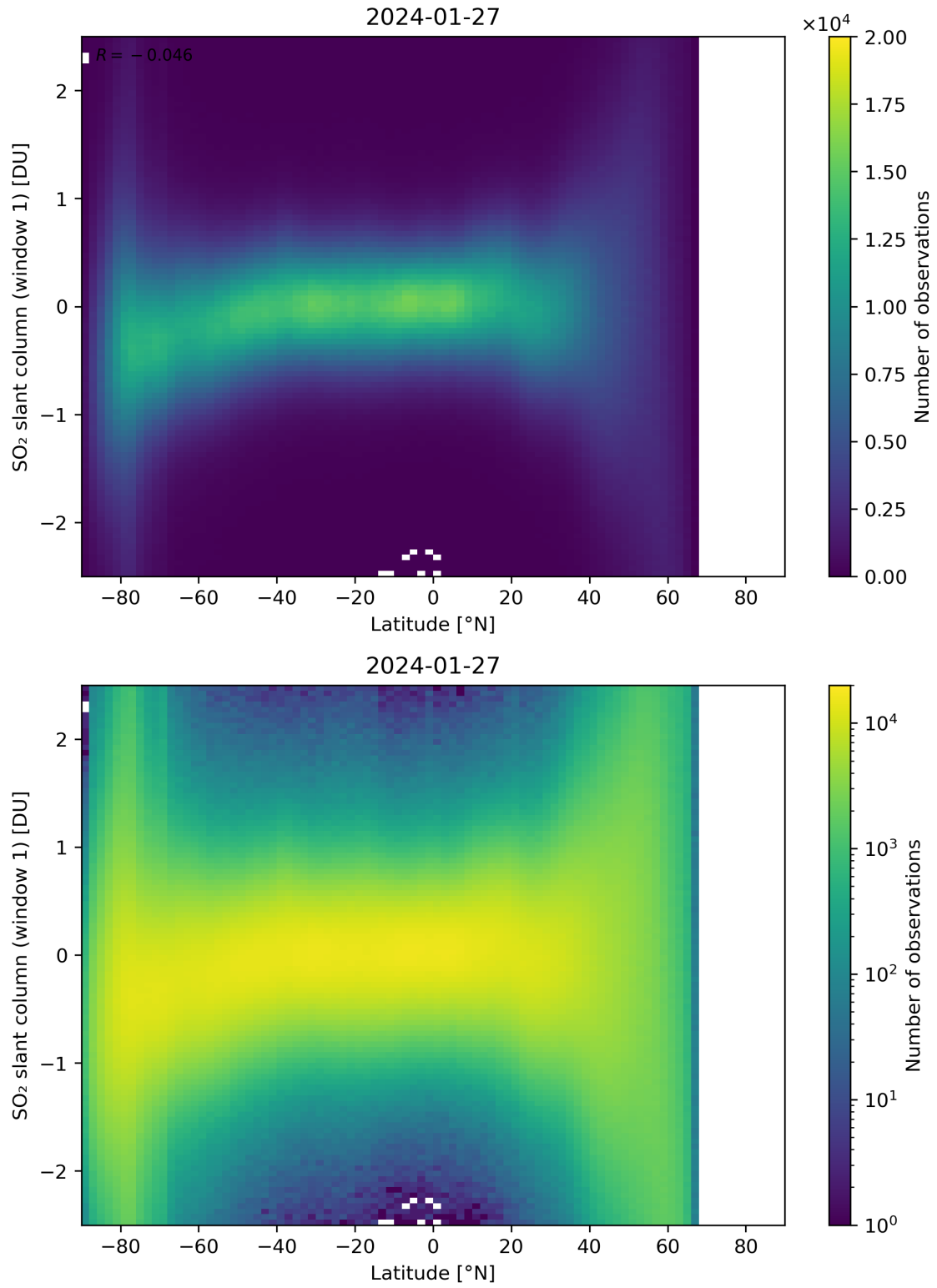
Figure 149: Scatter density plot of “Latitude” against “SO 2 slant column (window 1)” for 2024-01-26 to 2024-01-28.
