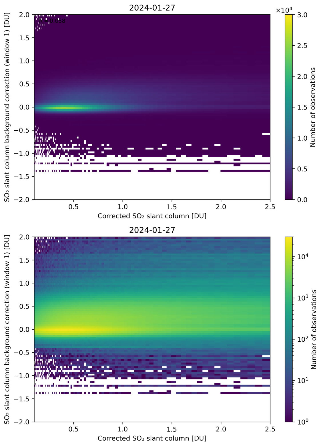
Figure 178: Scatter density plot of “Corrected SO 2 slant column” against “SO 2 slant column background correction (window 1)” for 2024-01-26 to 2024-01-28.
