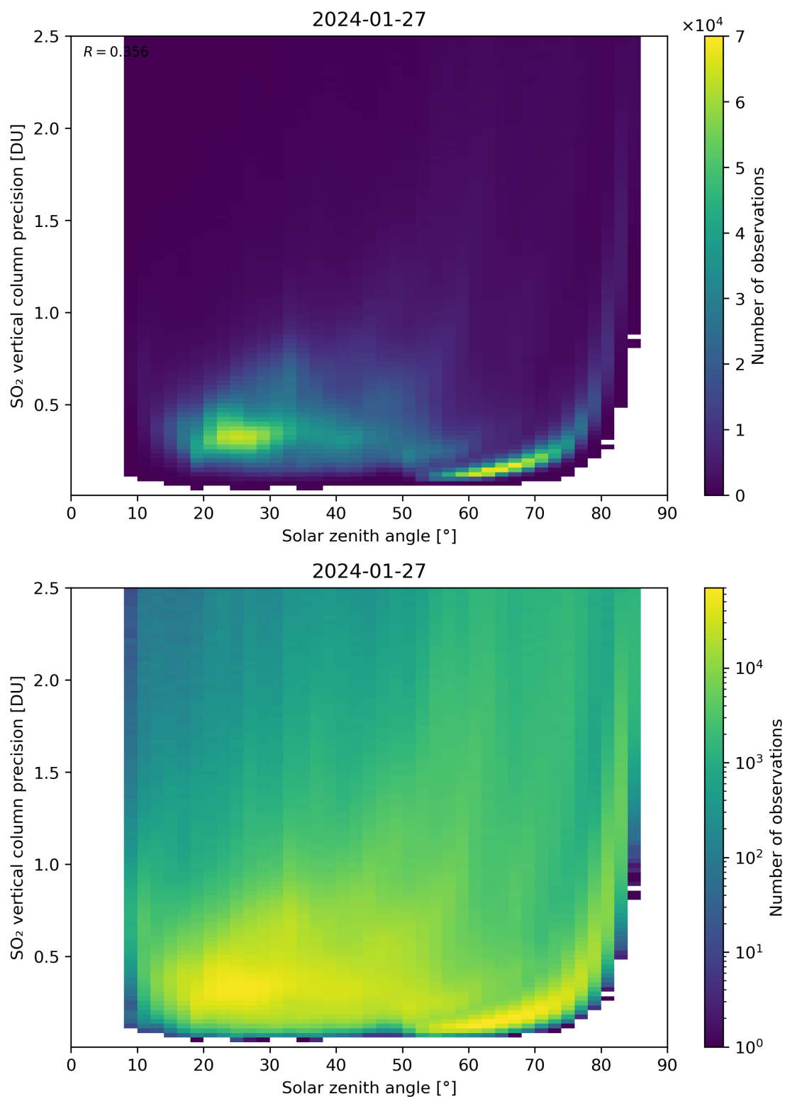
Figure 177: Scatter density plot of “Solar zenith angle” against “SO 2 vertical column precision” for 2024-01-26 to 2024-01-28.
