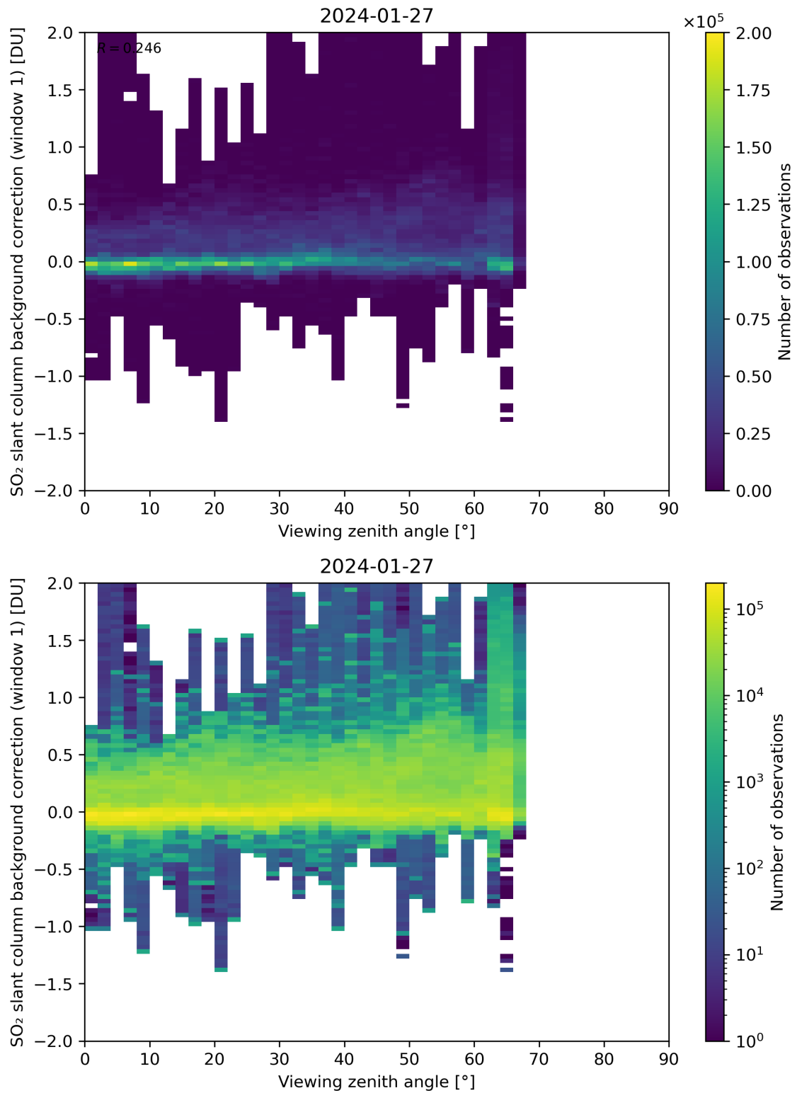
Figure 308: Scatter density plot of “Viewing zenith angle” against “SO 2 slant column background correction (window 1)” for 2024-01-26 to 2024-01-28.
