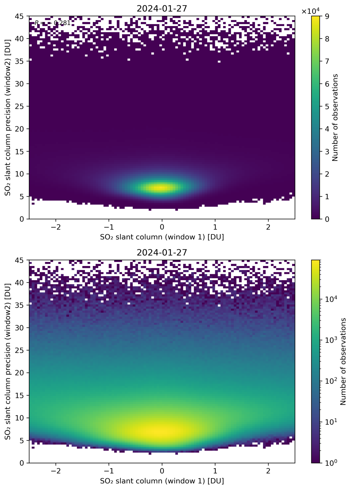
Figure 236: Scatter density plot of “SO 2 slant column (window 1)” against “SO 2 slant column precision (window2)” for 2024-01-26 to 2024-01-28.
