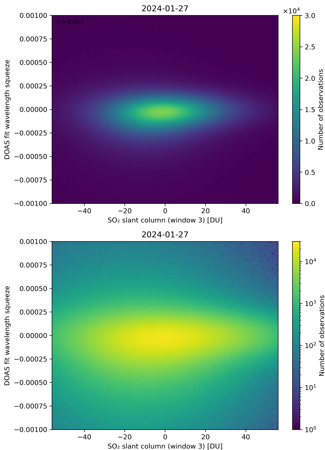
Figure 255: Scatter density plot of “SO 2 slant column (window 3)” against “DOAS fit wavelength squeeze” for 2024-01-26 to 2024-01-28.
