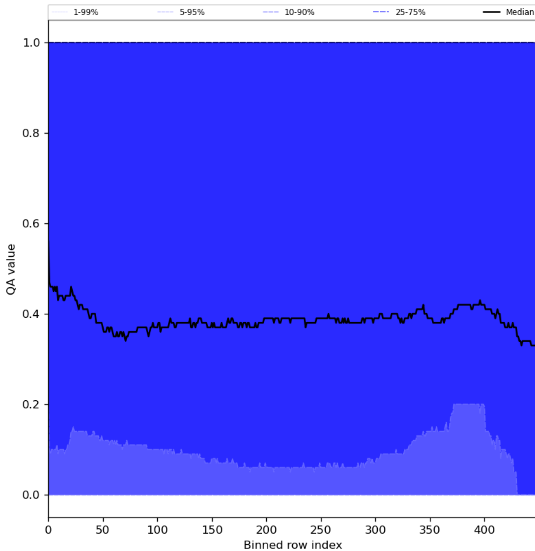
Figure 75: Along track statistics of “QA value” for 2024-01-26 to 2024-01-28
