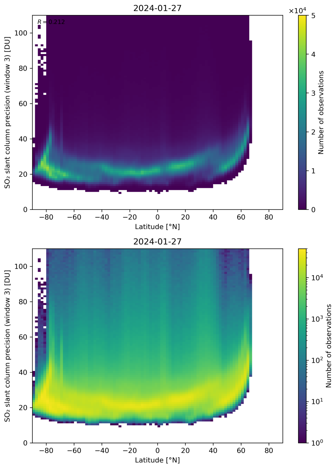
Figure 153: Scatter density plot of “Latitude” against “SO 2 slant column precision (window 3)” for 2024-01-26 to 2024-01-28.
