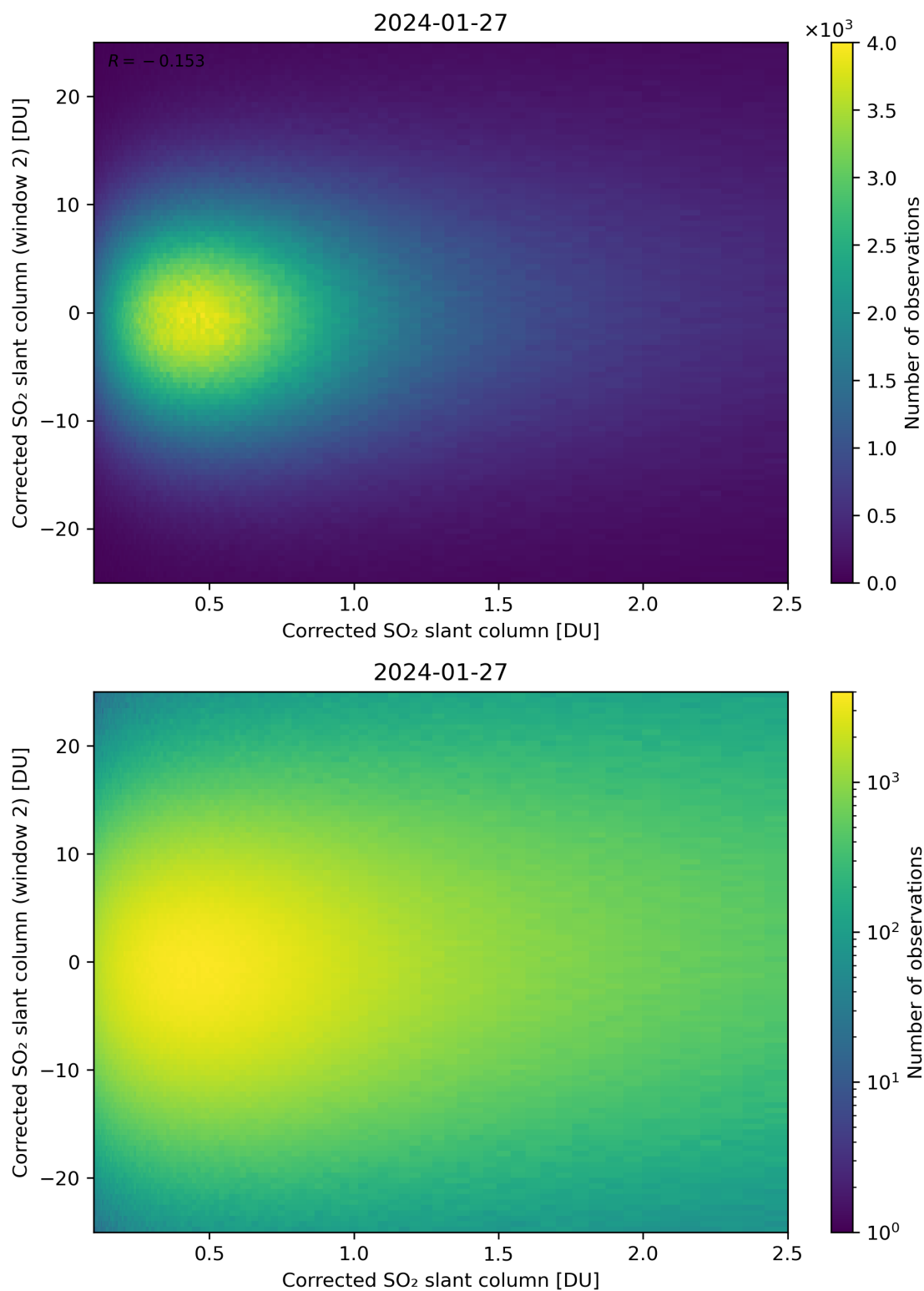
Figure 185: Scatter density plot of “Corrected SO 2 slant column” against “Corrected SO 2 slant column (window 2)” for 2024-01-26 to 2024-01-28.
