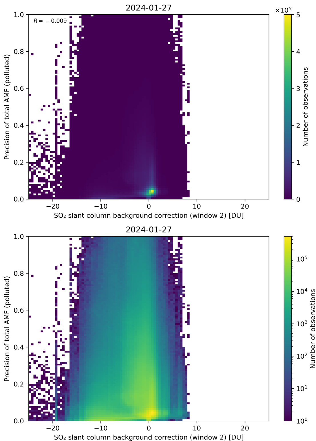
Figure 120: Scatter density plot of “SO 2 slant column background correction (window 2)” against “Precision of total AMF (polluted)” for 2024-01-26 to 2024-01-28.
