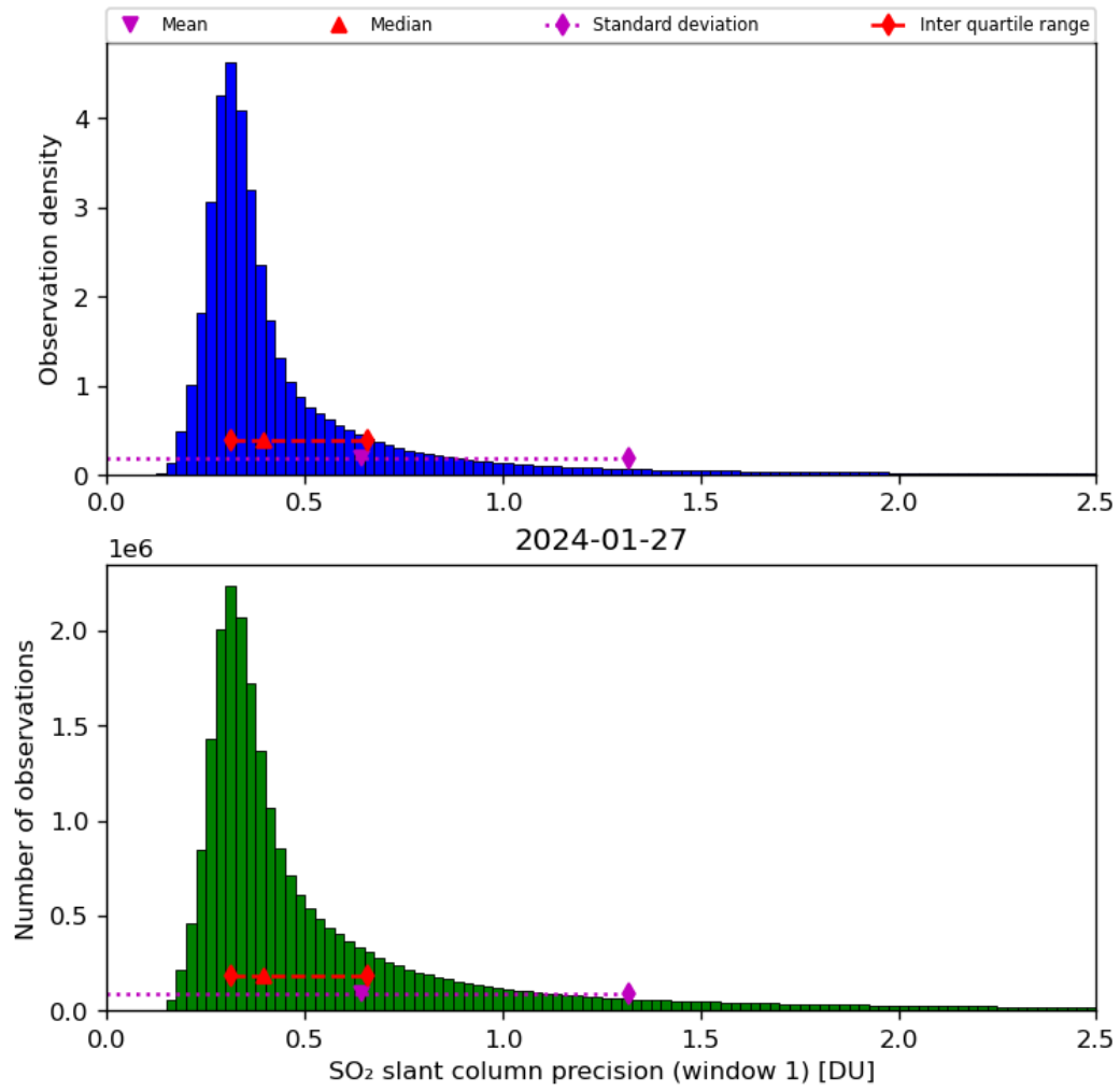
Figure 57: Histogram of “SO 2 slant column precision (window 1)” for 2024-01-26 to 2024-01-28
