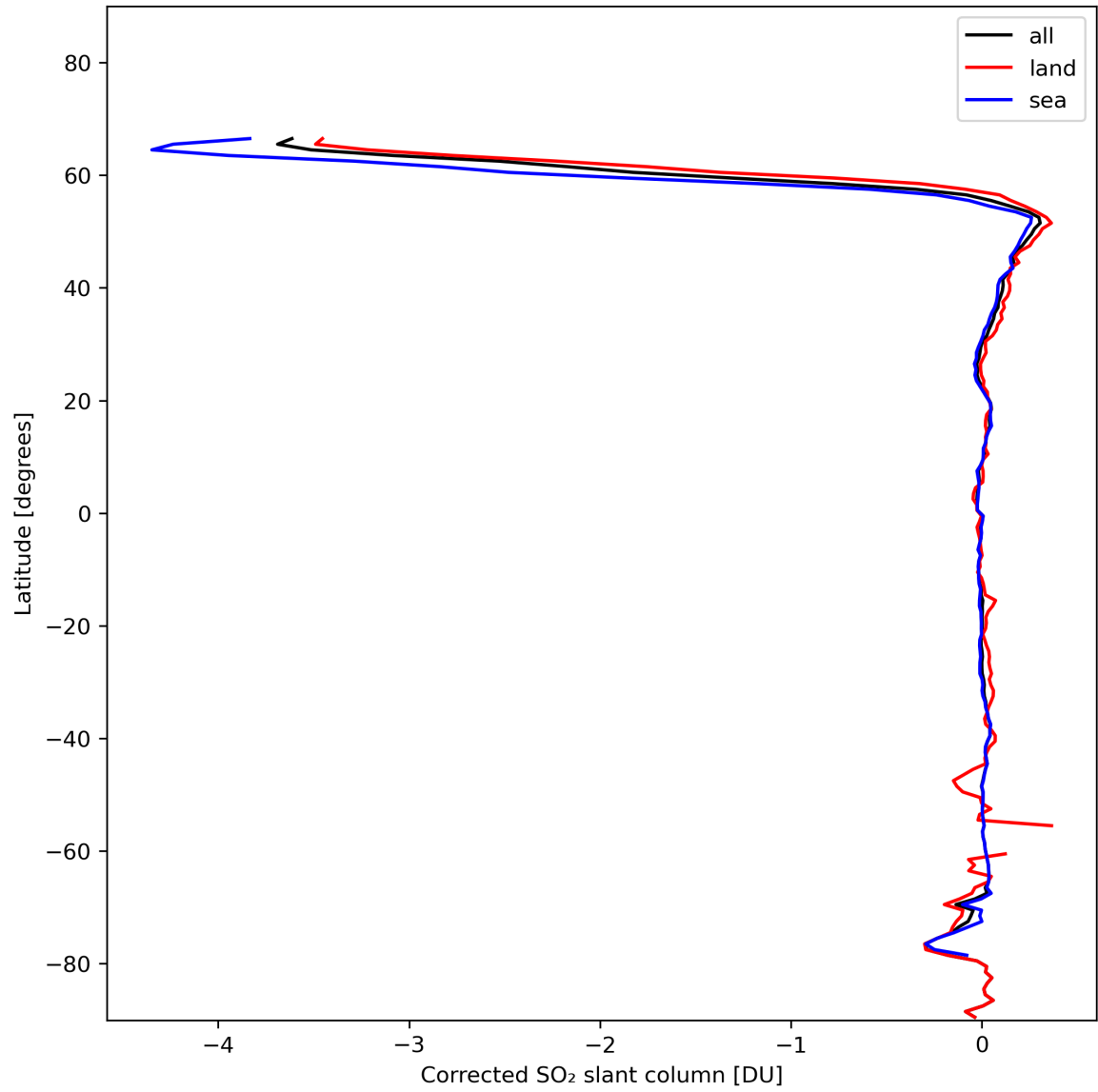
Figure 32: Zonal average of “Corrected SO 2 slant column” for 2024-01-26 to 2024-01-28.
