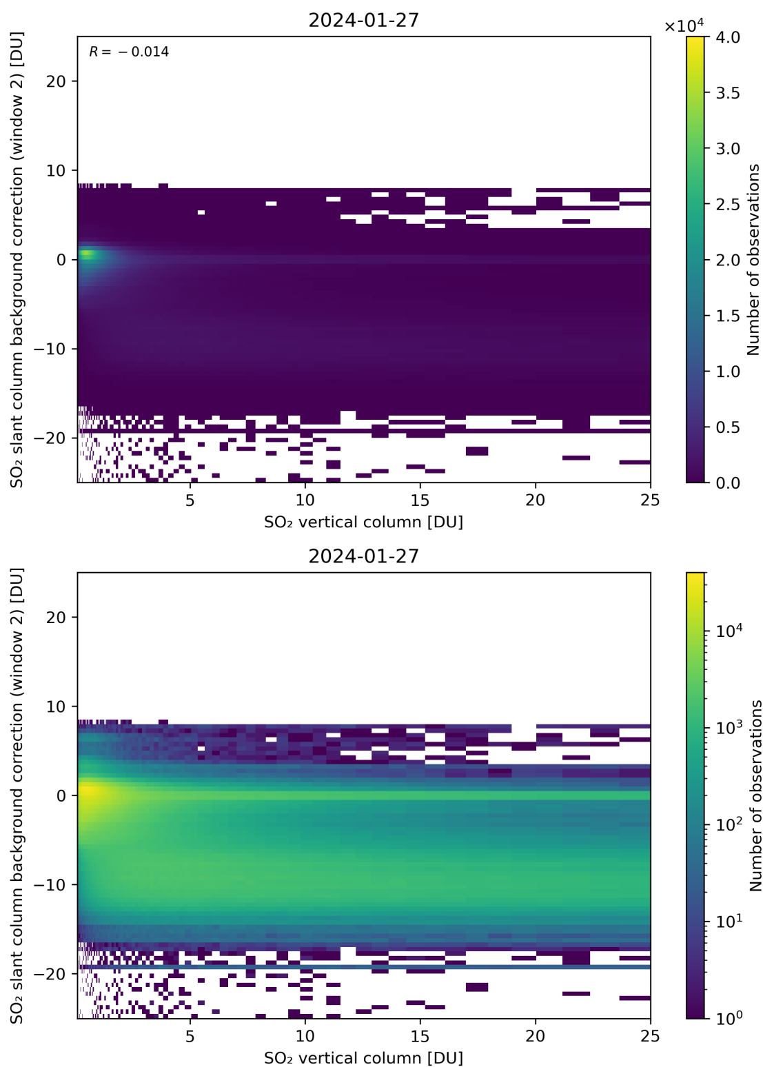
Figure 274: Scatter density plot of “SO 2 vertical column” against “SO 2 slant column background correction (window 2)” for 2024-01-26 to 2024-01-28.
