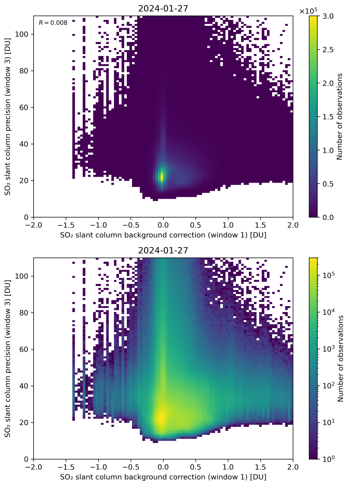
Figure 108: Scatter density plot of “SO 2 slant column background correction (window 1)” against “SO 2 slant column precision (window 3)” for 2024-01-26 to 2024-01-28.
