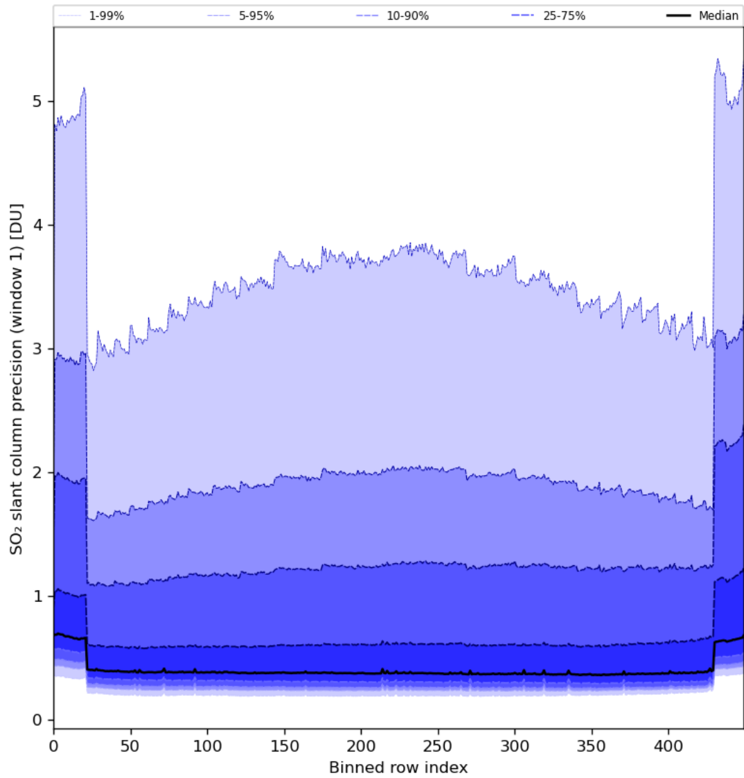
Figure 80: Along track statistics of “SO 2 slant column precision (window 1)” for 2024-01-26 to 2024-01-28
