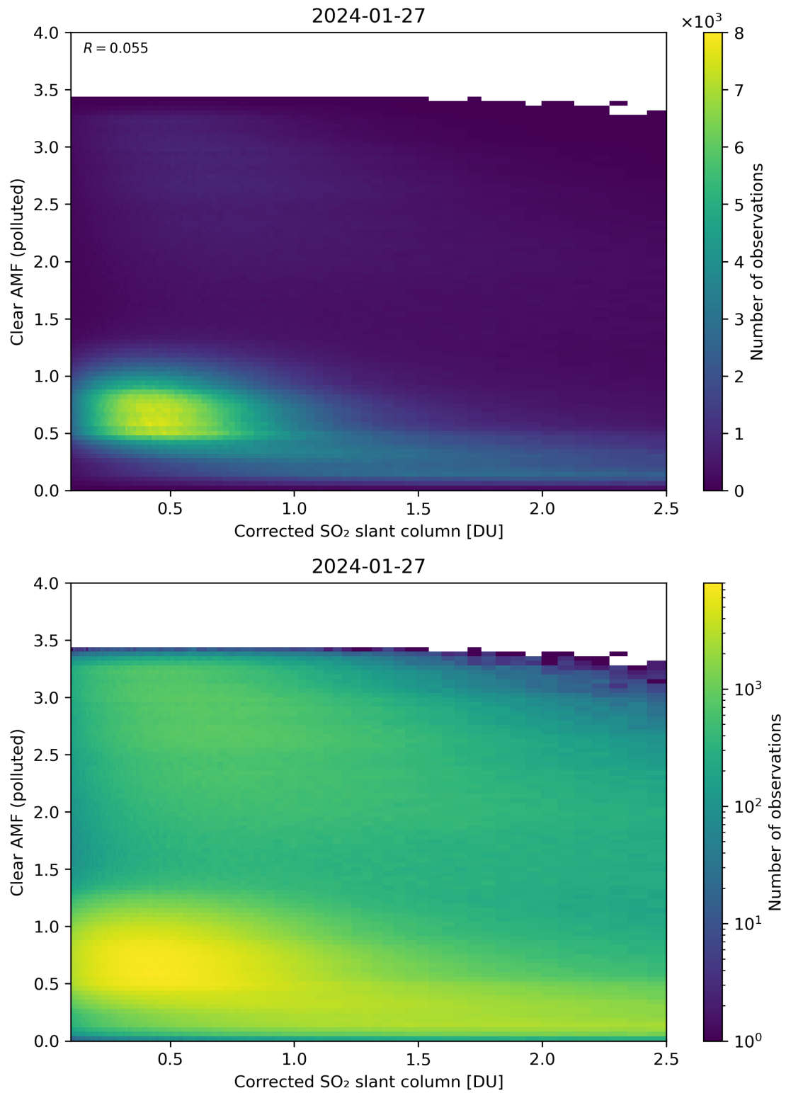
Figure 184: Scatter density plot of “Corrected SO 2 slant column” against “Clear AMF (polluted)” for 2024-01-26 to 2024-01-28.
