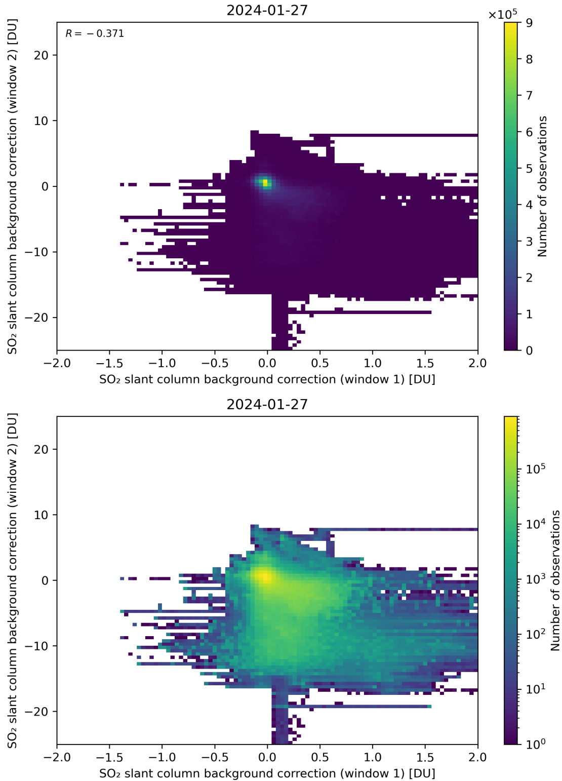
Figure 98: Scatter density plot of “SO 2 slant column background correction (window 1)” against “SO 2 slant column background correction (window 2)” for 2024-01-26 to 2024-01-28.
