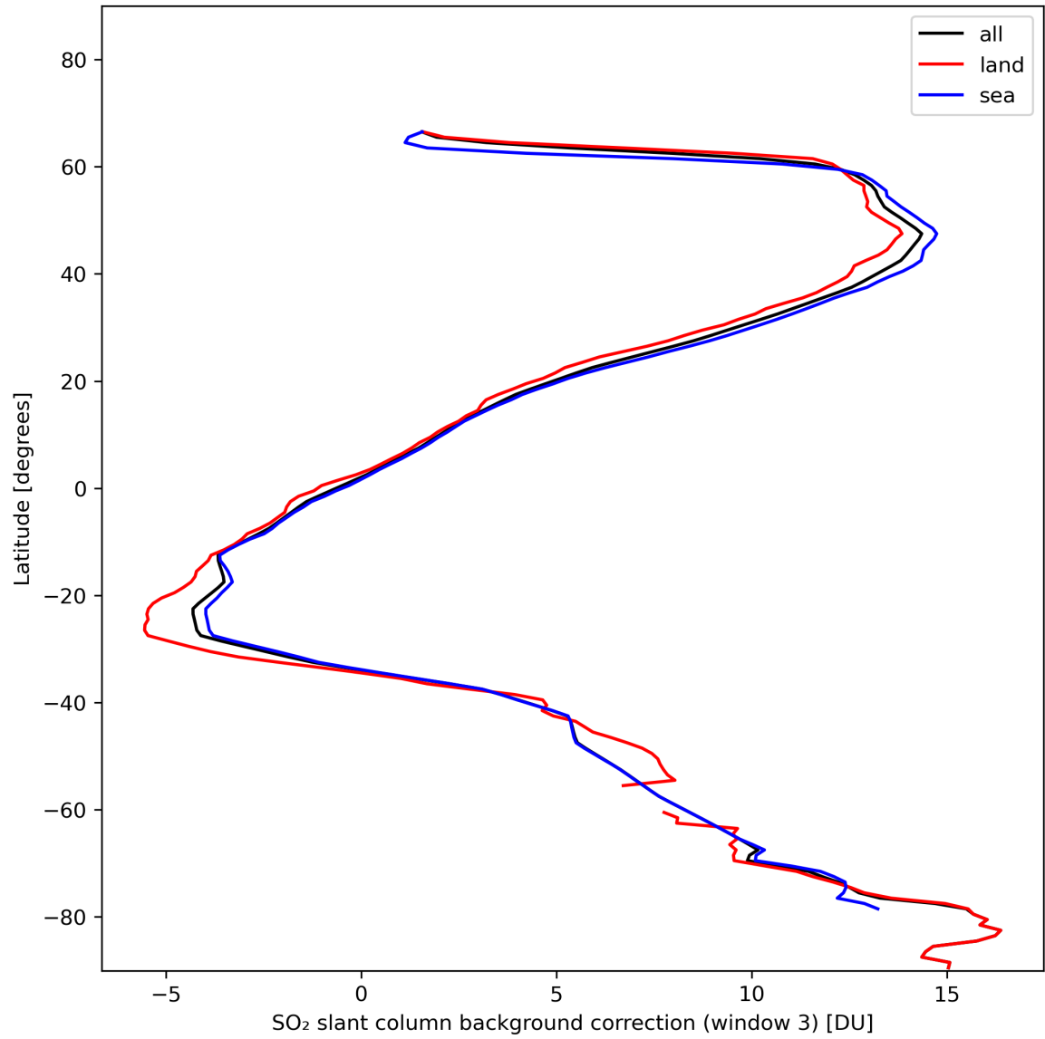
Figure 44: Zonal average of “SO 2 slant column background correction (window 3)” for 2024-01-26 to 2024-01-28.
