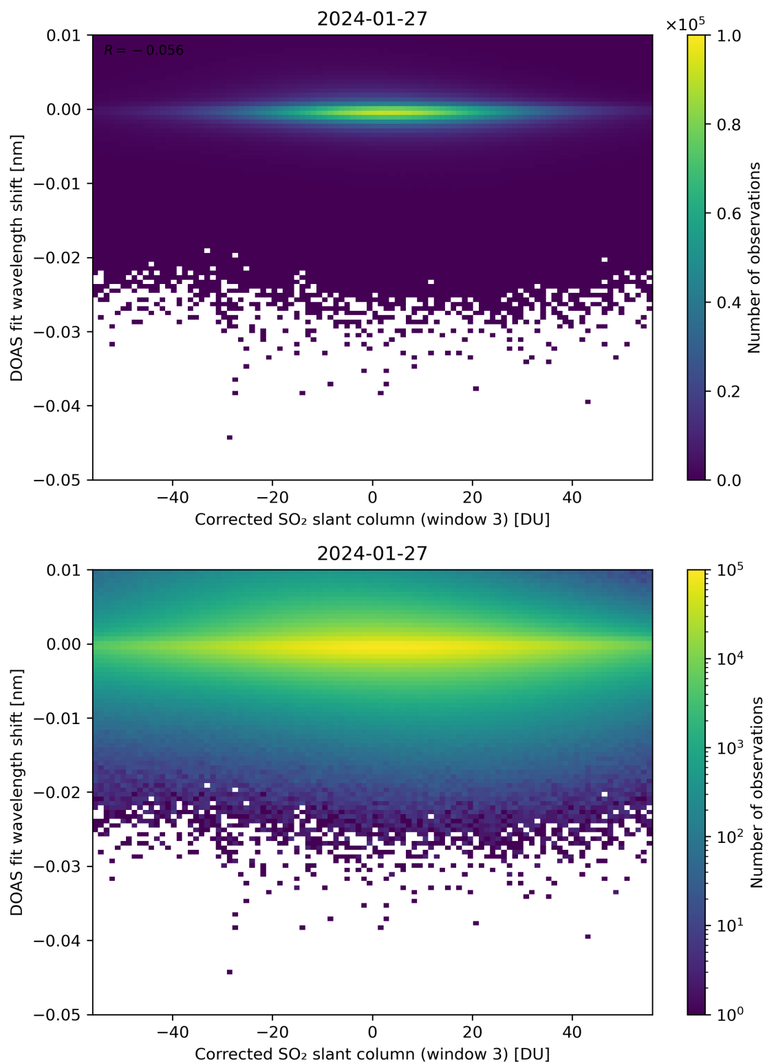
Figure 206: Scatter density plot of “Corrected SO 2 slant column (window 3)” against “DOAS fit wavelength shift” for 2024-01-26 to 2024-01-28.
