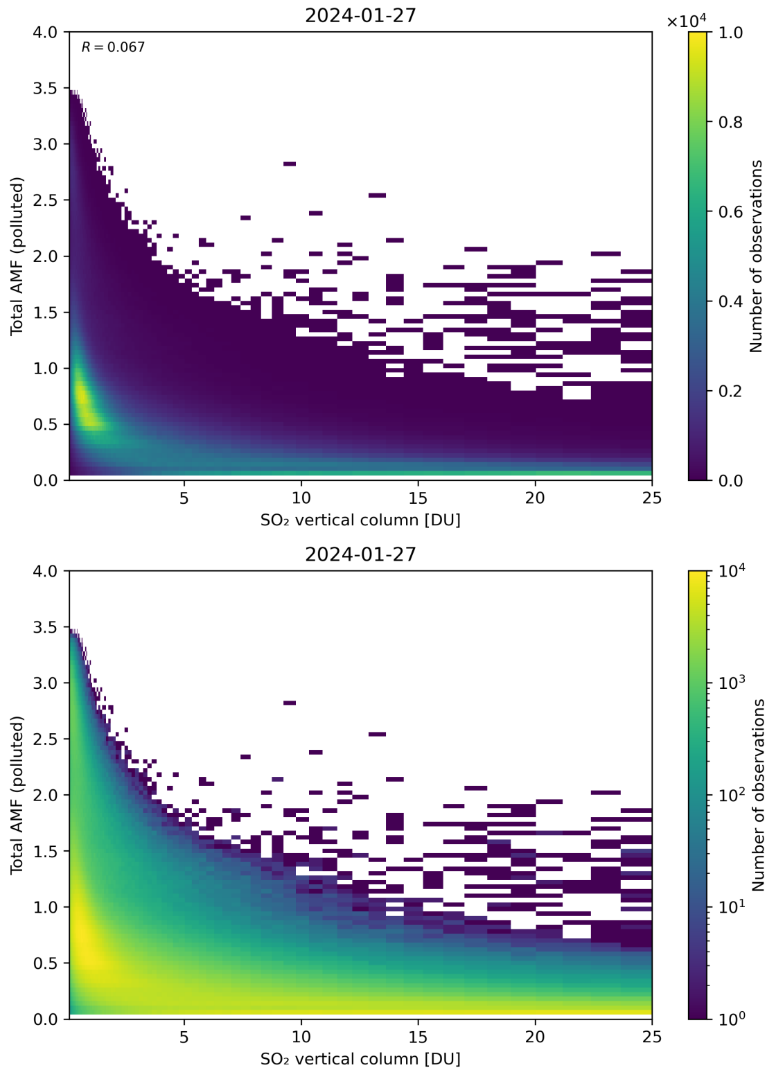
Figure 305: Scatter density plot of “SO 2 vertical column” against “Total AMF (polluted)” for 2024-01-26 to 2024-01-28.
