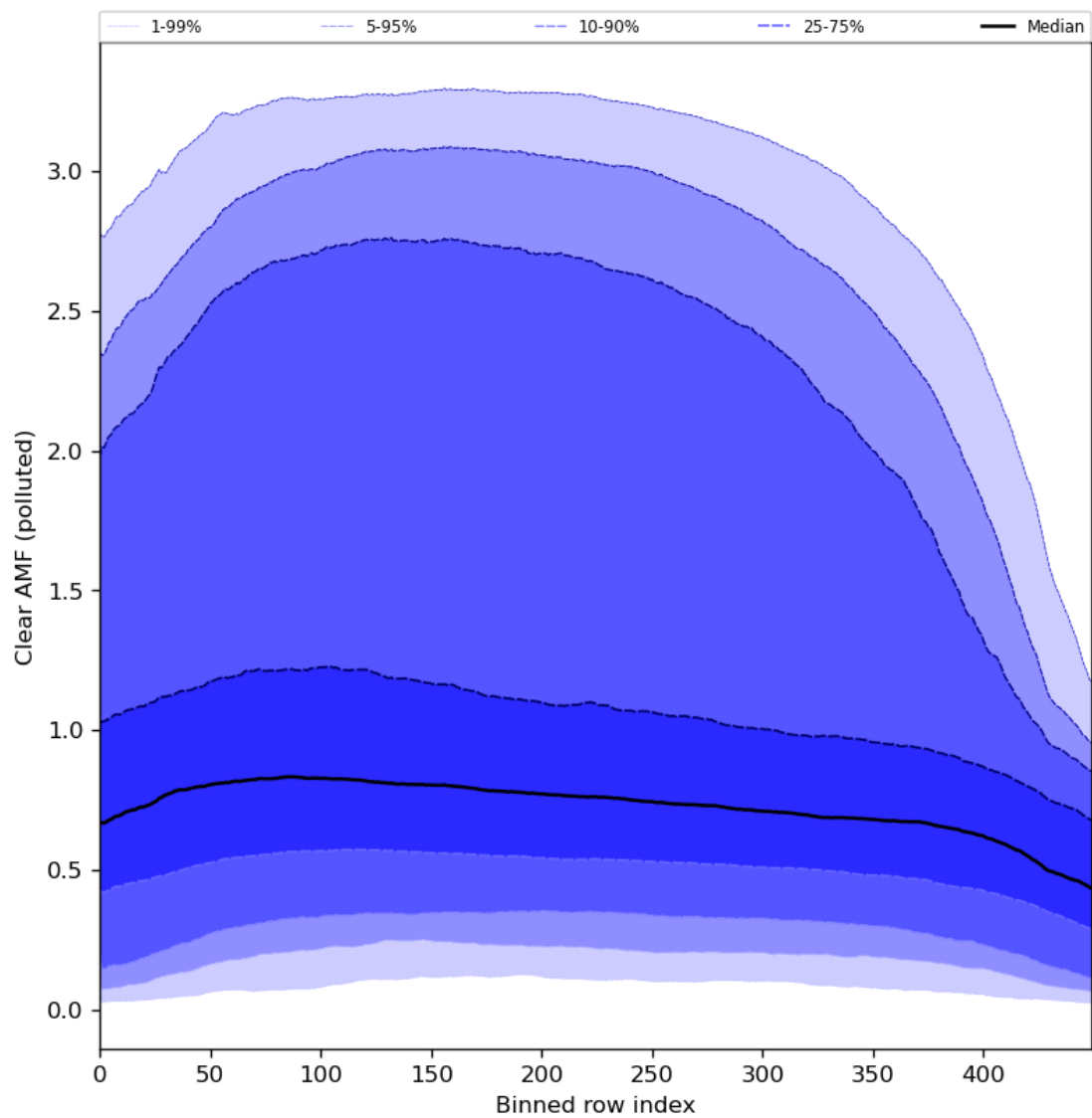
Figure 96: Along track statistics of “Clear AMF (polluted)” for 2024-01-26 to 2024-01-28
