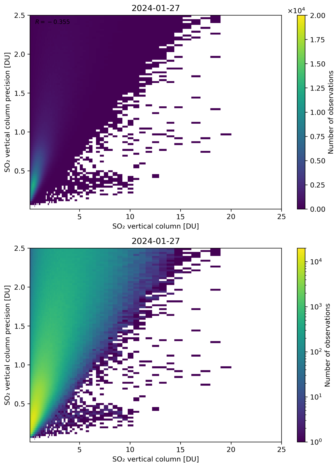
Figure 307: Scatter density plot of “SO 2 vertical column” against “SO 2 vertical column precision” for 2024-01-26 to 2024-01-28.
