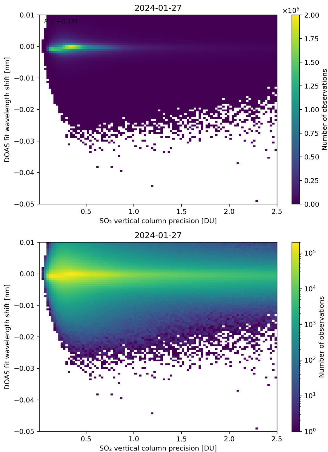
Figure 282: Scatter density plot of “SO 2 vertical column precision” against “DOAS fit wavelength shift” for 2024-01-26 to 2024-01-28.
