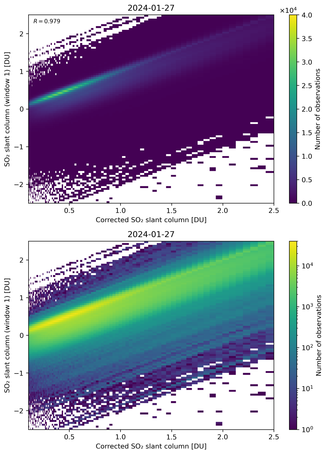
Figure 187: Scatter density plot of “Corrected SO 2 slant column” against “SO 2 slant column (window 1)” for 2024-01-26 to 2024-01-28.
