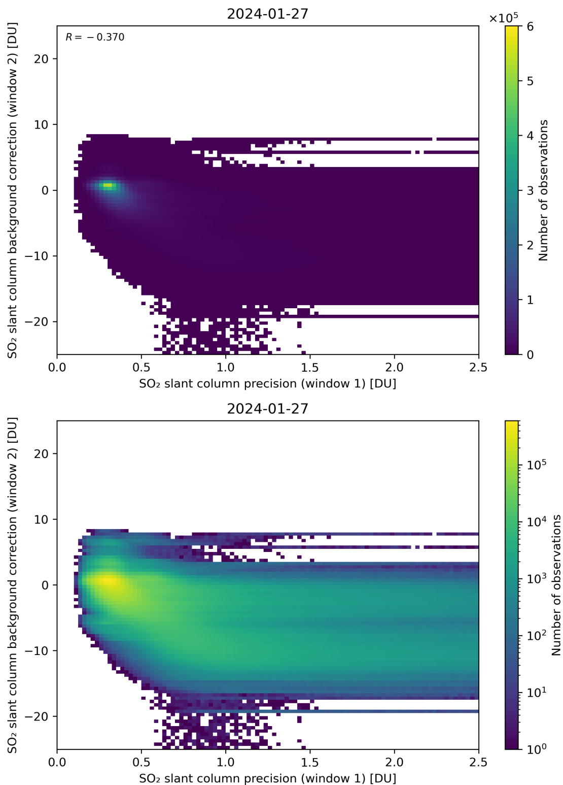
Figure 219: Scatter density plot of “SO 2 slant column precision (window 1)” against “SO 2 slant column background correction (window 2)” for 2024-01-26 to 2024-01-28.
