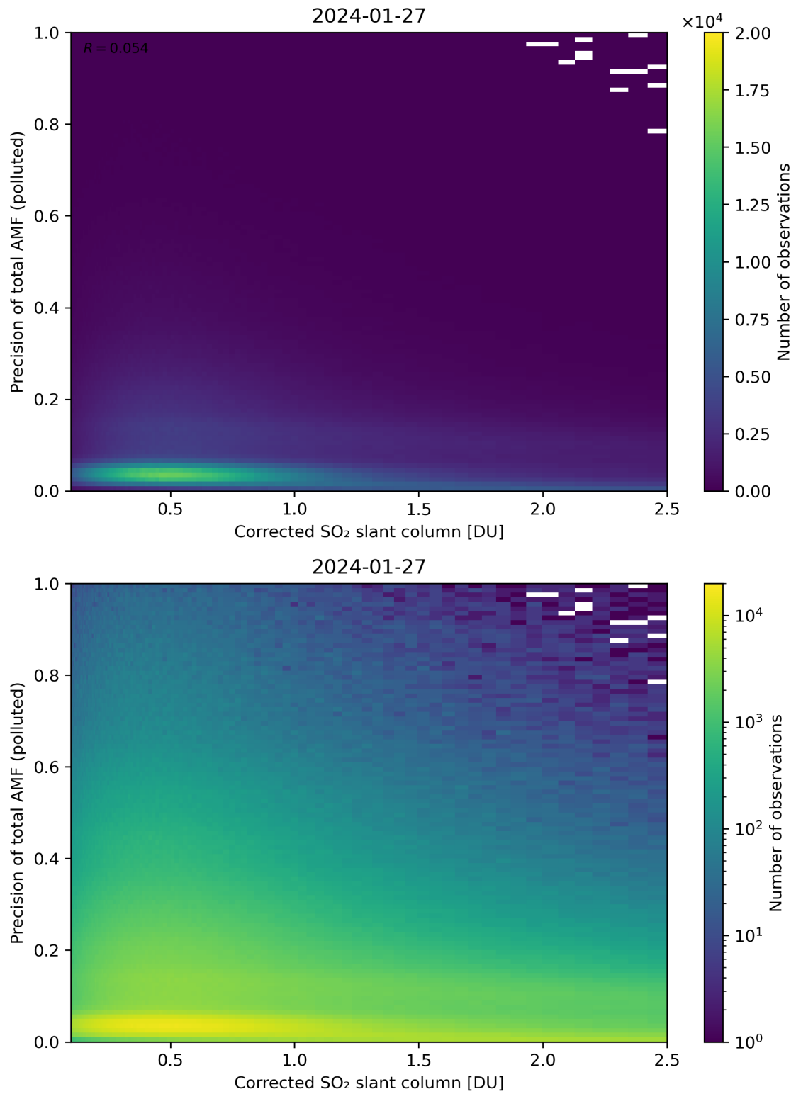
Figure 193: Scatter density plot of “Corrected SO 2 slant column” against “Precision of total AMF (polluted)” for 2024-01-26 to 2024-01-28.
