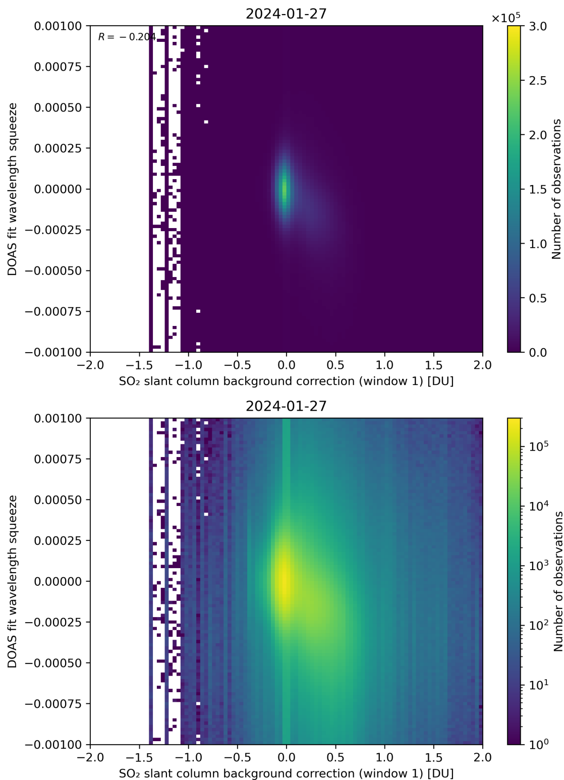
Figure 101: Scatter density plot of “SO 2 slant column background correction (window 1)” against “DOAS fit wavelength squeeze” for 2024-01-26 to 2024-01-28.
