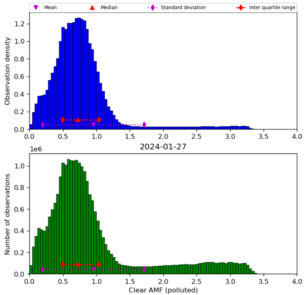
Figure 73: Histogram of “Clear AMF (polluted)” for 2024-01-26 to 2024-01-28
