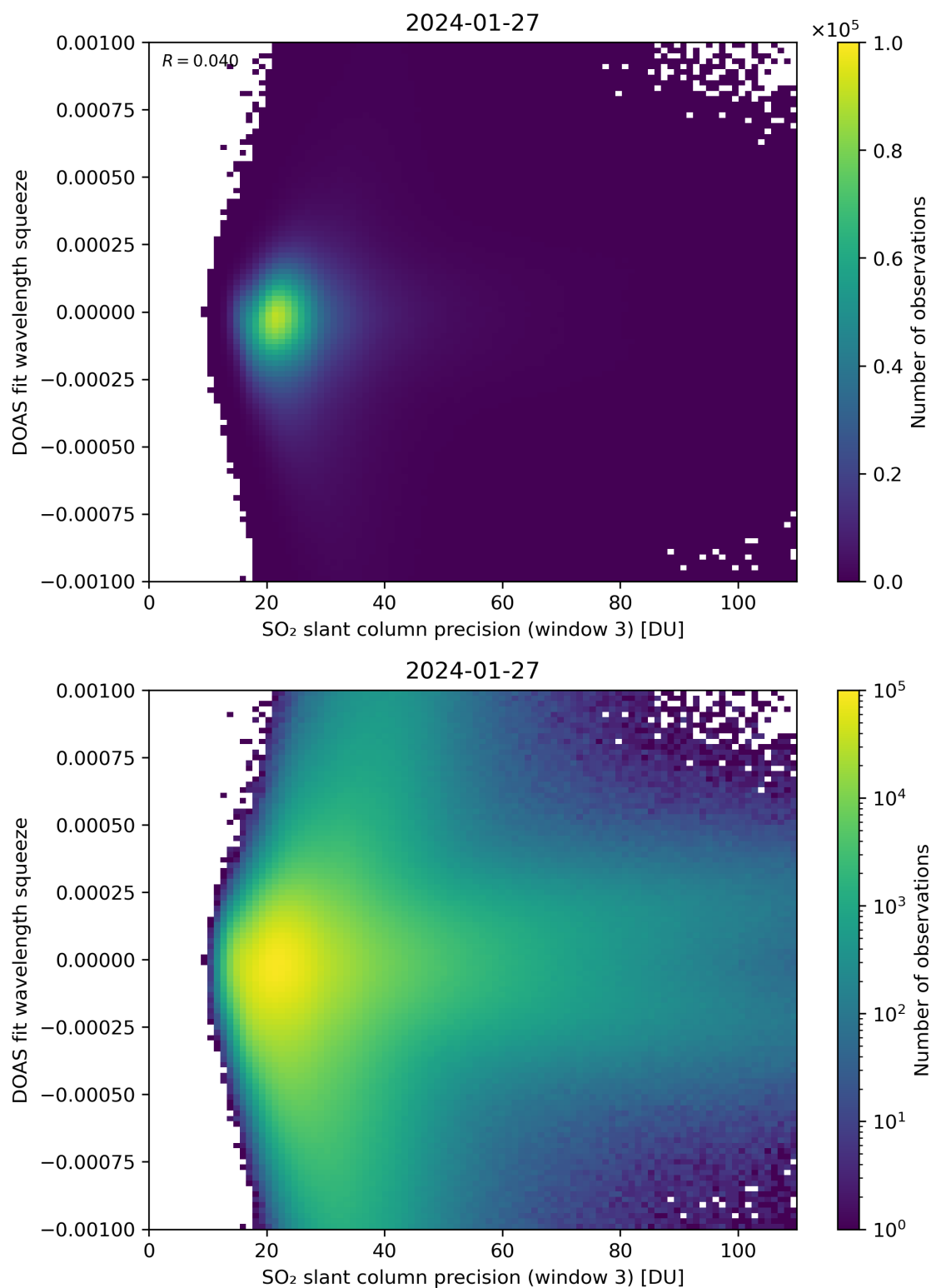
Figure 259: Scatter density plot of “SO 2 slant column precision (window 3)” against “DOAS fit wavelength squeeze” for 2024-01-26 to 2024-01-28.
