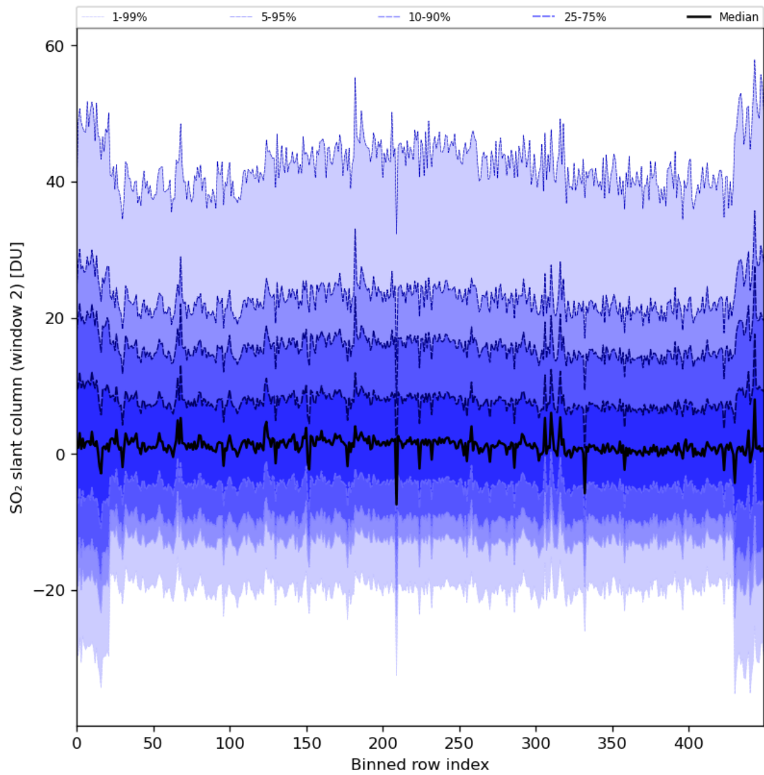
Figure 83: Along track statistics of “SO 2 slant column (window 2)” for 2024-01-26 to 2024-01-28
