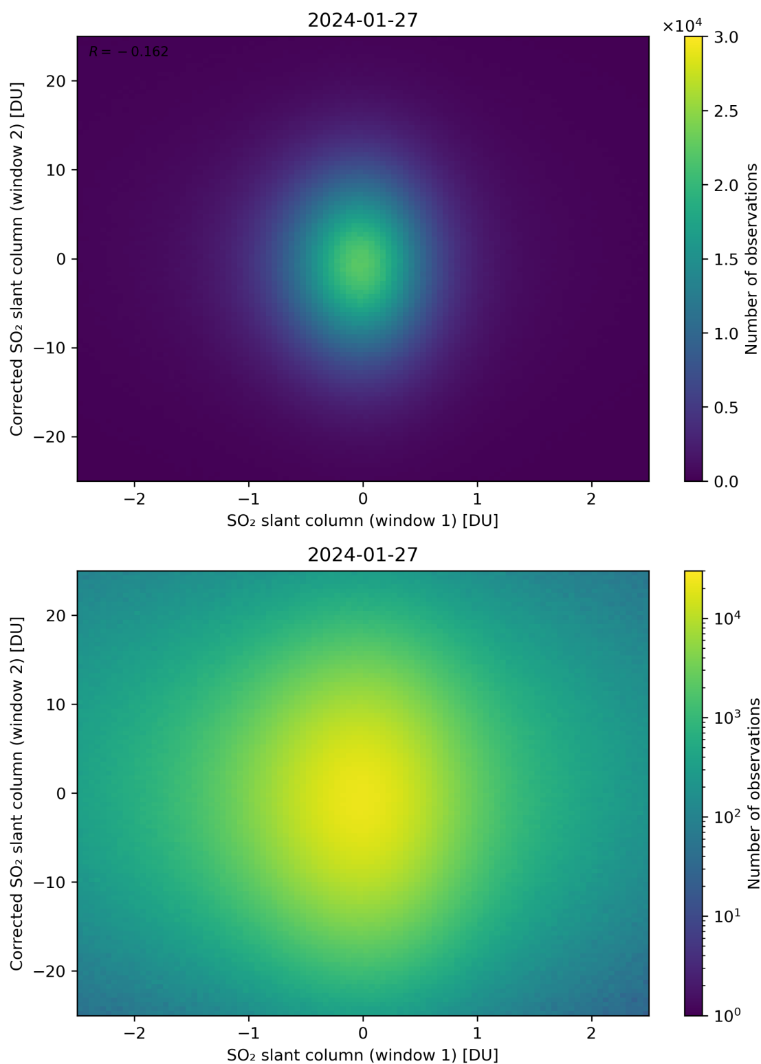
Figure 233: Scatter density plot of “SO 2 slant column (window 1)” against “Corrected SO 2 slant column (window 2)” for 2024-01-26 to 2024-01-28.
