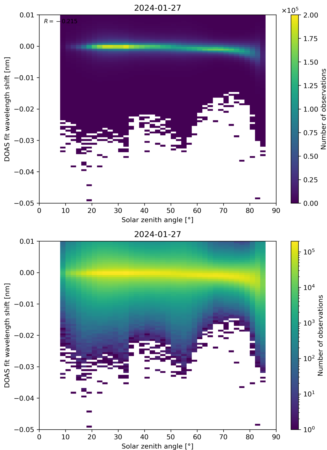
Figure 161: Scatter density plot of “Solar zenith angle” against “DOAS fit wavelength shift” for 2024-01-26 to 2024-01-28.
