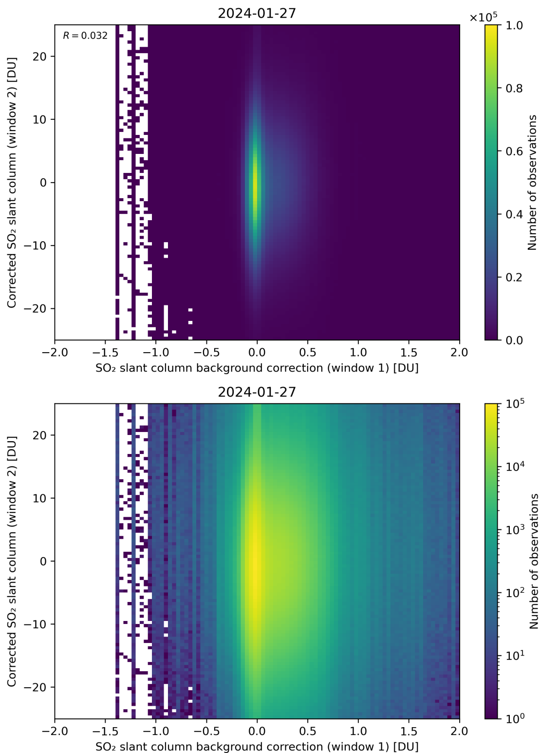
Figure 104: Scatter density plot of “SO 2 slant column background correction (window 1)” against “Corrected SO 2 slant column (window 2)” for 2024-01-26 to 2024-01-28.
