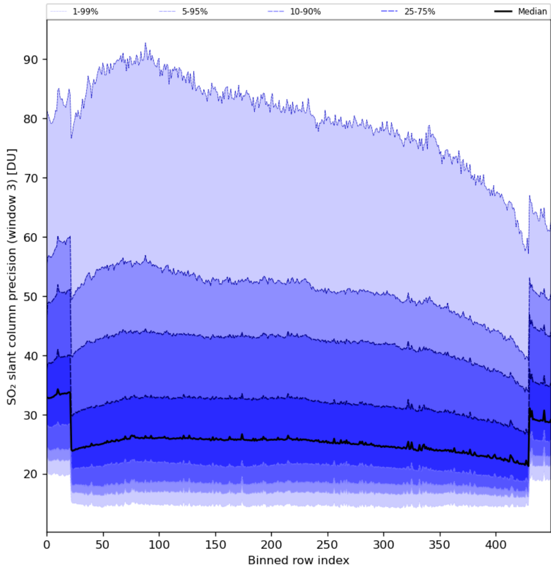
Figure 88: Along track statistics of “SO 2 slant column precision (window 3)” for 2024-01-26 to 2024-01-28
