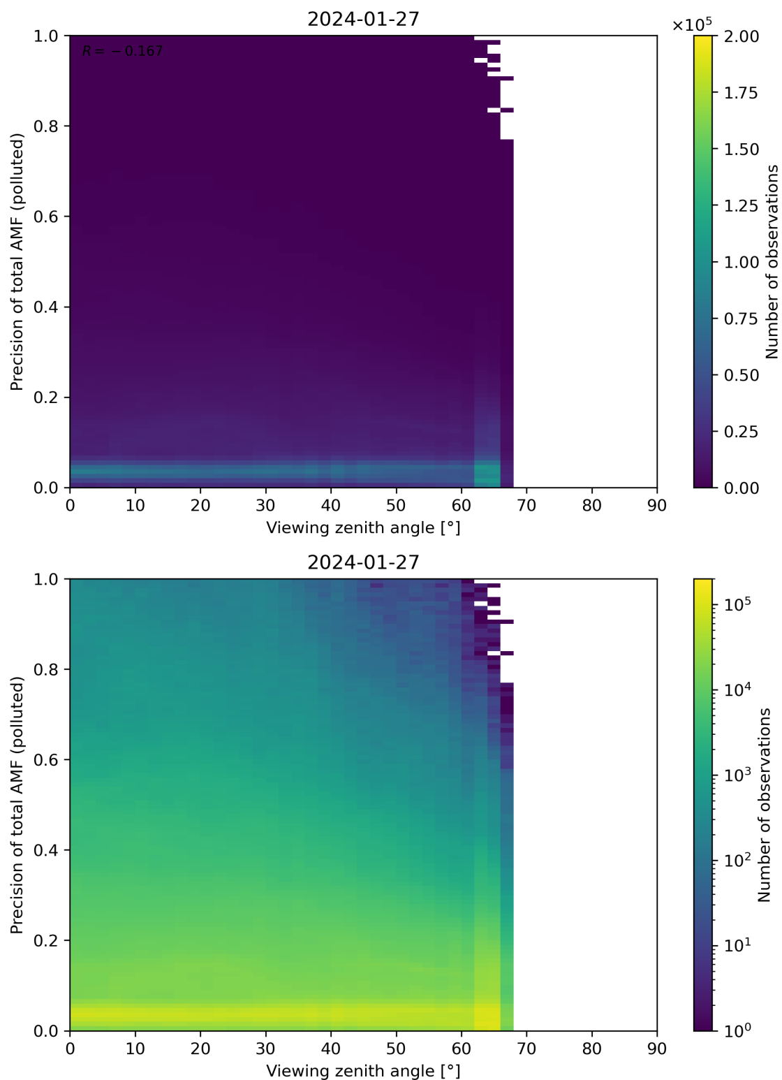
Figure 326: Scatter density plot of “Viewing zenith angle” against “Precision of total AMF (polluted)” for 2024-01-26 to 2024-01-28.
