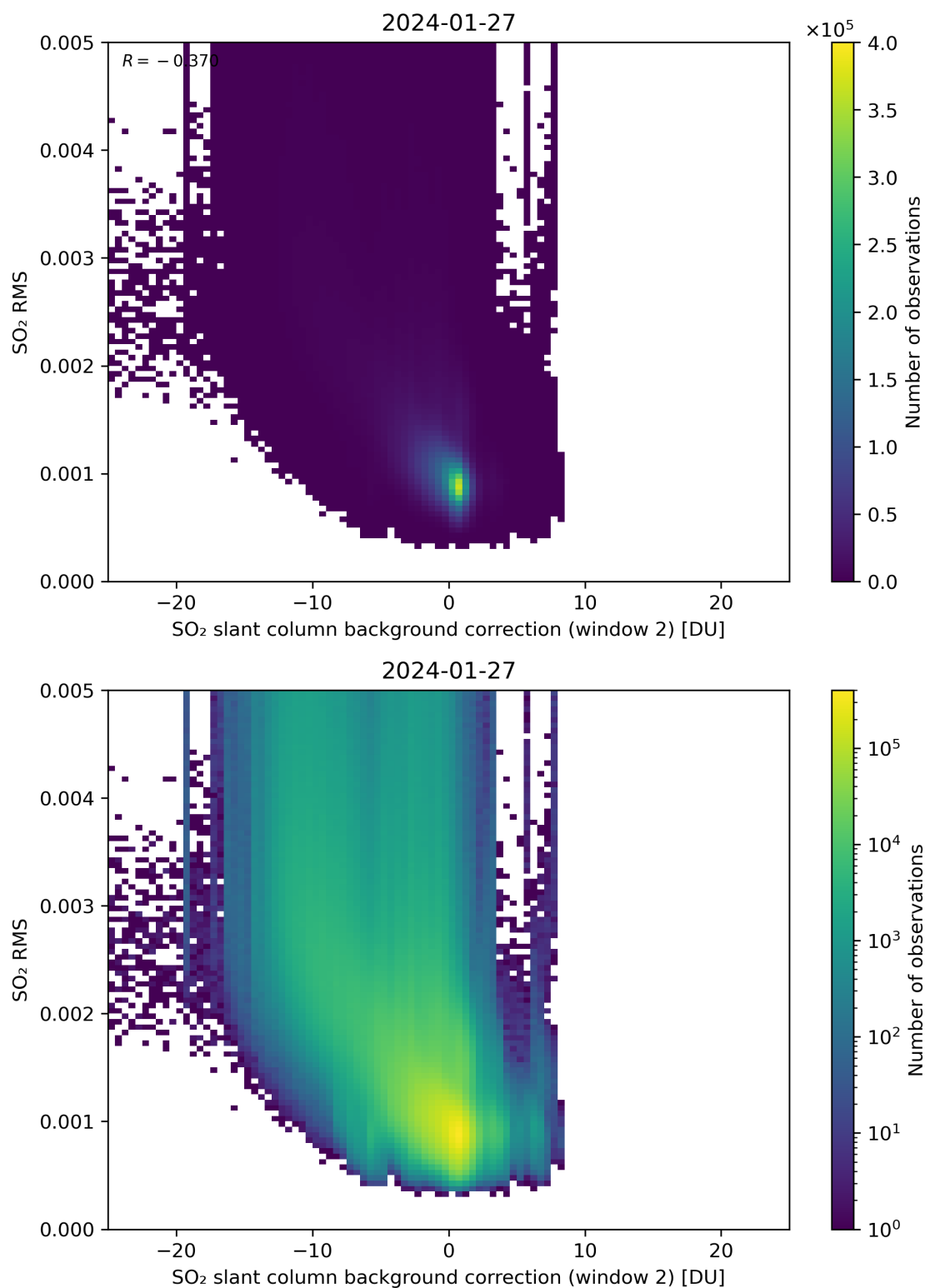
Figure 114: Scatter density plot of “SO 2 slant column background correction (window 2)” against “SO 2 RMS” for 2024-01-26 to 2024-01-28.
