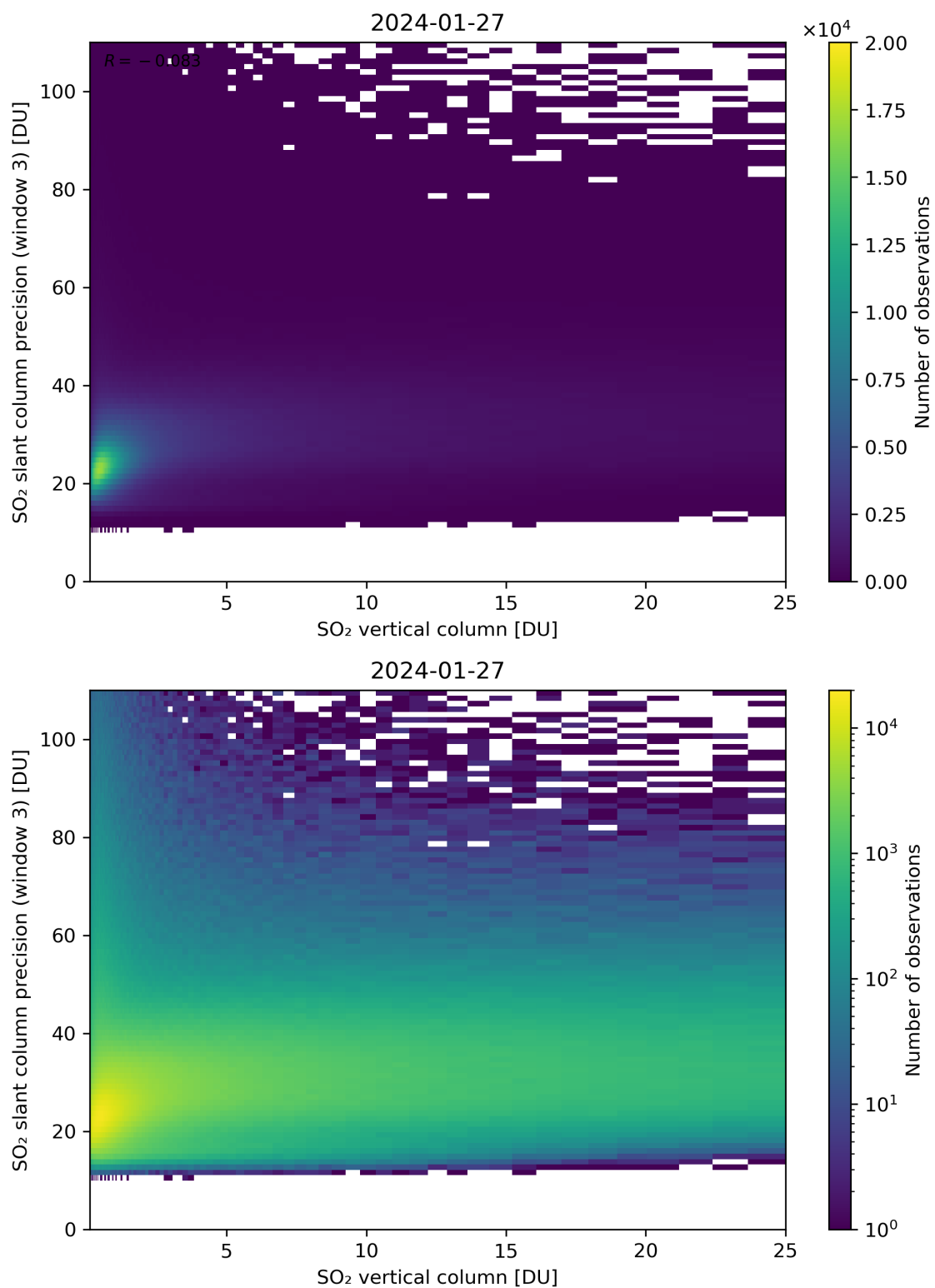
Figure 304: Scatter density plot of “SO 2 vertical column” against “SO 2 slant column precision (window 3)” for 2024-01-26 to 2024-01-28.
