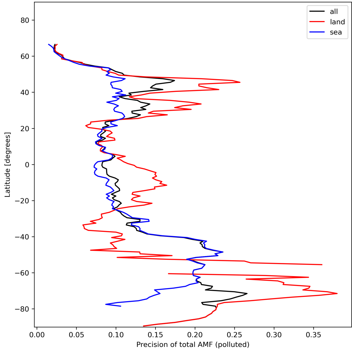
Figure 49: Zonal average of “Precision of total AMF (polluted)” for 2024-01-26 to 2024-01-28.
