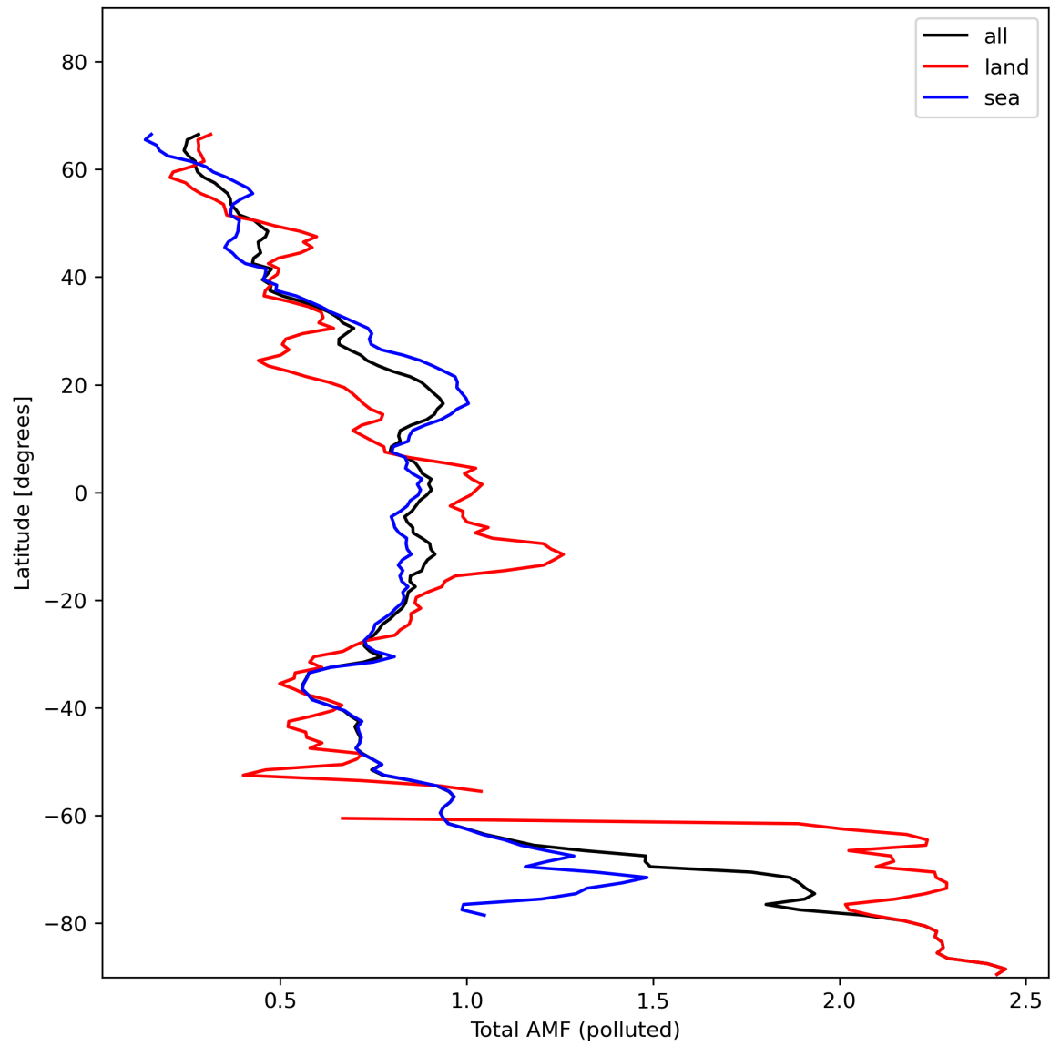
Figure 48: Zonal average of “Total AMF (polluted)” for 2024-01-26 to 2024-01-28.
