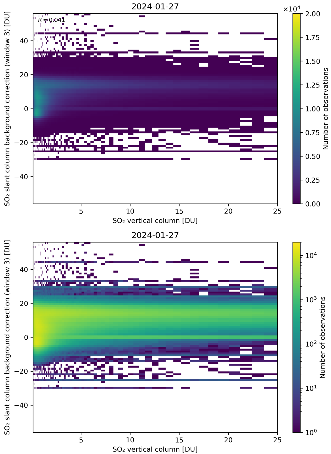
Figure 275: Scatter density plot of “SO 2 vertical column” against “SO 2 slant column background correction (window 3)” for 2024-01-26 to 2024-01-28.
