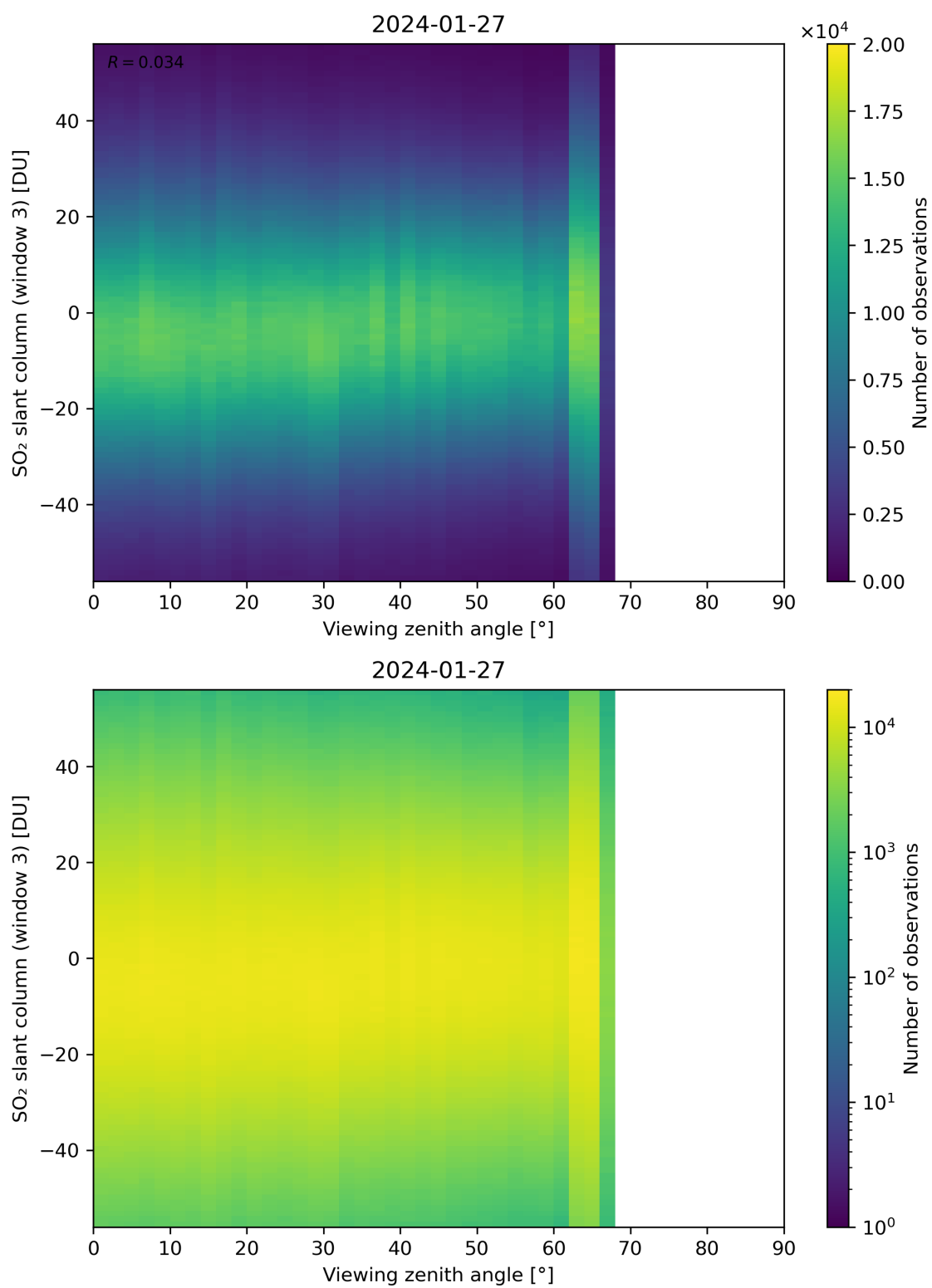
Figure 323: Scatter density plot of “Viewing zenith angle” against “SO 2 slant column (window 3)” for 2024-01-26 to 2024-01-28.
