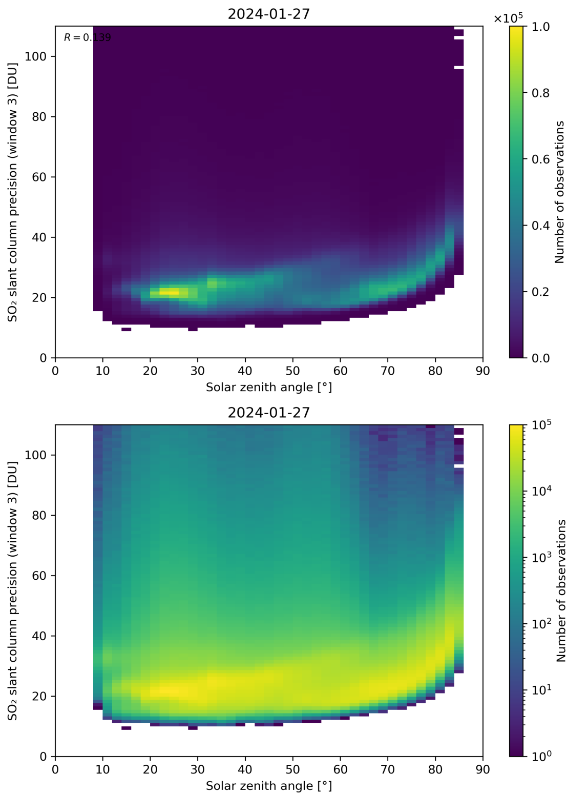
Figure 173: Scatter density plot of “Solar zenith angle” against “SO 2 slant column precision (window 3)” for 2024-01-26 to 2024-01-28.
