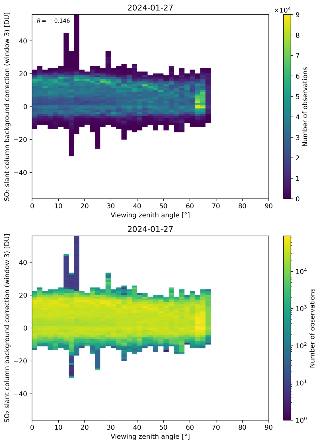
Figure 310: Scatter density plot of “Viewing zenith angle” against “SO 2 slant column background correction (window 3)” for 2024-01-26 to 2024-01-28.
