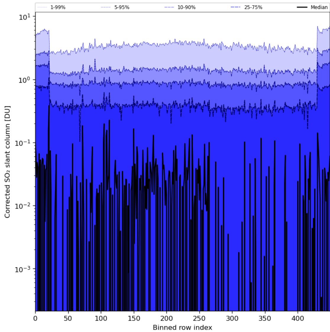
Figure 78: Along track statistics of “Corrected SO 2 slant column” for 2024-01-26 to 2024-01-28
