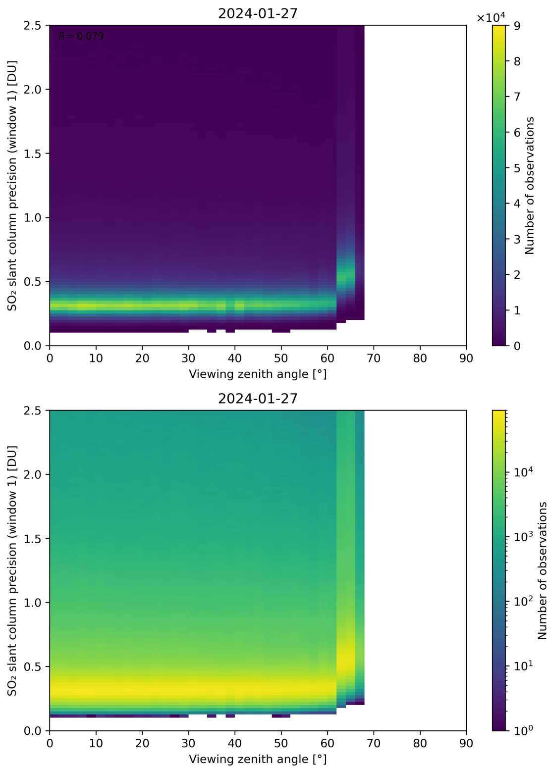
Figure 321: Scatter density plot of “Viewing zenith angle” against “SO 2 slant column precision (window 1)” for 2024-01-26 to 2024-01-28.
