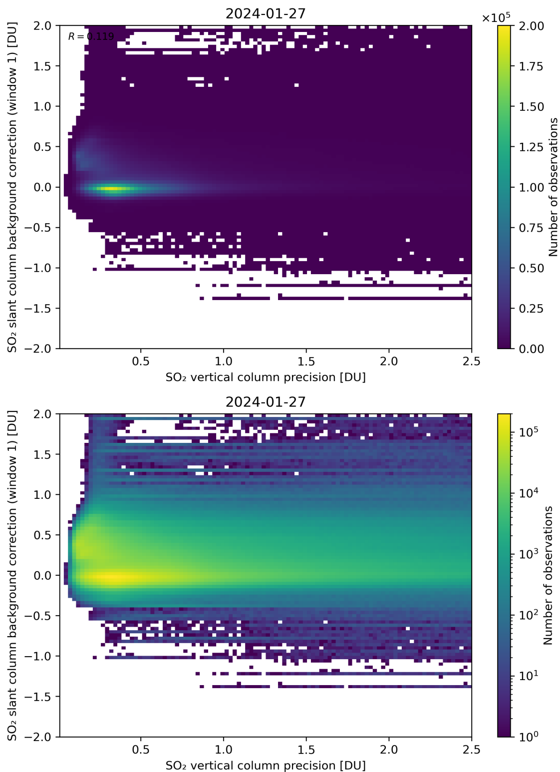
Figure 279: Scatter density plot of “SO 2 vertical column precision” against “SO 2 slant column background correction (window 1)” for 2024-01-26 to 2024-01-28.
