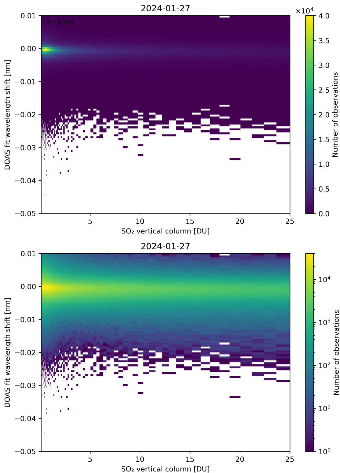
Figure 276: Scatter density plot of “SO 2 vertical column” against “DOAS fit wavelength shift” for 2024-01-26 to 2024-01-28.
