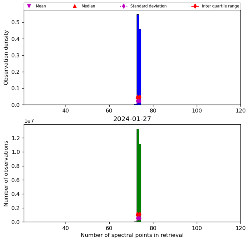
Figure 74: Histogram of “Number of spectral points in retrieval” for 2024-01-26 to 2024-01-28
