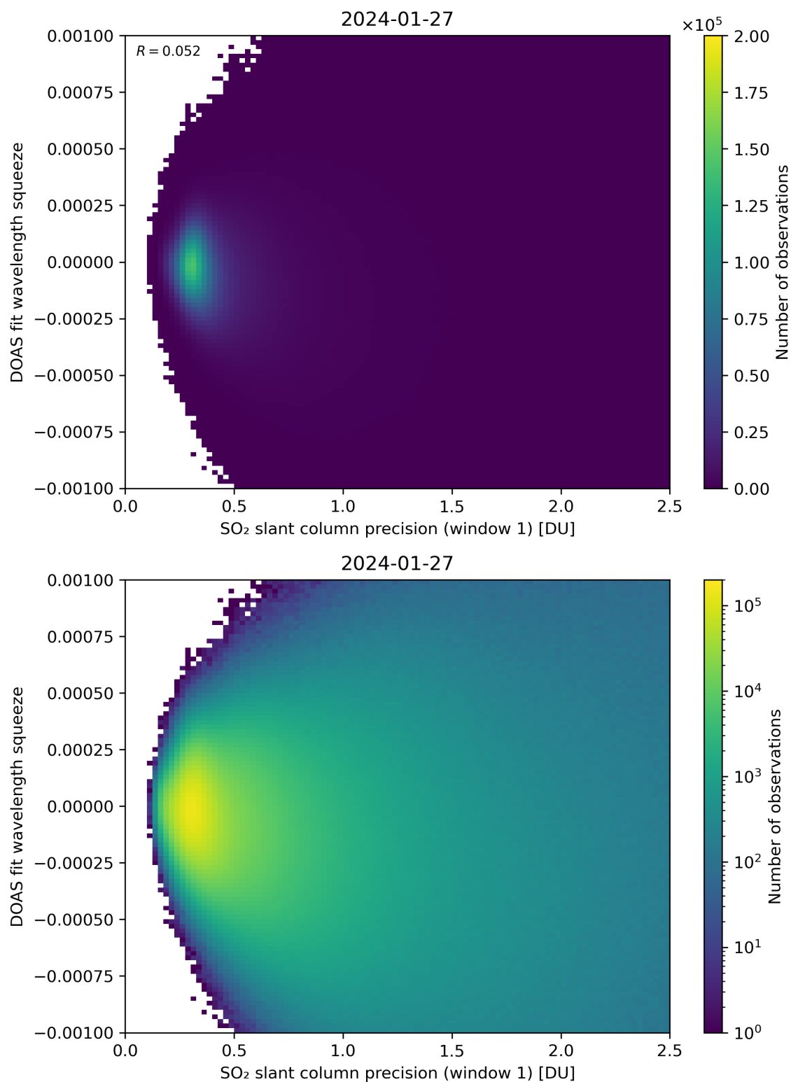
Figure 222: Scatter density plot of “SO 2 slant column precision (window 1)” against “DOAS fit wavelength squeeze” for 2024-01-26 to 2024-01-28.
