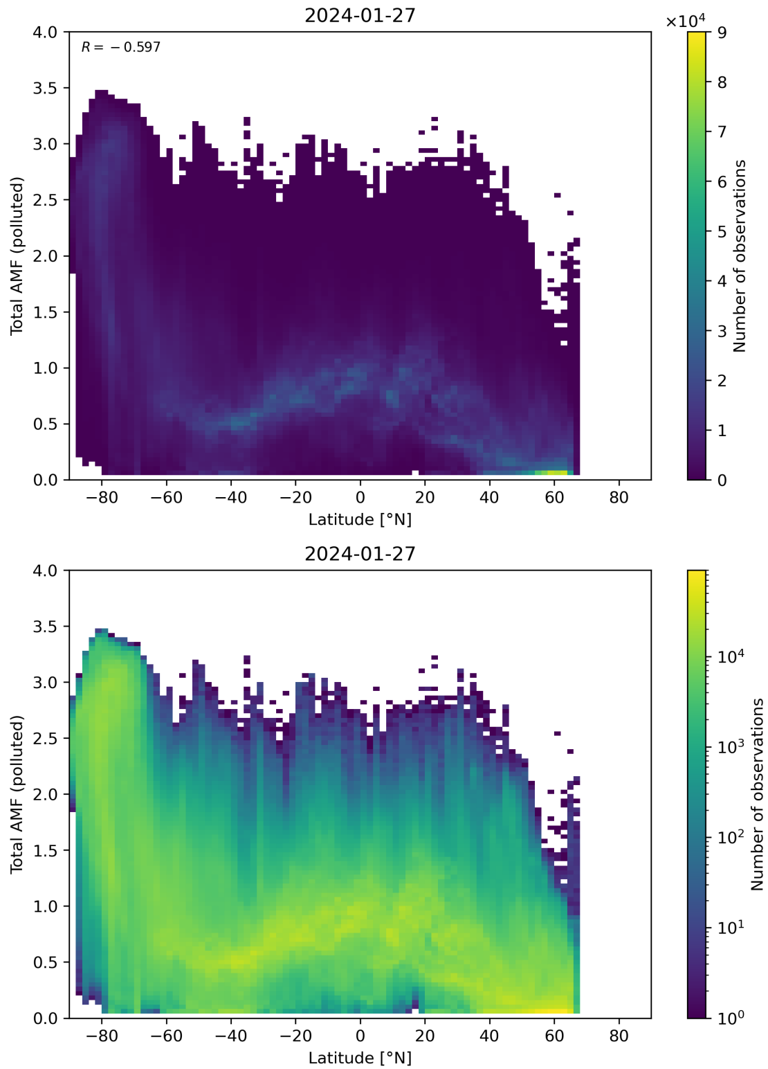
Figure 154: Scatter density plot of “Latitude” against “Total AMF (polluted)” for 2024-01-26 to 2024-01-28.
