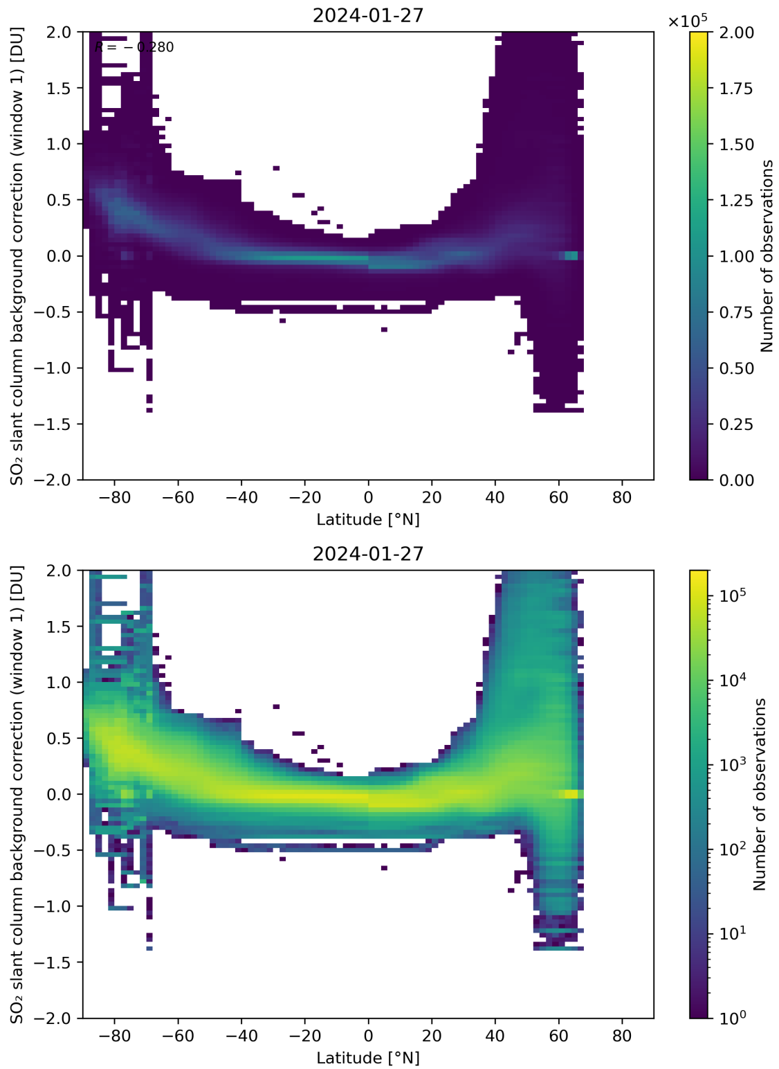
Figure 139: Scatter density plot of “Latitude” against “SO 2 slant column background correction (window 1)” for 2024-01-26 to 2024-01-28.
