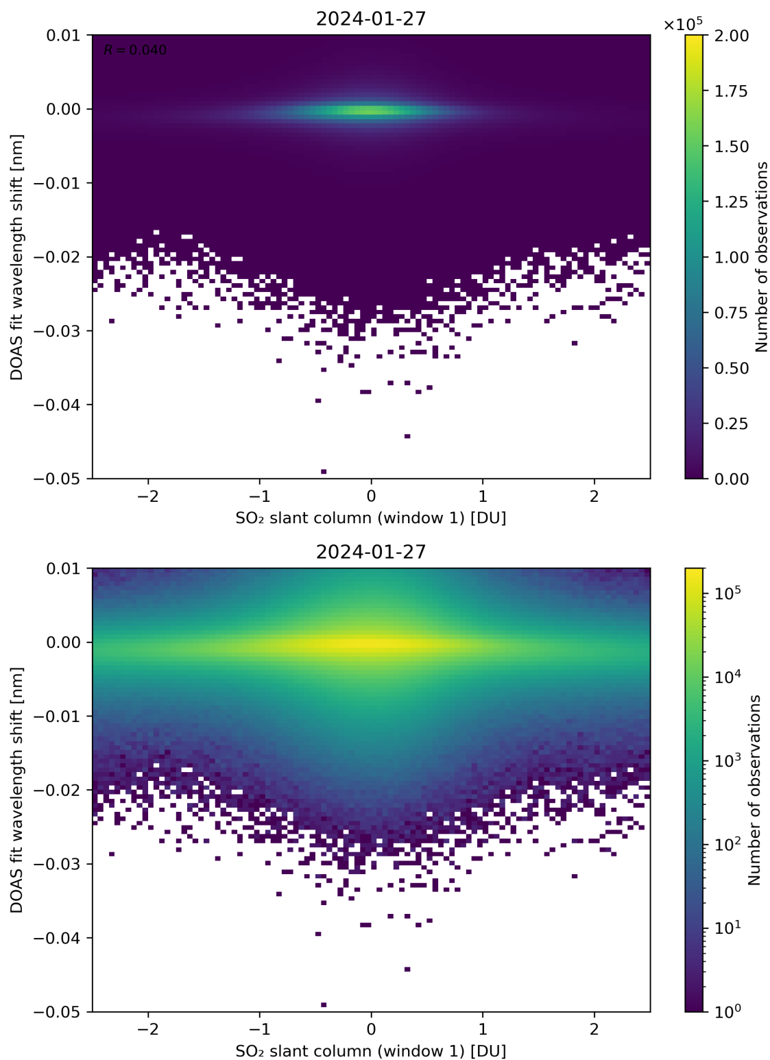
Figure 215: Scatter density plot of “SO 2 slant column (window 1)” against “DOAS fit wavelength shift” for 2024-01-26 to 2024-01-28.
