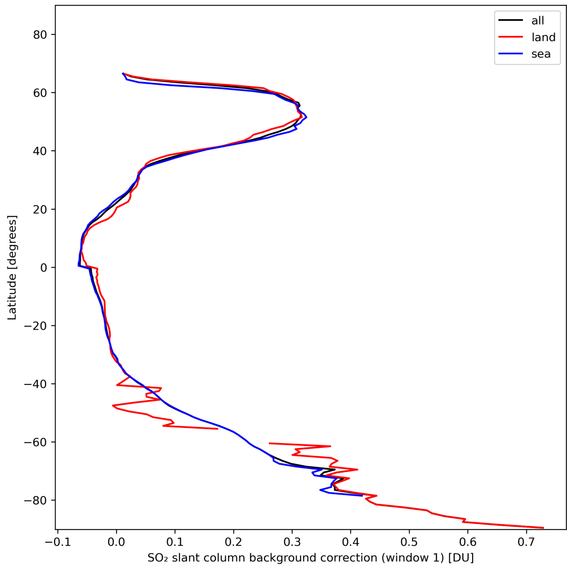
Figure 36: Zonal average of “SO 2 slant column background correction (window 1)” for 2024-01-26 to 2024-01-28.
