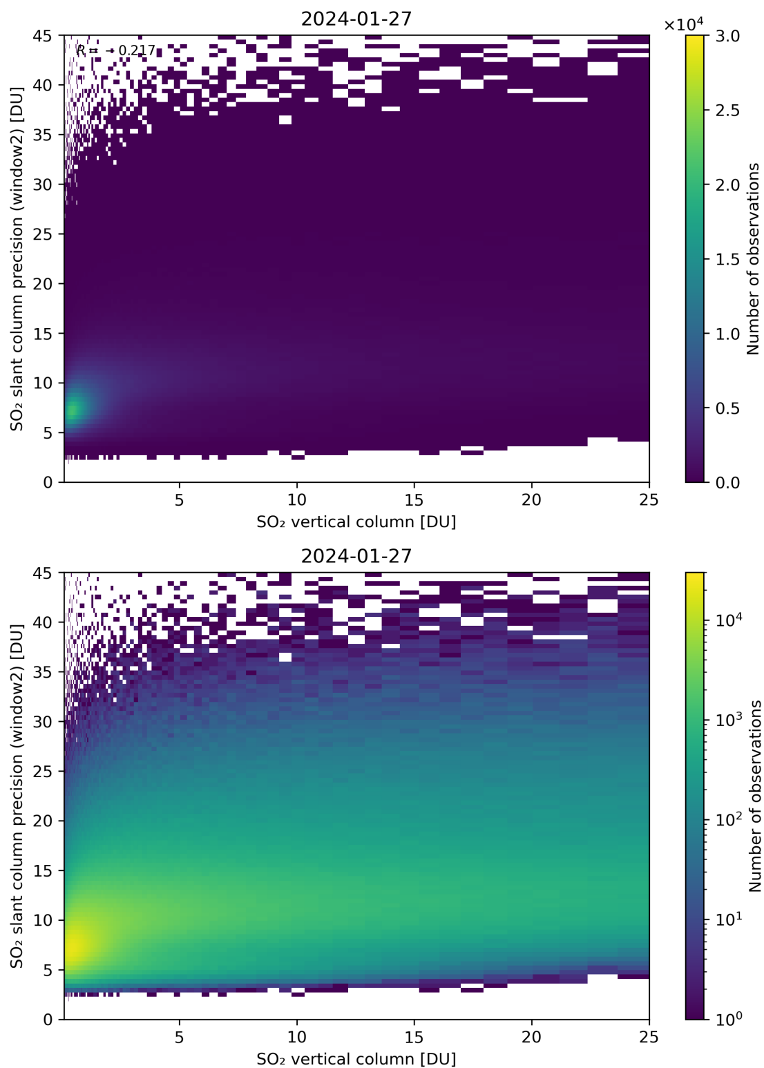
Figure 302: Scatter density plot of “SO 2 vertical column” against “SO 2 slant column precision (window2)” for 2024-01-26 to 2024-01-28.
