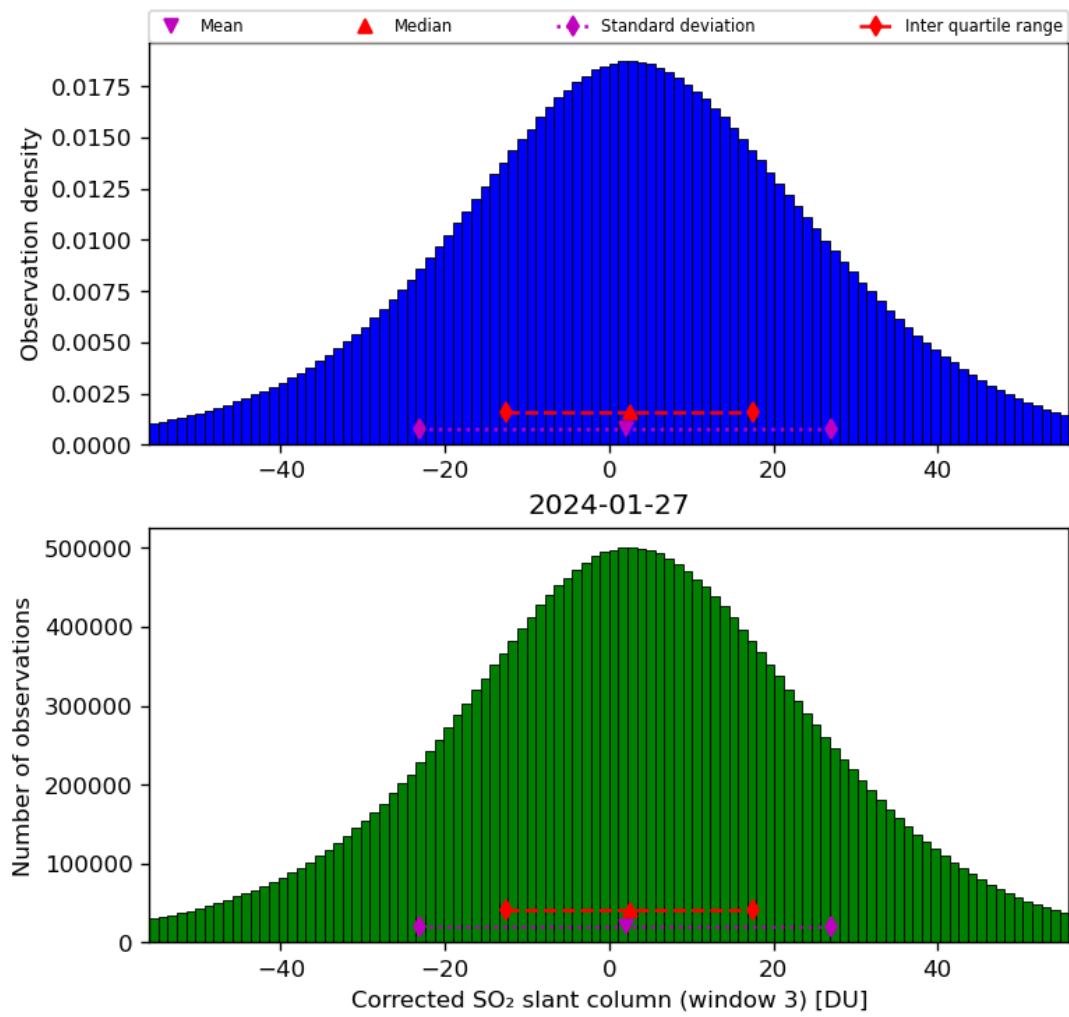
Figure 66: Histogram of "Corrected SO 2 slant column (window 3)" for 2024-01-26 to 2024-01-28
