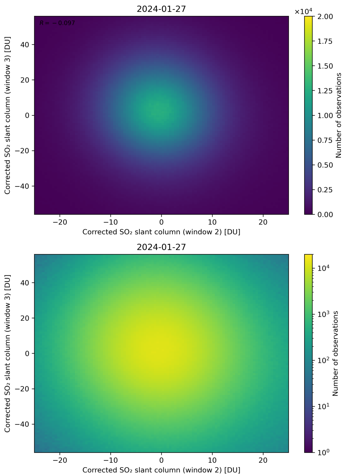
Figure 200: Scatter density plot of “Corrected SO 2 slant column (window 2)” against “Corrected SO 2 slant column (window 3)” for 2024-01-26 to 2024-01-28.
