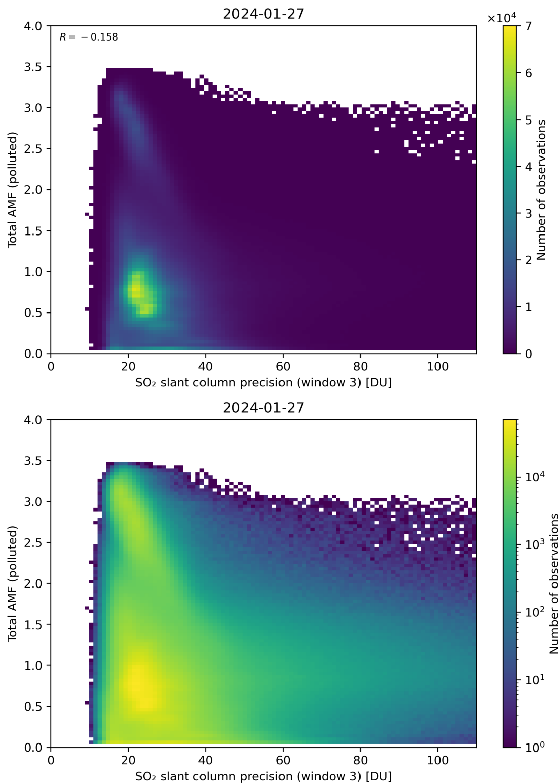
Figure 263: Scatter density plot of “SO 2 slant column precision (window 3)” against “Total AMF (polluted)” for 2024-01-26 to 2024-01-28.
