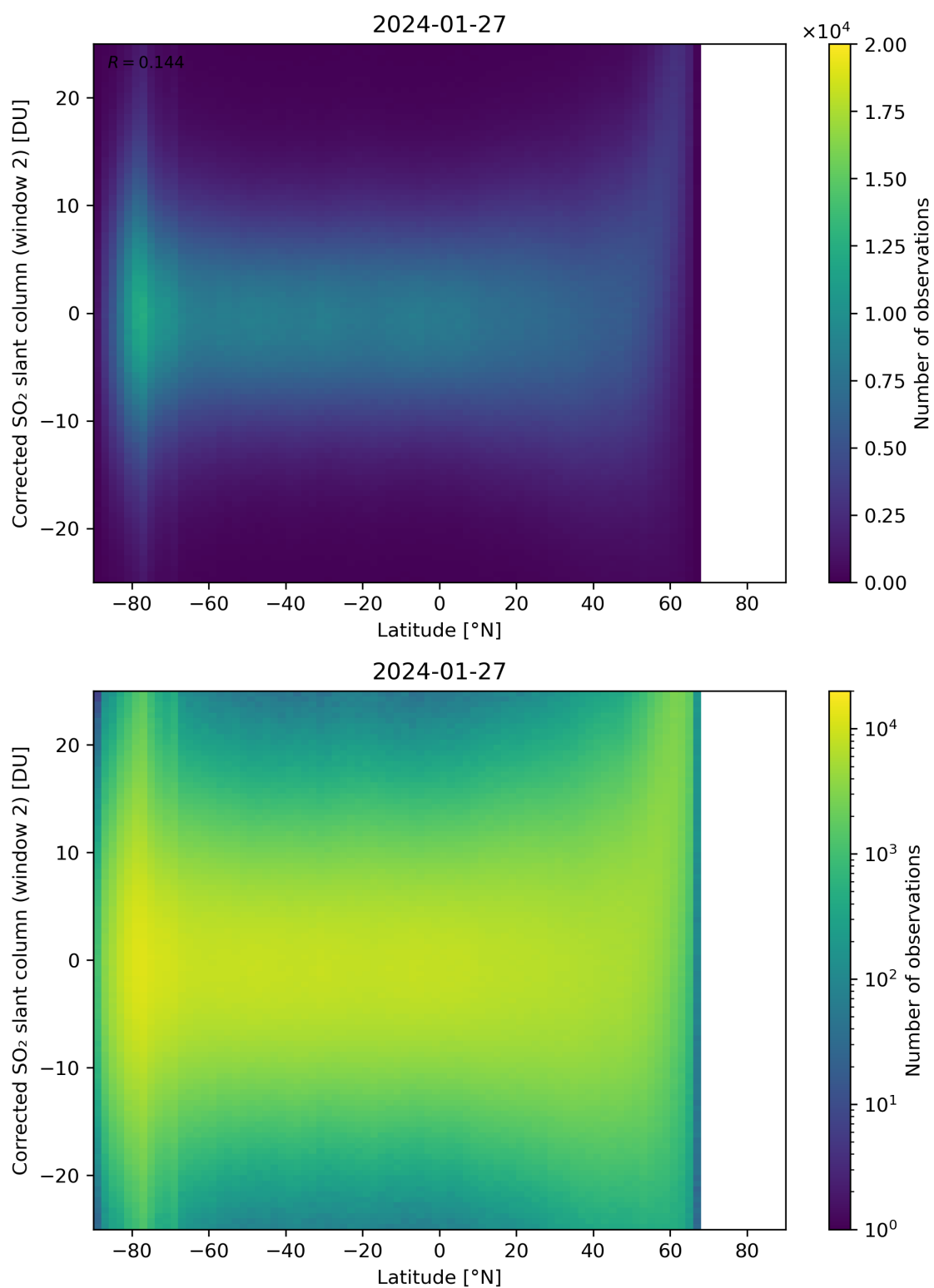
Figure 147: Scatter density plot of “Latitude” against “Corrected SO 2 slant column (window 2)” for 2024-01-26 to 2024-01-28.
