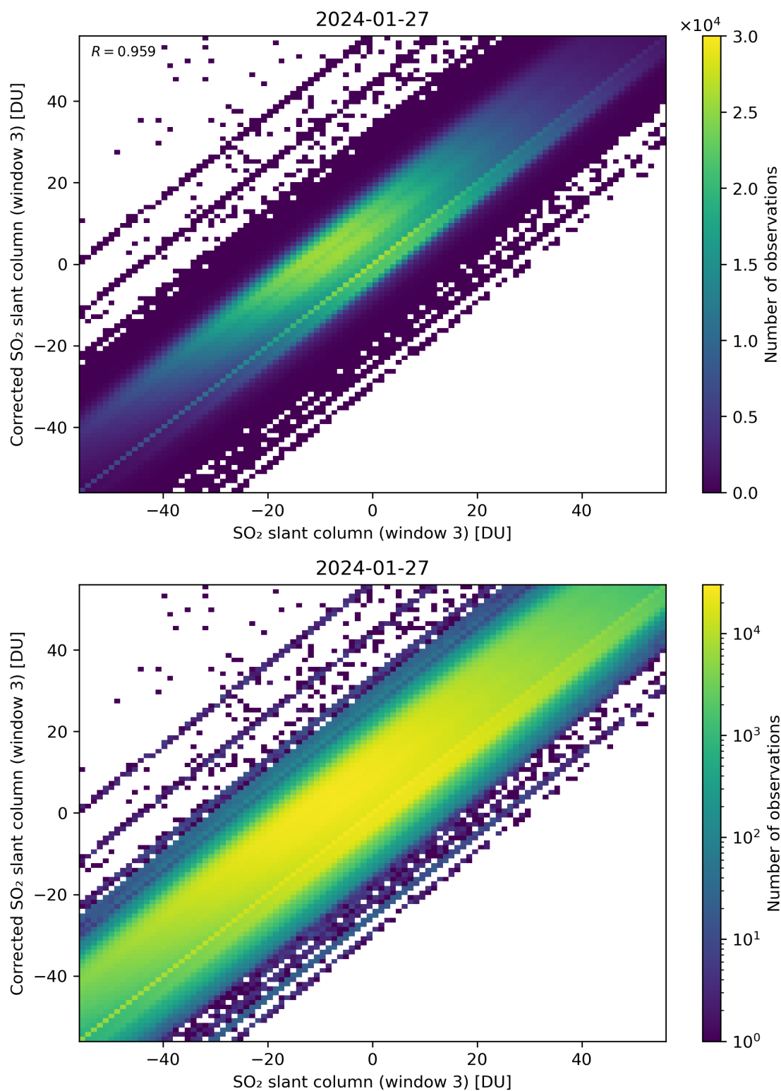
Figure 266: Scatter density plot of “SO 2 slant column (window 3)” against “Corrected SO 2 slant column (window 3)” for 2024-01-26 to 2024-01-28.
