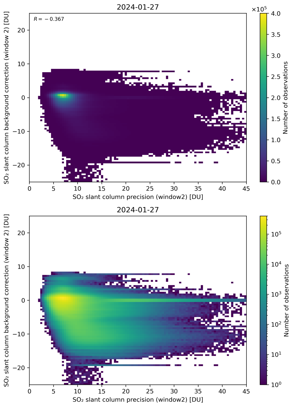
Figure 241: Scatter density plot of “SO 2 slant column precision (window2)” against “SO 2 slant column background correction (window 2)” for 2024-01-26 to 2024-01-28.
