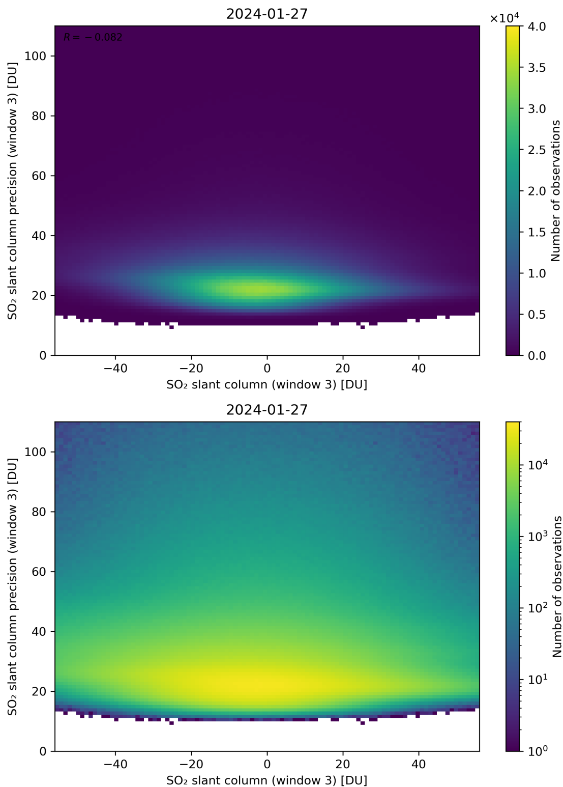
Figure 267: Scatter density plot of “SO 2 slant column (window 3)” against “SO 2 slant column precision (window 3)” for 2024-01-26 to 2024-01-28.
