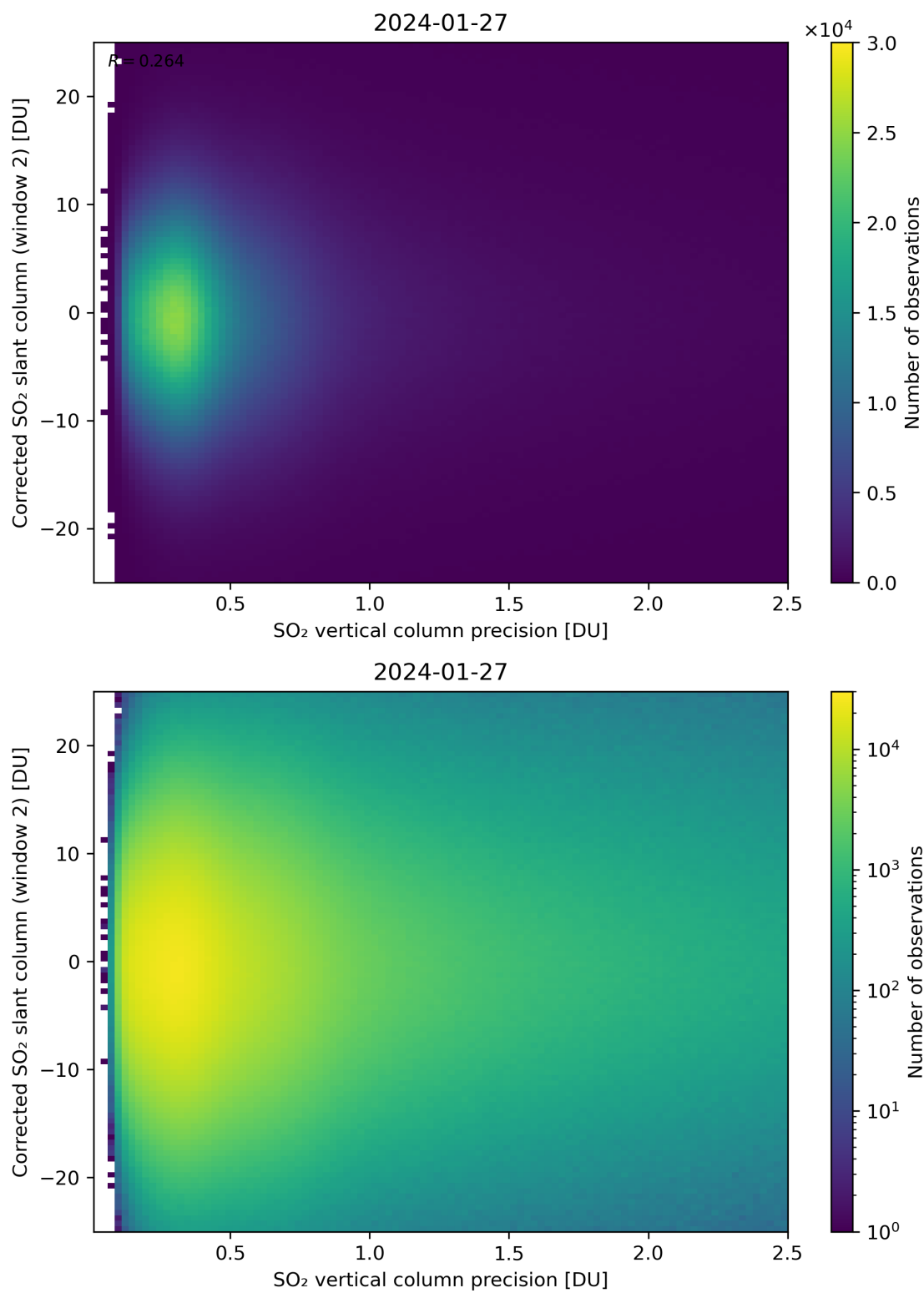
Figure 287: Scatter density plot of “SO 2 vertical column precision” against “Corrected SO 2 slant column (window 2)” for 2024-01-26 to 2024-01-28.
