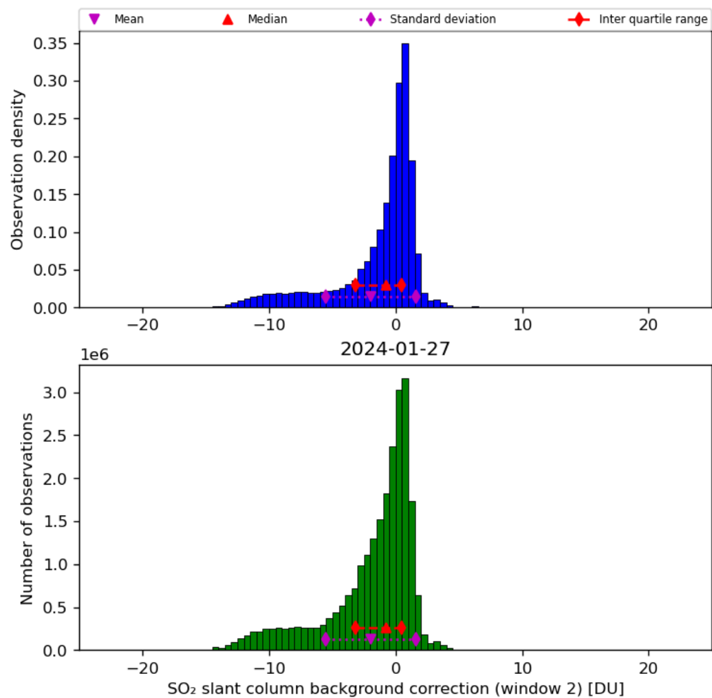
Figure 63: Histogram of “SO 2 slant column background correction (window 2)” for 2024-01-26 to 2024-01-28
