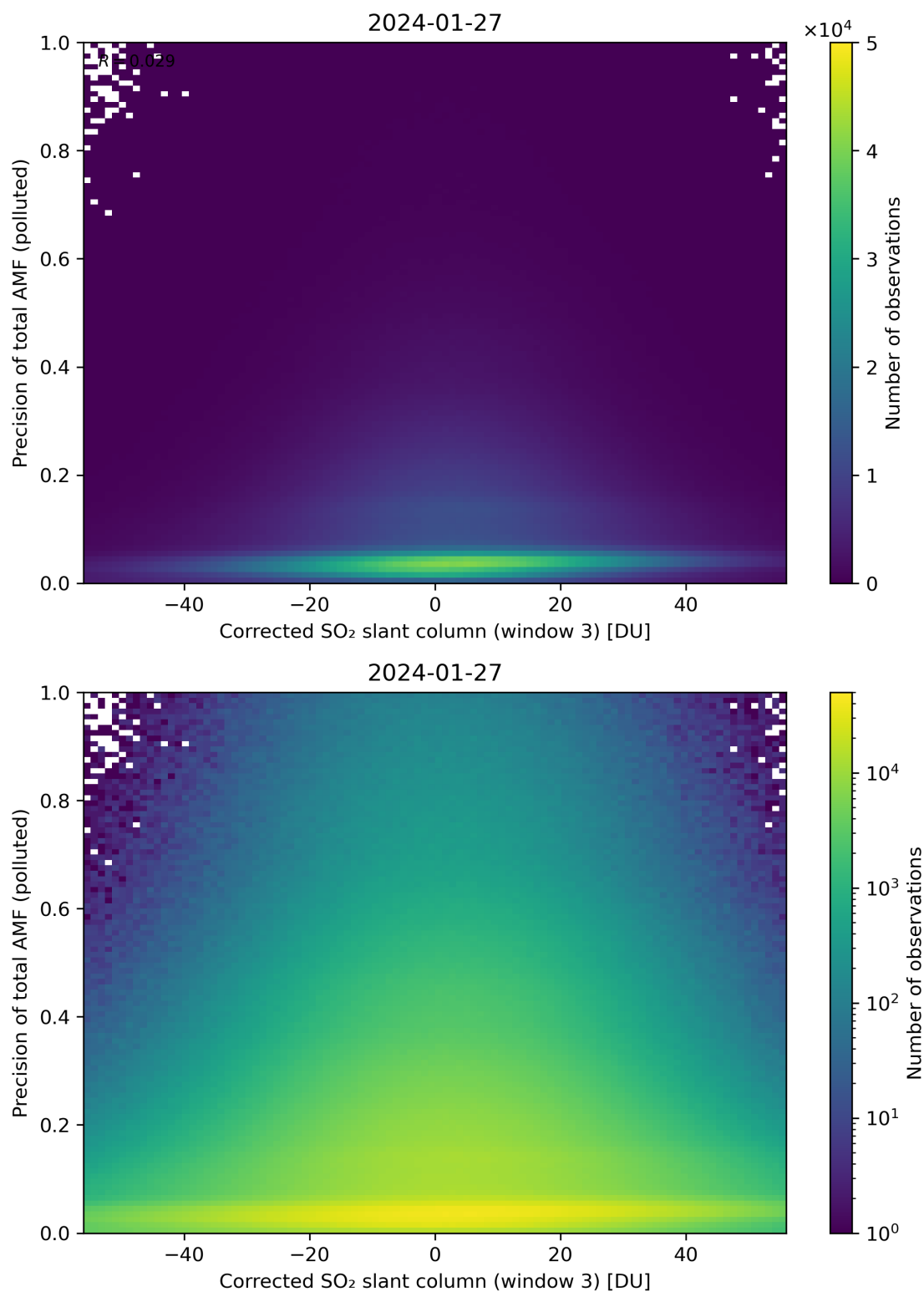
Figure 211: Scatter density plot of “Corrected SO 2 slant column (window 3)” against “Precision of total AMF (polluted)” for 2024-01-26 to 2024-01-28.
