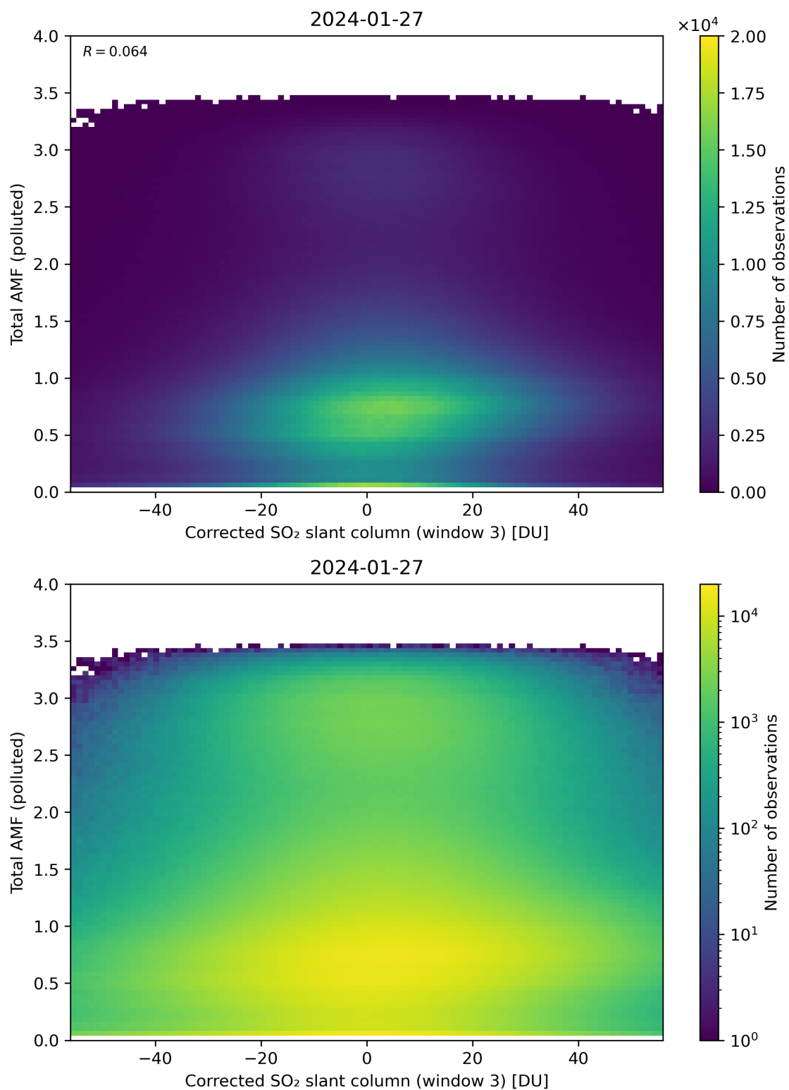
Figure 210: Scatter density plot of “Corrected SO 2 slant column (window 3)” against “Total AMF (polluted)” for 2024-01-26 to 2024-01-28.
