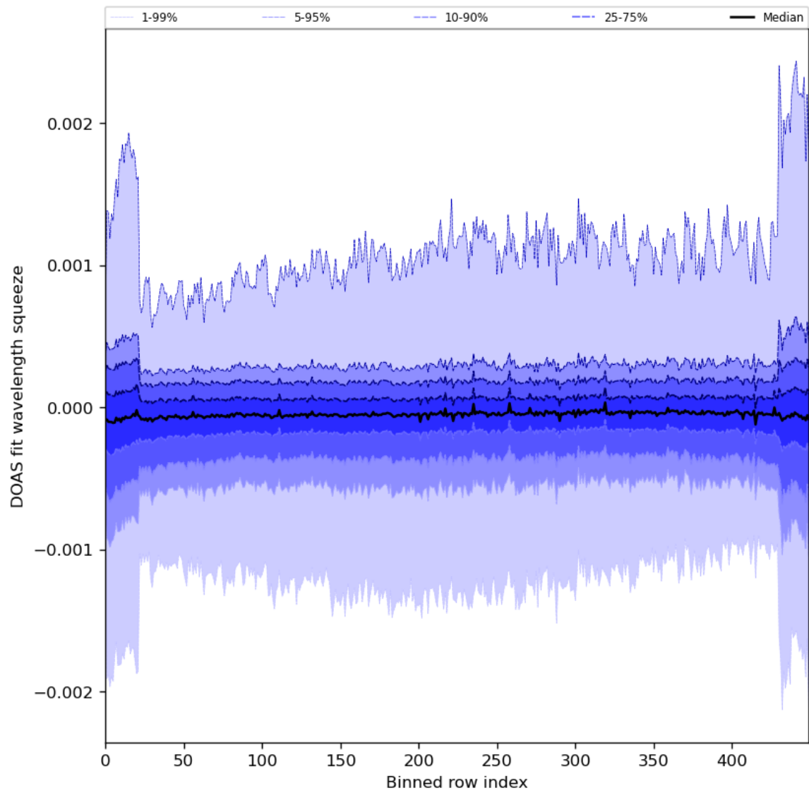
Figure 92: Along track statistics of “DOAS fit wavelength squeeze” for 2024-01-26 to 2024-01-28
