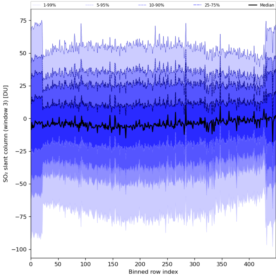
Figure 87: Along track statistics of “SO 2 slant column (window 3)” for 2024-01-26 to 2024-01-28
