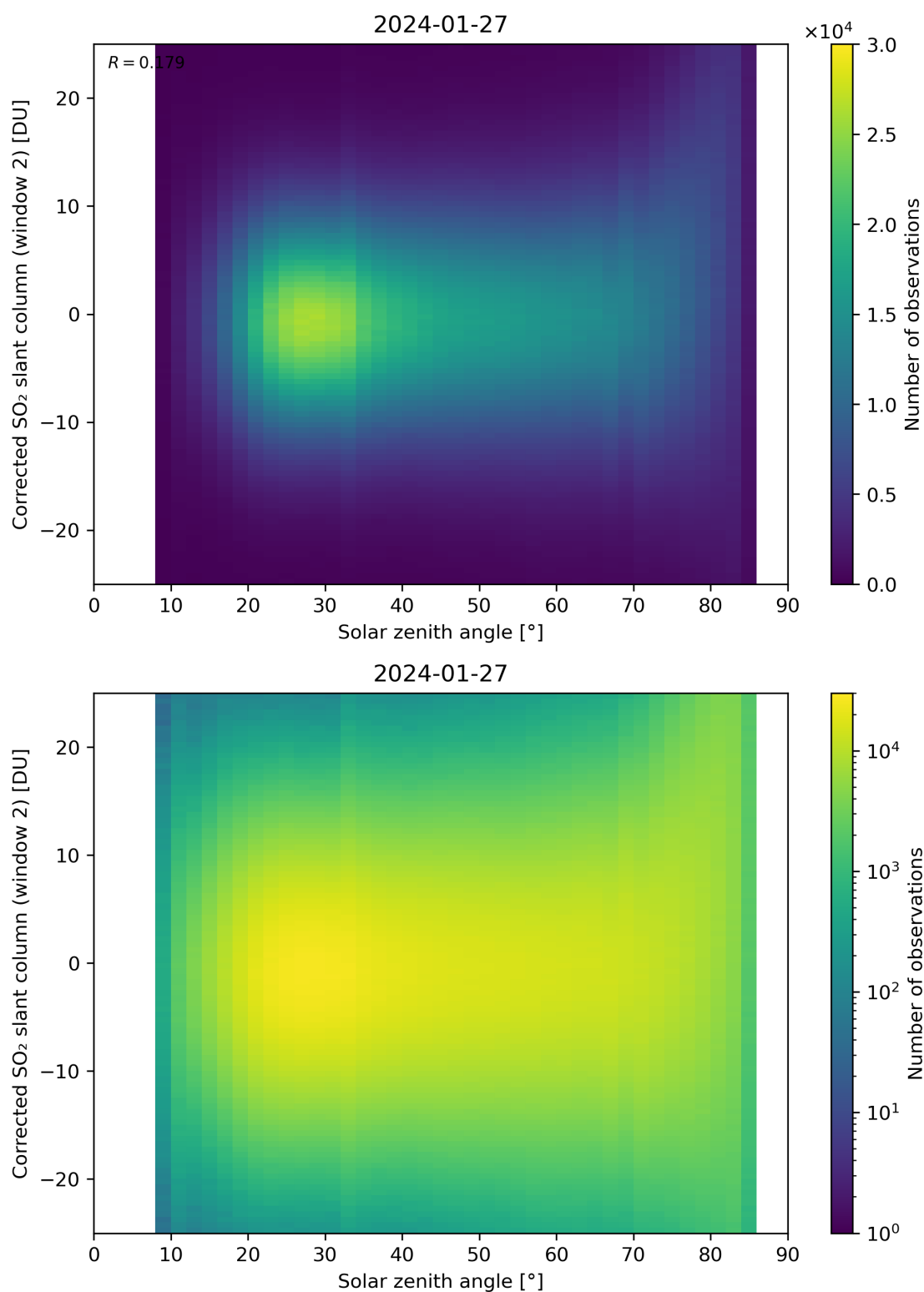
Figure 167: Scatter density plot of “Solar zenith angle” against “Corrected SO 2 slant column (window 2)” for 2024-01-26 to 2024-01-28.
