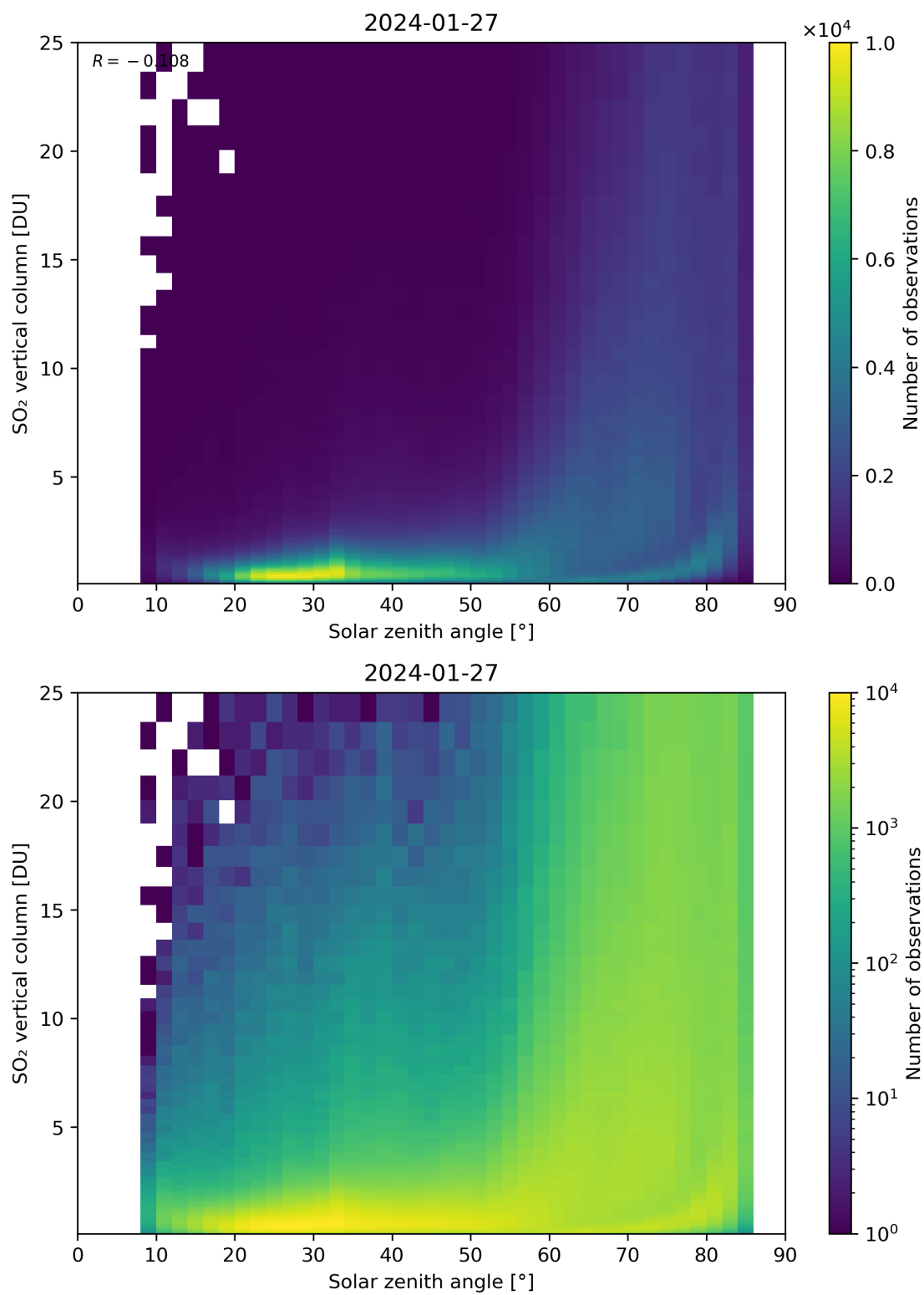
Figure 176: Scatter density plot of “Solar zenith angle” against “SO 2 vertical column” for 2024-01-26 to 2024-01-28.
