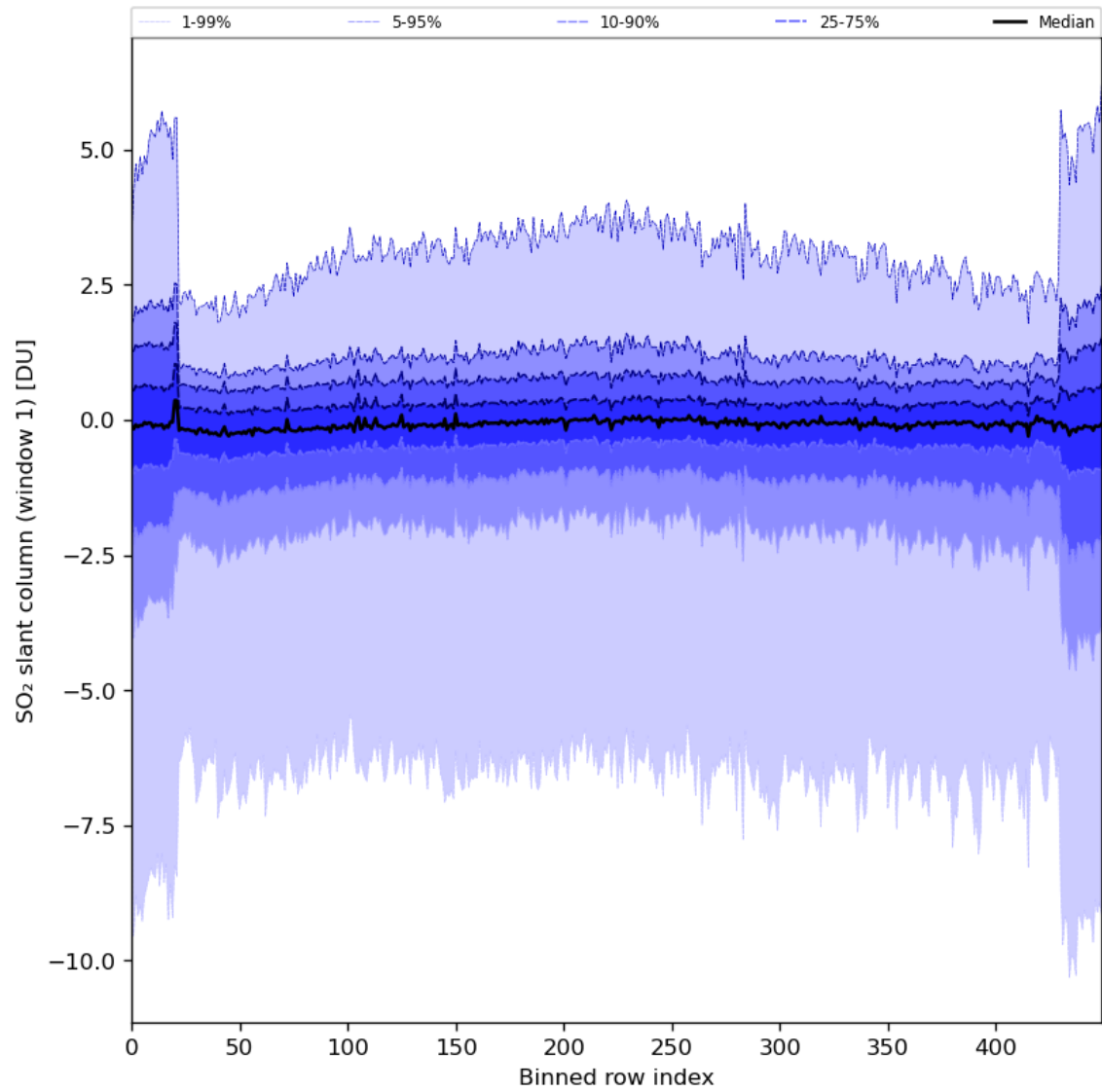
Figure 79: Along track statistics of “SO 2 slant column (window 1)” for 2024-01-26 to 2024-01-28
