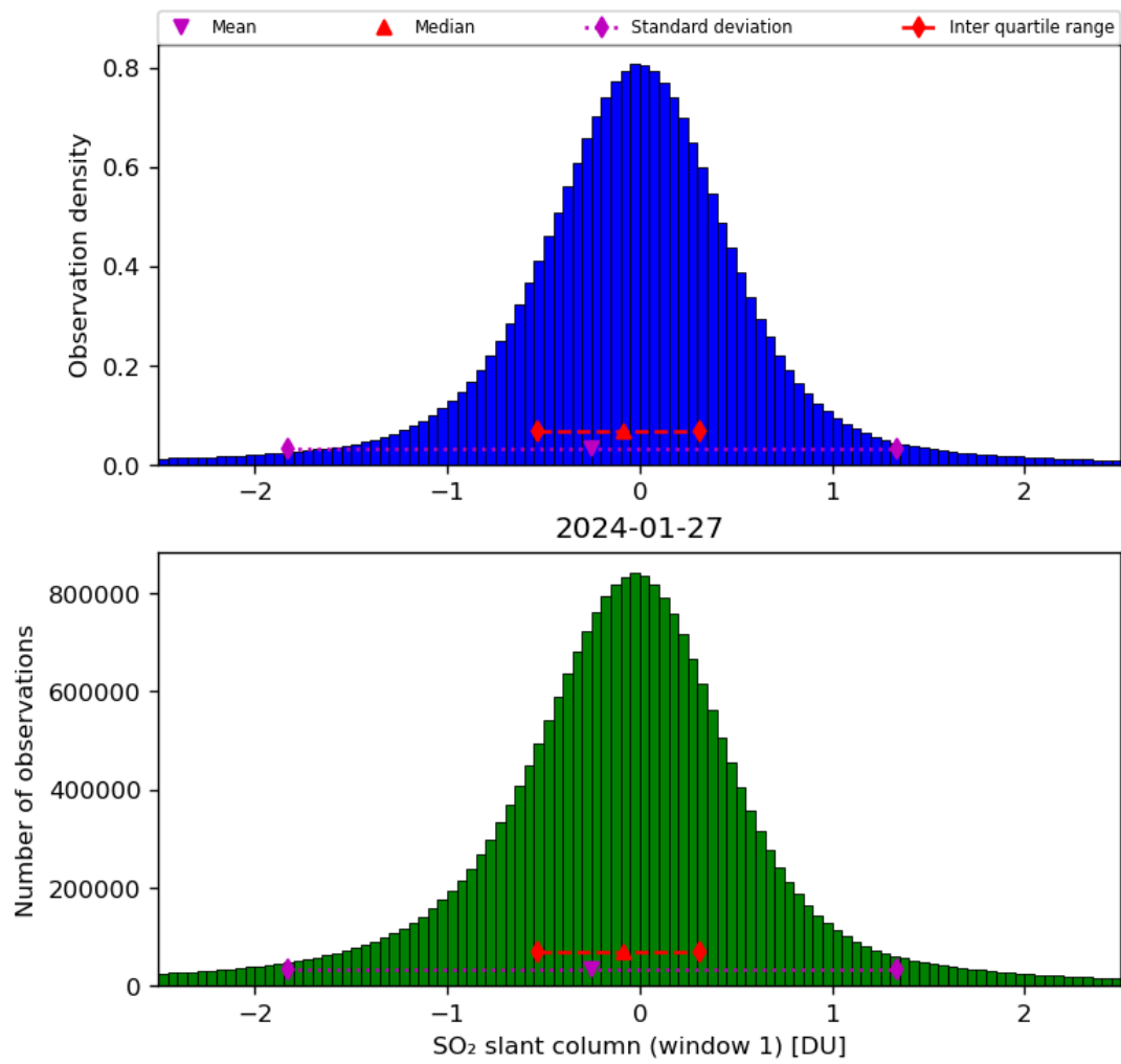
Figure 56: Histogram of “SO 2 slant column (window 1)” for 2024-01-26 to 2024-01-28
