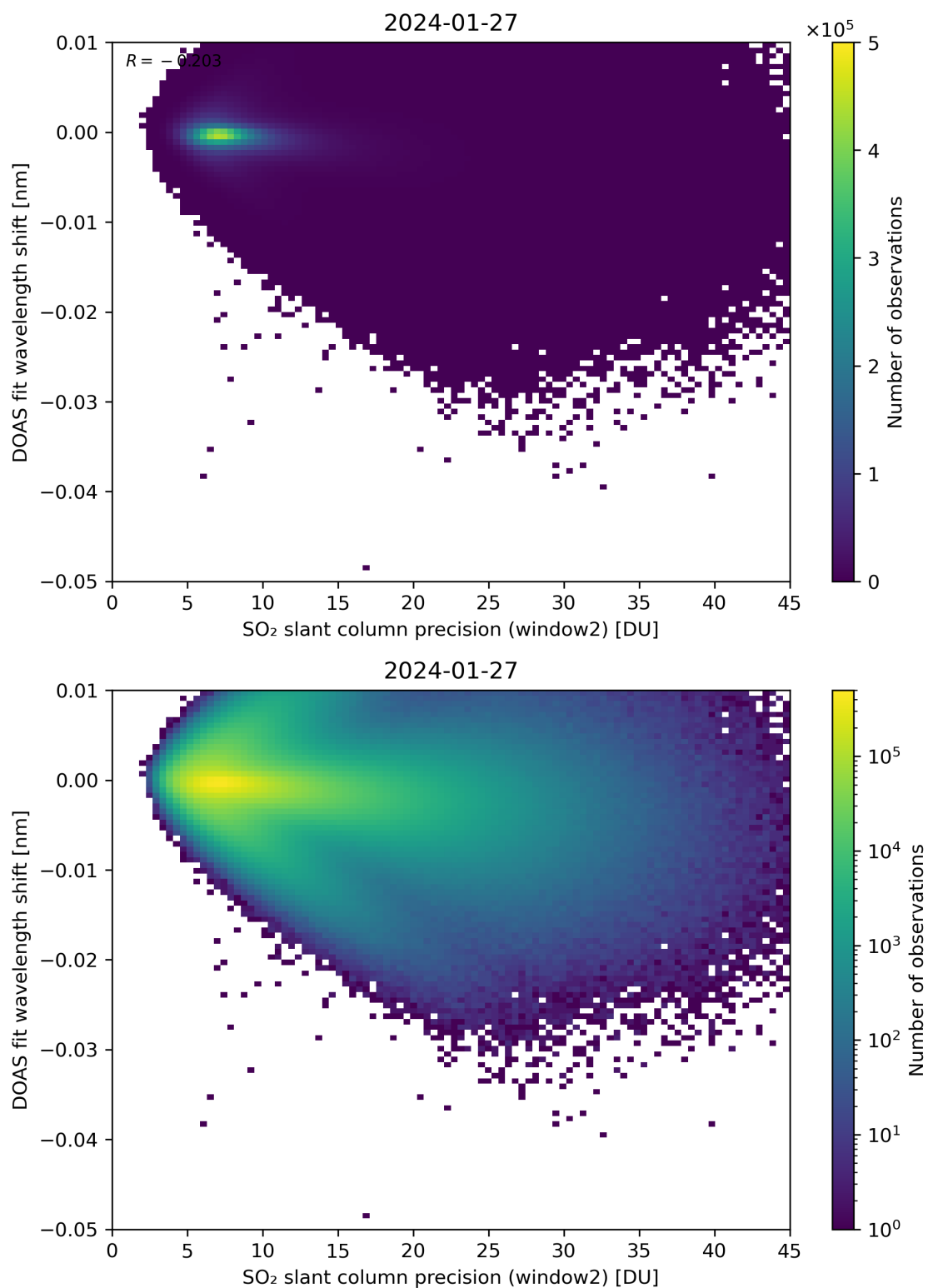
Figure 243: Scatter density plot of “SO 2 slant column precision (window2)” against “DOAS fit wavelength shift” for 2024-01-26 to 2024-01-28.
