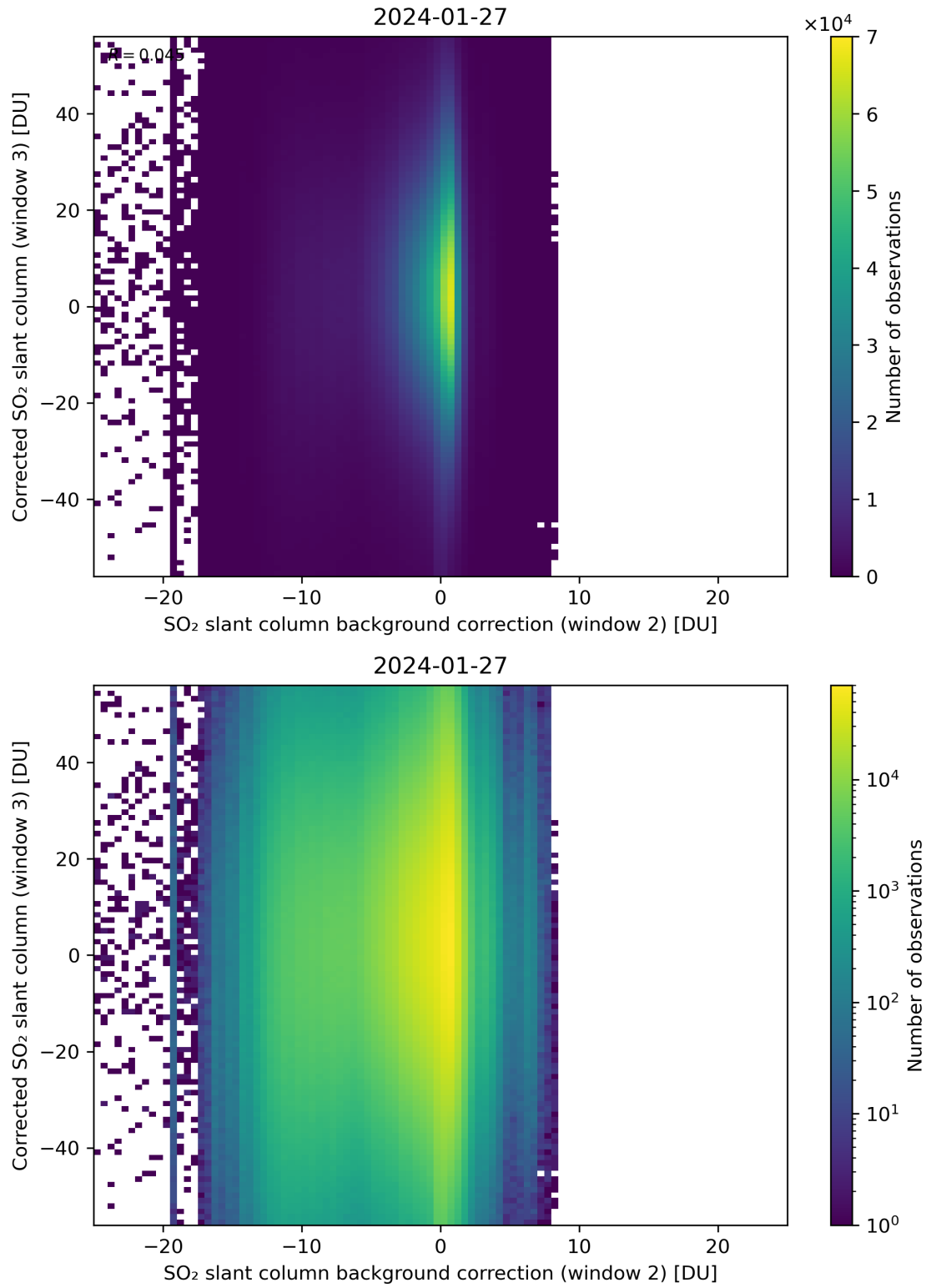
Figure 116: Scatter density plot of “SO 2 slant column background correction (window 2)” against “Corrected SO 2 slant column (window 3)” for 2024-01-26 to 2024-01-28.
