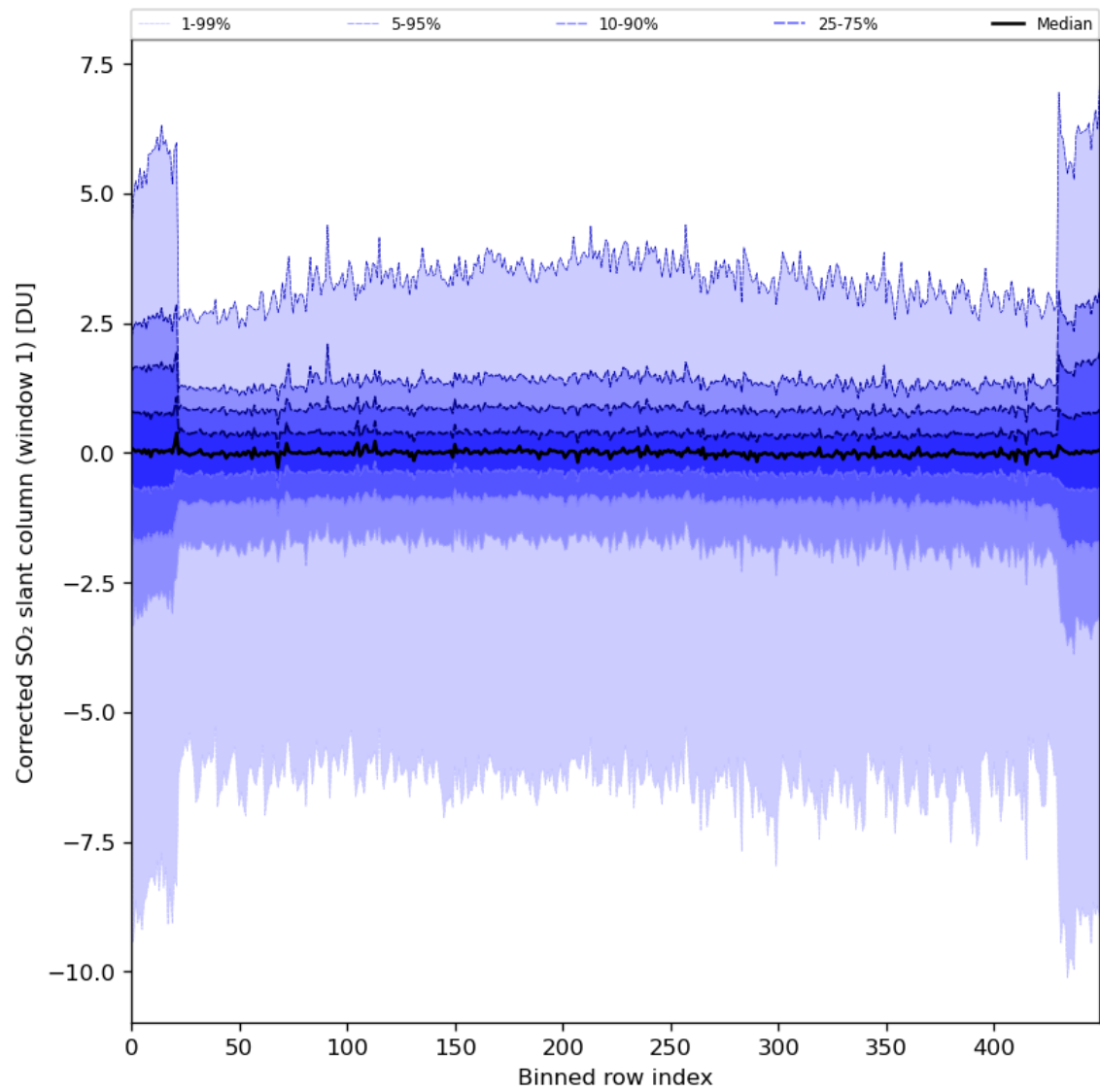
Figure 81: Along track statistics of “Corrected SO 2 slant column (window 1)” for 2024-01-26 to 2024-01-28
