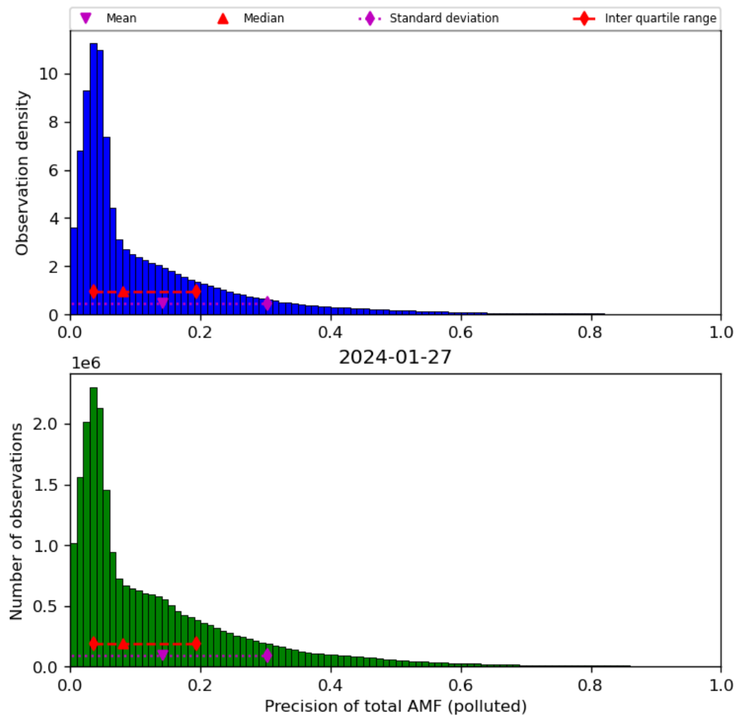
Figure 72: Histogram of “Precision of total AMF (polluted)” for 2024-01-26 to 2024-01-28
