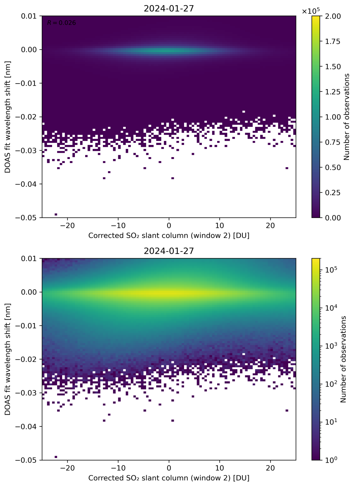
Figure 196: Scatter density plot of “Corrected SO 2 slant column (window 2)” against “DOAS fit wavelength shift” for 2024-01-26 to 2024-01-28.
