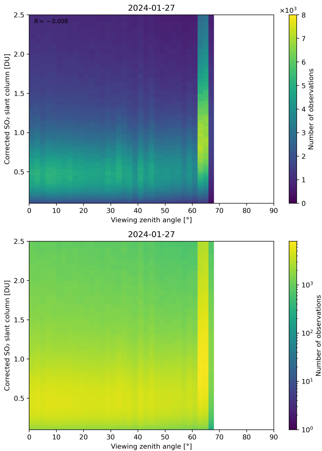
Figure 317: Scatter density plot of “Viewing zenith angle” against “Corrected SO 2 slant column” for 2024-01-26 to 2024-01-28.
