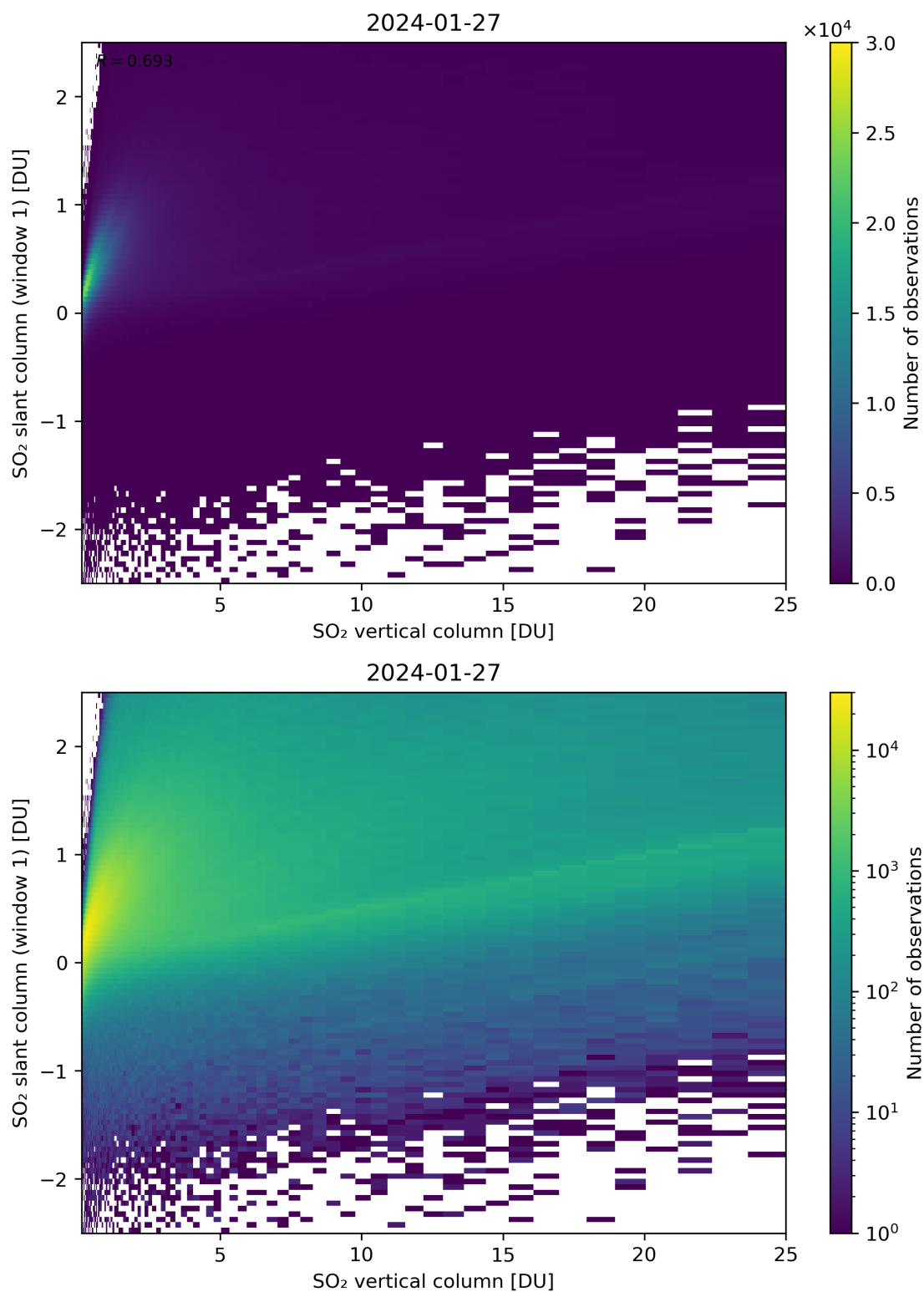
Figure 300: Scatter density plot of “SO 2 vertical column” against “SO 2 slant column (window 1)” for 2024-01-26 to 2024-01-28.
