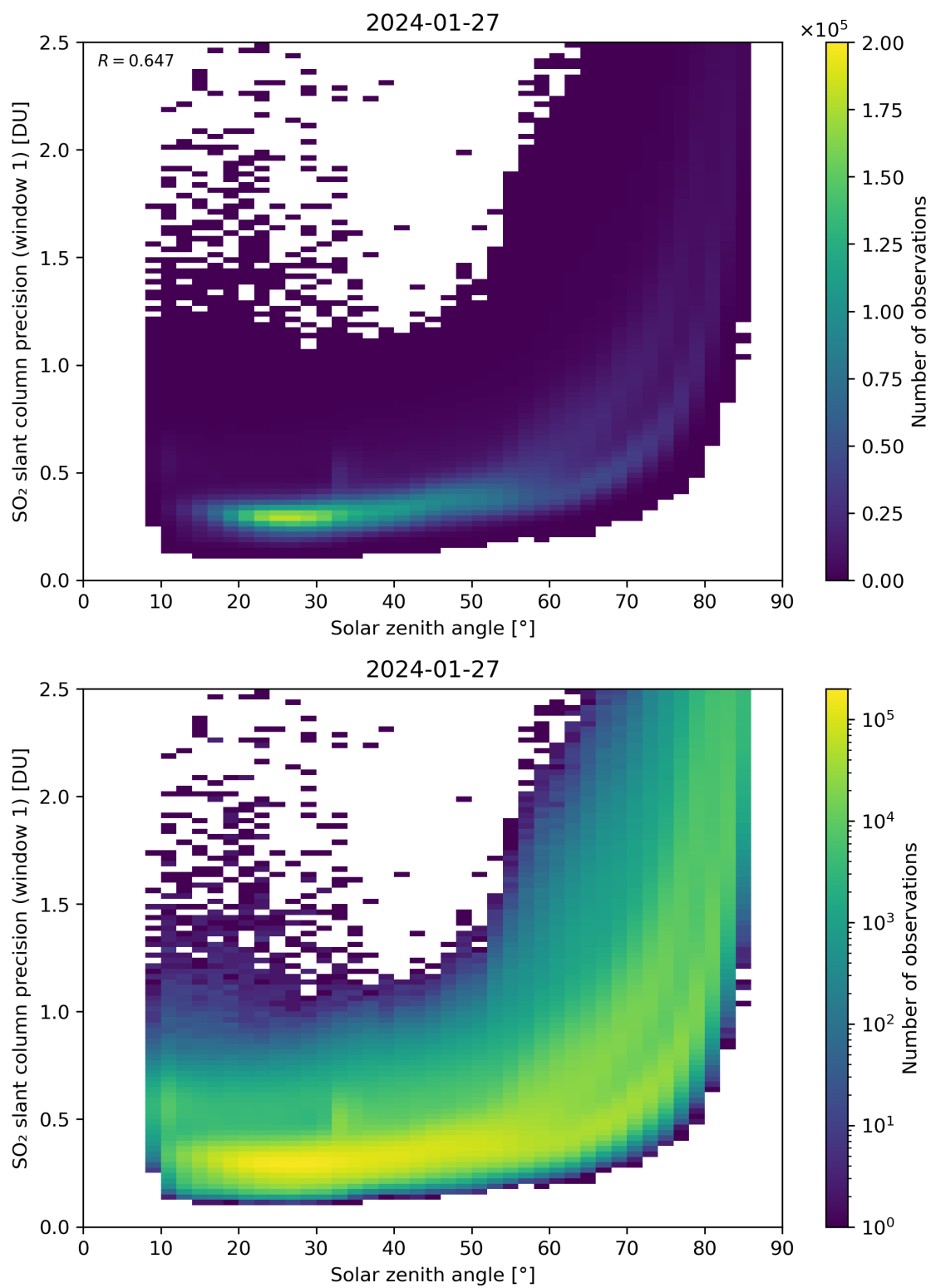
Figure 170: Scatter density plot of “Solar zenith angle” against “SO 2 slant column precision (window 1)” for 2024-01-26 to 2024-01-28.
