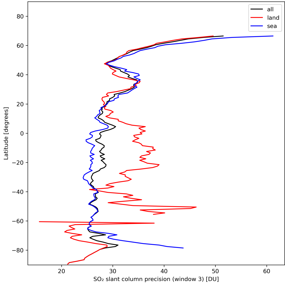
Figure 42: Zonal average of “SO 2 slant column precision (window 3)” for 2024-01-26 to 2024-01-28.
