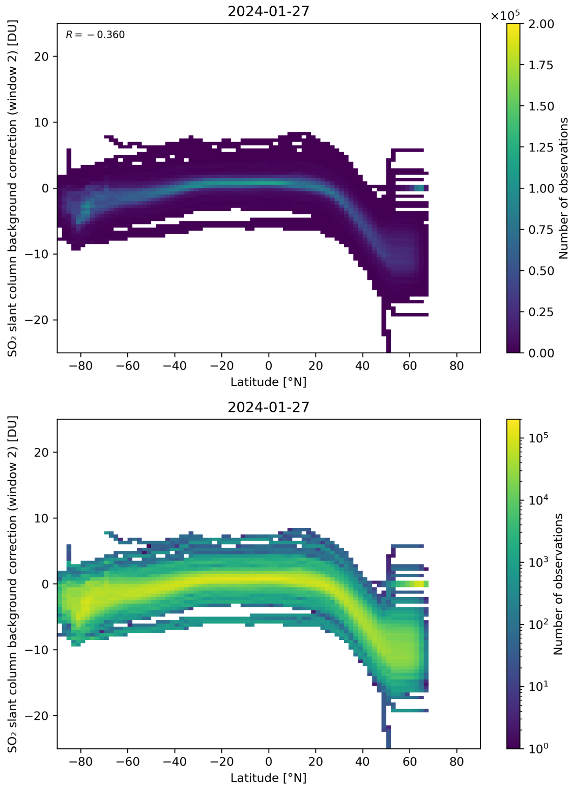
Figure 140: Scatter density plot of “Latitude” against “SO 2 slant column background correction (window 2)” for 2024-01-26 to 2024-01-28.
