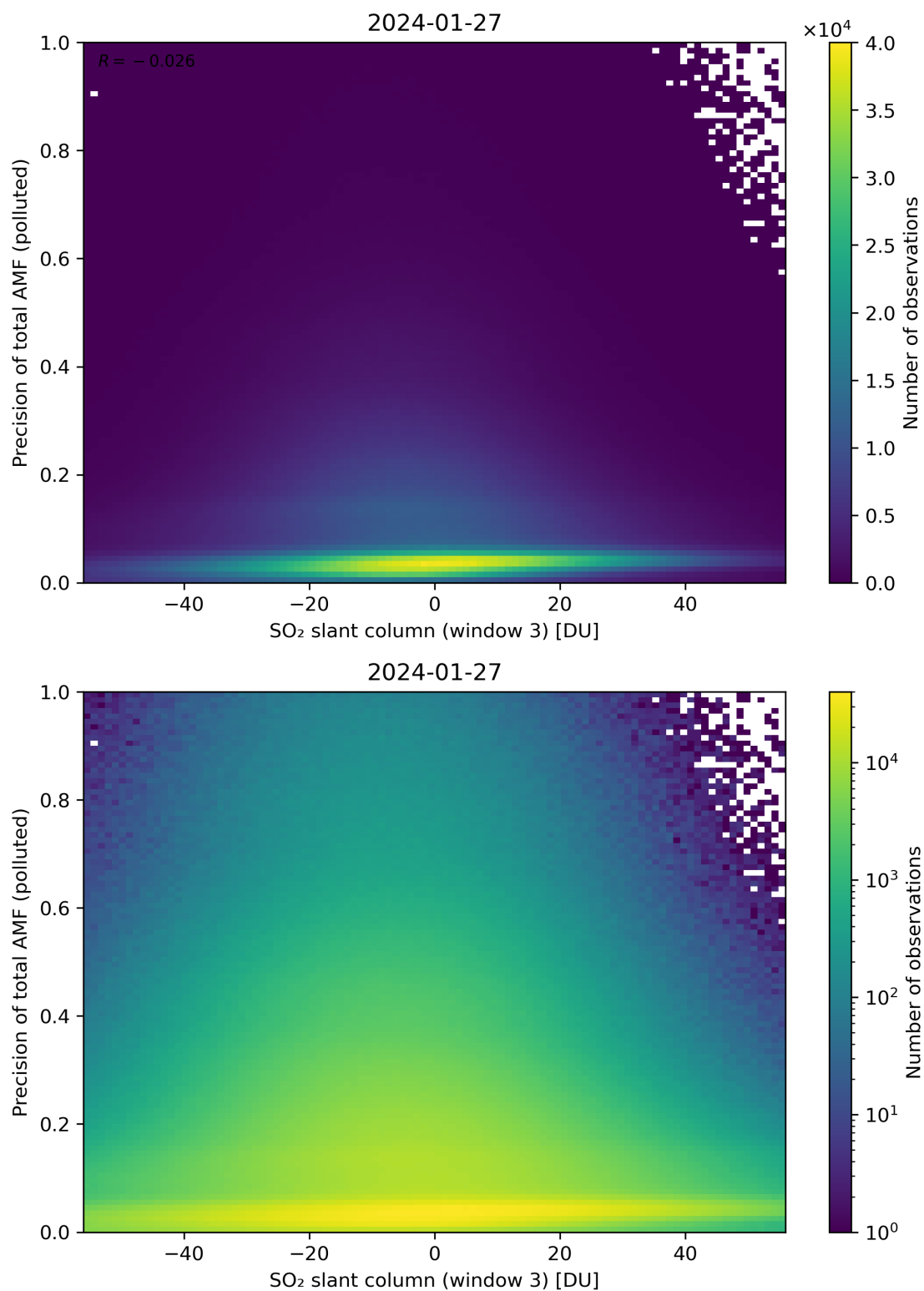
Figure 269: Scatter density plot of “SO 2 slant column (window 3)” against “Precision of total AMF (polluted)” for 2024-01-26 to 2024-01-28.
