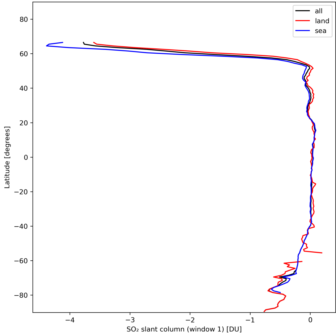
Figure 33: Zonal average of “SO 2 slant column (window 1)” for 2024-01-26 to 2024-01-28.
