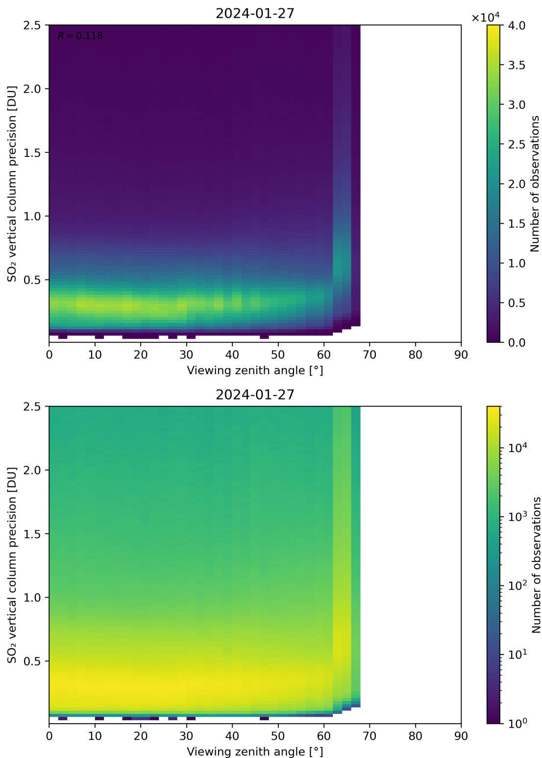
Figure 328: Scatter density plot of “Viewing zenith angle” against “SO 2 vertical column precision” for 2024-01-26 to 2024-01-28.
