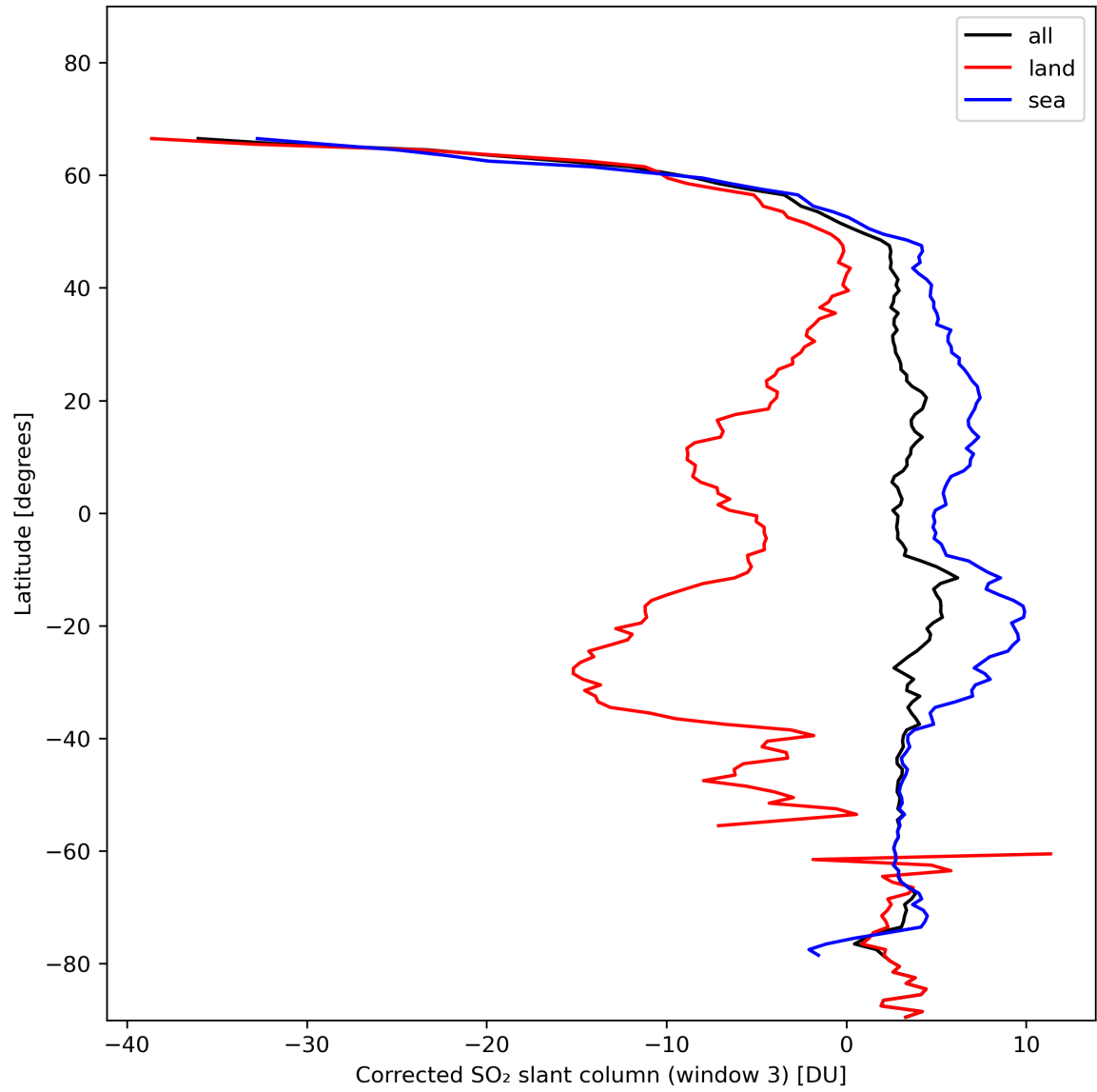
Figure 43: Zonal average of “Corrected SO 2 slant column (window 3)” for 2024-01-26 to 2024-01-28.
