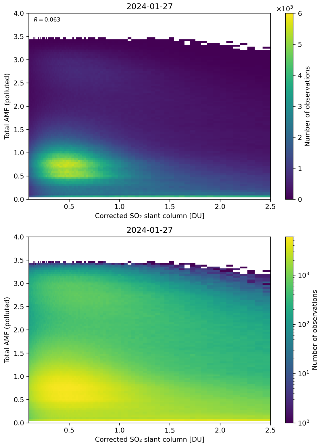
Figure 192: Scatter density plot of “Corrected SO 2 slant column” against “Total AMF (polluted)” for 2024-01-26 to 2024-01-28.
