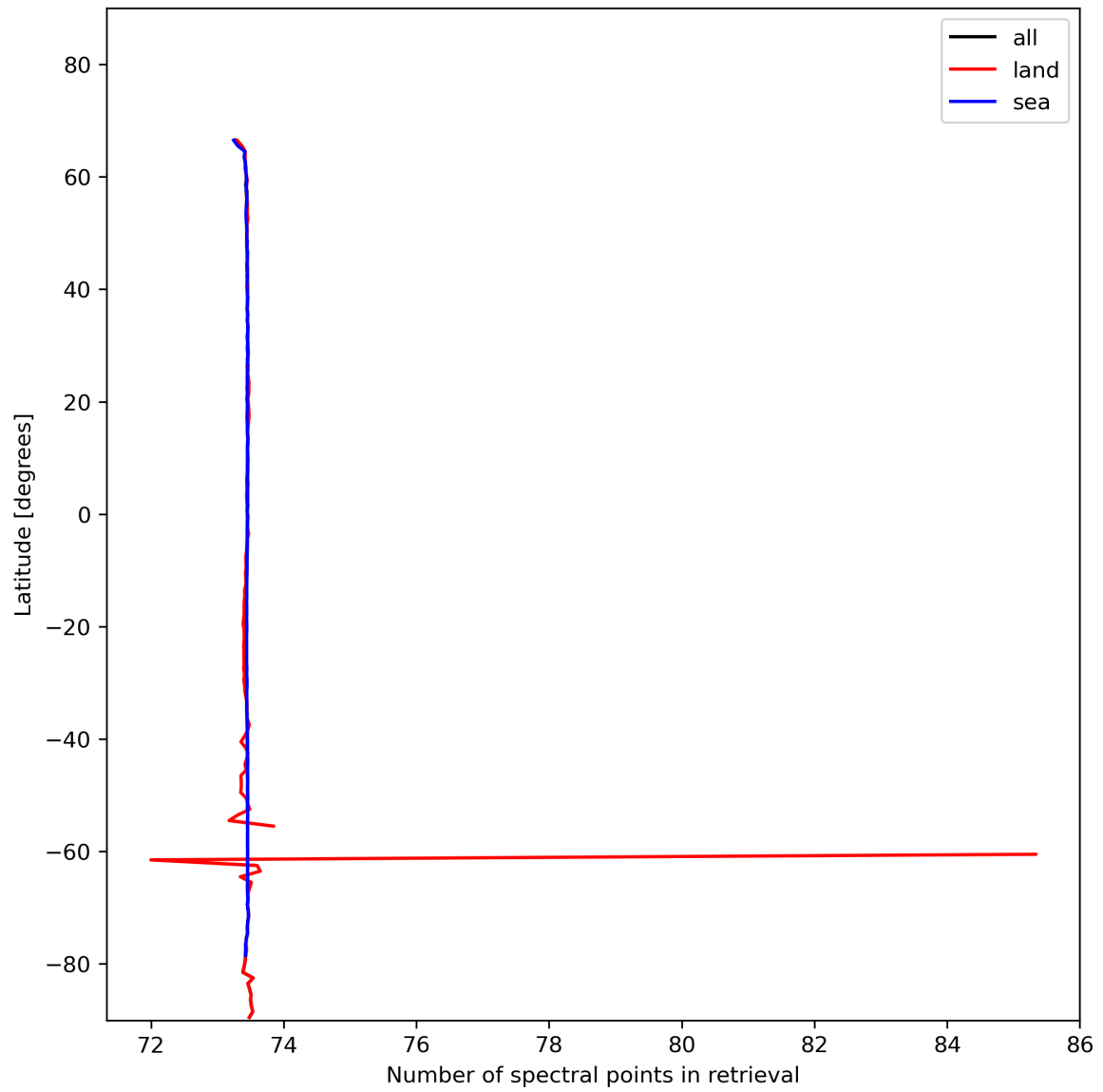
Figure 51: Zonal average of “Number of spectral points in retrieval” for 2024-01-26 to 2024-01-28.
