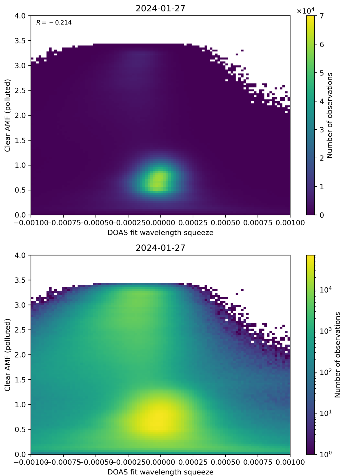
Figure 133: Scatter density plot of “DOAS fit wavelength squeeze” against “Clear AMF (polluted)” for 2024-01-26 to 2024-01-28.
