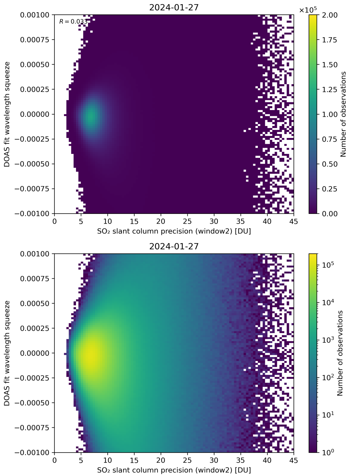
Figure 244: Scatter density plot of “SO 2 slant column precision (window2)” against “DOAS fit wavelength squeeze” for 2024-01-26 to 2024-01-28.
