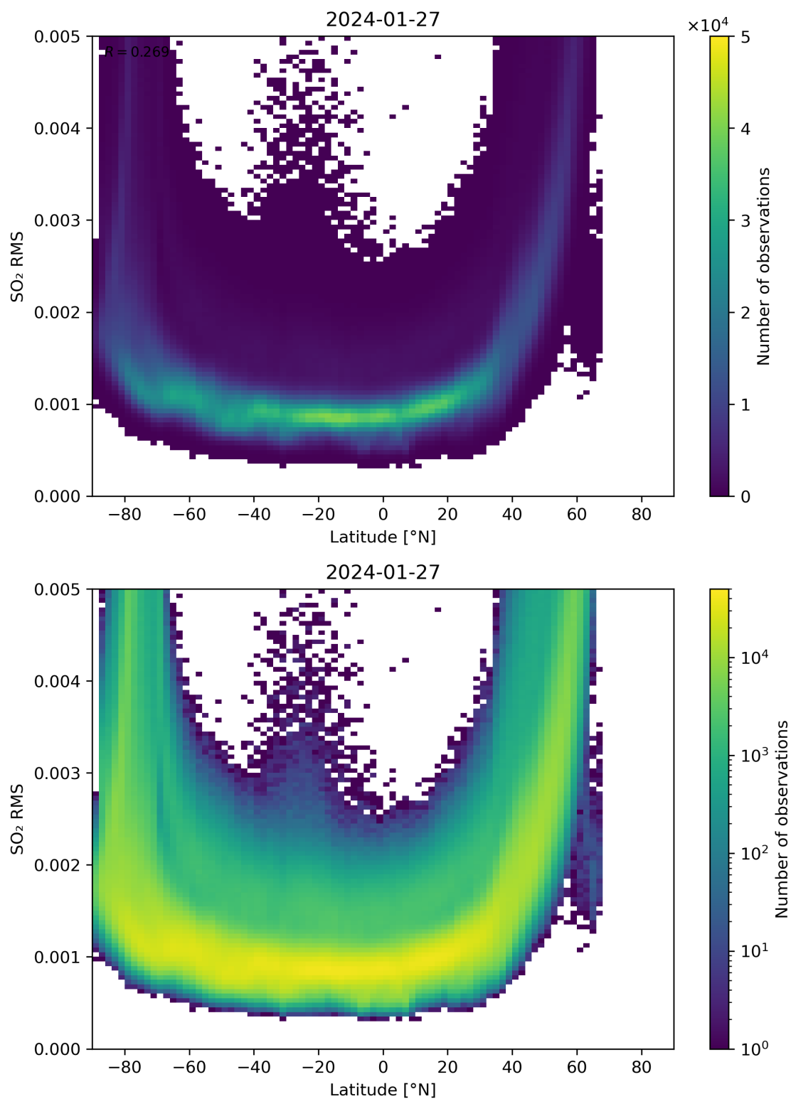
Figure 144: Scatter density plot of “Latitude” against “SO 2 RMS” for 2024-01-26 to 2024-01-28.
