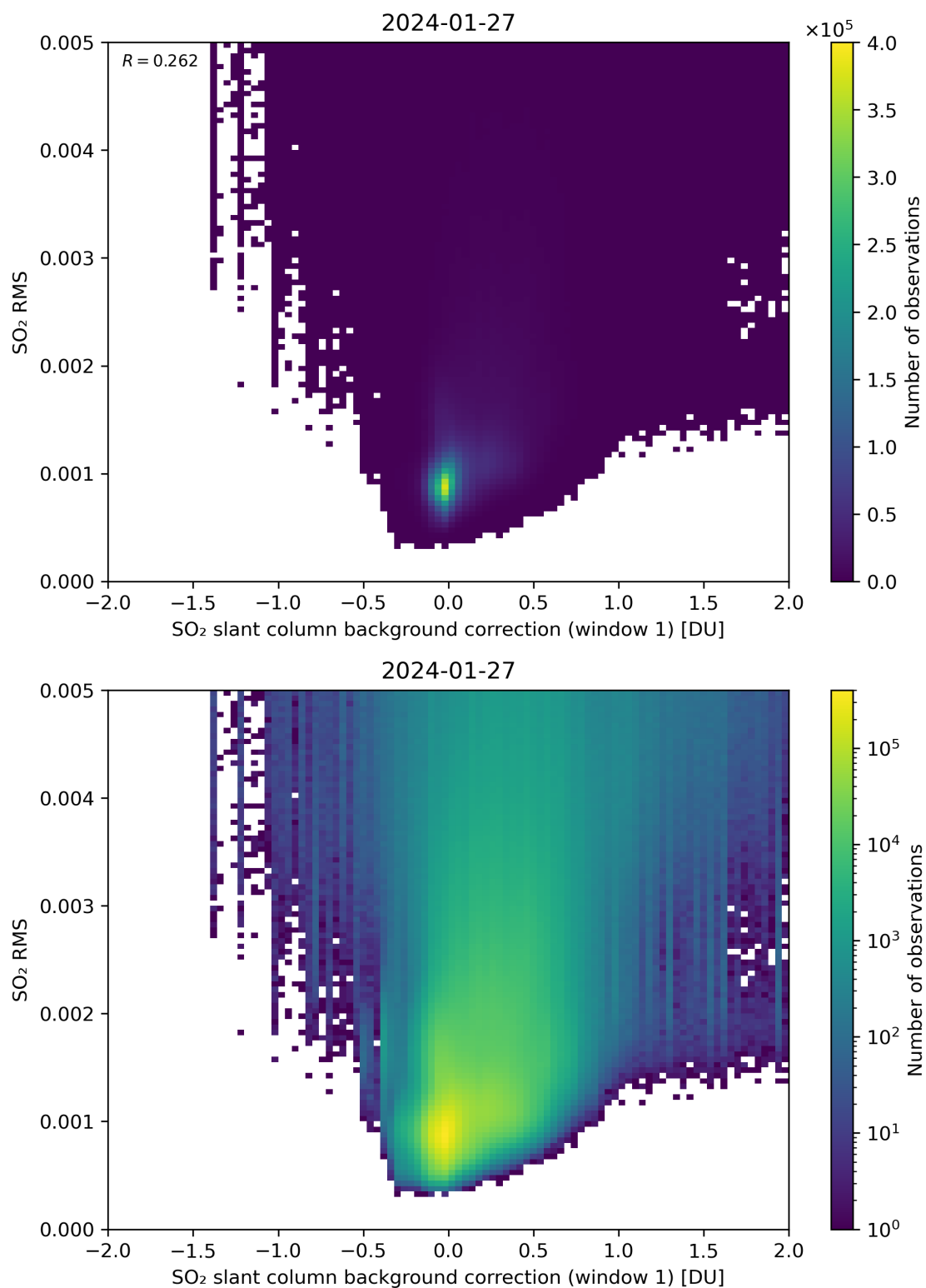
Figure 102: Scatter density plot of “SO 2 slant column background correction (window 1)” against “SO 2 RMS” for 2024-01-26 to 2024-01-28.
