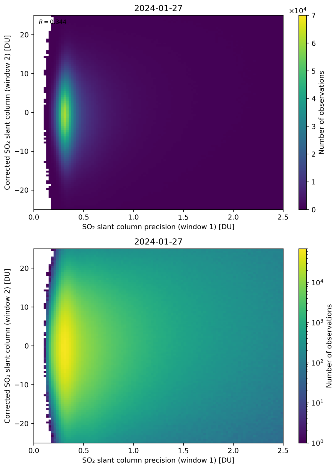
Figure 225: Scatter density plot of “SO 2 slant column precision (window 1)” against “Corrected SO 2 slant column (window 2)” for 2024-01-26 to 2024-01-28.
