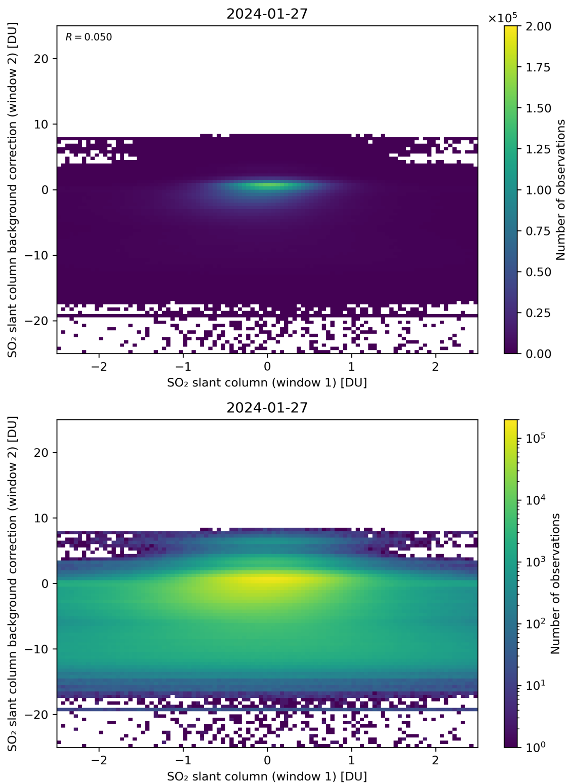
Figure 213: Scatter density plot of “SO 2 slant column (window 1)” against “SO 2 slant column background correction (window 2)” for 2024-01-26 to 2024-01-28.
