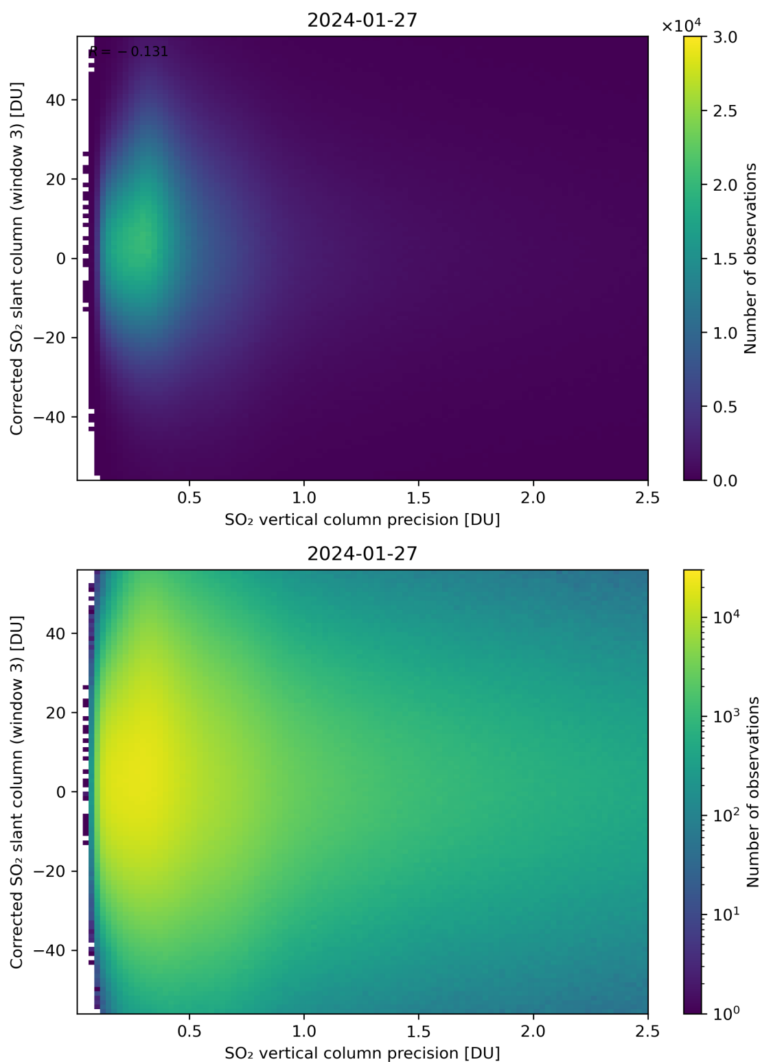
Figure 288: Scatter density plot of “SO 2 vertical column precision” against “Corrected SO 2 slant column (window 3)” for 2024-01-26 to 2024-01-28.
