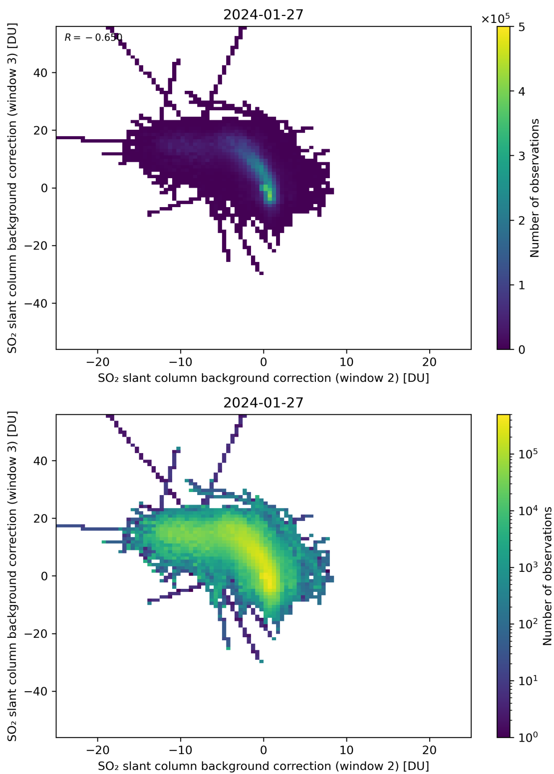
Figure 111: Scatter density plot of “SO 2 slant column background correction (window 2)” against “SO 2 slant column background correction (window 3)” for 2024-01-26 to 2024-01-28.
