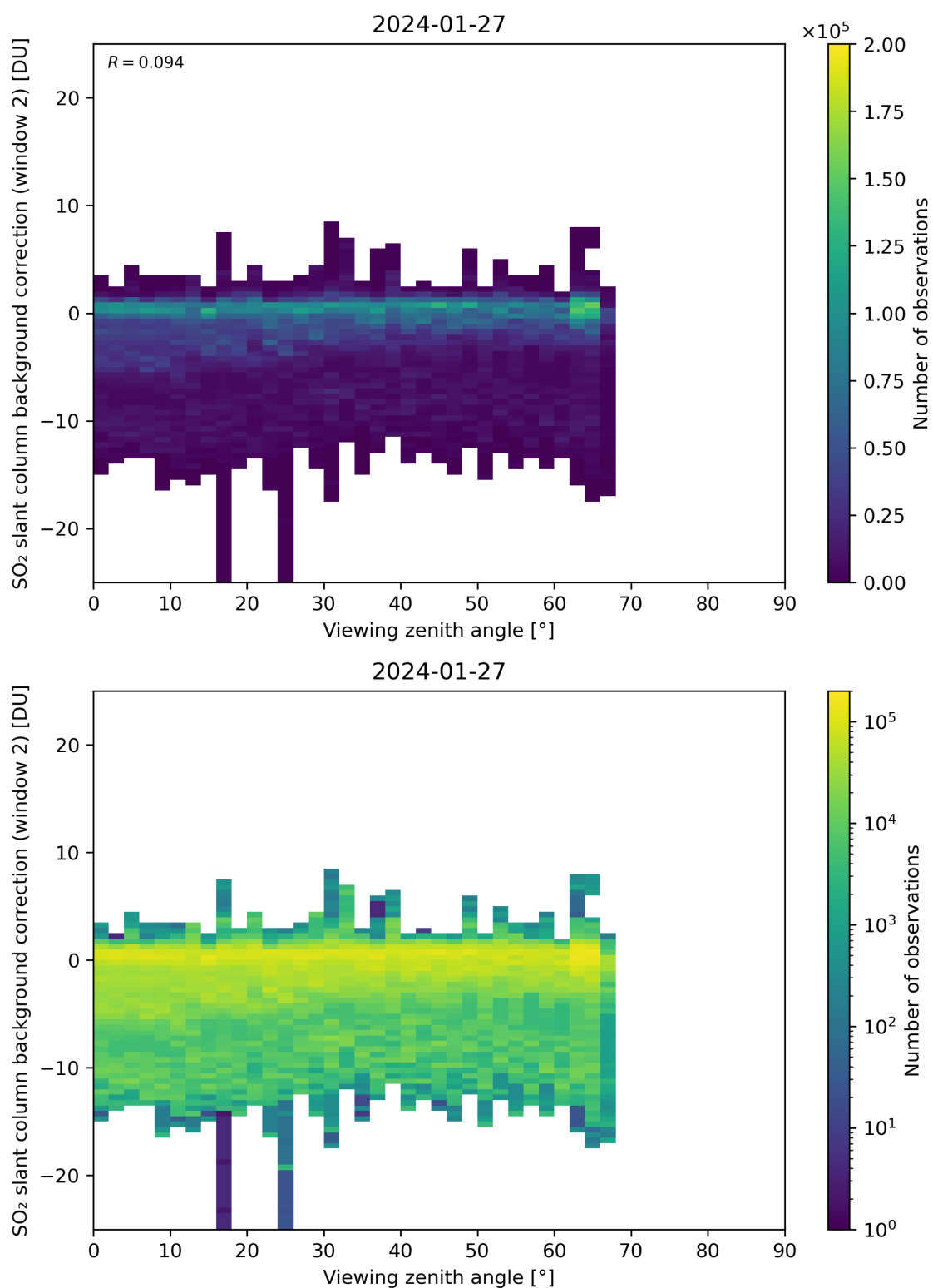
Figure 309: Scatter density plot of “Viewing zenith angle” against “SO 2 slant column background correction (window 2)” for 2024-01-26 to 2024-01-28.
