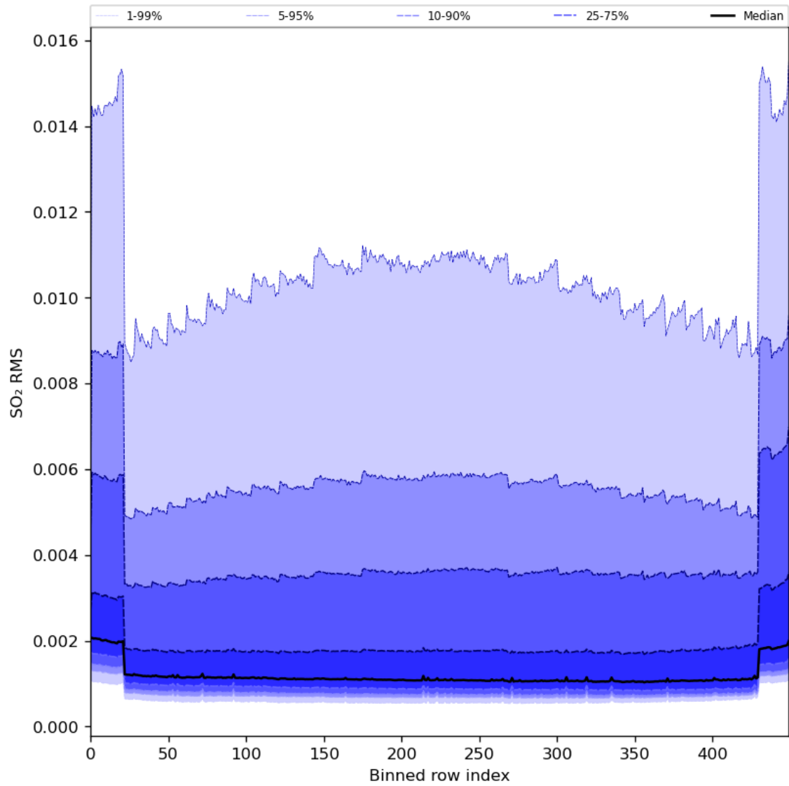
Figure 93: Along track statistics of "SO 2 RMS" for 2024-01-26 to 2024-01-28
