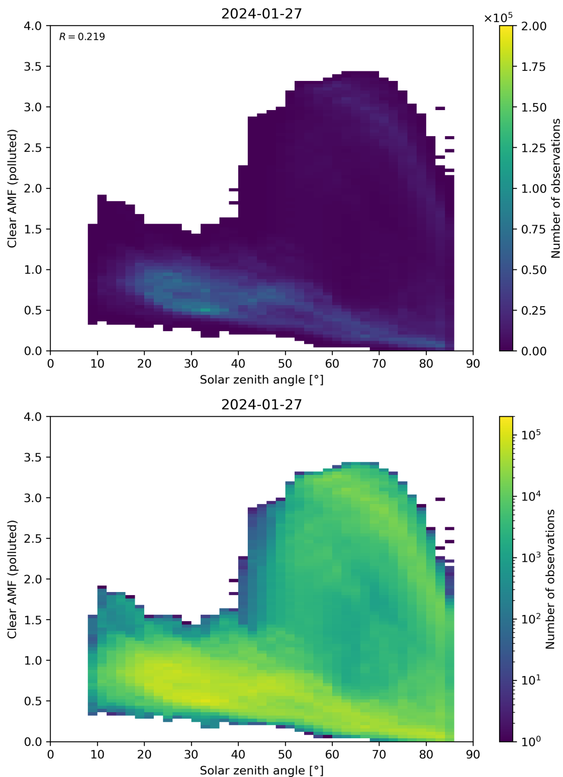
Figure 165: Scatter density plot of “Solar zenith angle” against “Clear AMF (polluted)” for 2024-01-26 to 2024-01-28.
