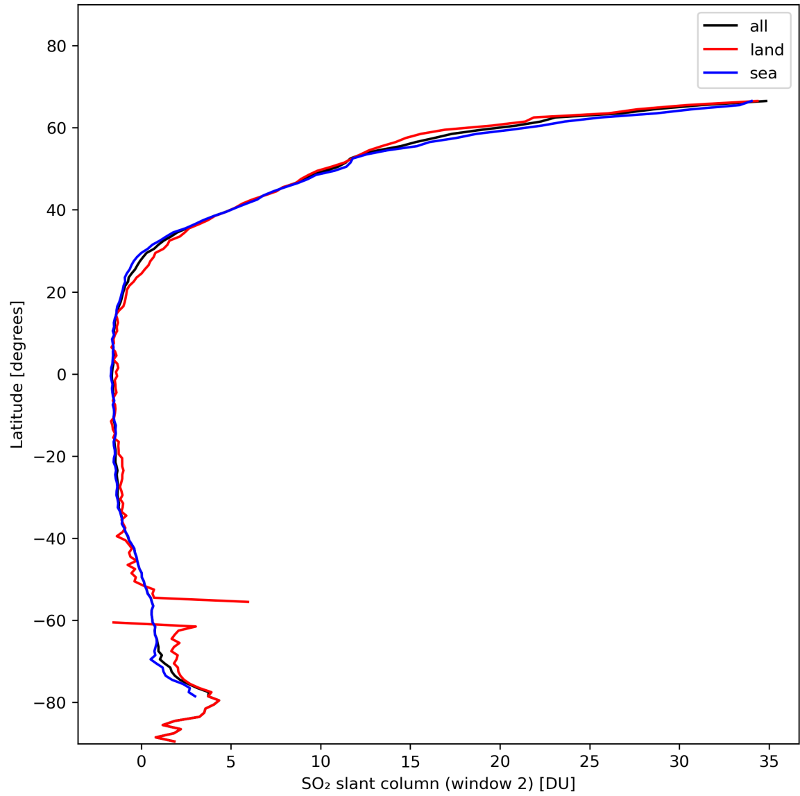
Figure 37: Zonal average of “SO 2 slant column (window 2)” for 2024-01-26 to 2024-01-28.
