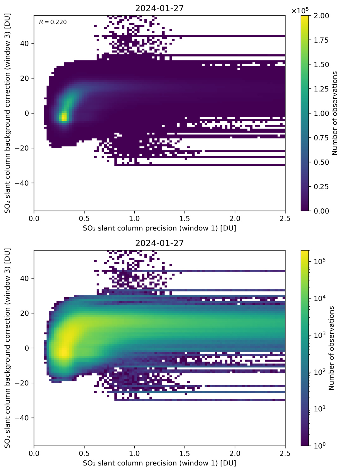
Figure 220: Scatter density plot of “SO 2 slant column precision (window 1)” against “SO 2 slant column background correction (window 3)” for 2024-01-26 to 2024-01-28.
