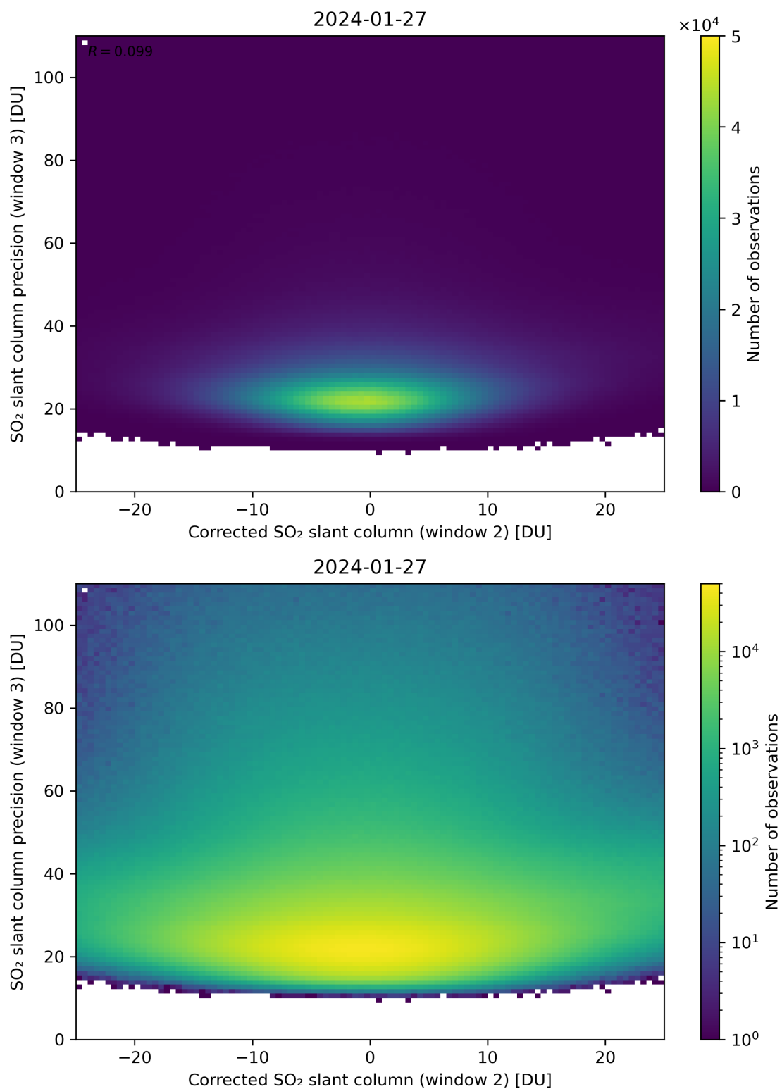
Figure 202: Scatter density plot of “Corrected SO 2 slant column (window 2)” against “SO 2 slant column precision (window 3)” for 2024-01-26 to 2024-01-28.
