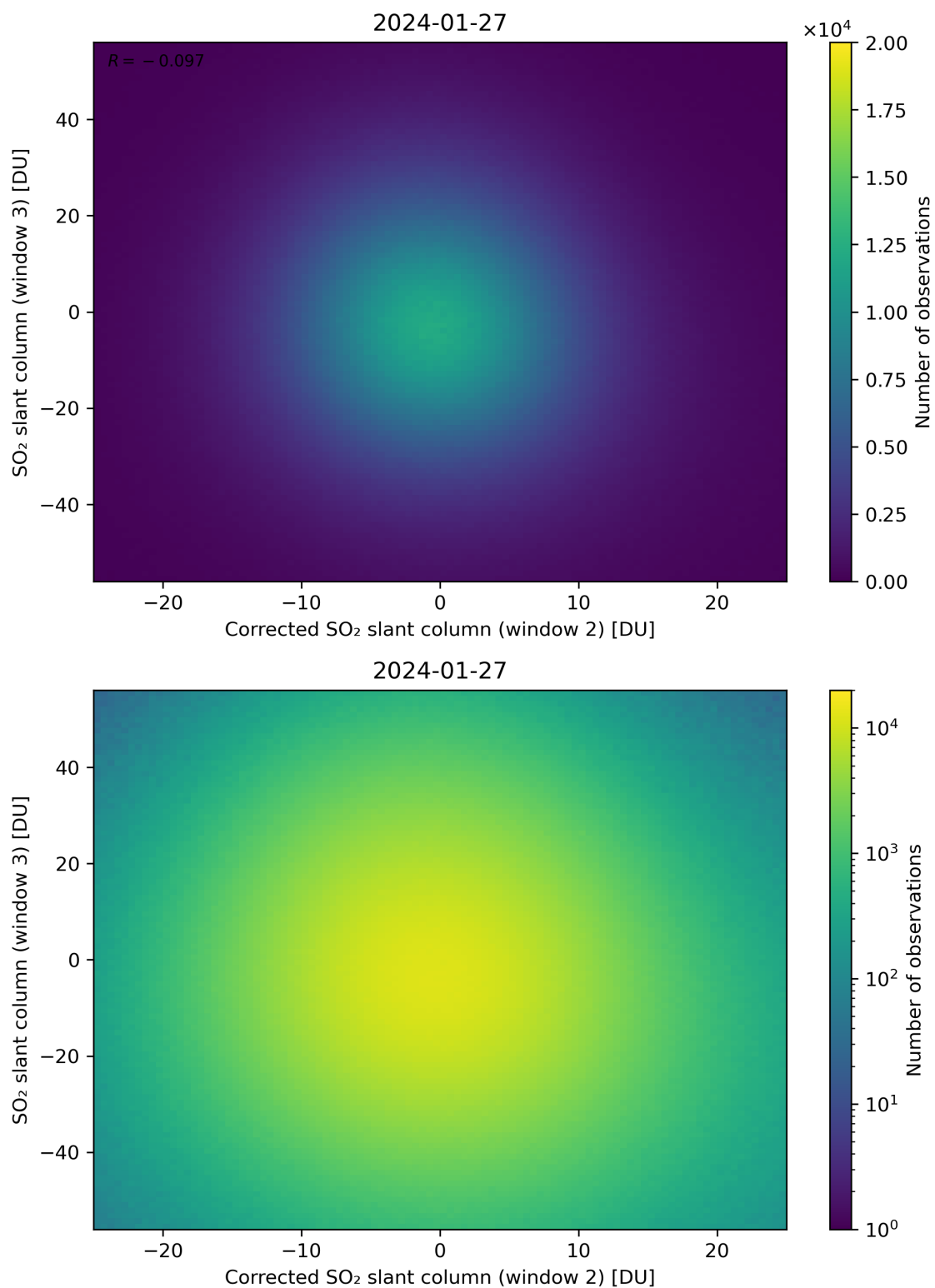
Figure 201: Scatter density plot of “Corrected SO 2 slant column (window 2)” against “SO 2 slant column (window 3)” for 2024-01-26 to 2024-01-28.
