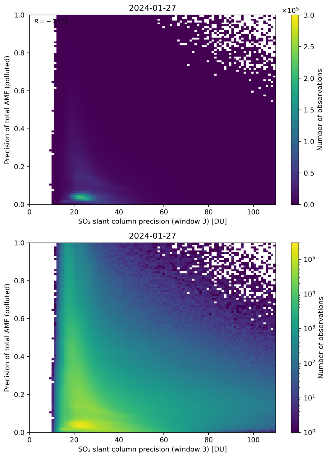
Figure 264: Scatter density plot of “SO 2 slant column precision (window 3)” against “Precision of total AMF (polluted)” for 2024-01-26 to 2024-01-28.
