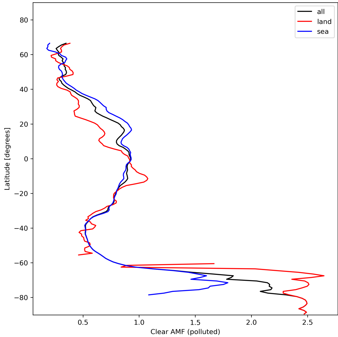
Figure 50: Zonal average of “Clear AMF (polluted)” for 2024-01-26 to 2024-01-28.
