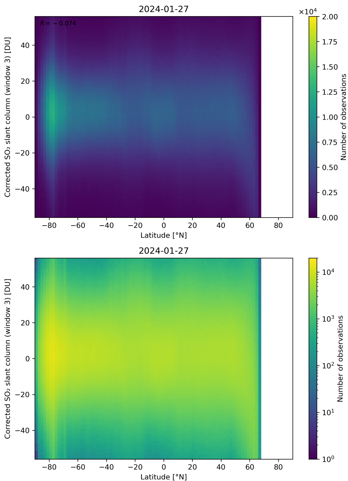
Figure 148: Scatter density plot of “Latitude” against “Corrected SO 2 slant column (window 3)” for 2024-01-26 to 2024-01-28.
