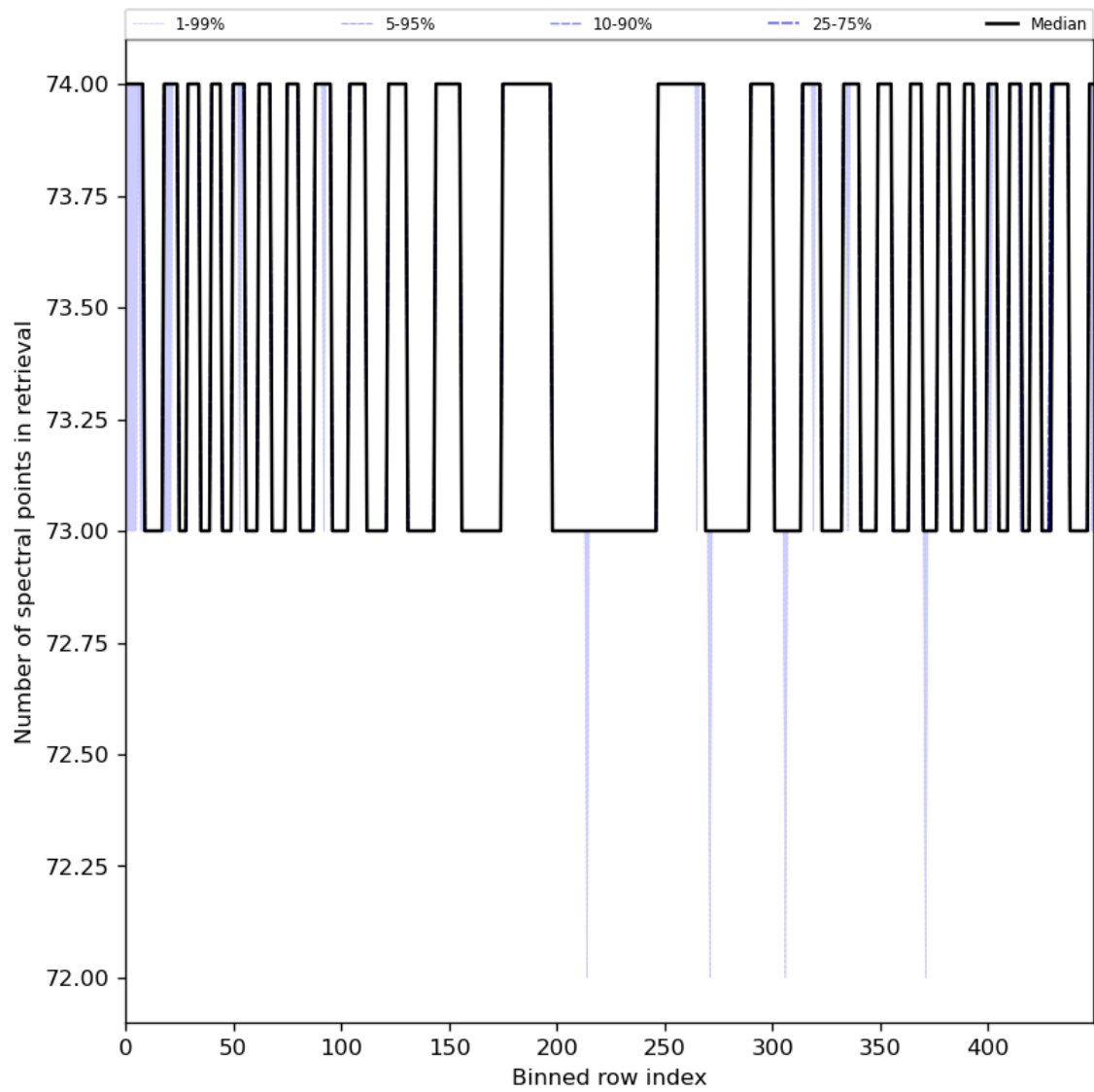
Figure 97: Along track statistics of “Number of spectral points in retrieval” for 2024-01-26 to 2024-01-28
