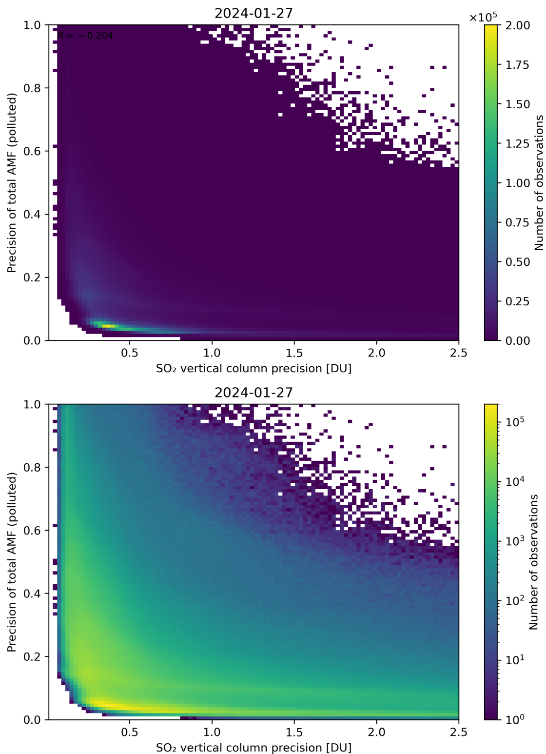
Figure 295: Scatter density plot of “SO 2 vertical column precision” against “Precision of total AMF (polluted)” for 2024-01-26 to 2024-01-28.
