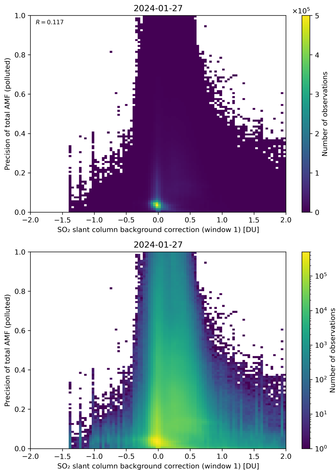
Figure 110: Scatter density plot of “SO 2 slant column background correction (window 1)” against “Precision of total AMF (polluted)” for 2024-01-26 to 2024-01-28.
