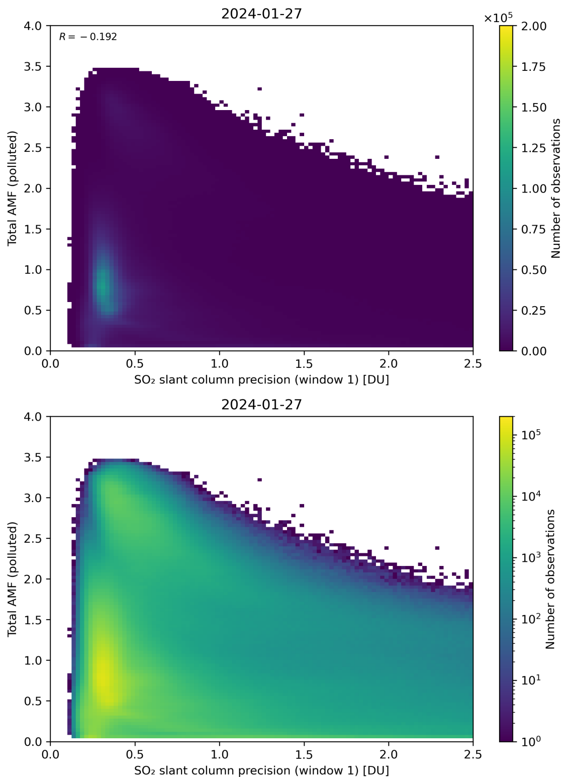
Figure 230: Scatter density plot of “SO 2 slant column precision (window 1)” against “Total AMF (polluted)” for 2024-01-26 to 2024-01-28.
