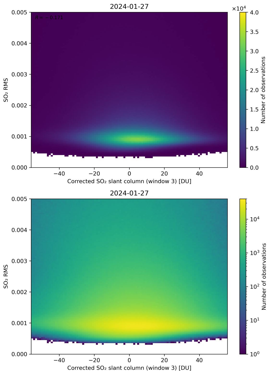
Figure 208: Scatter density plot of “Corrected SO 2 slant column (window 3)” against “SO 2 RMS” for 2024-01-26 to 2024-01-28.
