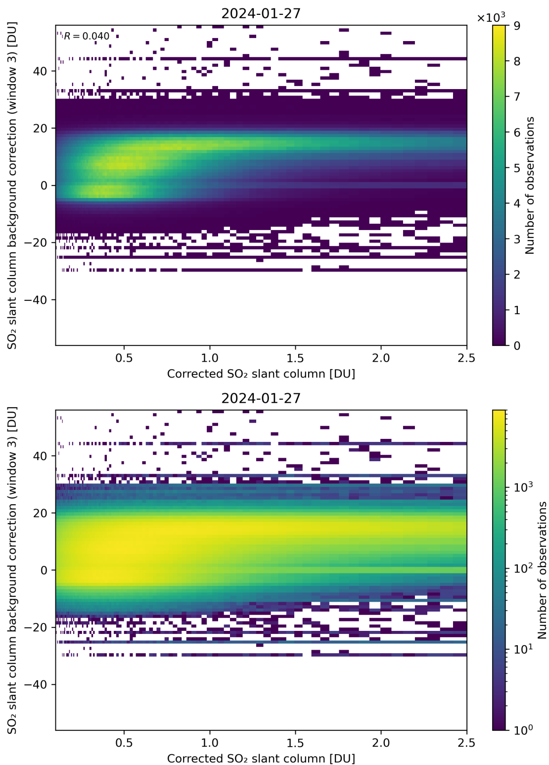
Figure 180: Scatter density plot of “Corrected SO 2 slant column” against “SO 2 slant column background correction (window 3)” for 2024-01-26 to 2024-01-28.
