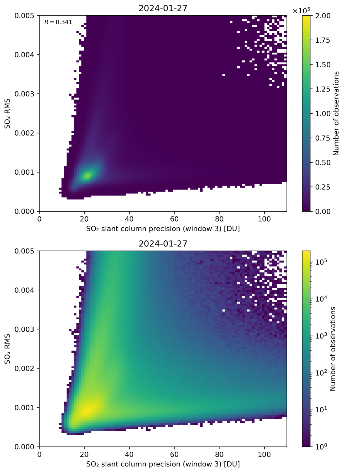
Figure 260: Scatter density plot of “SO 2 slant column precision (window 3)” against “SO 2 RMS” for 2024-01-26 to 2024-01-28.
