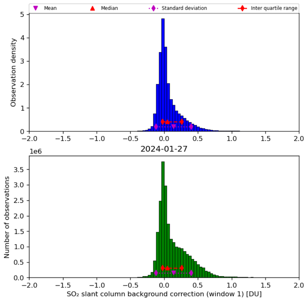
Figure 59: Histogram of “SO 2 slant column background correction (window 1)” for 2024-01-26 to 2024-01-28
