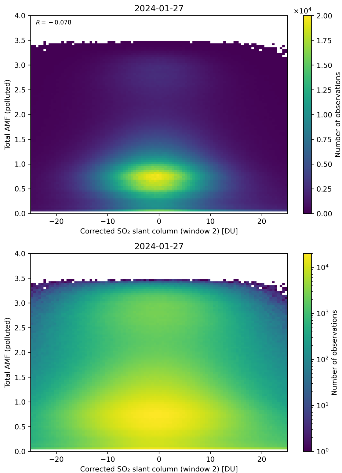
Figure 203: Scatter density plot of “Corrected SO 2 slant column (window 2)” against “Total AMF (polluted)” for 2024-01-26 to 2024-01-28.
