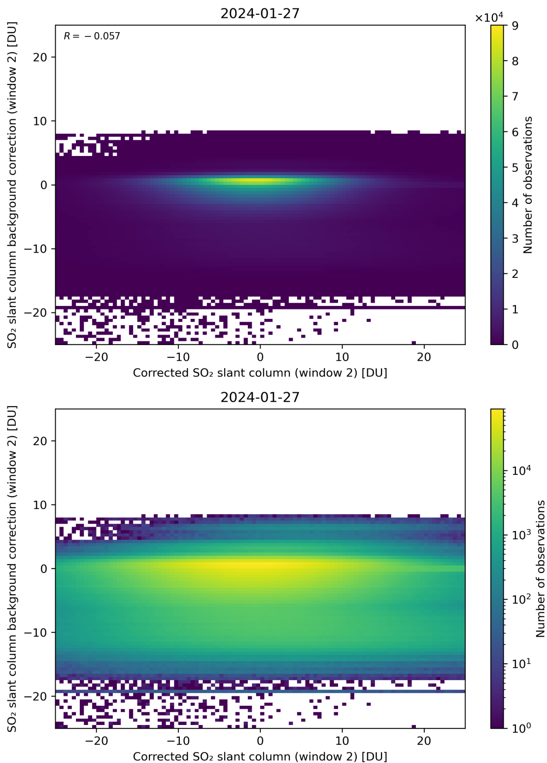
Figure 194: Scatter density plot of “Corrected SO 2 slant column (window 2)” against “SO 2 slant column background correction (window 2)” for 2024-01-26 to 2024-01-28.
