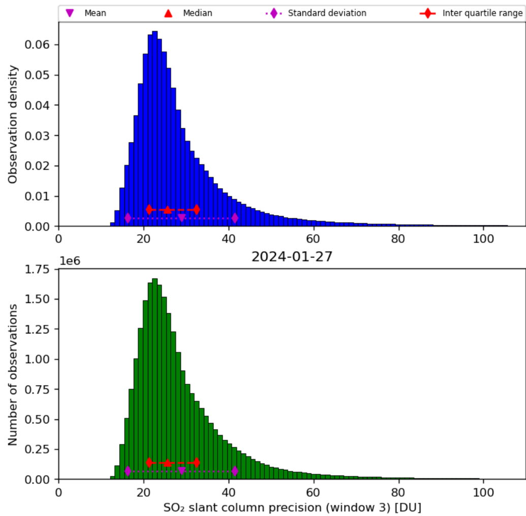
Figure 65: Histogram of “SO 2 slant column precision (window 3)” for 2024-01-26 to 2024-01-28
