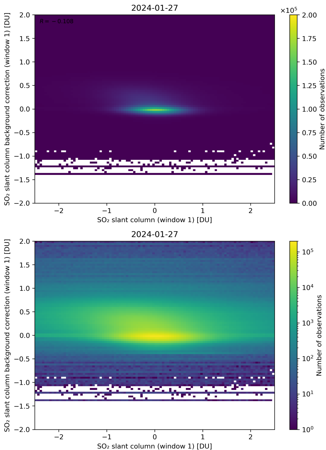
Figure 212: Scatter density plot of “SO 2 slant column (window 1)” against “SO 2 slant column background correction (window 1)” for 2024-01-26 to 2024-01-28.
