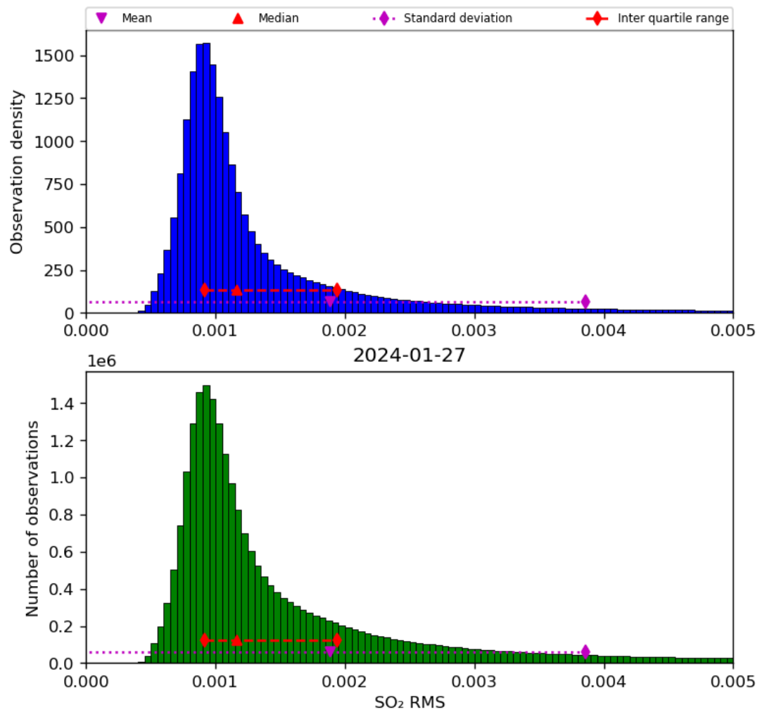
Figure 70: Histogram of “SO 2 RMS” for 2024-01-26 to 2024-01-28
