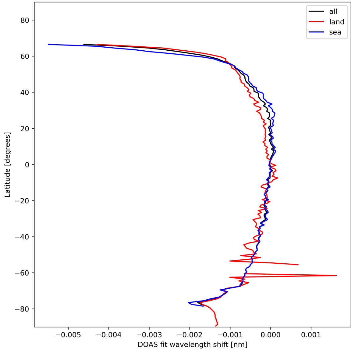
Figure 45: Zonal average of “DOAS fit wavelength shift” for 2024-01-26 to 2024-01-28.
