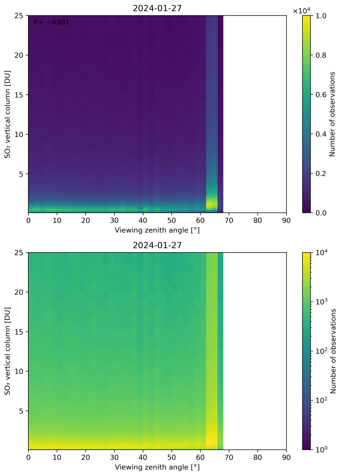
Figure 327: Scatter density plot of “Viewing zenith angle” against “SO 2 vertical column” for 2024-01-26 to 2024-01-28.
