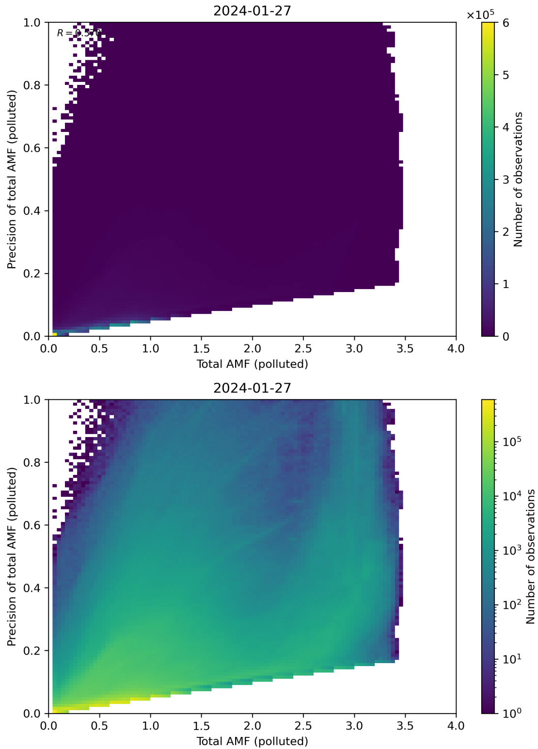
Figure 272: Scatter density plot of “Total AMF (polluted)” against “Precision of total AMF (polluted)” for 2024-01-26 to 2024-01-28.
