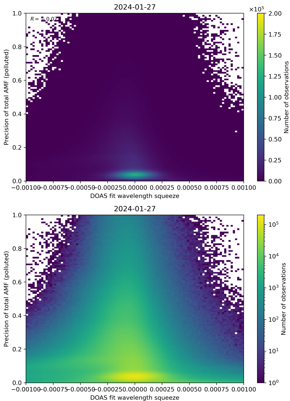
Figure 135: Scatter density plot of “DOAS fit wavelength squeeze” against “Precision of total AMF (polluted)” for 2024-01-26 to 2024-01-28.
