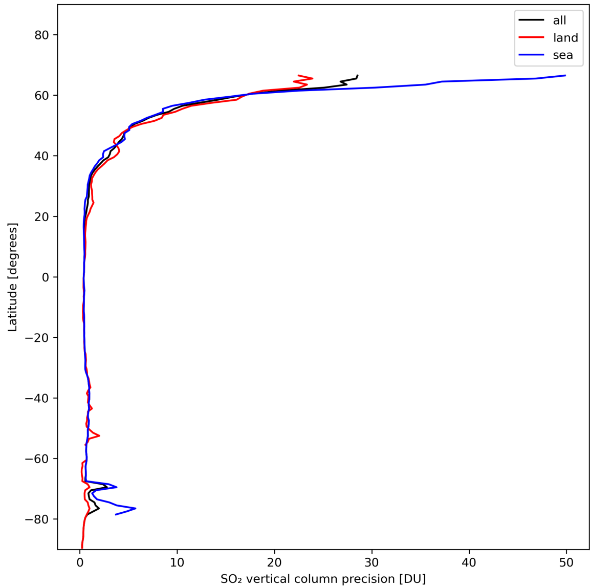
Figure 31: Zonal average of “SO 2 vertical column precision” for 2024-01-26 to 2024-01-28.
