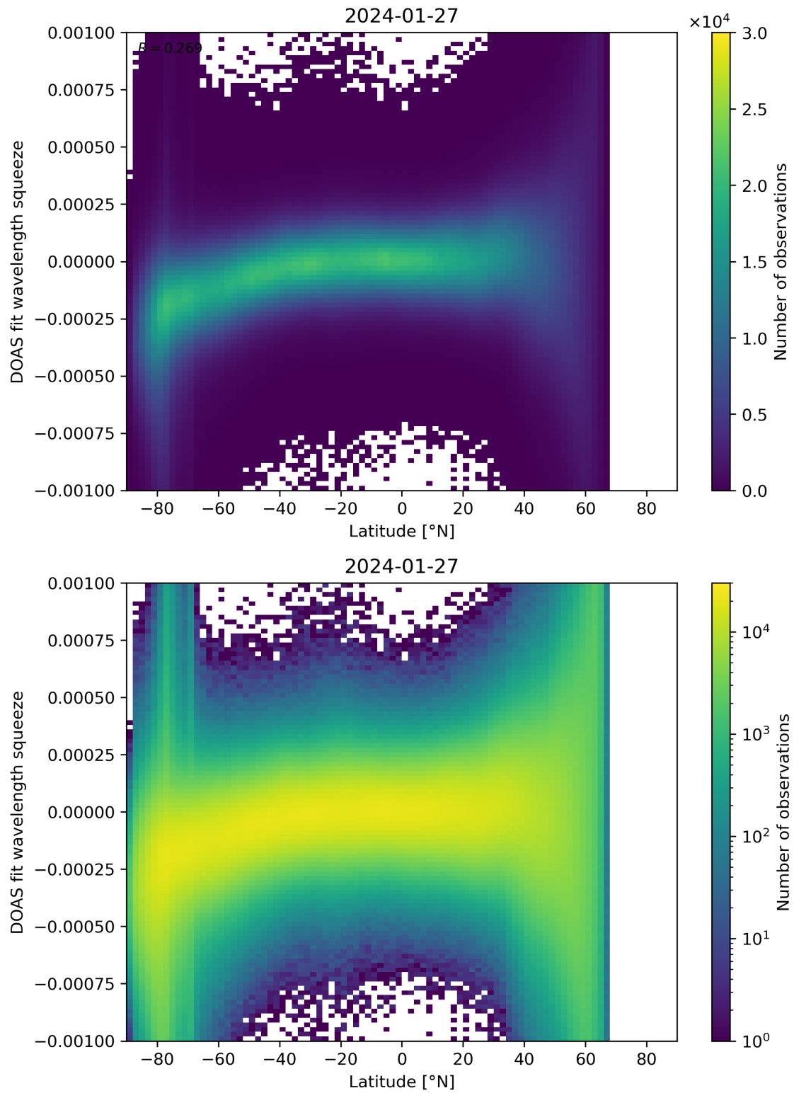
Figure 143: Scatter density plot of “Latitude” against “DOAS fit wavelength squeeze” for 2024-01-26 to 2024-01-28.
