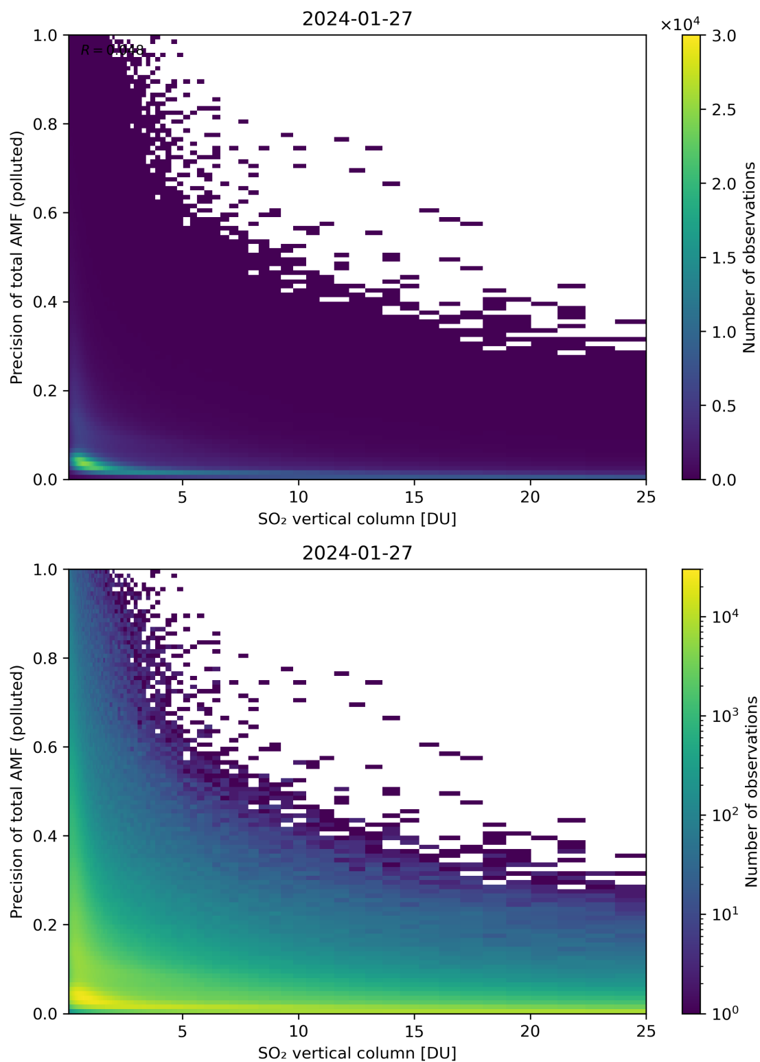
Figure 306: Scatter density plot of “SO 2 vertical column” against “Precision of total AMF (polluted)” for 2024-01-26 to 2024-01-28.
