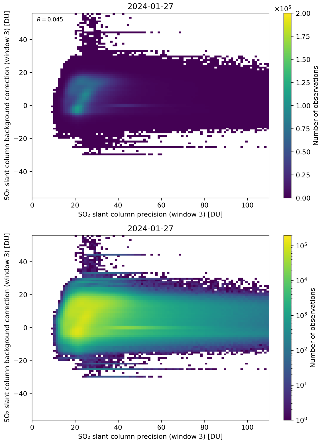
Figure 257: Scatter density plot of “SO 2 slant column precision (window 3)” against “SO 2 slant column background correction (window 3)” for 2024-01-26 to 2024-01-28.
