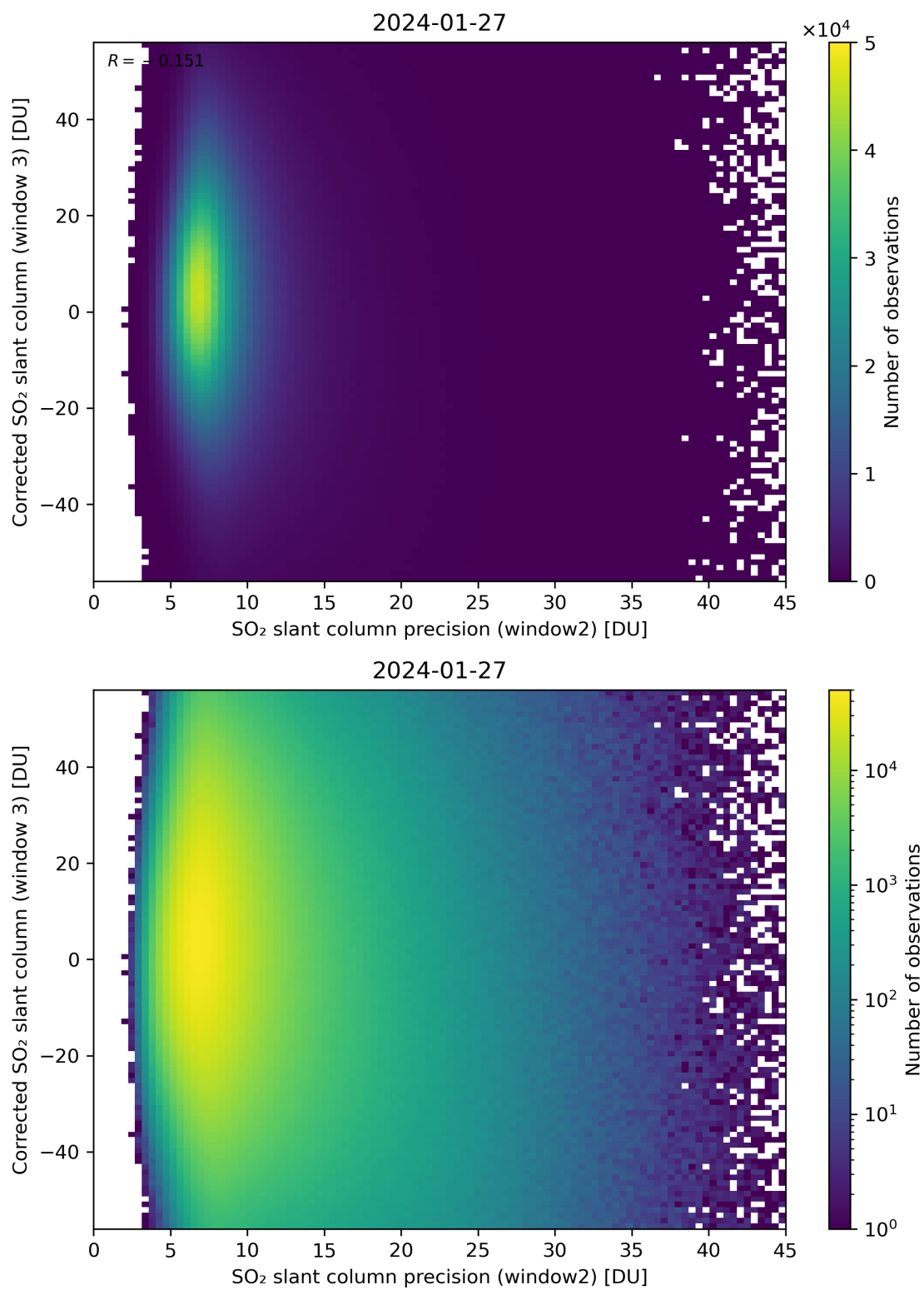
Figure 248: Scatter density plot of “SO 2 slant column precision (window2)” against “Corrected SO 2 slant column (window 3)” for 2024-01-26 to 2024-01-28.
