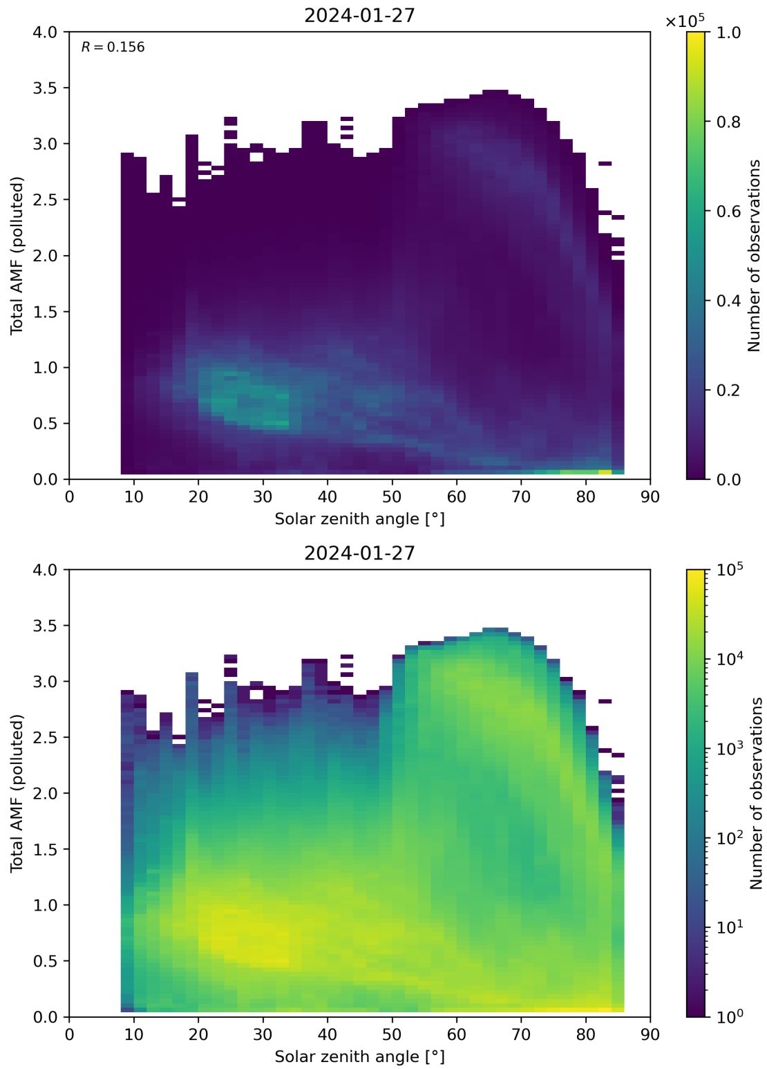
Figure 174: Scatter density plot of “Solar zenith angle” against “Total AMF (polluted)” for 2024-01-26 to 2024-01-28.
