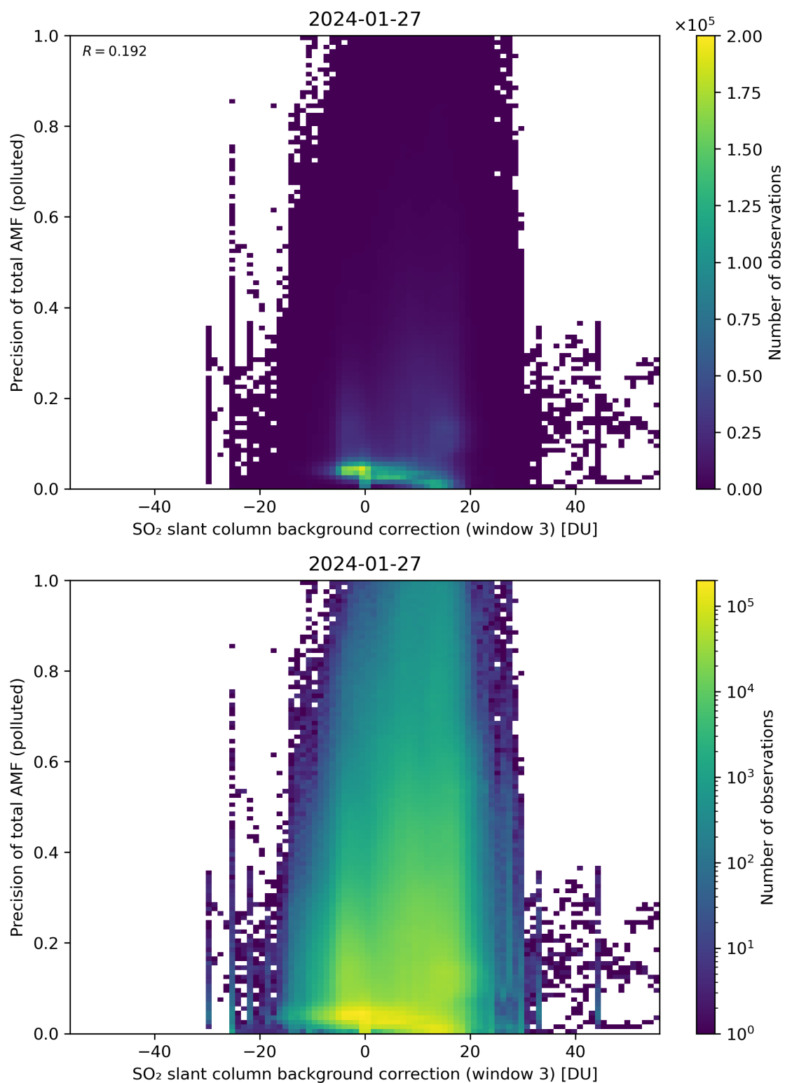
Figure 126: Scatter density plot of “SO 2 slant column background correction (window 3)” against “Precision of total AMF (polluted)” for 2024-01-26 to 2024-01-28.
