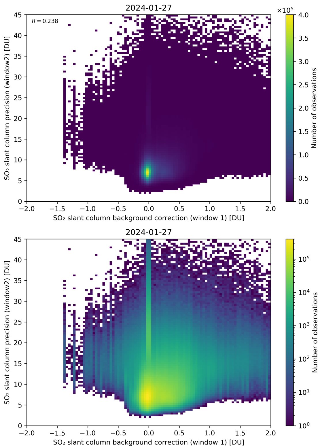
Figure 106: Scatter density plot of “SO 2 slant column background correction (window 1)” against “SO 2 slant column precision (window2)” for 2024-01-26 to 2024-01-28.
