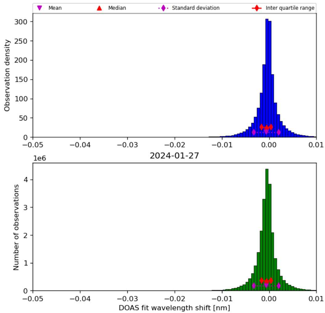
Figure 68: Histogram of “DOAS fit wavelength shift” for 2024-01-26 to 2024-01-28
