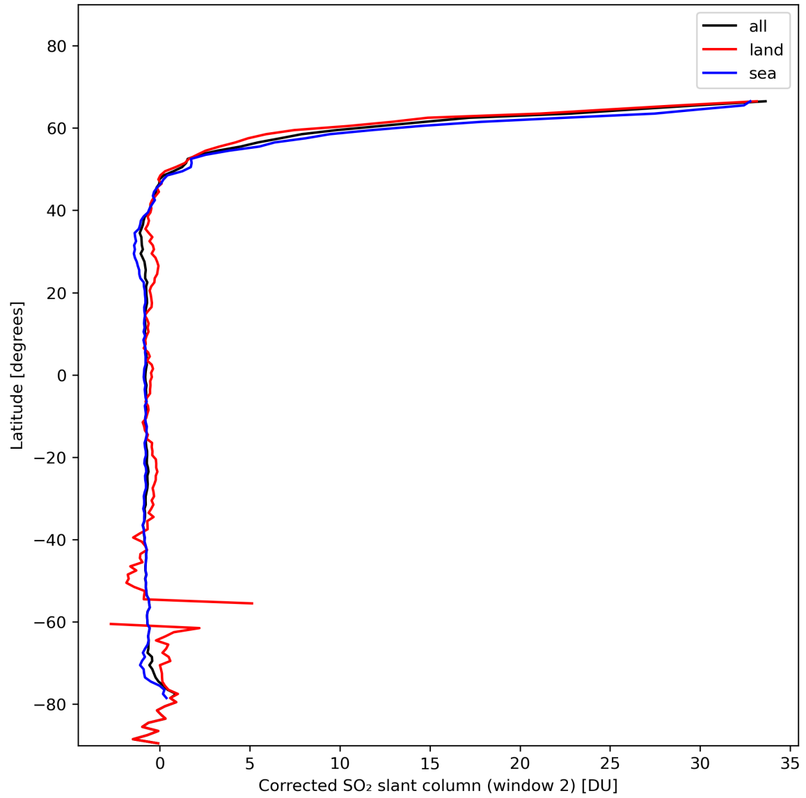
Figure 39: Zonal average of “Corrected SO 2 slant column (window 2)” for 2024-01-26 to 2024-01-28.
