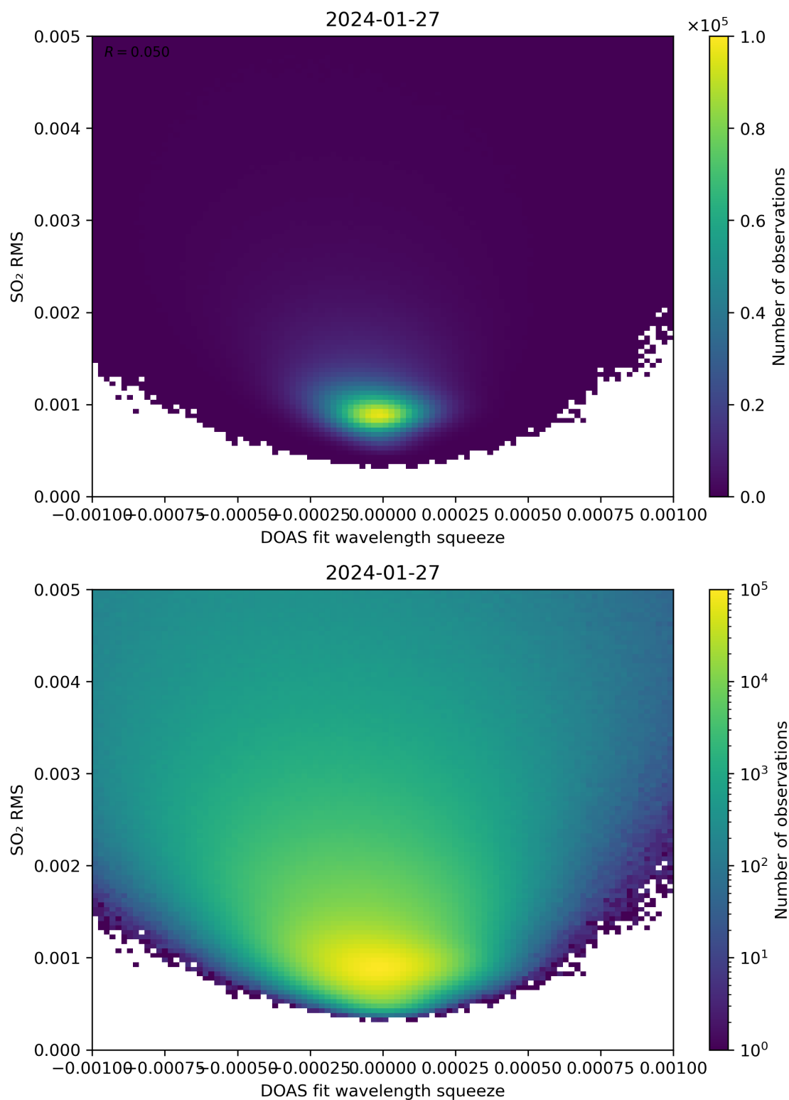
Figure 132: Scatter density plot of “DOAS fit wavelength squeeze” against “SO 2 RMS” for 2024-01-26 to 2024-01-28.
