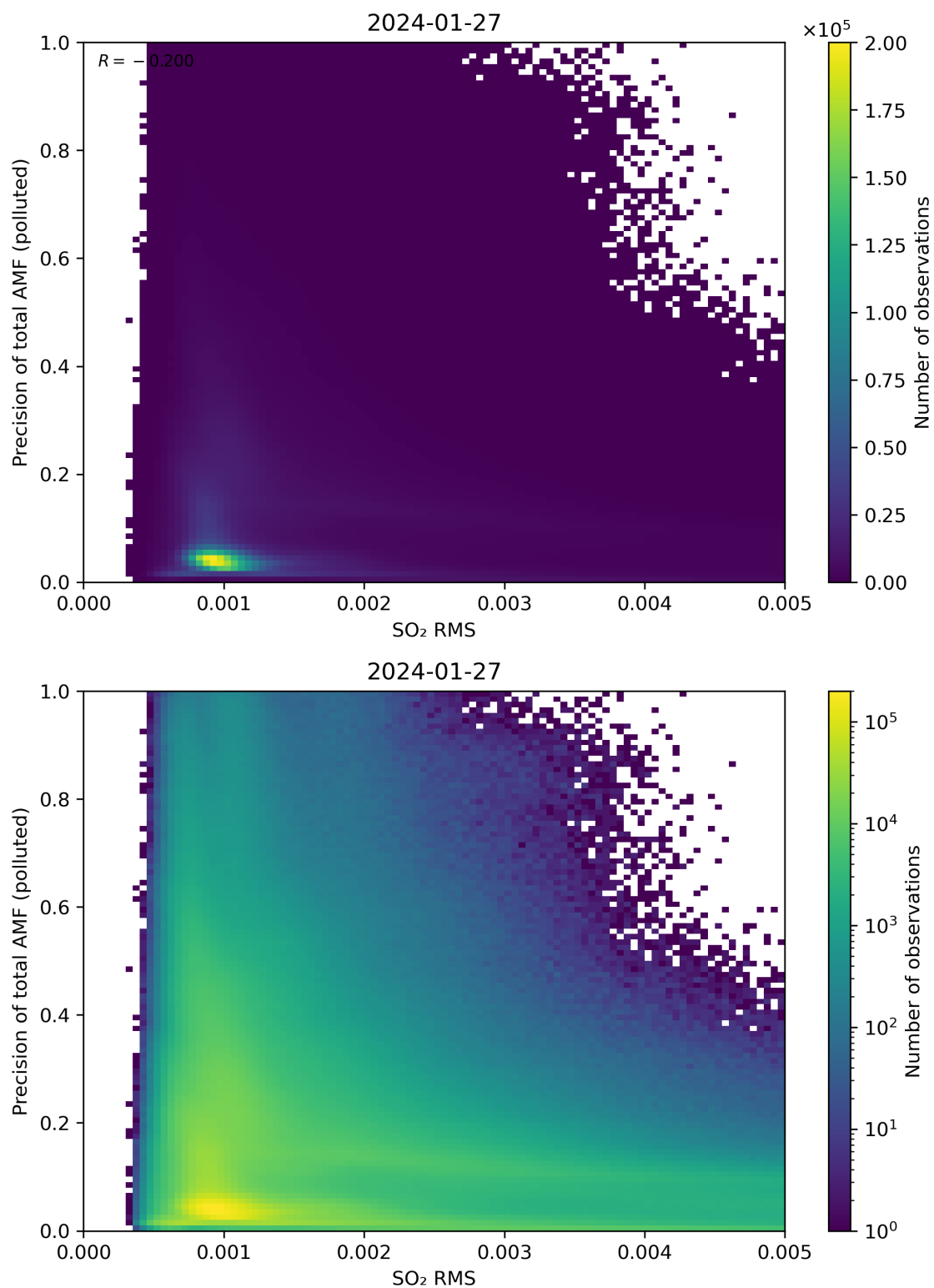
Figure 138: Scatter density plot of “SO 2 RMS” against “Precision of total AMF (polluted)” for 2024-01-26 to 2024-01-28.
