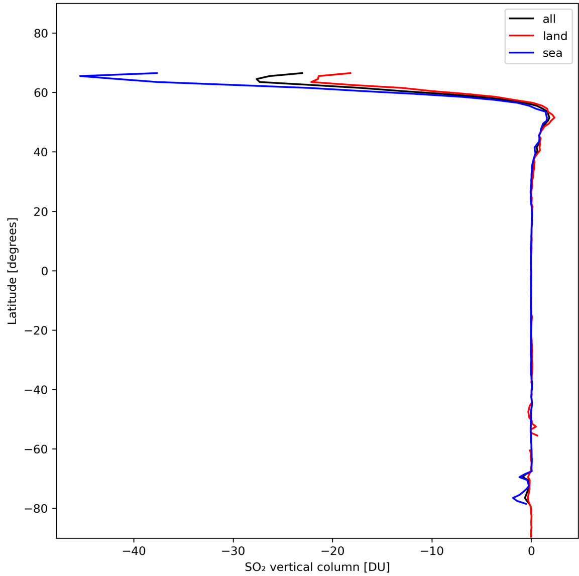
Figure 30: Zonal average of “SO 2 vertical column” for 2024-01-26 to 2024-01-28.
