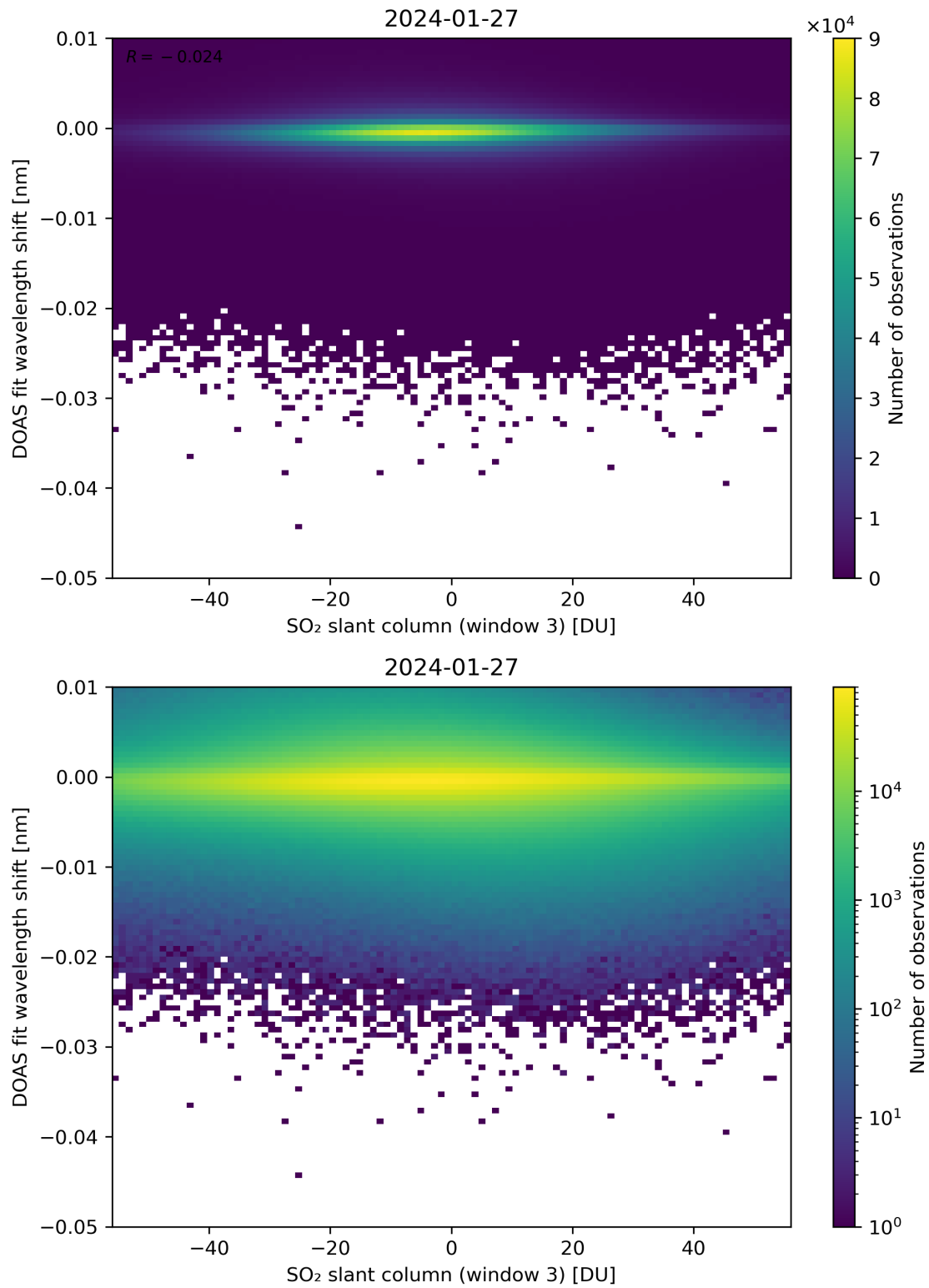
Figure 254: Scatter density plot of “SO 2 slant column (window 3)” against “DOAS fit wavelength shift” for 2024-01-26 to 2024-01-28.
