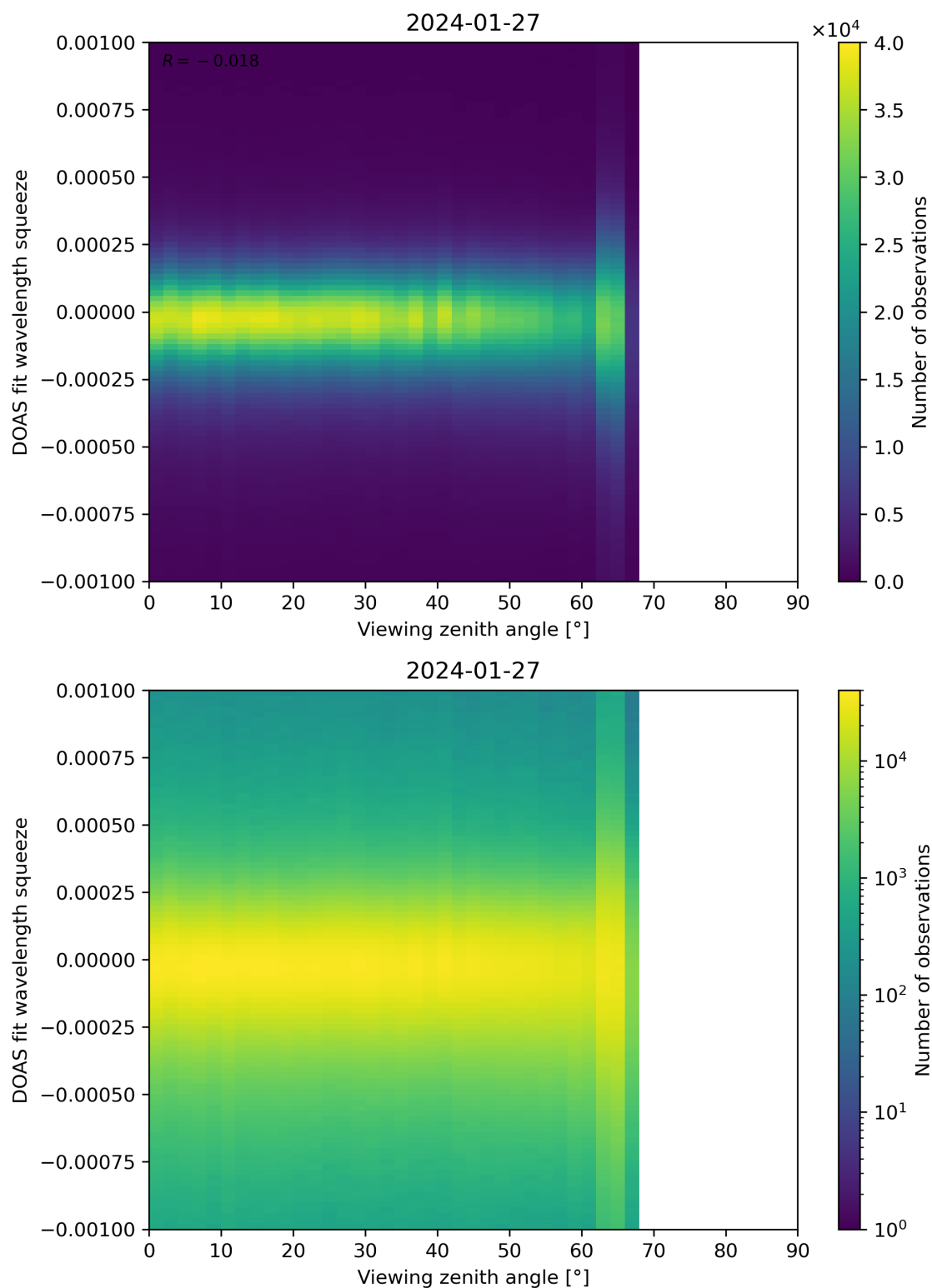
Figure 312: Scatter density plot of “Viewing zenith angle” against “DOAS fit wavelength squeeze” for 2024-01-26 to 2024-01-28.
