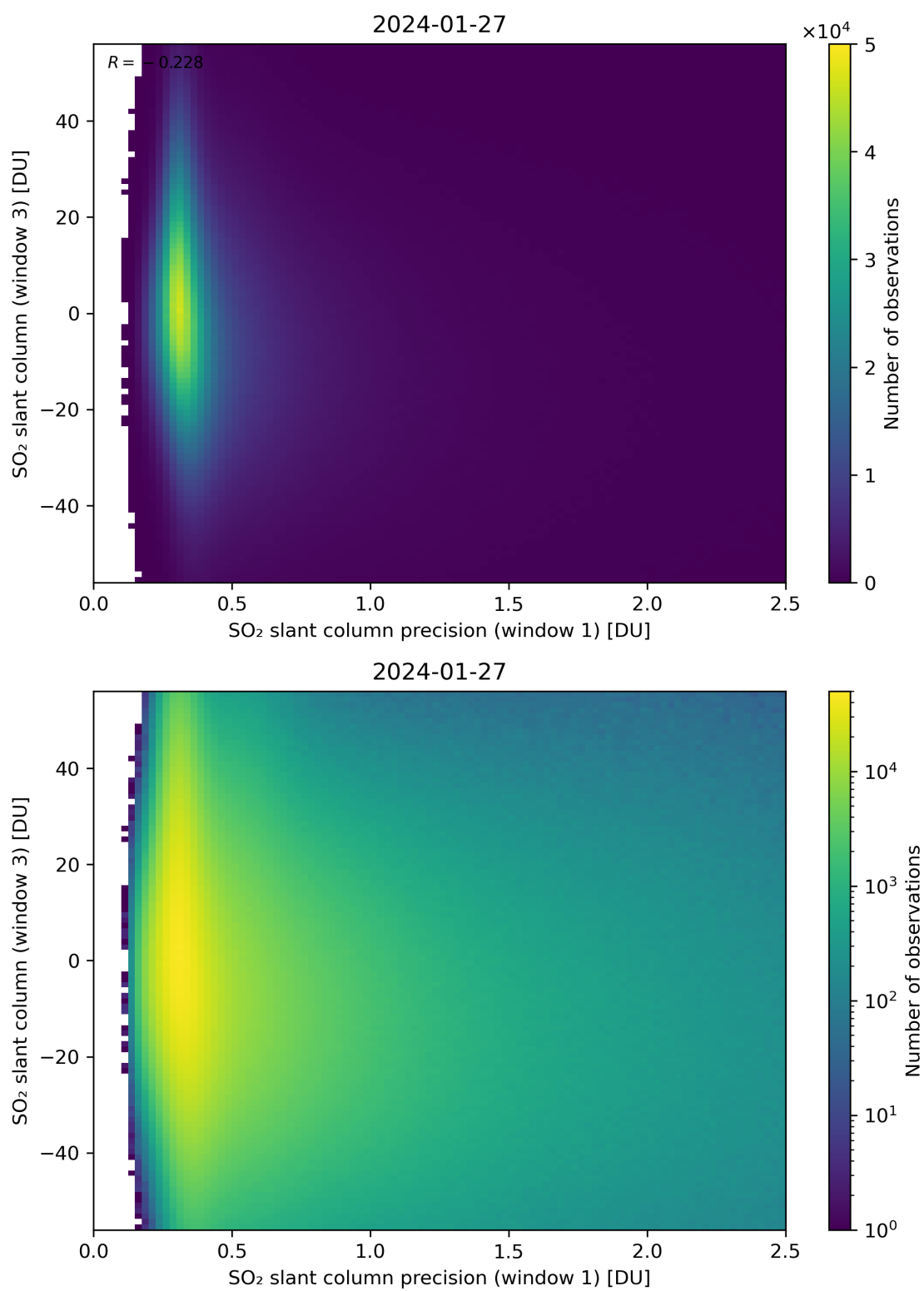
Figure 228: Scatter density plot of “SO 2 slant column precision (window 1)” against “SO 2 slant column (window 3)” for 2024-01-26 to 2024-01-28.
