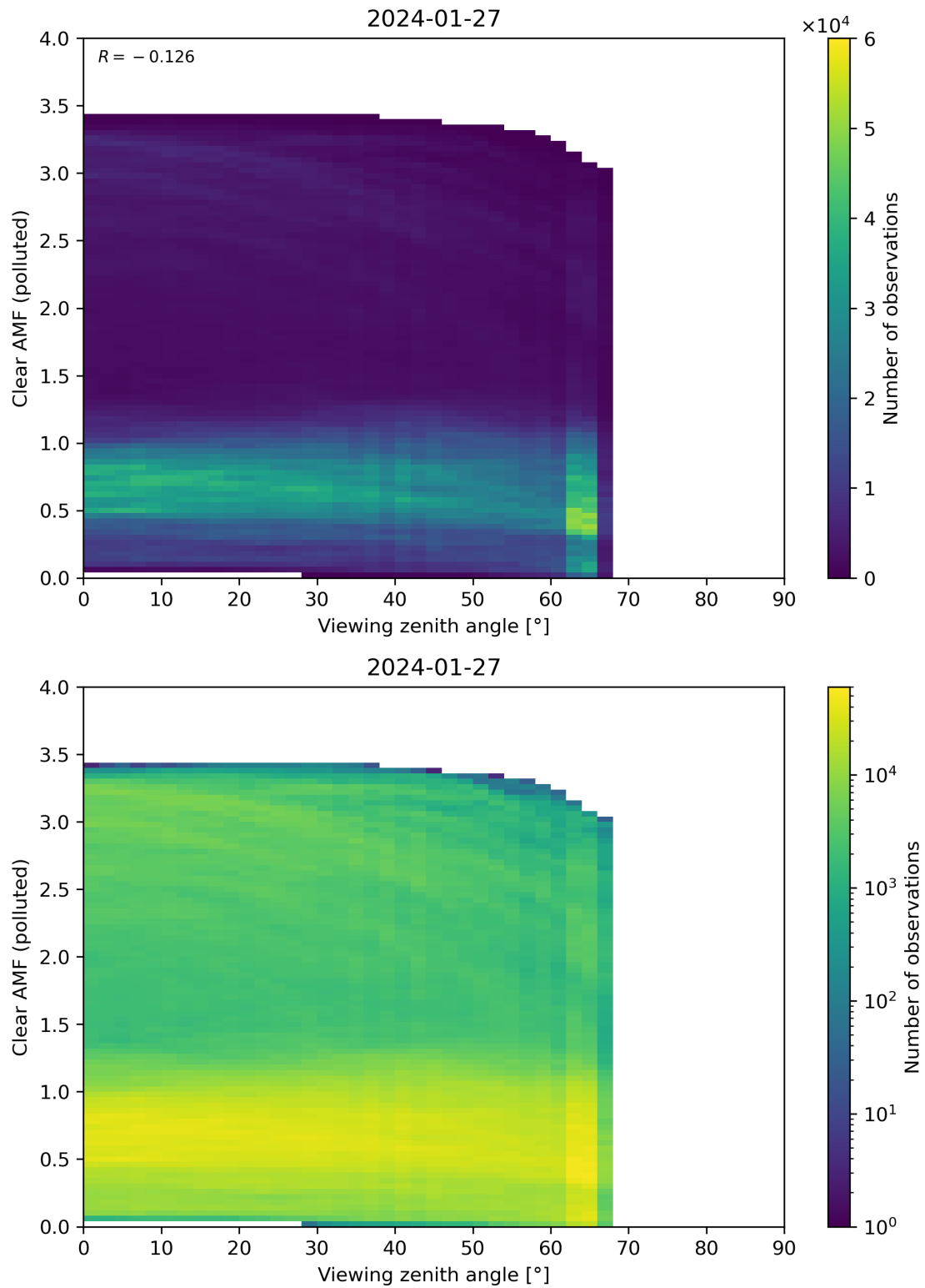
Figure 316: Scatter density plot of “Viewing zenith angle” against “Clear AMF (polluted)” for 2024-01-26 to 2024-01-28.
