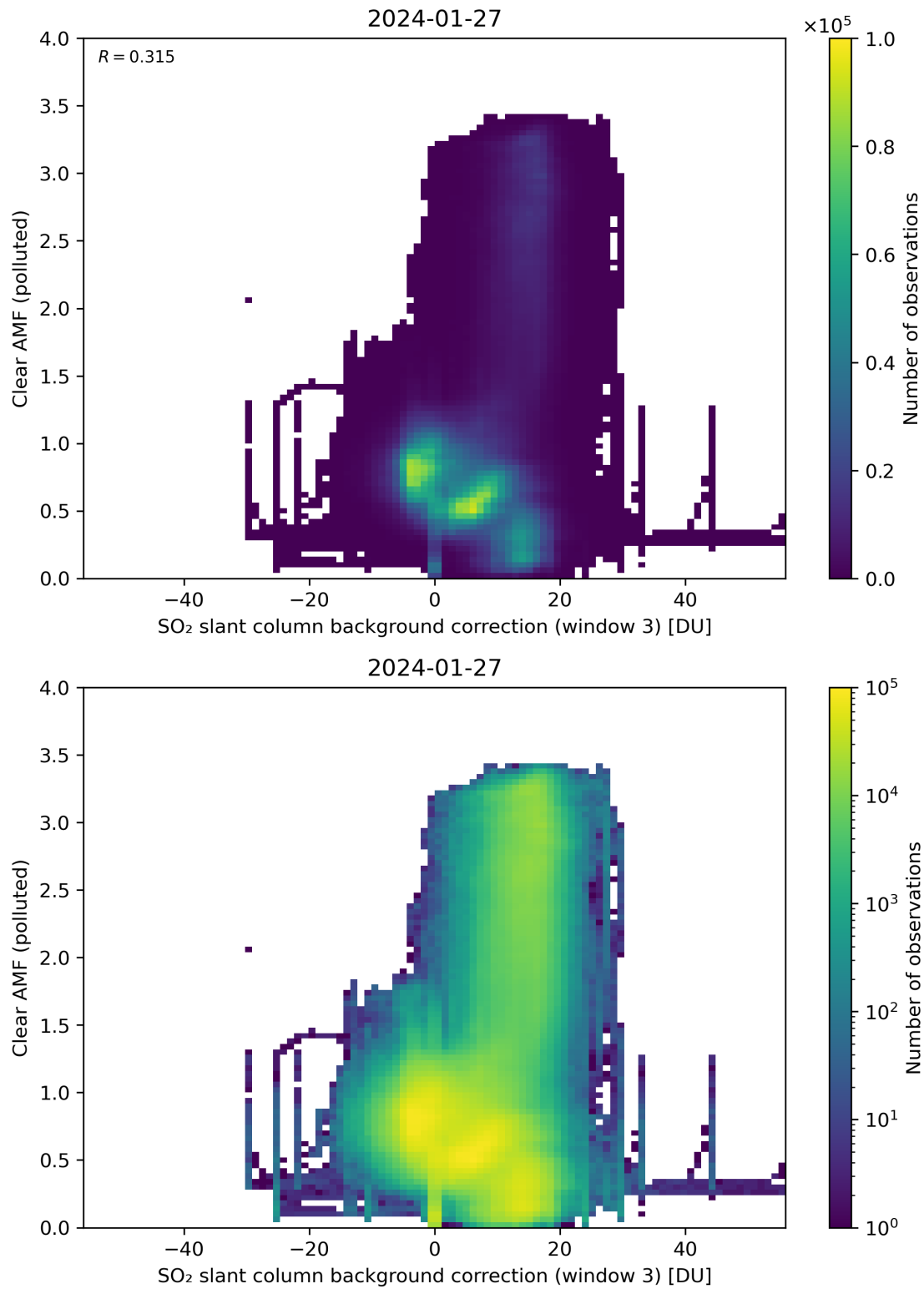
Figure 124: Scatter density plot of “SO 2 slant column background correction (window 3)” against “Clear AMF (polluted)” for 2024-01-26 to 2024-01-28.
