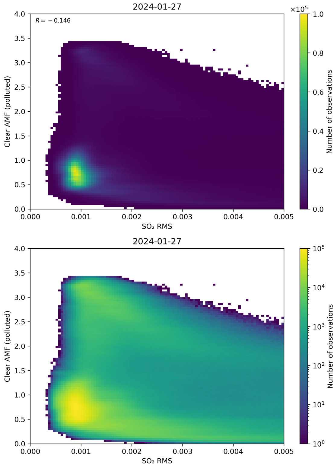
Figure 136: Scatter density plot of “SO 2 RMS” against “Clear AMF (polluted)” for 2024-01-26 to 2024-01-28.
