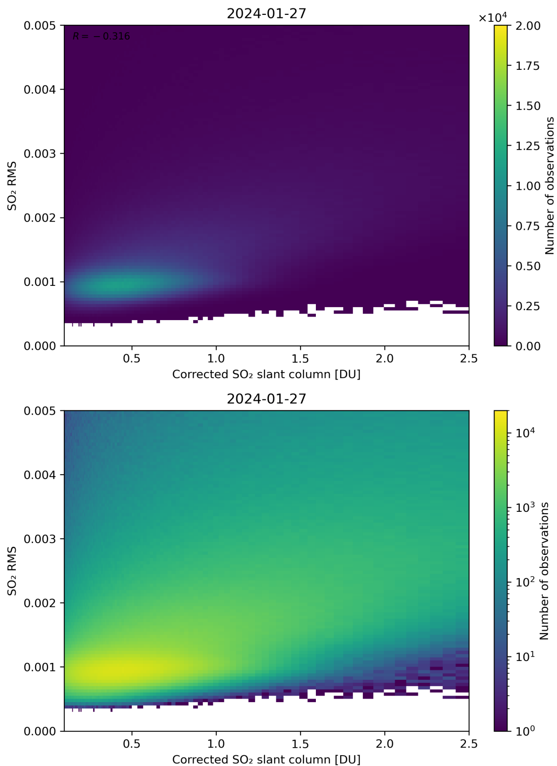
Figure 183: Scatter density plot of “Corrected SO 2 slant column” against “SO 2 RMS” for 2024-01-26 to 2024-01-28.
