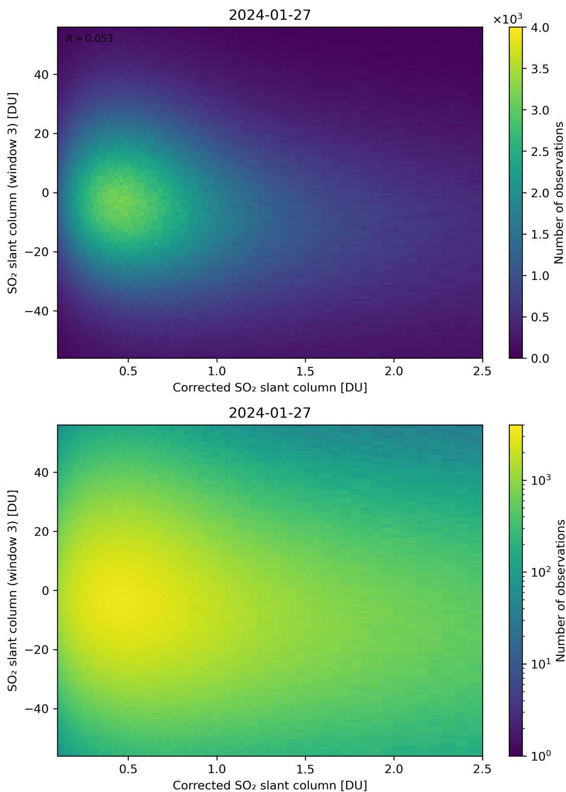
Figure 190: Scatter density plot of “Corrected SO 2 slant column” against “SO 2 slant column (window 3)” for 2024-01-26 to 2024-01-28.
