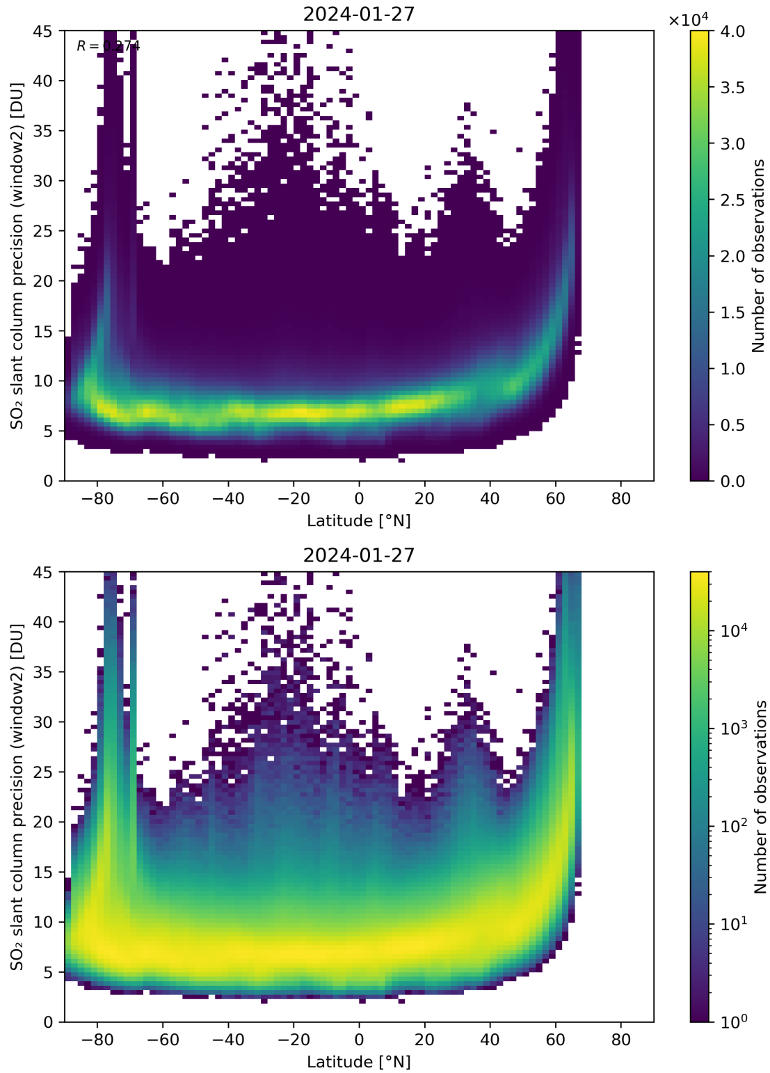
Figure 151: Scatter density plot of “Latitude” against “SO 2 slant column precision (window2)” for 2024-01-26 to 2024-01-28.
