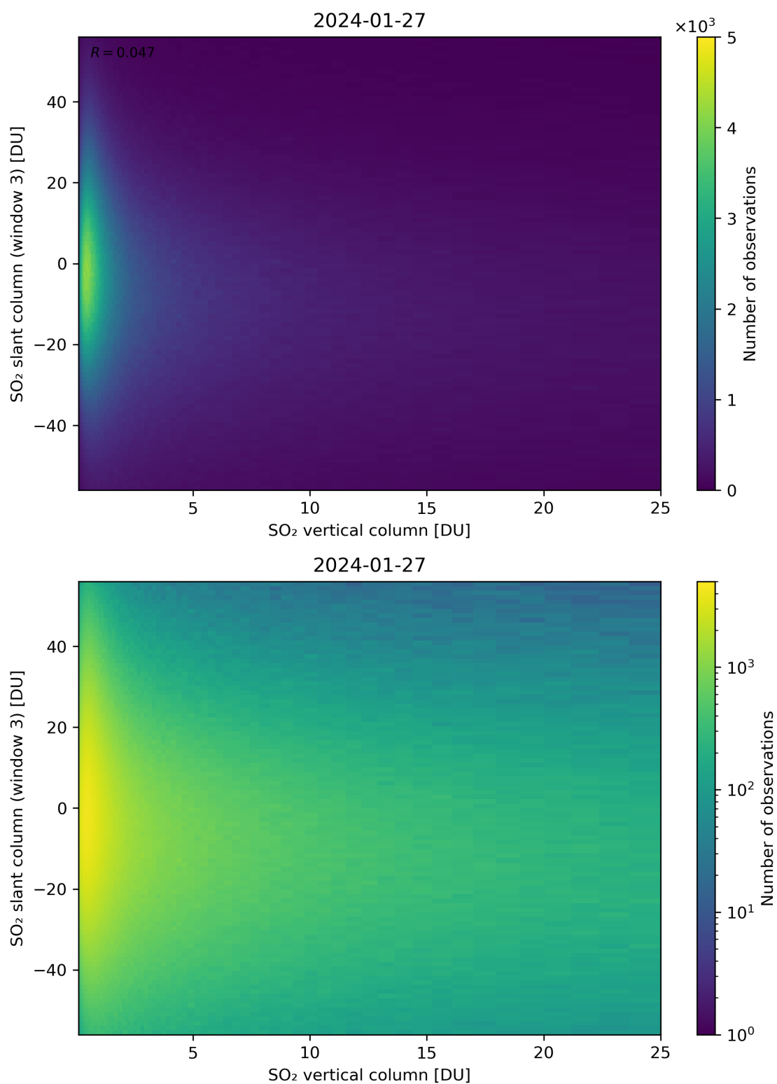
Figure 303: Scatter density plot of “SO 2 vertical column” against “SO 2 slant column (window 3)” for 2024-01-26 to 2024-01-28.
