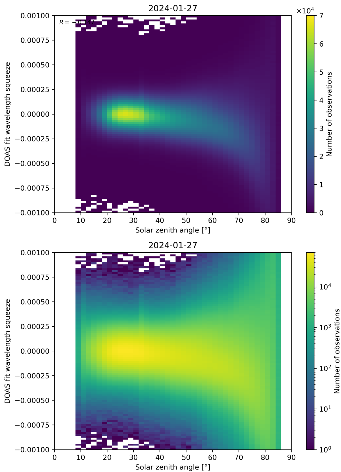
Figure 162: Scatter density plot of “Solar zenith angle” against “DOAS fit wavelength squeeze” for 2024-01-26 to 2024-01-28.
