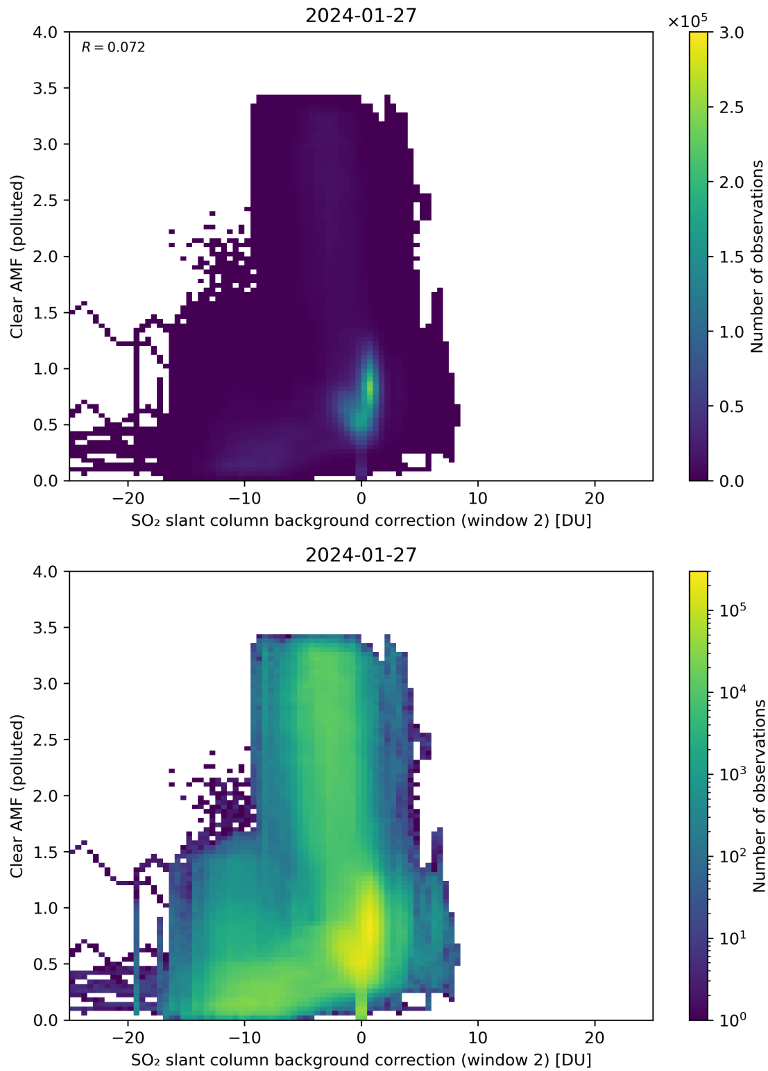
Figure 115: Scatter density plot of “SO 2 slant column background correction (window 2)” against “Clear AMF (polluted)” for 2024-01-26 to 2024-01-28.
