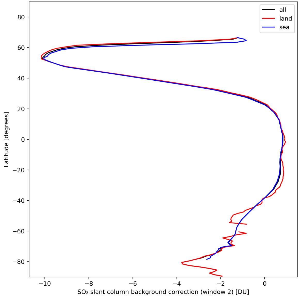
Figure 40: Zonal average of “SO 2 slant column background correction (window 2)” for 2024-01-26 to 2024-01-28.
