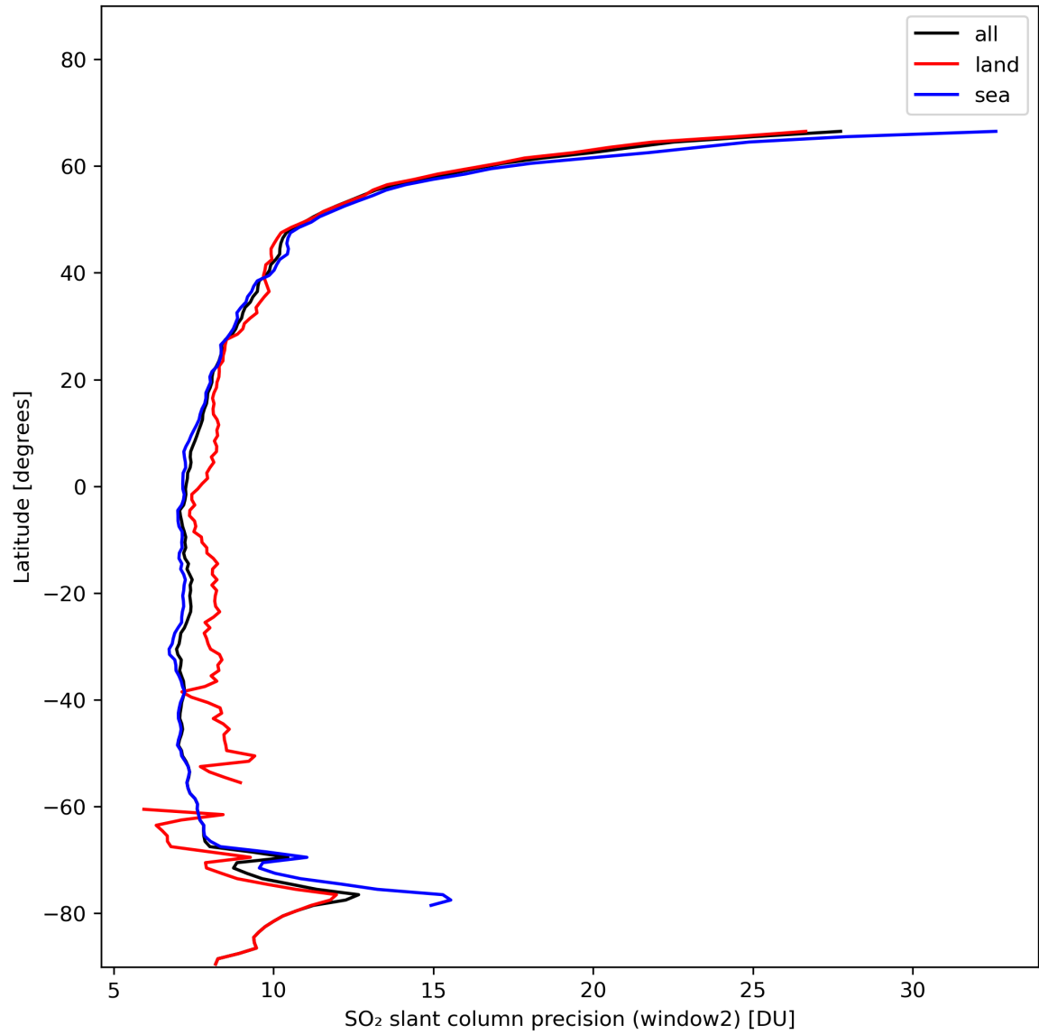
Figure 38: Zonal average of “SO 2 slant column precision (window2)” for 2024-01-26 to 2024-01-28.
