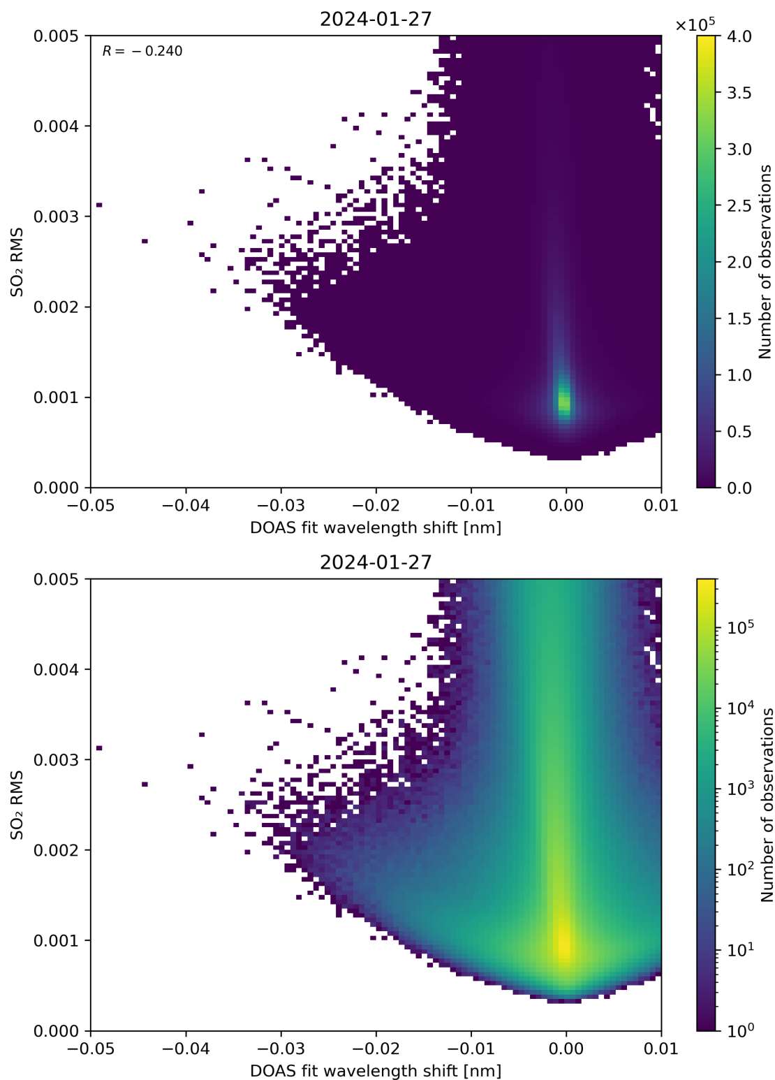
Figure 128: Scatter density plot of “DOAS fit wavelength shift” against “SO 2 RMS” for 2024-01-26 to 2024-01-28.
