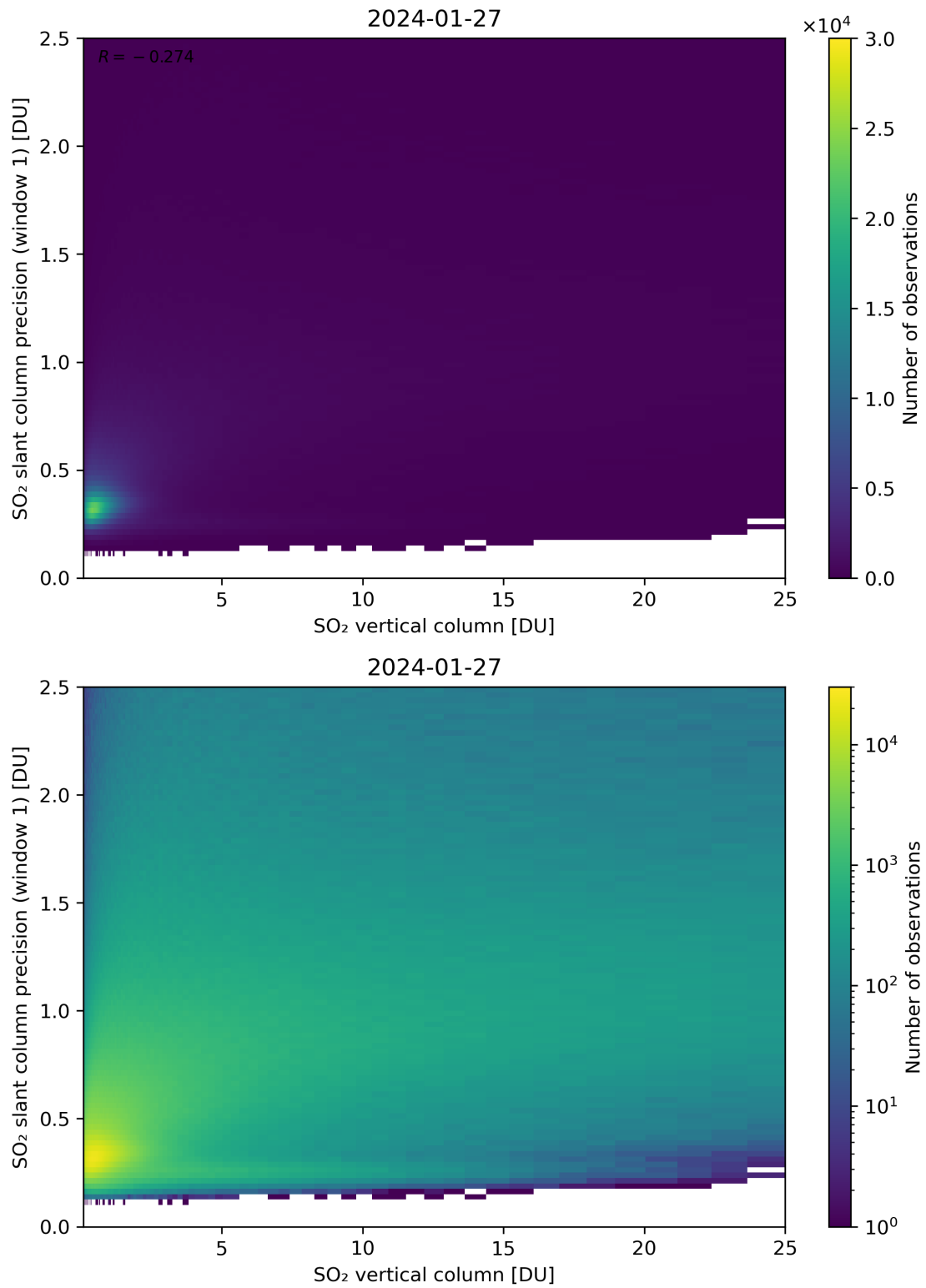
Figure 301: Scatter density plot of “SO 2 vertical column” against “SO 2 slant column precision (window 1)” for 2024-01-26 to 2024-01-28.
