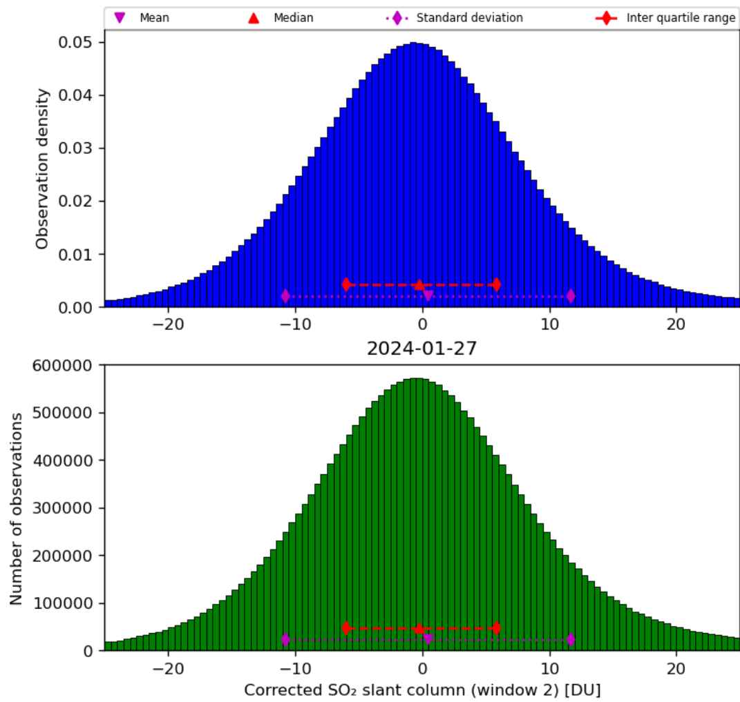
Figure 62: Histogram of “Corrected SO 2 slant column (window 2)” for 2024-01-26 to 2024-01-28
