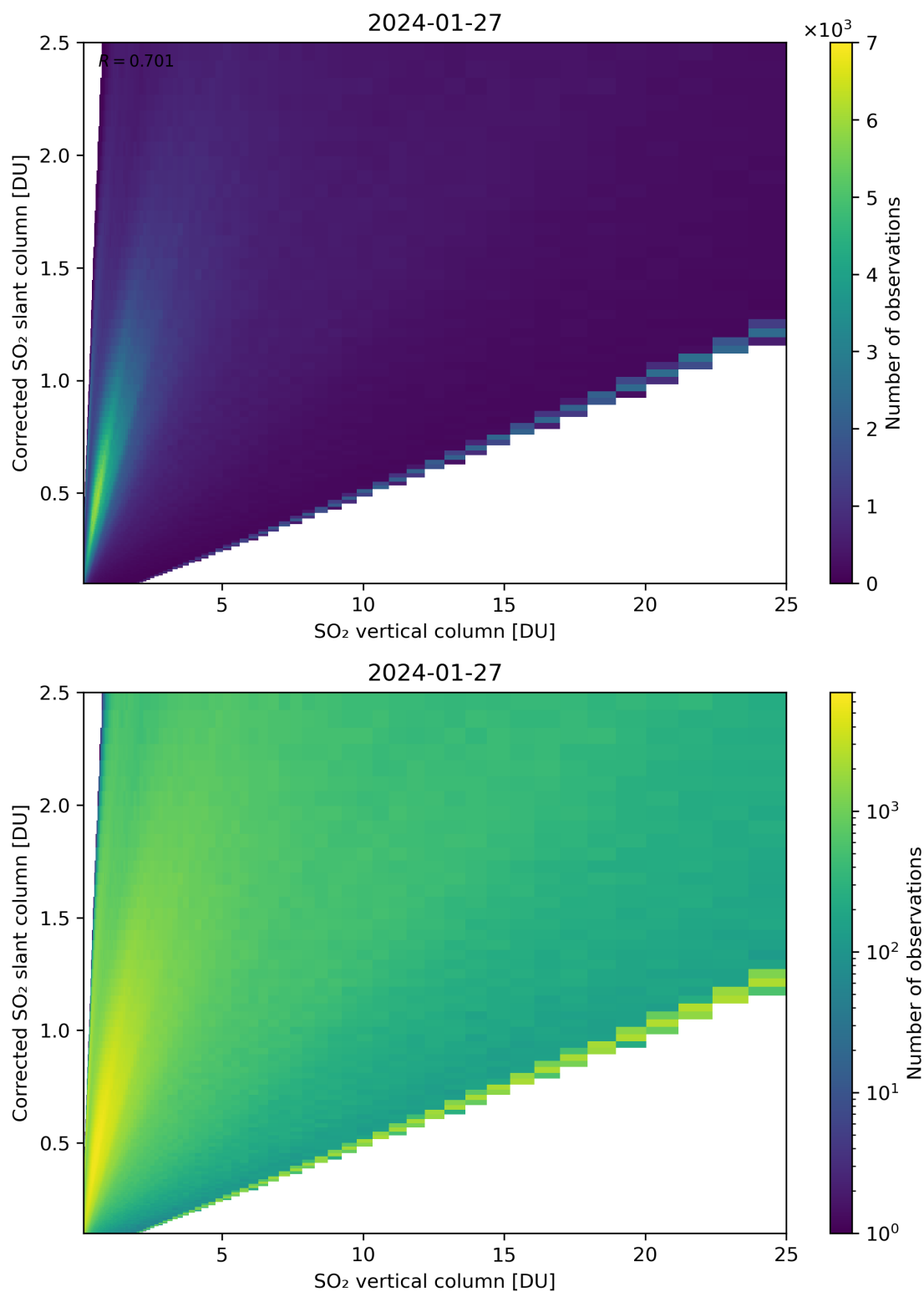
Figure 297: Scatter density plot of “SO 2 vertical column” against “Corrected SO 2 slant column” for 2024-01-26 to 2024-01-28.
