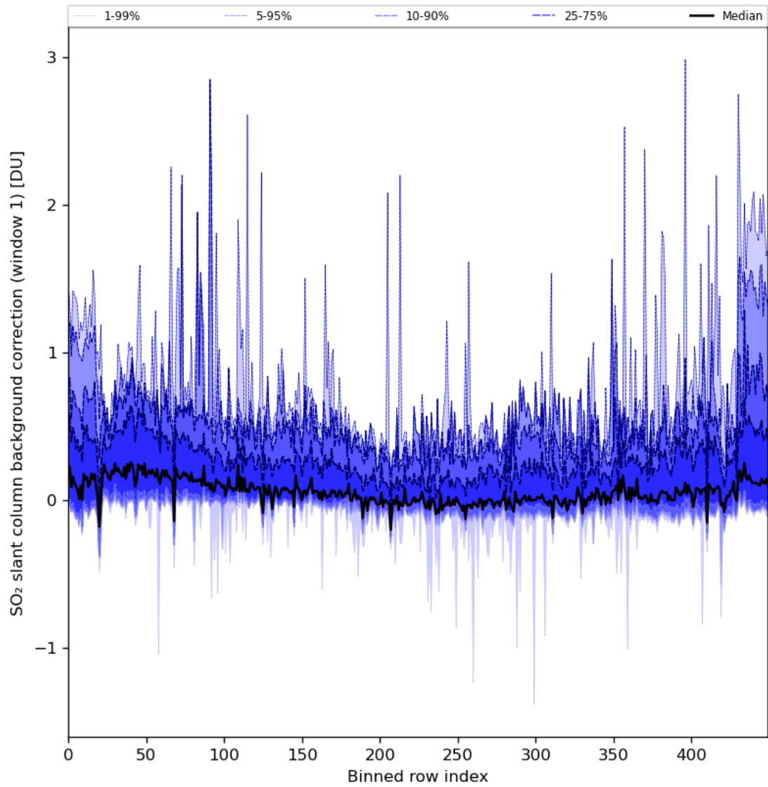
Figure 82: Along track statistics of “SO 2 slant column background correction (window 1)” for 2024-01-26 to 2024-01-28
