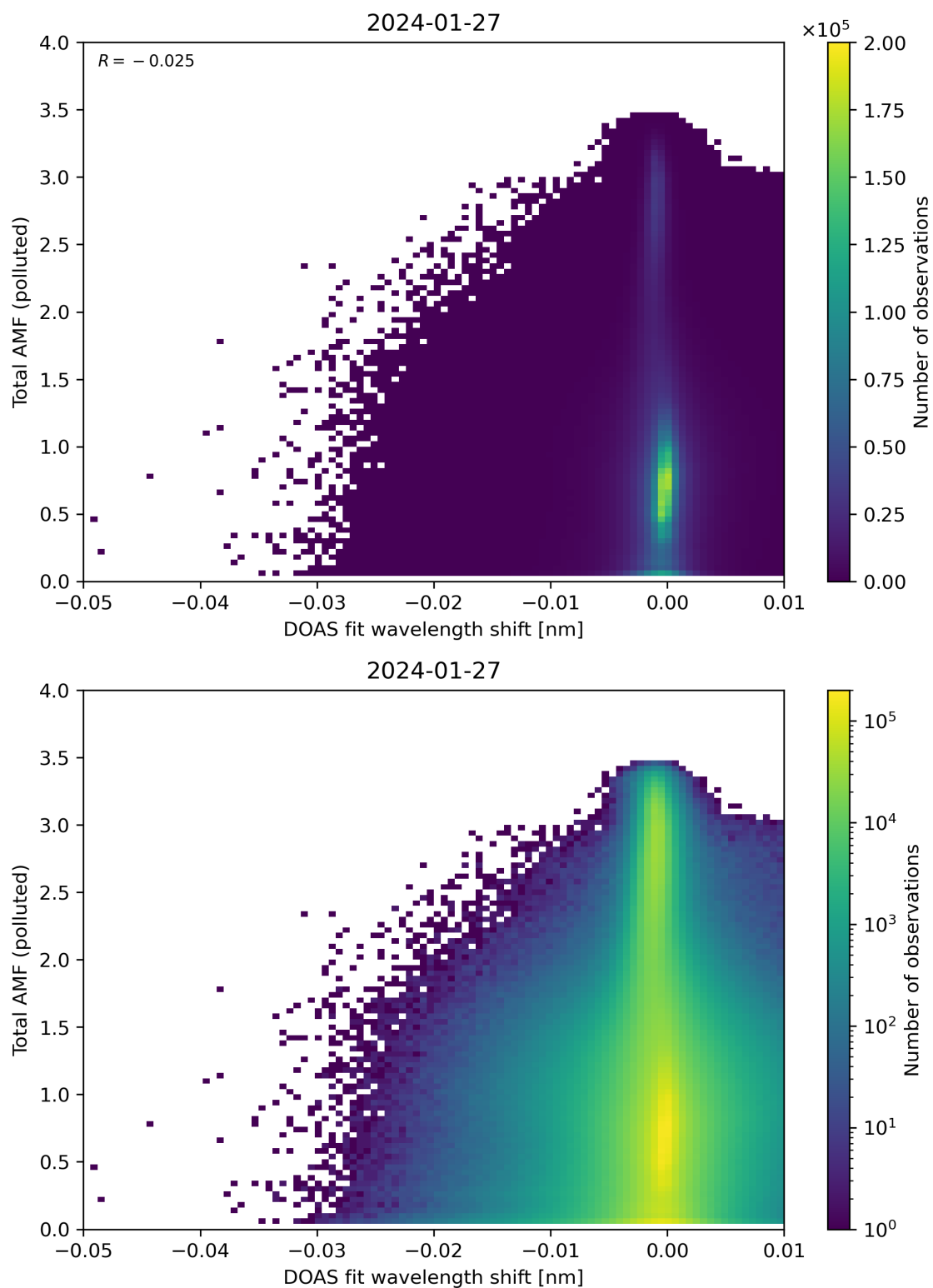
Figure 130: Scatter density plot of “DOAS fit wavelength shift” against “Total AMF (polluted)” for 2024-01-26 to 2024-01-28.
