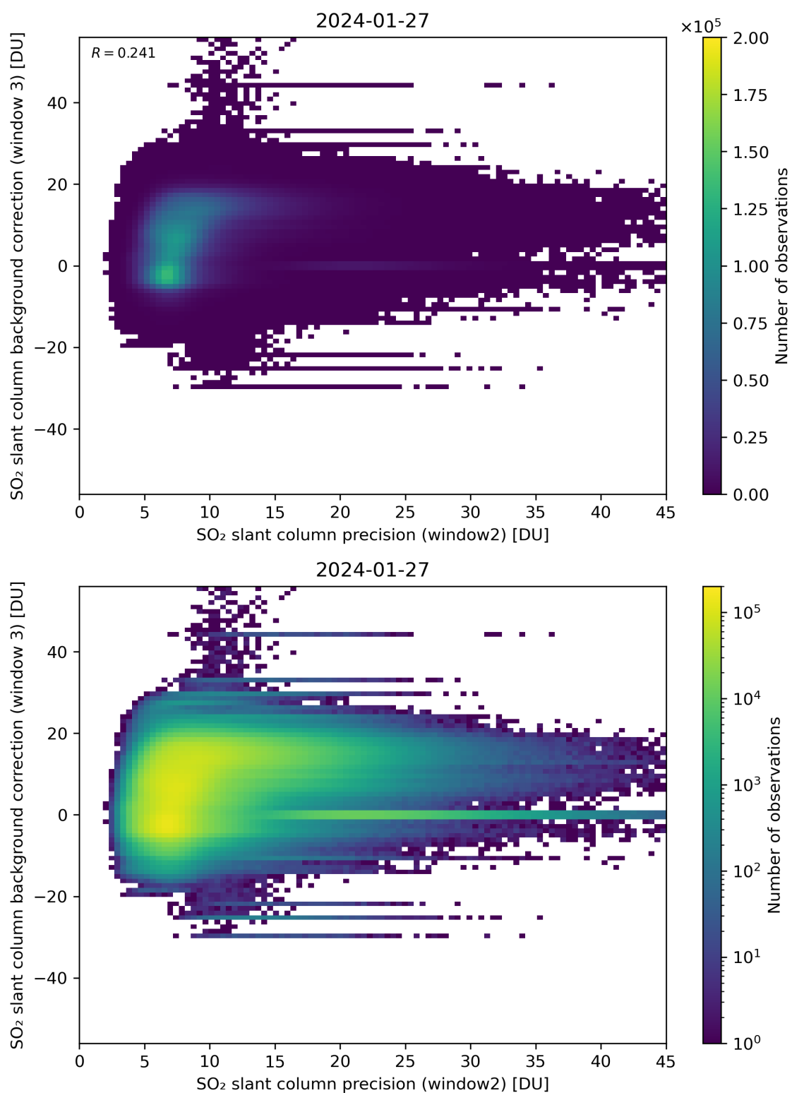
Figure 242: Scatter density plot of “SO 2 slant column precision (window2)” against “SO 2 slant column background correction (window 3)” for 2024-01-26 to 2024-01-28.
