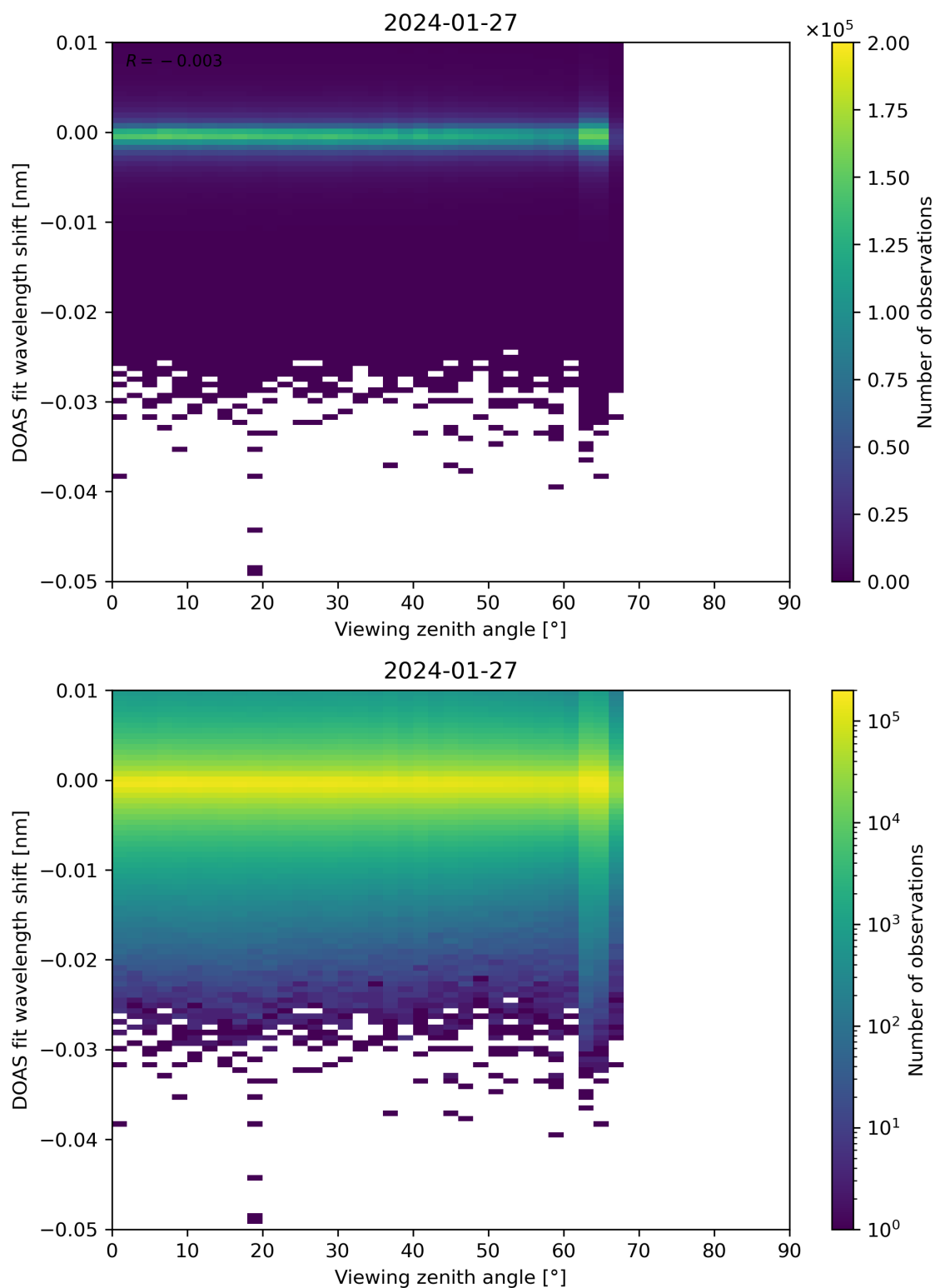
Figure 311: Scatter density plot of “Viewing zenith angle” against “DOAS fit wavelength shift” for 2024-01-26 to 2024-01-28.
