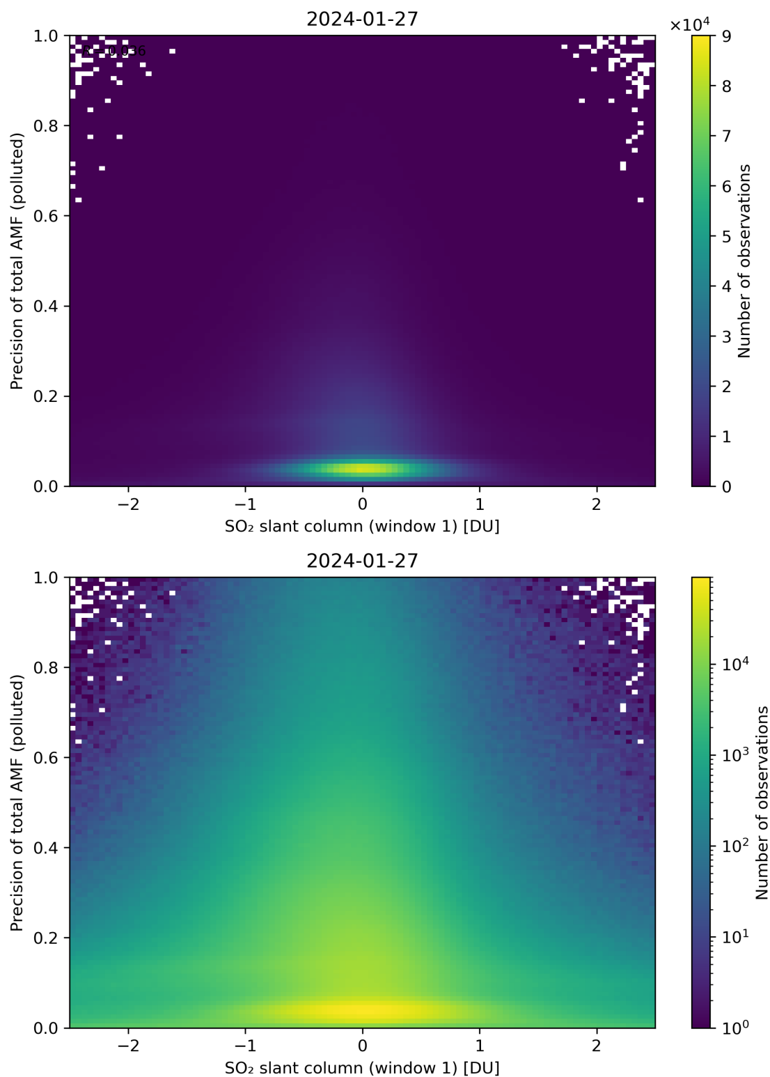
Figure 240: Scatter density plot of “SO 2 slant column (window 1)” against “Precision of total AMF (polluted)” for 2024-01-26 to 2024-01-28.
