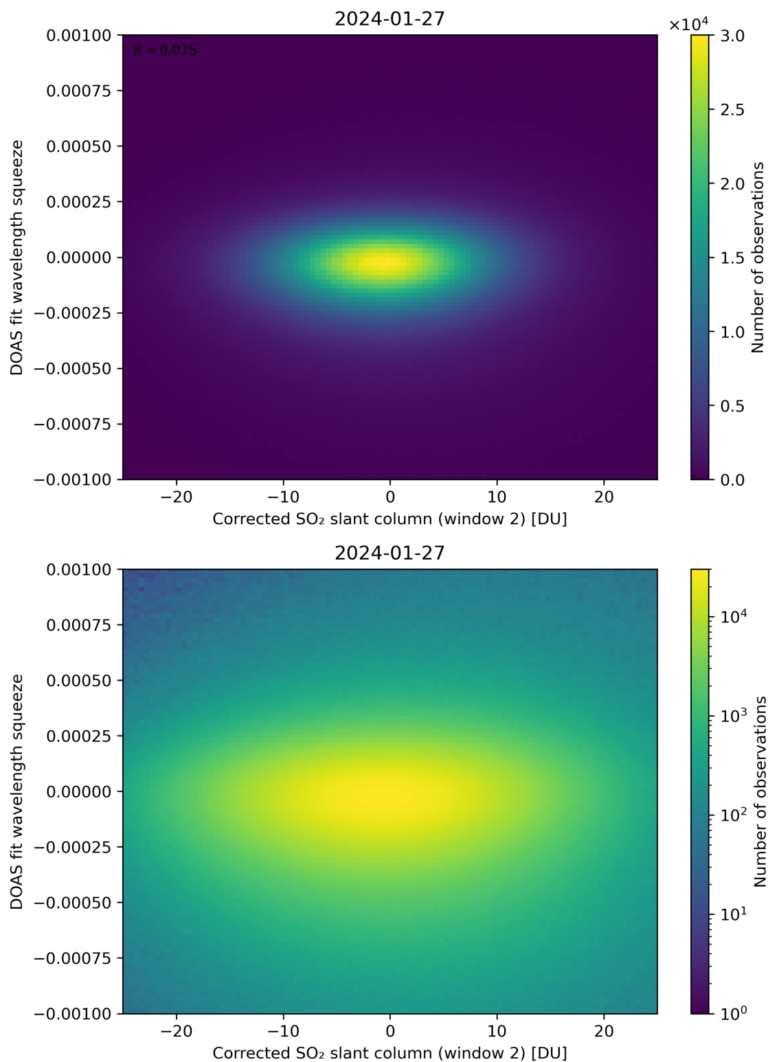
Figure 197: Scatter density plot of “Corrected SO 2 slant column (window 2)” against “DOAS fit wavelength squeeze” for 2024-01-26 to 2024-01-28.
