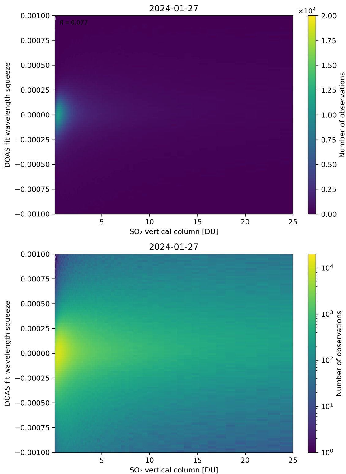
Figure 277: Scatter density plot of “SO 2 vertical column” against “DOAS fit wavelength squeeze” for 2024-01-26 to 2024-01-28.
