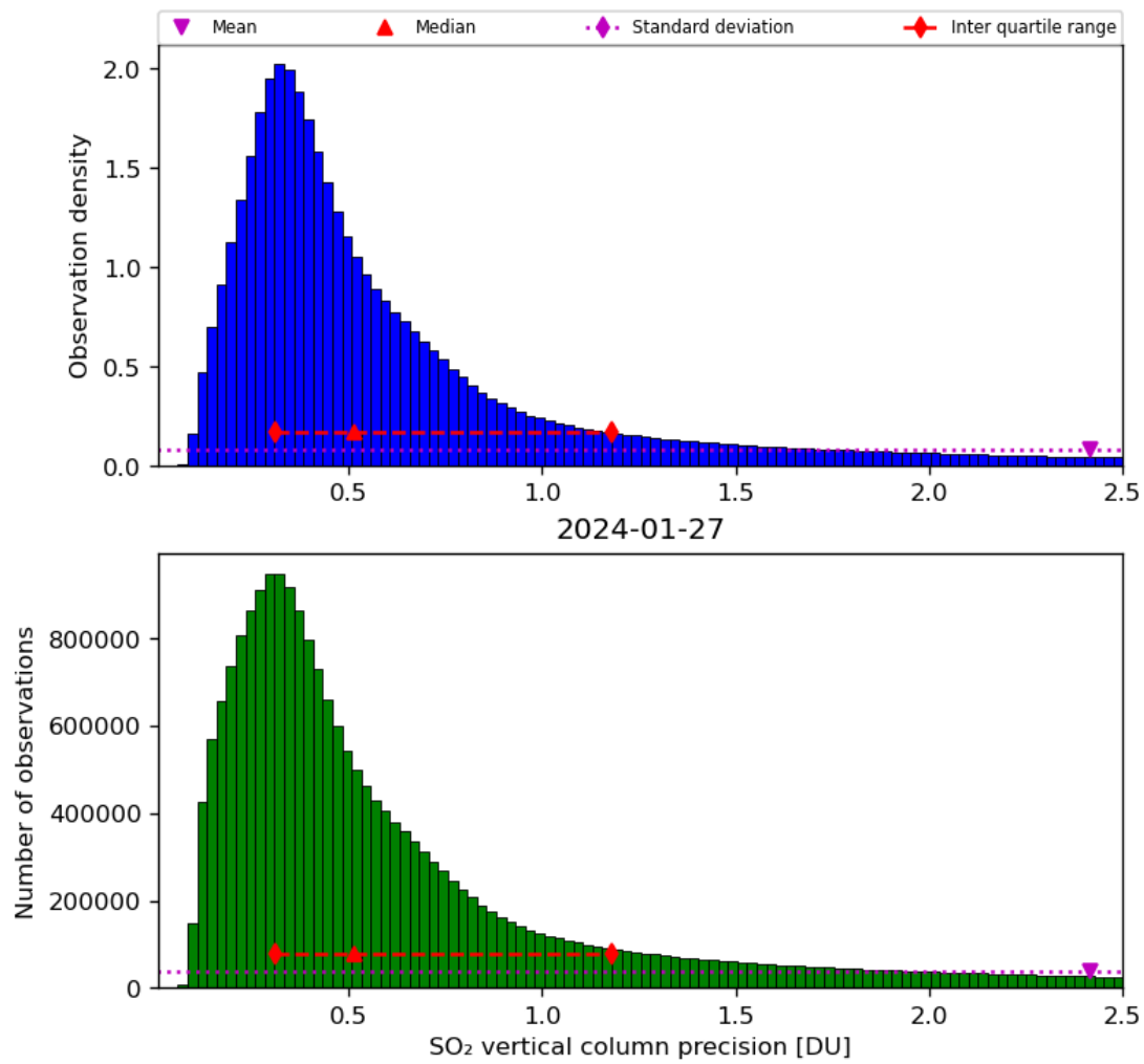
Figure 54: Histogram of “SO 2 vertical column precision” for 2024-01-26 to 2024-01-28
