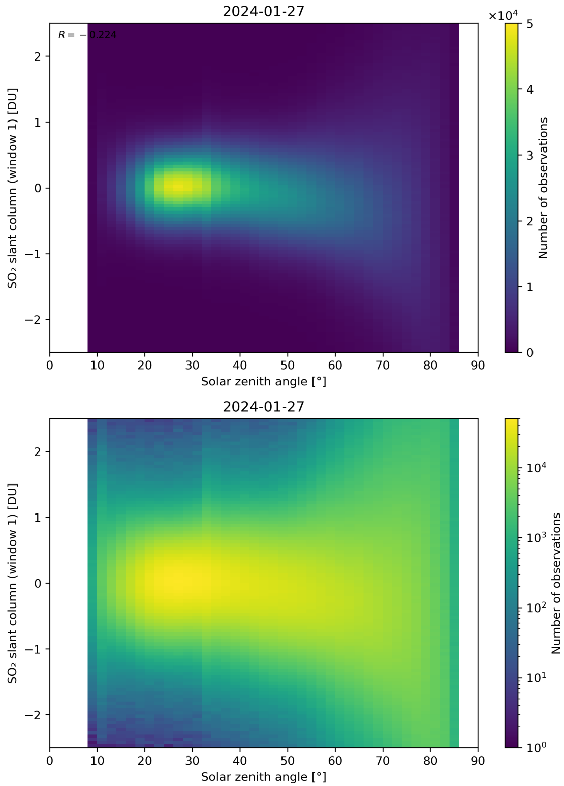
Figure 169: Scatter density plot of “Solar zenith angle” against “SO 2 slant column (window 1)” for 2024-01-26 to 2024-01-28.
