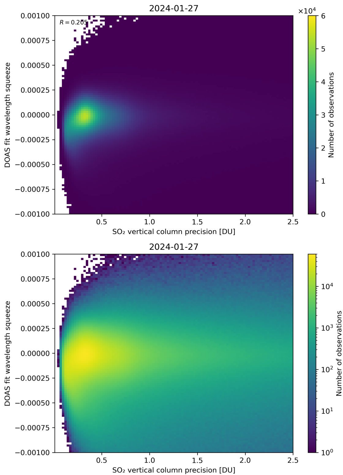
Figure 283: Scatter density plot of “SO 2 vertical column precision” against “DOAS fit wavelength squeeze” for 2024-01-26 to 2024-01-28.
