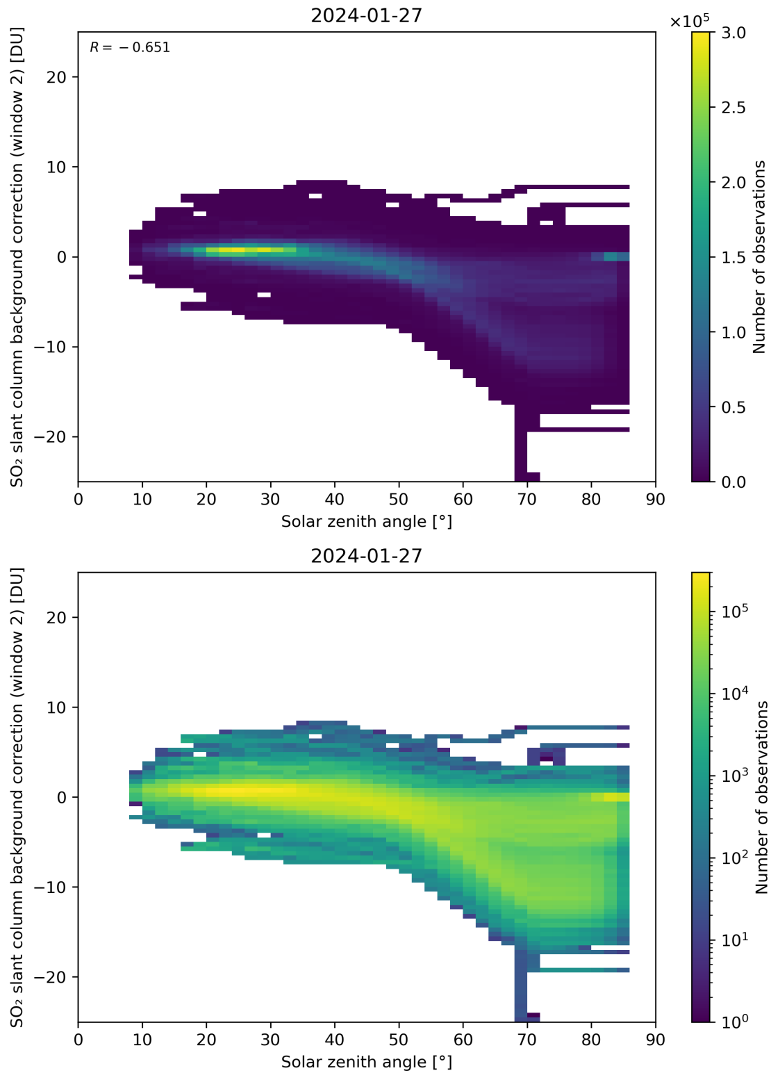
Figure 159: Scatter density plot of “Solar zenith angle” against “SO 2 slant column background correction (window 2)” for 2024-01-26 to 2024-01-28.
