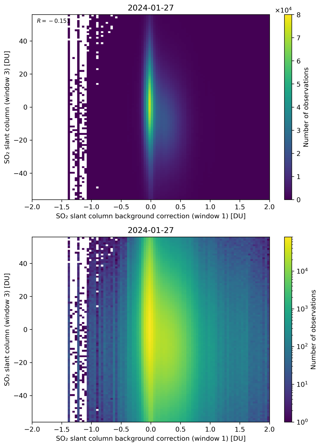
Figure 107: Scatter density plot of “SO 2 slant column background correction (window 1)” against “SO 2 slant column (window 3)” for 2024-01-26 to 2024-01-28.
