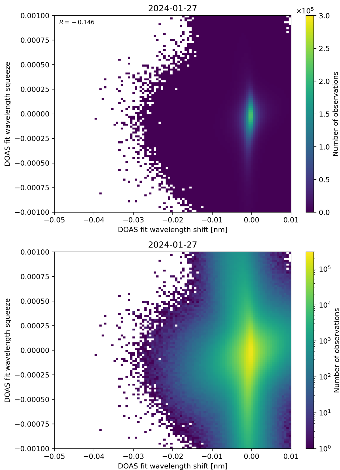
Figure 127: Scatter density plot of “DOAS fit wavelength shift” against “DOAS fit wavelength squeeze” for 2024-01-26 to 2024-01-28.
