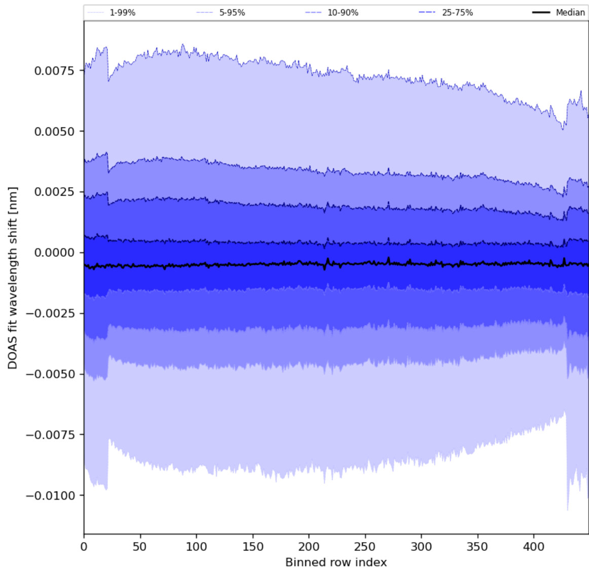
Figure 91: Along track statistics of “DOAS fit wavelength shift” for 2024-01-26 to 2024-01-28
