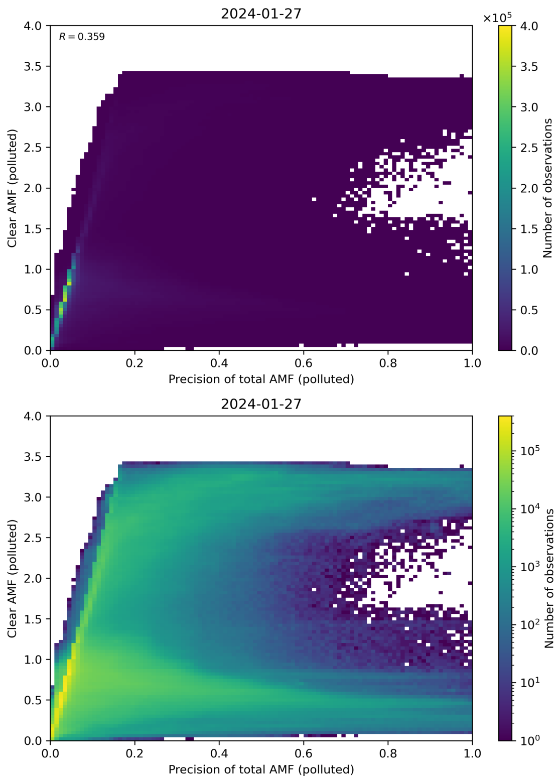
Figure 270: Scatter density plot of “Precision of total AMF (polluted)” against “Clear AMF (polluted)” for 2024-01-26 to 2024-01-28.
