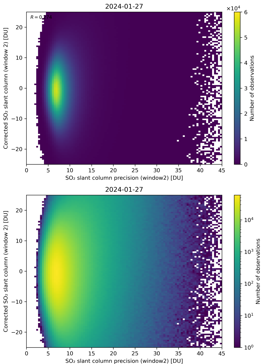
Figure 247: Scatter density plot of “SO 2 slant column precision (window2)” against “Corrected SO 2 slant column (window 2)” for 2024-01-26 to 2024-01-28.
