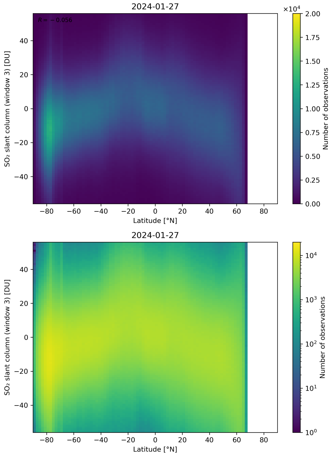
Figure 152: Scatter density plot of “Latitude” against “SO 2 slant column (window 3)” for 2024-01-26 to 2024-01-28.
