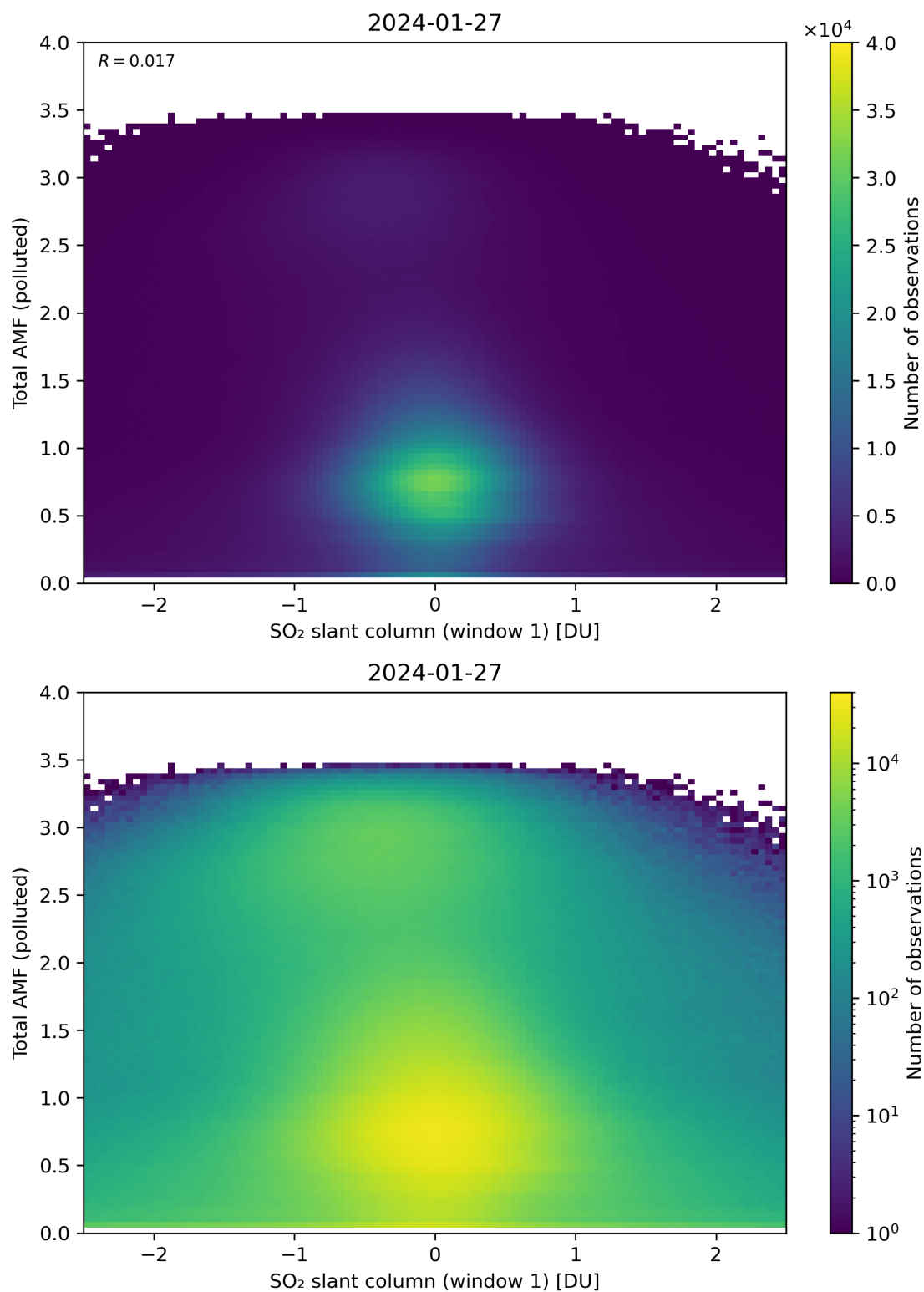
Figure 239: Scatter density plot of “SO 2 slant column (window 1)” against “Total AMF (polluted)” for 2024-01-26 to 2024-01-28.
