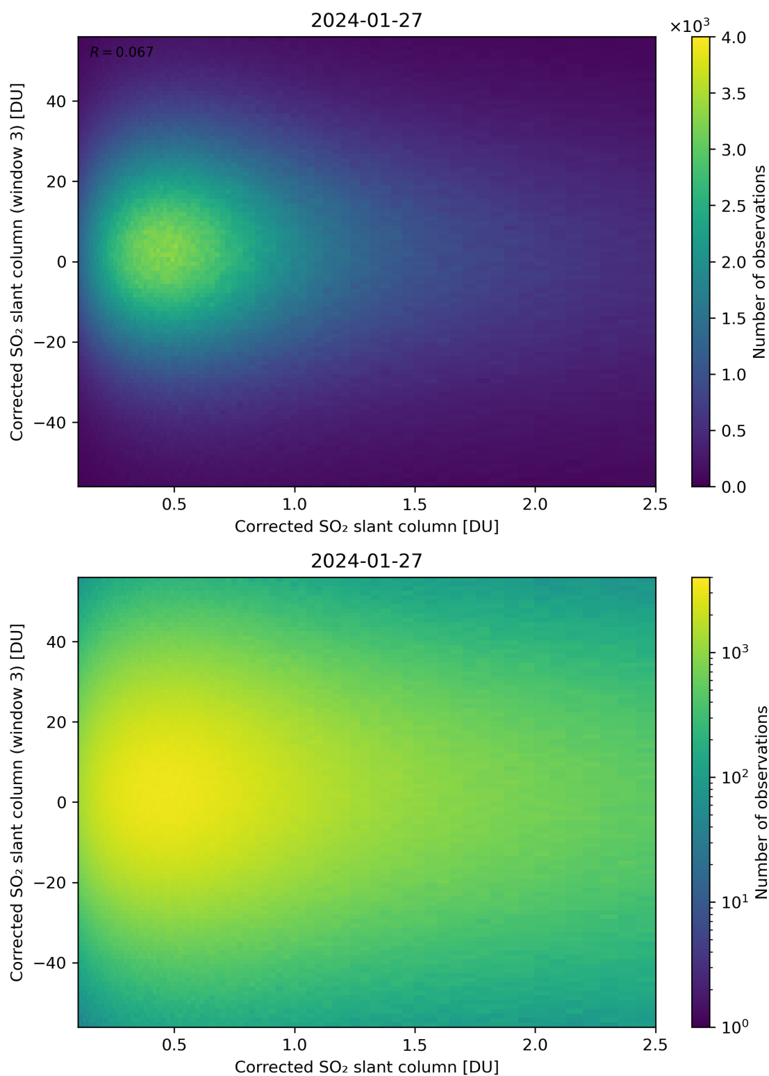
Figure 186: Scatter density plot of “Corrected SO 2 slant column” against “Corrected SO 2 slant column (window 3)” for 2024-01-26 to 2024-01-28.
