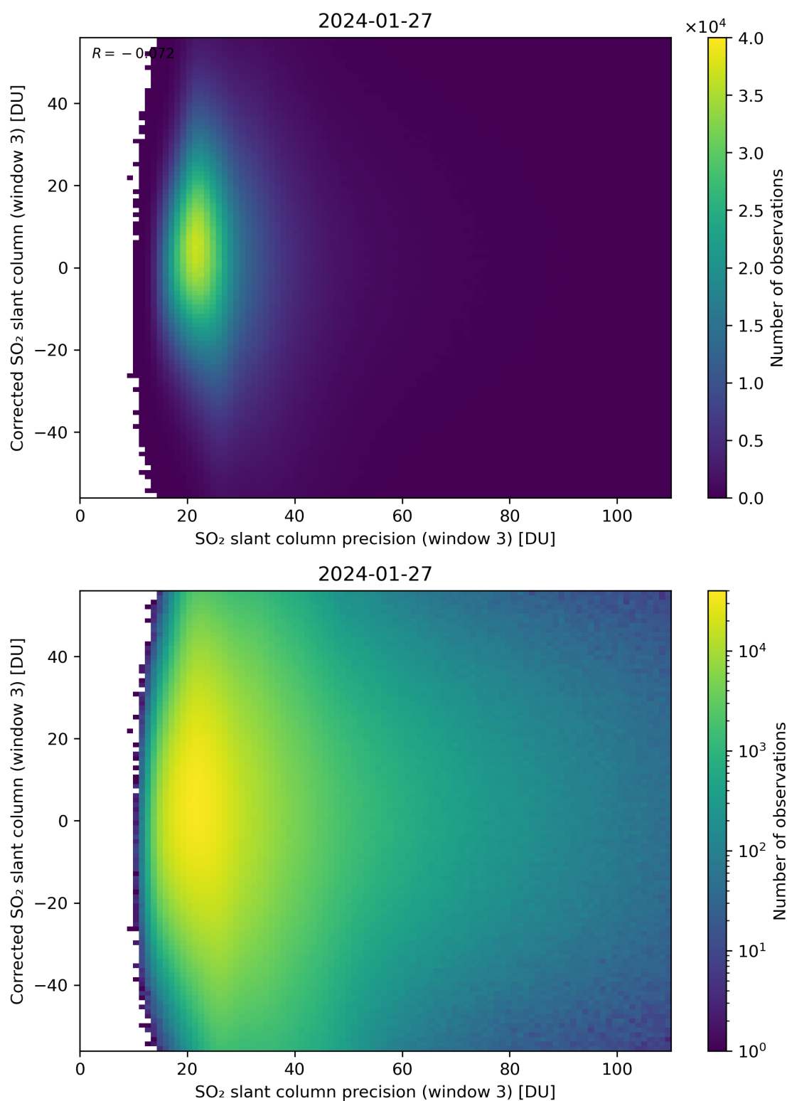
Figure 262: Scatter density plot of “SO 2 slant column precision (window 3)” against “Corrected SO 2 slant column (window 3)” for 2024-01-26 to 2024-01-28.
