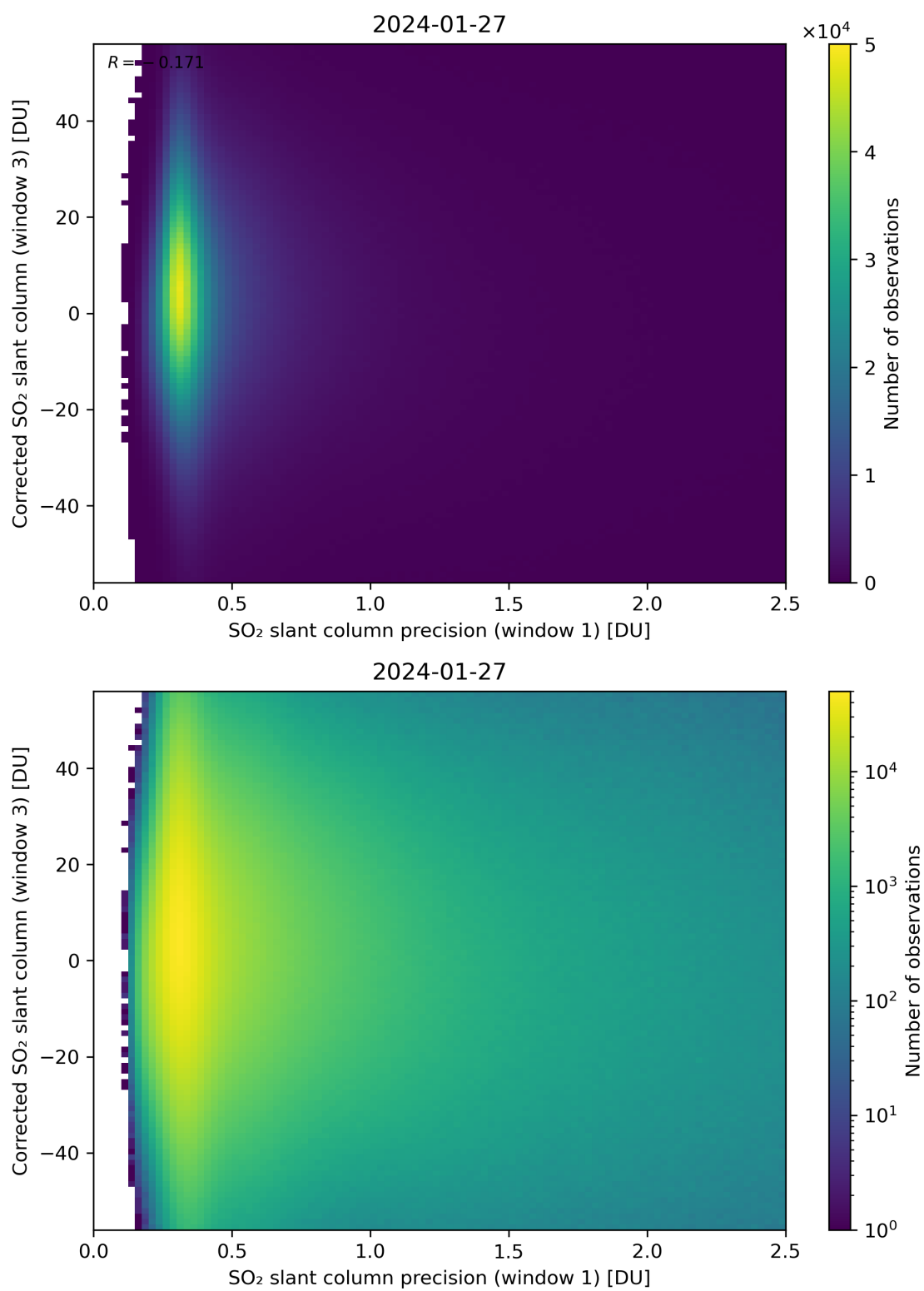
Figure 226: Scatter density plot of “SO 2 slant column precision (window 1)” against “Corrected SO 2 slant column (window 3)” for 2024-01-26 to 2024-01-28.
