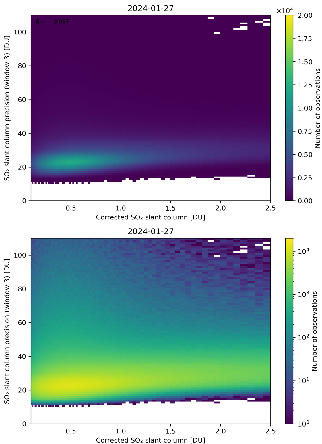
Figure 191: Scatter density plot of “Corrected SO 2 slant column” against “SO 2 slant column precision (window 3)” for 2024-01-26 to 2024-01-28.
