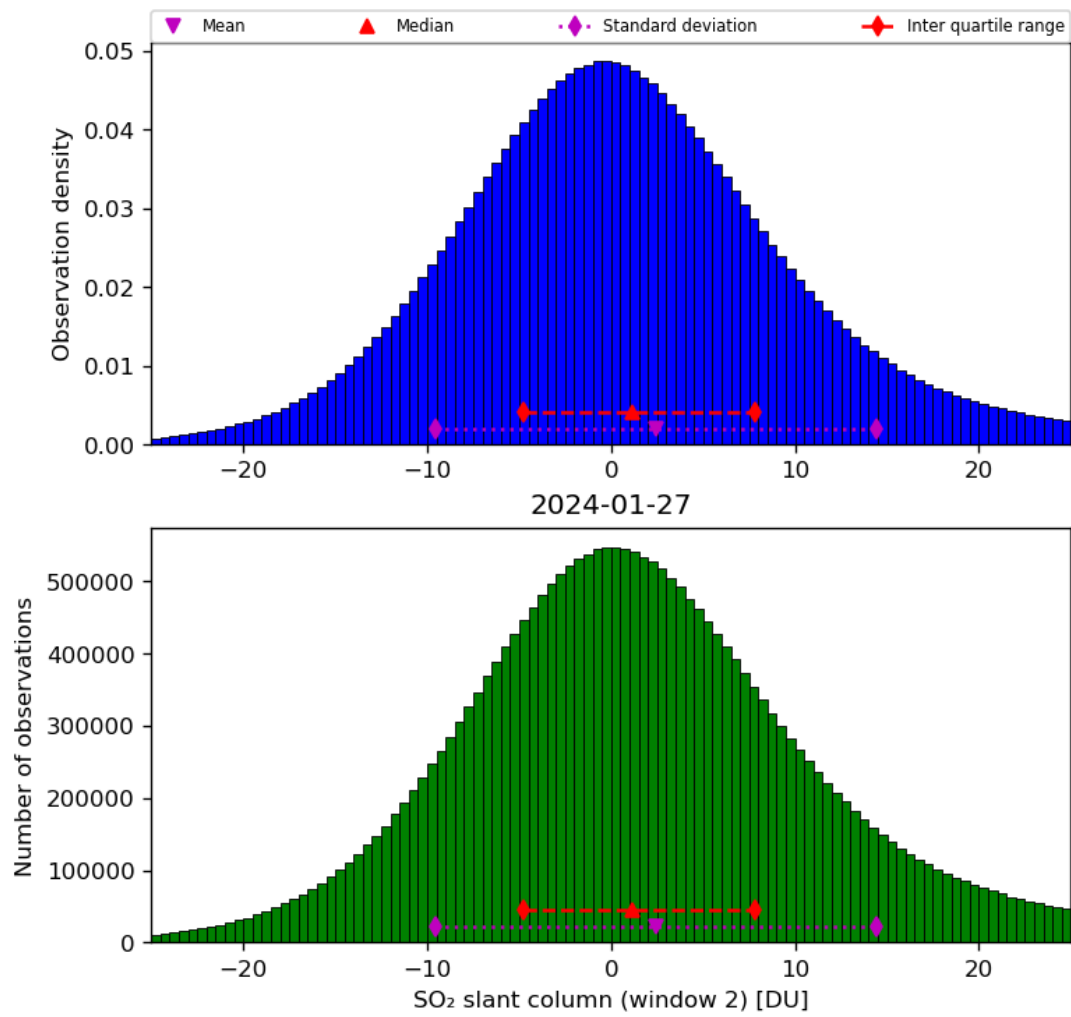
Figure 60: Histogram of “SO 2 slant column (window 2)” for 2024-01-26 to 2024-01-28
