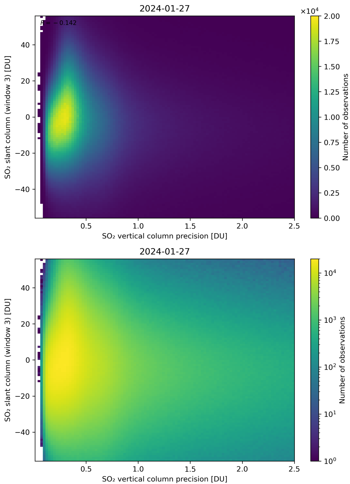
Figure 292: Scatter density plot of “SO 2 vertical column precision” against “SO 2 slant column (window 3)” for 2024-01-26 to 2024-01-28.
