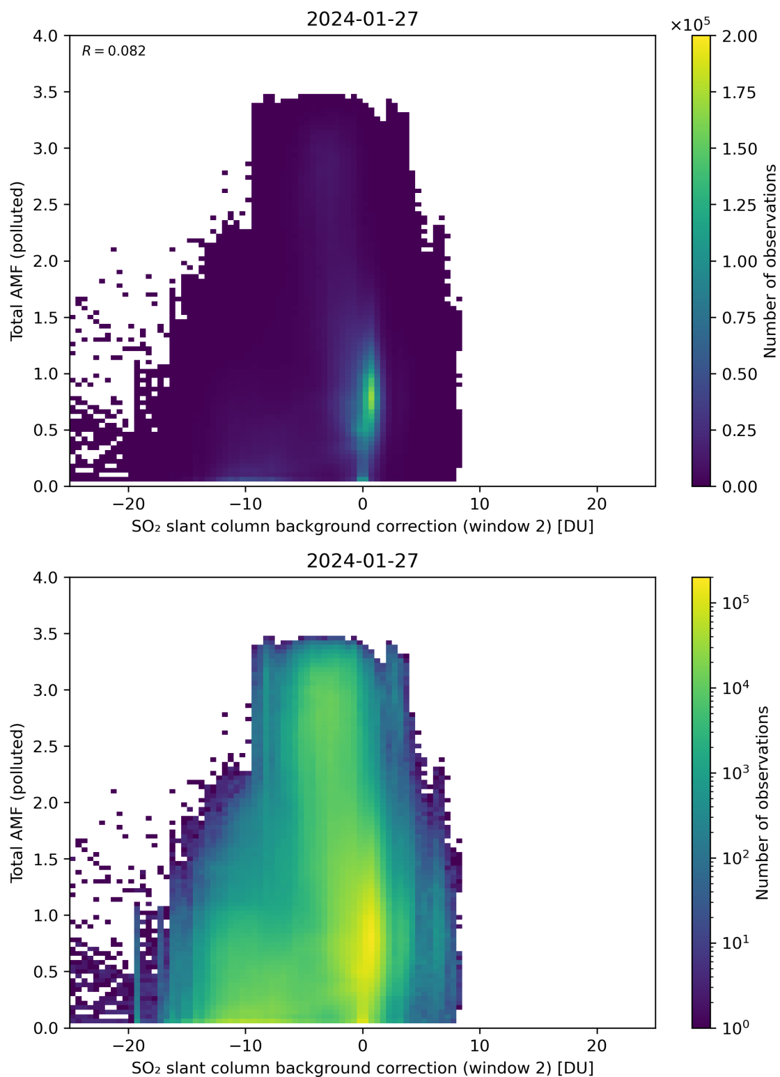
Figure 119: Scatter density plot of “SO 2 slant column background correction (window 2)” against “Total AMF (polluted)” for 2024-01-26 to 2024-01-28.
