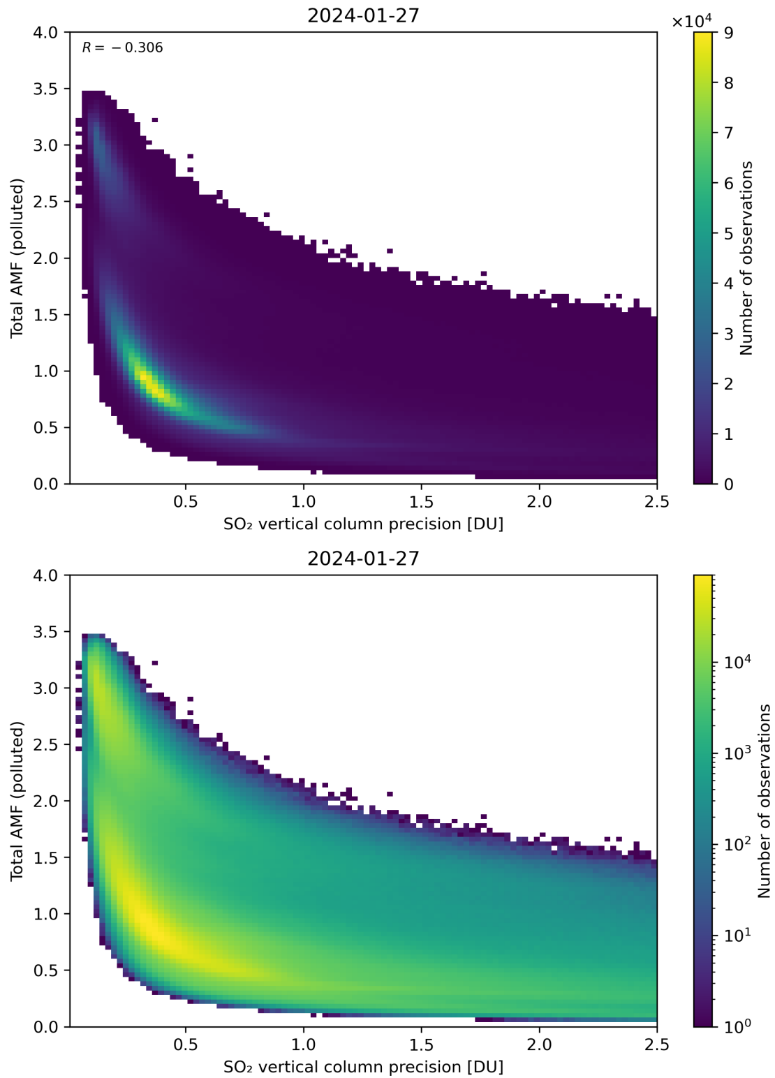
Figure 294: Scatter density plot of “SO 2 vertical column precision” against “Total AMF (polluted)” for 2024-01-26 to 2024-01-28.
