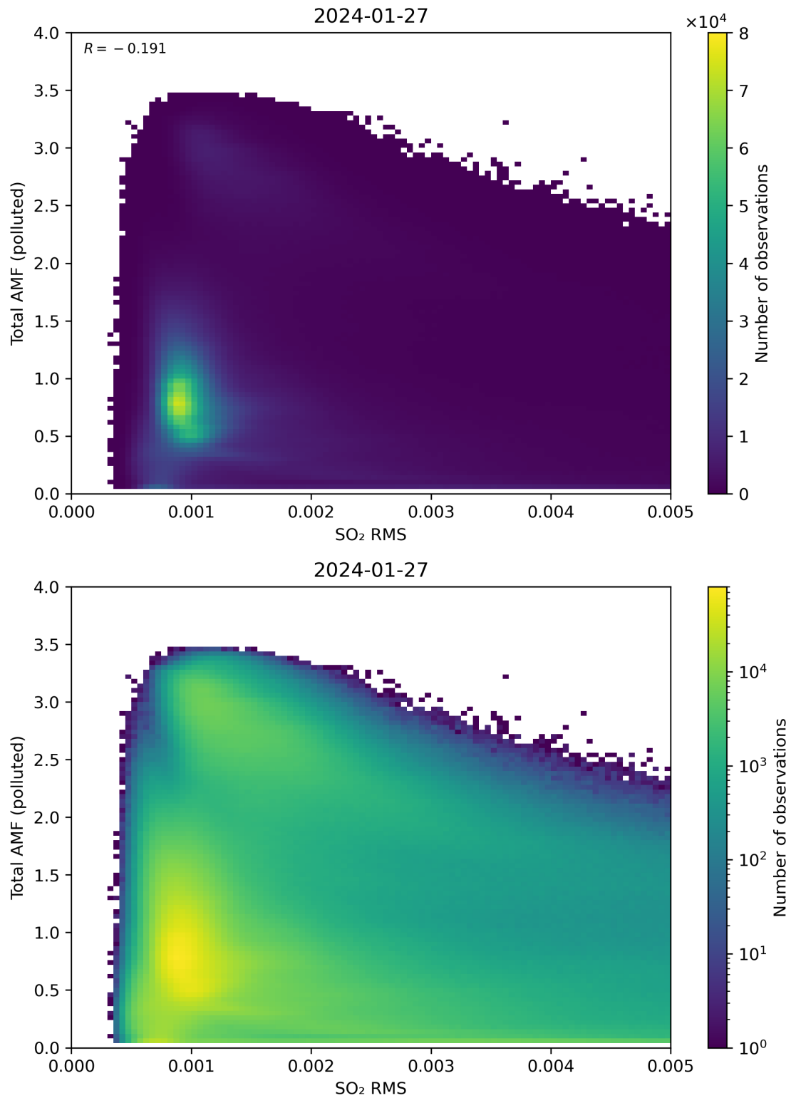
Figure 137: Scatter density plot of “SO 2 RMS” against “Total AMF (polluted)” for 2024-01-26 to 2024-01-28.
