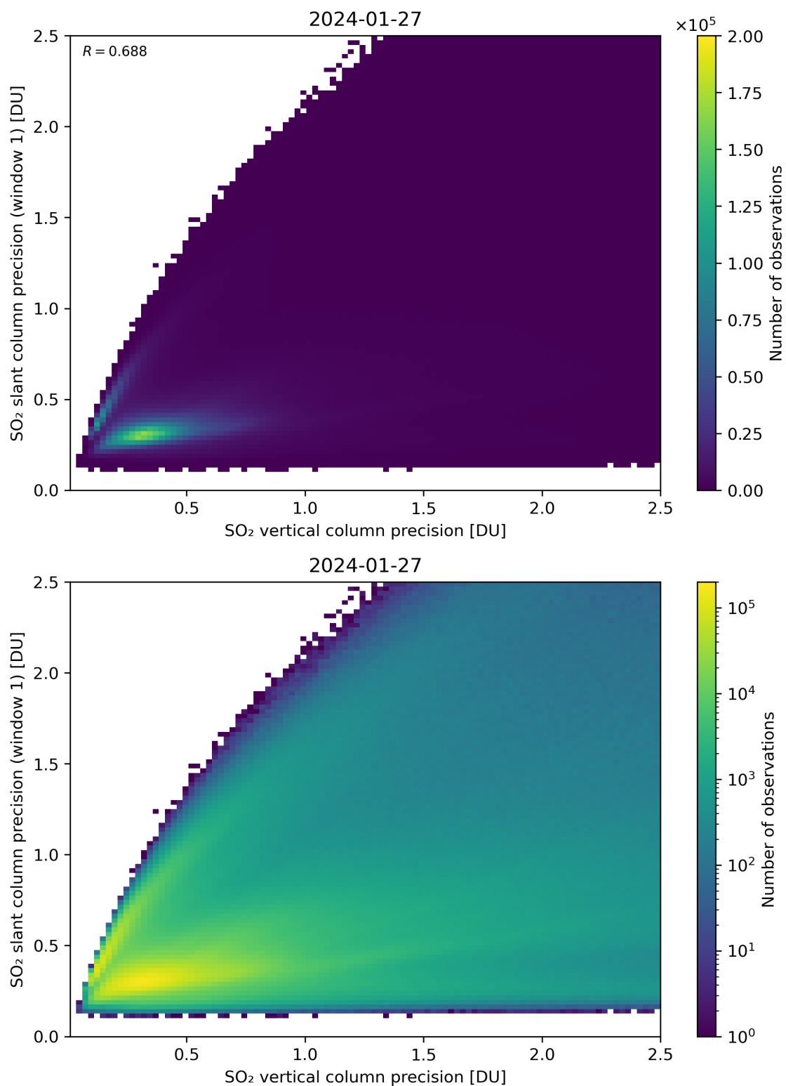
Figure 290: Scatter density plot of “SO 2 vertical column precision” against “SO 2 slant column precision (window 1)” for 2024-01-26 to 2024-01-28.
