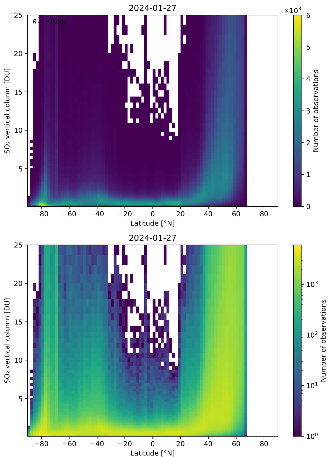
Figure 156: Scatter density plot of “Latitude” against “SO 2 vertical column” for 2024-01-26 to 2024-01-28.
