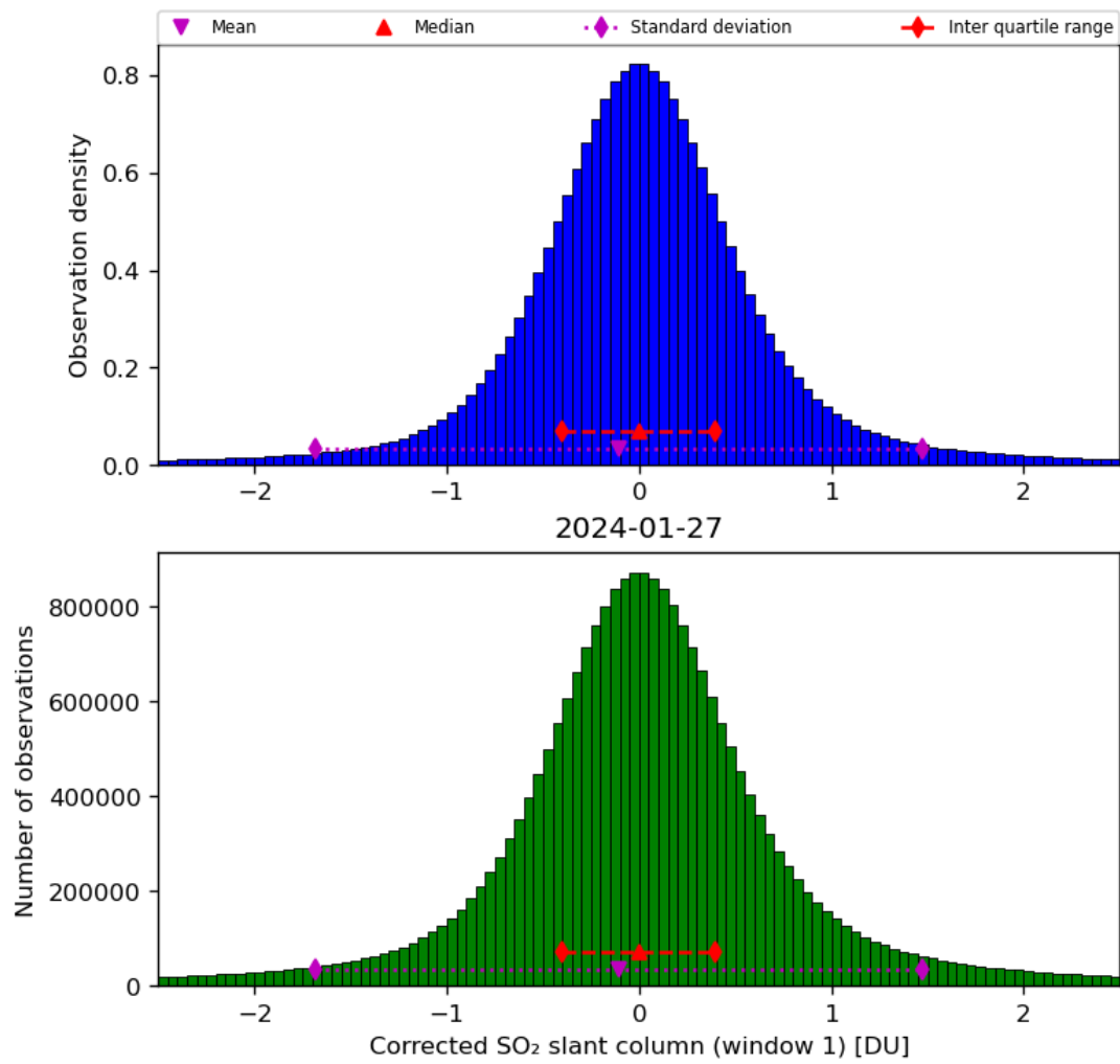
Figure 58: Histogram of “Corrected SO 2 slant column (window 1)” for 2024-01-26 to 2024-01-28
