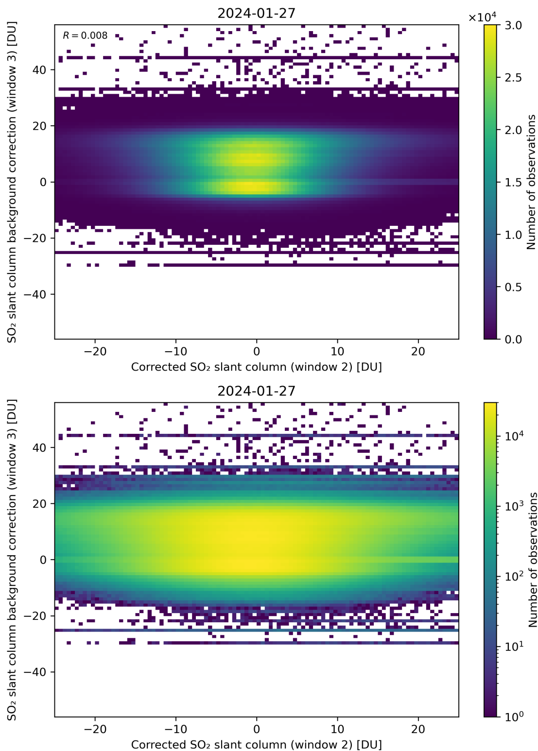
Figure 195: Scatter density plot of “Corrected SO 2 slant column (window 2)” against “SO 2 slant column background correction (window 3)” for 2024-01-26 to 2024-01-28.
