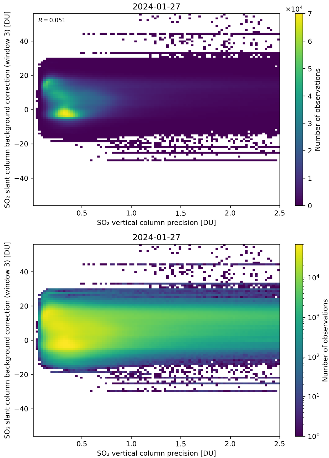
Figure 281: Scatter density plot of “SO 2 vertical column precision” against “SO 2 slant column background correction (window 3)” for 2024-01-26 to 2024-01-28.
