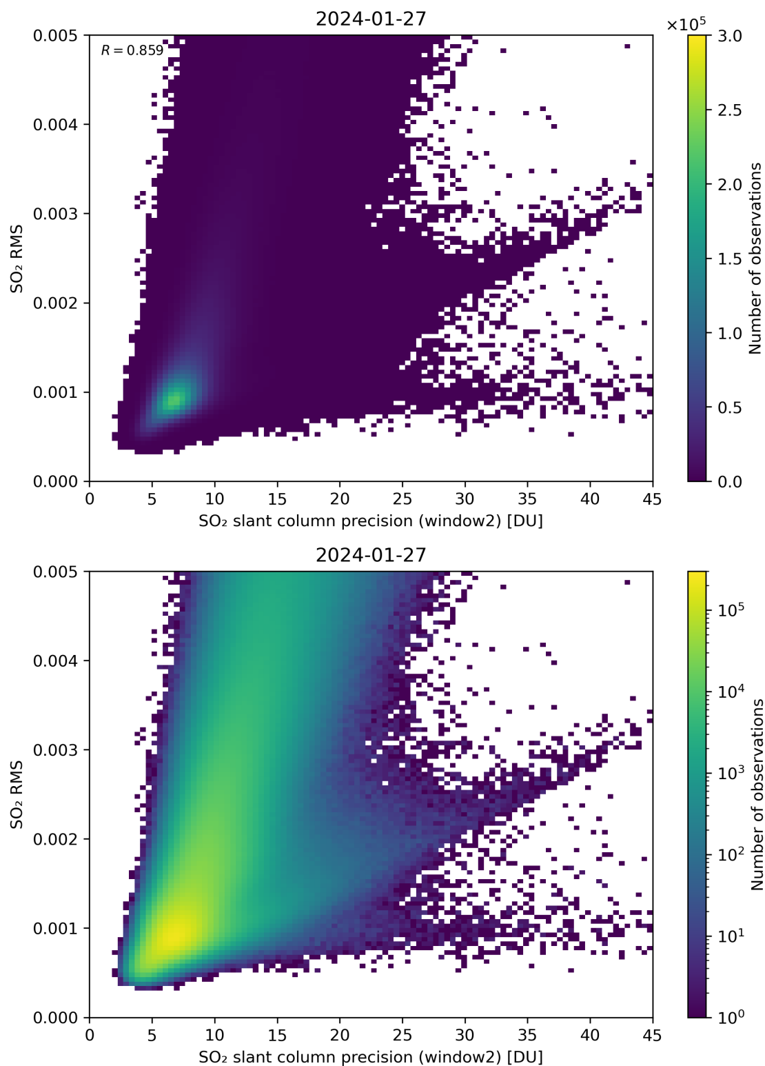
Figure 245: Scatter density plot of “SO 2 slant column precision (window2)” against “SO 2 RMS” for 2024-01-26 to 2024-01-28.
