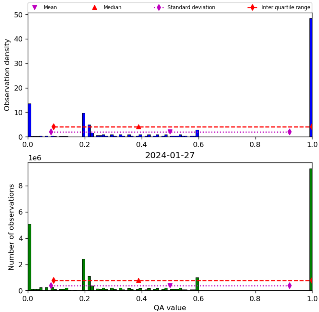
Figure 52: Histogram of “QA value” for 2024-01-26 to 2024-01-28
