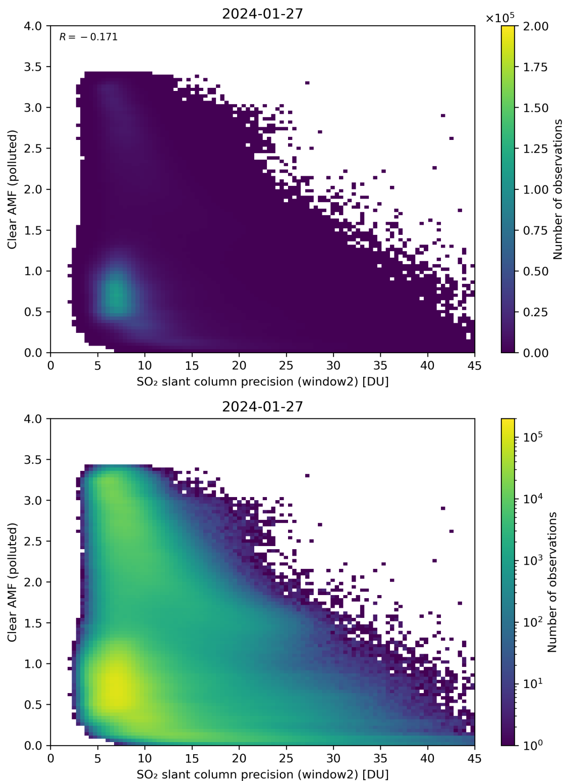
Figure 246: Scatter density plot of “SO 2 slant column precision (window2)” against “Clear AMF (polluted)” for 2024-01-26 to 2024-01-28.
