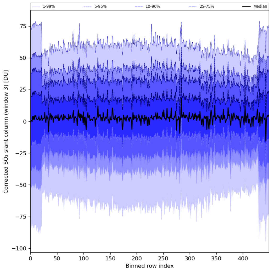
Figure 89: Along track statistics of “Corrected SO 2 slant column (window 3)” for 2024-01-26 to 2024-01-28
