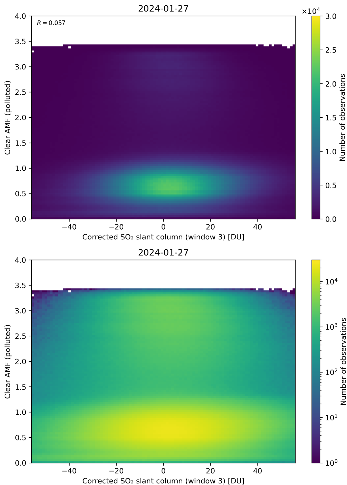
Figure 209: Scatter density plot of “Corrected SO 2 slant column (window 3)” against “Clear AMF (polluted)” for 2024-01-26 to 2024-01-28.
