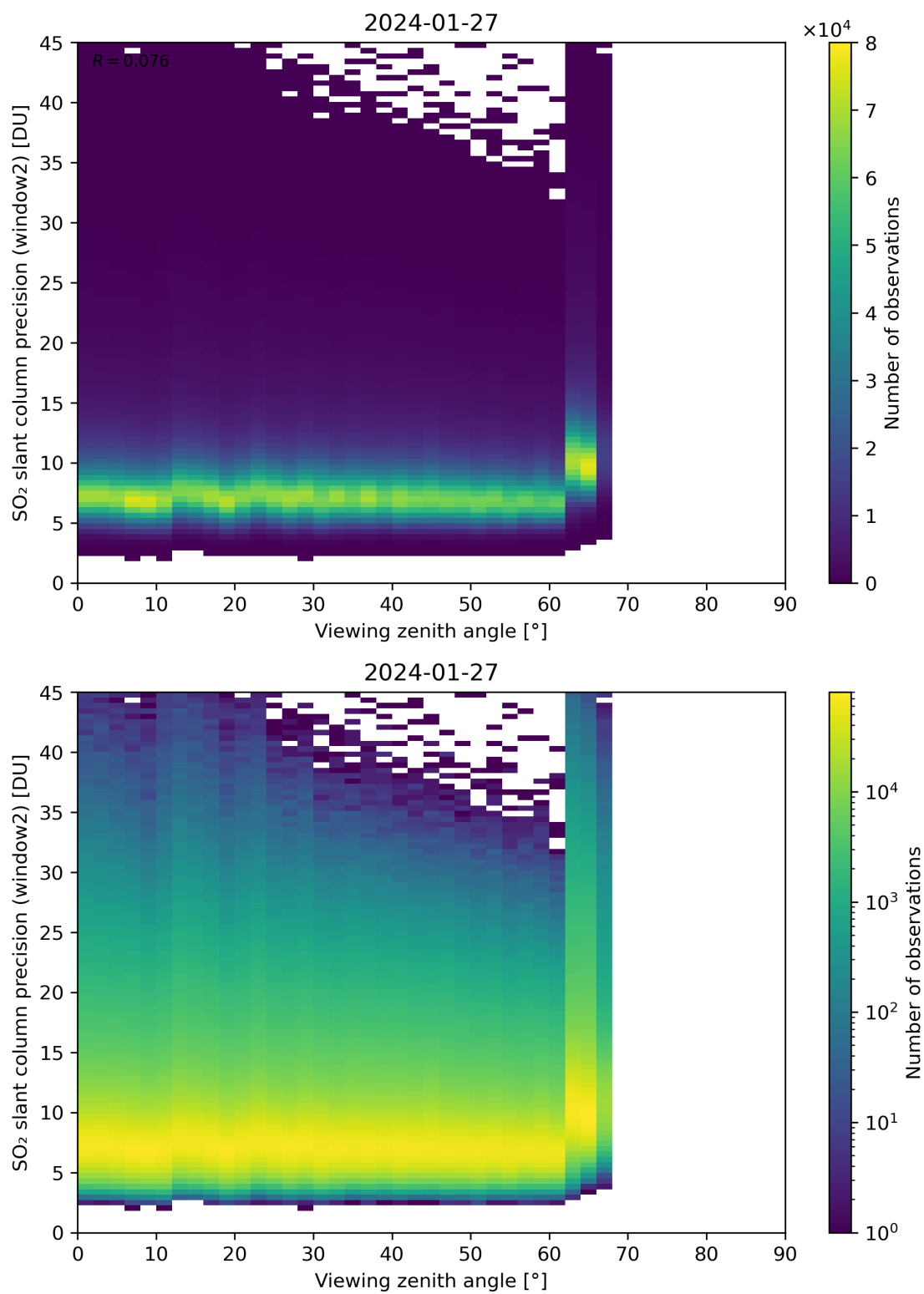
Figure 322: Scatter density plot of “Viewing zenith angle” against “SO 2 slant column precision (window2)” for 2024-01-26 to 2024-01-28.
