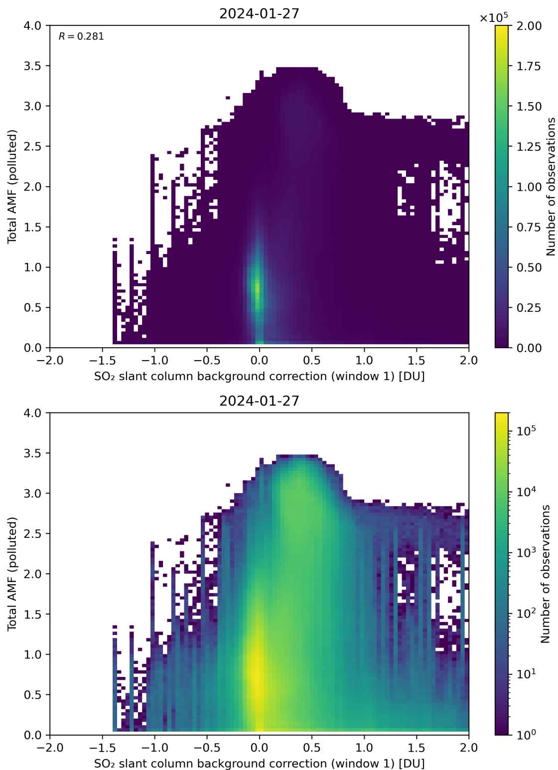
Figure 109: Scatter density plot of “SO 2 slant column background correction (window 1)” against “Total AMF (polluted)” for 2024-01-26 to 2024-01-28.
