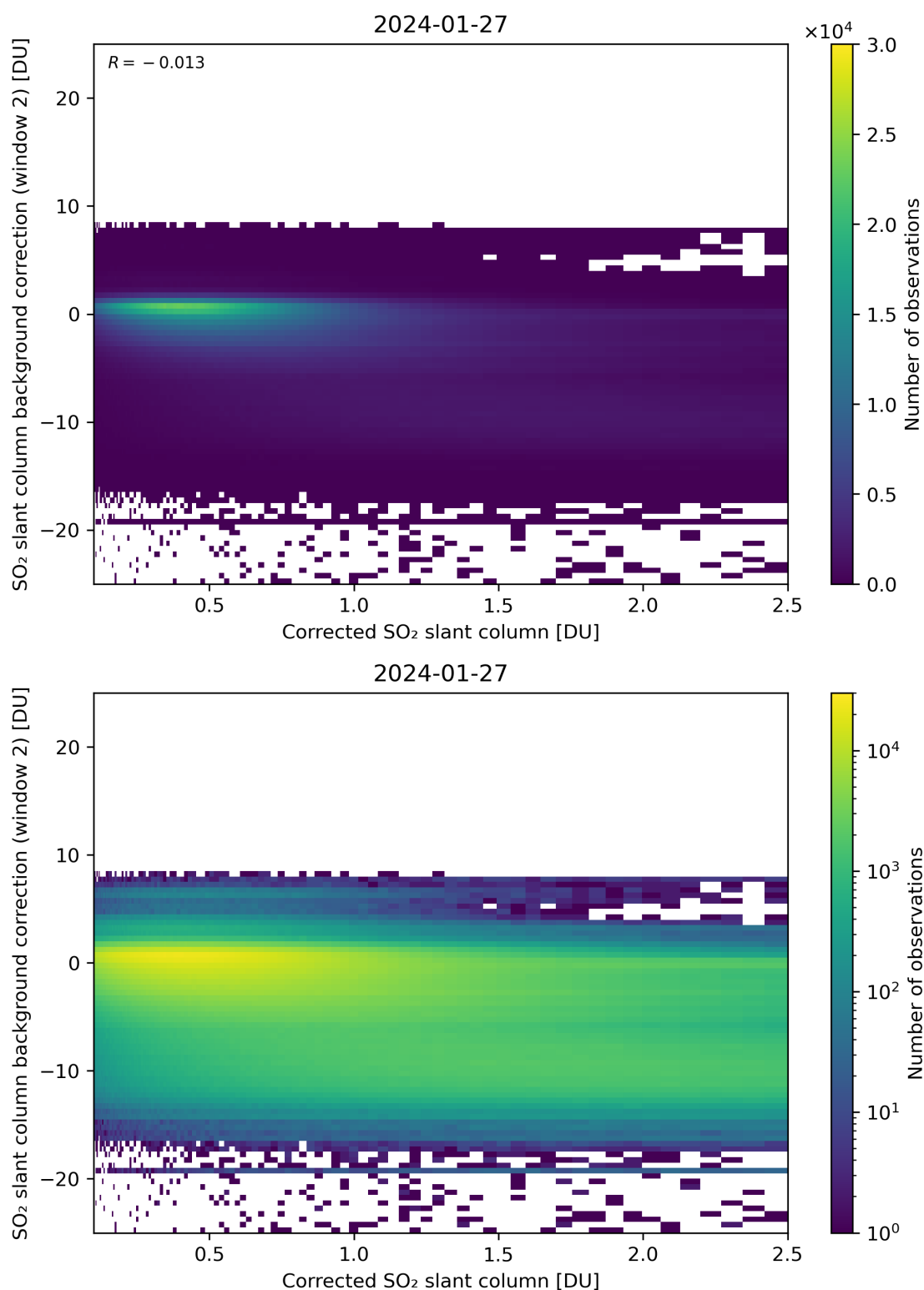
Figure 179: Scatter density plot of “Corrected SO 2 slant column” against “SO 2 slant column background correction (window 2)” for 2024-01-26 to 2024-01-28.
