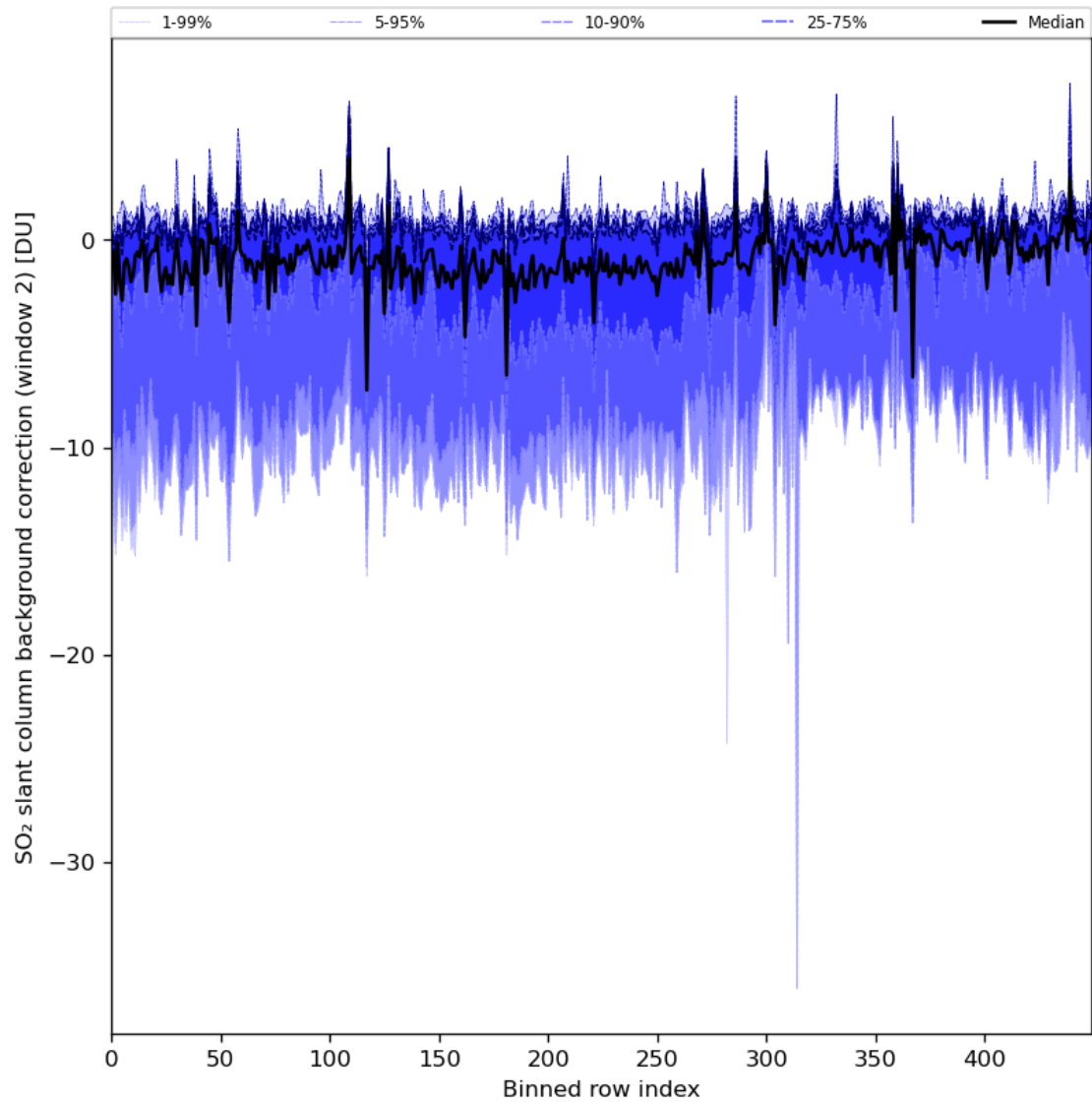
Figure 86: Along track statistics of “SO 2 slant column background correction (window 2)” for 2024-01-26 to 2024-01-28
