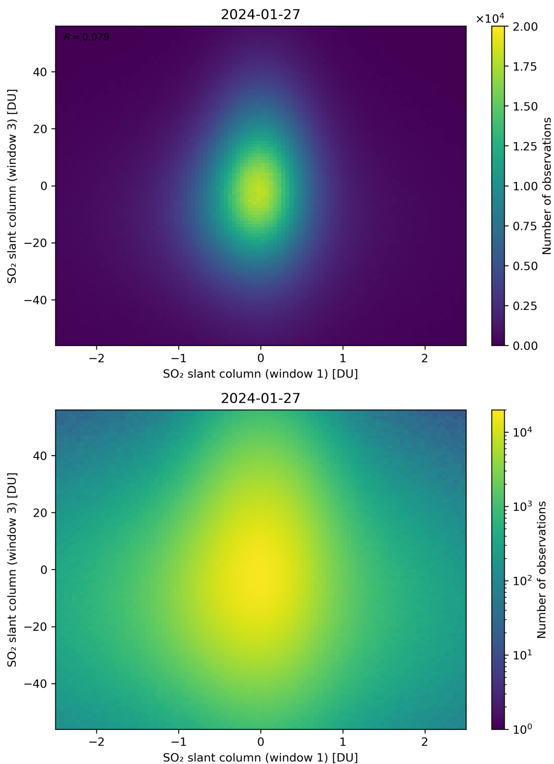
Figure 237: Scatter density plot of “SO 2 slant column (window 1)” against “SO 2 slant column (window 3)” for 2024-01-26 to 2024-01-28.
