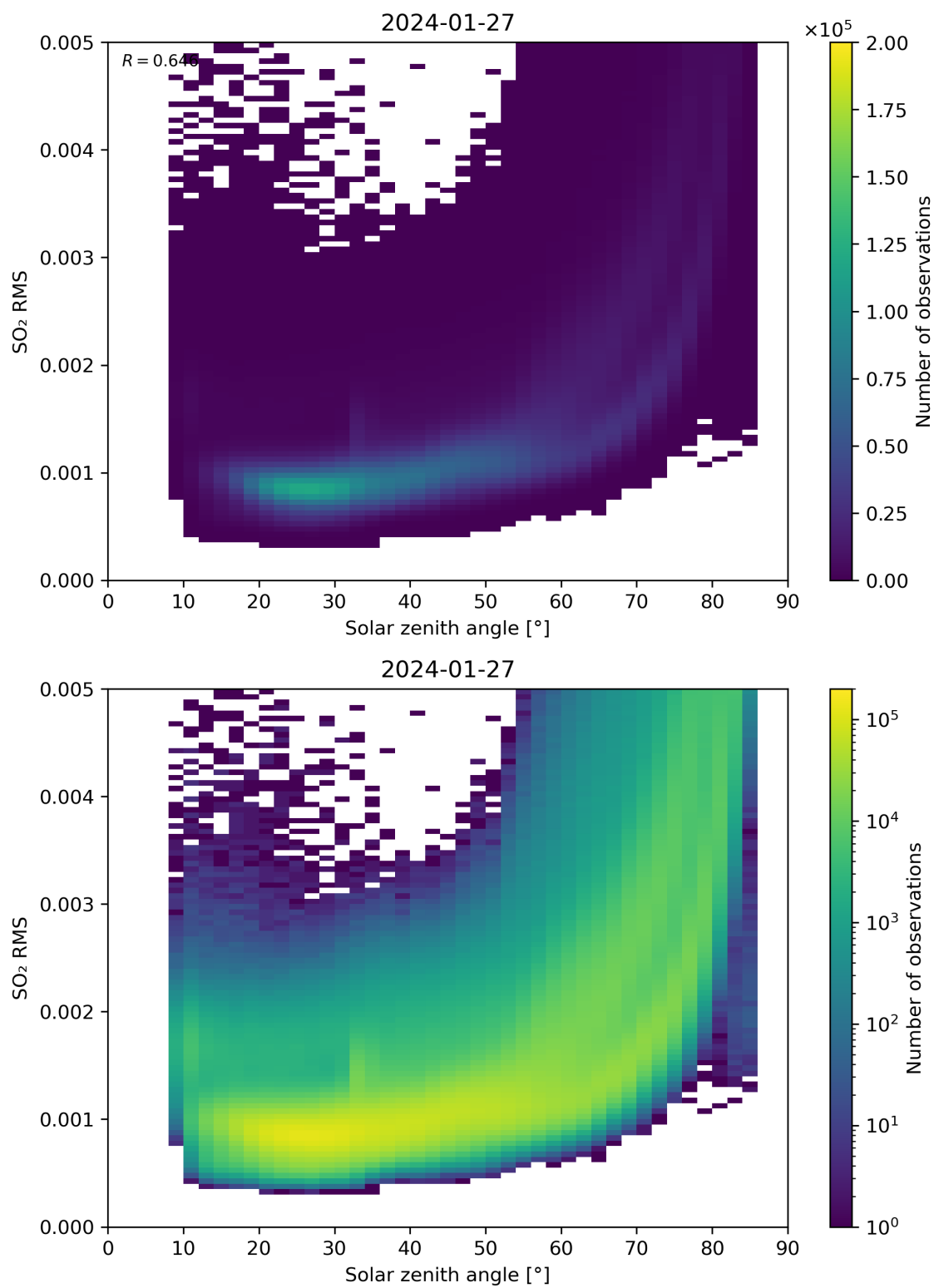
Figure 163: Scatter density plot of “Solar zenith angle” against “SO 2 RMS” for 2024-01-26 to 2024-01-28.
