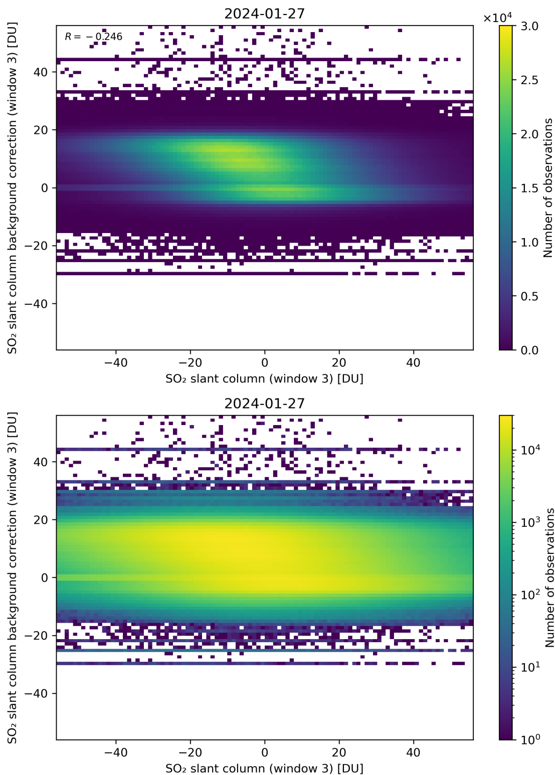
Figure 253: Scatter density plot of “SO 2 slant column (window 3)” against “SO 2 slant column background correction (window 3)” for 2024-01-26 to 2024-01-28.
