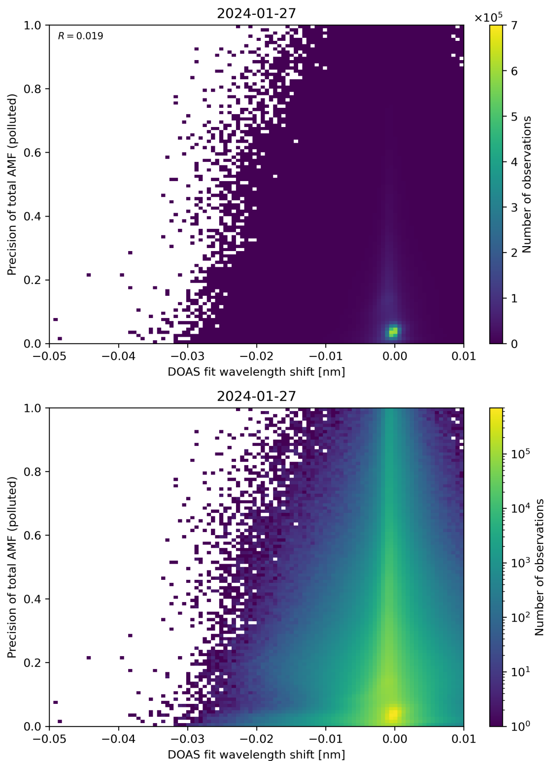
Figure 131: Scatter density plot of “DOAS fit wavelength shift” against “Precision of total AMF (polluted)” for 2024-01-26 to 2024-01-28.
