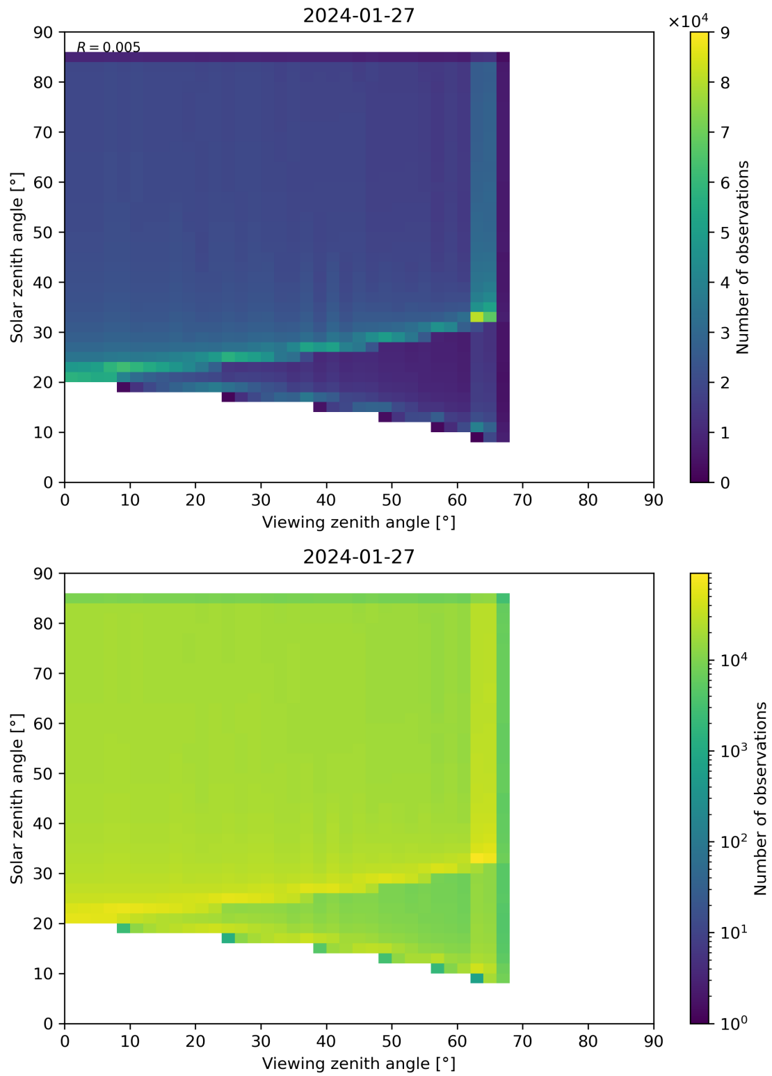
Figure 315: Scatter density plot of “Viewing zenith angle” against “Solar zenith angle” for 2024-01-26 to 2024-01-28.
