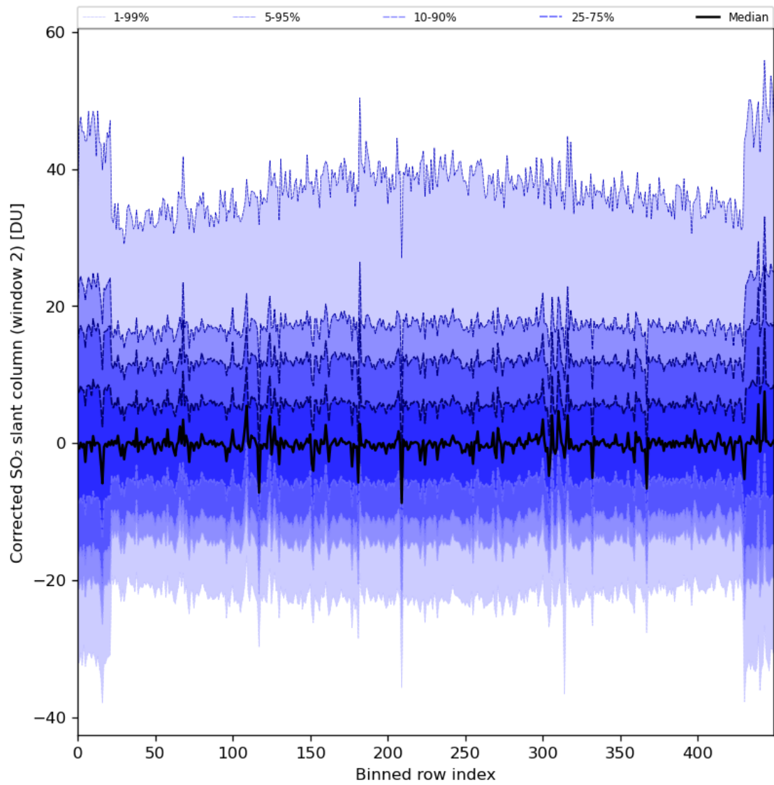
Figure 85: Along track statistics of “Corrected SO 2 slant column (window 2)” for 2024-01-26 to 2024-01-28
