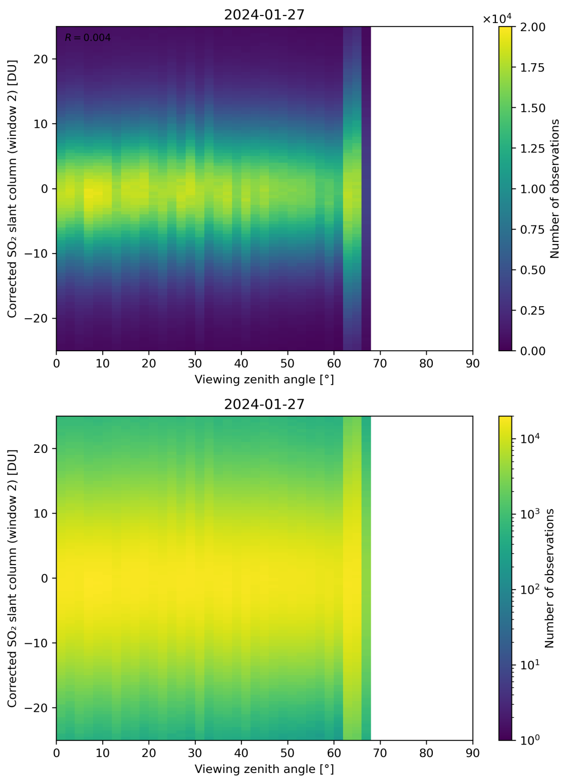
Figure 318: Scatter density plot of “Viewing zenith angle” against “Corrected SO 2 slant column (window 2)” for 2024-01-26 to 2024-01-28.
