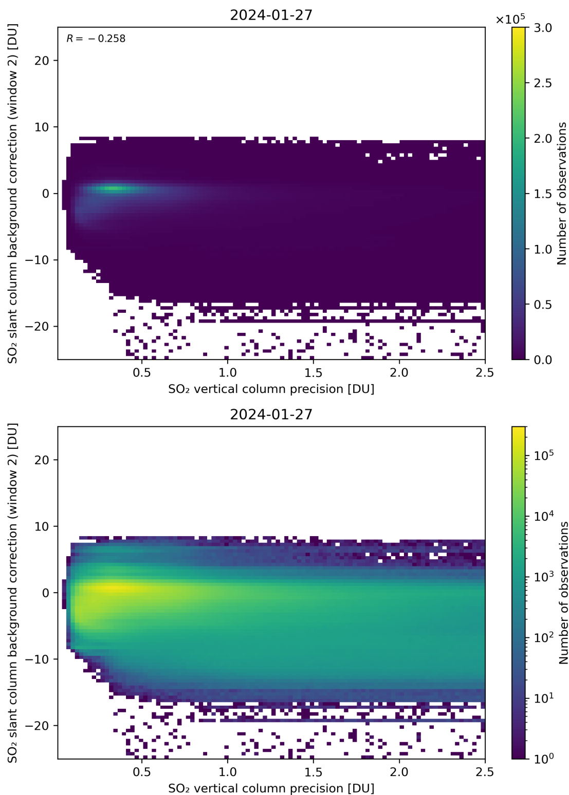
Figure 280: Scatter density plot of “SO 2 vertical column precision” against “SO 2 slant column background correction (window 2)” for 2024-01-26 to 2024-01-28.
