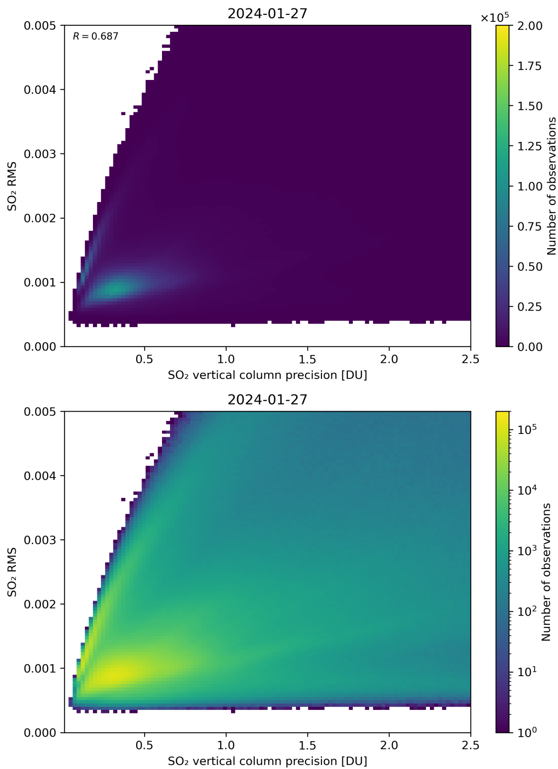
Figure 284: Scatter density plot of “SO 2 vertical column precision” against “SO 2 RMS” for 2024-01-26 to 2024-01-28.
