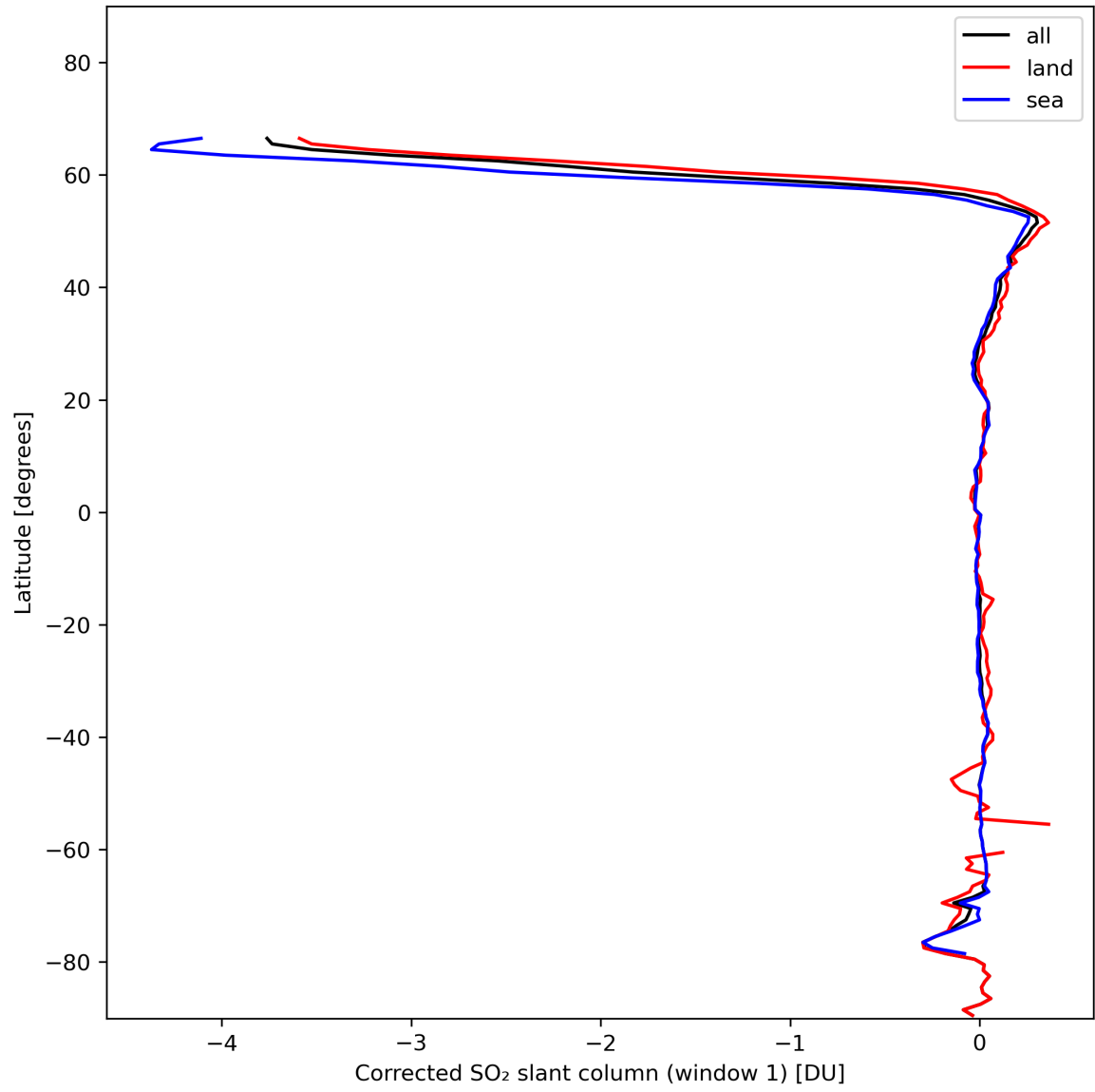
Figure 35: Zonal average of “Corrected SO 2 slant column (window 1)” for 2024-01-26 to 2024-01-28.
