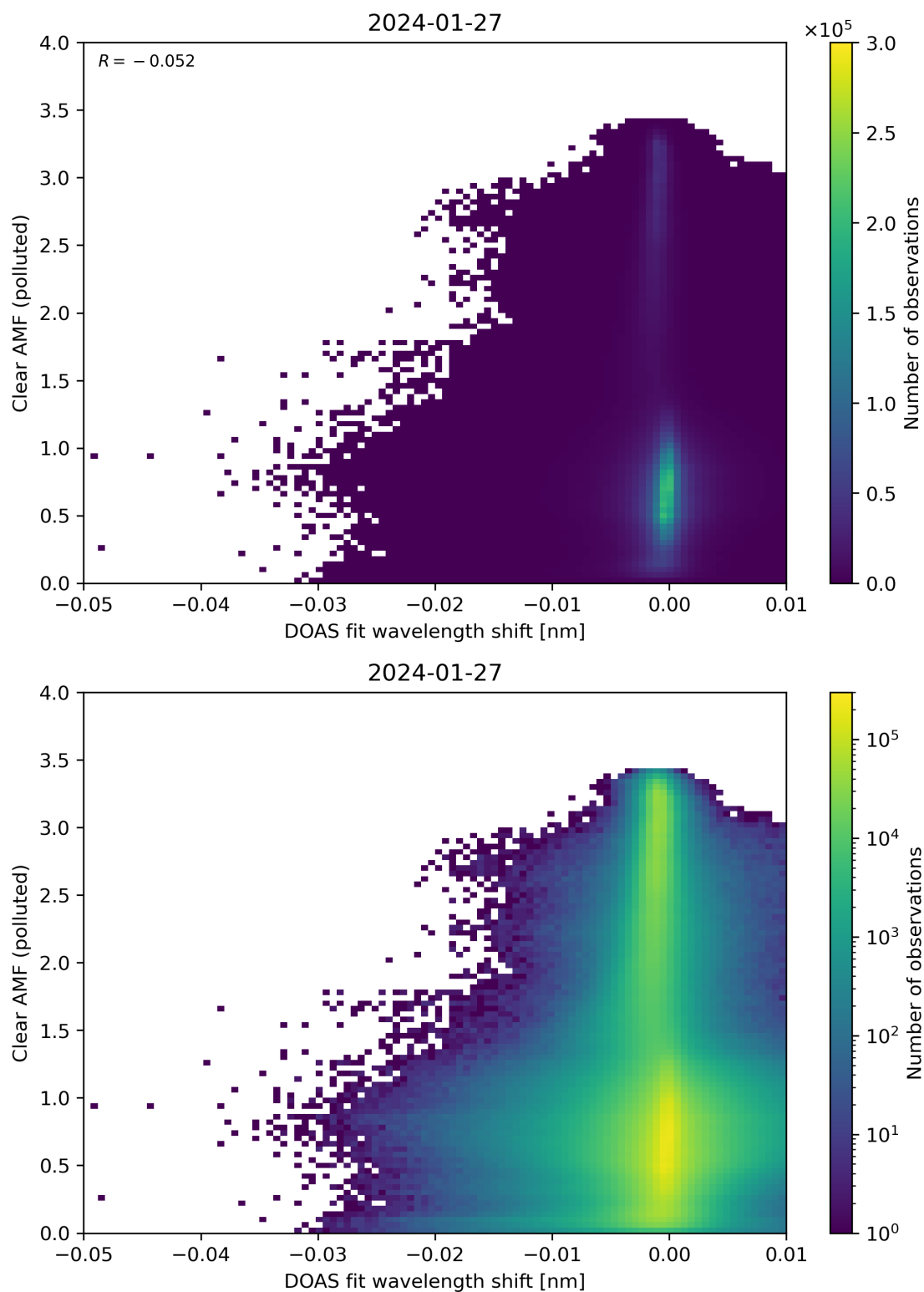
Figure 129: Scatter density plot of “DOAS fit wavelength shift” against “Clear AMF (polluted)” for 2024-01-26 to 2024-01-28.
