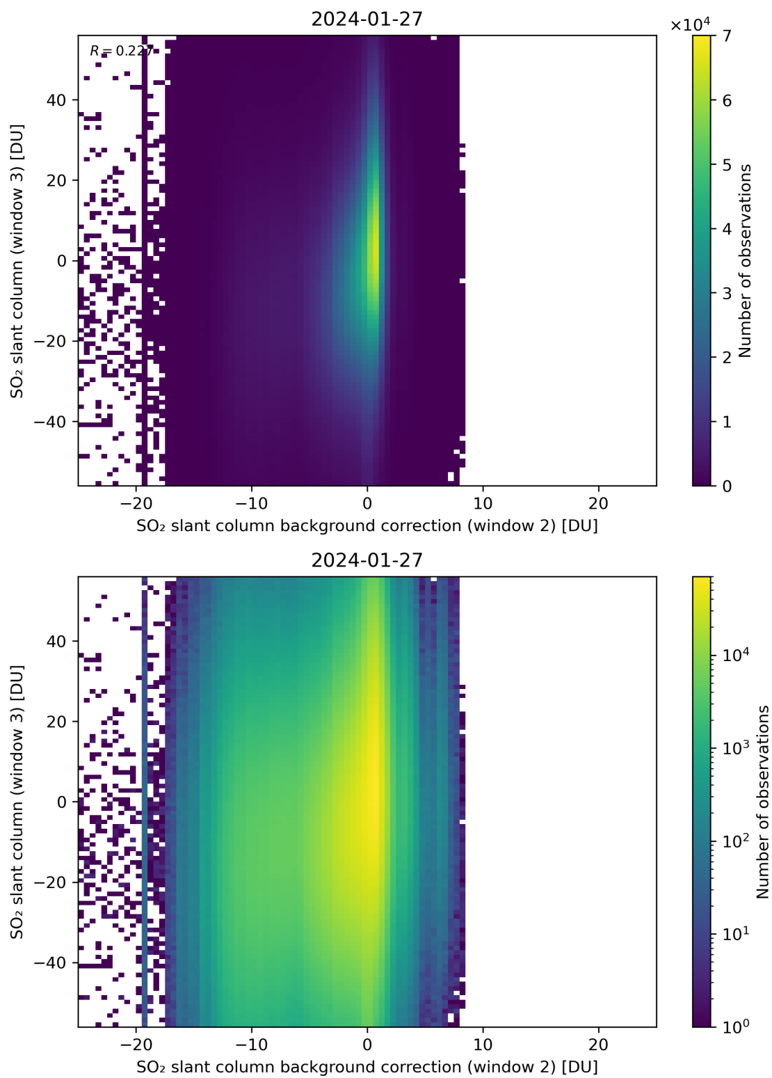
Figure 117: Scatter density plot of “SO 2 slant column background correction (window 2)” against “SO 2 slant column (window 3)” for 2024-01-26 to 2024-01-28.
