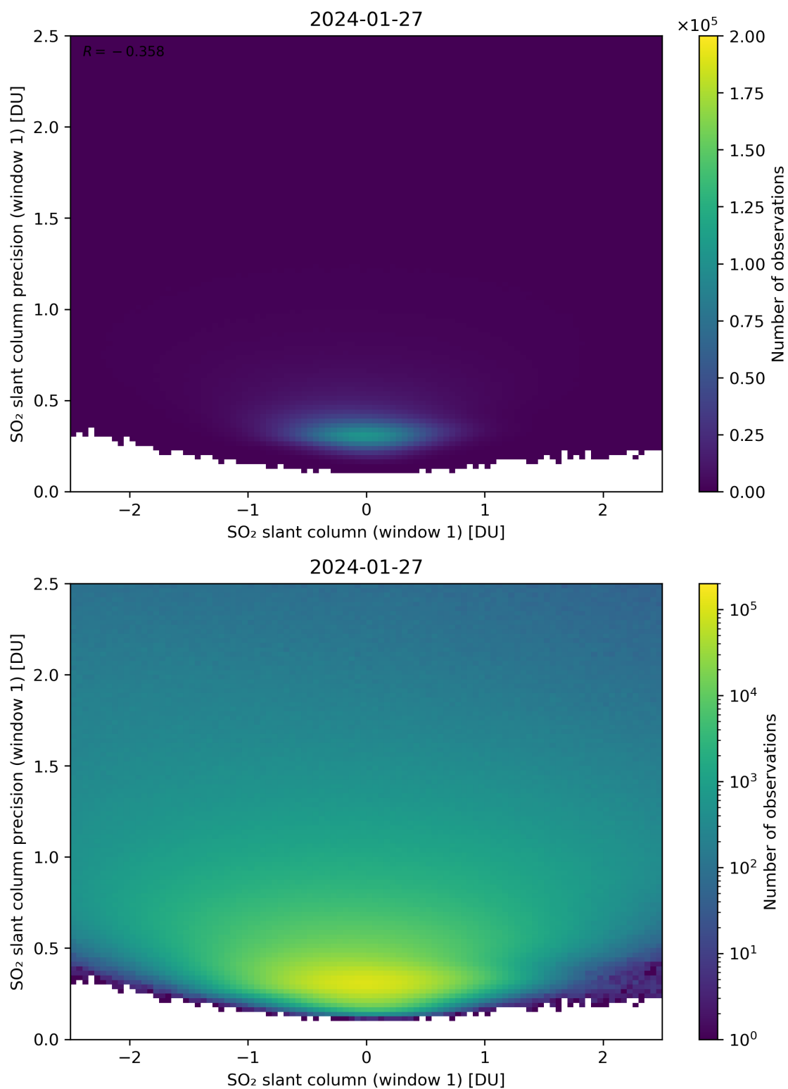
Figure 235: Scatter density plot of “SO 2 slant column (window 1)” against “SO 2 slant column precision (window 1)” for 2024-01-26 to 2024-01-28.
