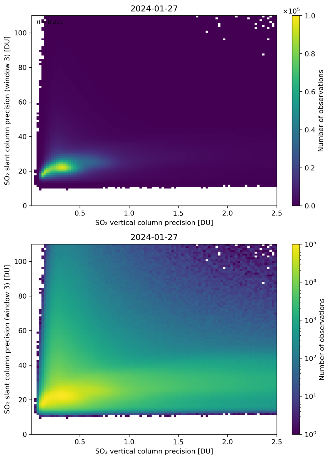
Figure 293: Scatter density plot of “SO 2 vertical column precision” against “SO 2 slant column precision (window 3)” for 2024-01-26 to 2024-01-28.
