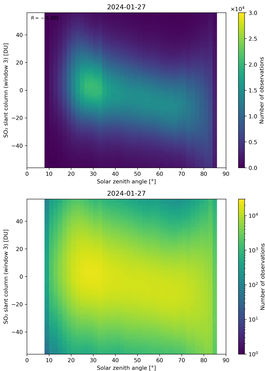
Figure 172: Scatter density plot of “Solar zenith angle” against “SO 2 slant column (window 3)” for 2024-01-26 to 2024-01-28.
