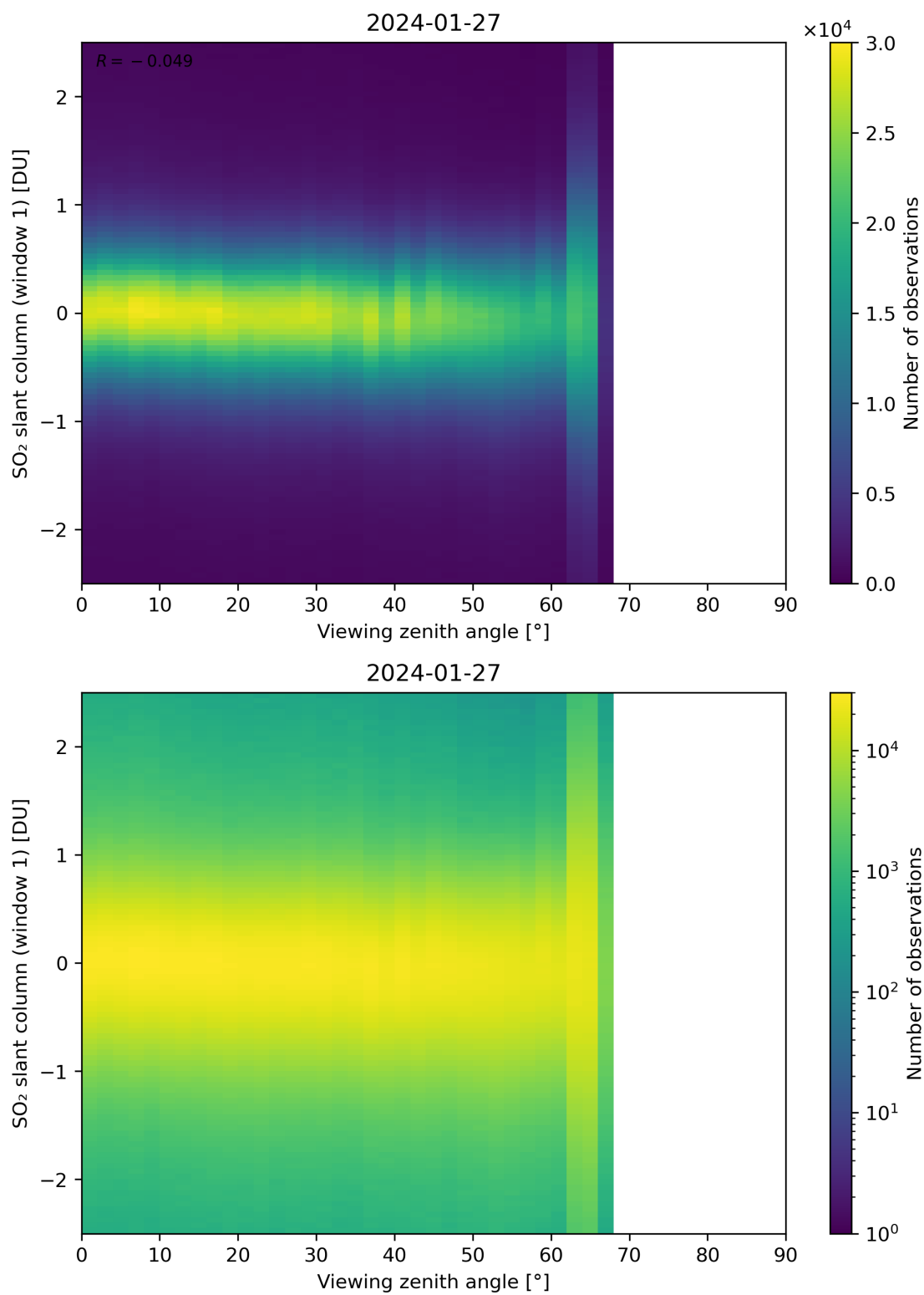
Figure 320: Scatter density plot of “Viewing zenith angle” against “SO 2 slant column (window 1)” for 2024-01-26 to 2024-01-28.
