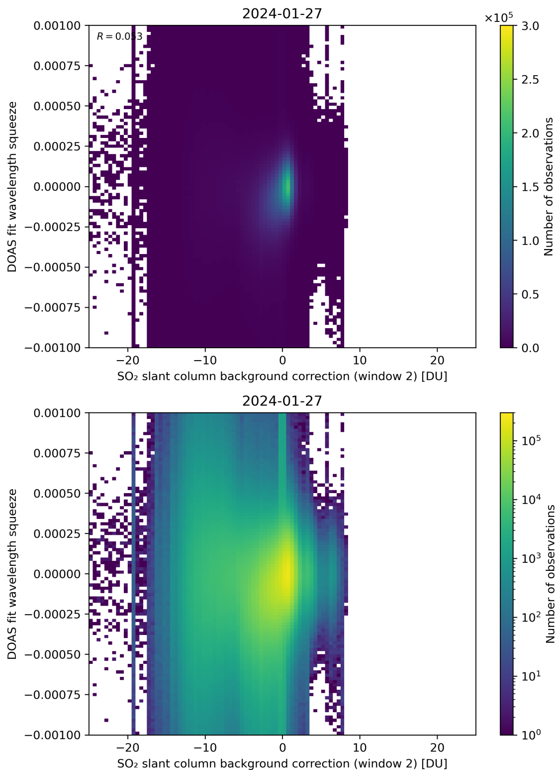
Figure 113: Scatter density plot of “SO 2 slant column background correction (window 2)” against “DOAS fit wavelength squeeze” for 2024-01-26 to 2024-01-28.
