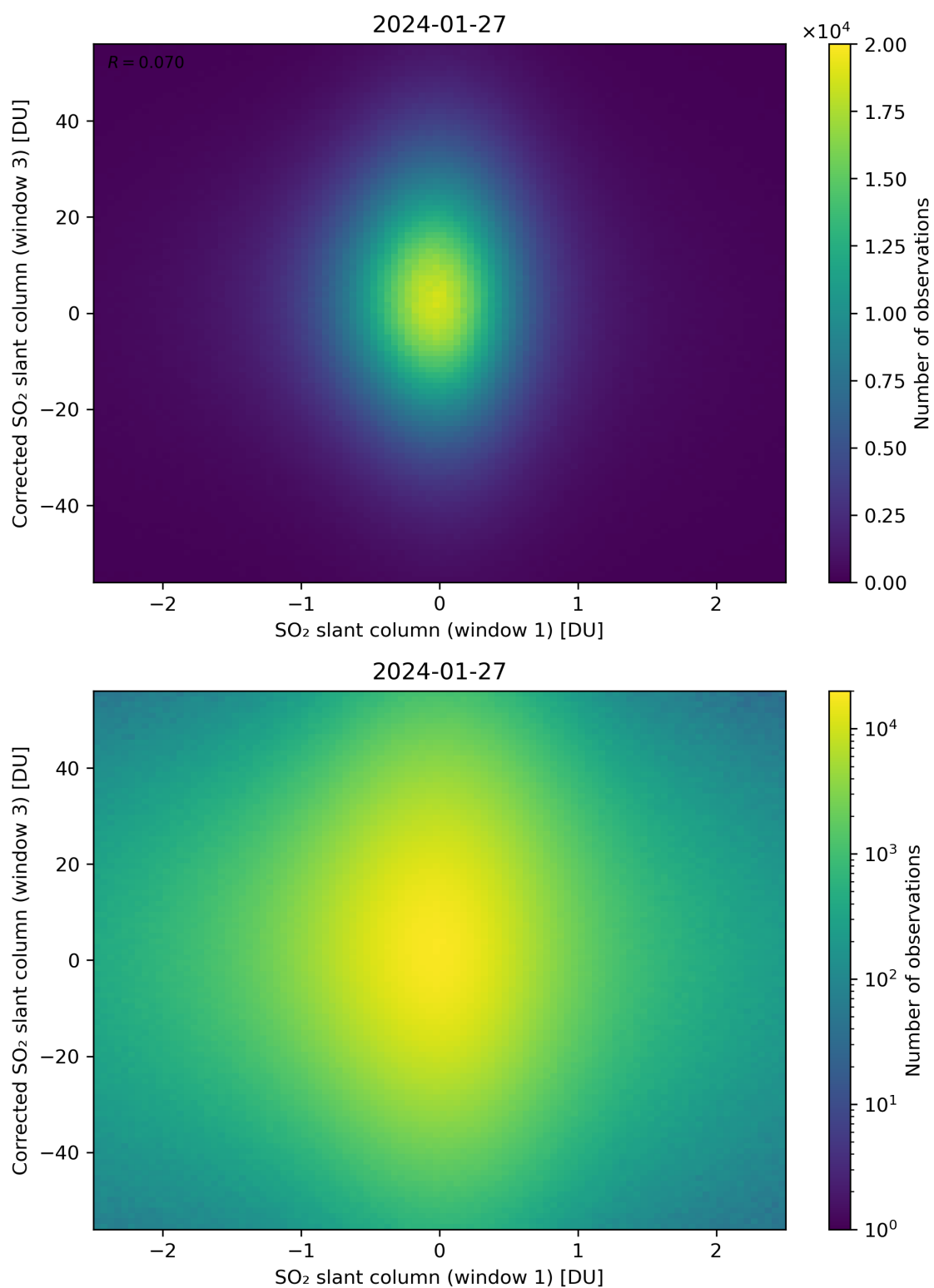
Figure 234: Scatter density plot of “SO 2 slant column (window 1)” against “Corrected SO 2 slant column (window 3)” for 2024-01-26 to 2024-01-28.
