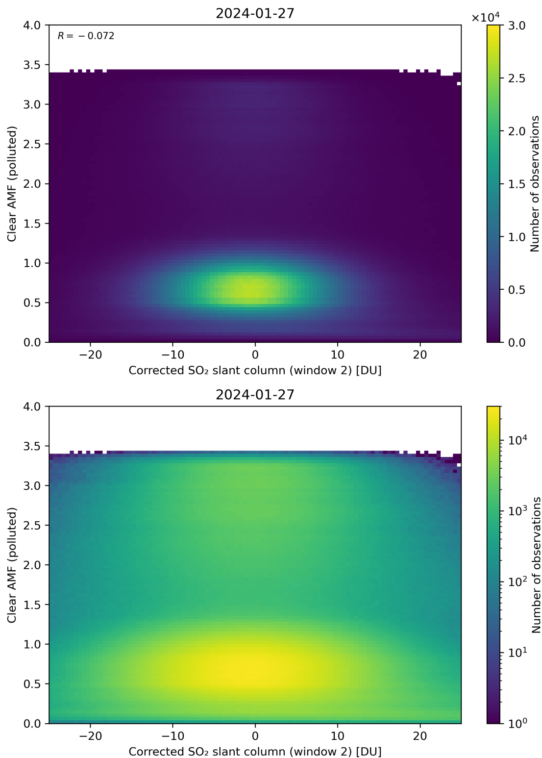
Figure 199: Scatter density plot of “Corrected SO 2 slant column (window 2)” against “Clear AMF (polluted)” for 2024-01-26 to 2024-01-28.
