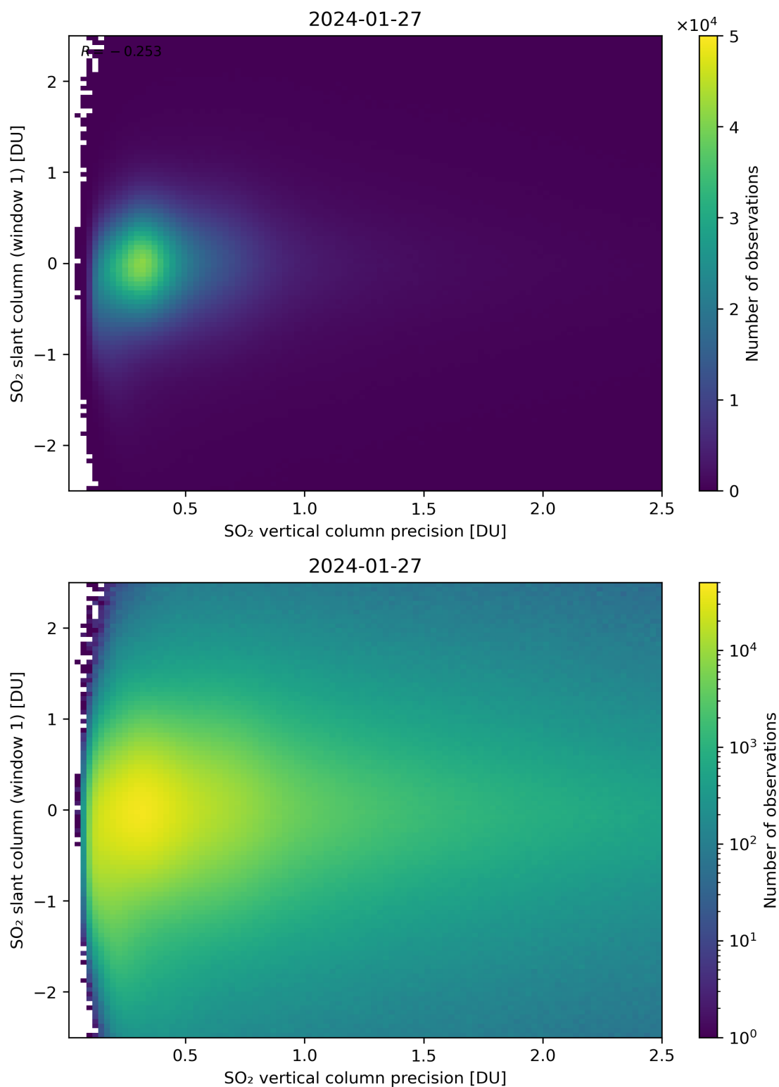
Figure 289: Scatter density plot of “SO 2 vertical column precision” against “SO 2 slant column (window 1)” for 2024-01-26 to 2024-01-28.
