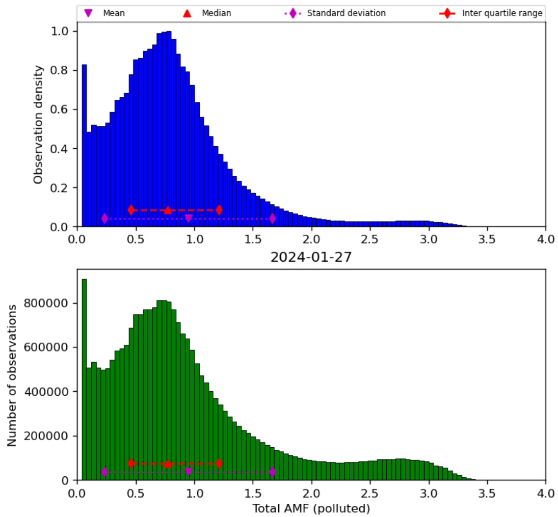
Figure 71: Histogram of “Total AMF (polluted)” for 2024-01-26 to 2024-01-28
