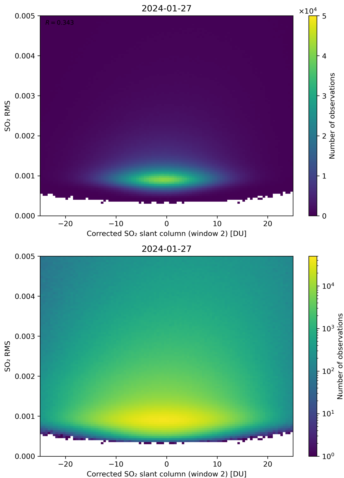
Figure 198: Scatter density plot of “Corrected SO 2 slant column (window 2)” against “SO 2 RMS” for 2024-01-26 to 2024-01-28.
