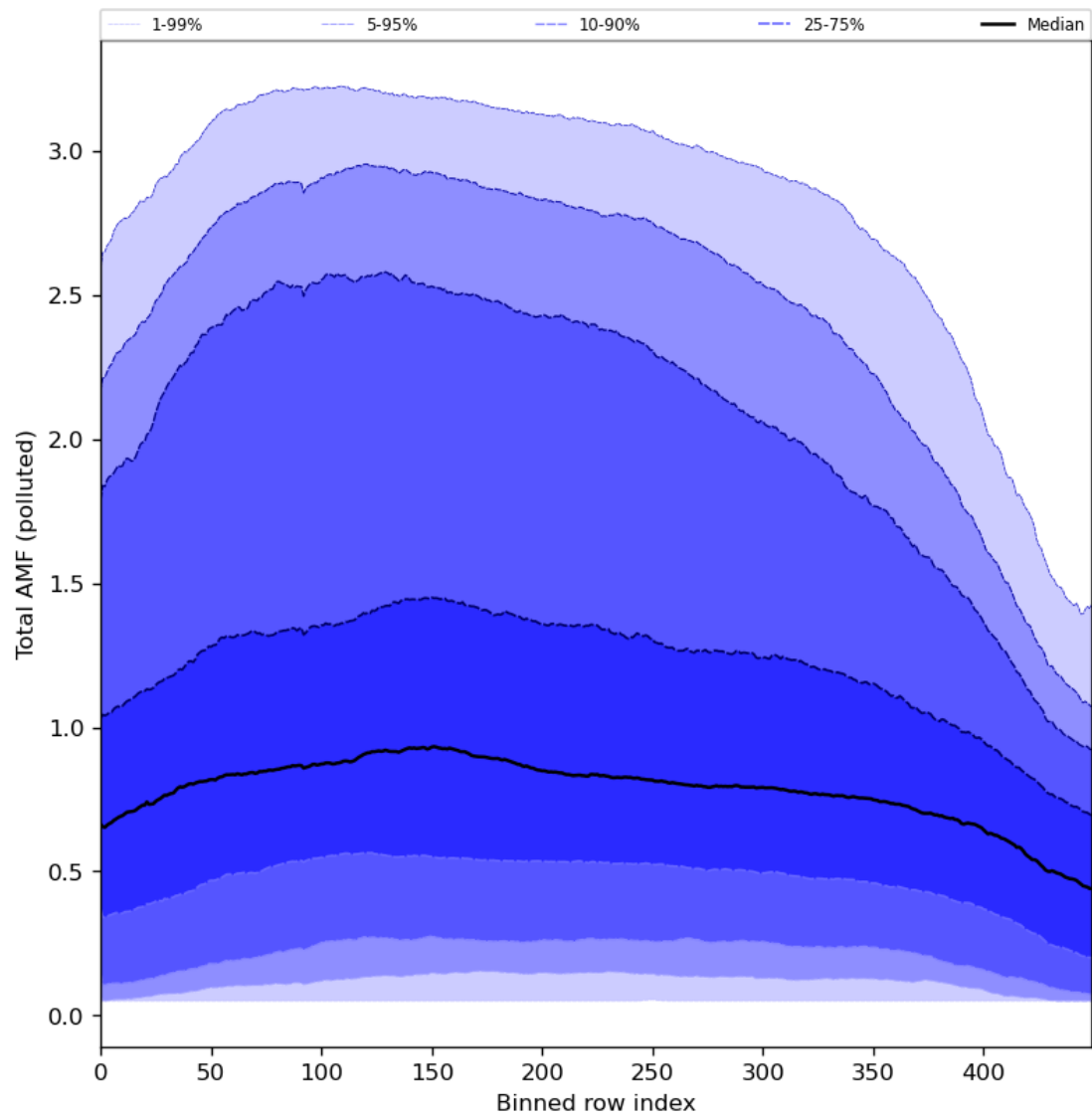
Figure 94: Along track statistics of “Total AMF (polluted)” for 2024-01-26 to 2024-01-28
