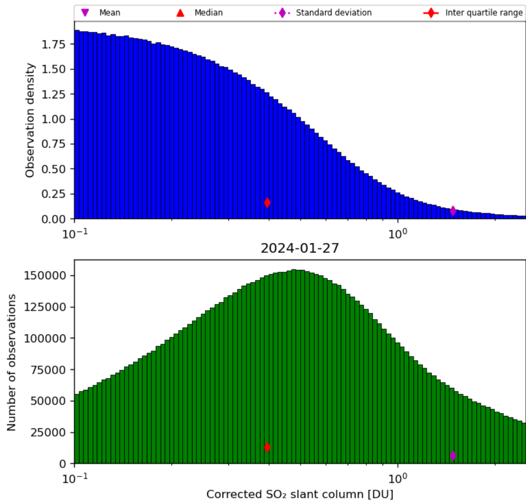
Figure 55: Histogram of “Corrected SO 2 slant column” for 2024-01-26 to 2024-01-28
