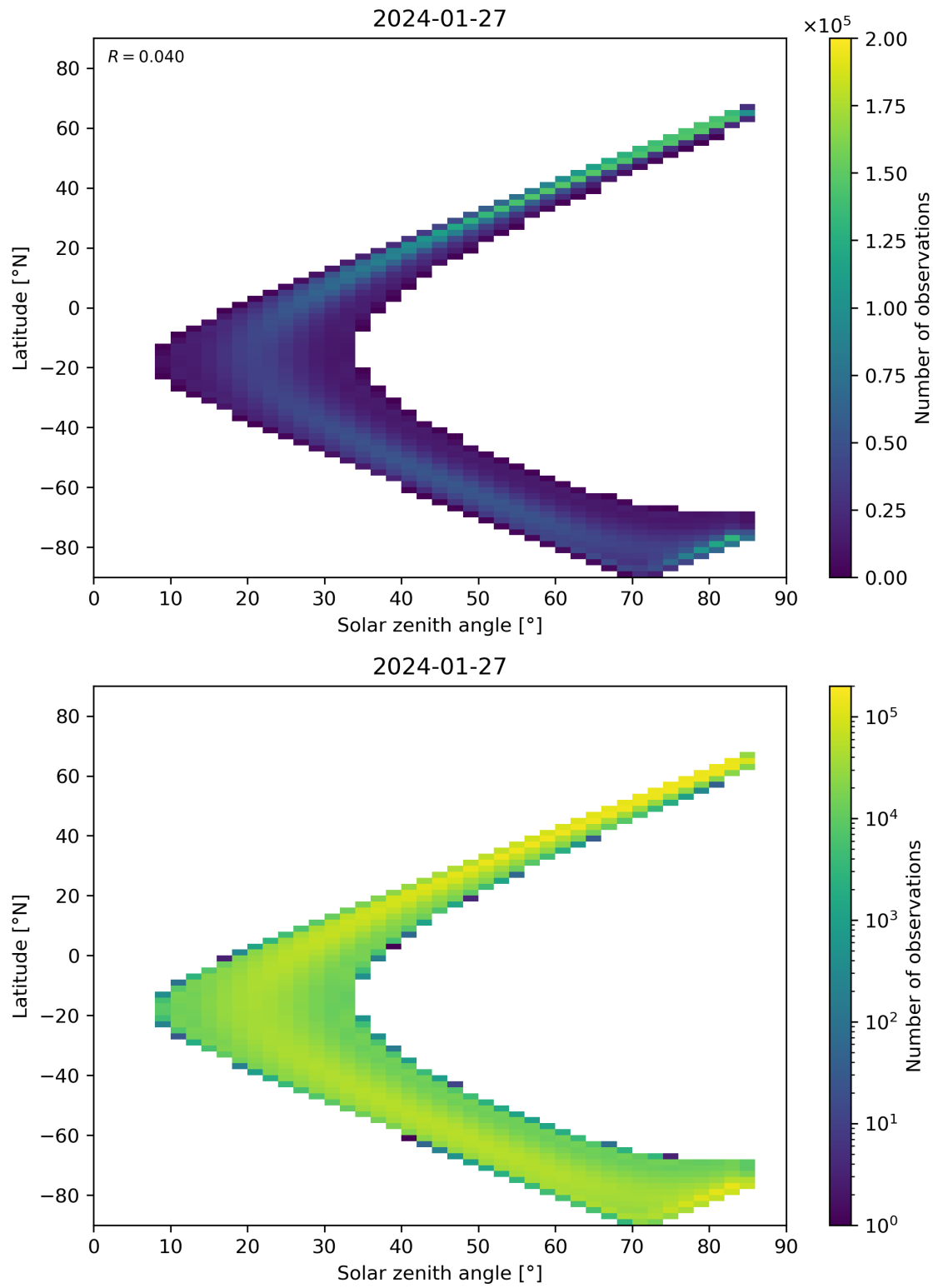
Figure 164: Scatter density plot of “Solar zenith angle” against “Latitude” for 2024-01-26 to 2024-01-28.
