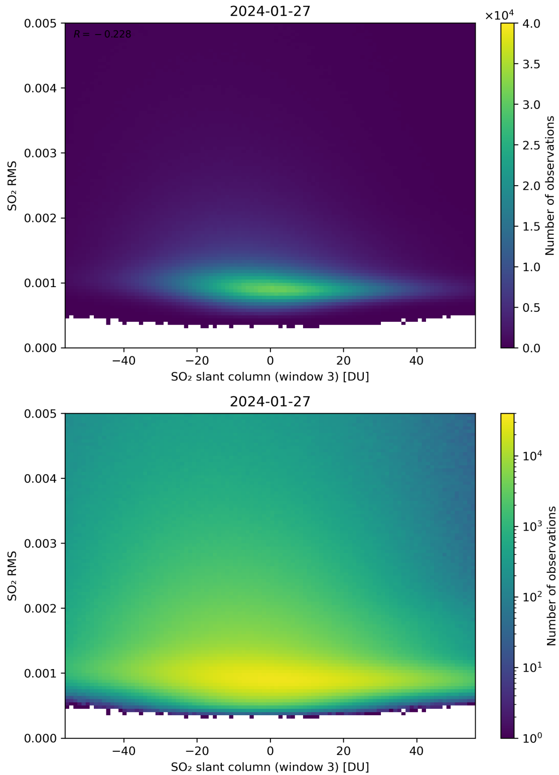
Figure 256: Scatter density plot of “SO 2 slant column (window 3)” against “SO 2 RMS” for 2024-01-26 to 2024-01-28.
