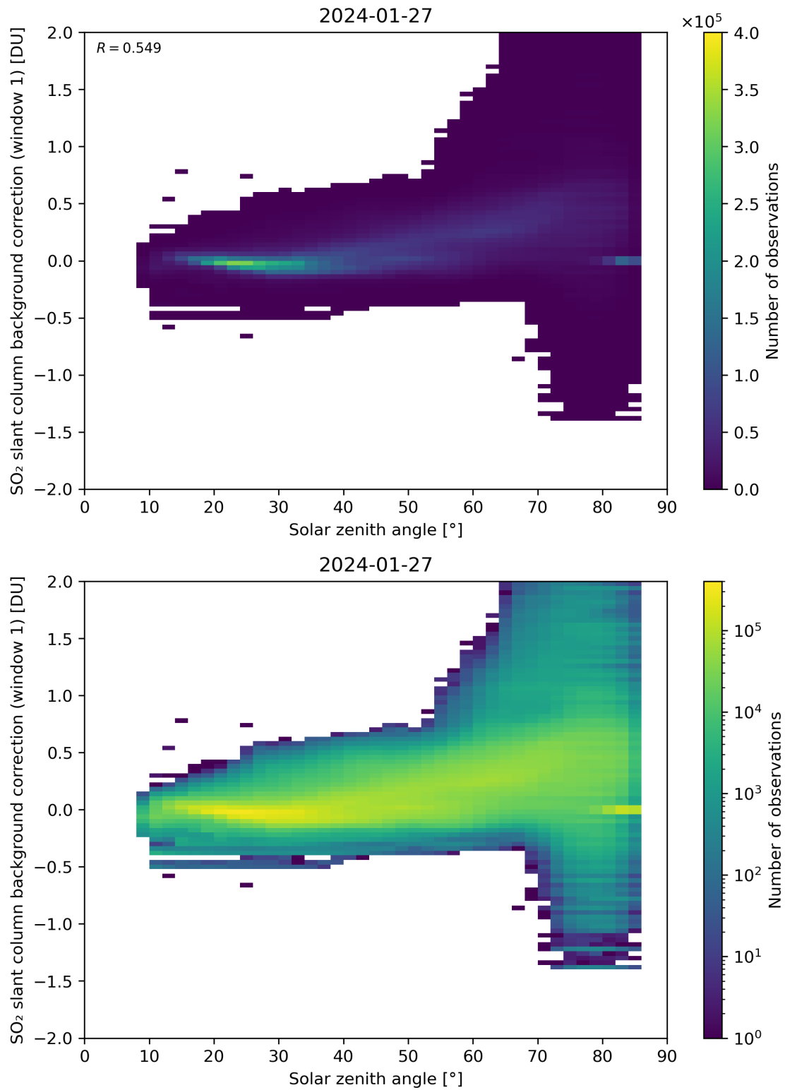
Figure 158: Scatter density plot of “Solar zenith angle” against “SO 2 slant column background correction (window 1)” for 2024-01-26 to 2024-01-28.
