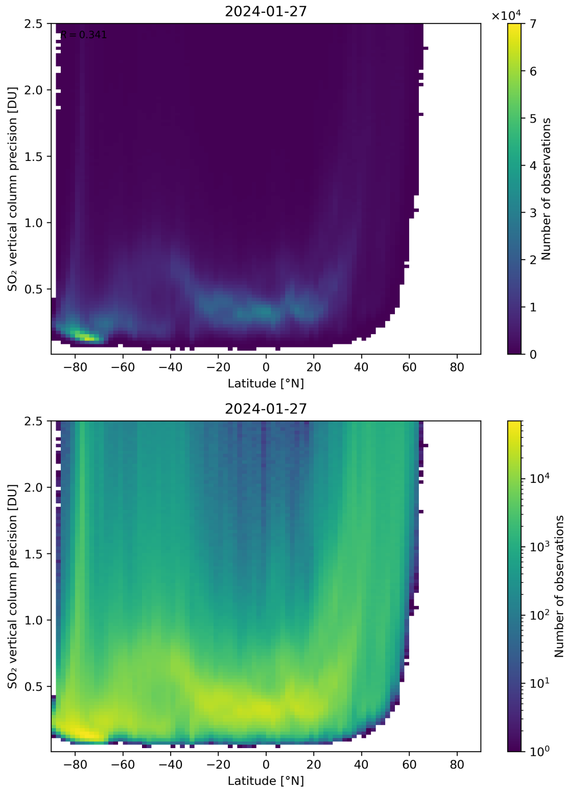
Figure 157: Scatter density plot of “Latitude” against “SO 2 vertical column precision” for 2024-01-26 to 2024-01-28.
