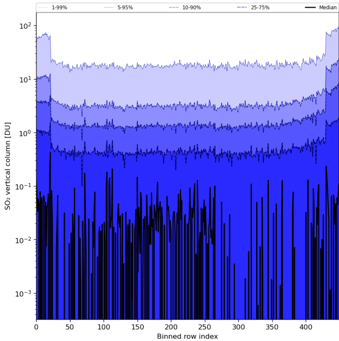
Figure 76: Along track statistics of “SO 2 vertical column” for 2024-01-26 to 2024-01-28
