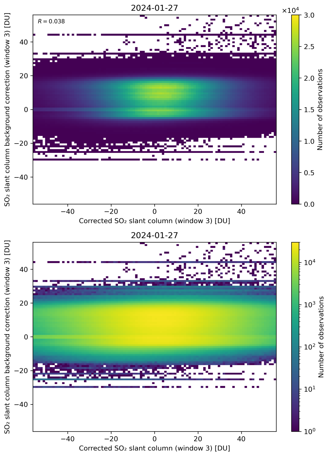
Figure 205: Scatter density plot of “Corrected SO 2 slant column (window 3)” against “SO 2 slant column background correction (window 3)” for 2024-01-26 to 2024-01-28.
