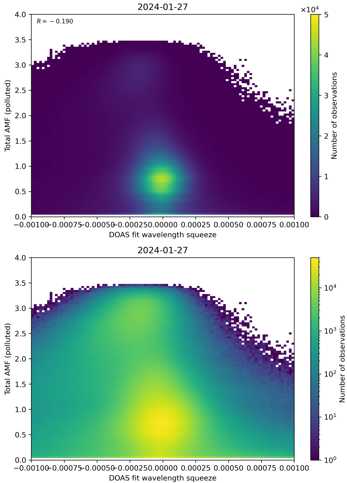
Figure 134: Scatter density plot of “DOAS fit wavelength squeeze” against “Total AMF (polluted)” for 2024-01-26 to 2024-01-28.
