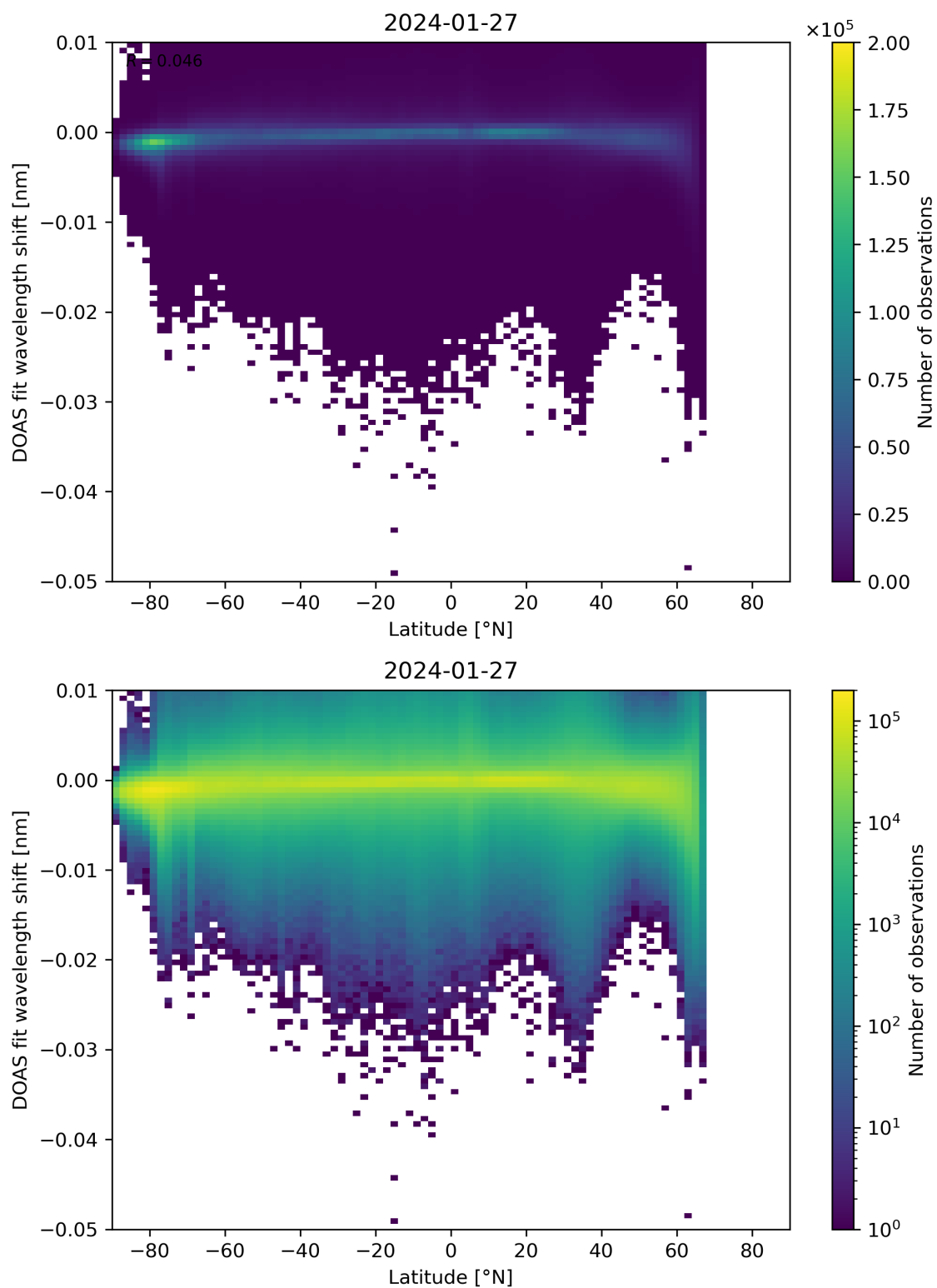
Figure 142: Scatter density plot of “Latitude” against “DOAS fit wavelength shift” for 2024-01-26 to 2024-01-28.
