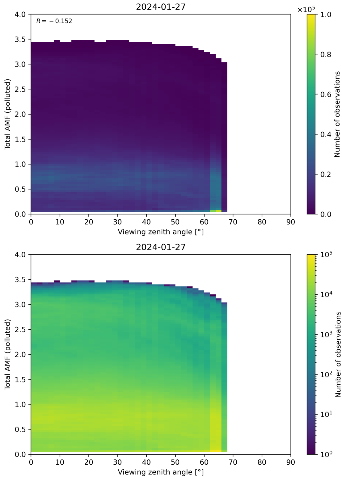
Figure 325: Scatter density plot of “Viewing zenith angle” against “Total AMF (polluted)” for 2024-01-26 to 2024-01-28.
