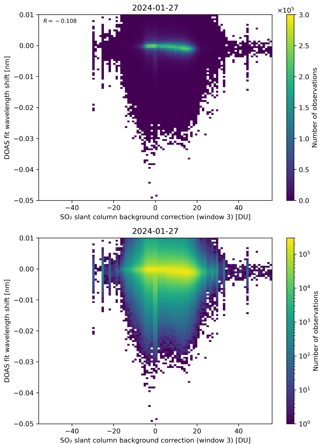
Figure 121: Scatter density plot of “SO 2 slant column background correction (window 3)” against “DOAS fit wavelength shift” for 2024-01-26 to 2024-01-28.
