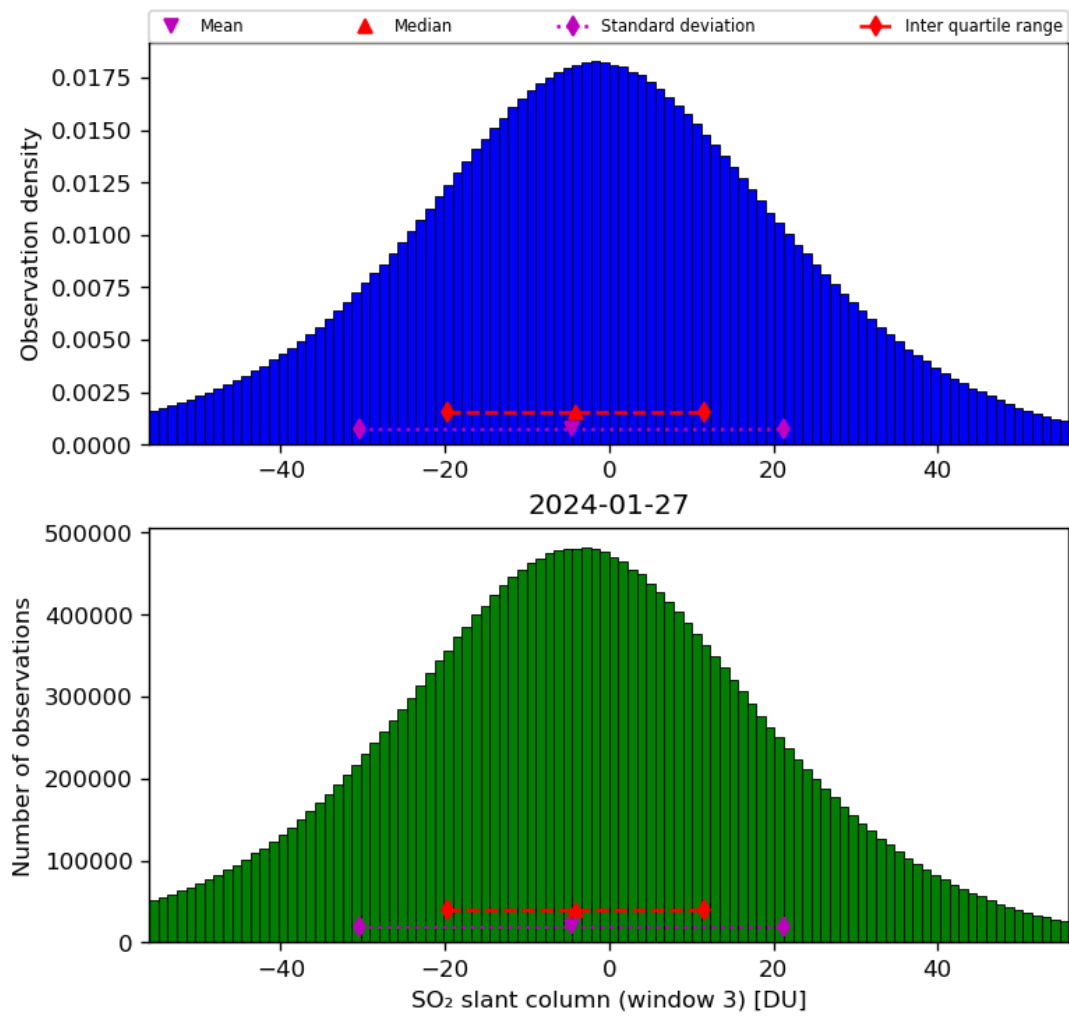
Figure 64: Histogram of “SO 2 slant column (window 3)” for 2024-01-26 to 2024-01-28
