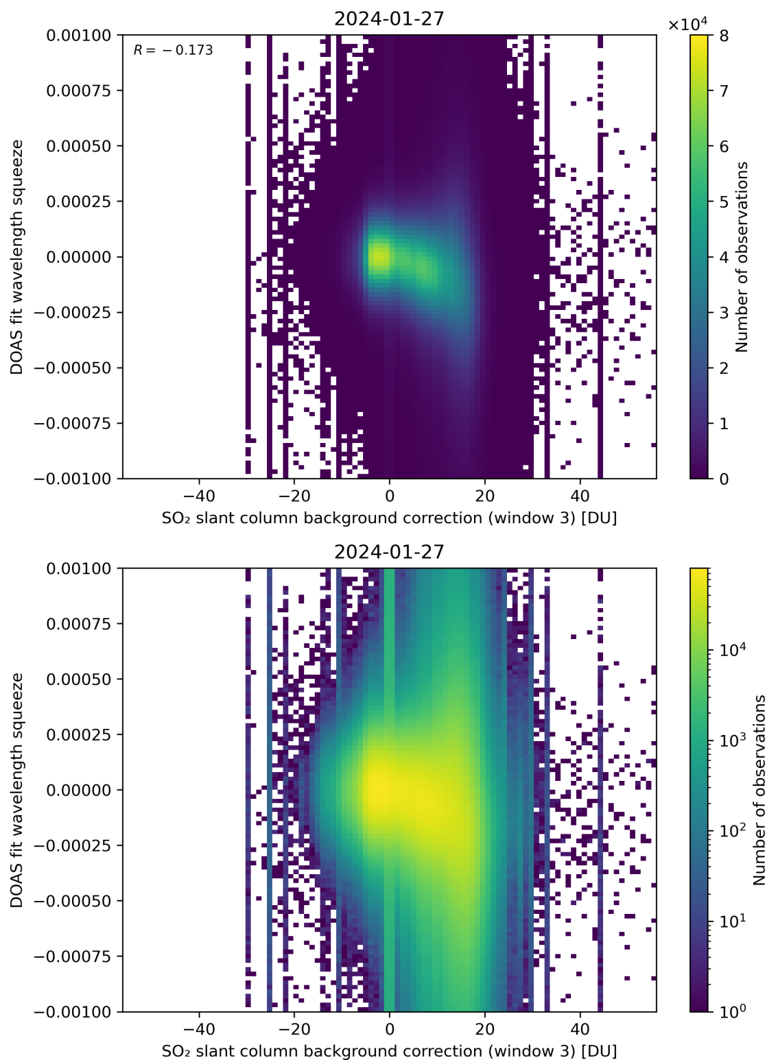
Figure 122: Scatter density plot of “SO 2 slant column background correction (window 3)” against “DOAS fit wavelength squeeze” for 2024-01-26 to 2024-01-28.
