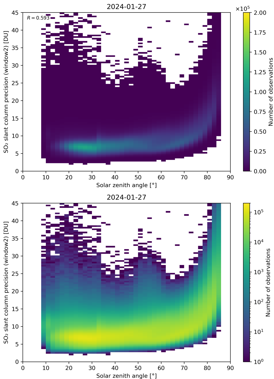
Figure 171: Scatter density plot of “Solar zenith angle” against “SO 2 slant column precision (window2)” for 2024-01-26 to 2024-01-28.
