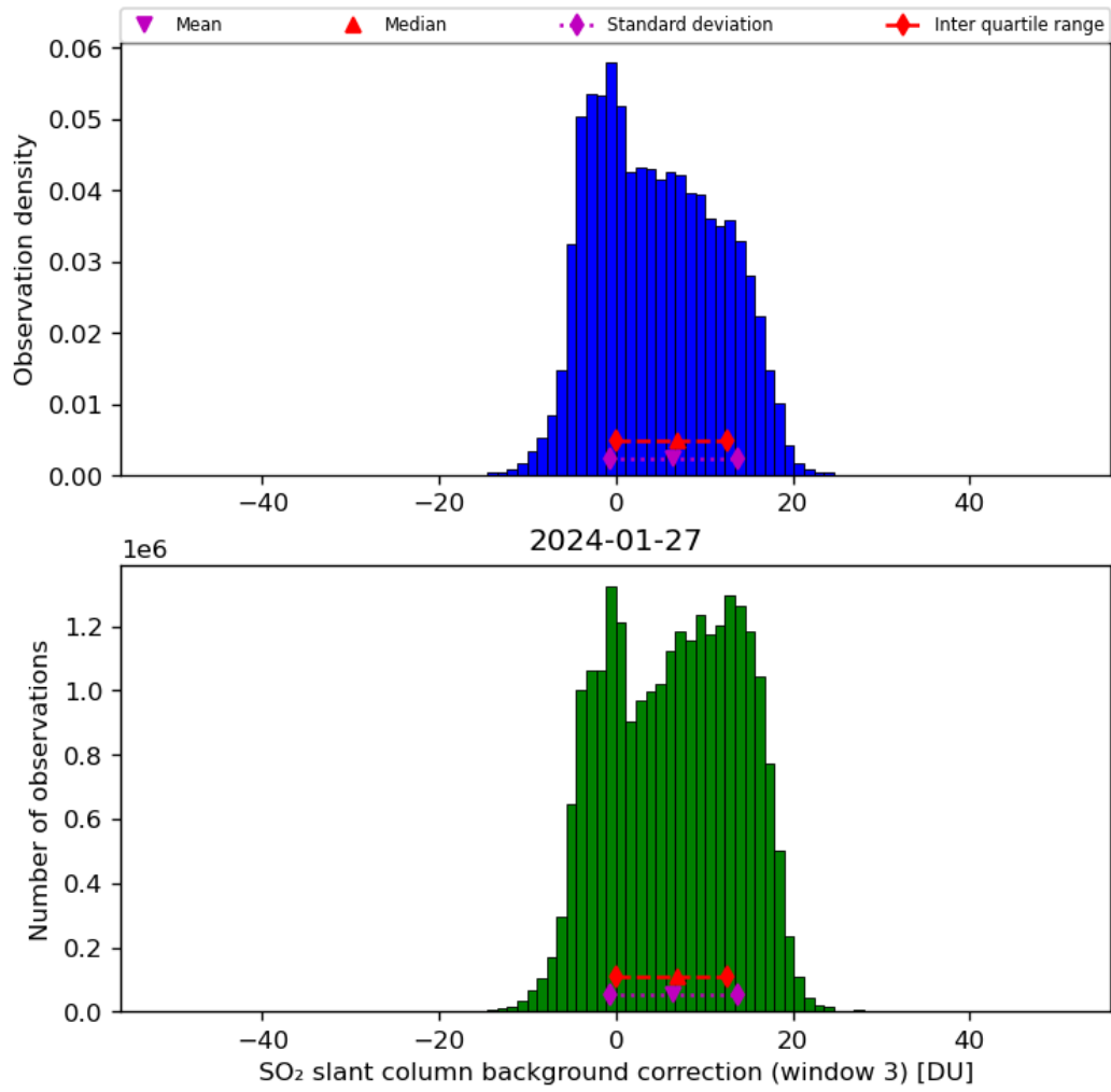
Figure 67: Histogram of “SO 2 slant column background correction (window 3)” for 2024-01-26 to 2024-01-28
