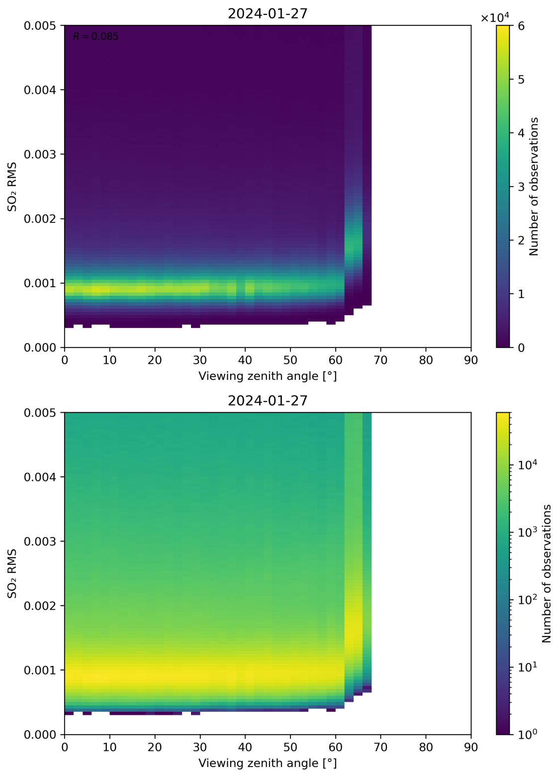
Figure 313: Scatter density plot of “Viewing zenith angle” against “SO 2 RMS” for 2024-01-26 to 2024-01-28.
