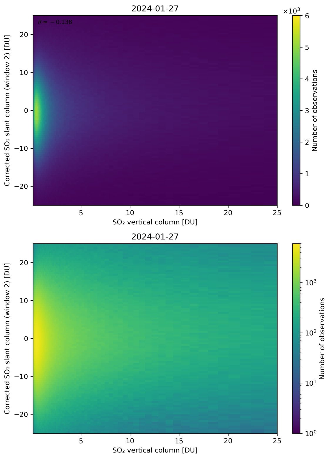
Figure 298: Scatter density plot of “SO 2 vertical column” against “Corrected SO 2 slant column (window 2)” for 2024-01-26 to 2024-01-28.
