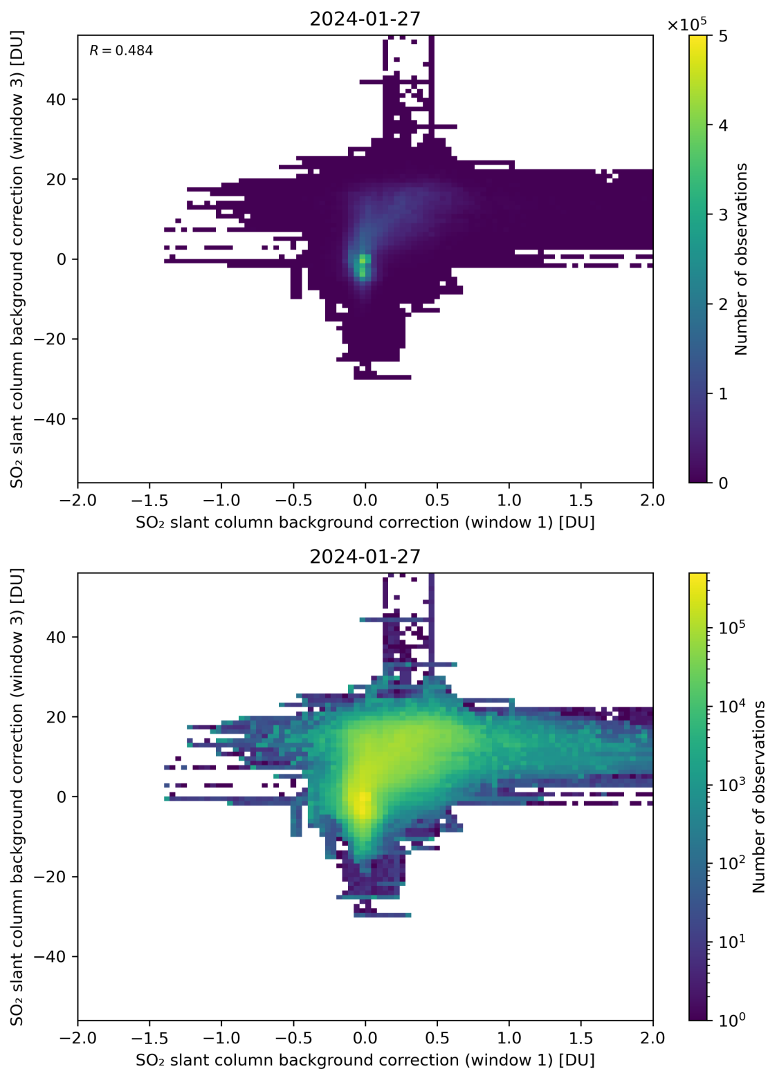
Figure 99: Scatter density plot of “SO 2 slant column background correction (window 1)” against “SO 2 slant column background correction (window 3)” for 2024-01-26 to 2024-01-28.
