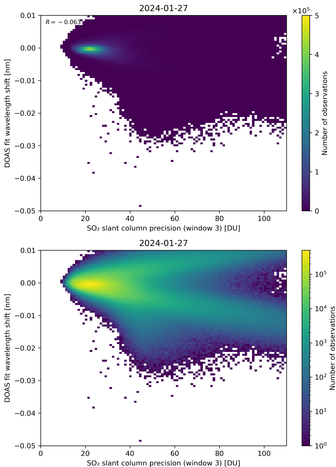
Figure 258: Scatter density plot of “SO 2 slant column precision (window 3)” against “DOAS fit wavelength shift” for 2024-01-26 to 2024-01-28.
