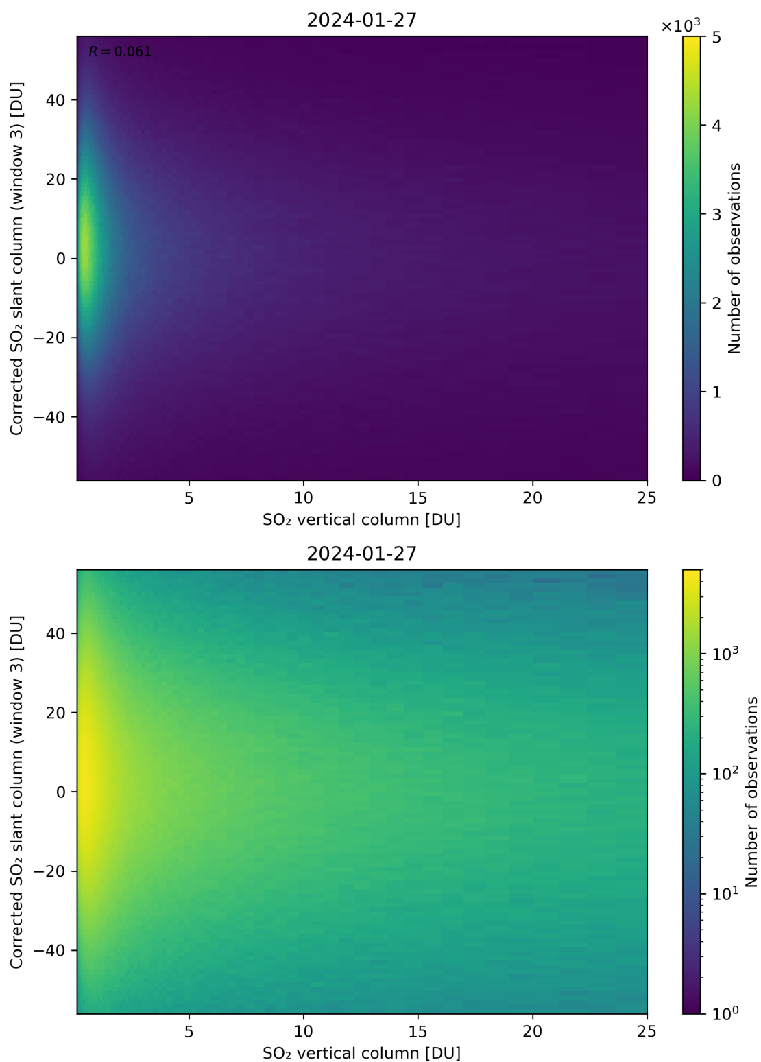
Figure 299: Scatter density plot of “SO 2 vertical column” against “Corrected SO 2 slant column (window 3)” for 2024-01-26 to 2024-01-28.
