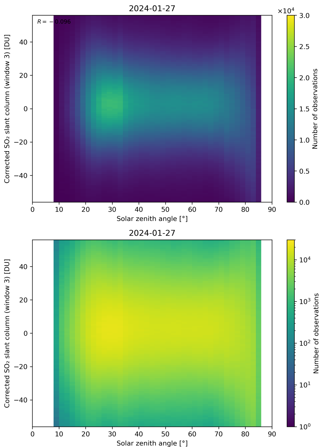
Figure 168: Scatter density plot of “Solar zenith angle” against “Corrected SO 2 slant column (window 3)” for 2024-01-26 to 2024-01-28.
