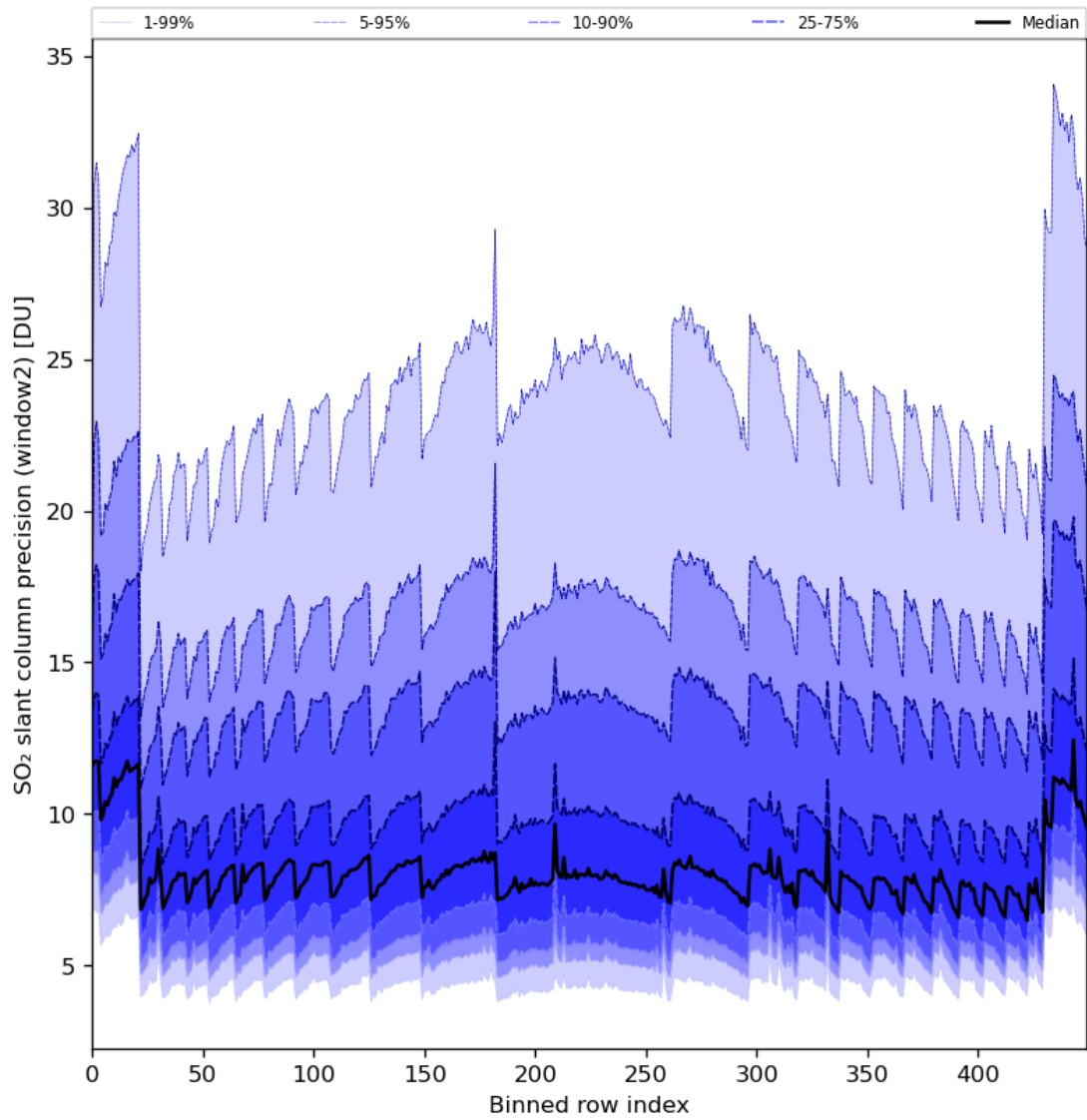
Figure 84: Along track statistics of “SO 2 slant column precision (window2)” for 2024-01-26 to 2024-01-28
