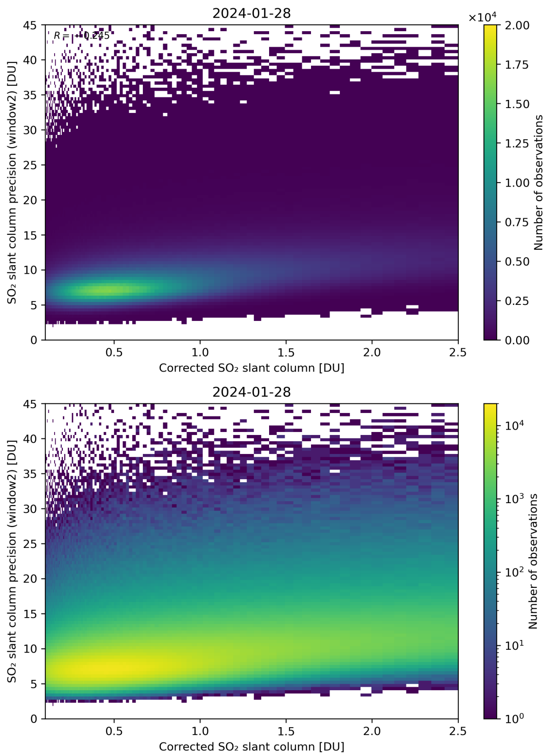
Figure 189: Scatter density plot of “Corrected SO 2 slant column” against “SO 2 slant column precision (window2)” for 2024-01-27 to 2024-01-29.
