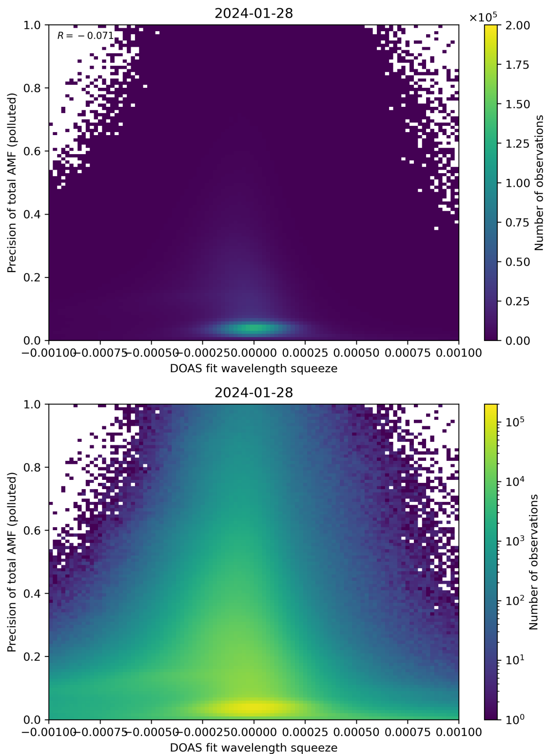
Figure 135: Scatter density plot of “DOAS fit wavelength squeeze” against “Precision of total AMF (polluted)” for 2024-01-27 to 2024-01-29.
