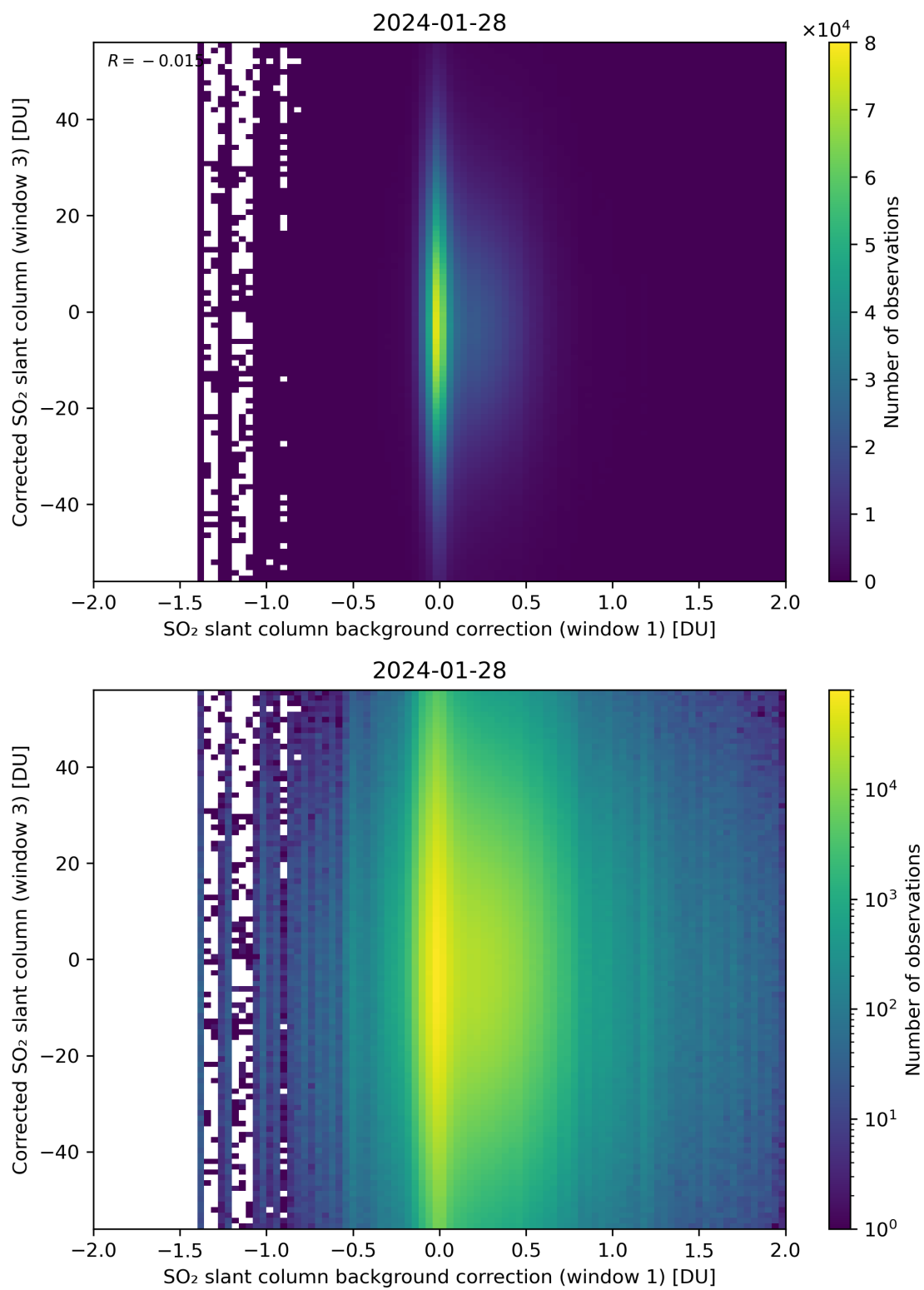
Figure 105: Scatter density plot of “SO 2 slant column background correction (window 1)” against “Corrected SO 2 slant column (window 3)” for 2024-01-27 to 2024-01-29.
