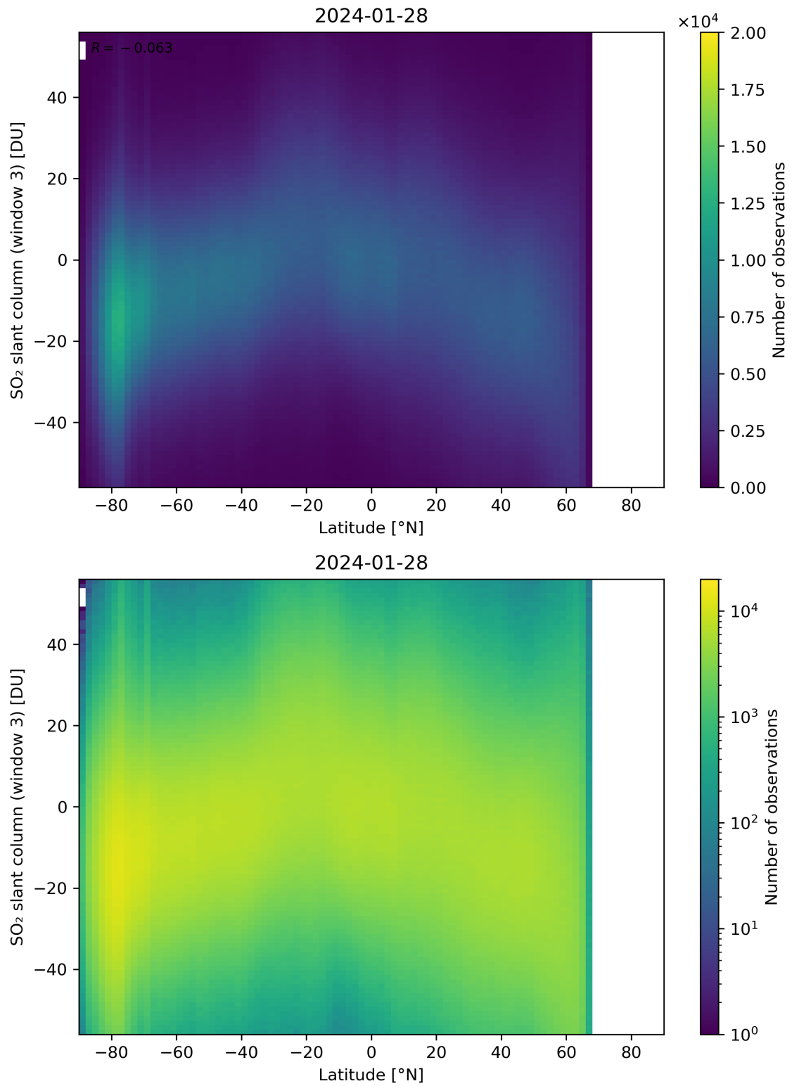
Figure 152: Scatter density plot of “Latitude” against “SO 2 slant column (window 3)” for 2024-01-27 to 2024-01-29.
