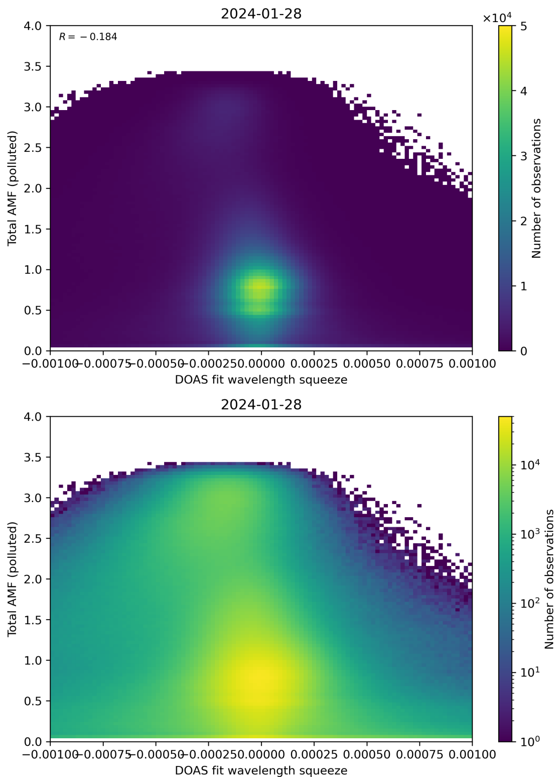
Figure 134: Scatter density plot of “DOAS fit wavelength squeeze” against “Total AMF (polluted)” for 2024-01-27 to 2024-01-29.
