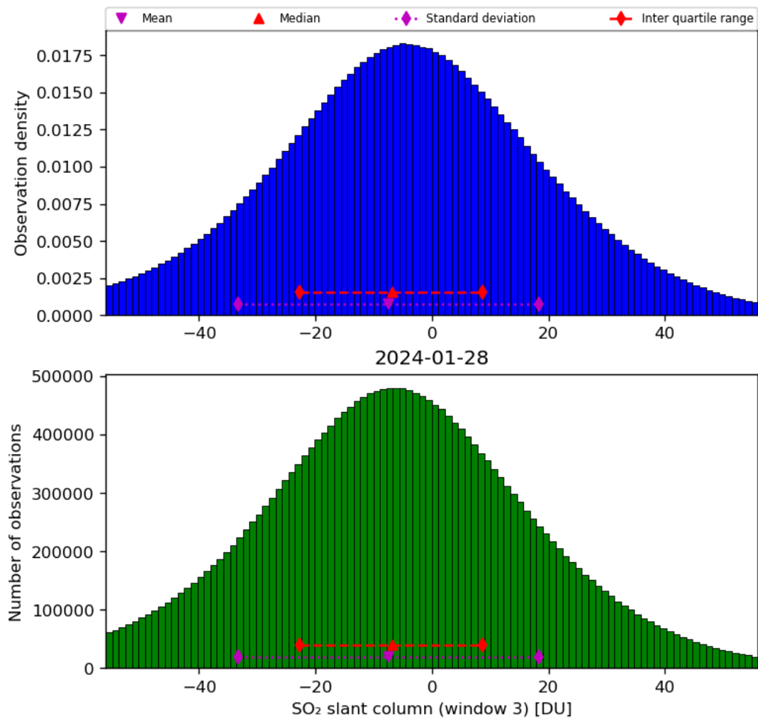
Figure 64: Histogram of “SO 2 slant column (window 3)” for 2024-01-27 to 2024-01-29
