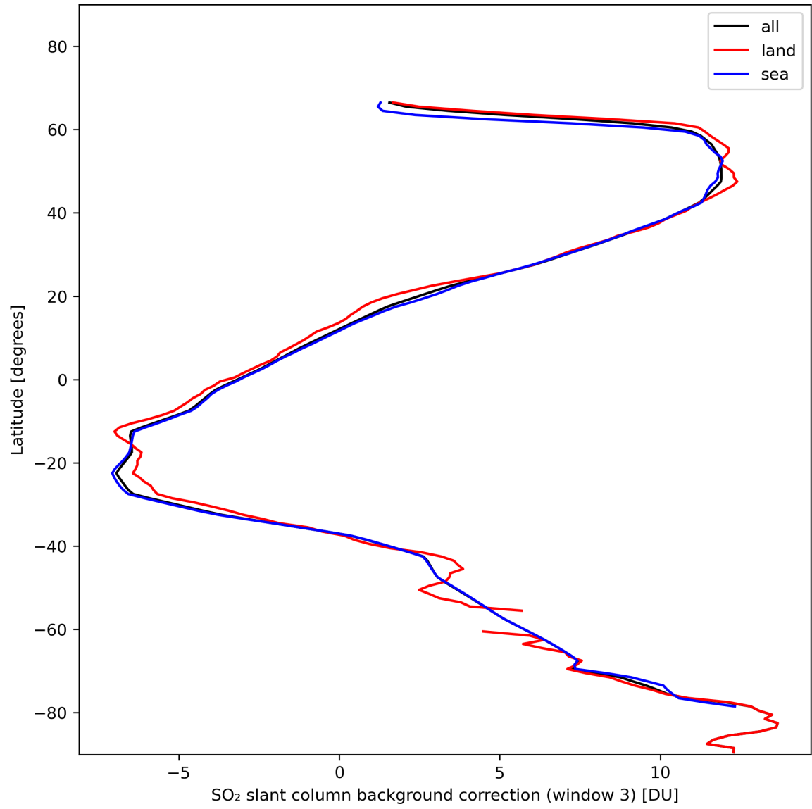
Figure 44: Zonal average of “SO 2 slant column background correction (window 3)” for 2024-01-27 to 2024-01-29.
