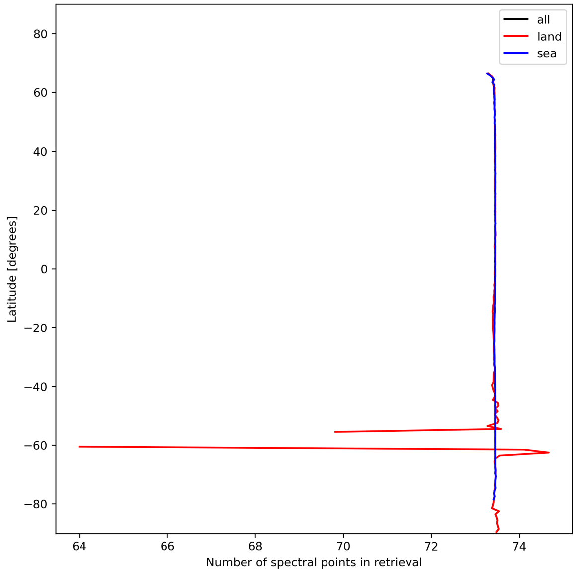
Figure 51: Zonal average of “Number of spectral points in retrieval” for 2024-01-27 to 2024-01-29.
