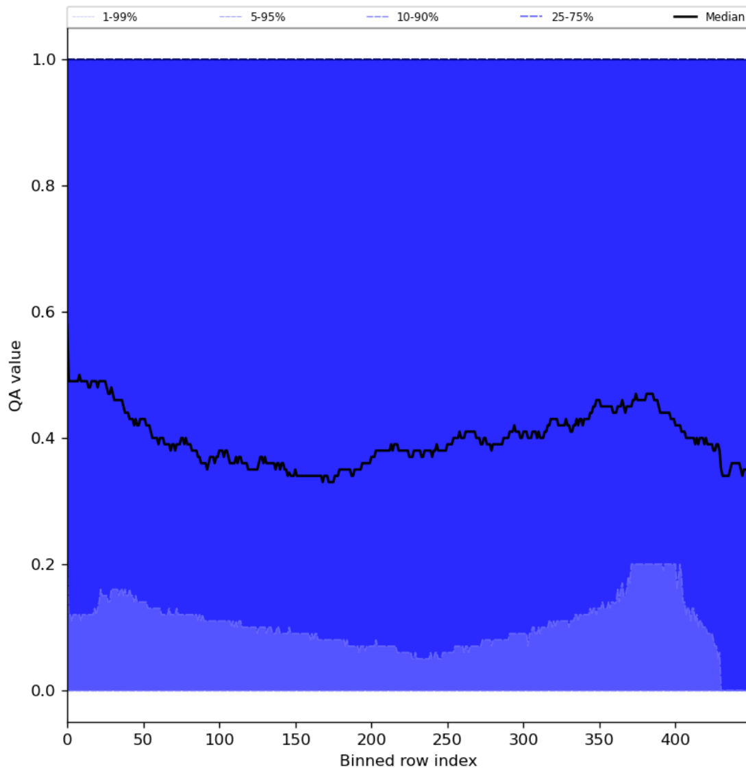
Figure 75: Along track statistics of “QA value” for 2024-01-27 to 2024-01-29
