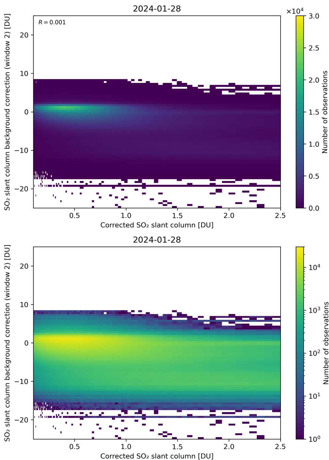
Figure 179: Scatter density plot of “Corrected SO 2 slant column” against “SO 2 slant column background correction (window 2)” for 2024-01-27 to 2024-01-29.
