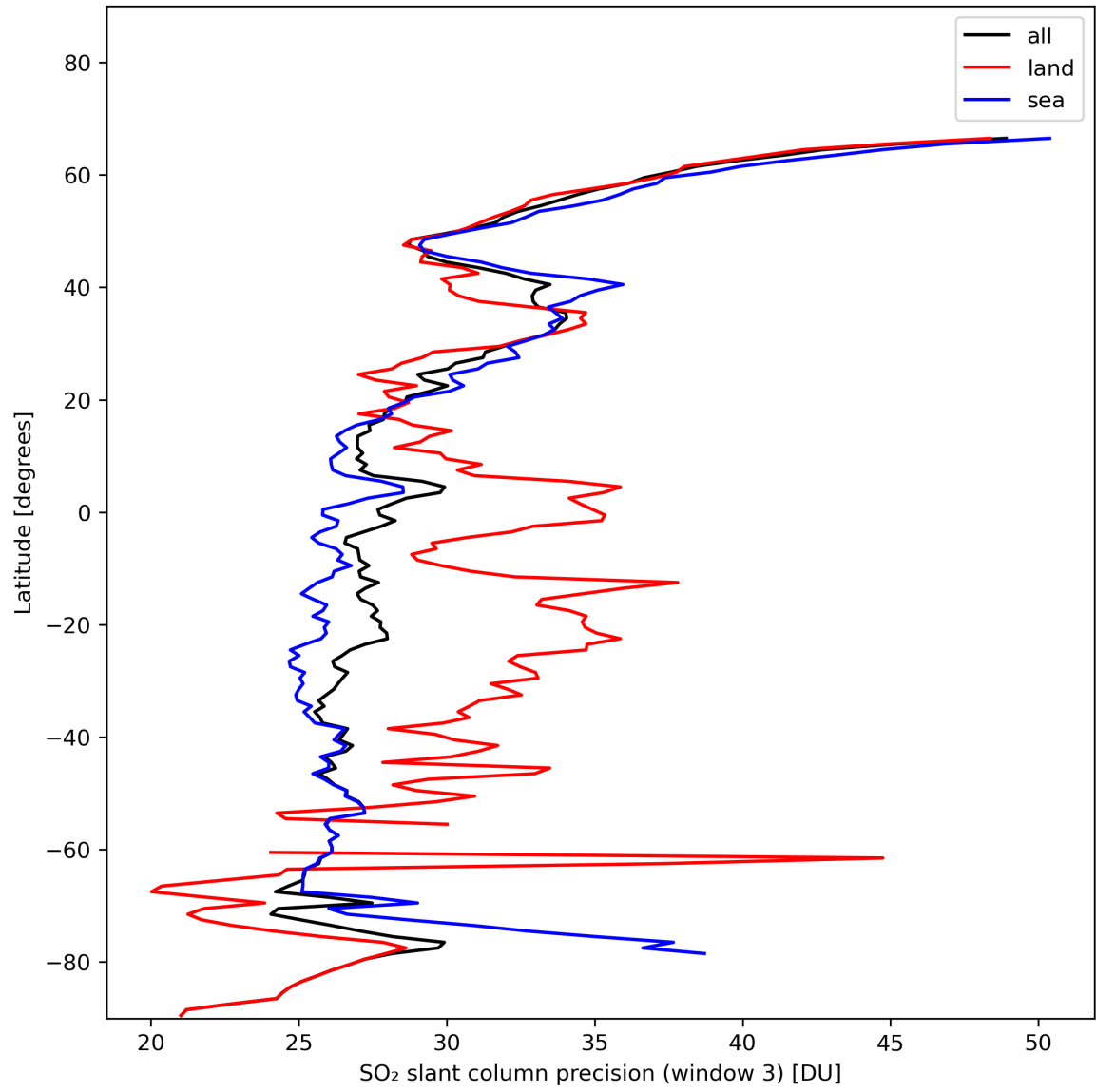
Figure 42: Zonal average of “SO 2 slant column precision (window 3)” for 2024-01-27 to 2024-01-29.
