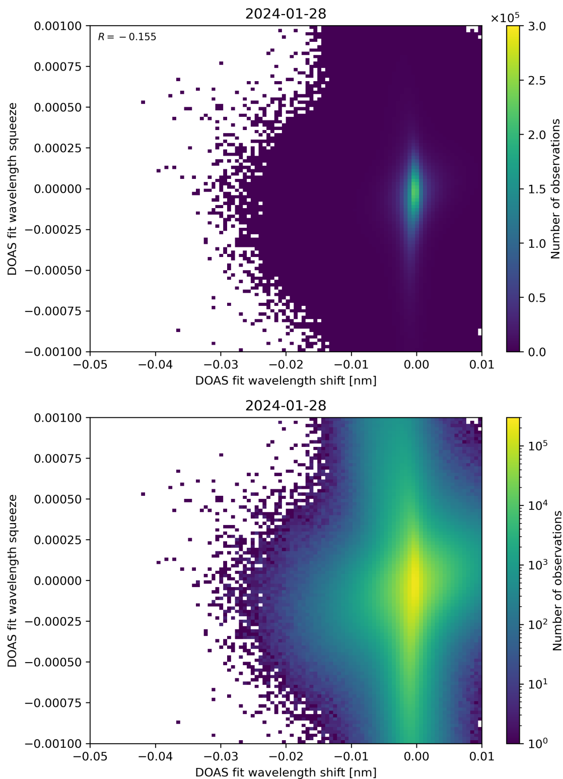
Figure 127: Scatter density plot of “DOAS fit wavelength shift” against “DOAS fit wavelength squeeze” for 2024-01-27 to 2024-01-29.
