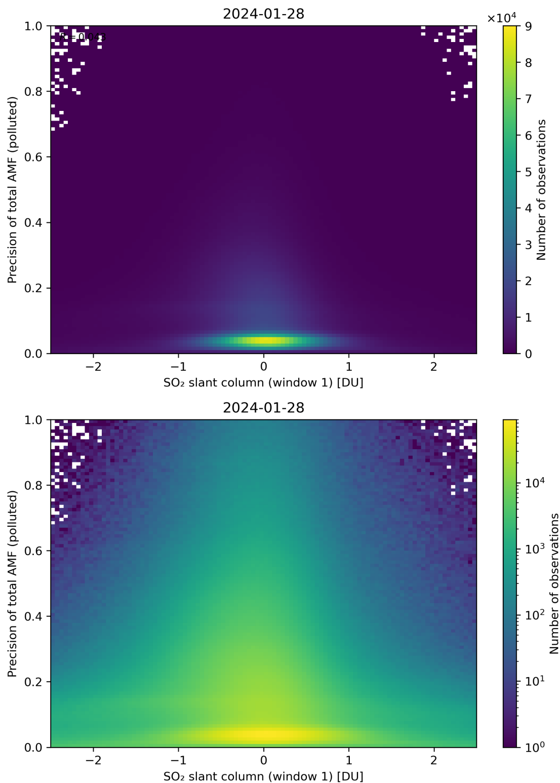
Figure 240: Scatter density plot of “SO 2 slant column (window 1)” against “Precision of total AMF (polluted)” for 2024-01-27 to 2024-01-29.
