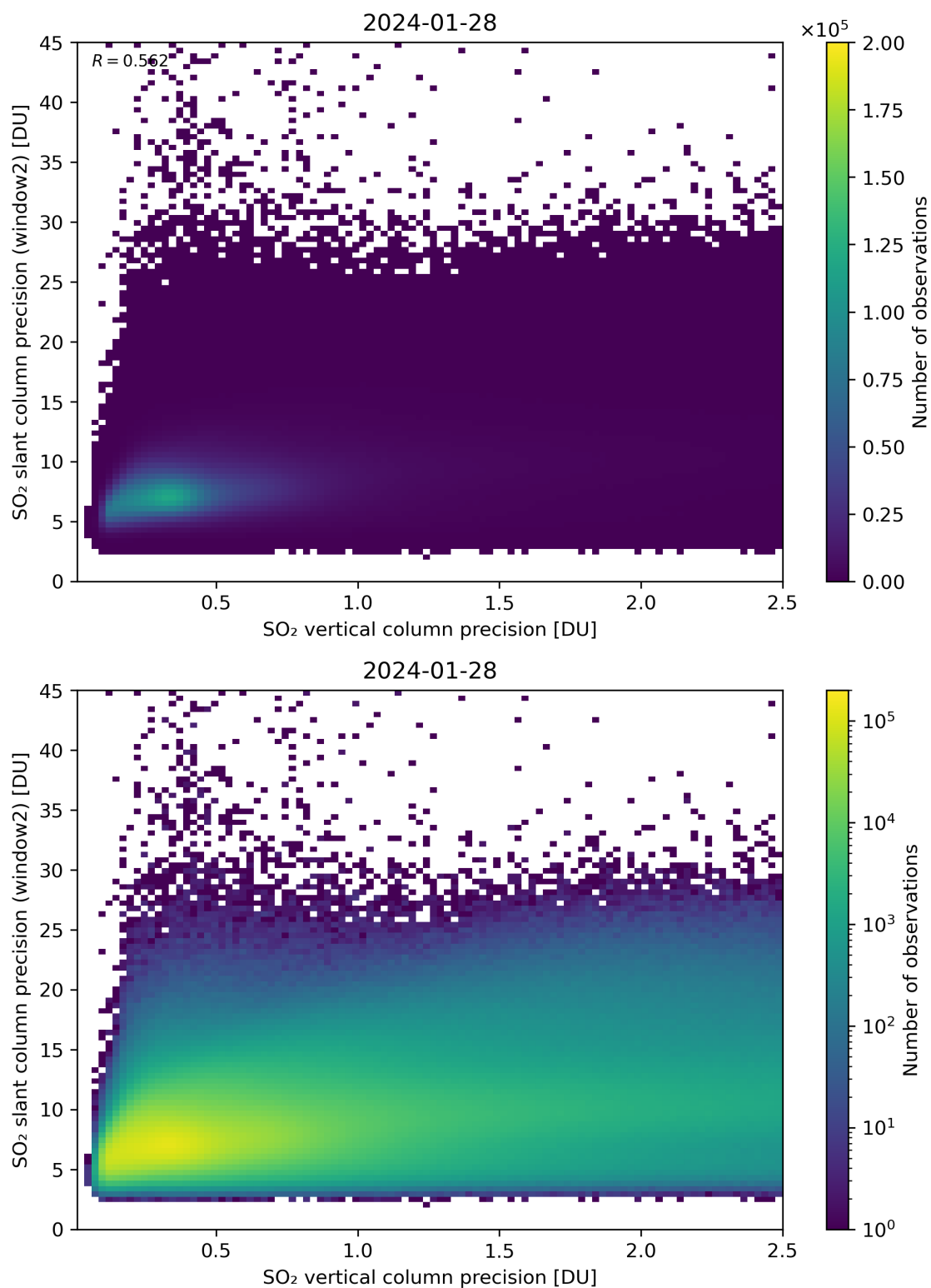
Figure 291: Scatter density plot of “SO 2 vertical column precision” against “SO 2 slant column precision (window2)” for 2024-01-27 to 2024-01-29.
