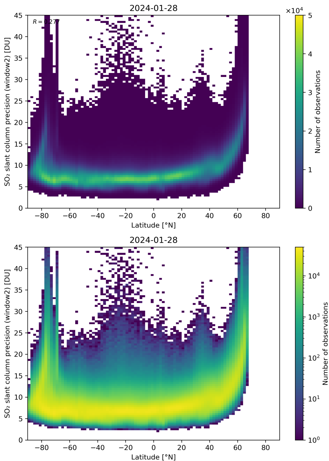
Figure 151: Scatter density plot of “Latitude” against “SO 2 slant column precision (window2)” for 2024-01-27 to 2024-01-29.
