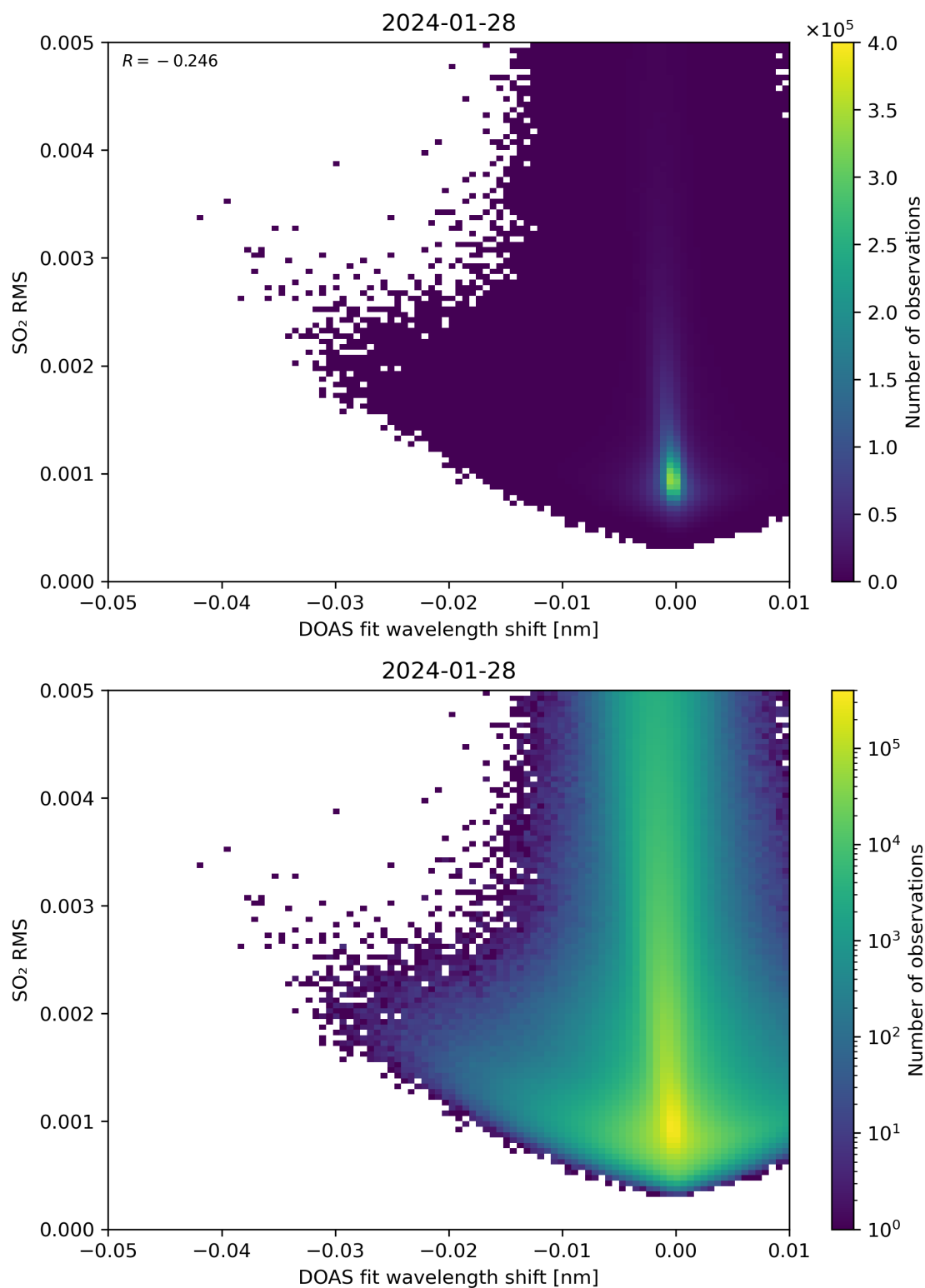
Figure 128: Scatter density plot of “DOAS fit wavelength shift” against “SO 2 RMS” for 2024-01-27 to 2024-01-29.
