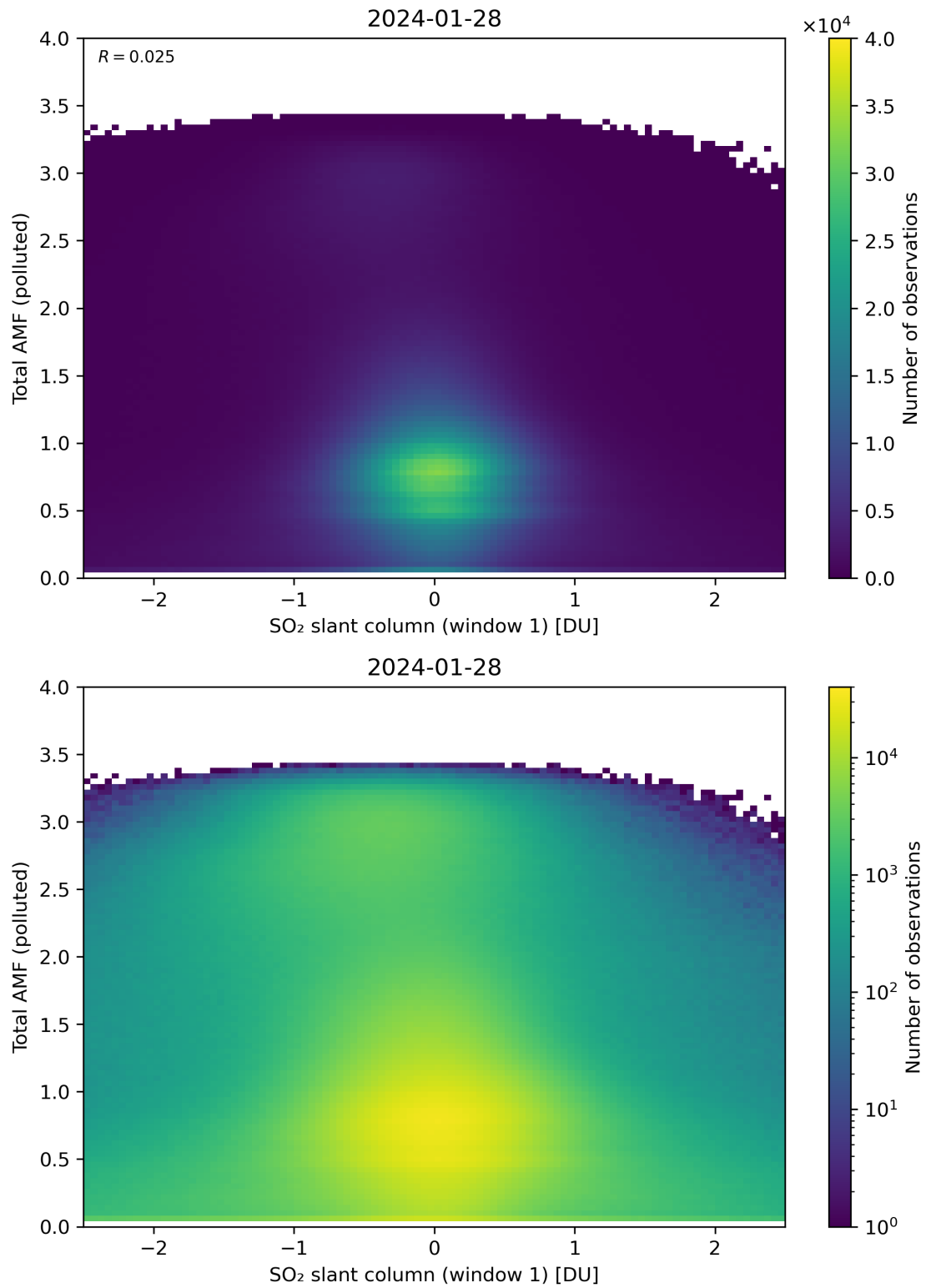
Figure 239: Scatter density plot of “SO 2 slant column (window 1)” against “Total AMF (polluted)” for 2024-01-27 to 2024-01-29.
