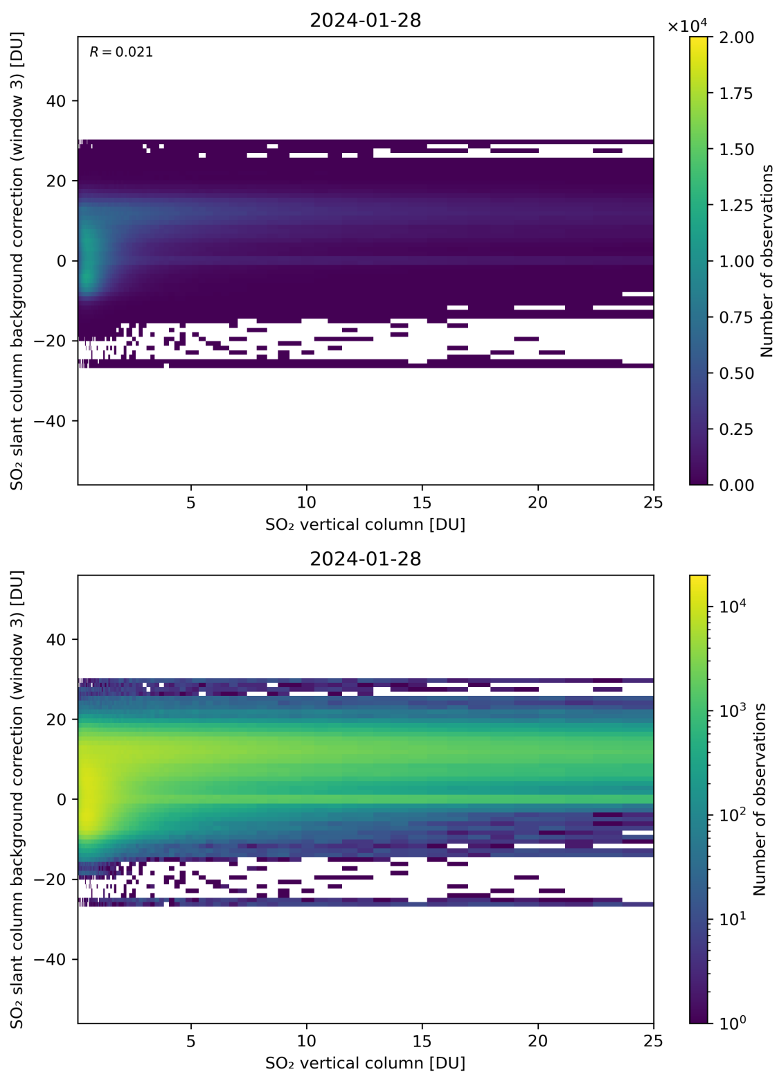
Figure 275: Scatter density plot of “SO 2 vertical column” against “SO 2 slant column background correction (window 3)” for 2024-01-27 to 2024-01-29.
