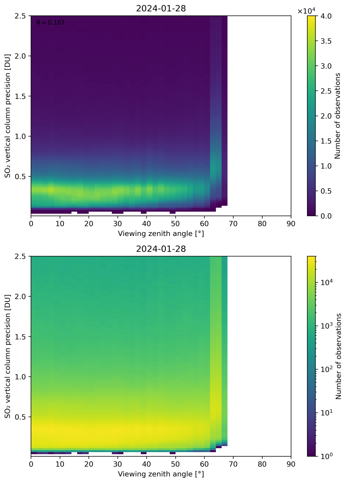
Figure 328: Scatter density plot of “Viewing zenith angle” against “SO 2 vertical column precision” for 2024-01-27 to 2024-01-29.
