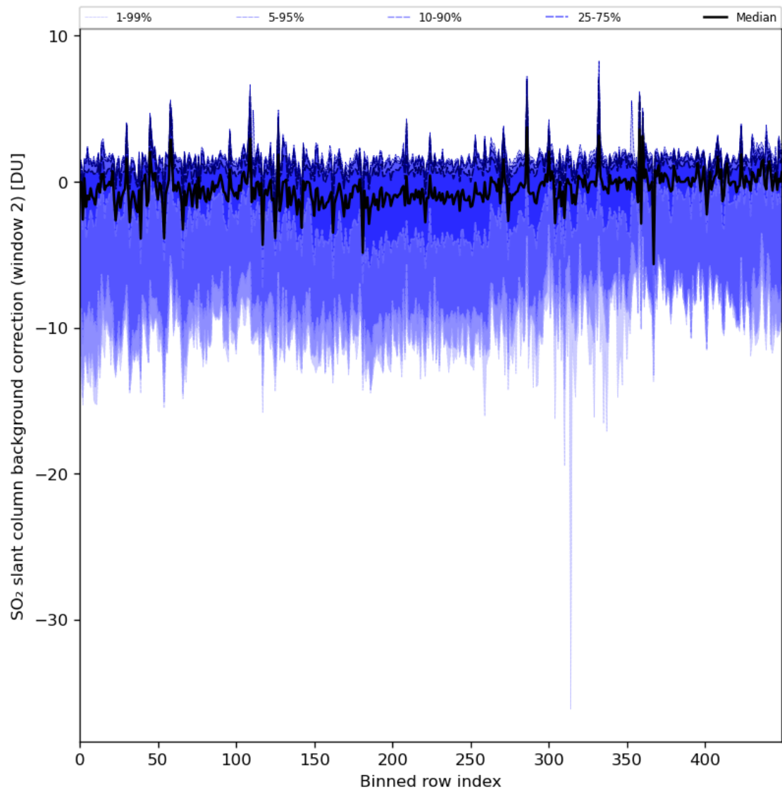
Figure 86: Along track statistics of “SO 2 slant column background correction (window 2)” for 2024-01-27 to 2024-01-29
