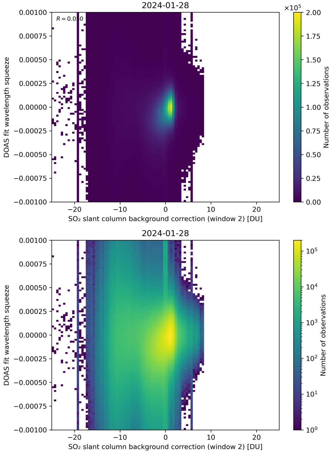
Figure 113: Scatter density plot of “SO 2 slant column background correction (window 2)” against “DOAS fit wavelength squeeze” for 2024-01-27 to 2024-01-29.
