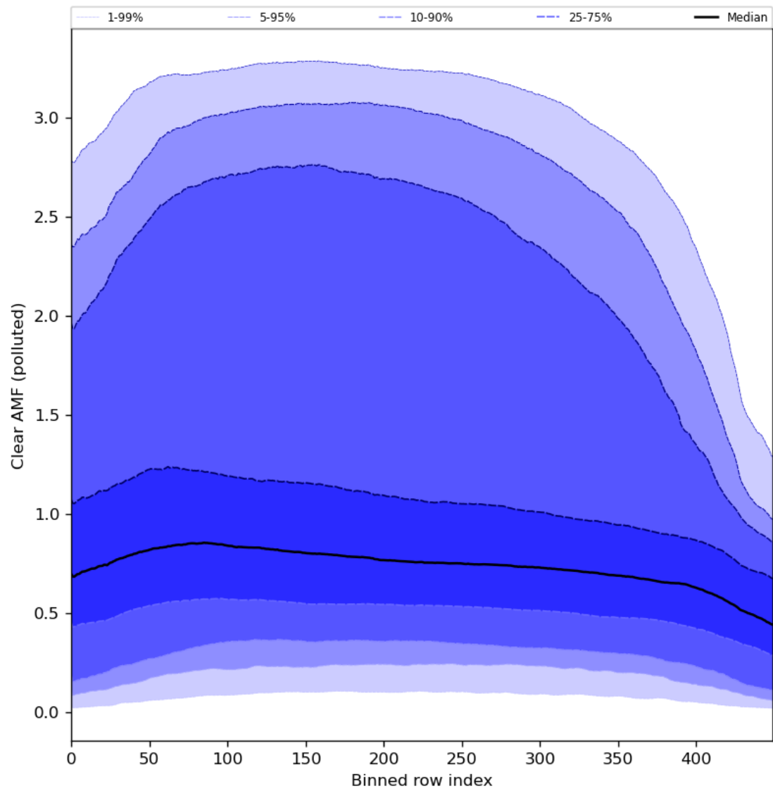
Figure 96: Along track statistics of “Clear AMF (polluted)” for 2024-01-27 to 2024-01-29
