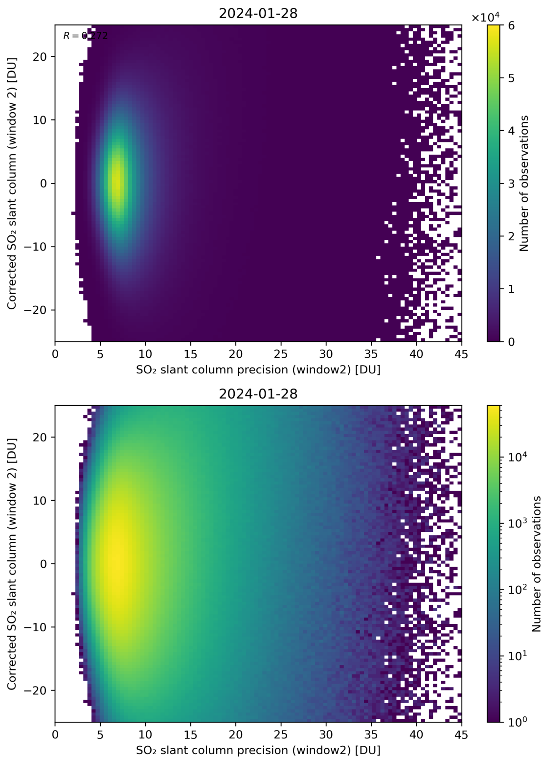
Figure 247: Scatter density plot of “SO 2 slant column precision (window2)” against “Corrected SO 2 slant column (window 2)” for 2024-01-27 to 2024-01-29.
