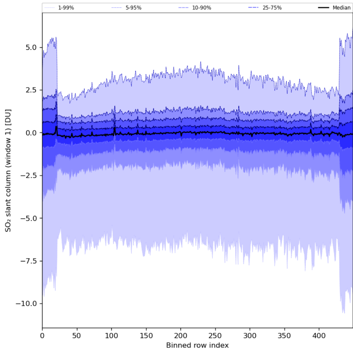
Figure 79: Along track statistics of “SO 2 slant column (window 1)” for 2024-01-27 to 2024-01-29
