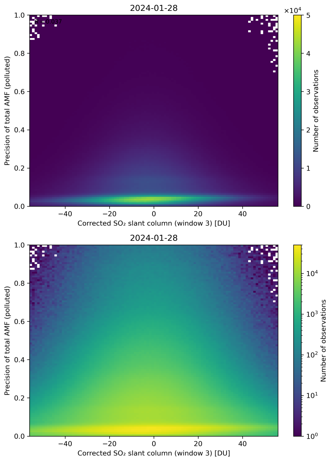
Figure 211: Scatter density plot of “Corrected SO 2 slant column (window 3)” against “Precision of total AMF (polluted)” for 2024-01-27 to 2024-01-29.
