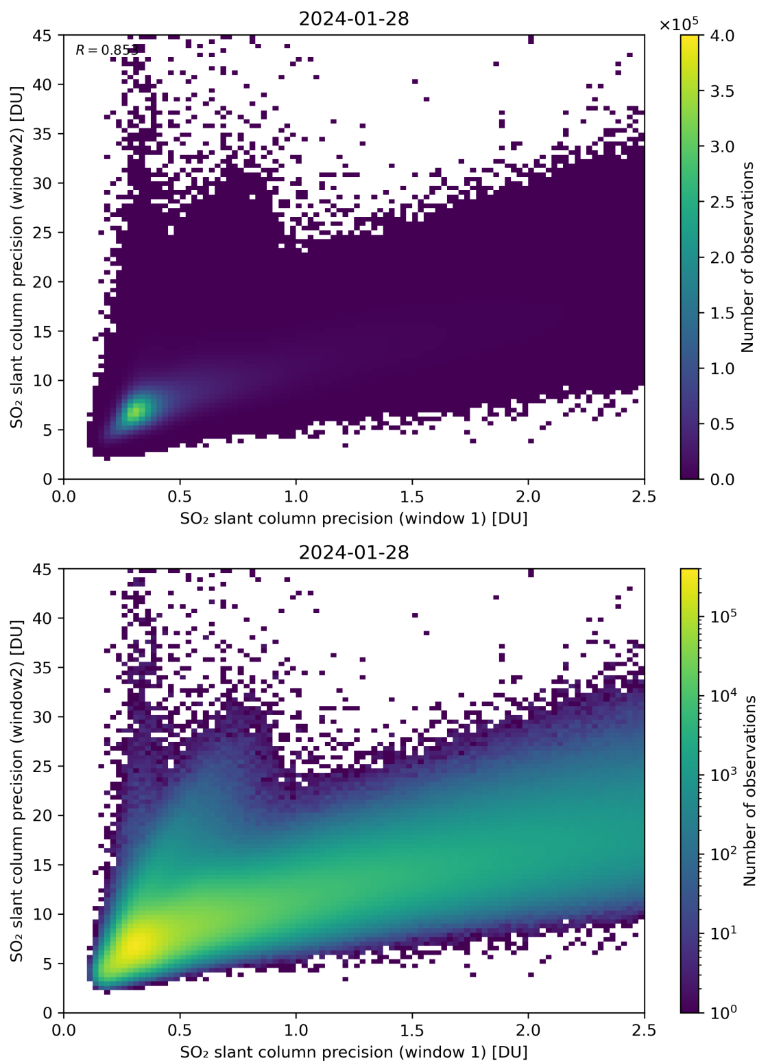
Figure 227: Scatter density plot of “SO 2 slant column precision (window 1)” against “SO 2 slant column precision (window 2)” for 2024-01-27 to 2024-01-29.
