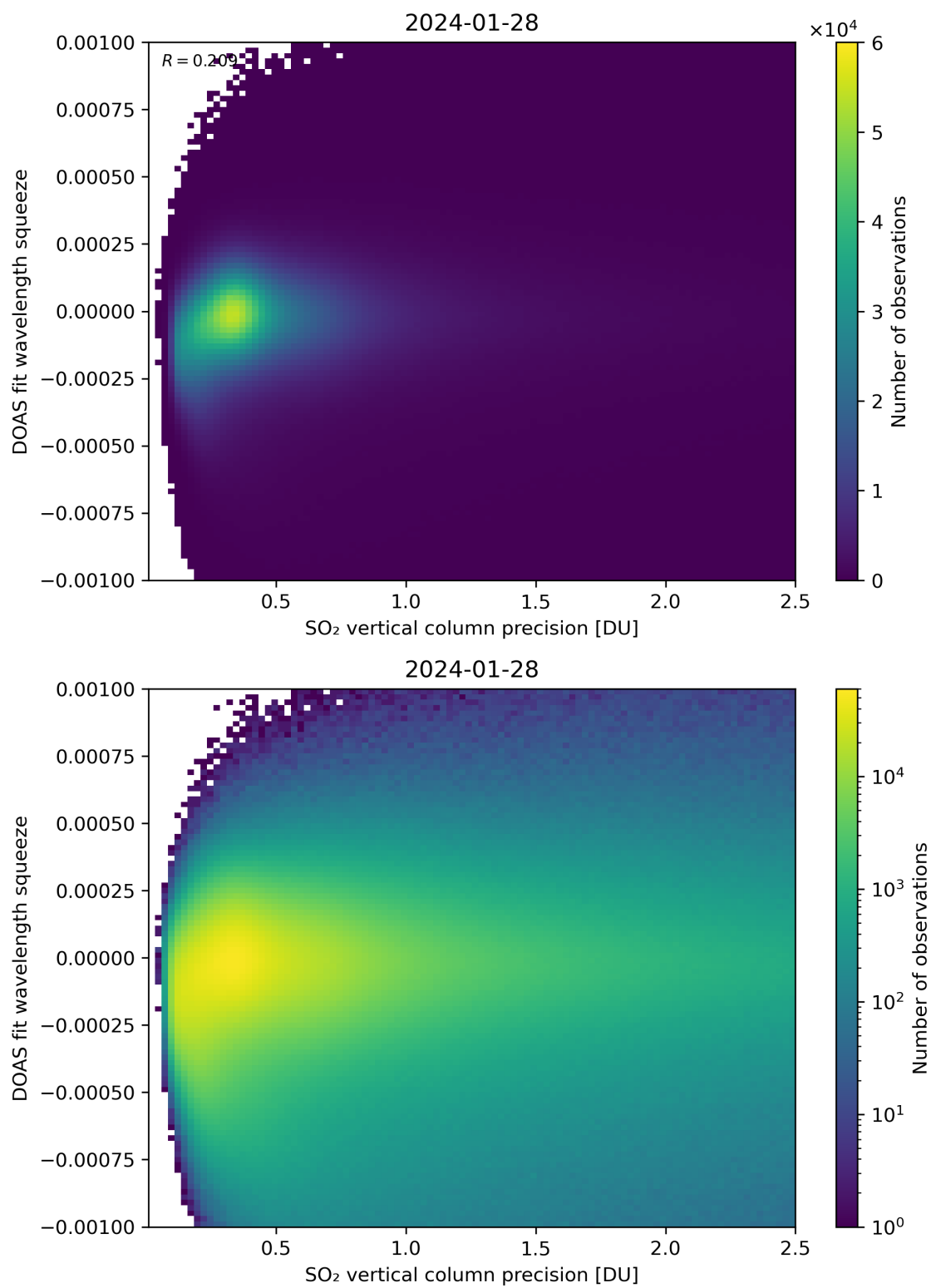
Figure 283: Scatter density plot of “SO 2 vertical column precision” against “DOAS fit wavelength squeeze” for 2024-01-27 to 2024-01-29.
