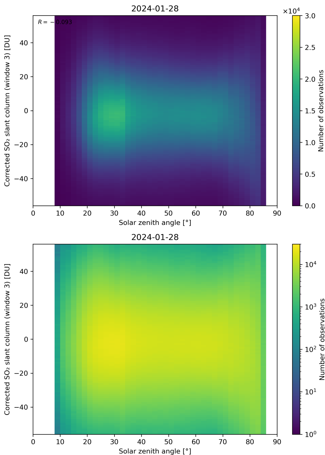
Figure 168: Scatter density plot of “Solar zenith angle” against “Corrected SO 2 slant column (window 3)” for 2024-01-27 to 2024-01-29.
