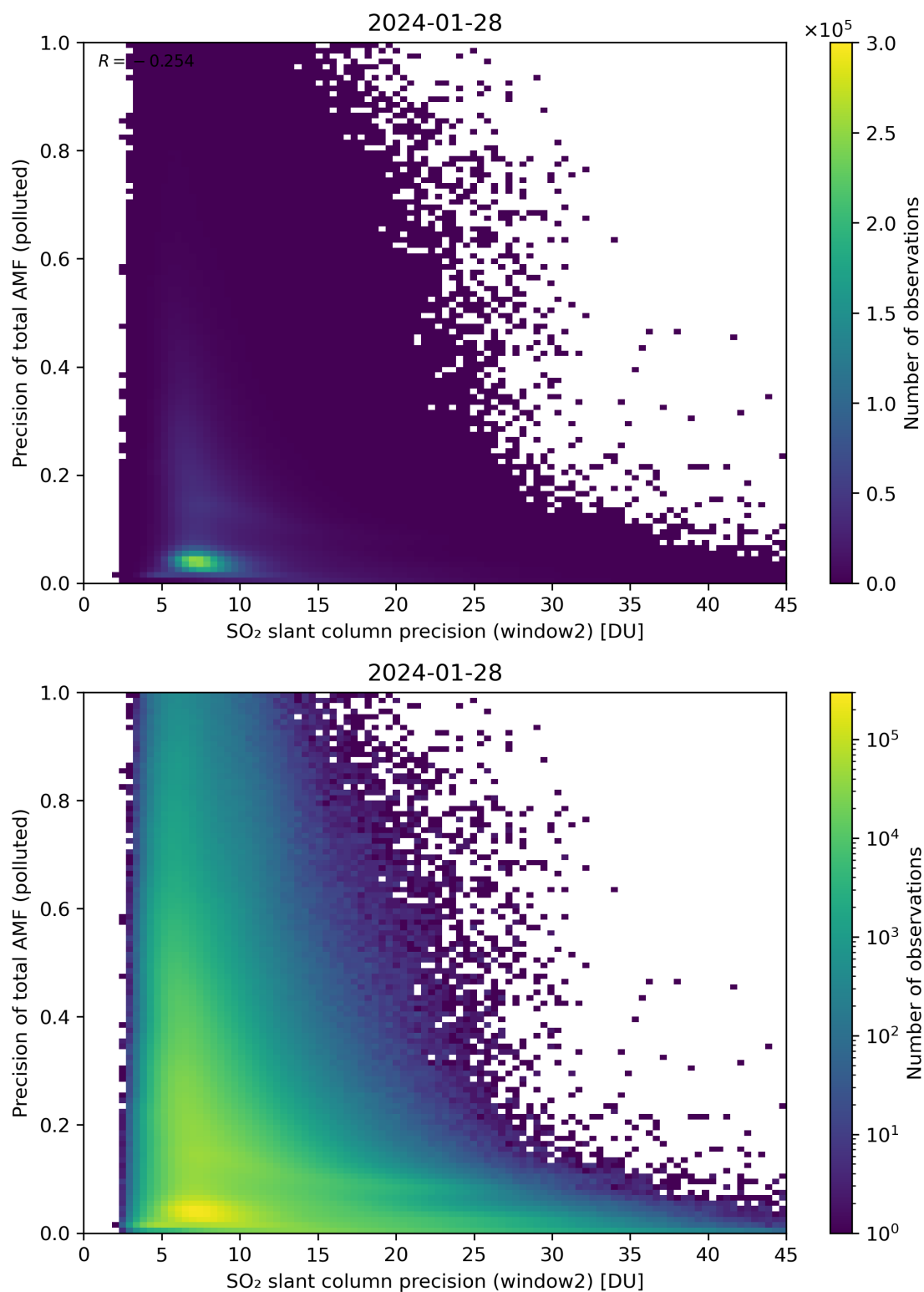
Figure 252: Scatter density plot of “SO 2 slant column precision (window2)” against “Precision of total AMF (polluted)” for 2024-01-27 to 2024-01-29.
