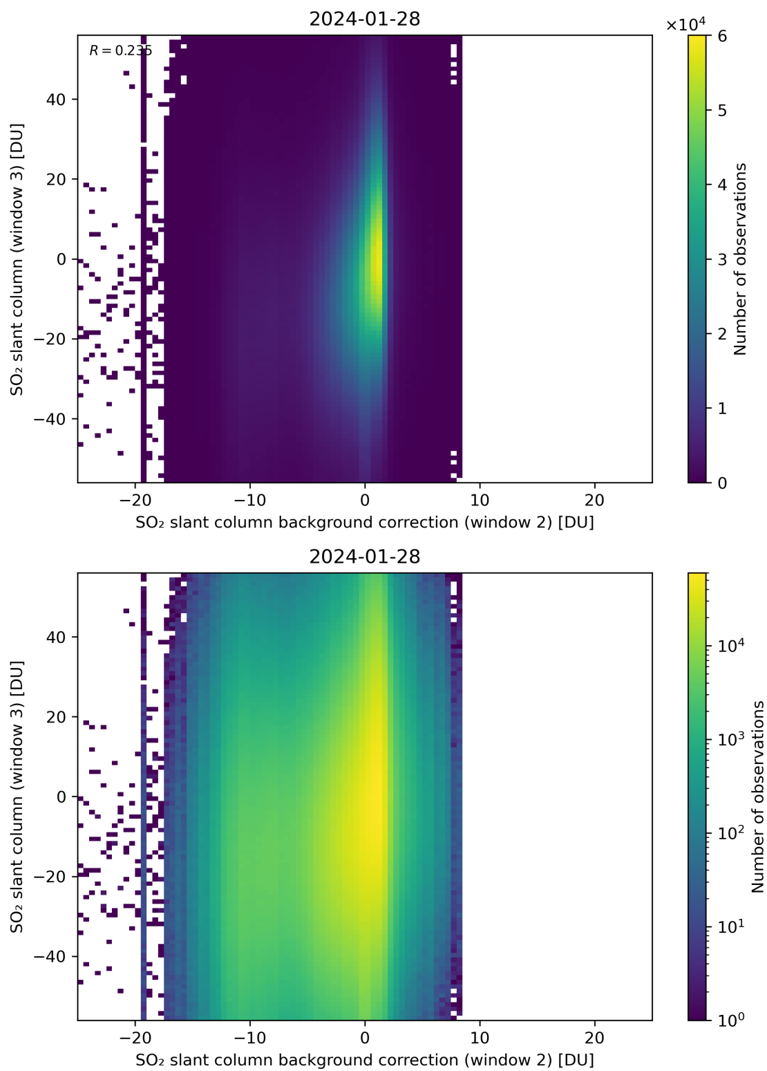
Figure 117: Scatter density plot of “SO 2 slant column background correction (window 2)” against “SO 2 slant column (window 3)” for 2024-01-27 to 2024-01-29.
