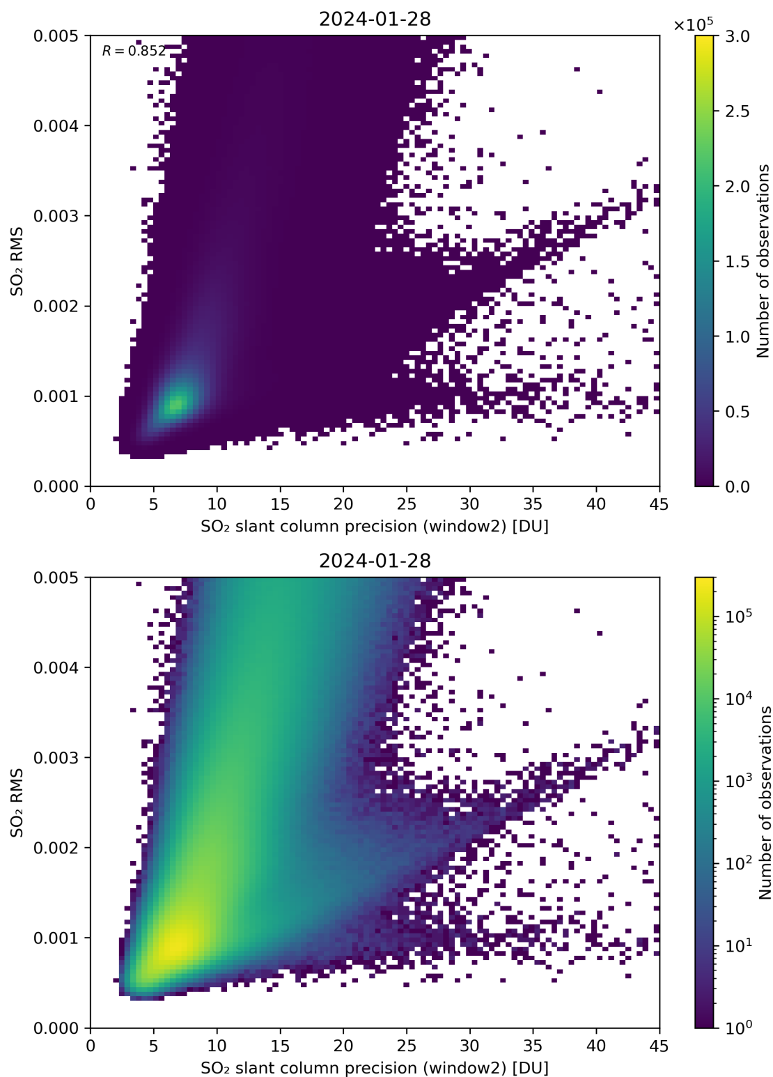
Figure 245: Scatter density plot of “SO 2 slant column precision (window2)” against “SO 2 RMS” for 2024-01-27 to 2024-01-29.
