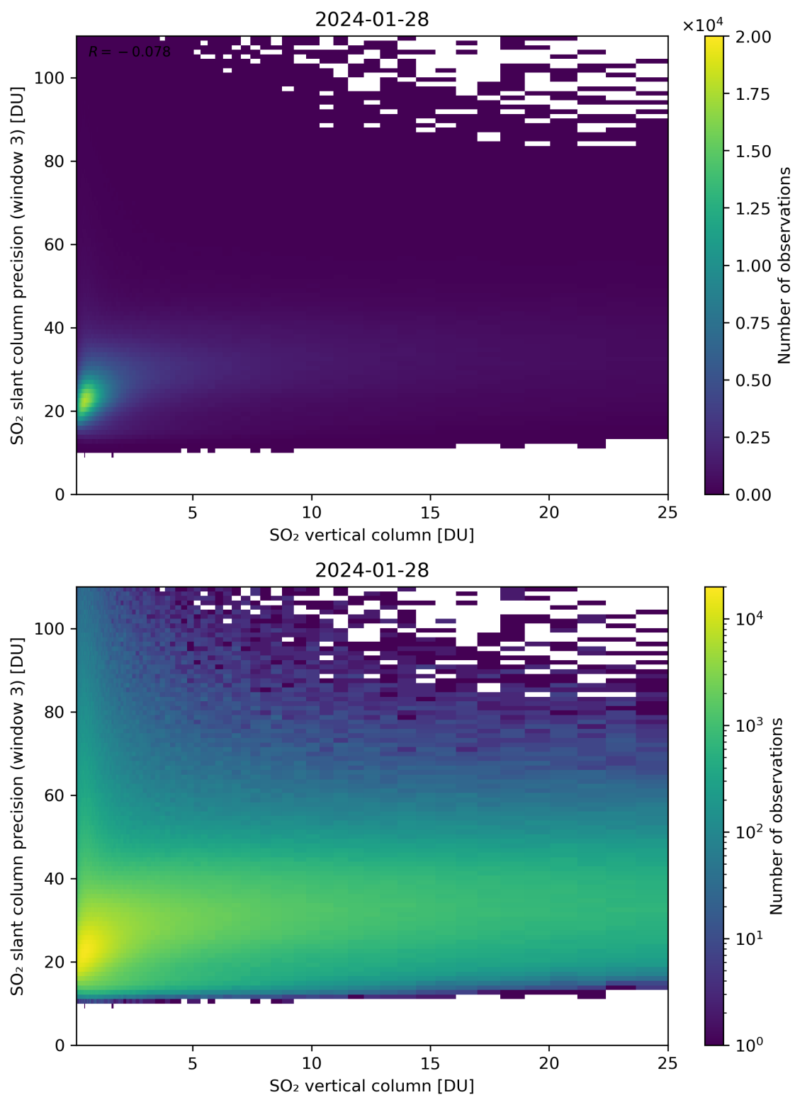
Figure 304: Scatter density plot of “SO 2 vertical column” against “SO 2 slant column precision (window 3)” for 2024-01-27 to 2024-01-29.
