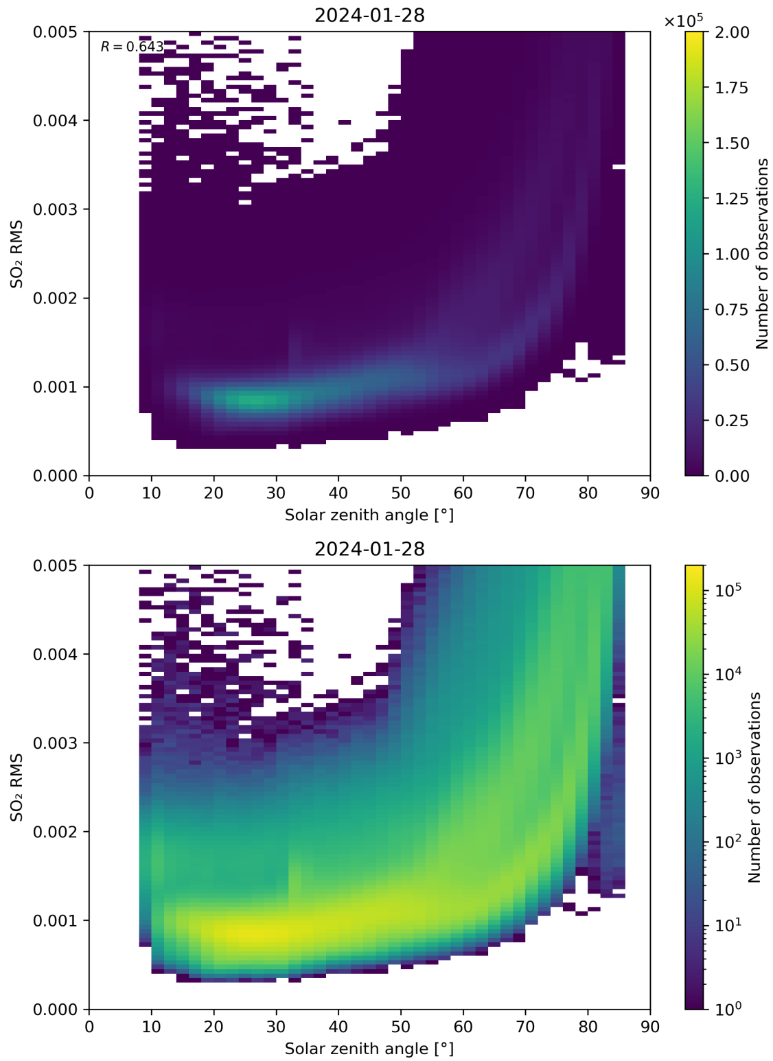
Figure 163: Scatter density plot of “Solar zenith angle” against “SO 2 RMS” for 2024-01-27 to 2024-01-29.
