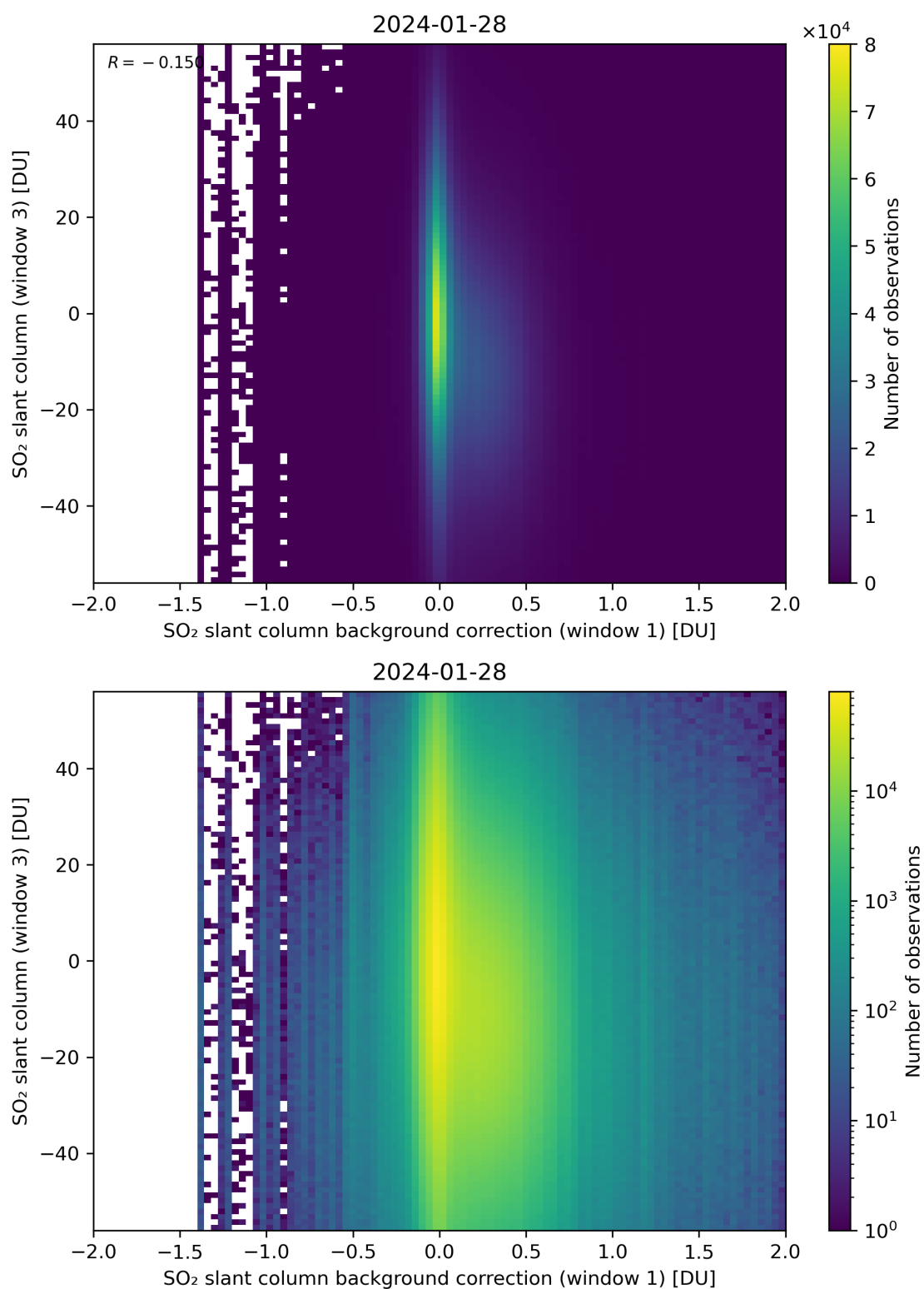
Figure 107: Scatter density plot of “SO 2 slant column background correction (window 1)” against “SO 2 slant column (window 3)” for 2024-01-27 to 2024-01-29.
