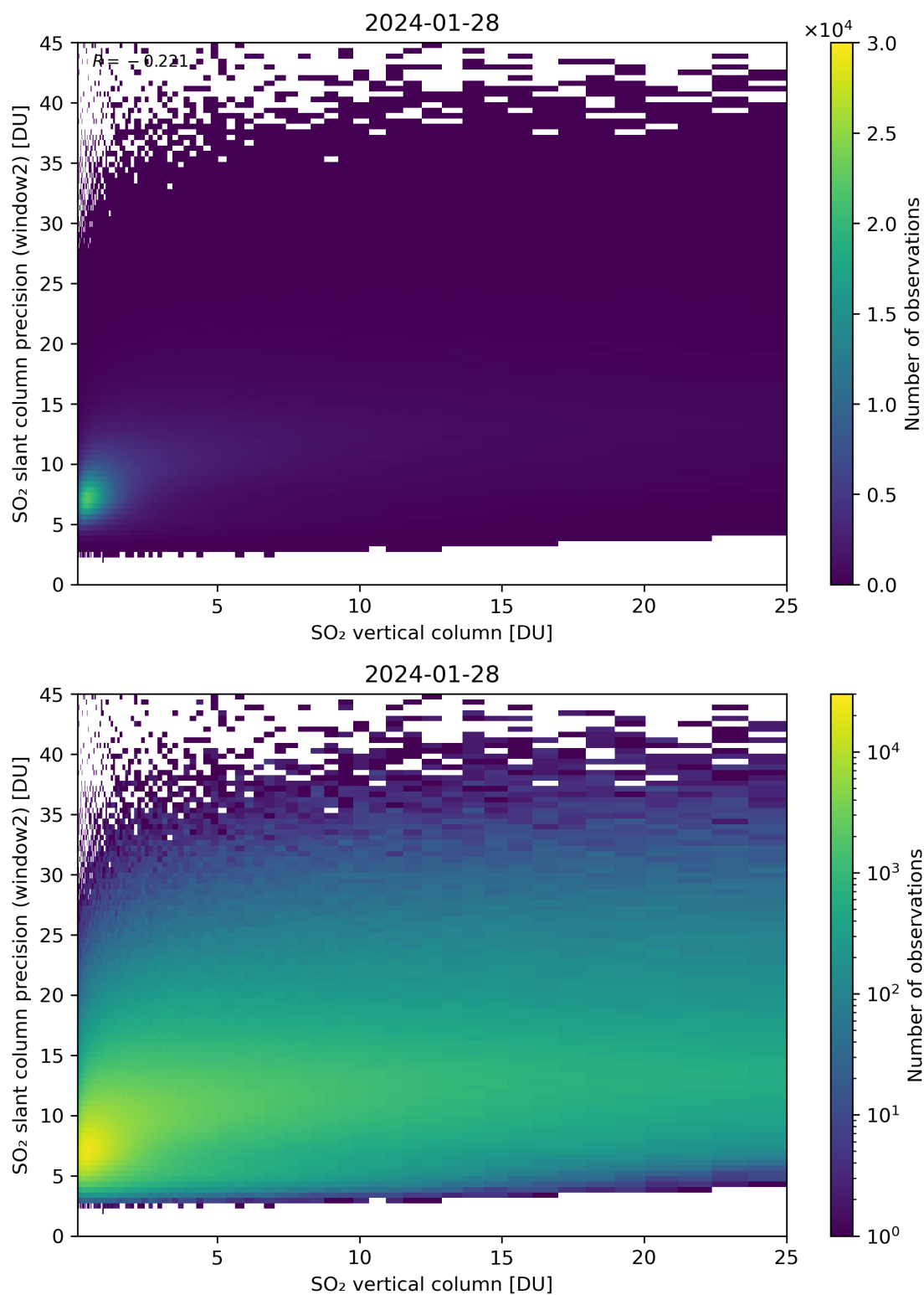
Figure 302: Scatter density plot of “SO 2 vertical column” against “SO 2 slant column precision (window2)” for 2024-01-27 to 2024-01-29.
