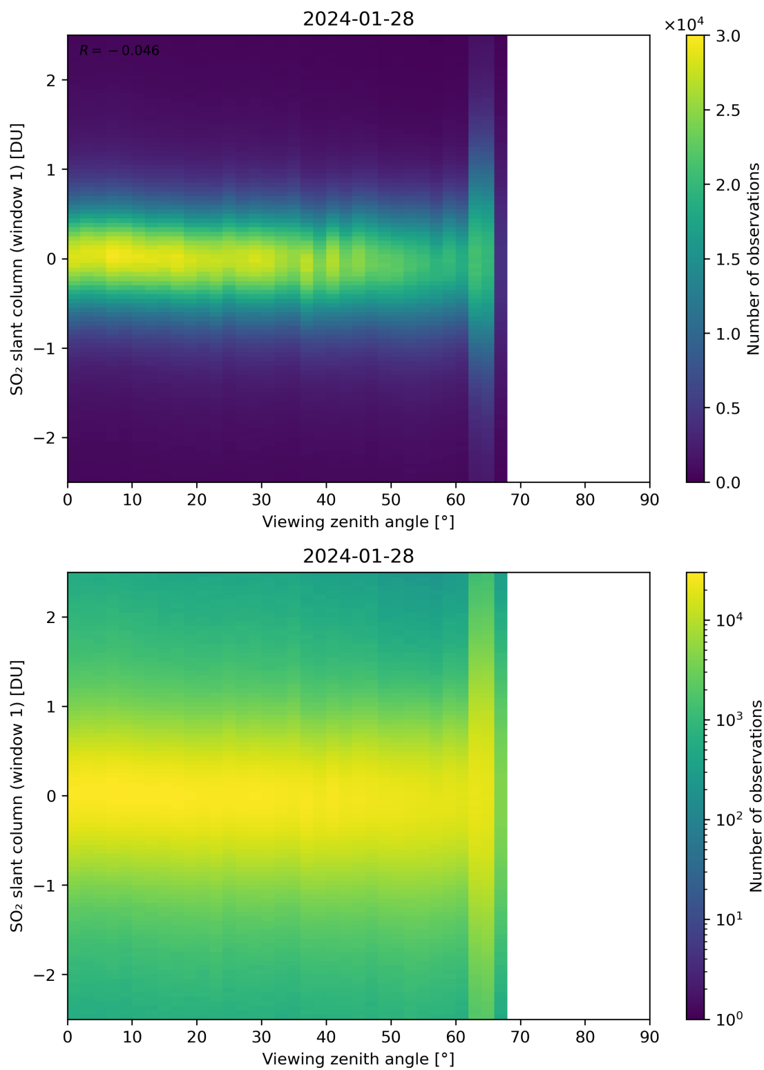
Figure 320: Scatter density plot of “Viewing zenith angle” against “SO 2 slant column (window 1)” for 2024-01-27 to 2024-01-29.
