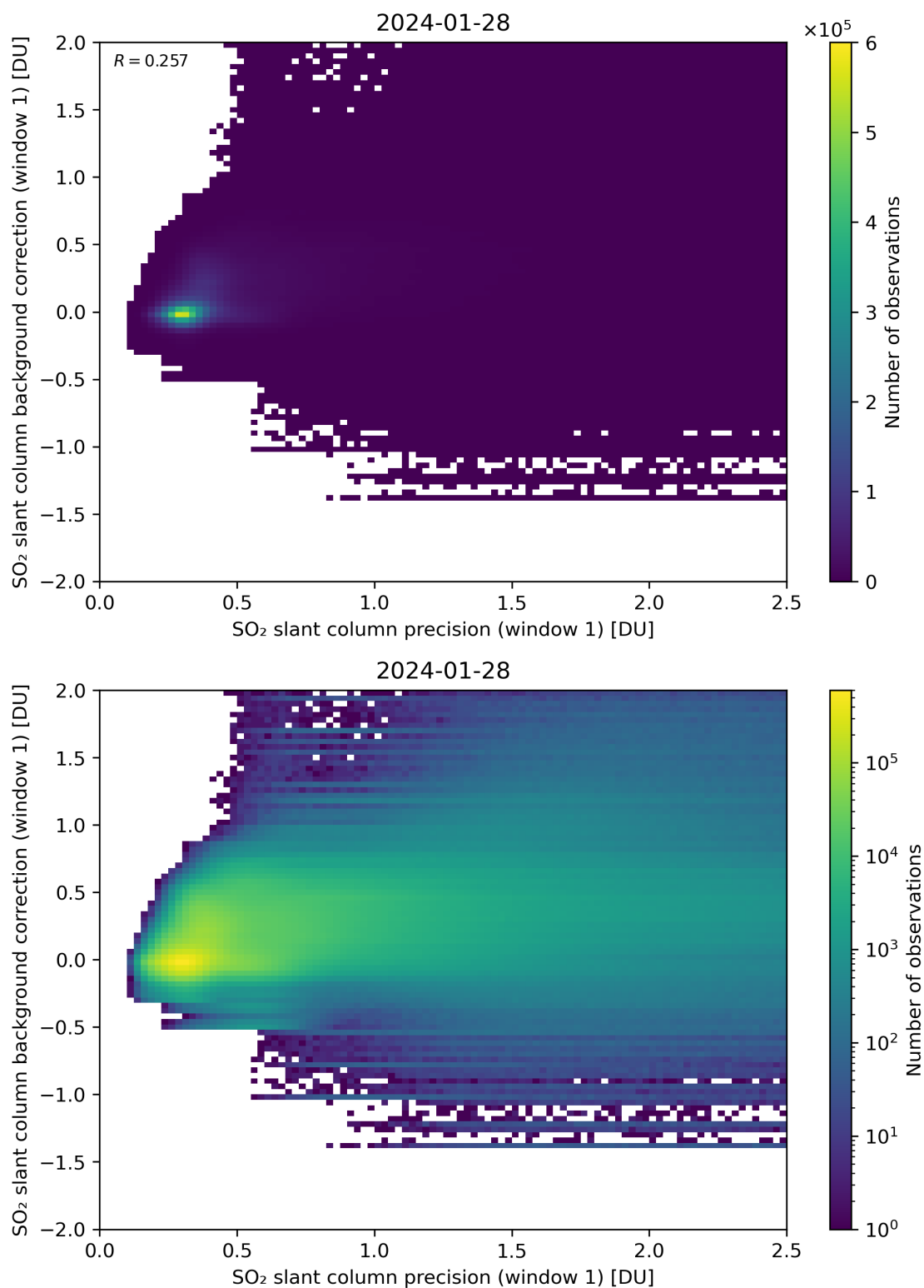
Figure 218: Scatter density plot of “SO 2 slant column precision (window 1)” against “SO 2 slant column background correction (window 1)” for 2024-01-27 to 2024-01-29.
