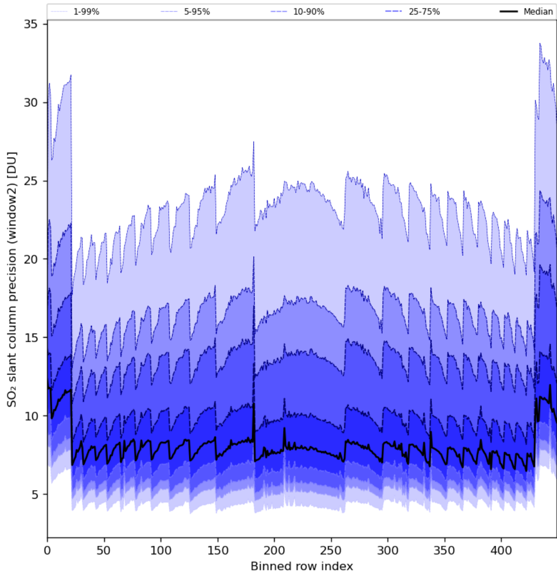
Figure 84: Along track statistics of “SO 2 slant column precision (window2)” for 2024-01-27 to 2024-01-29
