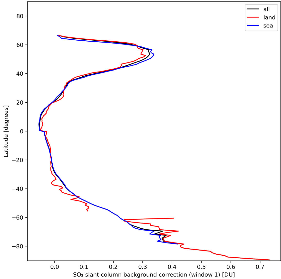
Figure 36: Zonal average of “SO 2 slant column background correction (window 1)” for 2024-01-27 to 2024-01-29.
