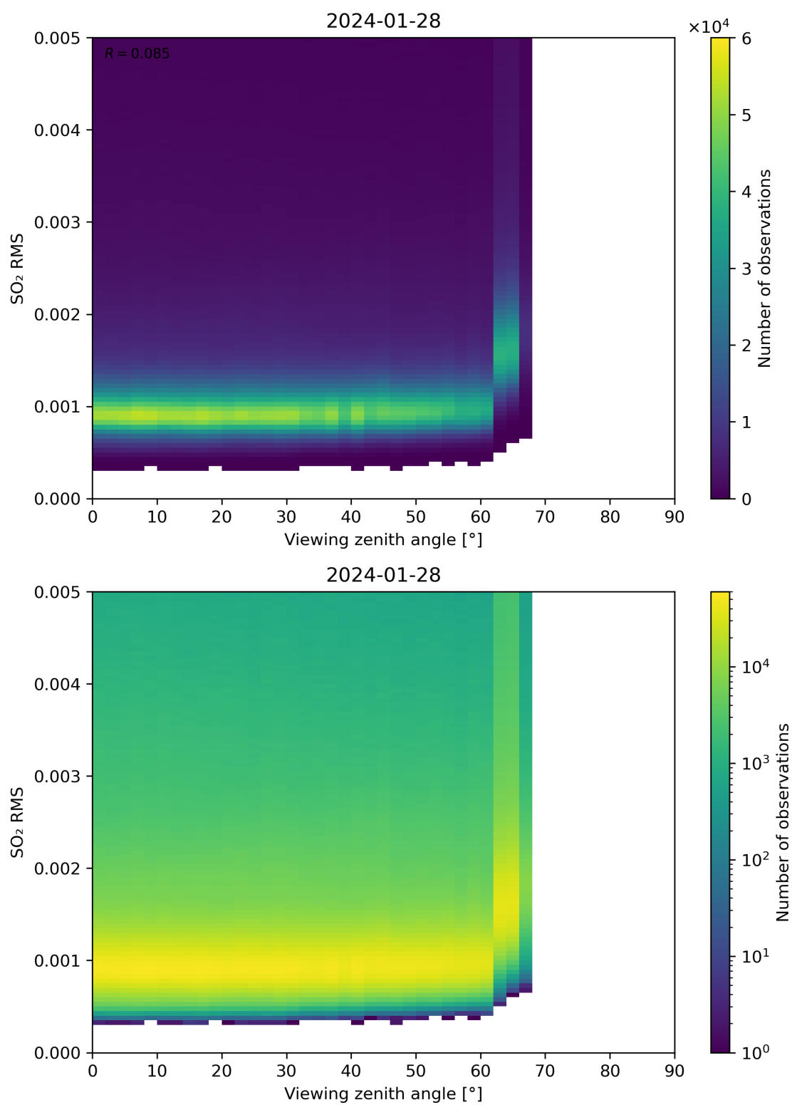
Figure 313: Scatter density plot of “Viewing zenith angle” against “SO 2 RMS” for 2024-01-27 to 2024-01-29.
