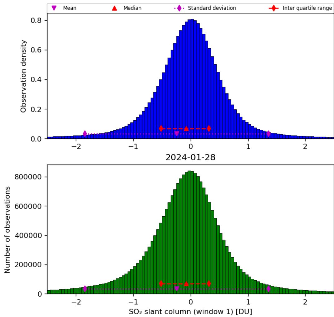
Figure 56: Histogram of “SO 2 slant column (window 1)” for 2024-01-27 to 2024-01-29
