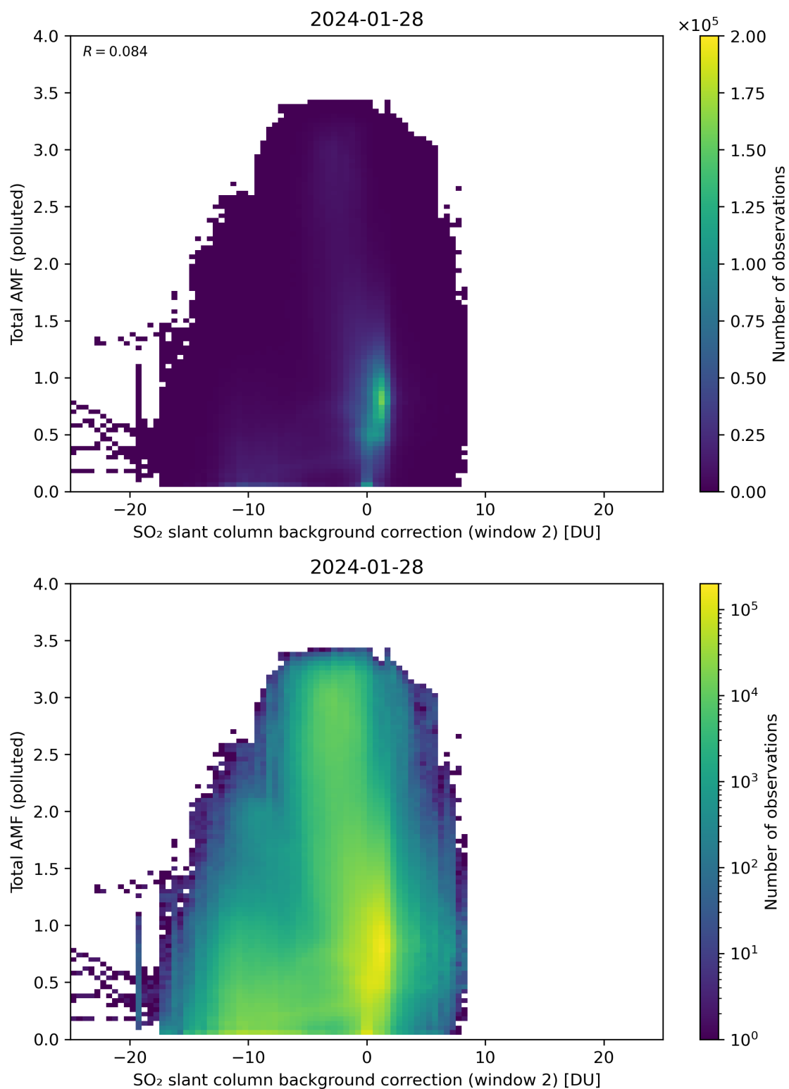
Figure 119: Scatter density plot of “SO 2 slant column background correction (window 2)” against “Total AMF (polluted)” for 2024-01-27 to 2024-01-29.
