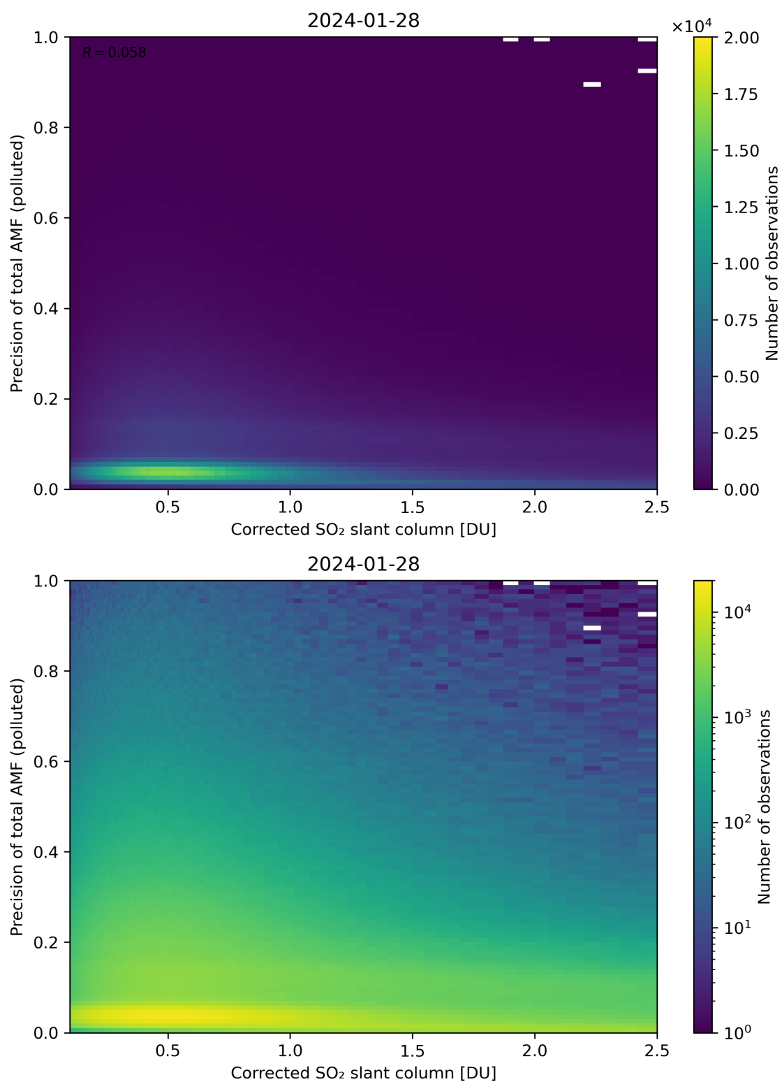
Figure 193: Scatter density plot of “Corrected SO 2 slant column” against “Precision of total AMF (polluted)” for 2024-01-27 to 2024-01-29.
