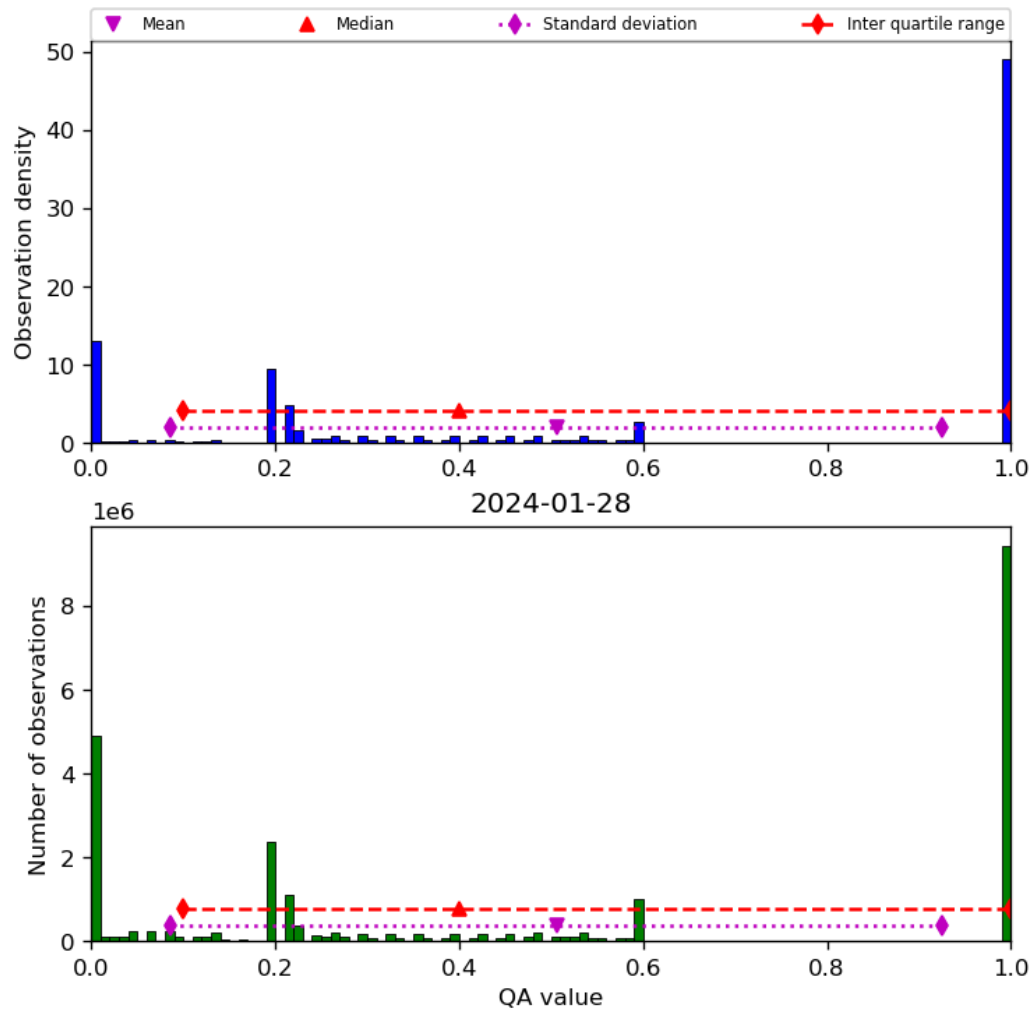
Figure 52: Histogram of “QA value” for 2024-01-27 to 2024-01-29
