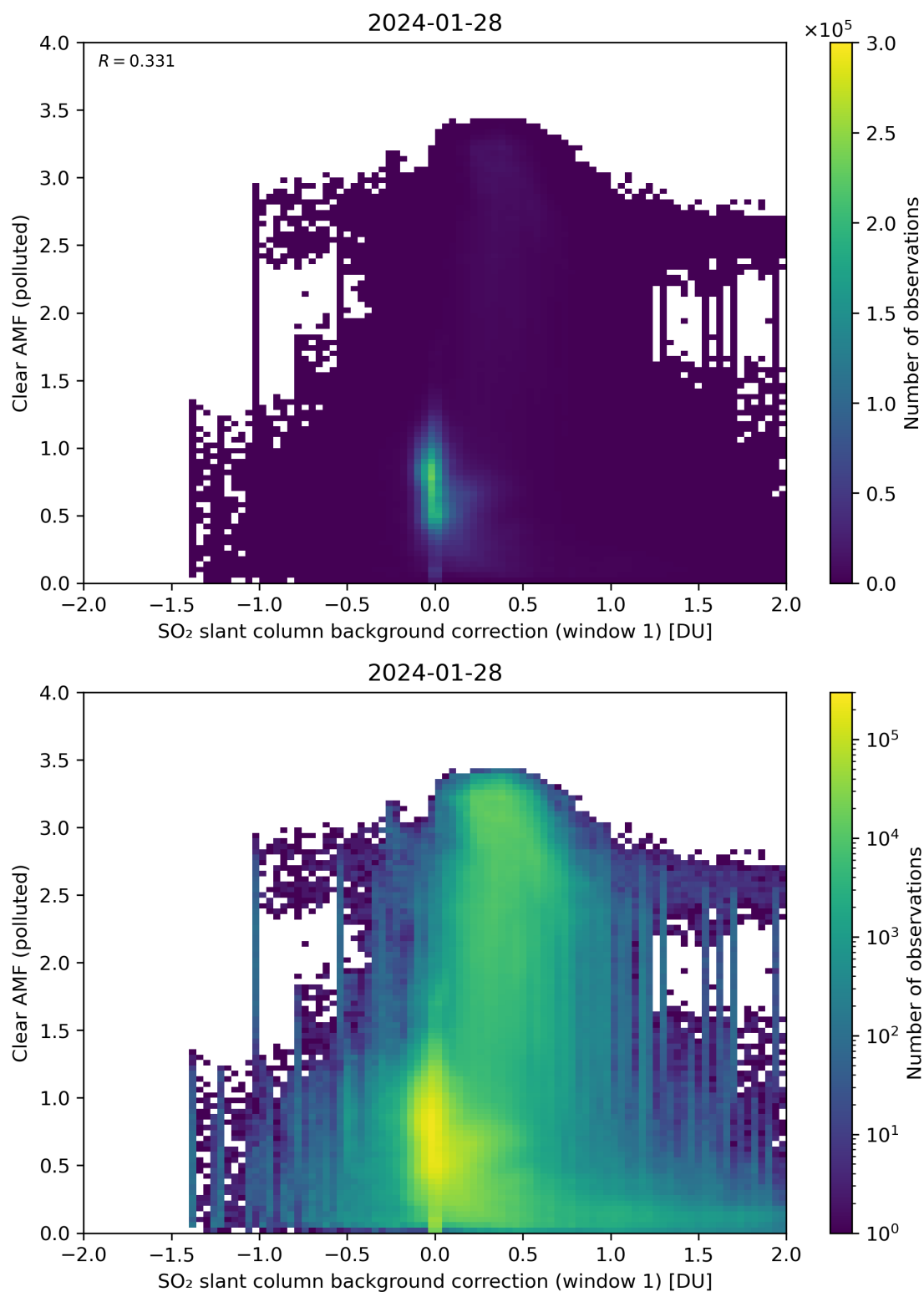
Figure 103: Scatter density plot of “SO 2 slant column background correction (window 1)” against “Clear AMF (polluted)” for 2024-01-27 to 2024-01-29.
