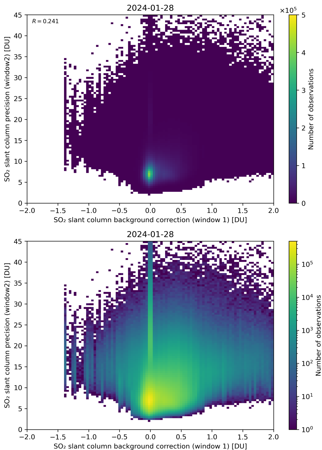
Figure 106: Scatter density plot of “SO 2 slant column background correction (window 1)” against “SO 2 slant column precision (window2)” for 2024-01-27 to 2024-01-29.
