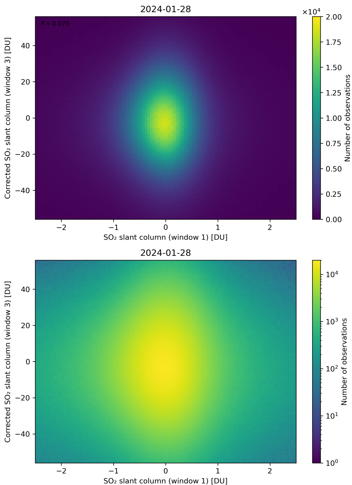
Figure 234: Scatter density plot of “SO 2 slant column (window 1)” against “Corrected SO 2 slant column (window 3)” for 2024-01-27 to 2024-01-29.
