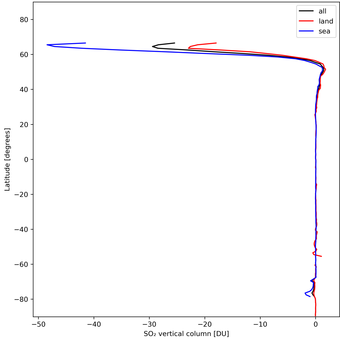
Figure 30: Zonal average of “SO 2 vertical column” for 2024-01-27 to 2024-01-29.
