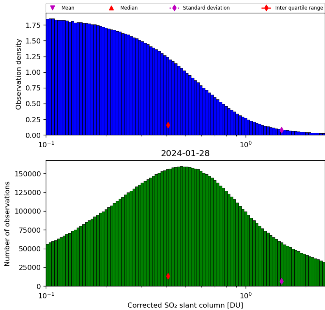
Figure 55: Histogram of “Corrected SO 2 slant column” for 2024-01-27 to 2024-01-29
