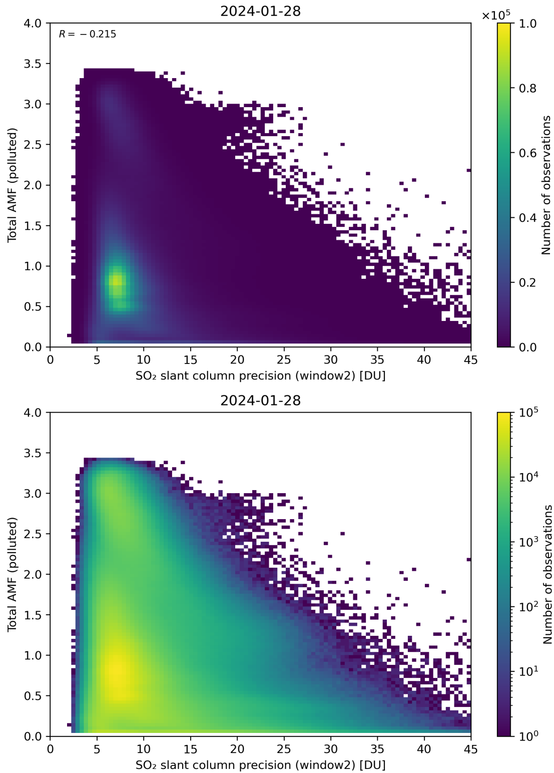
Figure 251: Scatter density plot of “SO 2 slant column precision (window2)” against “Total AMF (polluted)” for 2024-01-27 to 2024-01-29.
