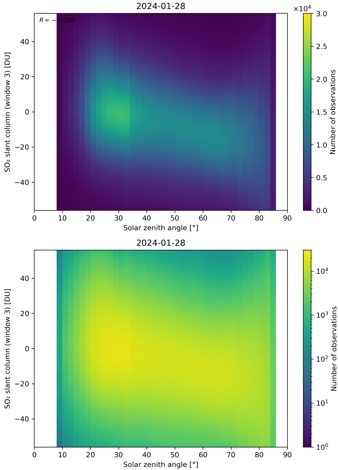
Figure 172: Scatter density plot of “Solar zenith angle” against “SO 2 slant column (window 3)” for 2024-01-27 to 2024-01-29.
