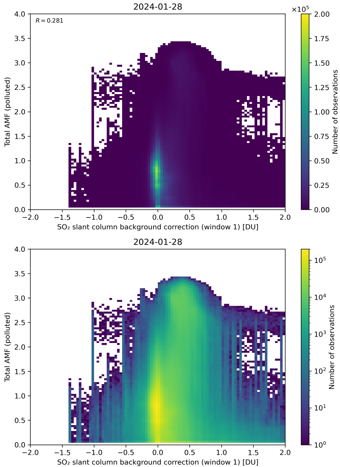
Figure 109: Scatter density plot of “SO 2 slant column background correction (window 1)” against “Total AMF (polluted)” for 2024-01-27 to 2024-01-29.
