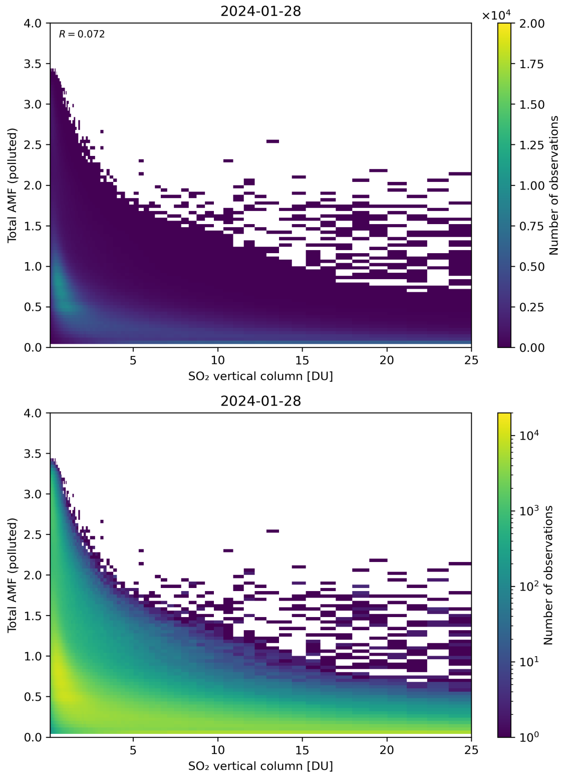
Figure 305: Scatter density plot of “SO 2 vertical column” against “Total AMF (polluted)” for 2024-01-27 to 2024-01-29.
