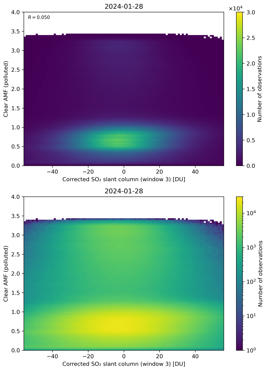
Figure 209: Scatter density plot of “Corrected SO 2 slant column (window 3)” against “Clear AMF (polluted)” for 2024-01-27 to 2024-01-29.
