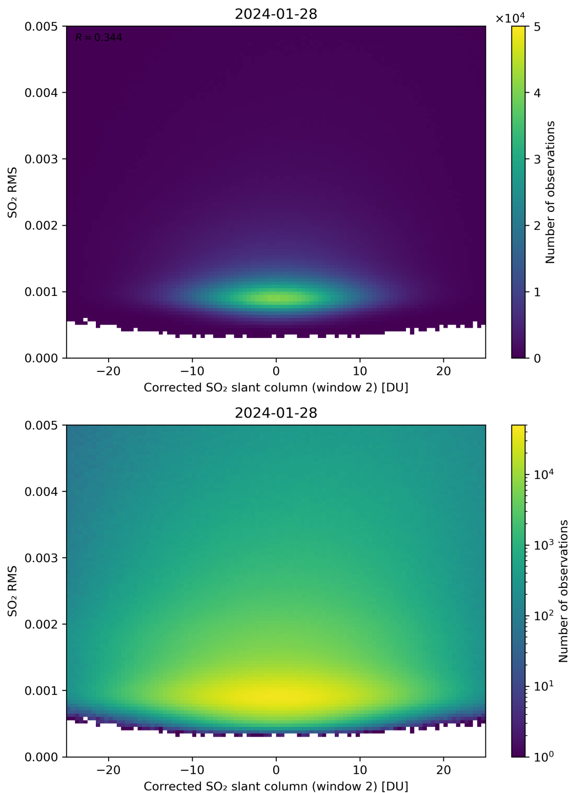
Figure 198: Scatter density plot of “Corrected SO 2 slant column (window 2)” against “SO 2 RMS” for 2024-01-27 to 2024-01-29.
