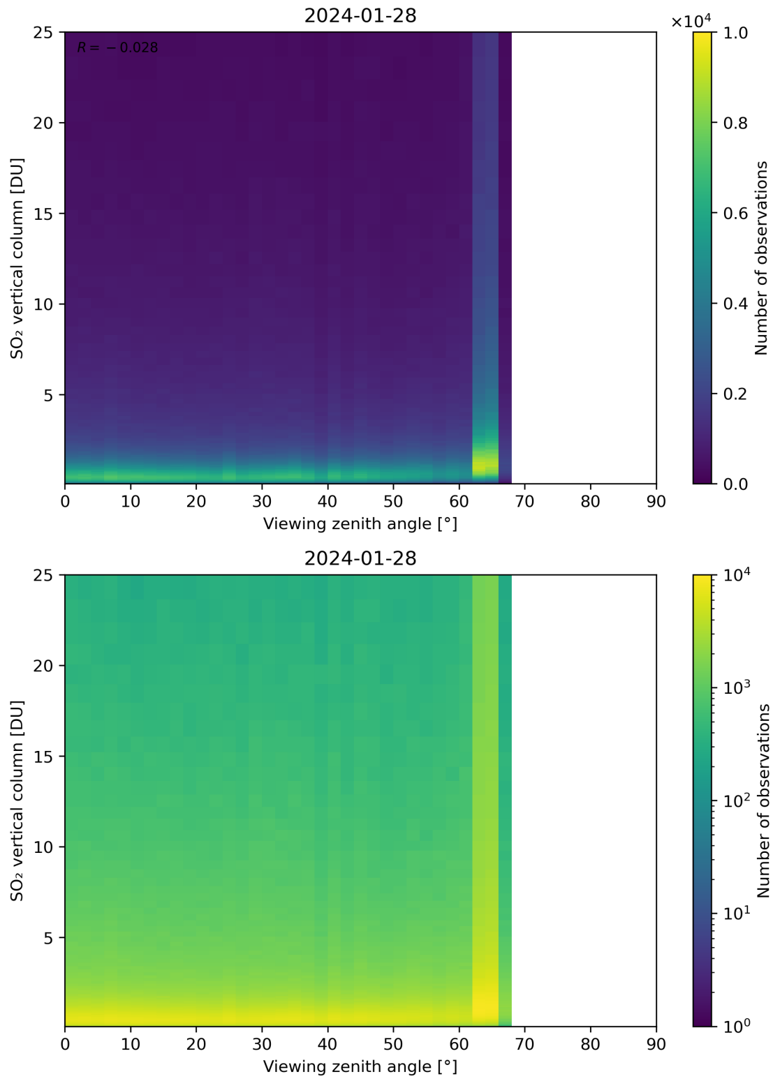
Figure 327: Scatter density plot of “Viewing zenith angle” against “SO 2 vertical column” for 2024-01-27 to 2024-01-29.
