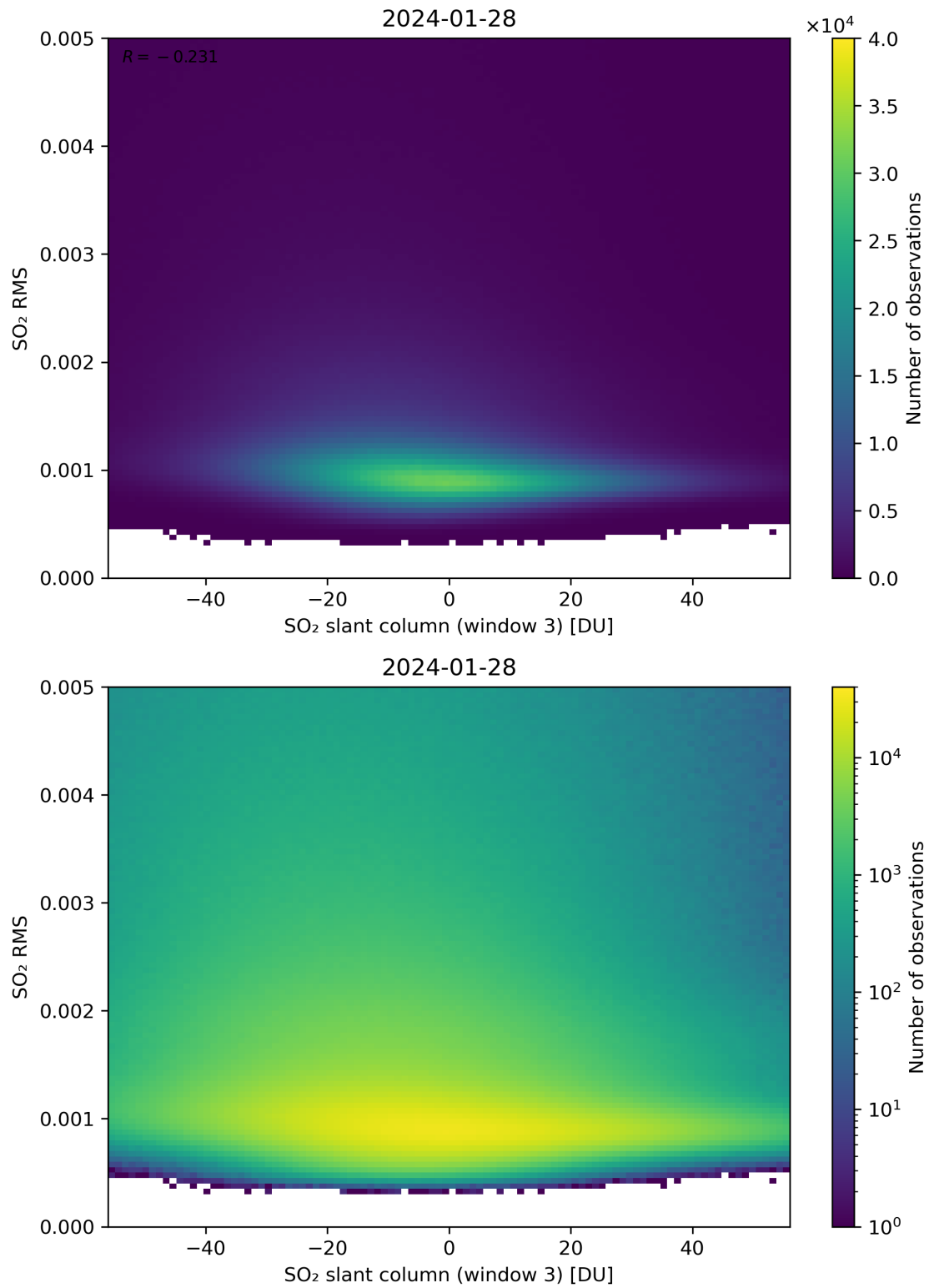
Figure 256: Scatter density plot of “SO 2 slant column (window 3)” against “SO 2 RMS” for 2024-01-27 to 2024-01-29.
