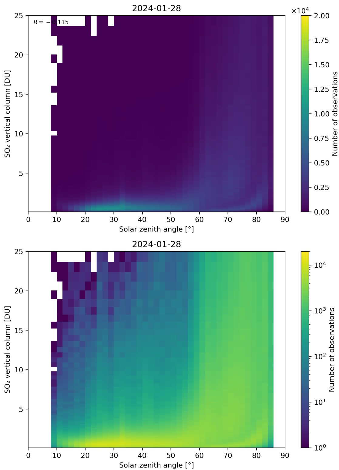
Figure 176: Scatter density plot of “Solar zenith angle” against “SO 2 vertical column” for 2024-01-27 to 2024-01-29.
