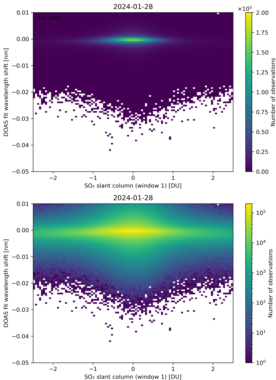
Figure 215: Scatter density plot of “SO 2 slant column (window 1)” against “DOAS fit wavelength shift” for 2024-01-27 to 2024-01-29.
