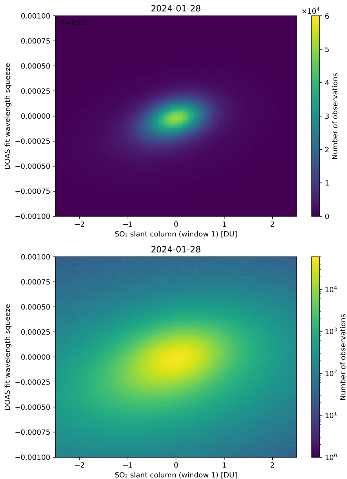
Figure 216: Scatter density plot of “SO 2 slant column (window 1)” against “DOAS fit wavelength squeeze” for 2024-01-27 to 2024-01-29.
