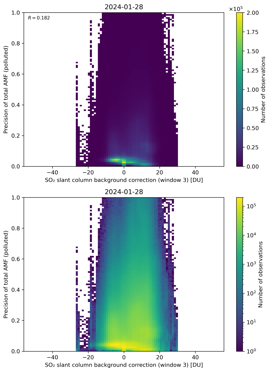
Figure 126: Scatter density plot of “SO 2 slant column background correction (window 3)” against “Precision of total AMF (polluted)” for 2024-01-27 to 2024-01-29.
