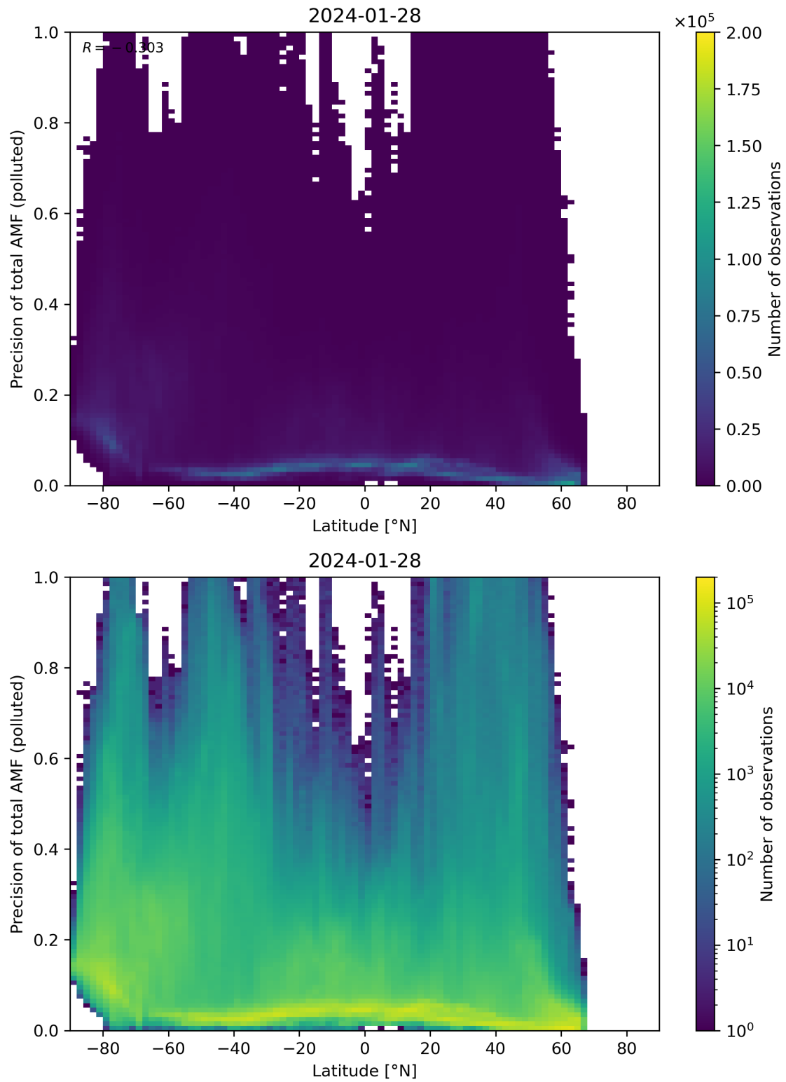
Figure 155: Scatter density plot of “Latitude” against “Precision of total AMF (polluted)” for 2024-01-27 to 2024-01-29.
