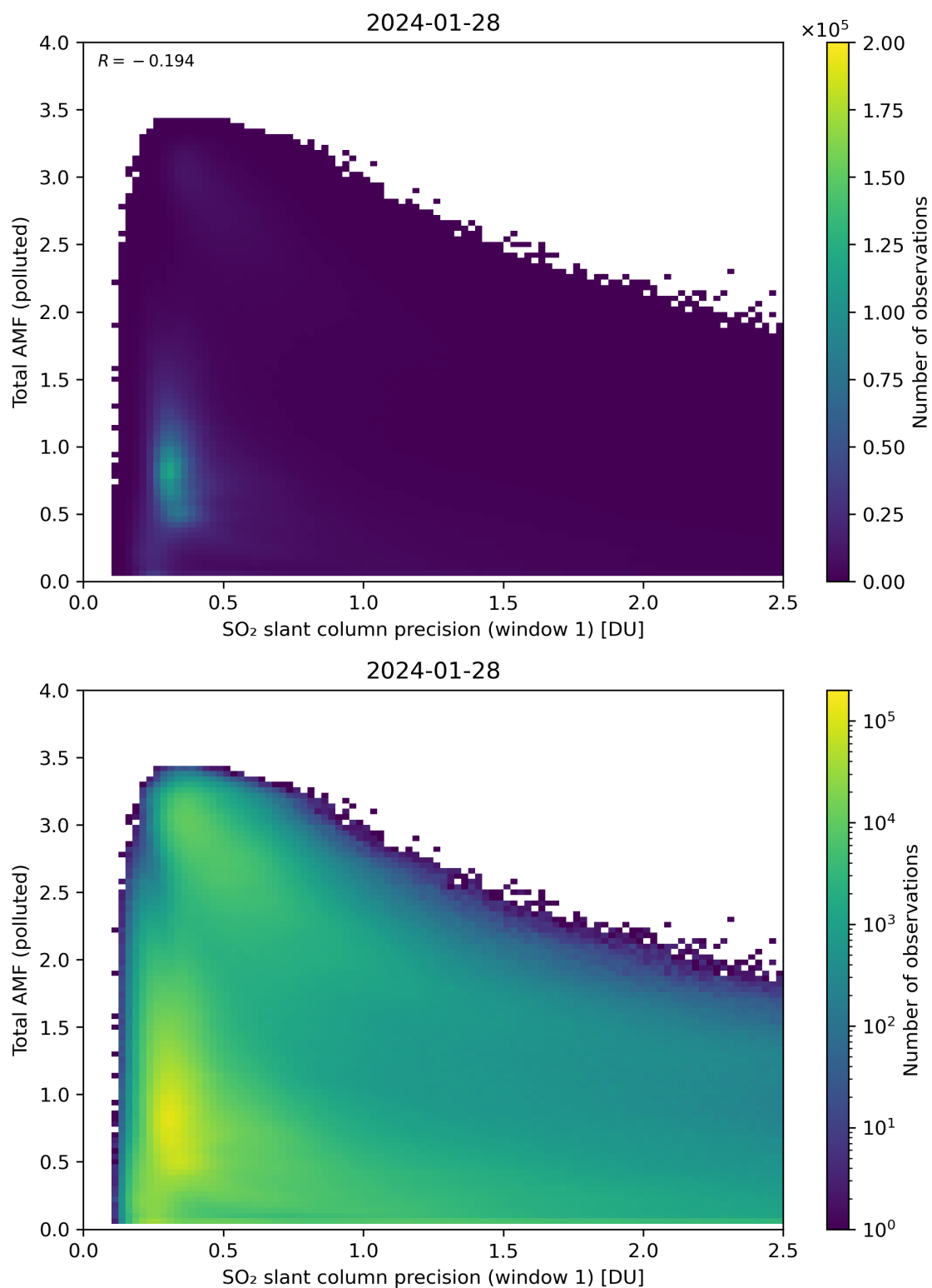
Figure 230: Scatter density plot of “SO 2 slant column precision (window 1)” against “Total AMF (polluted)” for 2024-01-27 to 2024-01-29.
