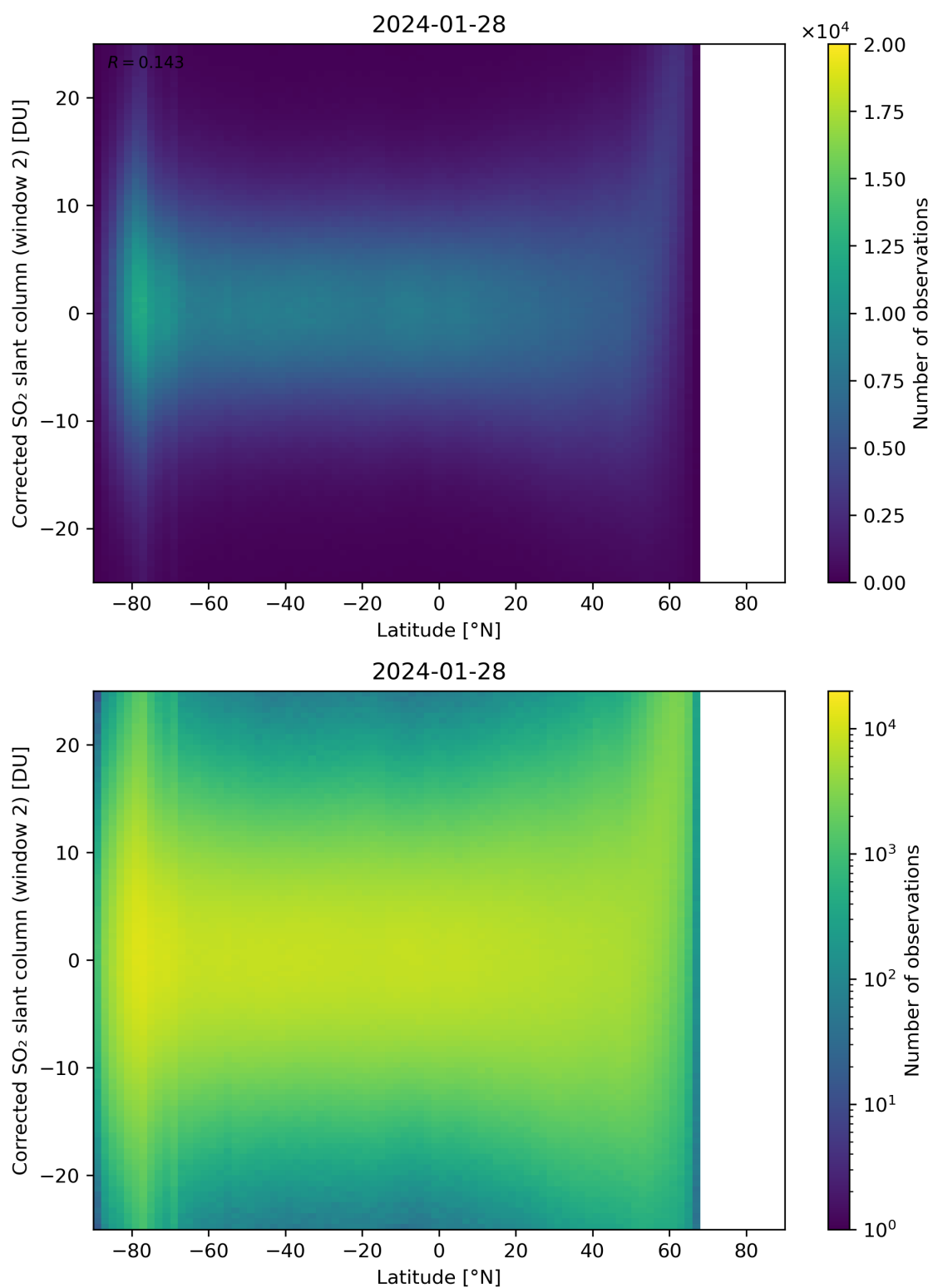
Figure 147: Scatter density plot of “Latitude” against “Corrected SO 2 slant column (window 2)” for 2024-01-27 to 2024-01-29.
