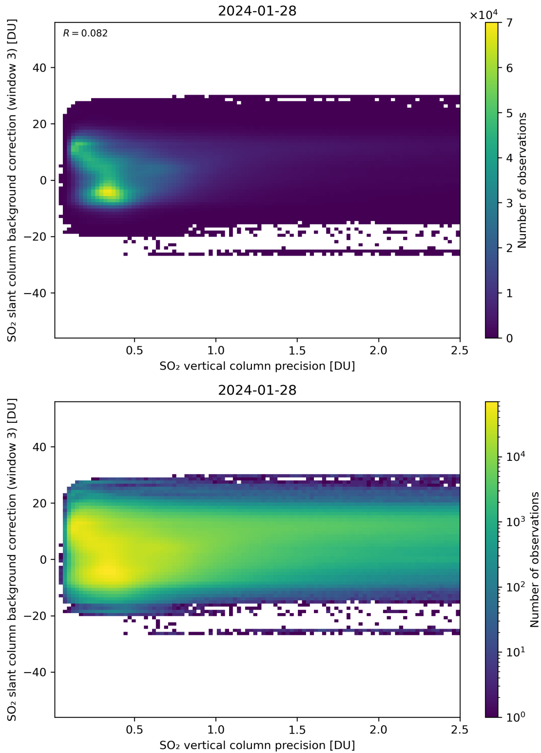
Figure 281: Scatter density plot of “SO 2 vertical column precision” against “SO 2 slant column background correction (window 3)” for 2024-01-27 to 2024-01-29.
