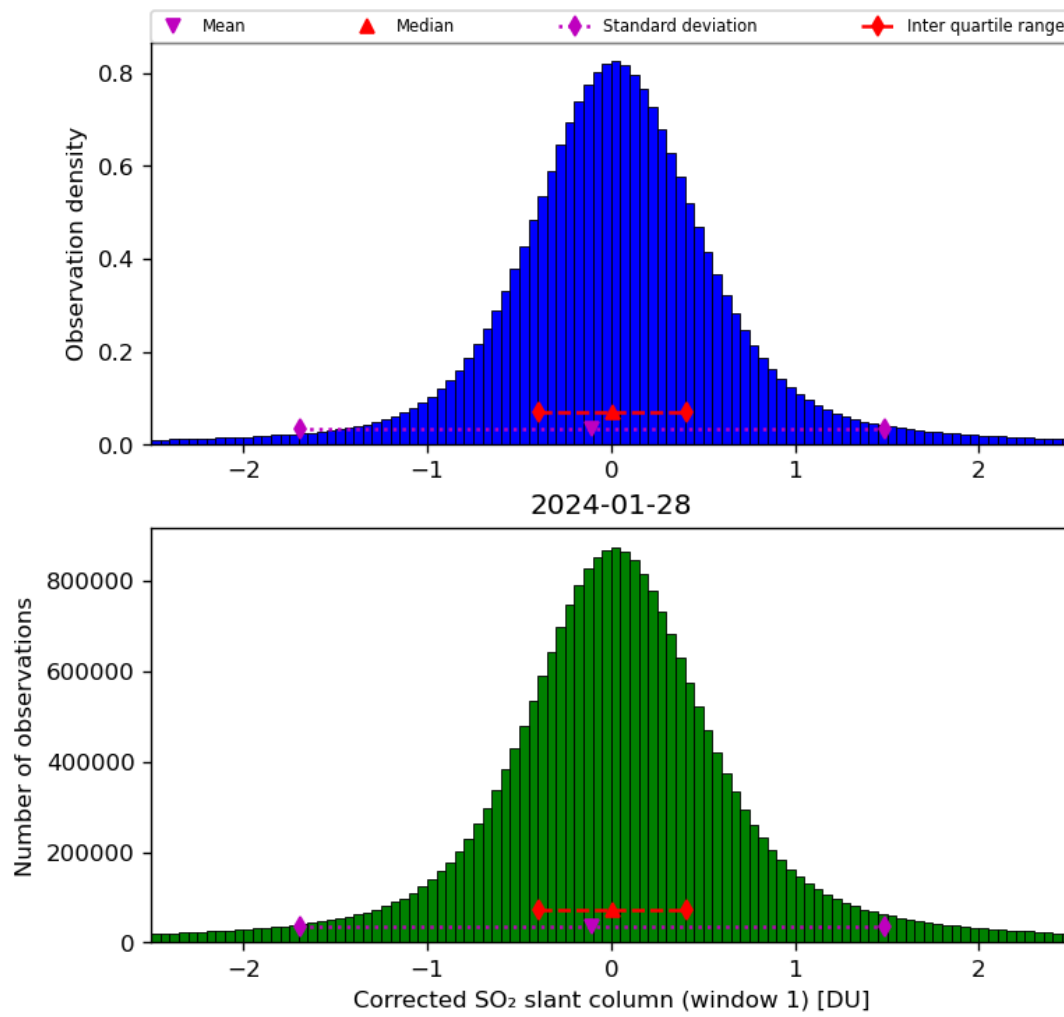
Figure 58: Histogram of “Corrected SO 2 slant column (window 1)” for 2024-01-27 to 2024-01-29
