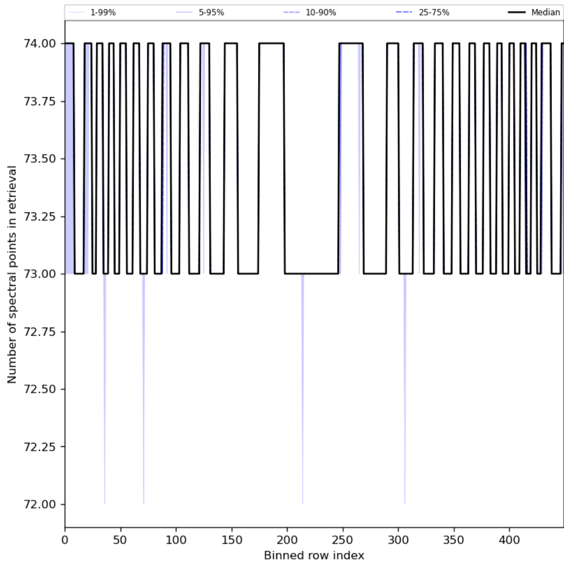
Figure 97: Along track statistics of “Number of spectral points in retrieval” for 2024-01-27 to 2024-01-29
