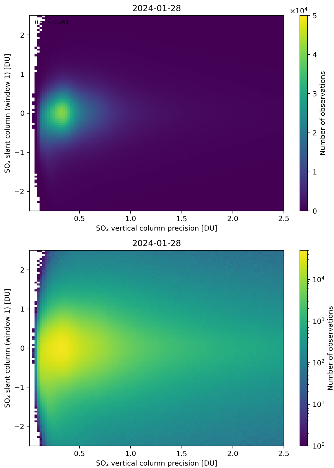
Figure 289: Scatter density plot of “SO 2 vertical column precision” against “SO 2 slant column (window 1)” for 2024-01-27 to 2024-01-29.
