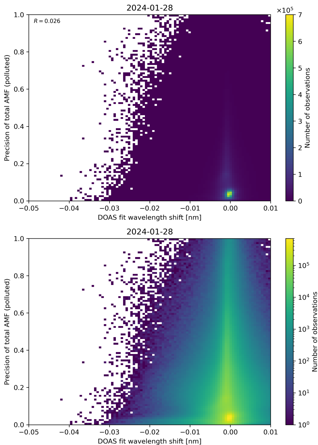
Figure 131: Scatter density plot of “DOAS fit wavelength shift” against “Precision of total AMF (polluted)” for 2024-01-27 to 2024-01-29.
