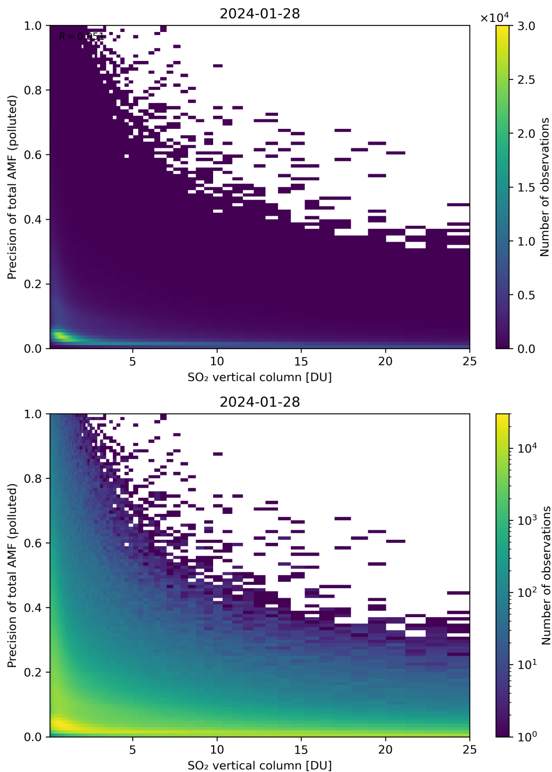
Figure 306: Scatter density plot of “SO 2 vertical column” against “Precision of total AMF (polluted)” for 2024-01-27 to 2024-01-29.
