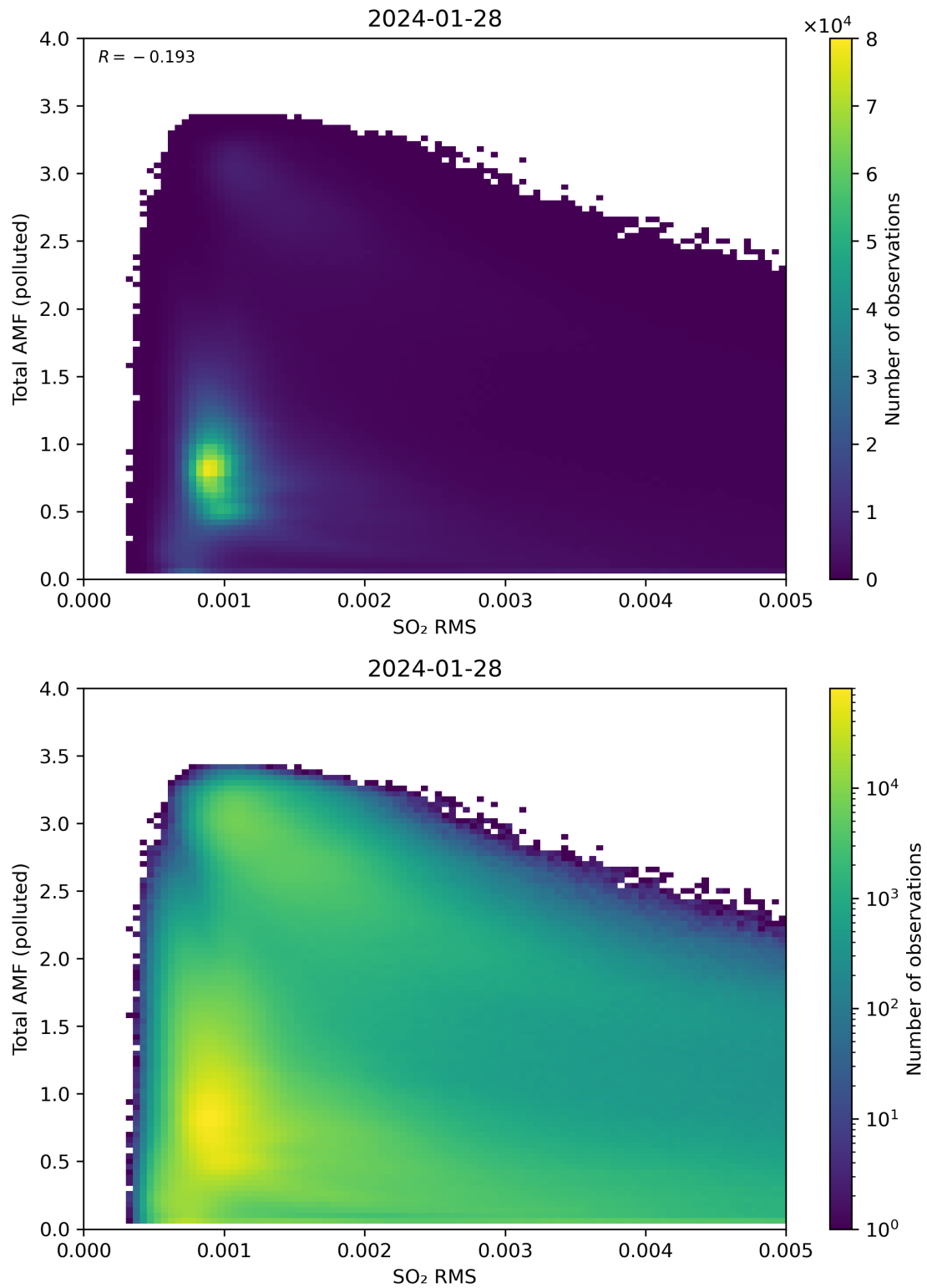
Figure 137: Scatter density plot of “SO 2 RMS” against “Total AMF (polluted)” for 2024-01-27 to 2024-01-29.
