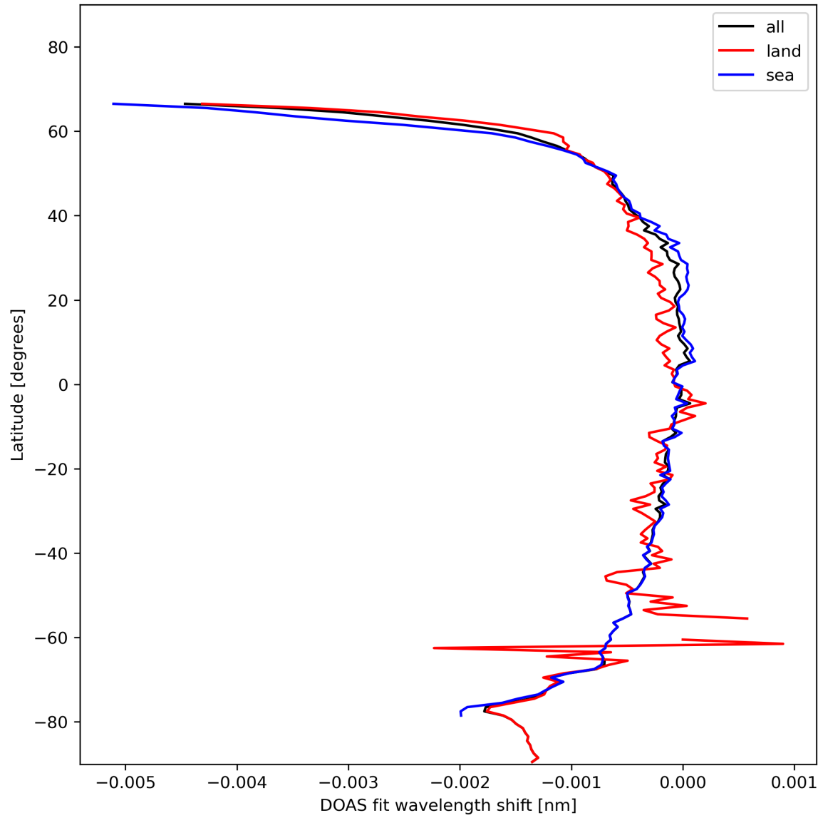
Figure 45: Zonal average of “DOAS fit wavelength shift” for 2024-01-27 to 2024-01-29.
