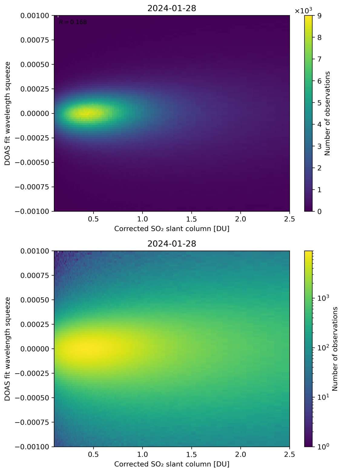
Figure 182: Scatter density plot of “Corrected SO 2 slant column” against “DOAS fit wavelength squeeze” for 2024-01-27 to 2024-01-29.
