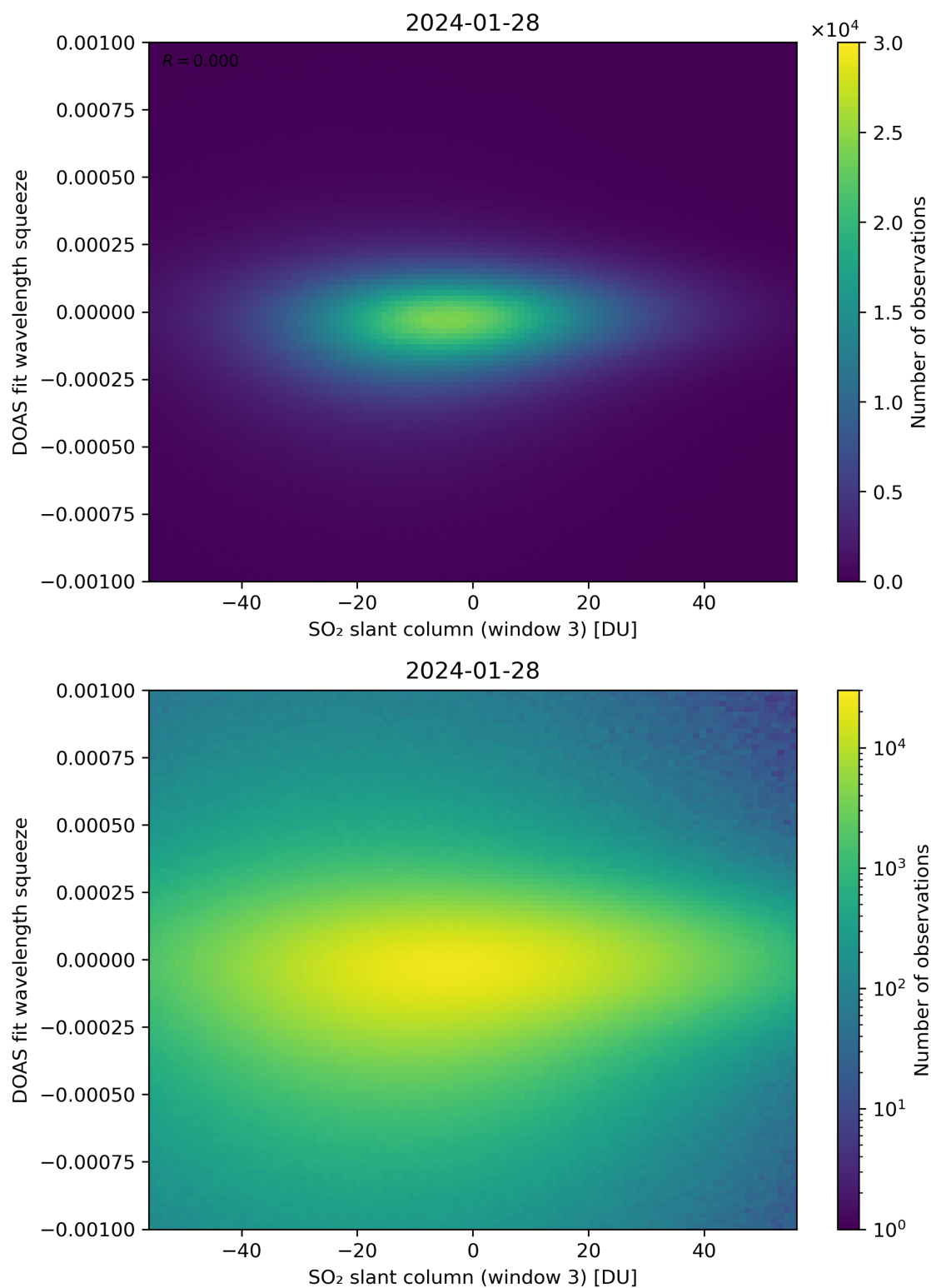
Figure 255: Scatter density plot of “SO 2 slant column (window 3)” against “DOAS fit wavelength squeeze” for 2024-01-27 to 2024-01-29.
