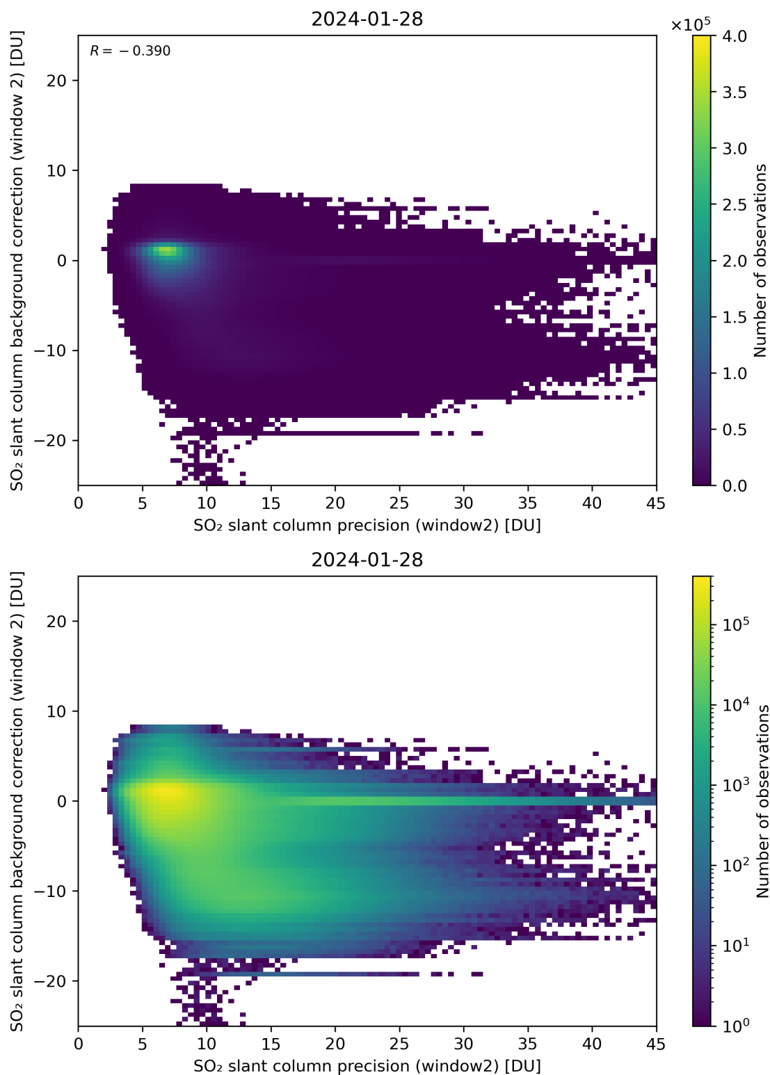
Figure 241: Scatter density plot of “SO 2 slant column precision (window2)” against “SO 2 slant column background correction (window 2)” for 2024-01-27 to 2024-01-29.
