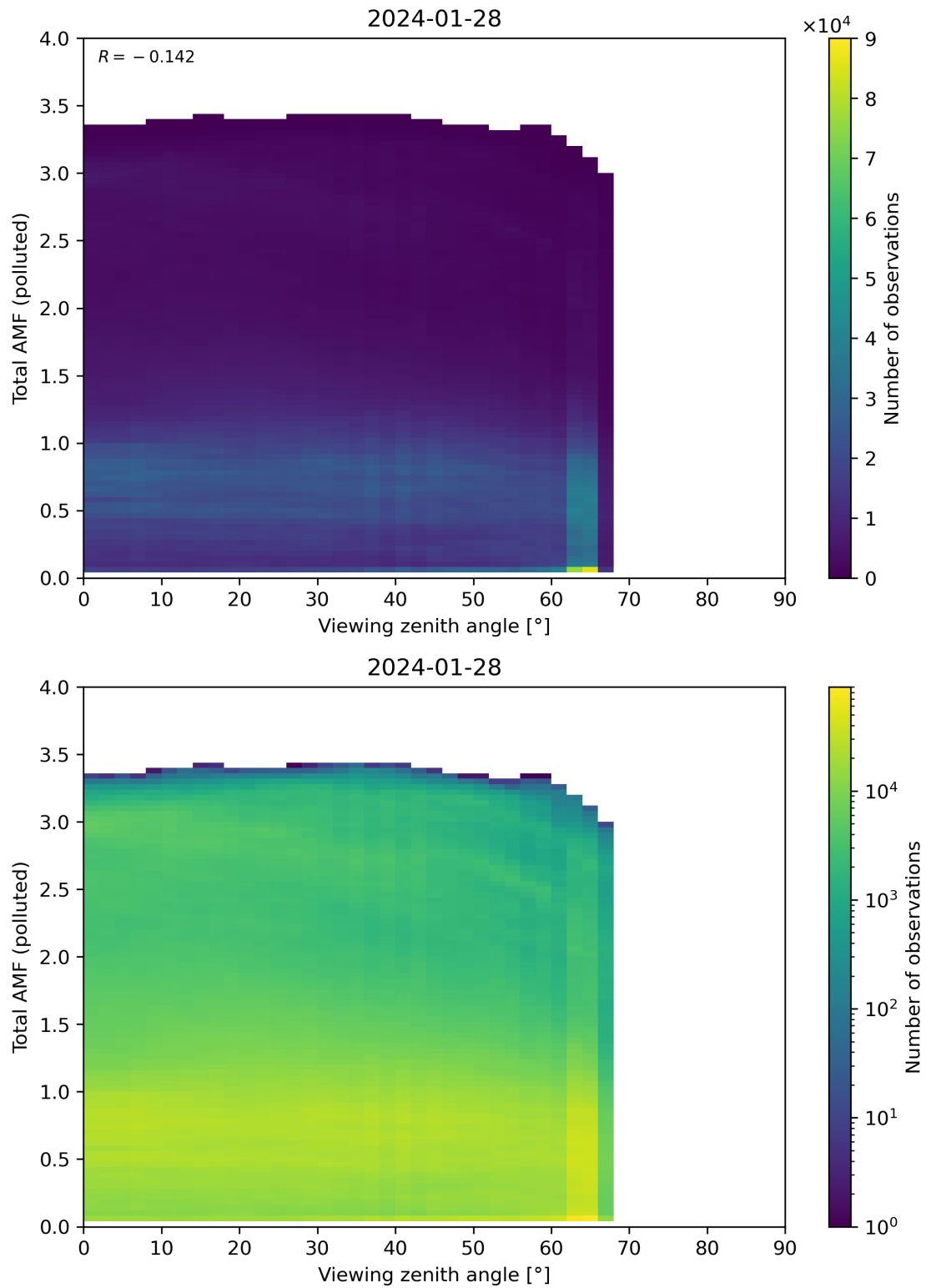
Figure 325: Scatter density plot of “Viewing zenith angle” against “Total AMF (polluted)” for 2024-01-27 to 2024-01-29.
