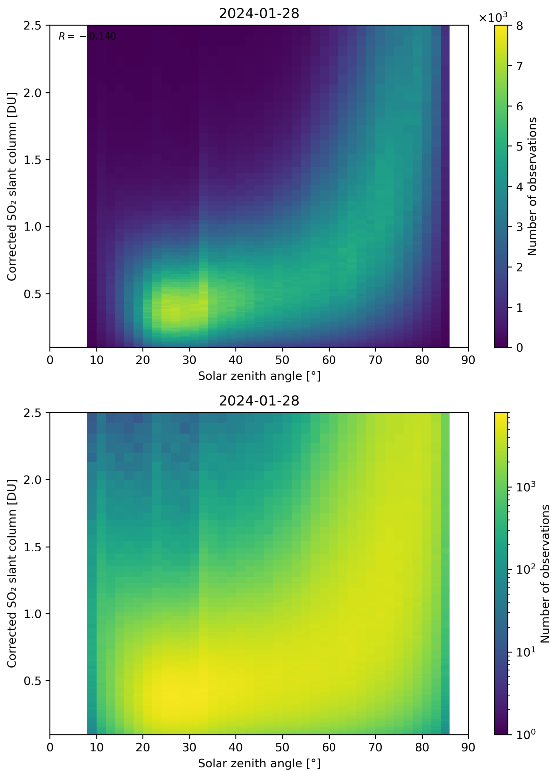
Figure 166: Scatter density plot of “Solar zenith angle” against “Corrected SO 2 slant column” for 2024-01-27 to 2024-01-29.
