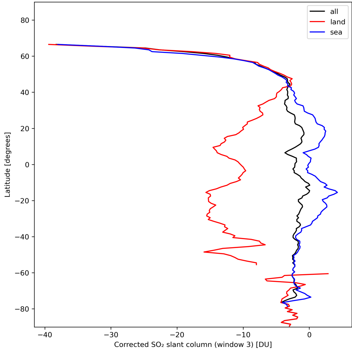
Figure 43: Zonal average of “Corrected SO 2 slant column (window 3)” for 2024-01-27 to 2024-01-29.
