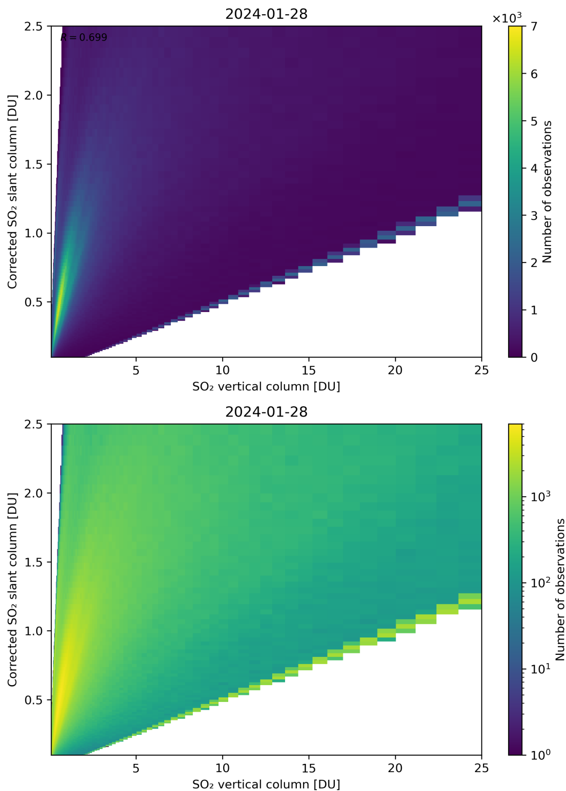
Figure 297: Scatter density plot of “SO 2 vertical column” against “Corrected SO 2 slant column” for 2024-01-27 to 2024-01-29.
