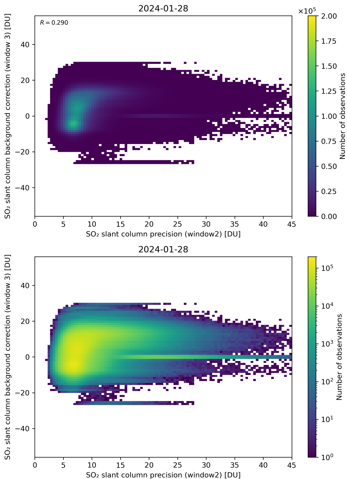
Figure 242: Scatter density plot of “SO 2 slant column precision (window2)” against “SO 2 slant column background correction (window 3)” for 2024-01-27 to 2024-01-29.
