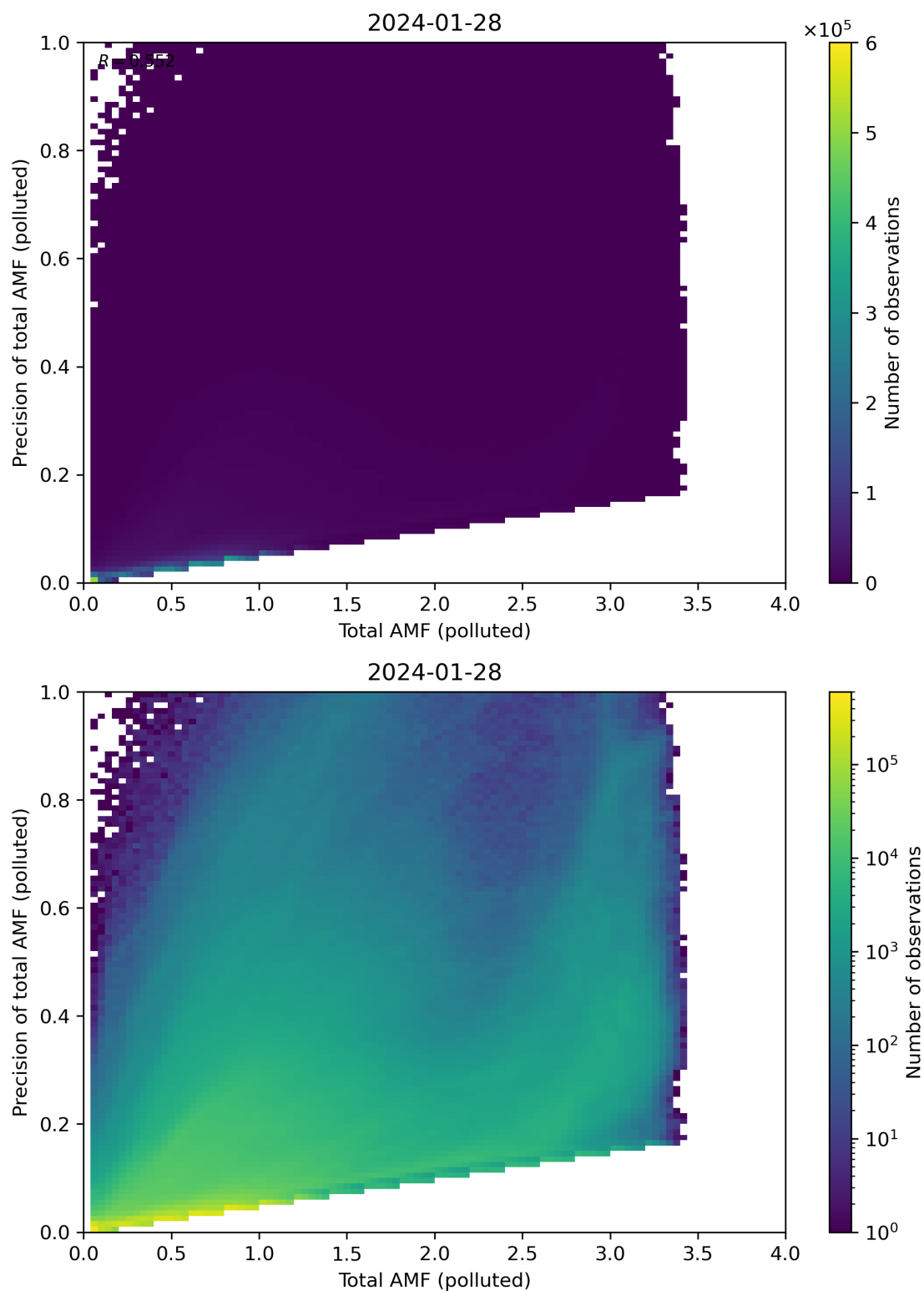
Figure 272: Scatter density plot of “Total AMF (polluted)” against “Precision of total AMF (polluted)” for 2024-01-27 to 2024-01-29.
