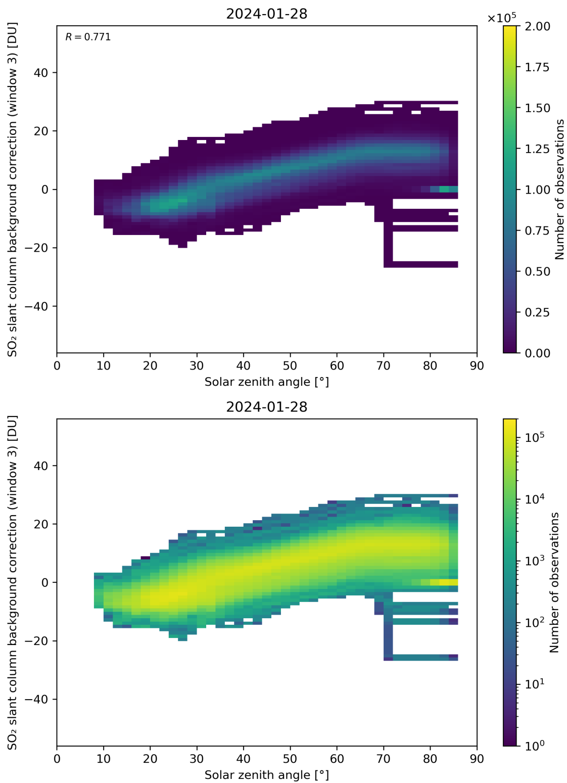
Figure 160: Scatter density plot of “Solar zenith angle” against “SO 2 slant column background correction (window 3)” for 2024-01-27 to 2024-01-29.
