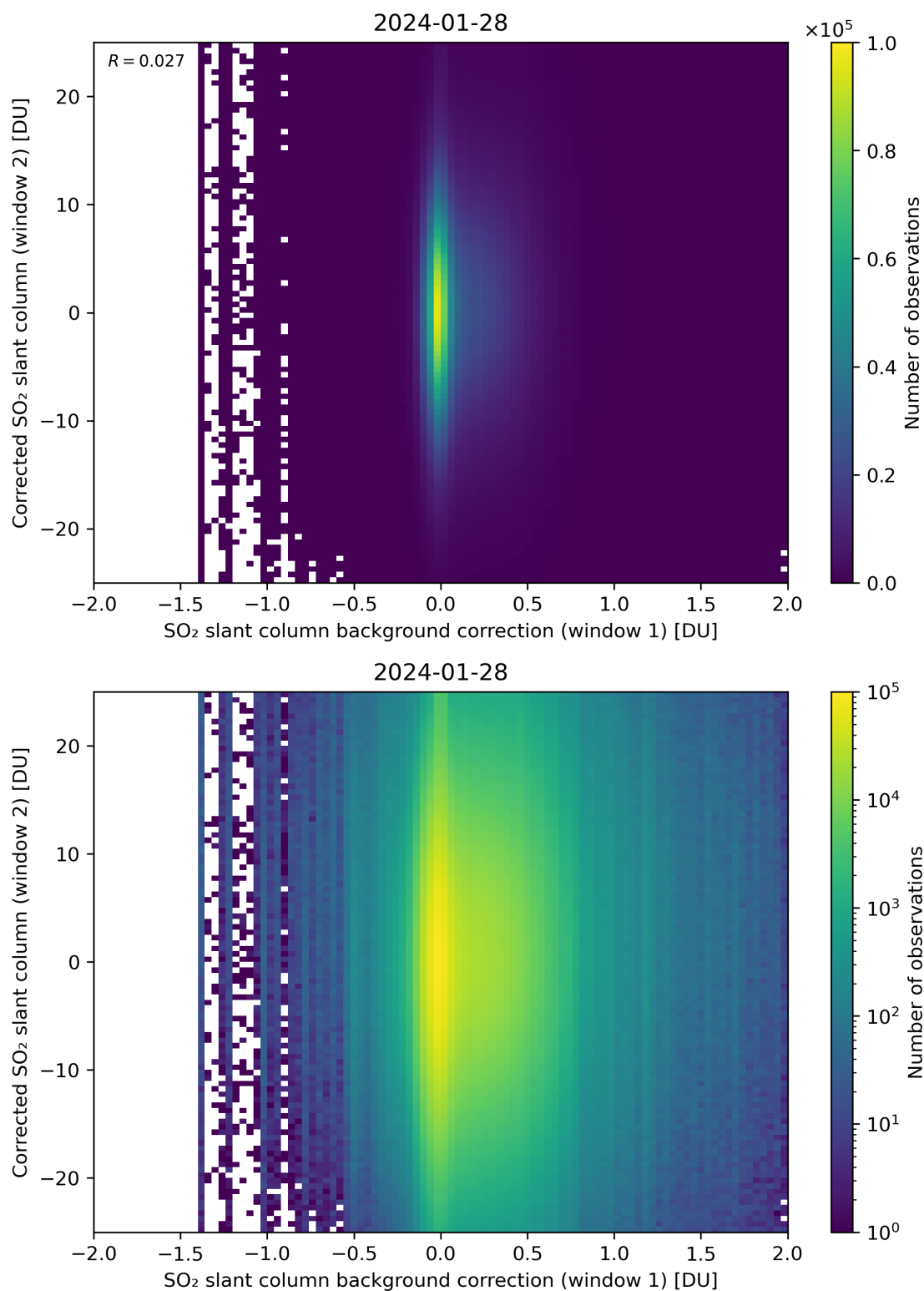
Figure 104: Scatter density plot of “SO 2 slant column background correction (window 1)” against “Corrected SO 2 slant column (window 2)” for 2024-01-27 to 2024-01-29.
