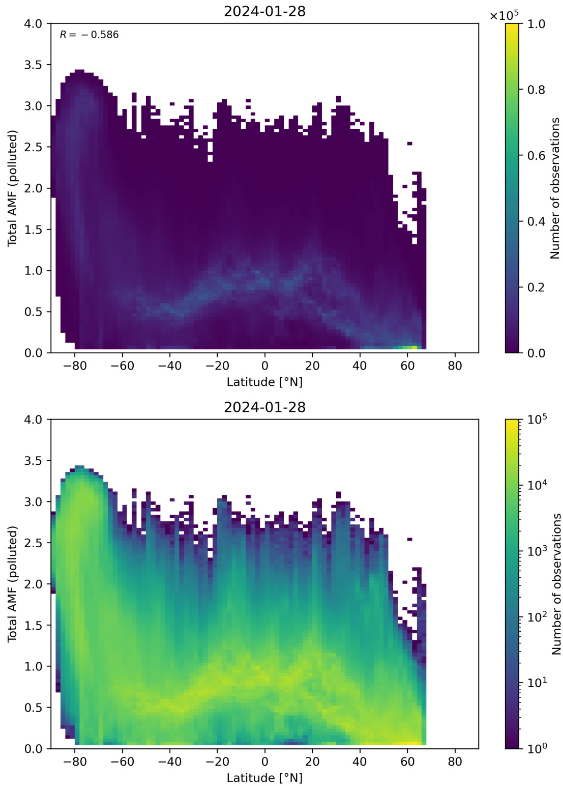
Figure 154: Scatter density plot of “Latitude” against “Total AMF (polluted)” for 2024-01-27 to 2024-01-29.
