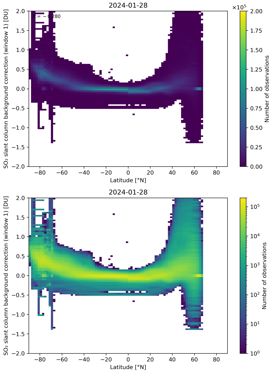
Figure 139: Scatter density plot of “Latitude” against “SO 2 slant column background correction (window 1)” for 2024-01-27 to 2024-01-29.
