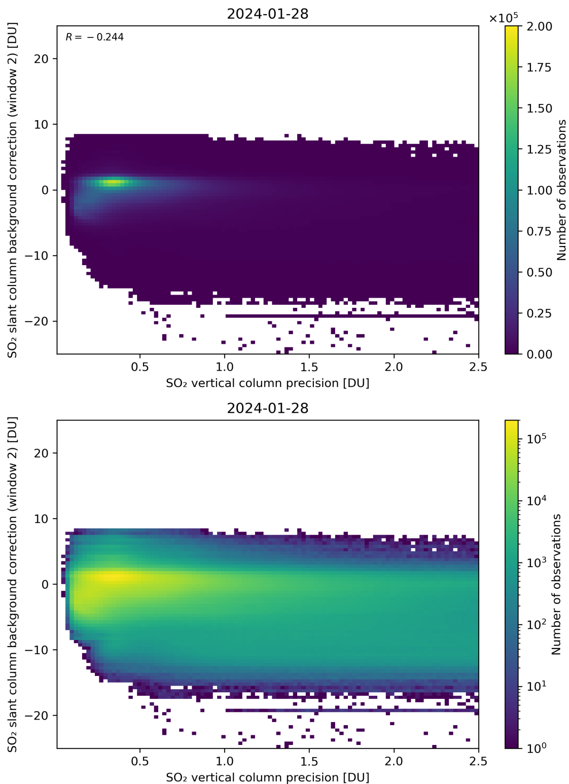
Figure 280: Scatter density plot of “SO 2 vertical column precision” against “SO 2 slant column background correction (window 2)” for 2024-01-27 to 2024-01-29.
