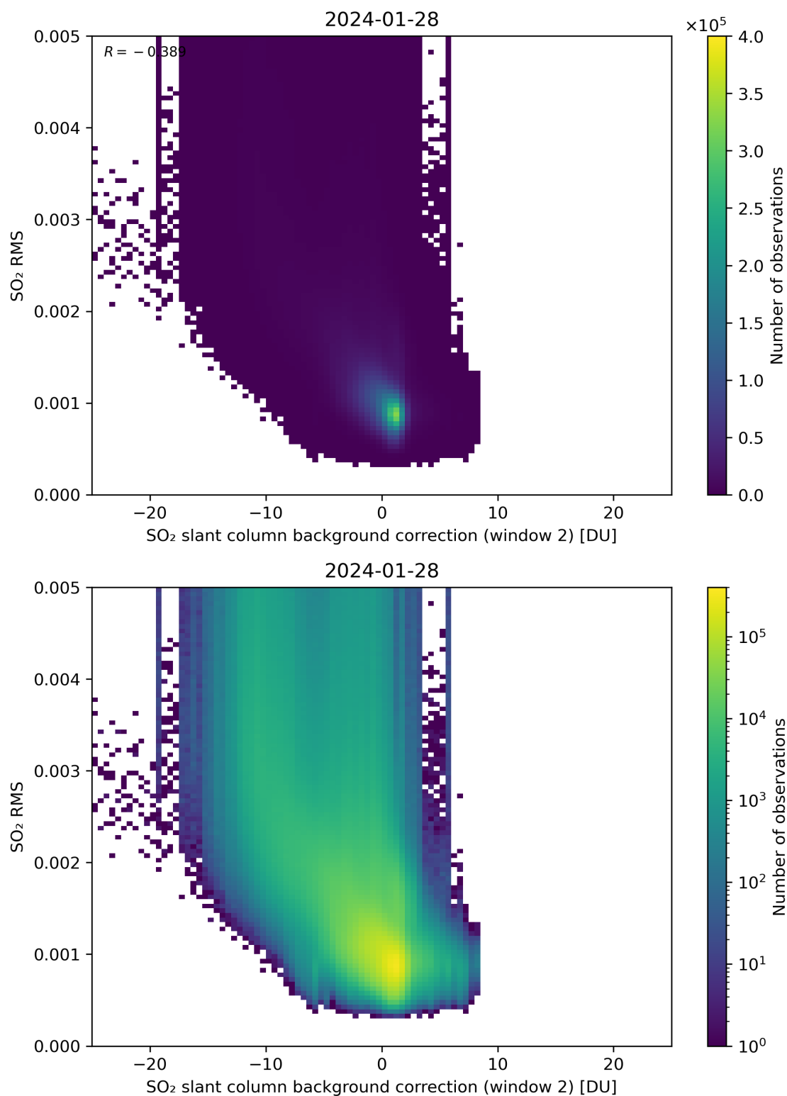
Figure 114: Scatter density plot of “SO 2 slant column background correction (window 2)” against “SO 2 RMS” for 2024-01-27 to 2024-01-29.
