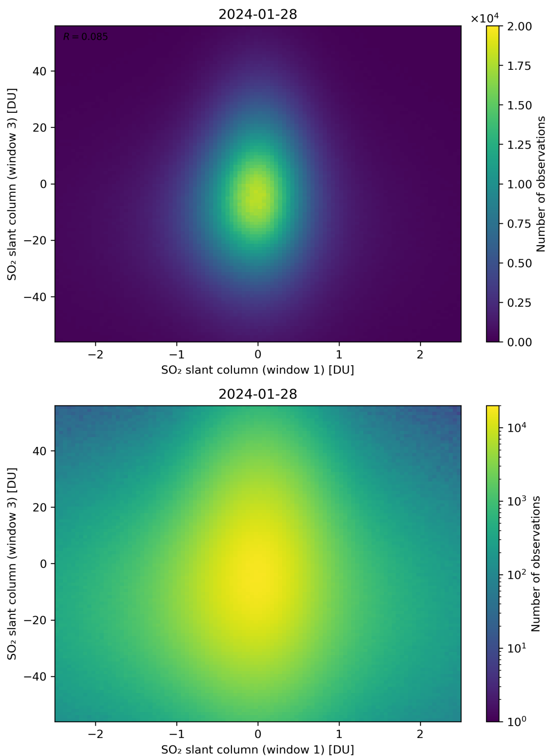
Figure 237: Scatter density plot of “SO 2 slant column (window 1)” against “SO 2 slant column (window 3)” for 2024-01-27 to 2024-01-29.
