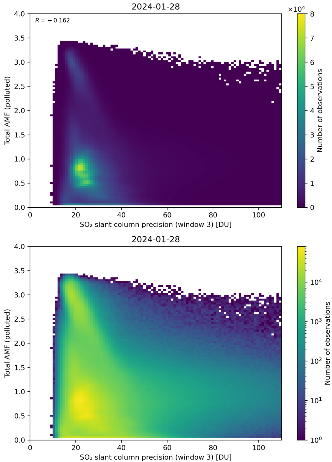
Figure 263: Scatter density plot of “SO 2 slant column precision (window 3)” against “Total AMF (polluted)” for 2024-01-27 to 2024-01-29.
