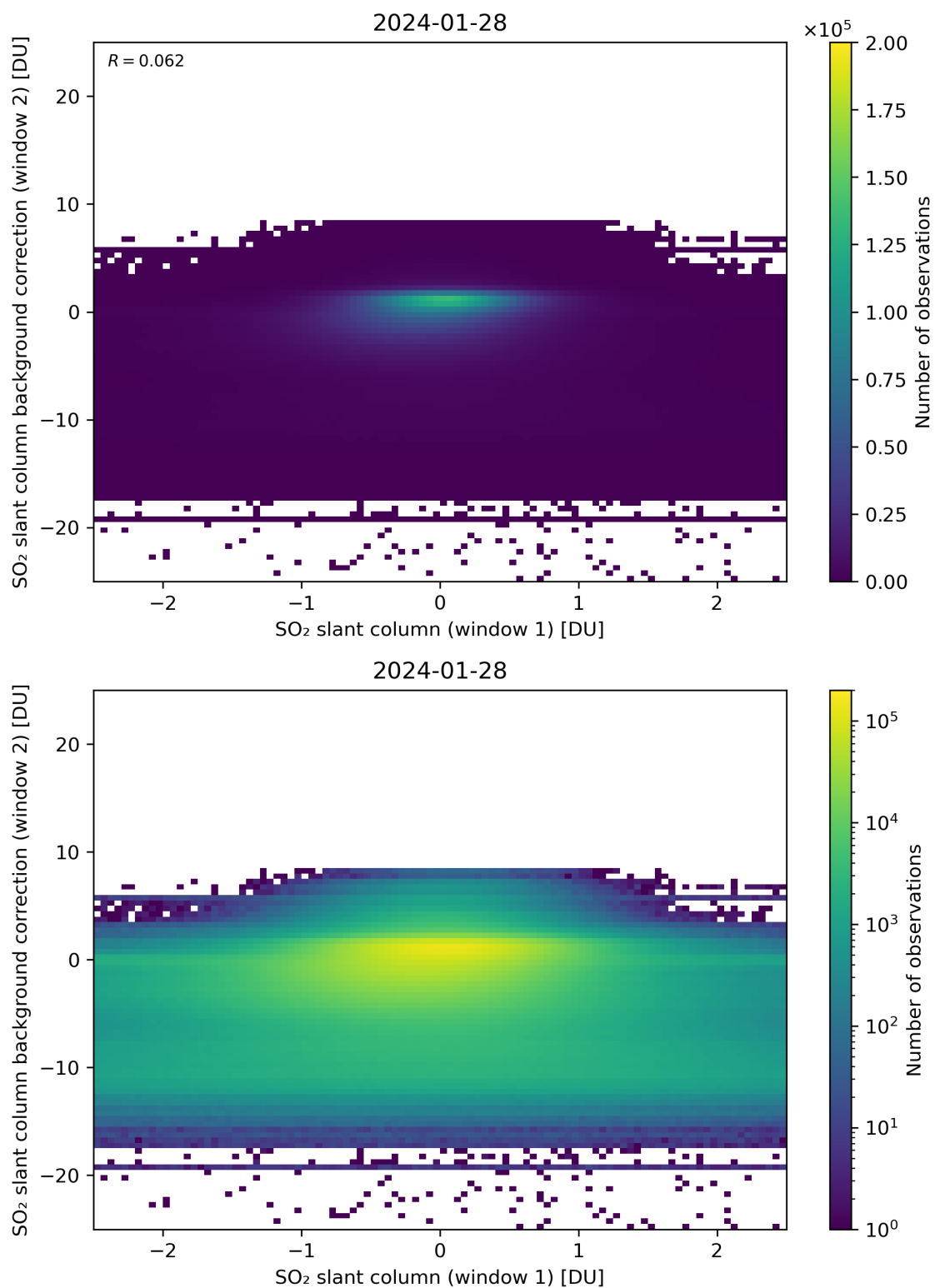
Figure 213: Scatter density plot of “SO 2 slant column (window 1)” against “SO 2 slant column background correction (window 2)” for 2024-01-27 to 2024-01-29.
