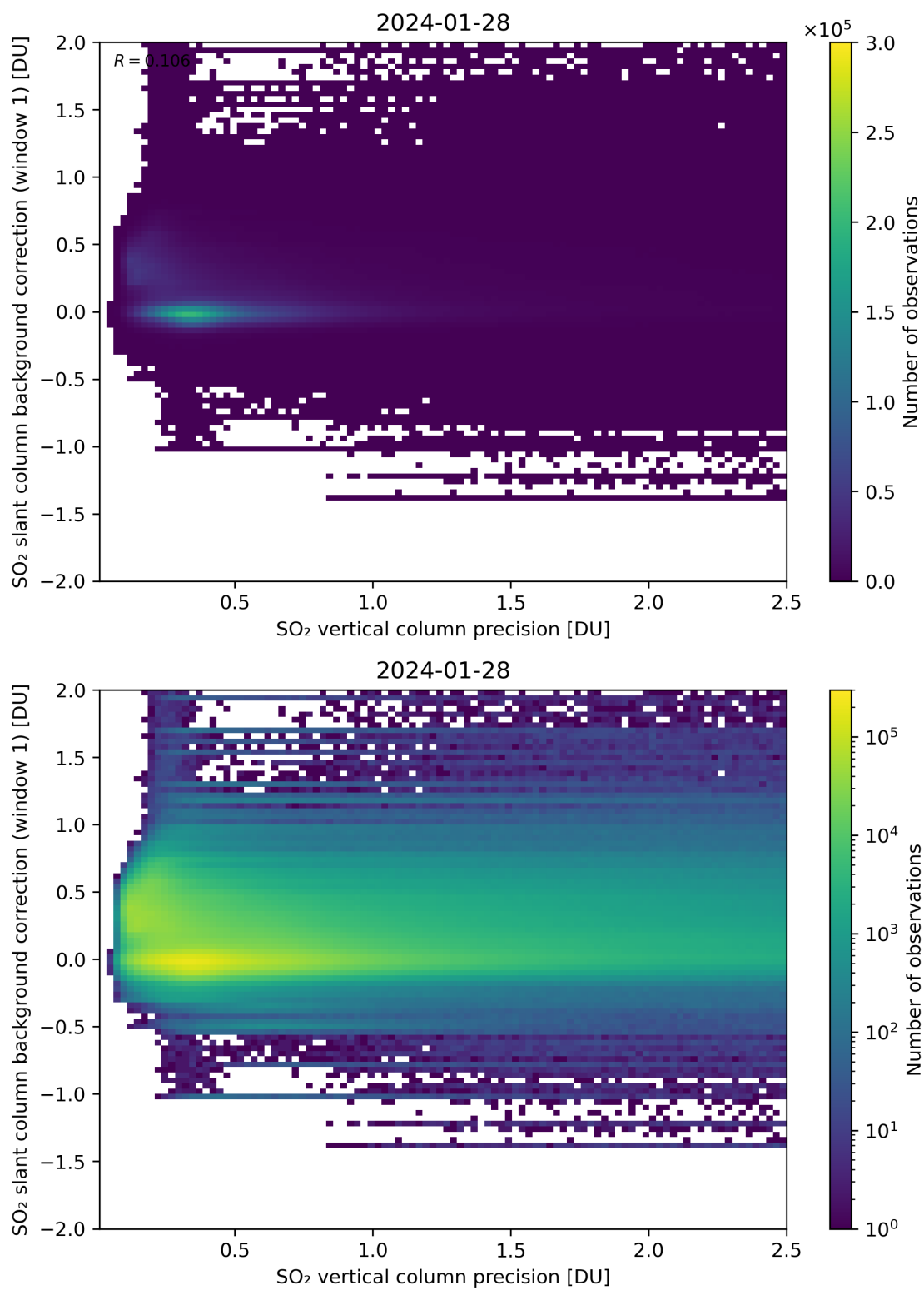
Figure 279: Scatter density plot of “SO 2 vertical column precision” against “SO 2 slant column background correction (window 1)” for 2024-01-27 to 2024-01-29.
