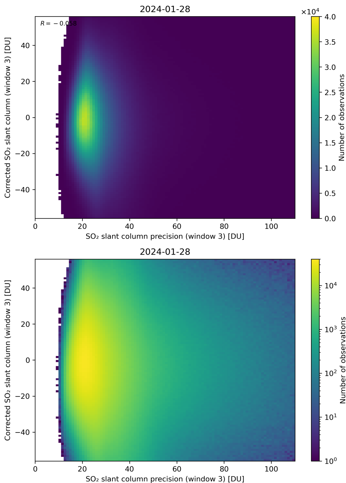
Figure 262: Scatter density plot of “SO 2 slant column precision (window 3)” against “Corrected SO 2 slant column (window 3)” for 2024-01-27 to 2024-01-29.
