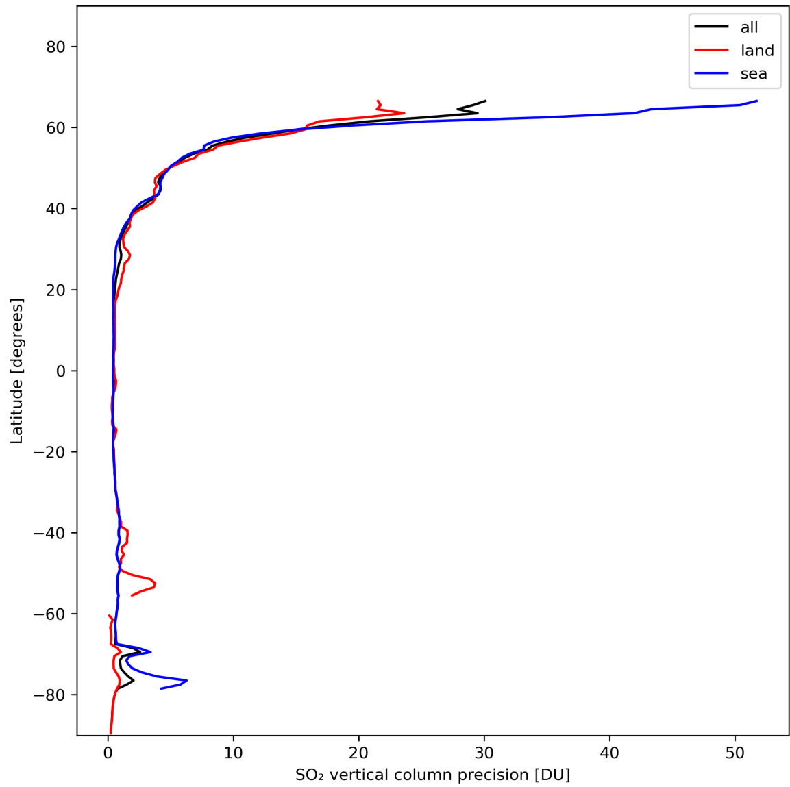
Figure 31: Zonal average of “SO 2 vertical column precision” for 2024-01-27 to 2024-01-29.
