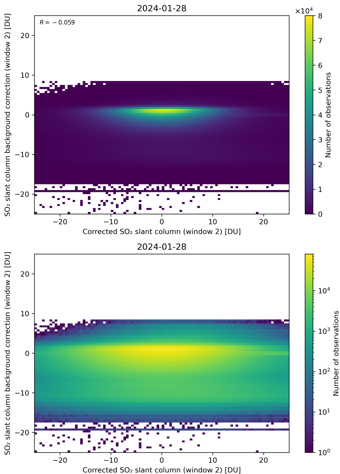
Figure 194: Scatter density plot of “Corrected SO 2 slant column (window 2)” against “SO 2 slant column background correction (window 2)” for 2024-01-27 to 2024-01-29.
