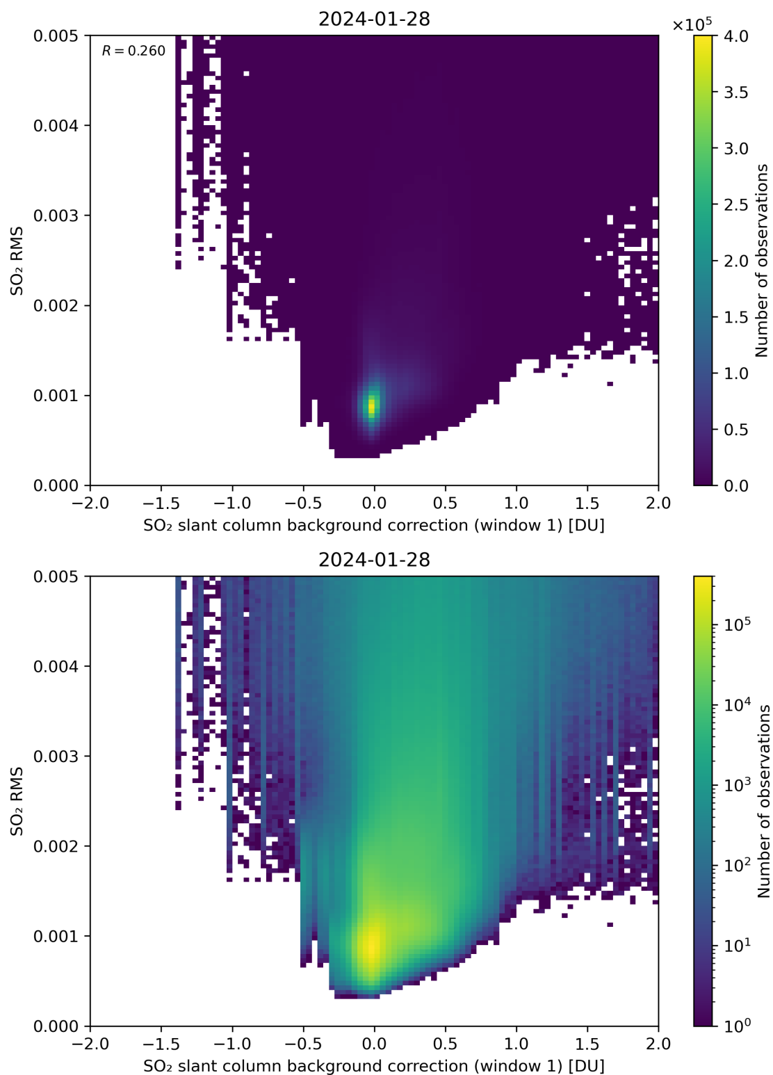
Figure 102: Scatter density plot of “SO 2 slant column background correction (window 1)” against “SO 2 RMS” for 2024-01-27 to 2024-01-29.
