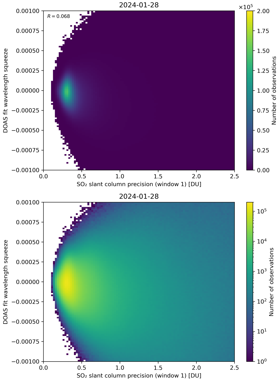
Figure 222: Scatter density plot of “SO 2 slant column precision (window 1)” against “DOAS fit wavelength squeeze” for 2024-01-27 to 2024-01-29.
