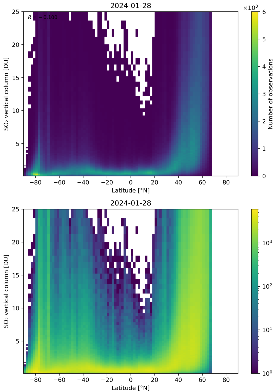
Figure 156: Scatter density plot of “Latitude” against “SO 2 vertical column” for 2024-01-27 to 2024-01-29.
