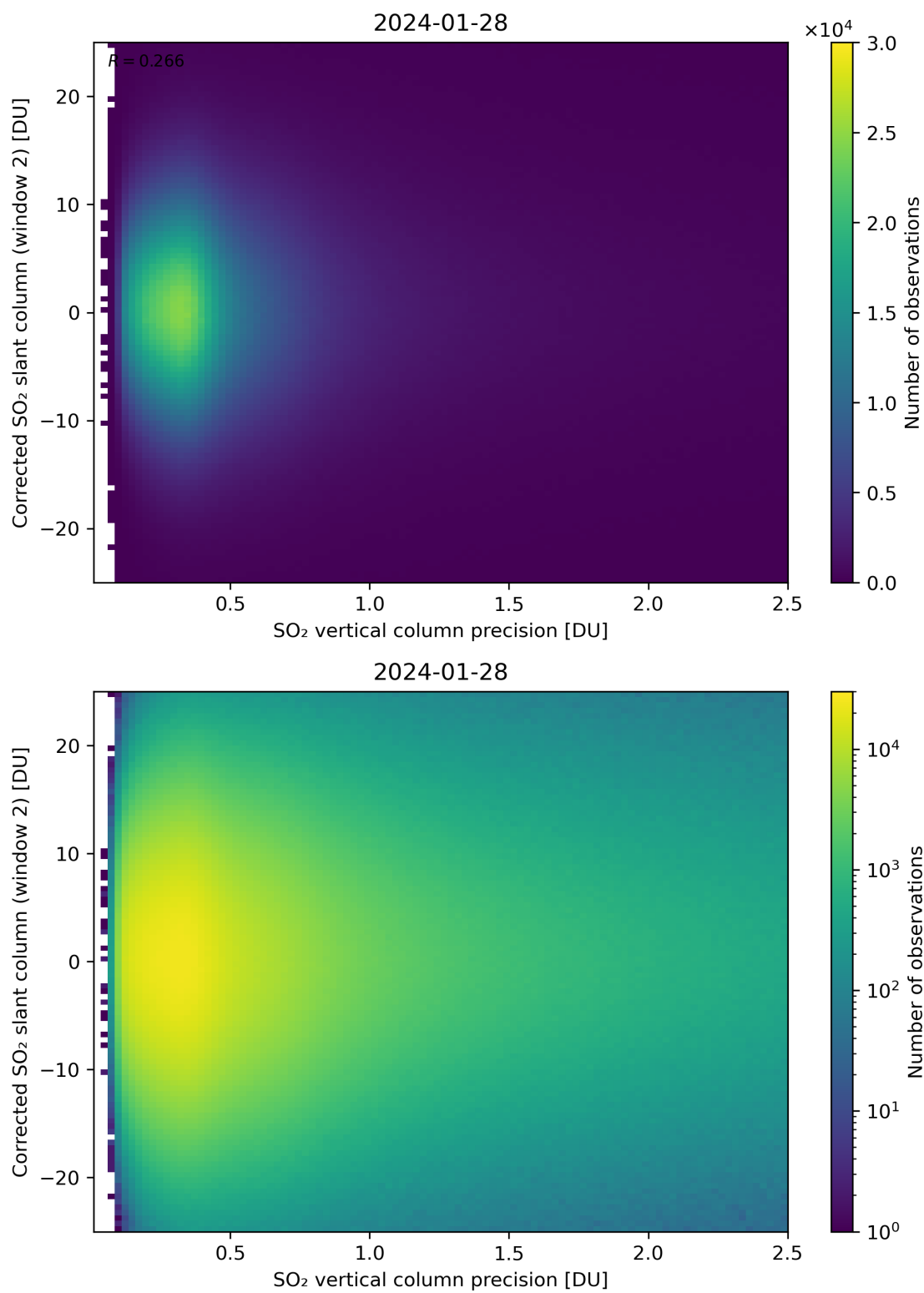
Figure 287: Scatter density plot of “SO 2 vertical column precision” against “Corrected SO 2 slant column (window 2)” for 2024-01-27 to 2024-01-29.
