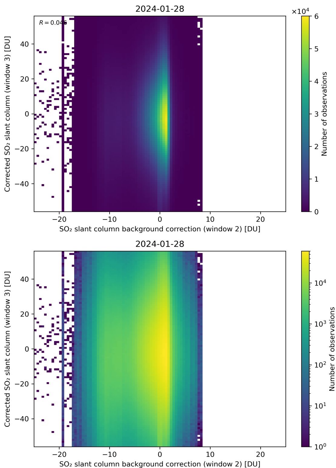
Figure 116: Scatter density plot of “SO 2 slant column background correction (window 2)” against “Corrected SO 2 slant column (window 3)” for 2024-01-27 to 2024-01-29.
