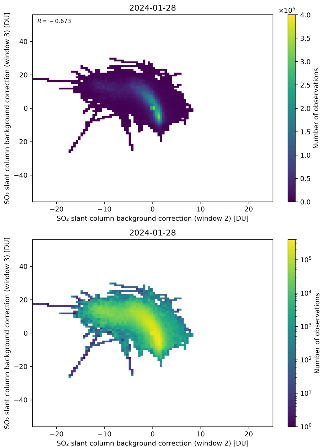
Figure 111: Scatter density plot of “SO 2 slant column background correction (window 2)” against “SO 2 slant column background correction (window 3)” for 2024-01-27 to 2024-01-29.
