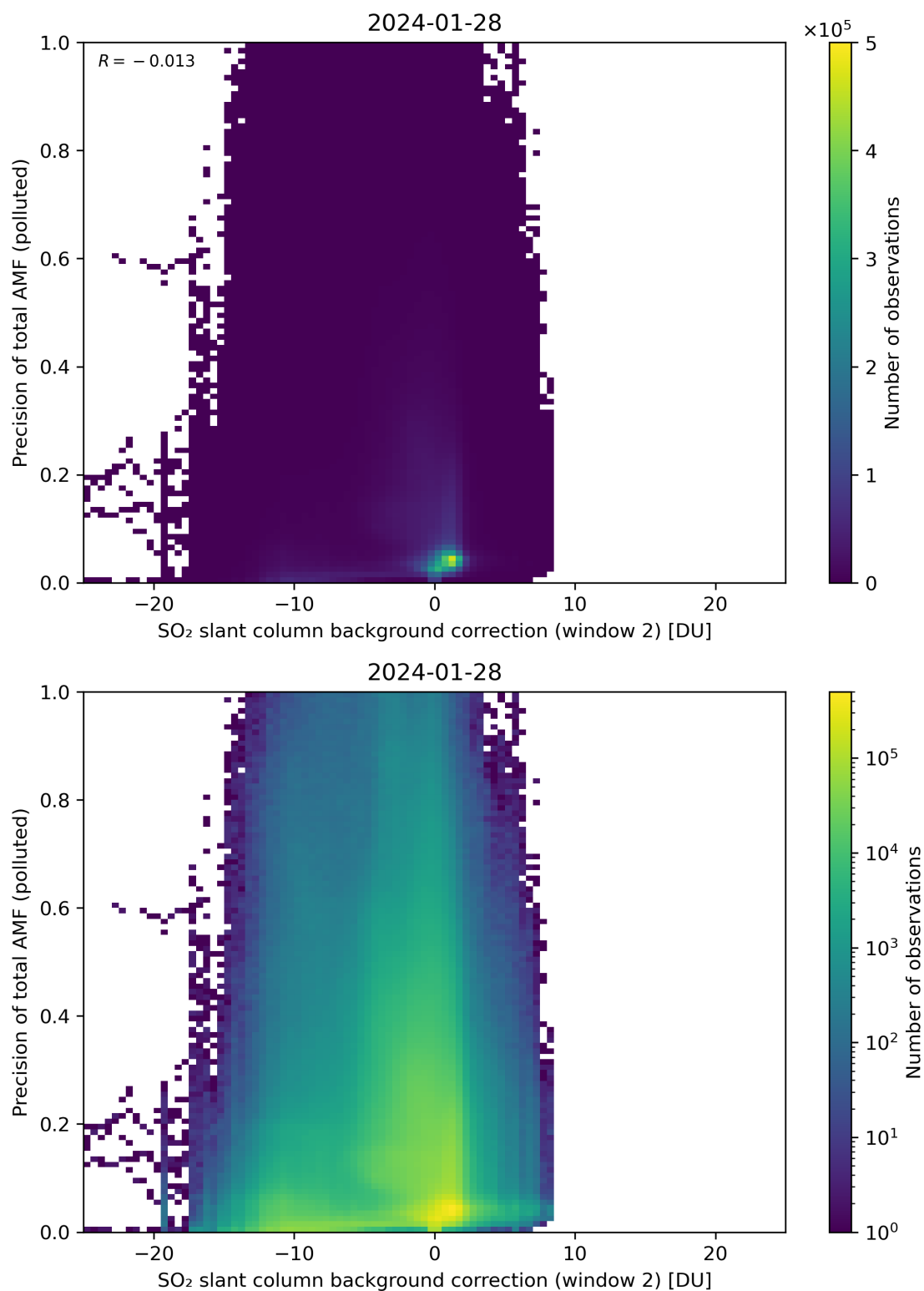
Figure 120: Scatter density plot of “SO 2 slant column background correction (window 2)” against “Precision of total AMF (polluted)” for 2024-01-27 to 2024-01-29.
