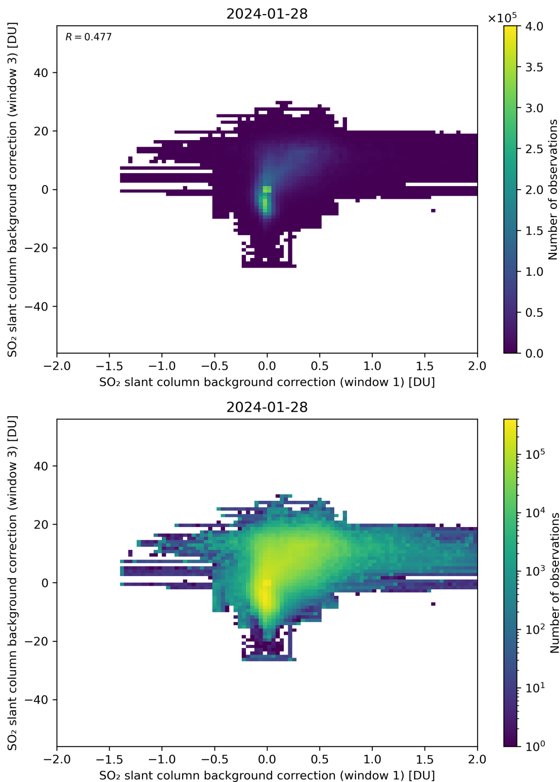
Figure 99: Scatter density plot of “SO 2 slant column background correction (window 1)” against “SO 2 slant column background correction (window 3)” for 2024-01-27 to 2024-01-29.
