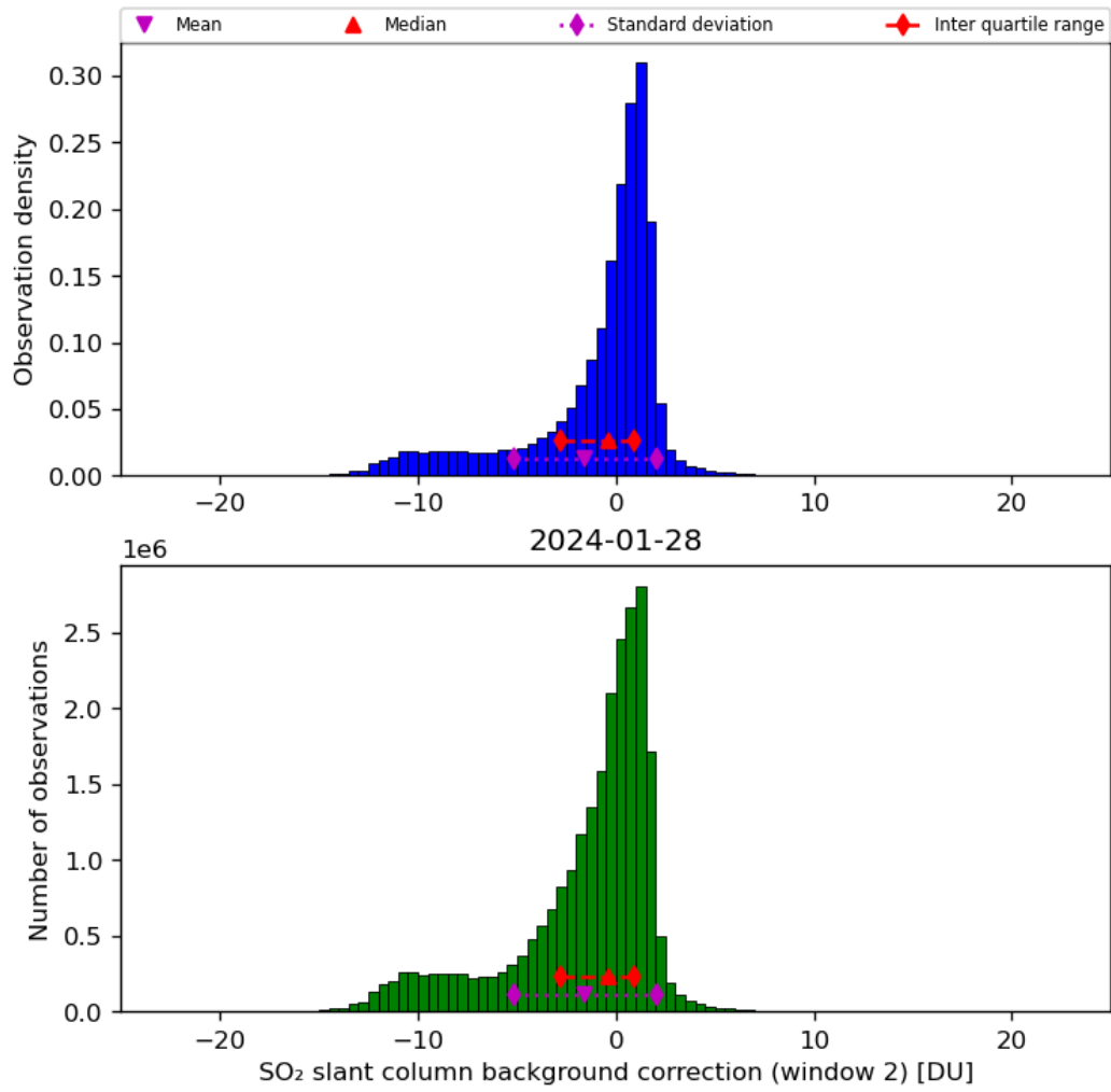
Figure 63: Histogram of “SO 2 slant column background correction (window 2)” for 2024-01-27 to 2024-01-29
