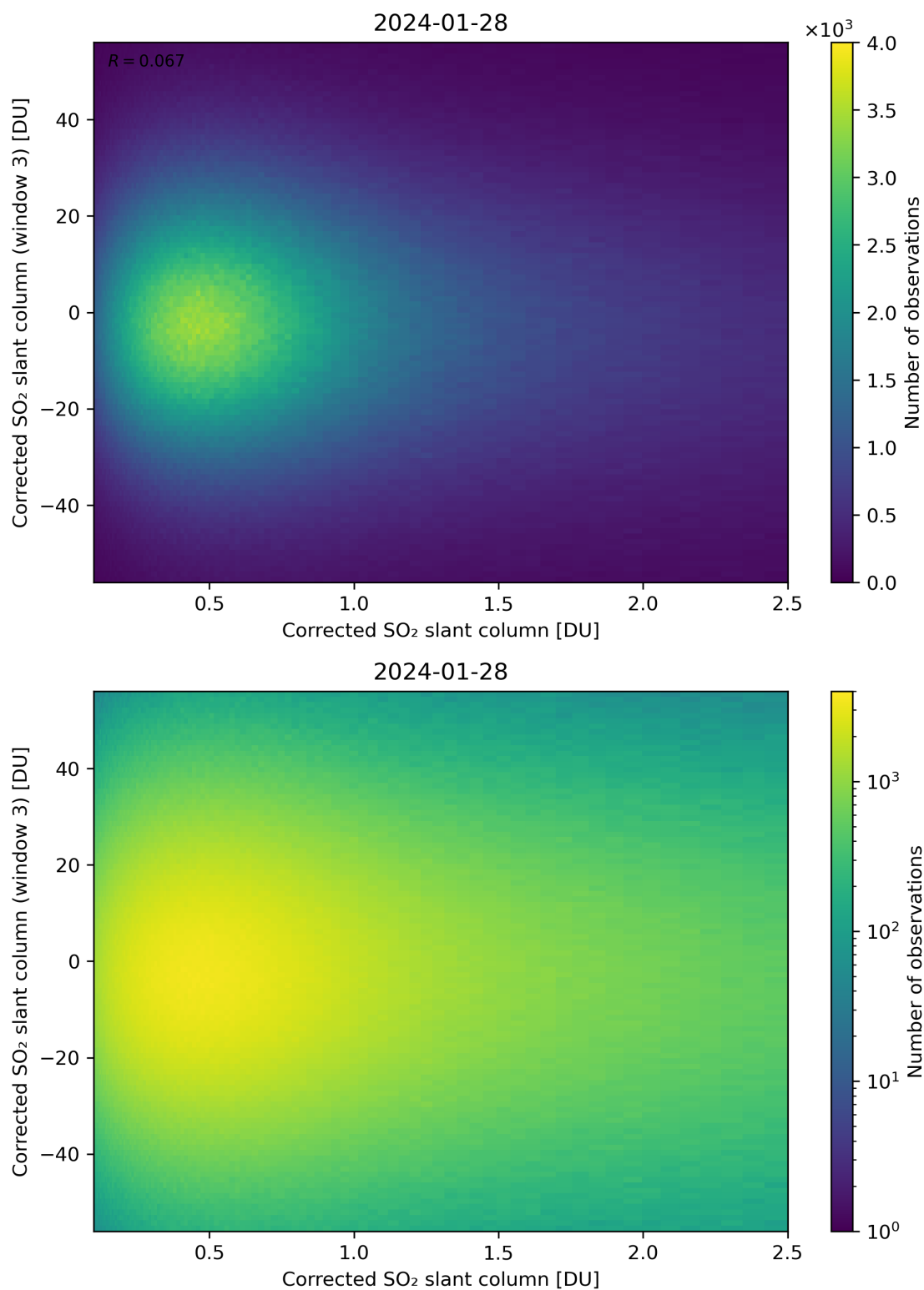
Figure 186: Scatter density plot of “Corrected SO 2 slant column” against “Corrected SO 2 slant column (window 3)” for 2024-01-27 to 2024-01-29.
