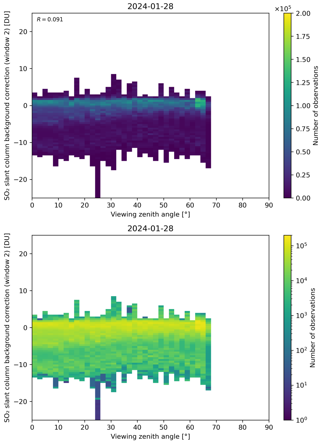
Figure 309: Scatter density plot of “Viewing zenith angle” against “SO 2 slant column background correction (window 2)” for 2024-01-27 to 2024-01-29.
