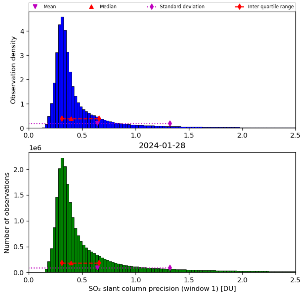
Figure 57: Histogram of “SO 2 slant column precision (window 1)” for 2024-01-27 to 2024-01-29
