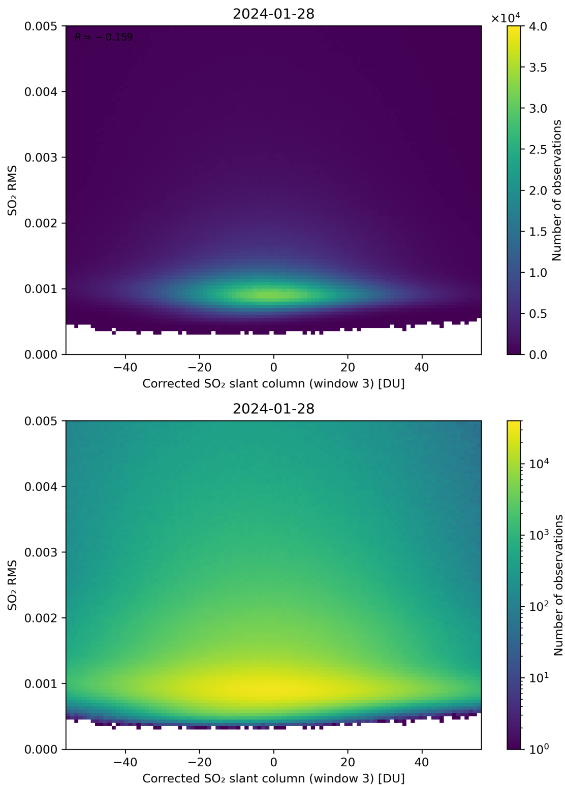
Figure 208: Scatter density plot of “Corrected SO 2 slant column (window 3)” against “SO 2 RMS” for 2024-01-27 to 2024-01-29.
