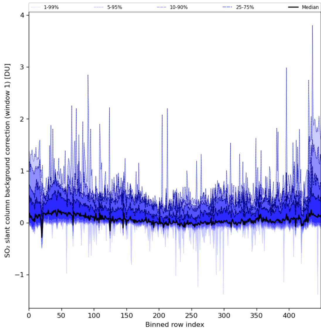
Figure 82: Along track statistics of “SO 2 slant column background correction (window 1)” for 2024-01-27 to 2024-01-29
