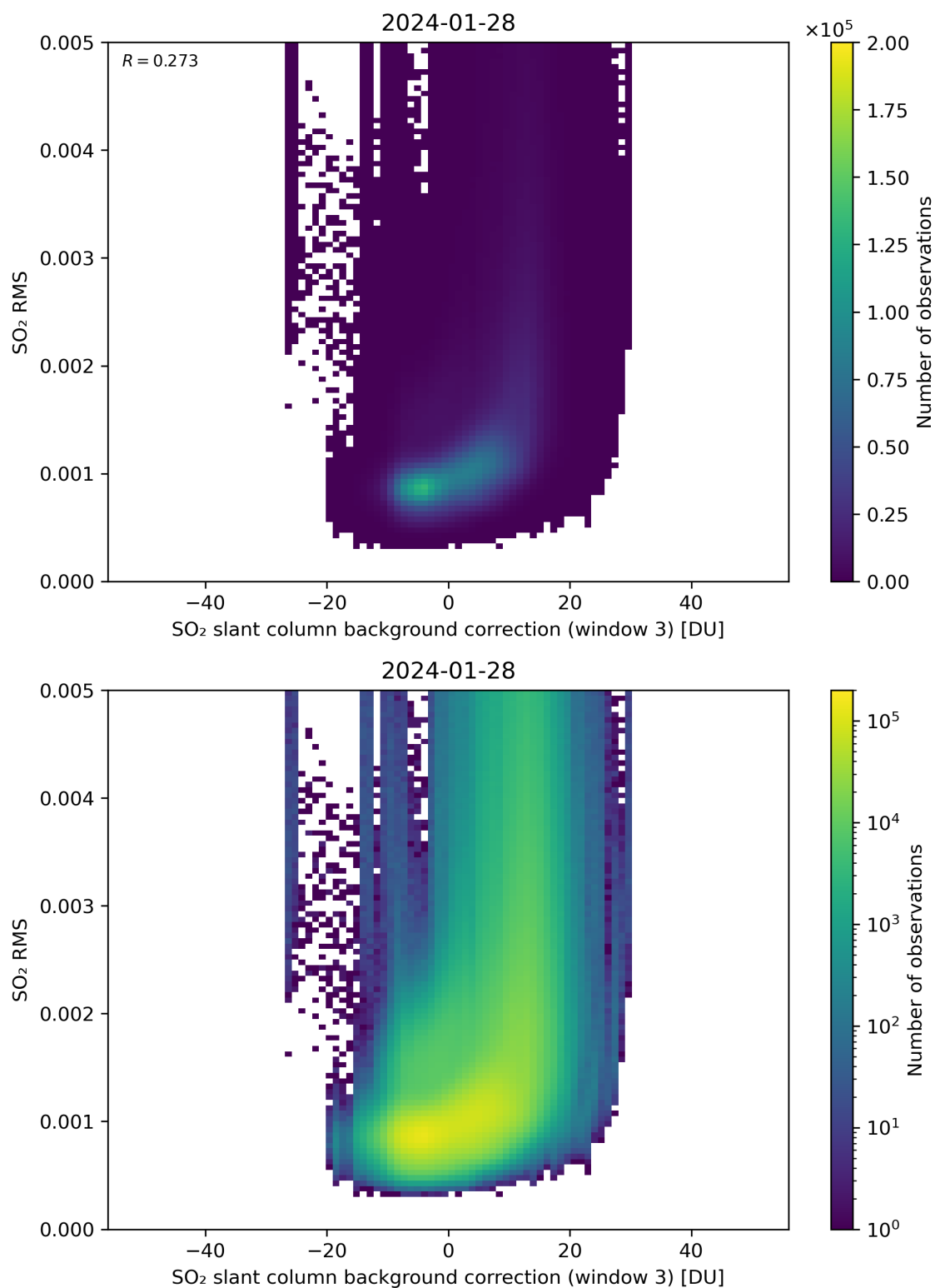
Figure 123: Scatter density plot of “SO 2 slant column background correction (window 3)” against “SO 2 RMS” for 2024-01-27 to 2024-01-29.
