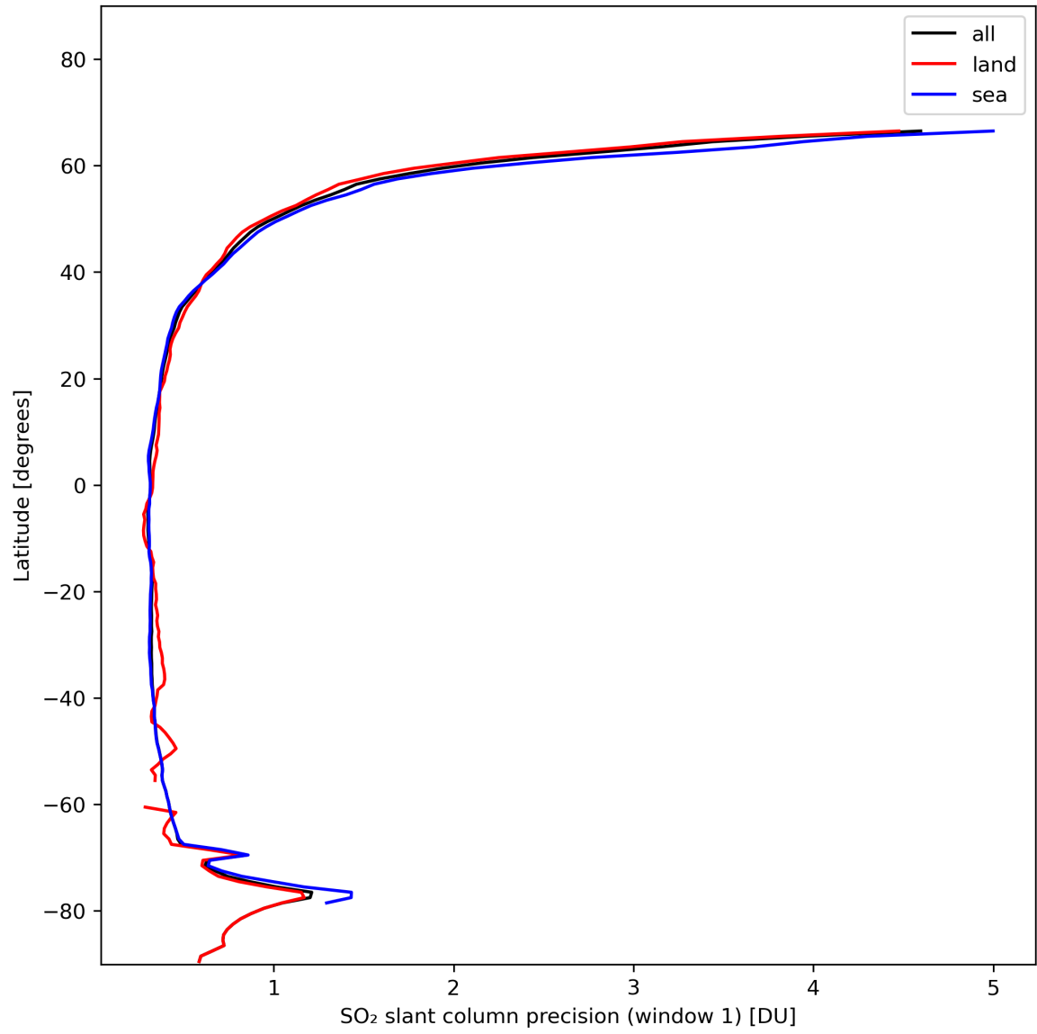
Figure 34: Zonal average of “SO 2 slant column precision (window 1)” for 2024-01-27 to 2024-01-29.
