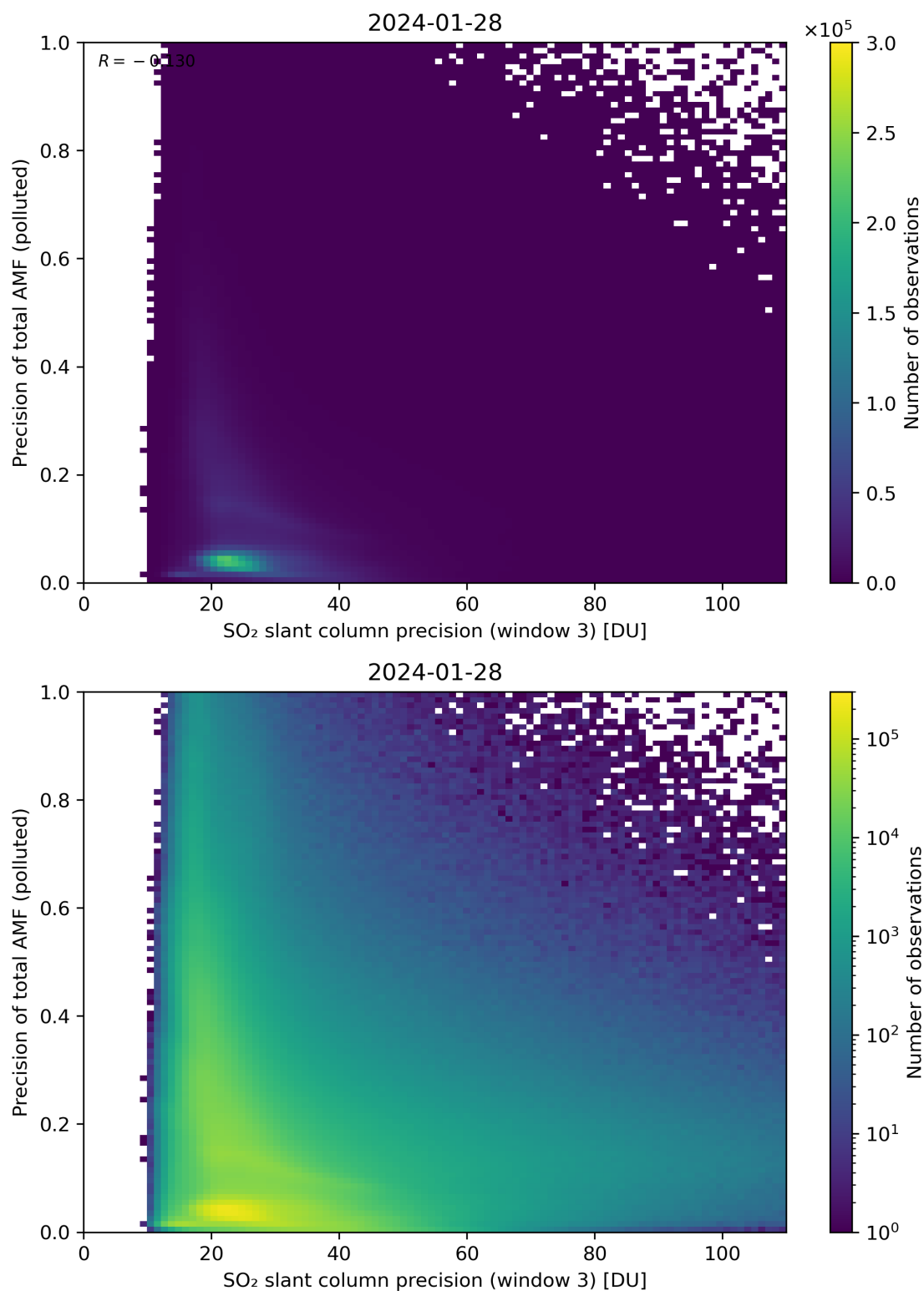
Figure 264: Scatter density plot of “SO 2 slant column precision (window 3)” against “Precision of total AMF (polluted)” for 2024-01-27 to 2024-01-29.
