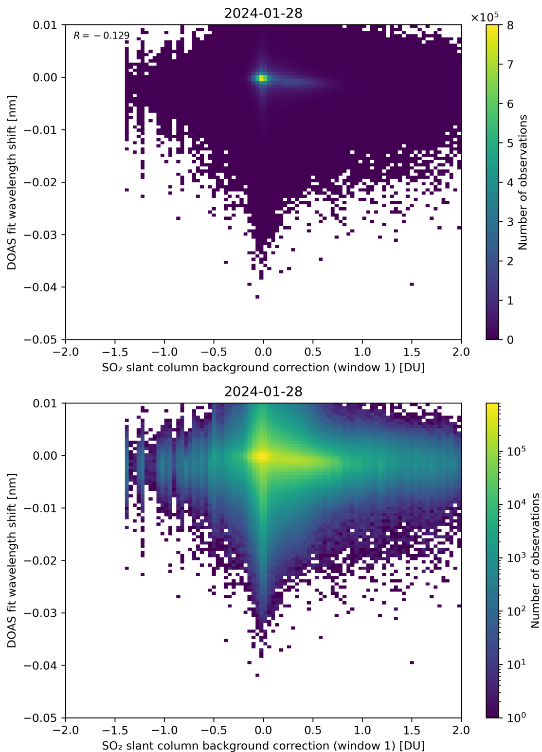
Figure 100: Scatter density plot of “SO 2 slant column background correction (window 1)” against “DOAS fit wavelength shift” for 2024-01-27 to 2024-01-29.
