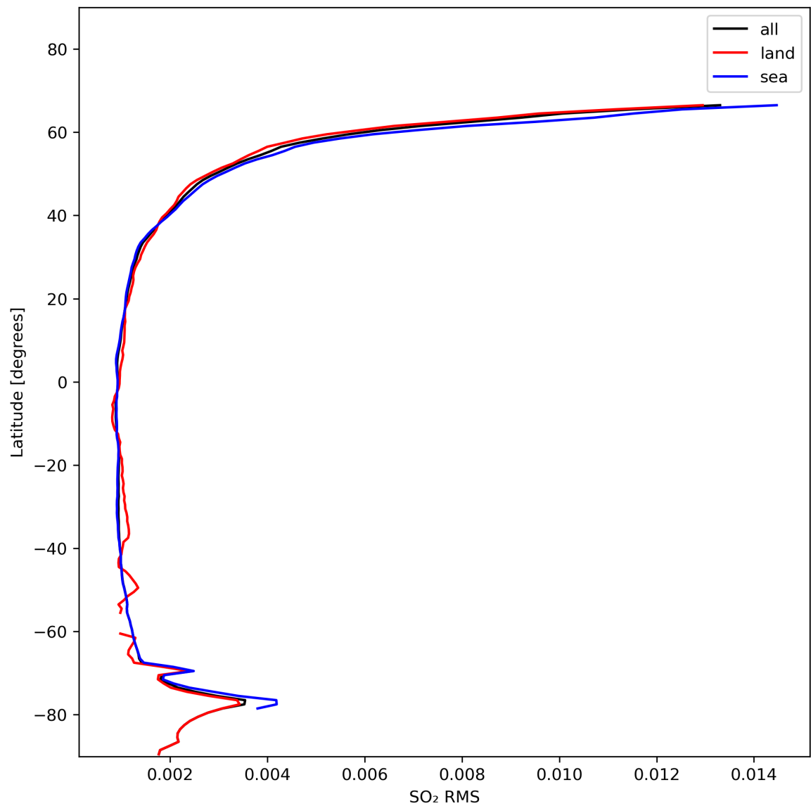
Figure 47: Zonal average of “SO 2 RMS” for 2024-01-27 to 2024-01-29.
