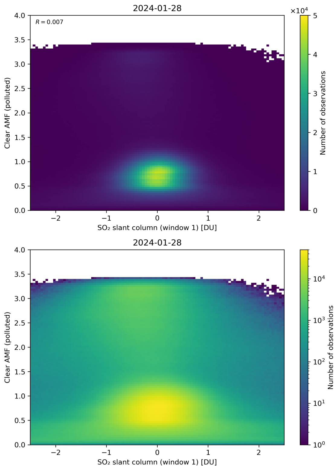
Figure 232: Scatter density plot of “SO 2 slant column (window 1)” against “Clear AMF (polluted)” for 2024-01-27 to 2024-01-29.
