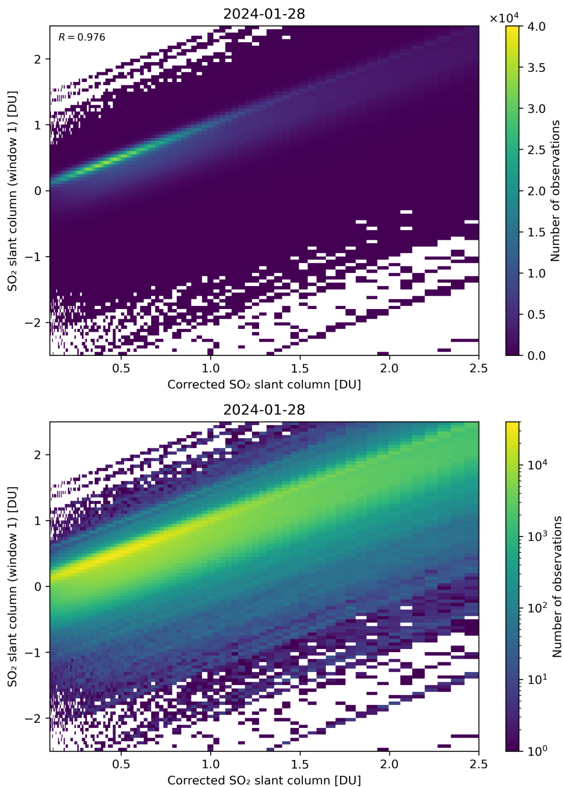
Figure 187: Scatter density plot of “Corrected SO 2 slant column” against “SO 2 slant column (window 1)” for 2024-01-27 to 2024-01-29.
