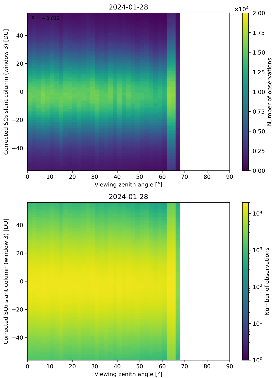
Figure 319: Scatter density plot of “Viewing zenith angle” against “Corrected SO 2 slant column (window 3)” for 2024-01-27 to 2024-01-29.
