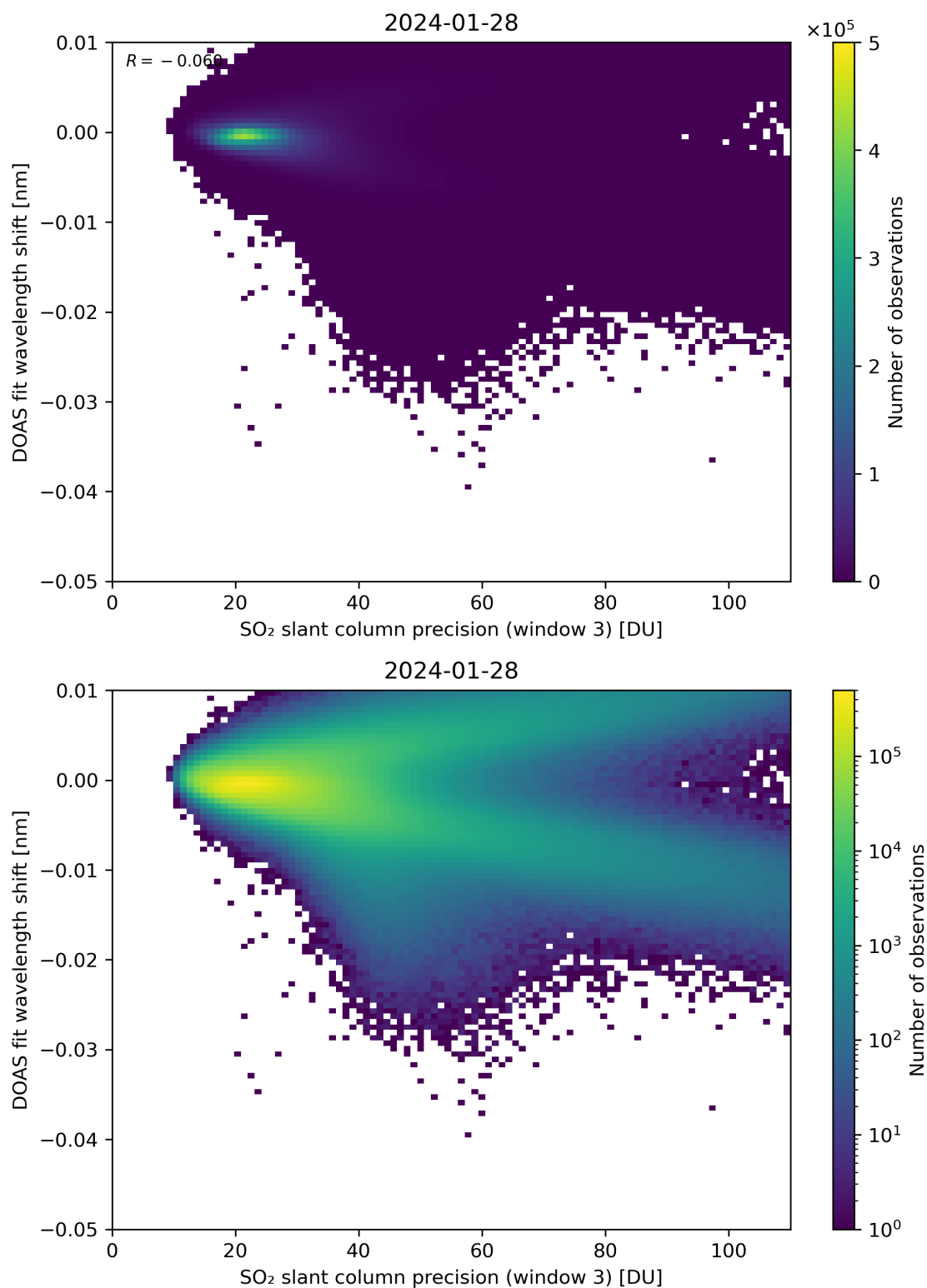
Figure 258: Scatter density plot of “SO 2 slant column precision (window 3)” against “DOAS fit wavelength shift” for 2024-01-27 to 2024-01-29.
