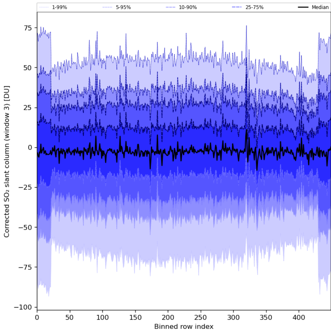
Figure 89: Along track statistics of “Corrected SO 2 slant column (window 3)” for 2024-01-27 to 2024-01-29
