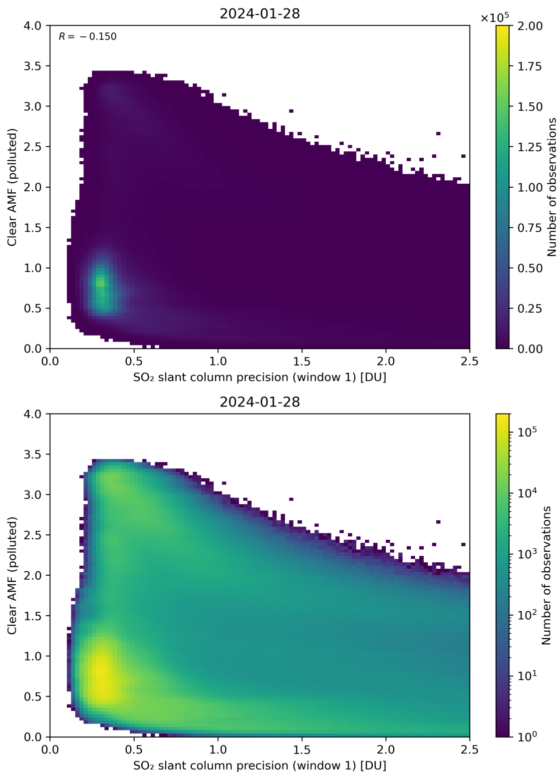
Figure 224: Scatter density plot of “SO 2 slant column precision (window 1)” against “Clear AMF (polluted)” for 2024-01-27 to 2024-01-29.
