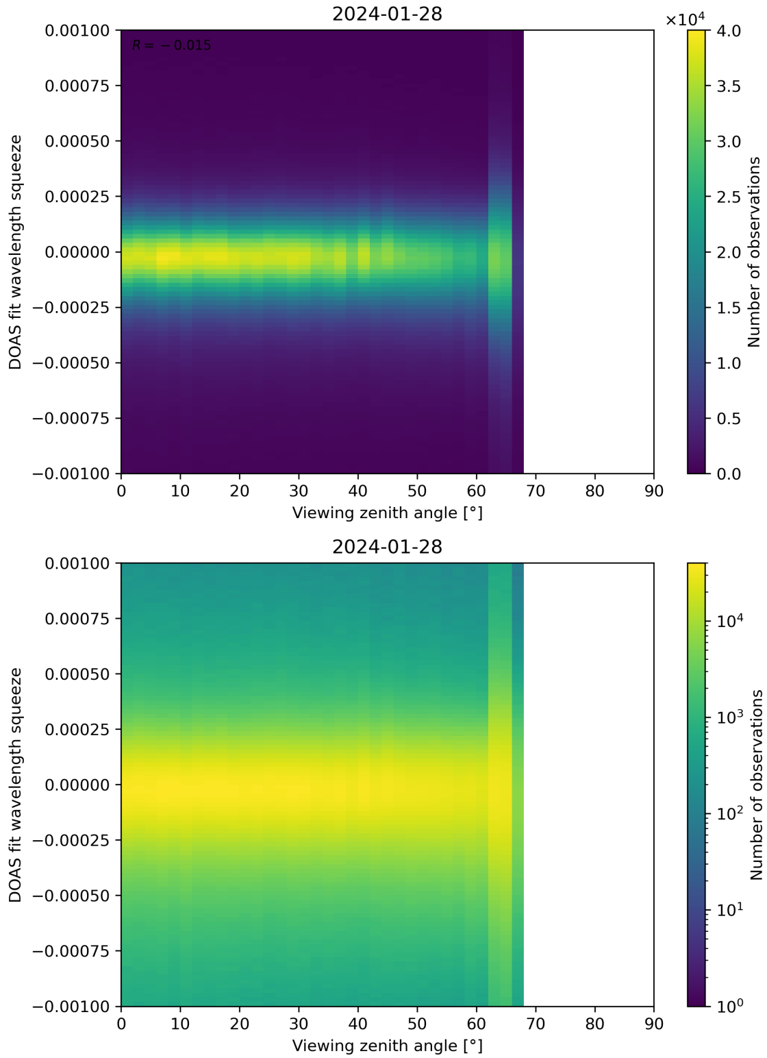
Figure 312: Scatter density plot of “Viewing zenith angle” against “DOAS fit wavelength squeeze” for 2024-01-27 to 2024-01-29.
