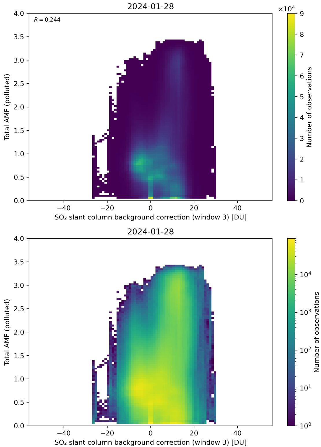
Figure 125: Scatter density plot of “SO 2 slant column background correction (window 3)” against “Total AMF (polluted)” for 2024-01-27 to 2024-01-29.
