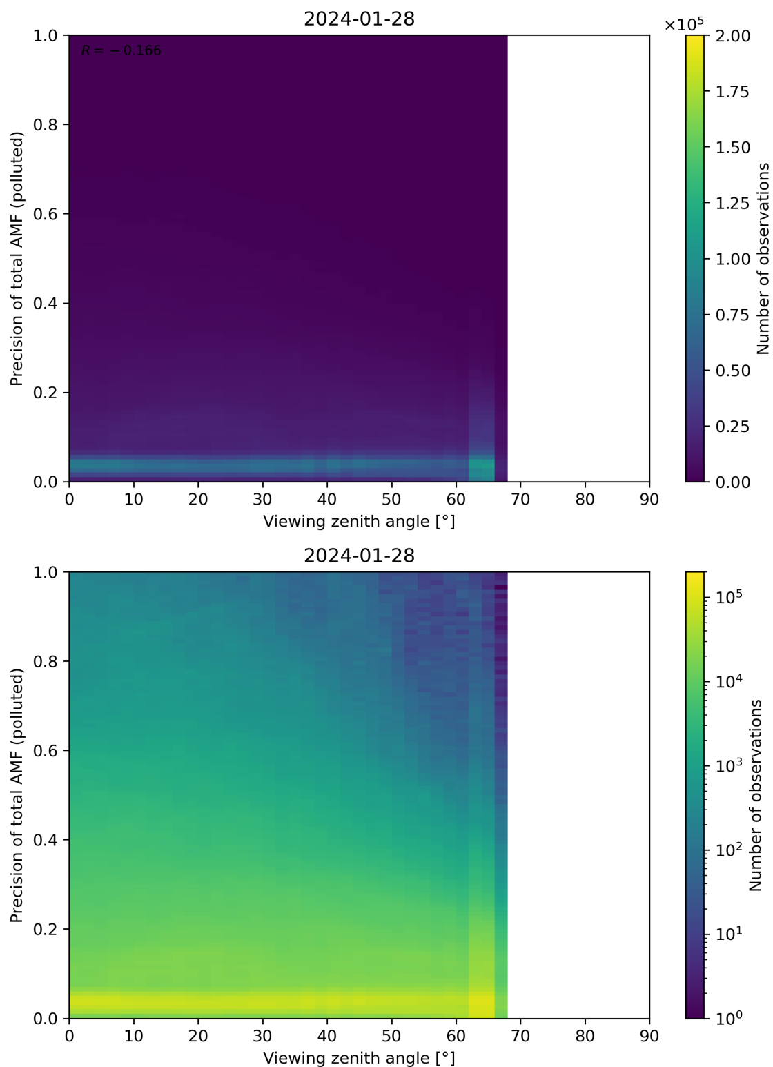
Figure 326: Scatter density plot of “Viewing zenith angle” against “Precision of total AMF (polluted)” for 2024-01-27 to 2024-01-29.
