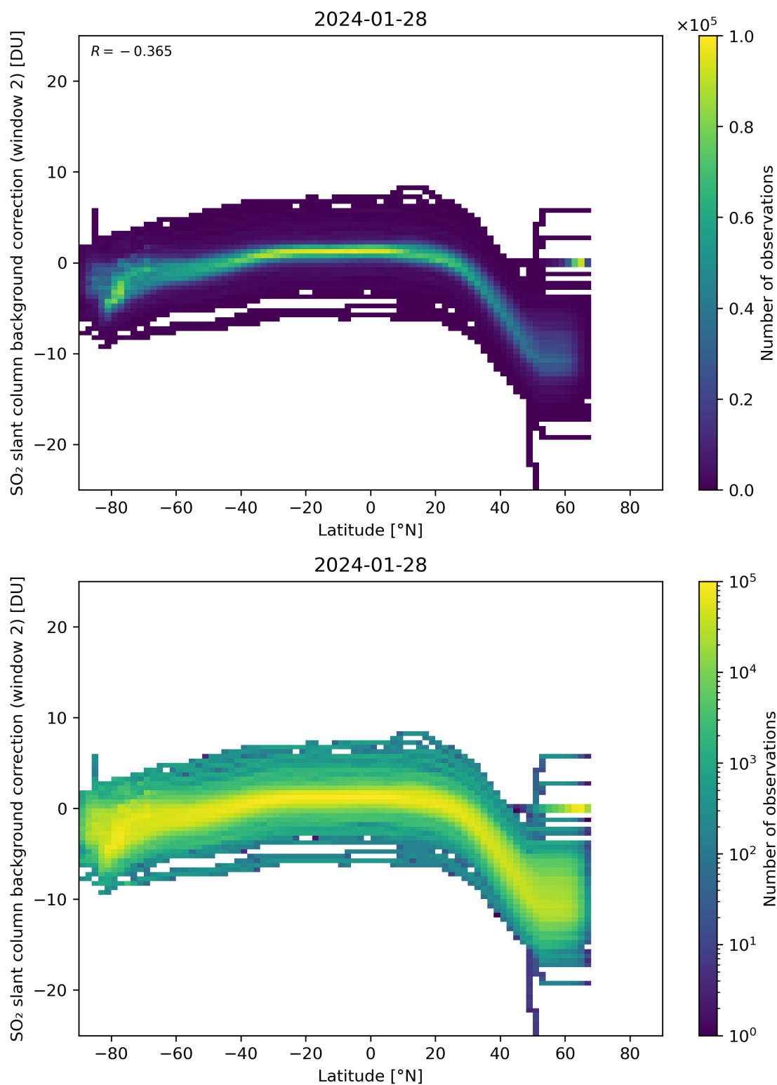
Figure 140: Scatter density plot of “Latitude” against “SO 2 slant column background correction (window 2)” for 2024-01-27 to 2024-01-29.
