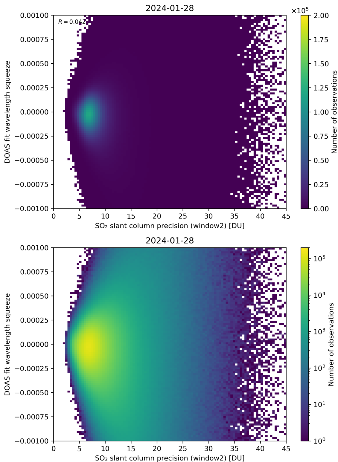
Figure 244: Scatter density plot of “SO 2 slant column precision (window2)” against “DOAS fit wavelength squeeze” for 2024-01-27 to 2024-01-29.
