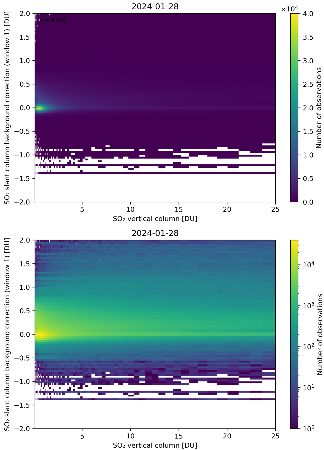
Figure 273: Scatter density plot of “SO 2 vertical column” against “SO 2 slant column background correction (window 1)” for 2024-01-27 to 2024-01-29.
