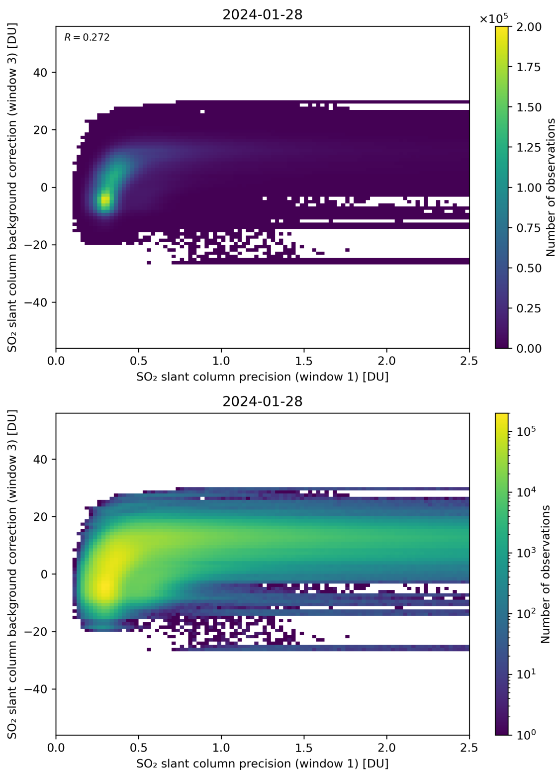
Figure 220: Scatter density plot of “SO 2 slant column precision (window 1)” against “SO 2 slant column background correction (window 3)” for 2024-01-27 to 2024-01-29.
