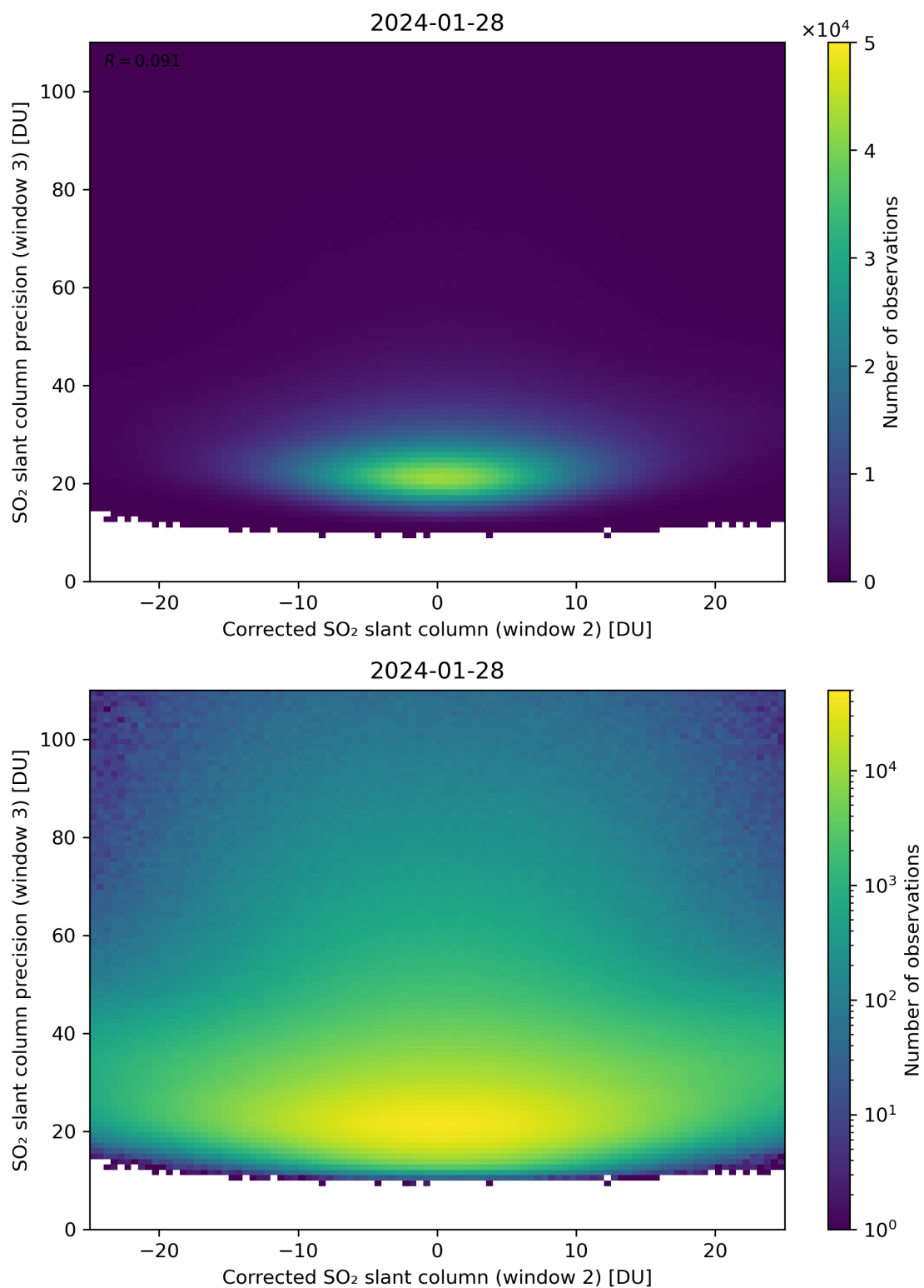
Figure 202: Scatter density plot of “Corrected SO 2 slant column (window 2)” against “SO 2 slant column precision (window 3)” for 2024-01-27 to 2024-01-29.
