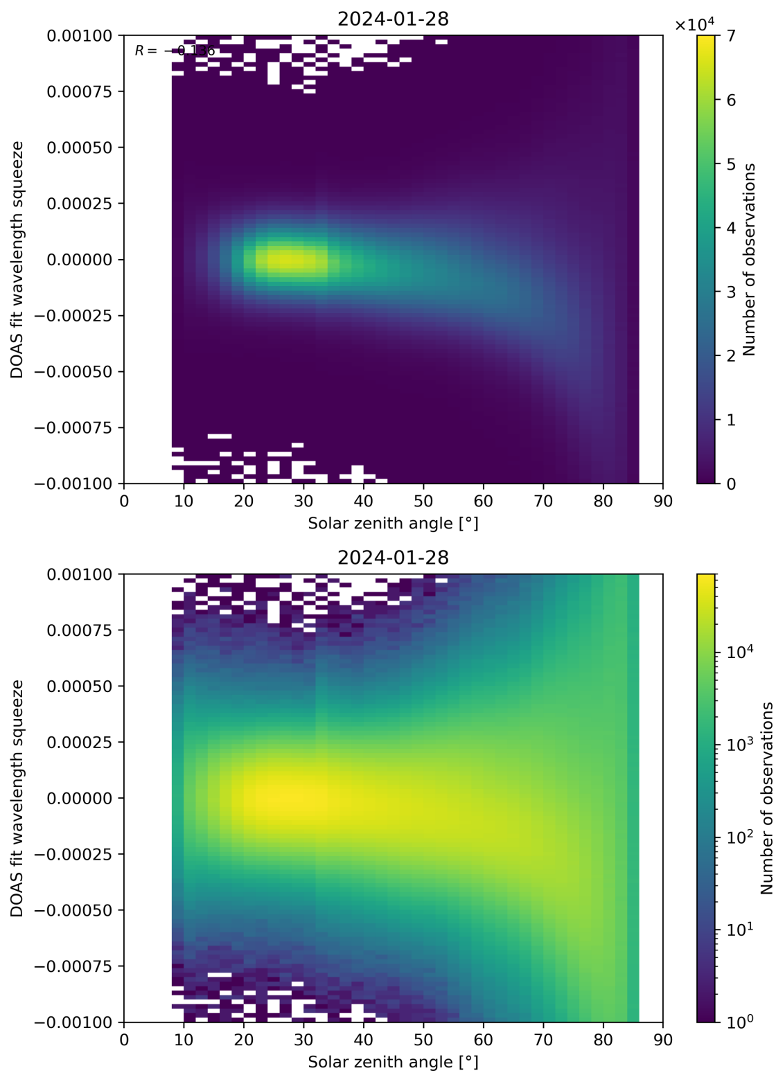
Figure 162: Scatter density plot of “Solar zenith angle” against “DOAS fit wavelength squeeze” for 2024-01-27 to 2024-01-29.
