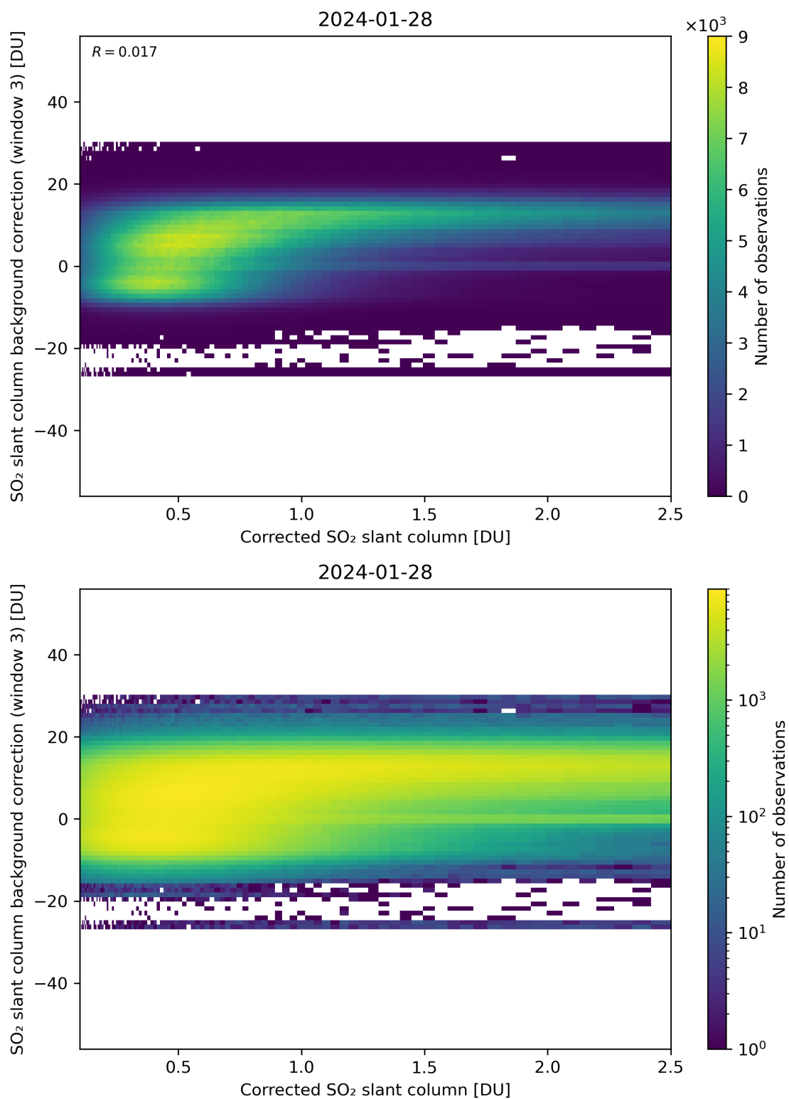
Figure 180: Scatter density plot of “Corrected SO 2 slant column” against “SO 2 slant column background correction (window 3)” for 2024-01-27 to 2024-01-29.
