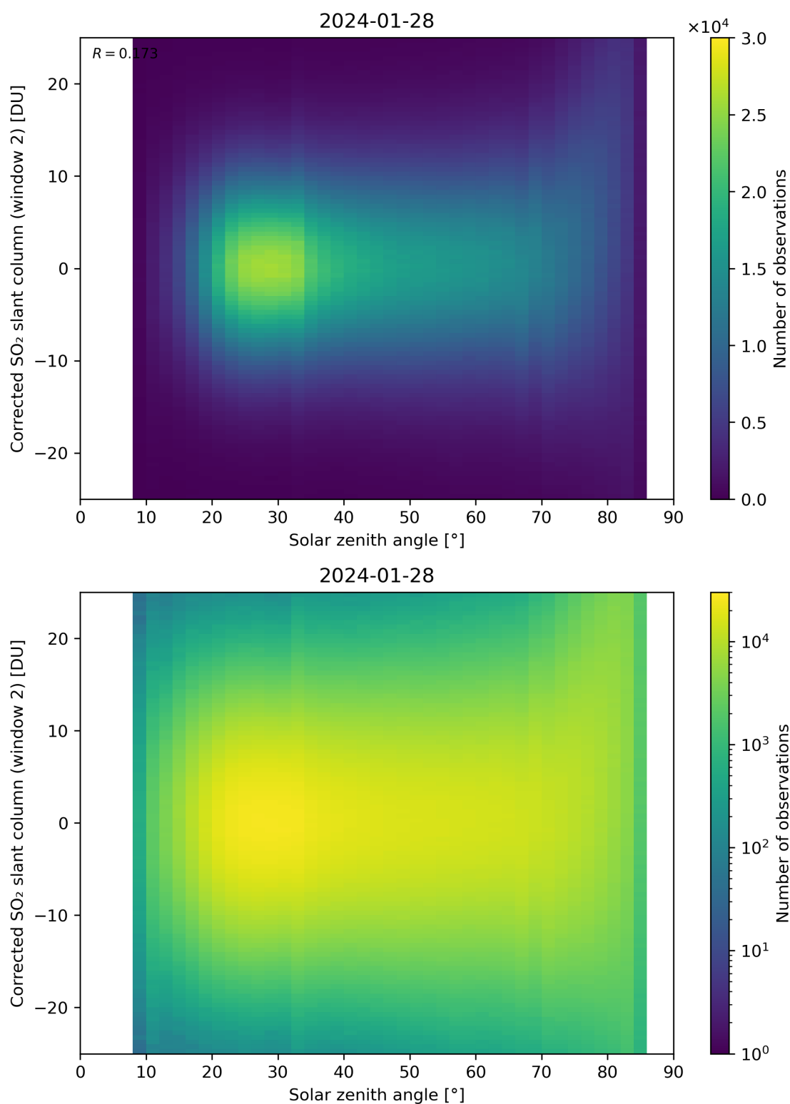
Figure 167: Scatter density plot of “Solar zenith angle” against “Corrected SO 2 slant column (window 2)” for 2024-01-27 to 2024-01-29.
