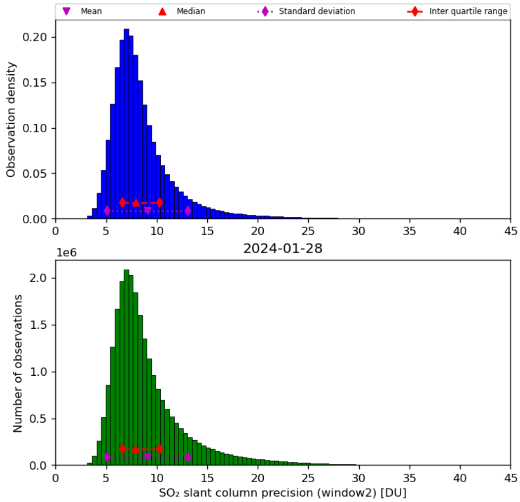
Figure 61: Histogram of “SO 2 slant column precision (window2)” for 2024-01-27 to 2024-01-29
