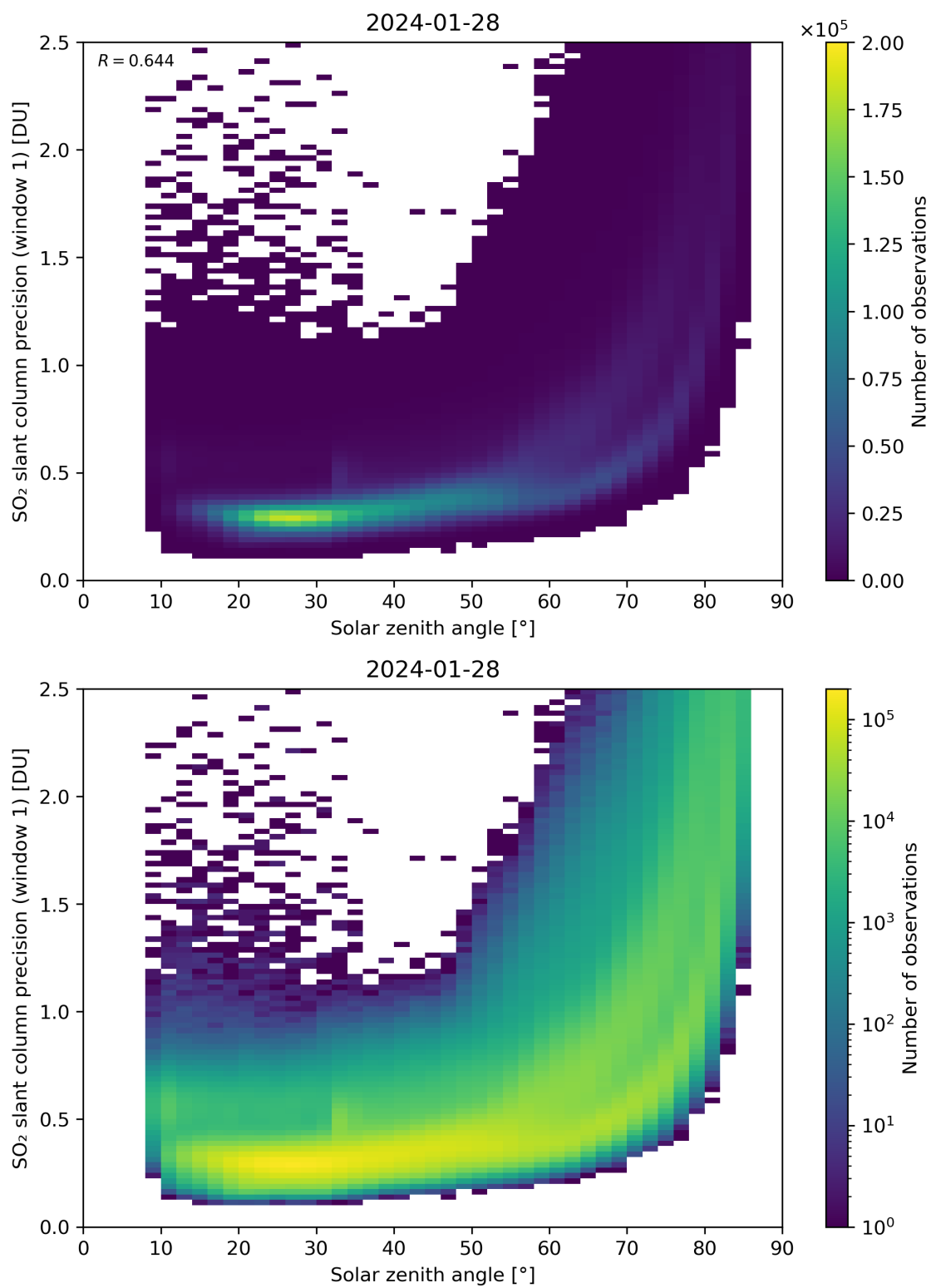
Figure 170: Scatter density plot of “Solar zenith angle” against “SO 2 slant column precision (window 1)” for 2024-01-27 to 2024-01-29.
