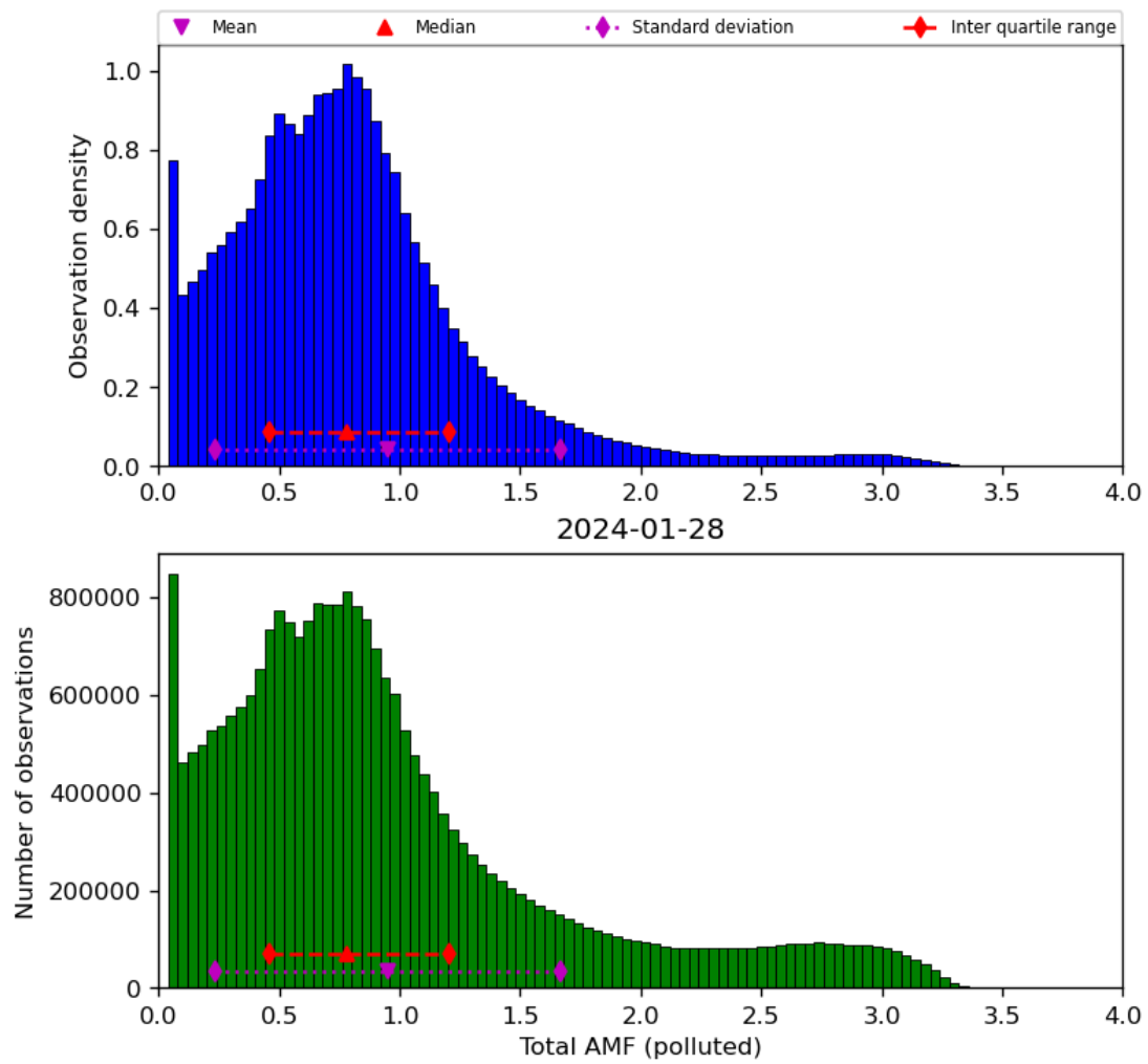
Figure 71: Histogram of “Total AMF (polluted)” for 2024-01-27 to 2024-01-29
