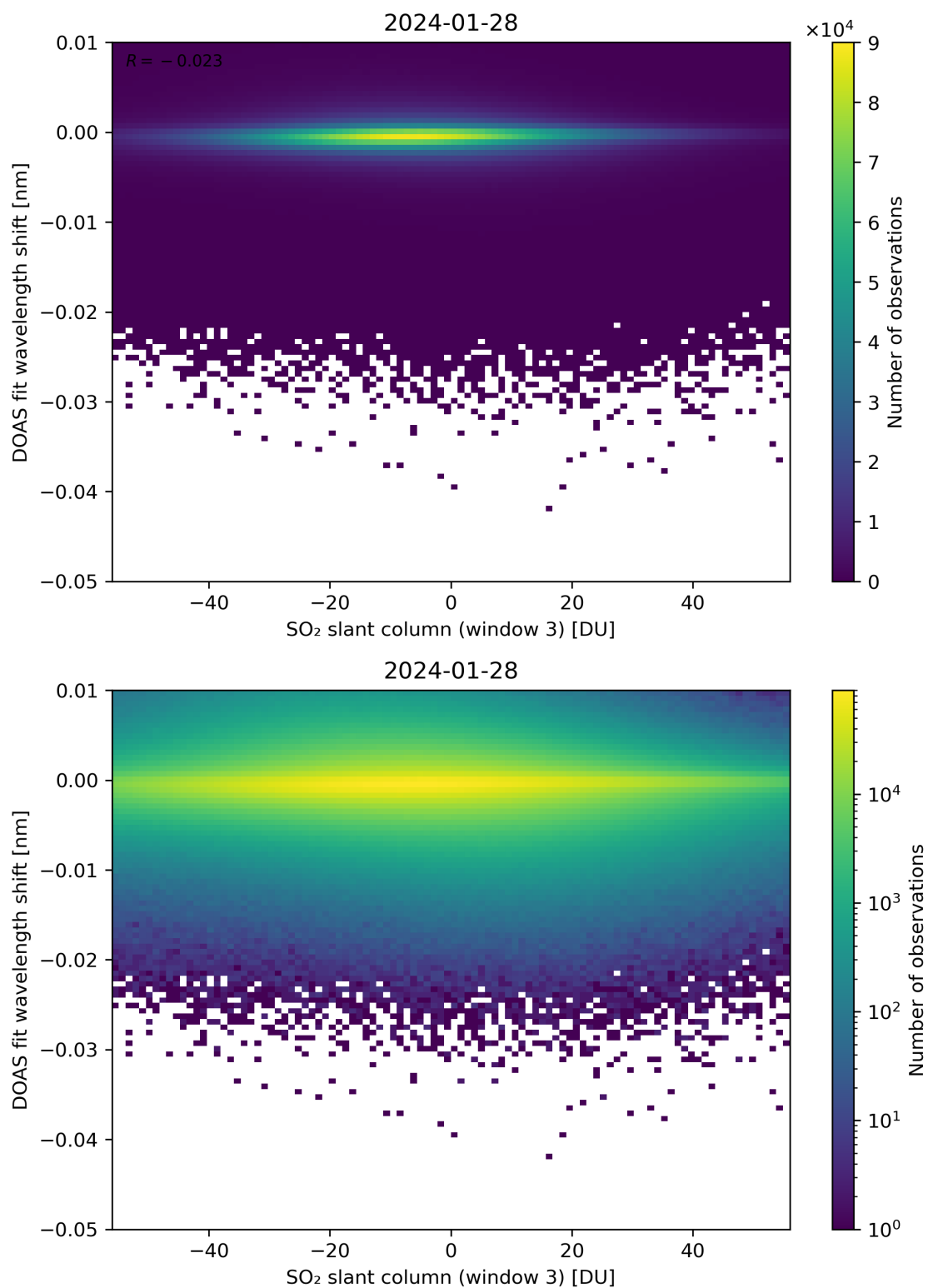
Figure 254: Scatter density plot of “SO 2 slant column (window 3)” against “DOAS fit wavelength shift” for 2024-01-27 to 2024-01-29.
