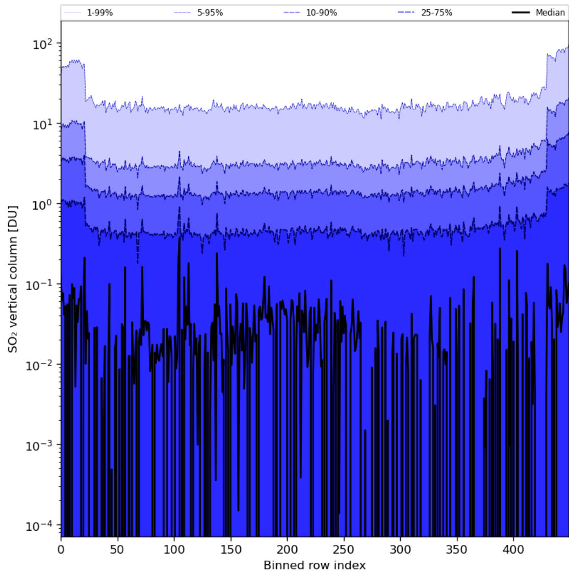
Figure 76: Along track statistics of “SO 2 vertical column” for 2024-01-27 to 2024-01-29
