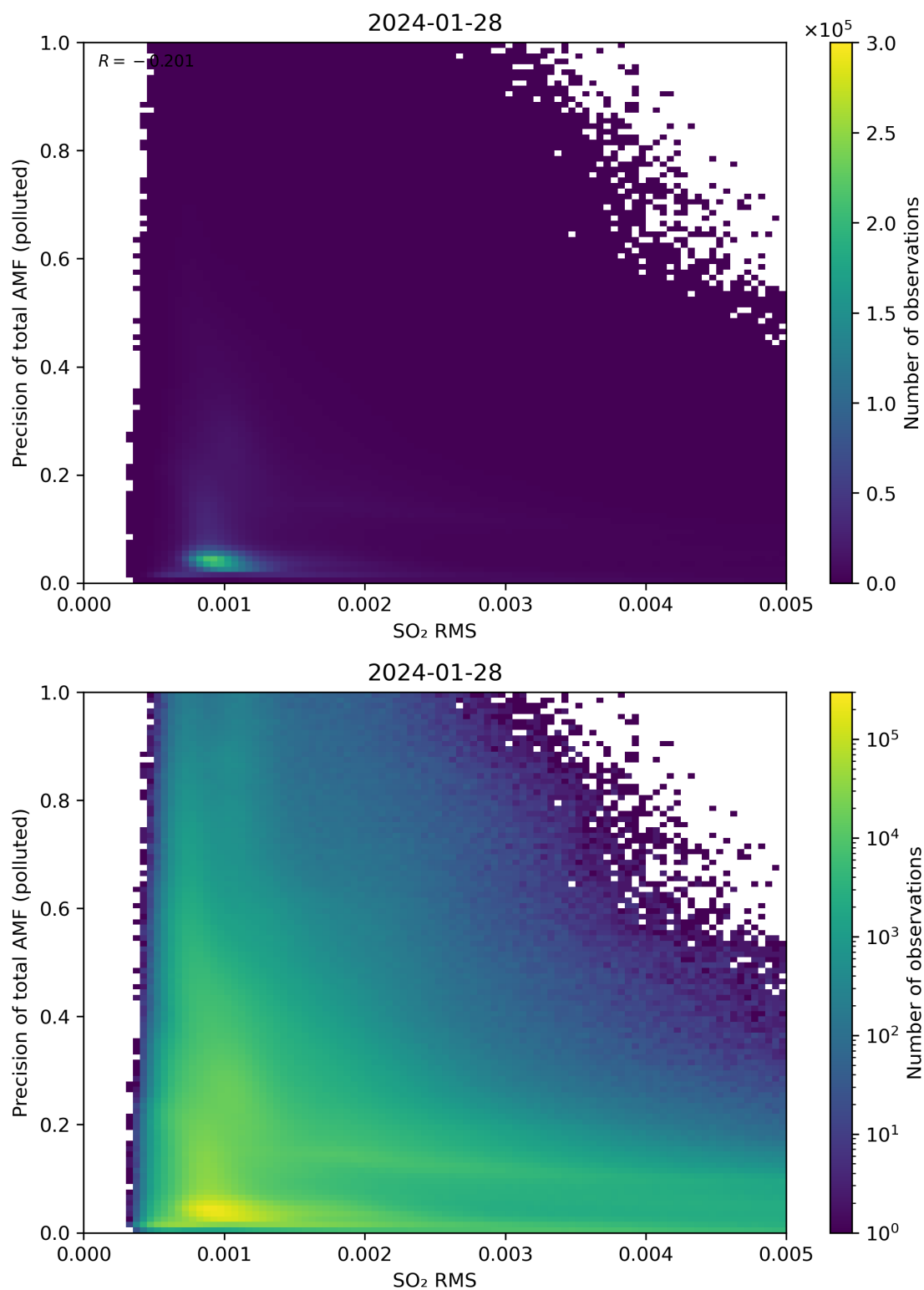
Figure 138: Scatter density plot of “SO 2 RMS” against “Precision of total AMF (polluted)” for 2024-01-27 to 2024-01-29.
