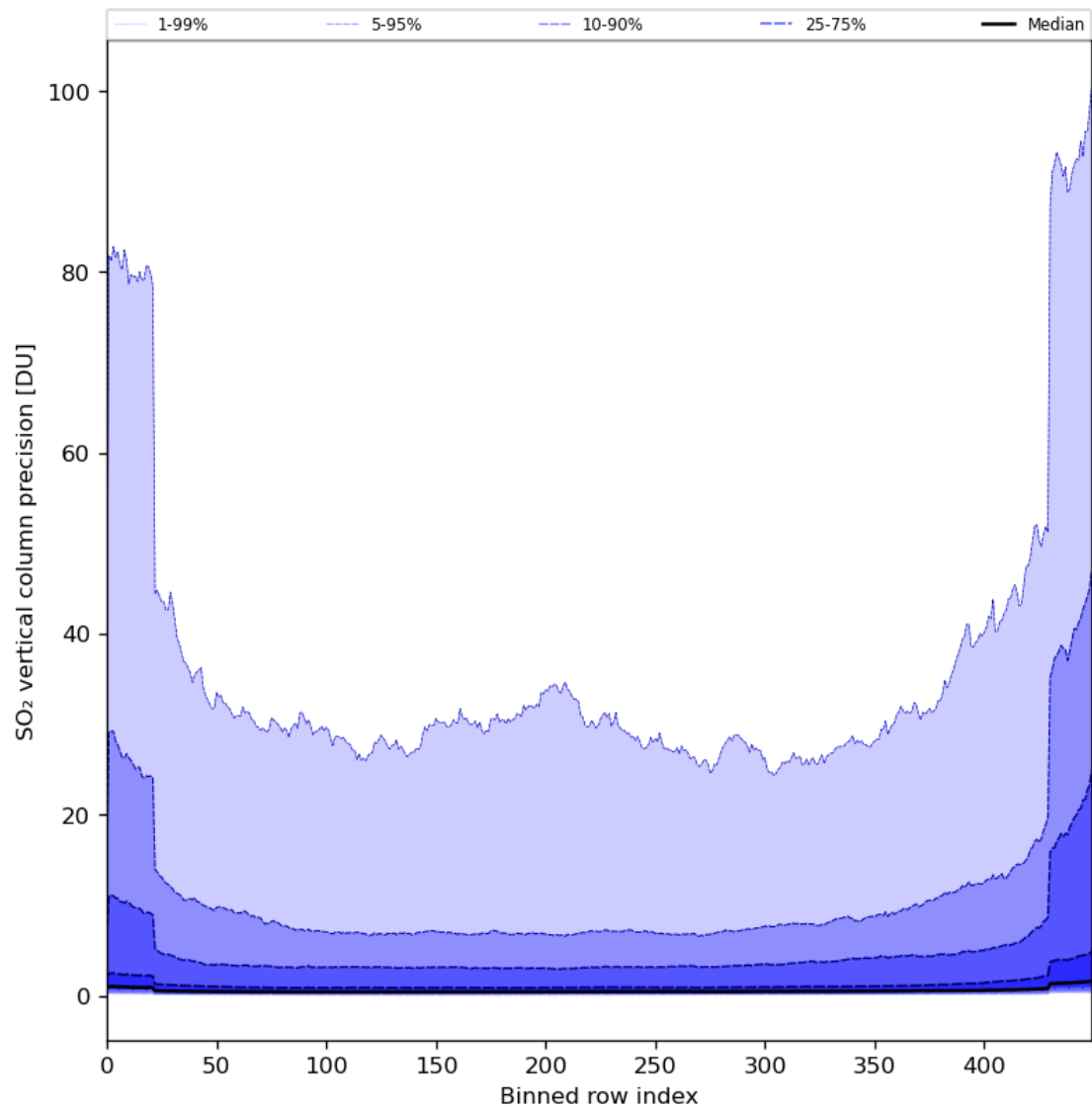
Figure 77: Along track statistics of “SO 2 vertical column precision” for 2024-01-27 to 2024-01-29
