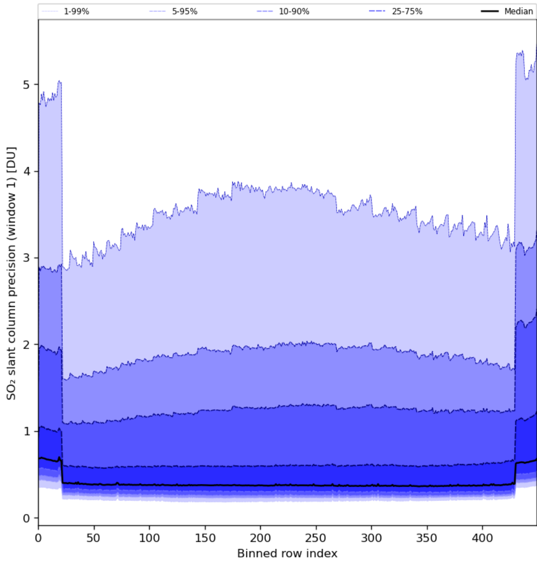
Figure 80: Along track statistics of “SO 2 slant column precision (window 1)” for 2024-01-27 to 2024-01-29
