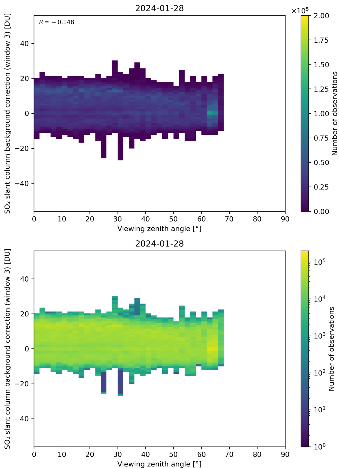
Figure 310: Scatter density plot of “Viewing zenith angle” against “SO 2 slant column background correction (window 3)” for 2024-01-27 to 2024-01-29.
