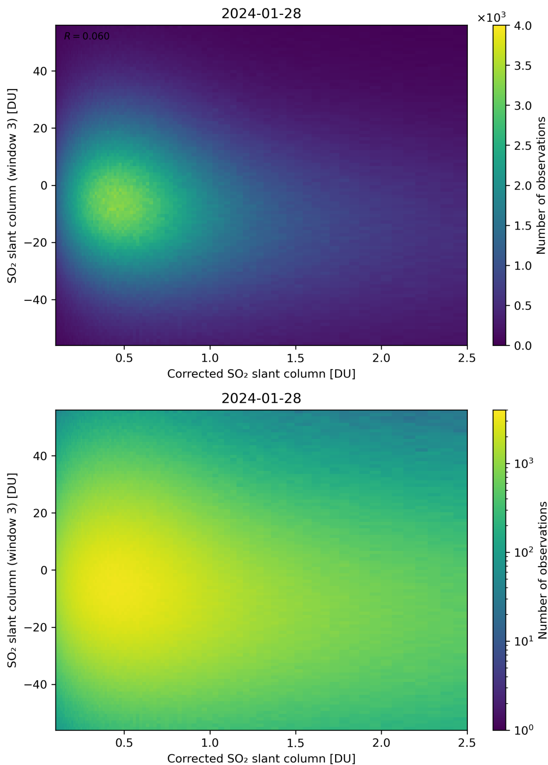
Figure 190: Scatter density plot of “Corrected SO 2 slant column” against “SO 2 slant column (window 3)” for 2024-01-27 to 2024-01-29.
