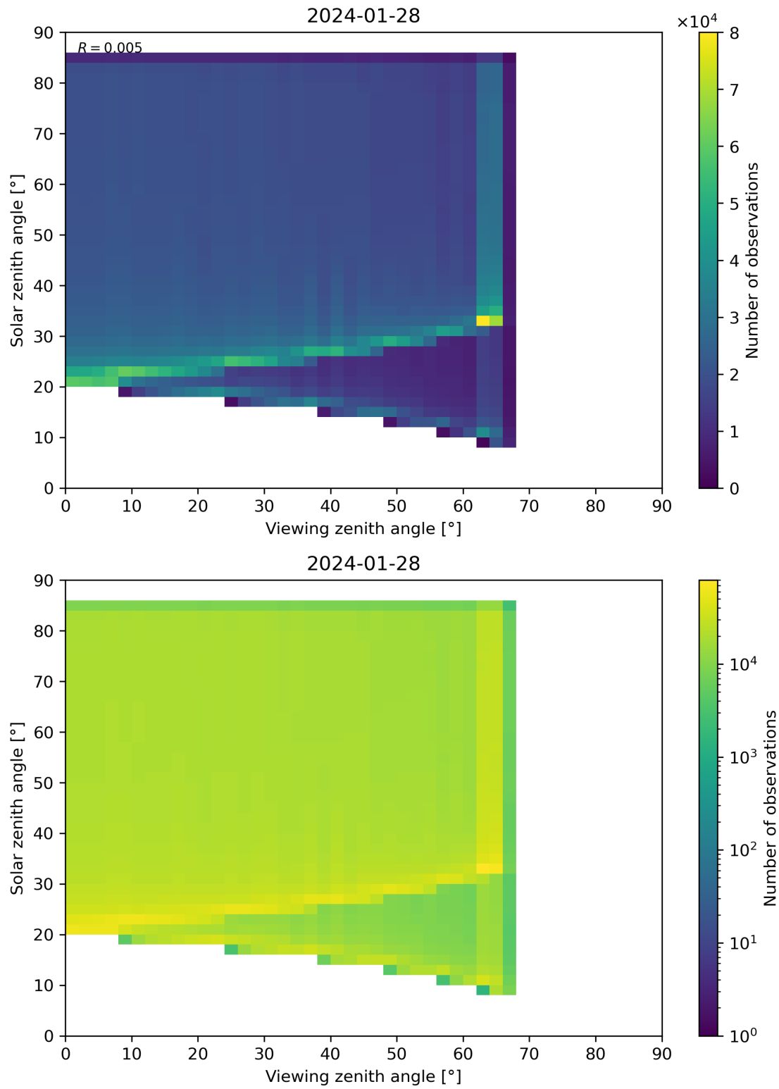
Figure 315: Scatter density plot of “Viewing zenith angle” against “Solar zenith angle” for 2024-01-27 to 2024-01-29.
