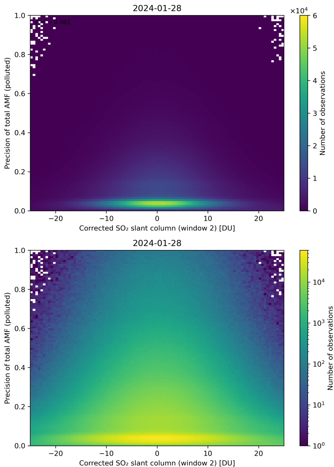
Figure 204: Scatter density plot of “Corrected SO 2 slant column (window 2)” against “Precision of total AMF (polluted)” for 2024-01-27 to 2024-01-29.
