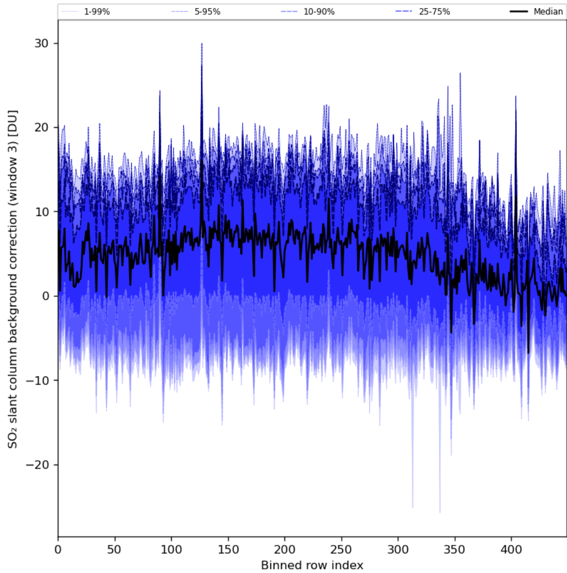
Figure 90: Along track statistics of “SO 2 slant column background correction (window 3)” for 2024-01-27 to 2024-01-29
