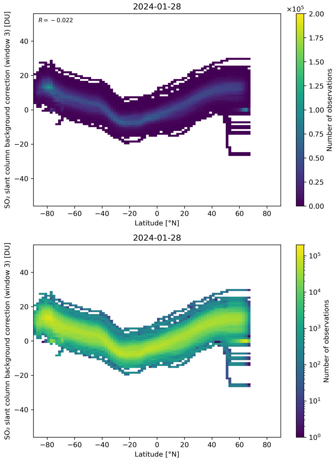
Figure 141: Scatter density plot of “Latitude” against “SO 2 slant column background correction (window 3)” for 2024-01-27 to 2024-01-29.
