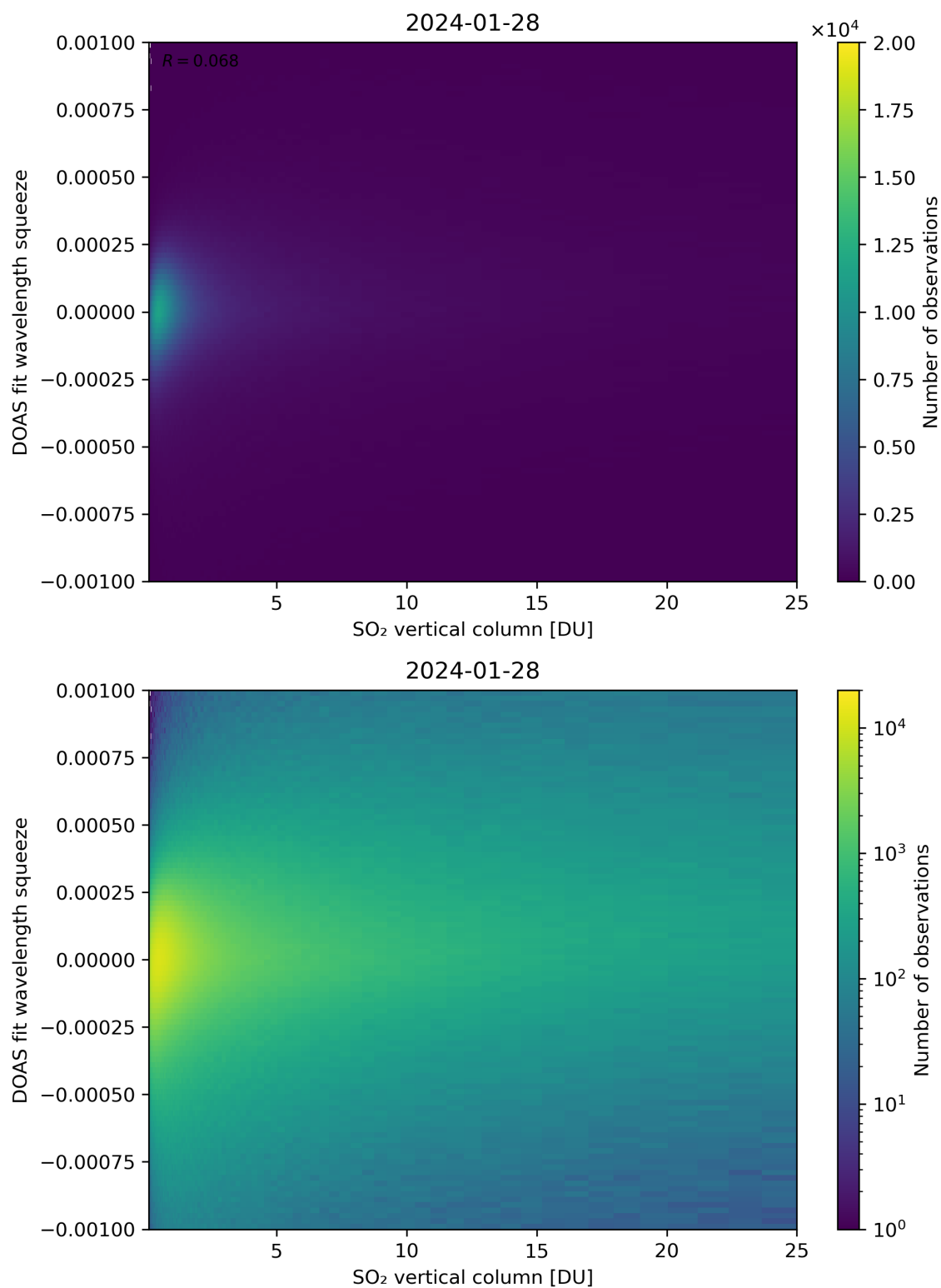
Figure 277: Scatter density plot of “SO 2 vertical column” against “DOAS fit wavelength squeeze” for 2024-01-27 to 2024-01-29.
