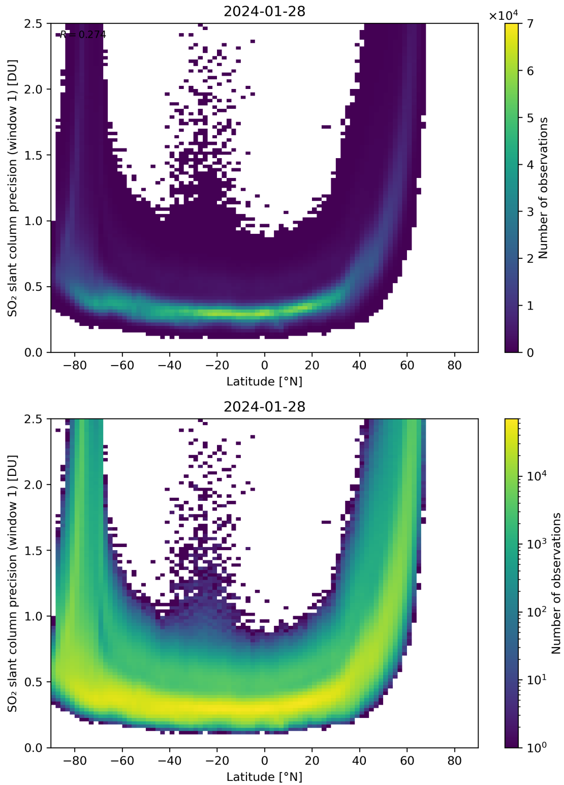
Figure 150: Scatter density plot of “Latitude” against “SO 2 slant column precision (window 1)” for 2024-01-27 to 2024-01-29.
