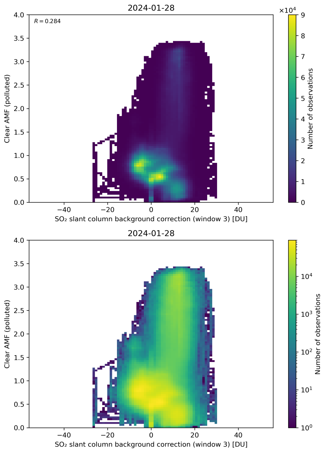
Figure 124: Scatter density plot of “SO 2 slant column background correction (window 3)” against “Clear AMF (polluted)” for 2024-01-27 to 2024-01-29.
