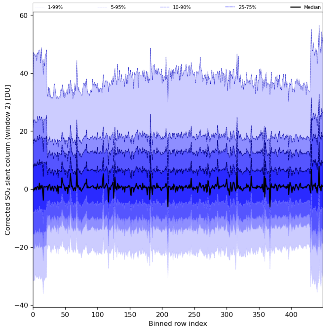
Figure 85: Along track statistics of “Corrected SO 2 slant column (window 2)” for 2024-01-27 to 2024-01-29
