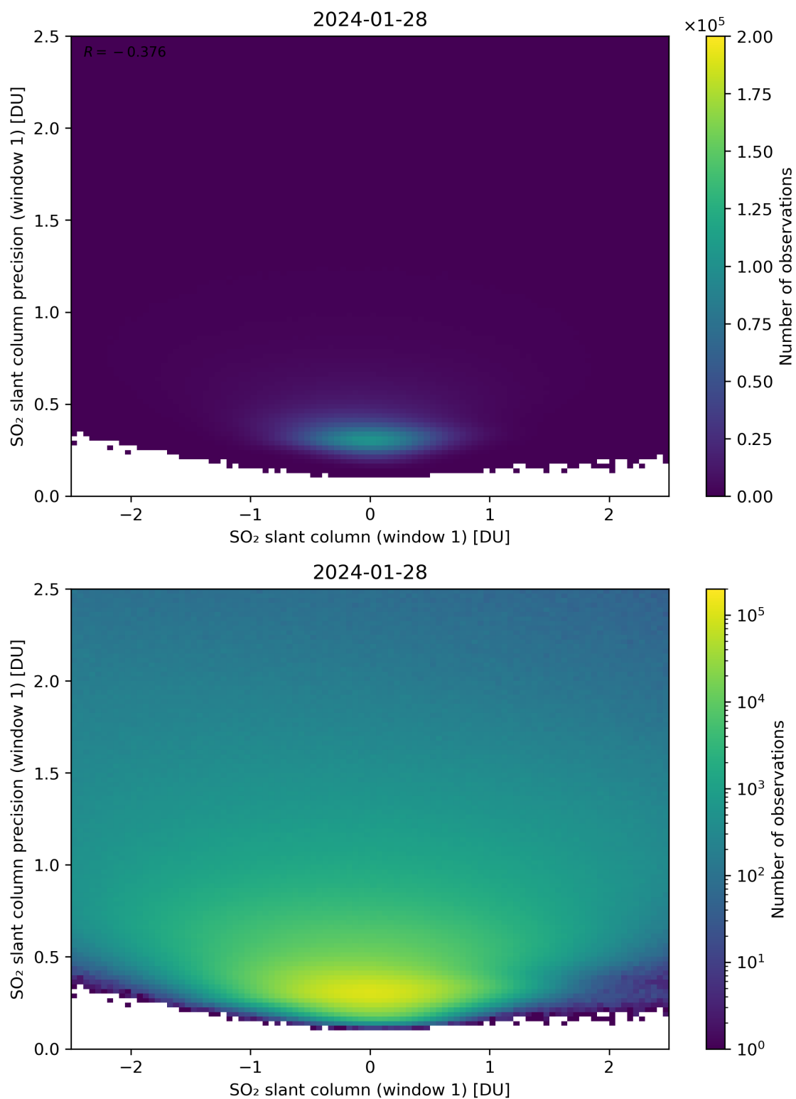
Figure 235: Scatter density plot of “SO 2 slant column (window 1)” against “SO 2 slant column precision (window 1)” for 2024-01-27 to 2024-01-29.
