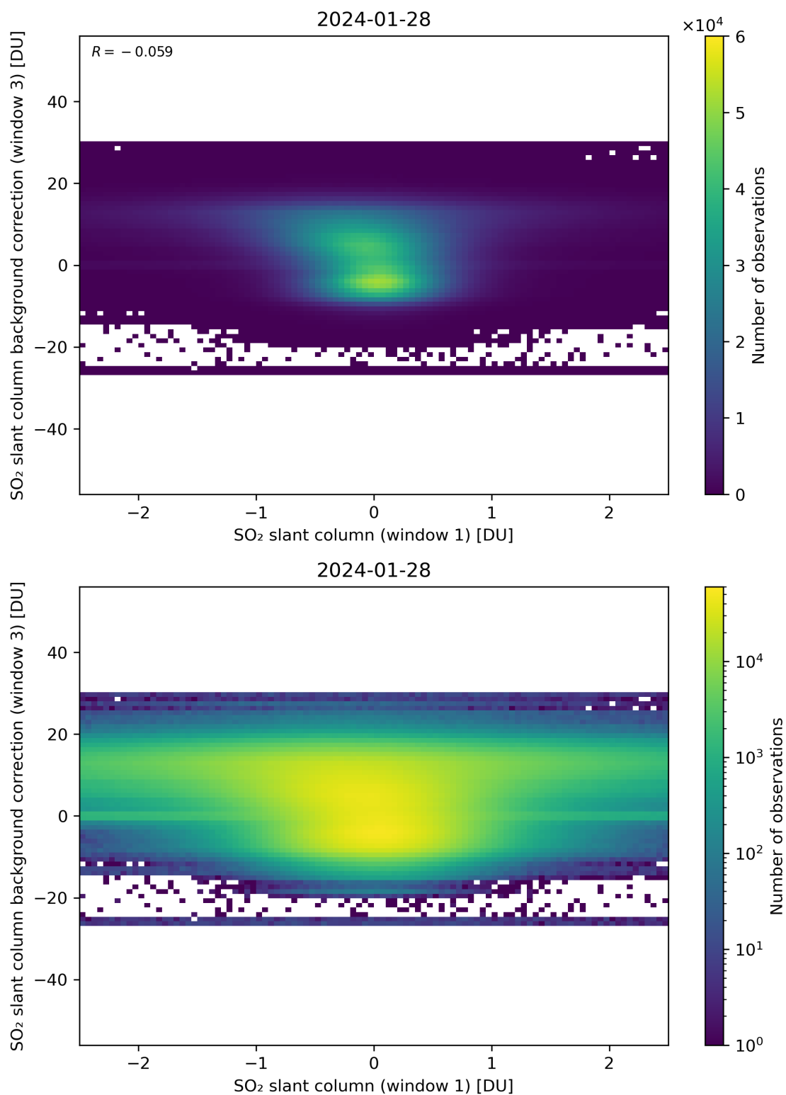
Figure 214: Scatter density plot of “SO 2 slant column (window 1)” against “SO 2 slant column background correction (window 3)” for 2024-01-27 to 2024-01-29.
