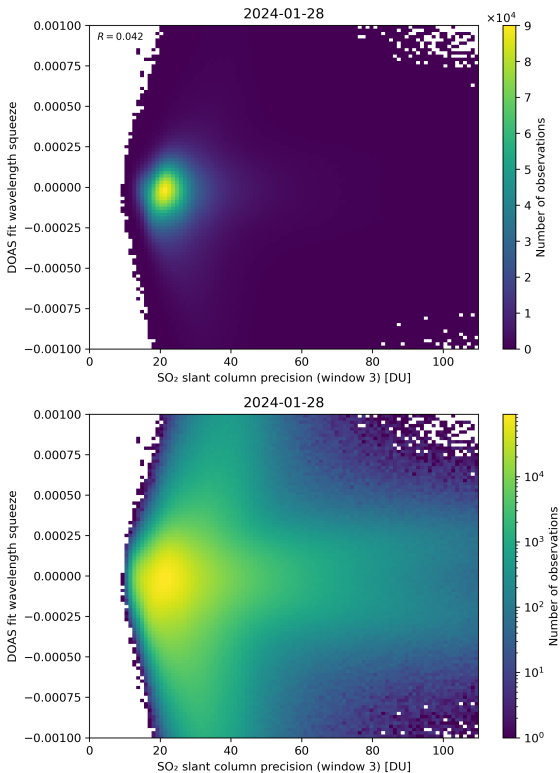
Figure 259: Scatter density plot of “SO 2 slant column precision (window 3)” against “DOAS fit wavelength squeeze” for 2024-01-27 to 2024-01-29.
