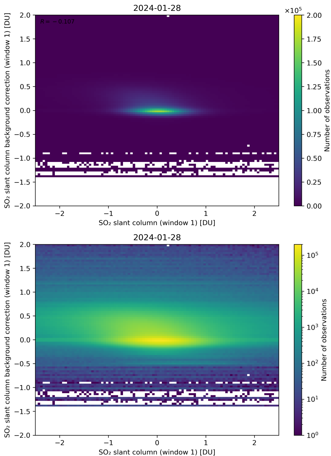
Figure 212: Scatter density plot of “SO 2 slant column (window 1)” against “SO 2 slant column background correction (window 1)” for 2024-01-27 to 2024-01-29.
