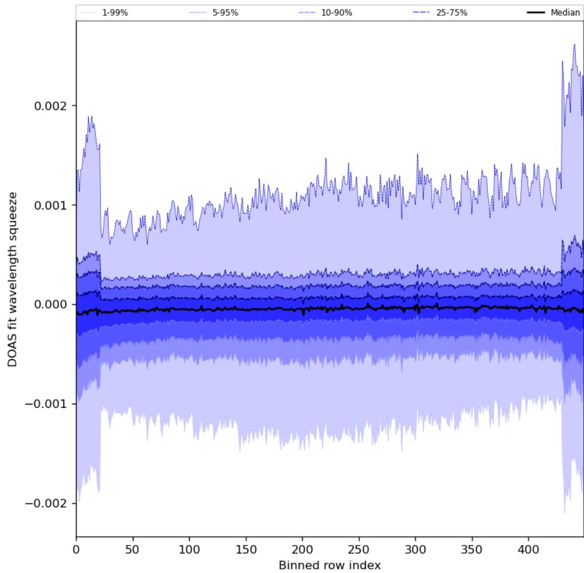
Figure 92: Along track statistics of “DOAS fit wavelength squeeze” for 2024-01-27 to 2024-01-29
