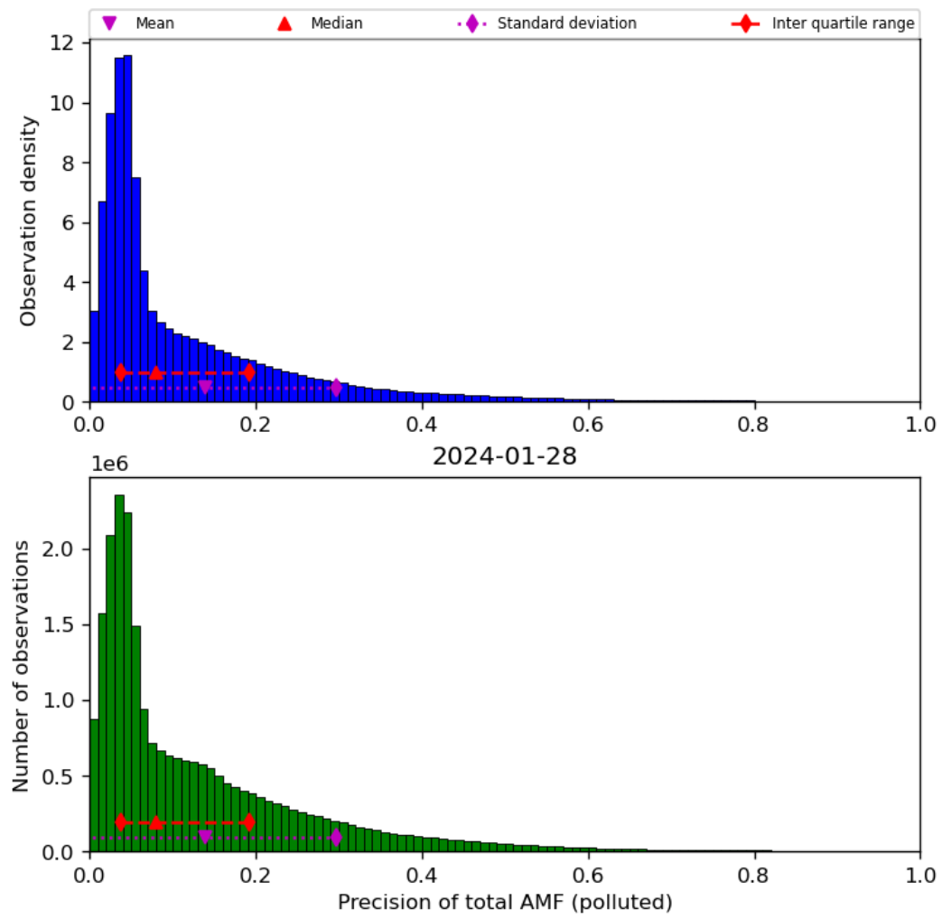
Figure 72: Histogram of “Precision of total AMF (polluted)” for 2024-01-27 to 2024-01-29
