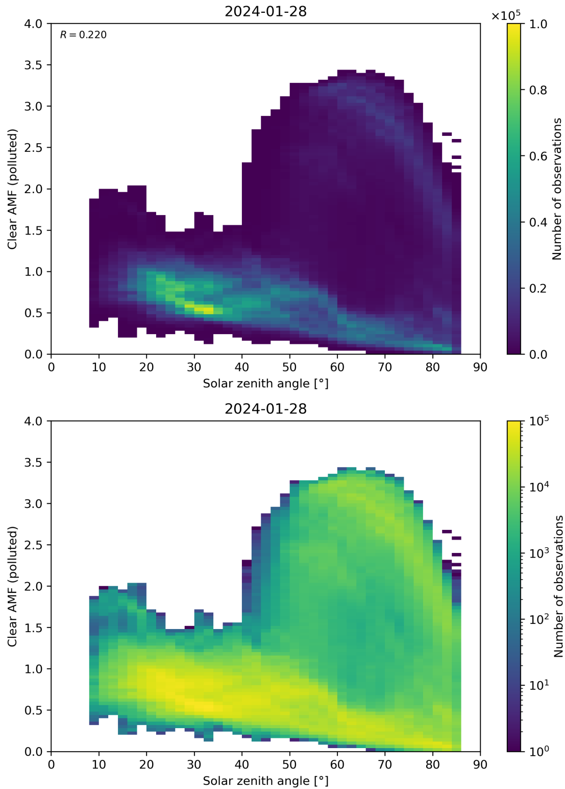
Figure 165: Scatter density plot of “Solar zenith angle” against “Clear AMF (polluted)” for 2024-01-27 to 2024-01-29.
