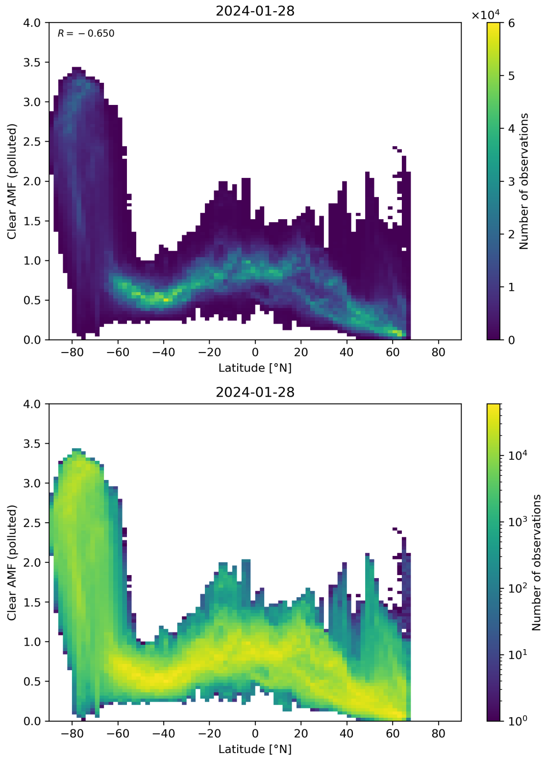
Figure 145: Scatter density plot of “Latitude” against “Clear AMF (polluted)” for 2024-01-27 to 2024-01-29.
