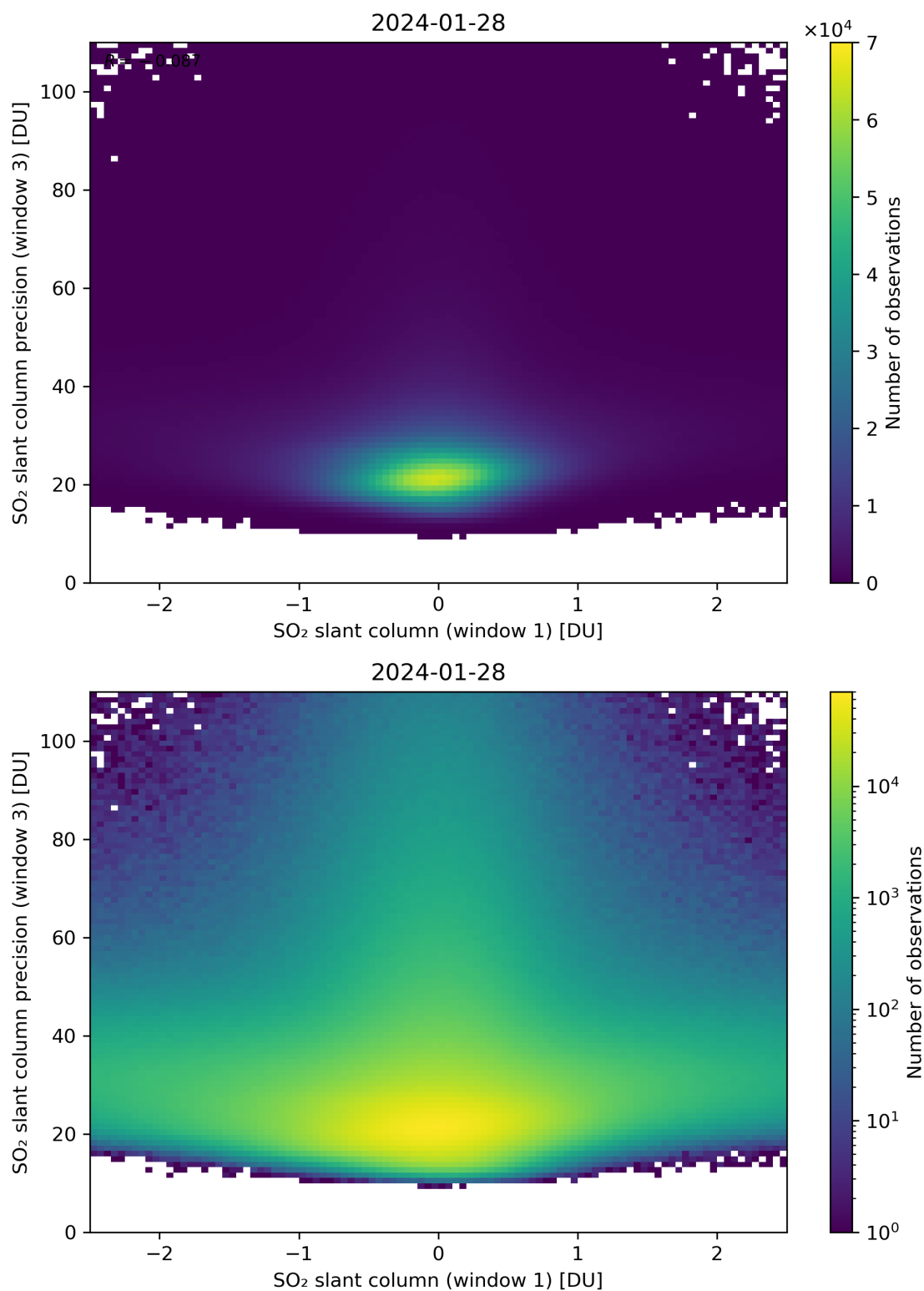
Figure 238: Scatter density plot of “SO 2 slant column (window 1)” against “SO 2 slant column precision (window 3)” for 2024-01-27 to 2024-01-29.
