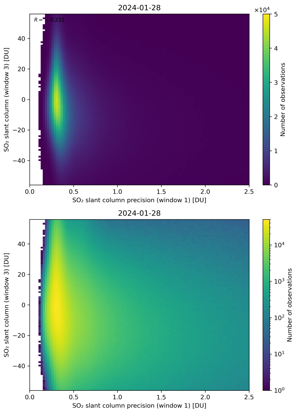
Figure 228: Scatter density plot of “SO 2 slant column precision (window 1)” against “SO 2 slant column (window 3)” for 2024-01-27 to 2024-01-29.
