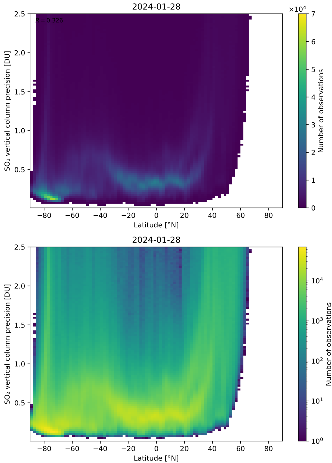
Figure 157: Scatter density plot of “Latitude” against “SO 2 vertical column precision” for 2024-01-27 to 2024-01-29.
