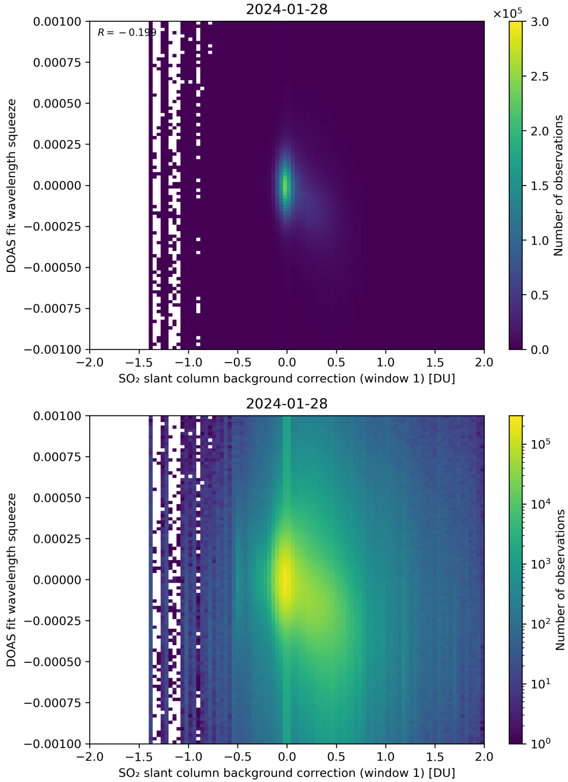
Figure 101: Scatter density plot of “SO 2 slant column background correction (window 1)” against “DOAS fit wavelength squeeze” for 2024-01-27 to 2024-01-29.
