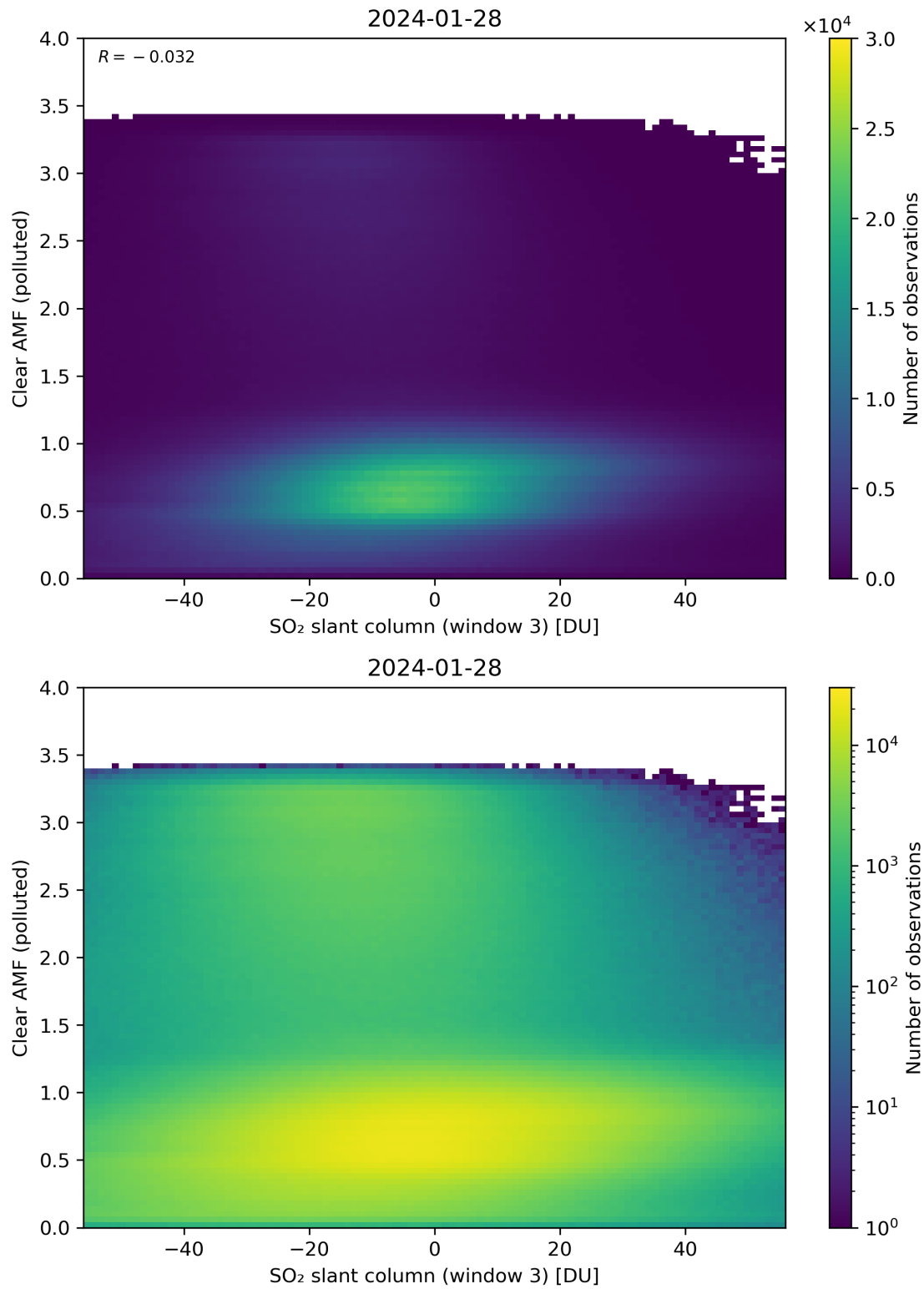
Figure 265: Scatter density plot of “SO 2 slant column (window 3)” against “Clear AMF (polluted)” for 2024-01-27 to 2024-01-29.
