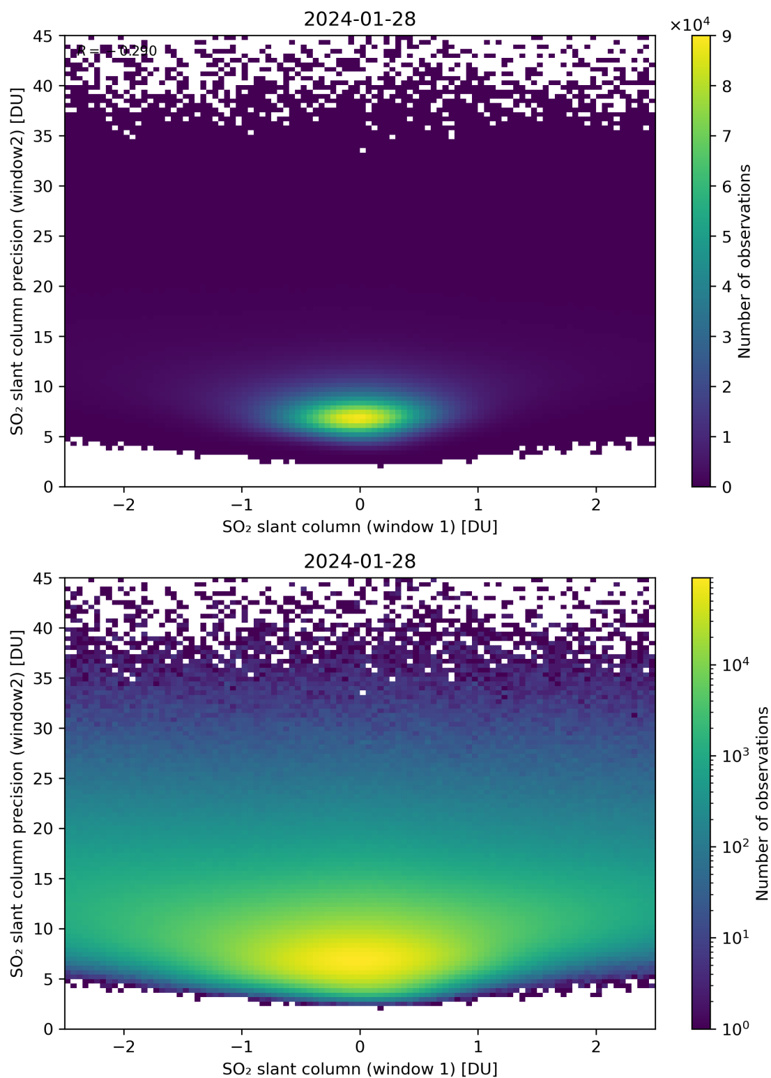
Figure 236: Scatter density plot of “SO 2 slant column (window 1)” against “SO 2 slant column precision (window2)” for 2024-01-27 to 2024-01-29.
