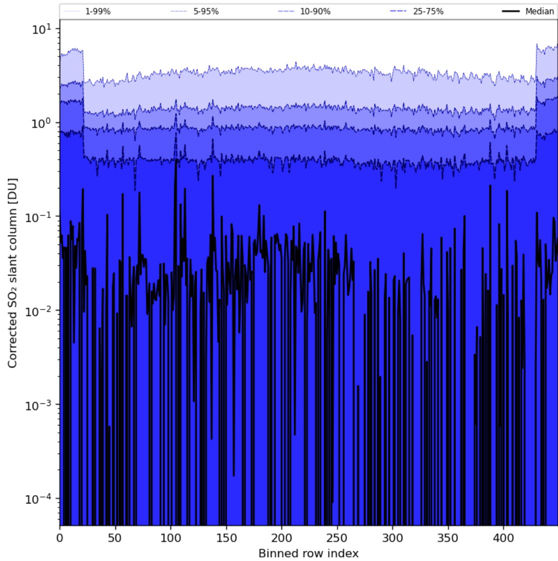
Figure 78: Along track statistics of “Corrected SO 2 slant column” for 2024-01-27 to 2024-01-29
