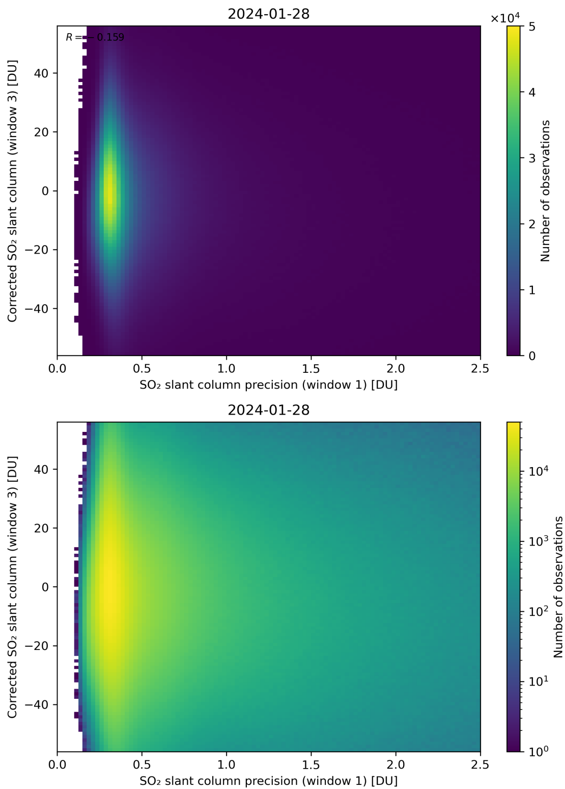
Figure 226: Scatter density plot of “SO 2 slant column precision (window 1)” against “Corrected SO 2 slant column (window 3)” for 2024-01-27 to 2024-01-29.
