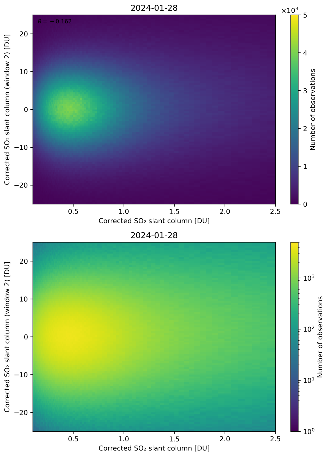
Figure 185: Scatter density plot of “Corrected SO 2 slant column” against “Corrected SO 2 slant column (window 2)” for 2024-01-27 to 2024-01-29.
