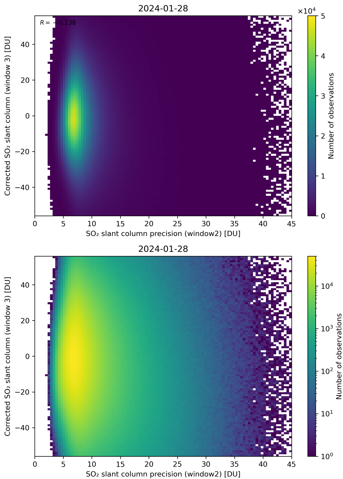
Figure 248: Scatter density plot of “SO 2 slant column precision (window2)” against “Corrected SO 2 slant column (window 3)” for 2024-01-27 to 2024-01-29.
