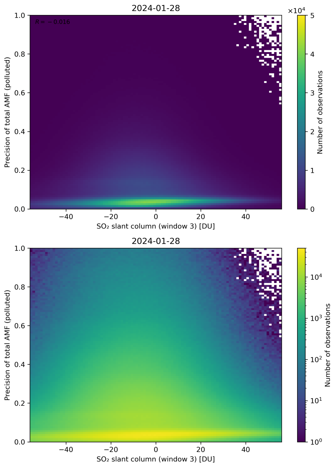
Figure 269: Scatter density plot of “SO 2 slant column (window 3)” against “Precision of total AMF (polluted)” for 2024-01-27 to 2024-01-29.
