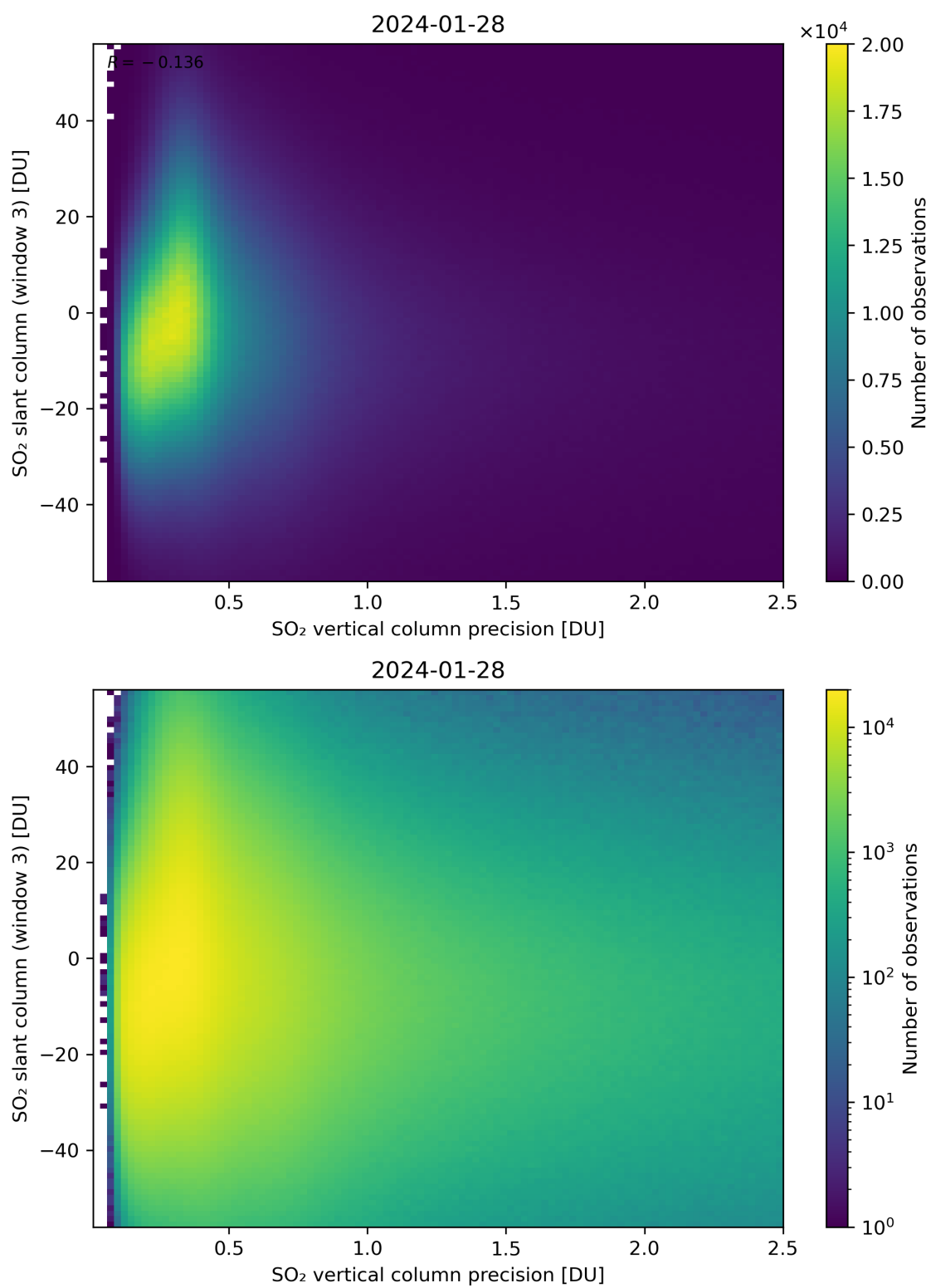
Figure 292: Scatter density plot of “SO 2 vertical column precision” against “SO 2 slant column (window 3)” for 2024-01-27 to 2024-01-29.
