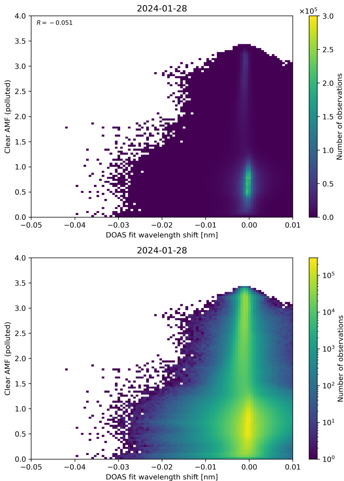
Figure 129: Scatter density plot of “DOAS fit wavelength shift” against “Clear AMF (polluted)” for 2024-01-27 to 2024-01-29.
