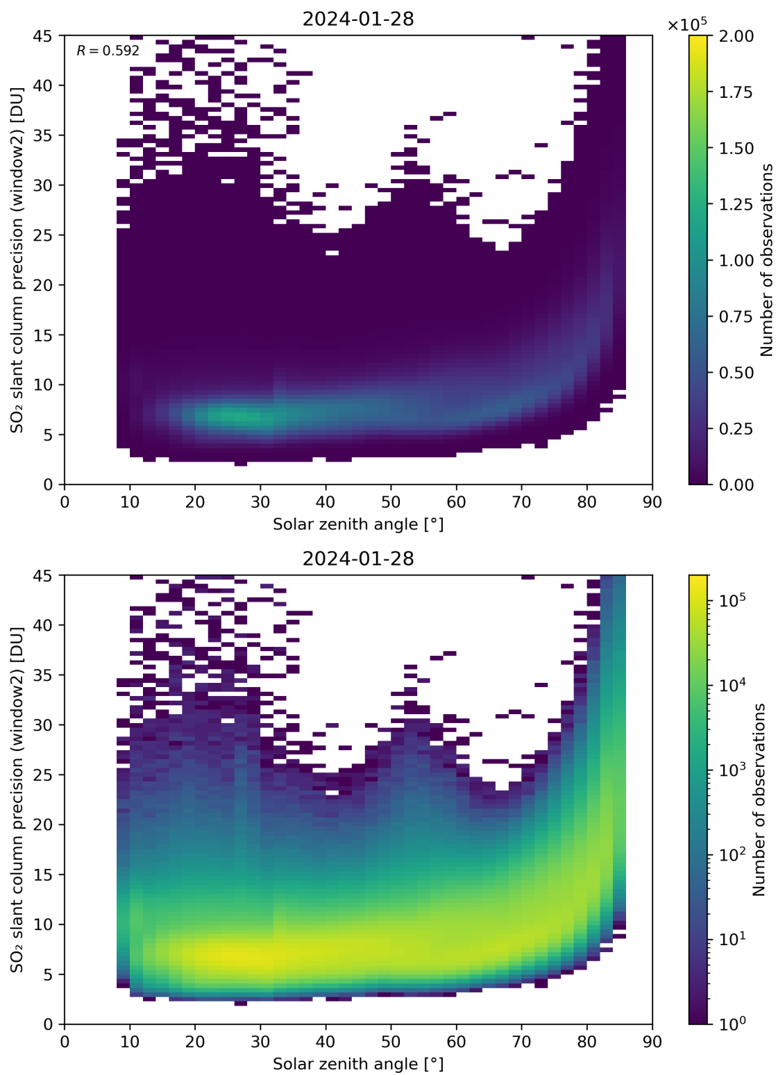
Figure 171: Scatter density plot of “Solar zenith angle” against “SO 2 slant column precision (window2)” for 2024-01-27 to 2024-01-29.
