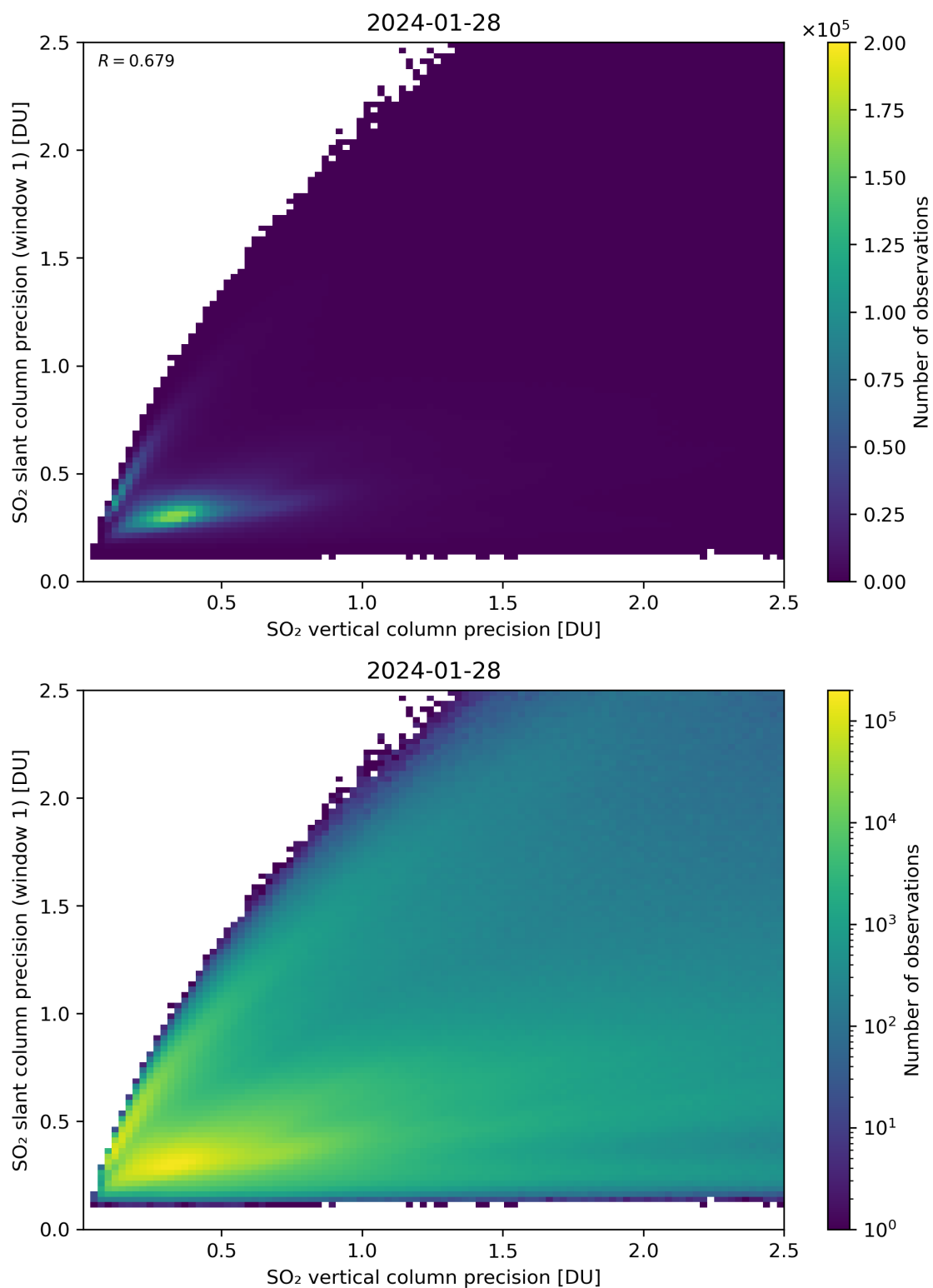
Figure 290: Scatter density plot of “SO 2 vertical column precision” against “SO 2 slant column precision (window 1)” for 2024-01-27 to 2024-01-29.
