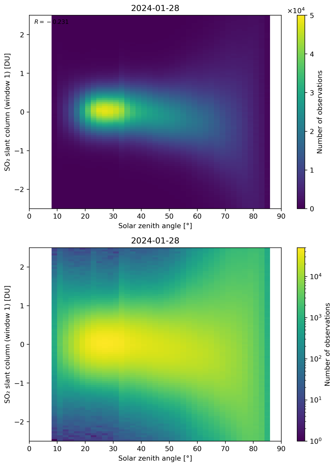
Figure 169: Scatter density plot of “Solar zenith angle” against “SO 2 slant column (window 1)” for 2024-01-27 to 2024-01-29.
