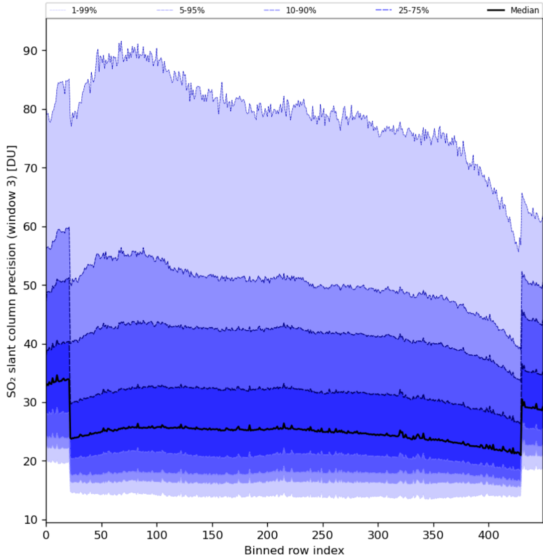
Figure 88: Along track statistics of “SO 2 slant column precision (window 3)” for 2024-01-27 to 2024-01-29
