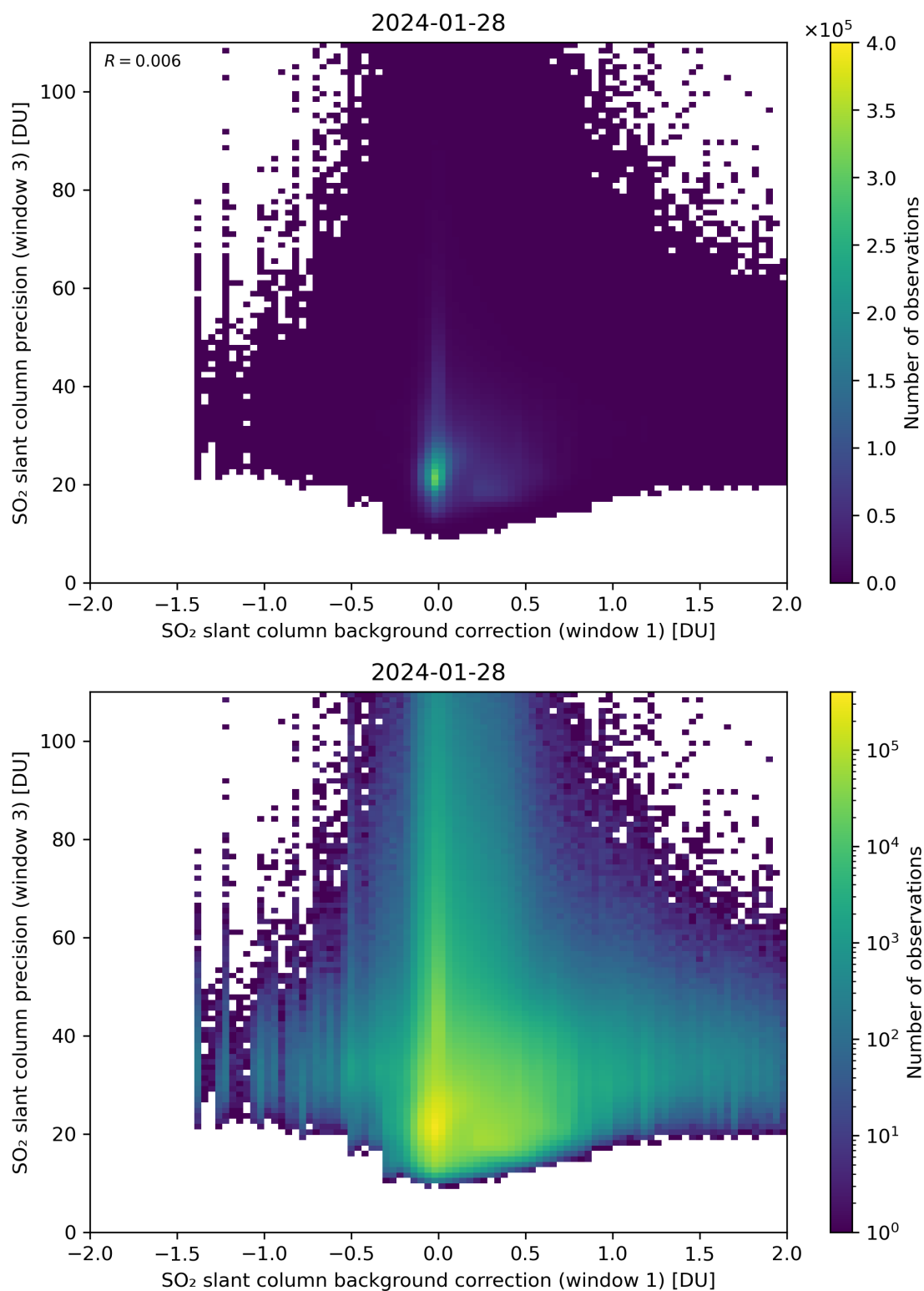
Figure 108: Scatter density plot of “SO 2 slant column background correction (window 1)” against “SO 2 slant column precision (window 3)” for 2024-01-27 to 2024-01-29.
