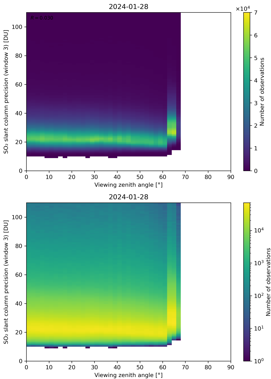
Figure 324: Scatter density plot of “Viewing zenith angle” against “SO 2 slant column precision (window 3)” for 2024-01-27 to 2024-01-29.
