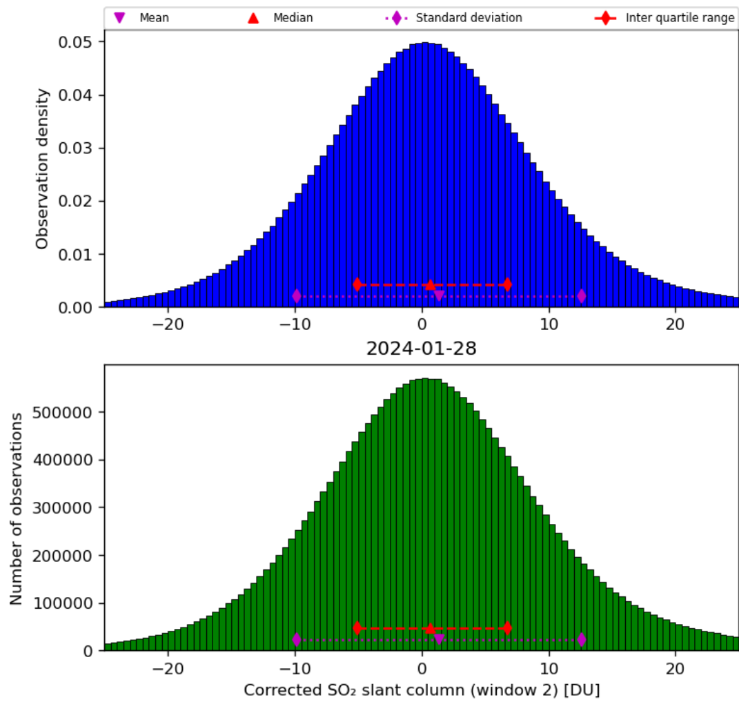
Figure 62: Histogram of “Corrected SO 2 slant column (window 2)” for 2024-01-27 to 2024-01-29
