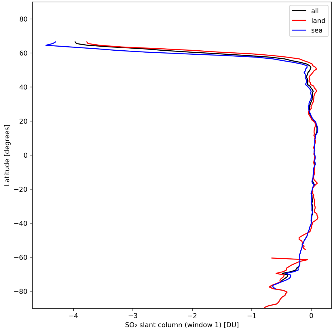
Figure 33: Zonal average of “SO 2 slant column (window 1)” for 2024-01-27 to 2024-01-29.
