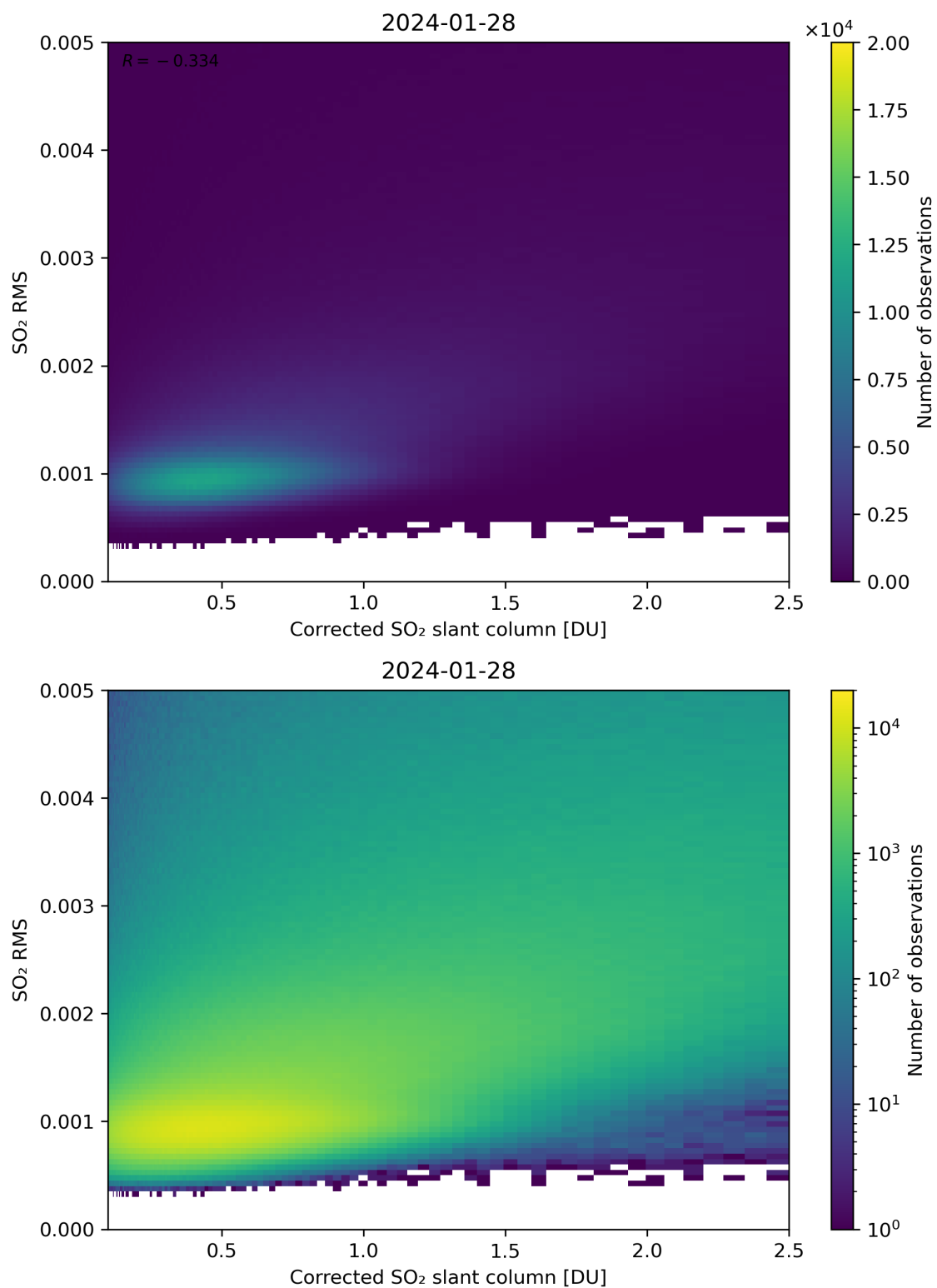
Figure 183: Scatter density plot of “Corrected SO 2 slant column” against “SO 2 RMS” for 2024-01-27 to 2024-01-29.
