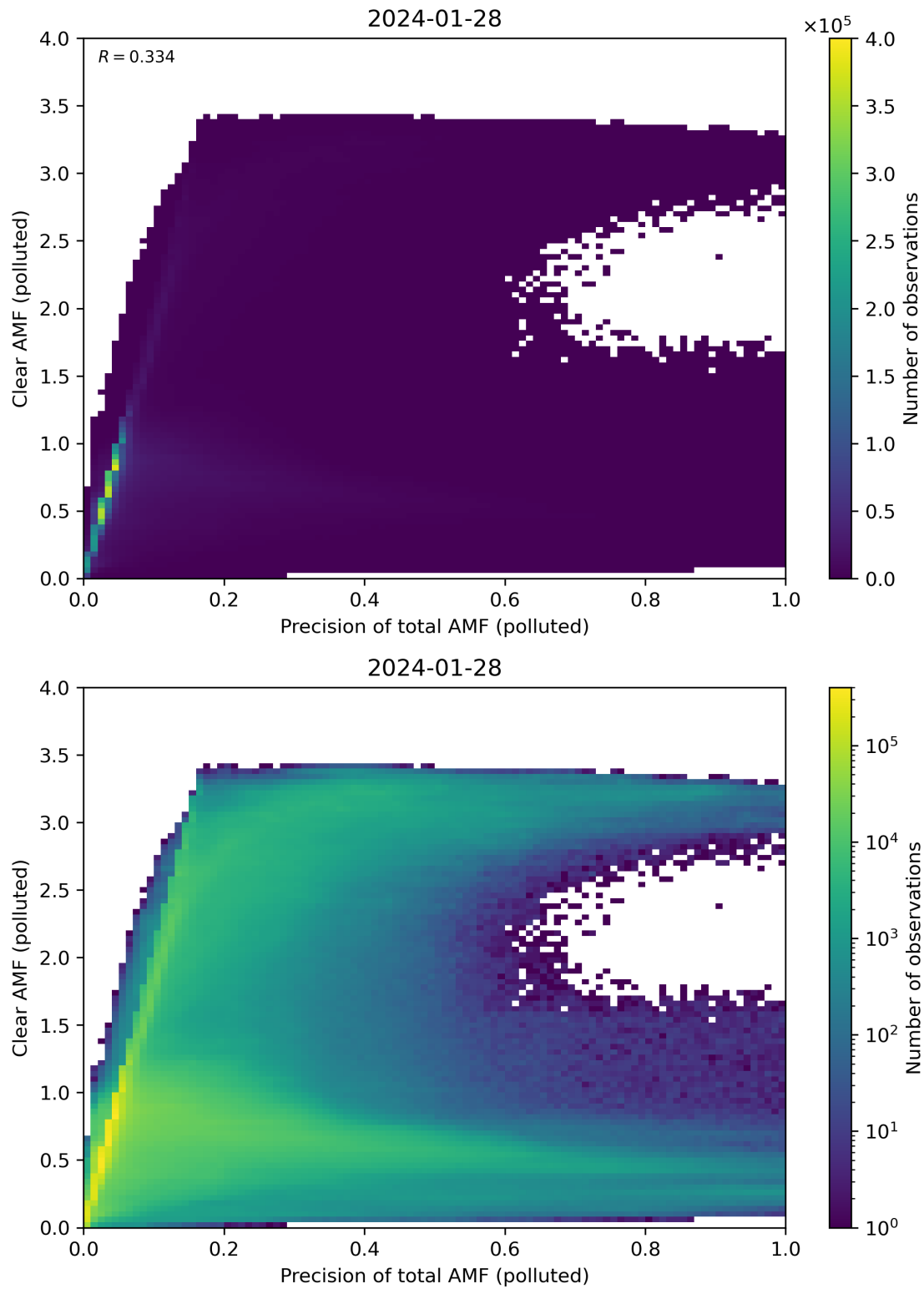
Figure 270: Scatter density plot of “Precision of total AMF (polluted)” against “Clear AMF (polluted)” for 2024-01-27 to 2024-01-29.
