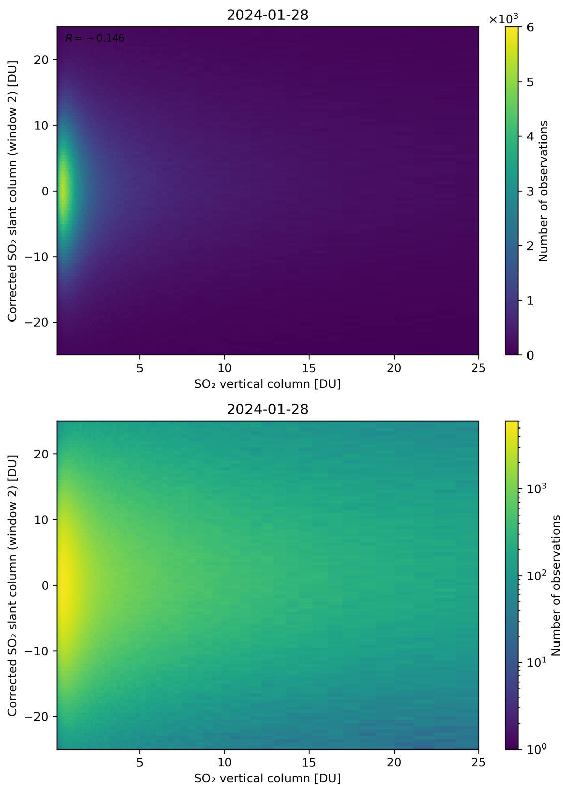
Figure 298: Scatter density plot of “SO 2 vertical column” against “Corrected SO 2 slant column (window 2)” for 2024-01-27 to 2024-01-29.
