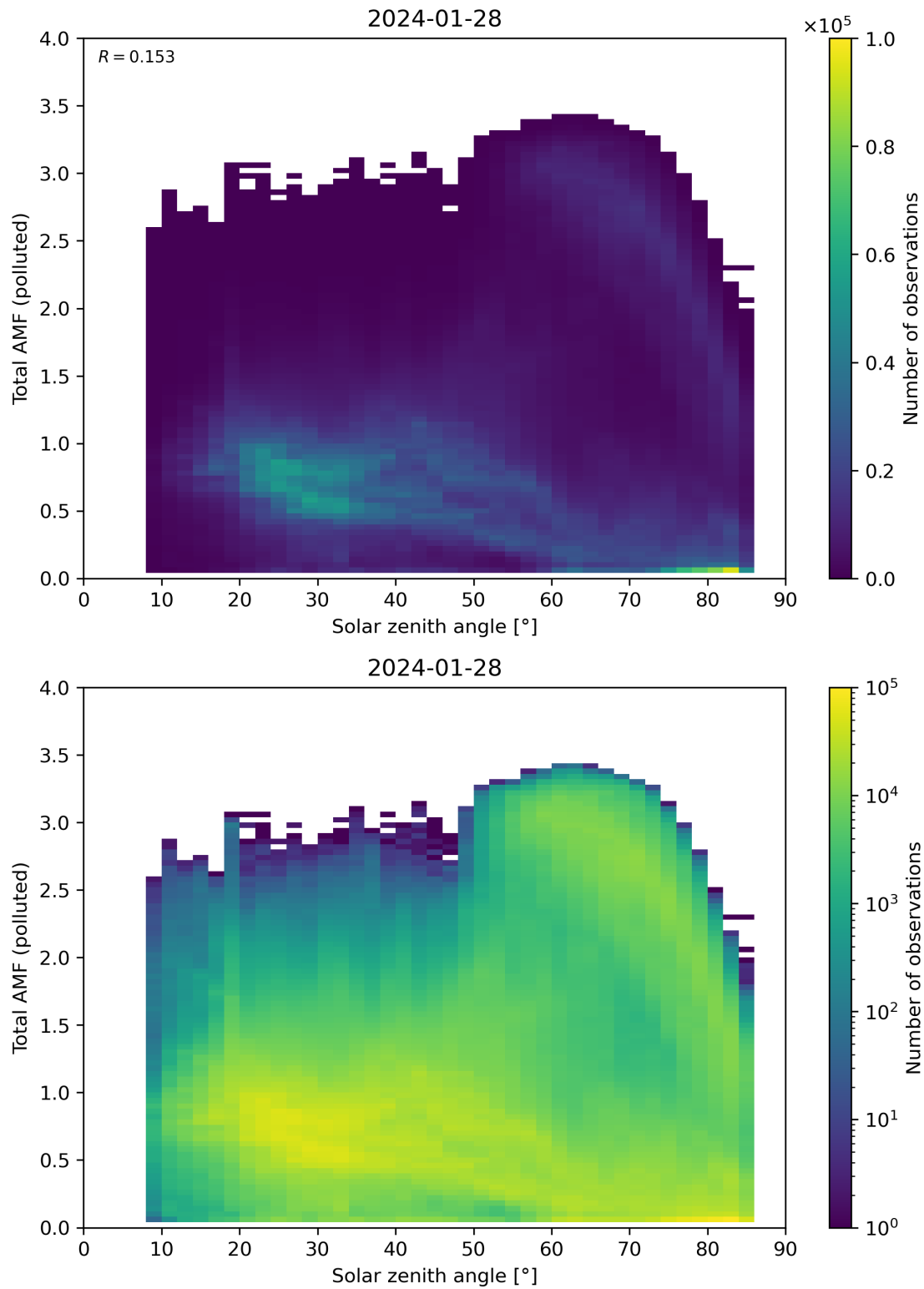
Figure 174: Scatter density plot of “Solar zenith angle” against “Total AMF (polluted)” for 2024-01-27 to 2024-01-29.
