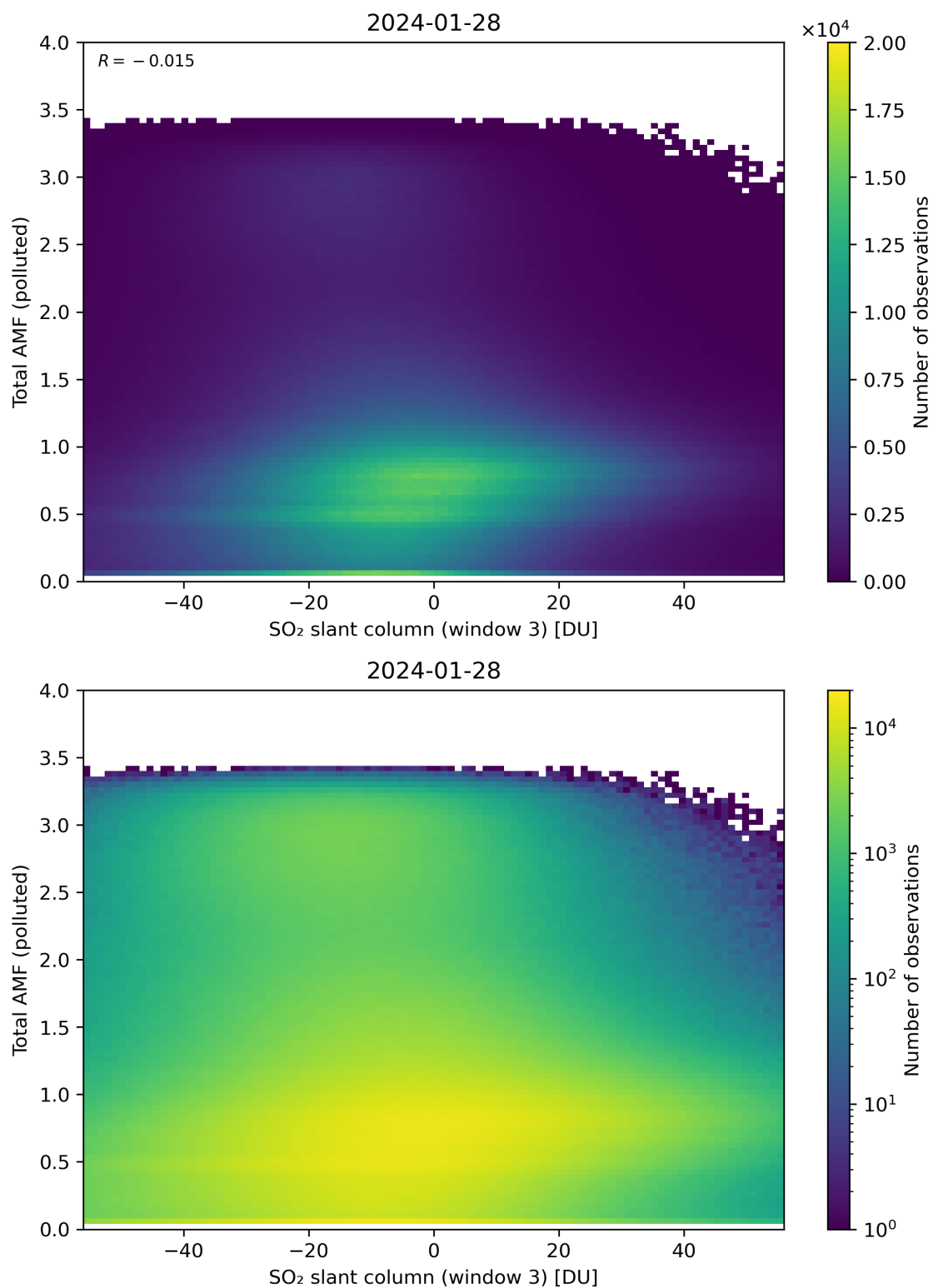
Figure 268: Scatter density plot of “SO 2 slant column (window 3)” against “Total AMF (polluted)” for 2024-01-27 to 2024-01-29.
