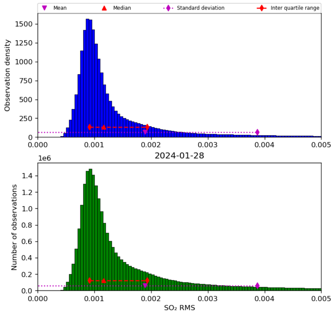
Figure 70: Histogram of “SO 2 RMS” for 2024-01-27 to 2024-01-29
