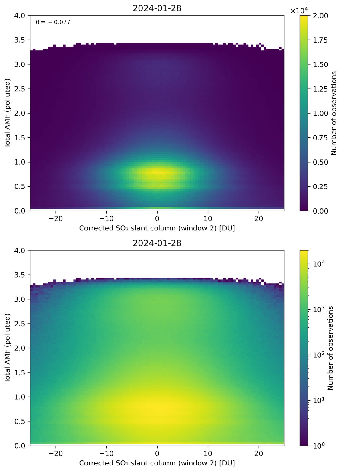
Figure 203: Scatter density plot of “Corrected SO 2 slant column (window 2)” against “Total AMF (polluted)” for 2024-01-27 to 2024-01-29.
