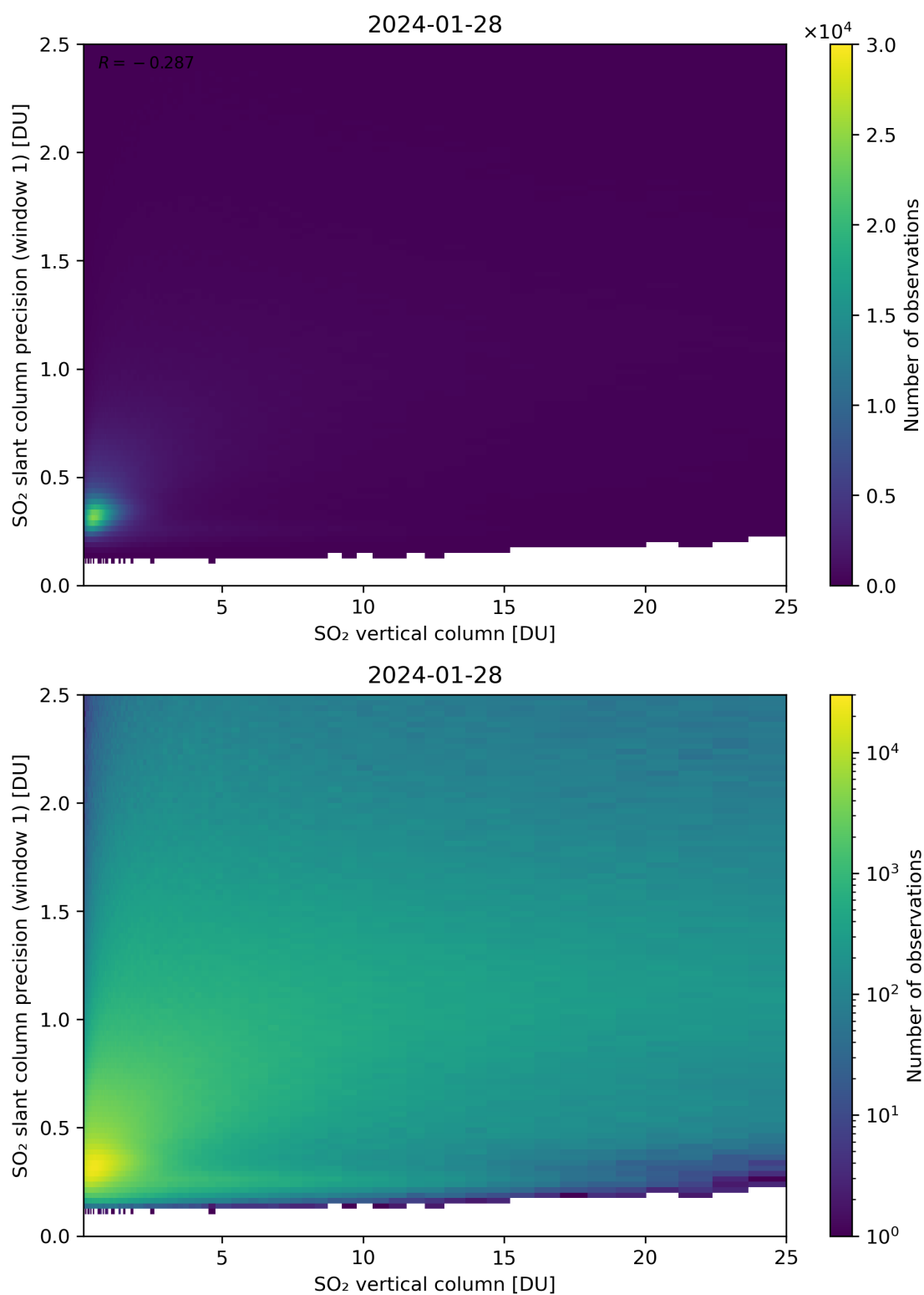
Figure 301: Scatter density plot of “SO 2 vertical column” against “SO 2 slant column precision (window 1)” for 2024-01-27 to 2024-01-29.
