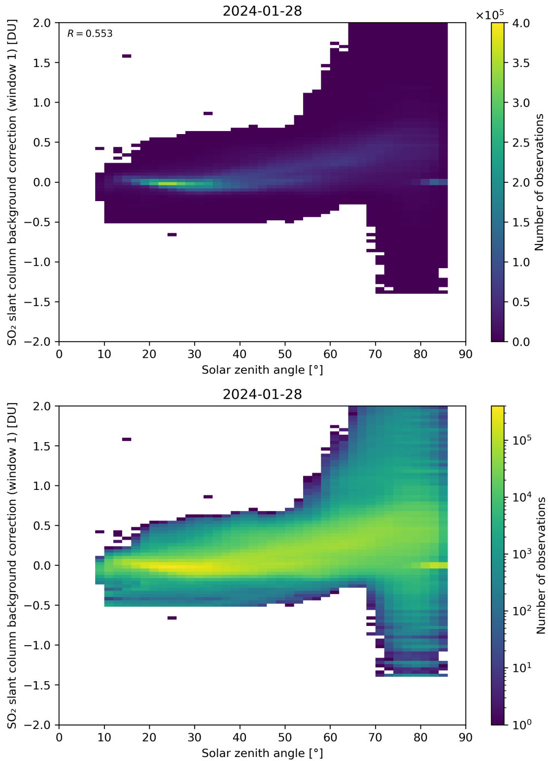
Figure 158: Scatter density plot of “Solar zenith angle” against “SO 2 slant column background correction (window 1)” for 2024-01-27 to 2024-01-29.
