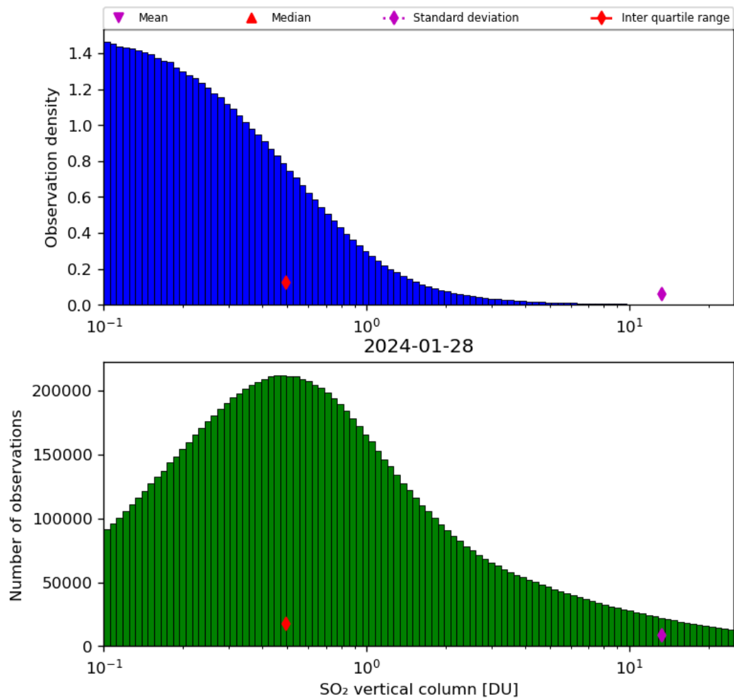
Figure 53: Histogram of “SO 2 vertical column” for 2024-01-27 to 2024-01-29
