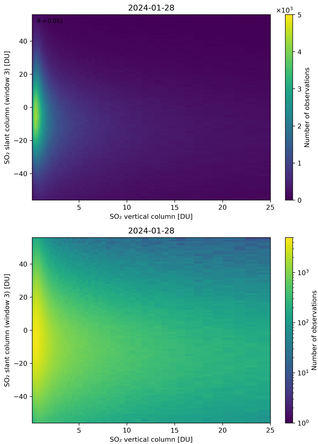
Figure 303: Scatter density plot of “SO 2 vertical column” against “SO 2 slant column (window 3)” for 2024-01-27 to 2024-01-29.
