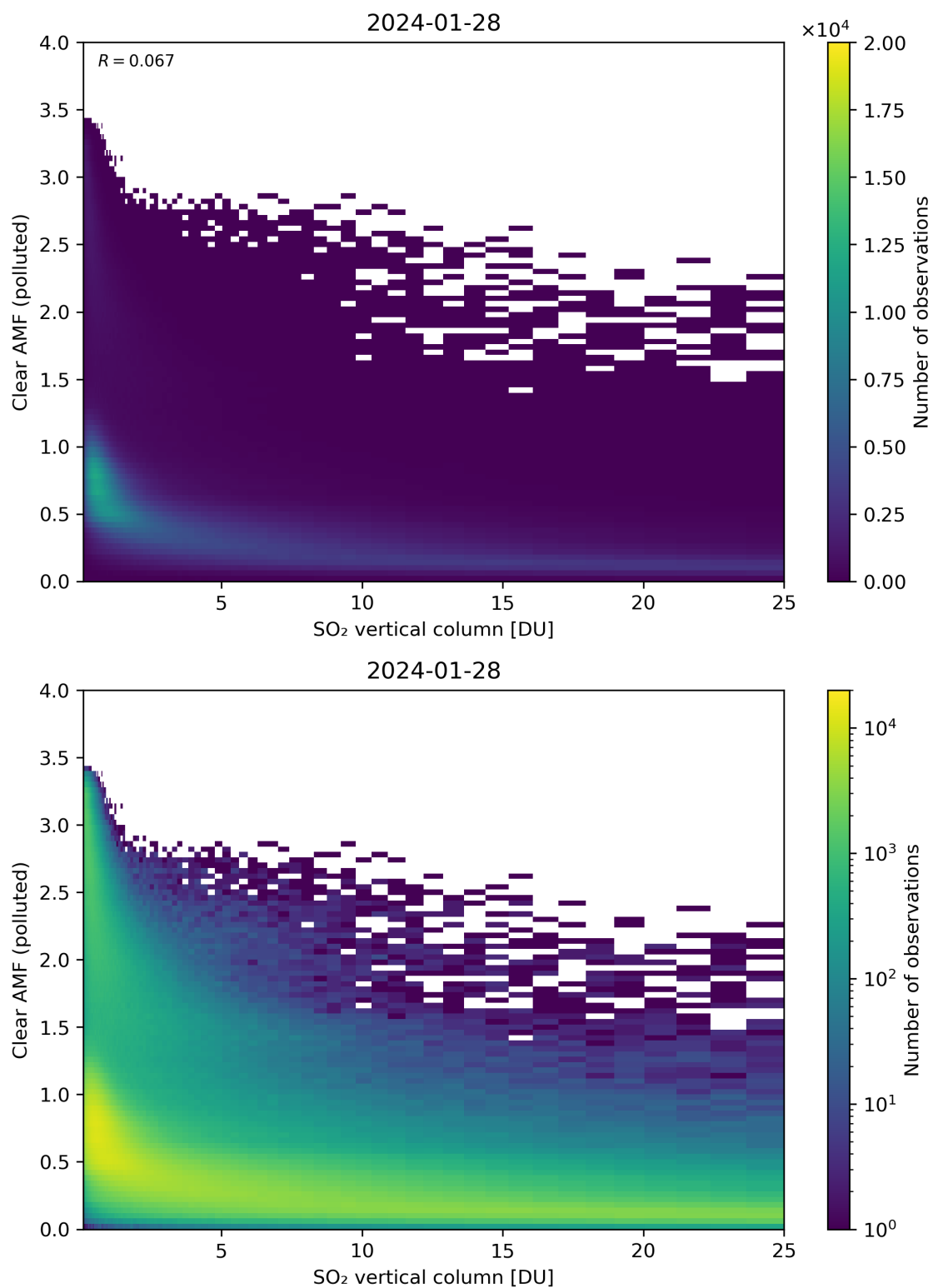
Figure 296: Scatter density plot of “SO 2 vertical column” against “Clear AMF (polluted)” for 2024-01-27 to 2024-01-29.
