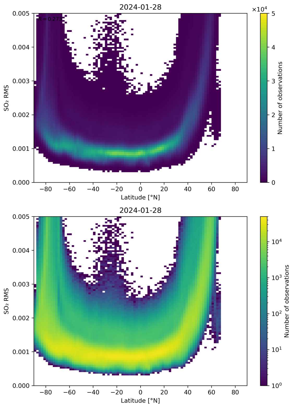
Figure 144: Scatter density plot of “Latitude” against “SO 2 RMS” for 2024-01-27 to 2024-01-29.
