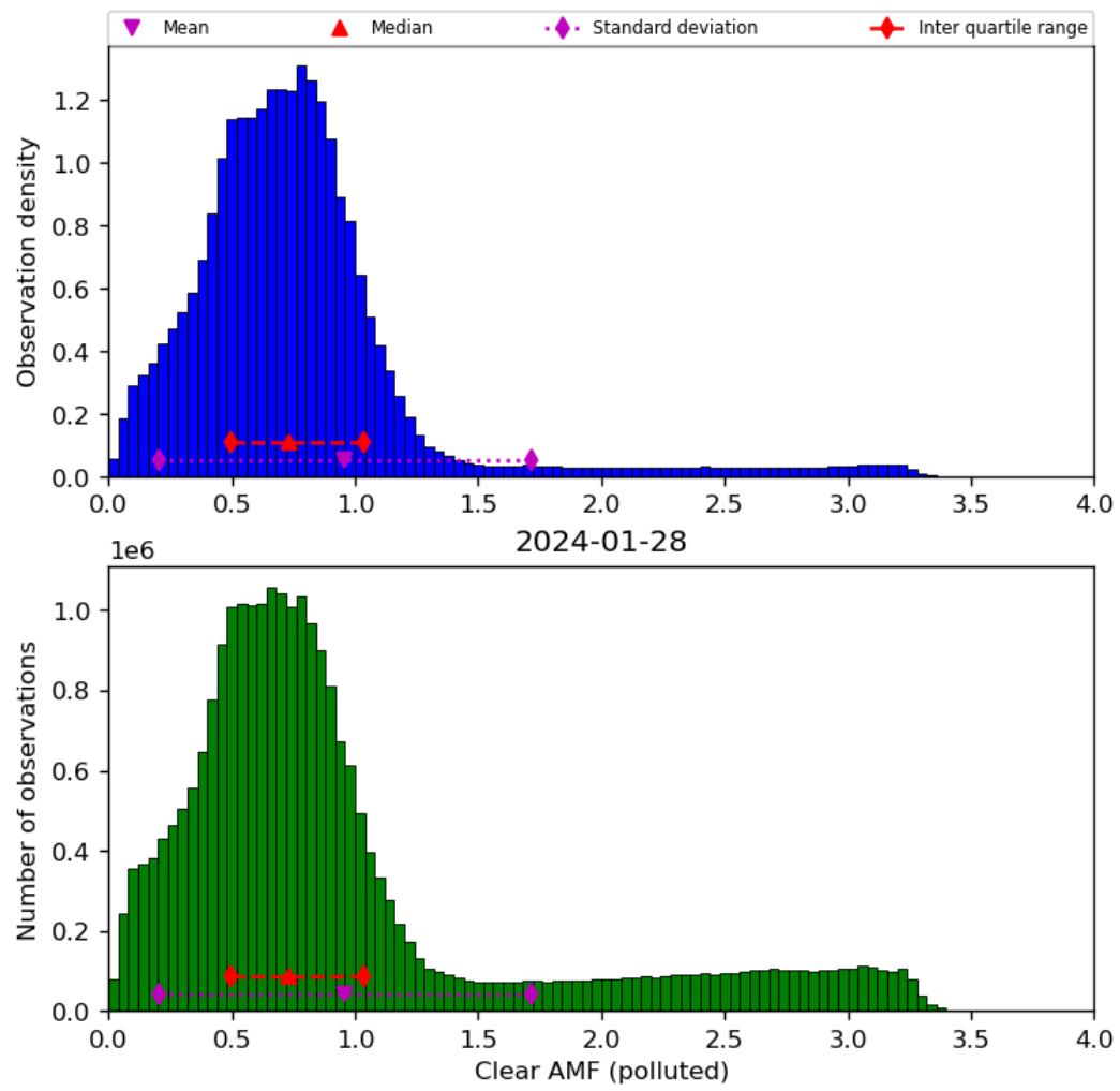
Figure 73: Histogram of “Clear AMF (polluted)” for 2024-01-27 to 2024-01-29
