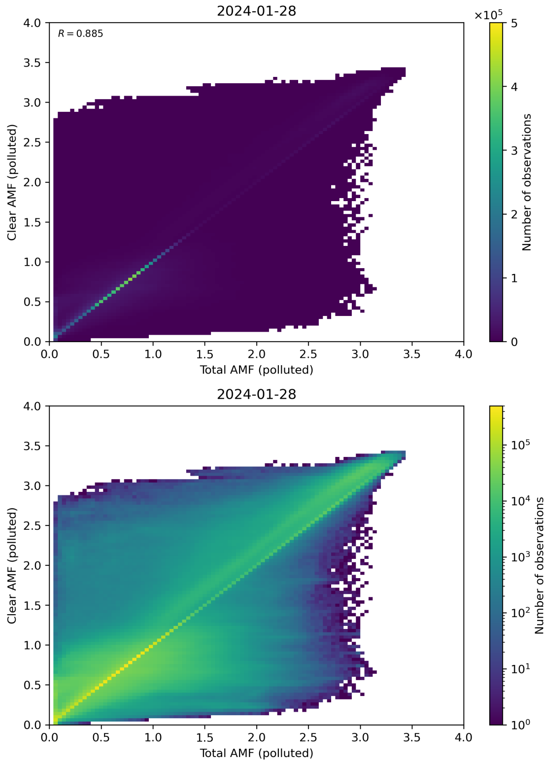
Figure 271: Scatter density plot of “Total AMF (polluted)” against “Clear AMF (polluted)” for 2024-01-27 to 2024-01-29.
