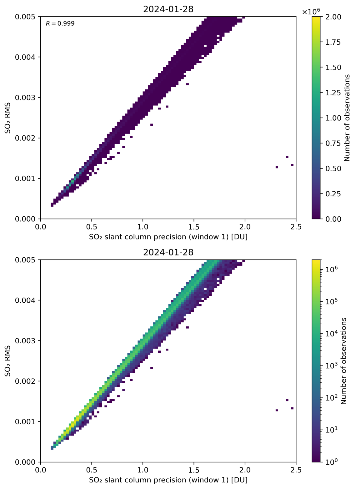
Figure 223: Scatter density plot of “SO 2 slant column precision (window 1)” against “SO 2 RMS” for 2024-01-27 to 2024-01-29.
