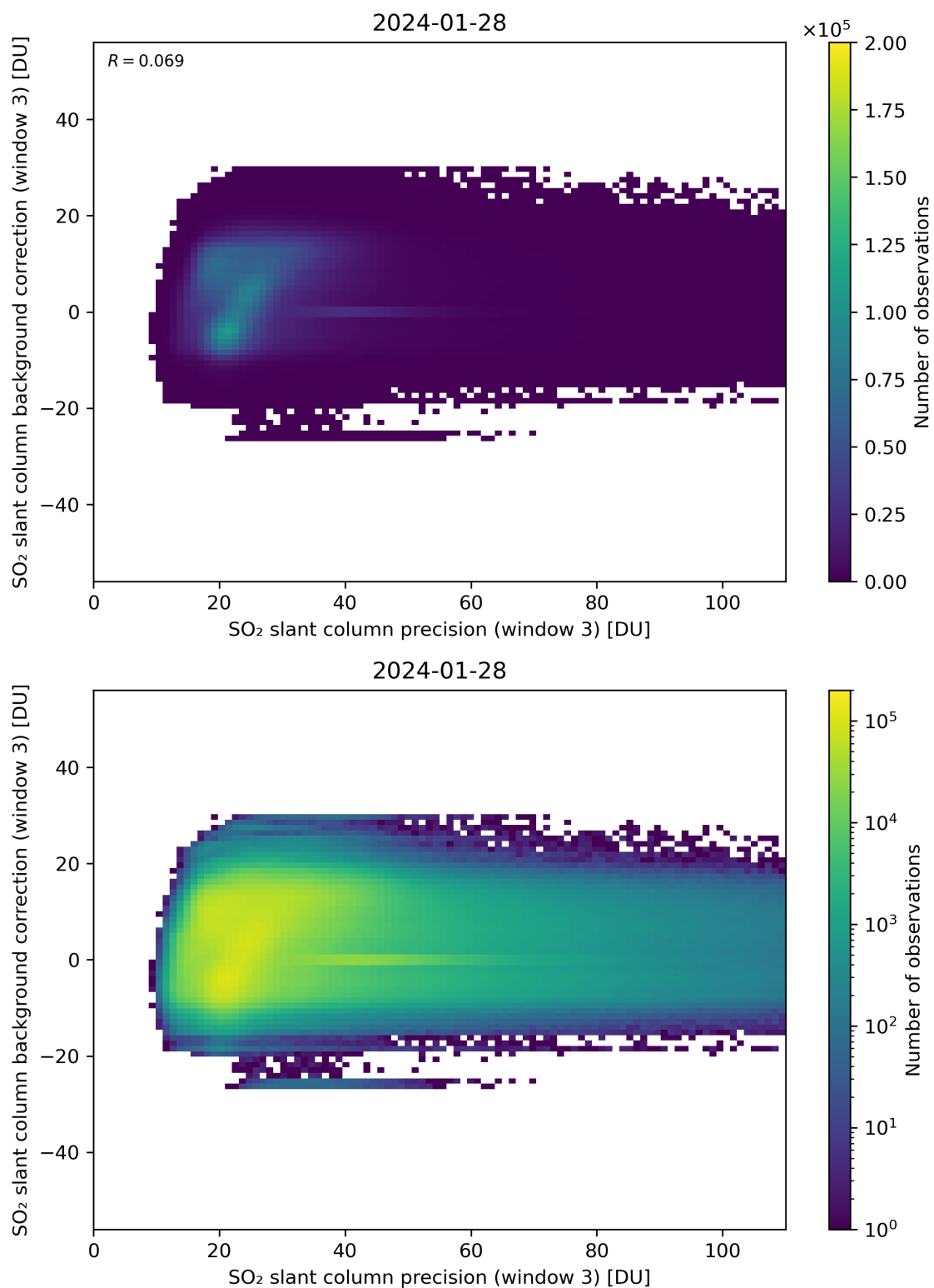
Figure 257: Scatter density plot of “SO 2 slant column precision (window 3)” against “SO 2 slant column background correction (window 3)” for 2024-01-27 to 2024-01-29.
