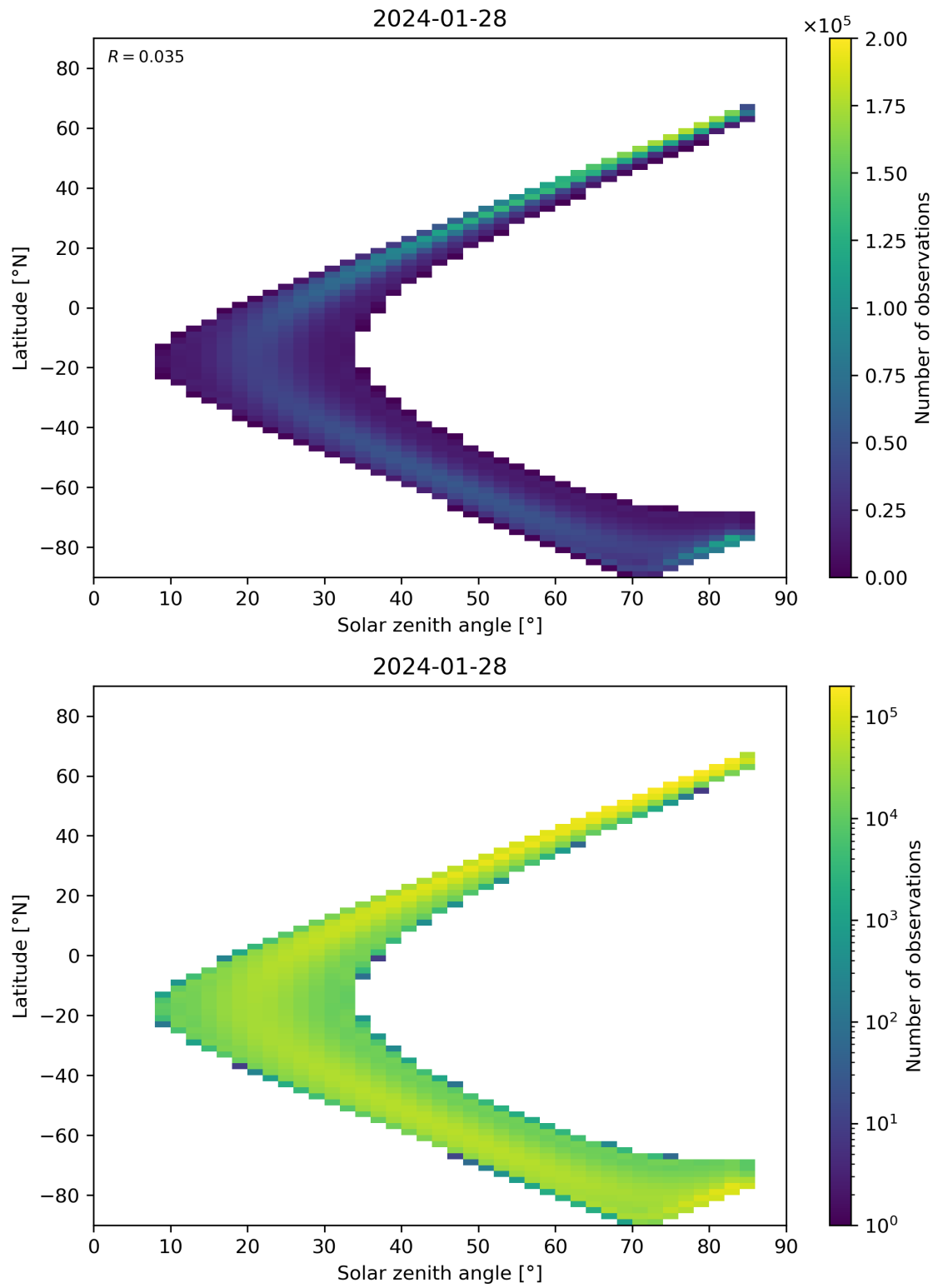
Figure 164: Scatter density plot of “Solar zenith angle” against “Latitude” for 2024-01-27 to 2024-01-29.
