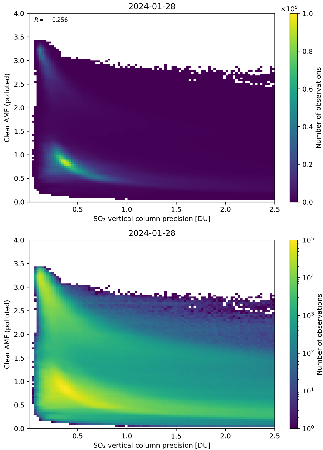
Figure 285: Scatter density plot of “SO 2 vertical column precision” against “Clear AMF (polluted)” for 2024-01-27 to 2024-01-29.
