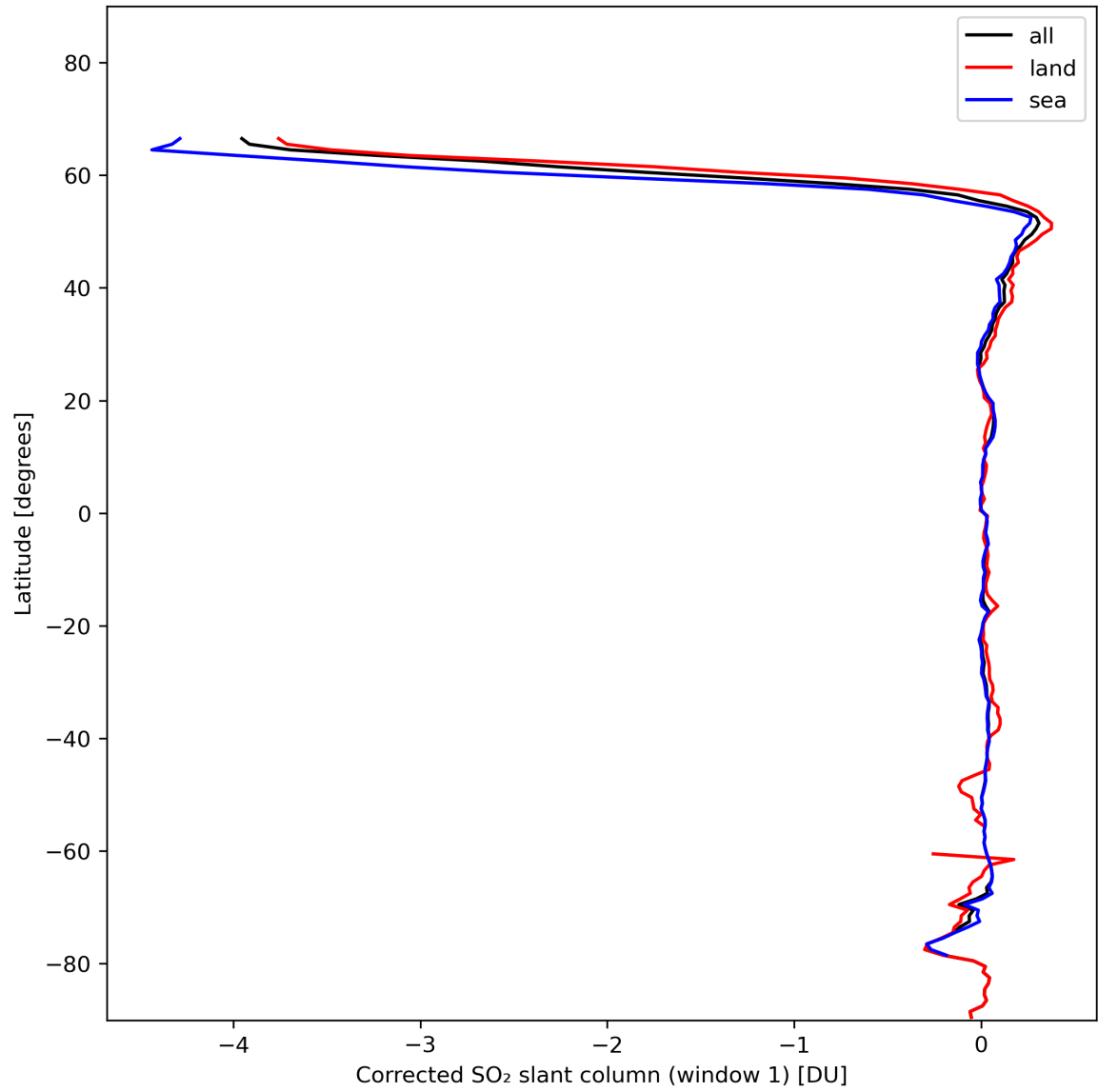
Figure 35: Zonal average of “Corrected SO 2 slant column (window 1)” for 2024-01-27 to 2024-01-29.
