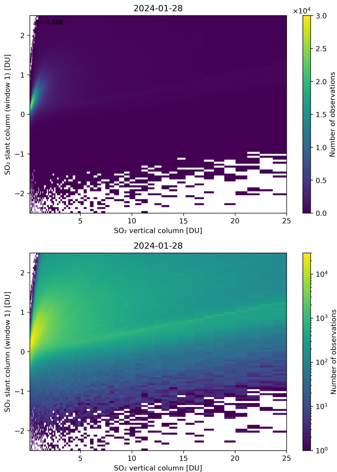
Figure 300: Scatter density plot of “SO 2 vertical column” against “SO 2 slant column (window 1)” for 2024-01-27 to 2024-01-29.
