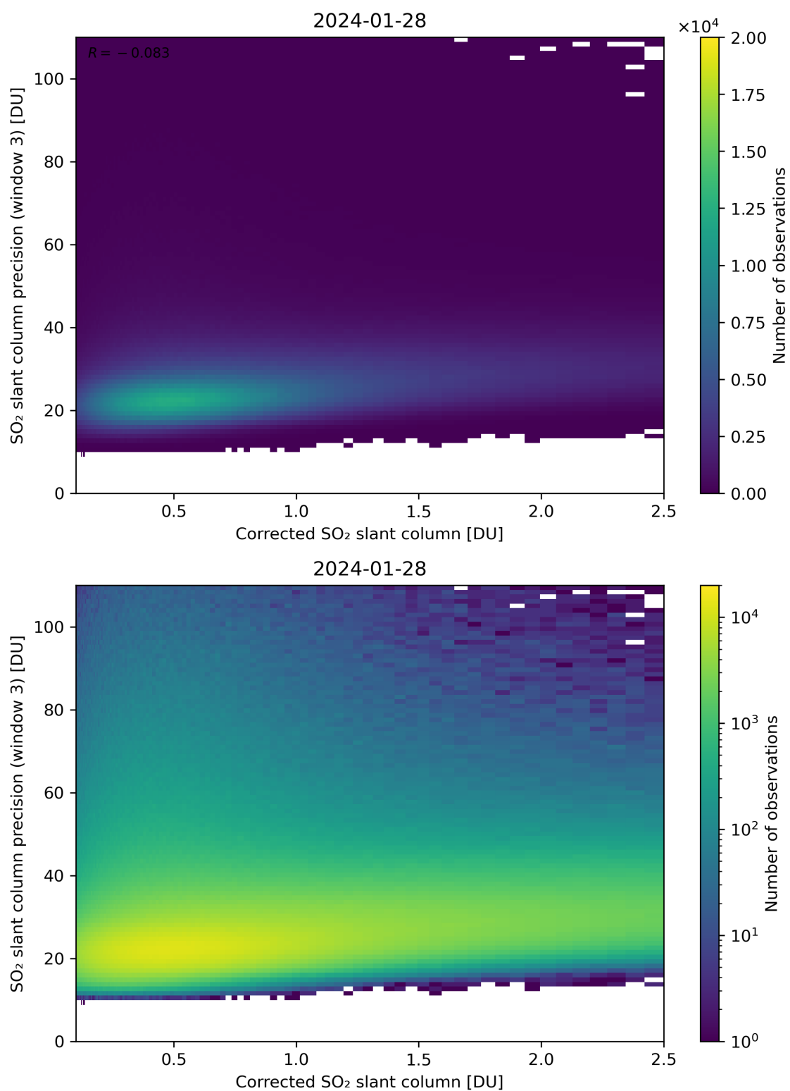
Figure 191: Scatter density plot of “Corrected SO 2 slant column” against “SO 2 slant column precision (window 3)” for 2024-01-27 to 2024-01-29.
