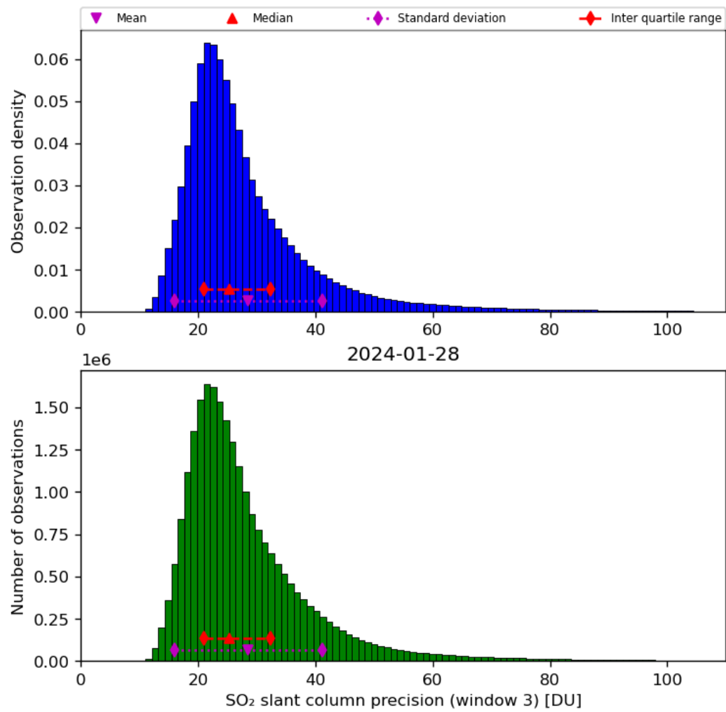
Figure 65: Histogram of “SO 2 slant column precision (window 3)” for 2024-01-27 to 2024-01-29
