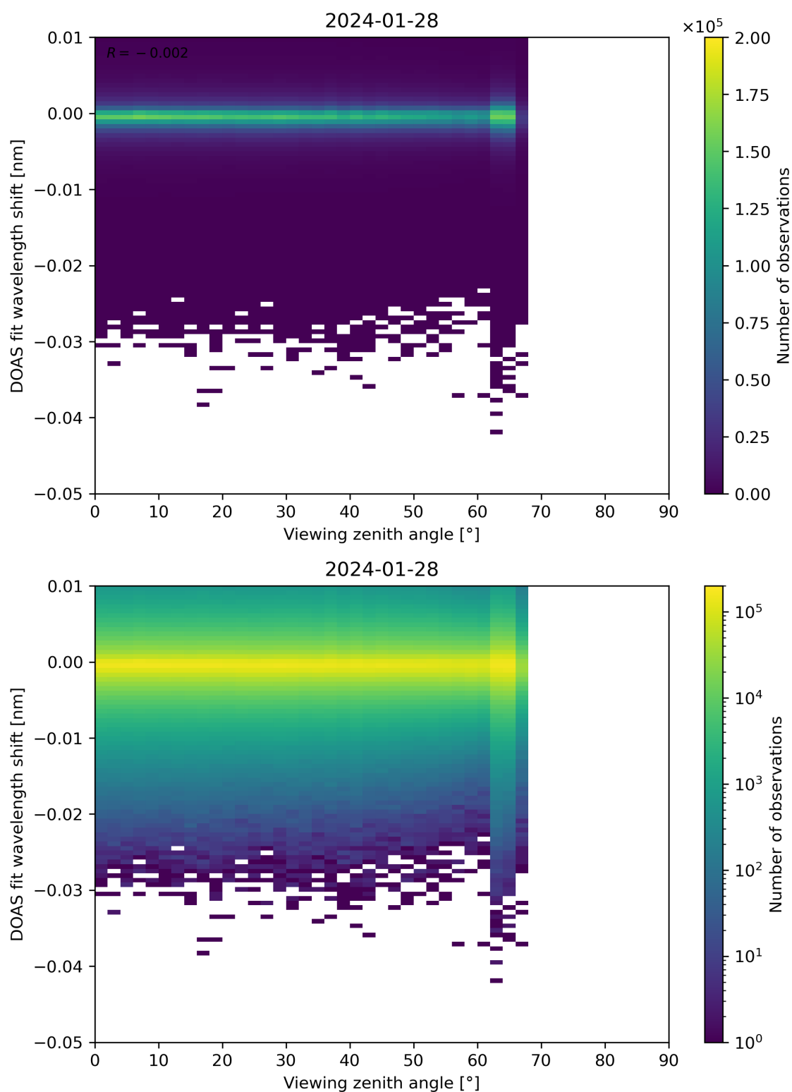
Figure 311: Scatter density plot of “Viewing zenith angle” against “DOAS fit wavelength shift” for 2024-01-27 to 2024-01-29.
