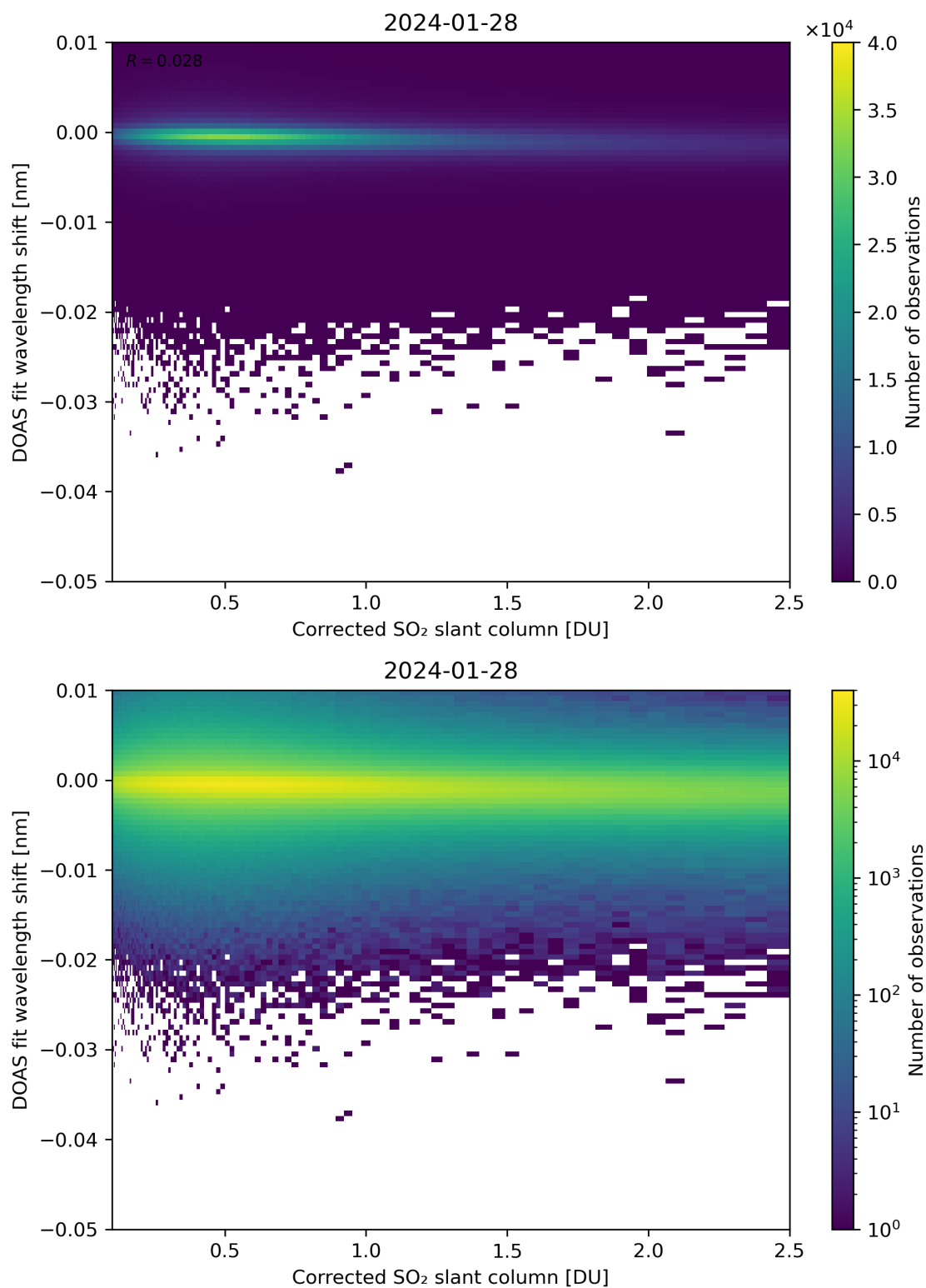
Figure 181: Scatter density plot of “Corrected SO 2 slant column” against “DOAS fit wavelength shift” for 2024-01-27 to 2024-01-29.
