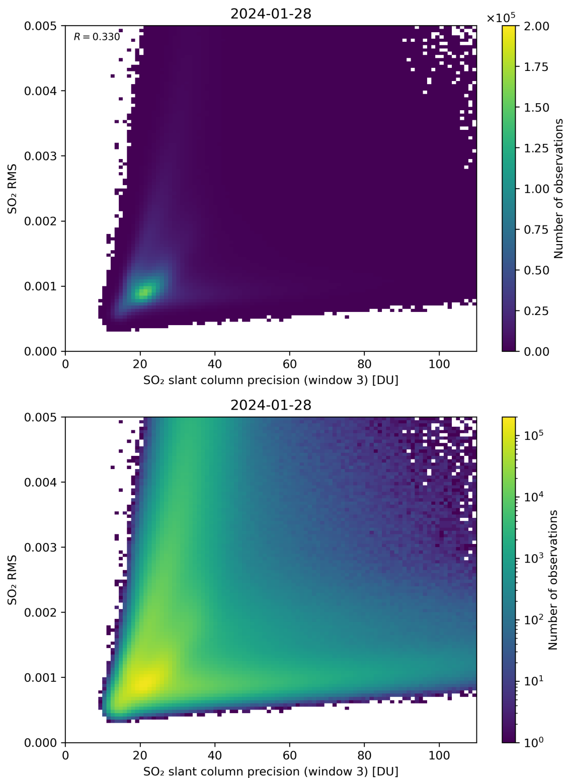
Figure 260: Scatter density plot of “SO 2 slant column precision (window 3)” against “SO 2 RMS” for 2024-01-27 to 2024-01-29.
