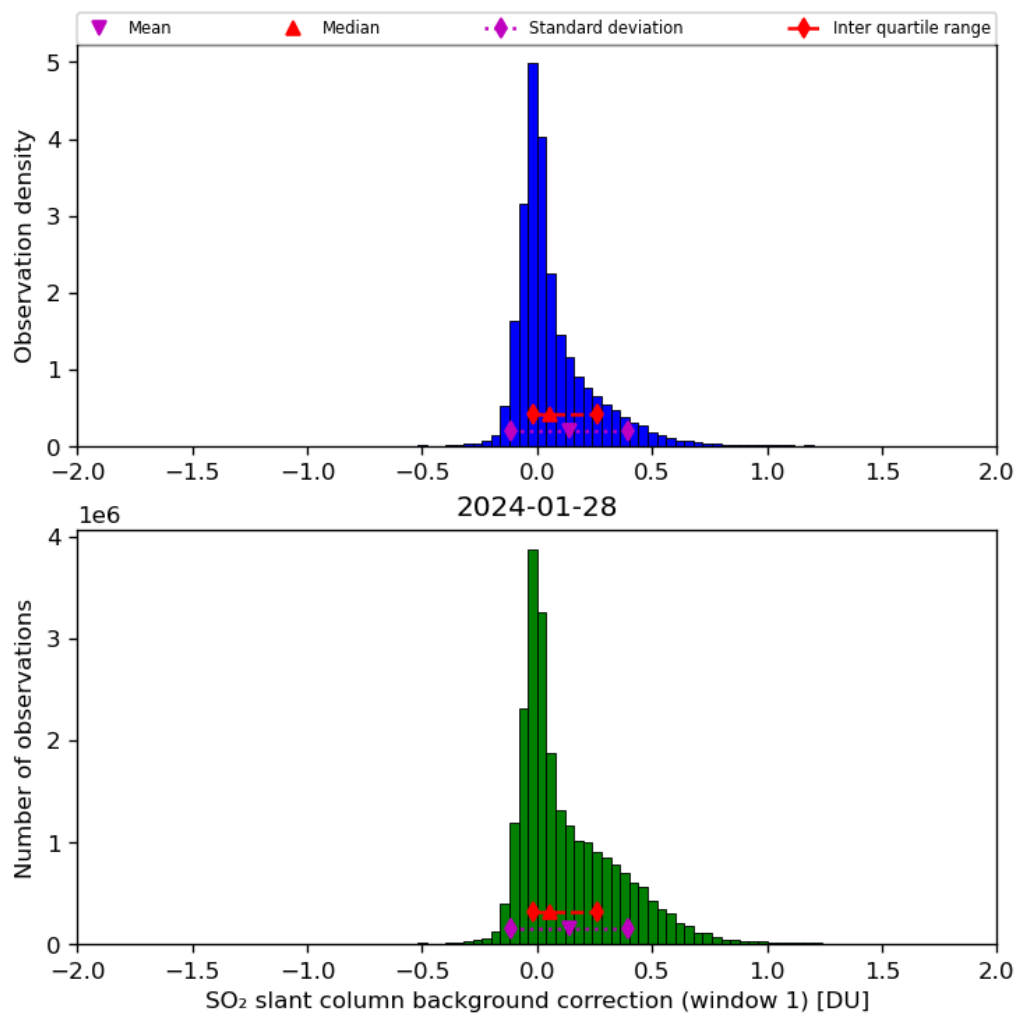
Figure 59: Histogram of “SO 2 slant column background correction (window 1)” for 2024-01-27 to 2024-01-29
