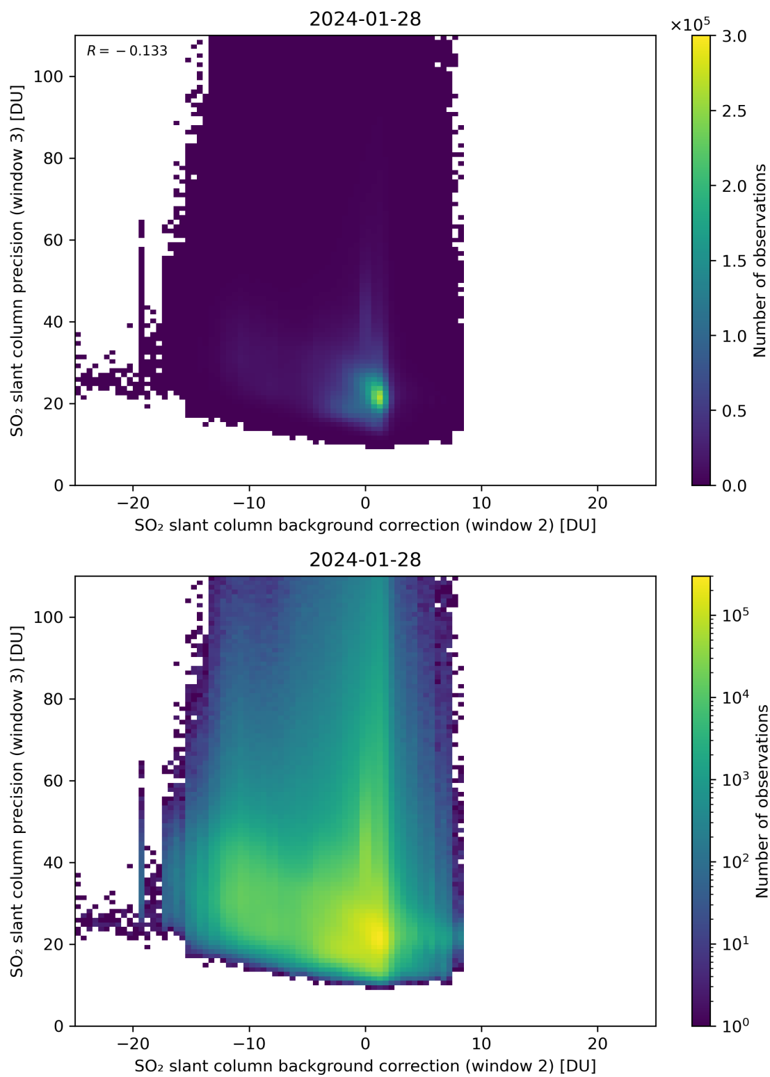
Figure 118: Scatter density plot of “SO 2 slant column background correction (window 2)” against “SO 2 slant column precision (window 3)” for 2024-01-27 to 2024-01-29.
