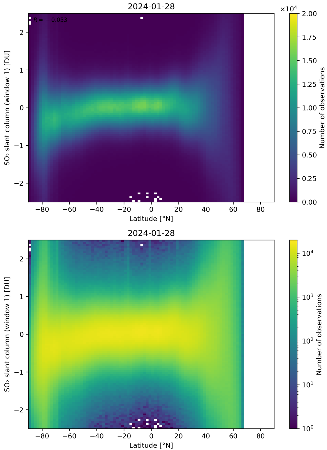
Figure 149: Scatter density plot of “Latitude” against “SO 2 slant column (window 1)” for 2024-01-27 to 2024-01-29.
