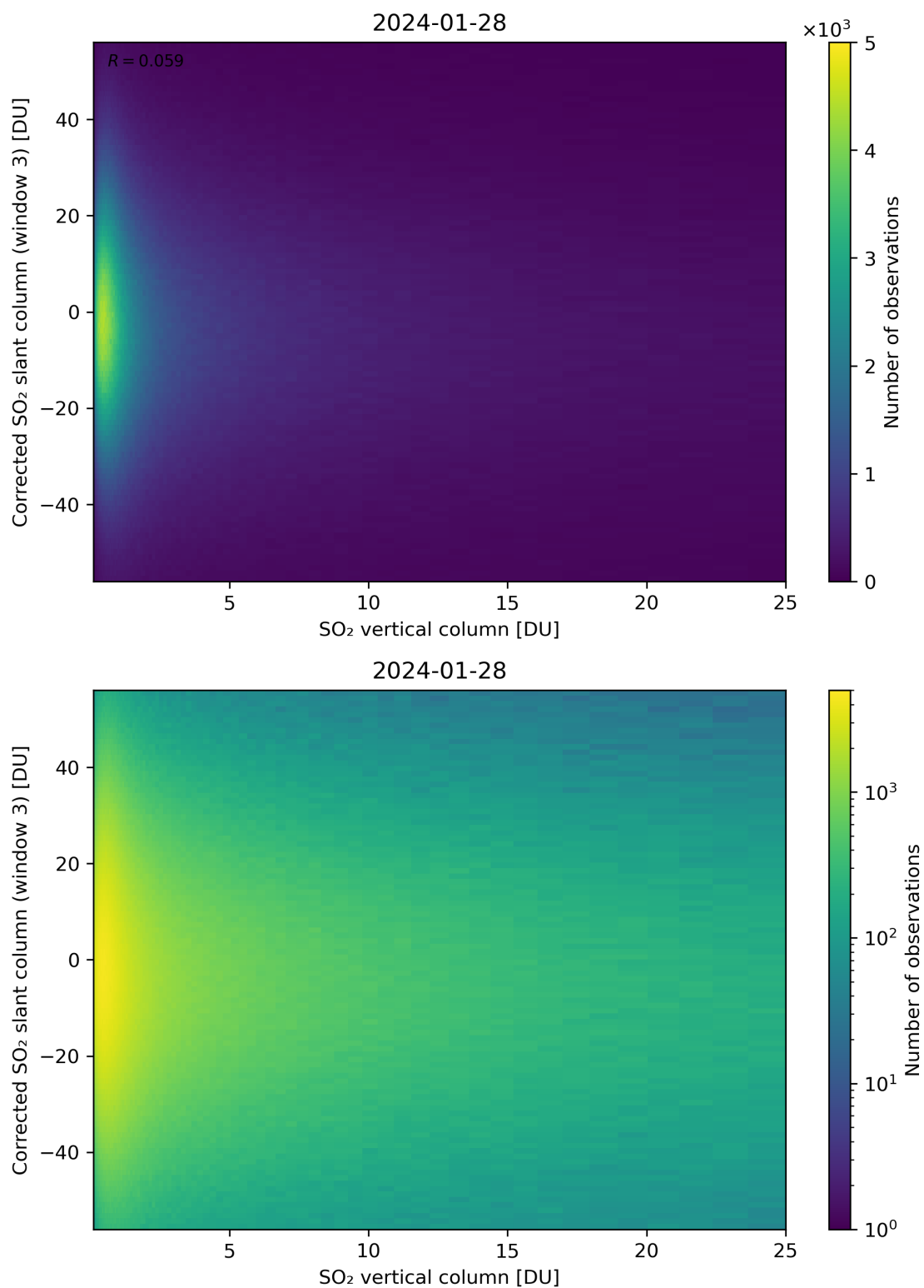
Figure 299: Scatter density plot of “SO 2 vertical column” against “Corrected SO 2 slant column (window 3)” for 2024-01-27 to 2024-01-29.
