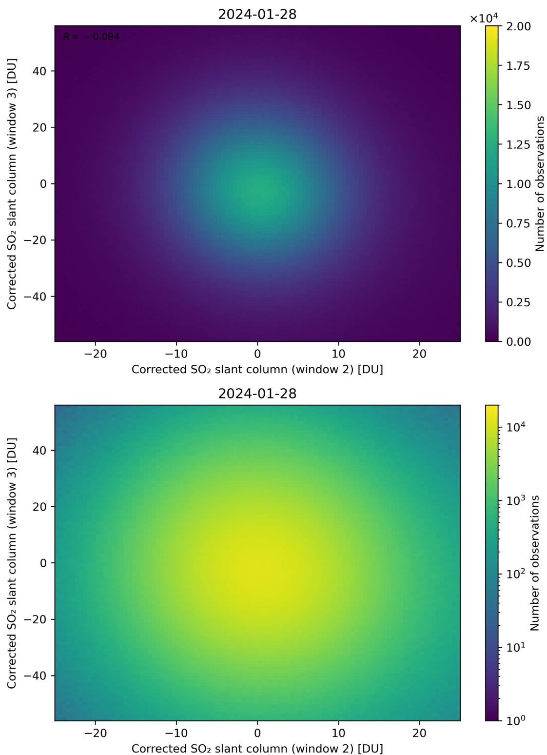
Figure 200: Scatter density plot of “Corrected SO 2 slant column (window 2)” against “Corrected SO 2 slant column (window 3)” for 2024-01-27 to 2024-01-29.
