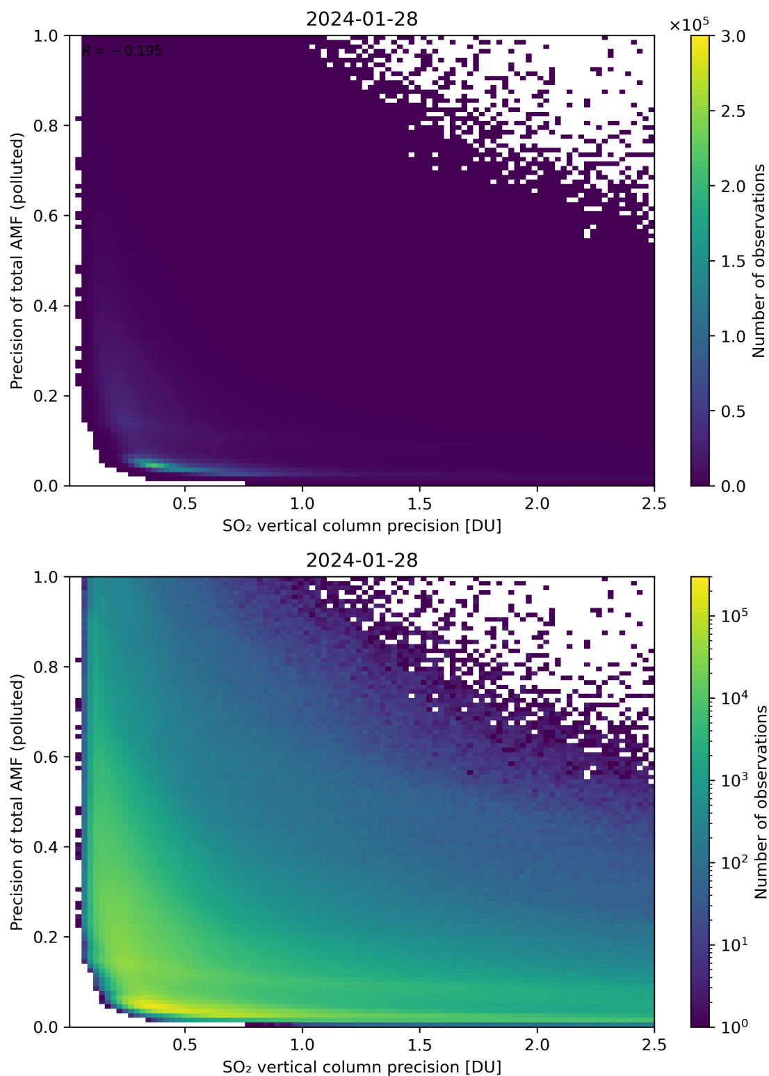
Figure 295: Scatter density plot of “SO 2 vertical column precision” against “Precision of total AMF (polluted)” for 2024-01-27 to 2024-01-29.
