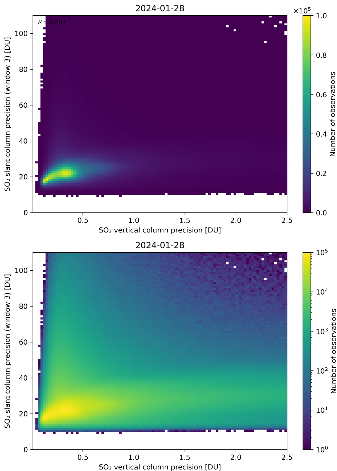
Figure 293: Scatter density plot of “SO 2 vertical column precision” against “SO 2 slant column precision (window 3)” for 2024-01-27 to 2024-01-29.
