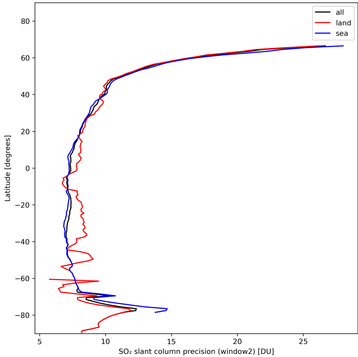
Figure 38: Zonal average of “SO 2 slant column precision (window2)” for 2024-01-27 to 2024-01-29.
