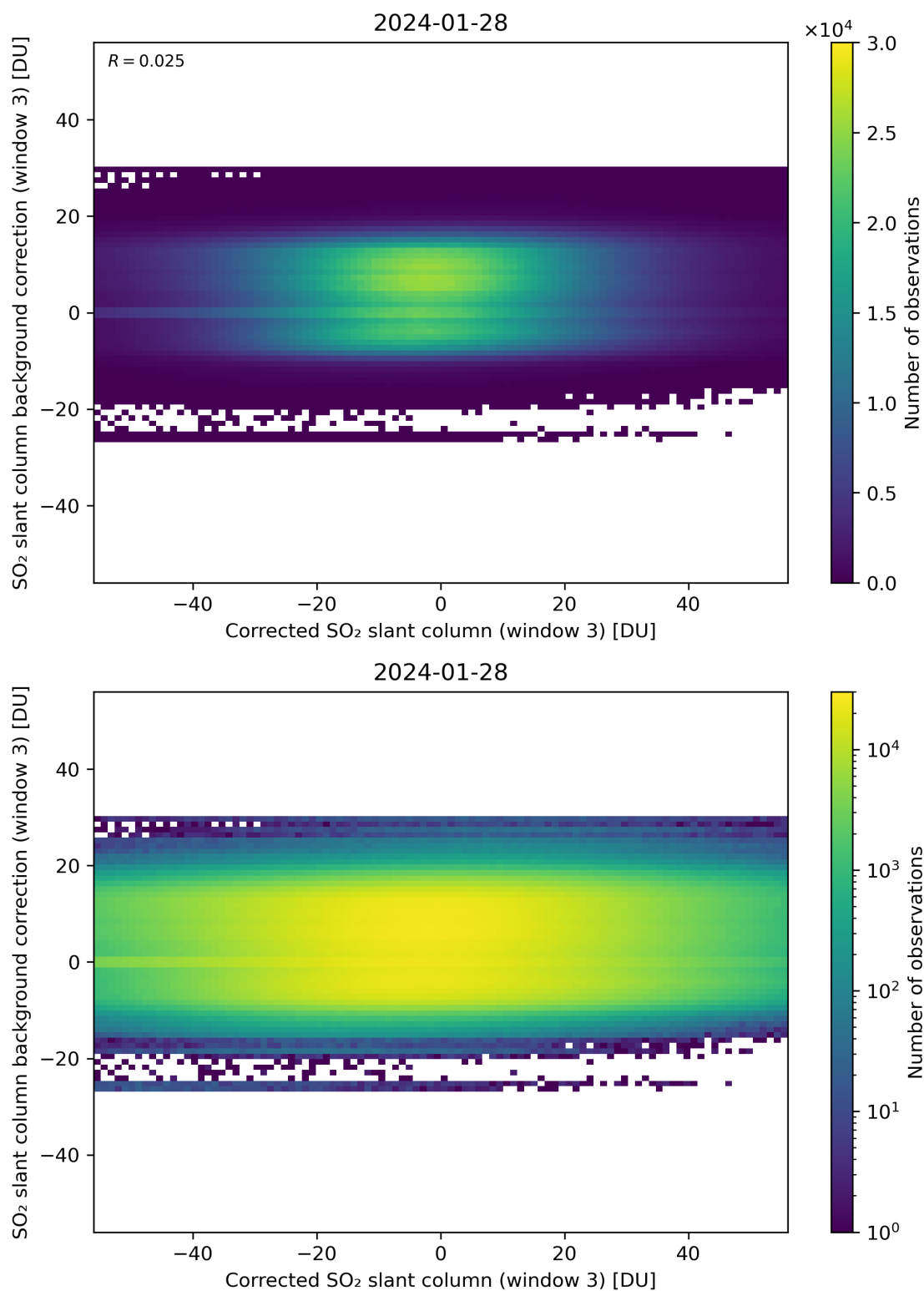
Figure 205: Scatter density plot of “Corrected SO 2 slant column (window 3)” against “SO 2 slant column background correction (window 3)” for 2024-01-27 to 2024-01-29.
