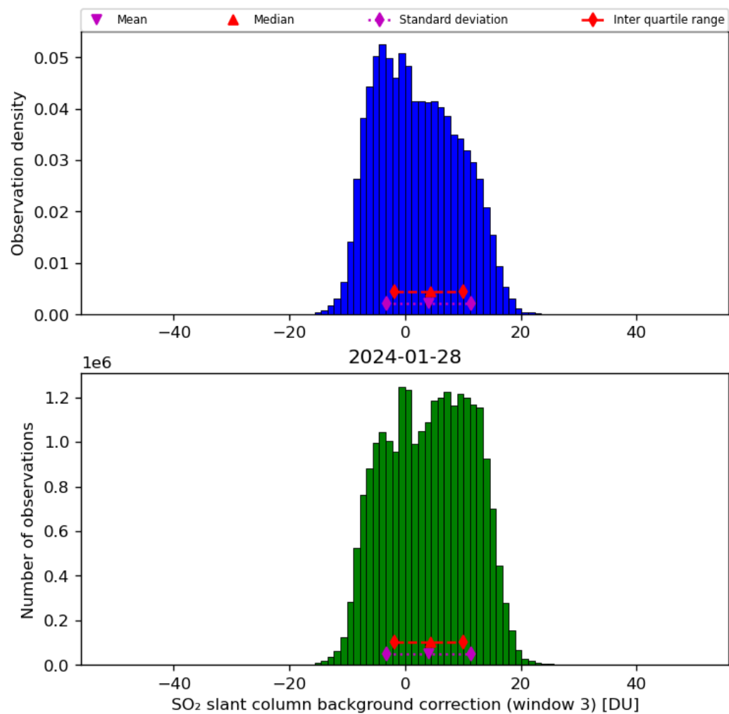
Figure 67: Histogram of “SO 2 slant column background correction (window 3)” for 2024-01-27 to 2024-01-29
