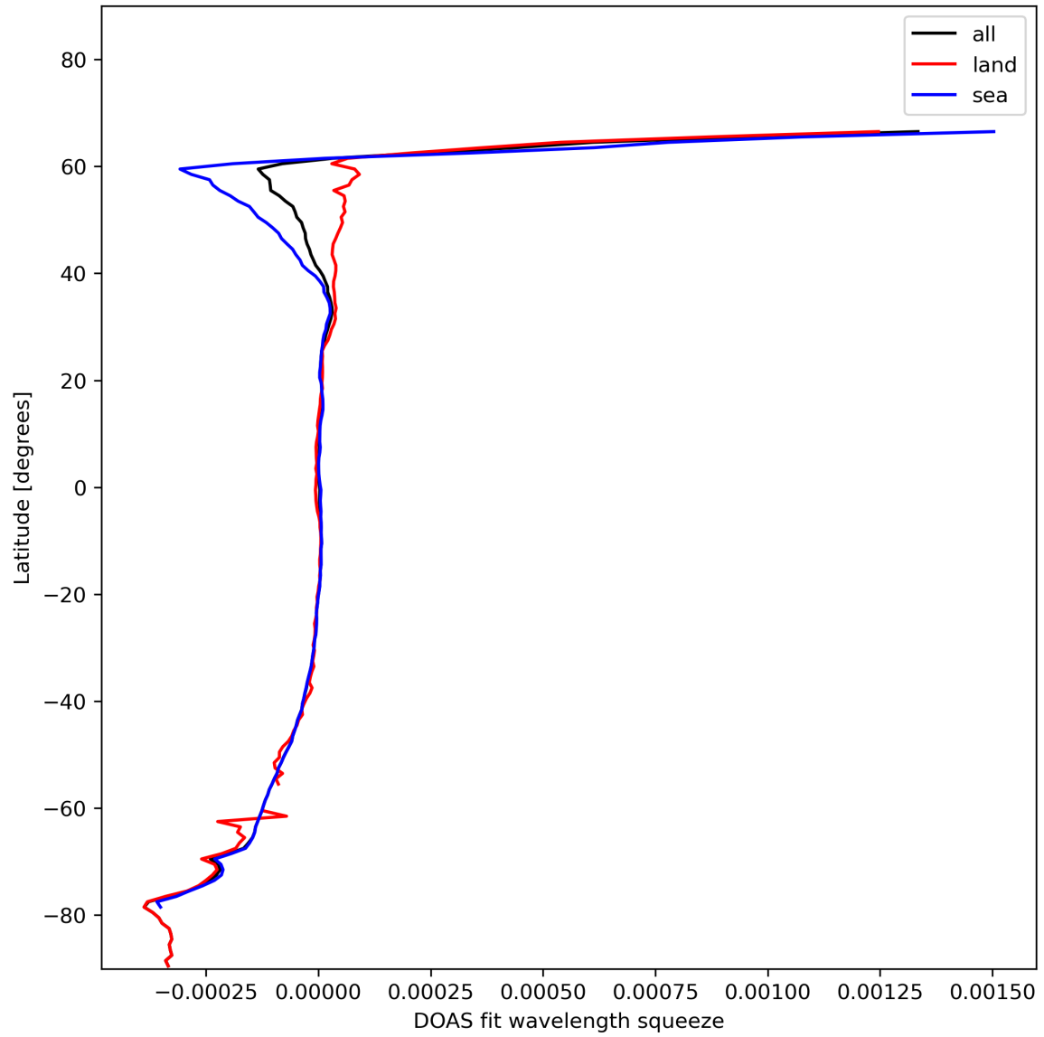
Figure 46: Zonal average of "DOAS fit wavelength squeeze" for 2024-01-27 to 2024-01-29.
