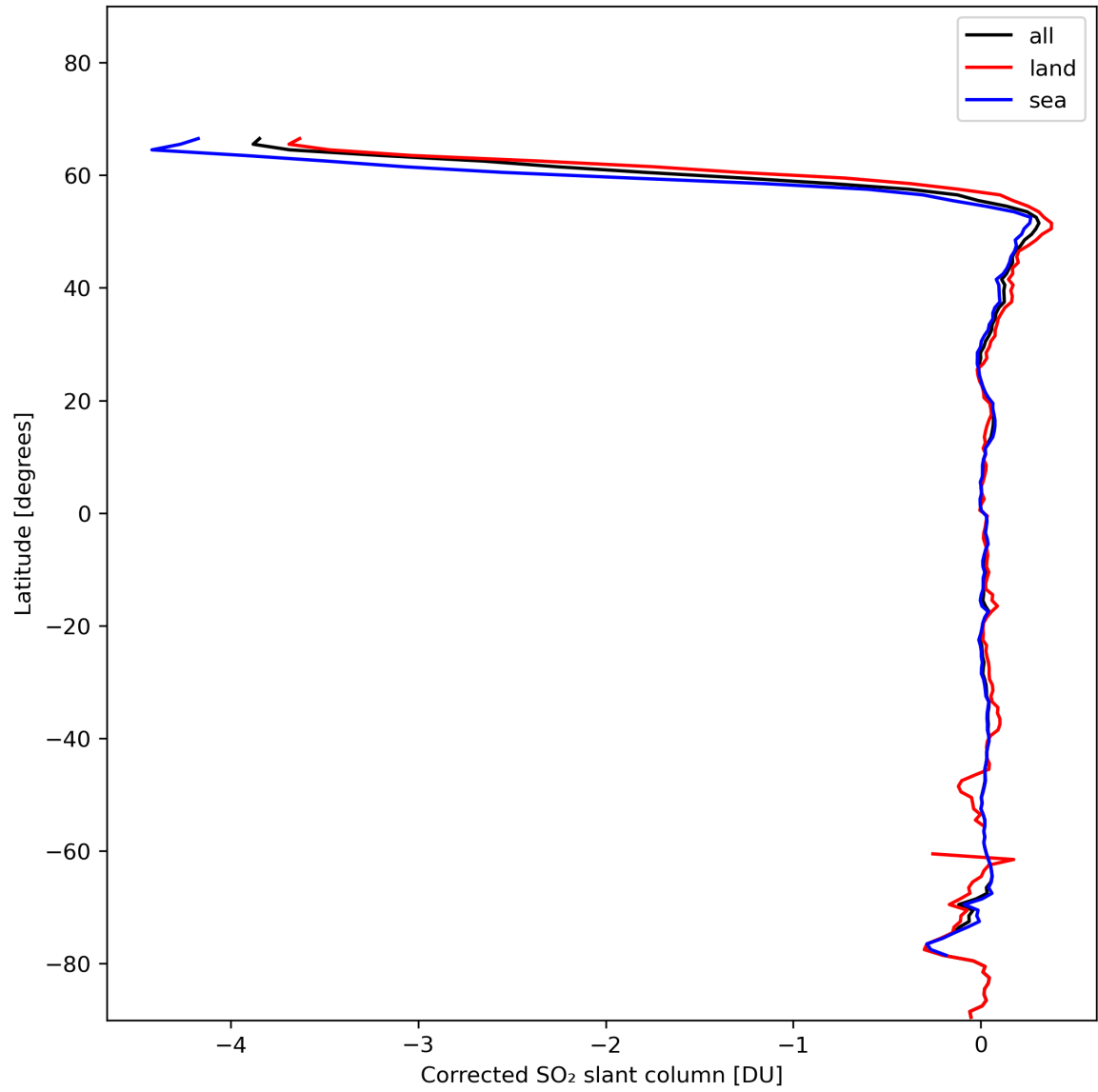
Figure 32: Zonal average of "Corrected SO 2 slant column" for 2024-01-27 to 2024-01-29.
