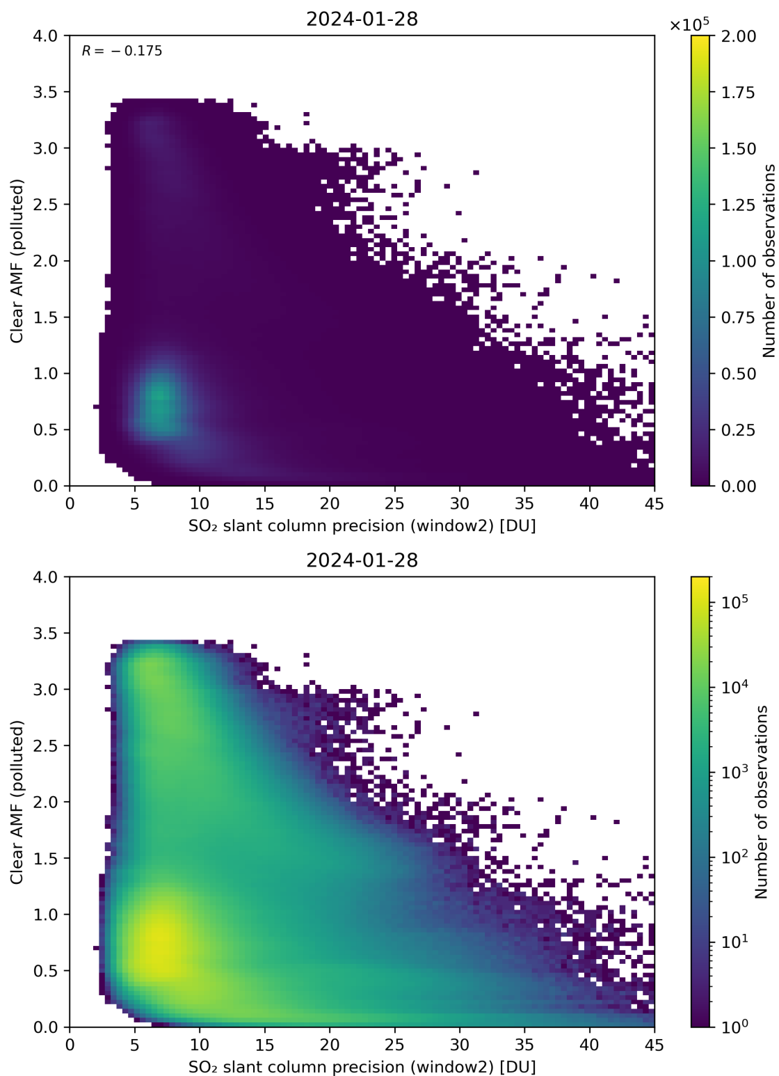
Figure 246: Scatter density plot of “SO 2 slant column precision (window2)” against “Clear AMF (polluted)” for 2024-01-27 to 2024-01-29.
