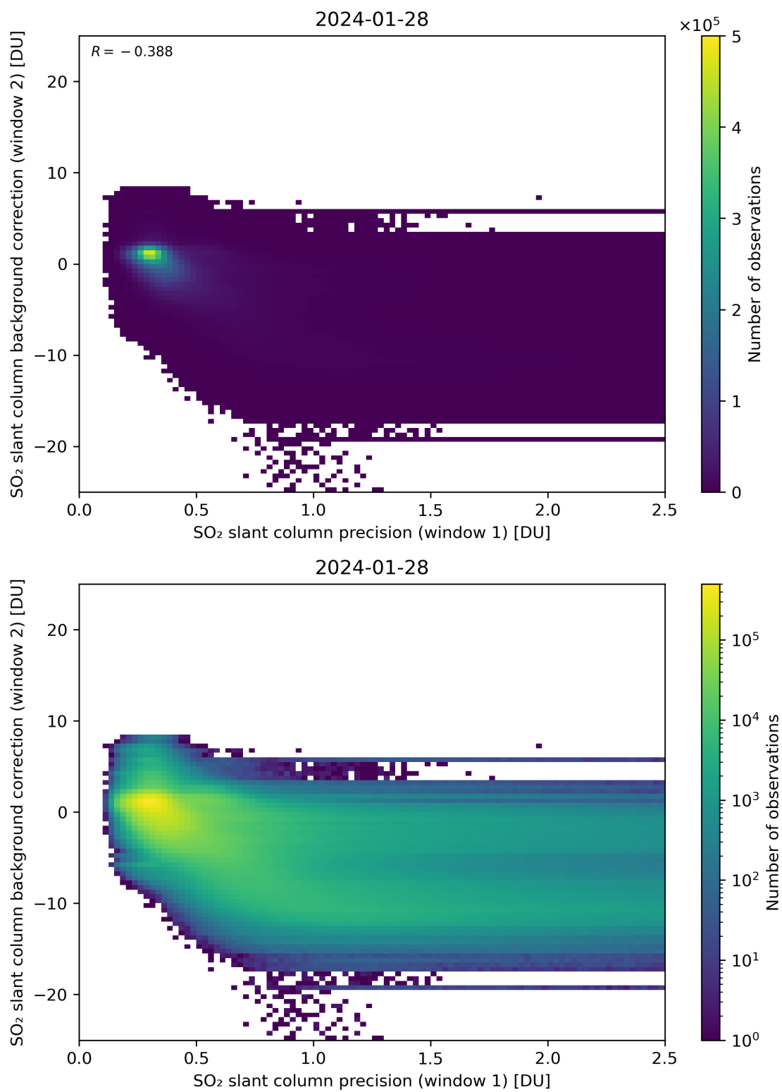
Figure 219: Scatter density plot of “SO 2 slant column precision (window 1)” against “SO 2 slant column background correction (window 2)” for 2024-01-27 to 2024-01-29.
