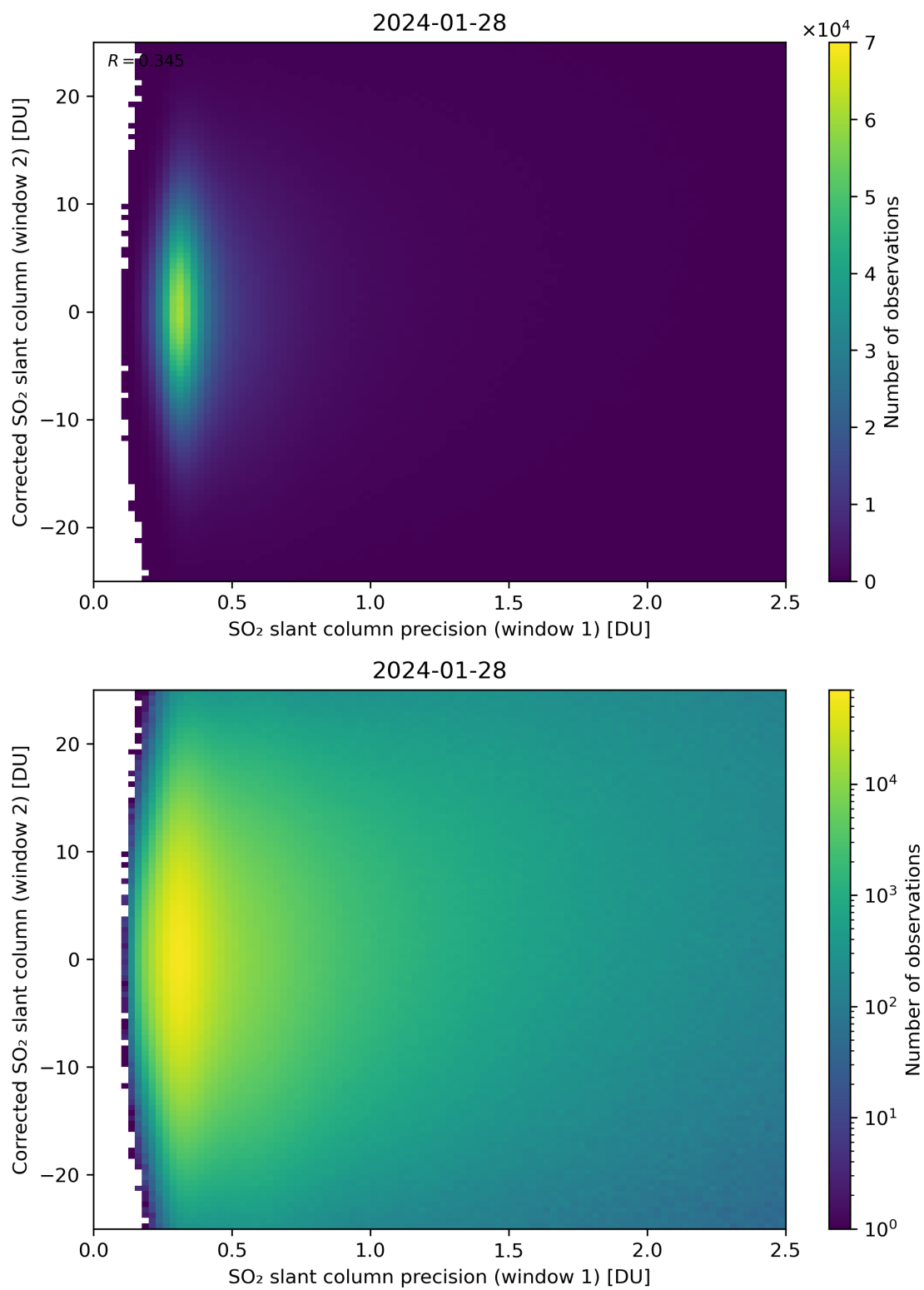
Figure 225: Scatter density plot of “SO 2 slant column precision (window 1)” against “Corrected SO 2 slant column (window 2)” for 2024-01-27 to 2024-01-29.
