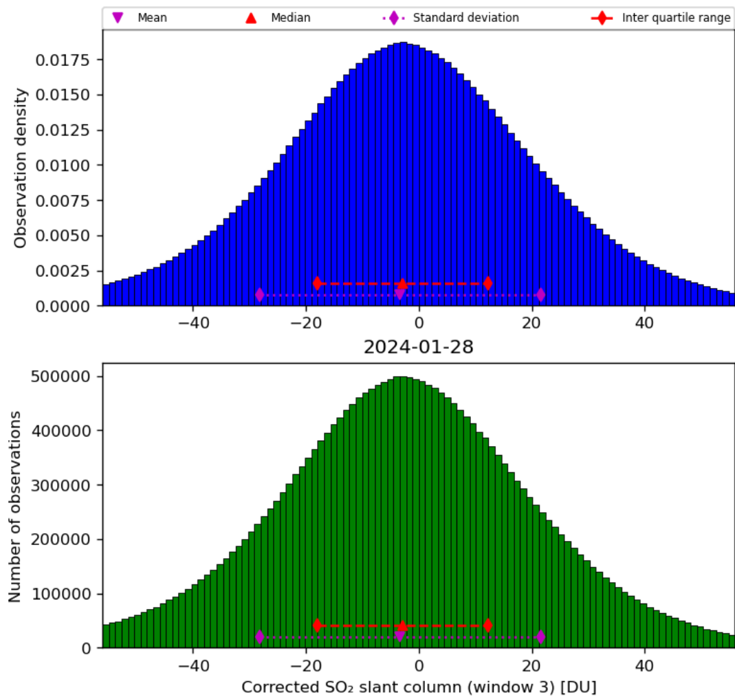
Figure 66: Histogram of “Corrected SO 2 slant column (window 3)” for 2024-01-27 to 2024-01-29
