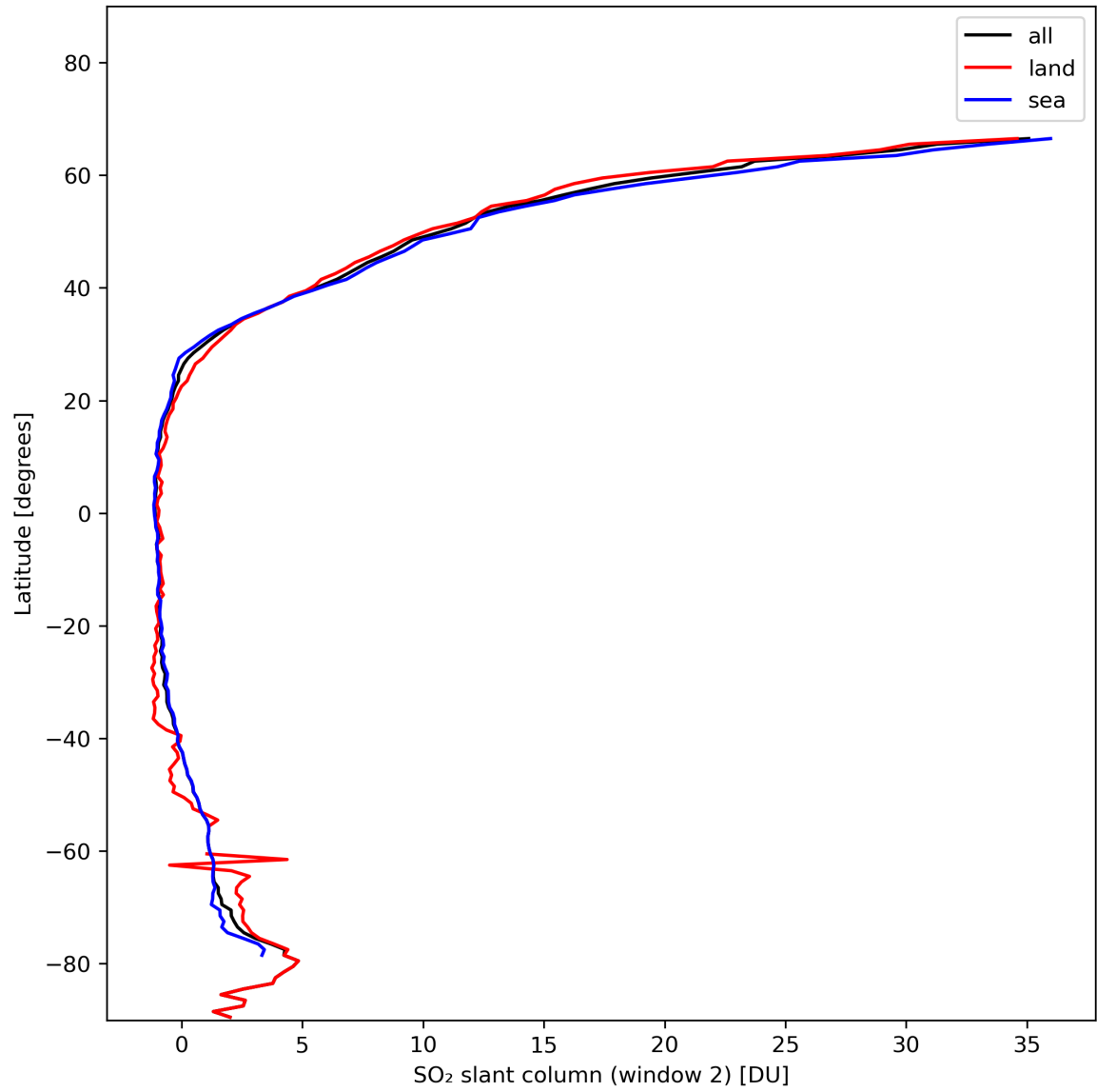
Figure 37: Zonal average of “SO 2 slant column (window 2)” for 2024-01-27 to 2024-01-29.
