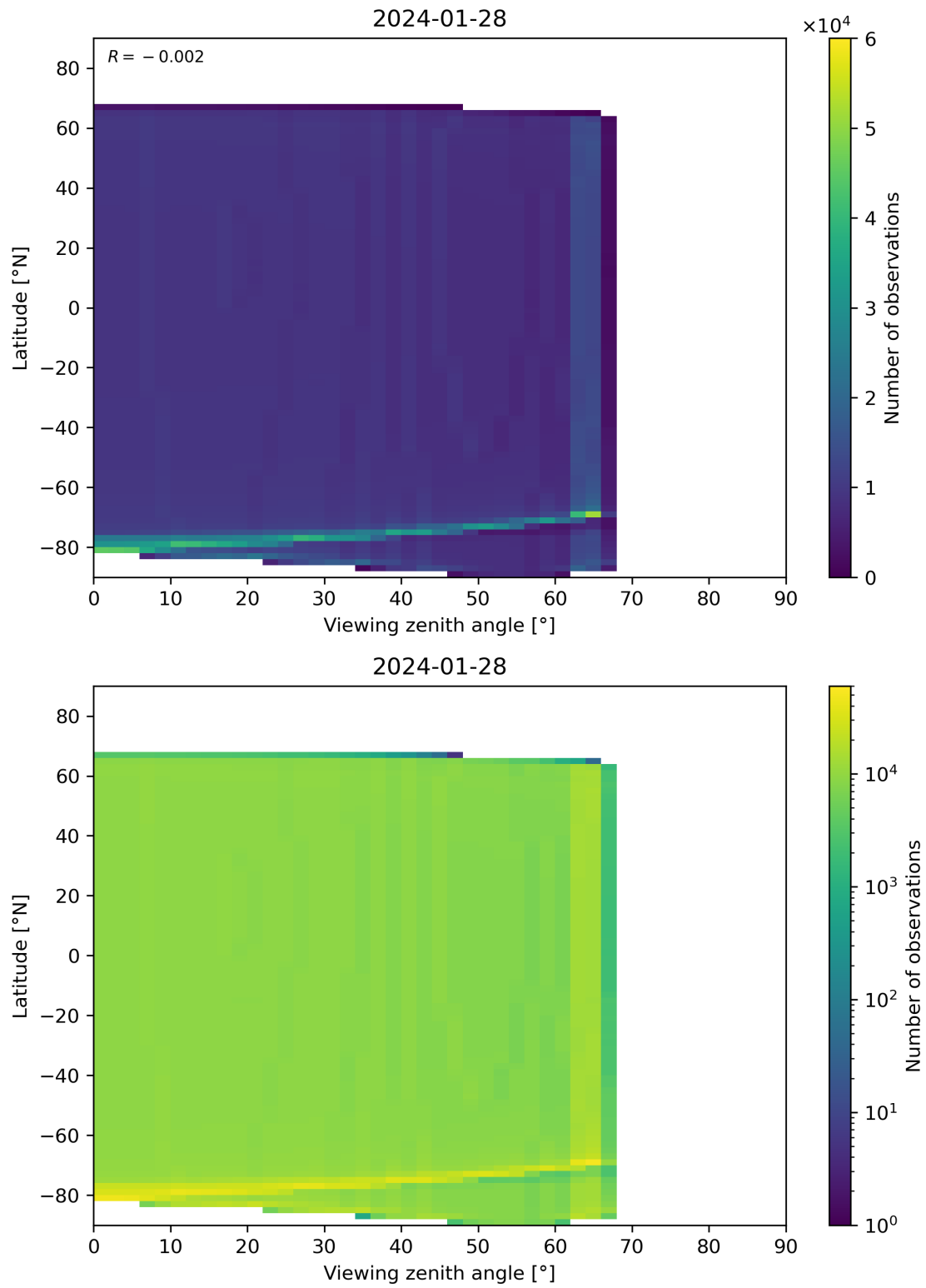
Figure 314: Scatter density plot of “Viewing zenith angle” against “Latitude” for 2024-01-27 to 2024-01-29.
