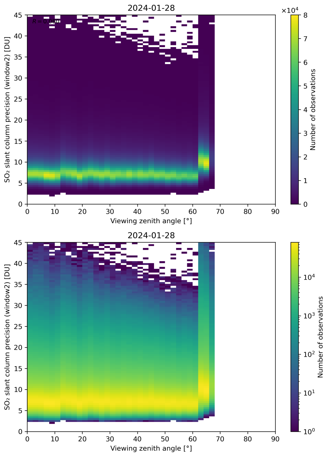
Figure 322: Scatter density plot of “Viewing zenith angle” against “SO 2 slant column precision (window2)” for 2024-01-27 to 2024-01-29.
