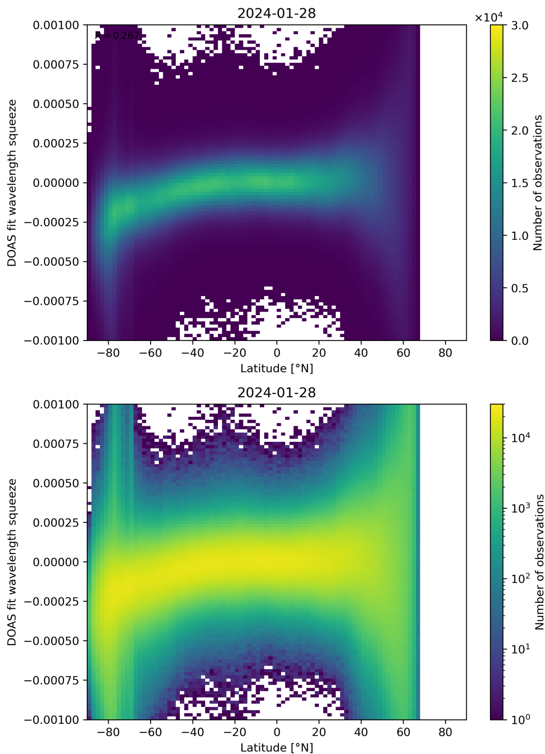
Figure 143: Scatter density plot of “Latitude” against “DOAS fit wavelength squeeze” for 2024-01-27 to 2024-01-29.
