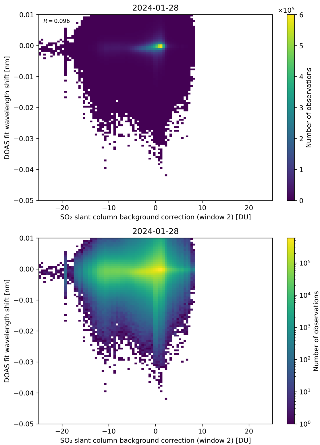
Figure 112: Scatter density plot of “SO 2 slant column background correction (window 2)” against “DOAS fit wavelength shift” for 2024-01-27 to 2024-01-29.
