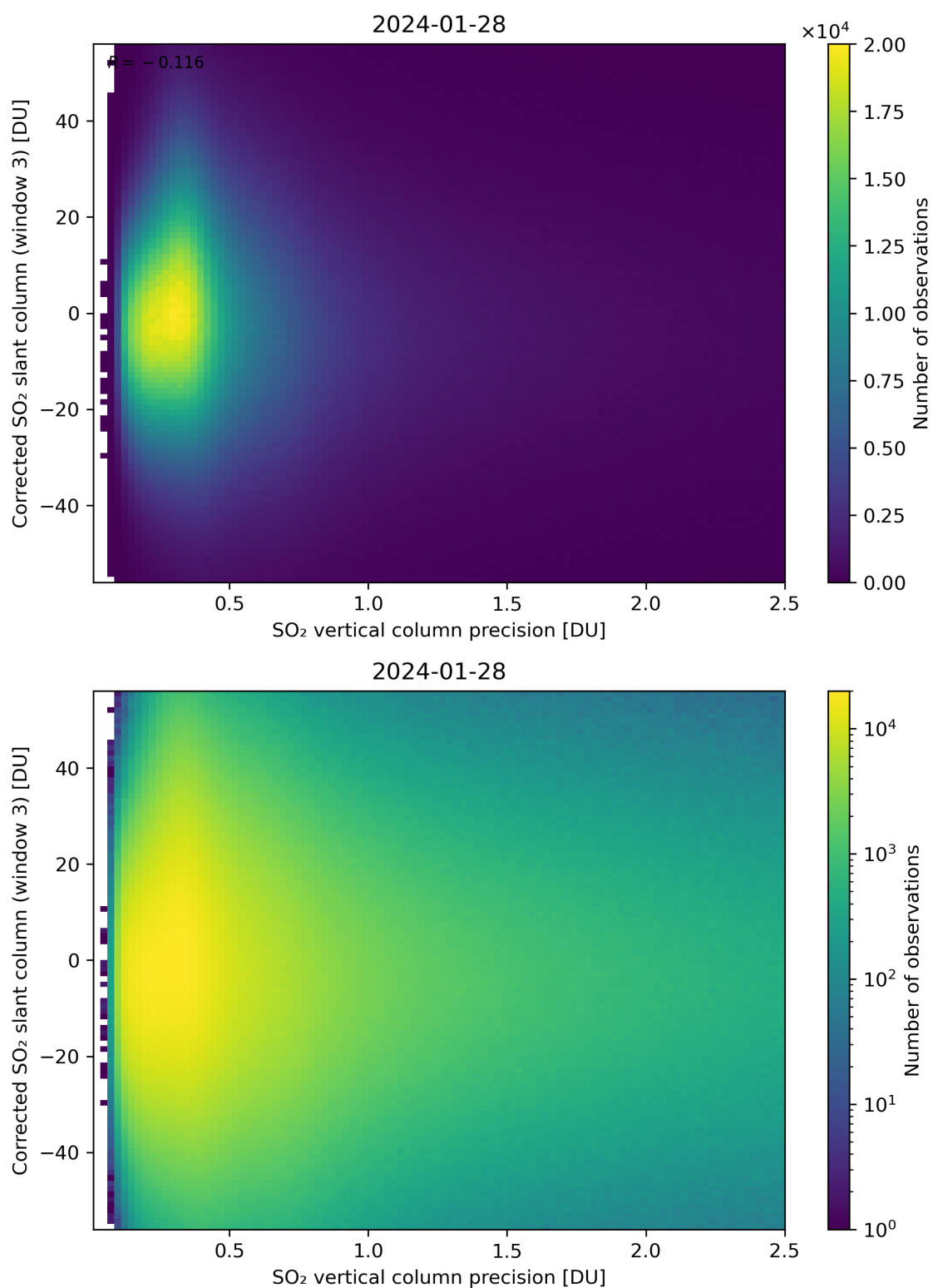
Figure 288: Scatter density plot of “SO 2 vertical column precision” against “Corrected SO 2 slant column (window 3)” for 2024-01-27 to 2024-01-29.
