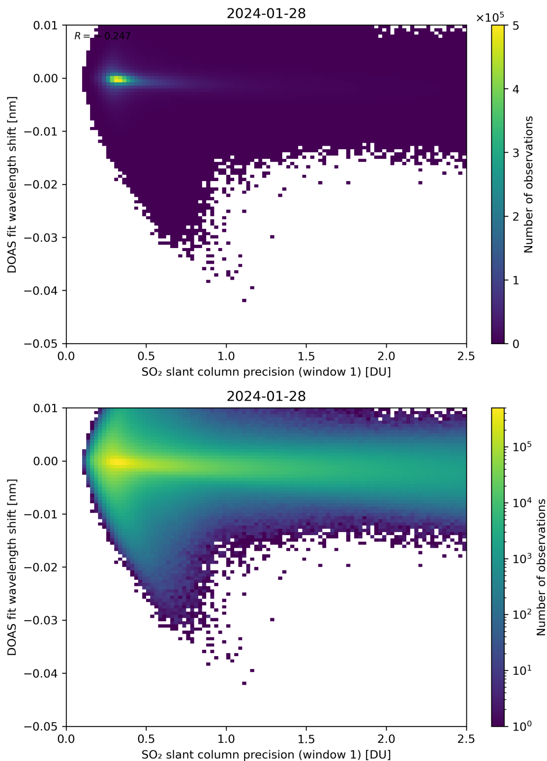
Figure 221: Scatter density plot of “SO 2 slant column precision (window 1)” against “DOAS fit wavelength shift” for 2024-01-27 to 2024-01-29.
