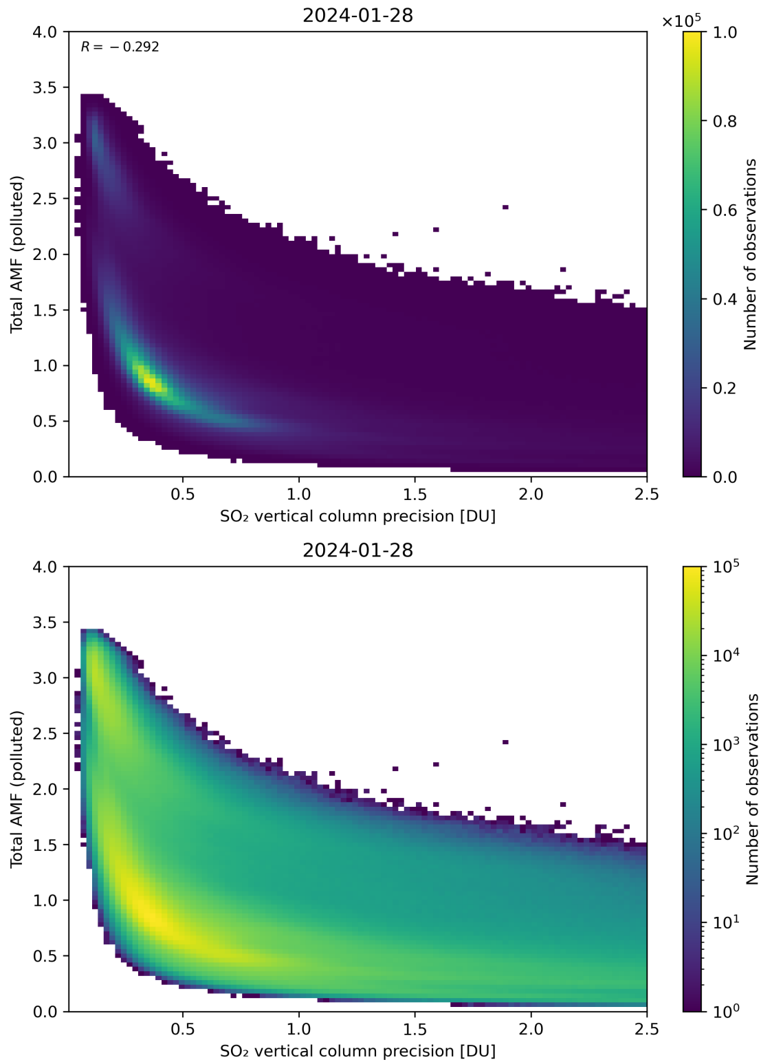
Figure 294: Scatter density plot of “SO 2 vertical column precision” against “Total AMF (polluted)” for 2024-01-27 to 2024-01-29.
