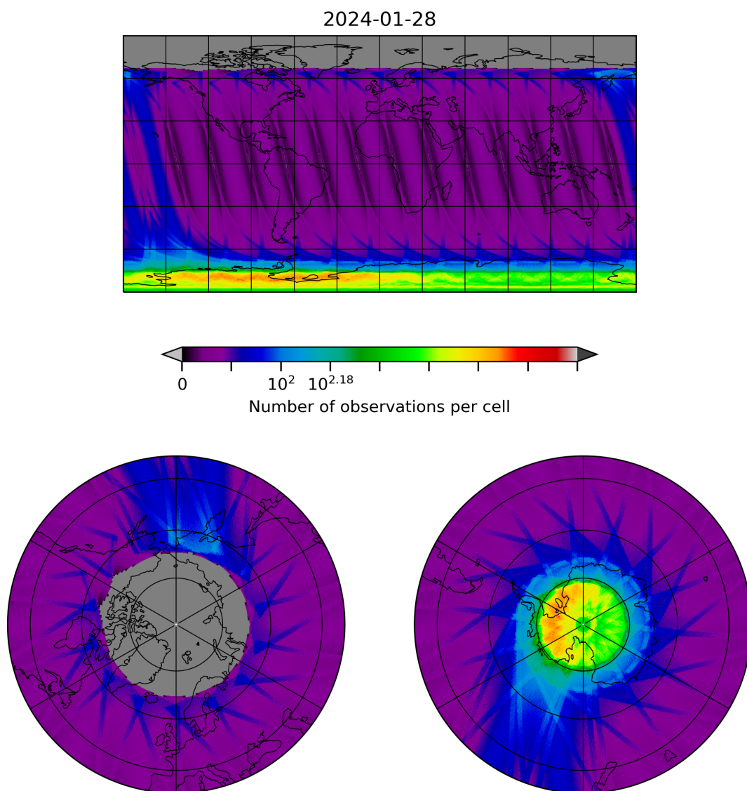
Figure 28: Map of the number of observations for 2024-01-27 to 2024-01-29
