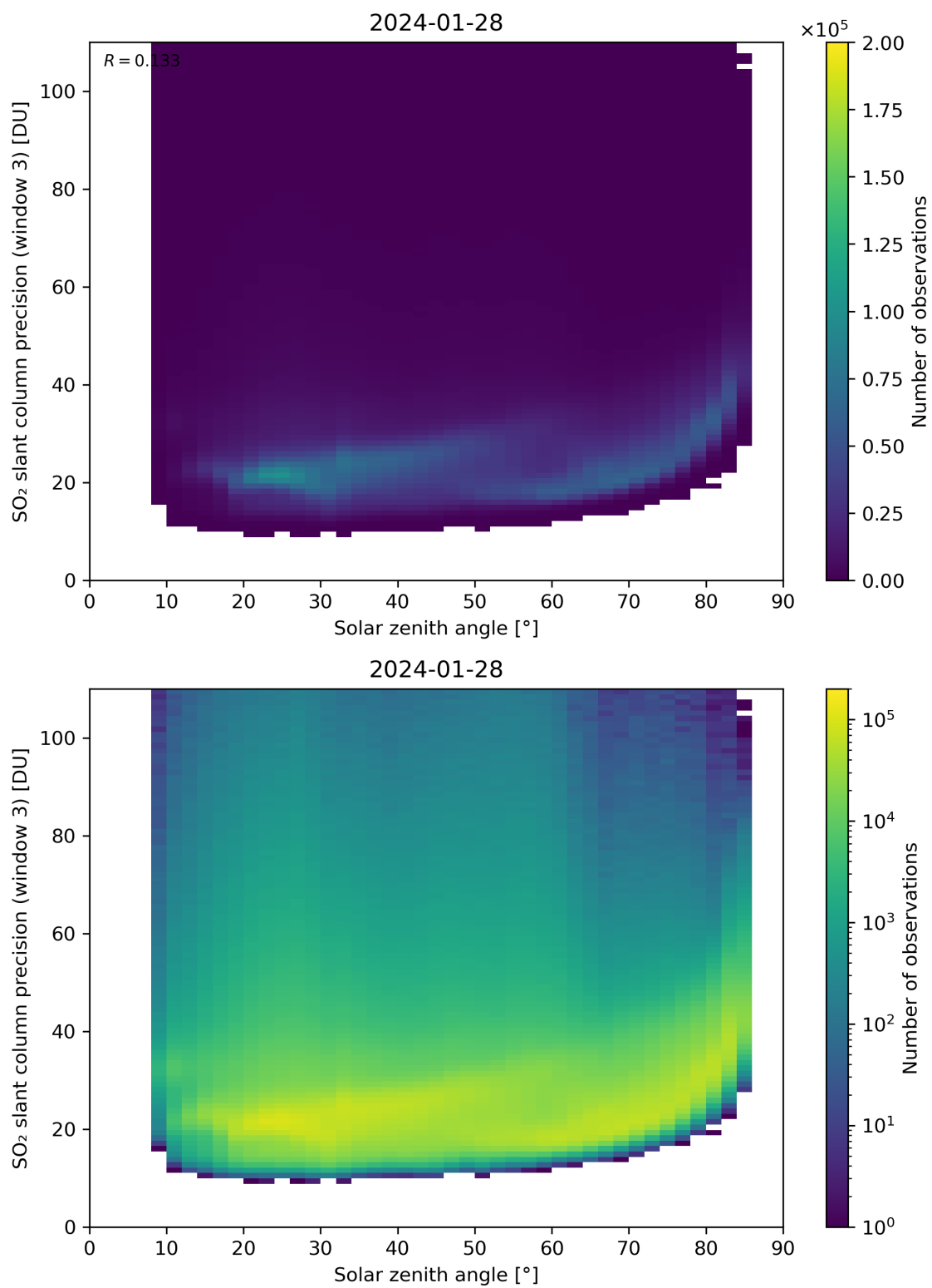
Figure 173: Scatter density plot of “Solar zenith angle” against “SO 2 slant column precision (window 3)” for 2024-01-27 to 2024-01-29.
