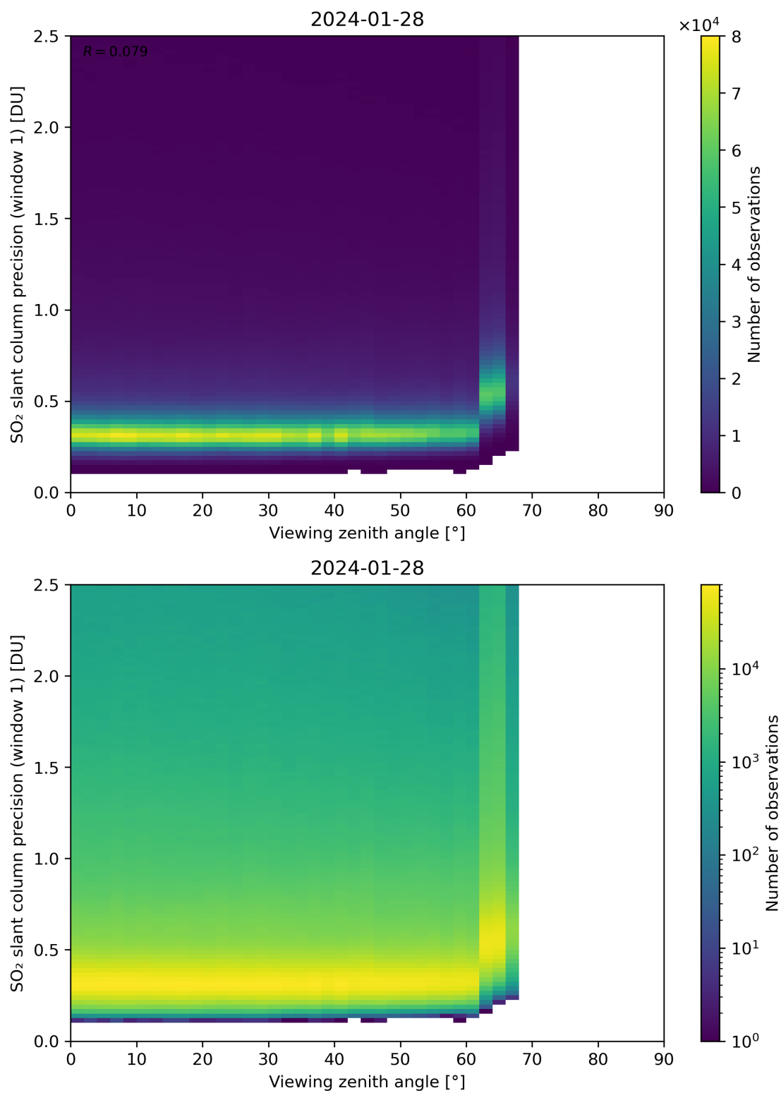
Figure 321: Scatter density plot of “Viewing zenith angle” against “SO 2 slant column precision (window 1)” for 2024-01-27 to 2024-01-29.
