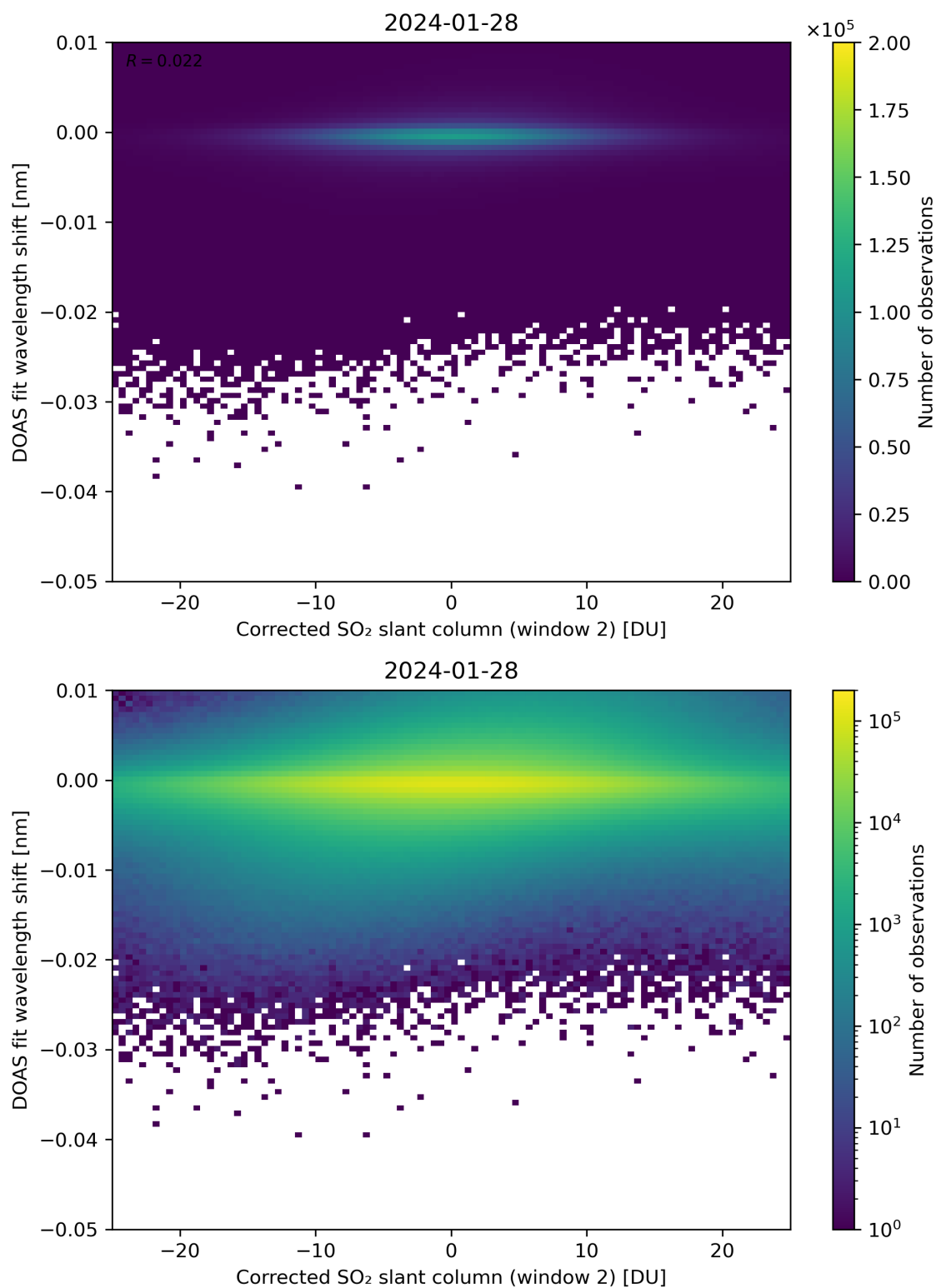
Figure 196: Scatter density plot of “Corrected SO 2 slant column (window 2)” against “DOAS fit wavelength shift” for 2024-01-27 to 2024-01-29.
