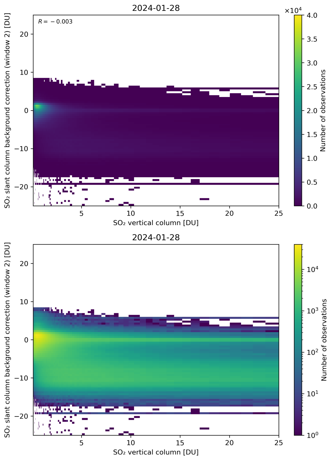
Figure 274: Scatter density plot of “SO 2 vertical column” against “SO 2 slant column background correction (window 2)” for 2024-01-27 to 2024-01-29.
