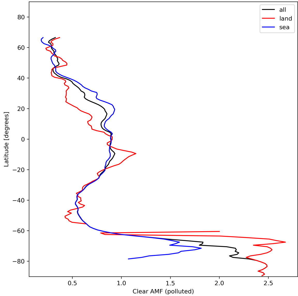
Figure 50: Zonal average of “Clear AMF (polluted)” for 2024-01-27 to 2024-01-29.
