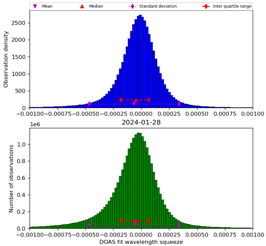
Figure 69: Histogram of “DOAS fit wavelength squeeze” for 2024-01-27 to 2024-01-29
