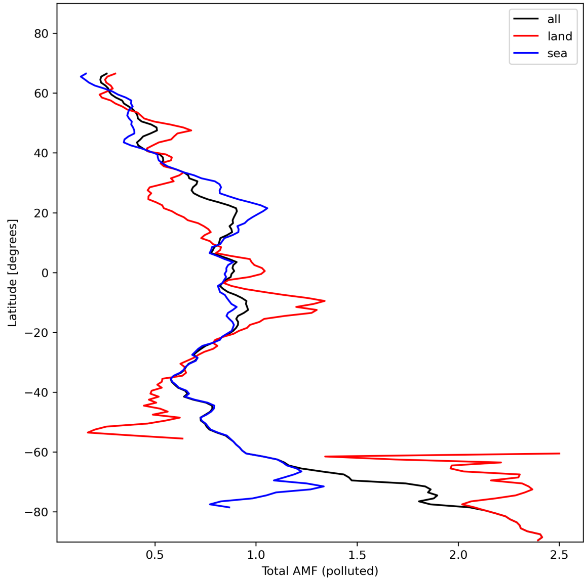
Figure 48: Zonal average of “Total AMF (polluted)” for 2024-01-27 to 2024-01-29.
