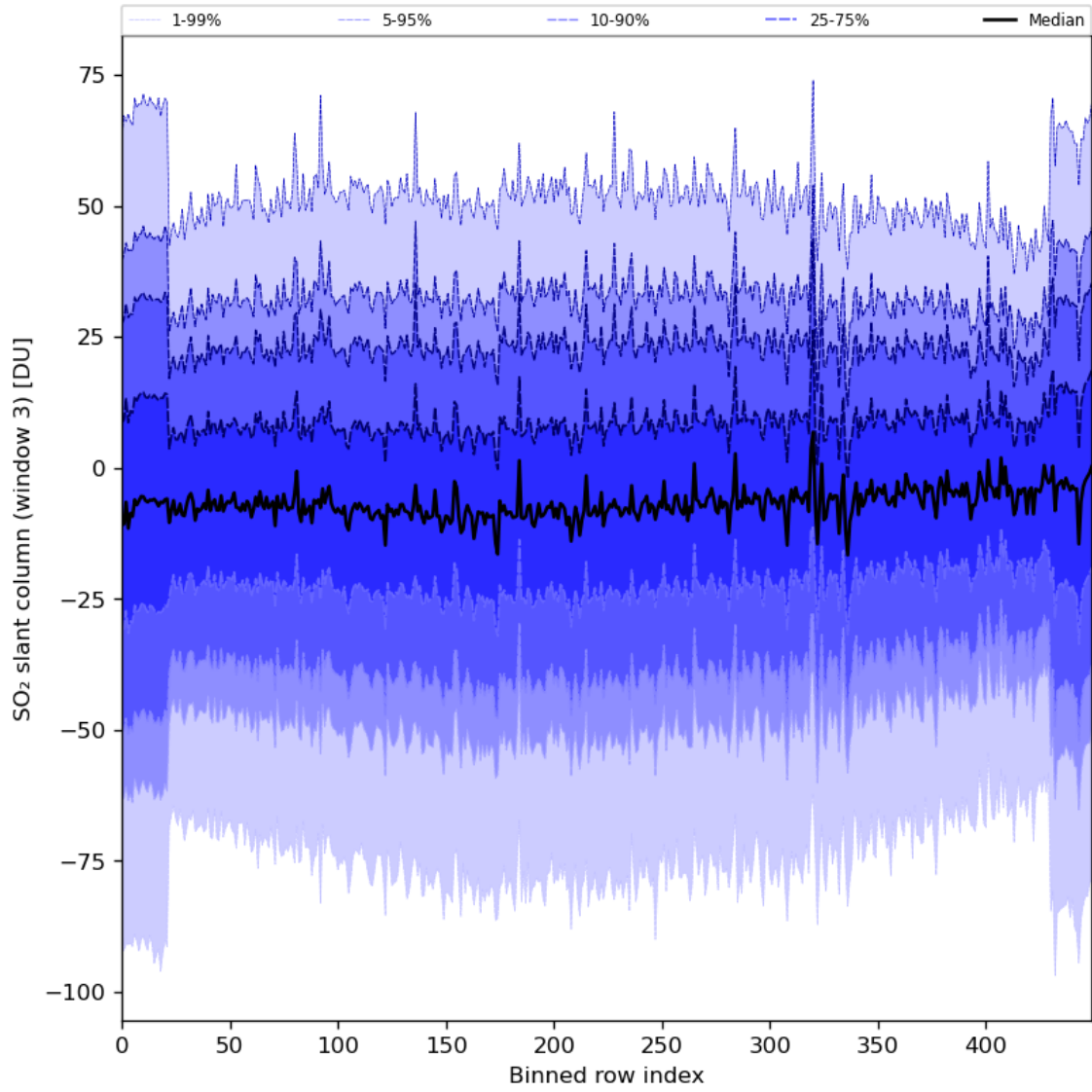
Figure 87: Along track statistics of “SO 2 slant column (window 3)” for 2024-01-27 to 2024-01-29
