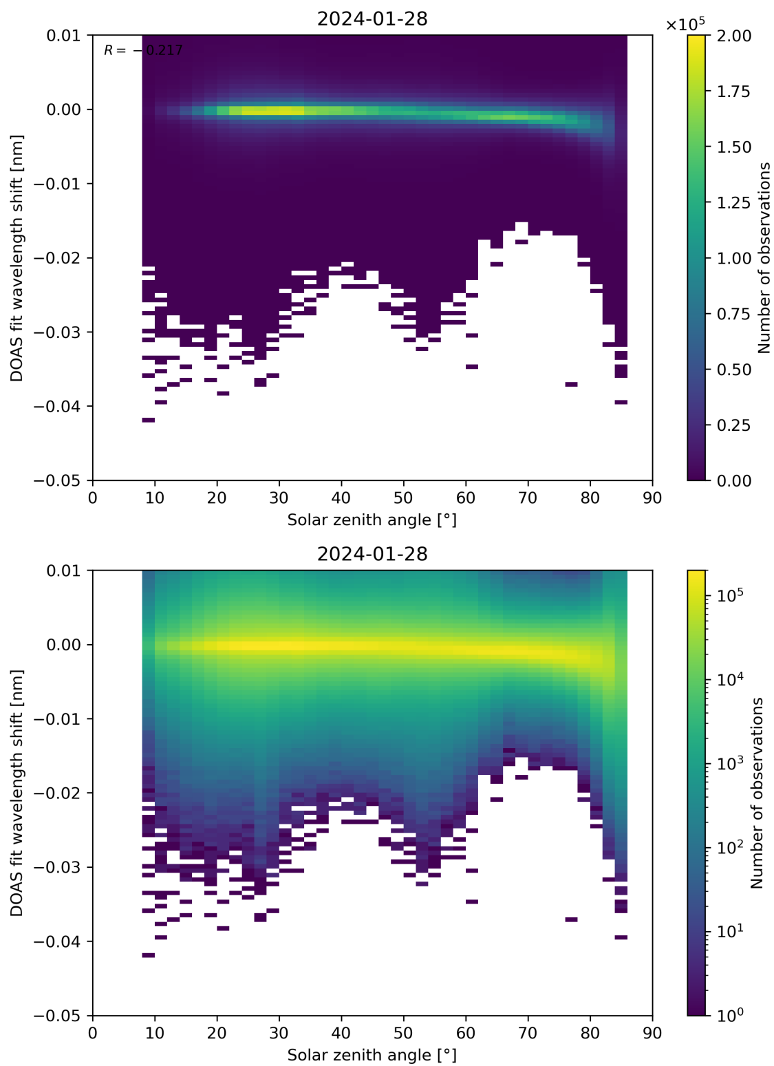
Figure 161: Scatter density plot of “Solar zenith angle” against “DOAS fit wavelength shift” for 2024-01-27 to 2024-01-29.
