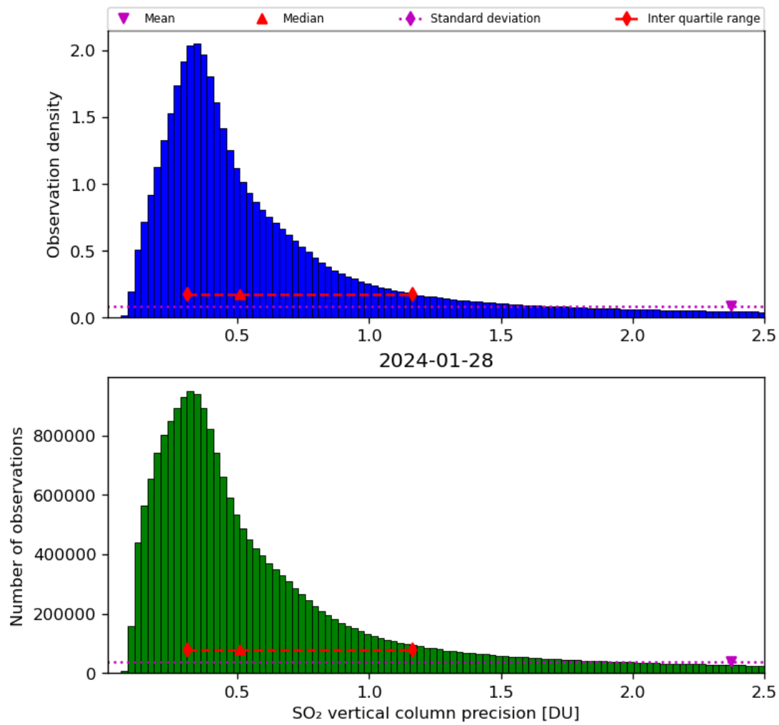
Figure 54: Histogram of “SO 2 vertical column precision” for 2024-01-27 to 2024-01-29
