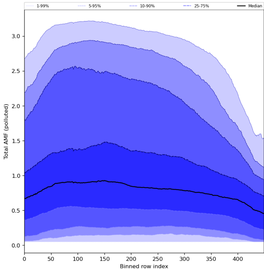
Figure 94: Along track statistics of “Total AMF (polluted)” for 2024-01-27 to 2024-01-29
