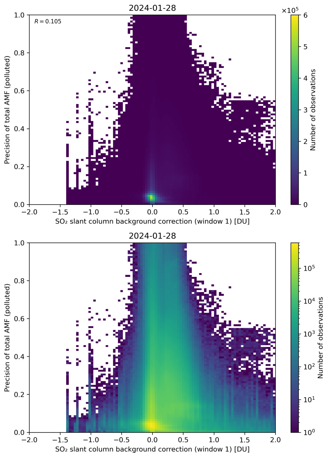
Figure 110: Scatter density plot of “SO 2 slant column background correction (window 1)” against “Precision of total AMF (polluted)” for 2024-01-27 to 2024-01-29.
