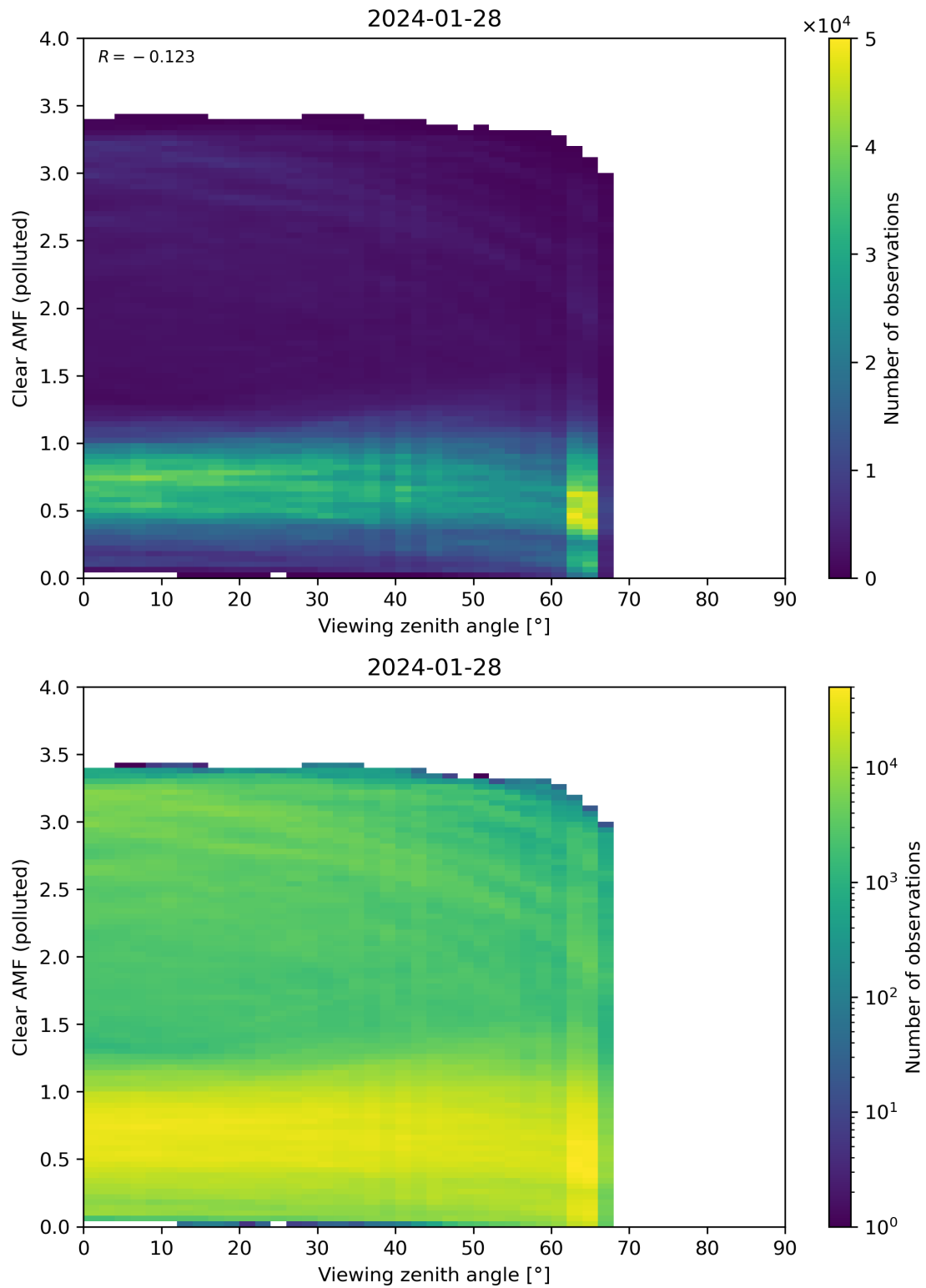
Figure 316: Scatter density plot of “Viewing zenith angle” against “Clear AMF (polluted)” for 2024-01-27 to 2024-01-29.
