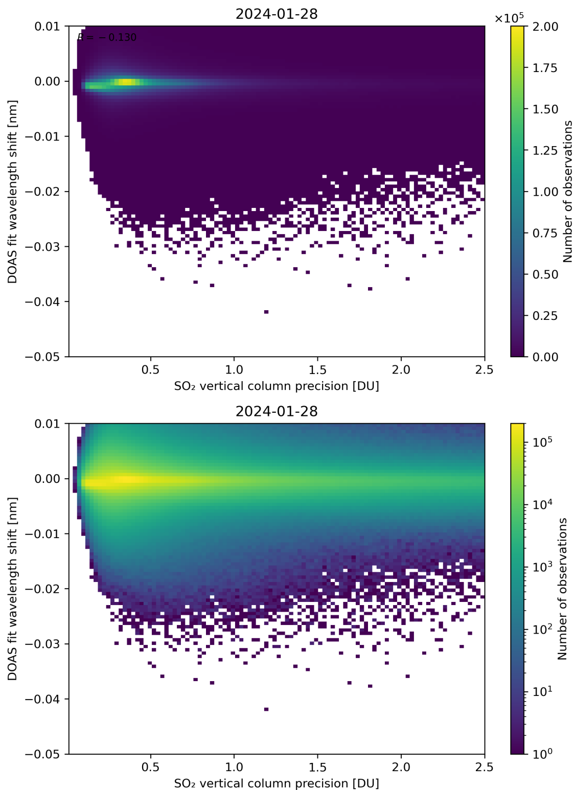
Figure 282: Scatter density plot of “SO 2 vertical column precision” against “DOAS fit wavelength shift” for 2024-01-27 to 2024-01-29.
