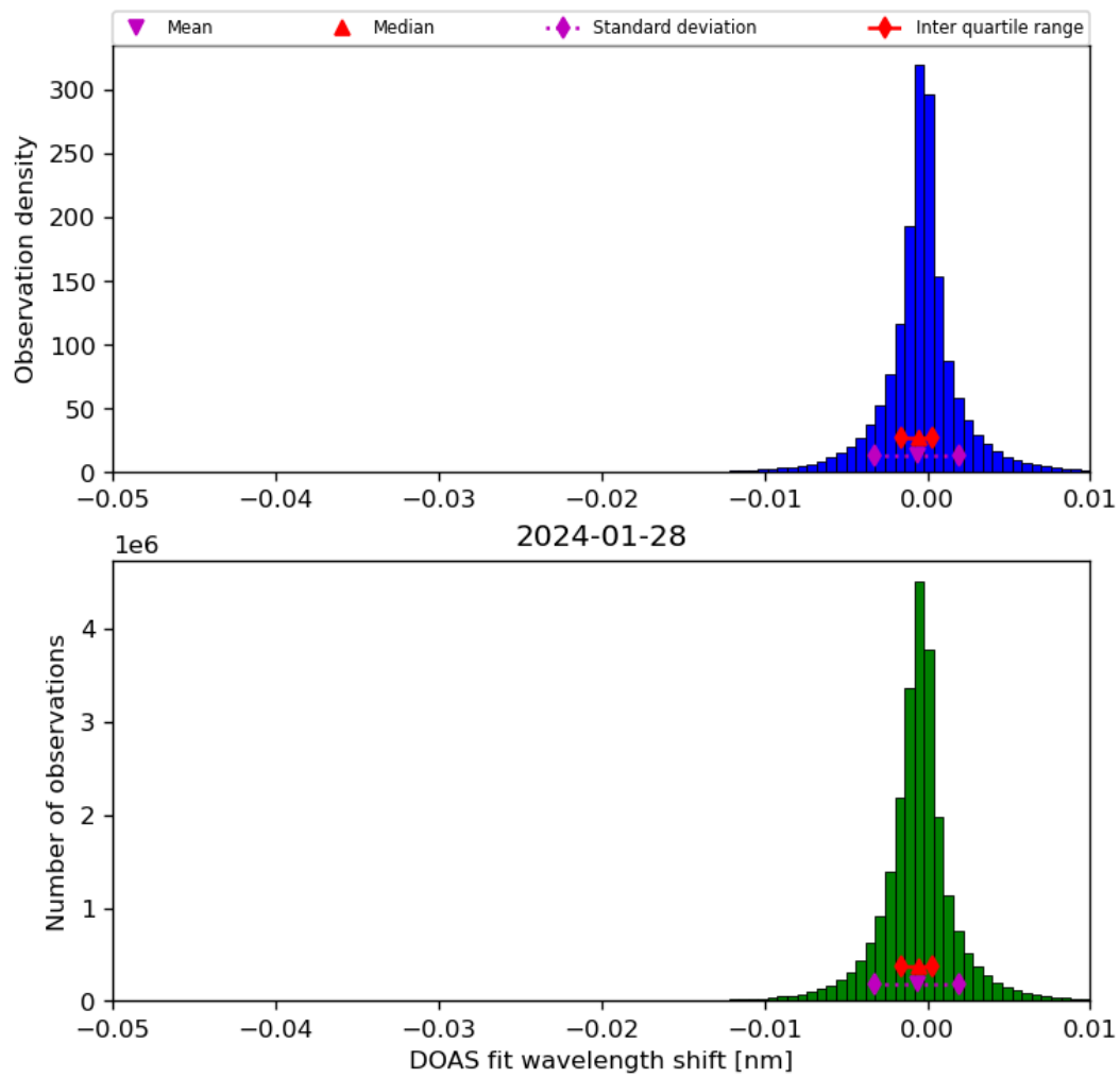
Figure 68: Histogram of “DOAS fit wavelength shift” for 2024-01-27 to 2024-01-29
