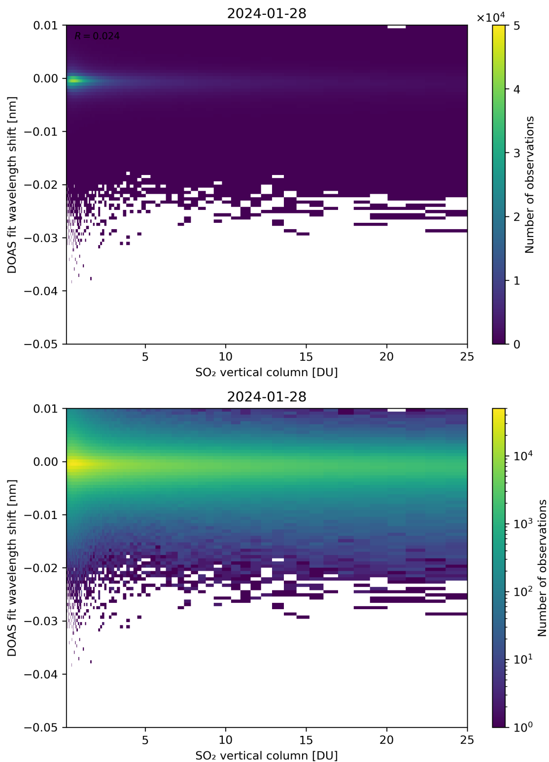
Figure 276: Scatter density plot of “SO 2 vertical column” against “DOAS fit wavelength shift” for 2024-01-27 to 2024-01-29.
