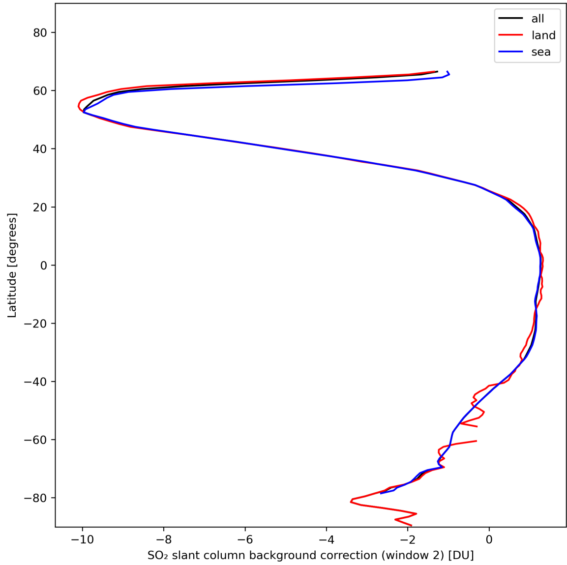
Figure 40: Zonal average of “SO 2 slant column background correction (window 2)” for 2024-01-27 to 2024-01-29.
