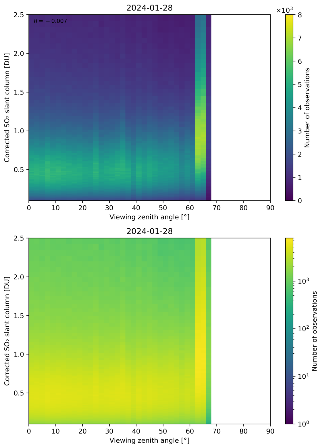
Figure 317: Scatter density plot of “Viewing zenith angle” against “Corrected SO 2 slant column” for 2024-01-27 to 2024-01-29.
