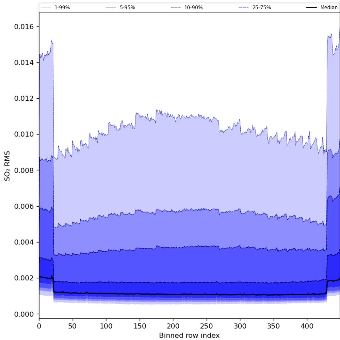
Figure 93: Along track statistics of “SO 2 RMS” for 2024-01-27 to 2024-01-29
