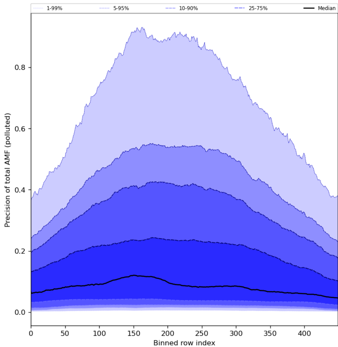
Figure 95: Along track statistics of “Precision of total AMF (polluted)” for 2024-01-27 to 2024-01-29
