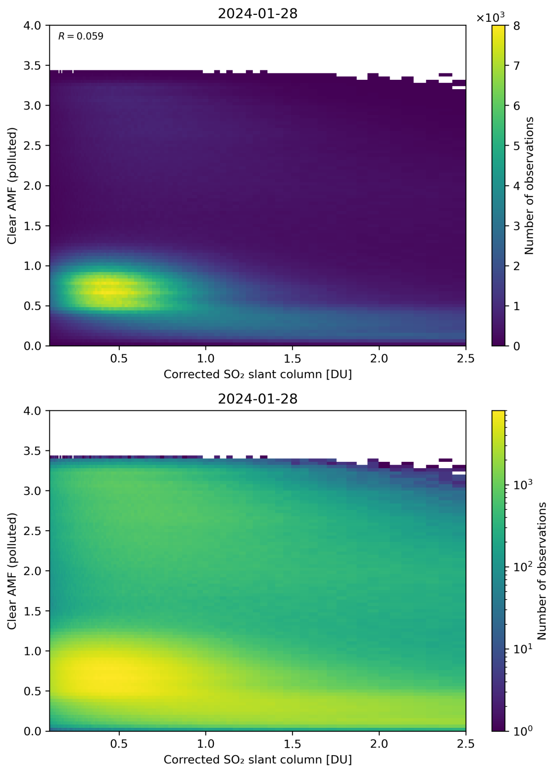
Figure 184: Scatter density plot of “Corrected SO 2 slant column” against “Clear AMF (polluted)” for 2024-01-27 to 2024-01-29.
