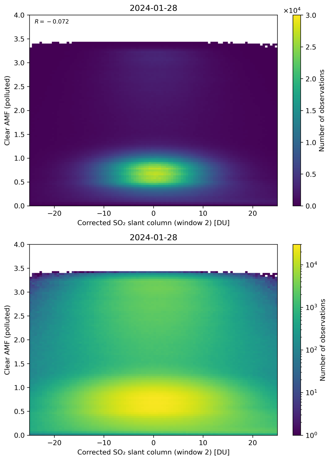
Figure 199: Scatter density plot of “Corrected SO 2 slant column (window 2)” against “Clear AMF (polluted)” for 2024-01-27 to 2024-01-29.
