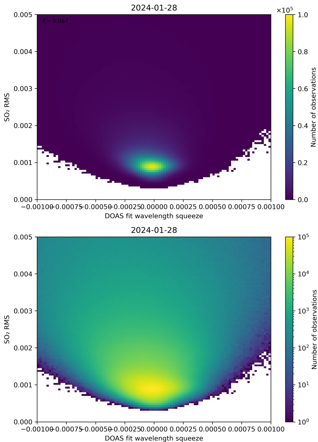
Figure 132: Scatter density plot of “DOAS fit wavelength squeeze” against “SO 2 RMS” for 2024-01-27 to 2024-01-29.
