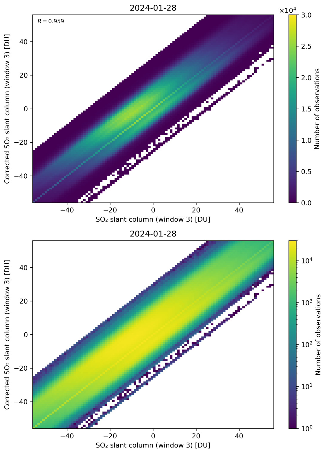
Figure 266: Scatter density plot of “SO 2 slant column (window 3)” against “Corrected SO 2 slant column (window 3)” for 2024-01-27 to 2024-01-29.
