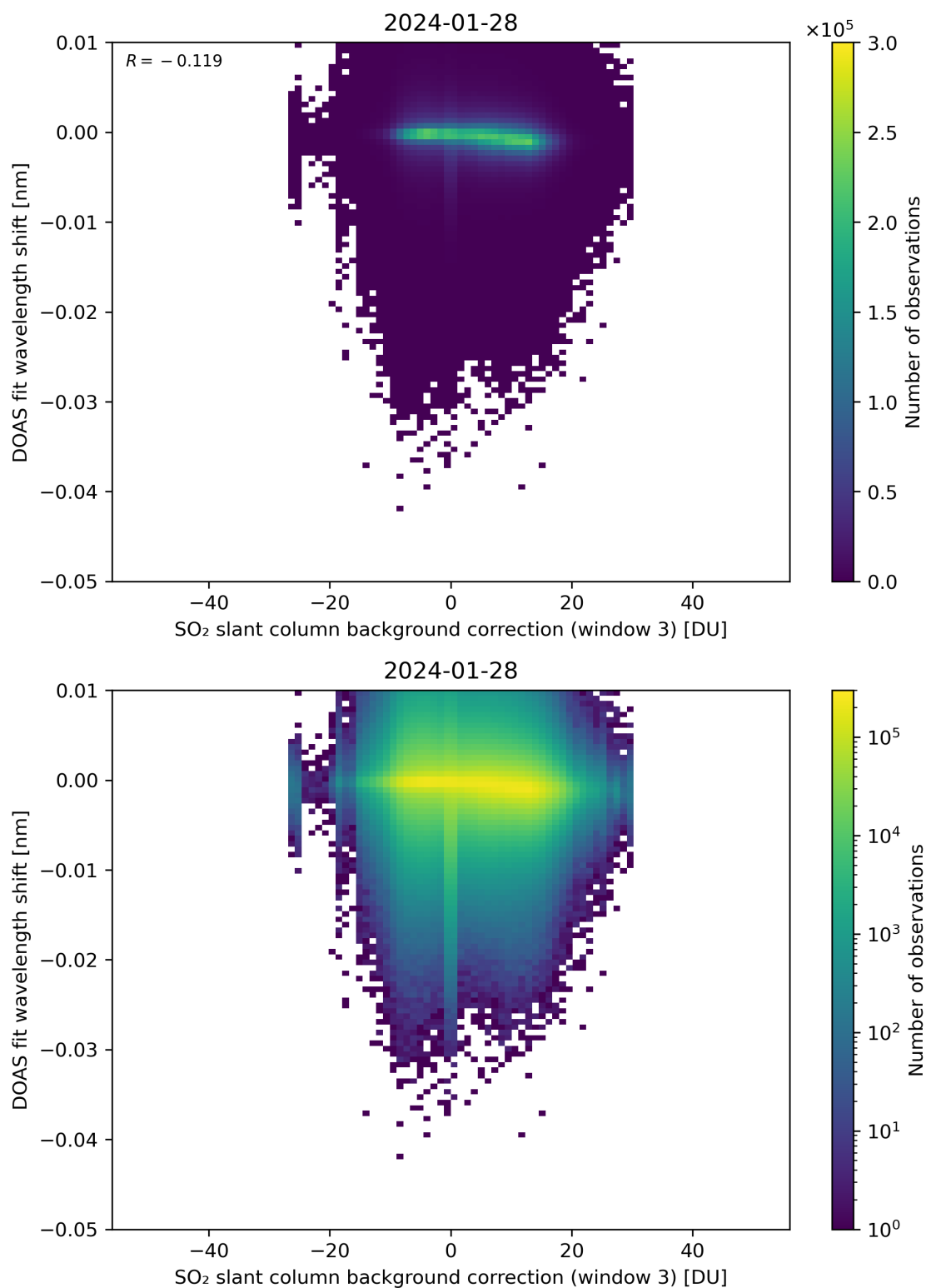
Figure 121: Scatter density plot of “SO 2 slant column background correction (window 3)” against “DOAS fit wavelength shift” for 2024-01-27 to 2024-01-29.
