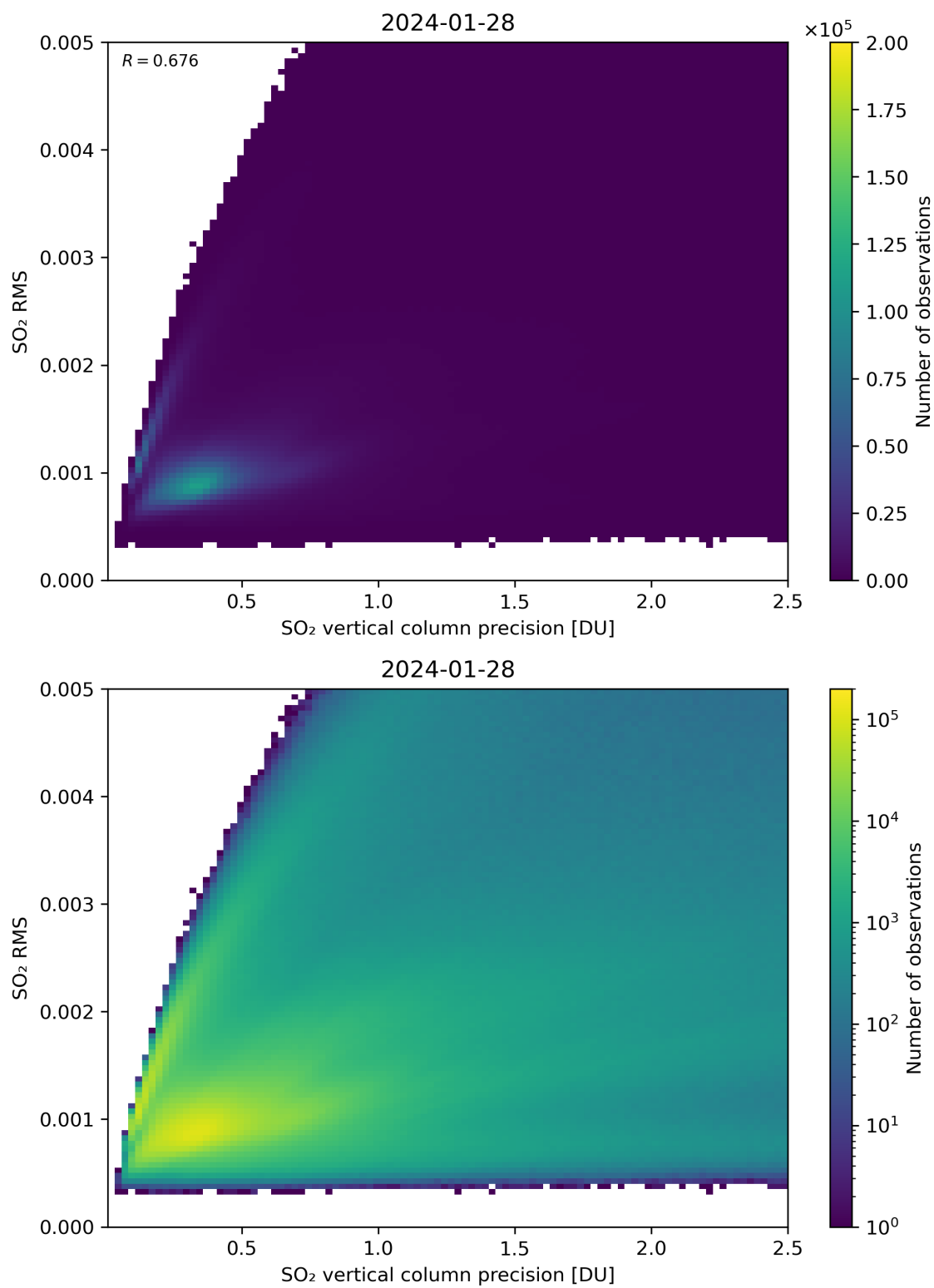
Figure 284: Scatter density plot of “SO 2 vertical column precision” against “SO 2 RMS” for 2024-01-27 to 2024-01-29.
