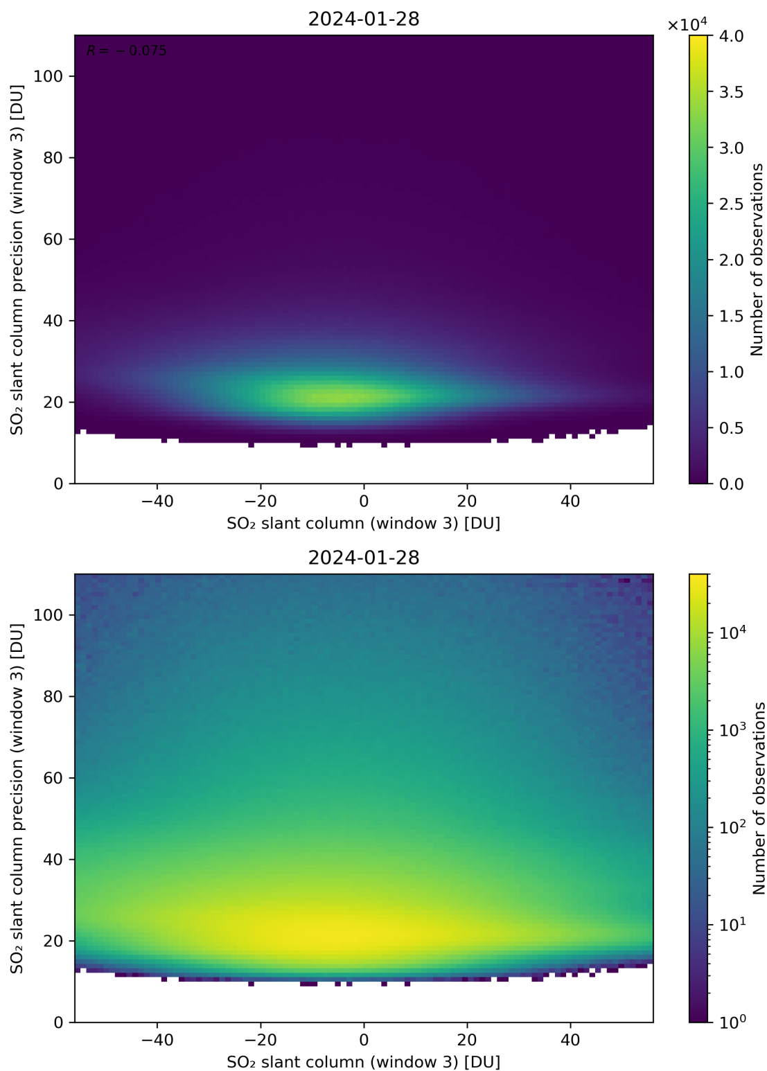
Figure 267: Scatter density plot of “SO 2 slant column (window 3)” against “SO 2 slant column precision (window 3)” for 2024-01-27 to 2024-01-29.
