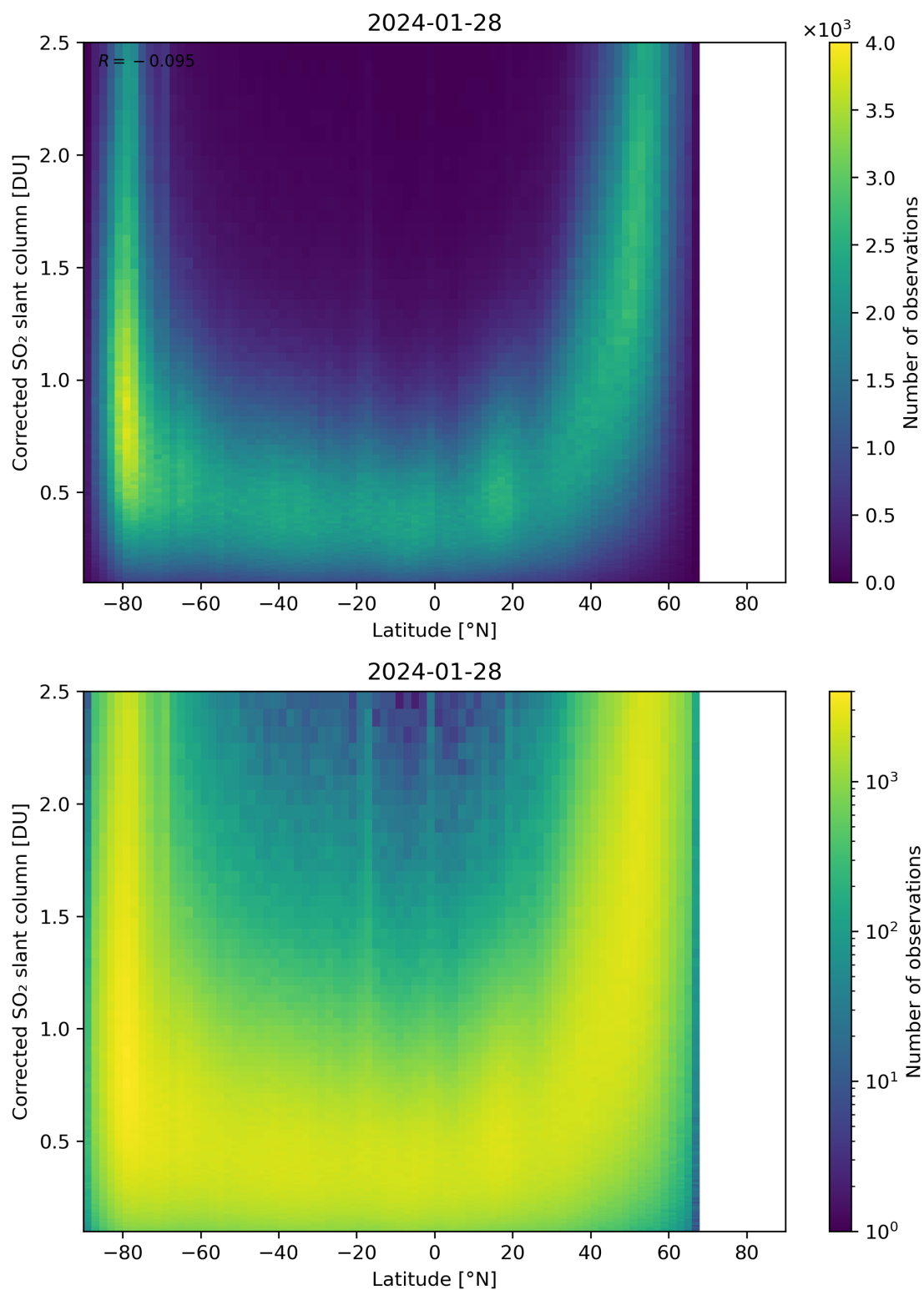
Figure 146: Scatter density plot of “Latitude” against “Corrected SO 2 slant column” for 2024-01-27 to 2024-01-29.
