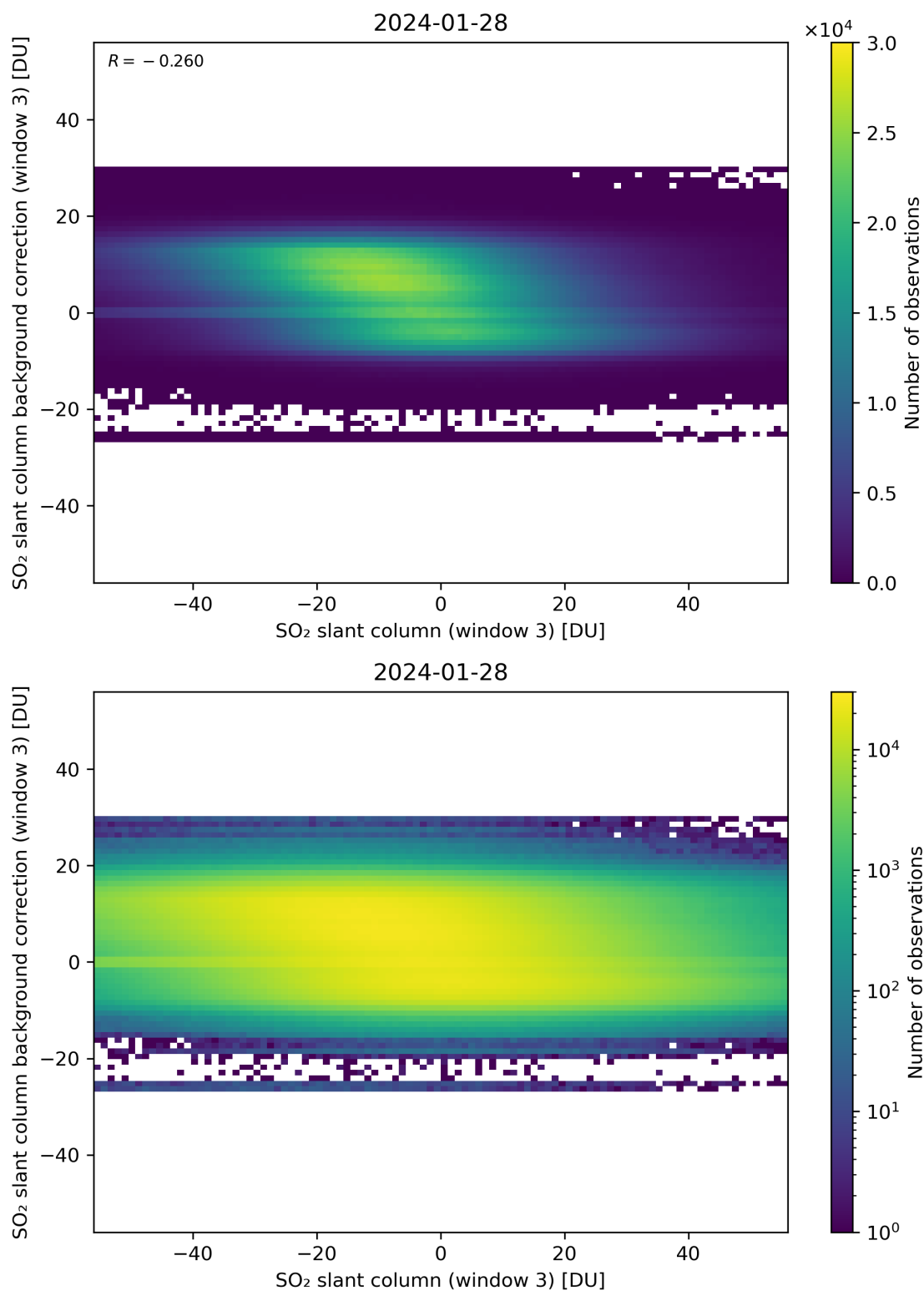
Figure 253: Scatter density plot of “SO 2 slant column (window 3)” against “SO 2 slant column background correction (window 3)” for 2024-01-27 to 2024-01-29.
