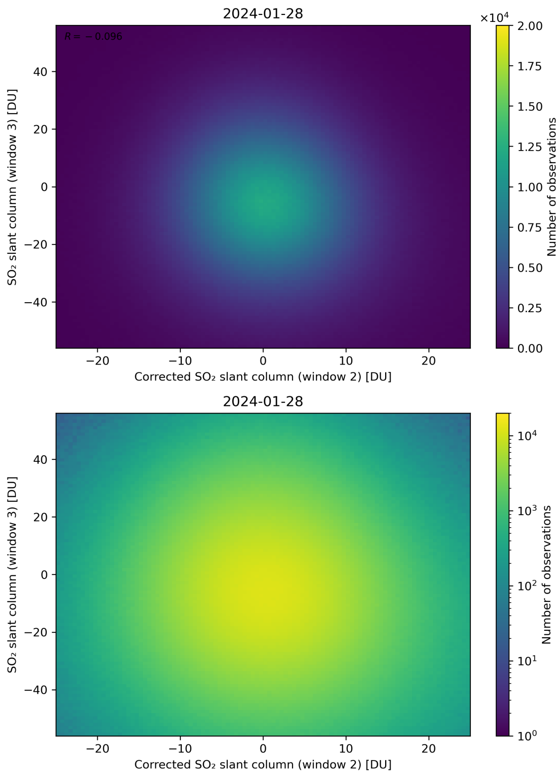
Figure 201: Scatter density plot of “Corrected SO 2 slant column (window 2)” against “SO 2 slant column (window 3)” for 2024-01-27 to 2024-01-29.
