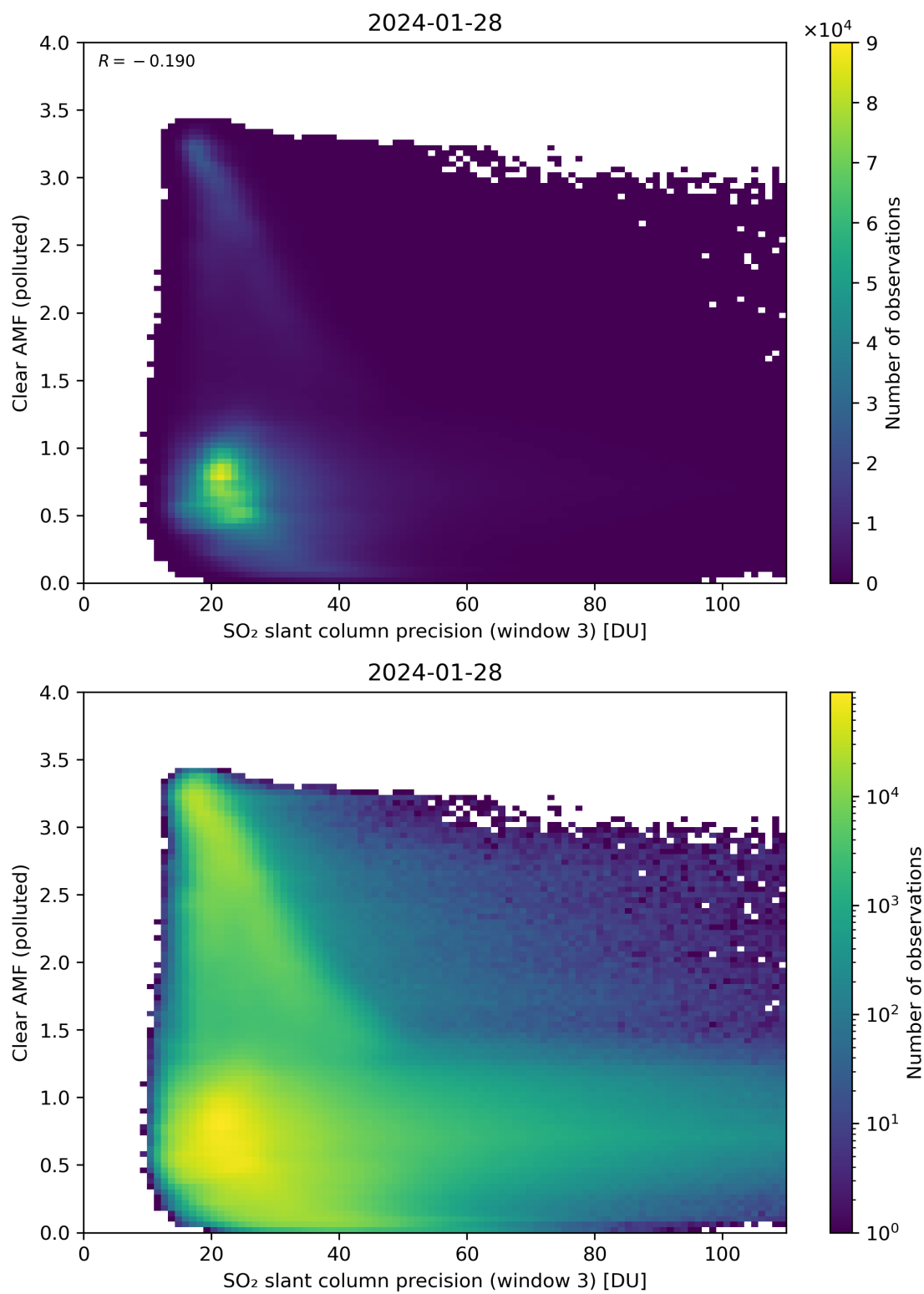
Figure 261: Scatter density plot of “SO 2 slant column precision (window 3)” against “Clear AMF (polluted)” for 2024-01-27 to 2024-01-29.
