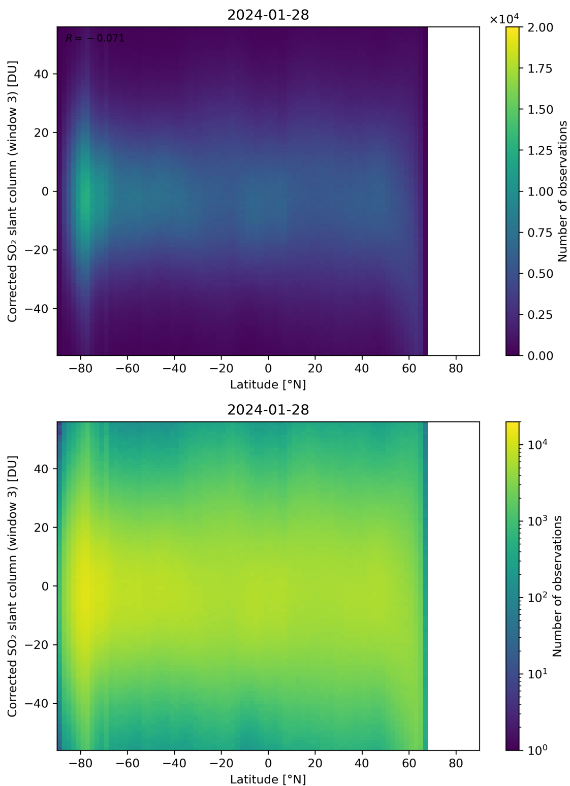
Figure 148: Scatter density plot of “Latitude” against “Corrected SO 2 slant column (window 3)” for 2024-01-27 to 2024-01-29.
