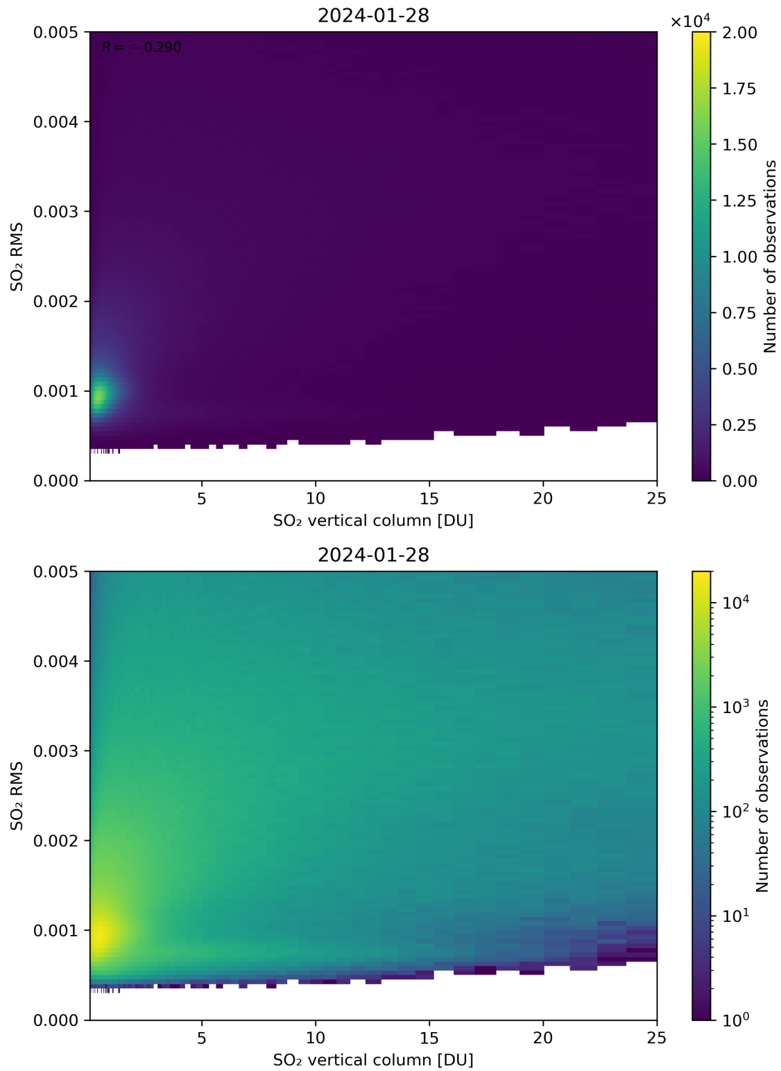
Figure 278: Scatter density plot of “SO 2 vertical column” against “SO 2 RMS” for 2024-01-27 to 2024-01-29.
