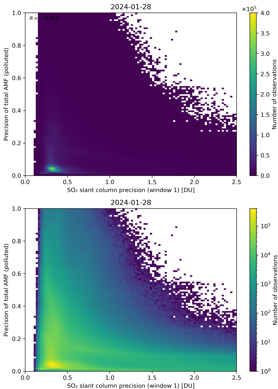
Figure 231: Scatter density plot of “SO 2 slant column precision (window 1)” against “Precision of total AMF (polluted)” for 2024-01-27 to 2024-01-29.
