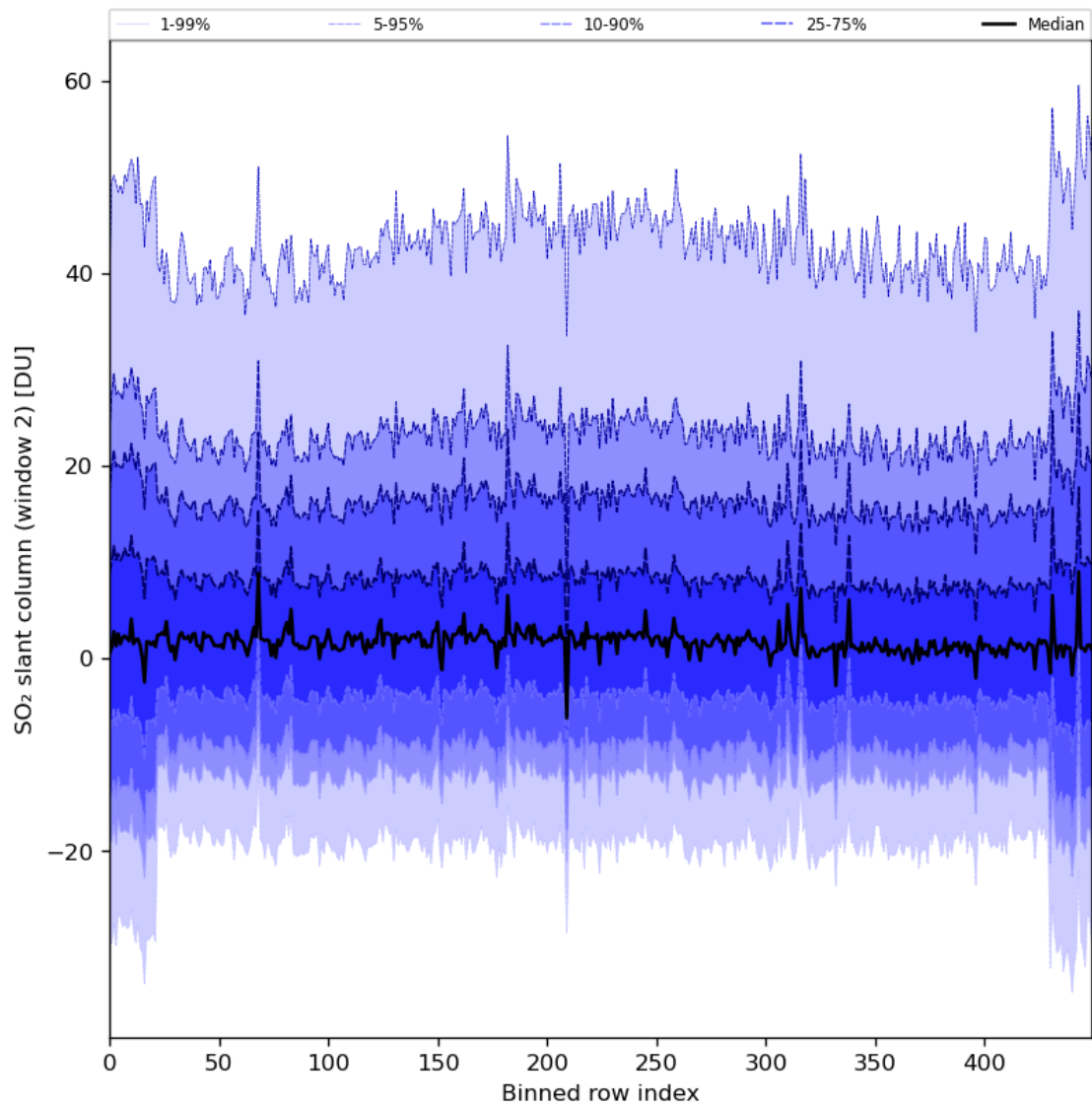
Figure 83: Along track statistics of “SO 2 slant column (window 2)” for 2024-01-27 to 2024-01-29
