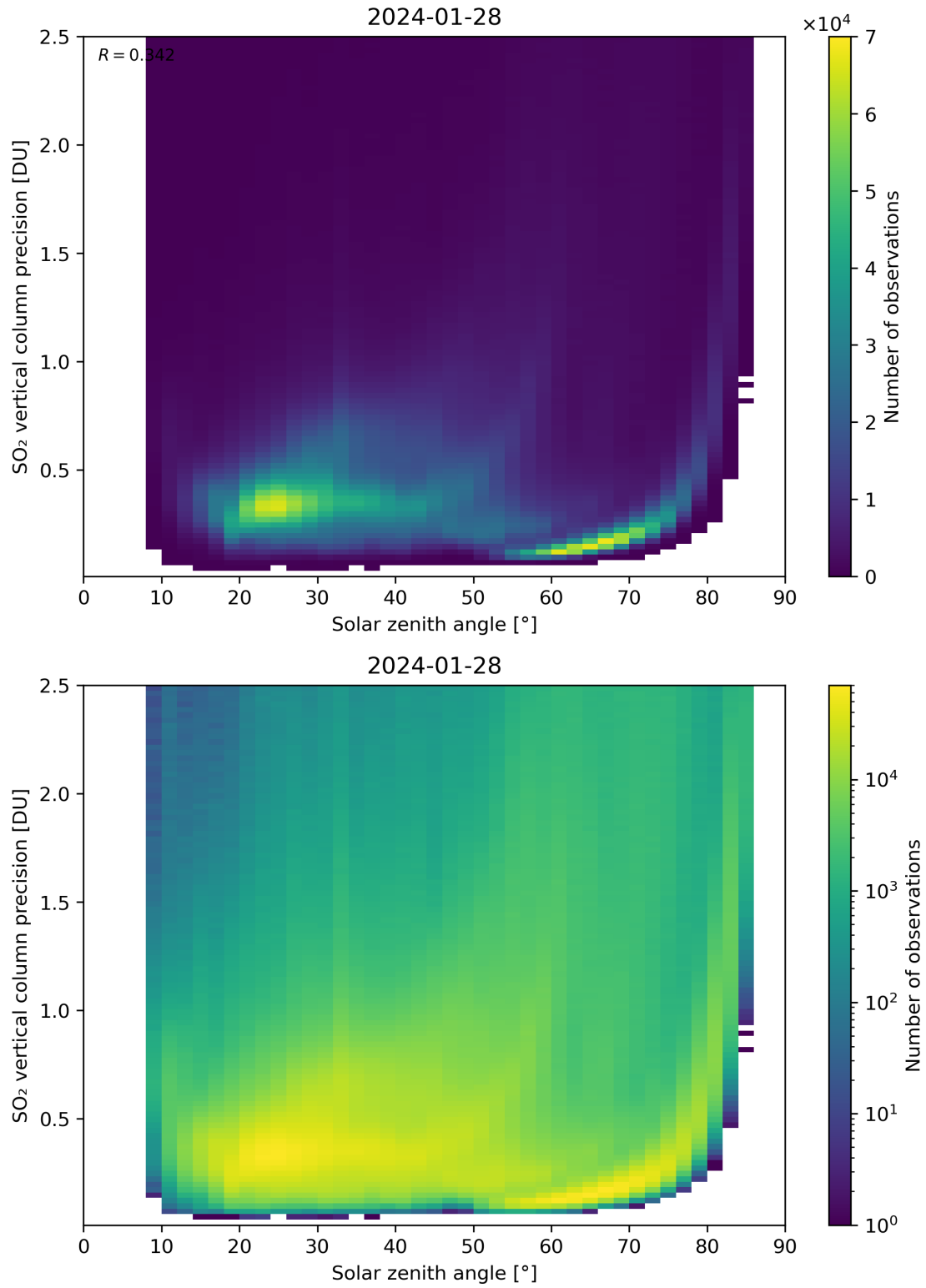
Figure 177: Scatter density plot of “Solar zenith angle” against “SO 2 vertical column precision” for 2024-01-27 to 2024-01-29.
