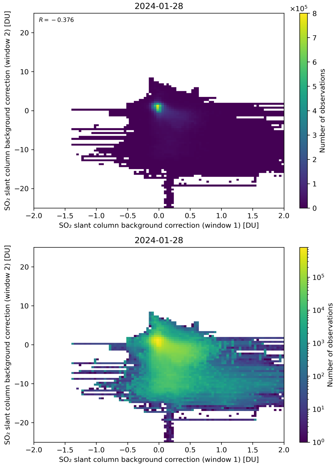
Figure 98: Scatter density plot of “SO 2 slant column background correction (window 1)” against “SO 2 slant column background correction (window 2)” for 2024-01-27 to 2024-01-29.
