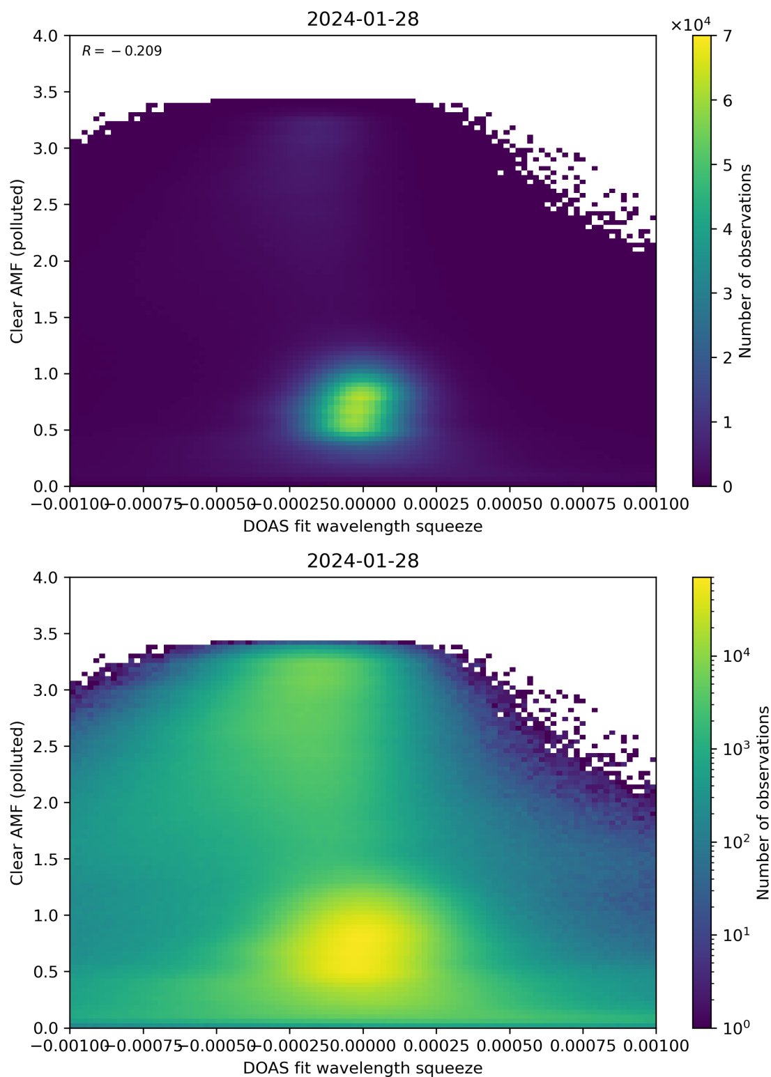
Figure 133: Scatter density plot of “DOAS fit wavelength squeeze” against “Clear AMF (polluted)” for 2024-01-27 to 2024-01-29.
