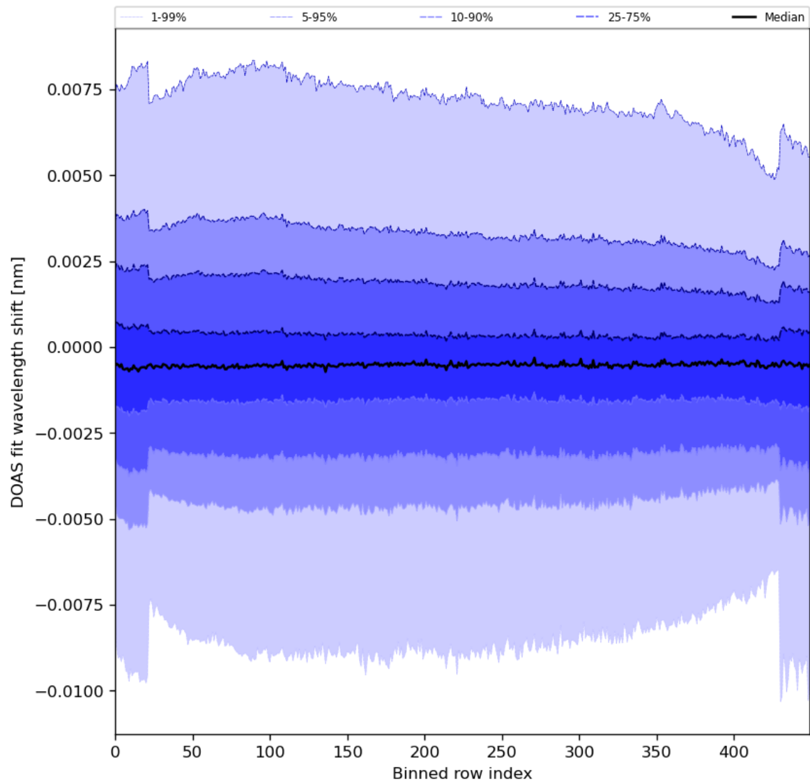
Figure 91: Along track statistics of “DOAS fit wavelength shift” for 2024-01-27 to 2024-01-29
