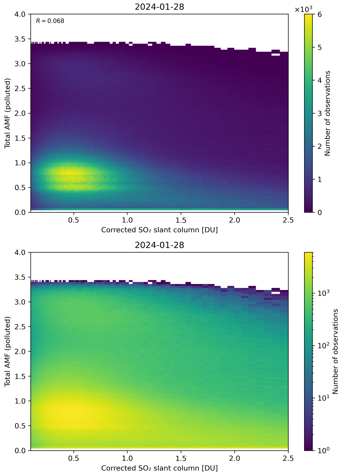
Figure 192: Scatter density plot of “Corrected SO 2 slant column” against “Total AMF (polluted)” for 2024-01-27 to 2024-01-29.
