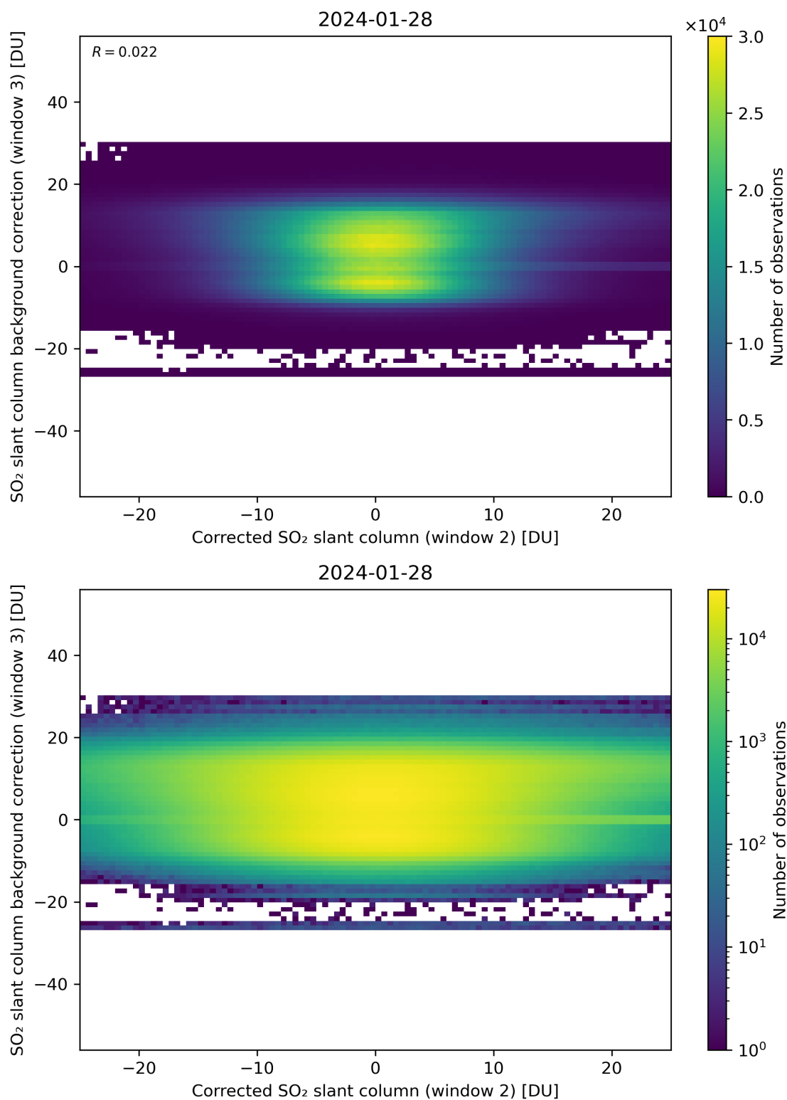
Figure 195: Scatter density plot of “Corrected SO 2 slant column (window 2)” against “SO 2 slant column background correction (window 3)” for 2024-01-27 to 2024-01-29.
