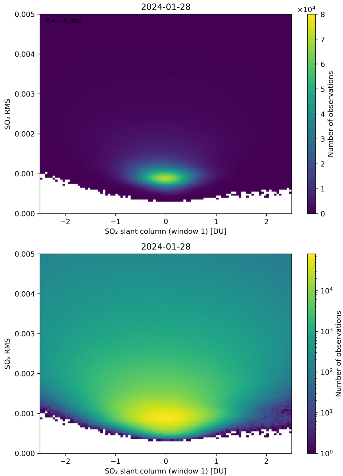
Figure 217: Scatter density plot of “SO 2 slant column (window 1)” against “SO 2 RMS” for 2024-01-27 to 2024-01-29.
