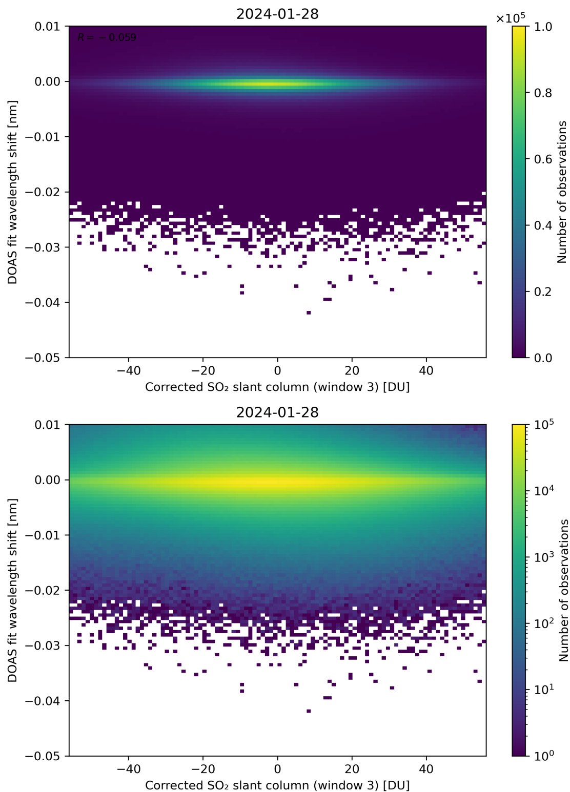
Figure 206: Scatter density plot of “Corrected SO 2 slant column (window 3)” against “DOAS fit wavelength shift” for 2024-01-27 to 2024-01-29.
