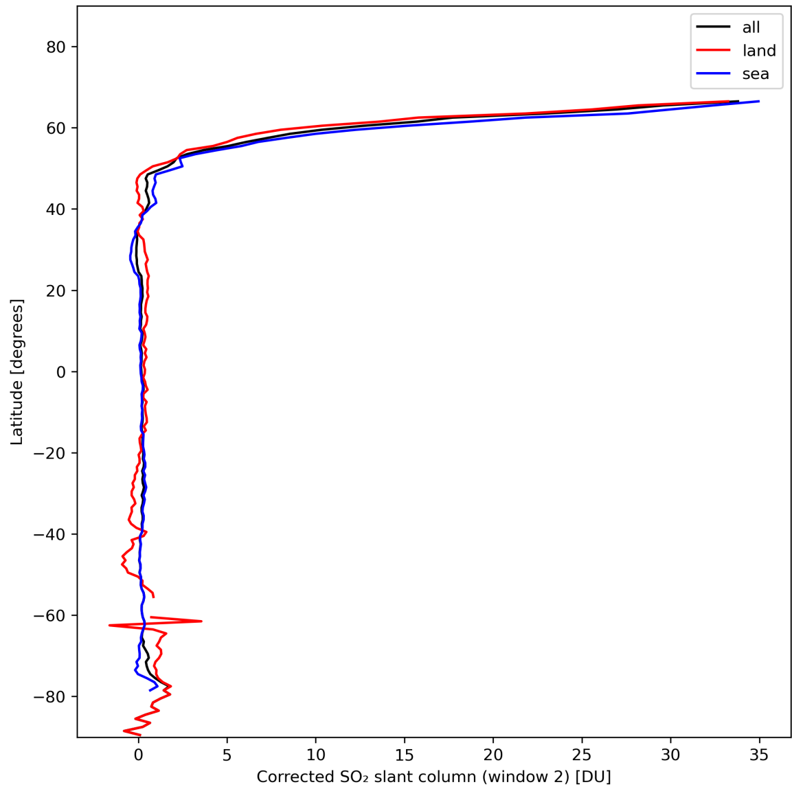
Figure 39: Zonal average of “Corrected SO 2 slant column (window 2)” for 2024-01-27 to 2024-01-29.
