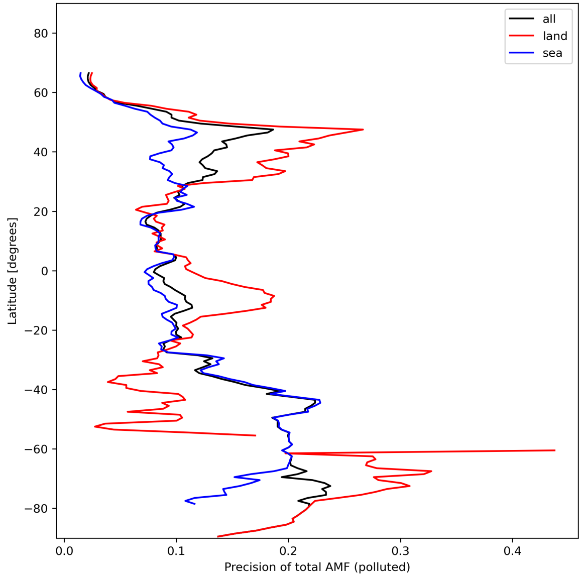
Figure 49: Zonal average of “Precision of total AMF (polluted)” for 2024-01-27 to 2024-01-29.
