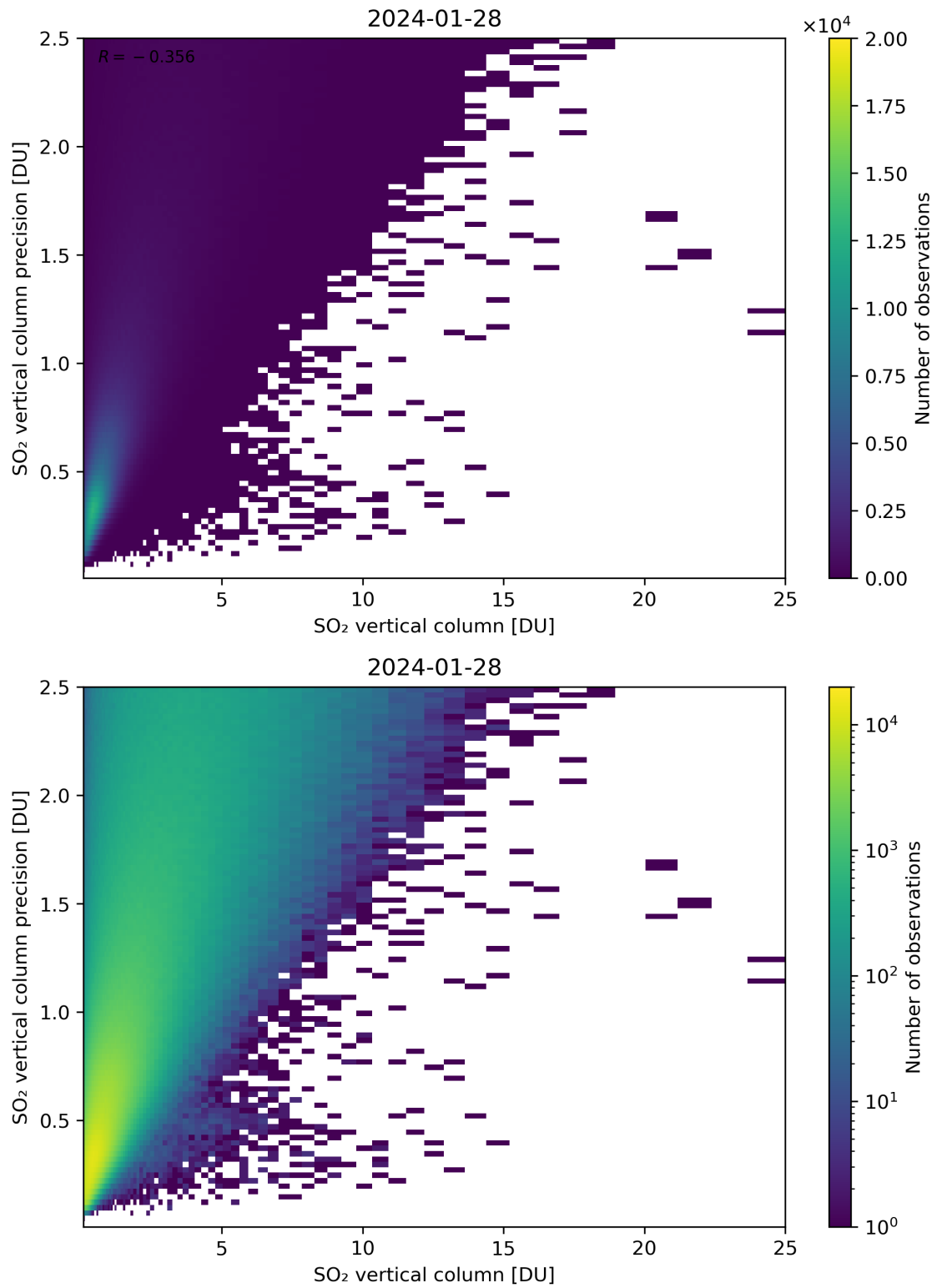
Figure 307: Scatter density plot of “SO 2 vertical column” against “SO 2 vertical column precision” for 2024-01-27 to 2024-01-29.
