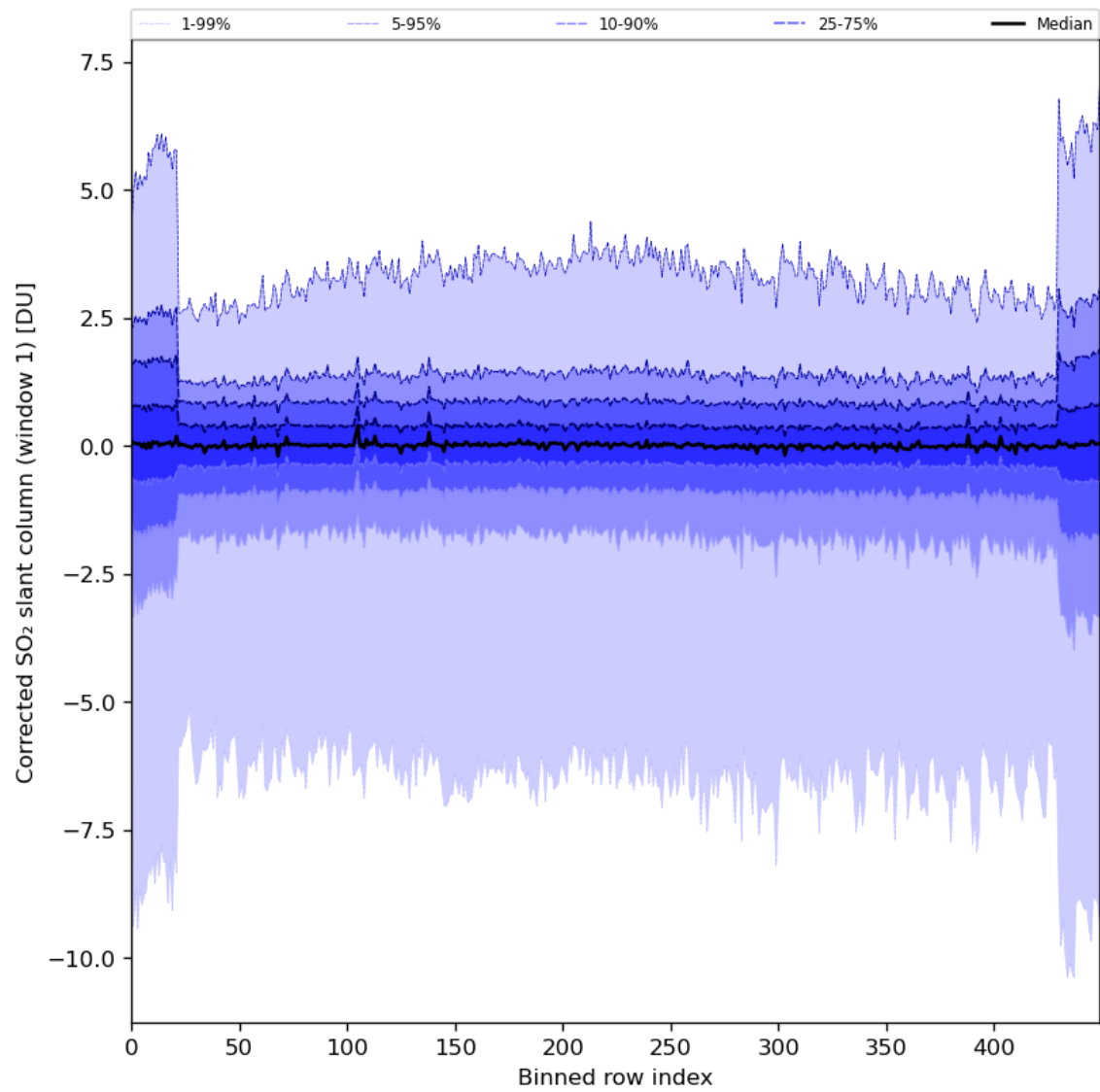
Figure 81: Along track statistics of “Corrected SO 2 slant column (window 1)” for 2024-01-27 to 2024-01-29
