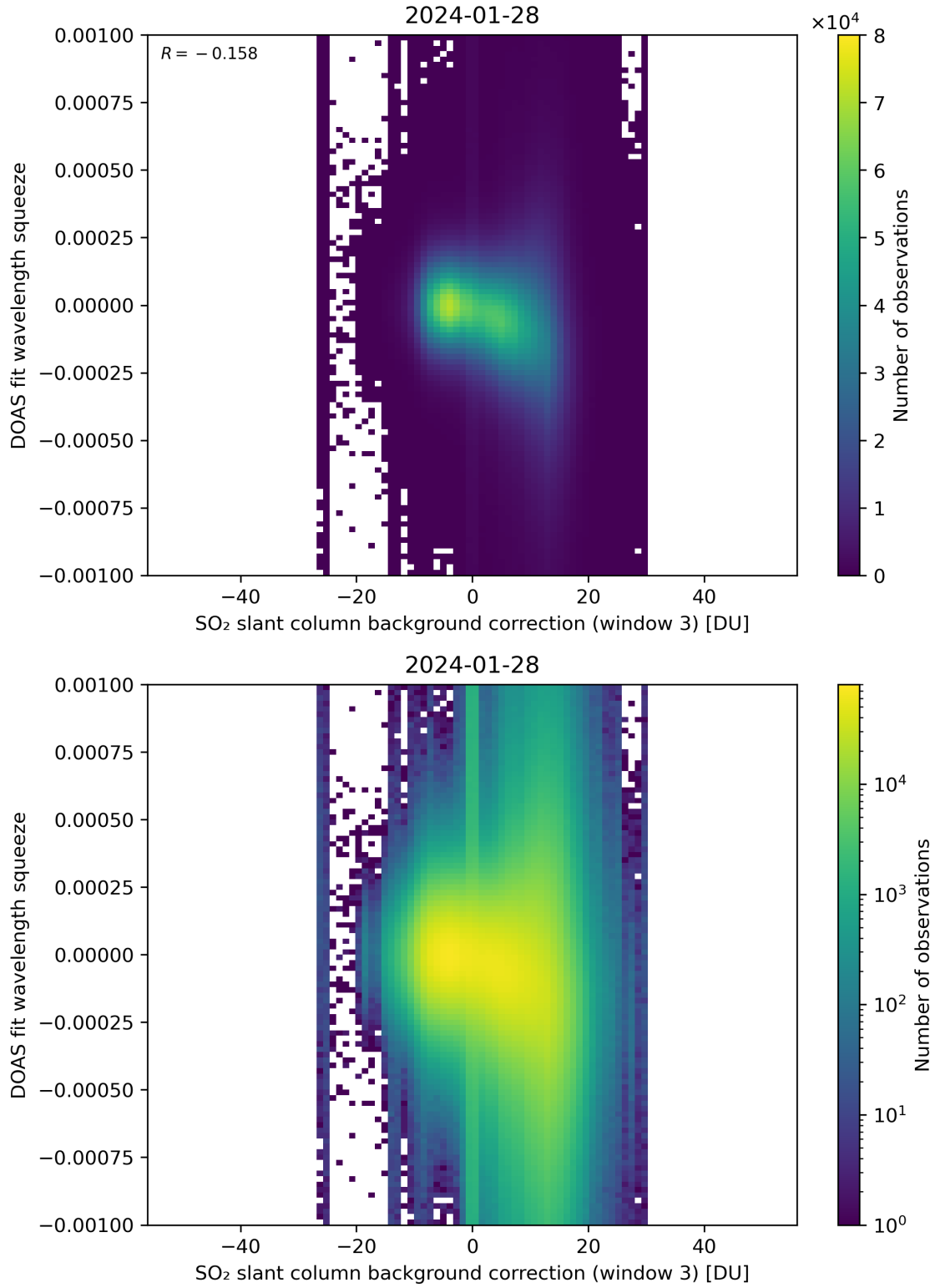
Figure 122: Scatter density plot of “SO 2 slant column background correction (window 3)” against “DOAS fit wavelength squeeze” for 2024-01-27 to 2024-01-29.
