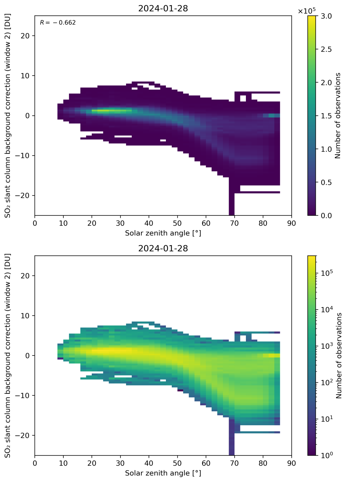
Figure 159: Scatter density plot of “Solar zenith angle” against “SO 2 slant column background correction (window 2)” for 2024-01-27 to 2024-01-29.
