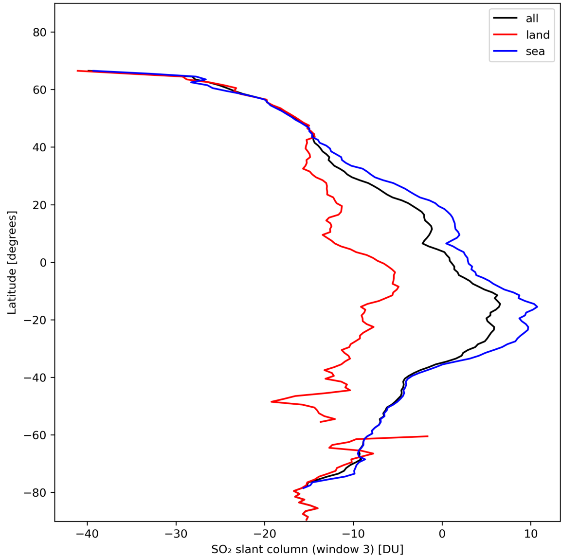
Figure 41: Zonal average of “SO 2 slant column (window 3)” for 2024-01-27 to 2024-01-29.
