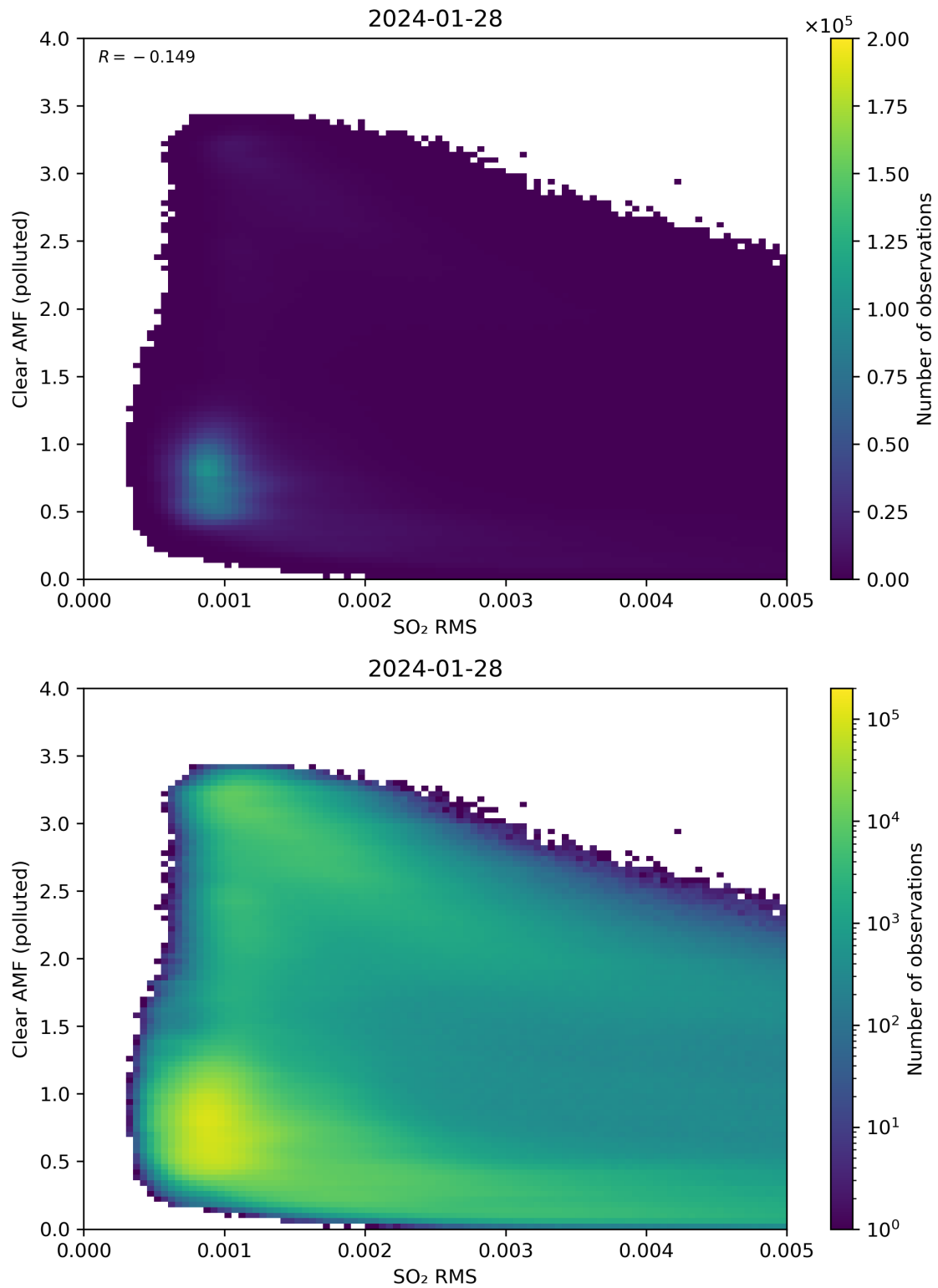
Figure 136: Scatter density plot of “SO 2 RMS” against “Clear AMF (polluted)” for 2024-01-27 to 2024-01-29.
