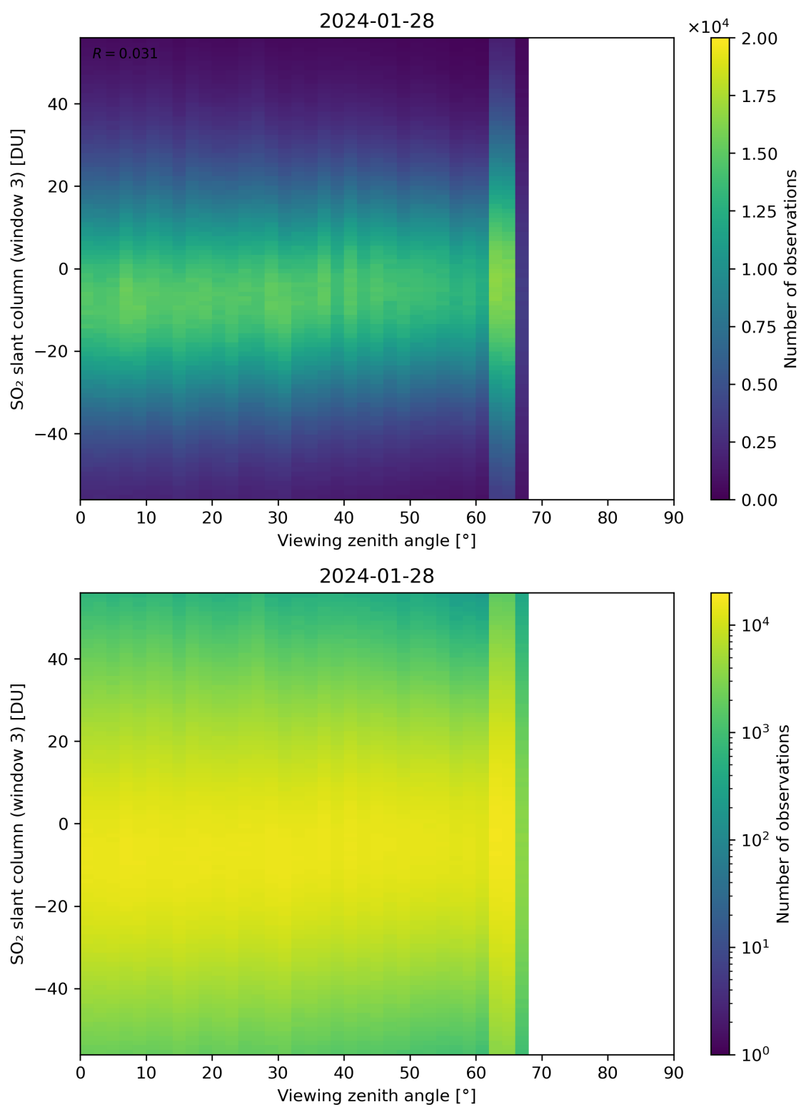
Figure 323: Scatter density plot of “Viewing zenith angle” against “SO 2 slant column (window 3)” for 2024-01-27 to 2024-01-29.
