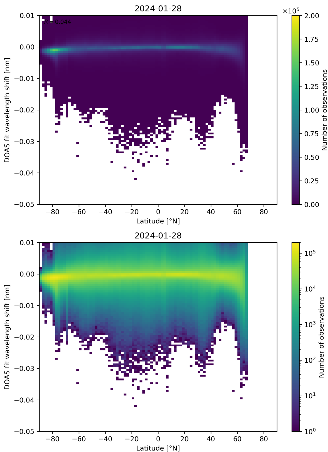
Figure 142: Scatter density plot of “Latitude” against “DOAS fit wavelength shift” for 2024-01-27 to 2024-01-29.
