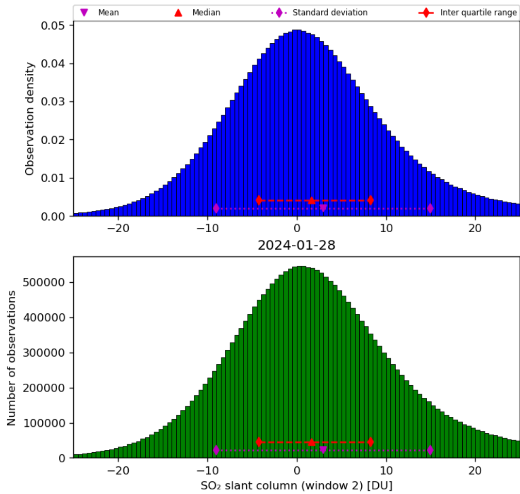
Figure 60: Histogram of “SO 2 slant column (window 2)” for 2024-01-27 to 2024-01-29
