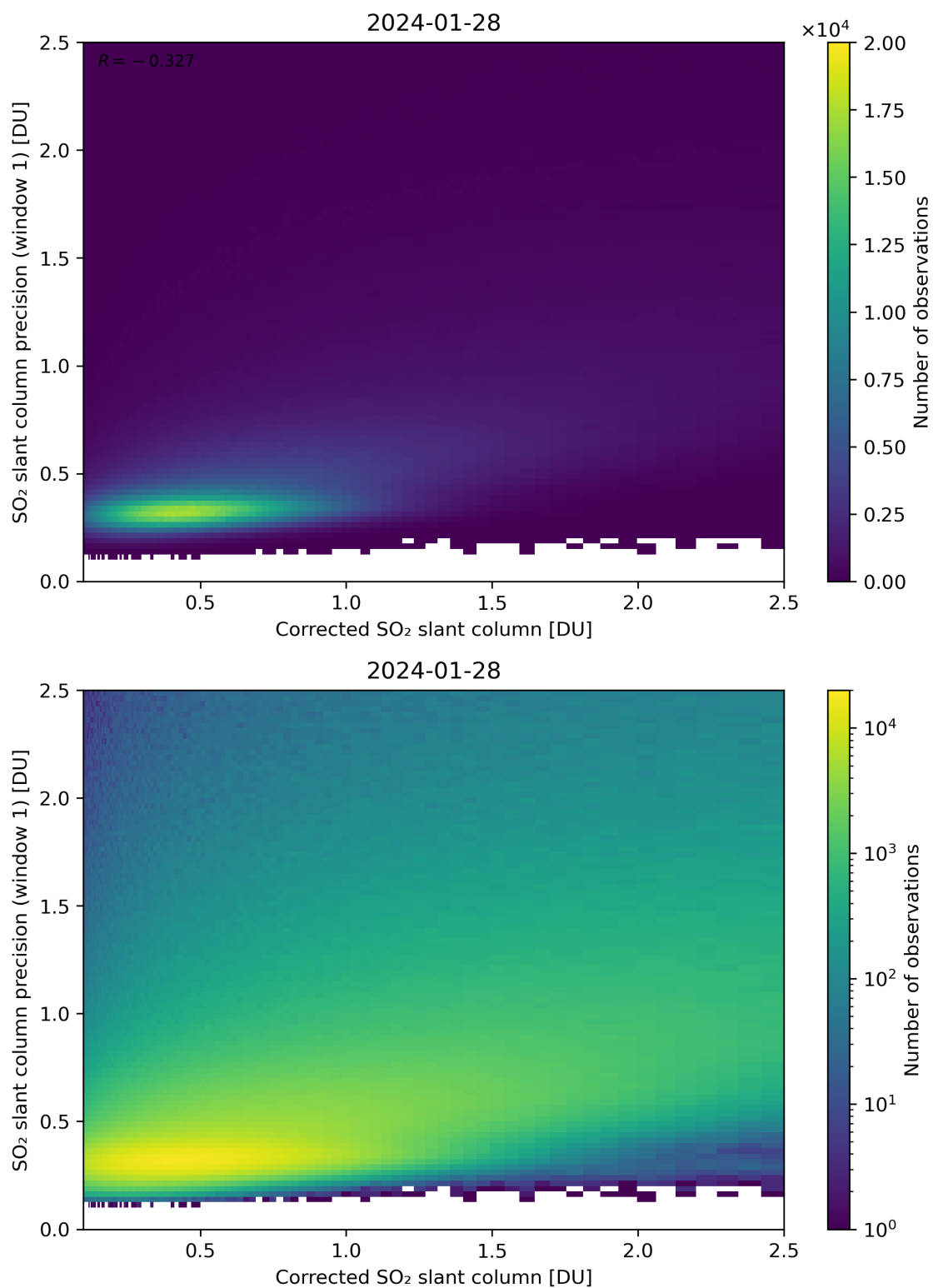
Figure 188: Scatter density plot of “Corrected SO 2 slant column” against “SO 2 slant column precision (window 1)” for 2024-01-27 to 2024-01-29.
