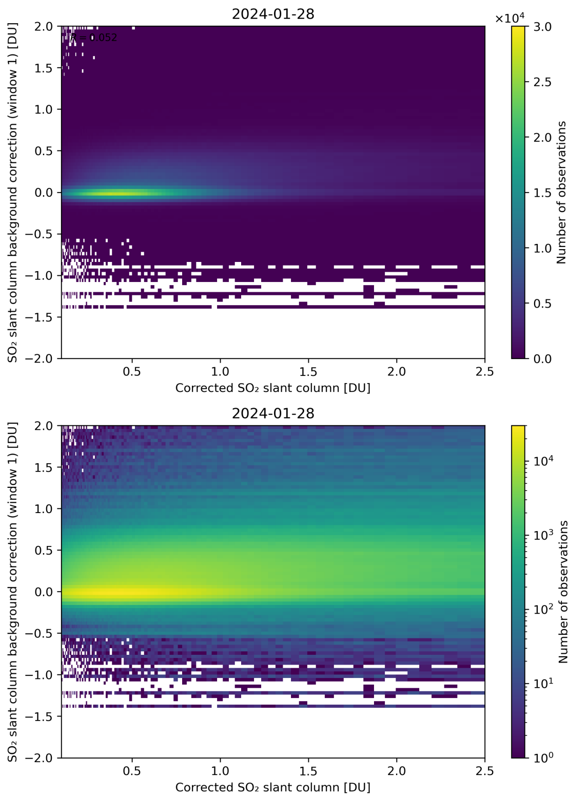
Figure 178: Scatter density plot of “Corrected SO 2 slant column” against “SO 2 slant column background correction (window 1)” for 2024-01-27 to 2024-01-29.
