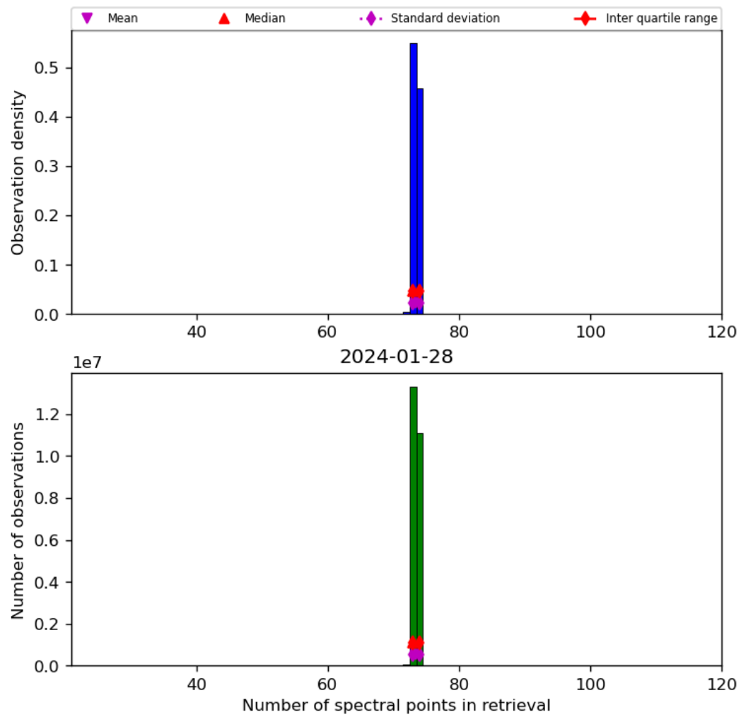
Figure 74: Histogram of “Number of spectral points in retrieval” for 2024-01-27 to 2024-01-29
