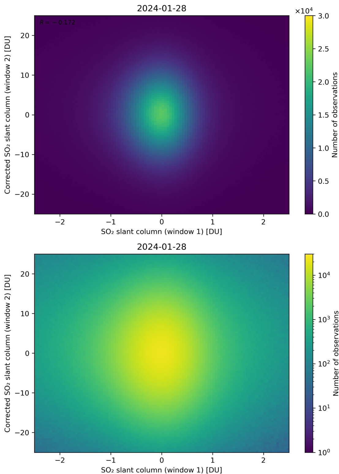
Figure 233: Scatter density plot of “SO 2 slant column (window 1)” against “Corrected SO 2 slant column (window 2)” for 2024-01-27 to 2024-01-29.
