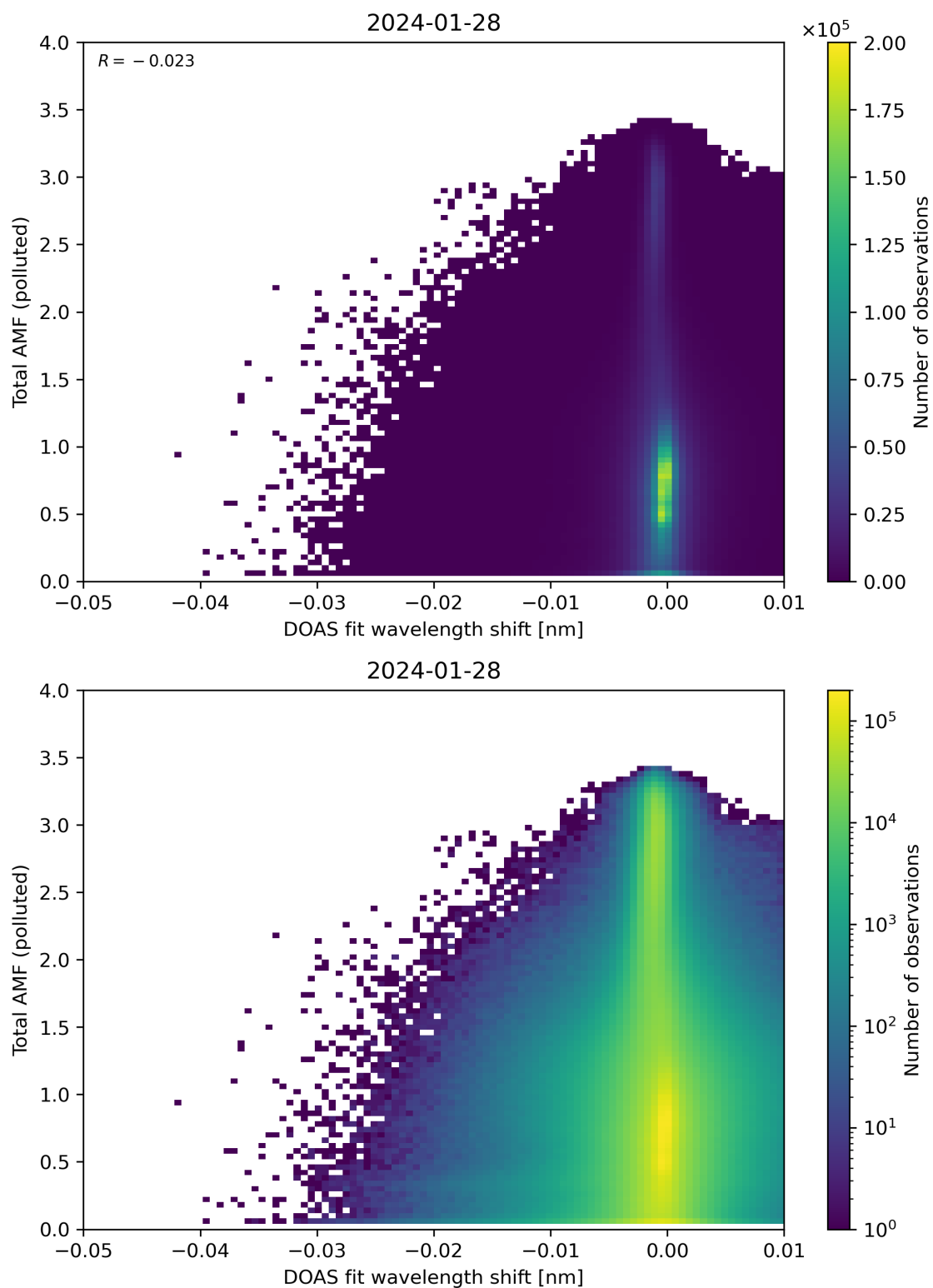
Figure 130: Scatter density plot of “DOAS fit wavelength shift” against “Total AMF (polluted)” for 2024-01-27 to 2024-01-29.
