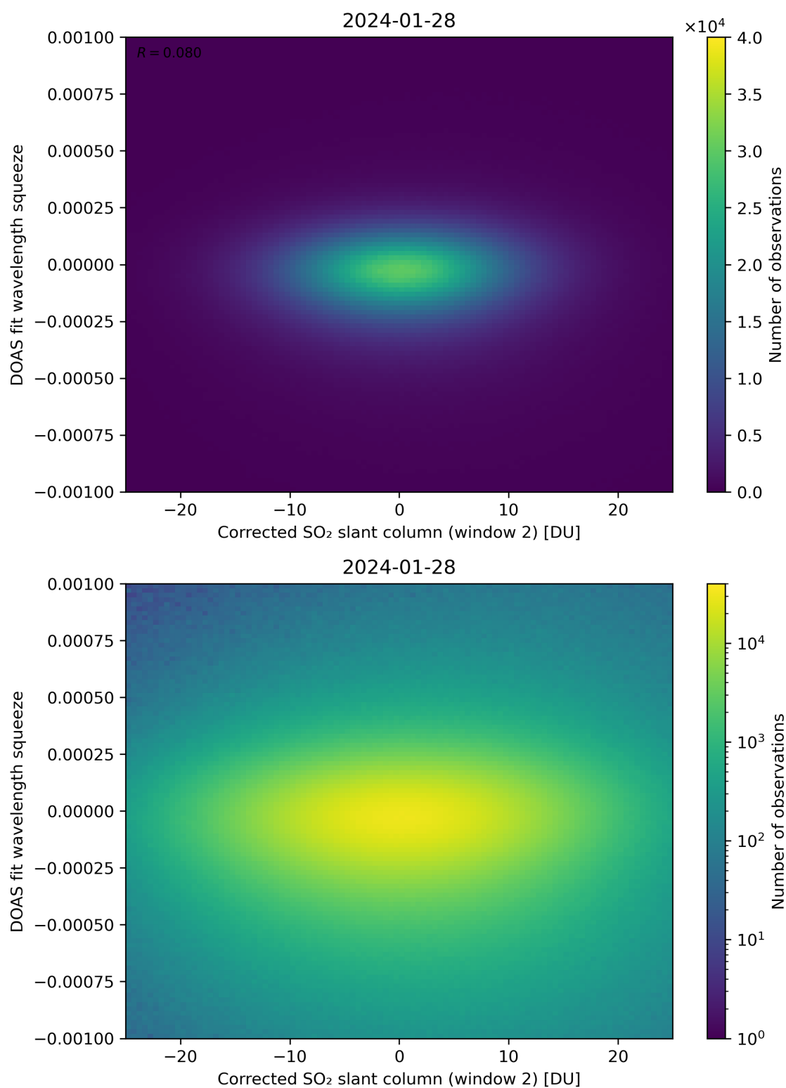
Figure 197: Scatter density plot of “Corrected SO 2 slant column (window 2)” against “DOAS fit wavelength squeeze” for 2024-01-27 to 2024-01-29.
