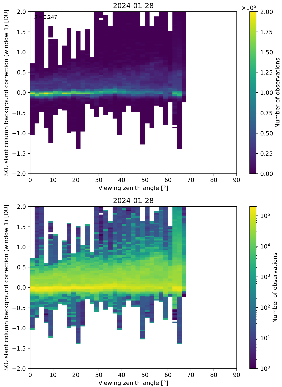
Figure 308: Scatter density plot of “Viewing zenith angle” against “SO 2 slant column background correction (window 1)” for 2024-01-27 to 2024-01-29.
