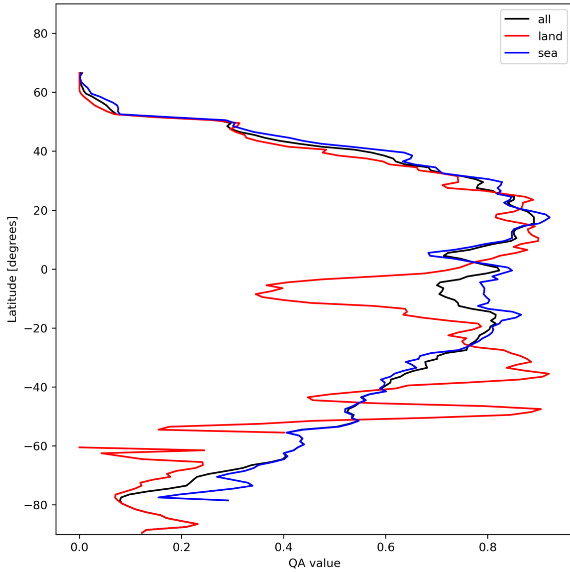
Figure 29: Zonal average of “QA value” for 2024-01-27 to 2024-01-29.
