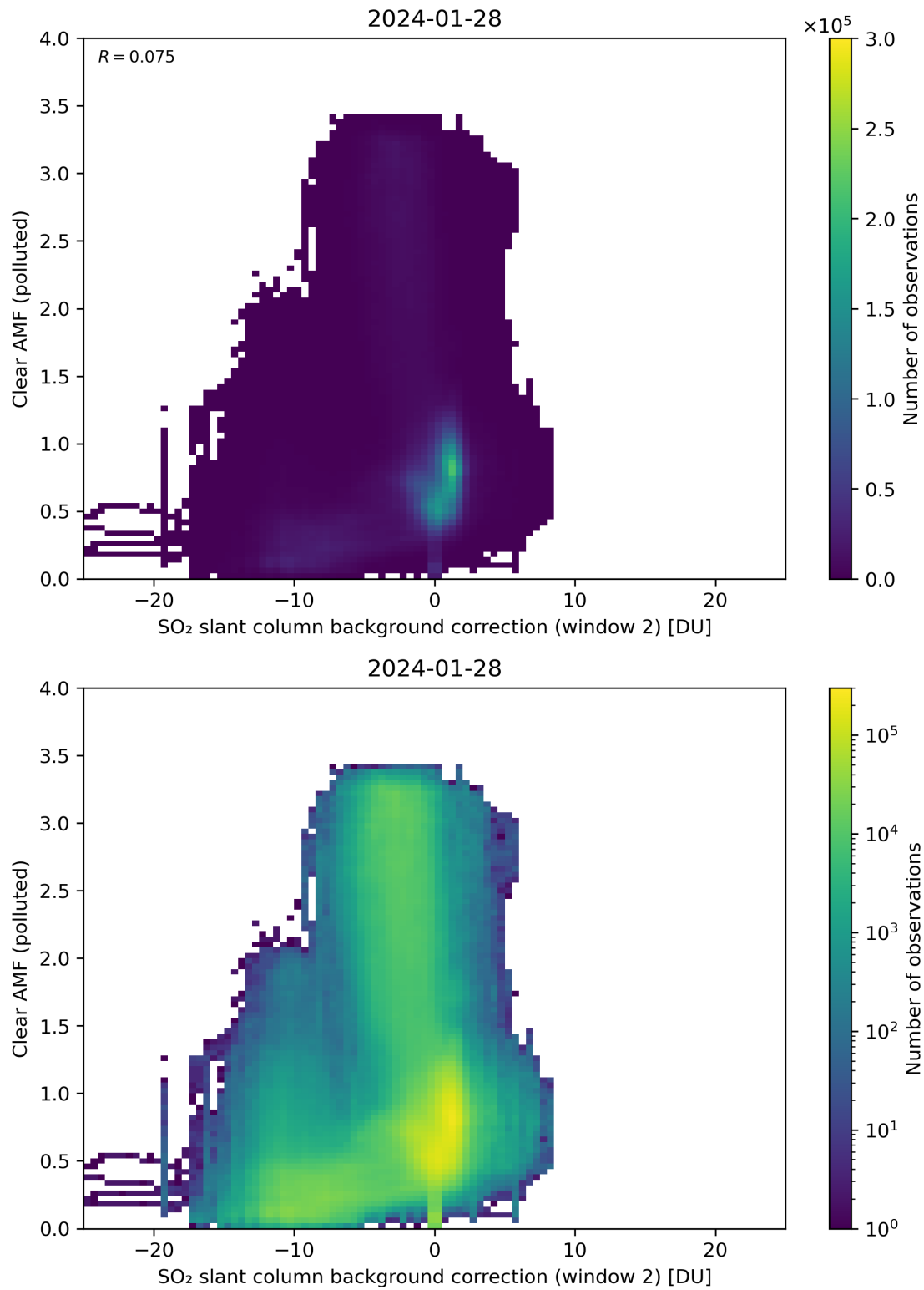
Figure 115: Scatter density plot of “SO 2 slant column background correction (window 2)” against “Clear AMF (polluted)” for 2024-01-27 to 2024-01-29.
