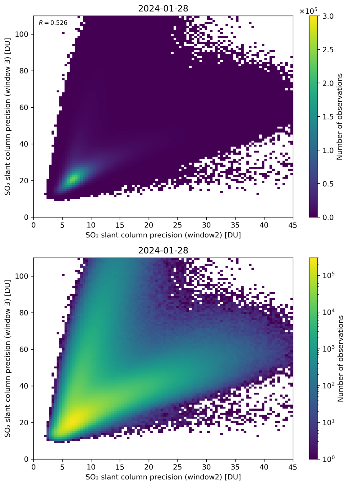
Figure 250: Scatter density plot of “SO 2 slant column precision (window2)” against “SO 2 slant column precision (window 3)” for 2024-01-27 to 2024-01-29.
