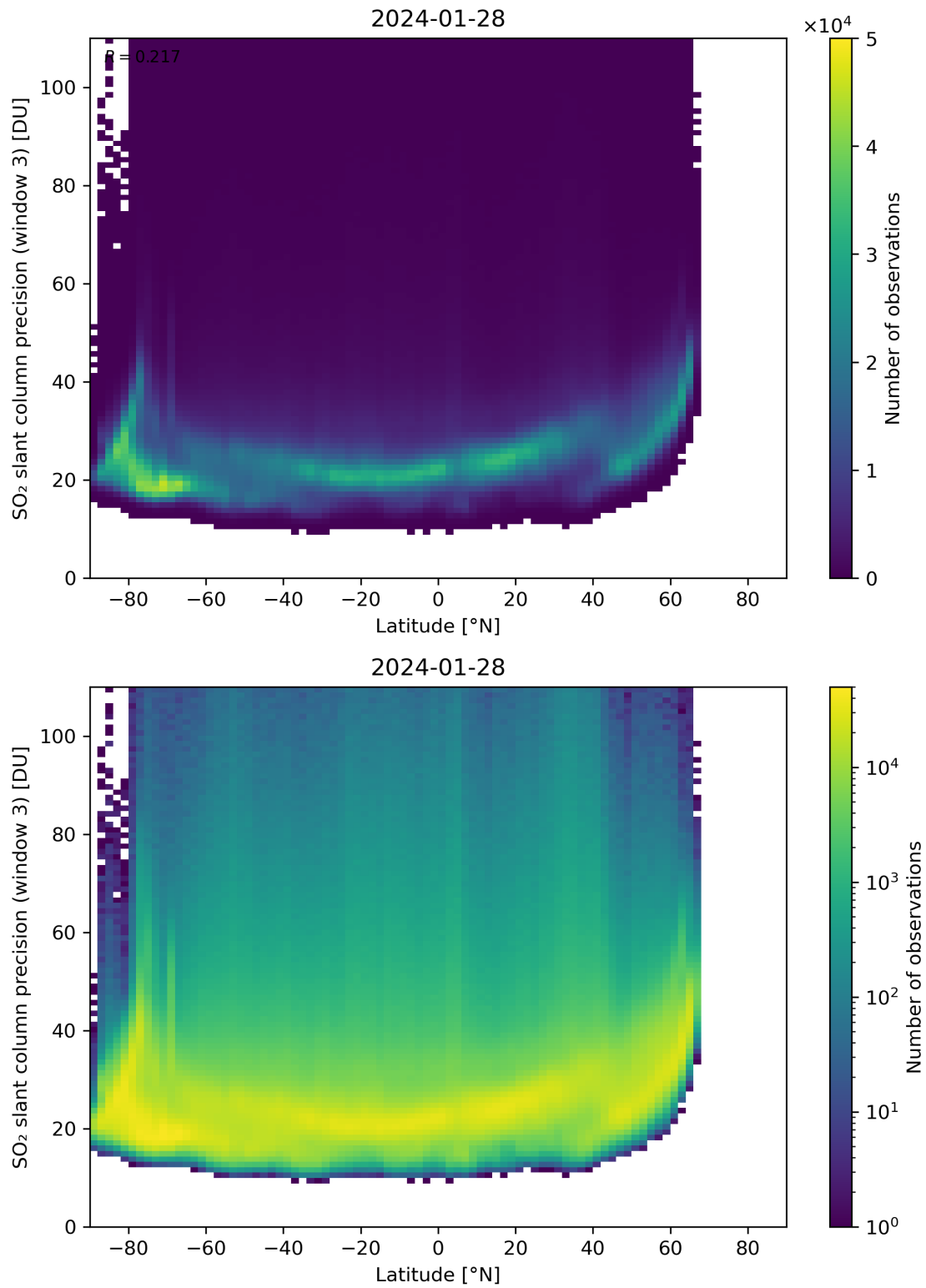
Figure 153: Scatter density plot of “Latitude” against “SO 2 slant column precision (window 3)” for 2024-01-27 to 2024-01-29.
