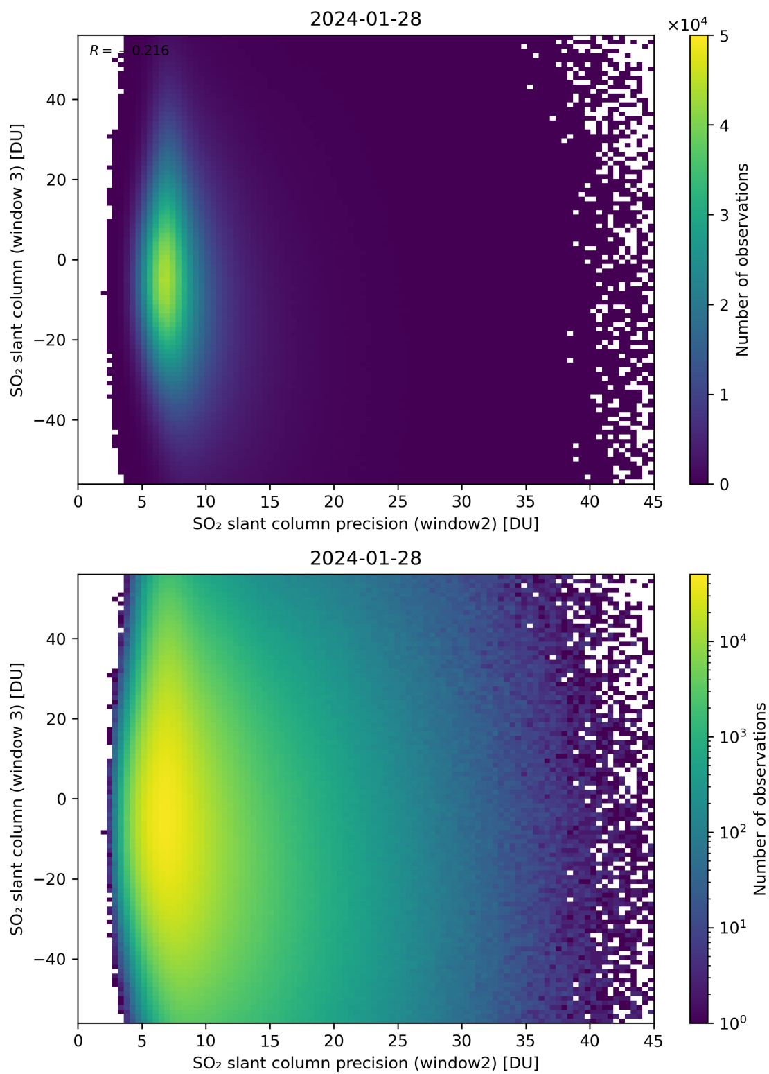
Figure 249: Scatter density plot of “SO 2 slant column precision (window2)” against “SO 2 slant column (window 3)” for 2024-01-27 to 2024-01-29.
