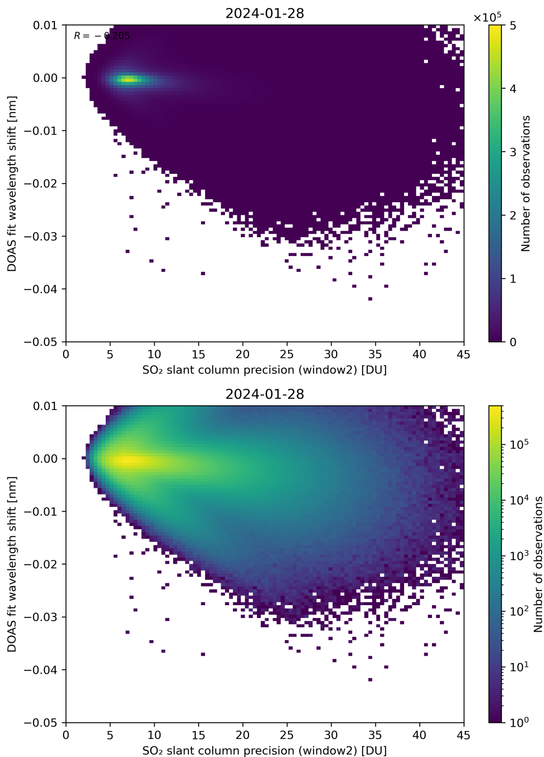
Figure 243: Scatter density plot of “SO 2 slant column precision (window2)” against “DOAS fit wavelength shift” for 2024-01-27 to 2024-01-29.
