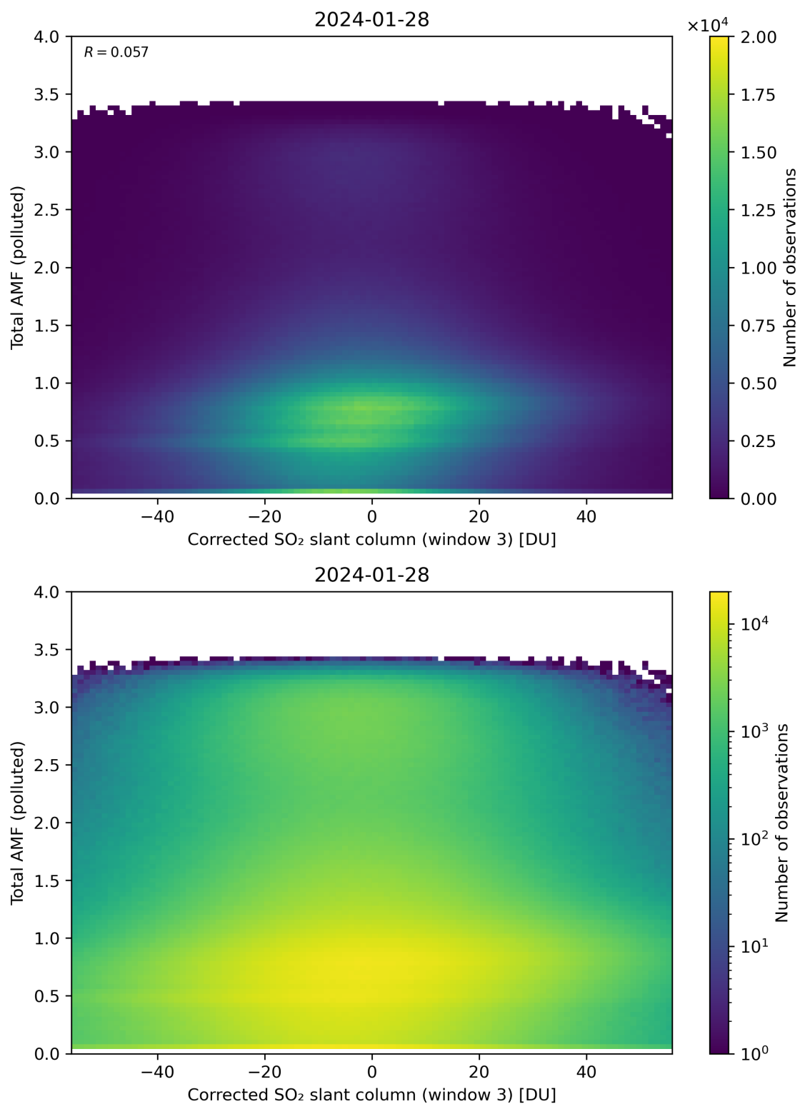
Figure 210: Scatter density plot of “Corrected SO 2 slant column (window 3)” against “Total AMF (polluted)” for 2024-01-27 to 2024-01-29.
