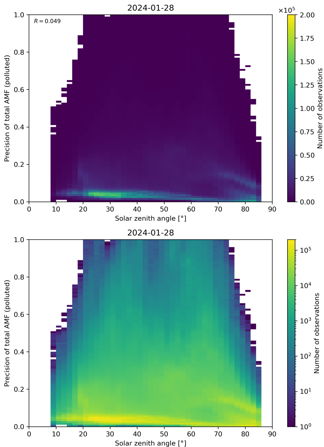
Figure 175: Scatter density plot of “Solar zenith angle” against “Precision of total AMF (polluted)” for 2024-01-27 to 2024-01-29.
