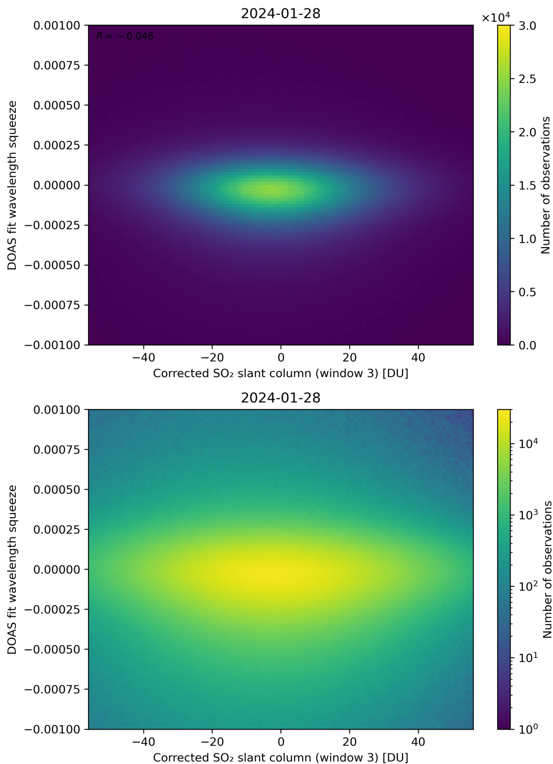
Figure 207: Scatter density plot of “Corrected SO 2 slant column (window 3)” against “DOAS fit wavelength squeeze” for 2024-01-27 to 2024-01-29.
