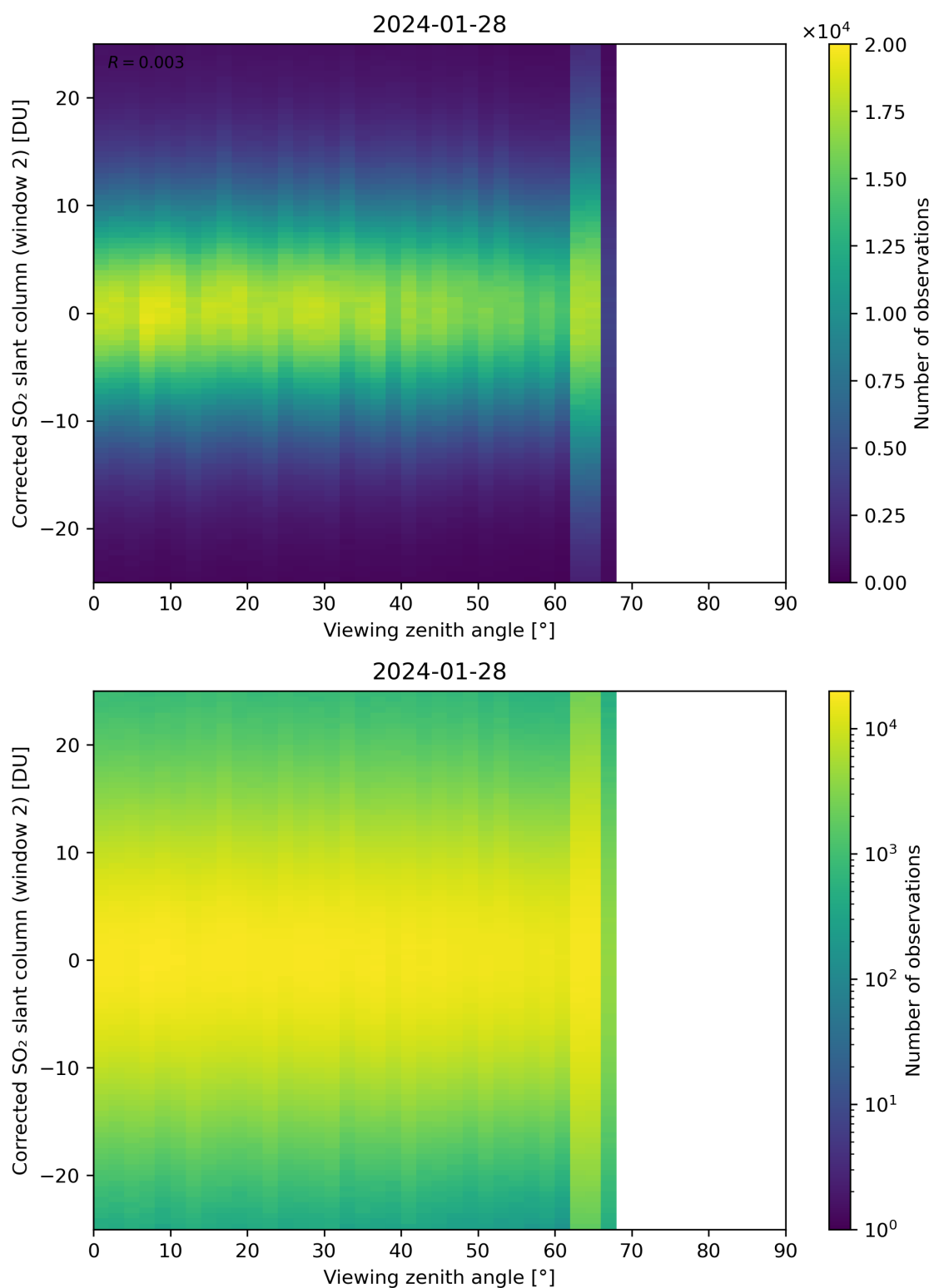
Figure 318: Scatter density plot of “Viewing zenith angle” against “Corrected SO 2 slant column (window 2)” for 2024-01-27 to 2024-01-29.
