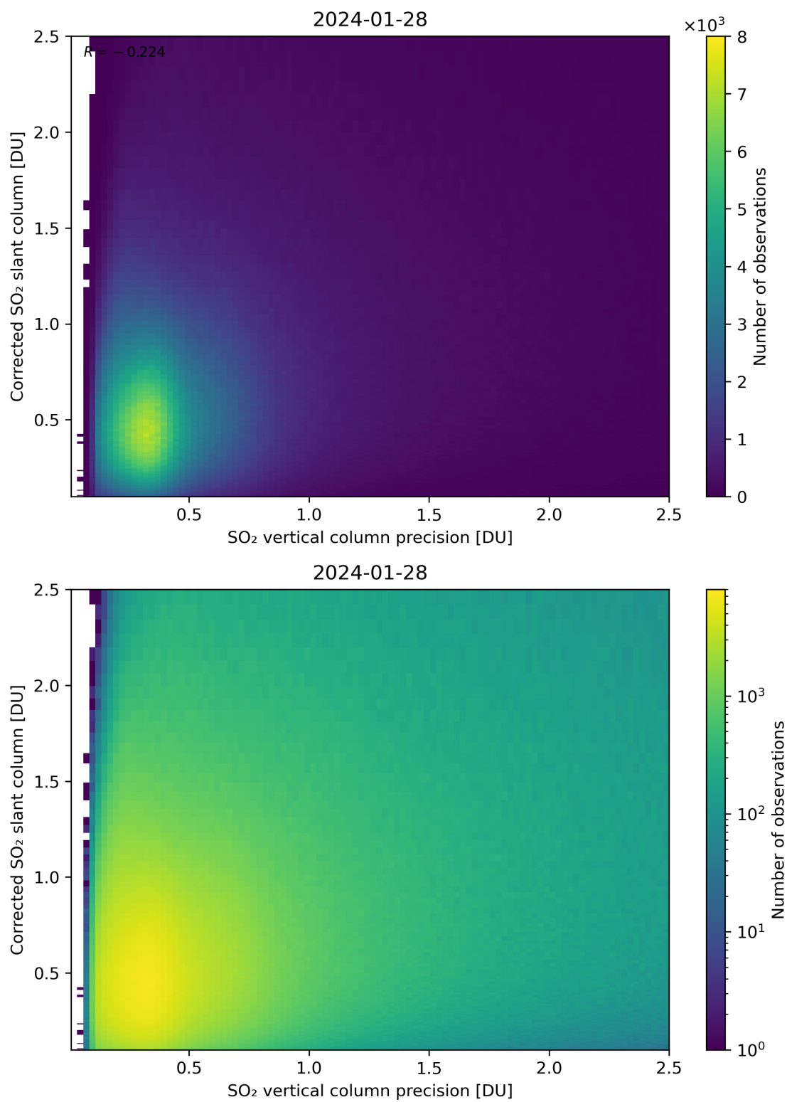
Figure 286: Scatter density plot of “SO 2 vertical column precision” against “Corrected SO 2 slant column” for 2024-01-27 to 2024-01-29.
