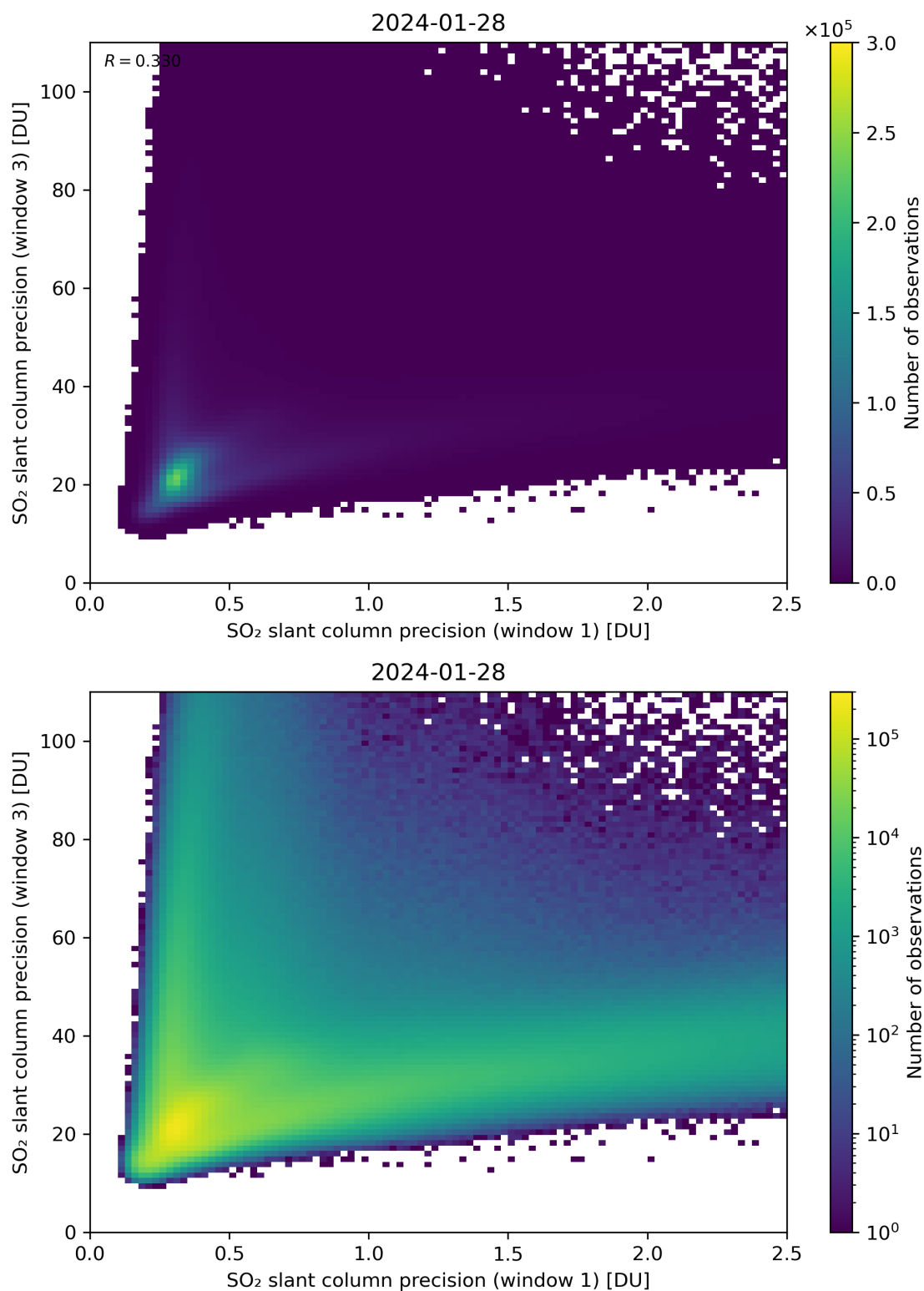
Figure 229: Scatter density plot of “SO 2 slant column precision (window 1)” against “SO 2 slant column precision (window 3)” for 2024-01-27 to 2024-01-29.
