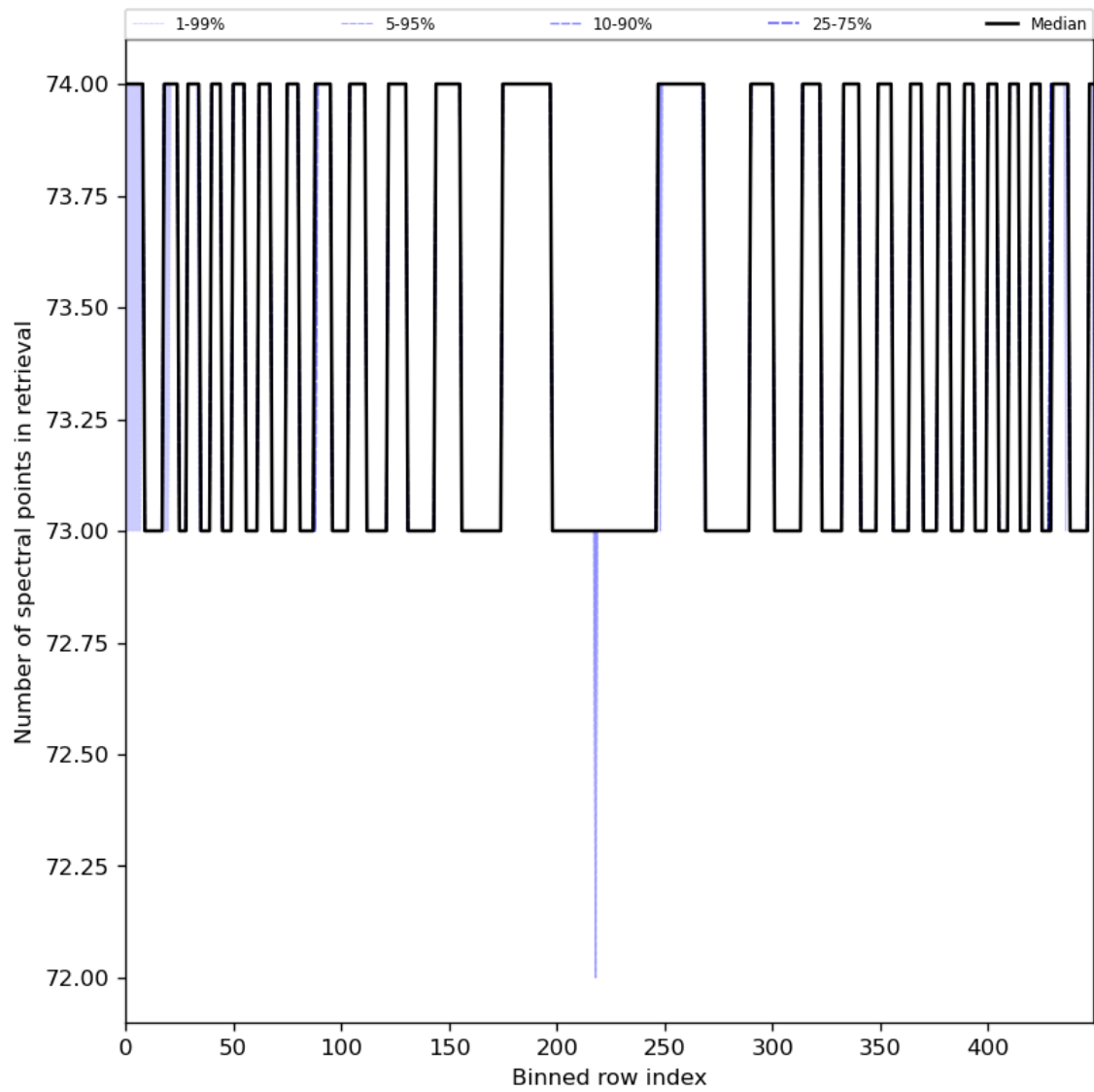
Figure 97: Along track statistics of “Number of spectral points in retrieval” for 2024-01-28 to 2024-01-30
