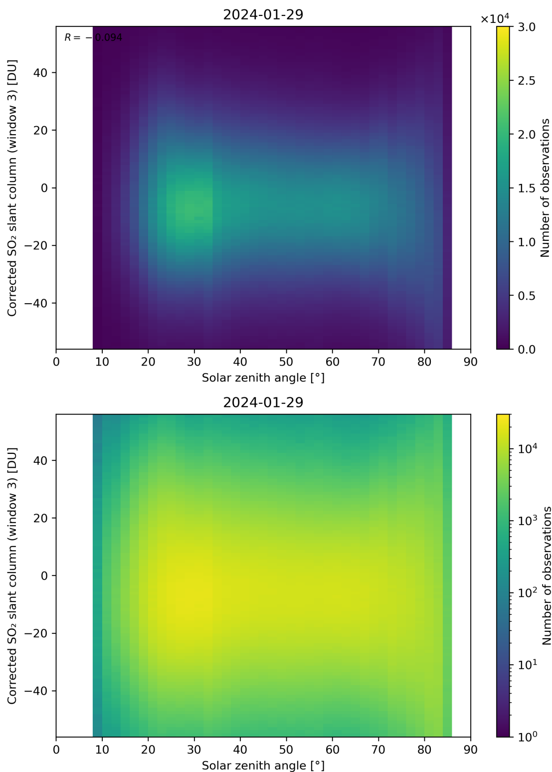
Figure 168: Scatter density plot of “Solar zenith angle” against “Corrected SO 2 slant column (window 3)” for 2024-01-28 to 2024-01-30.
