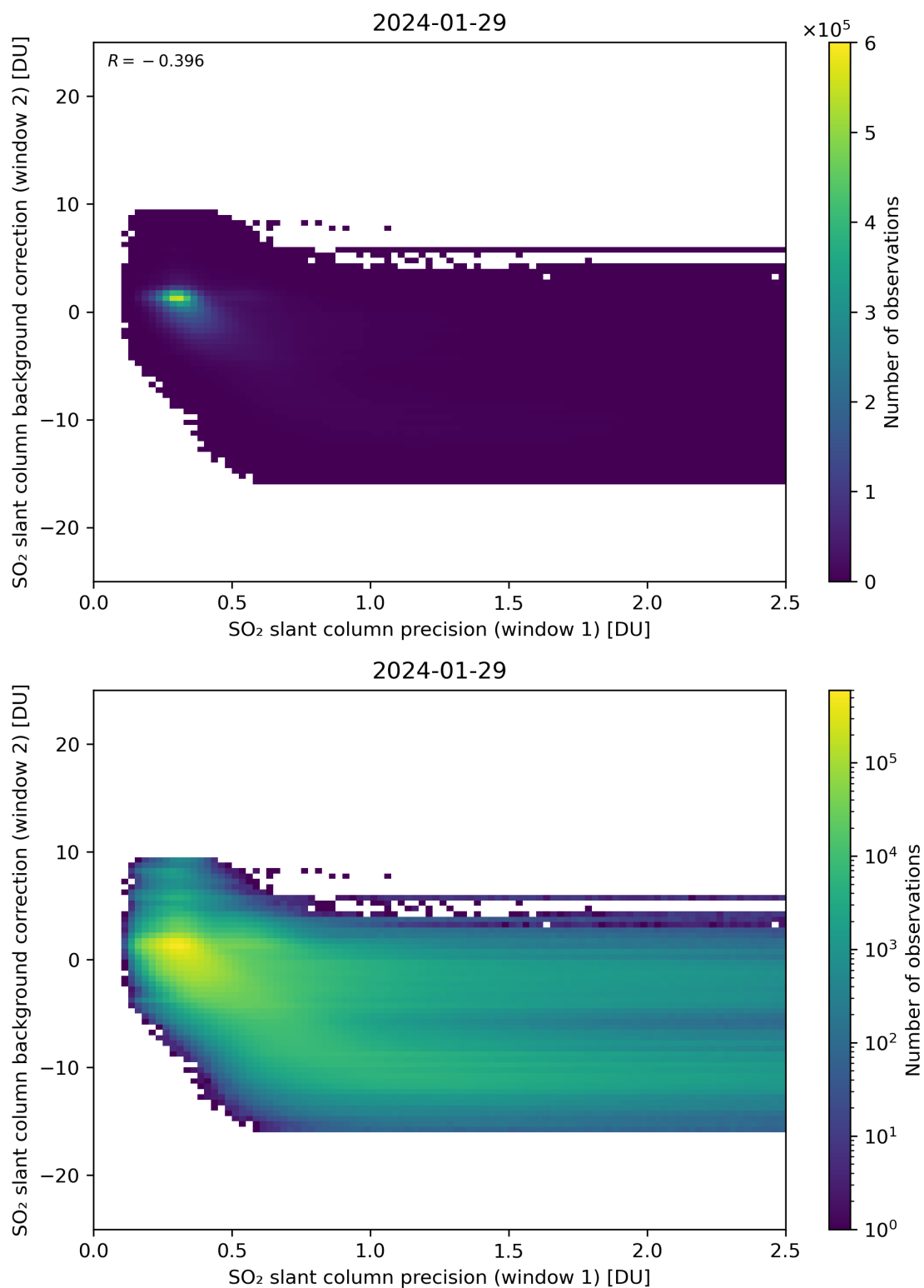
Figure 219: Scatter density plot of “SO 2 slant column precision (window 1)” against “SO 2 slant column background correction (window 2)” for 2024-01-28 to 2024-01-30.
