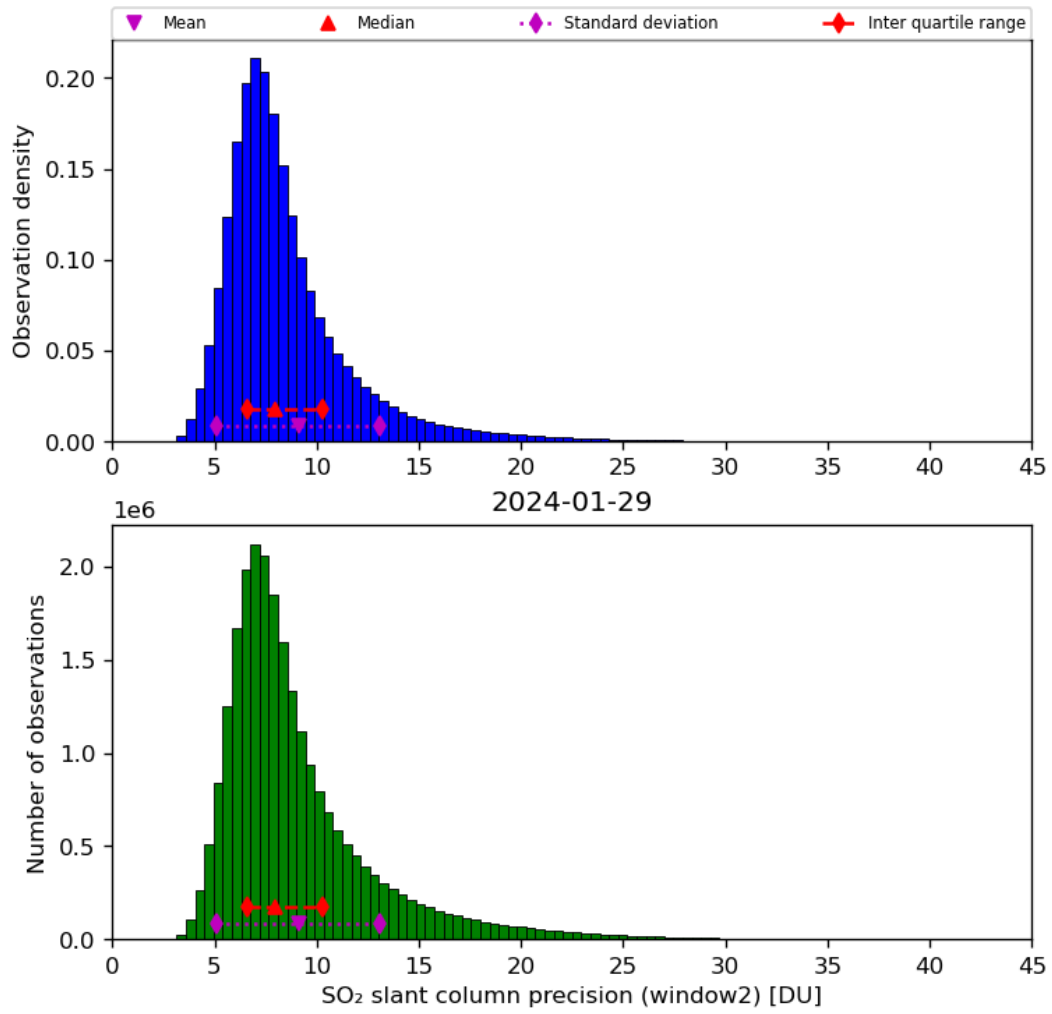
Figure 61: Histogram of “SO 2 slant column precision (window2)” for 2024-01-28 to 2024-01-30
