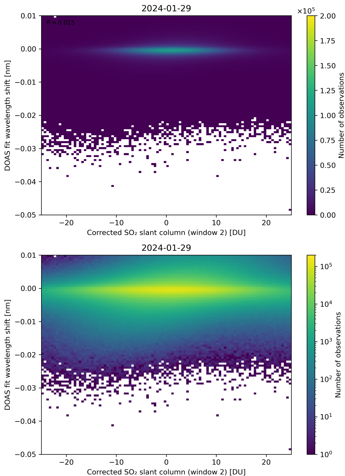
Figure 196: Scatter density plot of “Corrected SO 2 slant column (window 2)” against “DOAS fit wavelength shift” for 2024-01-28 to 2024-01-30.
