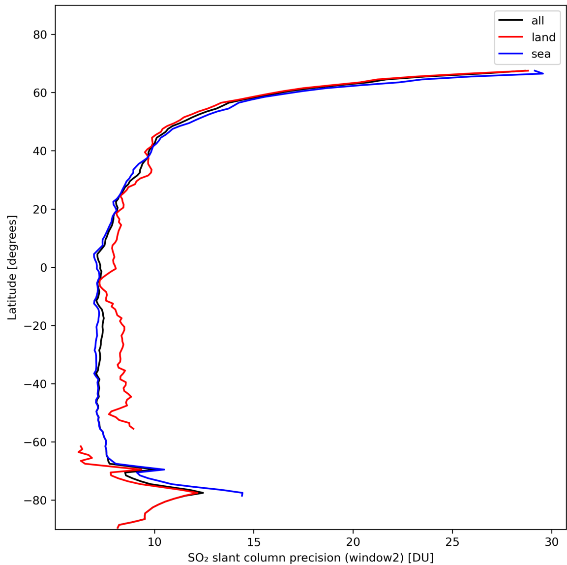
Figure 38: Zonal average of “SO 2 slant column precision (window2)” for 2024-01-28 to 2024-01-30.
