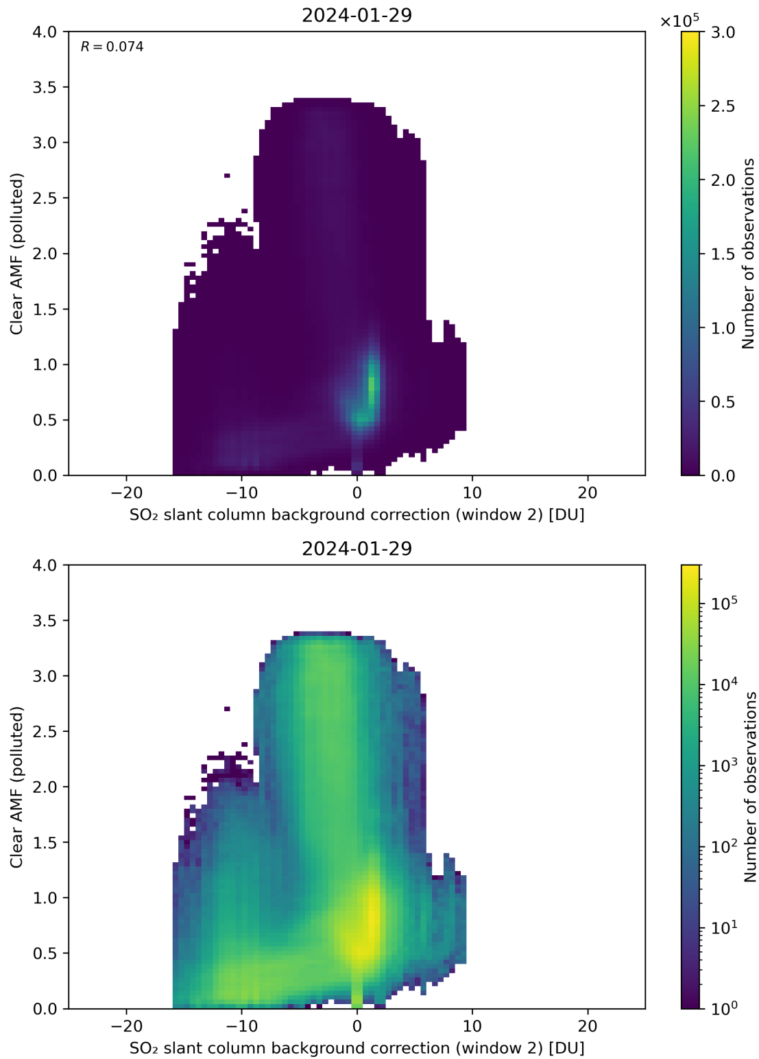
Figure 115: Scatter density plot of “SO 2 slant column background correction (window 2)” against “Clear AMF (polluted)” for 2024-01-28 to 2024-01-30.
