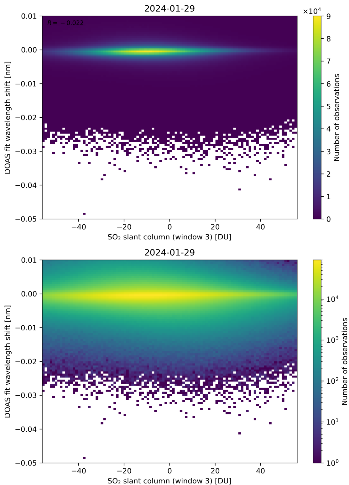
Figure 254: Scatter density plot of “SO 2 slant column (window 3)” against “DOAS fit wavelength shift” for 2024-01-28 to 2024-01-30.
