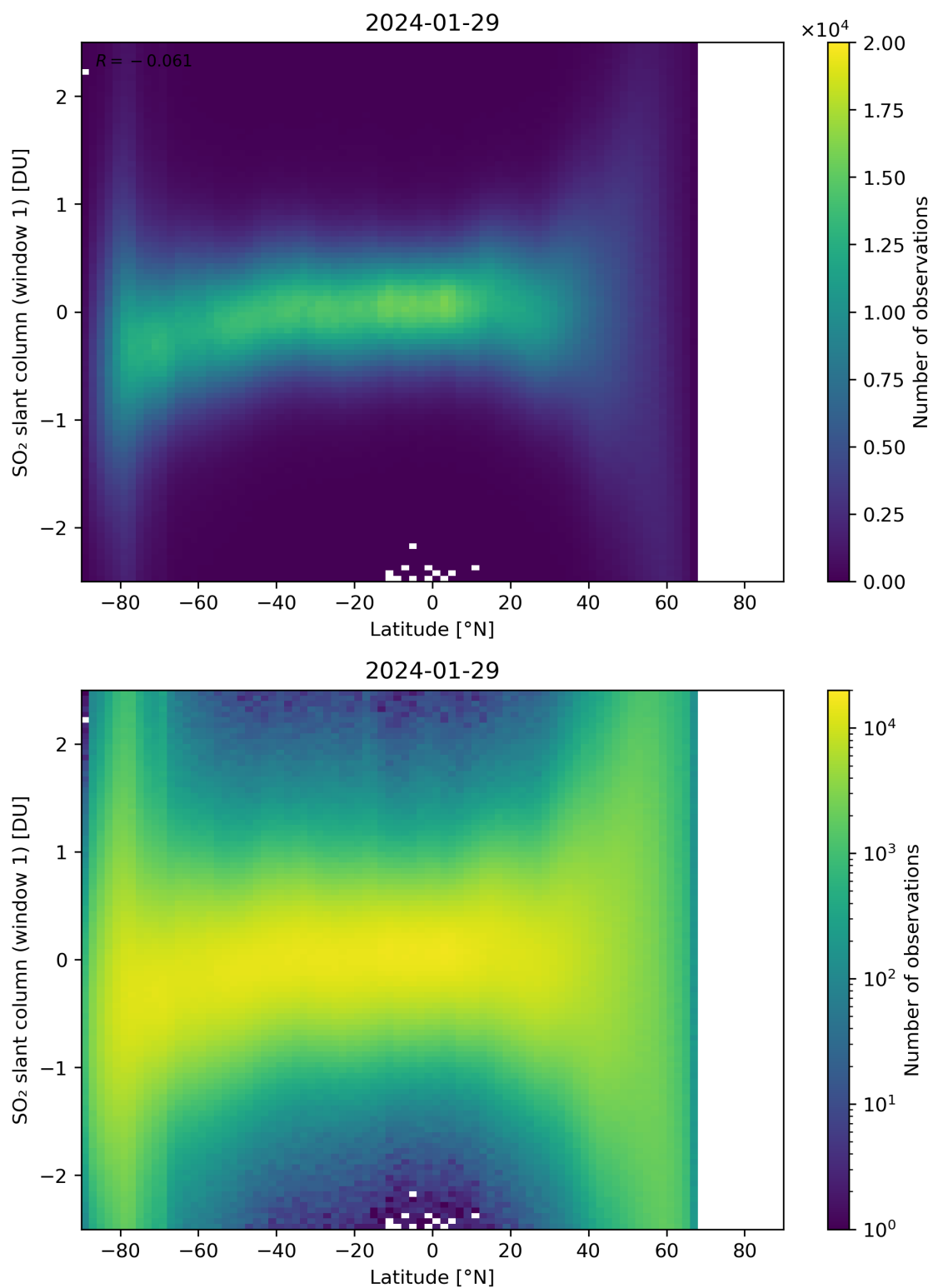
Figure 149: Scatter density plot of “Latitude” against “SO 2 slant column (window 1)” for 2024-01-28 to 2024-01-30.
