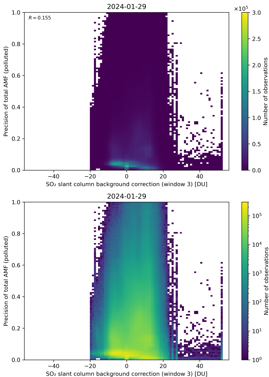
Figure 126: Scatter density plot of “SO 2 slant column background correction (window 3)” against “Precision of total AMF (polluted)” for 2024-01-28 to 2024-01-30.
