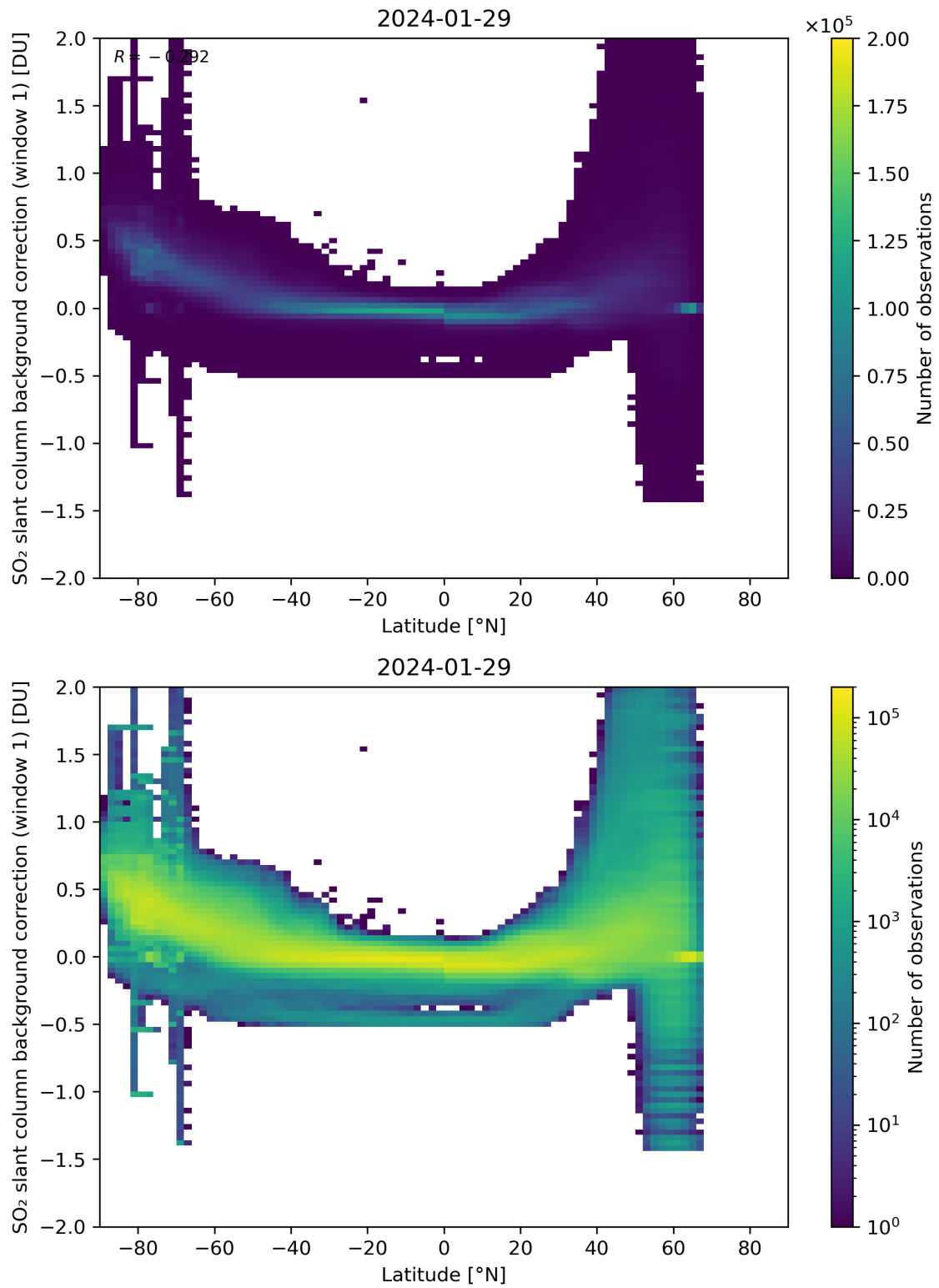
Figure 139: Scatter density plot of “Latitude” against “SO 2 slant column background correction (window 1)” for 2024-01-28 to 2024-01-30.
