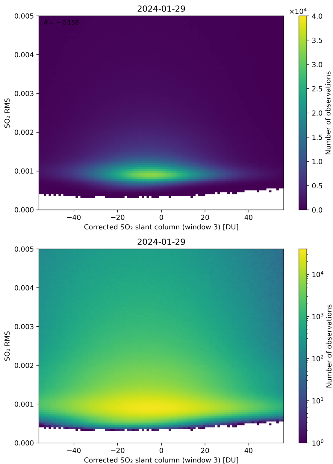
Figure 208: Scatter density plot of “Corrected SO 2 slant column (window 3)” against “SO 2 RMS” for 2024-01-28 to 2024-01-30.
