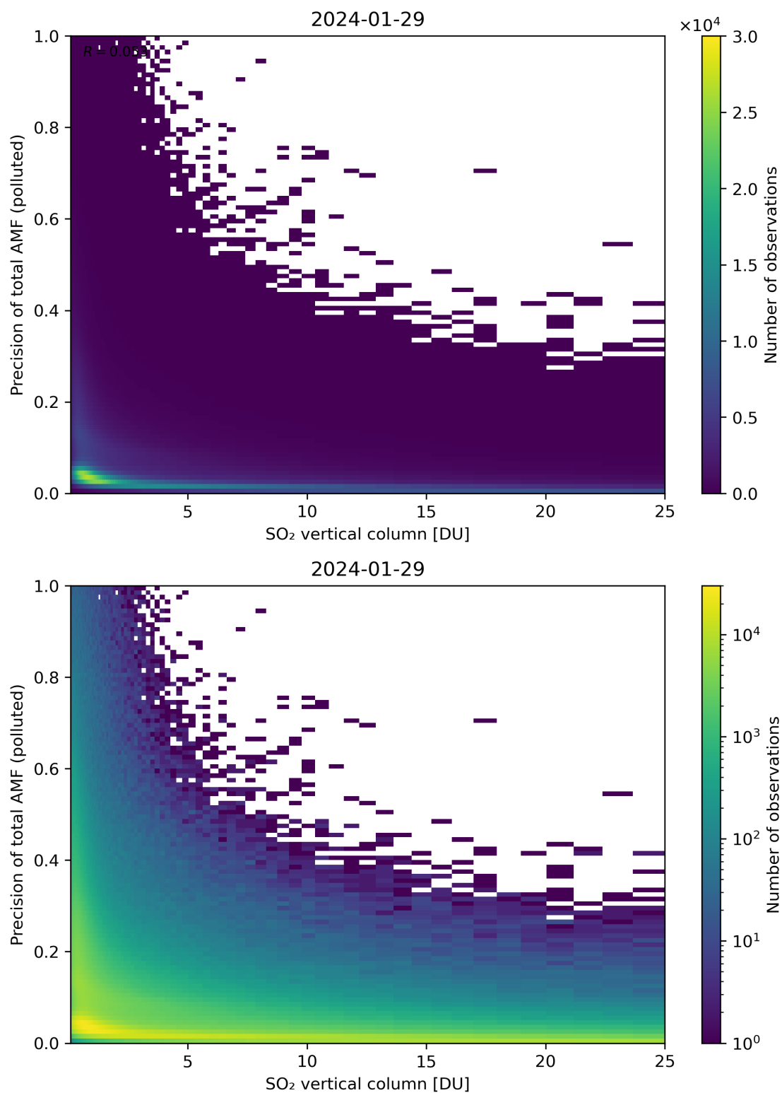
Figure 306: Scatter density plot of “SO 2 vertical column” against “Precision of total AMF (polluted)” for 2024-01-28 to 2024-01-30.
