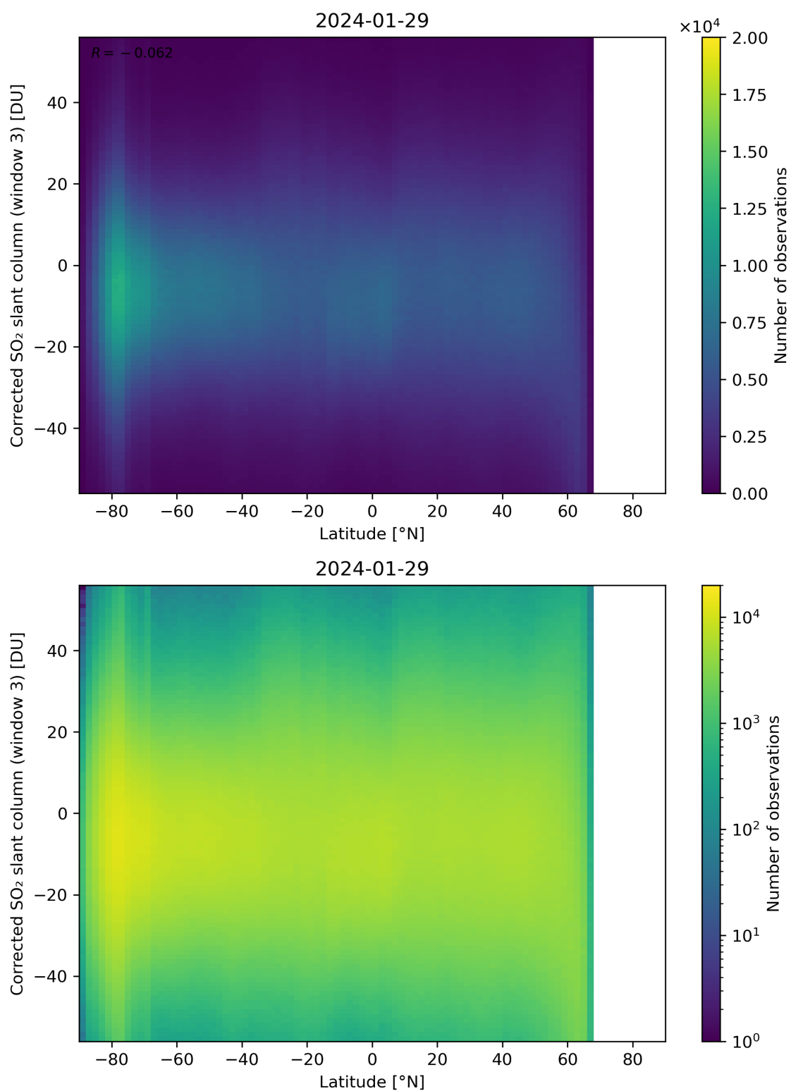
Figure 148: Scatter density plot of “Latitude” against “Corrected SO 2 slant column (window 3)” for 2024-01-28 to 2024-01-30.
