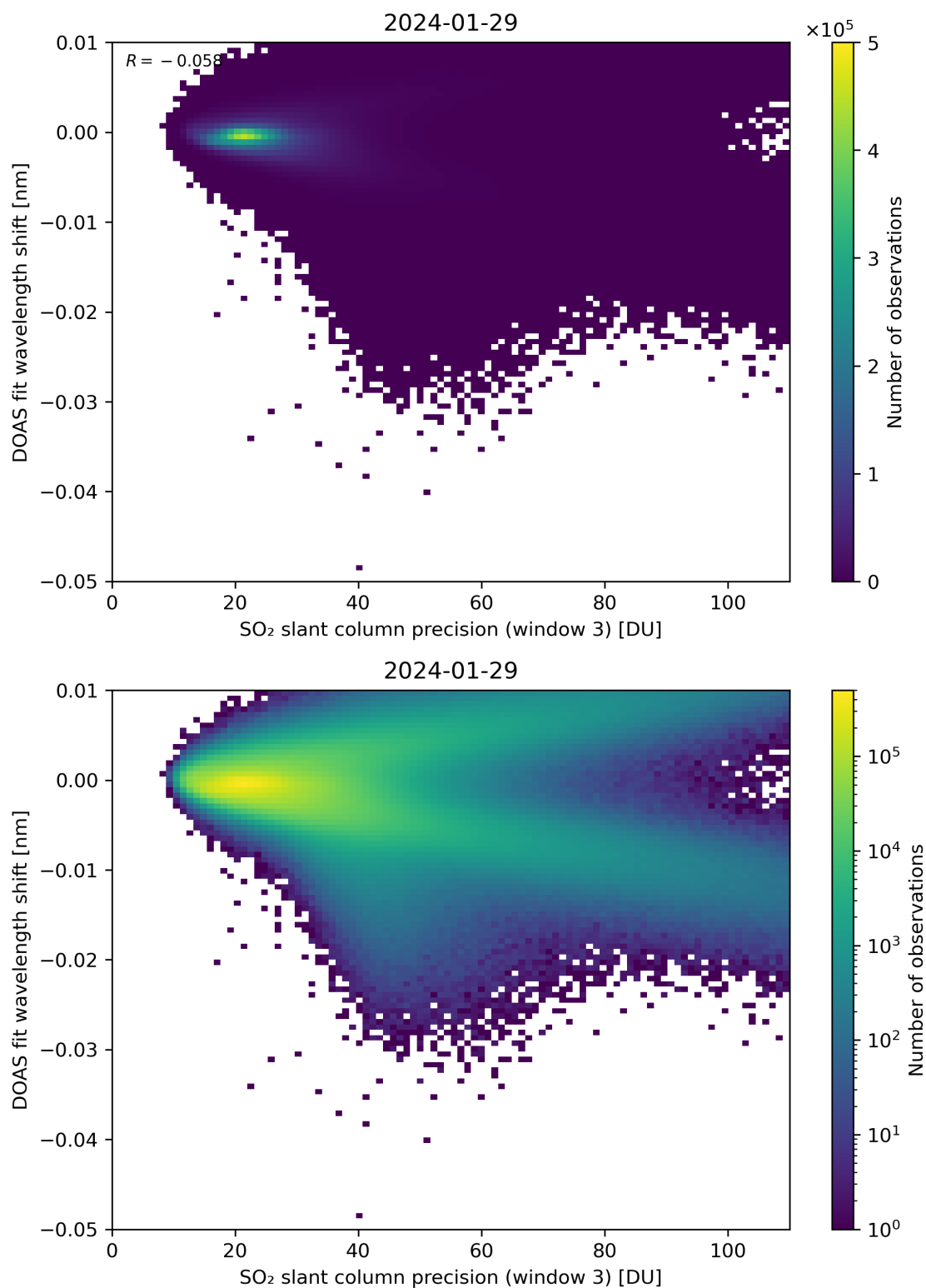
Figure 258: Scatter density plot of “SO 2 slant column precision (window 3)” against “DOAS fit wavelength shift” for 2024-01-28 to 2024-01-30.
