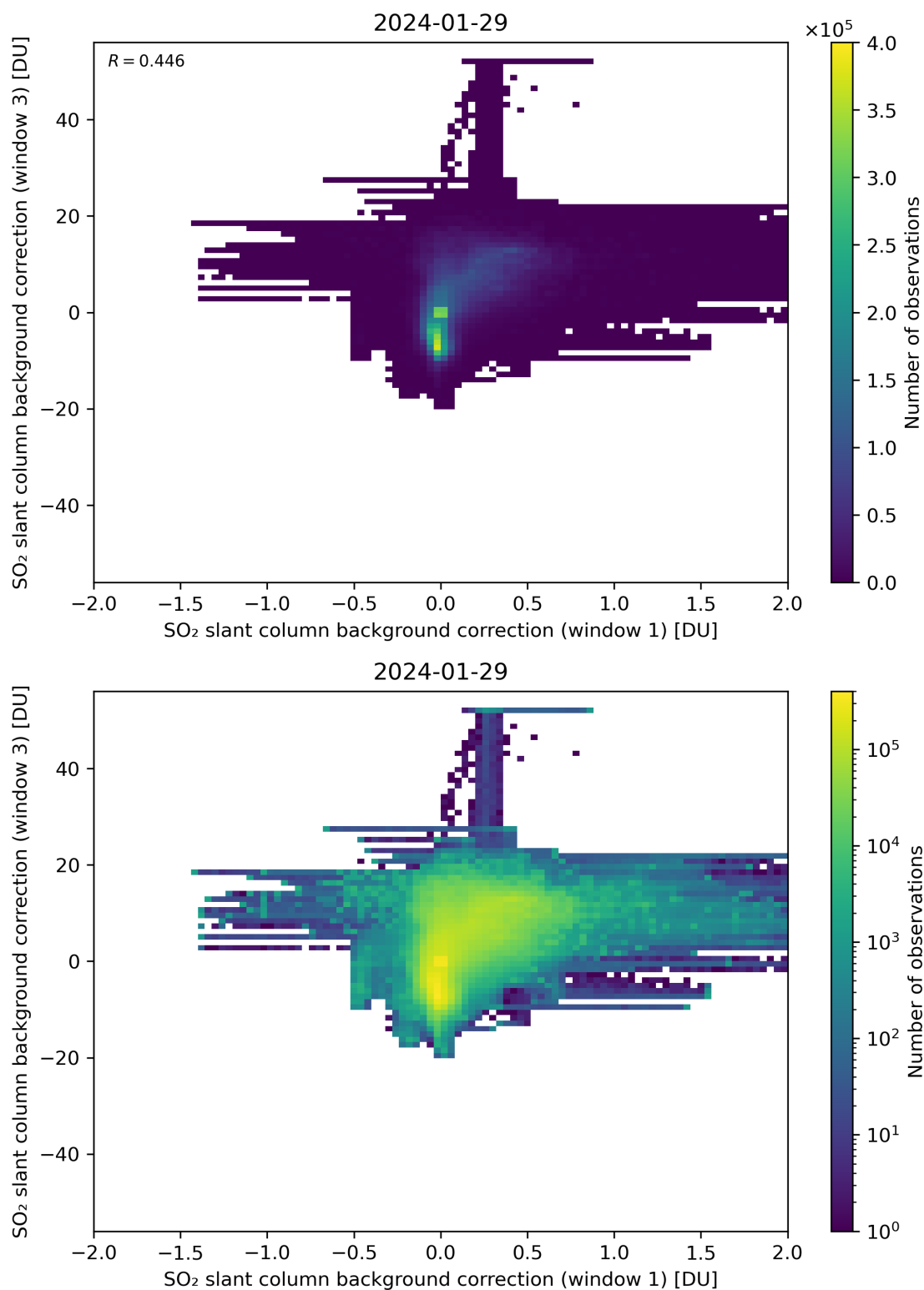
Figure 99: Scatter density plot of “SO 2 slant column background correction (window 1)” against “SO 2 slant column background correction (window 3)” for 2024-01-28 to 2024-01-30.
