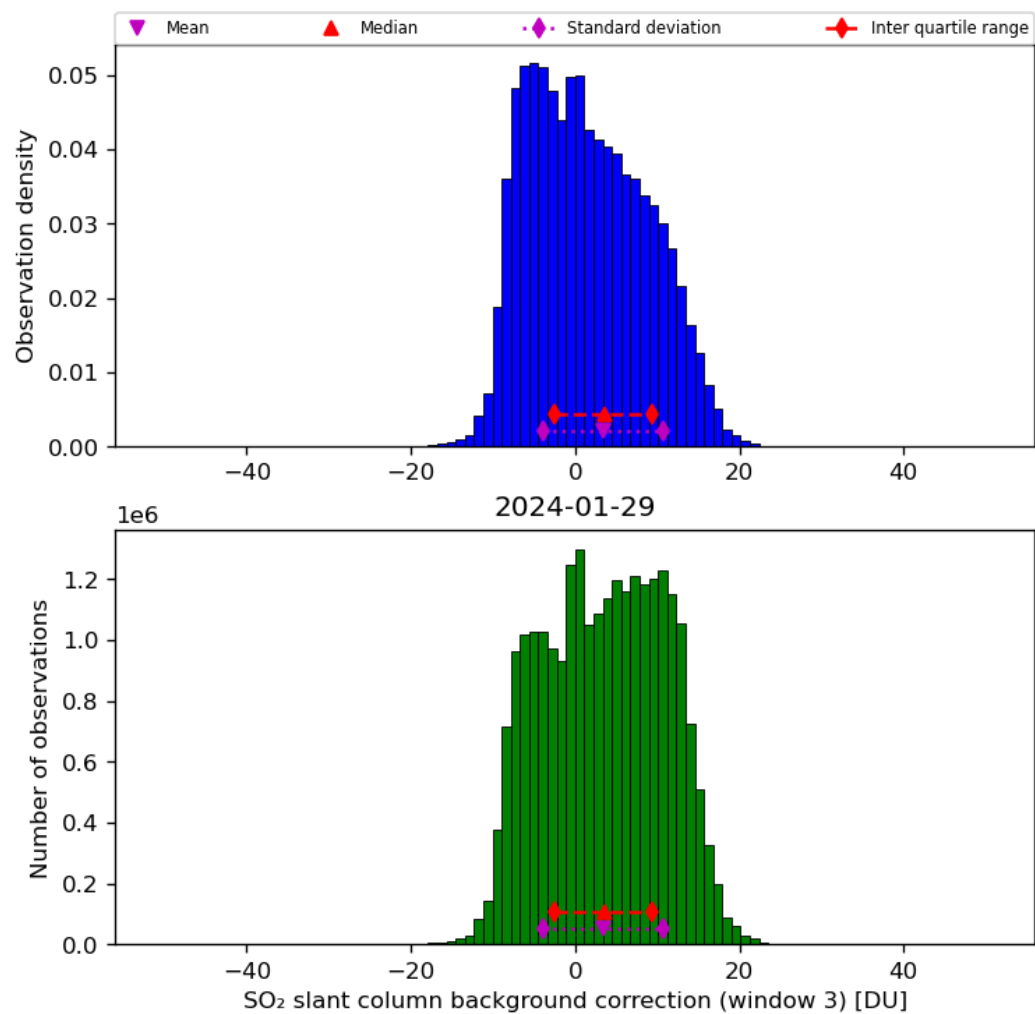
Figure 67: Histogram of “SO 2 slant column background correction (window 3)” for 2024-01-28 to 2024-01-30
