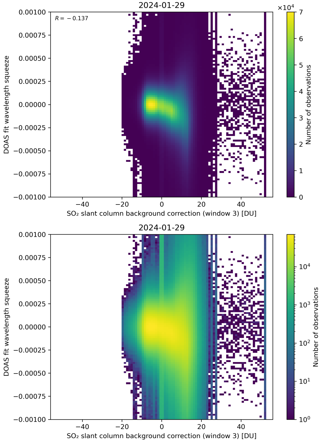
Figure 122: Scatter density plot of “SO 2 slant column background correction (window 3)” against “DOAS fit wavelength squeeze” for 2024-01-28 to 2024-01-30.
