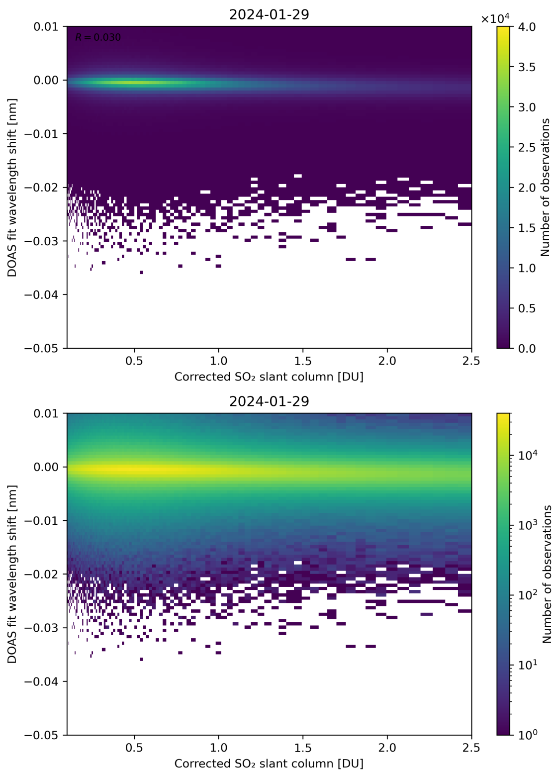
Figure 181: Scatter density plot of “Corrected SO 2 slant column” against “DOAS fit wavelength shift” for 2024-01-28 to 2024-01-30.
