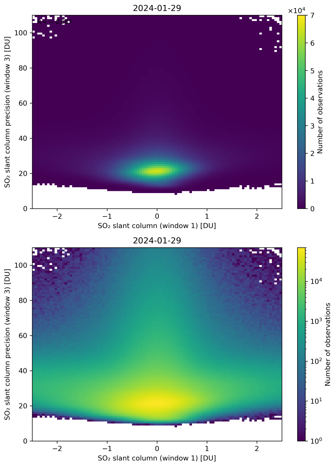
Figure 238: Scatter density plot of “SO 2 slant column (window 1)” against “SO 2 slant column precision (window 3)” for 2024-01-28 to 2024-01-30.
