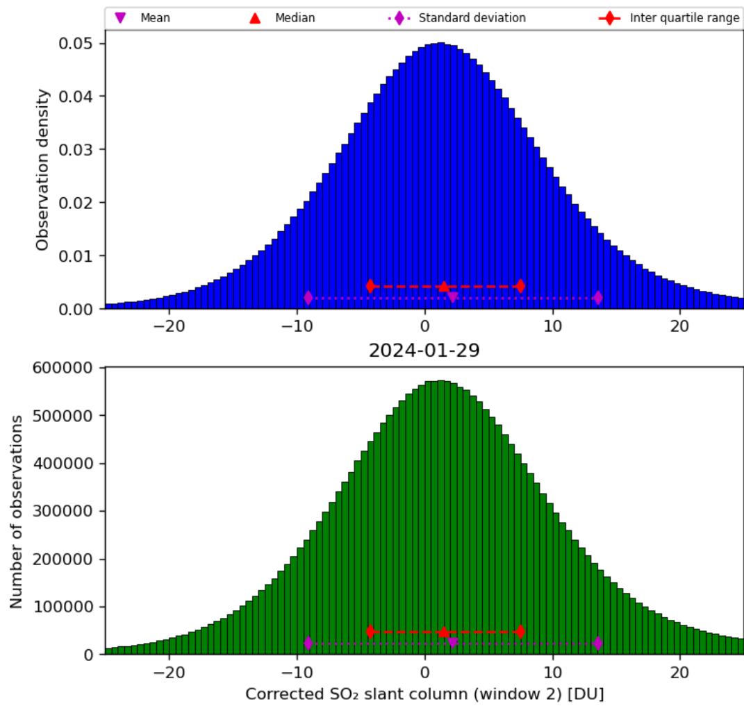
Figure 62: Histogram of “Corrected SO 2 slant column (window 2)” for 2024-01-28 to 2024-01-30
