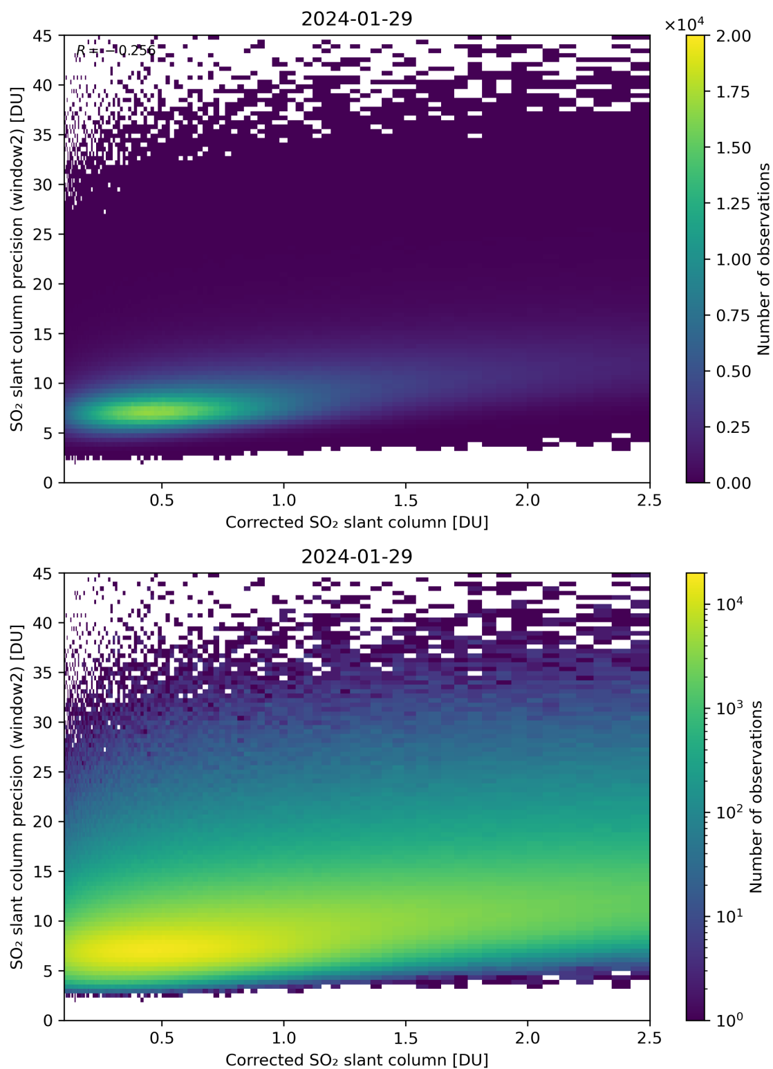
Figure 189: Scatter density plot of “Corrected SO 2 slant column” against “SO 2 slant column precision (window2)” for 2024-01-28 to 2024-01-30.
