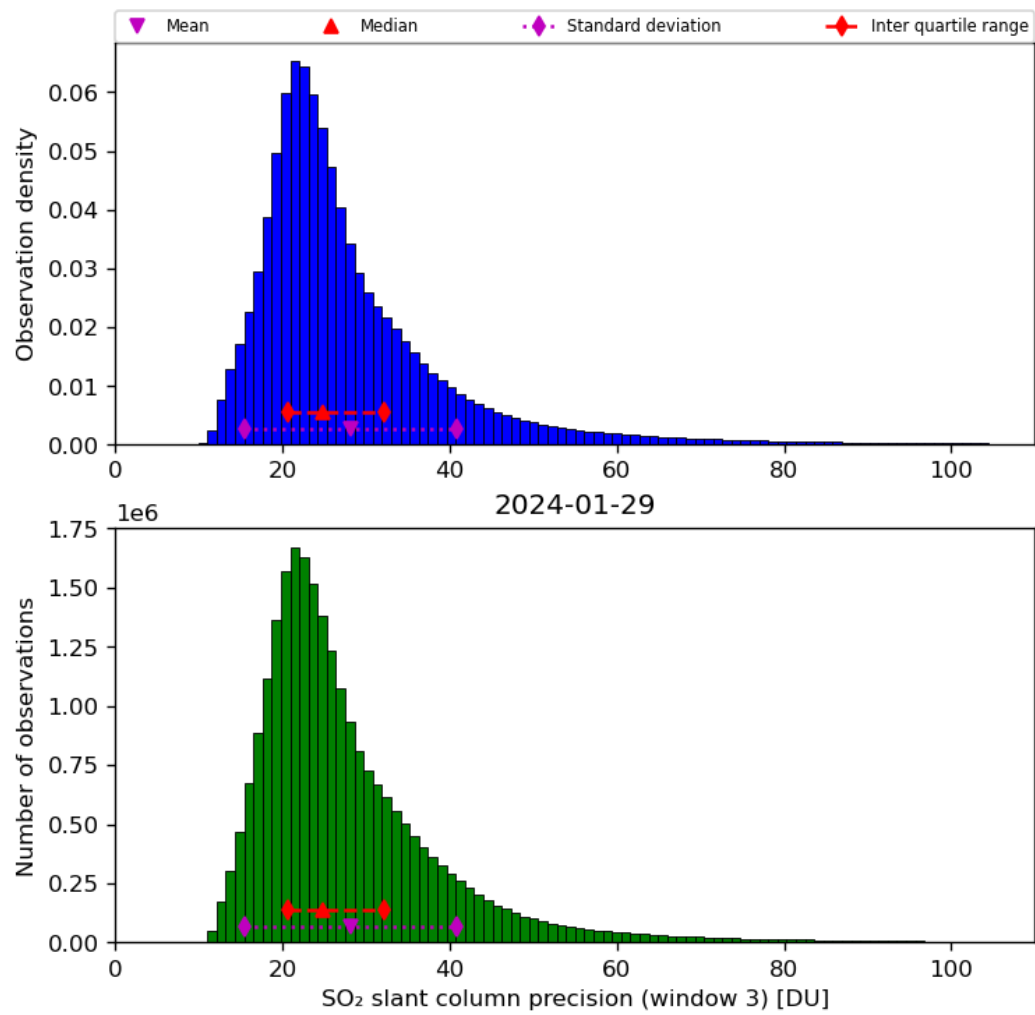
Figure 65: Histogram of “SO 2 slant column precision (window 3)” for 2024-01-28 to 2024-01-30
