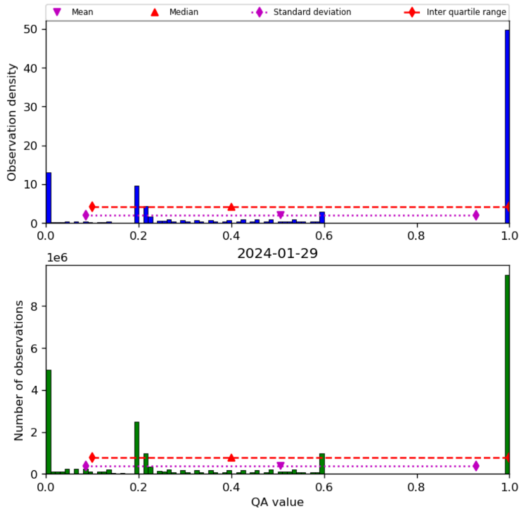
Figure 52: Histogram of “QA value” for 2024-01-28 to 2024-01-30
