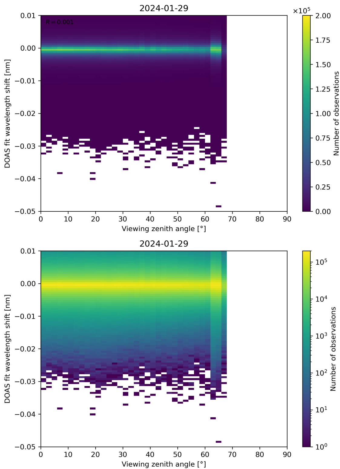
Figure 311: Scatter density plot of “Viewing zenith angle” against “DOAS fit wavelength shift” for 2024-01-28 to 2024-01-30.
