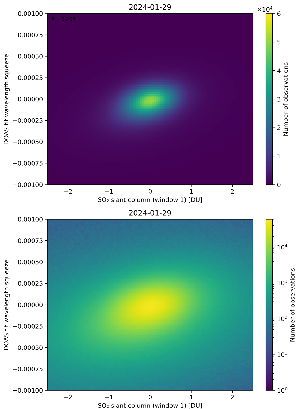
Figure 216: Scatter density plot of “SO 2 slant column (window 1)” against “DOAS fit wavelength squeeze” for 2024-01-28 to 2024-01-30.
