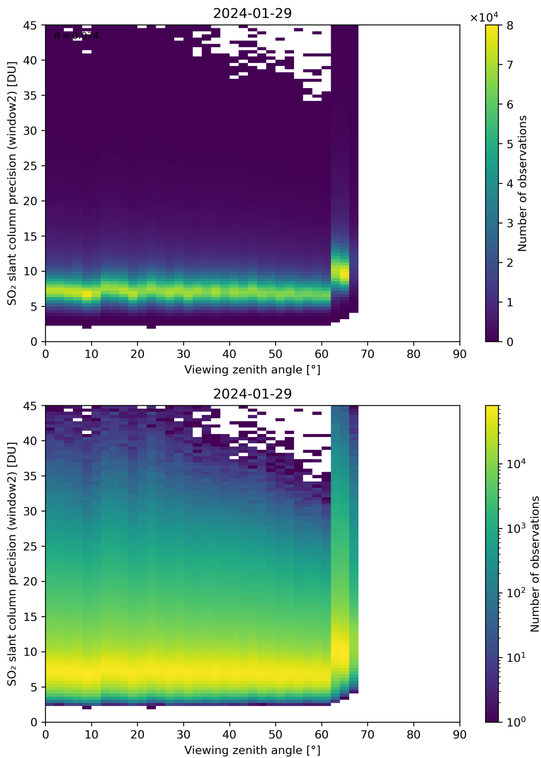
Figure 322: Scatter density plot of “Viewing zenith angle” against “SO 2 slant column precision (window2)” for 2024-01-28 to 2024-01-30.
