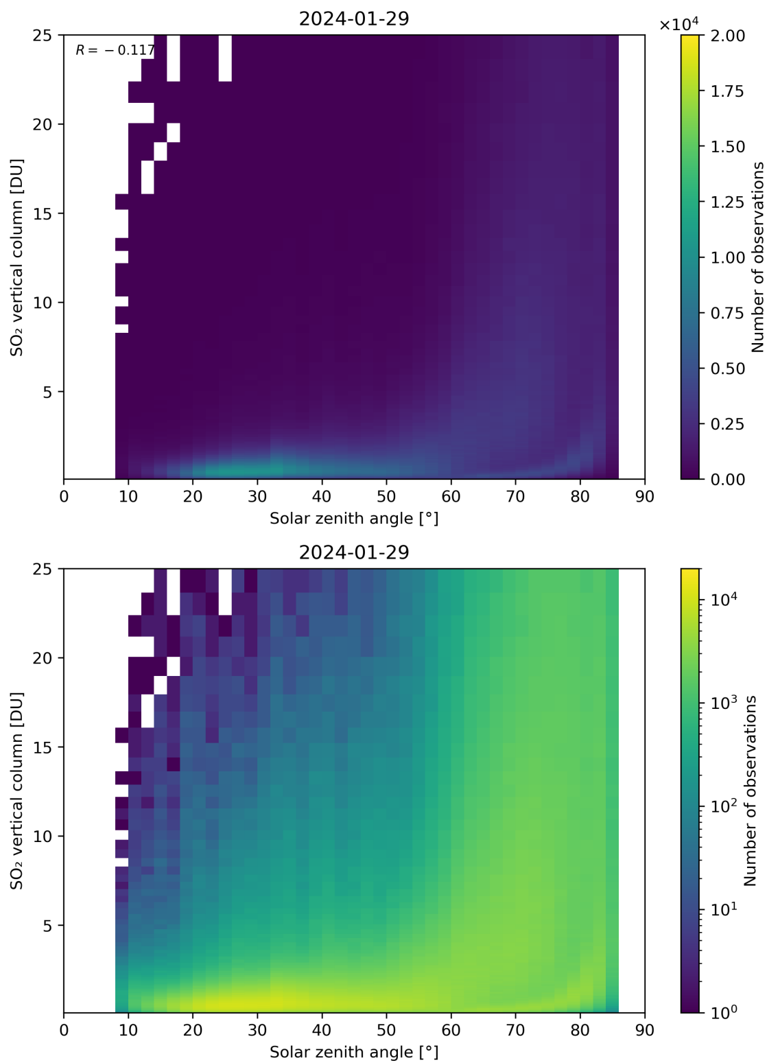
Figure 176: Scatter density plot of “Solar zenith angle” against “SO 2 vertical column” for 2024-01-28 to 2024-01-30.
