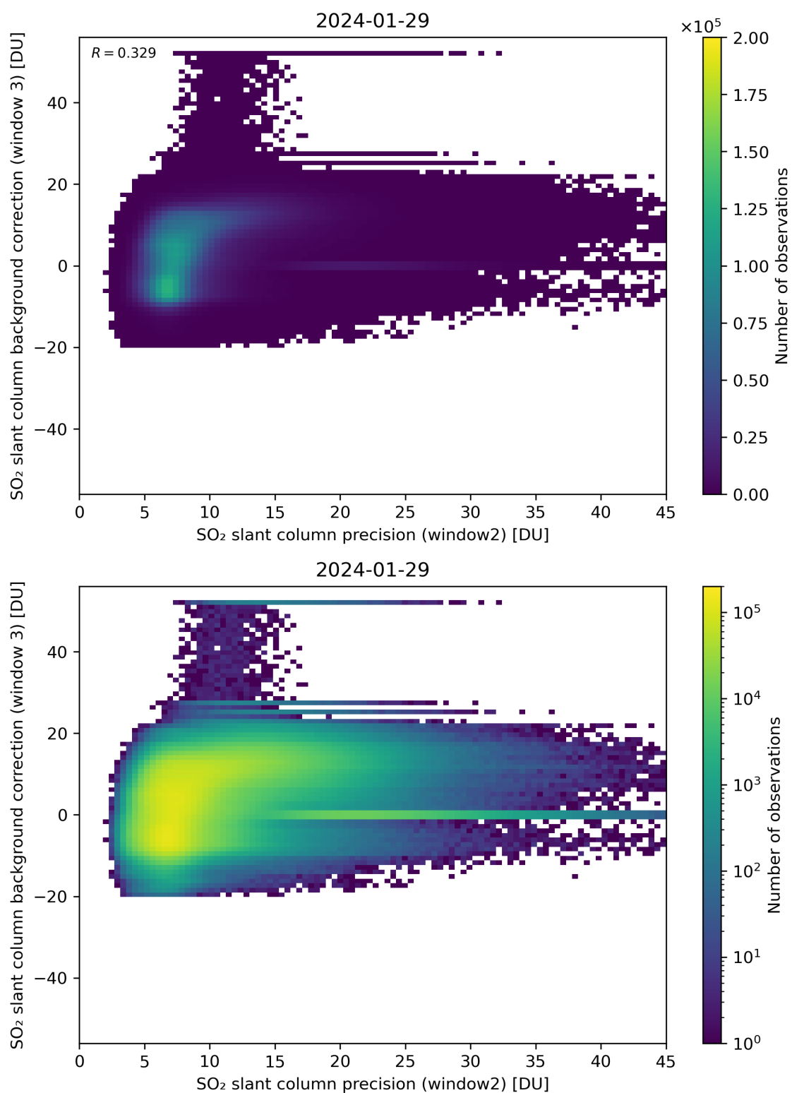
Figure 242: Scatter density plot of “SO 2 slant column precision (window2)” against “SO 2 slant column background correction (window 3)” for 2024-01-28 to 2024-01-30.
