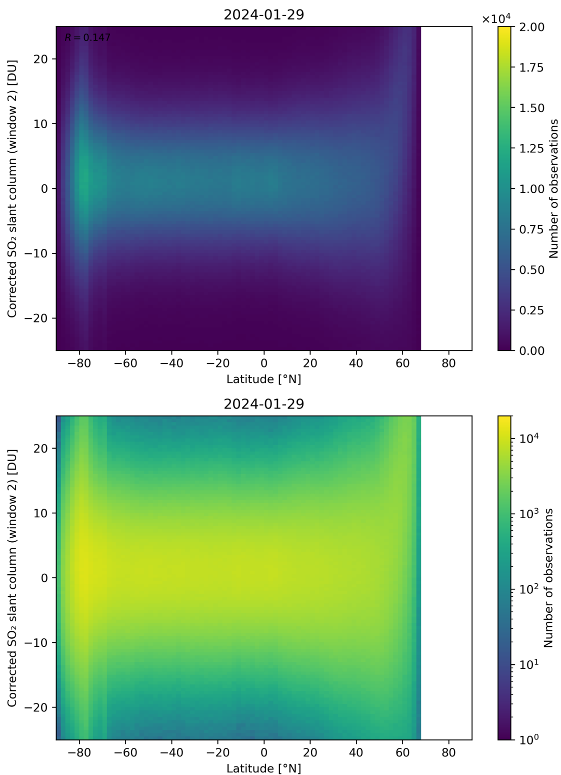
Figure 147: Scatter density plot of “Latitude” against “Corrected SO 2 slant column (window 2)” for 2024-01-28 to 2024-01-30.
