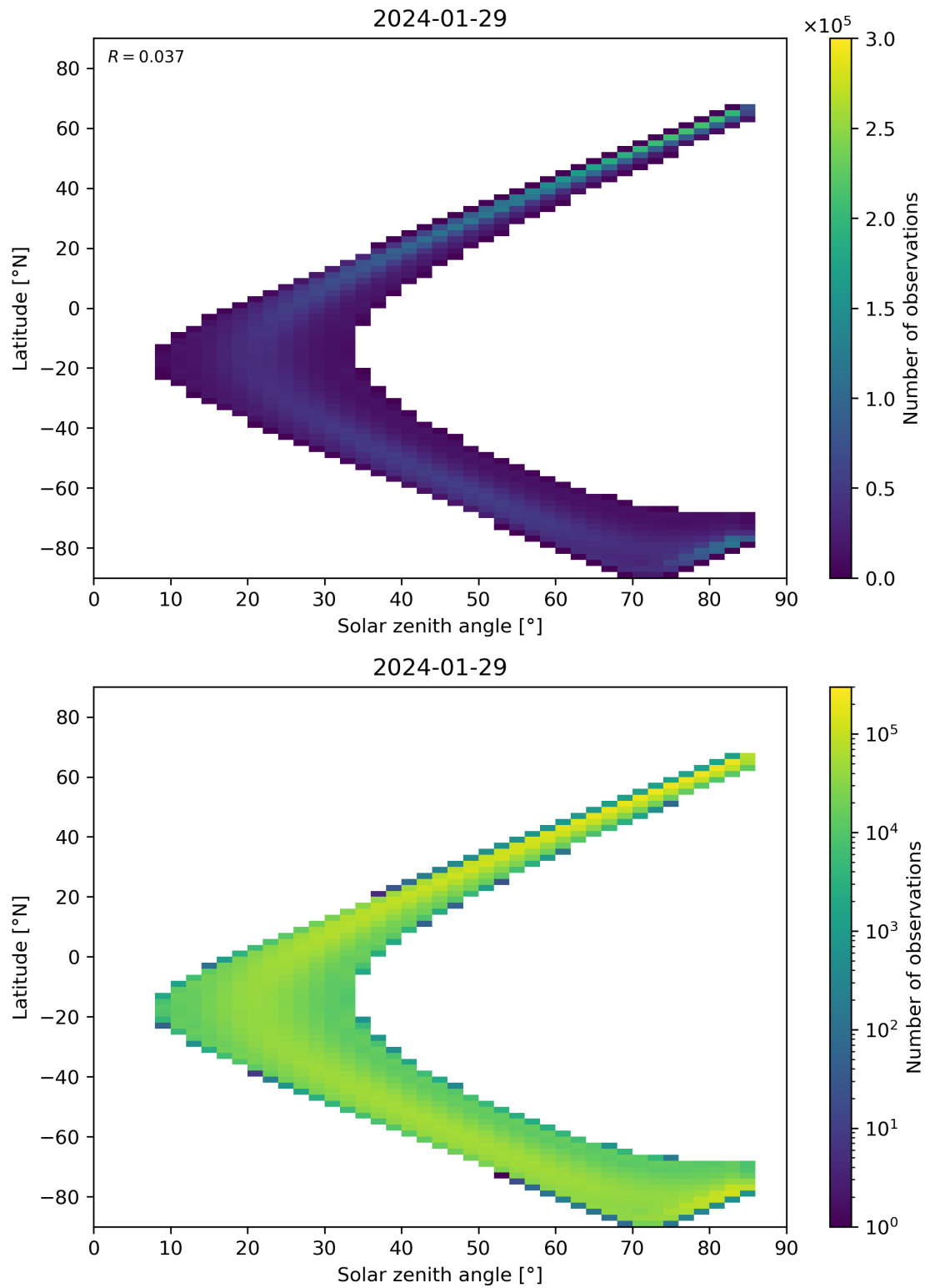
Figure 164: Scatter density plot of “Solar zenith angle” against “Latitude” for 2024-01-28 to 2024-01-30.
