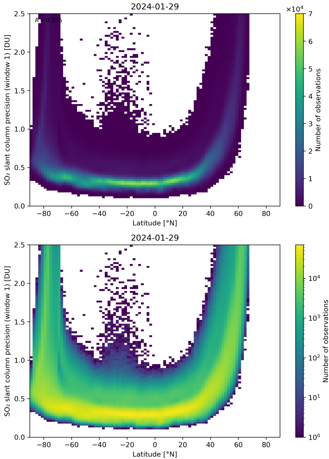
Figure 150: Scatter density plot of “Latitude” against “SO 2 slant column precision (window 1)” for 2024-01-28 to 2024-01-30.
