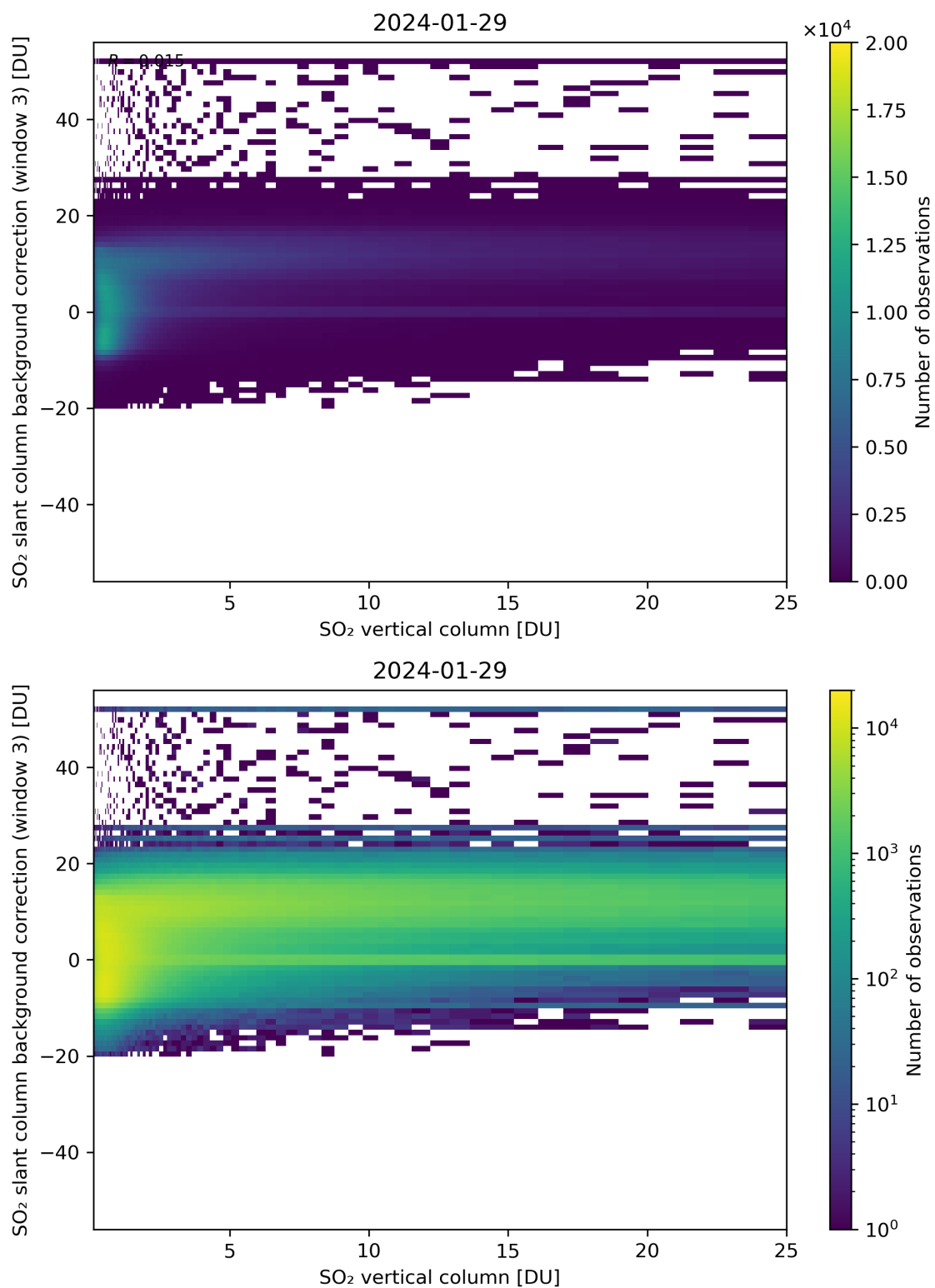
Figure 275: Scatter density plot of “SO 2 vertical column” against “SO 2 slant column background correction (window 3)” for 2024-01-28 to 2024-01-30.
