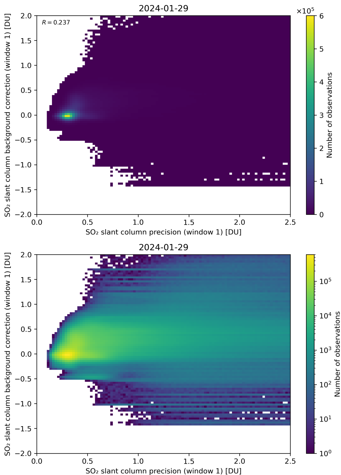
Figure 218: Scatter density plot of “SO 2 slant column precision (window 1)” against “SO 2 slant column background correction (window 1)” for 2024-01-28 to 2024-01-30.
