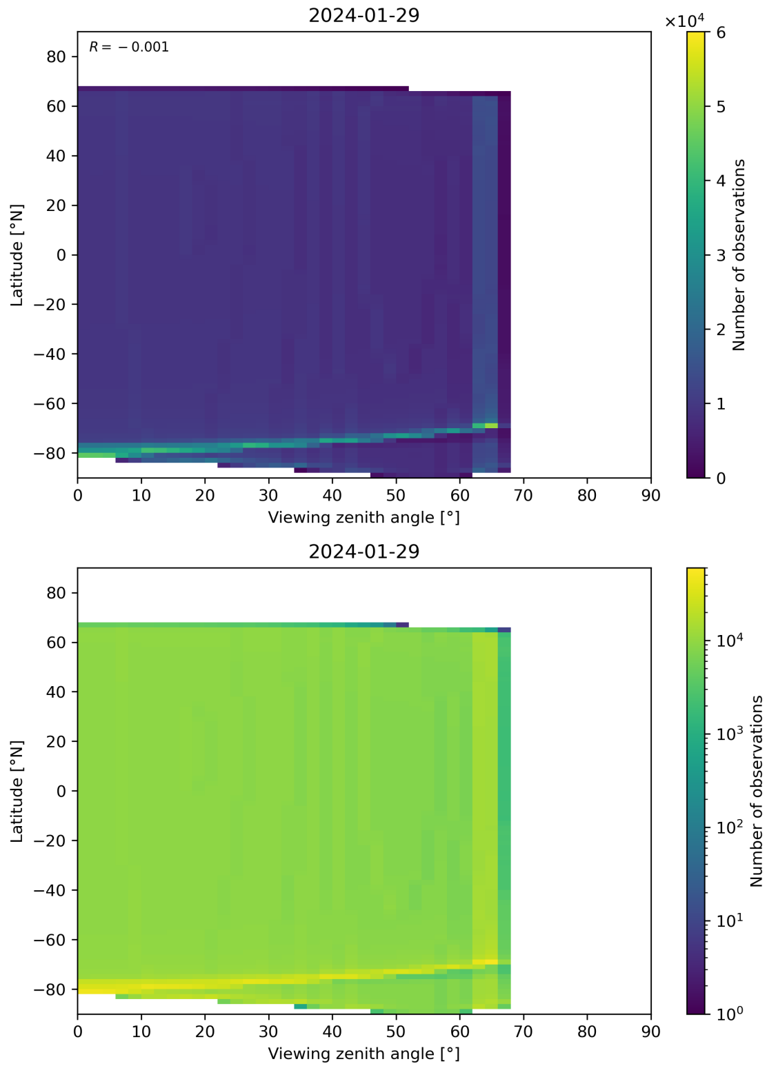
Figure 314: Scatter density plot of “Viewing zenith angle” against “Latitude” for 2024-01-28 to 2024-01-30.
