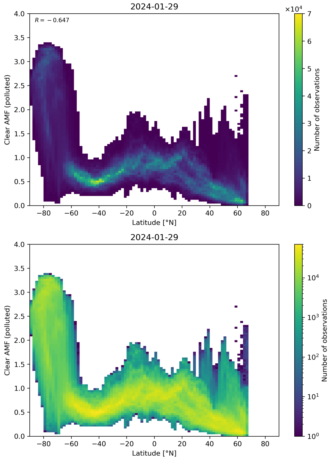
Figure 145: Scatter density plot of “Latitude” against “Clear AMF (polluted)” for 2024-01-28 to 2024-01-30.
