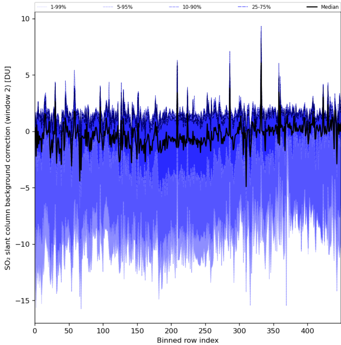
Figure 86: Along track statistics of “SO 2 slant column background correction (window 2)” for 2024-01-28 to 2024-01-30
