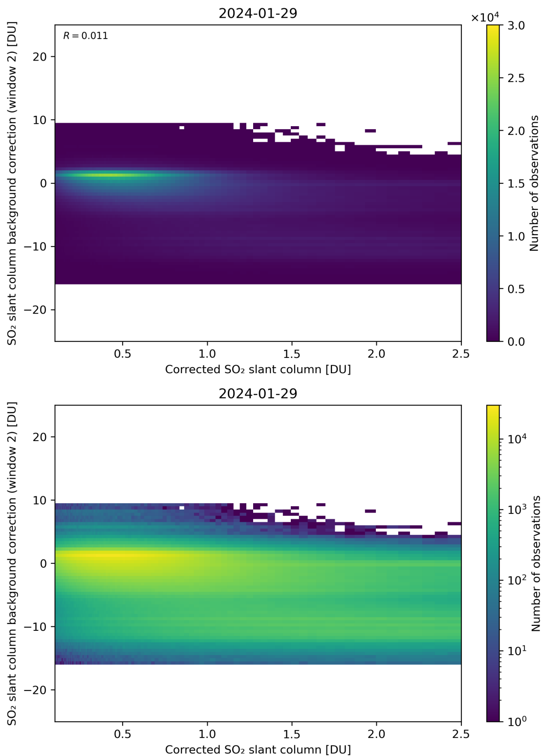
Figure 179: Scatter density plot of “Corrected SO 2 slant column” against “SO 2 slant column background correction (window 2)” for 2024-01-28 to 2024-01-30.
