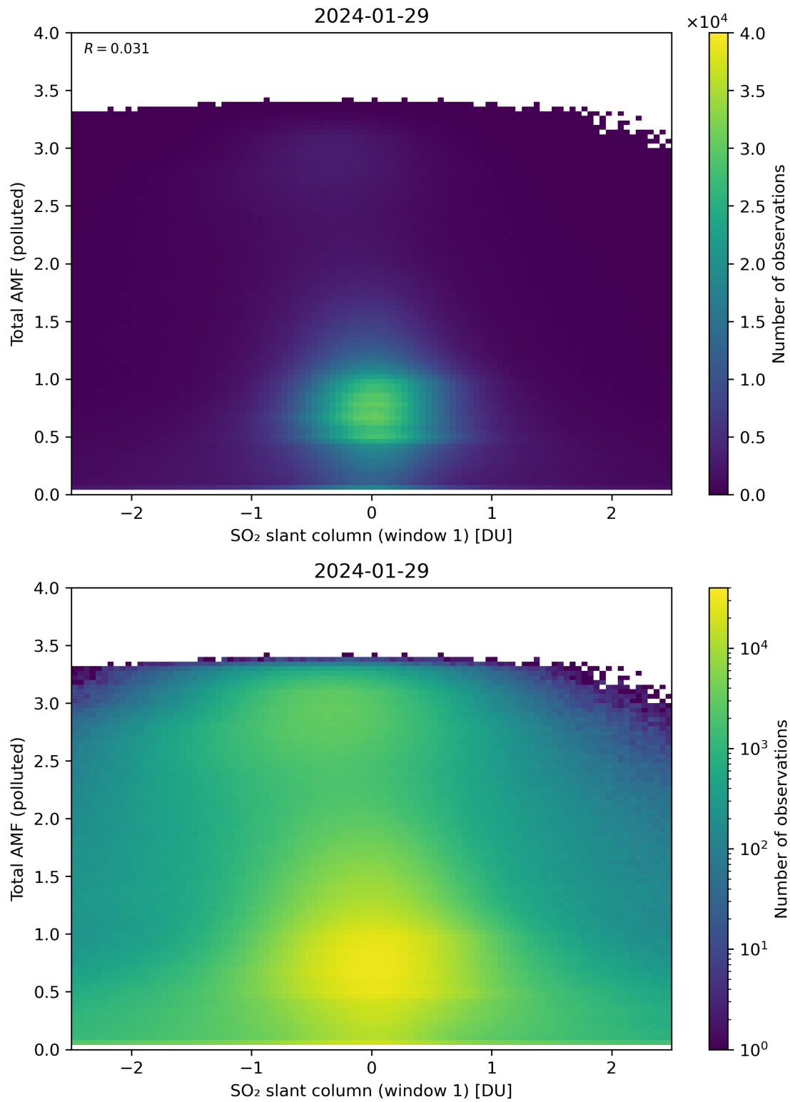
Figure 239: Scatter density plot of “SO 2 slant column (window 1)” against “Total AMF (polluted)” for 2024-01-28 to 2024-01-30.
