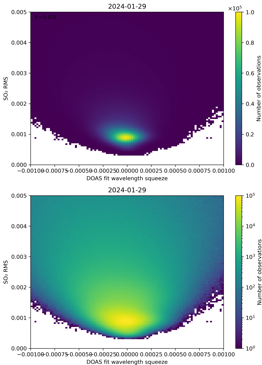
Figure 132: Scatter density plot of “DOAS fit wavelength squeeze” against “SO 2 RMS” for 2024-01-28 to 2024-01-30.
