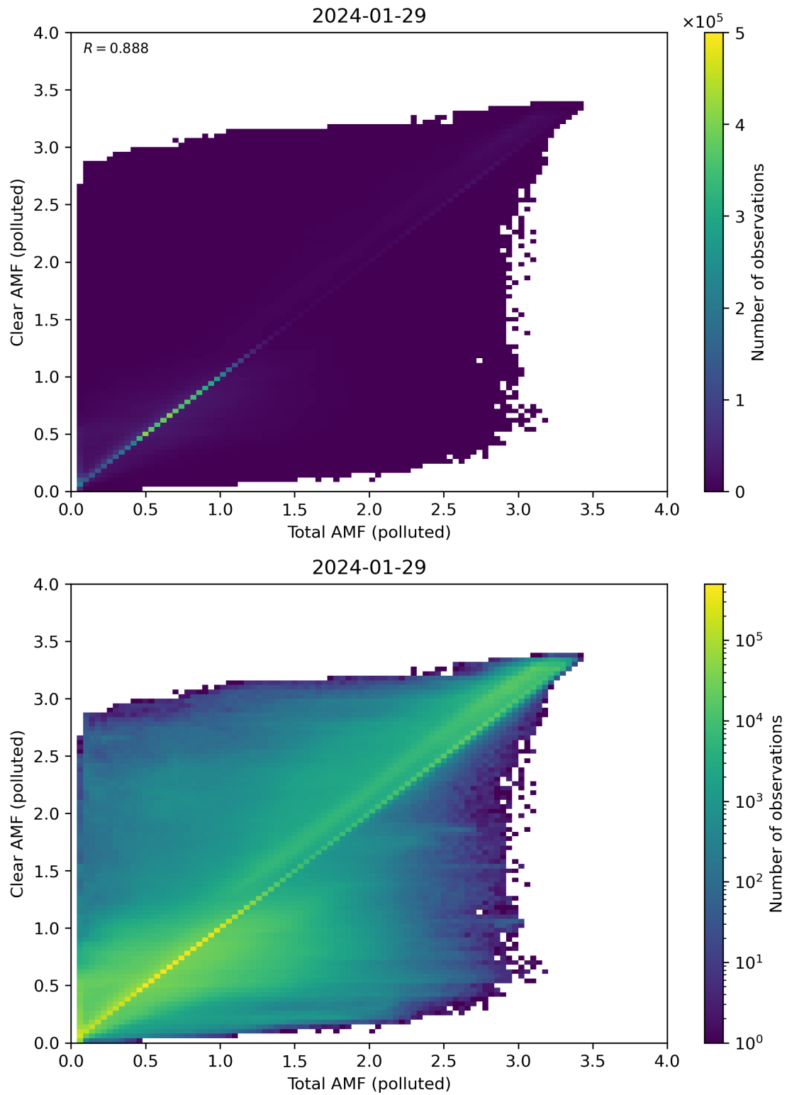
Figure 271: Scatter density plot of “Total AMF (polluted)” against “Clear AMF (polluted)” for 2024-01-28 to 2024-01-30.
