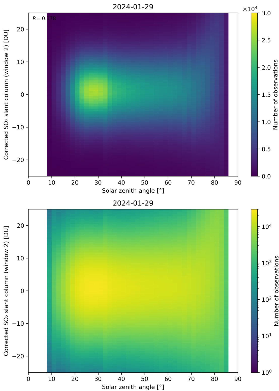
Figure 167: Scatter density plot of “Solar zenith angle” against “Corrected SO 2 slant column (window 2)” for 2024-01-28 to 2024-01-30.
