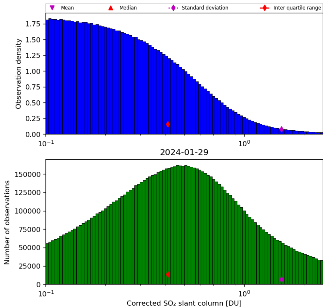
Figure 55: Histogram of “Corrected SO 2 slant column” for 2024-01-28 to 2024-01-30
