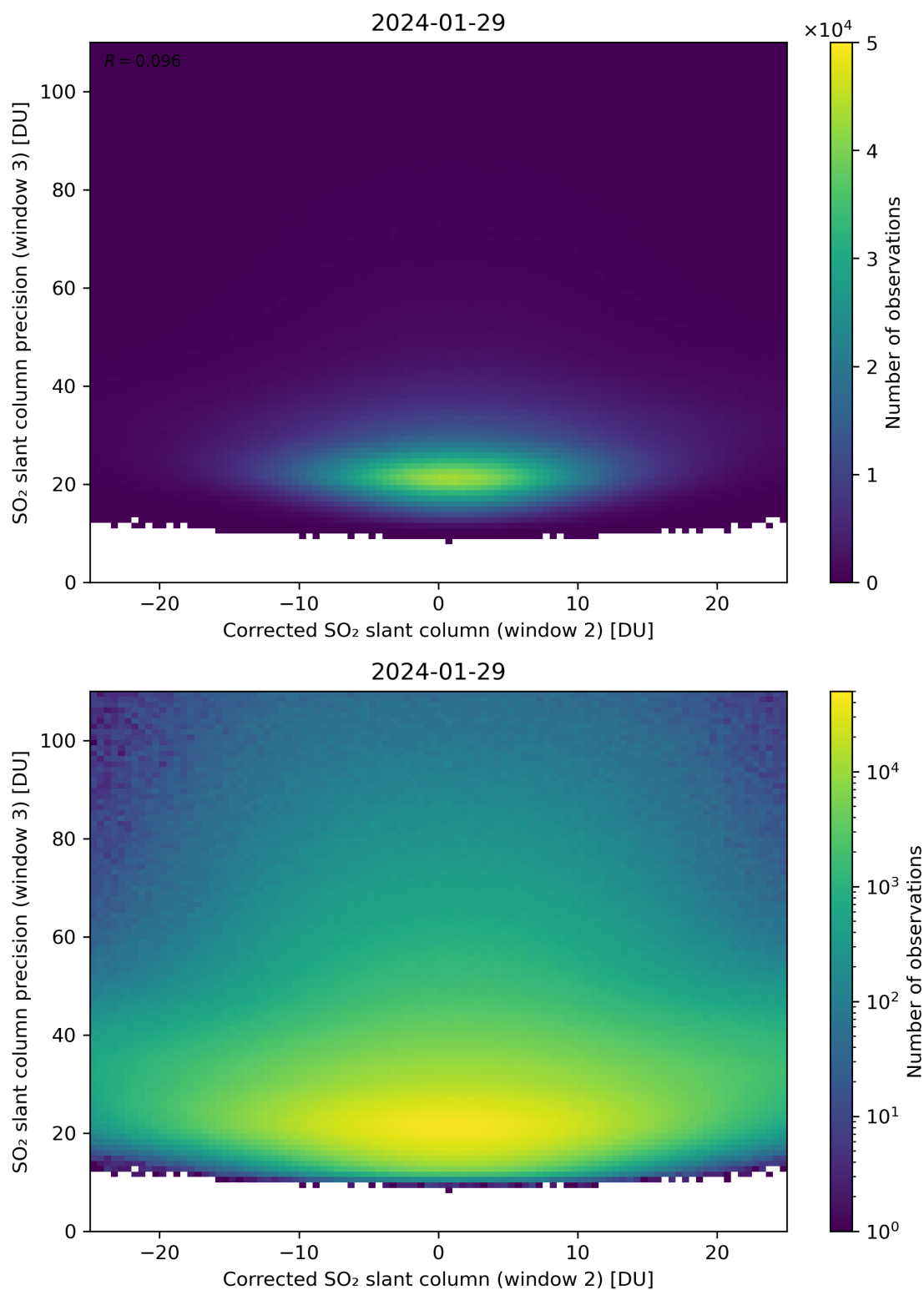
Figure 202: Scatter density plot of “Corrected SO 2 slant column (window 2)” against “SO 2 slant column precision (window 3)” for 2024-01-28 to 2024-01-30.
