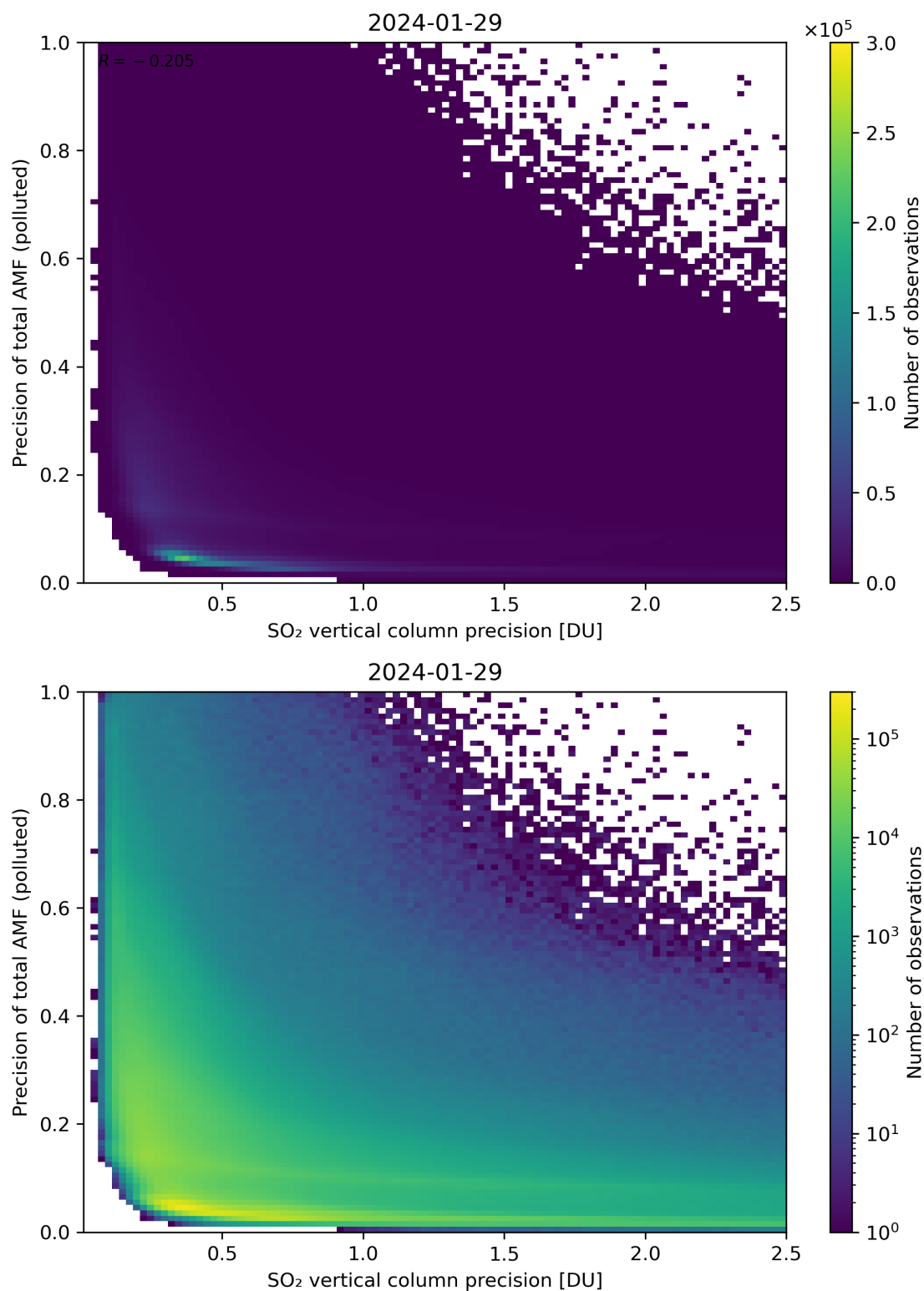
Figure 295: Scatter density plot of “SO 2 vertical column precision” against “Precision of total AMF (polluted)” for 2024-01-28 to 2024-01-30.
