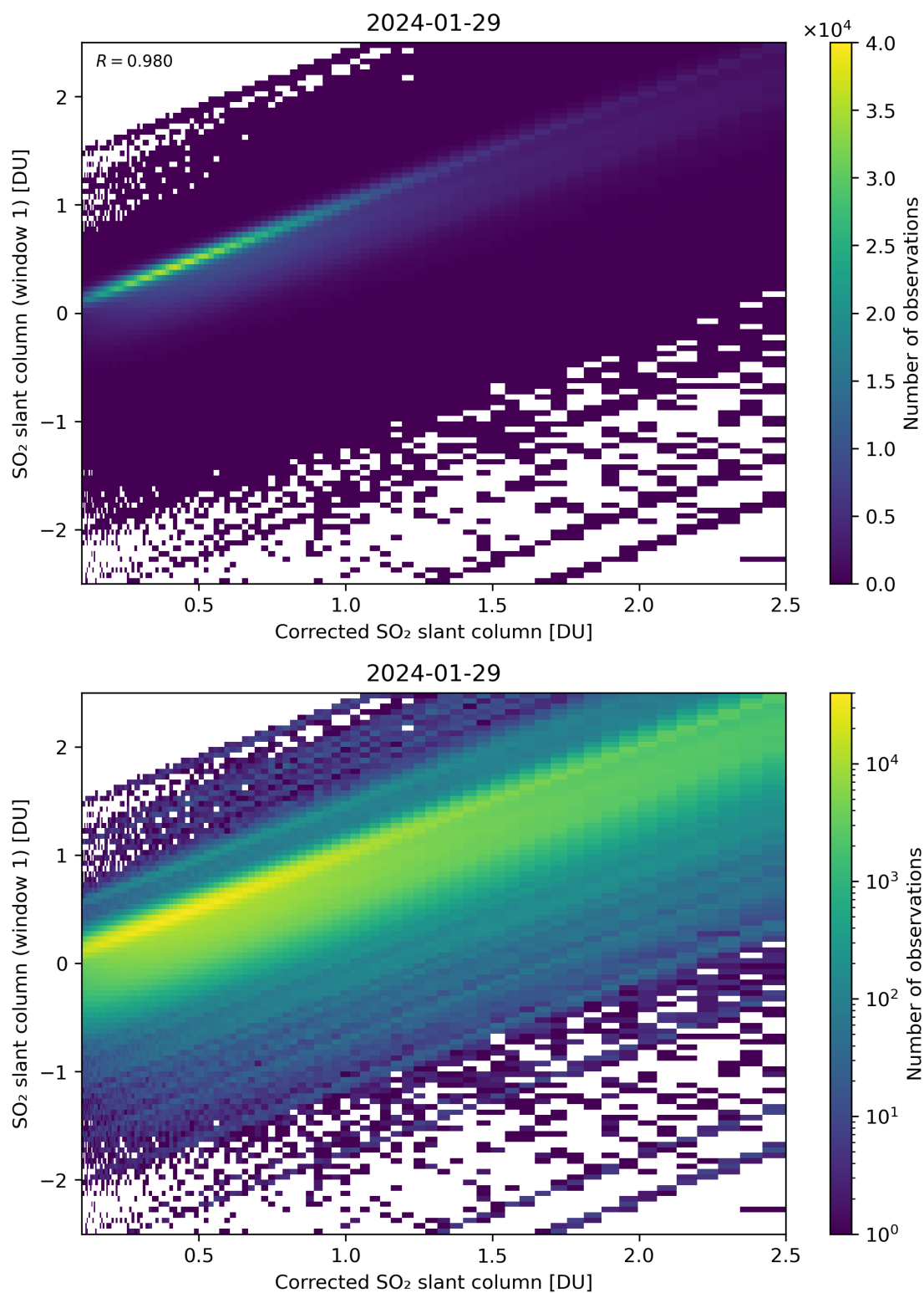
Figure 187: Scatter density plot of “Corrected SO 2 slant column” against “SO 2 slant column (window 1)” for 2024-01-28 to 2024-01-30.
