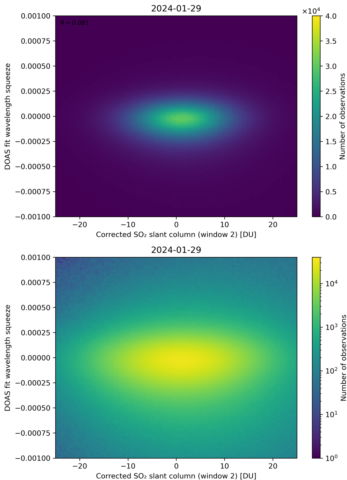
Figure 197: Scatter density plot of “Corrected SO 2 slant column (window 2)” against “DOAS fit wavelength squeeze” for 2024-01-28 to 2024-01-30.
