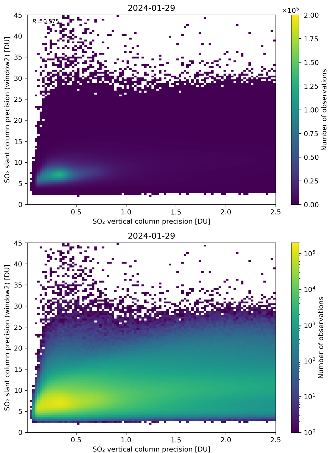
Figure 291: Scatter density plot of “SO 2 vertical column precision” against “SO 2 slant column precision (window2)” for 2024-01-28 to 2024-01-30.
