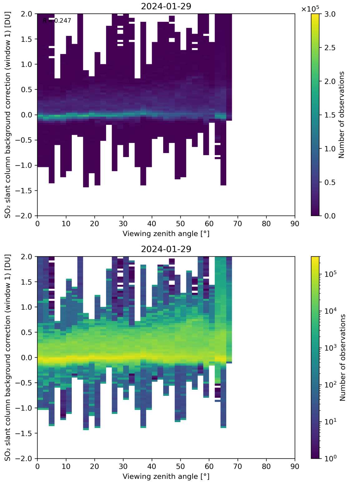
Figure 308: Scatter density plot of “Viewing zenith angle” against “SO 2 slant column background correction (window 1)” for 2024-01-28 to 2024-01-30.
