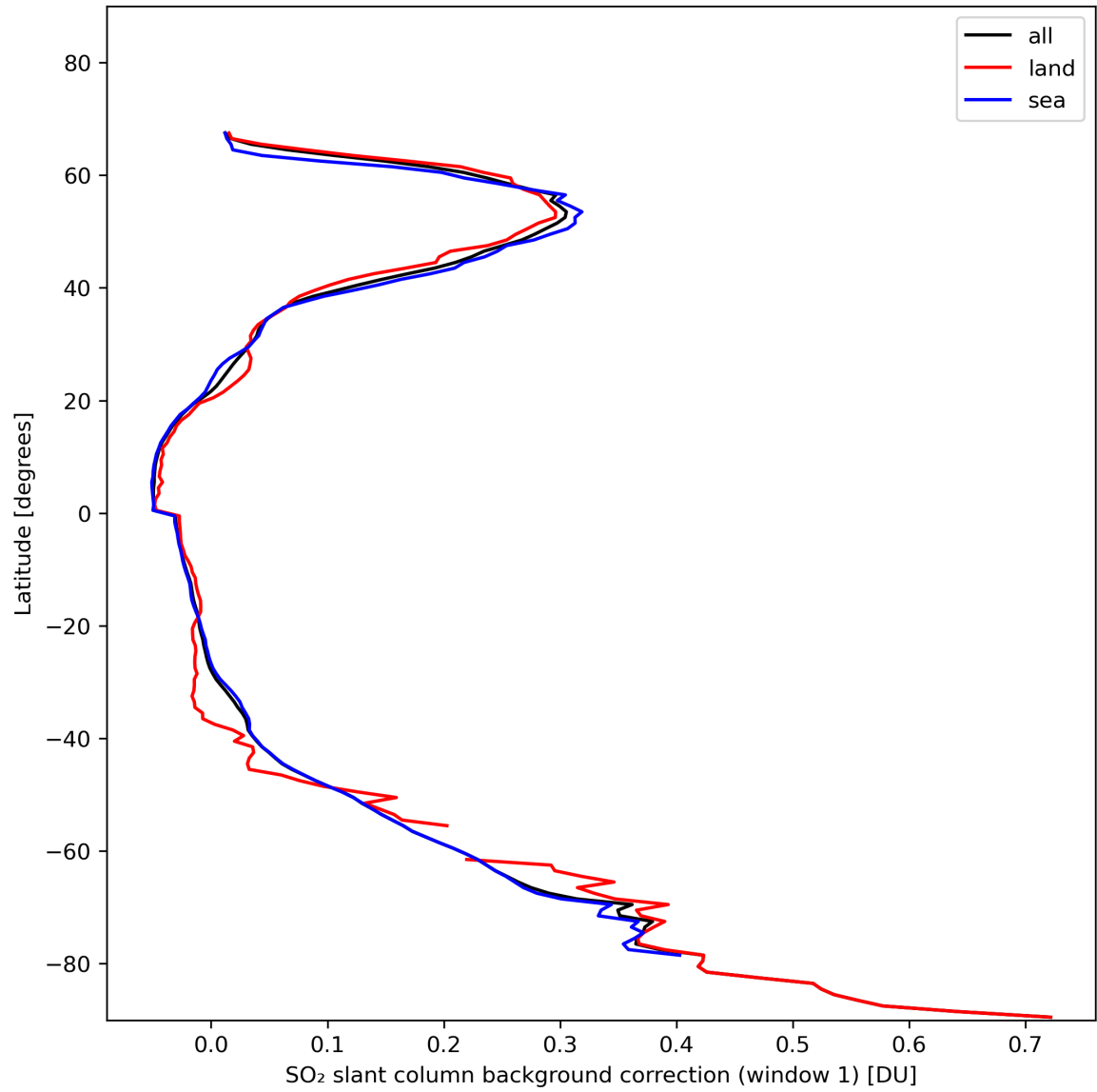
Figure 36: Zonal average of “SO 2 slant column background correction (window 1)” for 2024-01-28 to 2024-01-30.
