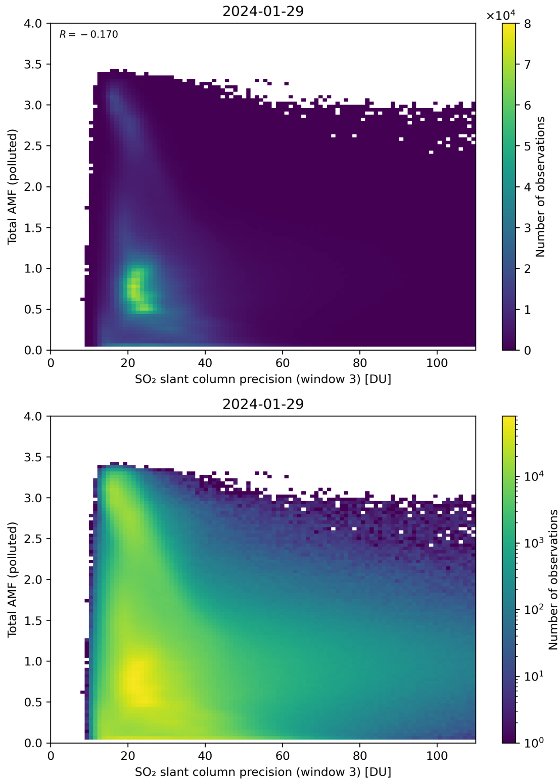
Figure 263: Scatter density plot of “SO 2 slant column precision (window 3)” against “Total AMF (polluted)” for 2024-01-28 to 2024-01-30.
