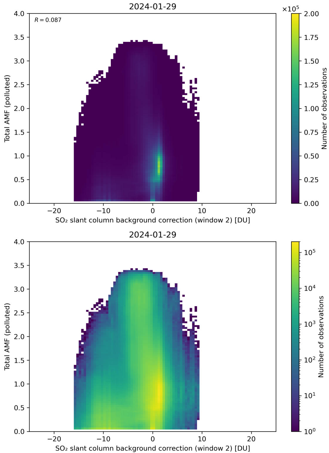
Figure 119: Scatter density plot of “SO 2 slant column background correction (window 2)” against “Total AMF (polluted)” for 2024-01-28 to 2024-01-30.
