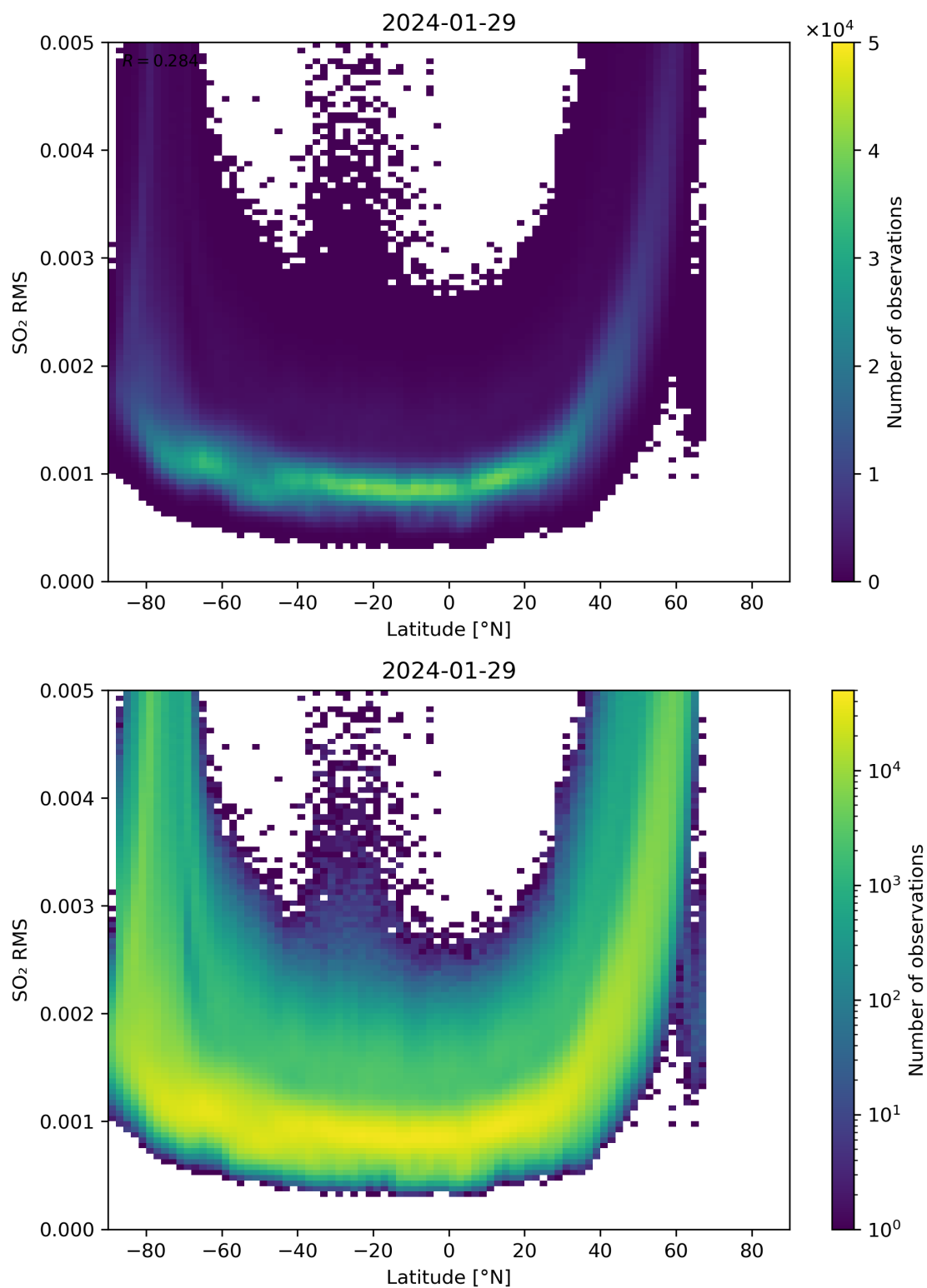
Figure 144: Scatter density plot of “Latitude” against “SO 2 RMS” for 2024-01-28 to 2024-01-30.
