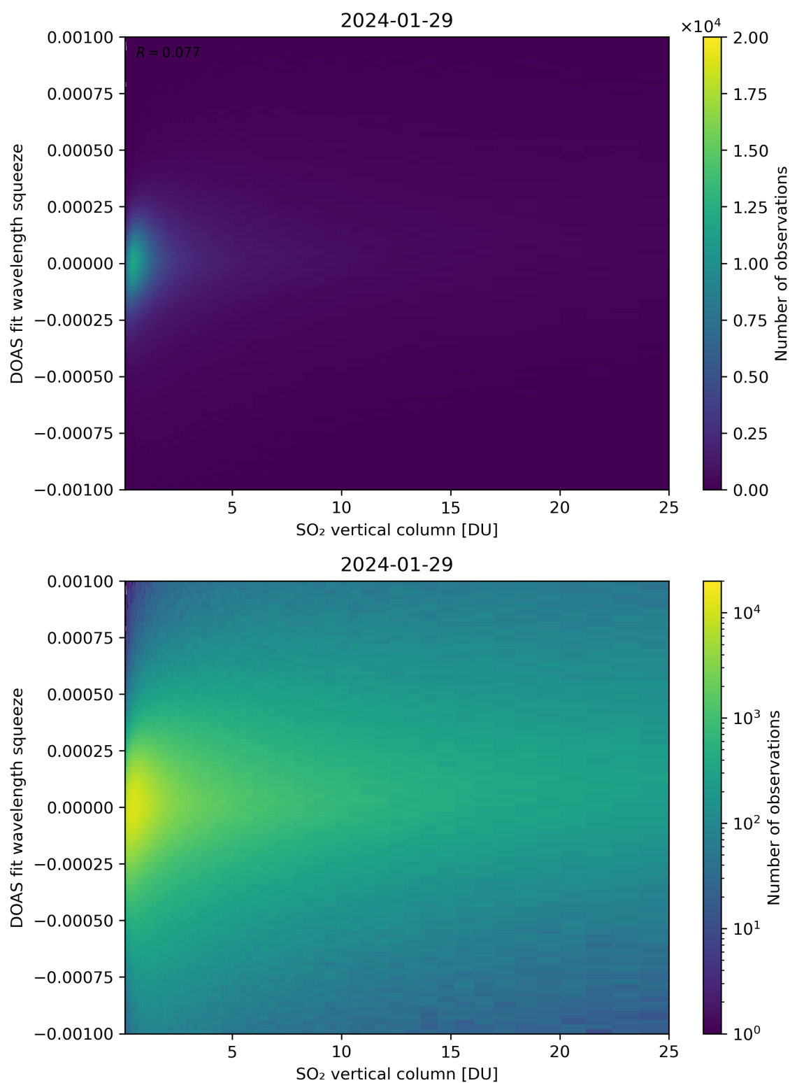
Figure 277: Scatter density plot of “SO 2 vertical column” against “DOAS fit wavelength squeeze” for 2024-01-28 to 2024-01-30.
