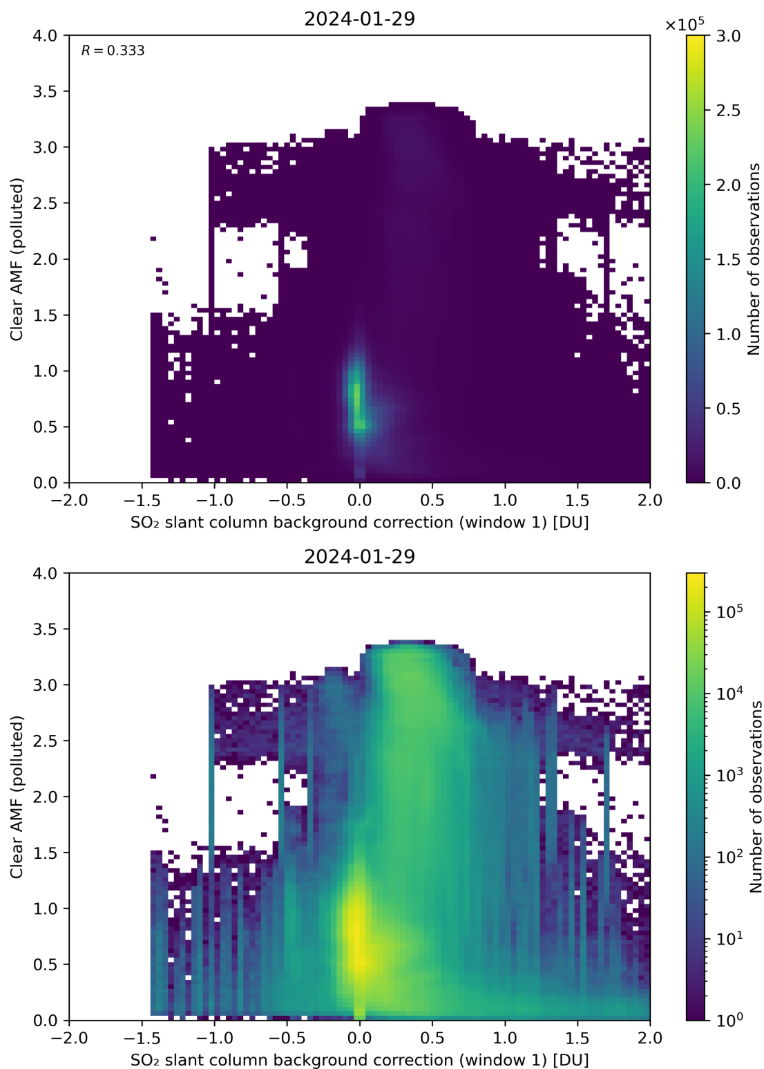
Figure 103: Scatter density plot of “SO 2 slant column background correction (window 1)” against “Clear AMF (polluted)” for 2024-01-28 to 2024-01-30.
