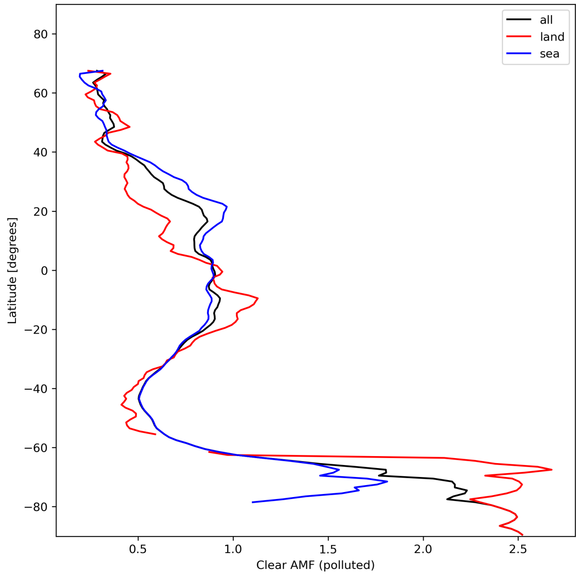
Figure 50: Zonal average of “Clear AMF (polluted)” for 2024-01-28 to 2024-01-30.
