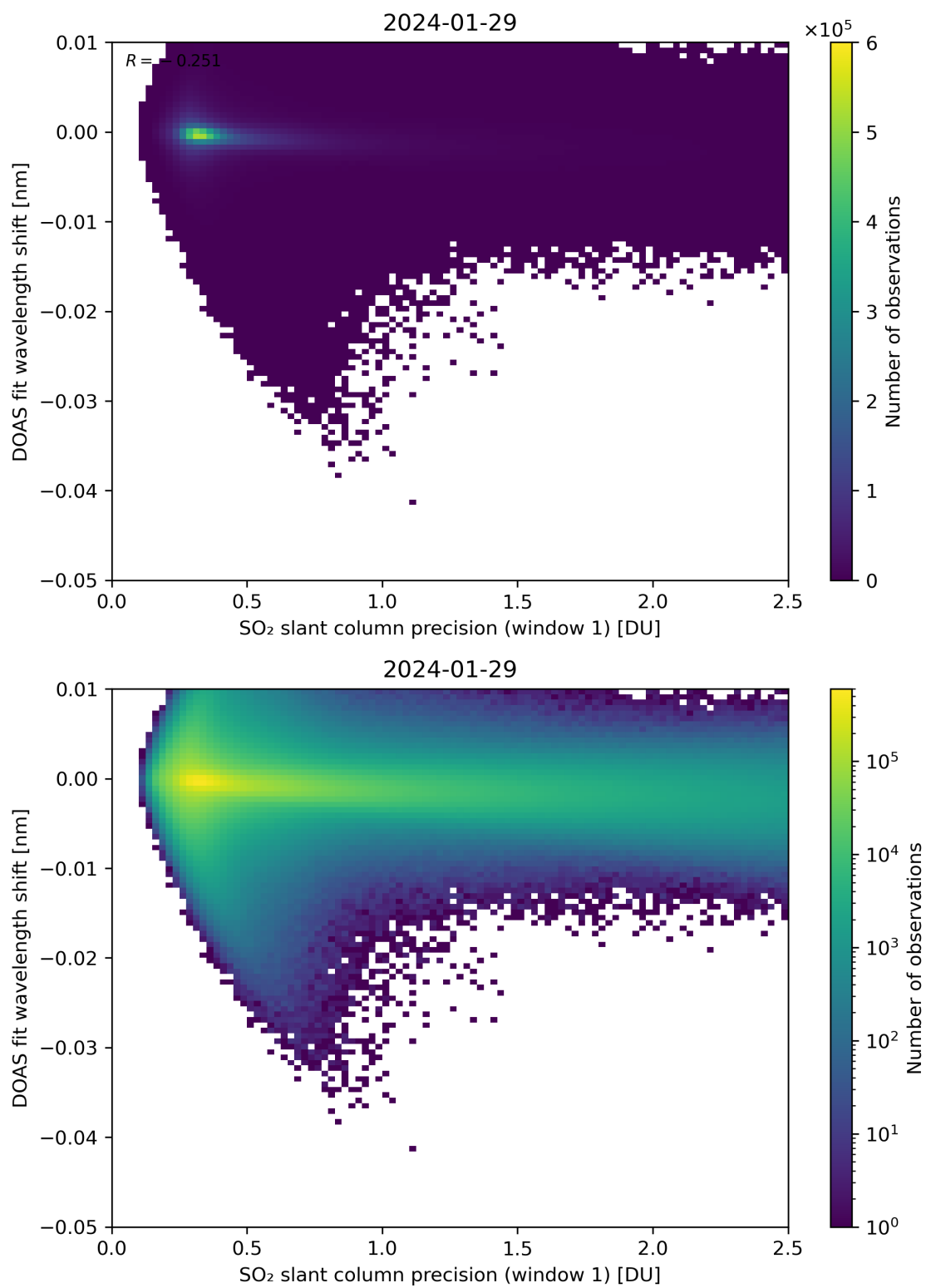
Figure 221: Scatter density plot of “SO 2 slant column precision (window 1)” against “DOAS fit wavelength shift” for 2024-01-28 to 2024-01-30.
