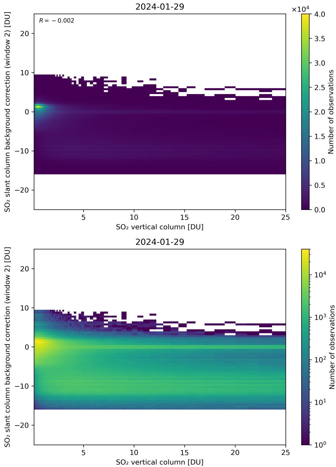
Figure 274: Scatter density plot of “SO 2 vertical column” against “SO 2 slant column background correction (window 2)” for 2024-01-28 to 2024-01-30.
