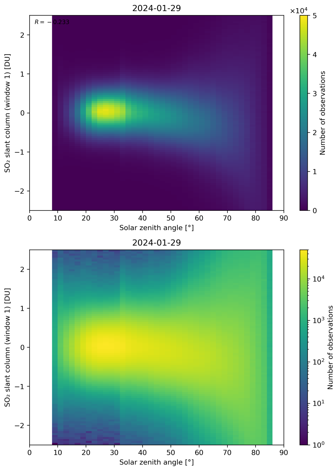
Figure 169: Scatter density plot of “Solar zenith angle” against “SO 2 slant column (window 1)” for 2024-01-28 to 2024-01-30.
