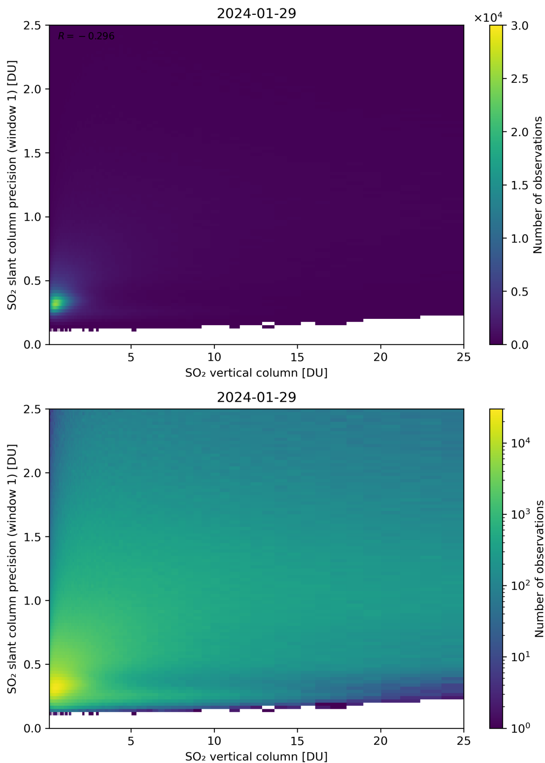
Figure 301: Scatter density plot of “SO 2 vertical column” against “SO 2 slant column precision (window 1)” for 2024-01-28 to 2024-01-30.
