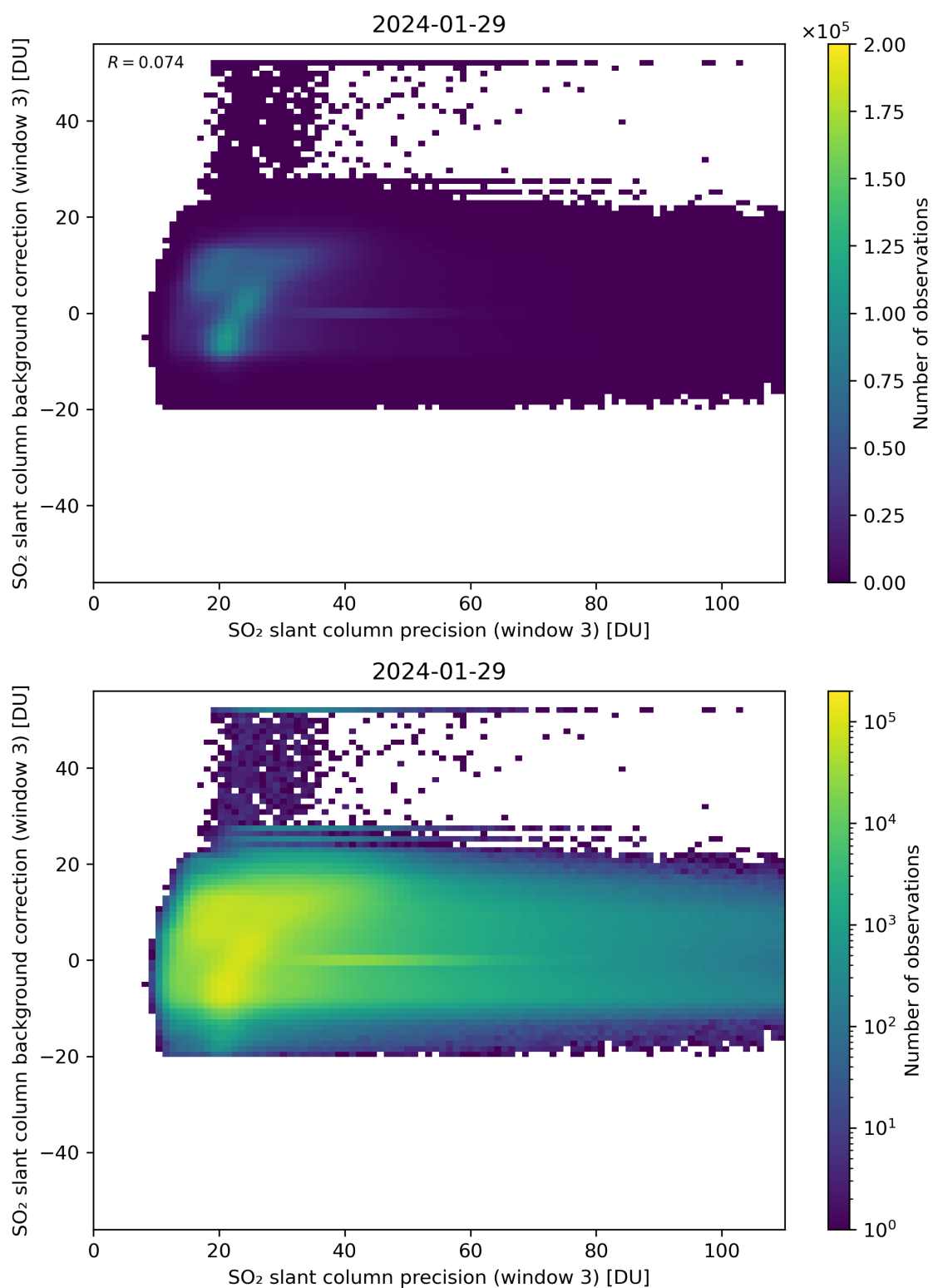
Figure 257: Scatter density plot of “SO 2 slant column precision (window 3)” against “SO 2 slant column background correction (window 3)” for 2024-01-28 to 2024-01-30.
