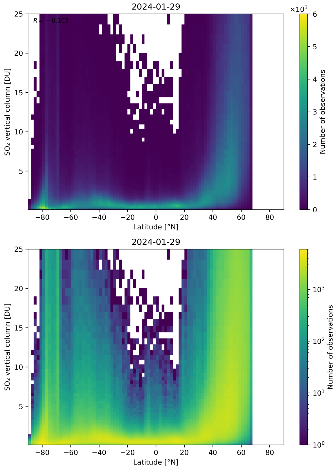
Figure 156: Scatter density plot of “Latitude” against “SO 2 vertical column” for 2024-01-28 to 2024-01-30.
