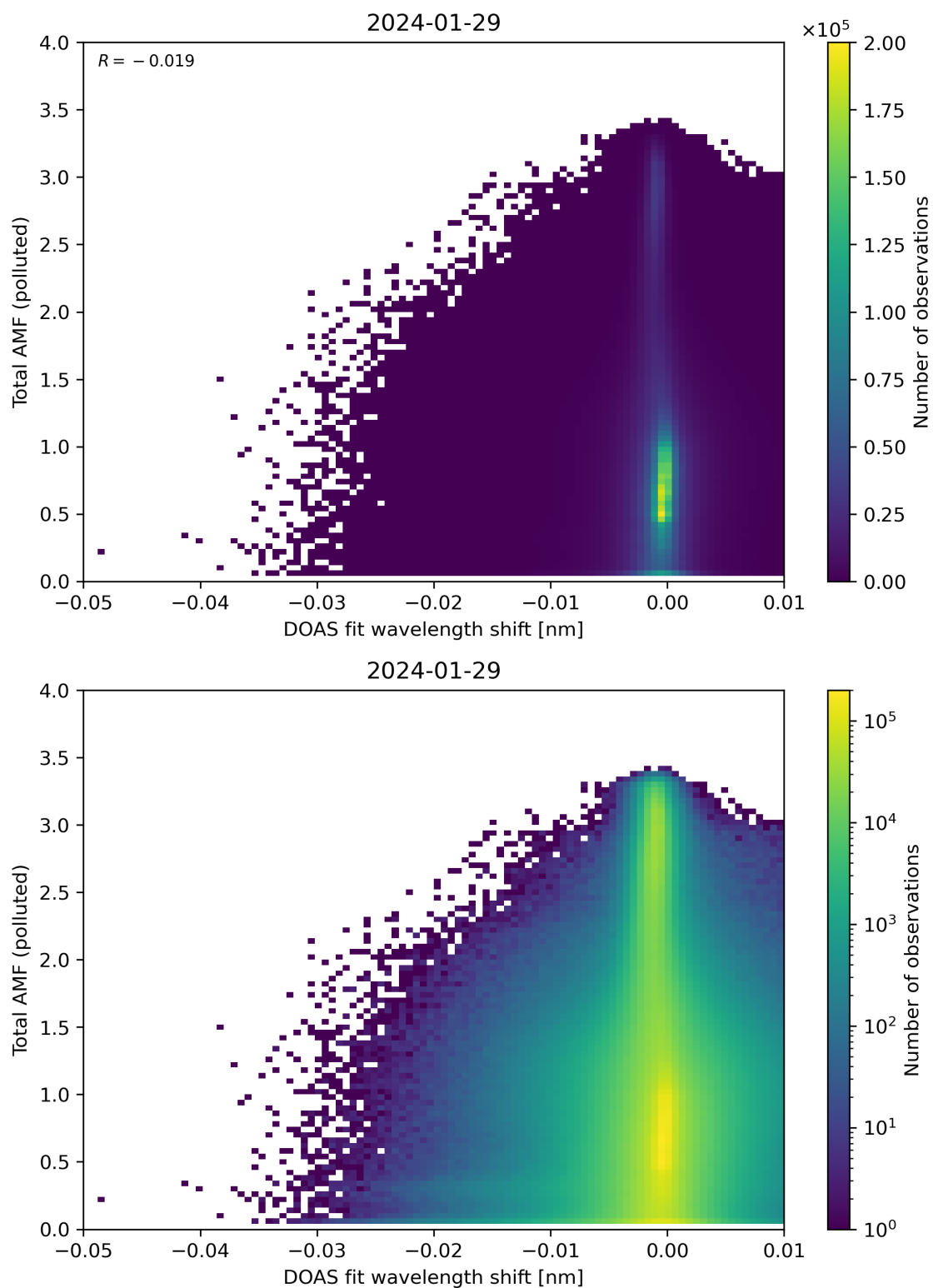
Figure 130: Scatter density plot of “DOAS fit wavelength shift” against “Total AMF (polluted)” for 2024-01-28 to 2024-01-30.
