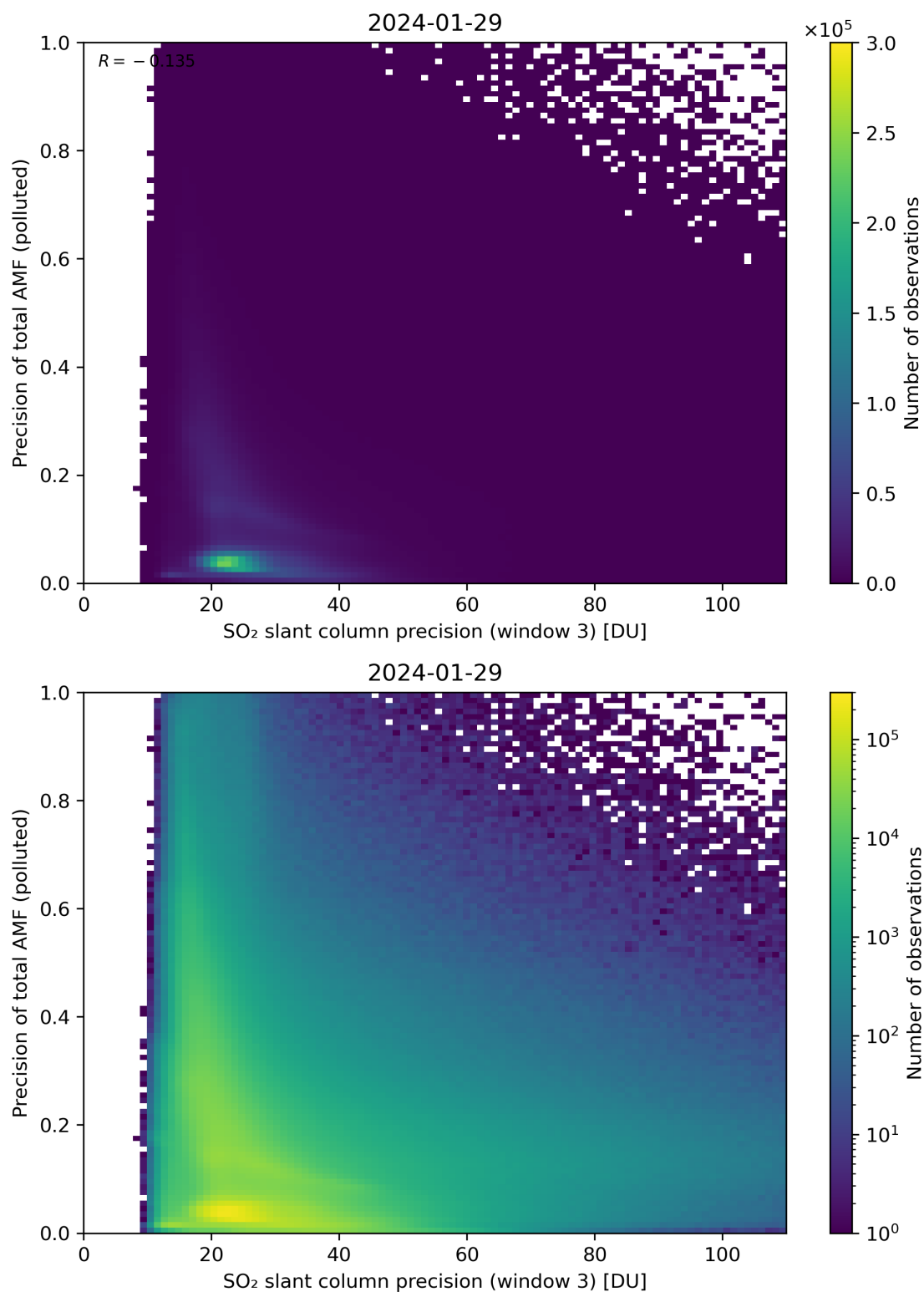
Figure 264: Scatter density plot of “SO 2 slant column precision (window 3)” against “Precision of total AMF (polluted)” for 2024-01-28 to 2024-01-30.
