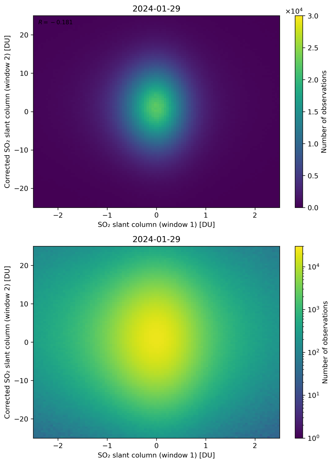
Figure 233: Scatter density plot of “SO 2 slant column (window 1)” against “Corrected SO 2 slant column (window 2)” for 2024-01-28 to 2024-01-30.
