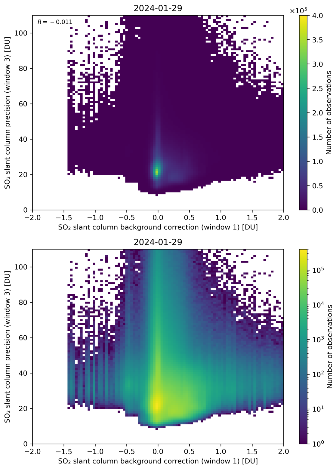
Figure 108: Scatter density plot of “SO 2 slant column background correction (window 1)” against “SO 2 slant column precision (window 3)” for 2024-01-28 to 2024-01-30.
