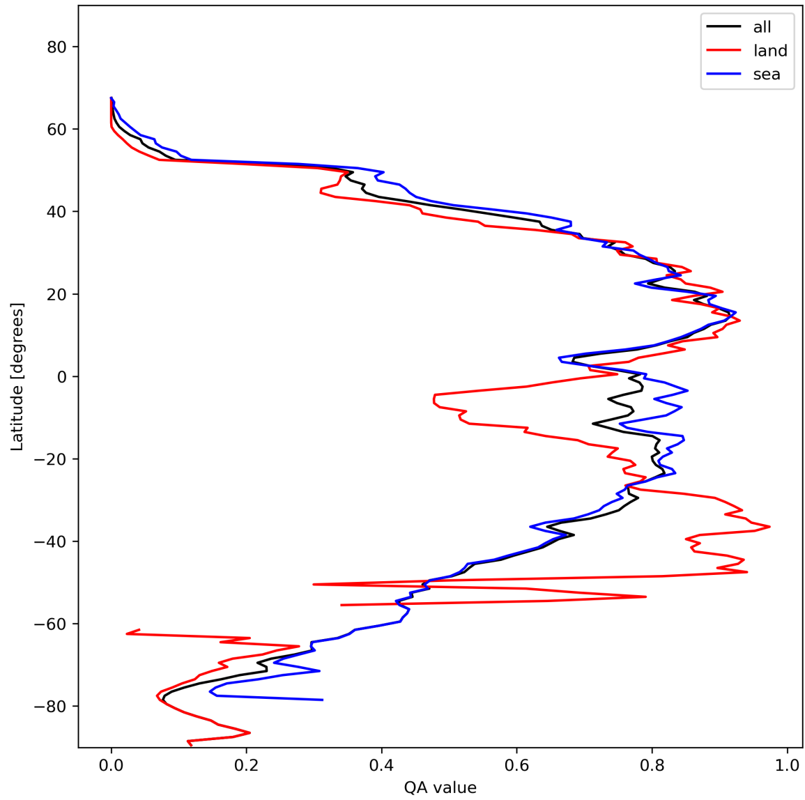
Figure 29: Zonal average of “QA value” for 2024-01-28 to 2024-01-30.
