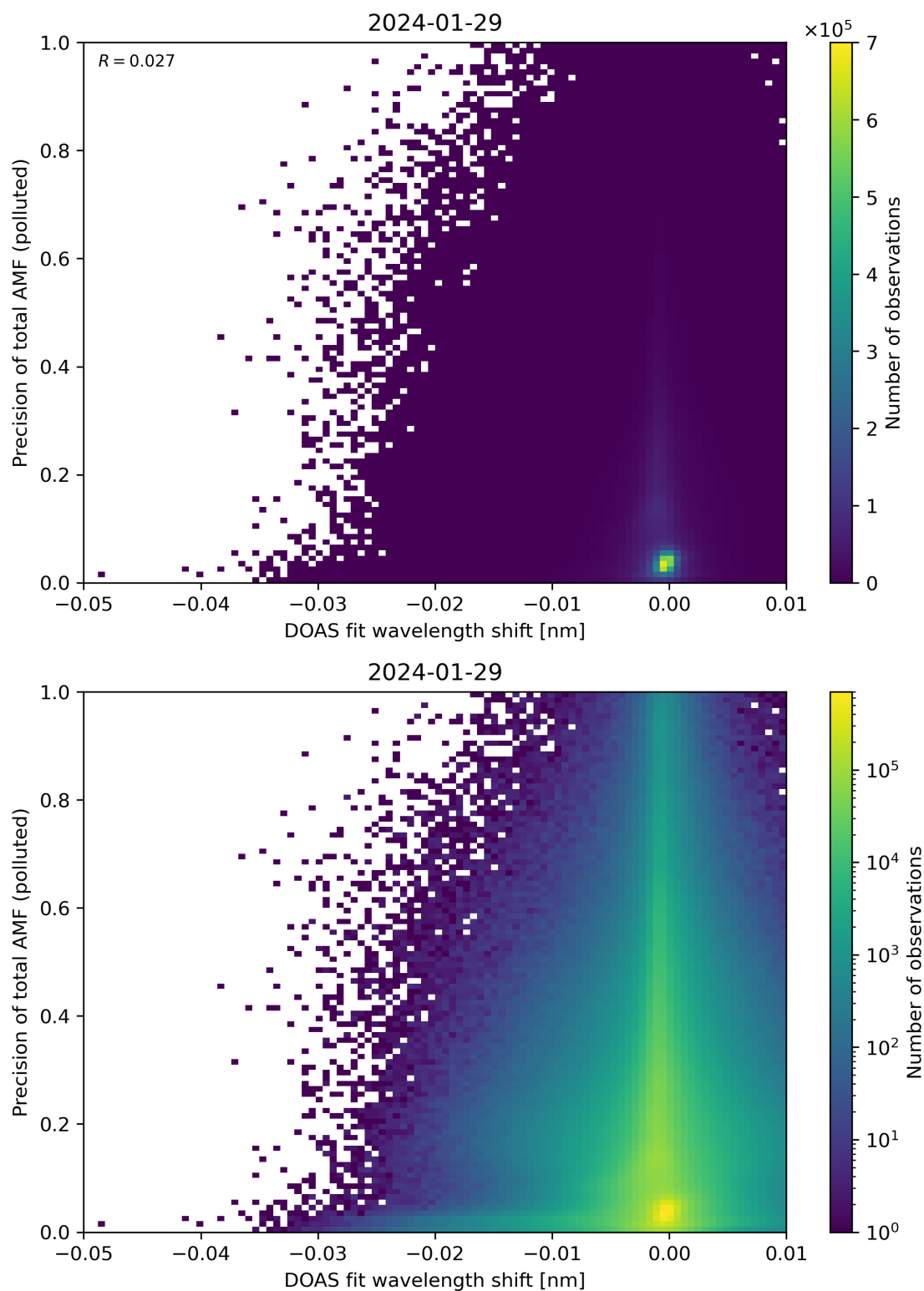
Figure 131: Scatter density plot of “DOAS fit wavelength shift” against “Precision of total AMF (polluted)” for 2024-01-28 to 2024-01-30.
