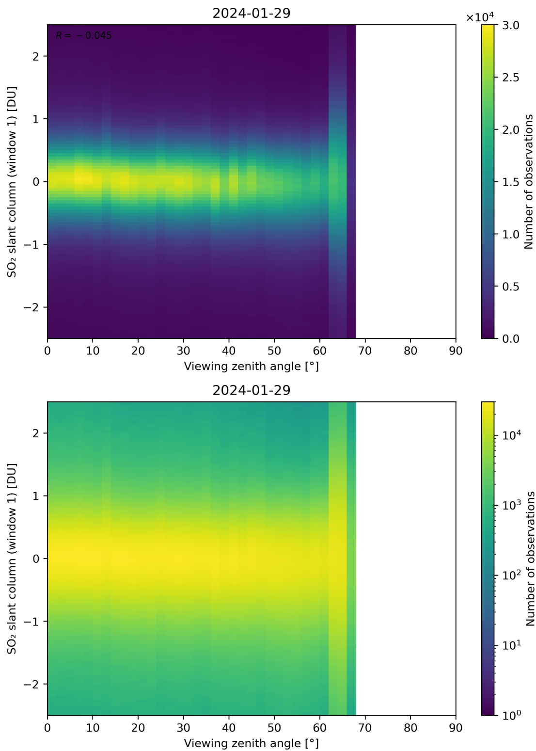
Figure 320: Scatter density plot of “Viewing zenith angle” against “SO 2 slant column (window 1)” for 2024-01-28 to 2024-01-30.
