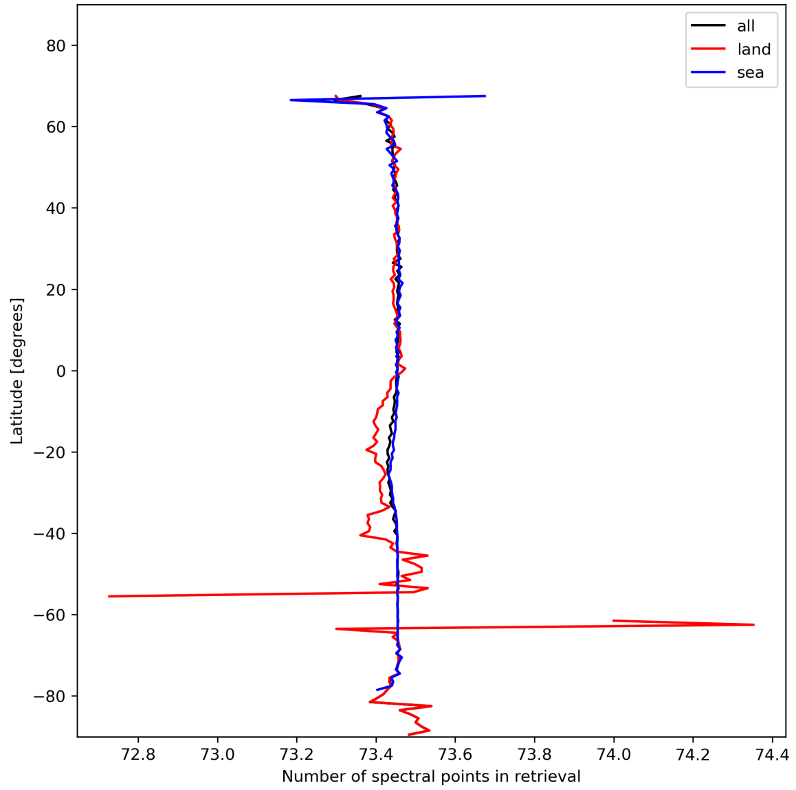
Figure 51: Zonal average of “Number of spectral points in retrieval” for 2024-01-28 to 2024-01-30.
