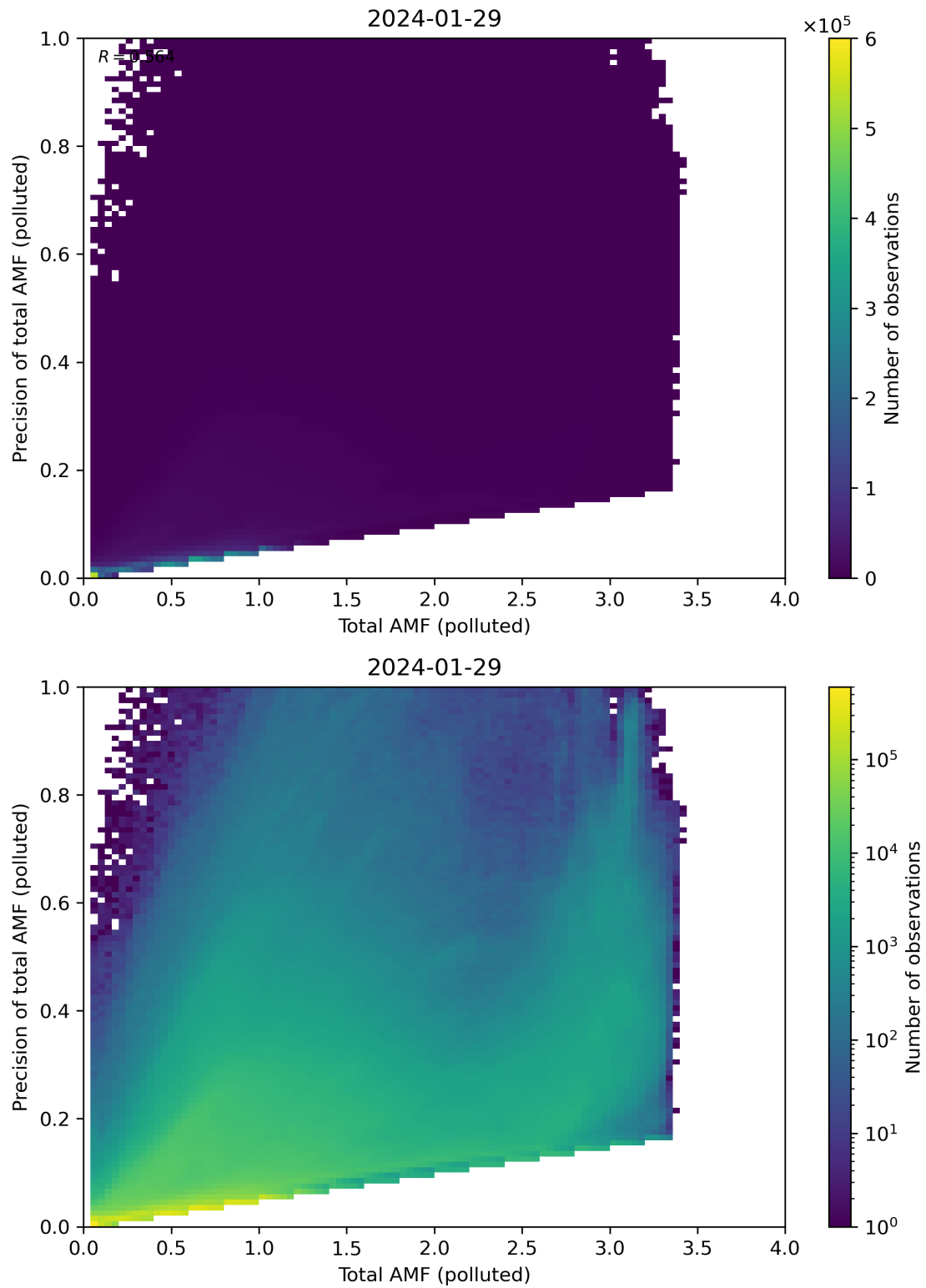
Figure 272: Scatter density plot of “Total AMF (polluted)” against “Precision of total AMF (polluted)” for 2024-01-28 to 2024-01-30.
