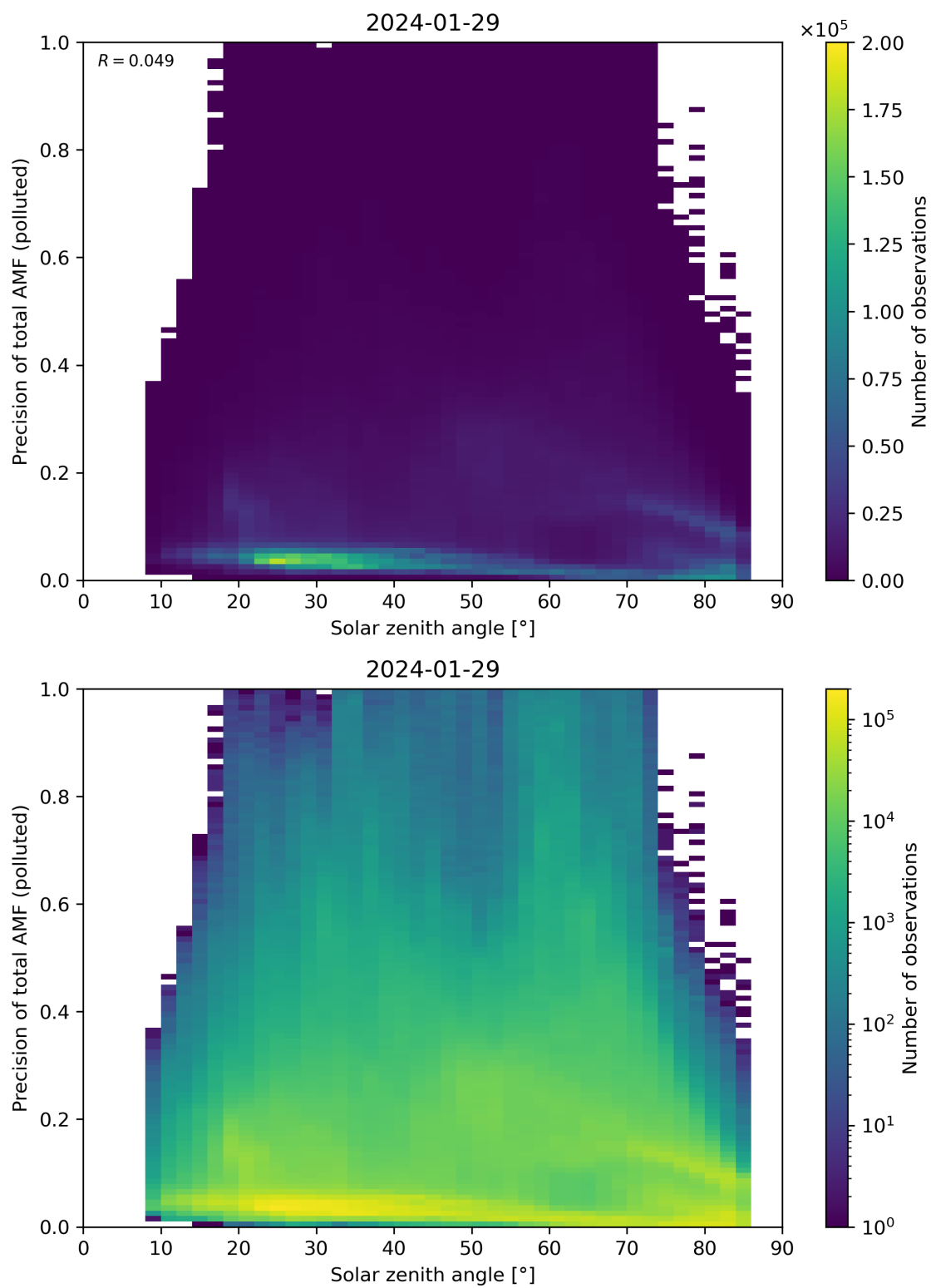
Figure 175: Scatter density plot of “Solar zenith angle” against “Precision of total AMF (polluted)” for 2024-01-28 to 2024-01-30.
