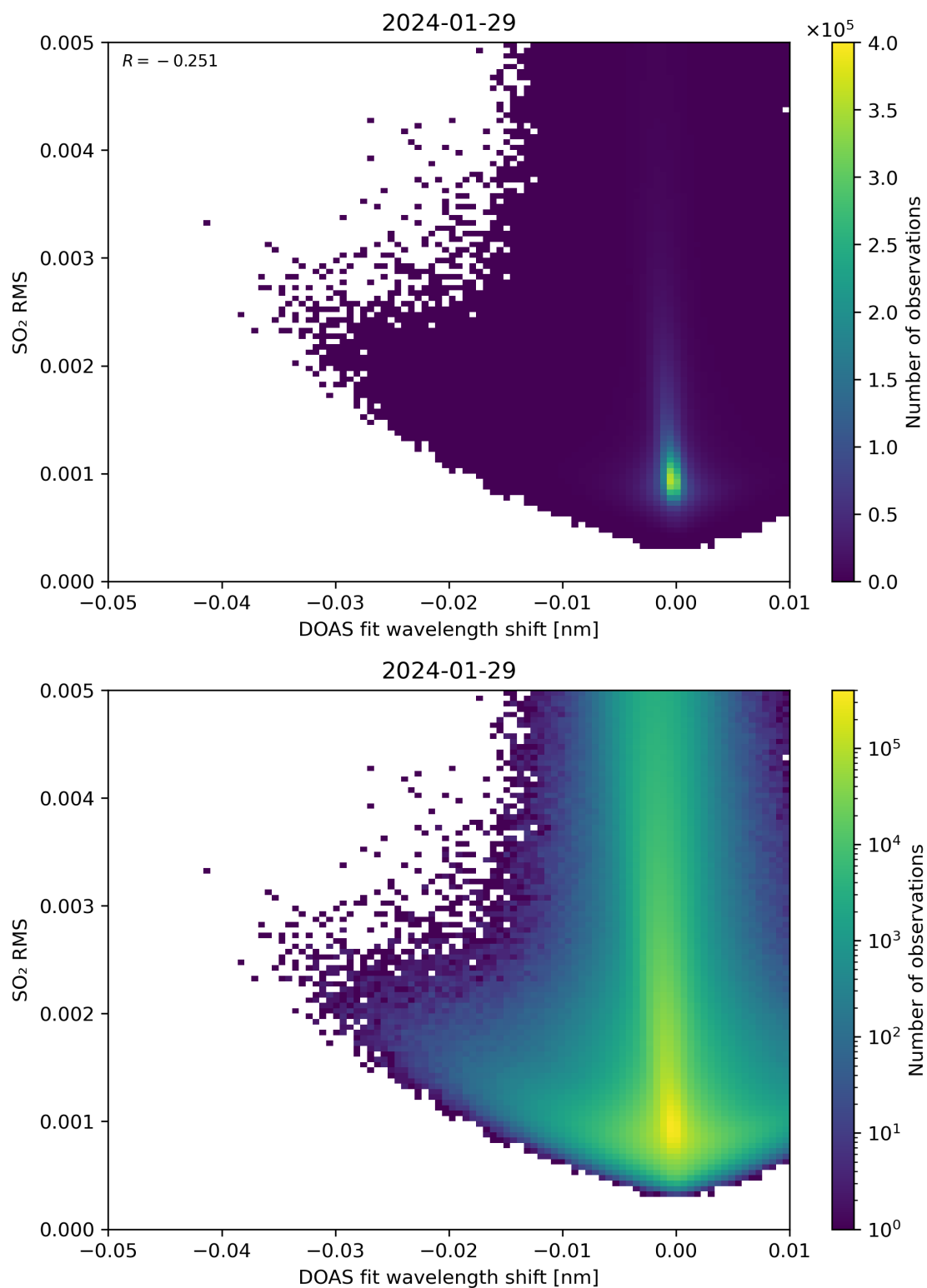
Figure 128: Scatter density plot of “DOAS fit wavelength shift” against “SO 2 RMS” for 2024-01-28 to 2024-01-30.
