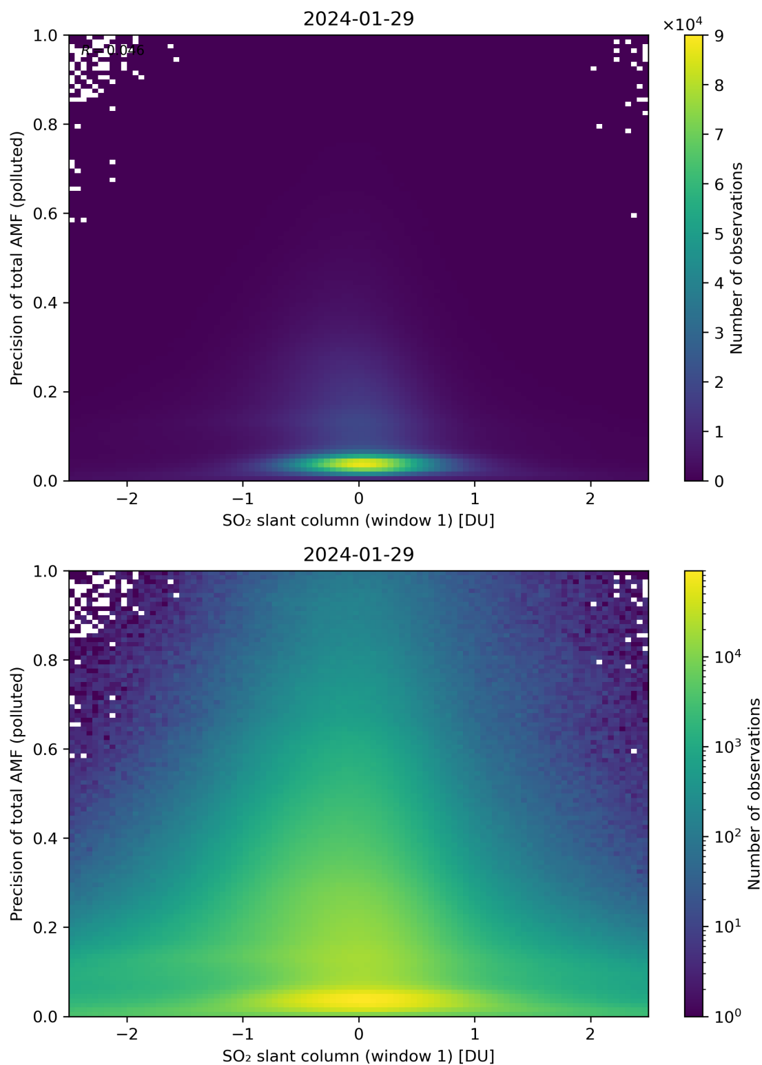
Figure 240: Scatter density plot of “SO 2 slant column (window 1)” against “Precision of total AMF (polluted)” for 2024-01-28 to 2024-01-30.
