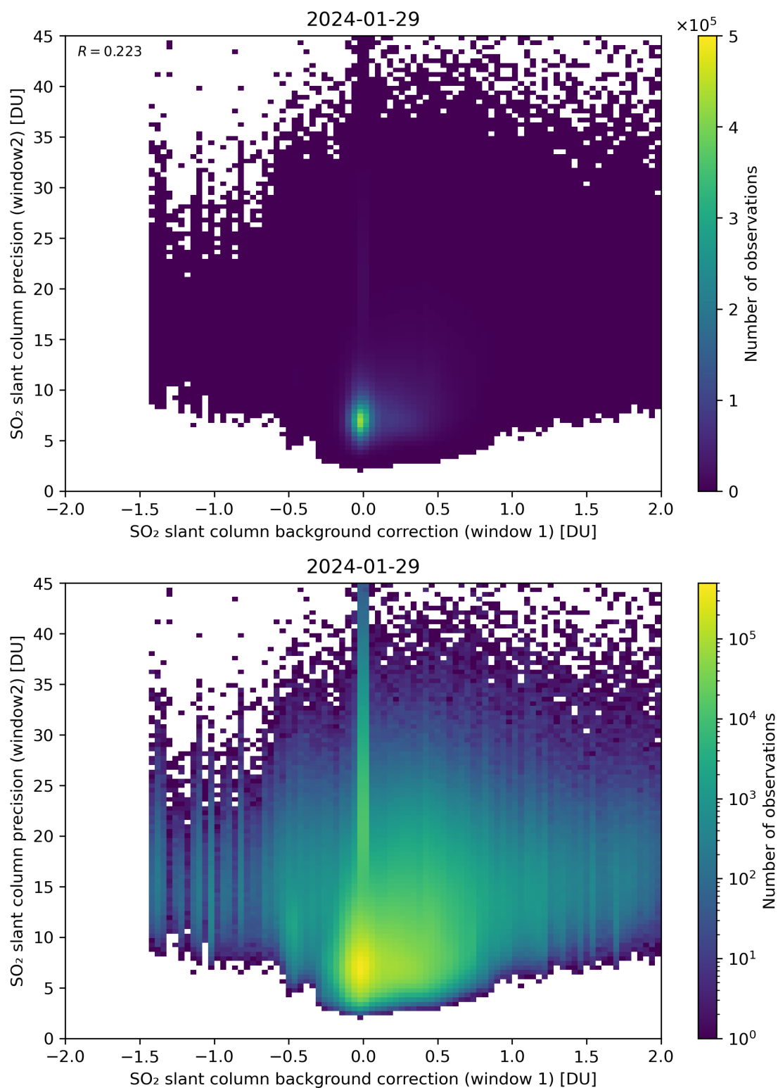
Figure 106: Scatter density plot of “SO 2 slant column background correction (window 1)” against “SO 2 slant column precision (window2)” for 2024-01-28 to 2024-01-30.
