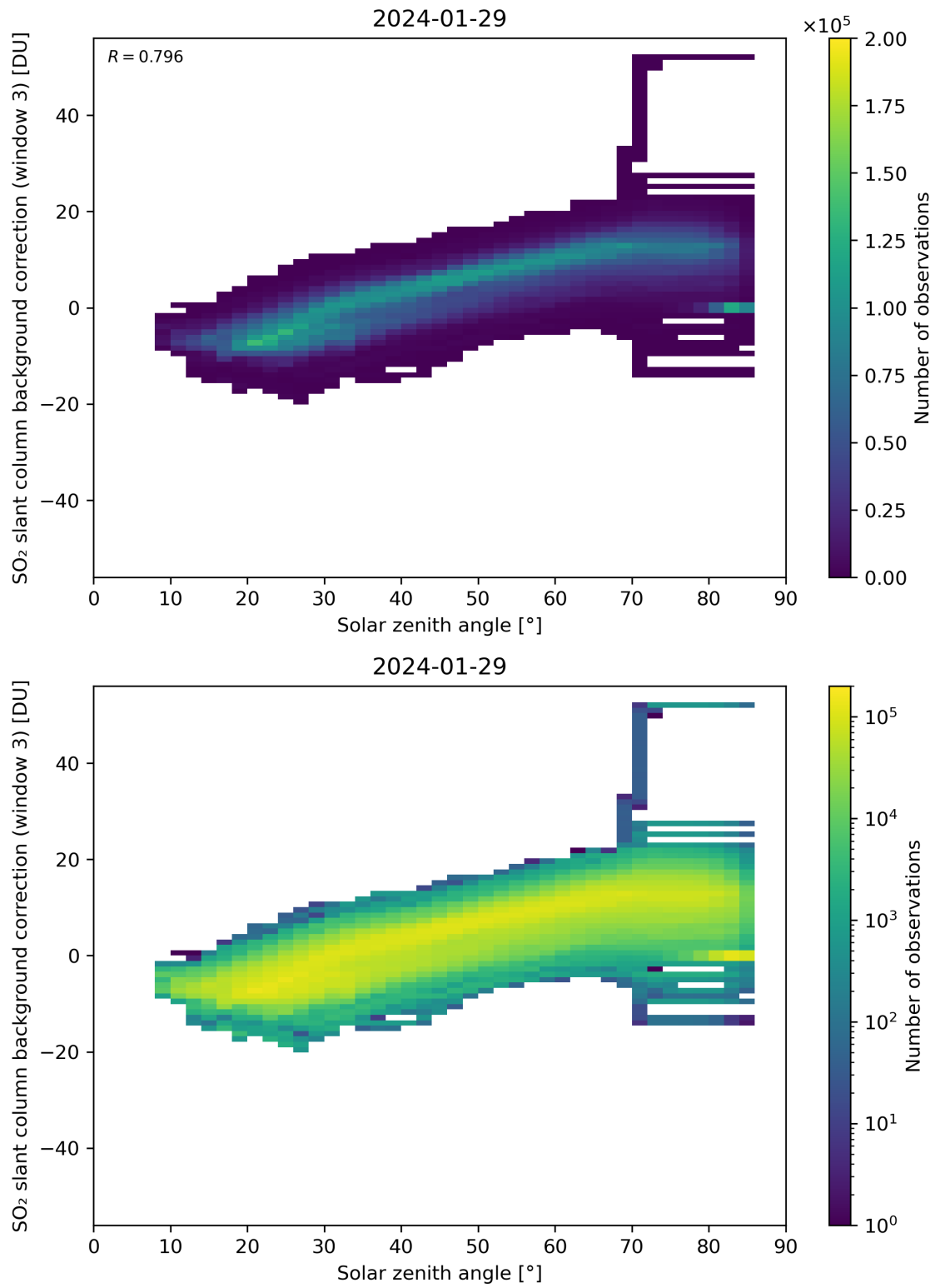
Figure 160: Scatter density plot of “Solar zenith angle” against “SO 2 slant column background correction (window 3)” for 2024-01-28 to 2024-01-30.
