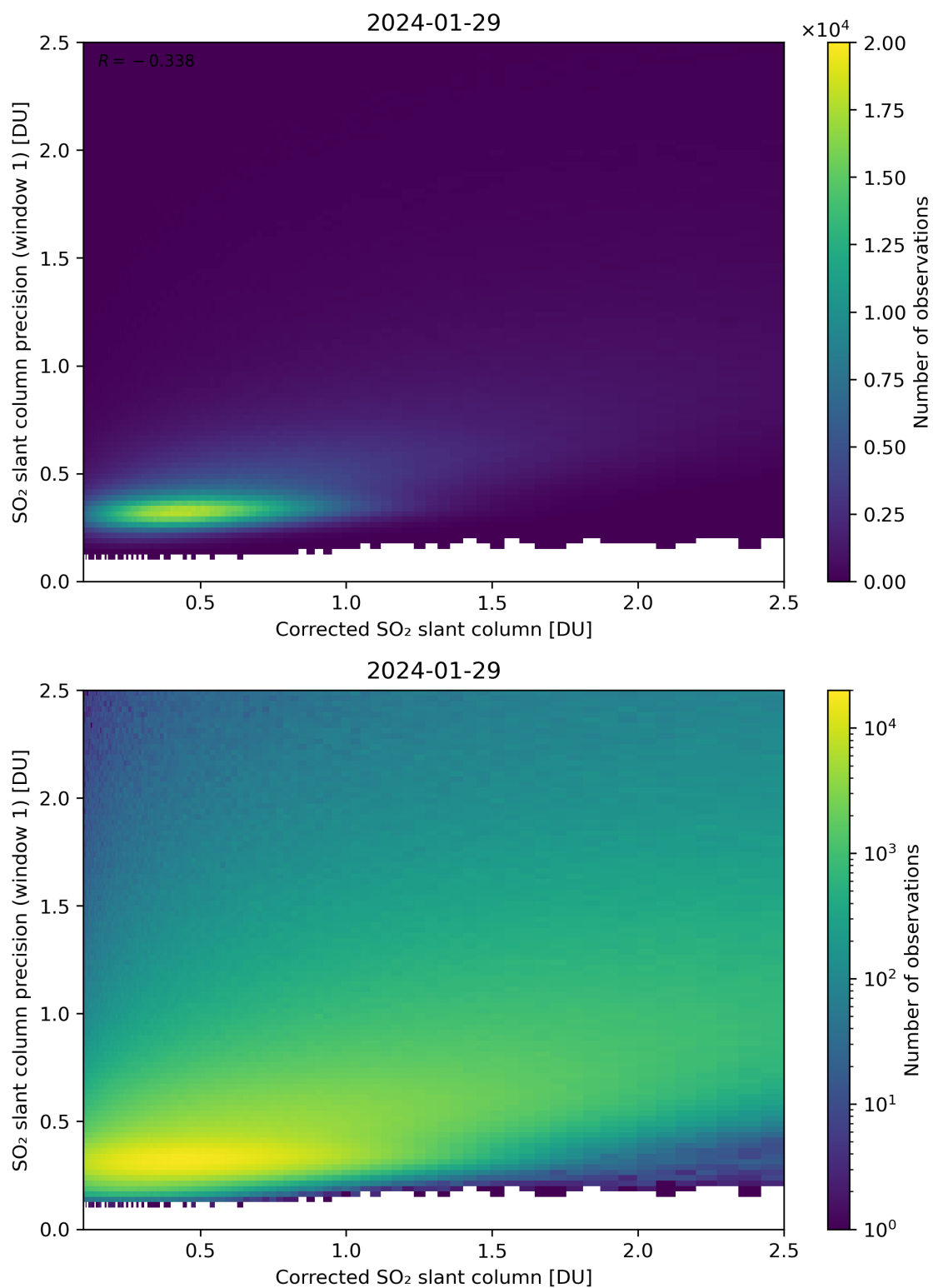
Figure 188: Scatter density plot of “Corrected SO 2 slant column” against “SO 2 slant column precision (window 1)” for 2024-01-28 to 2024-01-30.
