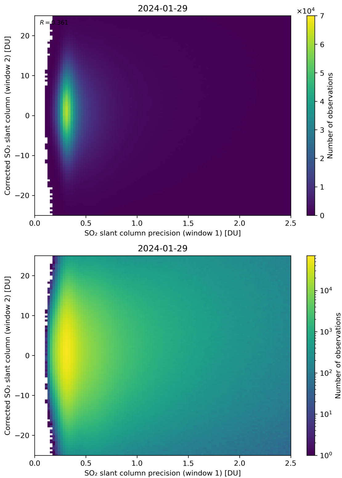
Figure 225: Scatter density plot of “SO 2 slant column precision (window 1)” against “Corrected SO 2 slant column (window 2)” for 2024-01-28 to 2024-01-30.
