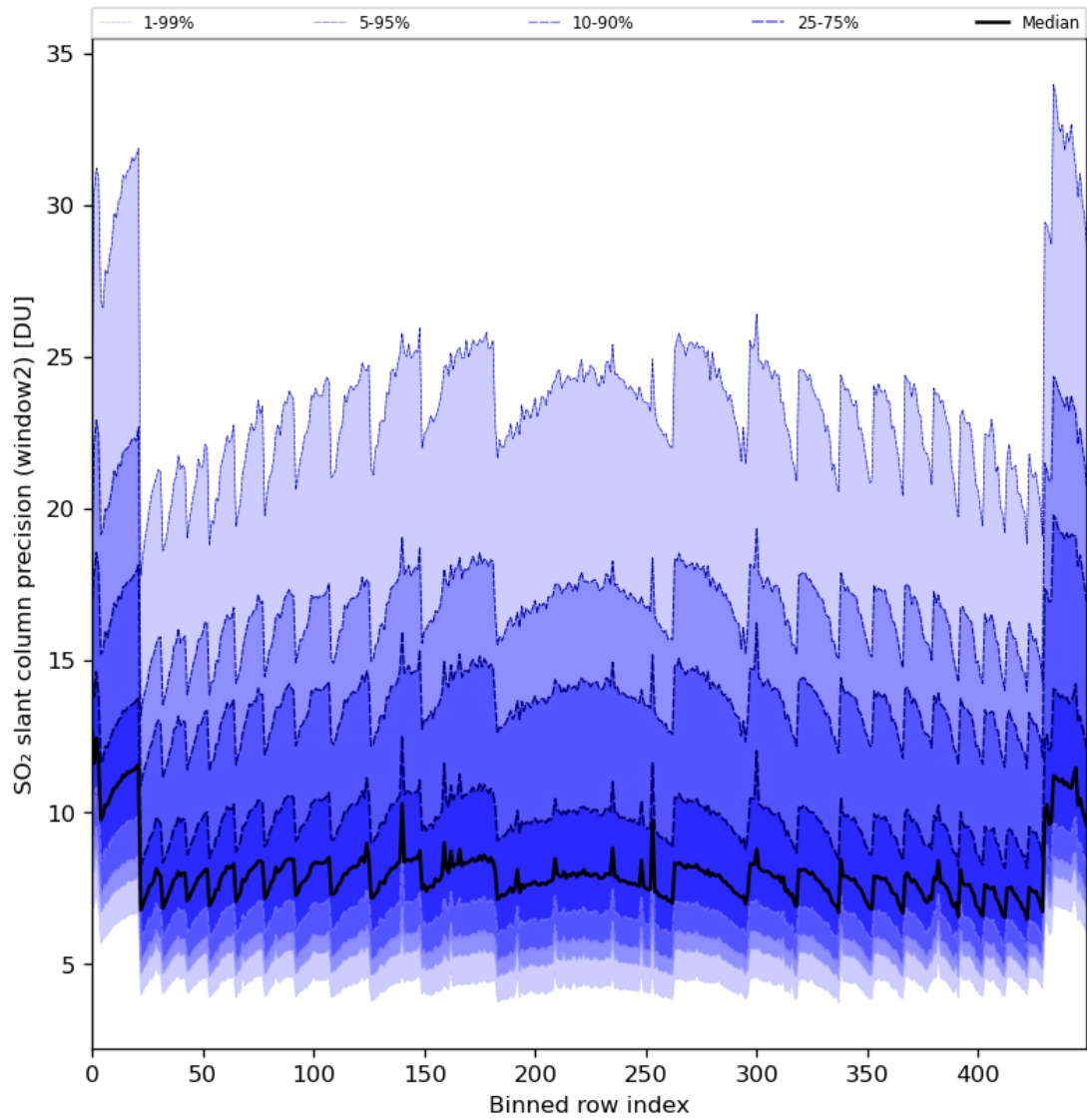
Figure 84: Along track statistics of “SO 2 slant column precision (window2)” for 2024-01-28 to 2024-01-30
