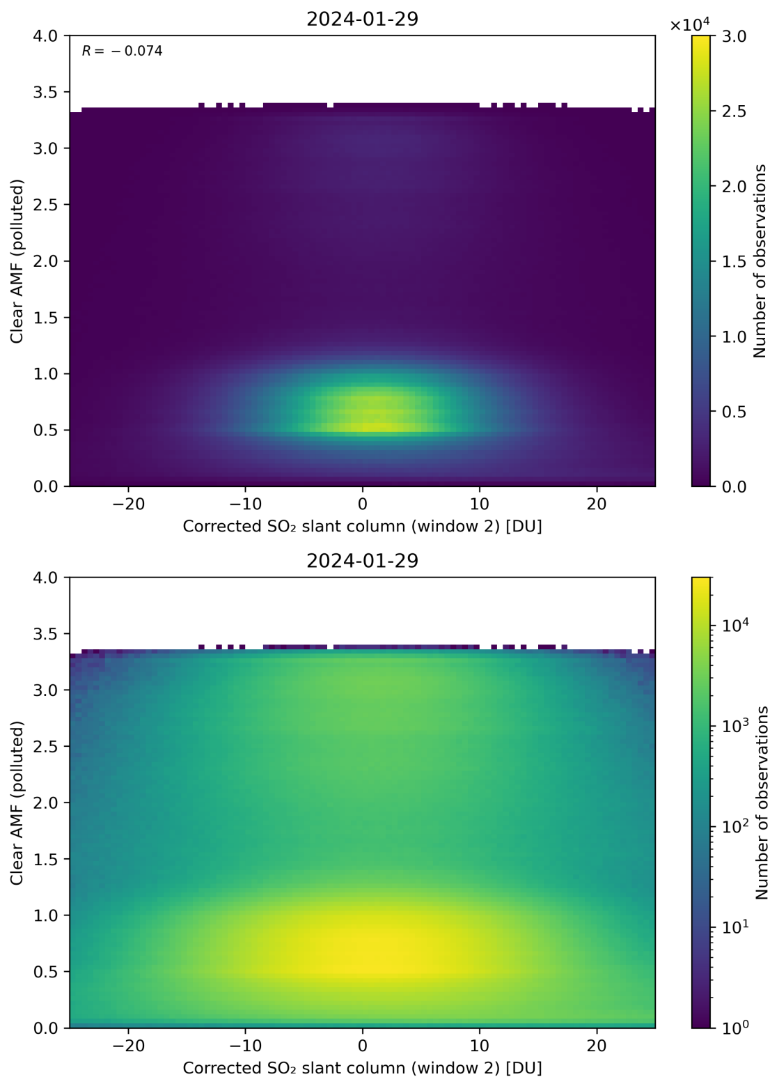
Figure 199: Scatter density plot of “Corrected SO 2 slant column (window 2)” against “Clear AMF (polluted)” for 2024-01-28 to 2024-01-30.
