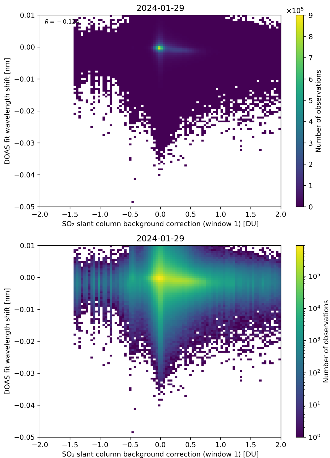
Figure 100: Scatter density plot of “SO 2 slant column background correction (window 1)” against “DOAS fit wavelength shift” for 2024-01-28 to 2024-01-30.
