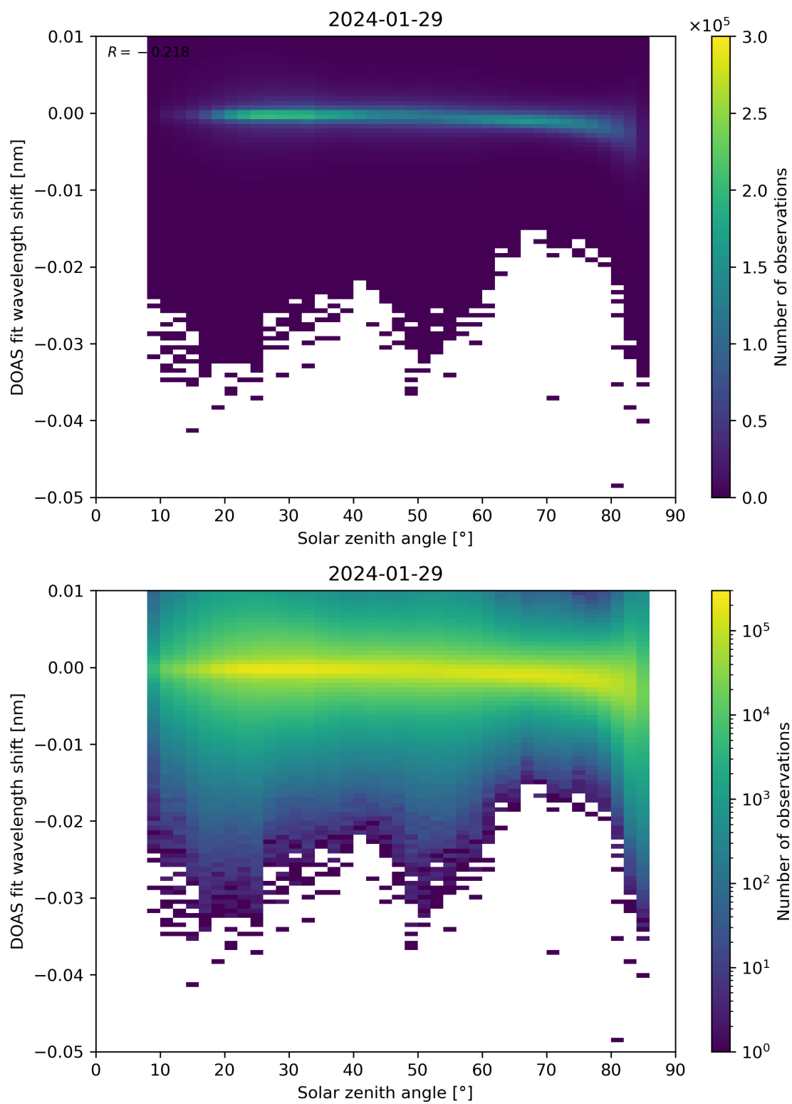
Figure 161: Scatter density plot of “Solar zenith angle” against “DOAS fit wavelength shift” for 2024-01-28 to 2024-01-30.
