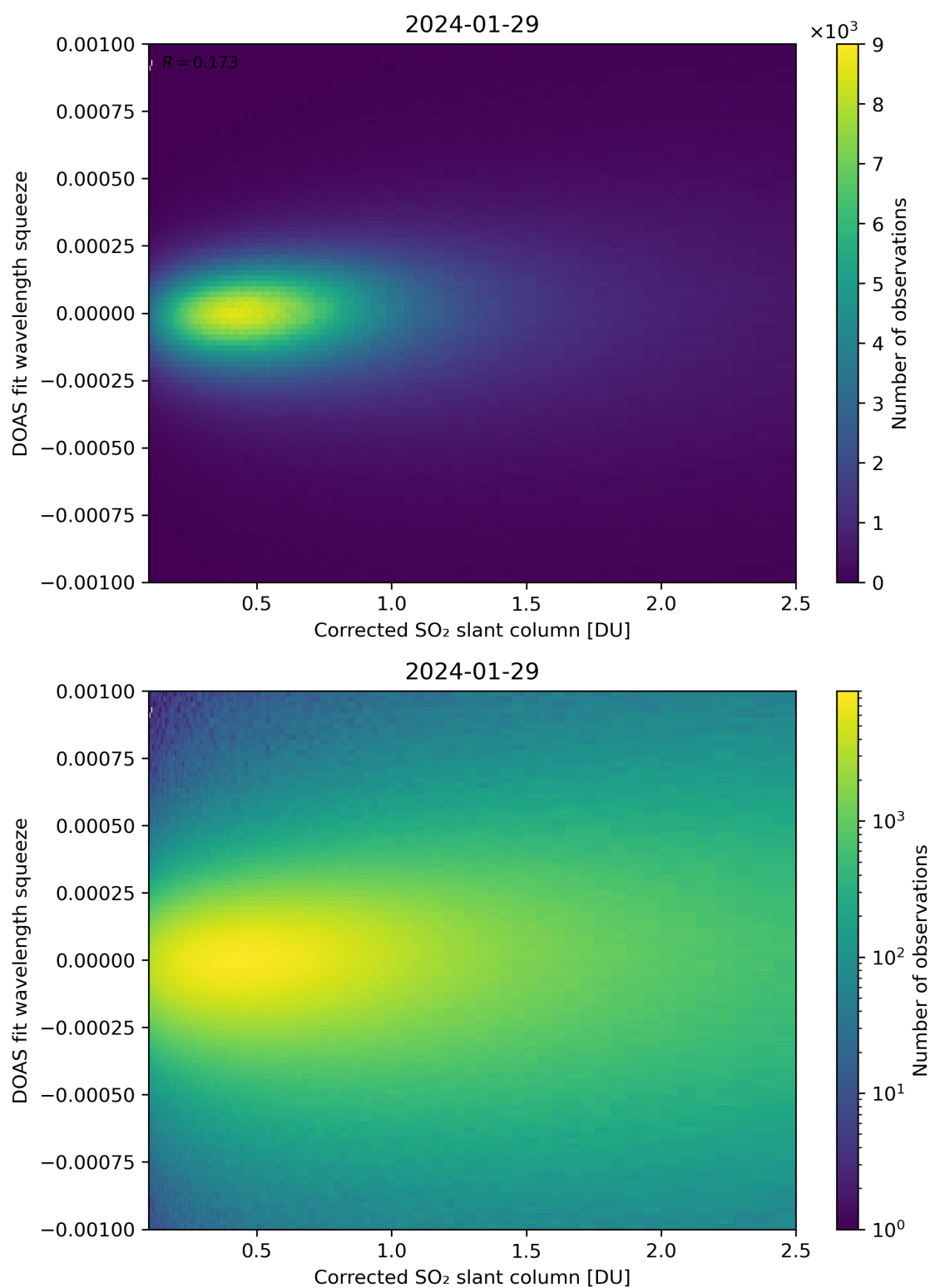
Figure 182: Scatter density plot of “Corrected SO 2 slant column” against “DOAS fit wavelength squeeze” for 2024-01-28 to 2024-01-30.
