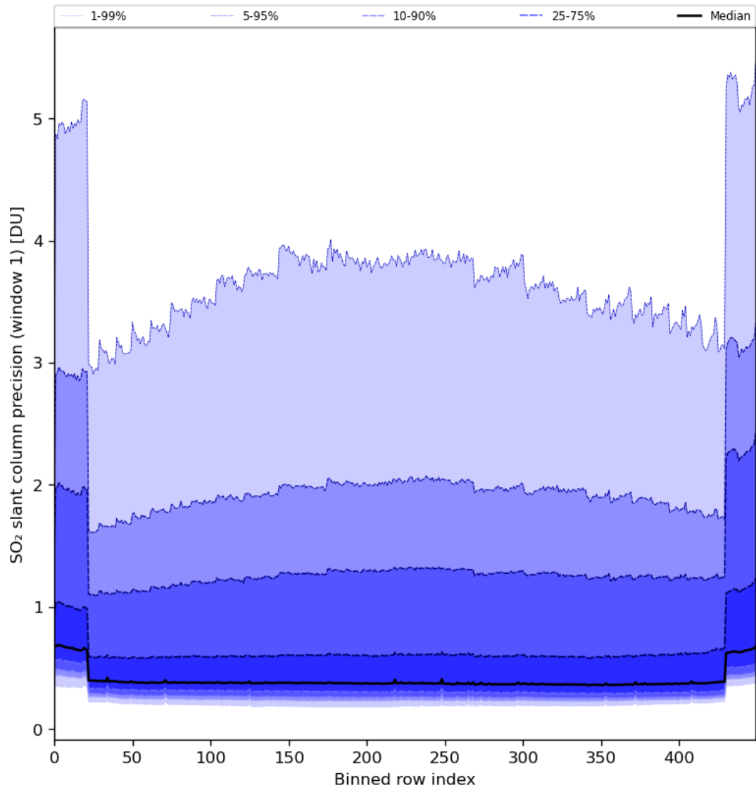
Figure 80: Along track statistics of “SO 2 slant column precision (window 1)” for 2024-01-28 to 2024-01-30
