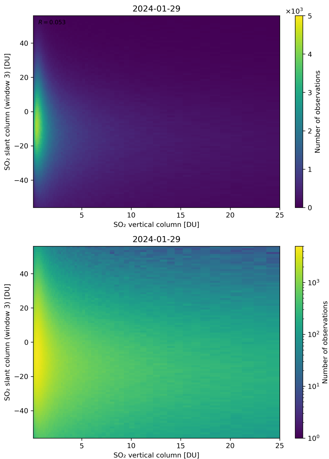
Figure 303: Scatter density plot of “SO 2 vertical column” against “SO 2 slant column (window 3)” for 2024-01-28 to 2024-01-30.
