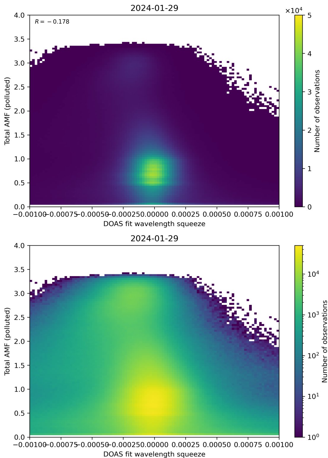
Figure 134: Scatter density plot of “DOAS fit wavelength squeeze” against “Total AMF (polluted)” for 2024-01-28 to 2024-01-30.
