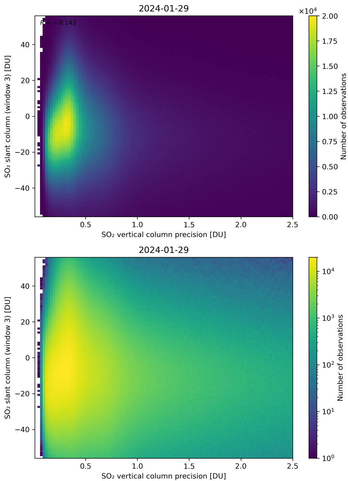
Figure 292: Scatter density plot of “SO 2 vertical column precision” against “SO 2 slant column (window 3)” for 2024-01-28 to 2024-01-30.
