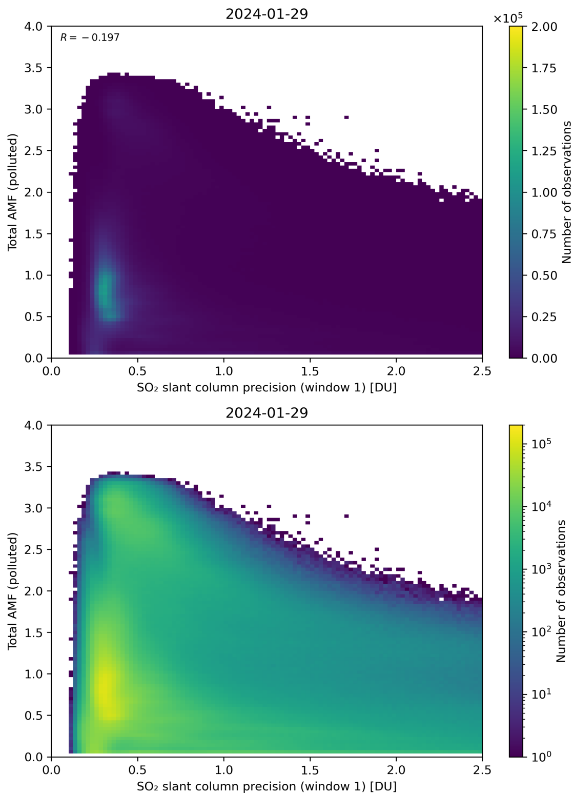
Figure 230: Scatter density plot of “SO 2 slant column precision (window 1)” against “Total AMF (polluted)” for 2024-01-28 to 2024-01-30.
