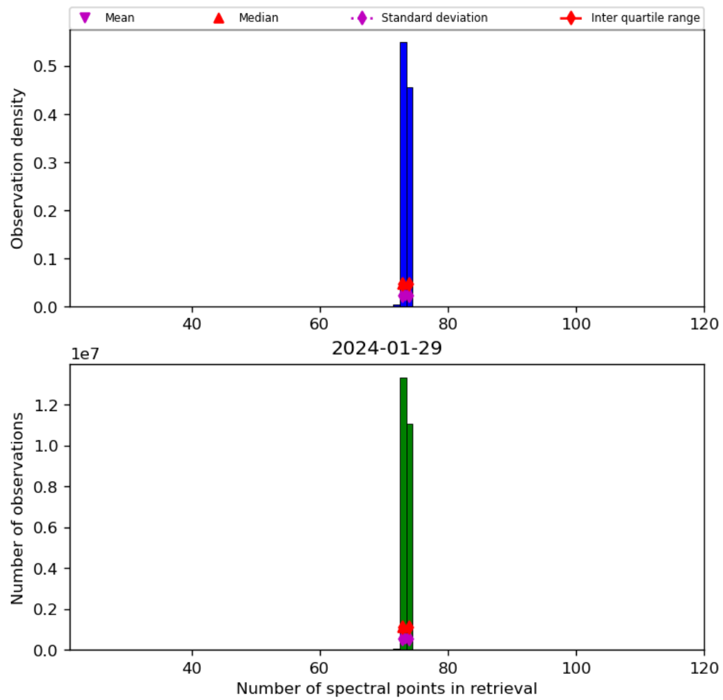
Figure 74: Histogram of “Number of spectral points in retrieval” for 2024-01-28 to 2024-01-30
