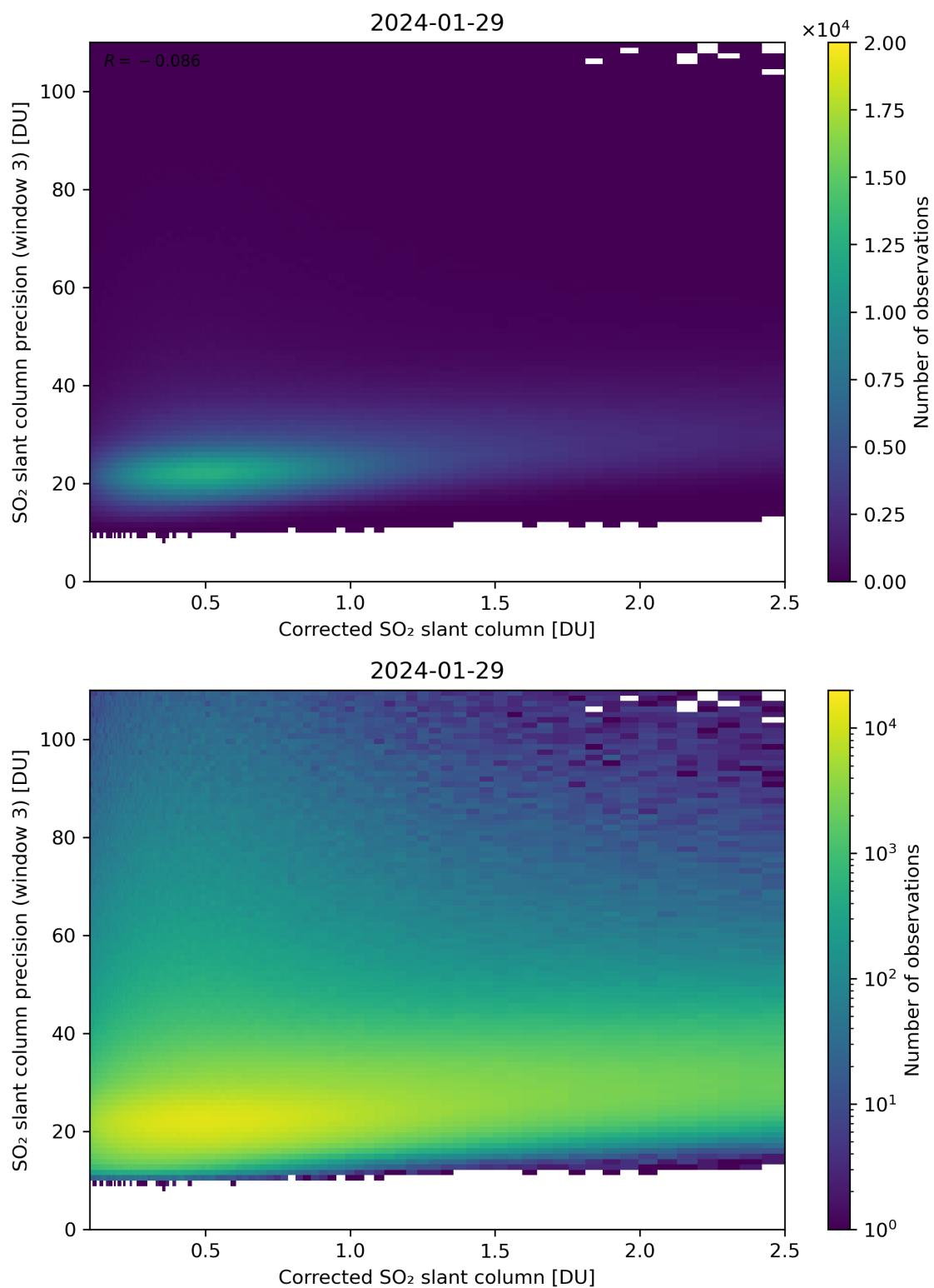
Figure 191: Scatter density plot of “Corrected SO 2 slant column” against “SO 2 slant column precision (window 3)” for 2024-01-28 to 2024-01-30.
