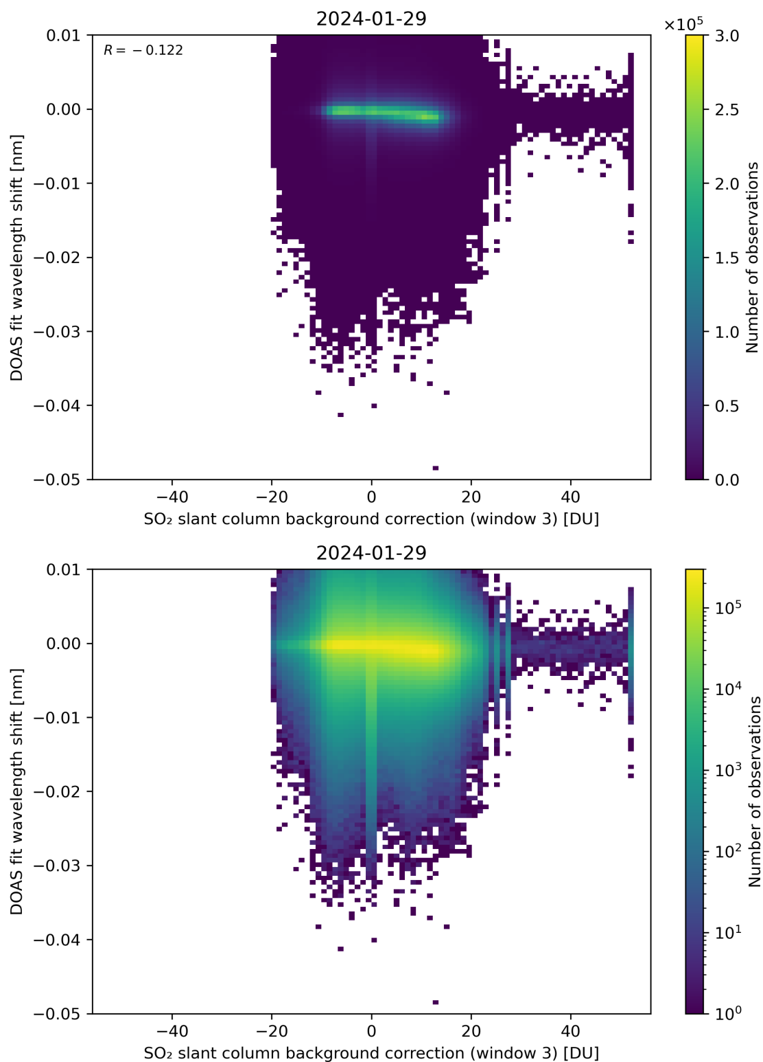
Figure 121: Scatter density plot of “SO 2 slant column background correction (window 3)” against “DOAS fit wavelength shift” for 2024-01-28 to 2024-01-30.
