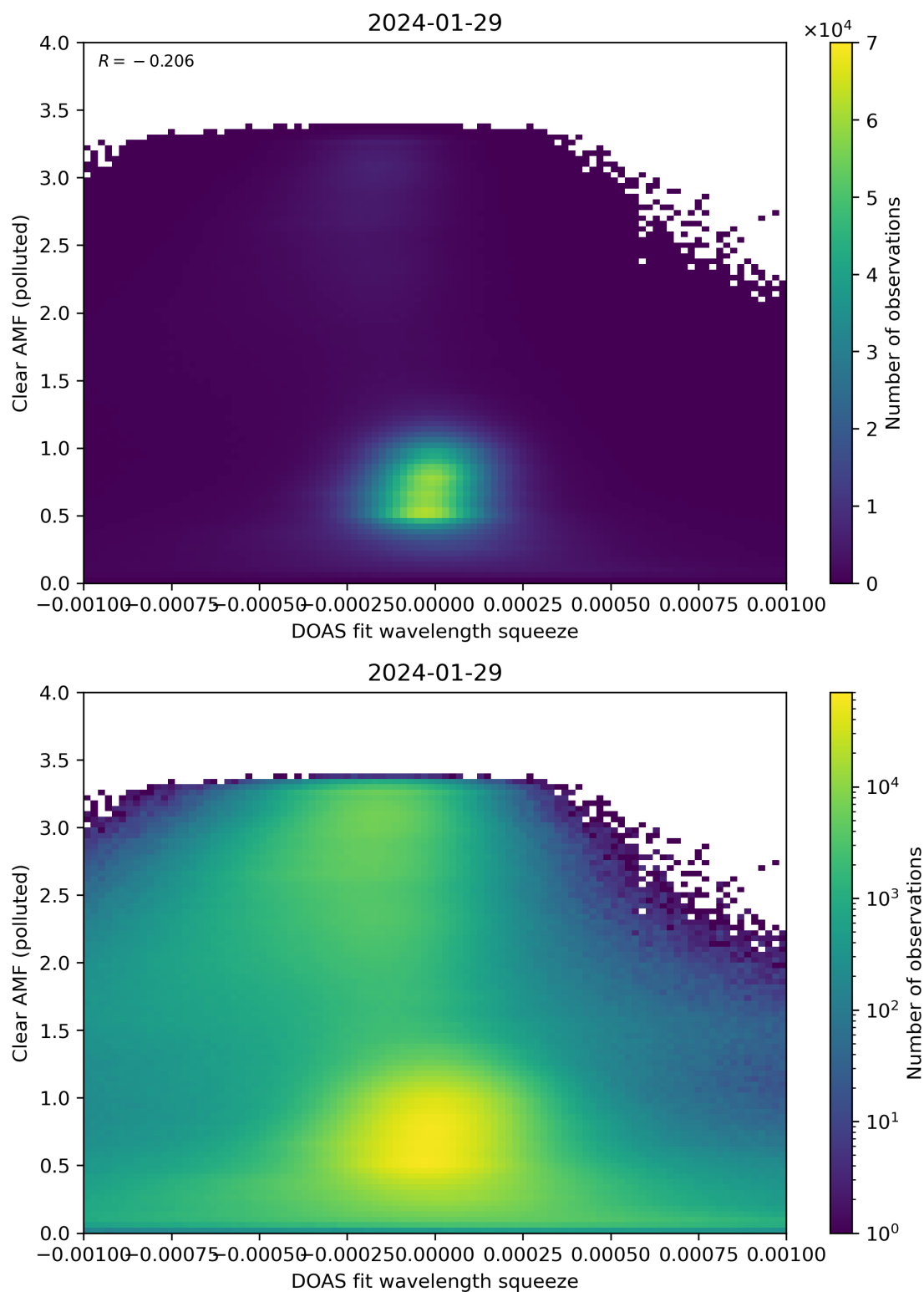
Figure 133: Scatter density plot of “DOAS fit wavelength squeeze” against “Clear AMF (polluted)” for 2024-01-28 to 2024-01-30.
