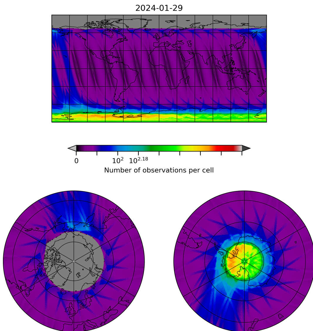
Figure 28: Map of the number of observations for 2024-01-28 to 2024-01-30
