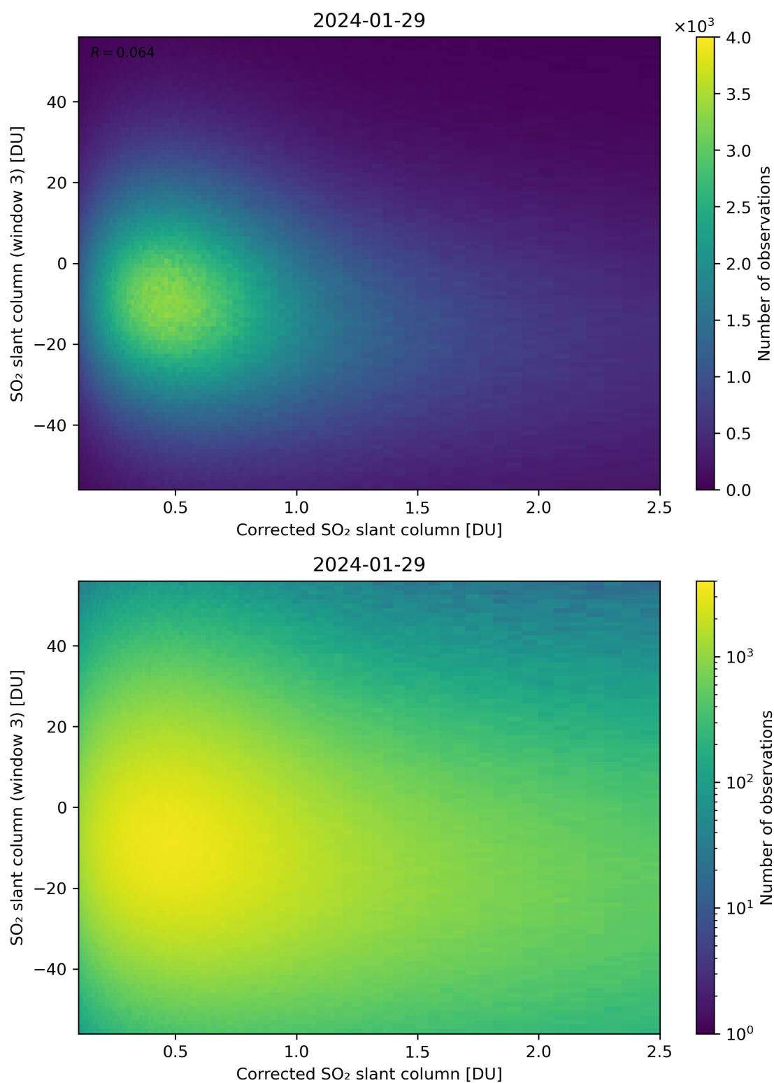
Figure 190: Scatter density plot of “Corrected SO 2 slant column” against “SO 2 slant column (window 3)” for 2024-01-28 to 2024-01-30.
