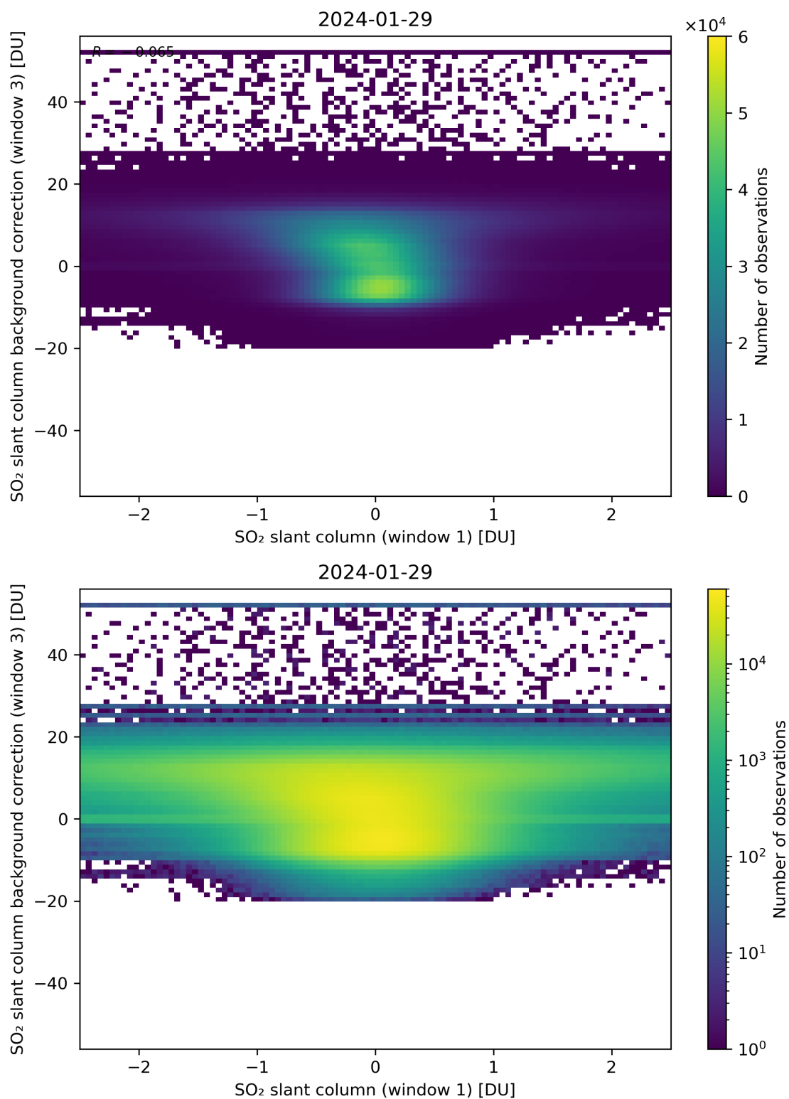
Figure 214: Scatter density plot of “SO 2 slant column (window 1)” against “SO 2 slant column background correction (window 3)” for 2024-01-28 to 2024-01-30.
