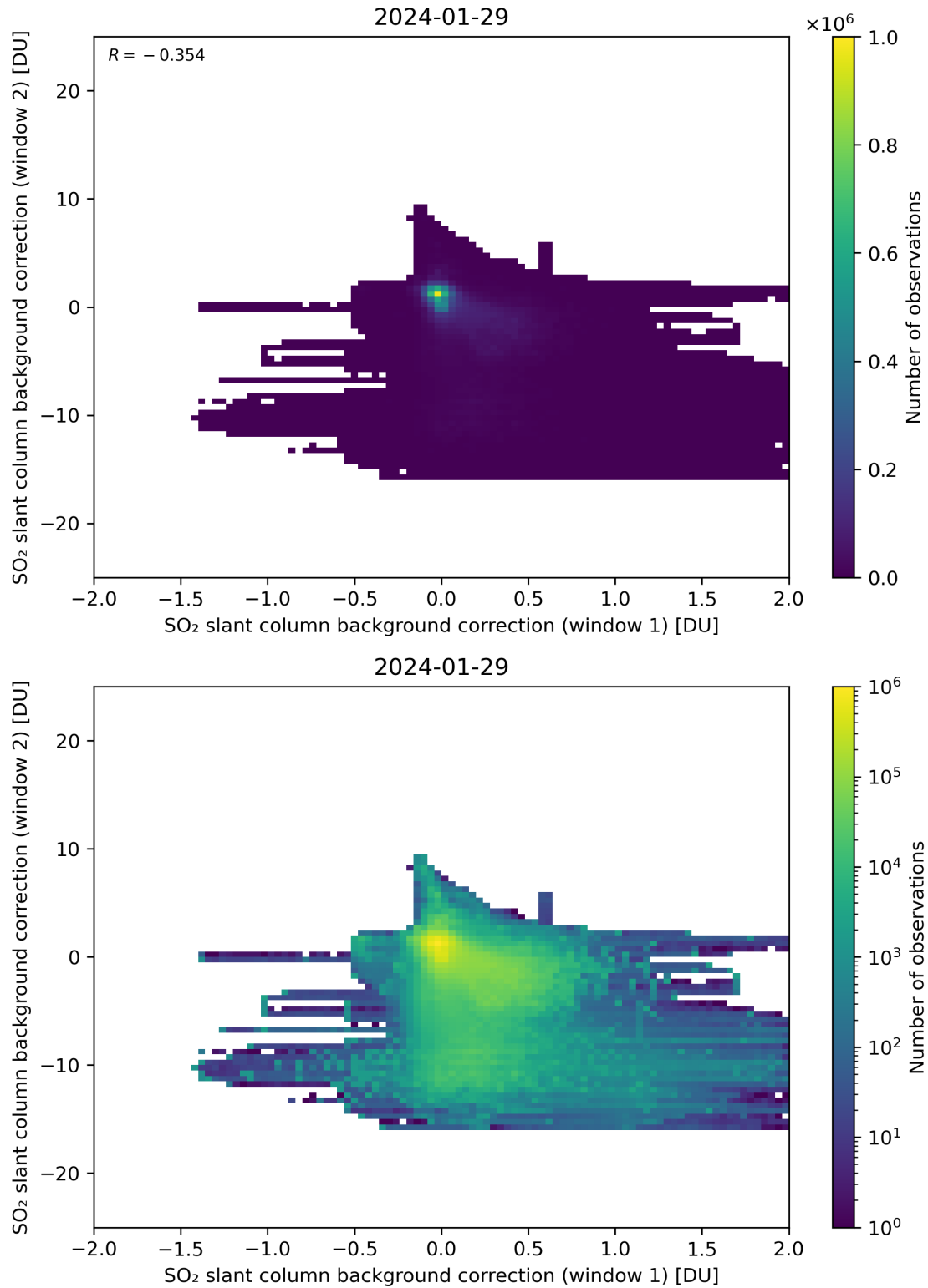
Figure 98: Scatter density plot of “SO 2 slant column background correction (window 1)” against “SO 2 slant column background correction (window 2)” for 2024-01-28 to 2024-01-30.
