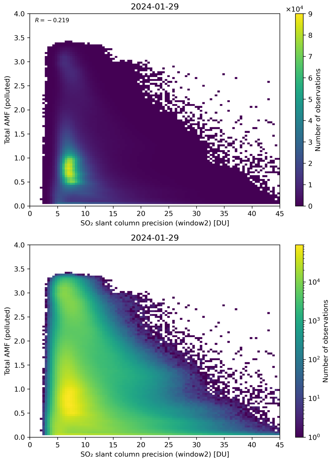
Figure 251: Scatter density plot of “SO 2 slant column precision (window2)” against “Total AMF (polluted)” for 2024-01-28 to 2024-01-30.
