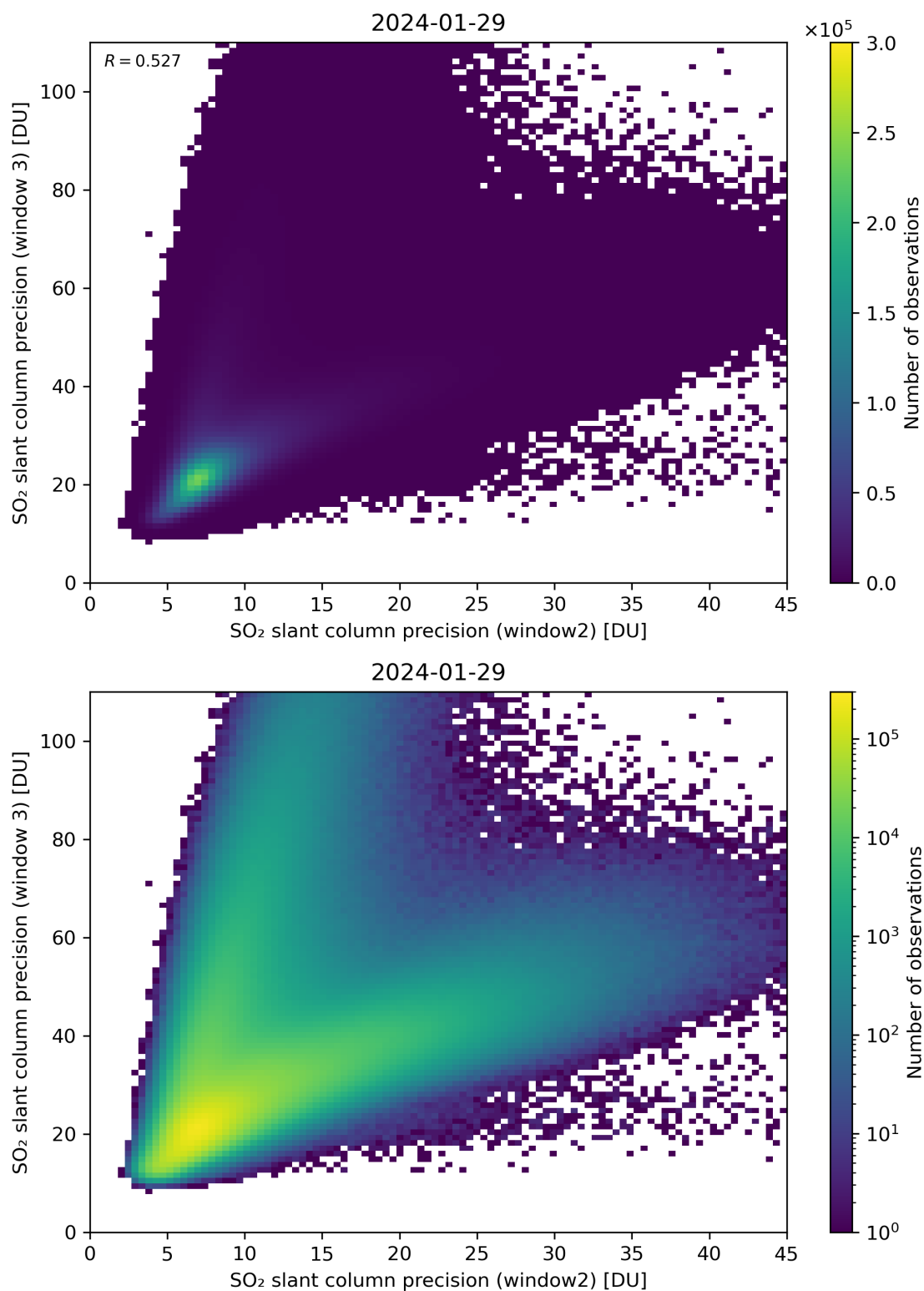
Figure 250: Scatter density plot of “SO 2 slant column precision (window2)” against “SO 2 slant column precision (window 3)” for 2024-01-28 to 2024-01-30.
