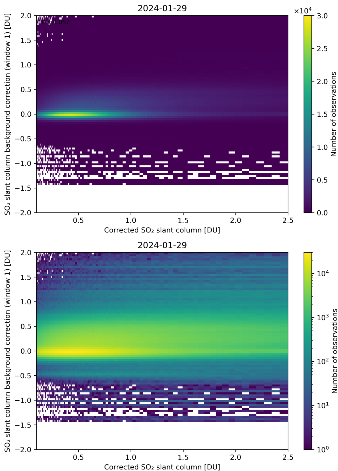
Figure 178: Scatter density plot of “Corrected SO 2 slant column” against “SO 2 slant column background correction (window 1)” for 2024-01-28 to 2024-01-30.
