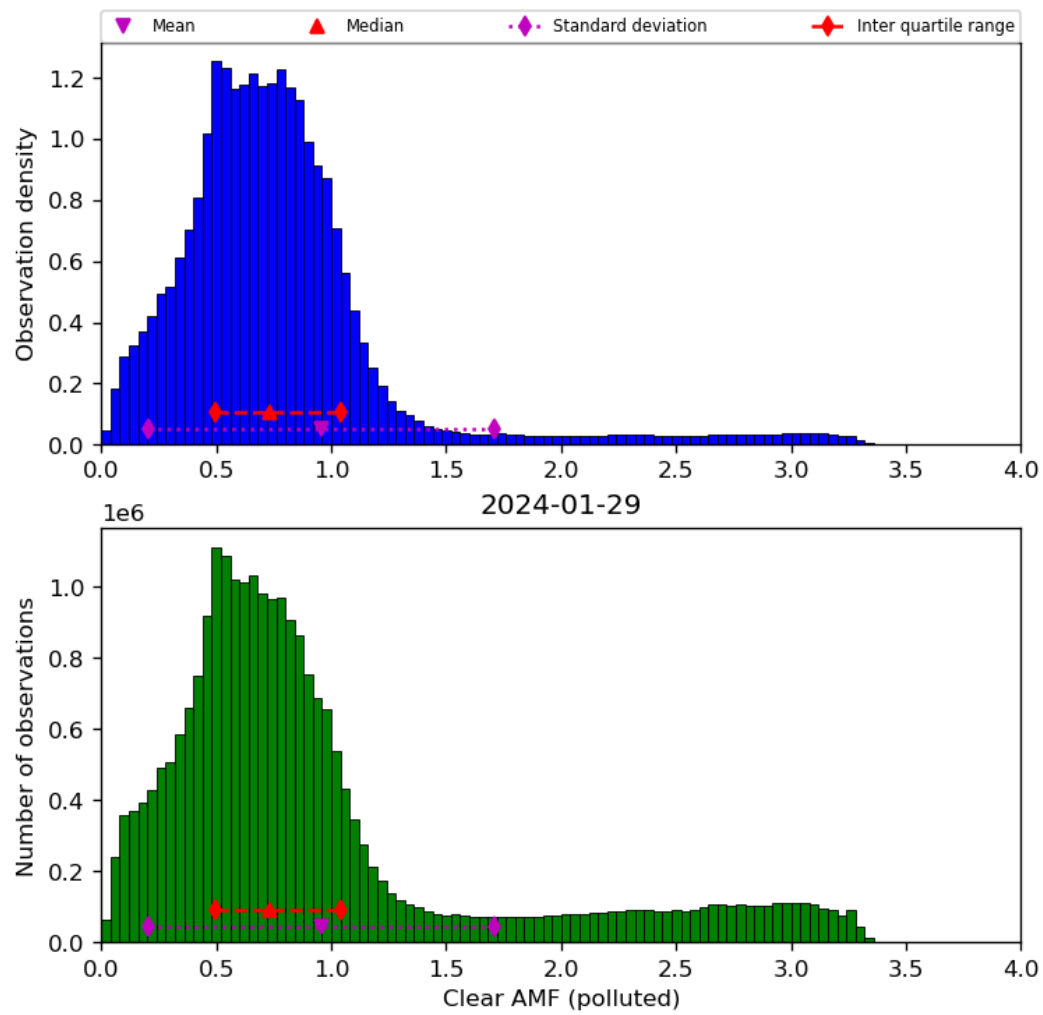
Figure 73: Histogram of “Clear AMF (polluted)” for 2024-01-28 to 2024-01-30
