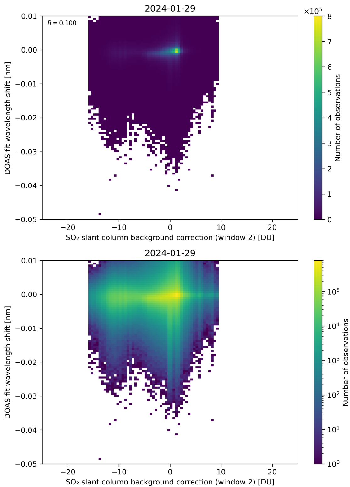
Figure 112: Scatter density plot of “SO 2 slant column background correction (window 2)” against “DOAS fit wavelength shift” for 2024-01-28 to 2024-01-30.
