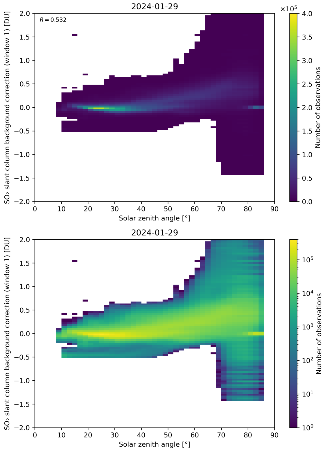
Figure 158: Scatter density plot of “Solar zenith angle” against “SO 2 slant column background correction (window 1)” for 2024-01-28 to 2024-01-30.
