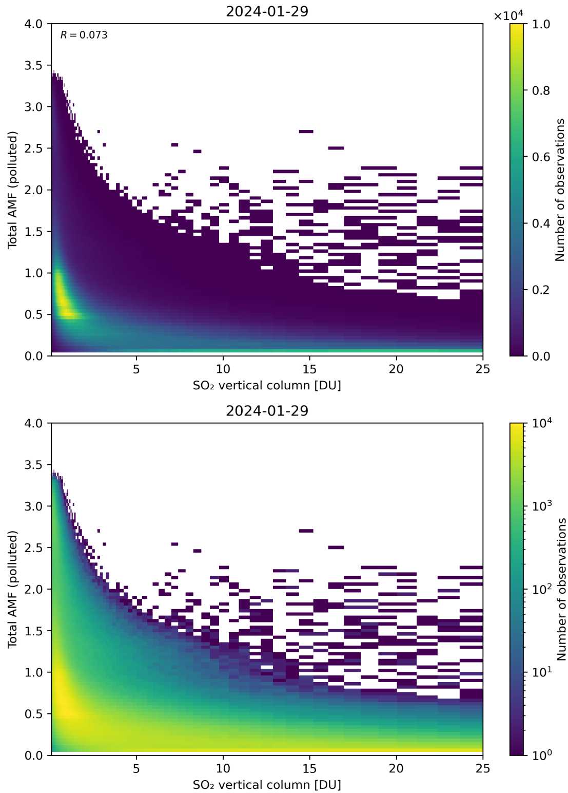
Figure 305: Scatter density plot of “SO 2 vertical column” against “Total AMF (polluted)” for 2024-01-28 to 2024-01-30.
