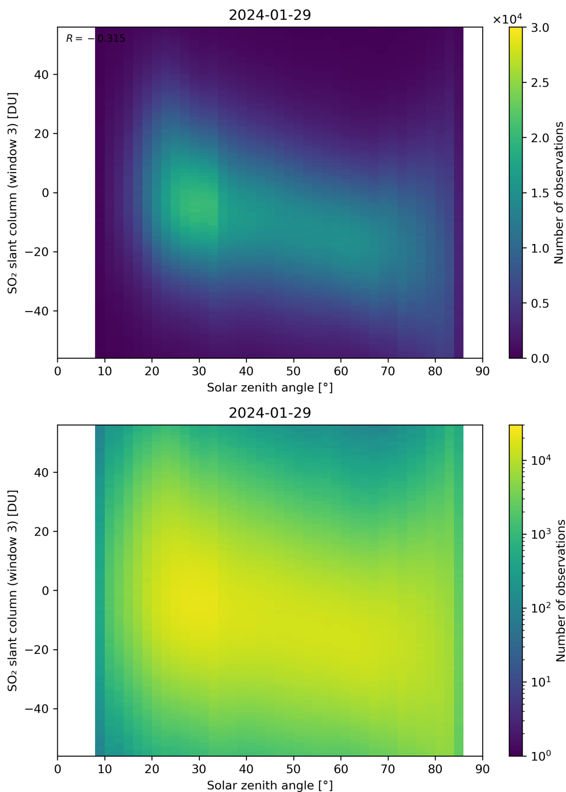
Figure 172: Scatter density plot of “Solar zenith angle” against “SO 2 slant column (window 3)” for 2024-01-28 to 2024-01-30.
