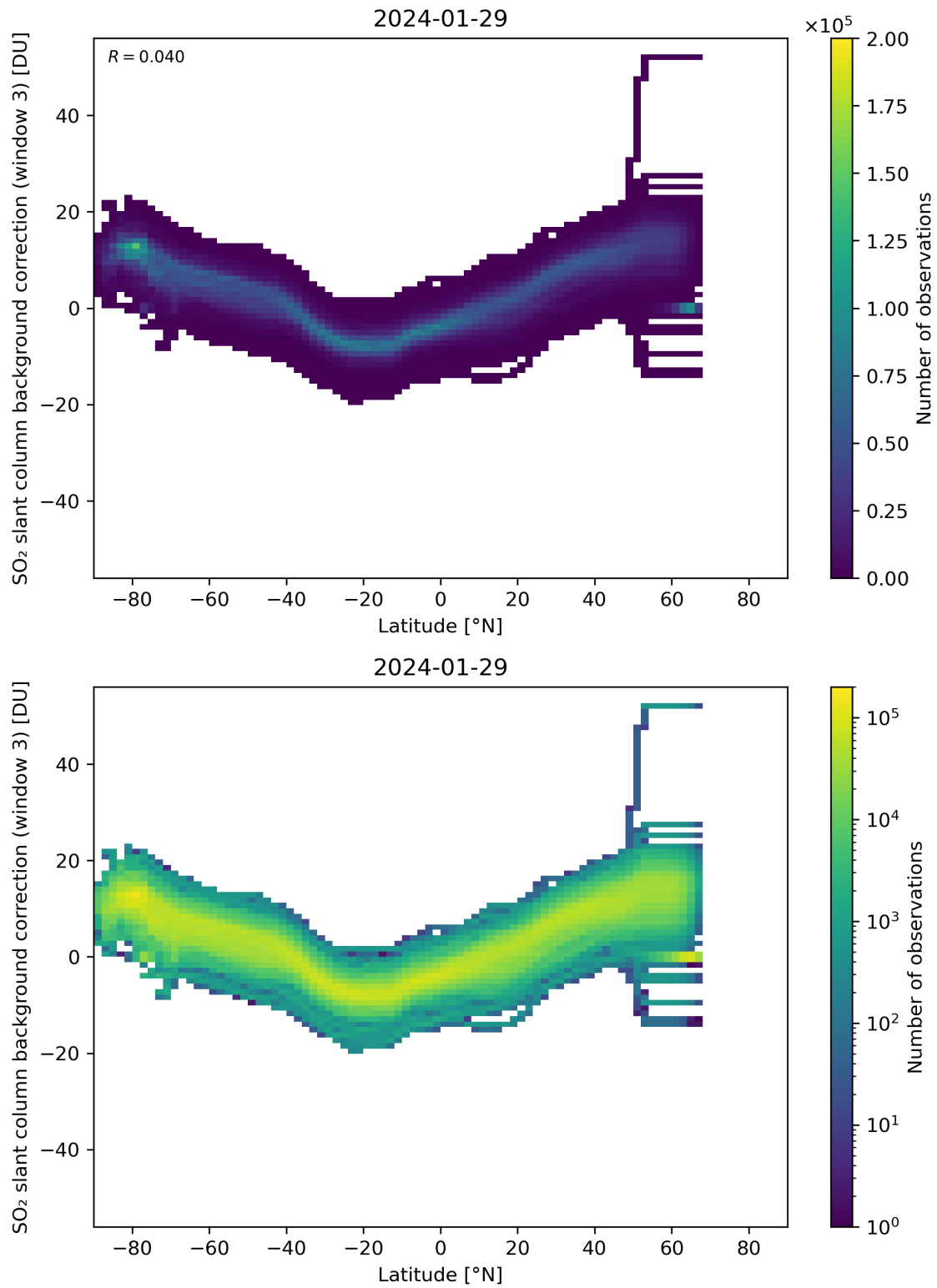
Figure 141: Scatter density plot of “Latitude” against “SO 2 slant column background correction (window 3)” for 2024-01-28 to 2024-01-30.
