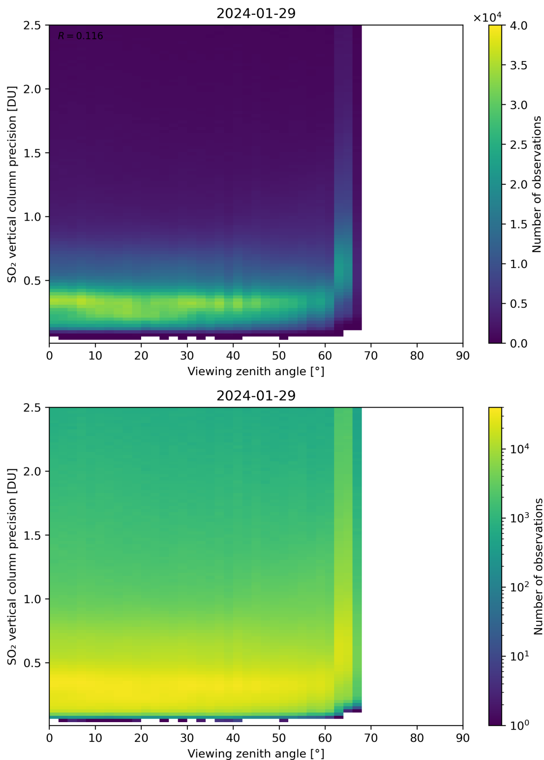
Figure 328: Scatter density plot of “Viewing zenith angle” against “SO 2 vertical column precision” for 2024-01-28 to 2024-01-30.
