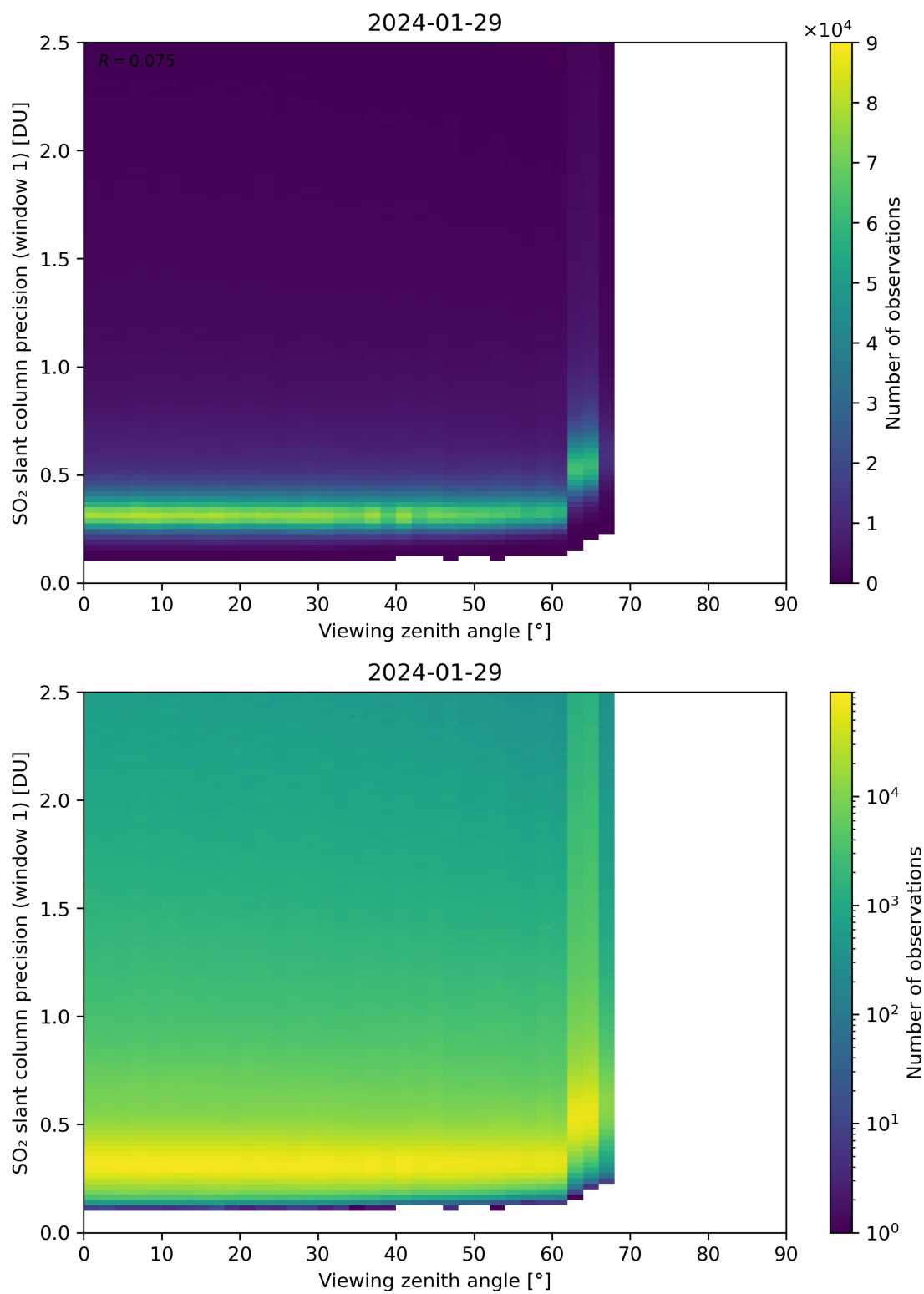
Figure 321: Scatter density plot of “Viewing zenith angle” against “SO 2 slant column precision (window 1)” for 2024-01-28 to 2024-01-30.
