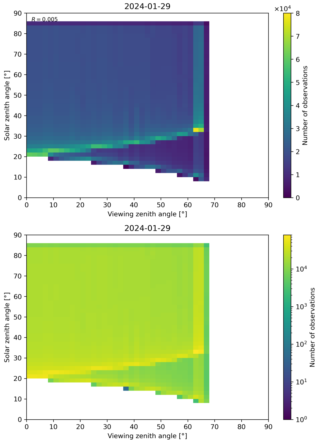
Figure 315: Scatter density plot of “Viewing zenith angle” against “Solar zenith angle” for 2024-01-28 to 2024-01-30.
