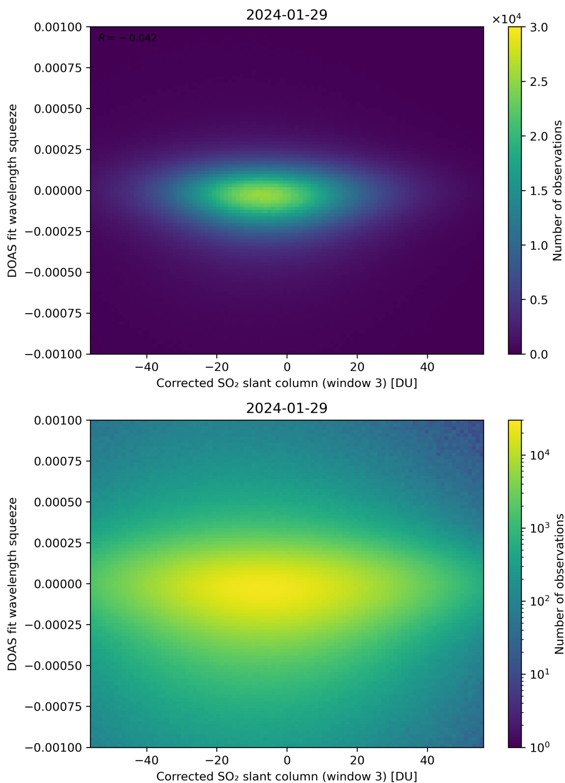
Figure 207: Scatter density plot of “Corrected SO 2 slant column (window 3)” against “DOAS fit wavelength squeeze” for 2024-01-28 to 2024-01-30.
