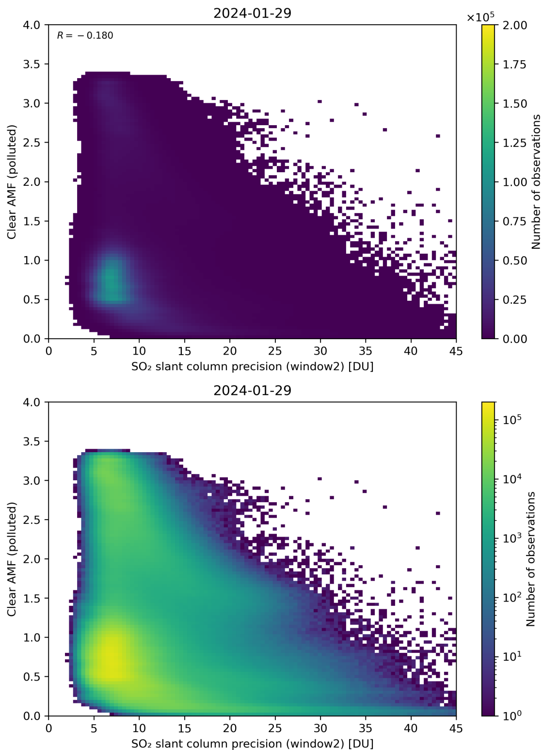
Figure 246: Scatter density plot of “SO 2 slant column precision (window2)” against “Clear AMF (polluted)” for 2024-01-28 to 2024-01-30.
