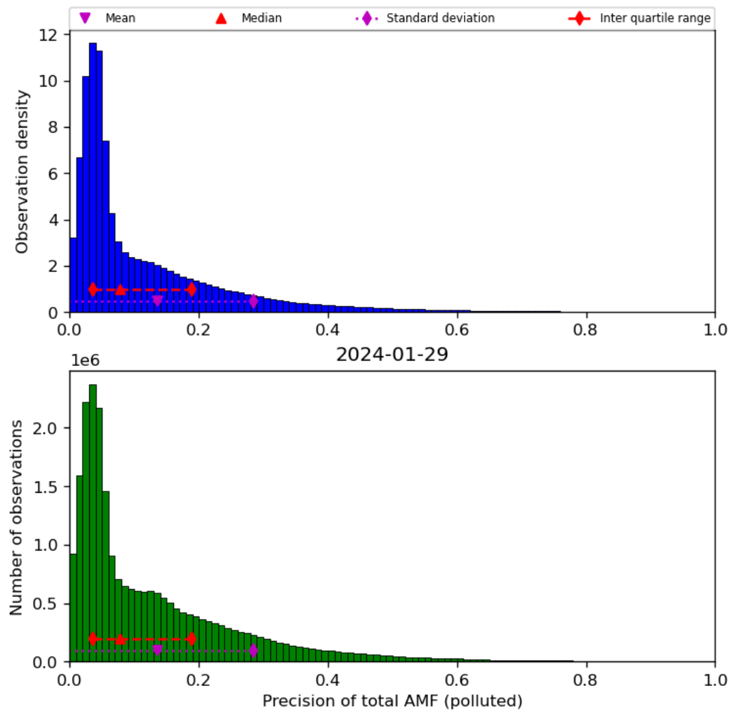
Figure 72: Histogram of “Precision of total AMF (polluted)” for 2024-01-28 to 2024-01-30
