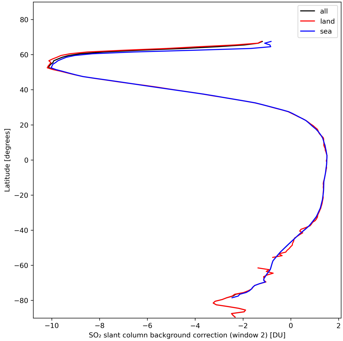
Figure 40: Zonal average of “SO 2 slant column background correction (window 2)” for 2024-01-28 to 2024-01-30.
