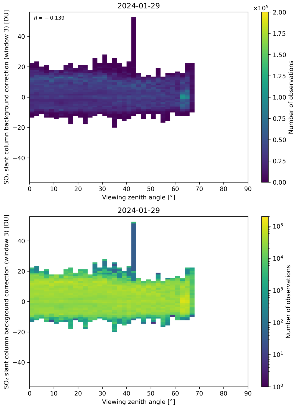
Figure 310: Scatter density plot of “Viewing zenith angle” against “SO 2 slant column background correction (window 3)” for 2024-01-28 to 2024-01-30.
