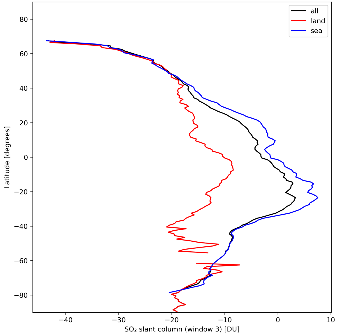
Figure 41: Zonal average of “SO 2 slant column (window 3)” for 2024-01-28 to 2024-01-30.
