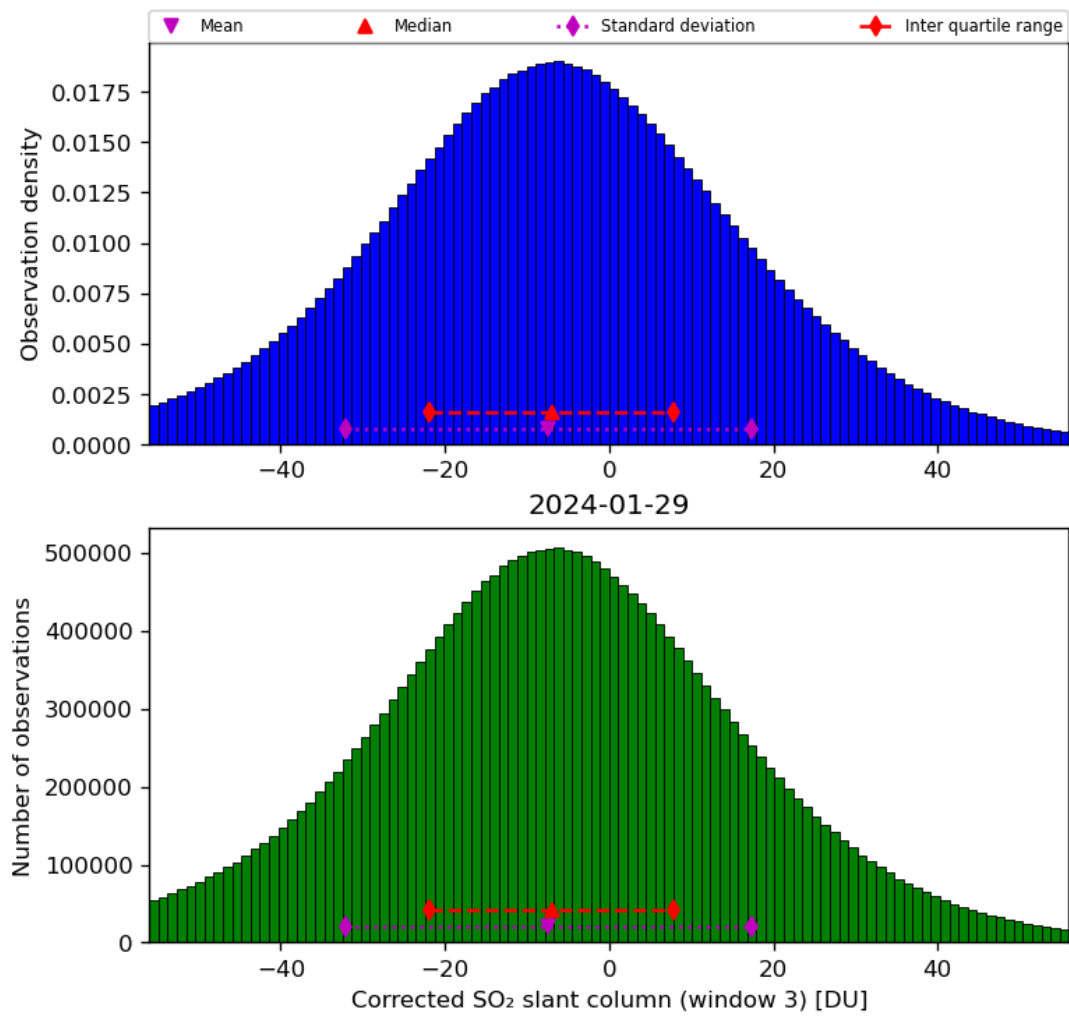
Figure 66: Histogram of “Corrected SO 2 slant column (window 3)” for 2024-01-28 to 2024-01-30
