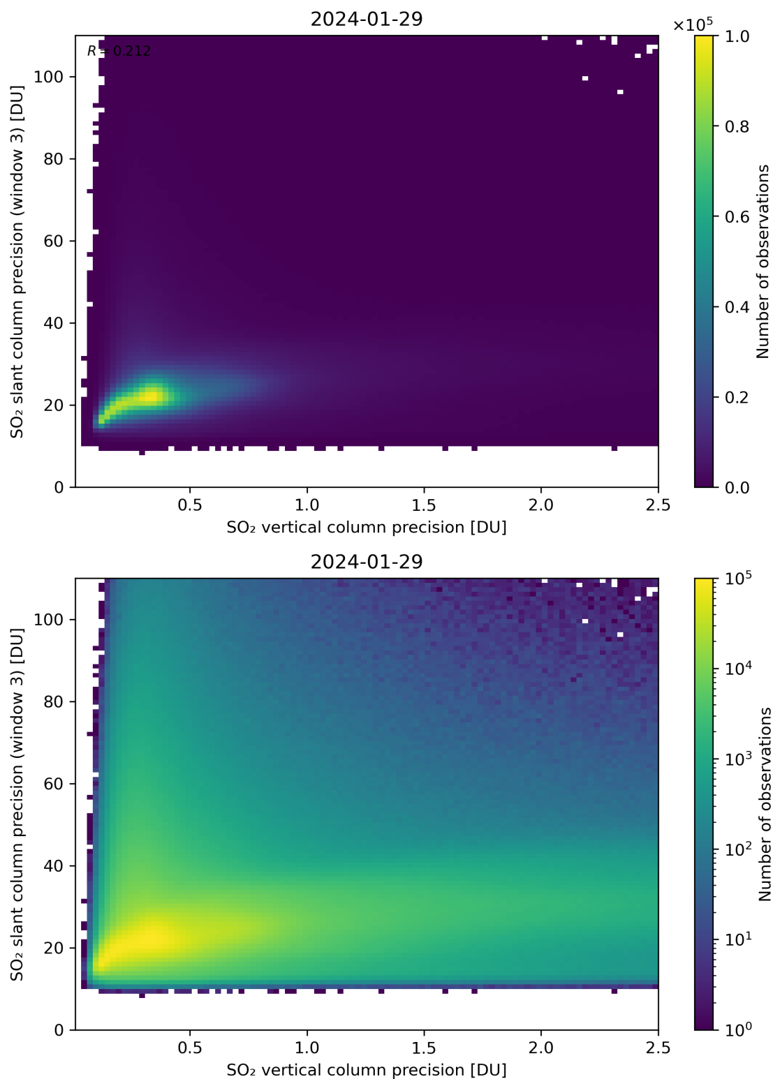
Figure 293: Scatter density plot of “SO 2 vertical column precision” against “SO 2 slant column precision (window 3)” for 2024-01-28 to 2024-01-30.
