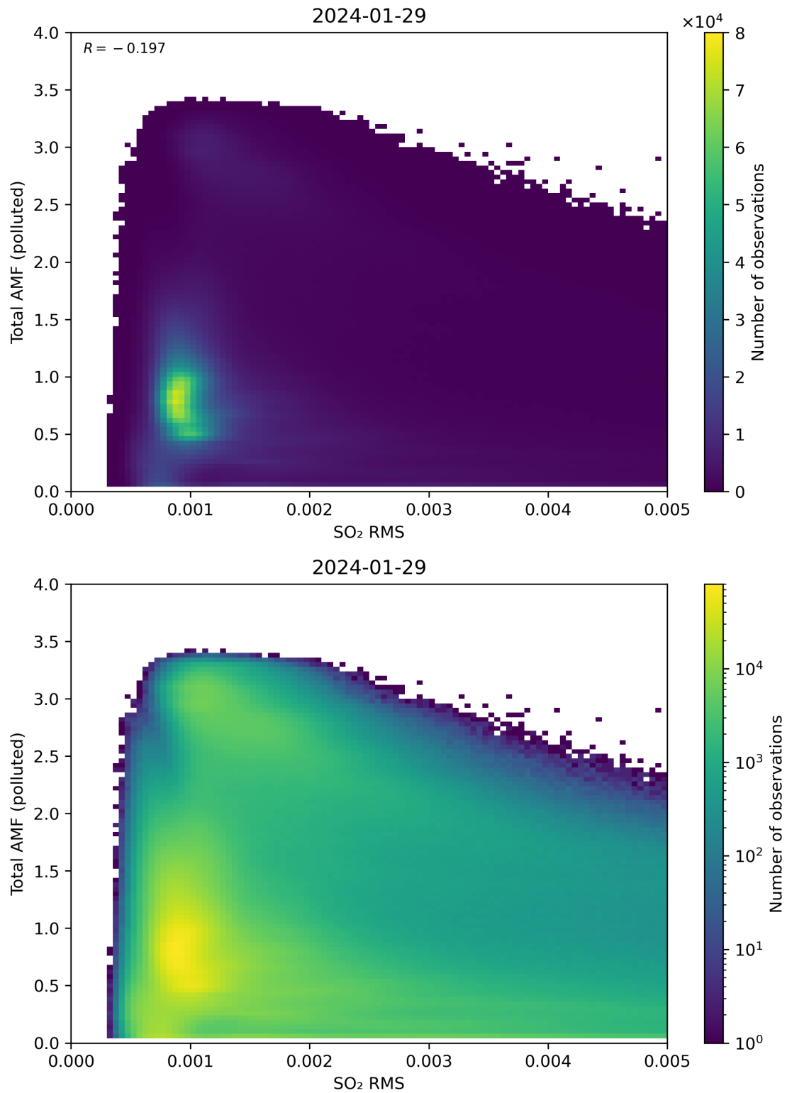
Figure 137: Scatter density plot of “SO 2 RMS” against “Total AMF (polluted)” for 2024-01-28 to 2024-01-30.
