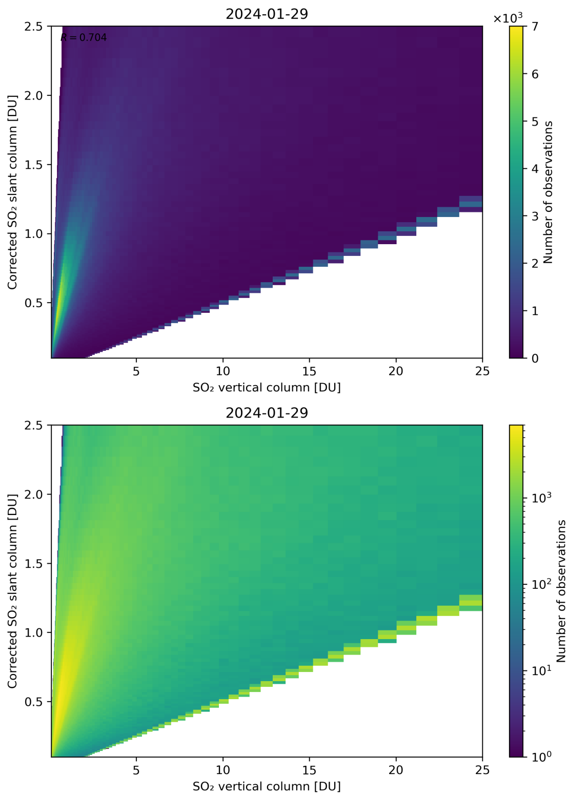
Figure 297: Scatter density plot of “SO 2 vertical column” against “Corrected SO 2 slant column” for 2024-01-28 to 2024-01-30.
