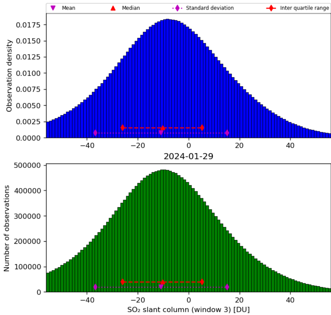
Figure 64: Histogram of “SO 2 slant column (window 3)” for 2024-01-28 to 2024-01-30
