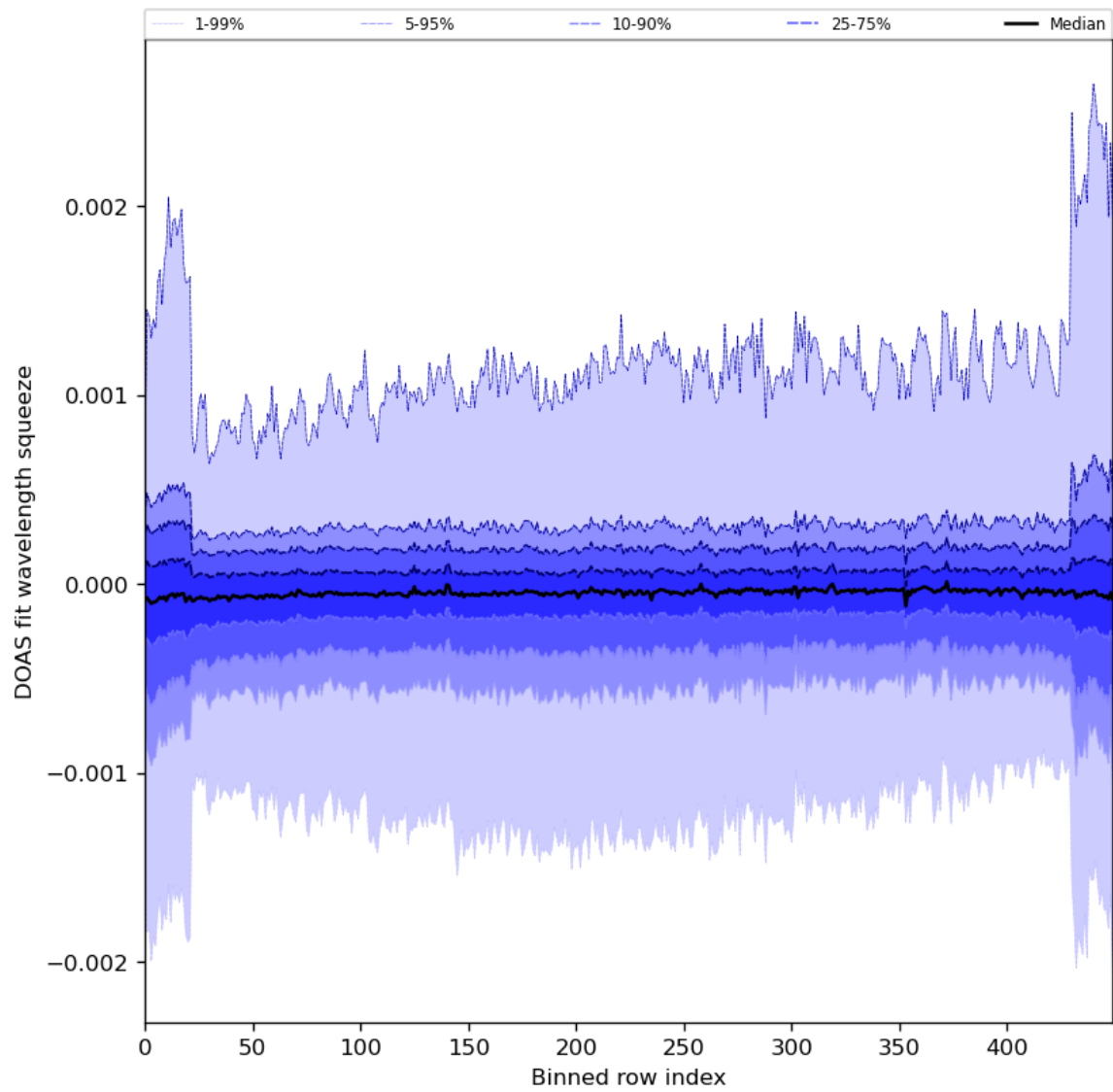
Figure 92: Along track statistics of “DOAS fit wavelength squeeze” for 2024-01-28 to 2024-01-30
