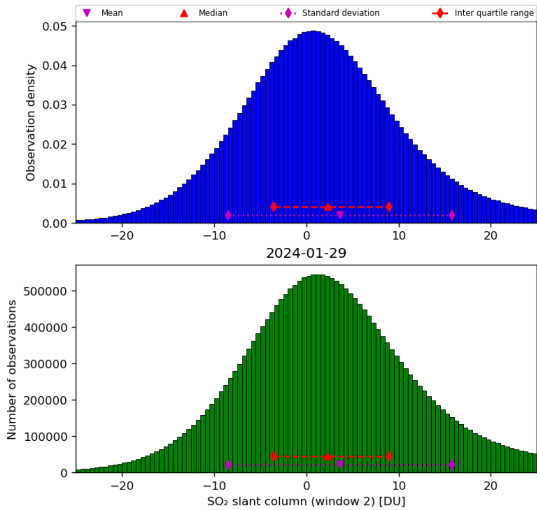
Figure 60: Histogram of “SO 2 slant column (window 2)” for 2024-01-28 to 2024-01-30
