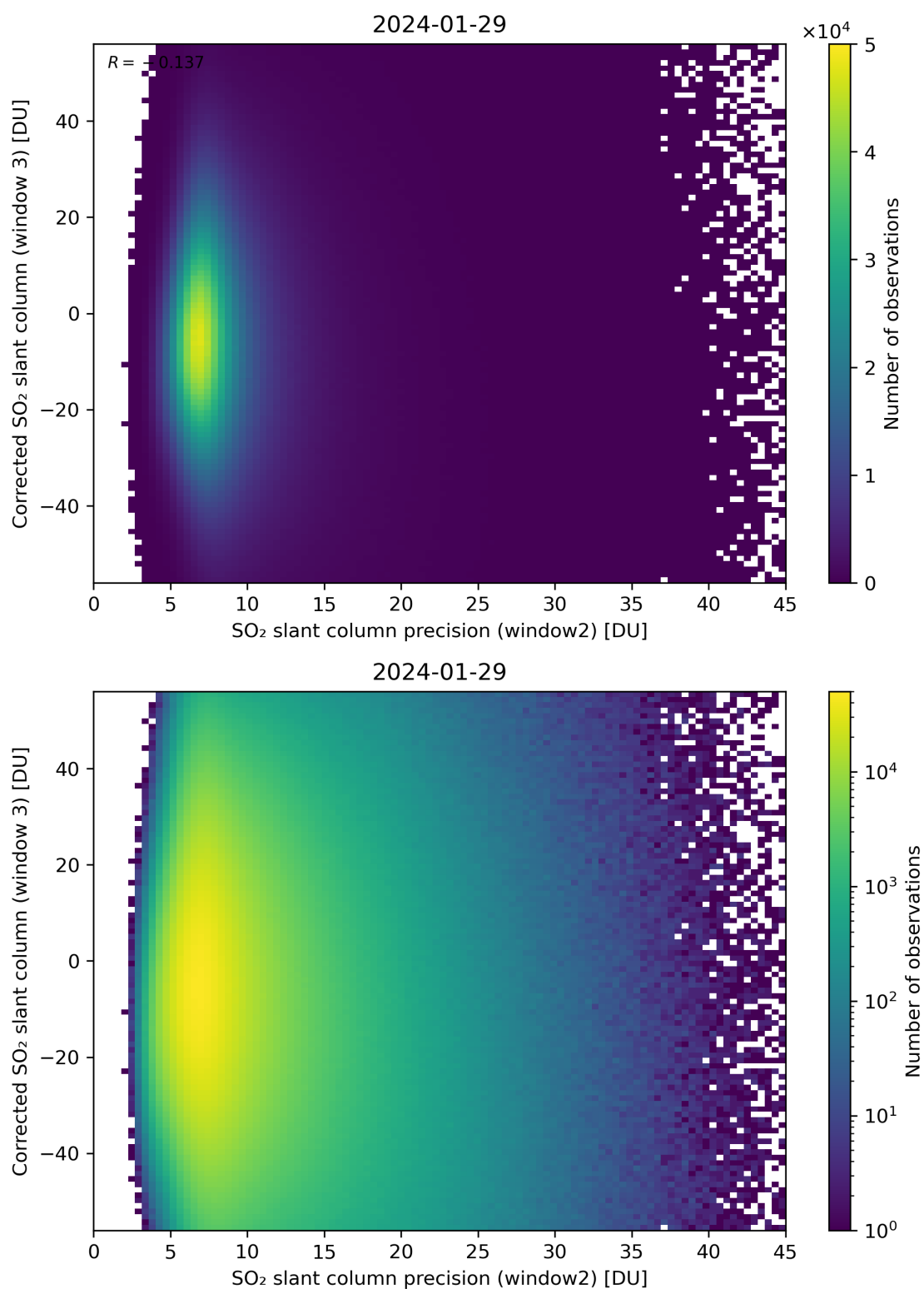
Figure 248: Scatter density plot of “SO 2 slant column precision (window2)” against “Corrected SO 2 slant column (window 3)” for 2024-01-28 to 2024-01-30.
