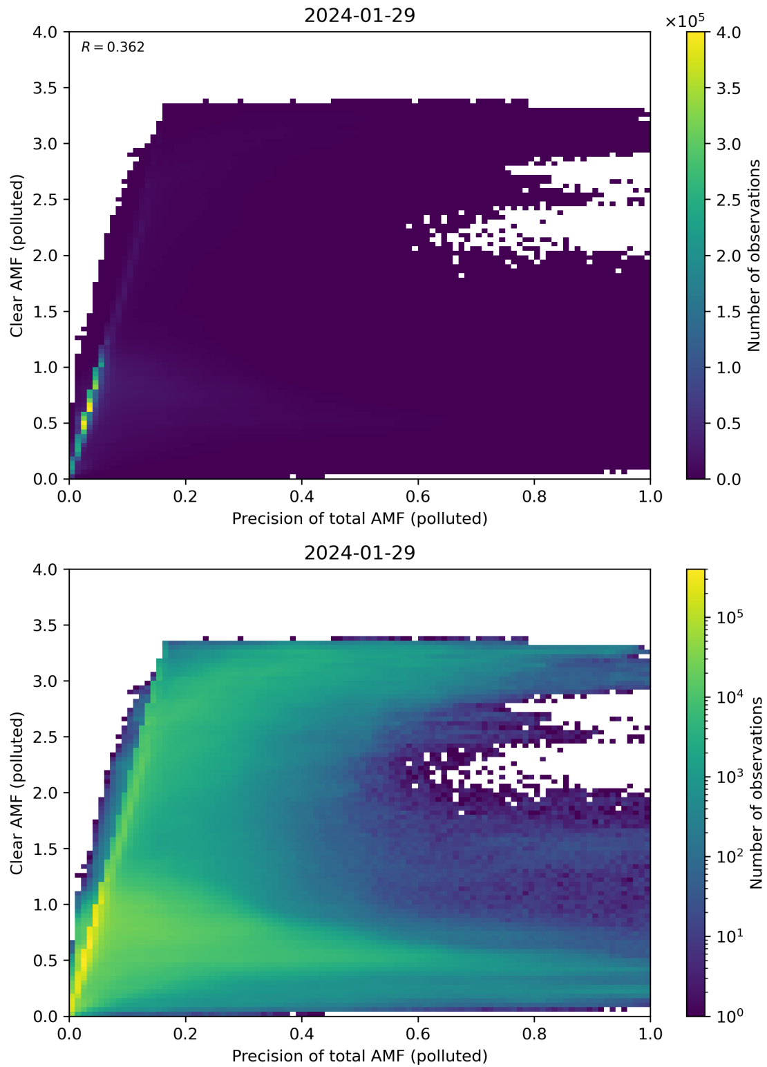
Figure 270: Scatter density plot of “Precision of total AMF (polluted)” against “Clear AMF (polluted)” for 2024-01-28 to 2024-01-30.
