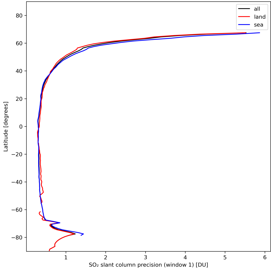
Figure 34: Zonal average of “SO 2 slant column precision (window 1)” for 2024-01-28 to 2024-01-30.
