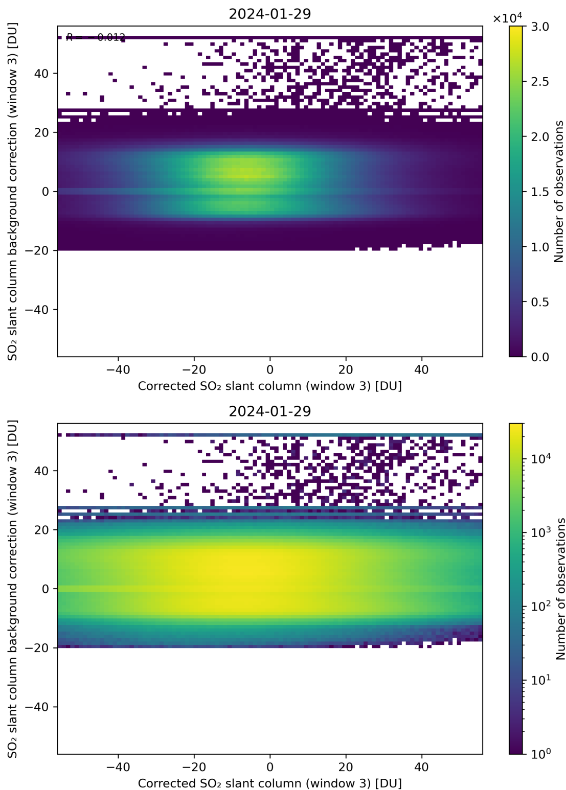
Figure 205: Scatter density plot of “Corrected SO 2 slant column (window 3)” against “SO 2 slant column background correction (window 3)” for 2024-01-28 to 2024-01-30.
