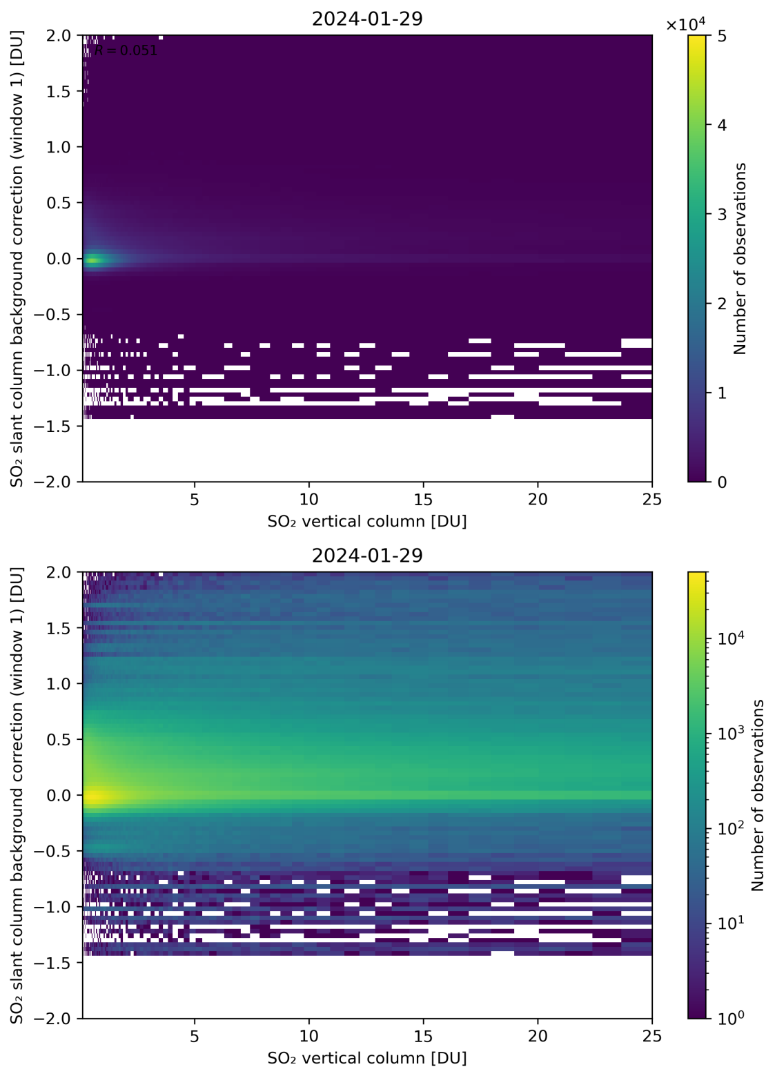
Figure 273: Scatter density plot of “SO 2 vertical column” against “SO 2 slant column background correction (window 1)” for 2024-01-28 to 2024-01-30.
