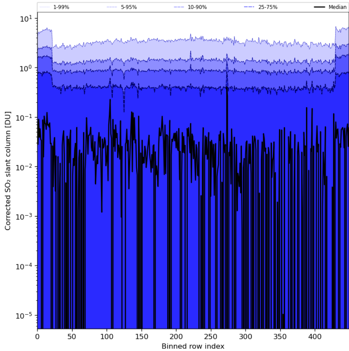
Figure 78: Along track statistics of “Corrected SO 2 slant column” for 2024-01-28 to 2024-01-30
