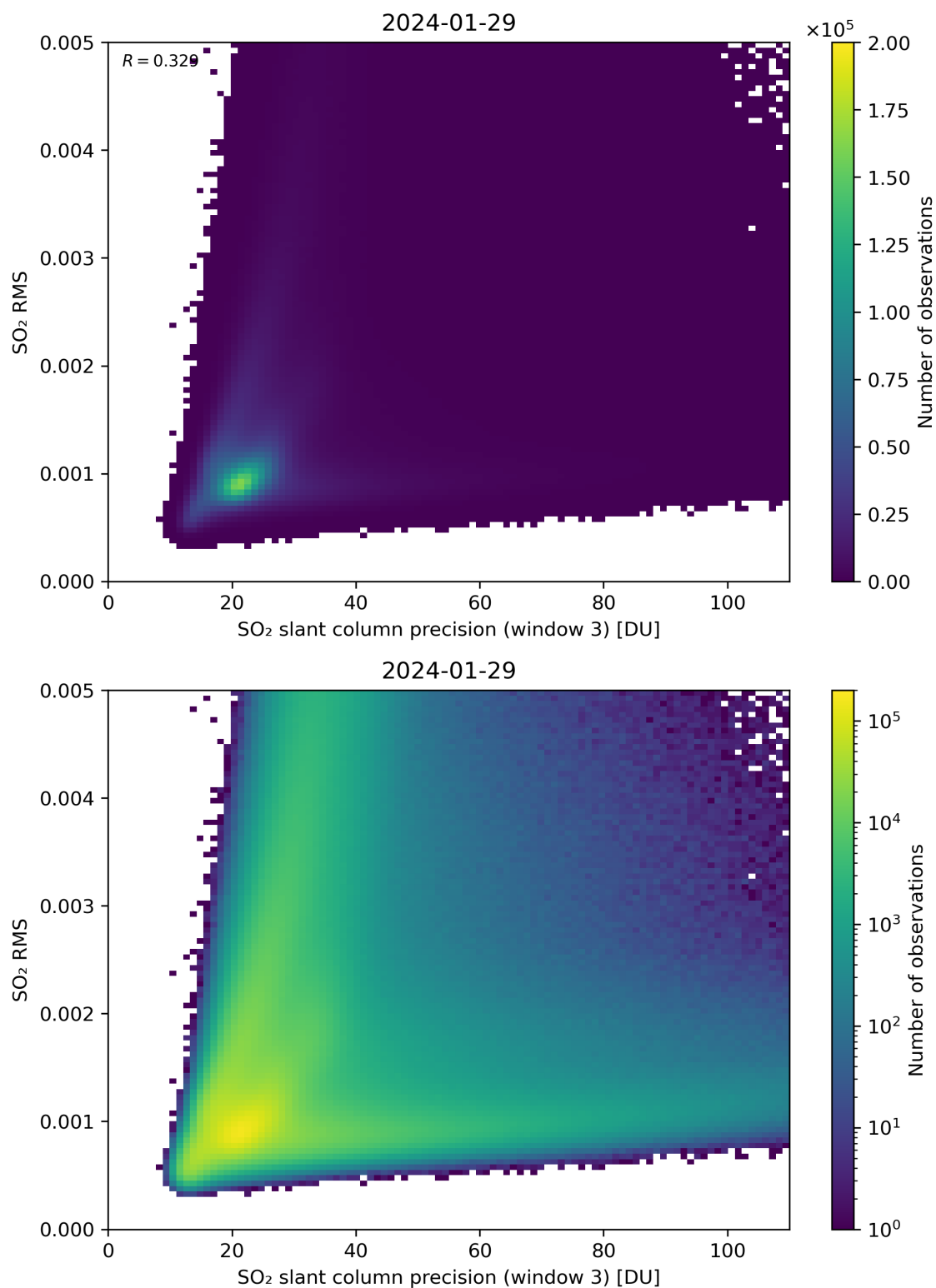
Figure 260: Scatter density plot of “SO 2 slant column precision (window 3)” against “SO 2 RMS” for 2024-01-28 to 2024-01-30.
