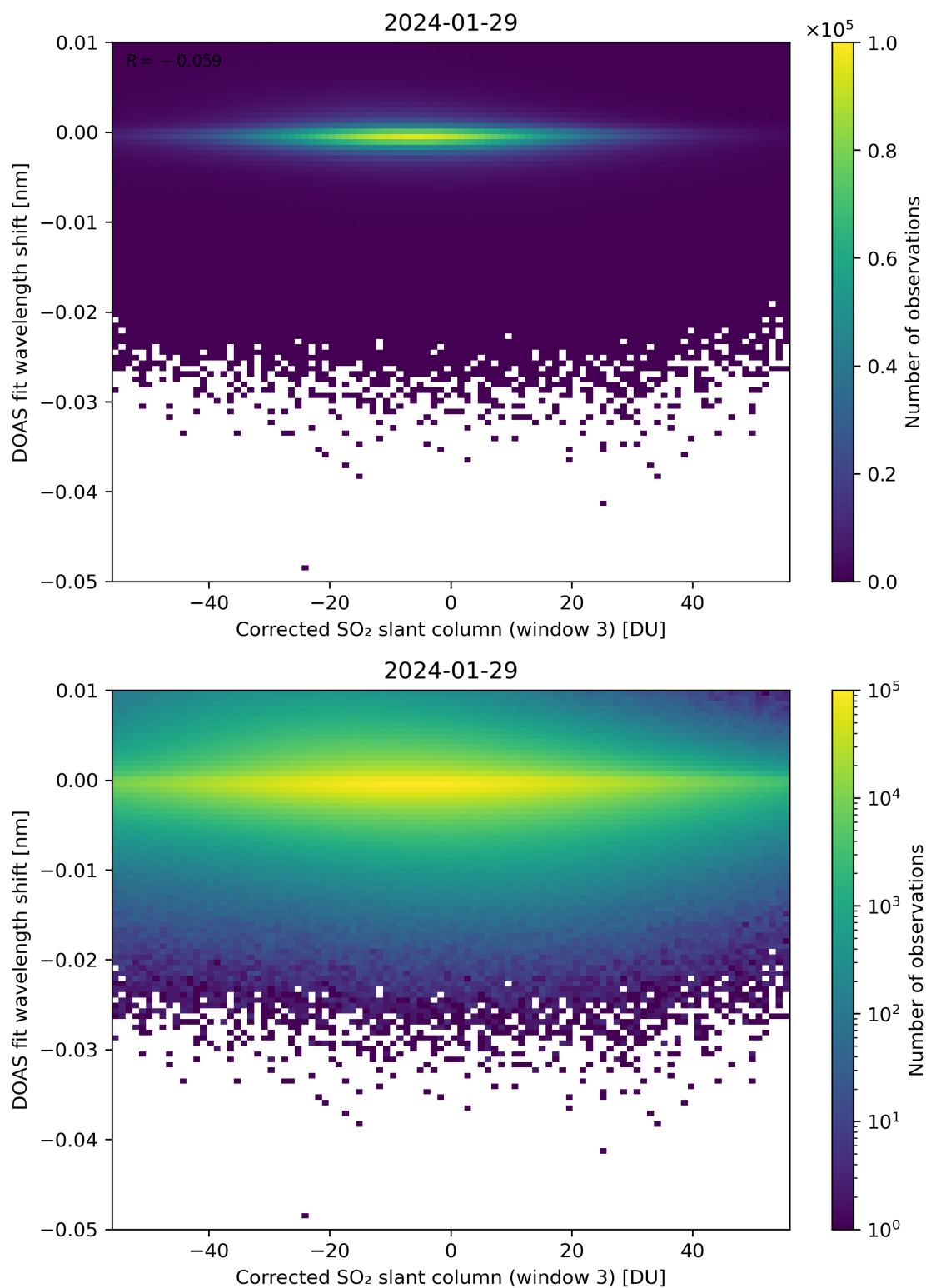
Figure 206: Scatter density plot of “Corrected SO 2 slant column (window 3)” against “DOAS fit wavelength shift” for 2024-01-28 to 2024-01-30.
