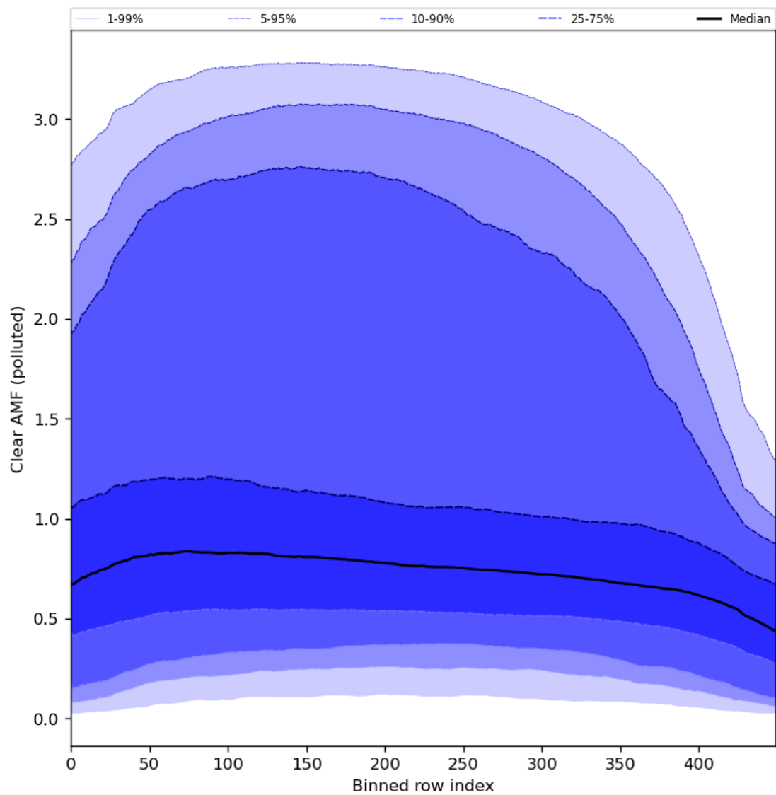
Figure 96: Along track statistics of “Clear AMF (polluted)” for 2024-01-28 to 2024-01-30
