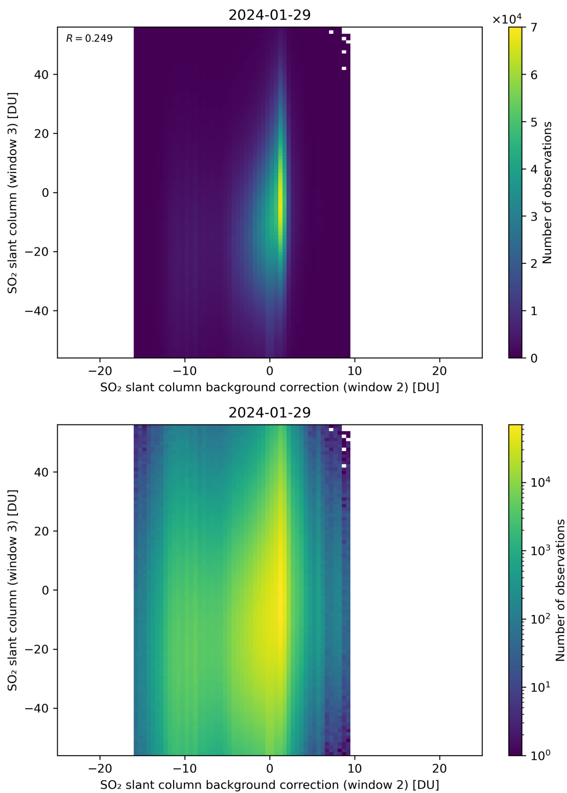
Figure 117: Scatter density plot of “SO 2 slant column background correction (window 2)” against “SO 2 slant column (window 3)” for 2024-01-28 to 2024-01-30.
