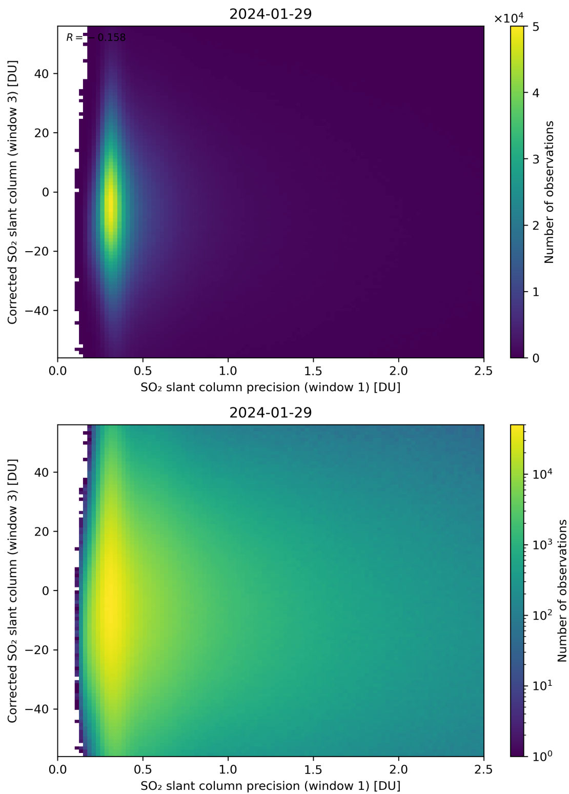
Figure 226: Scatter density plot of “SO 2 slant column precision (window 1)” against “Corrected SO 2 slant column (window 3)” for 2024-01-28 to 2024-01-30.
