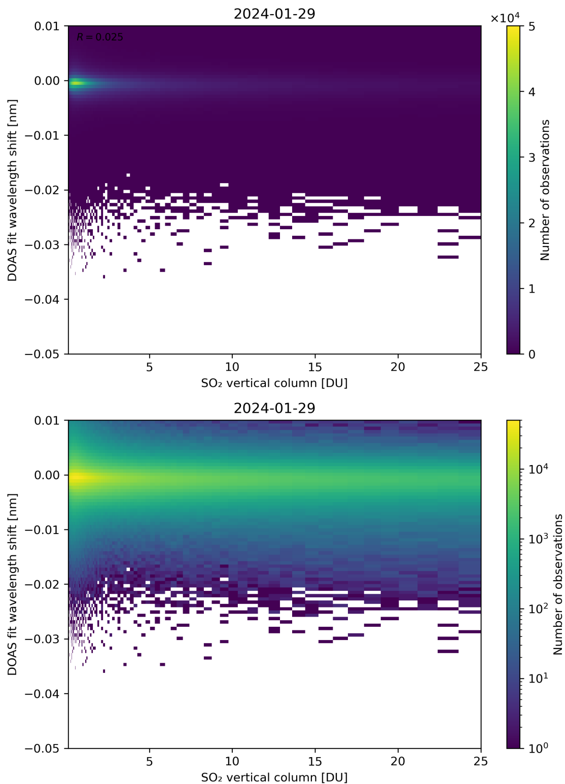
Figure 276: Scatter density plot of “SO 2 vertical column” against “DOAS fit wavelength shift” for 2024-01-28 to 2024-01-30.
