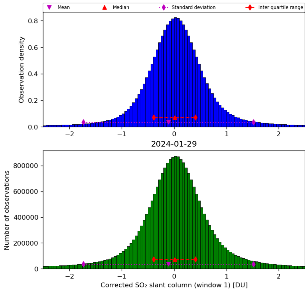
Figure 58: Histogram of “Corrected SO 2 slant column (window 1)” for 2024-01-28 to 2024-01-30
