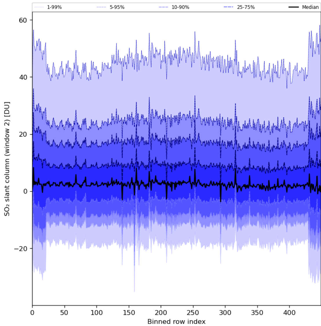
Figure 83: Along track statistics of “SO 2 slant column (window 2)” for 2024-01-28 to 2024-01-30
