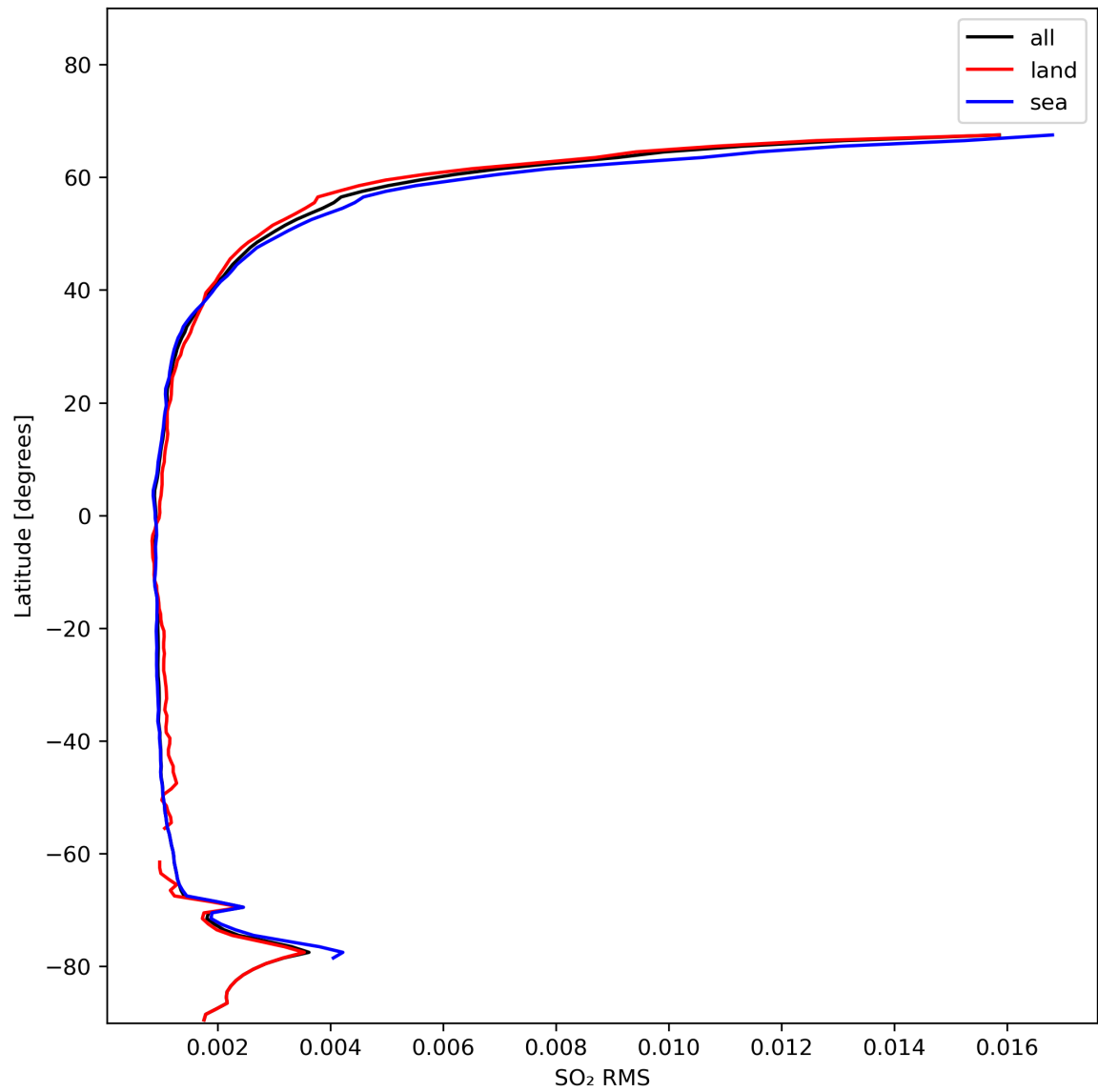
Figure 47: Zonal average of “SO 2 RMS” for 2024-01-28 to 2024-01-30.
