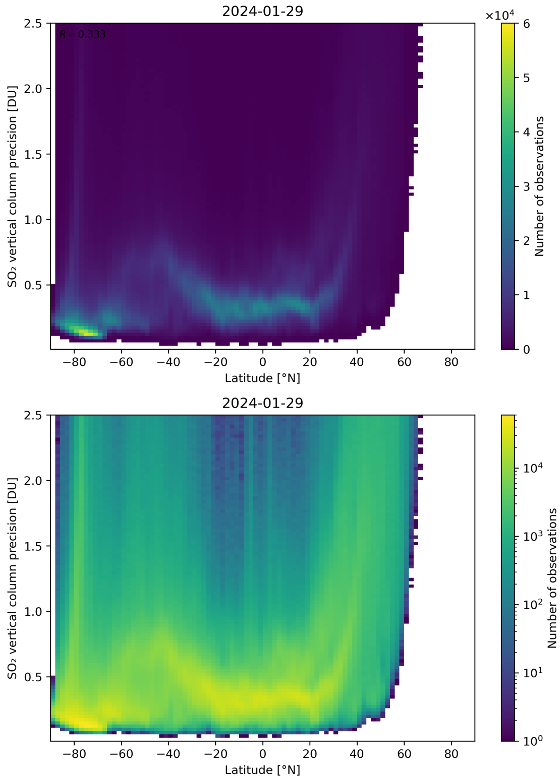
Figure 157: Scatter density plot of “Latitude” against “SO 2 vertical column precision” for 2024-01-28 to 2024-01-30.
