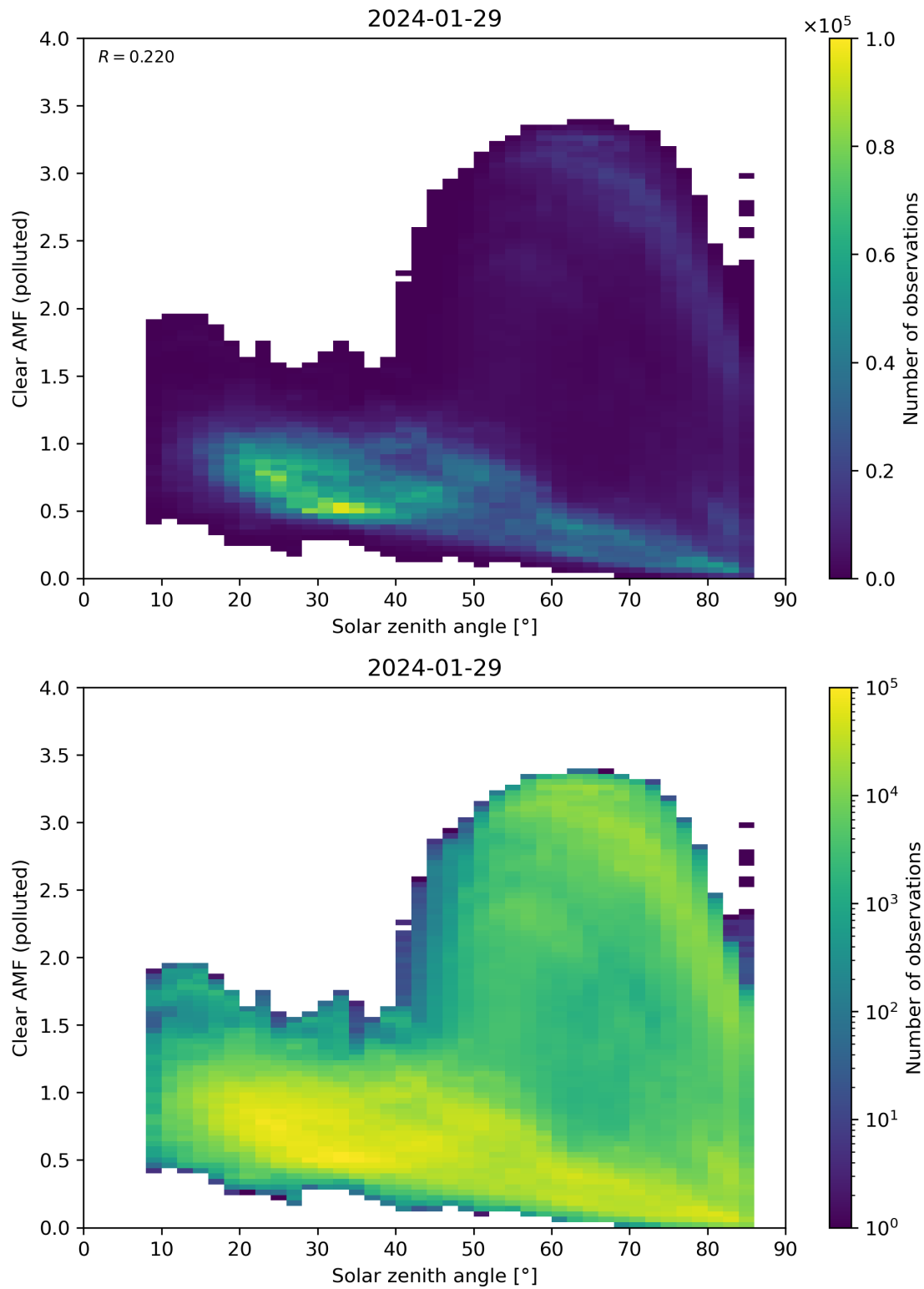
Figure 165: Scatter density plot of “Solar zenith angle” against “Clear AMF (polluted)” for 2024-01-28 to 2024-01-30.
