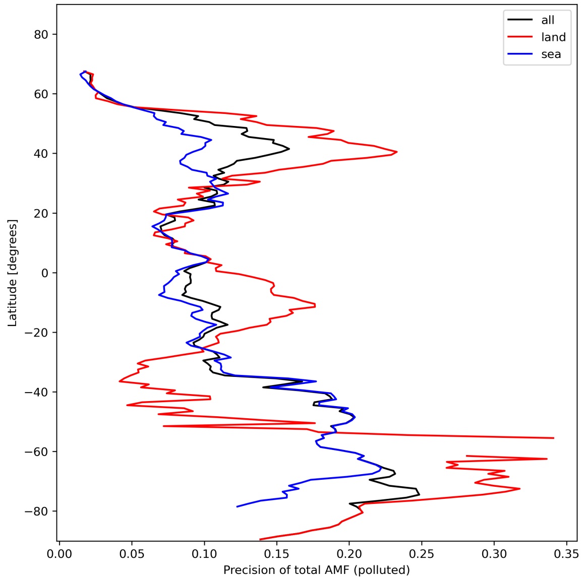
Figure 49: Zonal average of “Precision of total AMF (polluted)” for 2024-01-28 to 2024-01-30.
