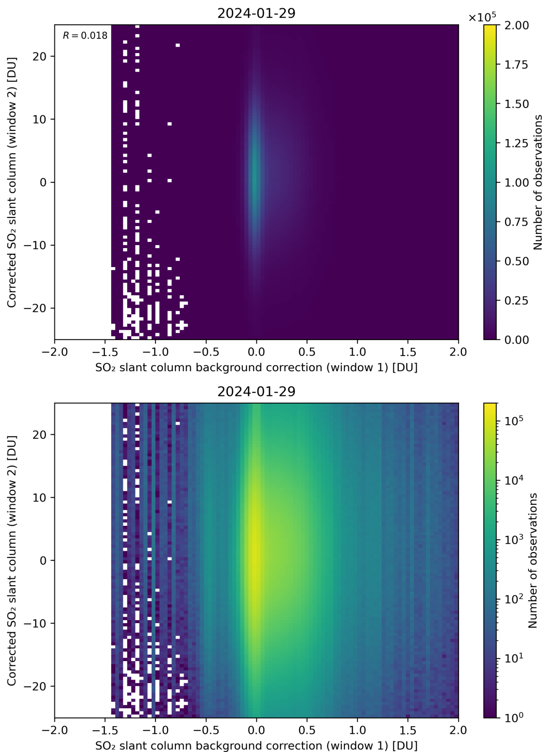
Figure 104: Scatter density plot of “SO 2 slant column background correction (window 1)” against “Corrected SO 2 slant column (window 2)” for 2024-01-28 to 2024-01-30.
