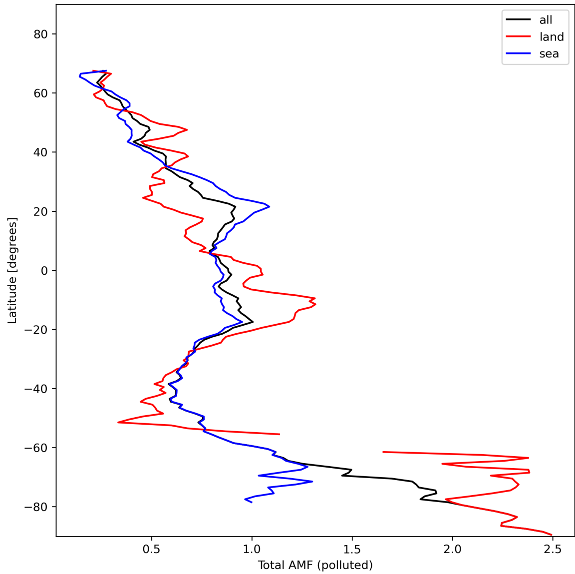
Figure 48: Zonal average of “Total AMF (polluted)” for 2024-01-28 to 2024-01-30.
