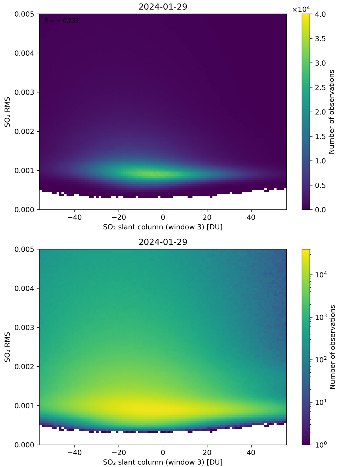
Figure 256: Scatter density plot of “SO 2 slant column (window 3)” against “SO 2 RMS” for 2024-01-28 to 2024-01-30.
