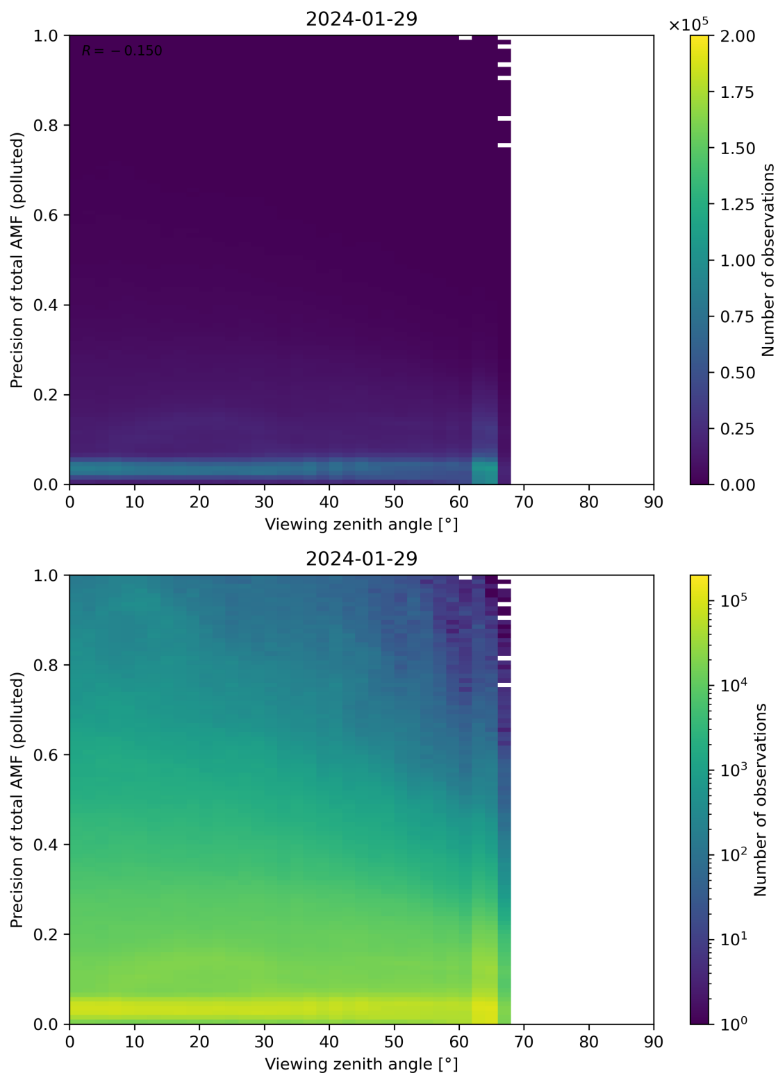
Figure 326: Scatter density plot of “Viewing zenith angle” against “Precision of total AMF (polluted)” for 2024-01-28 to 2024-01-30.
