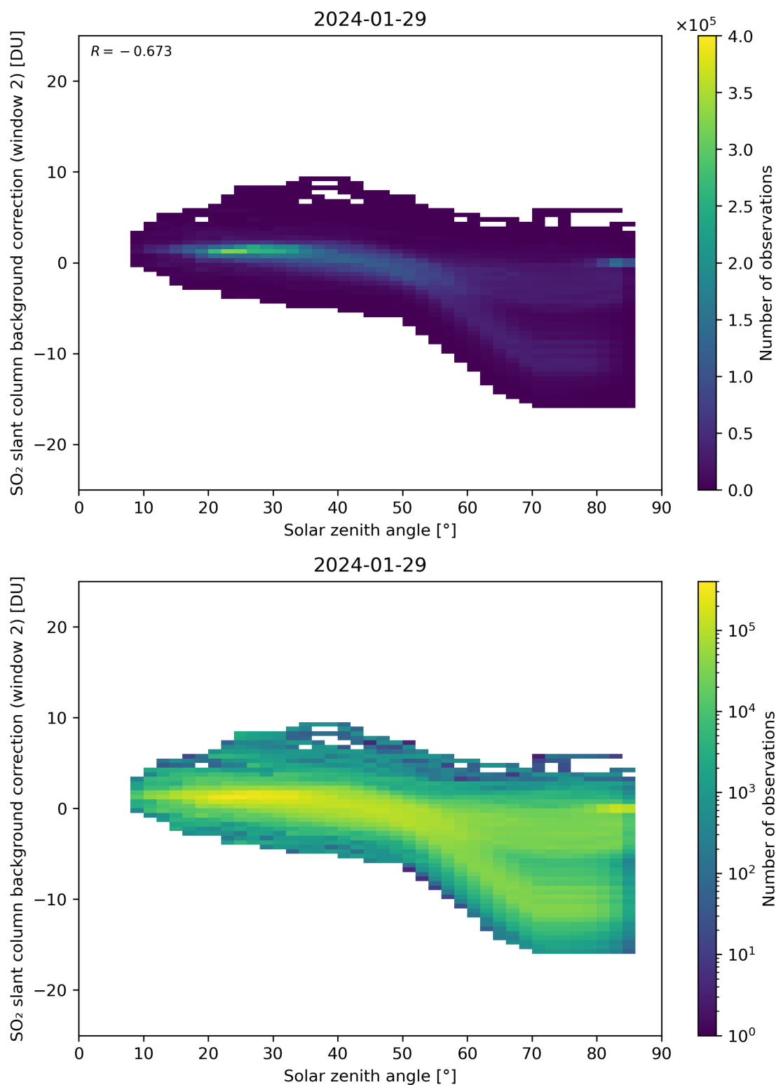
Figure 159: Scatter density plot of “Solar zenith angle” against “SO 2 slant column background correction (window 2)” for 2024-01-28 to 2024-01-30.
