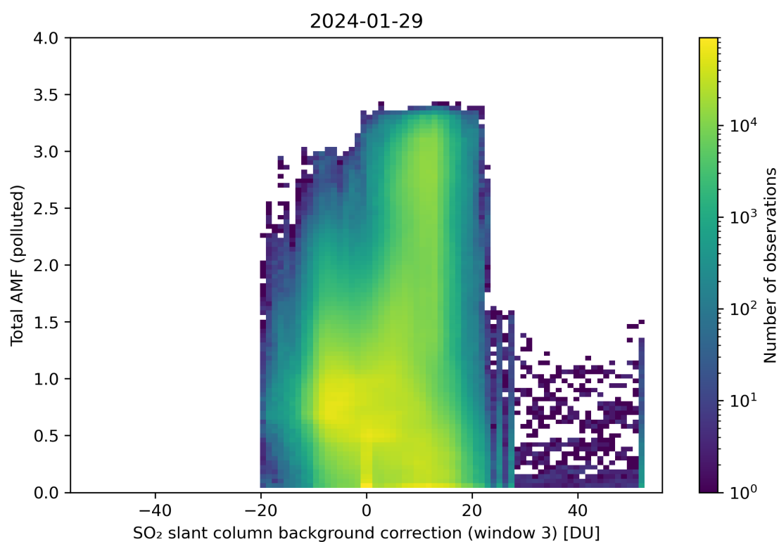
Figure 125: Scatter density plot of “SO 2 slant column background correction (window 3)” against “Total AMF (polluted)” for 2024-01-28 to 2024-01-30.
