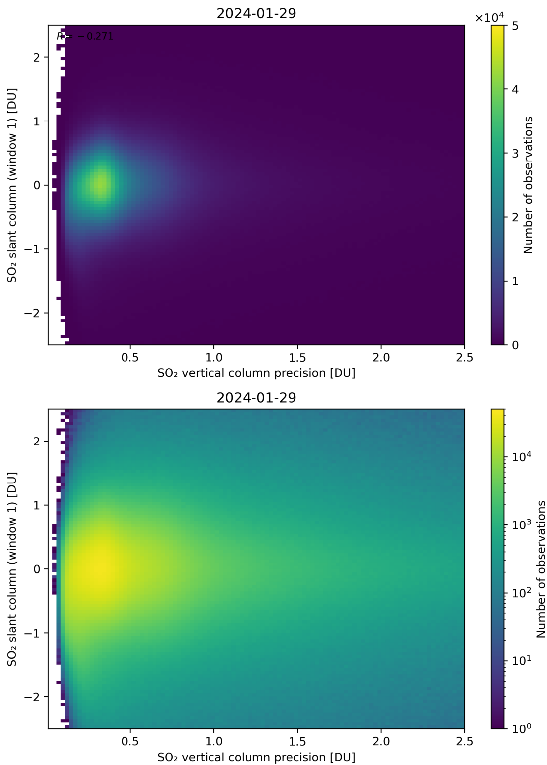
Figure 289: Scatter density plot of “SO 2 vertical column precision” against “SO 2 slant column (window 1)” for 2024-01-28 to 2024-01-30.
