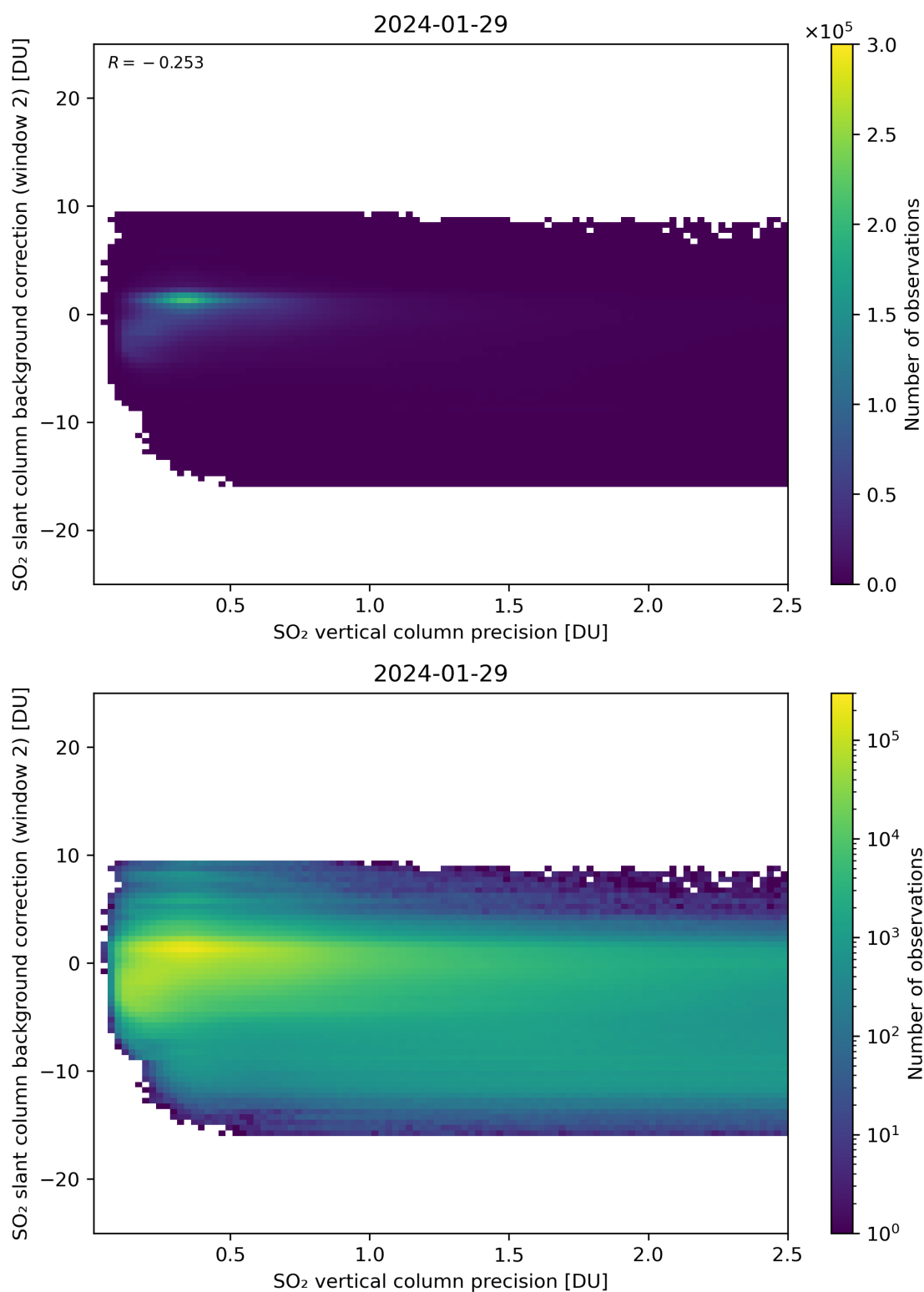
Figure 280: Scatter density plot of “SO 2 vertical column precision” against “SO 2 slant column background correction (window 2)” for 2024-01-28 to 2024-01-30.
