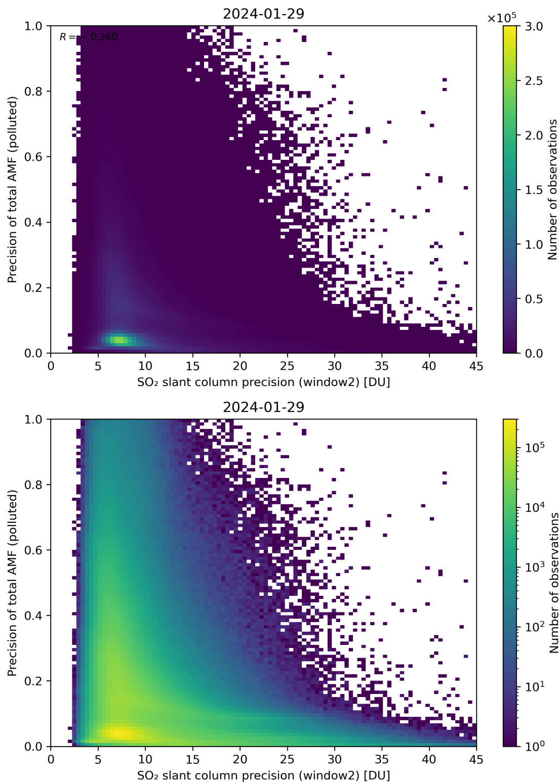
Figure 252: Scatter density plot of “SO 2 slant column precision (window2)” against “Precision of total AMF (polluted)” for 2024-01-28 to 2024-01-30.
