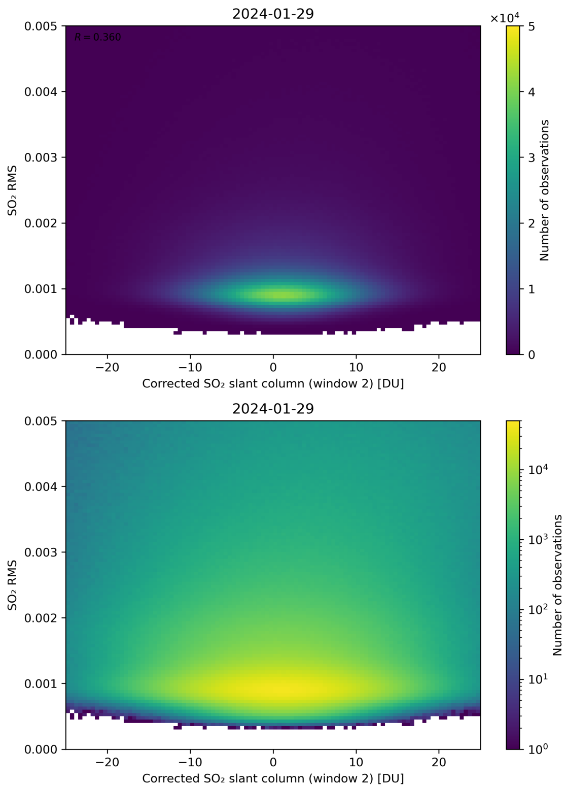
Figure 198: Scatter density plot of “Corrected SO 2 slant column (window 2)” against “SO 2 RMS” for 2024-01-28 to 2024-01-30.
