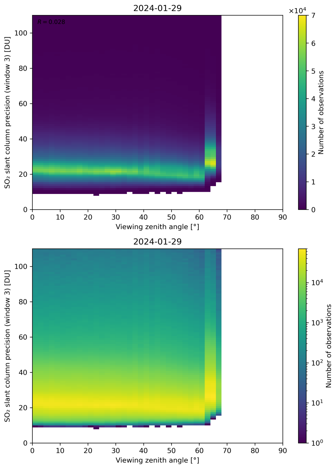
Figure 324: Scatter density plot of “Viewing zenith angle” against “SO 2 slant column precision (window 3)” for 2024-01-28 to 2024-01-30.
