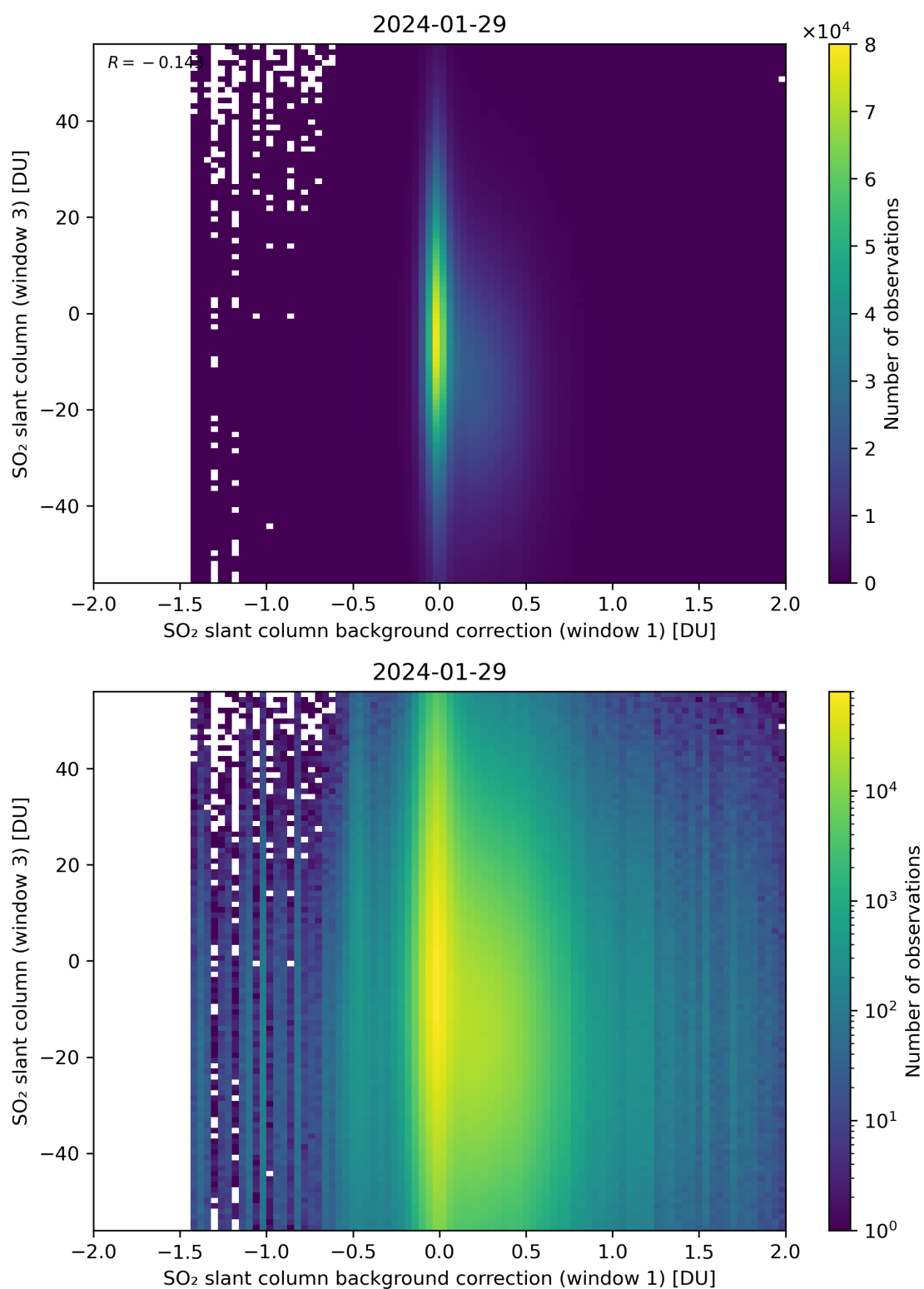
Figure 107: Scatter density plot of “SO 2 slant column background correction (window 1)” against “SO 2 slant column (window 3)” for 2024-01-28 to 2024-01-30.
