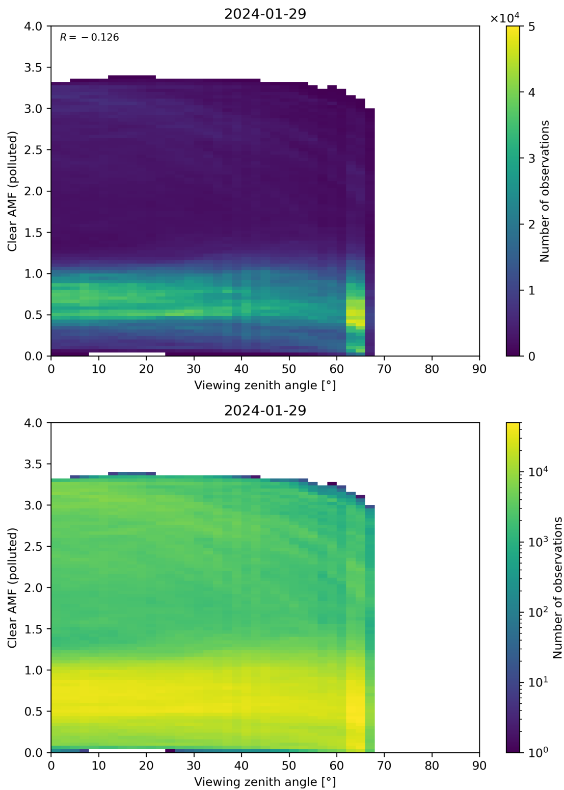
Figure 316: Scatter density plot of “Viewing zenith angle” against “Clear AMF (polluted)” for 2024-01-28 to 2024-01-30.
