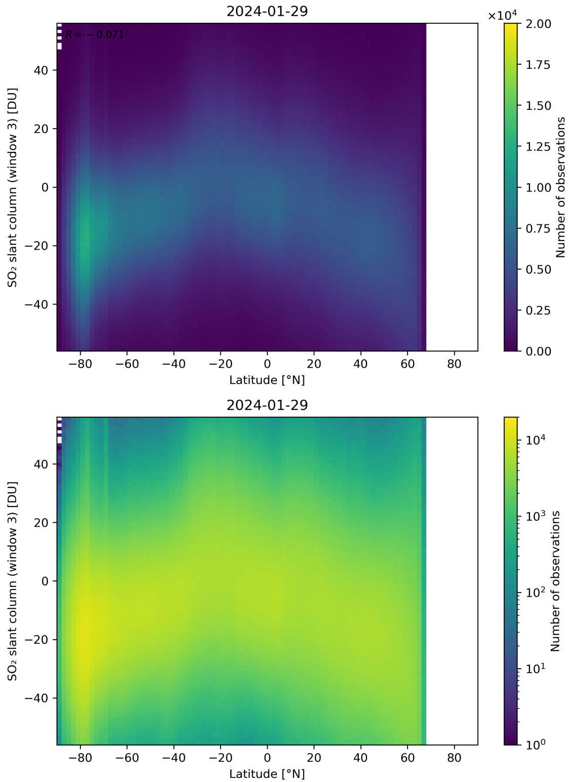
Figure 152: Scatter density plot of “Latitude” against “SO 2 slant column (window 3)” for 2024-01-28 to 2024-01-30.
