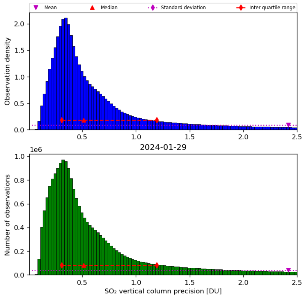
Figure 54: Histogram of “SO 2 vertical column precision” for 2024-01-28 to 2024-01-30
