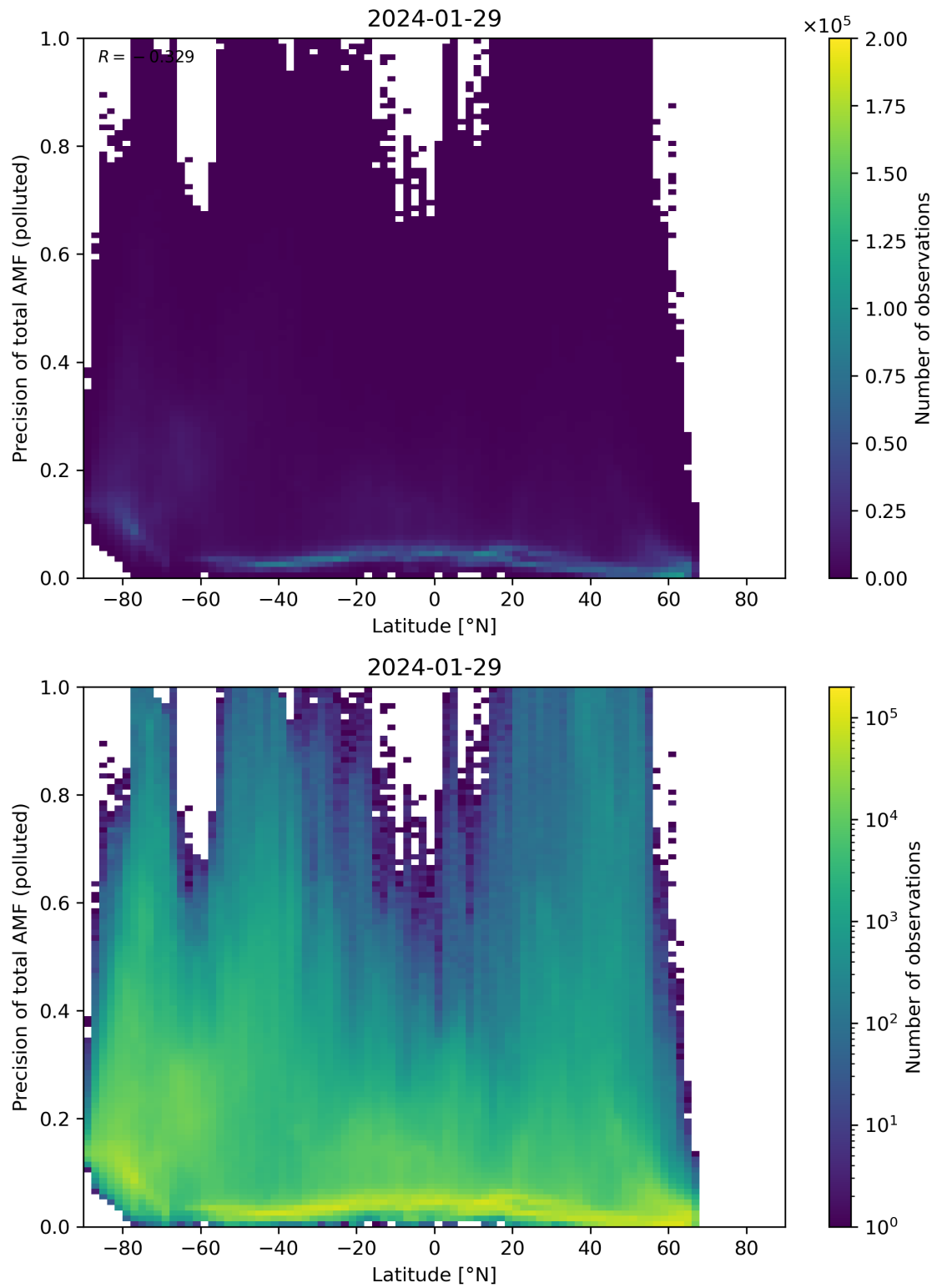
Figure 155: Scatter density plot of “Latitude” against “Precision of total AMF (polluted)” for 2024-01-28 to 2024-01-30.
