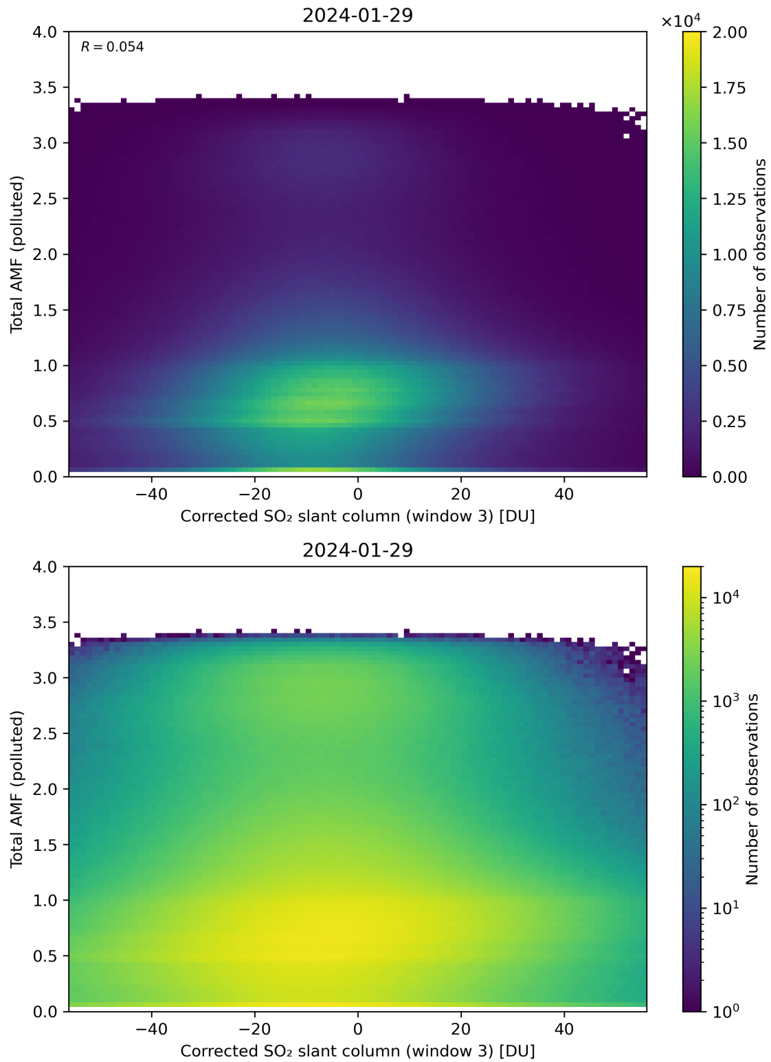
Figure 210: Scatter density plot of “Corrected SO 2 slant column (window 3)” against “Total AMF (polluted)” for 2024-01-28 to 2024-01-30.
