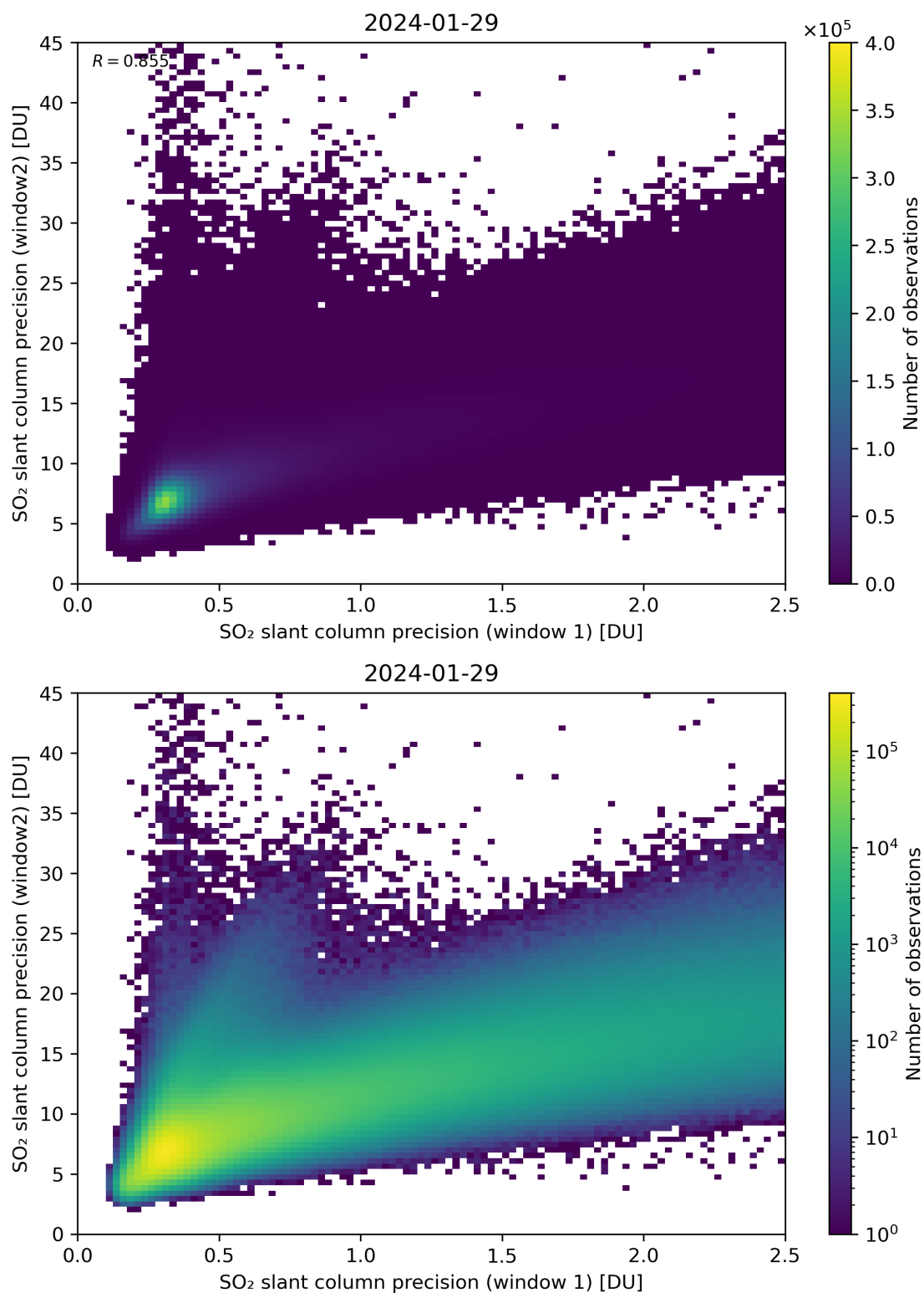
Figure 227: Scatter density plot of “SO 2 slant column precision (window 1)” against “SO 2 slant column precision (window2)” for 2024-01-28 to 2024-01-30.
