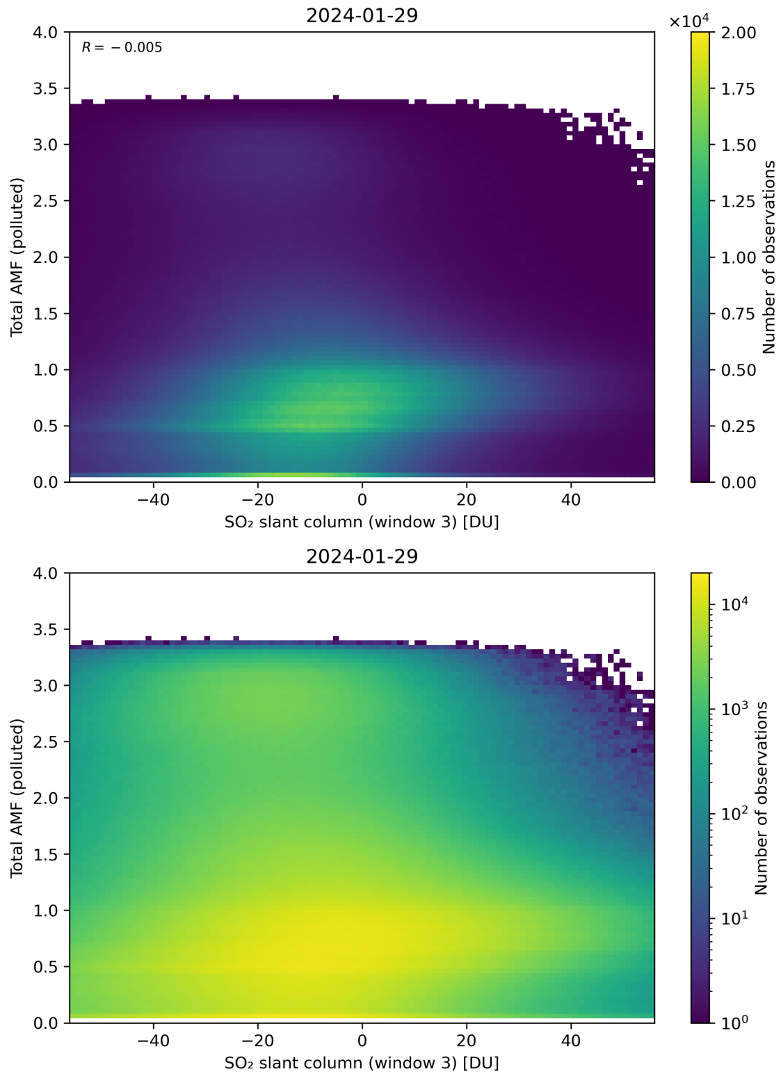
Figure 268: Scatter density plot of “SO 2 slant column (window 3)” against “Total AMF (polluted)” for 2024-01-28 to 2024-01-30.
