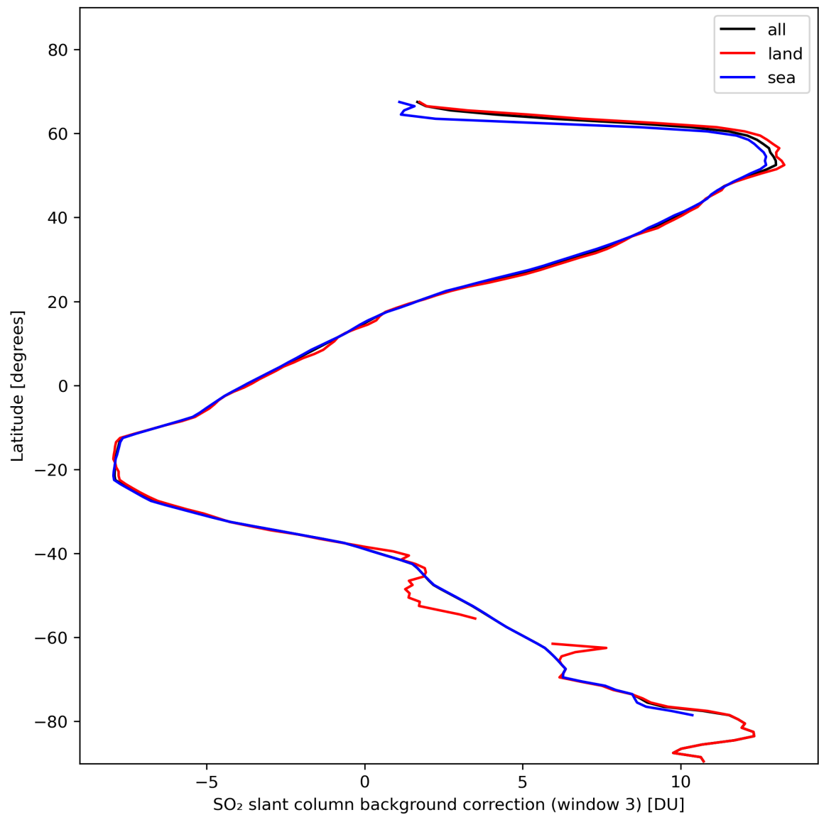
Figure 44: Zonal average of “SO 2 slant column background correction (window 3)” for 2024-01-28 to 2024-01-30.
