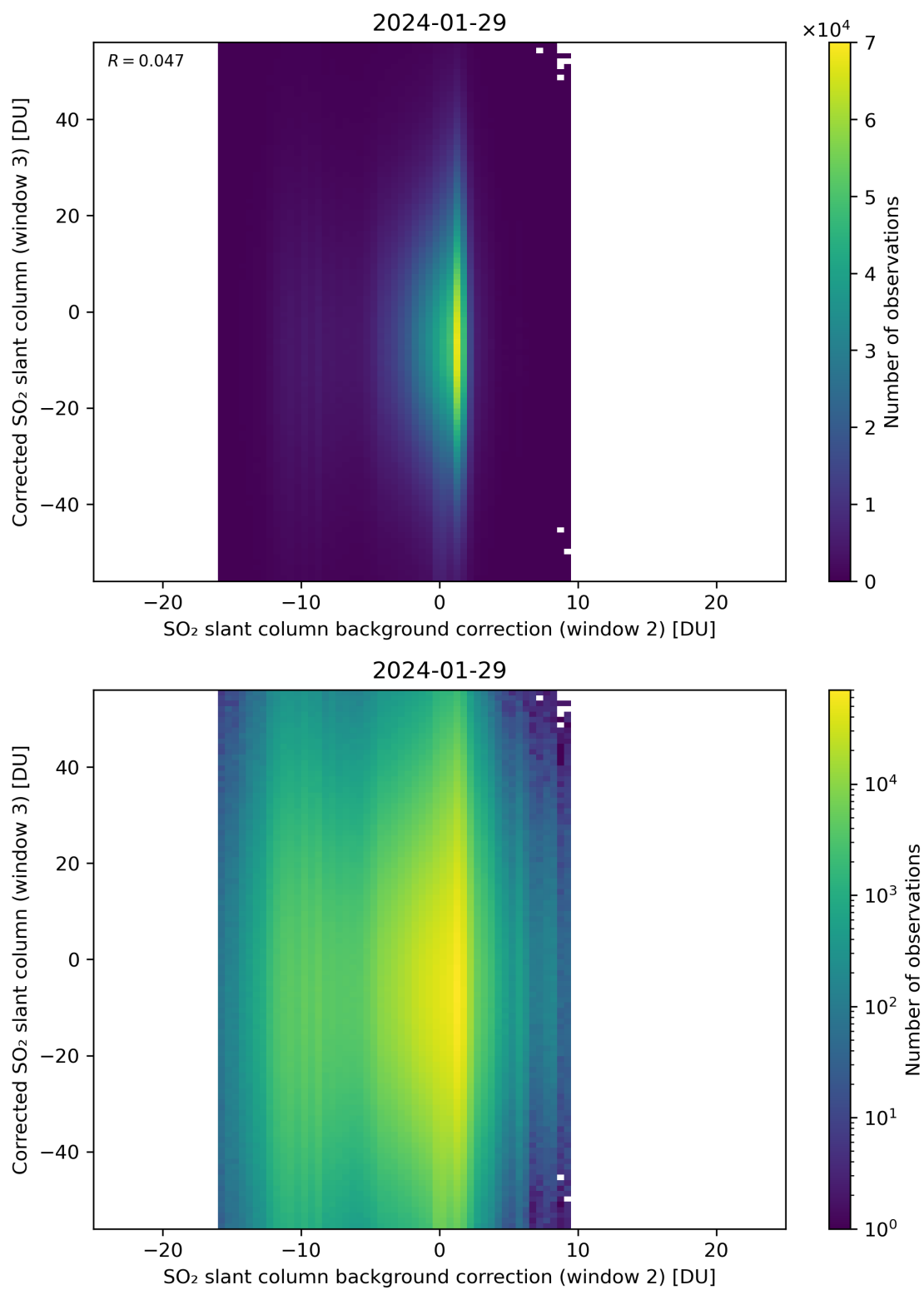
Figure 116: Scatter density plot of “SO 2 slant column background correction (window 2)” against “Corrected SO 2 slant column (window 3)” for 2024-01-28 to 2024-01-30.
