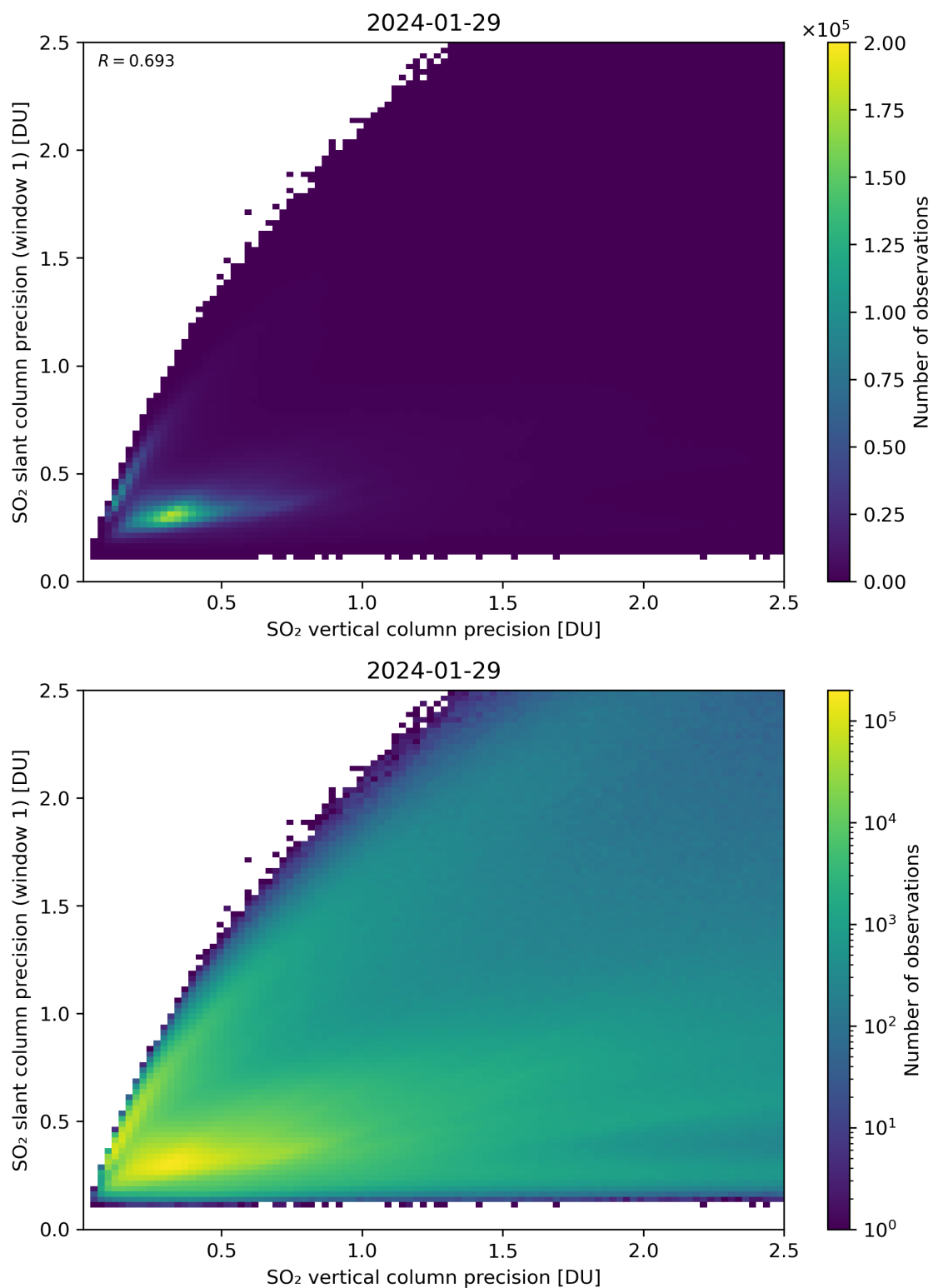
Figure 290: Scatter density plot of “SO 2 vertical column precision” against “SO 2 slant column precision (window 1)” for 2024-01-28 to 2024-01-30.
