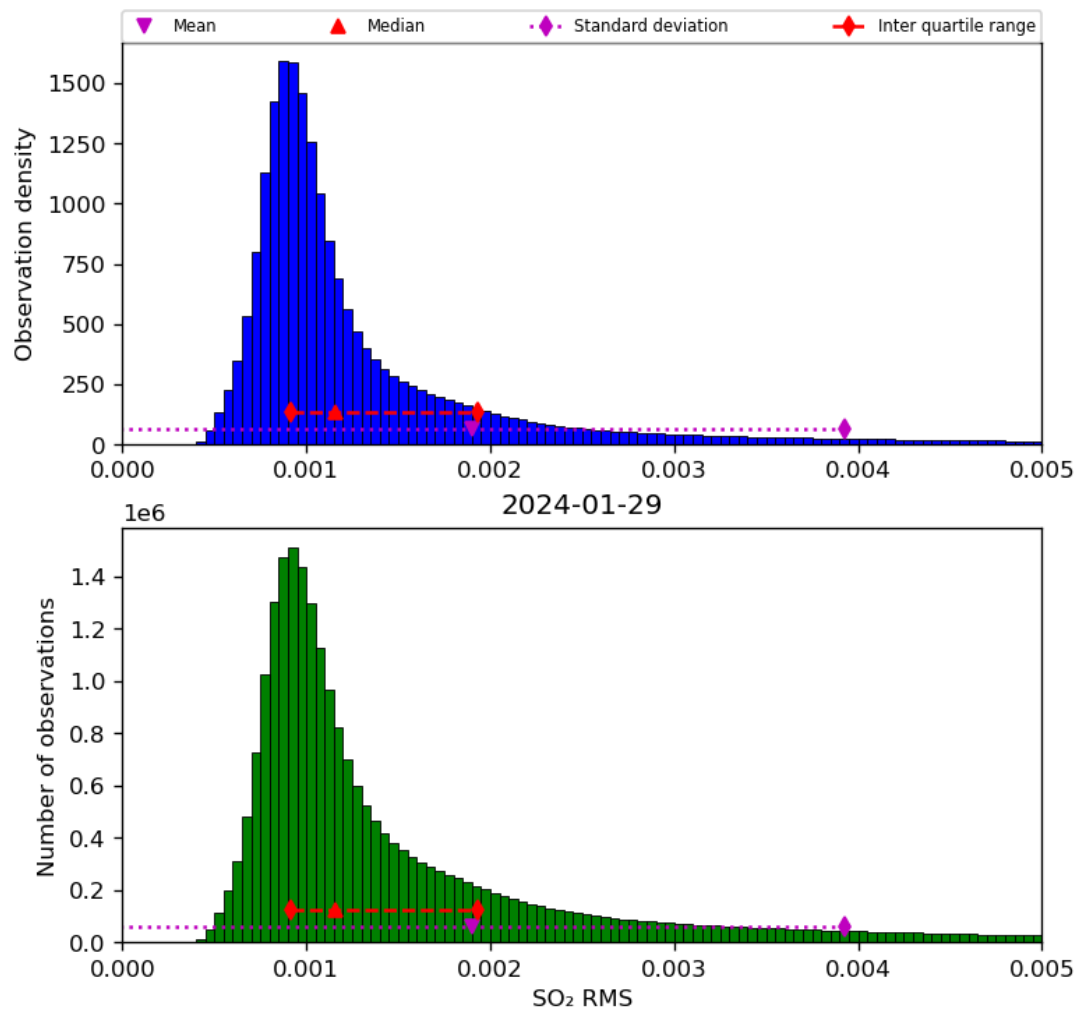
Figure 70: Histogram of “SO 2 RMS” for 2024-01-28 to 2024-01-30
