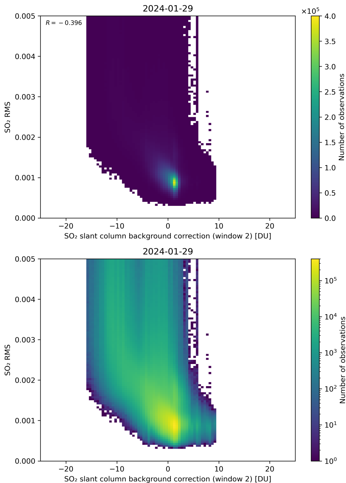
Figure 114: Scatter density plot of “SO 2 slant column background correction (window 2)” against “SO 2 RMS” for 2024-01-28 to 2024-01-30.
