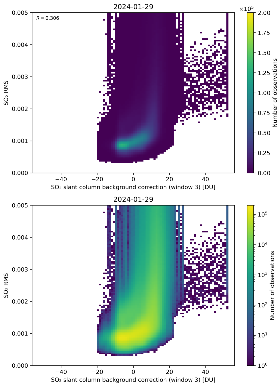
Figure 123: Scatter density plot of “SO 2 slant column background correction (window 3)” against “SO 2 RMS” for 2024-01-28 to 2024-01-30.
