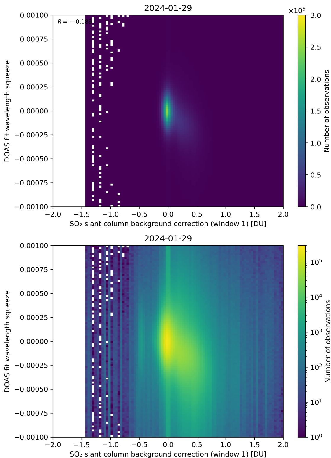
Figure 101: Scatter density plot of “SO 2 slant column background correction (window 1)” against “DOAS fit wavelength squeeze” for 2024-01-28 to 2024-01-30.
