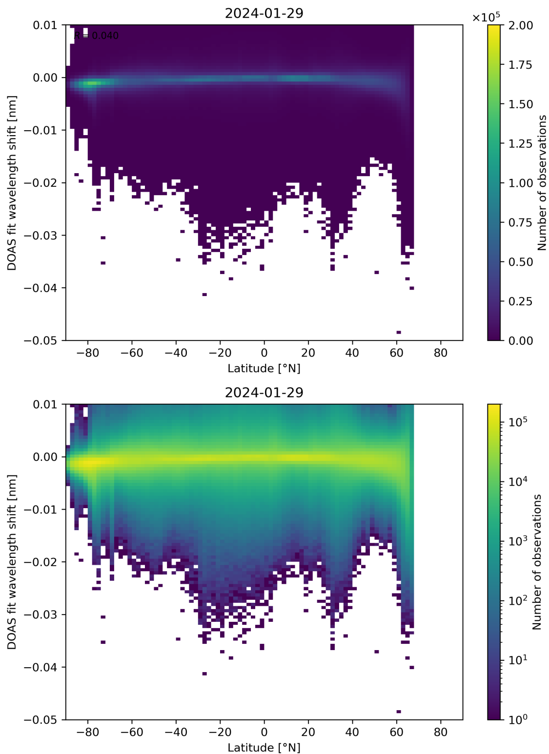
Figure 142: Scatter density plot of “Latitude” against “DOAS fit wavelength shift” for 2024-01-28 to 2024-01-30.
