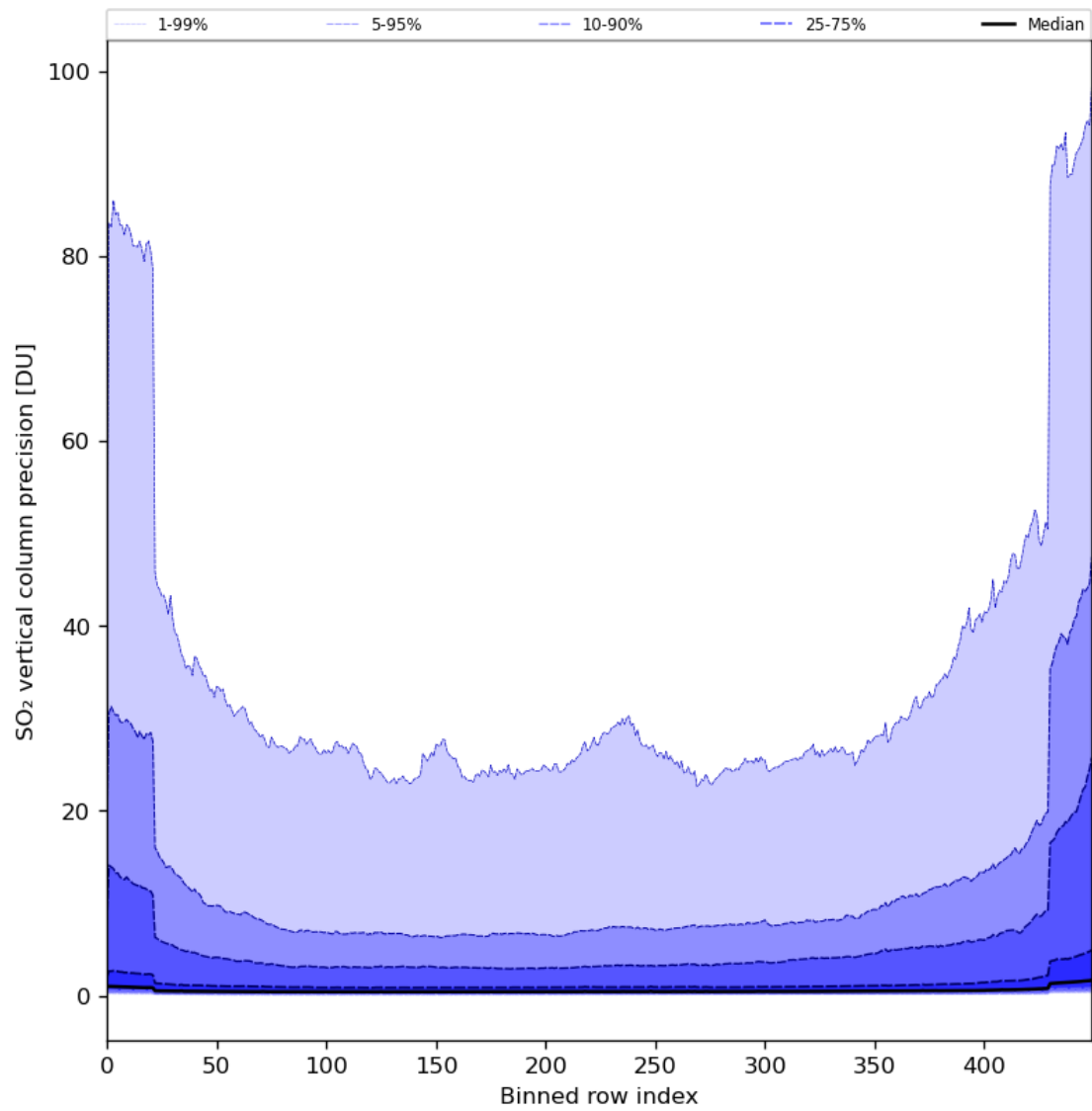
Figure 77: Along track statistics of “SO 2 vertical column precision” for 2024-01-28 to 2024-01-30
