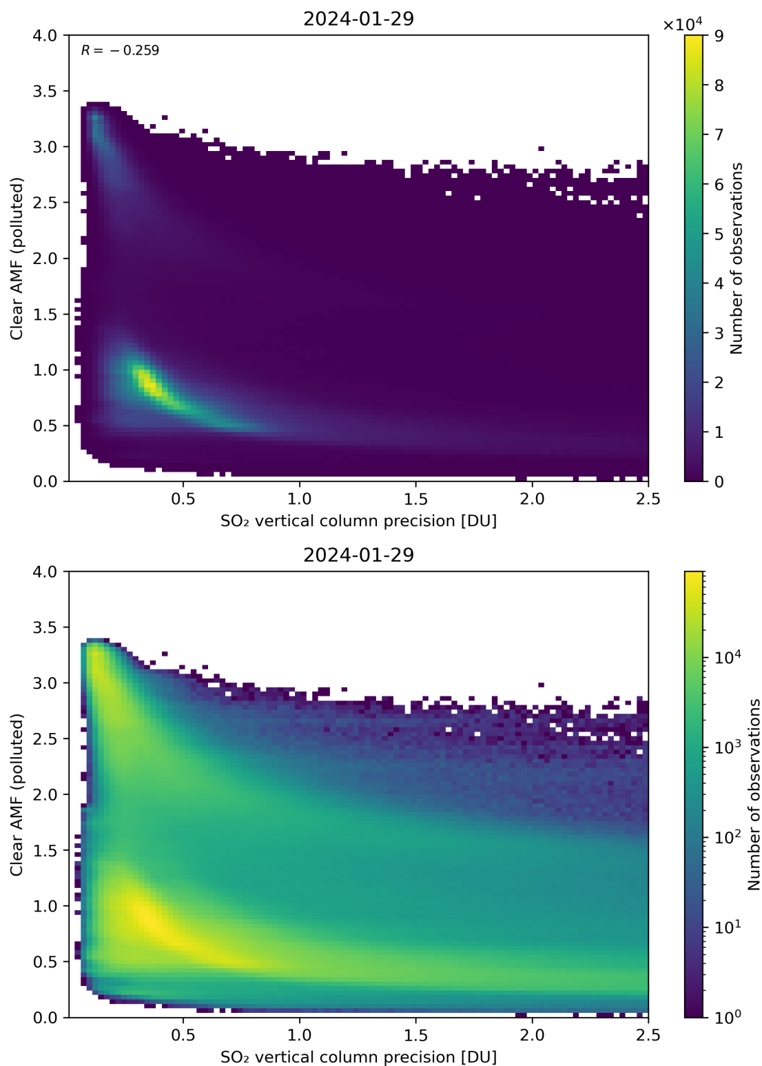
Figure 285: Scatter density plot of “SO 2 vertical column precision” against “Clear AMF (polluted)” for 2024-01-28 to 2024-01-30.
