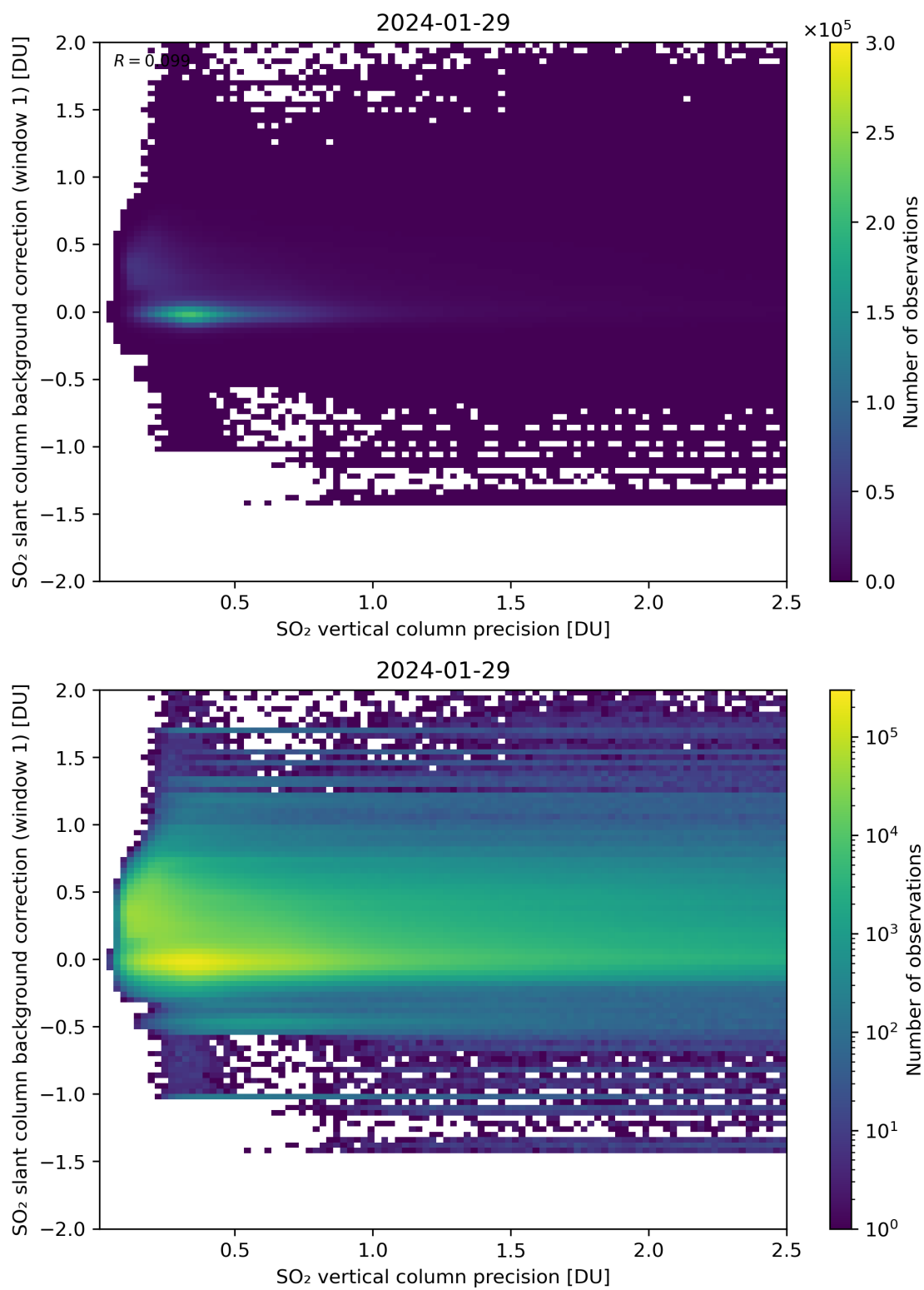
Figure 279: Scatter density plot of “SO 2 vertical column precision” against “SO 2 slant column background correction (window 1)” for 2024-01-28 to 2024-01-30.
