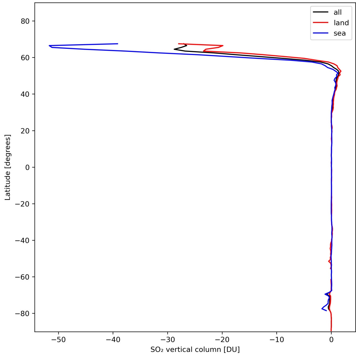
Figure 30: Zonal average of “SO 2 vertical column” for 2024-01-28 to 2024-01-30.
