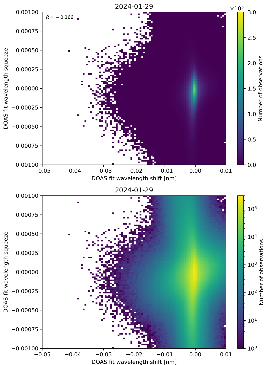
Figure 127: Scatter density plot of “DOAS fit wavelength shift” against “DOAS fit wavelength squeeze” for 2024-01-28 to 2024-01-30.
