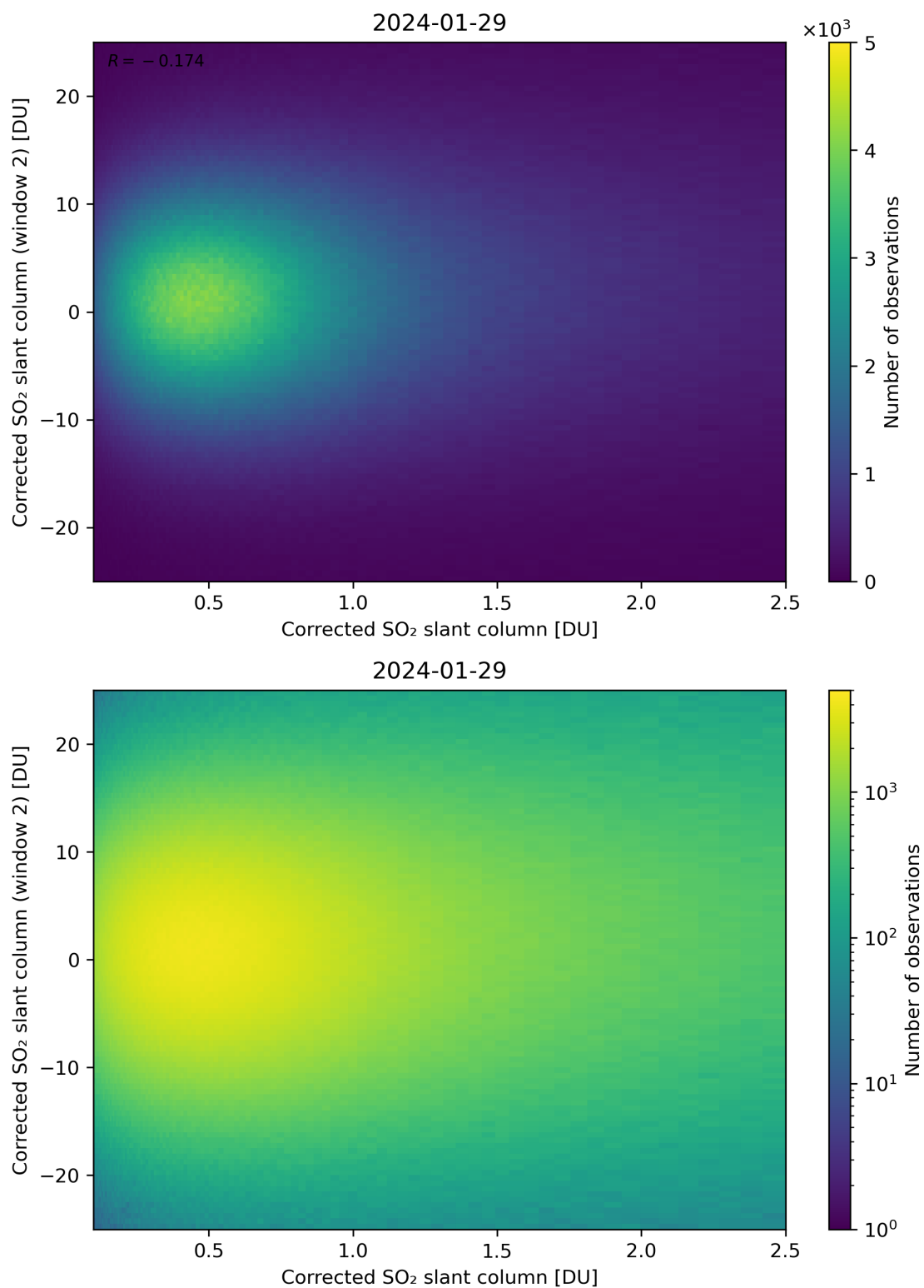
Figure 185: Scatter density plot of “Corrected SO 2 slant column” against “Corrected SO 2 slant column (window 2)” for 2024-01-28 to 2024-01-30.
