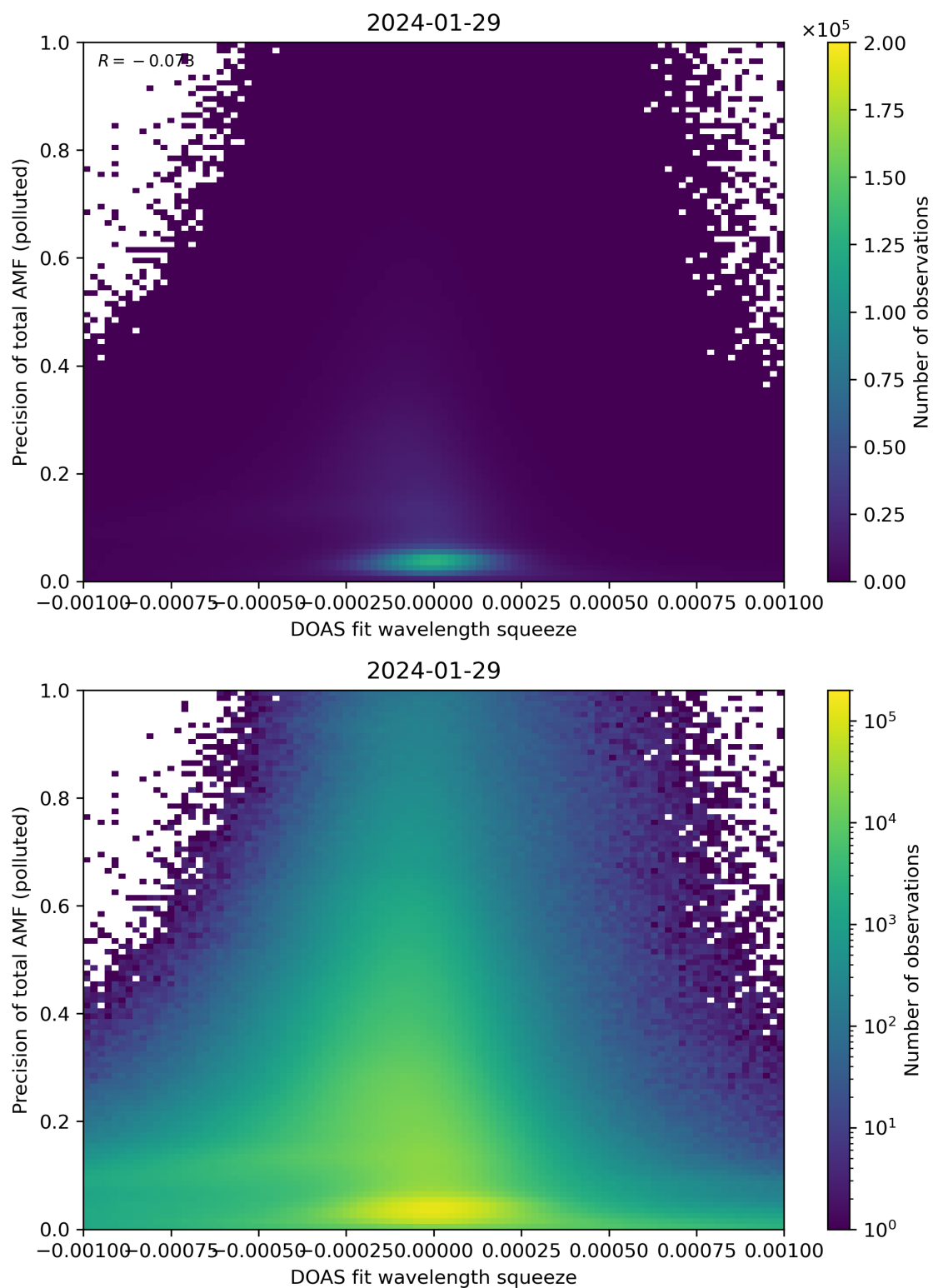
Figure 135: Scatter density plot of “DOAS fit wavelength squeeze” against “Precision of total AMF (polluted)” for 2024-01-28 to 2024-01-30.
