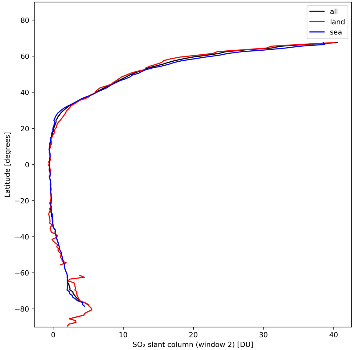
Figure 37: Zonal average of “SO 2 slant column (window 2)” for 2024-01-28 to 2024-01-30.
