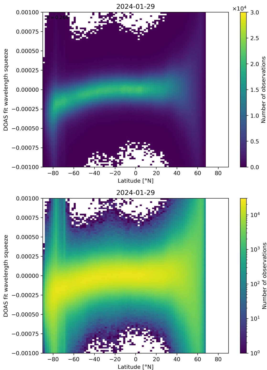
Figure 143: Scatter density plot of “Latitude” against “DOAS fit wavelength squeeze” for 2024-01-28 to 2024-01-30.
