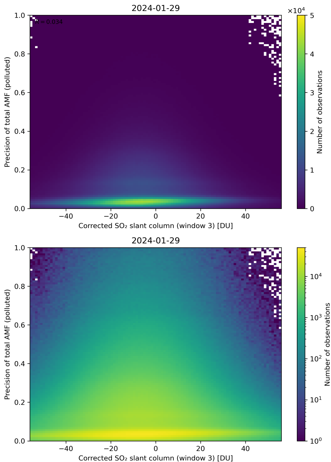
Figure 211: Scatter density plot of “Corrected SO 2 slant column (window 3)” against “Precision of total AMF (polluted)” for 2024-01-28 to 2024-01-30.
