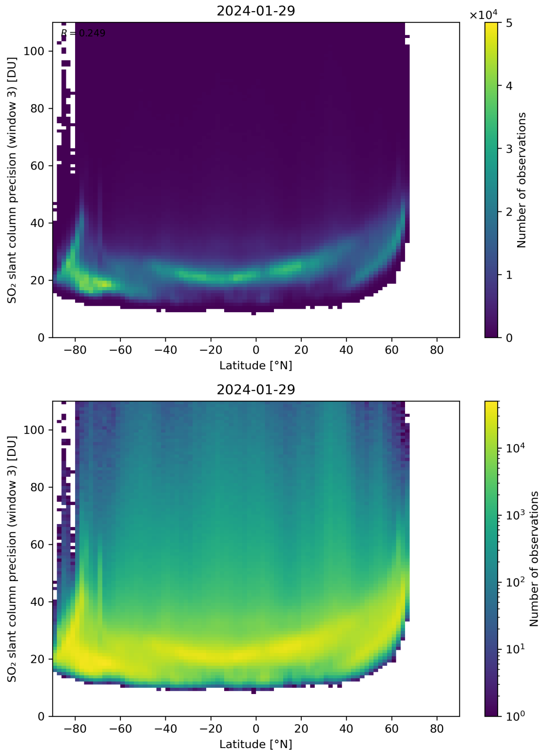
Figure 153: Scatter density plot of “Latitude” against “SO 2 slant column precision (window 3)” for 2024-01-28 to 2024-01-30.
