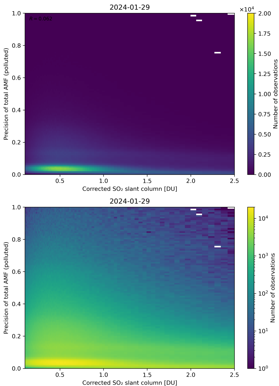
Figure 193: Scatter density plot of “Corrected SO 2 slant column” against “Precision of total AMF (polluted)” for 2024-01-28 to 2024-01-30.
