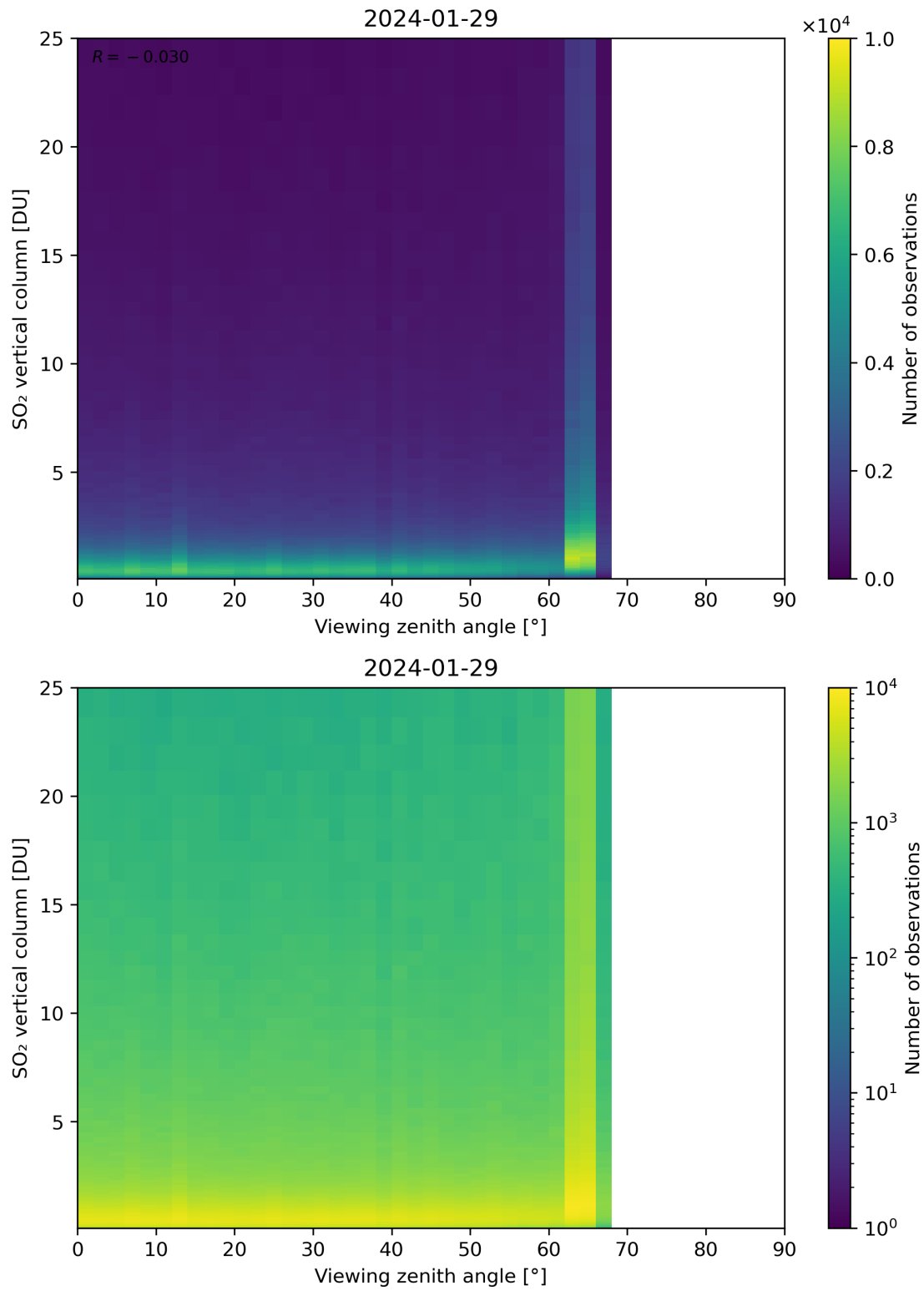
Figure 327: Scatter density plot of “Viewing zenith angle” against “SO 2 vertical column” for 2024-01-28 to 2024-01-30.
