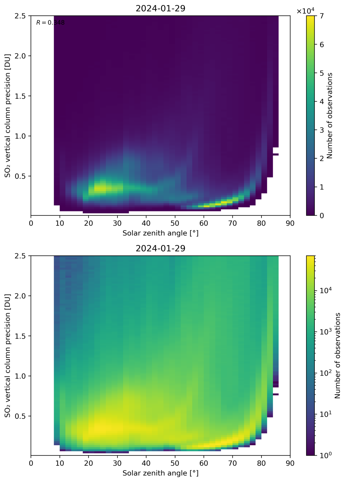
Figure 177: Scatter density plot of “Solar zenith angle” against “SO 2 vertical column precision” for 2024-01-28 to 2024-01-30.
