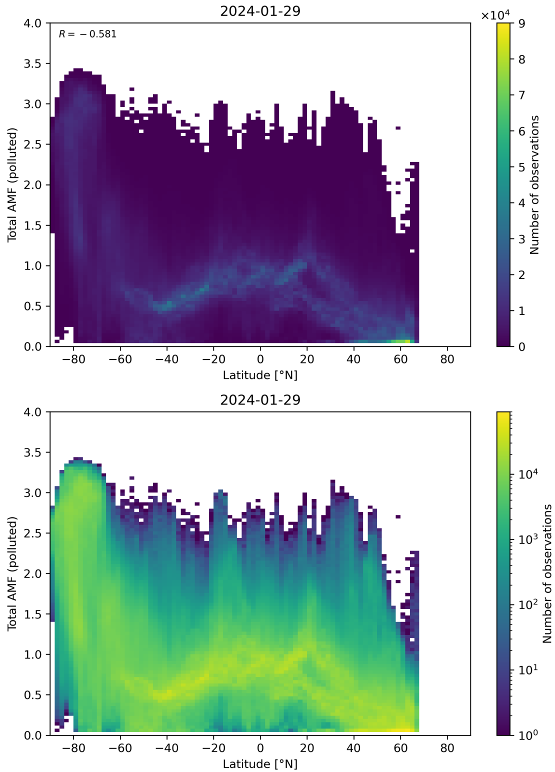
Figure 154: Scatter density plot of “Latitude” against “Total AMF (polluted)” for 2024-01-28 to 2024-01-30.
