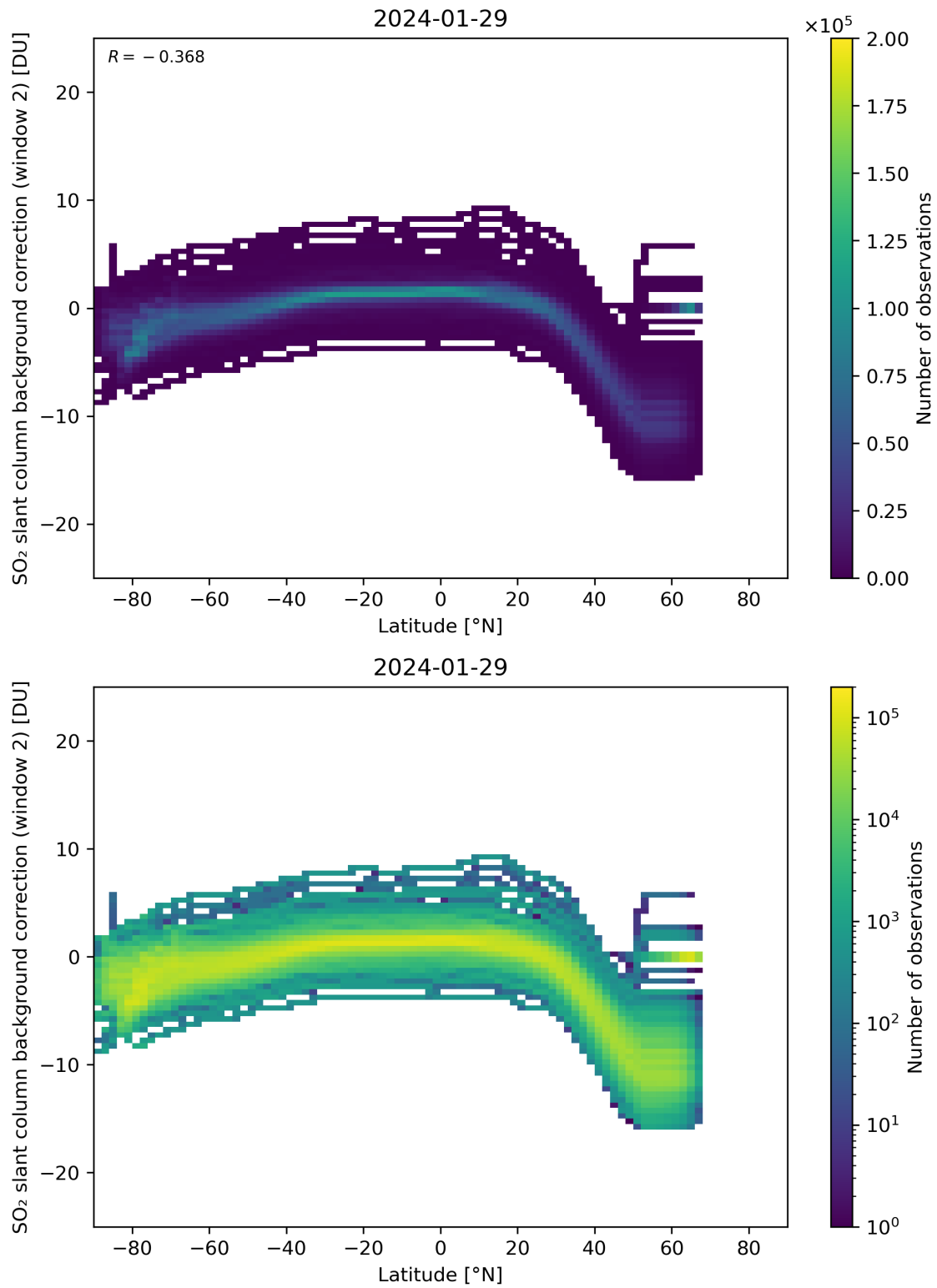
Figure 140: Scatter density plot of “Latitude” against “SO 2 slant column background correction (window 2)” for 2024-01-28 to 2024-01-30.
