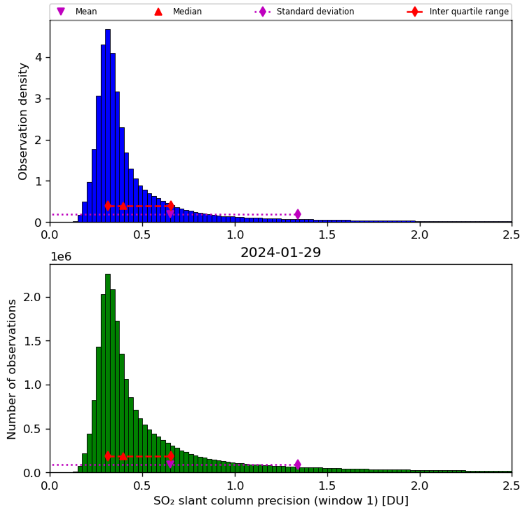
Figure 57: Histogram of “SO 2 slant column precision (window 1)” for 2024-01-28 to 2024-01-30
