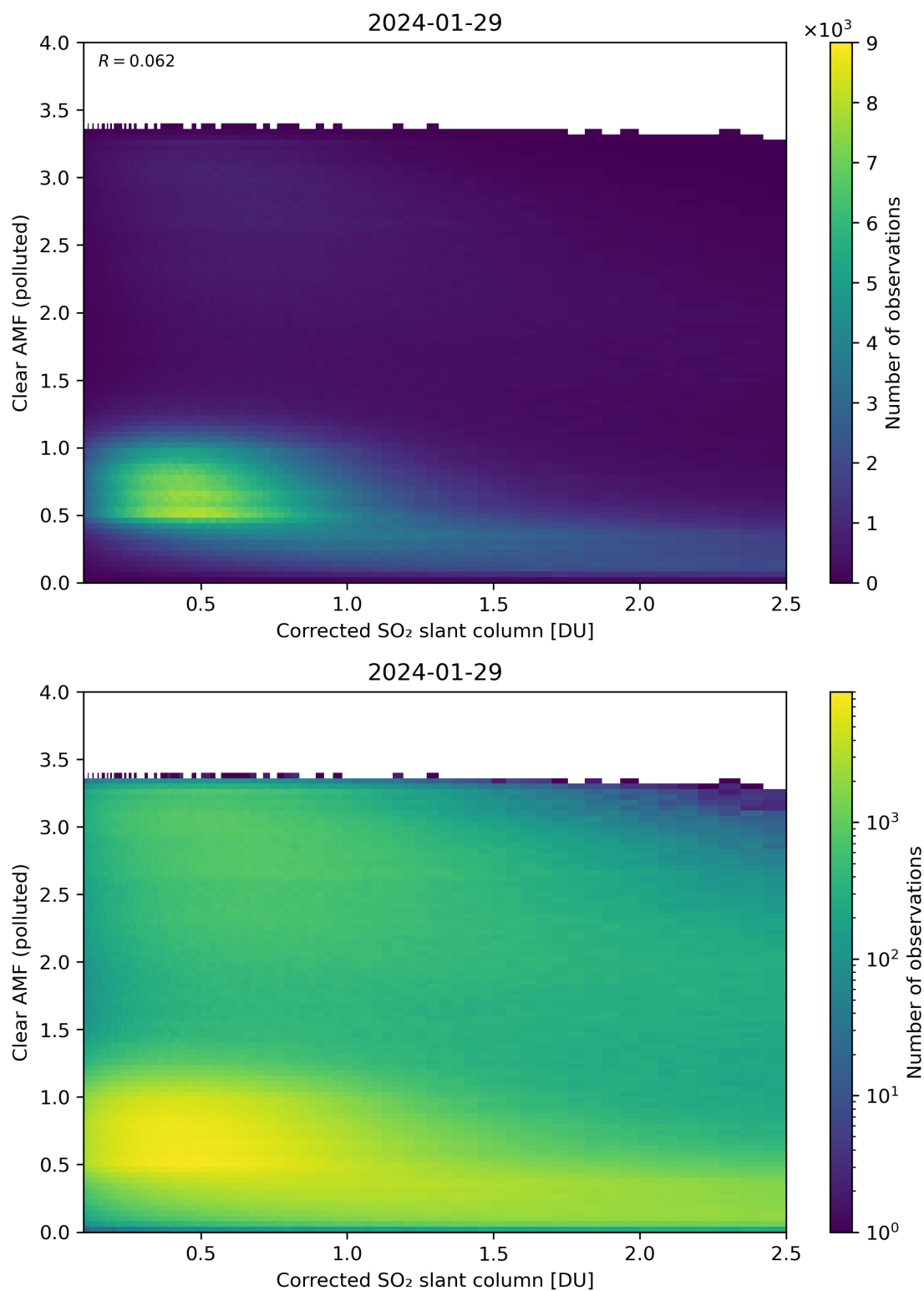
Figure 184: Scatter density plot of “Corrected SO 2 slant column” against “Clear AMF (polluted)” for 2024-01-28 to 2024-01-30.
