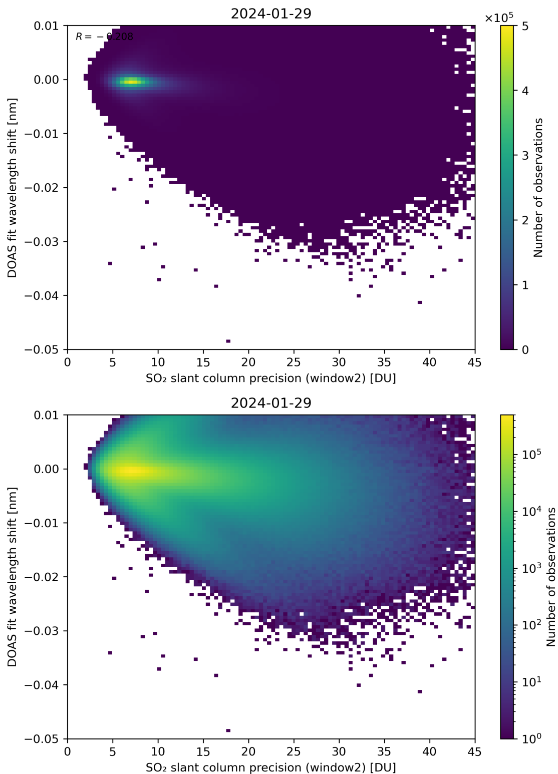
Figure 243: Scatter density plot of “SO 2 slant column precision (window2)” against “DOAS fit wavelength shift” for 2024-01-28 to 2024-01-30.
