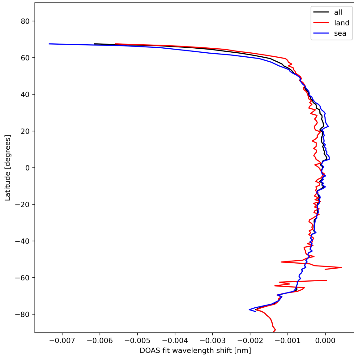
Figure 45: Zonal average of “DOAS fit wavelength shift” for 2024-01-28 to 2024-01-30.
