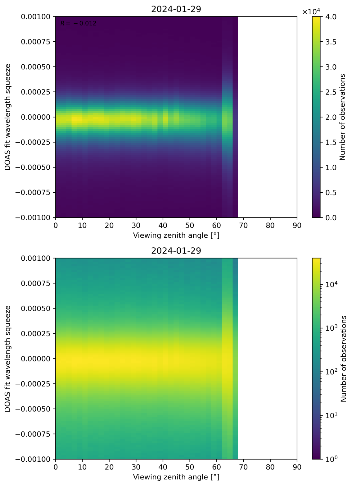
Figure 312: Scatter density plot of “Viewing zenith angle” against “DOAS fit wavelength squeeze” for 2024-01-28 to 2024-01-30.
