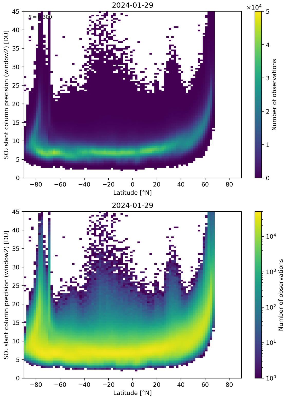
Figure 151: Scatter density plot of “Latitude” against “SO 2 slant column precision (window2)” for 2024-01-28 to 2024-01-30.
