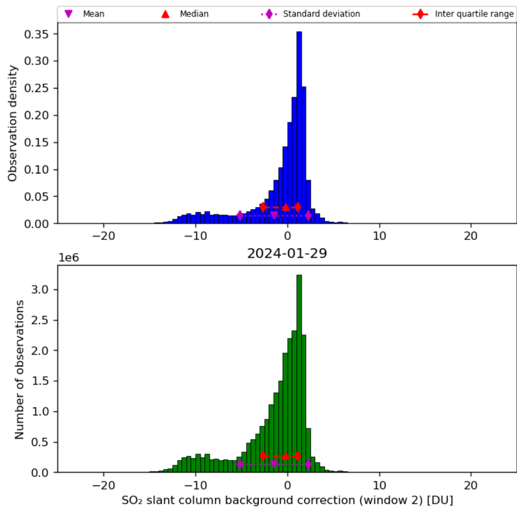
Figure 63: Histogram of “SO 2 slant column background correction (window 2)” for 2024-01-28 to 2024-01-30
