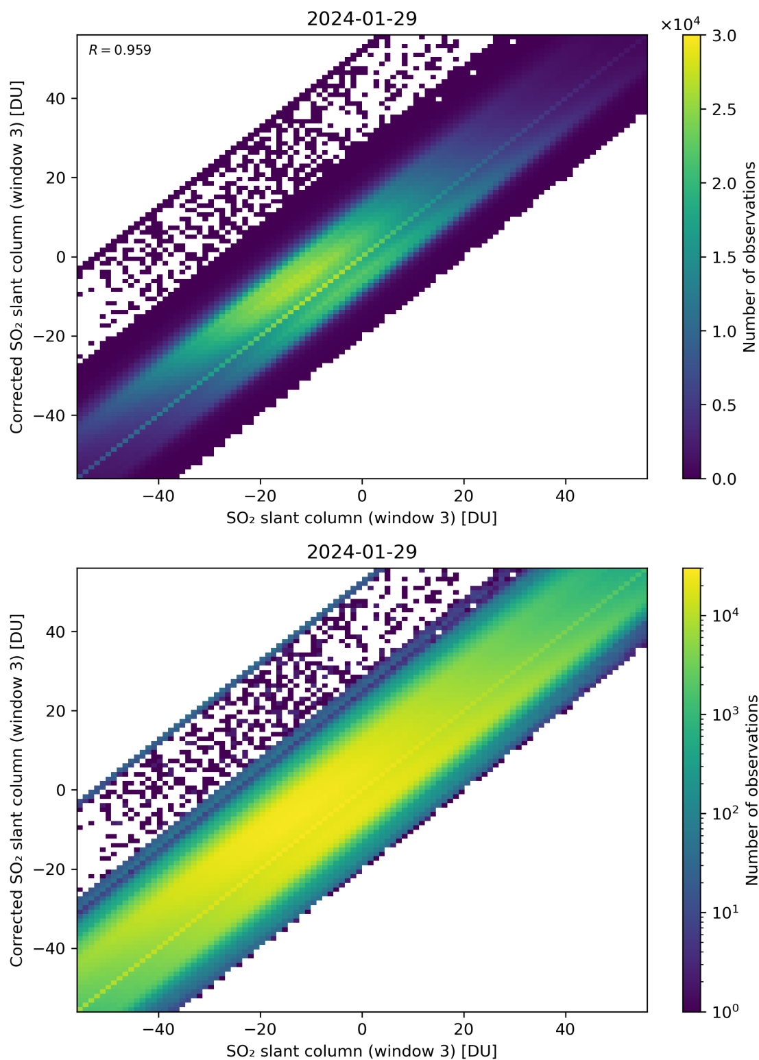
Figure 266: Scatter density plot of “SO 2 slant column (window 3)” against “Corrected SO 2 slant column (window 3)” for 2024-01-28 to 2024-01-30.
