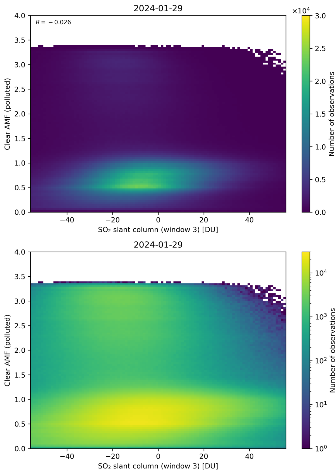
Figure 265: Scatter density plot of “SO 2 slant column (window 3)” against “Clear AMF (polluted)” for 2024-01-28 to 2024-01-30.
