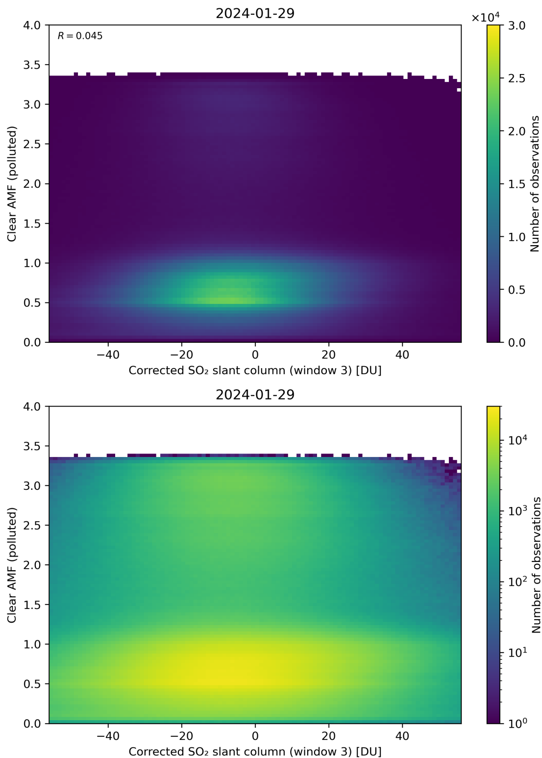
Figure 209: Scatter density plot of “Corrected SO 2 slant column (window 3)” against “Clear AMF (polluted)” for 2024-01-28 to 2024-01-30.
