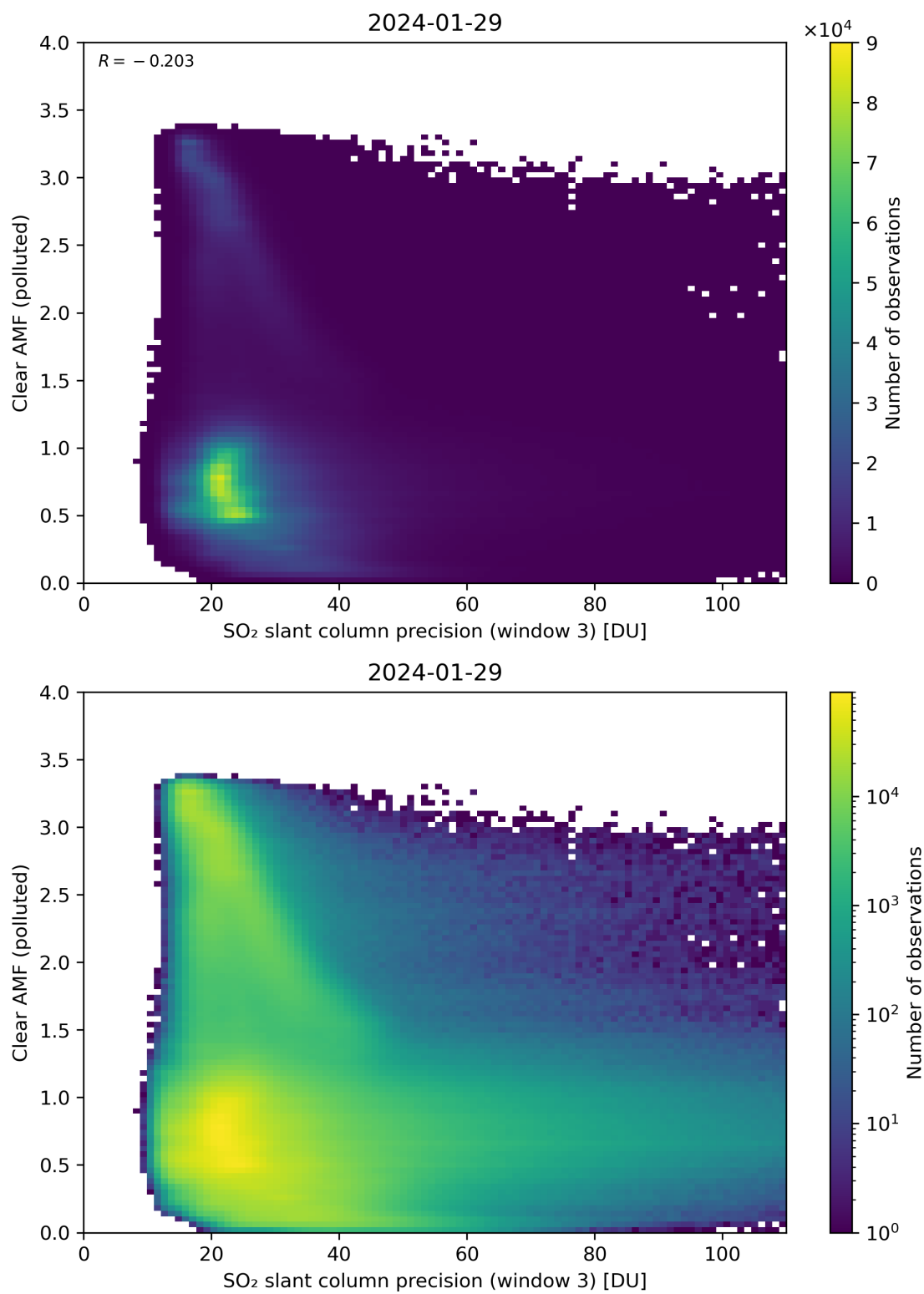
Figure 261: Scatter density plot of “SO 2 slant column precision (window 3)” against “Clear AMF (polluted)” for 2024-01-28 to 2024-01-30.
