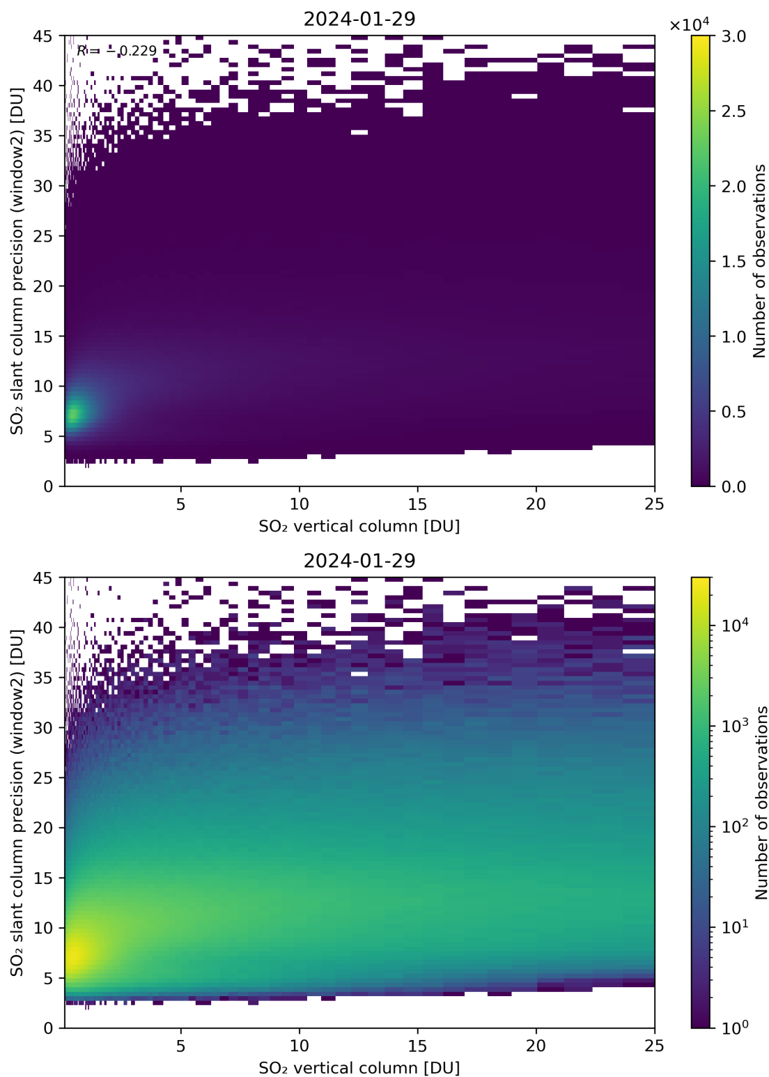
Figure 302: Scatter density plot of “SO 2 vertical column” against “SO 2 slant column precision (window2)” for 2024-01-28 to 2024-01-30.
