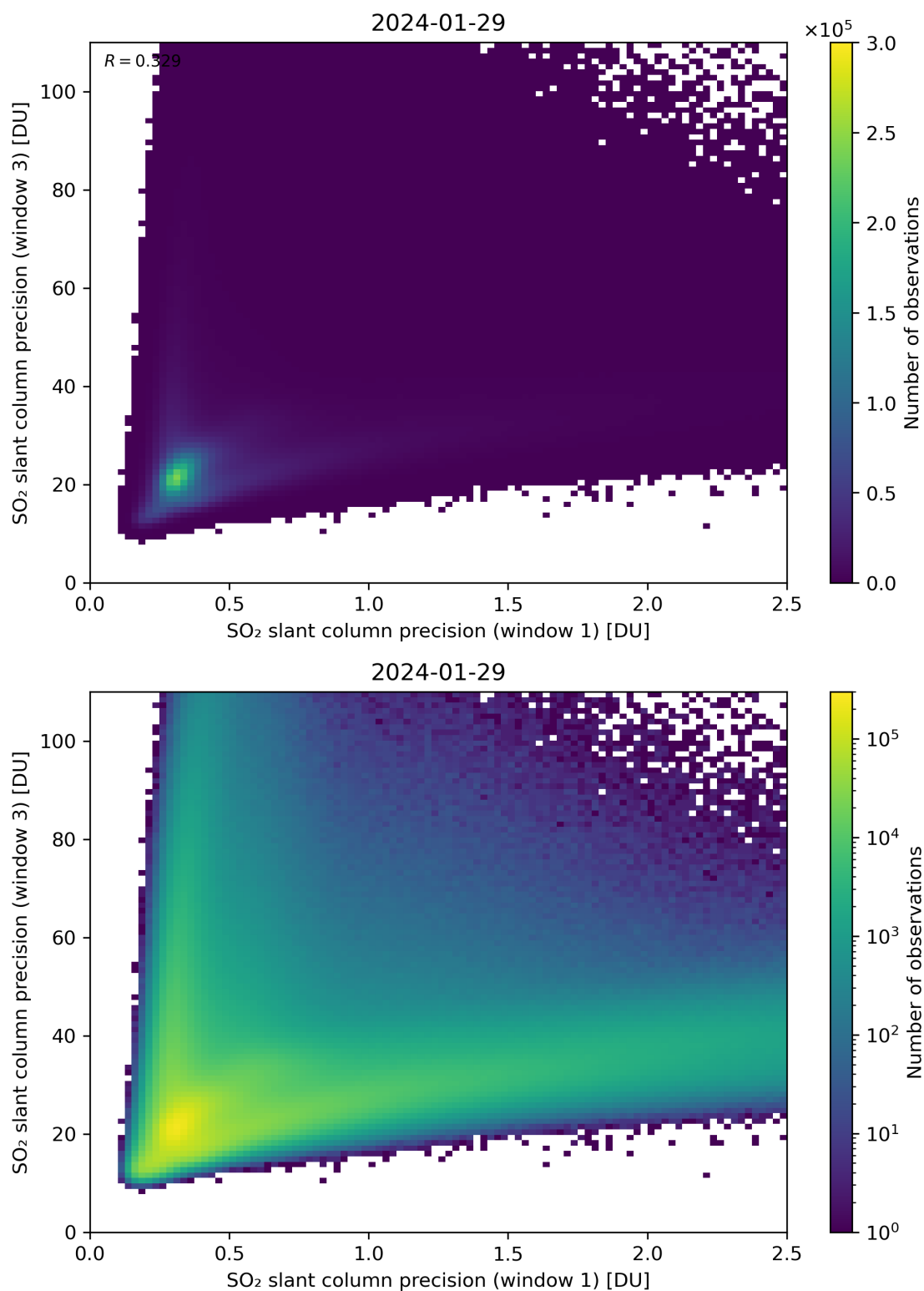
Figure 229: Scatter density plot of “SO 2 slant column precision (window 1)” against “SO 2 slant column precision (window 3)” for 2024-01-28 to 2024-01-30.
