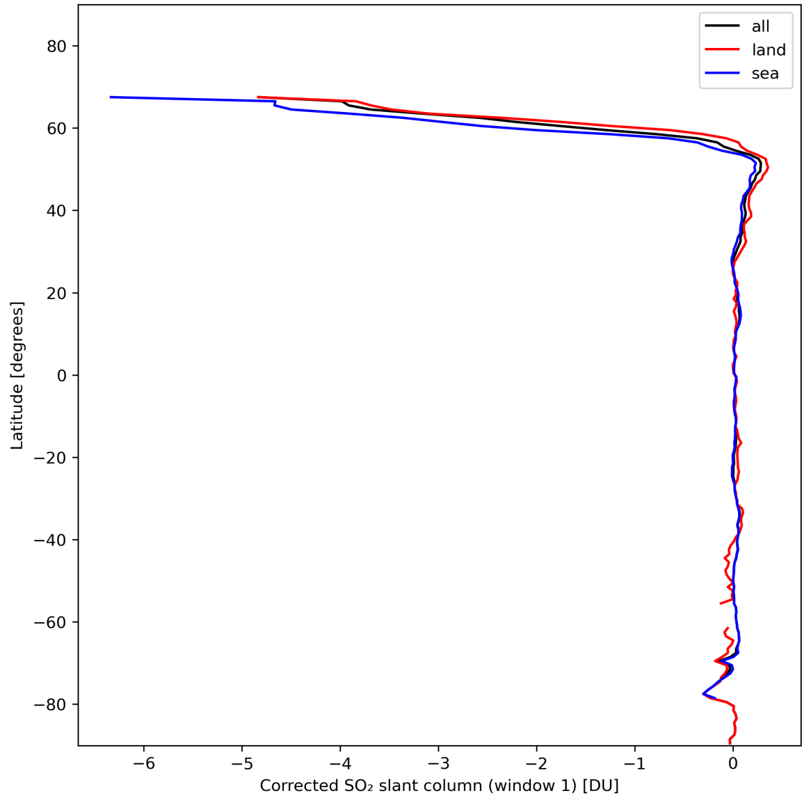
Figure 35: Zonal average of “Corrected SO 2 slant column (window 1)” for 2024-01-28 to 2024-01-30.
