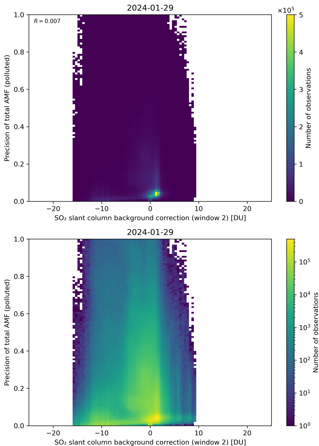
Figure 120: Scatter density plot of “SO 2 slant column background correction (window 2)” against “Precision of total AMF (polluted)” for 2024-01-28 to 2024-01-30.
