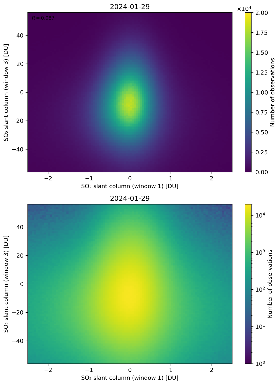
Figure 237: Scatter density plot of “SO 2 slant column (window 1)” against “SO 2 slant column (window 3)” for 2024-01-28 to 2024-01-30.
