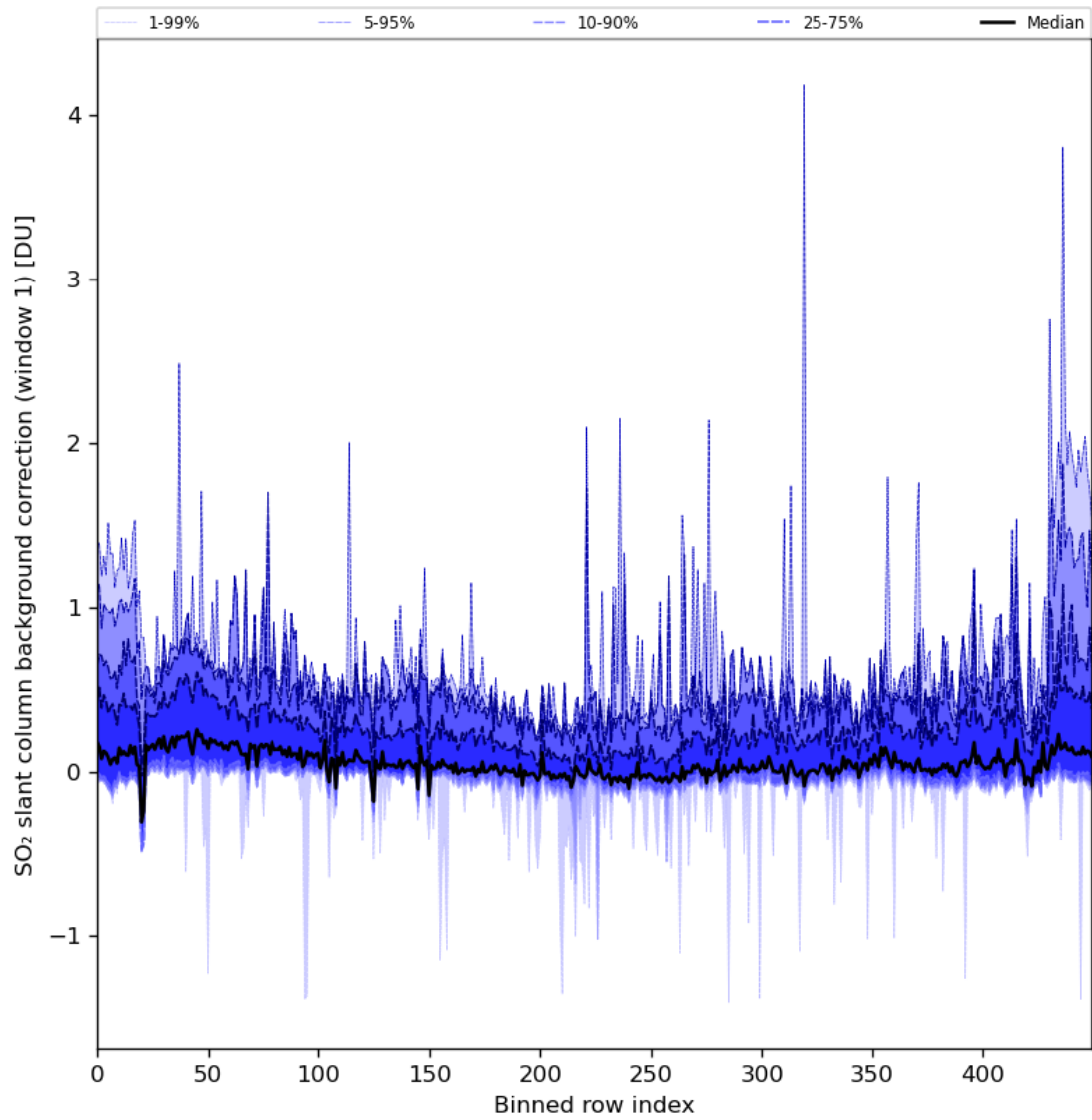
Figure 82: Along track statistics of “SO 2 slant column background correction (window 1)” for 2024-01-28 to 2024-01-30
