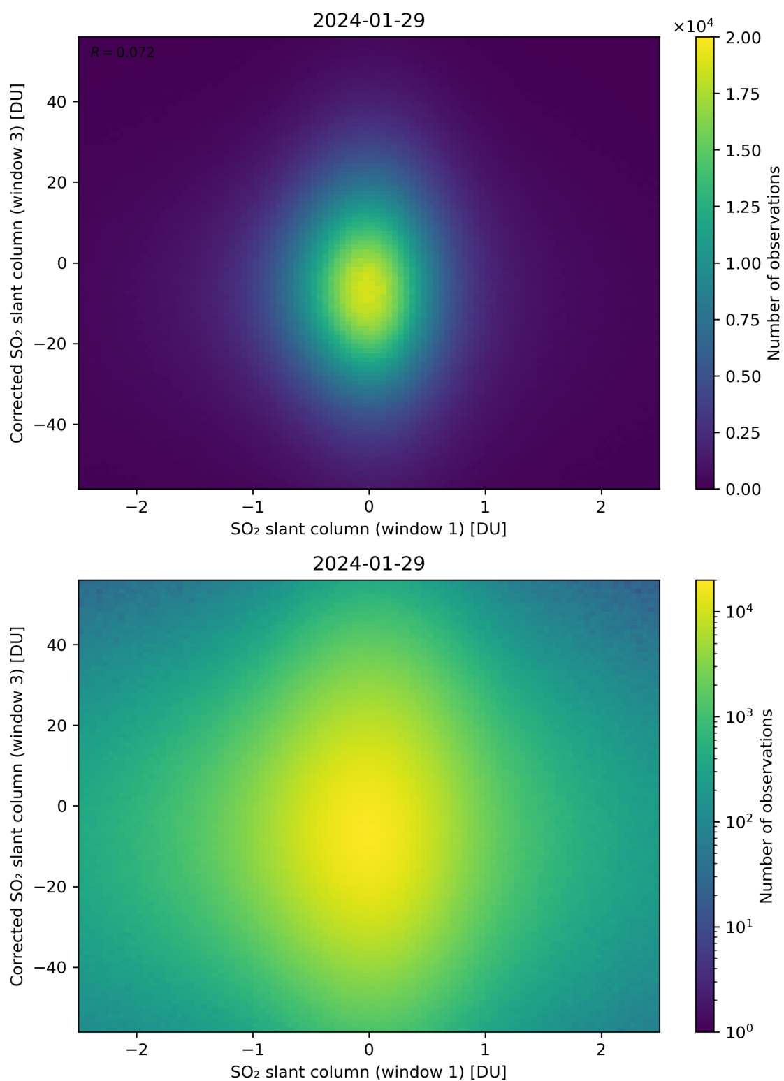
Figure 234: Scatter density plot of “SO 2 slant column (window 1)” against “Corrected SO 2 slant column (window 3)” for 2024-01-28 to 2024-01-30.
