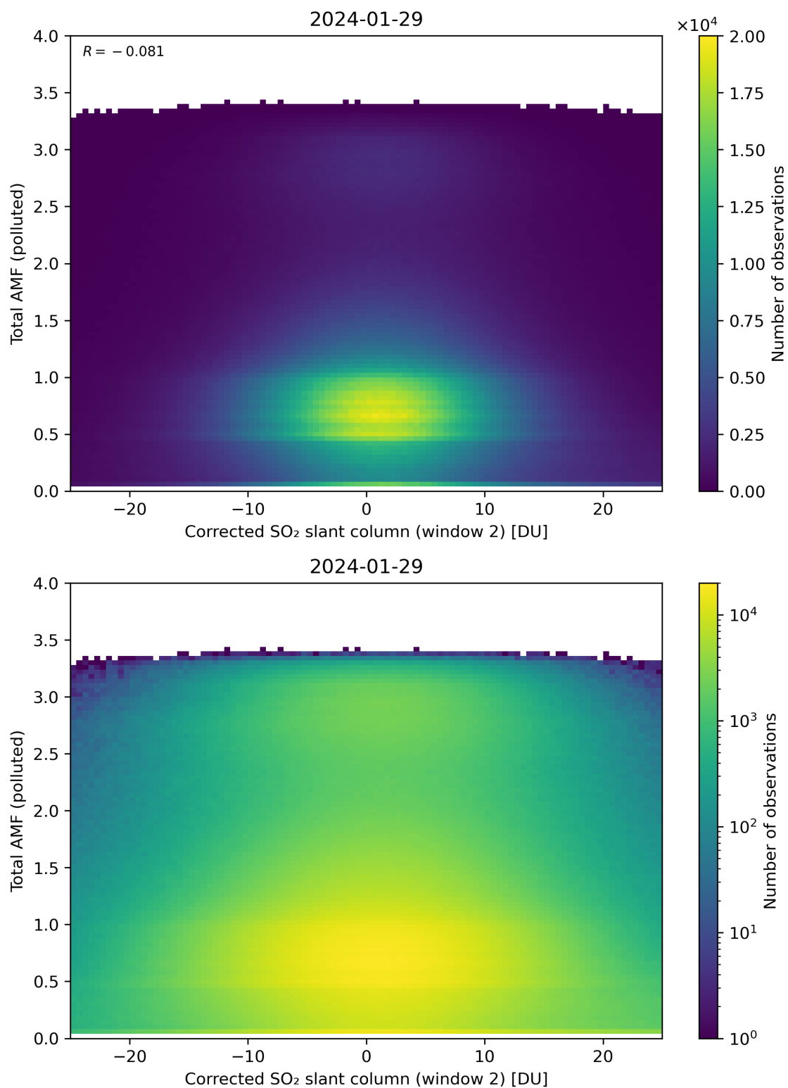
Figure 203: Scatter density plot of “Corrected SO 2 slant column (window 2)” against “Total AMF (polluted)” for 2024-01-28 to 2024-01-30.
