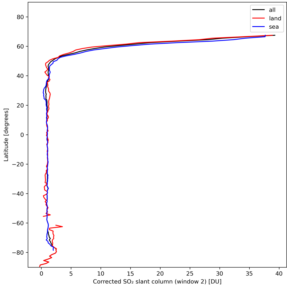
Figure 39: Zonal average of “Corrected SO 2 slant column (window 2)” for 2024-01-28 to 2024-01-30.
