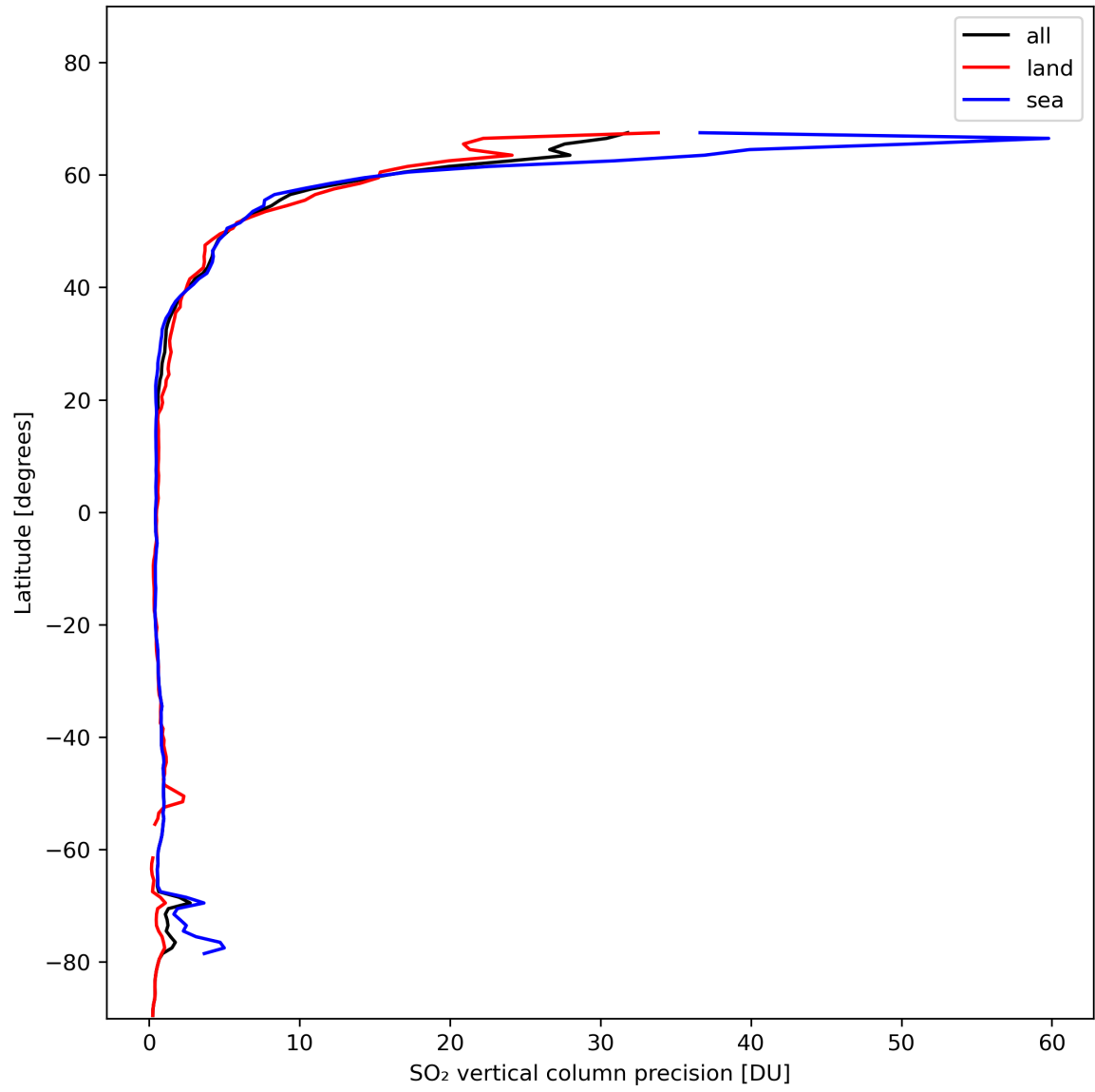
Figure 31: Zonal average of “SO 2 vertical column precision” for 2024-01-28 to 2024-01-30.
