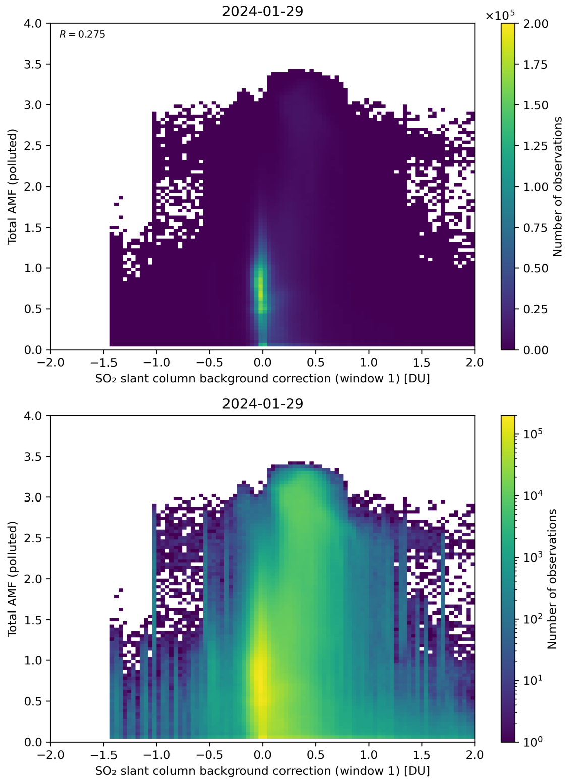
Figure 109: Scatter density plot of “SO 2 slant column background correction (window 1)” against “Total AMF (polluted)” for 2024-01-28 to 2024-01-30.
