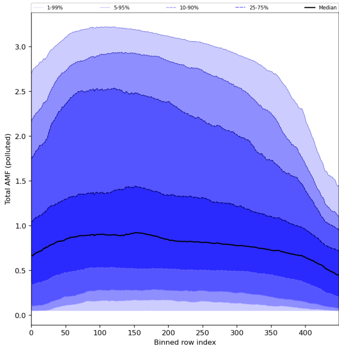
Figure 94: Along track statistics of “Total AMF (polluted)” for 2024-01-28 to 2024-01-30
