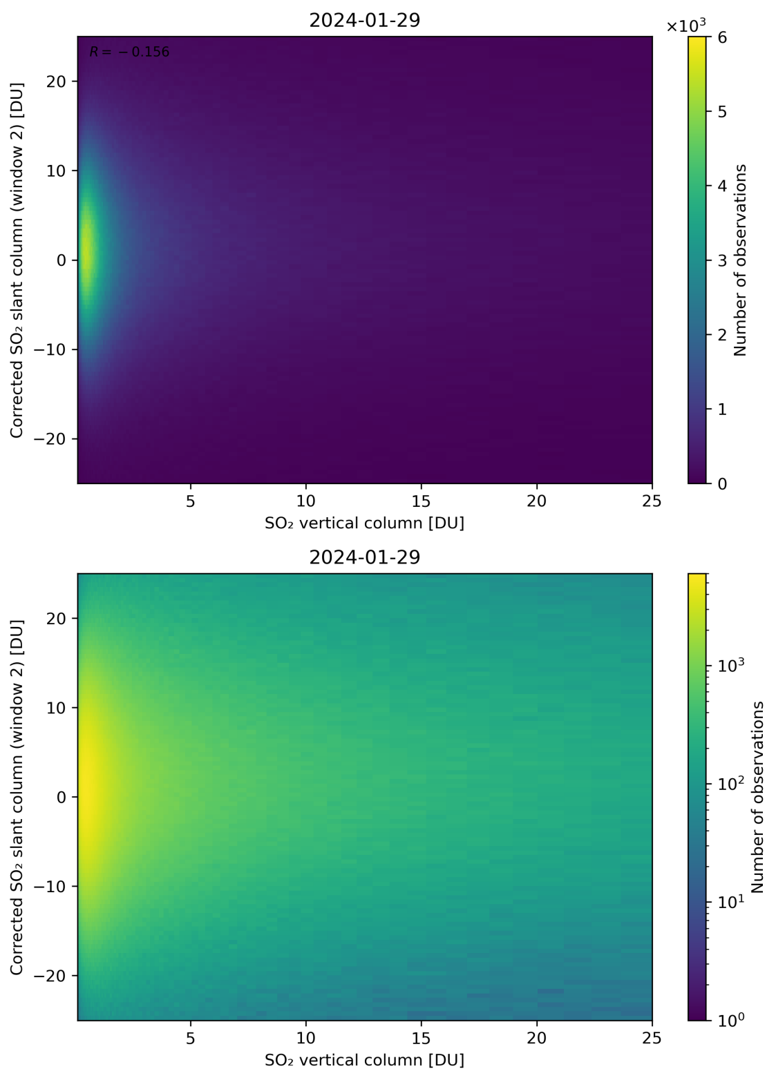
Figure 298: Scatter density plot of “SO 2 vertical column” against “Corrected SO 2 slant column (window 2)” for 2024-01-28 to 2024-01-30.
