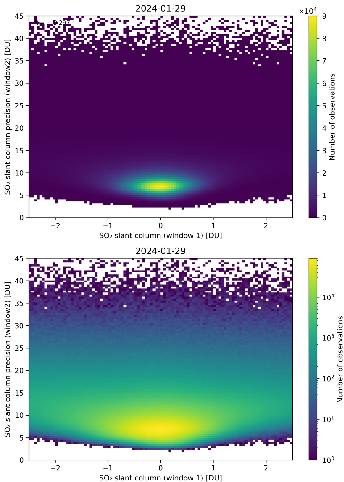
Figure 236: Scatter density plot of “SO 2 slant column (window 1)” against “SO 2 slant column precision (window2)” for 2024-01-28 to 2024-01-30.
