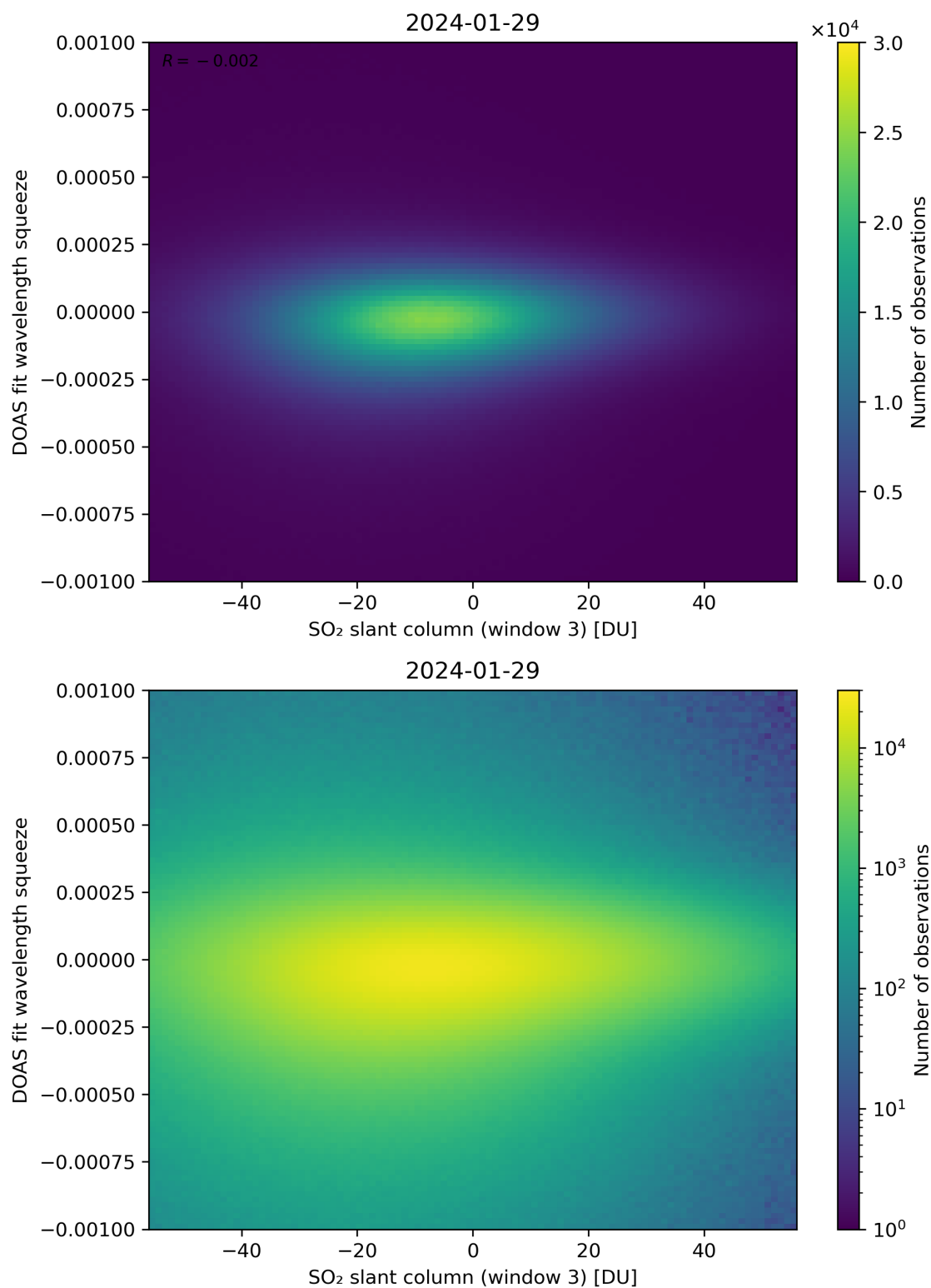
Figure 255: Scatter density plot of “SO 2 slant column (window 3)” against “DOAS fit wavelength squeeze” for 2024-01-28 to 2024-01-30.
