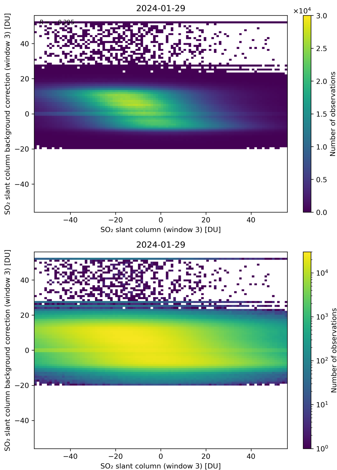
Figure 253: Scatter density plot of “SO 2 slant column (window 3)” against “SO 2 slant column background correction (window 3)” for 2024-01-28 to 2024-01-30.
