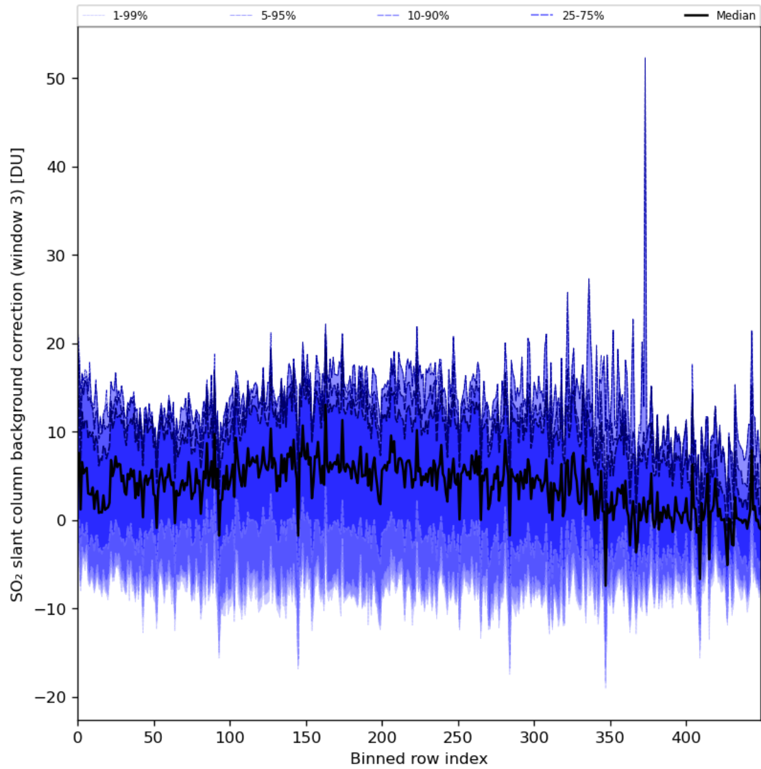
Figure 90: Along track statistics of “SO 2 slant column background correction (window 3)” for 2024-01-28 to 2024-01-30
