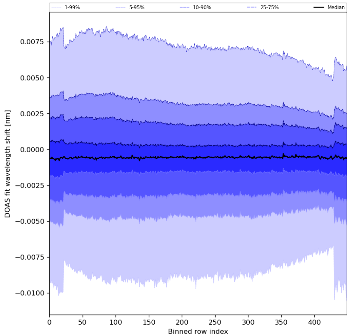
Figure 91: Along track statistics of “DOAS fit wavelength shift” for 2024-01-28 to 2024-01-30
