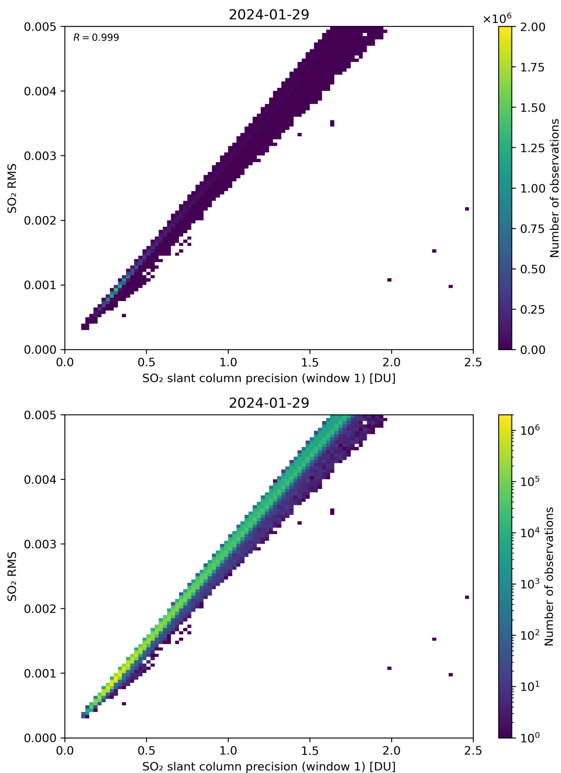
Figure 223: Scatter density plot of “SO 2 slant column precision (window 1)” against “SO 2 RMS” for 2024-01-28 to 2024-01-30.
