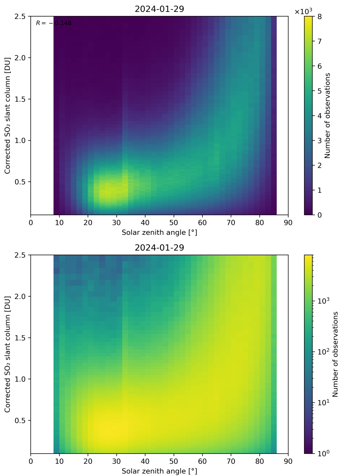
Figure 166: Scatter density plot of “Solar zenith angle” against “Corrected SO 2 slant column” for 2024-01-28 to 2024-01-30.
