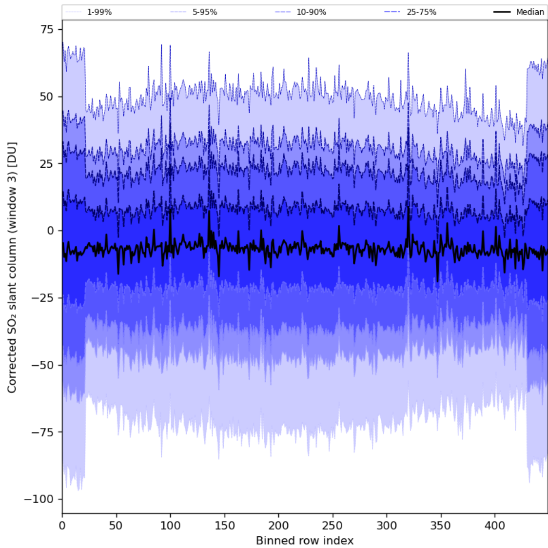
Figure 89: Along track statistics of “Corrected SO 2 slant column (window 3)” for 2024-01-28 to 2024-01-30
