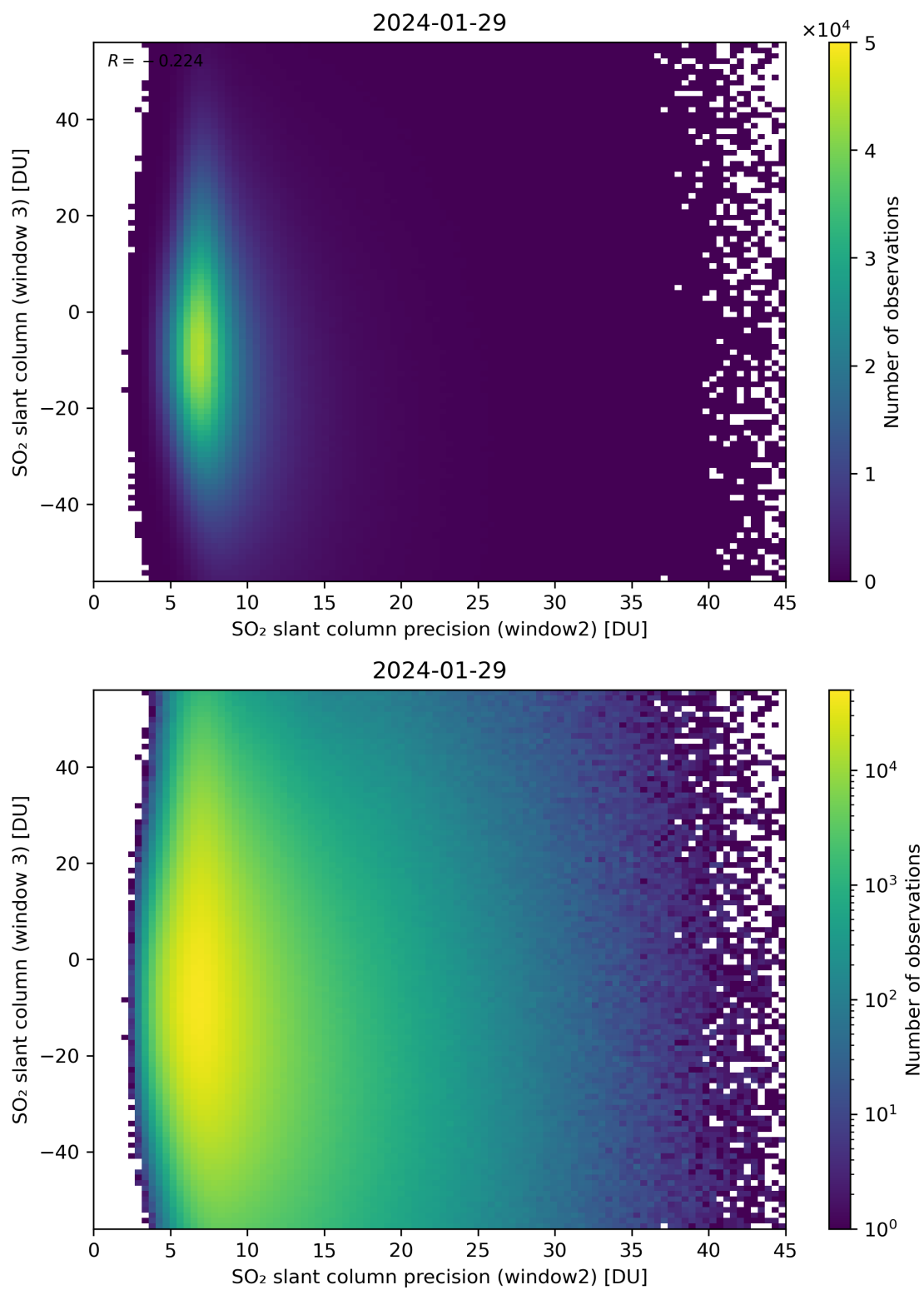
Figure 249: Scatter density plot of “SO 2 slant column precision (window2)” against “SO 2 slant column (window 3)” for 2024-01-28 to 2024-01-30.
