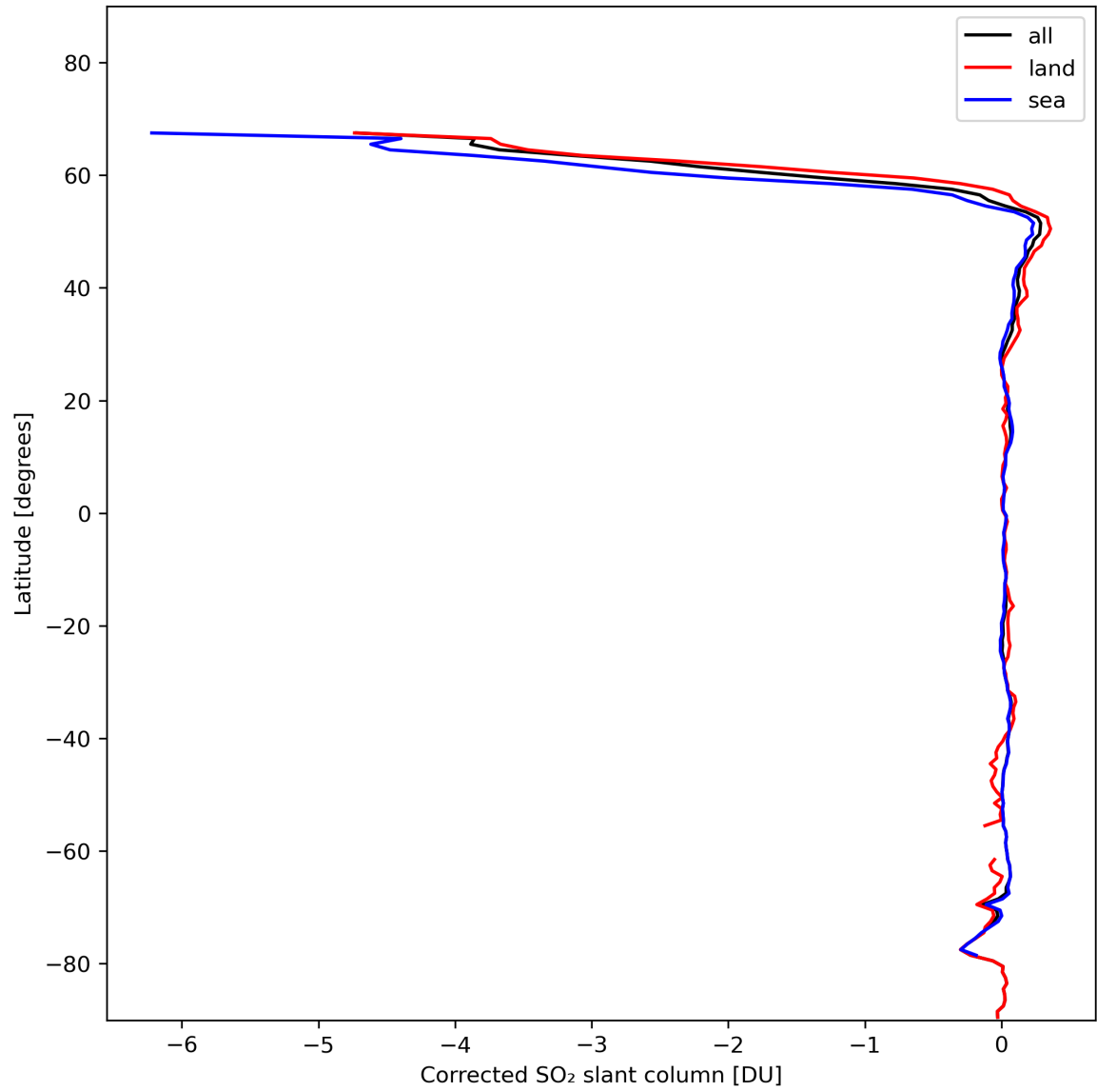
Figure 32: Zonal average of “Corrected SO 2 slant column” for 2024-01-28 to 2024-01-30.
