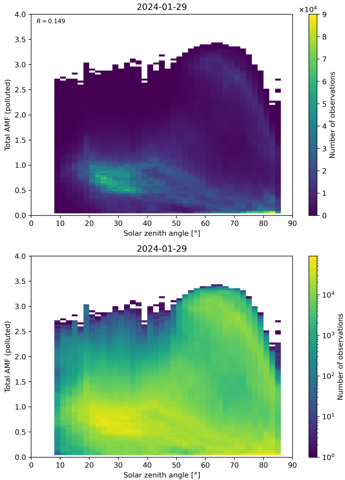
Figure 174: Scatter density plot of “Solar zenith angle” against “Total AMF (polluted)” for 2024-01-28 to 2024-01-30.
