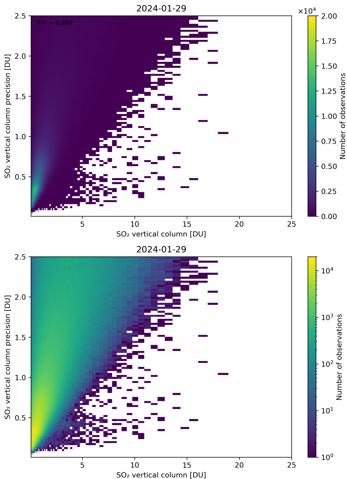
Figure 307: Scatter density plot of “SO 2 vertical column” against “SO 2 vertical column precision” for 2024-01-28 to 2024-01-30.
