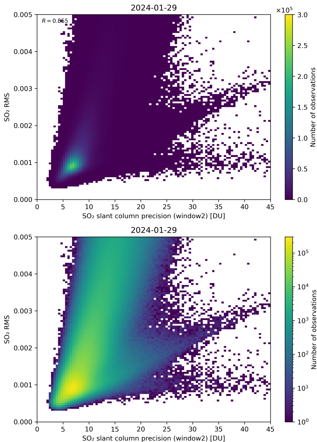
Figure 245: Scatter density plot of “SO 2 slant column precision (window2)” against “SO 2 RMS” for 2024-01-28 to 2024-01-30.
