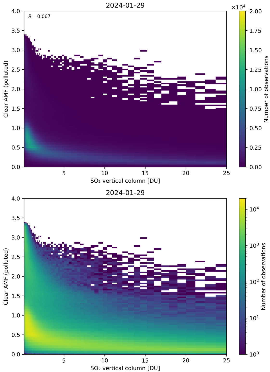
Figure 296: Scatter density plot of “SO 2 vertical column” against “Clear AMF (polluted)” for 2024-01-28 to 2024-01-30.
