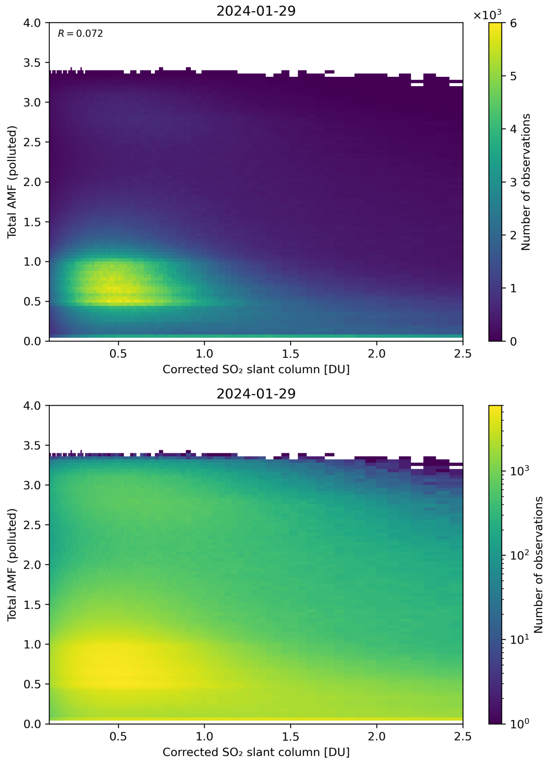
Figure 192: Scatter density plot of “Corrected SO 2 slant column” against “Total AMF (polluted)” for 2024-01-28 to 2024-01-30.
