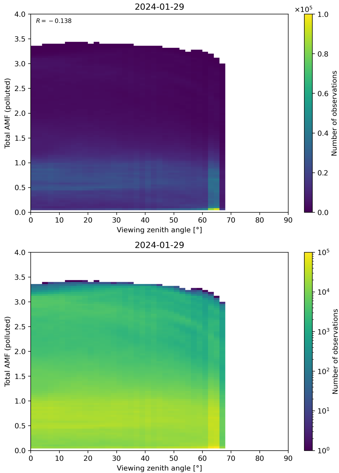
Figure 325: Scatter density plot of “Viewing zenith angle” against “Total AMF (polluted)” for 2024-01-28 to 2024-01-30.
