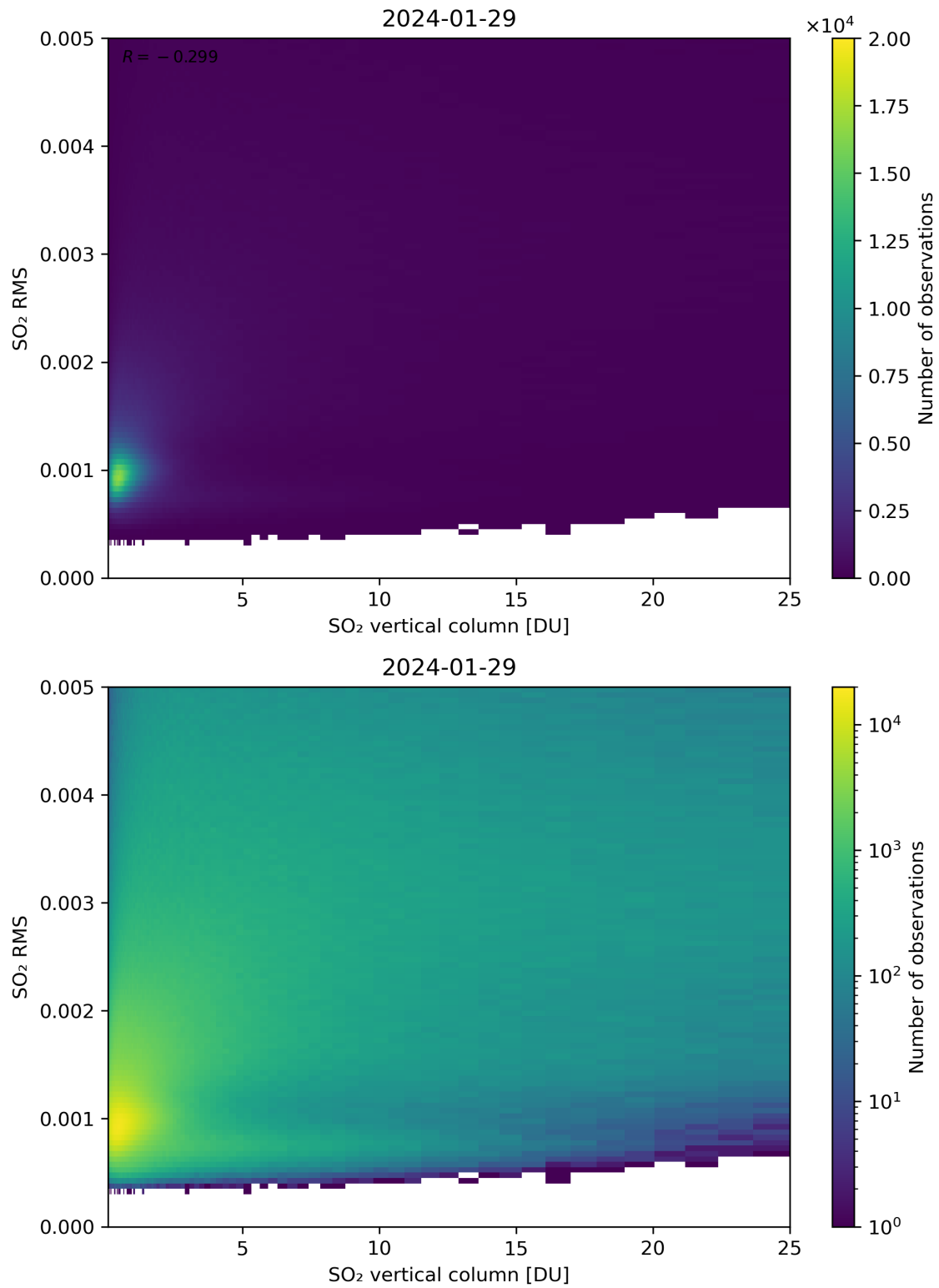
Figure 278: Scatter density plot of “SO 2 vertical column” against “SO 2 RMS” for 2024-01-28 to 2024-01-30.
