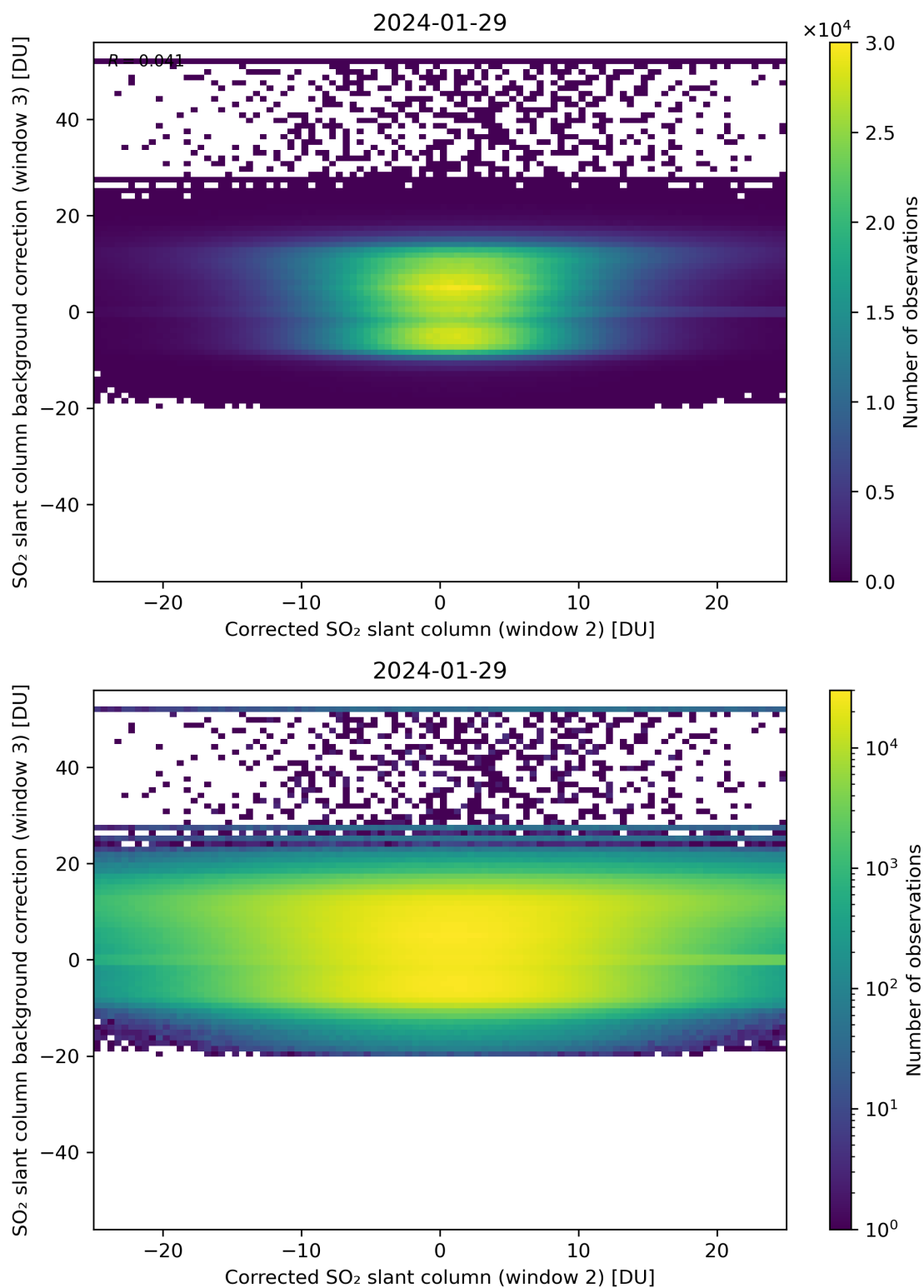
Figure 195: Scatter density plot of “Corrected SO 2 slant column (window 2)” against “SO 2 slant column background correction (window 3)” for 2024-01-28 to 2024-01-30.
