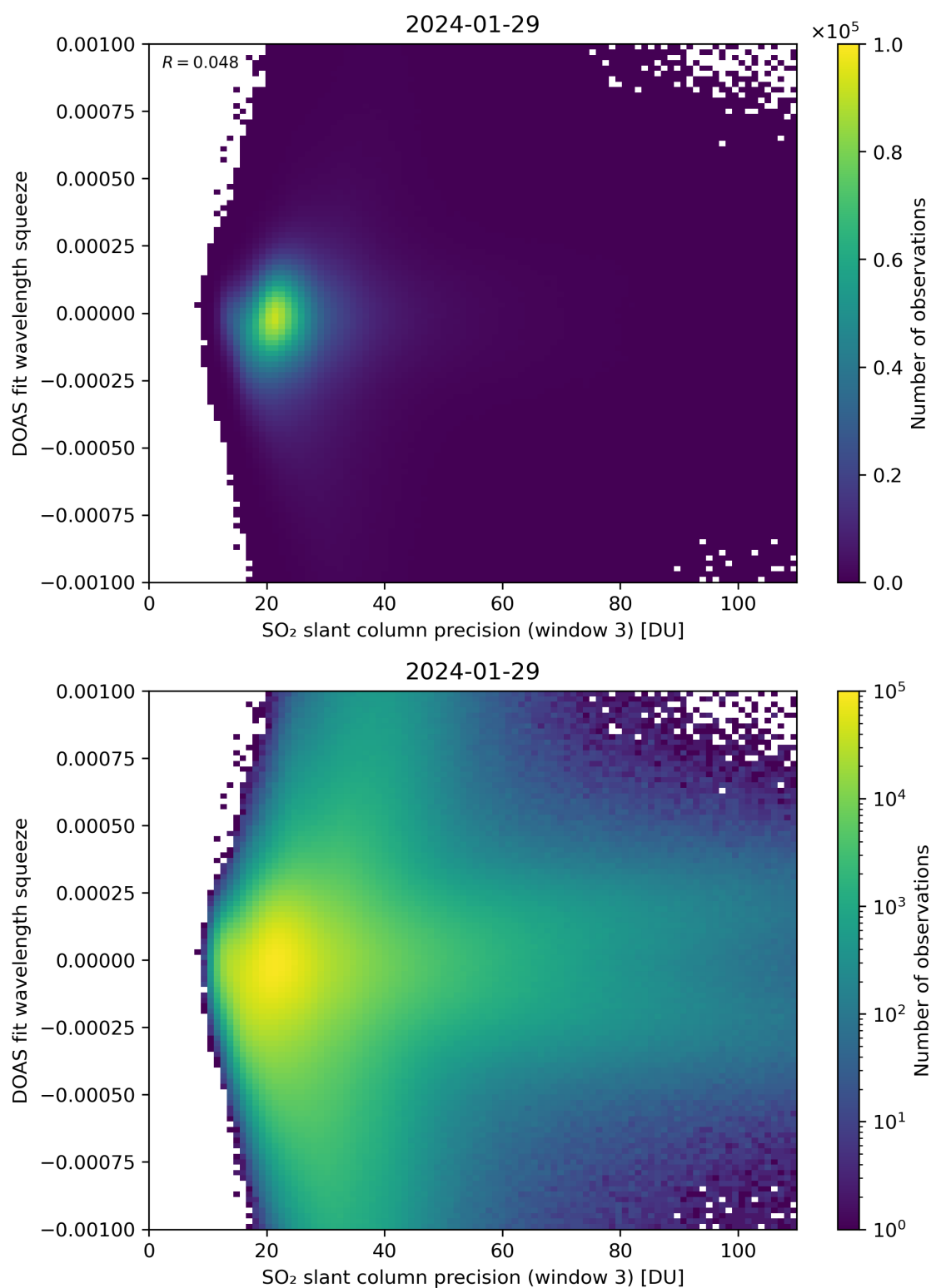
Figure 259: Scatter density plot of “SO 2 slant column precision (window 3)” against “DOAS fit wavelength squeeze” for 2024-01-28 to 2024-01-30.
