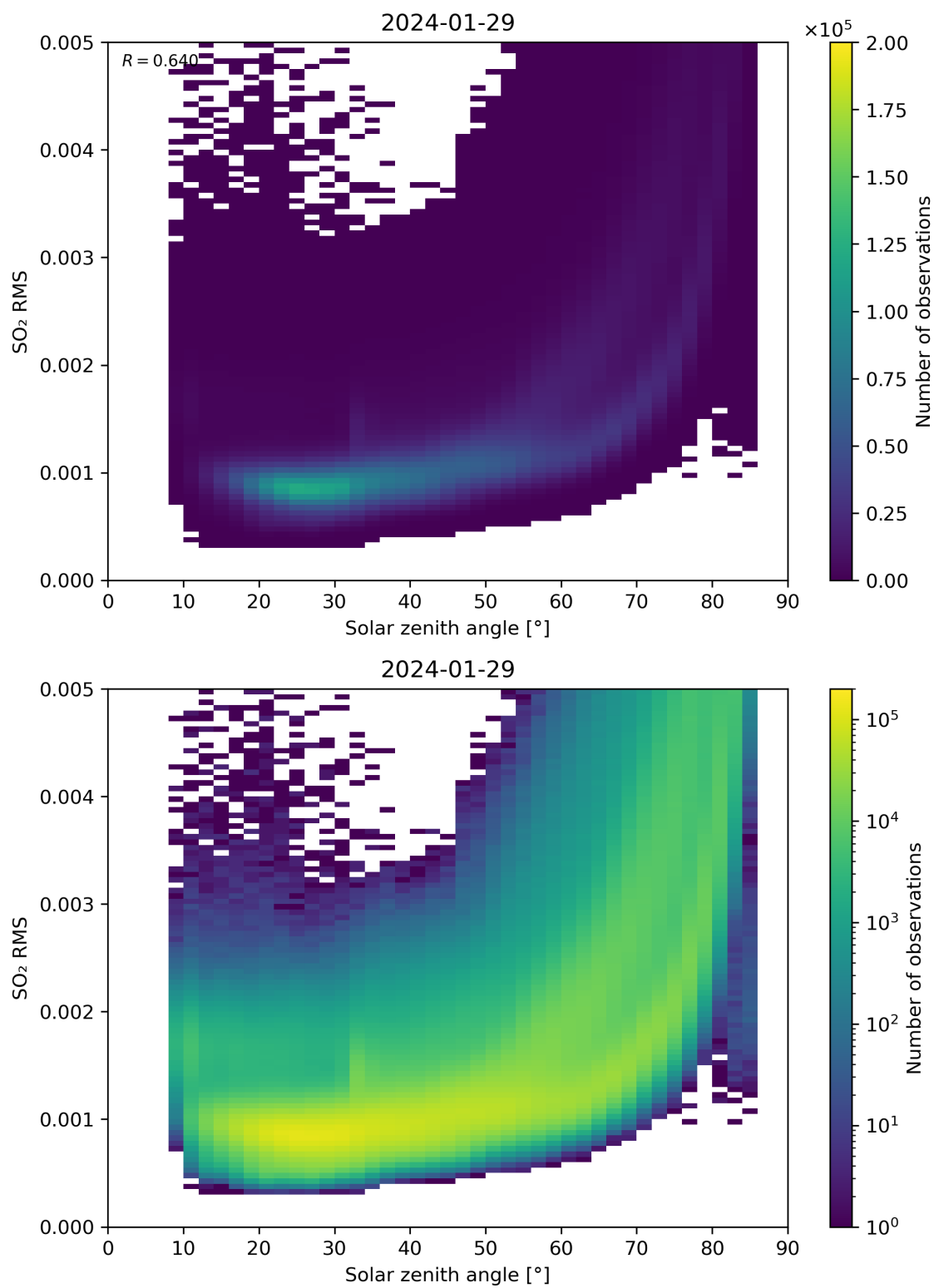
Figure 163: Scatter density plot of “Solar zenith angle” against “SO 2 RMS” for 2024-01-28 to 2024-01-30.
