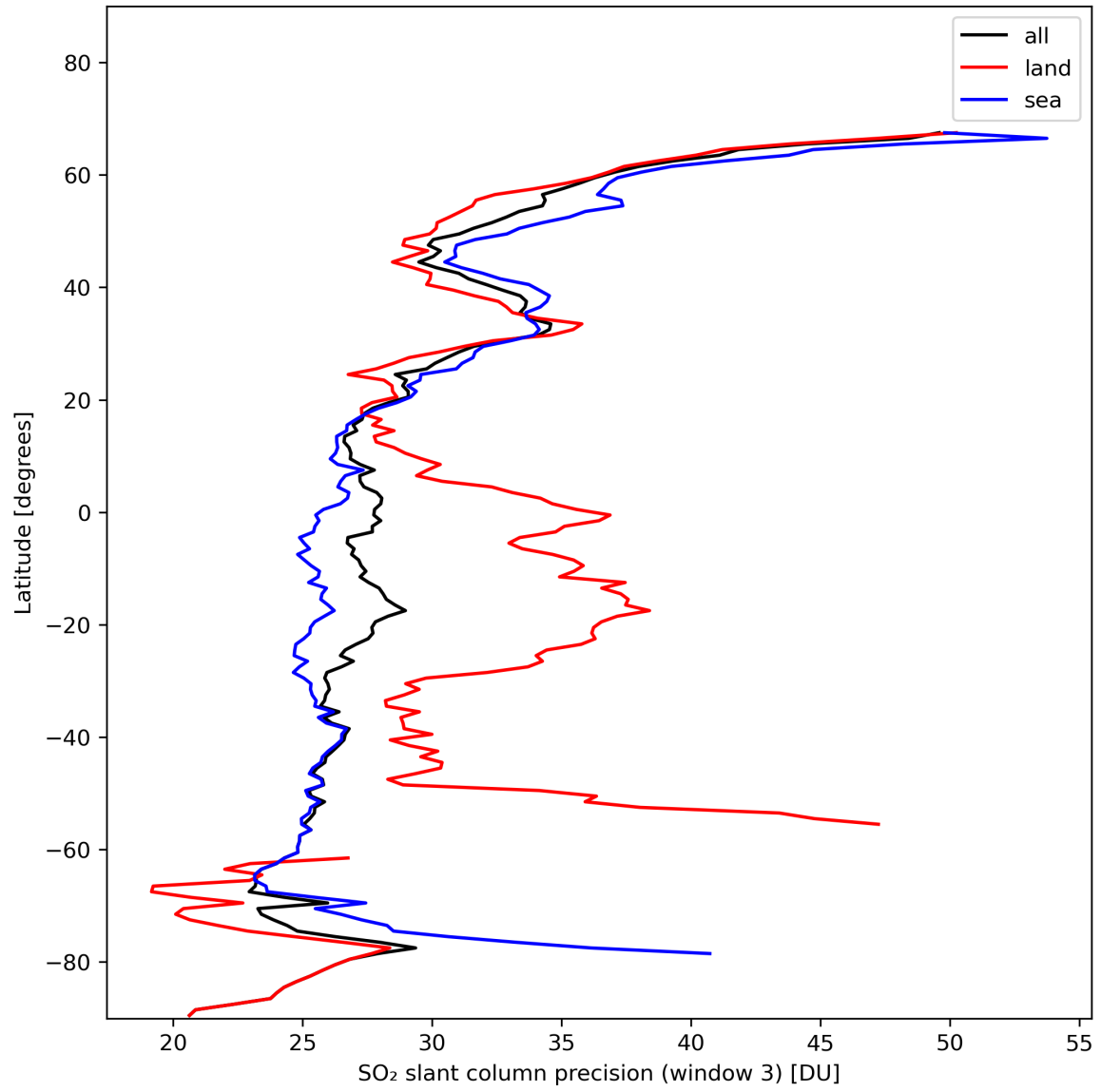
Figure 42: Zonal average of “SO 2 slant column precision (window 3)” for 2024-01-28 to 2024-01-30.
