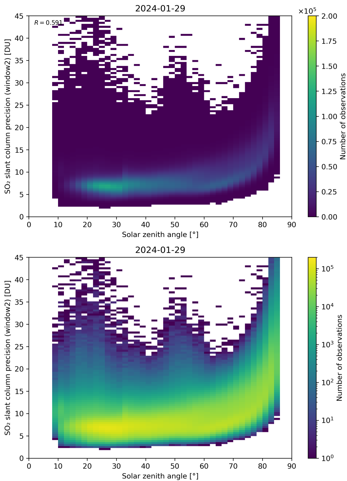
Figure 171: Scatter density plot of “Solar zenith angle” against “SO 2 slant column precision (window2)” for 2024-01-28 to 2024-01-30.
