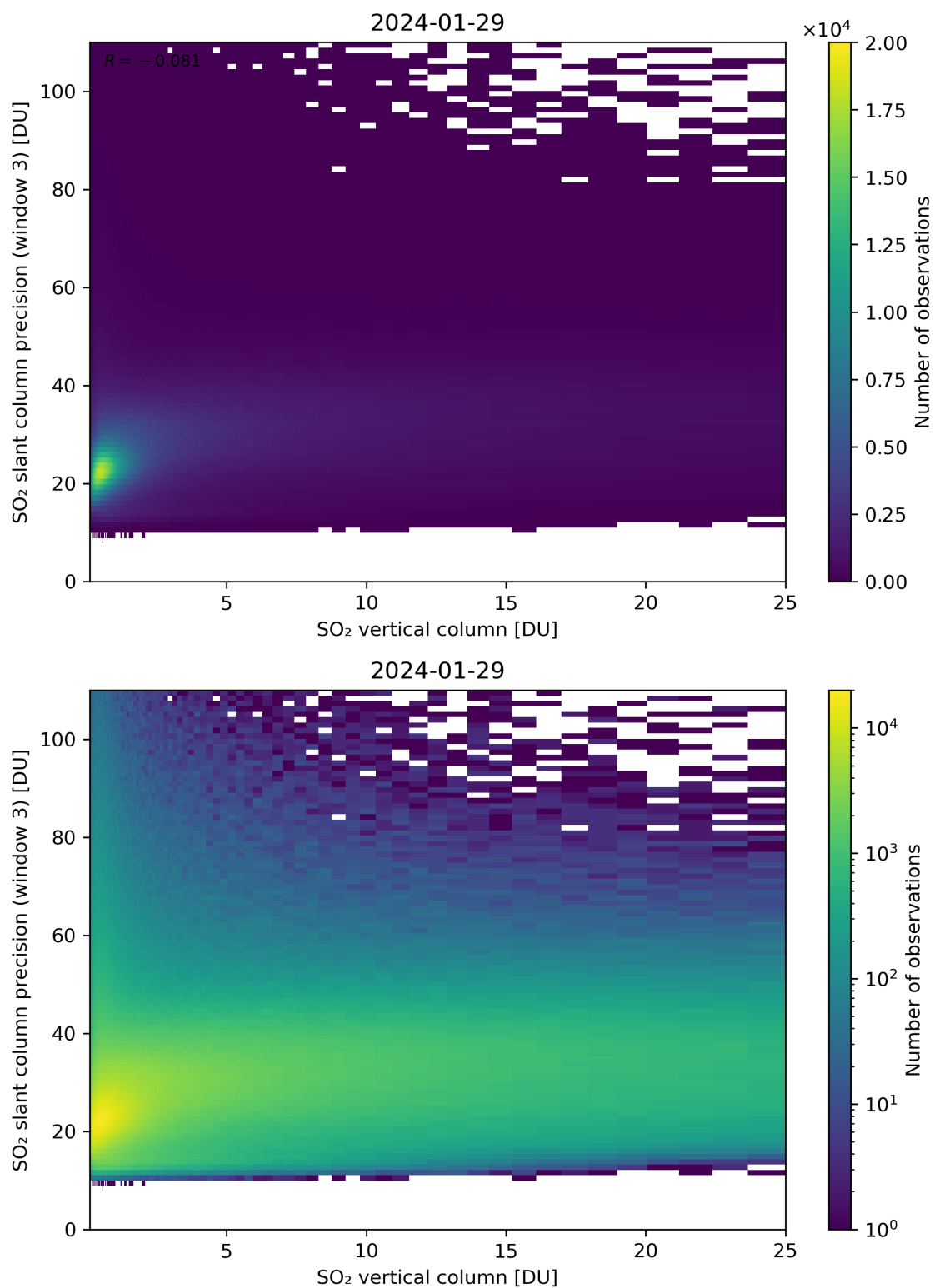
Figure 304: Scatter density plot of “SO 2 vertical column” against “SO 2 slant column precision (window 3)” for 2024-01-28 to 2024-01-30.
