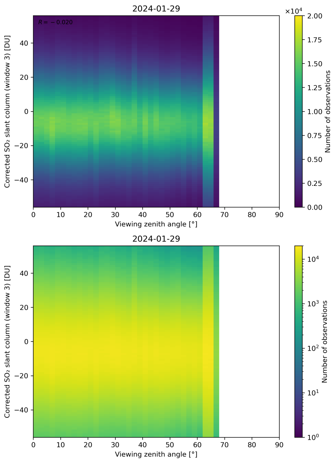
Figure 319: Scatter density plot of “Viewing zenith angle” against “Corrected SO 2 slant column (window 3)” for 2024-01-28 to 2024-01-30.
