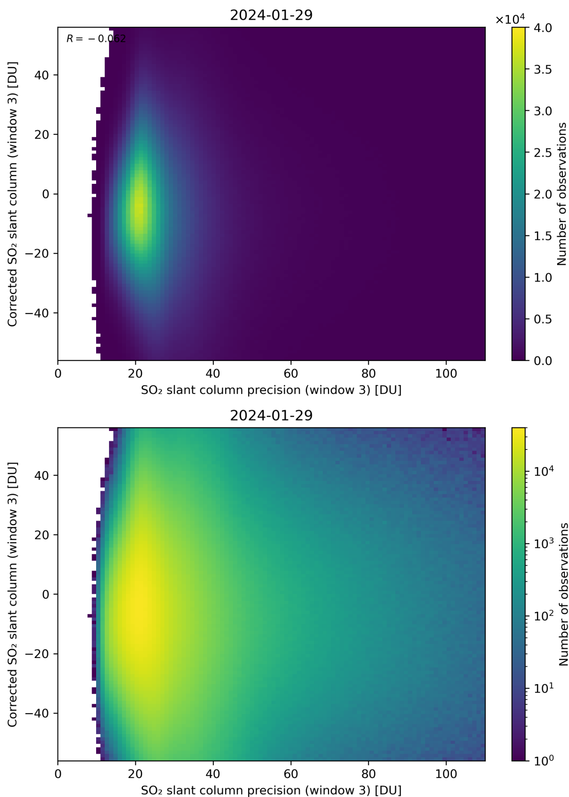
Figure 262: Scatter density plot of “SO 2 slant column precision (window 3)” against “Corrected SO 2 slant column (window 3)” for 2024-01-28 to 2024-01-30.
