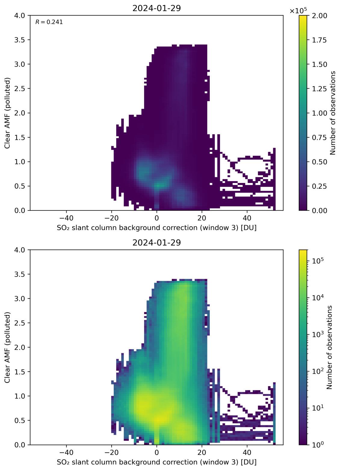
Figure 124: Scatter density plot of “SO 2 slant column background correction (window 3)” against “Clear AMF (polluted)” for 2024-01-28 to 2024-01-30.
