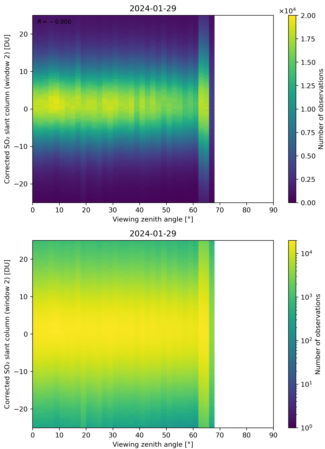
Figure 318: Scatter density plot of “Viewing zenith angle” against “Corrected SO 2 slant column (window 2)” for 2024-01-28 to 2024-01-30.
