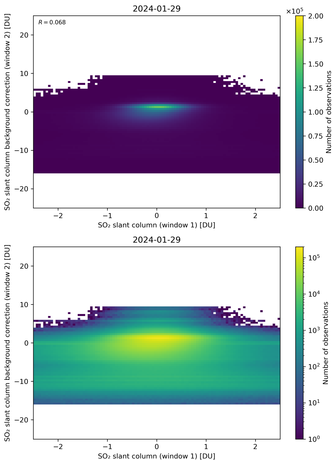
Figure 213: Scatter density plot of “SO 2 slant column (window 1)” against “SO 2 slant column background correction (window 2)” for 2024-01-28 to 2024-01-30.
