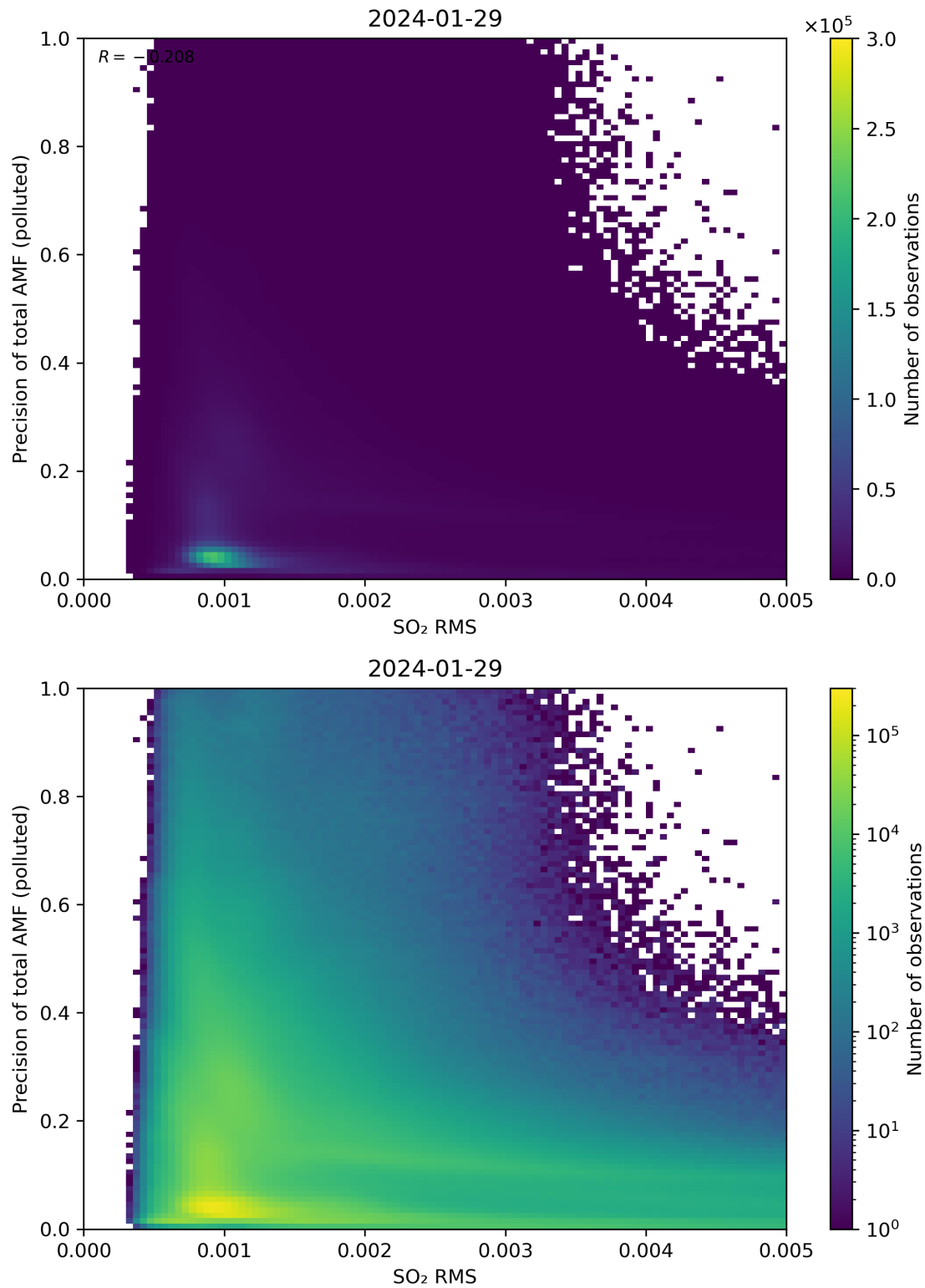
Figure 138: Scatter density plot of “SO 2 RMS” against “Precision of total AMF (polluted)” for 2024-01-28 to 2024-01-30.
