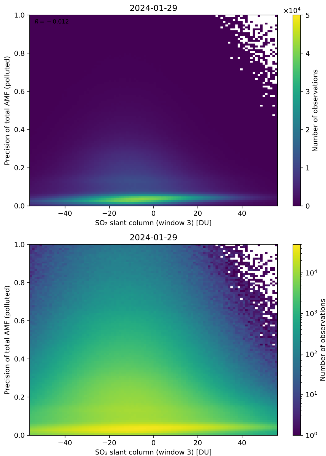
Figure 269: Scatter density plot of “SO 2 slant column (window 3)” against “Precision of total AMF (polluted)” for 2024-01-28 to 2024-01-30.
