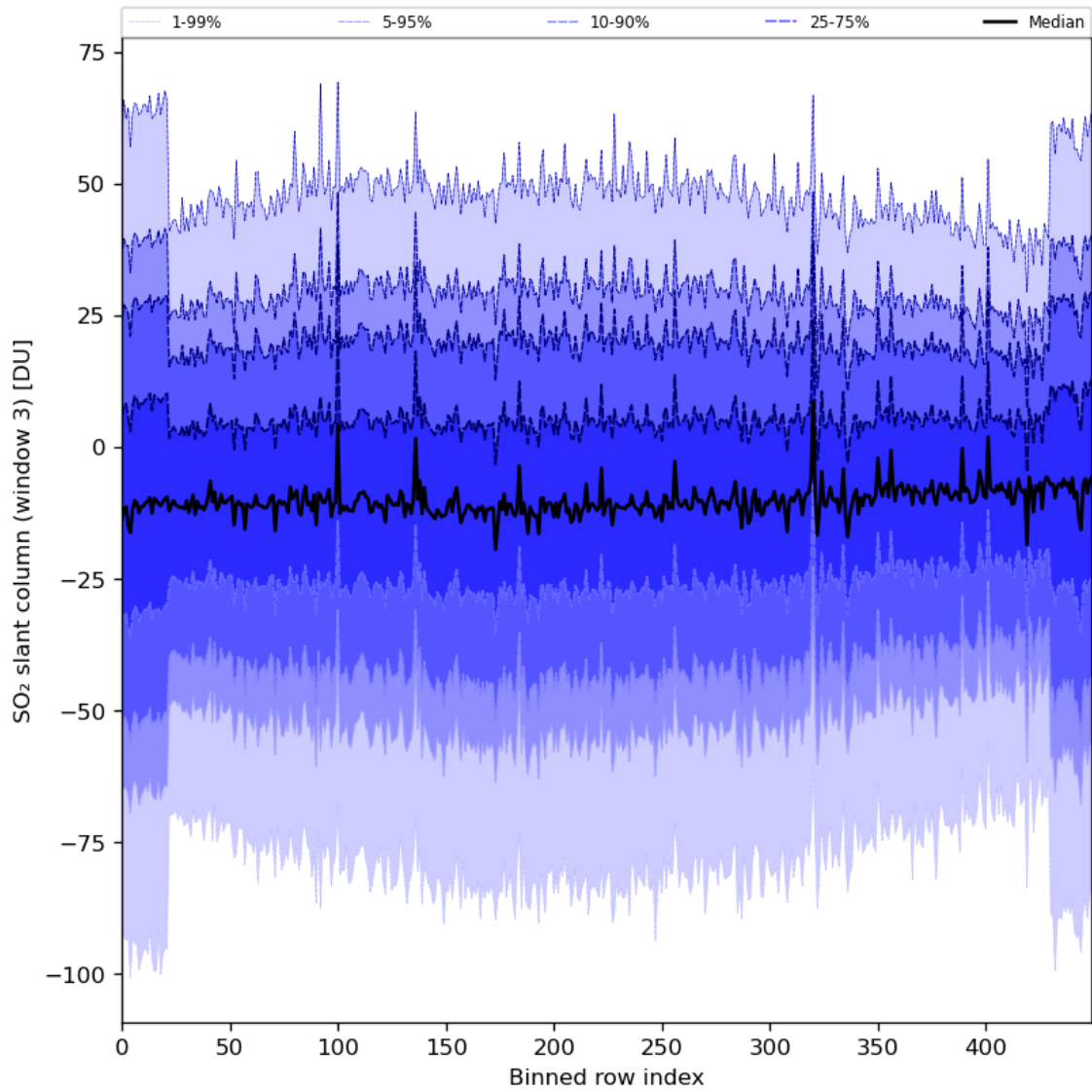
Figure 87: Along track statistics of “SO 2 slant column (window 3)” for 2024-01-28 to 2024-01-30
