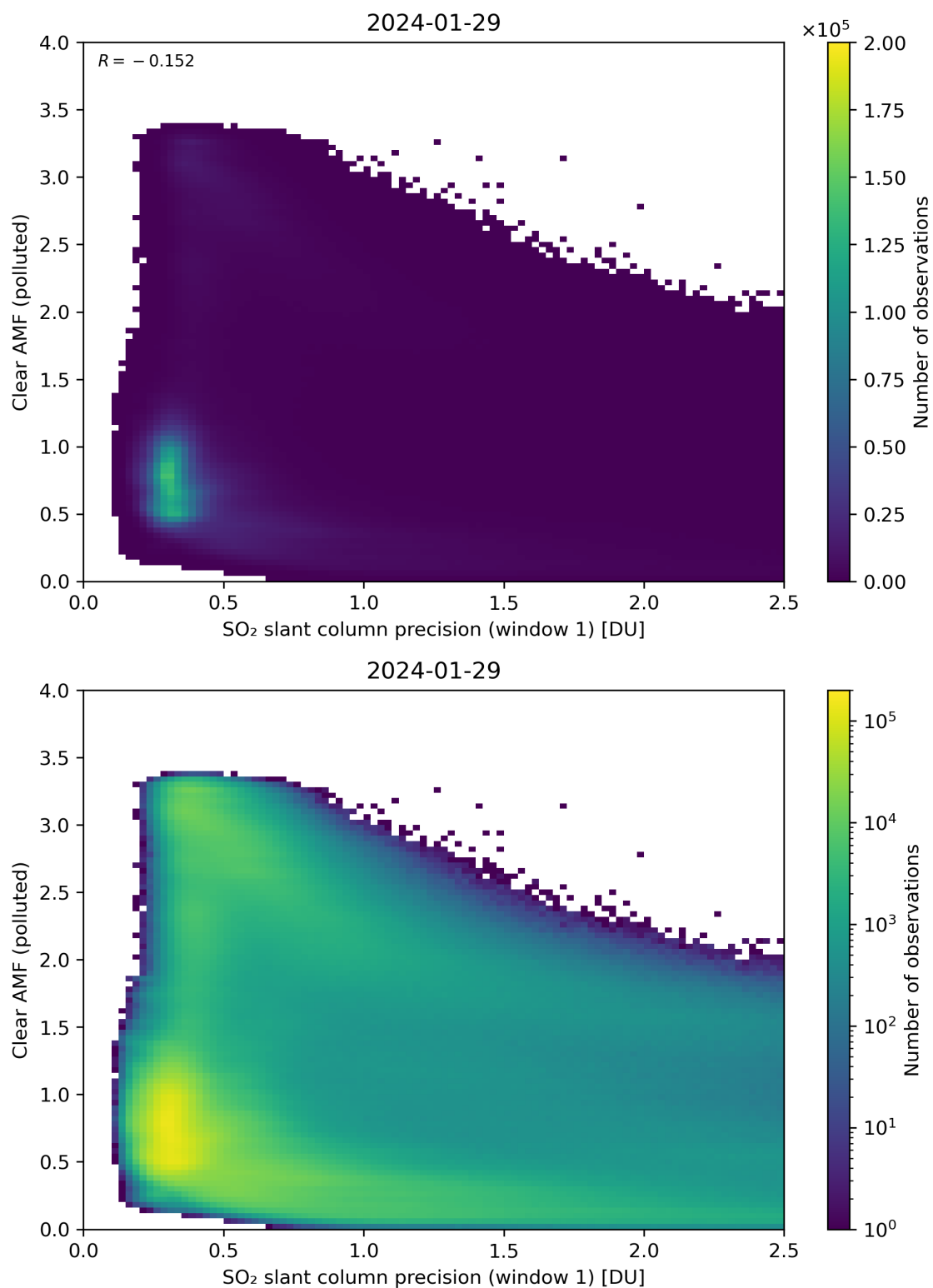
Figure 224: Scatter density plot of “SO 2 slant column precision (window 1)” against “Clear AMF (polluted)” for 2024-01-28 to 2024-01-30.
