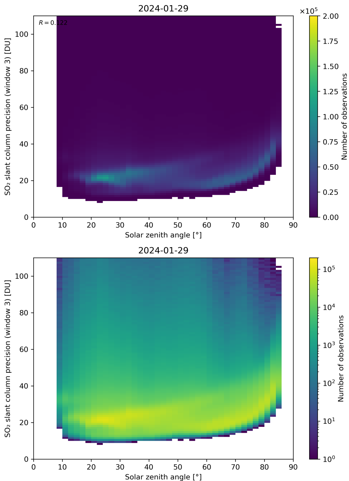
Figure 173: Scatter density plot of “Solar zenith angle” against “SO 2 slant column precision (window 3)” for 2024-01-28 to 2024-01-30.
