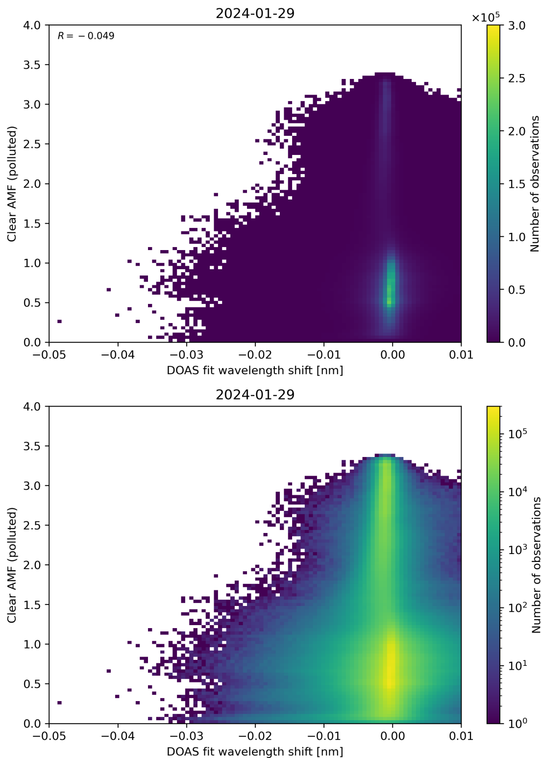
Figure 129: Scatter density plot of “DOAS fit wavelength shift” against “Clear AMF (polluted)” for 2024-01-28 to 2024-01-30.
