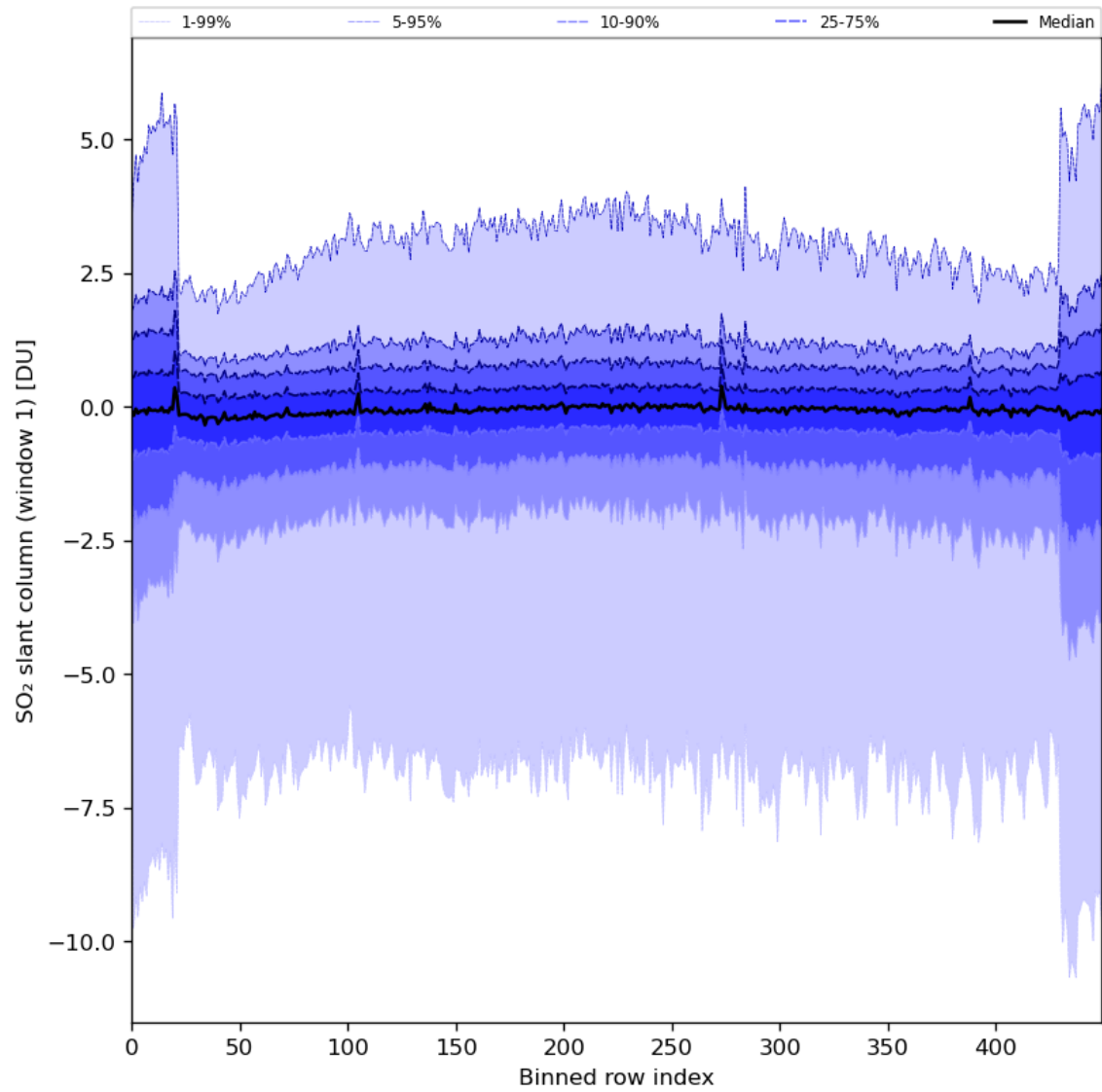
Figure 79: Along track statistics of “SO 2 slant column (window 1)” for 2024-01-28 to 2024-01-30
