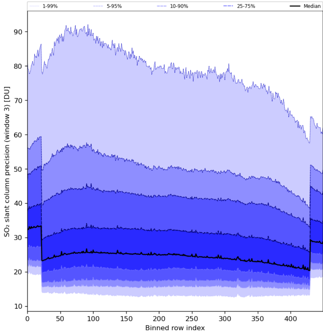
Figure 88: Along track statistics of “SO 2 slant column precision (window 3)” for 2024-01-28 to 2024-01-30
