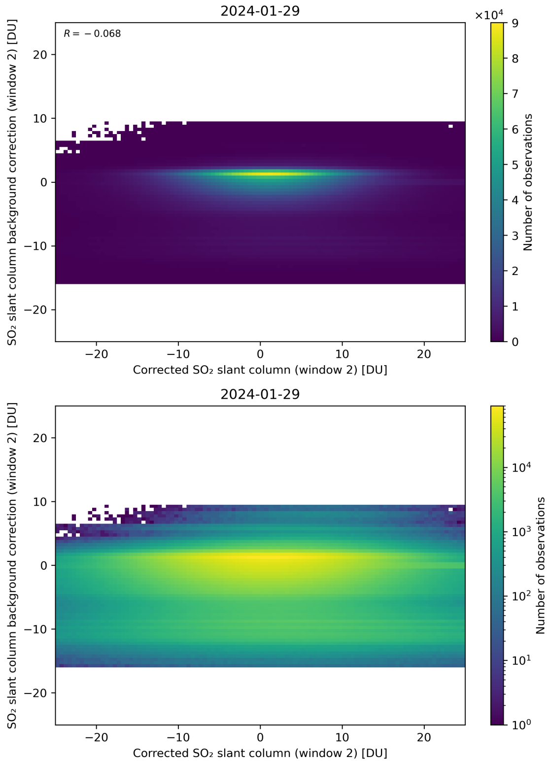
Figure 194: Scatter density plot of “Corrected SO 2 slant column (window 2)” against “SO 2 slant column background correction (window 2)” for 2024-01-28 to 2024-01-30.
