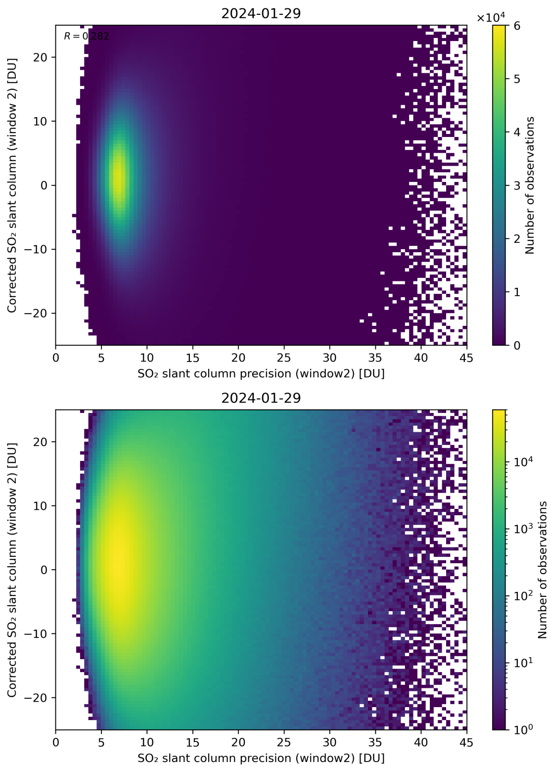
Figure 247: Scatter density plot of “SO 2 slant column precision (window2)” against “Corrected SO 2 slant column (window 2)” for 2024-01-28 to 2024-01-30.
