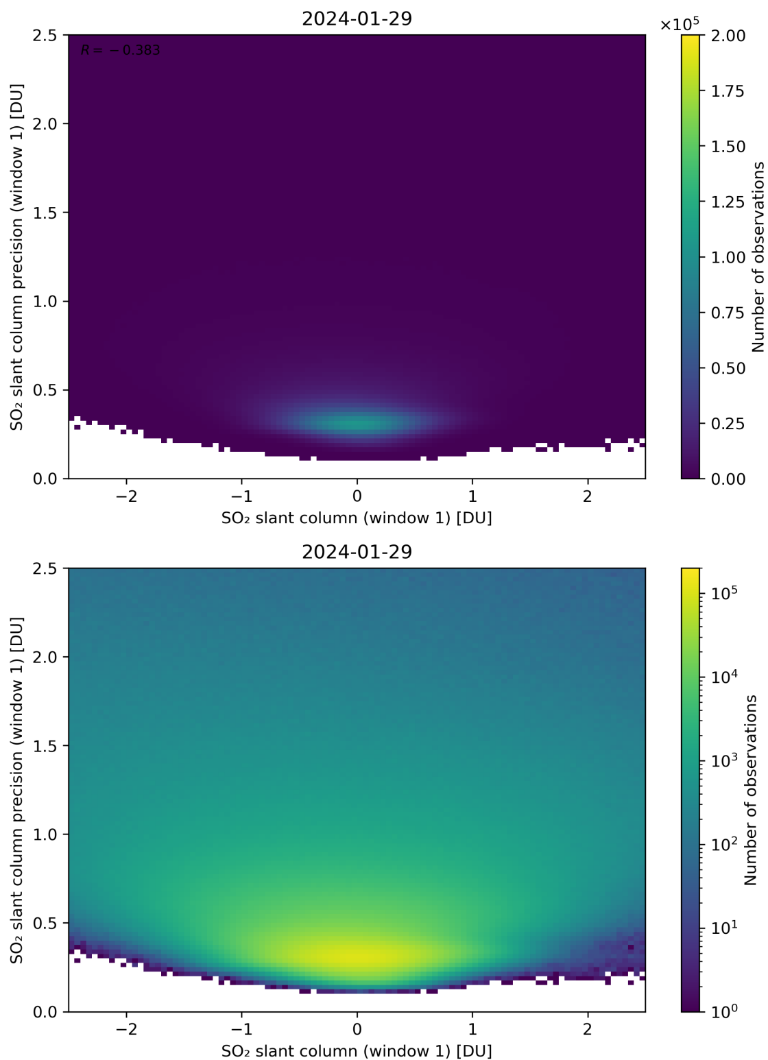
Figure 235: Scatter density plot of “SO 2 slant column (window 1)” against “SO 2 slant column precision (window 1)” for 2024-01-28 to 2024-01-30.
