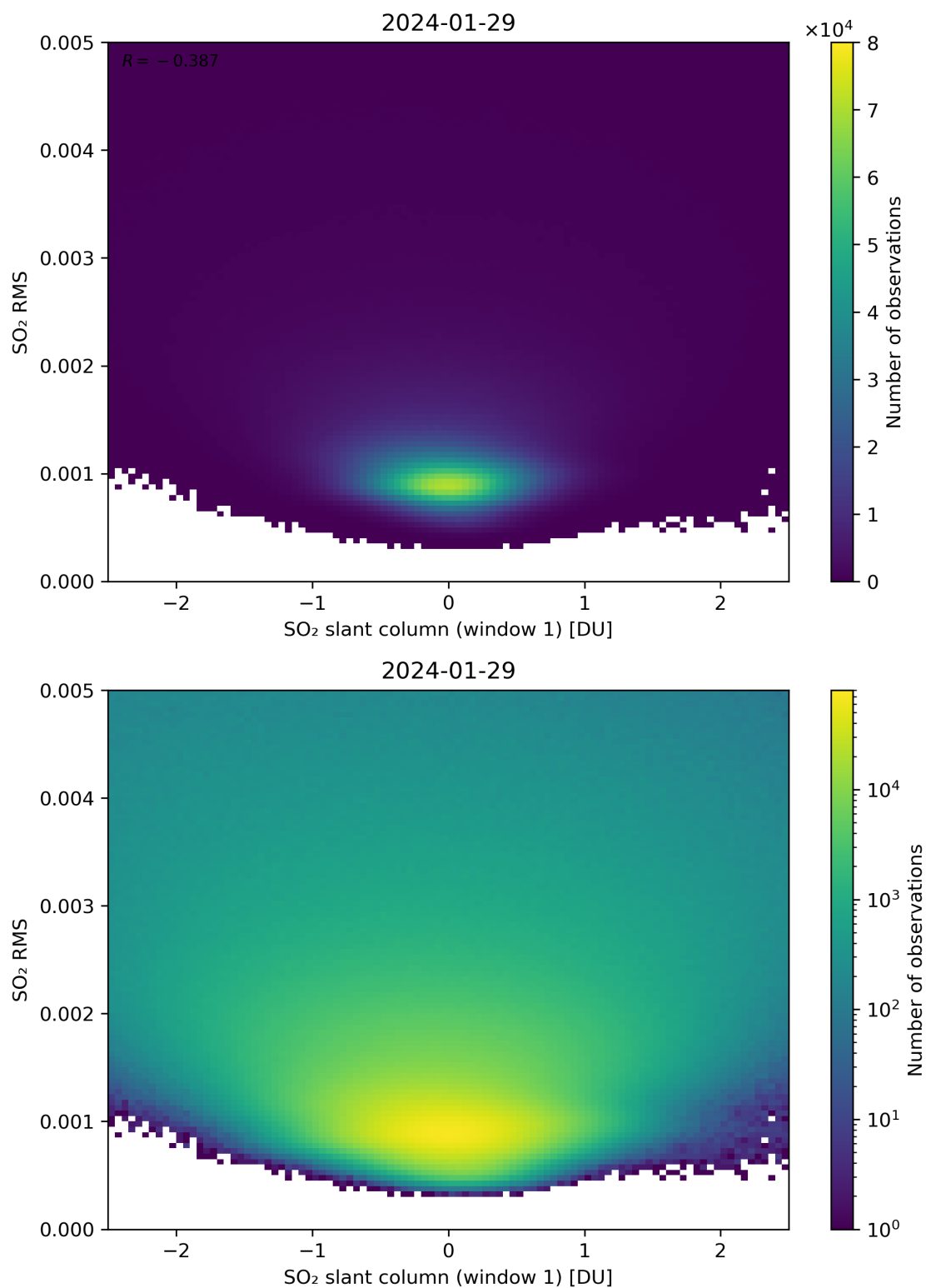
Figure 217: Scatter density plot of “SO 2 slant column (window 1)” against “SO 2 RMS” for 2024-01-28 to 2024-01-30.
