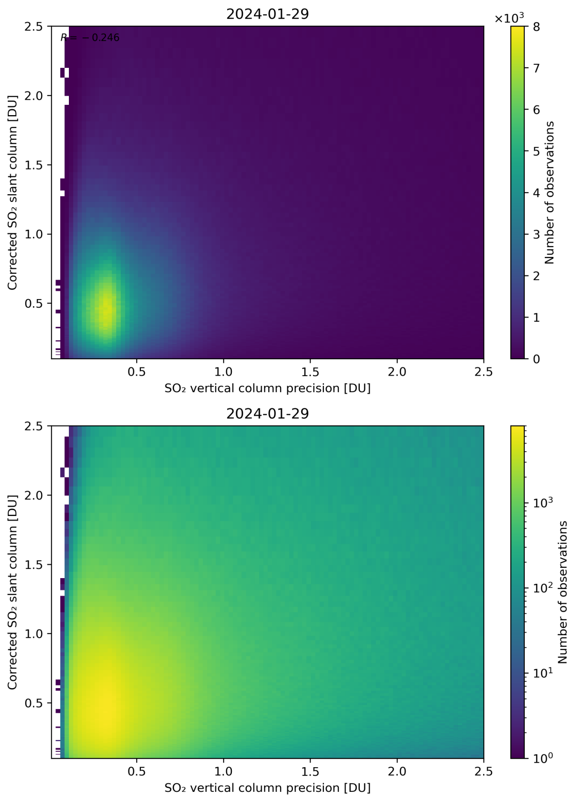
Figure 286: Scatter density plot of “SO 2 vertical column precision” against “Corrected SO 2 slant column” for 2024-01-28 to 2024-01-30.
