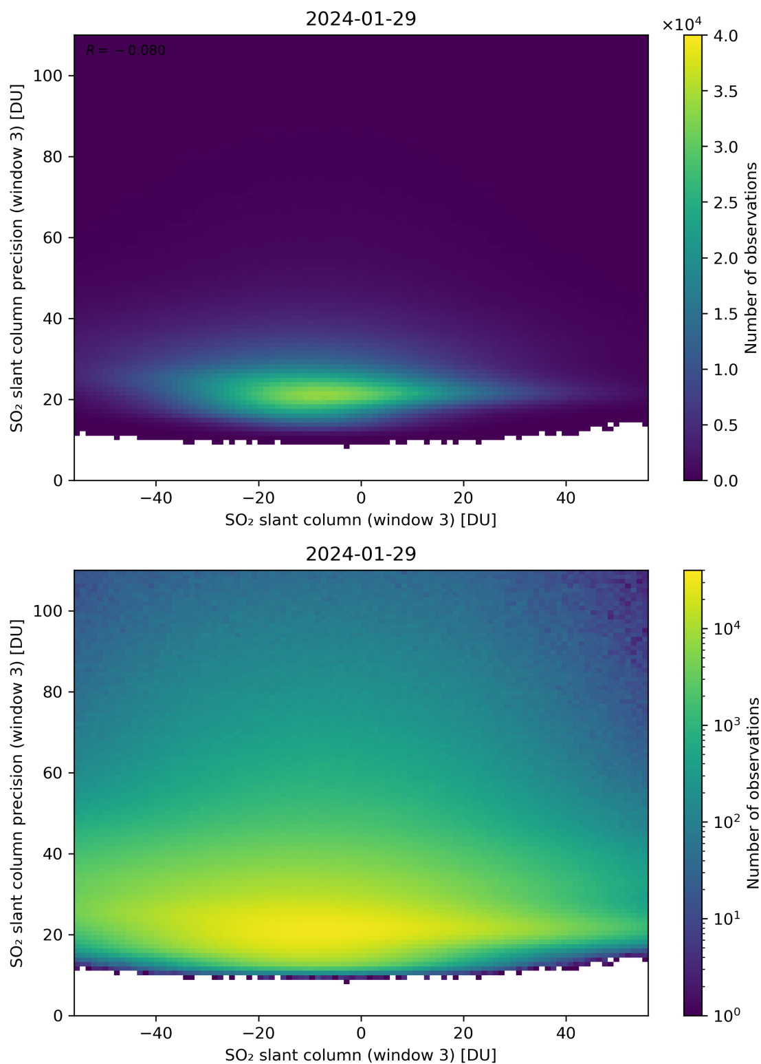
Figure 267: Scatter density plot of “SO 2 slant column (window 3)” against “SO 2 slant column precision (window 3)” for 2024-01-28 to 2024-01-30.
