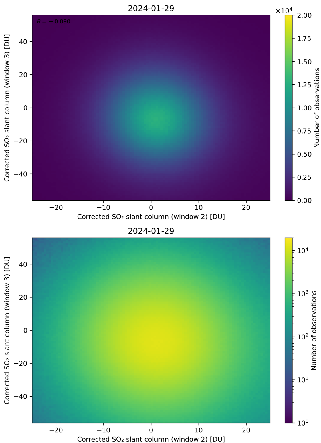
Figure 200: Scatter density plot of “Corrected SO 2 slant column (window 2)” against “Corrected SO 2 slant column (window 3)” for 2024-01-28 to 2024-01-30.
