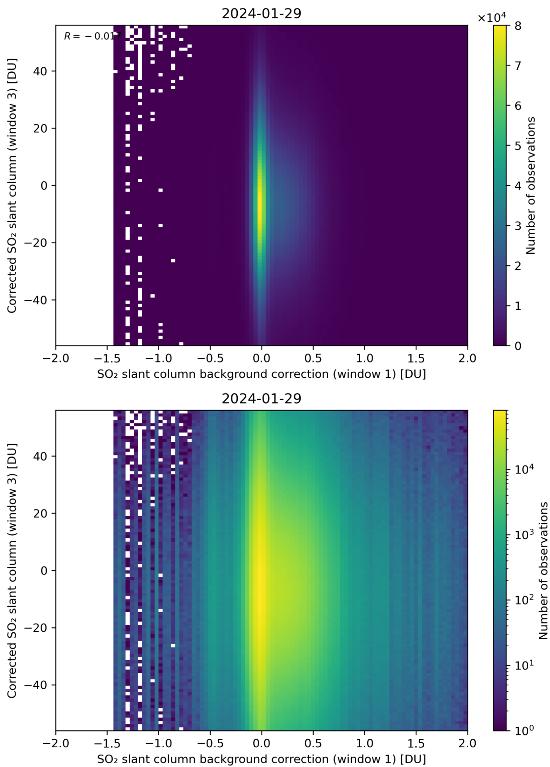
Figure 105: Scatter density plot of “SO 2 slant column background correction (window 1)” against “Corrected SO 2 slant column (window 3)” for 2024-01-28 to 2024-01-30.
