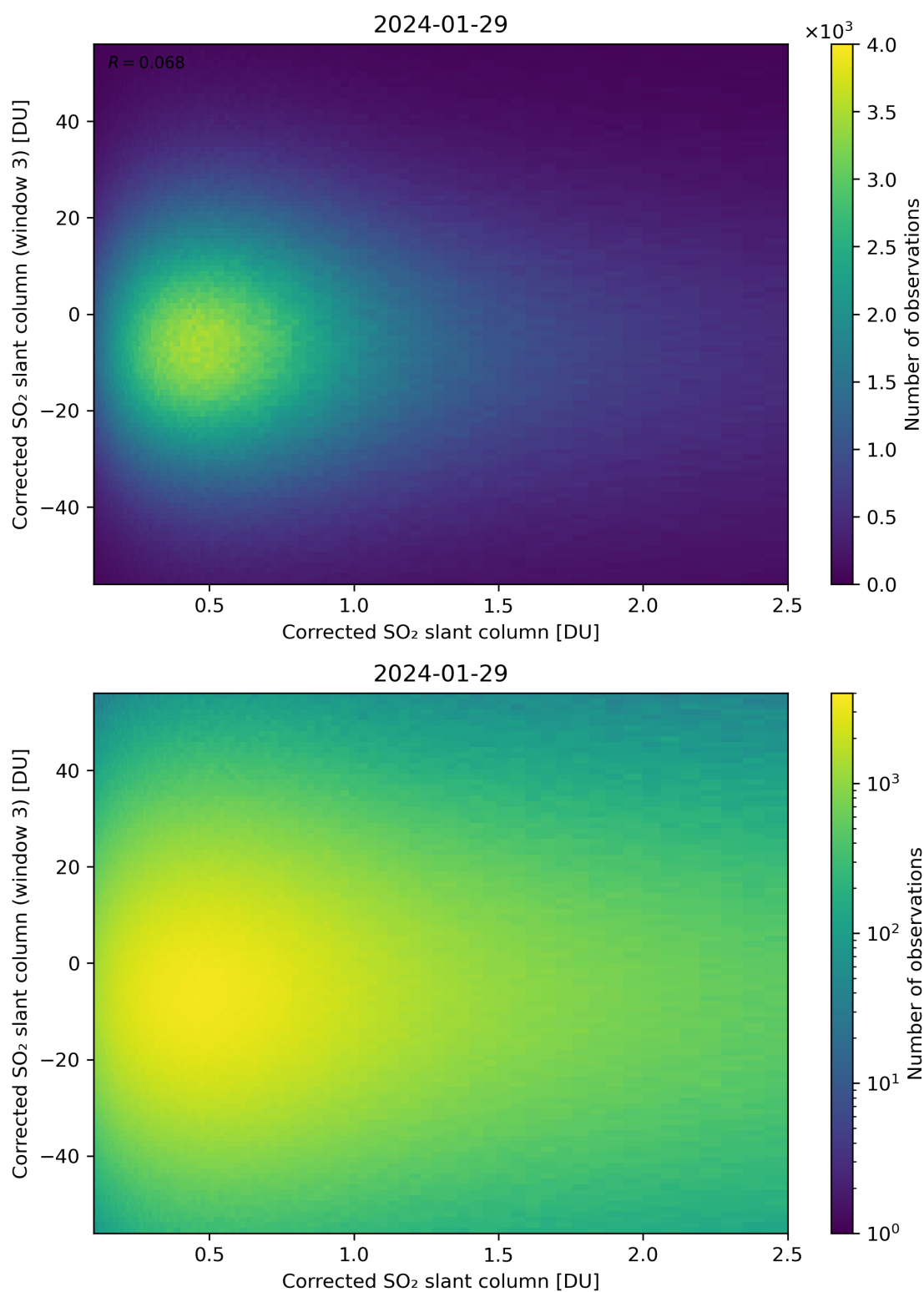
Figure 186: Scatter density plot of “Corrected SO 2 slant column” against “Corrected SO 2 slant column (window 3)” for 2024-01-28 to 2024-01-30.
