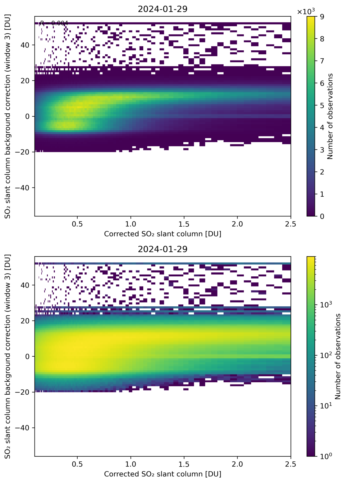
Figure 180: Scatter density plot of “Corrected SO 2 slant column” against “SO 2 slant column background correction (window 3)” for 2024-01-28 to 2024-01-30.
