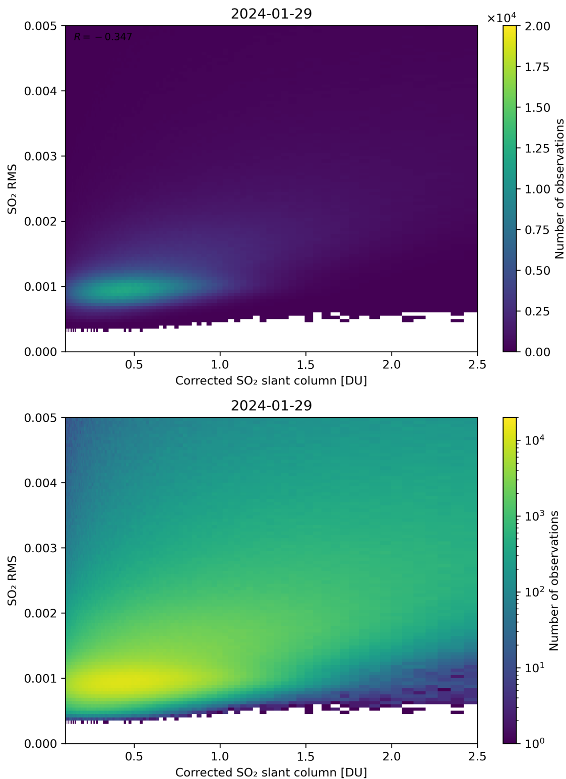
Figure 183: Scatter density plot of “Corrected SO 2 slant column” against “SO 2 RMS” for 2024-01-28 to 2024-01-30.
