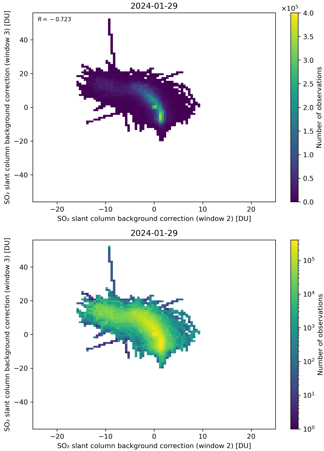
Figure 111: Scatter density plot of “SO 2 slant column background correction (window 2)” against “SO 2 slant column background correction (window 3)” for 2024-01-28 to 2024-01-30.
