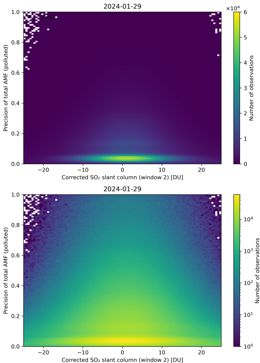
Figure 204: Scatter density plot of “Corrected SO 2 slant column (window 2)” against “Precision of total AMF (polluted)” for 2024-01-28 to 2024-01-30.
