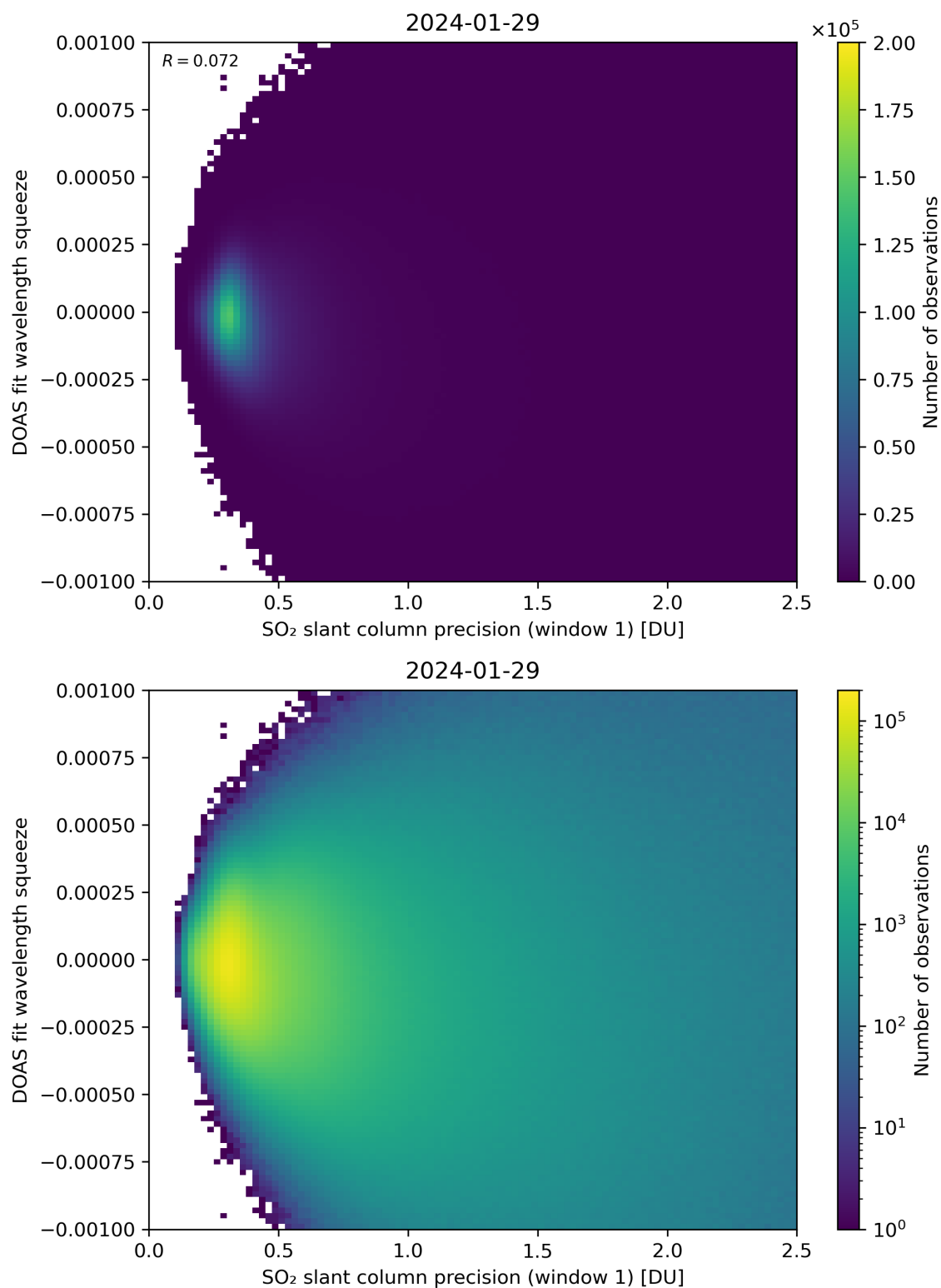
Figure 222: Scatter density plot of “SO 2 slant column precision (window 1)” against “DOAS fit wavelength squeeze” for 2024-01-28 to 2024-01-30.
