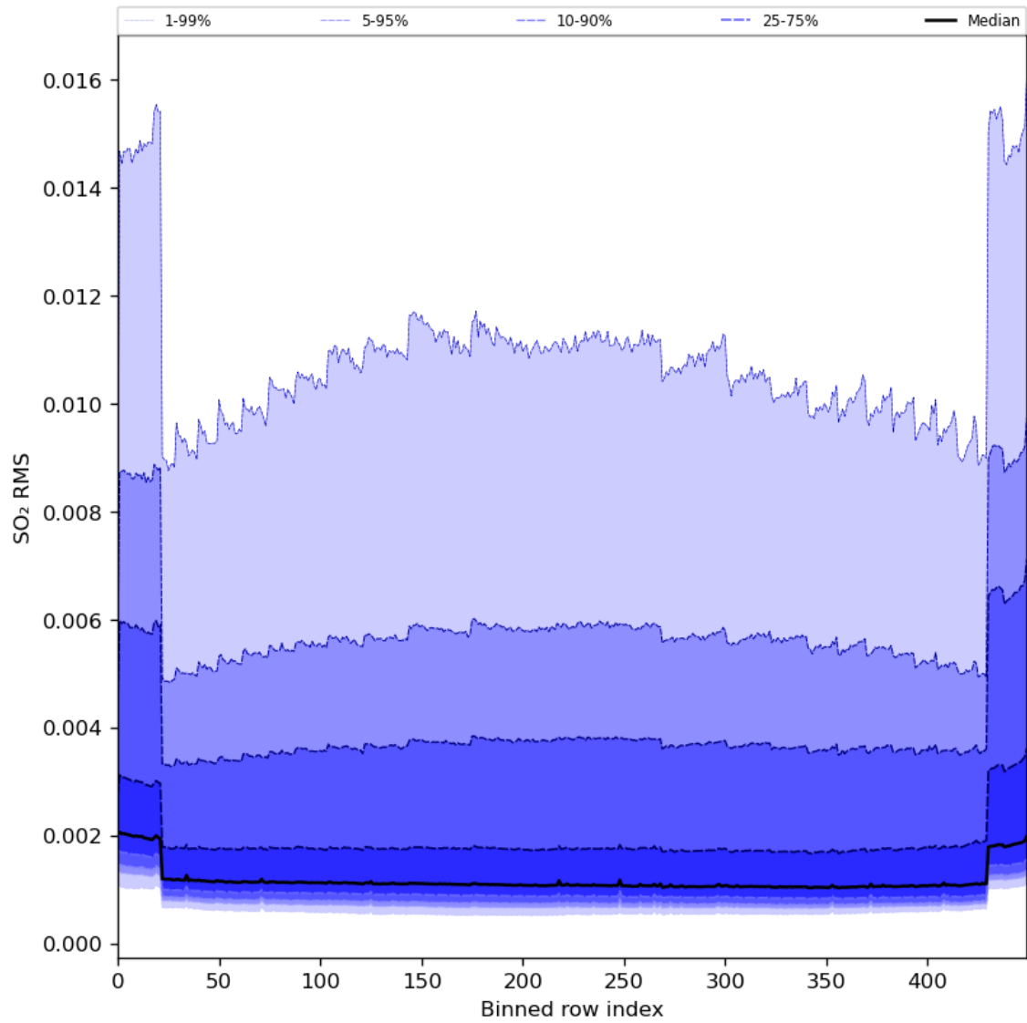
Figure 93: Along track statistics of “SO 2 RMS” for 2024-01-28 to 2024-01-30
