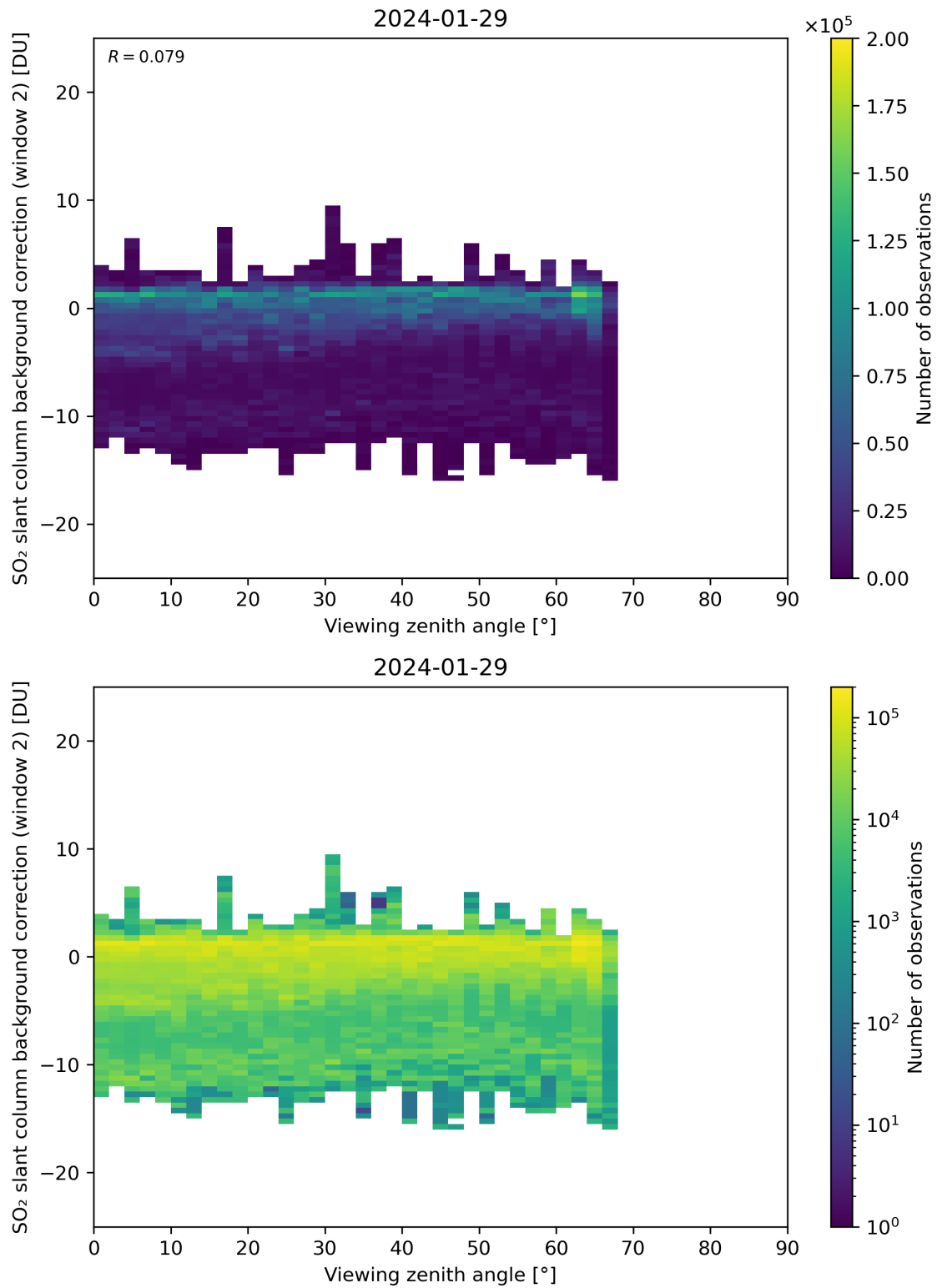
Figure 309: Scatter density plot of “Viewing zenith angle” against “SO 2 slant column background correction (window 2)” for 2024-01-28 to 2024-01-30.
