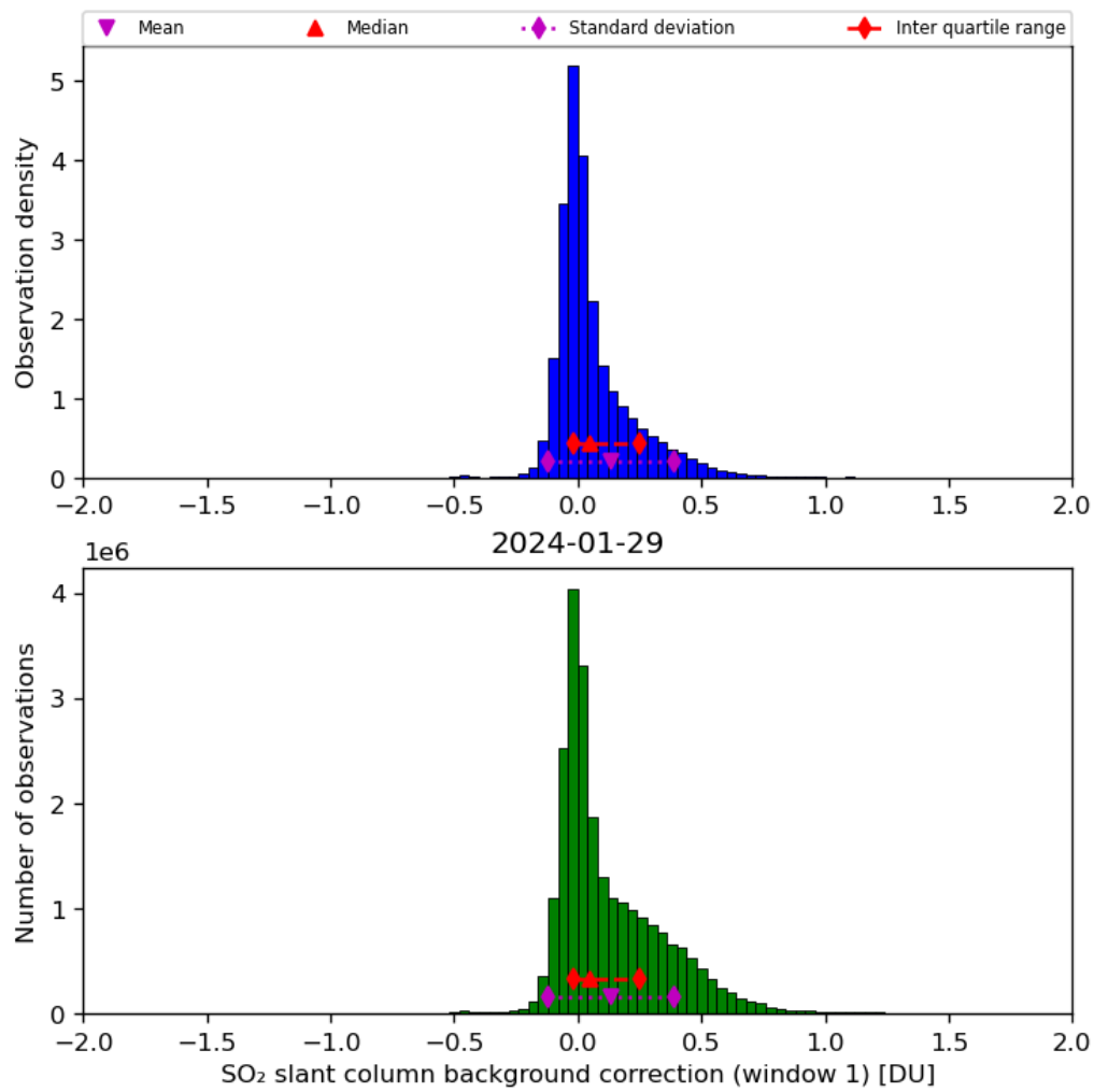
Figure 59: Histogram of “SO 2 slant column background correction (window 1)” for 2024-01-28 to 2024-01-30
