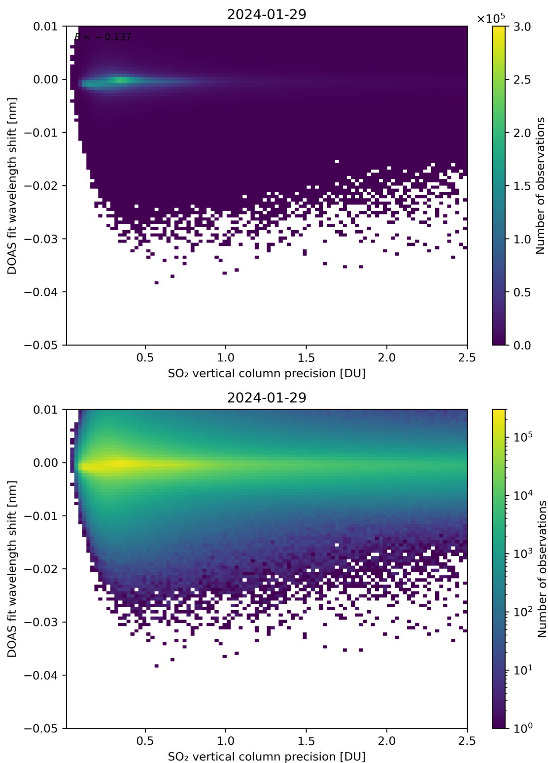
Figure 282: Scatter density plot of “SO 2 vertical column precision” against “DOAS fit wavelength shift” for 2024-01-28 to 2024-01-30.
