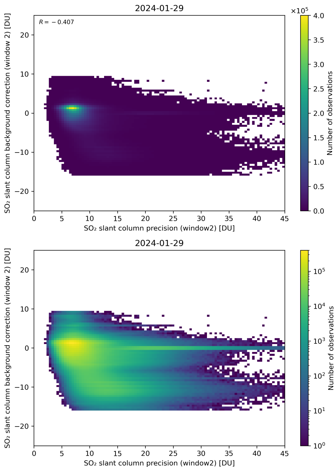
Figure 241: Scatter density plot of “SO 2 slant column precision (window2)” against “SO 2 slant column background correction (window 2)” for 2024-01-28 to 2024-01-30.
