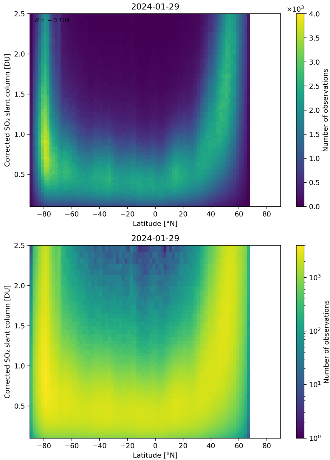
Figure 146: Scatter density plot of “Latitude” against “Corrected SO 2 slant column” for 2024-01-28 to 2024-01-30.
