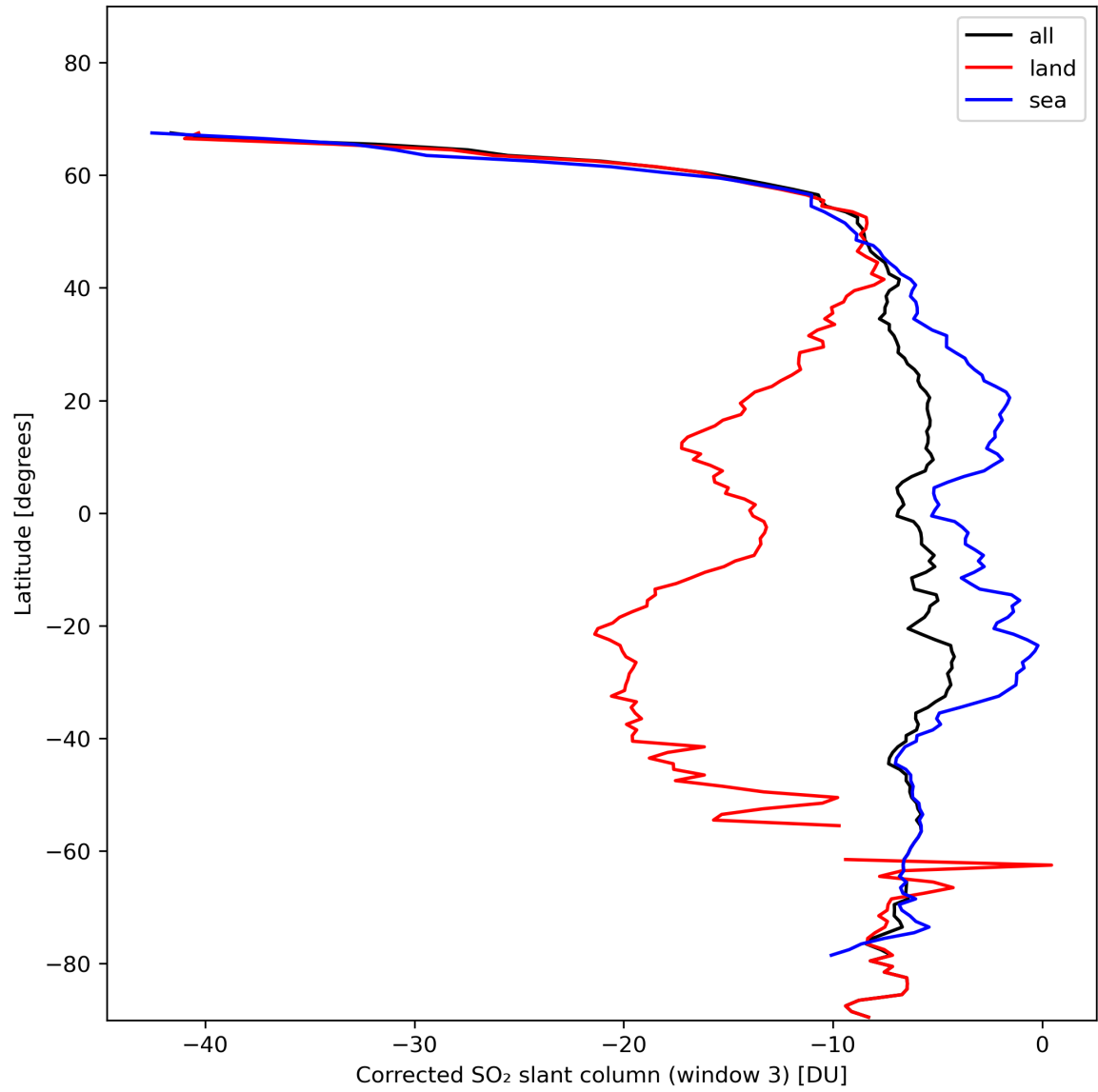
Figure 43: Zonal average of “Corrected SO 2 slant column (window 3)” for 2024-01-28 to 2024-01-30.
