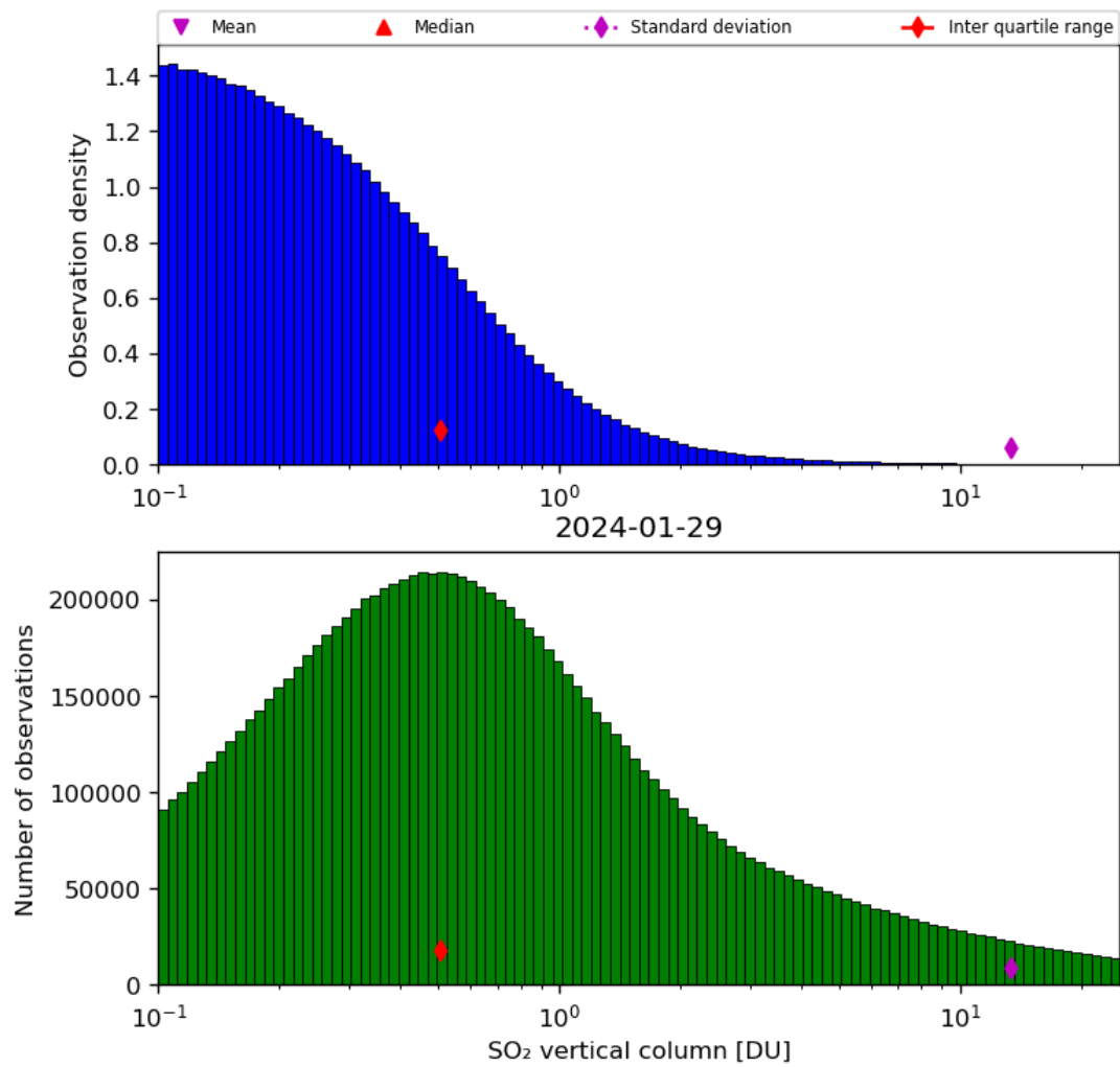
Figure 53: Histogram of “SO 2 vertical column” for 2024-01-28 to 2024-01-30
