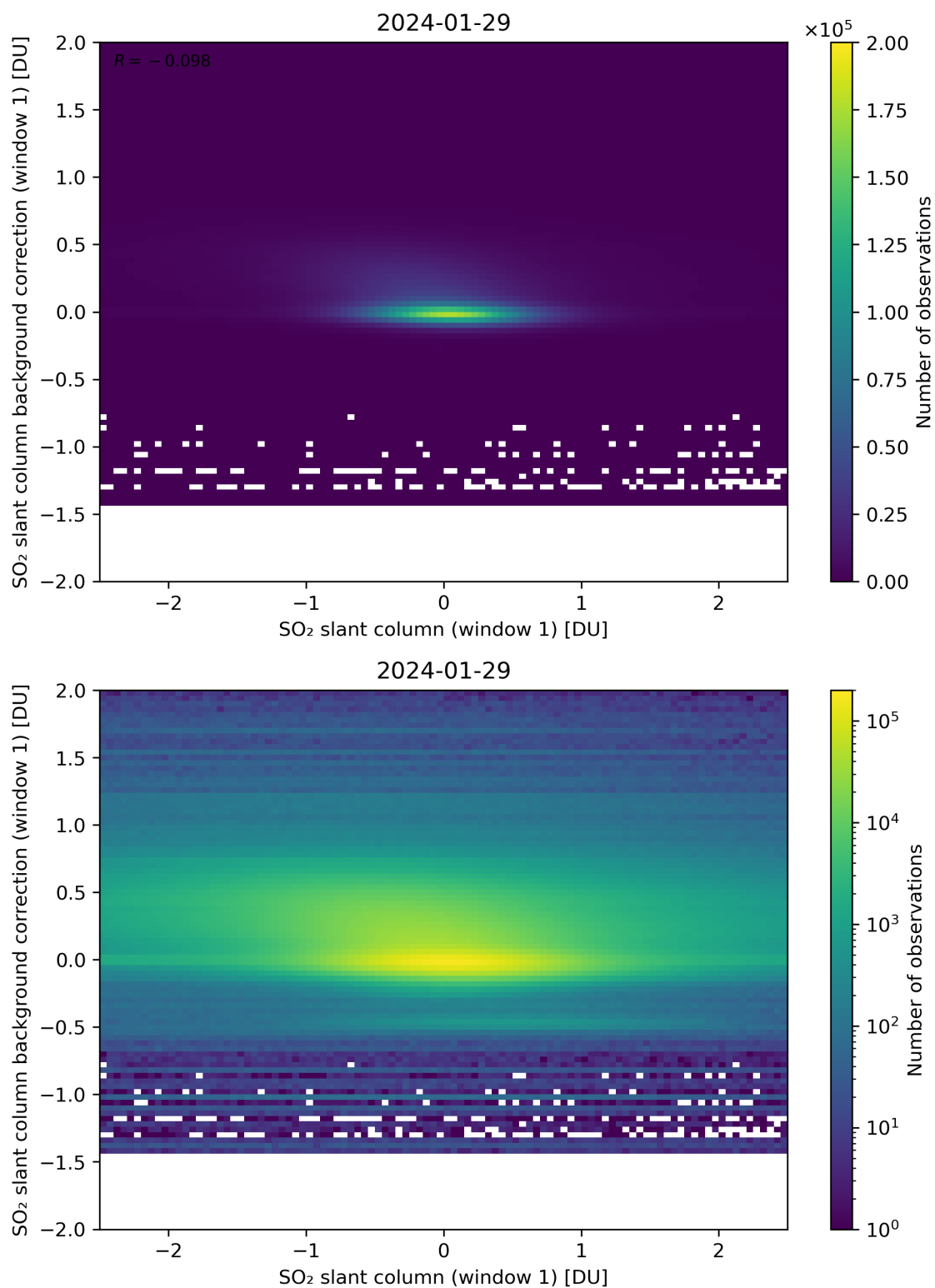
Figure 212: Scatter density plot of “SO 2 slant column (window 1)” against “SO 2 slant column background correction (window 1)” for 2024-01-28 to 2024-01-30.
