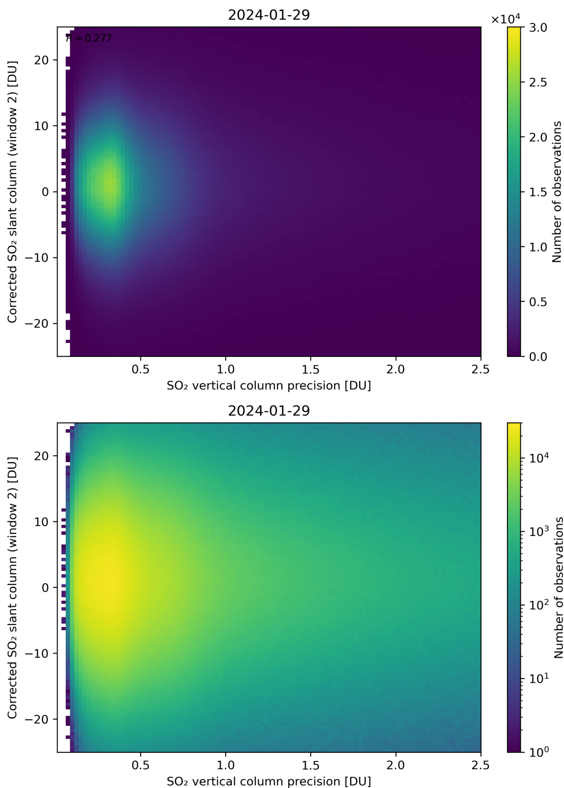
Figure 287: Scatter density plot of “SO 2 vertical column precision” against “Corrected SO 2 slant column (window 2)” for 2024-01-28 to 2024-01-30.
