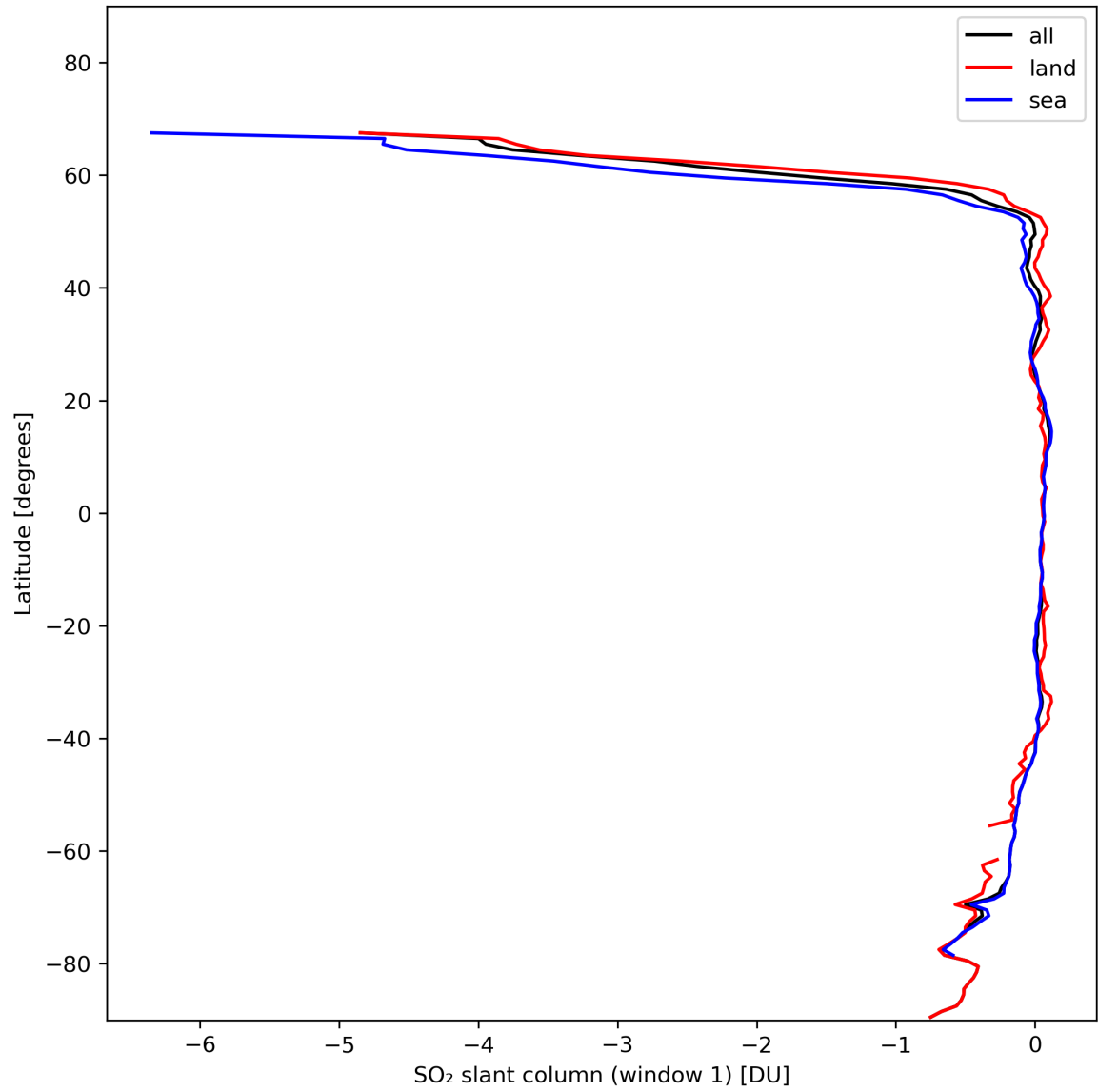
Figure 33: Zonal average of “SO 2 slant column (window 1)” for 2024-01-28 to 2024-01-30.
