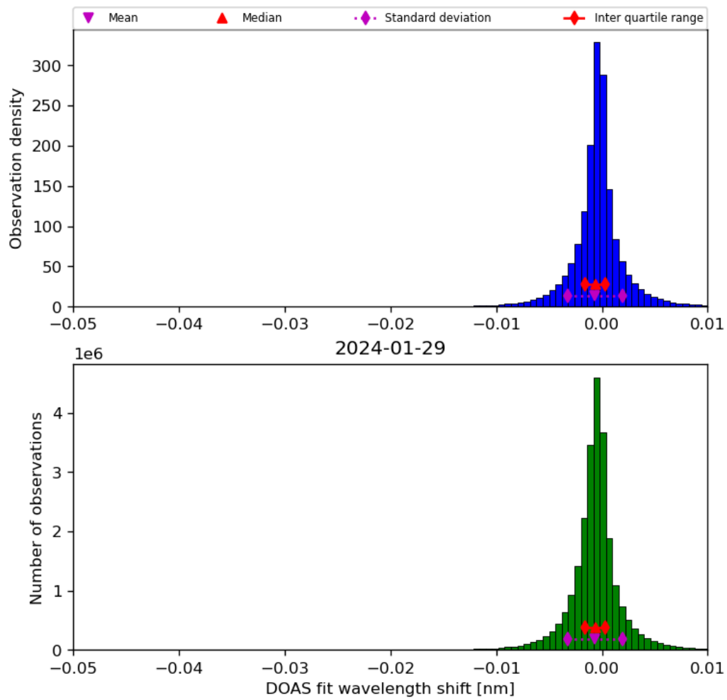
Figure 68: Histogram of “DOAS fit wavelength shift” for 2024-01-28 to 2024-01-30
