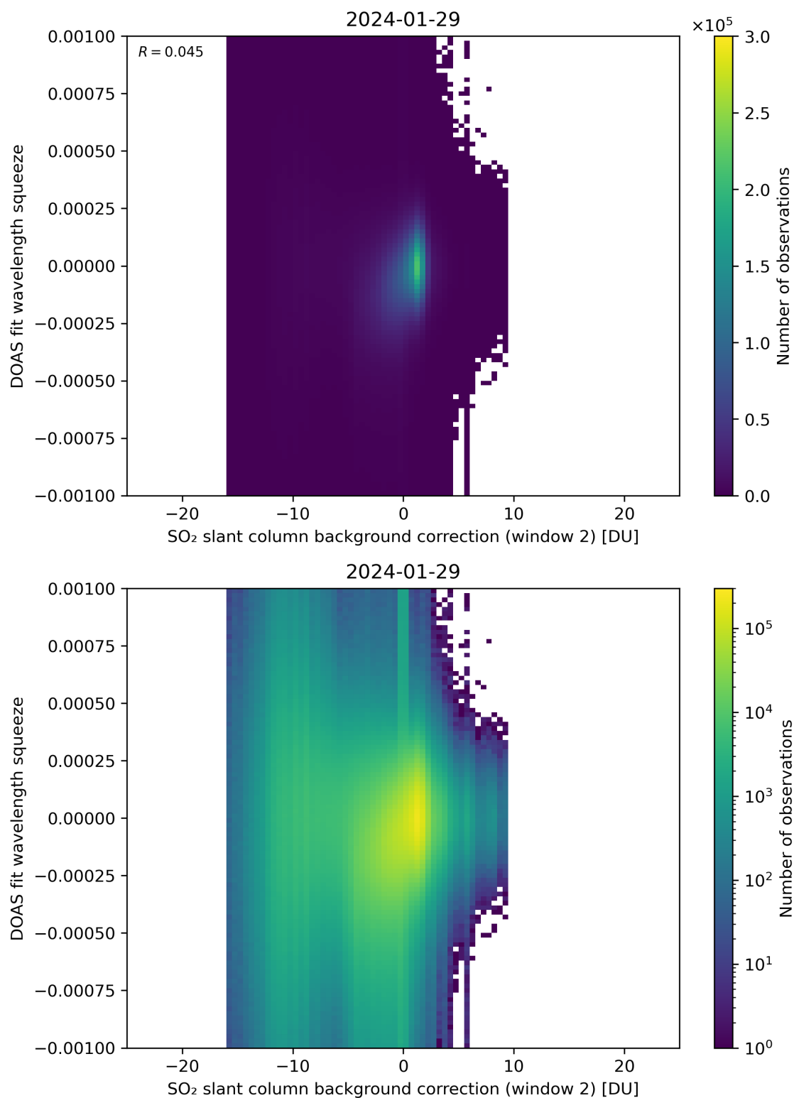
Figure 113: Scatter density plot of “SO 2 slant column background correction (window 2)” against “DOAS fit wavelength squeeze” for 2024-01-28 to 2024-01-30.
