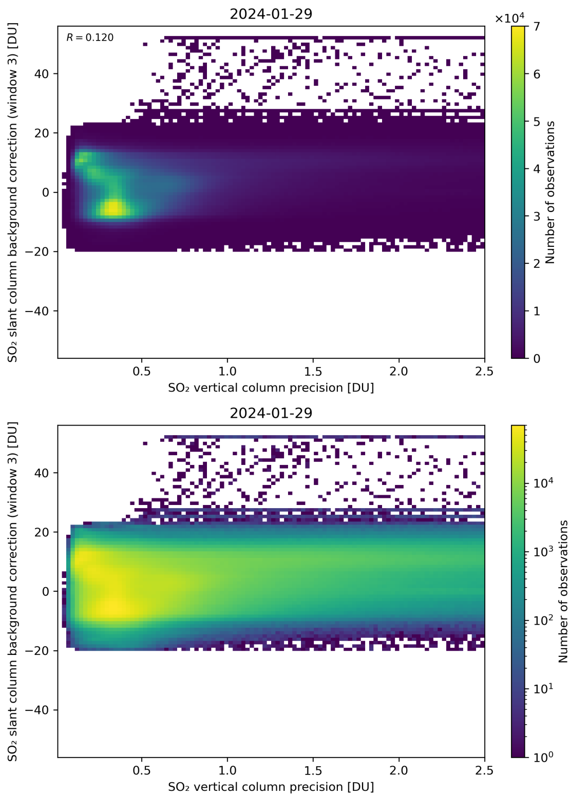
Figure 281: Scatter density plot of “SO 2 vertical column precision” against “SO 2 slant column background correction (window 3)” for 2024-01-28 to 2024-01-30.
