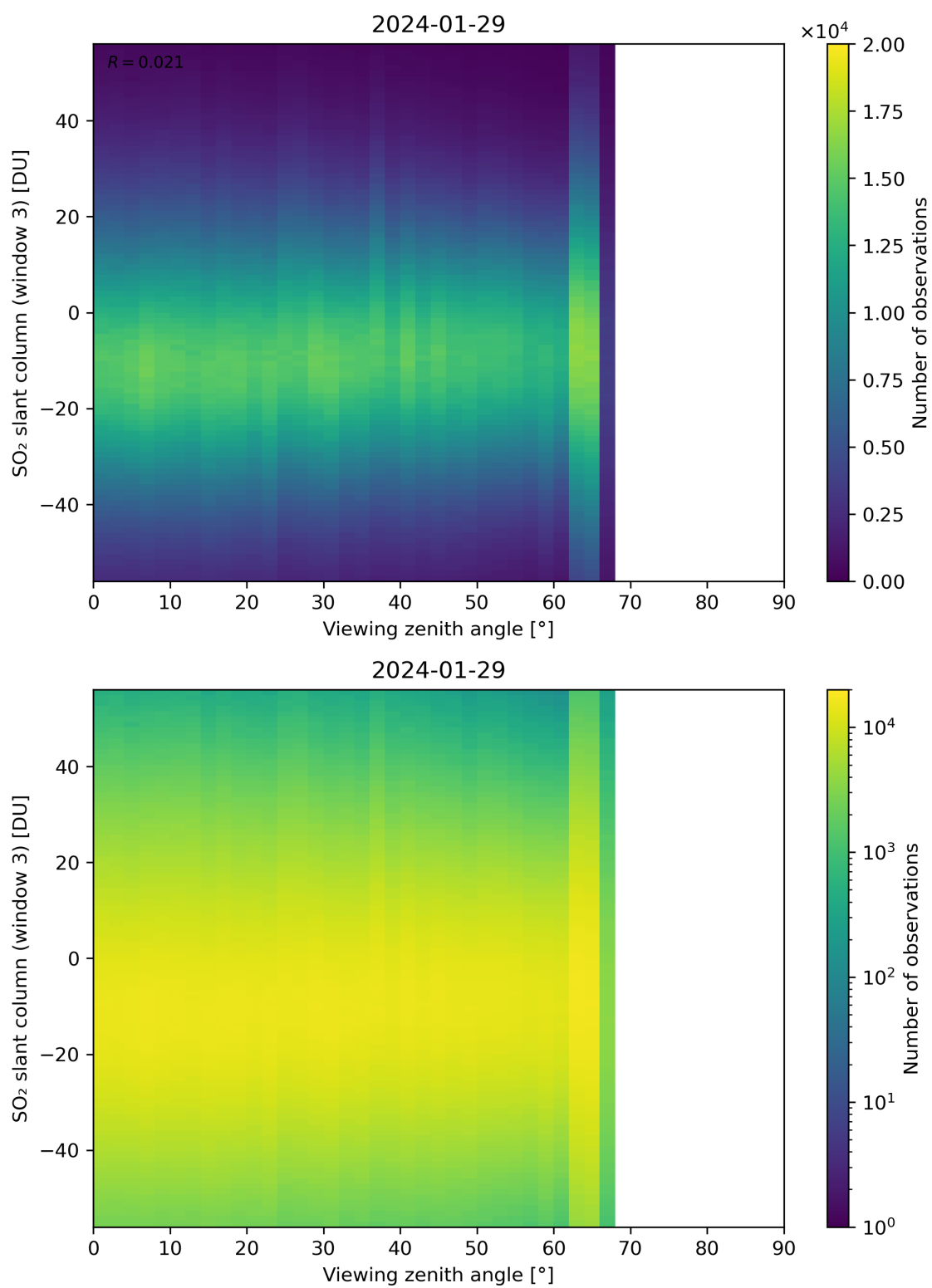
Figure 323: Scatter density plot of “Viewing zenith angle” against “SO 2 slant column (window 3)” for 2024-01-28 to 2024-01-30.
