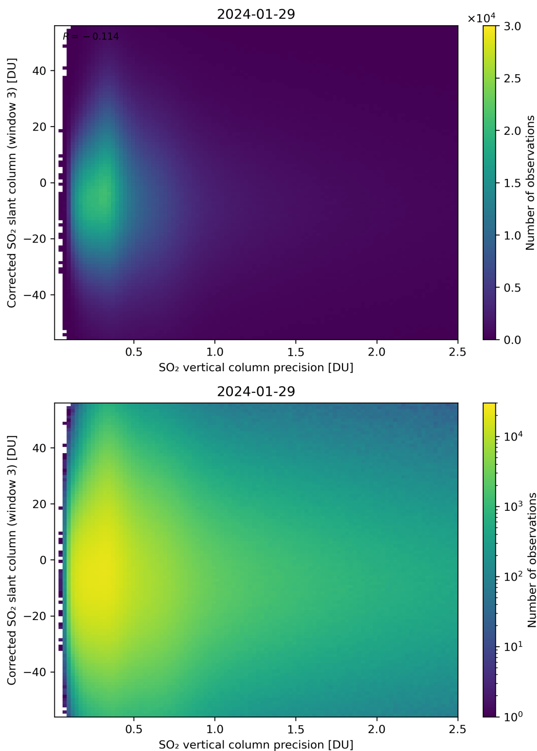
Figure 288: Scatter density plot of “SO 2 vertical column precision” against “Corrected SO 2 slant column (window 3)” for 2024-01-28 to 2024-01-30.
