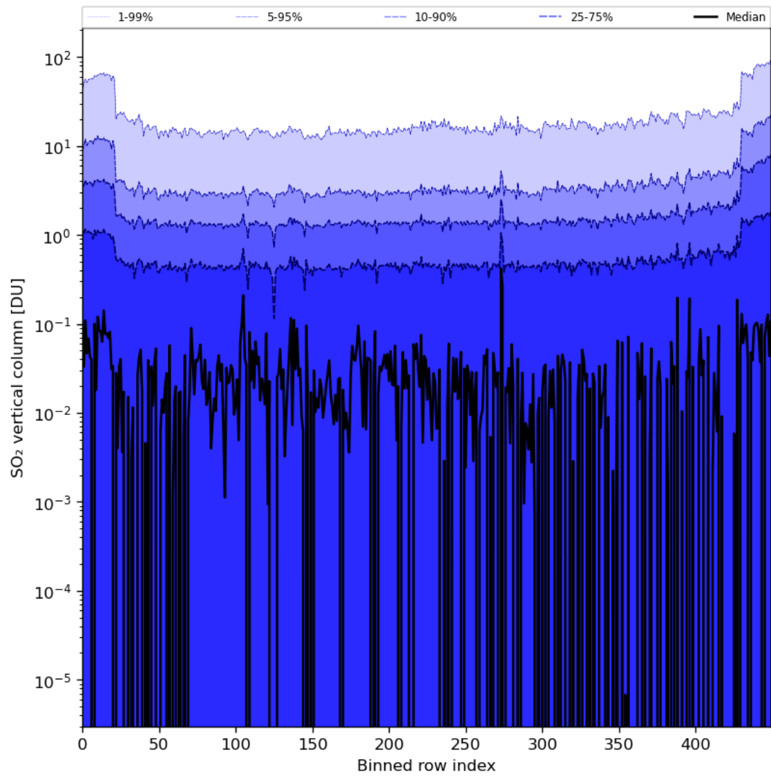
Figure 76: Along track statistics of “SO 2 vertical column” for 2024-01-28 to 2024-01-30
