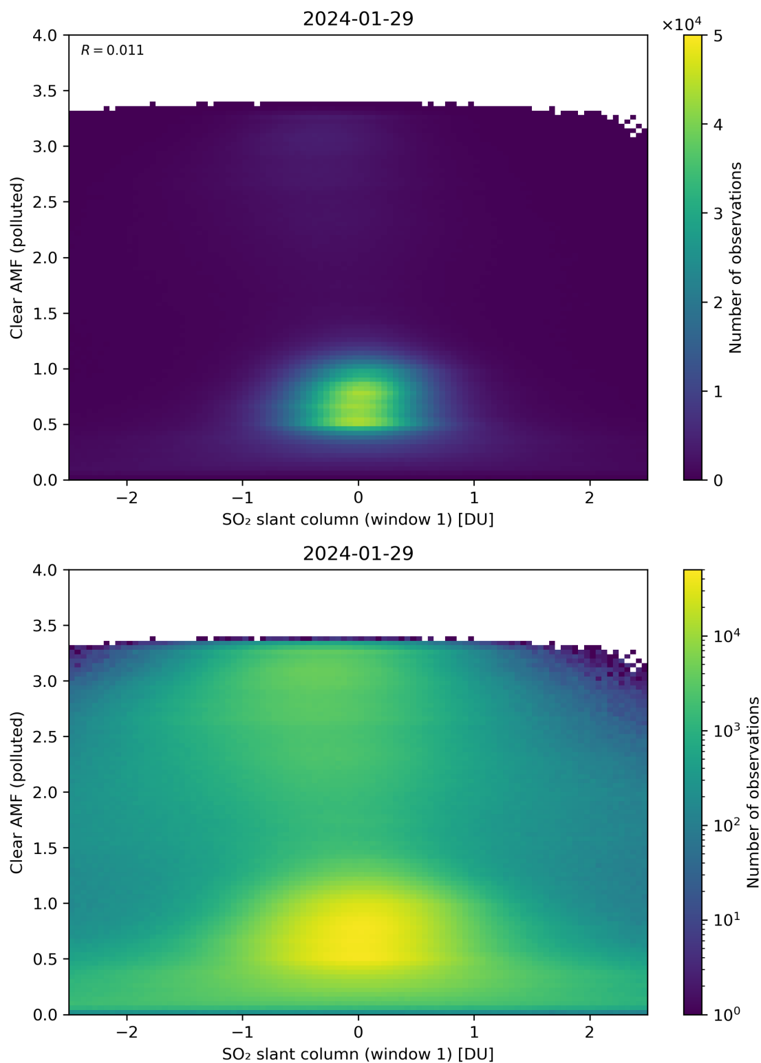
Figure 232: Scatter density plot of “SO 2 slant column (window 1)” against “Clear AMF (polluted)” for 2024-01-28 to 2024-01-30.
