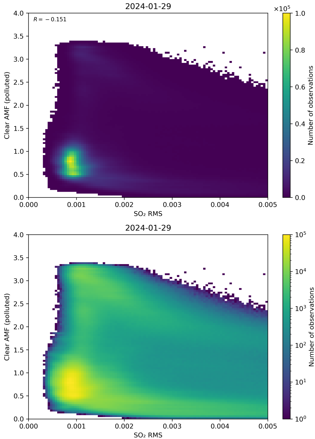
Figure 136: Scatter density plot of “SO 2 RMS” against “Clear AMF (polluted)” for 2024-01-28 to 2024-01-30.
