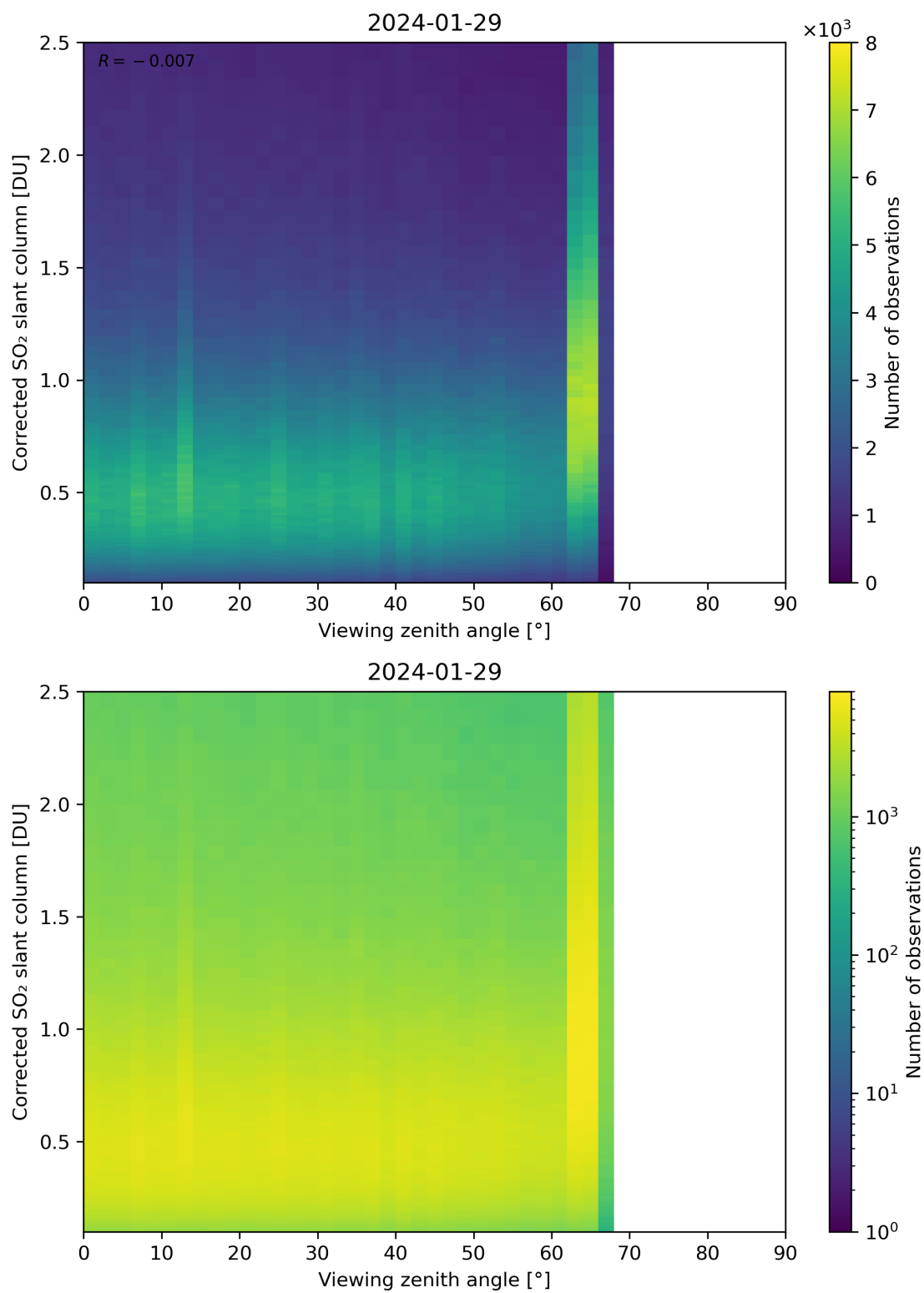
Figure 317: Scatter density plot of “Viewing zenith angle” against “Corrected SO 2 slant column” for 2024-01-28 to 2024-01-30.
