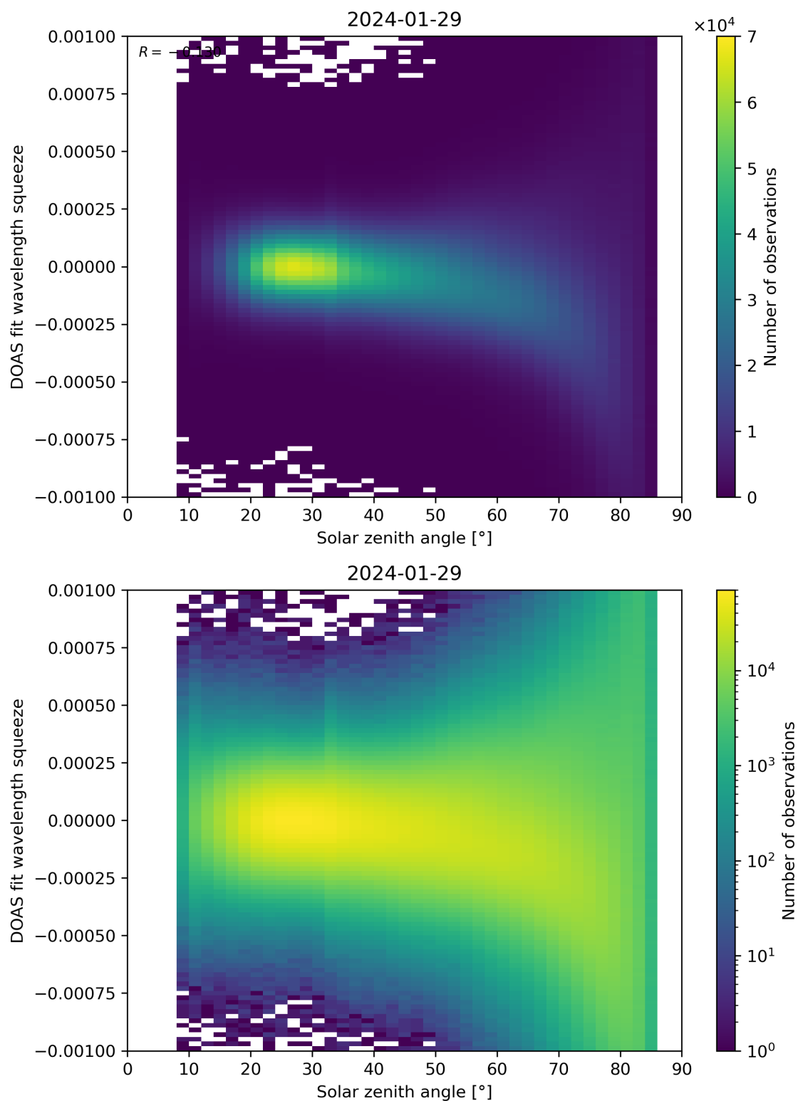
Figure 162: Scatter density plot of “Solar zenith angle” against “DOAS fit wavelength squeeze” for 2024-01-28 to 2024-01-30.
