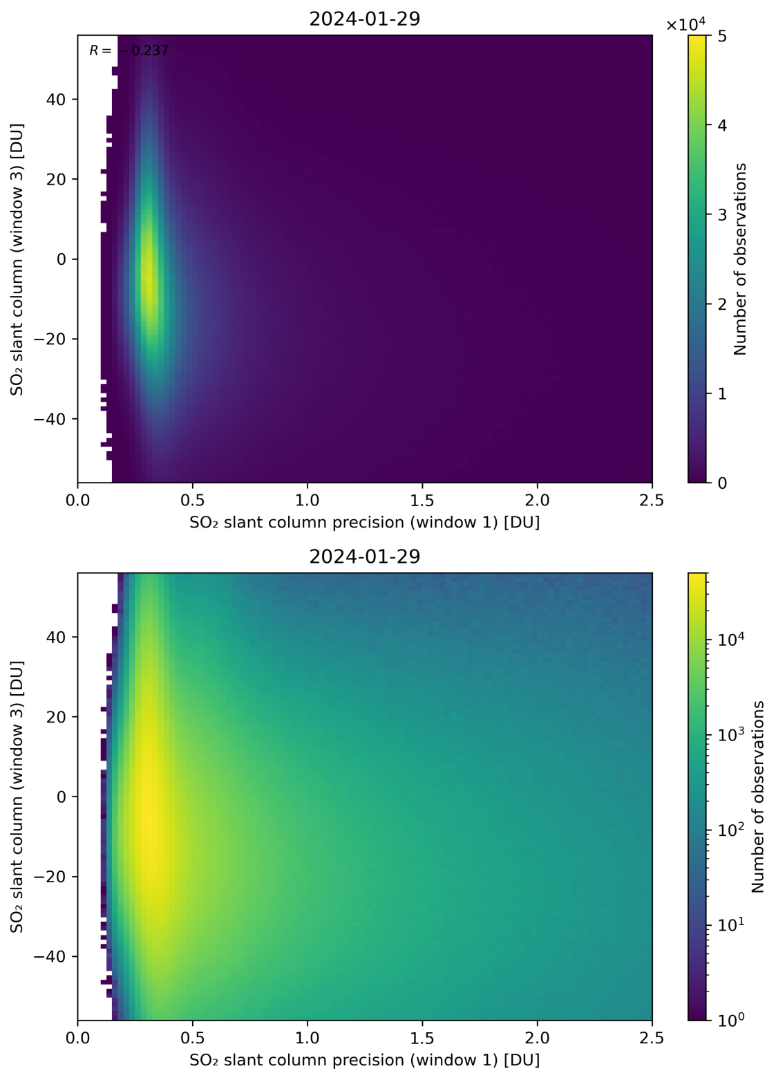
Figure 228: Scatter density plot of “SO 2 slant column precision (window 1)” against “SO 2 slant column (window 3)” for 2024-01-28 to 2024-01-30.
