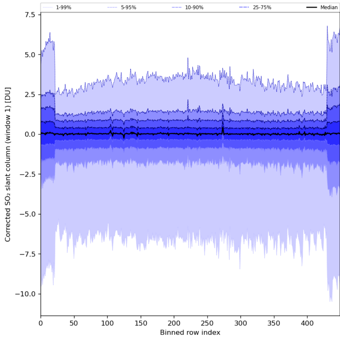
Figure 81: Along track statistics of “Corrected SO 2 slant column (window 1)” for 2024-01-28 to 2024-01-30
