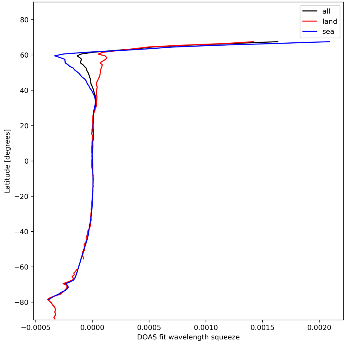
Figure 46: Zonal average of “DOAS fit wavelength squeeze” for 2024-01-28 to 2024-01-30.
