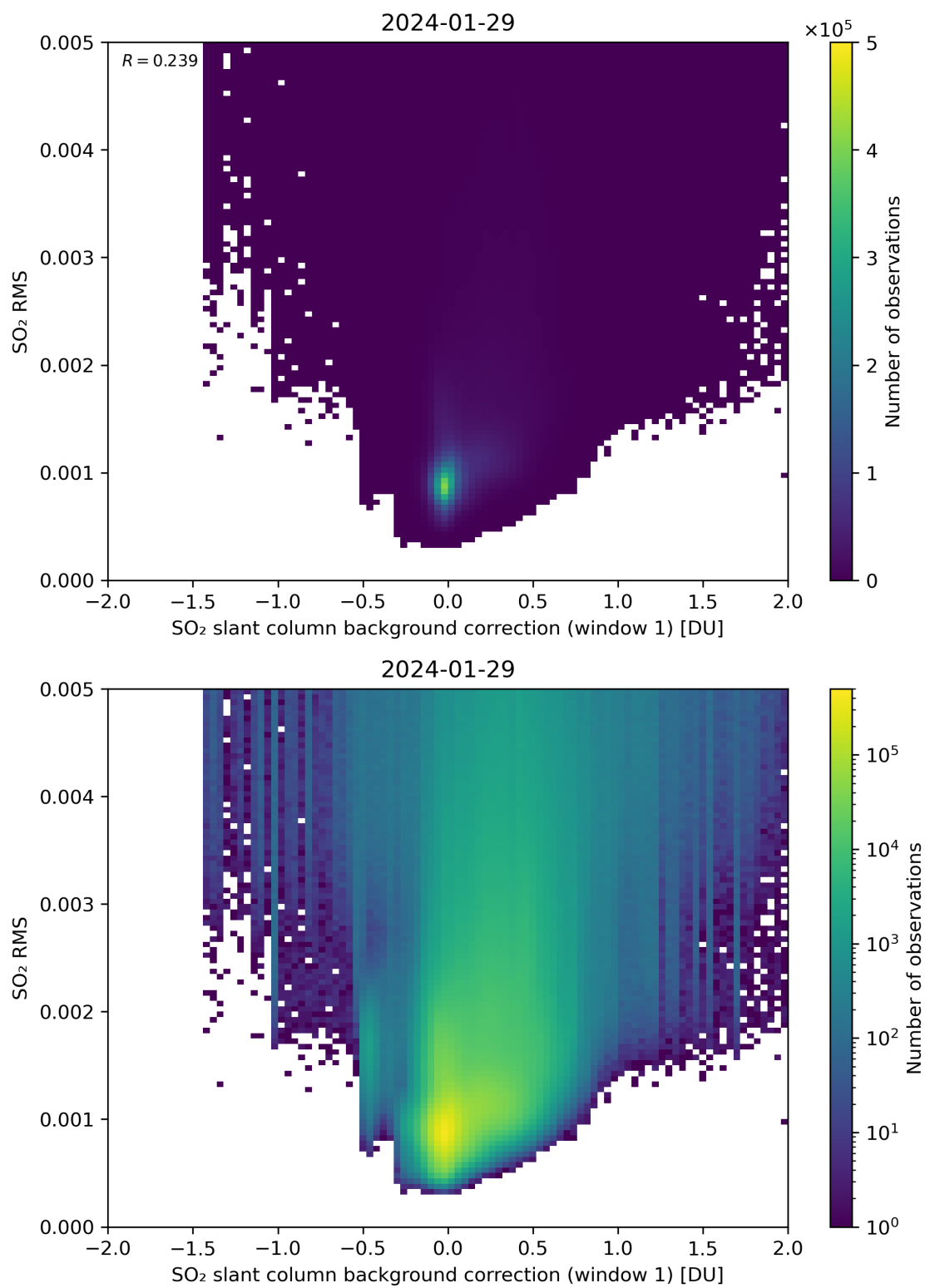
Figure 102: Scatter density plot of “SO 2 slant column background correction (window 1)” against “SO 2 RMS” for 2024-01-28 to 2024-01-30.
