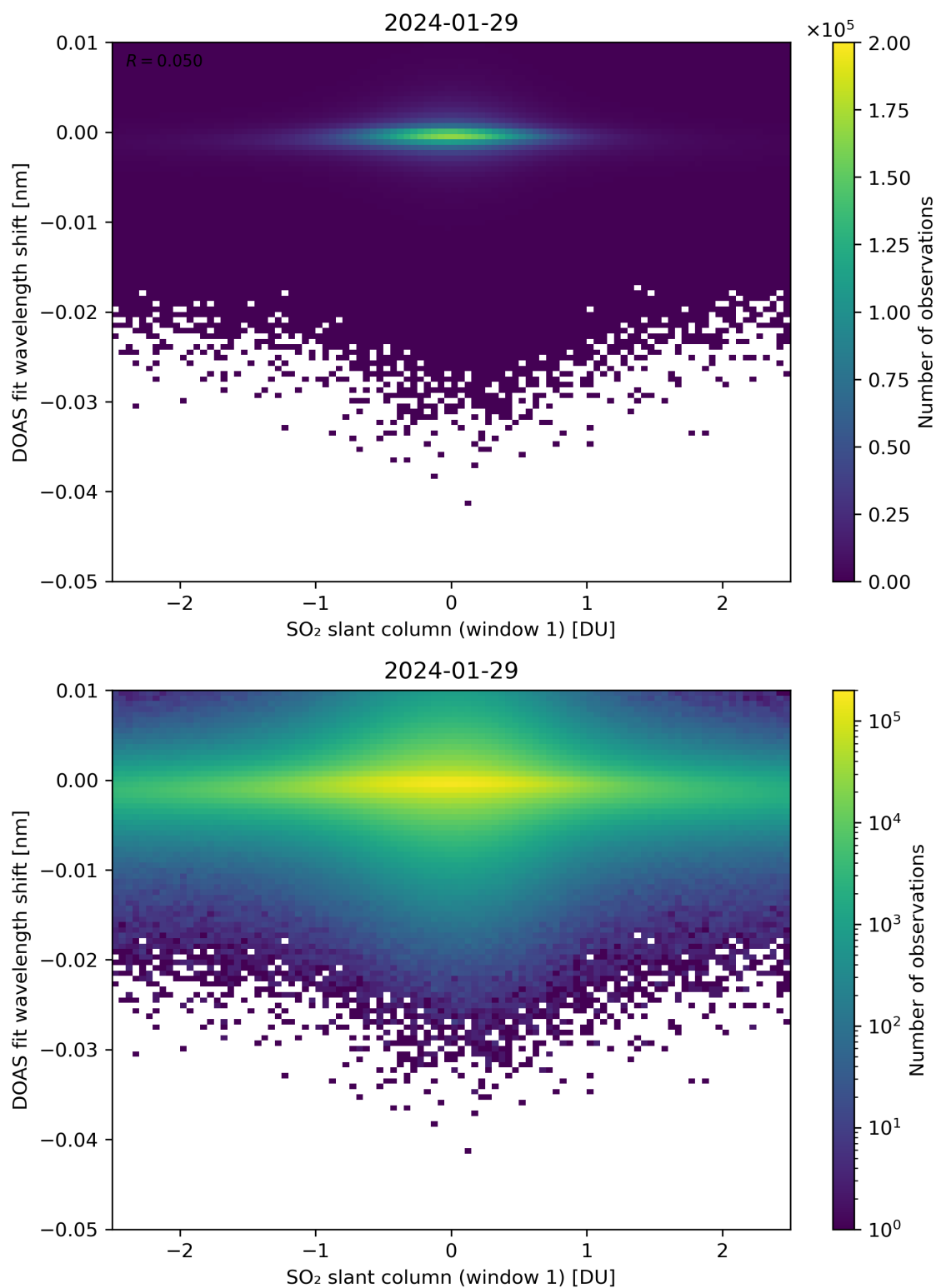
Figure 215: Scatter density plot of “SO 2 slant column (window 1)” against “DOAS fit wavelength shift” for 2024-01-28 to 2024-01-30.
