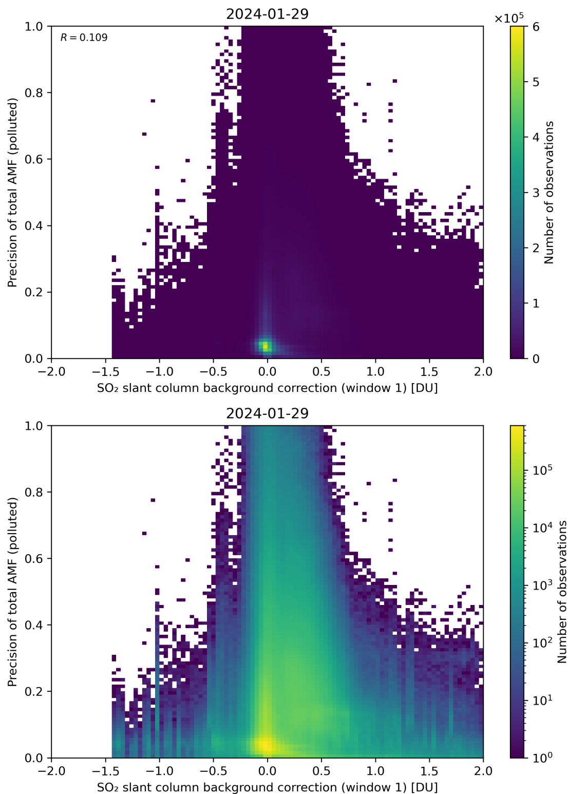
Figure 110: Scatter density plot of “SO 2 slant column background correction (window 1)” against “Precision of total AMF (polluted)” for 2024-01-28 to 2024-01-30.
