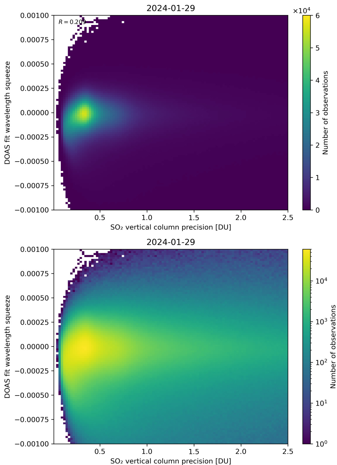
Figure 283: Scatter density plot of “SO 2 vertical column precision” against “DOAS fit wavelength squeeze” for 2024-01-28 to 2024-01-30.
