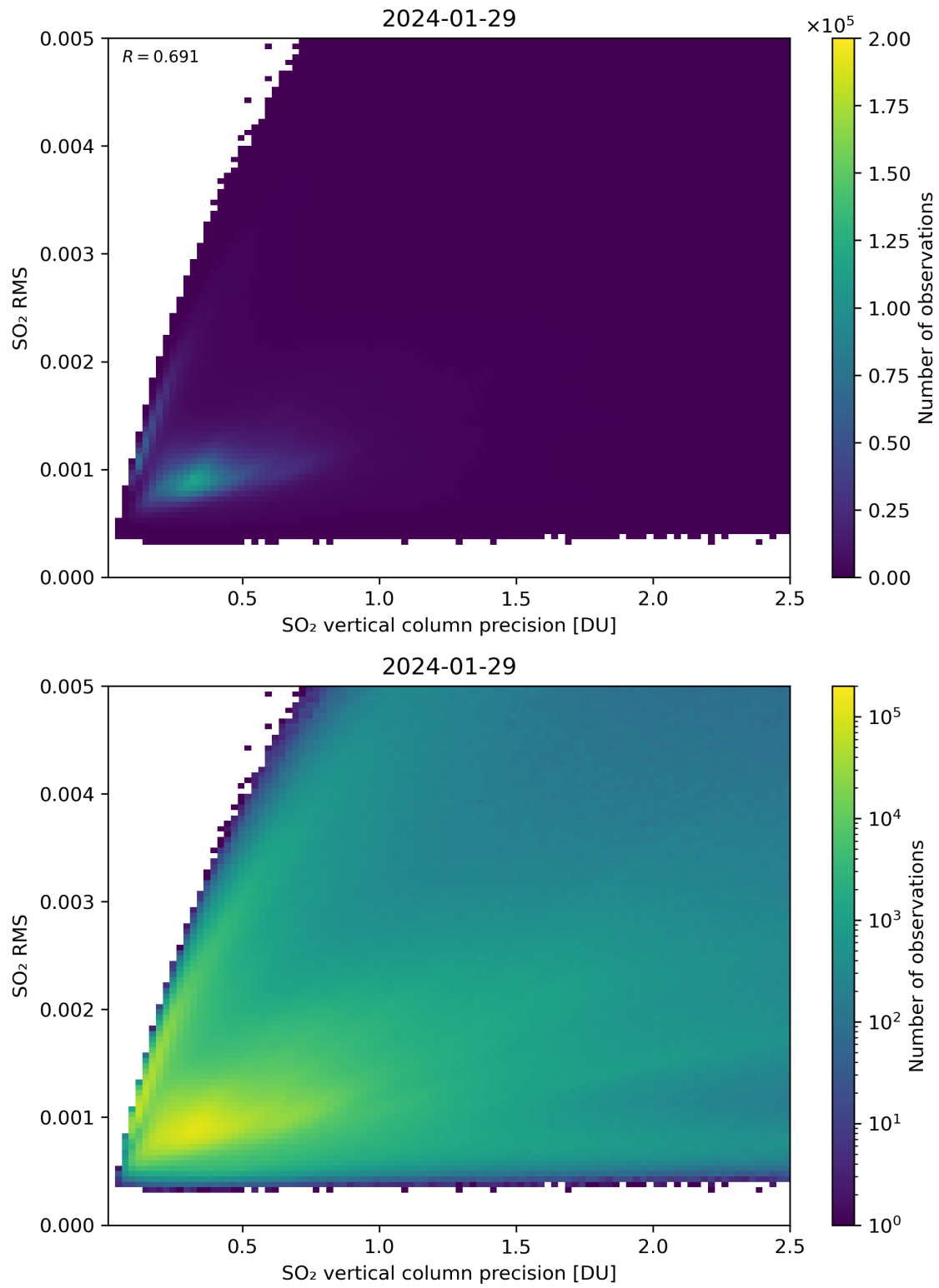
Figure 284: Scatter density plot of “SO 2 vertical column precision” against “SO 2 RMS” for 2024-01-28 to 2024-01-30.
