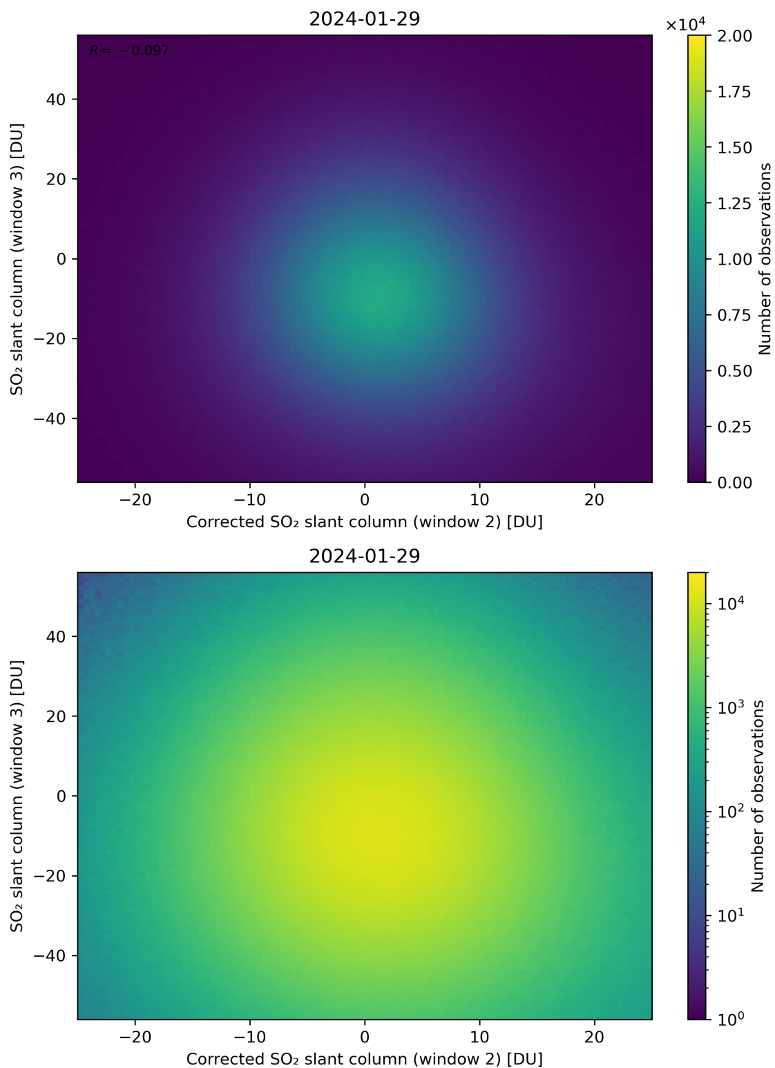
Figure 201: Scatter density plot of “Corrected SO 2 slant column (window 2)” against “SO 2 slant column (window 3)” for 2024-01-28 to 2024-01-30.
