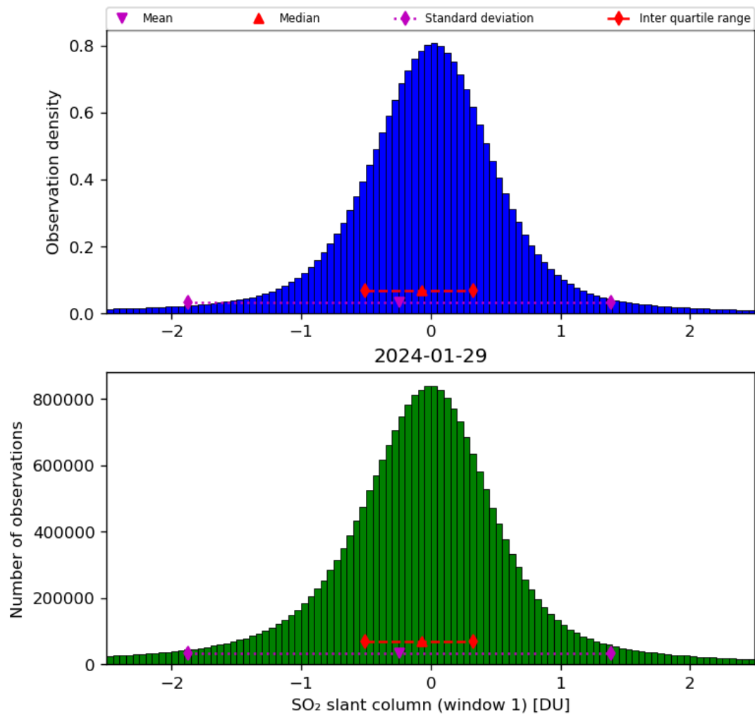
Figure 56: Histogram of “SO 2 slant column (window 1)” for 2024-01-28 to 2024-01-30
