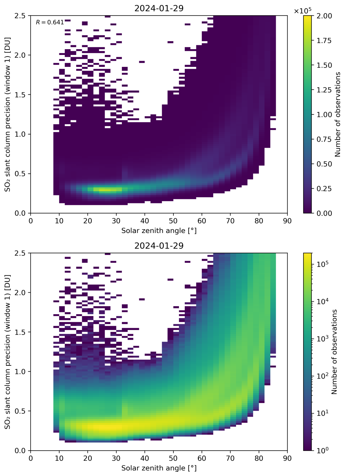
Figure 170: Scatter density plot of “Solar zenith angle” against “SO 2 slant column precision (window 1)” for 2024-01-28 to 2024-01-30.
