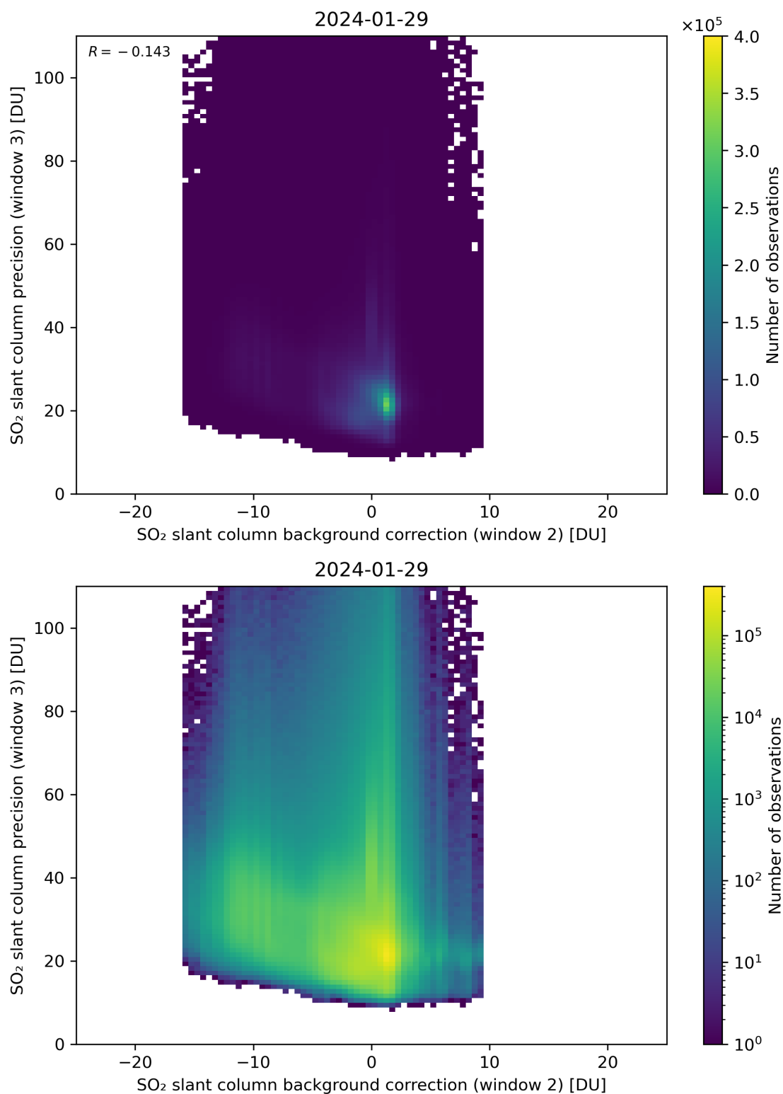
Figure 118: Scatter density plot of “SO 2 slant column background correction (window 2)” against “SO 2 slant column precision (window 3)” for 2024-01-28 to 2024-01-30.
