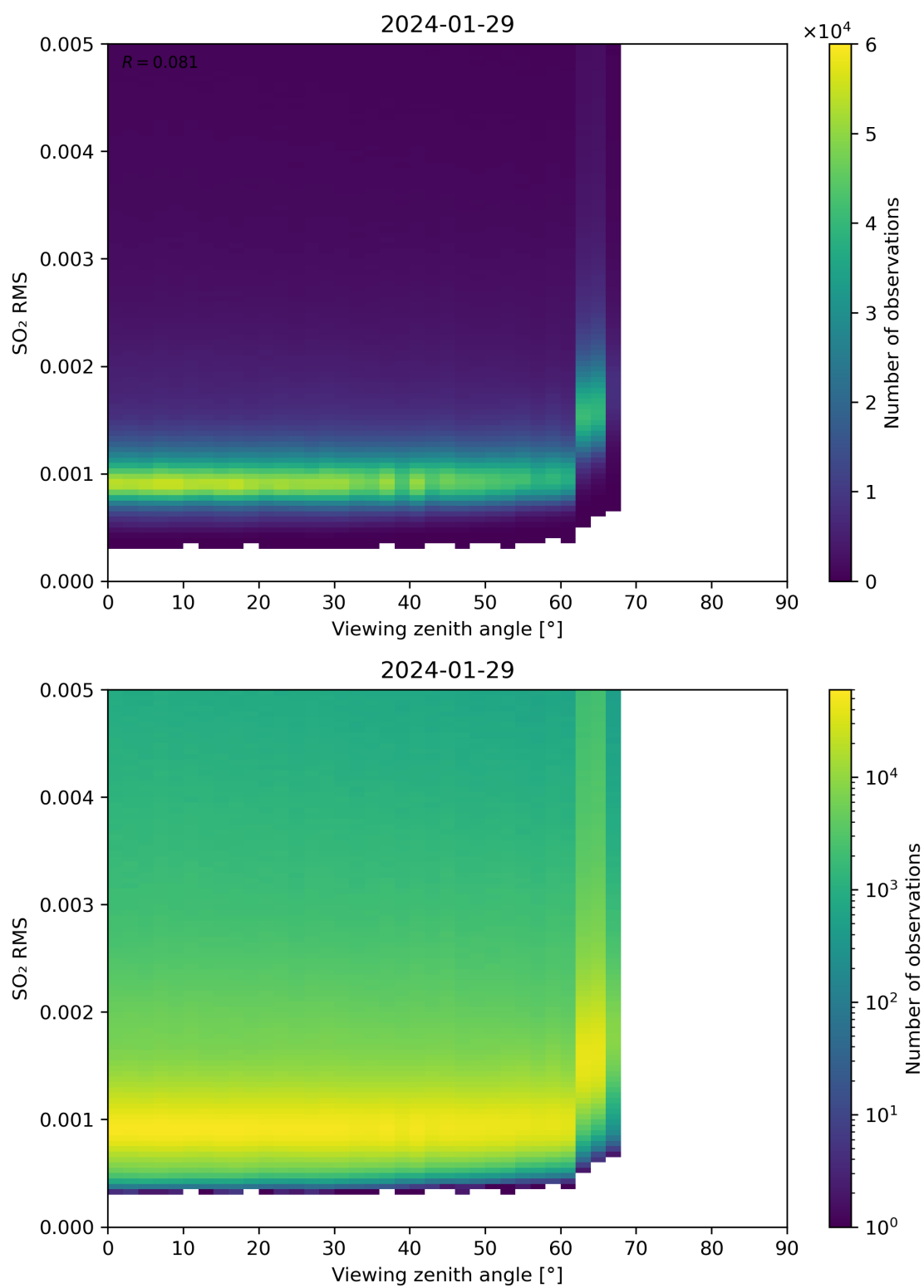
Figure 313: Scatter density plot of “Viewing zenith angle” against “SO 2 RMS” for 2024-01-28 to 2024-01-30.
