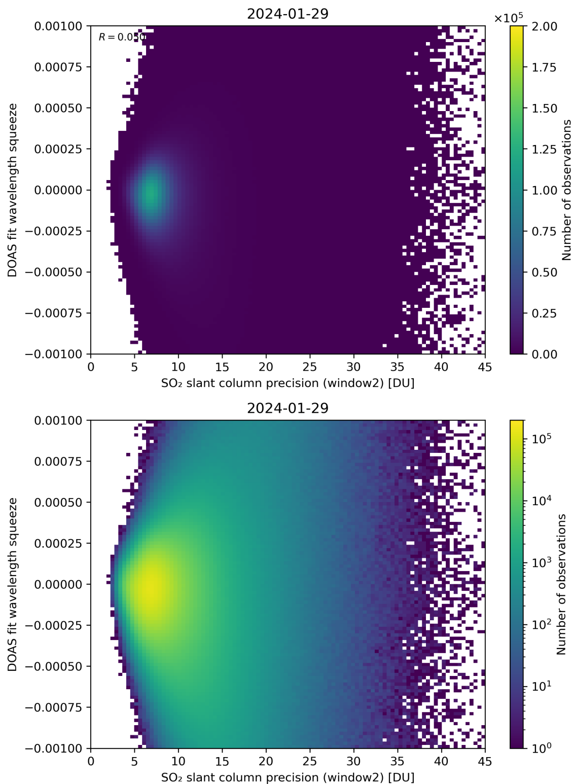
Figure 244: Scatter density plot of “SO 2 slant column precision (window2)” against “DOAS fit wavelength squeeze” for 2024-01-28 to 2024-01-30.
