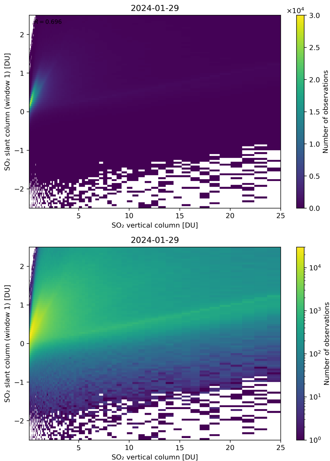
Figure 300: Scatter density plot of “SO 2 vertical column” against “SO 2 slant column (window 1)” for 2024-01-28 to 2024-01-30.
