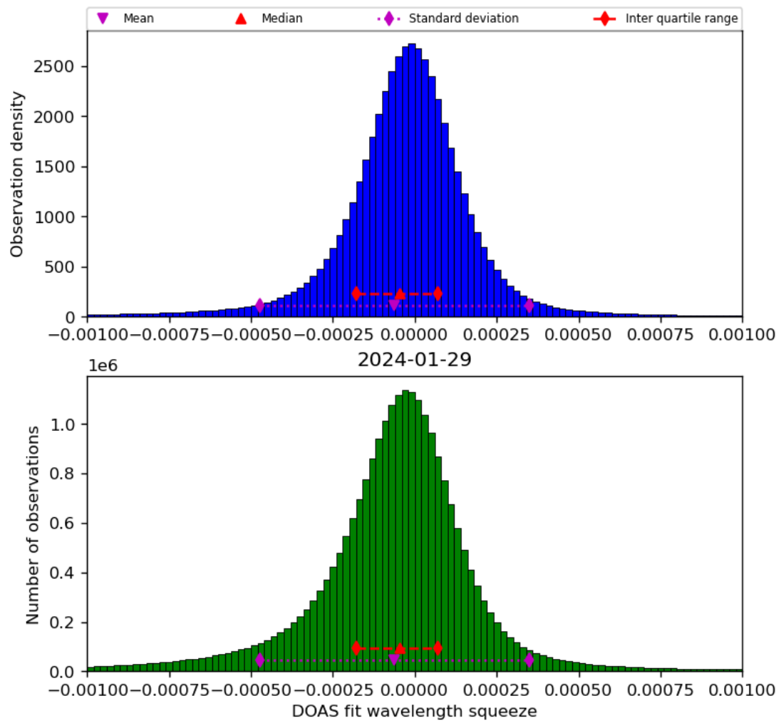
Figure 69: Histogram of “DOAS fit wavelength squeeze” for 2024-01-28 to 2024-01-30
