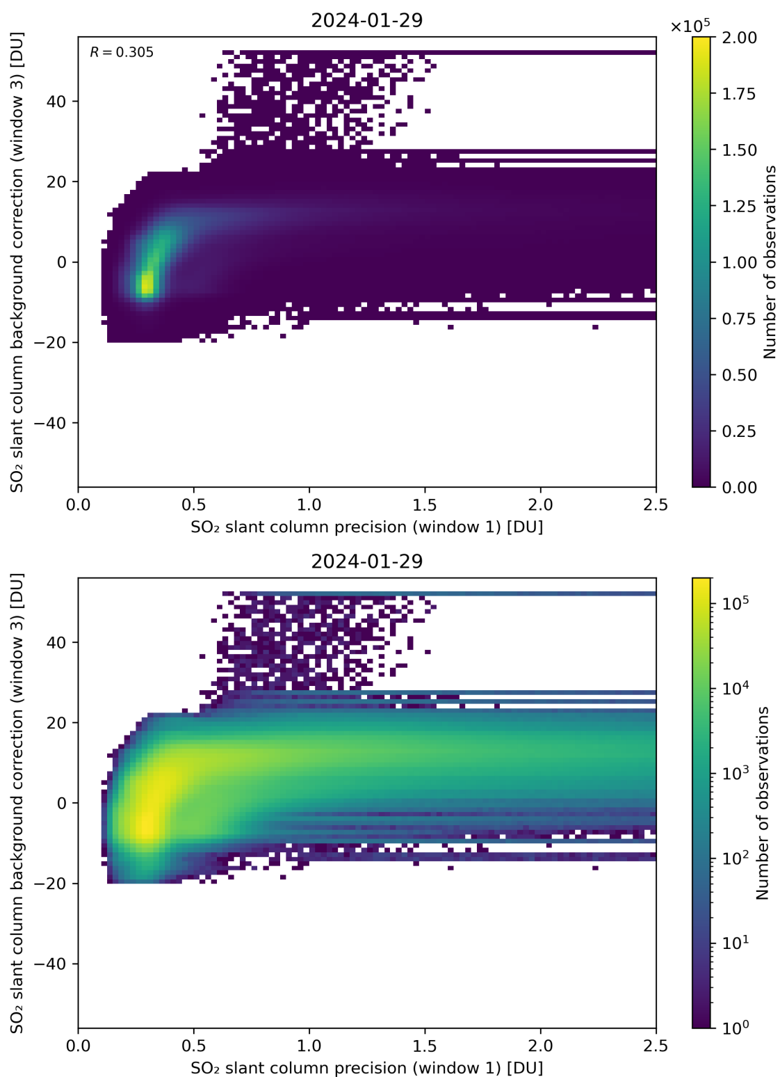
Figure 220: Scatter density plot of “SO 2 slant column precision (window 1)” against “SO 2 slant column background correction (window 3)” for 2024-01-28 to 2024-01-30.
