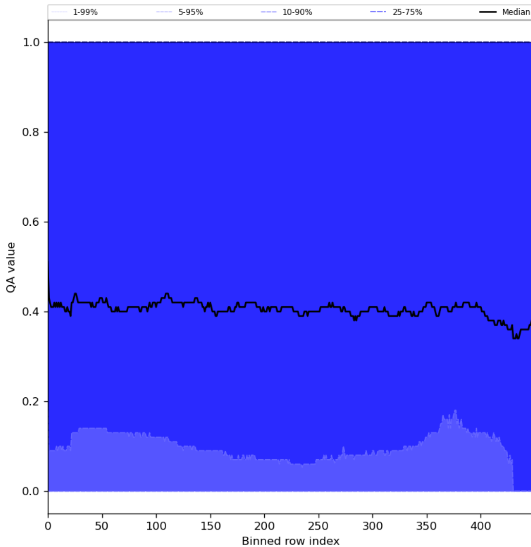
Figure 75: Along track statistics of “QA value” for 2024-01-28 to 2024-01-30
