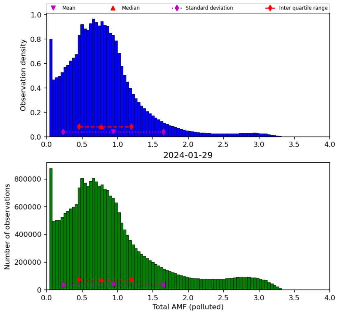
Figure 71: Histogram of “Total AMF (polluted)” for 2024-01-28 to 2024-01-30
