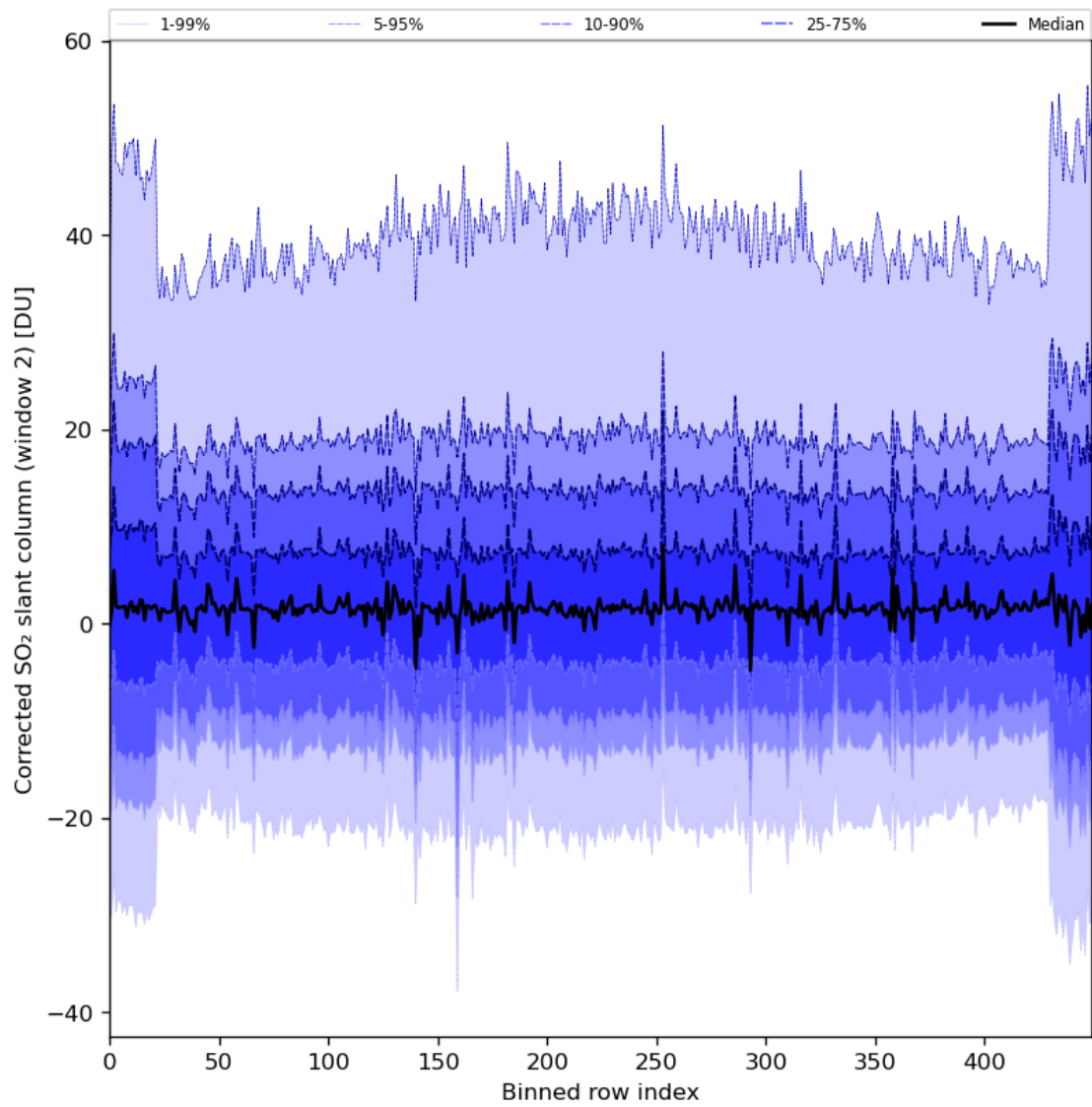
Figure 85: Along track statistics of “Corrected SO 2 slant column (window 2)” for 2024-01-28 to 2024-01-30
