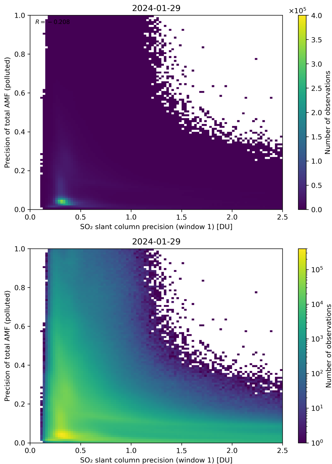
Figure 231: Scatter density plot of “SO 2 slant column precision (window 1)” against “Precision of total AMF (polluted)” for 2024-01-28 to 2024-01-30.
