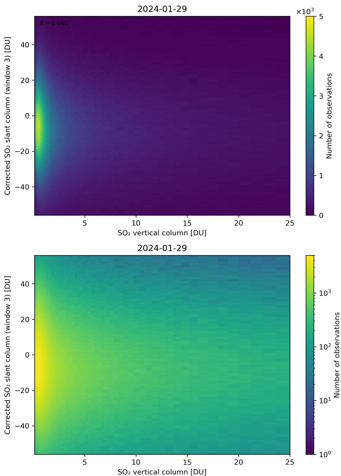
Figure 299: Scatter density plot of “SO 2 vertical column” against “Corrected SO 2 slant column (window 3)” for 2024-01-28 to 2024-01-30.
