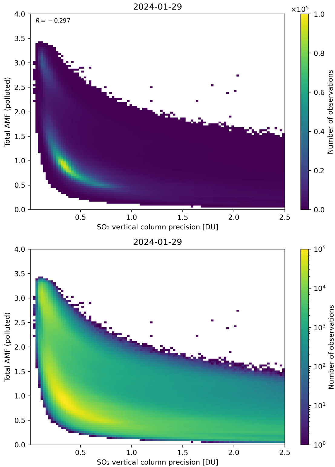
Figure 294: Scatter density plot of “SO 2 vertical column precision” against “Total AMF (polluted)” for 2024-01-28 to 2024-01-30.
