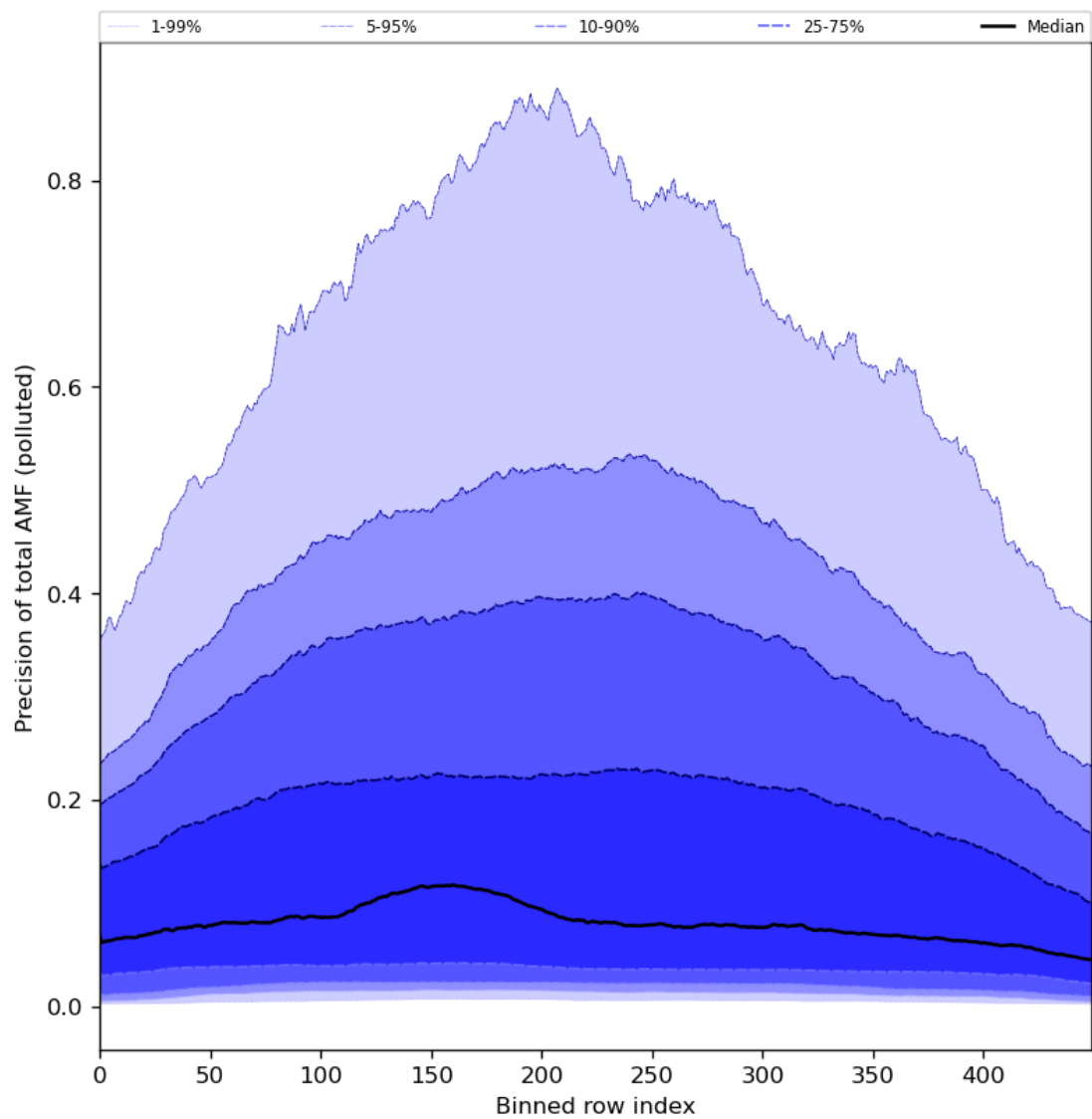
Figure 95: Along track statistics of “Precision of total AMF (polluted)” for 2024-01-28 to 2024-01-30
