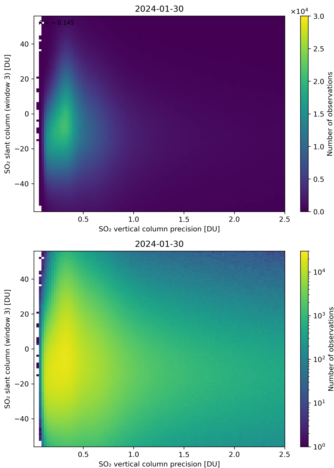
Figure 292: Scatter density plot of “SO 2 vertical column precision” against “SO 2 slant column (window 3)” for 2024-01-29 to 2024-01-31.
