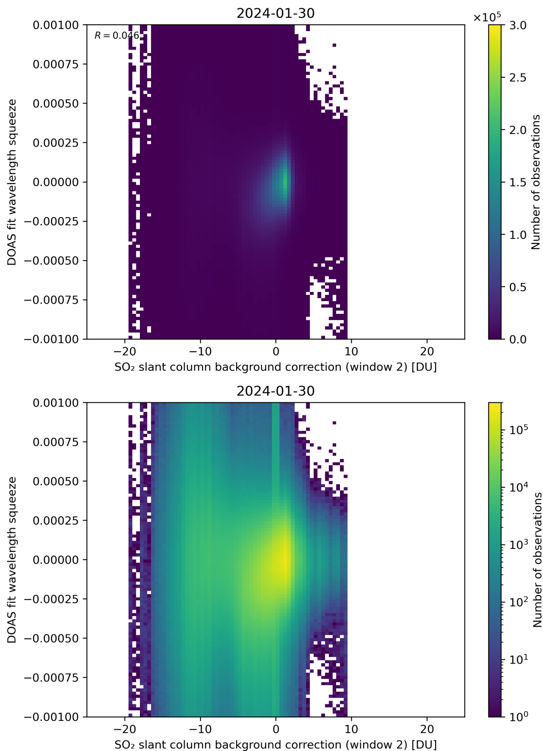
Figure 113: Scatter density plot of “SO 2 slant column background correction (window 2)” against “DOAS fit wavelength squeeze” for 2024-01-29 to 2024-01-31.
