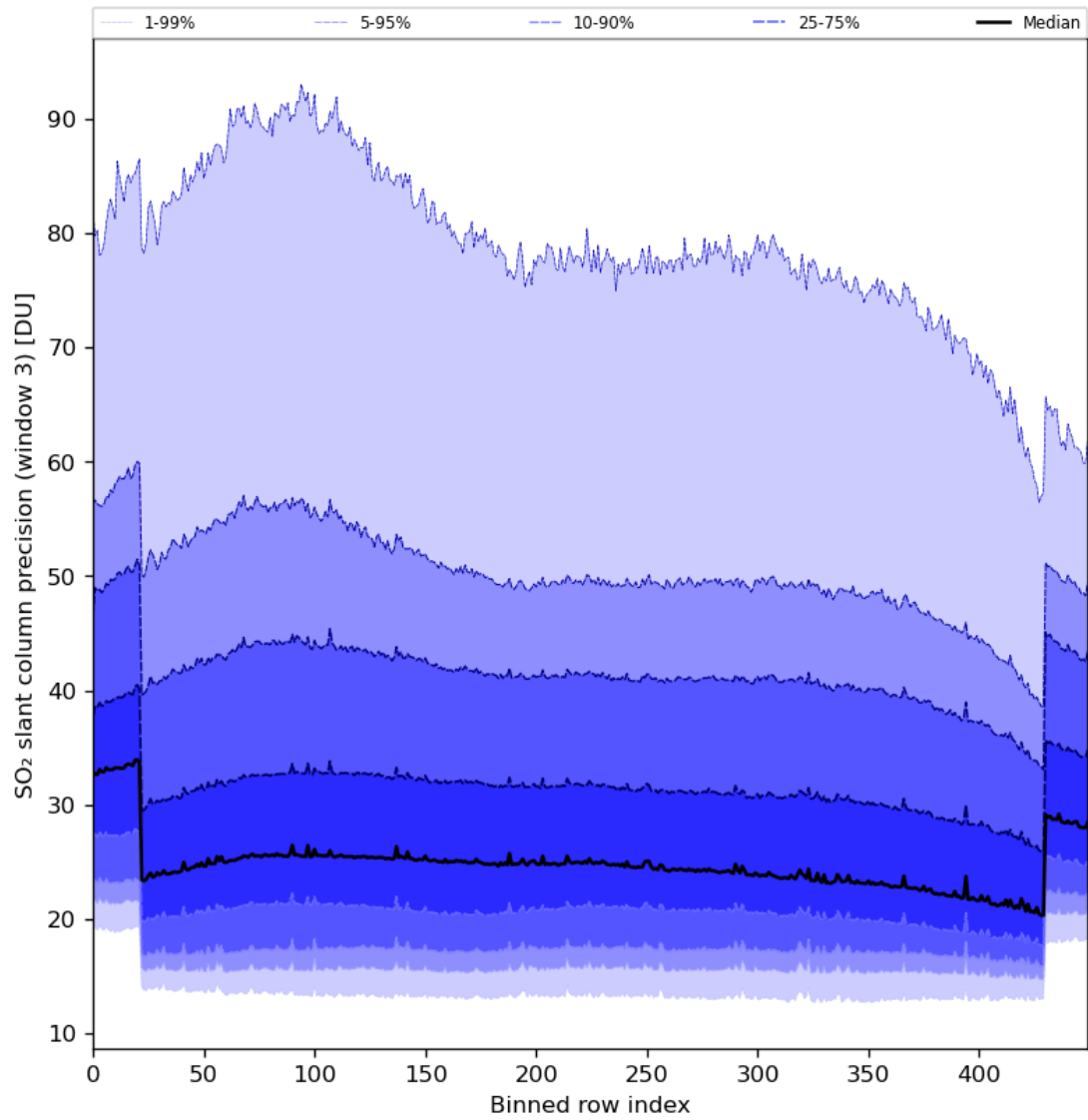
Figure 88: Along track statistics of “SO 2 slant column precision (window 3)” for 2024-01-29 to 2024-01-31
