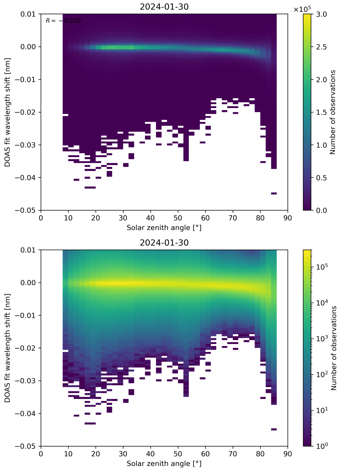
Figure 161: Scatter density plot of “Solar zenith angle” against “DOAS fit wavelength shift” for 2024-01-29 to 2024-01-31.
