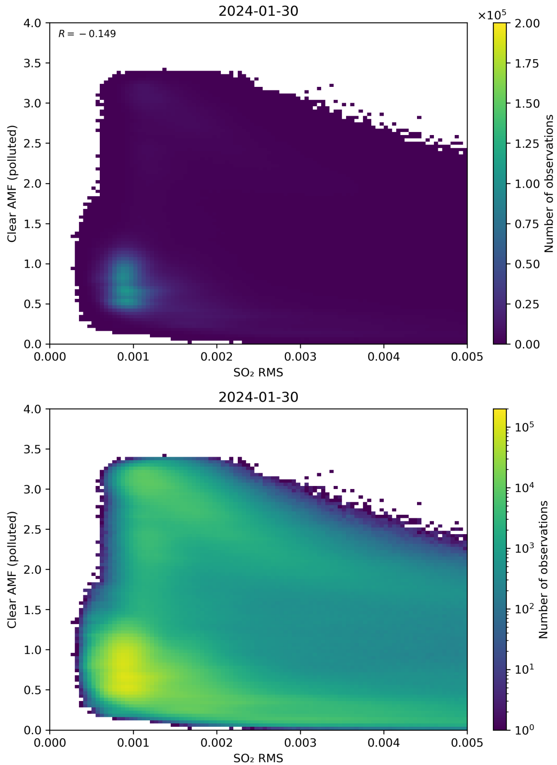
Figure 136: Scatter density plot of “SO 2 RMS” against “Clear AMF (polluted)” for 2024-01-29 to 2024-01-31.
