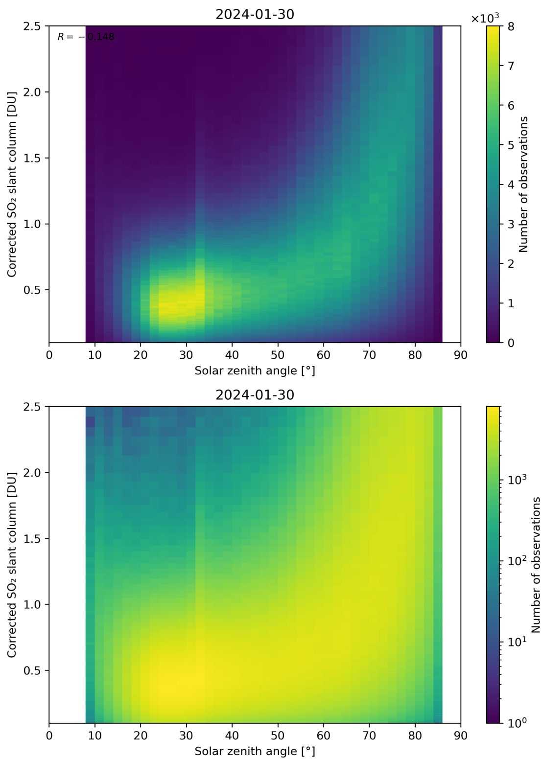
Figure 166: Scatter density plot of “Solar zenith angle” against “Corrected SO 2 slant column” for 2024-01-29 to 2024-01-31.
