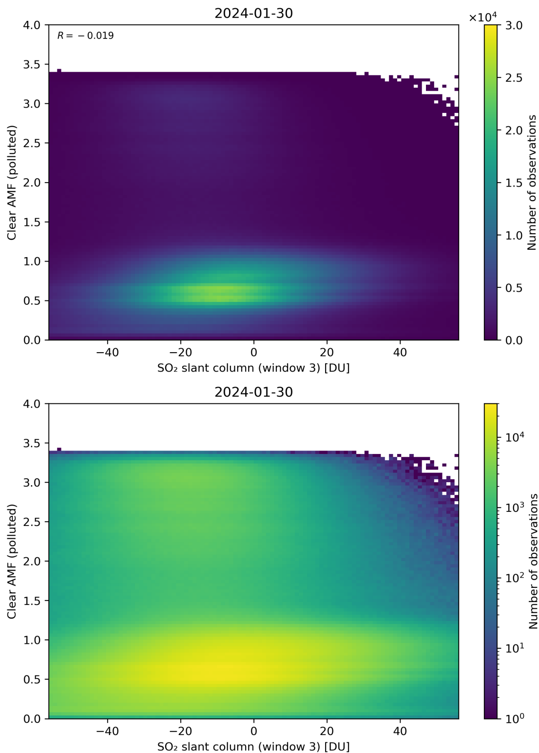
Figure 265: Scatter density plot of “SO 2 slant column (window 3)” against “Clear AMF (polluted)” for 2024-01-29 to 2024-01-31.
