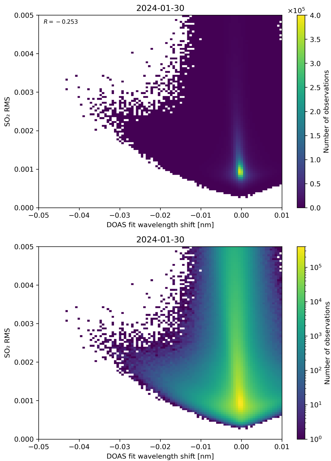
Figure 128: Scatter density plot of “DOAS fit wavelength shift” against “SO 2 RMS” for 2024-01-29 to 2024-01-31.
