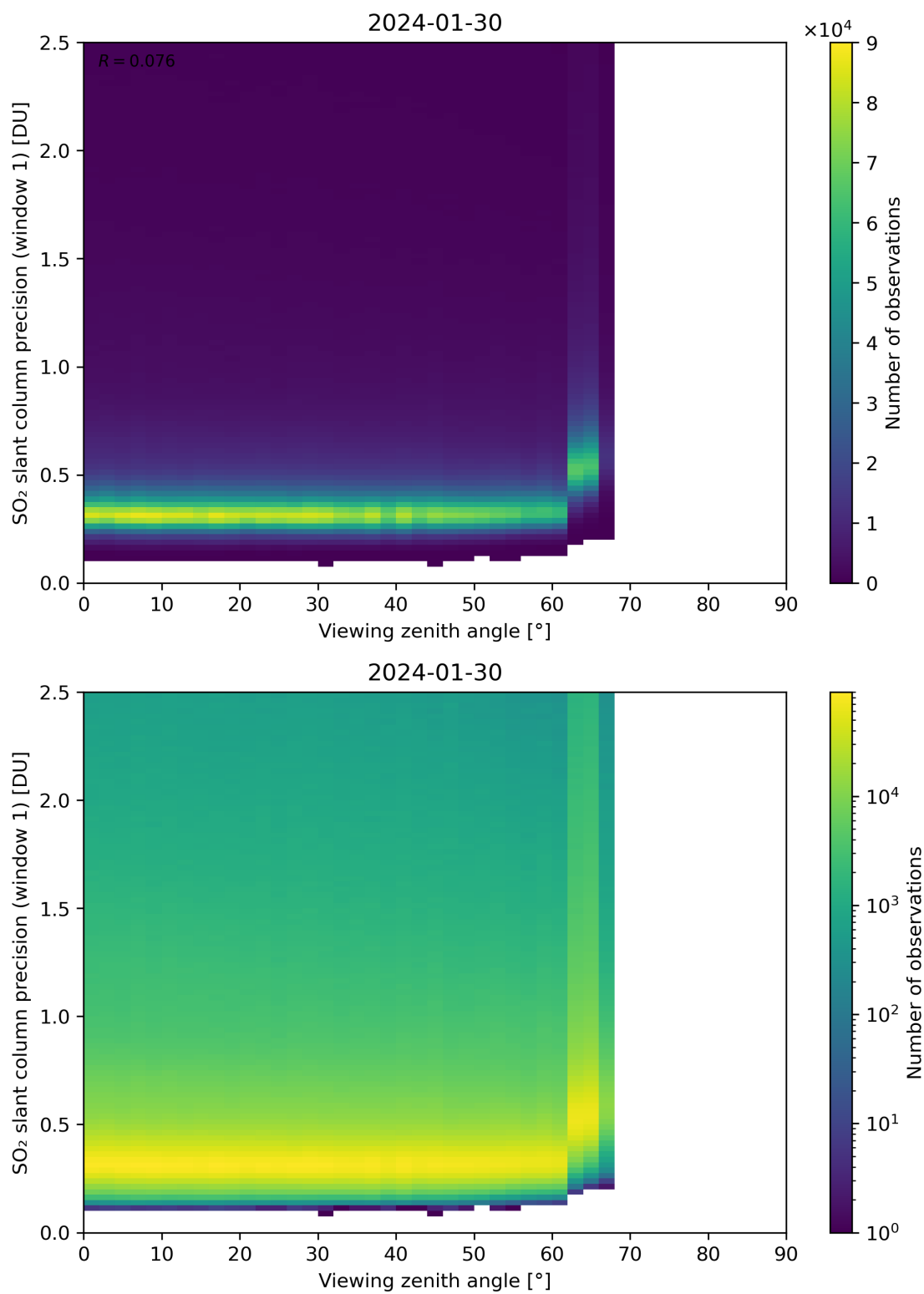
Figure 321: Scatter density plot of “Viewing zenith angle” against “SO 2 slant column precision (window 1)” for 2024-01-29 to 2024-01-31.
