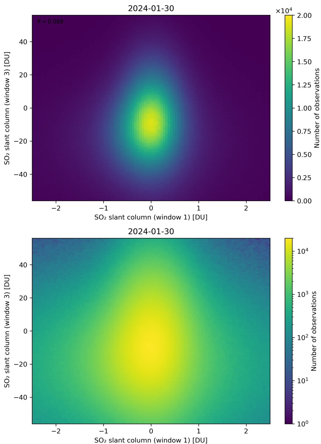
Figure 237: Scatter density plot of “SO 2 slant column (window 1)” against “SO 2 slant column (window 3)” for 2024-01-29 to 2024-01-31.
