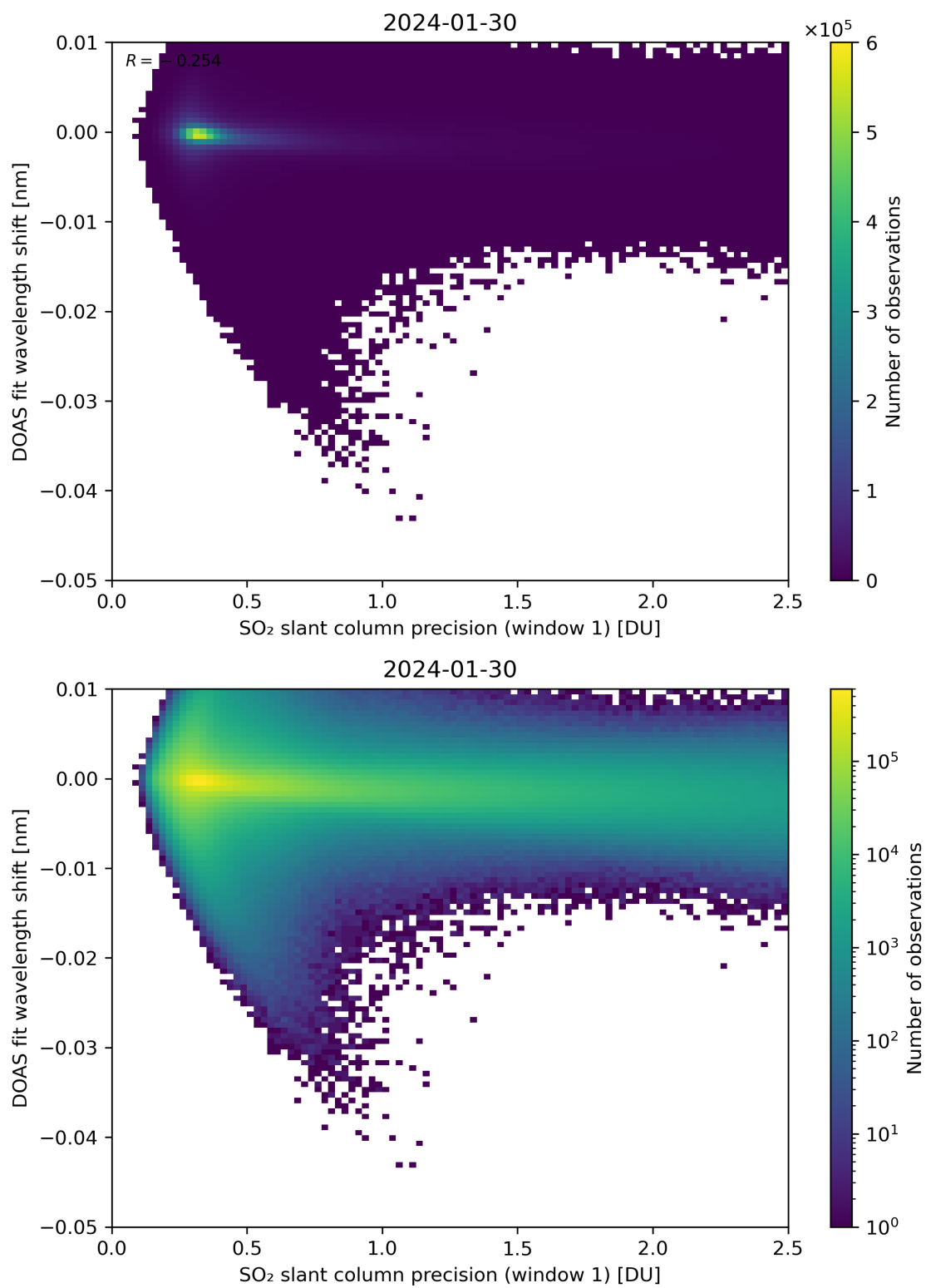
Figure 221: Scatter density plot of “SO 2 slant column precision (window 1)” against “DOAS fit wavelength shift” for 2024-01-29 to 2024-01-31.
