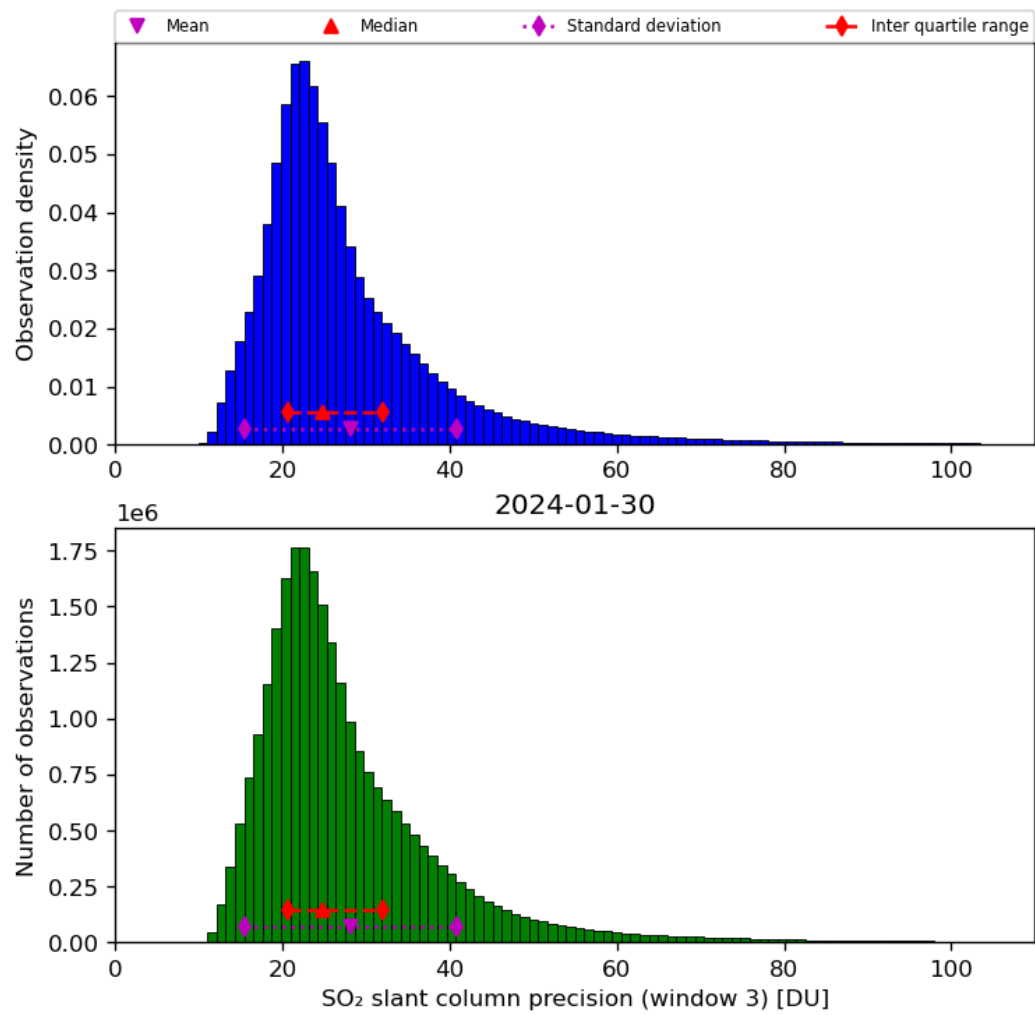
Figure 65: Histogram of “SO 2 slant column precision (window 3)” for 2024-01-29 to 2024-01-31
