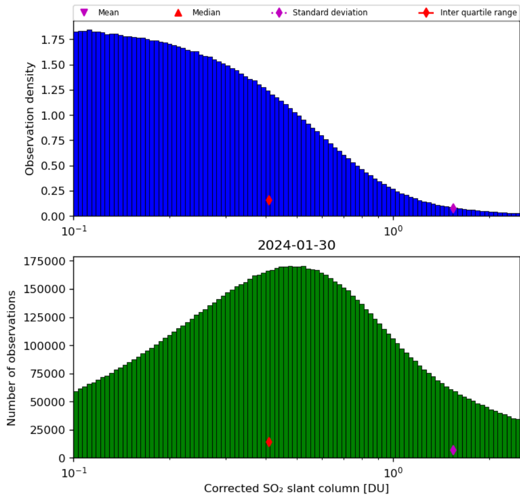
Figure 55: Histogram of “Corrected SO 2 slant column” for 2024-01-29 to 2024-01-31
