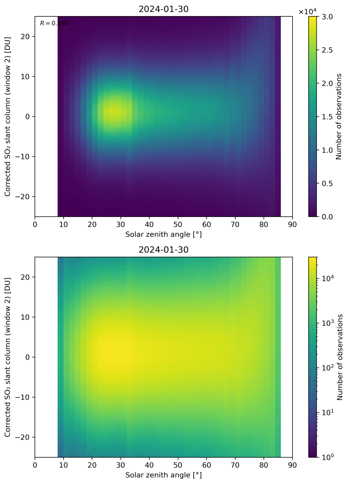
Figure 167: Scatter density plot of “Solar zenith angle” against “Corrected SO 2 slant column (window 2)” for 2024-01-29 to 2024-01-31.
