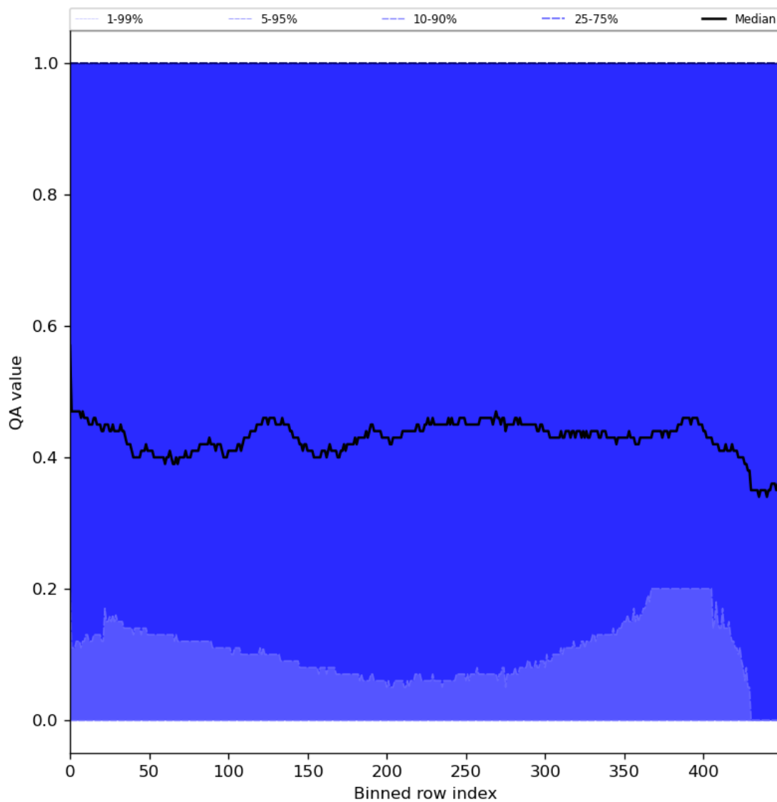
Figure 75: Along track statistics of “QA value” for 2024-01-29 to 2024-01-31
