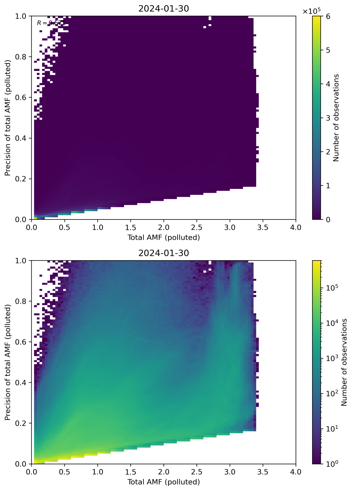
Figure 272: Scatter density plot of “Total AMF (polluted)” against “Precision of total AMF (polluted)” for 2024-01-29 to 2024-01-31.
