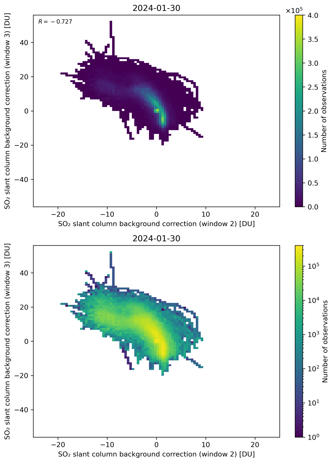
Figure 111: Scatter density plot of “SO 2 slant column background correction (window 2)” against “SO 2 slant column background correction (window 3)” for 2024-01-29 to 2024-01-31.
