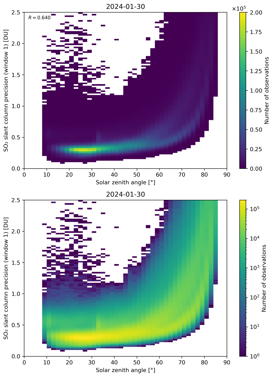
Figure 170: Scatter density plot of “Solar zenith angle” against “SO 2 slant column precision (window 1)” for 2024-01-29 to 2024-01-31.
