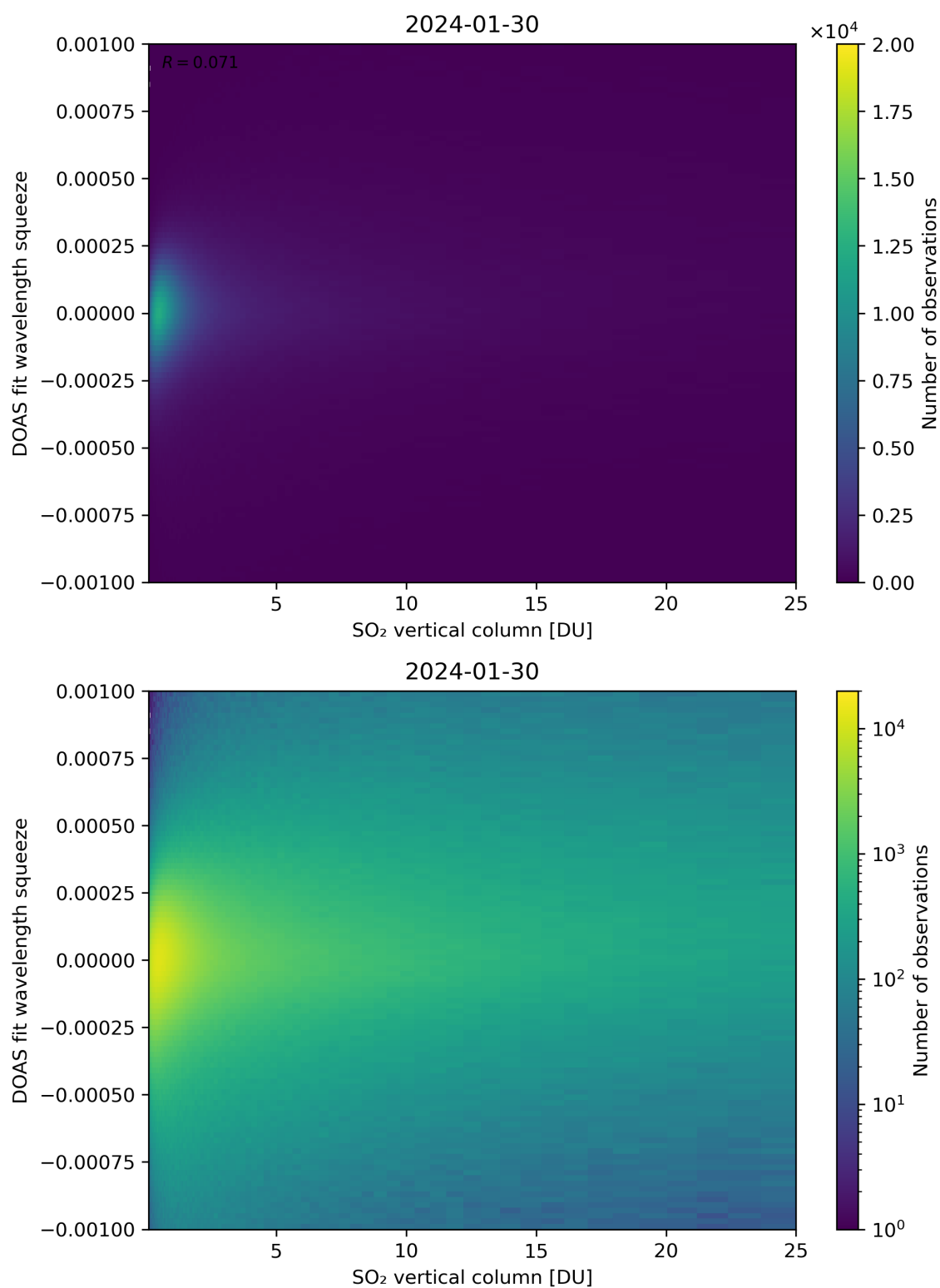
Figure 277: Scatter density plot of “SO 2 vertical column” against “DOAS fit wavelength squeeze” for 2024-01-29 to 2024-01-31.
