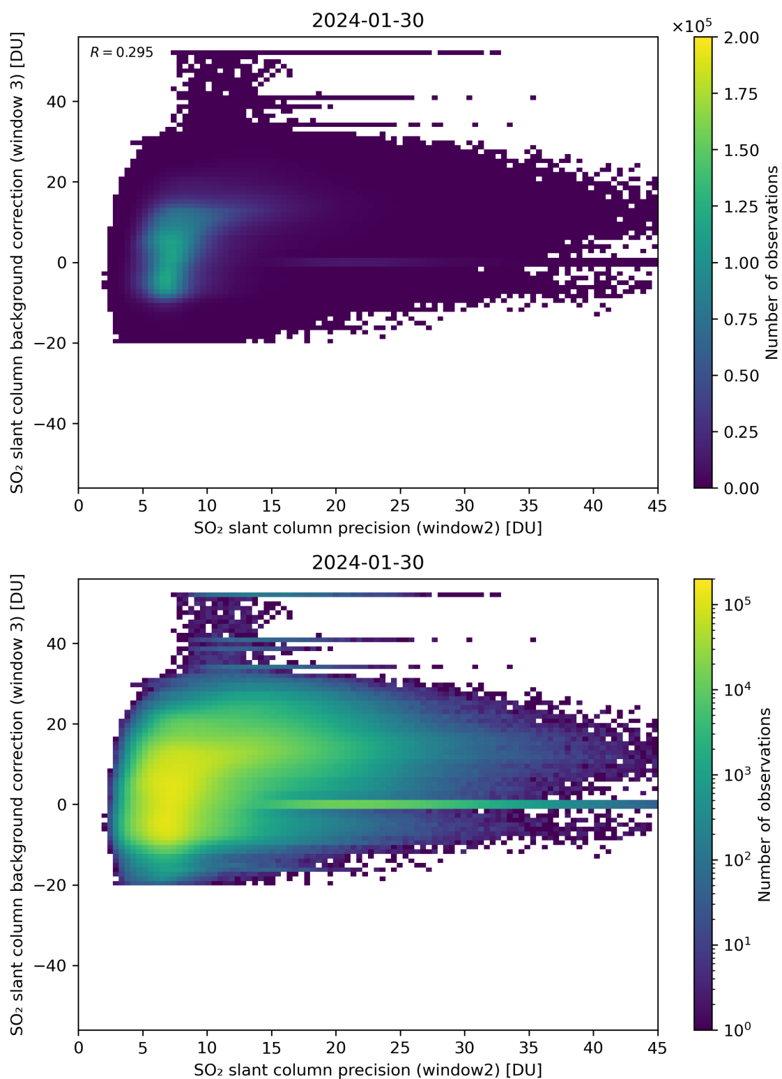
Figure 242: Scatter density plot of “SO 2 slant column precision (window2)” against “SO 2 slant column background correction (window 3)” for 2024-01-29 to 2024-01-31.
