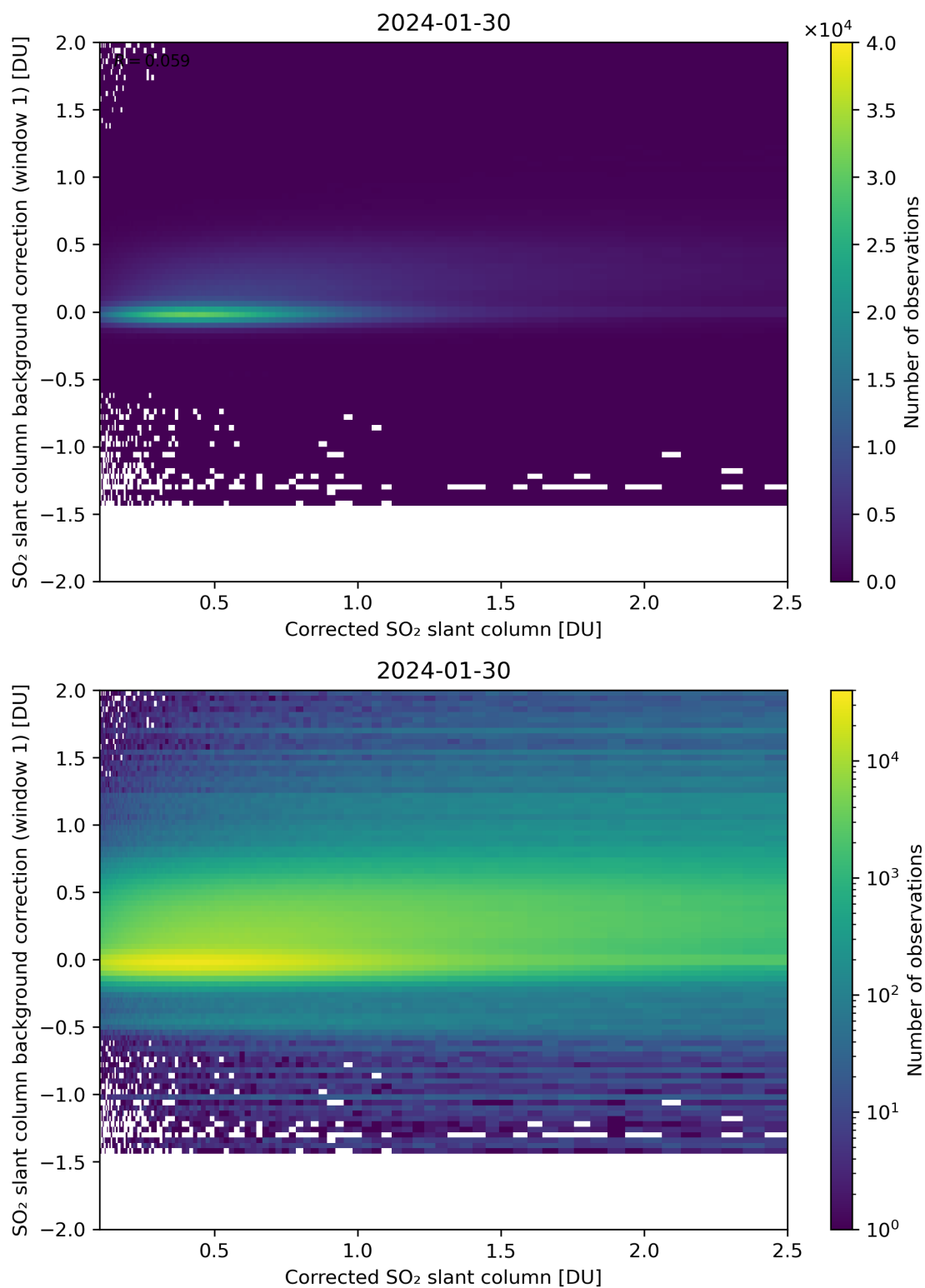
Figure 178: Scatter density plot of “Corrected SO 2 slant column” against “SO 2 slant column background correction (window 1)” for 2024-01-29 to 2024-01-31.
