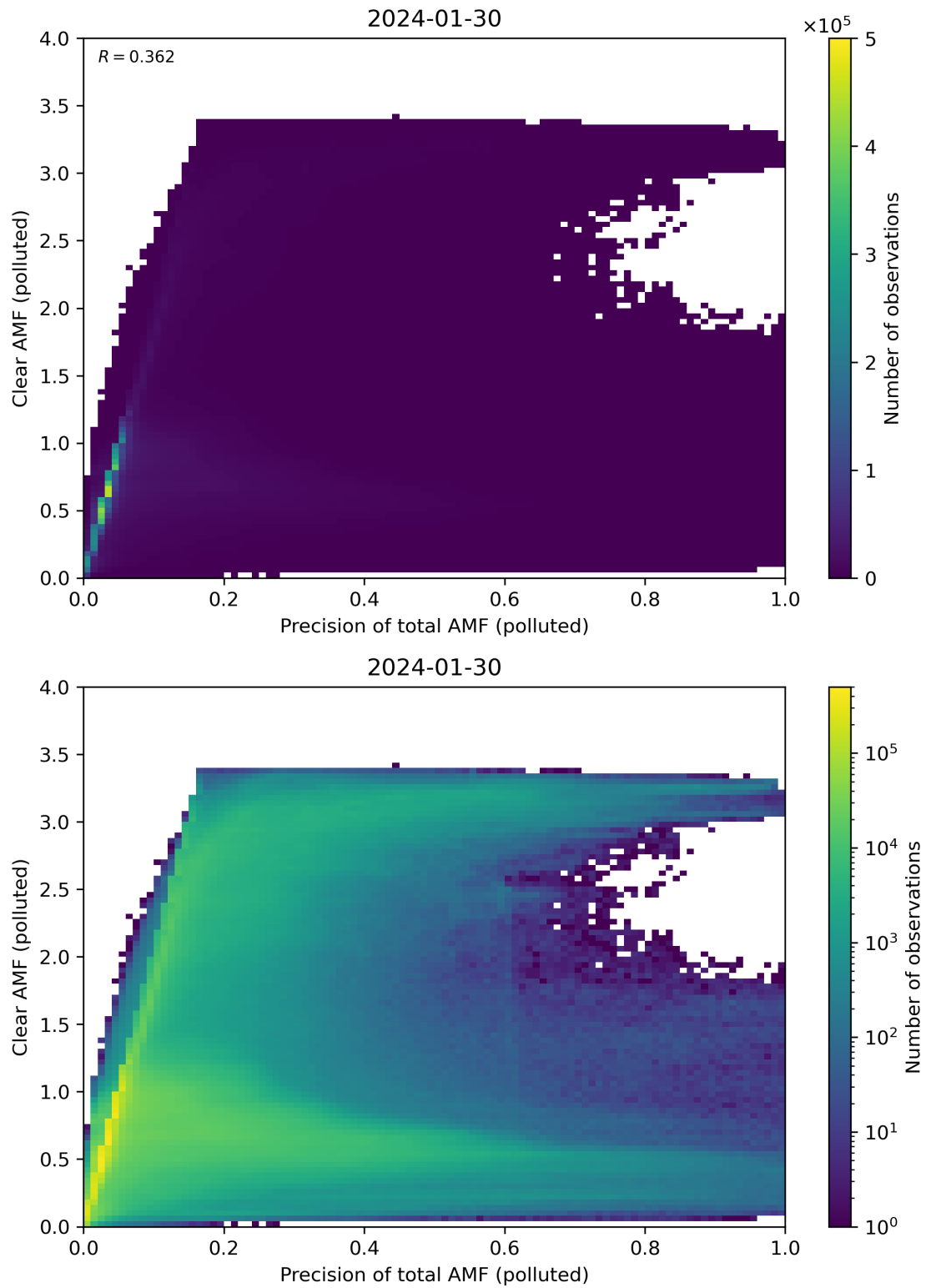
Figure 270: Scatter density plot of “Precision of total AMF (polluted)” against “Clear AMF (polluted)” for 2024-01-29 to 2024-01-31.
