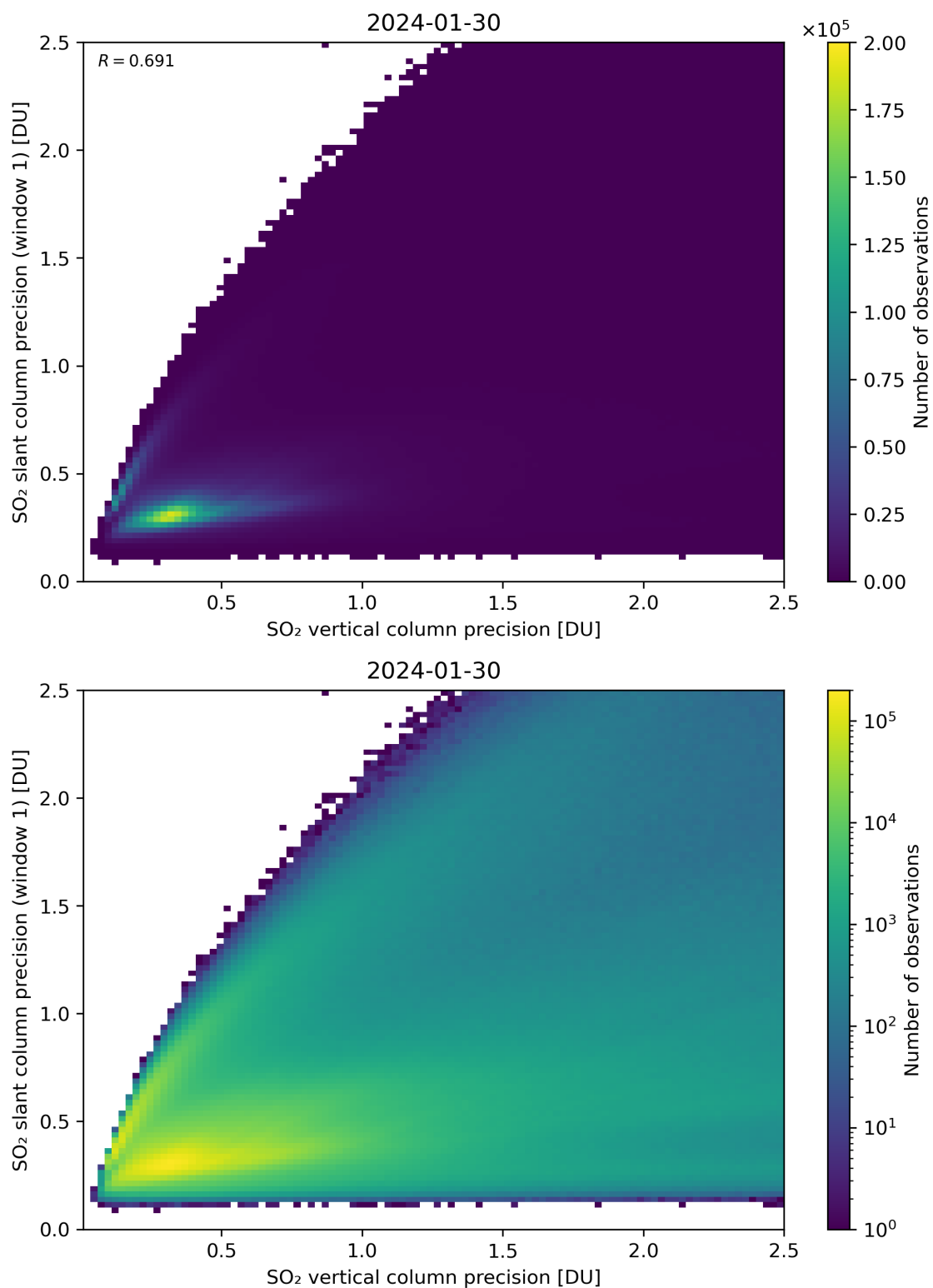
Figure 290: Scatter density plot of “SO 2 vertical column precision” against “SO 2 slant column precision (window 1)” for 2024-01-29 to 2024-01-31.
