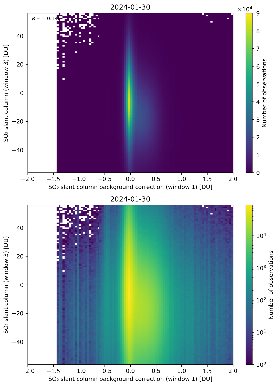
Figure 107: Scatter density plot of “SO 2 slant column background correction (window 1)” against “SO 2 slant column (window 3)” for 2024-01-29 to 2024-01-31.
