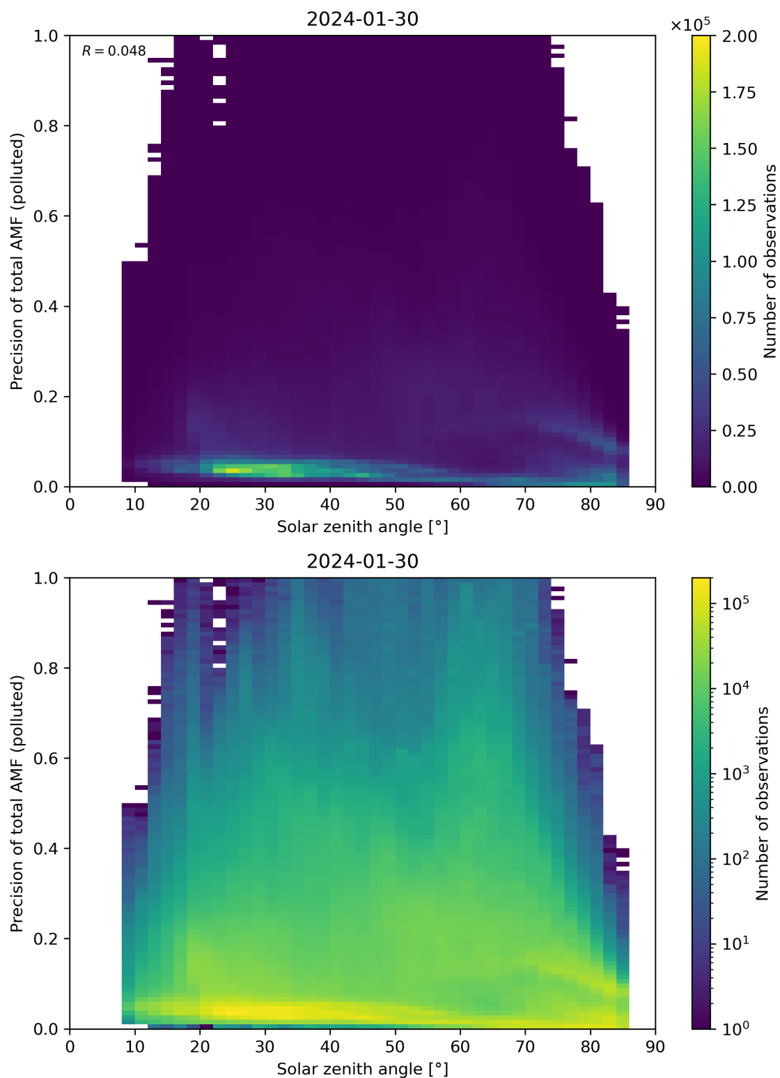
Figure 175: Scatter density plot of “Solar zenith angle” against “Precision of total AMF (polluted)” for 2024-01-29 to 2024-01-31.
