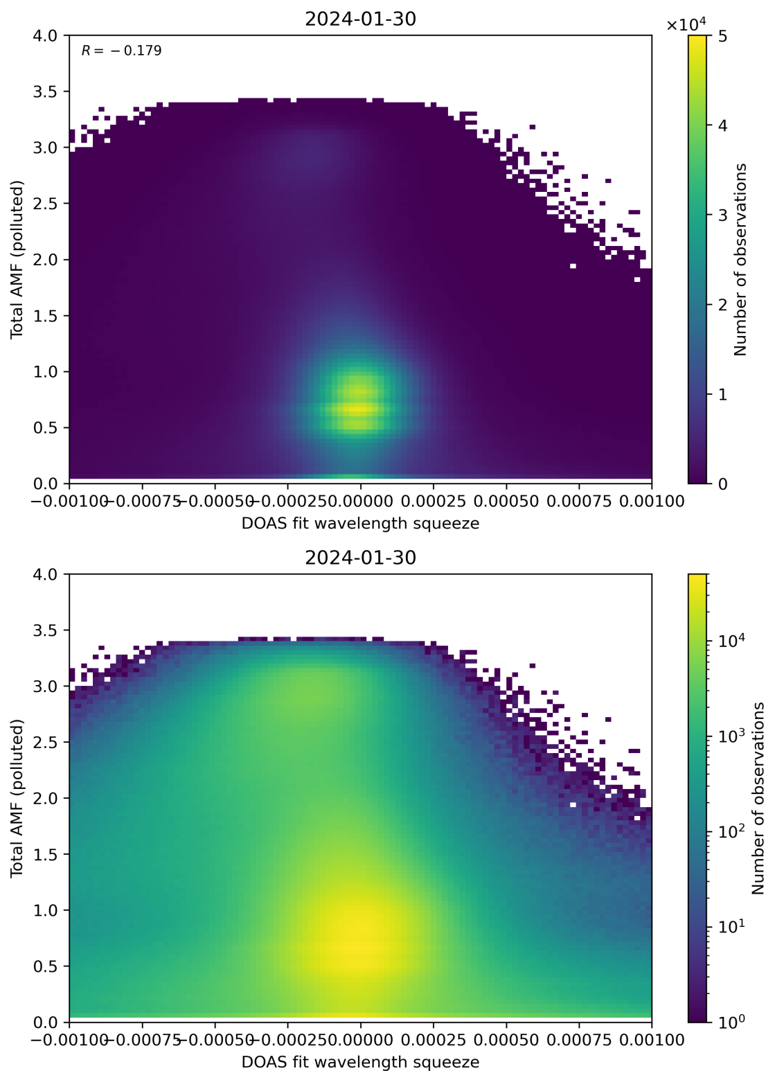
Figure 134: Scatter density plot of “DOAS fit wavelength squeeze” against “Total AMF (polluted)” for 2024-01-29 to 2024-01-31.
