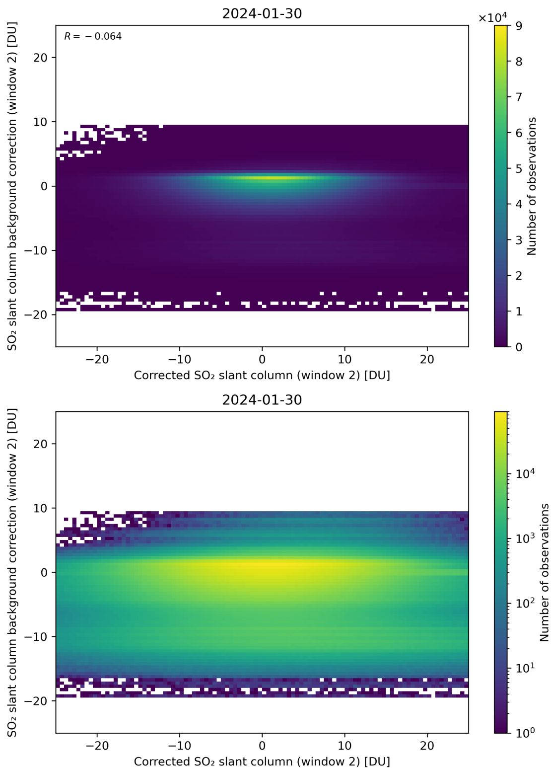
Figure 194: Scatter density plot of “Corrected SO 2 slant column (window 2)” against “SO 2 slant column background correction (window 2)” for 2024-01-29 to 2024-01-31.
