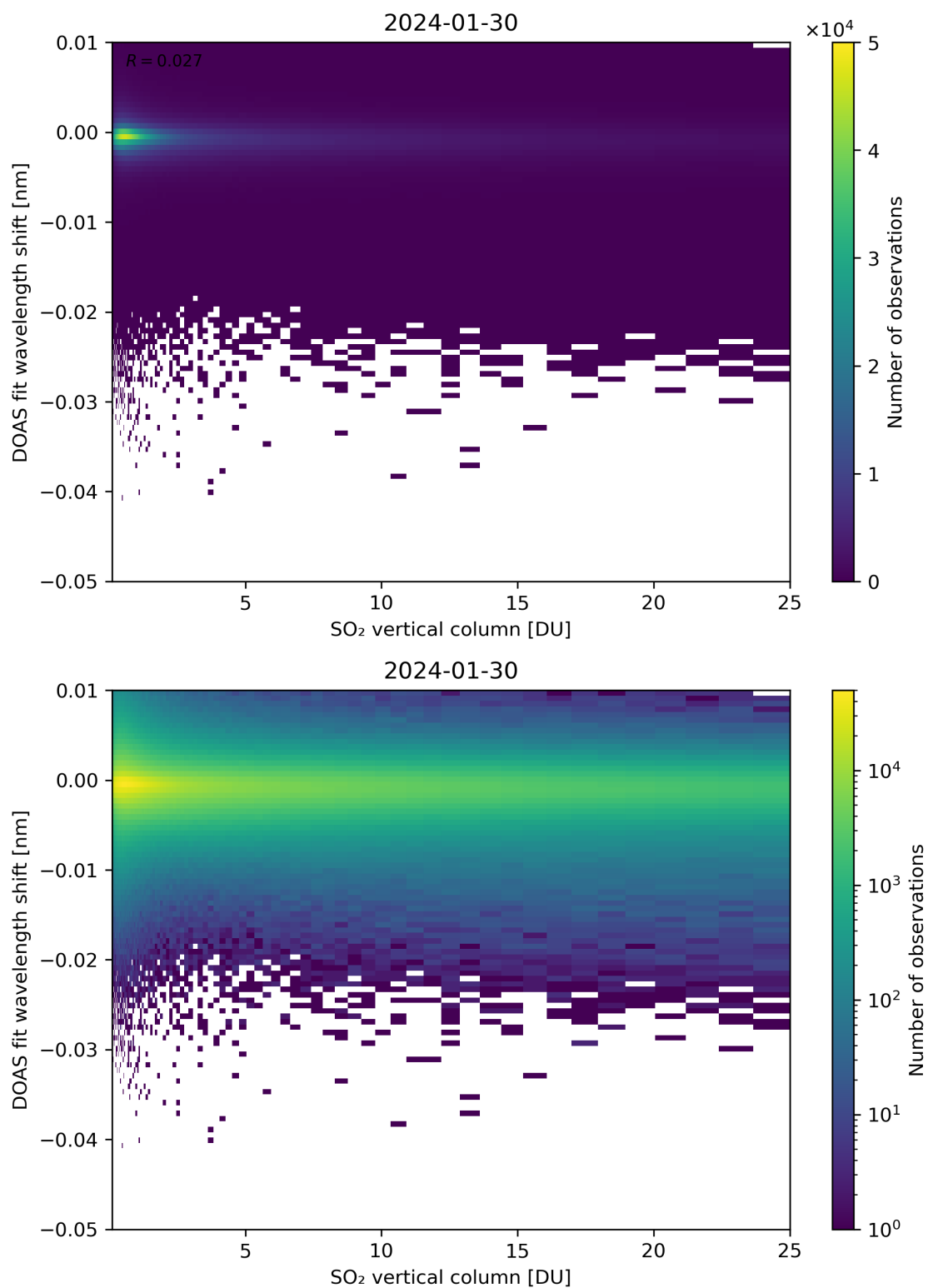
Figure 276: Scatter density plot of “SO 2 vertical column” against “DOAS fit wavelength shift” for 2024-01-29 to 2024-01-31.
