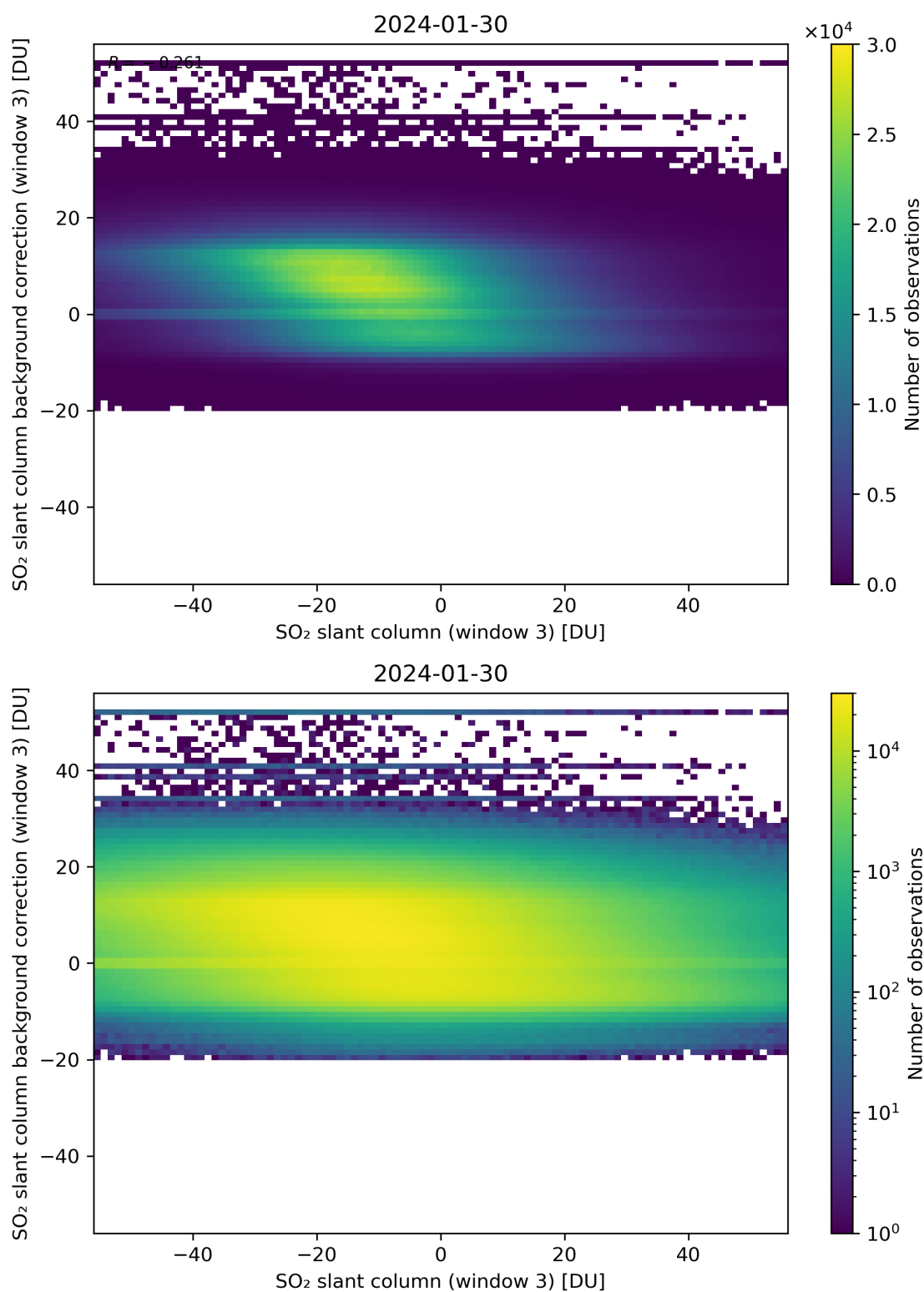
Figure 253: Scatter density plot of “SO 2 slant column (window 3)” against “SO 2 slant column background correction (window 3)” for 2024-01-29 to 2024-01-31.
