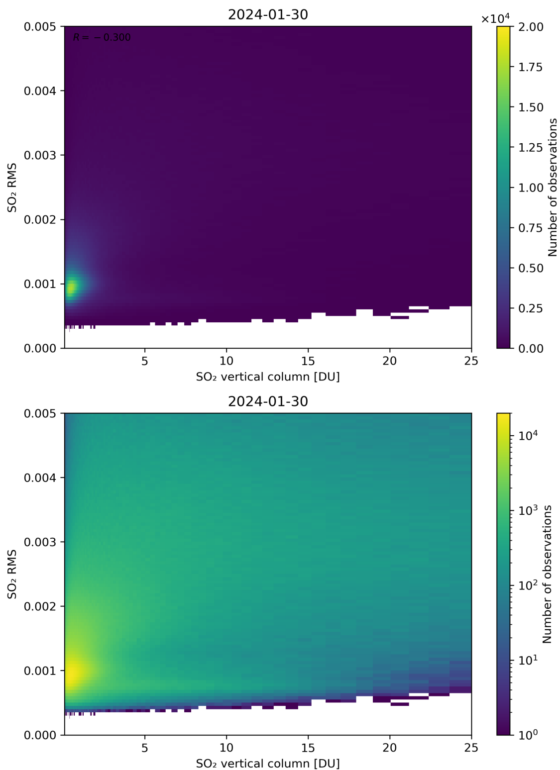
Figure 278: Scatter density plot of “SO 2 vertical column” against “SO 2 RMS” for 2024-01-29 to 2024-01-31.
