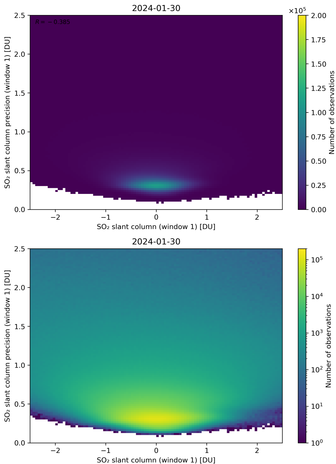
Figure 235: Scatter density plot of “SO 2 slant column (window 1)” against “SO 2 slant column precision (window 1)” for 2024-01-29 to 2024-01-31.
