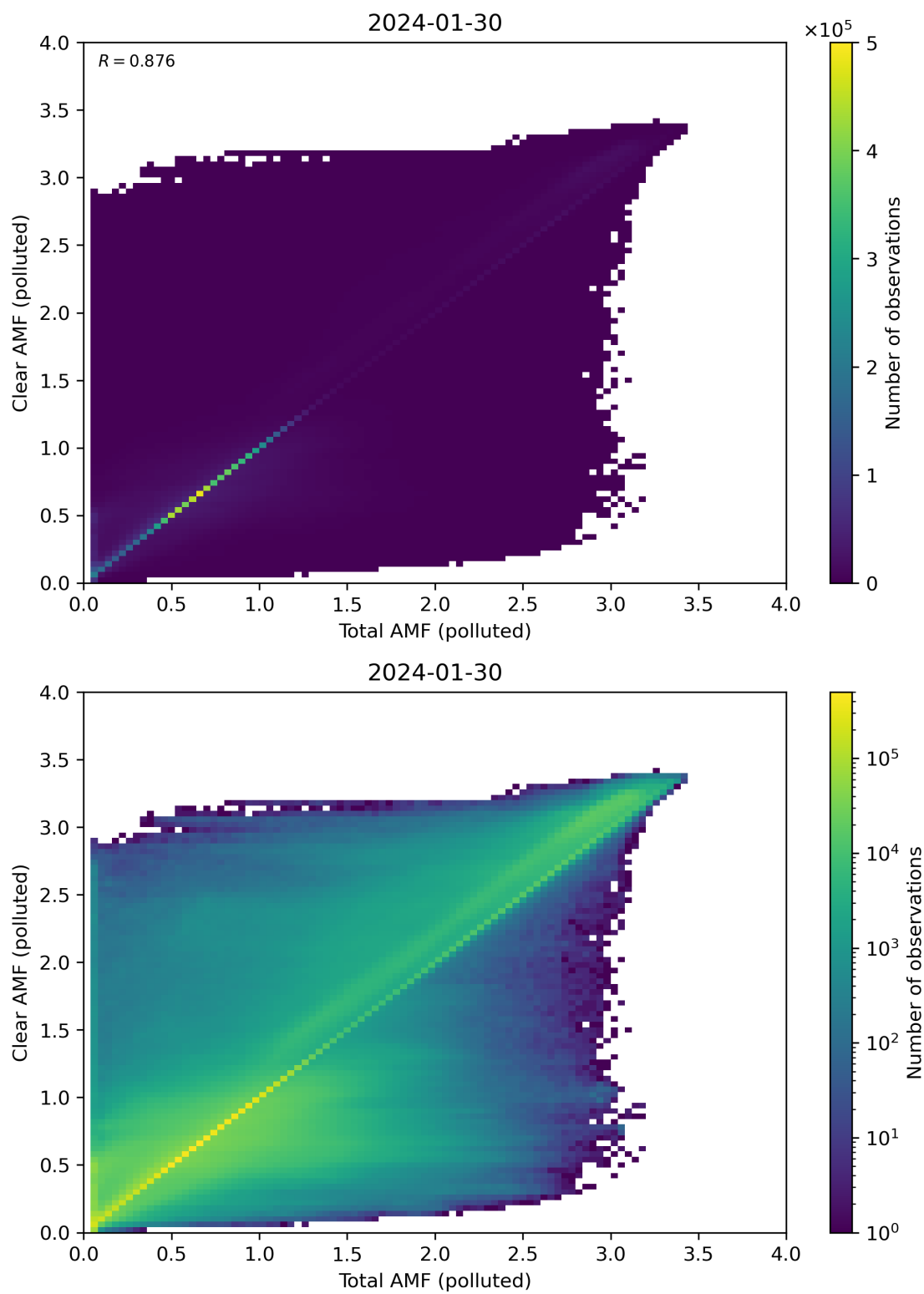
Figure 271: Scatter density plot of “Total AMF (polluted)” against “Clear AMF (polluted)” for 2024-01-29 to 2024-01-31.
