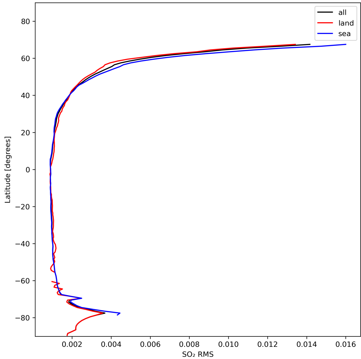
Figure 47: Zonal average of “SO 2 RMS” for 2024-01-29 to 2024-01-31.
