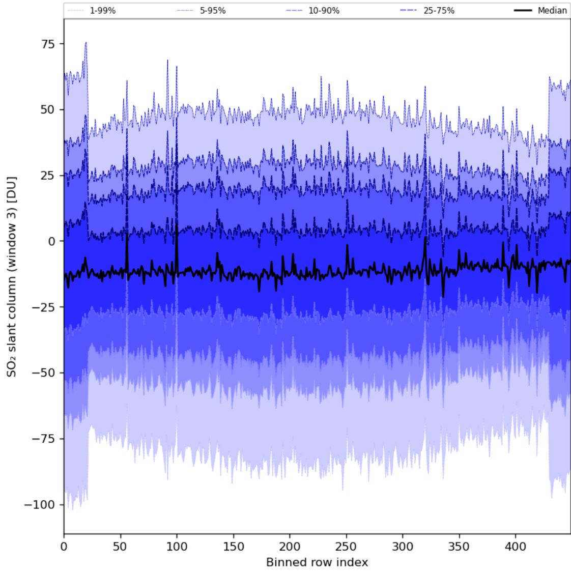
Figure 87: Along track statistics of “SO 2 slant column (window 3)” for 2024-01-29 to 2024-01-31
