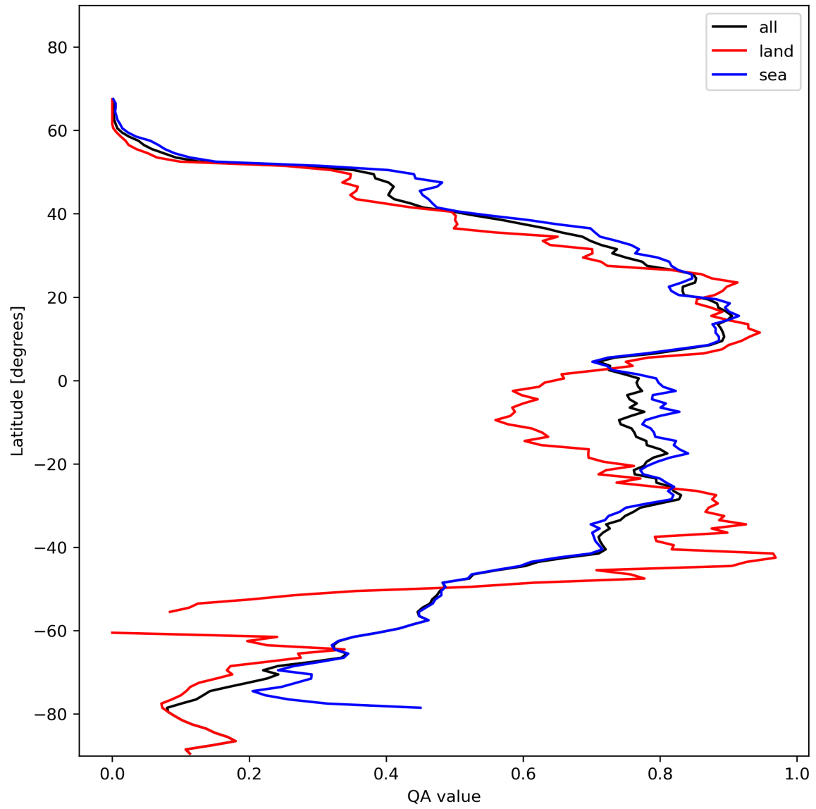
Figure 29: Zonal average of “QA value” for 2024-01-29 to 2024-01-31.
