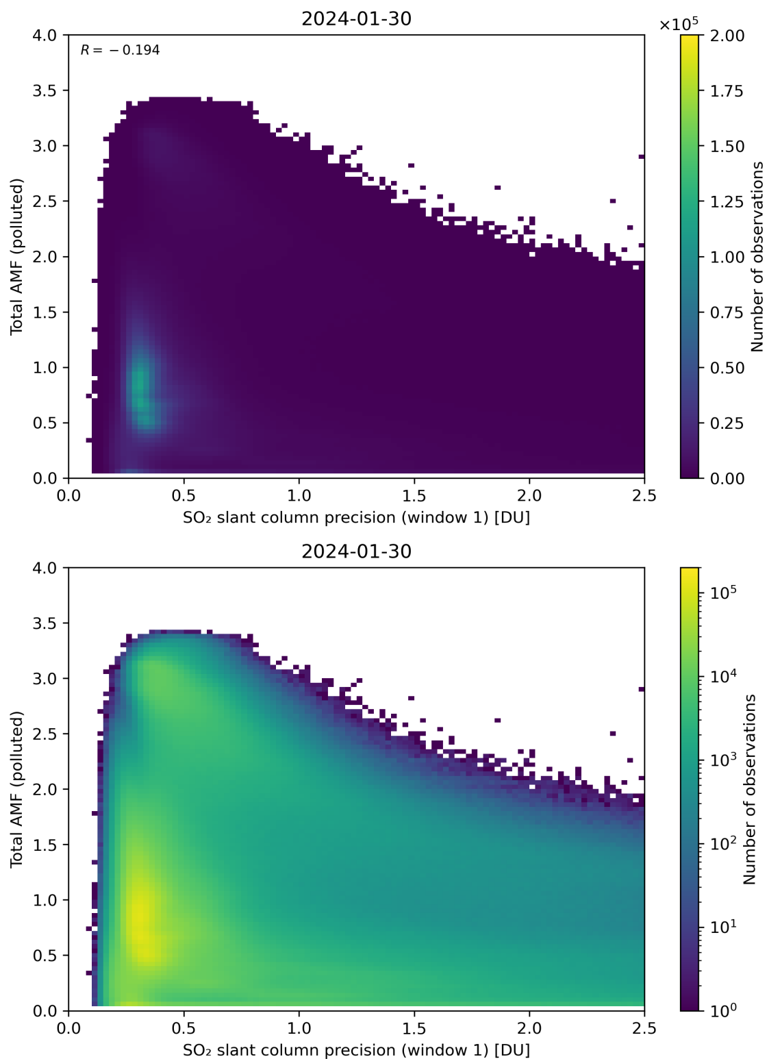
Figure 230: Scatter density plot of “SO 2 slant column precision (window 1)” against “Total AMF (polluted)” for 2024-01-29 to 2024-01-31.
