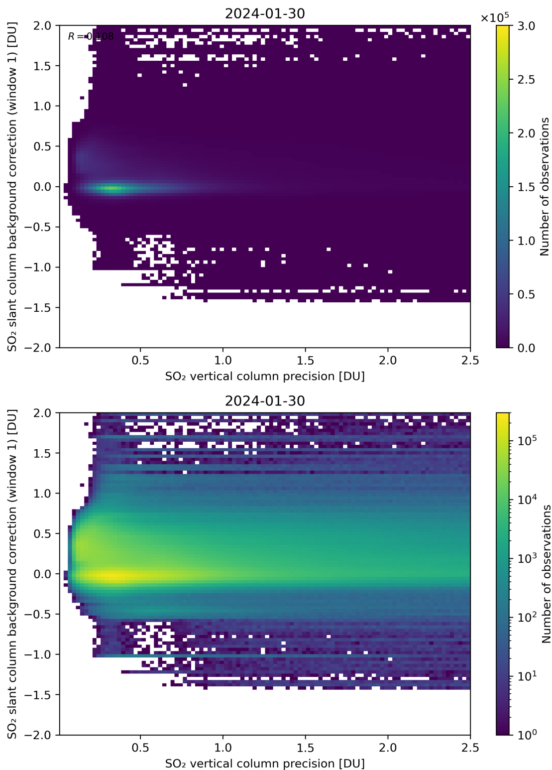
Figure 279: Scatter density plot of “SO 2 vertical column precision” against “SO 2 slant column background correction (window 1)” for 2024-01-29 to 2024-01-31.
