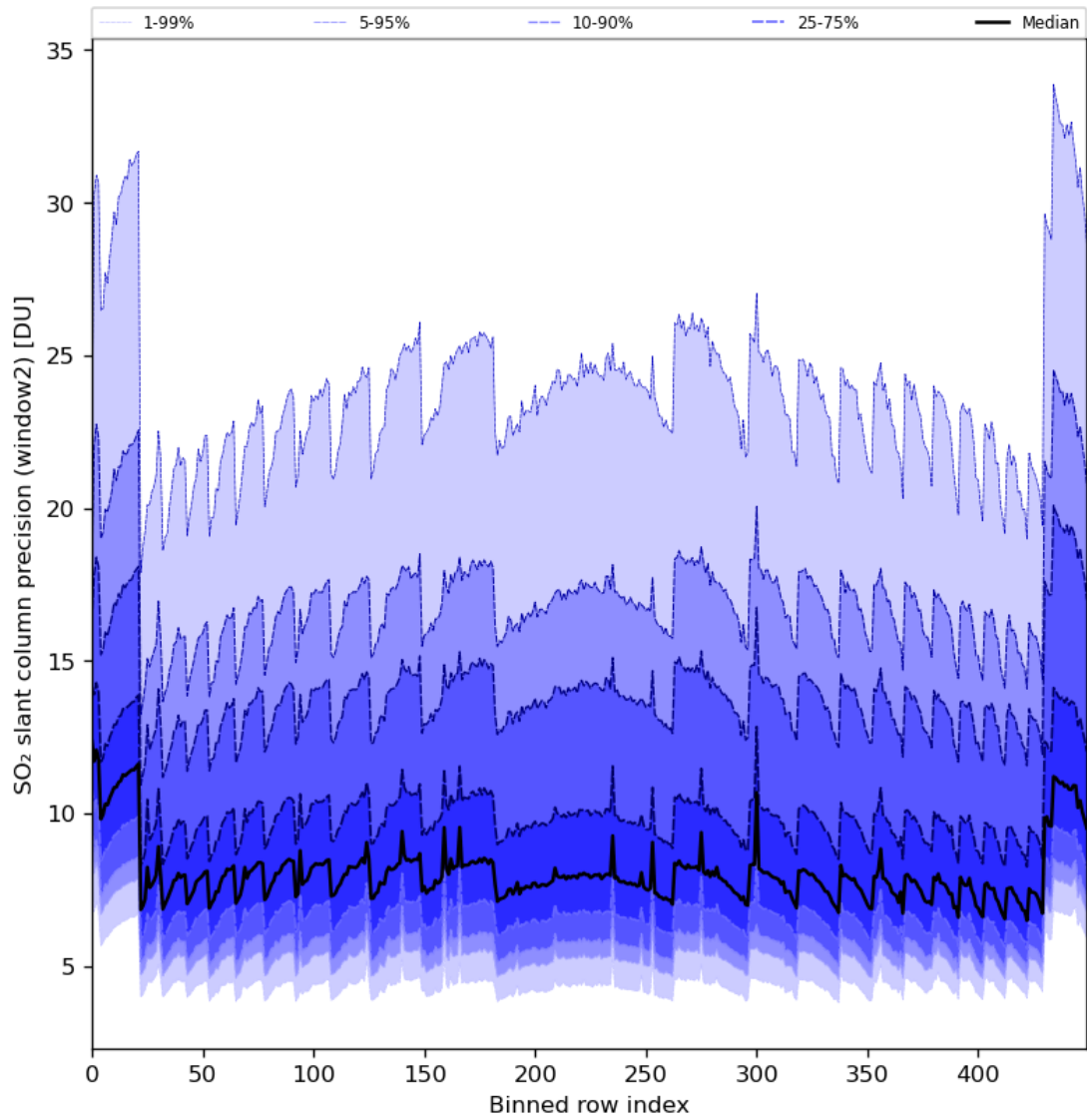
Figure 84: Along track statistics of “SO 2 slant column precision (window2)” for 2024-01-29 to 2024-01-31
