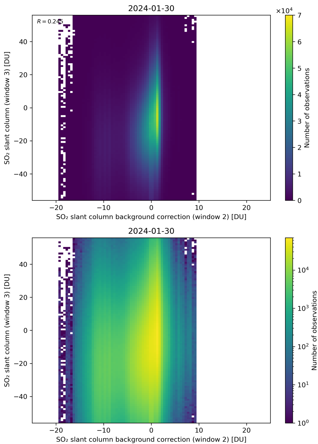
Figure 117: Scatter density plot of “SO 2 slant column background correction (window 2)” against “SO 2 slant column (window 3)” for 2024-01-29 to 2024-01-31.
