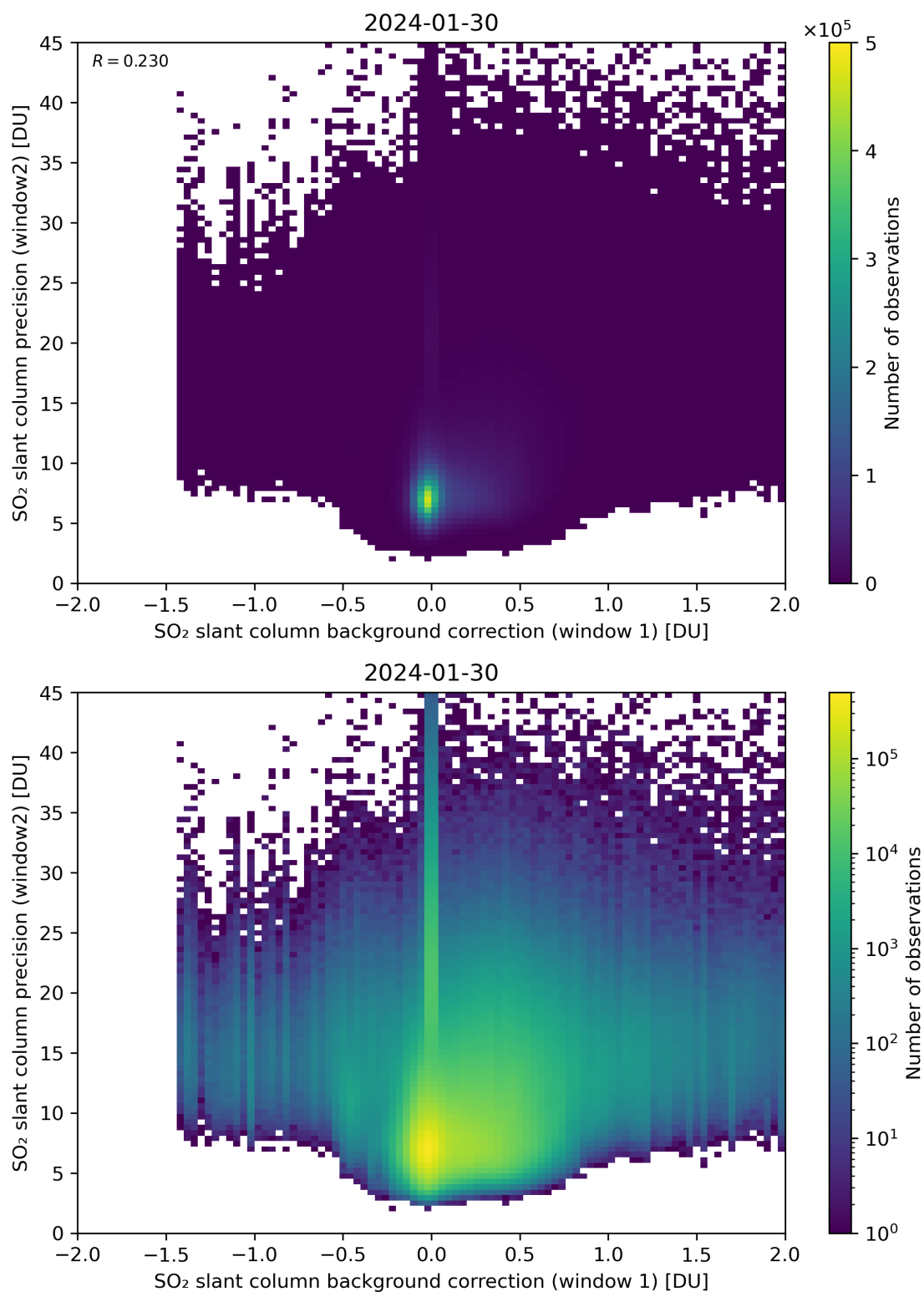
Figure 106: Scatter density plot of “SO 2 slant column background correction (window 1)” against “SO 2 slant column precision (window2)” for 2024-01-29 to 2024-01-31.
