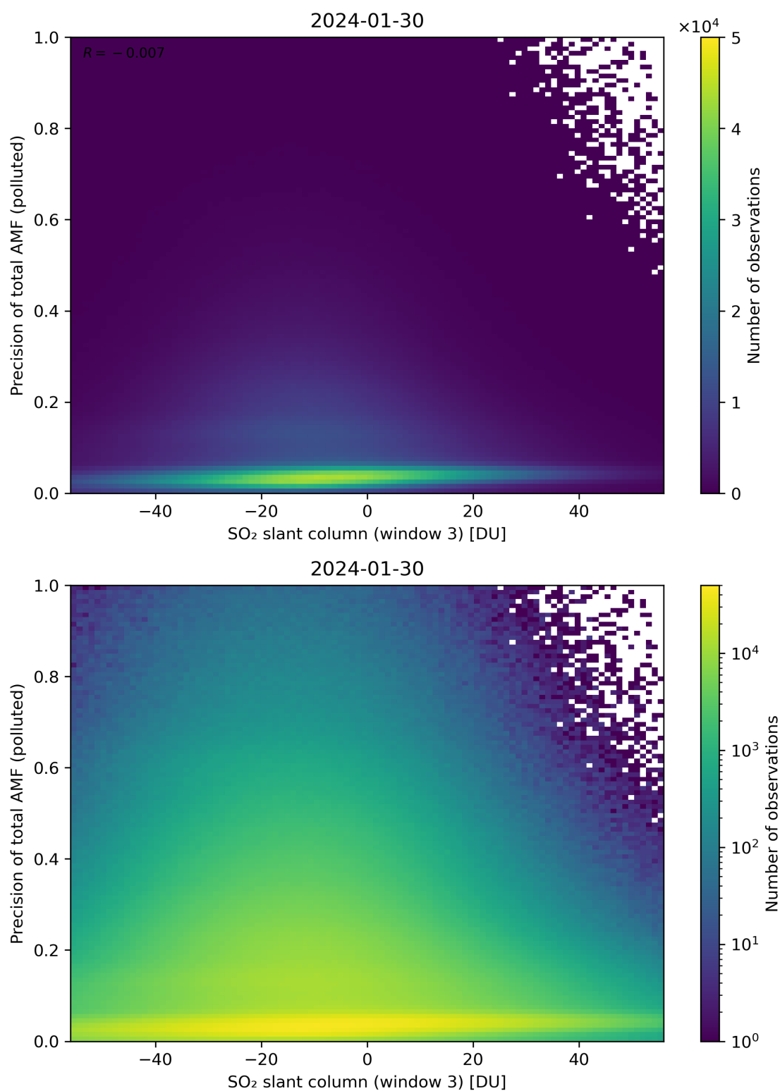
Figure 269: Scatter density plot of “SO 2 slant column (window 3)” against “Precision of total AMF (polluted)” for 2024-01-29 to 2024-01-31.
