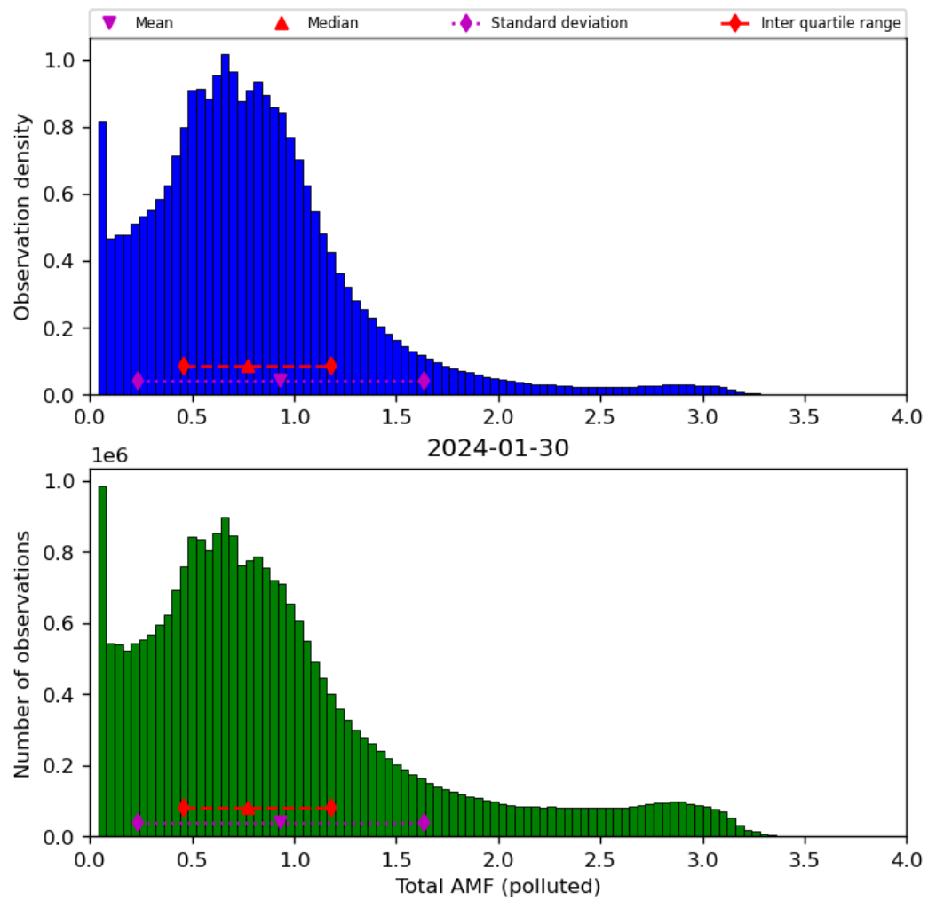
Figure 71: Histogram of “Total AMF (polluted)” for 2024-01-29 to 2024-01-31
