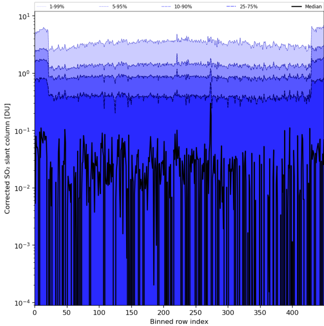
Figure 78: Along track statistics of “Corrected SO 2 slant column” for 2024-01-29 to 2024-01-31
