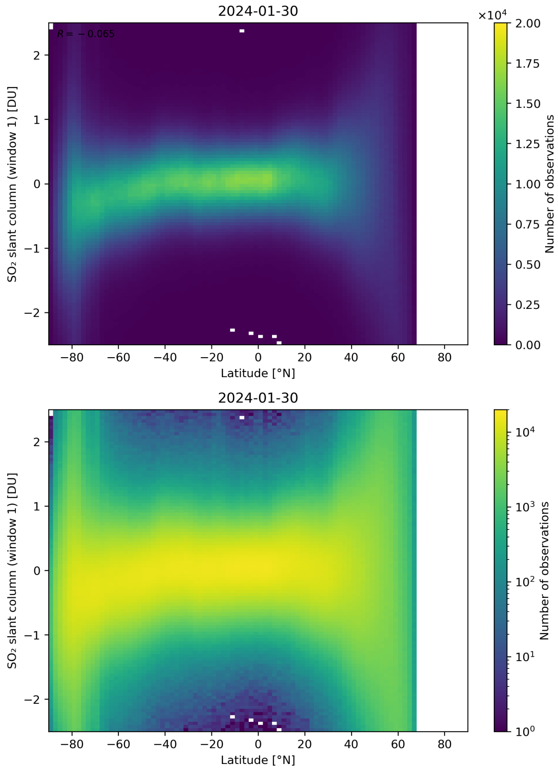
Figure 149: Scatter density plot of “Latitude” against “SO 2 slant column (window 1)” for 2024-01-29 to 2024-01-31.
