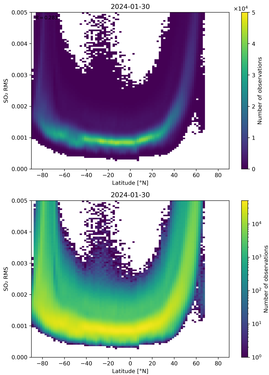
Figure 144: Scatter density plot of “Latitude” against “SO 2 RMS” for 2024-01-29 to 2024-01-31.
