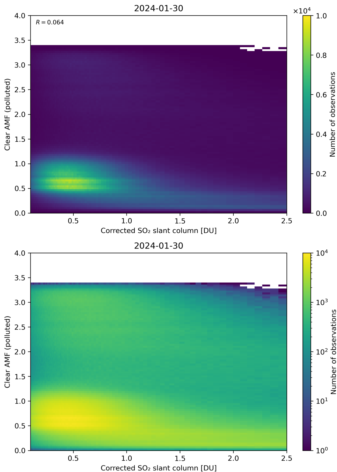
Figure 184: Scatter density plot of “Corrected SO 2 slant column” against “Clear AMF (polluted)” for 2024-01-29 to 2024-01-31.
