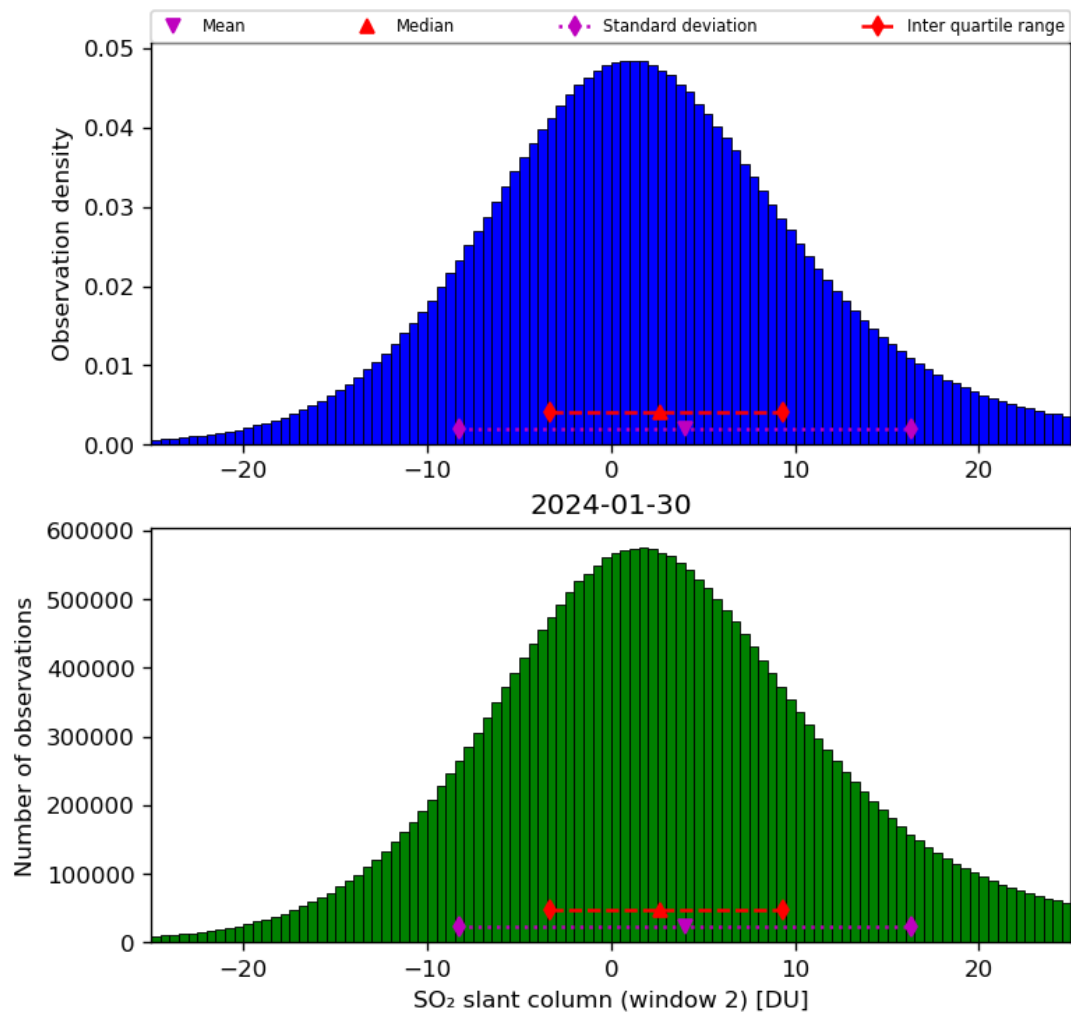
Figure 60: Histogram of “SO 2 slant column (window 2)” for 2024-01-29 to 2024-01-31
