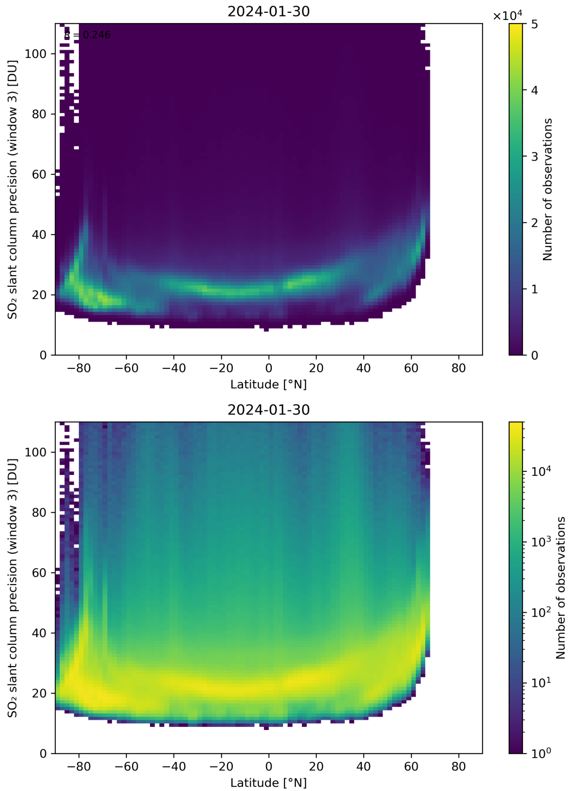
Figure 153: Scatter density plot of “Latitude” against “SO 2 slant column precision (window 3)” for 2024-01-29 to 2024-01-31.
