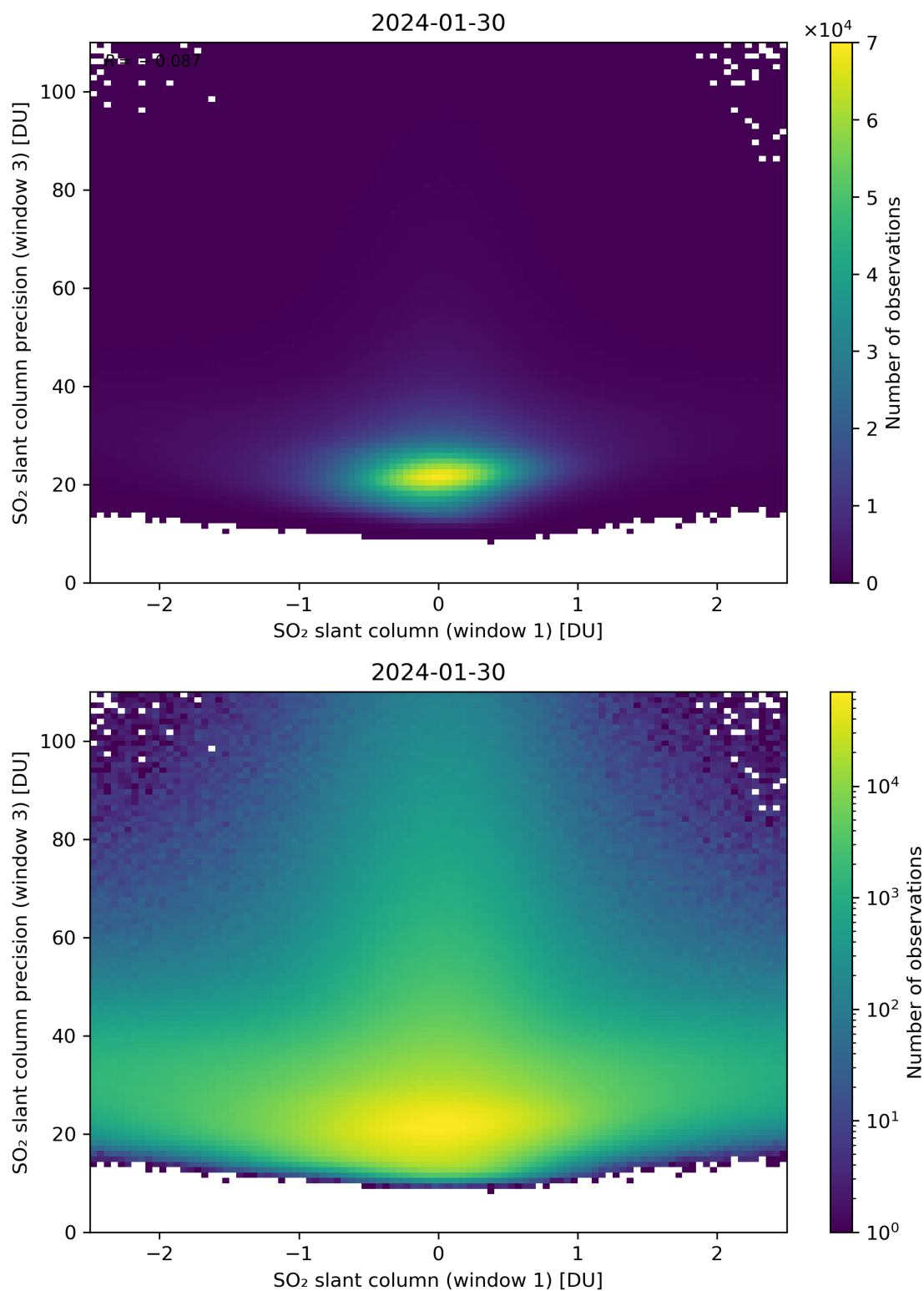
Figure 238: Scatter density plot of “SO 2 slant column (window 1)” against “SO 2 slant column precision (window 3)” for 2024-01-29 to 2024-01-31.
