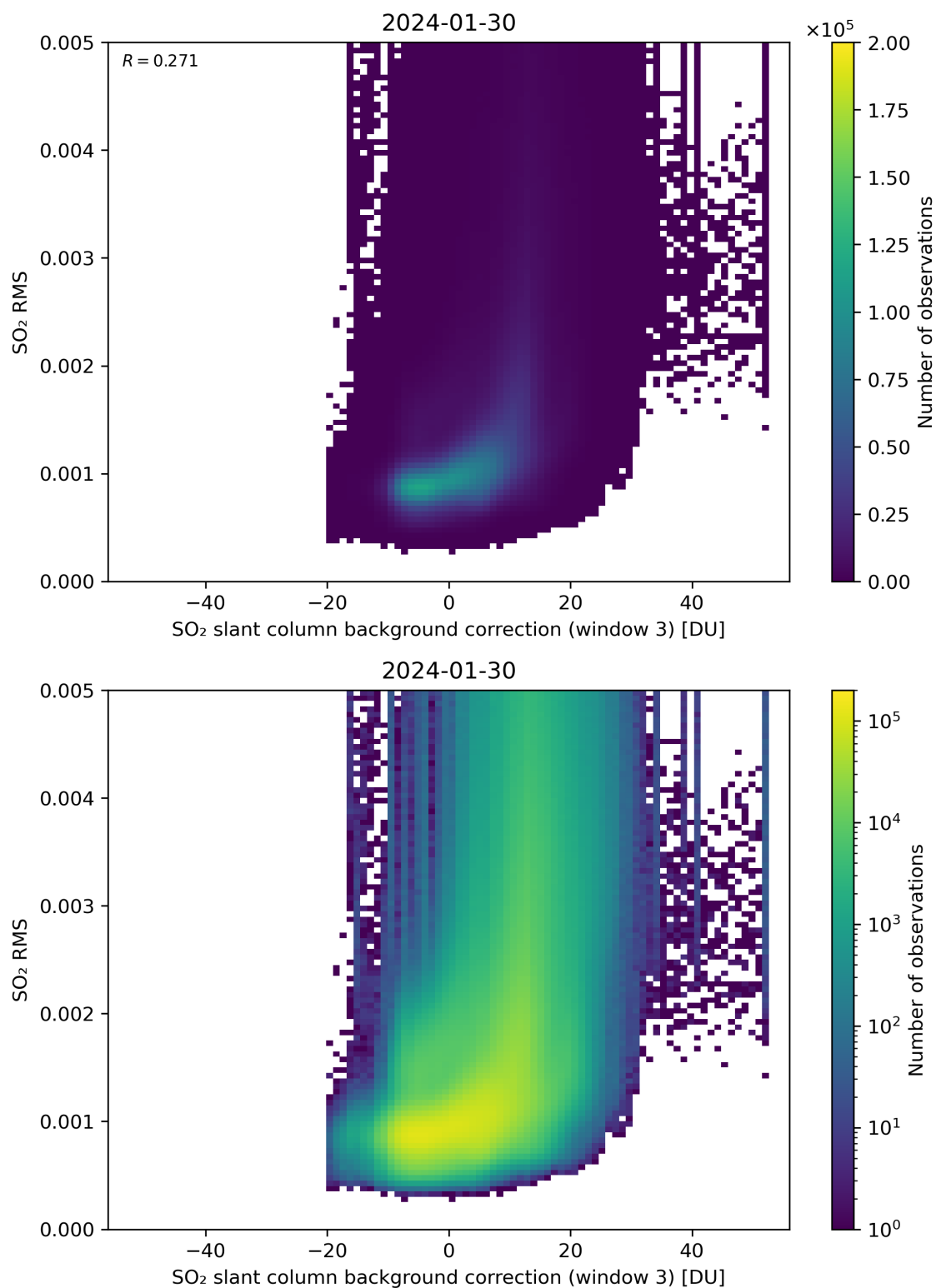
Figure 123: Scatter density plot of “SO 2 slant column background correction (window 3)” against “SO 2 RMS” for 2024-01-29 to 2024-01-31.
