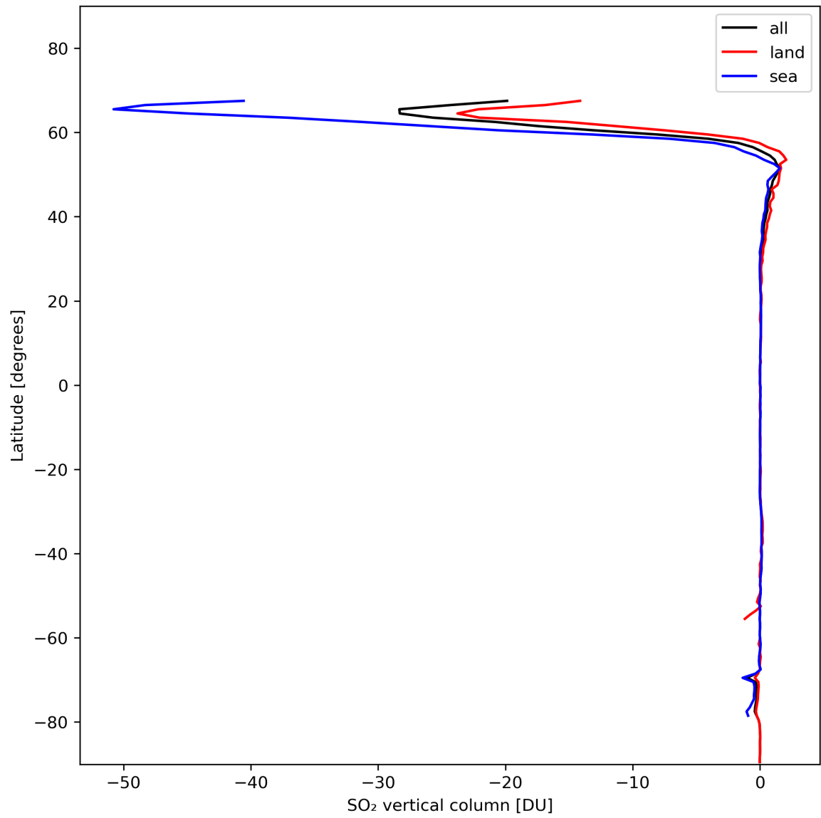
Figure 30: Zonal average of “SO 2 vertical column” for 2024-01-29 to 2024-01-31.
