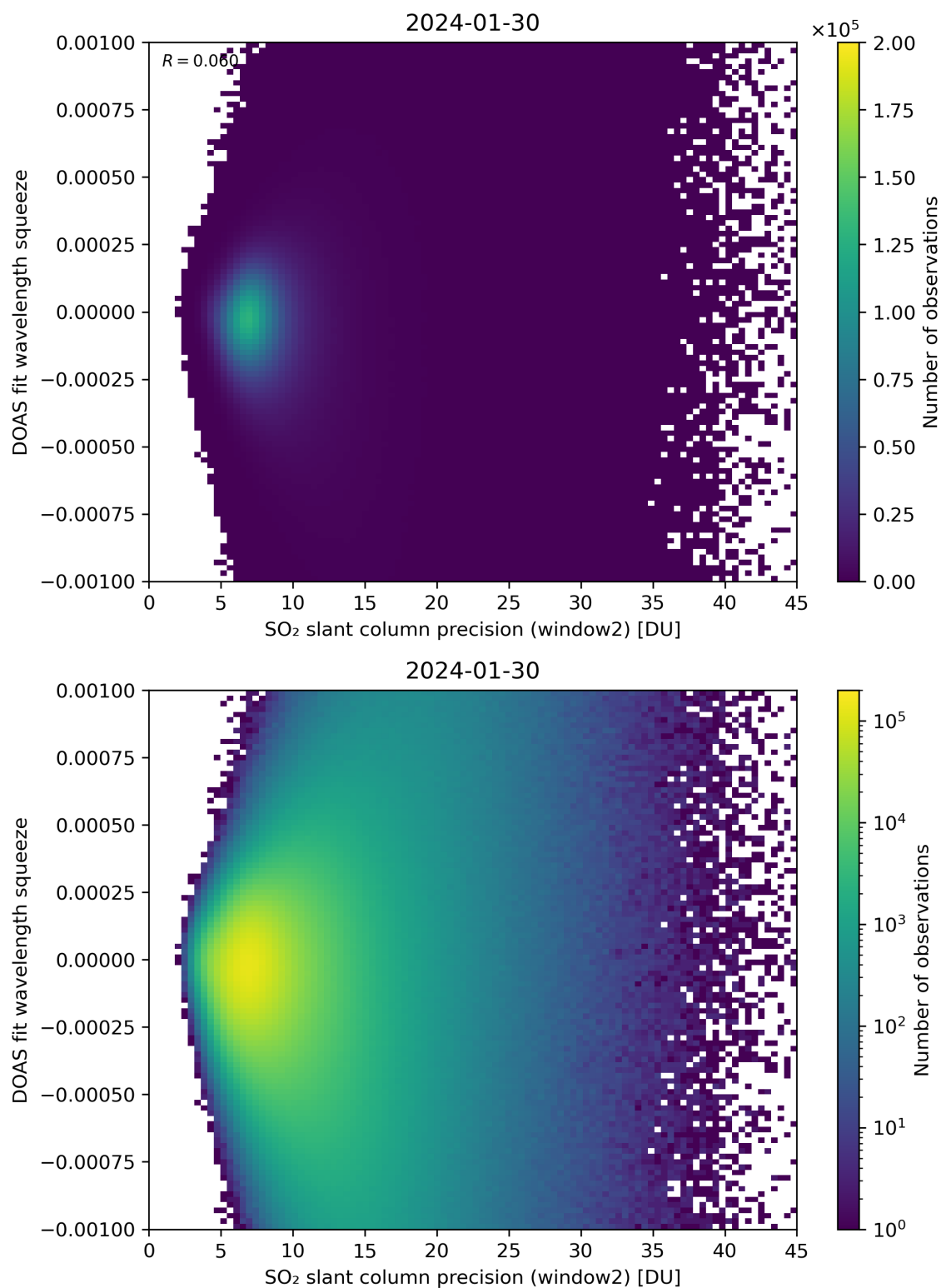
Figure 244: Scatter density plot of “SO 2 slant column precision (window2)” against “DOAS fit wavelength squeeze” for 2024-01-29 to 2024-01-31.
