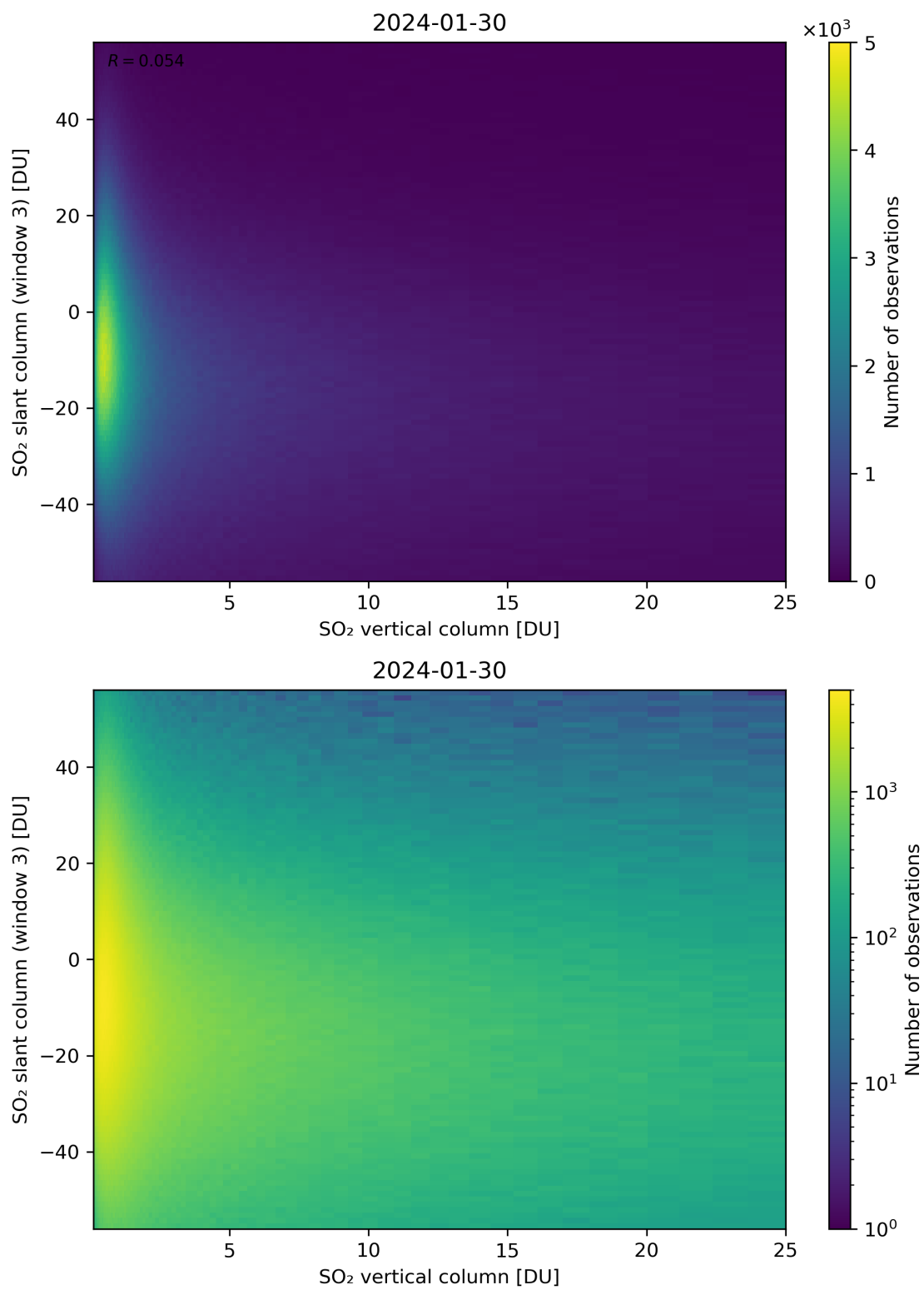
Figure 303: Scatter density plot of “SO 2 vertical column” against “SO 2 slant column (window 3)” for 2024-01-29 to 2024-01-31.
