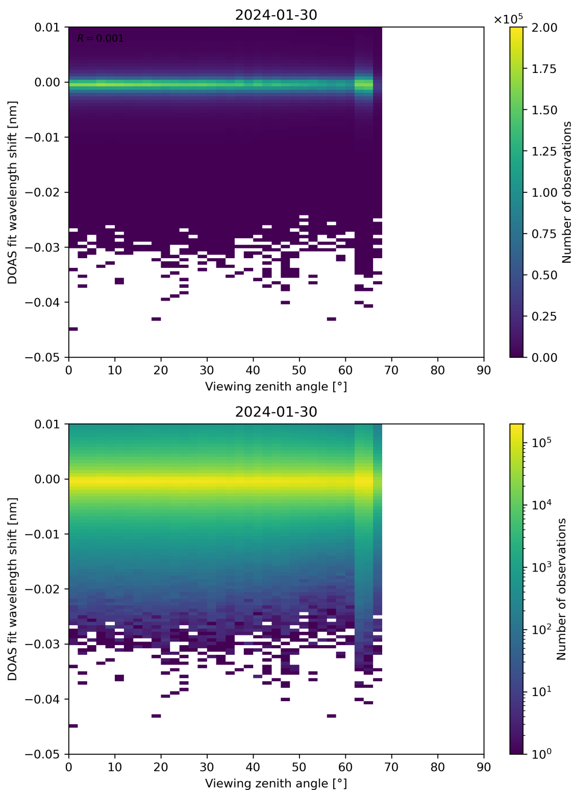
Figure 311: Scatter density plot of “Viewing zenith angle” against “DOAS fit wavelength shift” for 2024-01-29 to 2024-01-31.
