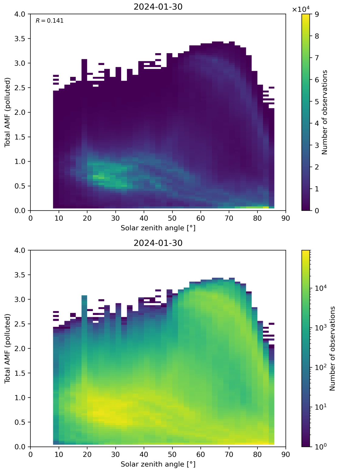
Figure 174: Scatter density plot of “Solar zenith angle” against “Total AMF (polluted)” for 2024-01-29 to 2024-01-31.
