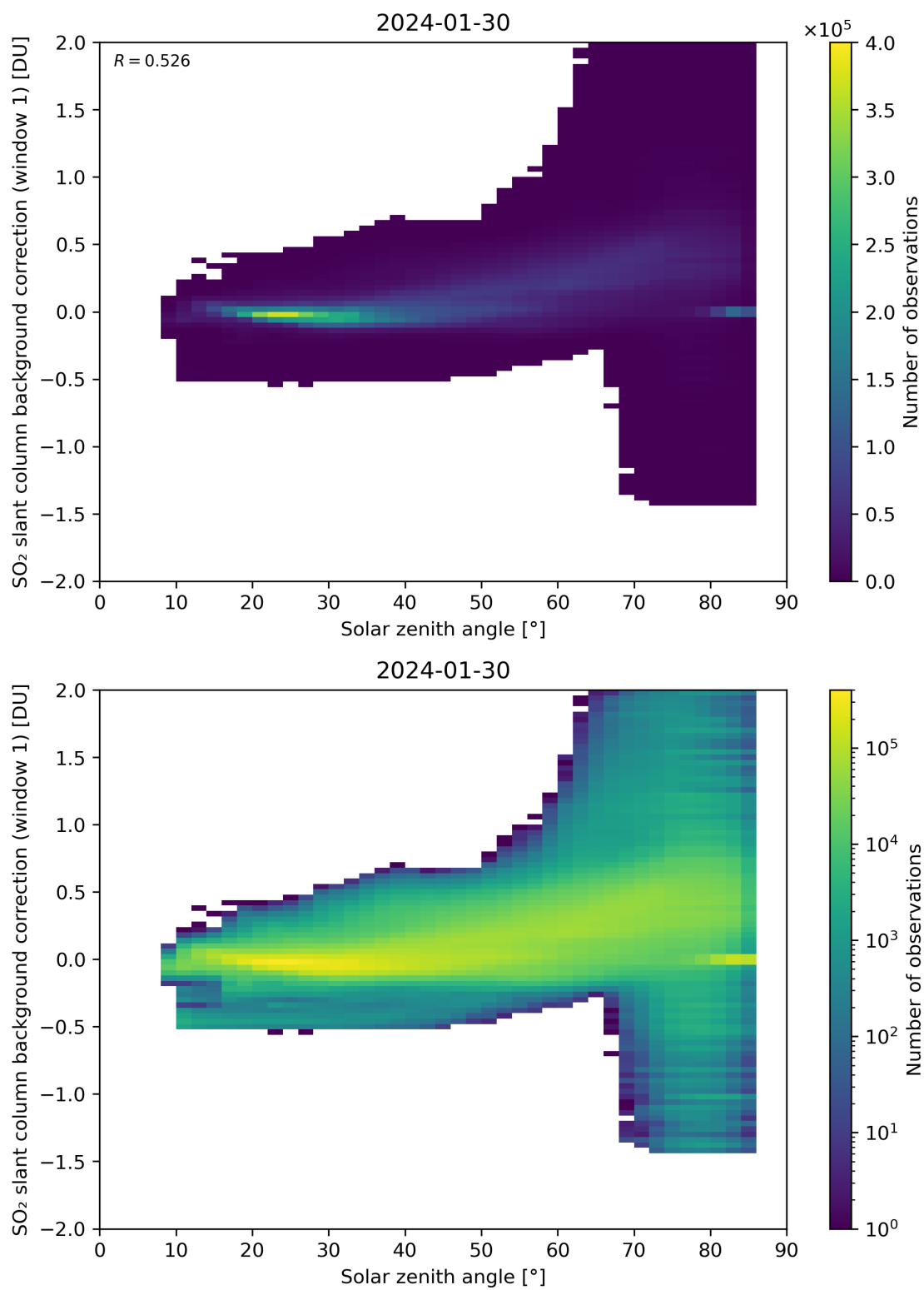
Figure 158: Scatter density plot of “Solar zenith angle” against “SO 2 slant column background correction (window 1)” for 2024-01-29 to 2024-01-31.
