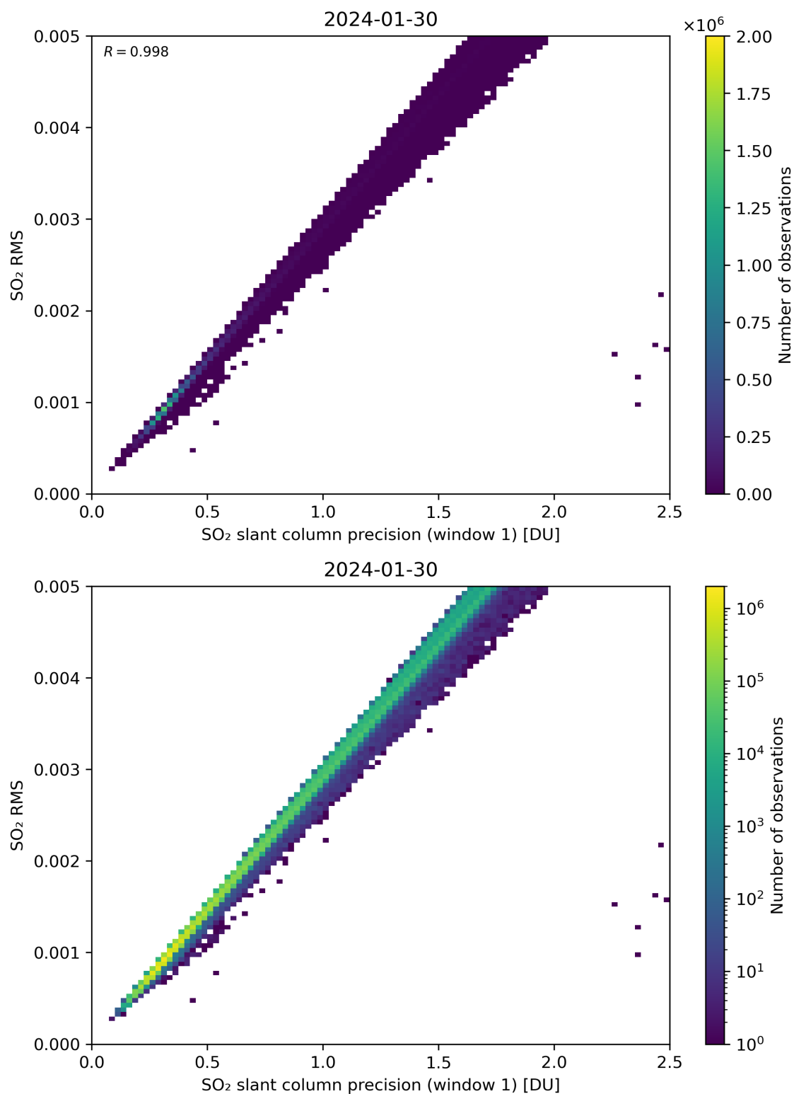
Figure 223: Scatter density plot of “SO 2 slant column precision (window 1)” against “SO 2 RMS” for 2024-01-29 to 2024-01-31.
