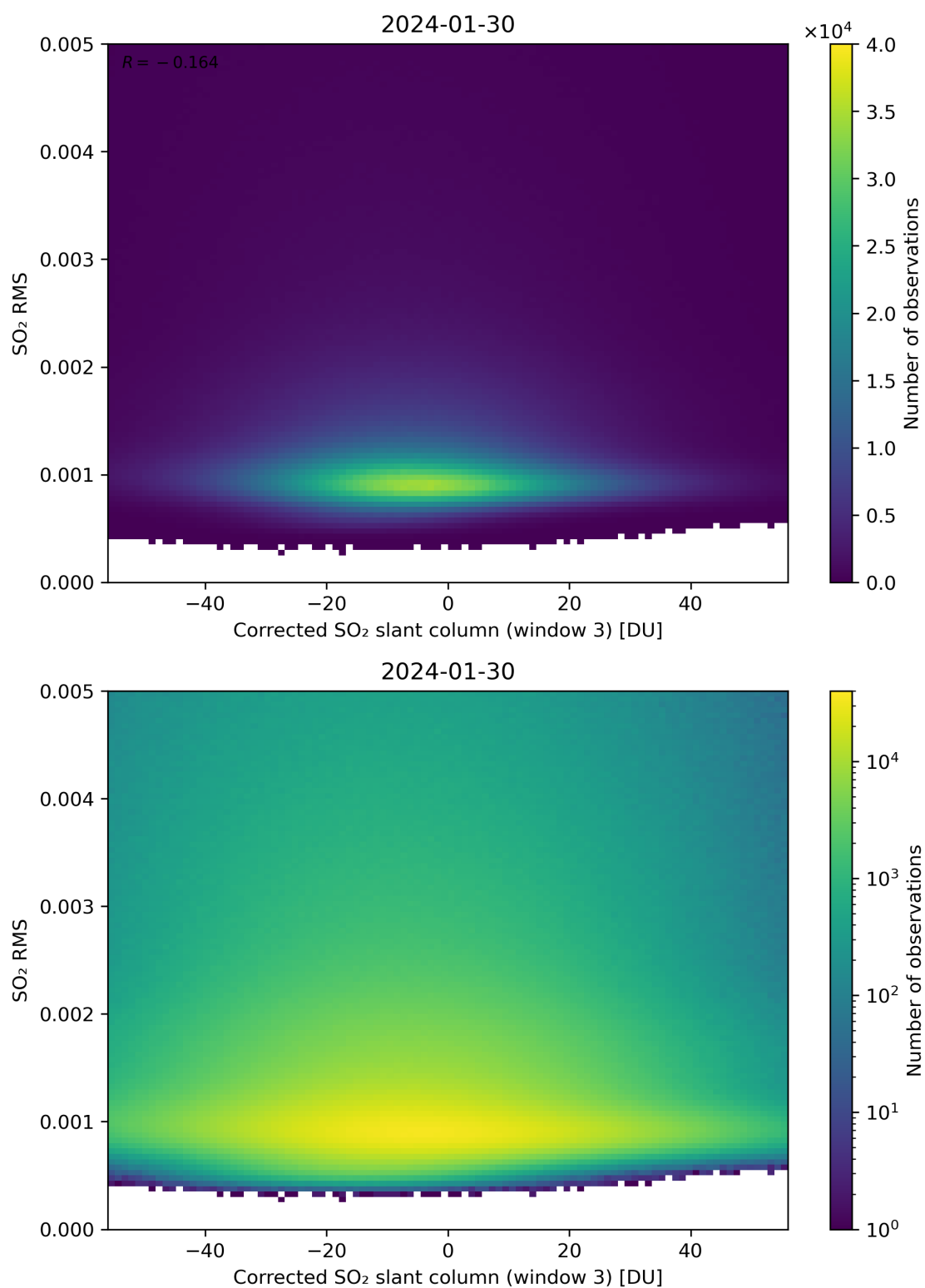
Figure 208: Scatter density plot of “Corrected SO 2 slant column (window 3)” against “SO 2 RMS” for 2024-01-29 to 2024-01-31.
