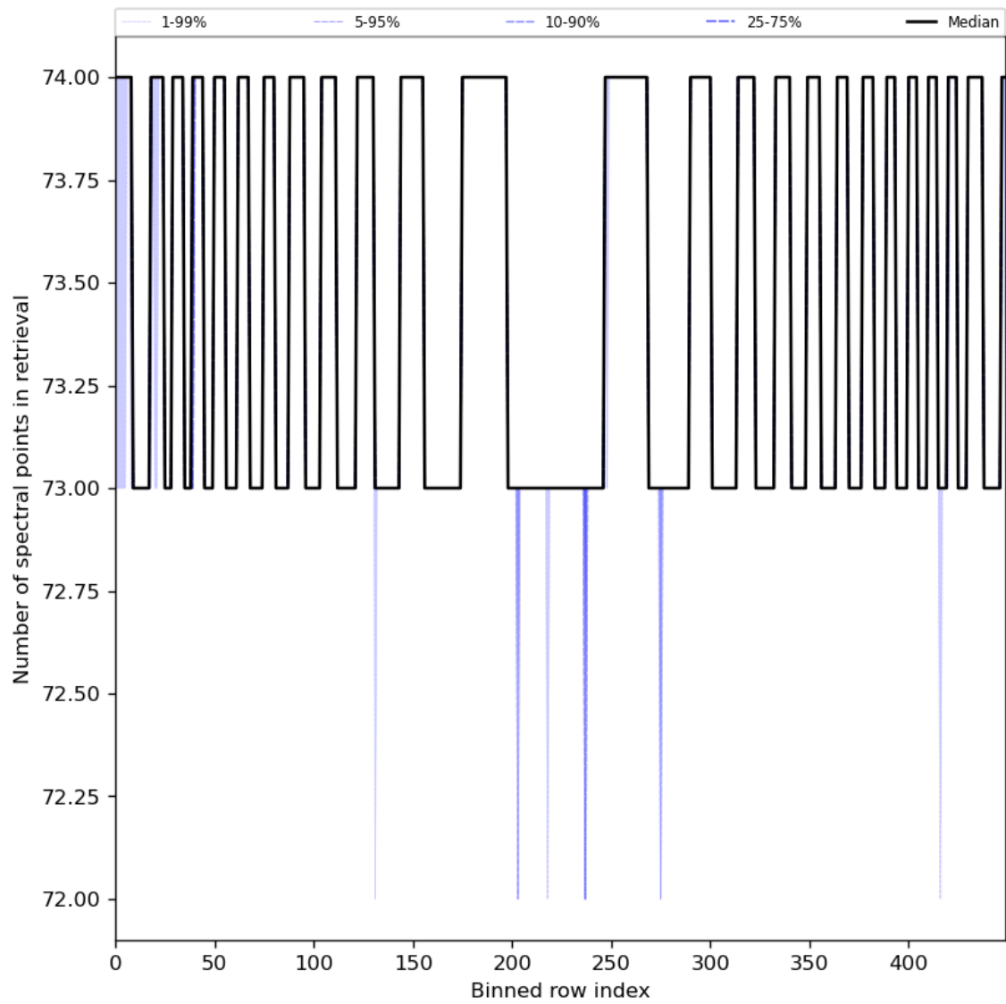
Figure 97: Along track statistics of “Number of spectral points in retrieval” for 2024-01-29 to 2024-01-31
