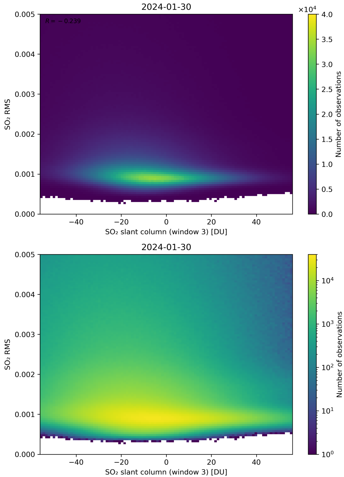
Figure 256: Scatter density plot of “SO 2 slant column (window 3)” against “SO 2 RMS” for 2024-01-29 to 2024-01-31.
