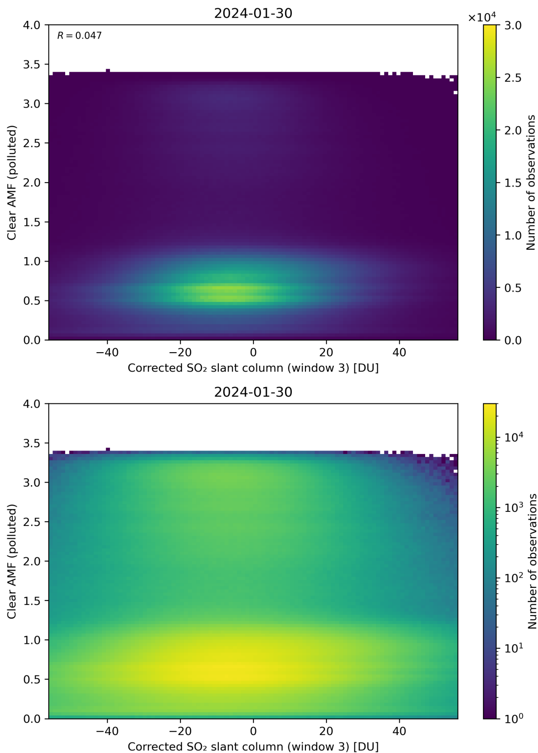
Figure 209: Scatter density plot of “Corrected SO 2 slant column (window 3)” against “Clear AMF (polluted)” for 2024-01-29 to 2024-01-31.
