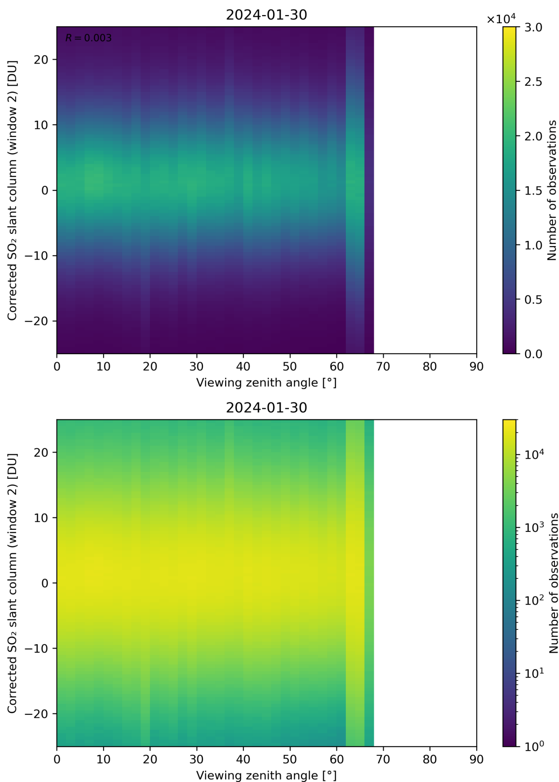
Figure 318: Scatter density plot of “Viewing zenith angle” against “Corrected SO 2 slant column (window 2)” for 2024-01-29 to 2024-01-31.
