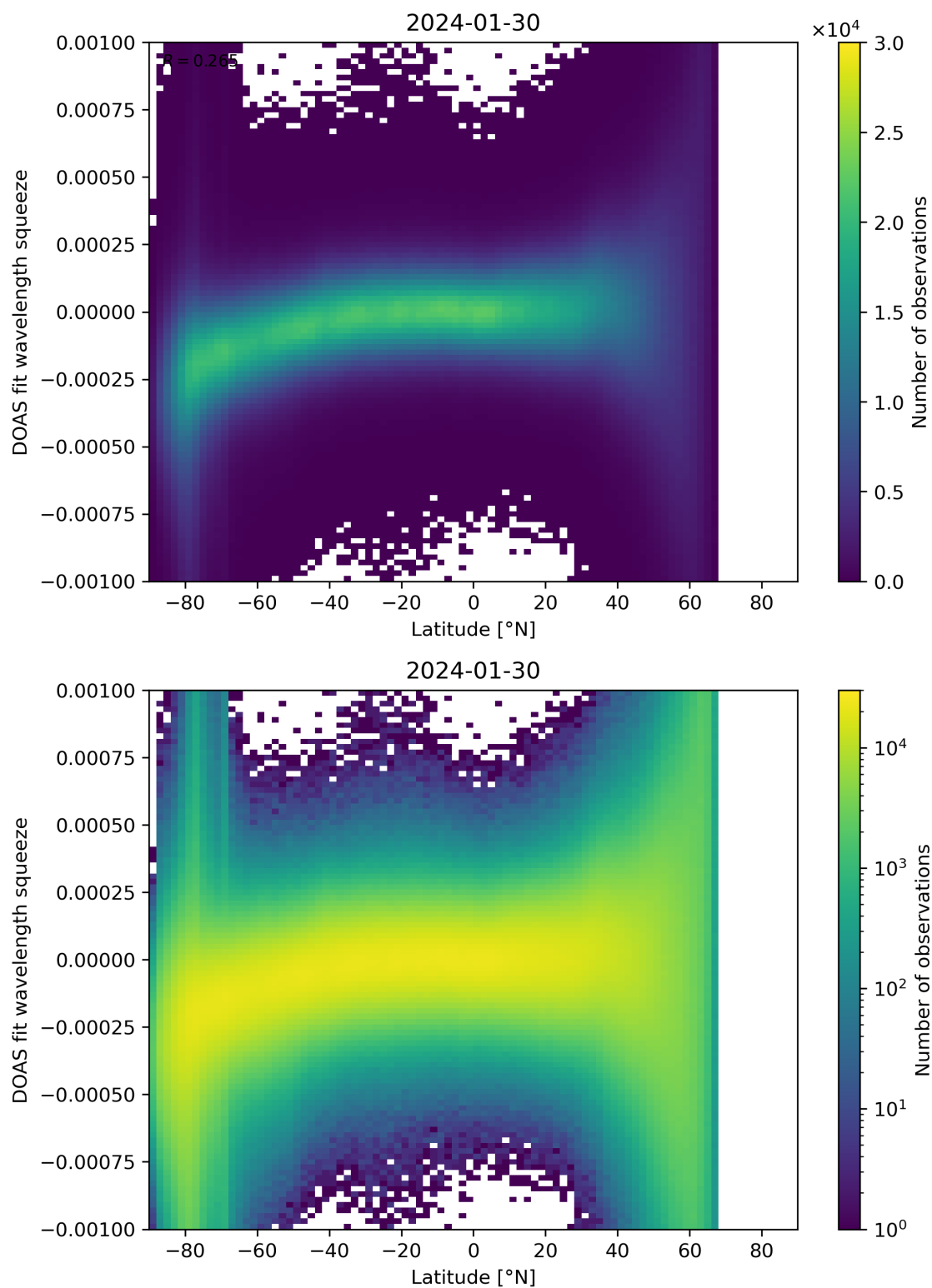
Figure 143: Scatter density plot of “Latitude” against “DOAS fit wavelength squeeze” for 2024-01-29 to 2024-01-31.
