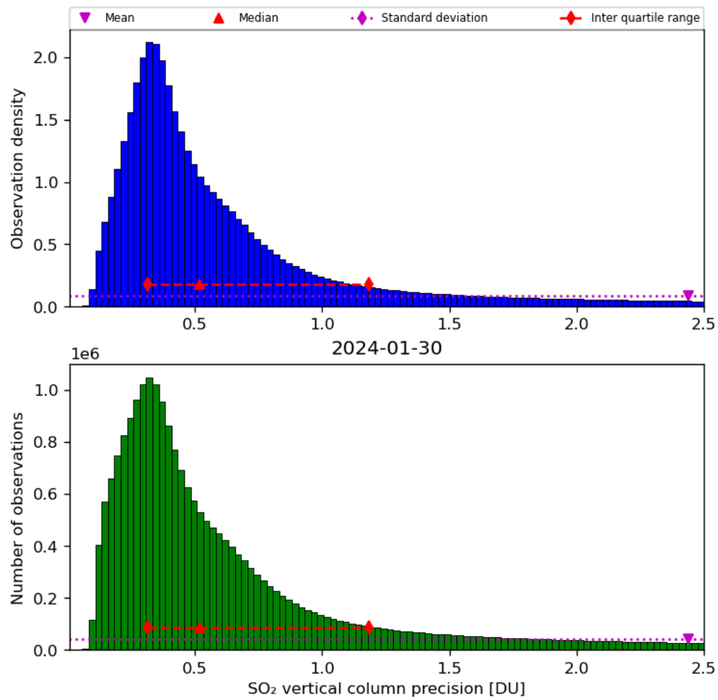
Figure 54: Histogram of “SO 2 vertical column precision” for 2024-01-29 to 2024-01-31
