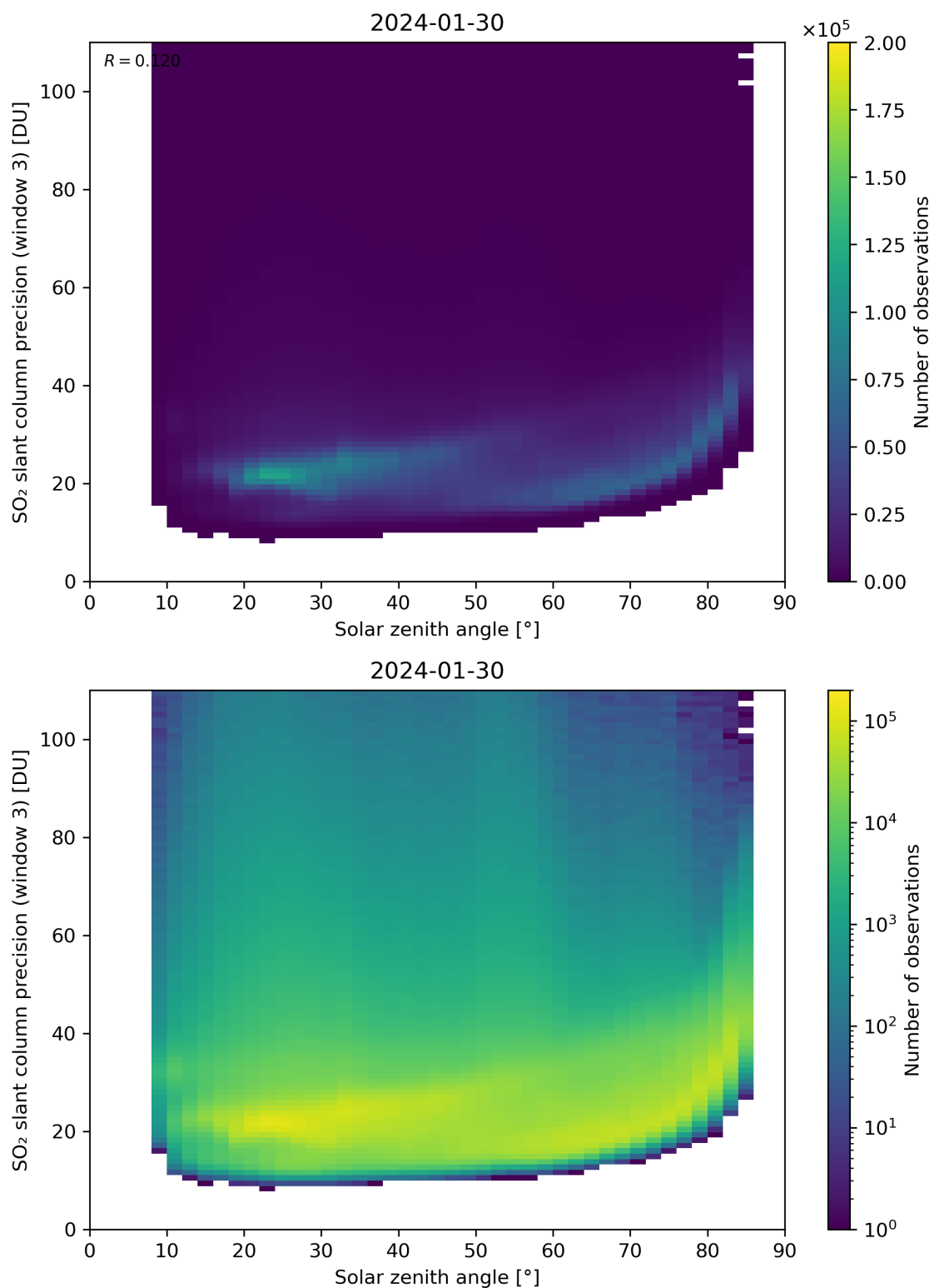
Figure 173: Scatter density plot of “Solar zenith angle” against “SO 2 slant column precision (window 3)” for 2024-01-29 to 2024-01-31.
