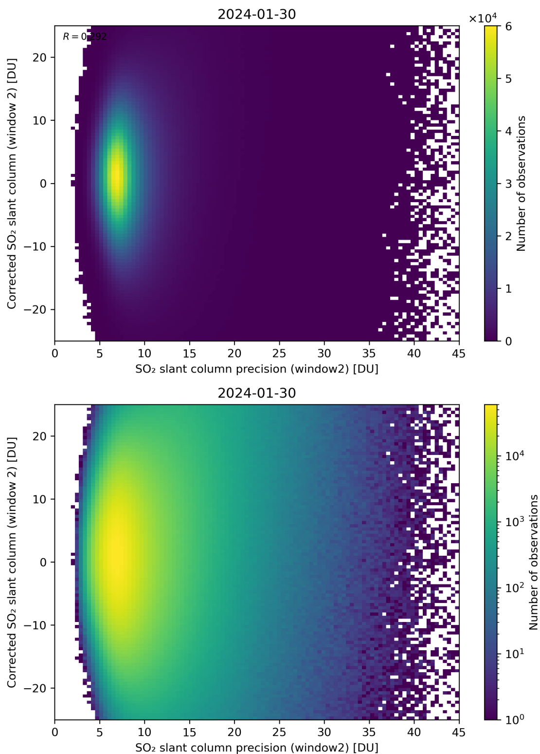
Figure 247: Scatter density plot of “SO 2 slant column precision (window2)” against “Corrected SO 2 slant column (window 2)” for 2024-01-29 to 2024-01-31.
