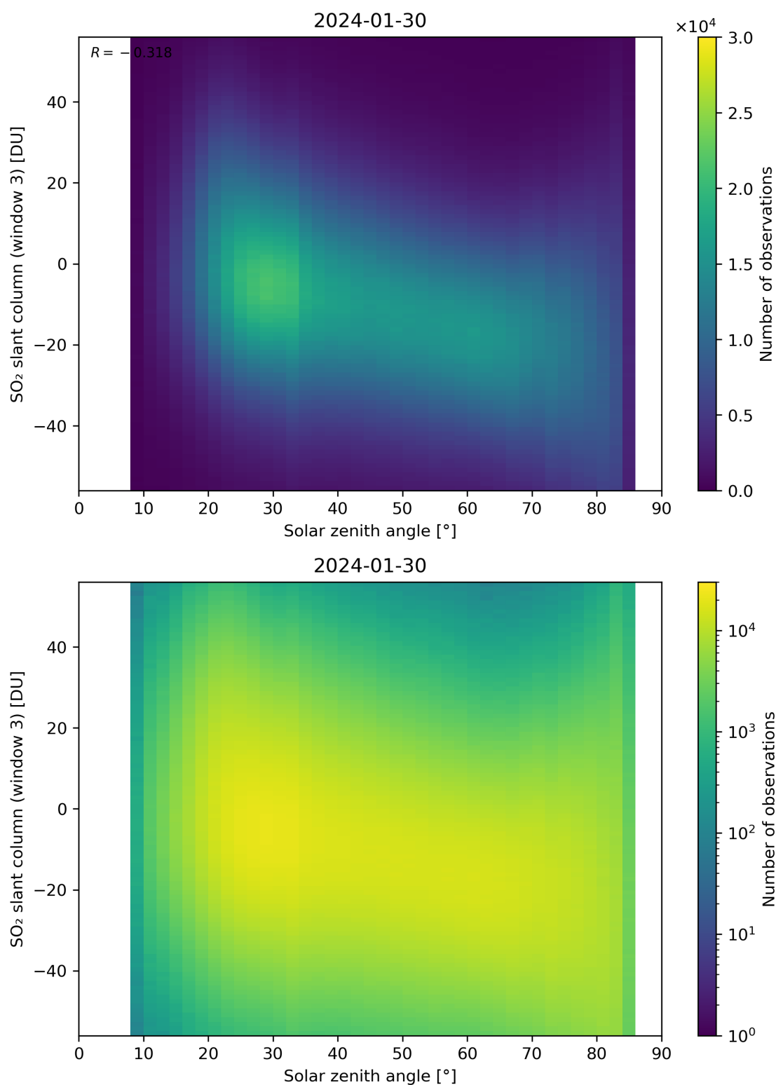
Figure 172: Scatter density plot of “Solar zenith angle” against “SO 2 slant column (window 3)” for 2024-01-29 to 2024-01-31.
