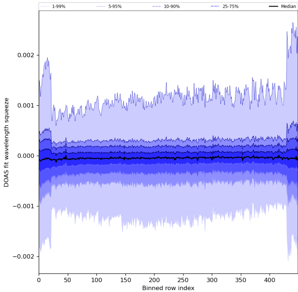
Figure 92: Along track statistics of “DOAS fit wavelength squeeze” for 2024-01-29 to 2024-01-31
