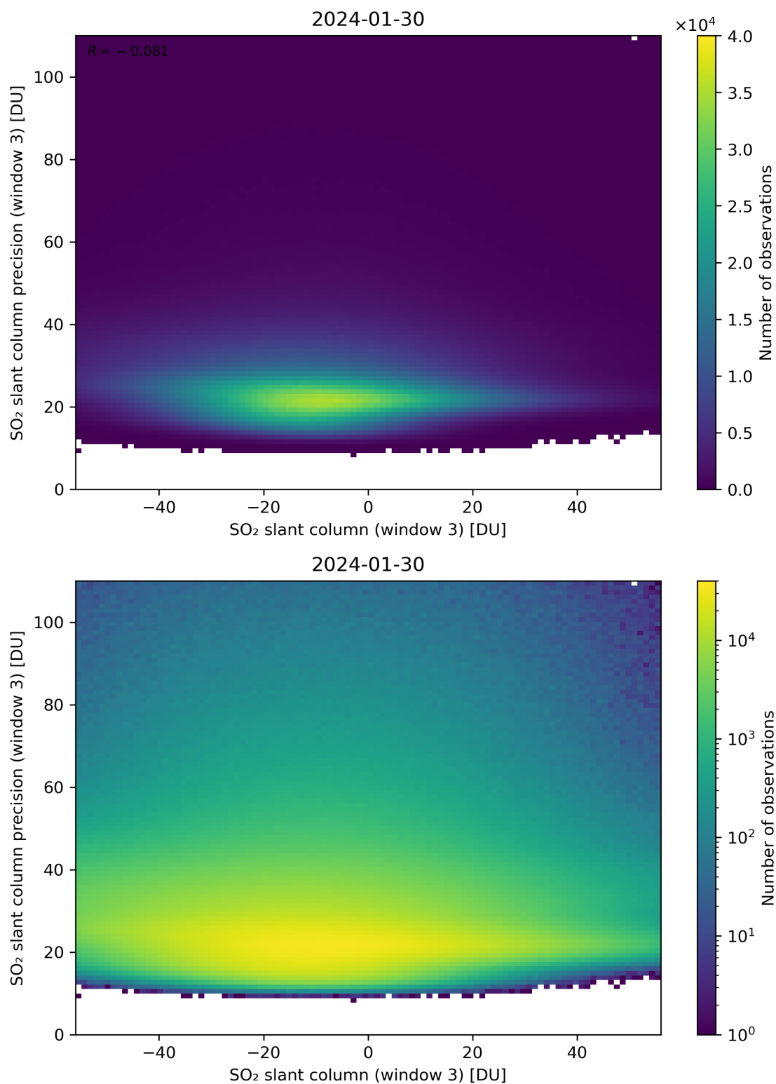
Figure 267: Scatter density plot of “SO 2 slant column (window 3)” against “SO 2 slant column precision (window 3)” for 2024-01-29 to 2024-01-31.
