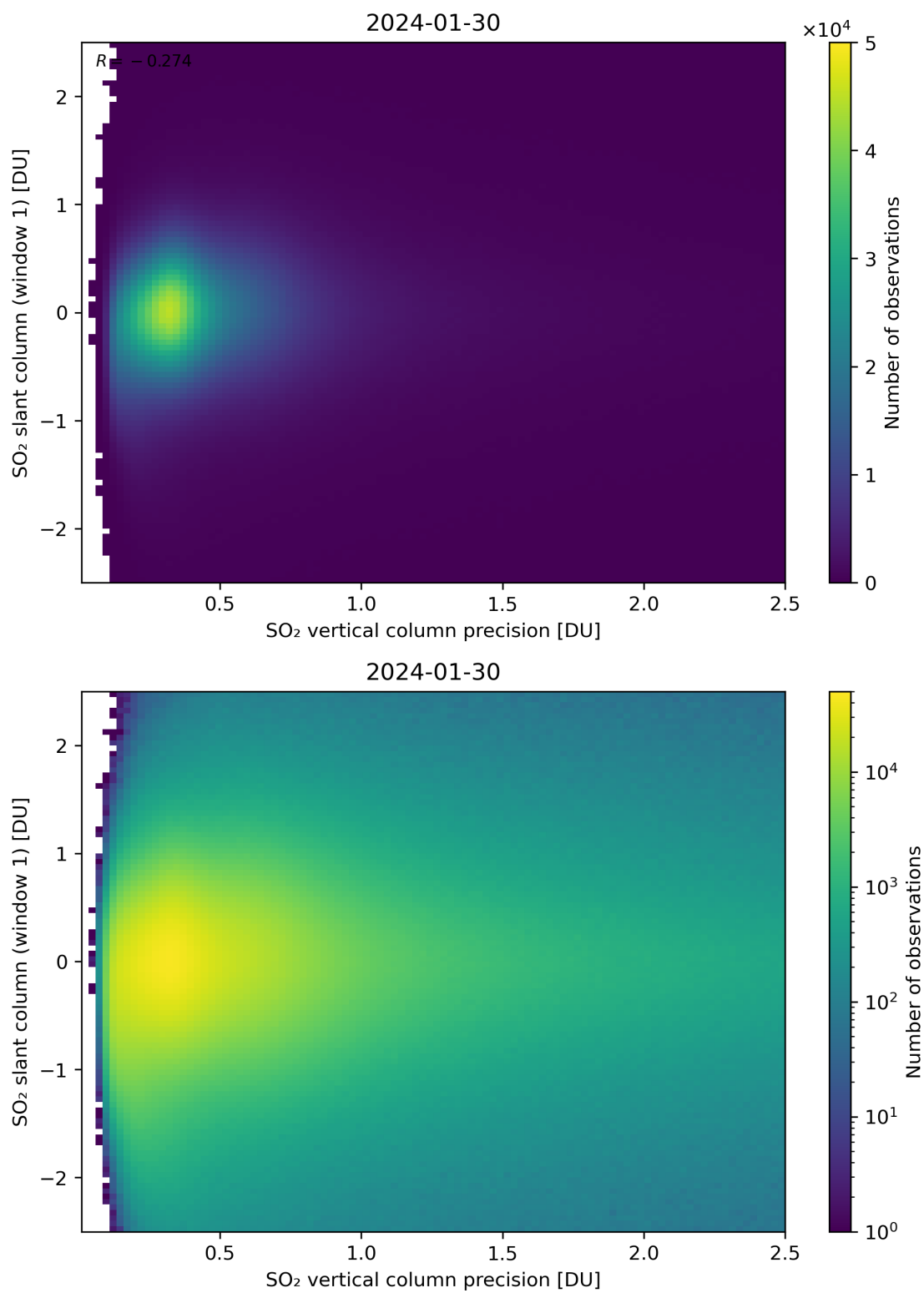
Figure 289: Scatter density plot of “SO 2 vertical column precision” against “SO 2 slant column (window 1)” for 2024-01-29 to 2024-01-31.
