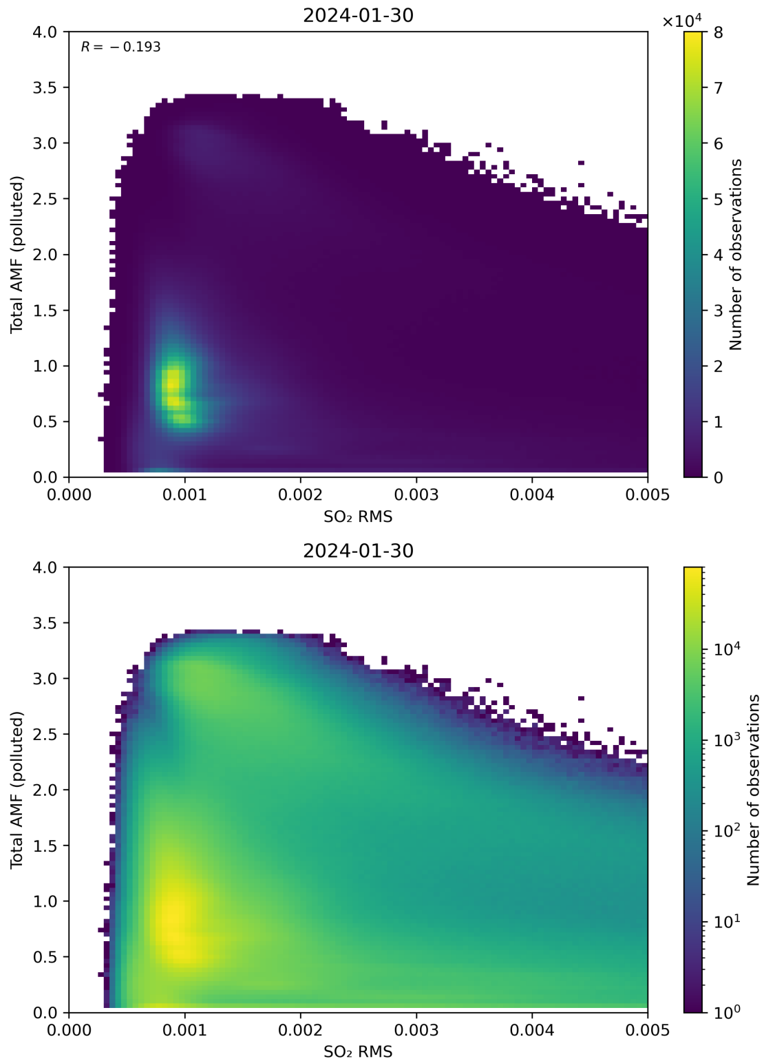
Figure 137: Scatter density plot of “SO 2 RMS” against “Total AMF (polluted)” for 2024-01-29 to 2024-01-31.
