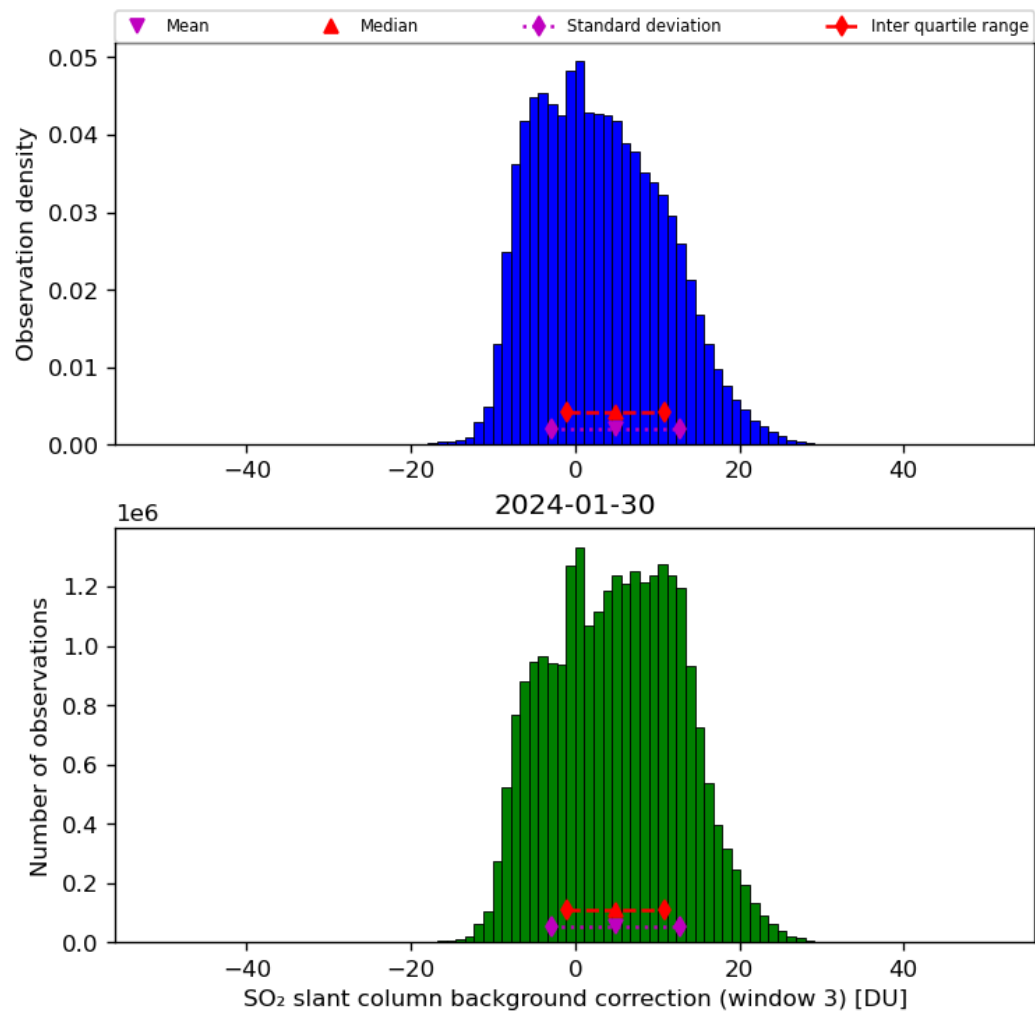
Figure 67: Histogram of “SO 2 slant column background correction (window 3)” for 2024-01-29 to 2024-01-31
