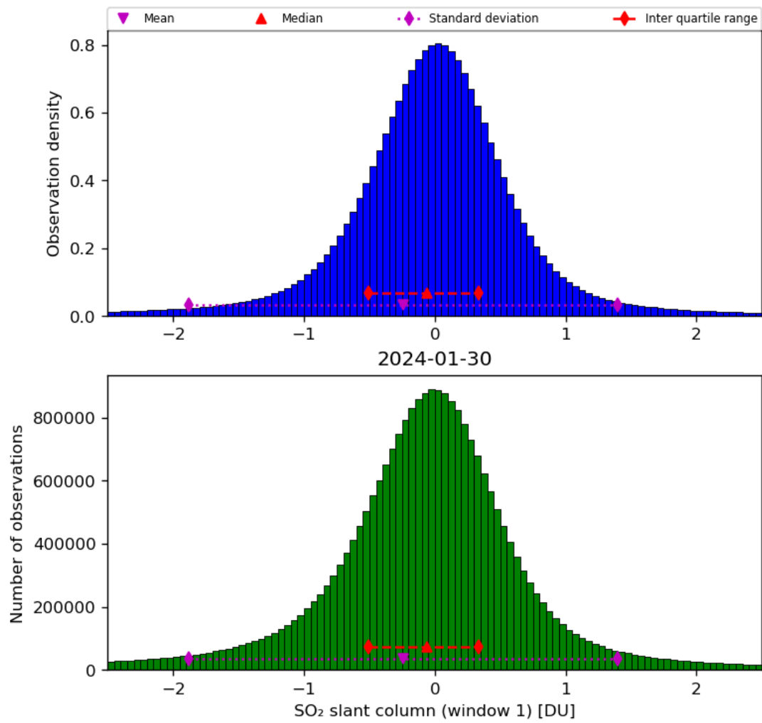
Figure 56: Histogram of “SO 2 slant column (window 1)” for 2024-01-29 to 2024-01-31
