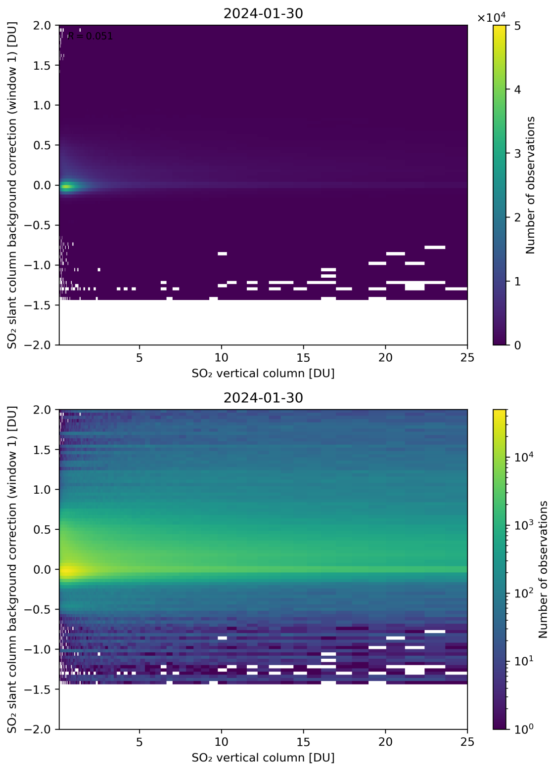
Figure 273: Scatter density plot of “SO 2 vertical column” against “SO 2 slant column background correction (window 1)” for 2024-01-29 to 2024-01-31.
