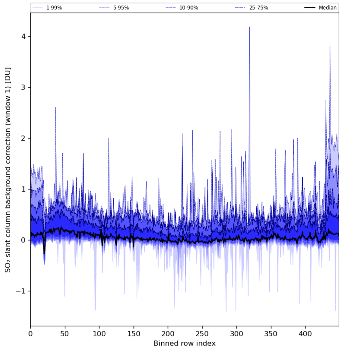
Figure 82: Along track statistics of “SO 2 slant column background correction (window 1)” for 2024-01-29 to 2024-01-31
