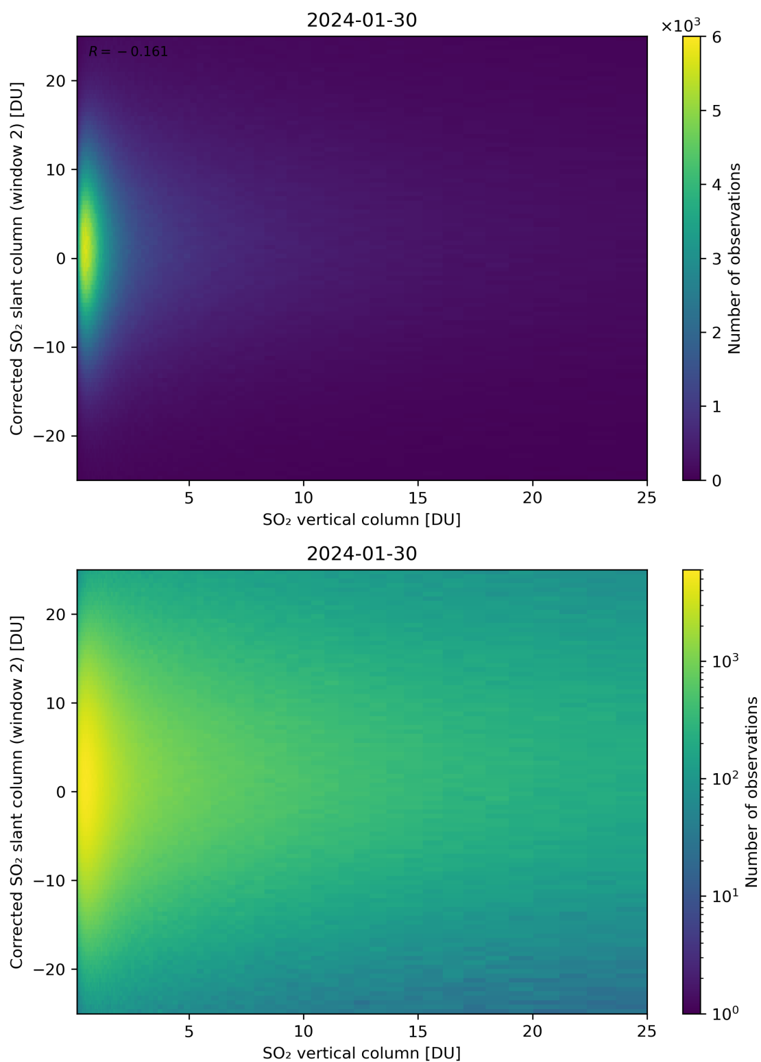
Figure 298: Scatter density plot of “SO 2 vertical column” against “Corrected SO 2 slant column (window 2)” for 2024-01-29 to 2024-01-31.
