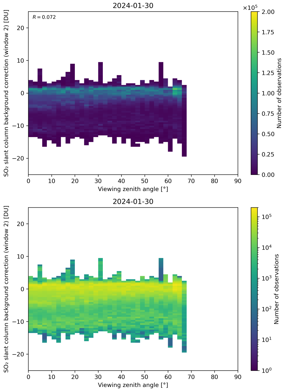
Figure 309: Scatter density plot of “Viewing zenith angle” against “SO 2 slant column background correction (window 2)” for 2024-01-29 to 2024-01-31.
