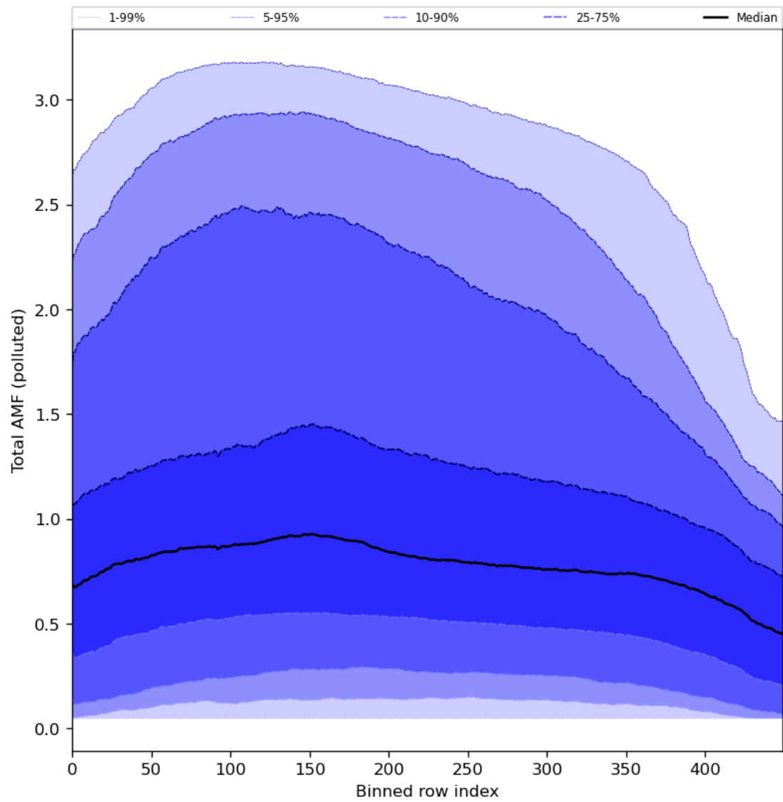
Figure 94: Along track statistics of “Total AMF (polluted)” for 2024-01-29 to 2024-01-31
