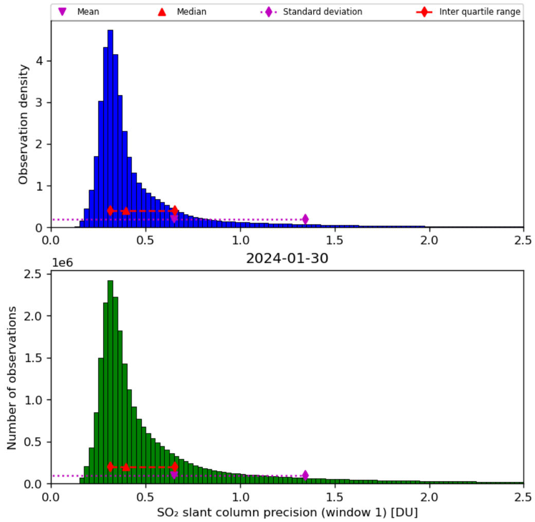
Figure 57: Histogram of “SO 2 slant column precision (window 1)” for 2024-01-29 to 2024-01-31
