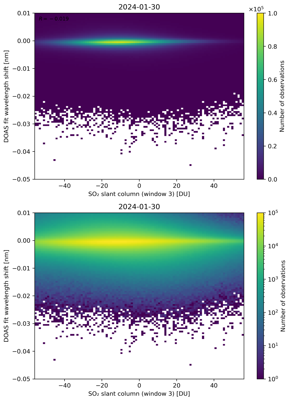
Figure 254: Scatter density plot of “SO 2 slant column (window 3)” against “DOAS fit wavelength shift” for 2024-01-29 to 2024-01-31.
