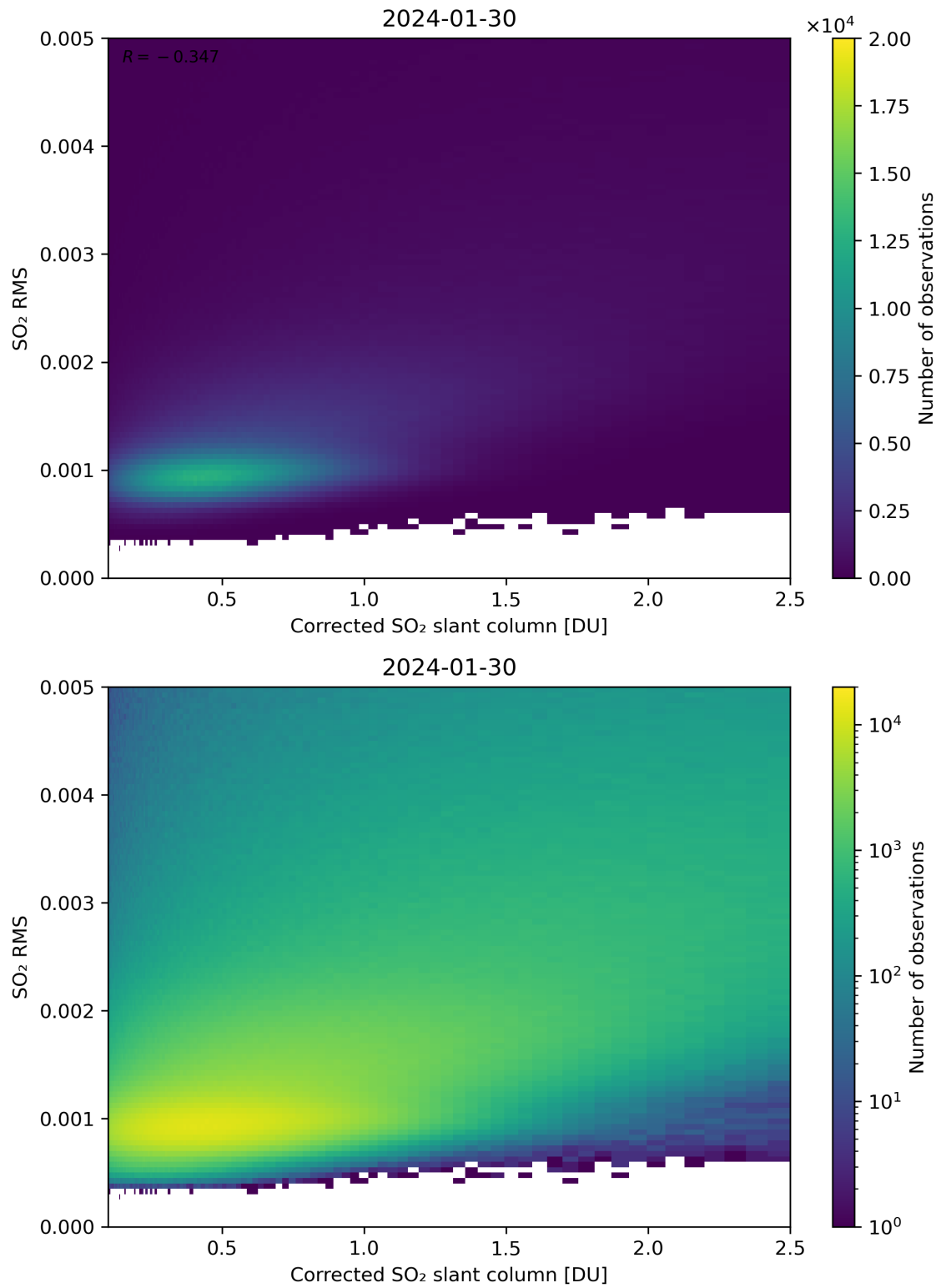
Figure 183: Scatter density plot of “Corrected SO 2 slant column” against “SO 2 RMS” for 2024-01-29 to 2024-01-31.
