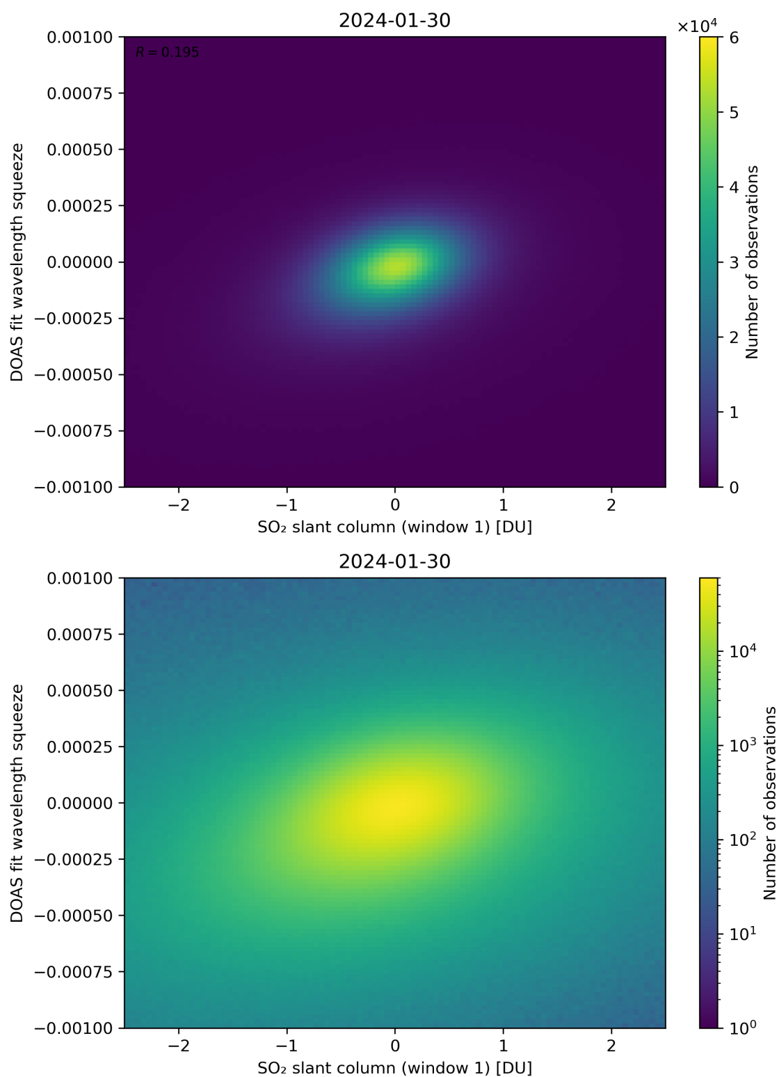
Figure 216: Scatter density plot of “SO 2 slant column (window 1)” against “DOAS fit wavelength squeeze” for 2024-01-29 to 2024-01-31.
