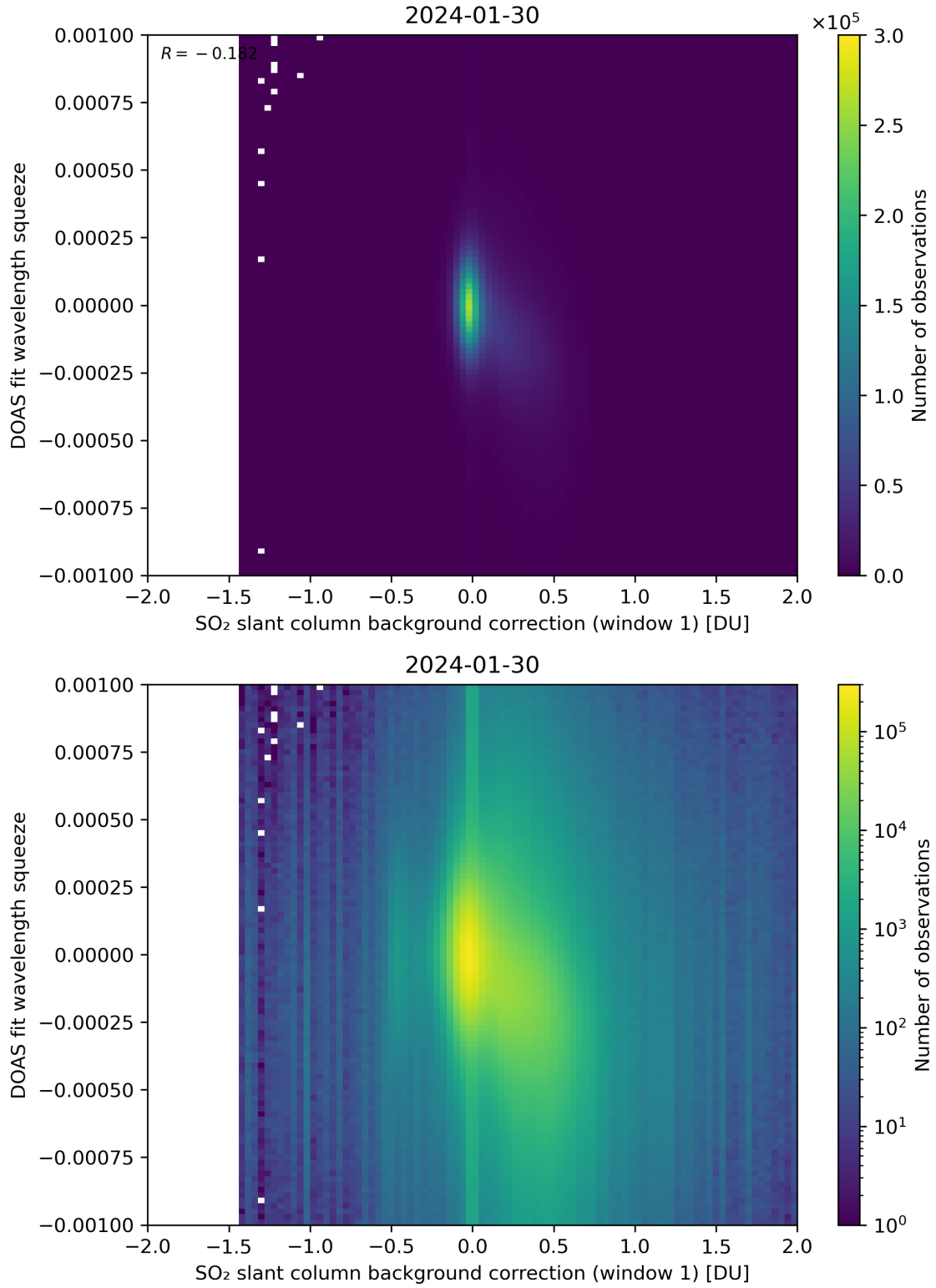
Figure 101: Scatter density plot of “SO 2 slant column background correction (window 1)” against “DOAS fit wavelength squeeze” for 2024-01-29 to 2024-01-31.
