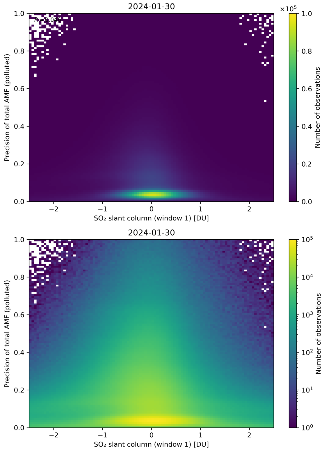
Figure 240: Scatter density plot of “SO 2 slant column (window 1)” against “Precision of total AMF (polluted)” for 2024-01-29 to 2024-01-31.
