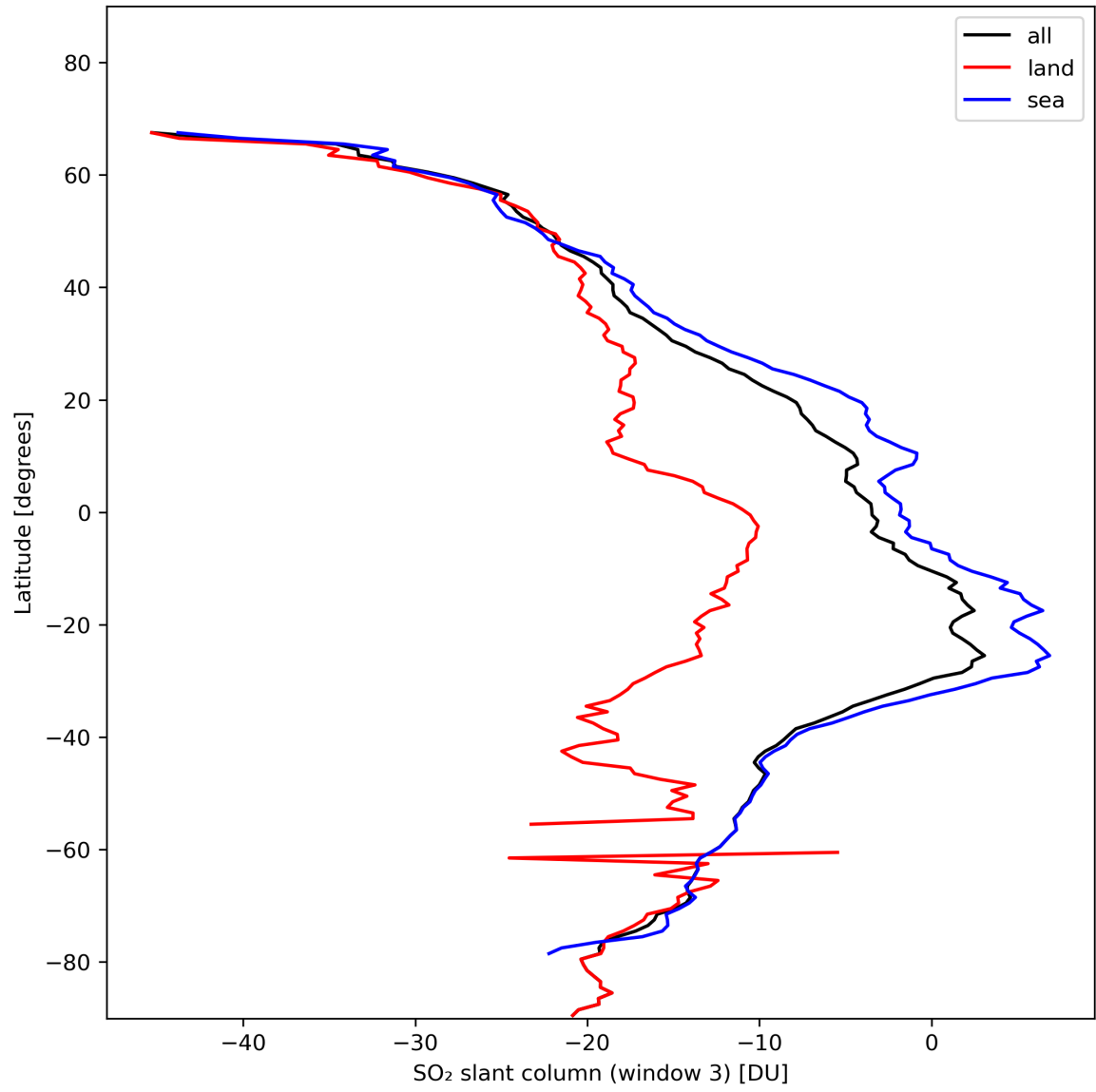
Figure 41: Zonal average of “SO 2 slant column (window 3)” for 2024-01-29 to 2024-01-31.
