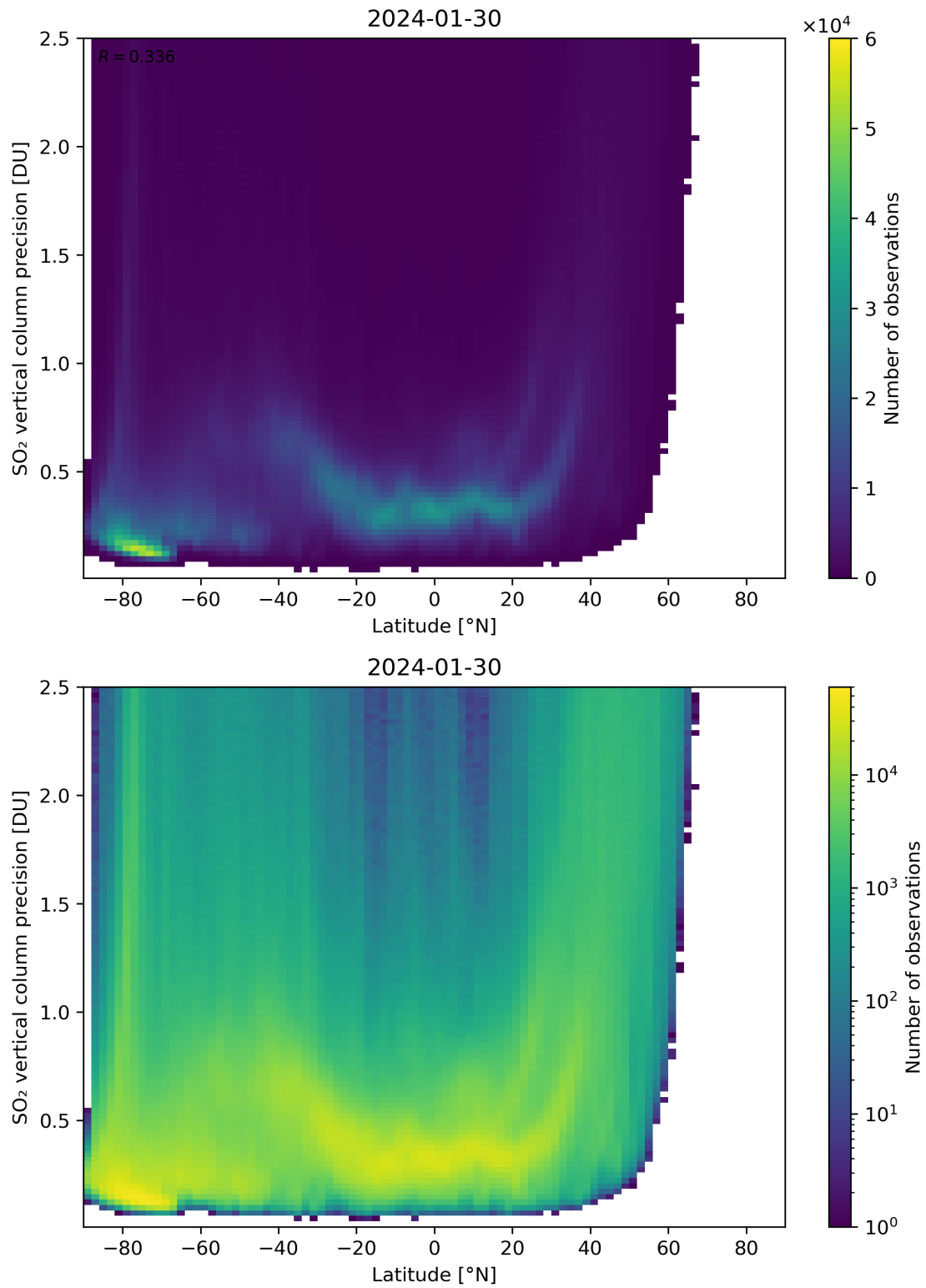
Figure 157: Scatter density plot of “Latitude” against “SO 2 vertical column precision” for 2024-01-29 to 2024-01-31.
