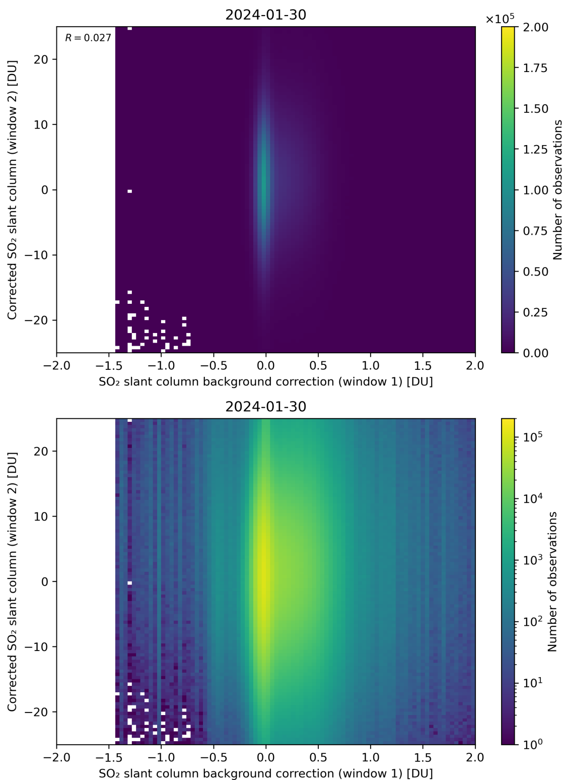
Figure 104: Scatter density plot of “SO 2 slant column background correction (window 1)” against “Corrected SO 2 slant column (window 2)” for 2024-01-29 to 2024-01-31.
