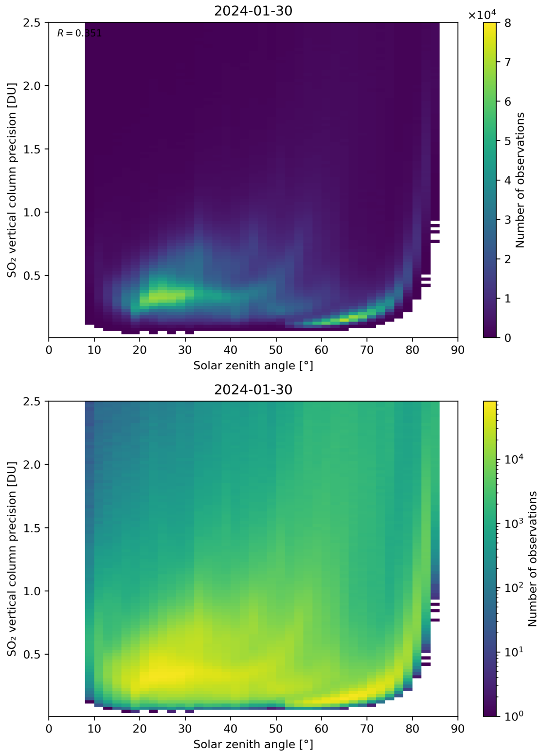
Figure 177: Scatter density plot of “Solar zenith angle” against “SO 2 vertical column precision” for 2024-01-29 to 2024-01-31.
