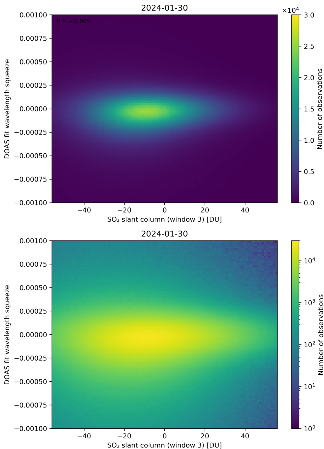
Figure 255: Scatter density plot of “SO 2 slant column (window 3)” against “DOAS fit wavelength squeeze” for 2024-01-29 to 2024-01-31.
