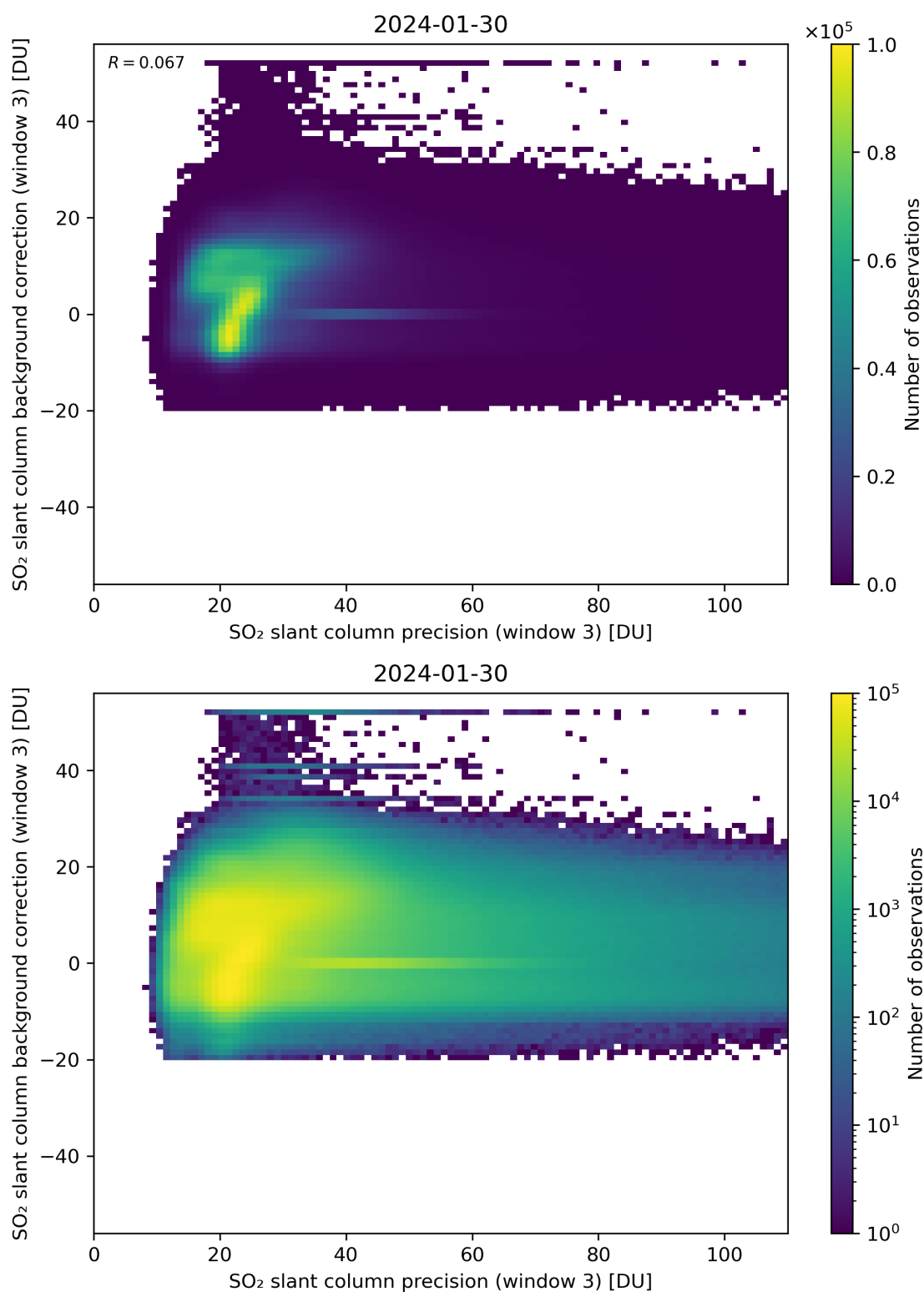
Figure 257: Scatter density plot of “SO 2 slant column precision (window 3)” against “SO 2 slant column background correction (window 3)” for 2024-01-29 to 2024-01-31.
