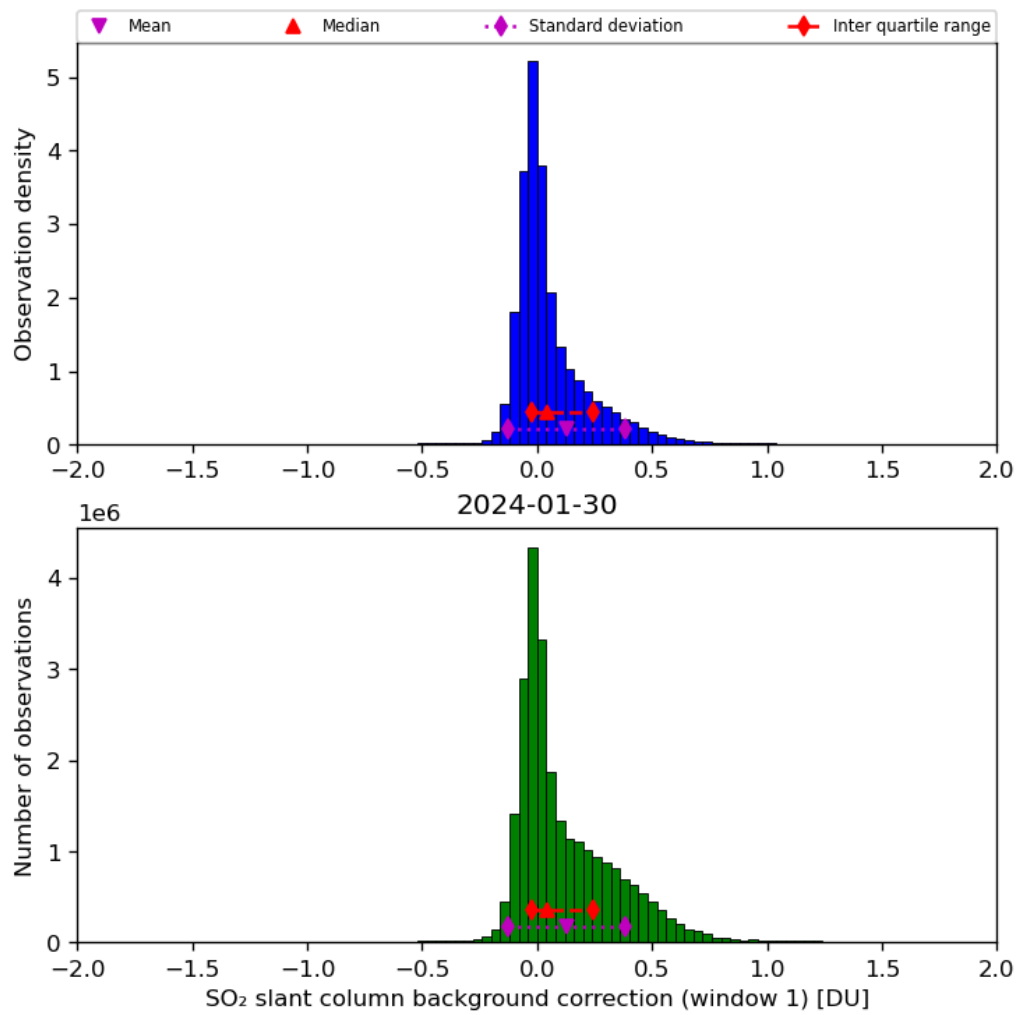
Figure 59: Histogram of “SO 2 slant column background correction (window 1)” for 2024-01-29 to 2024-01-31
