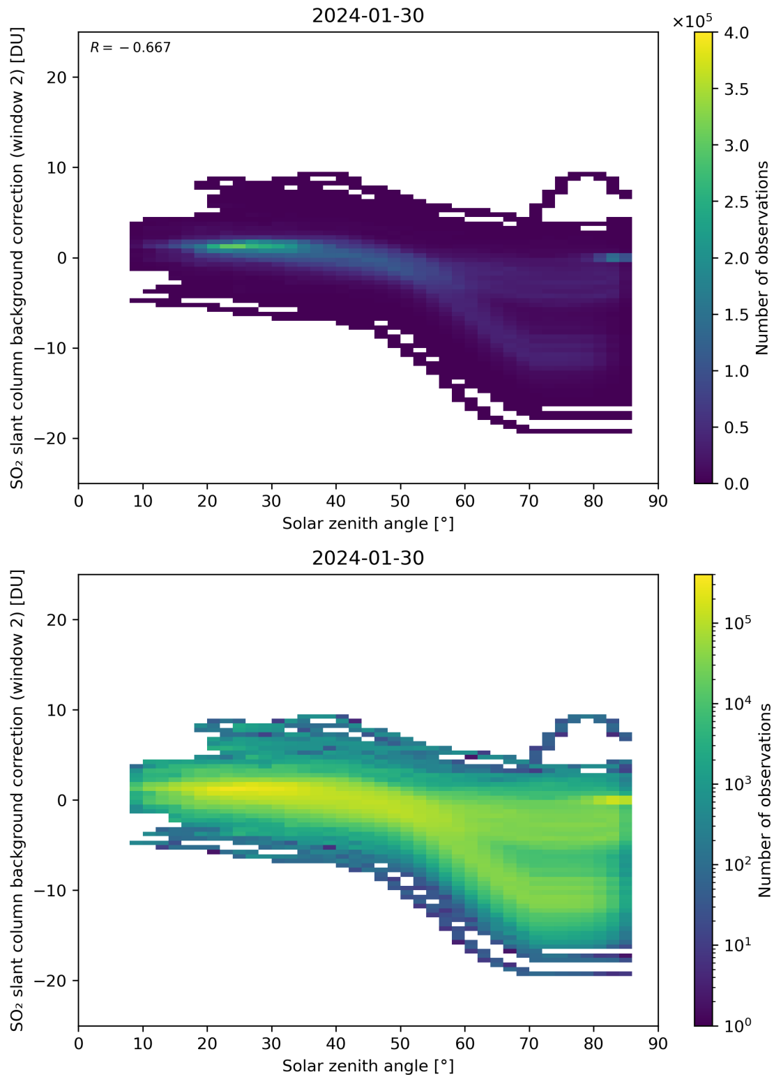
Figure 159: Scatter density plot of “Solar zenith angle” against “SO 2 slant column background correction (window 2)” for 2024-01-29 to 2024-01-31.
