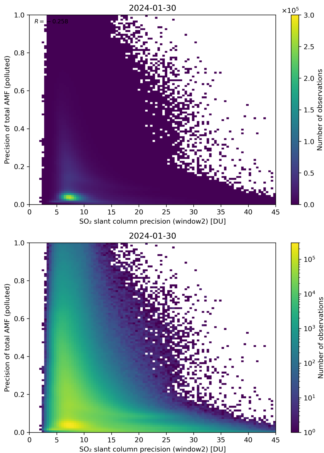
Figure 252: Scatter density plot of “SO 2 slant column precision (window2)” against “Precision of total AMF (polluted)” for 2024-01-29 to 2024-01-31.
