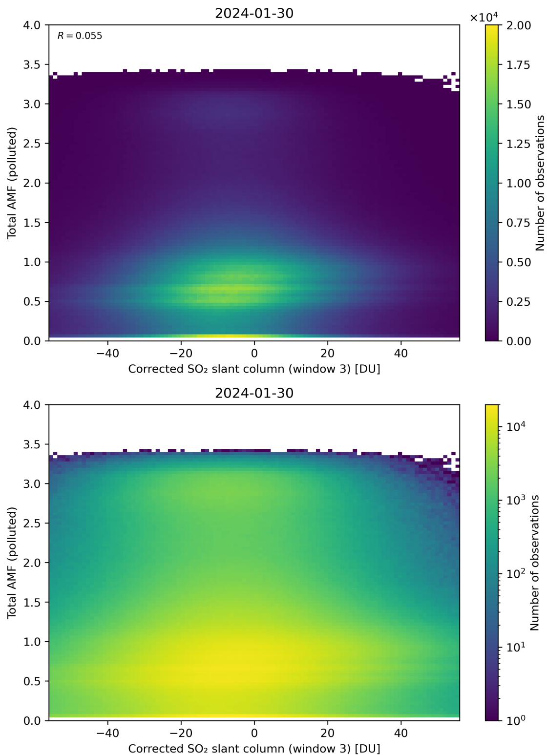
Figure 210: Scatter density plot of “Corrected SO 2 slant column (window 3)” against “Total AMF (polluted)” for 2024-01-29 to 2024-01-31.
