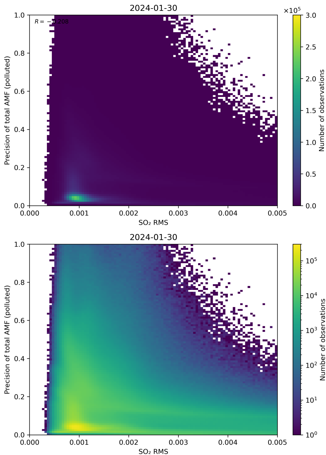
Figure 138: Scatter density plot of “SO 2 RMS” against “Precision of total AMF (polluted)” for 2024-01-29 to 2024-01-31.
