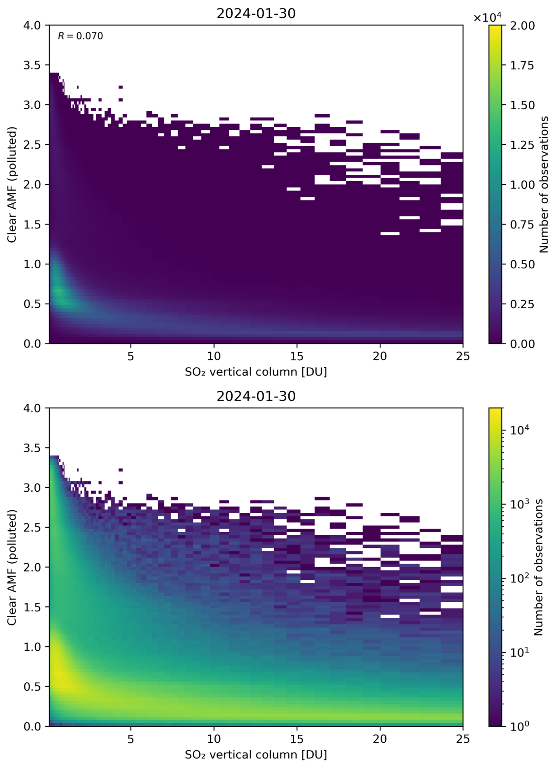
Figure 296: Scatter density plot of “SO 2 vertical column” against “Clear AMF (polluted)” for 2024-01-29 to 2024-01-31.
