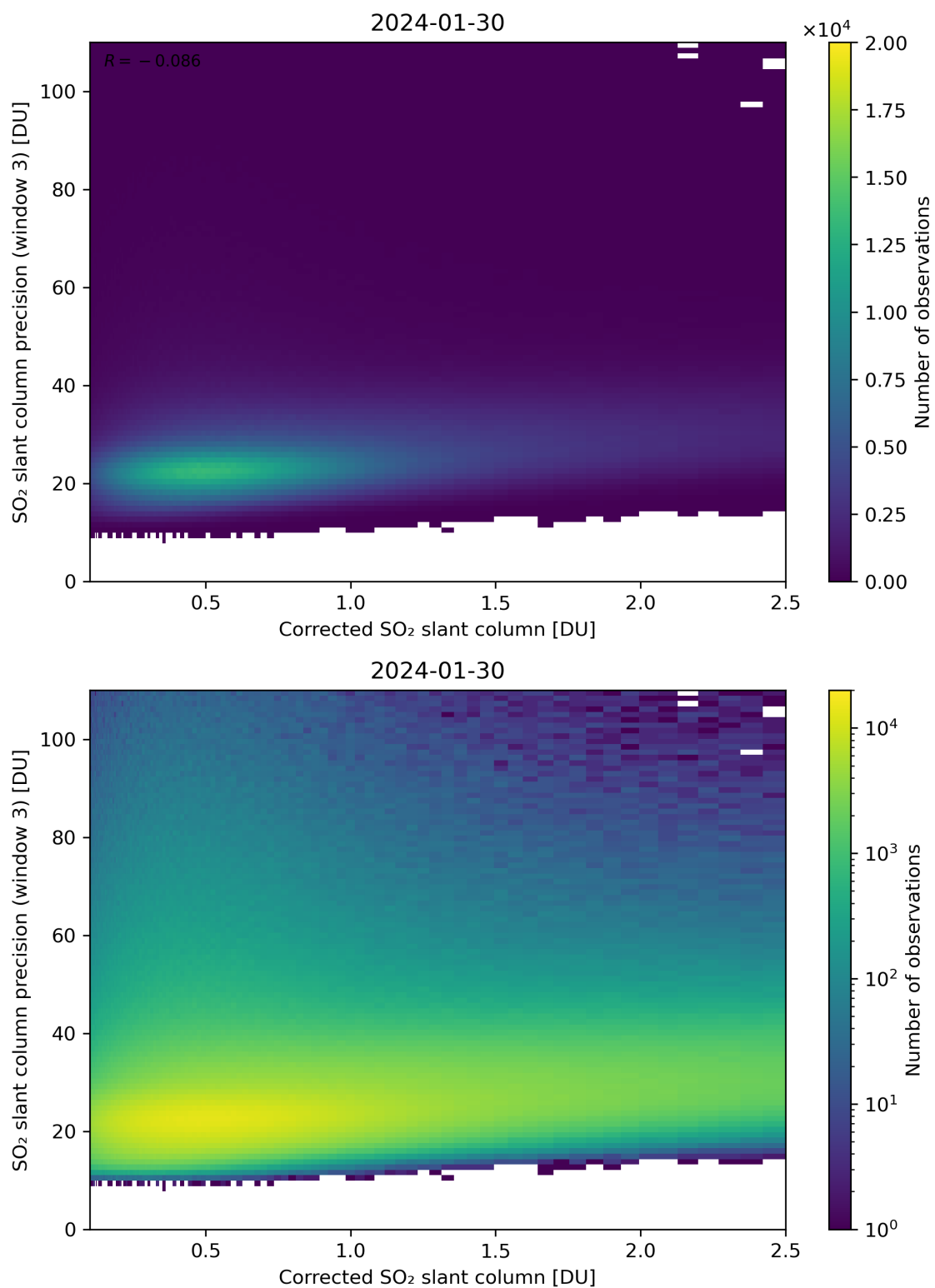
Figure 191: Scatter density plot of “Corrected SO 2 slant column” against “SO 2 slant column precision (window 3)” for 2024-01-29 to 2024-01-31.
