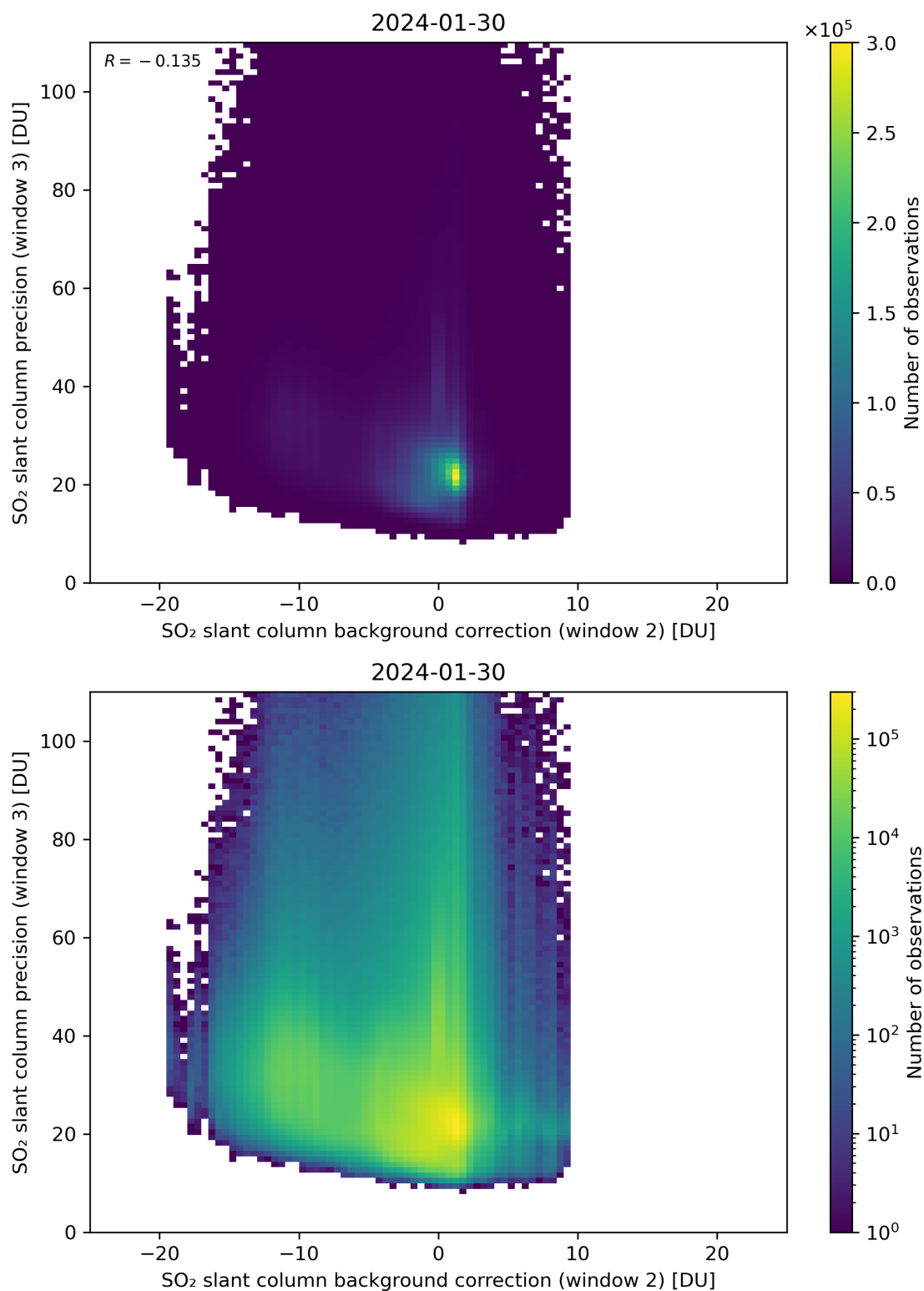
Figure 118: Scatter density plot of “SO 2 slant column background correction (window 2)” against “SO 2 slant column precision (window 3)” for 2024-01-29 to 2024-01-31.
