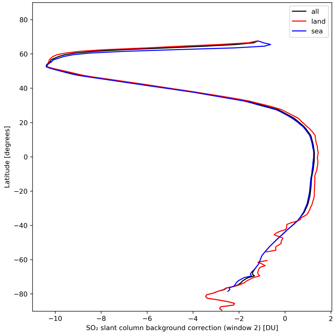
Figure 40: Zonal average of “SO 2 slant column background correction (window 2)” for 2024-01-29 to 2024-01-31.
