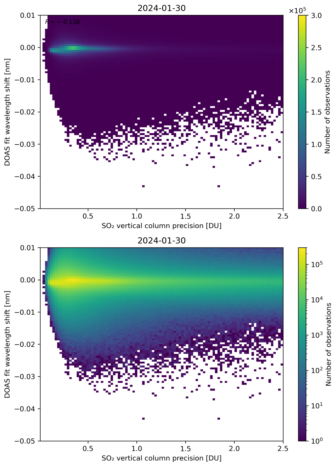
Figure 282: Scatter density plot of “SO 2 vertical column precision” against “DOAS fit wavelength shift” for 2024-01-29 to 2024-01-31.
