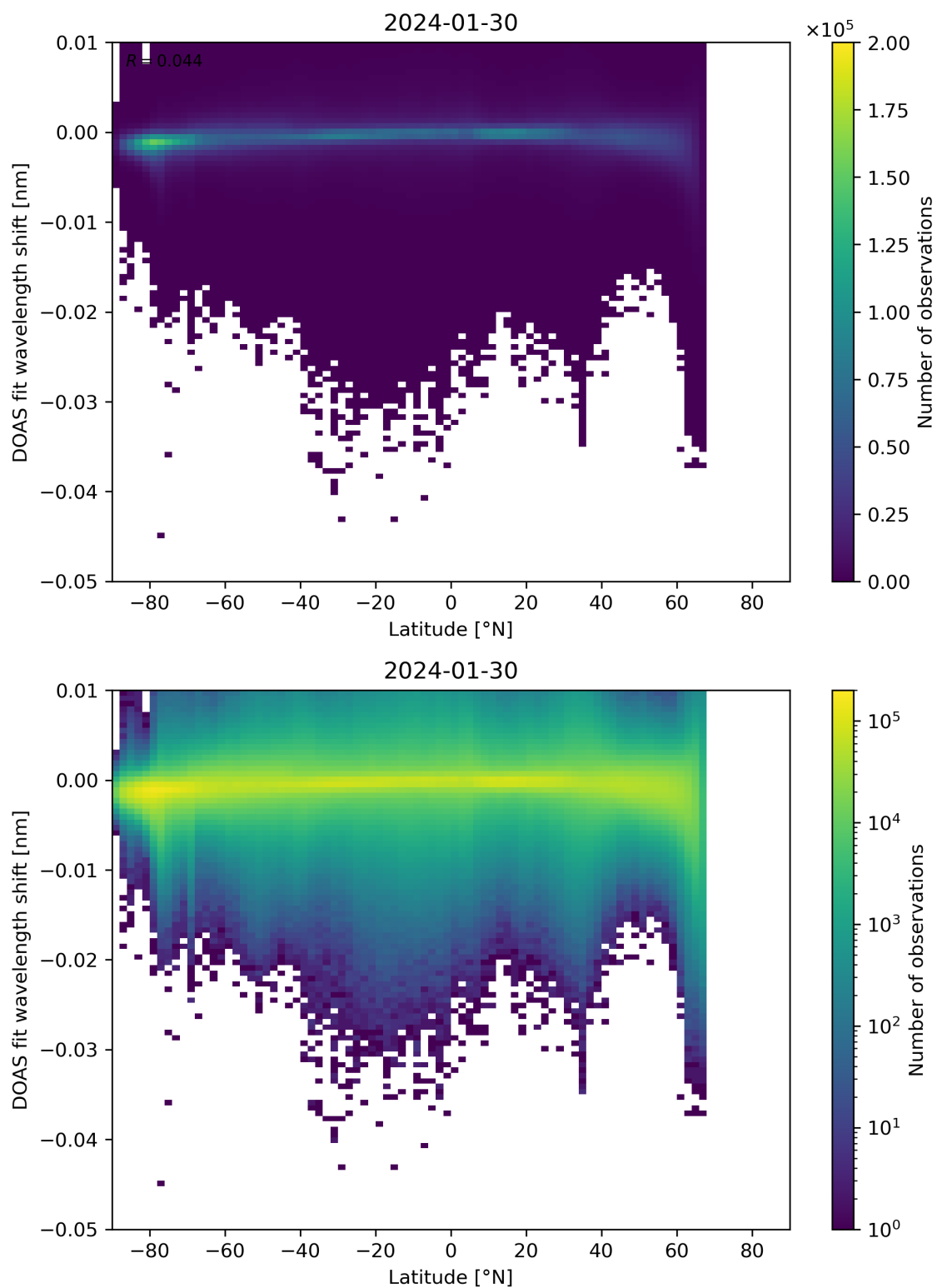
Figure 142: Scatter density plot of “Latitude” against “DOAS fit wavelength shift” for 2024-01-29 to 2024-01-31.
