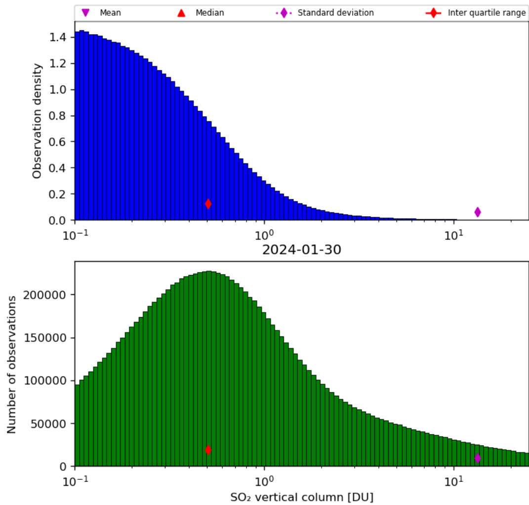
Figure 53: Histogram of “SO 2 vertical column” for 2024-01-29 to 2024-01-31
