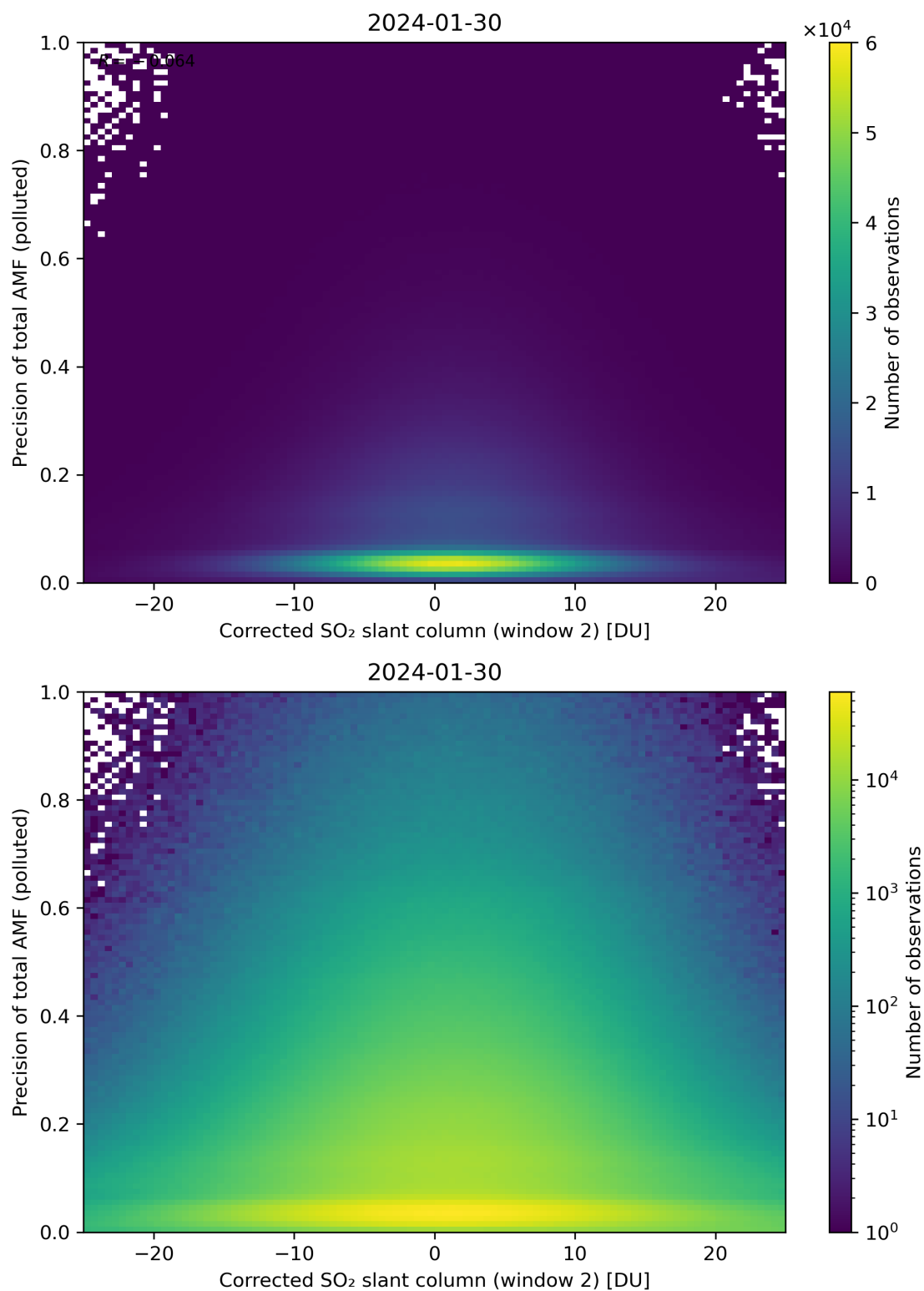
Figure 204: Scatter density plot of “Corrected SO 2 slant column (window 2)” against “Precision of total AMF (polluted)” for 2024-01-29 to 2024-01-31.
