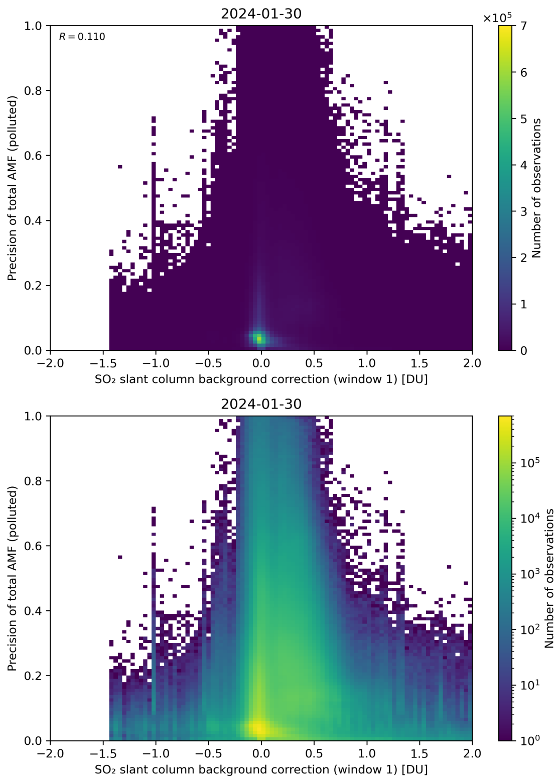
Figure 110: Scatter density plot of “SO 2 slant column background correction (window 1)” against “Precision of total AMF (polluted)” for 2024-01-29 to 2024-01-31.
