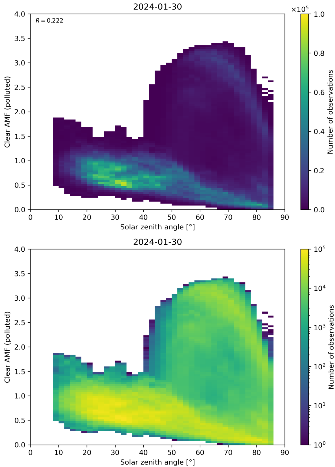
Figure 165: Scatter density plot of “Solar zenith angle” against “Clear AMF (polluted)” for 2024-01-29 to 2024-01-31.
