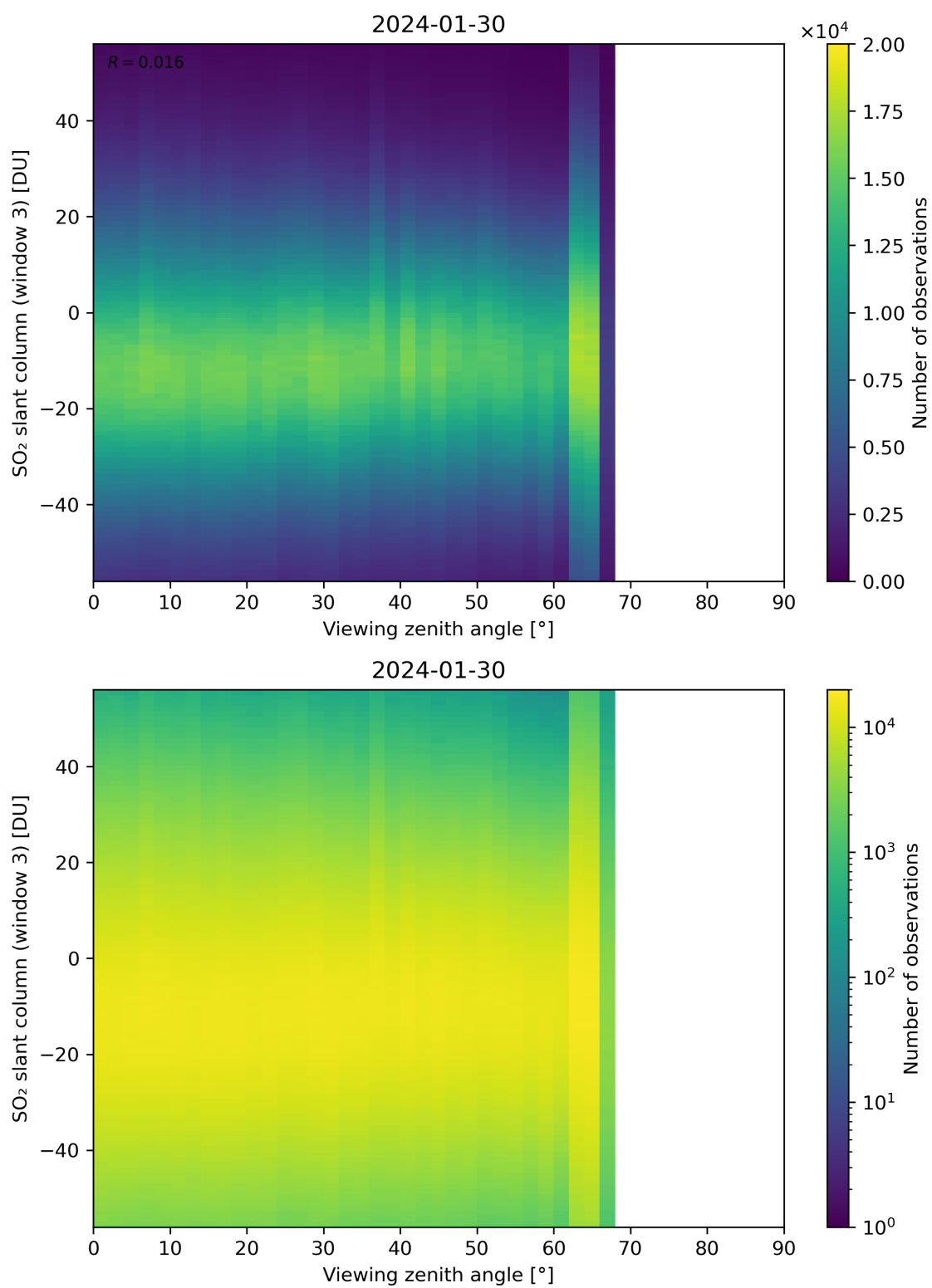
Figure 323: Scatter density plot of “Viewing zenith angle” against “SO 2 slant column (window 3)” for 2024-01-29 to 2024-01-31.
