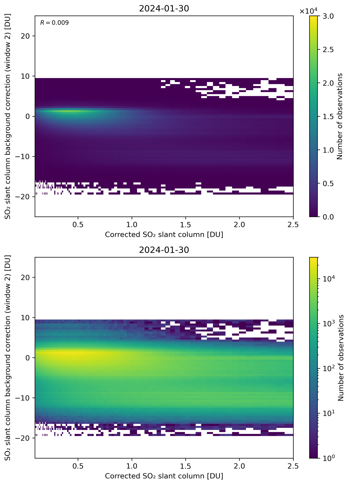
Figure 179: Scatter density plot of “Corrected SO 2 slant column” against “SO 2 slant column background correction (window 2)” for 2024-01-29 to 2024-01-31.
