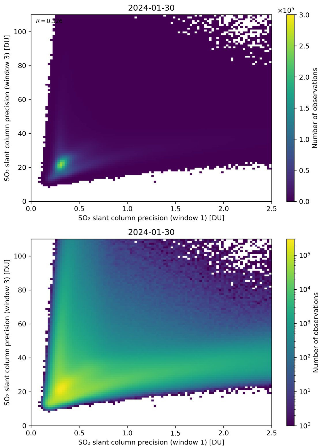
Figure 229: Scatter density plot of “SO 2 slant column precision (window 1)” against “SO 2 slant column precision (window 3)” for 2024-01-29 to 2024-01-31.
