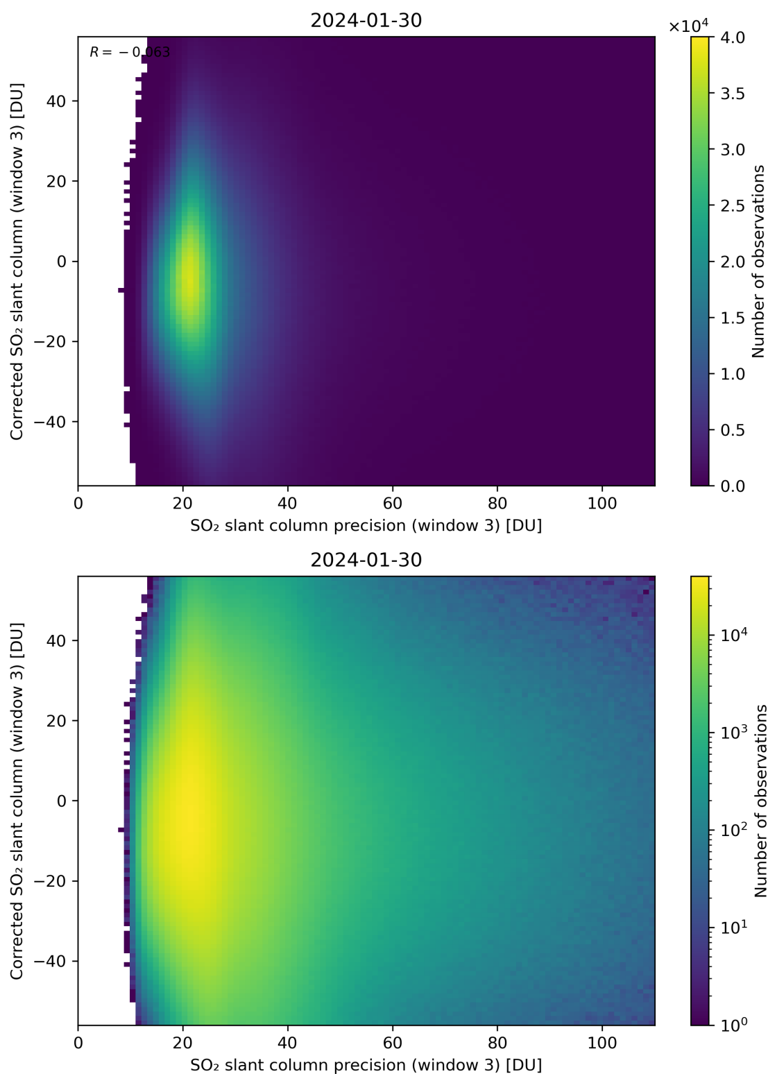
Figure 262: Scatter density plot of “SO 2 slant column precision (window 3)” against “Corrected SO 2 slant column (window 3)” for 2024-01-29 to 2024-01-31.
