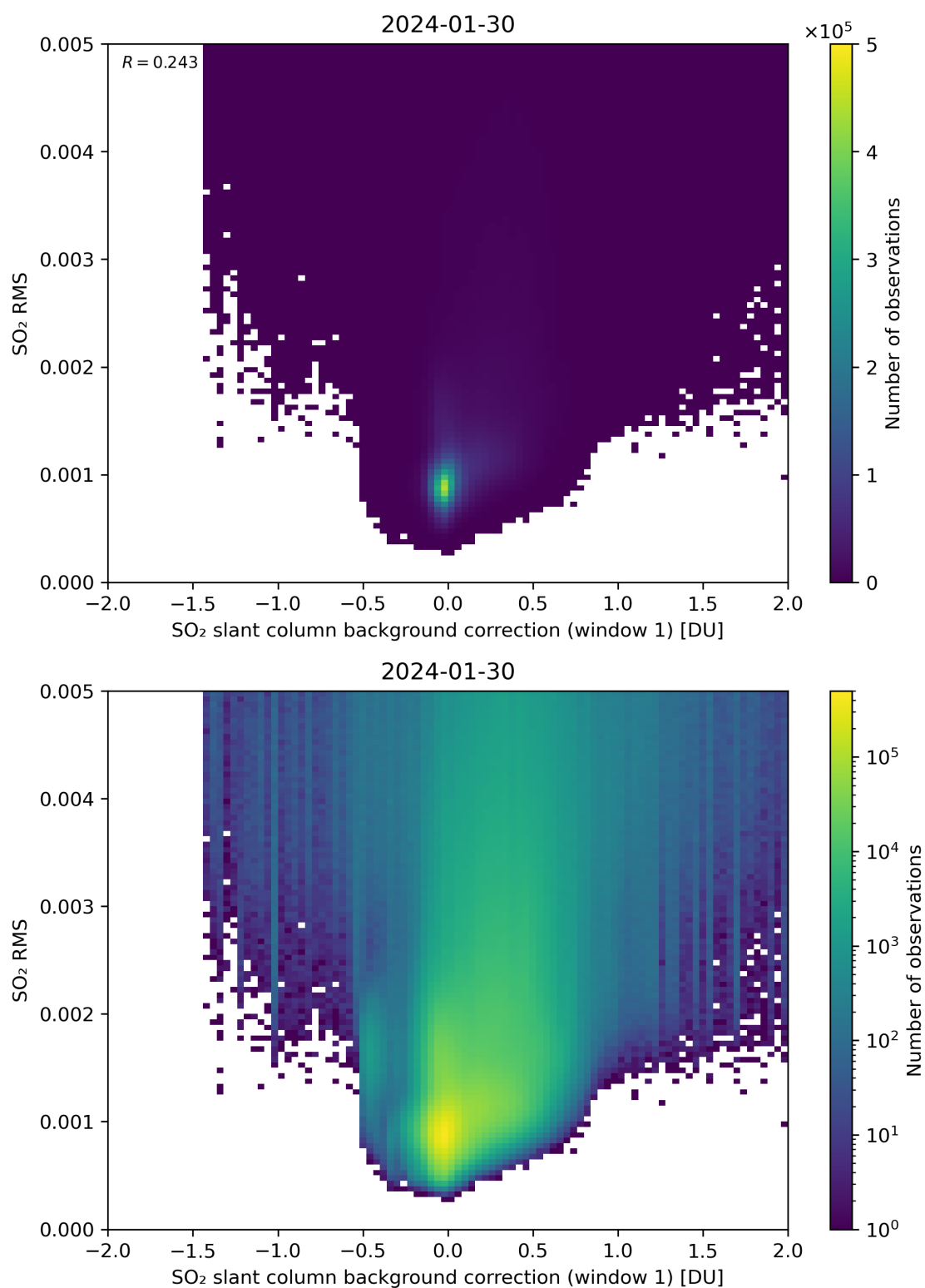
Figure 102: Scatter density plot of “SO 2 slant column background correction (window 1)” against “SO 2 RMS” for 2024-01-29 to 2024-01-31.
