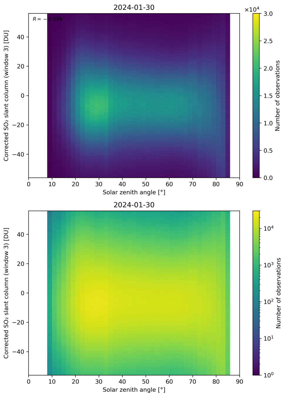
Figure 168: Scatter density plot of “Solar zenith angle” against “Corrected SO 2 slant column (window 3)” for 2024-01-29 to 2024-01-31.
