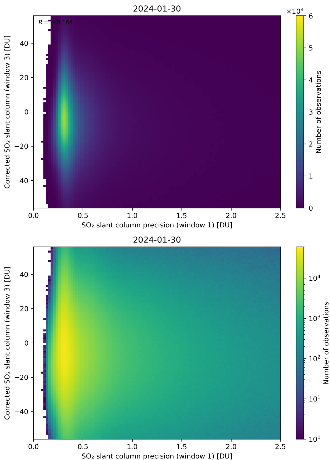
Figure 226: Scatter density plot of “SO 2 slant column precision (window 1)” against “Corrected SO 2 slant column (window 3)” for 2024-01-29 to 2024-01-31.
