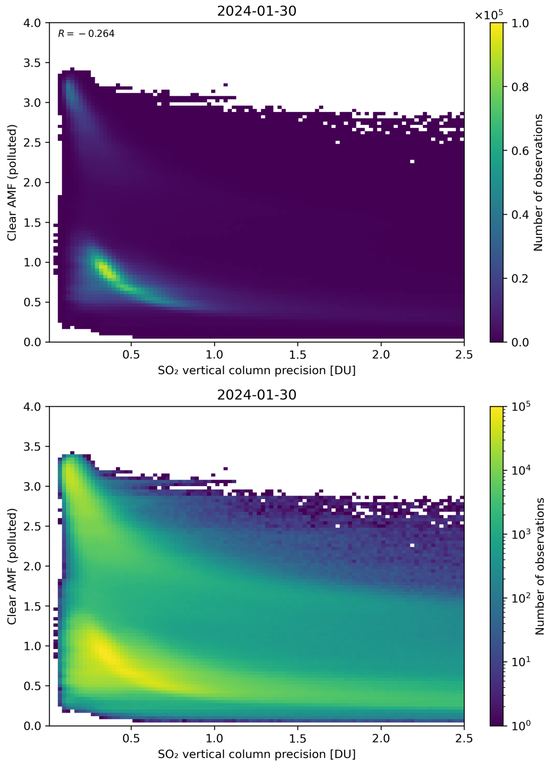
Figure 285: Scatter density plot of “SO 2 vertical column precision” against “Clear AMF (polluted)” for 2024-01-29 to 2024-01-31.
