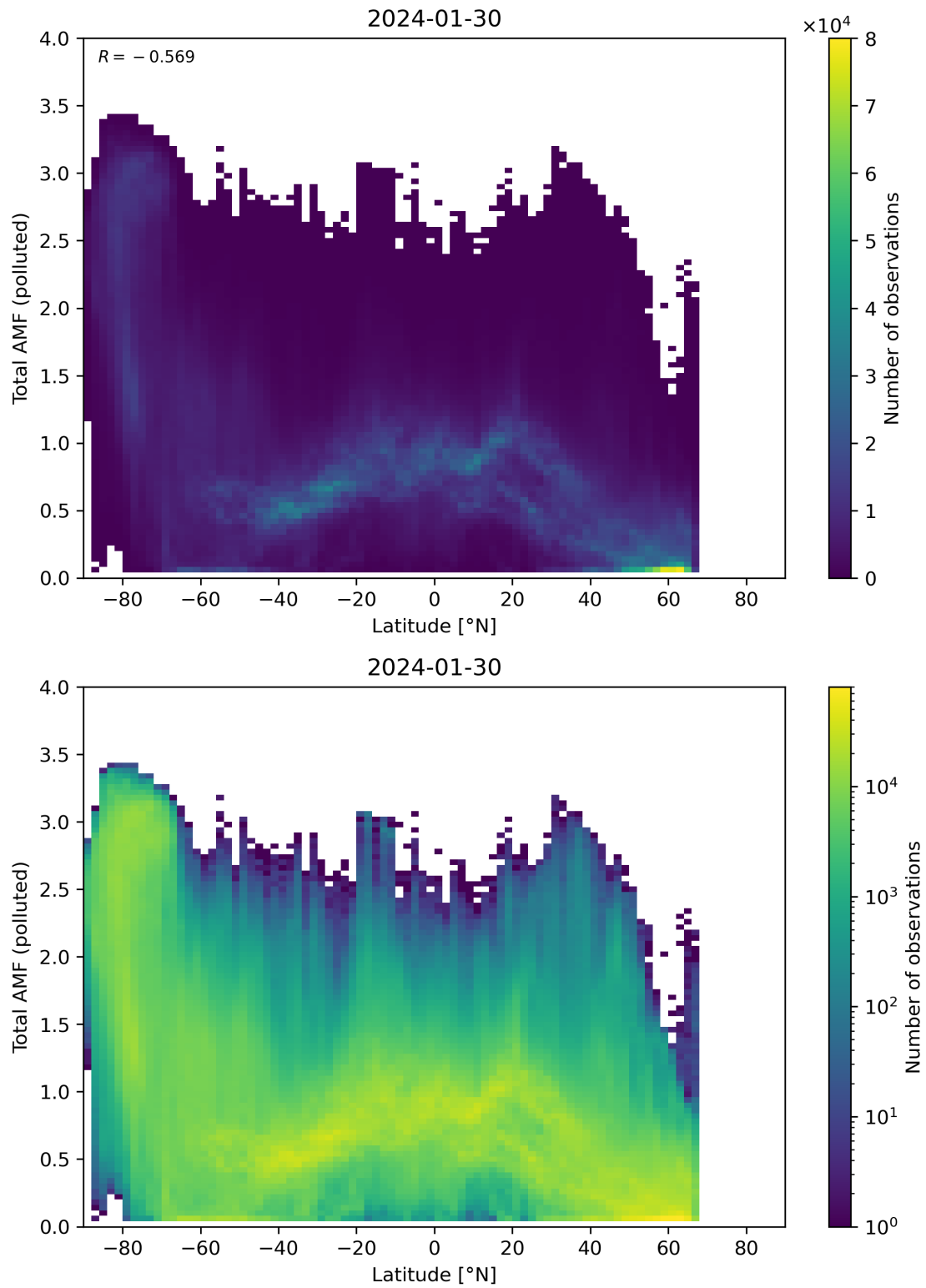
Figure 154: Scatter density plot of “Latitude” against “Total AMF (polluted)” for 2024-01-29 to 2024-01-31.
