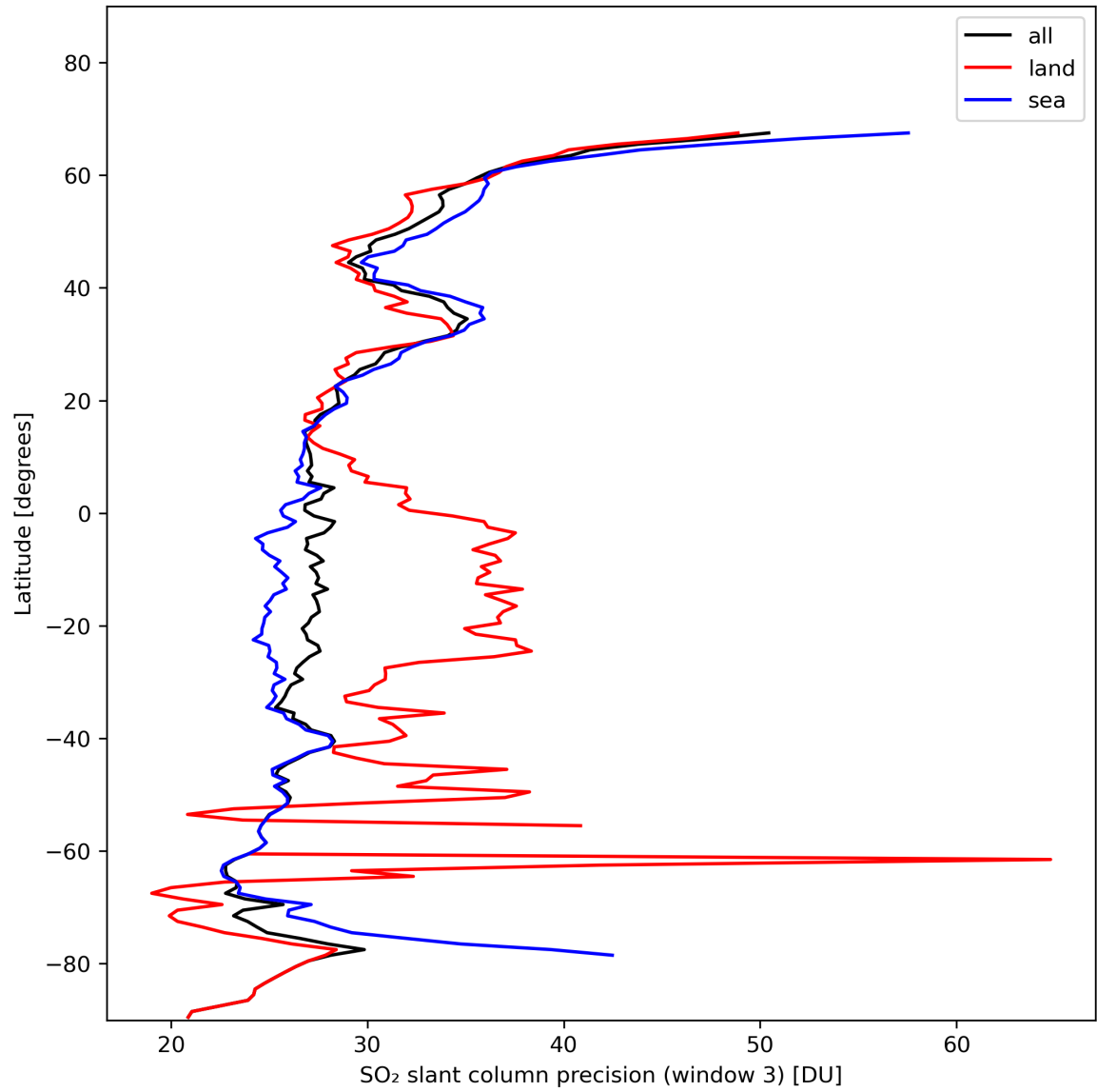
Figure 42: Zonal average of “SO 2 slant column precision (window 3)” for 2024-01-29 to 2024-01-31.
