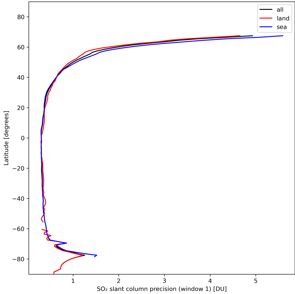
Figure 34: Zonal average of “SO 2 slant column precision (window 1)” for 2024-01-29 to 2024-01-31.
