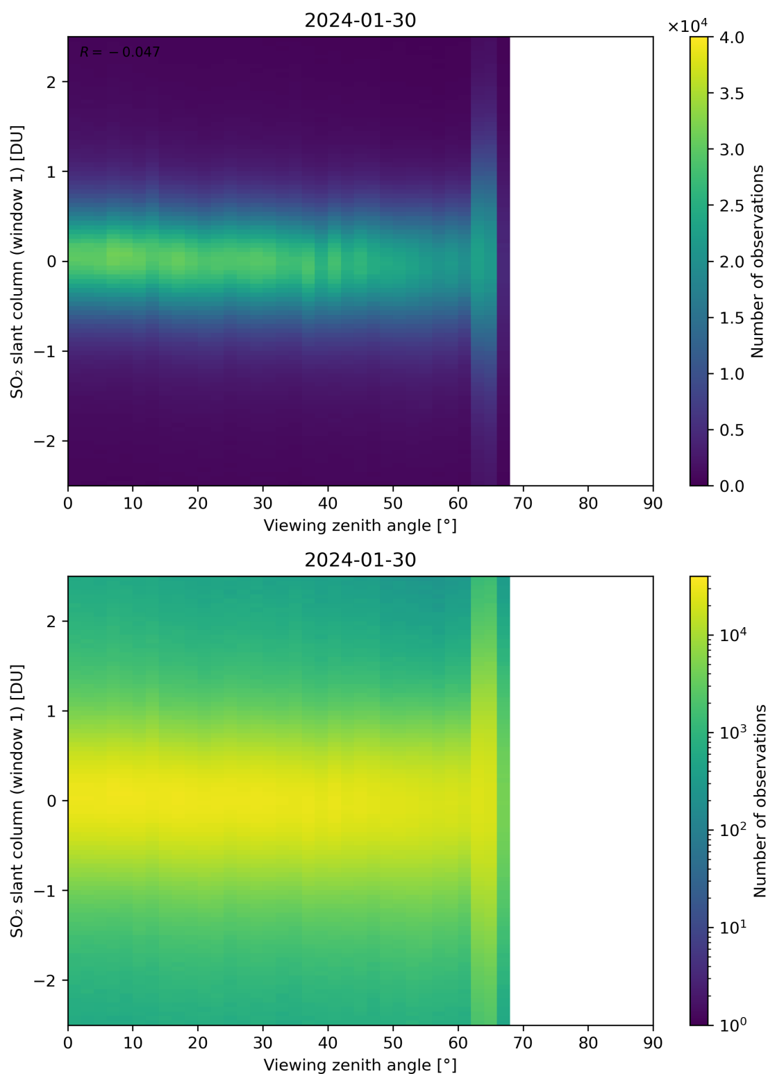
Figure 320: Scatter density plot of “Viewing zenith angle” against “SO 2 slant column (window 1)” for 2024-01-29 to 2024-01-31.
