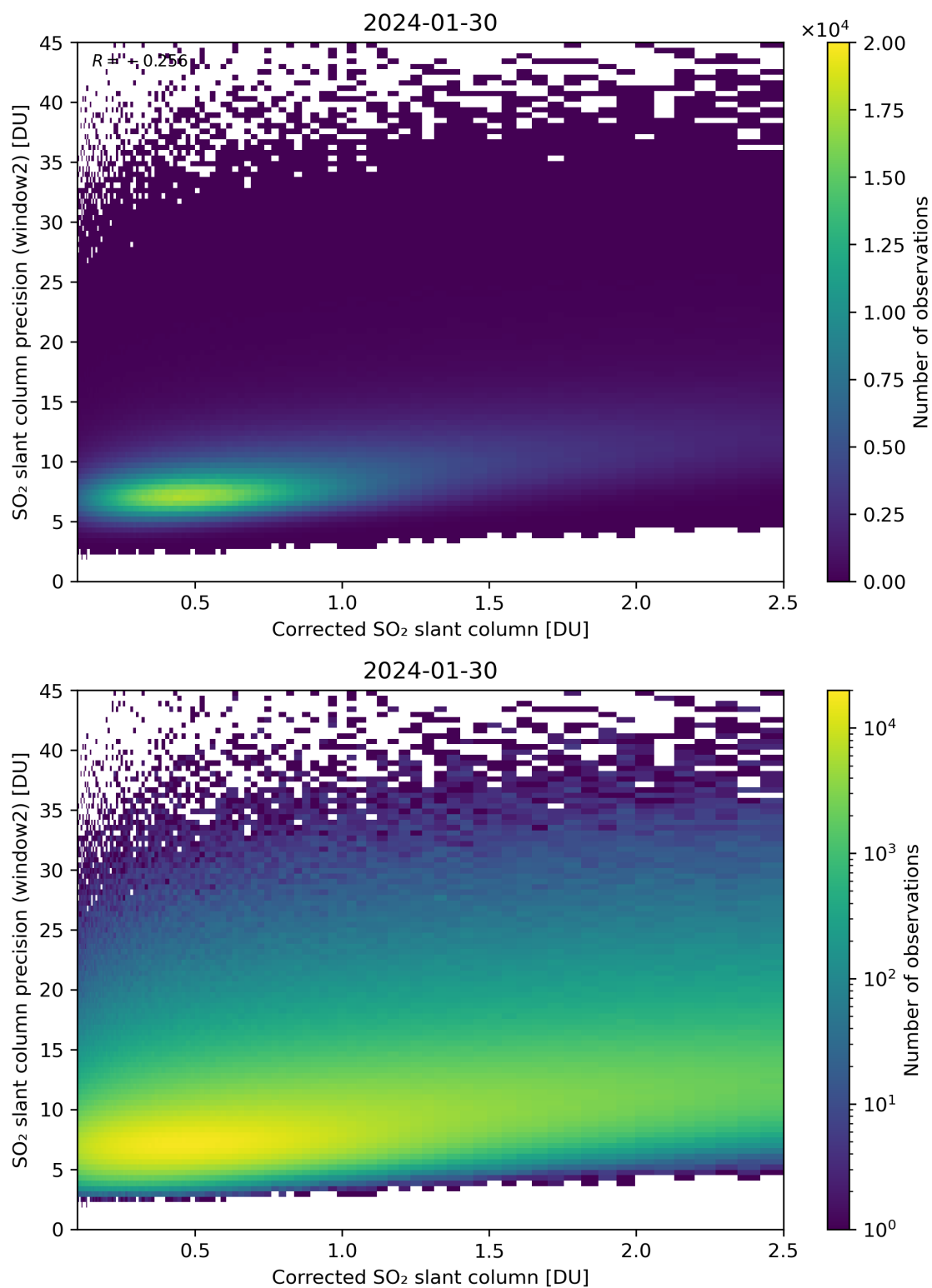
Figure 189: Scatter density plot of “Corrected SO 2 slant column” against “SO 2 slant column precision (window2)” for 2024-01-29 to 2024-01-31.
