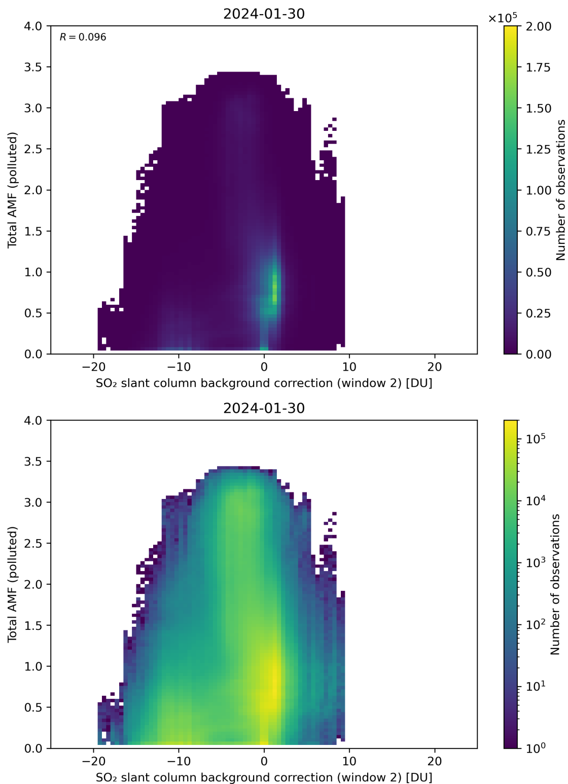
Figure 119: Scatter density plot of “SO 2 slant column background correction (window 2)” against “Total AMF (polluted)” for 2024-01-29 to 2024-01-31.
