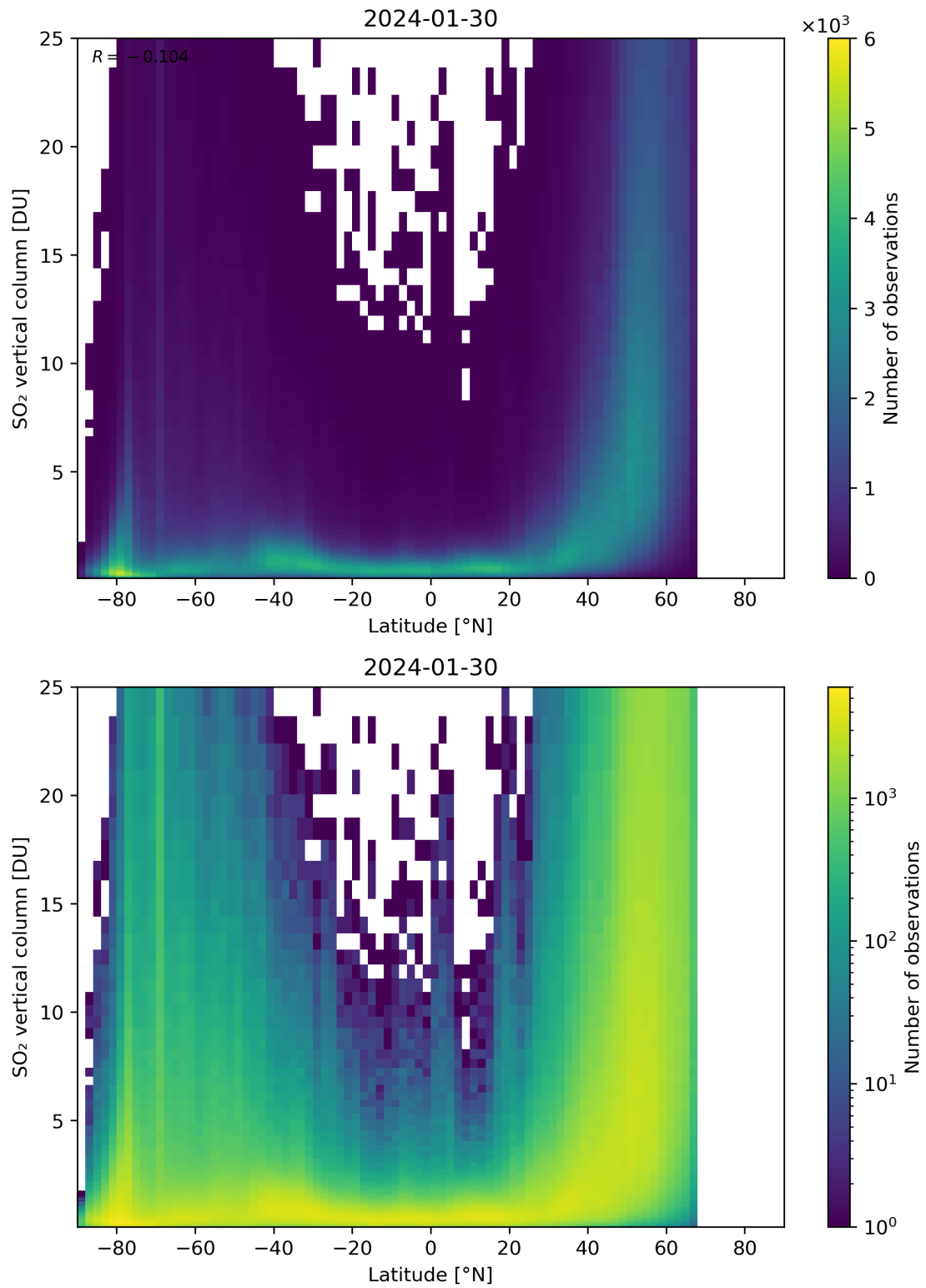
Figure 156: Scatter density plot of “Latitude” against “SO 2 vertical column” for 2024-01-29 to 2024-01-31.
