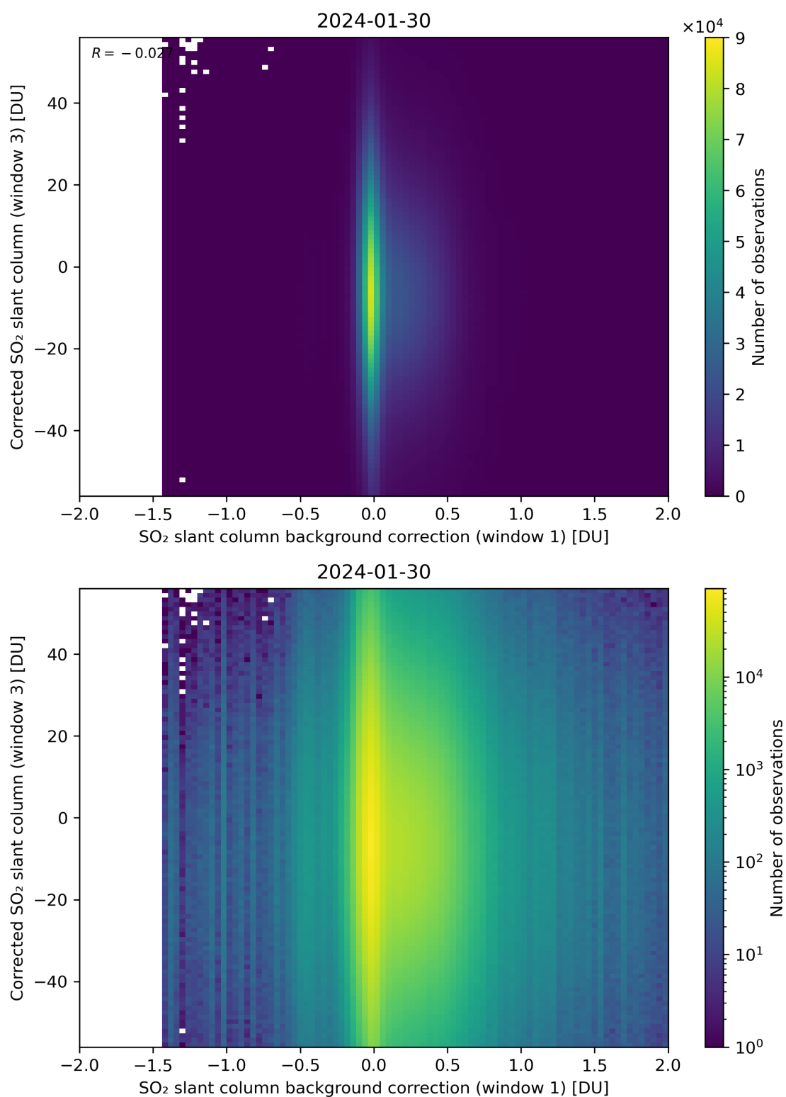
Figure 105: Scatter density plot of “SO 2 slant column background correction (window 1)” against “Corrected SO 2 slant column (window 3)” for 2024-01-29 to 2024-01-31.
