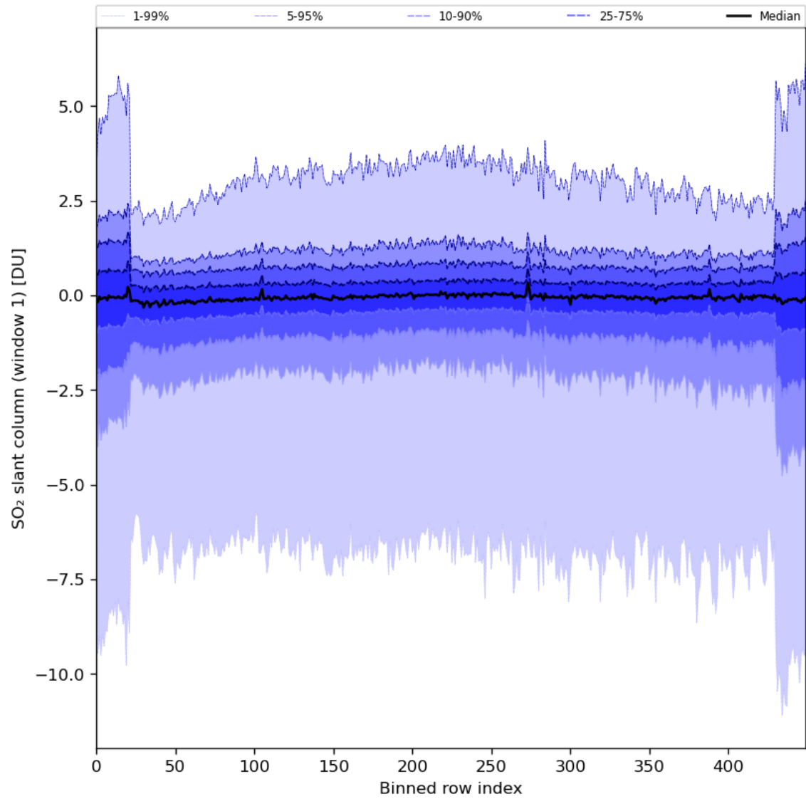
Figure 79: Along track statistics of “SO 2 slant column (window 1)” for 2024-01-29 to 2024-01-31
