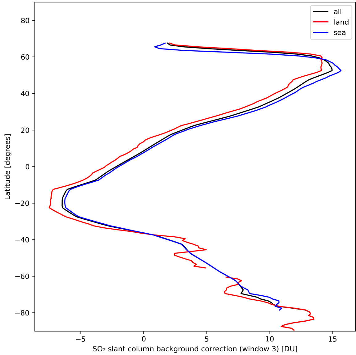
Figure 44: Zonal average of “SO 2 slant column background correction (window 3)” for 2024-01-29 to 2024-01-31.
