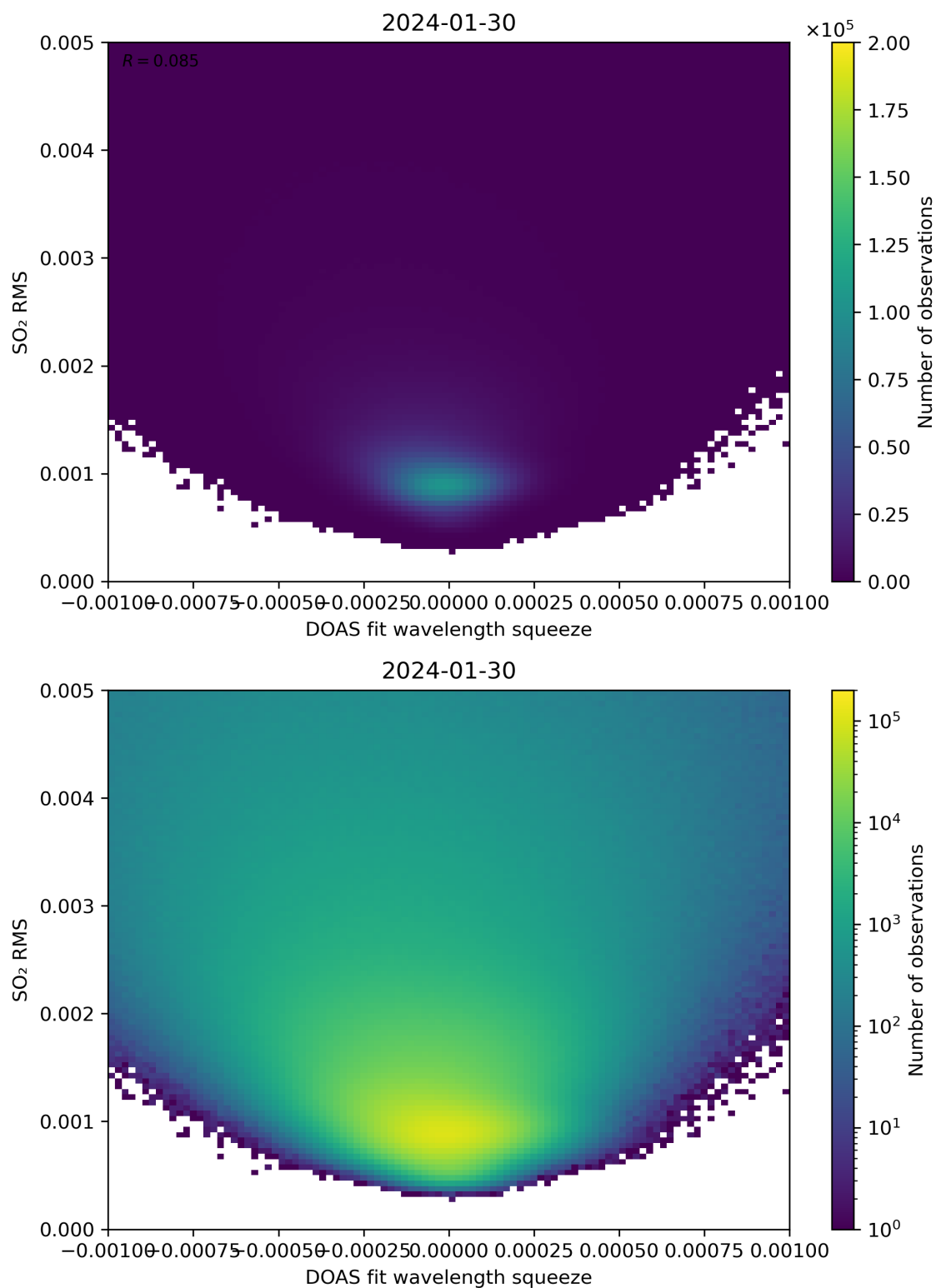
Figure 132: Scatter density plot of “DOAS fit wavelength squeeze” against “SO 2 RMS” for 2024-01-29 to 2024-01-31.
