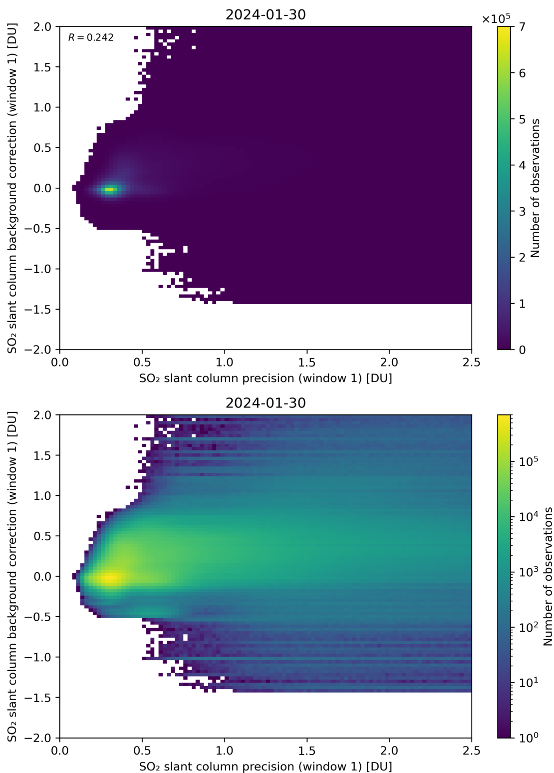
Figure 218: Scatter density plot of “SO 2 slant column precision (window 1)” against “SO 2 slant column background correction (window 1)” for 2024-01-29 to 2024-01-31.
