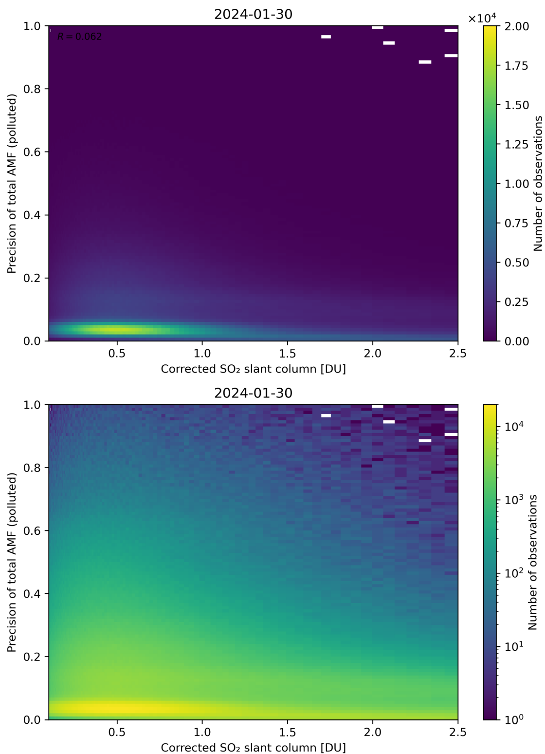
Figure 193: Scatter density plot of “Corrected SO 2 slant column” against “Precision of total AMF (polluted)” for 2024-01-29 to 2024-01-31.
