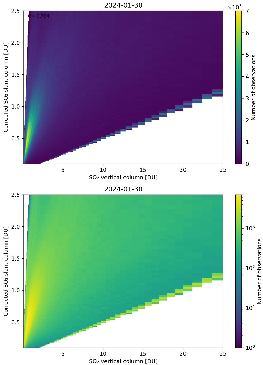
Figure 297: Scatter density plot of “SO 2 vertical column” against “Corrected SO 2 slant column” for 2024-01-29 to 2024-01-31.
