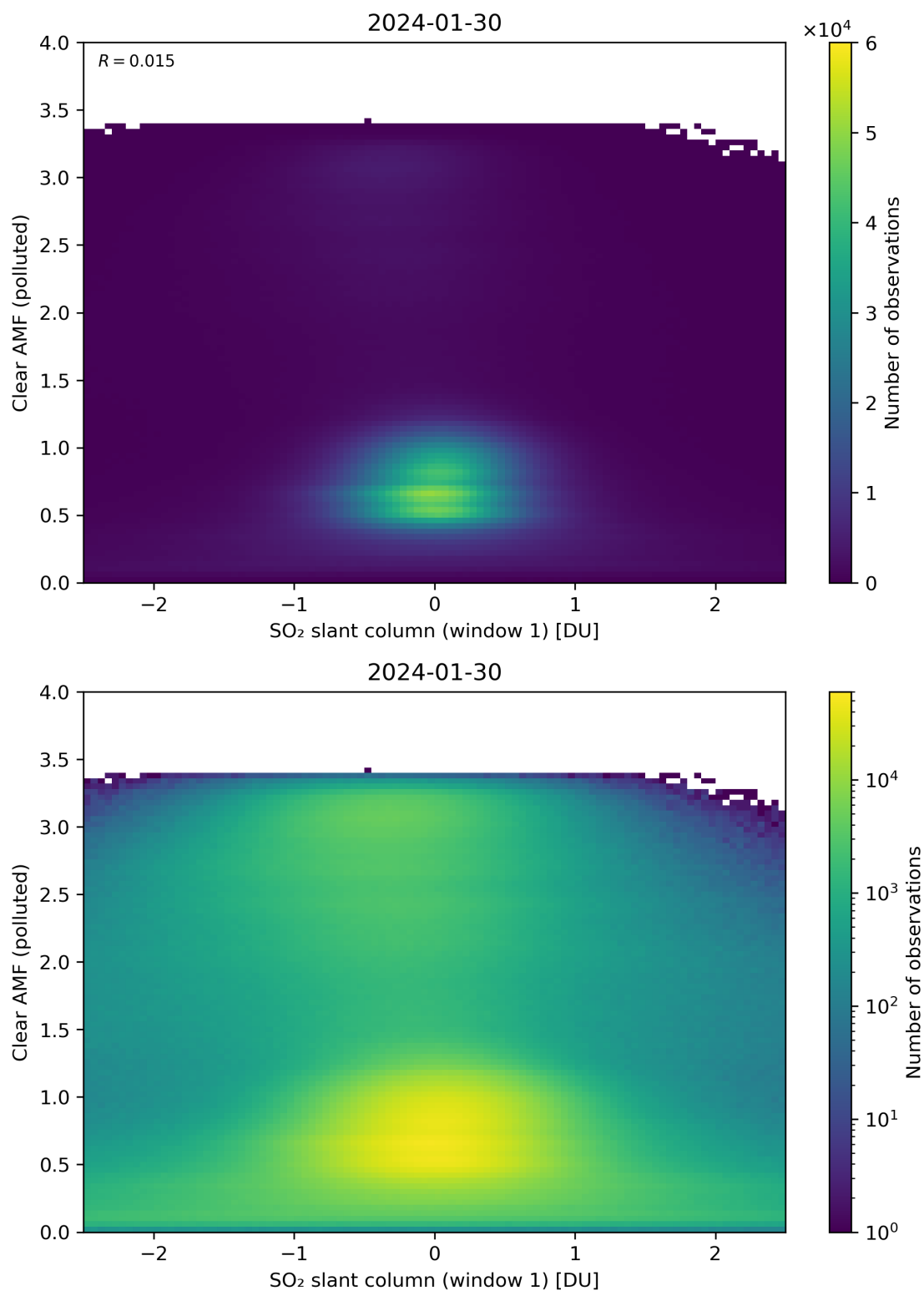
Figure 232: Scatter density plot of “SO 2 slant column (window 1)” against “Clear AMF (polluted)” for 2024-01-29 to 2024-01-31.
