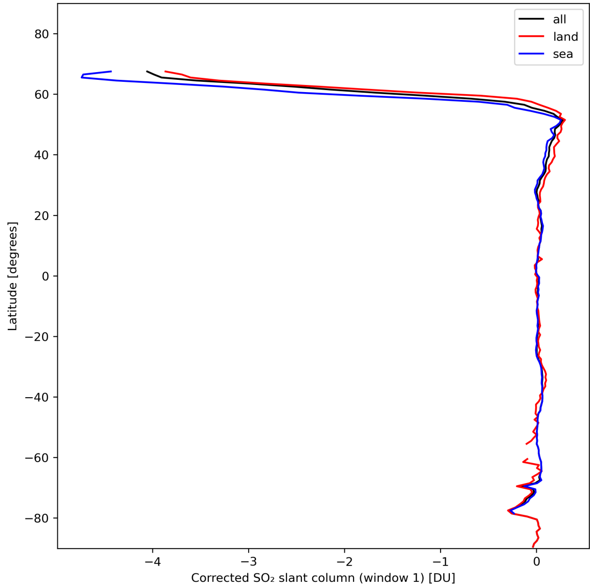
Figure 35: Zonal average of “Corrected SO 2 slant column (window 1)” for 2024-01-29 to 2024-01-31.
