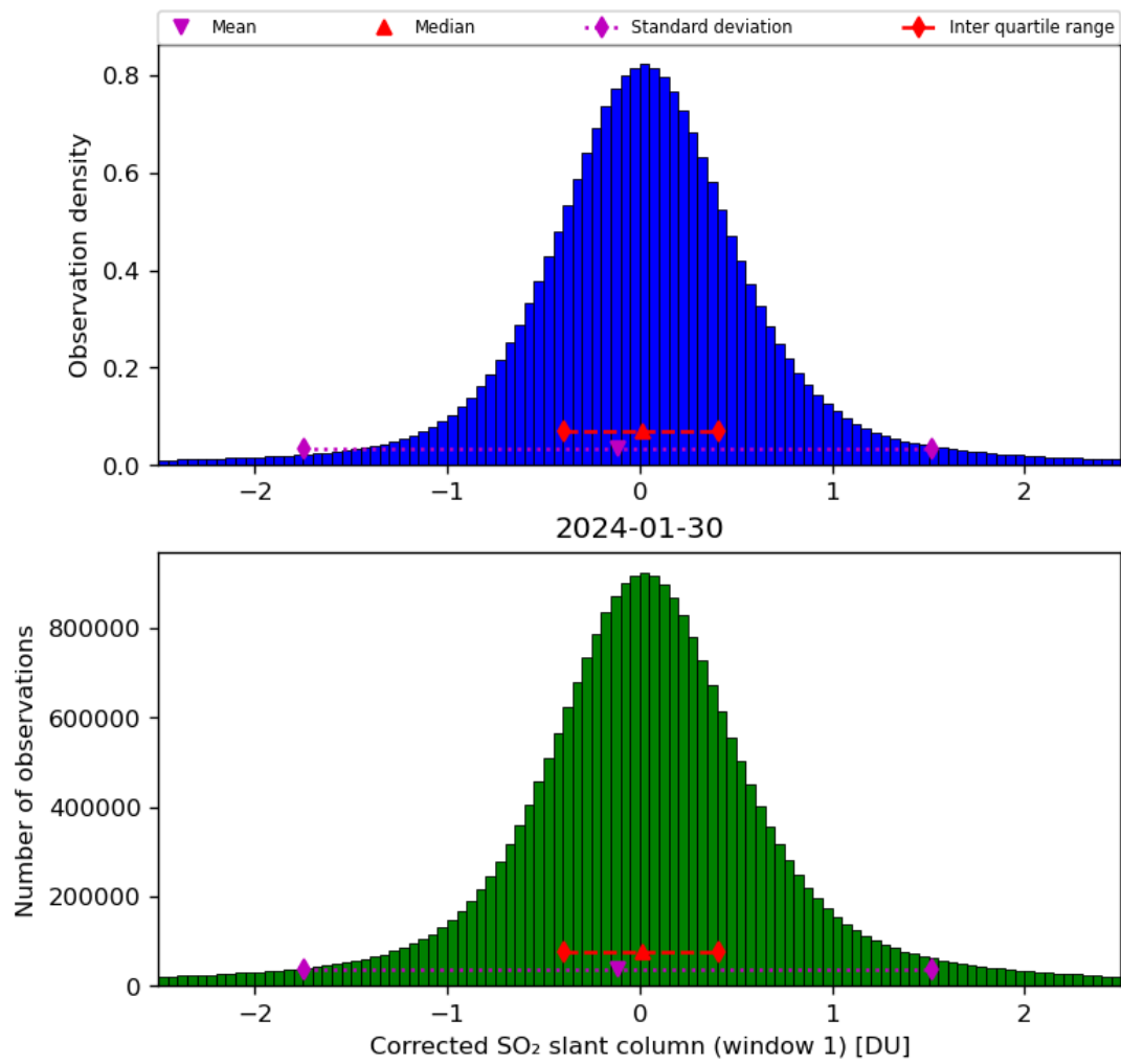
Figure 58: Histogram of “Corrected SO 2 slant column (window 1)” for 2024-01-29 to 2024-01-31
