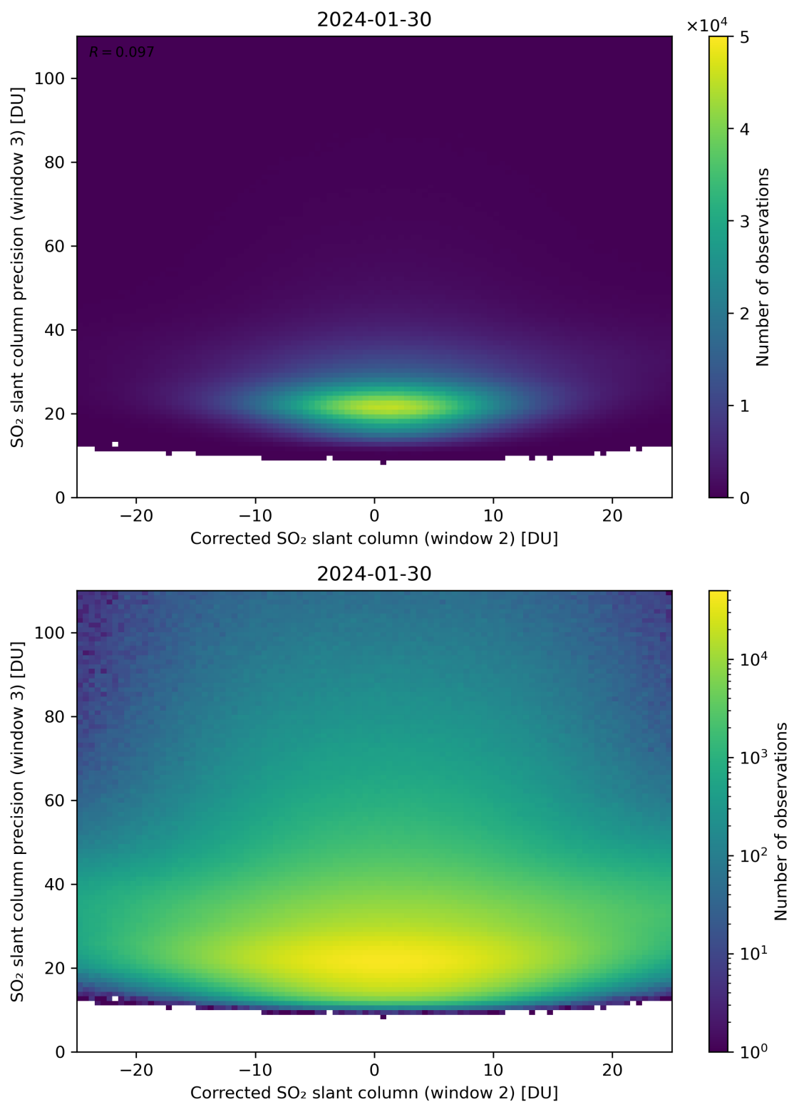
Figure 202: Scatter density plot of “Corrected SO 2 slant column (window 2)” against “SO 2 slant column precision (window 3)” for 2024-01-29 to 2024-01-31.
