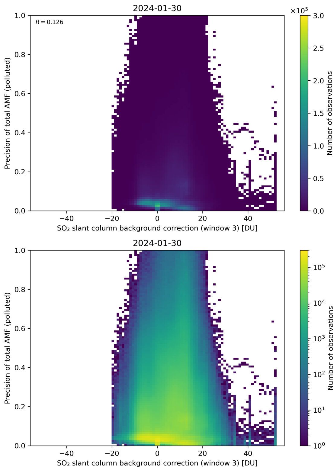
Figure 126: Scatter density plot of “SO 2 slant column background correction (window 3)” against “Precision of total AMF (polluted)” for 2024-01-29 to 2024-01-31.
