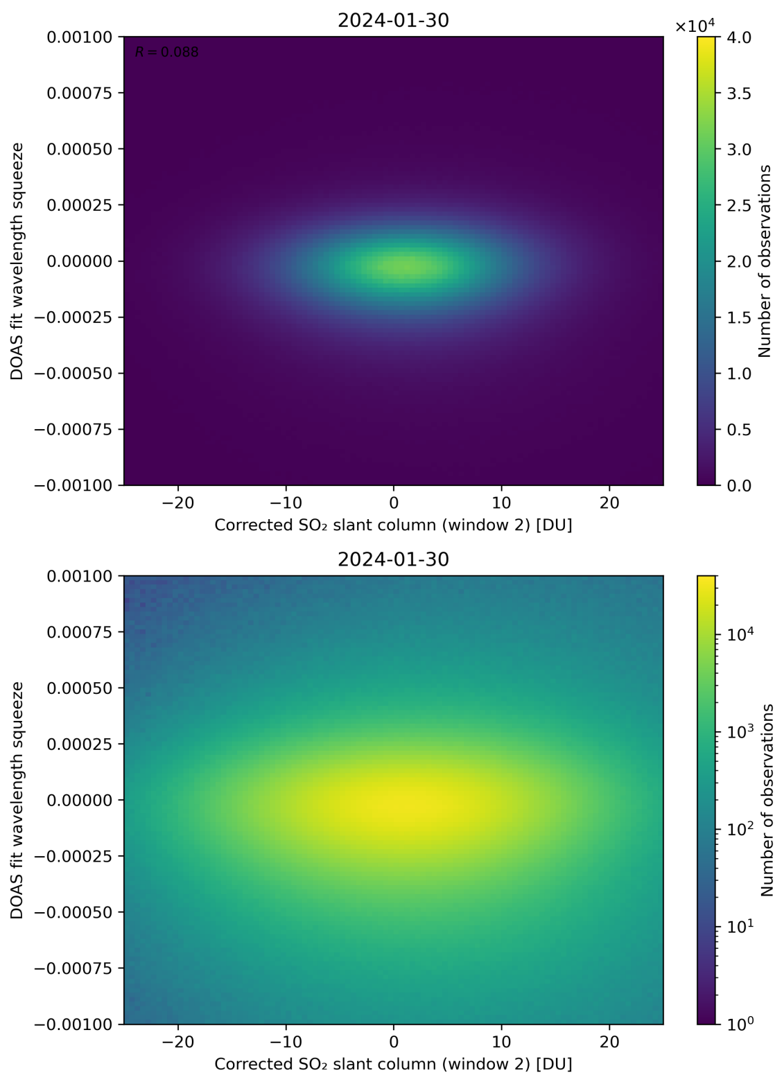
Figure 197: Scatter density plot of “Corrected SO 2 slant column (window 2)” against “DOAS fit wavelength squeeze” for 2024-01-29 to 2024-01-31.
