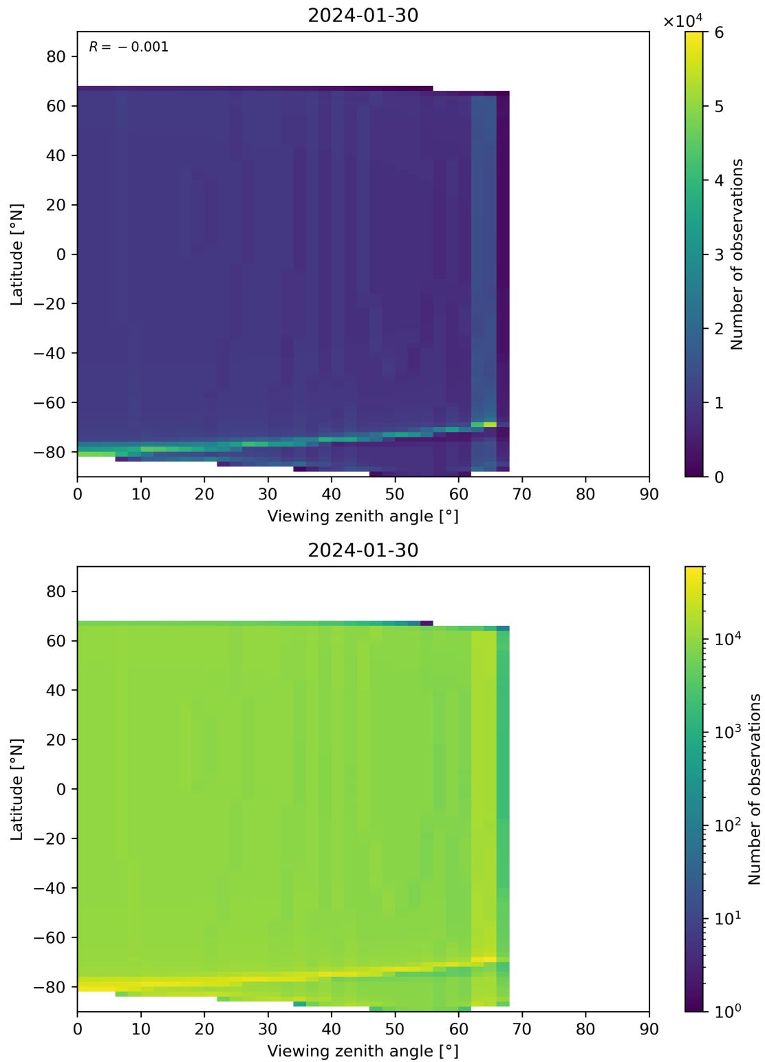
Figure 314: Scatter density plot of “Viewing zenith angle” against “Latitude” for 2024-01-29 to 2024-01-31.
