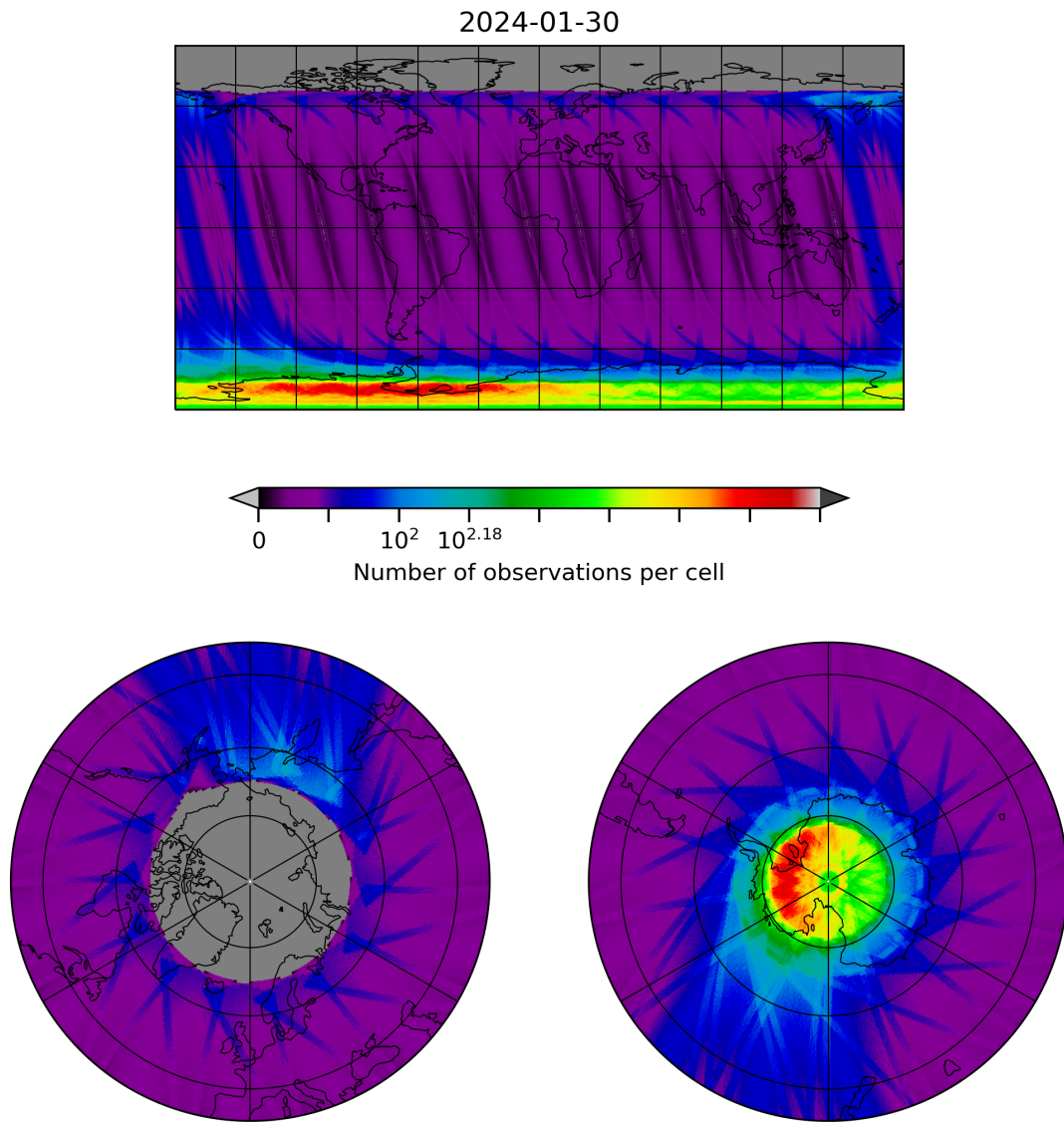
Figure 28: Map of the number of observations for 2024-01-29 to 2024-01-31
