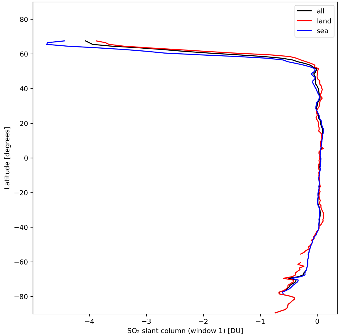
Figure 33: Zonal average of “SO 2 slant column (window 1)” for 2024-01-29 to 2024-01-31.
