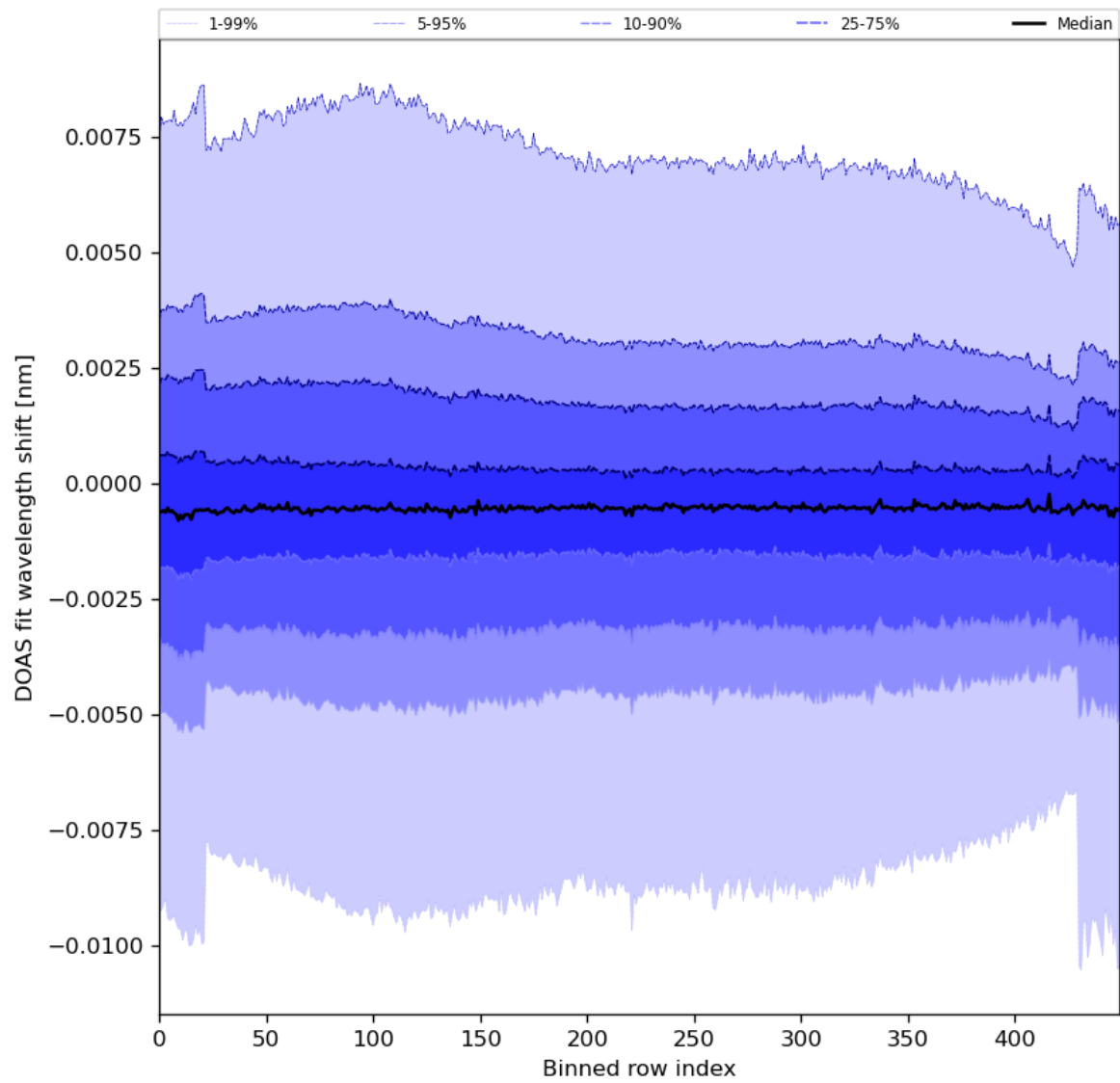
Figure 91: Along track statistics of “DOAS fit wavelength shift” for 2024-01-29 to 2024-01-31
