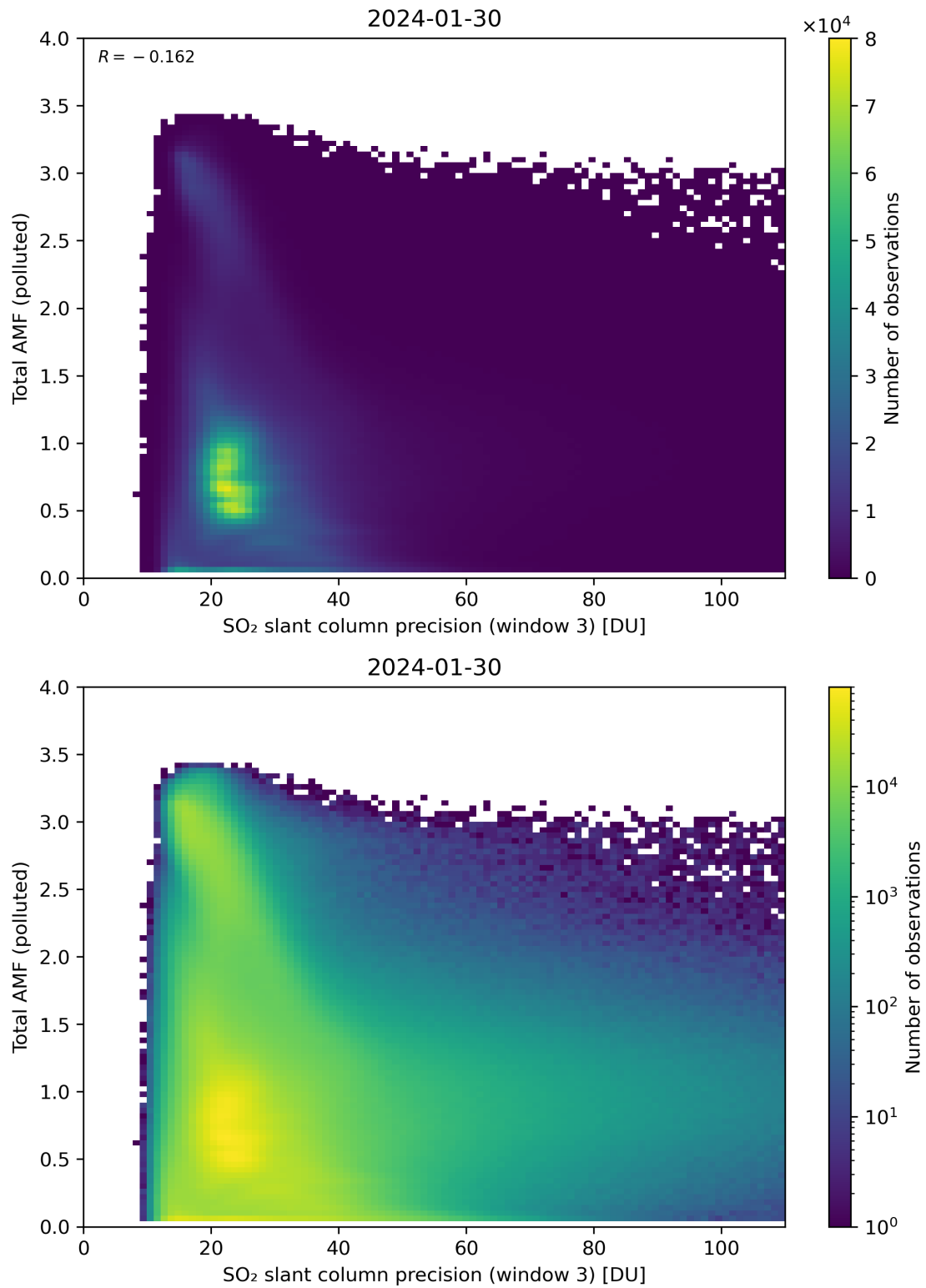
Figure 263: Scatter density plot of “SO 2 slant column precision (window 3)” against “Total AMF (polluted)” for 2024-01-29 to 2024-01-31.
