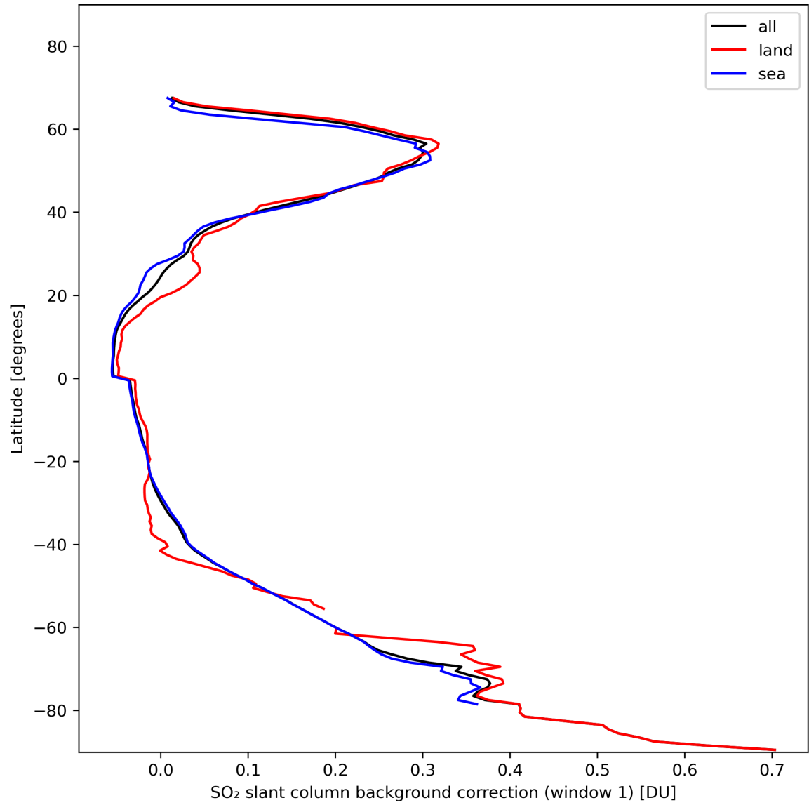
Figure 36: Zonal average of “SO 2 slant column background correction (window 1)” for 2024-01-29 to 2024-01-31.
