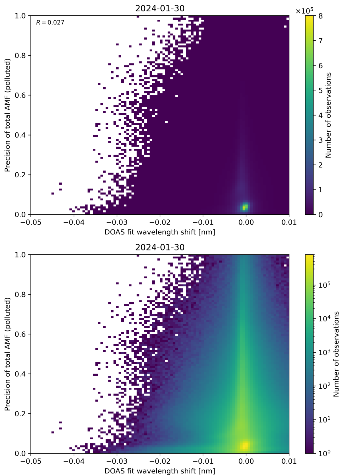
Figure 131: Scatter density plot of “DOAS fit wavelength shift” against “Precision of total AMF (polluted)” for 2024-01-29 to 2024-01-31.
