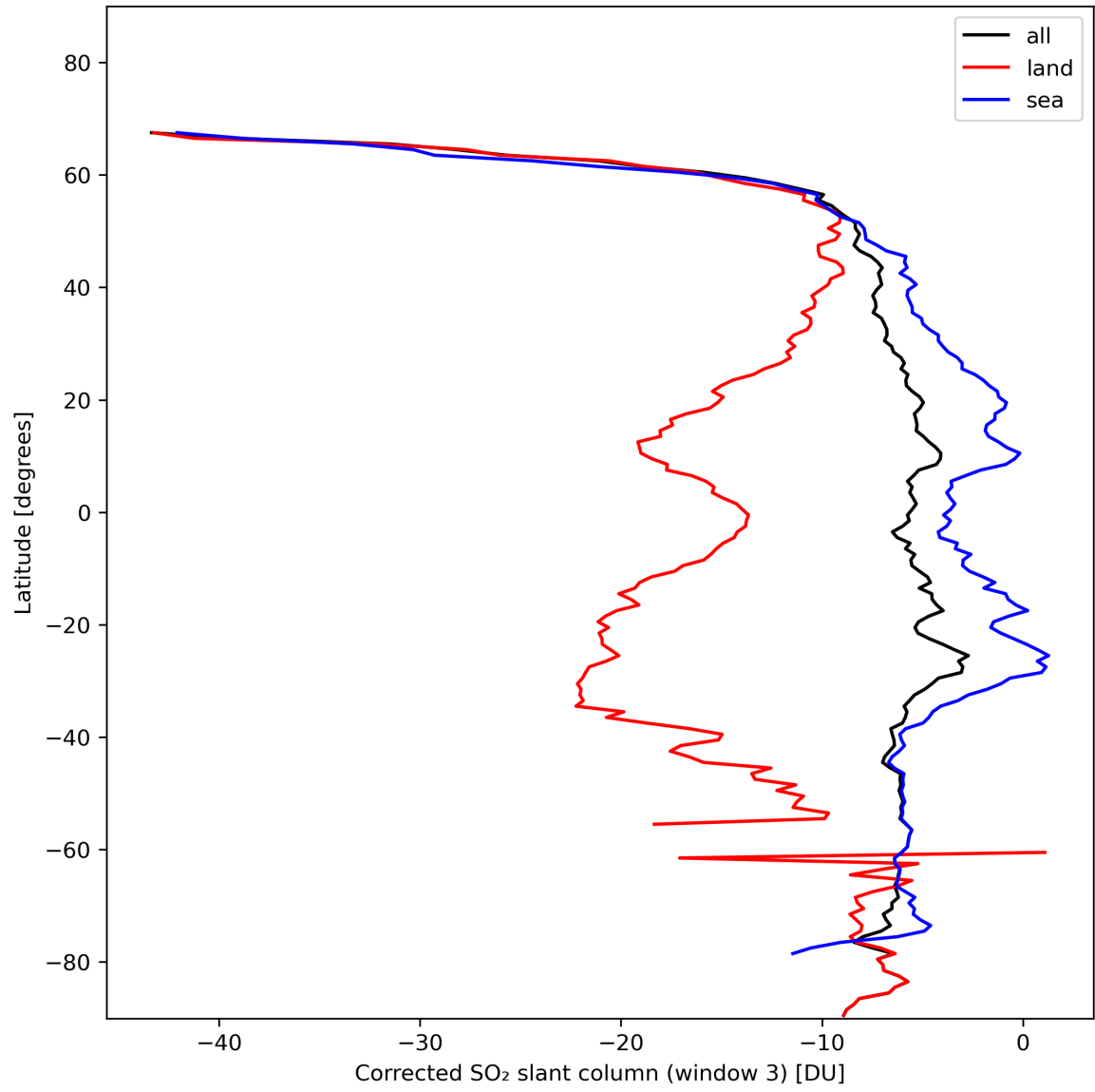
Figure 43: Zonal average of “Corrected SO 2 slant column (window 3)” for 2024-01-29 to 2024-01-31.
