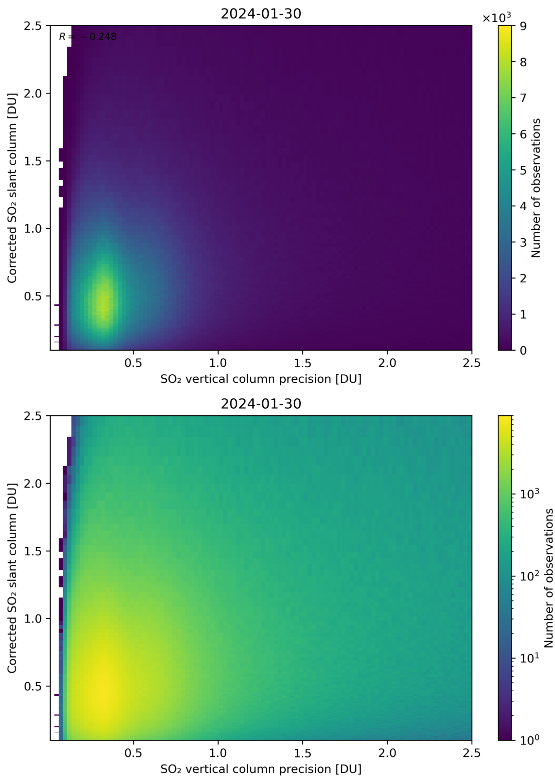
Figure 286: Scatter density plot of “SO 2 vertical column precision” against “Corrected SO 2 slant column” for 2024-01-29 to 2024-01-31.
