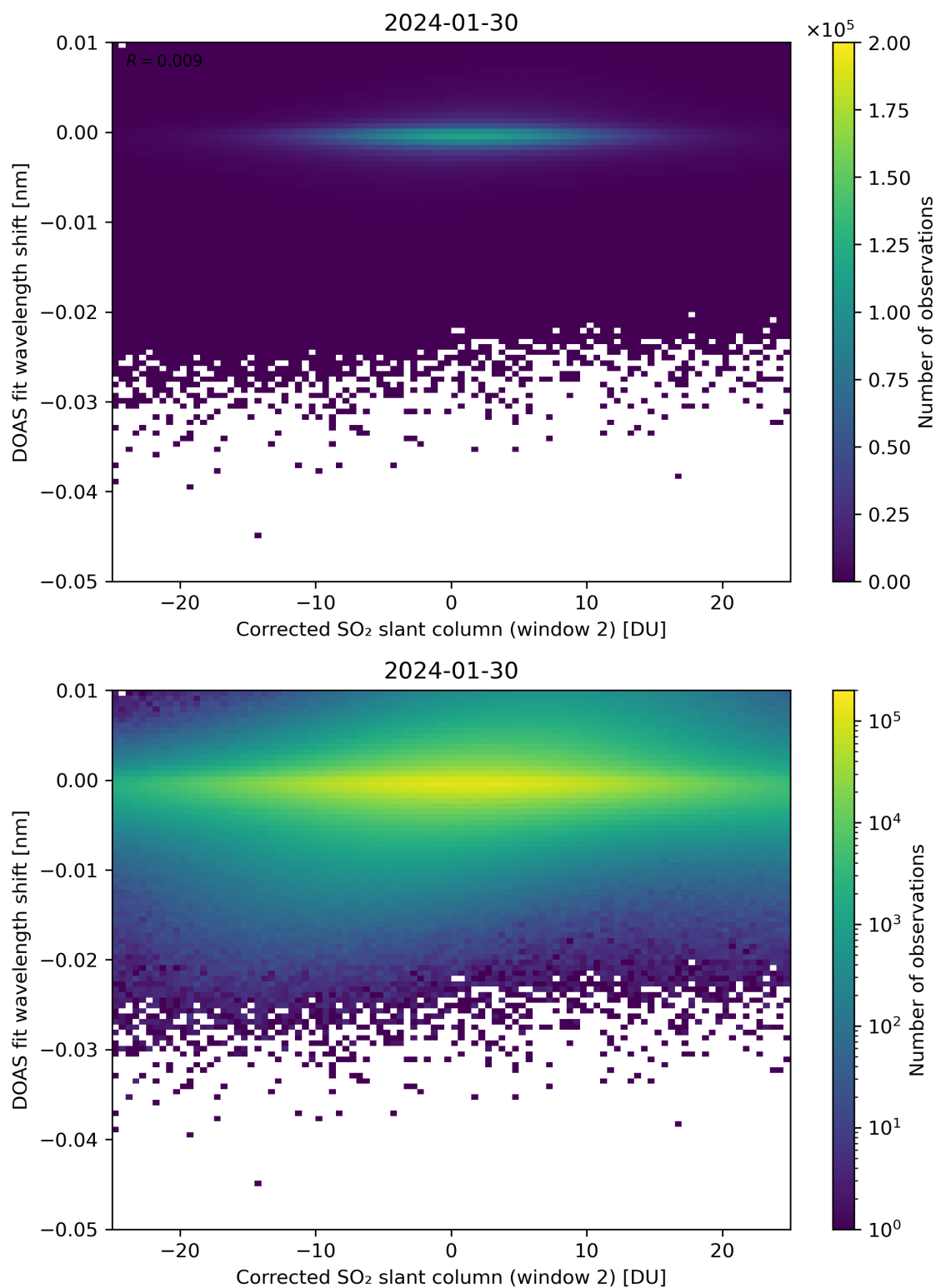
Figure 196: Scatter density plot of “Corrected SO 2 slant column (window 2)” against “DOAS fit wavelength shift” for 2024-01-29 to 2024-01-31.
