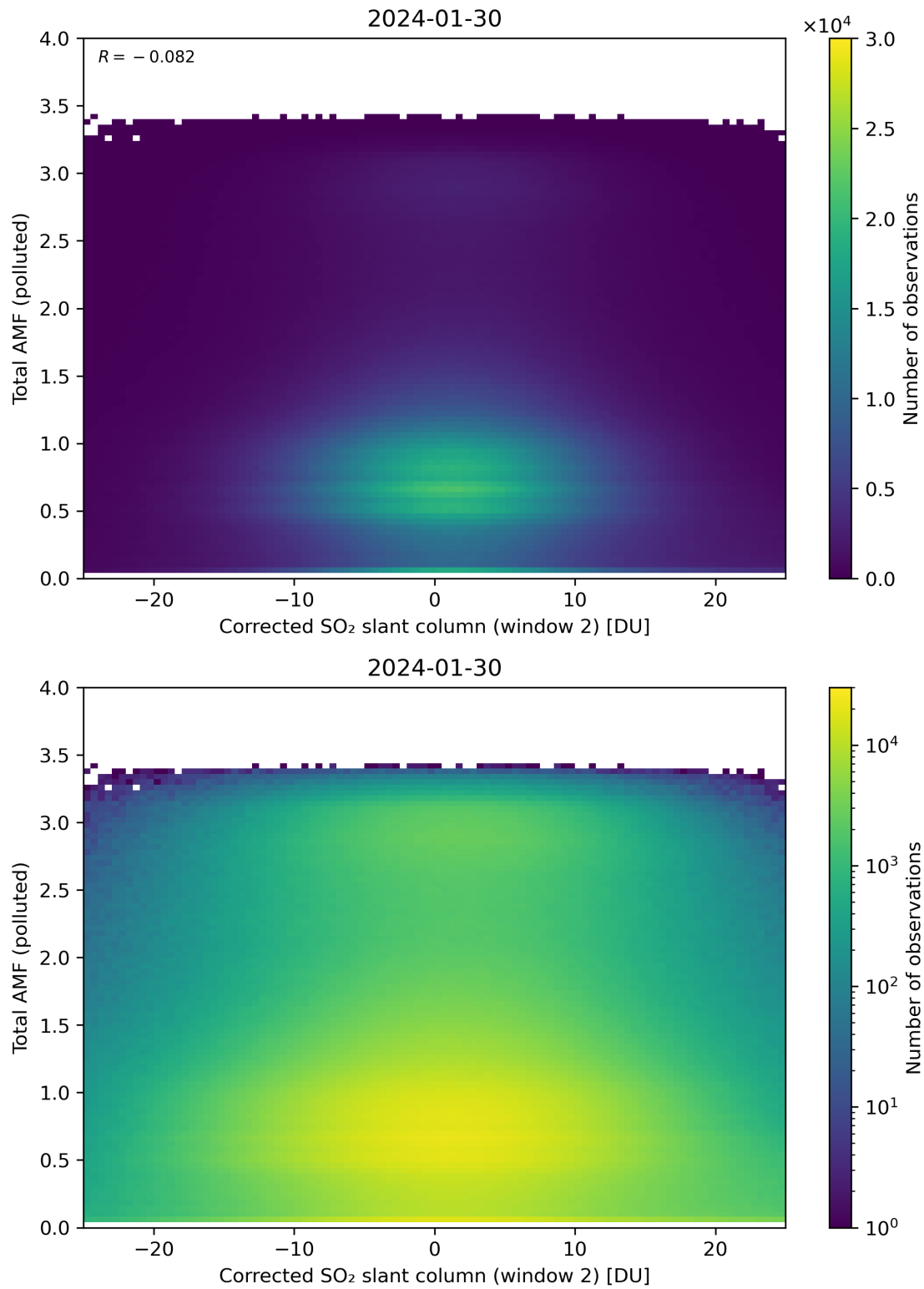
Figure 203: Scatter density plot of “Corrected SO 2 slant column (window 2)” against “Total AMF (polluted)” for 2024-01-29 to 2024-01-31.
