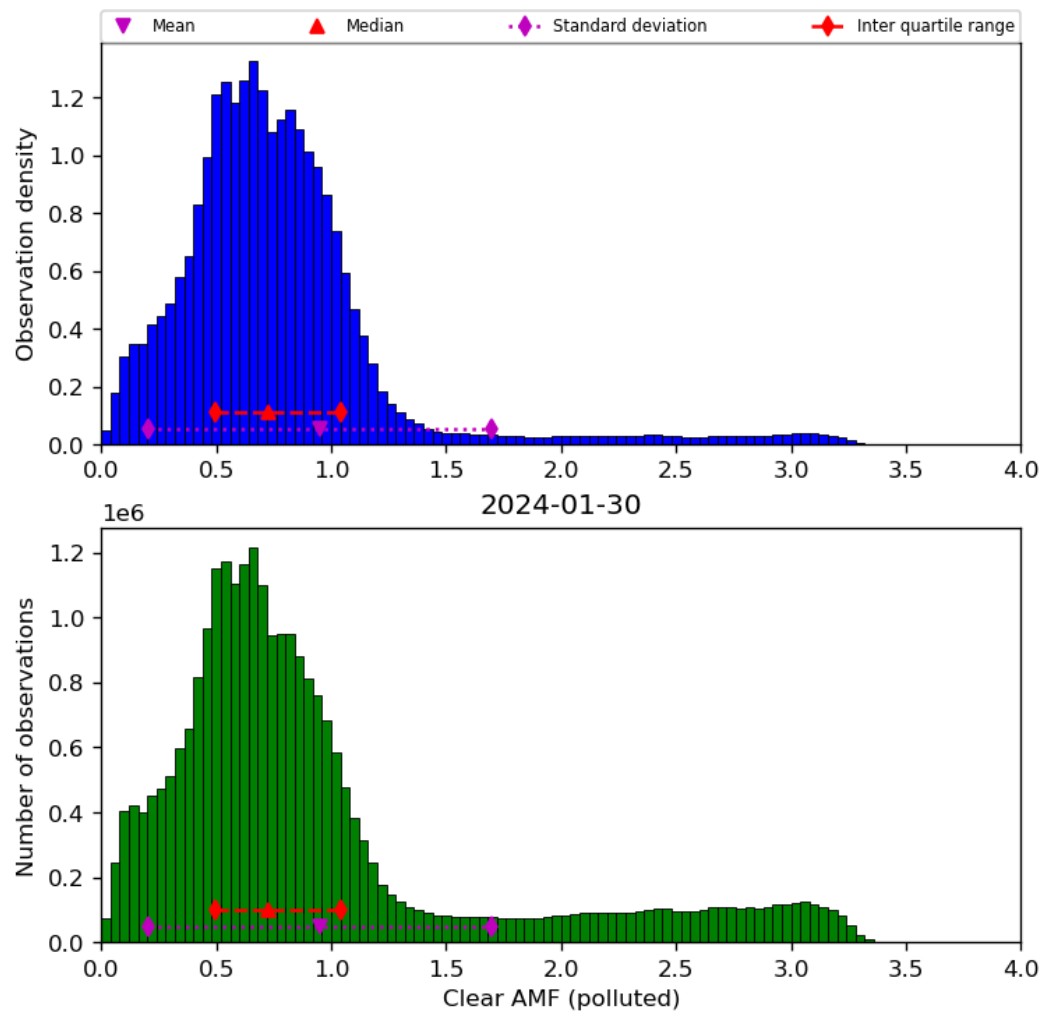
Figure 73: Histogram of “Clear AMF (polluted)” for 2024-01-29 to 2024-01-31
