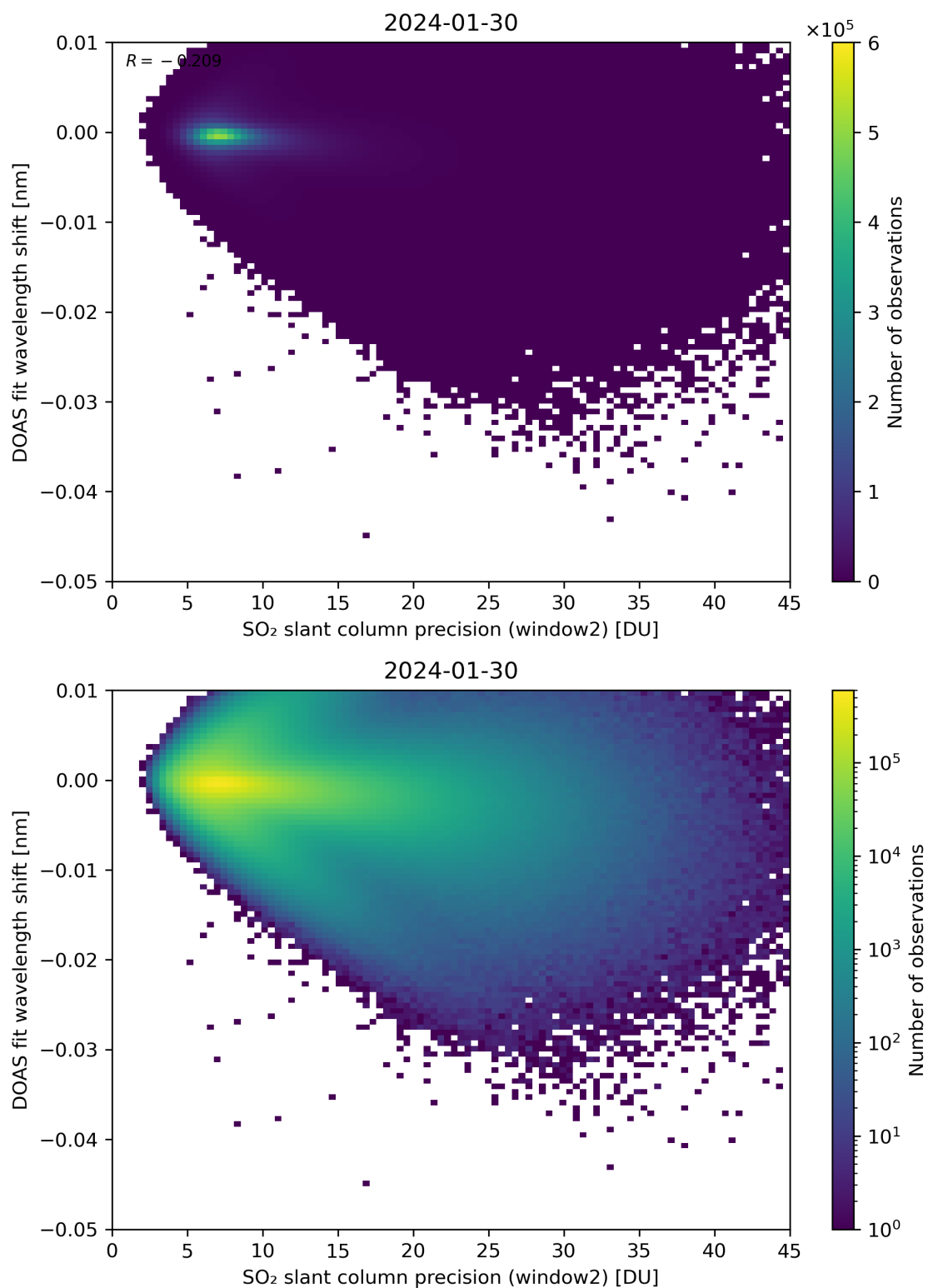
Figure 243: Scatter density plot of “SO 2 slant column precision (window2)” against “DOAS fit wavelength shift” for 2024-01-29 to 2024-01-31.
