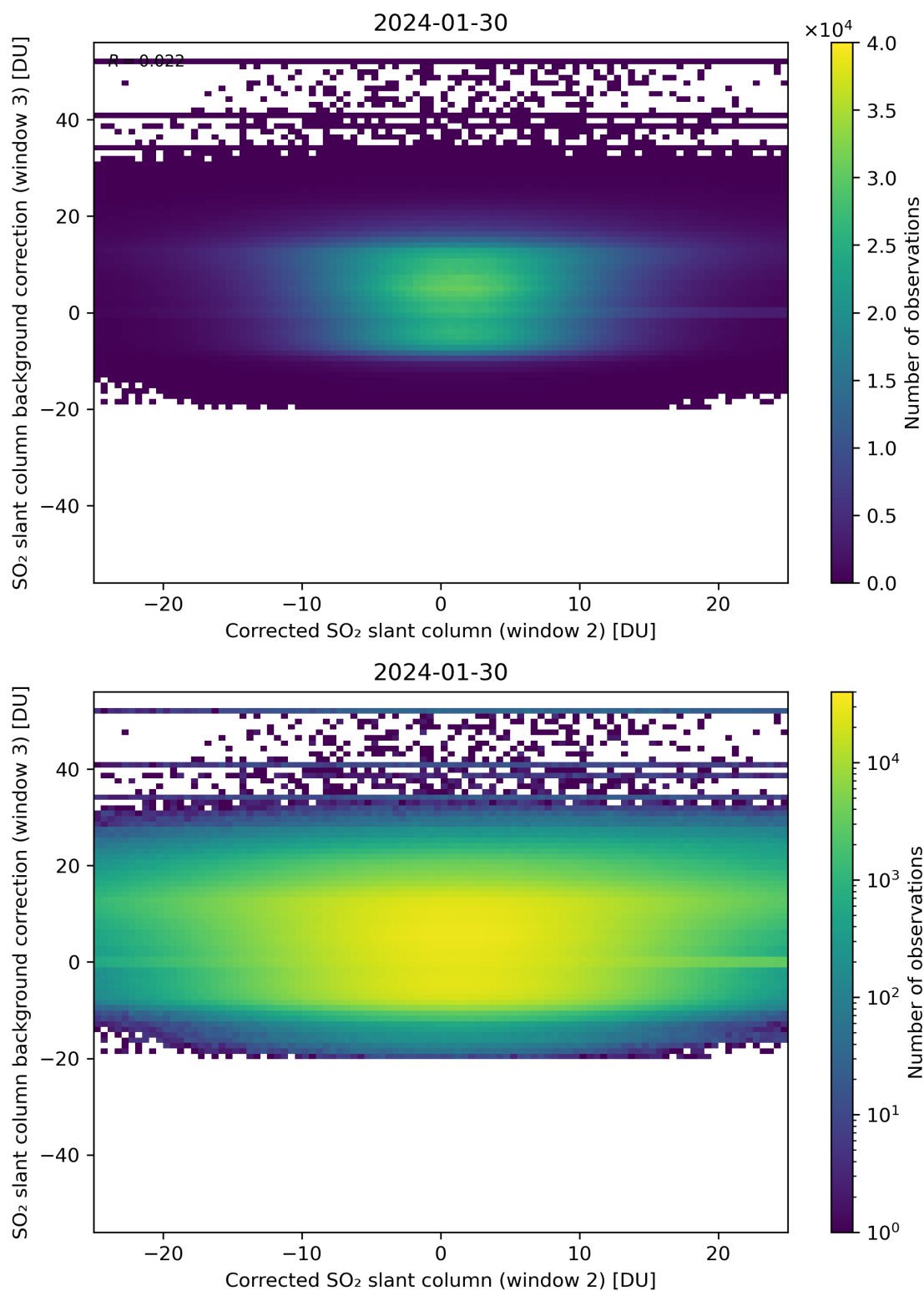
Figure 195: Scatter density plot of “Corrected SO 2 slant column (window 2)” against “SO 2 slant column background correction (window 3)” for 2024-01-29 to 2024-01-31.
