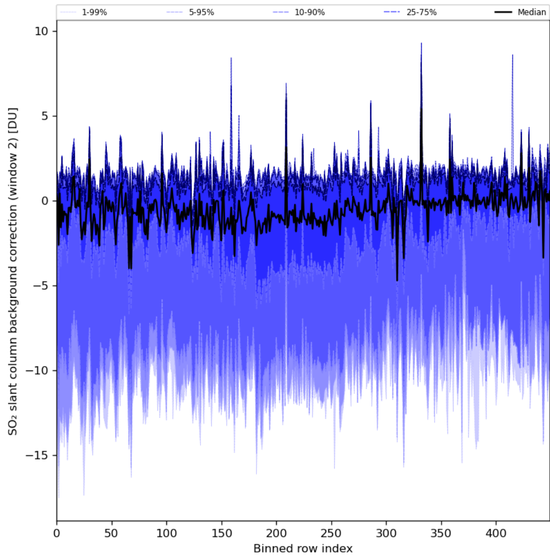
Figure 86: Along track statistics of “SO 2 slant column background correction (window 2)” for 2024-01-29 to 2024-01-31
