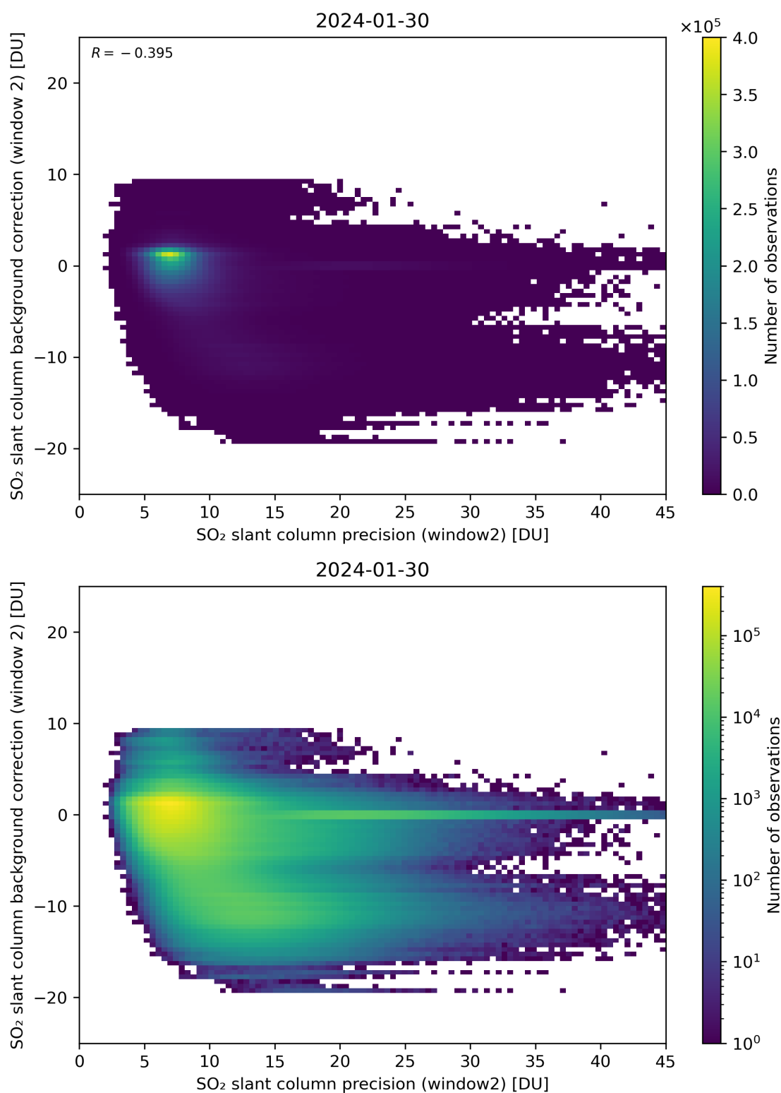
Figure 241: Scatter density plot of “SO 2 slant column precision (window2)” against “SO 2 slant column background correction (window 2)” for 2024-01-29 to 2024-01-31.
