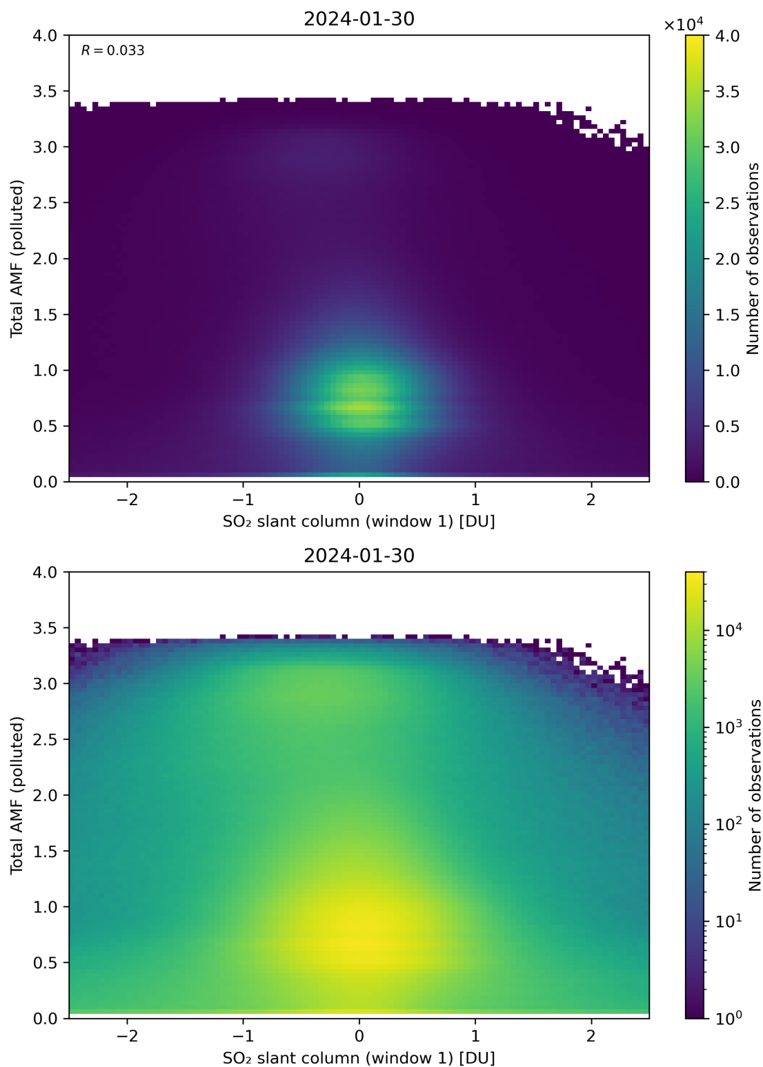
Figure 239: Scatter density plot of “SO 2 slant column (window 1)” against “Total AMF (polluted)” for 2024-01-29 to 2024-01-31.
