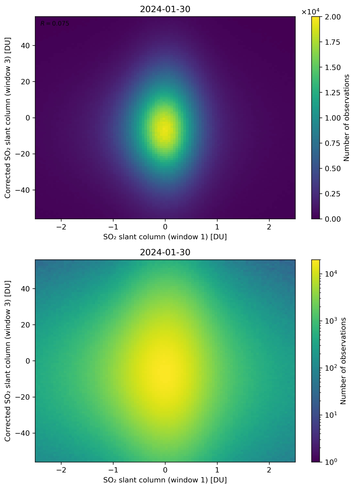
Figure 234: Scatter density plot of “SO 2 slant column (window 1)” against “Corrected SO 2 slant column (window 3)” for 2024-01-29 to 2024-01-31.
