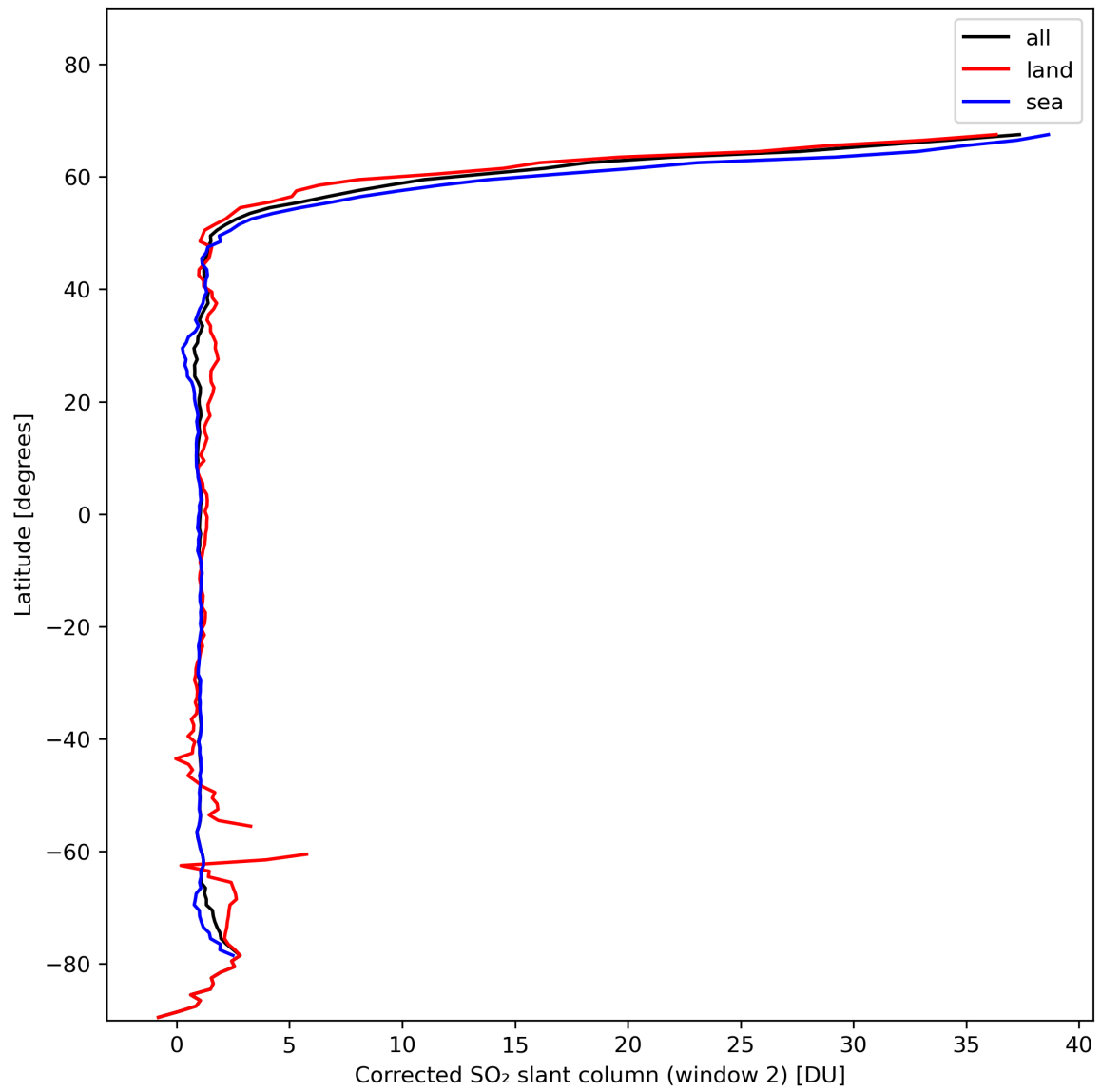
Figure 39: Zonal average of “Corrected SO 2 slant column (window 2)” for 2024-01-29 to 2024-01-31.
