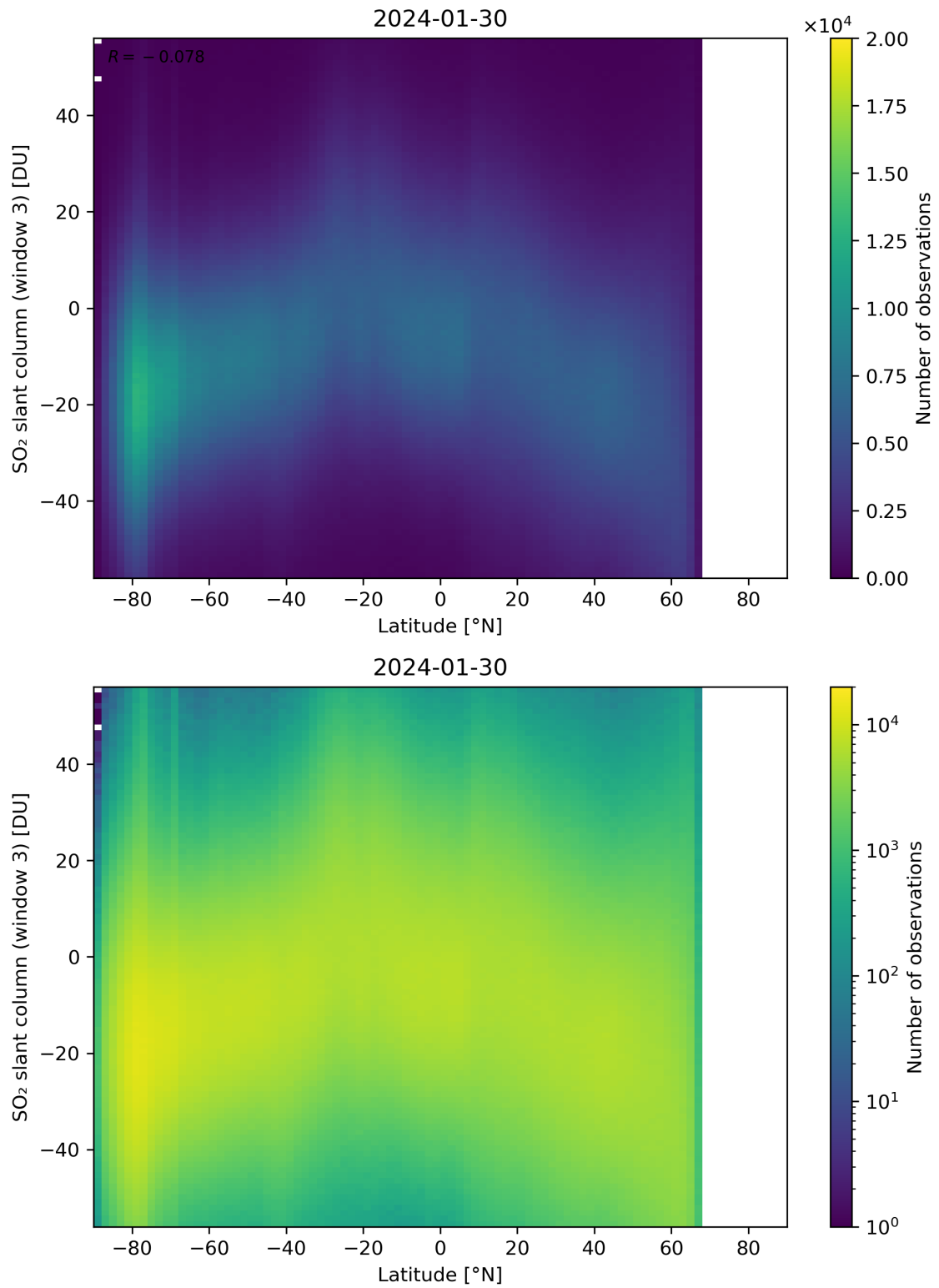
Figure 152: Scatter density plot of “Latitude” against “SO 2 slant column (window 3)” for 2024-01-29 to 2024-01-31.
