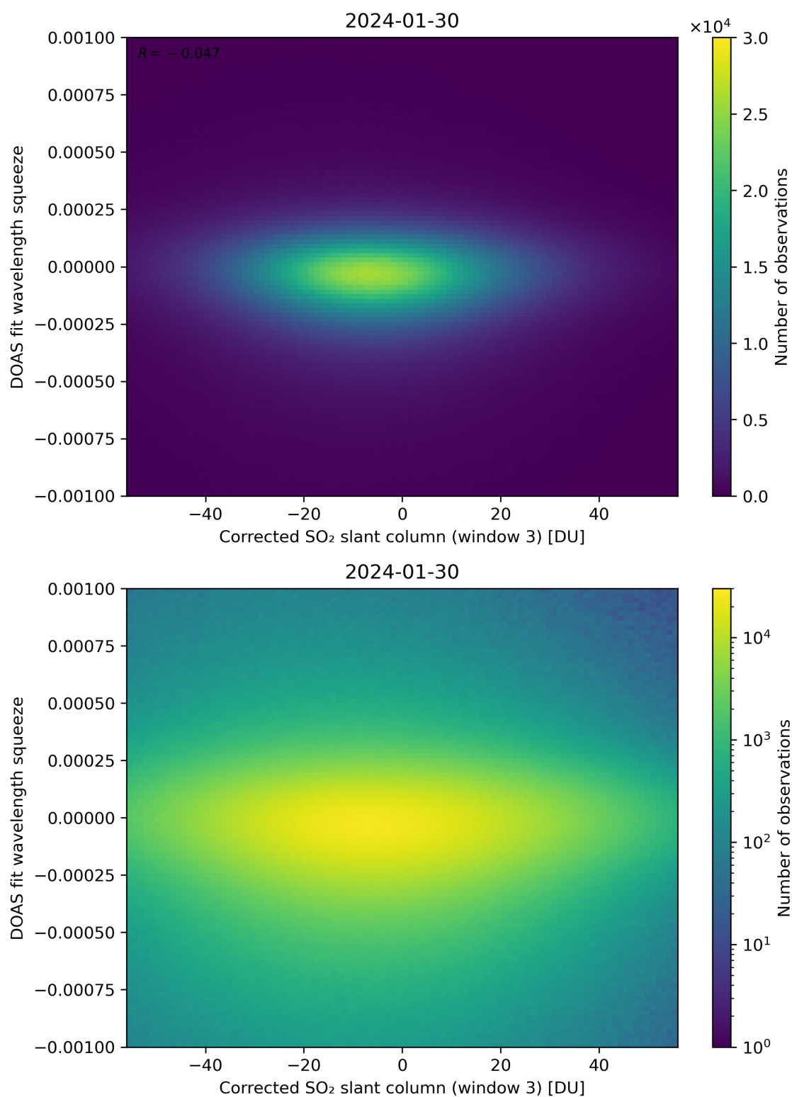
Figure 207: Scatter density plot of “Corrected SO 2 slant column (window 3)” against “DOAS fit wavelength squeeze” for 2024-01-29 to 2024-01-31.
