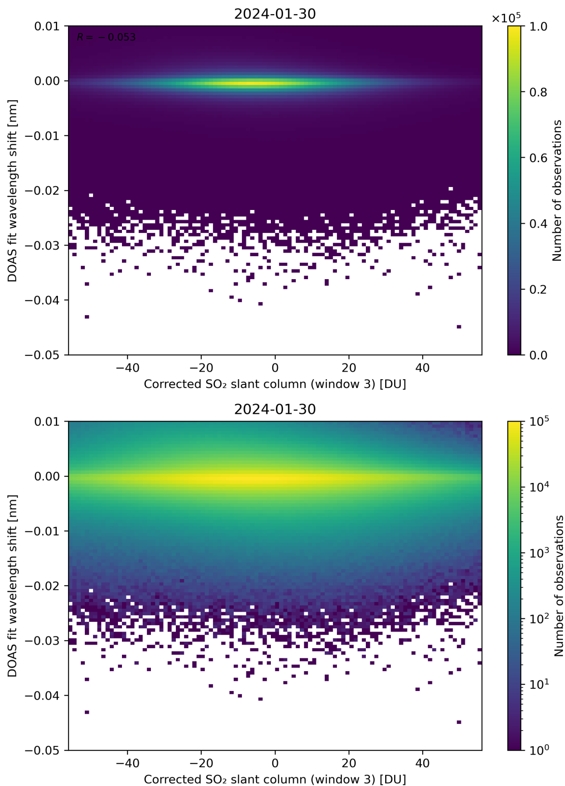
Figure 206: Scatter density plot of “Corrected SO 2 slant column (window 3)” against “DOAS fit wavelength shift” for 2024-01-29 to 2024-01-31.
