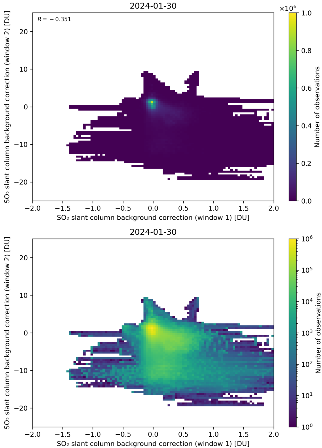
Figure 98: Scatter density plot of “SO 2 slant column background correction (window 1)” against “SO 2 slant column background correction (window 2)” for 2024-01-29 to 2024-01-31.
