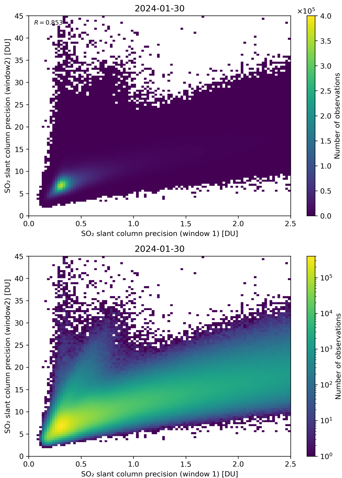
Figure 227: Scatter density plot of “SO 2 slant column precision (window 1)” against “SO 2 slant column precision (window2)” for 2024-01-29 to 2024-01-31.
