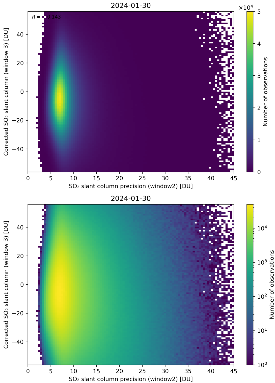
Figure 248: Scatter density plot of “SO 2 slant column precision (window2)” against “Corrected SO 2 slant column (window 3)” for 2024-01-29 to 2024-01-31.
