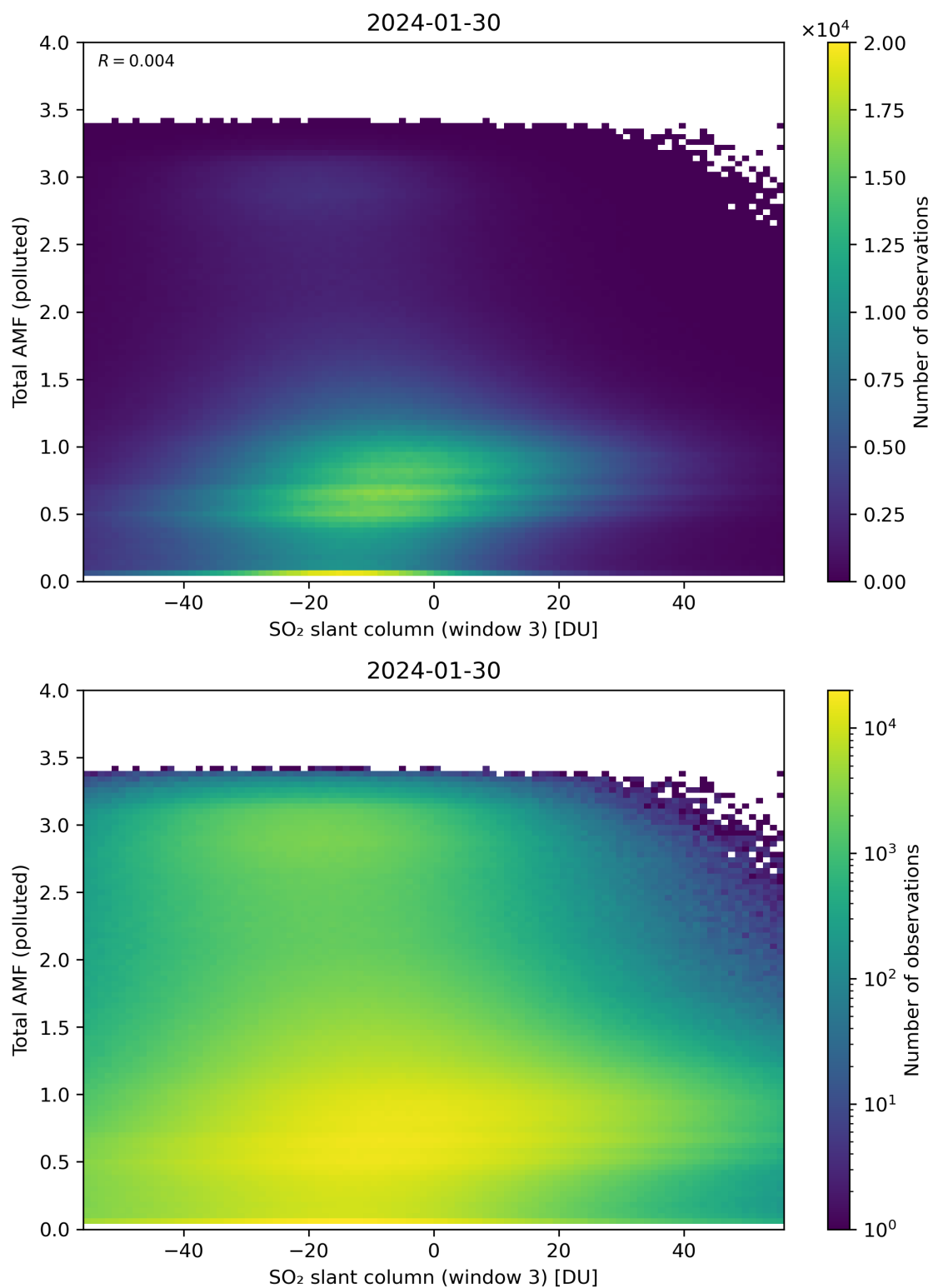
Figure 268: Scatter density plot of “SO 2 slant column (window 3)” against “Total AMF (polluted)” for 2024-01-29 to 2024-01-31.
