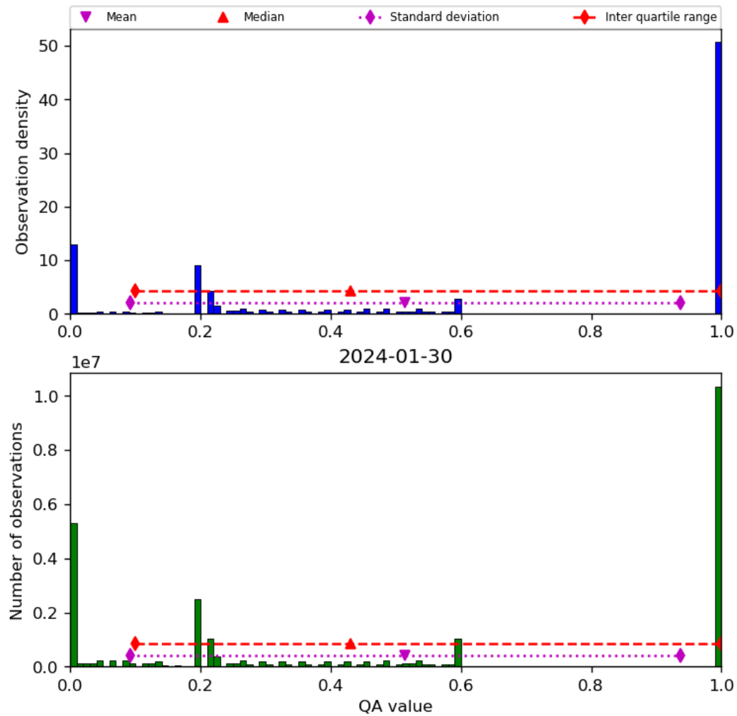
Figure 52: Histogram of “QA value” for 2024-01-29 to 2024-01-31
