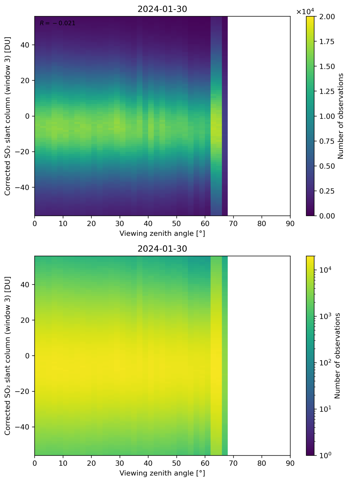
Figure 319: Scatter density plot of “Viewing zenith angle” against “Corrected SO 2 slant column (window 3)” for 2024-01-29 to 2024-01-31.
