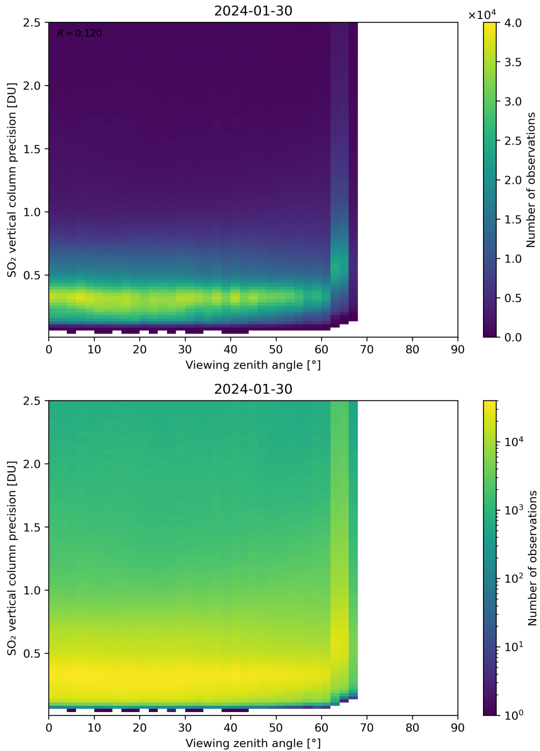
Figure 328: Scatter density plot of “Viewing zenith angle” against “SO 2 vertical column precision” for 2024-01-29 to 2024-01-31.
