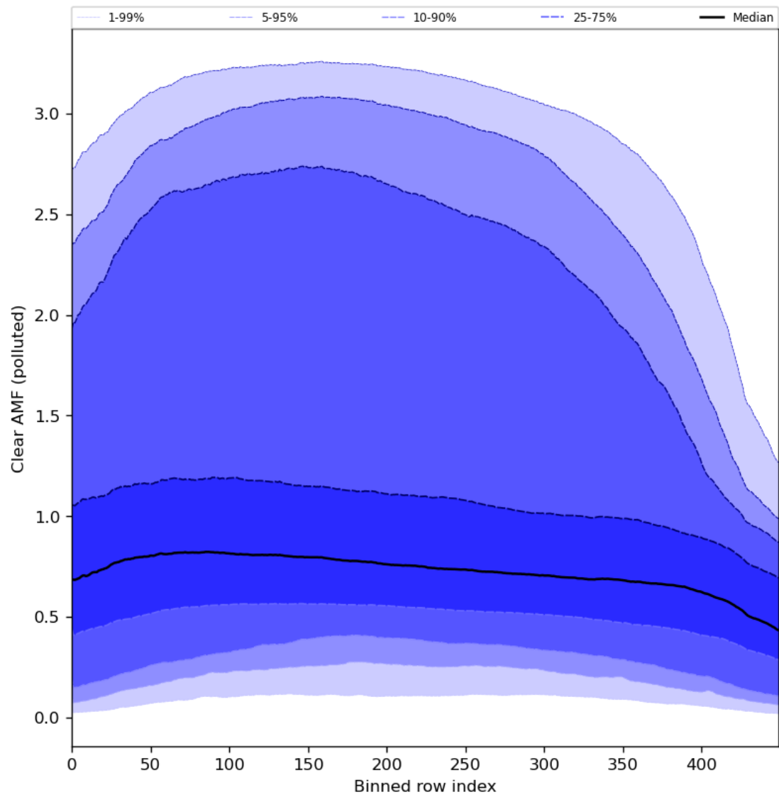
Figure 96: Along track statistics of “Clear AMF (polluted)” for 2024-01-29 to 2024-01-31
