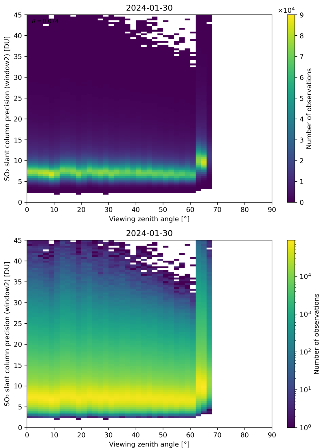
Figure 322: Scatter density plot of “Viewing zenith angle” against “SO 2 slant column precision (window2)” for 2024-01-29 to 2024-01-31.
