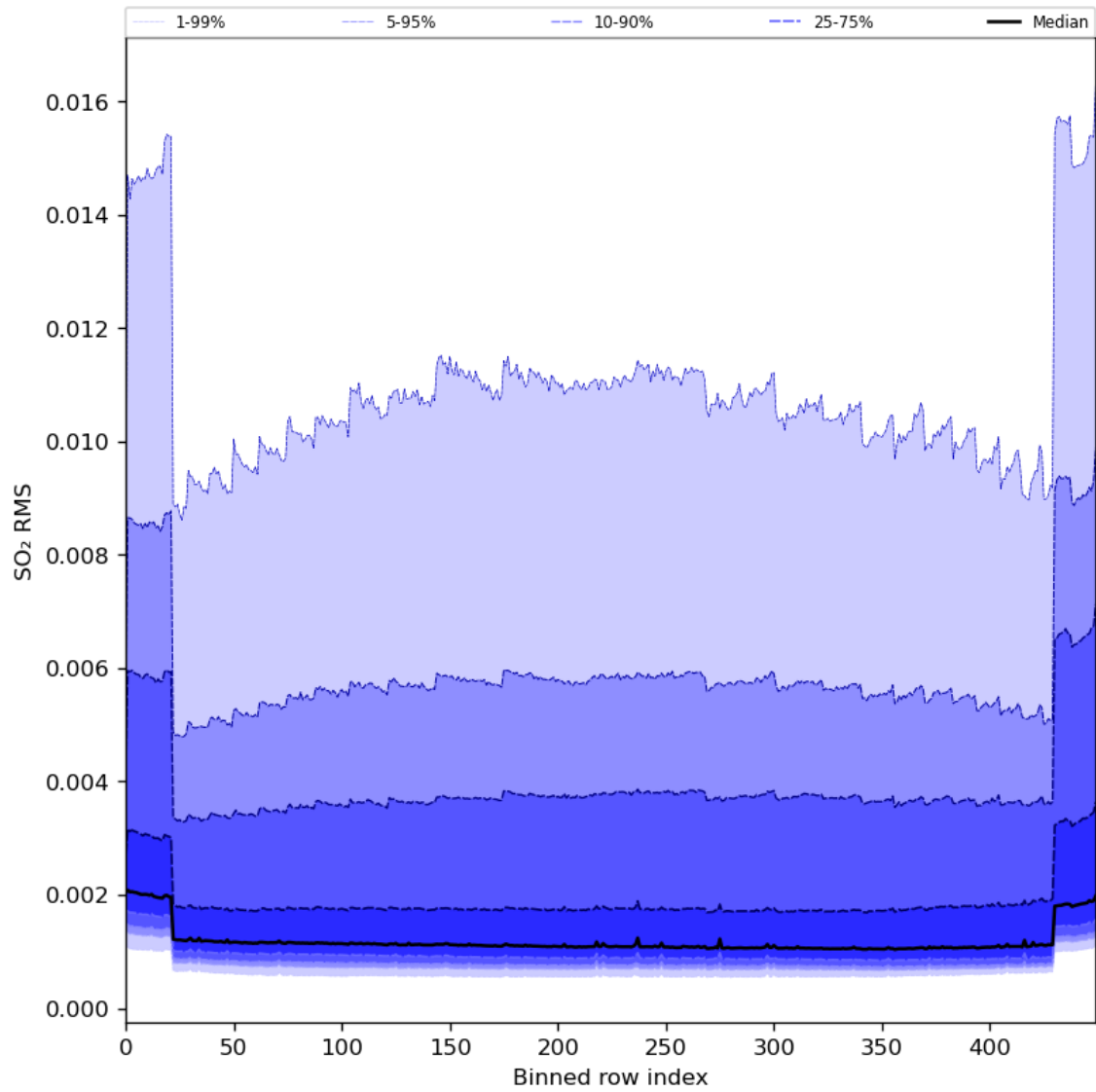
Figure 93: Along track statistics of “SO 2 RMS” for 2024-01-29 to 2024-01-31
