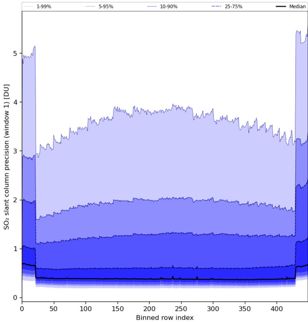
Figure 80: Along track statistics of “SO 2 slant column precision (window 1)” for 2024-01-29 to 2024-01-31
