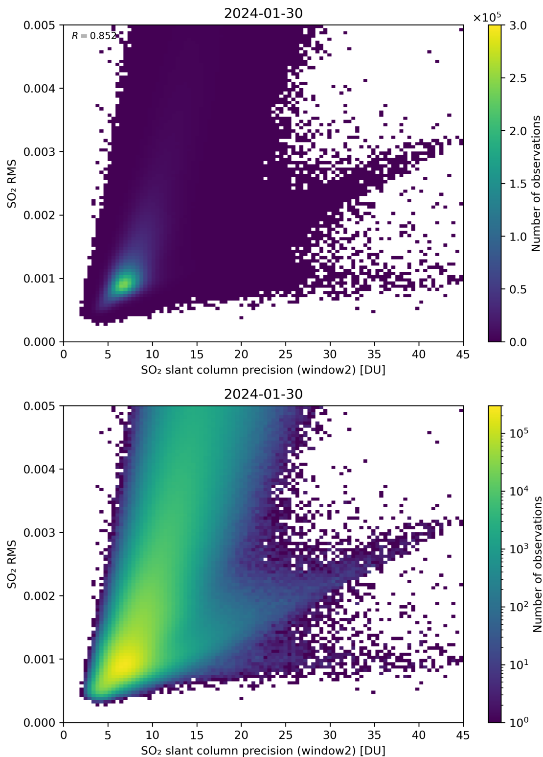
Figure 245: Scatter density plot of “SO 2 slant column precision (window2)” against “SO 2 RMS” for 2024-01-29 to 2024-01-31.
