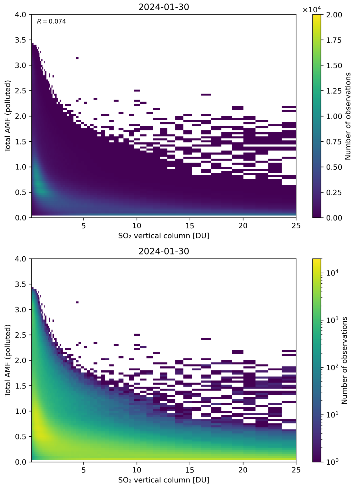
Figure 305: Scatter density plot of “SO 2 vertical column” against “Total AMF (polluted)” for 2024-01-29 to 2024-01-31.
