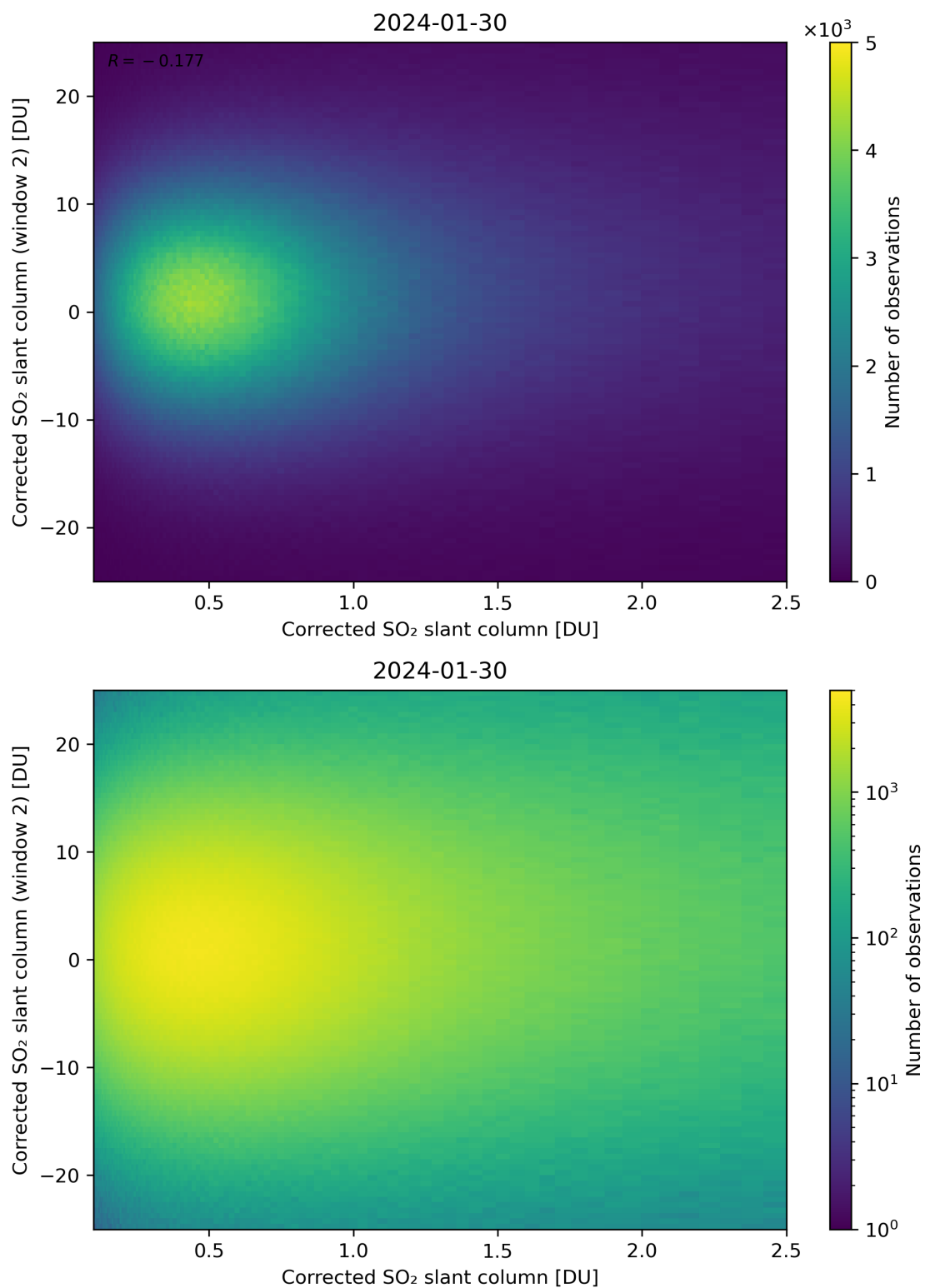
Figure 185: Scatter density plot of “Corrected SO 2 slant column” against “Corrected SO 2 slant column (window 2)” for 2024-01-29 to 2024-01-31.
