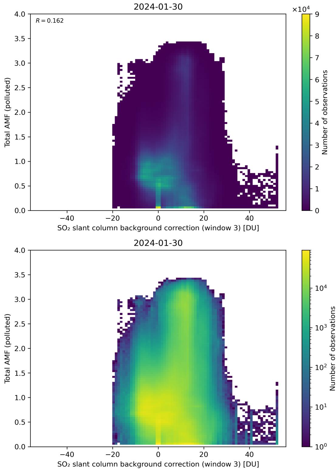
Figure 125: Scatter density plot of “SO 2 slant column background correction (window 3)” against “Total AMF (polluted)” for 2024-01-29 to 2024-01-31.
