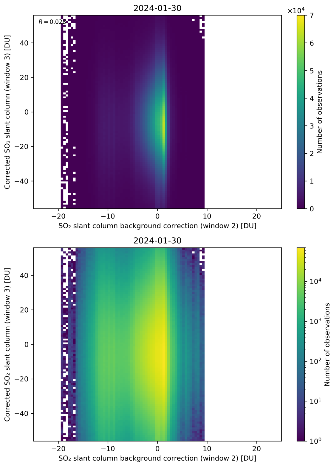
Figure 116: Scatter density plot of “SO 2 slant column background correction (window 2)” against “Corrected SO 2 slant column (window 3)” for 2024-01-29 to 2024-01-31.
