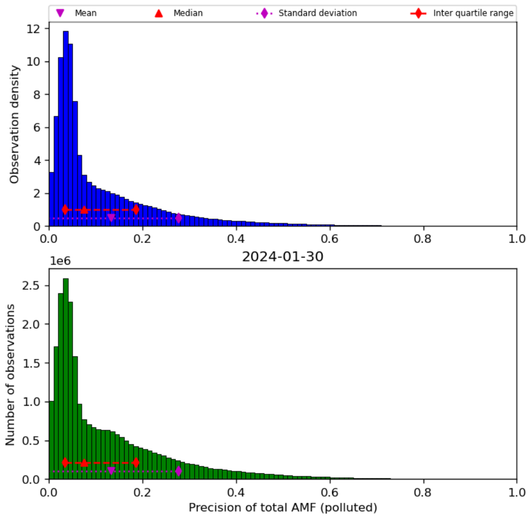
Figure 72: Histogram of “Precision of total AMF (polluted)” for 2024-01-29 to 2024-01-31
