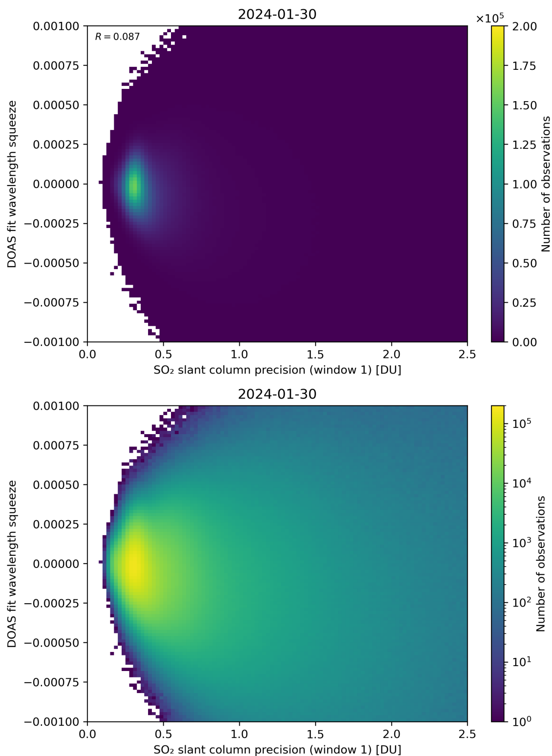
Figure 222: Scatter density plot of “SO 2 slant column precision (window 1)” against “DOAS fit wavelength squeeze” for 2024-01-29 to 2024-01-31.
