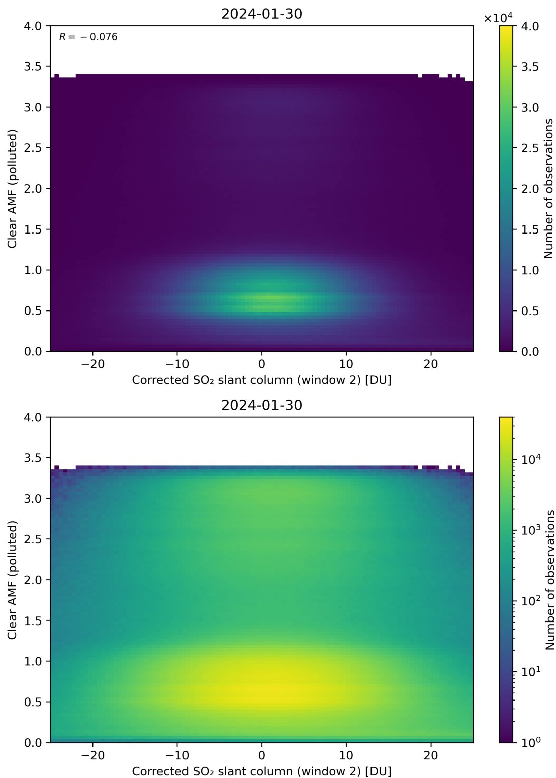
Figure 199: Scatter density plot of “Corrected SO 2 slant column (window 2)” against “Clear AMF (polluted)” for 2024-01-29 to 2024-01-31.
