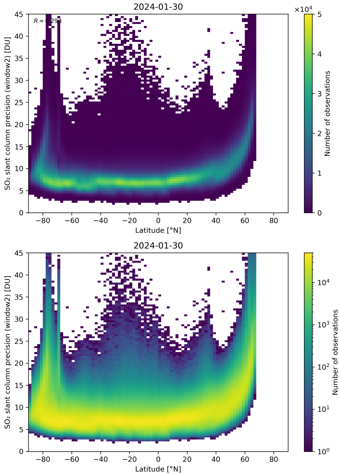
Figure 151: Scatter density plot of “Latitude” against “SO 2 slant column precision (window2)” for 2024-01-29 to 2024-01-31.
