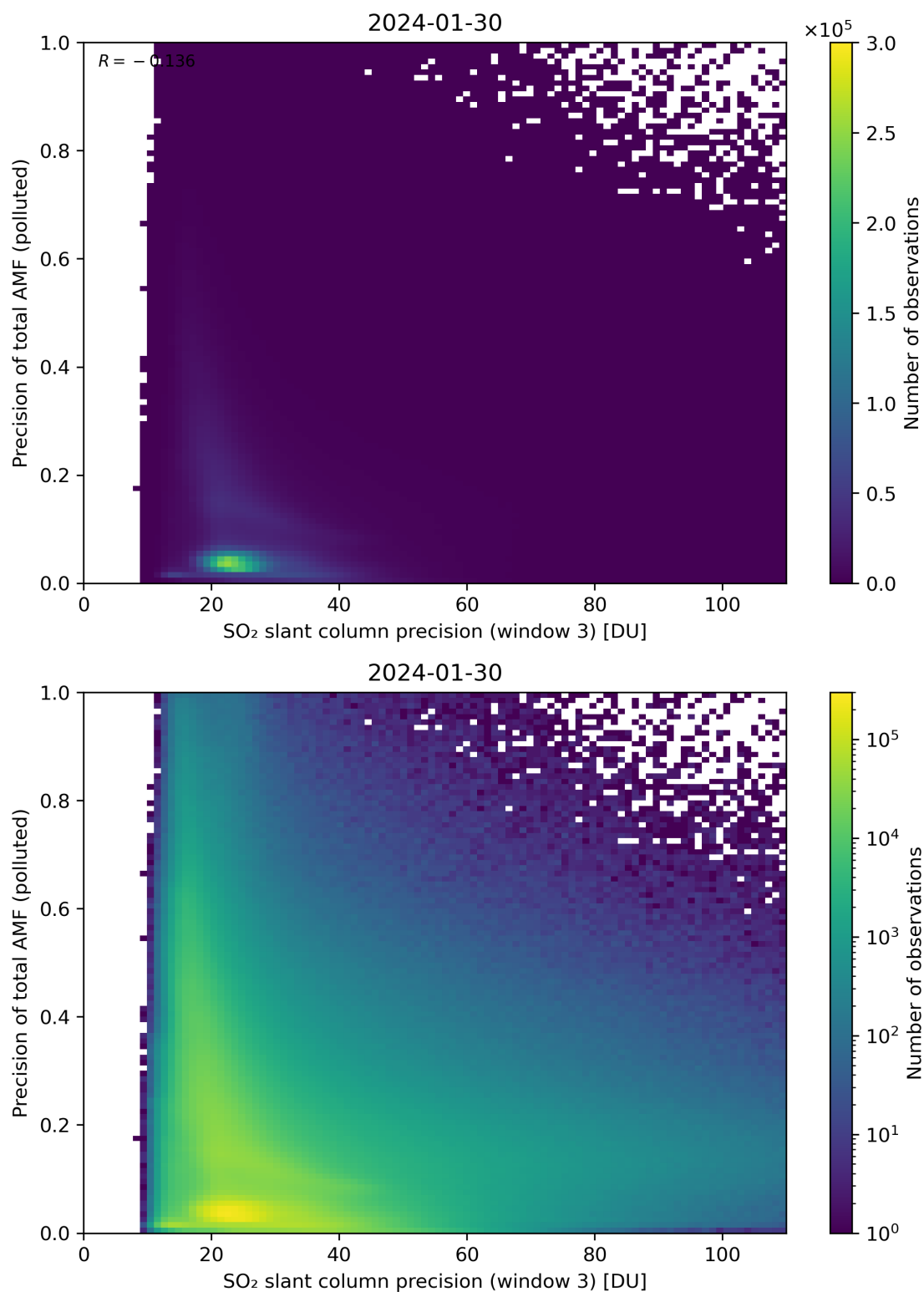
Figure 264: Scatter density plot of “SO 2 slant column precision (window 3)” against “Precision of total AMF (polluted)” for 2024-01-29 to 2024-01-31.
