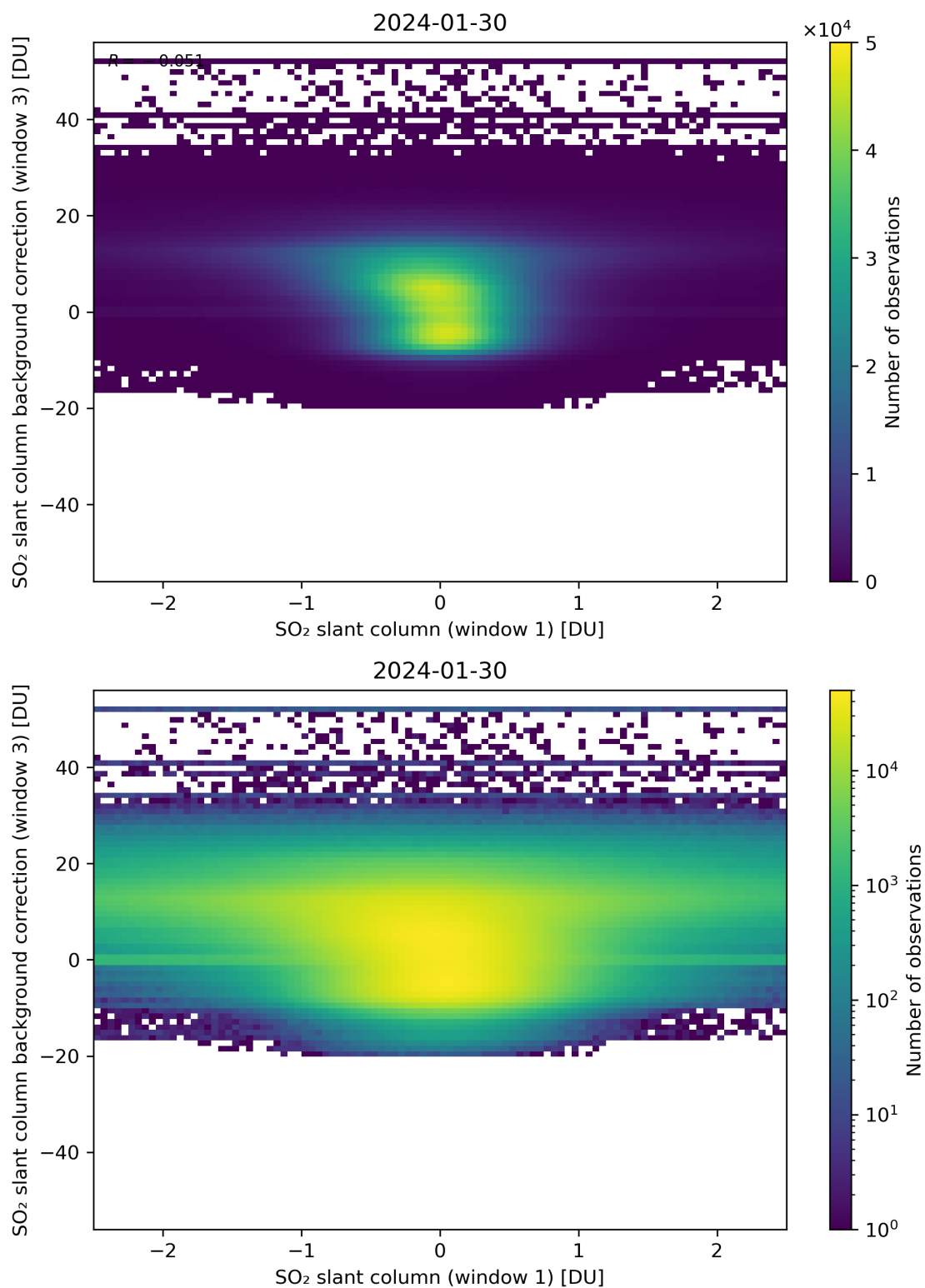
Figure 214: Scatter density plot of "SO 2 slant column (window 1)" against "SO 2 slant column background correction (window 3)" for 2024-01-29 to 2024-01-31.
