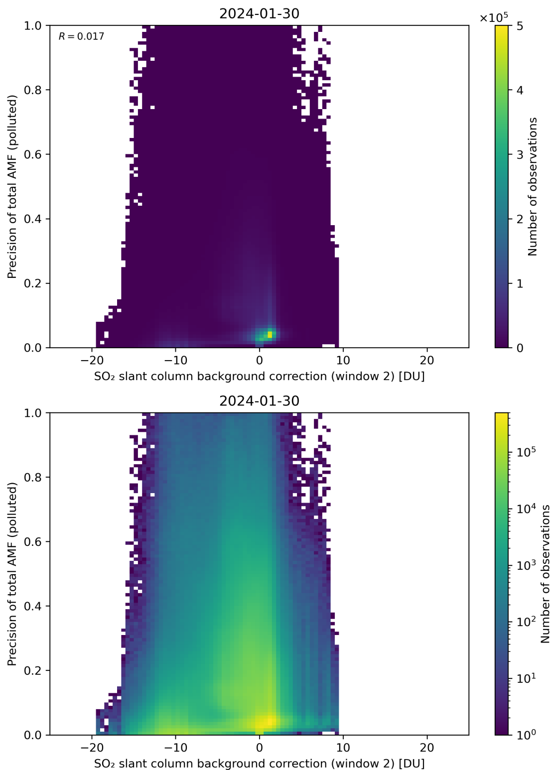
Figure 120: Scatter density plot of “SO 2 slant column background correction (window 2)” against “Precision of total AMF (polluted)” for 2024-01-29 to 2024-01-31.
