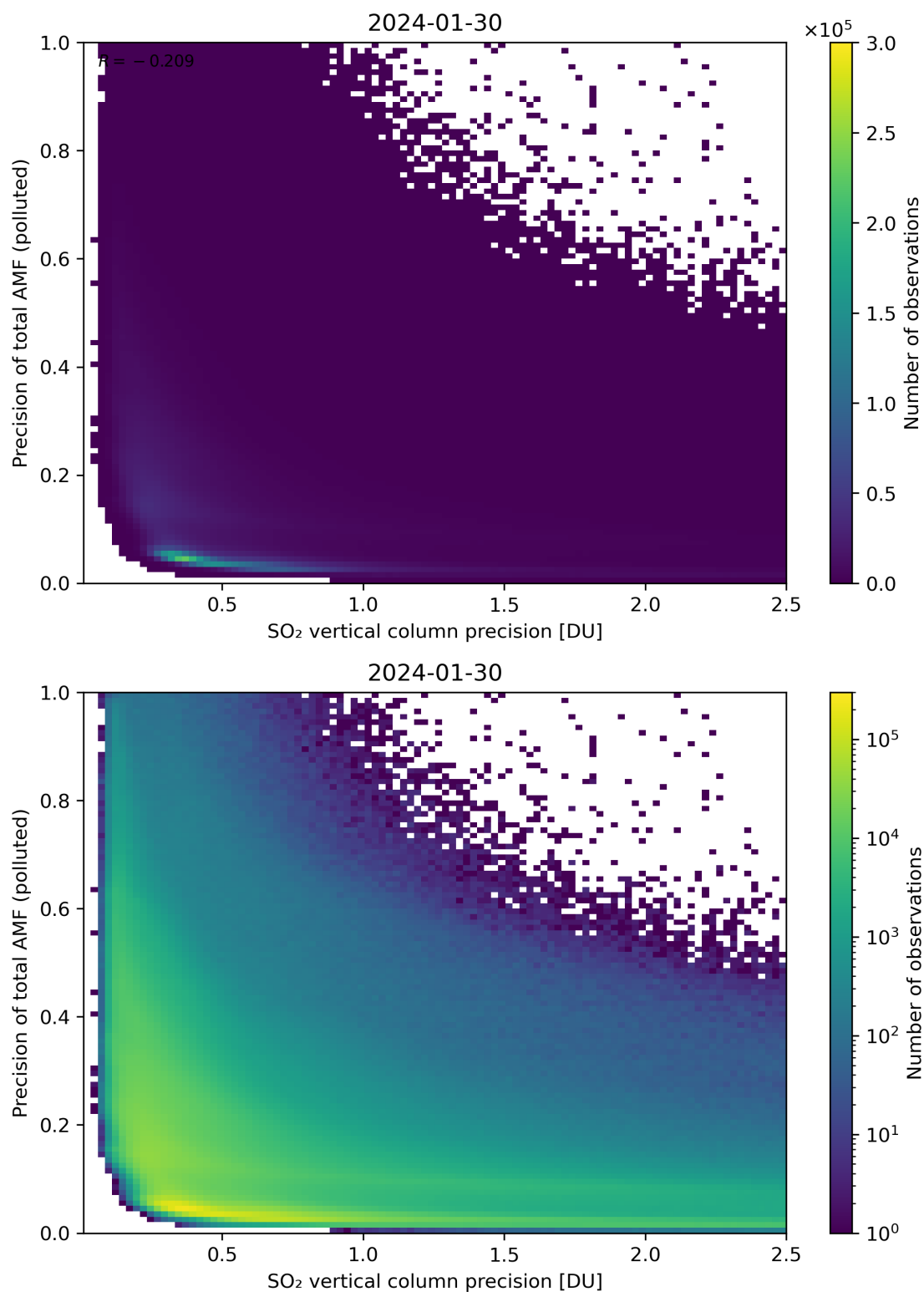
Figure 295: Scatter density plot of “SO 2 vertical column precision” against “Precision of total AMF (polluted)” for 2024-01-29 to 2024-01-31.
