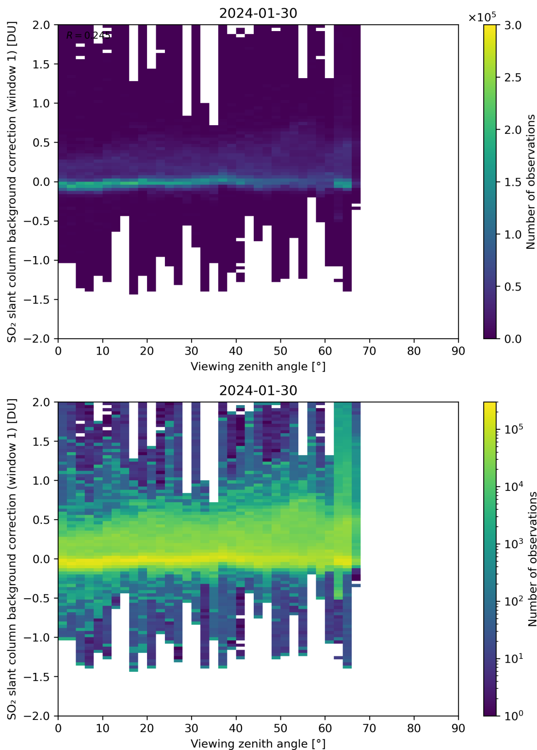
Figure 308: Scatter density plot of “Viewing zenith angle” against “SO 2 slant column background correction (window 1)” for 2024-01-29 to 2024-01-31.
