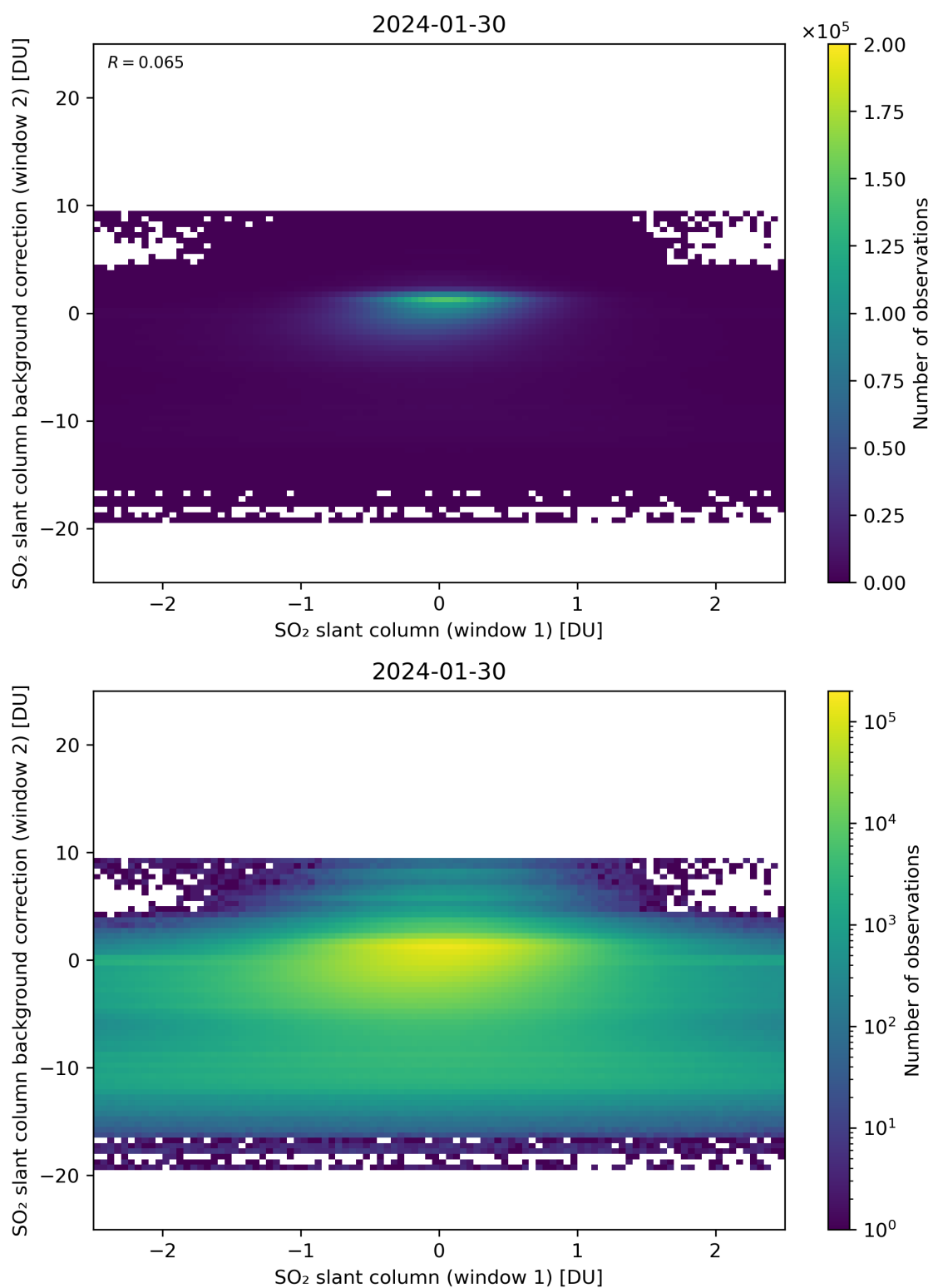
Figure 213: Scatter density plot of “SO 2 slant column (window 1)” against “SO 2 slant column background correction (window 2)” for 2024-01-29 to 2024-01-31.
