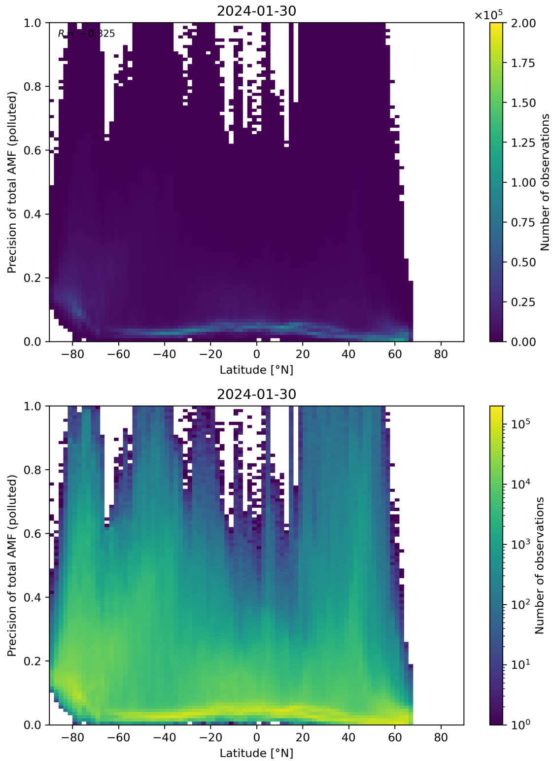
Figure 155: Scatter density plot of “Latitude” against “Precision of total AMF (polluted)” for 2024-01-29 to 2024-01-31.
