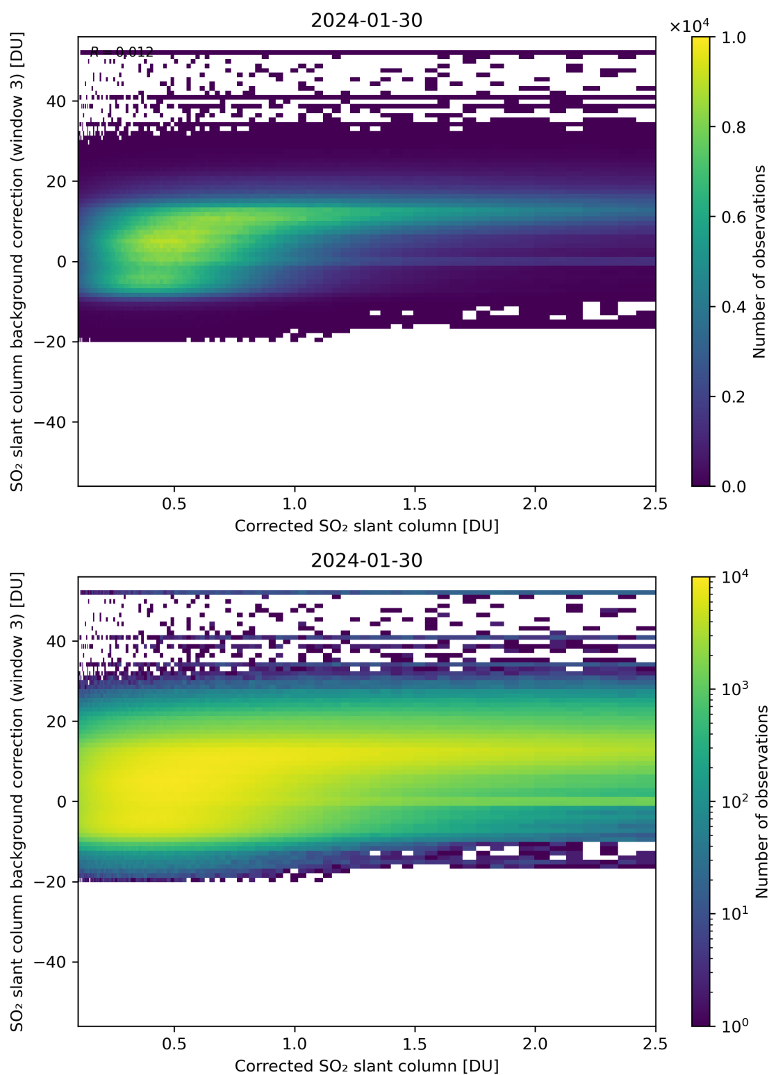
Figure 180: Scatter density plot of “Corrected SO 2 slant column” against “SO 2 slant column background correction (window 3)” for 2024-01-29 to 2024-01-31.
