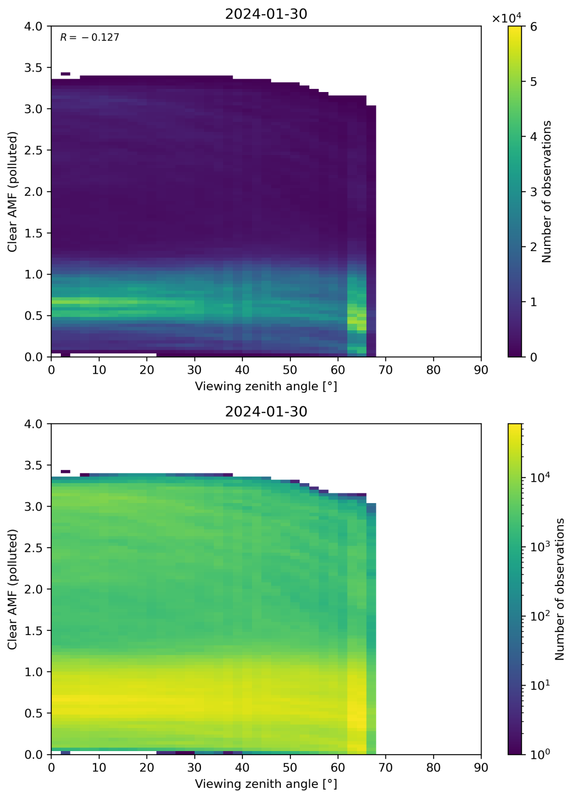
Figure 316: Scatter density plot of “Viewing zenith angle” against “Clear AMF (polluted)” for 2024-01-29 to 2024-01-31.
