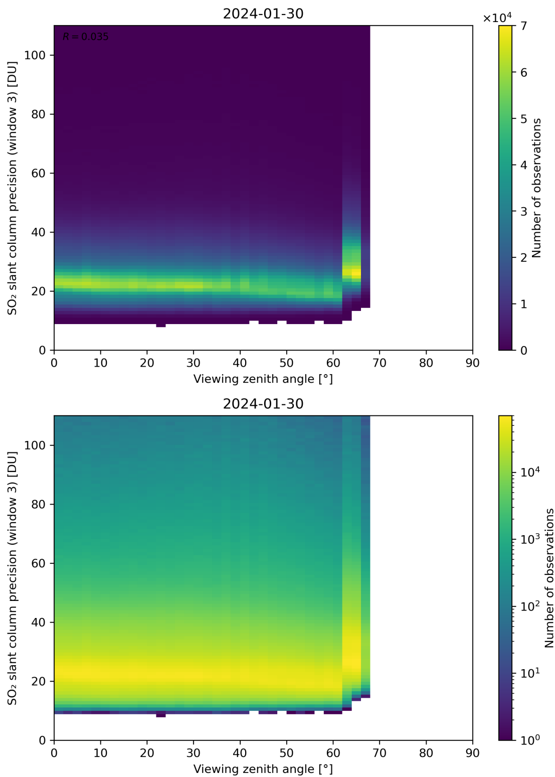
Figure 324: Scatter density plot of “Viewing zenith angle” against “SO 2 slant column precision (window 3)” for 2024-01-29 to 2024-01-31.
