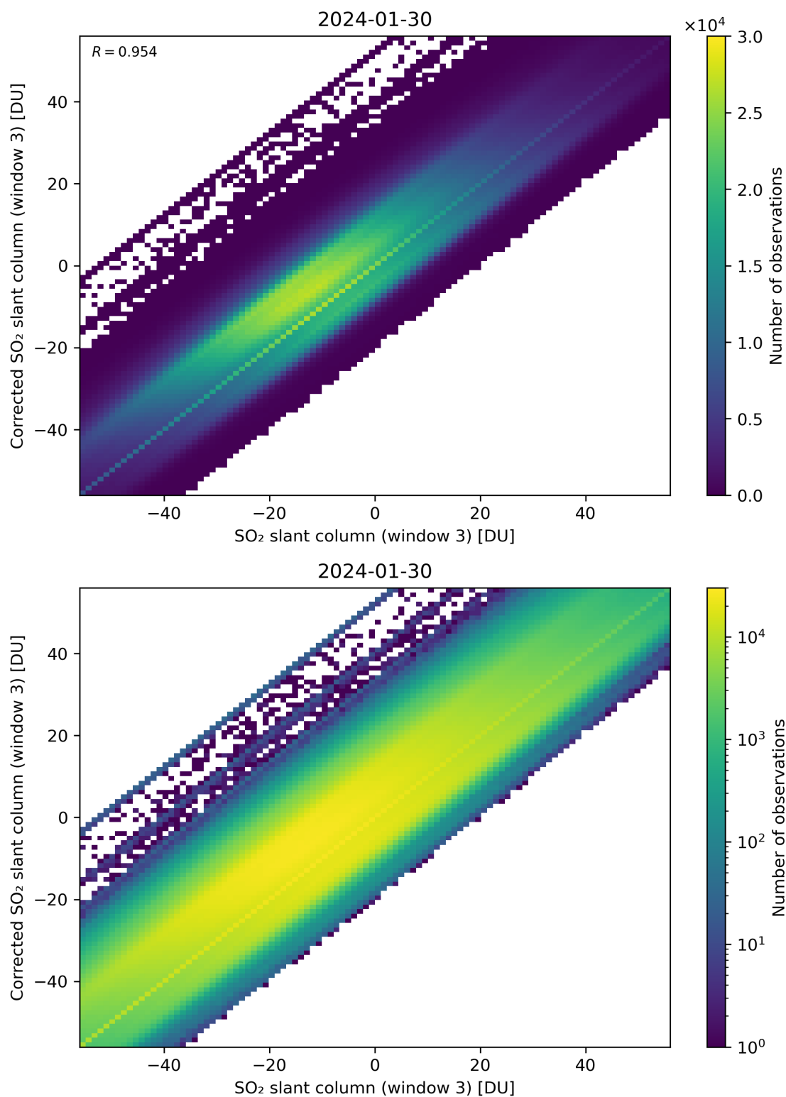
Figure 266: Scatter density plot of “SO 2 slant column (window 3)” against “Corrected SO 2 slant column (window 3)” for 2024-01-29 to 2024-01-31.
