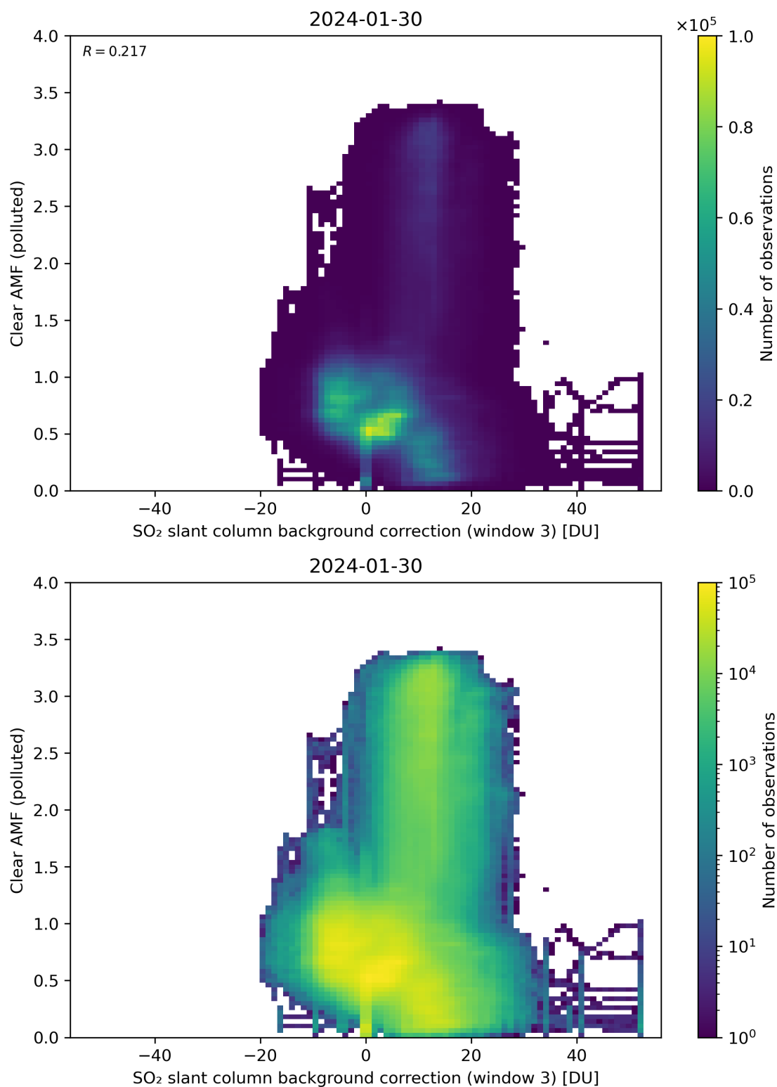
Figure 124: Scatter density plot of “SO 2 slant column background correction (window 3)” against “Clear AMF (polluted)” for 2024-01-29 to 2024-01-31.
