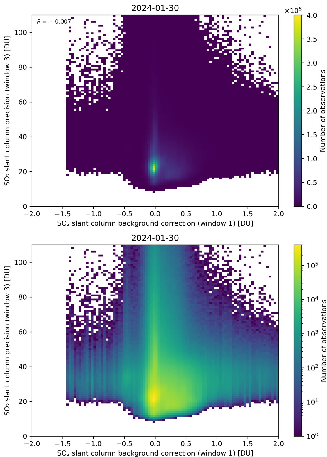
Figure 108: Scatter density plot of “SO 2 slant column background correction (window 1)” against “SO 2 slant column precision (window 3)” for 2024-01-29 to 2024-01-31.
