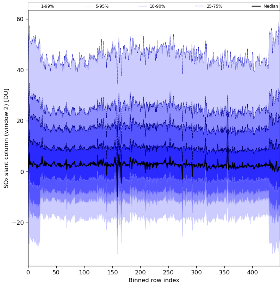
Figure 83: Along track statistics of “SO 2 slant column (window 2)” for 2024-01-29 to 2024-01-31
