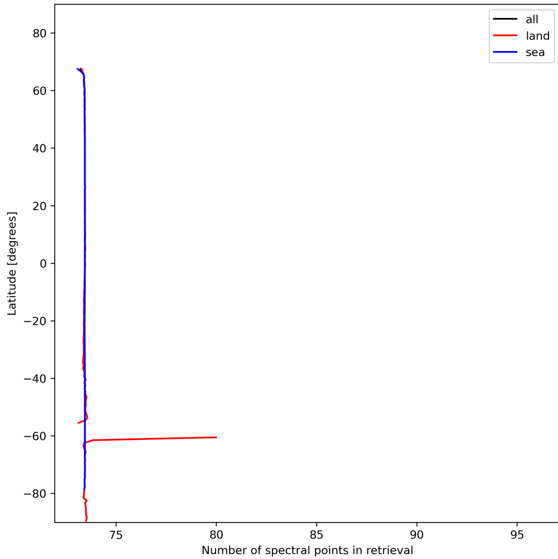
Figure 51: Zonal average of “Number of spectral points in retrieval” for 2024-01-29 to 2024-01-31.
