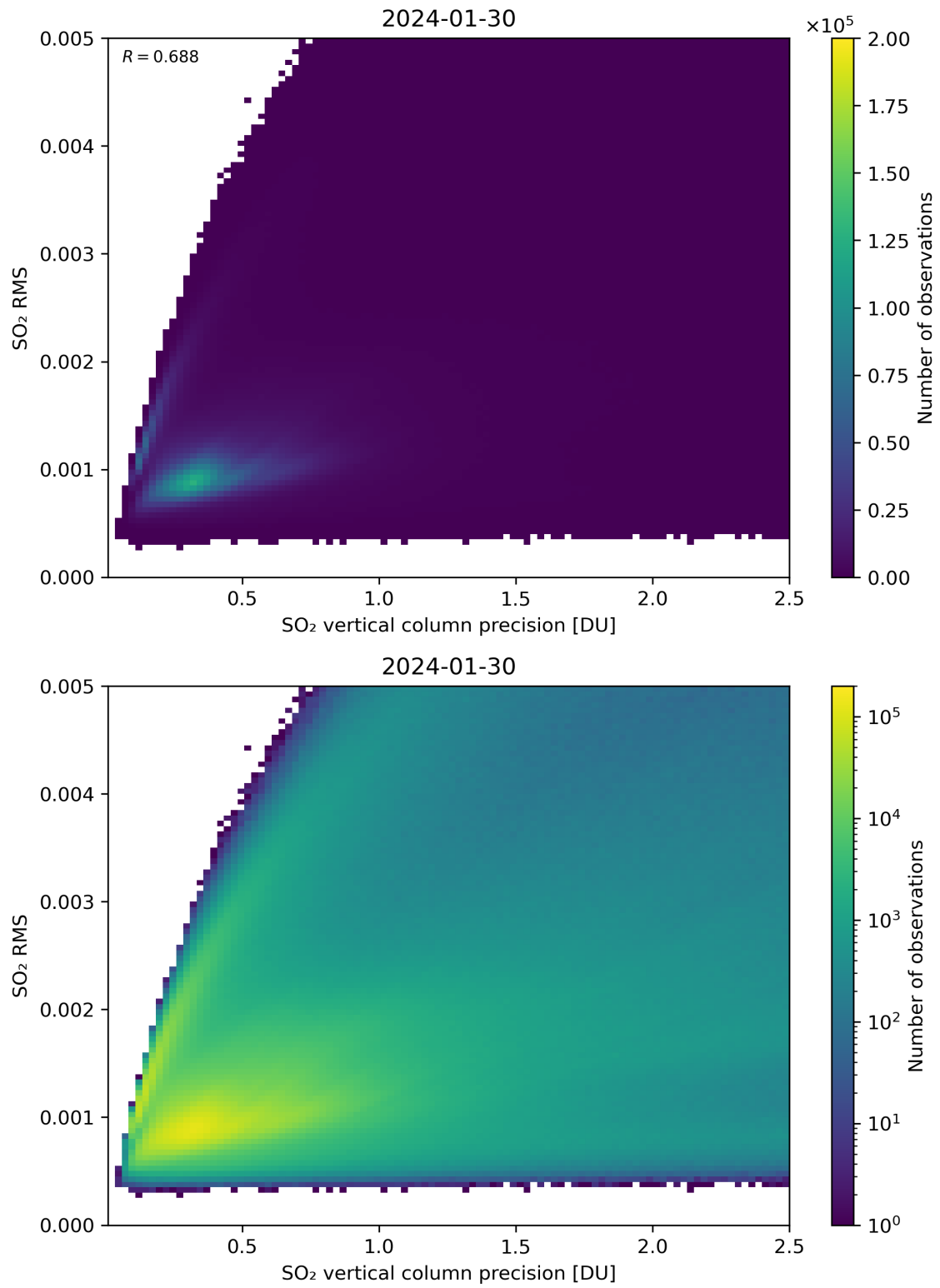
Figure 284: Scatter density plot of “SO 2 vertical column precision” against “SO 2 RMS” for 2024-01-29 to 2024-01-31.
