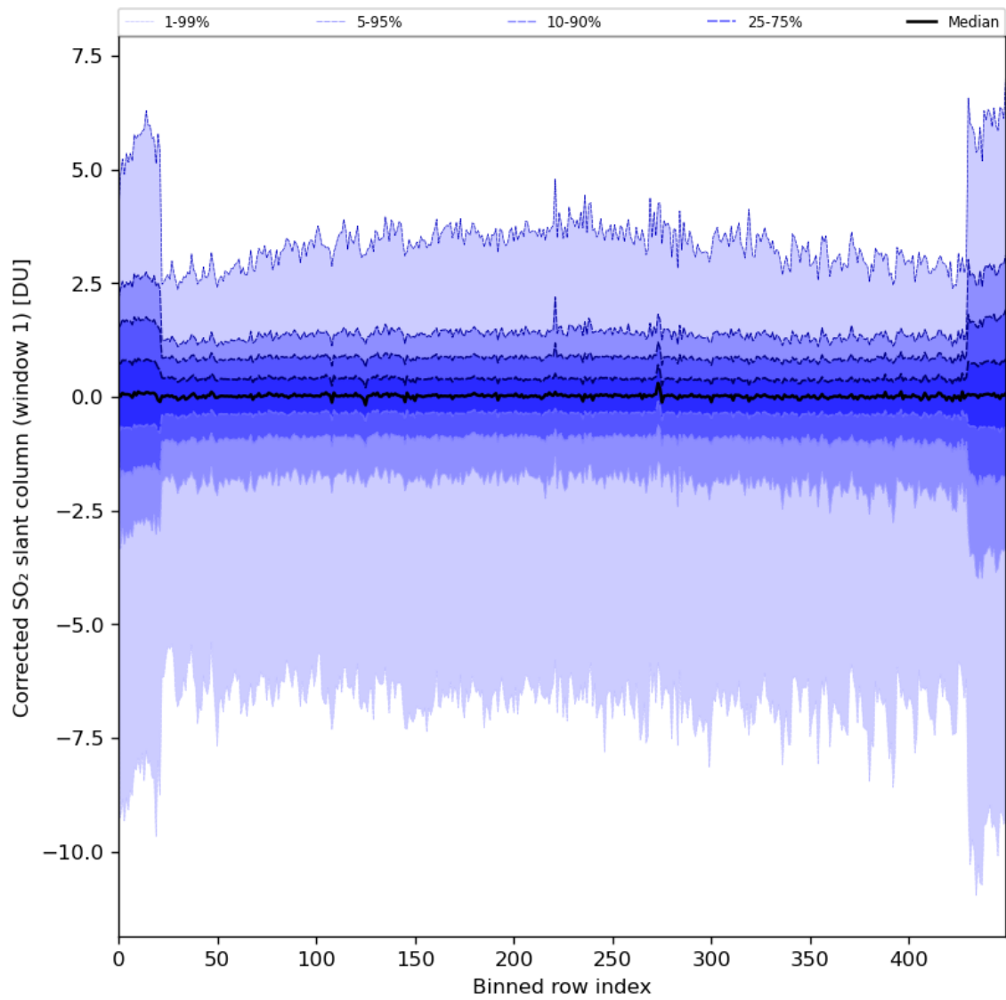
Figure 81: Along track statistics of “Corrected SO 2 slant column (window 1)” for 2024-01-29 to 2024-01-31
