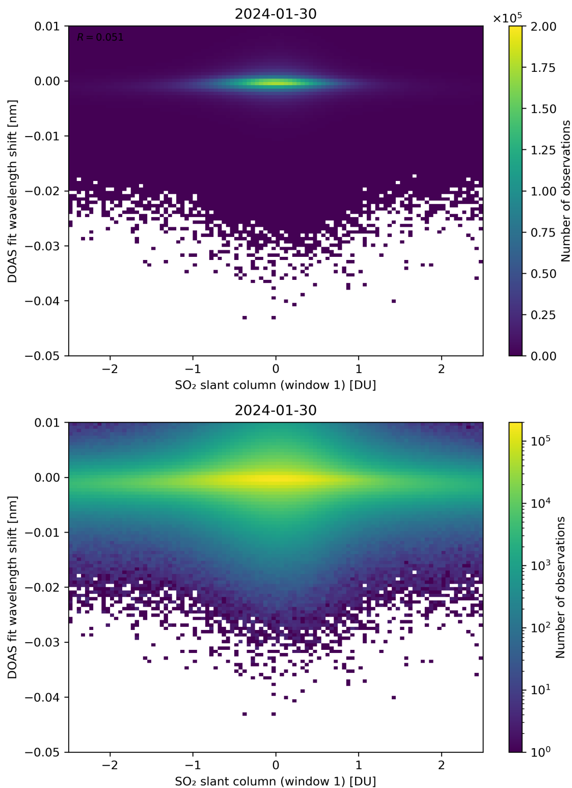
Figure 215: Scatter density plot of “SO 2 slant column (window 1)” against “DOAS fit wavelength shift” for 2024-01-29 to 2024-01-31.
