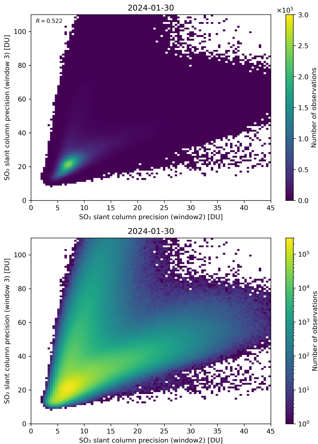
Figure 250: Scatter density plot of “SO 2 slant column precision (window2)” against “SO 2 slant column precision (window 3)” for 2024-01-29 to 2024-01-31.
