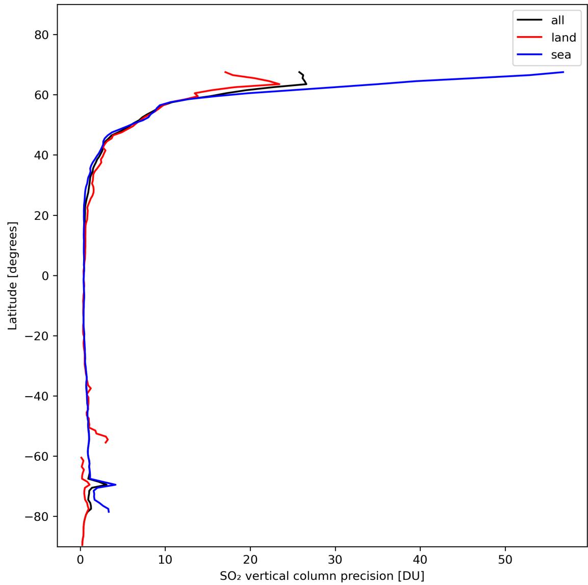
Figure 31: Zonal average of “SO 2 vertical column precision” for 2024-01-29 to 2024-01-31.
