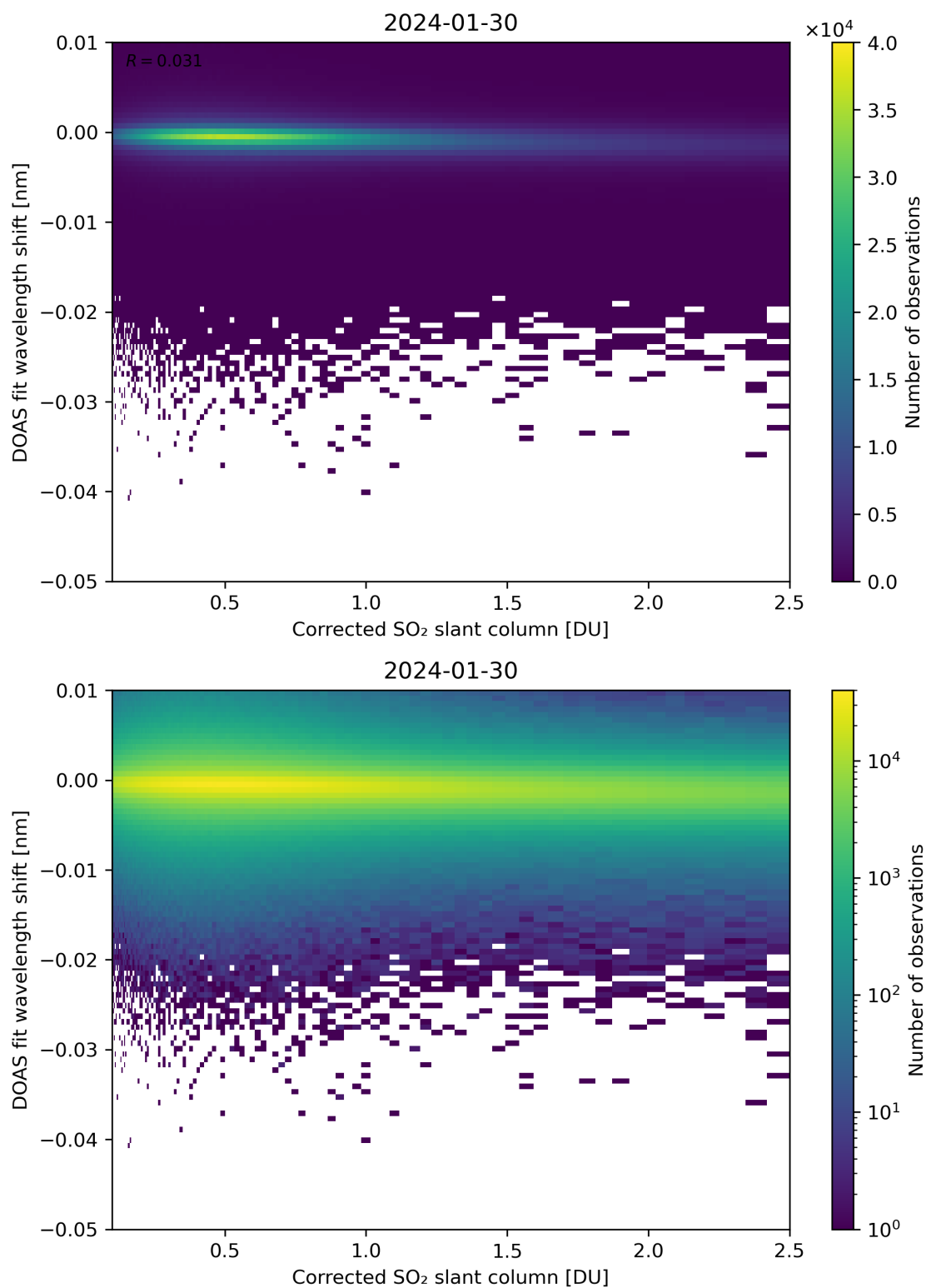
Figure 181: Scatter density plot of “Corrected SO 2 slant column” against “DOAS fit wavelength shift” for 2024-01-29 to 2024-01-31.
