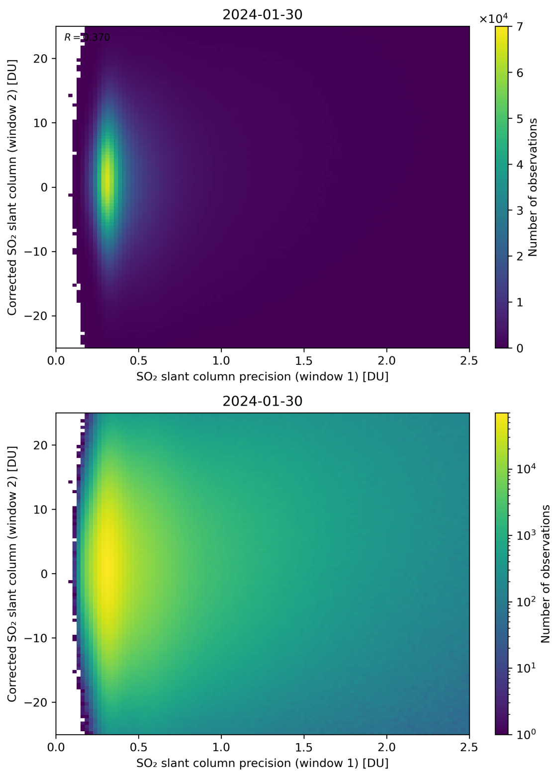
Figure 225: Scatter density plot of “SO 2 slant column precision (window 1)” against “Corrected SO 2 slant column (window 2)” for 2024-01-29 to 2024-01-31.
