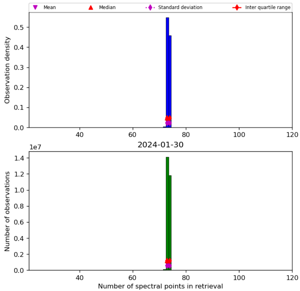
Figure 74: Histogram of “Number of spectral points in retrieval” for 2024-01-29 to 2024-01-31
