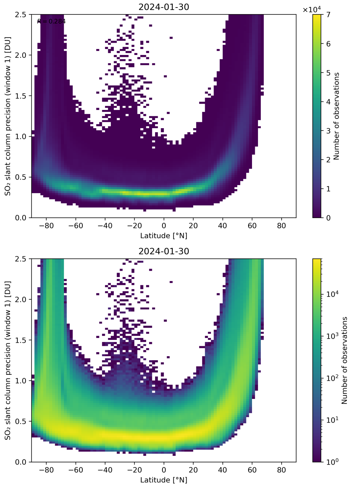
Figure 150: Scatter density plot of “Latitude” against “SO 2 slant column precision (window 1)” for 2024-01-29 to 2024-01-31.
