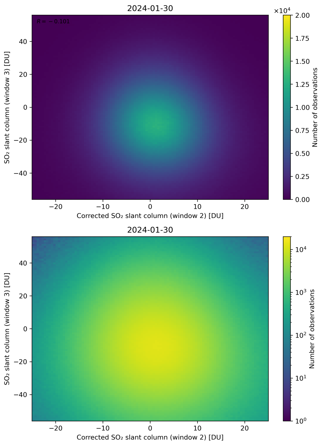
Figure 201: Scatter density plot of “Corrected SO 2 slant column (window 2)” against “SO 2 slant column (window 3)” for 2024-01-29 to 2024-01-31.
