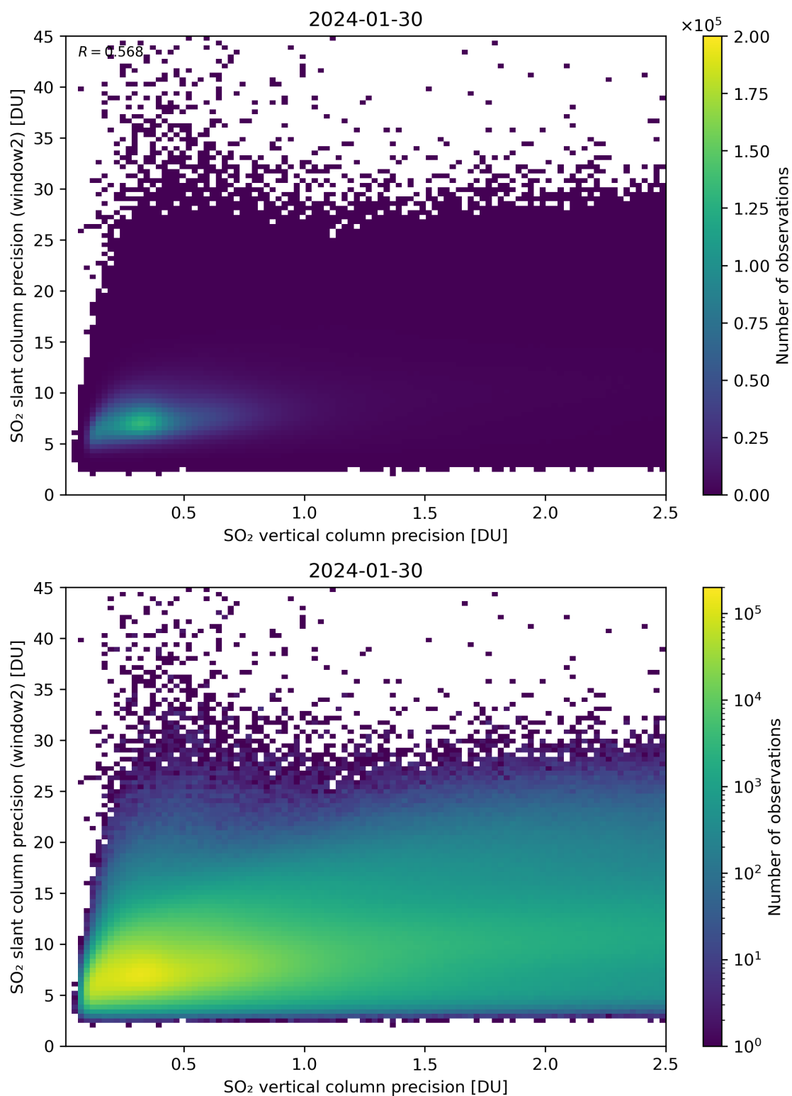
Figure 291: Scatter density plot of “SO 2 vertical column precision” against “SO 2 slant column precision (window2)” for 2024-01-29 to 2024-01-31.
