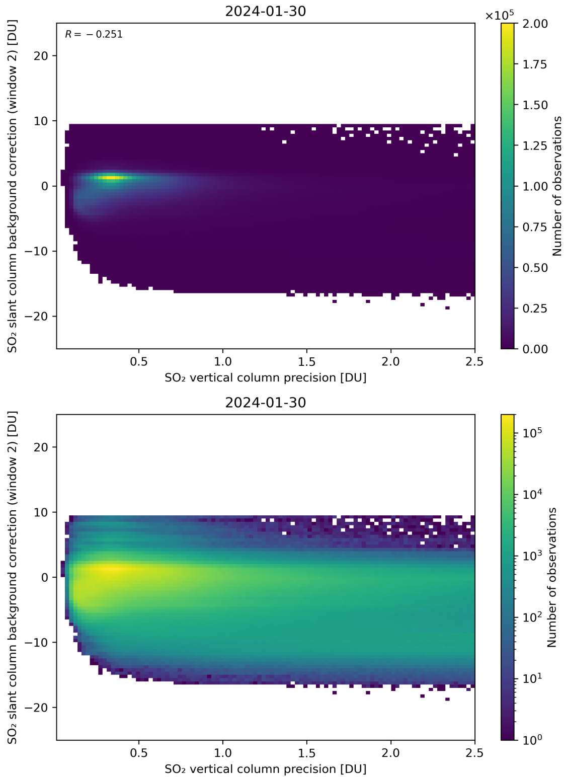
Figure 280: Scatter density plot of “SO 2 vertical column precision” against “SO 2 slant column background correction (window 2)” for 2024-01-29 to 2024-01-31.
