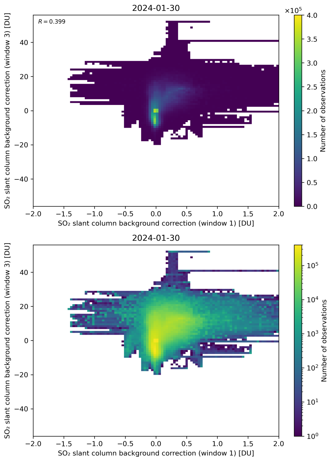
Figure 99: Scatter density plot of “SO 2 slant column background correction (window 1)” against “SO 2 slant column background correction (window 3)” for 2024-01-29 to 2024-01-31.
