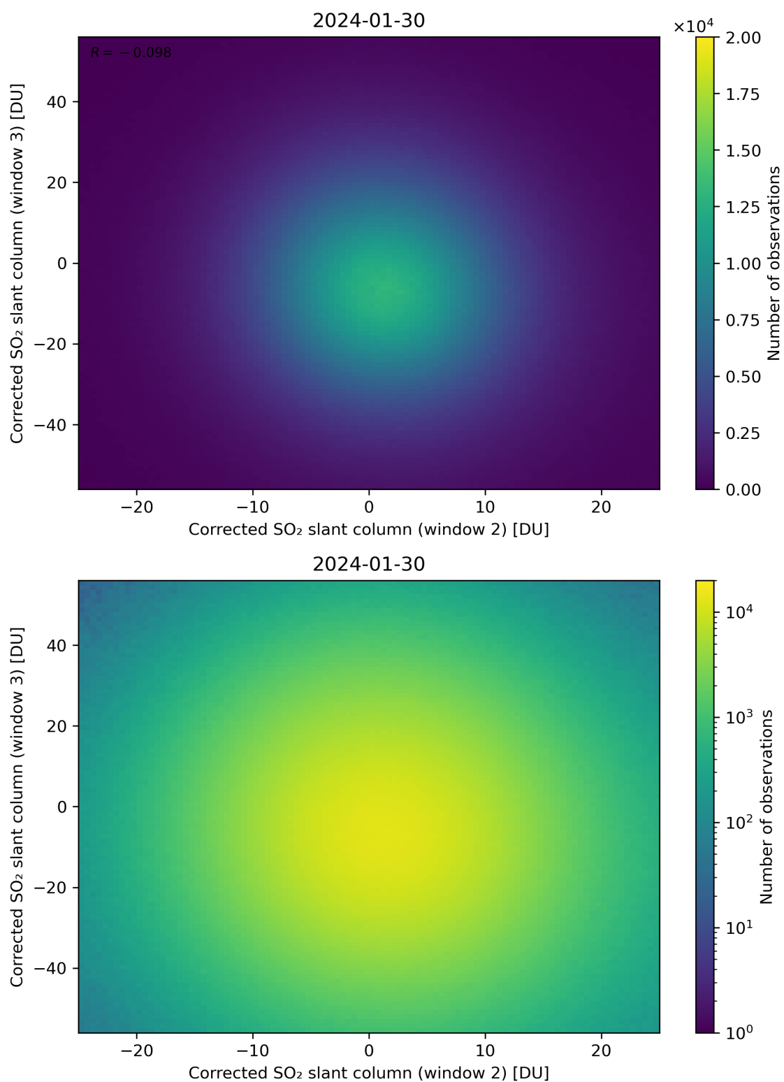
Figure 200: Scatter density plot of “Corrected SO 2 slant column (window 2)” against “Corrected SO 2 slant column (window 3)” for 2024-01-29 to 2024-01-31.
