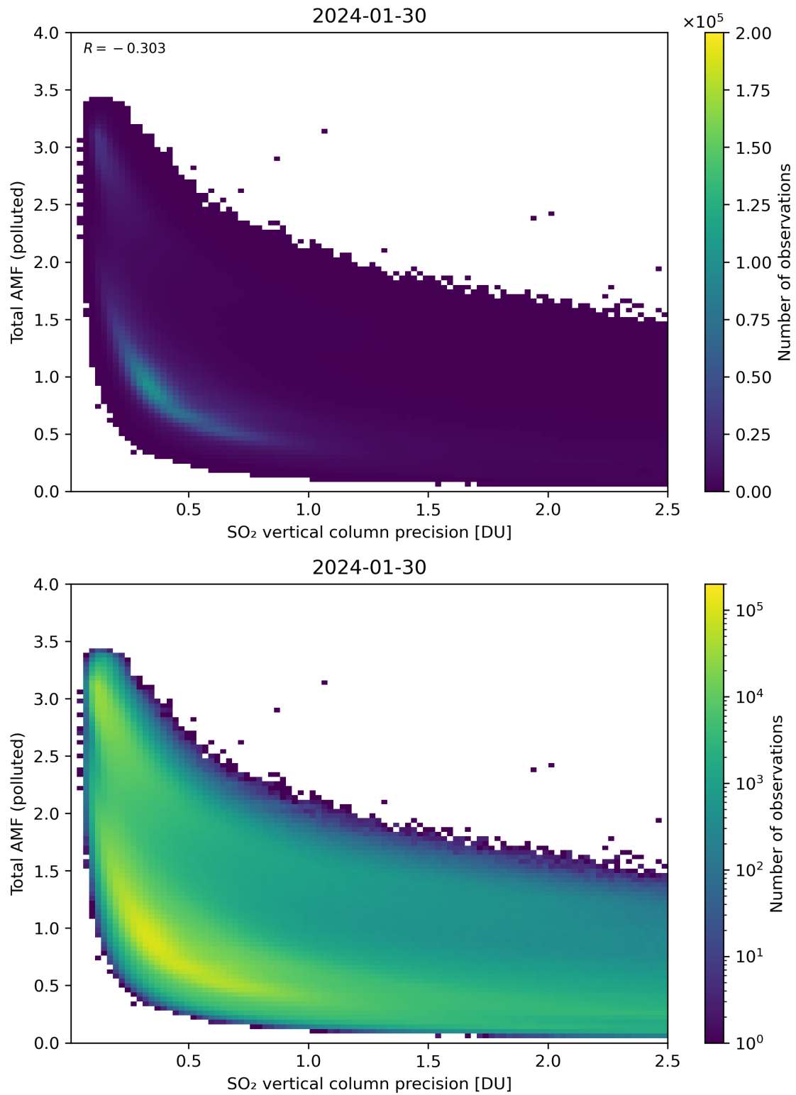
Figure 294: Scatter density plot of “SO 2 vertical column precision” against “Total AMF (polluted)” for 2024-01-29 to 2024-01-31.
