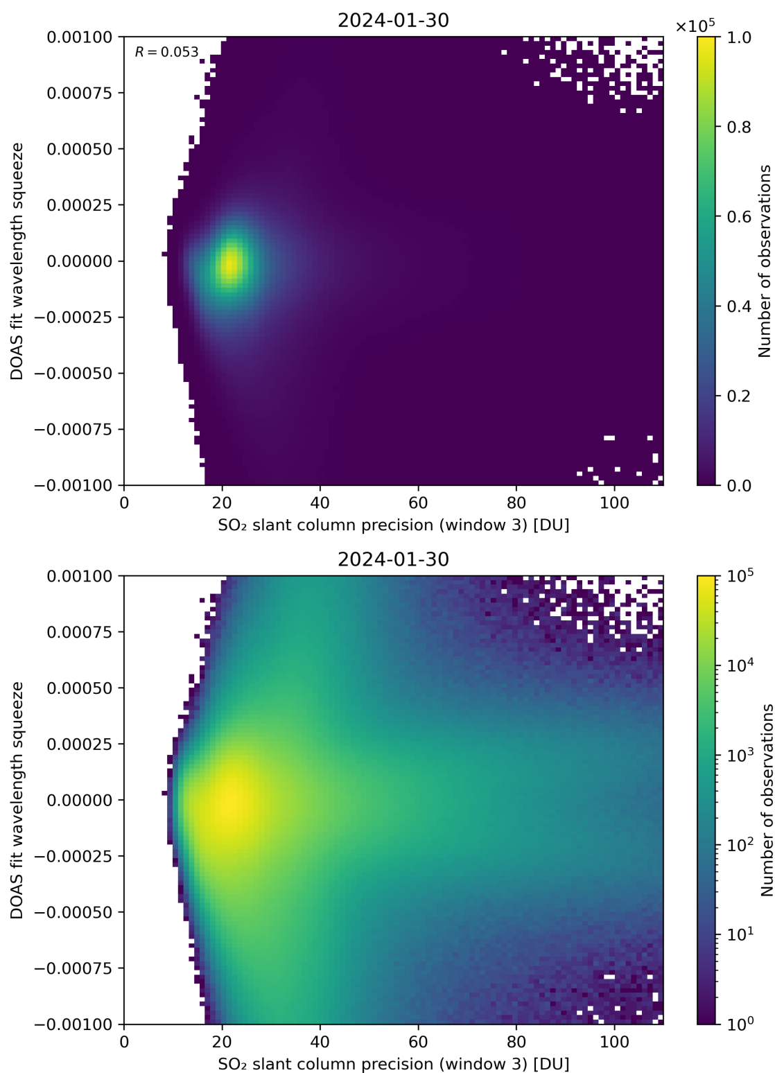
Figure 259: Scatter density plot of “SO 2 slant column precision (window 3)” against “DOAS fit wavelength squeeze” for 2024-01-29 to 2024-01-31.
