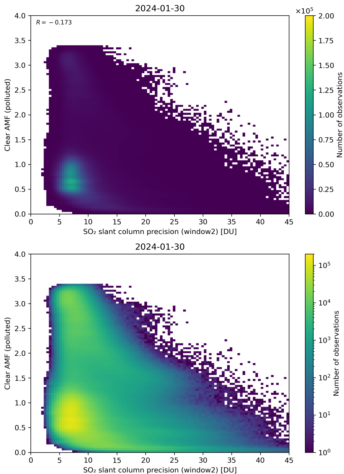
Figure 246: Scatter density plot of “SO 2 slant column precision (window2)” against “Clear AMF (polluted)” for 2024-01-29 to 2024-01-31.
