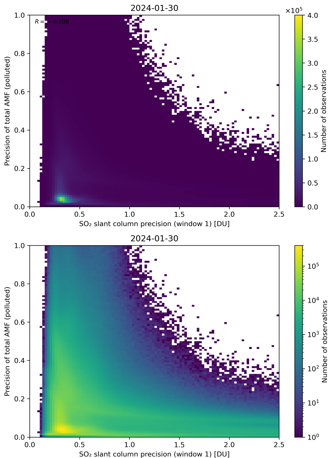
Figure 231: Scatter density plot of “SO 2 slant column precision (window 1)” against “Precision of total AMF (polluted)” for 2024-01-29 to 2024-01-31.
