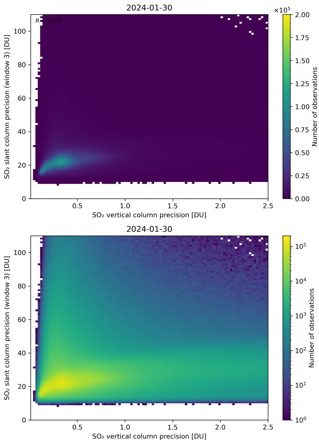
Figure 293: Scatter density plot of “SO 2 vertical column precision” against “SO 2 slant column precision (window 3)” for 2024-01-29 to 2024-01-31.
