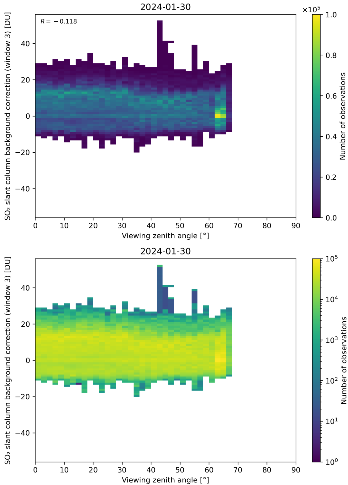
Figure 310: Scatter density plot of “Viewing zenith angle” against “SO 2 slant column background correction (window 3)” for 2024-01-29 to 2024-01-31.
