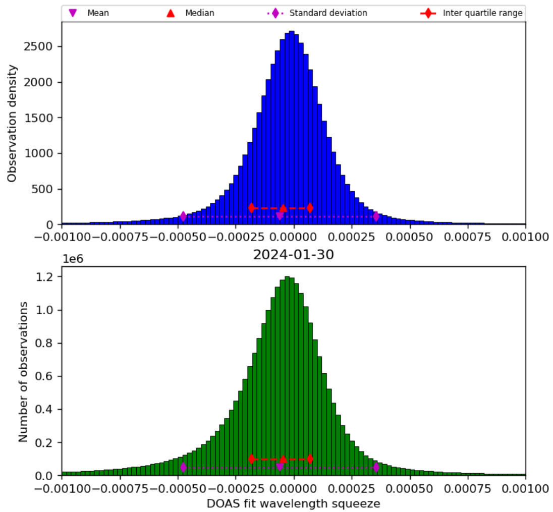
Figure 69: Histogram of “DOAS fit wavelength squeeze” for 2024-01-29 to 2024-01-31
