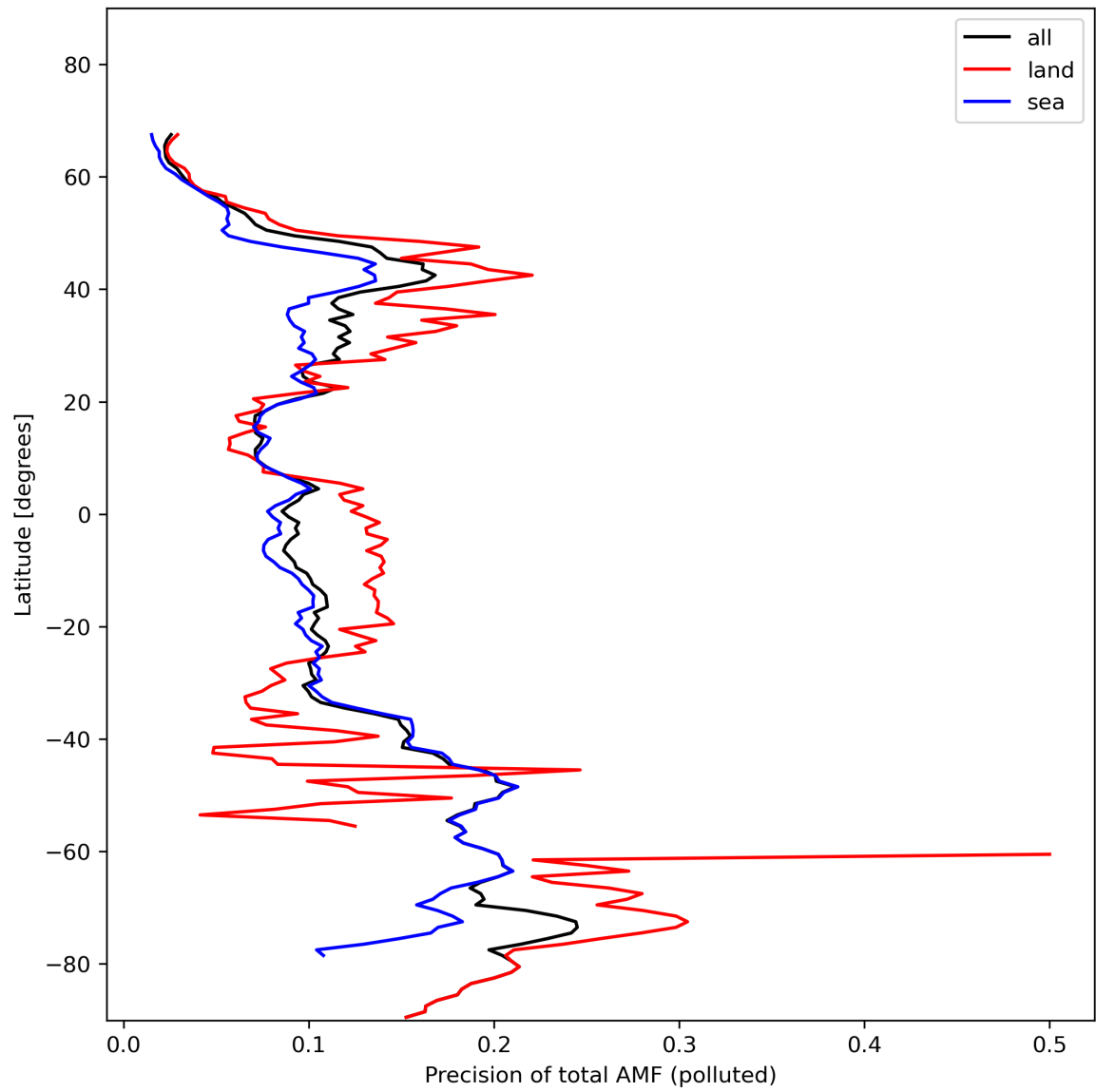
Figure 49: Zonal average of “Precision of total AMF (polluted)” for 2024-01-29 to 2024-01-31.
