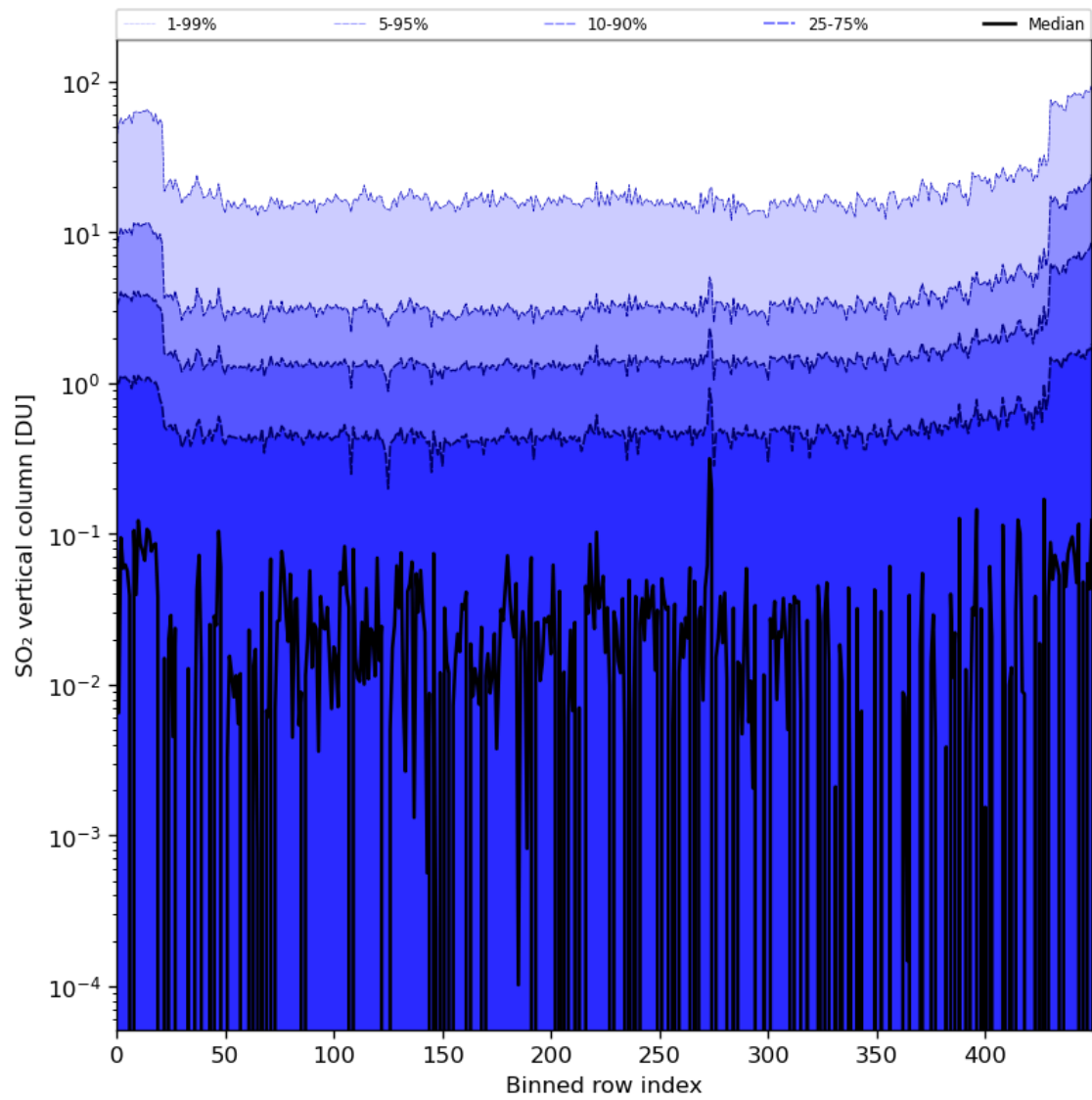
Figure 76: Along track statistics of “SO 2 vertical column” for 2024-01-29 to 2024-01-31
