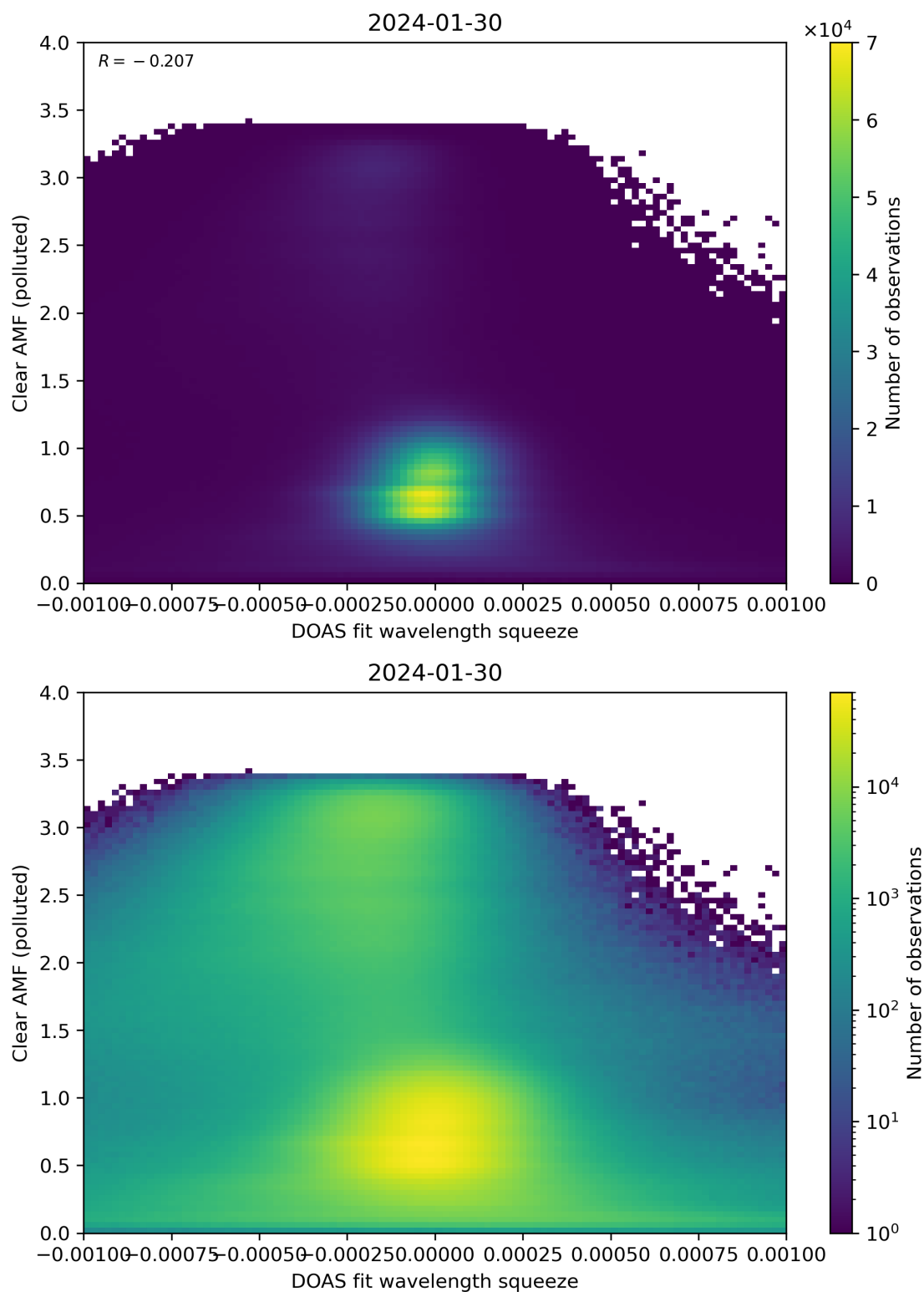
Figure 133: Scatter density plot of “DOAS fit wavelength squeeze” against “Clear AMF (polluted)” for 2024-01-29 to 2024-01-31.
