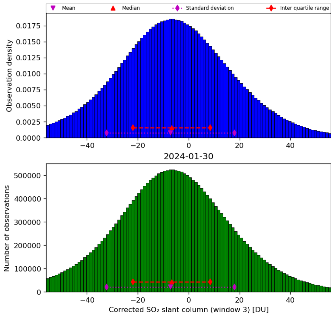
Figure 66: Histogram of “Corrected SO 2 slant column (window 3)” for 2024-01-29 to 2024-01-31
