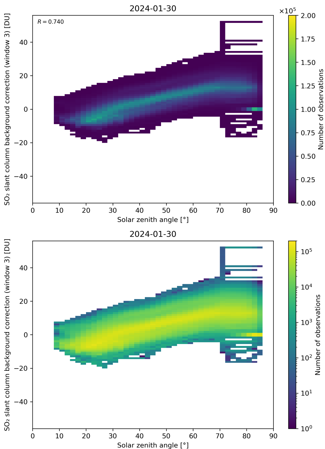
Figure 160: Scatter density plot of “Solar zenith angle” against “SO 2 slant column background correction (window 3)” for 2024-01-29 to 2024-01-31.
