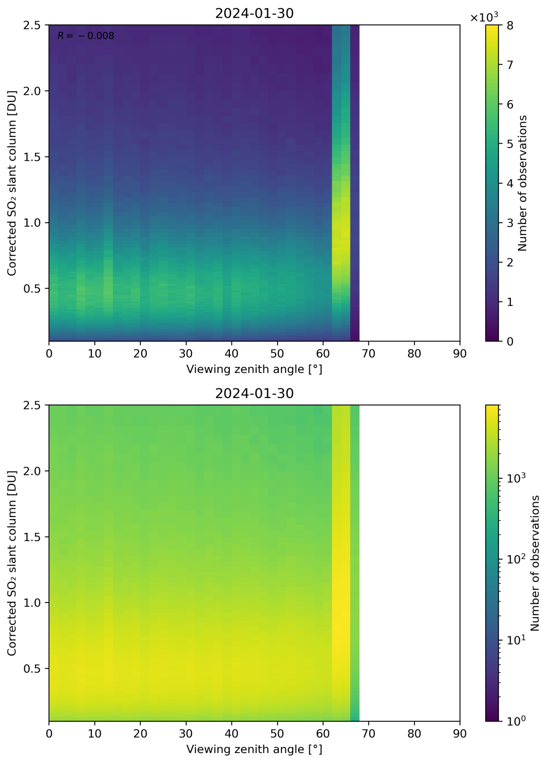
Figure 317: Scatter density plot of “Viewing zenith angle” against “Corrected SO 2 slant column” for 2024-01-29 to 2024-01-31.
