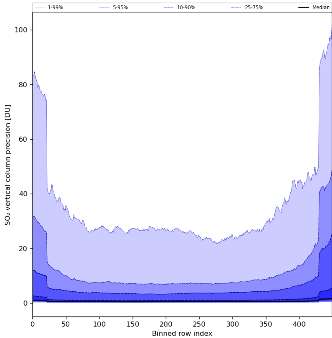
Figure 77: Along track statistics of “SO 2 vertical column precision” for 2024-01-29 to 2024-01-31
