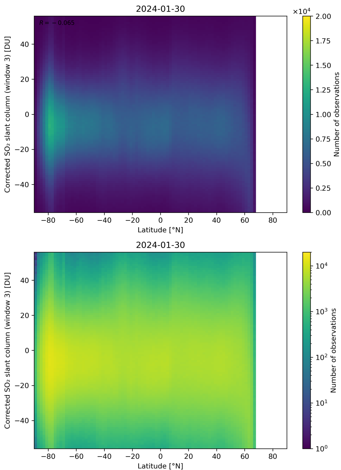
Figure 148: Scatter density plot of “Latitude” against “Corrected SO 2 slant column (window 3)” for 2024-01-29 to 2024-01-31.
