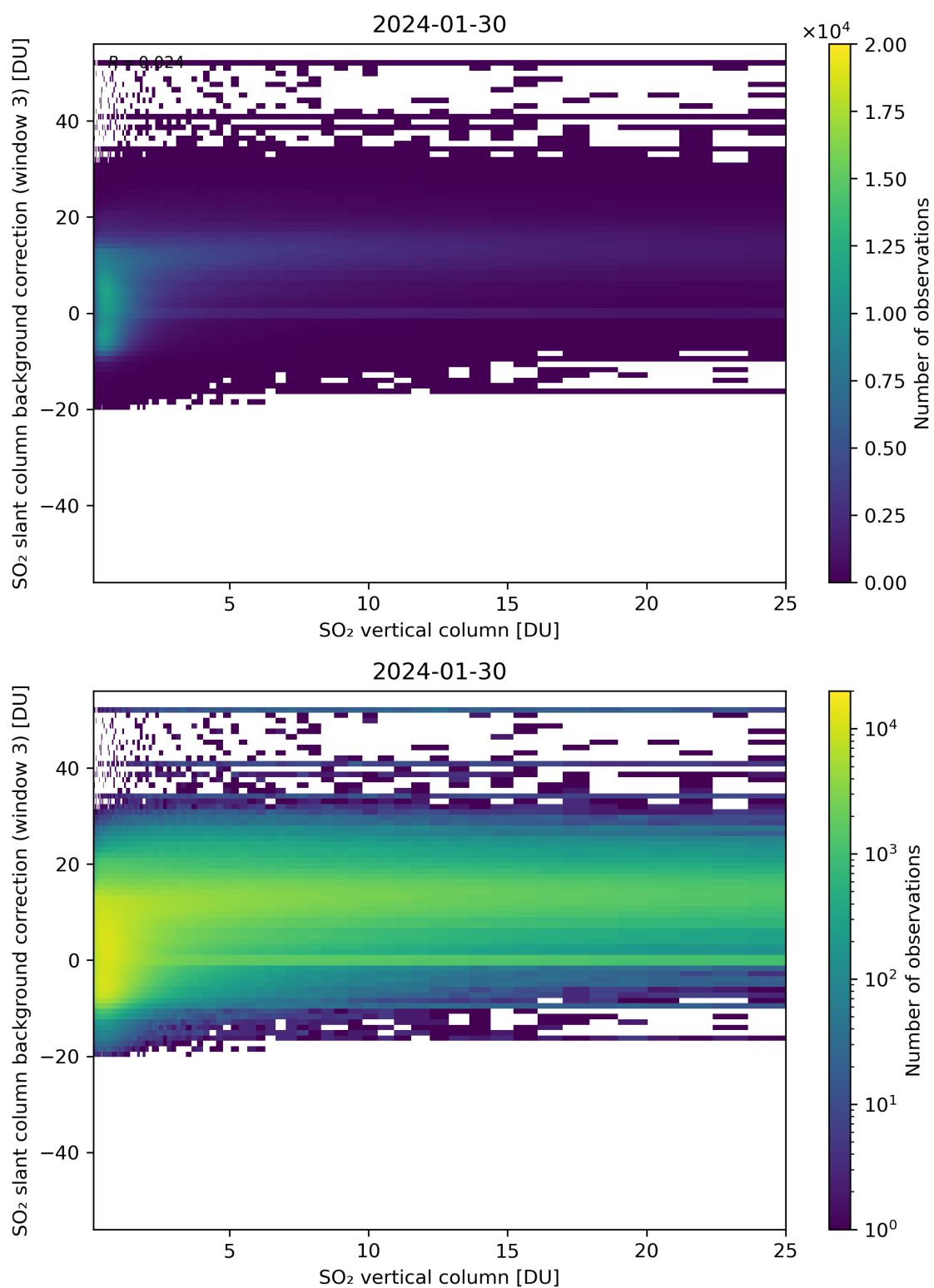
Figure 275: Scatter density plot of “SO 2 vertical column” against “SO 2 slant column background correction (window 3)” for 2024-01-29 to 2024-01-31.
