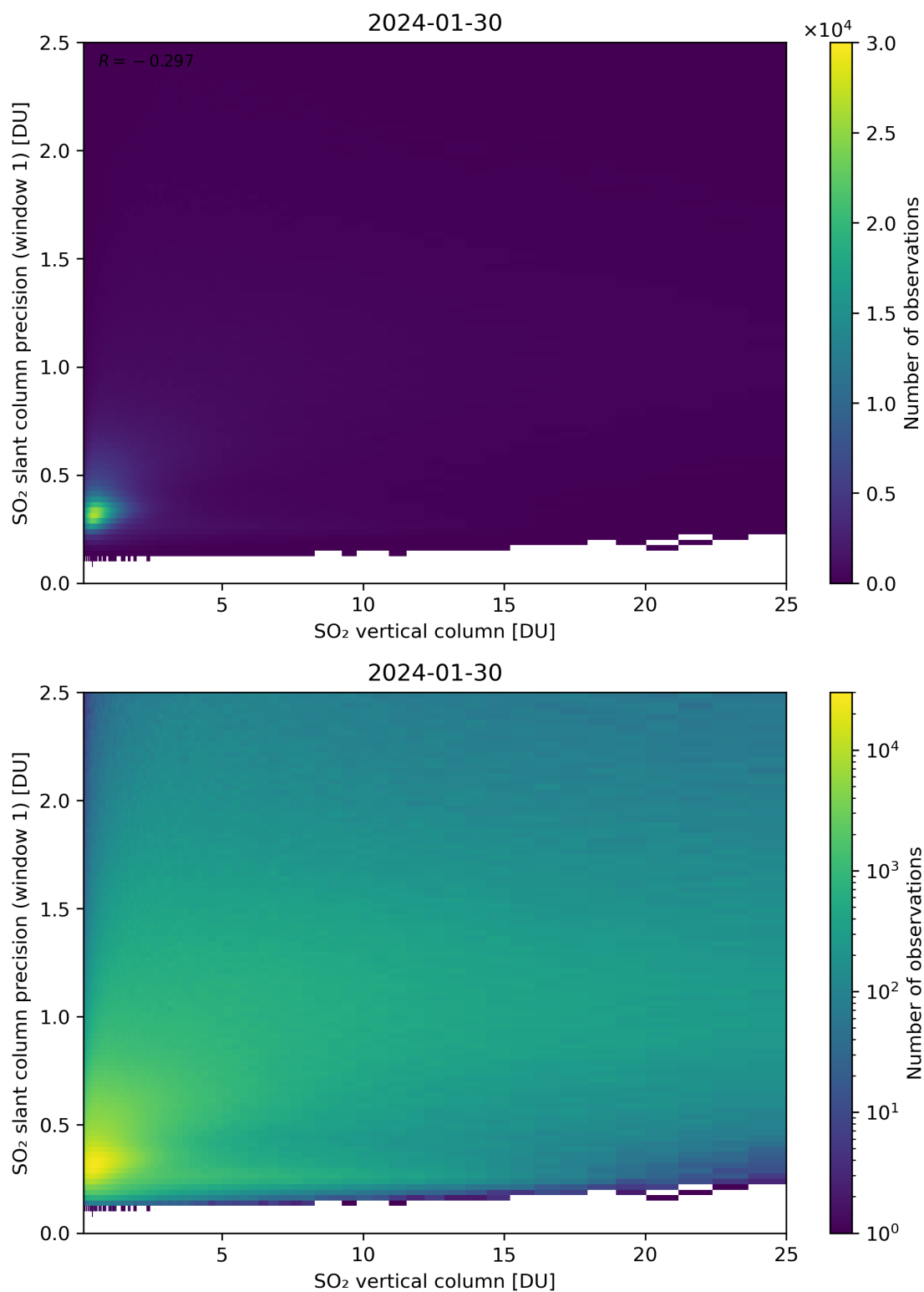
Figure 301: Scatter density plot of “SO 2 vertical column” against “SO 2 slant column precision (window 1)” for 2024-01-29 to 2024-01-31.
