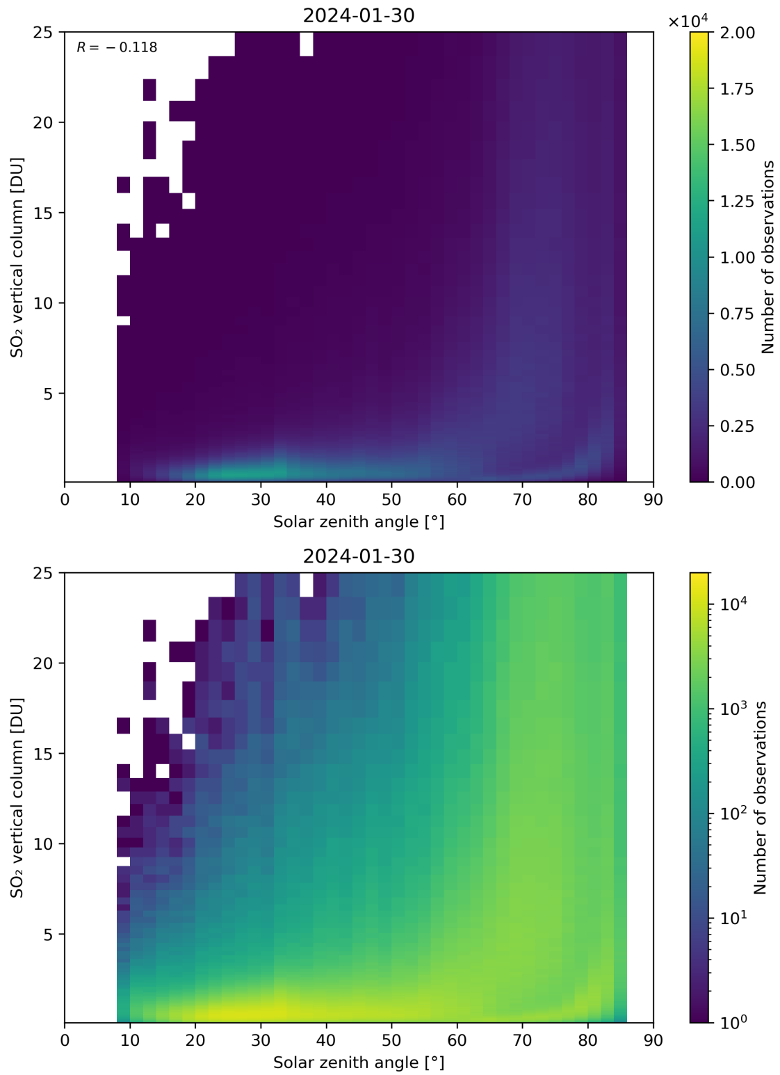
Figure 176: Scatter density plot of “Solar zenith angle” against “SO 2 vertical column” for 2024-01-29 to 2024-01-31.
