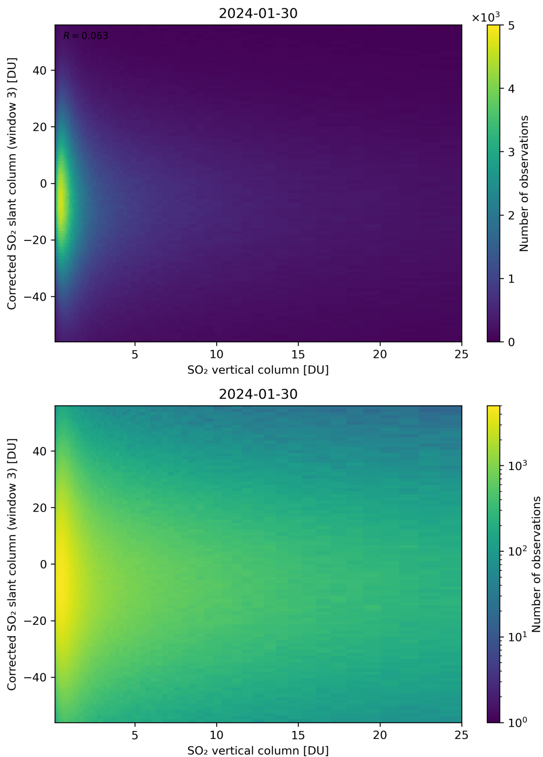
Figure 299: Scatter density plot of “SO 2 vertical column” against “Corrected SO 2 slant column (window 3)” for 2024-01-29 to 2024-01-31.
