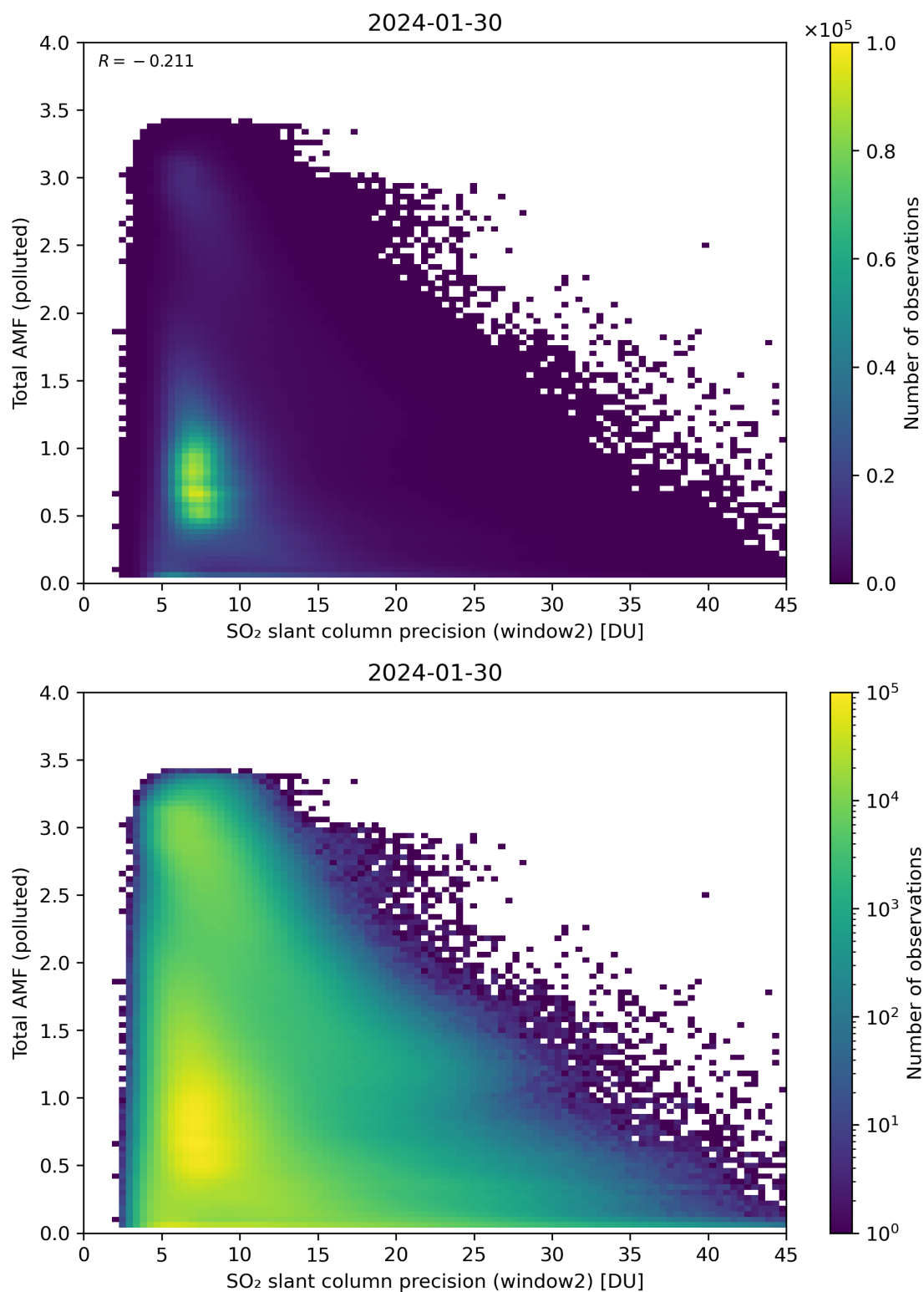
Figure 251: Scatter density plot of “SO 2 slant column precision (window2)” against “Total AMF (polluted)” for 2024-01-29 to 2024-01-31.
