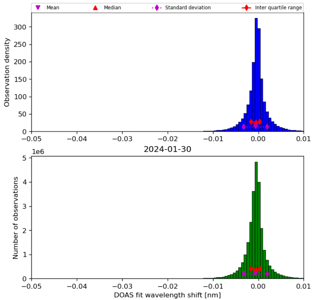
Figure 68: Histogram of “DOAS fit wavelength shift” for 2024-01-29 to 2024-01-31
