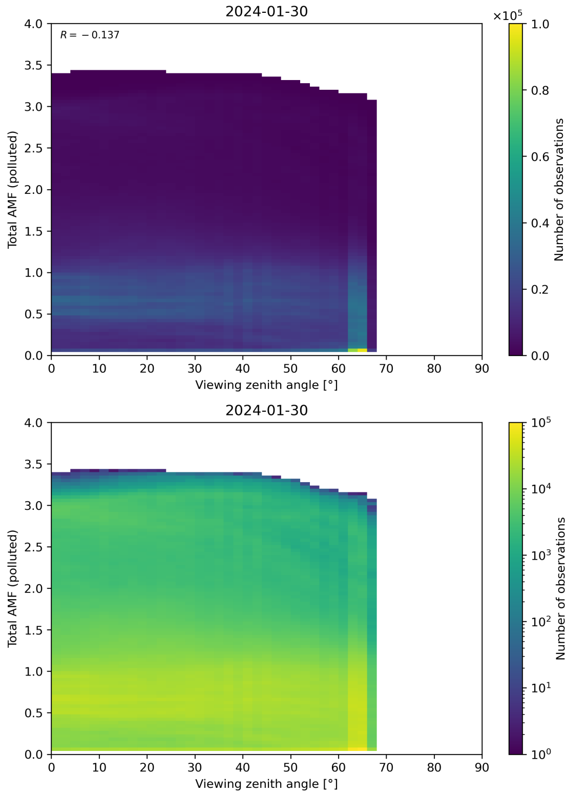
Figure 325: Scatter density plot of “Viewing zenith angle” against “Total AMF (polluted)” for 2024-01-29 to 2024-01-31.
