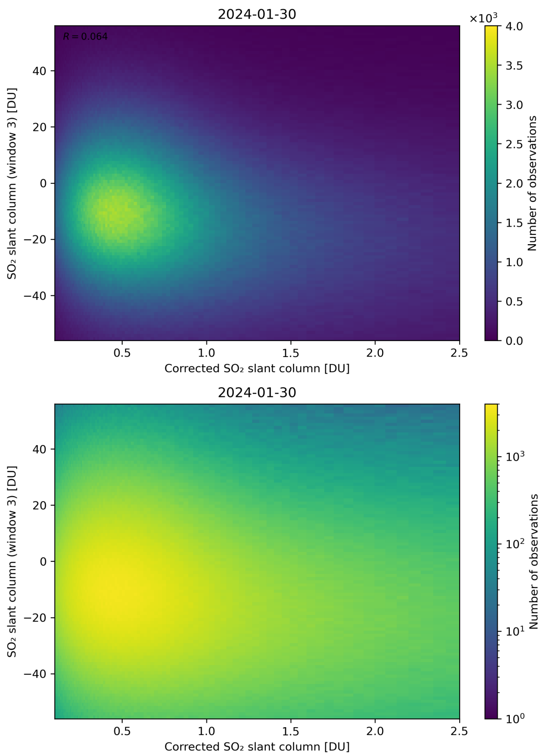
Figure 190: Scatter density plot of “Corrected SO 2 slant column” against “SO 2 slant column (window 3)” for 2024-01-29 to 2024-01-31.
