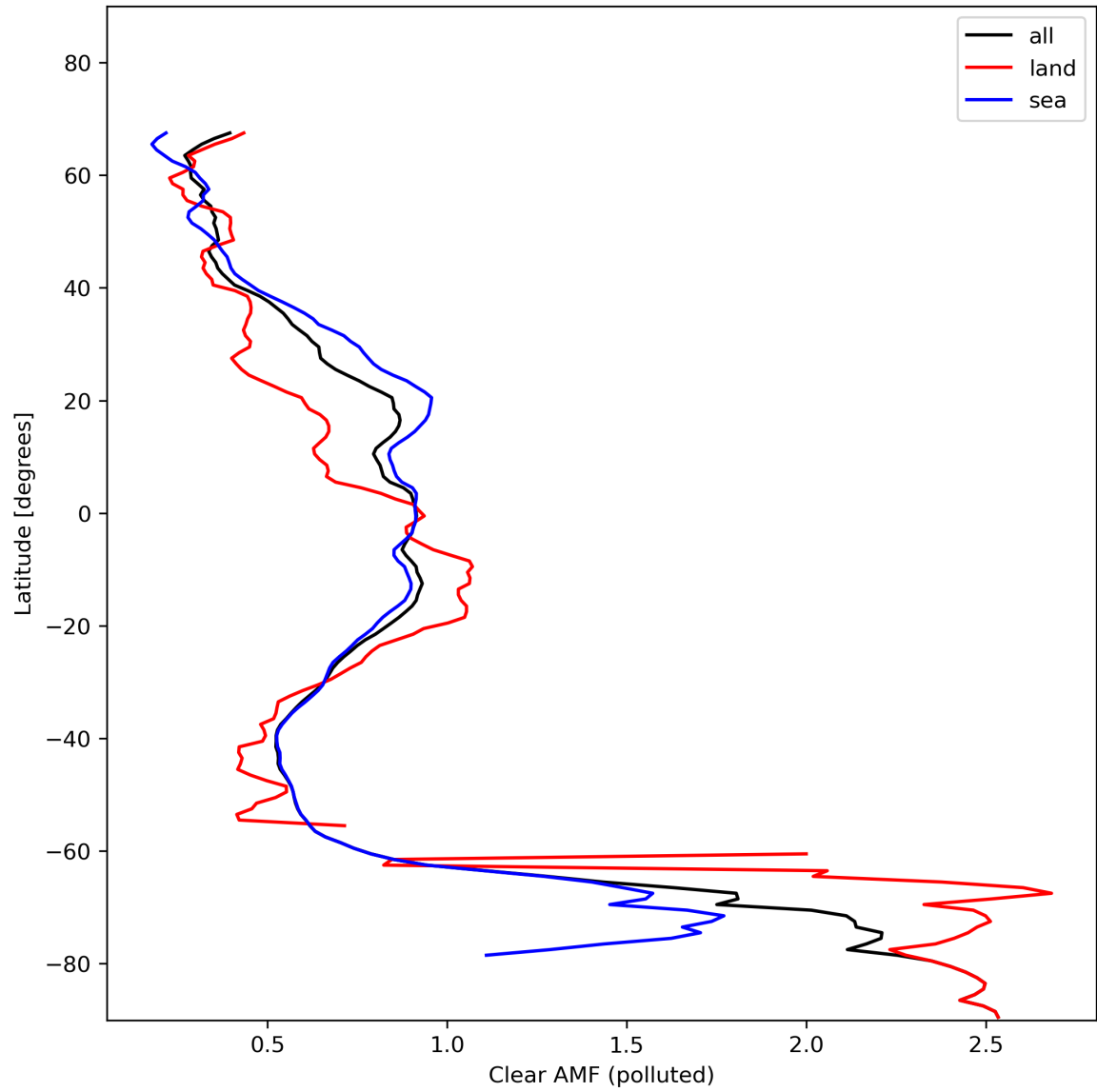
Figure 50: Zonal average of “Clear AMF (polluted)” for 2024-01-29 to 2024-01-31.
