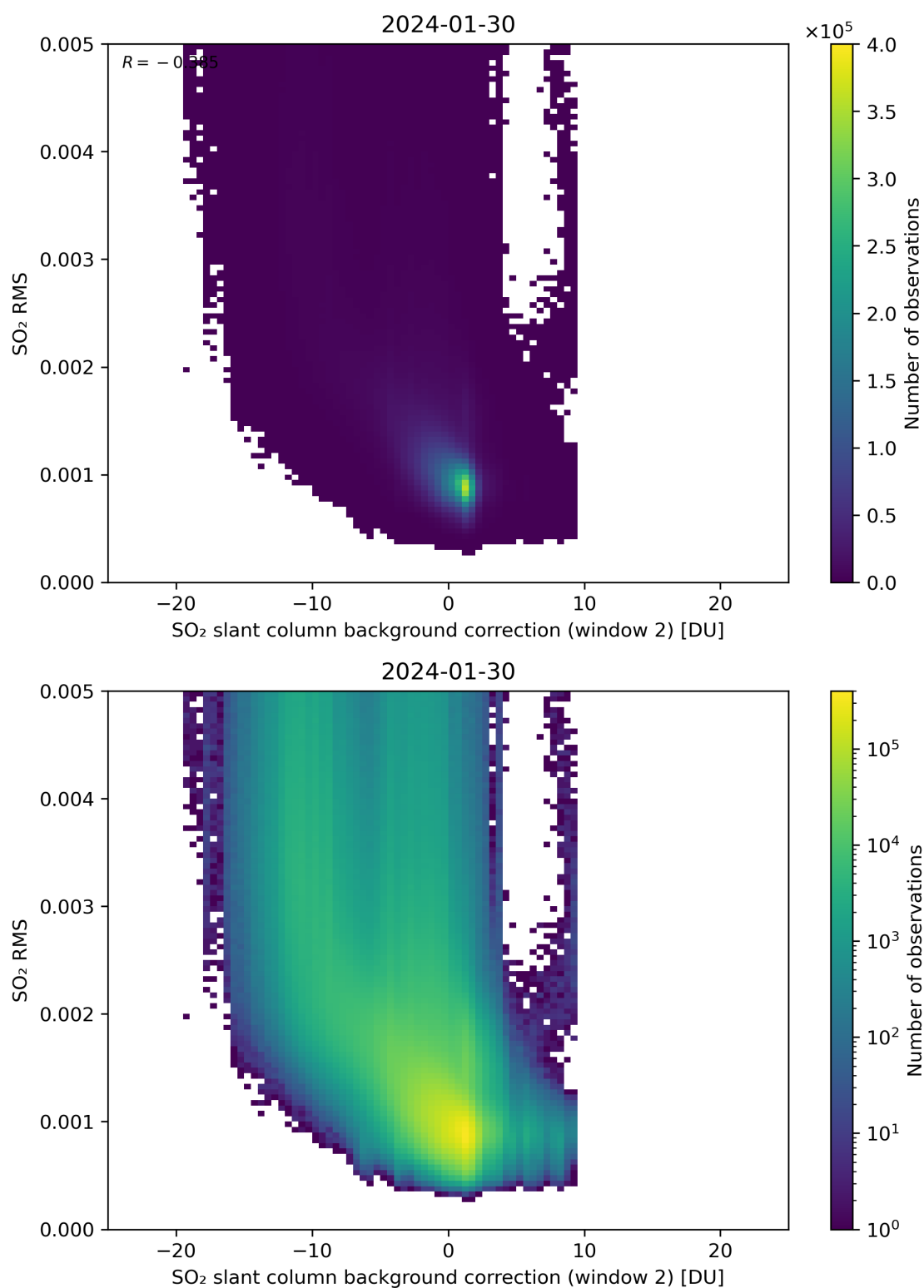
Figure 114: Scatter density plot of “SO 2 slant column background correction (window 2)” against “SO 2 RMS” for 2024-01-29 to 2024-01-31.
