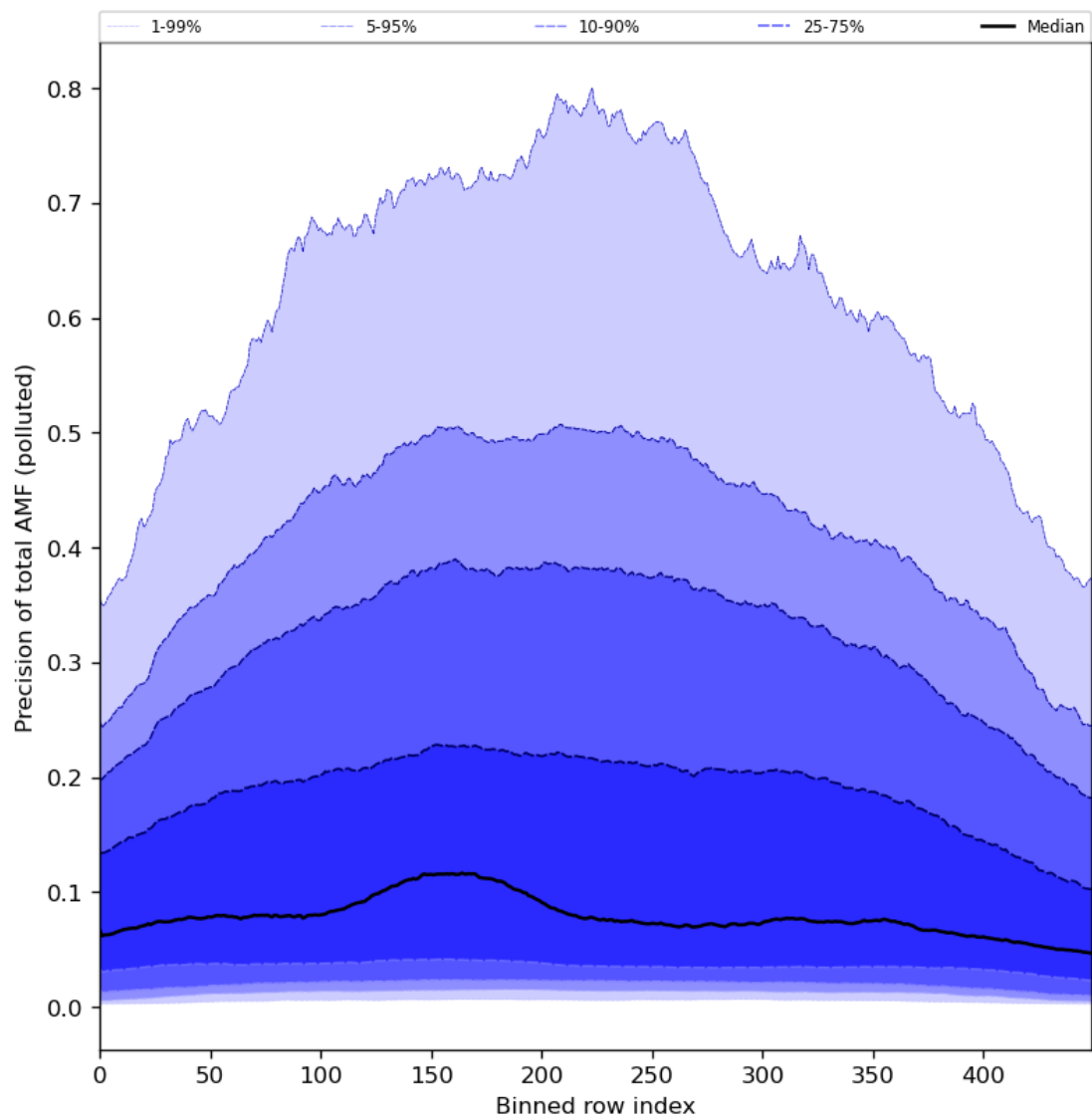
Figure 95: Along track statistics of “Precision of total AMF (polluted)” for 2024-01-29 to 2024-01-31
