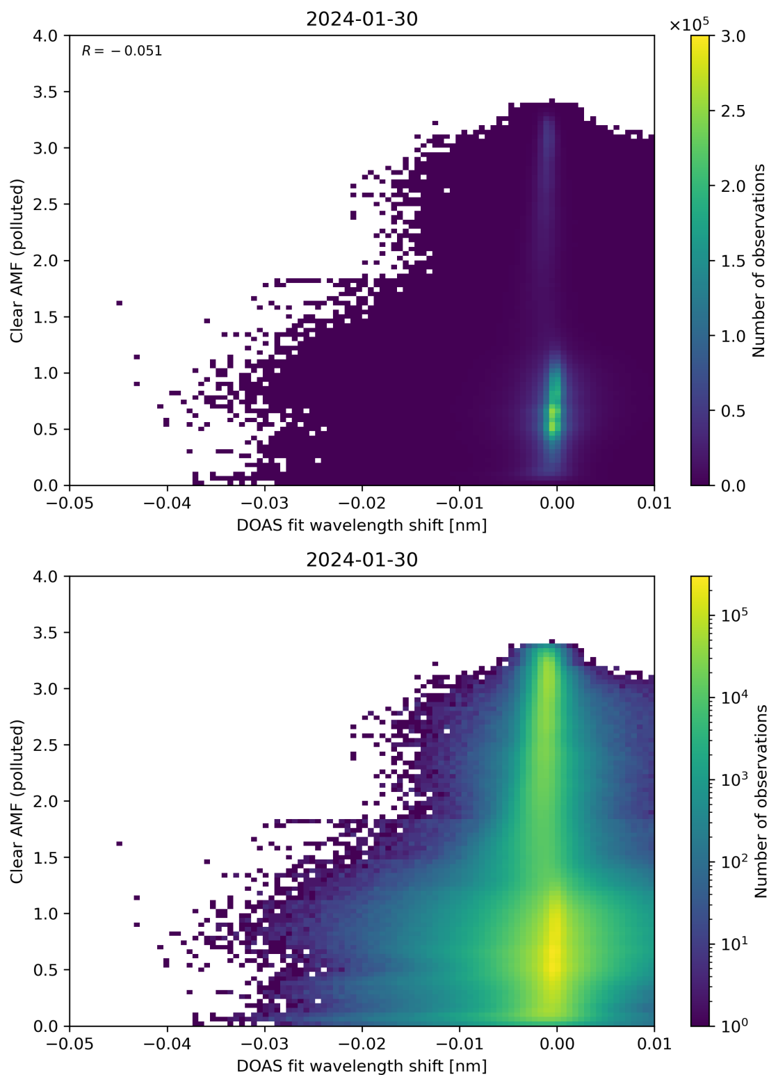
Figure 129: Scatter density plot of “DOAS fit wavelength shift” against “Clear AMF (polluted)” for 2024-01-29 to 2024-01-31.
