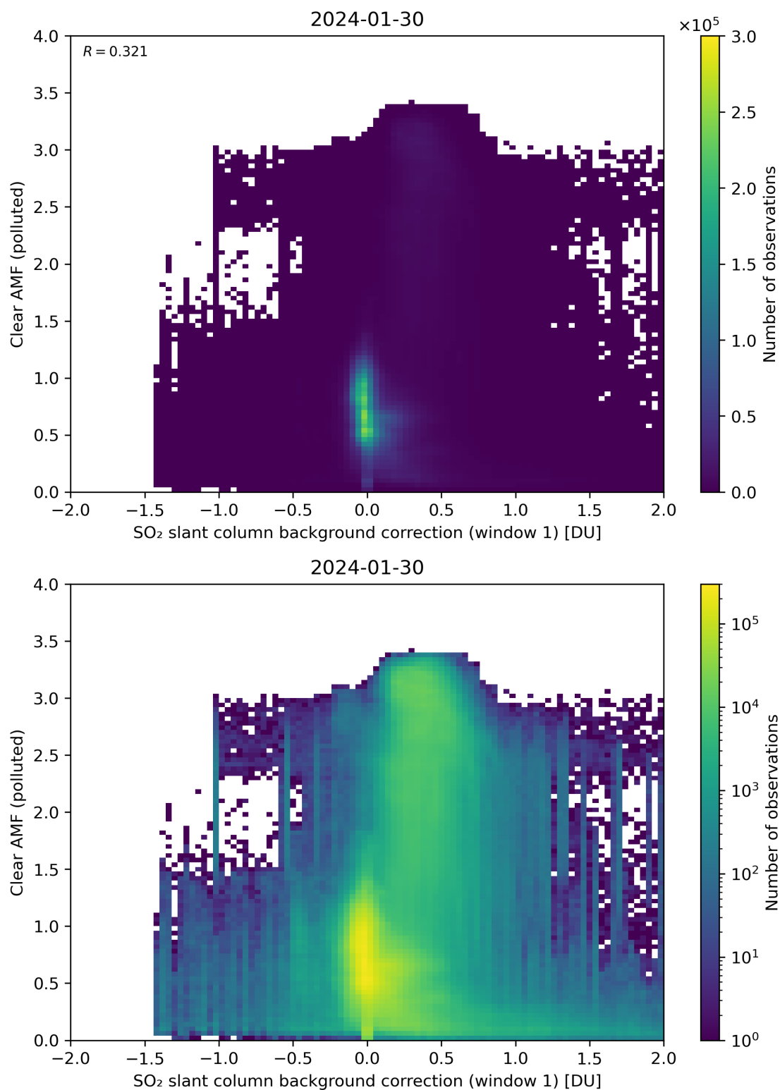
Figure 103: Scatter density plot of “SO 2 slant column background correction (window 1)” against “Clear AMF (polluted)” for 2024-01-29 to 2024-01-31.
