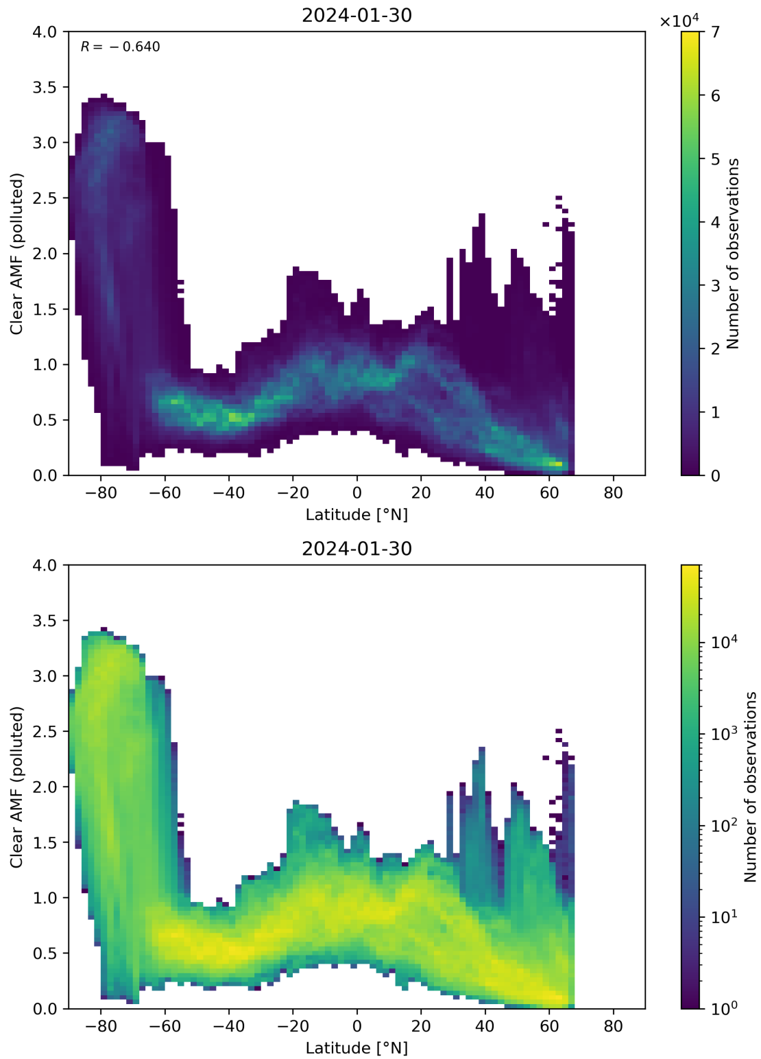
Figure 145: Scatter density plot of “Latitude” against “Clear AMF (polluted)” for 2024-01-29 to 2024-01-31.
