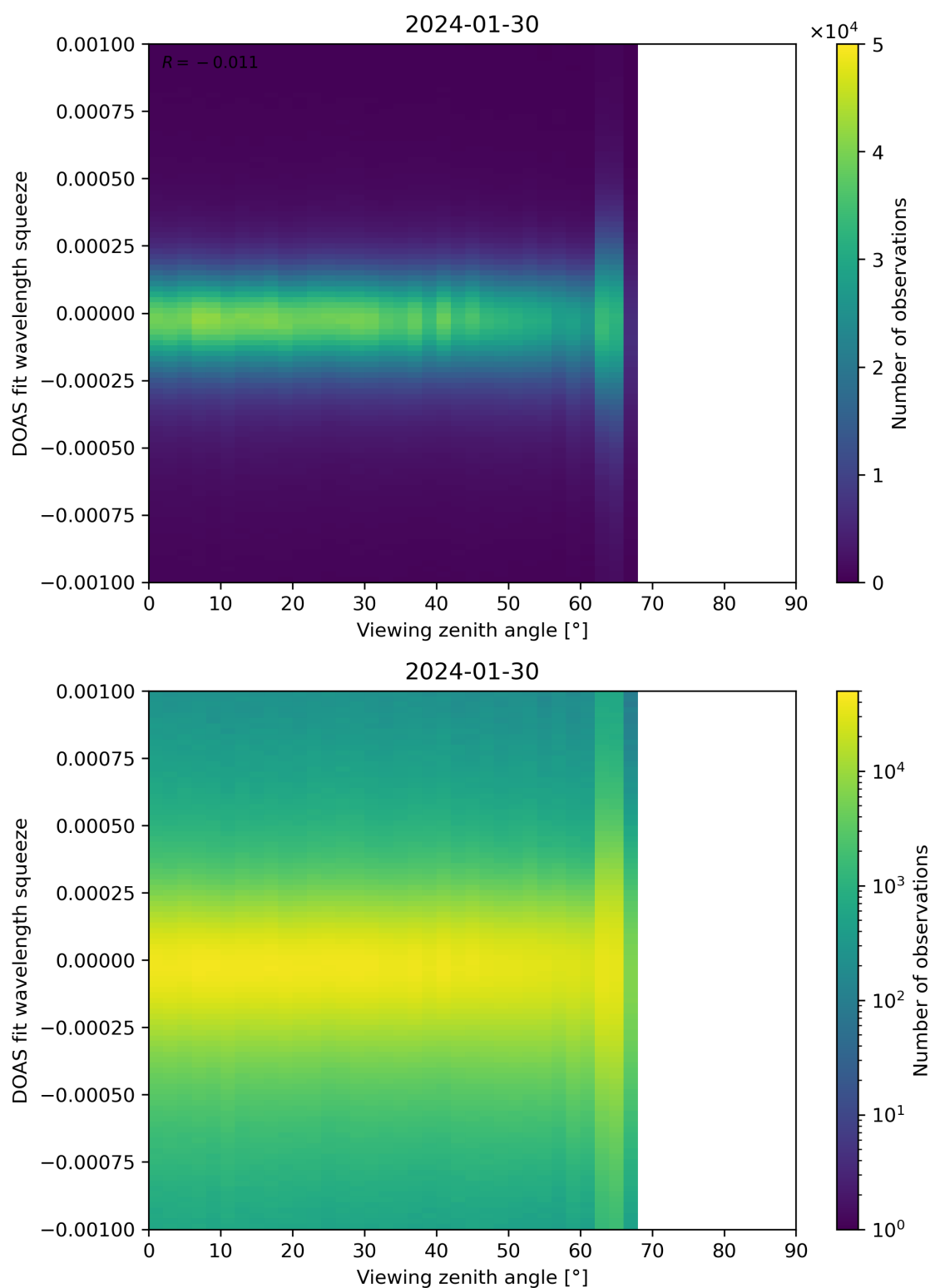
Figure 312: Scatter density plot of “Viewing zenith angle” against “DOAS fit wavelength squeeze” for 2024-01-29 to 2024-01-31.
