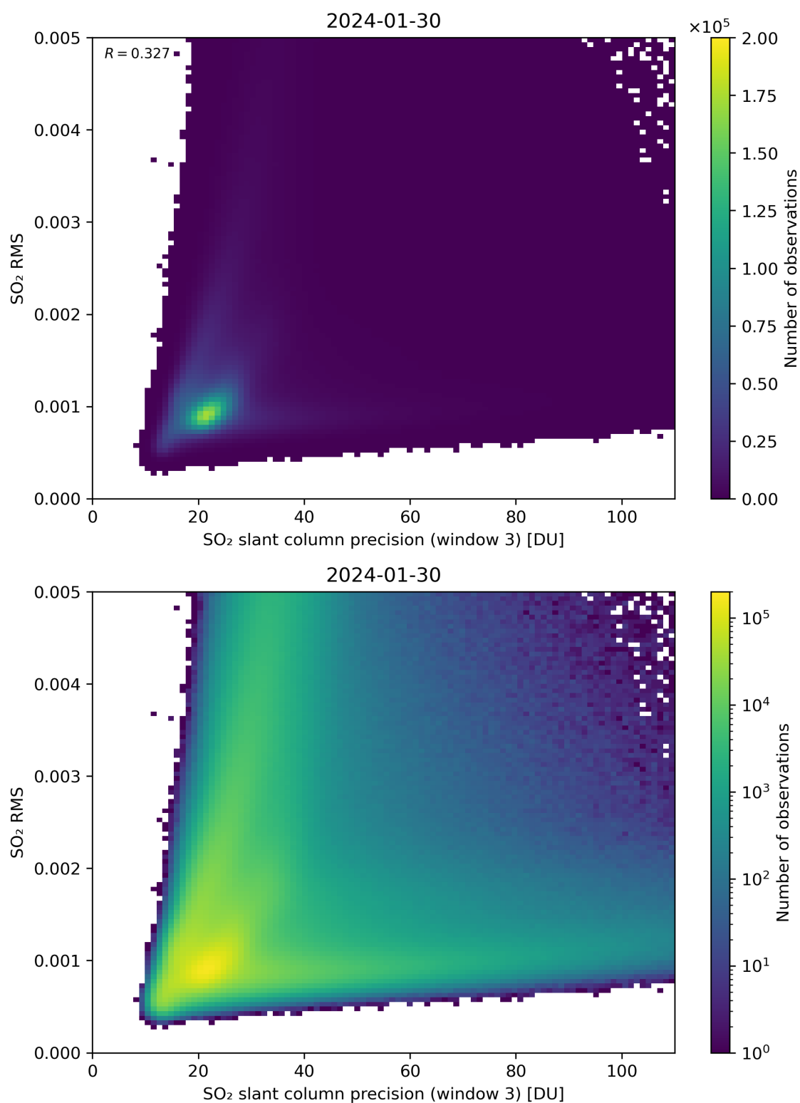
Figure 260: Scatter density plot of “SO 2 slant column precision (window 3)” against “SO 2 RMS” for 2024-01-29 to 2024-01-31.
