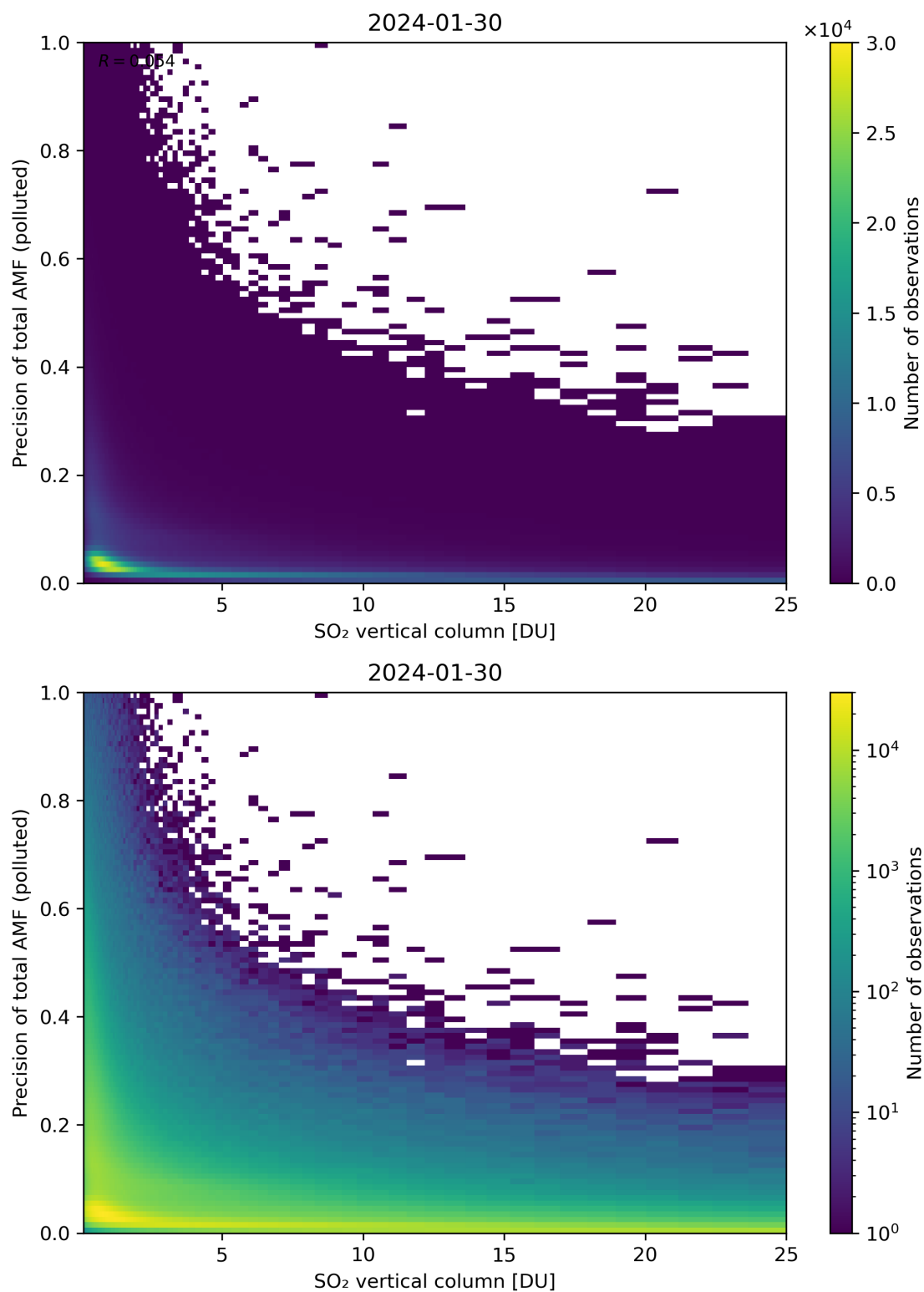
Figure 306: Scatter density plot of “SO 2 vertical column” against “Precision of total AMF (polluted)” for 2024-01-29 to 2024-01-31.
