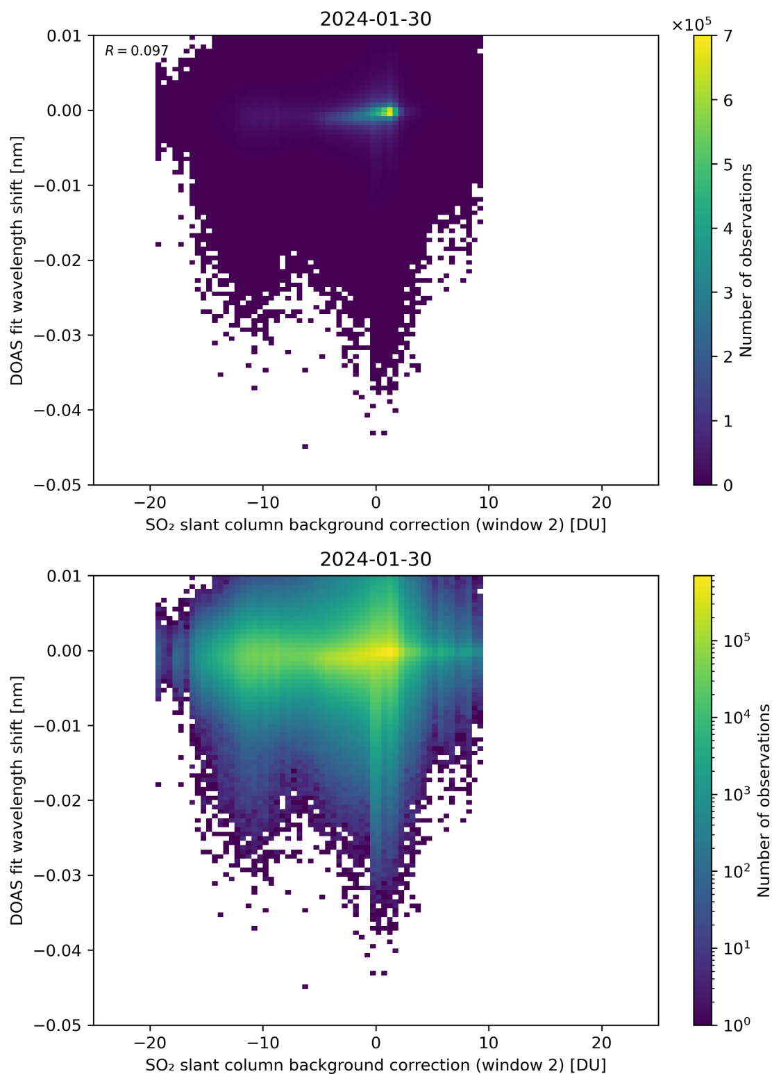
Figure 112: Scatter density plot of “SO 2 slant column background correction (window 2)” against “DOAS fit wavelength shift” for 2024-01-29 to 2024-01-31.
