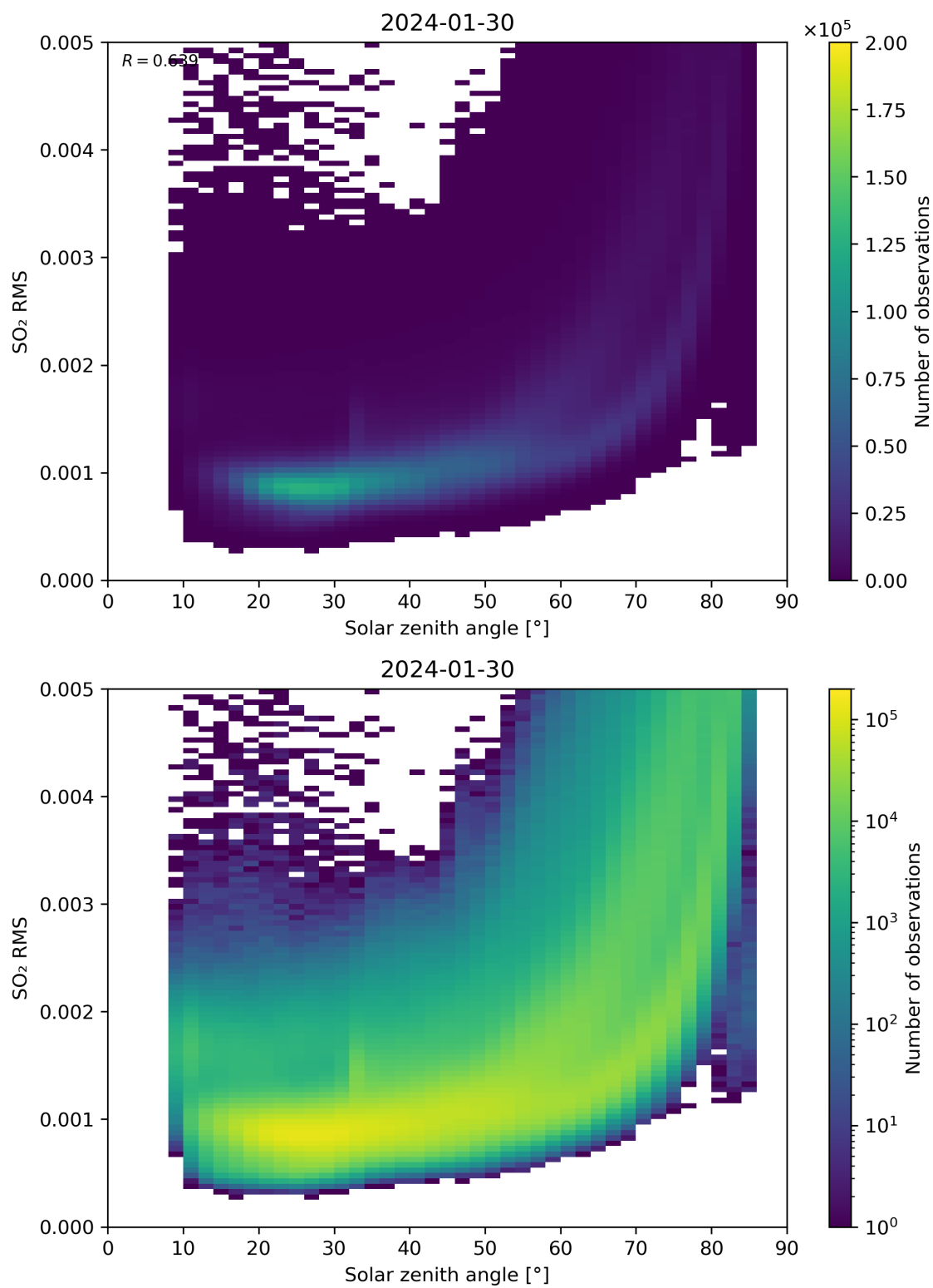
Figure 163: Scatter density plot of “Solar zenith angle” against “SO 2 RMS” for 2024-01-29 to 2024-01-31.
