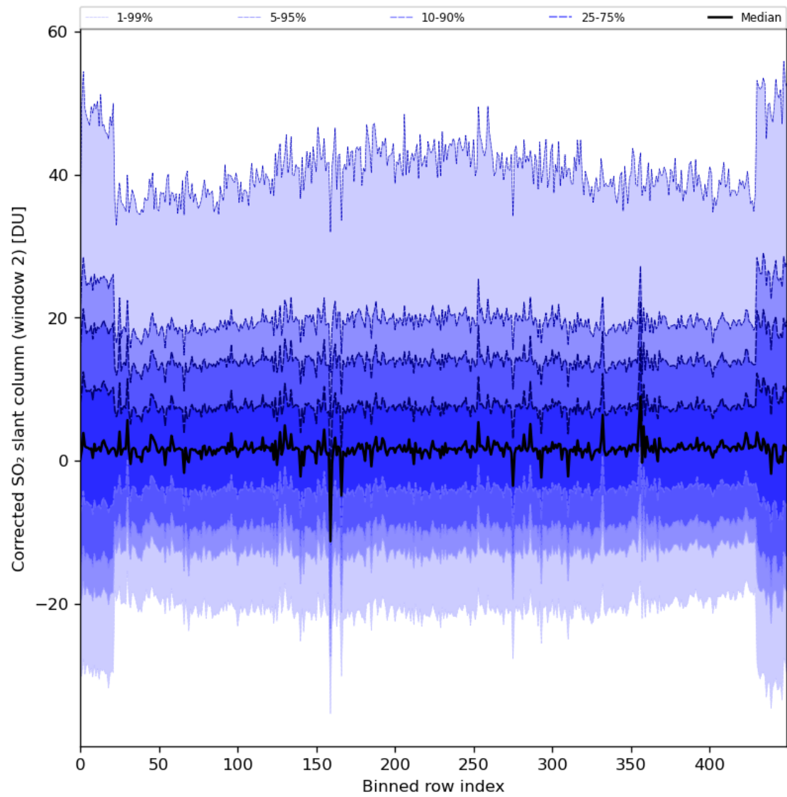
Figure 85: Along track statistics of “Corrected SO 2 slant column (window 2)” for 2024-01-29 to 2024-01-31
