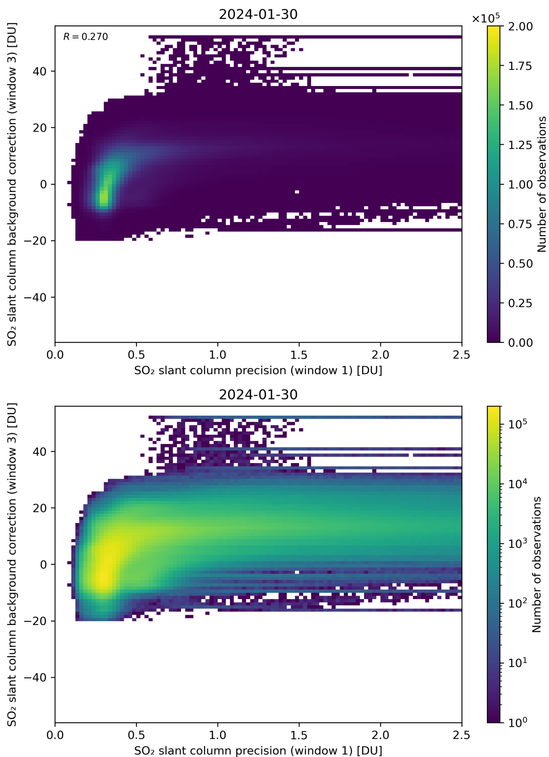
Figure 220: Scatter density plot of “SO 2 slant column precision (window 1)” against “SO 2 slant column background correction (window 3)” for 2024-01-29 to 2024-01-31.
