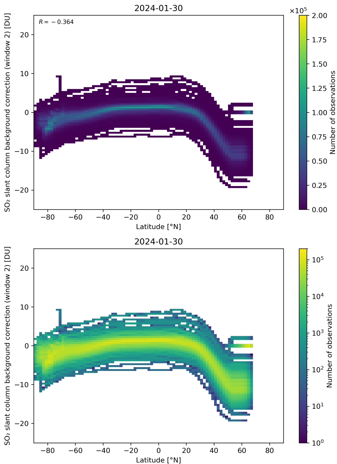
Figure 140: Scatter density plot of “Latitude” against “SO 2 slant column background correction (window 2)” for 2024-01-29 to 2024-01-31.
