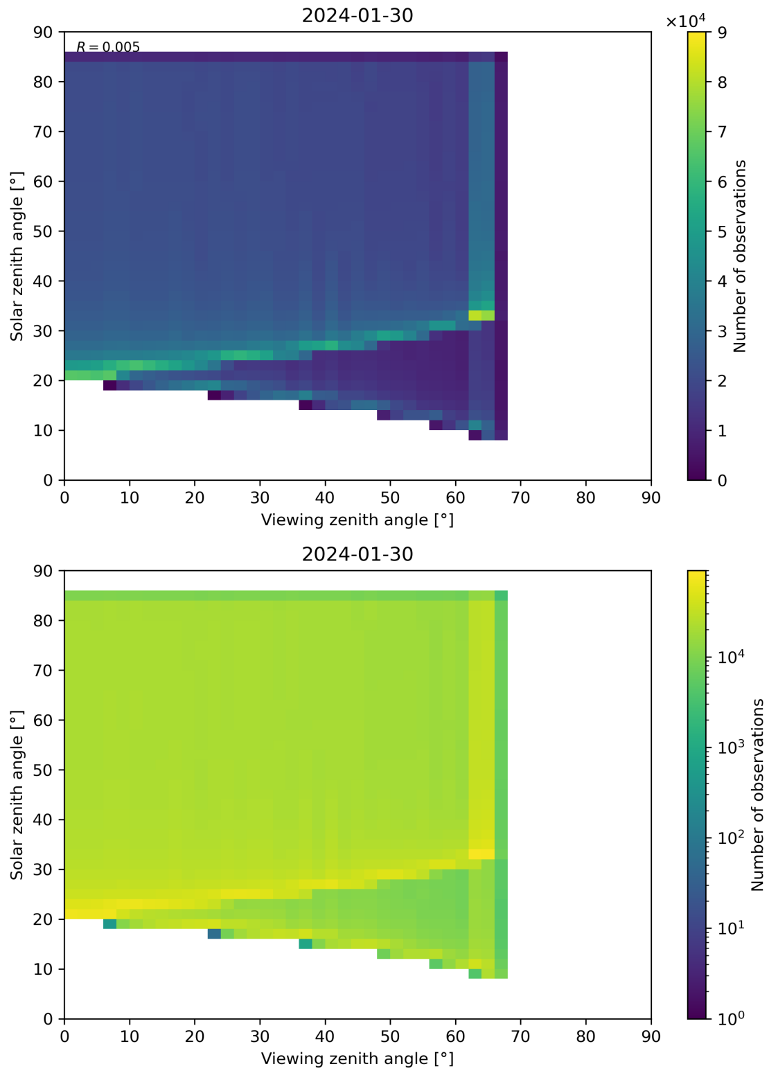
Figure 315: Scatter density plot of “Viewing zenith angle” against “Solar zenith angle” for 2024-01-29 to 2024-01-31.
