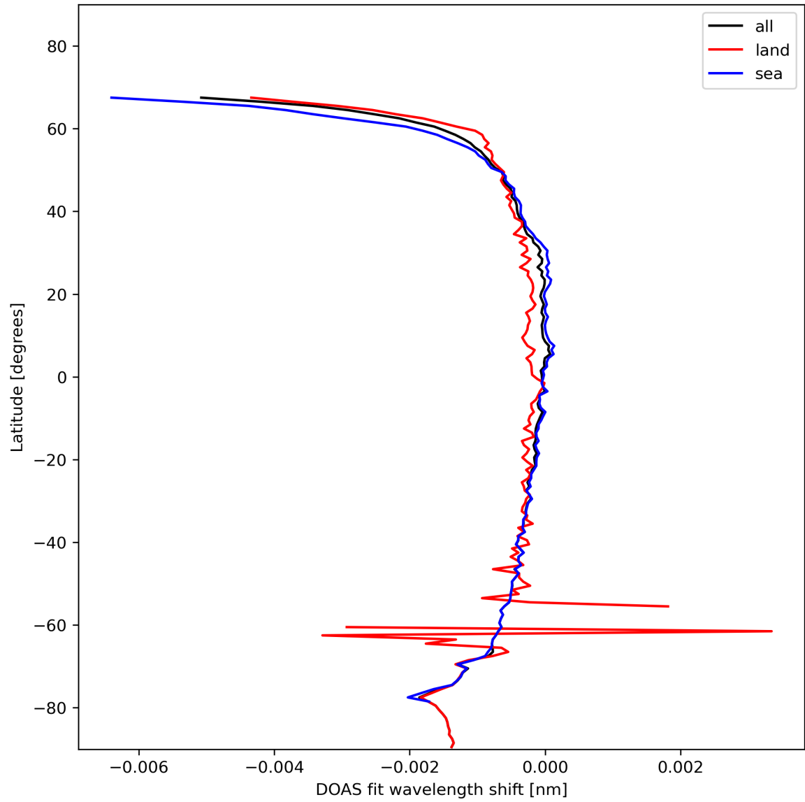
Figure 45: Zonal average of “DOAS fit wavelength shift” for 2024-01-29 to 2024-01-31.
