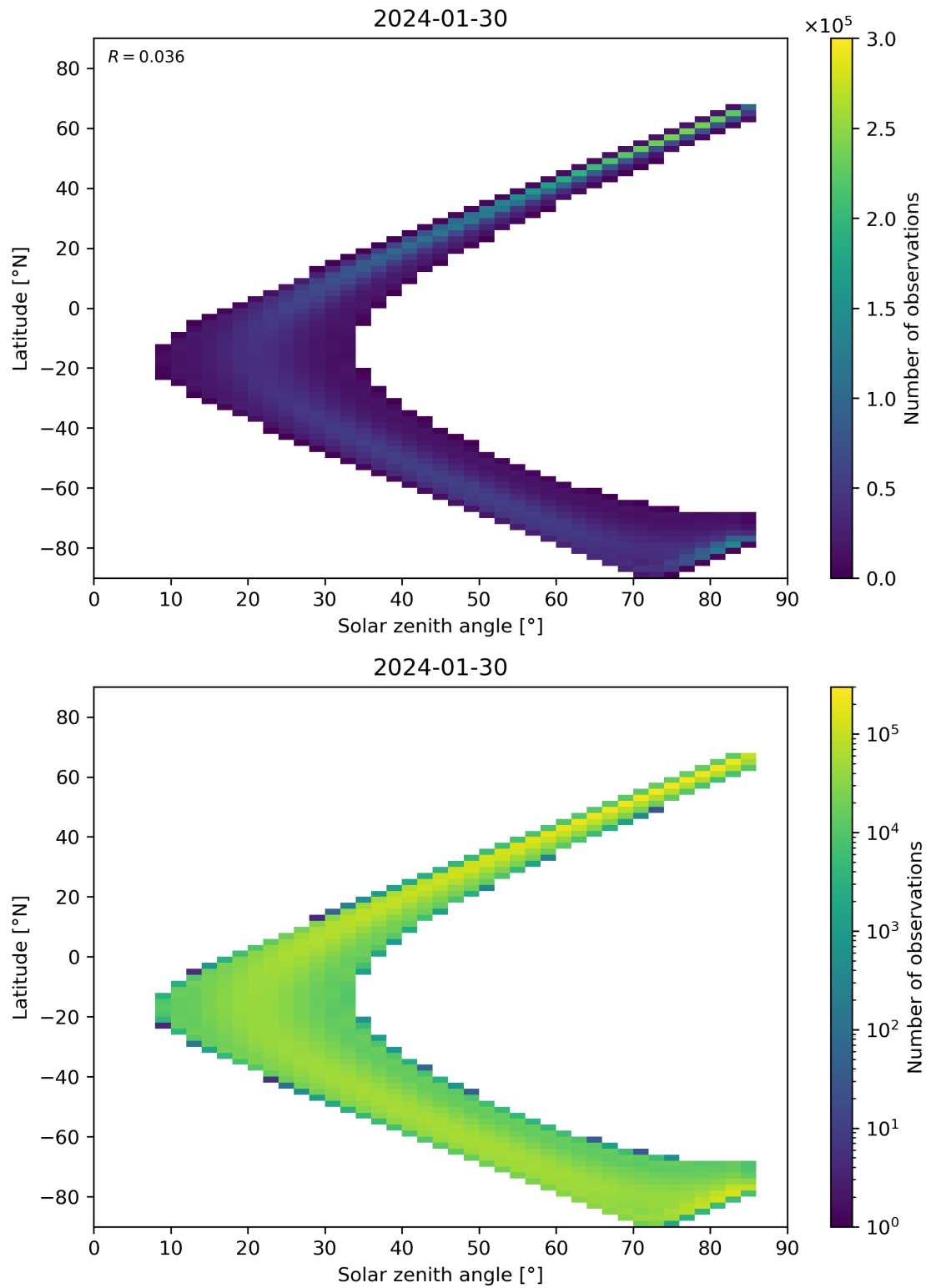
Figure 164: Scatter density plot of “Solar zenith angle” against “Latitude” for 2024-01-29 to 2024-01-31.
