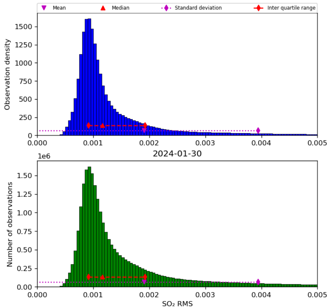
Figure 70: Histogram of “SO 2 RMS” for 2024-01-29 to 2024-01-31
