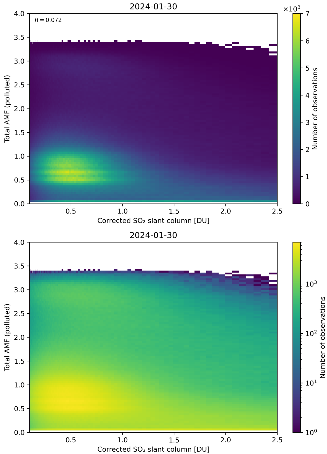
Figure 192: Scatter density plot of “Corrected SO 2 slant column” against “Total AMF (polluted)” for 2024-01-29 to 2024-01-31.
