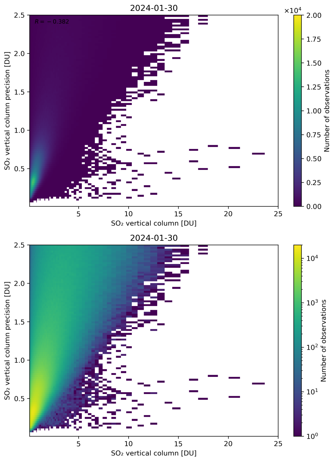
Figure 307: Scatter density plot of “SO 2 vertical column” against “SO 2 vertical column precision” for 2024-01-29 to 2024-01-31.
