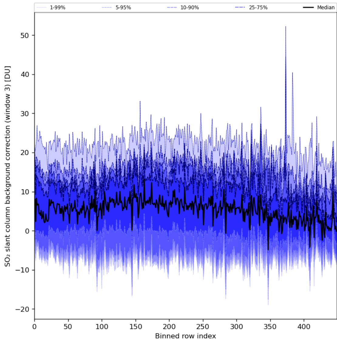
Figure 90: Along track statistics of “SO 2 slant column background correction (window 3)” for 2024-01-29 to 2024-01-31
