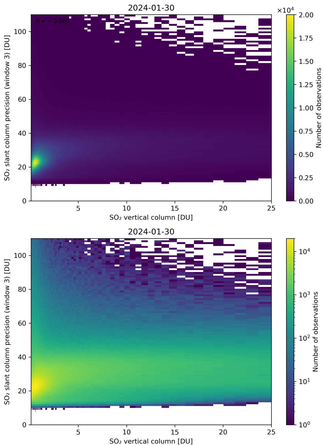
Figure 304: Scatter density plot of “SO 2 vertical column” against “SO 2 slant column precision (window 3)” for 2024-01-29 to 2024-01-31.
