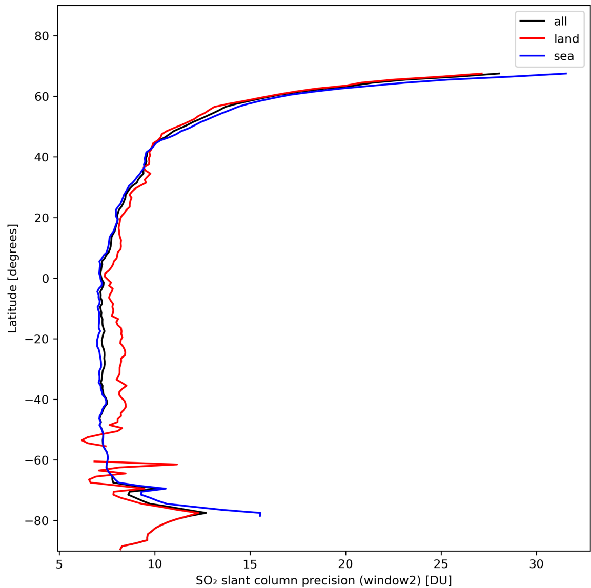
Figure 38: Zonal average of “SO 2 slant column precision (window2)” for 2024-01-29 to 2024-01-31.
