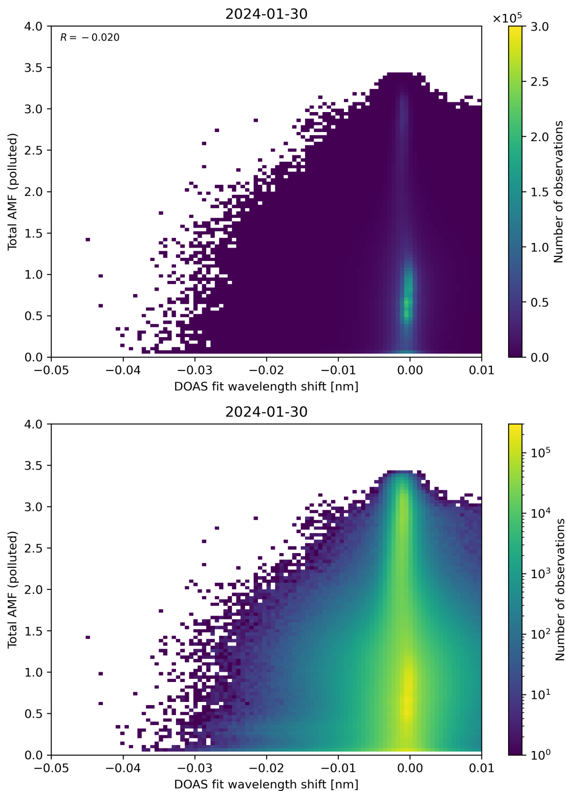
Figure 130: Scatter density plot of “DOAS fit wavelength shift” against “Total AMF (polluted)” for 2024-01-29 to 2024-01-31.
