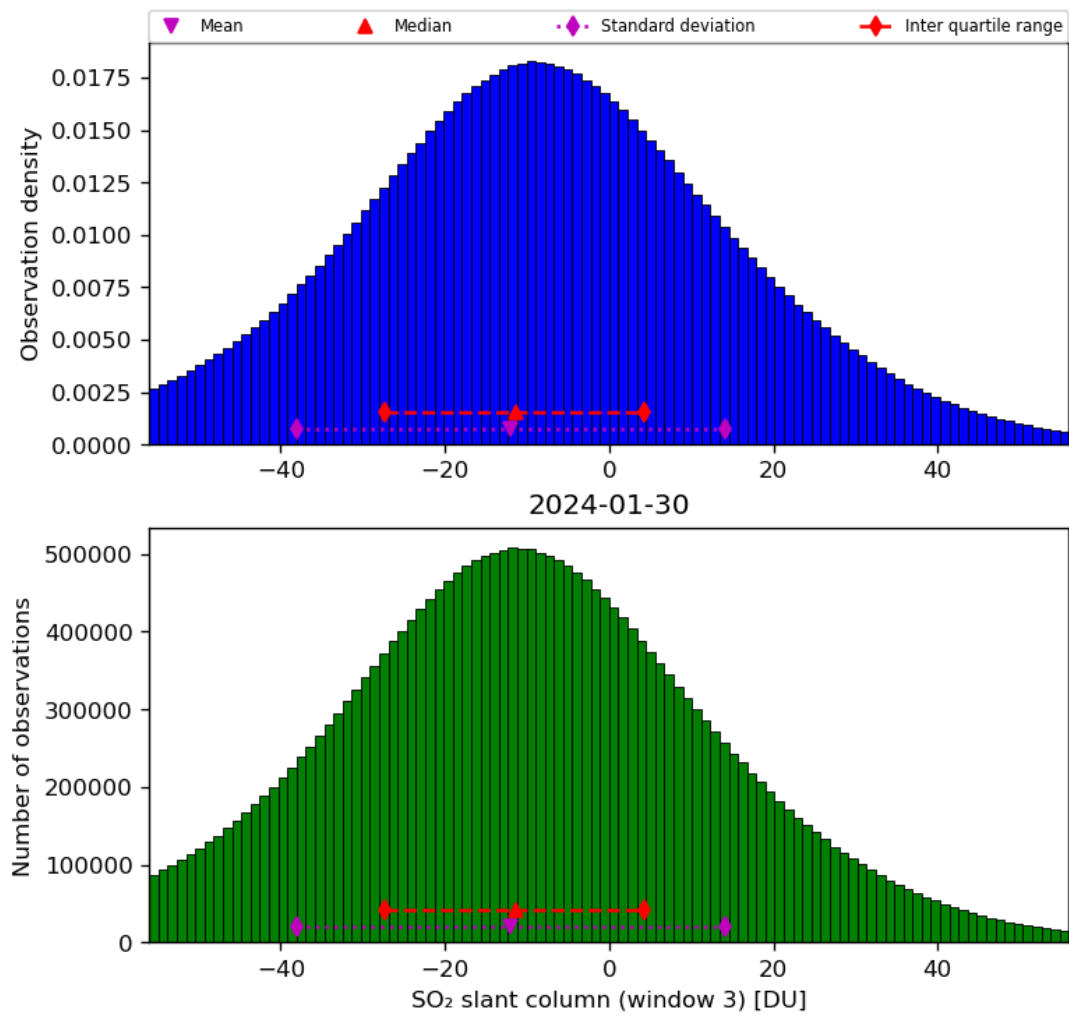
Figure 64: Histogram of “SO 2 slant column (window 3)” for 2024-01-29 to 2024-01-31
