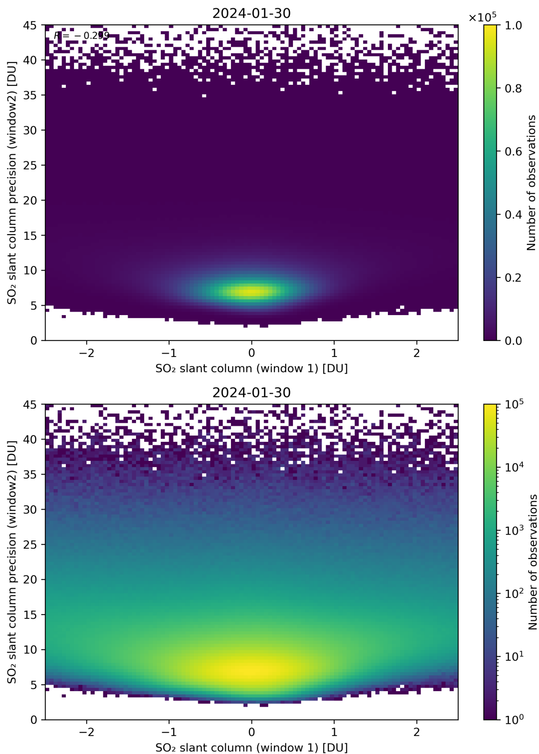
Figure 236: Scatter density plot of “SO 2 slant column (window 1)” against “SO 2 slant column precision (window2)” for 2024-01-29 to 2024-01-31.
