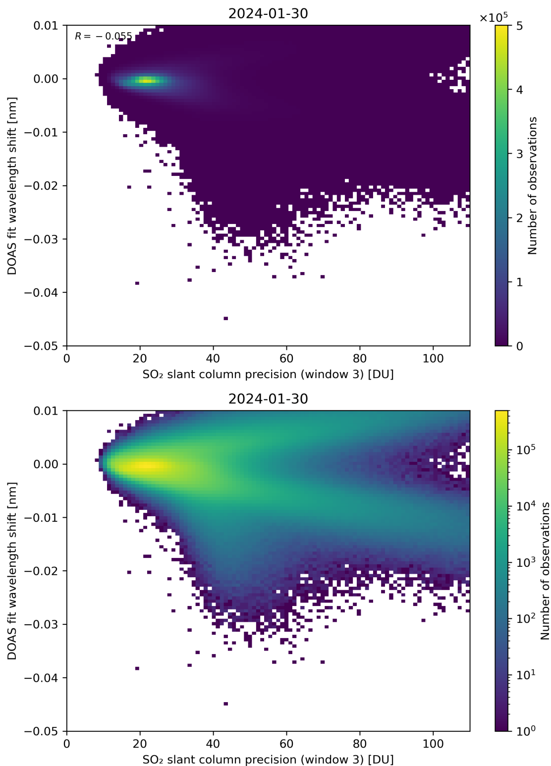
Figure 258: Scatter density plot of “SO 2 slant column precision (window 3)” against “DOAS fit wavelength shift” for 2024-01-29 to 2024-01-31.
