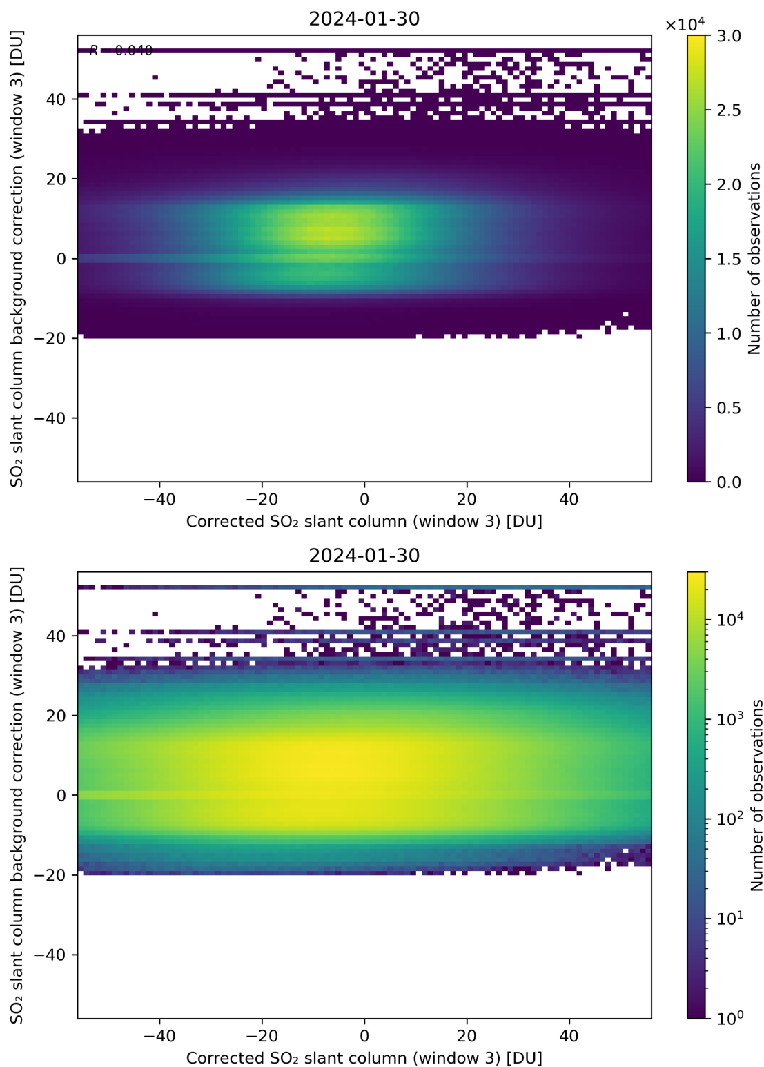
Figure 205: Scatter density plot of “Corrected SO 2 slant column (window 3)” against “SO 2 slant column background correction (window 3)” for 2024-01-29 to 2024-01-31.
