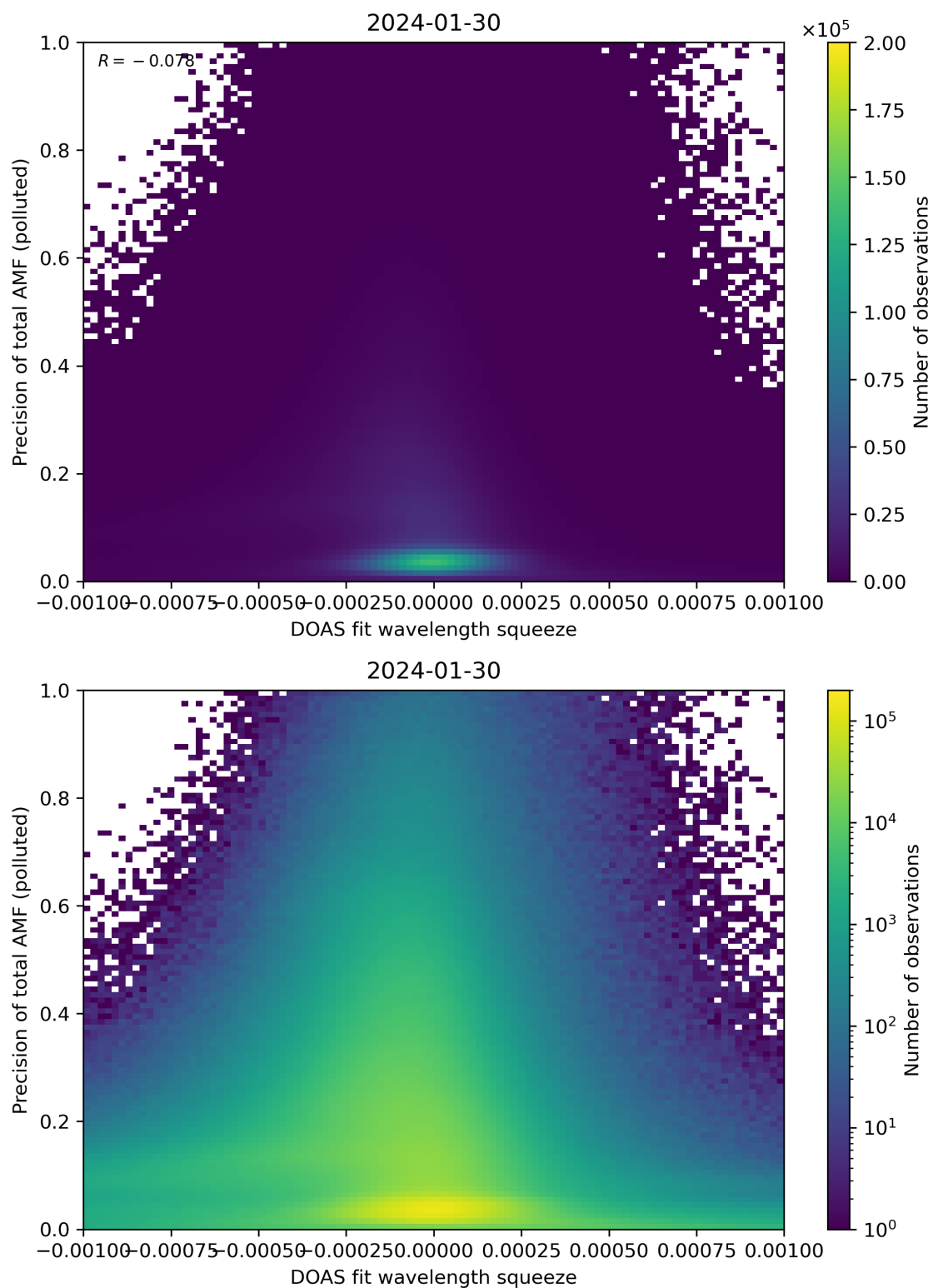
Figure 135: Scatter density plot of “DOAS fit wavelength squeeze” against “Precision of total AMF (polluted)” for 2024-01-29 to 2024-01-31.
