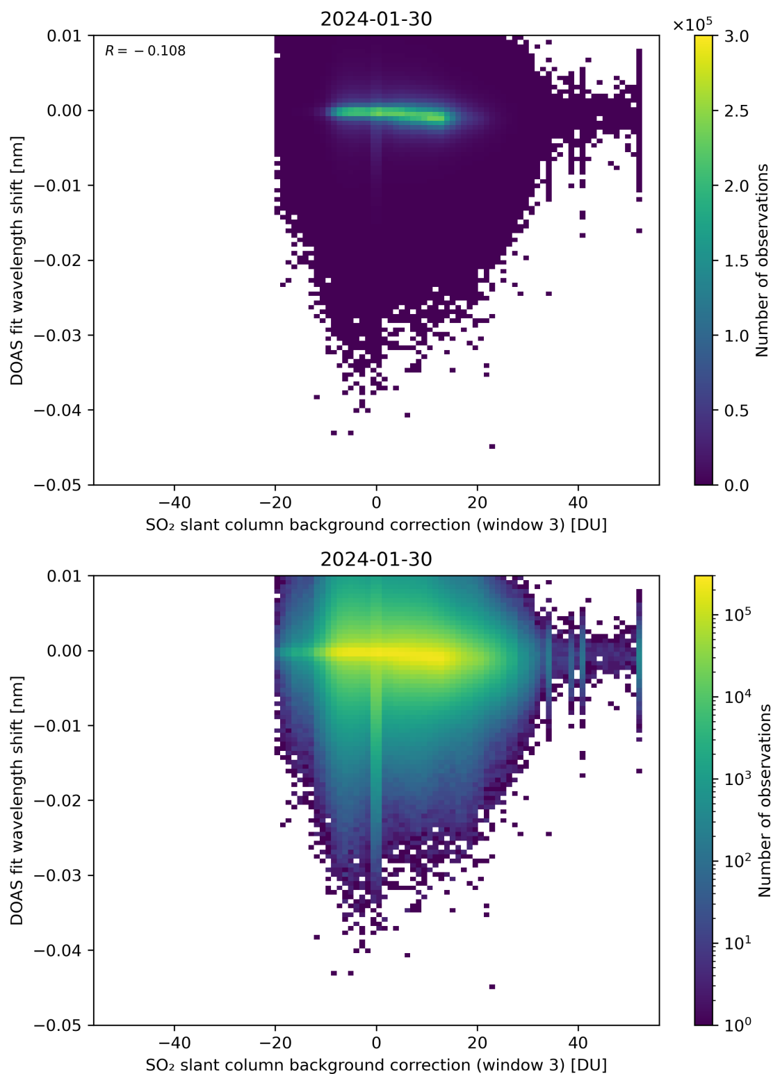
Figure 121: Scatter density plot of “SO 2 slant column background correction (window 3)” against “DOAS fit wavelength shift” for 2024-01-29 to 2024-01-31.
