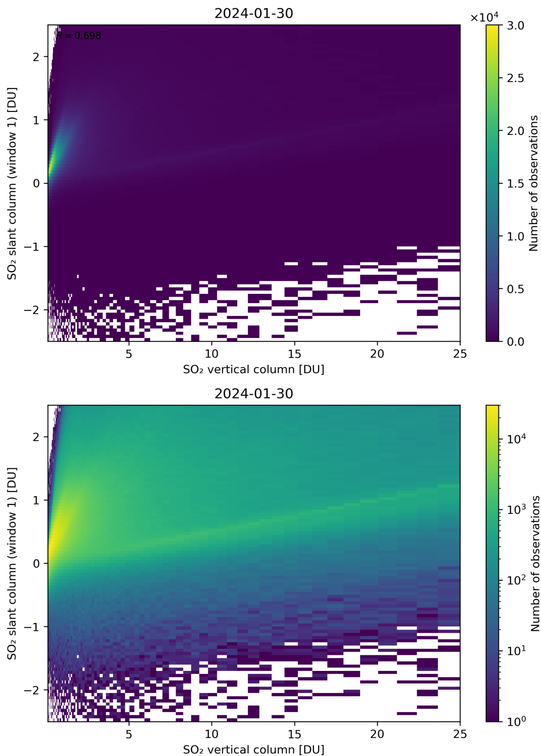
Figure 300: Scatter density plot of “SO 2 vertical column” against “SO 2 slant column (window 1)” for 2024-01-29 to 2024-01-31.
