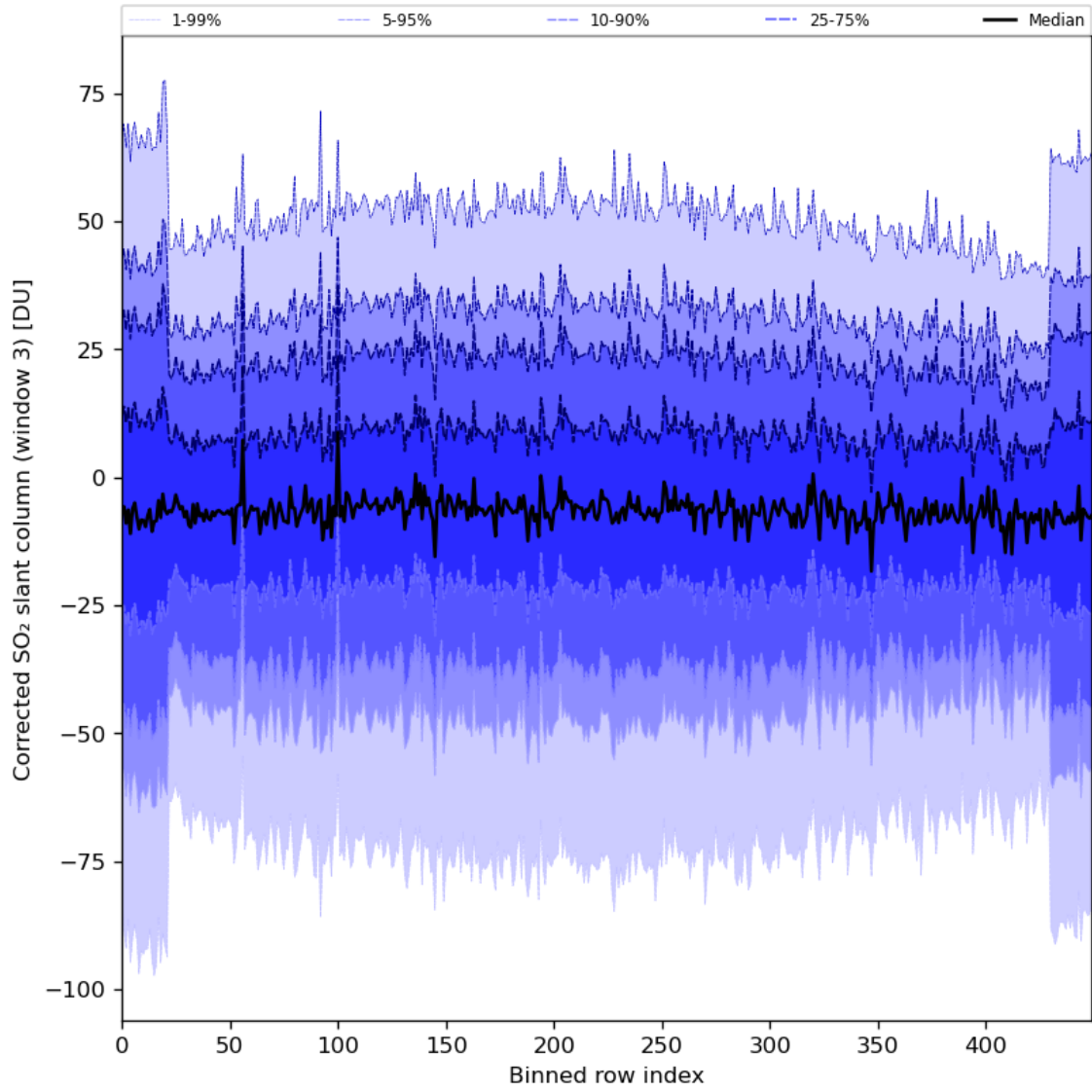
Figure 89: Along track statistics of “Corrected SO 2 slant column (window 3)” for 2024-01-29 to 2024-01-31
