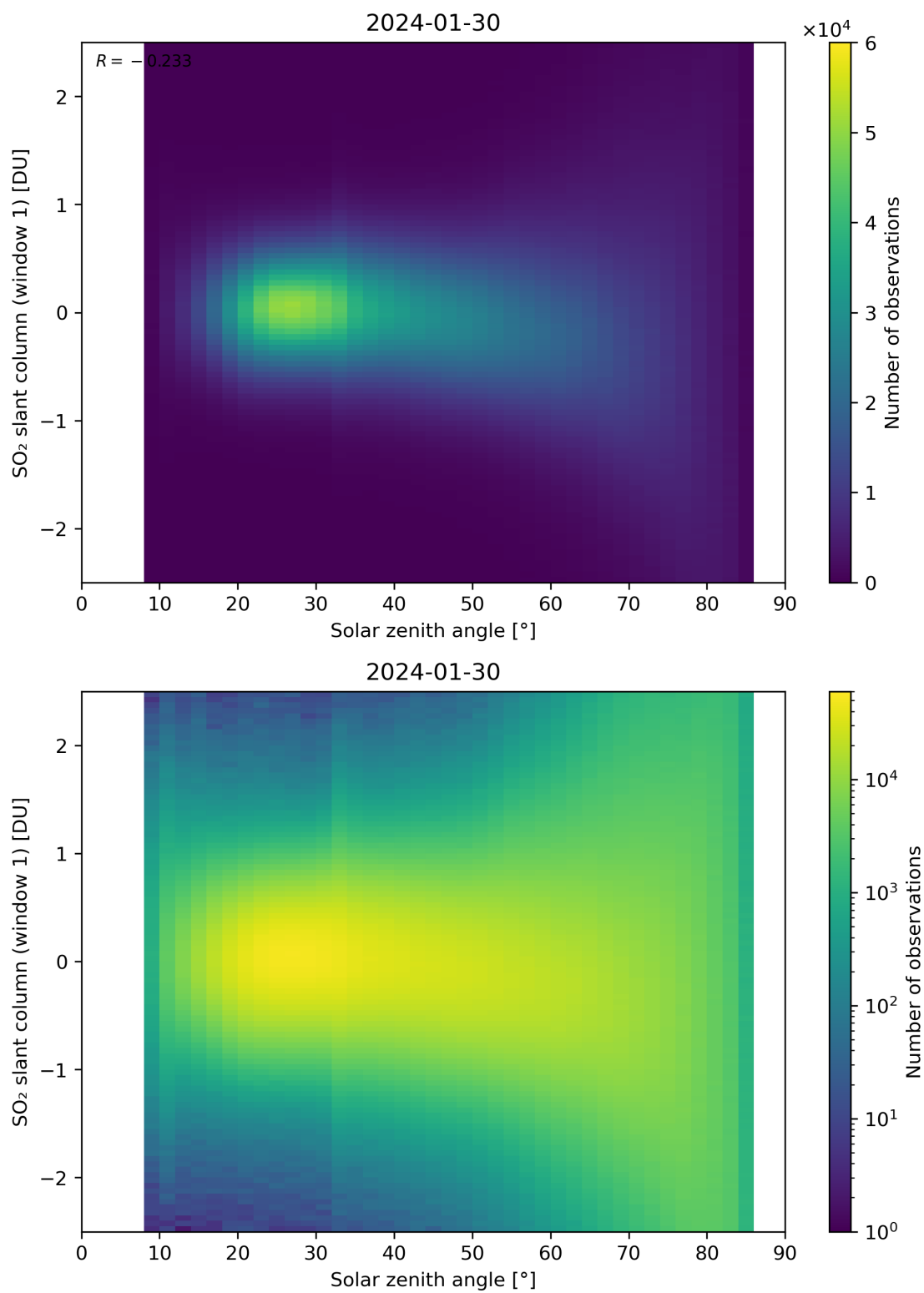
Figure 169: Scatter density plot of “Solar zenith angle” against “SO 2 slant column (window 1)” for 2024-01-29 to 2024-01-31.
