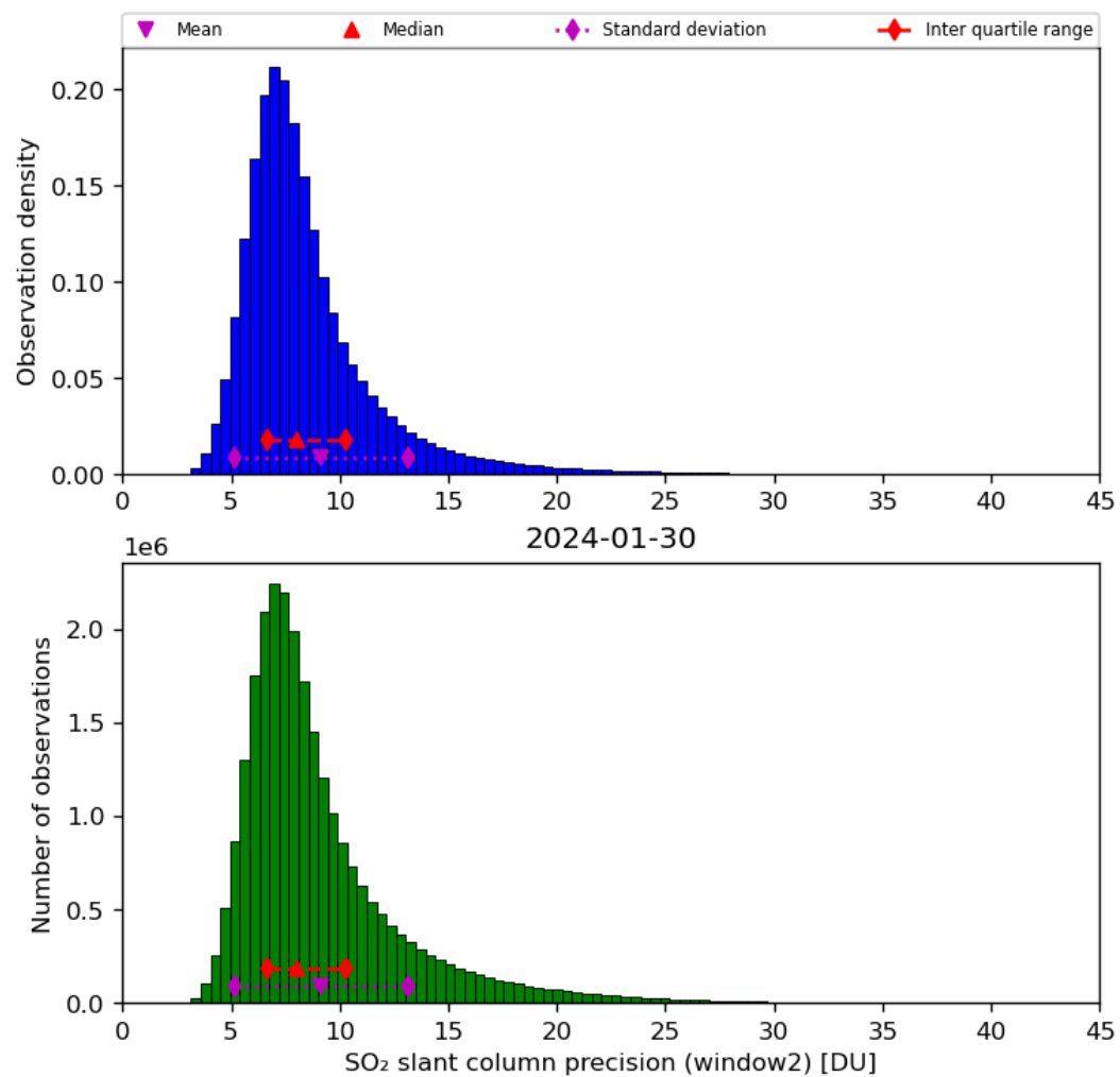
Figure 61: Histogram of “SO 2 slant column precision (window2)” for 2024-01-29 to 2024-01-31
