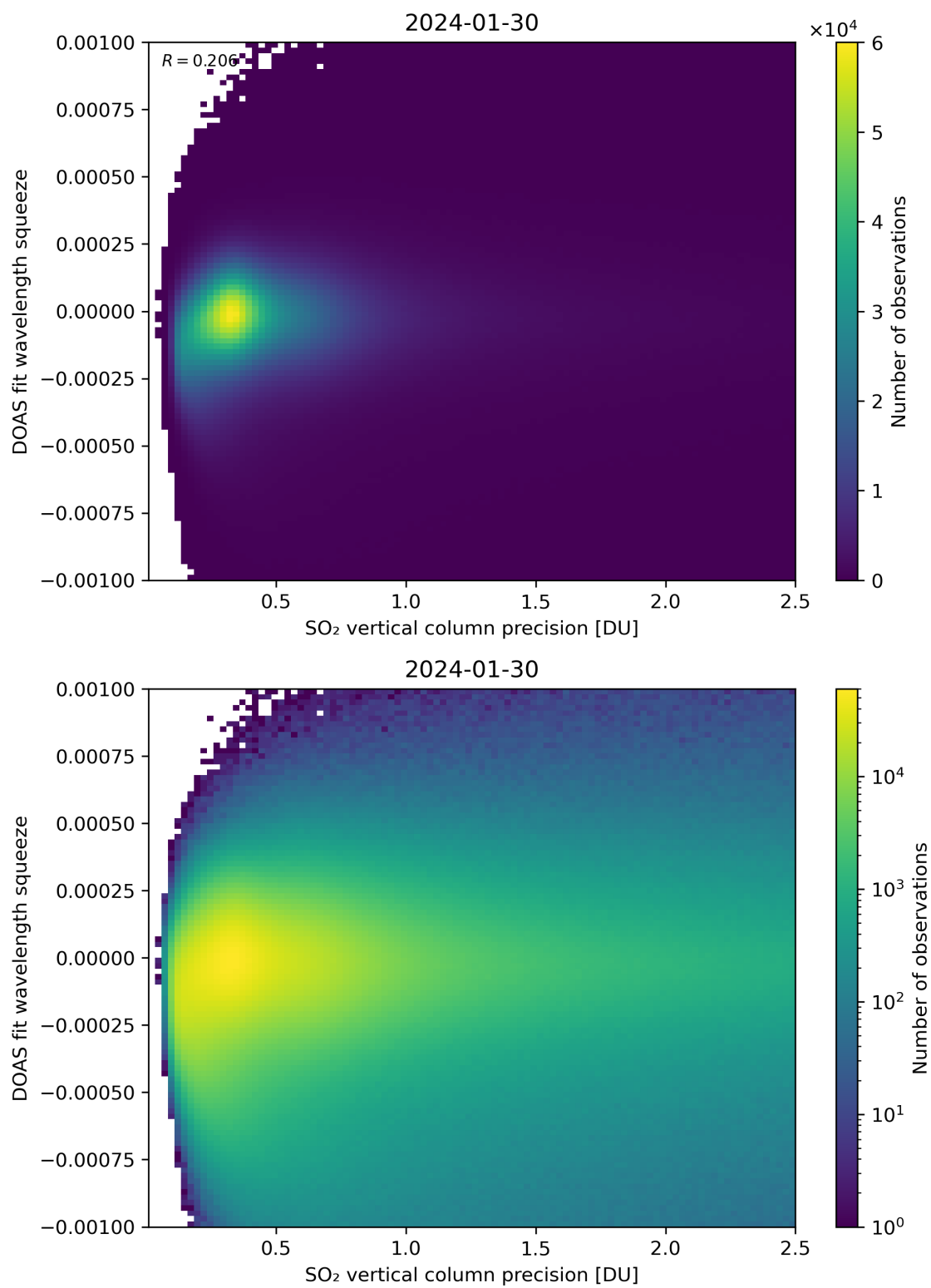
Figure 283: Scatter density plot of “SO 2 vertical column precision” against “DOAS fit wavelength squeeze” for 2024-01-29 to 2024-01-31.
