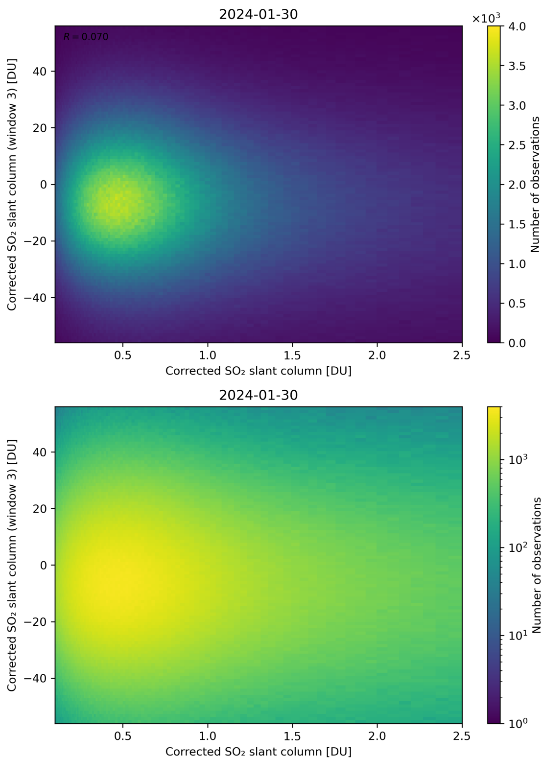
Figure 186: Scatter density plot of “Corrected SO 2 slant column” against “Corrected SO 2 slant column (window 3)” for 2024-01-29 to 2024-01-31.
