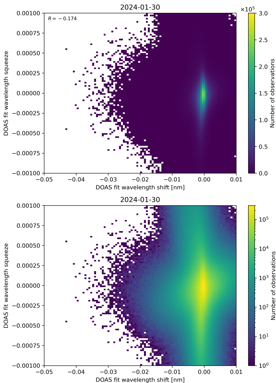
Figure 127: Scatter density plot of “DOAS fit wavelength shift” against “DOAS fit wavelength squeeze” for 2024-01-29 to 2024-01-31.
