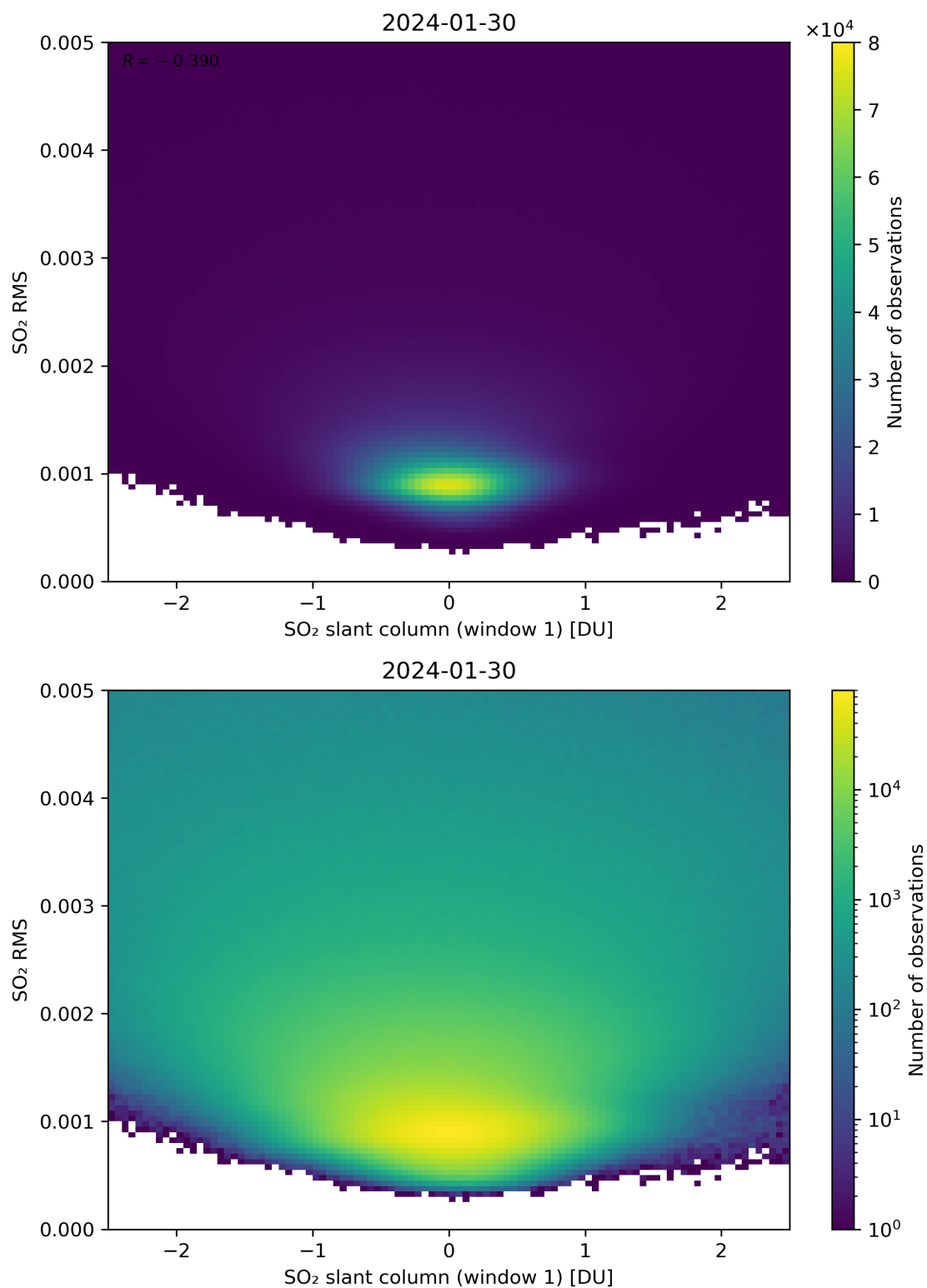
Figure 217: Scatter density plot of “SO 2 slant column (window 1)” against “SO 2 RMS” for 2024-01-29 to 2024-01-31.
