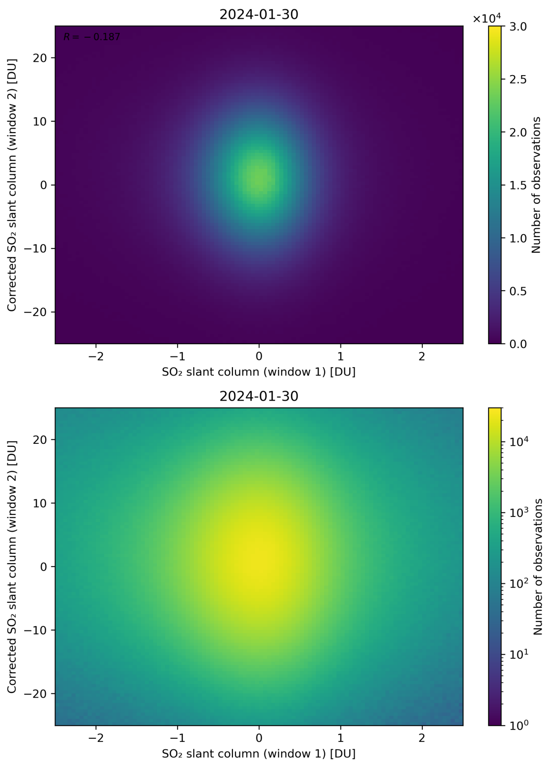
Figure 233: Scatter density plot of “SO 2 slant column (window 1)” against “Corrected SO 2 slant column (window 2)” for 2024-01-29 to 2024-01-31.
