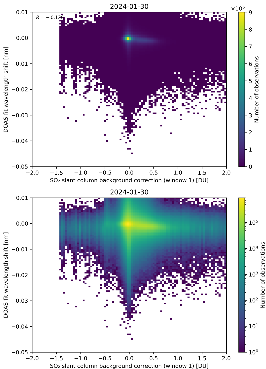
Figure 100: Scatter density plot of “SO 2 slant column background correction (window 1)” against “DOAS fit wavelength shift” for 2024-01-29 to 2024-01-31.
