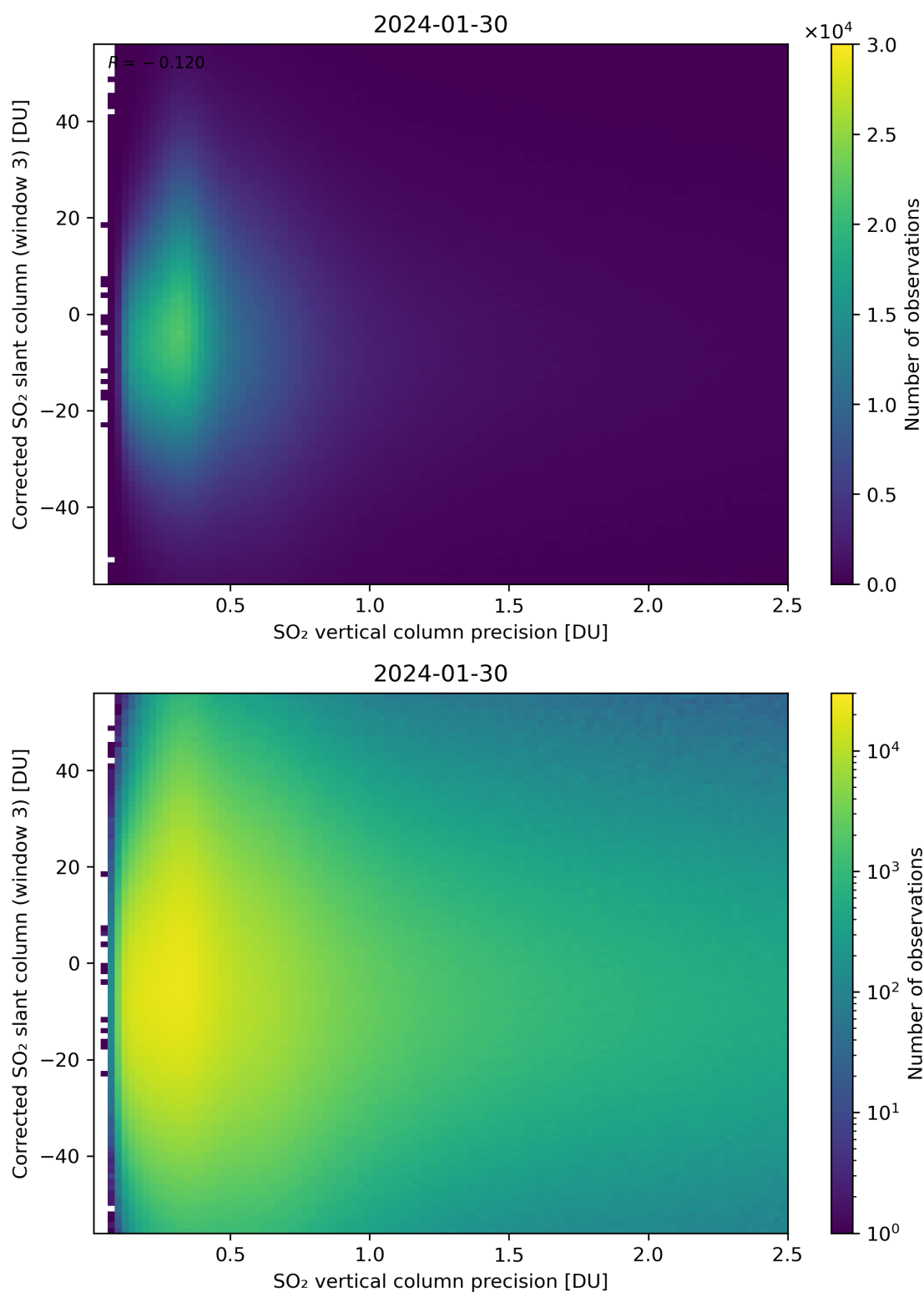
Figure 288: Scatter density plot of “SO 2 vertical column precision” against “Corrected SO 2 slant column (window 3)” for 2024-01-29 to 2024-01-31.
