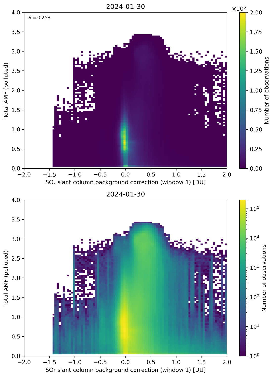
Figure 109: Scatter density plot of “SO 2 slant column background correction (window 1)” against “Total AMF (polluted)” for 2024-01-29 to 2024-01-31.
