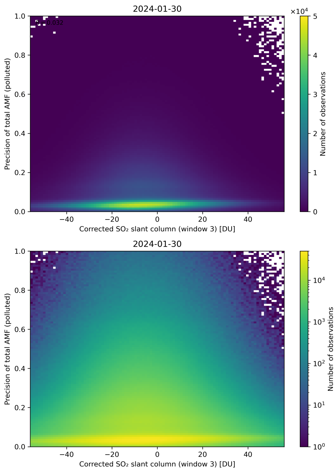
Figure 211: Scatter density plot of “Corrected SO 2 slant column (window 3)” against “Precision of total AMF (polluted)” for 2024-01-29 to 2024-01-31.
