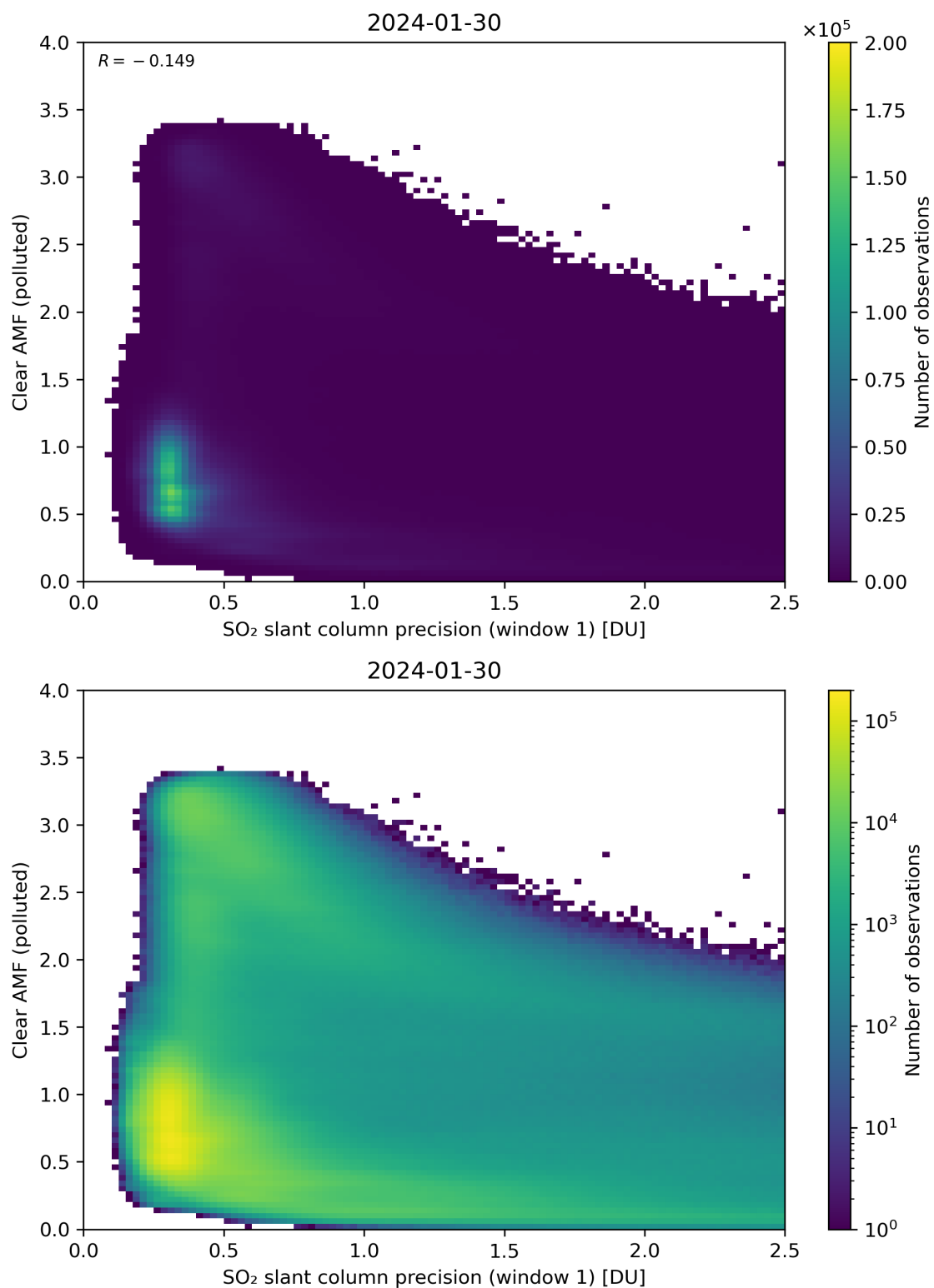
Figure 224: Scatter density plot of “SO 2 slant column precision (window 1)” against “Clear AMF (polluted)” for 2024-01-29 to 2024-01-31.
