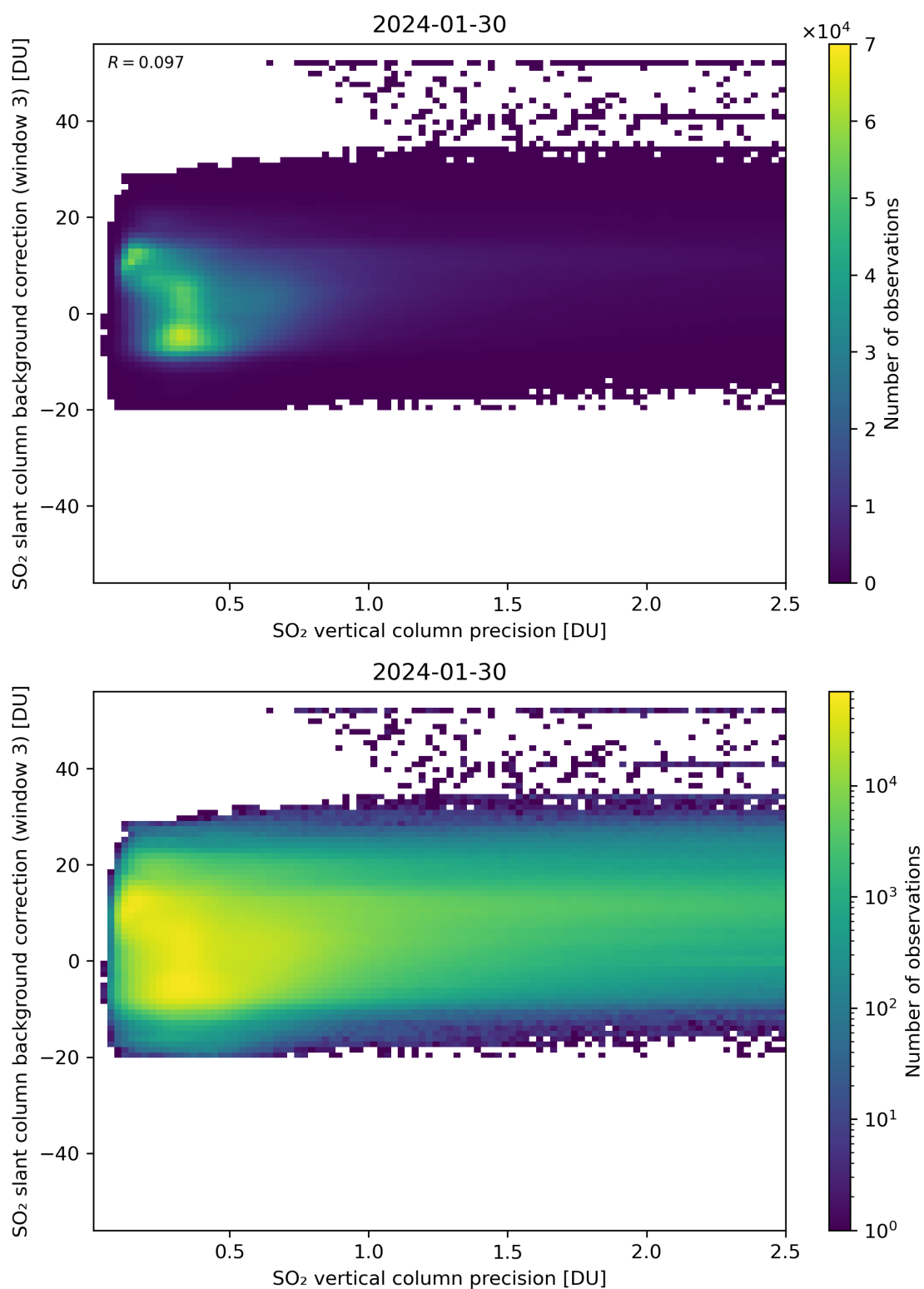
Figure 281: Scatter density plot of “SO 2 vertical column precision” against “SO 2 slant column background correction (window 3)” for 2024-01-29 to 2024-01-31.
