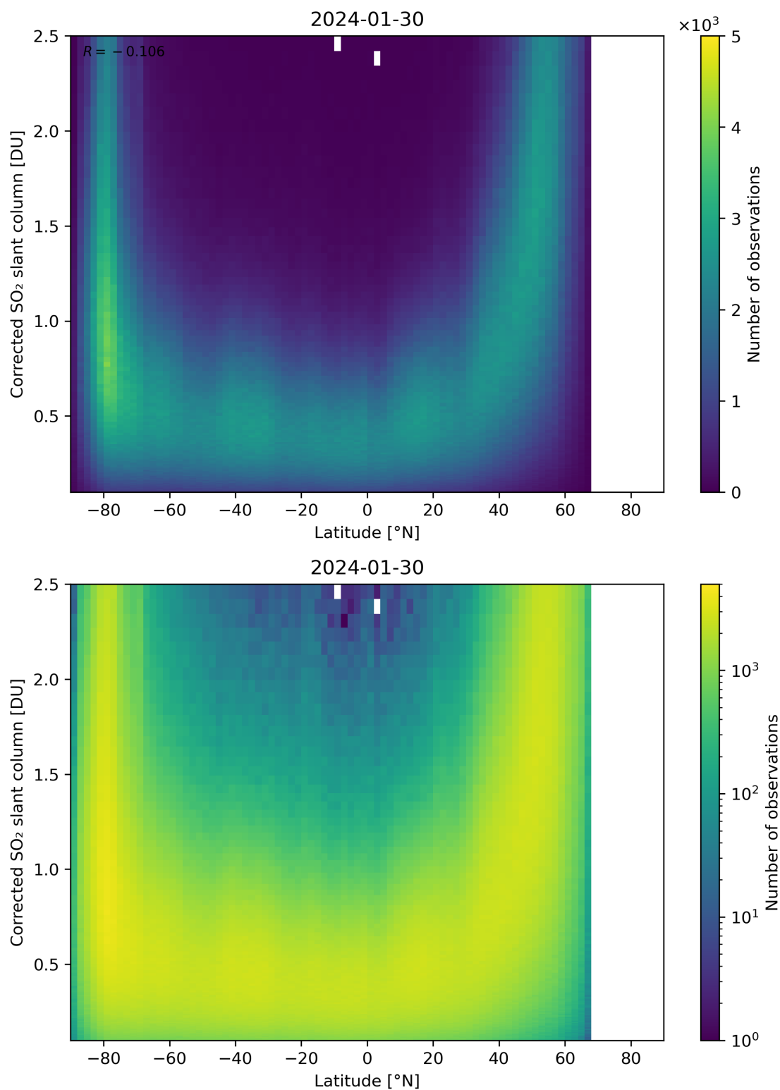
Figure 146: Scatter density plot of “Latitude” against “Corrected SO 2 slant column” for 2024-01-29 to 2024-01-31.
