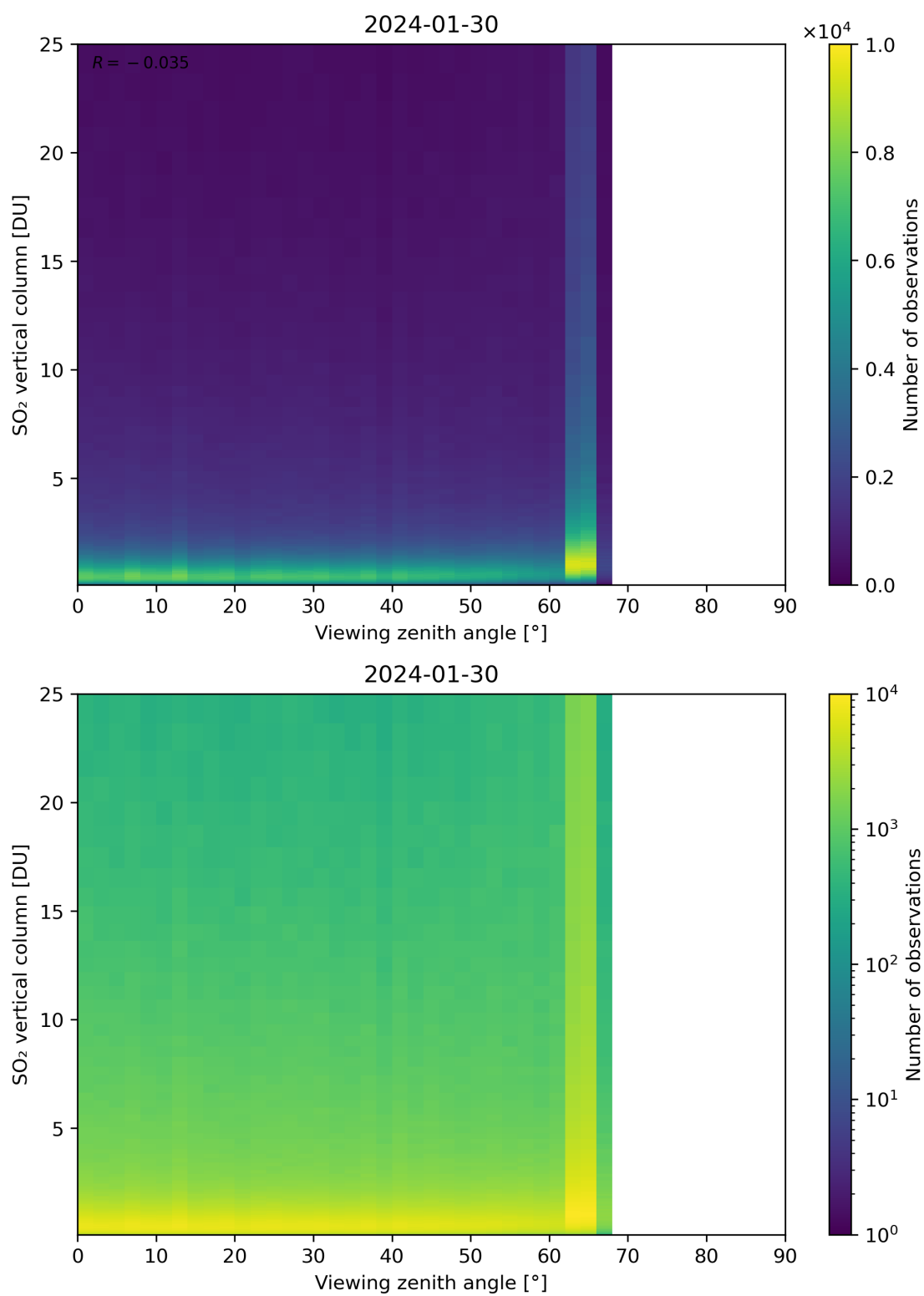
Figure 327: Scatter density plot of “Viewing zenith angle” against “SO 2 vertical column” for 2024-01-29 to 2024-01-31.
