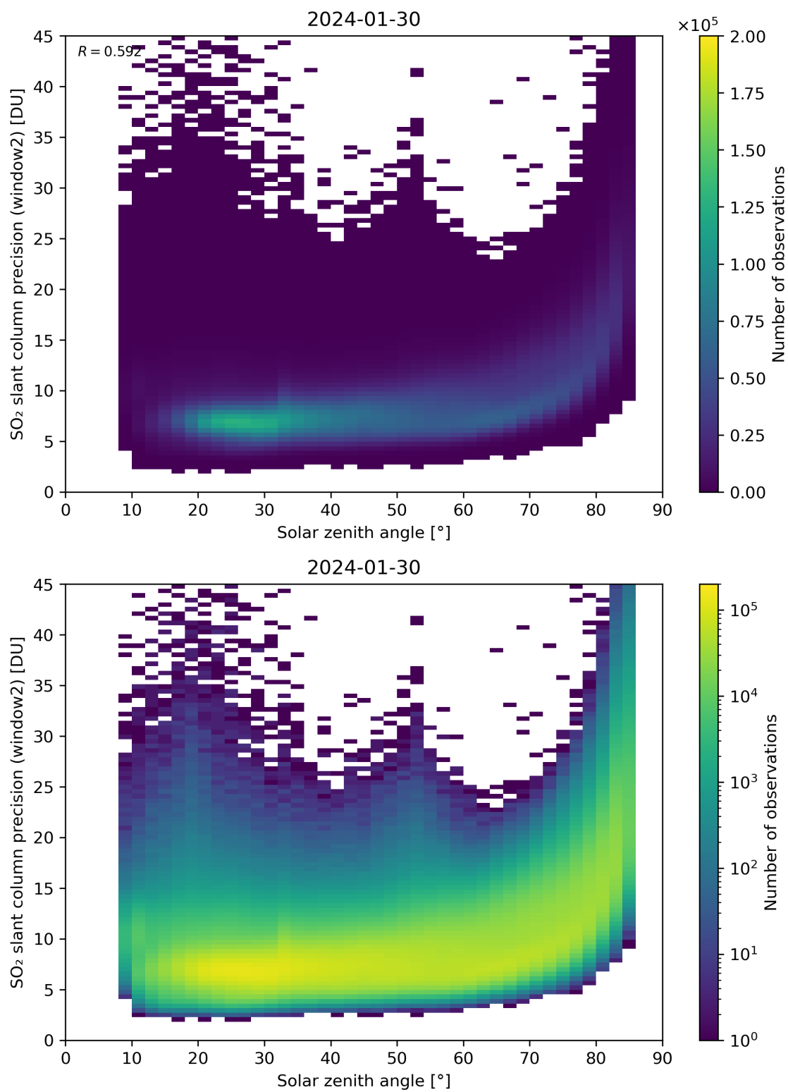
Figure 171: Scatter density plot of “Solar zenith angle” against “SO 2 slant column precision (window2)” for 2024-01-29 to 2024-01-31.
