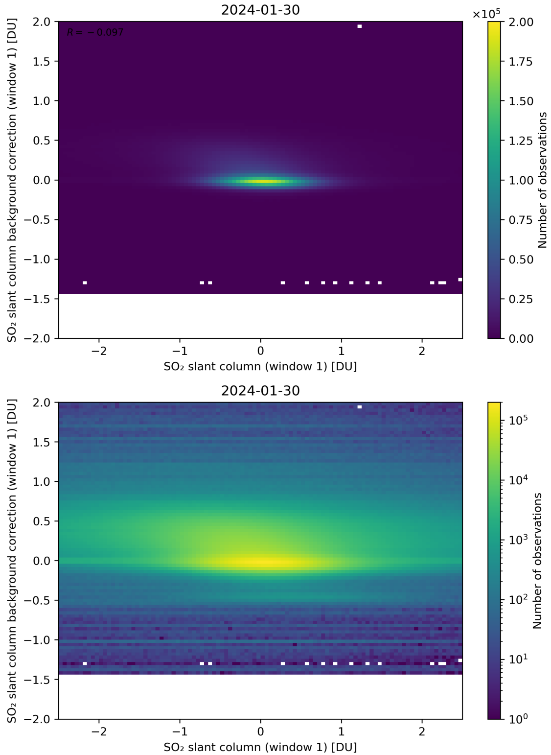
Figure 212: Scatter density plot of “SO 2 slant column (window 1)” against “SO 2 slant column background correction (window 1)” for 2024-01-29 to 2024-01-31.
