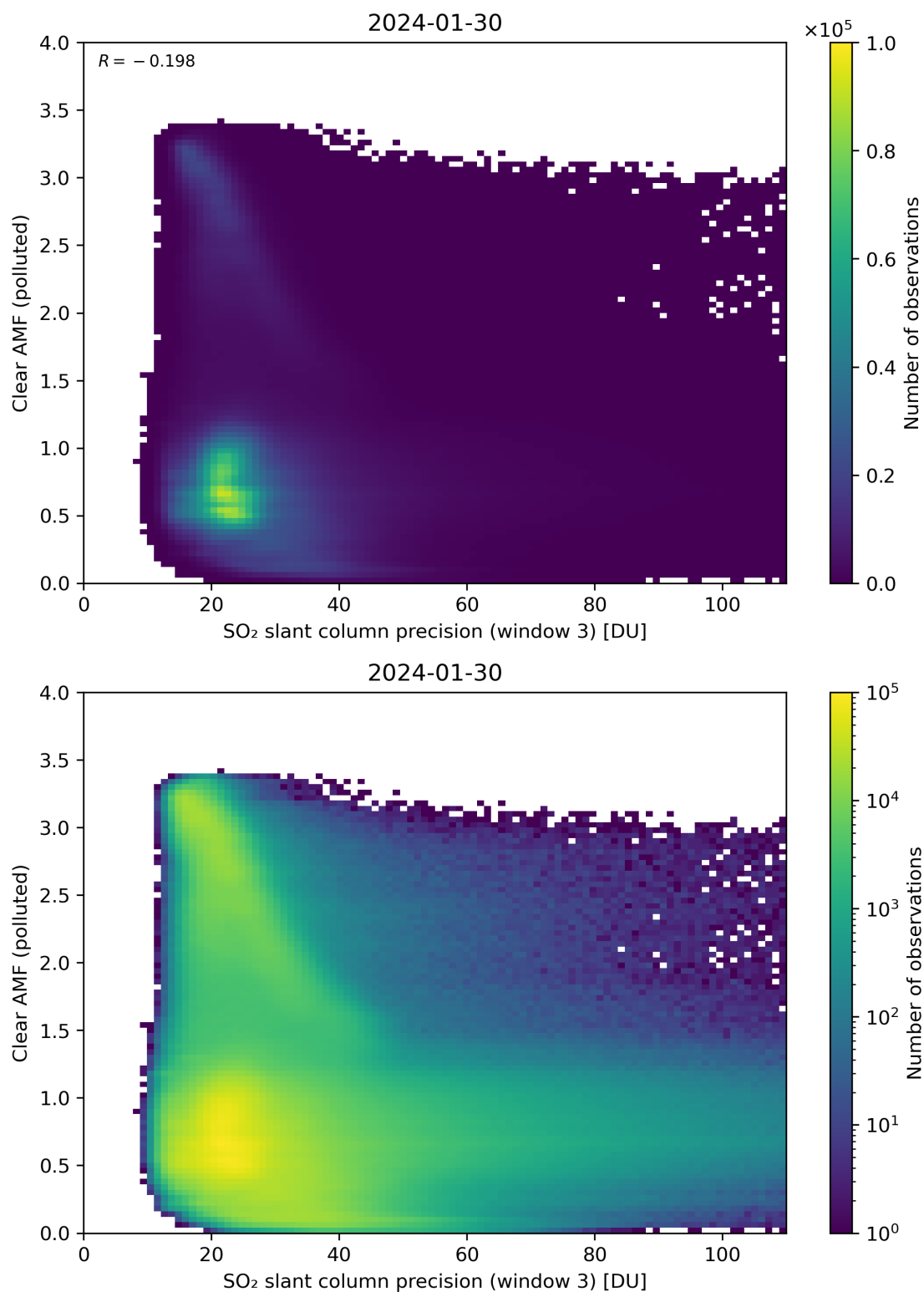
Figure 261: Scatter density plot of “SO 2 slant column precision (window 3)” against “Clear AMF (polluted)” for 2024-01-29 to 2024-01-31.
