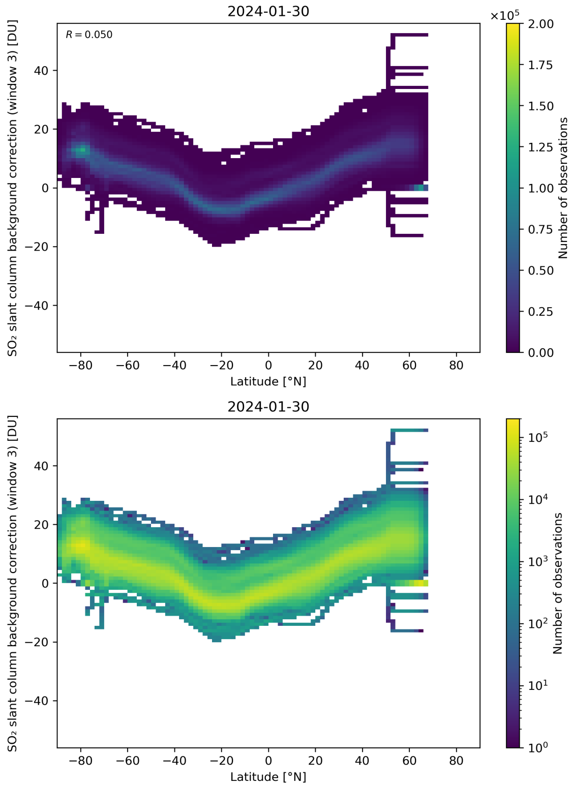
Figure 141: Scatter density plot of “Latitude” against “SO 2 slant column background correction (window 3)” for 2024-01-29 to 2024-01-31.
