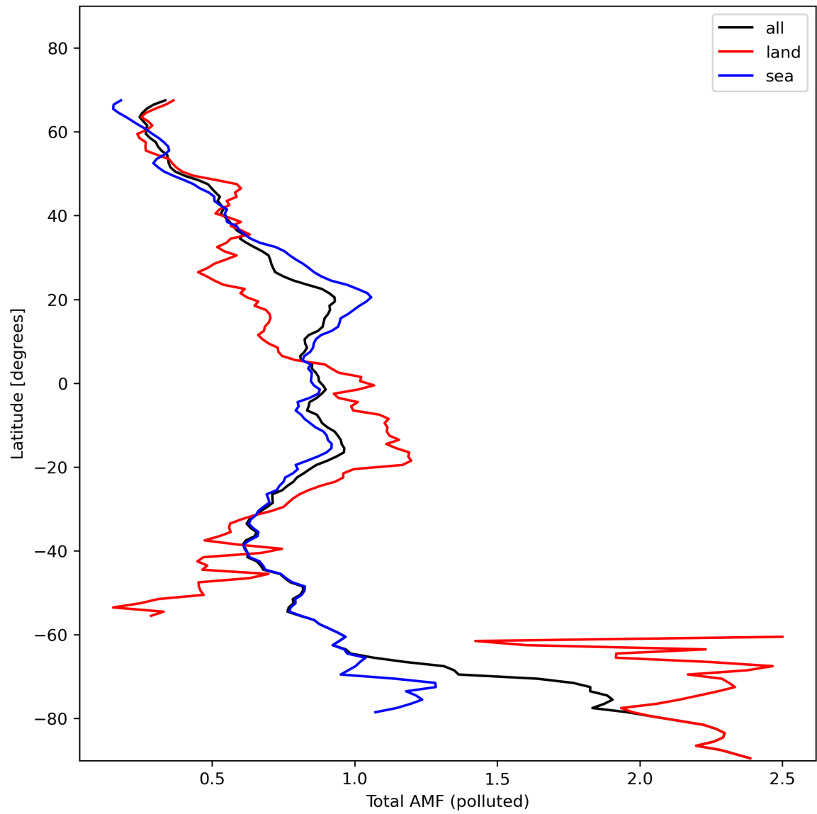
Figure 48: Zonal average of “Total AMF (polluted)” for 2024-01-29 to 2024-01-31.
