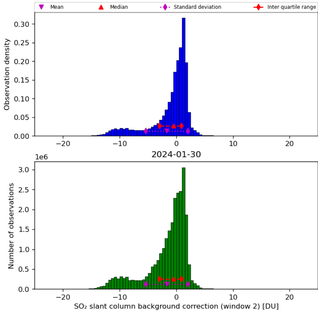
Figure 63: Histogram of “SO 2 slant column background correction (window 2)” for 2024-01-29 to 2024-01-31
