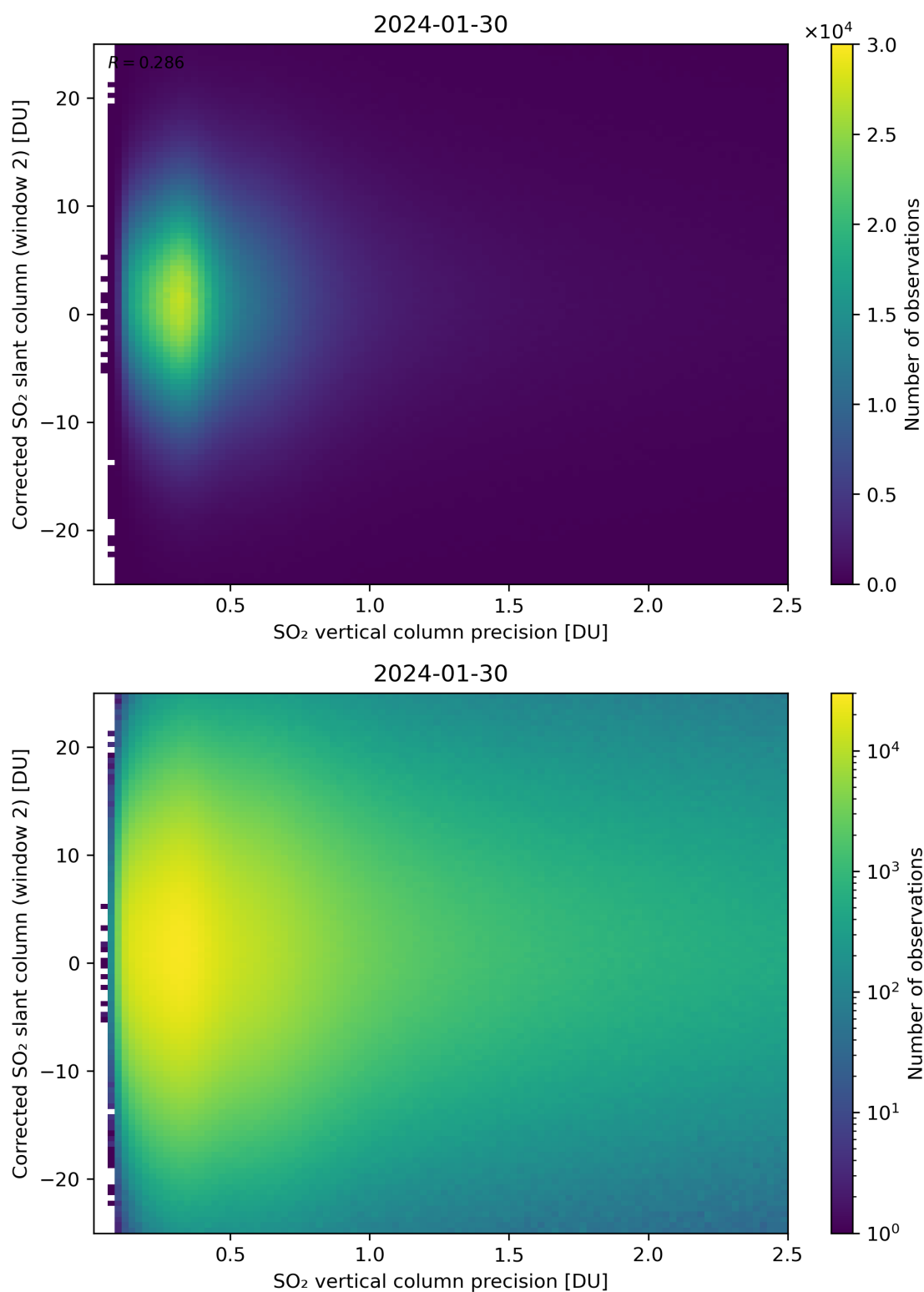
Figure 287: Scatter density plot of “SO 2 vertical column precision” against “Corrected SO 2 slant column (window 2)” for 2024-01-29 to 2024-01-31.
