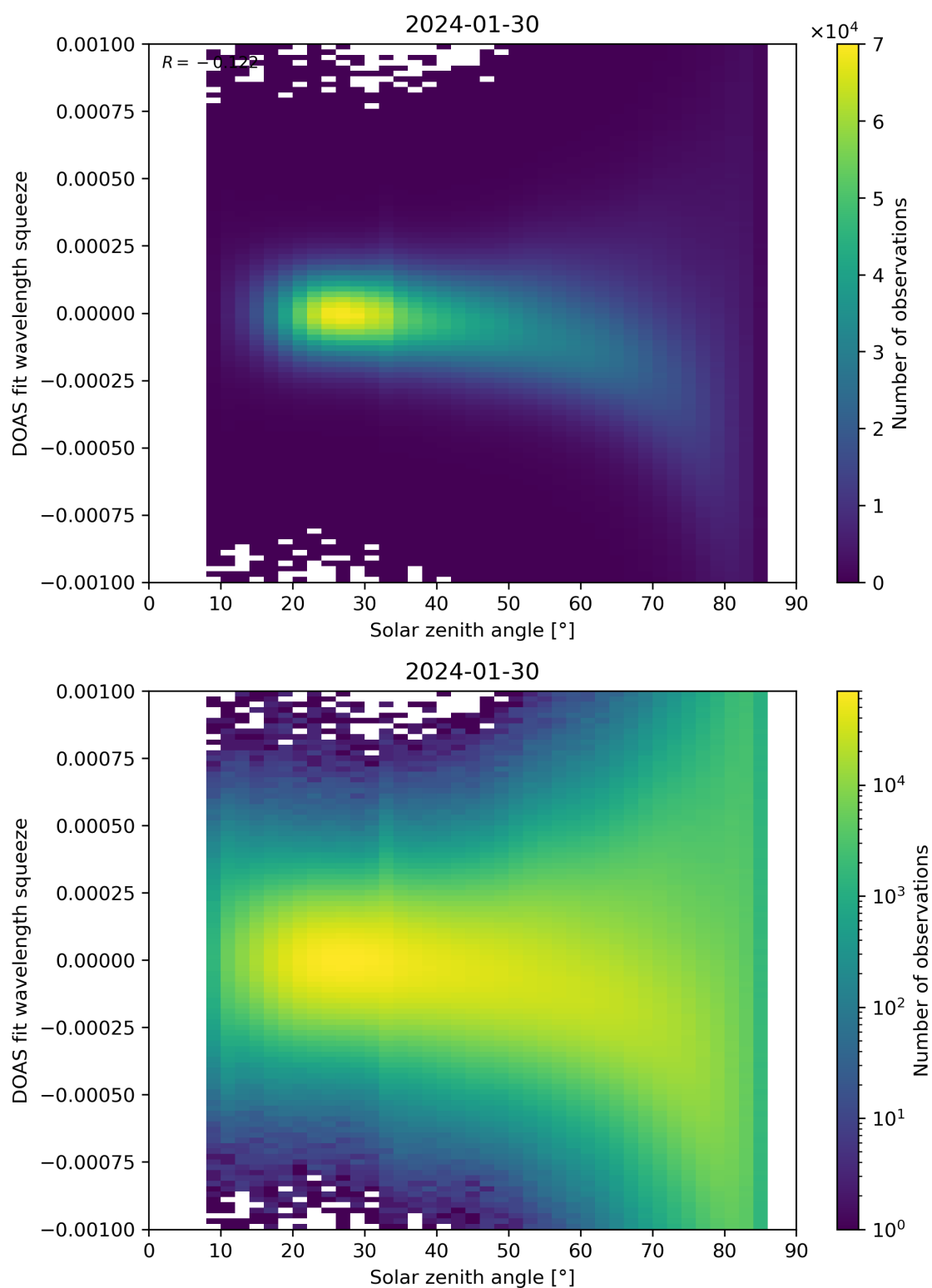
Figure 162: Scatter density plot of “Solar zenith angle” against “DOAS fit wavelength squeeze” for 2024-01-29 to 2024-01-31.
