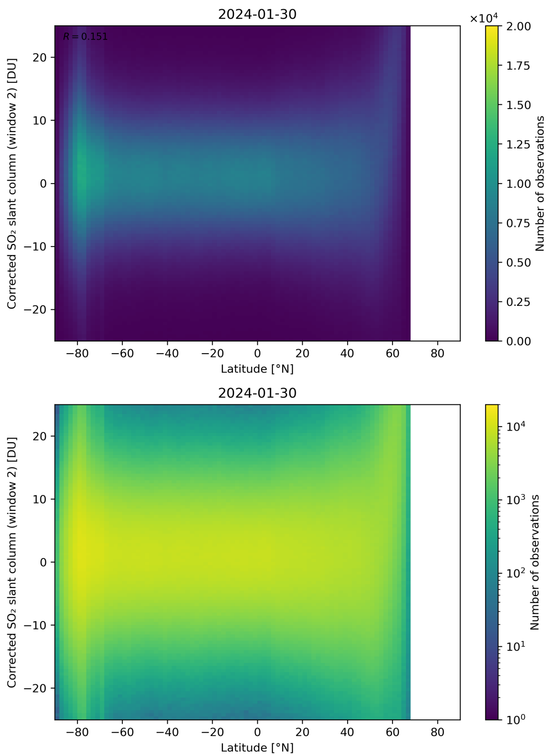
Figure 147: Scatter density plot of “Latitude” against “Corrected SO 2 slant column (window 2)” for 2024-01-29 to 2024-01-31.
