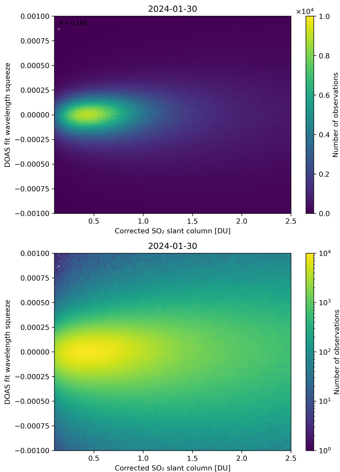
Figure 182: Scatter density plot of “Corrected SO 2 slant column” against “DOAS fit wavelength squeeze” for 2024-01-29 to 2024-01-31.
