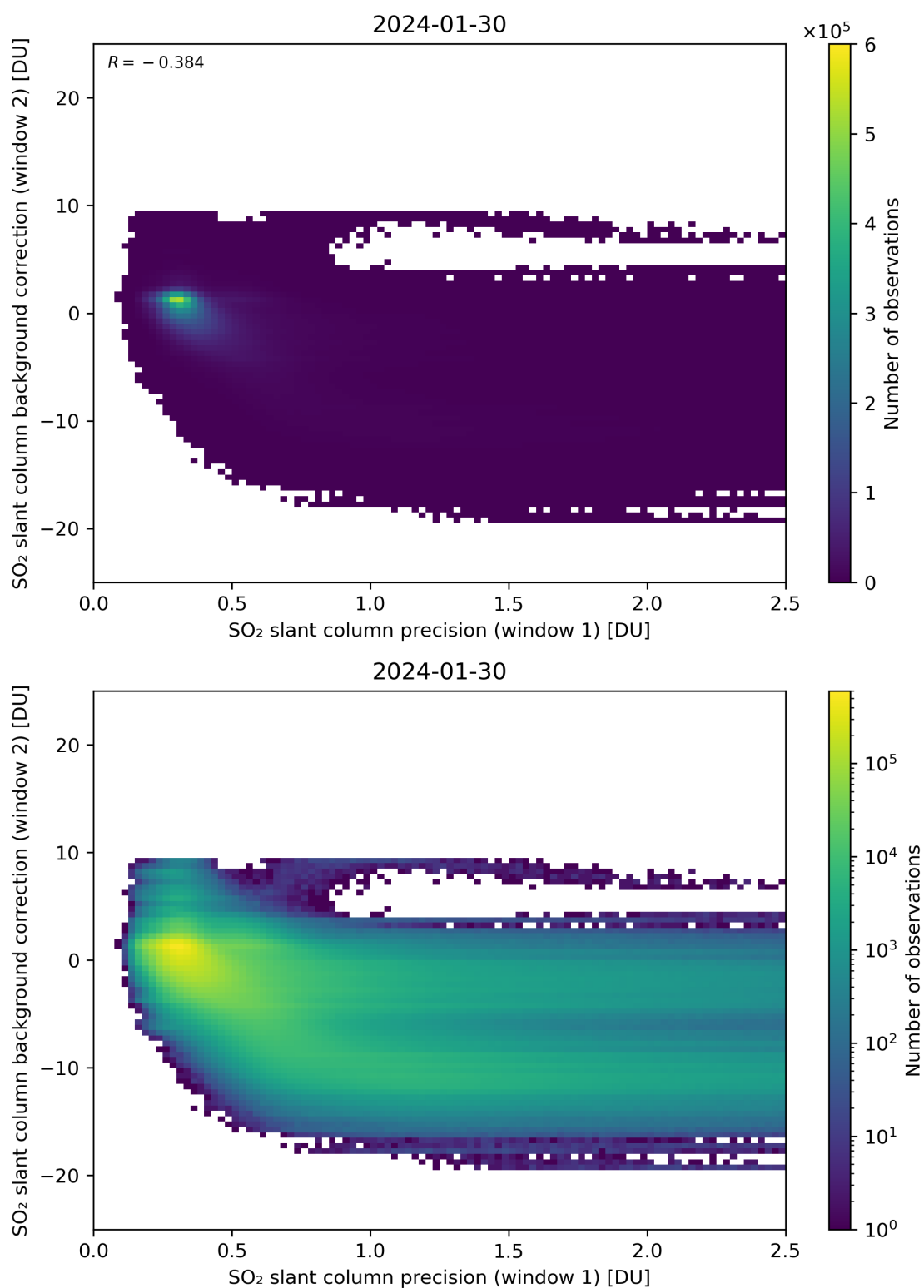
Figure 219: Scatter density plot of “SO 2 slant column precision (window 1)” against “SO 2 slant column background correction (window 2)” for 2024-01-29 to 2024-01-31.
