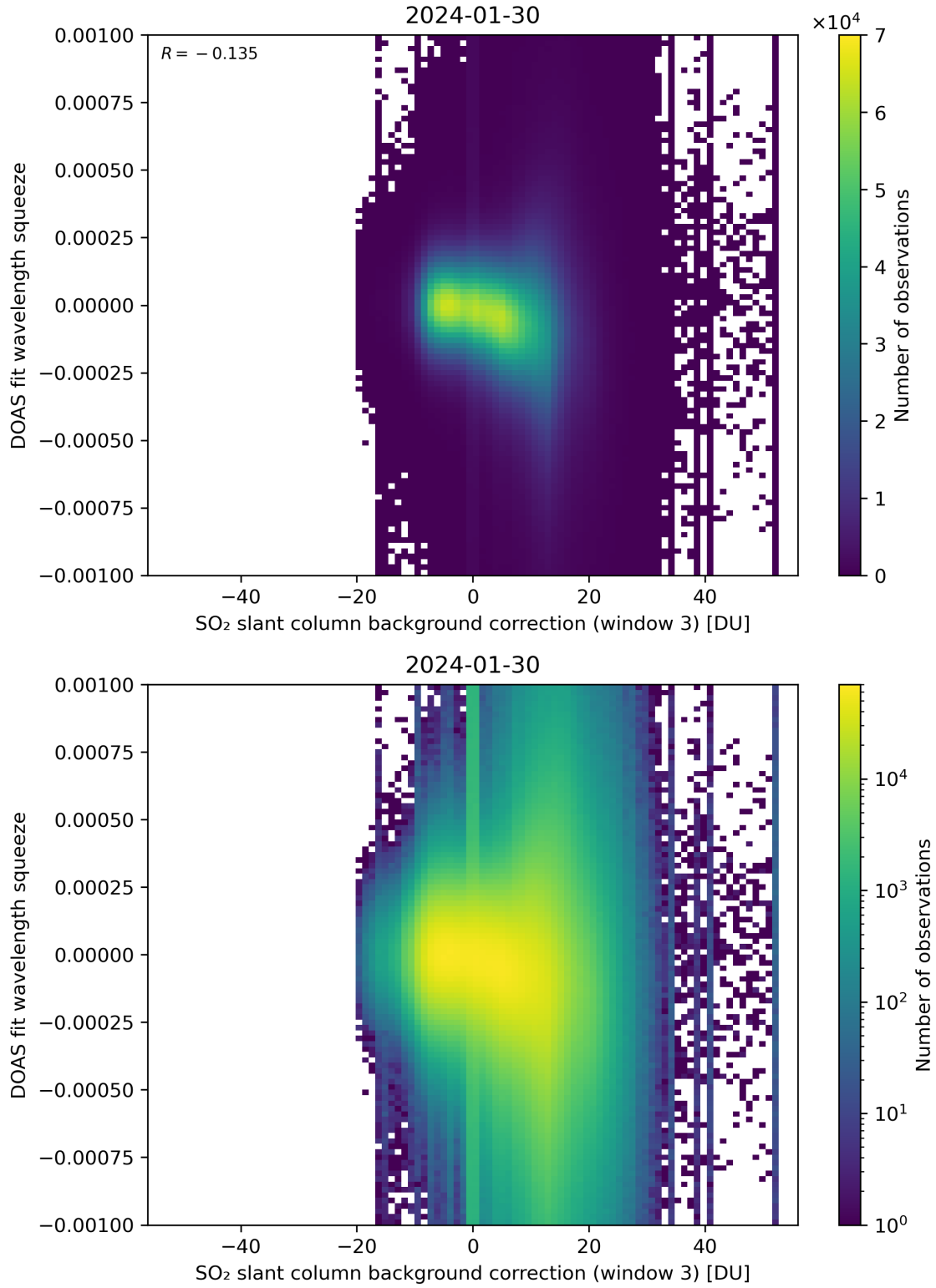
Figure 122: Scatter density plot of “SO 2 slant column background correction (window 3)” against “DOAS fit wavelength squeeze” for 2024-01-29 to 2024-01-31.
