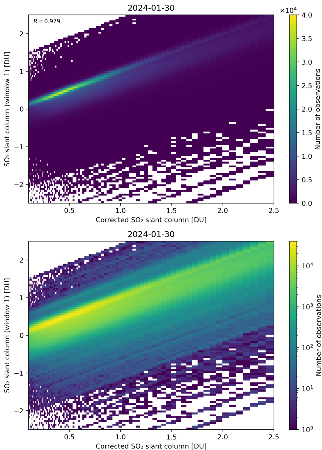
Figure 187: Scatter density plot of “Corrected SO 2 slant column” against “SO 2 slant column (window 1)” for 2024-01-29 to 2024-01-31.
