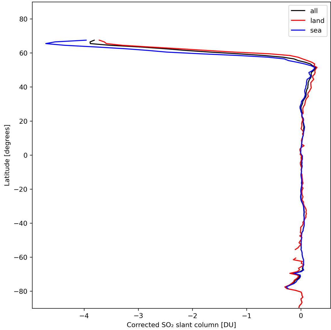
Figure 32: Zonal average of “Corrected SO 2 slant column” for 2024-01-29 to 2024-01-31.
