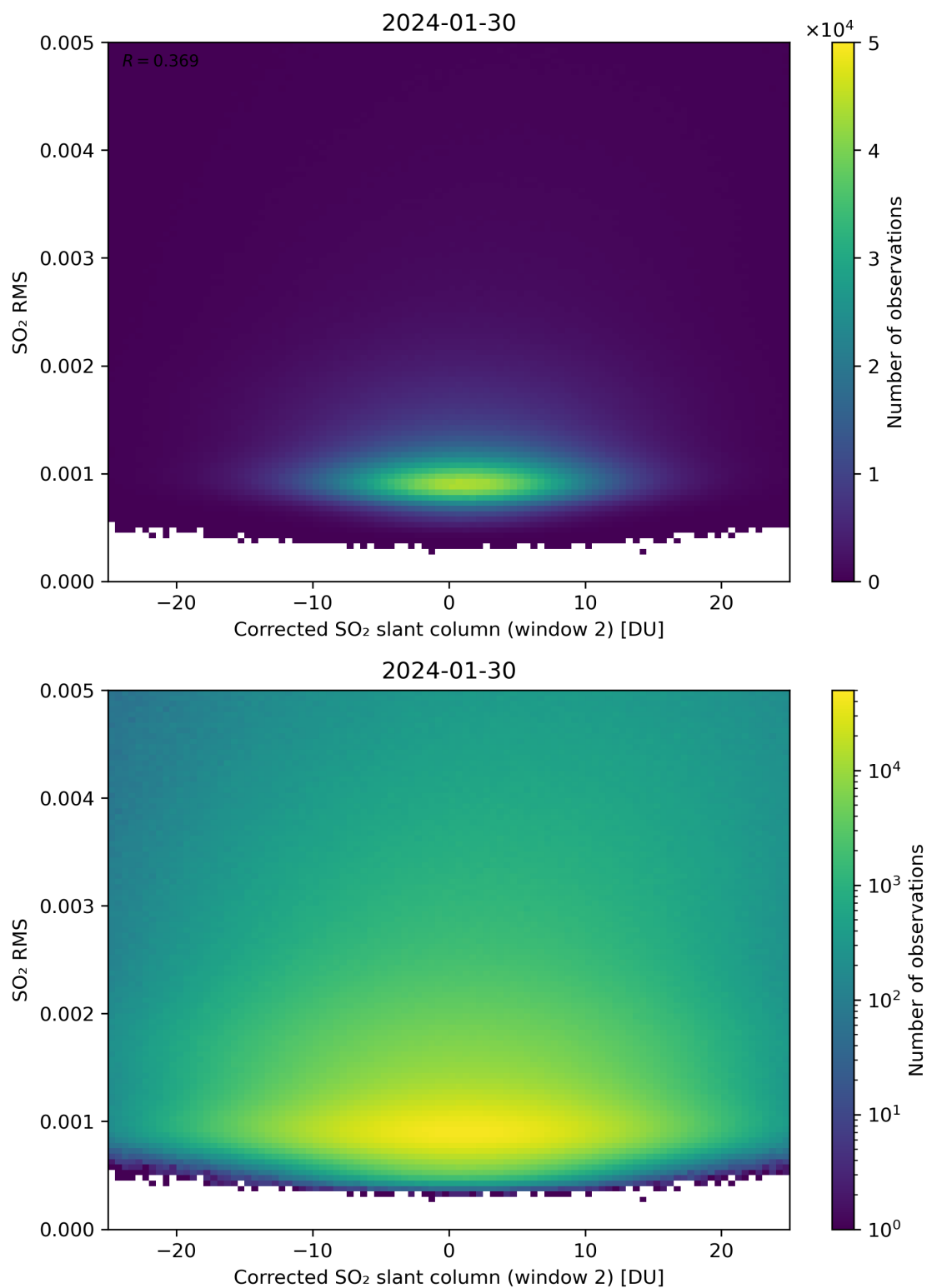
Figure 198: Scatter density plot of “Corrected SO 2 slant column (window 2)” against “SO 2 RMS” for 2024-01-29 to 2024-01-31.
