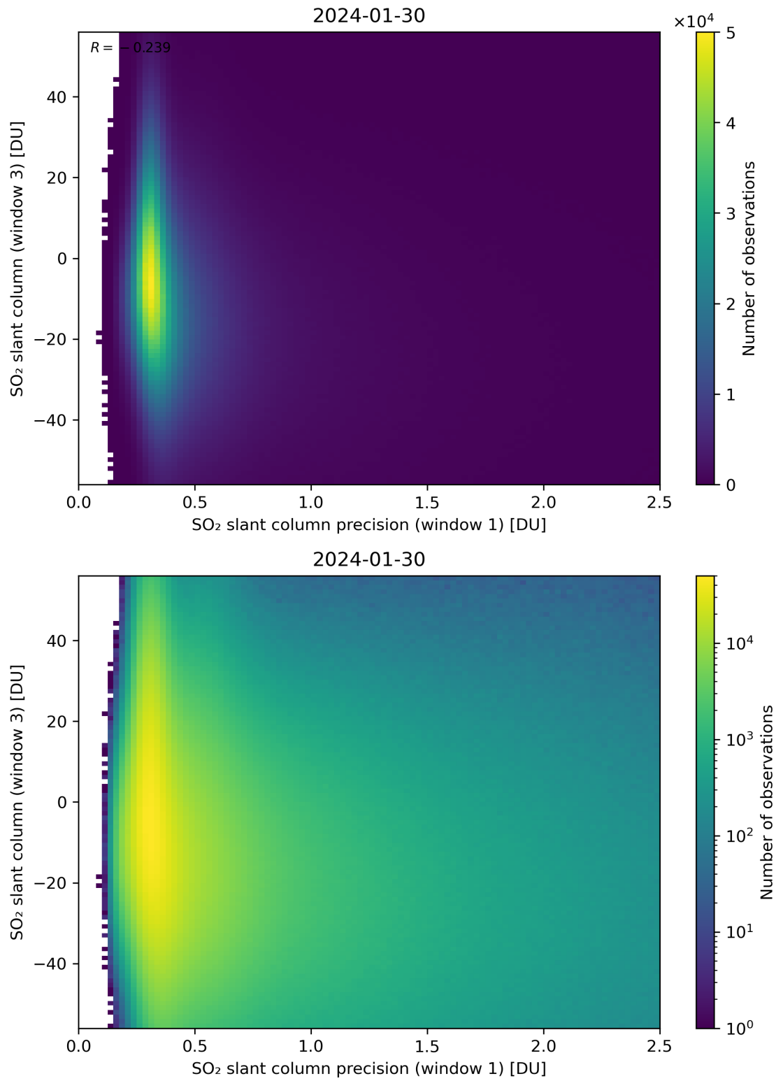
Figure 228: Scatter density plot of “SO 2 slant column precision (window 1)” against “SO 2 slant column (window 3)” for 2024-01-29 to 2024-01-31.
