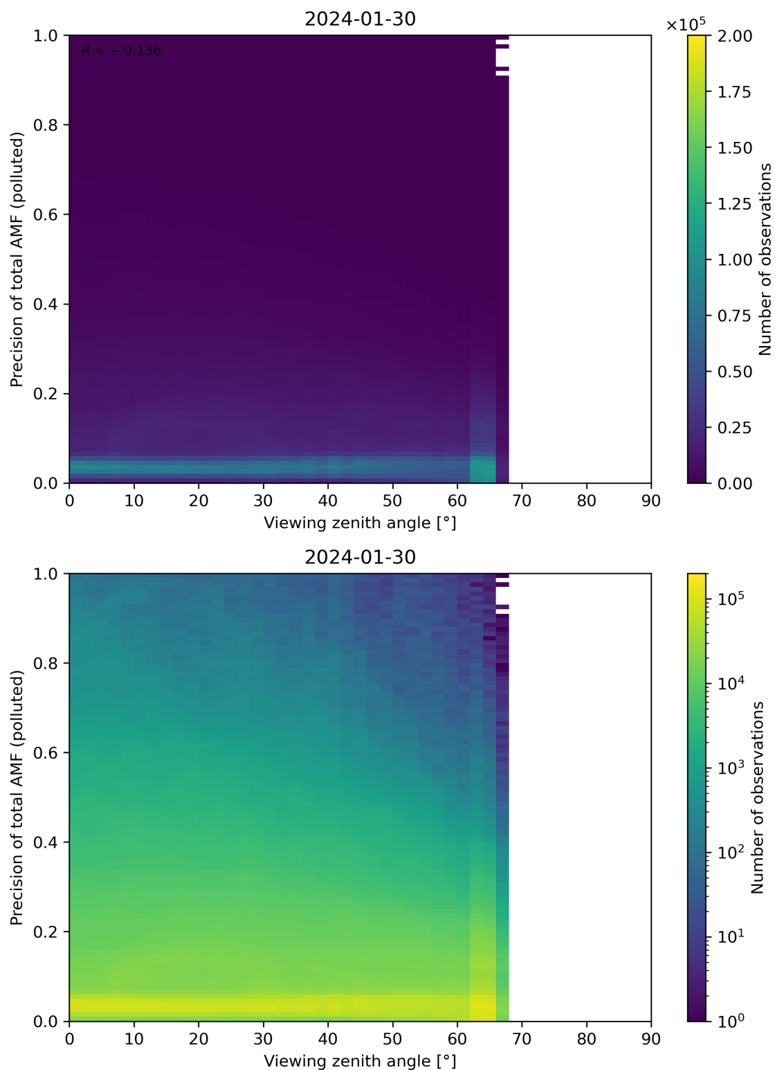
Figure 326: Scatter density plot of “Viewing zenith angle” against “Precision of total AMF (polluted)” for 2024-01-29 to 2024-01-31.
