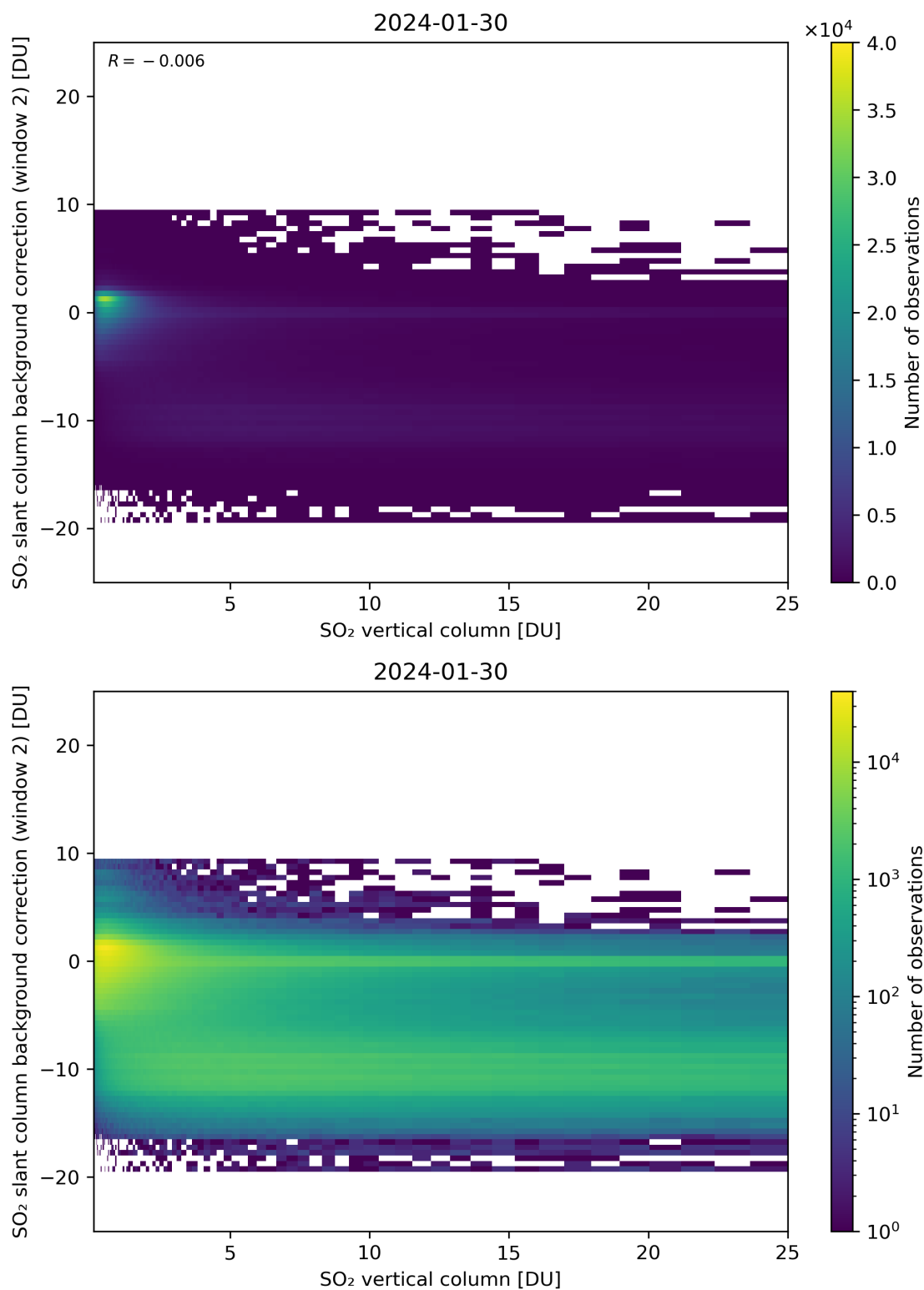
Figure 274: Scatter density plot of “SO 2 vertical column” against “SO 2 slant column background correction (window 2)” for 2024-01-29 to 2024-01-31.
