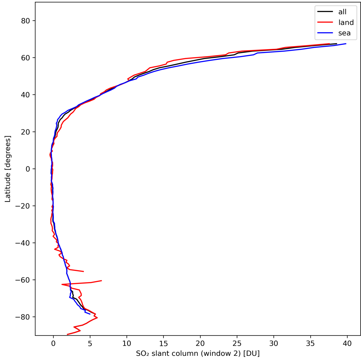
Figure 37: Zonal average of “SO 2 slant column (window 2)” for 2024-01-29 to 2024-01-31.
