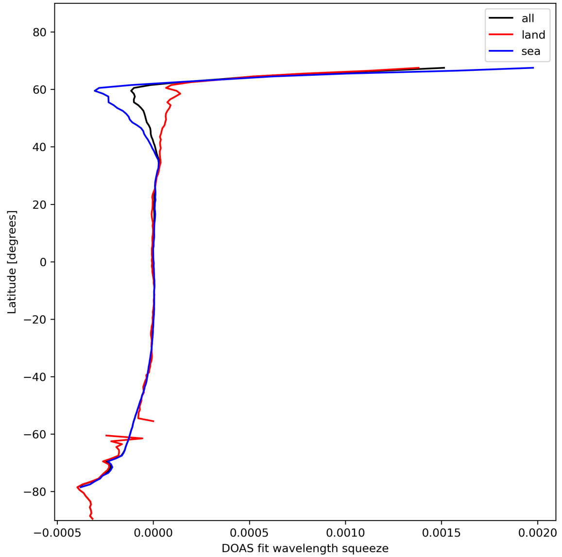
Figure 46: Zonal average of “DOAS fit wavelength squeeze” for 2024-01-29 to 2024-01-31.
