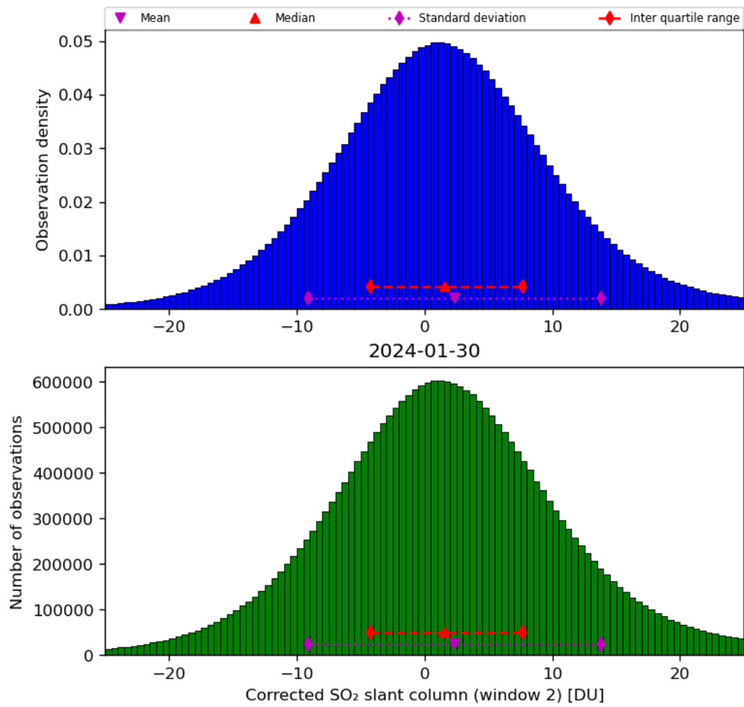
Figure 62: Histogram of “Corrected SO 2 slant column (window 2)” for 2024-01-29 to 2024-01-31
