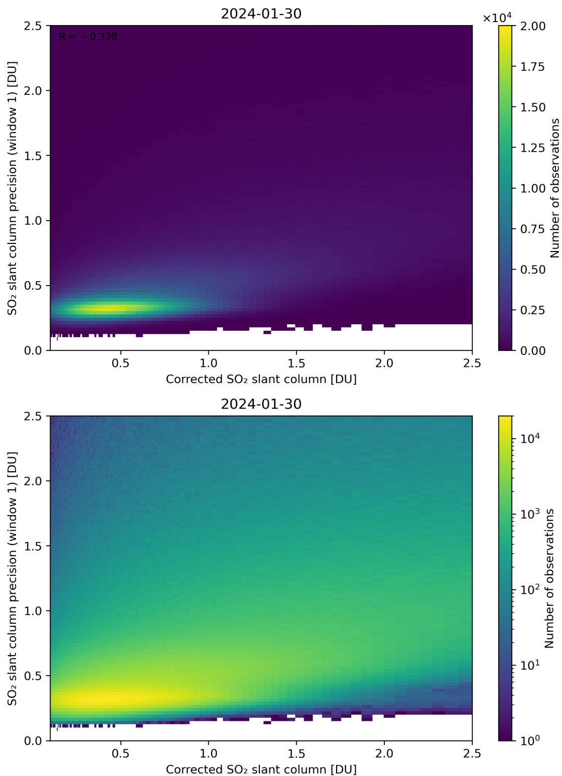
Figure 188: Scatter density plot of “Corrected SO 2 slant column” against “SO 2 slant column precision (window 1)” for 2024-01-29 to 2024-01-31.
