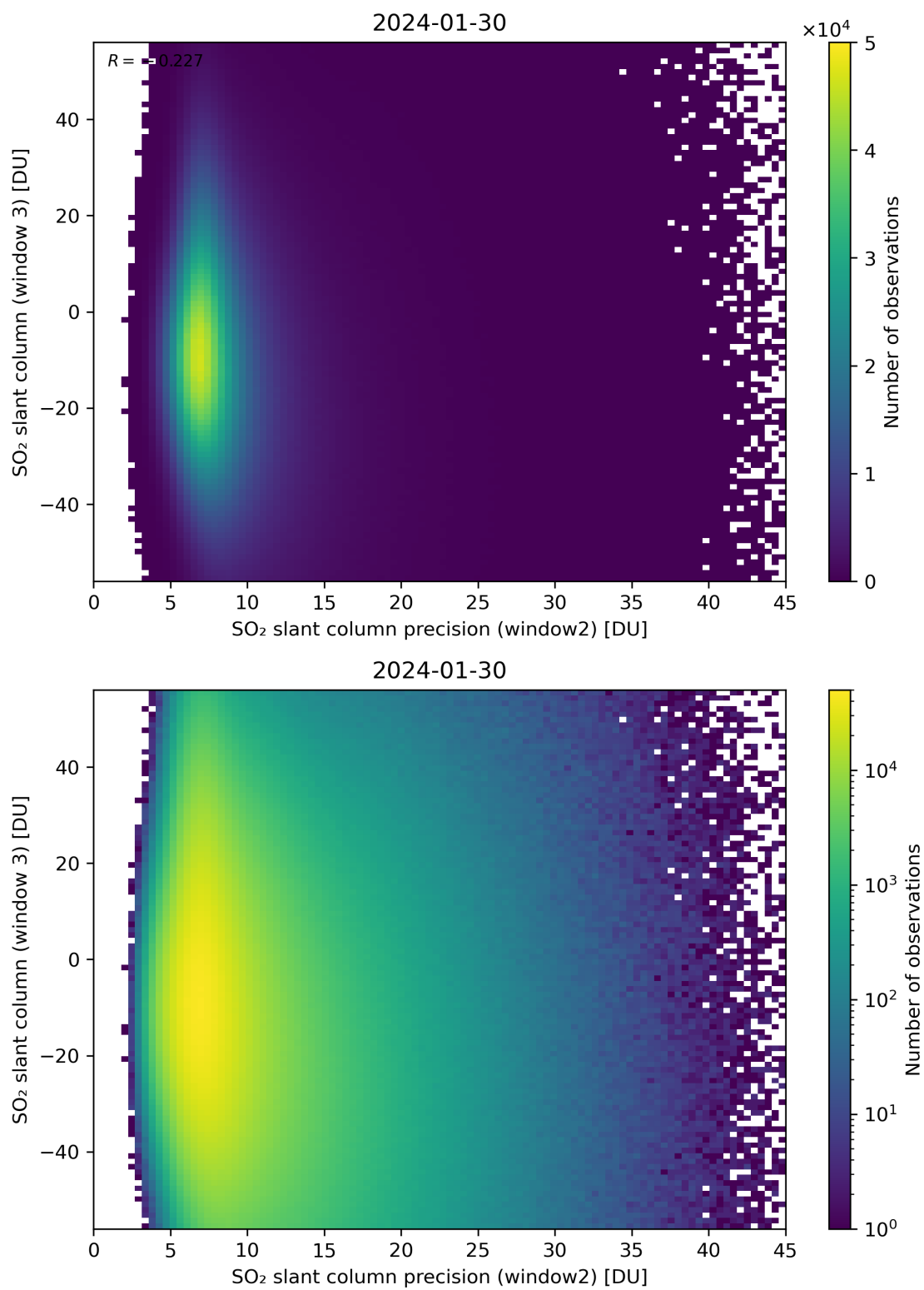
Figure 249: Scatter density plot of “SO 2 slant column precision (window2)” against “SO 2 slant column (window 3)” for 2024-01-29 to 2024-01-31.
