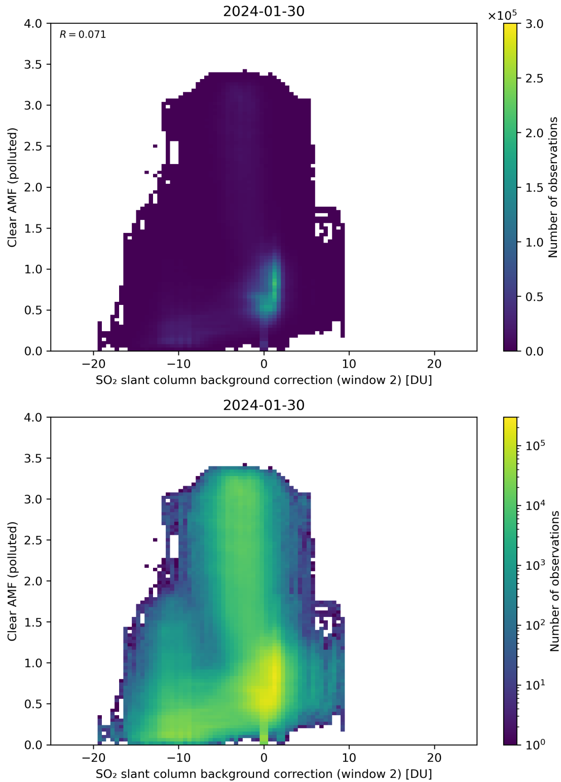
Figure 115: Scatter density plot of “SO 2 slant column background correction (window 2)” against “Clear AMF (polluted)” for 2024-01-29 to 2024-01-31.
