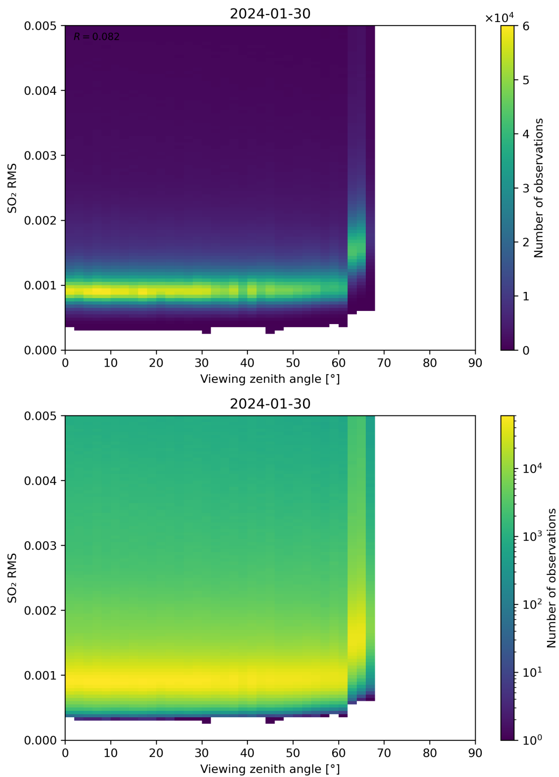
Figure 313: Scatter density plot of “Viewing zenith angle” against “SO 2 RMS” for 2024-01-29 to 2024-01-31.
