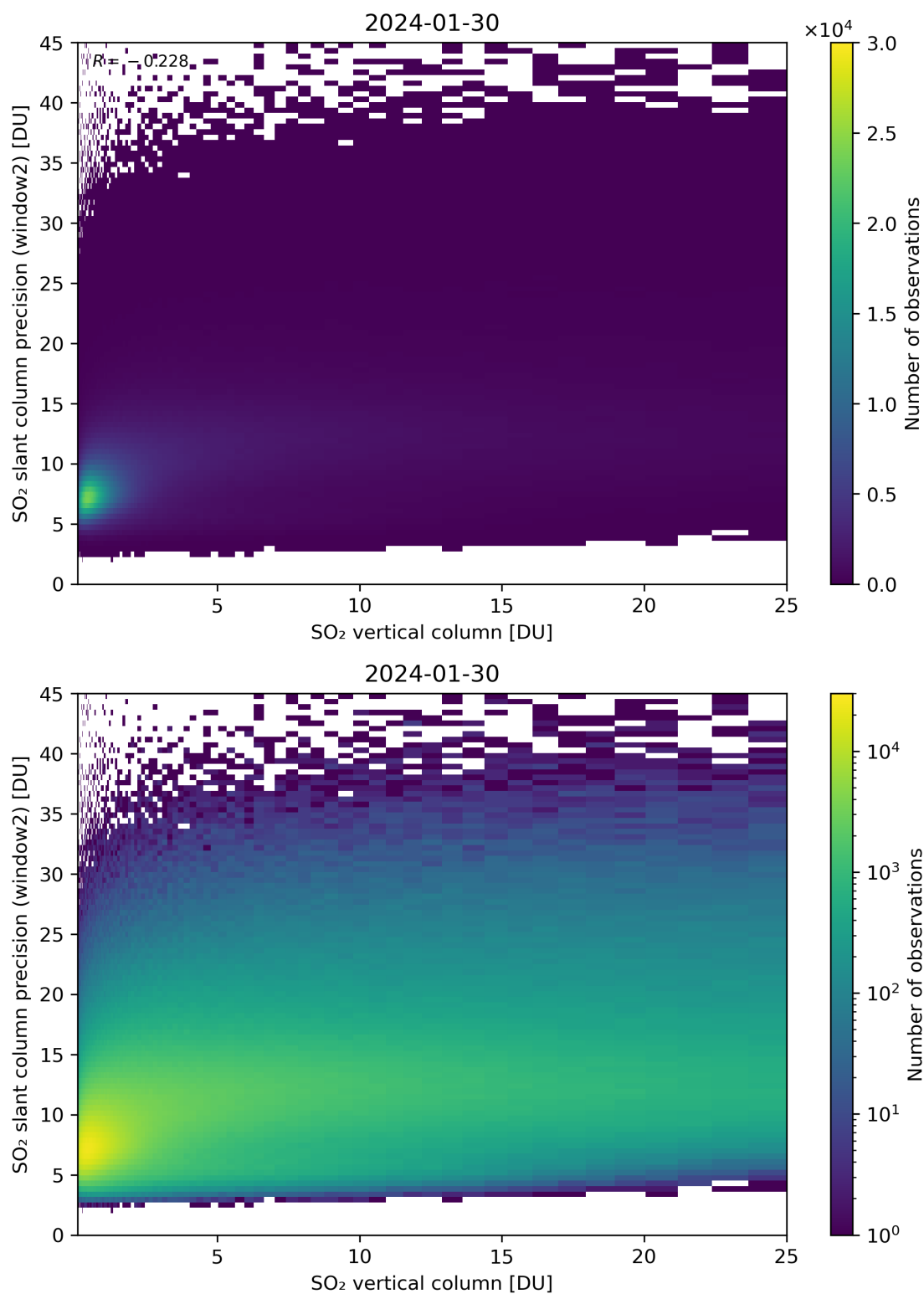
Figure 302: Scatter density plot of “SO 2 vertical column” against “SO 2 slant column precision (window2)” for 2024-01-29 to 2024-01-31.
