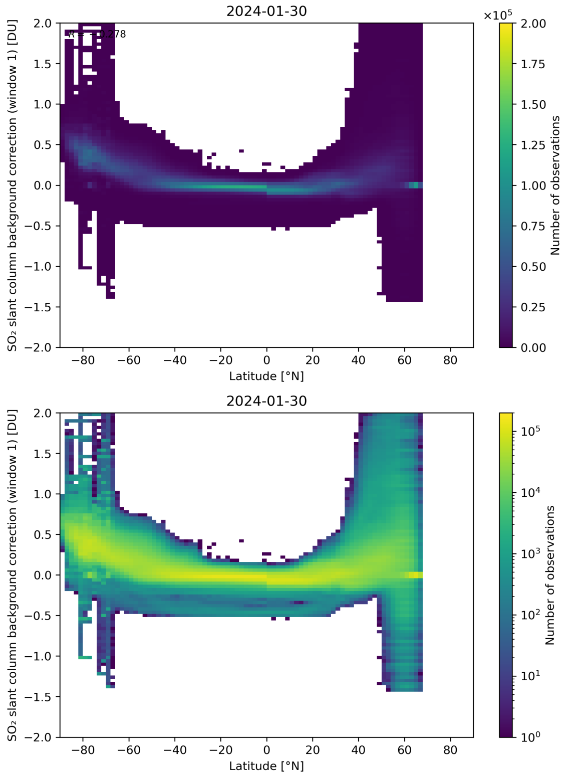
Figure 139: Scatter density plot of “Latitude” against “SO 2 slant column background correction (window 1)” for 2024-01-29 to 2024-01-31.
