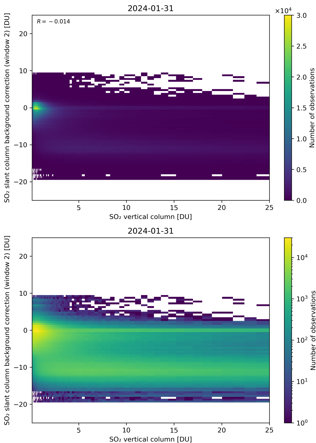
Figure 274: Scatter density plot of “SO 2 vertical column” against “SO 2 slant column background correction (window 2)” for 2024-01-31 to 2024-02-01.
