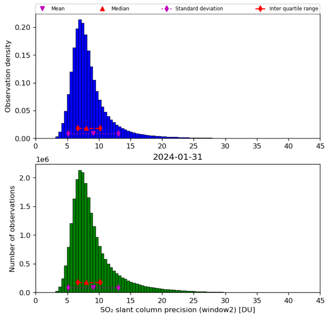
Figure 61: Histogram of “SO 2 slant column precision (window2)” for 2024-01-31 to 2024-02-01
