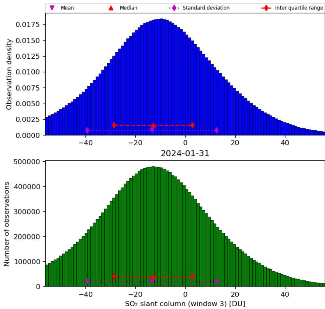
Figure 64: Histogram of “SO 2 slant column (window 3)” for 2024-01-31 to 2024-02-01
