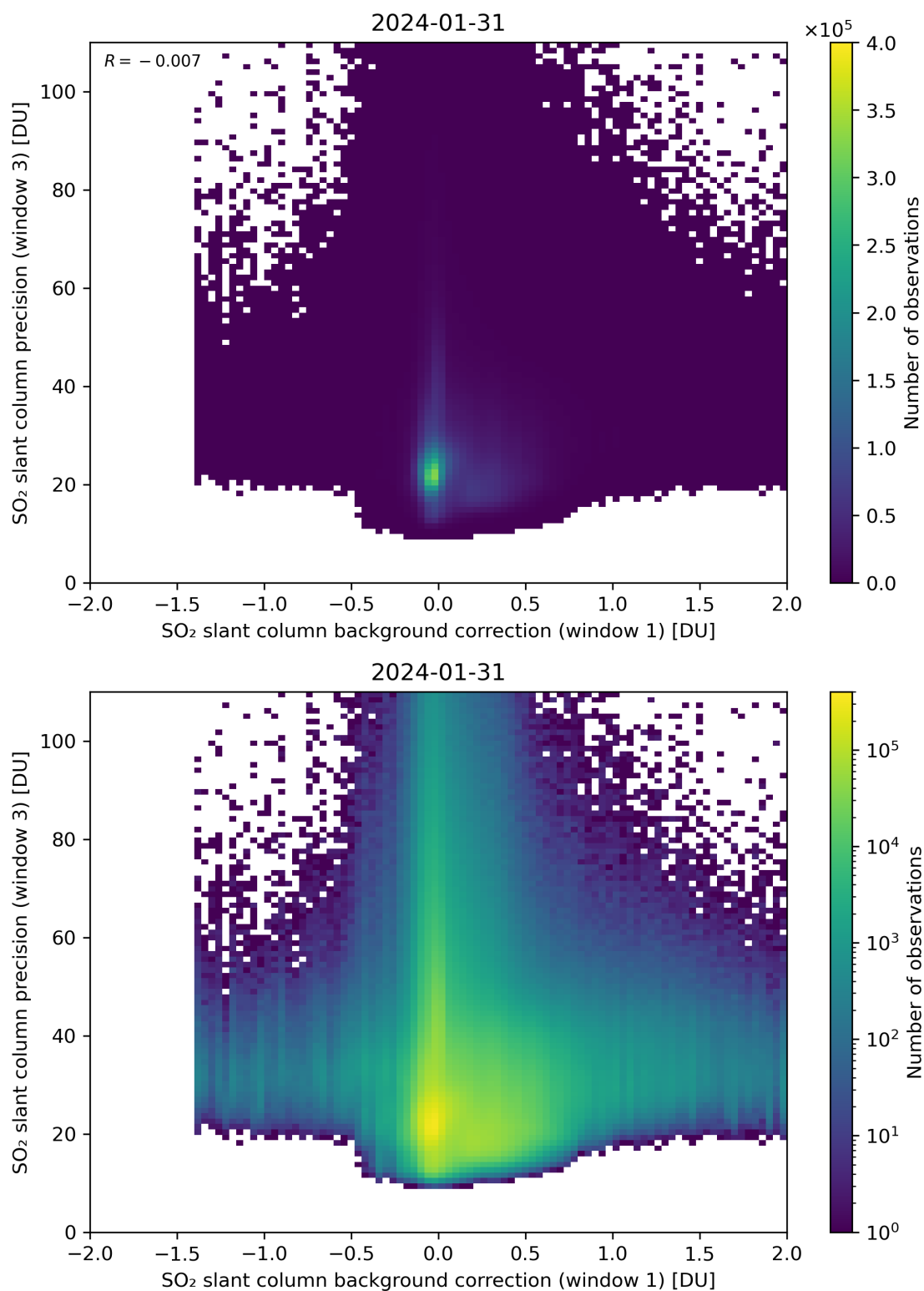
Figure 108: Scatter density plot of “SO 2 slant column background correction (window 1)” against “SO 2 slant column precision (window 3)” for 2024-01-31 to 2024-02-01.
