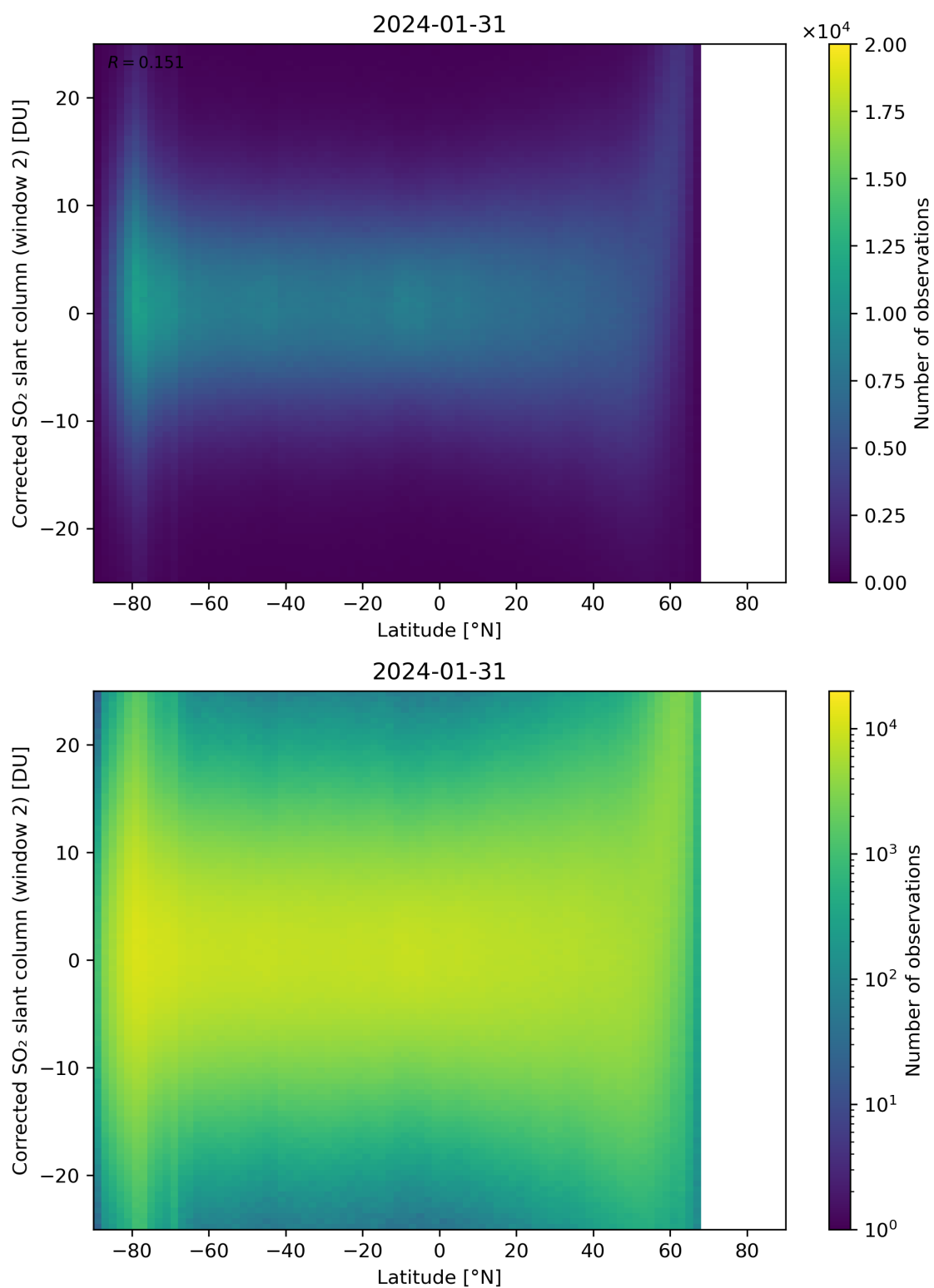
Figure 147: Scatter density plot of “Latitude” against “Corrected SO 2 slant column (window 2)” for 2024-01-31 to 2024-02-01.
