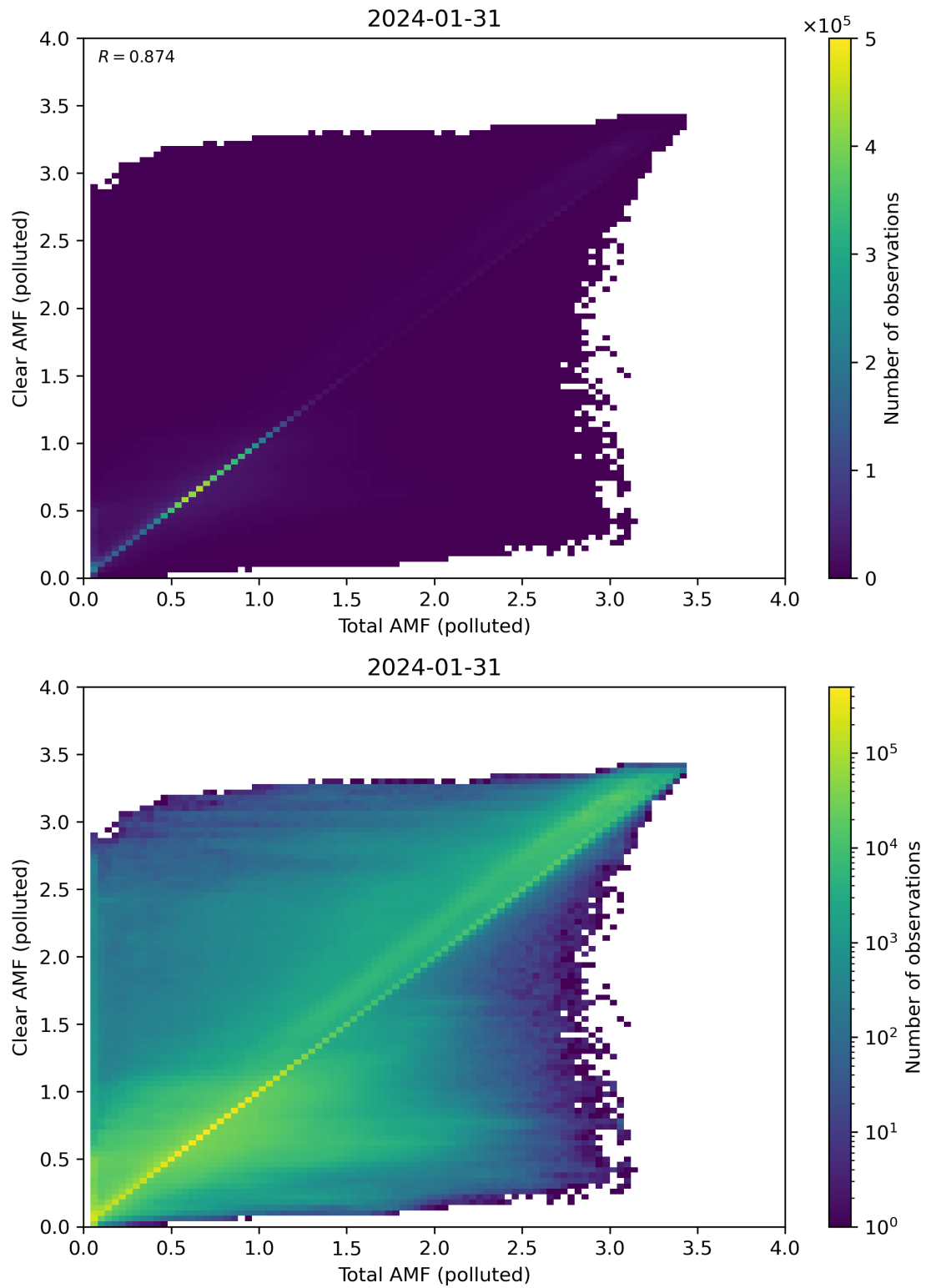
Figure 271: Scatter density plot of “Total AMF (polluted)” against “Clear AMF (polluted)” for 2024-01-31 to 2024-02-01.
