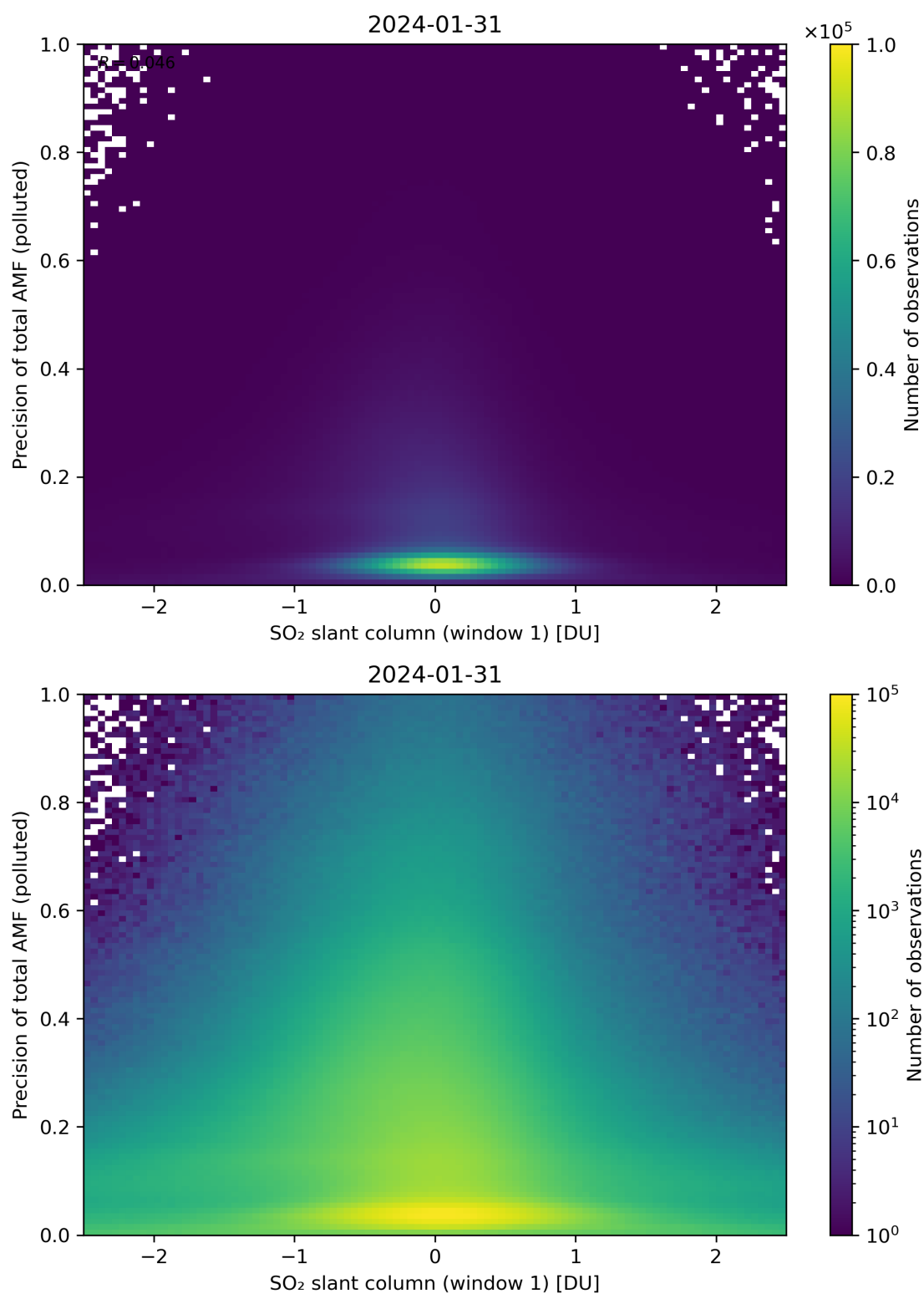
Figure 240: Scatter density plot of “SO 2 slant column (window 1)” against “Precision of total AMF (polluted)” for 2024-01-31 to 2024-02-01.
