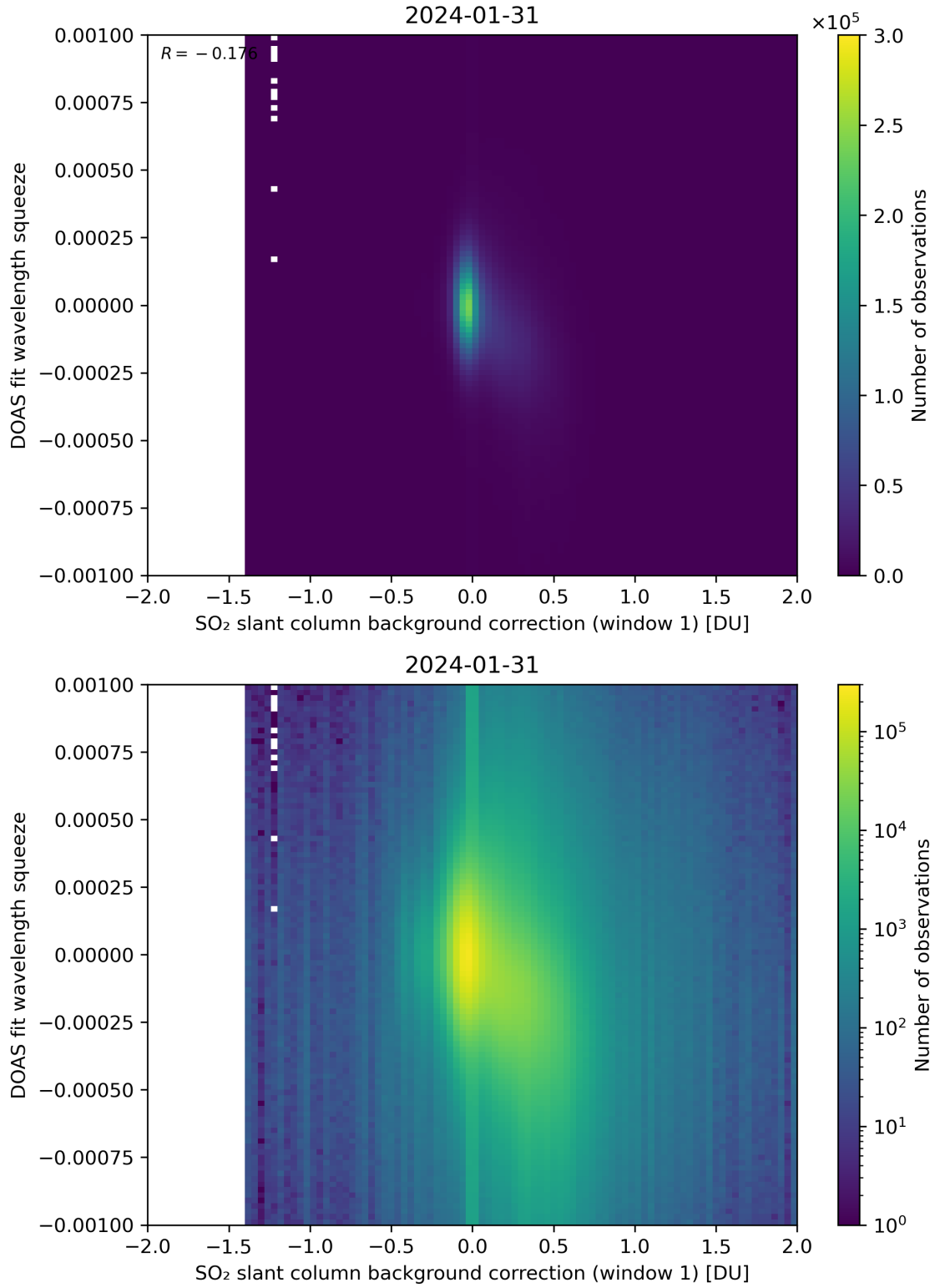
Figure 101: Scatter density plot of “SO 2 slant column background correction (window 1)” against “DOAS fit wavelength squeeze” for 2024-01-31 to 2024-02-01.
