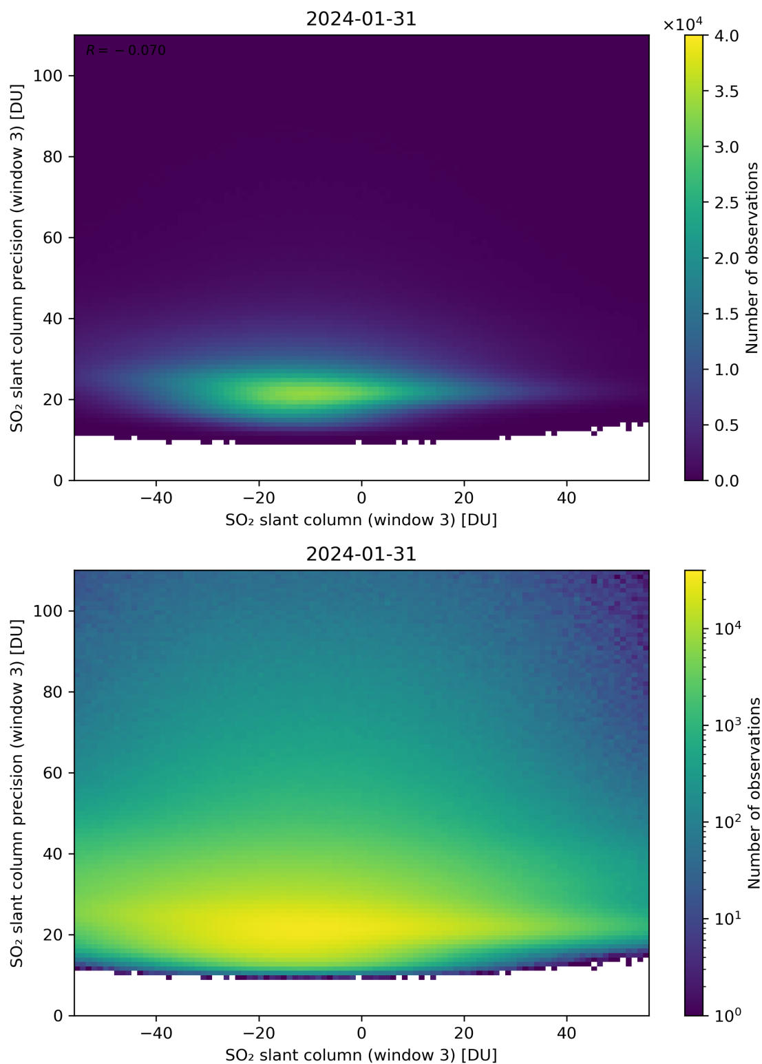
Figure 267: Scatter density plot of “SO 2 slant column (window 3)” against “SO 2 slant column precision (window 3)” for 2024-01-31 to 2024-02-01.
