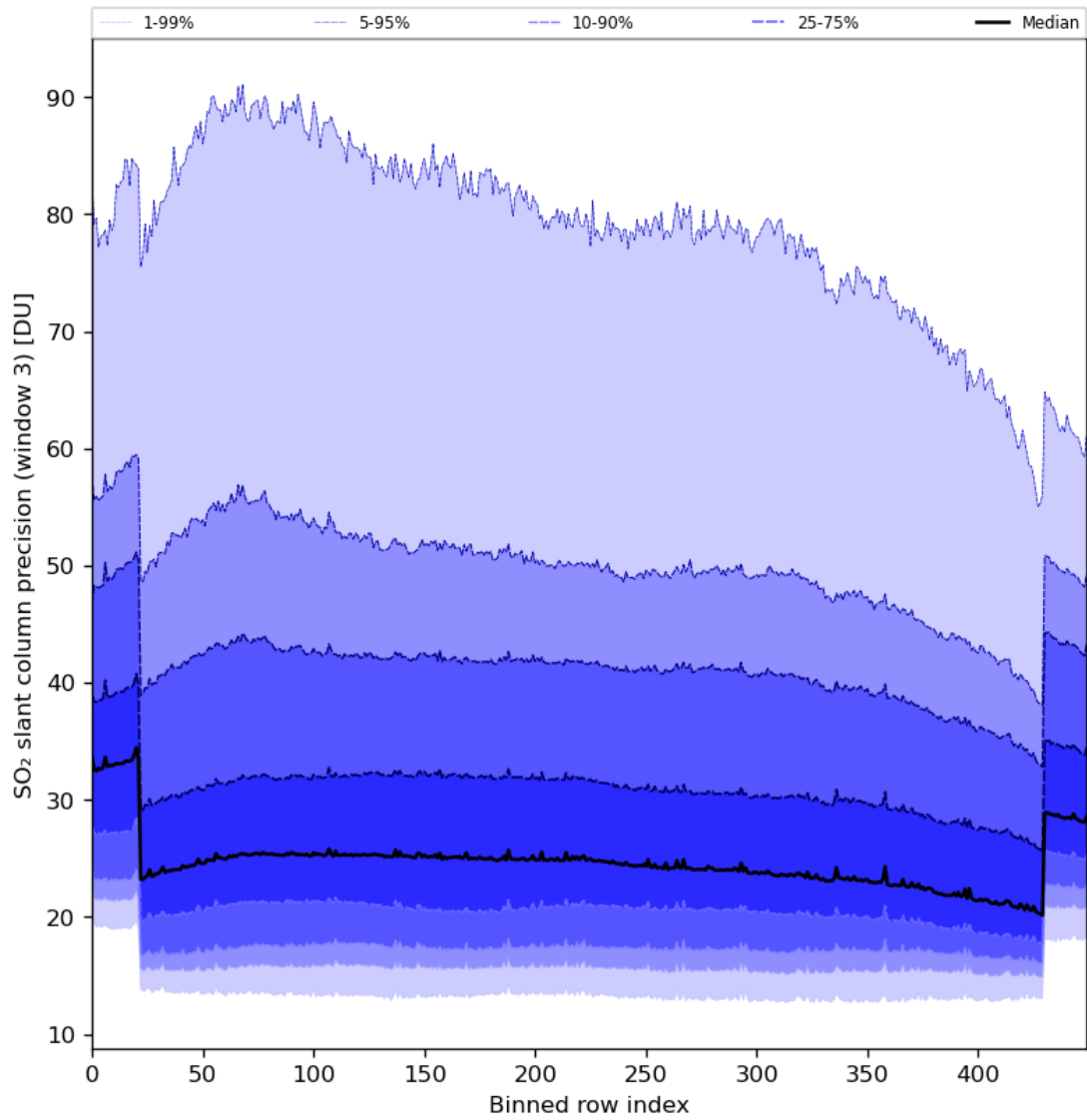
Figure 88: Along track statistics of “SO 2 slant column precision (window 3)” for 2024-01-31 to 2024-02-01
