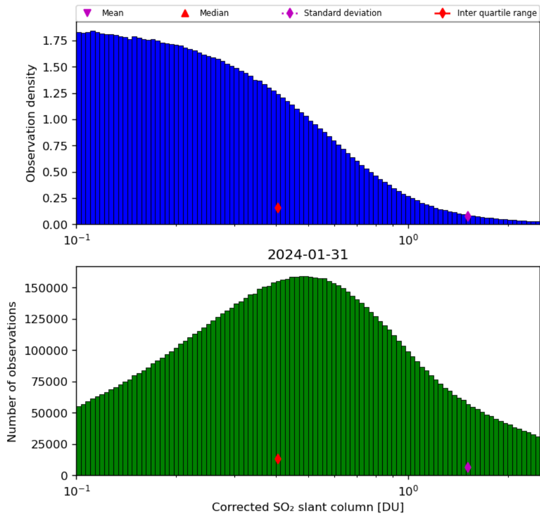
Figure 55: Histogram of “Corrected SO 2 slant column” for 2024-01-31 to 2024-02-01
