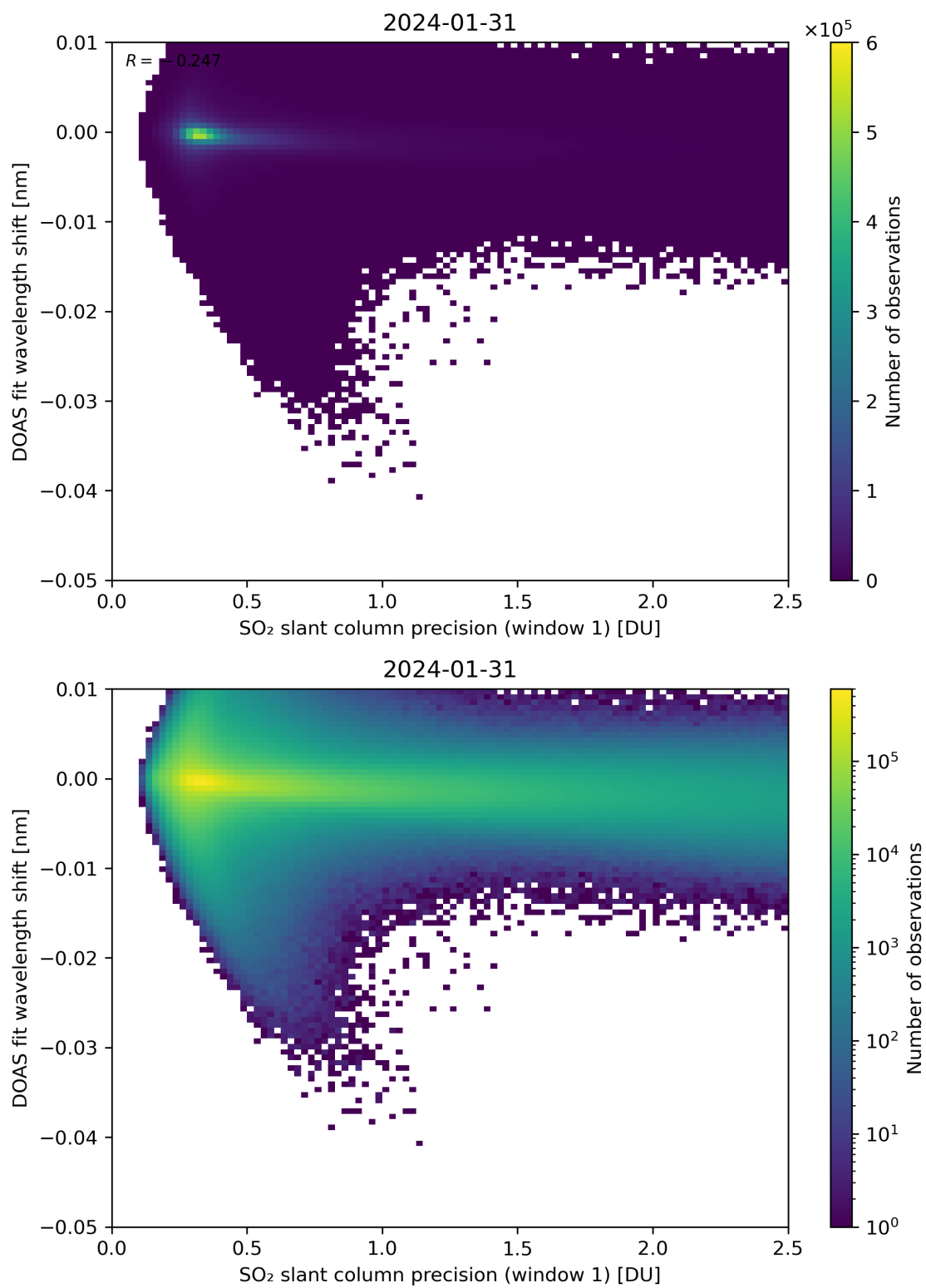
Figure 221: Scatter density plot of “SO 2 slant column precision (window 1)” against “DOAS fit wavelength shift” for 2024-01-31 to 2024-02-01.
