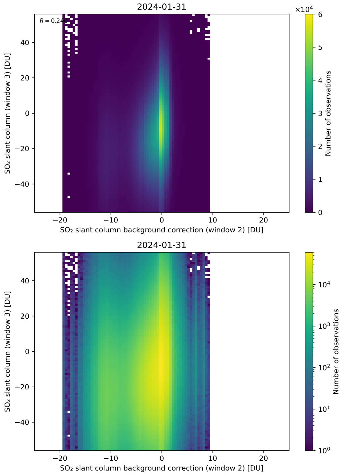
Figure 117: Scatter density plot of “SO 2 slant column background correction (window 2)” against “SO 2 slant column (window 3)” for 2024-01-31 to 2024-02-01.
