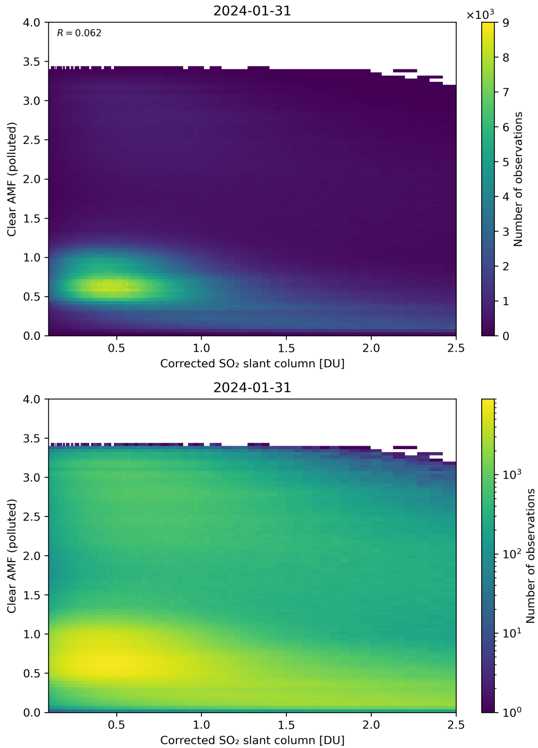
Figure 184: Scatter density plot of “Corrected SO 2 slant column” against “Clear AMF (polluted)” for 2024-01-31 to 2024-02-01.
