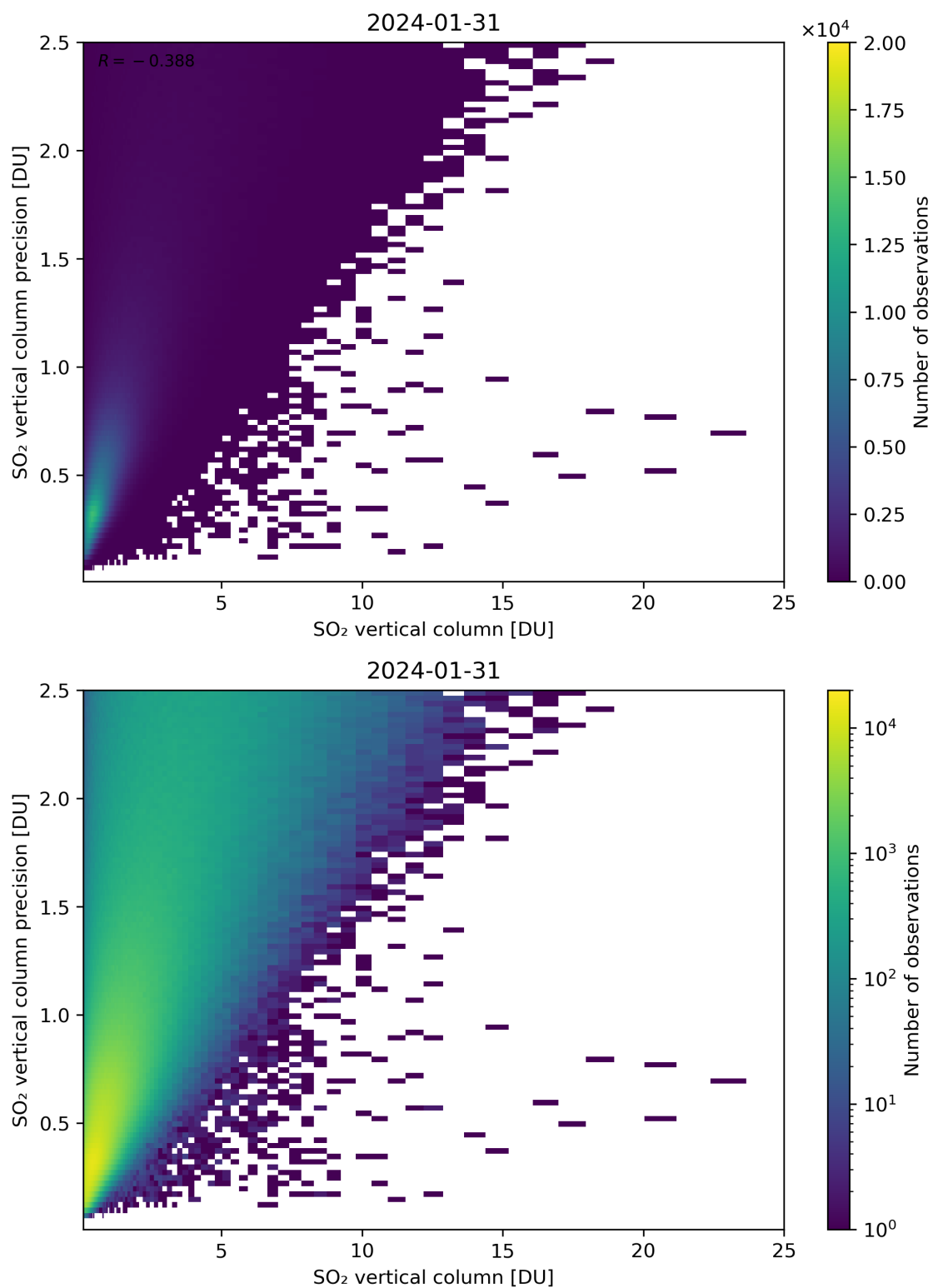
Figure 307: Scatter density plot of “SO 2 vertical column” against “SO 2 vertical column precision” for 2024-01-31 to 2024-02-01.
