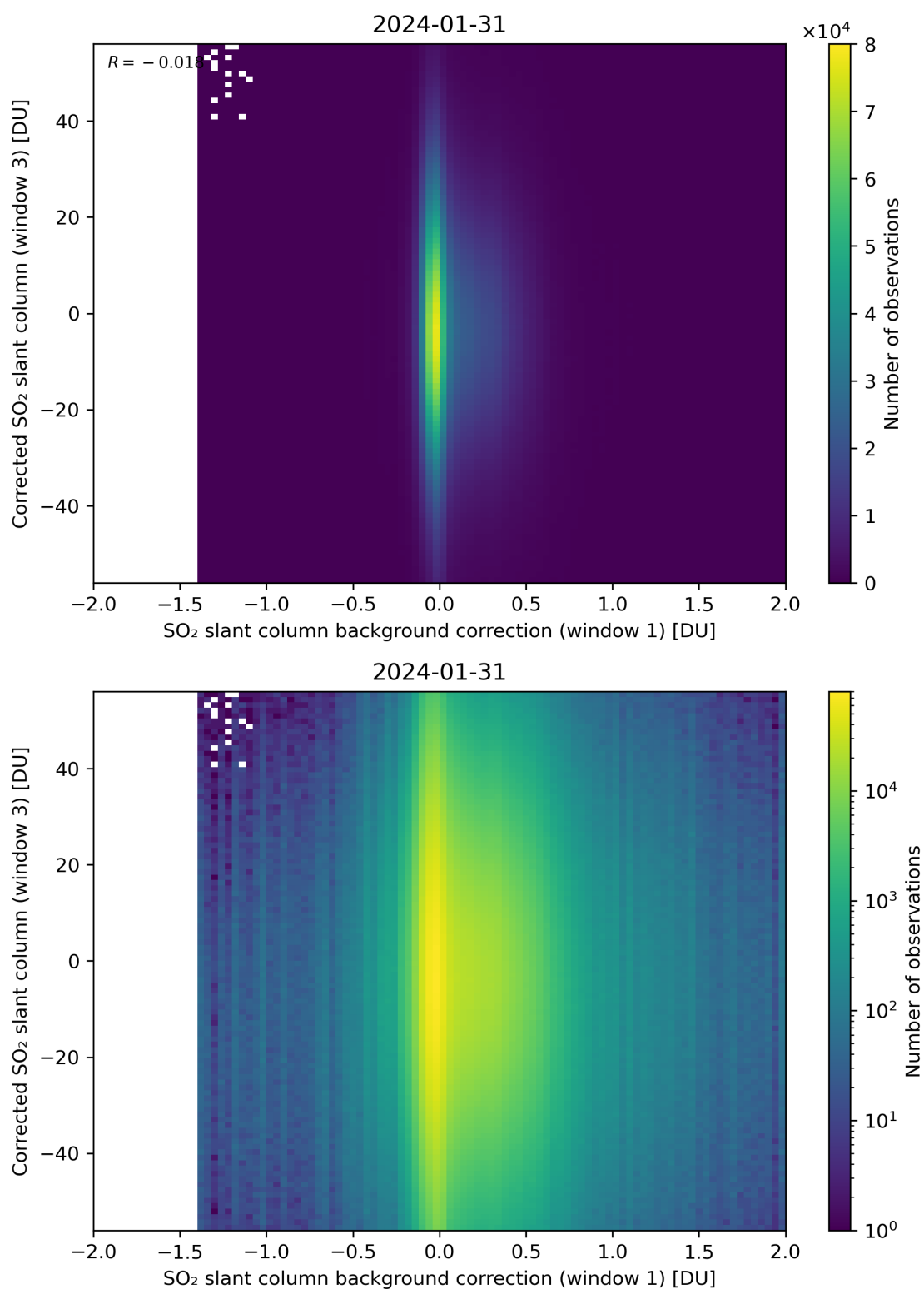
Figure 105: Scatter density plot of “SO 2 slant column background correction (window 1)” against “Corrected SO 2 slant column (window 3)” for 2024-01-31 to 2024-02-01.
