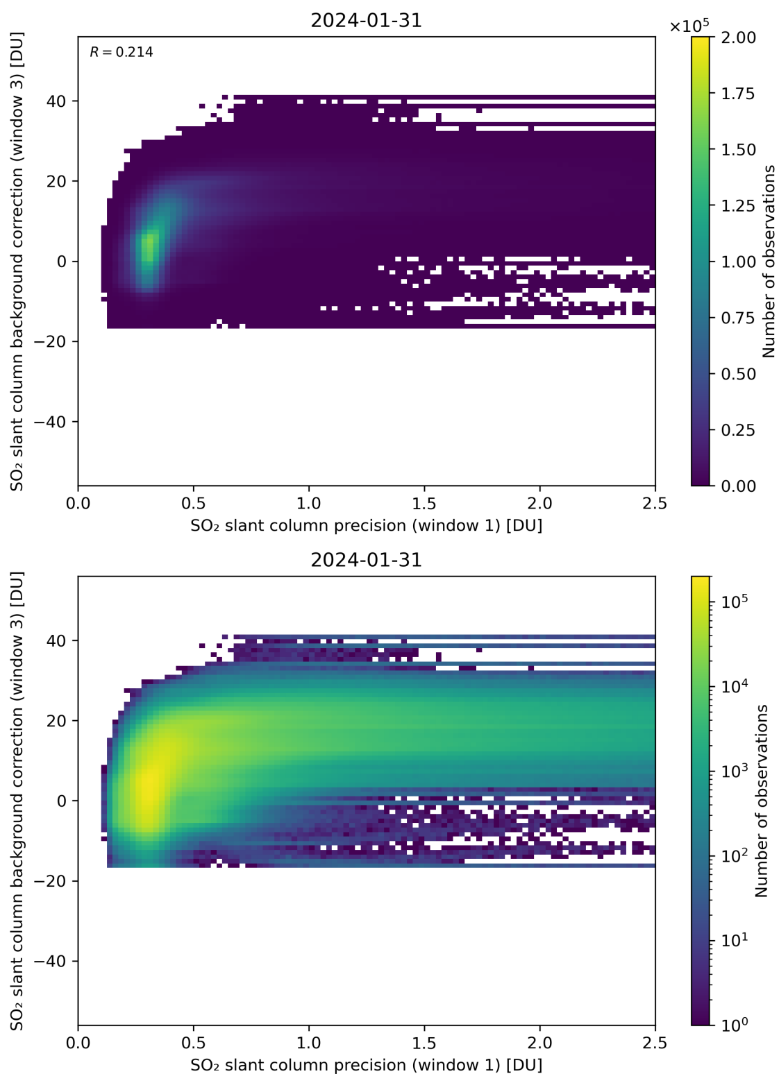
Figure 220: Scatter density plot of “SO 2 slant column precision (window 1)” against “SO 2 slant column background correction (window 3)” for 2024-01-31 to 2024-02-01.
