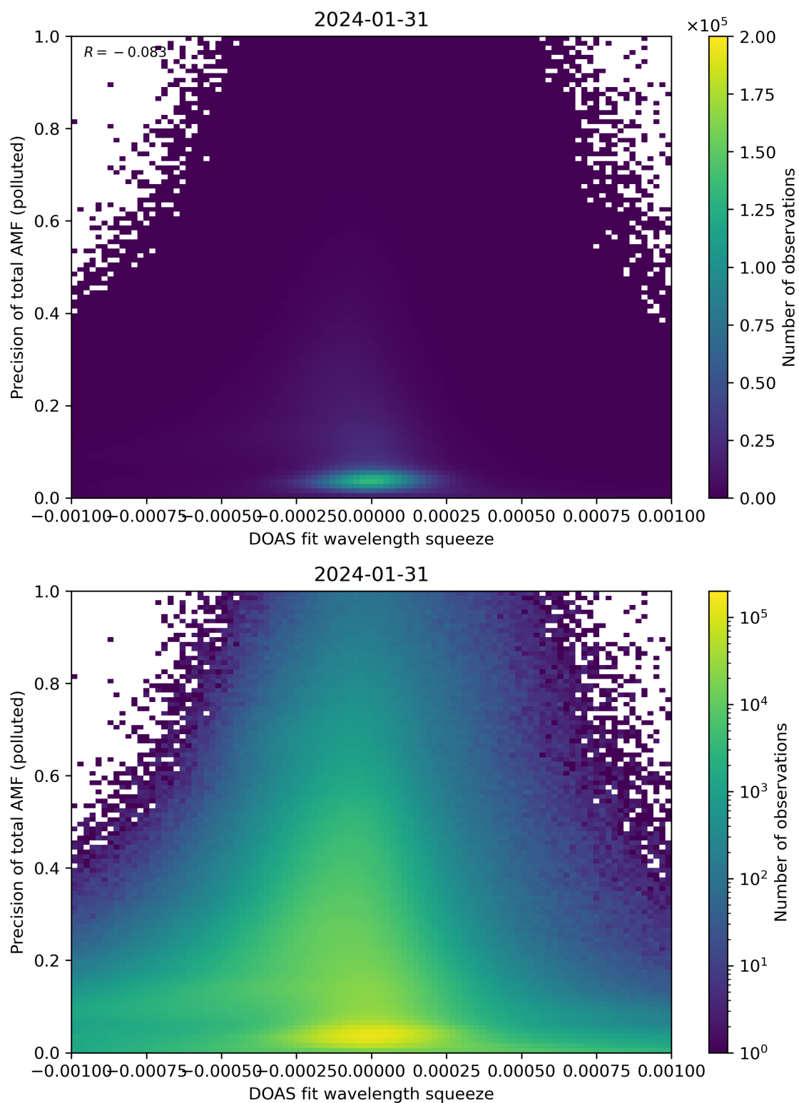
Figure 135: Scatter density plot of “DOAS fit wavelength squeeze” against “Precision of total AMF (polluted)” for 2024-01-31 to 2024-02-01.
