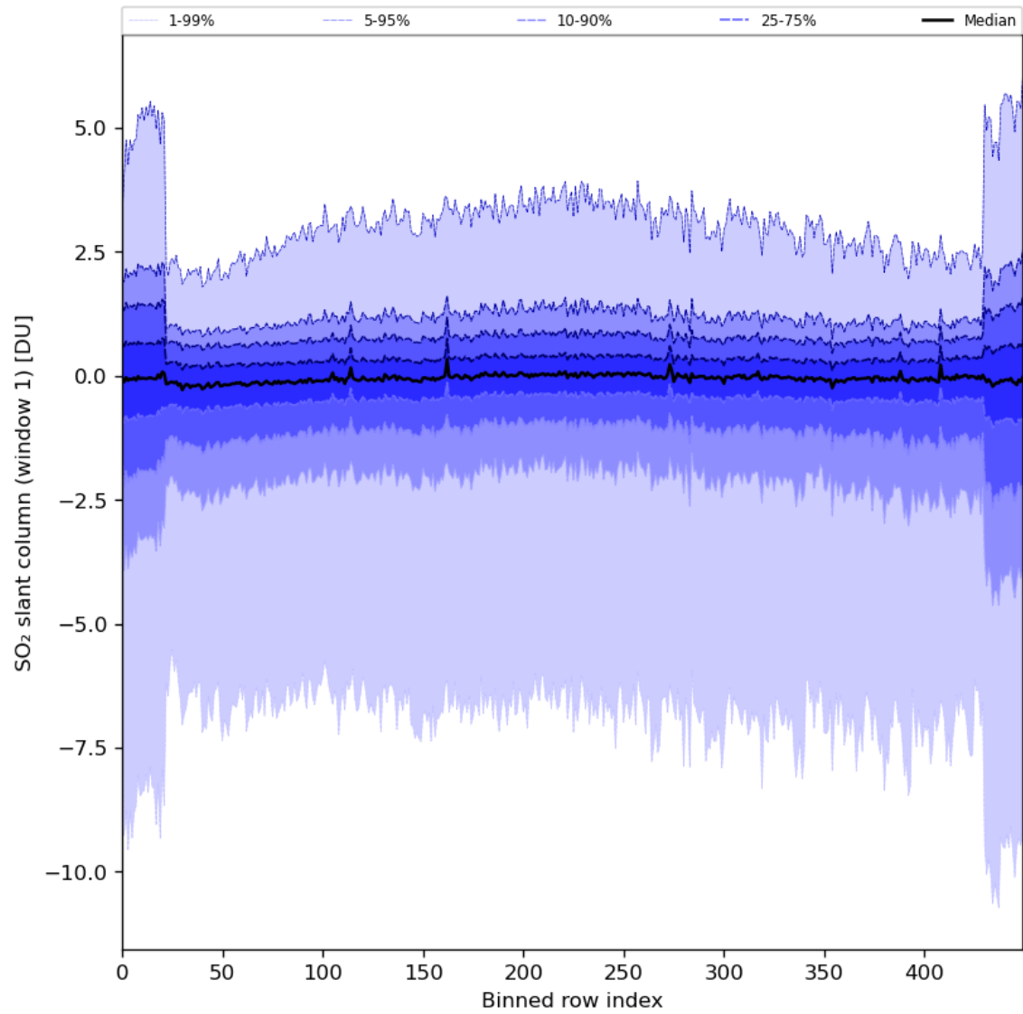
Figure 79: Along track statistics of “SO 2 slant column (window 1)” for 2024-01-31 to 2024-02-01
