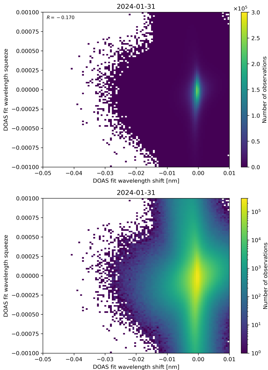
Figure 127: Scatter density plot of “DOAS fit wavelength shift” against “DOAS fit wavelength squeeze” for 2024-01-31 to 2024-02-01.
