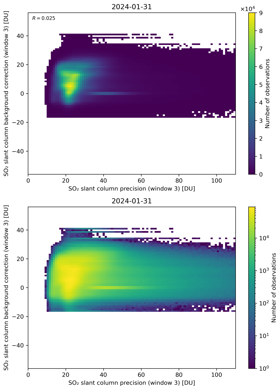
Figure 257: Scatter density plot of “SO 2 slant column precision (window 3)” against “SO 2 slant column background correction (window 3)” for 2024-01-31 to 2024-02-01.
