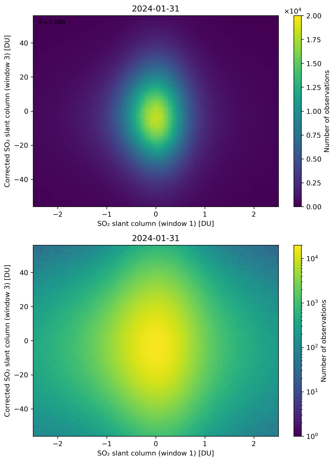
Figure 234: Scatter density plot of “SO 2 slant column (window 1)” against “Corrected SO 2 slant column (window 3)” for 2024-01-31 to 2024-02-01.
