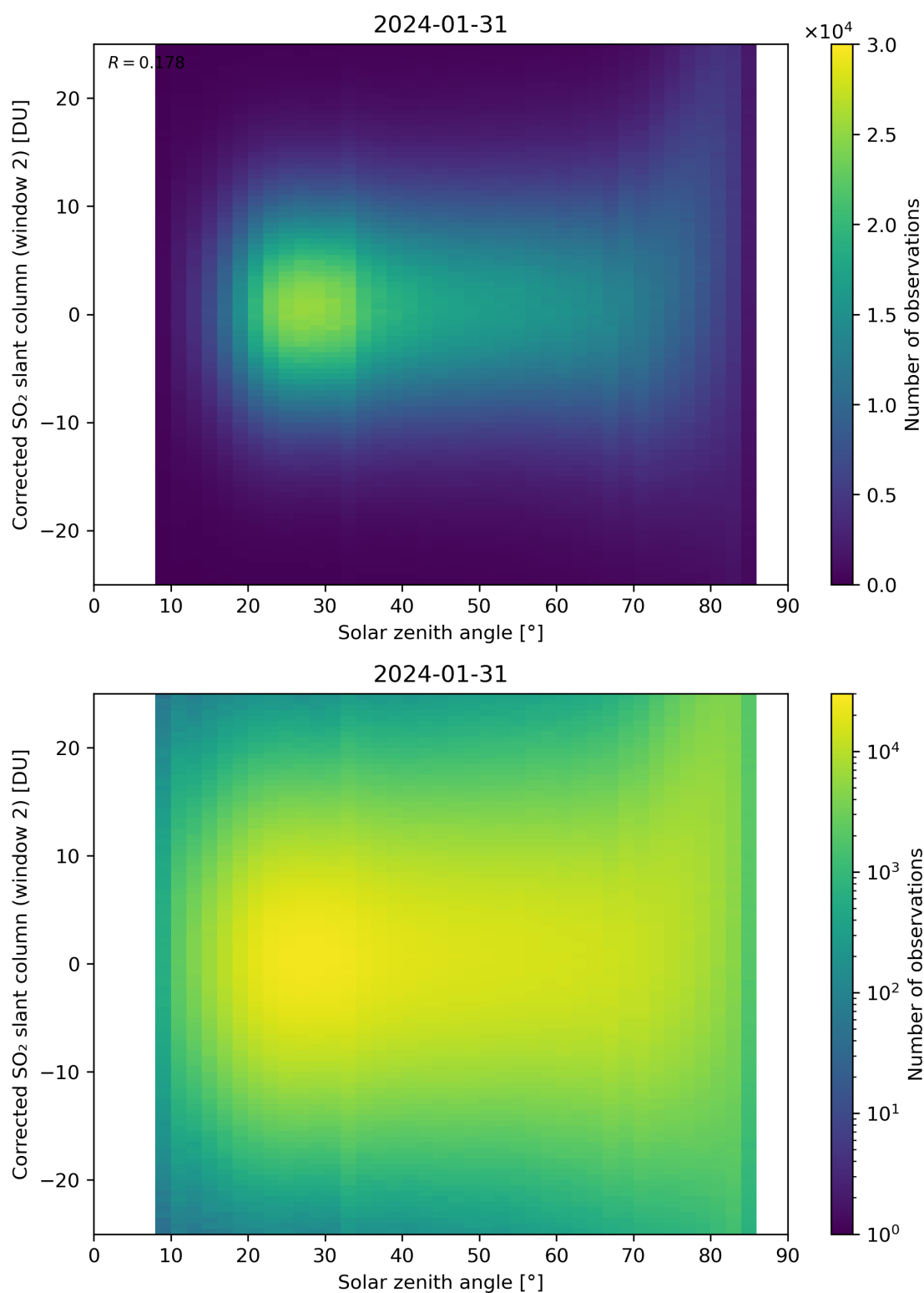
Figure 167: Scatter density plot of “Solar zenith angle” against “Corrected SO 2 slant column (window 2)” for 2024-01-31 to 2024-02-01.
