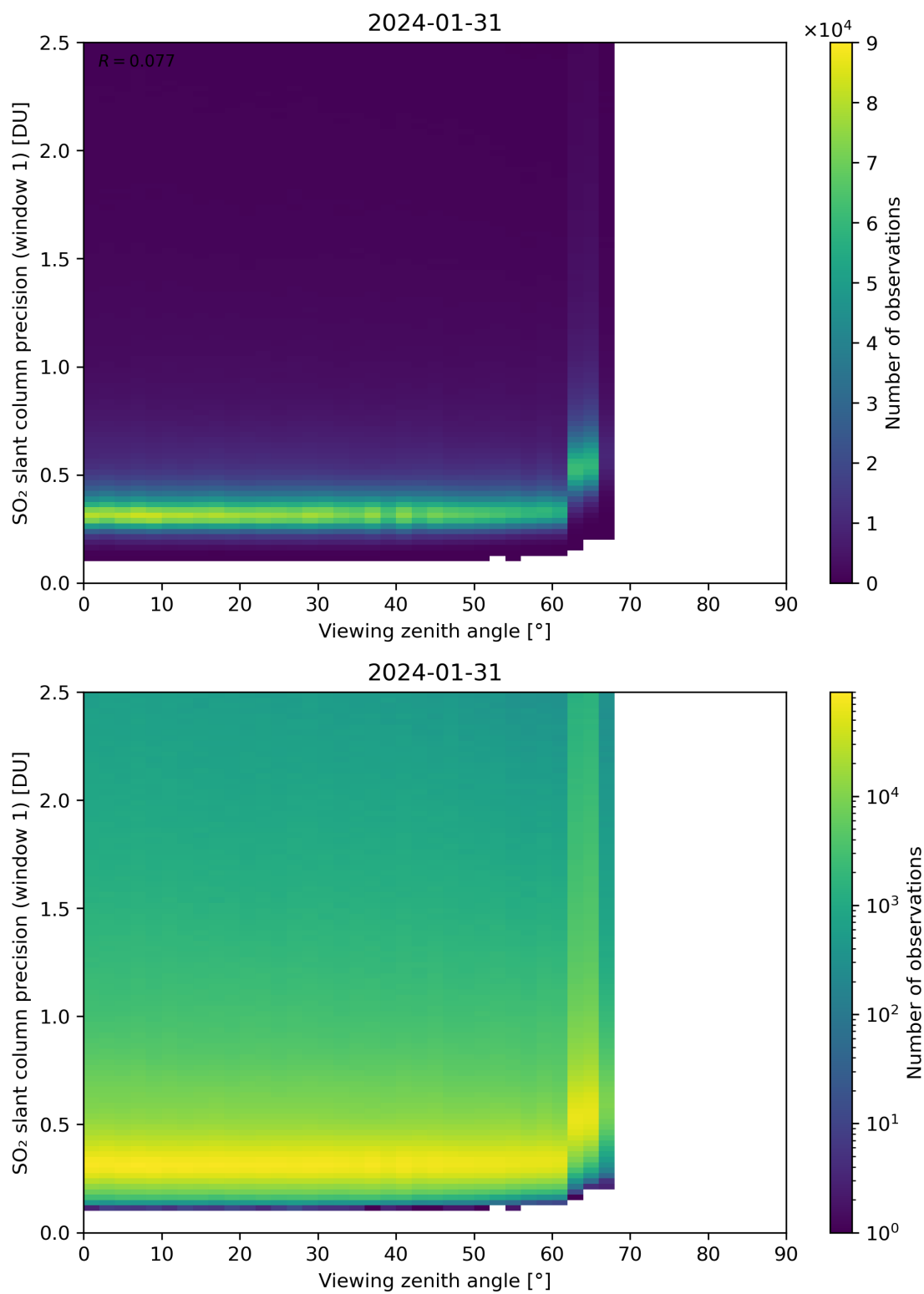
Figure 321: Scatter density plot of “Viewing zenith angle” against “SO 2 slant column precision (window 1)” for 2024-01-31 to 2024-02-01.
