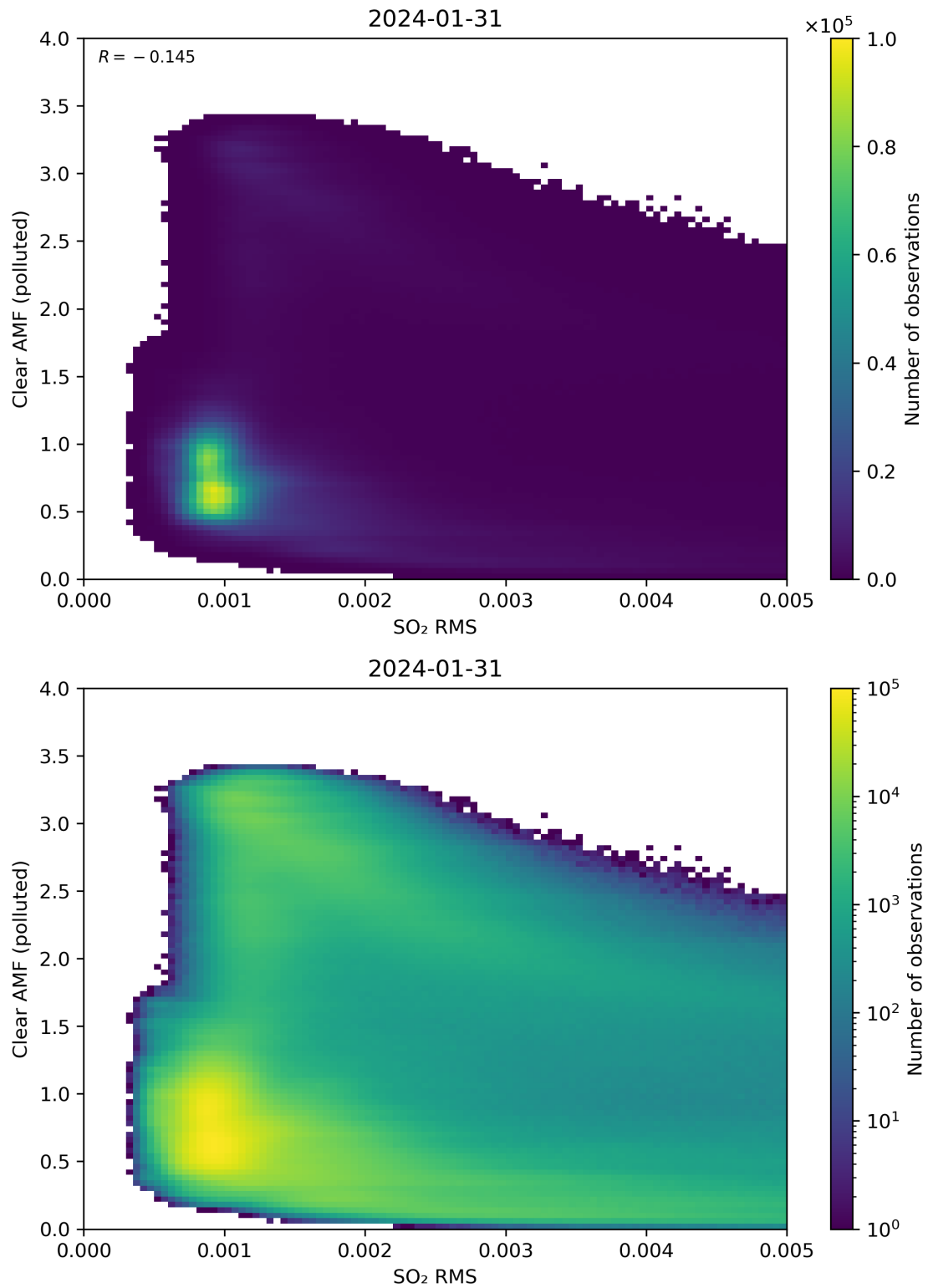
Figure 136: Scatter density plot of “SO 2 RMS” against “Clear AMF (polluted)” for 2024-01-31 to 2024-02-01.
