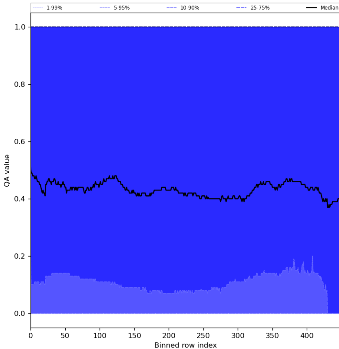
Figure 75: Along track statistics of “QA value” for 2024-01-31 to 2024-02-01
