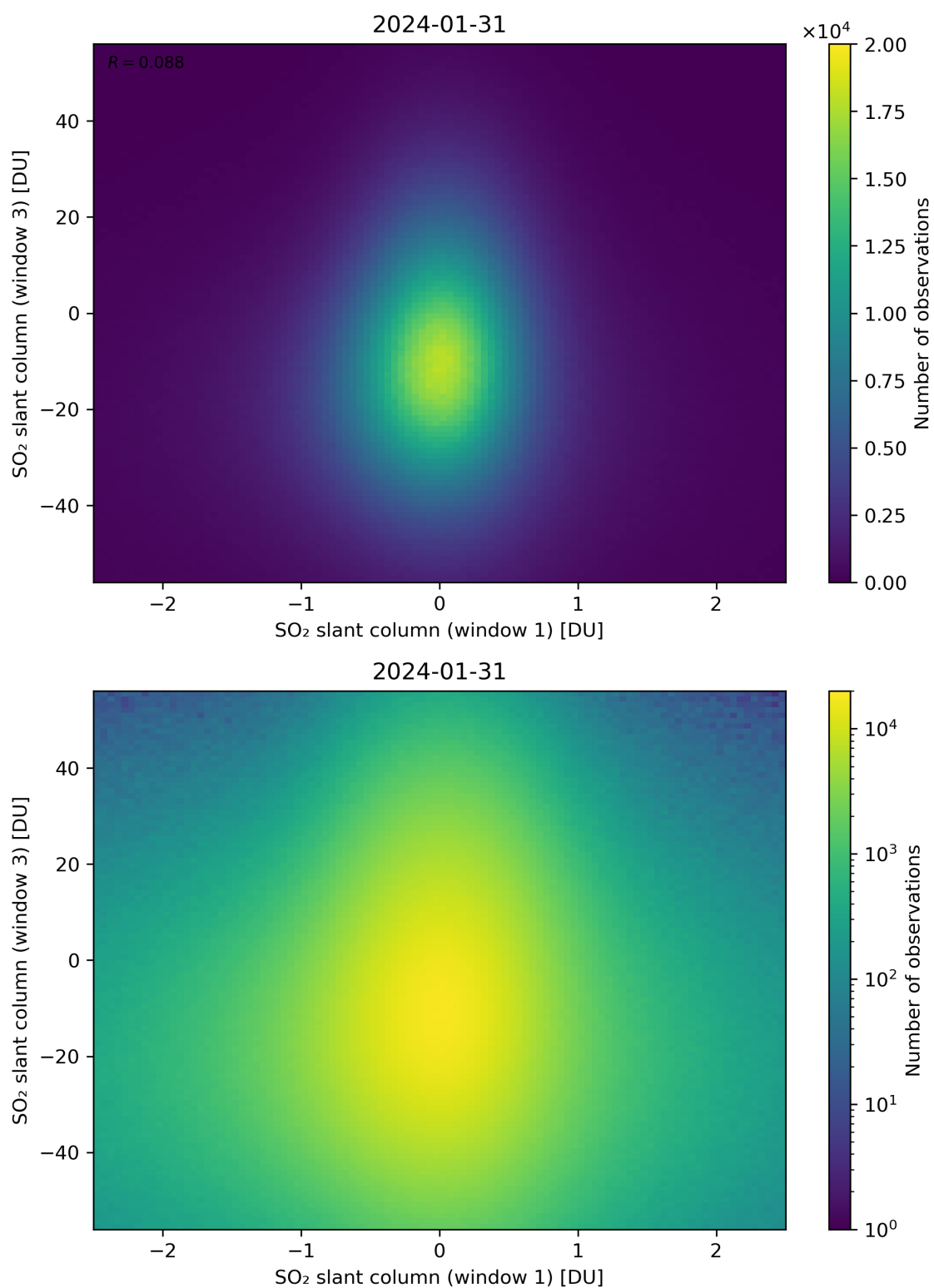
Figure 237: Scatter density plot of “SO 2 slant column (window 1)” against “SO 2 slant column (window 3)” for 2024-01-31 to 2024-02-01.
