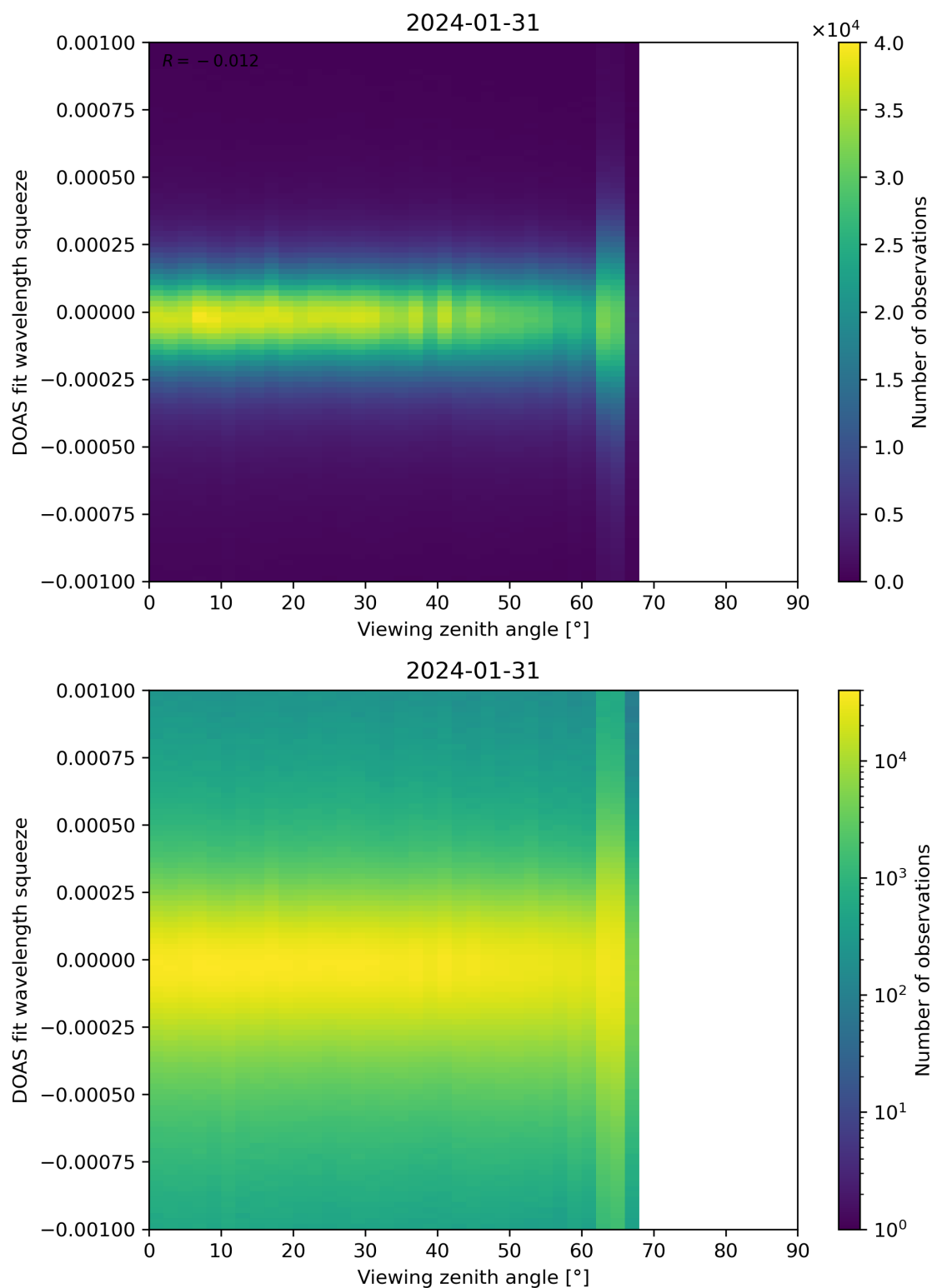
Figure 312: Scatter density plot of “Viewing zenith angle” against “DOAS fit wavelength squeeze” for 2024-01-31 to 2024-02-01.
