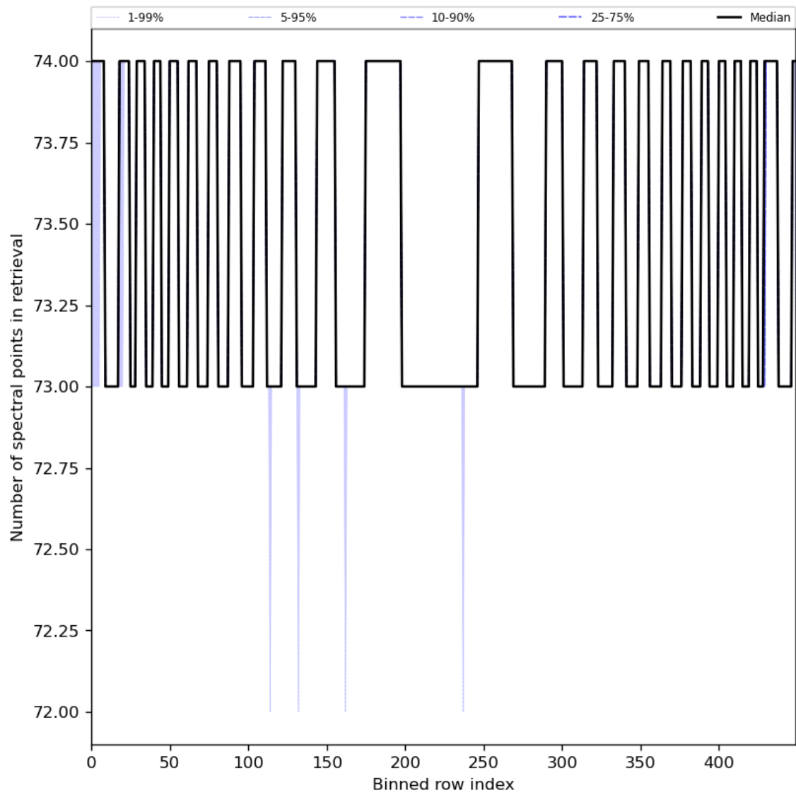
Figure 97: Along track statistics of “Number of spectral points in retrieval” for 2024-01-31 to 2024-02-01
