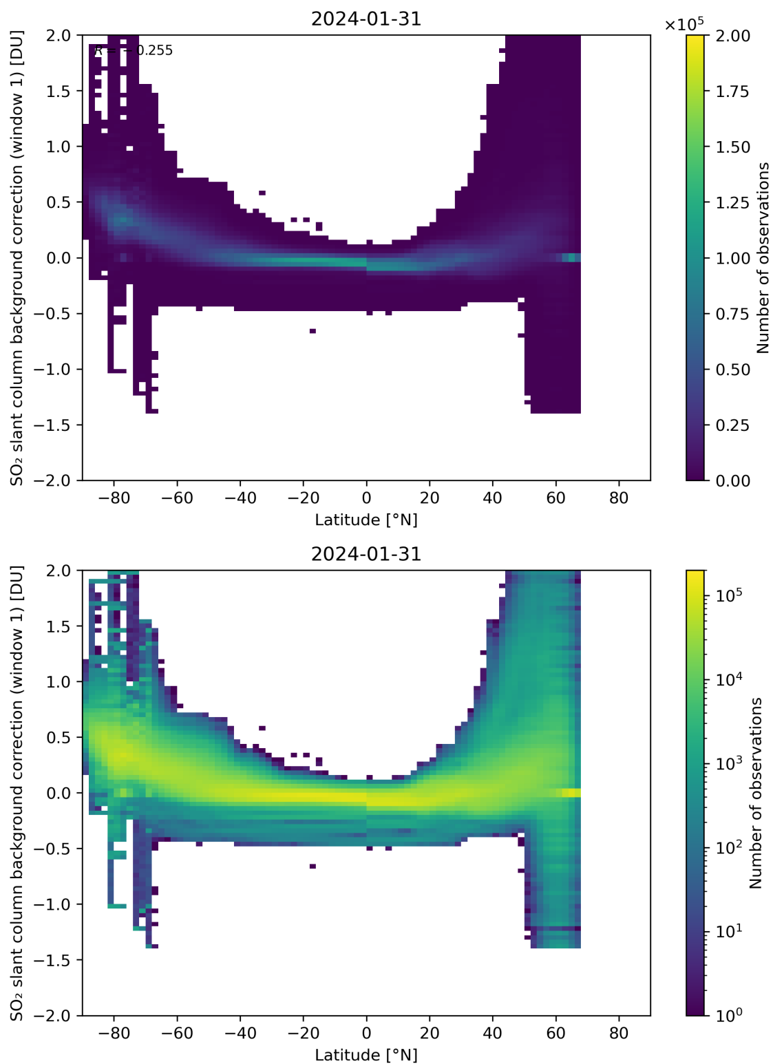
Figure 139: Scatter density plot of “Latitude” against “SO 2 slant column background correction (window 1)” for 2024-01-31 to 2024-02-01.
