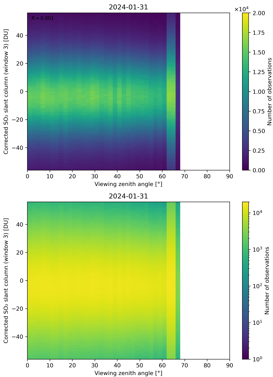
Figure 319: Scatter density plot of “Viewing zenith angle” against “Corrected SO 2 slant column (window 3)” for 2024-01-31 to 2024-02-01.
