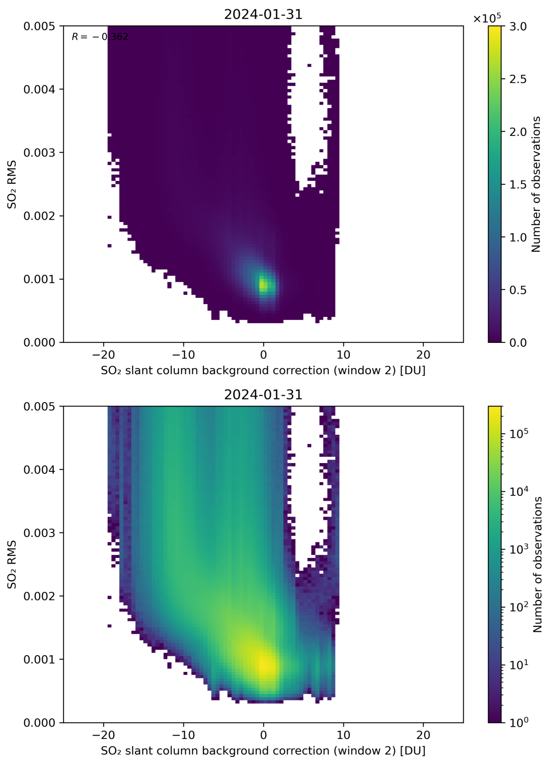
Figure 114: Scatter density plot of “SO 2 slant column background correction (window 2)” against “SO 2 RMS” for 2024-01-31 to 2024-02-01.
