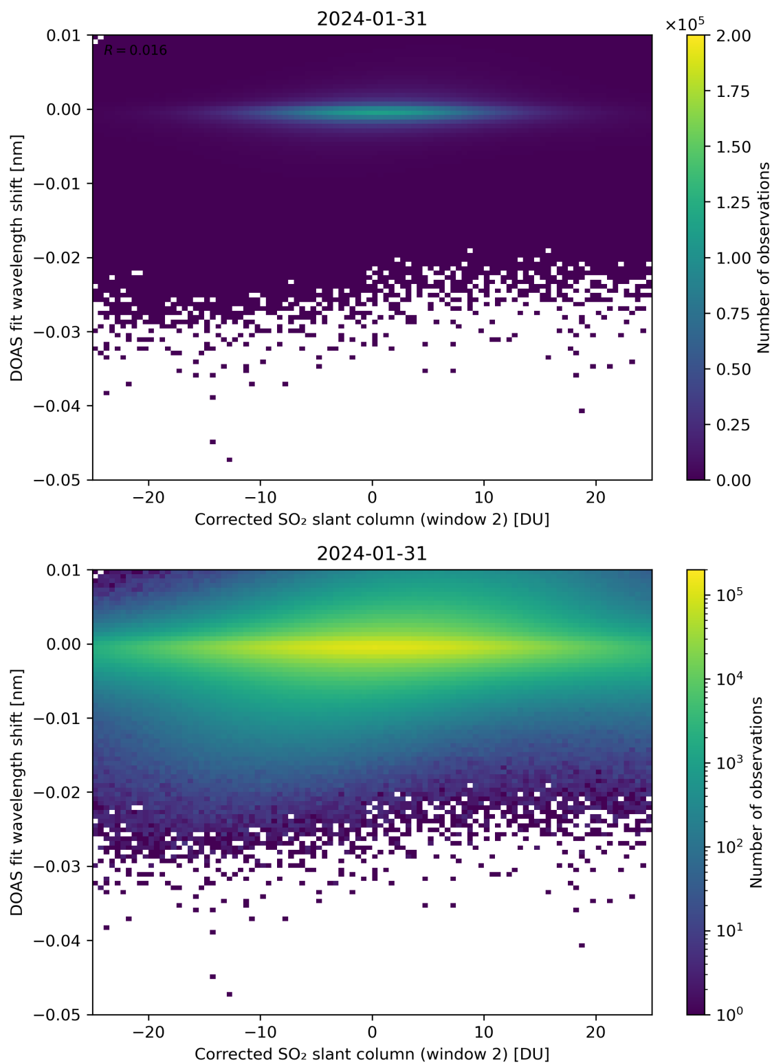
Figure 196: Scatter density plot of “Corrected SO 2 slant column (window 2)” against “DOAS fit wavelength shift” for 2024-01-31 to 2024-02-01.
