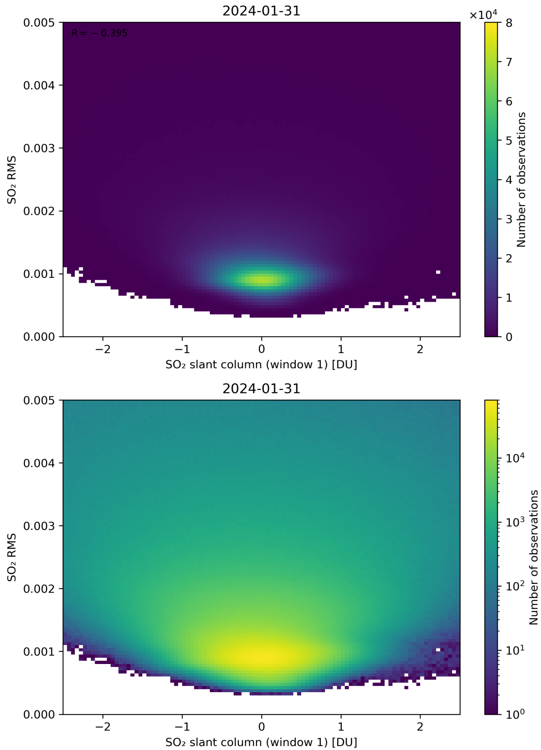
Figure 217: Scatter density plot of “SO 2 slant column (window 1)” against “SO 2 RMS” for 2024-01-31 to 2024-02-01.
