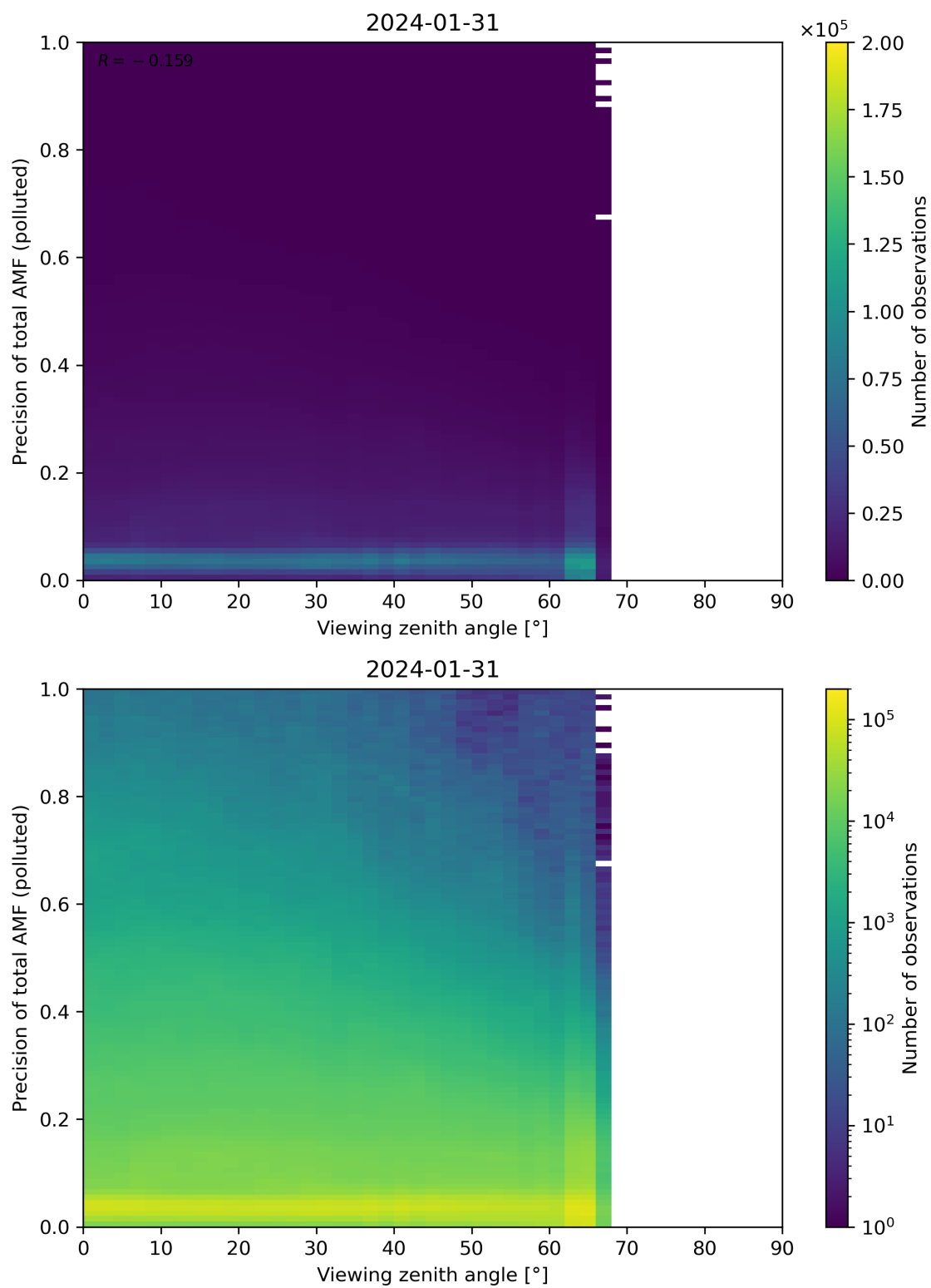
Figure 326: Scatter density plot of “Viewing zenith angle” against “Precision of total AMF (polluted)” for 2024-01-31 to 2024-02-01.
