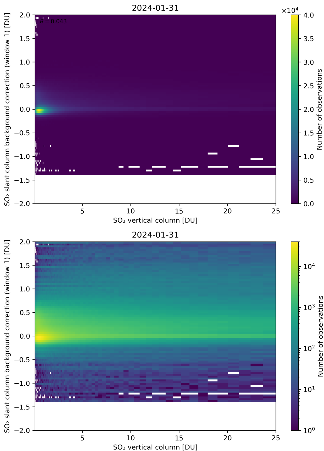
Figure 273: Scatter density plot of “SO 2 vertical column” against “SO 2 slant column background correction (window 1)” for 2024-01-31 to 2024-02-01.
