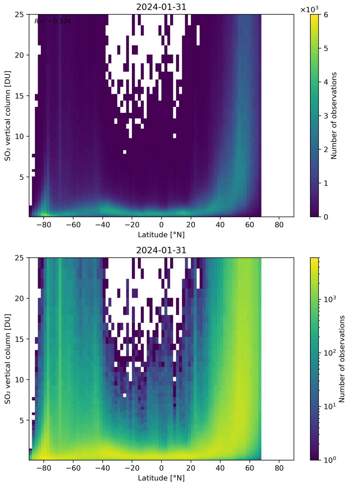
Figure 156: Scatter density plot of “Latitude” against “SO 2 vertical column” for 2024-01-31 to 2024-02-01.
