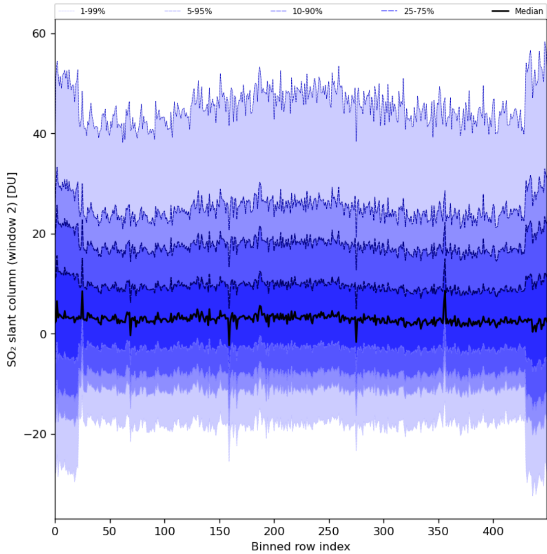
Figure 83: Along track statistics of “SO 2 slant column (window 2)” for 2024-01-31 to 2024-02-01
