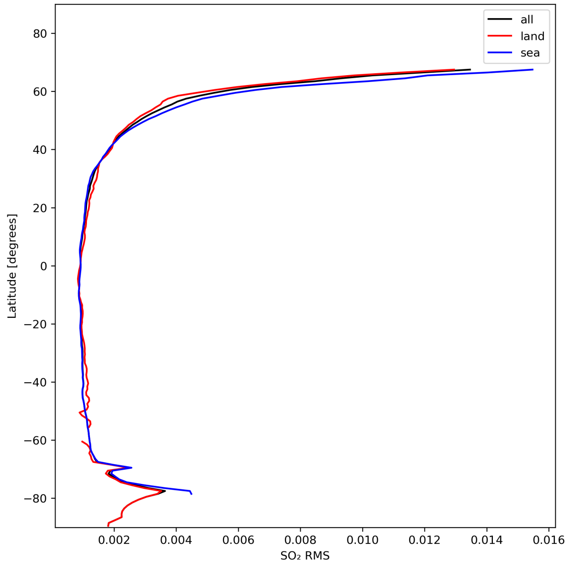
Figure 47: Zonal average of “SO 2 RMS” for 2024-01-31 to 2024-02-01.
