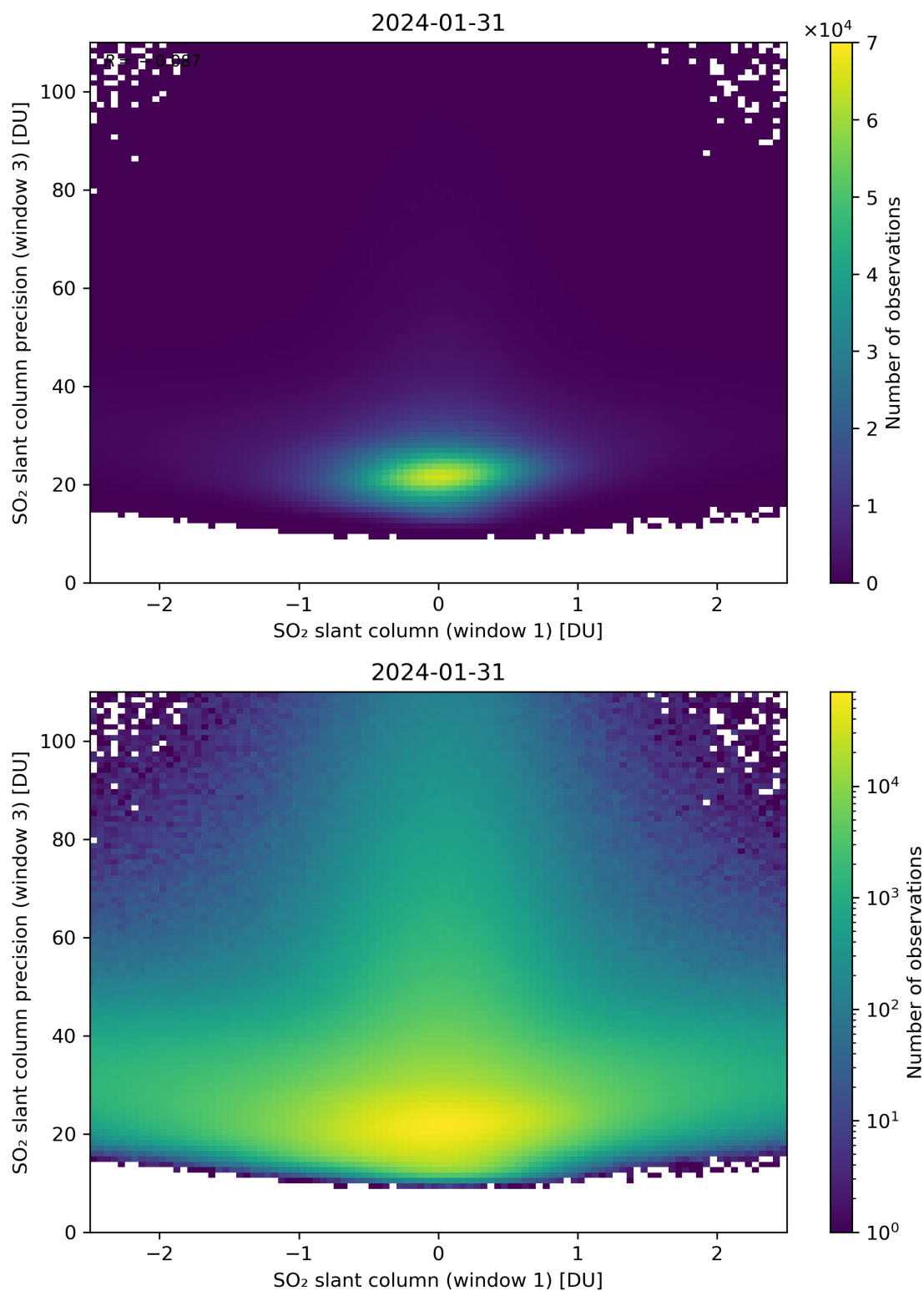
Figure 238: Scatter density plot of “SO 2 slant column (window 1)” against “SO 2 slant column precision (window 3)” for 2024-01-31 to 2024-02-01.
