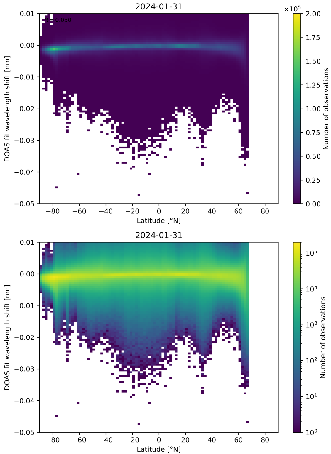
Figure 142: Scatter density plot of “Latitude” against “DOAS fit wavelength shift” for 2024-01-31 to 2024-02-01.
