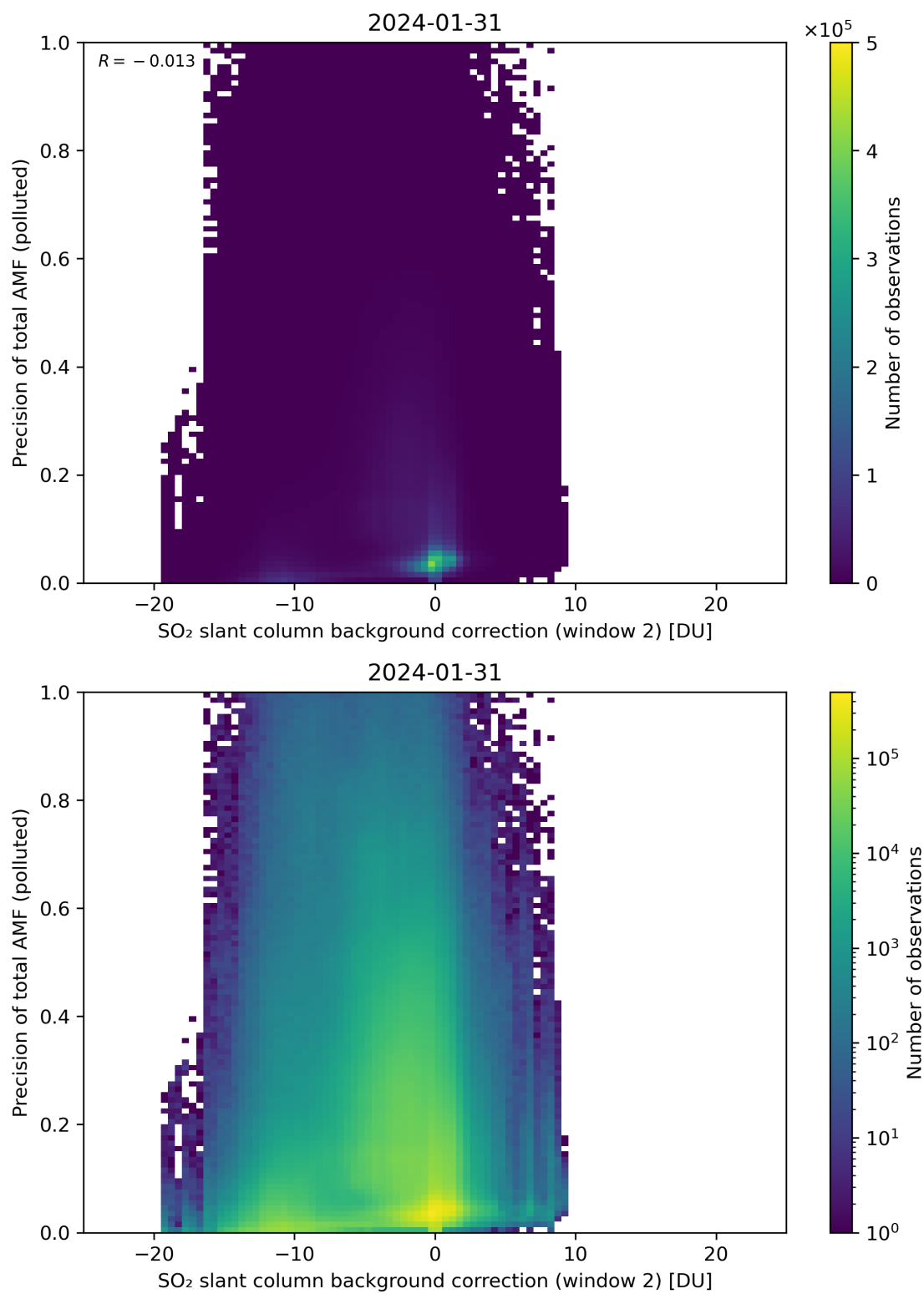
Figure 120: Scatter density plot of “SO 2 slant column background correction (window 2)” against “Precision of total AMF (polluted)” for 2024-01-31 to 2024-02-01.
