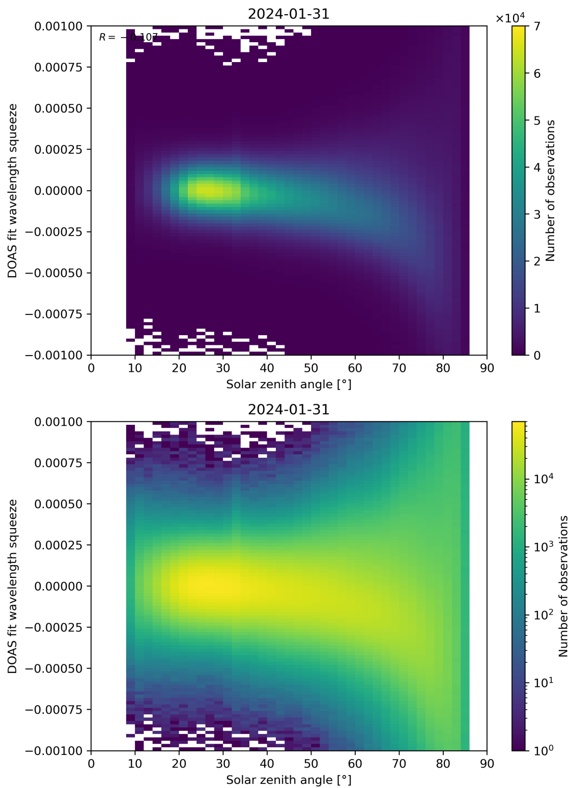
Figure 162: Scatter density plot of “Solar zenith angle” against “DOAS fit wavelength squeeze” for 2024-01-31 to 2024-02-01.
