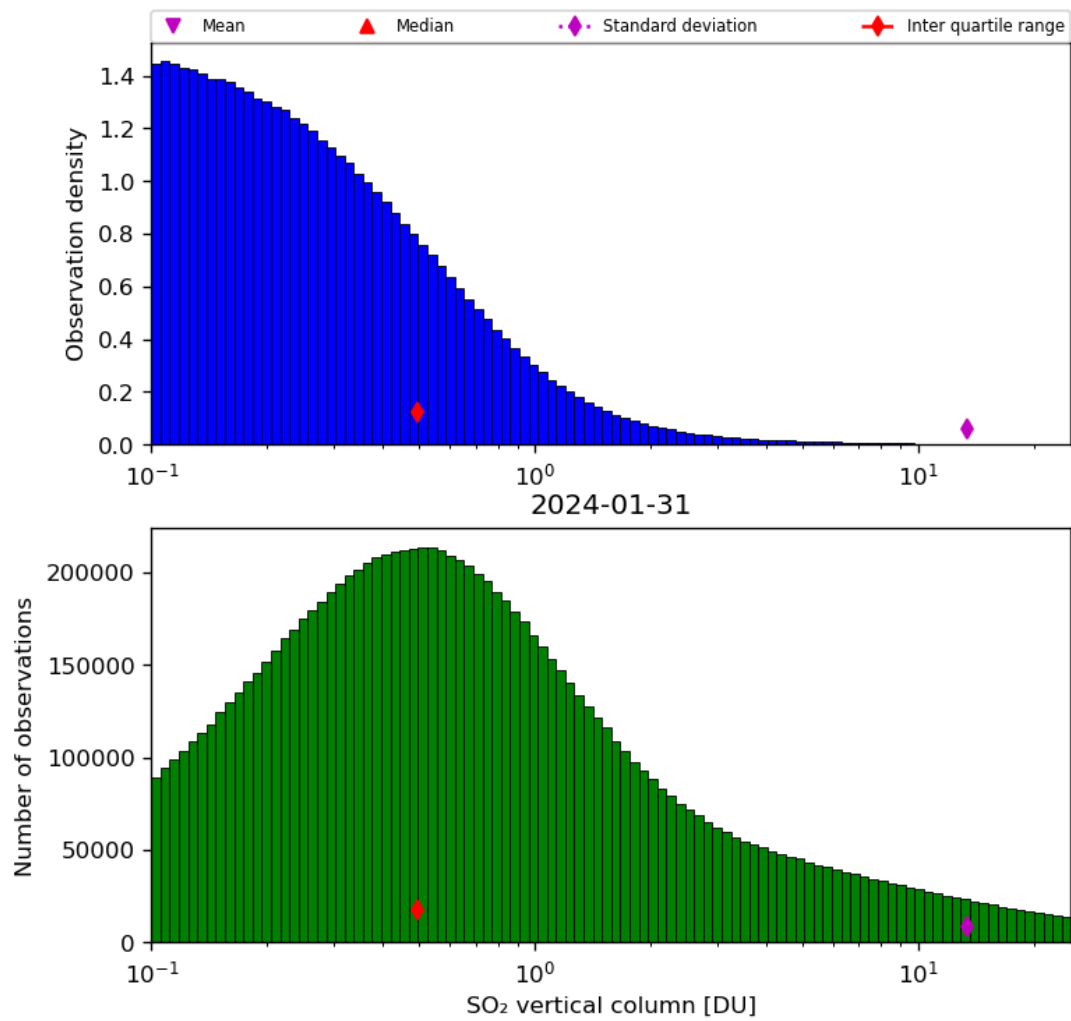
Figure 53: Histogram of “SO 2 vertical column” for 2024-01-31 to 2024-02-01
