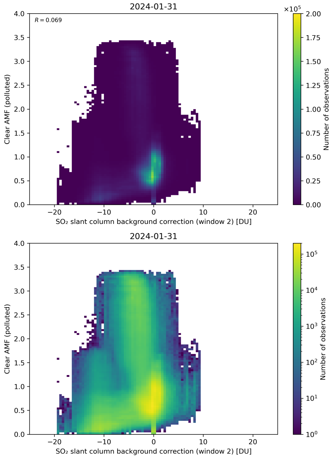
Figure 115: Scatter density plot of “SO 2 slant column background correction (window 2)” against “Clear AMF (polluted)” for 2024-01-31 to 2024-02-01.
