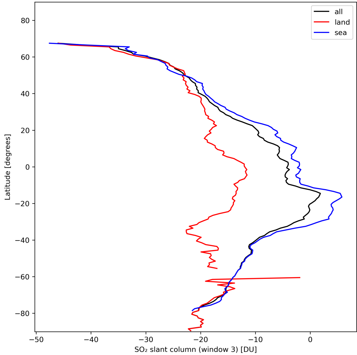
Figure 41: Zonal average of “SO 2 slant column (window 3)” for 2024-01-31 to 2024-02-01.
