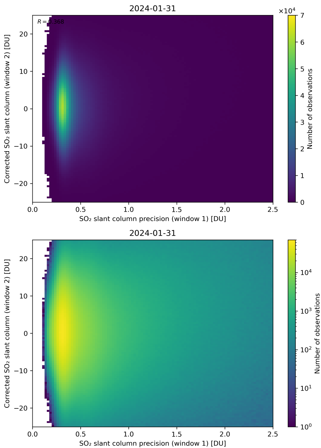
Figure 225: Scatter density plot of “SO 2 slant column precision (window 1)” against “Corrected SO 2 slant column (window 2)” for 2024-01-31 to 2024-02-01.
