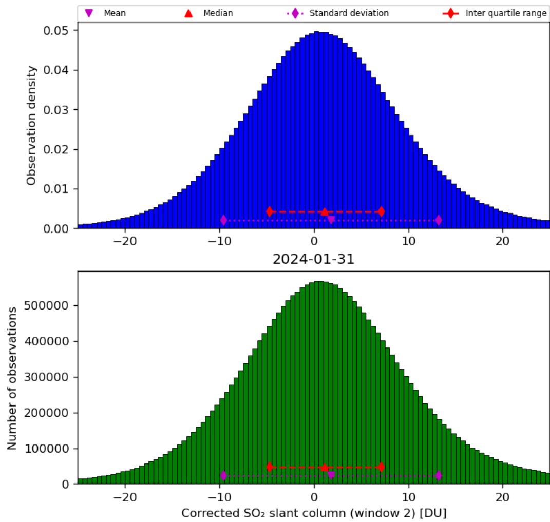
Figure 62: Histogram of “Corrected SO 2 slant column (window 2)” for 2024-01-31 to 2024-02-01
