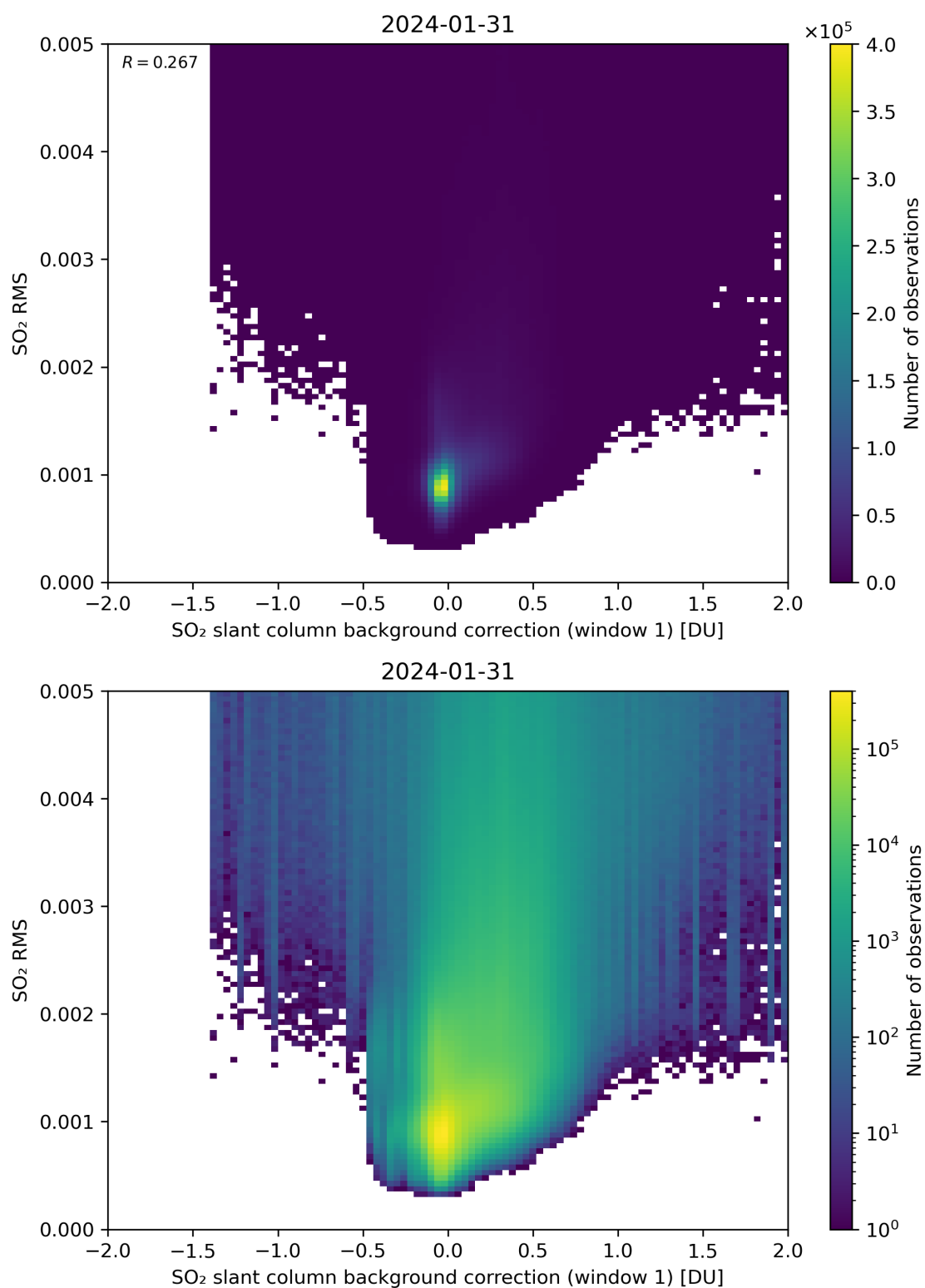
Figure 102: Scatter density plot of “SO 2 slant column background correction (window 1)” against “SO 2 RMS” for 2024-01-31 to 2024-02-01.
