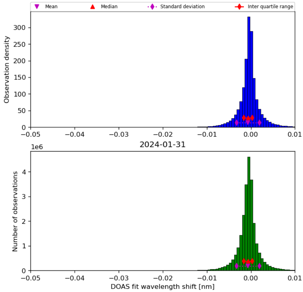
Figure 68: Histogram of “DOAS fit wavelength shift” for 2024-01-31 to 2024-02-01
