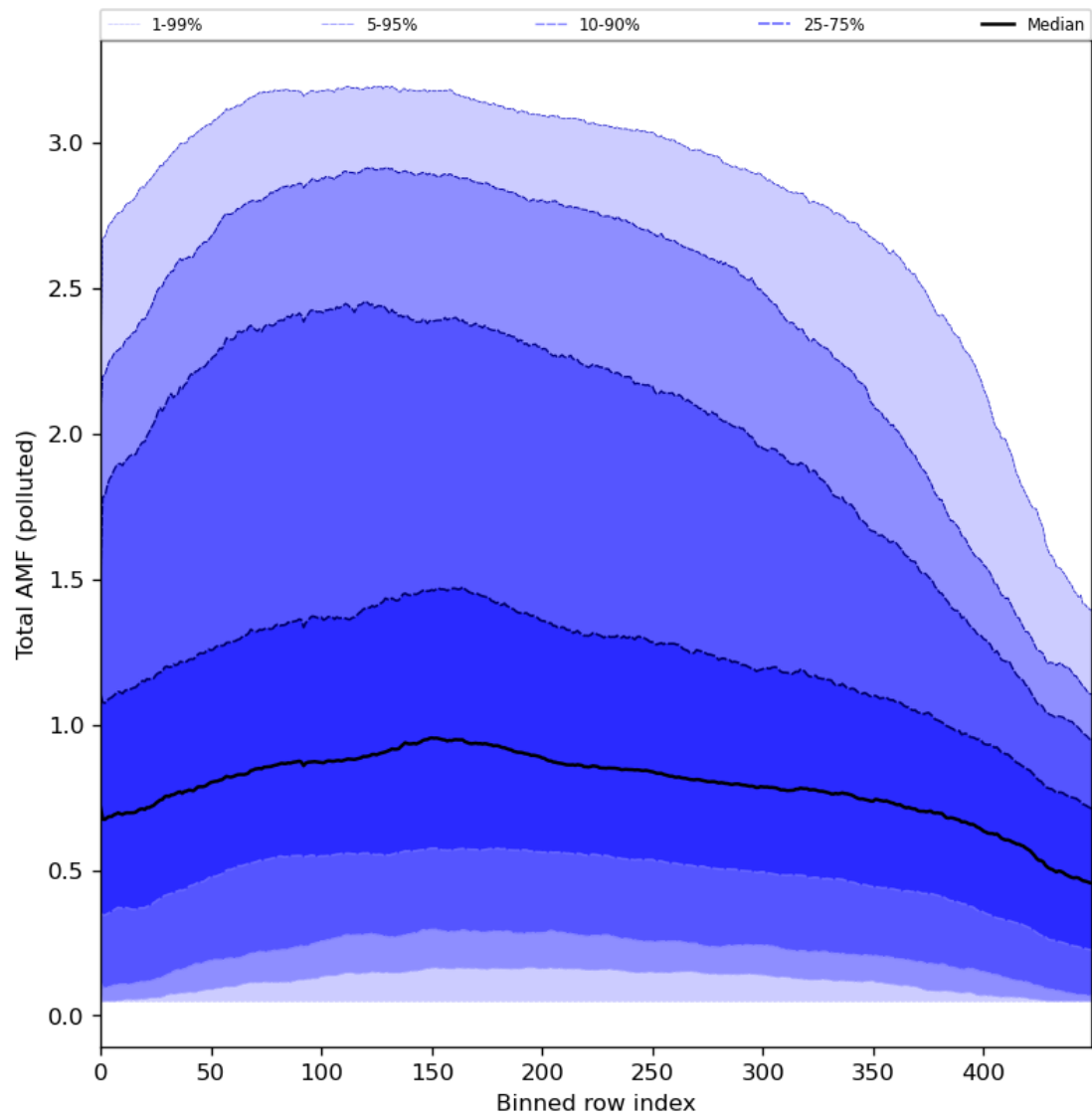
Figure 94: Along track statistics of “Total AMF (polluted)” for 2024-01-31 to 2024-02-01
