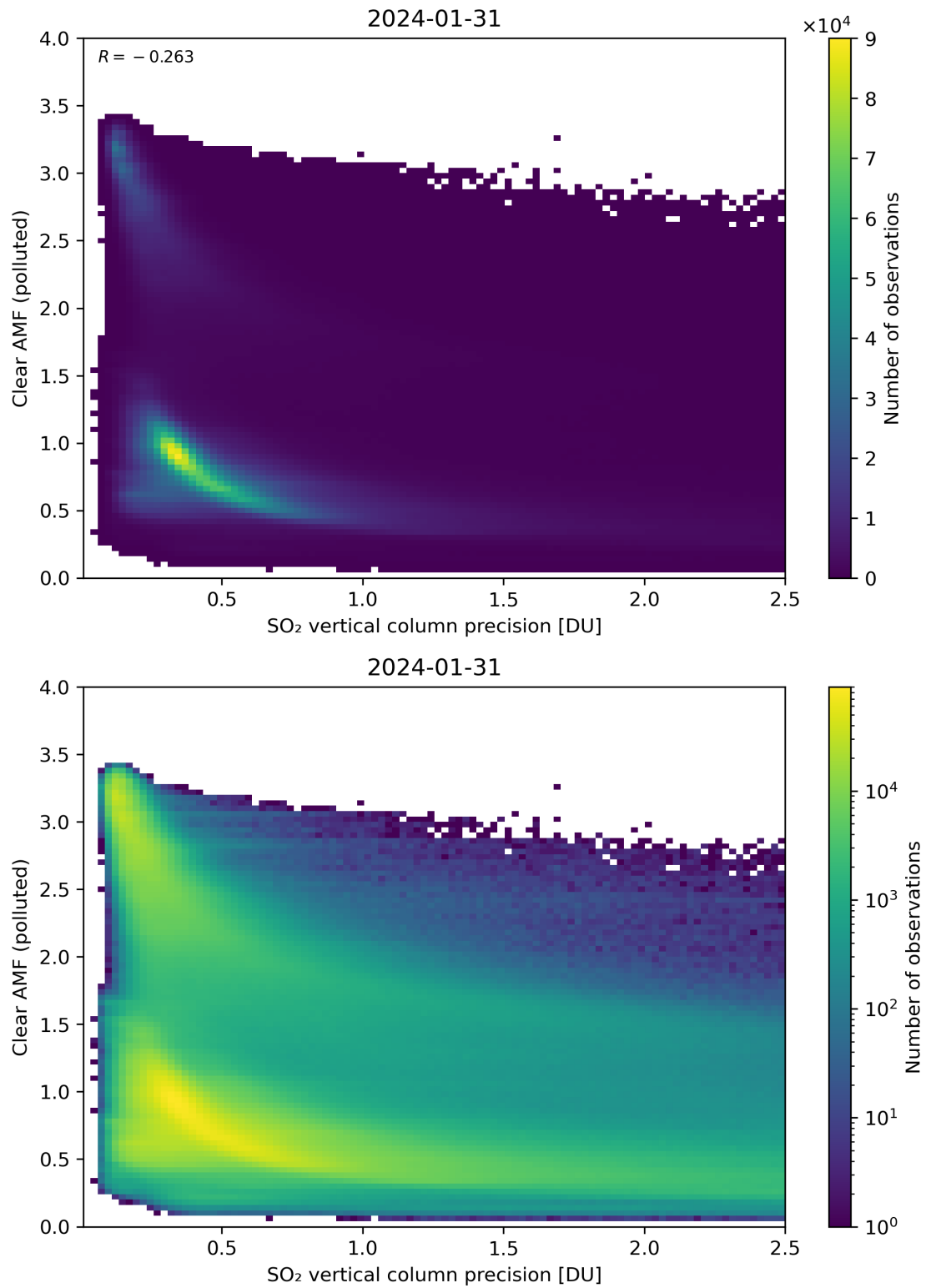
Figure 285: Scatter density plot of “SO 2 vertical column precision” against “Clear AMF (polluted)” for 2024-01-31 to 2024-02-01.
