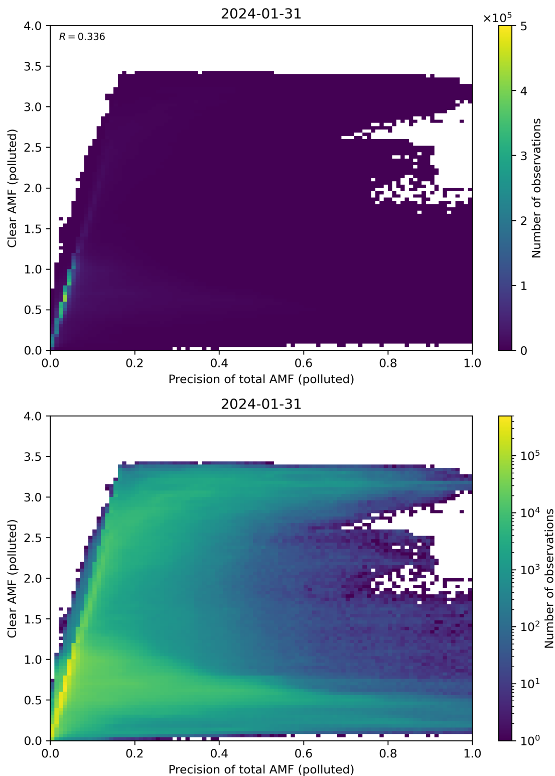
Figure 270: Scatter density plot of “Precision of total AMF (polluted)” against “Clear AMF (polluted)” for 2024-01-31 to 2024-02-01.
