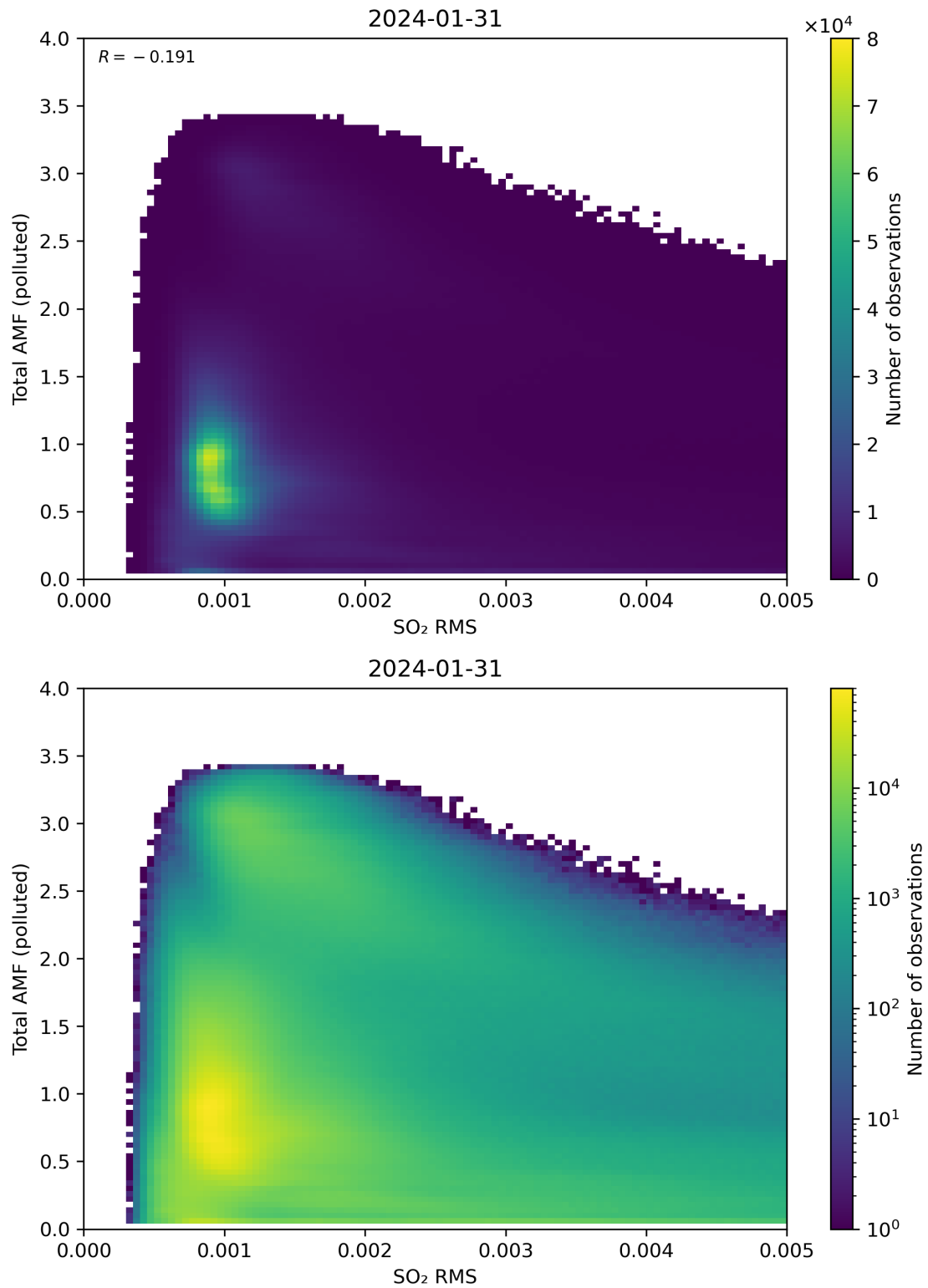
Figure 137: Scatter density plot of “SO 2 RMS” against “Total AMF (polluted)” for 2024-01-31 to 2024-02-01.
