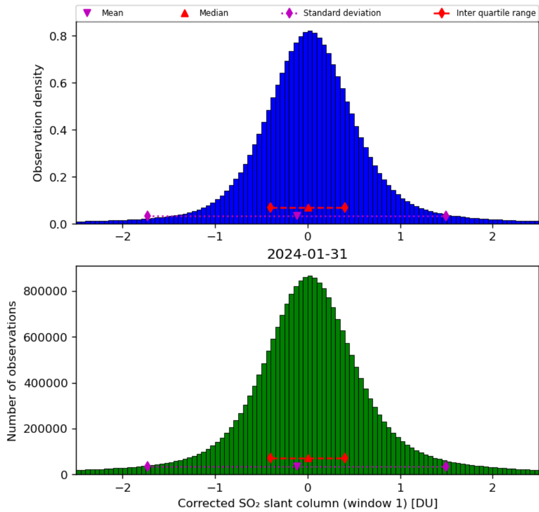
Figure 58: Histogram of “Corrected SO 2 slant column (window 1)” for 2024-01-31 to 2024-02-01
