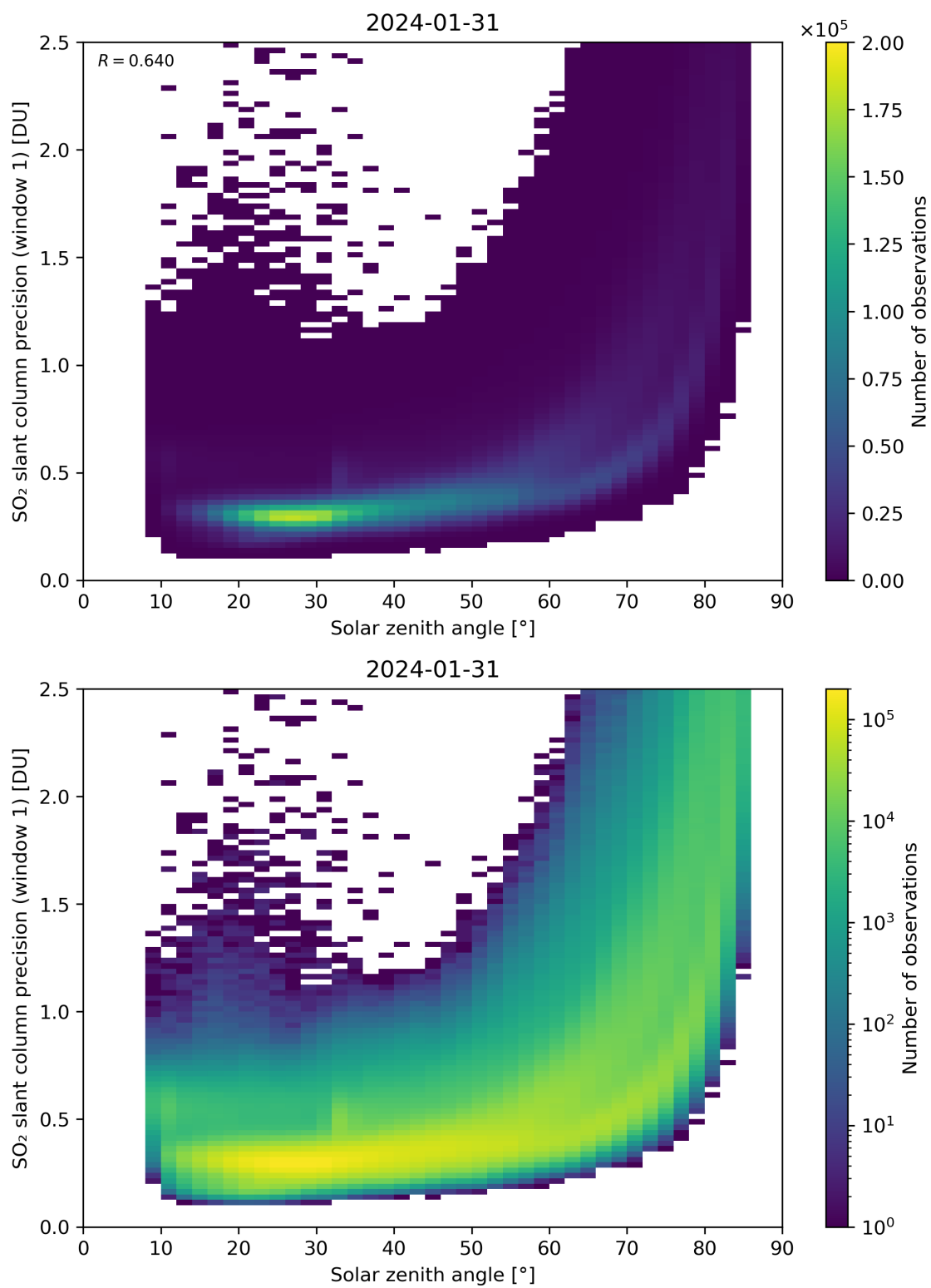
Figure 170: Scatter density plot of “Solar zenith angle” against “SO 2 slant column precision (window 1)” for 2024-01-31 to 2024-02-01.
