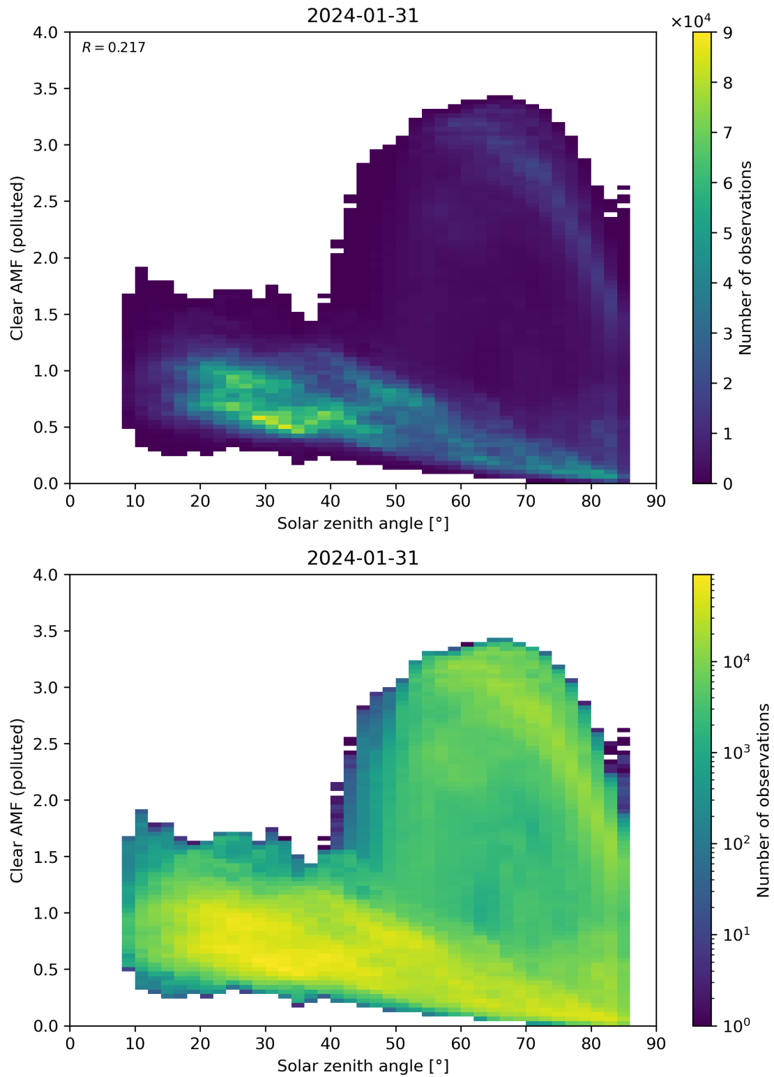
Figure 165: Scatter density plot of “Solar zenith angle” against “Clear AMF (polluted)” for 2024-01-31 to 2024-02-01.
