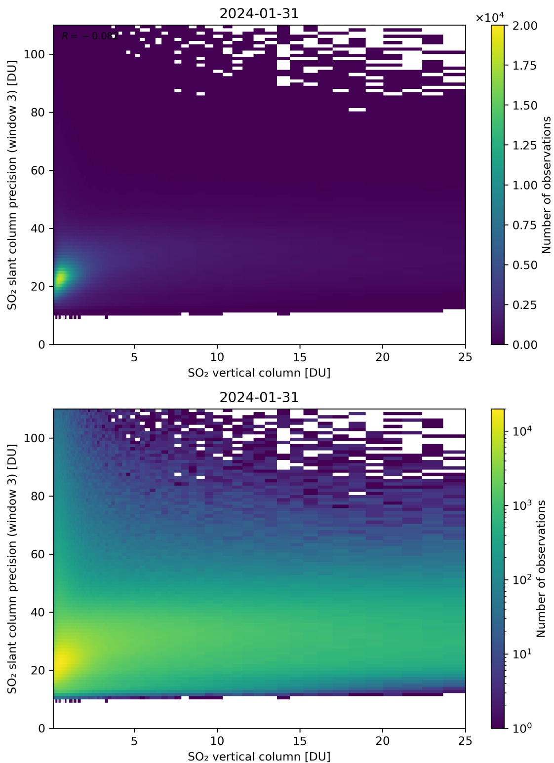
Figure 304: Scatter density plot of “SO 2 vertical column” against “SO 2 slant column precision (window 3)” for 2024-01-31 to 2024-02-01.
