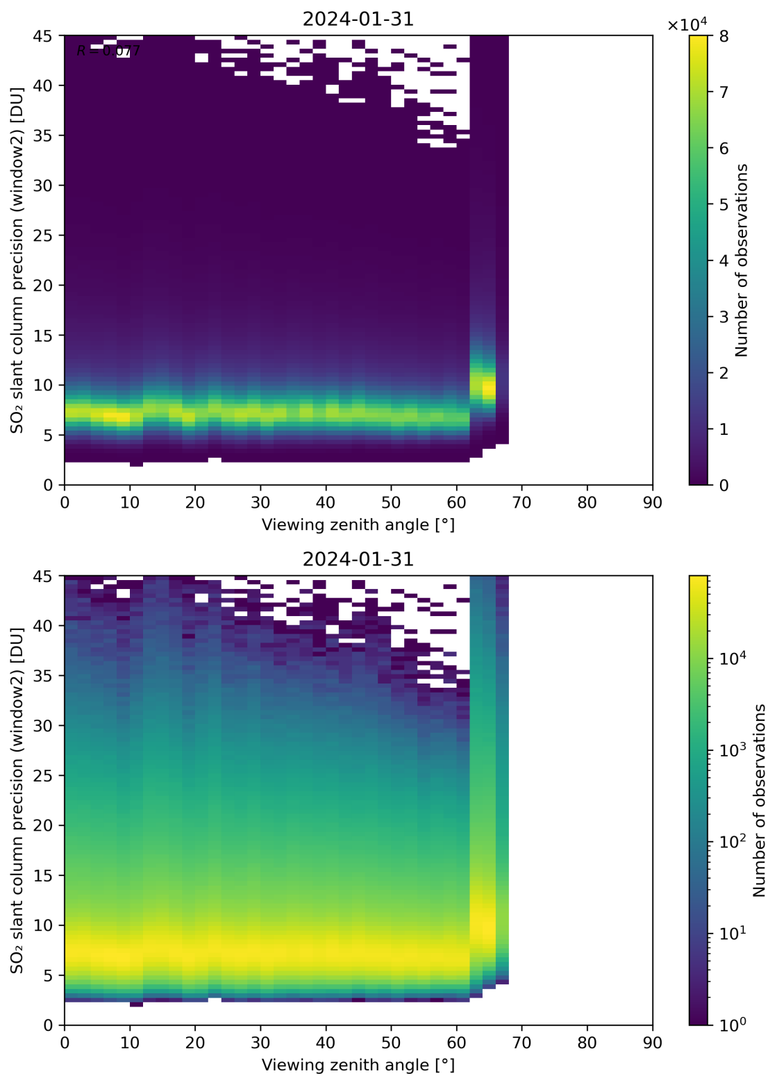
Figure 322: Scatter density plot of “Viewing zenith angle” against “SO 2 slant column precision (window2)” for 2024-01-31 to 2024-02-01.
