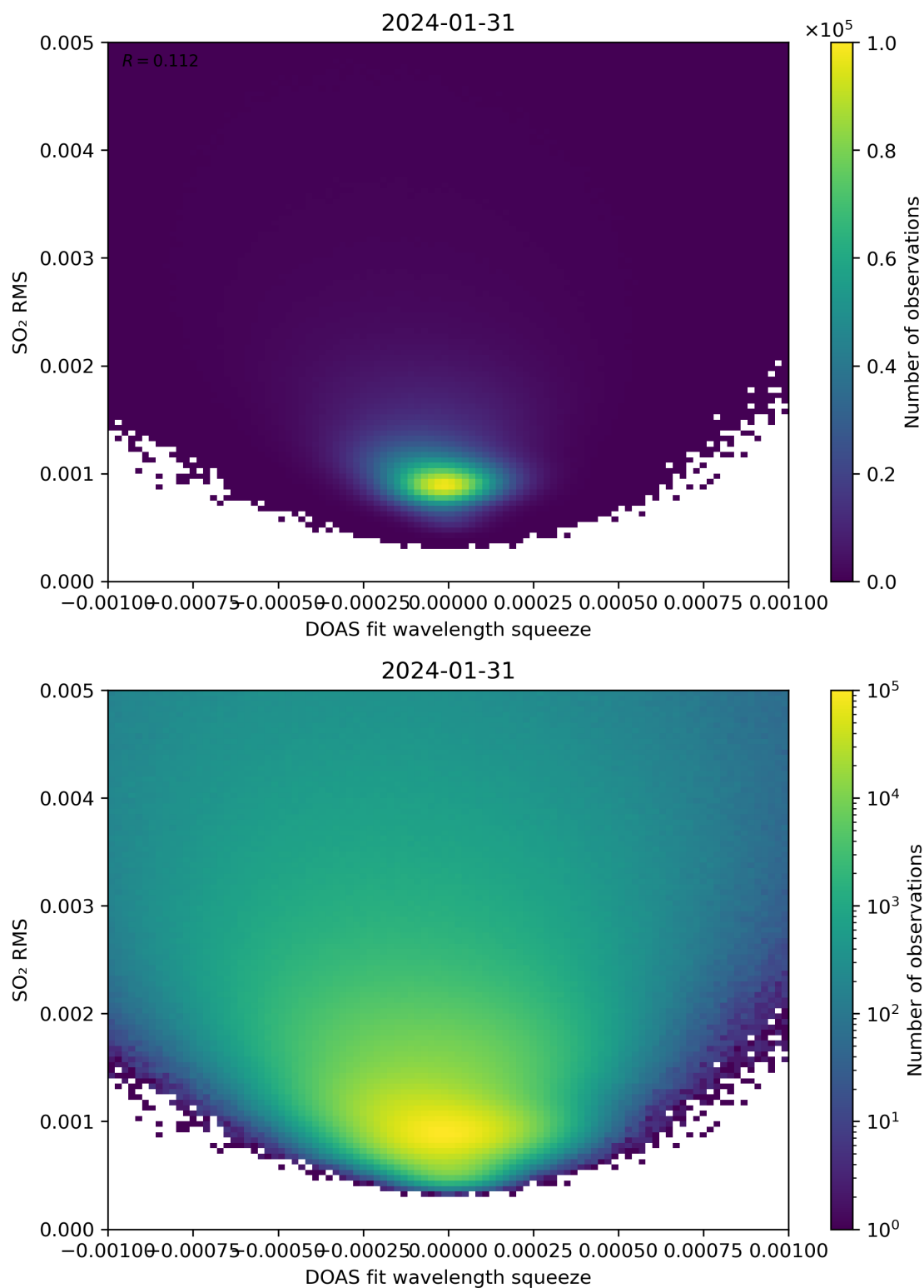
Figure 132: Scatter density plot of “DOAS fit wavelength squeeze” against “SO 2 RMS” for 2024-01-31 to 2024-02-01.
