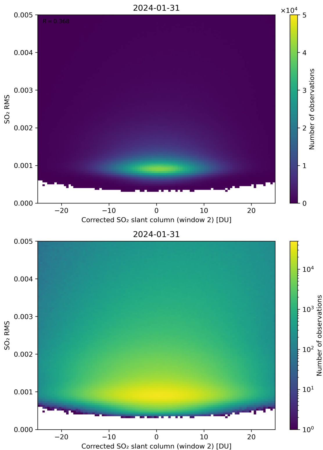
Figure 198: Scatter density plot of “Corrected SO 2 slant column (window 2)” against “SO 2 RMS” for 2024-01-31 to 2024-02-01.
