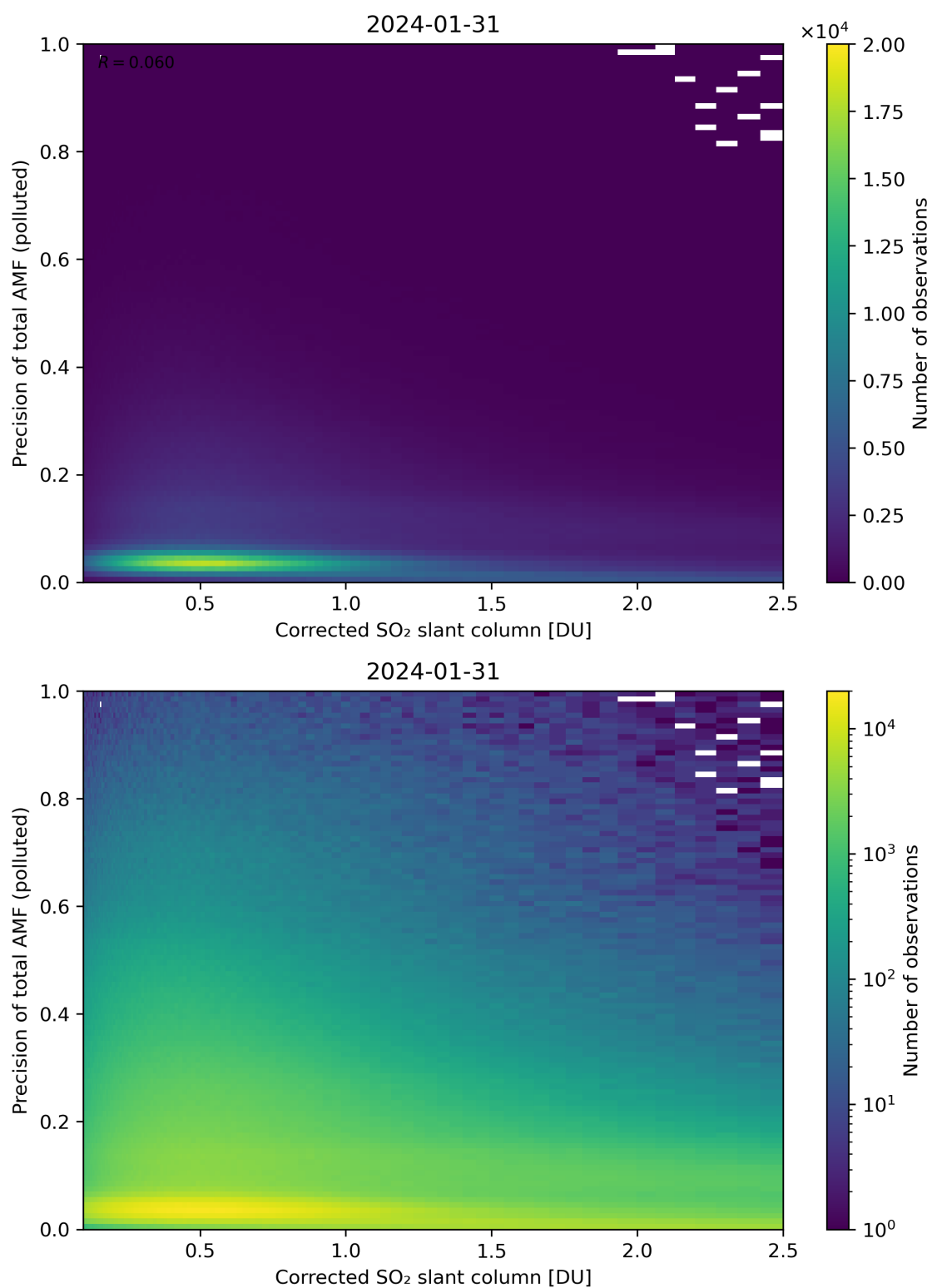
Figure 193: Scatter density plot of “Corrected SO 2 slant column” against “Precision of total AMF (polluted)” for 2024-01-31 to 2024-02-01.
