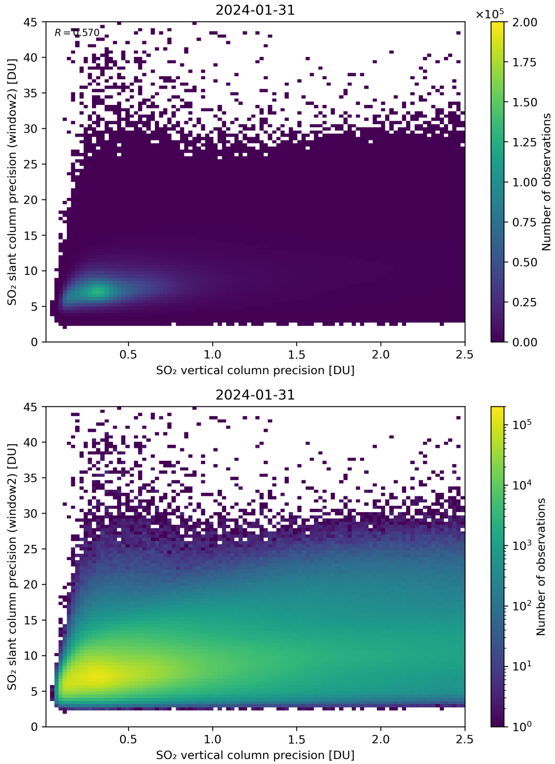
Figure 291: Scatter density plot of “SO 2 vertical column precision” against “SO 2 slant column precision (window2)” for 2024-01-31 to 2024-02-01.
