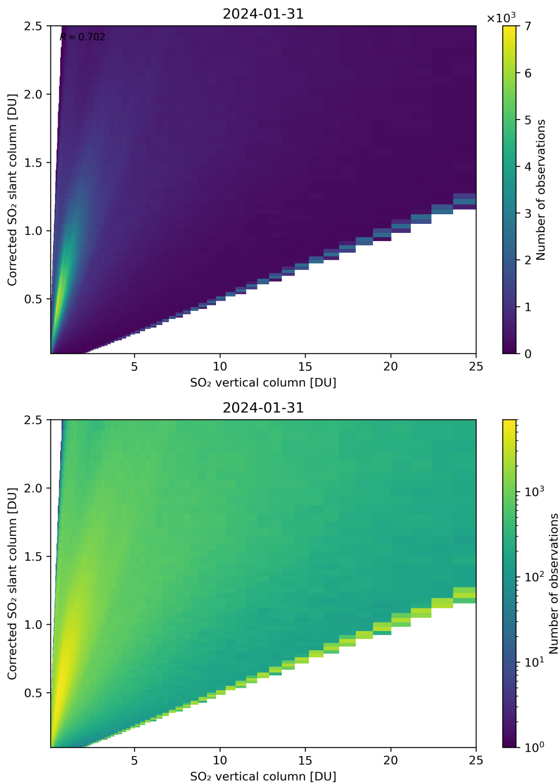
Figure 297: Scatter density plot of “SO 2 vertical column” against “Corrected SO 2 slant column” for 2024-01-31 to 2024-02-01.
