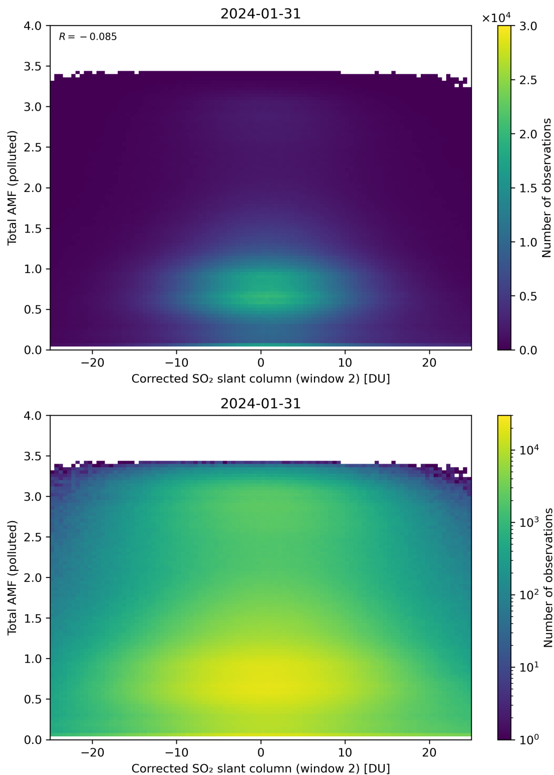
Figure 203: Scatter density plot of “Corrected SO 2 slant column (window 2)” against “Total AMF (polluted)” for 2024-01-31 to 2024-02-01.
