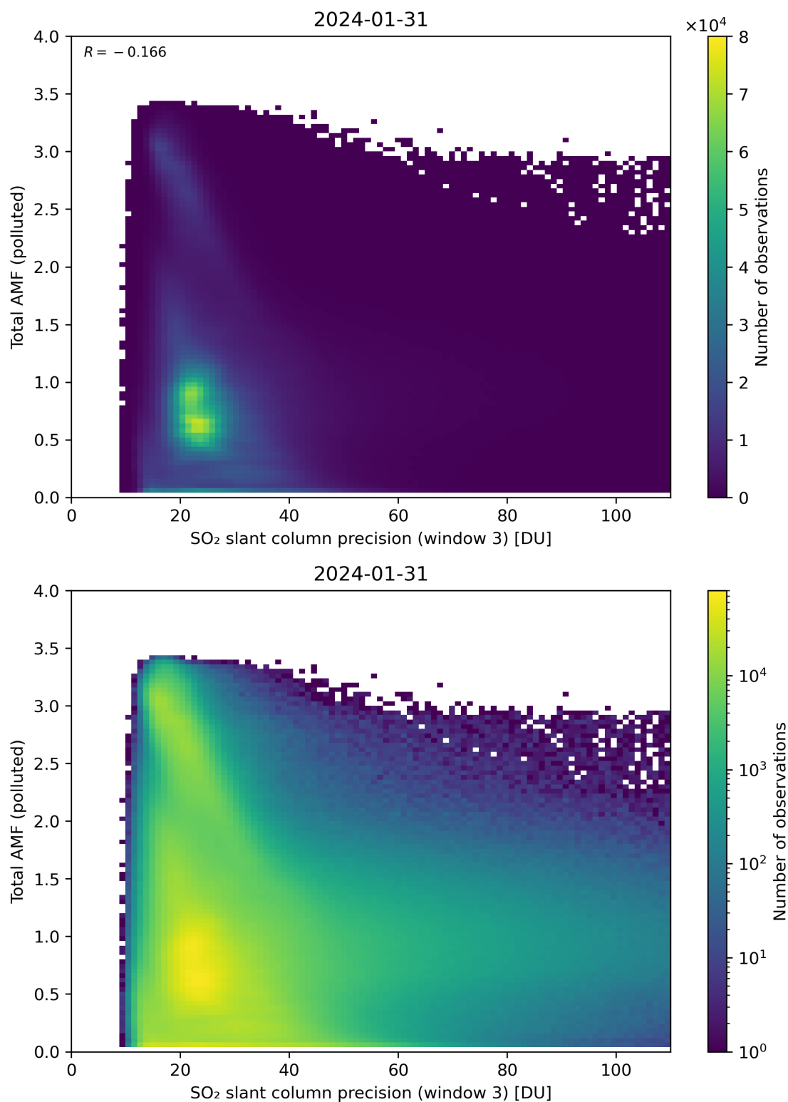
Figure 263: Scatter density plot of “SO 2 slant column precision (window 3)” against “Total AMF (polluted)” for 2024-01-31 to 2024-02-01.
