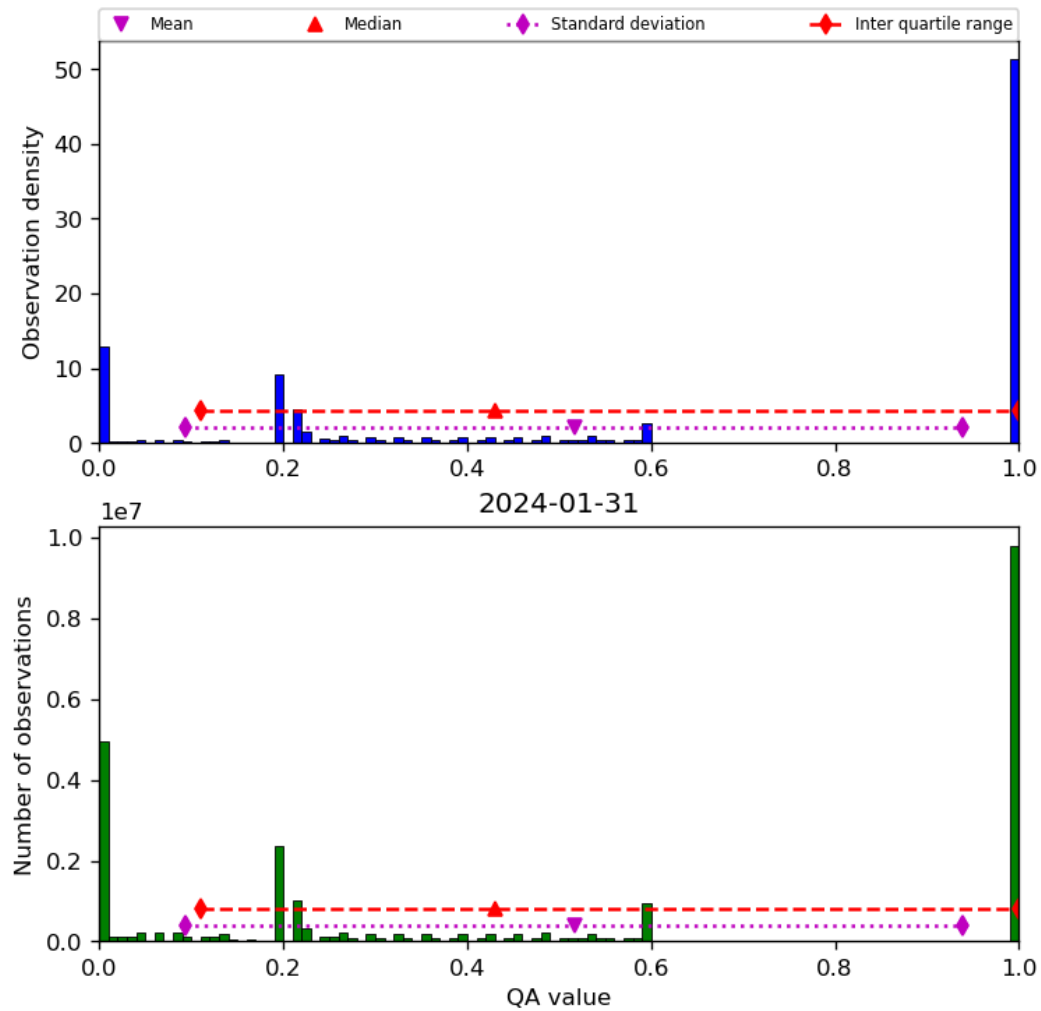
Figure 52: Histogram of “QA value” for 2024-01-31 to 2024-02-01
