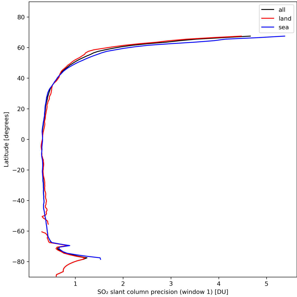
Figure 34: Zonal average of “SO 2 slant column precision (window 1)” for 2024-01-31 to 2024-02-01.
