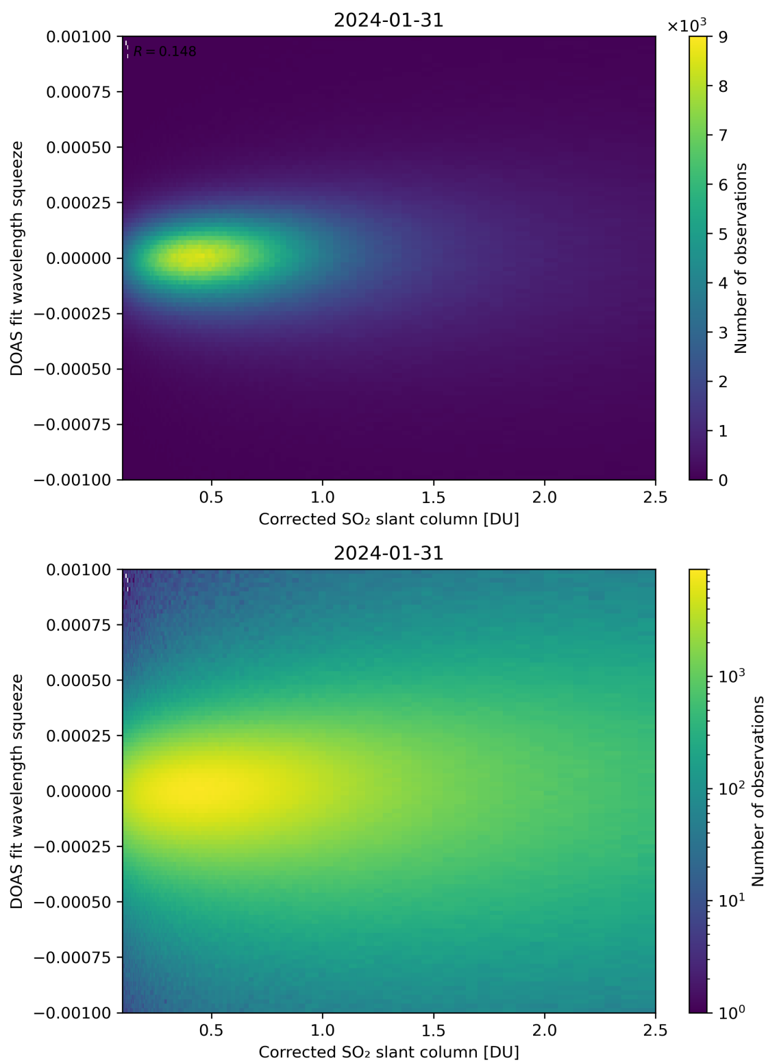
Figure 182: Scatter density plot of “Corrected SO 2 slant column” against “DOAS fit wavelength squeeze” for 2024-01-31 to 2024-02-01.
