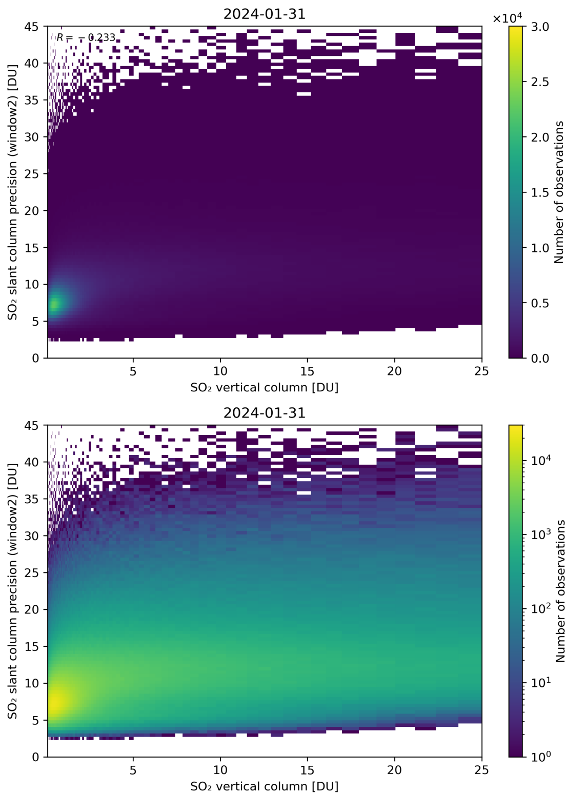
Figure 302: Scatter density plot of “SO 2 vertical column” against “SO 2 slant column precision (window2)” for 2024-01-31 to 2024-02-01.
