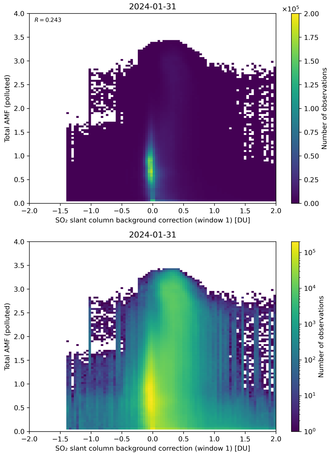
Figure 109: Scatter density plot of “SO 2 slant column background correction (window 1)” against “Total AMF (polluted)” for 2024-01-31 to 2024-02-01.
