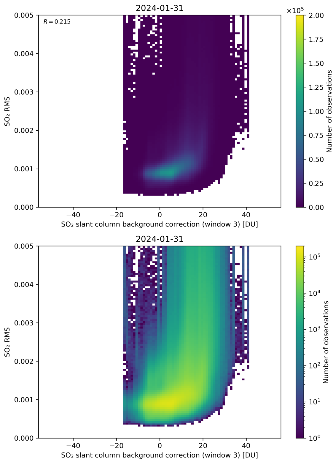
Figure 123: Scatter density plot of “SO 2 slant column background correction (window 3)” against “SO 2 RMS” for 2024-01-31 to 2024-02-01.
