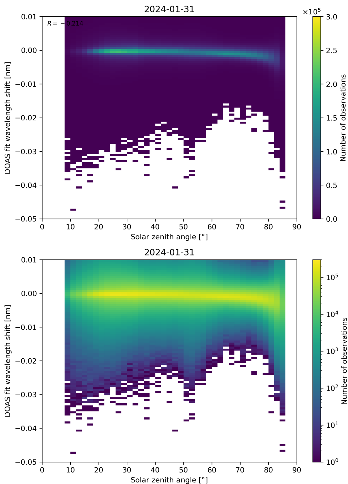
Figure 161: Scatter density plot of “Solar zenith angle” against “DOAS fit wavelength shift” for 2024-01-31 to 2024-02-01.
