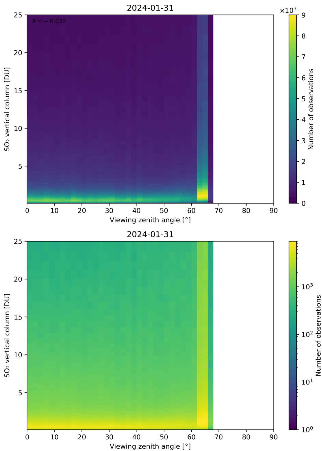
Figure 327: Scatter density plot of “Viewing zenith angle” against “SO 2 vertical column” for 2024-01-31 to 2024-02-01.
