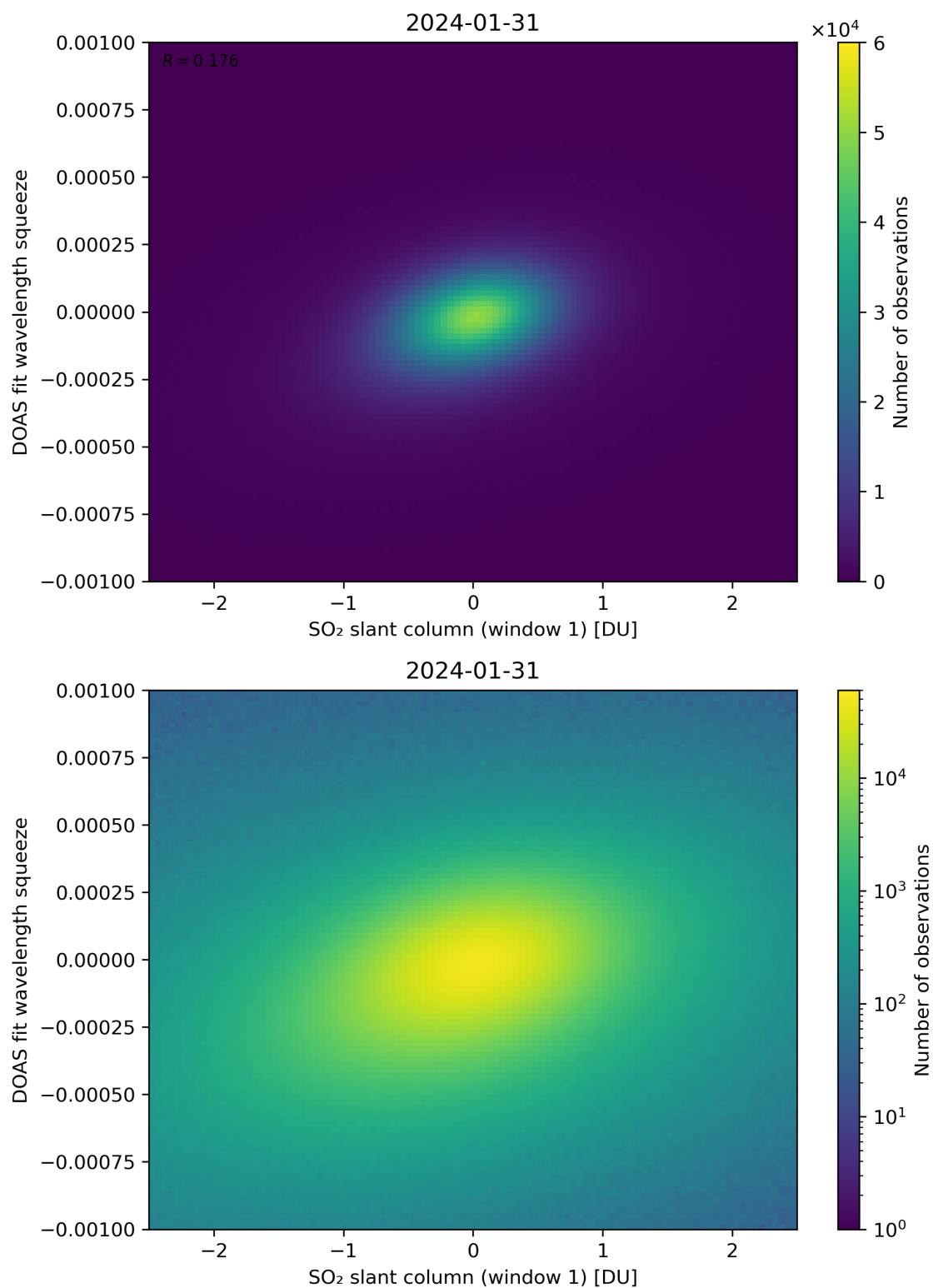
Figure 216: Scatter density plot of “SO 2 slant column (window 1)” against “DOAS fit wavelength squeeze” for 2024-01-31 to 2024-02-01.
