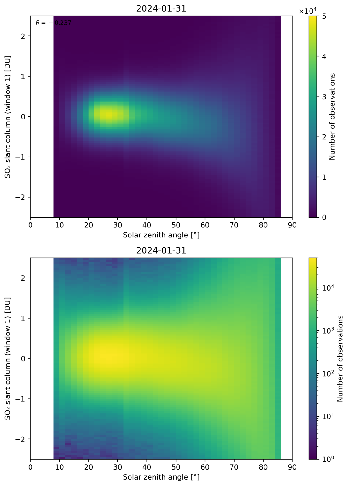
Figure 169: Scatter density plot of “Solar zenith angle” against “SO 2 slant column (window 1)” for 2024-01-31 to 2024-02-01.
