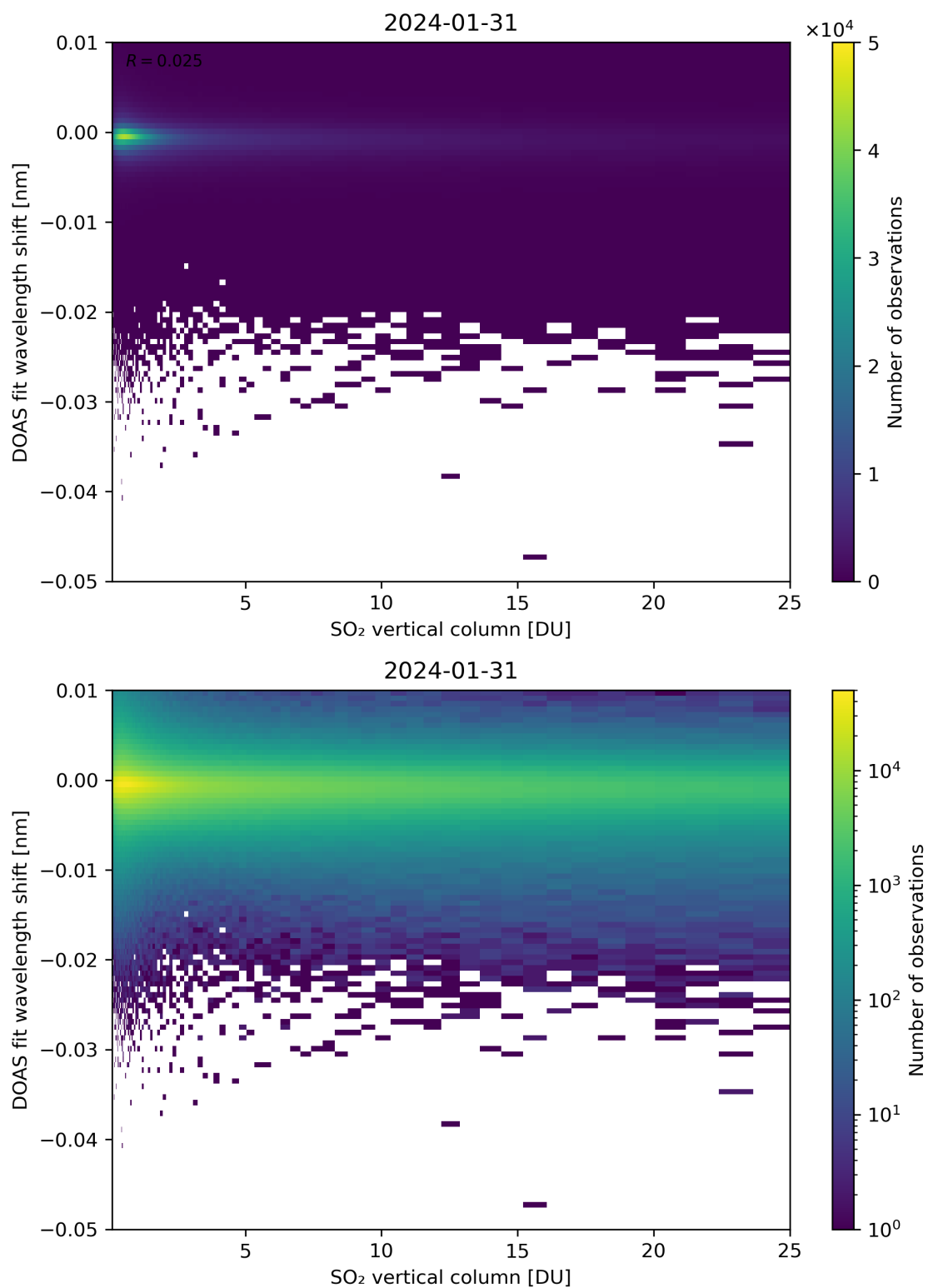
Figure 276: Scatter density plot of “SO 2 vertical column” against “DOAS fit wavelength shift” for 2024-01-31 to 2024-02-01.
