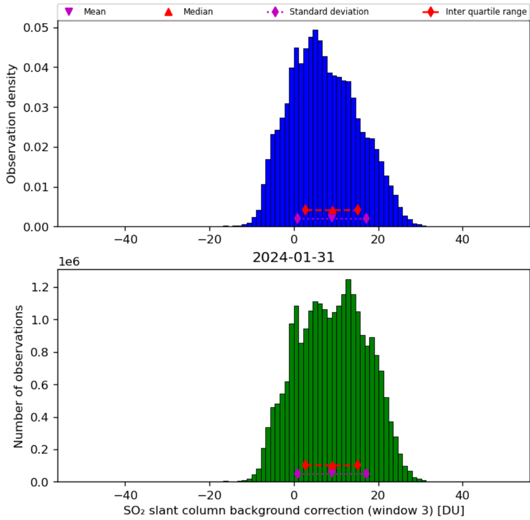
Figure 67: Histogram of “SO 2 slant column background correction (window 3)” for 2024-01-31 to 2024-02-01
