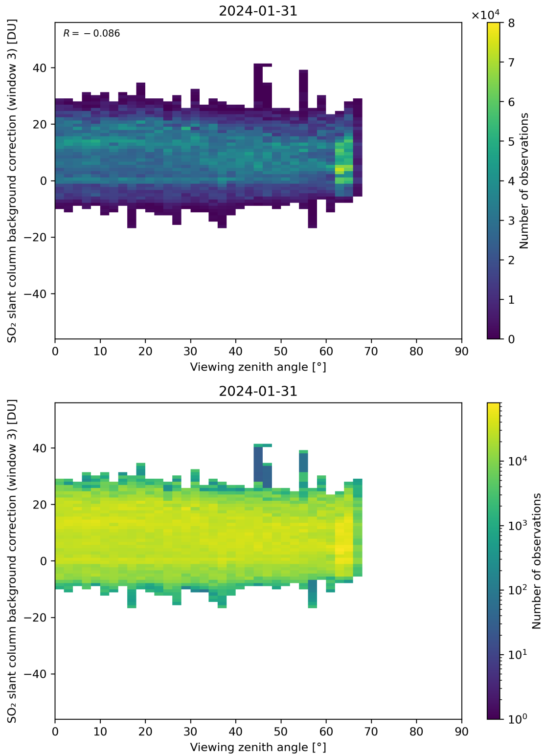
Figure 310: Scatter density plot of “Viewing zenith angle” against “SO 2 slant column background correction (window 3)” for 2024-01-31 to 2024-02-01.
