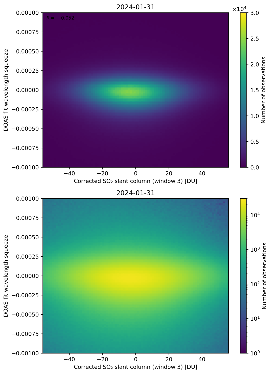
Figure 207: Scatter density plot of “Corrected SO 2 slant column (window 3)” against “DOAS fit wavelength squeeze” for 2024-01-31 to 2024-02-01.
