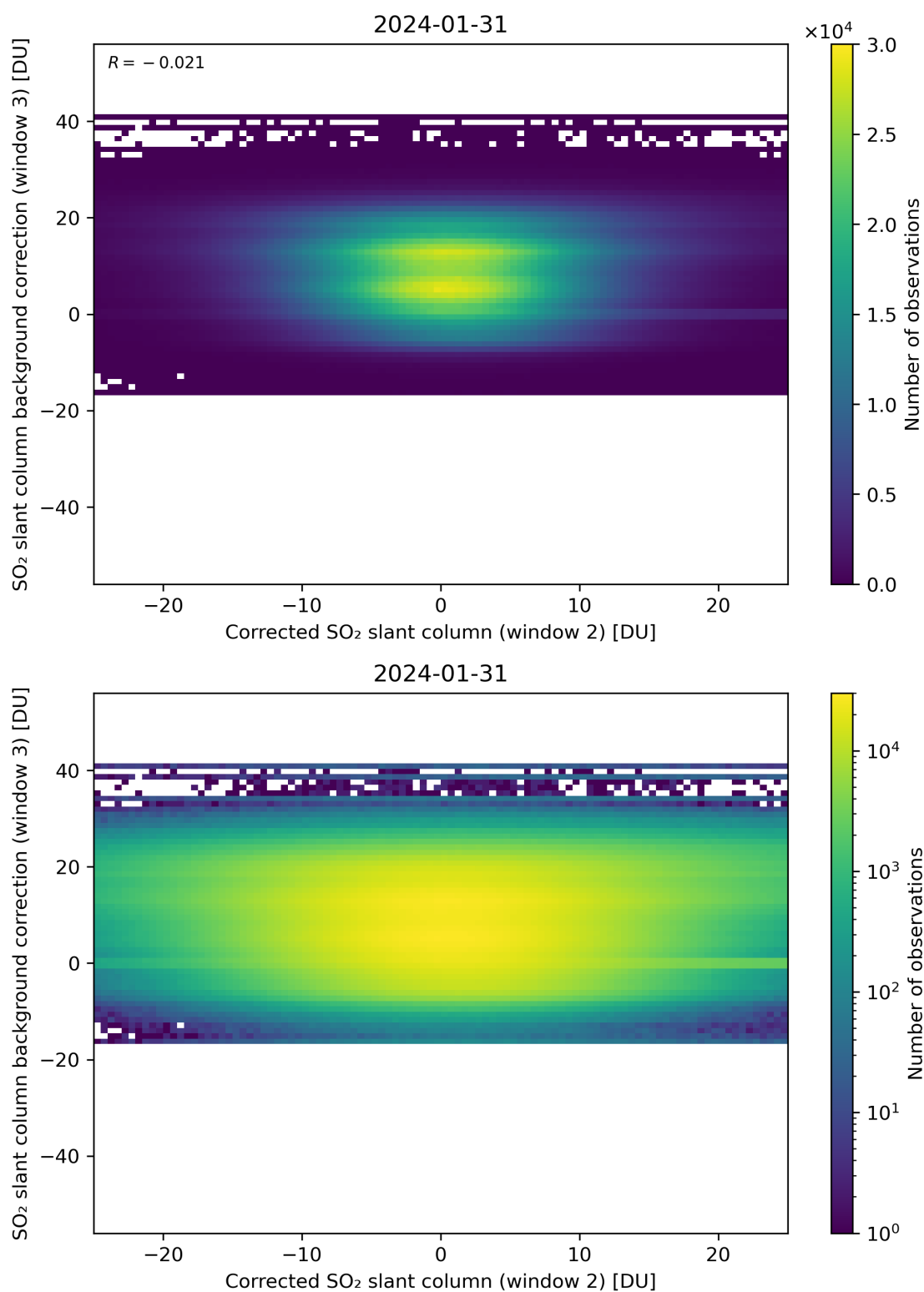
Figure 195: Scatter density plot of “Corrected SO 2 slant column (window 2)” against “SO 2 slant column background correction (window 3)” for 2024-01-31 to 2024-02-01.
