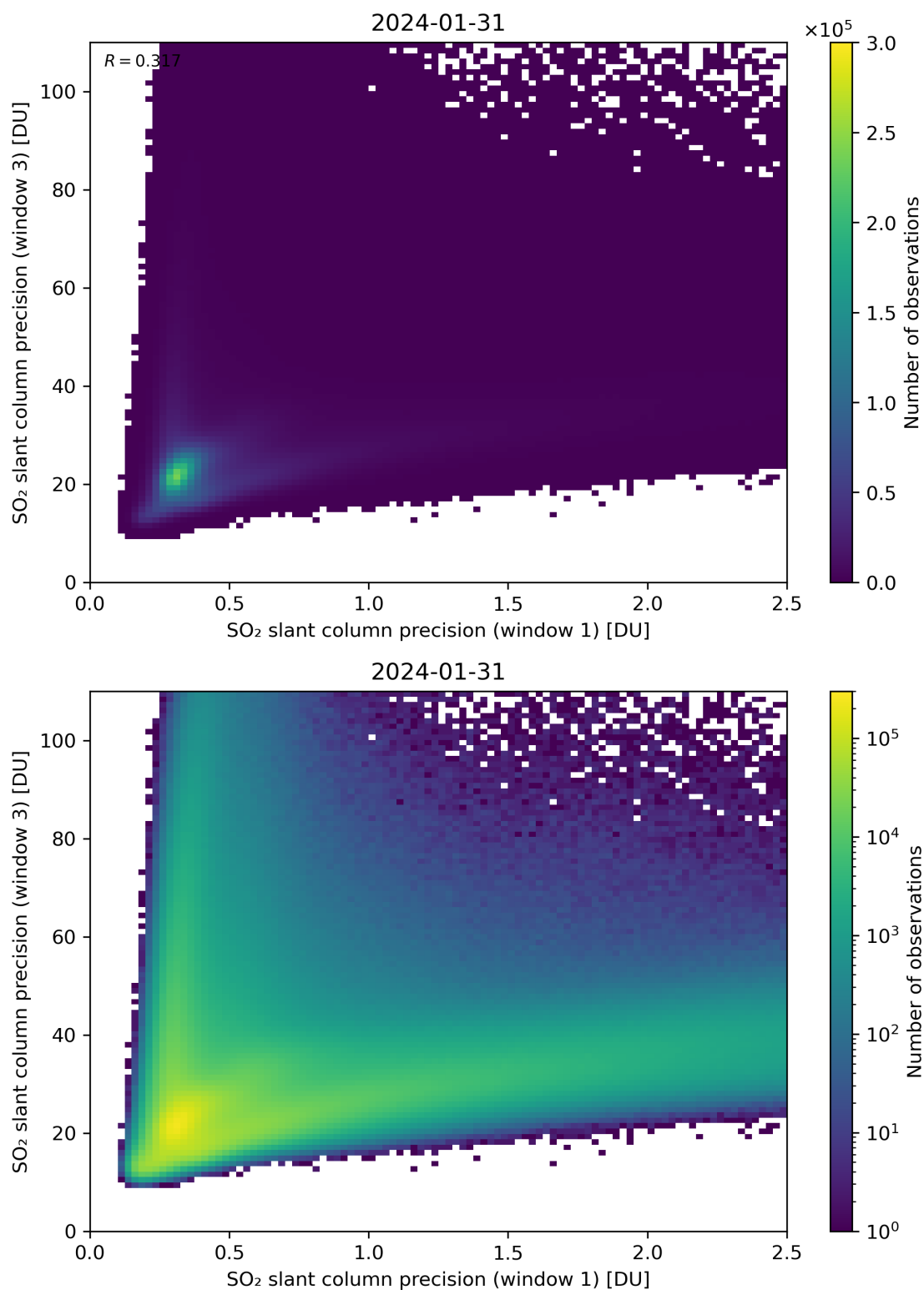
Figure 229: Scatter density plot of “SO 2 slant column precision (window 1)” against “SO 2 slant column precision (window 3)” for 2024-01-31 to 2024-02-01.
