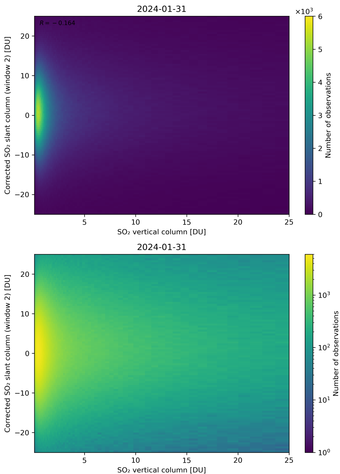
Figure 298: Scatter density plot of “SO 2 vertical column” against “Corrected SO 2 slant column (window 2)” for 2024-01-31 to 2024-02-01.
