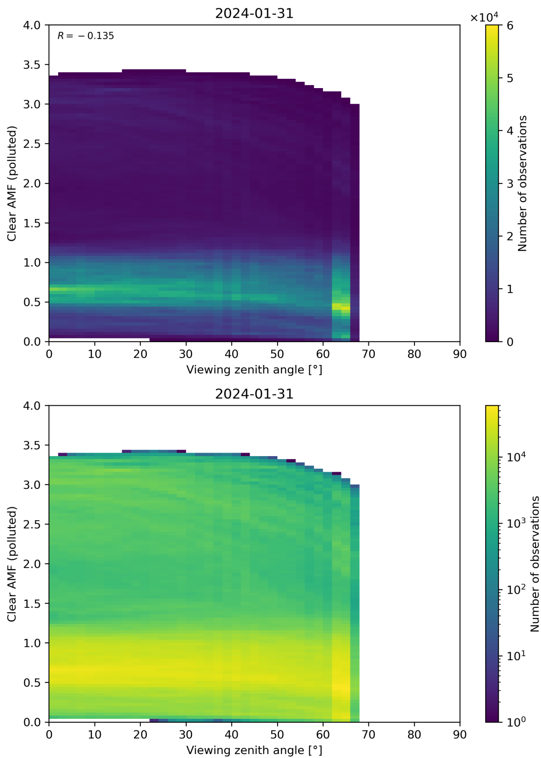
Figure 316: Scatter density plot of “Viewing zenith angle” against “Clear AMF (polluted)” for 2024-01-31 to 2024-02-01.
