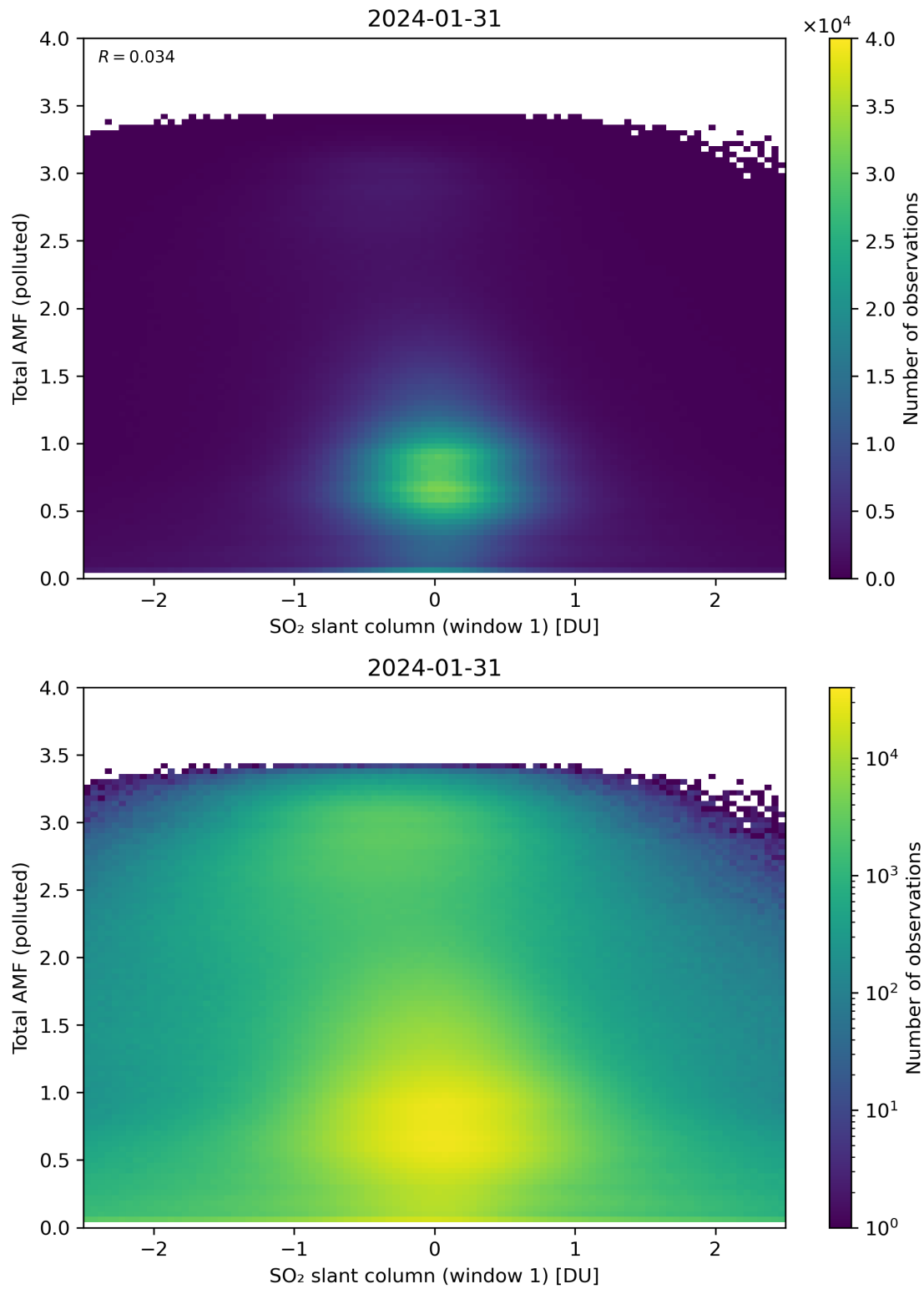
Figure 239: Scatter density plot of “SO 2 slant column (window 1)” against “Total AMF (polluted)” for 2024-01-31 to 2024-02-01.
