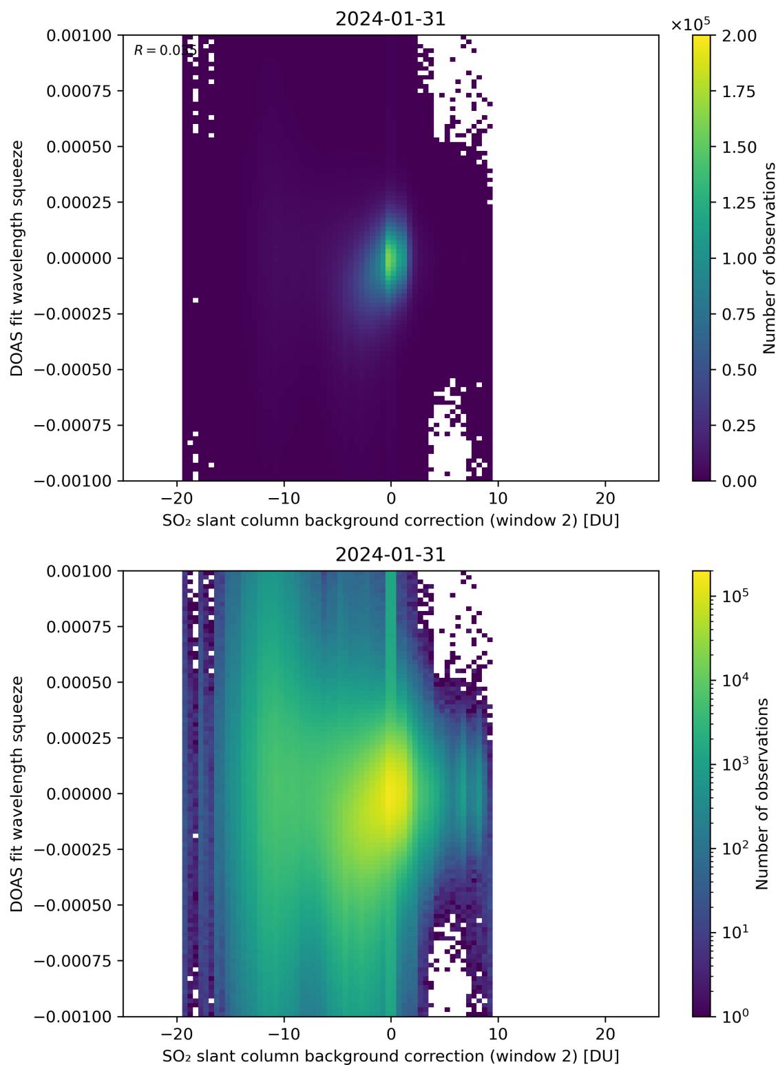
Figure 113: Scatter density plot of "SO 2 slant column background correction (window 2)" against "DOAS fit wavelength squeeze" for 2024-01-31 to 2024-02-01.
