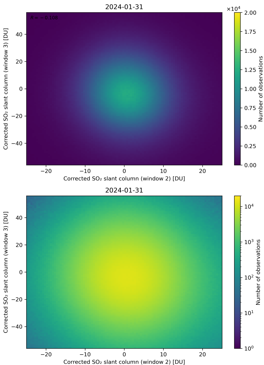
Figure 200: Scatter density plot of “Corrected SO 2 slant column (window 2)” against “Corrected SO 2 slant column (window 3)” for 2024-01-31 to 2024-02-01.
