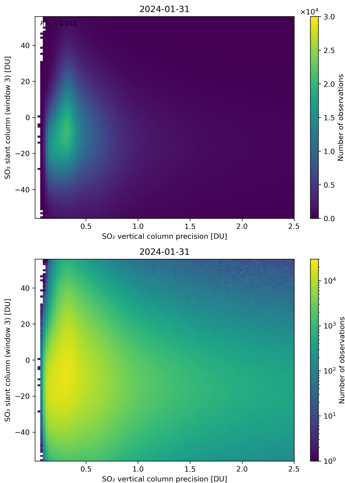
Figure 292: Scatter density plot of “SO 2 vertical column precision” against “SO 2 slant column (window 3)” for 2024-01-31 to 2024-02-01.
