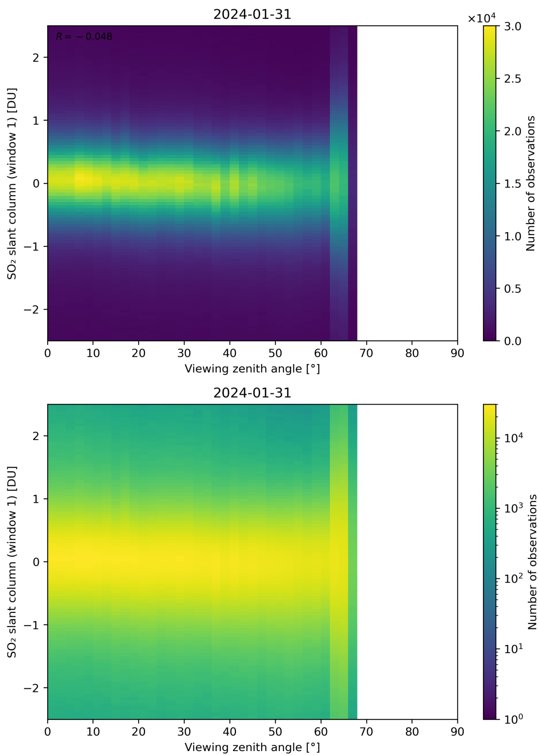
Figure 320: Scatter density plot of “Viewing zenith angle” against “SO 2 slant column (window 1)” for 2024-01-31 to 2024-02-01.
