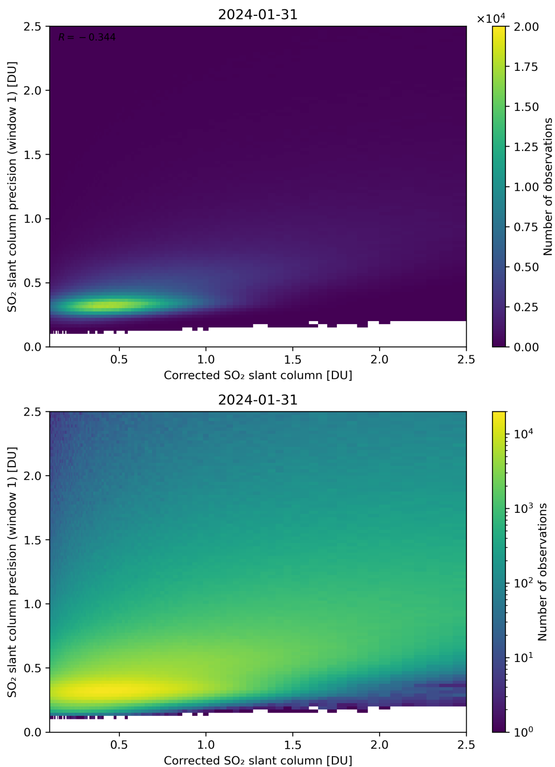
Figure 188: Scatter density plot of “Corrected SO 2 slant column” against “SO 2 slant column precision (window 1)” for 2024-01-31 to 2024-02-01.
