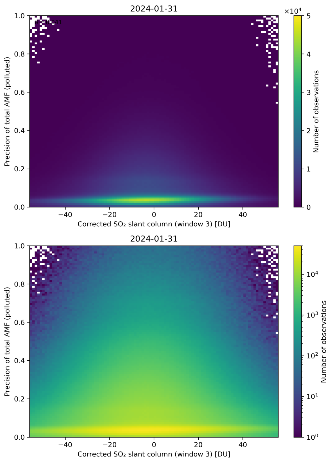
Figure 211: Scatter density plot of “Corrected SO 2 slant column (window 3)” against “Precision of total AMF (polluted)” for 2024-01-31 to 2024-02-01.
