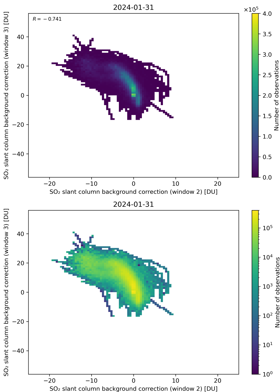
Figure 111: Scatter density plot of “SO 2 slant column background correction (window 2)” against “SO 2 slant column background correction (window 3)” for 2024-01-31 to 2024-02-01.
