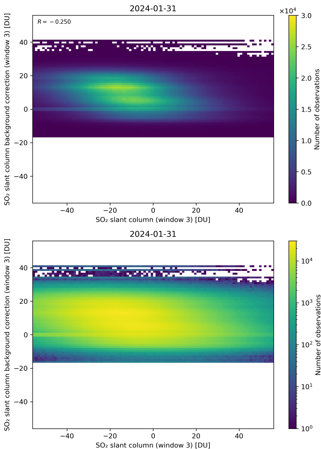
Figure 253: Scatter density plot of “SO 2 slant column (window 3)” against “SO 2 slant column background correction (window 3)” for 2024-01-31 to 2024-02-01.
