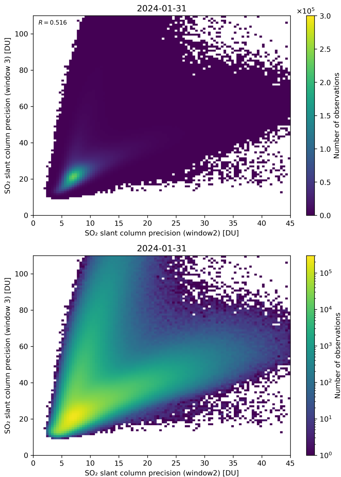
Figure 250: Scatter density plot of “SO 2 slant column precision (window2)” against “SO 2 slant column precision (window 3)” for 2024-01-31 to 2024-02-01.
