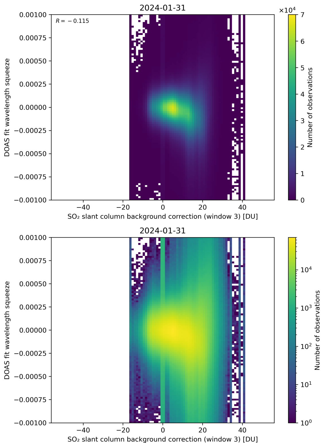
Figure 122: Scatter density plot of “SO 2 slant column background correction (window 3)” against “DOAS fit wavelength squeeze” for 2024-01-31 to 2024-02-01.
