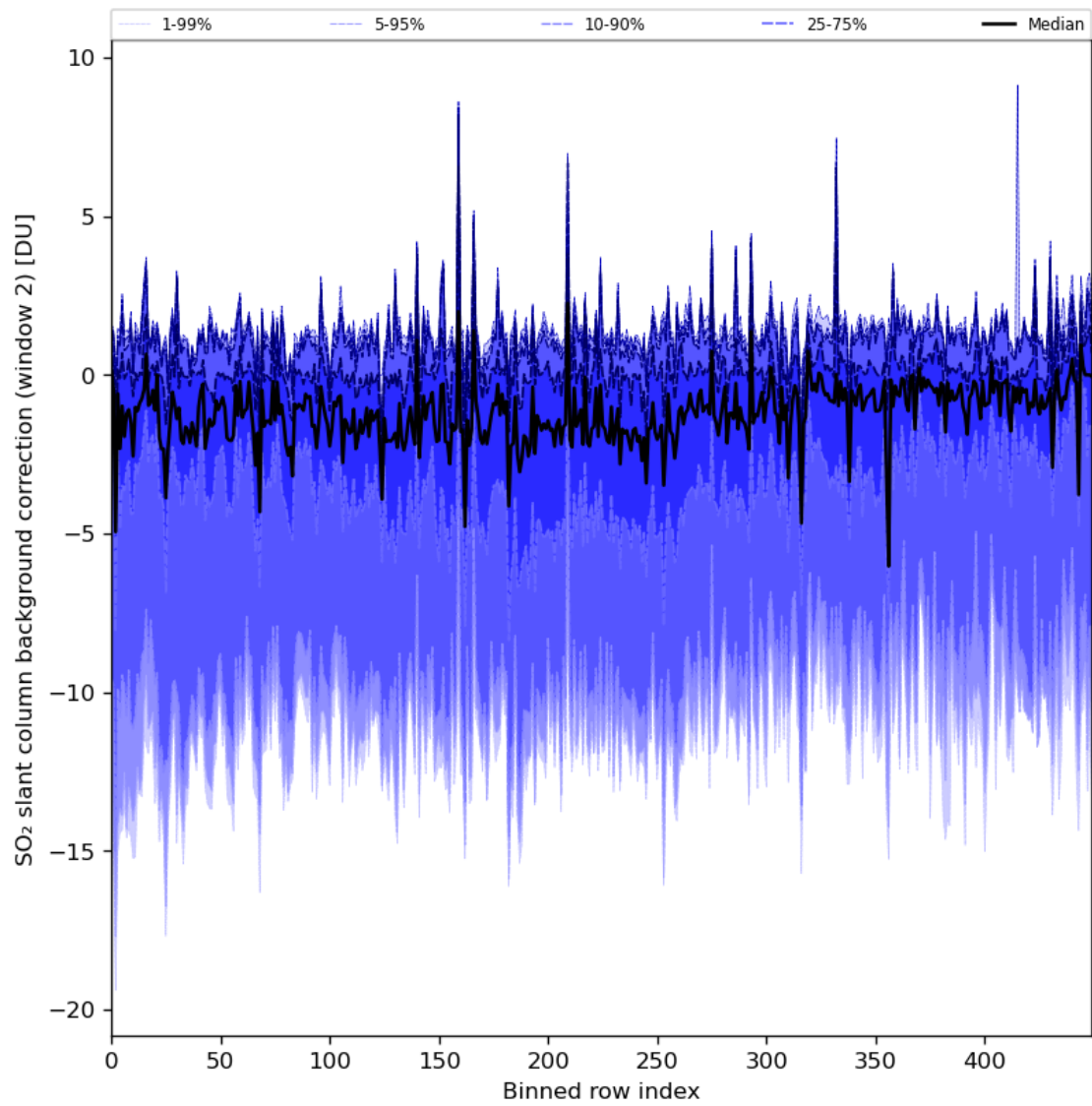
Figure 86: Along track statistics of “SO 2 slant column background correction (window 2)” for 2024-01-31 to 2024-02-01
