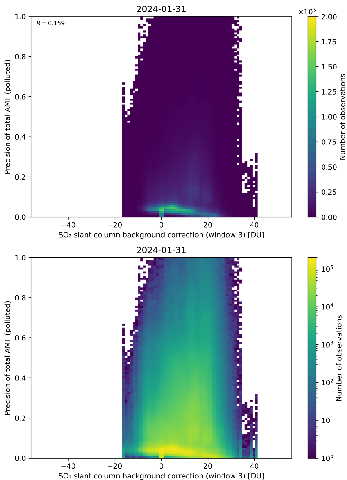
Figure 126: Scatter density plot of “SO 2 slant column background correction (window 3)” against “Precision of total AMF (polluted)” for 2024-01-31 to 2024-02-01.
