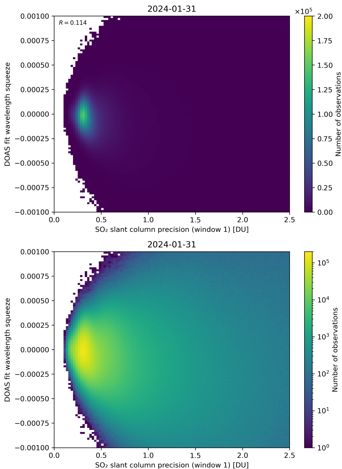
Figure 222: Scatter density plot of “SO 2 slant column precision (window 1)” against “DOAS fit wavelength squeeze” for 2024-01-31 to 2024-02-01.
