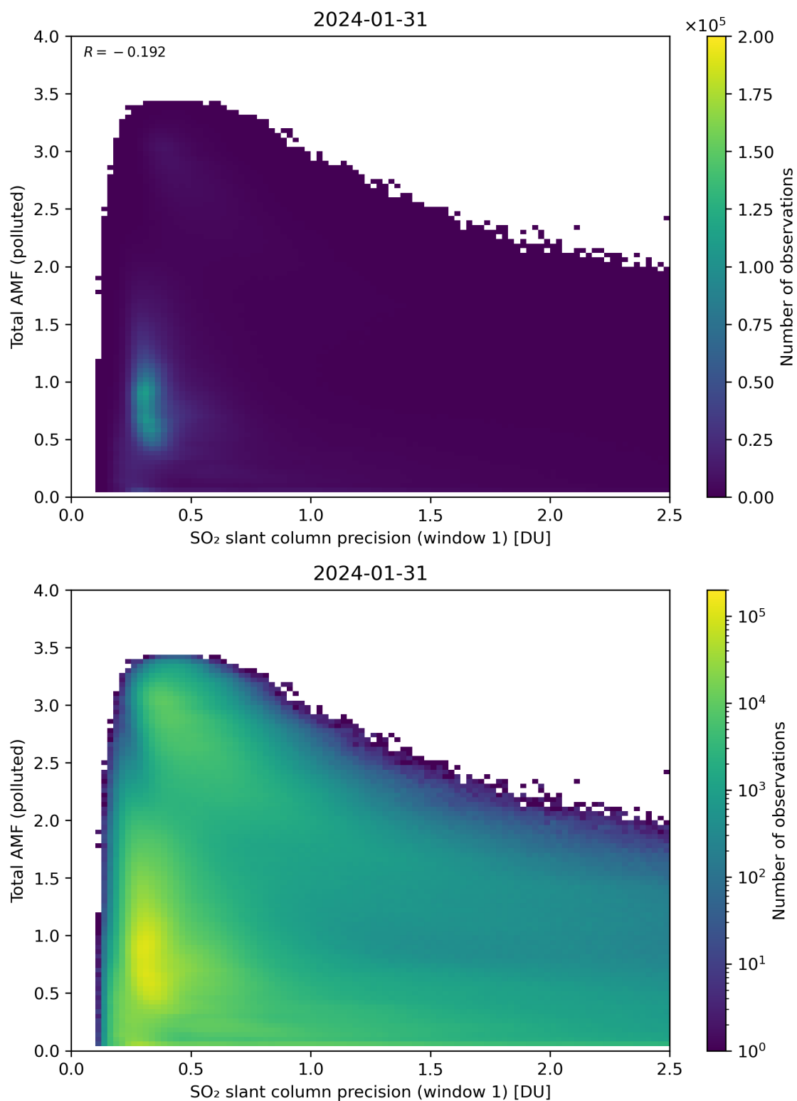
Figure 230: Scatter density plot of “SO 2 slant column precision (window 1)” against “Total AMF (polluted)” for 2024-01-31 to 2024-02-01.
