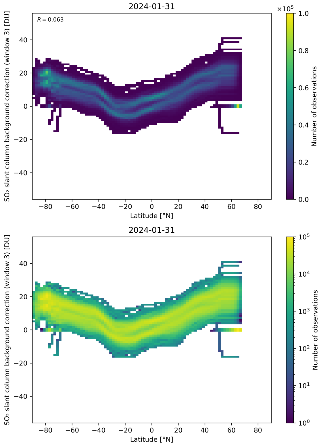
Figure 141: Scatter density plot of “Latitude” against “SO 2 slant column background correction (window 3)” for 2024-01-31 to 2024-02-01.
