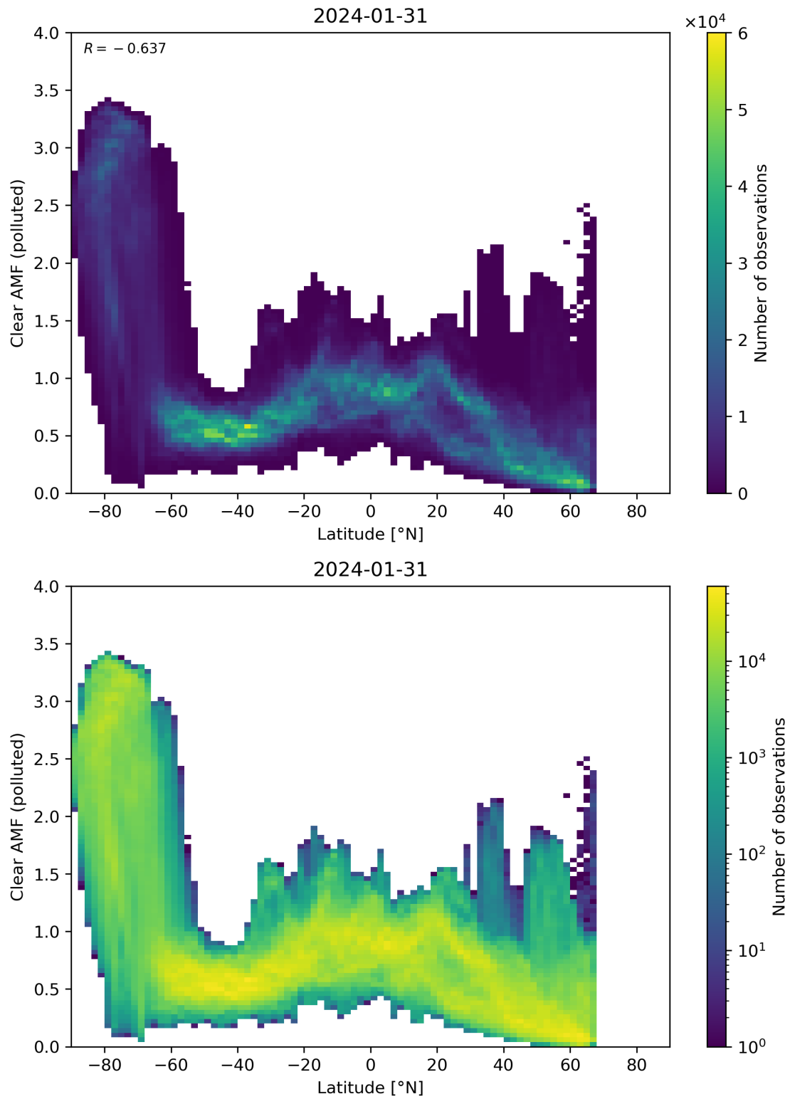
Figure 145: Scatter density plot of “Latitude” against “Clear AMF (polluted)” for 2024-01-31 to 2024-02-01.
