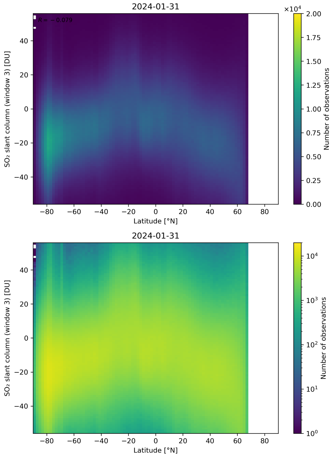
Figure 152: Scatter density plot of “Latitude” against “SO 2 slant column (window 3)” for 2024-01-31 to 2024-02-01.
