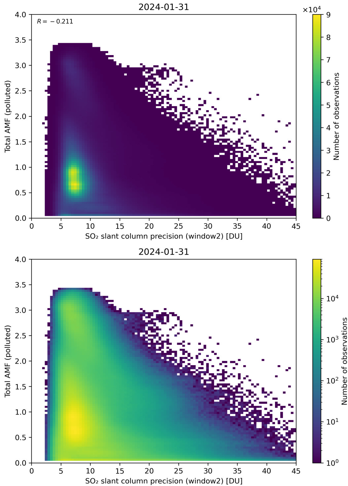
Figure 251: Scatter density plot of “SO 2 slant column precision (window2)” against “Total AMF (polluted)” for 2024-01-31 to 2024-02-01.
