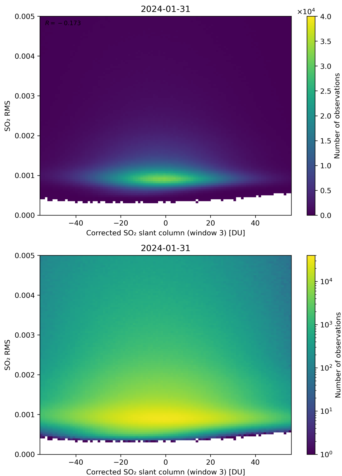
Figure 208: Scatter density plot of “Corrected SO 2 slant column (window 3)” against “SO 2 RMS” for 2024-01-31 to 2024-02-01.
