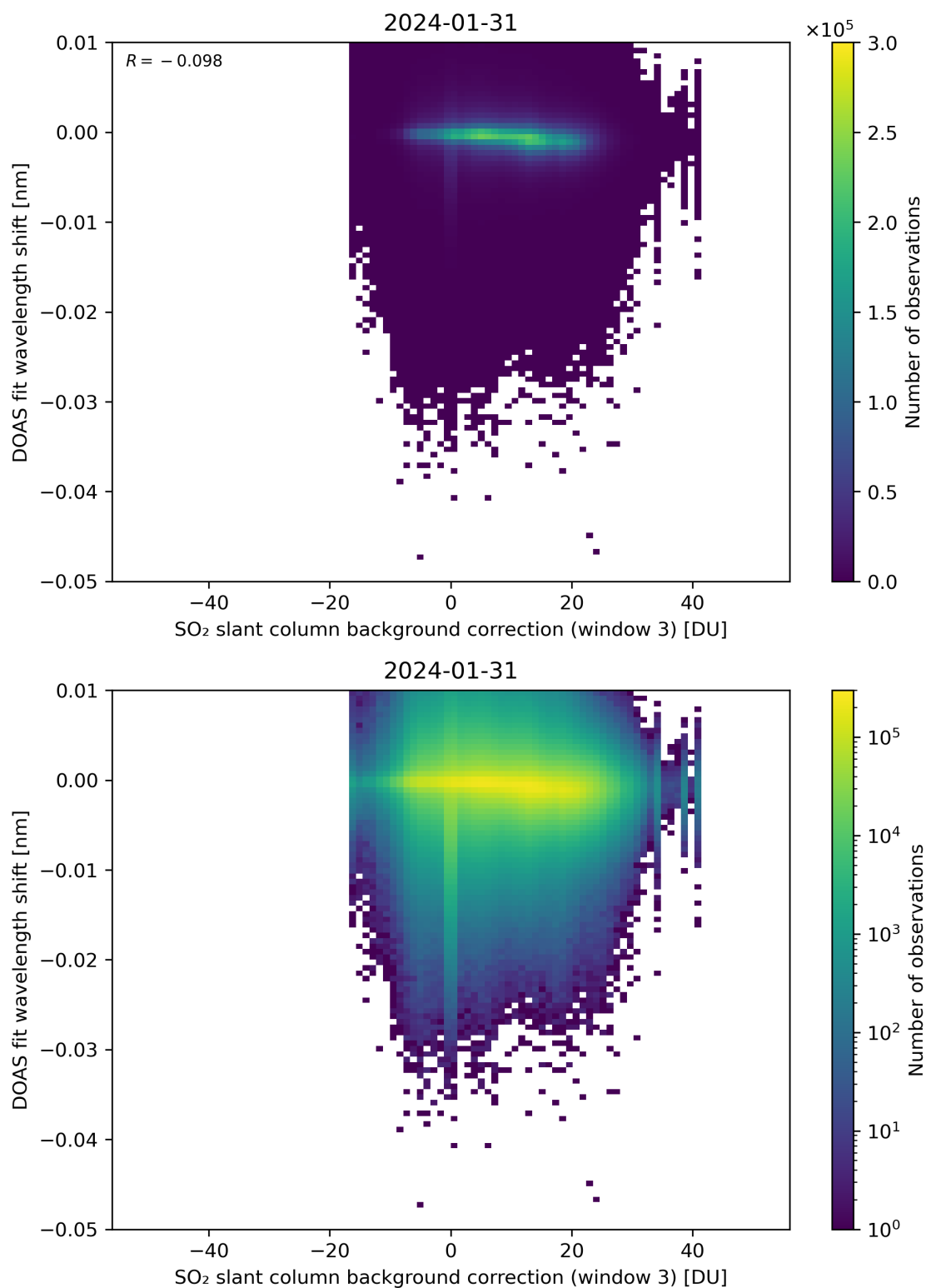
Figure 121: Scatter density plot of “SO 2 slant column background correction (window 3)” against “DOAS fit wavelength shift” for 2024-01-31 to 2024-02-01.
