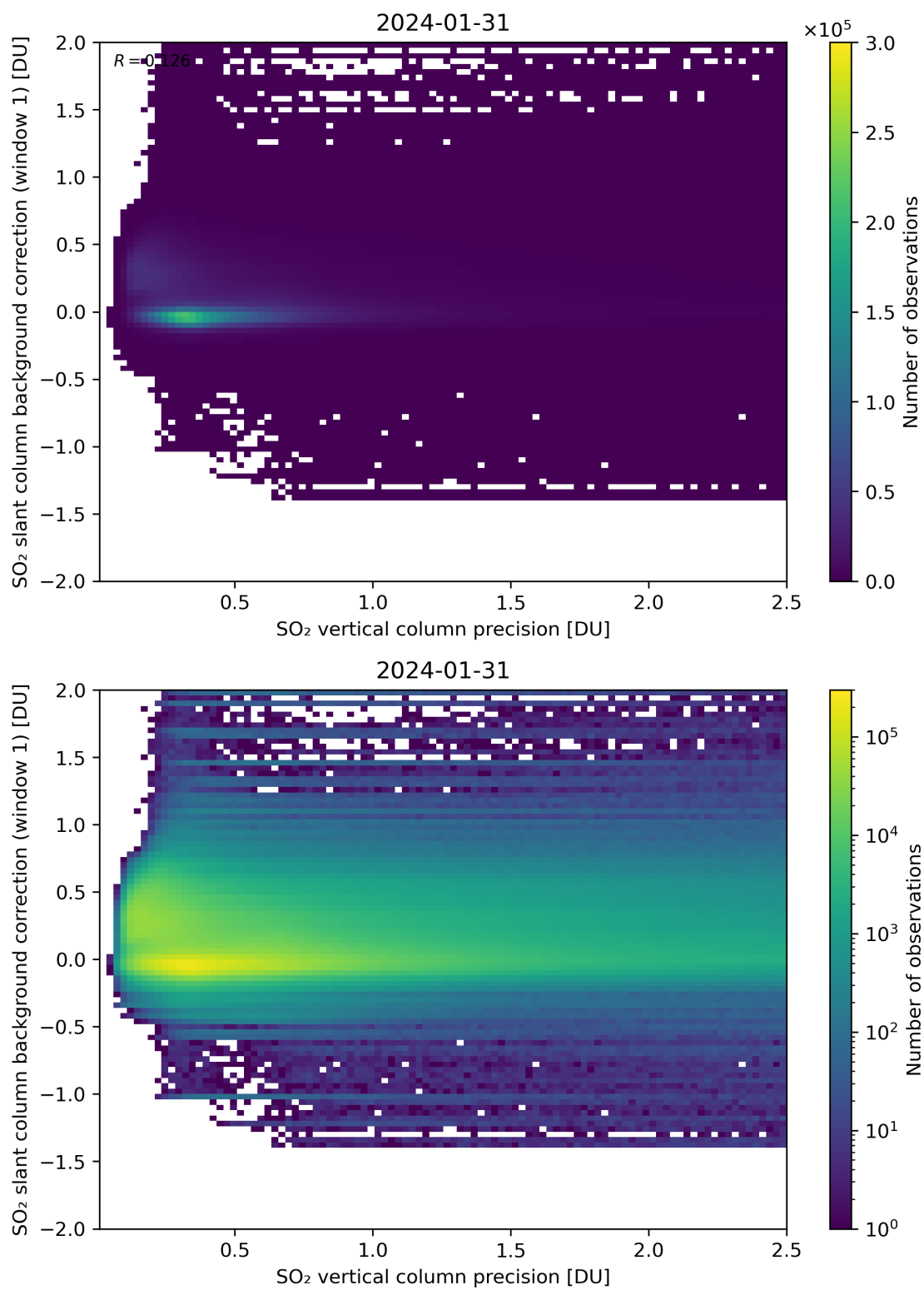
Figure 279: Scatter density plot of “SO 2 vertical column precision” against “SO 2 slant column background correction (window 1)” for 2024-01-31 to 2024-02-01.
