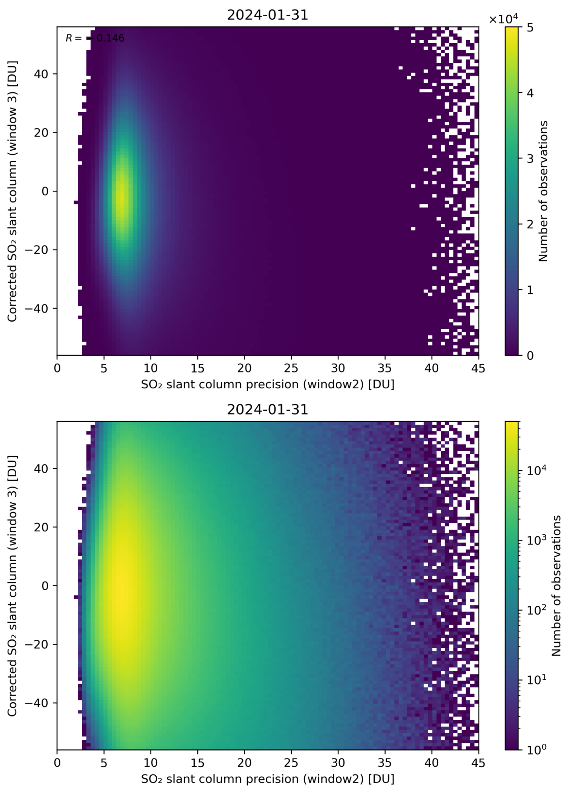
Figure 248: Scatter density plot of “SO 2 slant column precision (window2)” against “Corrected SO 2 slant column (window 3)” for 2024-01-31 to 2024-02-01.
