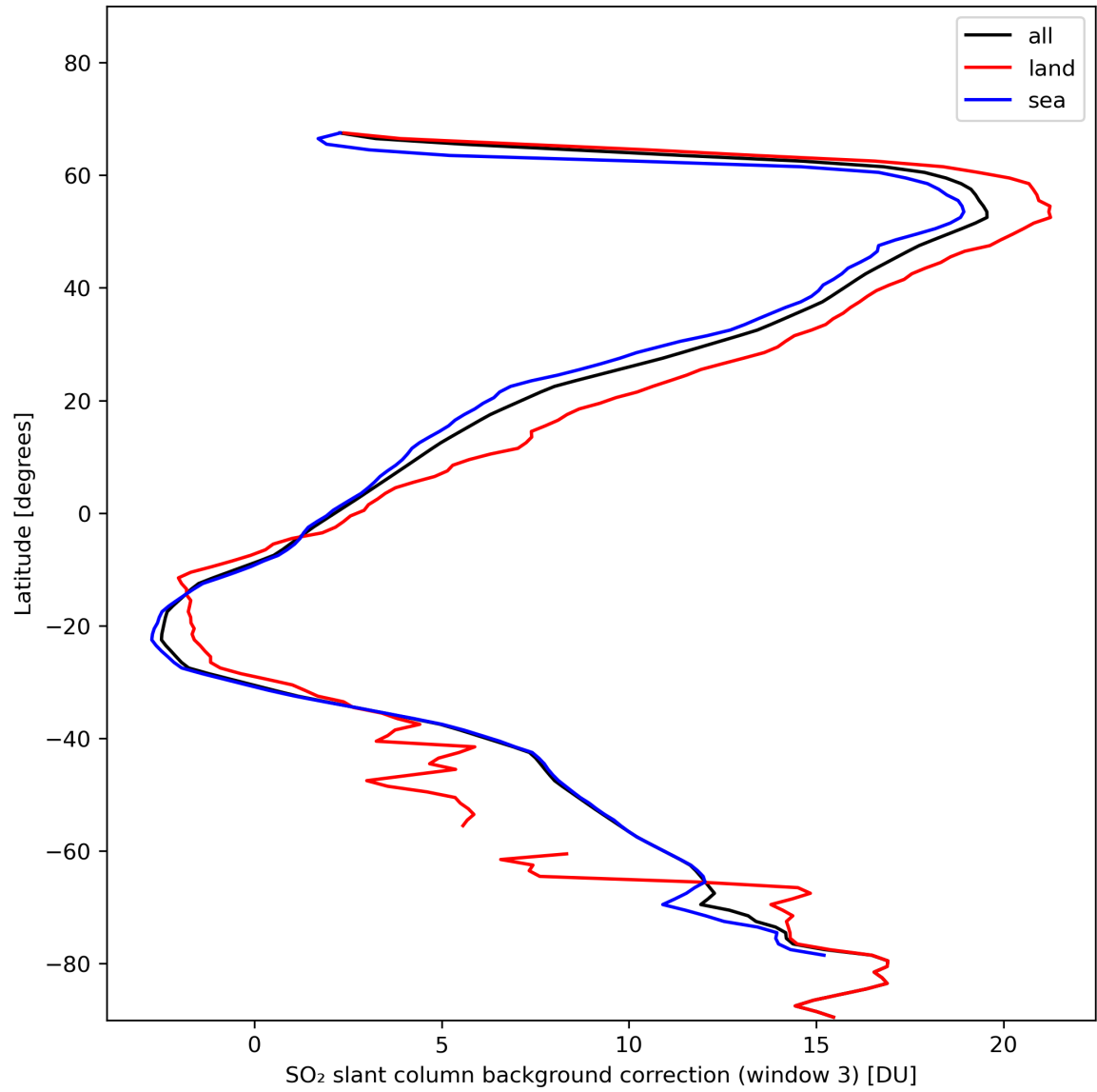
Figure 44: Zonal average of “SO 2 slant column background correction (window 3)” for 2024-01-31 to 2024-02-01.
