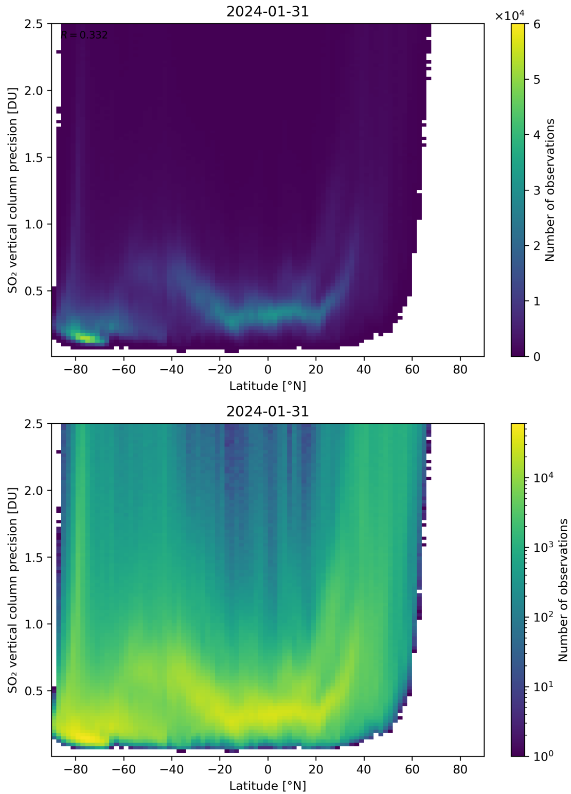
Figure 157: Scatter density plot of “Latitude” against “SO 2 vertical column precision” for 2024-01-31 to 2024-02-01.
