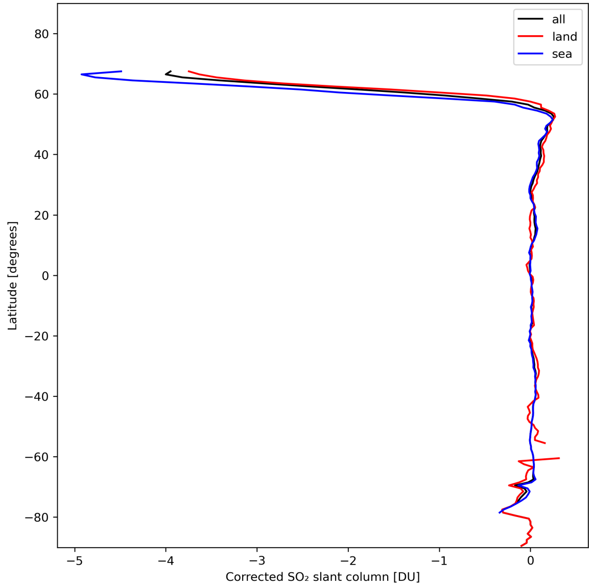
Figure 32: Zonal average of “Corrected SO 2 slant column” for 2024-01-31 to 2024-02-01.
