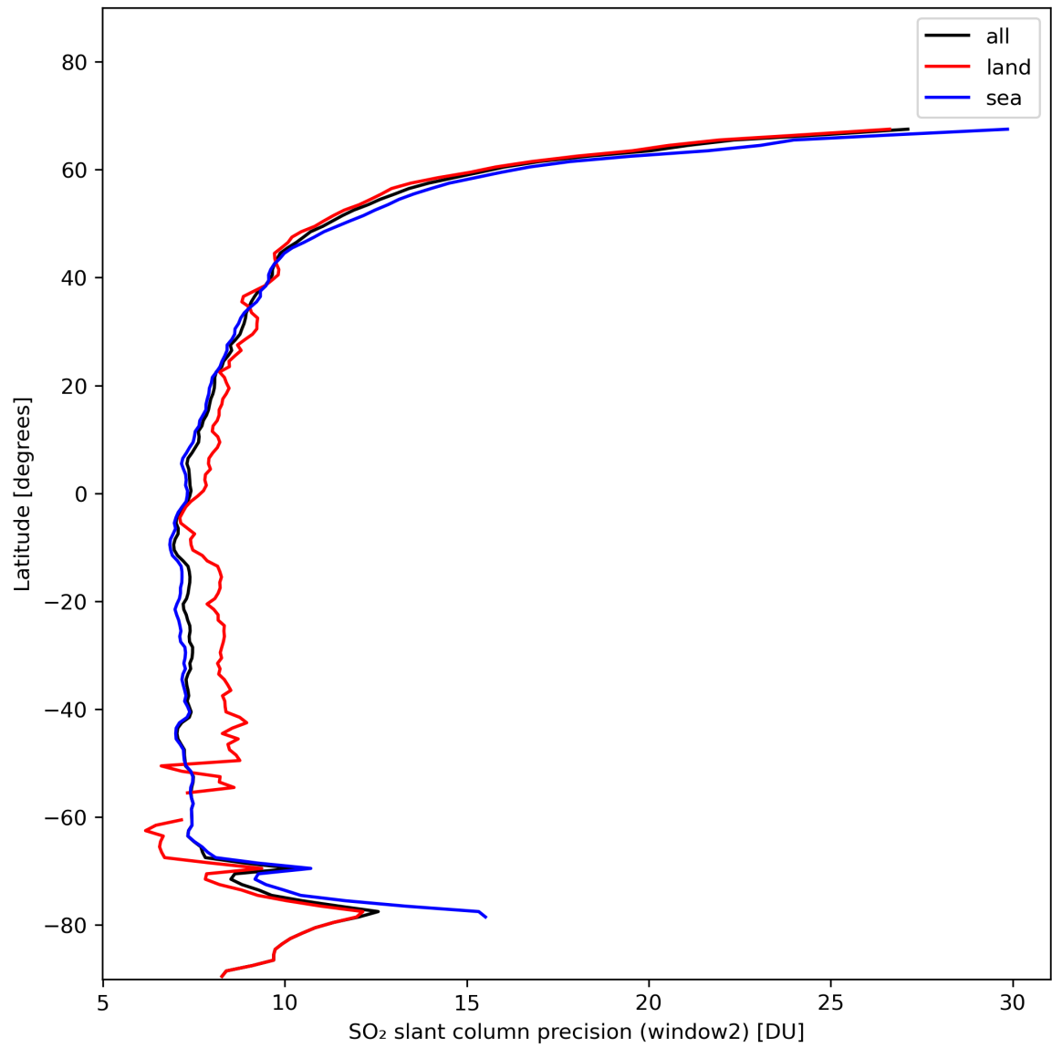
Figure 38: Zonal average of “SO 2 slant column precision (window2)” for 2024-01-31 to 2024-02-01.
