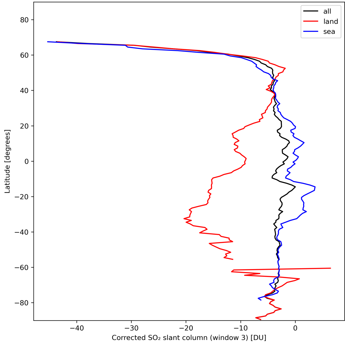
Figure 43: Zonal average of “Corrected SO 2 slant column (window 3)” for 2024-01-31 to 2024-02-01.
