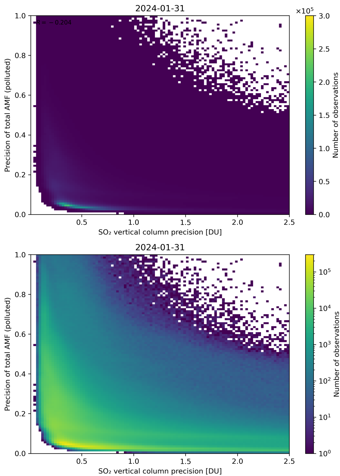
Figure 295: Scatter density plot of “SO 2 vertical column precision” against “Precision of total AMF (polluted)” for 2024-01-31 to 2024-02-01.
