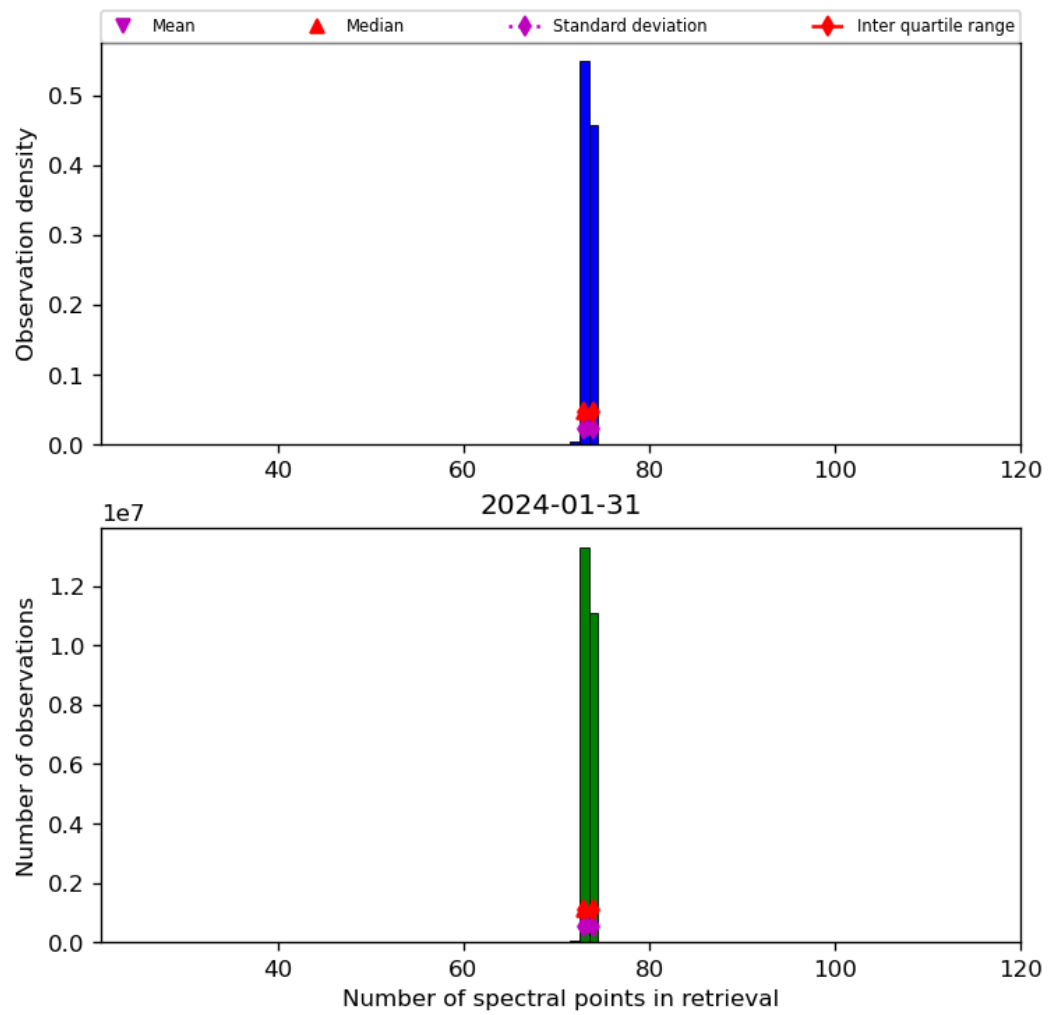
Figure 74: Histogram of “Number of spectral points in retrieval” for 2024-01-31 to 2024-02-01
