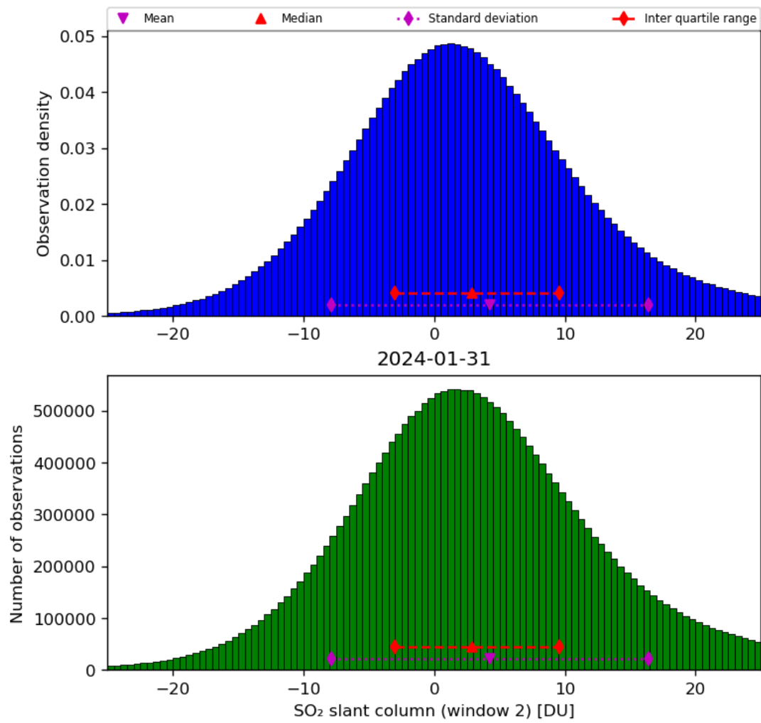
Figure 60: Histogram of “SO 2 slant column (window 2)” for 2024-01-31 to 2024-02-01
