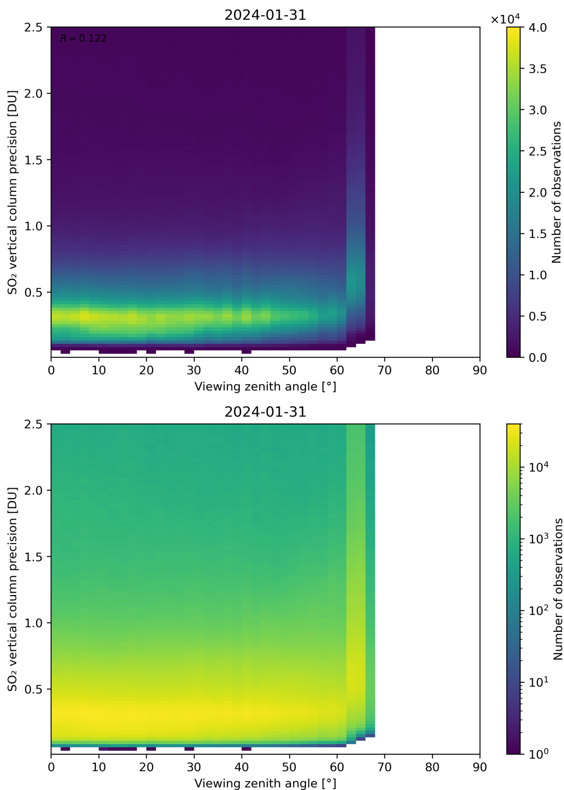
Figure 328: Scatter density plot of “Viewing zenith angle” against “SO 2 vertical column precision” for 2024-01-31 to 2024-02-01.
