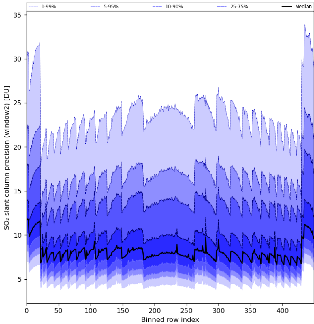
Figure 84: Along track statistics of “SO 2 slant column precision (window2)” for 2024-01-31 to 2024-02-01
