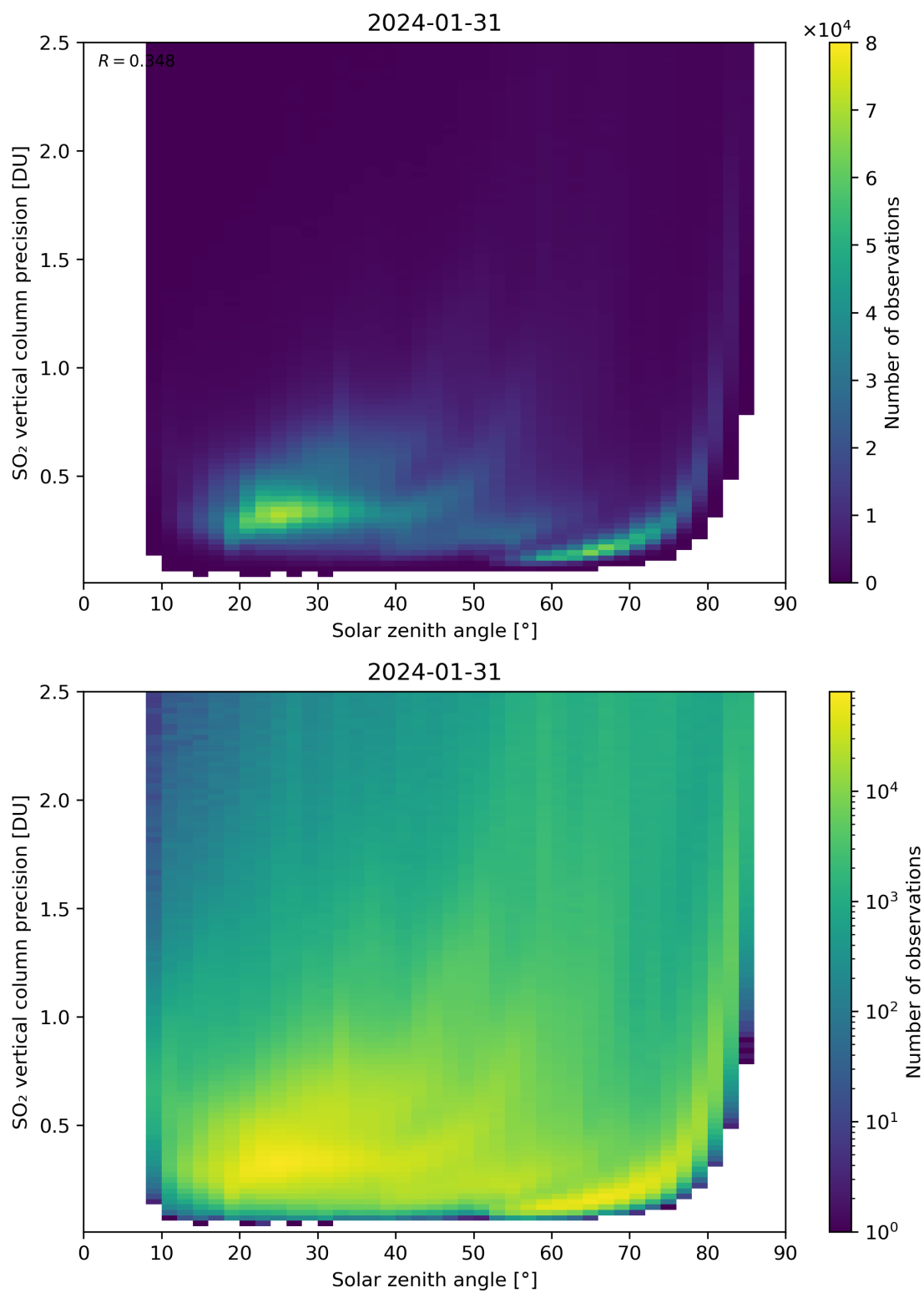
Figure 177: Scatter density plot of “Solar zenith angle” against “SO 2 vertical column precision” for 2024-01-31 to 2024-02-01.
