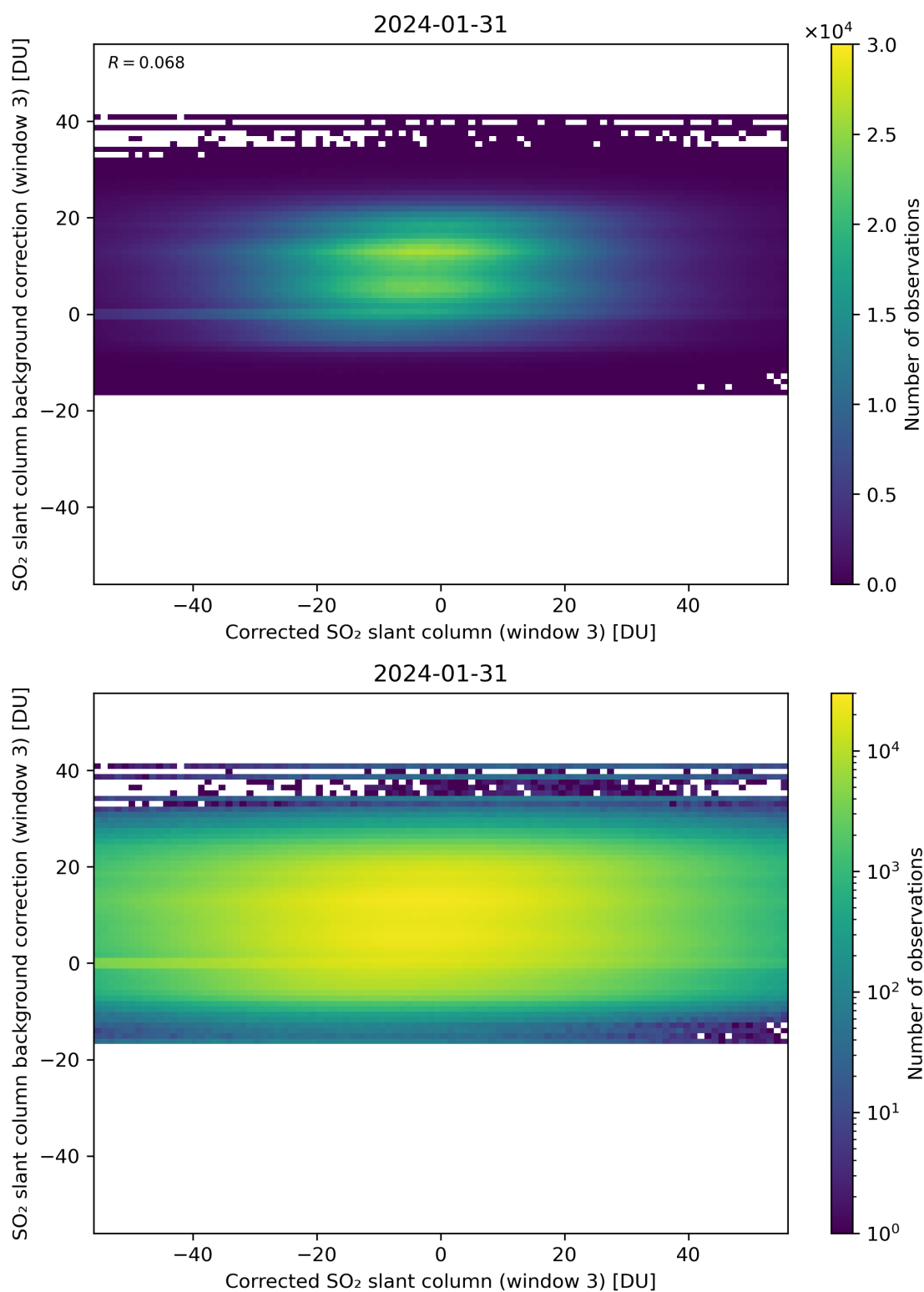
Figure 205: Scatter density plot of “Corrected SO 2 slant column (window 3)” against “SO 2 slant column background correction (window 3)” for 2024-01-31 to 2024-02-01.
