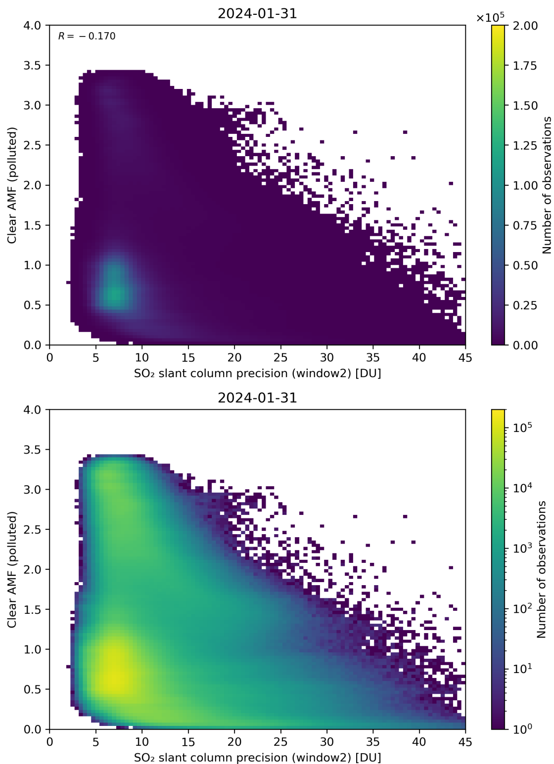
Figure 246: Scatter density plot of “SO 2 slant column precision (window2)” against “Clear AMF (polluted)” for 2024-01-31 to 2024-02-01.
