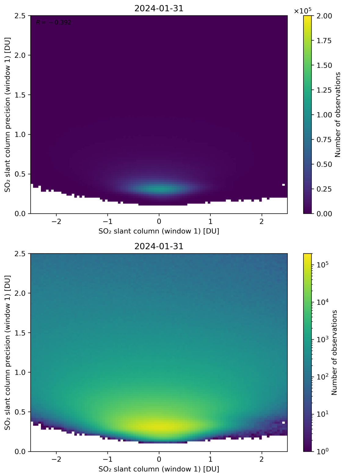
Figure 235: Scatter density plot of “SO 2 slant column (window 1)” against “SO 2 slant column precision (window 1)” for 2024-01-31 to 2024-02-01.
