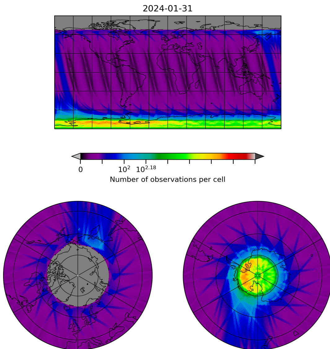
Figure 28: Map of the number of observations for 2024-01-31 to 2024-02-01
