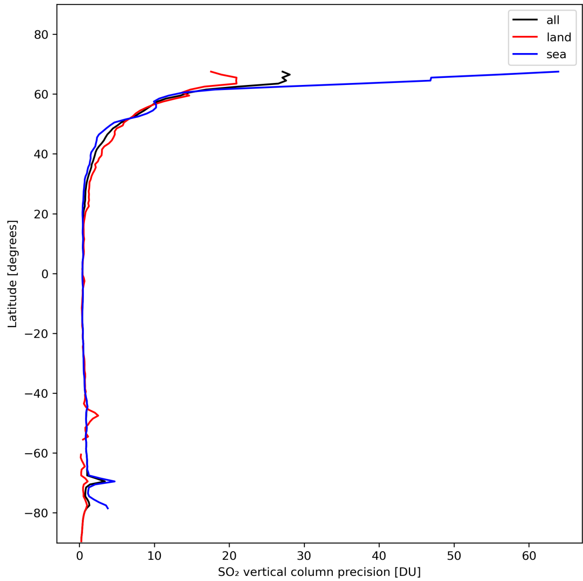
Figure 31: Zonal average of “SO 2 vertical column precision” for 2024-01-31 to 2024-02-01.
