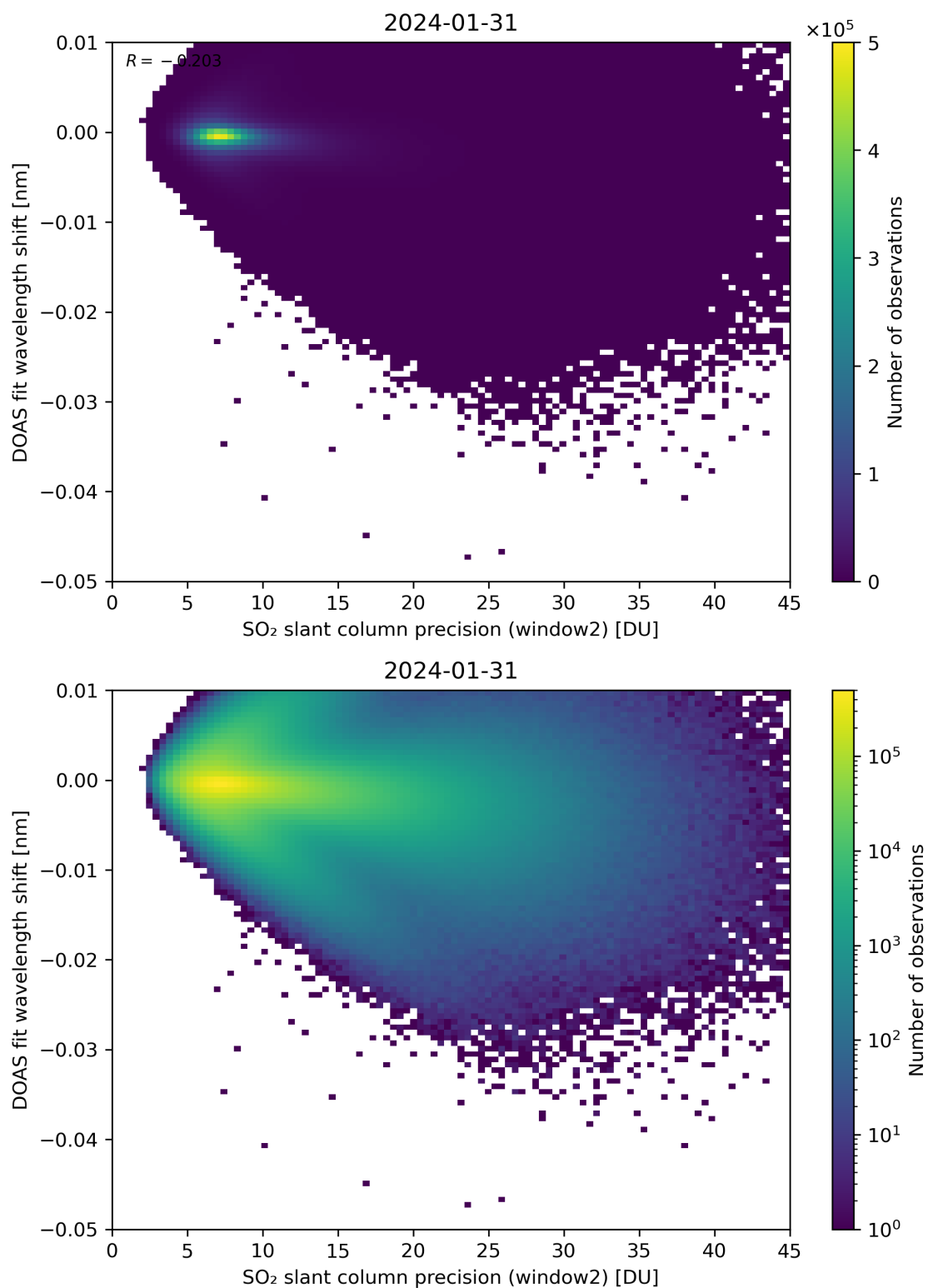
Figure 243: Scatter density plot of “SO 2 slant column precision (window2)” against “DOAS fit wavelength shift” for 2024-01-31 to 2024-02-01.
