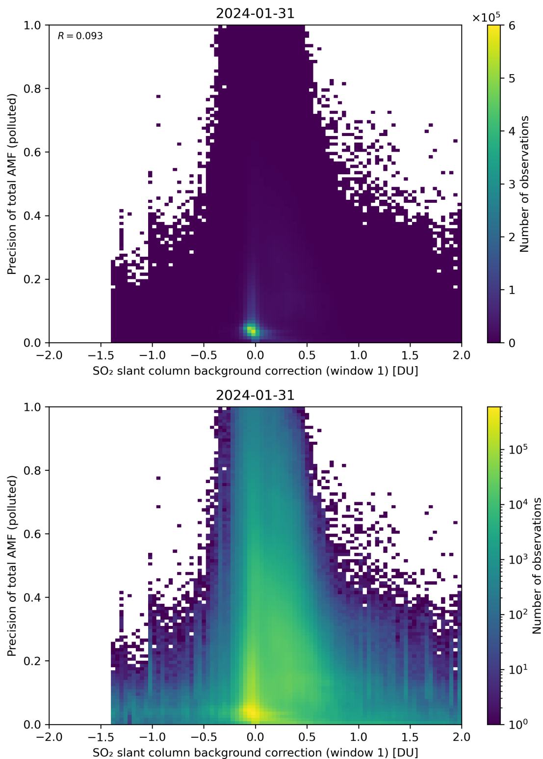
Figure 110: Scatter density plot of “SO 2 slant column background correction (window 1)” against “Precision of total AMF (polluted)” for 2024-01-31 to 2024-02-01.
