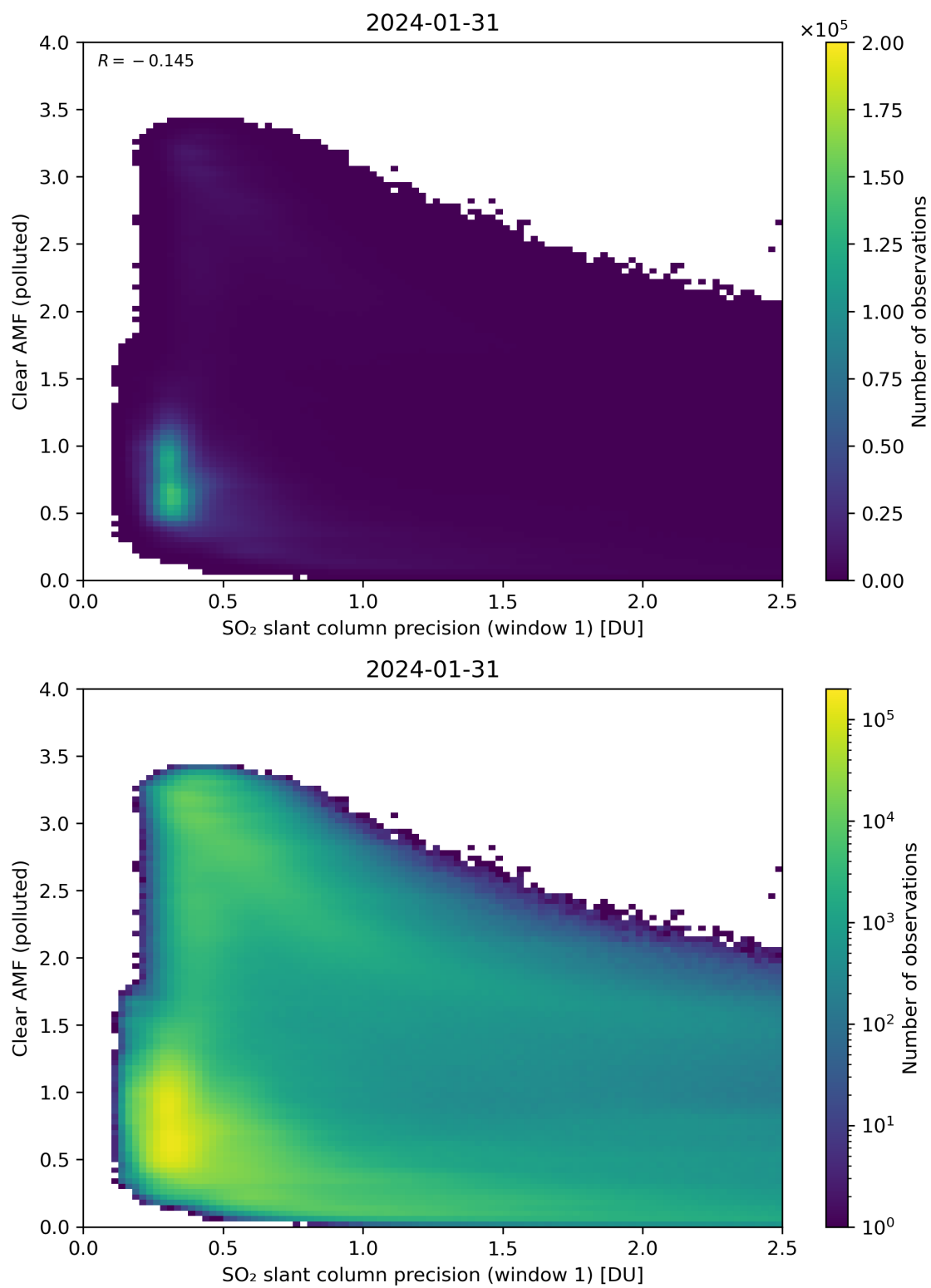
Figure 224: Scatter density plot of “SO 2 slant column precision (window 1)” against “Clear AMF (polluted)” for 2024-01-31 to 2024-02-01.
