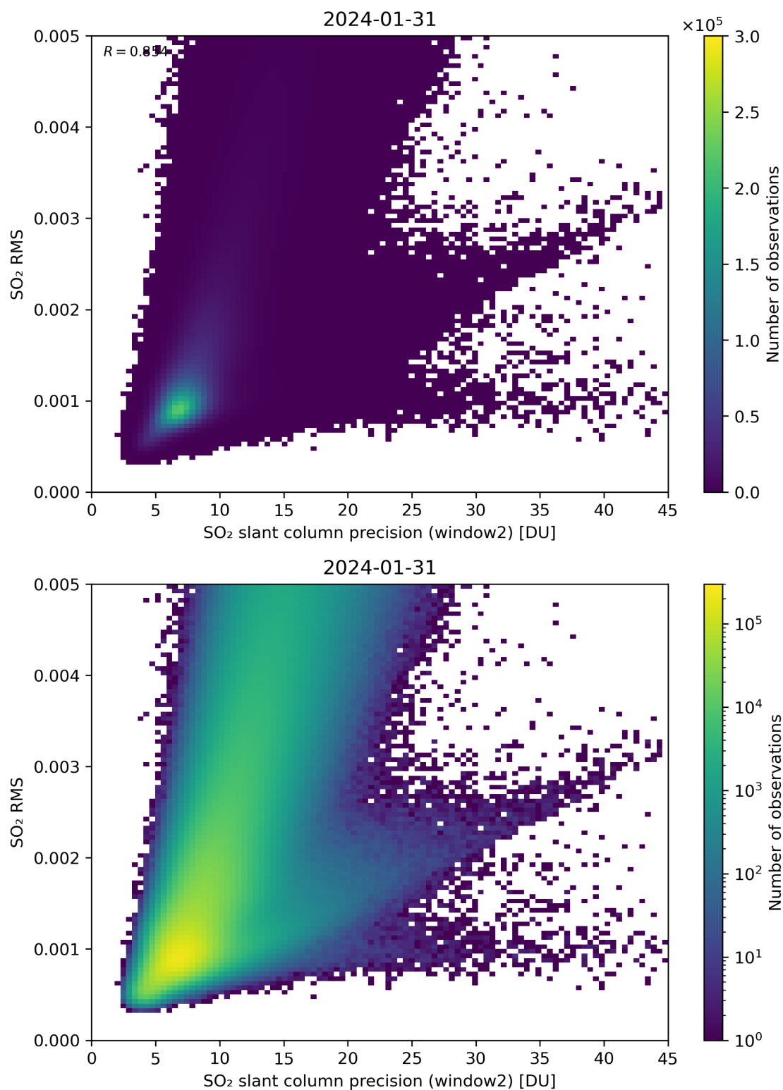
Figure 245: Scatter density plot of “SO 2 slant column precision (window2)” against “SO 2 RMS” for 2024-01-31 to 2024-02-01.
