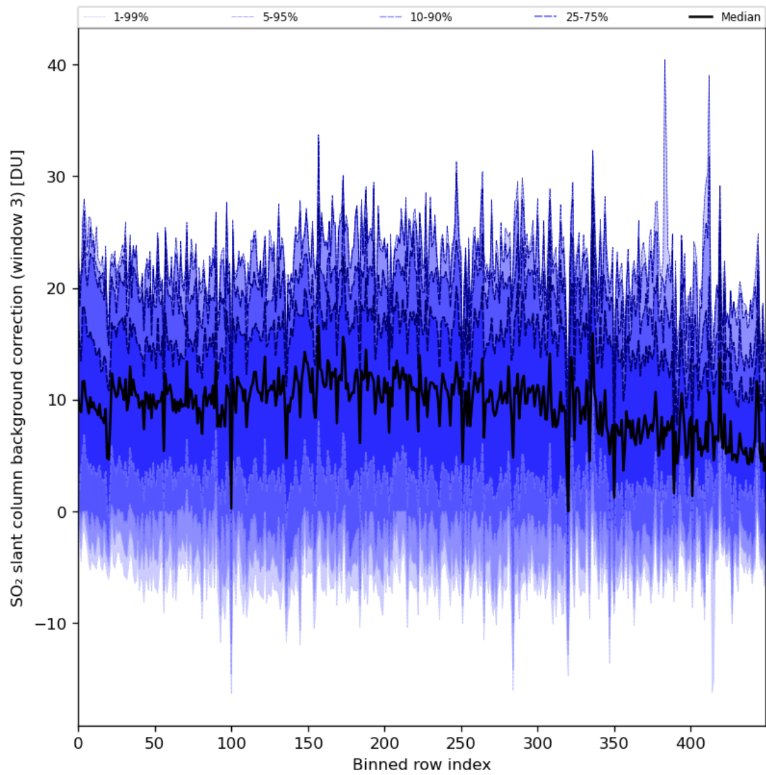
Figure 90: Along track statistics of “SO 2 slant column background correction (window 3)” for 2024-01-31 to 2024-02-01
