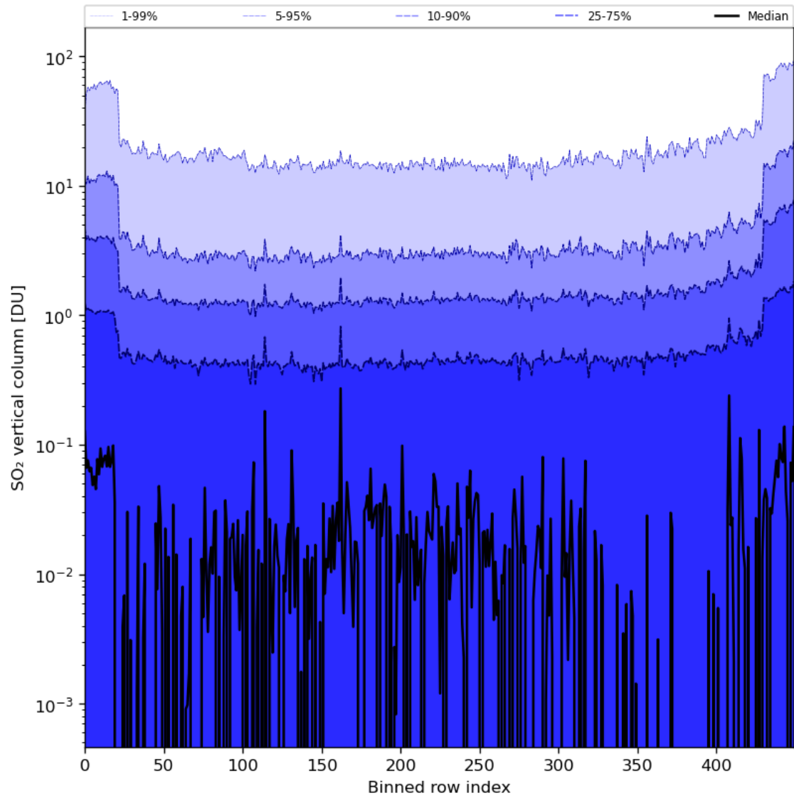
Figure 76: Along track statistics of “SO 2 vertical column” for 2024-01-31 to 2024-02-01
