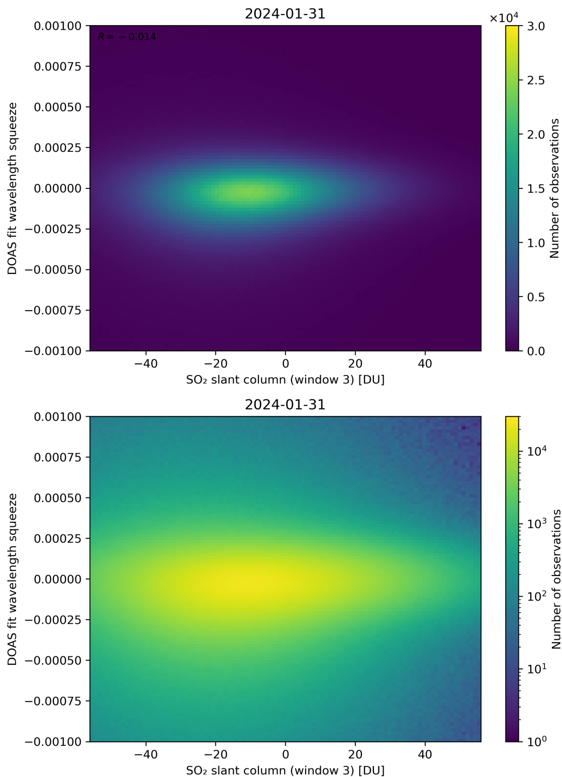
Figure 255: Scatter density plot of “SO 2 slant column (window 3)” against “DOAS fit wavelength squeeze” for 2024-01-31 to 2024-02-01.
