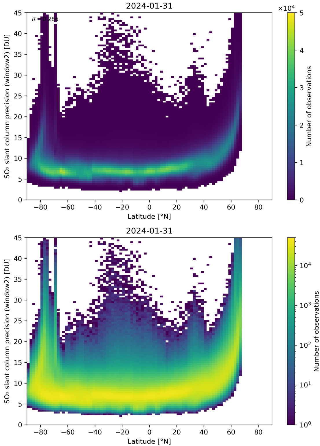
Figure 151: Scatter density plot of “Latitude” against “SO 2 slant column precision (window2)” for 2024-01-31 to 2024-02-01.
