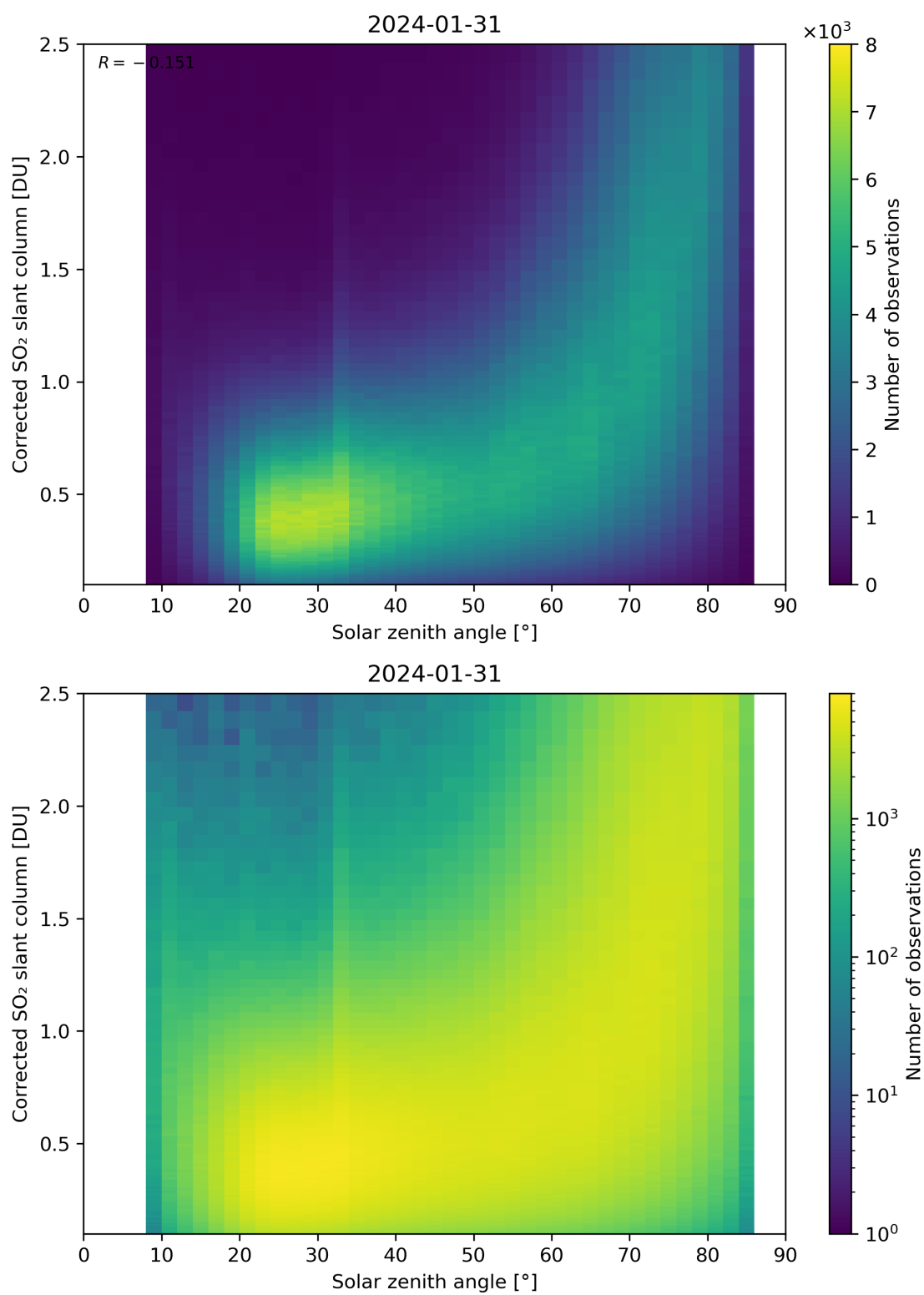
Figure 166: Scatter density plot of “Solar zenith angle” against “Corrected SO 2 slant column” for 2024-01-31 to 2024-02-01.
