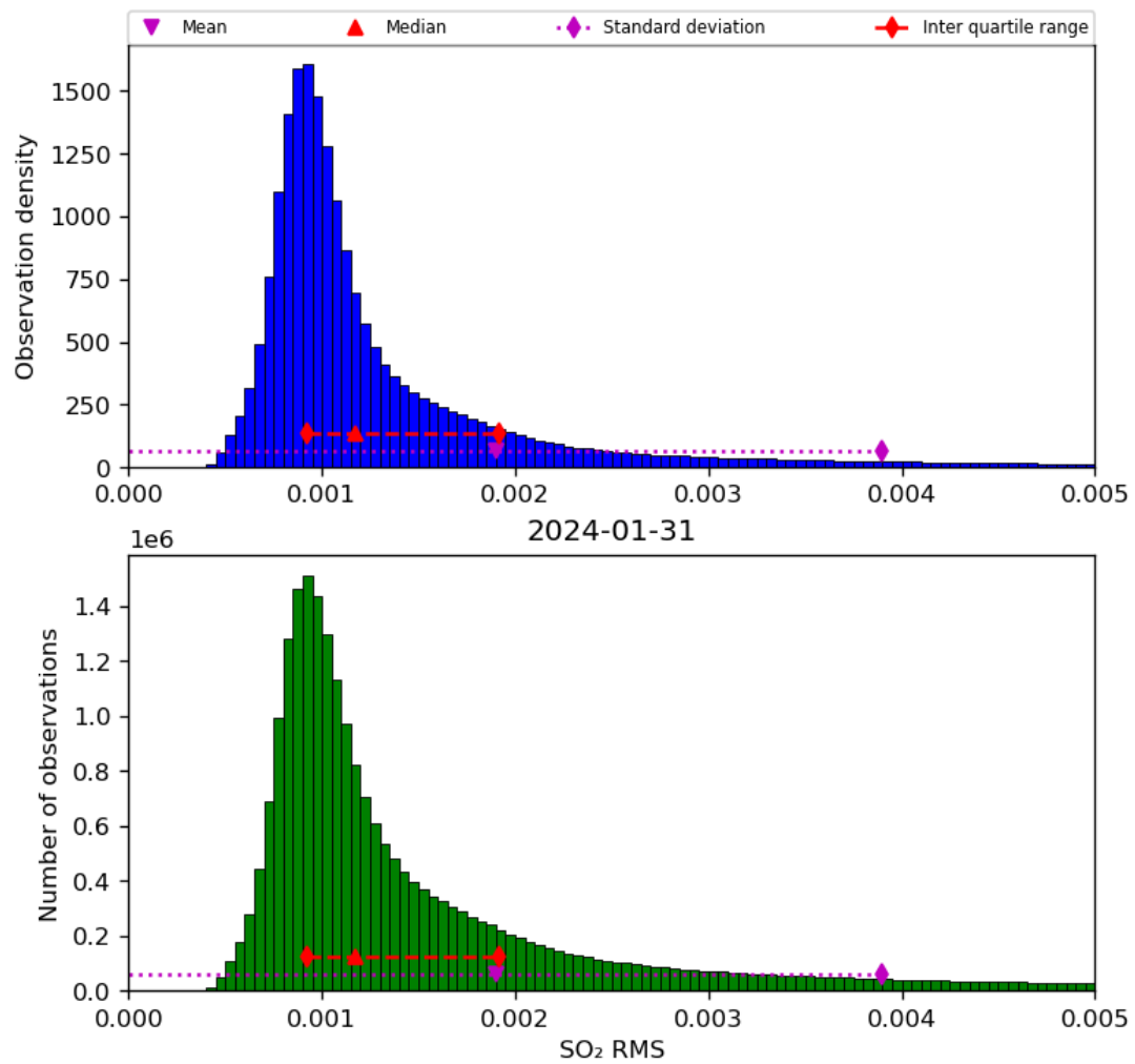
Figure 70: Histogram of “SO 2 RMS” for 2024-01-31 to 2024-02-01
