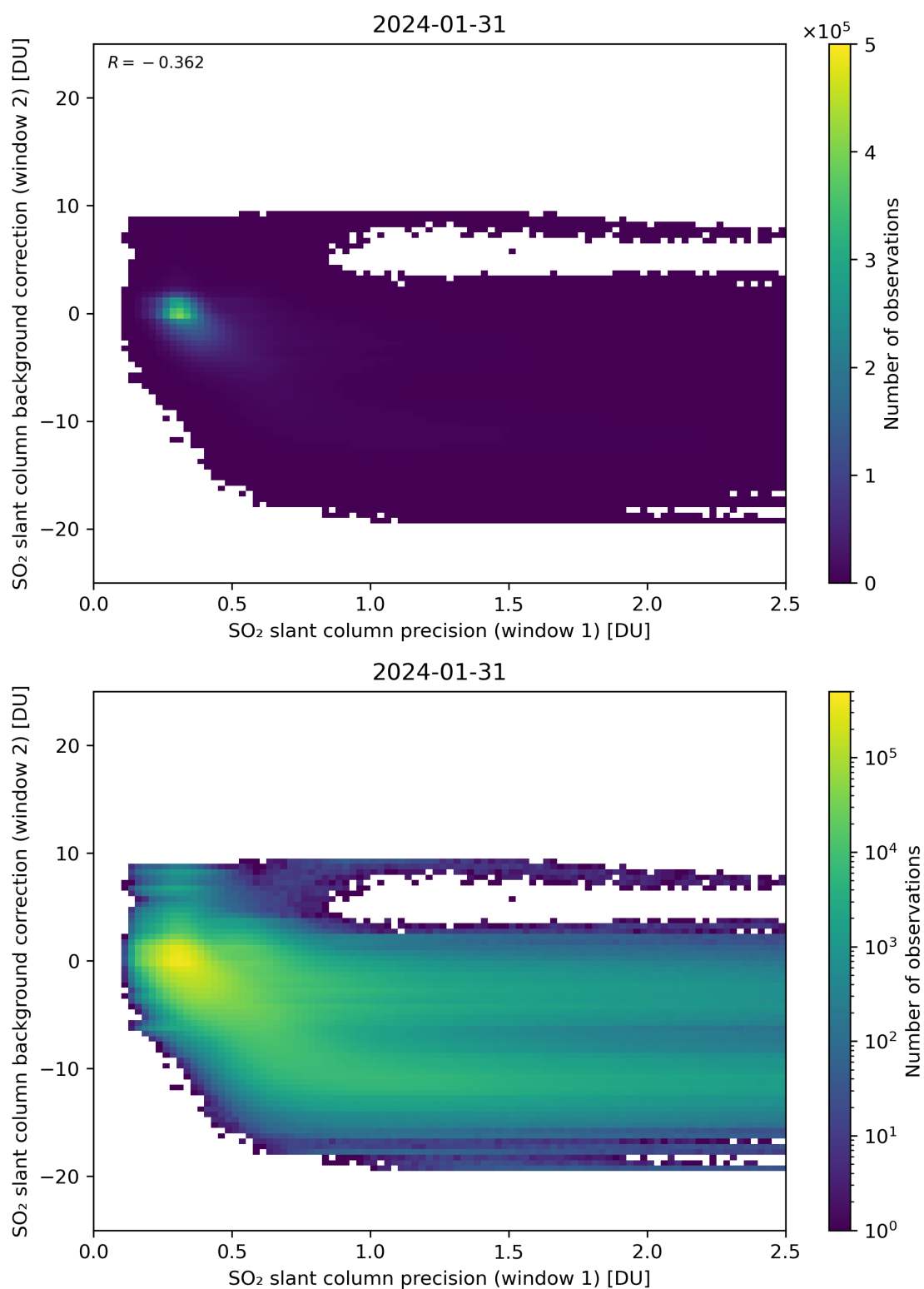
Figure 219: Scatter density plot of “SO 2 slant column precision (window 1)” against “SO 2 slant column background correction (window 2)” for 2024-01-31 to 2024-02-01.
