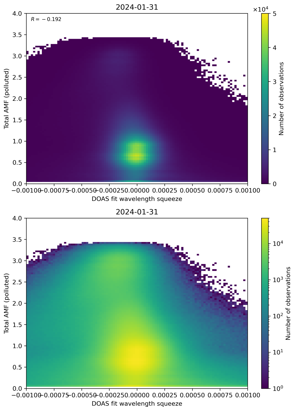
Figure 134: Scatter density plot of “DOAS fit wavelength squeeze” against “Total AMF (polluted)” for 2024-01-31 to 2024-02-01.
