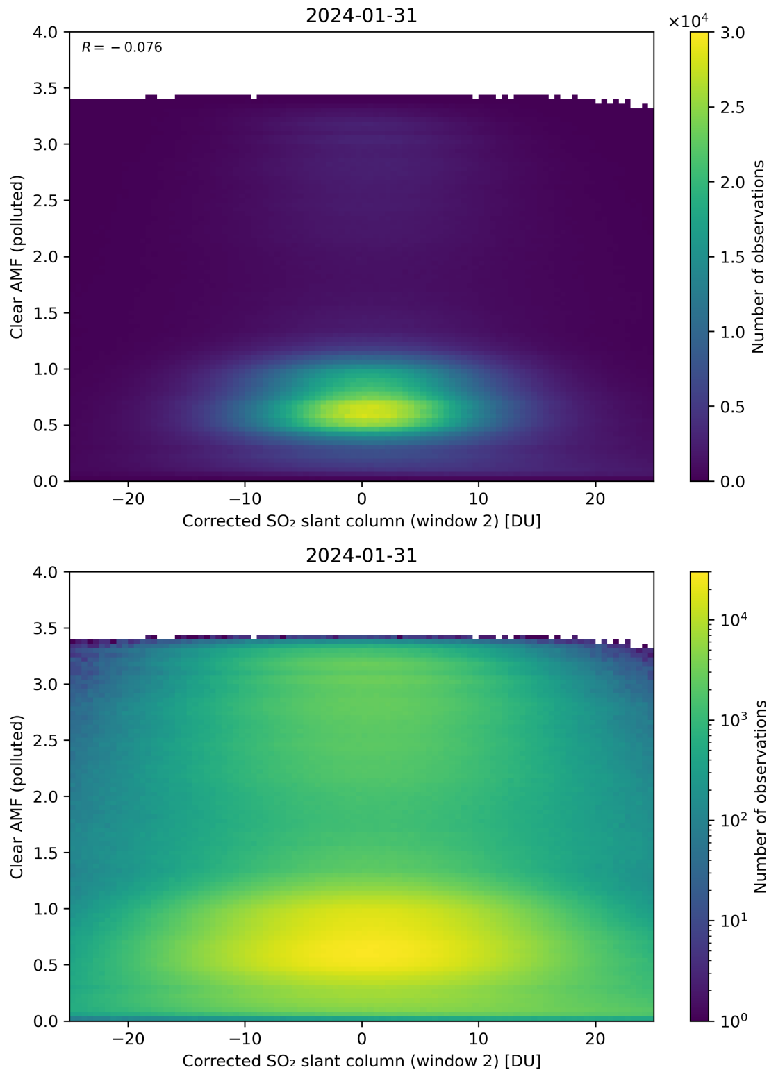
Figure 199: Scatter density plot of “Corrected SO 2 slant column (window 2)” against “Clear AMF (polluted)” for 2024-01-31 to 2024-02-01.
