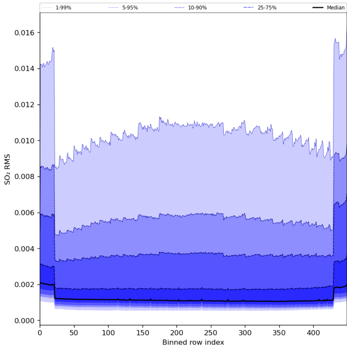
Figure 93: Along track statistics of “SO 2 RMS” for 2024-01-31 to 2024-02-01
