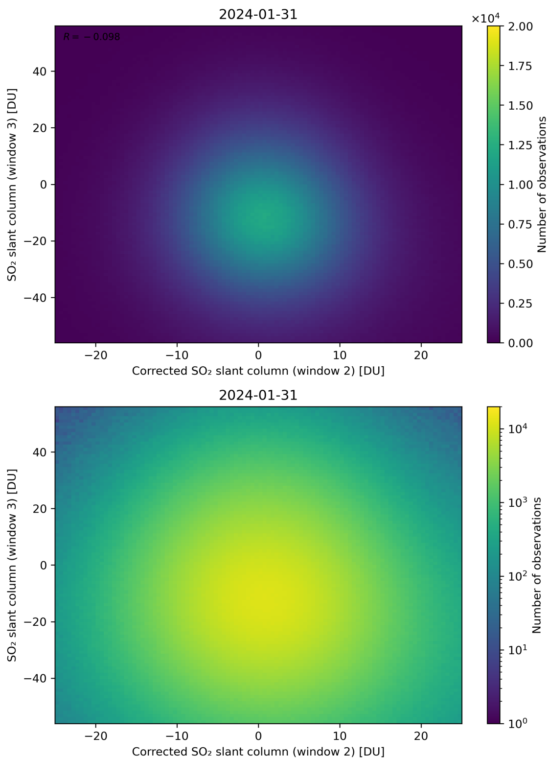
Figure 201: Scatter density plot of “Corrected SO 2 slant column (window 2)” against “SO 2 slant column (window 3)” for 2024-01-31 to 2024-02-01.
