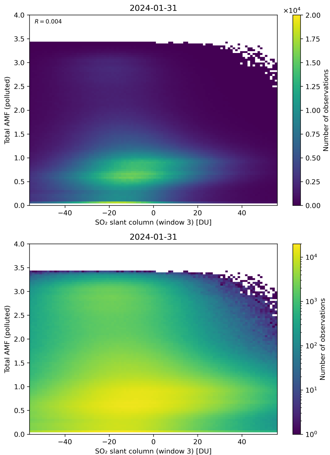
Figure 268: Scatter density plot of “SO 2 slant column (window 3)” against “Total AMF (polluted)” for 2024-01-31 to 2024-02-01.
