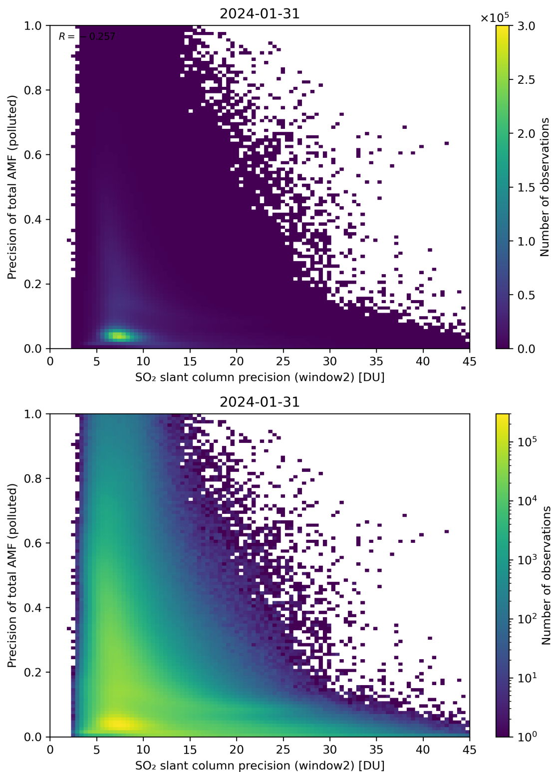
Figure 252: Scatter density plot of “SO 2 slant column precision (window2)” against “Precision of total AMF (polluted)” for 2024-01-31 to 2024-02-01.
