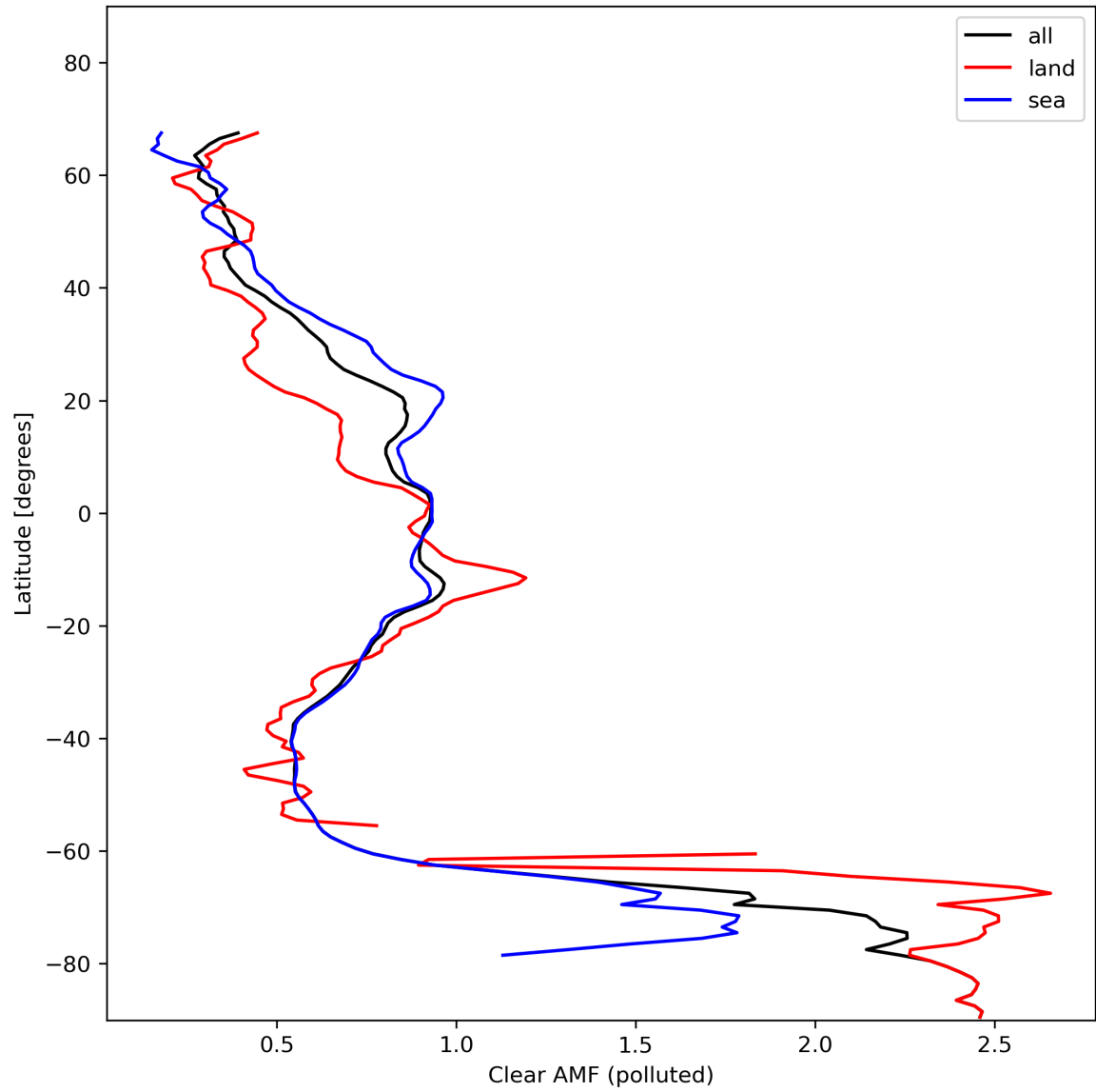
Figure 50: Zonal average of “Clear AMF (polluted)” for 2024-01-31 to 2024-02-01.
