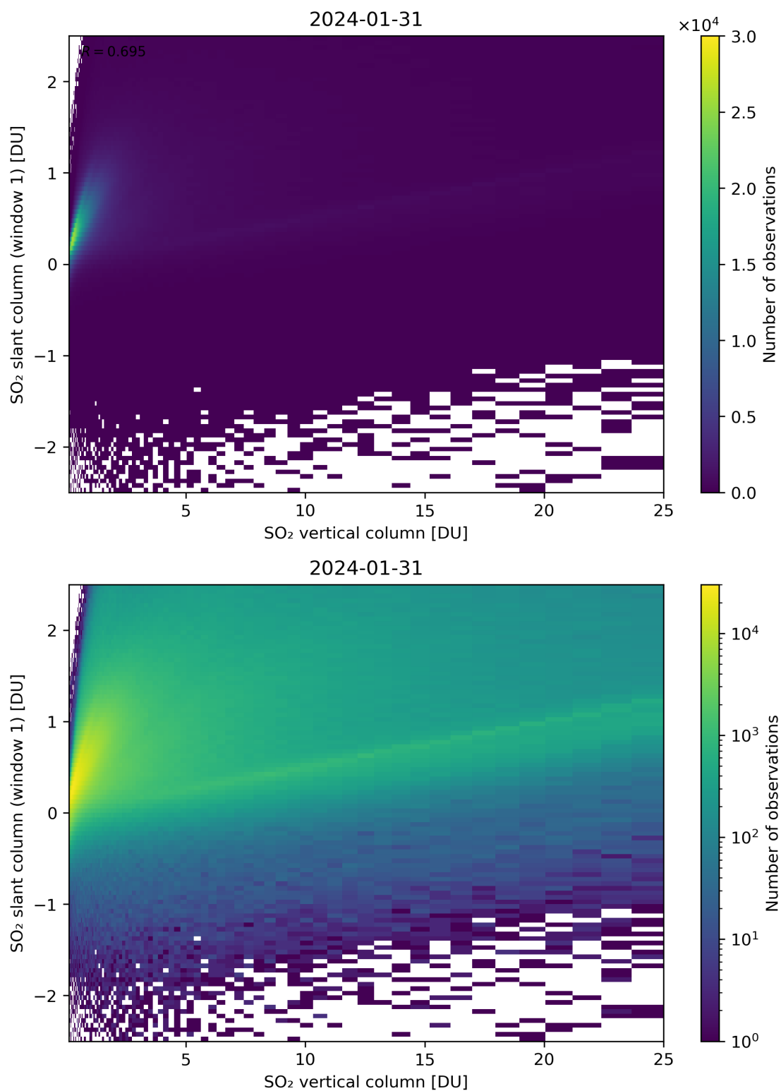
Figure 300: Scatter density plot of “SO 2 vertical column” against “SO 2 slant column (window 1)” for 2024-01-31 to 2024-02-01.
