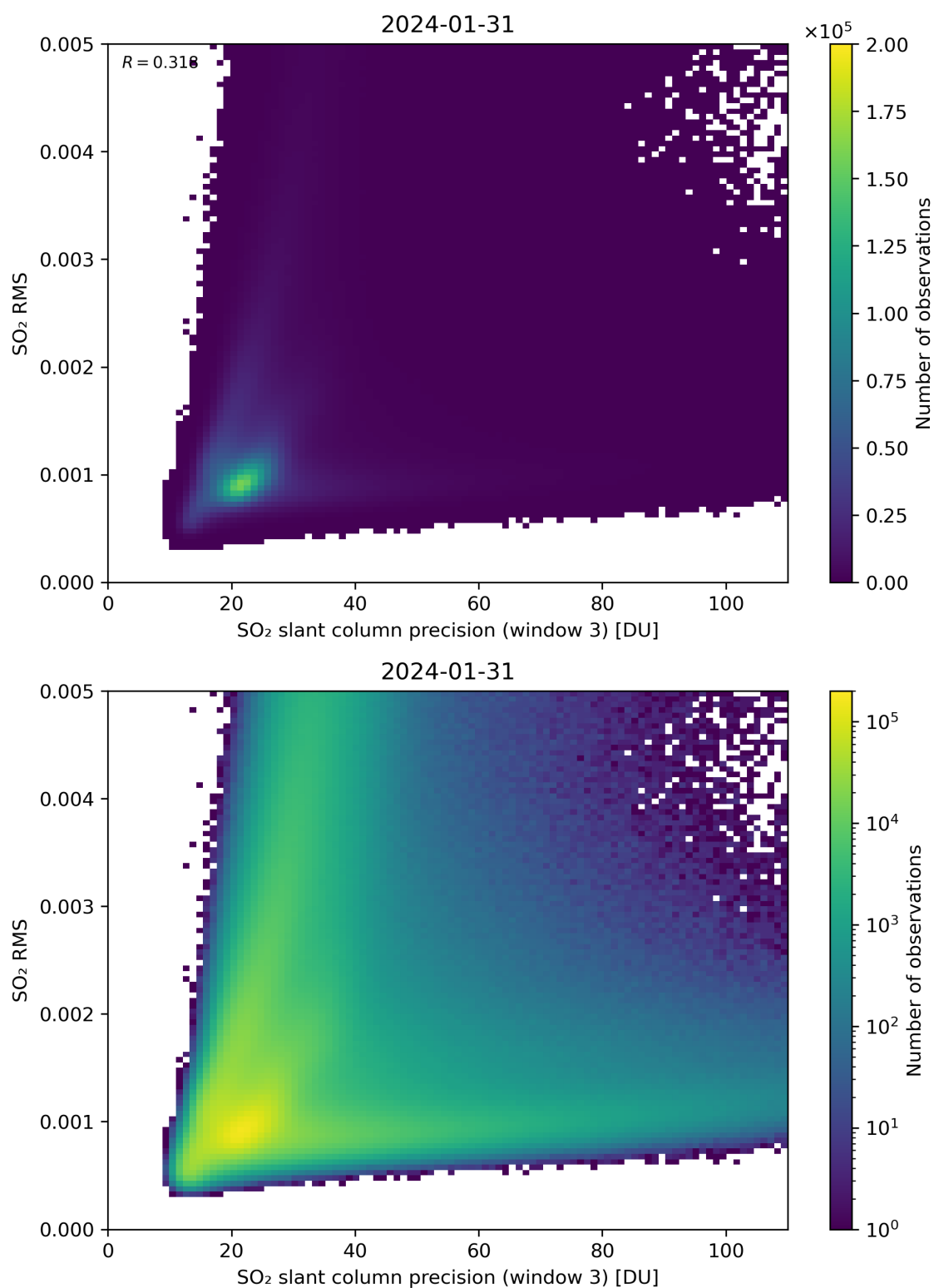
Figure 260: Scatter density plot of “SO 2 slant column precision (window 3)” against “SO 2 RMS” for 2024-01-31 to 2024-02-01.
