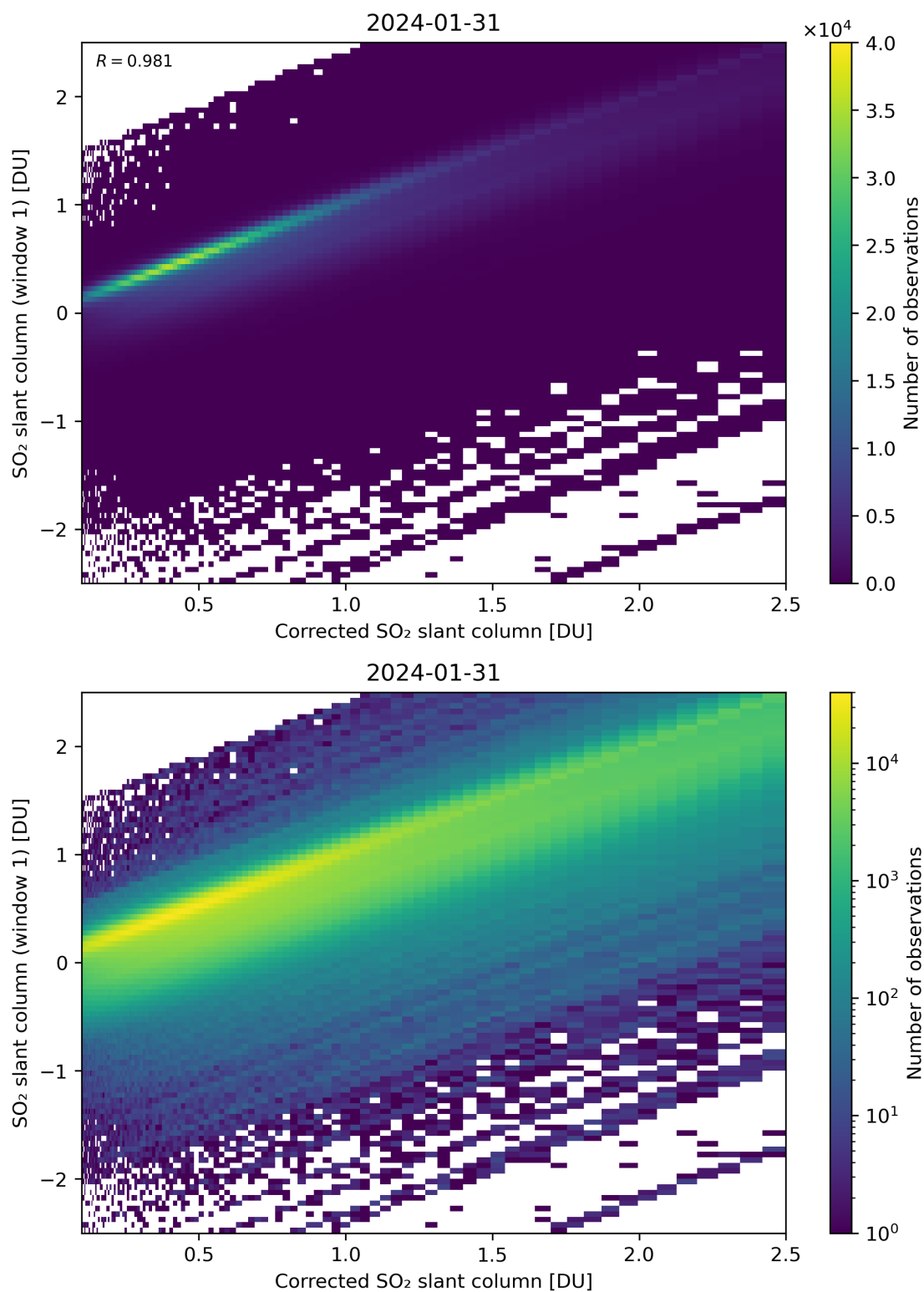
Figure 187: Scatter density plot of “Corrected SO 2 slant column” against “SO 2 slant column (window 1)” for 2024-01-31 to 2024-02-01.
