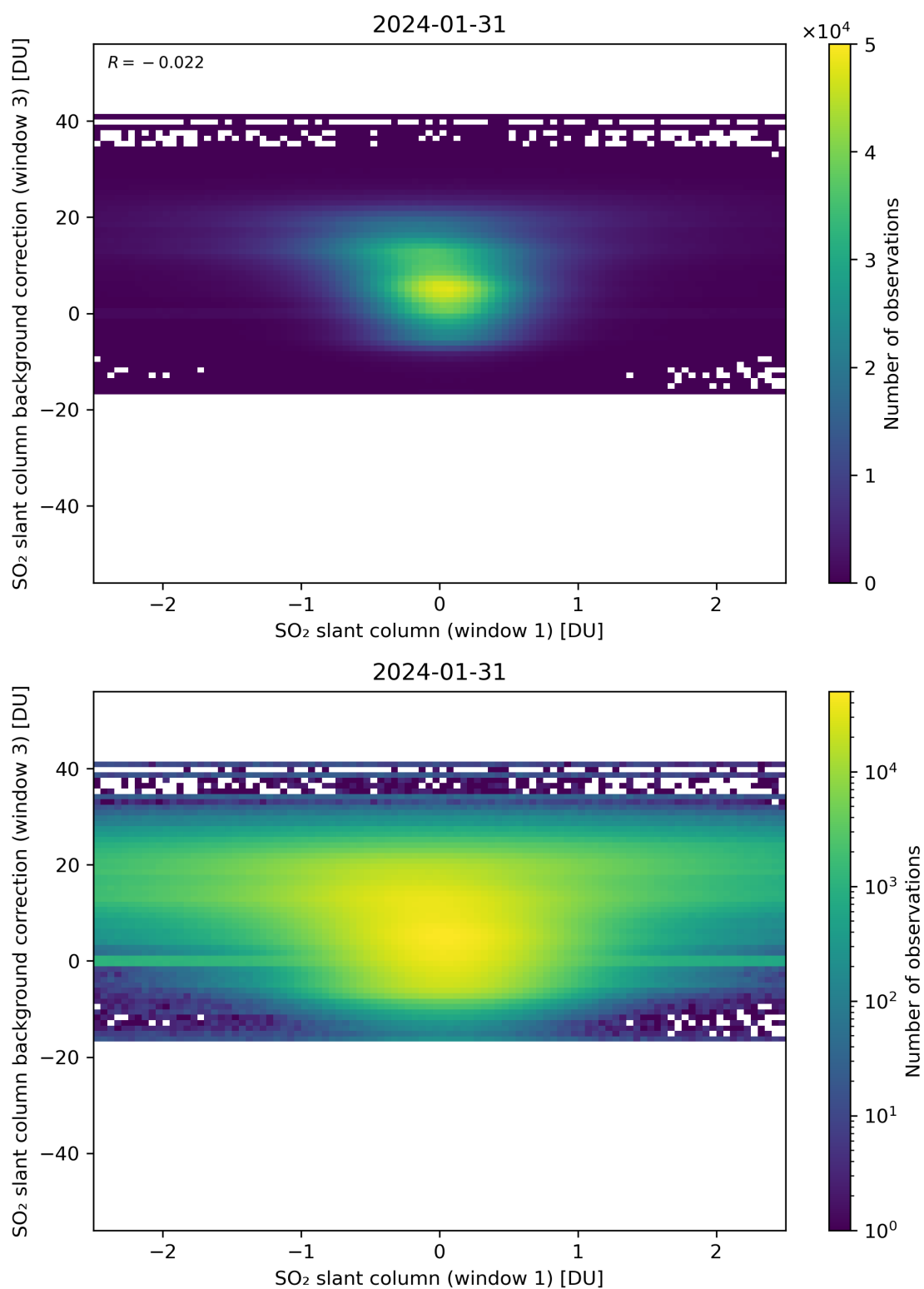
Figure 214: Scatter density plot of “SO 2 slant column (window 1)” against “SO 2 slant column background correction (window 3)” for 2024-01-31 to 2024-02-01.
