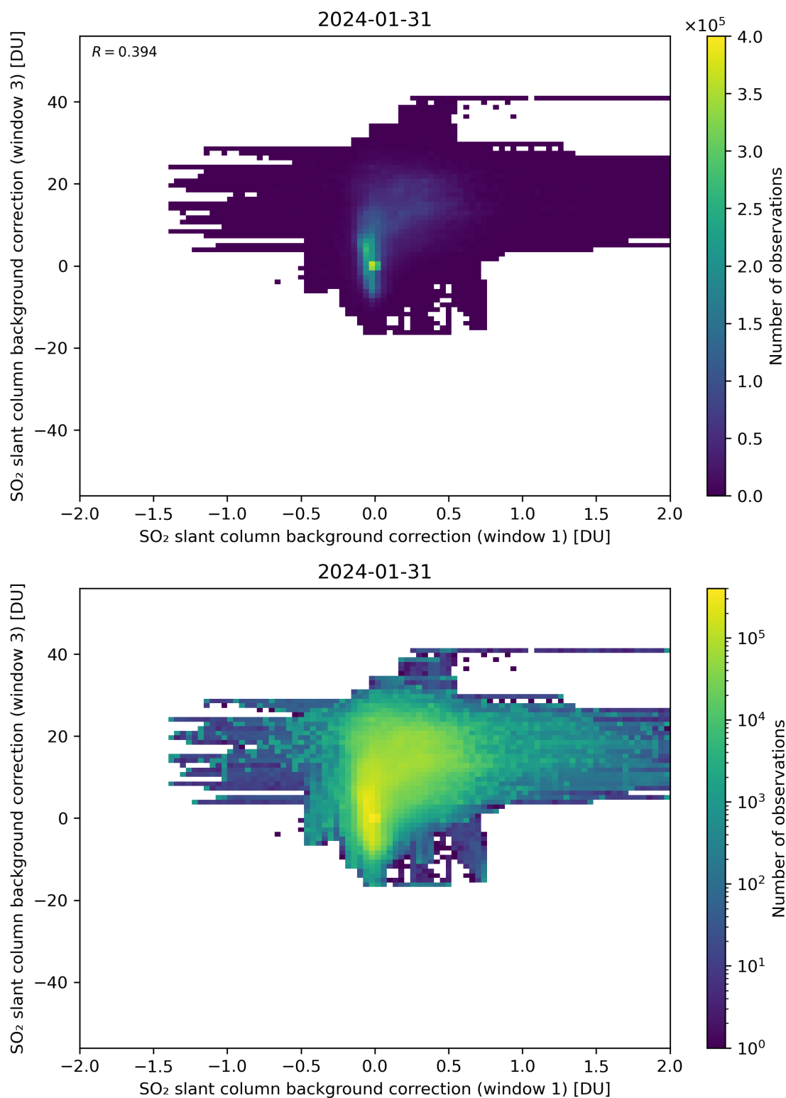
Figure 99: Scatter density plot of “SO 2 slant column background correction (window 1)” against “SO 2 slant column background correction (window 3)” for 2024-01-31 to 2024-02-01.
