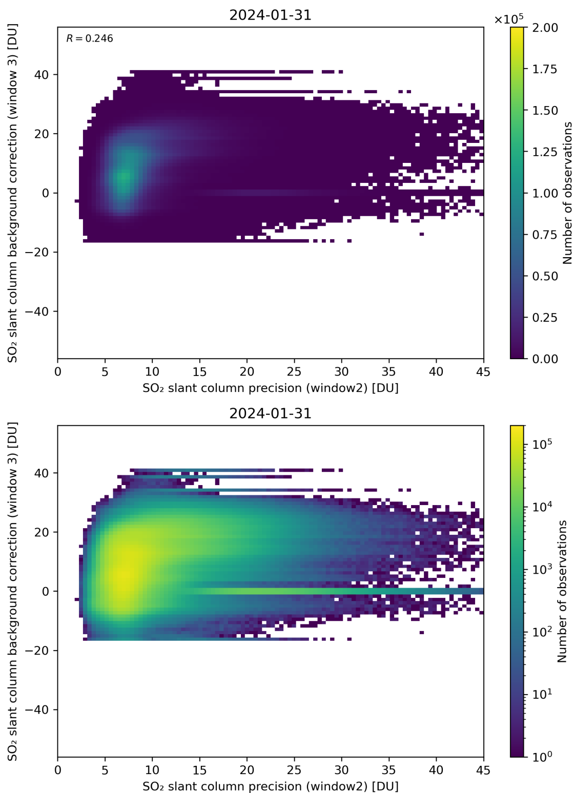
Figure 242: Scatter density plot of “SO 2 slant column precision (window2)” against “SO 2 slant column background correction (window 3)” for 2024-01-31 to 2024-02-01.
