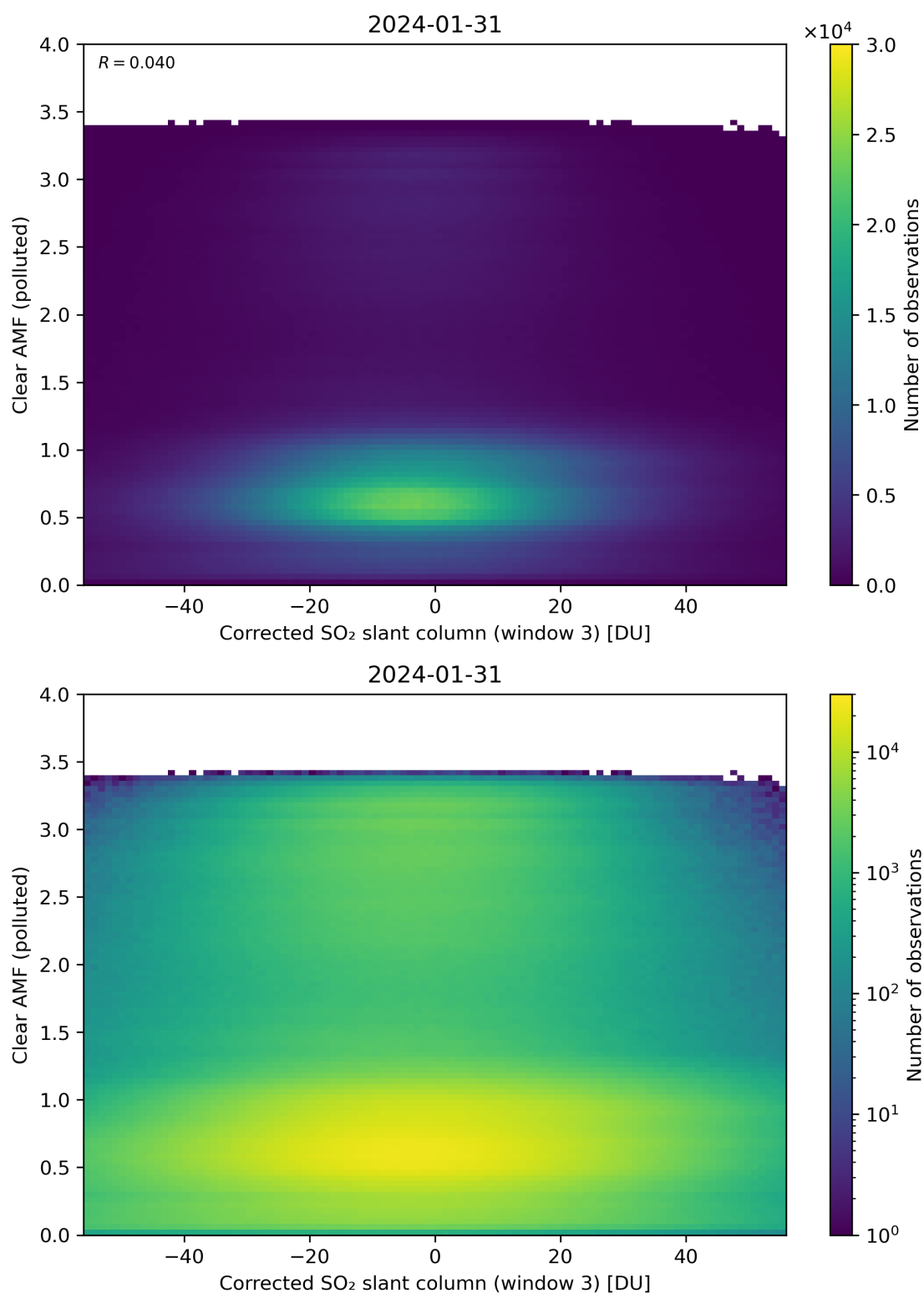
Figure 209: Scatter density plot of “Corrected SO 2 slant column (window 3)” against “Clear AMF (polluted)” for 2024-01-31 to 2024-02-01.
