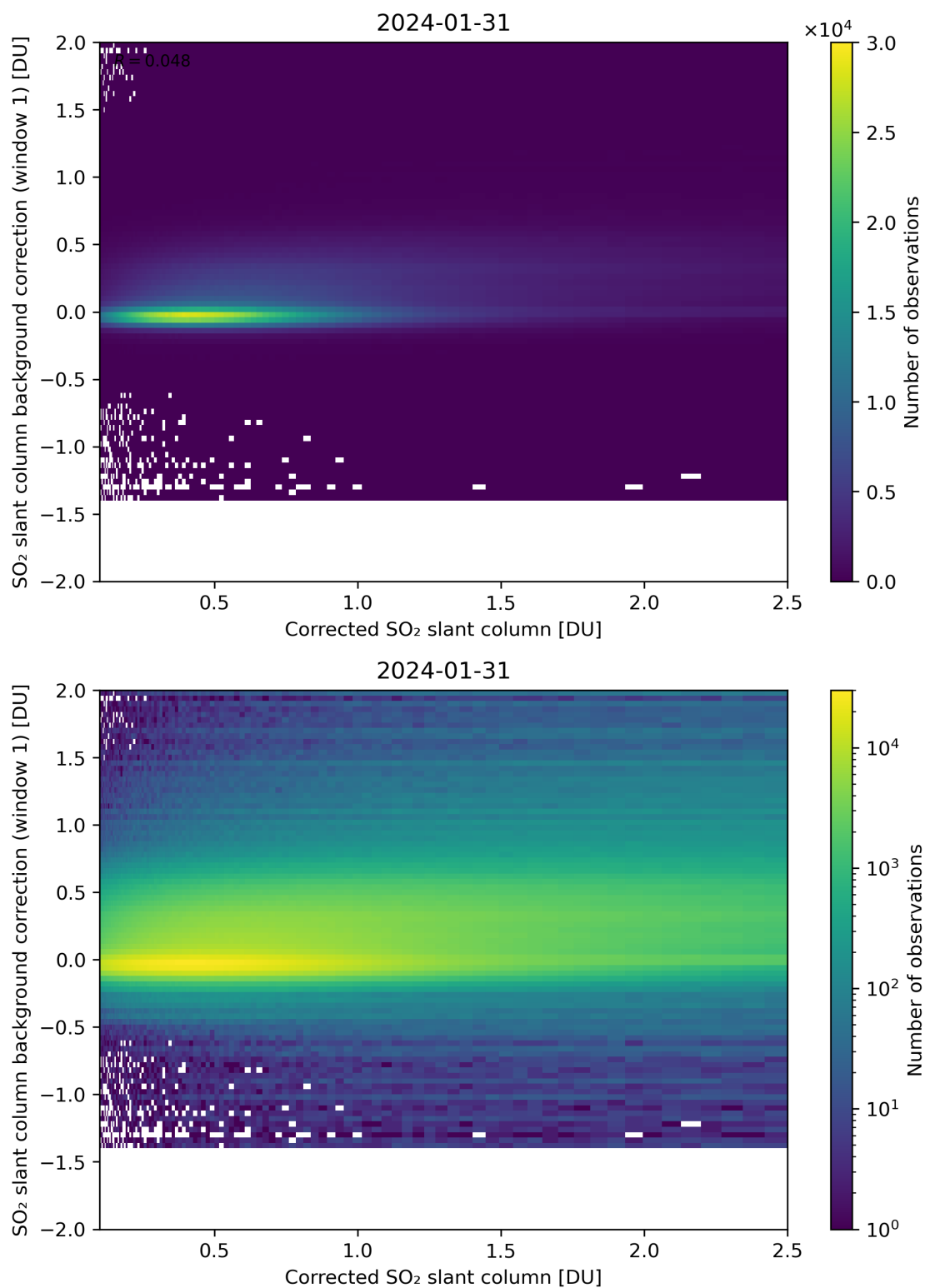
Figure 178: Scatter density plot of “Corrected SO 2 slant column” against “SO 2 slant column background correction (window 1)” for 2024-01-31 to 2024-02-01.
