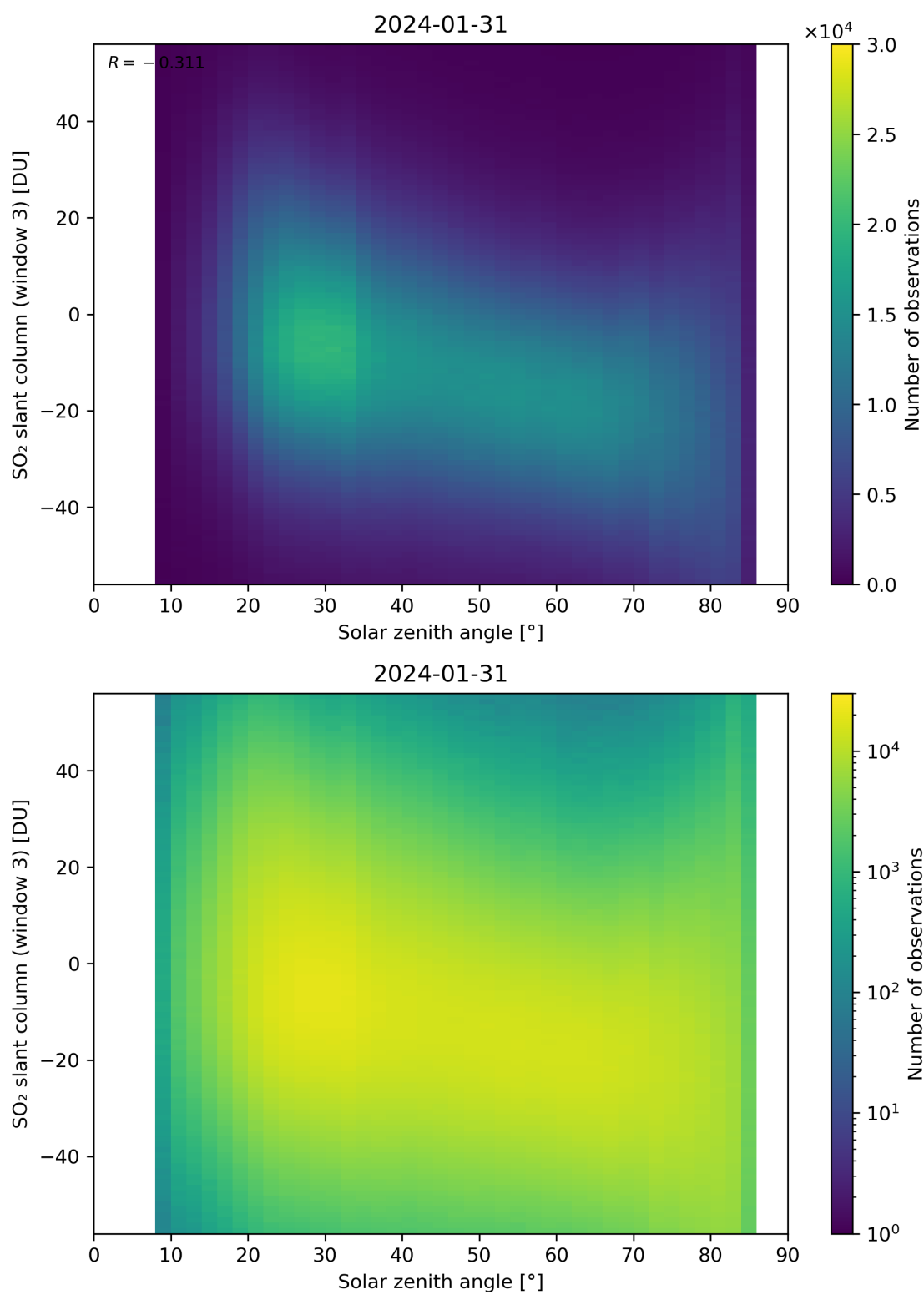
Figure 172: Scatter density plot of “Solar zenith angle” against “SO 2 slant column (window 3)” for 2024-01-31 to 2024-02-01.
