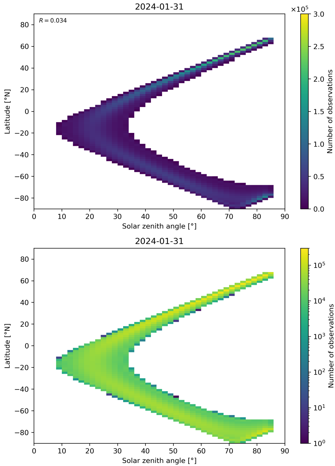
Figure 164: Scatter density plot of “Solar zenith angle” against “Latitude” for 2024-01-31 to 2024-02-01.
