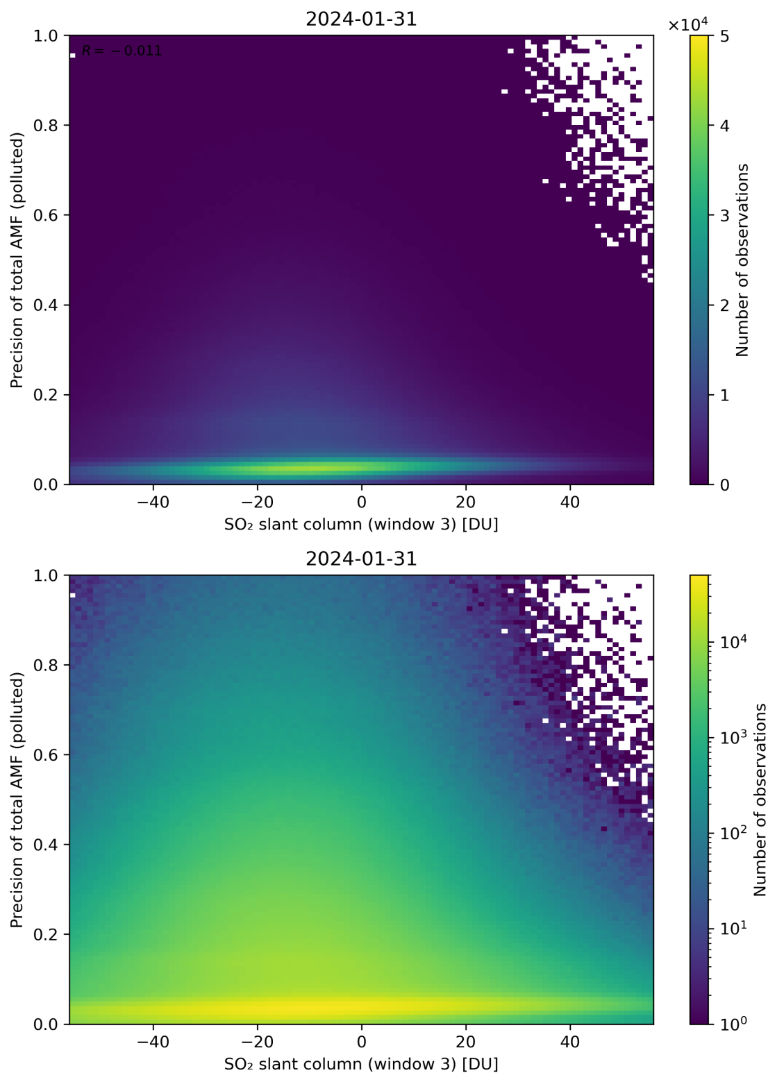
Figure 269: Scatter density plot of “SO 2 slant column (window 3)” against “Precision of total AMF (polluted)” for 2024-01-31 to 2024-02-01.
