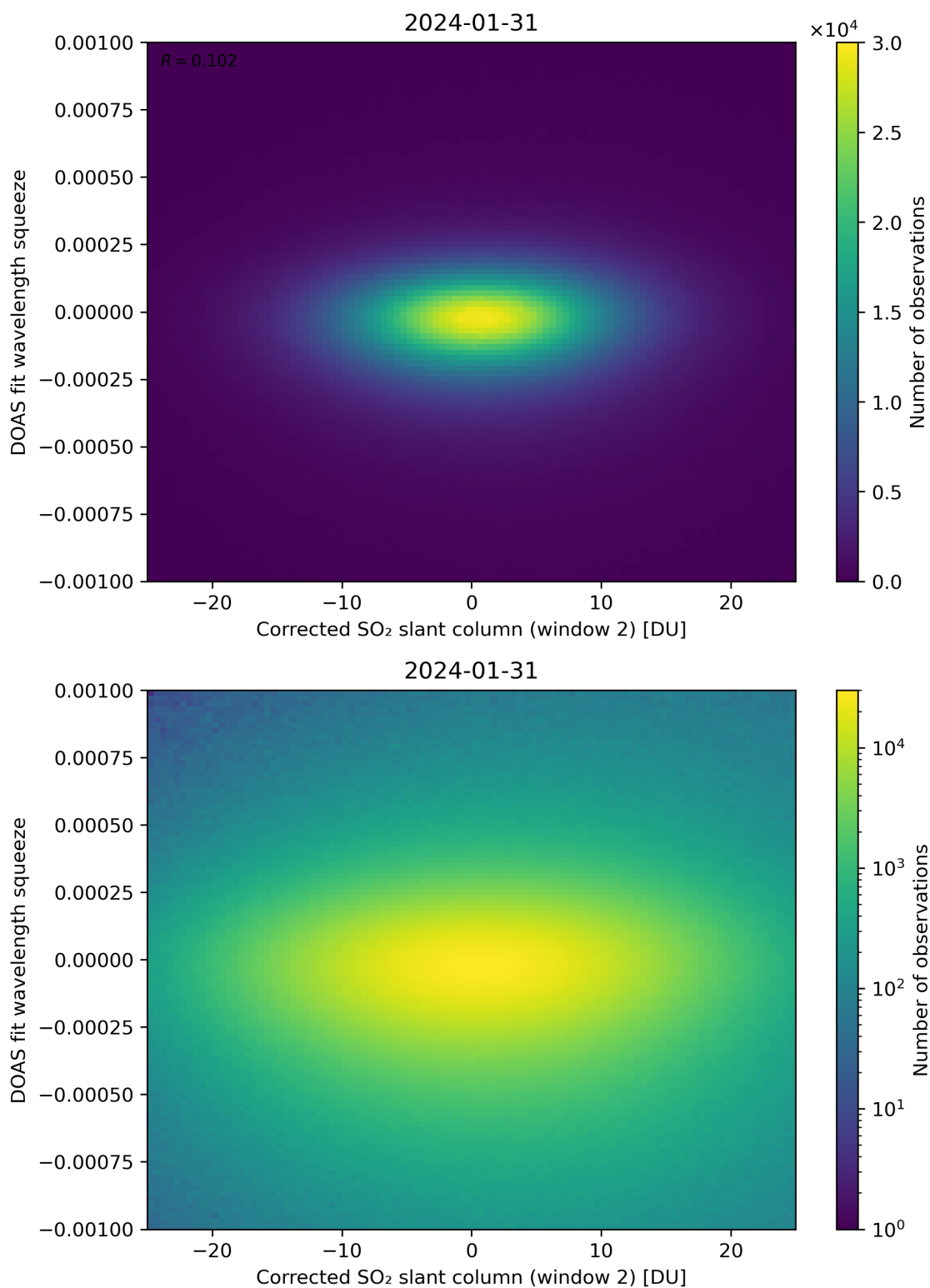
Figure 197: Scatter density plot of “Corrected SO 2 slant column (window 2)” against “DOAS fit wavelength squeeze” for 2024-01-31 to 2024-02-01.
