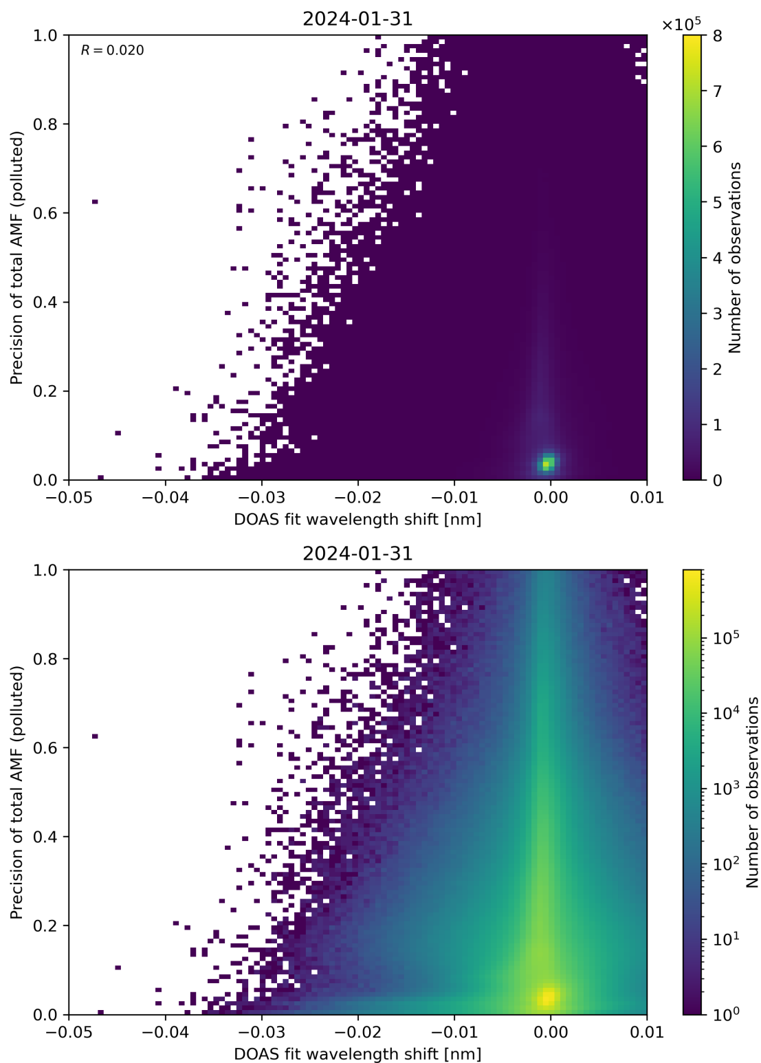
Figure 131: Scatter density plot of “DOAS fit wavelength shift” against “Precision of total AMF (polluted)” for 2024-01-31 to 2024-02-01.
