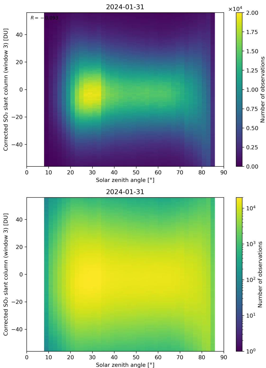
Figure 168: Scatter density plot of “Solar zenith angle” against “Corrected SO 2 slant column (window 3)” for 2024-01-31 to 2024-02-01.
