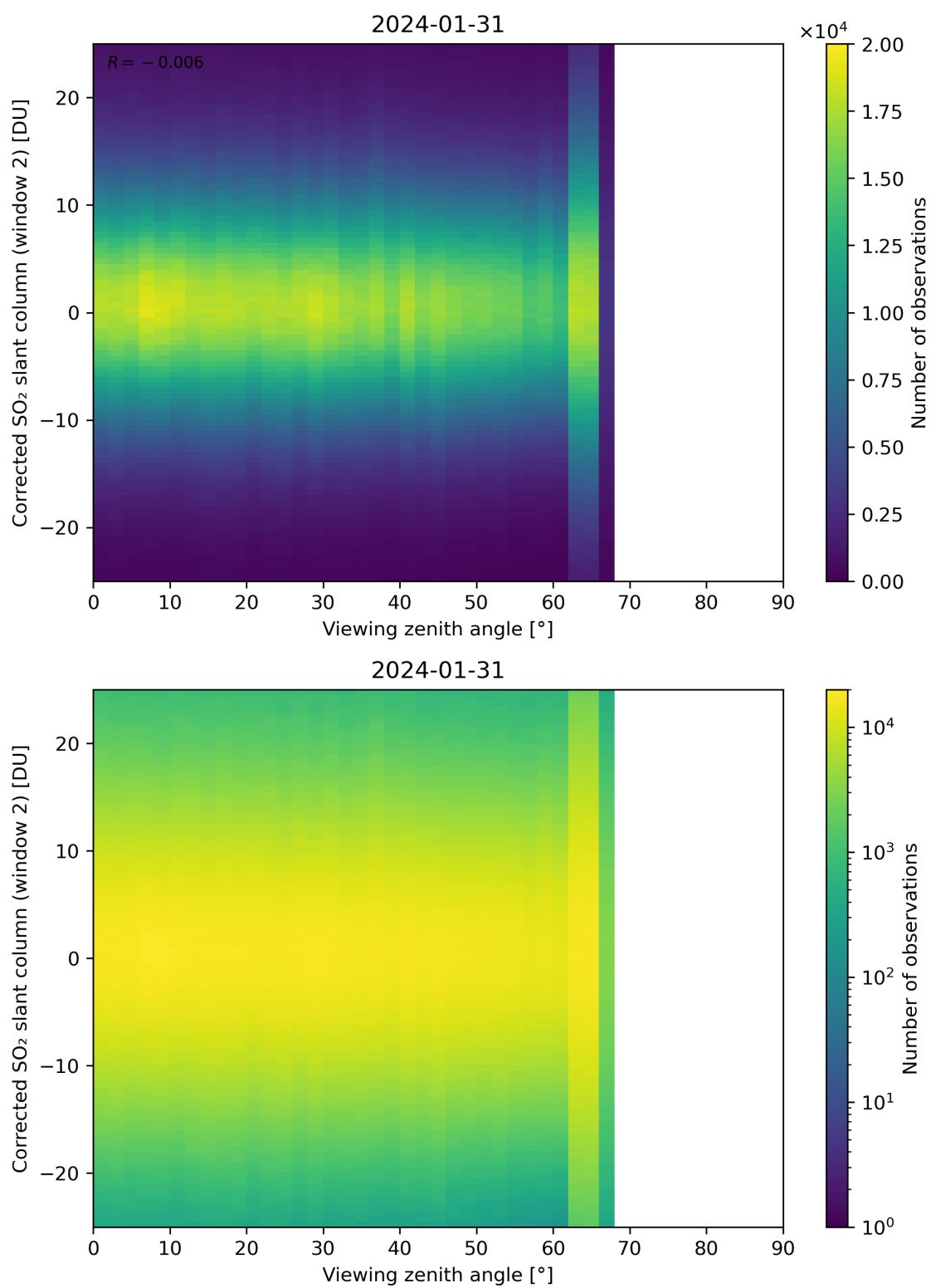
Figure 318: Scatter density plot of “Viewing zenith angle” against “Corrected SO 2 slant column (window 2)” for 2024-01-31 to 2024-02-01.
