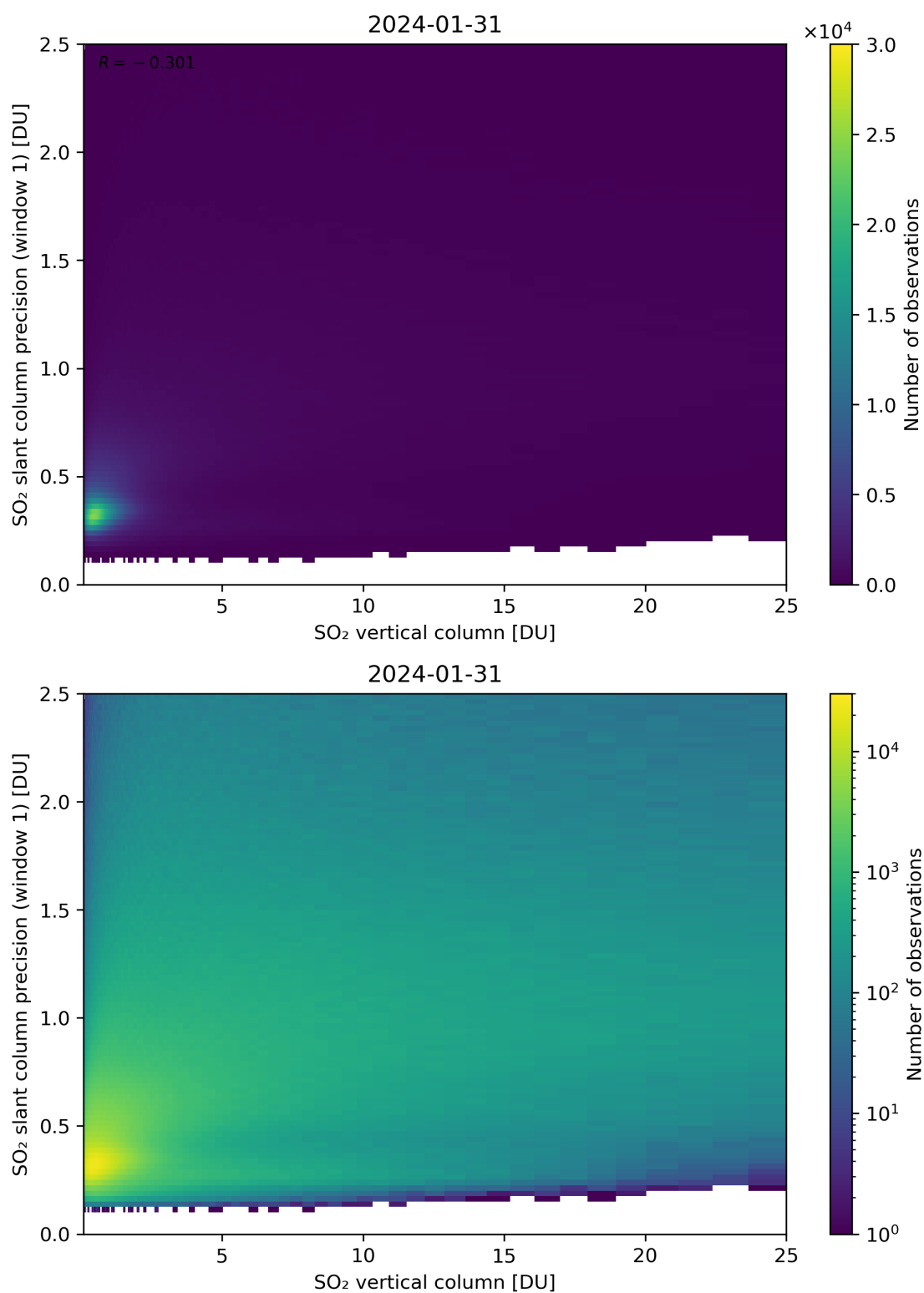
Figure 301: Scatter density plot of “SO 2 vertical column” against “SO 2 slant column precision (window 1)” for 2024-01-31 to 2024-02-01.
