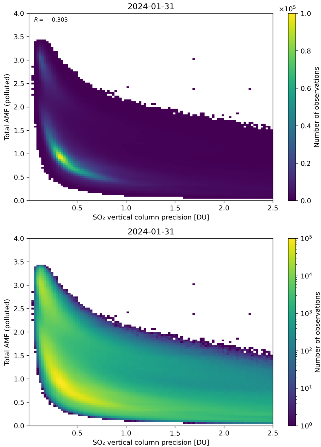
Figure 294: Scatter density plot of “SO 2 vertical column precision” against “Total AMF (polluted)” for 2024-01-31 to 2024-02-01.
