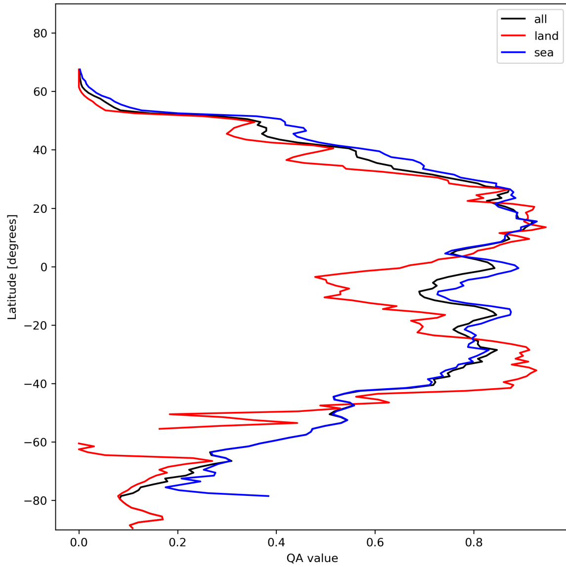
Figure 29: Zonal average of “QA value” for 2024-01-31 to 2024-02-01.
