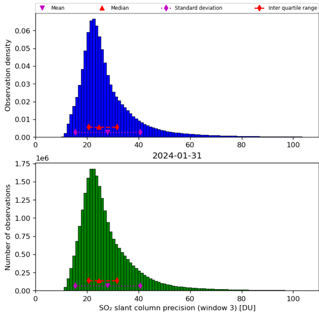
Figure 65: Histogram of “SO 2 slant column precision (window 3)” for 2024-01-31 to 2024-02-01
