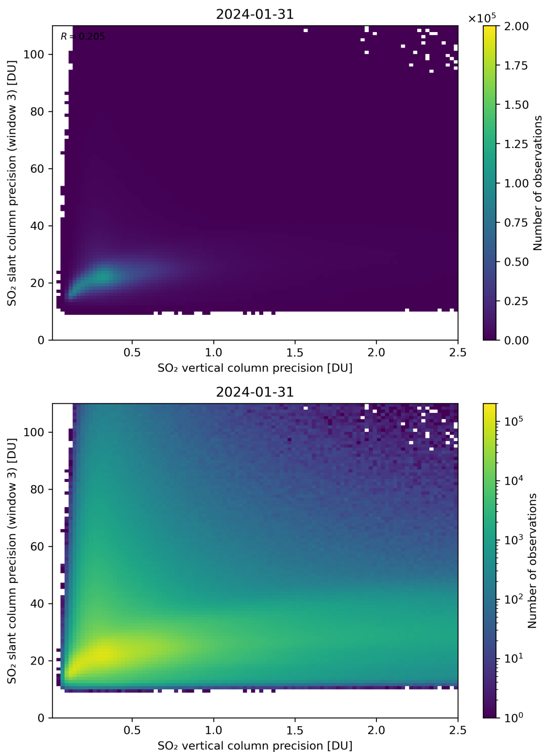
Figure 293: Scatter density plot of “SO 2 vertical column precision” against “SO 2 slant column precision (window 3)” for 2024-01-31 to 2024-02-01.
