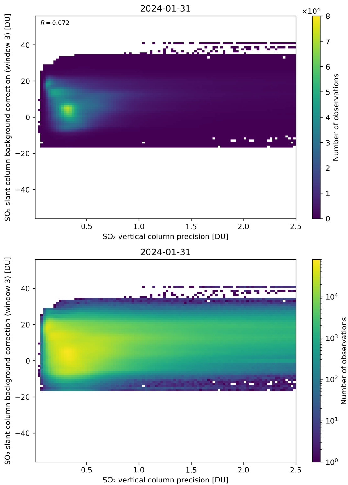
Figure 281: Scatter density plot of “SO 2 vertical column precision” against “SO 2 slant column background correction (window 3)” for 2024-01-31 to 2024-02-01.
