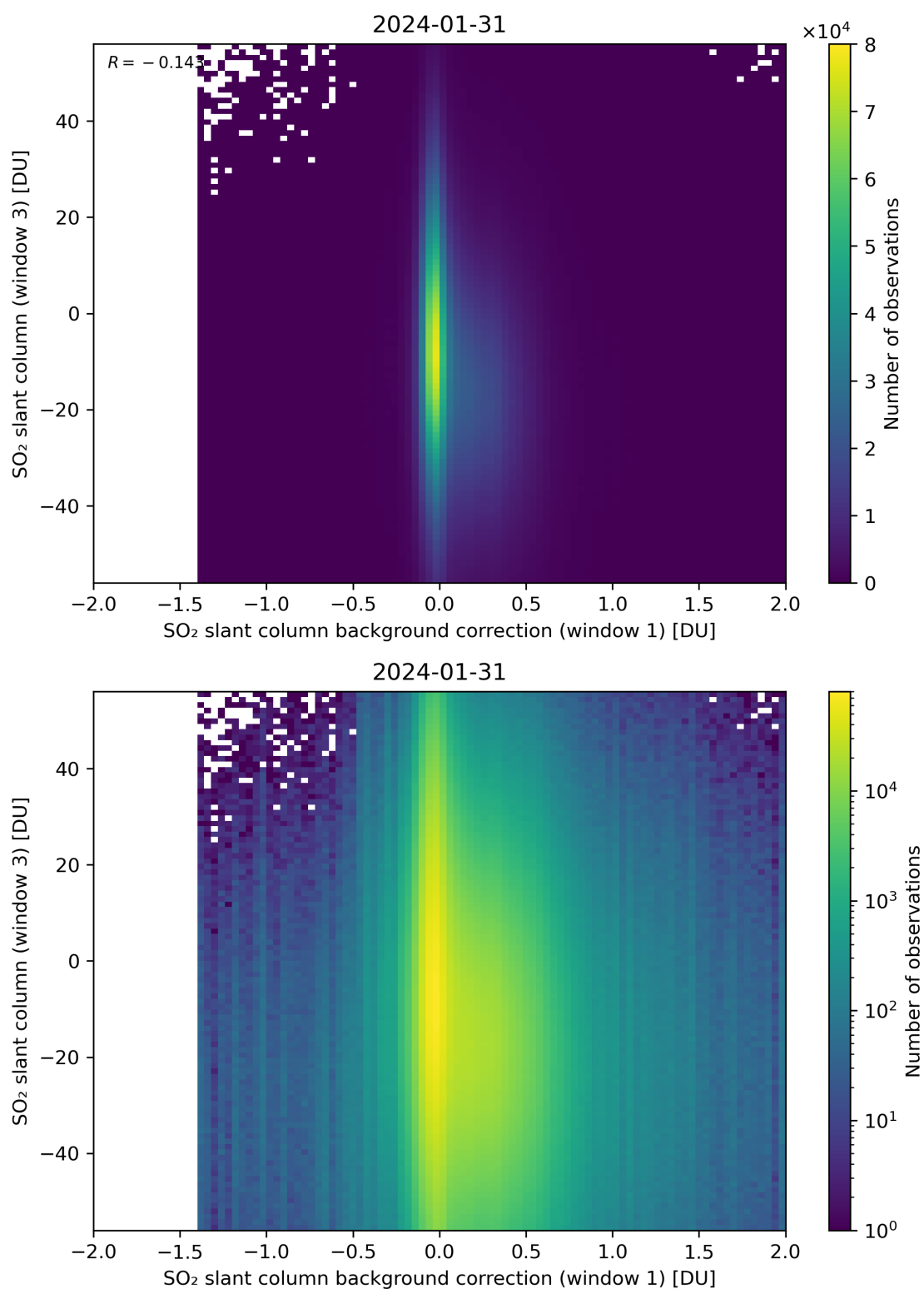
Figure 107: Scatter density plot of “SO 2 slant column background correction (window 1)” against “SO 2 slant column (window 3)” for 2024-01-31 to 2024-02-01.
