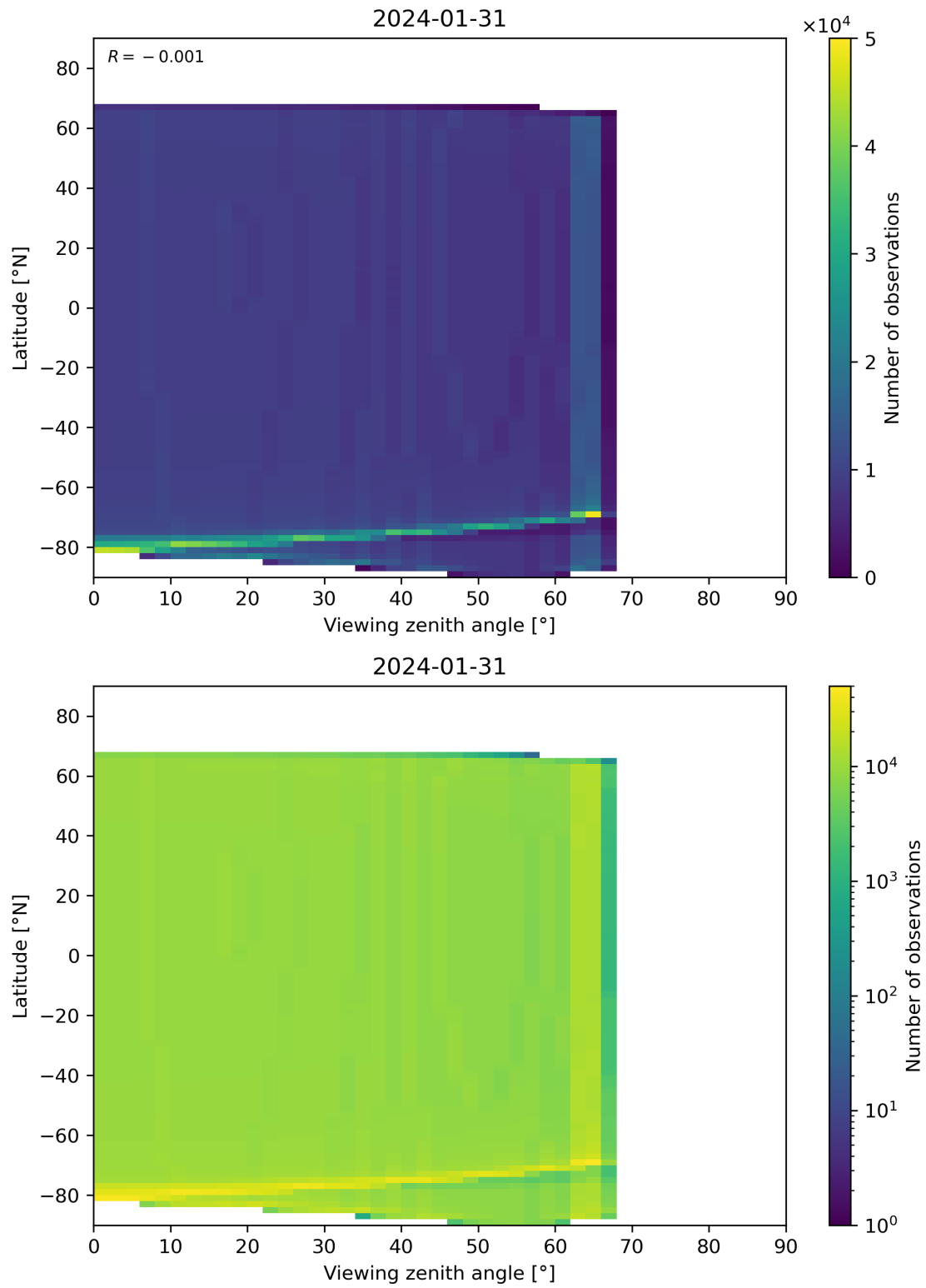
Figure 314: Scatter density plot of “Viewing zenith angle” against “Latitude” for 2024-01-31 to 2024-02-01.
