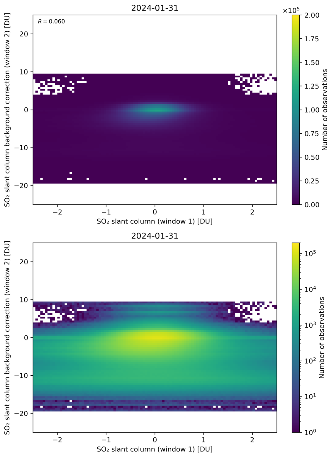
Figure 213: Scatter density plot of “SO 2 slant column (window 1)” against “SO 2 slant column background correction (window 2)” for 2024-01-31 to 2024-02-01.
