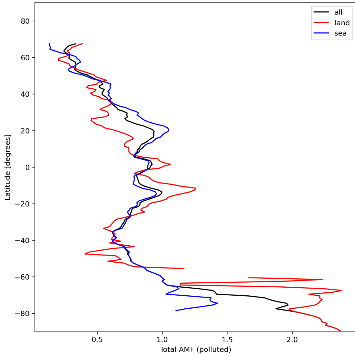
Figure 48: Zonal average of “Total AMF (polluted)” for 2024-01-31 to 2024-02-01.
