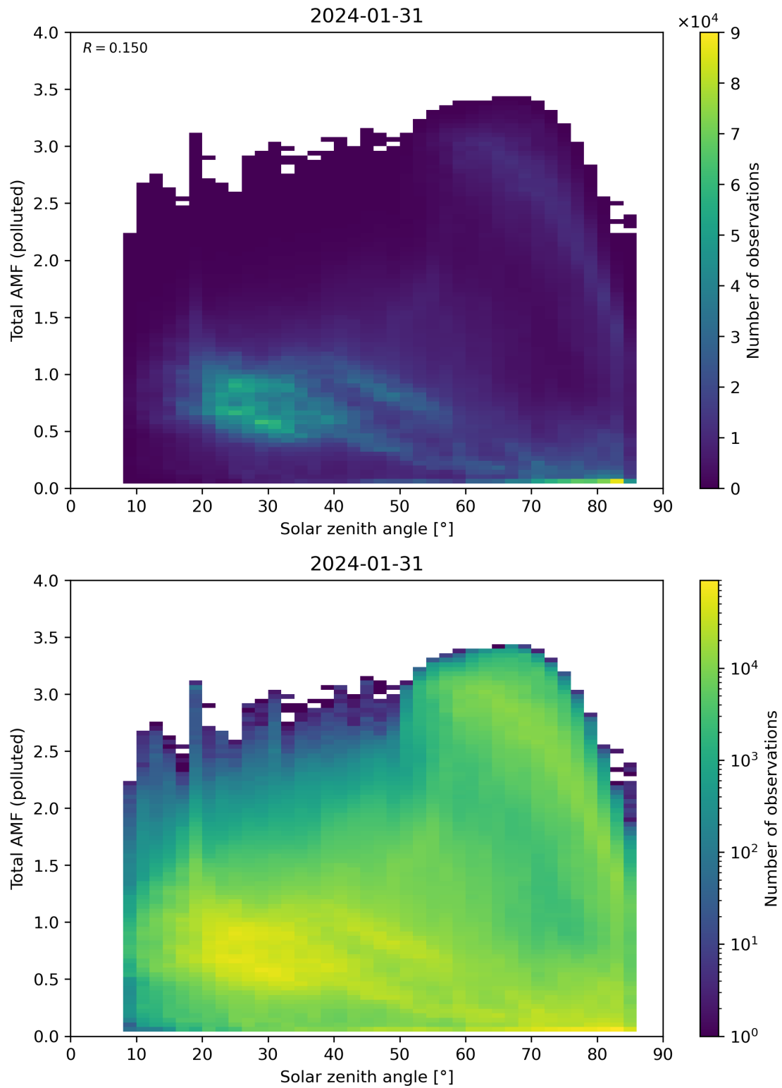
Figure 174: Scatter density plot of “Solar zenith angle” against “Total AMF (polluted)” for 2024-01-31 to 2024-02-01.
