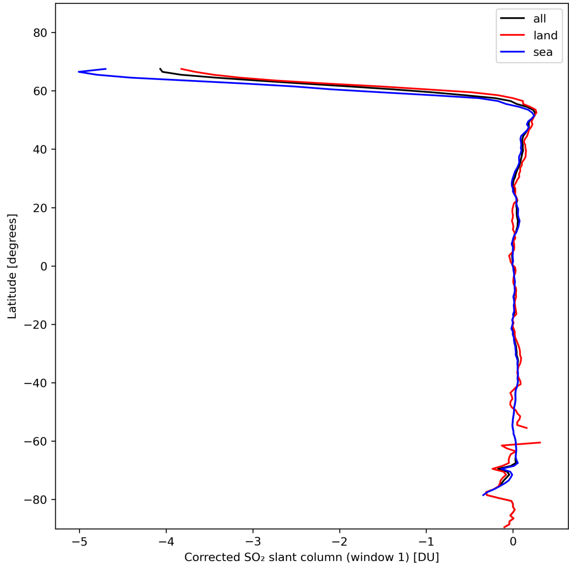
Figure 35: Zonal average of “Corrected SO 2 slant column (window 1)” for 2024-01-31 to 2024-02-01.
