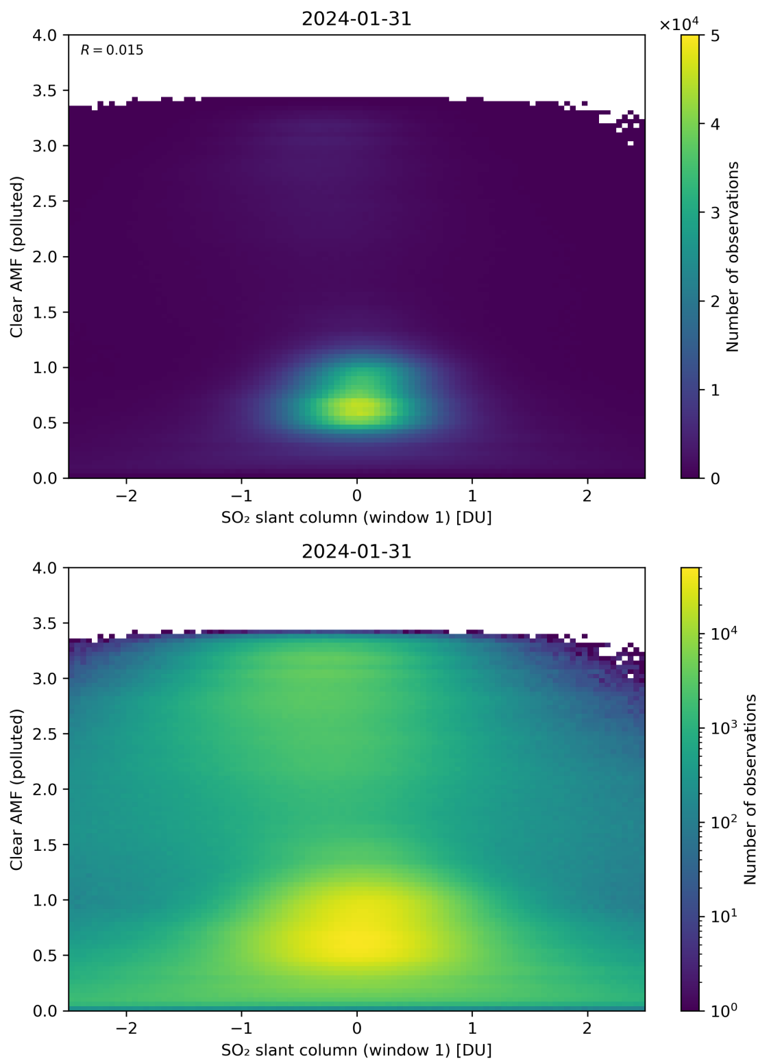
Figure 232: Scatter density plot of “SO 2 slant column (window 1)” against “Clear AMF (polluted)” for 2024-01-31 to 2024-02-01.
