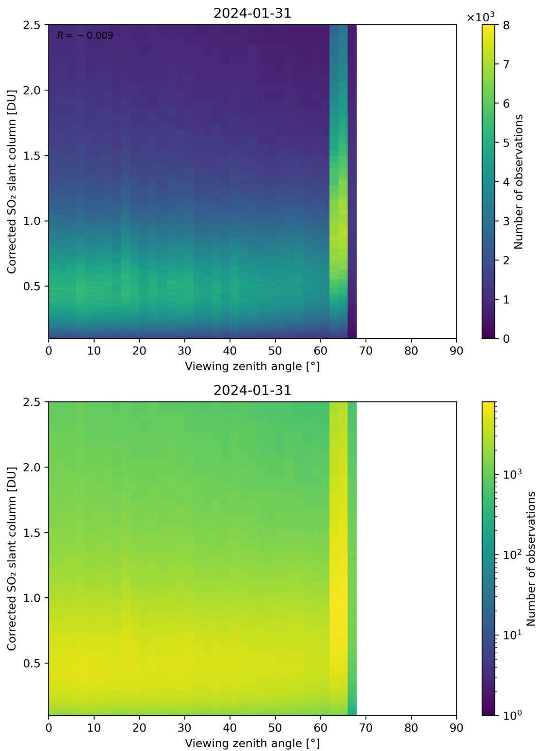
Figure 317: Scatter density plot of “Viewing zenith angle” against “Corrected SO 2 slant column” for 2024-01-31 to 2024-02-01.
