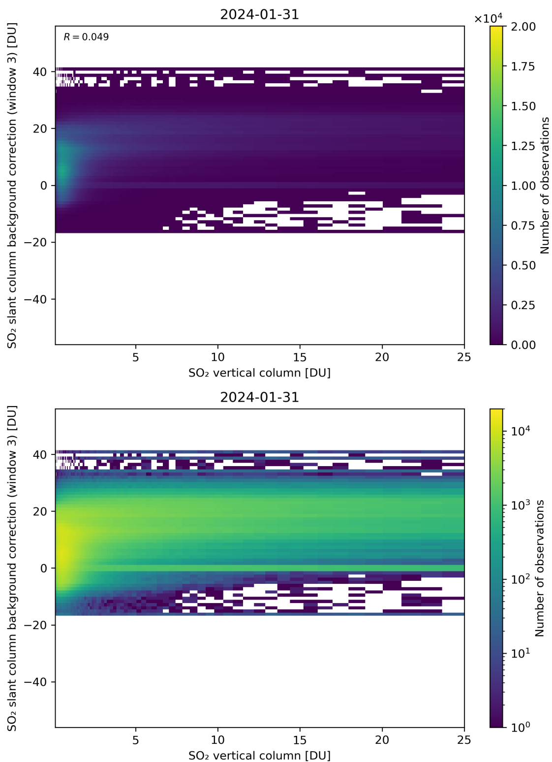
Figure 275: Scatter density plot of “SO 2 vertical column” against “SO 2 slant column background correction (window 3)” for 2024-01-31 to 2024-02-01.
