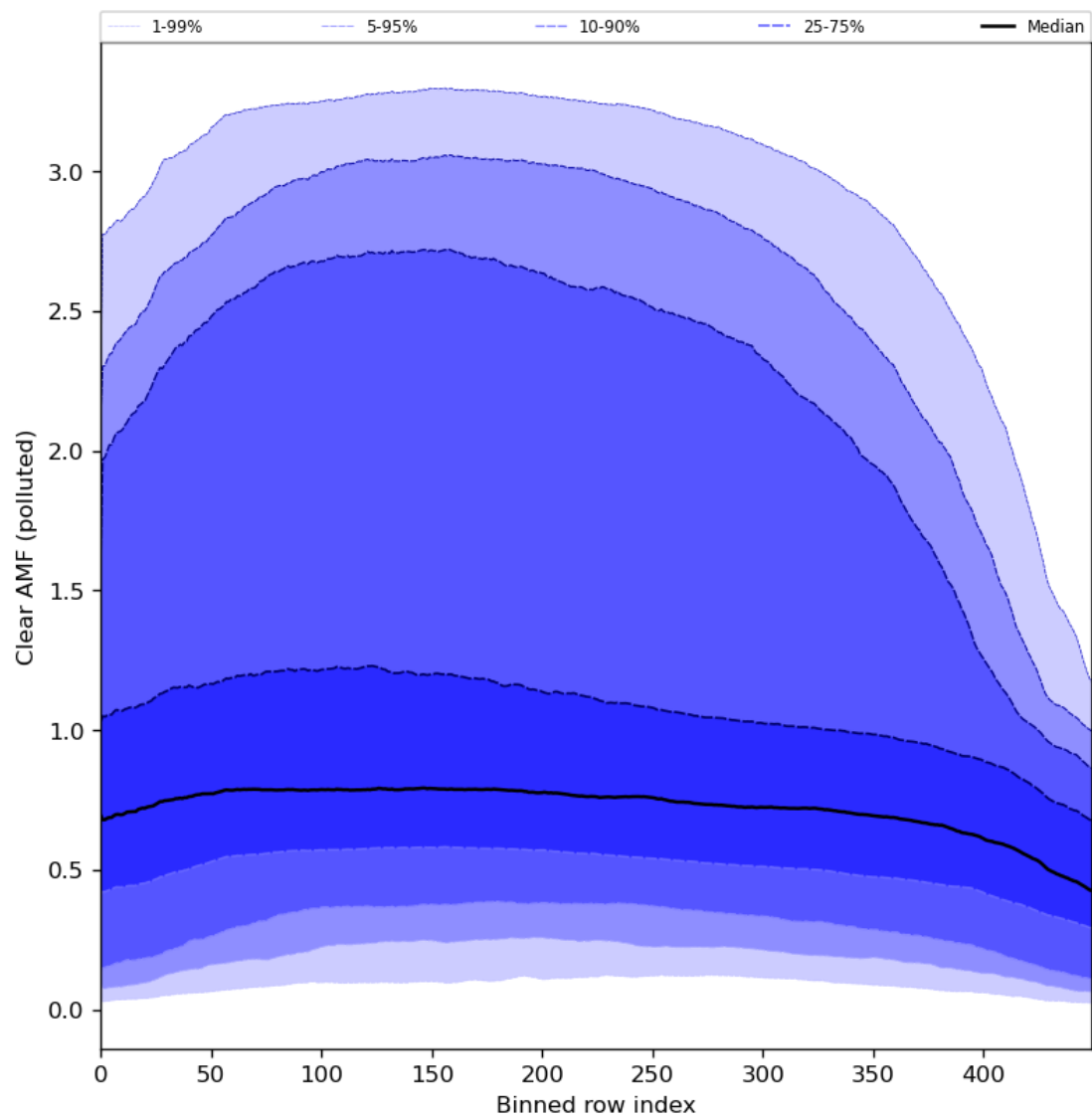
Figure 96: Along track statistics of “Clear AMF (polluted)” for 2024-01-31 to 2024-02-01
