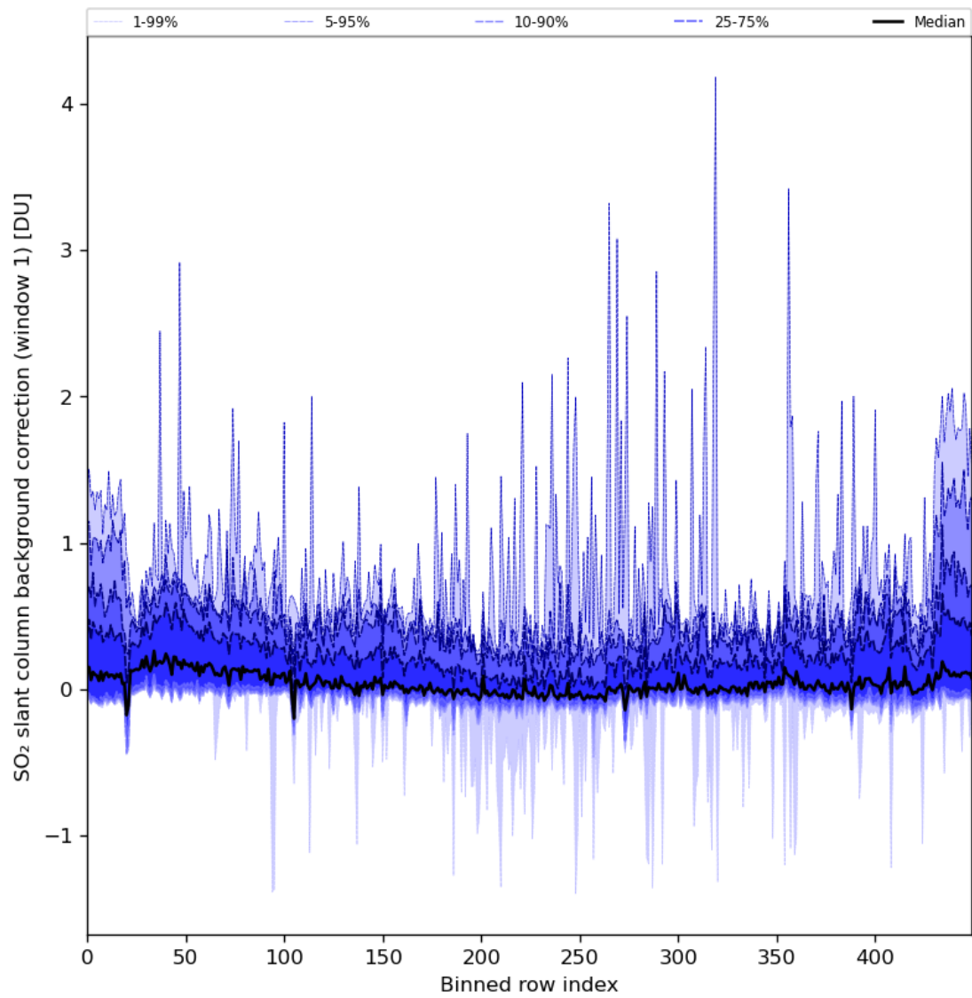
Figure 82: Along track statistics of “SO 2 slant column background correction (window 1)” for 2024-01-31 to 2024-02-01
