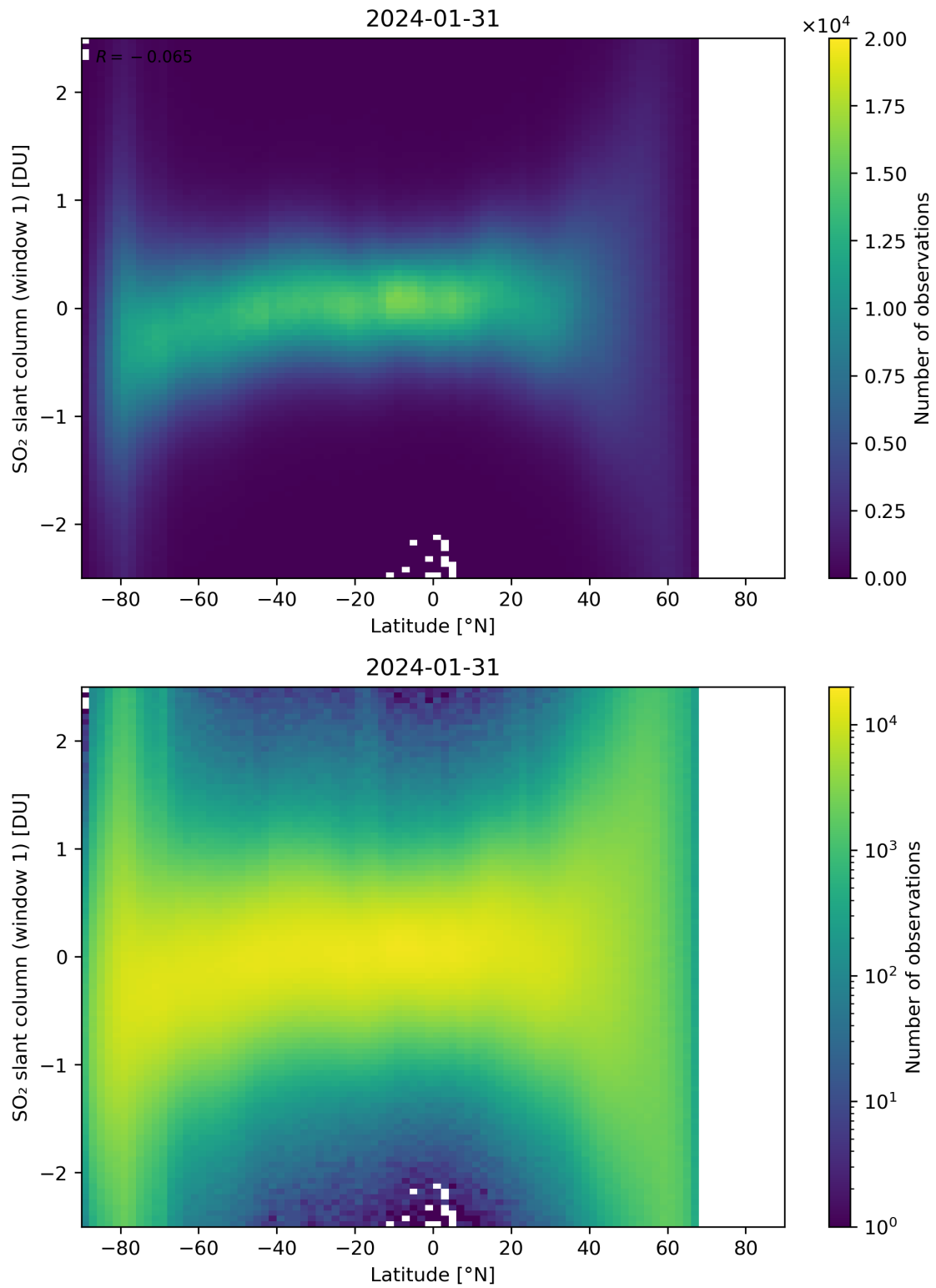
Figure 149: Scatter density plot of “Latitude” against “SO 2 slant column (window 1)” for 2024-01-31 to 2024-02-01.
