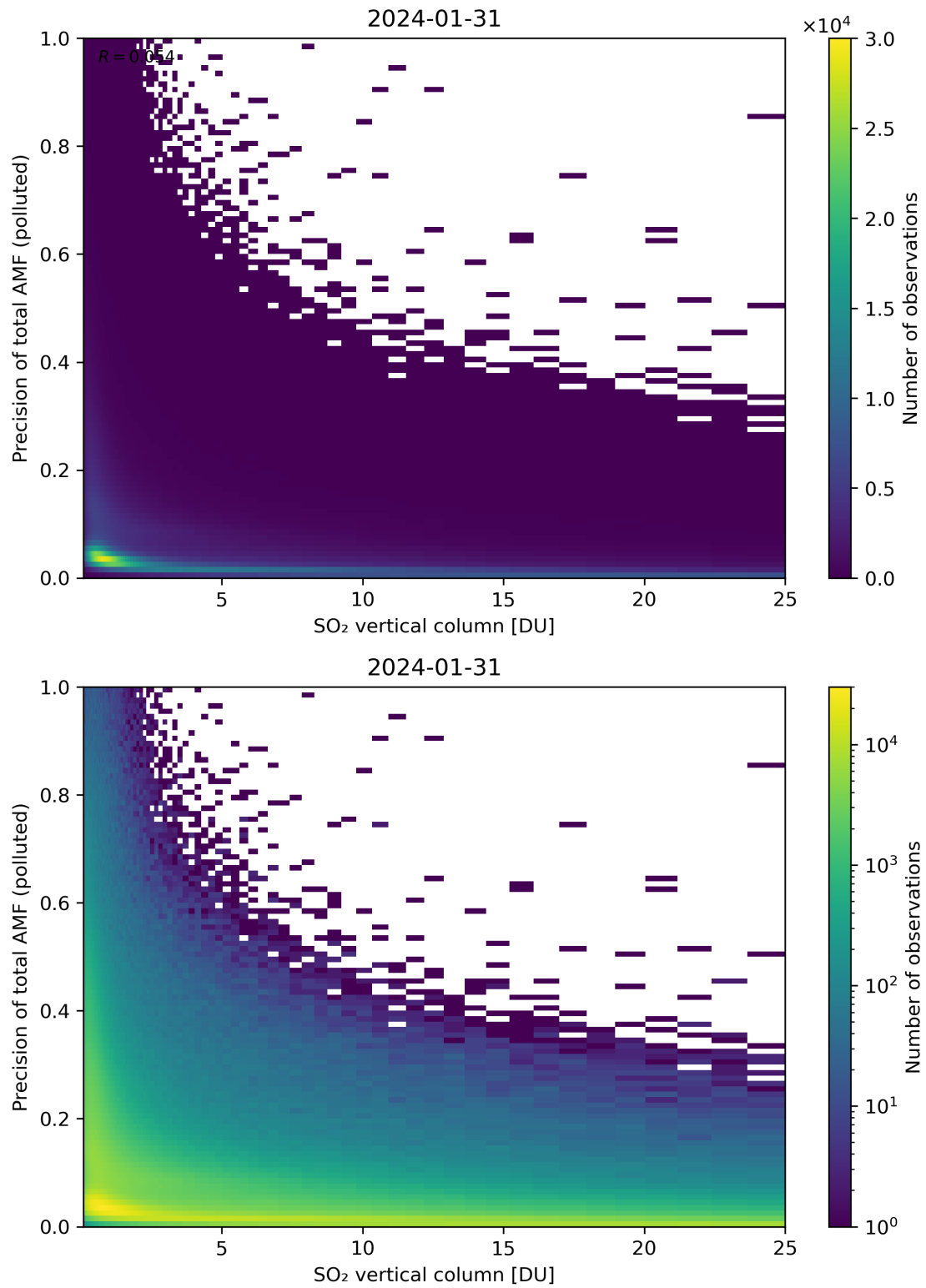
Figure 306: Scatter density plot of “SO 2 vertical column” against “Precision of total AMF (polluted)” for 2024-01-31 to 2024-02-01.
