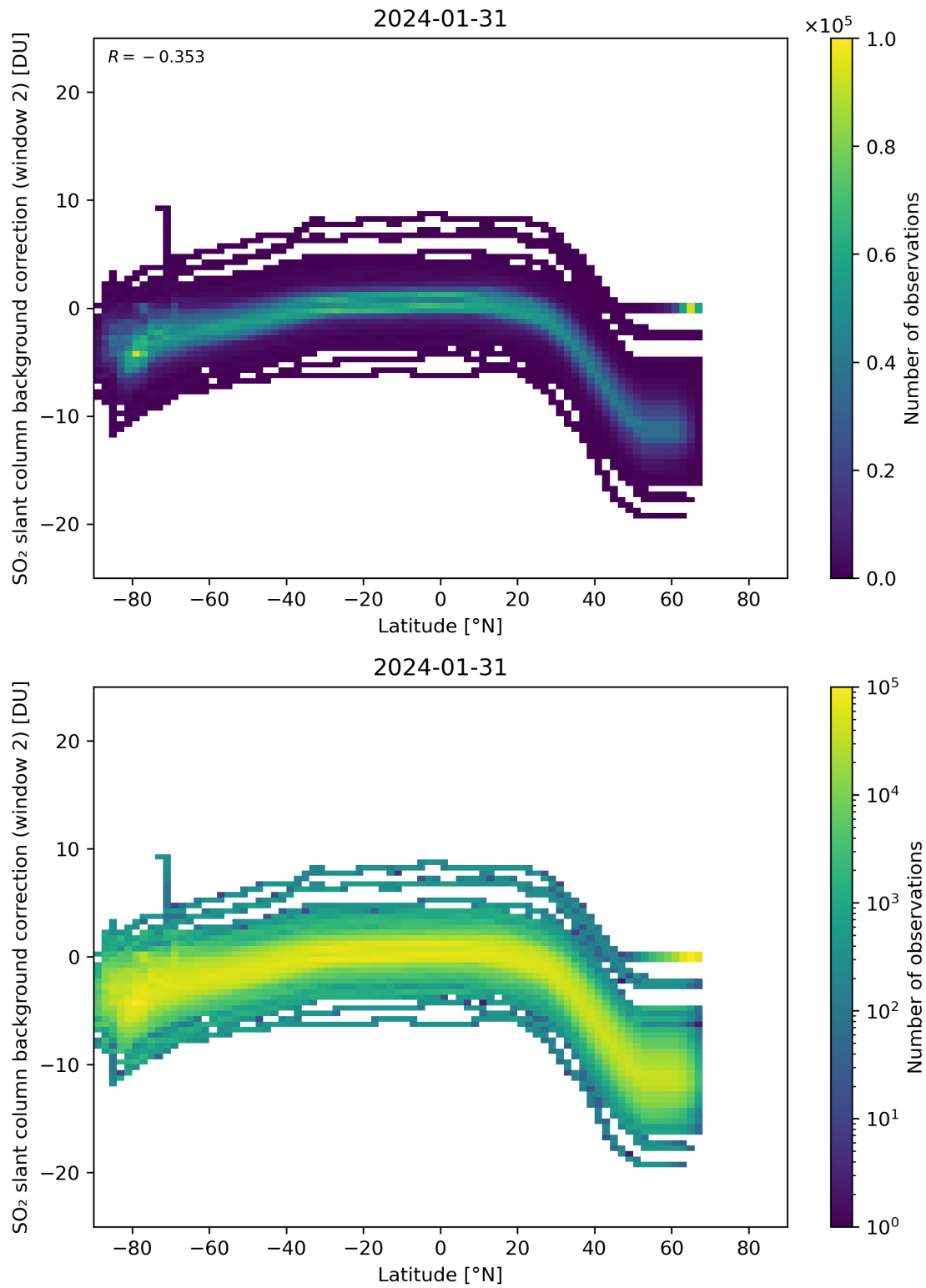
Figure 140: Scatter density plot of “Latitude” against “SO 2 slant column background correction (window 2)” for 2024-01-31 to 2024-02-01.
