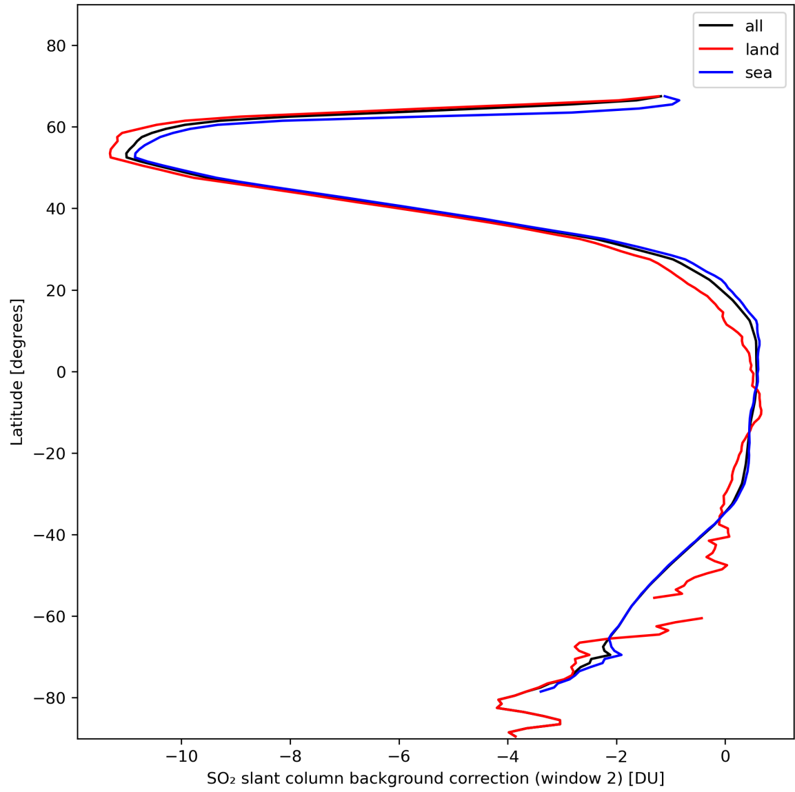
Figure 40: Zonal average of "SO 2 slant column background correction (window 2)" for 2024-01-31 to 2024-02-01.
