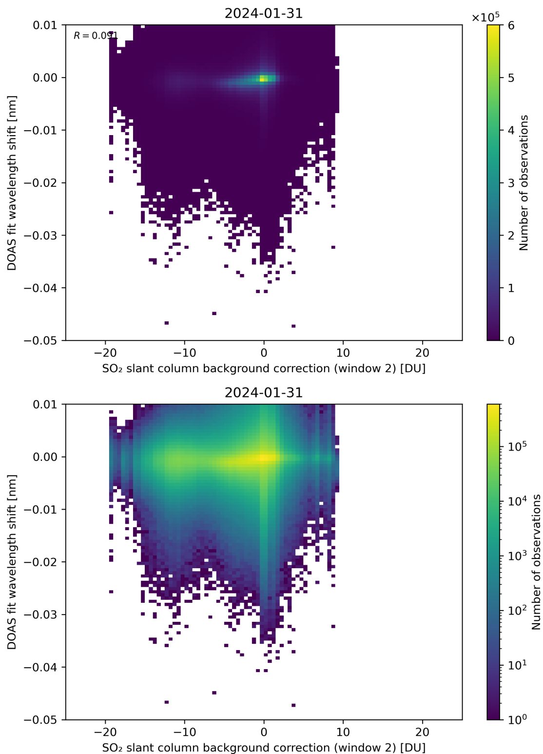
Figure 112: Scatter density plot of “SO 2 slant column background correction (window 2)” against “DOAS fit wavelength shift” for 2024-01-31 to 2024-02-01.
