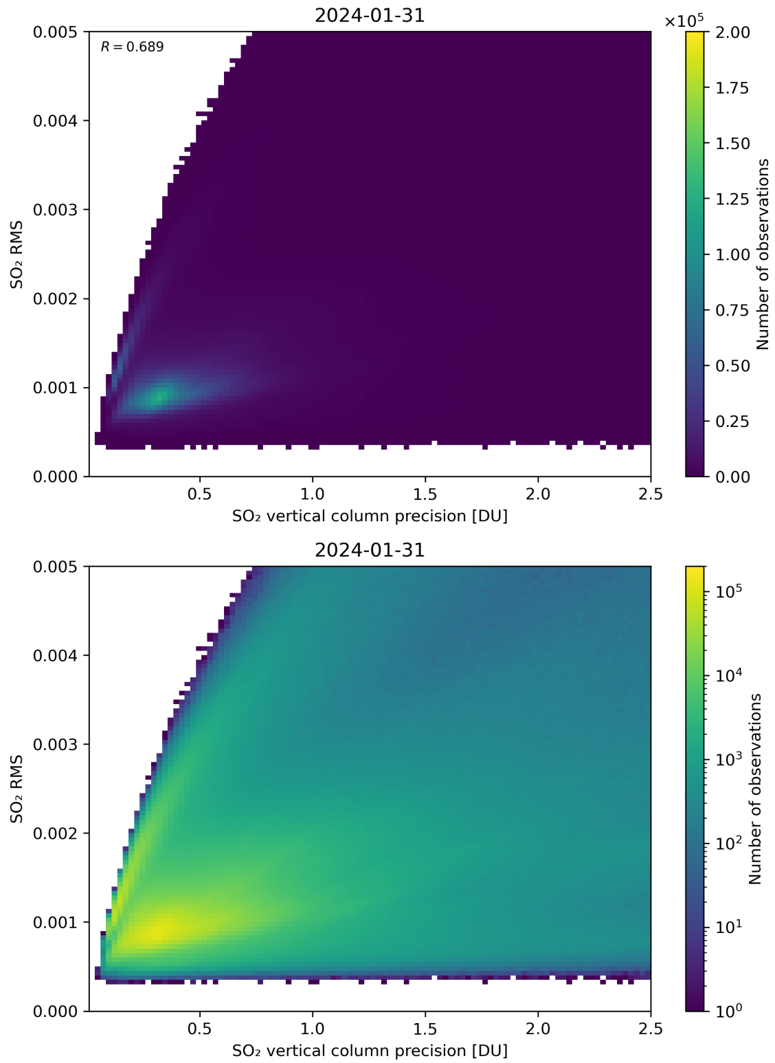
Figure 284: Scatter density plot of “SO 2 vertical column precision” against “SO 2 RMS” for 2024-01-31 to 2024-02-01.
