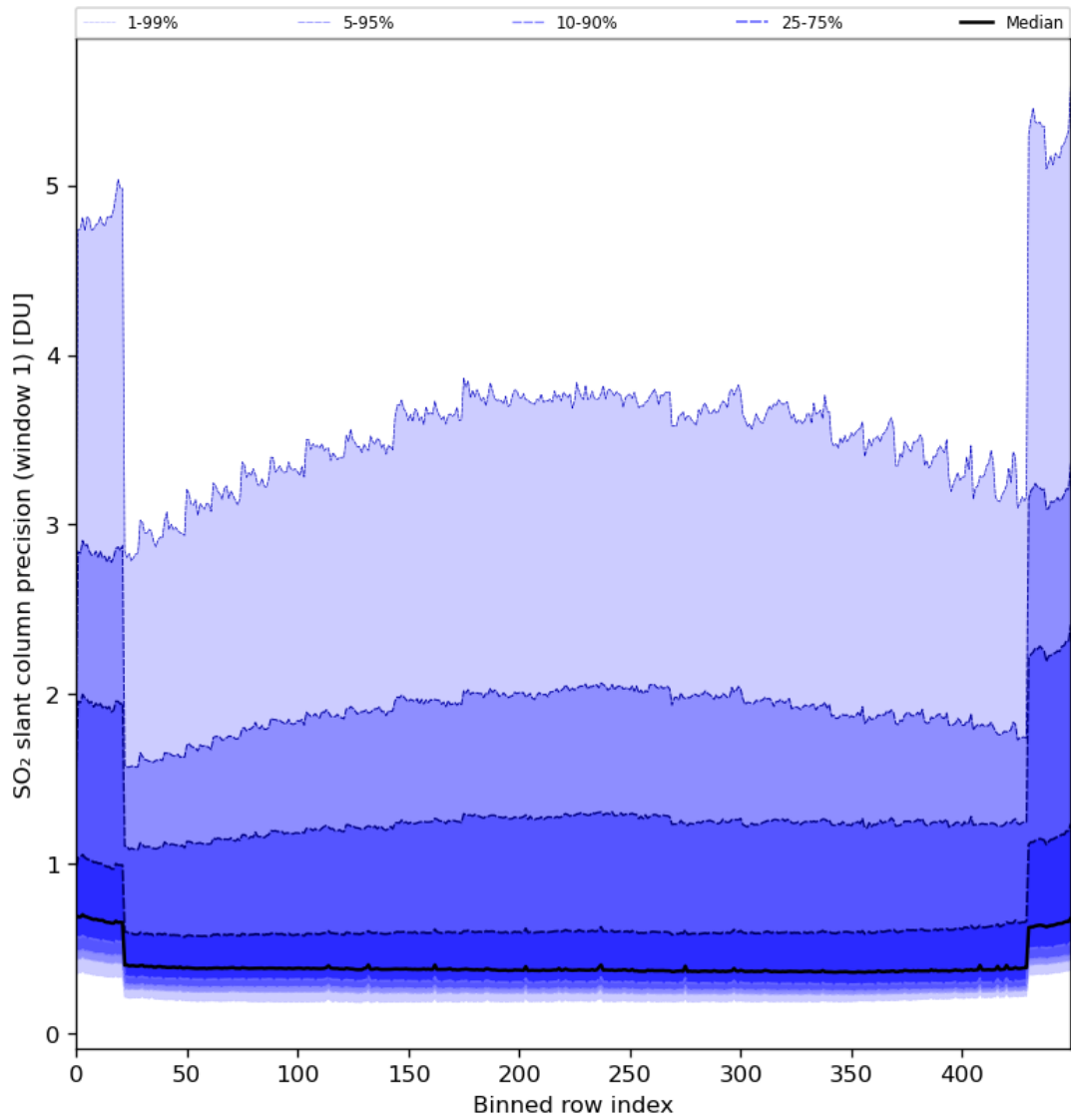
Figure 80: Along track statistics of “SO 2 slant column precision (window 1)” for 2024-01-31 to 2024-02-01
