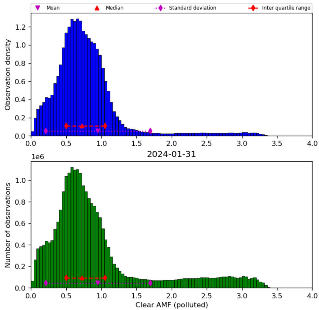
Figure 73: Histogram of “Clear AMF (polluted)” for 2024-01-31 to 2024-02-01
