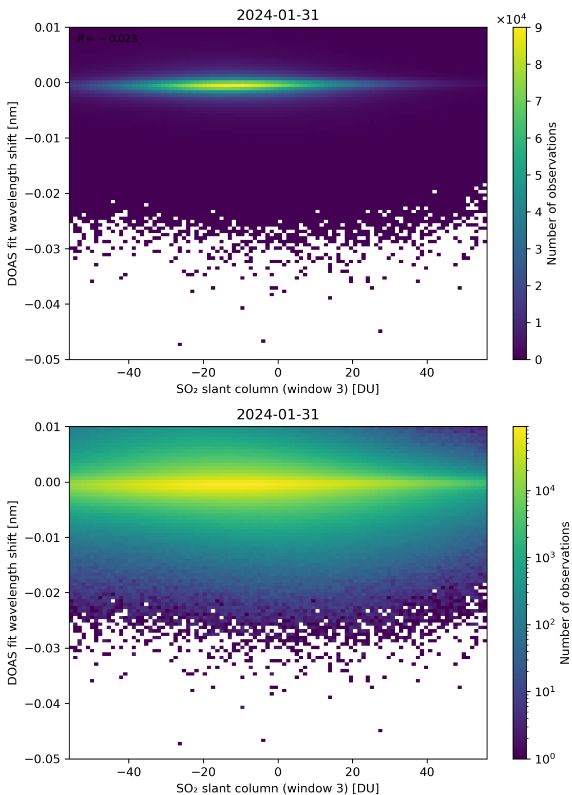
Figure 254: Scatter density plot of “SO 2 slant column (window 3)” against “DOAS fit wavelength shift” for 2024-01-31 to 2024-02-01.
