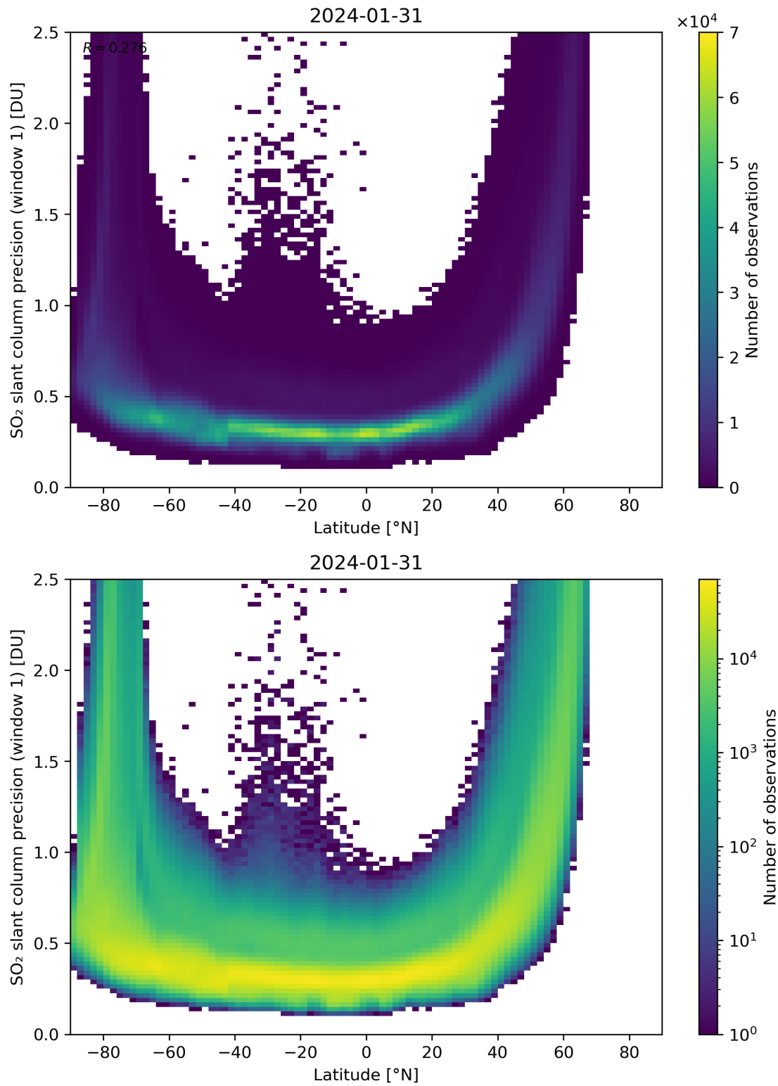
Figure 150: Scatter density plot of “Latitude” against “SO 2 slant column precision (window 1)” for 2024-01-31 to 2024-02-01.
