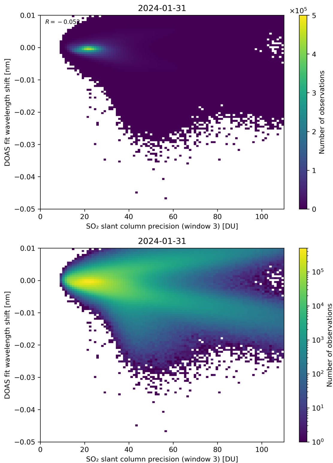
Figure 258: Scatter density plot of “SO 2 slant column precision (window 3)” against “DOAS fit wavelength shift” for 2024-01-31 to 2024-02-01.
