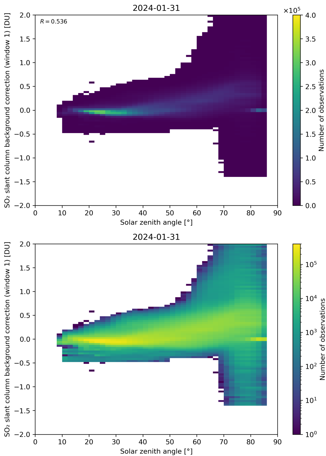
Figure 158: Scatter density plot of “Solar zenith angle” against “SO 2 slant column background correction (window 1)” for 2024-01-31 to 2024-02-01.
