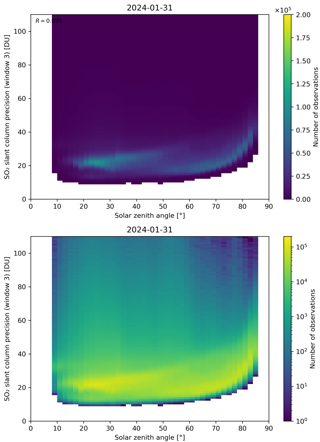
Figure 173: Scatter density plot of “Solar zenith angle” against “SO 2 slant column precision (window 3)” for 2024-01-31 to 2024-02-01.
