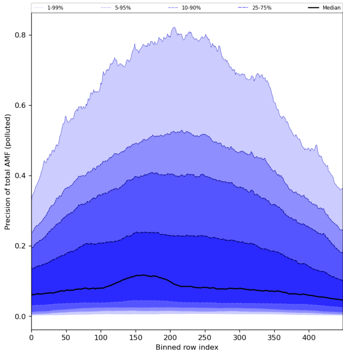
Figure 95: Along track statistics of “Precision of total AMF (polluted)” for 2024-01-31 to 2024-02-01
