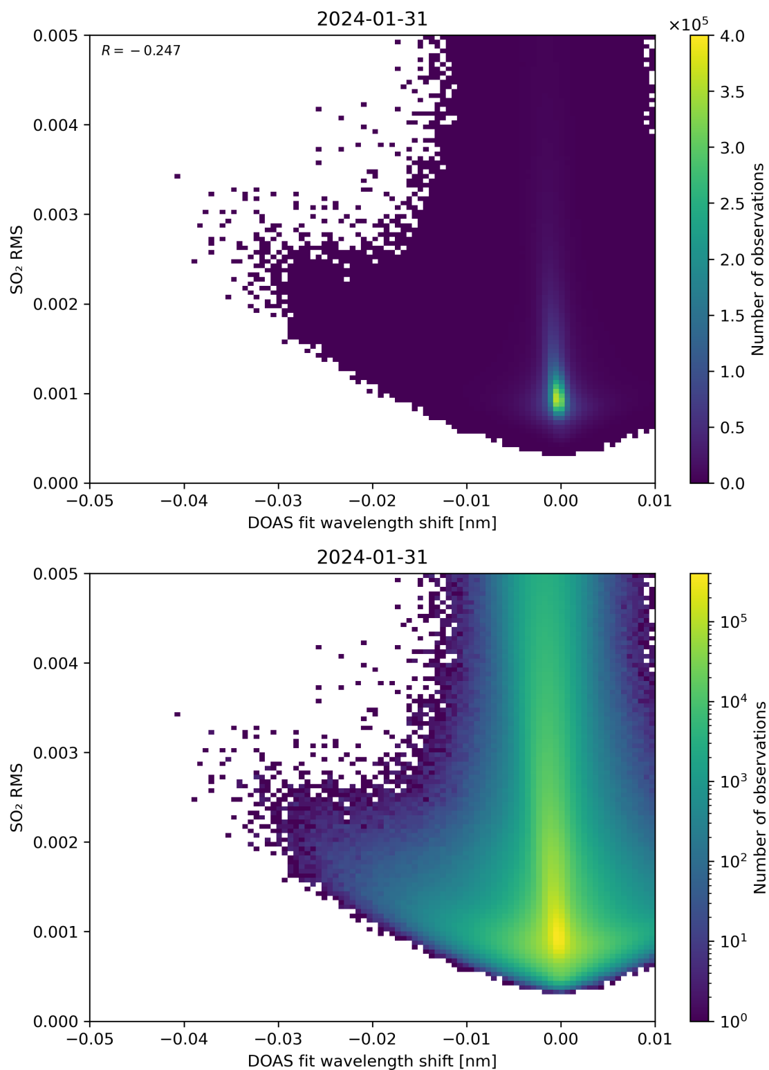
Figure 128: Scatter density plot of “DOAS fit wavelength shift” against “SO 2 RMS” for 2024-01-31 to 2024-02-01.
