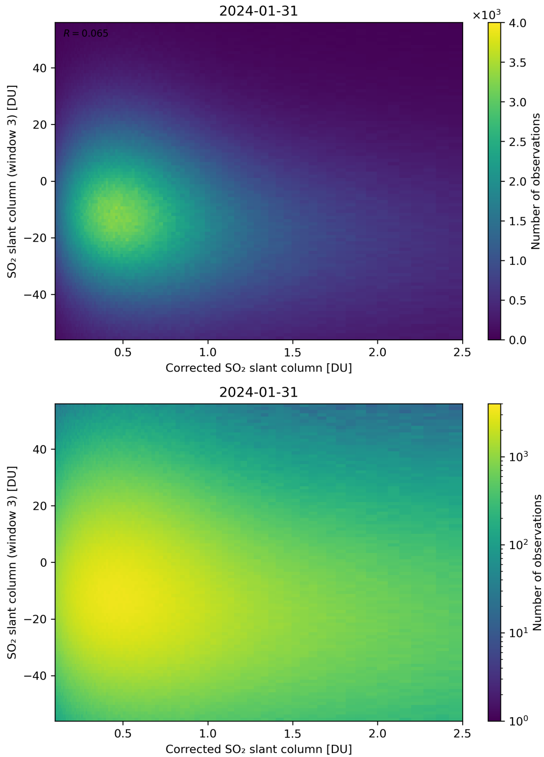
Figure 190: Scatter density plot of “Corrected SO 2 slant column” against “SO 2 slant column (window 3)” for 2024-01-31 to 2024-02-01.
