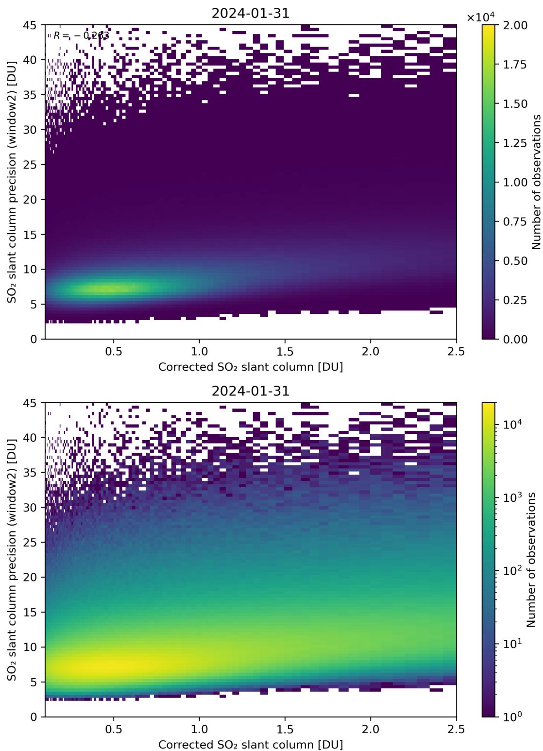
Figure 189: Scatter density plot of “Corrected SO 2 slant column” against “SO 2 slant column precision (window2)” for 2024-01-31 to 2024-02-01.
