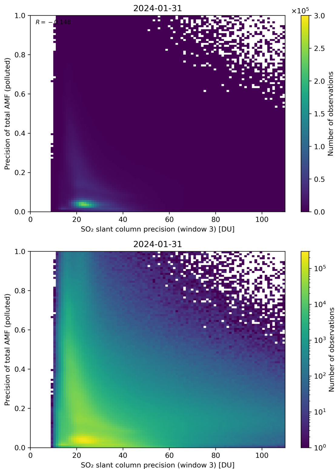
Figure 264: Scatter density plot of “SO 2 slant column precision (window 3)” against “Precision of total AMF (polluted)” for 2024-01-31 to 2024-02-01.
