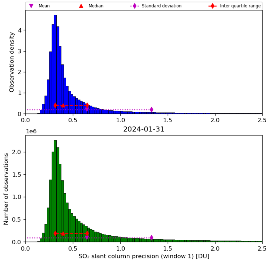
Figure 57: Histogram of “SO 2 slant column precision (window 1)” for 2024-01-31 to 2024-02-01
