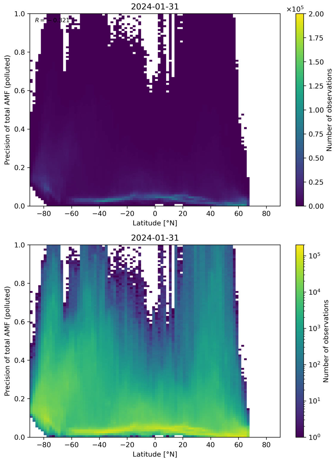
Figure 155: Scatter density plot of “Latitude” against “Precision of total AMF (polluted)” for 2024-01-31 to 2024-02-01.
