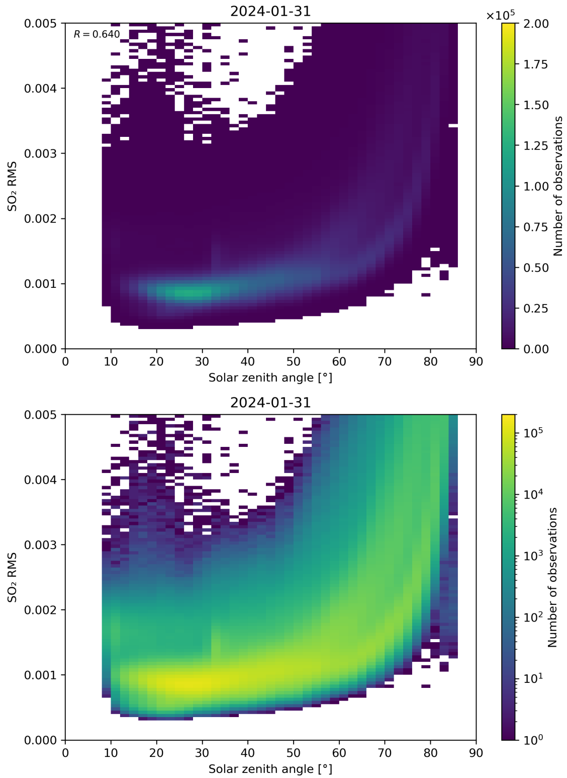
Figure 163: Scatter density plot of “Solar zenith angle” against “SO 2 RMS” for 2024-01-31 to 2024-02-01.
