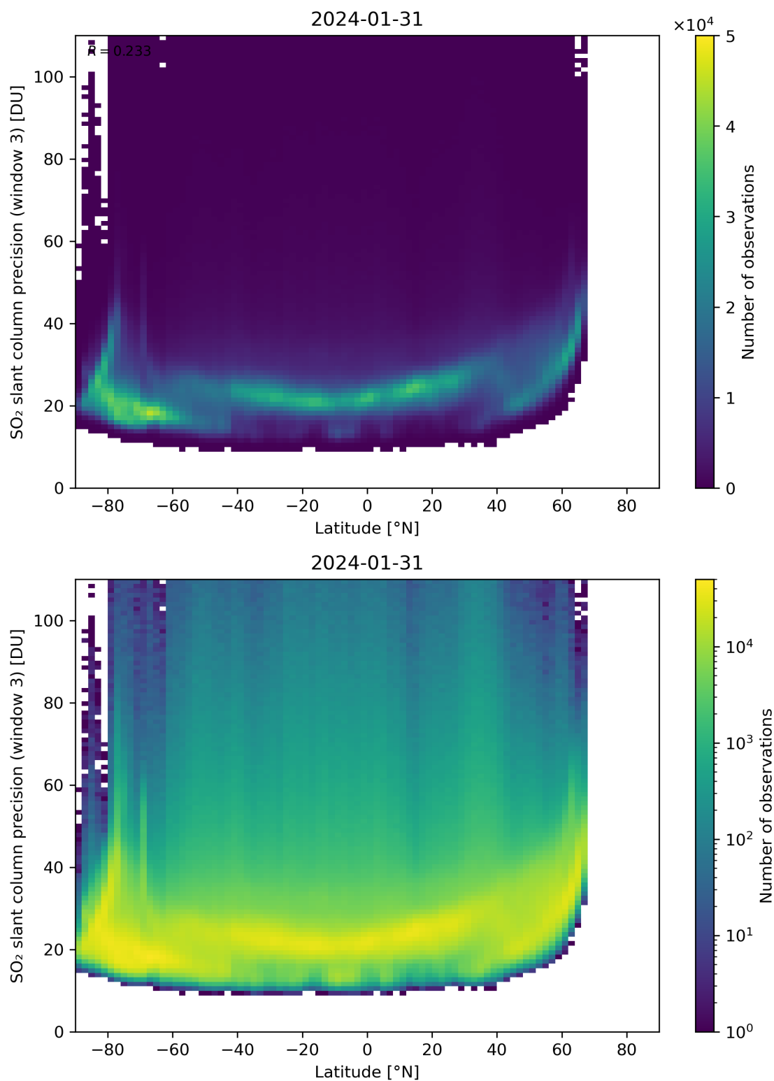
Figure 153: Scatter density plot of “Latitude” against “SO 2 slant column precision (window 3)” for 2024-01-31 to 2024-02-01.
