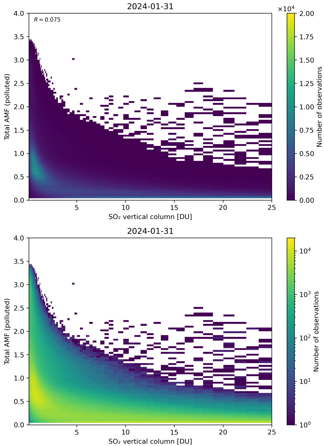
Figure 305: Scatter density plot of “SO 2 vertical column” against “Total AMF (polluted)” for 2024-01-31 to 2024-02-01.
