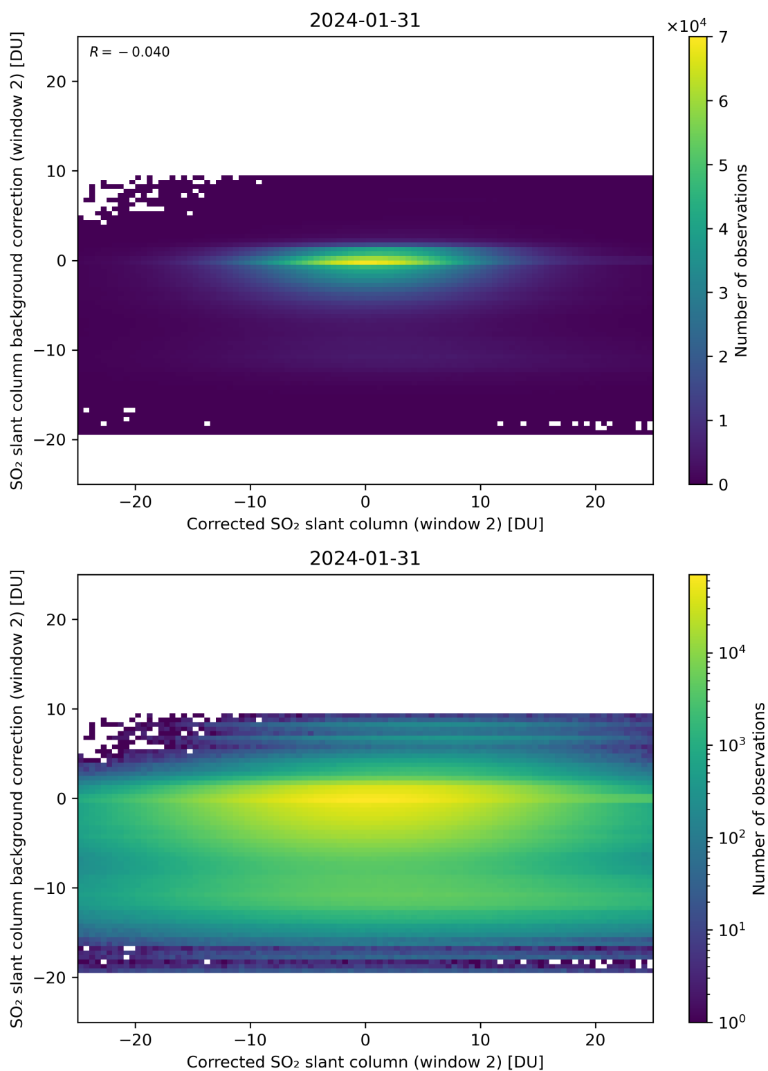
Figure 194: Scatter density plot of “Corrected SO 2 slant column (window 2)” against “SO 2 slant column background correction (window 2)” for 2024-01-31 to 2024-02-01.
