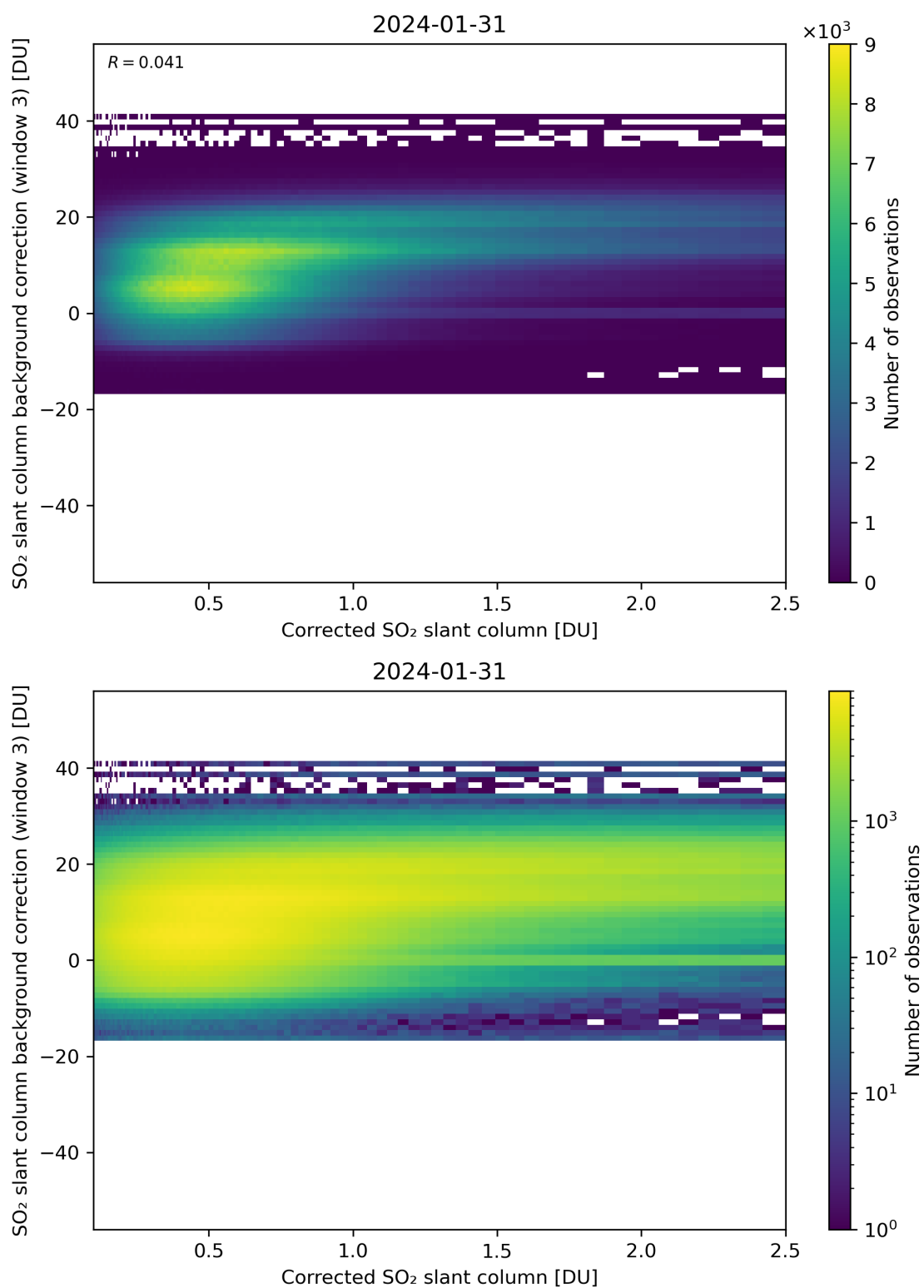
Figure 180: Scatter density plot of “Corrected SO 2 slant column” against “SO 2 slant column background correction (window 3)” for 2024-01-31 to 2024-02-01.
