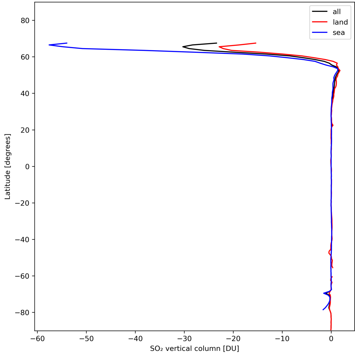
Figure 30: Zonal average of “SO 2 vertical column” for 2024-01-31 to 2024-02-01.
