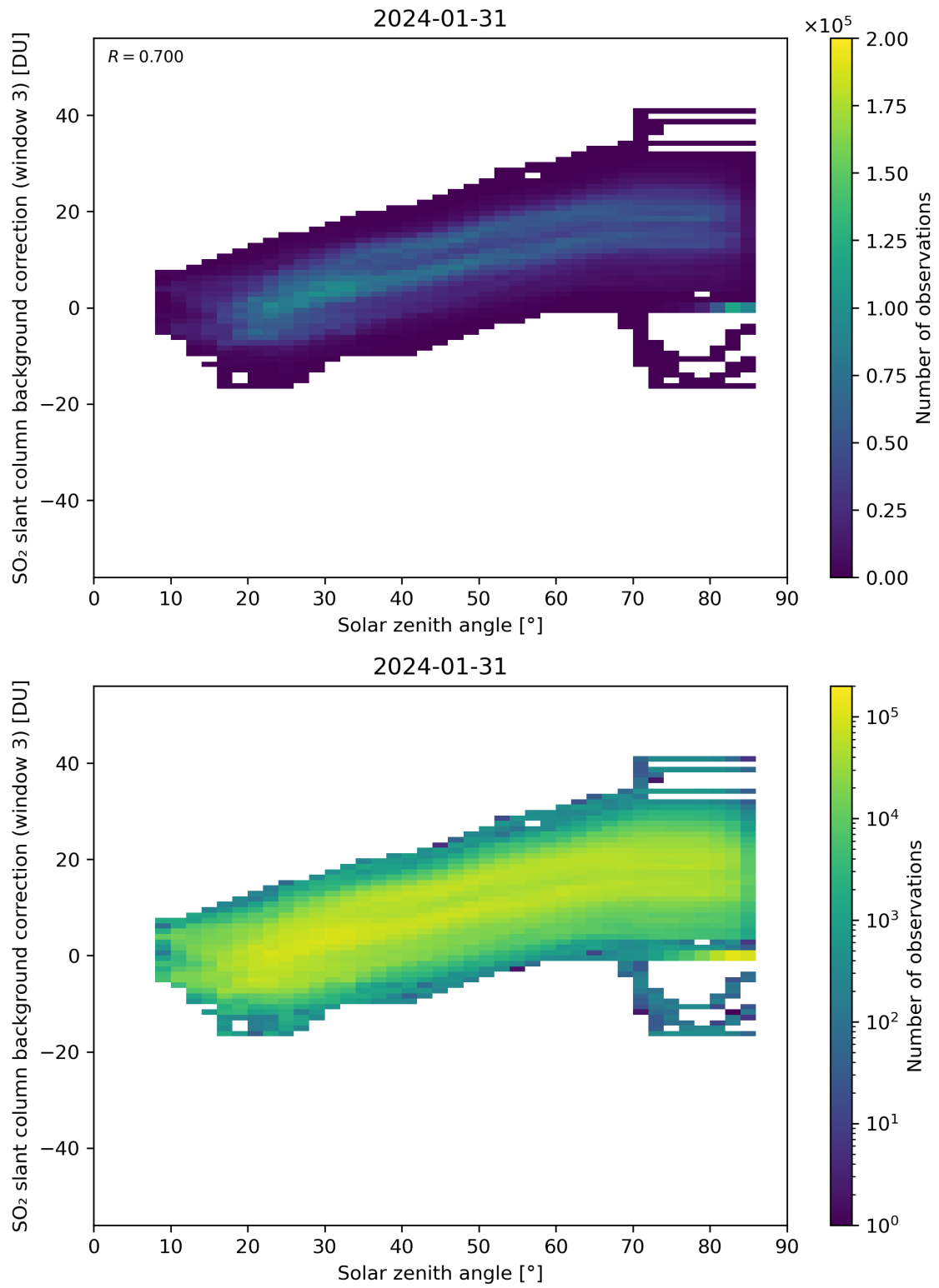
Figure 160: Scatter density plot of “Solar zenith angle” against “SO 2 slant column background correction (window 3)” for 2024-01-31 to 2024-02-01.
