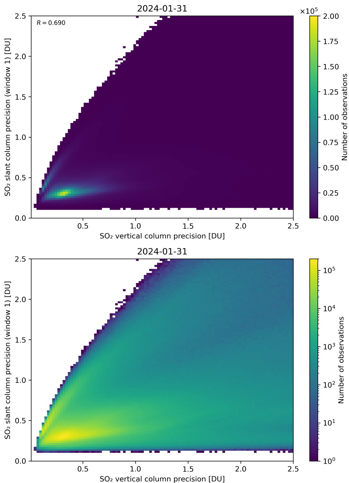
Figure 290: Scatter density plot of “SO 2 vertical column precision” against “SO 2 slant column precision (window 1)” for 2024-01-31 to 2024-02-01.
