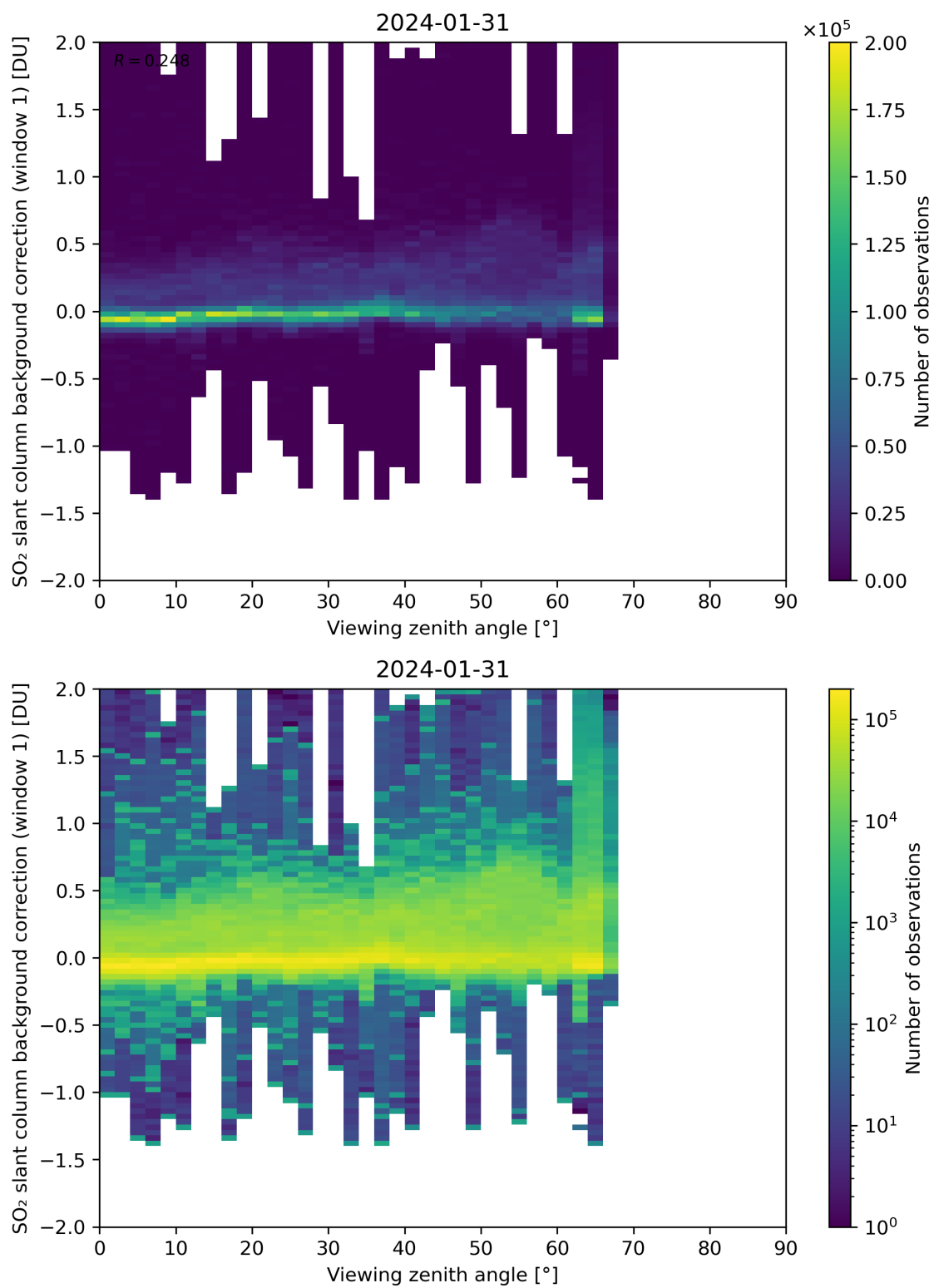
Figure 308: Scatter density plot of “Viewing zenith angle” against “SO 2 slant column background correction (window 1)” for 2024-01-31 to 2024-02-01.
