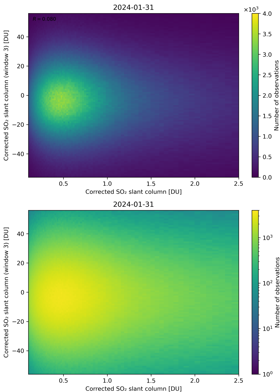
Figure 186: Scatter density plot of “Corrected SO 2 slant column” against “Corrected SO 2 slant column (window 3)” for 2024-01-31 to 2024-02-01.
