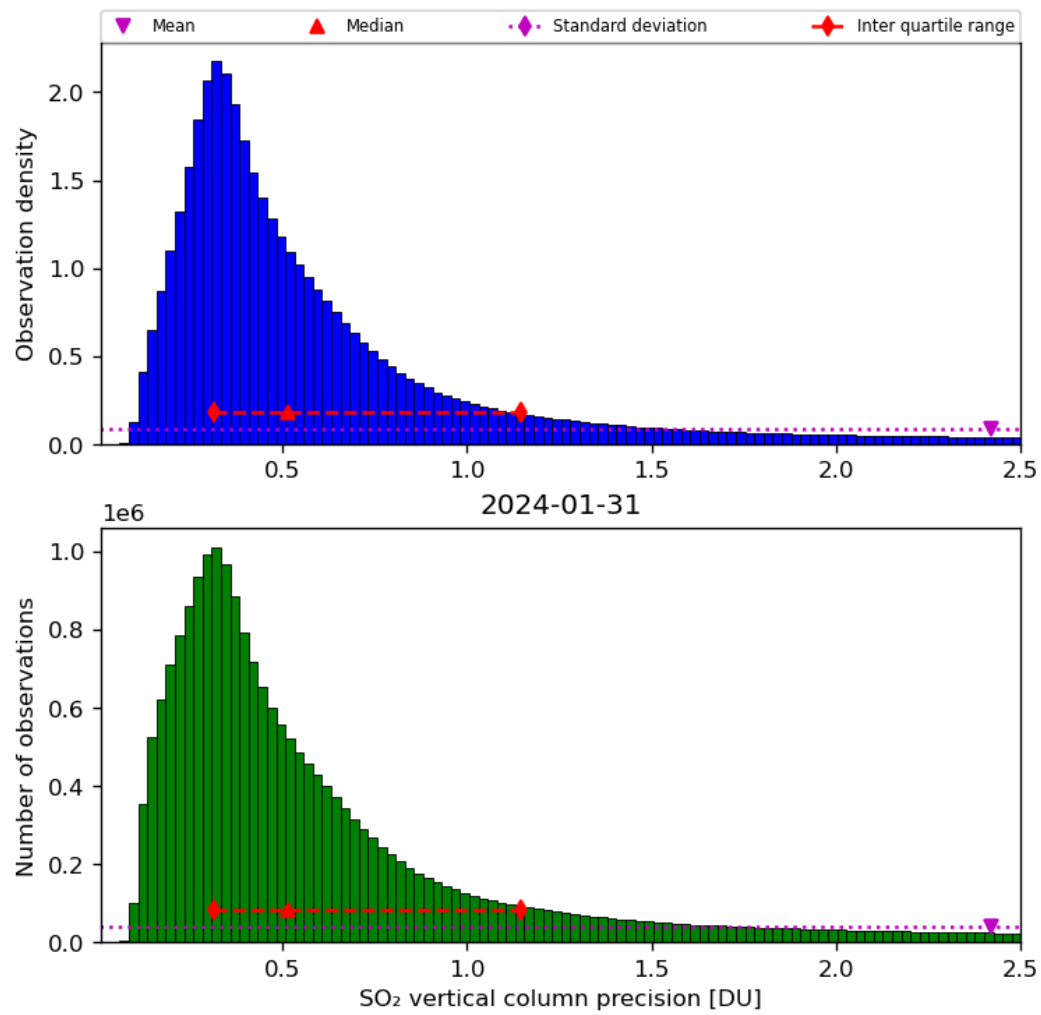
Figure 54: Histogram of "SO 2 vertical column precision" for 2024-01-31 to 2024-02-01
