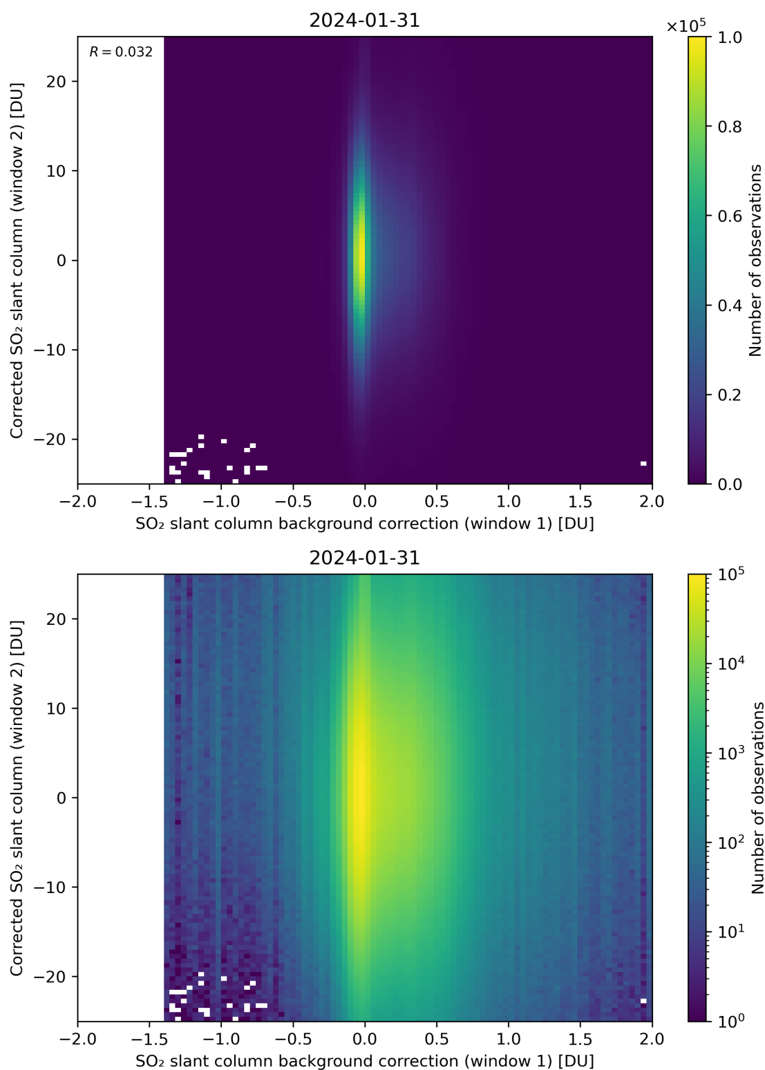
Figure 104: Scatter density plot of “SO 2 slant column background correction (window 1)” against “Corrected SO 2 slant column (window 2)” for 2024-01-31 to 2024-02-01.
