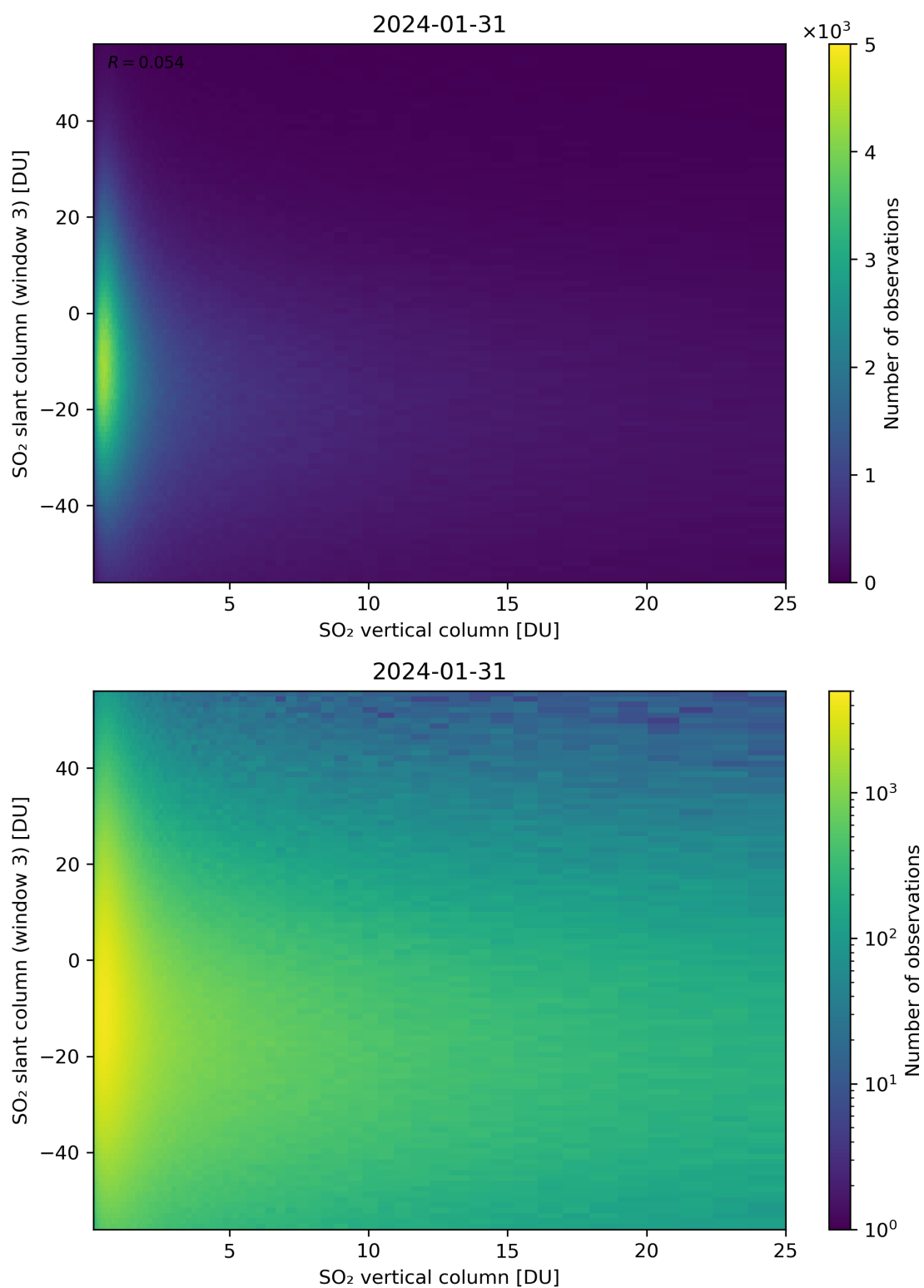
Figure 303: Scatter density plot of “SO 2 vertical column” against “SO 2 slant column (window 3)” for 2024-01-31 to 2024-02-01.
