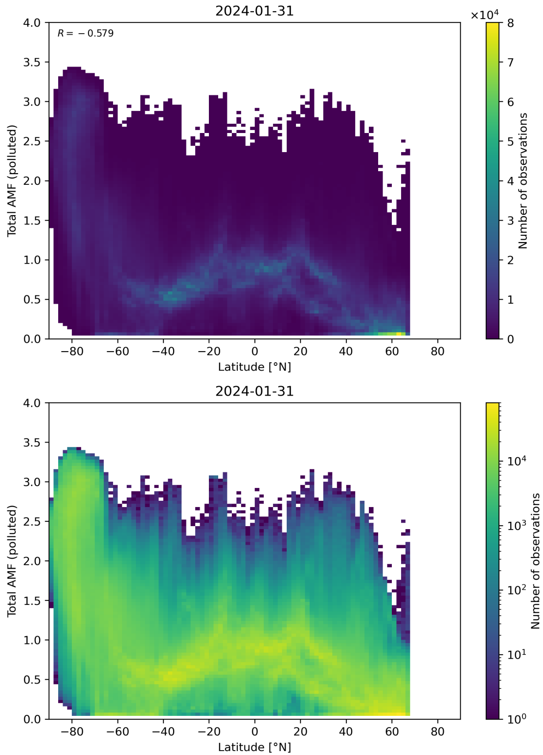
Figure 154: Scatter density plot of “Latitude” against “Total AMF (polluted)” for 2024-01-31 to 2024-02-01.
