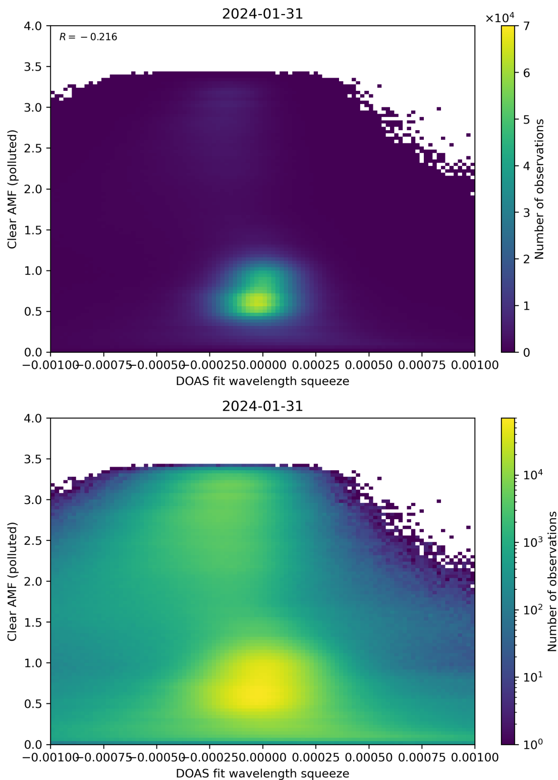
Figure 133: Scatter density plot of “DOAS fit wavelength squeeze” against “Clear AMF (polluted)” for 2024-01-31 to 2024-02-01.
