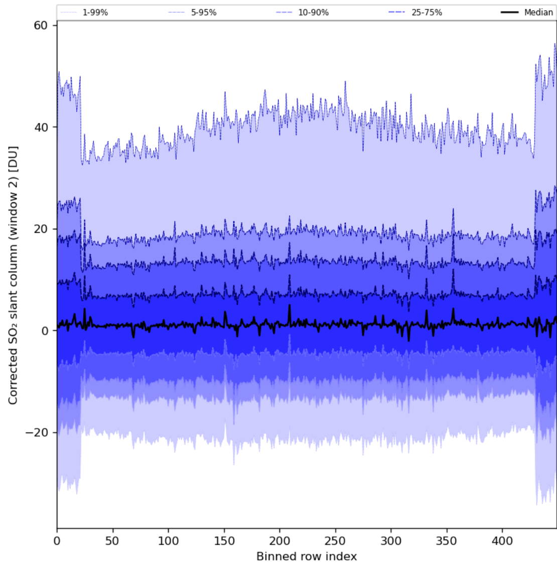
Figure 85: Along track statistics of “Corrected SO 2 slant column (window 2)” for 2024-01-31 to 2024-02-01
