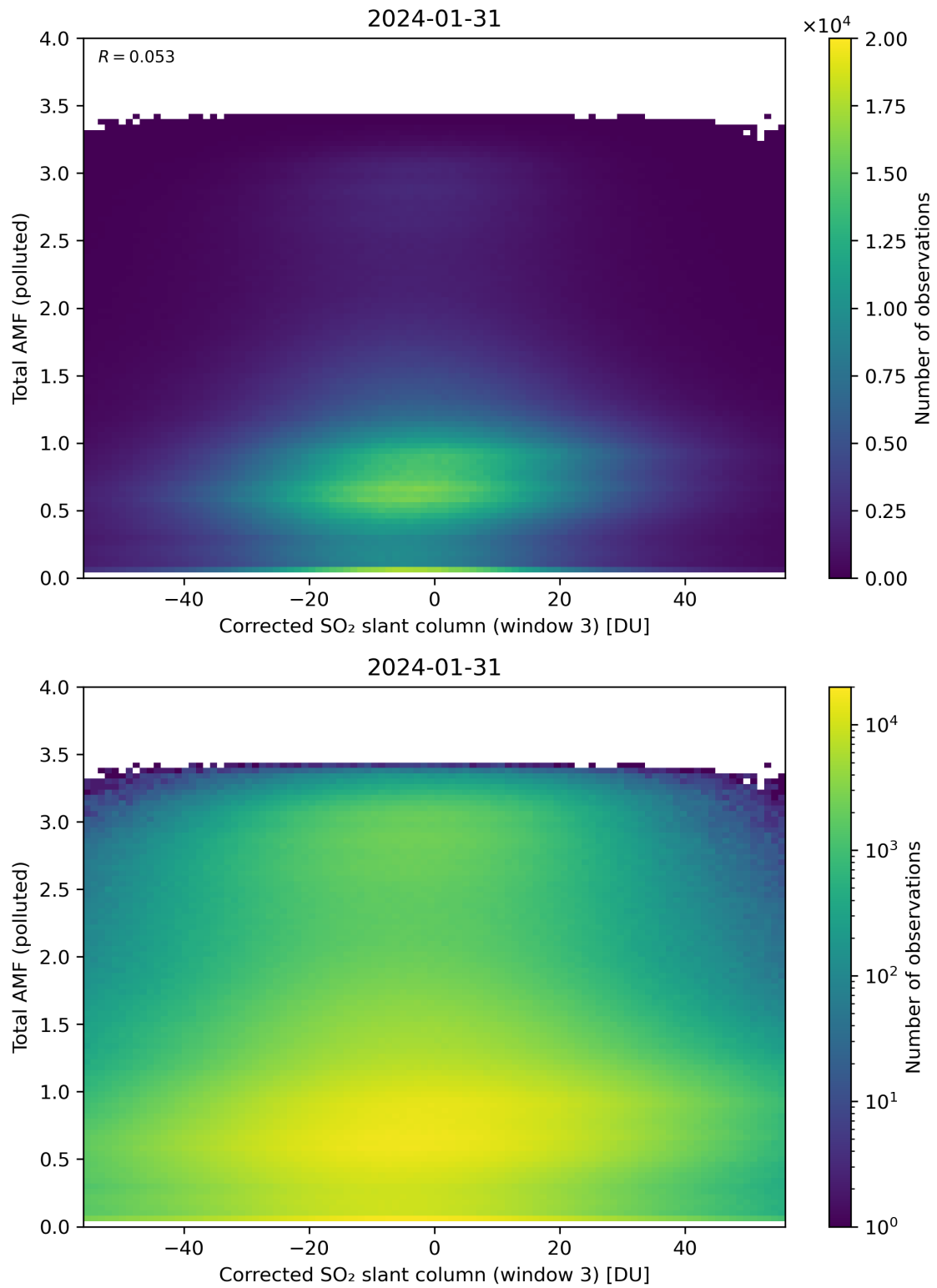
Figure 210: Scatter density plot of “Corrected SO 2 slant column (window 3)” against “Total AMF (polluted)” for 2024-01-31 to 2024-02-01.
