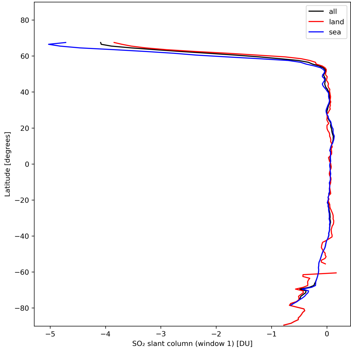
Figure 33: Zonal average of “SO 2 slant column (window 1)” for 2024-01-31 to 2024-02-01.
