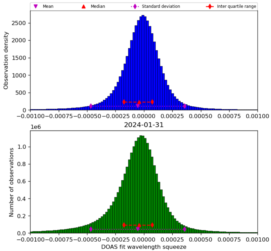
Figure 69: Histogram of “DOAS fit wavelength squeeze” for 2024-01-31 to 2024-02-01
