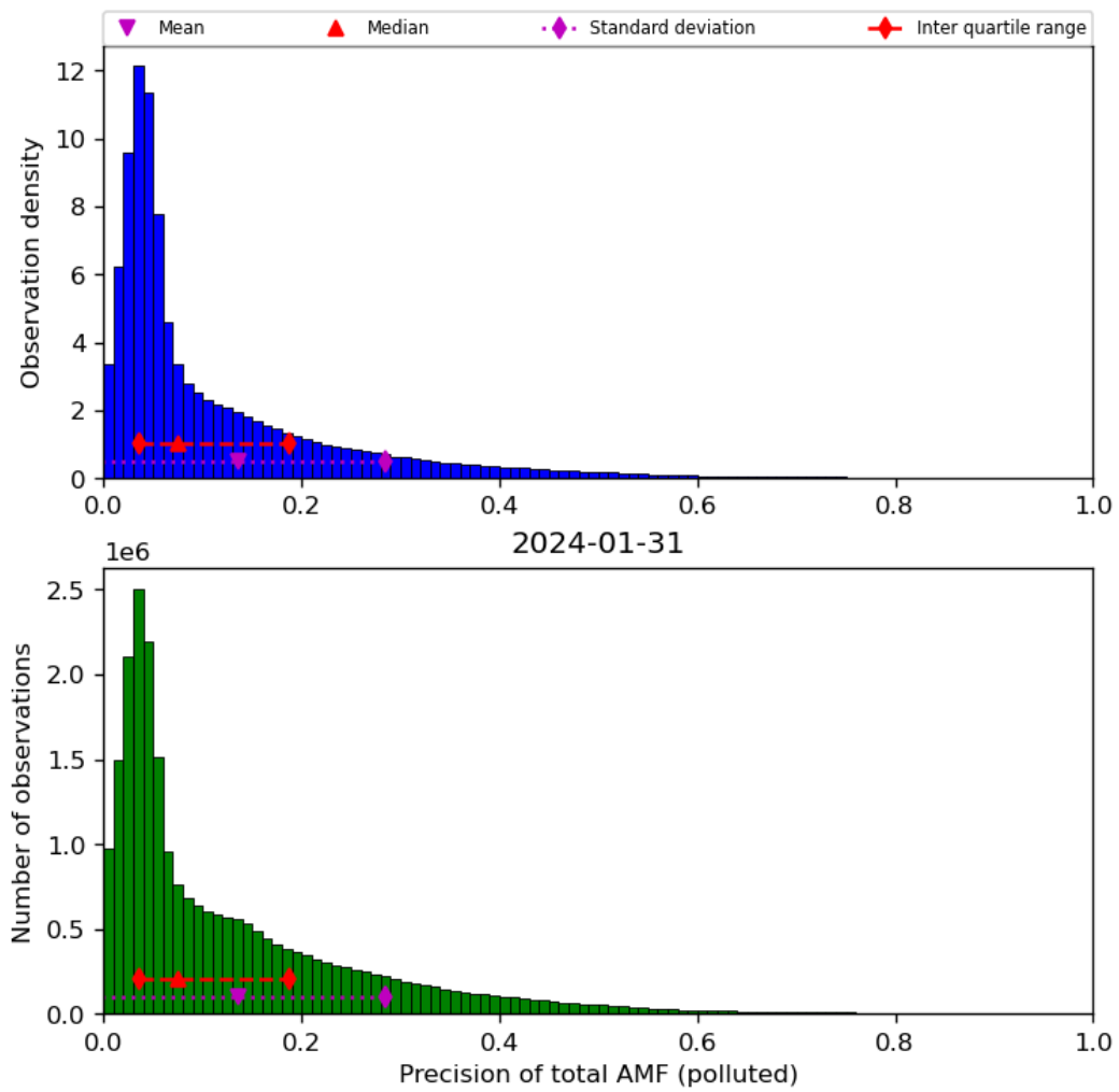
Figure 72: Histogram of “Precision of total AMF (polluted)” for 2024-01-31 to 2024-02-01
