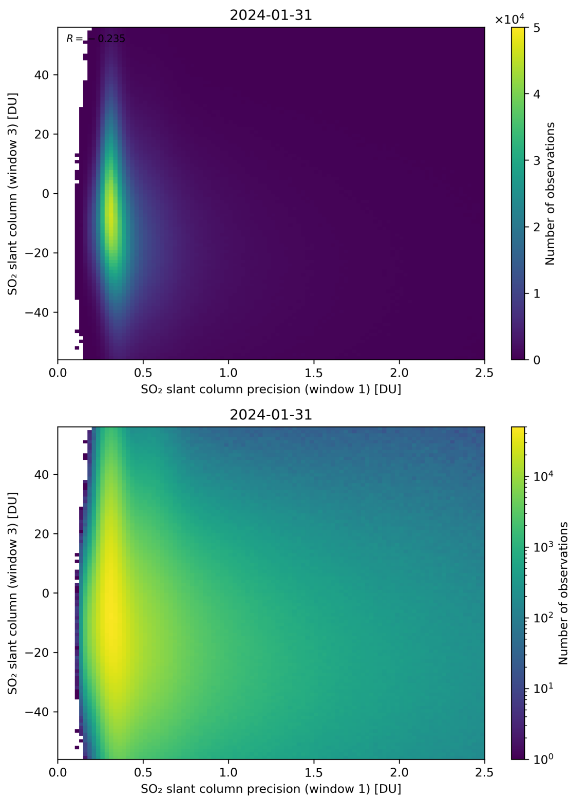
Figure 228: Scatter density plot of “SO 2 slant column precision (window 1)” against “SO 2 slant column (window 3)” for 2024-01-31 to 2024-02-01.
