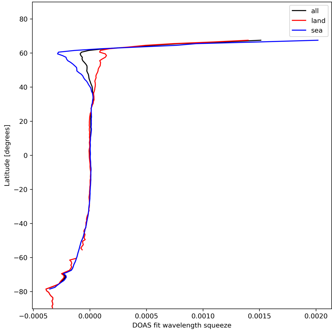
Figure 46: Zonal average of "DOAS fit wavelength squeeze" for 2024-01-31 to 2024-02-01.
