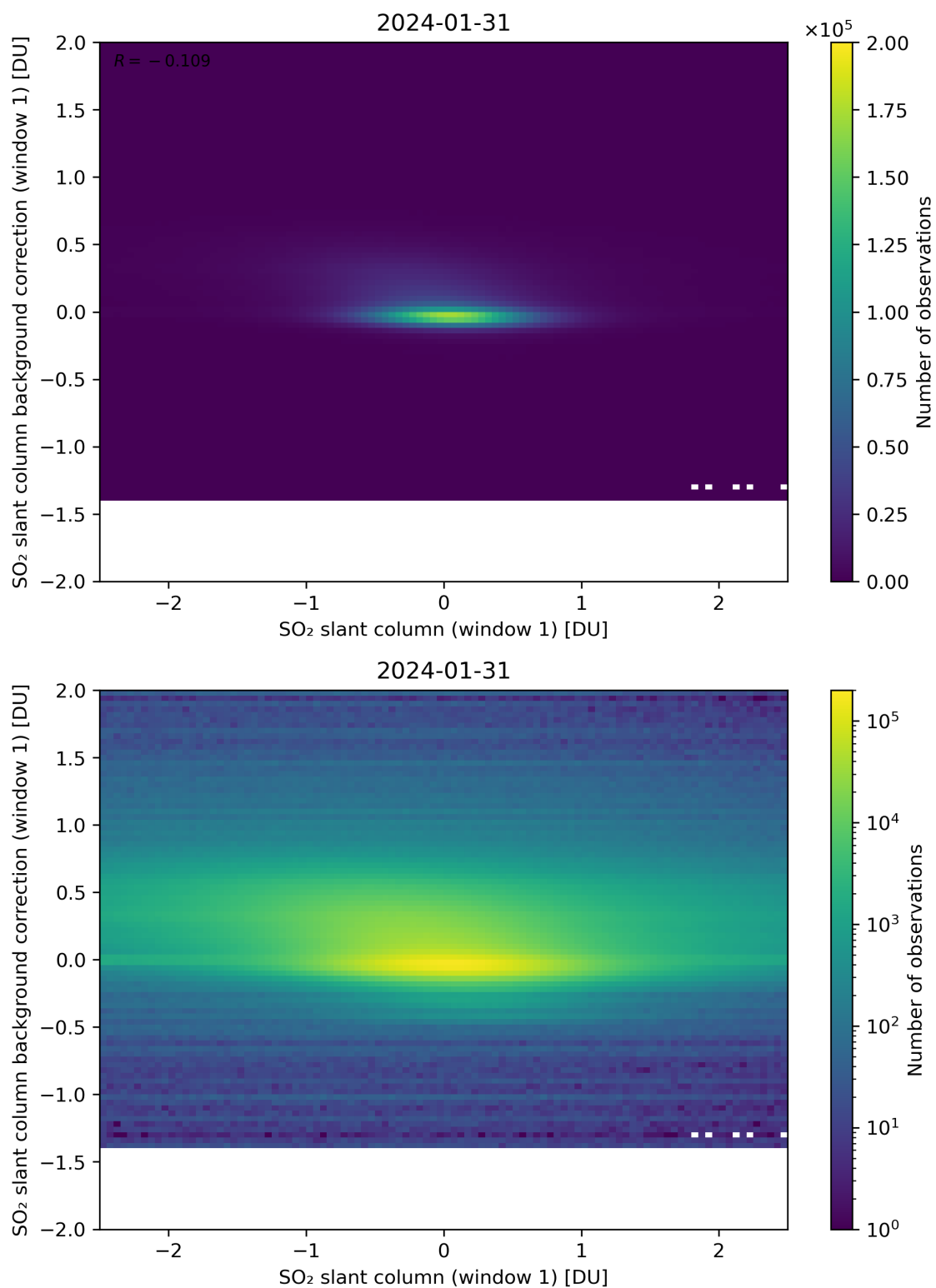
Figure 212: Scatter density plot of “SO 2 slant column (window 1)” against “SO 2 slant column background correction (window 1)” for 2024-01-31 to 2024-02-01.
