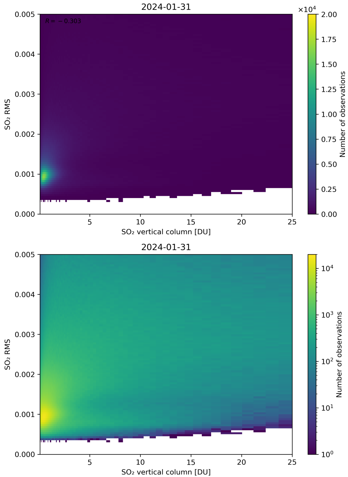
Figure 278: Scatter density plot of “SO 2 vertical column” against “SO 2 RMS” for 2024-01-31 to 2024-02-01.
