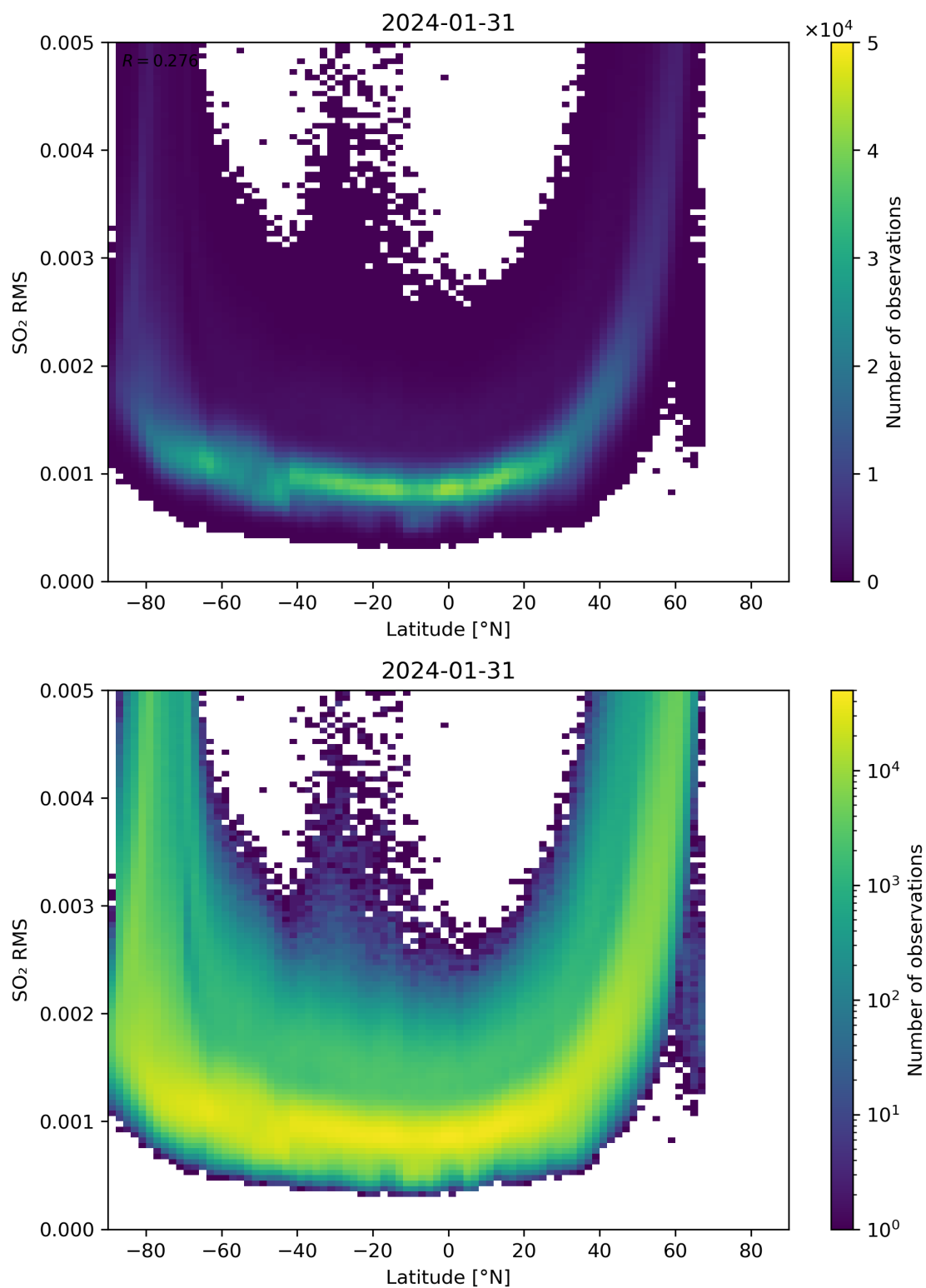
Figure 144: Scatter density plot of “Latitude” against “SO 2 RMS” for 2024-01-31 to 2024-02-01.
