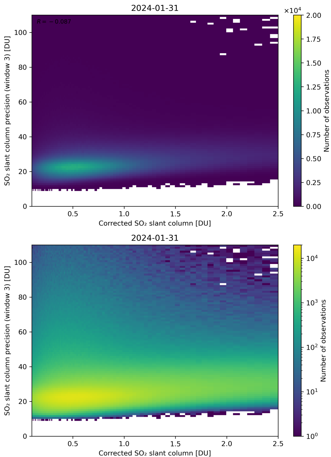
Figure 191: Scatter density plot of “Corrected SO 2 slant column” against “SO 2 slant column precision (window 3)” for 2024-01-31 to 2024-02-01.
