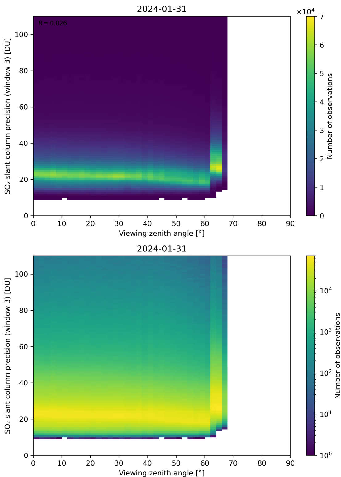
Figure 324: Scatter density plot of “Viewing zenith angle” against “SO 2 slant column precision (window 3)” for 2024-01-31 to 2024-02-01.
