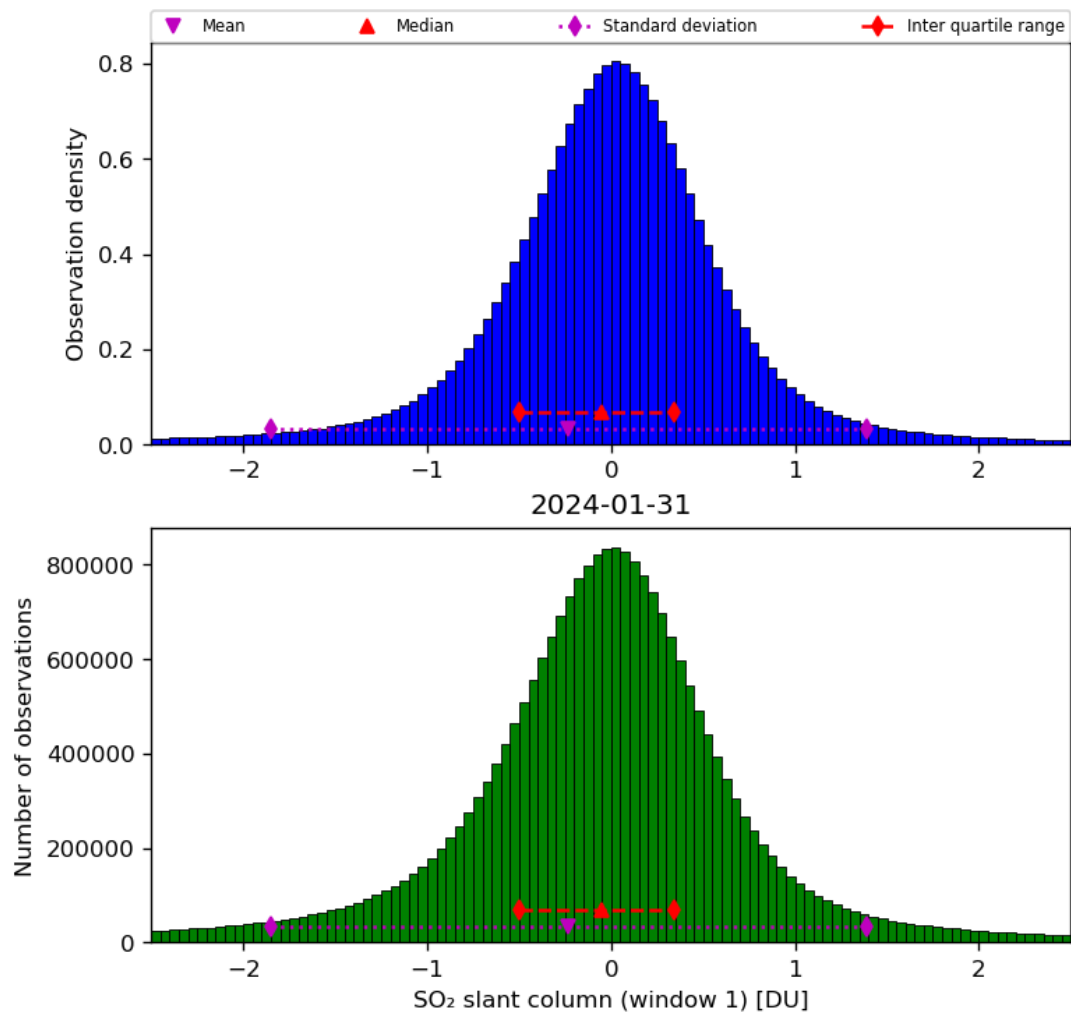
Figure 56: Histogram of “SO 2 slant column (window 1)” for 2024-01-31 to 2024-02-01
