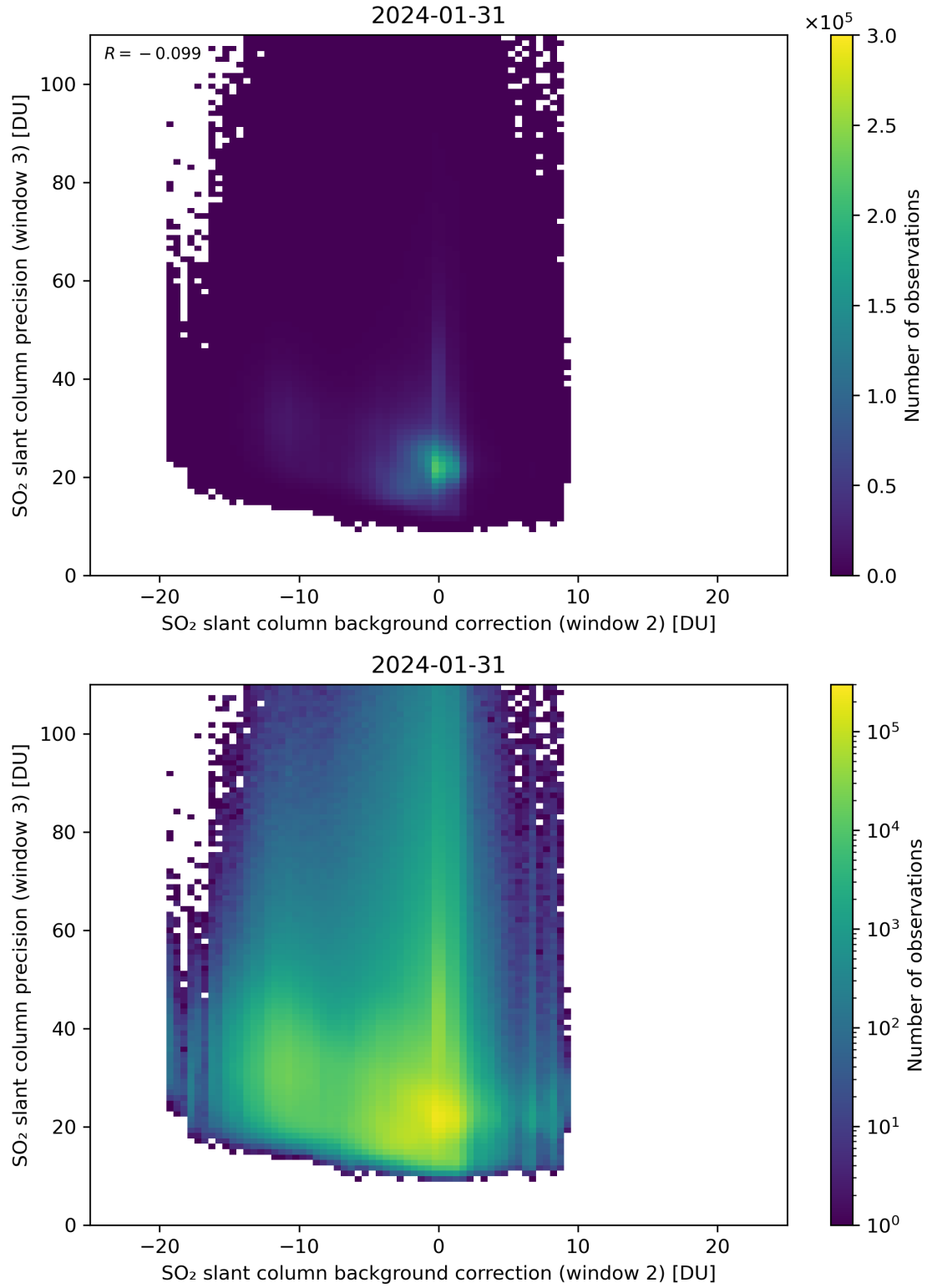
Figure 118: Scatter density plot of “SO 2 slant column background correction (window 2)” against “SO 2 slant column precision (window 3)” for 2024-01-31 to 2024-02-01.
