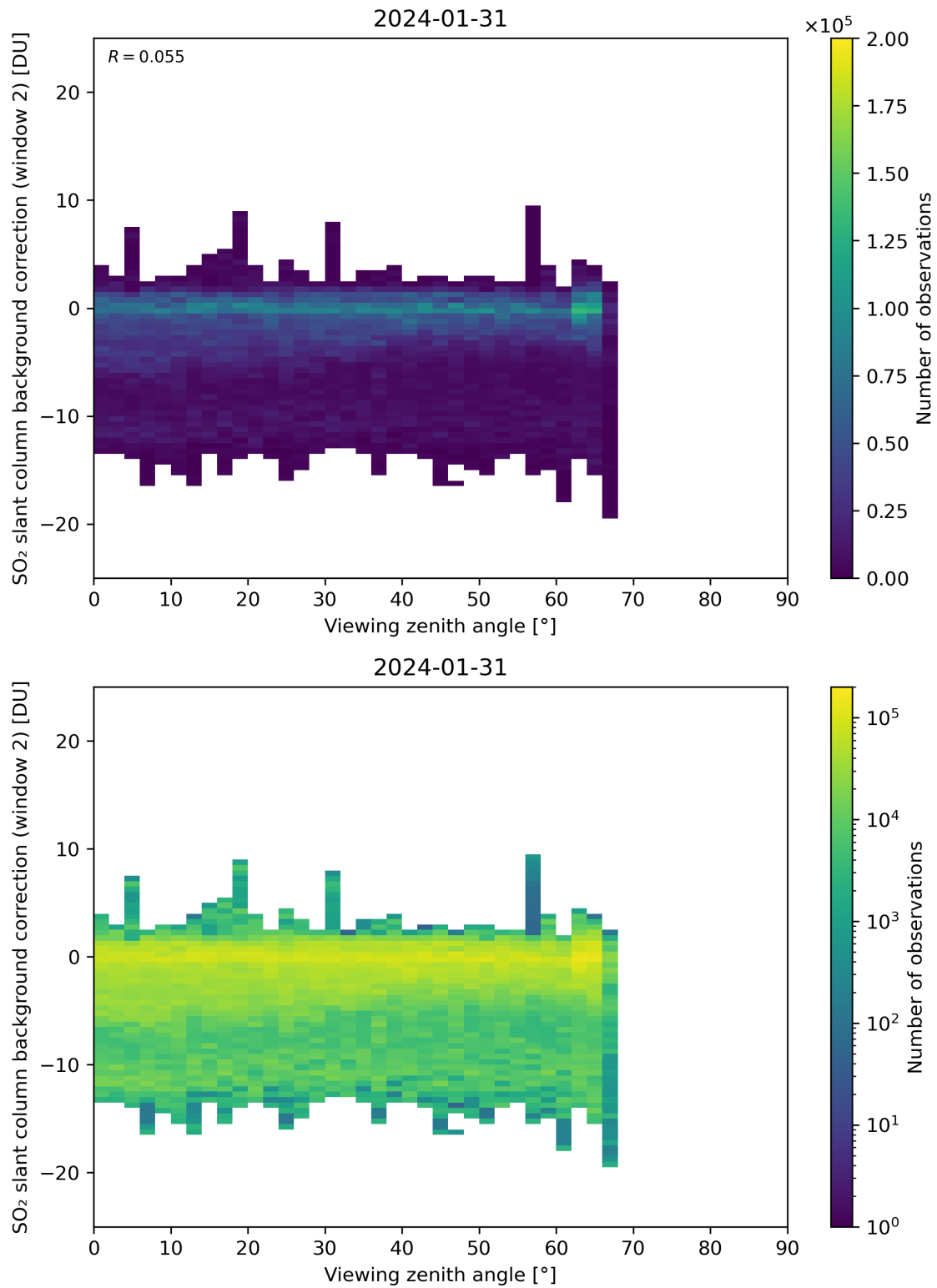
Figure 309: Scatter density plot of “Viewing zenith angle” against “SO 2 slant column background correction (window 2)” for 2024-01-31 to 2024-02-01.
