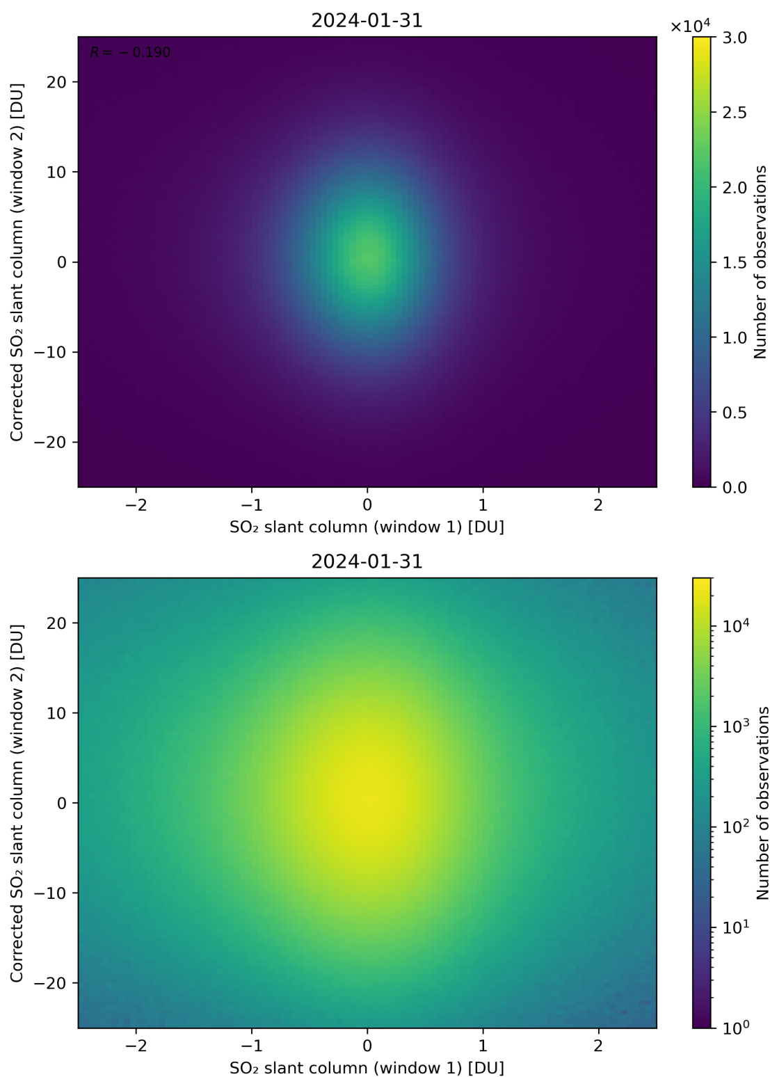
Figure 233: Scatter density plot of “SO 2 slant column (window 1)” against “Corrected SO 2 slant column (window 2)” for 2024-01-31 to 2024-02-01.
