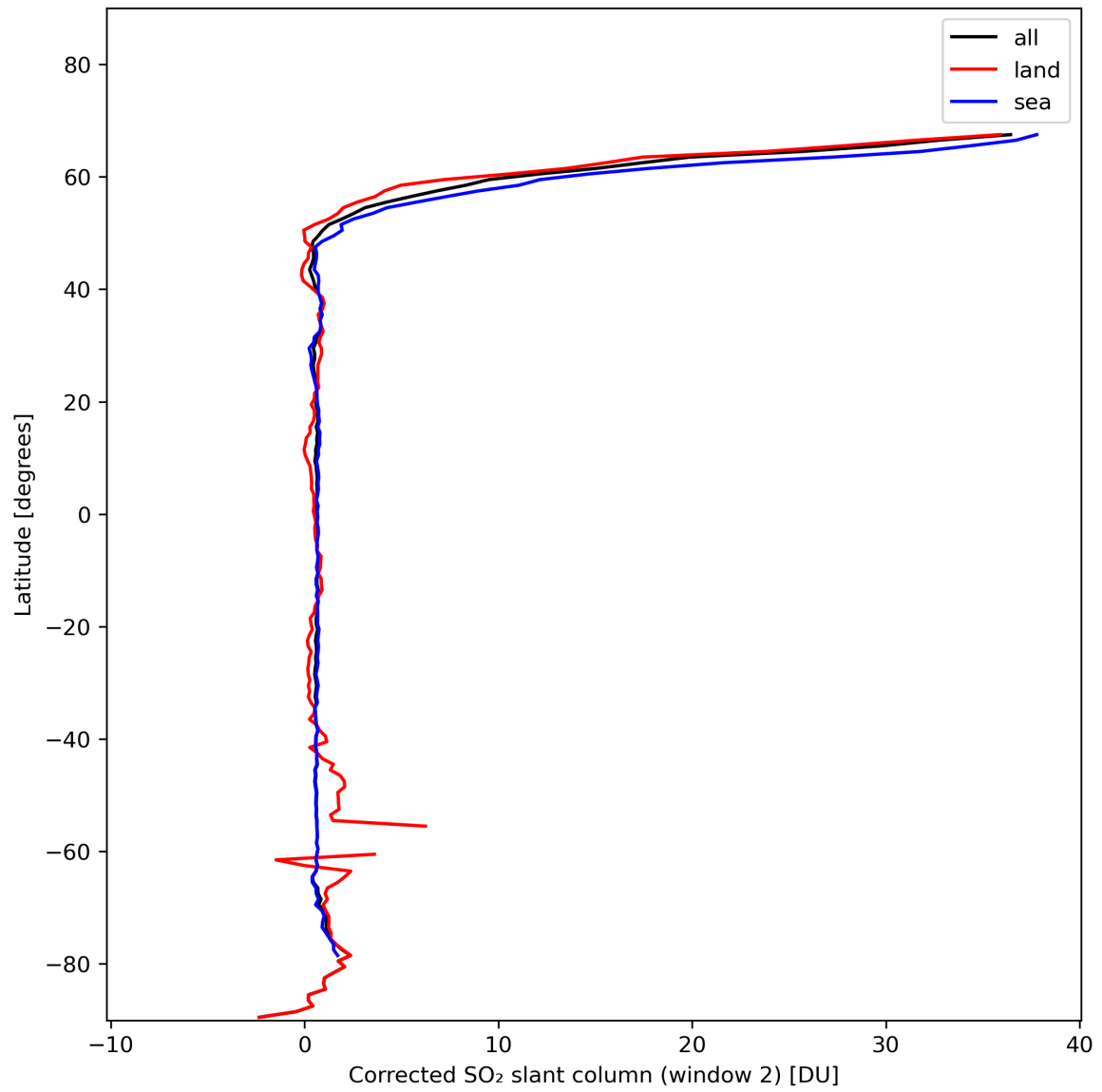
Figure 39: Zonal average of “Corrected SO 2 slant column (window 2)” for 2024-01-31 to 2024-02-01.
