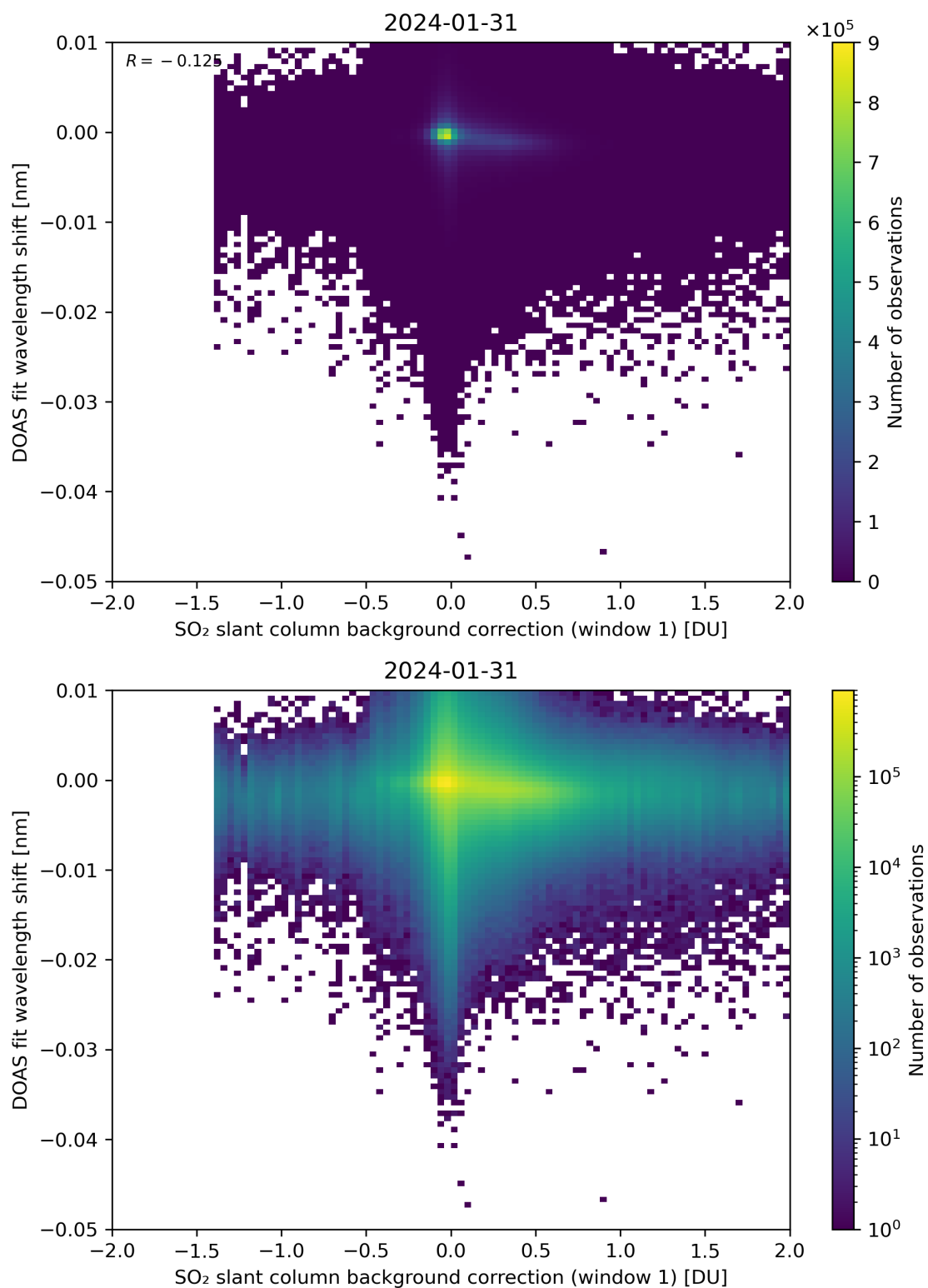
Figure 100: Scatter density plot of “SO 2 slant column background correction (window 1)” against “DOAS fit wavelength shift” for 2024-01-31 to 2024-02-01.
