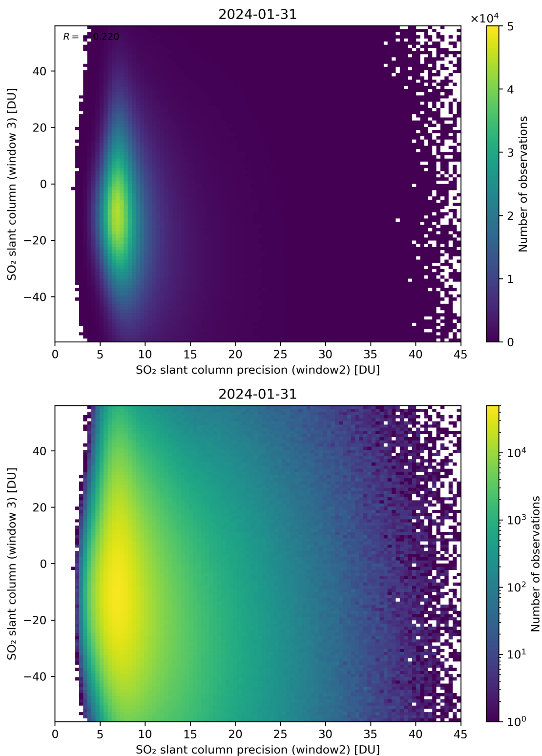
Figure 249: Scatter density plot of “SO 2 slant column precision (window2)” against “SO 2 slant column (window 3)” for 2024-01-31 to 2024-02-01.
