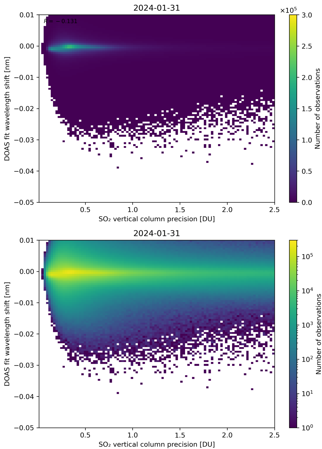
Figure 282: Scatter density plot of “SO 2 vertical column precision” against “DOAS fit wavelength shift” for 2024-01-31 to 2024-02-01.
