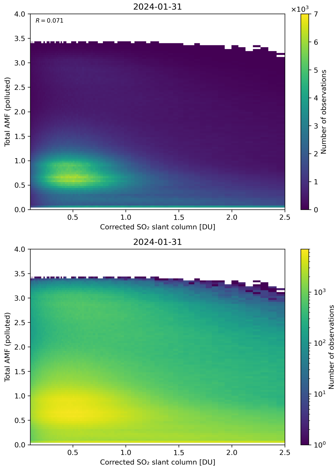
Figure 192: Scatter density plot of “Corrected SO 2 slant column” against “Total AMF (polluted)” for 2024-01-31 to 2024-02-01.
