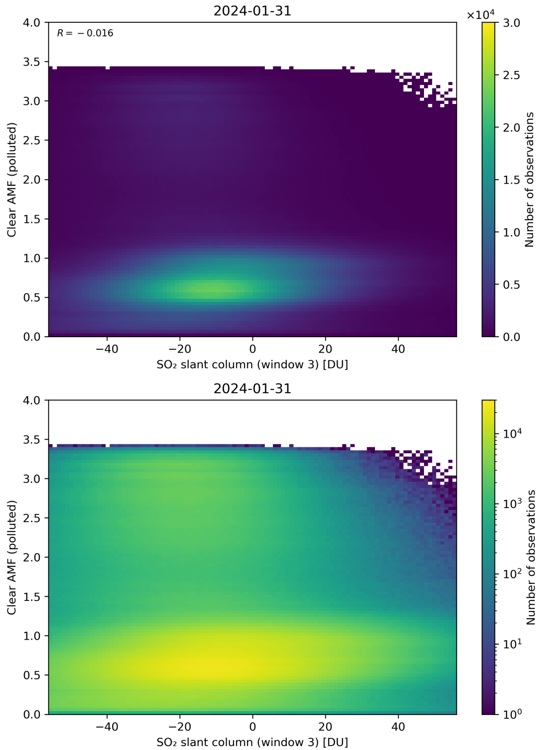
Figure 265: Scatter density plot of “SO 2 slant column (window 3)” against “Clear AMF (polluted)” for 2024-01-31 to 2024-02-01.
