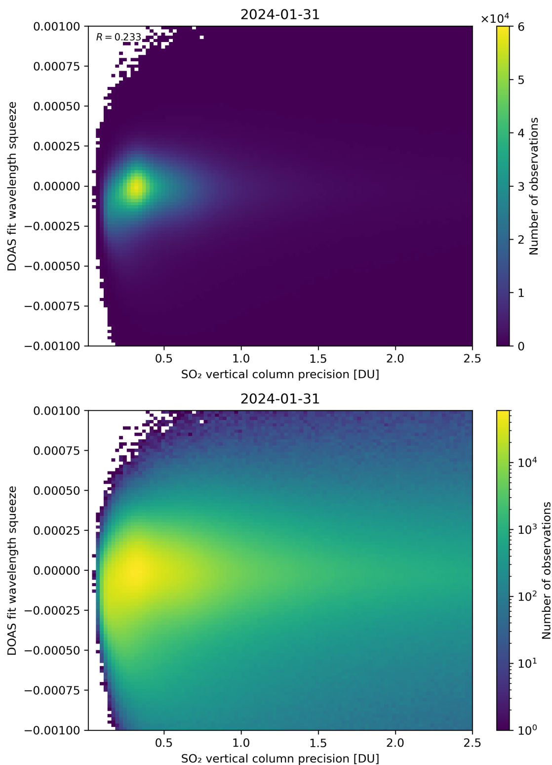
Figure 283: Scatter density plot of “SO 2 vertical column precision” against “DOAS fit wavelength squeeze” for 2024-01-31 to 2024-02-01.
