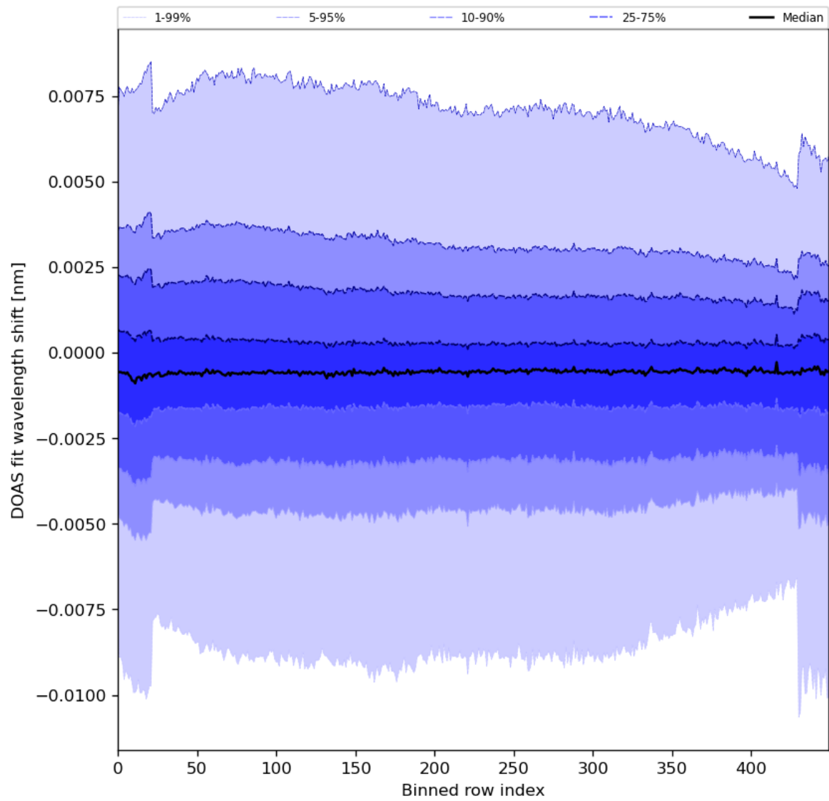
Figure 91: Along track statistics of “DOAS fit wavelength shift” for 2024-01-31 to 2024-02-01
