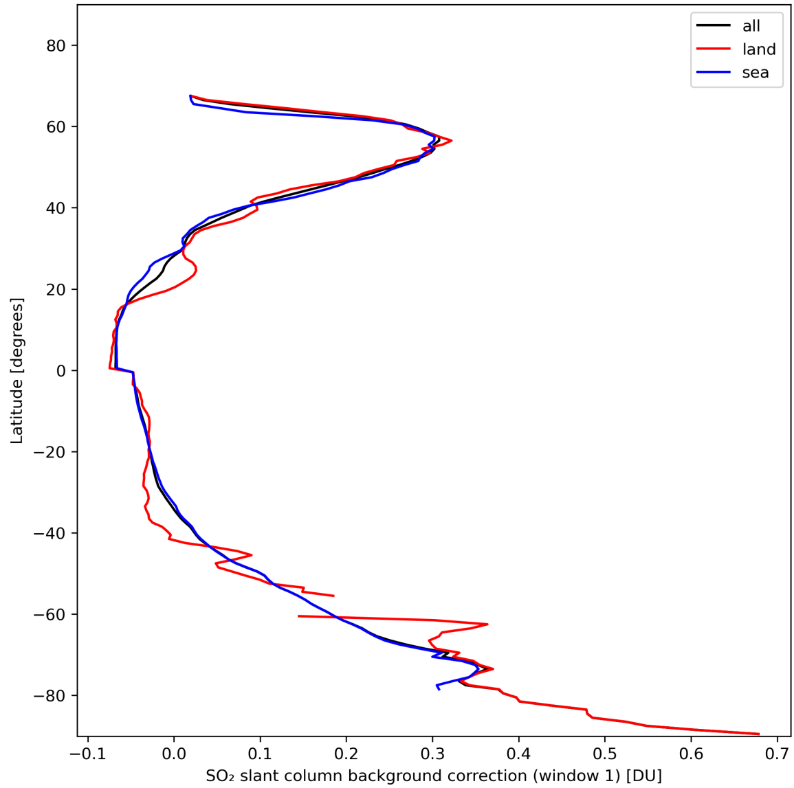
Figure 36: Zonal average of “SO 2 slant column background correction (window 1)” for 2024-01-31 to 2024-02-01.
