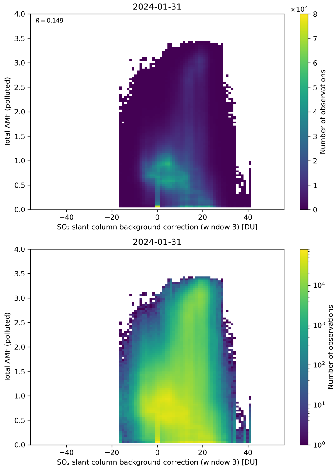
Figure 125: Scatter density plot of “SO 2 slant column background correction (window 3)” against “Total AMF (polluted)” for 2024-01-31 to 2024-02-01.
