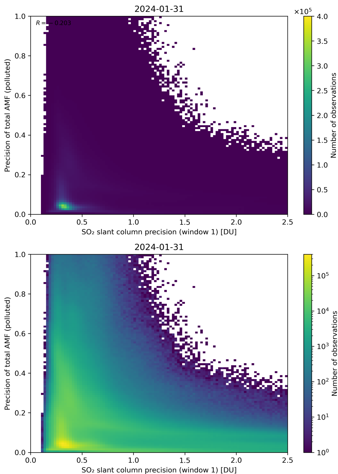
Figure 231: Scatter density plot of “SO 2 slant column precision (window 1)” against “Precision of total AMF (polluted)” for 2024-01-31 to 2024-02-01.
