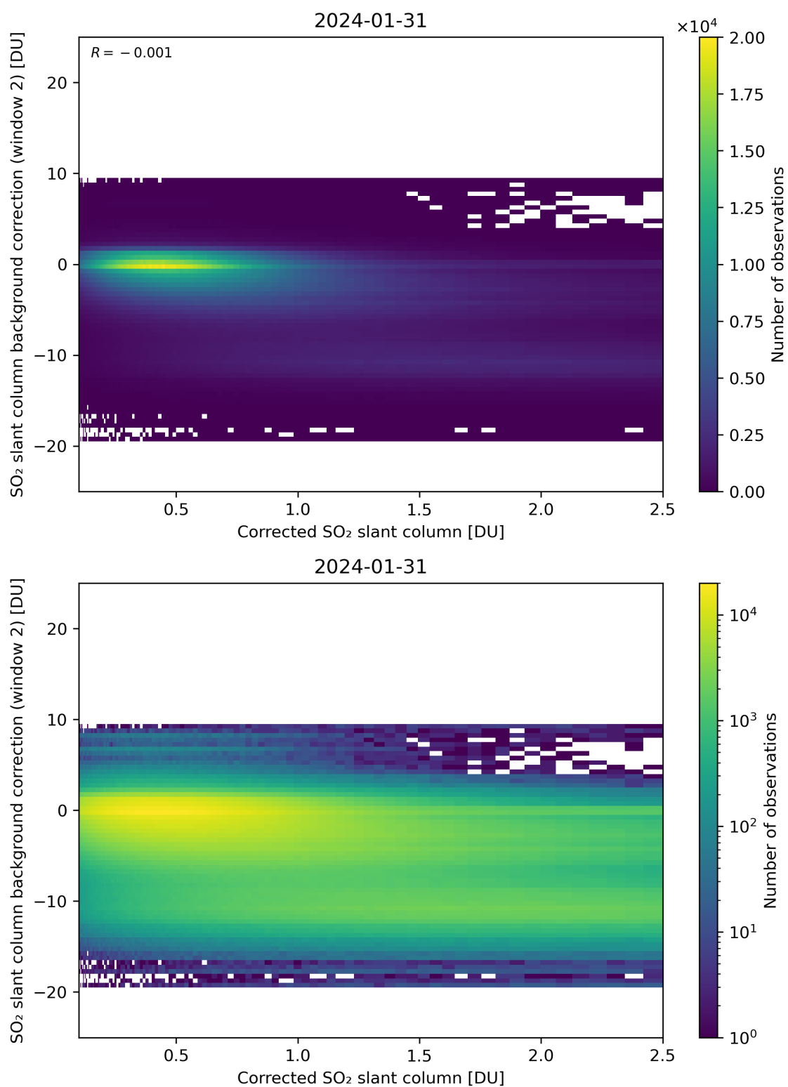
Figure 179: Scatter density plot of “Corrected SO 2 slant column” against “SO 2 slant column background correction (window 2)” for 2024-01-31 to 2024-02-01.
