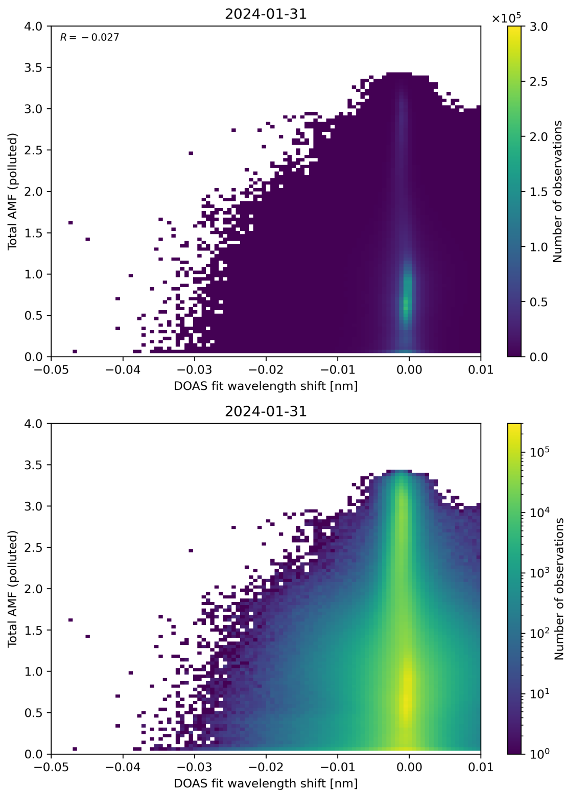
Figure 130: Scatter density plot of “DOAS fit wavelength shift” against “Total AMF (polluted)” for 2024-01-31 to 2024-02-01.
