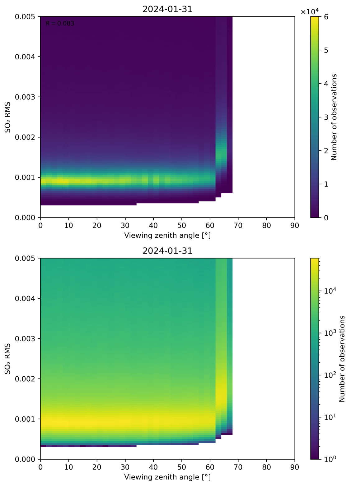
Figure 313: Scatter density plot of “Viewing zenith angle” against “SO 2 RMS” for 2024-01-31 to 2024-02-01.
