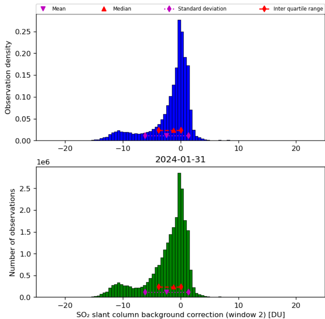
Figure 63: Histogram of “SO 2 slant column background correction (window 2)” for 2024-01-31 to 2024-02-01
