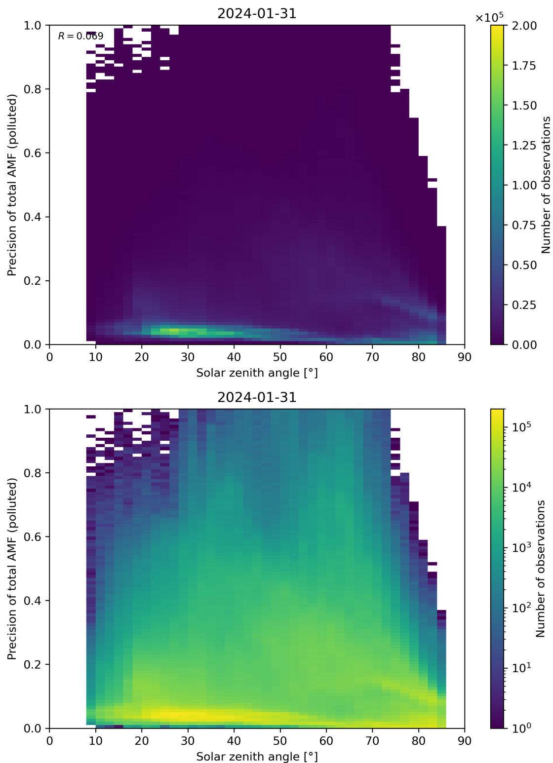
Figure 175: Scatter density plot of “Solar zenith angle” against “Precision of total AMF (polluted)” for 2024-01-31 to 2024-02-01.
