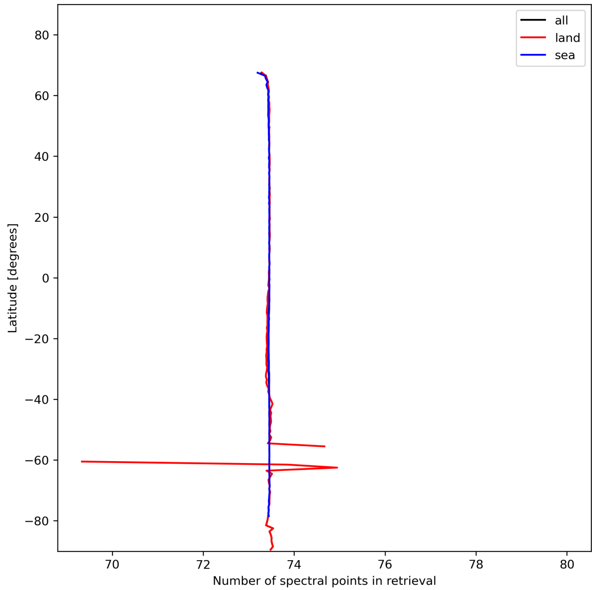
Figure 51: Zonal average of “Number of spectral points in retrieval” for 2024-01-31 to 2024-02-01.
