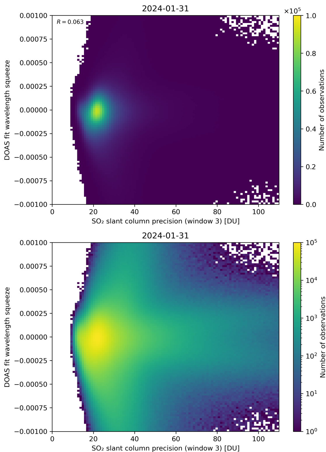
Figure 259: Scatter density plot of “SO 2 slant column precision (window 3)” against “DOAS fit wavelength squeeze” for 2024-01-31 to 2024-02-01.
