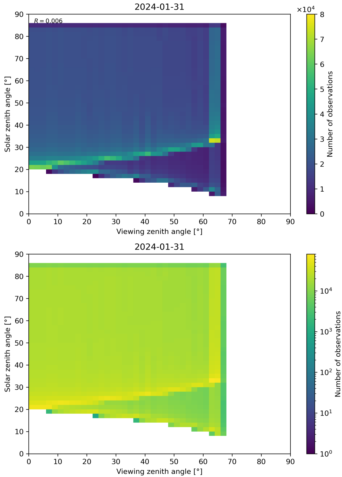
Figure 315: Scatter density plot of “Viewing zenith angle” against “Solar zenith angle” for 2024-01-31 to 2024-02-01.
