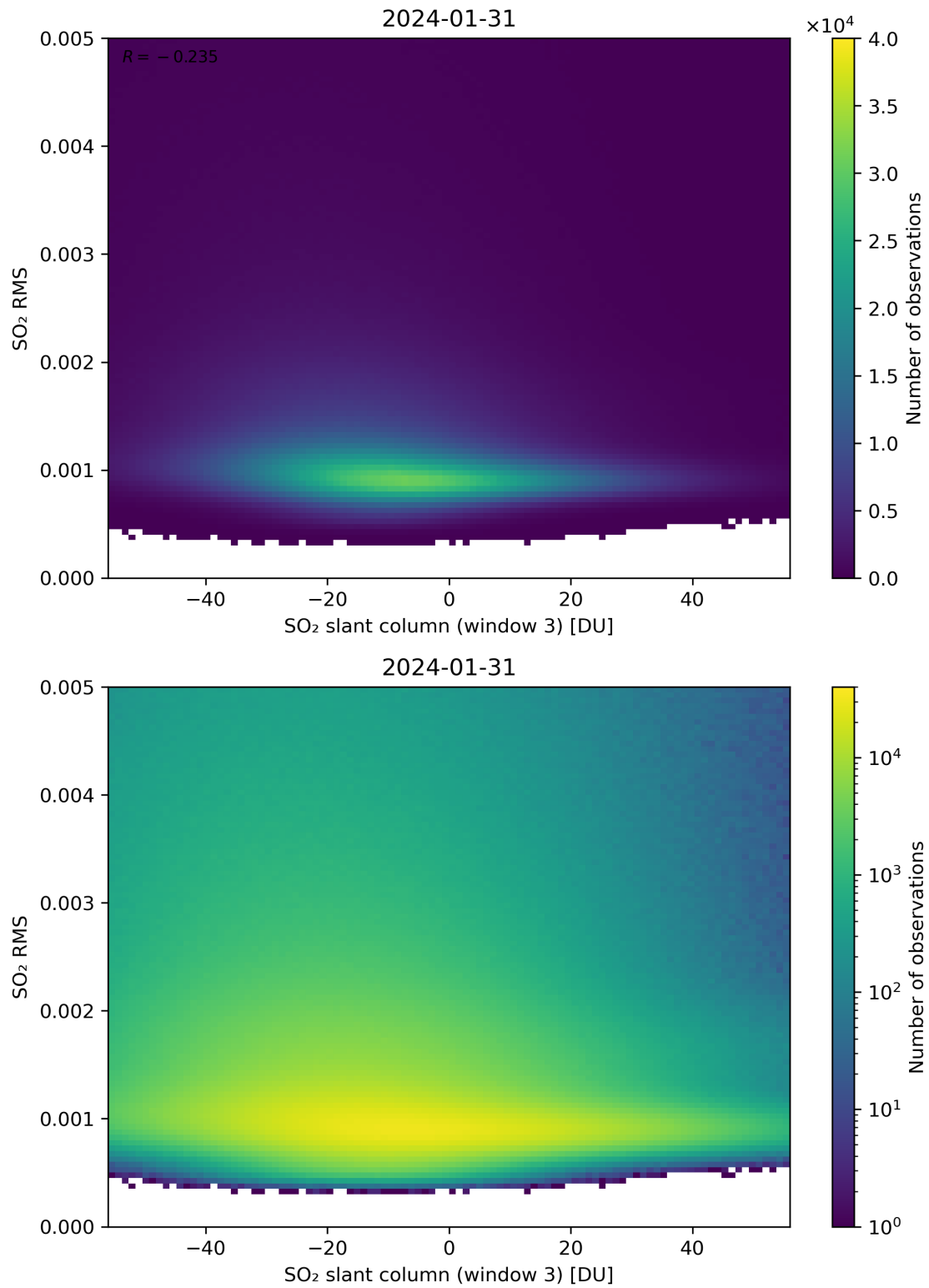
Figure 256: Scatter density plot of “SO 2 slant column (window 3)” against “SO 2 RMS” for 2024-01-31 to 2024-02-01.
