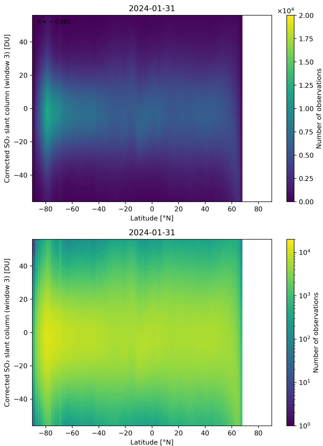
Figure 148: Scatter density plot of “Latitude” against “Corrected SO 2 slant column (window 3)” for 2024-01-31 to 2024-02-01.
