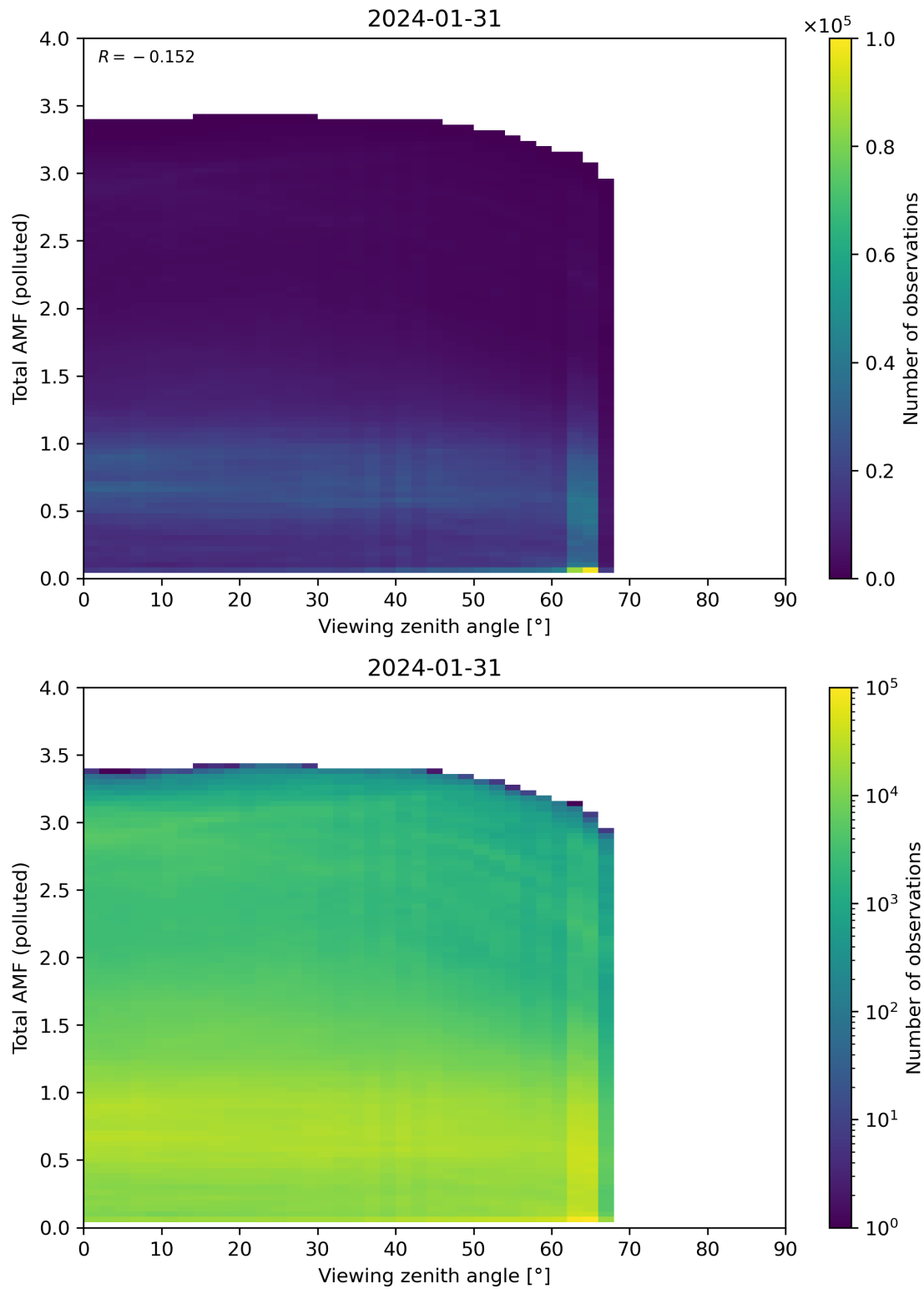
Figure 325: Scatter density plot of “Viewing zenith angle” against “Total AMF (polluted)” for 2024-01-31 to 2024-02-01.
