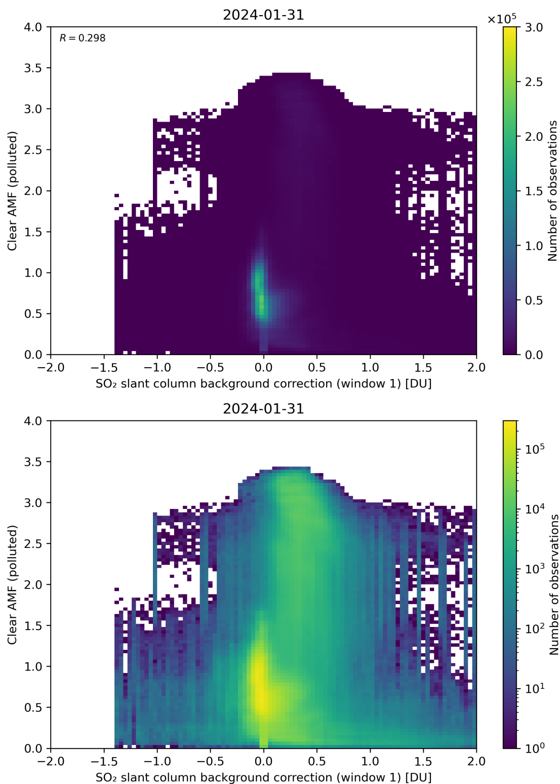
Figure 103: Scatter density plot of “SO 2 slant column background correction (window 1)” against “Clear AMF (polluted)” for 2024-01-31 to 2024-02-01.
