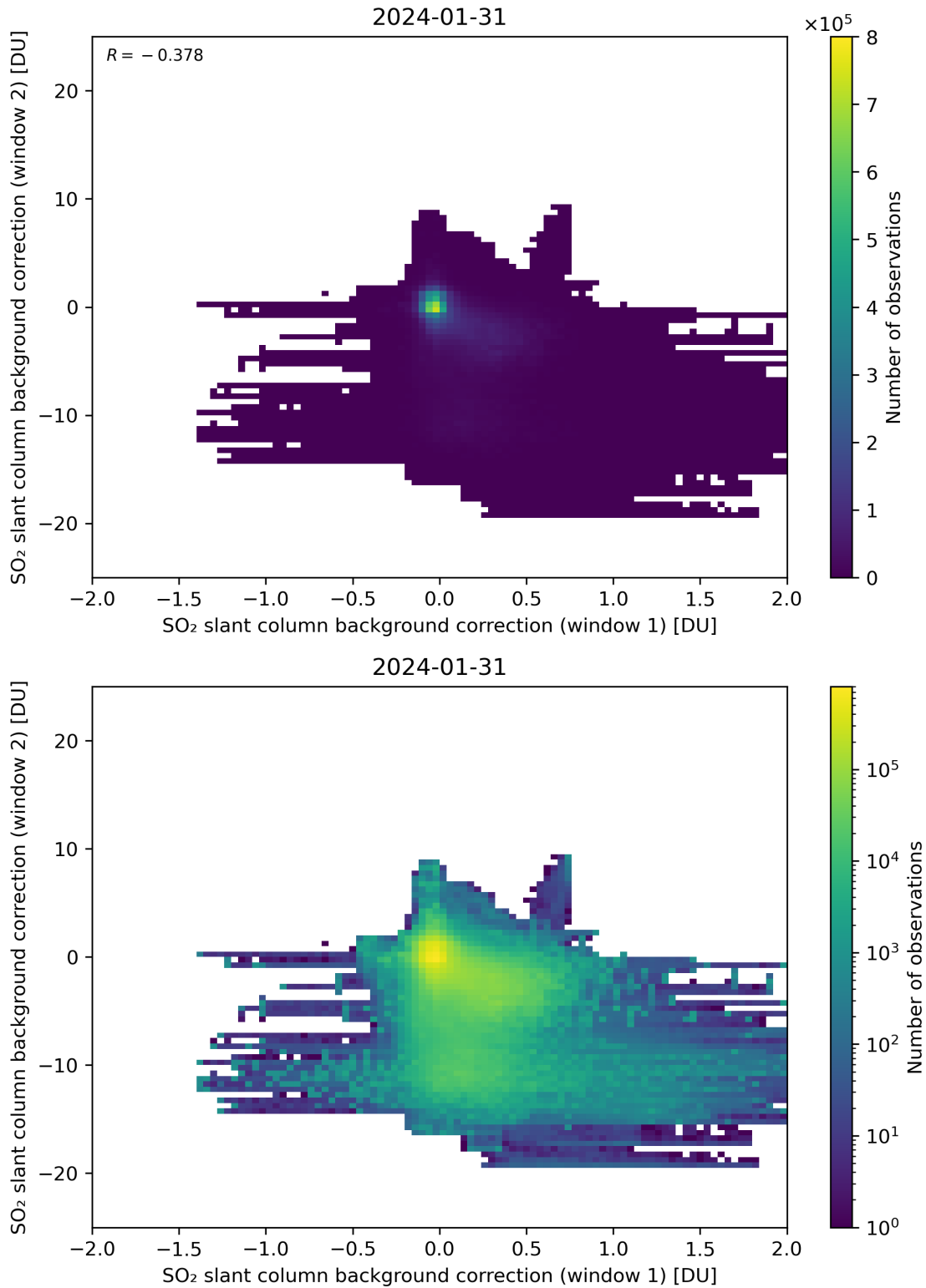
Figure 98: Scatter density plot of “SO 2 slant column background correction (window 1)” against “SO 2 slant column background correction (window 2)” for 2024-01-31 to 2024-02-01.
