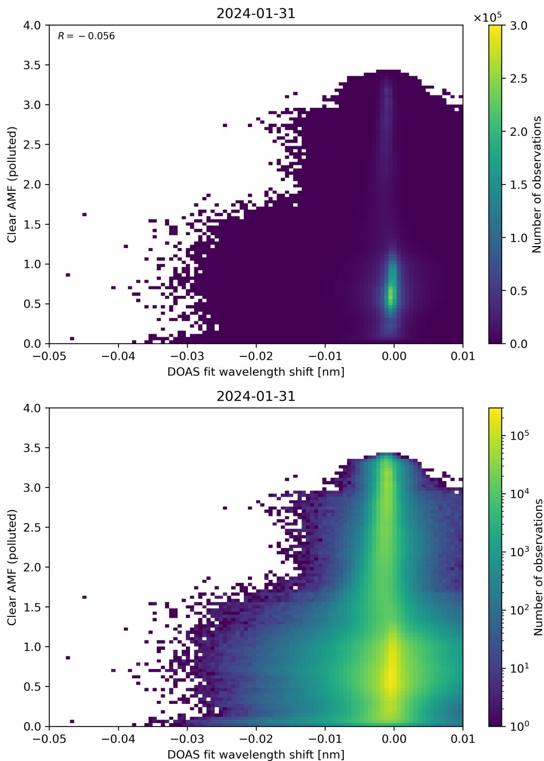
Figure 129: Scatter density plot of “DOAS fit wavelength shift” against “Clear AMF (polluted)” for 2024-01-31 to 2024-02-01.
