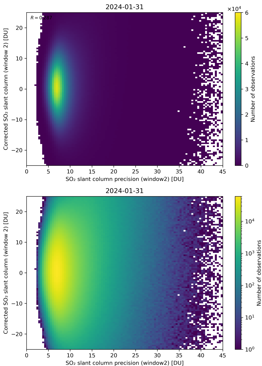
Figure 247: Scatter density plot of “SO 2 slant column precision (window2)” against “Corrected SO 2 slant column (window 2)” for 2024-01-31 to 2024-02-01.
