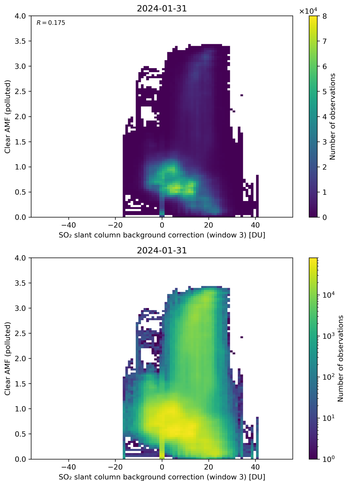
Figure 124: Scatter density plot of “SO 2 slant column background correction (window 3)” against “Clear AMF (polluted)” for 2024-01-31 to 2024-02-01.
