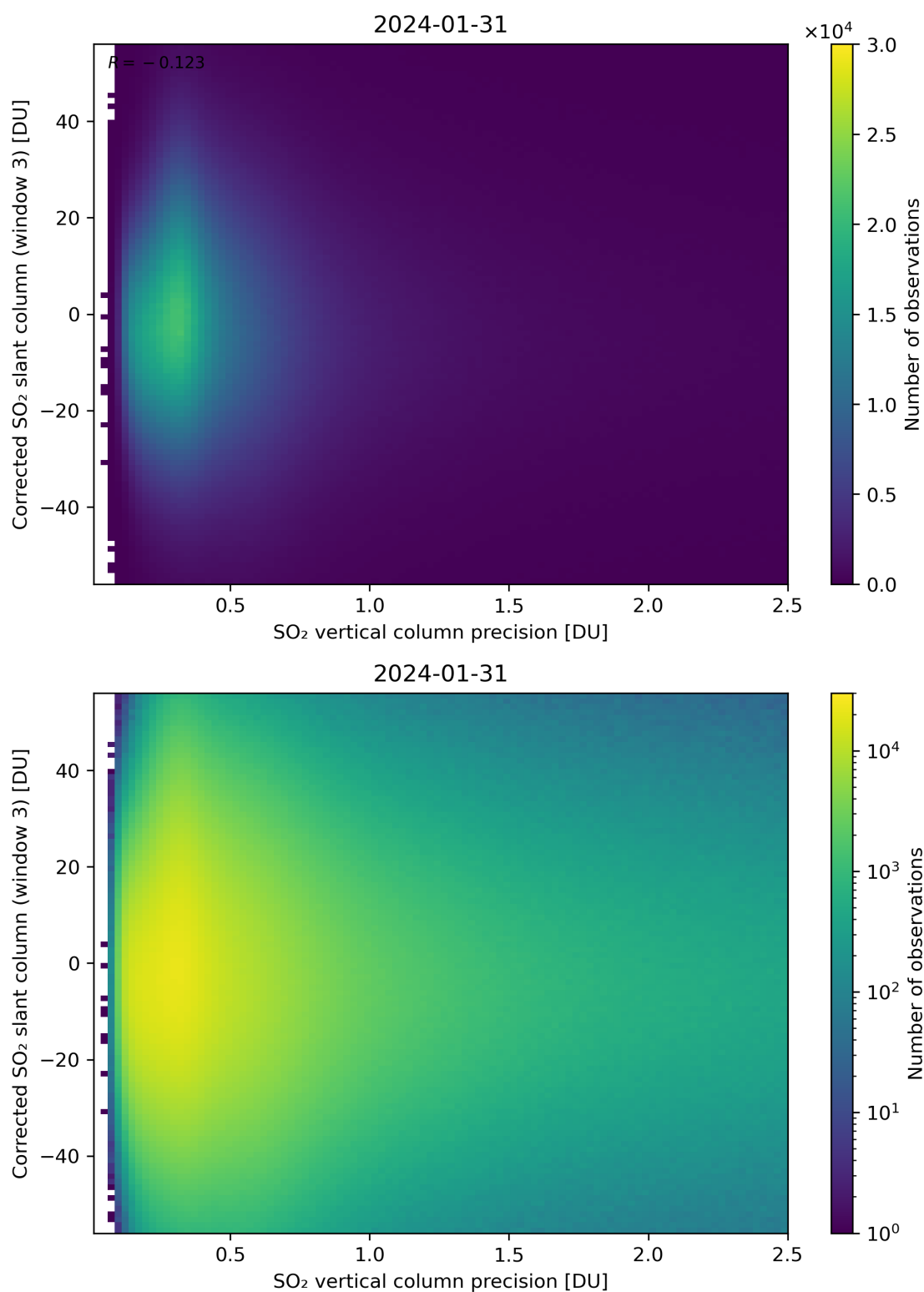
Figure 288: Scatter density plot of “SO 2 vertical column precision” against “Corrected SO 2 slant column (window 3)” for 2024-01-31 to 2024-02-01.
