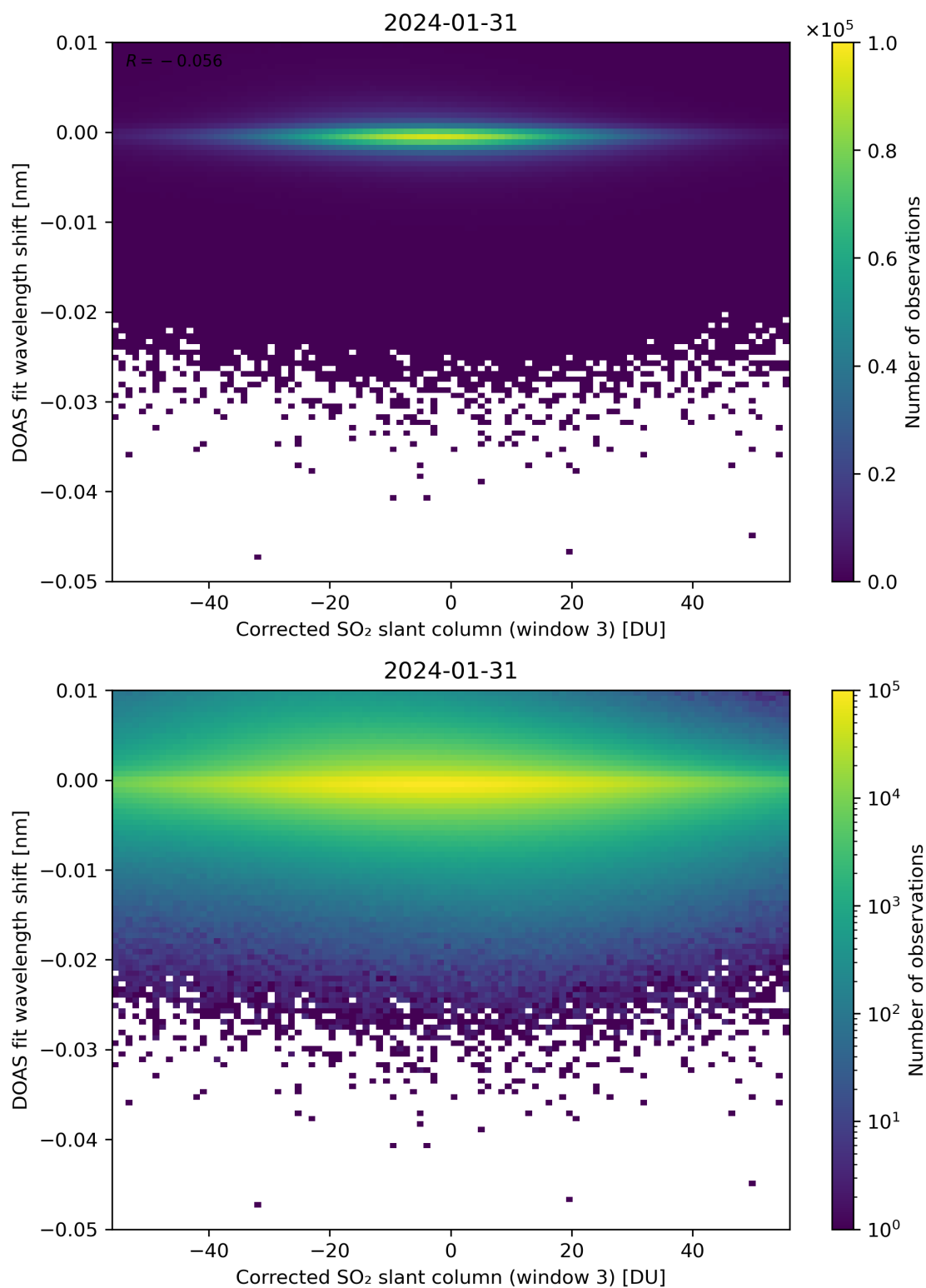
Figure 206: Scatter density plot of “Corrected SO 2 slant column (window 3)” against “DOAS fit wavelength shift” for 2024-01-31 to 2024-02-01.
