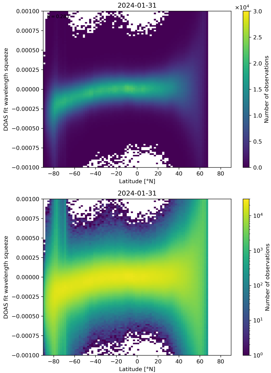
Figure 143: Scatter density plot of “Latitude” against “DOAS fit wavelength squeeze” for 2024-01-31 to 2024-02-01.
