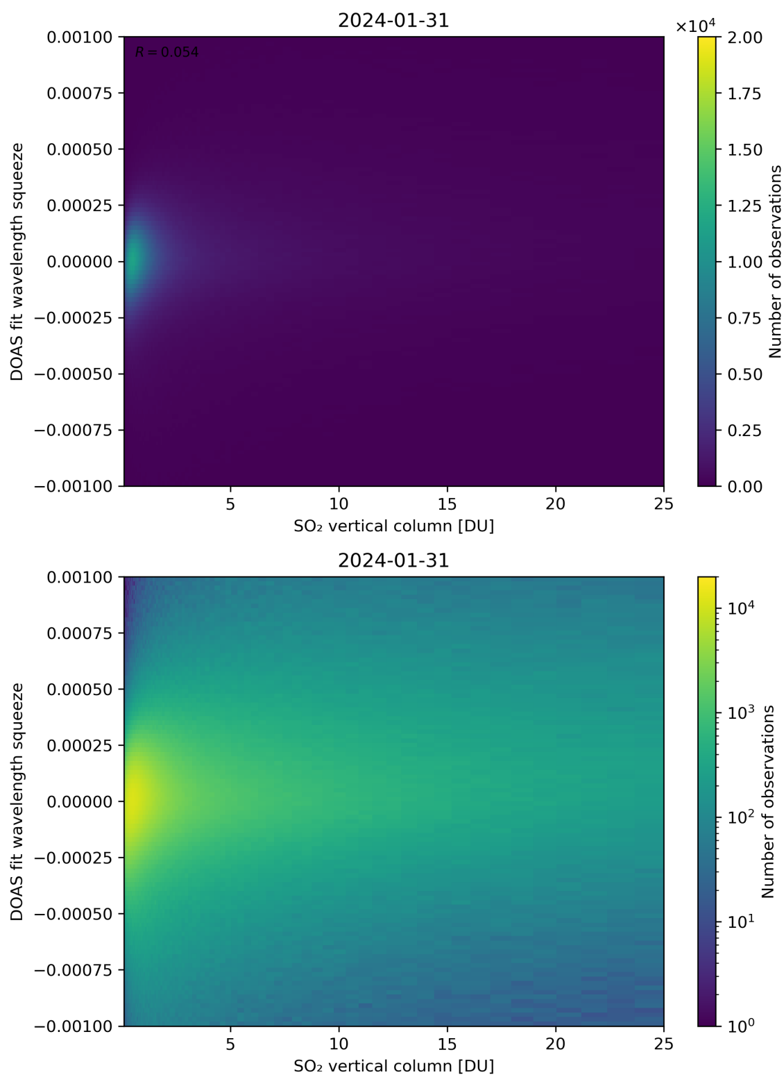
Figure 277: Scatter density plot of “SO 2 vertical column” against “DOAS fit wavelength squeeze” for 2024-01-31 to 2024-02-01.
