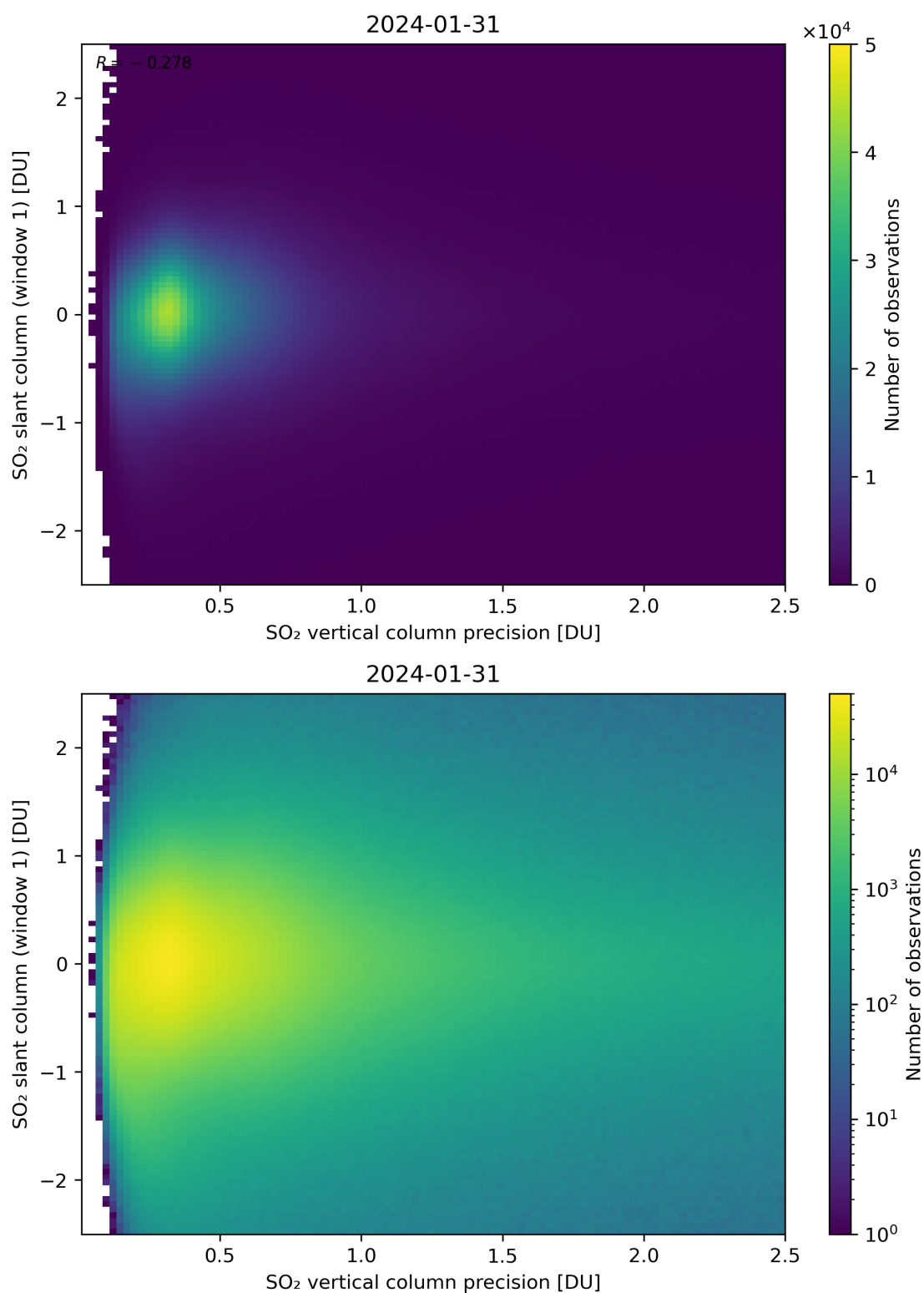
Figure 289: Scatter density plot of “SO 2 vertical column precision” against “SO 2 slant column (window 1)” for 2024-01-31 to 2024-02-01.
