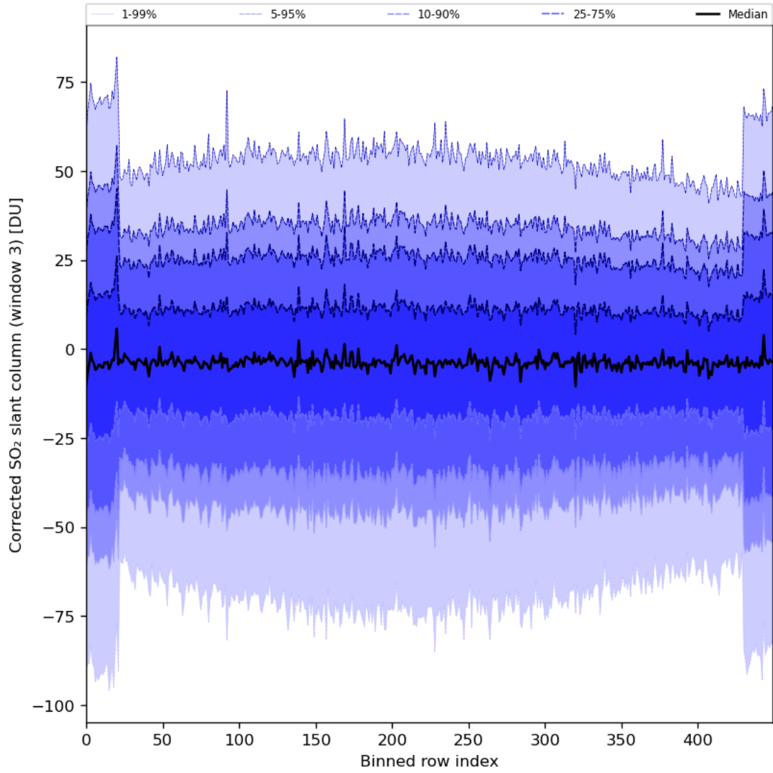
Figure 89: Along track statistics of “Corrected SO 2 slant column (window 3)” for 2024-01-31 to 2024-02-01
