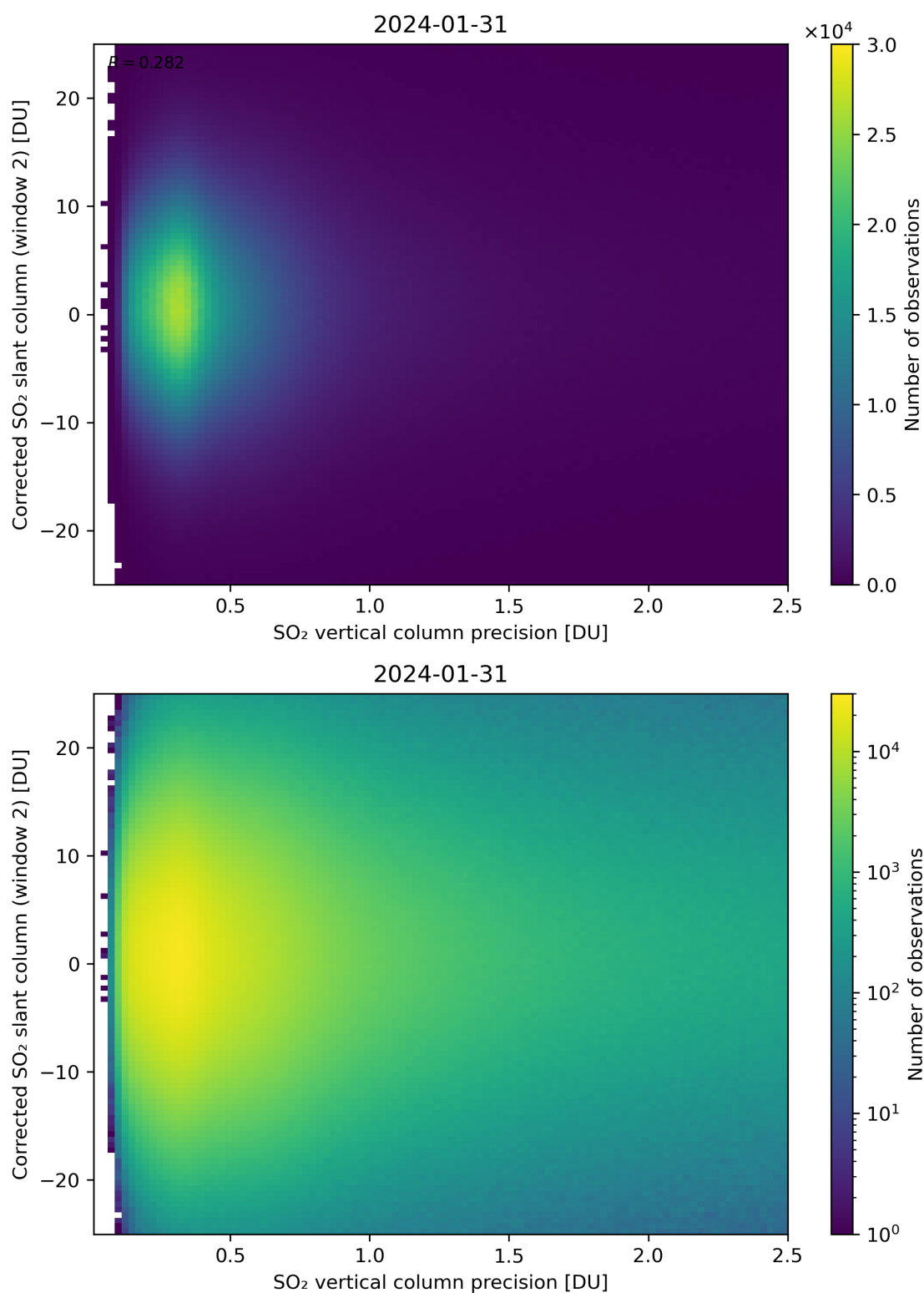
Figure 287: Scatter density plot of “SO 2 vertical column precision” against “Corrected SO 2 slant column (window 2)” for 2024-01-31 to 2024-02-01.
