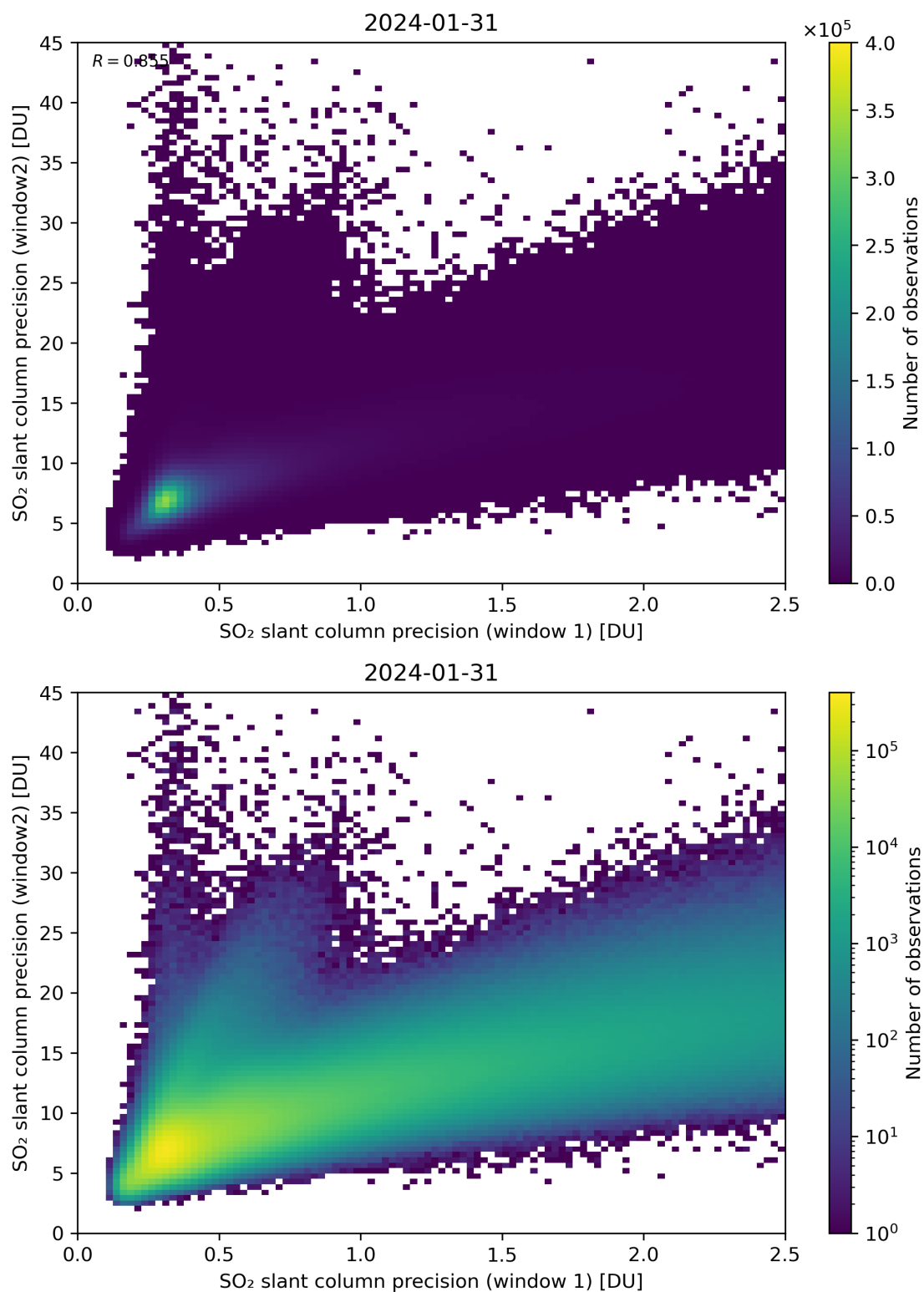
Figure 227: Scatter density plot of “SO 2 slant column precision (window 1)” against “SO 2 slant column precision (window2)” for 2024-01-31 to 2024-02-01.
