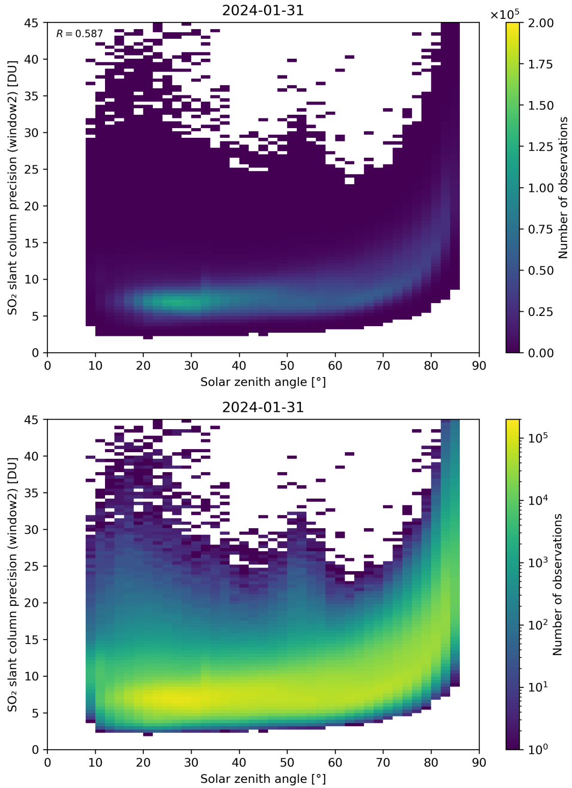
Figure 171: Scatter density plot of “Solar zenith angle” against “SO 2 slant column precision (window2)” for 2024-01-31 to 2024-02-01.
