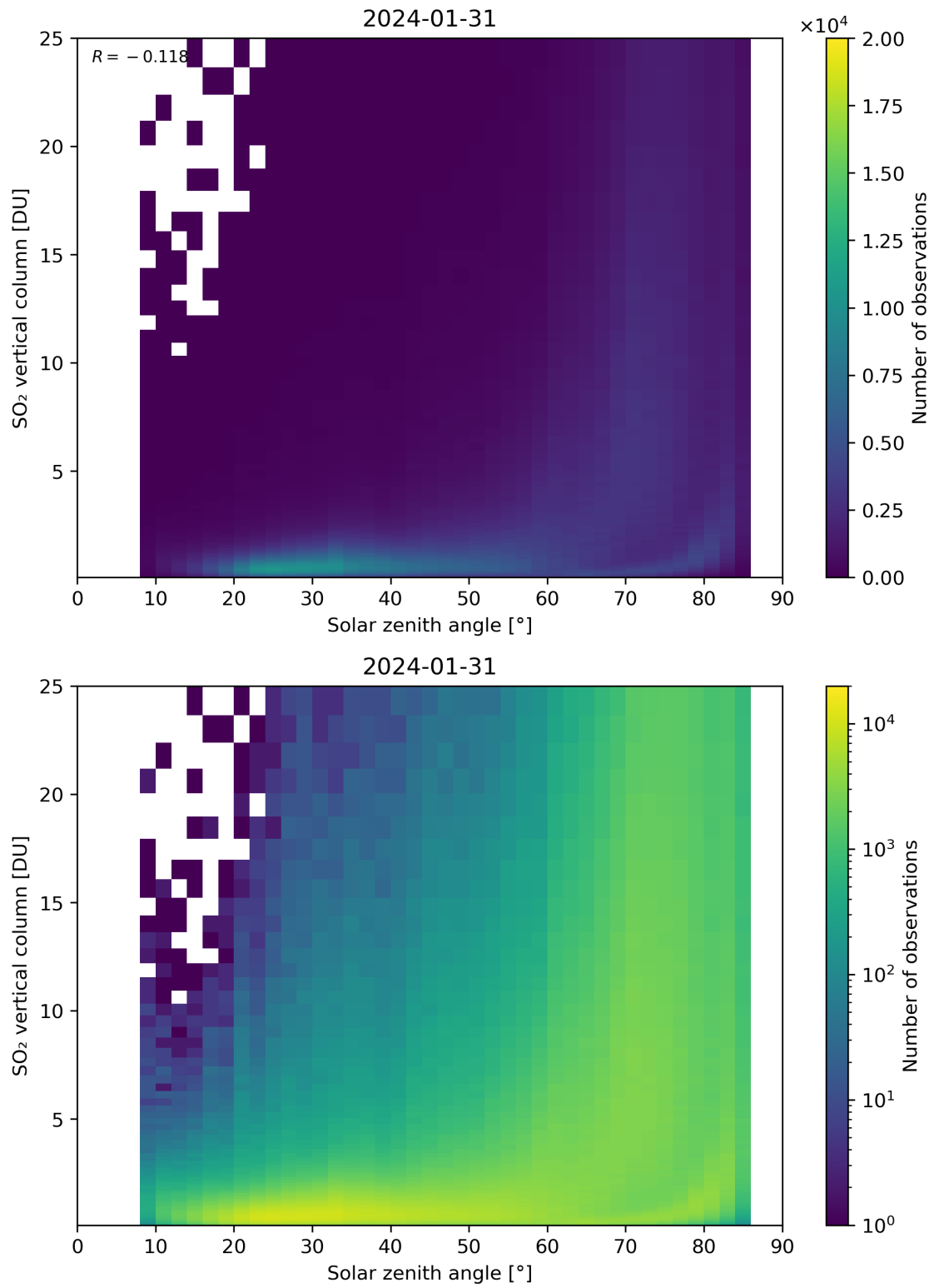
Figure 176: Scatter density plot of “Solar zenith angle” against “SO 2 vertical column” for 2024-01-31 to 2024-02-01.
