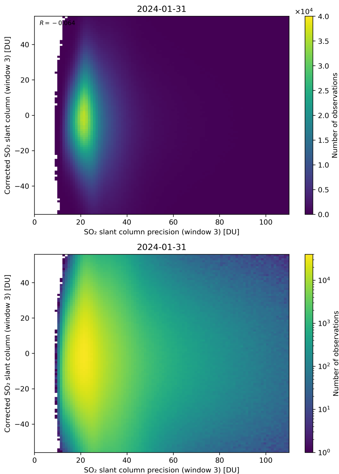
Figure 262: Scatter density plot of “SO 2 slant column precision (window 3)” against “Corrected SO 2 slant column (window 3)” for 2024-01-31 to 2024-02-01.
