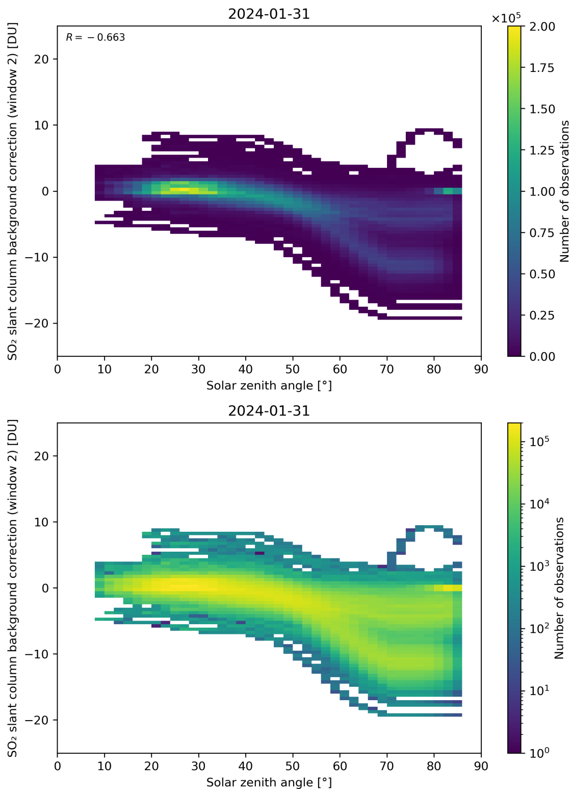
Figure 159: Scatter density plot of “Solar zenith angle” against “SO 2 slant column background correction (window 2)” for 2024-01-31 to 2024-02-01.
