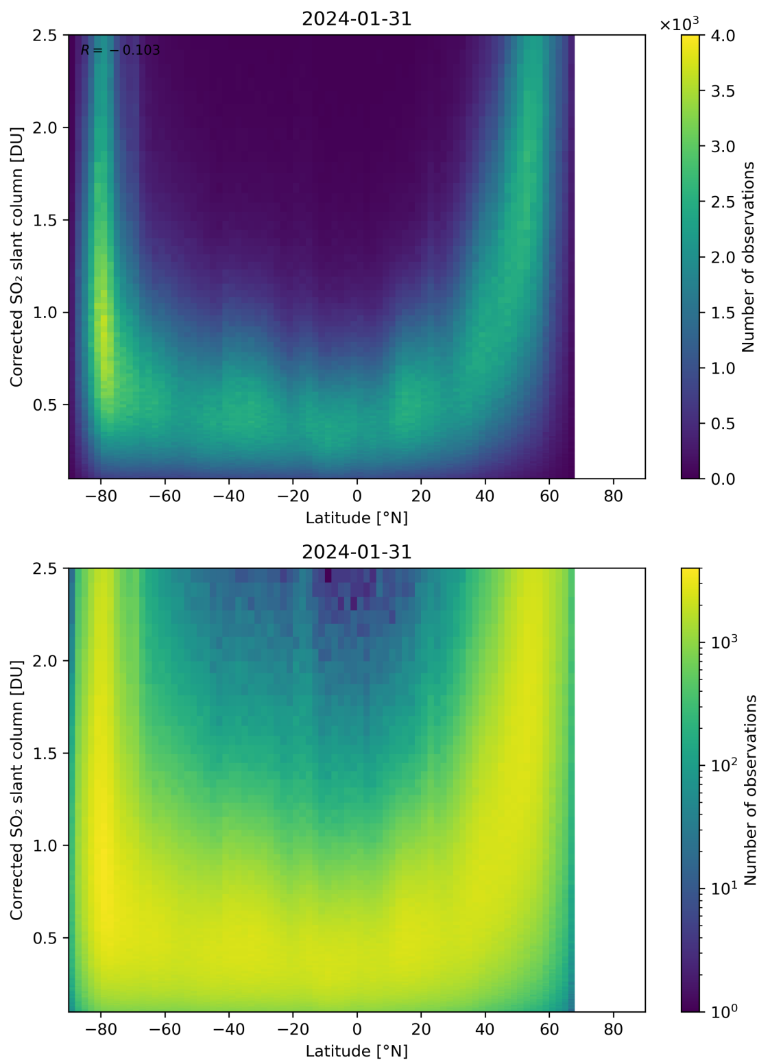
Figure 146: Scatter density plot of “Latitude” against “Corrected SO 2 slant column” for 2024-01-31 to 2024-02-01.
