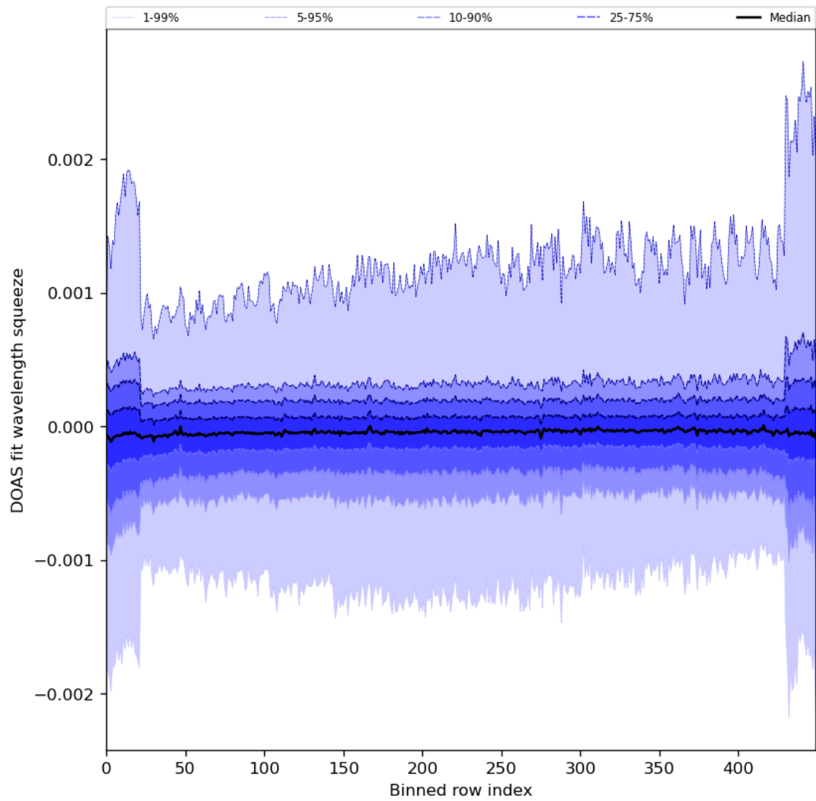
Figure 92: Along track statistics of “DOAS fit wavelength squeeze” for 2024-01-31 to 2024-02-01
