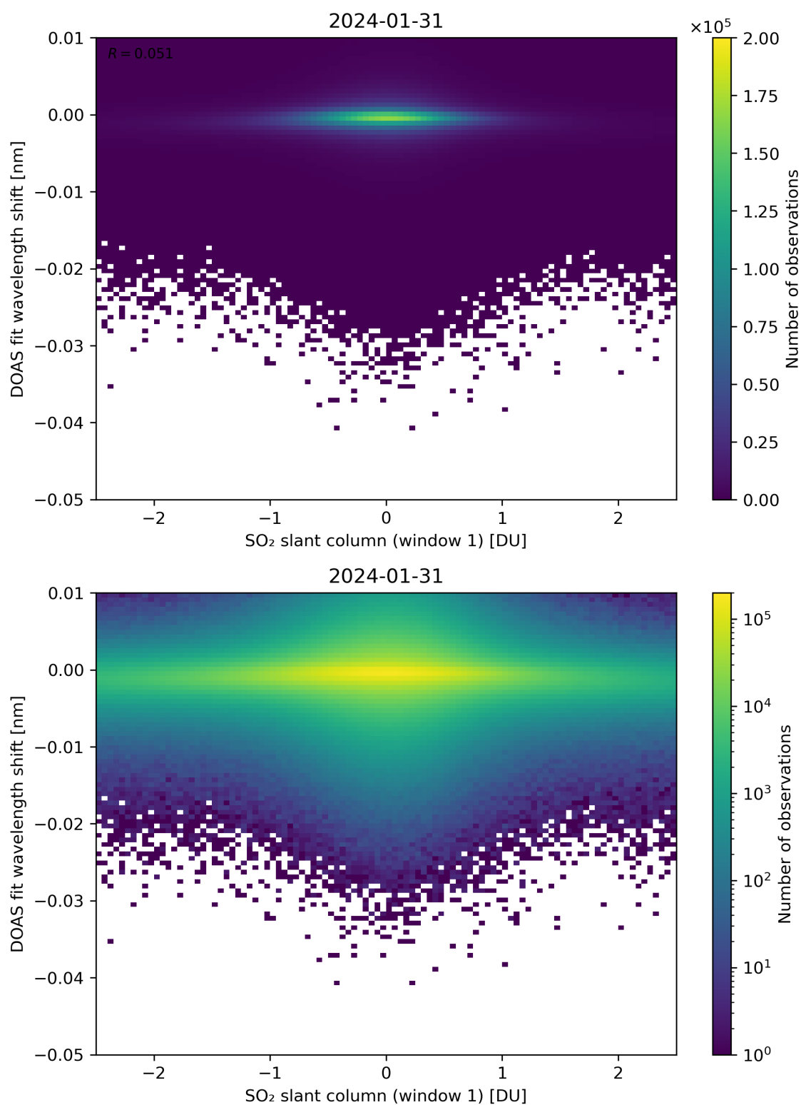
Figure 215: Scatter density plot of “SO 2 slant column (window 1)” against “DOAS fit wavelength shift” for 2024-01-31 to 2024-02-01.
