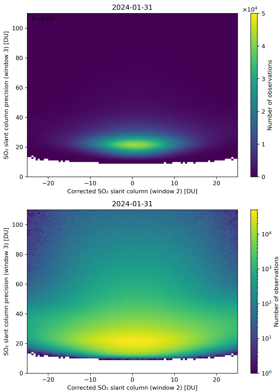
Figure 202: Scatter density plot of “Corrected SO 2 slant column (window 2)” against “SO 2 slant column precision (window 3)” for 2024-01-31 to 2024-02-01.
