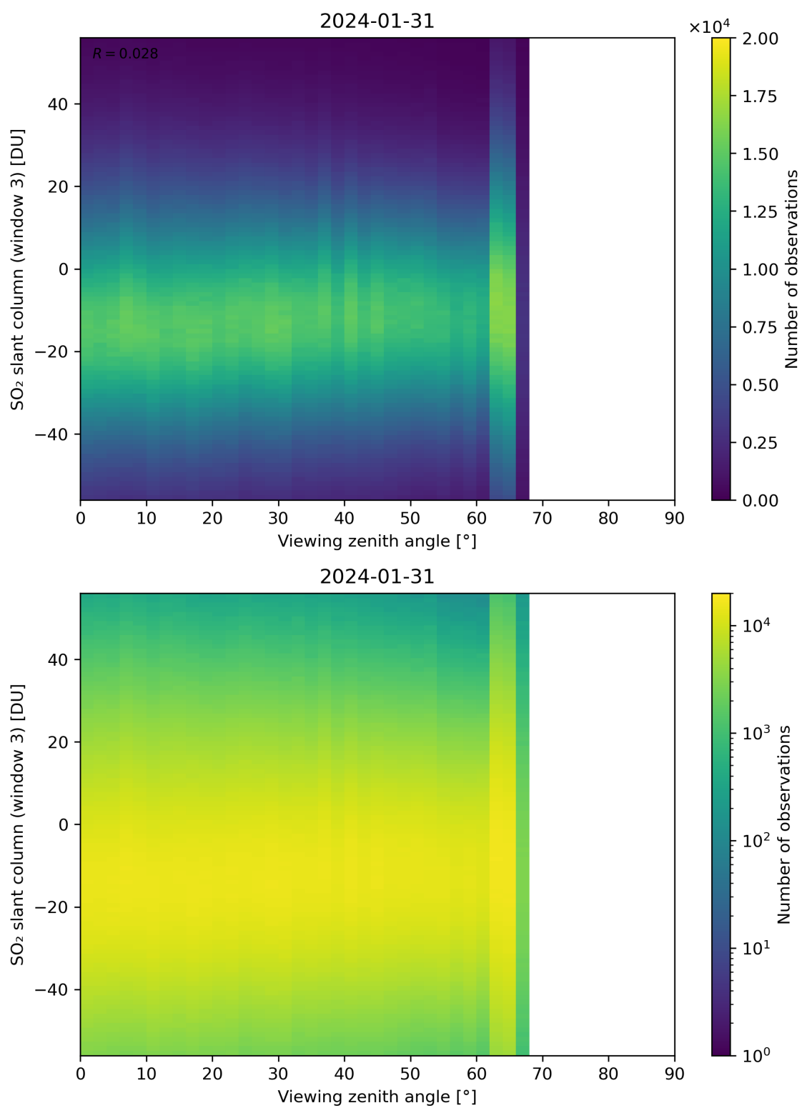
Figure 323: Scatter density plot of “Viewing zenith angle” against “SO 2 slant column (window 3)” for 2024-01-31 to 2024-02-01.
