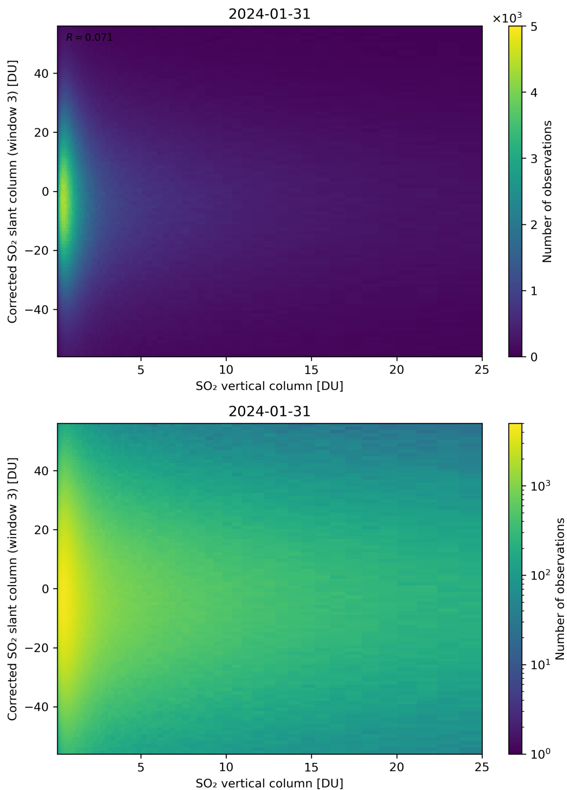
Figure 299: Scatter density plot of “SO 2 vertical column” against “Corrected SO 2 slant column (window 3)” for 2024-01-31 to 2024-02-01.
