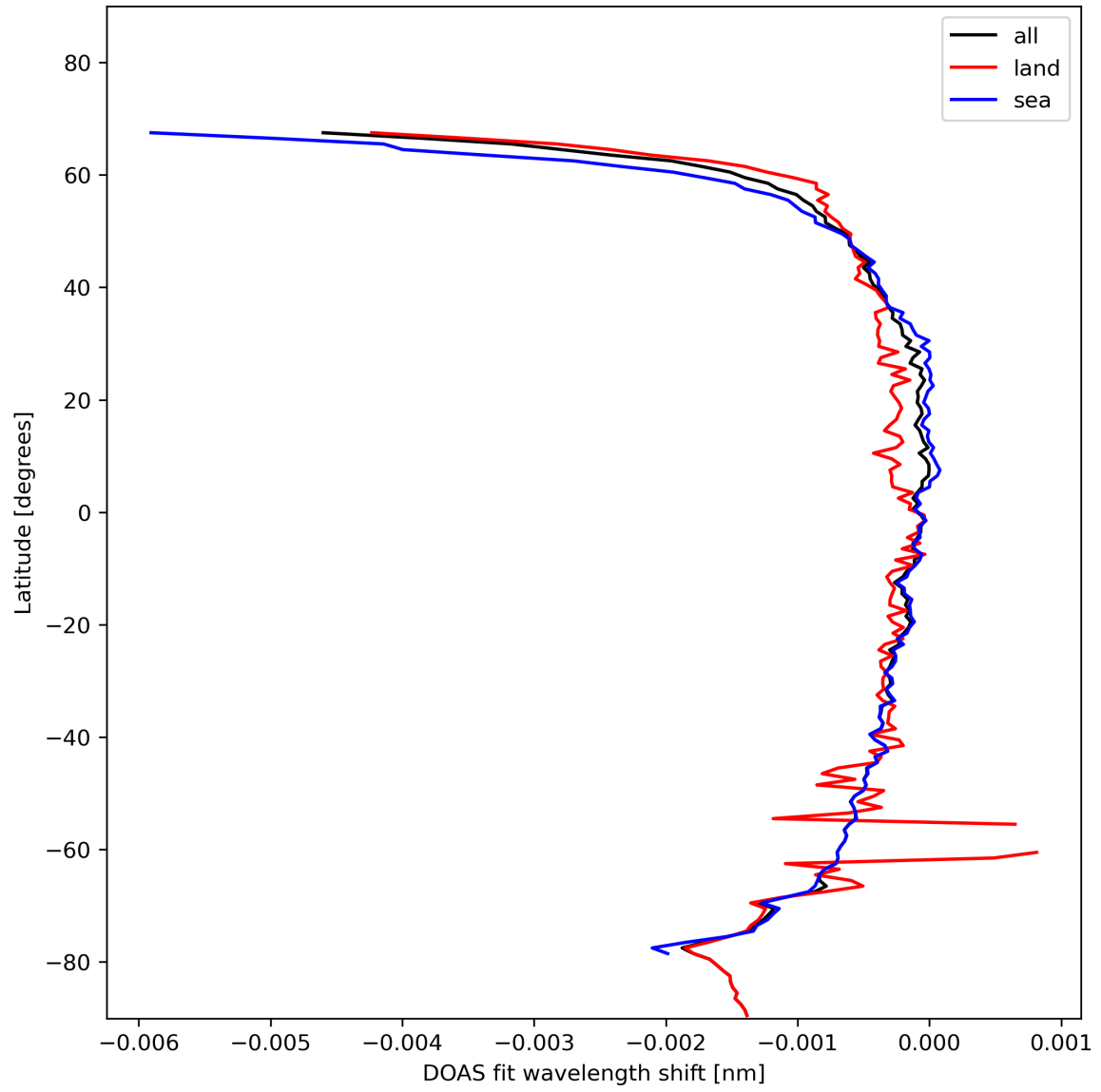
Figure 45: Zonal average of “DOAS fit wavelength shift” for 2024-01-31 to 2024-02-01.
