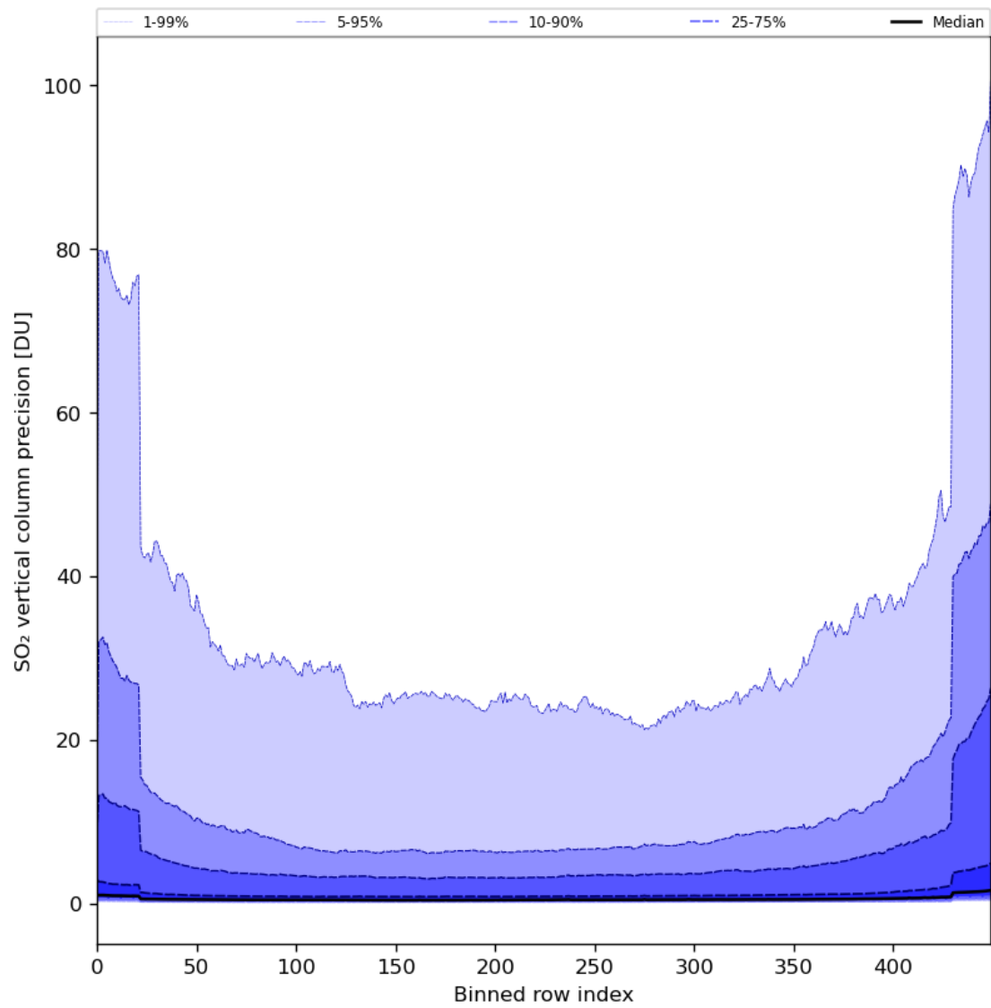
Figure 77: Along track statistics of “SO 2 vertical column precision” for 2024-01-31 to 2024-02-01
