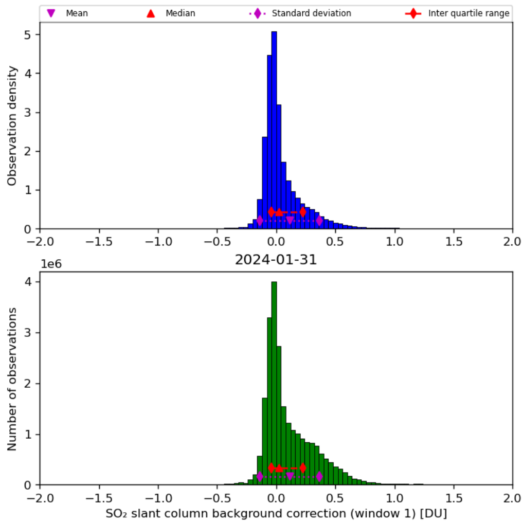
Figure 59: Histogram of “SO 2 slant column background correction (window 1)” for 2024-01-31 to 2024-02-01
