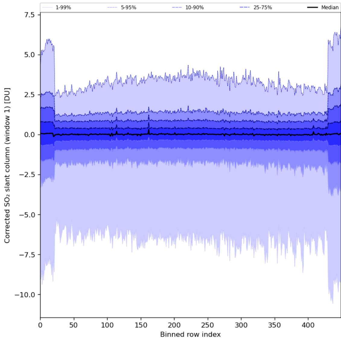
Figure 81: Along track statistics of “Corrected SO 2 slant column (window 1)” for 2024-01-31 to 2024-02-01
