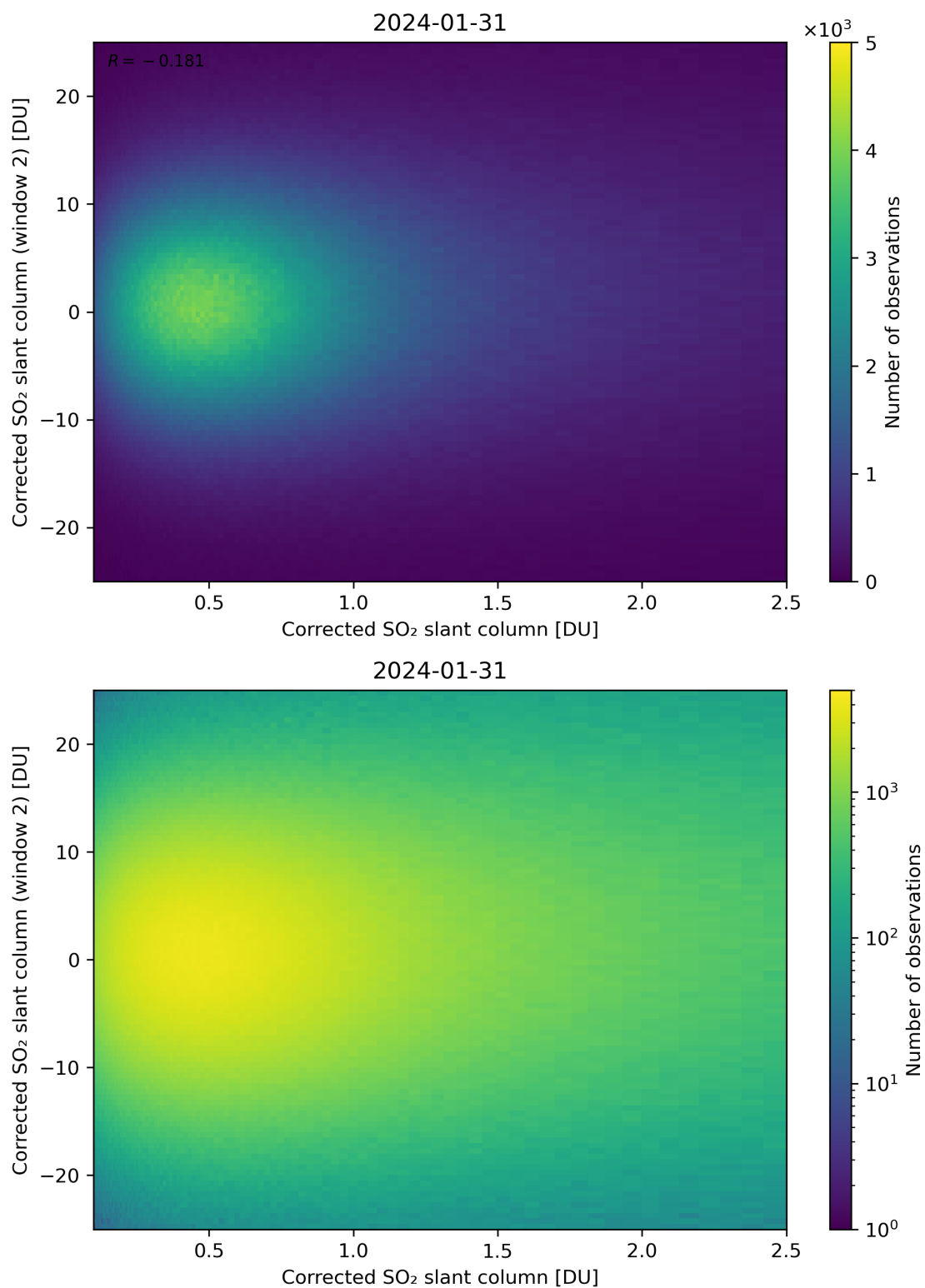
Figure 185: Scatter density plot of “Corrected SO 2 slant column” against “Corrected SO 2 slant column (window 2)” for 2024-01-31 to 2024-02-01.
