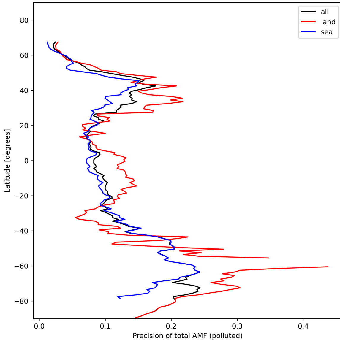
Figure 49: Zonal average of “Precision of total AMF (polluted)” for 2024-01-31 to 2024-02-01.
