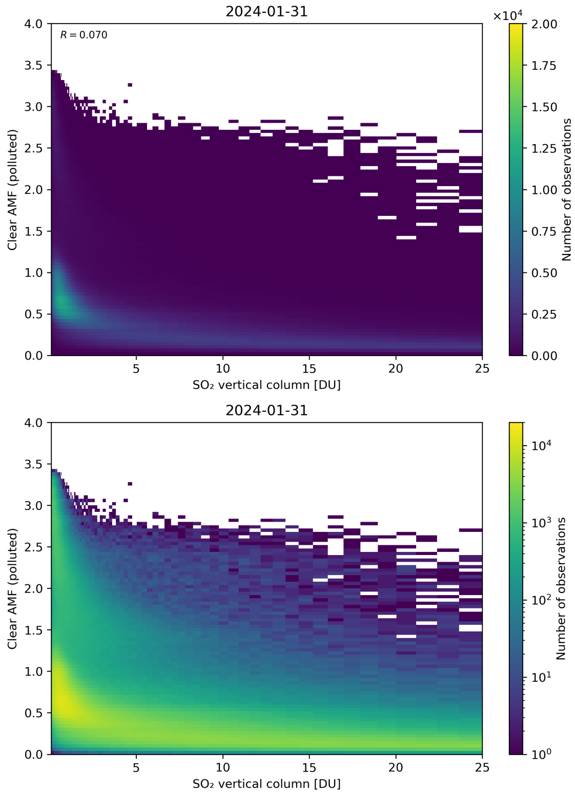
Figure 296: Scatter density plot of “SO 2 vertical column” against “Clear AMF (polluted)” for 2024-01-31 to 2024-02-01.
