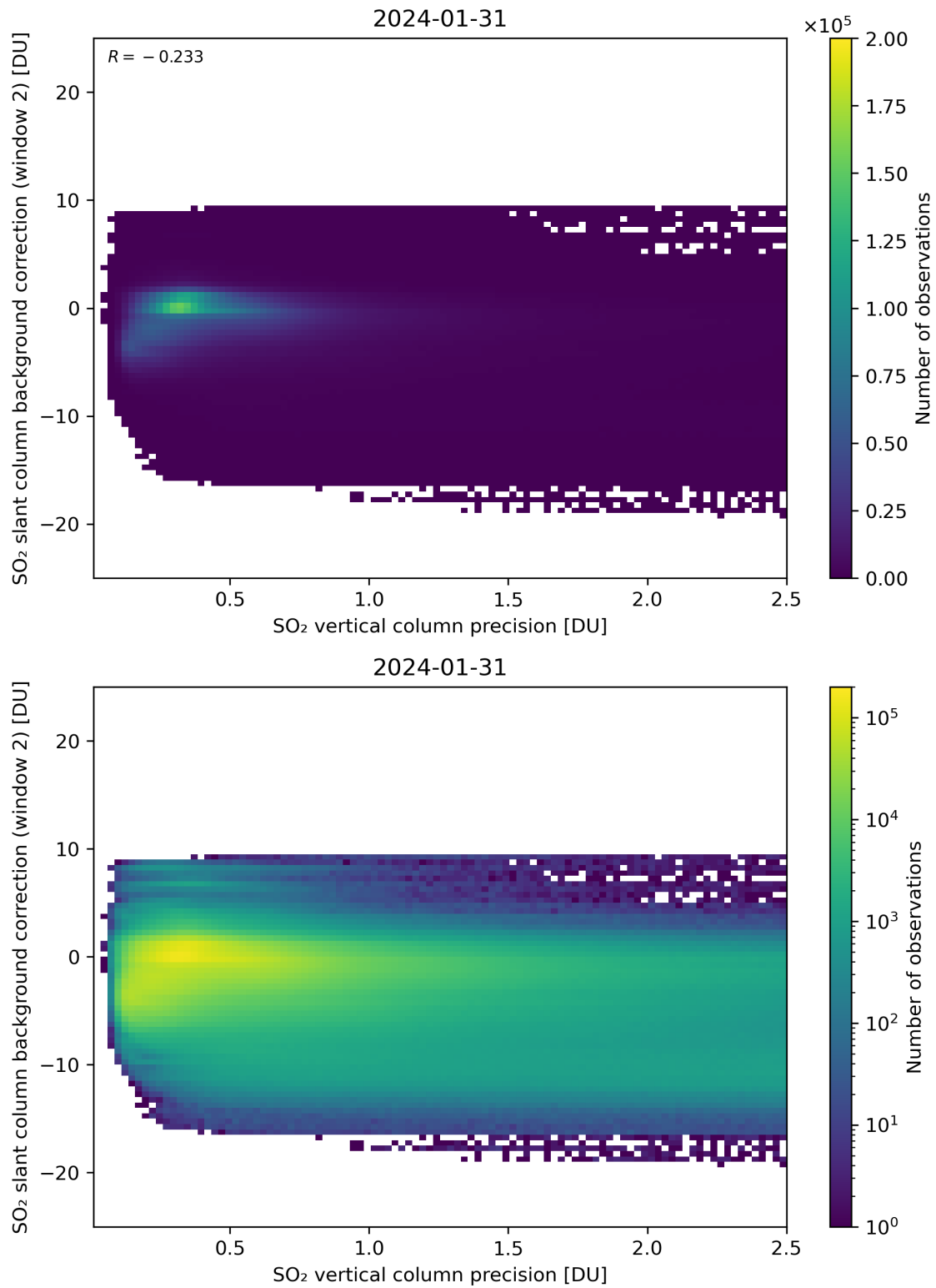
Figure 280: Scatter density plot of “SO 2 vertical column precision” against “SO 2 slant column background correction (window 2)” for 2024-01-31 to 2024-02-01.
