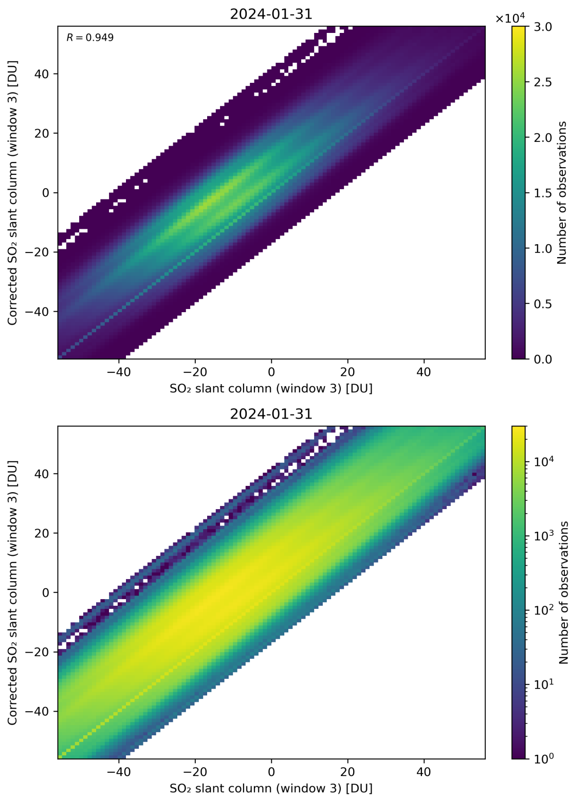
Figure 266: Scatter density plot of “SO 2 slant column (window 3)” against “Corrected SO 2 slant column (window 3)” for 2024-01-31 to 2024-02-01.
