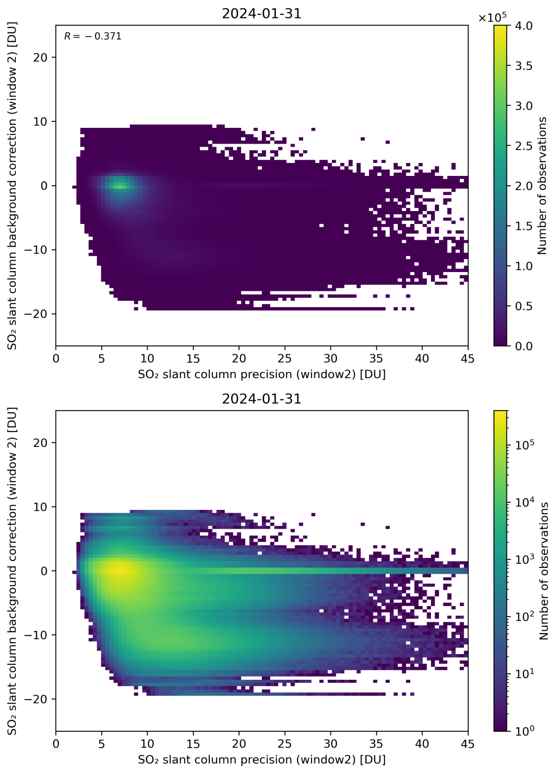
Figure 241: Scatter density plot of “SO 2 slant column precision (window2)” against “SO 2 slant column background correction (window 2)” for 2024-01-31 to 2024-02-01.
