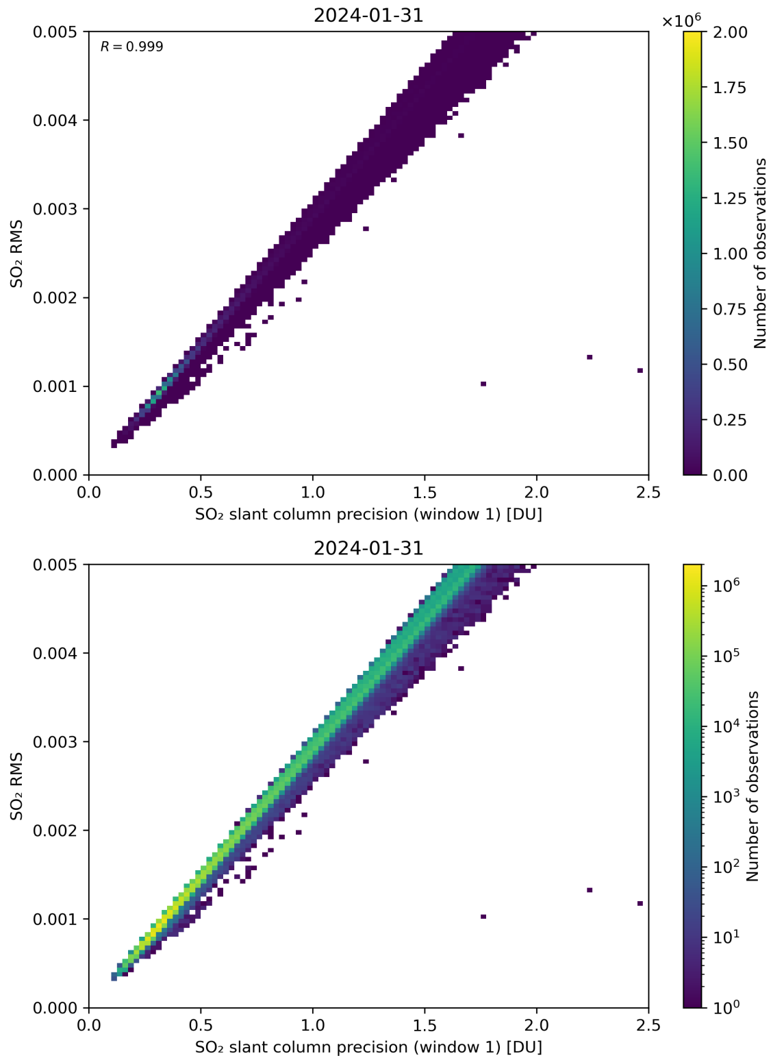
Figure 223: Scatter density plot of “SO 2 slant column precision (window 1)” against “SO 2 RMS” for 2024-01-31 to 2024-02-01.
