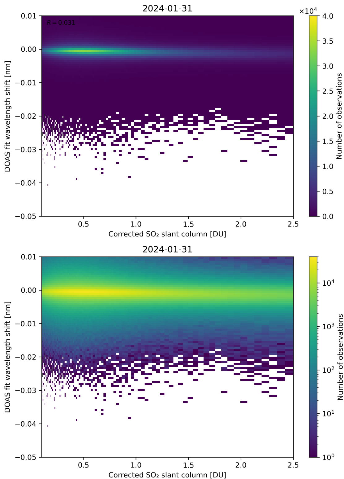
Figure 181: Scatter density plot of “Corrected SO 2 slant column” against “DOAS fit wavelength shift” for 2024-01-31 to 2024-02-01.
