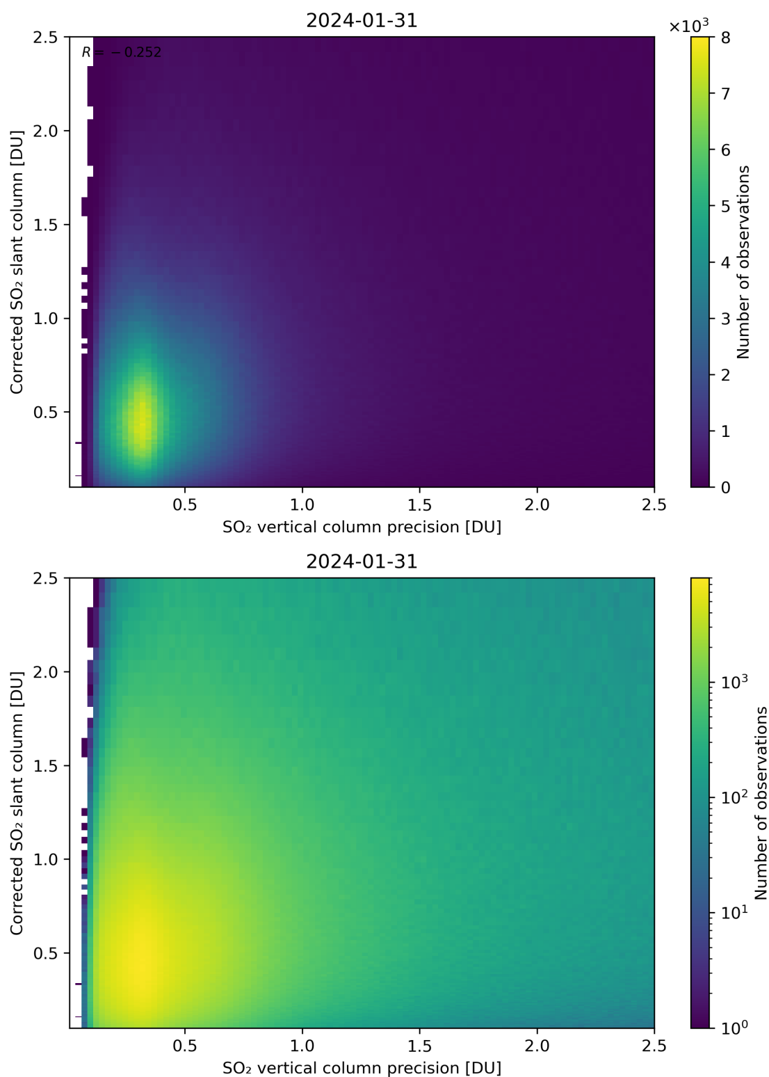
Figure 286: Scatter density plot of “SO 2 vertical column precision” against “Corrected SO 2 slant column” for 2024-01-31 to 2024-02-01.
