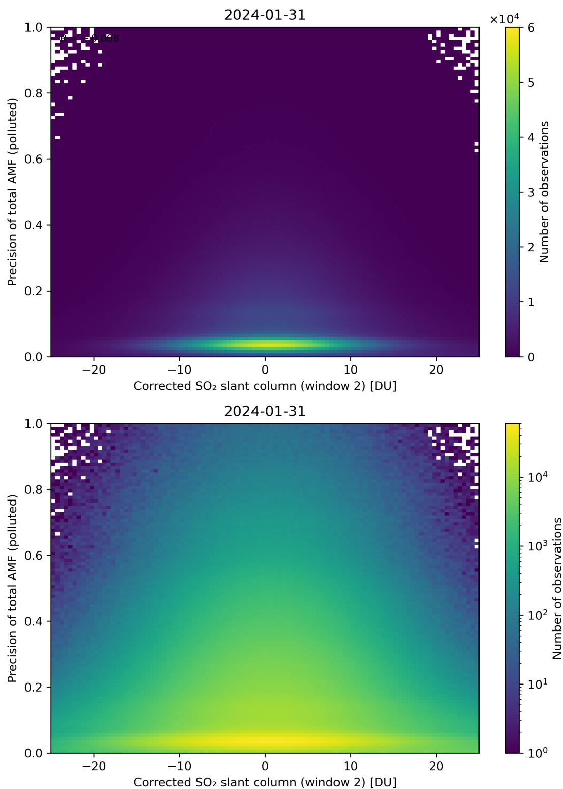
Figure 204: Scatter density plot of “Corrected SO 2 slant column (window 2)” against “Precision of total AMF (polluted)” for 2024-01-31 to 2024-02-01.
