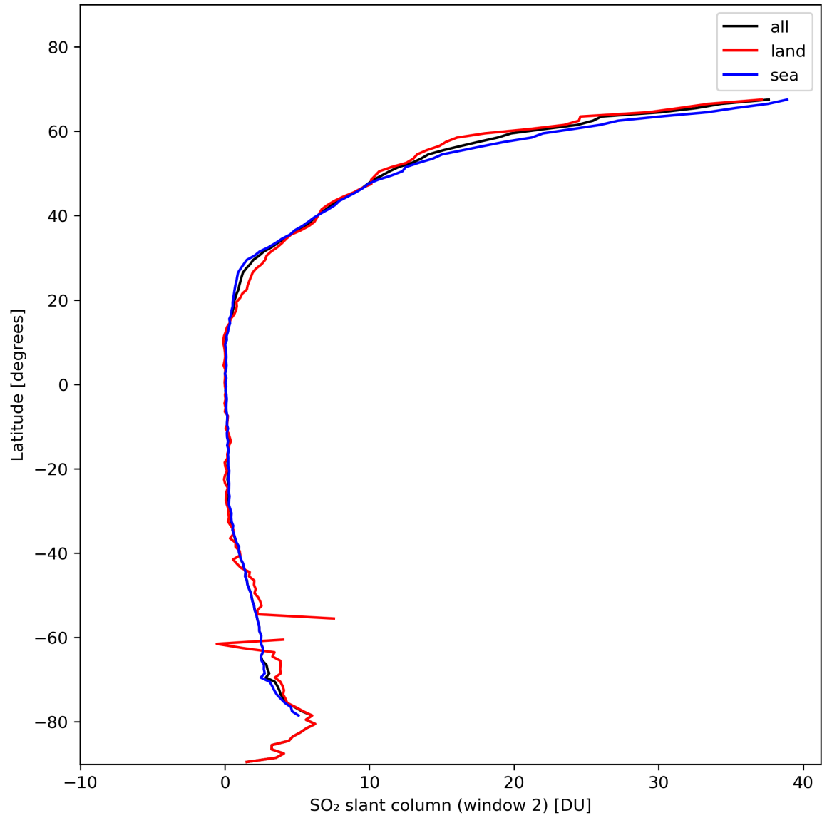
Figure 37: Zonal average of “SO 2 slant column (window 2)” for 2024-01-31 to 2024-02-01.
