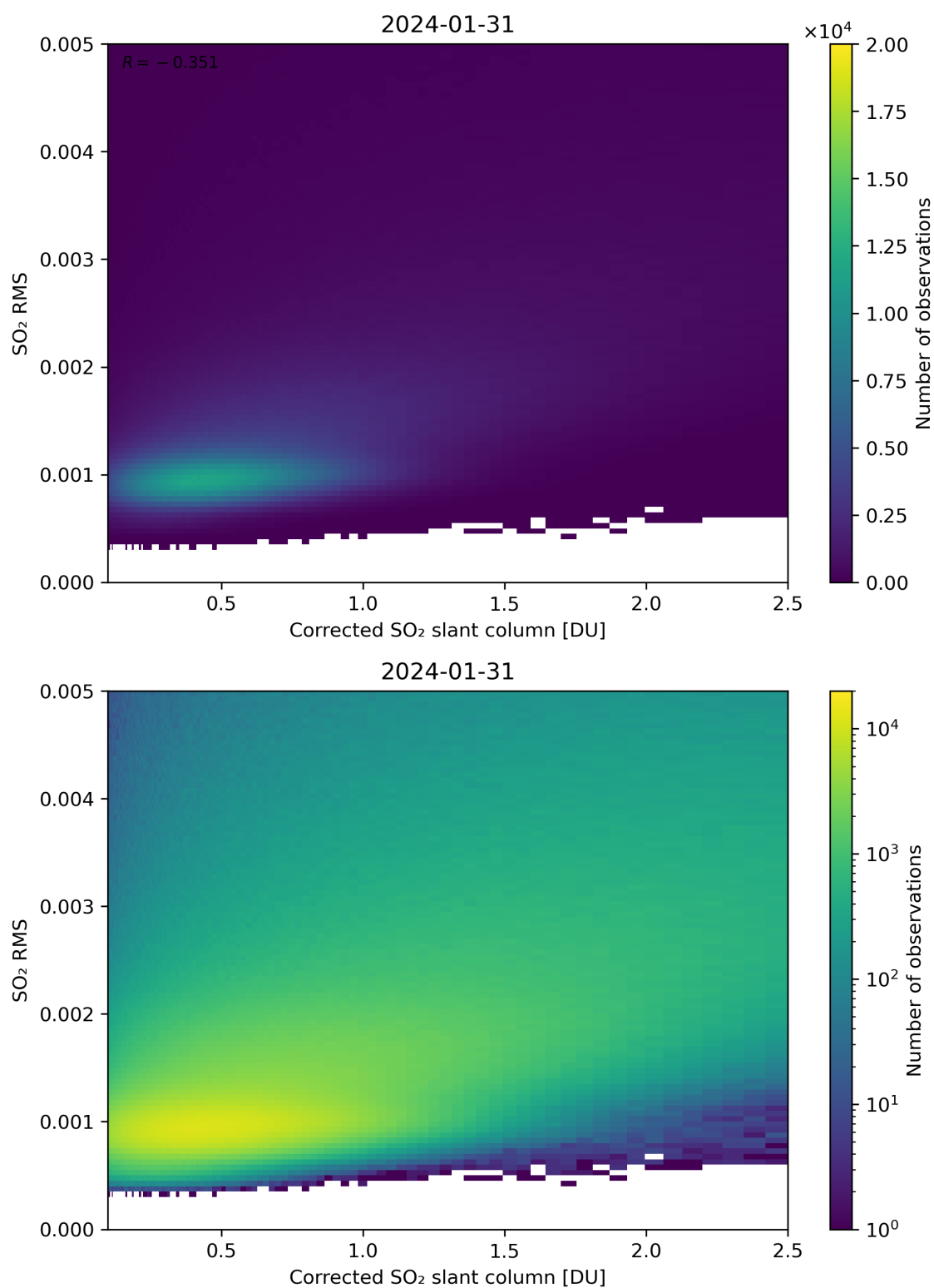
Figure 183: Scatter density plot of “Corrected SO 2 slant column” against “SO 2 RMS” for 2024-01-31 to 2024-02-01.
