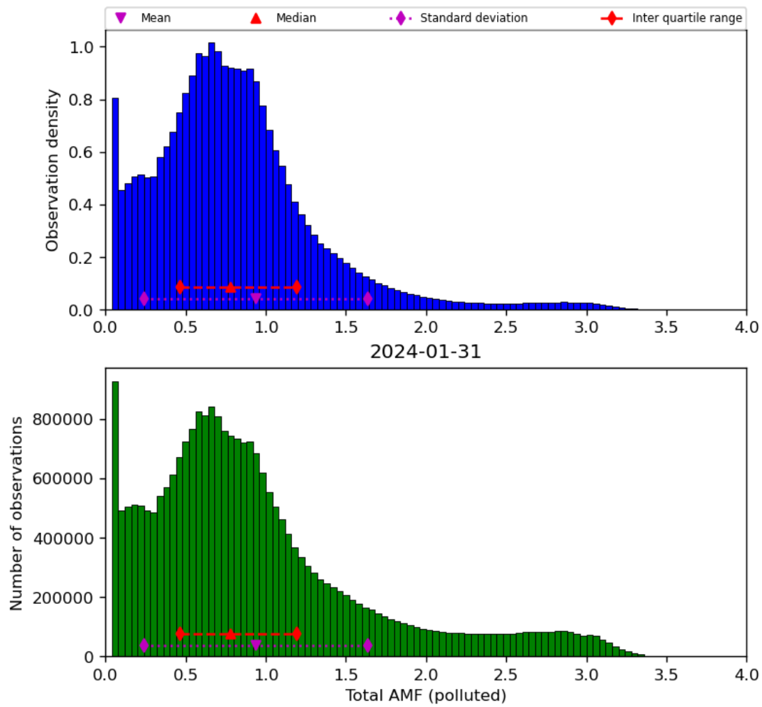
Figure 71: Histogram of “Total AMF (polluted)” for 2024-01-31 to 2024-02-01
