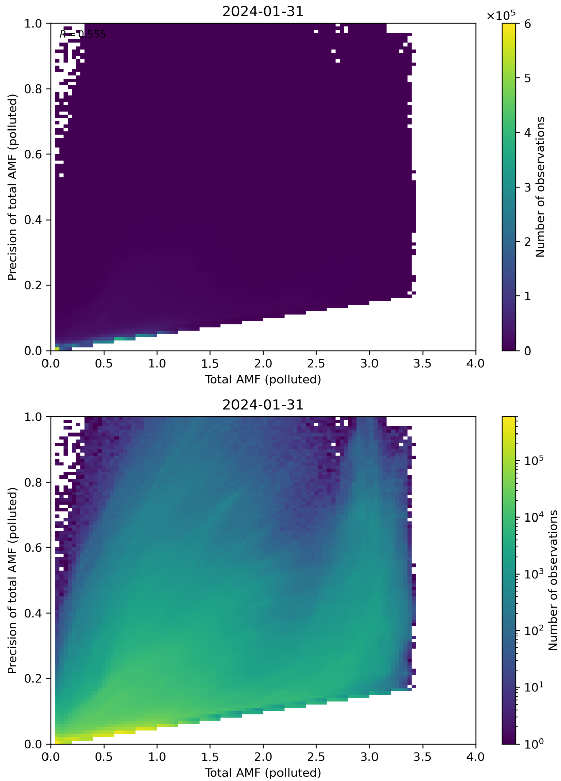
Figure 272: Scatter density plot of “Total AMF (polluted)” against “Precision of total AMF (polluted)” for 2024-01-31 to 2024-02-01.
