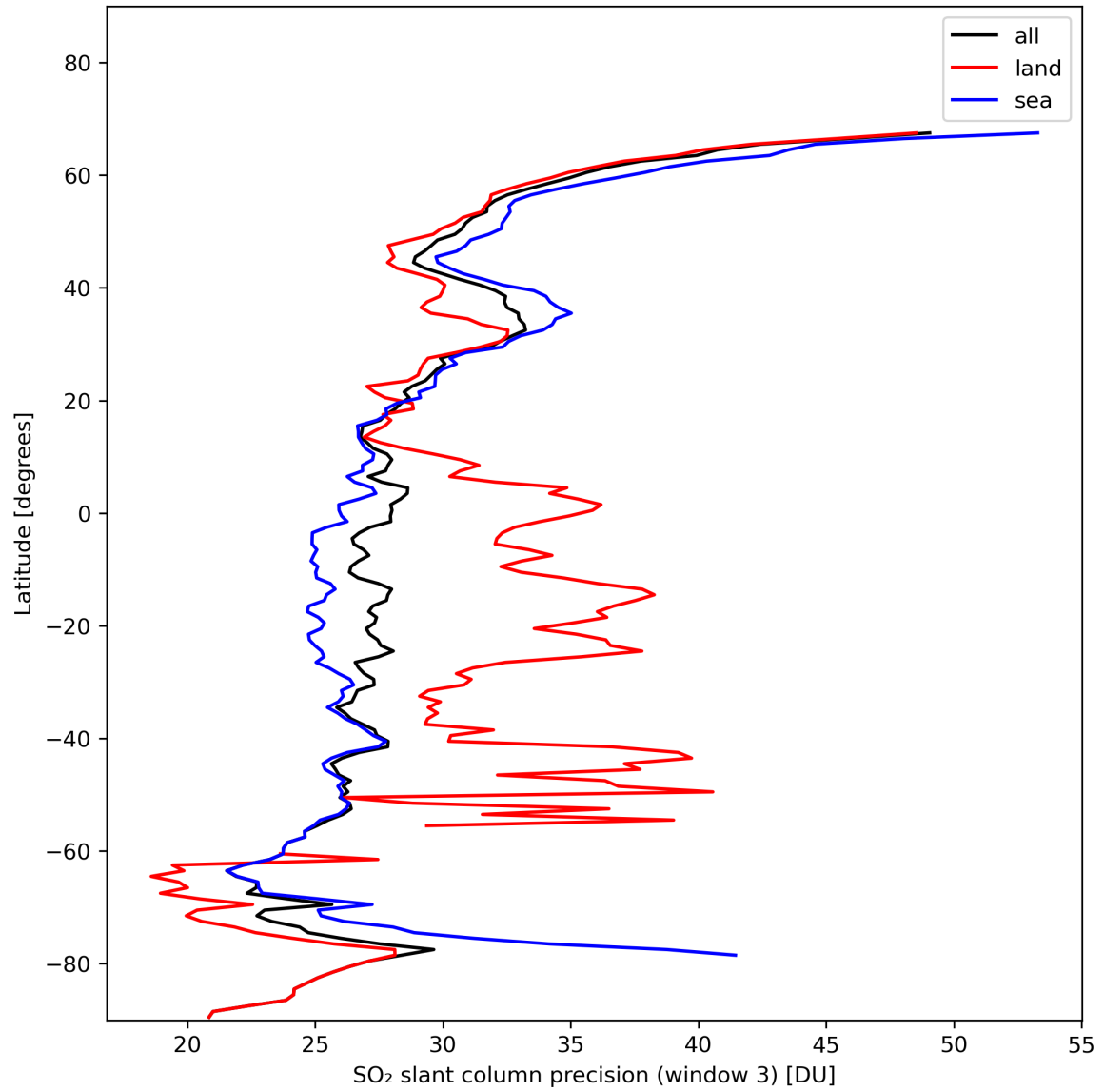
Figure 42: Zonal average of “SO 2 slant column precision (window 3)” for 2024-01-31 to 2024-02-01.
