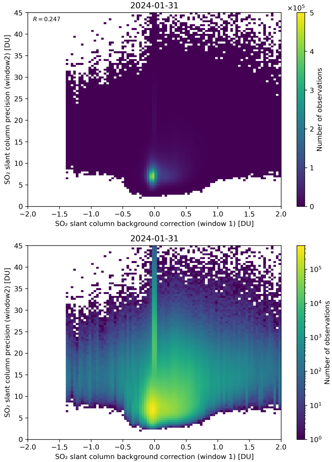
Figure 106: Scatter density plot of “SO 2 slant column background correction (window 1)” against “SO 2 slant column precision (window2)” for 2024-01-31 to 2024-02-01.
