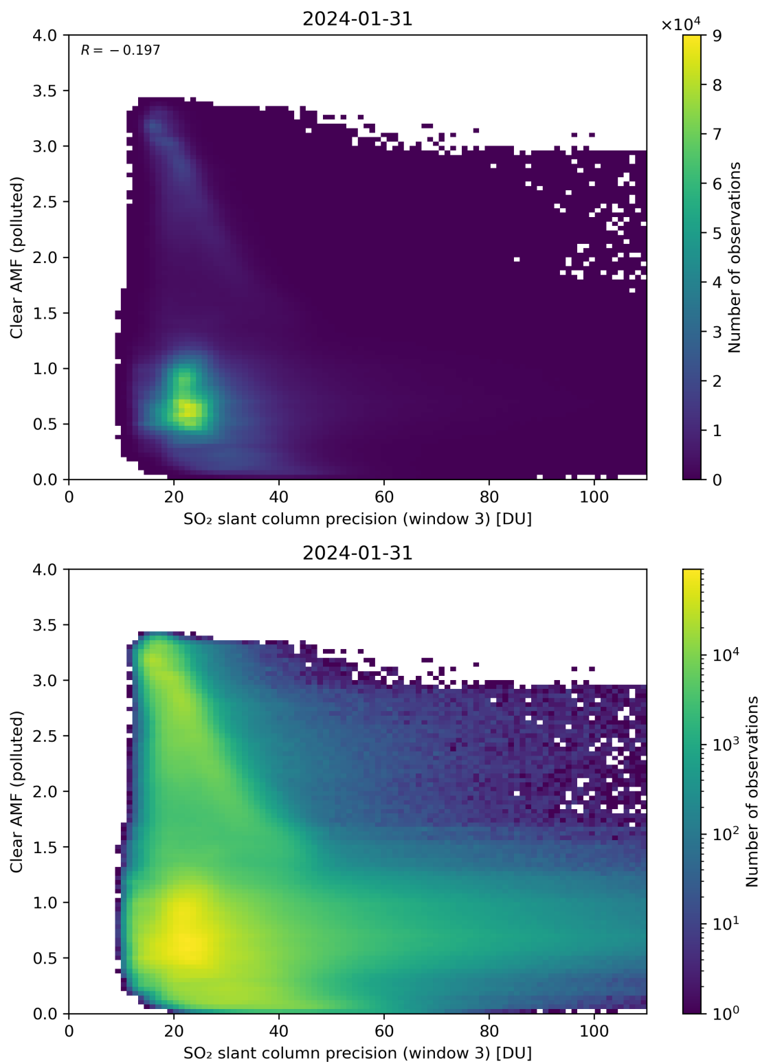
Figure 261: Scatter density plot of “SO 2 slant column precision (window 3)” against “Clear AMF (polluted)” for 2024-01-31 to 2024-02-01.
