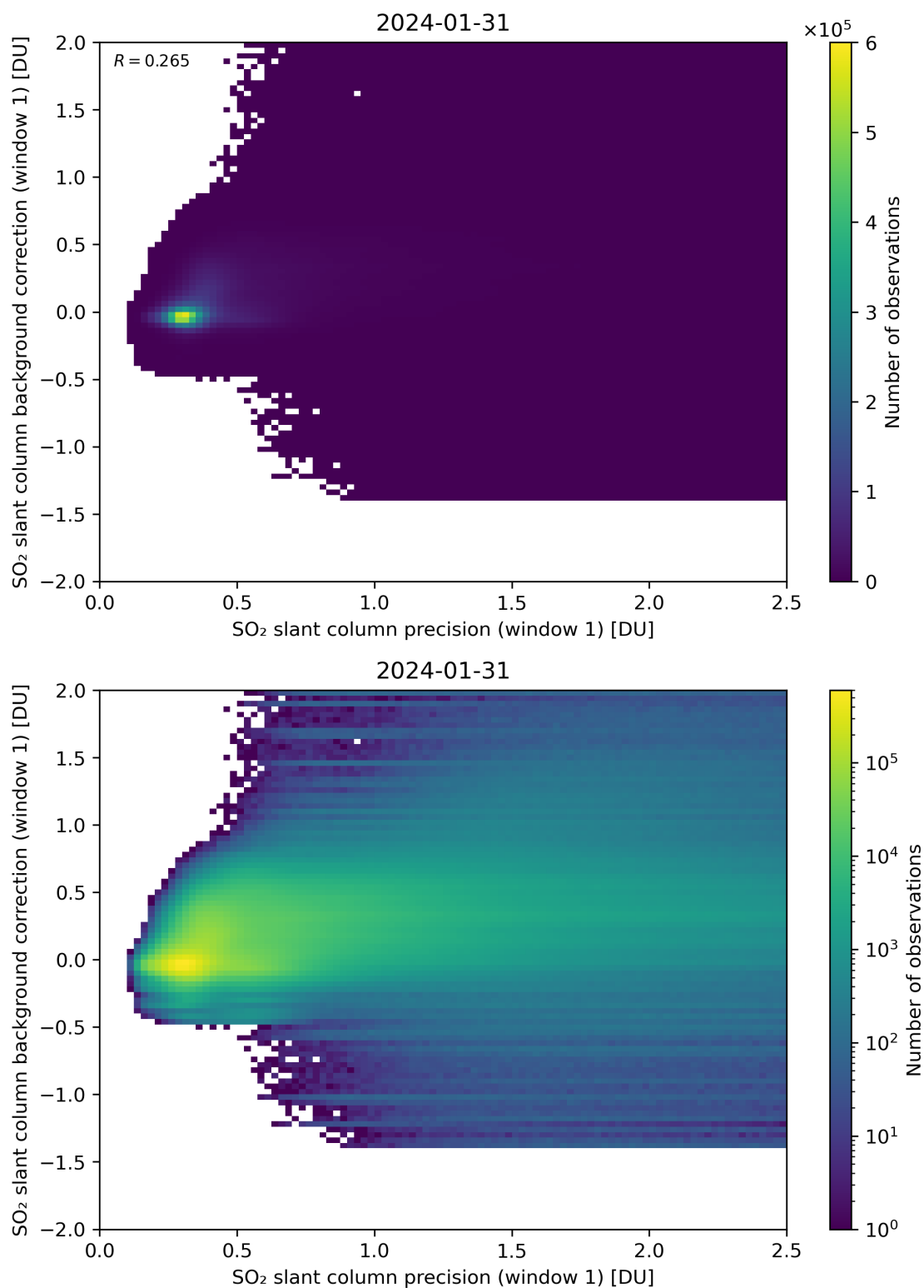
Figure 218: Scatter density plot of “SO 2 slant column precision (window 1)” against “SO 2 slant column background correction (window 1)” for 2024-01-31 to 2024-02-01.
