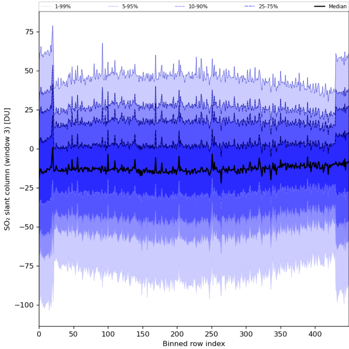
Figure 87: Along track statistics of “SO 2 slant column (window 3)” for 2024-01-31 to 2024-02-01
