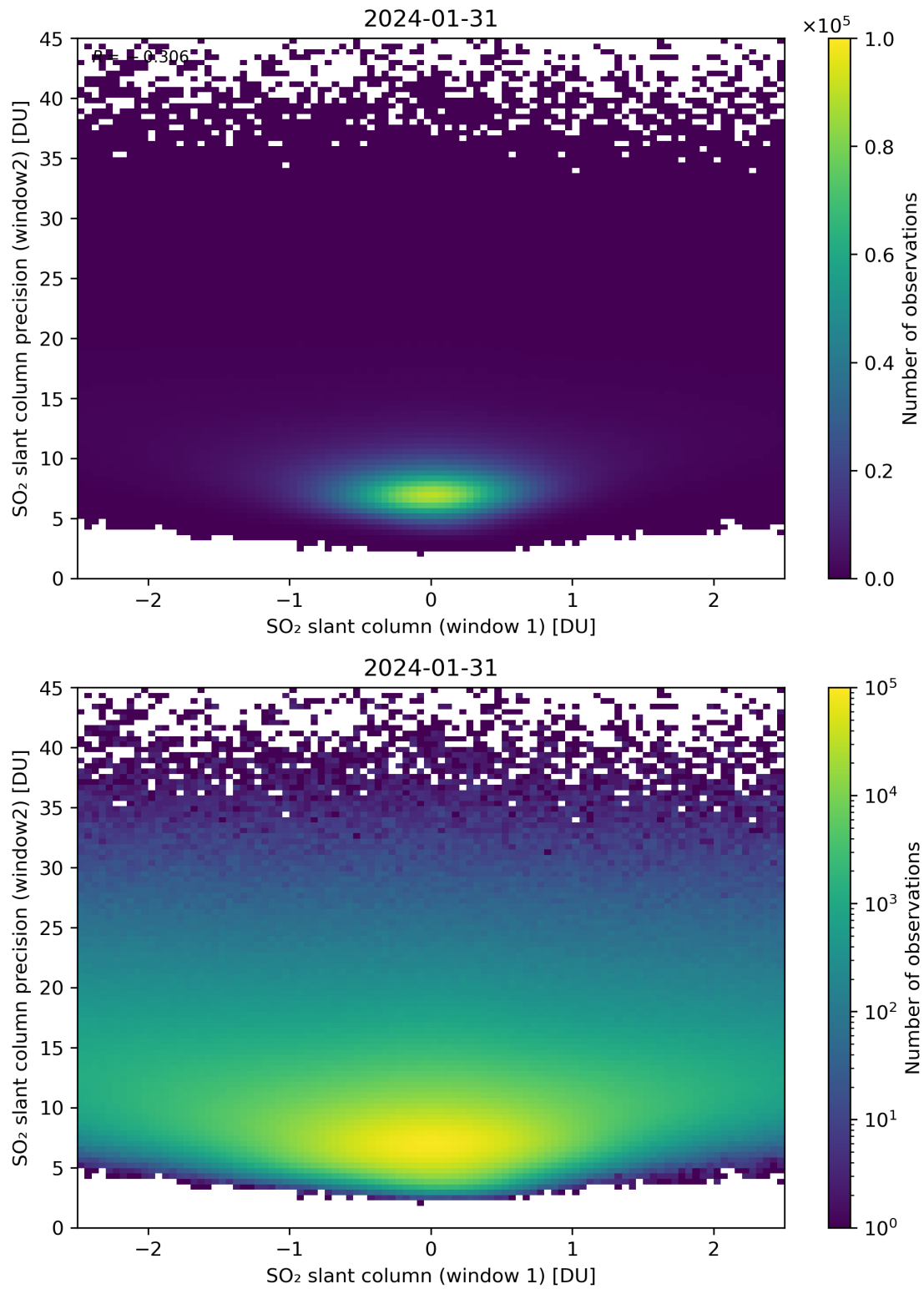
Figure 236: Scatter density plot of “SO 2 slant column (window 1)” against “SO 2 slant column precision (window2)” for 2024-01-31 to 2024-02-01.
