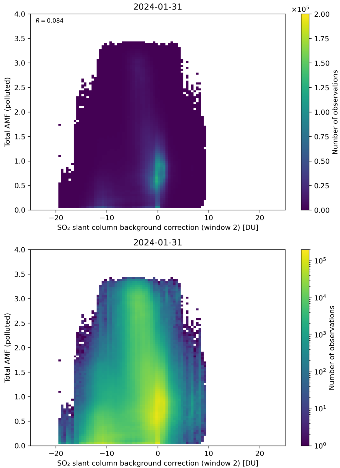
Figure 119: Scatter density plot of “SO 2 slant column background correction (window 2)” against “Total AMF (polluted)” for 2024-01-31 to 2024-02-01.
