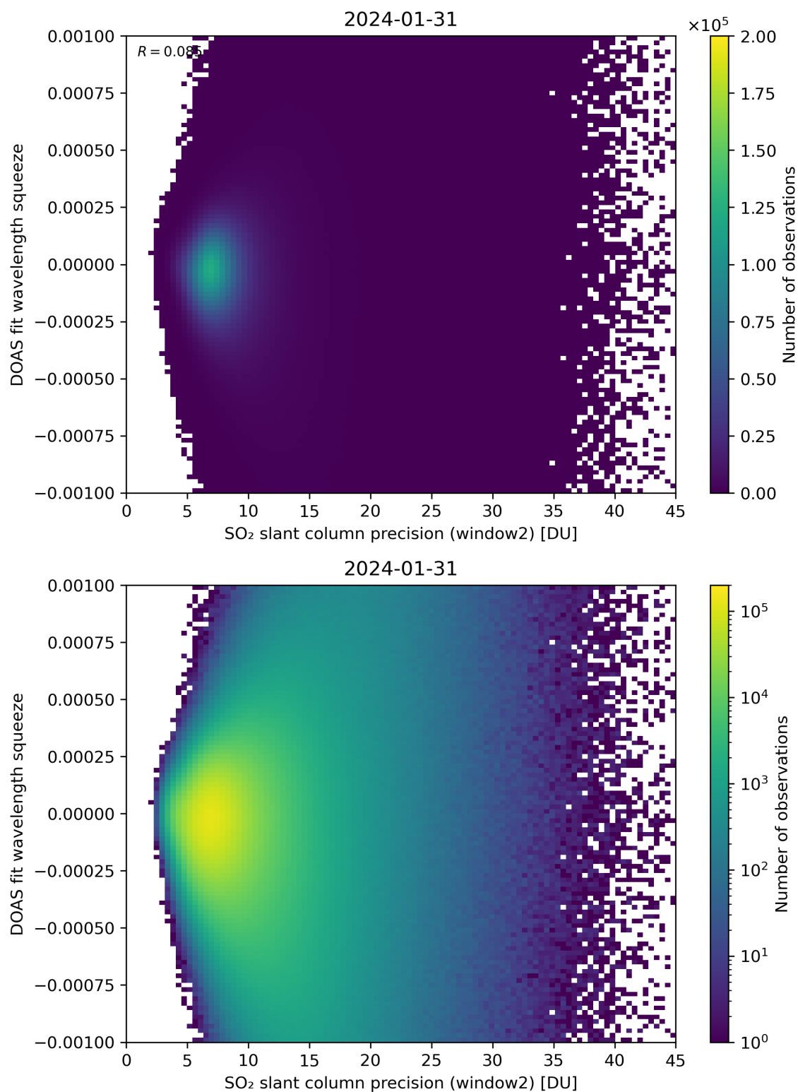
Figure 244: Scatter density plot of “SO 2 slant column precision (window2)” against “DOAS fit wavelength squeeze” for 2024-01-31 to 2024-02-01.
