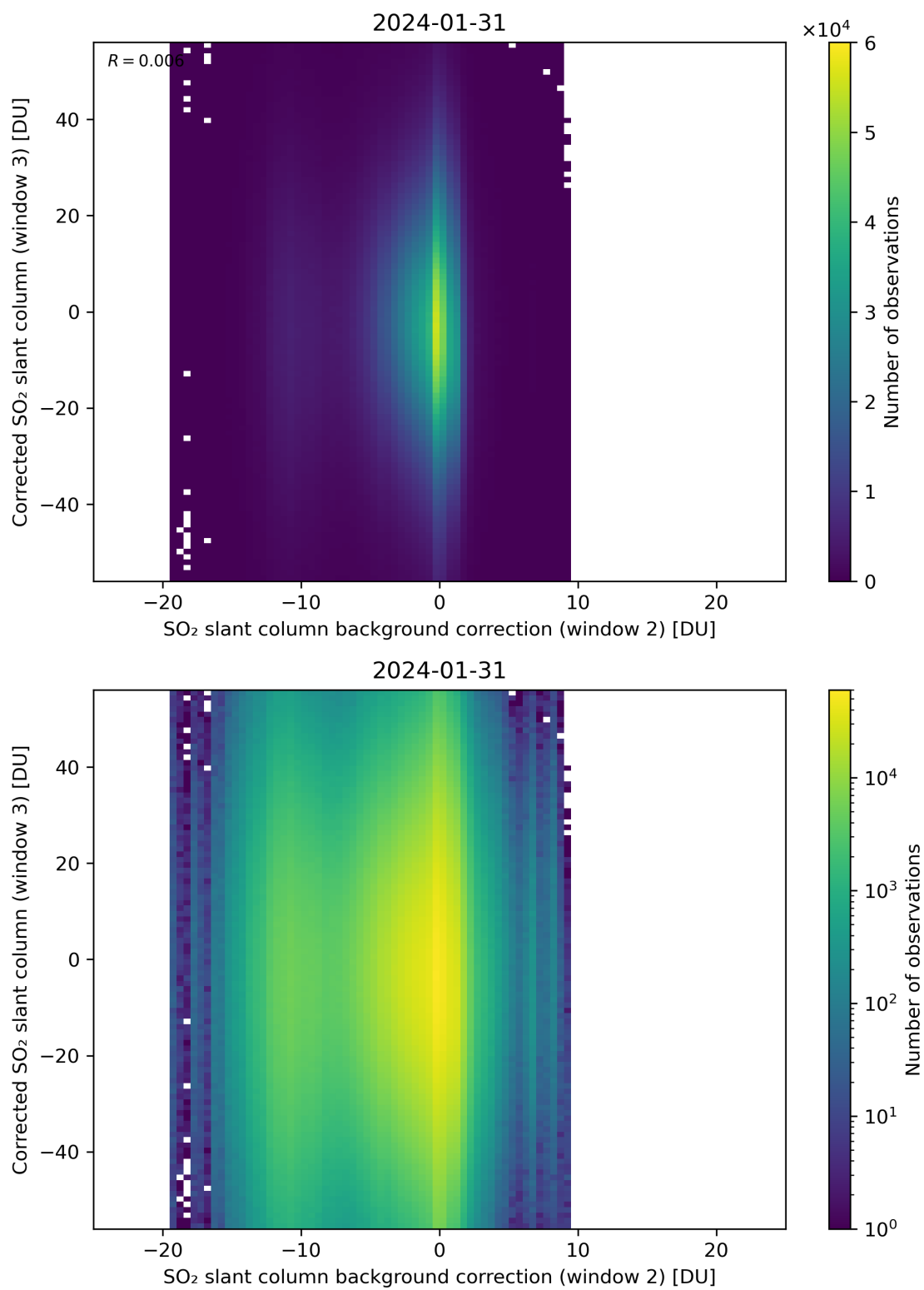
Figure 116: Scatter density plot of “SO 2 slant column background correction (window 2)” against “Corrected SO 2 slant column (window 3)” for 2024-01-31 to 2024-02-01.
