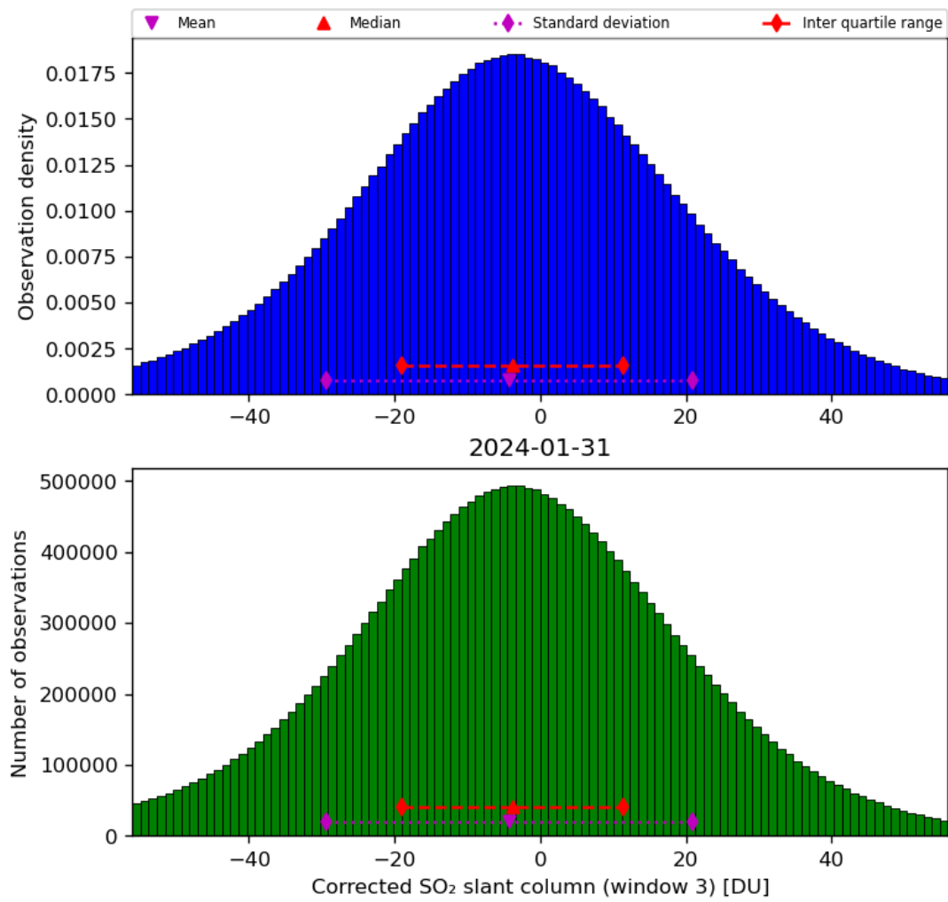
Figure 66: Histogram of “Corrected SO 2 slant column (window 3)” for 2024-01-31 to 2024-02-01
