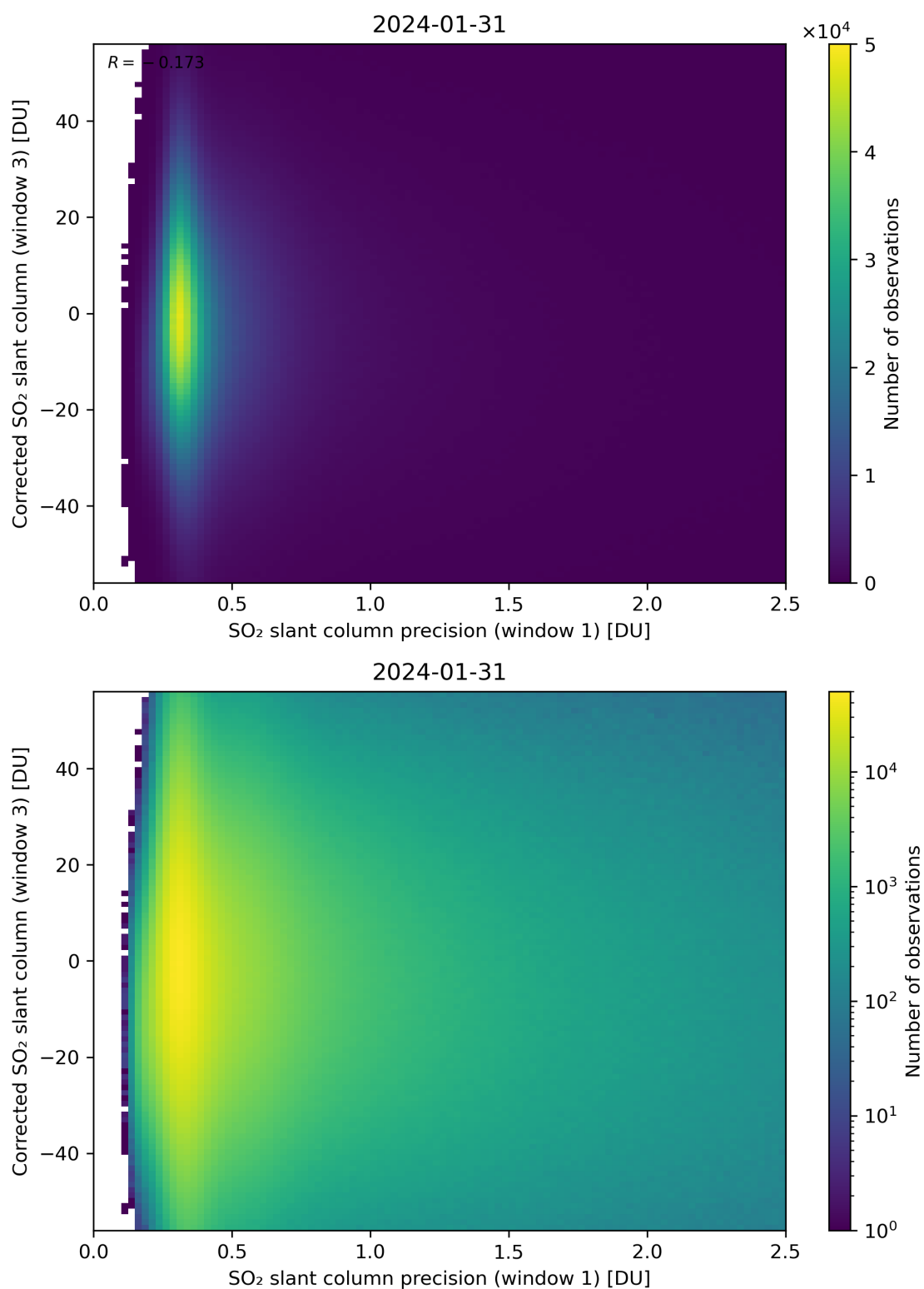
Figure 226: Scatter density plot of “SO 2 slant column precision (window 1)” against “Corrected SO 2 slant column (window 3)” for 2024-01-31 to 2024-02-01.
