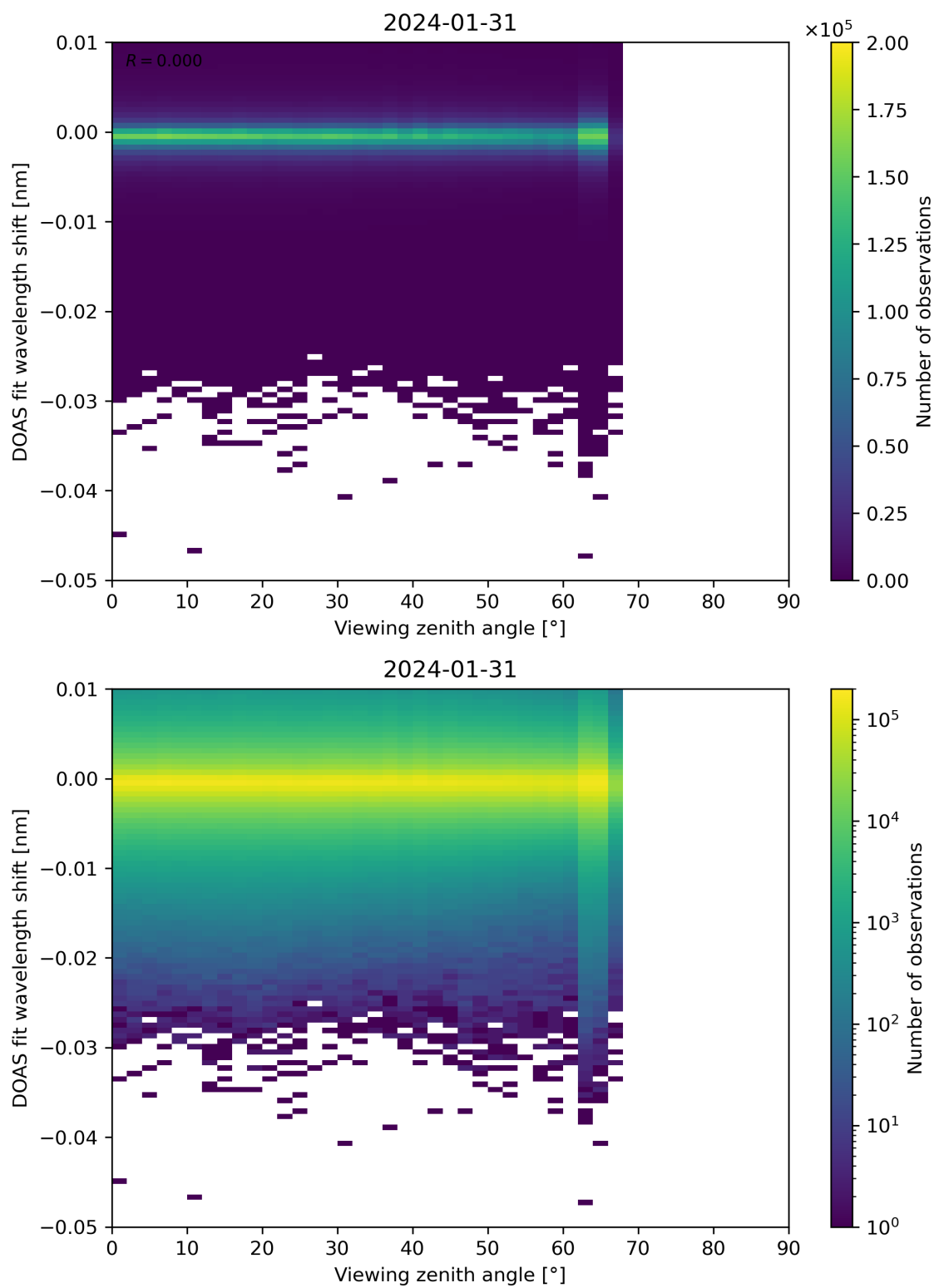
Figure 311: Scatter density plot of “Viewing zenith angle” against “DOAS fit wavelength shift” for 2024-01-31 to 2024-02-01.
