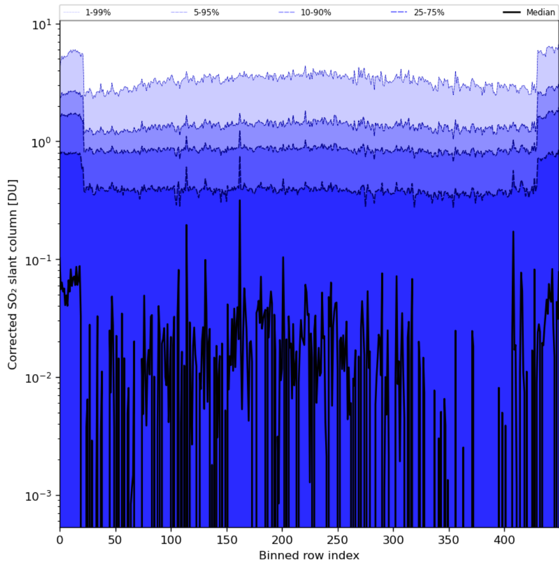
Figure 78: Along track statistics of “Corrected SO 2 slant column” for 2024-01-31 to 2024-02-01
