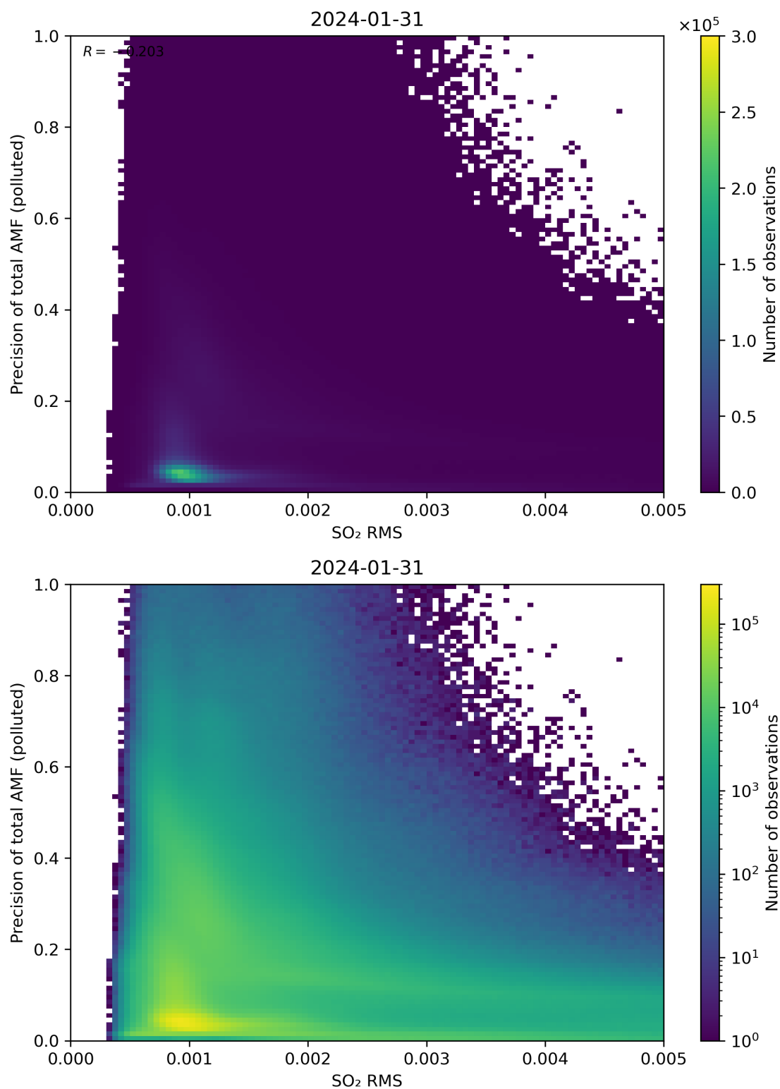
Figure 138: Scatter density plot of “SO 2 RMS” against “Precision of total AMF (polluted)” for 2024-01-31 to 2024-02-01.
