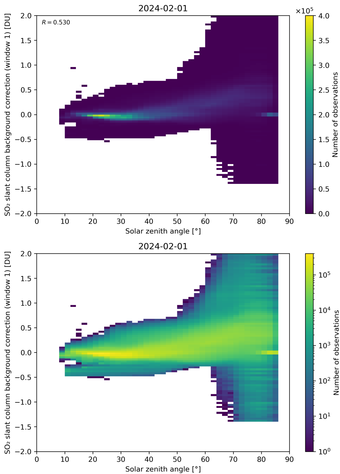
Figure 158: Scatter density plot of “Solar zenith angle” against “SO 2 slant column background correction (window 1)” for 2024-01-31 to 2024-02-02.
