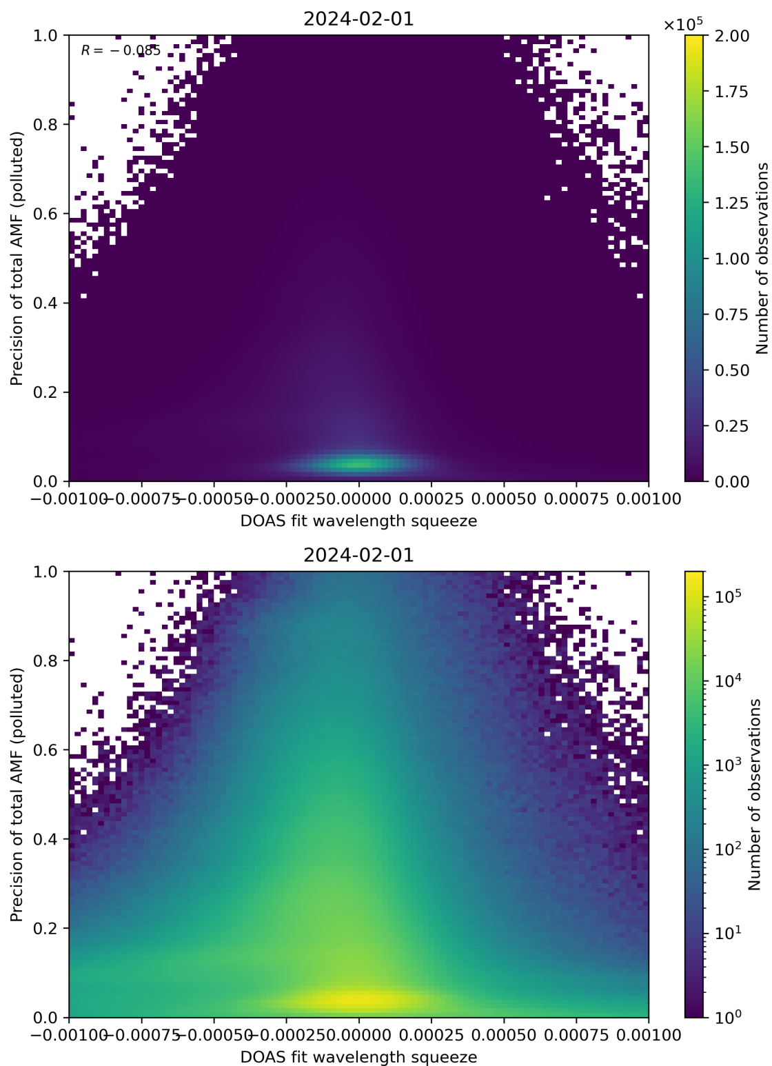
Figure 135: Scatter density plot of “DOAS fit wavelength squeeze” against “Precision of total AMF (polluted)” for 2024-01-31 to 2024-02-02.
