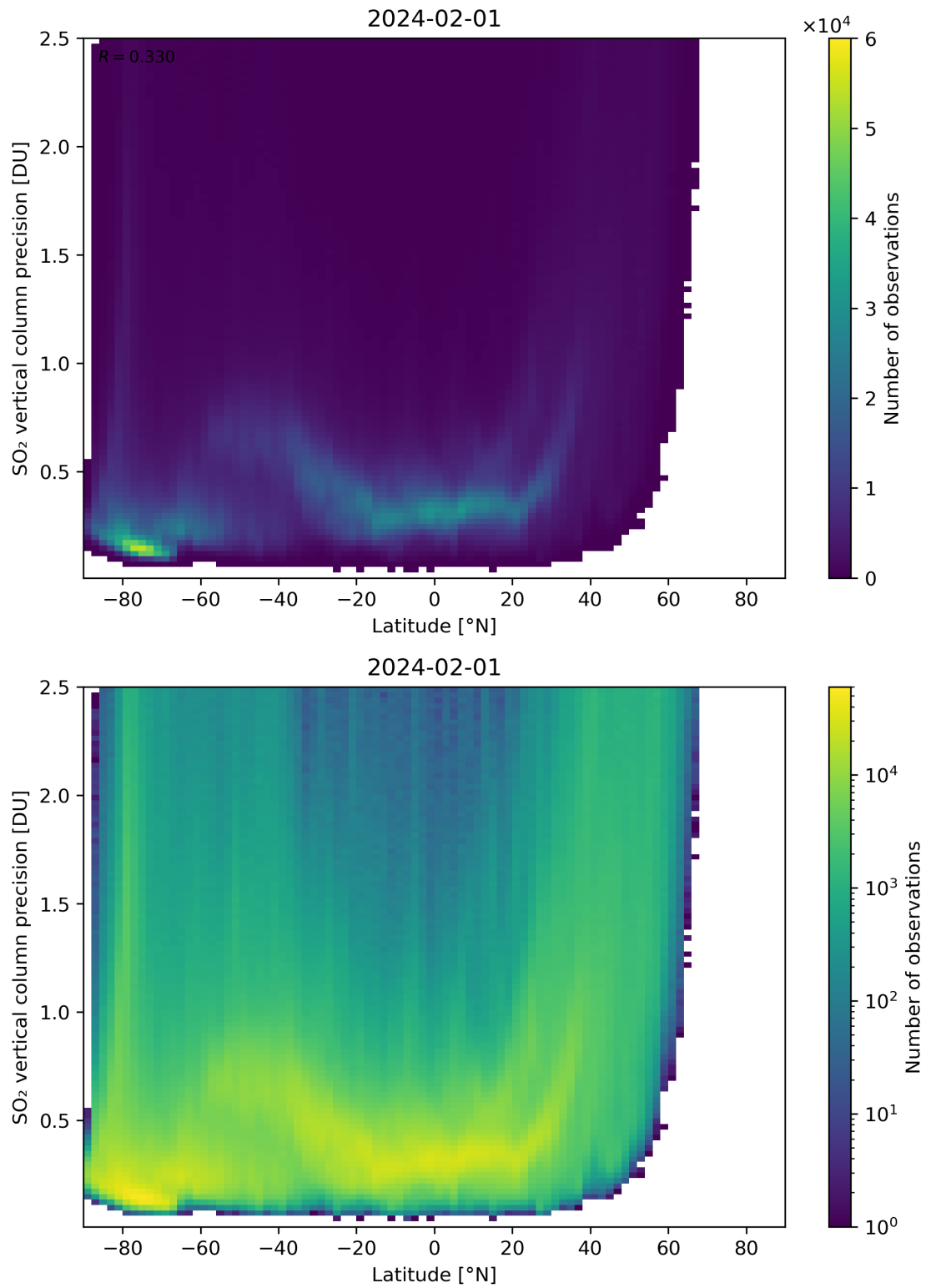
Figure 157: Scatter density plot of “Latitude” against “SO 2 vertical column precision” for 2024-01-31 to 2024-02-02.
