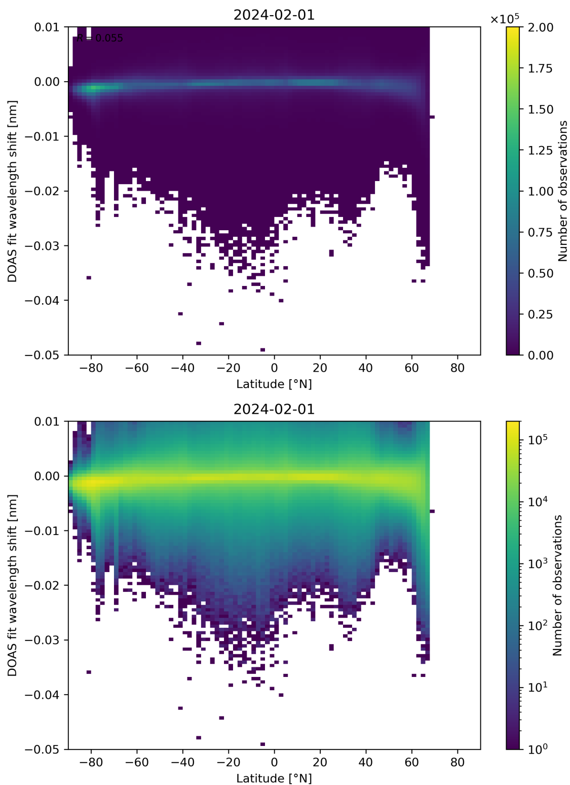
Figure 142: Scatter density plot of “Latitude” against “DOAS fit wavelength shift” for 2024-01-31 to 2024-02-02.
