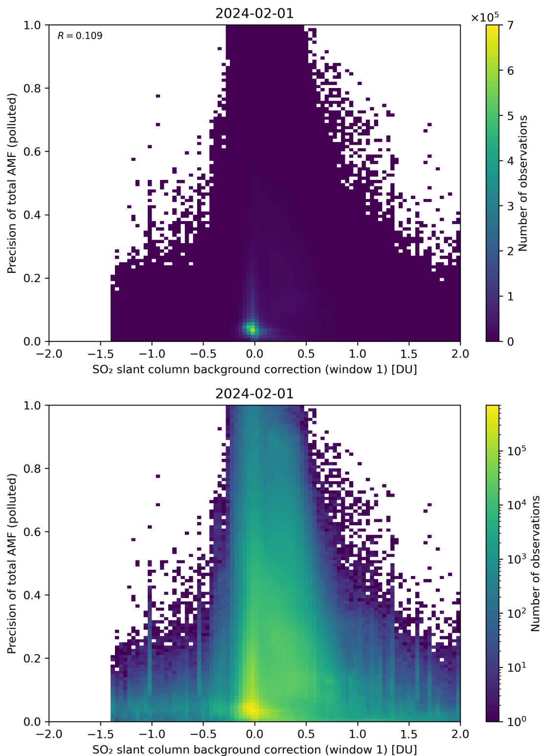
Figure 110: Scatter density plot of “SO 2 slant column background correction (window 1)” against “Precision of total AMF (polluted)” for 2024-01-31 to 2024-02-02.
