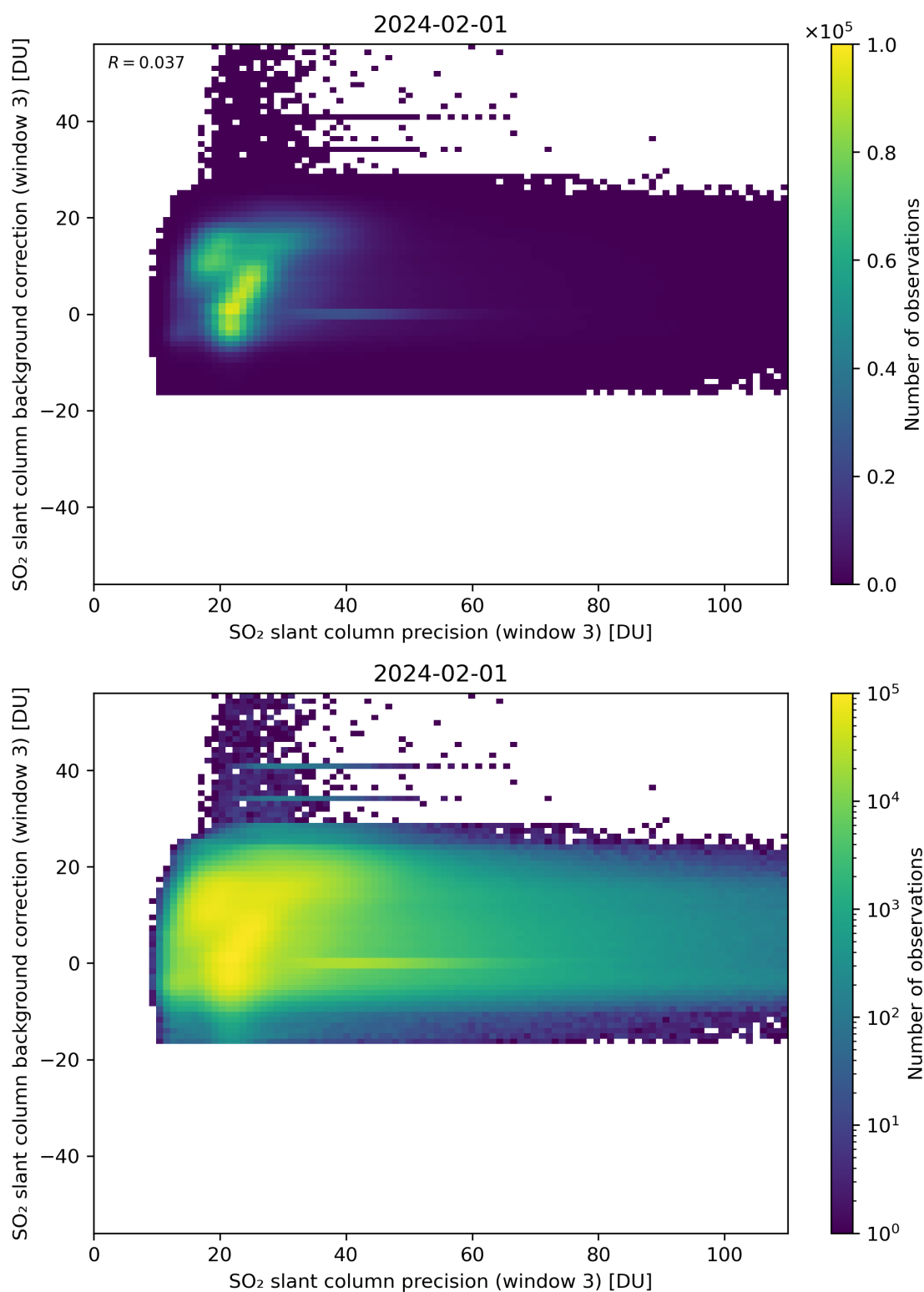
Figure 257: Scatter density plot of “SO 2 slant column precision (window 3)” against “SO 2 slant column background correction (window 3)” for 2024-01-31 to 2024-02-02.
