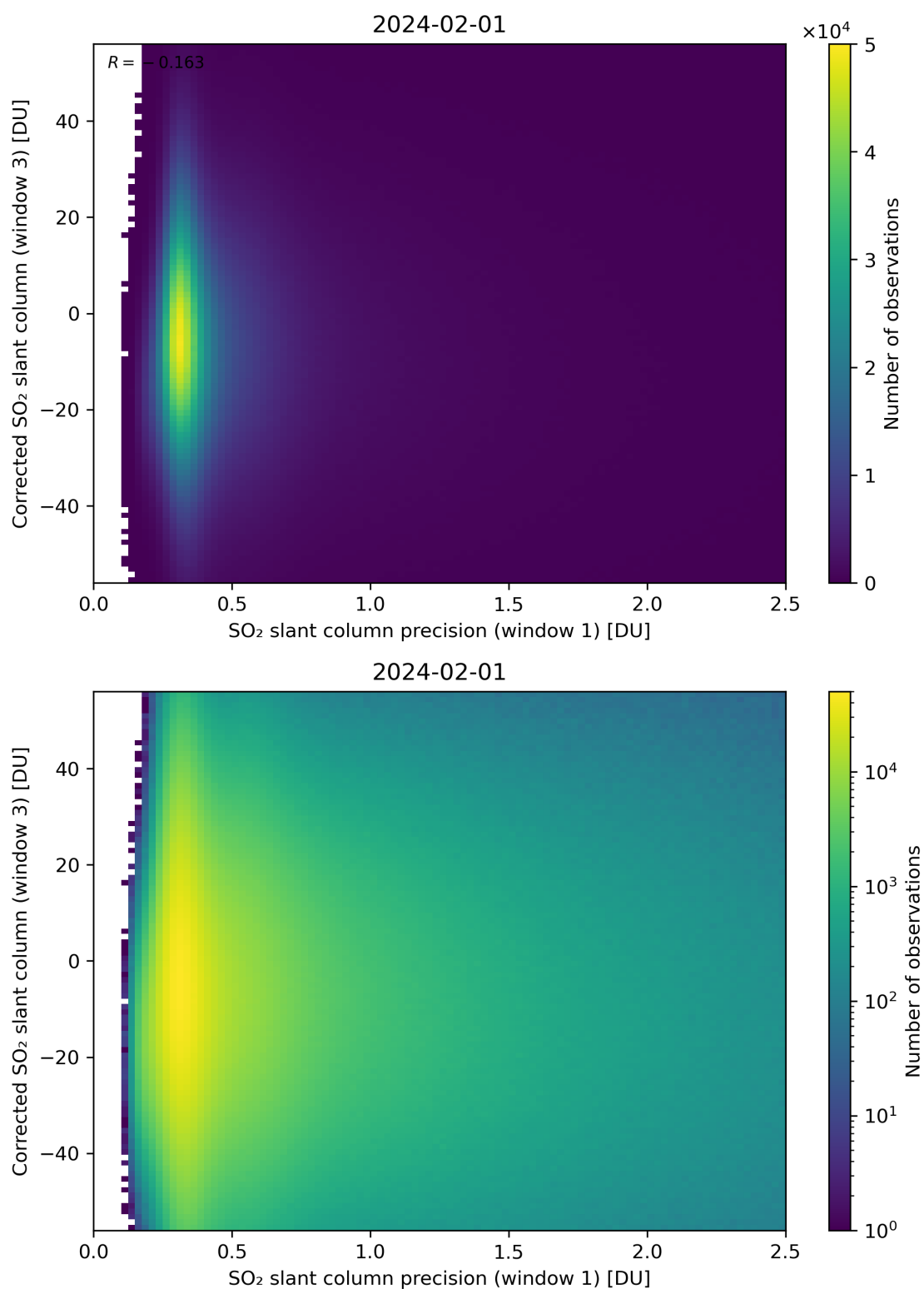
Figure 226: Scatter density plot of “SO 2 slant column precision (window 1)” against “Corrected SO 2 slant column (window 3)” for 2024-01-31 to 2024-02-02.
