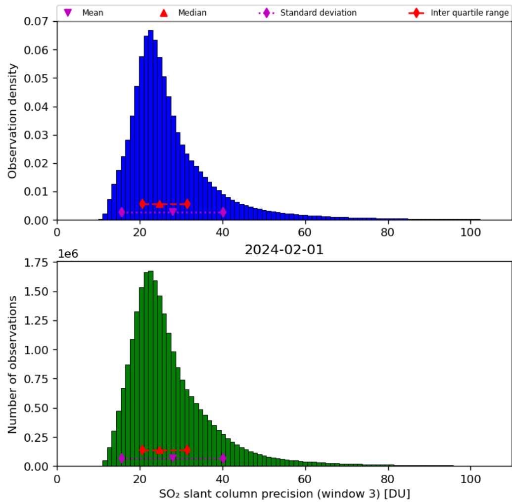
Figure 65: Histogram of “SO 2 slant column precision (window 3)” for 2024-01-31 to 2024-02-02
