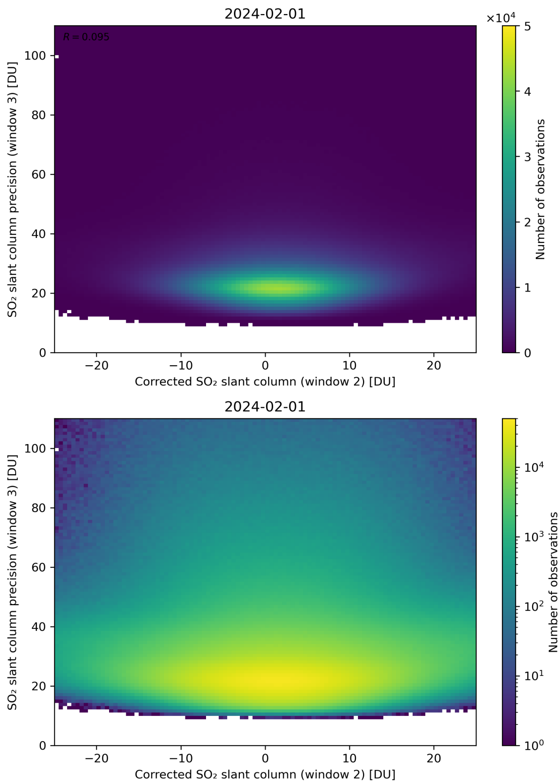
Figure 202: Scatter density plot of “Corrected SO 2 slant column (window 2)” against “SO 2 slant column precision (window 3)” for 2024-01-31 to 2024-02-02.
