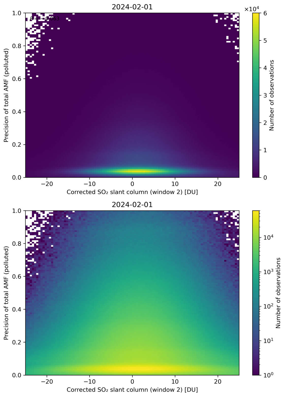
Figure 204: Scatter density plot of “Corrected SO 2 slant column (window 2)” against “Precision of total AMF (polluted)” for 2024-01-31 to 2024-02-02.
