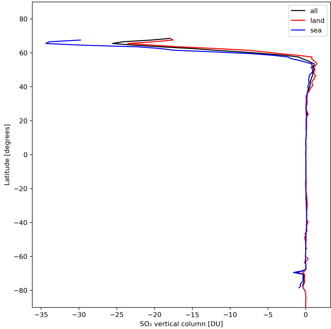
Figure 30: Zonal average of “SO 2 vertical column” for 2024-01-31 to 2024-02-02.
