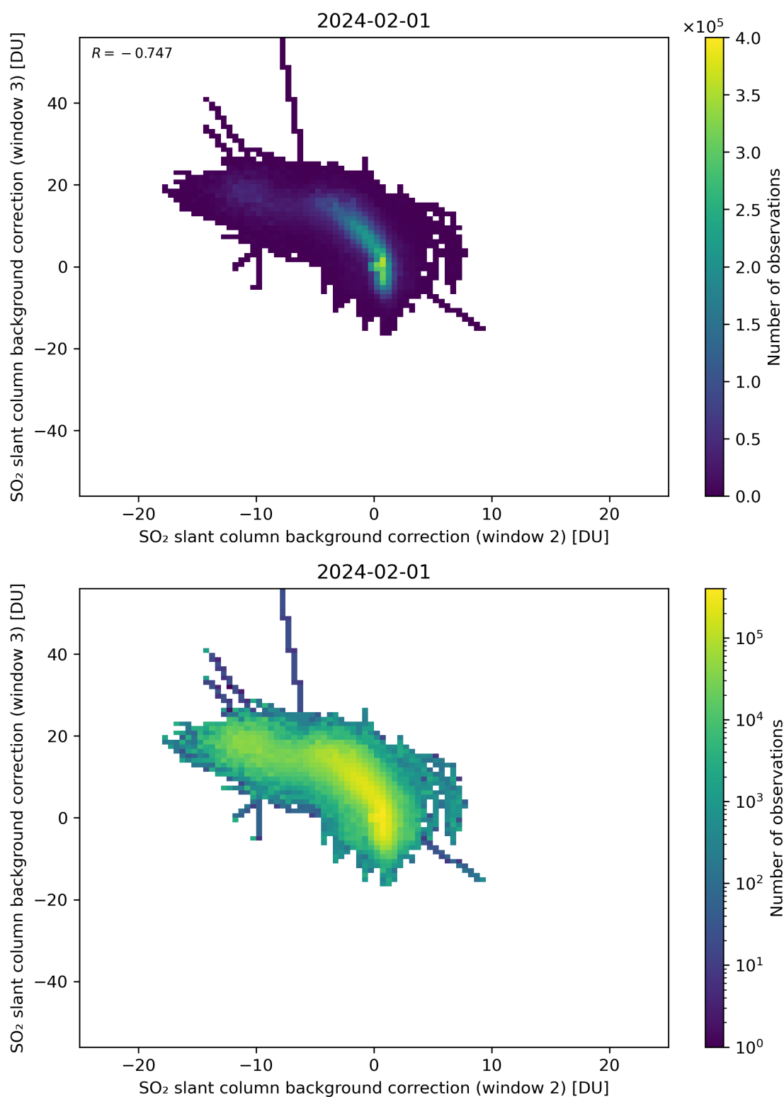
Figure 111: Scatter density plot of “SO 2 slant column background correction (window 2)” against “SO 2 slant column background correction (window 3)” for 2024-01-31 to 2024-02-02.
