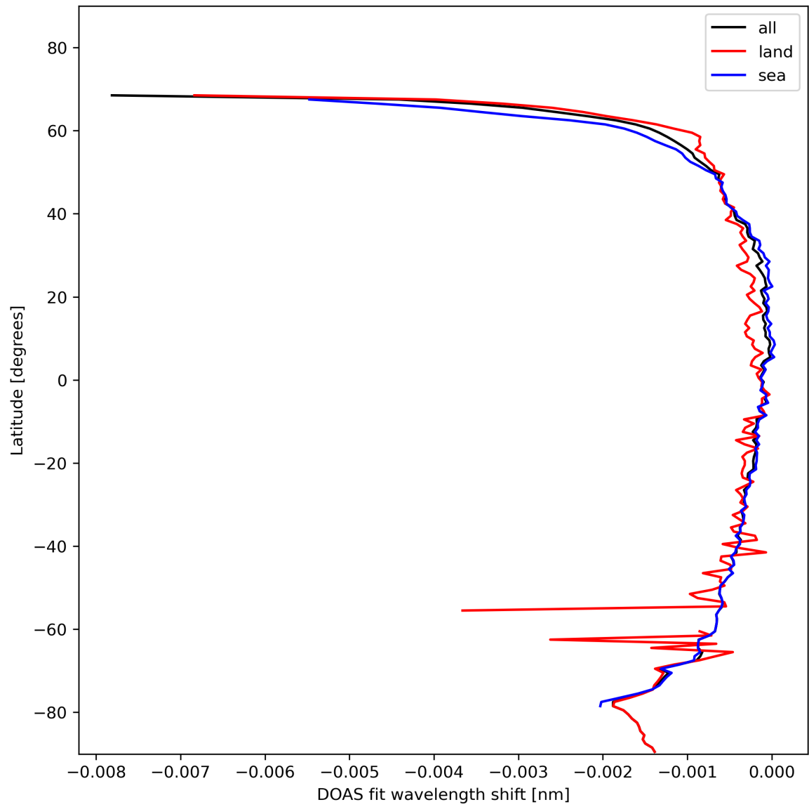
Figure 45: Zonal average of “DOAS fit wavelength shift” for 2024-01-31 to 2024-02-02.
