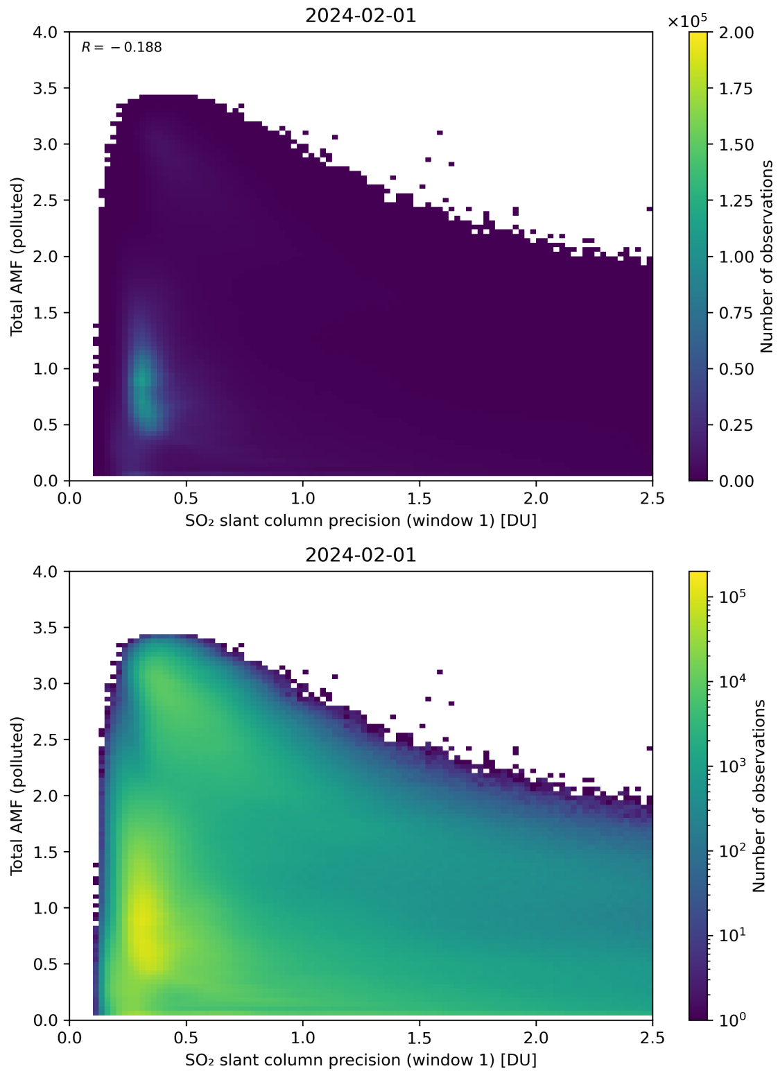
Figure 230: Scatter density plot of “SO 2 slant column precision (window 1)” against “Total AMF (polluted)” for 2024-01-31 to 2024-02-02.
