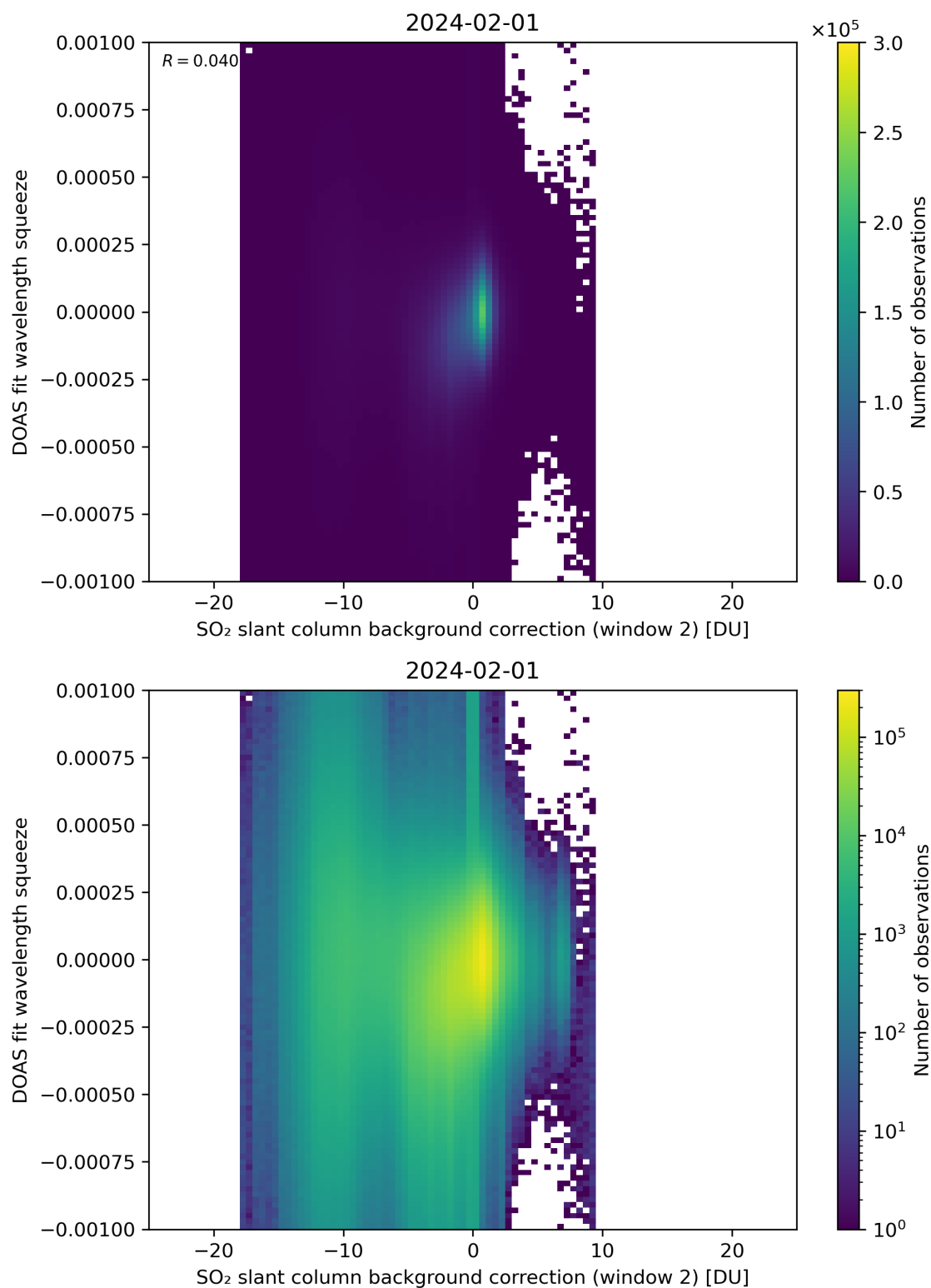
Figure 113: Scatter density plot of “SO 2 slant column background correction (window 2)” against “DOAS fit wavelength squeeze” for 2024-01-31 to 2024-02-02.
