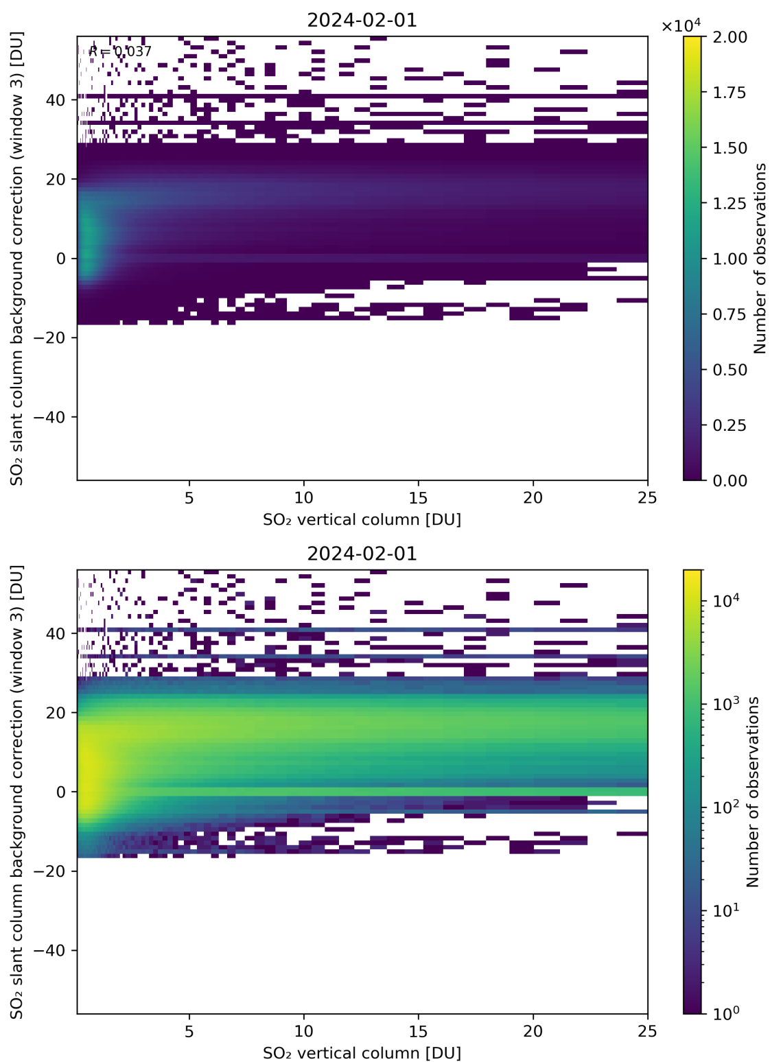
Figure 275: Scatter density plot of “SO 2 vertical column” against “SO 2 slant column background correction (window 3)” for 2024-01-31 to 2024-02-02.
