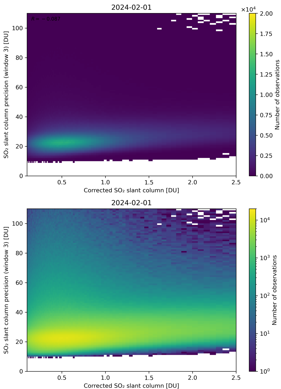
Figure 191: Scatter density plot of “Corrected SO 2 slant column” against “SO 2 slant column precision (window 3)” for 2024-01-31 to 2024-02-02.
