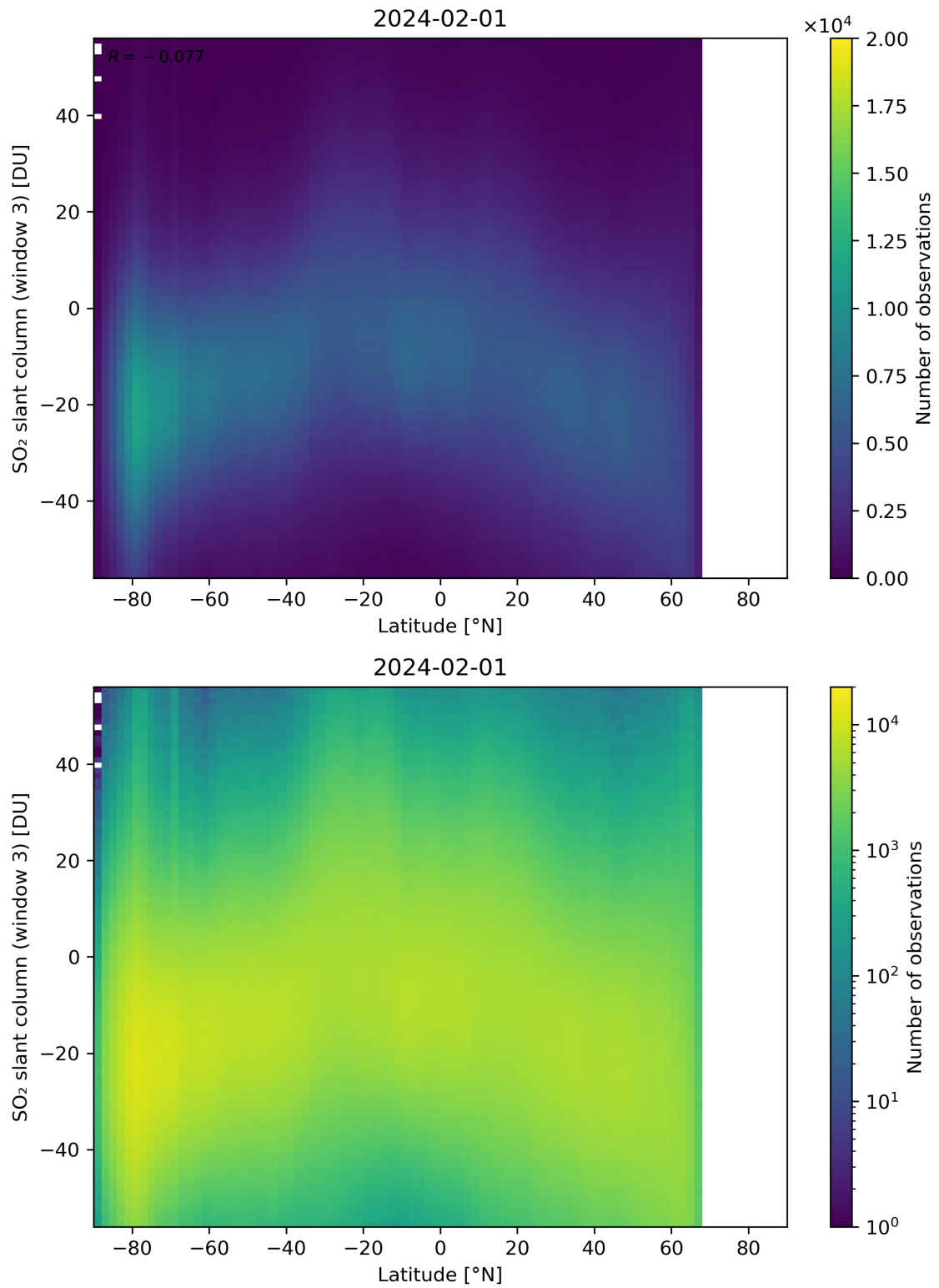
Figure 152: Scatter density plot of “Latitude” against “SO 2 slant column (window 3)” for 2024-01-31 to 2024-02-02.
