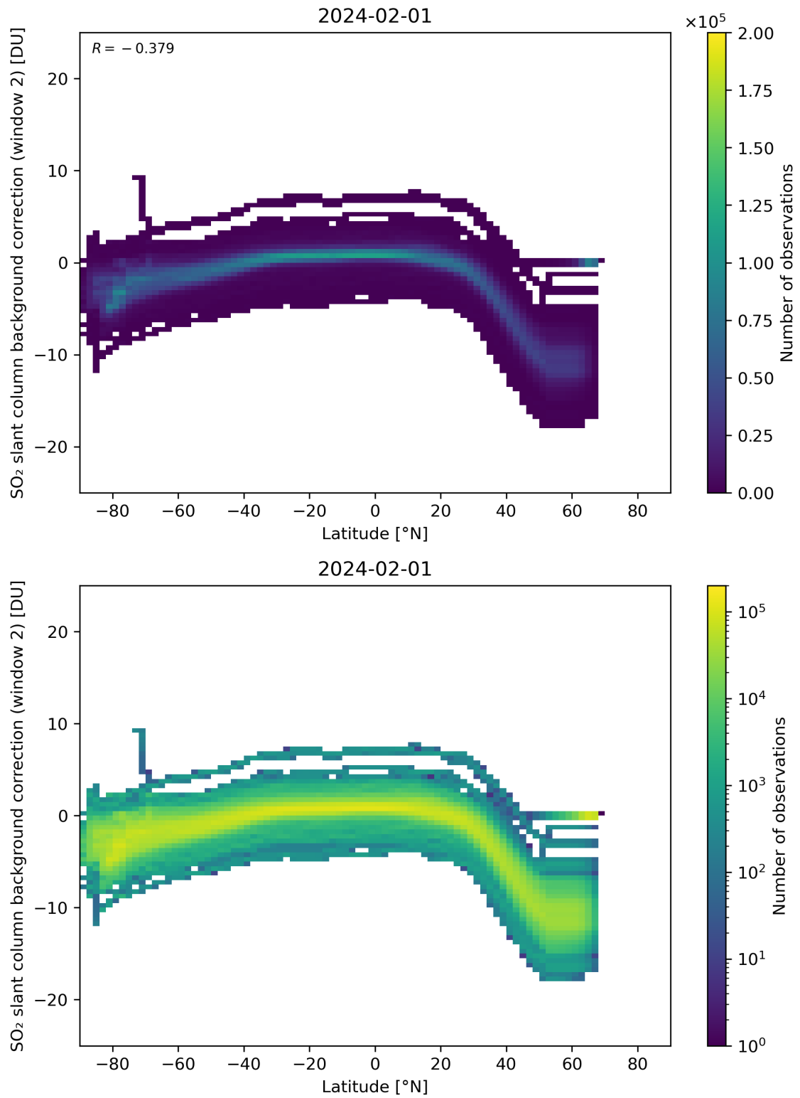
Figure 140: Scatter density plot of “Latitude” against “SO 2 slant column background correction (window 2)” for 2024-01-31 to 2024-02-02.
