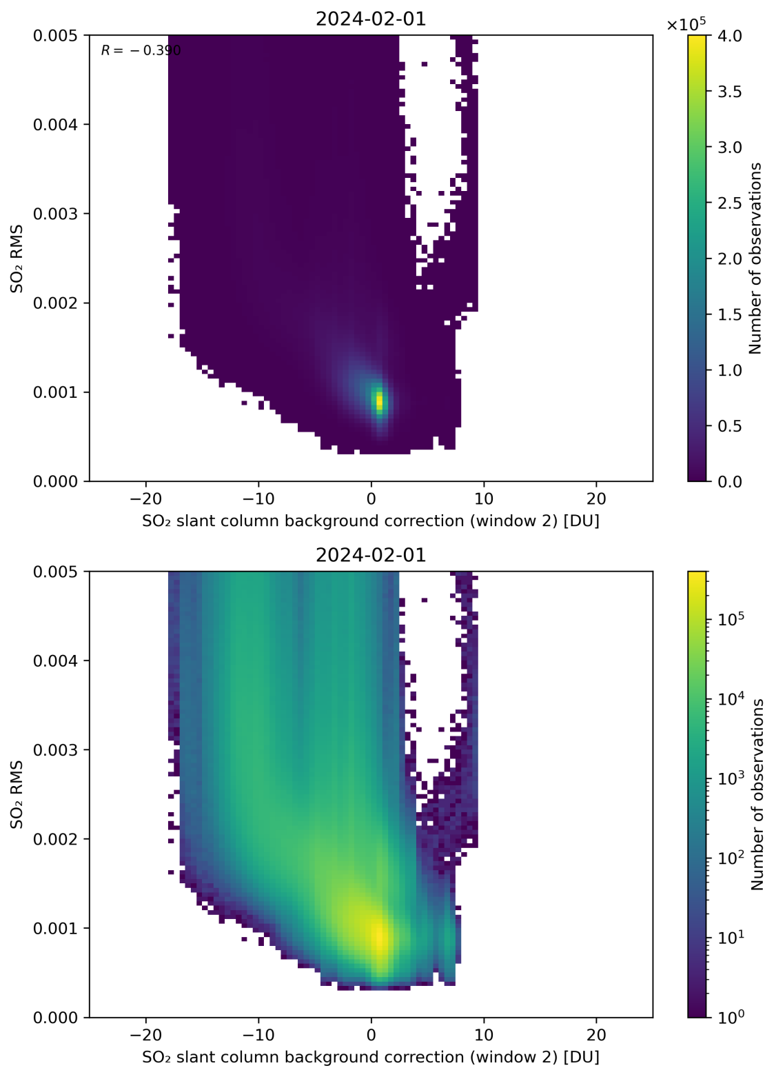
Figure 114: Scatter density plot of “SO 2 slant column background correction (window 2)” against “SO 2 RMS” for 2024-01-31 to 2024-02-02.
