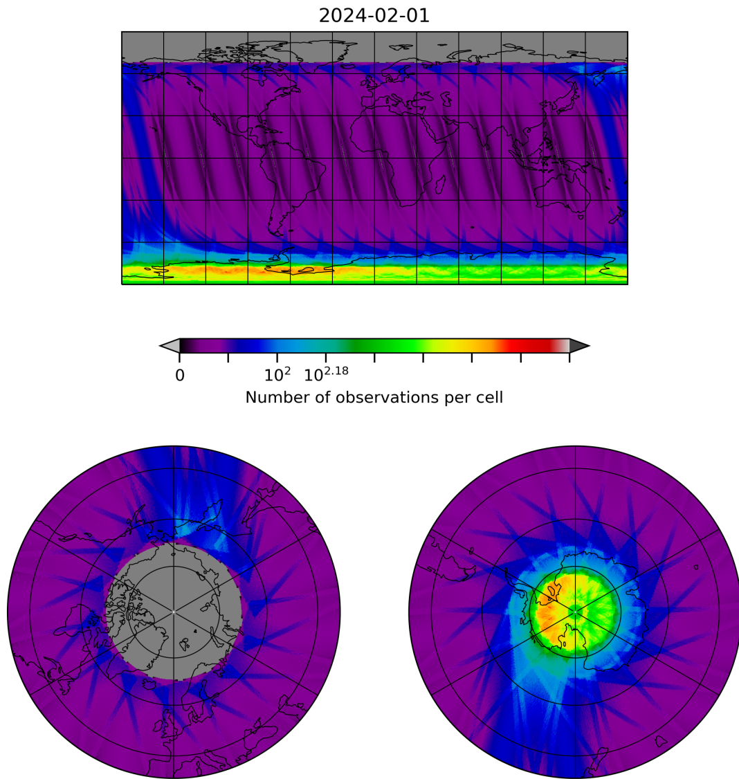
Figure 28: Map of the number of observations for 2024-01-31 to 2024-02-02
