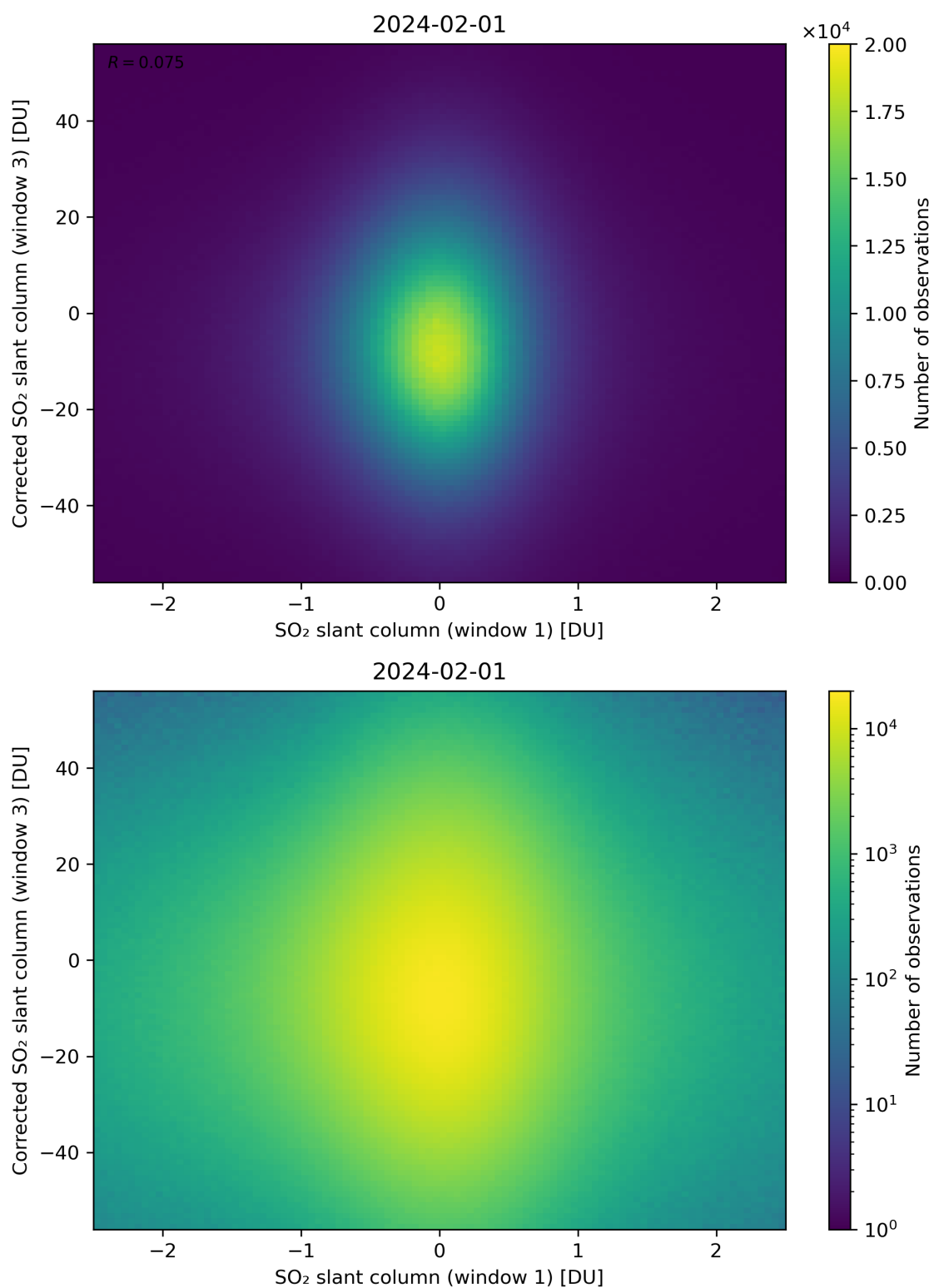
Figure 234: Scatter density plot of “SO 2 slant column (window 1)” against “Corrected SO 2 slant column (window 3)” for 2024-01-31 to 2024-02-02.
