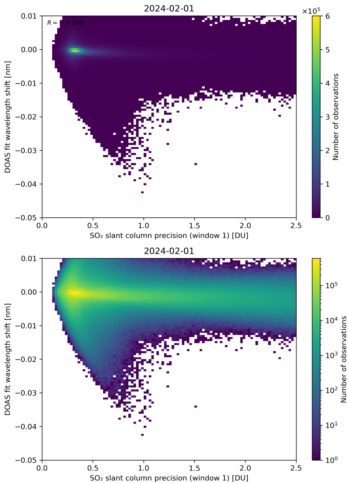
Figure 221: Scatter density plot of “SO 2 slant column precision (window 1)” against “DOAS fit wavelength shift” for 2024-01-31 to 2024-02-02.
