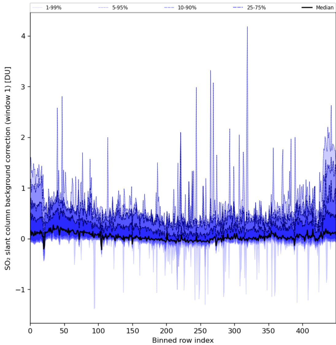
Figure 82: Along track statistics of “SO 2 slant column background correction (window 1)” for 2024-01-31 to 2024-02-02
