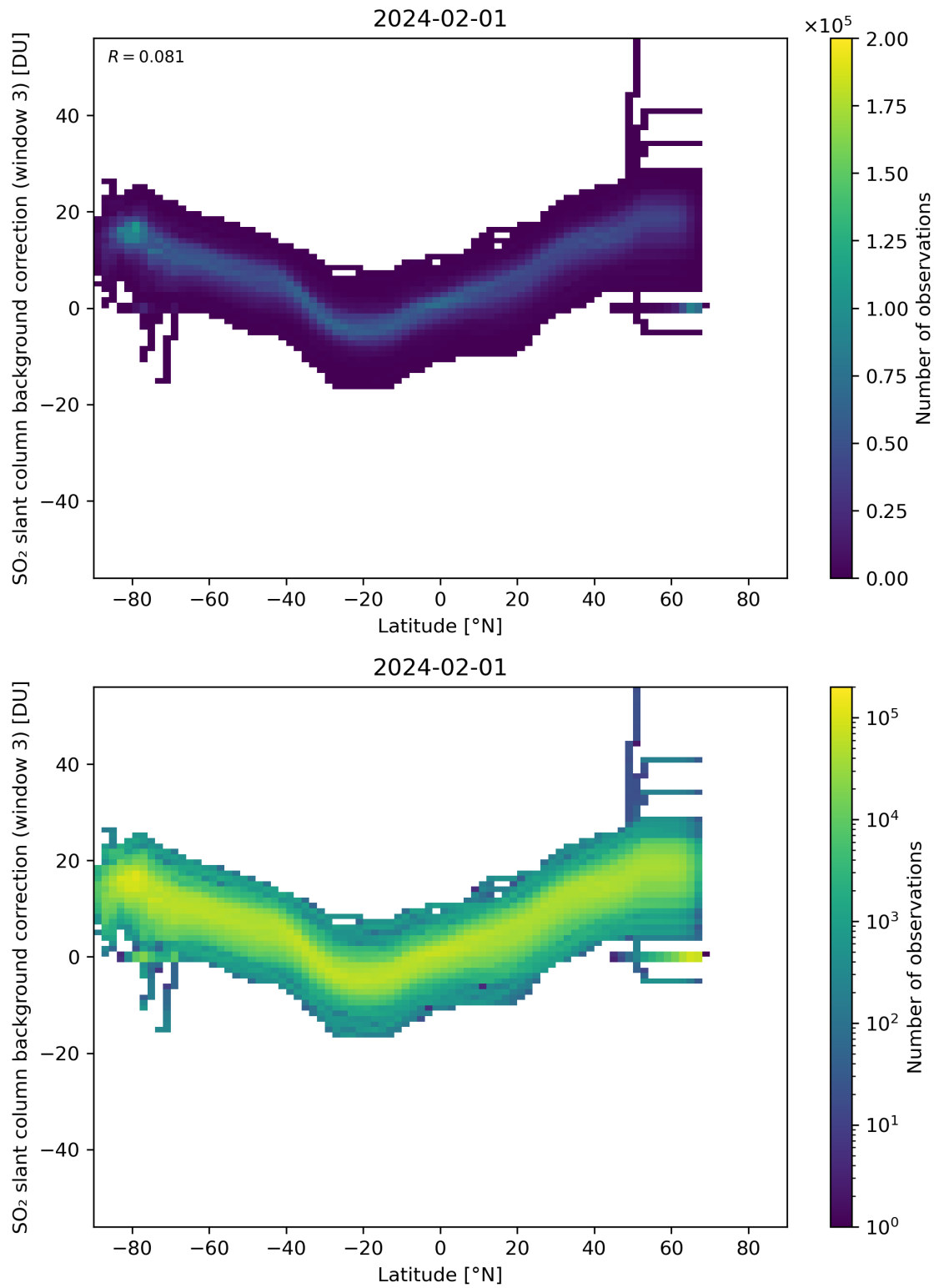
Figure 141: Scatter density plot of “Latitude” against “SO 2 slant column background correction (window 3)” for 2024-01-31 to 2024-02-02.
