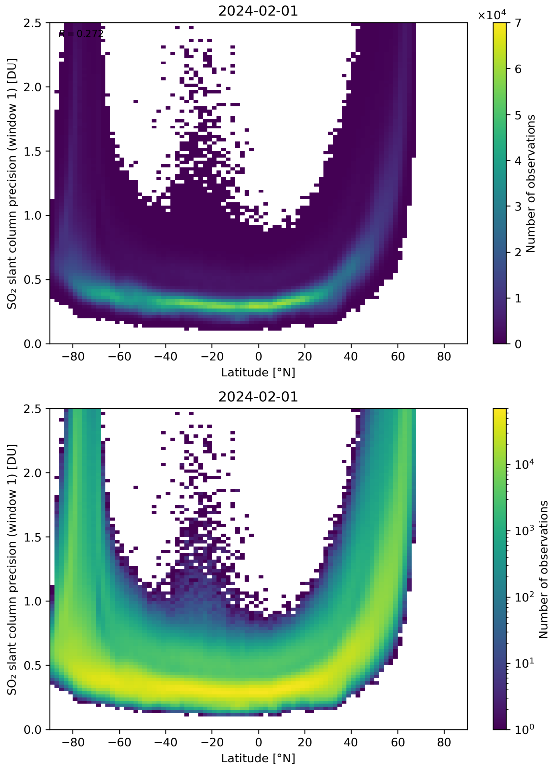
Figure 150: Scatter density plot of “Latitude” against “SO 2 slant column precision (window 1)” for 2024-01-31 to 2024-02-02.
