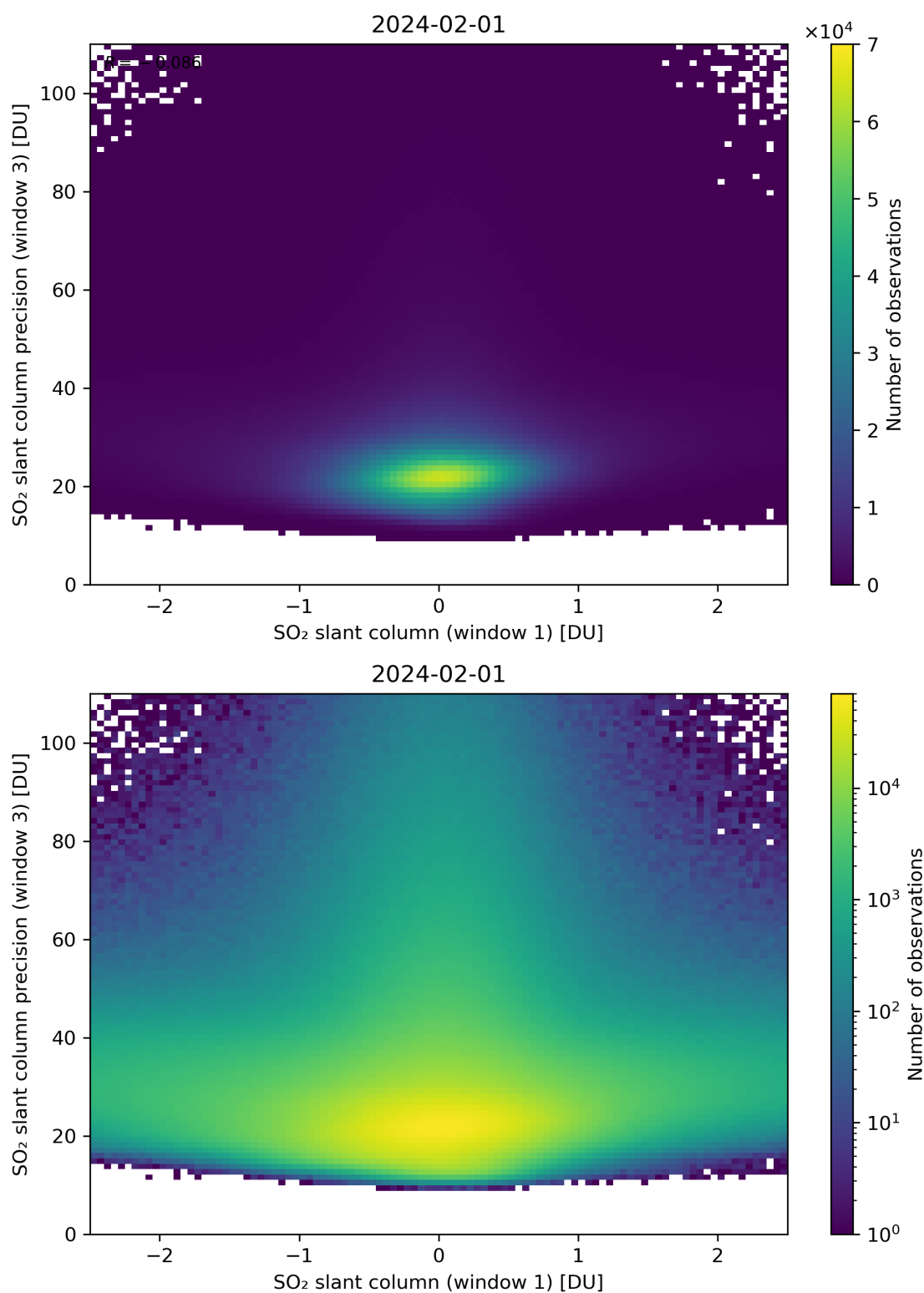
Figure 238: Scatter density plot of “SO 2 slant column (window 1)” against “SO 2 slant column precision (window 3)” for 2024-01-31 to 2024-02-02.
