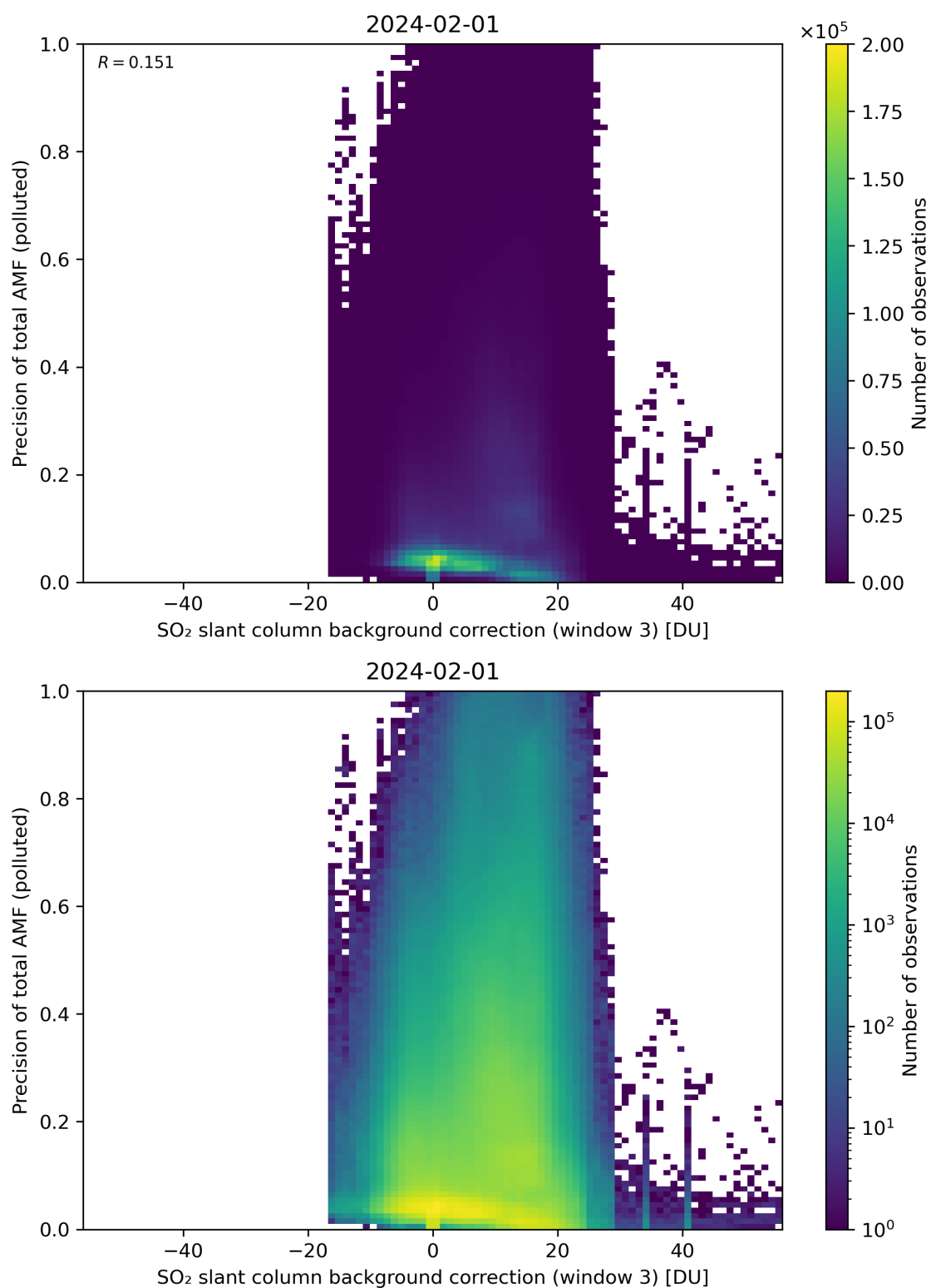
Figure 126: Scatter density plot of “SO 2 slant column background correction (window 3)” against “Precision of total AMF (polluted)” for 2024-01-31 to 2024-02-02.
