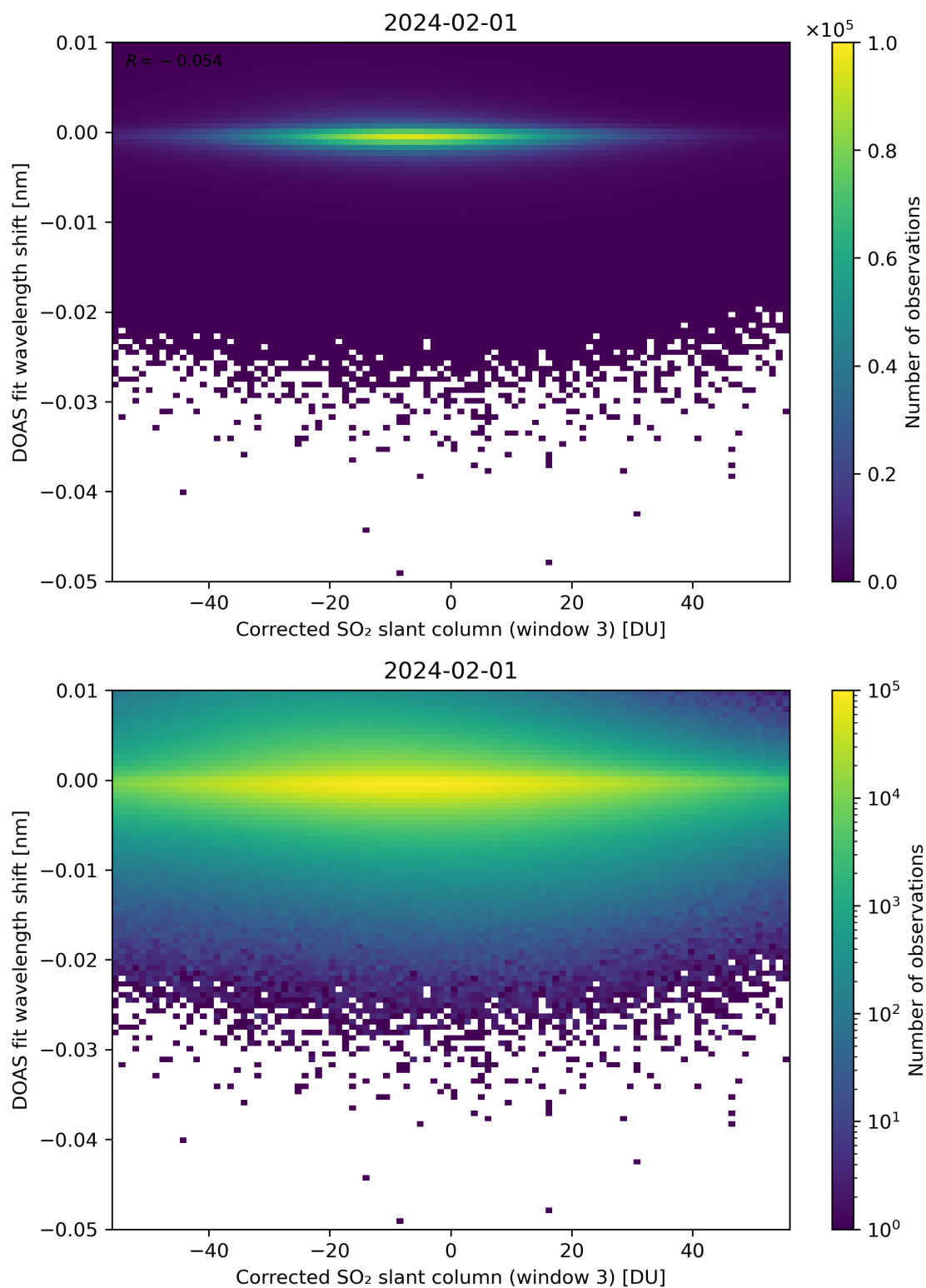
Figure 206: Scatter density plot of “Corrected SO 2 slant column (window 3)” against “DOAS fit wavelength shift” for 2024-01-31 to 2024-02-02.
