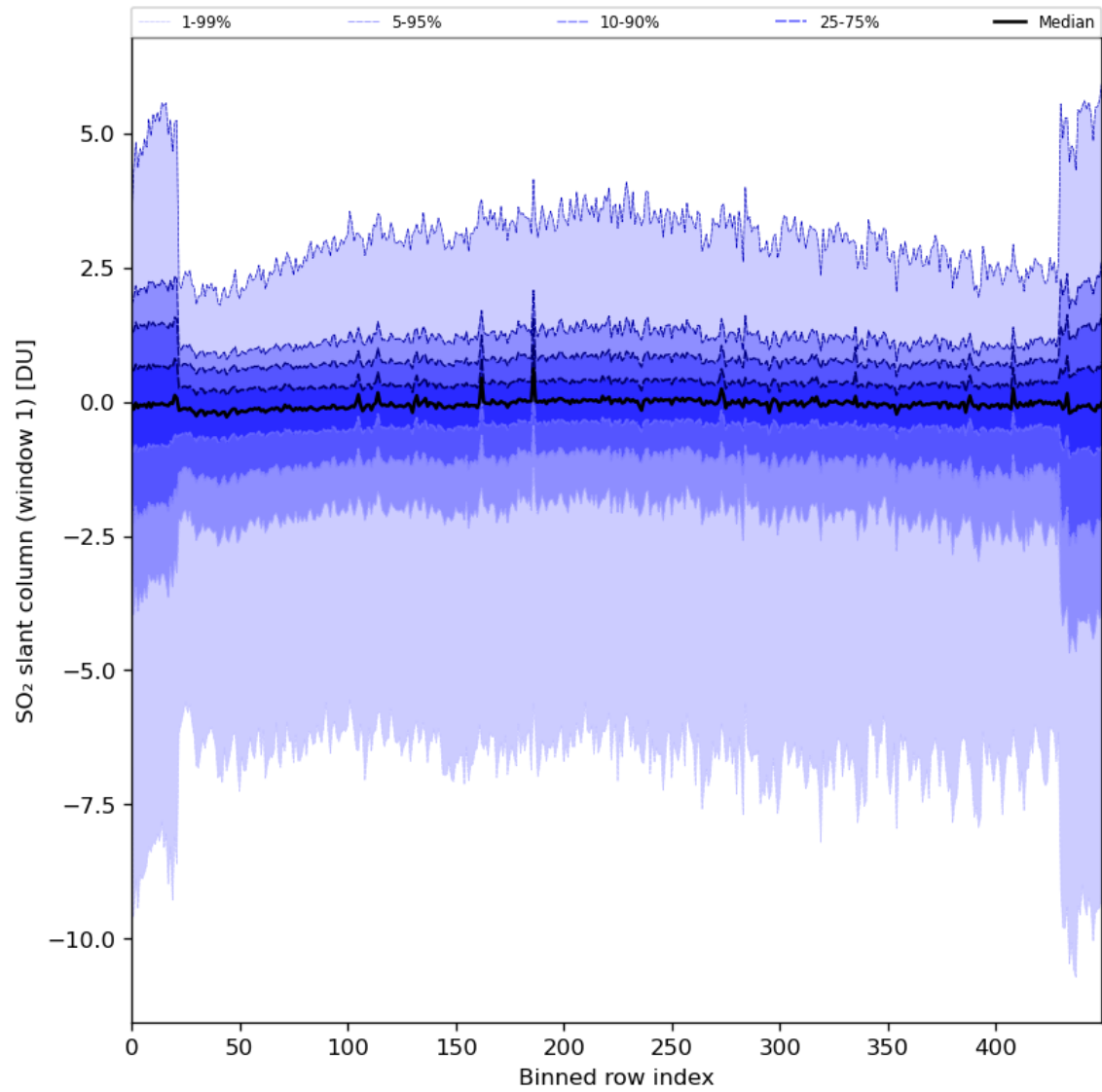
Figure 79: Along track statistics of “SO 2 slant column (window 1)” for 2024-01-31 to 2024-02-02
