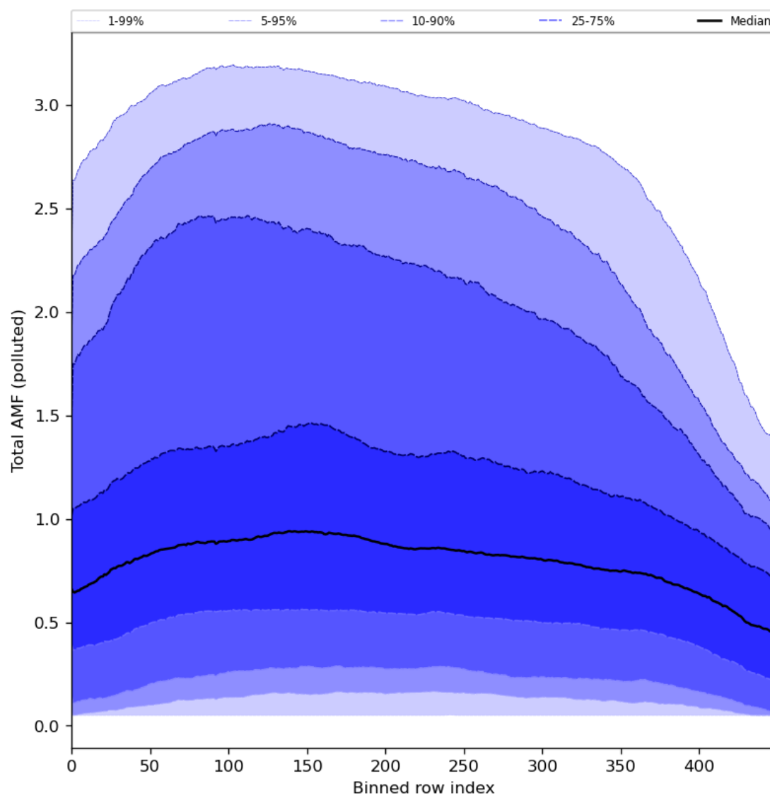
Figure 94: Along track statistics of “Total AMF (polluted)” for 2024-01-31 to 2024-02-02
