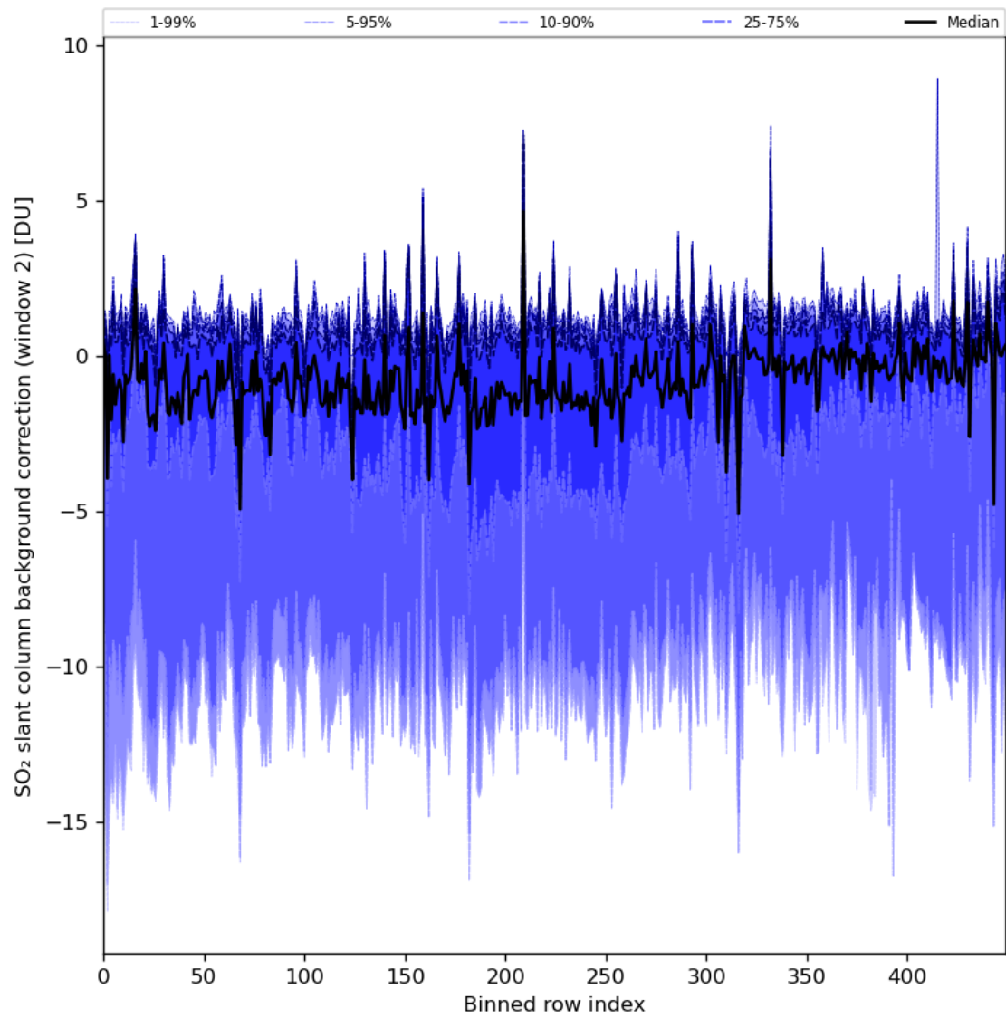
Figure 86: Along track statistics of “SO 2 slant column background correction (window 2)” for 2024-01-31 to 2024-02-02
