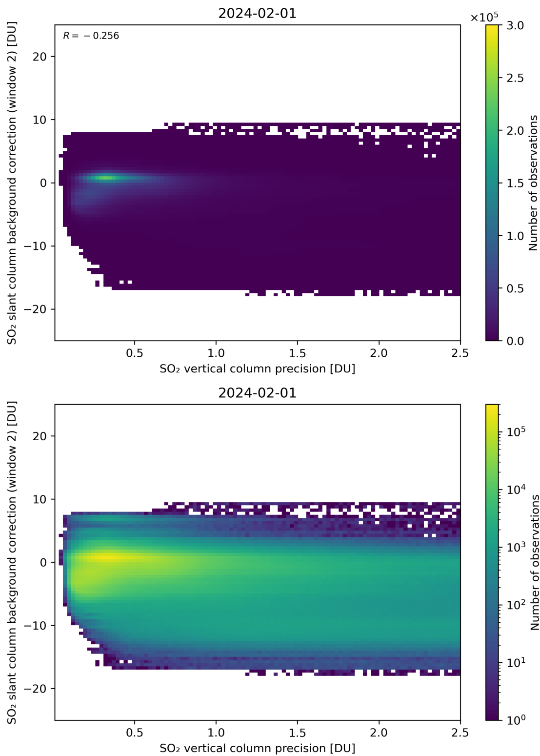
Figure 280: Scatter density plot of “SO 2 vertical column precision” against “SO 2 slant column background correction (window 2)” for 2024-01-31 to 2024-02-02.
