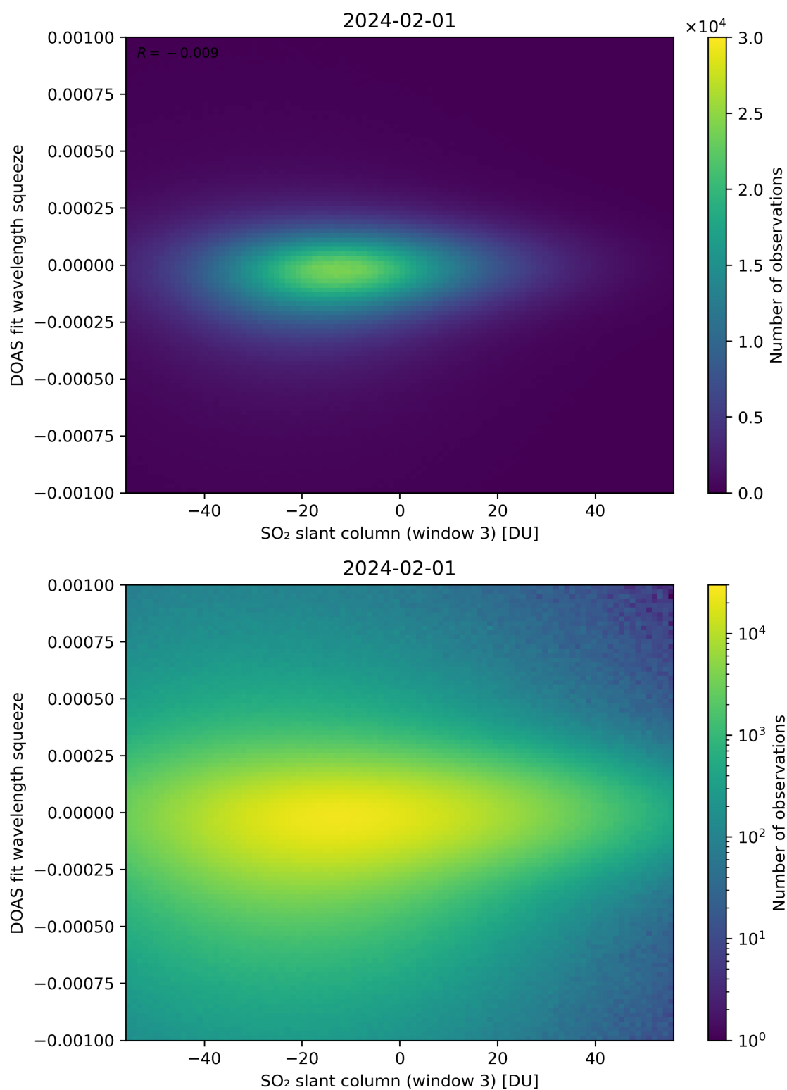
Figure 255: Scatter density plot of “SO 2 slant column (window 3)” against “DOAS fit wavelength squeeze” for 2024-01-31 to 2024-02-02.
