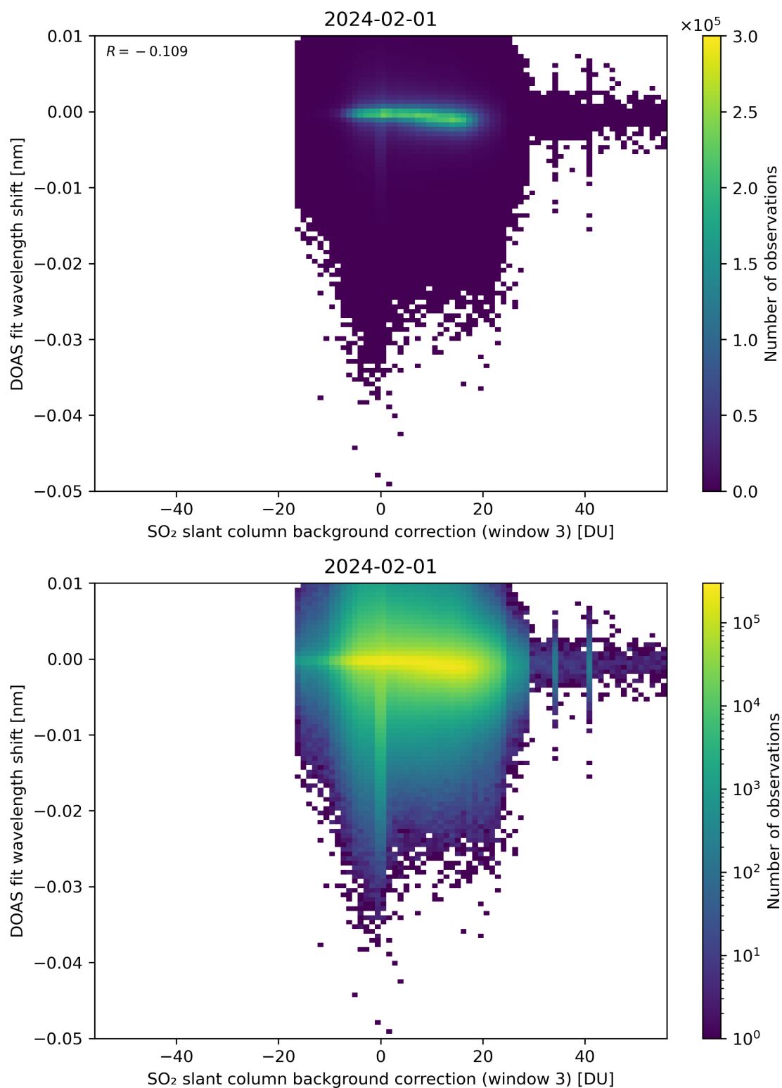
Figure 121: Scatter density plot of “SO 2 slant column background correction (window 3)” against “DOAS fit wavelength shift” for 2024-01-31 to 2024-02-02.
