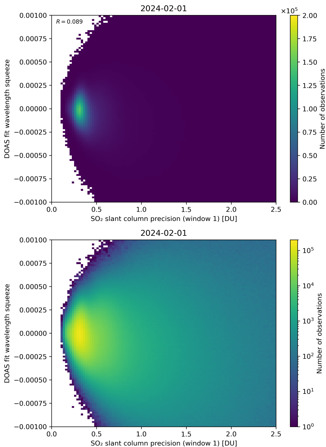
Figure 222: Scatter density plot of “SO 2 slant column precision (window 1)” against “DOAS fit wavelength squeeze” for 2024-01-31 to 2024-02-02.
