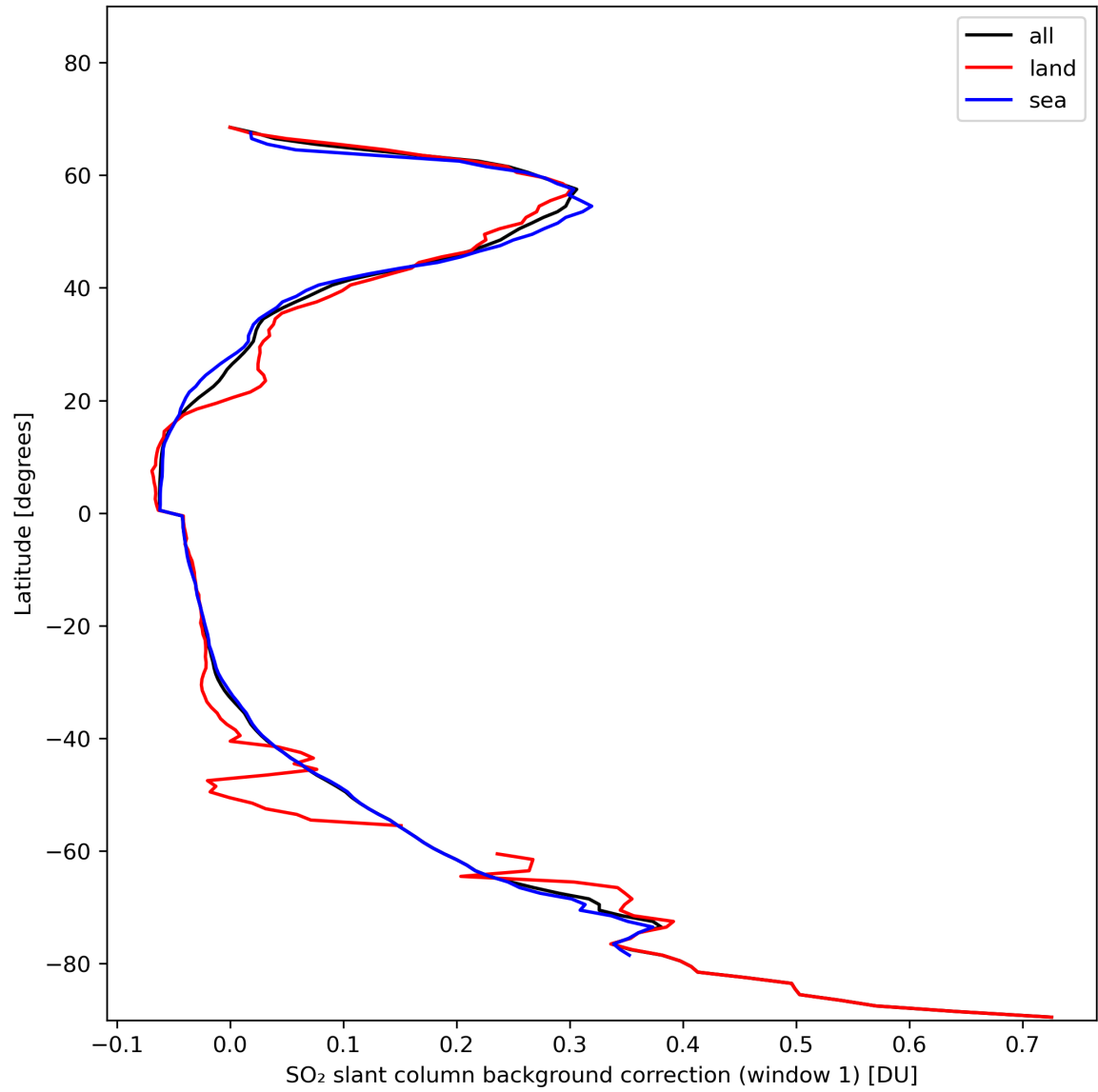
Figure 36: Zonal average of “SO 2 slant column background correction (window 1)” for 2024-01-31 to 2024-02-02.
