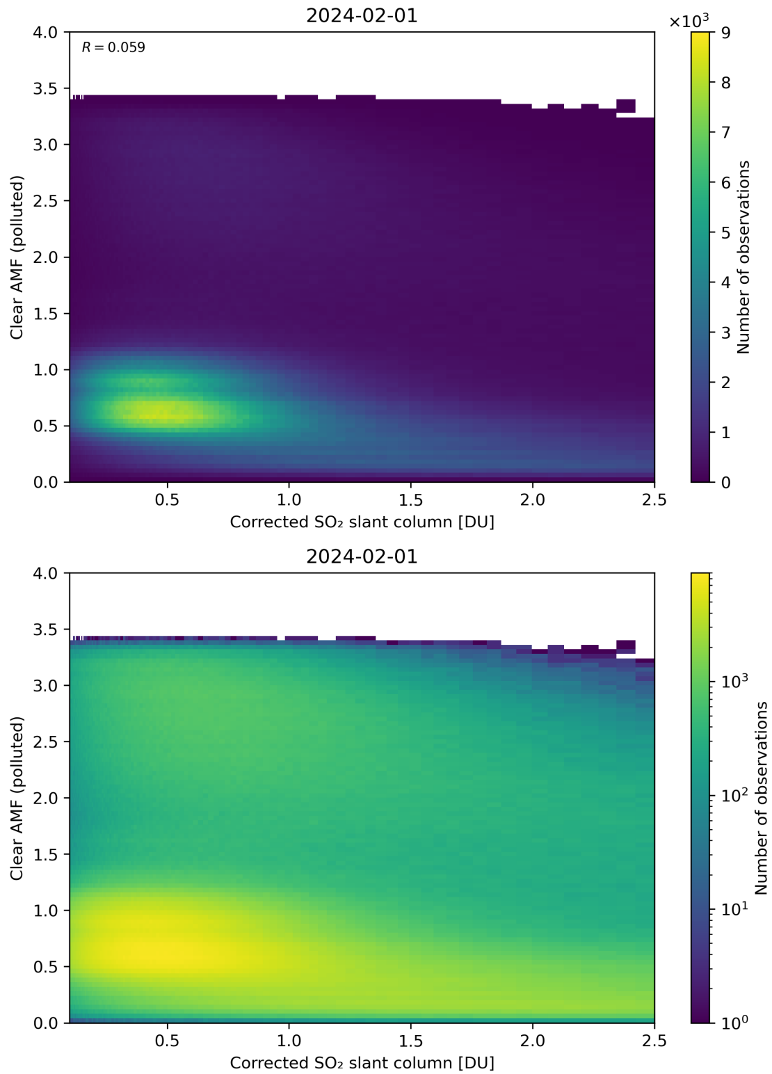
Figure 184: Scatter density plot of “Corrected SO 2 slant column” against “Clear AMF (polluted)” for 2024-01-31 to 2024-02-02.
