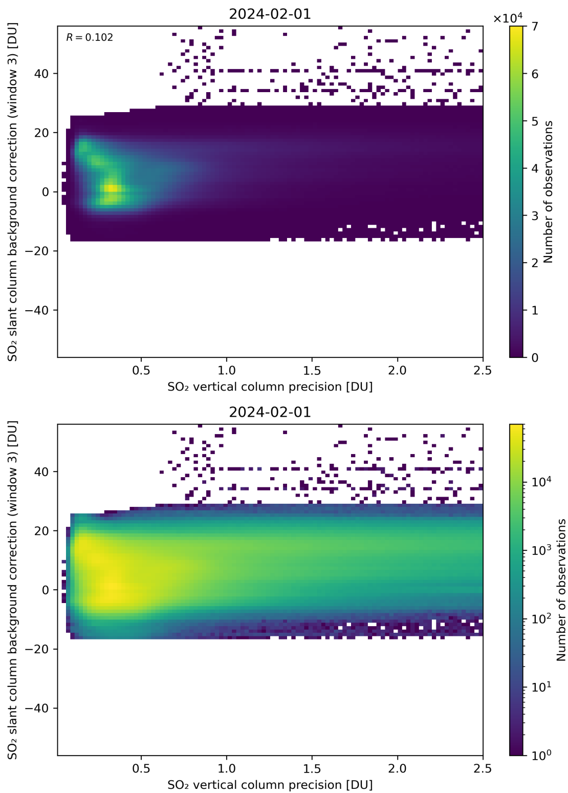
Figure 281: Scatter density plot of “SO 2 vertical column precision” against “SO 2 slant column background correction (window 3)” for 2024-01-31 to 2024-02-02.
