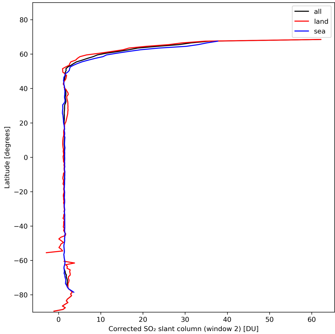
Figure 39: Zonal average of “Corrected SO 2 slant column (window 2)” for 2024-01-31 to 2024-02-02.
