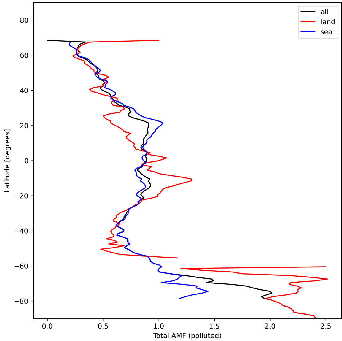
Figure 48: Zonal average of “Total AMF (polluted)” for 2024-01-31 to 2024-02-02.
