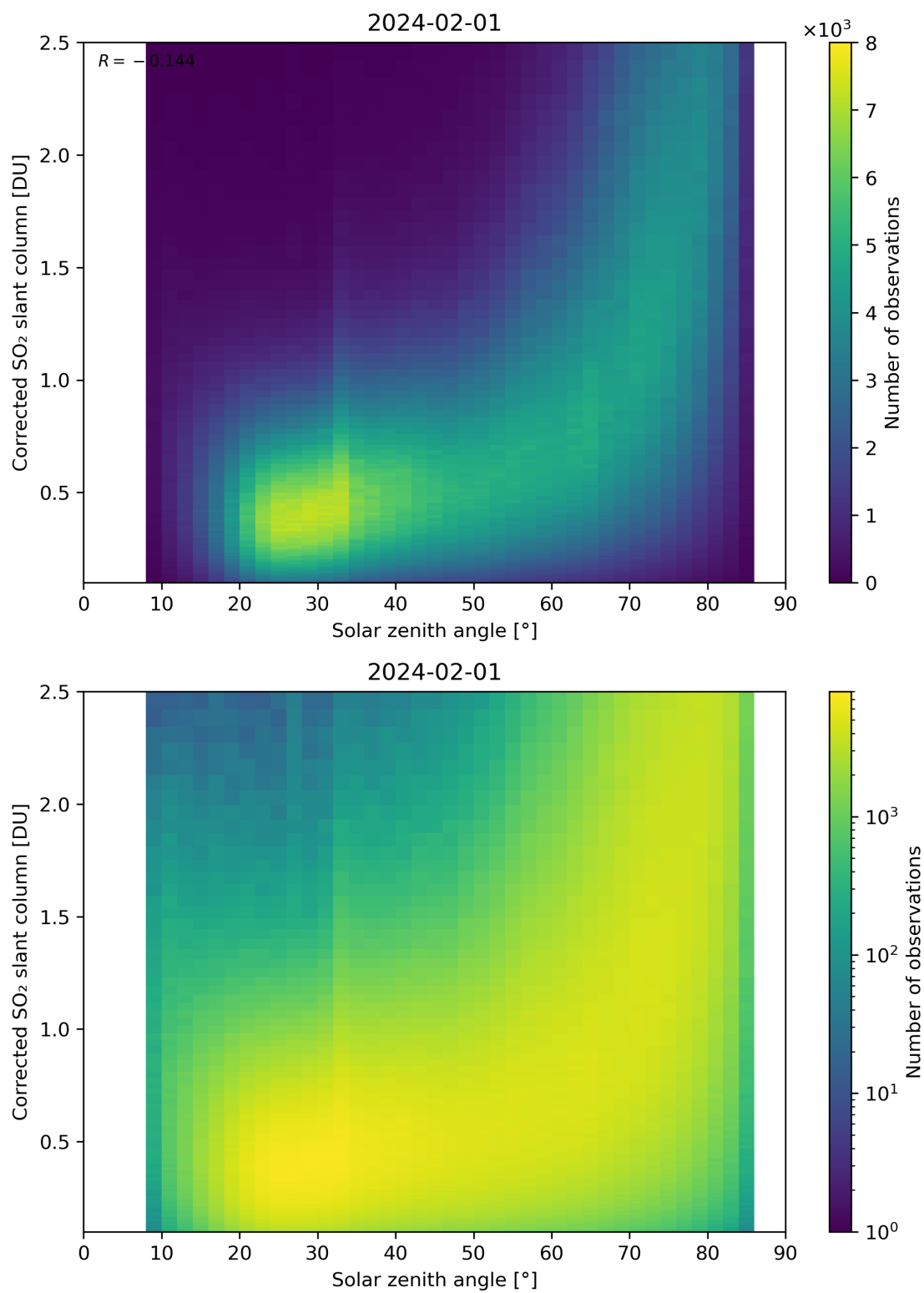
Figure 166: Scatter density plot of “Solar zenith angle” against “Corrected SO 2 slant column” for 2024-01-31 to 2024-02-02.
