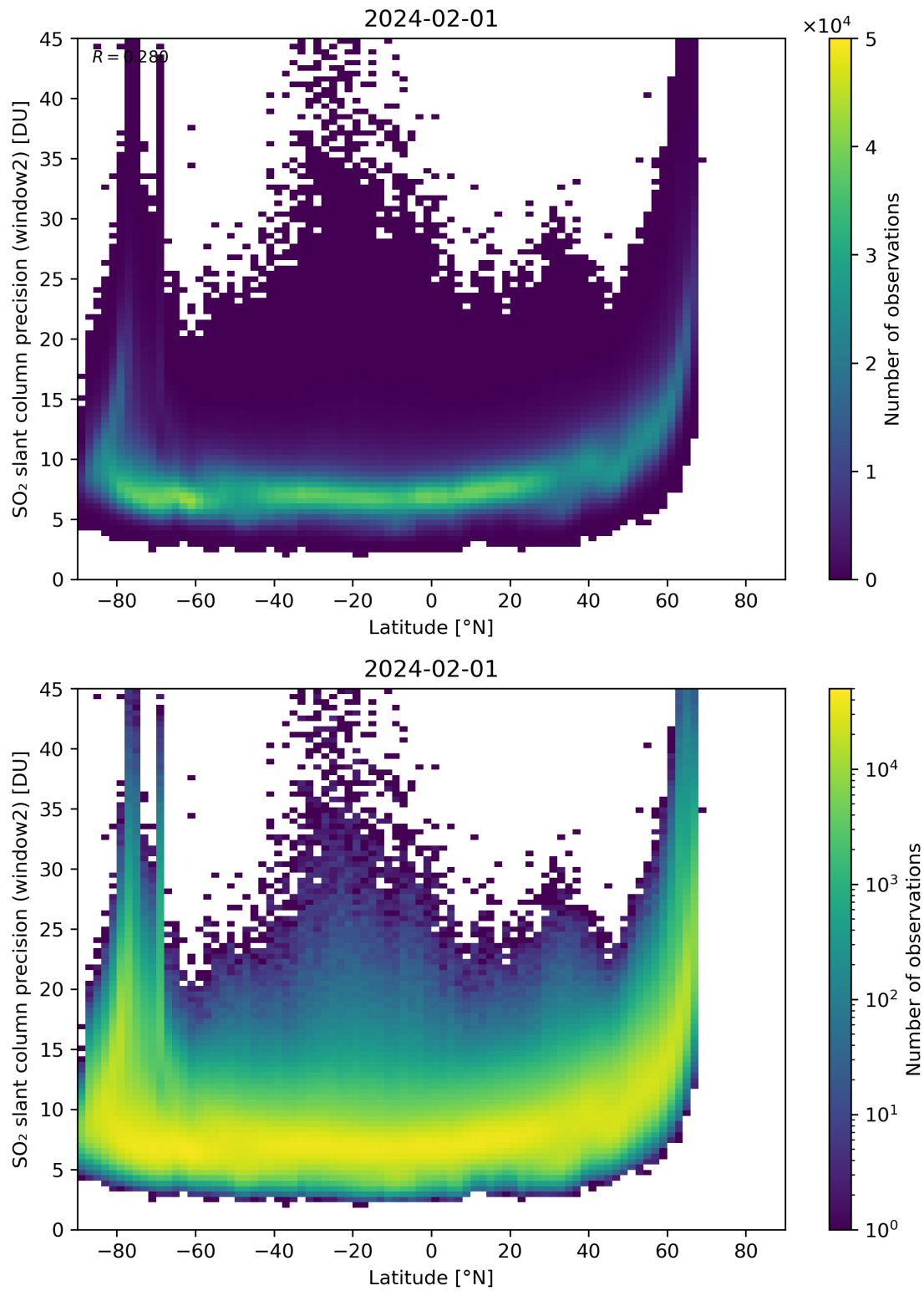
Figure 151: Scatter density plot of “Latitude” against “SO 2 slant column precision (window2)” for 2024-01-31 to 2024-02-02.
