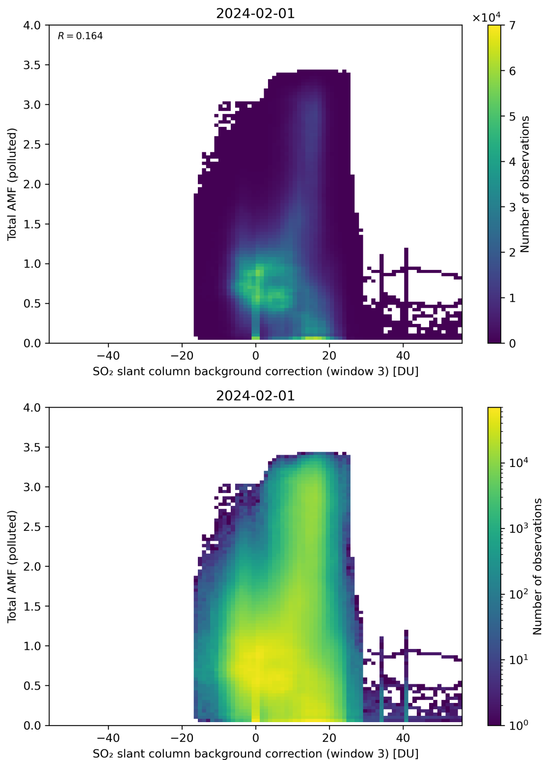
Figure 125: Scatter density plot of “SO 2 slant column background correction (window 3)” against “Total AMF (polluted)” for 2024-01-31 to 2024-02-02.
