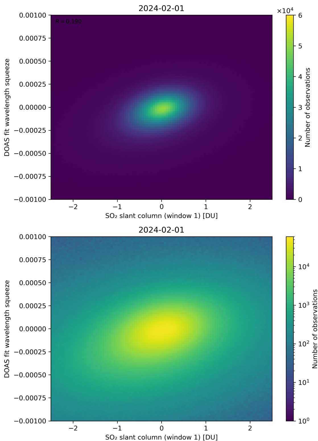
Figure 216: Scatter density plot of “SO 2 slant column (window 1)” against “DOAS fit wavelength squeeze” for 2024-01-31 to 2024-02-02.
