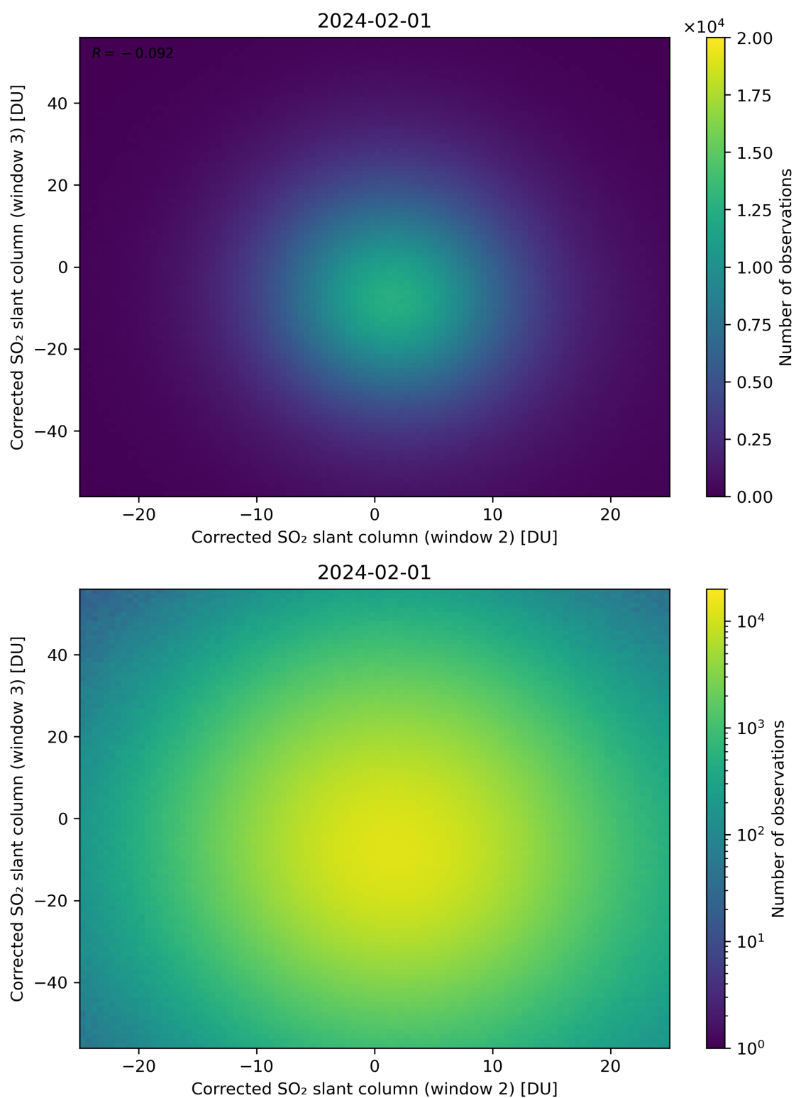
Figure 200: Scatter density plot of “Corrected SO 2 slant column (window 2)” against “Corrected SO 2 slant column (window 3)” for 2024-01-31 to 2024-02-02.
