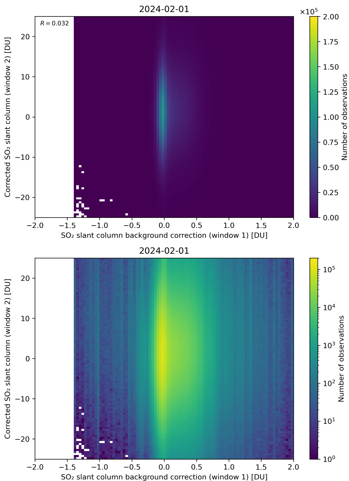
Figure 104: Scatter density plot of “SO 2 slant column background correction (window 1)” against “Corrected SO 2 slant column (window 2)” for 2024-01-31 to 2024-02-02.
