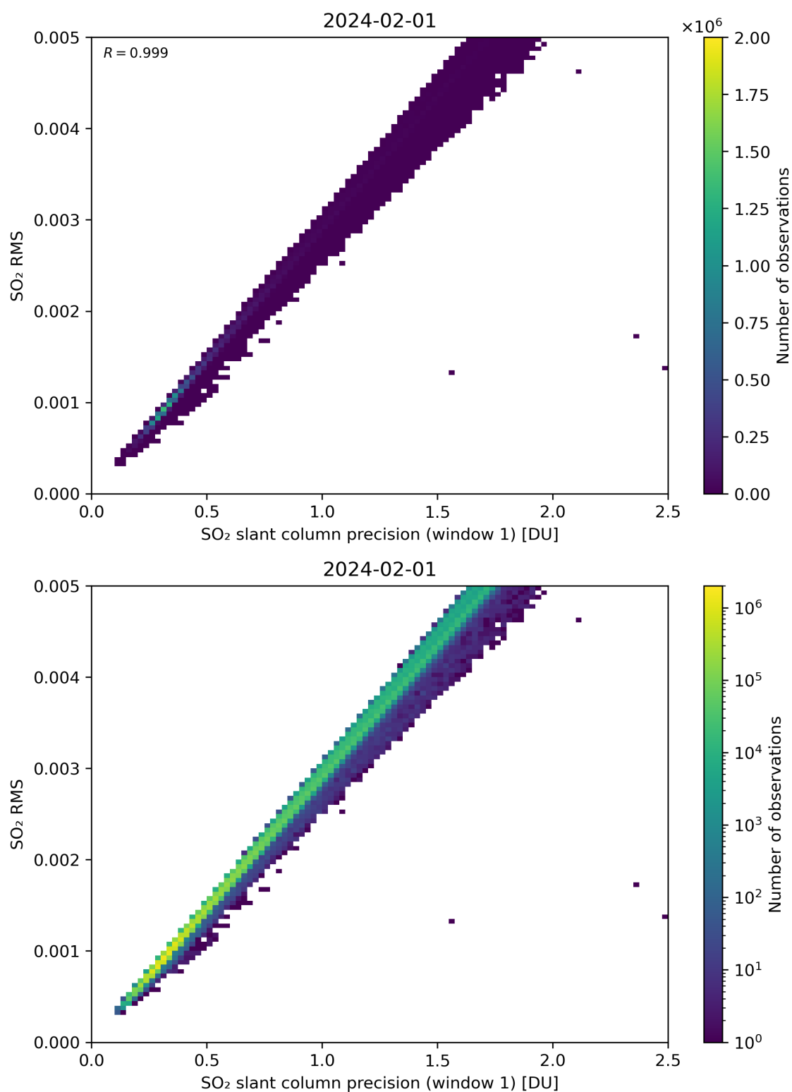
Figure 223: Scatter density plot of “SO 2 slant column precision (window 1)” against “SO 2 RMS” for 2024-01-31 to 2024-02-02.
