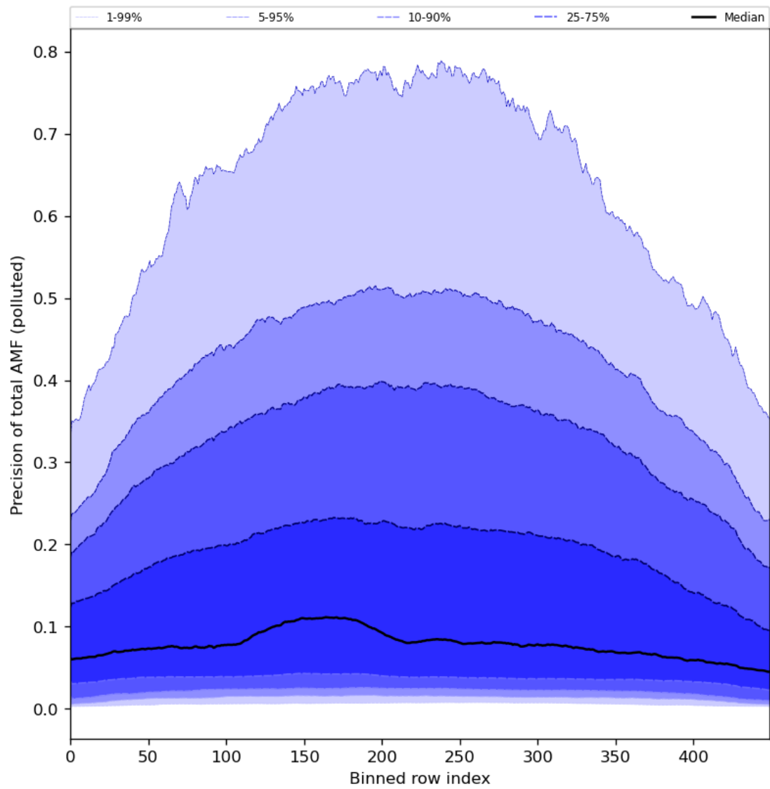
Figure 95: Along track statistics of “Precision of total AMF (polluted)” for 2024-01-31 to 2024-02-02
