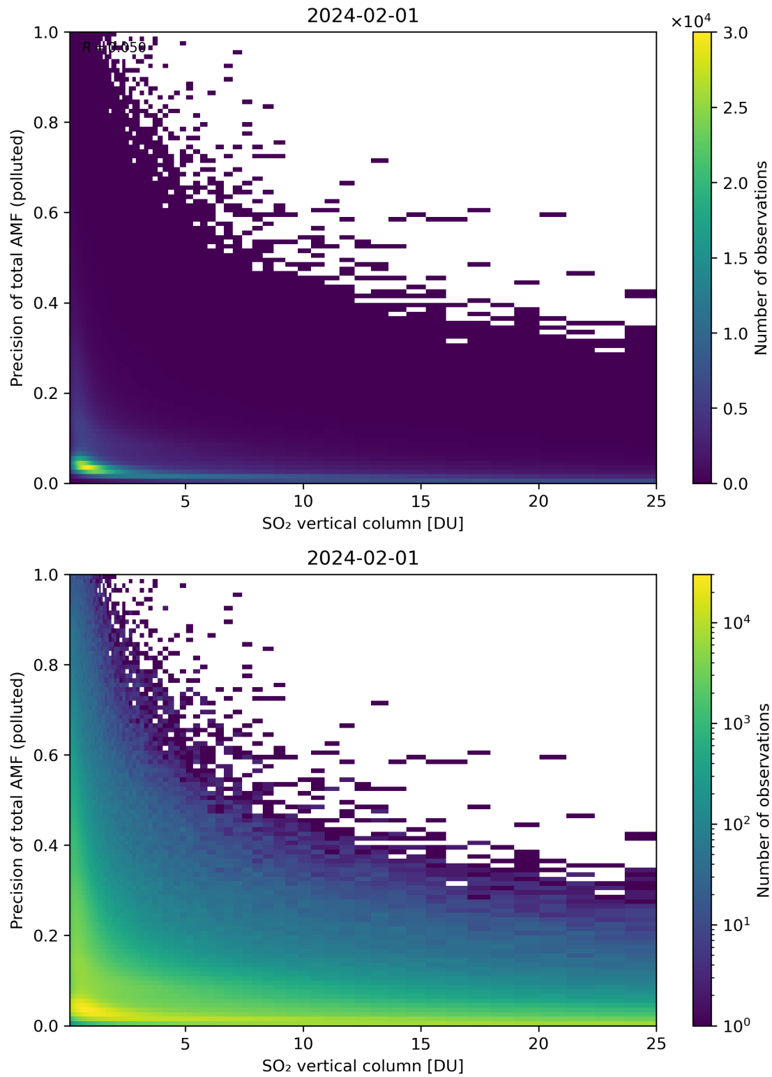
Figure 306: Scatter density plot of “SO 2 vertical column” against “Precision of total AMF (polluted)” for 2024-01-31 to 2024-02-02.
