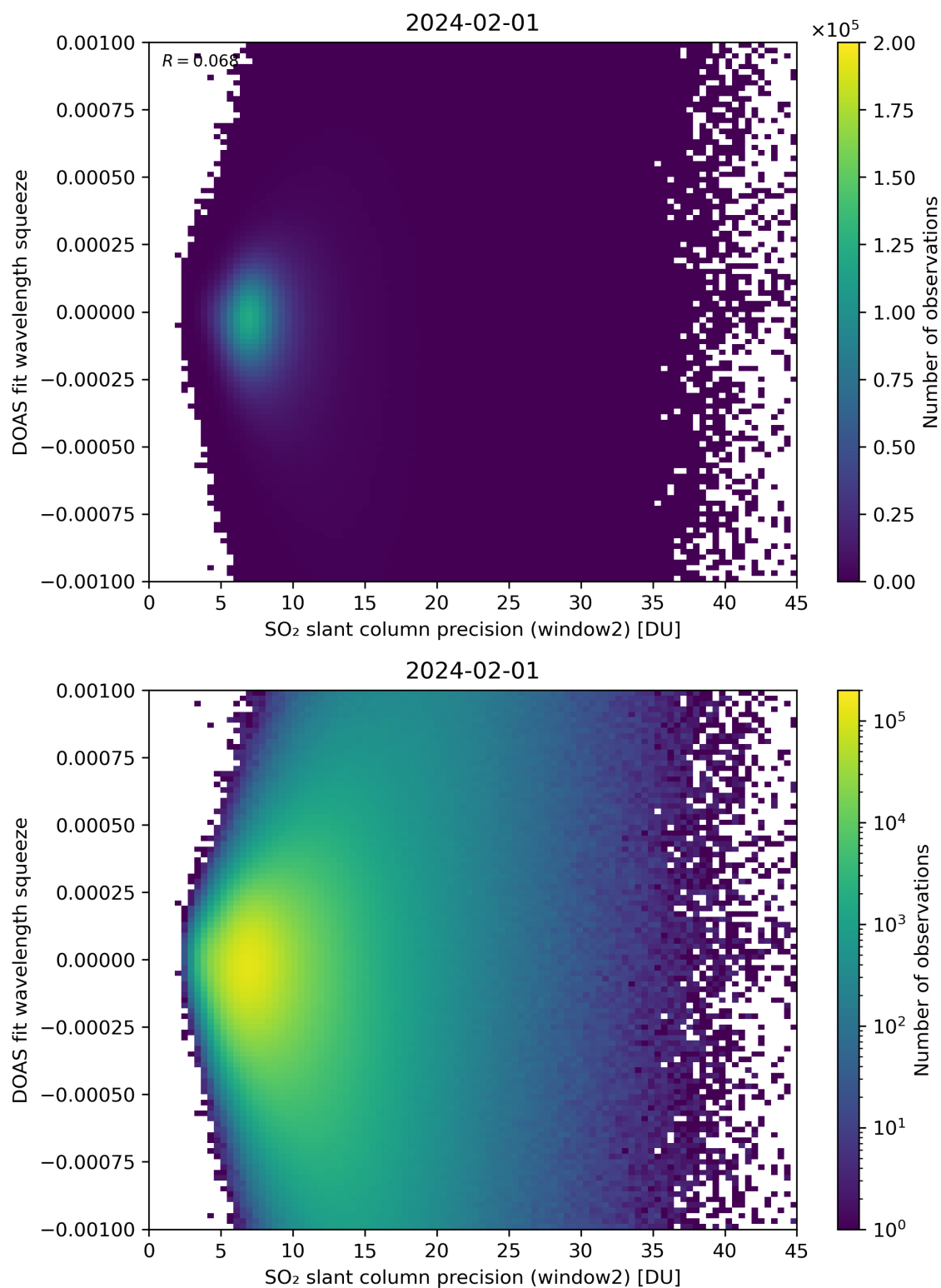
Figure 244: Scatter density plot of “SO 2 slant column precision (window2)” against “DOAS fit wavelength squeeze” for 2024-01-31 to 2024-02-02.
