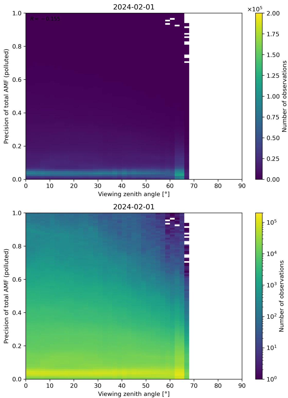
Figure 326: Scatter density plot of “Viewing zenith angle” against “Precision of total AMF (polluted)” for 2024-01-31 to 2024-02-02.
