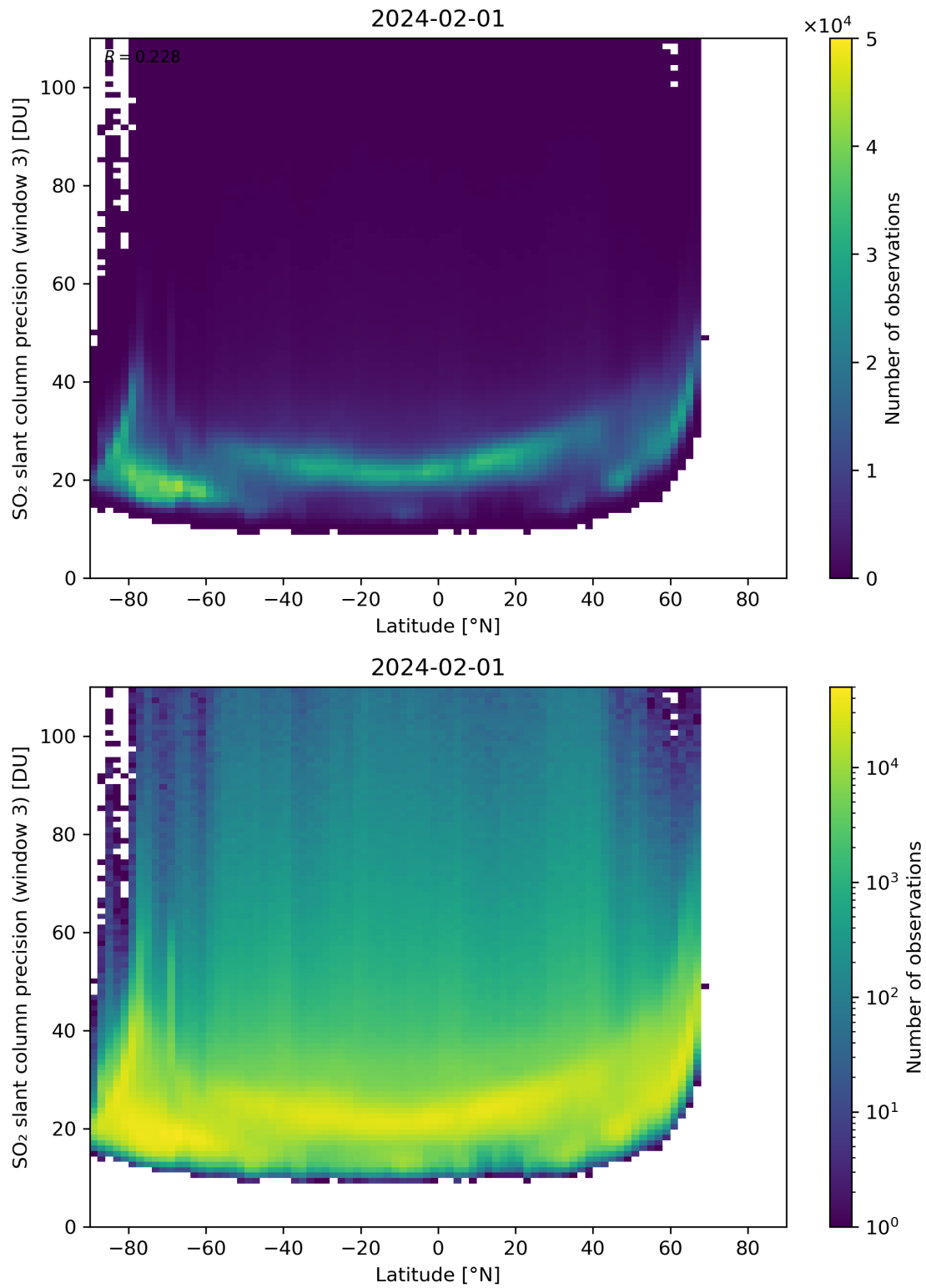
Figure 153: Scatter density plot of “Latitude” against “SO 2 slant column precision (window 3)” for 2024-01-31 to 2024-02-02.
