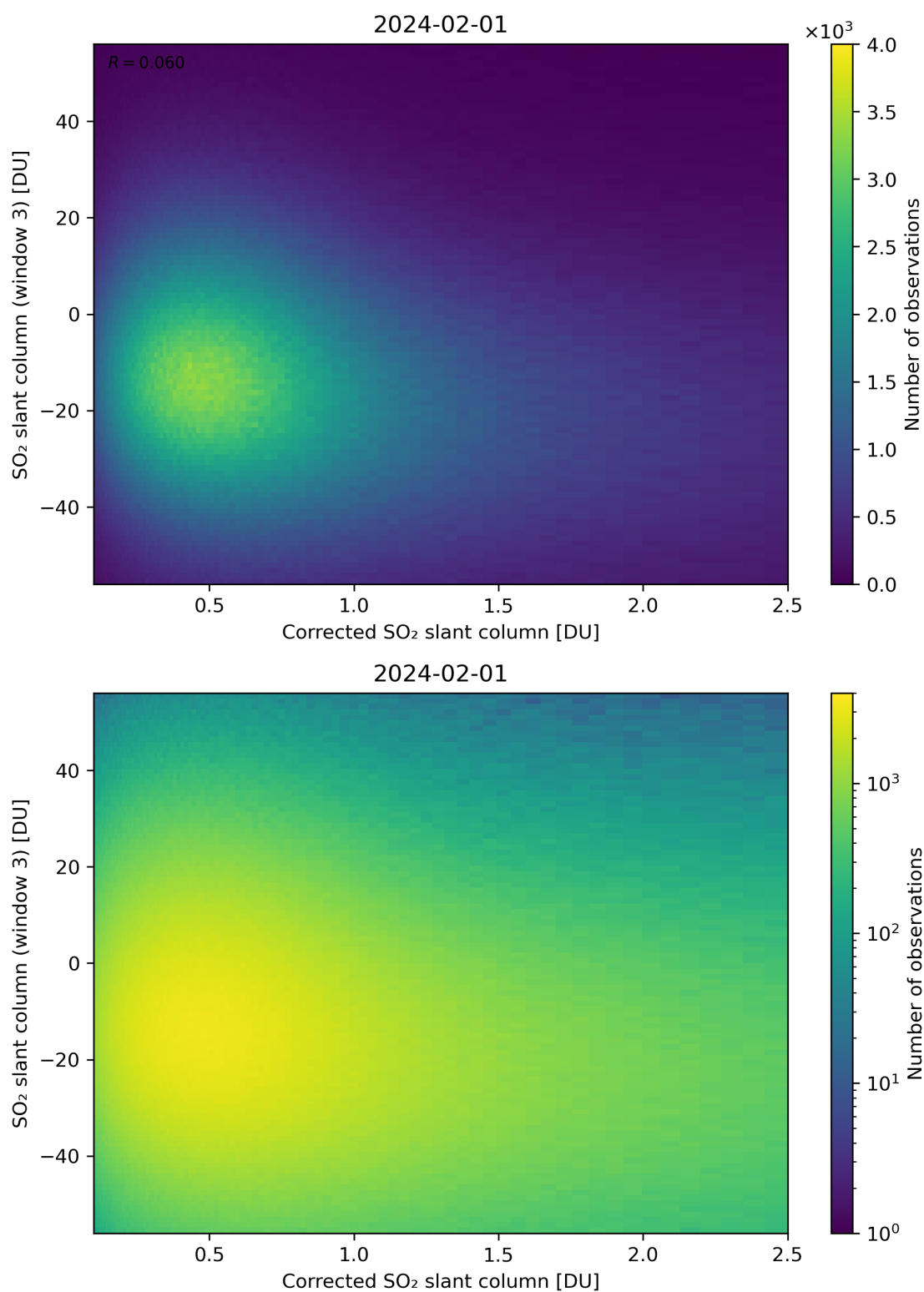
Figure 190: Scatter density plot of “Corrected SO 2 slant column” against “SO 2 slant column (window 3)” for 2024-01-31 to 2024-02-02.
