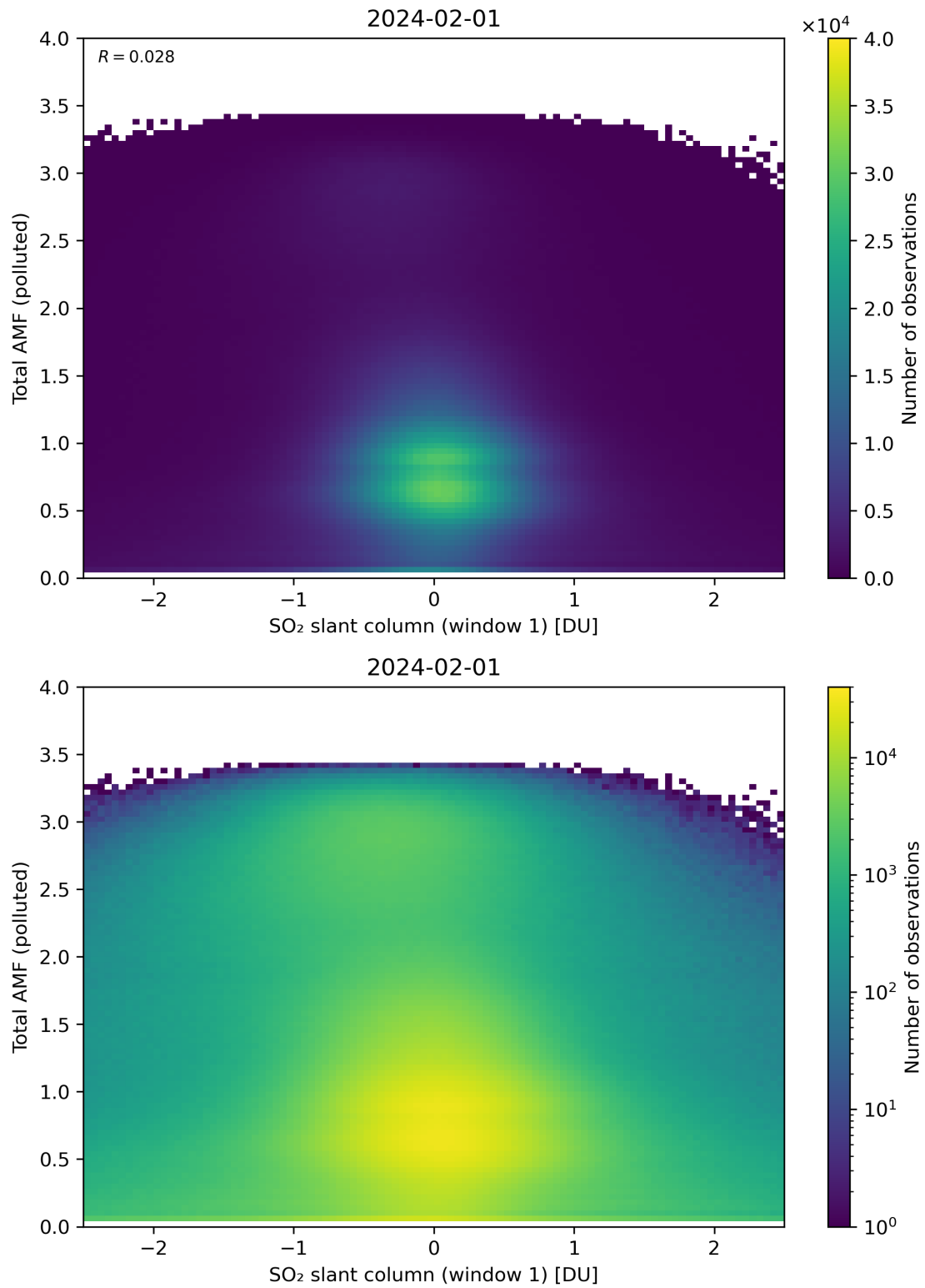
Figure 239: Scatter density plot of “SO 2 slant column (window 1)” against “Total AMF (polluted)” for 2024-01-31 to 2024-02-02.
