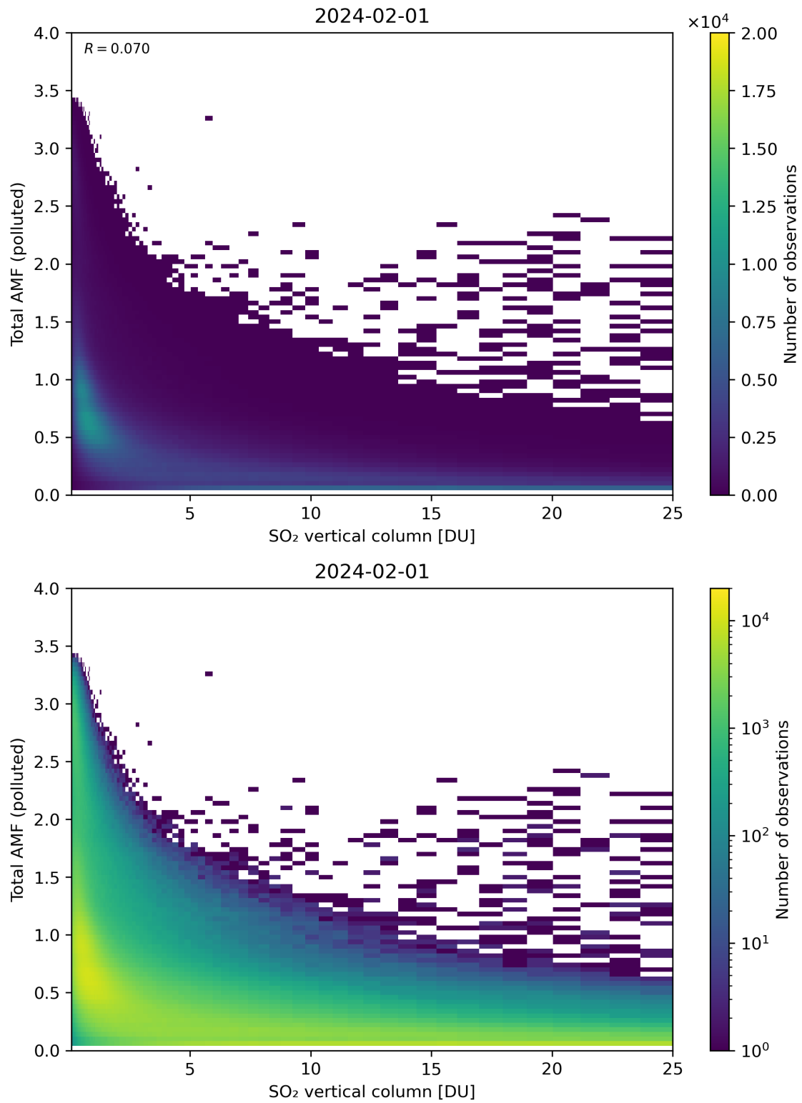
Figure 305: Scatter density plot of “SO 2 vertical column” against “Total AMF (polluted)” for 2024-01-31 to 2024-02-02.
