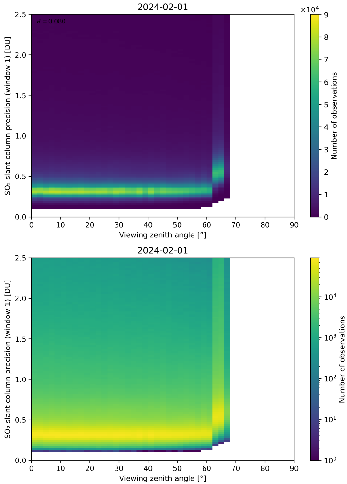
Figure 321: Scatter density plot of “Viewing zenith angle” against “SO 2 slant column precision (window 1)” for 2024-01-31 to 2024-02-02.
