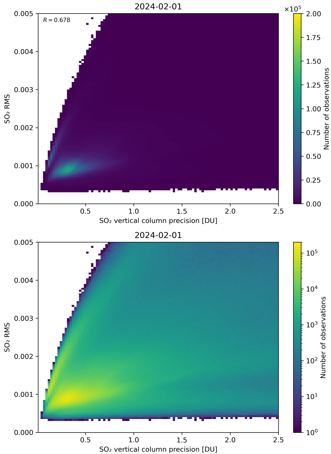
Figure 284: Scatter density plot of “SO 2 vertical column precision” against “SO 2 RMS” for 2024-01-31 to 2024-02-02.
