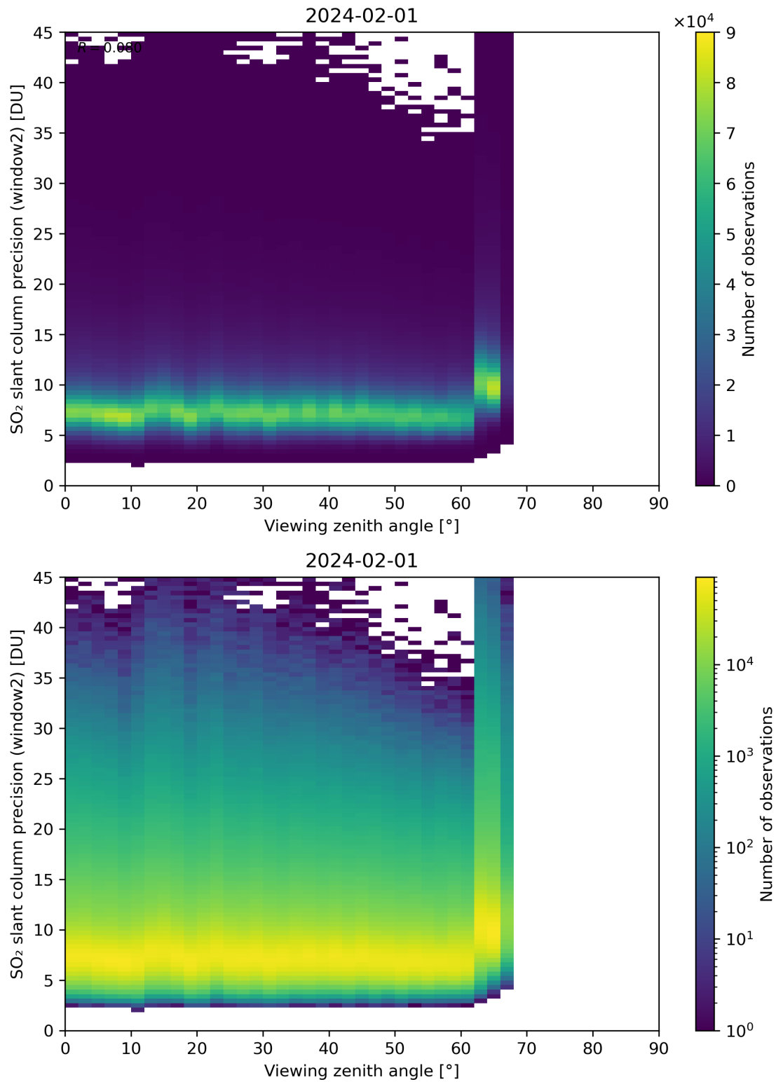
Figure 322: Scatter density plot of “Viewing zenith angle” against “SO 2 slant column precision (window2)” for 2024-01-31 to 2024-02-02.
