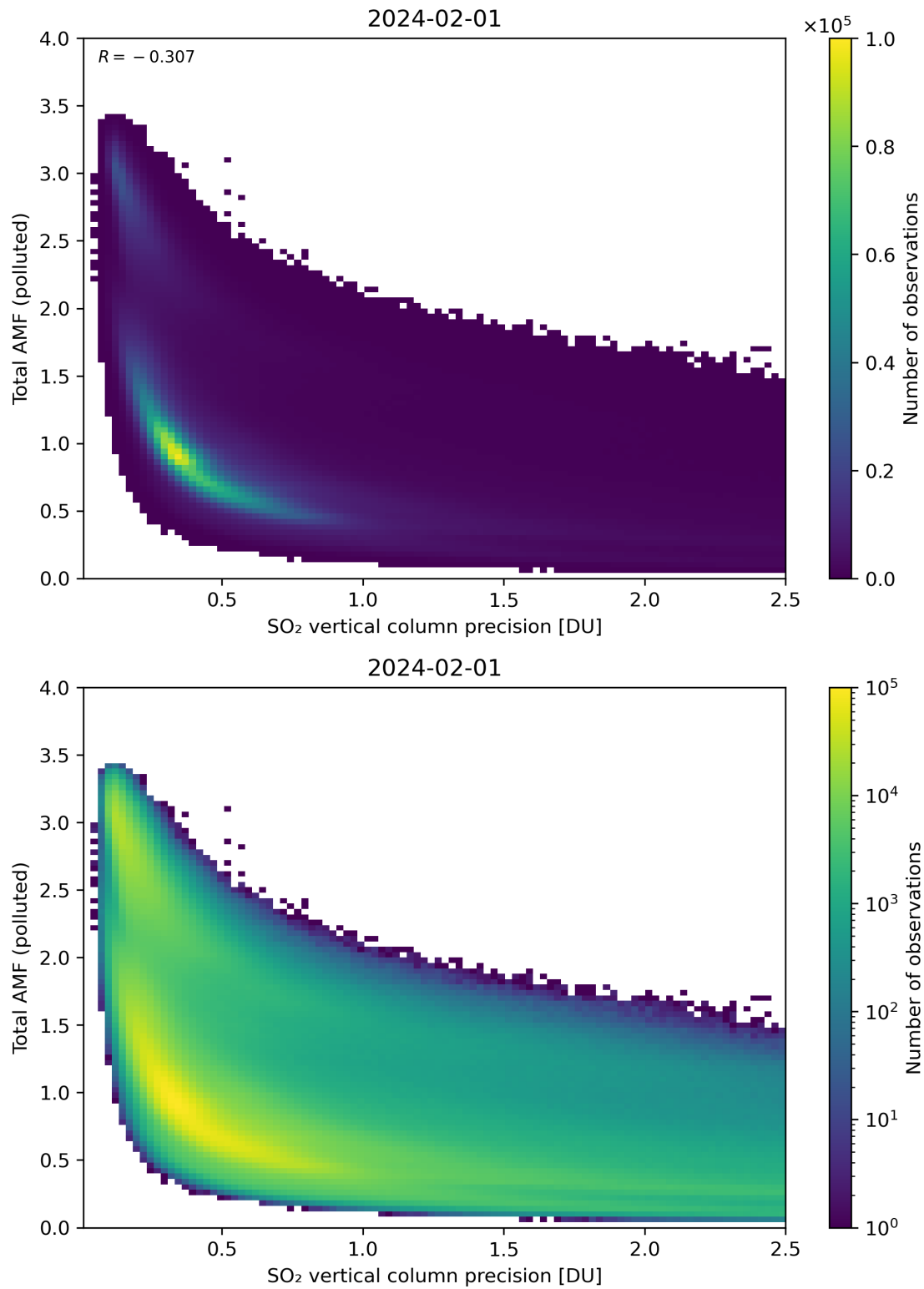
Figure 294: Scatter density plot of “SO 2 vertical column precision” against “Total AMF (polluted)” for 2024-01-31 to 2024-02-02.
