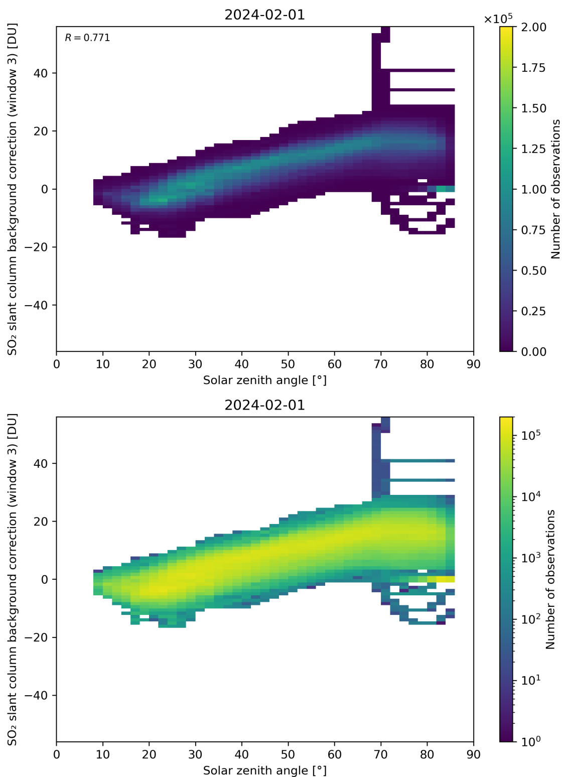
Figure 160: Scatter density plot of “Solar zenith angle” against “SO 2 slant column background correction (window 3)” for 2024-01-31 to 2024-02-02.
