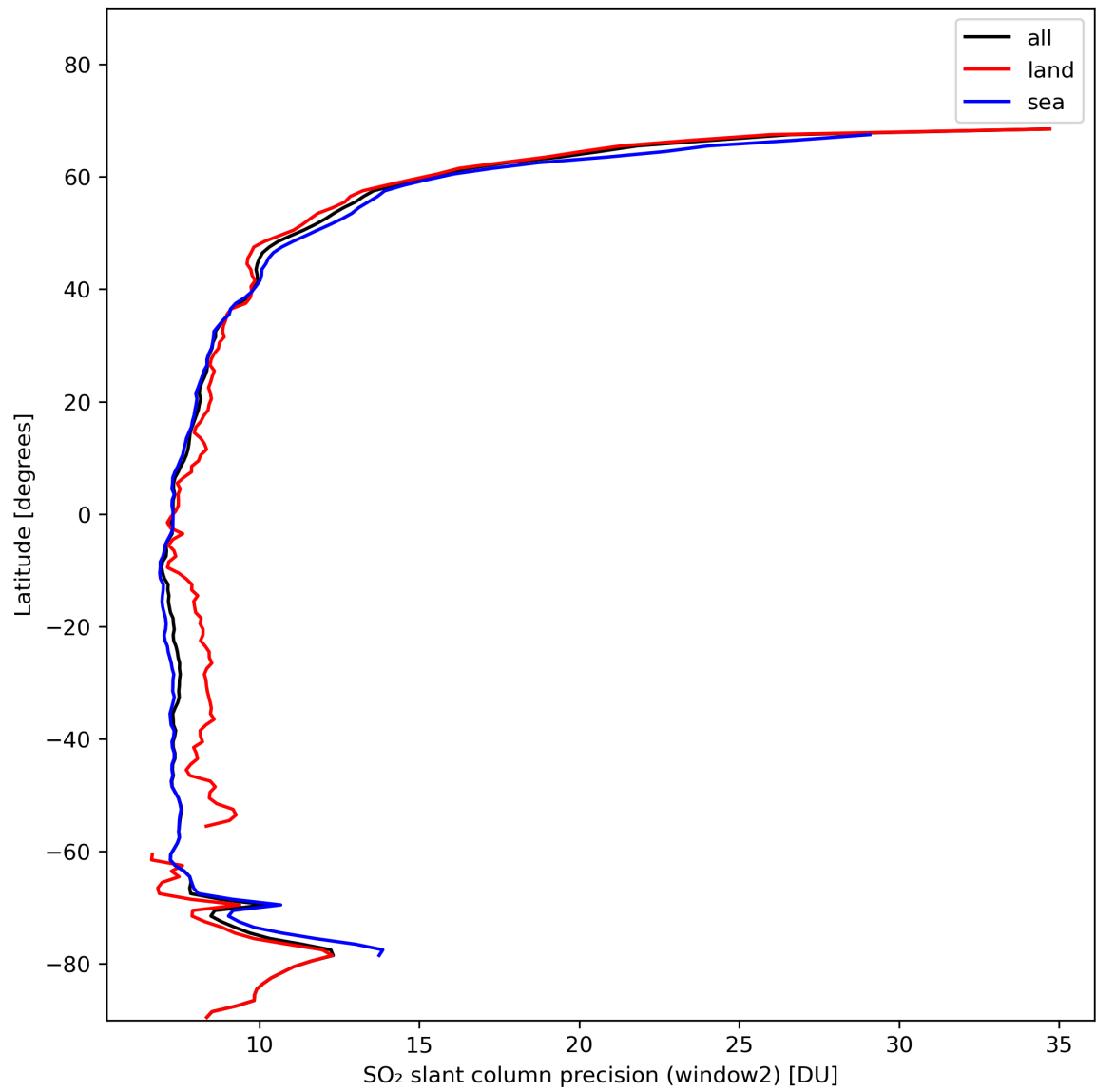
Figure 38: Zonal average of “SO 2 slant column precision (window2)” for 2024-01-31 to 2024-02-02.
