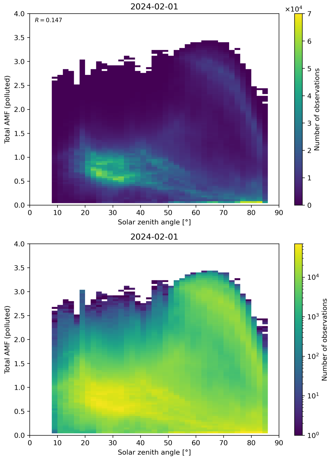
Figure 174: Scatter density plot of “Solar zenith angle” against “Total AMF (polluted)” for 2024-01-31 to 2024-02-02.
