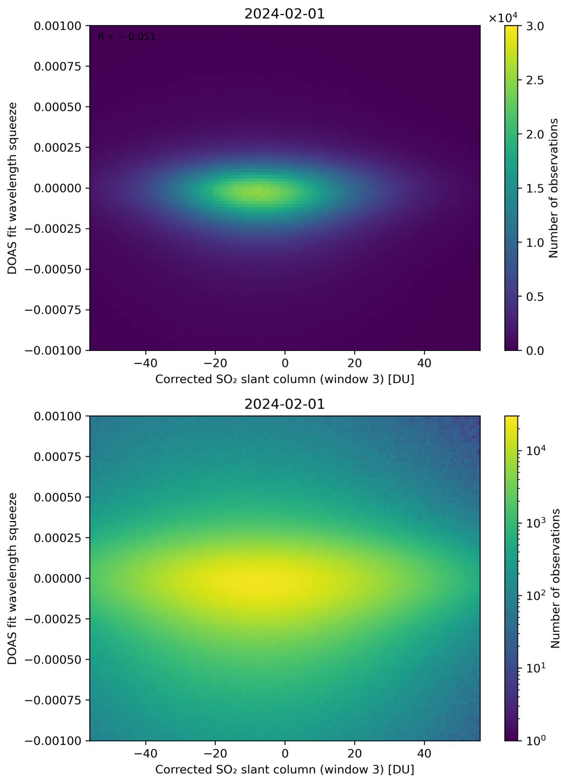
Figure 207: Scatter density plot of “Corrected SO 2 slant column (window 3)” against “DOAS fit wavelength squeeze” for 2024-01-31 to 2024-02-02.
