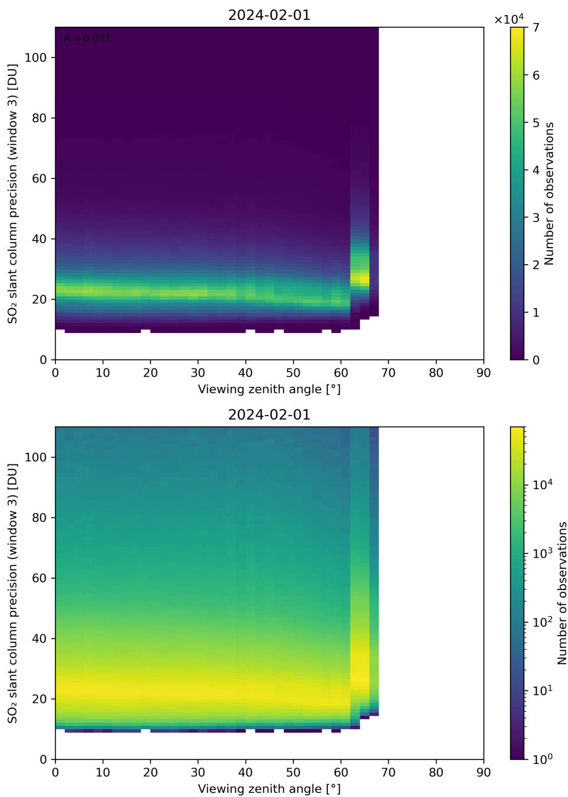
Figure 324: Scatter density plot of “Viewing zenith angle” against “SO 2 slant column precision (window 3)” for 2024-01-31 to 2024-02-02.
