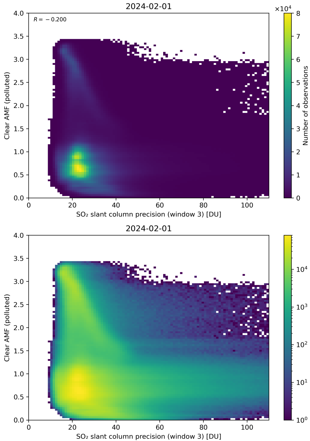
Figure 261: Scatter density plot of “SO 2 slant column precision (window 3)” against “Clear AMF (polluted)” for 2024-01-31 to 2024-02-02.
