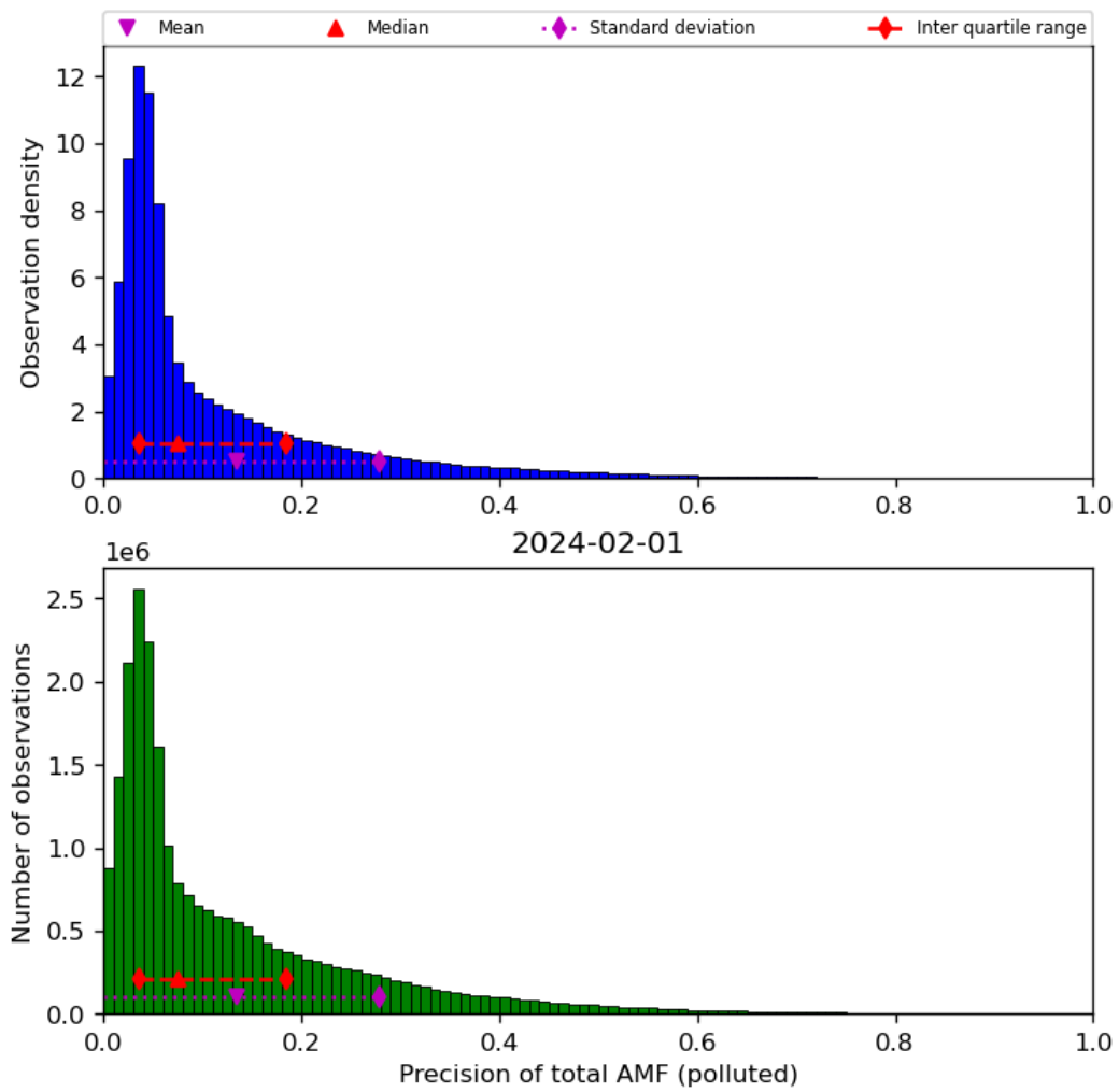
Figure 72: Histogram of “Precision of total AMF (polluted)” for 2024-01-31 to 2024-02-02
