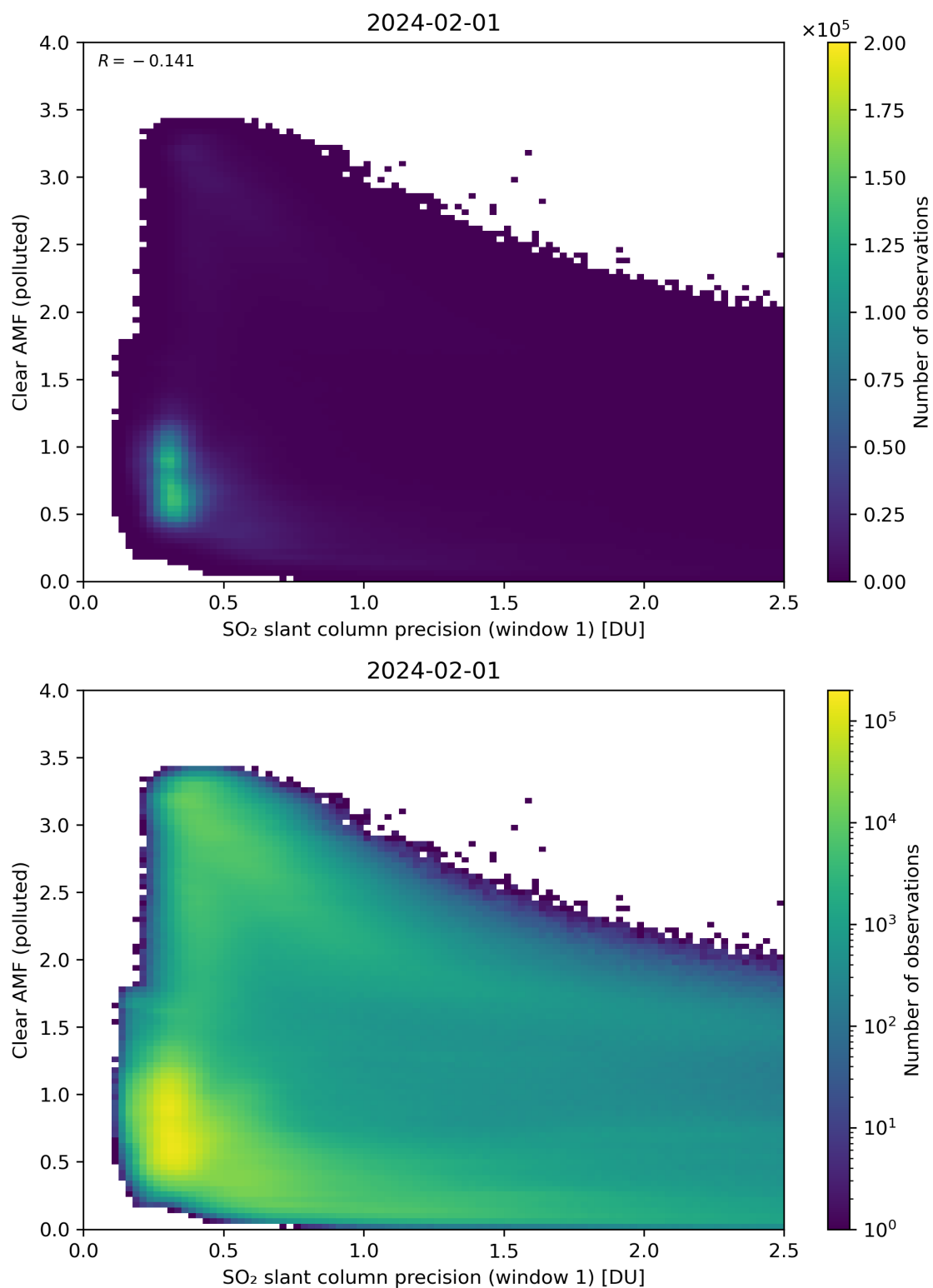
Figure 224: Scatter density plot of “SO 2 slant column precision (window 1)” against “Clear AMF (polluted)” for 2024-01-31 to 2024-02-02.
