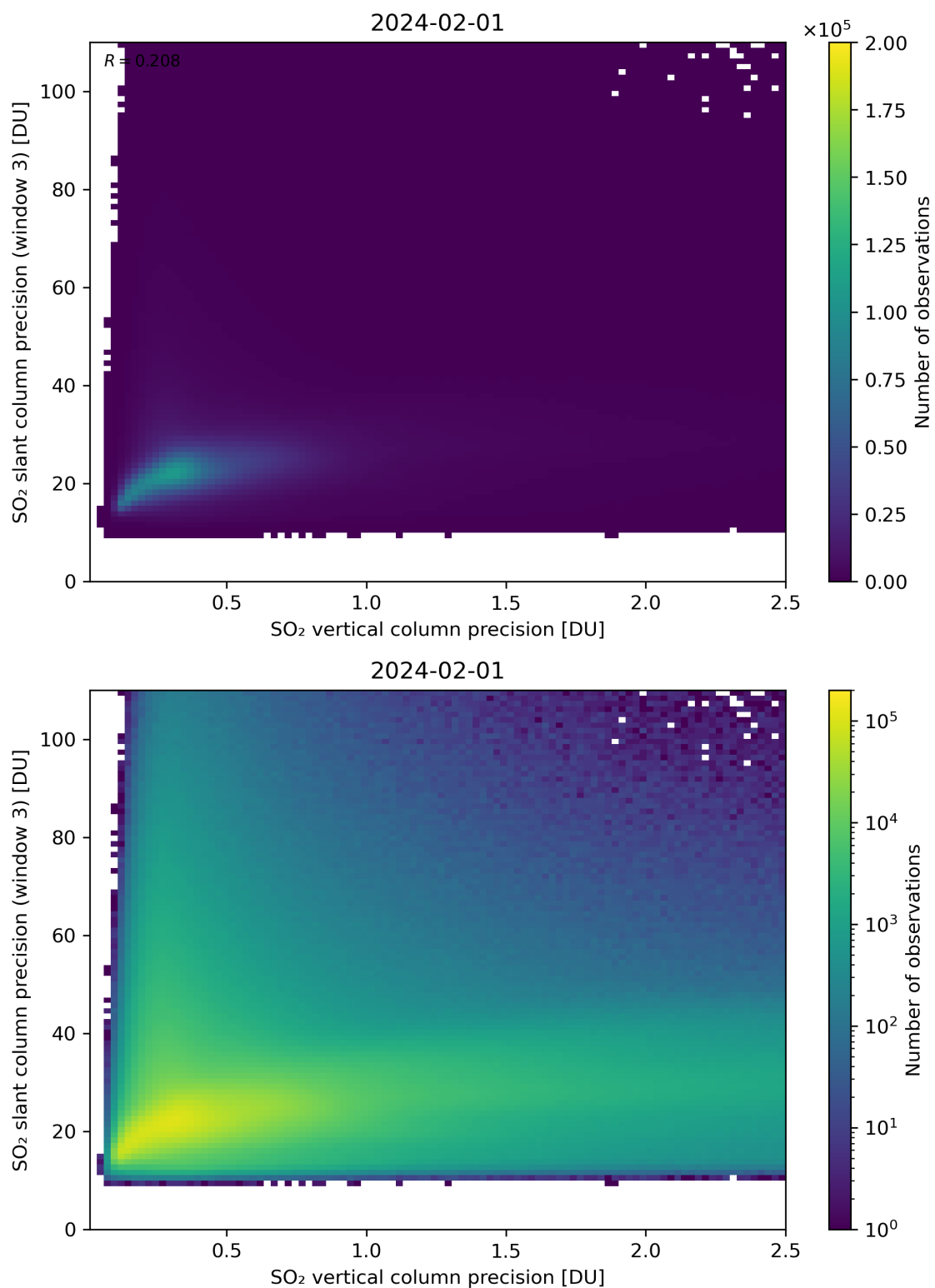
Figure 293: Scatter density plot of “SO 2 vertical column precision” against “SO 2 slant column precision (window 3)” for 2024-01-31 to 2024-02-02.
