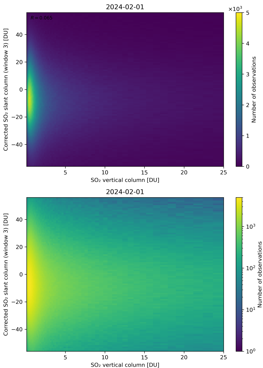
Figure 299: Scatter density plot of “SO 2 vertical column” against “Corrected SO 2 slant column (window 3)” for 2024-01-31 to 2024-02-02.
