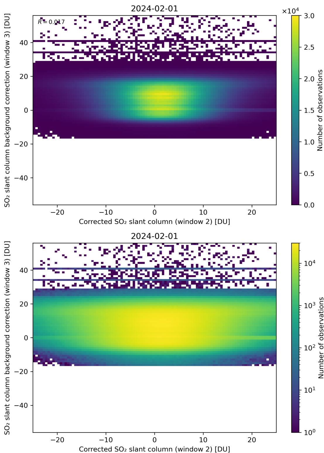
Figure 195: Scatter density plot of “Corrected SO 2 slant column (window 2)” against “SO 2 slant column background correction (window 3)” for 2024-01-31 to 2024-02-02.
