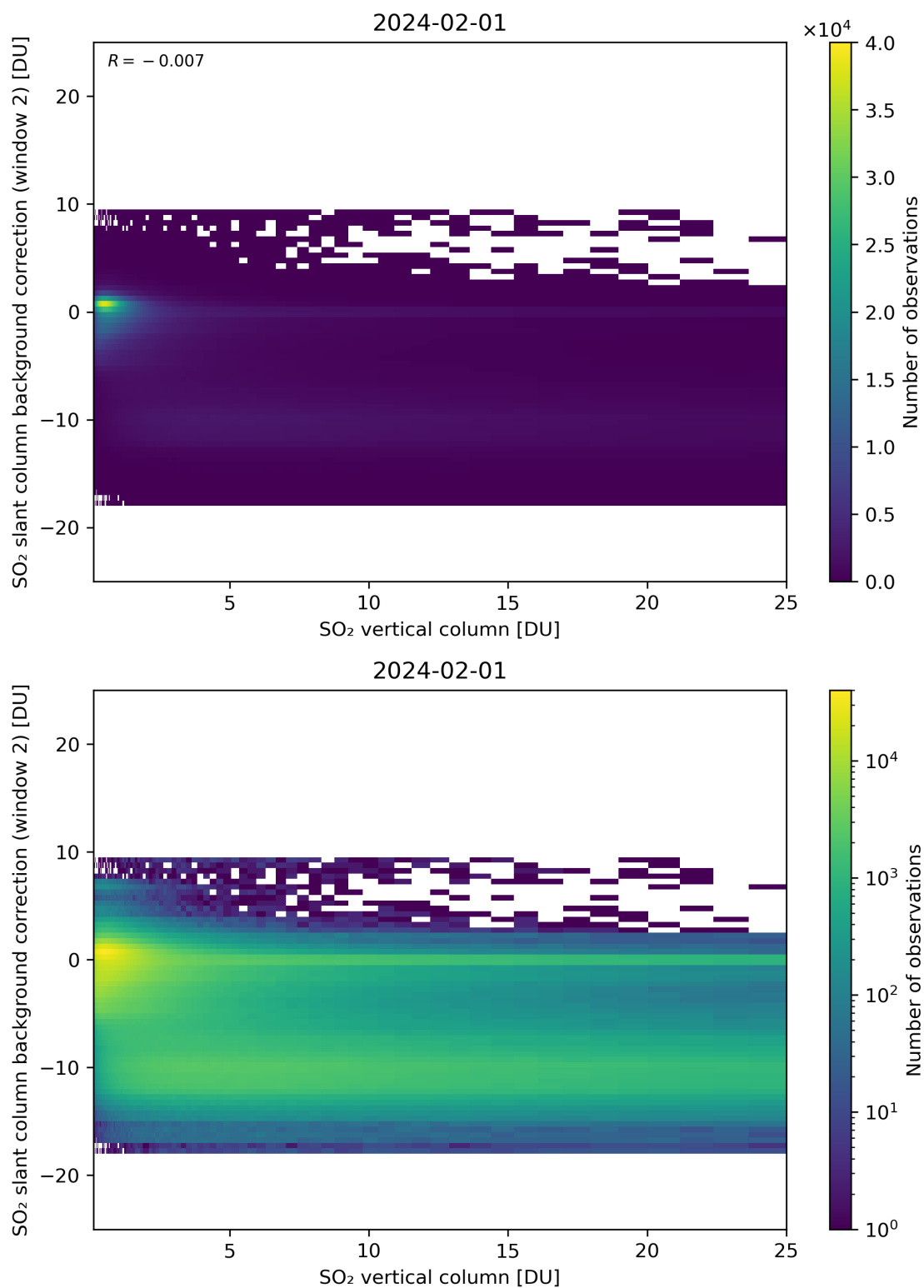
Figure 274: Scatter density plot of “SO 2 vertical column” against “SO 2 slant column background correction (window 2)” for 2024-01-31 to 2024-02-02.
