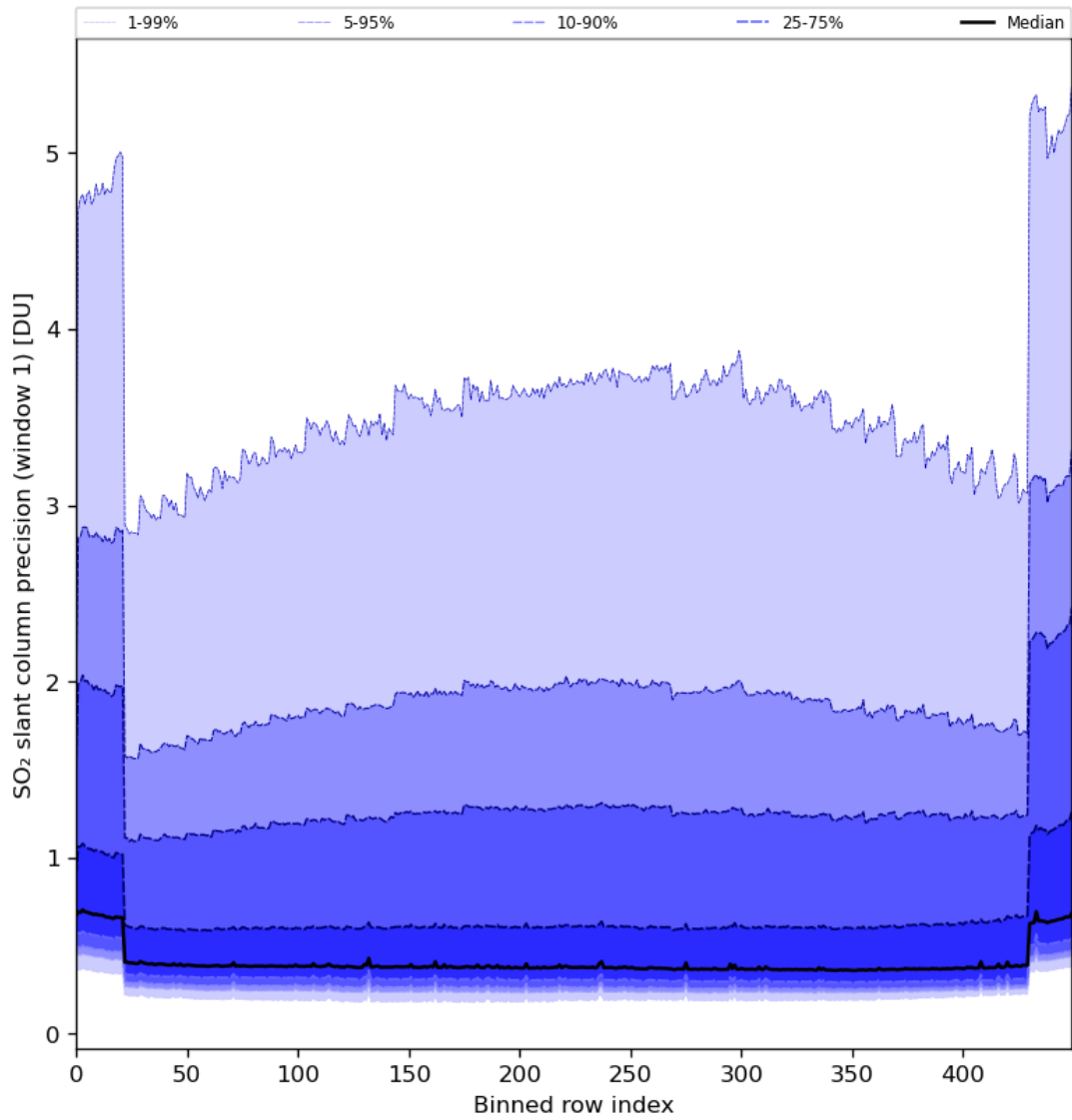
Figure 80: Along track statistics of “SO 2 slant column precision (window 1)” for 2024-01-31 to 2024-02-02
