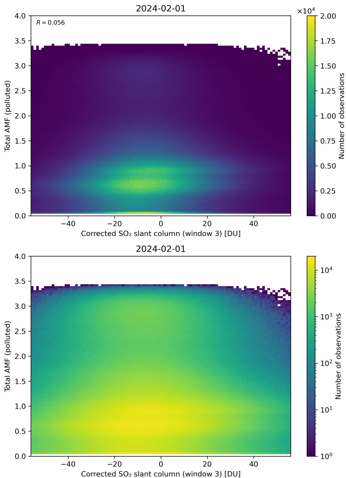
Figure 210: Scatter density plot of “Corrected SO 2 slant column (window 3)” against “Total AMF (polluted)” for 2024-01-31 to 2024-02-02.
