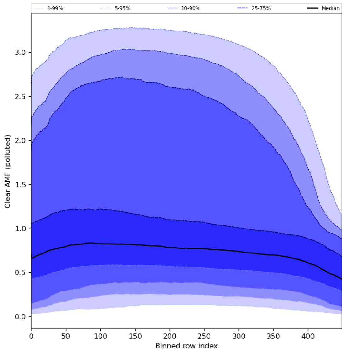
Figure 96: Along track statistics of “Clear AMF (polluted)” for 2024-01-31 to 2024-02-02
