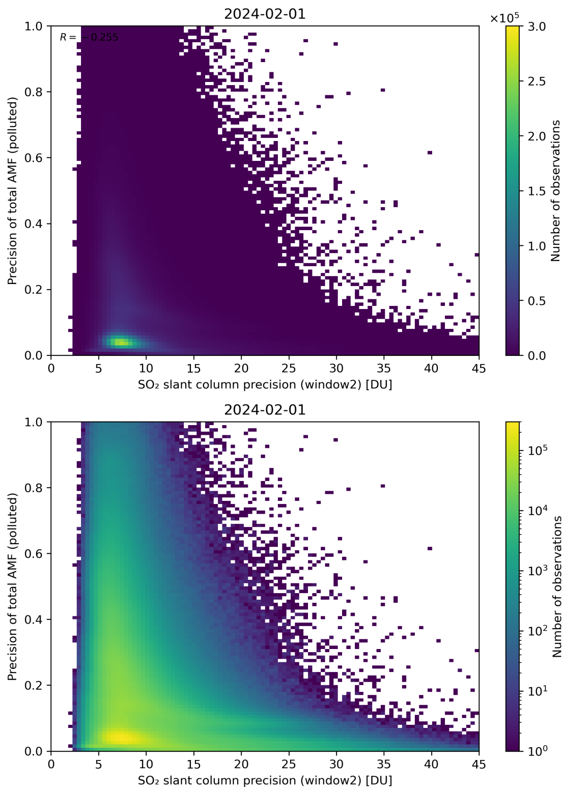
Figure 252: Scatter density plot of “SO 2 slant column precision (window2)” against “Precision of total AMF (polluted)” for 2024-01-31 to 2024-02-02.
