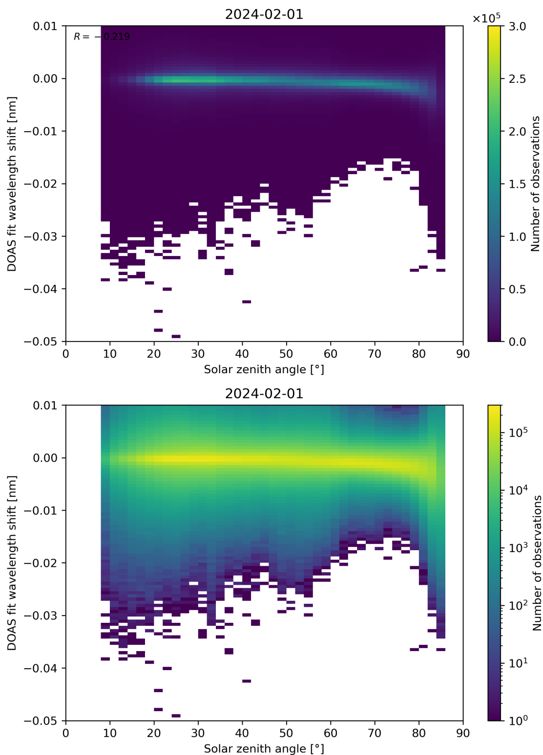
Figure 161: Scatter density plot of “Solar zenith angle” against “DOAS fit wavelength shift” for 2024-01-31 to 2024-02-02.
