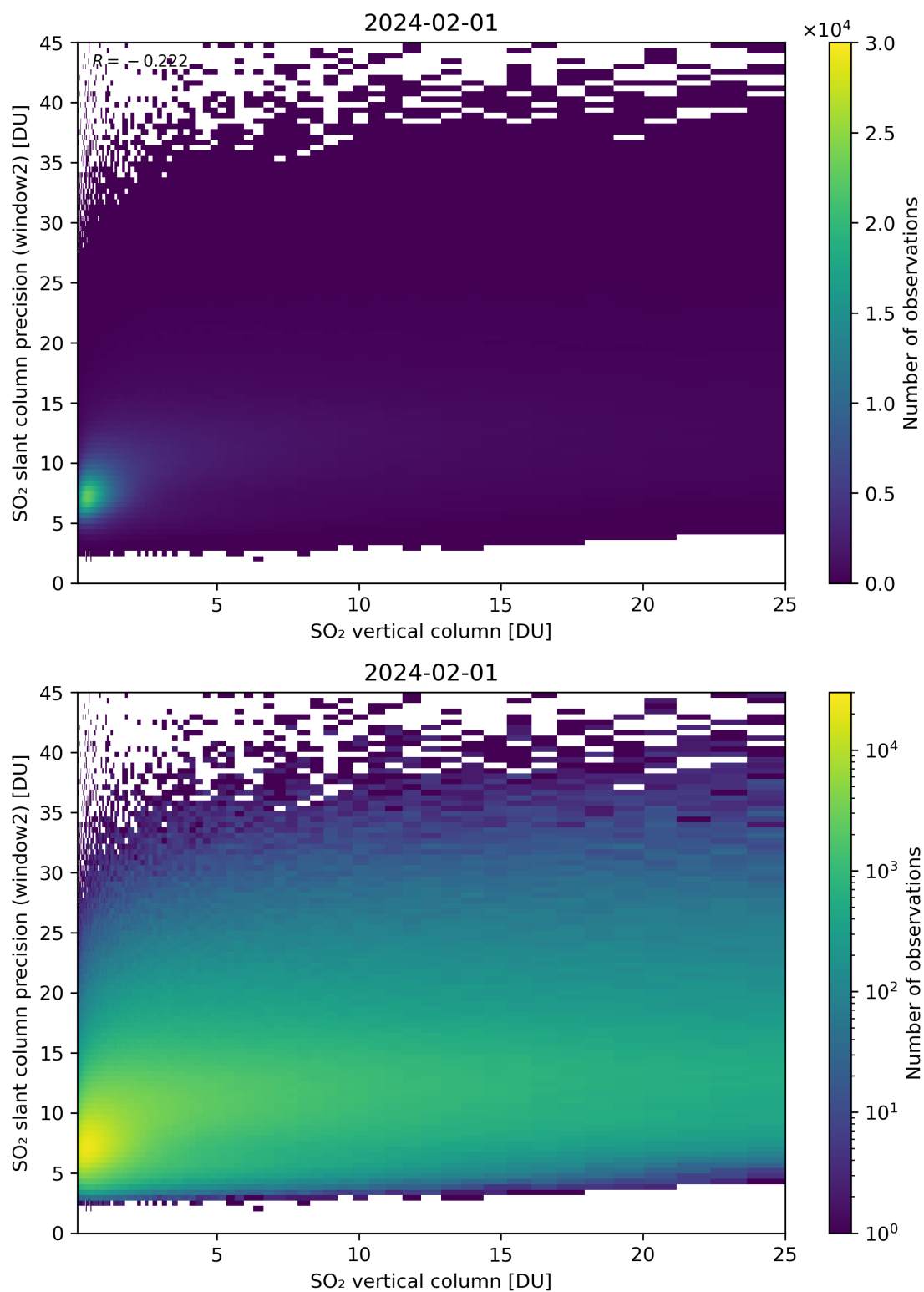
Figure 302: Scatter density plot of “SO 2 vertical column” against “SO 2 slant column precision (window2)” for 2024-01-31 to 2024-02-02.
