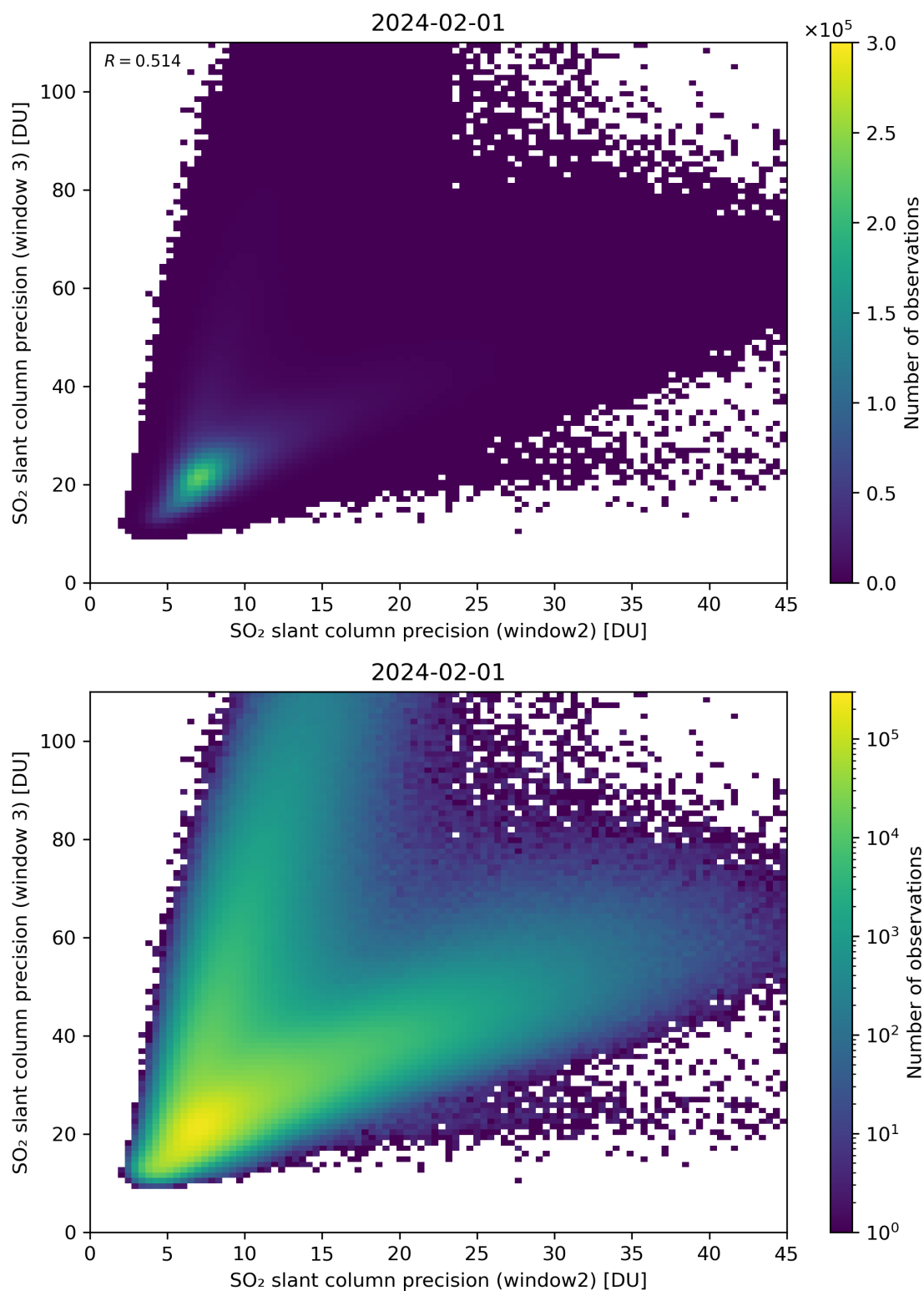
Figure 250: Scatter density plot of “SO 2 slant column precision (window2)” against “SO 2 slant column precision (window 3)” for 2024-01-31 to 2024-02-02.
