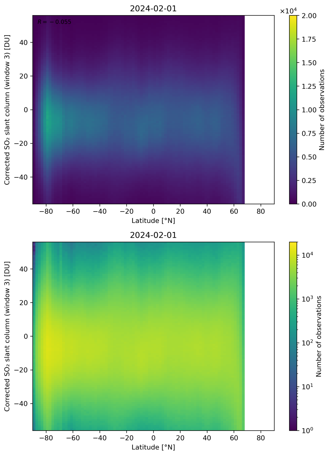
Figure 148: Scatter density plot of “Latitude” against “Corrected SO 2 slant column (window 3)” for 2024-01-31 to 2024-02-02.
