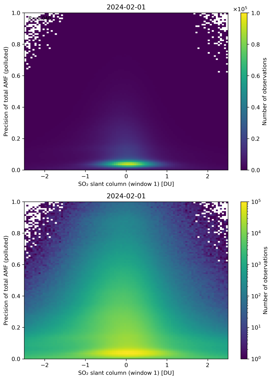
Figure 240: Scatter density plot of “SO 2 slant column (window 1)” against “Precision of total AMF (polluted)” for 2024-01-31 to 2024-02-02.
