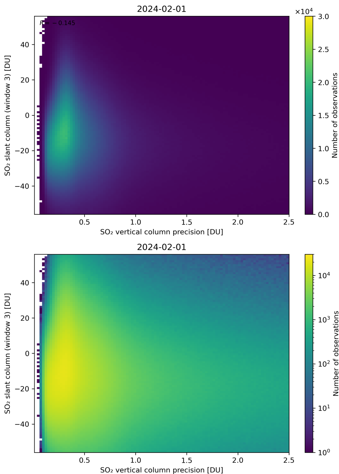
Figure 292: Scatter density plot of “SO 2 vertical column precision” against “SO 2 slant column (window 3)” for 2024-01-31 to 2024-02-02.
