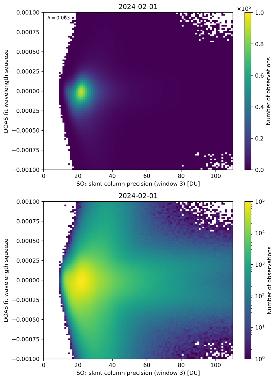
Figure 259: Scatter density plot of “SO 2 slant column precision (window 3)” against “DOAS fit wavelength squeeze” for 2024-01-31 to 2024-02-02.
