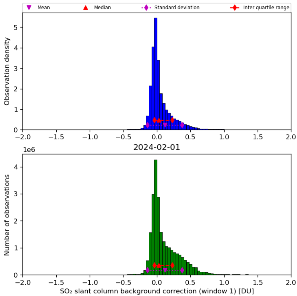
Figure 59: Histogram of “SO 2 slant column background correction (window 1)” for 2024-01-31 to 2024-02-02
