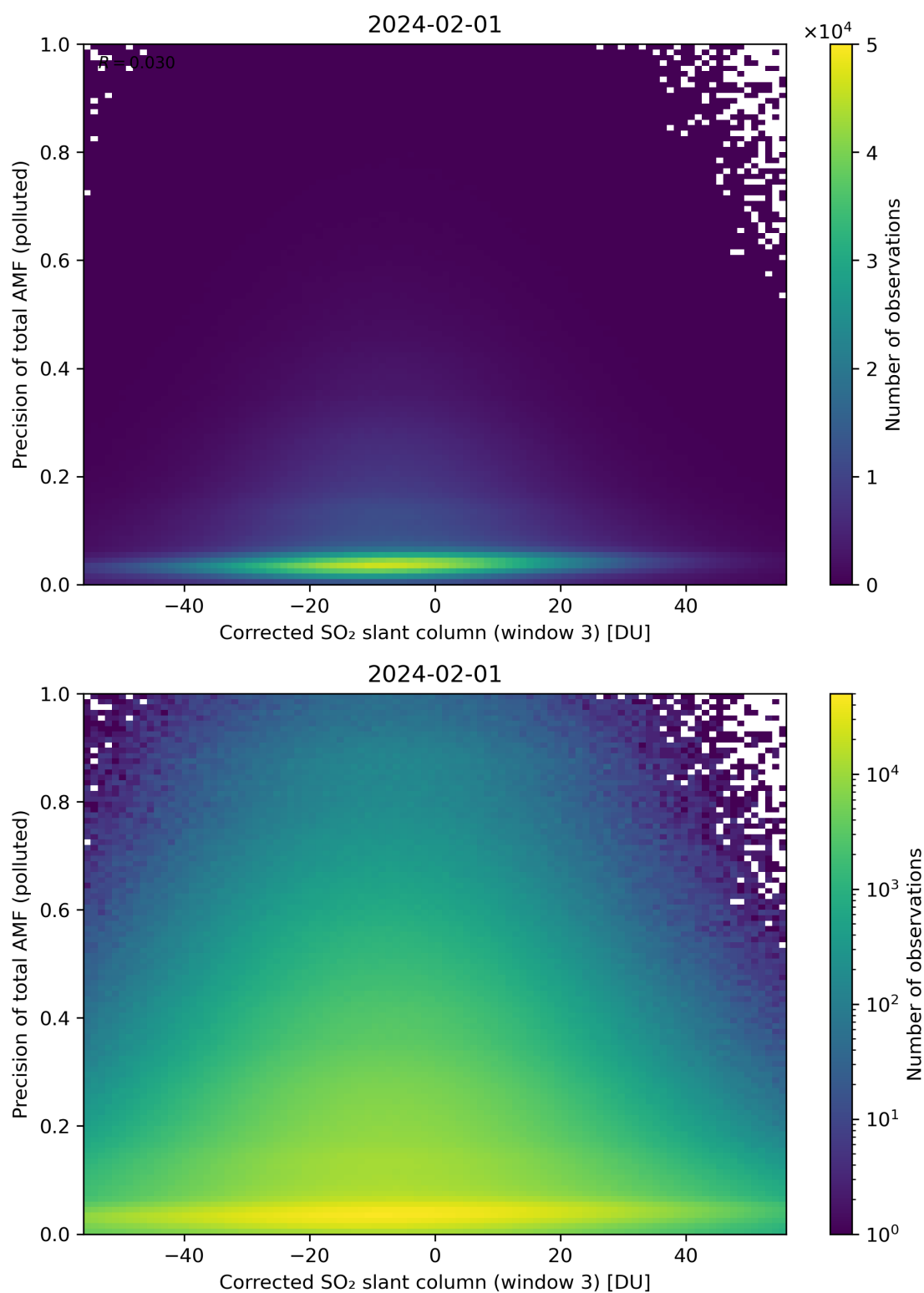
Figure 211: Scatter density plot of “Corrected SO 2 slant column (window 3)” against “Precision of total AMF (polluted)” for 2024-01-31 to 2024-02-02.
