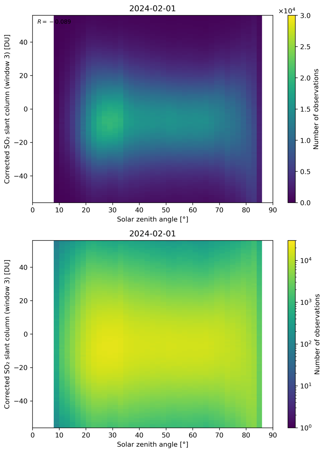
Figure 168: Scatter density plot of “Solar zenith angle” against “Corrected SO 2 slant column (window 3)” for 2024-01-31 to 2024-02-02.
