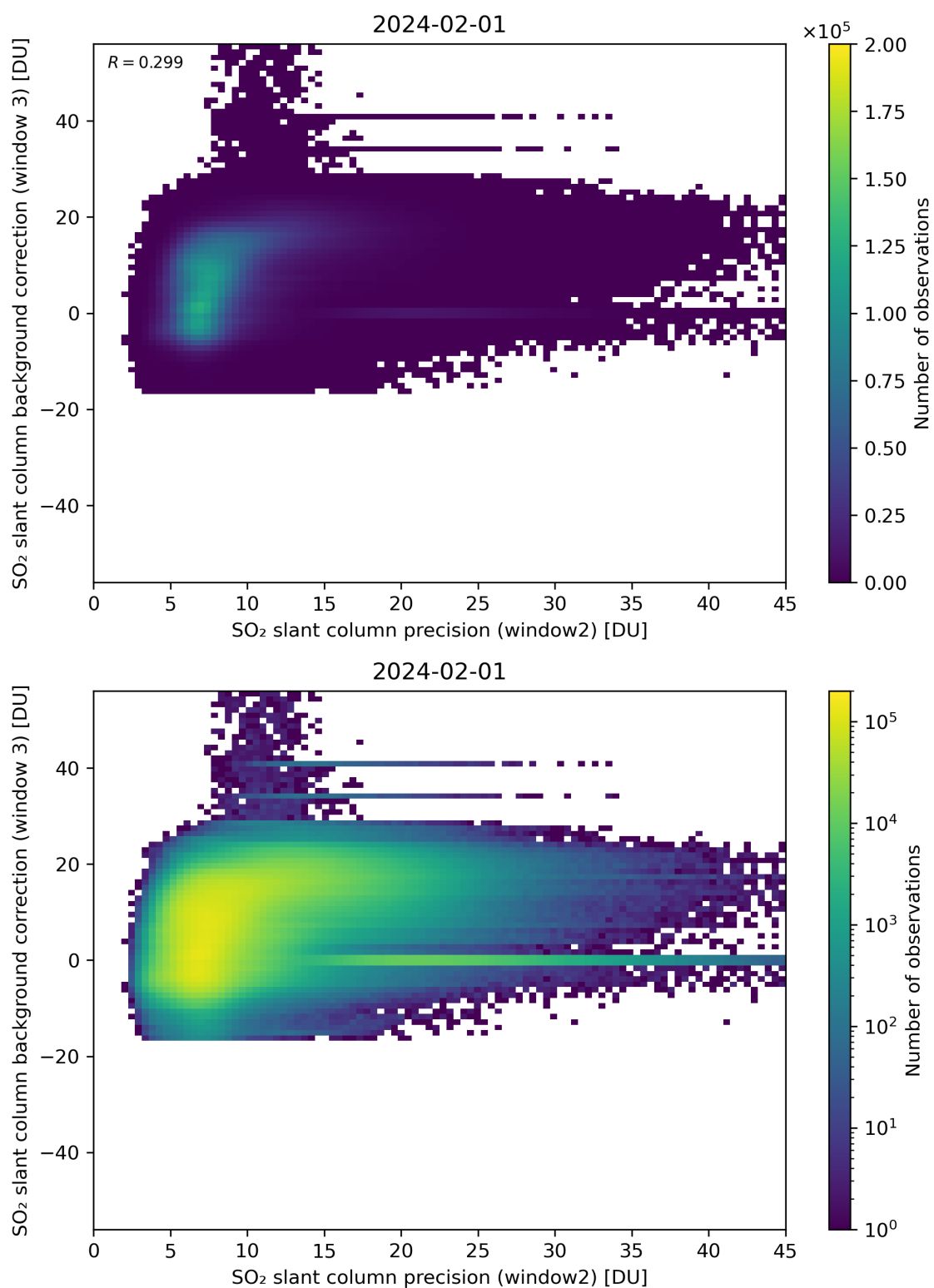
Figure 242: Scatter density plot of “SO 2 slant column precision (window2)” against “SO 2 slant column background correction (window 3)” for 2024-01-31 to 2024-02-02.
