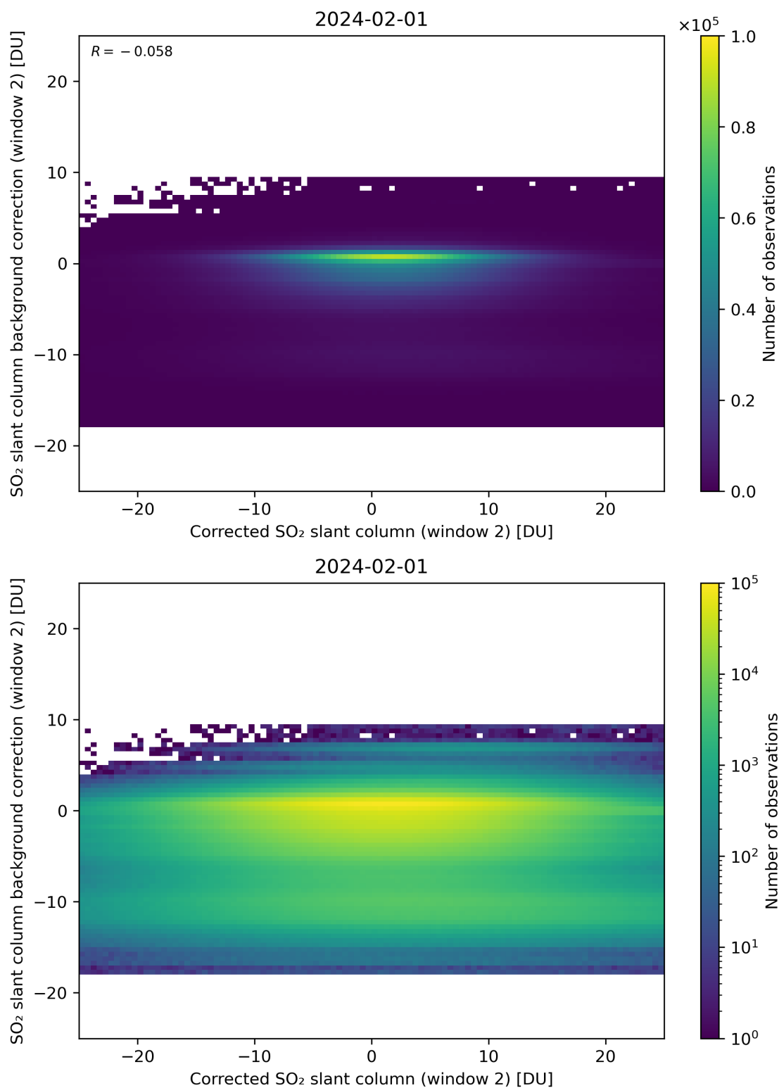
Figure 194: Scatter density plot of “Corrected SO 2 slant column (window 2)” against “SO 2 slant column background correction (window 2)” for 2024-01-31 to 2024-02-02.
