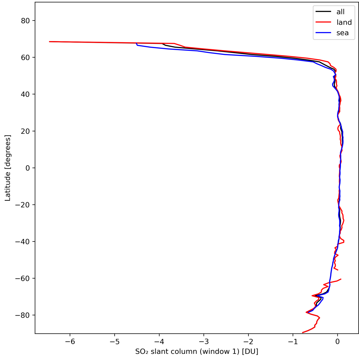
Figure 33: Zonal average of “SO 2 slant column (window 1)” for 2024-01-31 to 2024-02-02.
