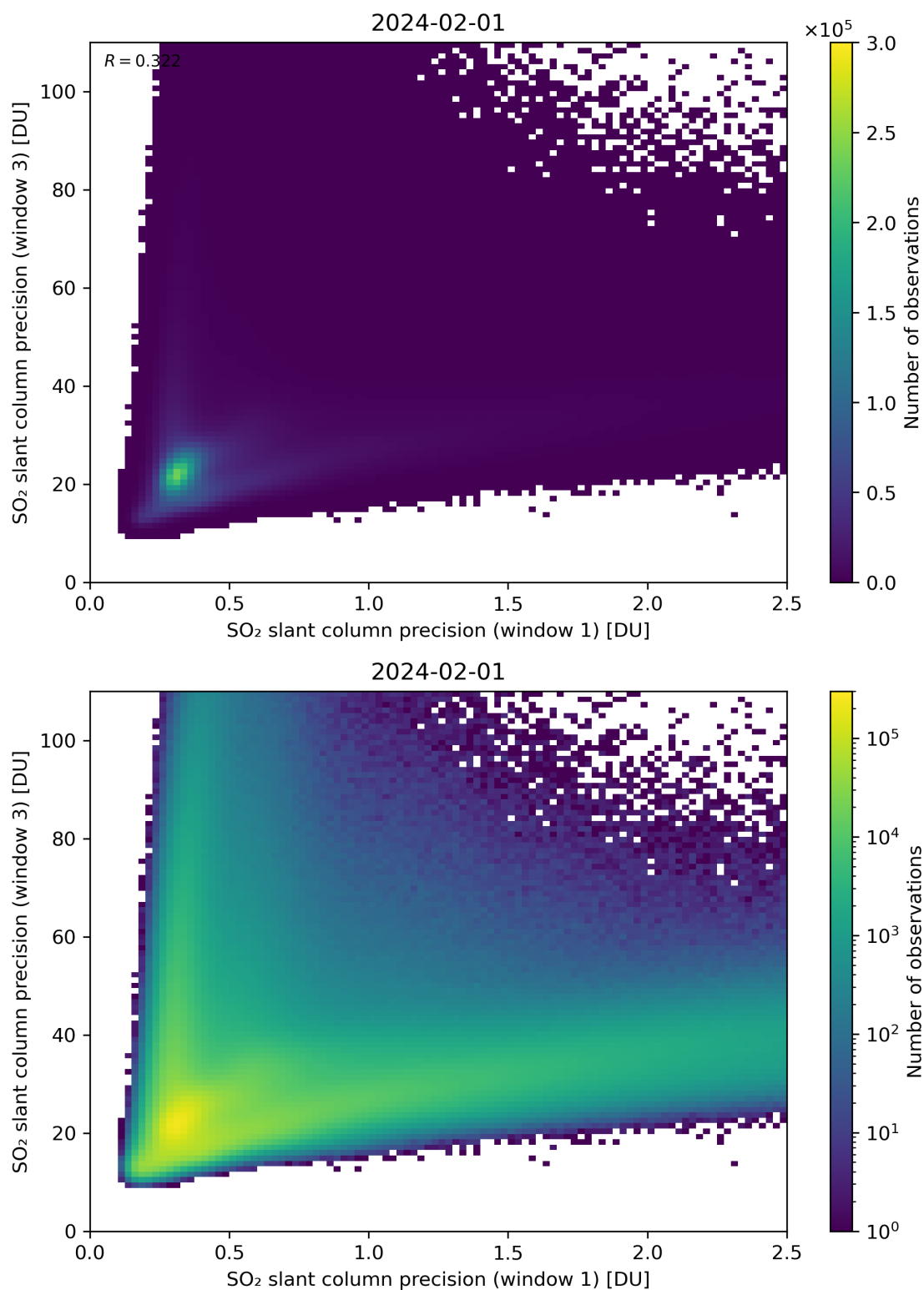
Figure 229: Scatter density plot of “SO 2 slant column precision (window 1)” against “SO 2 slant column precision (window 3)” for 2024-01-31 to 2024-02-02.
