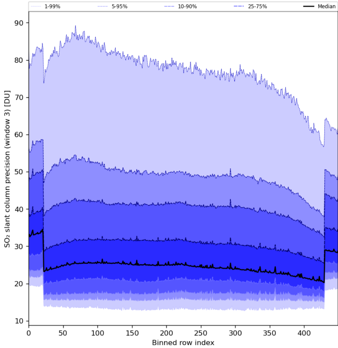
Figure 88: Along track statistics of “SO 2 slant column precision (window 3)” for 2024-01-31 to 2024-02-02
