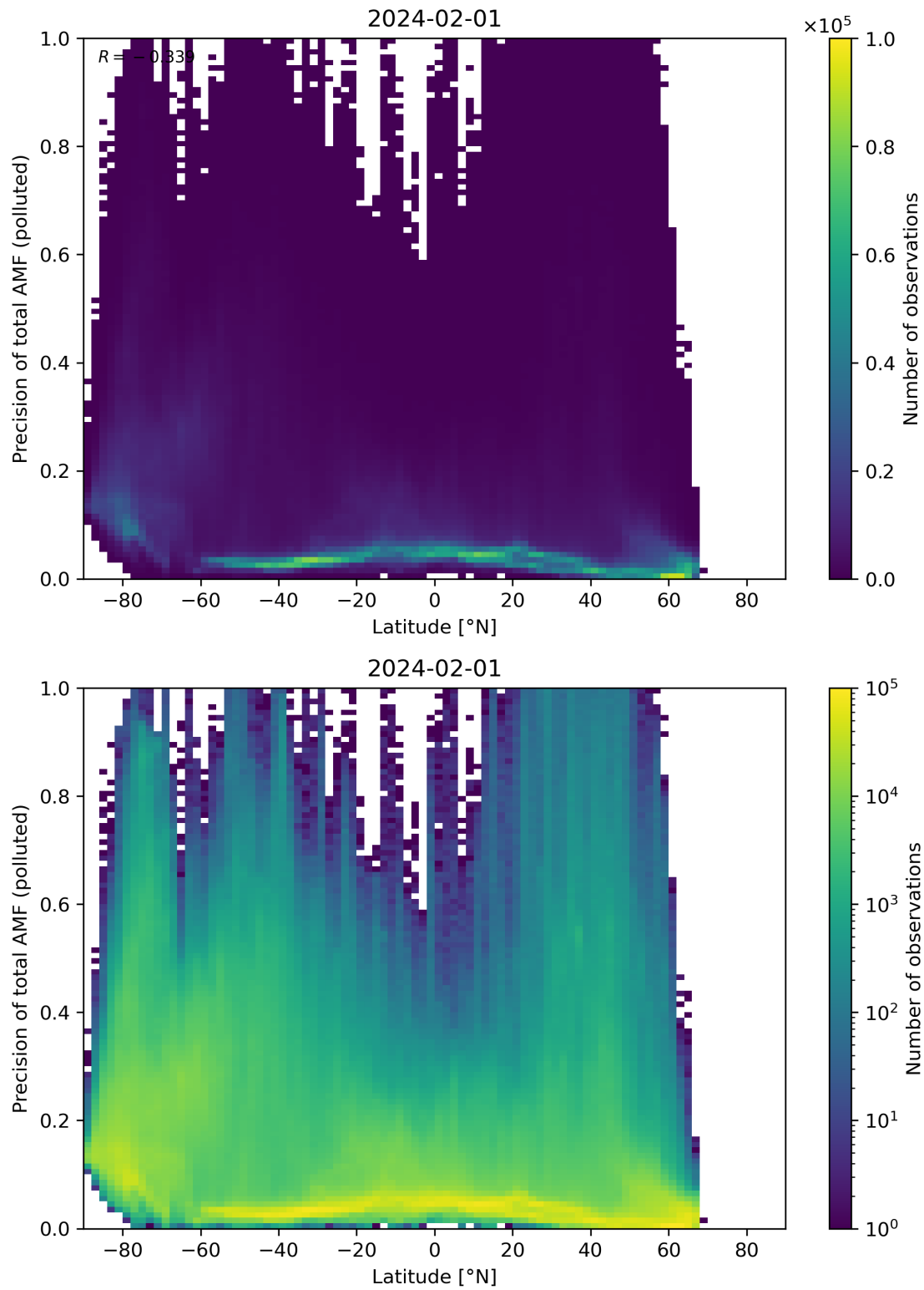
Figure 155: Scatter density plot of “Latitude” against “Precision of total AMF (polluted)” for 2024-01-31 to 2024-02-02.
