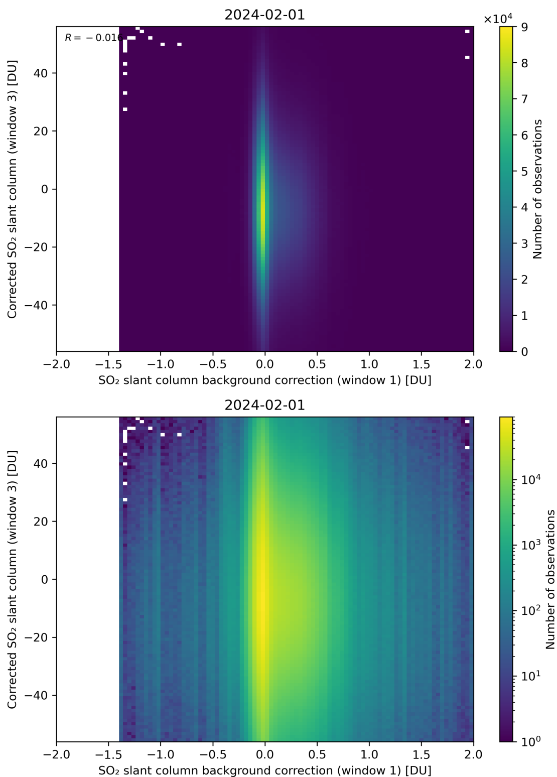
Figure 105: Scatter density plot of “SO 2 slant column background correction (window 1)” against “Corrected SO 2 slant column (window 3)” for 2024-01-31 to 2024-02-02.
