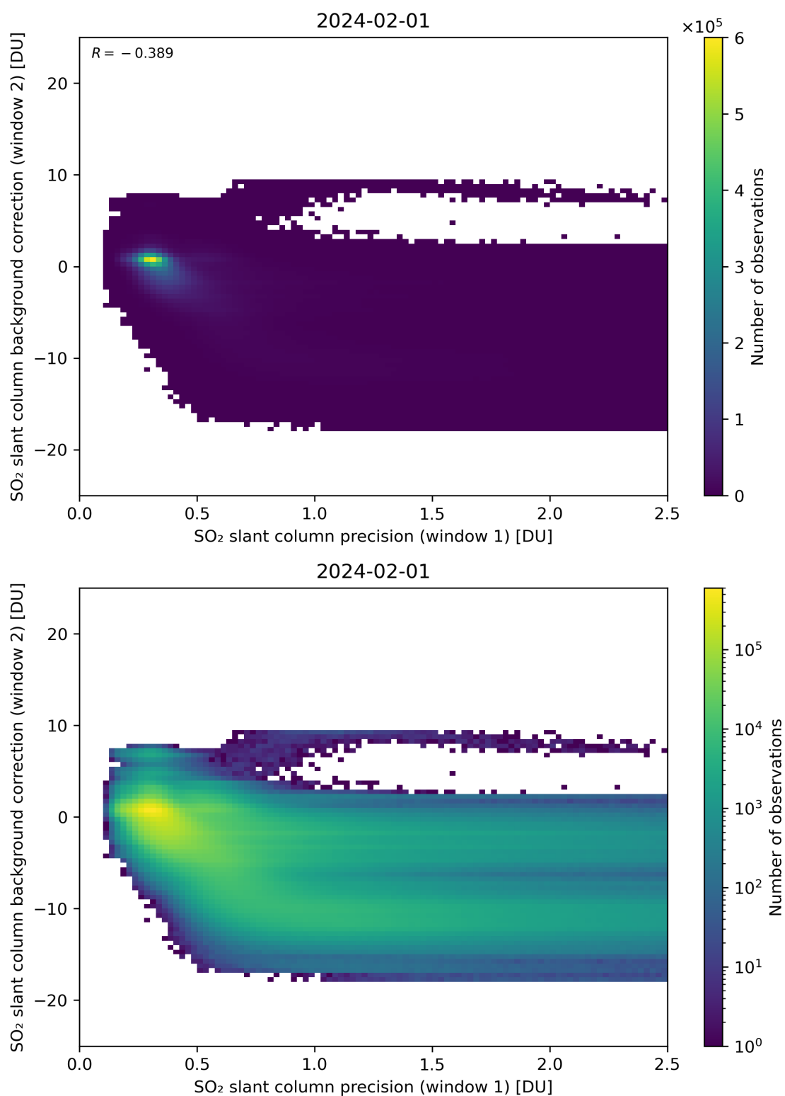
Figure 219: Scatter density plot of “SO 2 slant column precision (window 1)” against “SO 2 slant column background correction (window 2)” for 2024-01-31 to 2024-02-02.
