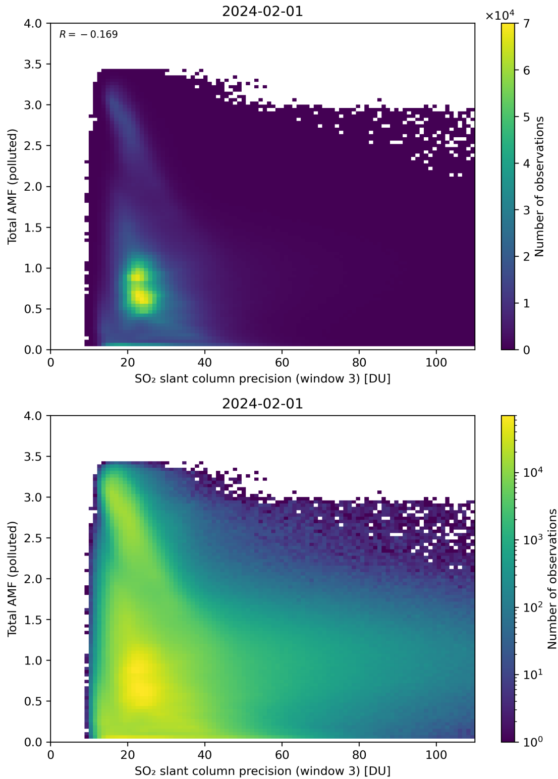
Figure 263: Scatter density plot of “SO 2 slant column precision (window 3)” against “Total AMF (polluted)” for 2024-01-31 to 2024-02-02.
