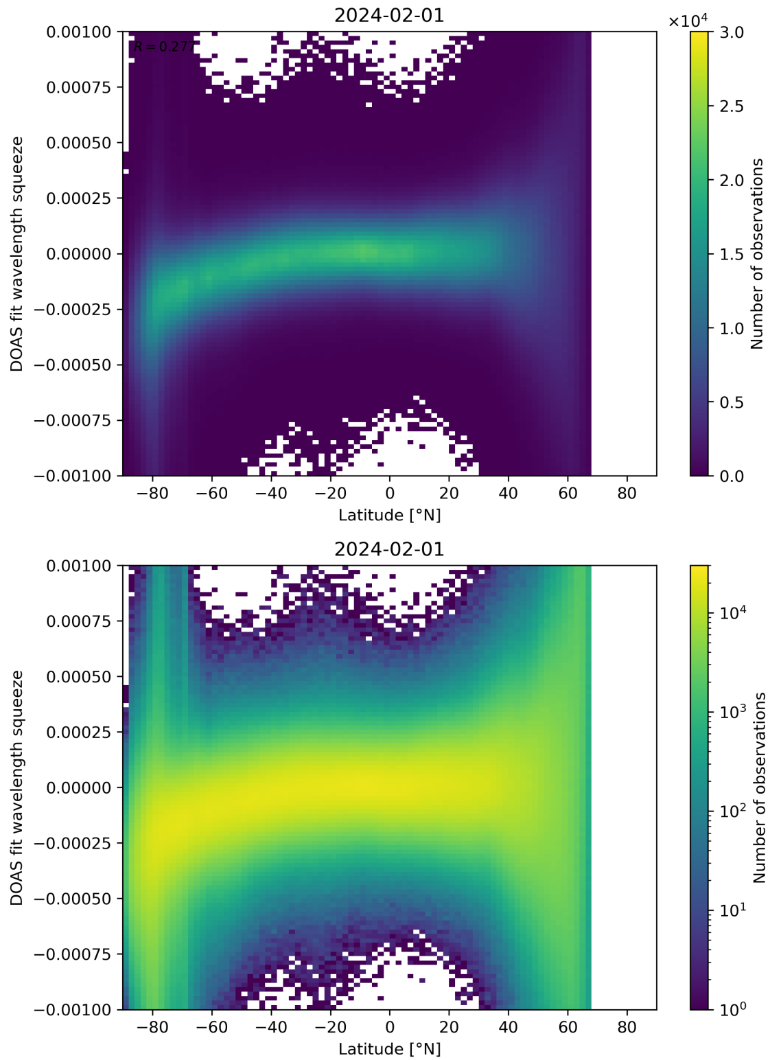
Figure 143: Scatter density plot of “Latitude” against “DOAS fit wavelength squeeze” for 2024-01-31 to 2024-02-02.
