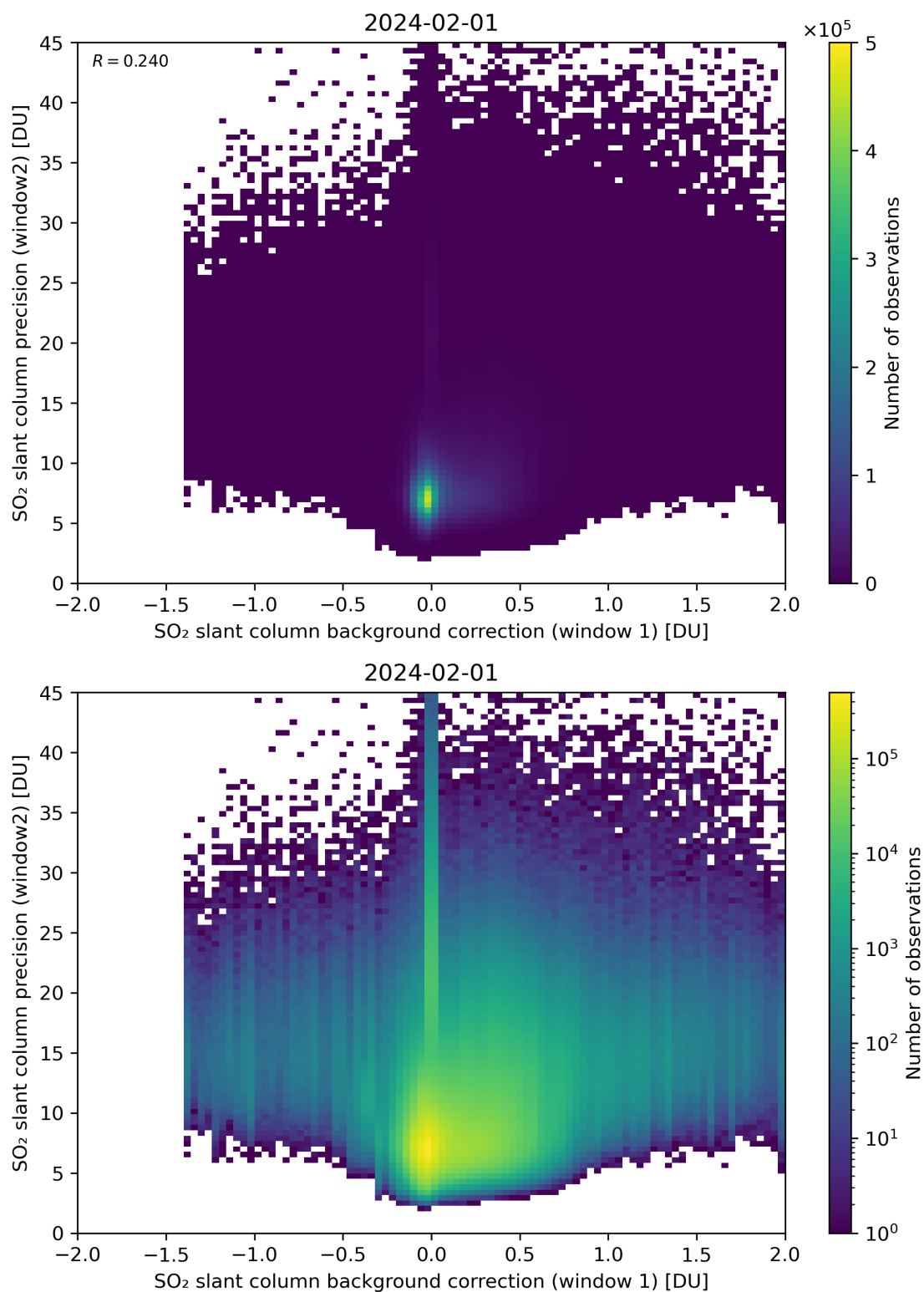
Figure 106: Scatter density plot of “SO 2 slant column background correction (window 1)” against “SO 2 slant column precision (window2)” for 2024-01-31 to 2024-02-02.
