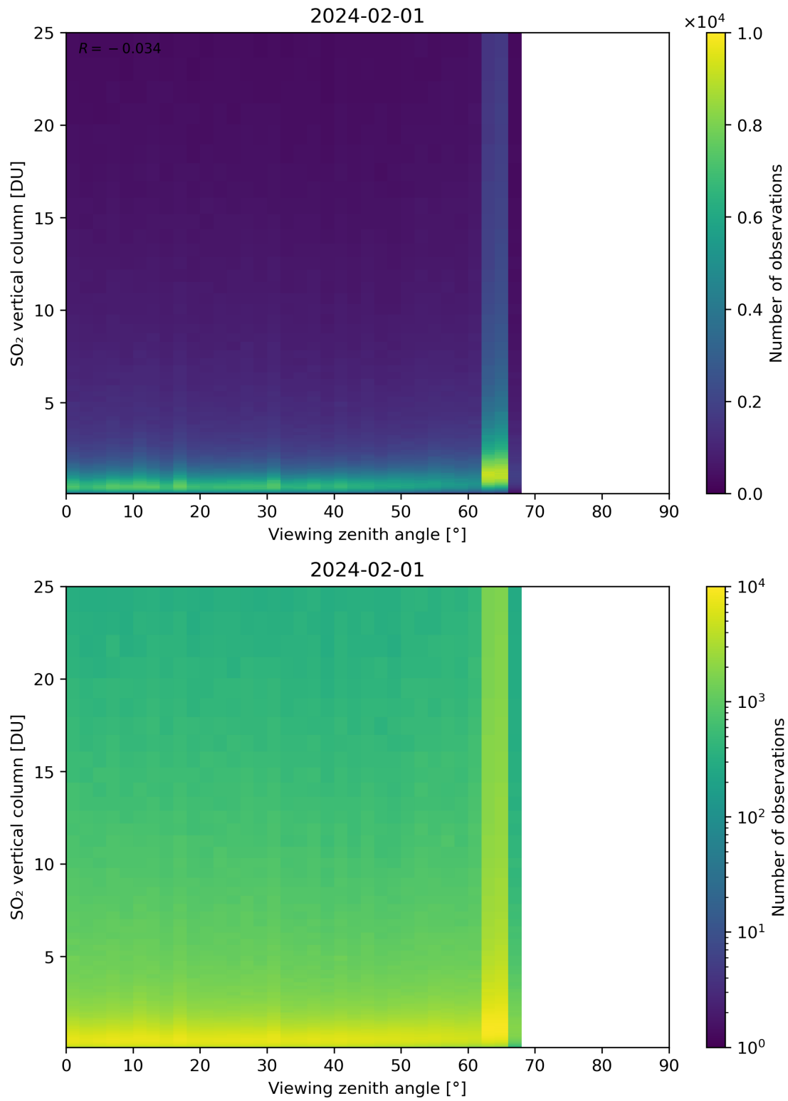
Figure 327: Scatter density plot of “Viewing zenith angle” against “SO 2 vertical column” for 2024-01-31 to 2024-02-02.
