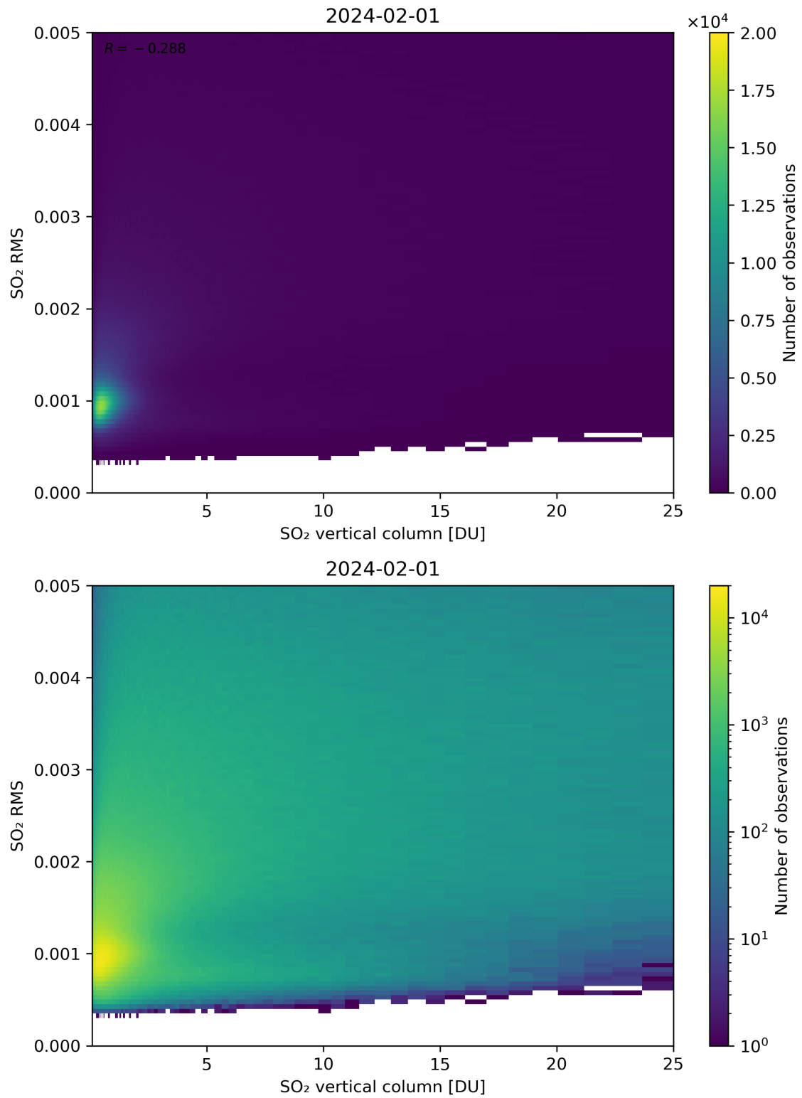
Figure 278: Scatter density plot of “SO 2 vertical column” against “SO 2 RMS” for 2024-01-31 to 2024-02-02.
