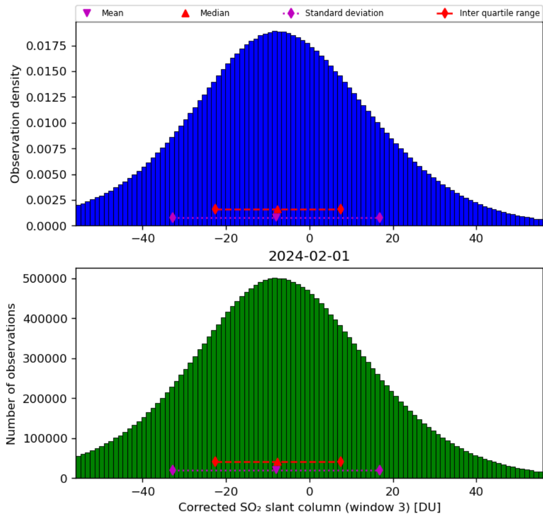
Figure 66: Histogram of “Corrected SO 2 slant column (window 3)” for 2024-01-31 to 2024-02-02
