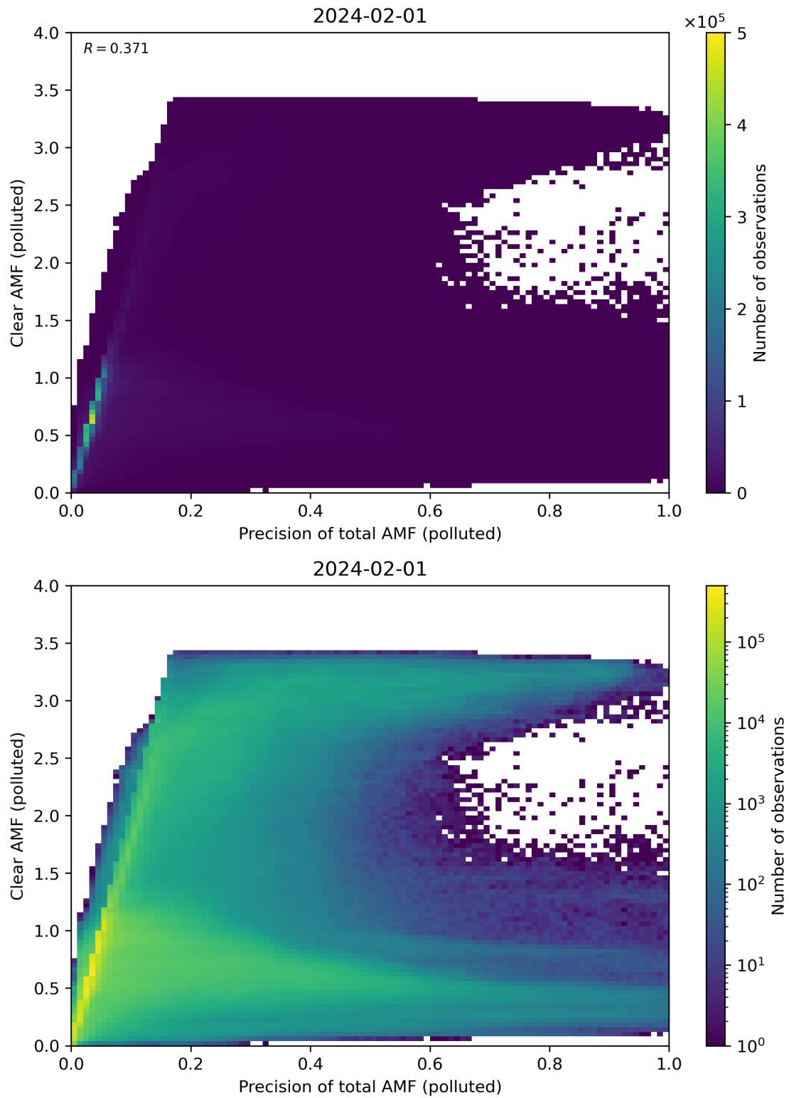
Figure 270: Scatter density plot of “Precision of total AMF (polluted)” against “Clear AMF (polluted)” for 2024-01-31 to 2024-02-02.
