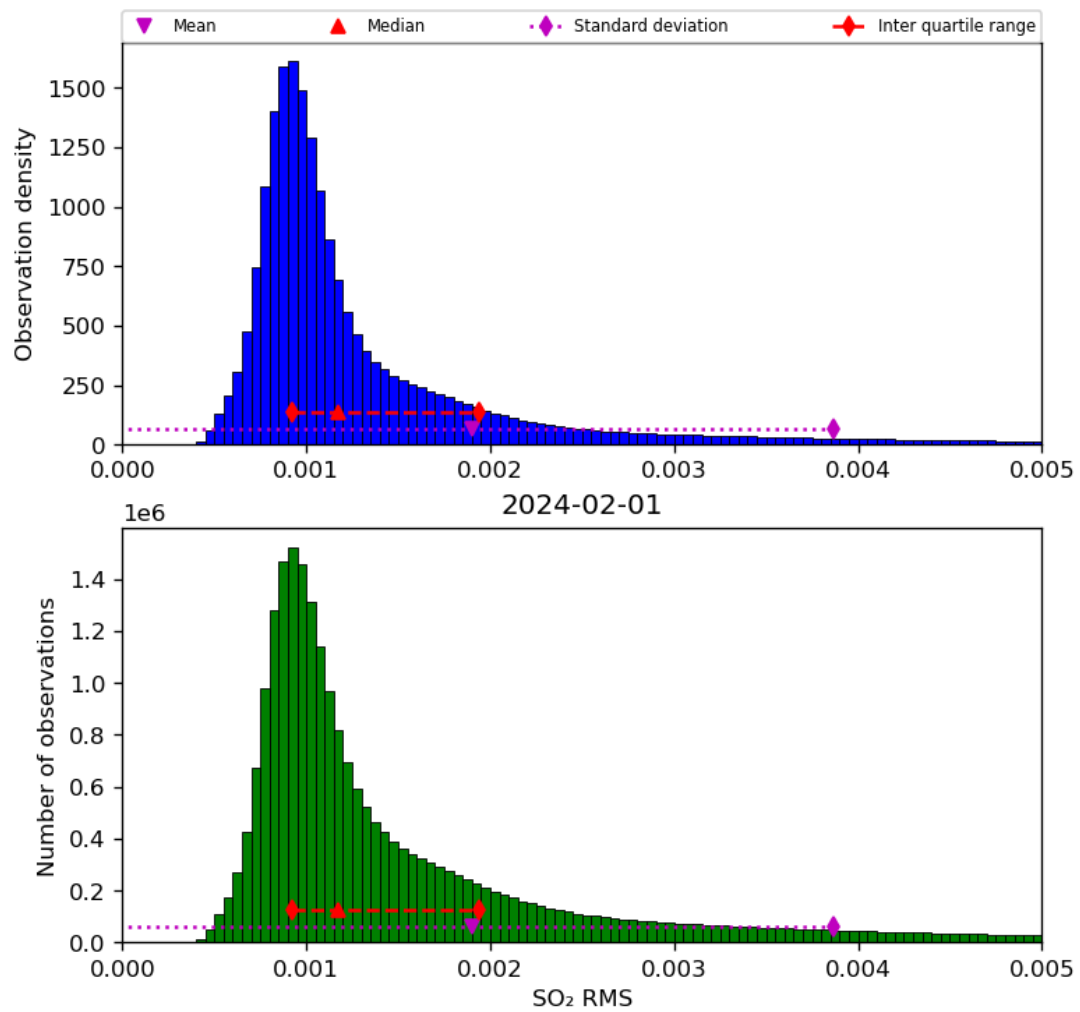
Figure 70: Histogram of “SO 2 RMS” for 2024-01-31 to 2024-02-02
