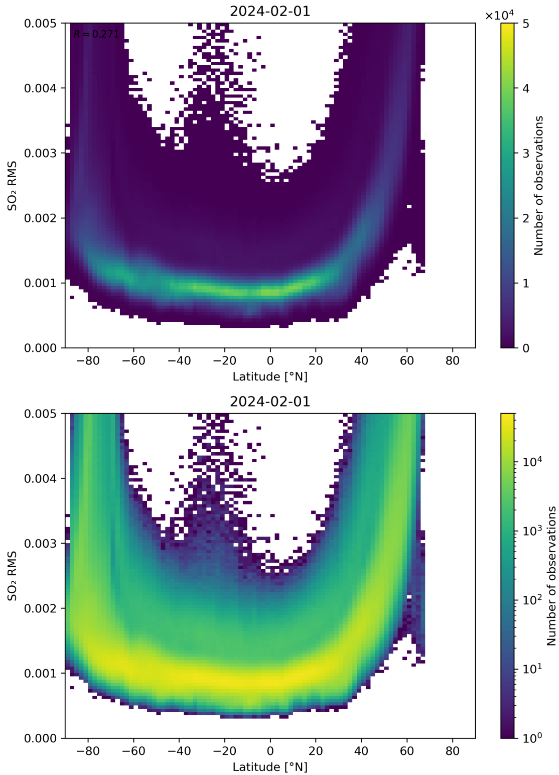
Figure 144: Scatter density plot of “Latitude” against “SO 2 RMS” for 2024-01-31 to 2024-02-02.
