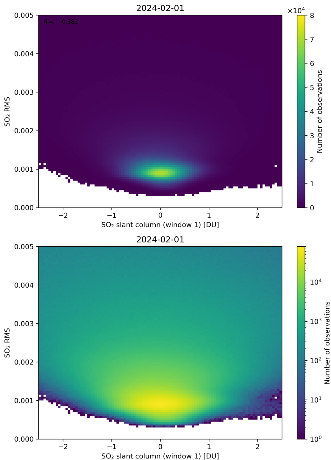
Figure 217: Scatter density plot of “SO 2 slant column (window 1)” against “SO 2 RMS” for 2024-01-31 to 2024-02-02.
