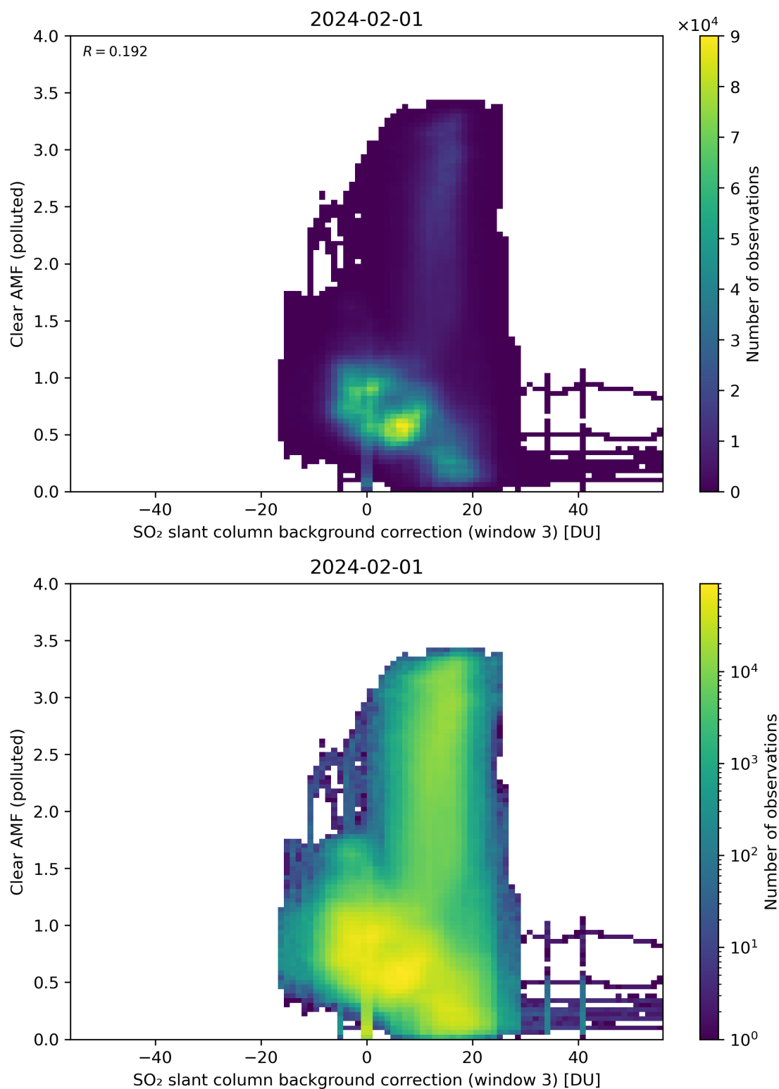
Figure 124: Scatter density plot of “SO 2 slant column background correction (window 3)” against “Clear AMF (polluted)” for 2024-01-31 to 2024-02-02.
