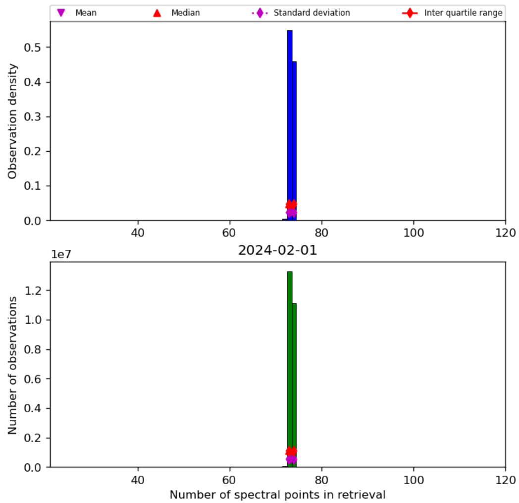
Figure 74: Histogram of “Number of spectral points in retrieval” for 2024-01-31 to 2024-02-02
