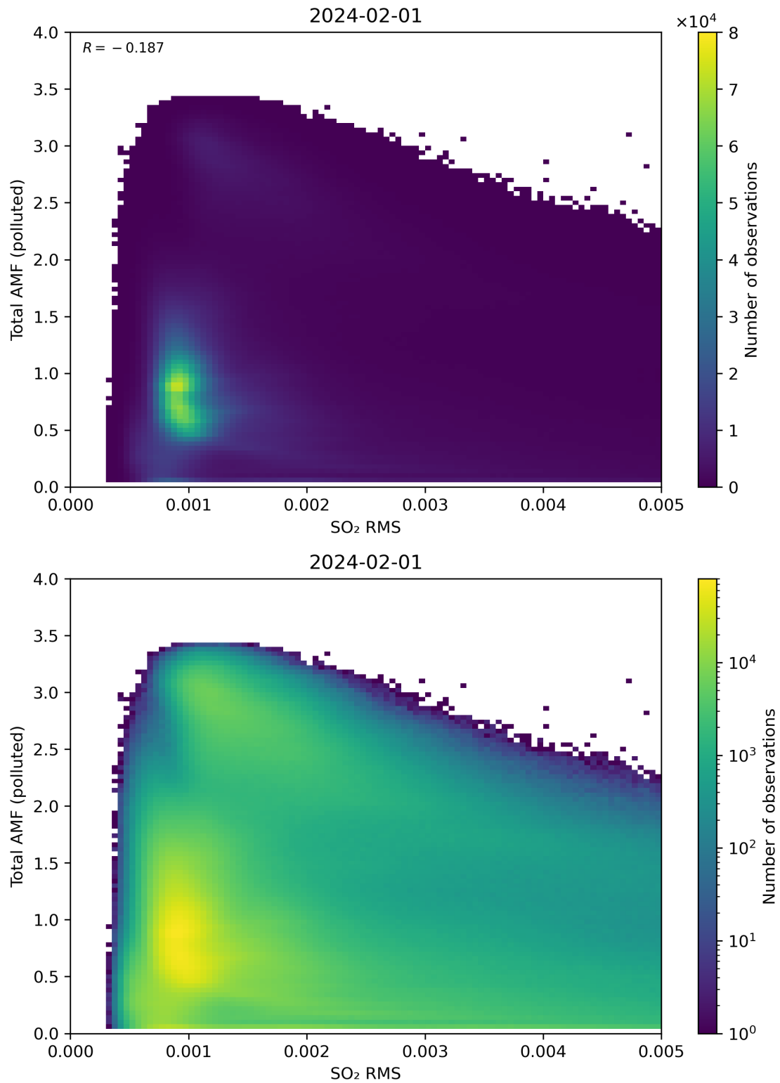
Figure 137: Scatter density plot of “SO 2 RMS” against “Total AMF (polluted)” for 2024-01-31 to 2024-02-02.
