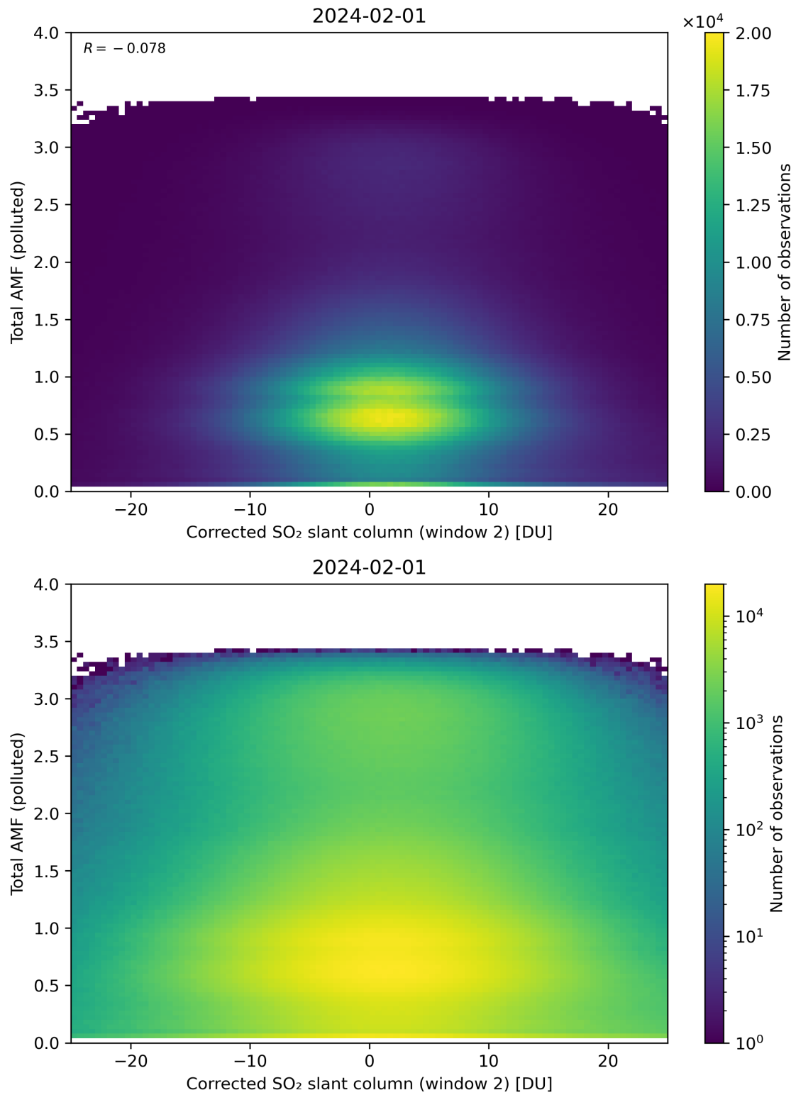
Figure 203: Scatter density plot of “Corrected SO 2 slant column (window 2)” against “Total AMF (polluted)” for 2024-01-31 to 2024-02-02.
