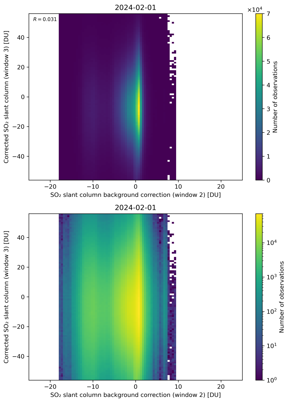
Figure 116: Scatter density plot of “SO 2 slant column background correction (window 2)” against “Corrected SO 2 slant column (window 3)” for 2024-01-31 to 2024-02-02.
