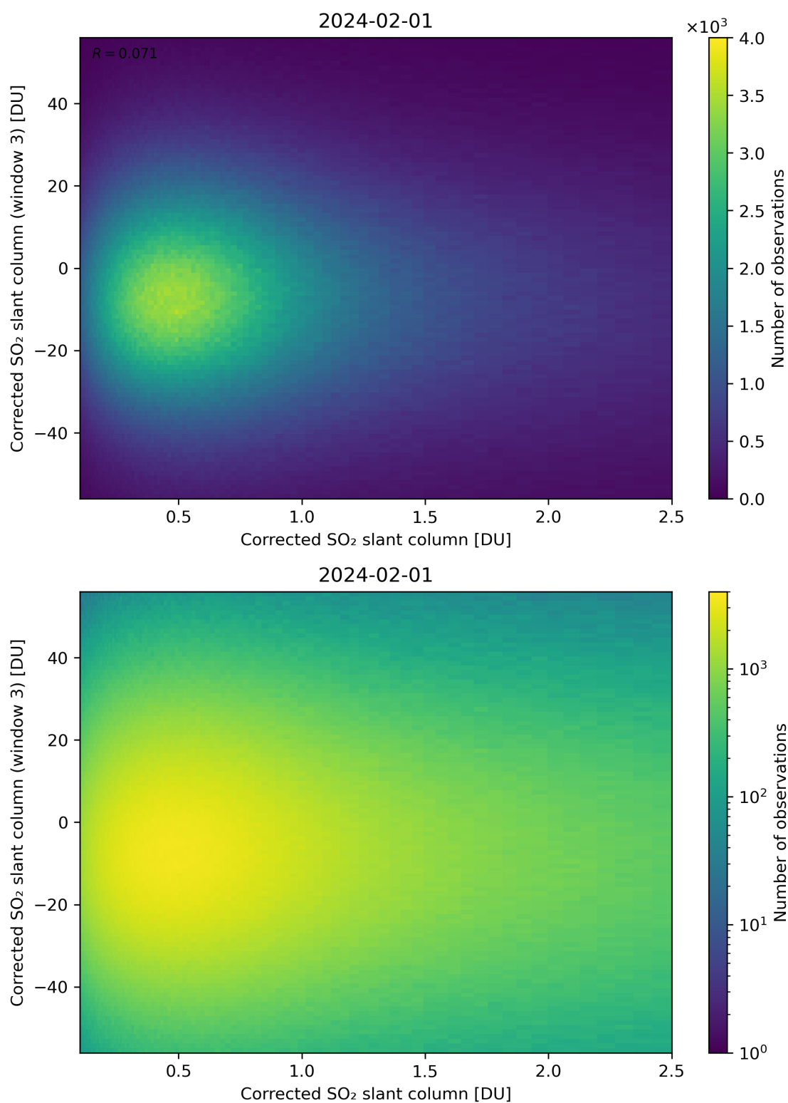
Figure 186: Scatter density plot of “Corrected SO 2 slant column” against “Corrected SO 2 slant column (window 3)” for 2024-01-31 to 2024-02-02.
