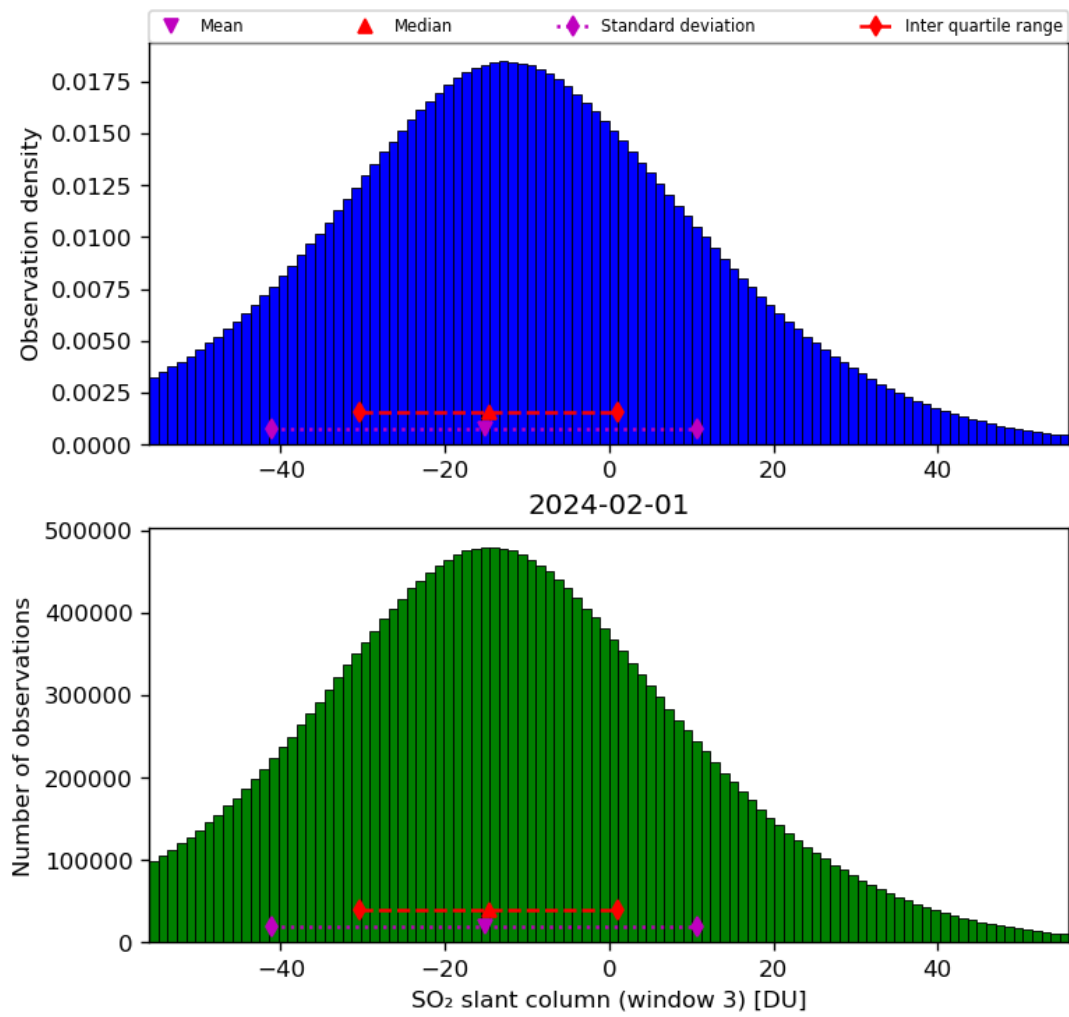
Figure 64: Histogram of “SO 2 slant column (window 3)” for 2024-01-31 to 2024-02-02
