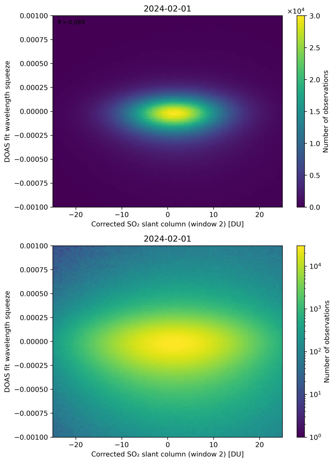
Figure 197: Scatter density plot of “Corrected SO 2 slant column (window 2)” against “DOAS fit wavelength squeeze” for 2024-01-31 to 2024-02-02.
