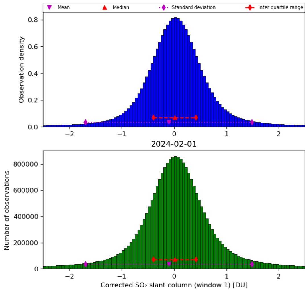
Figure 58: Histogram of “Corrected SO 2 slant column (window 1)” for 2024-01-31 to 2024-02-02
