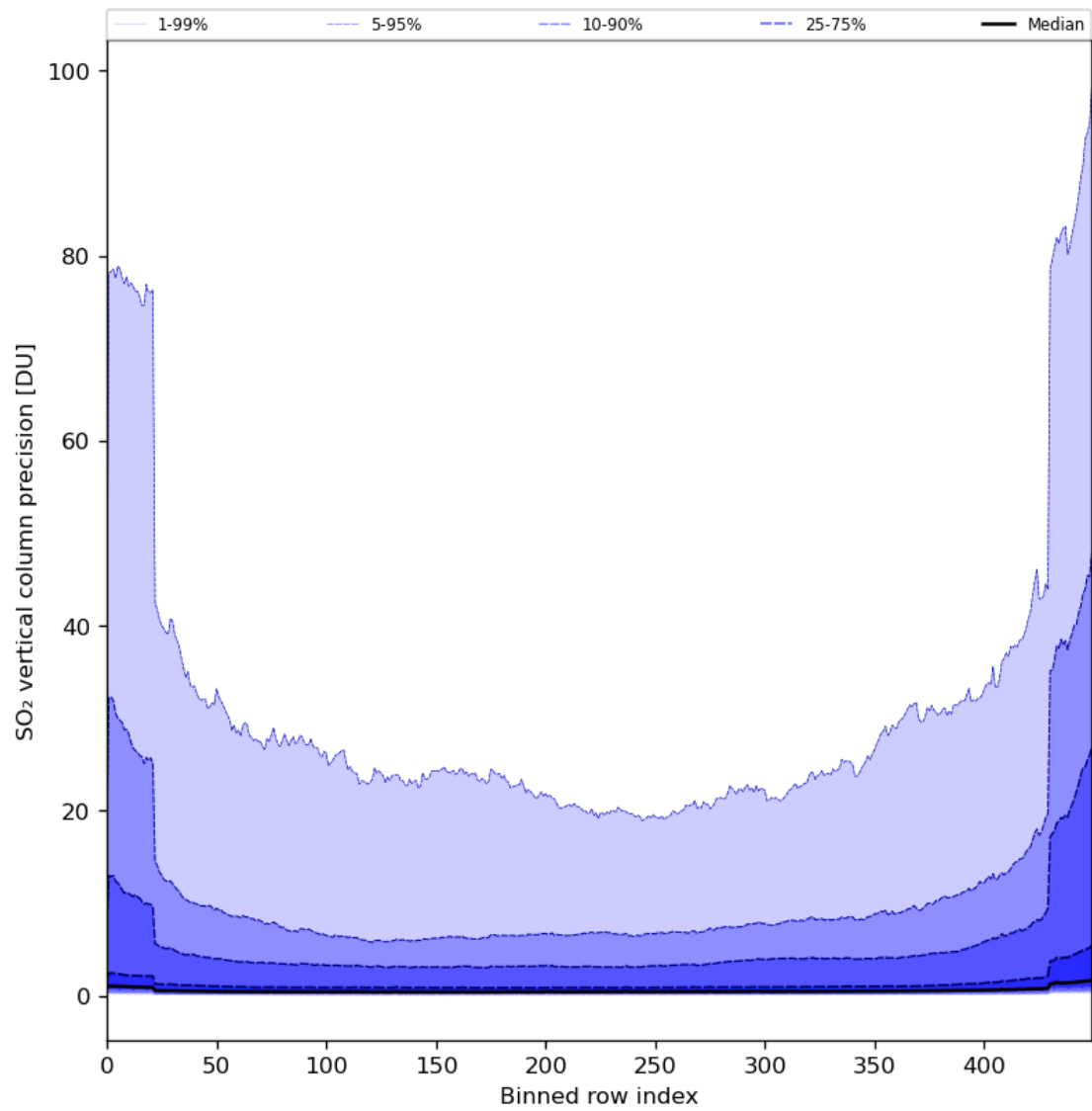
Figure 77: Along track statistics of “SO 2 vertical column precision” for 2024-01-31 to 2024-02-02
