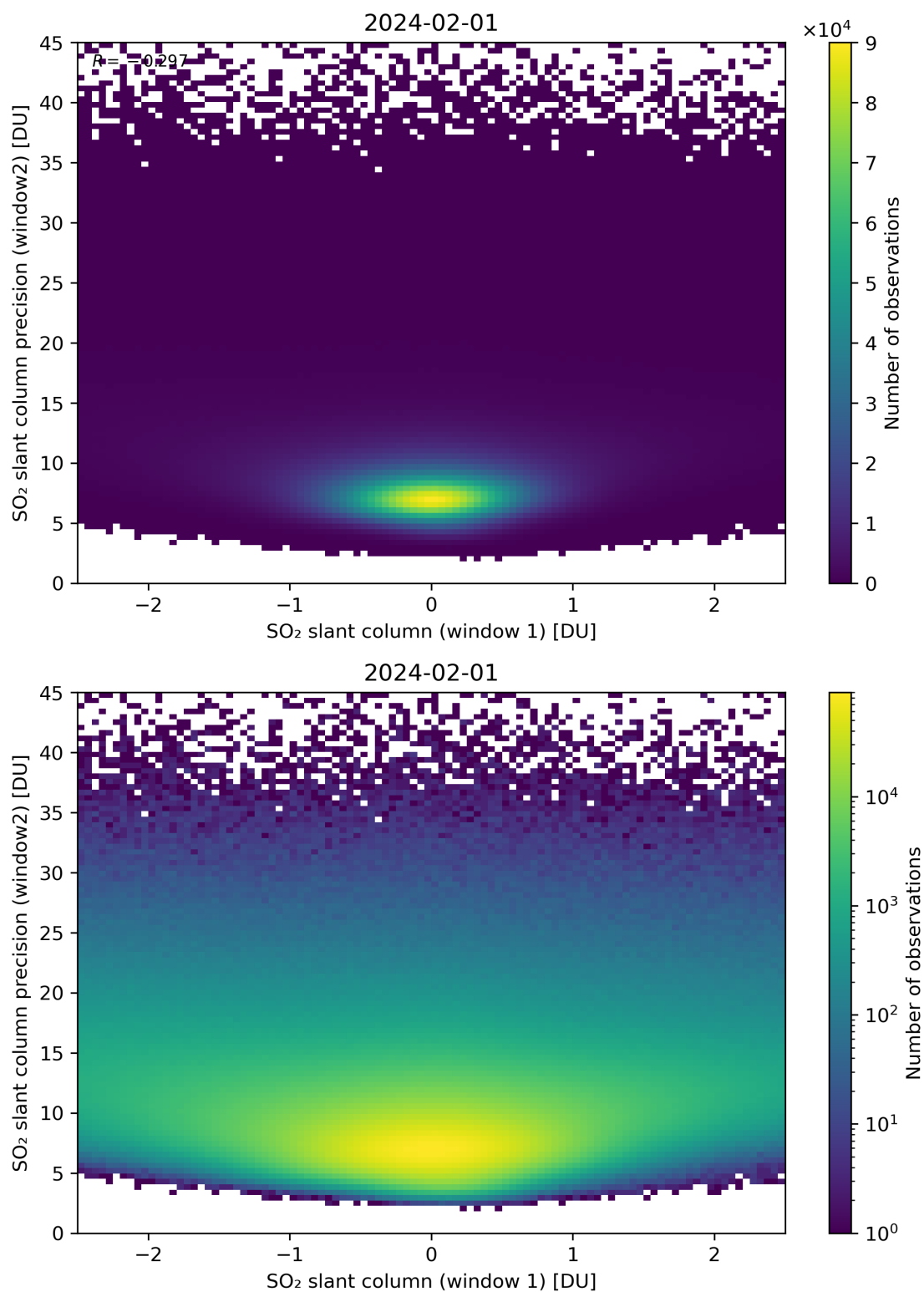
Figure 236: Scatter density plot of “SO 2 slant column (window 1)” against “SO 2 slant column precision (window2)” for 2024-01-31 to 2024-02-02.
