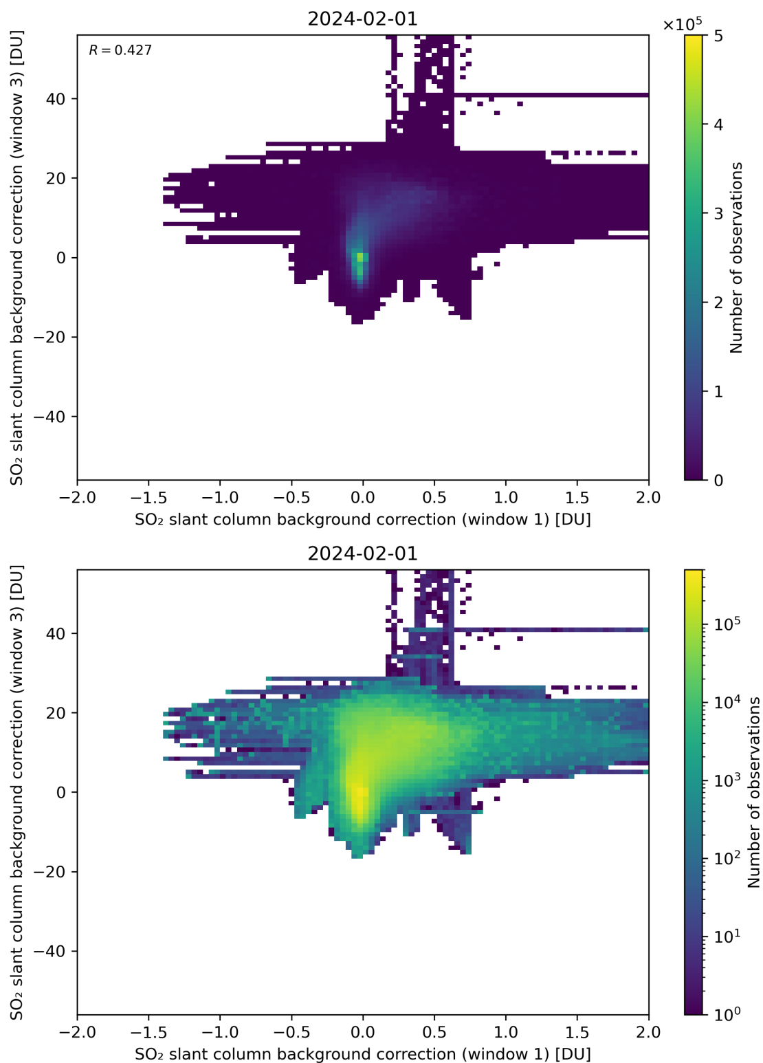
Figure 99: Scatter density plot of “SO 2 slant column background correction (window 1)” against “SO 2 slant column background correction (window 3)” for 2024-01-31 to 2024-02-02.
