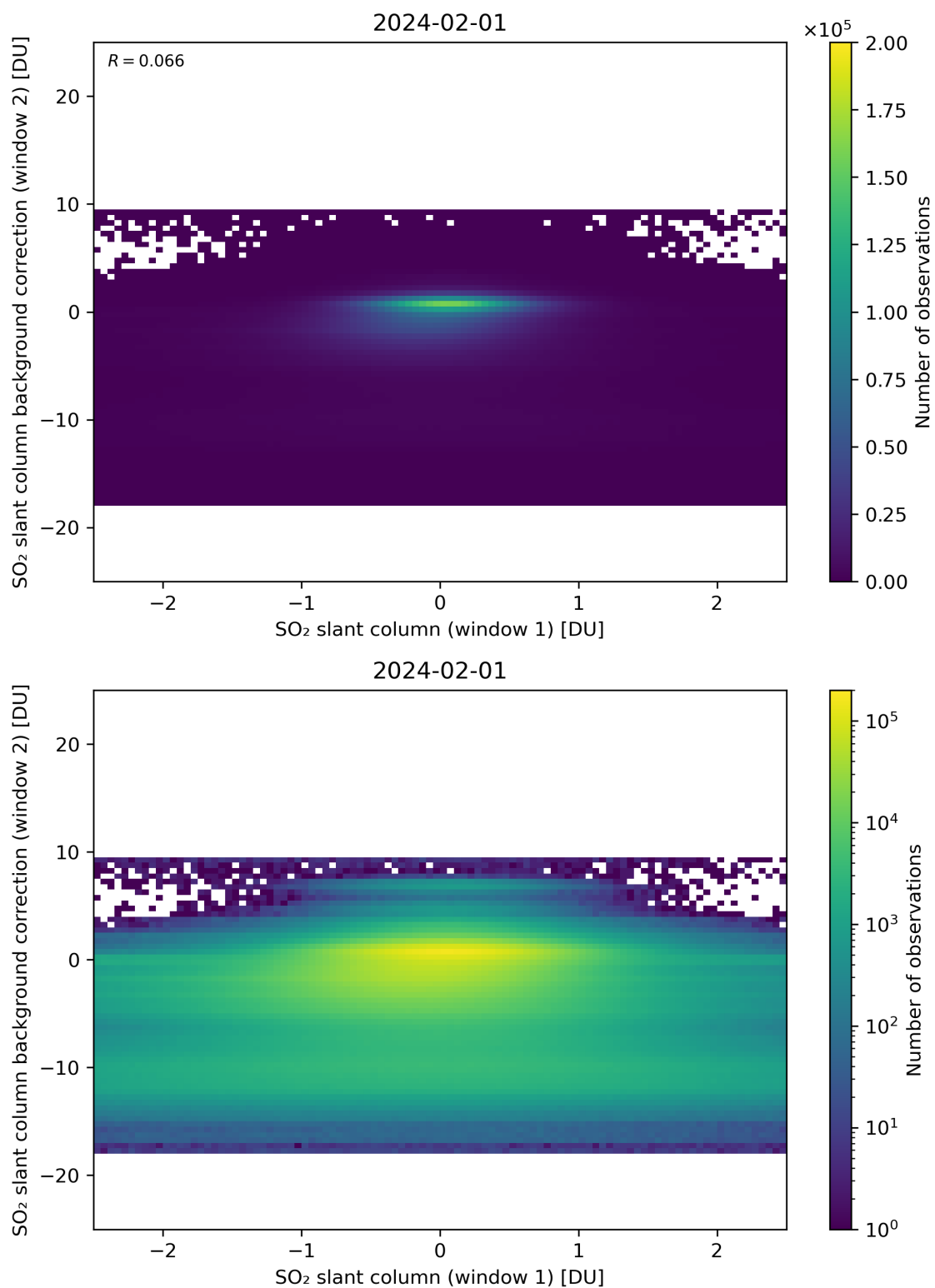
Figure 213: Scatter density plot of “SO 2 slant column (window 1)” against “SO 2 slant column background correction (window 2)” for 2024-01-31 to 2024-02-02.
