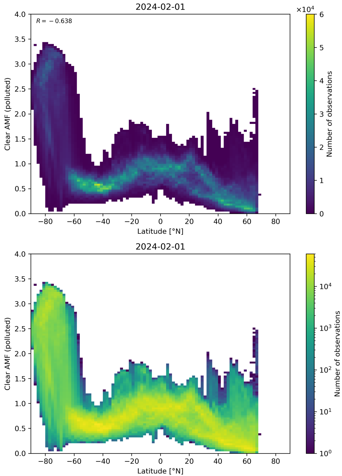
Figure 145: Scatter density plot of “Latitude” against “Clear AMF (polluted)” for 2024-01-31 to 2024-02-02.
