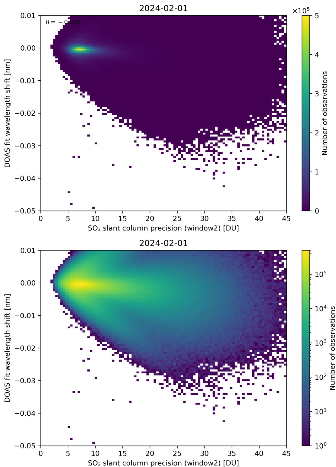
Figure 243: Scatter density plot of “SO 2 slant column precision (window2)” against “DOAS fit wavelength shift” for 2024-01-31 to 2024-02-02.
