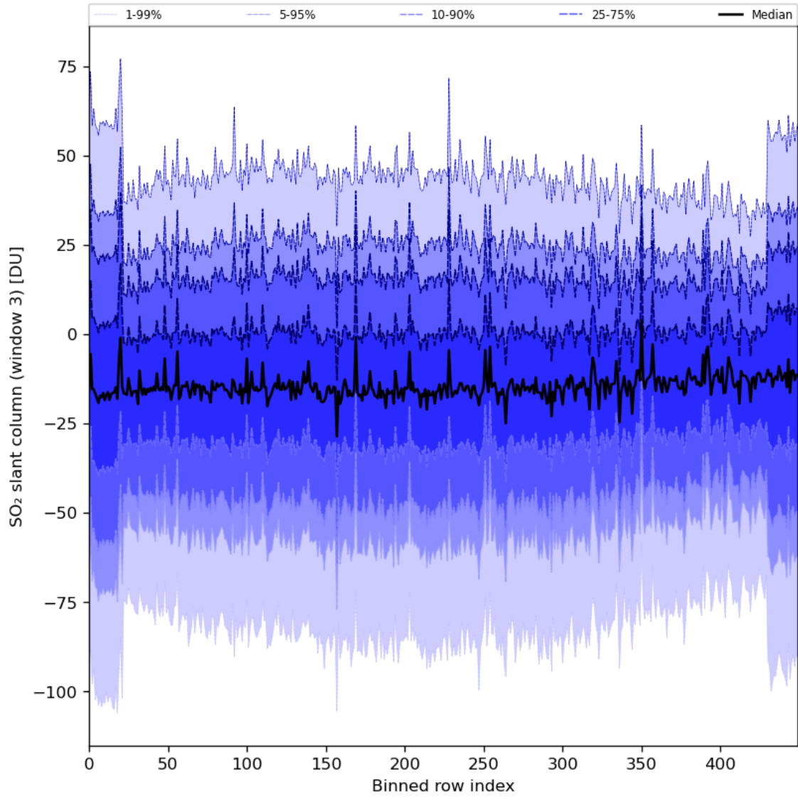
Figure 87: Along track statistics of “SO 2 slant column (window 3)” for 2024-01-31 to 2024-02-02
