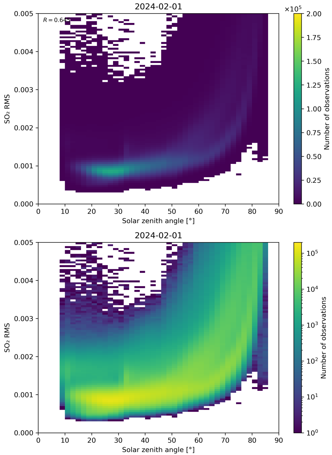
Figure 163: Scatter density plot of “Solar zenith angle” against “SO 2 RMS” for 2024-01-31 to 2024-02-02.
