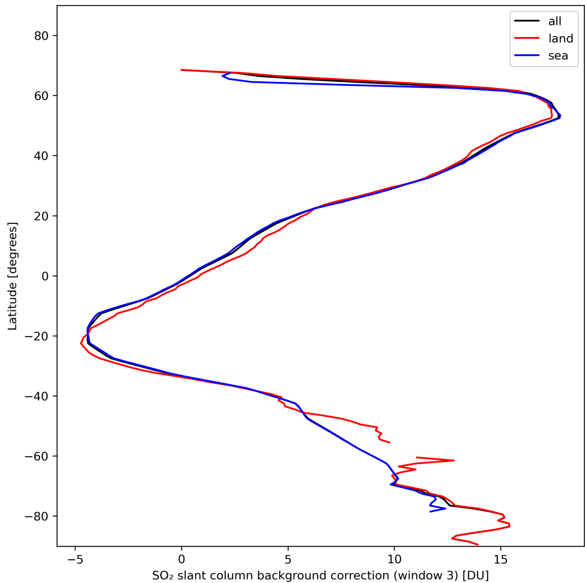
Figure 44: Zonal average of “SO 2 slant column background correction (window 3)” for 2024-01-31 to 2024-02-02.
