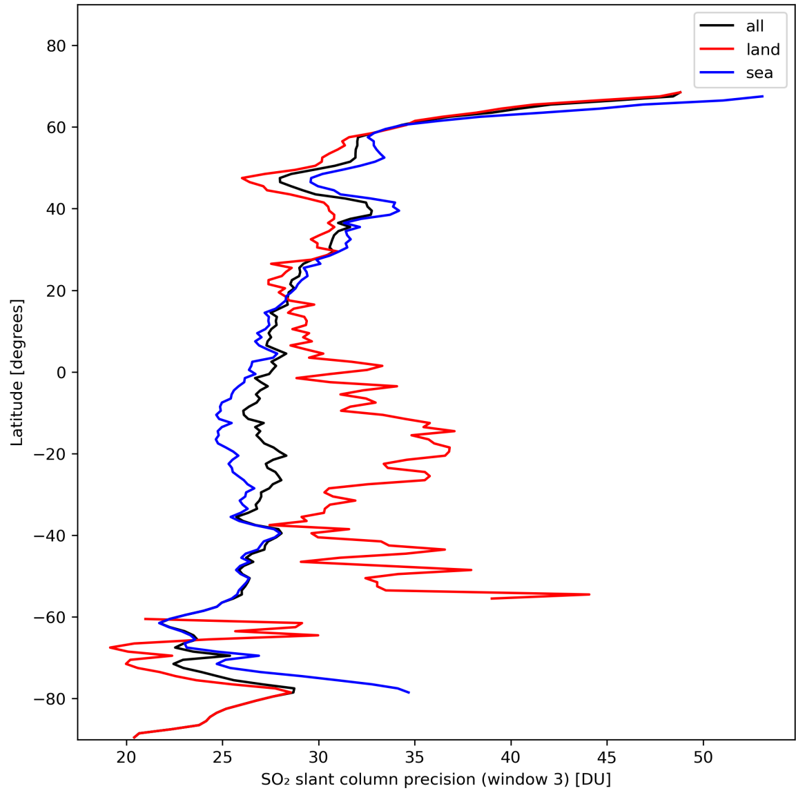
Figure 42: Zonal average of “SO 2 slant column precision (window 3)” for 2024-01-31 to 2024-02-02.
