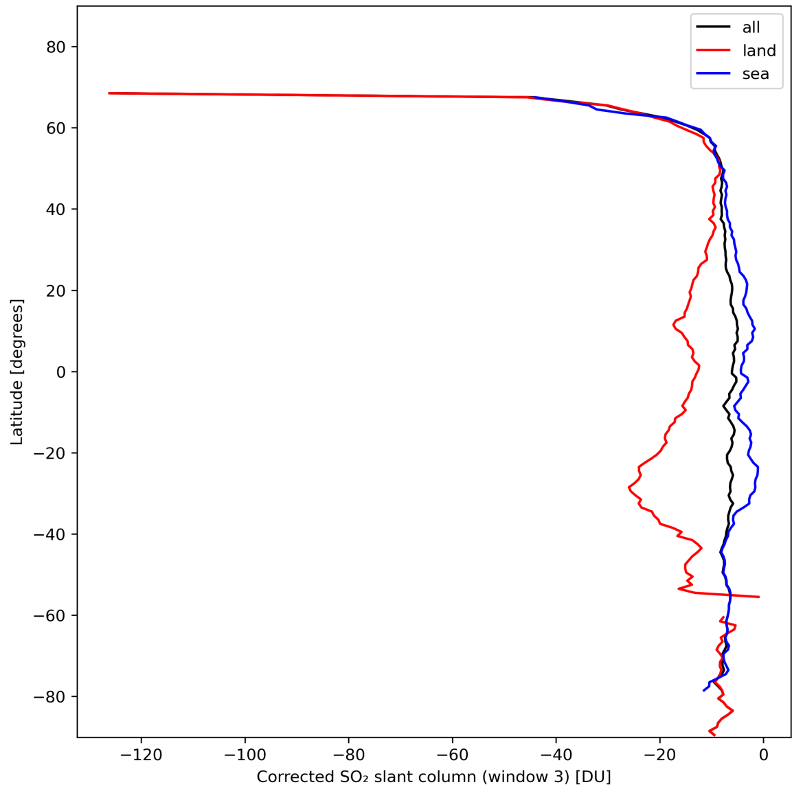
Figure 43: Zonal average of “Corrected SO 2 slant column (window 3)” for 2024-01-31 to 2024-02-02.
