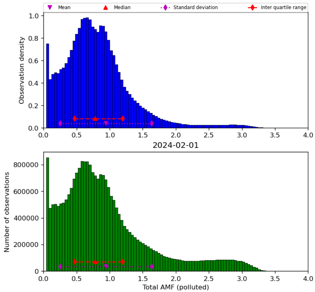
Figure 71: Histogram of “Total AMF (polluted)” for 2024-01-31 to 2024-02-02
