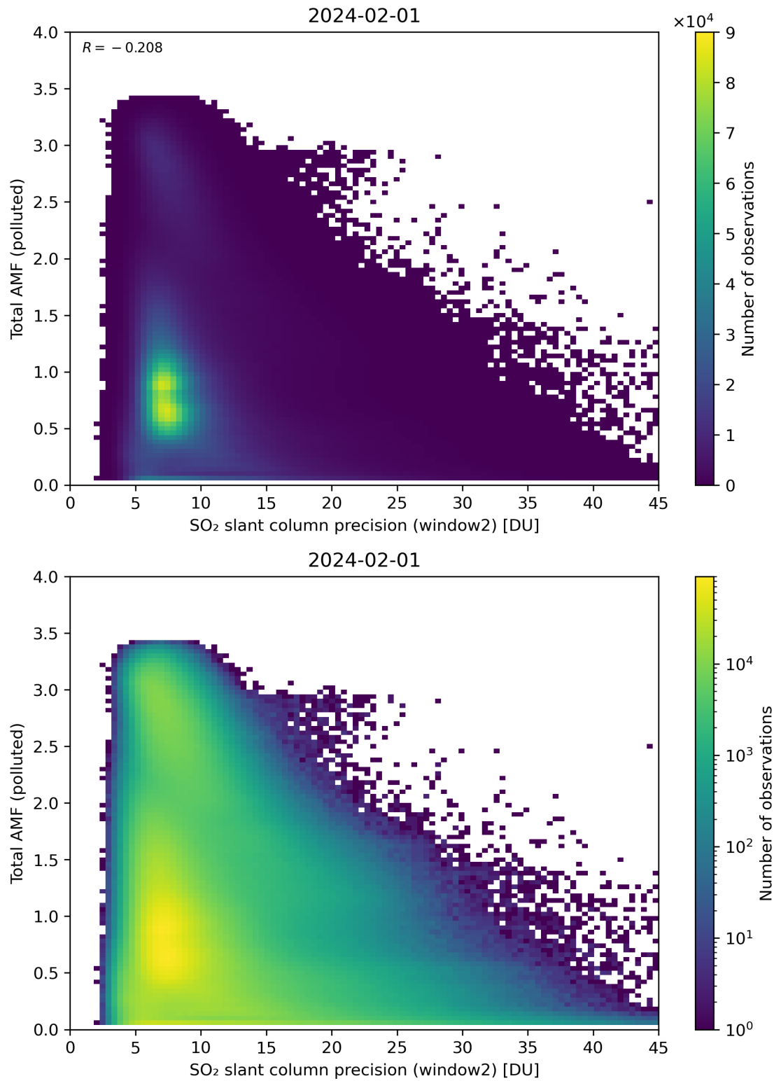
Figure 251: Scatter density plot of “SO 2 slant column precision (window2)” against “Total AMF (polluted)” for 2024-01-31 to 2024-02-02.
