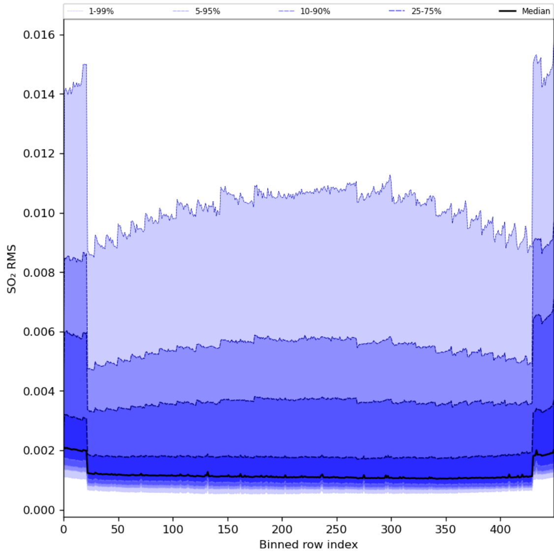
Figure 93: Along track statistics of “SO 2 RMS” for 2024-01-31 to 2024-02-02
