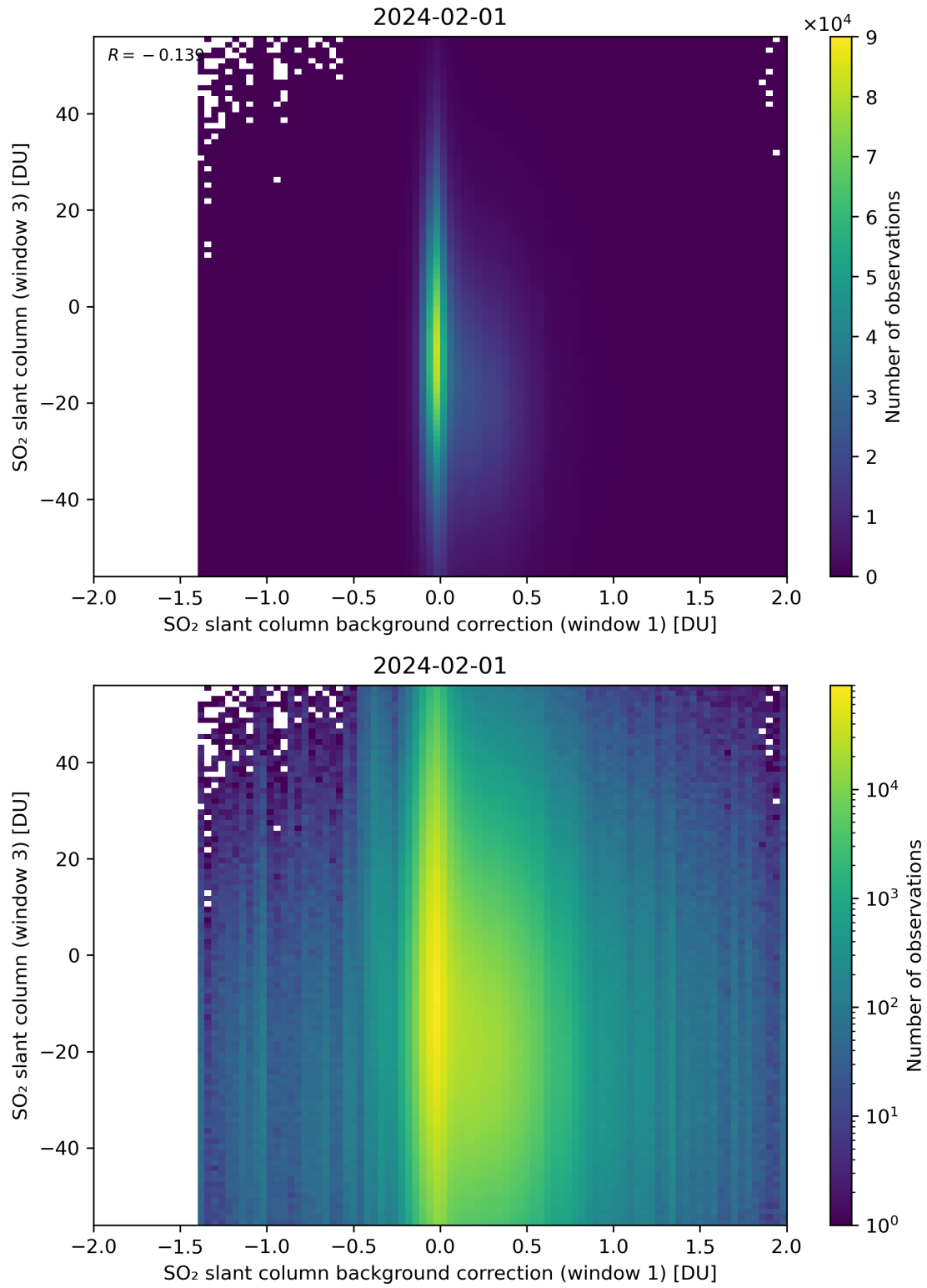
Figure 107: Scatter density plot of “SO 2 slant column background correction (window 1)” against “SO 2 slant column (window 3)” for 2024-01-31 to 2024-02-02.
