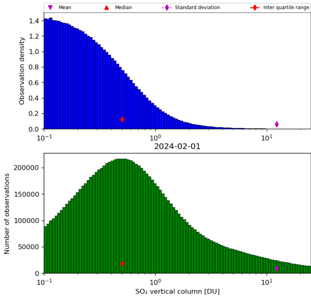
Figure 53: Histogram of “SO 2 vertical column” for 2024-01-31 to 2024-02-02
