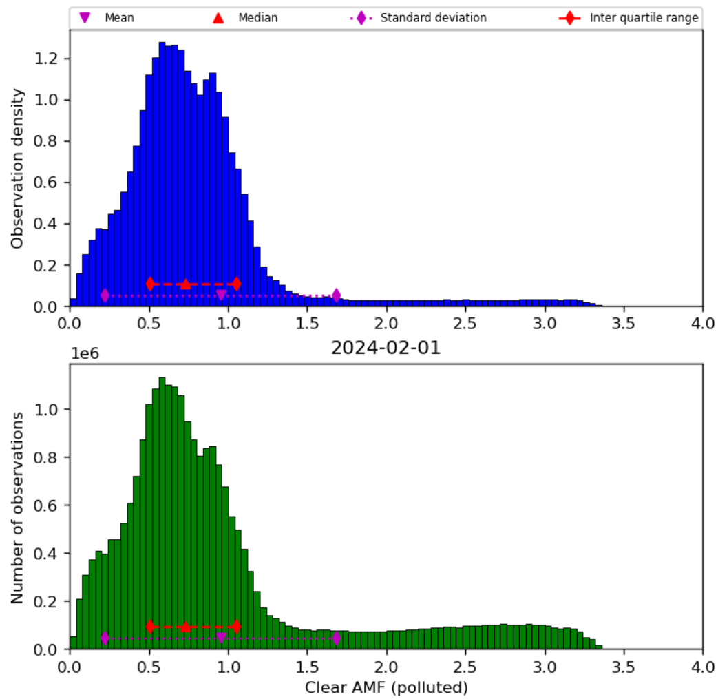
Figure 73: Histogram of “Clear AMF (polluted)” for 2024-01-31 to 2024-02-02
