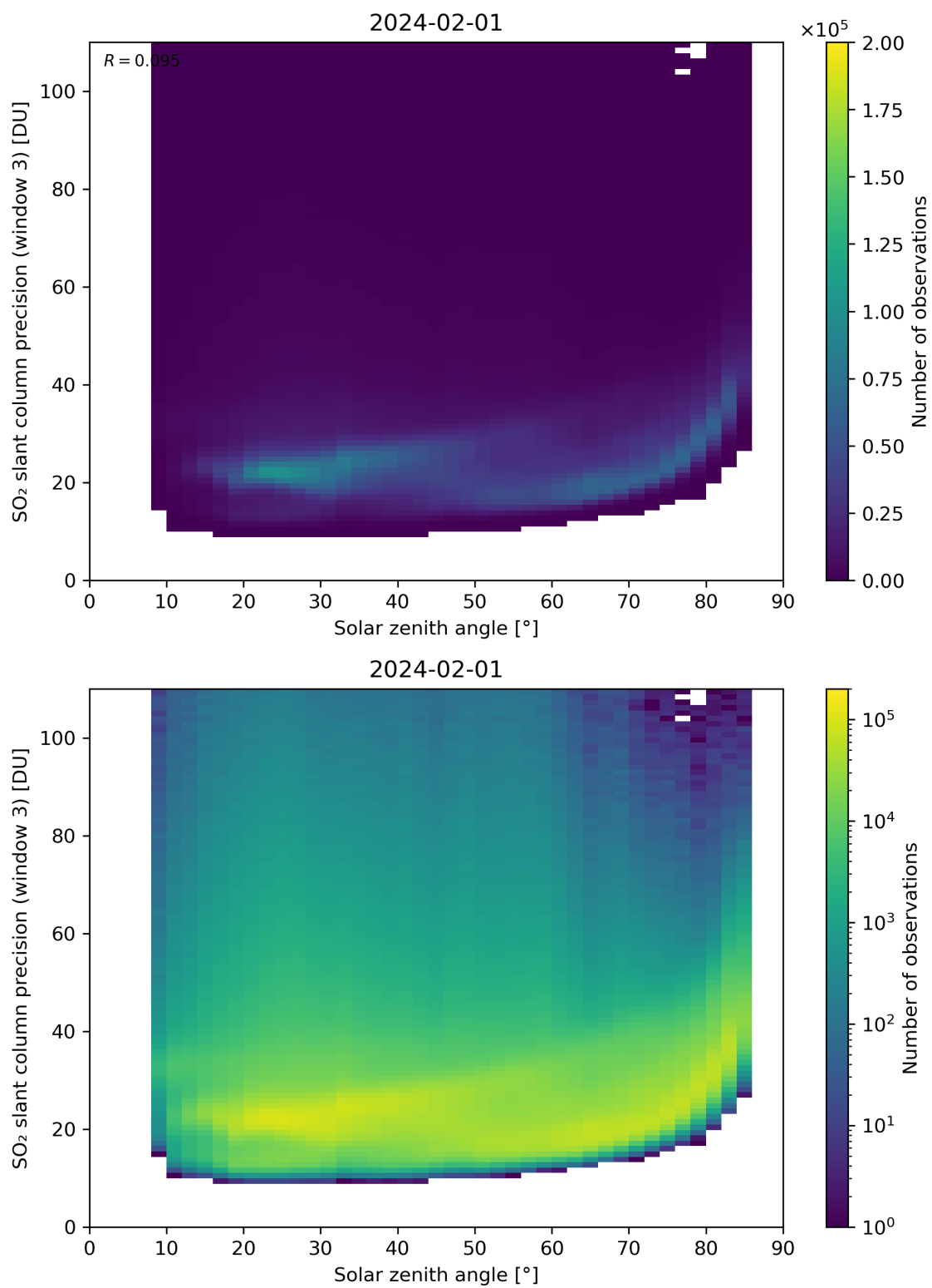
Figure 173: Scatter density plot of “Solar zenith angle” against “SO 2 slant column precision (window 3)” for 2024-01-31 to 2024-02-02.
