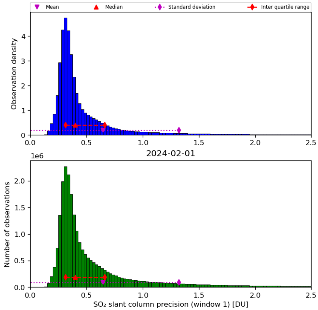
Figure 57: Histogram of “SO 2 slant column precision (window 1)” for 2024-01-31 to 2024-02-02
