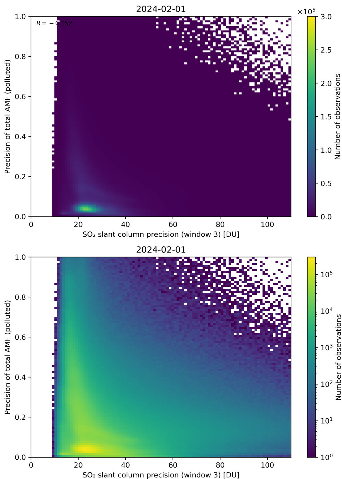
Figure 264: Scatter density plot of “SO 2 slant column precision (window 3)” against “Precision of total AMF (polluted)” for 2024-01-31 to 2024-02-02.
