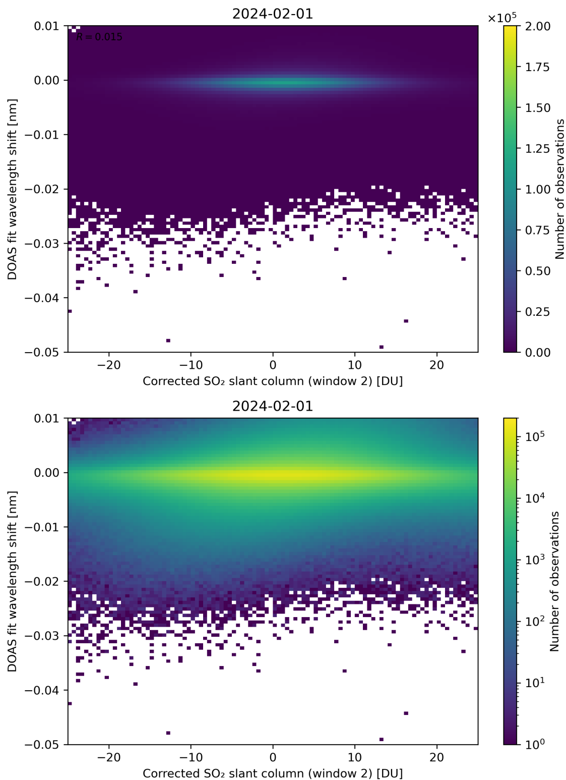
Figure 196: Scatter density plot of “Corrected SO 2 slant column (window 2)” against “DOAS fit wavelength shift” for 2024-01-31 to 2024-02-02.
