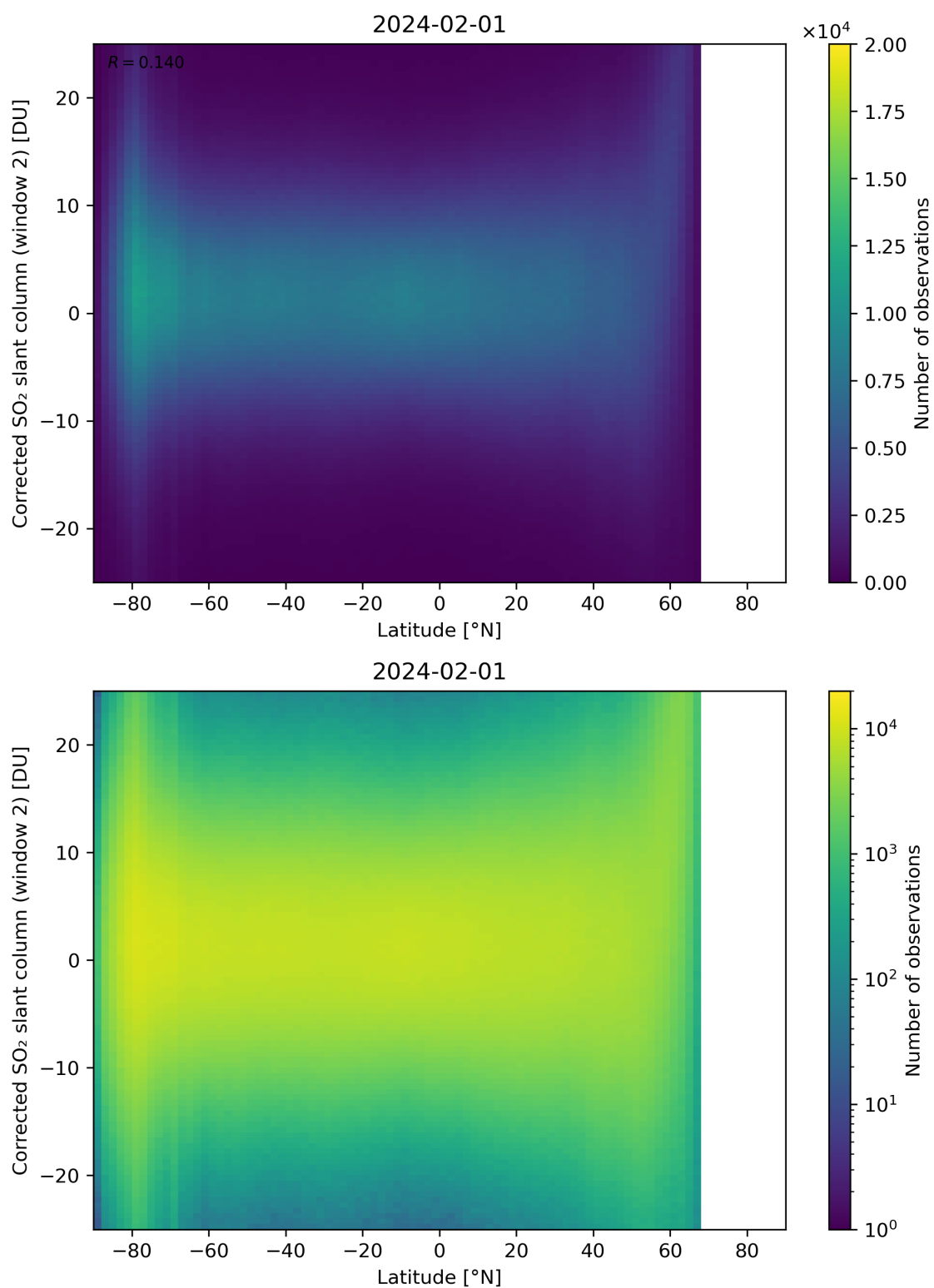
Figure 147: Scatter density plot of “Latitude” against “Corrected SO 2 slant column (window 2)” for 2024-01-31 to 2024-02-02.
