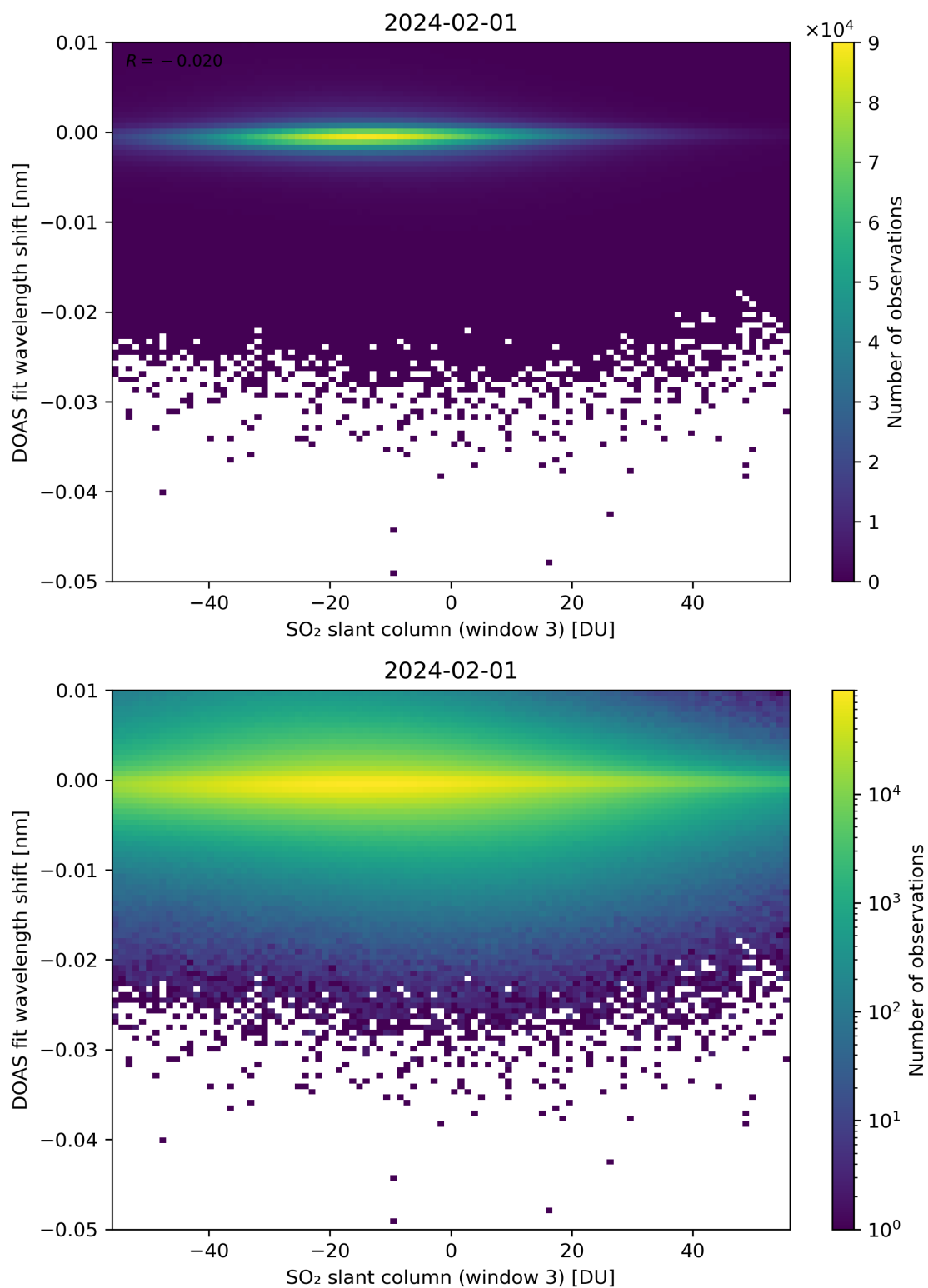
Figure 254: Scatter density plot of “SO 2 slant column (window 3)” against “DOAS fit wavelength shift” for 2024-01-31 to 2024-02-02.
