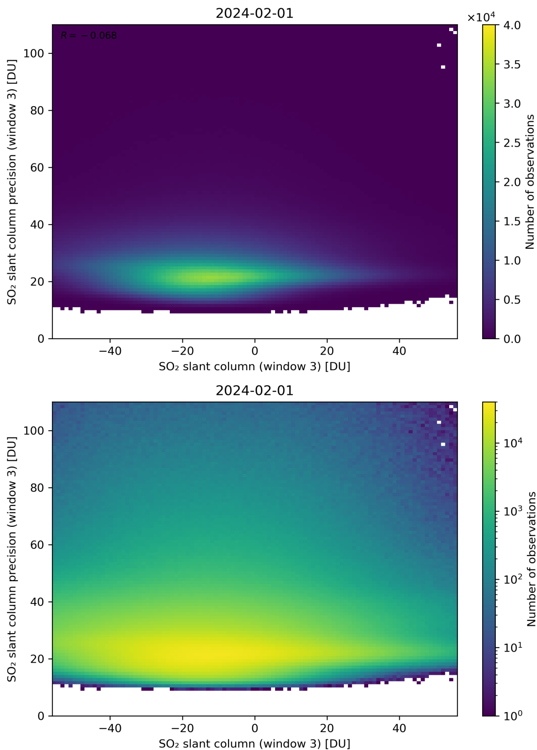
Figure 267: Scatter density plot of “SO 2 slant column (window 3)” against “SO 2 slant column precision (window 3)” for 2024-01-31 to 2024-02-02.
