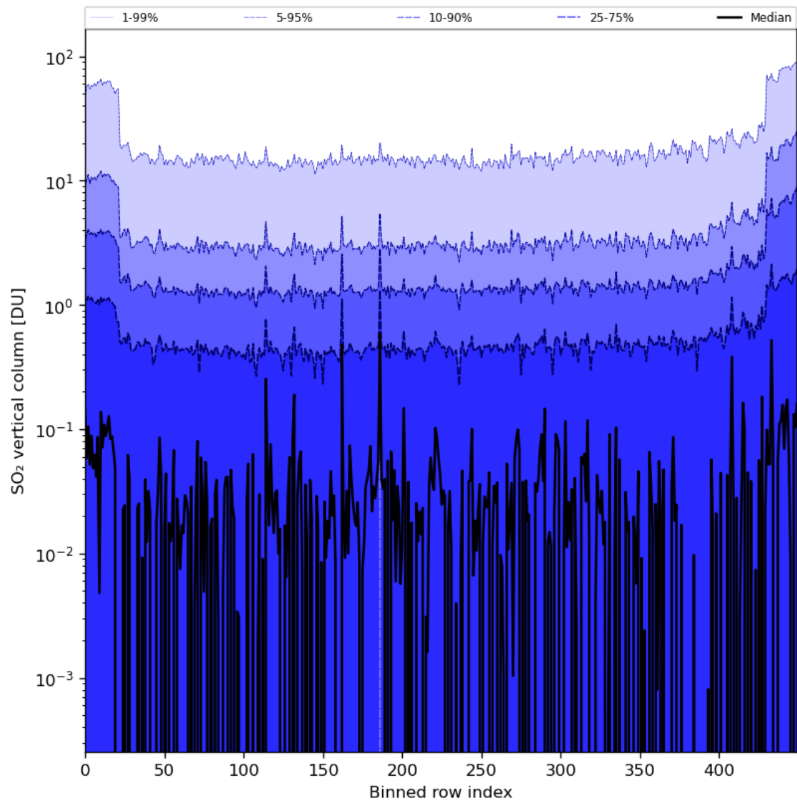
Figure 76: Along track statistics of “SO 2 vertical column” for 2024-01-31 to 2024-02-02
