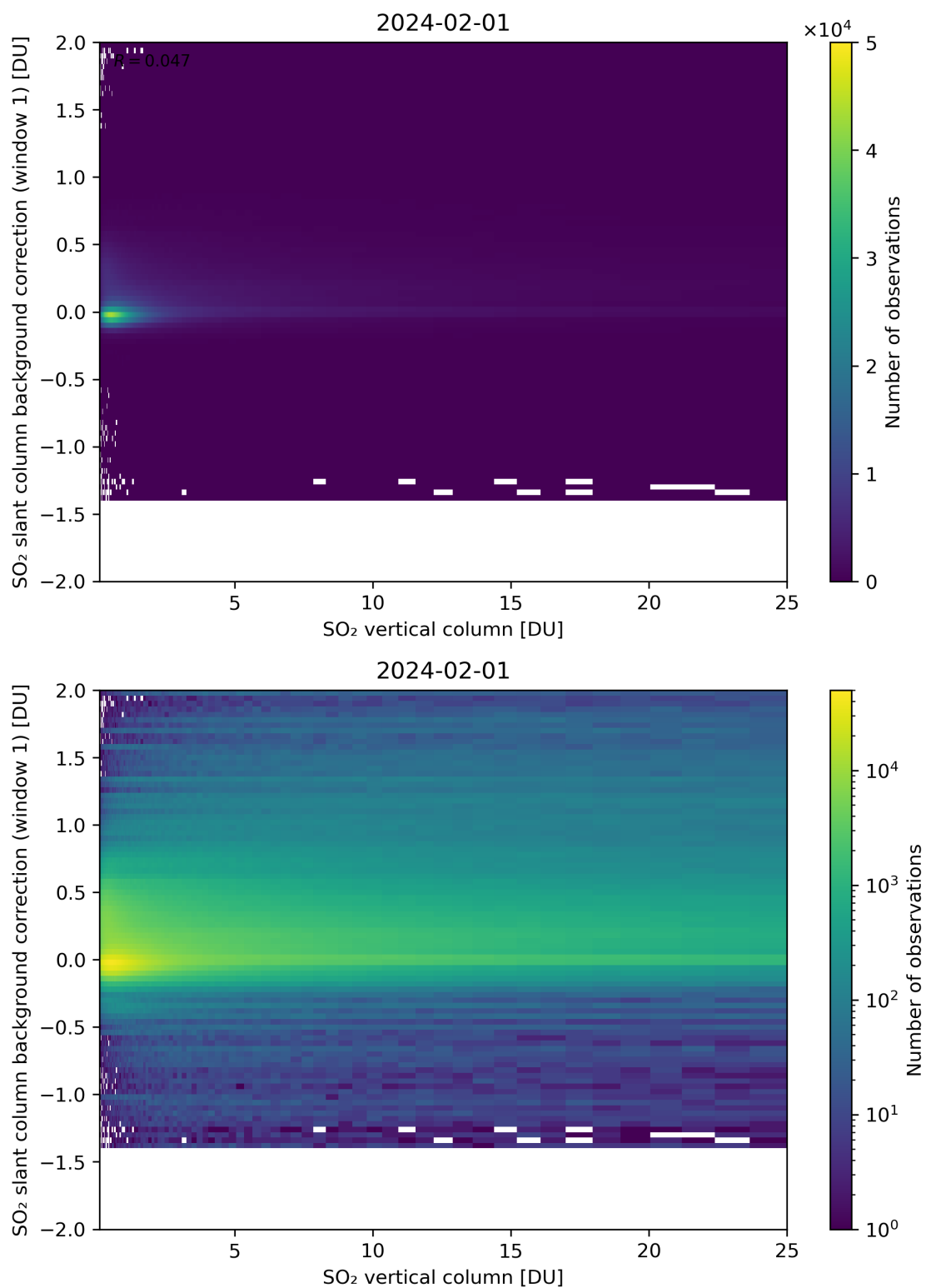
Figure 273: Scatter density plot of “SO 2 vertical column” against “SO 2 slant column background correction (window 1)” for 2024-01-31 to 2024-02-02.
