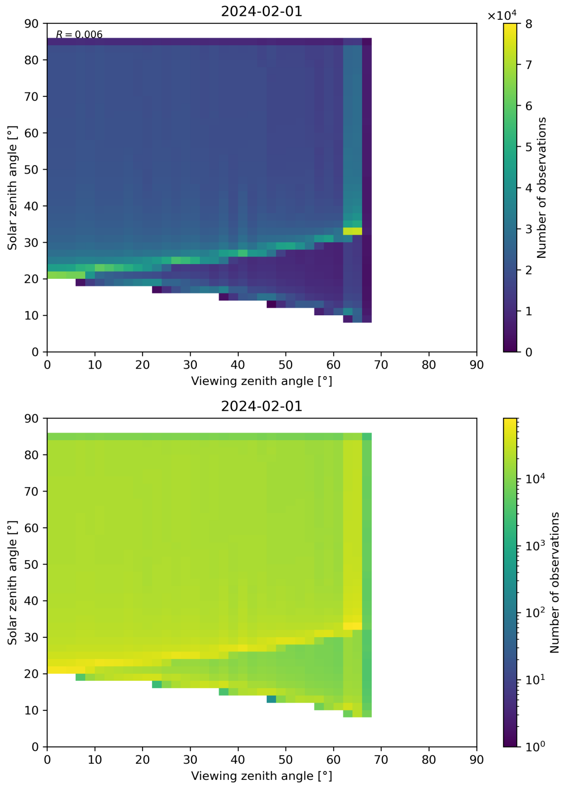
Figure 315: Scatter density plot of “Viewing zenith angle” against “Solar zenith angle” for 2024-01-31 to 2024-02-02.
