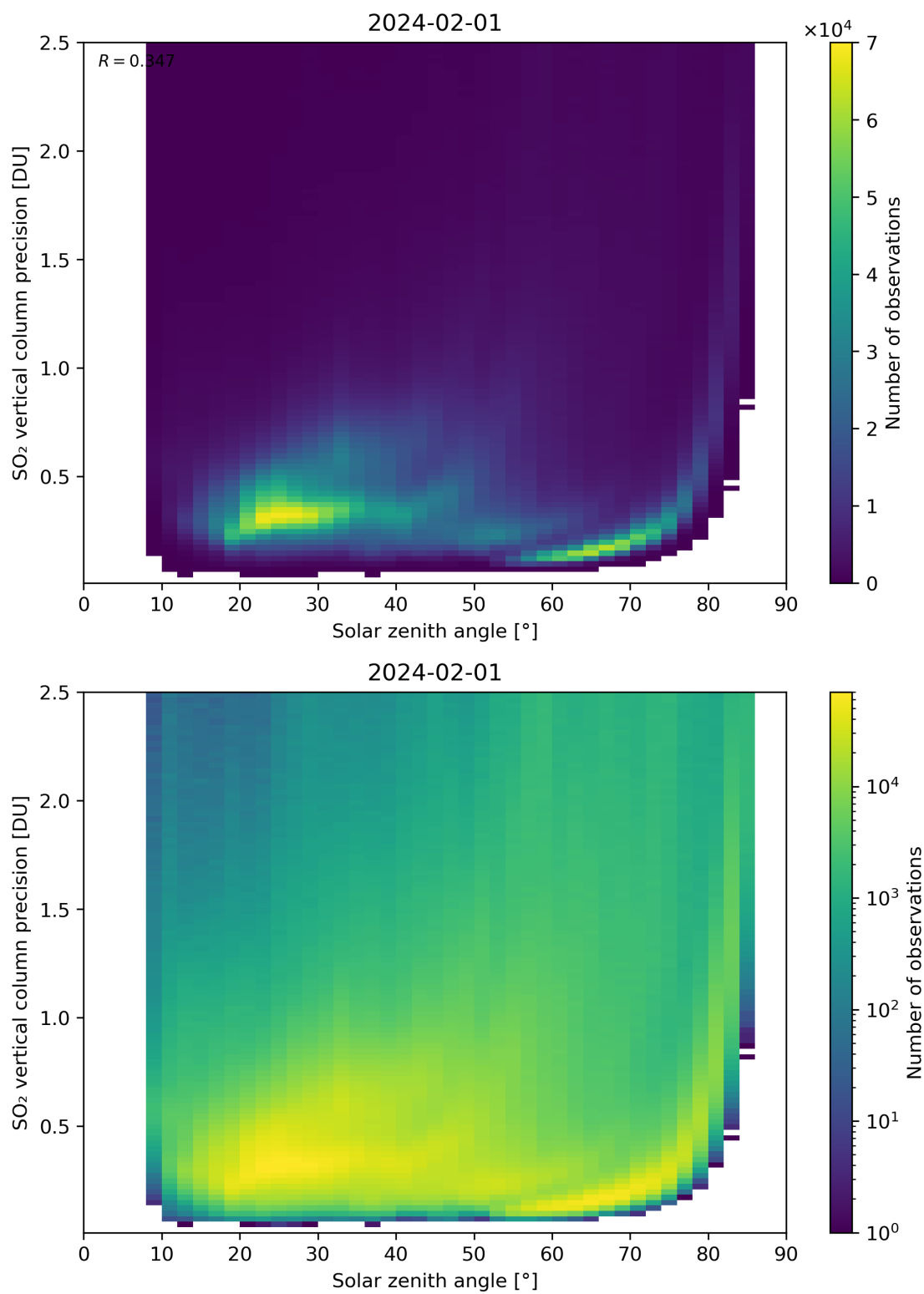
Figure 177: Scatter density plot of “Solar zenith angle” against “SO 2 vertical column precision” for 2024-01-31 to 2024-02-02.
