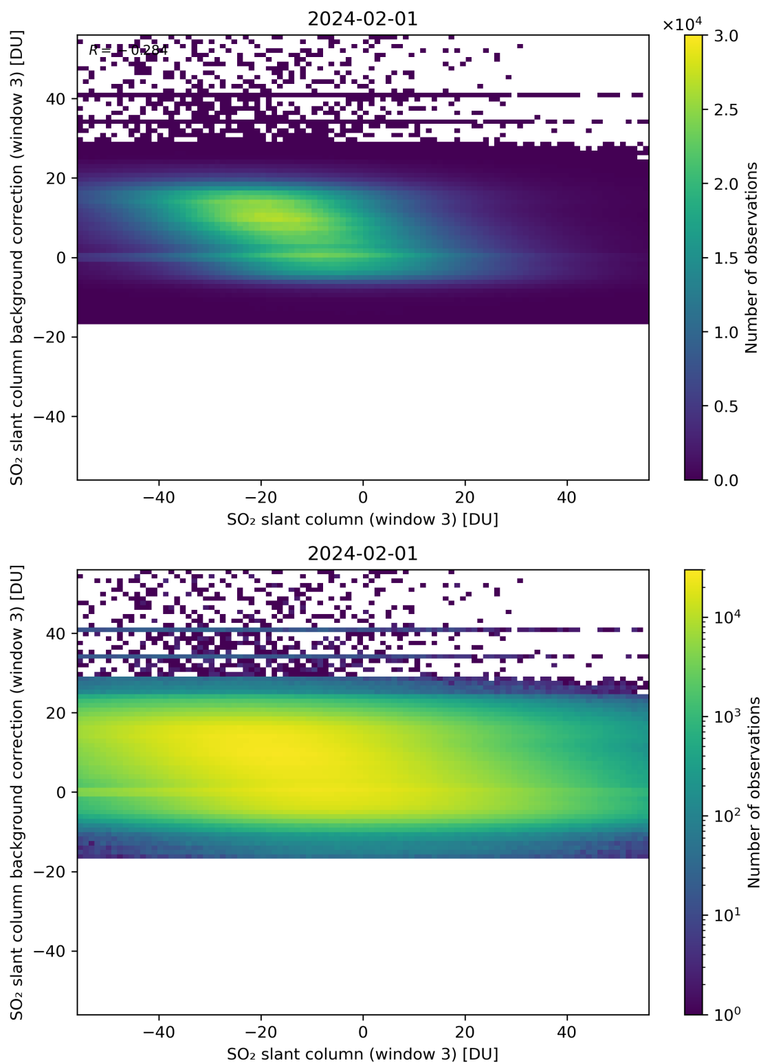
Figure 253: Scatter density plot of “SO 2 slant column (window 3)” against “SO 2 slant column background correction (window 3)” for 2024-01-31 to 2024-02-02.
