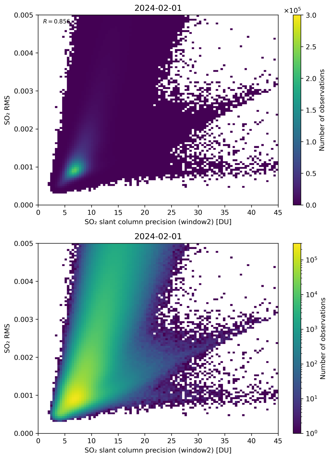
Figure 245: Scatter density plot of “SO 2 slant column precision (window2)” against “SO 2 RMS” for 2024-01-31 to 2024-02-02.
