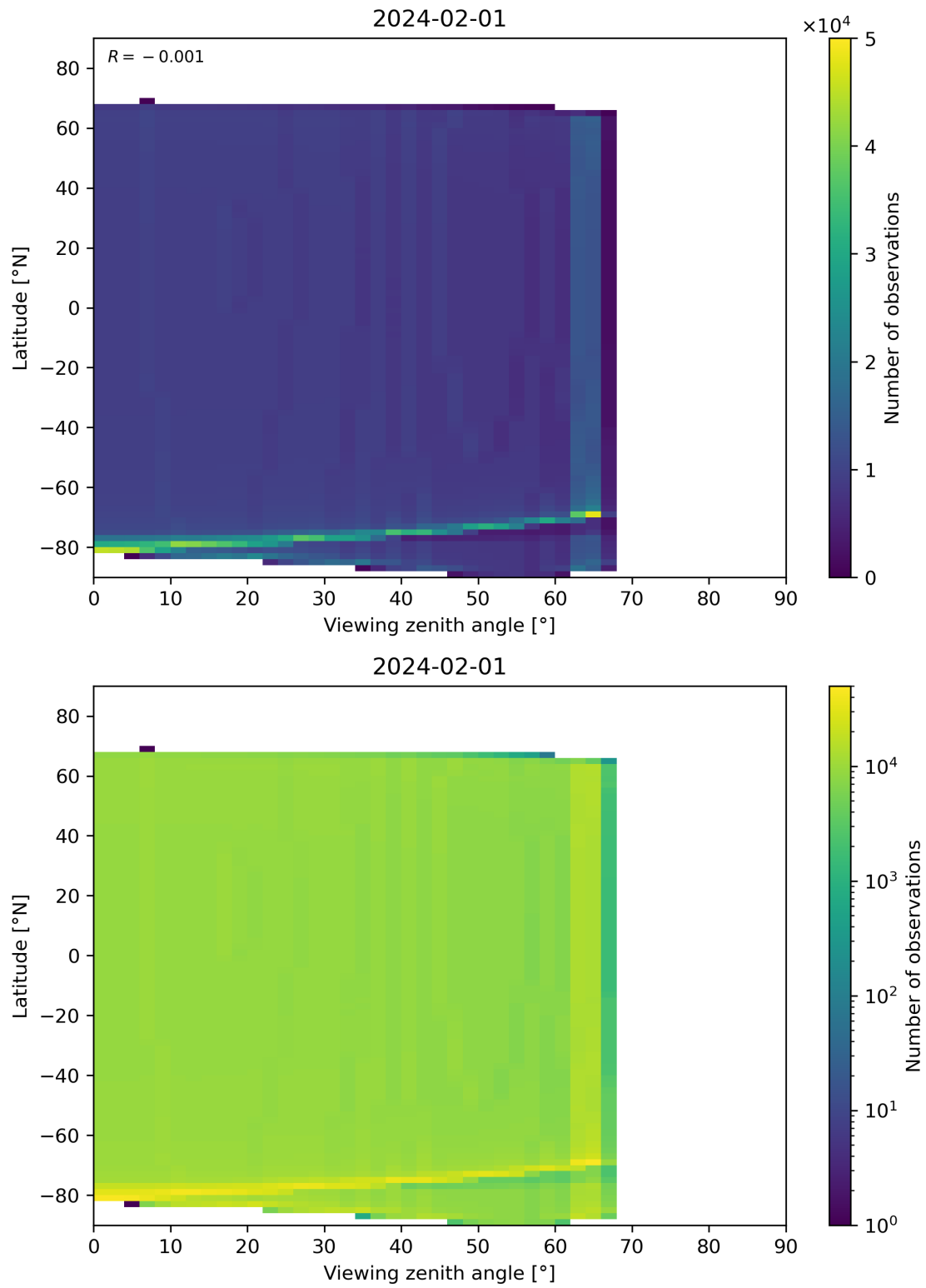
Figure 314: Scatter density plot of “Viewing zenith angle” against “Latitude” for 2024-01-31 to 2024-02-02.
