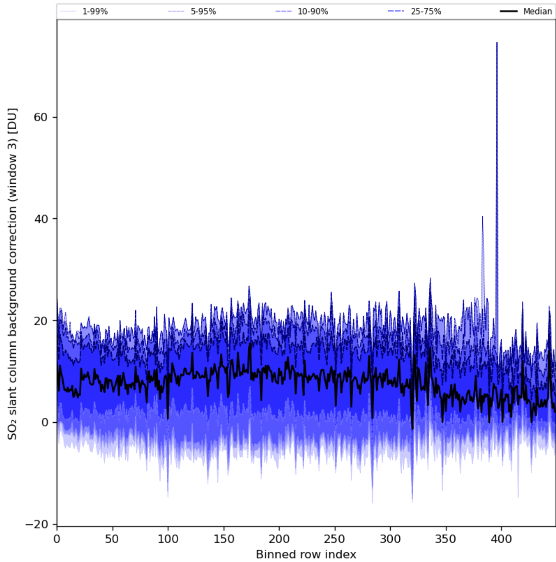
Figure 90: Along track statistics of “SO 2 slant column background correction (window 3)” for 2024-01-31 to 2024-02-02
