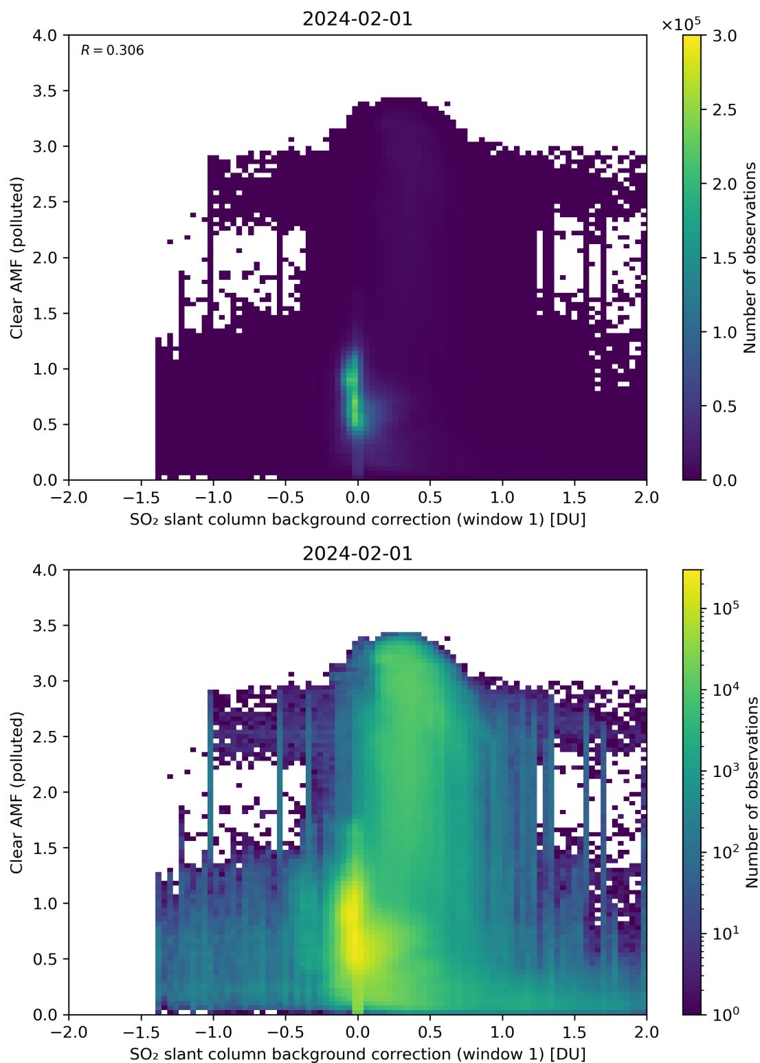
Figure 103: Scatter density plot of “SO 2 slant column background correction (window 1)” against “Clear AMF (polluted)” for 2024-01-31 to 2024-02-02.
