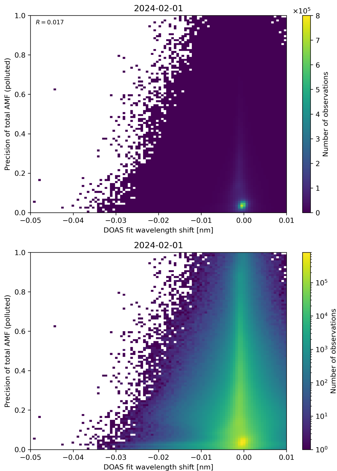
Figure 131: Scatter density plot of “DOAS fit wavelength shift” against “Precision of total AMF (polluted)” for 2024-01-31 to 2024-02-02.
