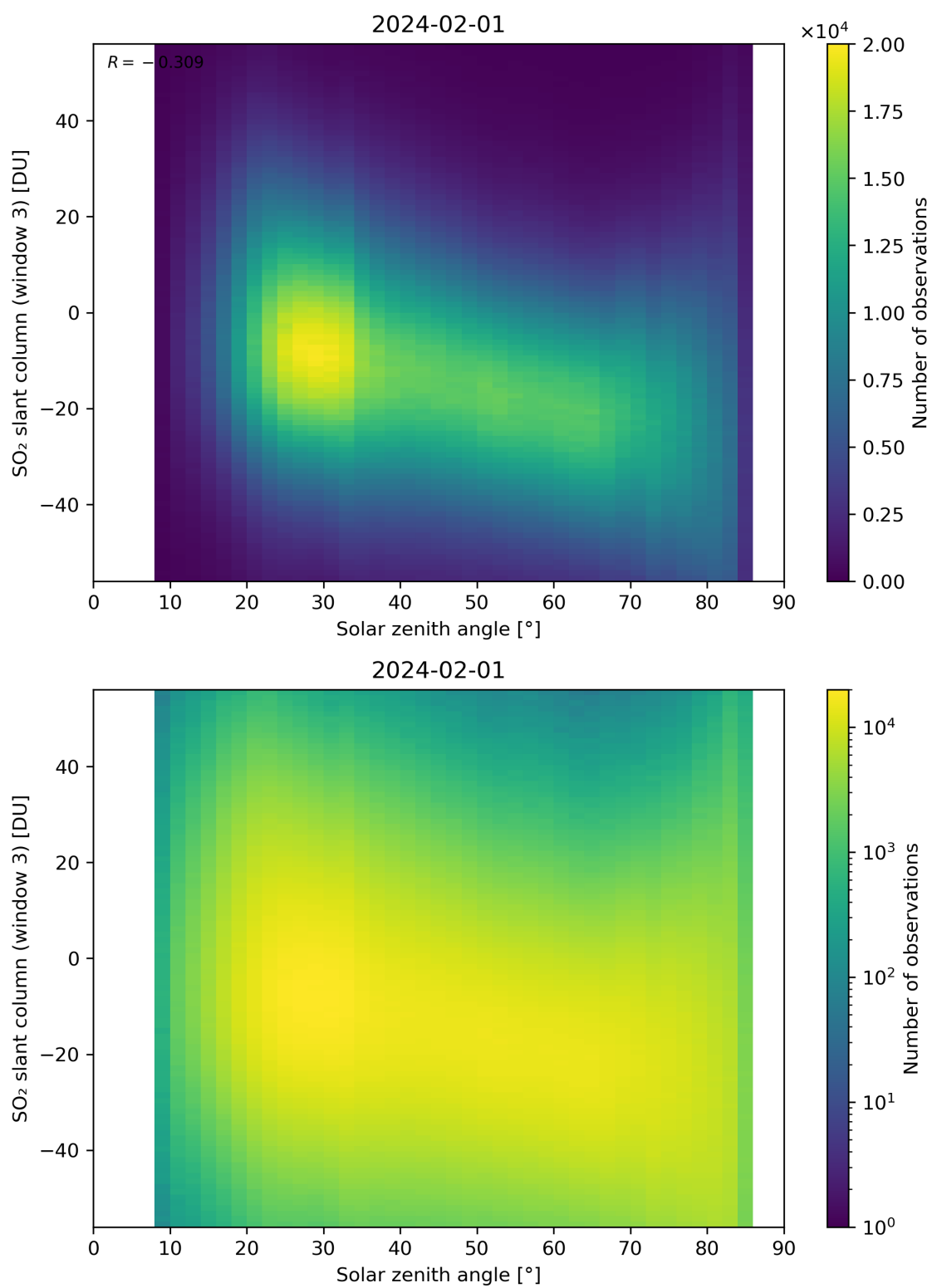
Figure 172: Scatter density plot of “Solar zenith angle” against “SO 2 slant column (window 3)” for 2024-01-31 to 2024-02-02.
