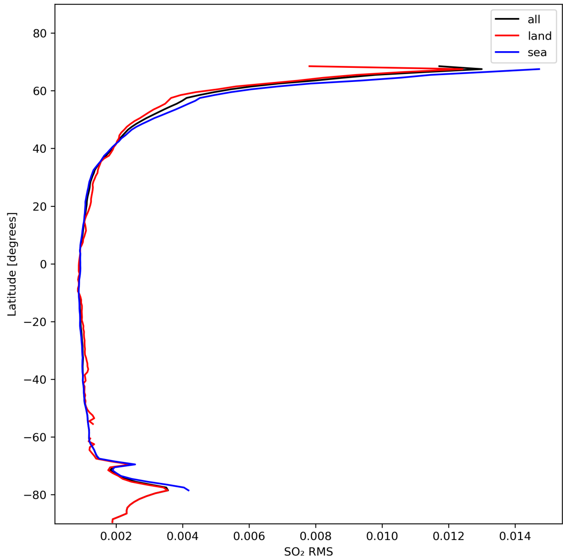
Figure 47: Zonal average of “SO 2 RMS” for 2024-01-31 to 2024-02-02.
