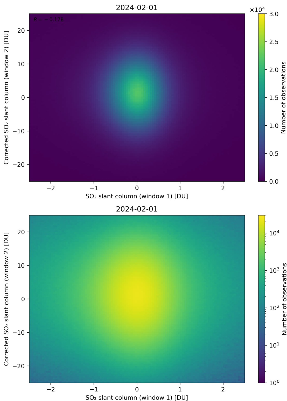
Figure 233: Scatter density plot of “SO 2 slant column (window 1)” against “Corrected SO 2 slant column (window 2)” for 2024-01-31 to 2024-02-02.
