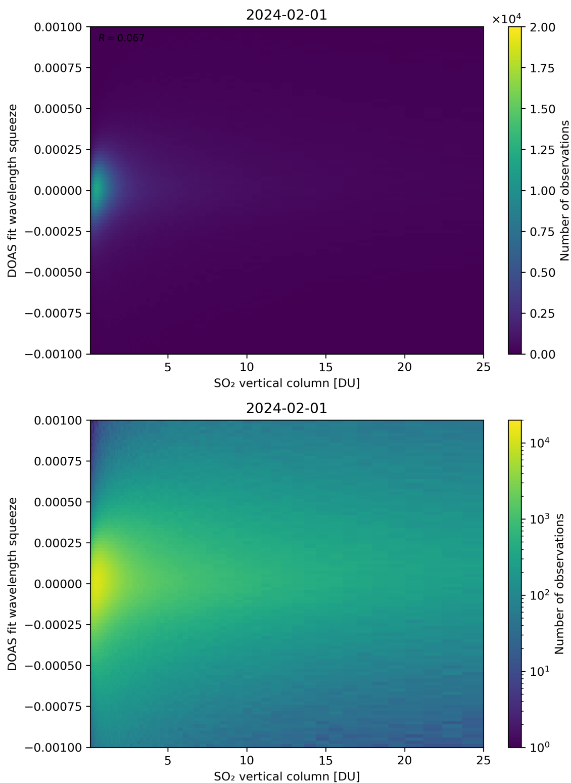
Figure 277: Scatter density plot of “SO 2 vertical column” against “DOAS fit wavelength squeeze” for 2024-01-31 to 2024-02-02.
