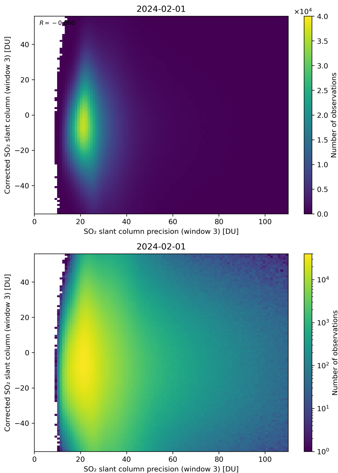
Figure 262: Scatter density plot of “SO 2 slant column precision (window 3)” against “Corrected SO 2 slant column (window 3)” for 2024-01-31 to 2024-02-02.
