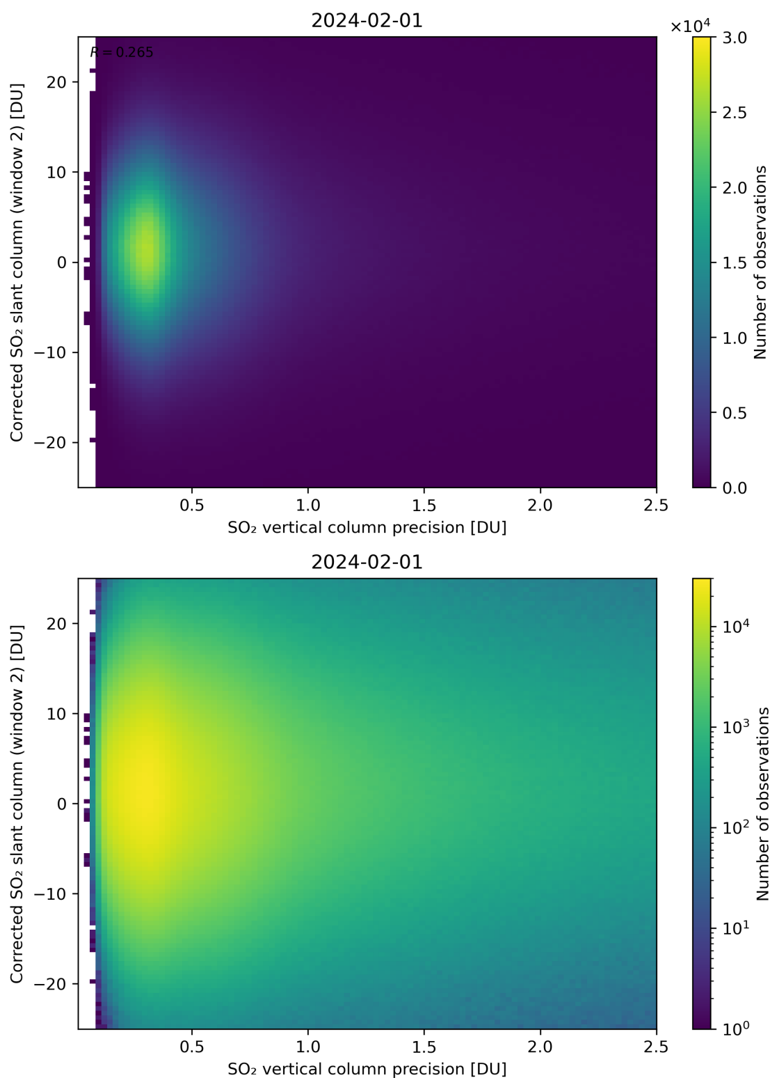
Figure 287: Scatter density plot of “SO 2 vertical column precision” against “Corrected SO 2 slant column (window 2)” for 2024-01-31 to 2024-02-02.
