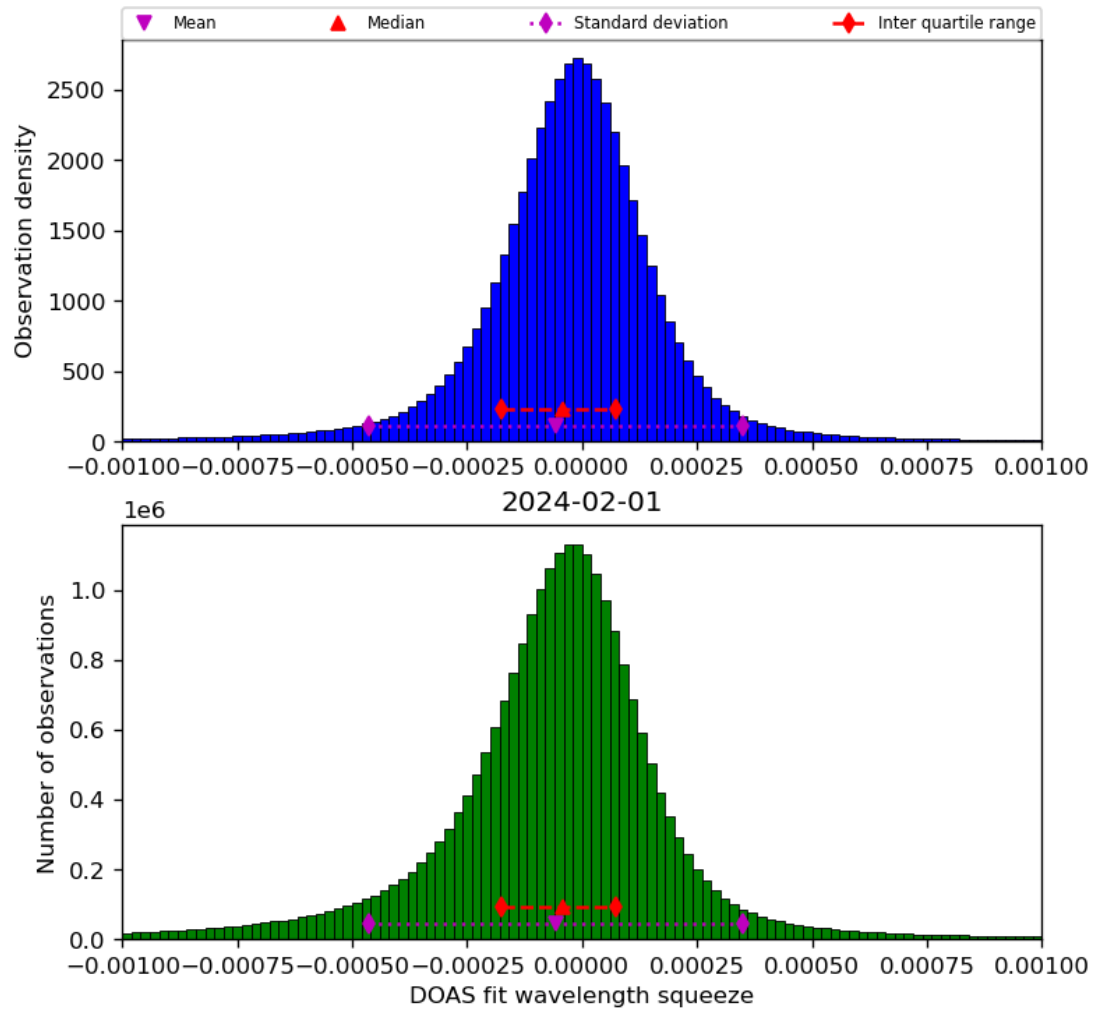
Figure 69: Histogram of “DOAS fit wavelength squeeze” for 2024-01-31 to 2024-02-02
