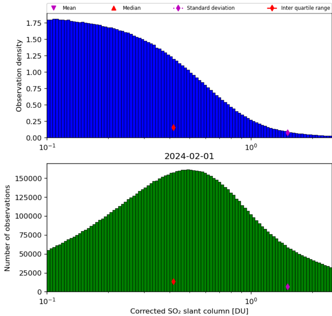
Figure 55: Histogram of “Corrected SO 2 slant column” for 2024-01-31 to 2024-02-02
