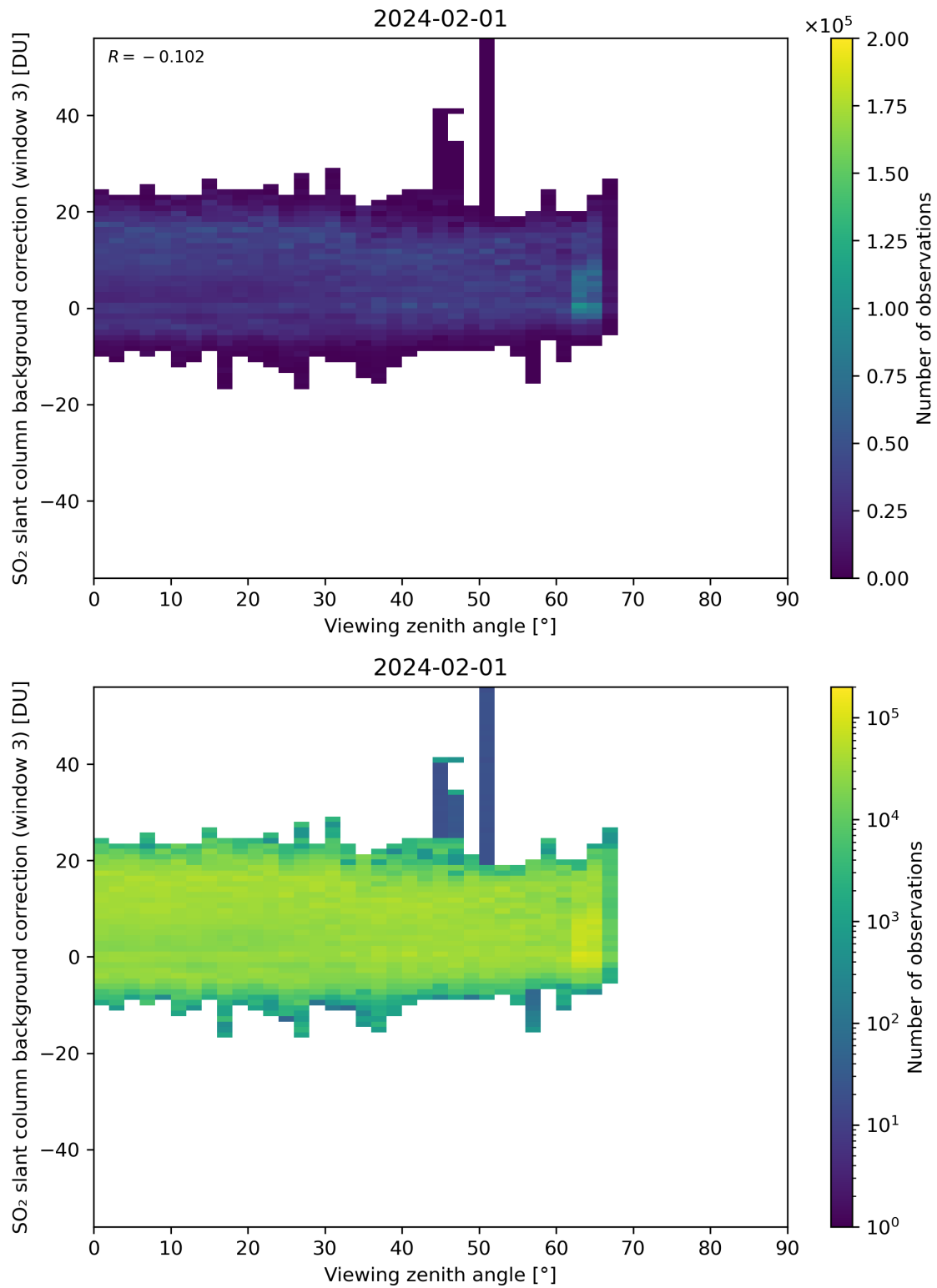
Figure 310: Scatter density plot of “Viewing zenith angle” against “SO 2 slant column background correction (window 3)” for 2024-01-31 to 2024-02-02.
