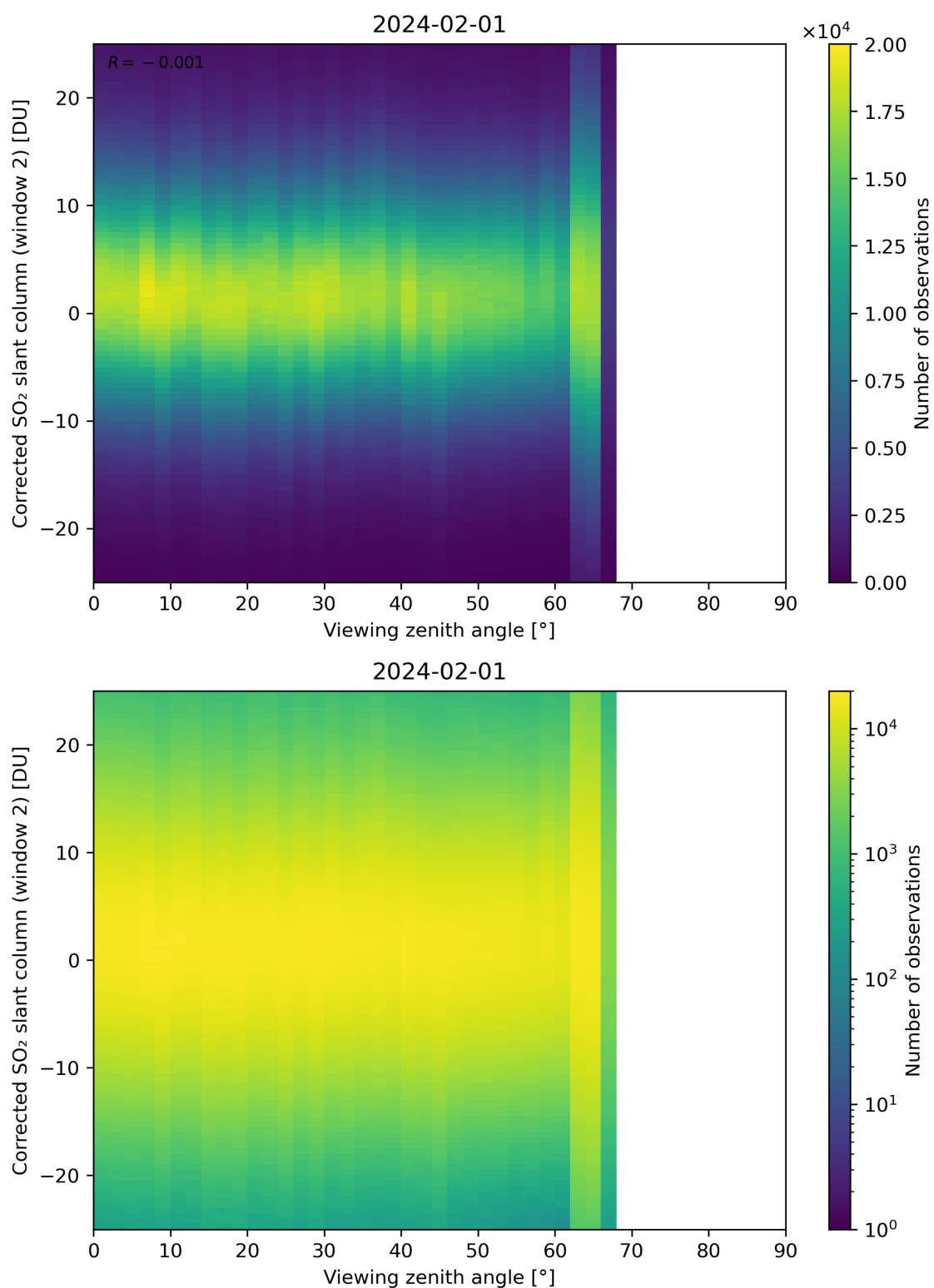
Figure 318: Scatter density plot of “Viewing zenith angle” against “Corrected SO 2 slant column (window 2)” for 2024-01-31 to 2024-02-02.
