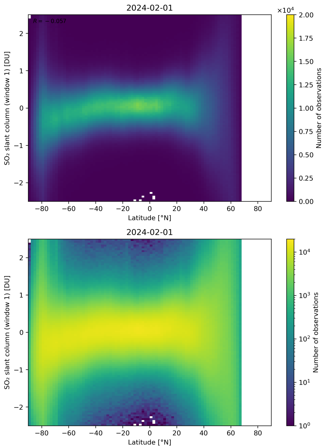
Figure 149: Scatter density plot of “Latitude” against “SO 2 slant column (window 1)” for 2024-01-31 to 2024-02-02.
