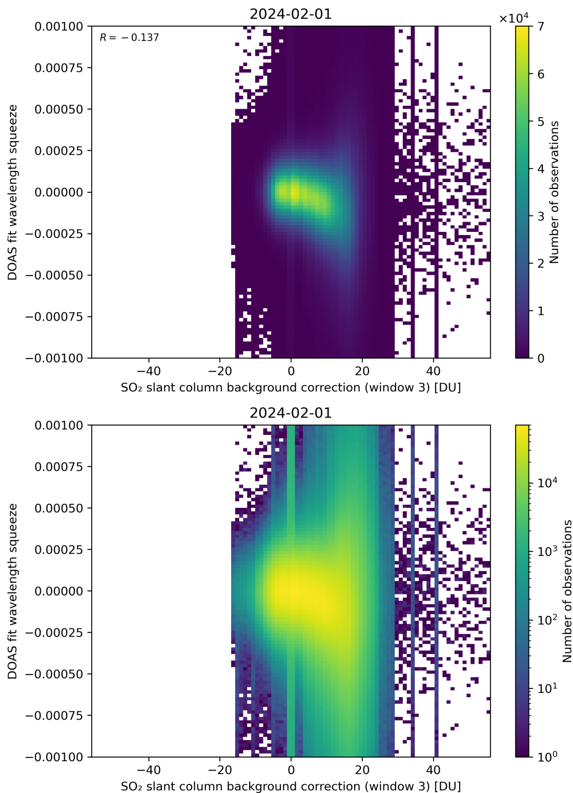
Figure 122: Scatter density plot of “SO 2 slant column background correction (window 3)” against “DOAS fit wavelength squeeze” for 2024-01-31 to 2024-02-02.
