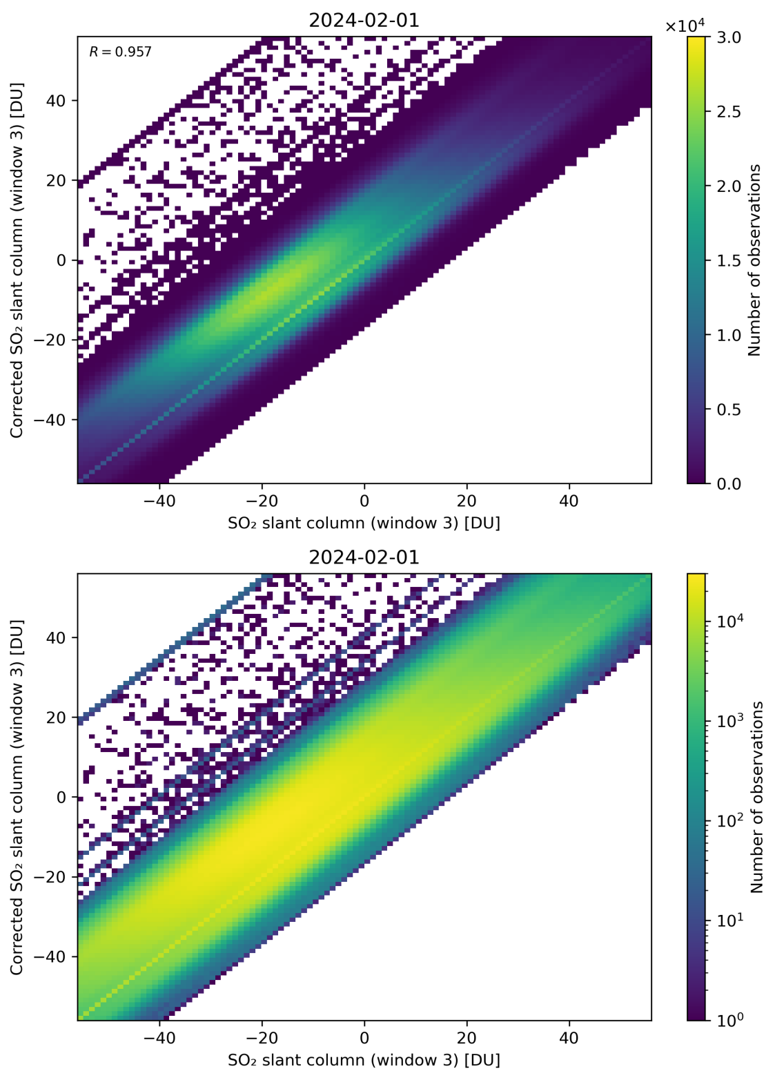
Figure 266: Scatter density plot of “SO 2 slant column (window 3)” against “Corrected SO 2 slant column (window 3)” for 2024-01-31 to 2024-02-02.
