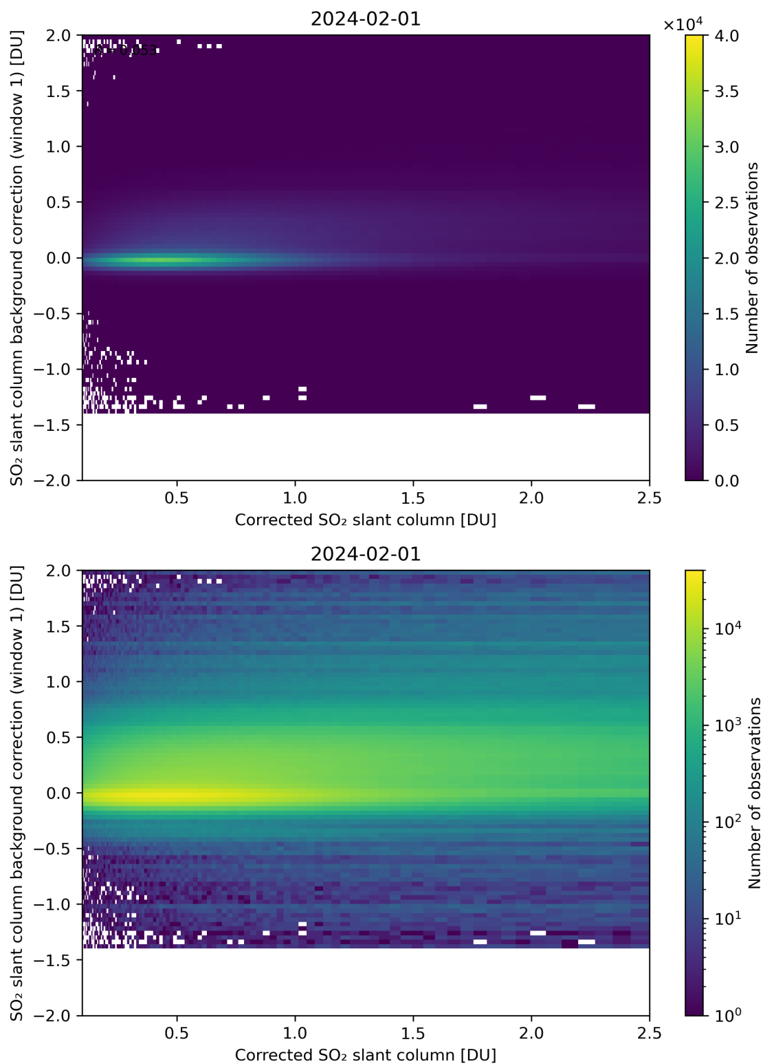
Figure 178: Scatter density plot of “Corrected SO 2 slant column” against “SO 2 slant column background correction (window 1)” for 2024-01-31 to 2024-02-02.
