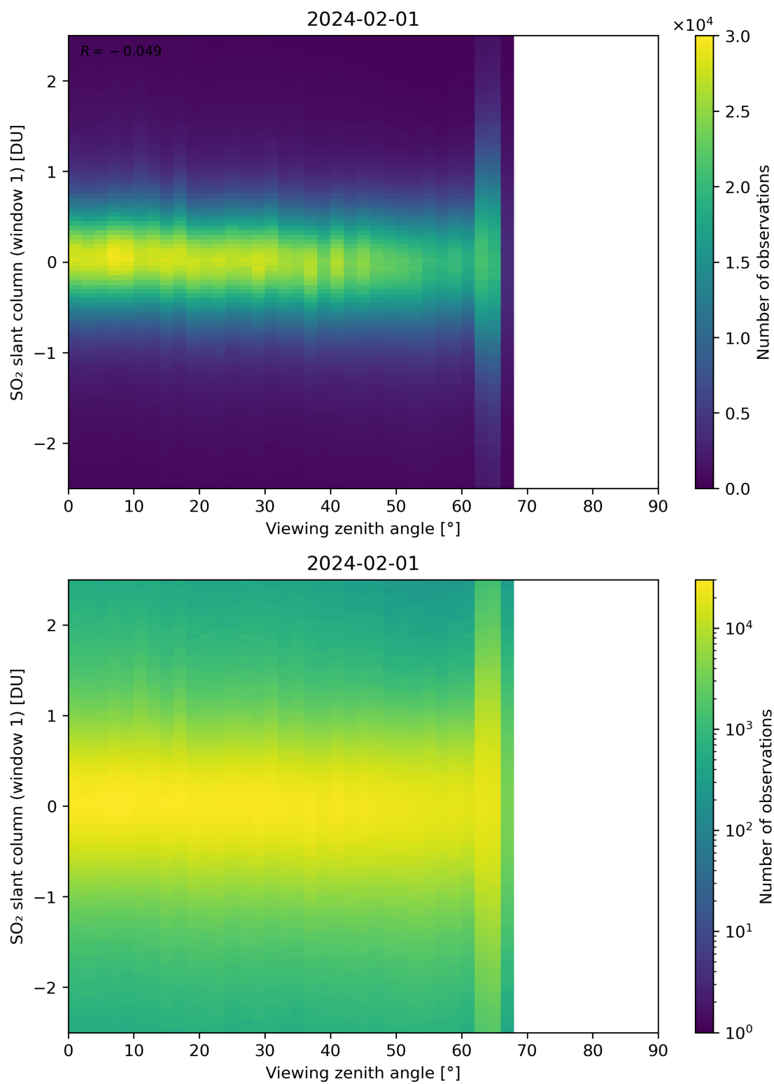
Figure 320: Scatter density plot of “Viewing zenith angle” against “SO 2 slant column (window 1)” for 2024-01-31 to 2024-02-02.
