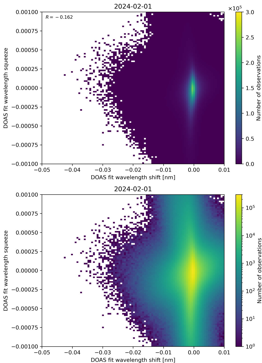
Figure 127: Scatter density plot of “DOAS fit wavelength shift” against “DOAS fit wavelength squeeze” for 2024-01-31 to 2024-02-02.
