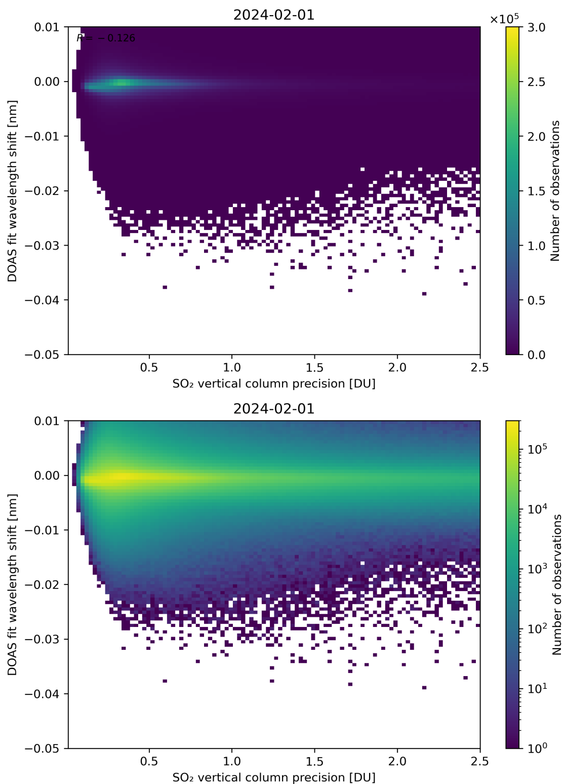
Figure 282: Scatter density plot of “SO 2 vertical column precision” against “DOAS fit wavelength shift” for 2024-01-31 to 2024-02-02.
