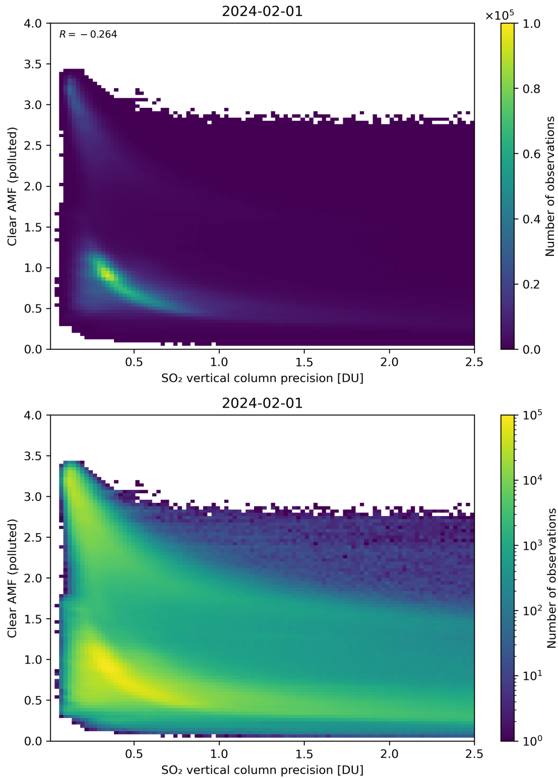
Figure 285: Scatter density plot of “SO 2 vertical column precision” against “Clear AMF (polluted)” for 2024-01-31 to 2024-02-02.
