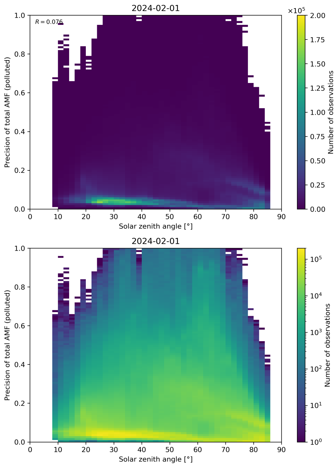
Figure 175: Scatter density plot of “Solar zenith angle” against “Precision of total AMF (polluted)” for 2024-01-31 to 2024-02-02.
