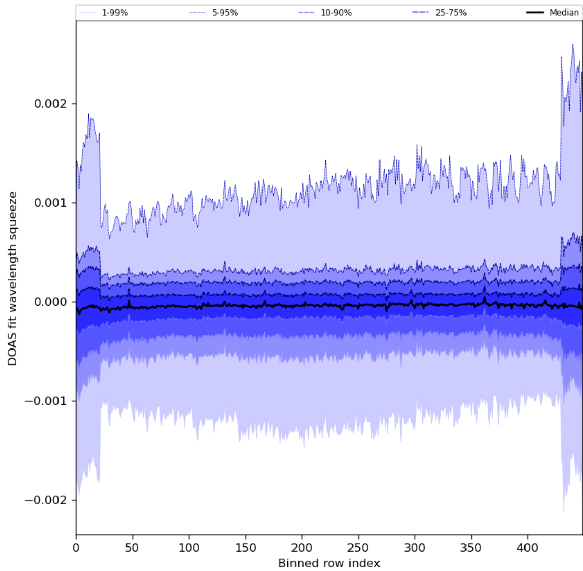
Figure 92: Along track statistics of “DOAS fit wavelength squeeze” for 2024-01-31 to 2024-02-02
