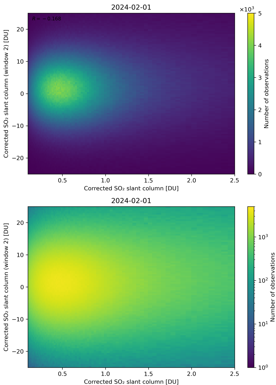
Figure 185: Scatter density plot of “Corrected SO 2 slant column” against “Corrected SO 2 slant column (window 2)” for 2024-01-31 to 2024-02-02.
