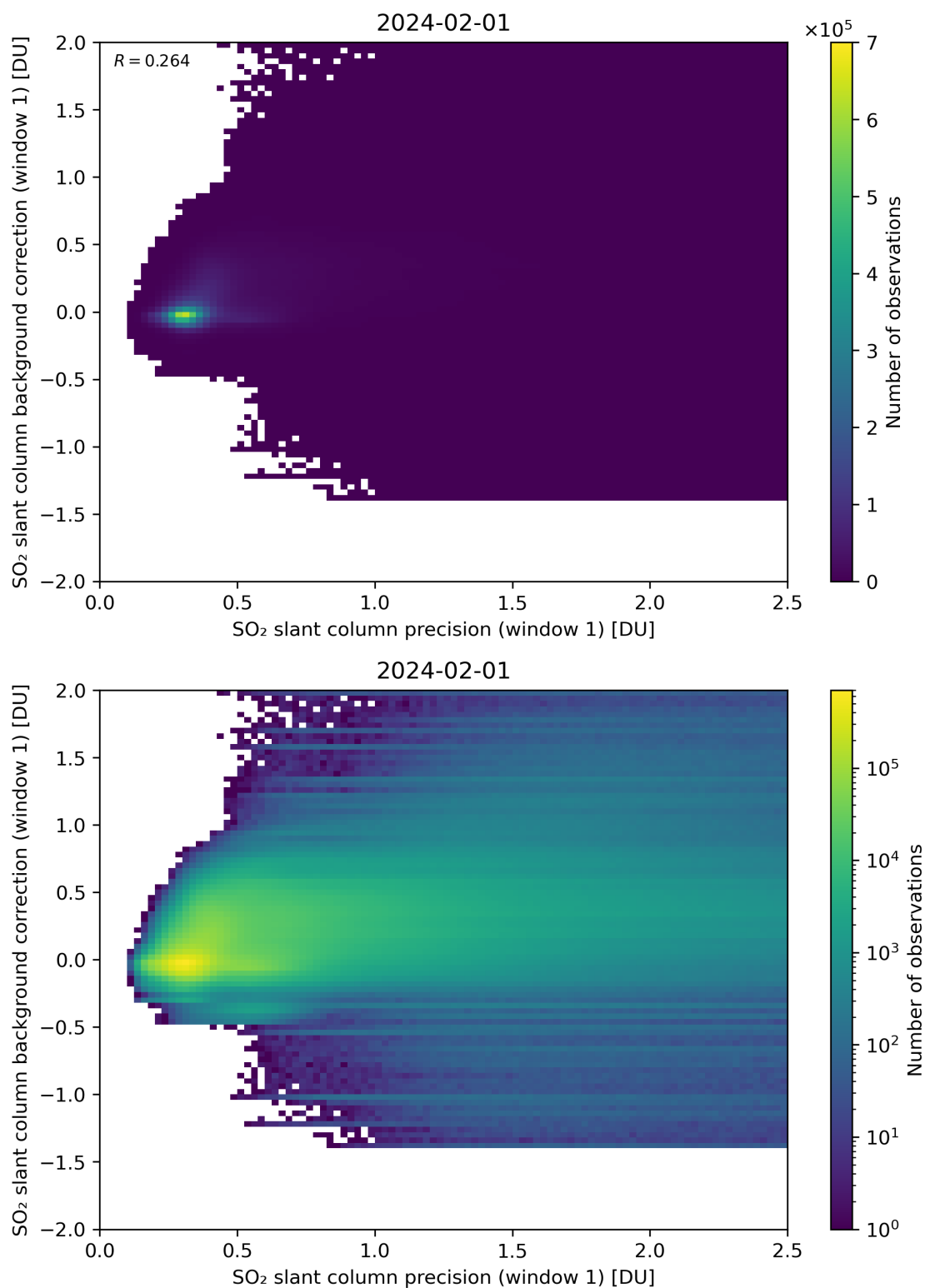
Figure 218: Scatter density plot of “SO 2 slant column precision (window 1)” against “SO 2 slant column background correction (window 1)” for 2024-01-31 to 2024-02-02.
