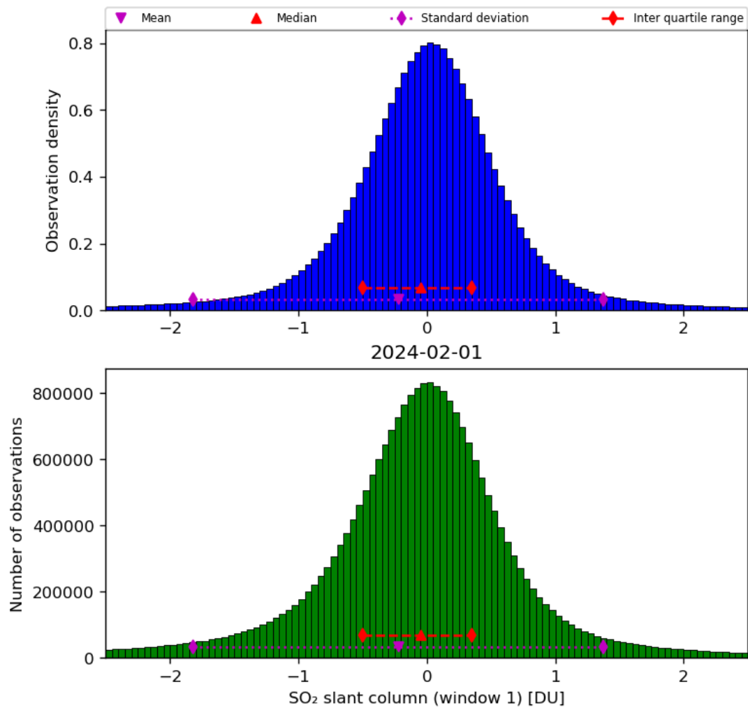
Figure 56: Histogram of “SO 2 slant column (window 1)” for 2024-01-31 to 2024-02-02
