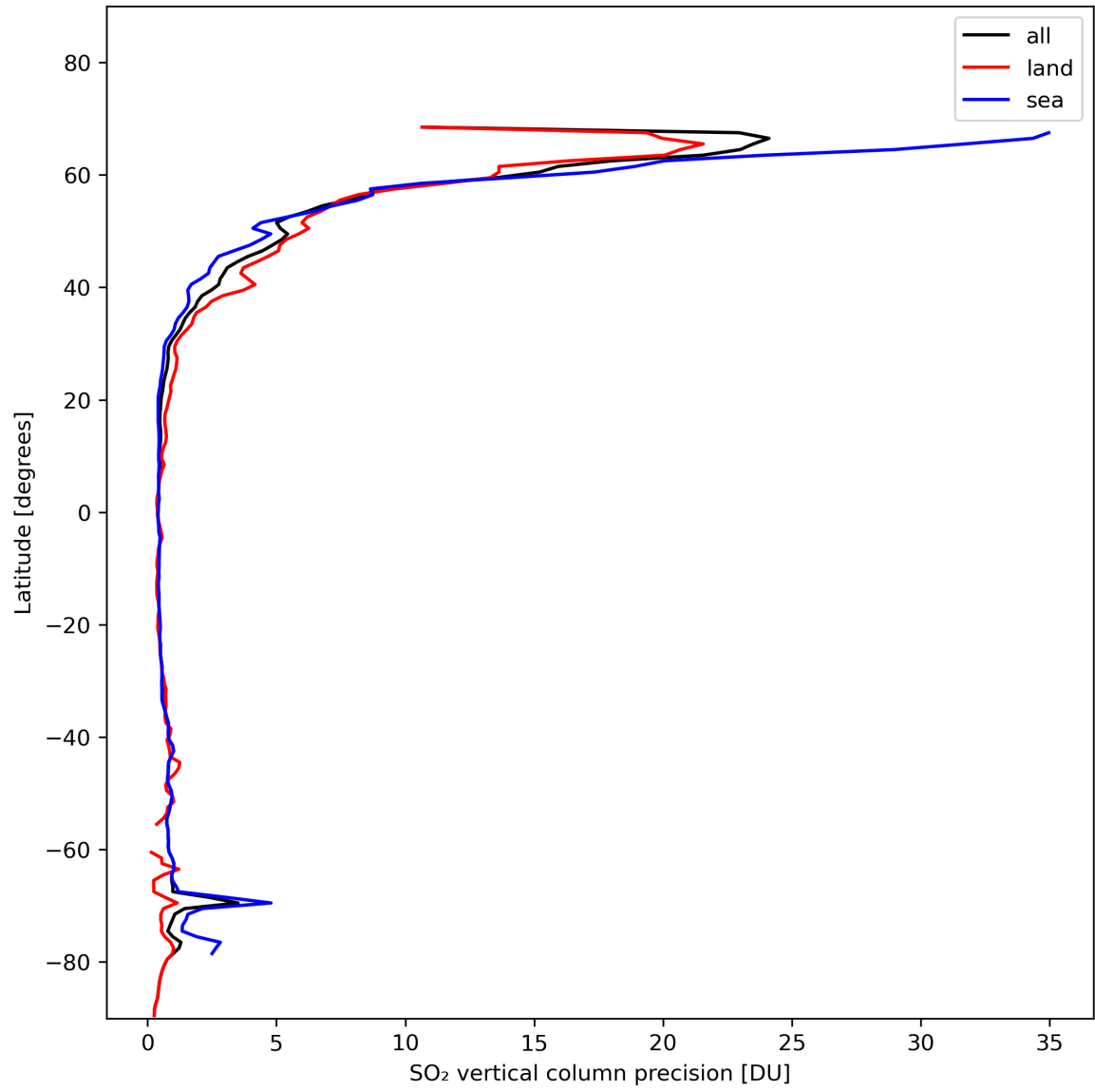
Figure 31: Zonal average of “SO 2 vertical column precision” for 2024-01-31 to 2024-02-02.
