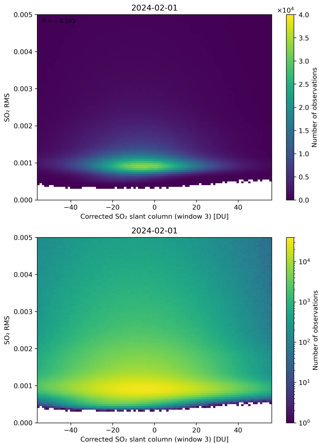
Figure 208: Scatter density plot of “Corrected SO 2 slant column (window 3)” against “SO 2 RMS” for 2024-01-31 to 2024-02-02.
