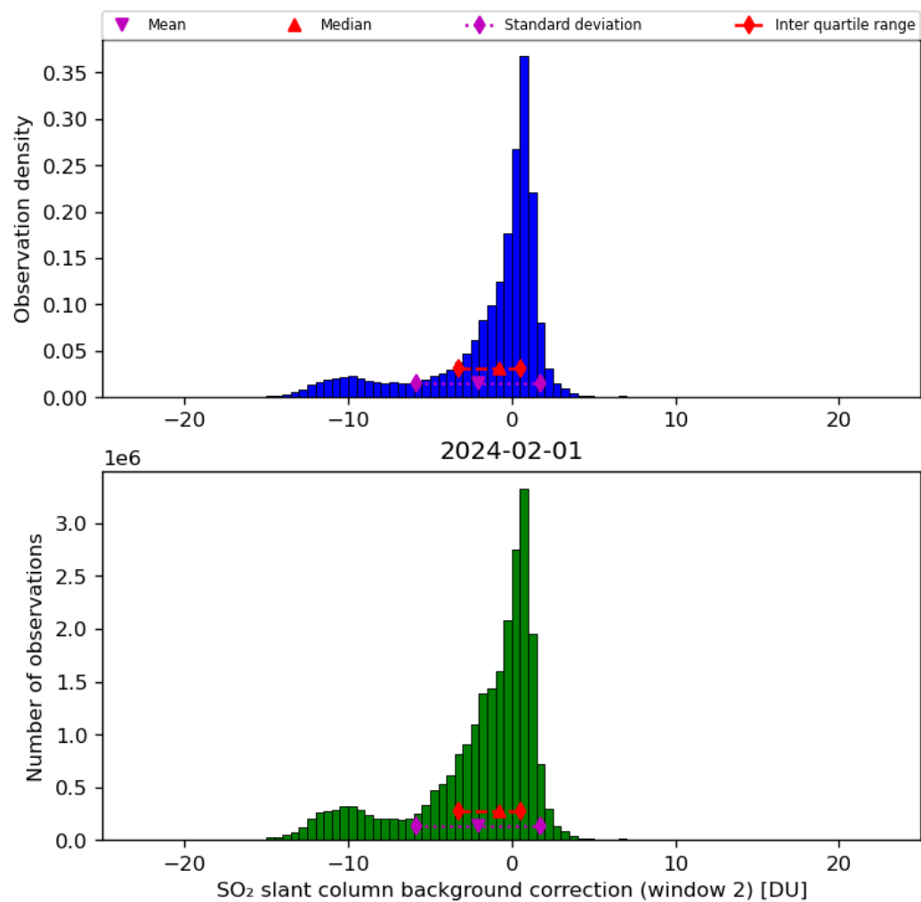
Figure 63: Histogram of “SO 2 slant column background correction (window 2)” for 2024-01-31 to 2024-02-02
