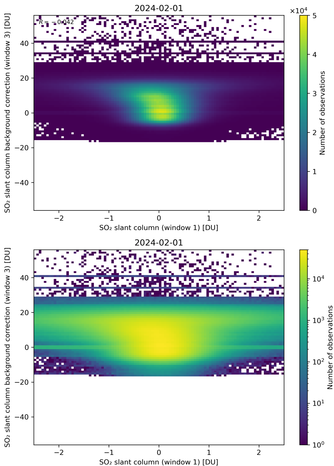
Figure 214: Scatter density plot of “SO 2 slant column (window 1)” against “SO 2 slant column background correction (window 3)” for 2024-01-31 to 2024-02-02.
