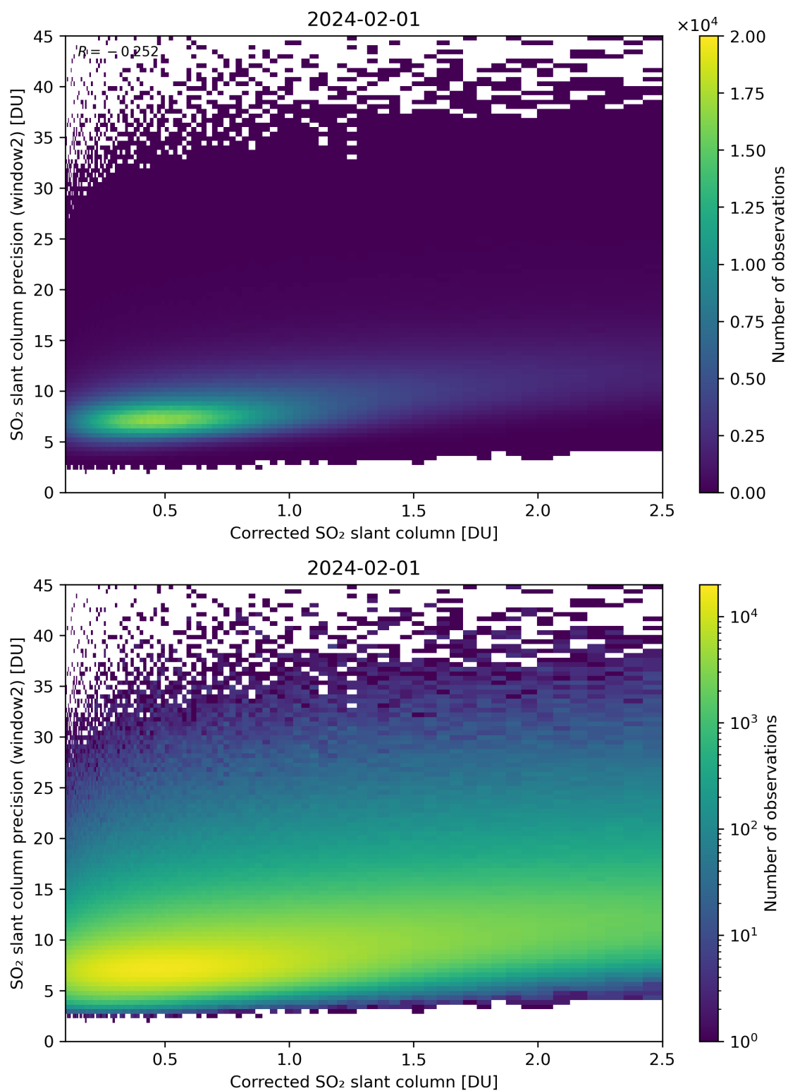
Figure 189: Scatter density plot of “Corrected SO 2 slant column” against “SO 2 slant column precision (window2)” for 2024-01-31 to 2024-02-02.
