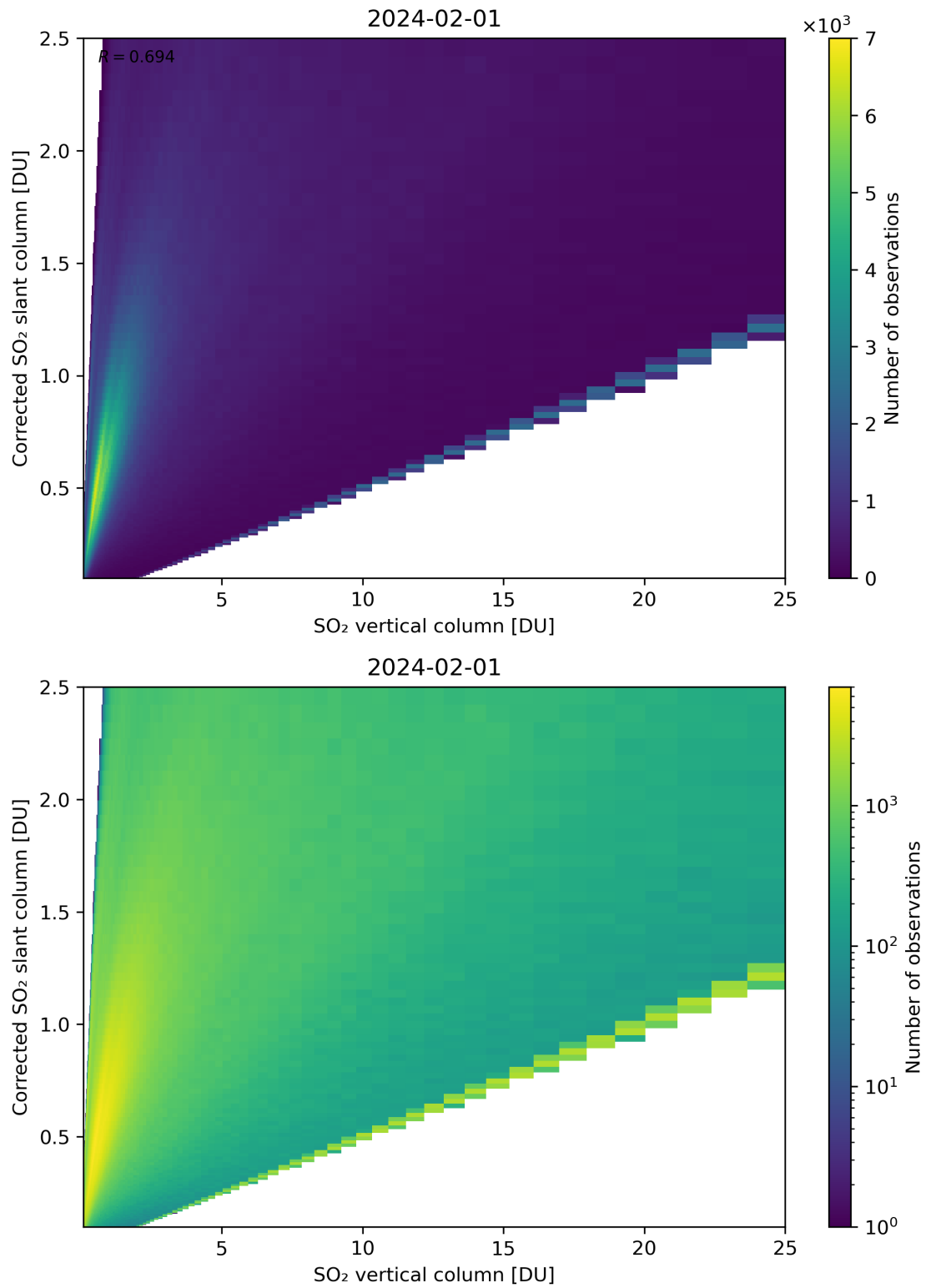
Figure 297: Scatter density plot of “SO 2 vertical column” against “Corrected SO 2 slant column” for 2024-01-31 to 2024-02-02.
