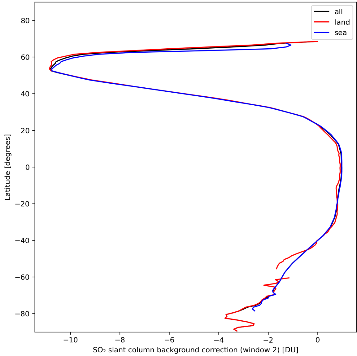
Figure 40: Zonal average of “SO 2 slant column background correction (window 2)” for 2024-01-31 to 2024-02-02.
