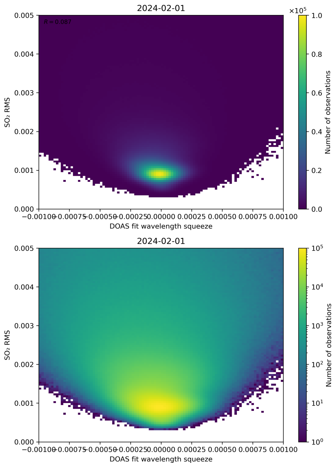
Figure 132: Scatter density plot of “DOAS fit wavelength squeeze” against “SO 2 RMS” for 2024-01-31 to 2024-02-02.
