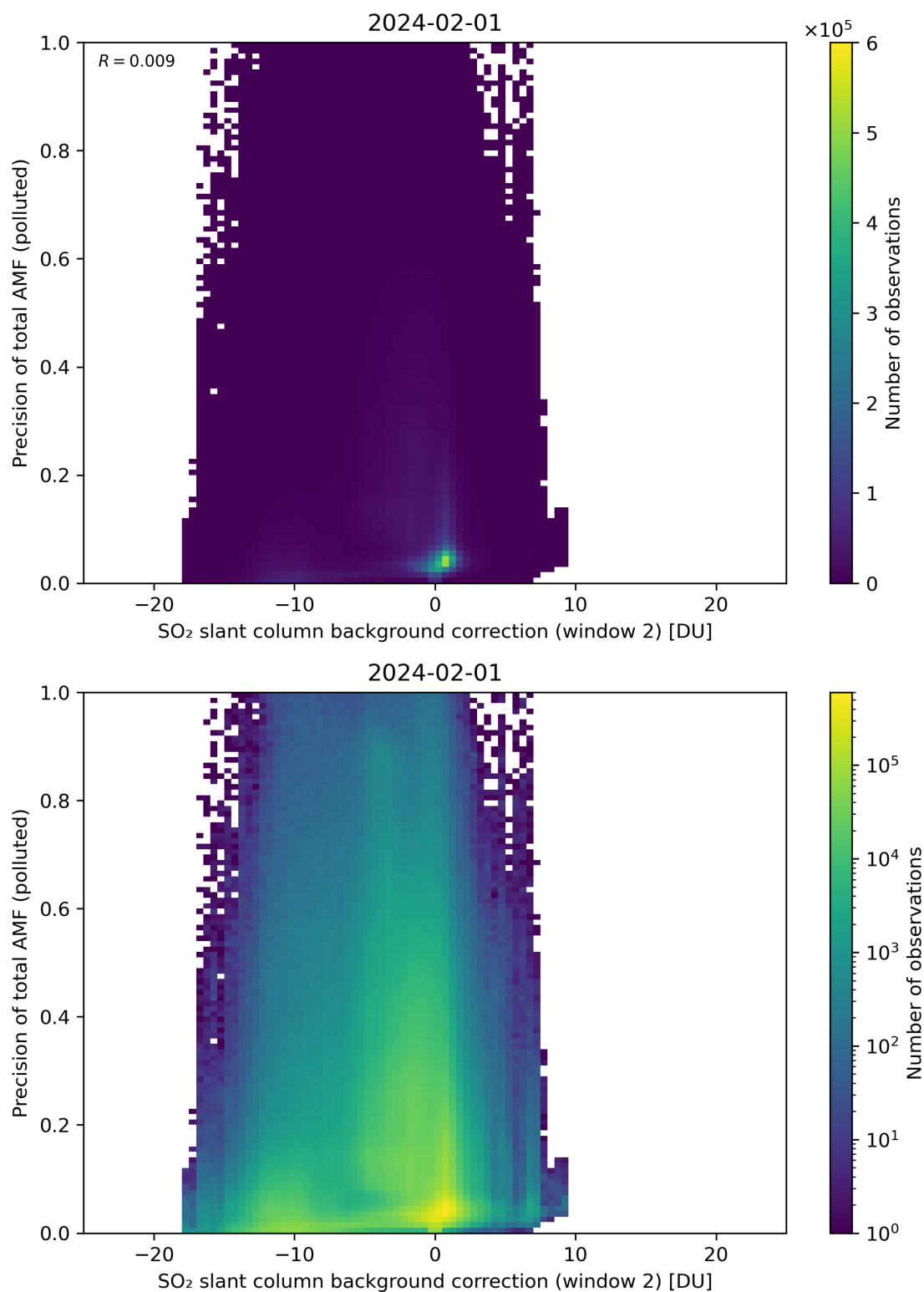
Figure 120: Scatter density plot of “SO 2 slant column background correction (window 2)” against “Precision of total AMF (polluted)” for 2024-01-31 to 2024-02-02.
