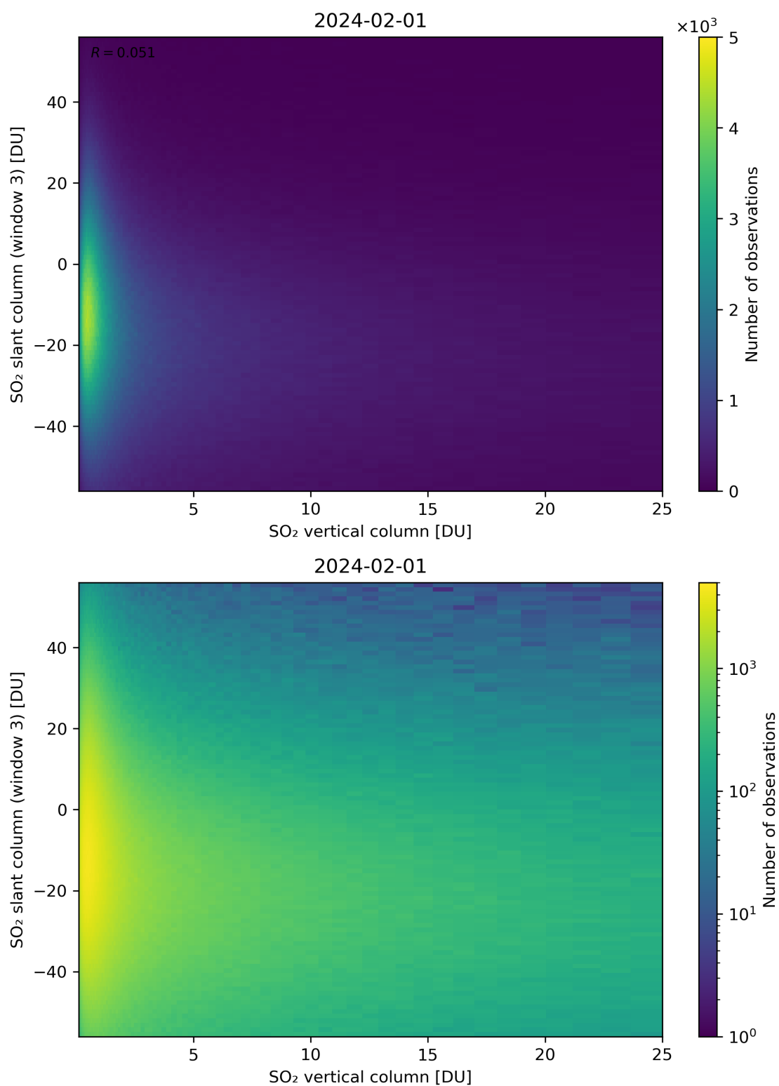
Figure 303: Scatter density plot of “SO 2 vertical column” against “SO 2 slant column (window 3)” for 2024-01-31 to 2024-02-02.
