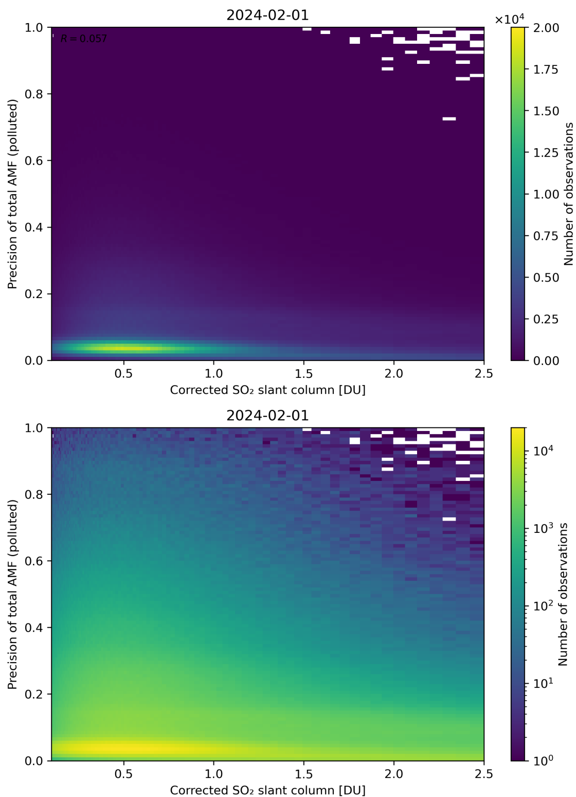
Figure 193: Scatter density plot of “Corrected SO 2 slant column” against “Precision of total AMF (polluted)” for 2024-01-31 to 2024-02-02.
