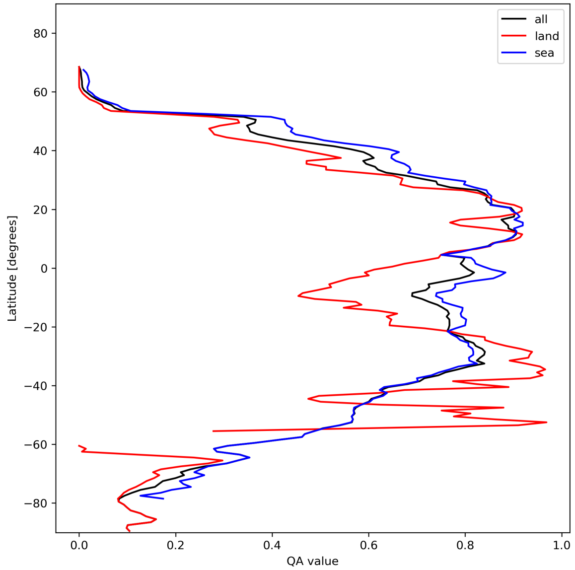
Figure 29: Zonal average of “QA value” for 2024-01-31 to 2024-02-02.
