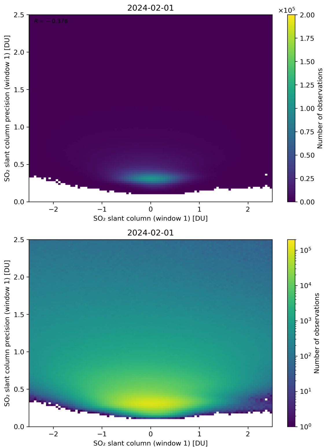
Figure 235: Scatter density plot of “SO 2 slant column (window 1)” against “SO 2 slant column precision (window 1)” for 2024-01-31 to 2024-02-02.
