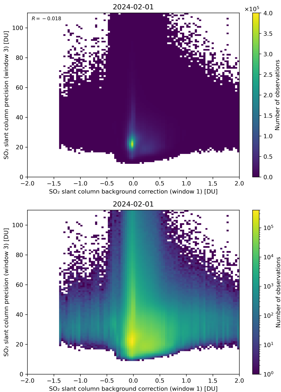
Figure 108: Scatter density plot of “SO 2 slant column background correction (window 1)” against “SO 2 slant column precision (window 3)” for 2024-01-31 to 2024-02-02.
