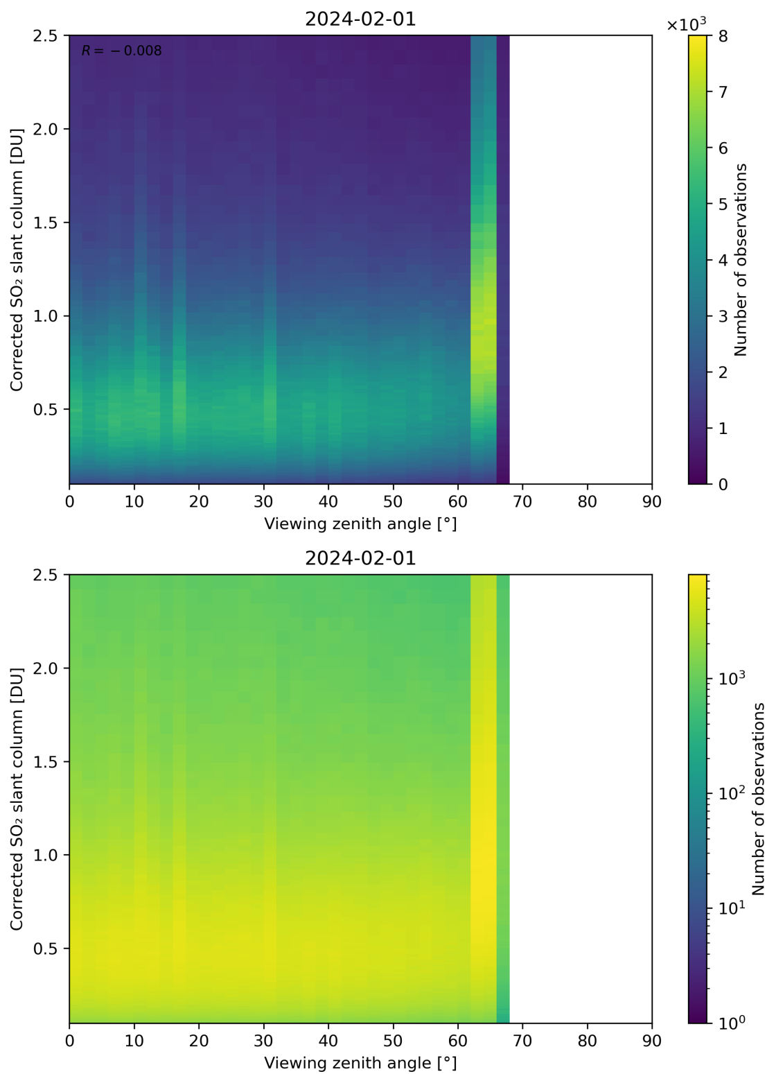
Figure 317: Scatter density plot of “Viewing zenith angle” against “Corrected SO 2 slant column” for 2024-01-31 to 2024-02-02.
