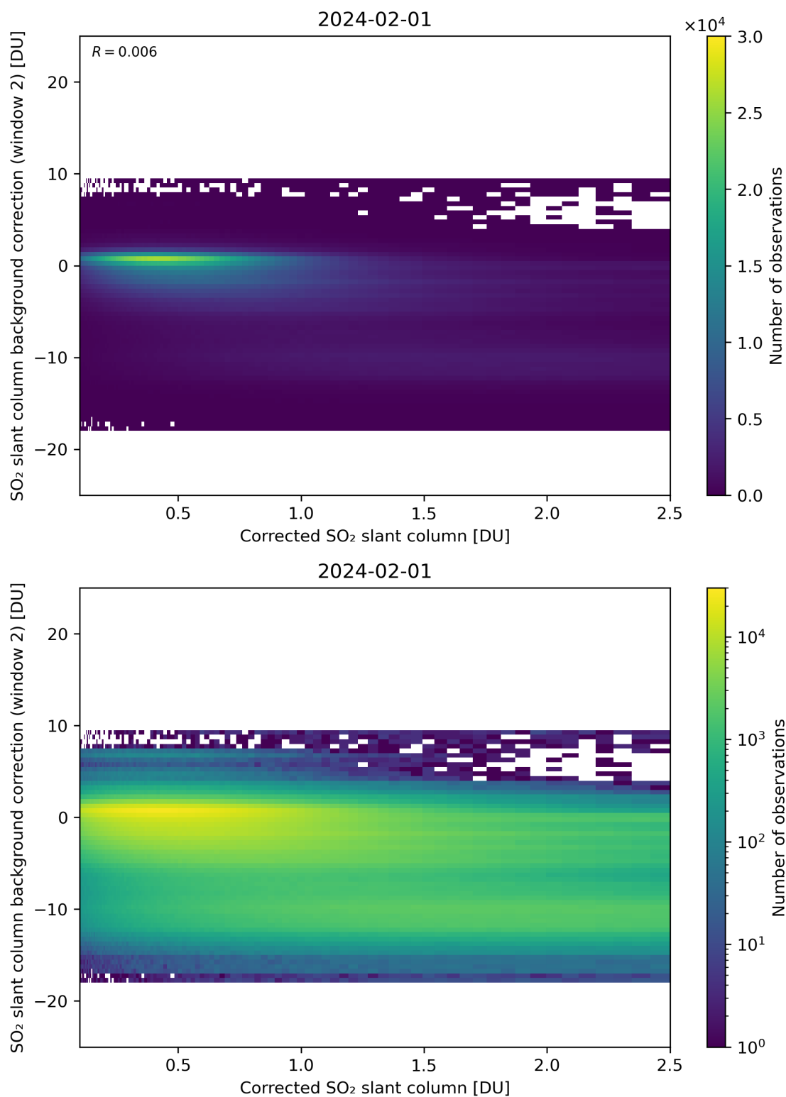
Figure 179: Scatter density plot of “Corrected SO 2 slant column” against “SO 2 slant column background correction (window 2)” for 2024-01-31 to 2024-02-02.
