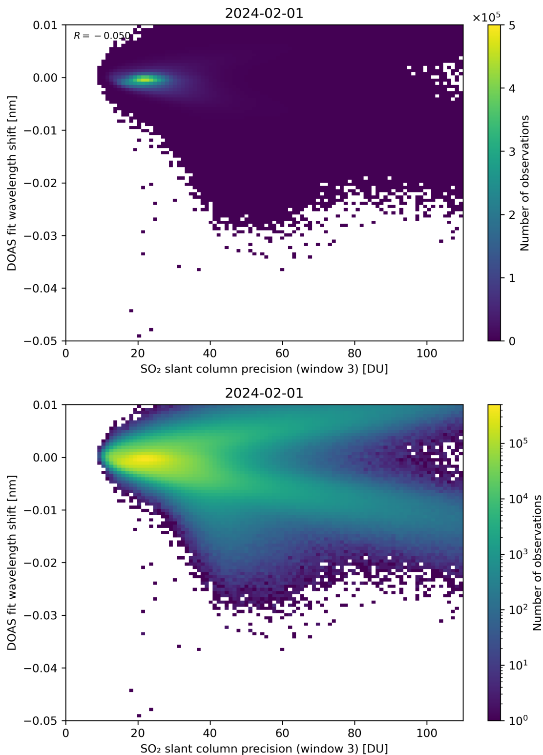
Figure 258: Scatter density plot of “SO 2 slant column precision (window 3)” against “DOAS fit wavelength shift” for 2024-01-31 to 2024-02-02.
