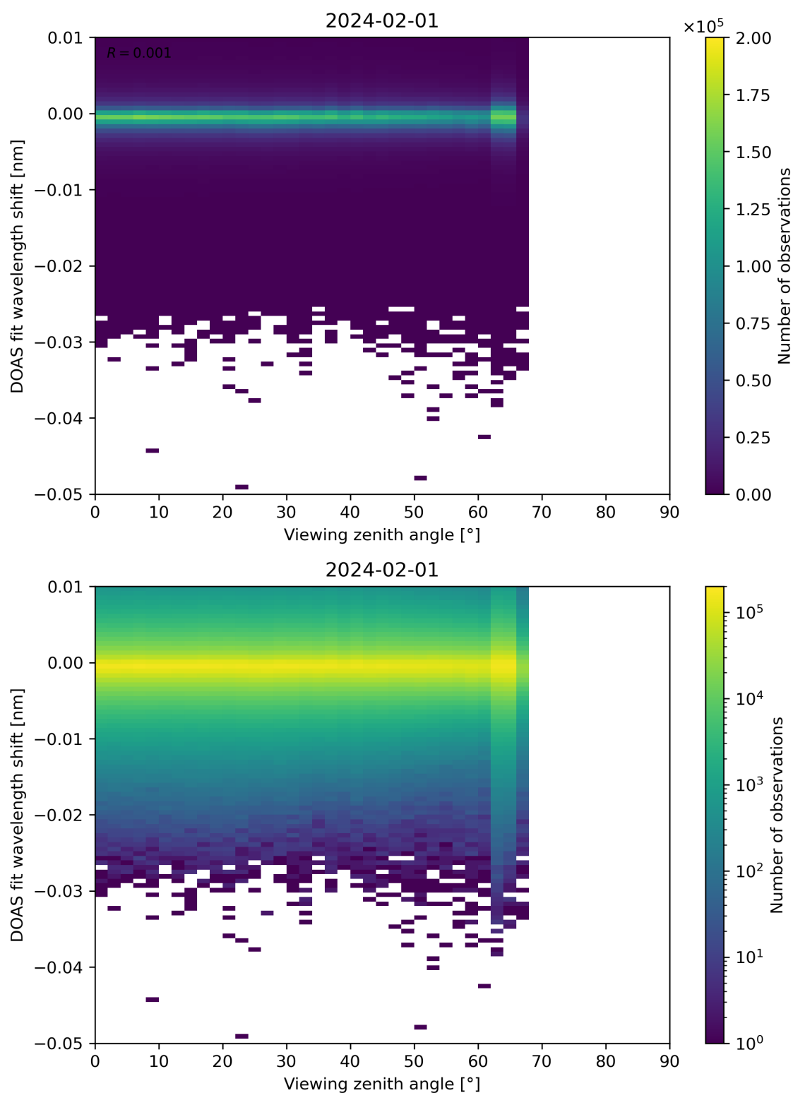
Figure 311: Scatter density plot of “Viewing zenith angle” against “DOAS fit wavelength shift” for 2024-01-31 to 2024-02-02.
