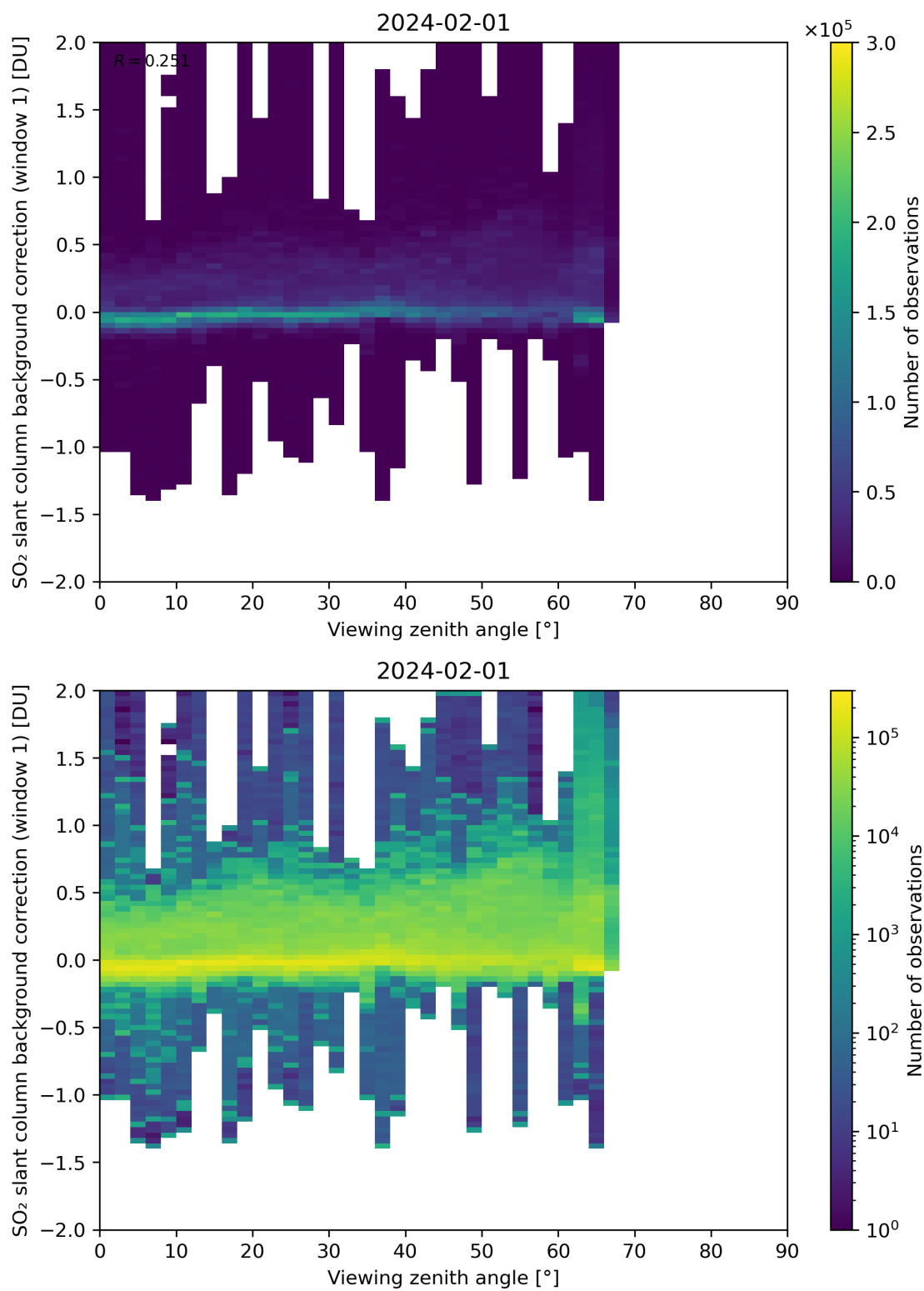
Figure 308: Scatter density plot of “Viewing zenith angle” against “SO 2 slant column background correction (window 1)” for 2024-01-31 to 2024-02-02.
