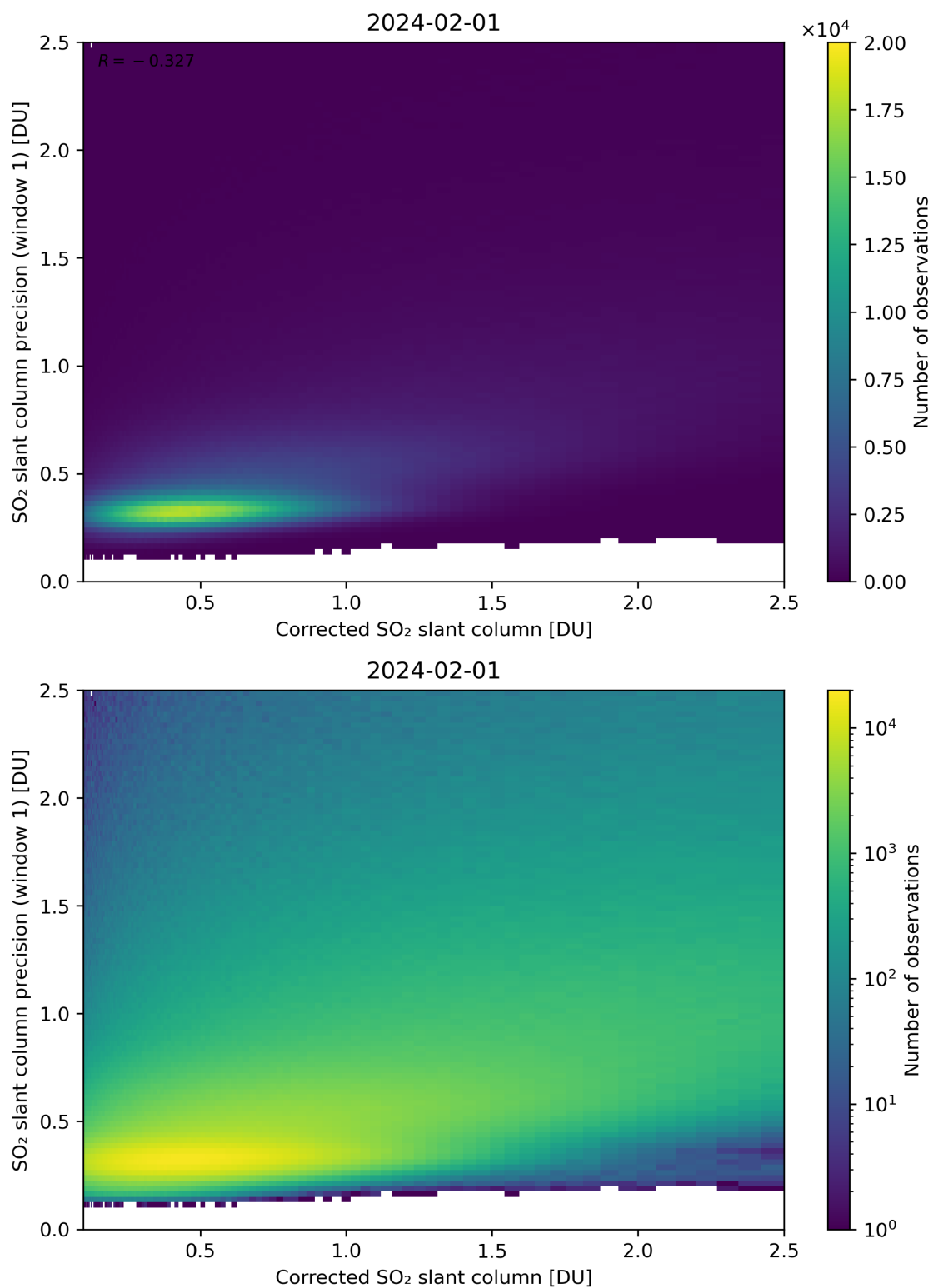
Figure 188: Scatter density plot of “Corrected SO 2 slant column” against “SO 2 slant column precision (window 1)” for 2024-01-31 to 2024-02-02.
