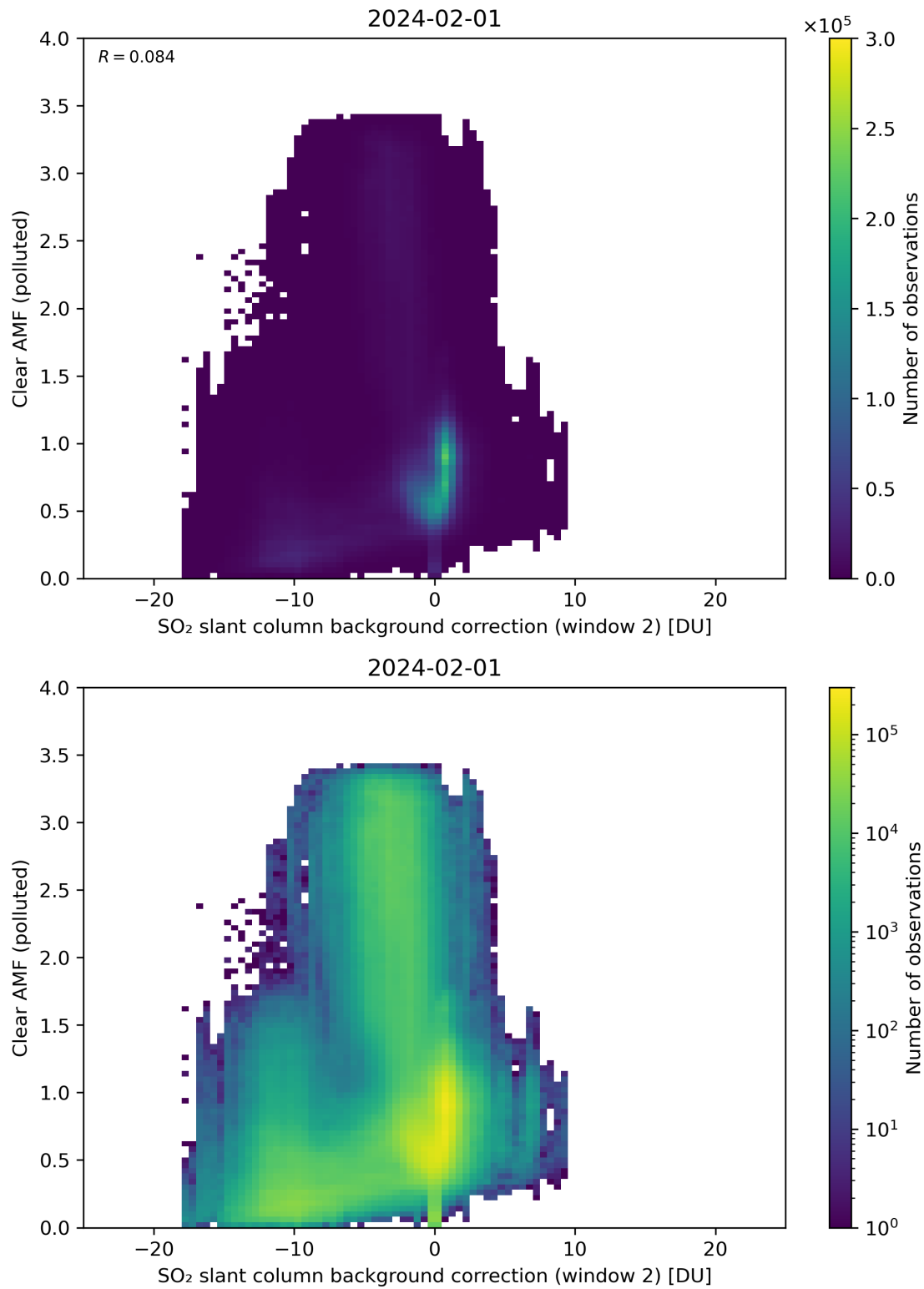
Figure 115: Scatter density plot of “SO 2 slant column background correction (window 2)” against “Clear AMF (polluted)” for 2024-01-31 to 2024-02-02.
