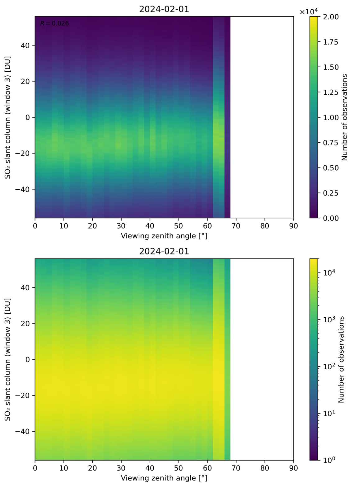
Figure 323: Scatter density plot of “Viewing zenith angle” against “SO 2 slant column (window 3)” for 2024-01-31 to 2024-02-02.
