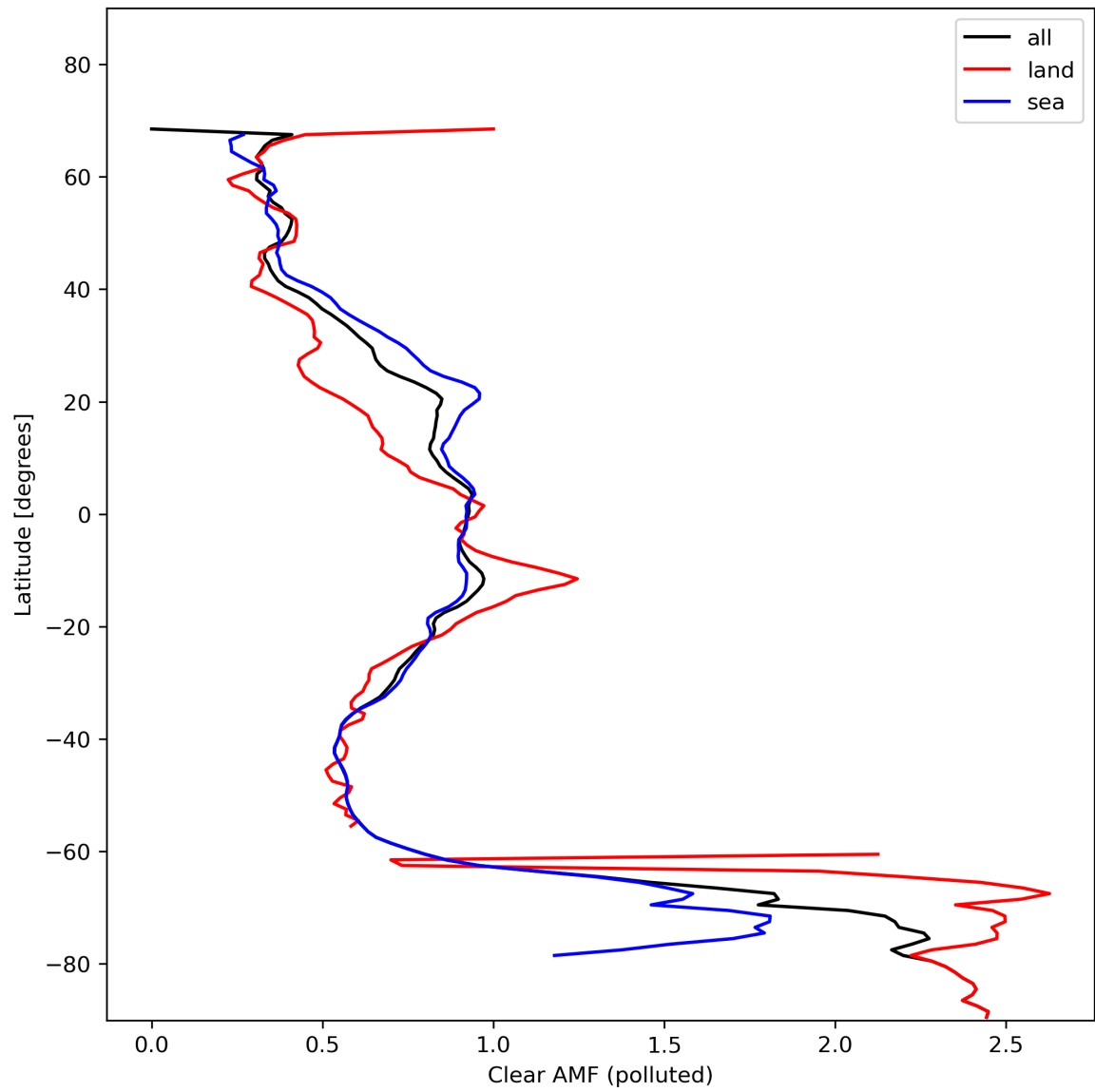
Figure 50: Zonal average of “Clear AMF (polluted)” for 2024-01-31 to 2024-02-02.
