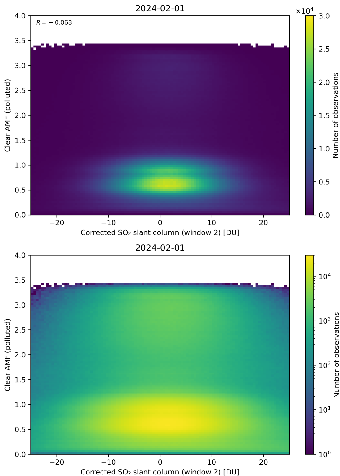
Figure 199: Scatter density plot of “Corrected SO 2 slant column (window 2)” against “Clear AMF (polluted)” for 2024-01-31 to 2024-02-02.
