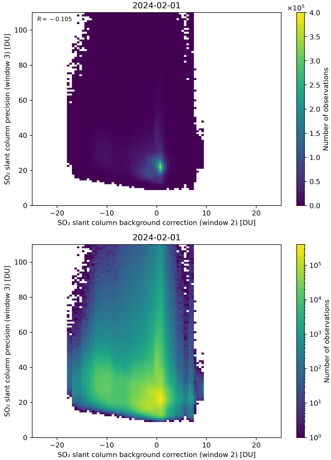
Figure 118: Scatter density plot of “SO 2 slant column background correction (window 2)” against “SO 2 slant column precision (window 3)” for 2024-01-31 to 2024-02-02.
