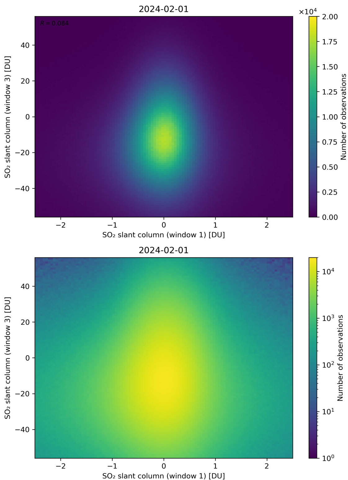
Figure 237: Scatter density plot of “SO 2 slant column (window 1)” against “SO 2 slant column (window 3)” for 2024-01-31 to 2024-02-02.
