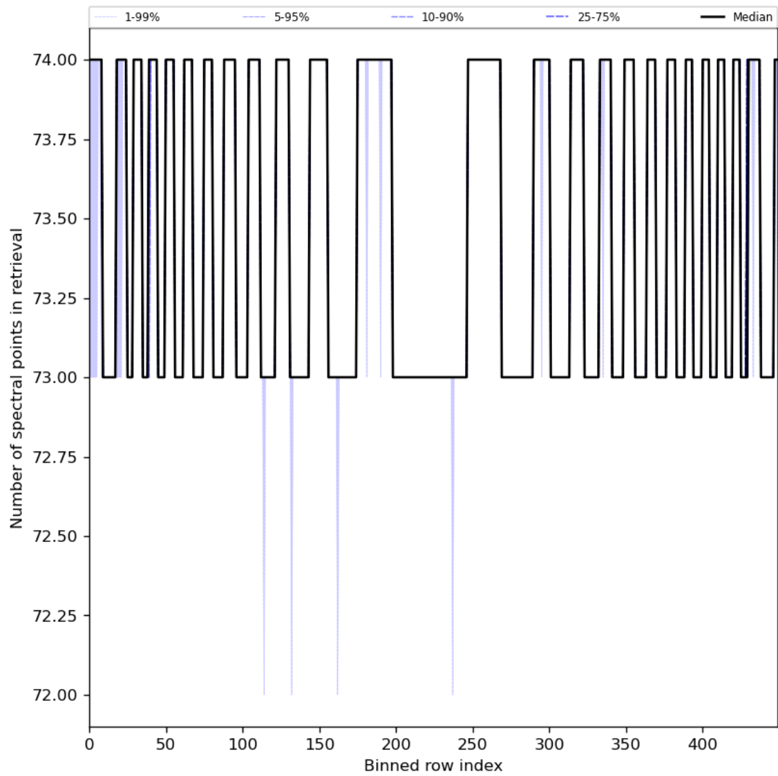
Figure 97: Along track statistics of “Number of spectral points in retrieval” for 2024-01-31 to 2024-02-02
