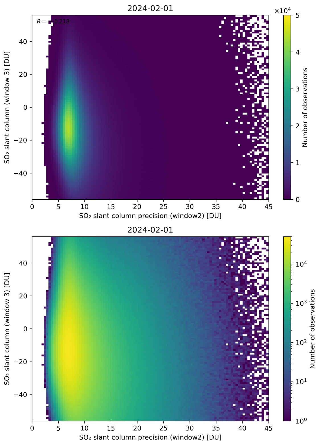
Figure 249: Scatter density plot of “SO 2 slant column precision (window2)” against “SO 2 slant column (window 3)” for 2024-01-31 to 2024-02-02.
