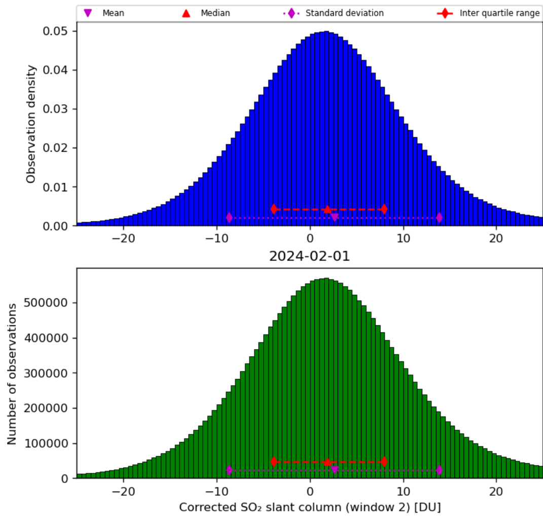
Figure 62: Histogram of “Corrected SO 2 slant column (window 2)” for 2024-01-31 to 2024-02-02
