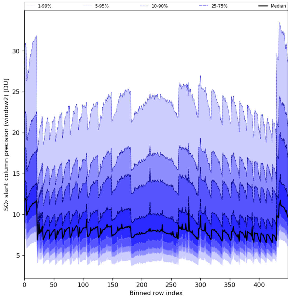
Figure 84: Along track statistics of “SO 2 slant column precision (window2)” for 2024-01-31 to 2024-02-02
