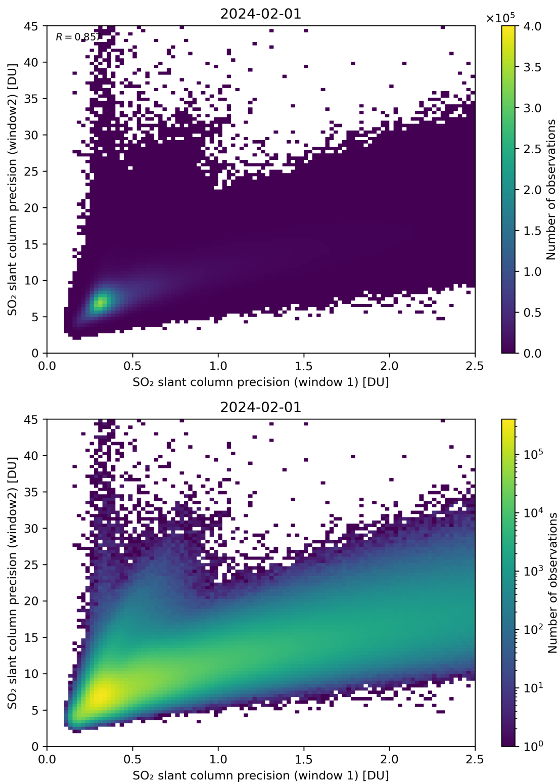
Figure 227: Scatter density plot of “SO 2 slant column precision (window 1)” against “SO 2 slant column precision (window2)” for 2024-01-31 to 2024-02-02.
