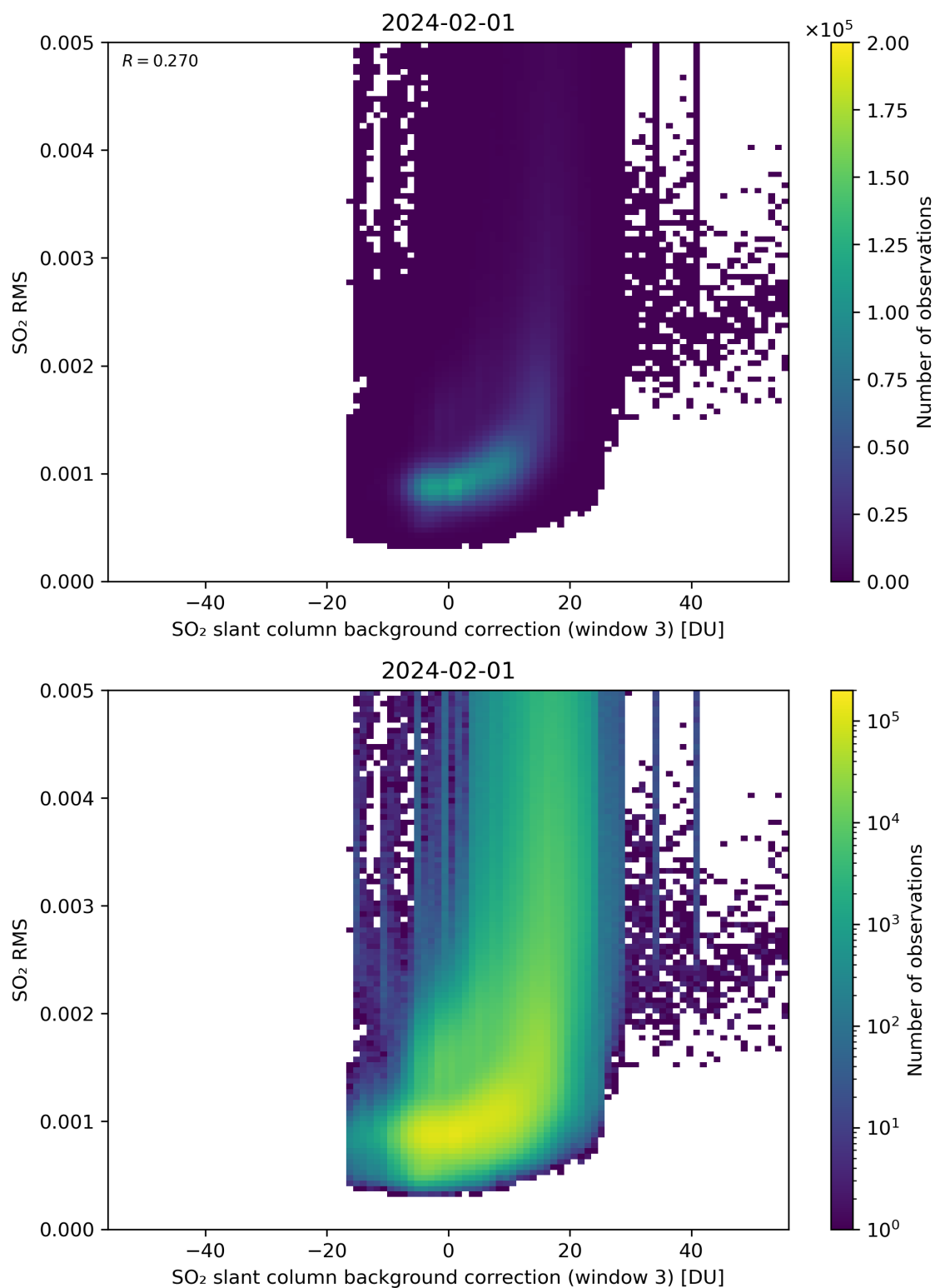
Figure 123: Scatter density plot of “SO 2 slant column background correction (window 3)” against “SO 2 RMS” for 2024-01-31 to 2024-02-02.
