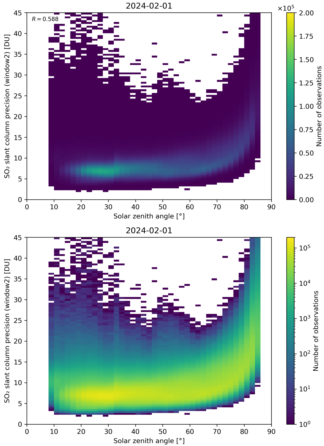
Figure 171: Scatter density plot of “Solar zenith angle” against “SO 2 slant column precision (window2)” for 2024-01-31 to 2024-02-02.
