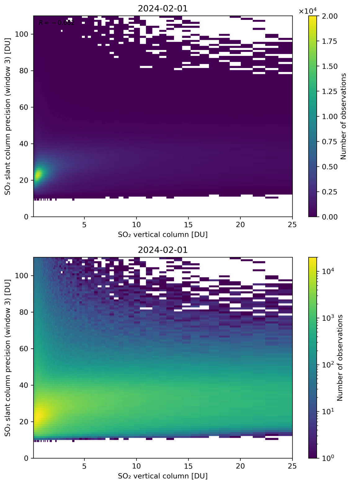
Figure 304: Scatter density plot of “SO 2 vertical column” against “SO 2 slant column precision (window 3)” for 2024-01-31 to 2024-02-02.
