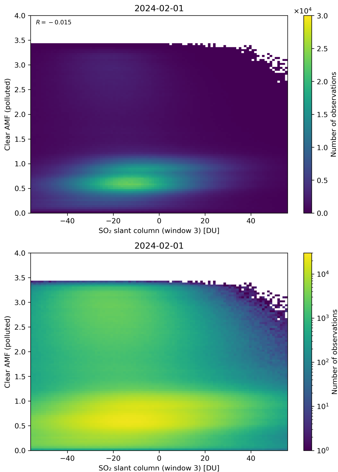
Figure 265: Scatter density plot of “SO 2 slant column (window 3)” against “Clear AMF (polluted)” for 2024-01-31 to 2024-02-02.
