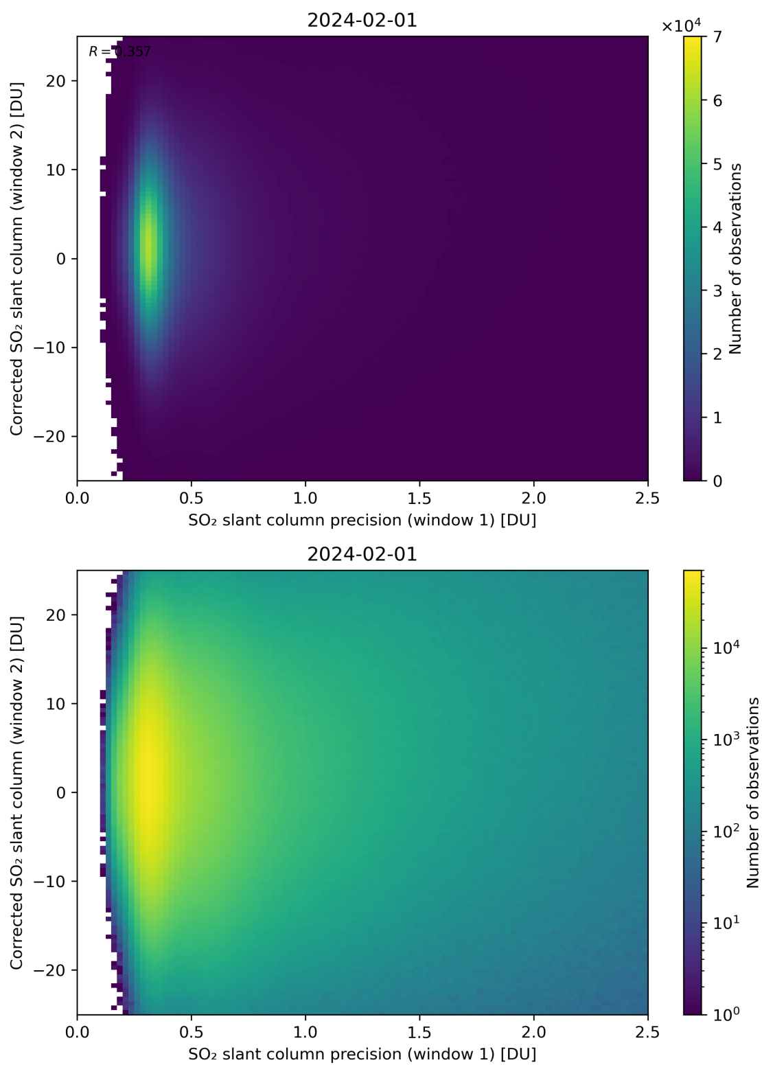
Figure 225: Scatter density plot of “SO 2 slant column precision (window 1)” against “Corrected SO 2 slant column (window 2)” for 2024-01-31 to 2024-02-02.
