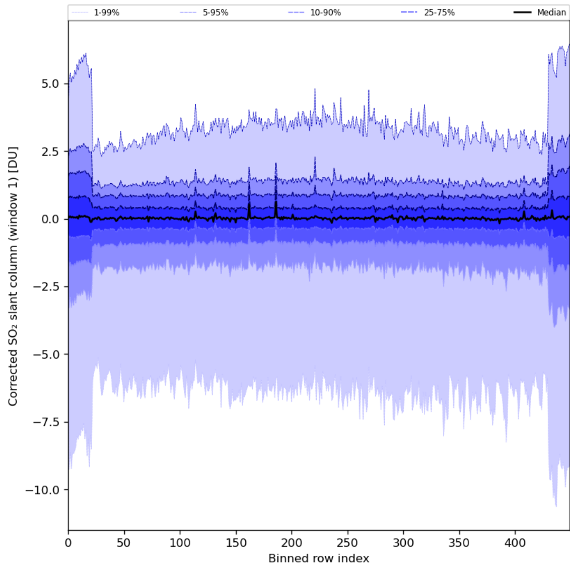
Figure 81: Along track statistics of “Corrected SO 2 slant column (window 1)” for 2024-01-31 to 2024-02-02
