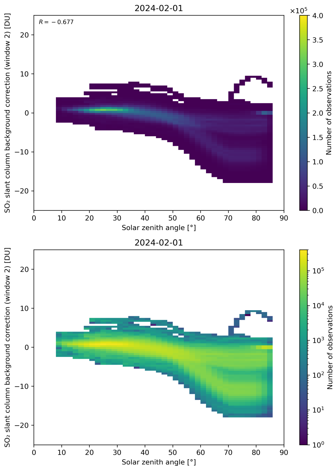
Figure 159: Scatter density plot of “Solar zenith angle” against “SO 2 slant column background correction (window 2)” for 2024-01-31 to 2024-02-02.
