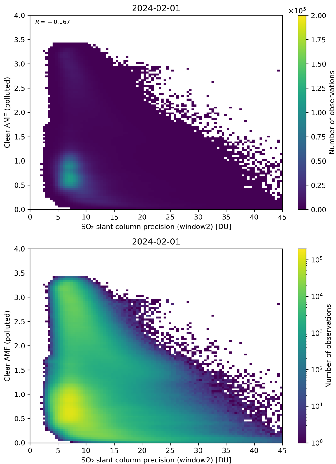
Figure 246: Scatter density plot of “SO 2 slant column precision (window2)” against “Clear AMF (polluted)” for 2024-01-31 to 2024-02-02.
