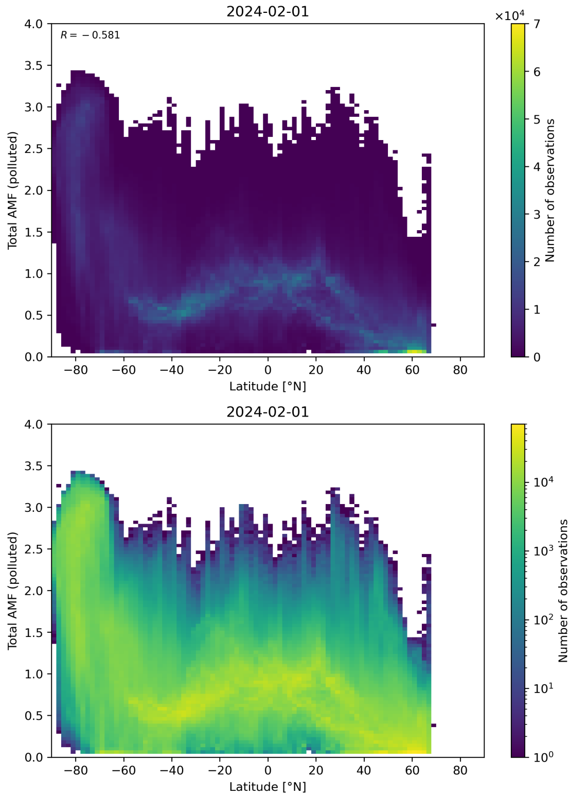
Figure 154: Scatter density plot of “Latitude” against “Total AMF (polluted)” for 2024-01-31 to 2024-02-02.
