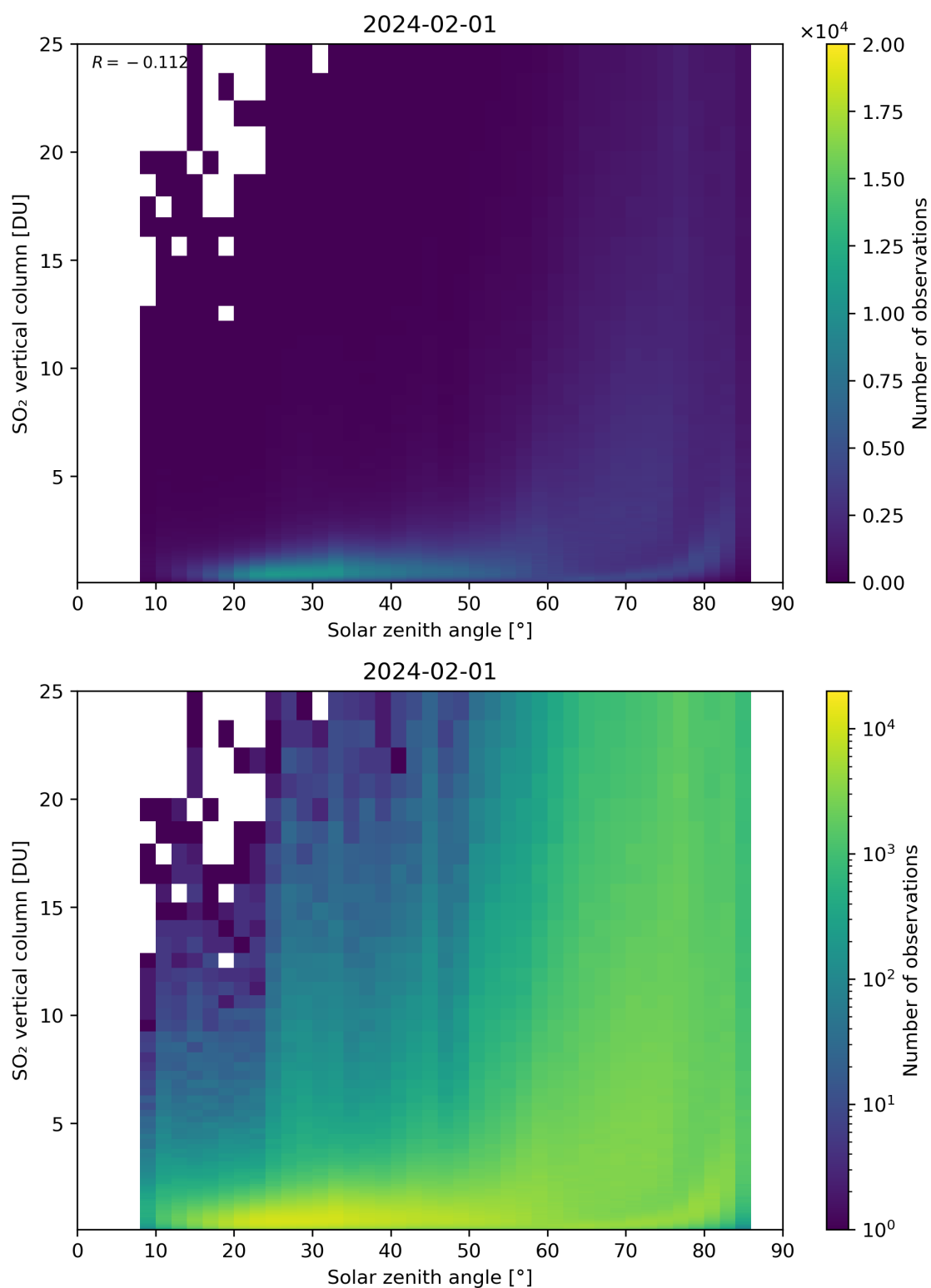
Figure 176: Scatter density plot of “Solar zenith angle” against “SO 2 vertical column” for 2024-01-31 to 2024-02-02.
