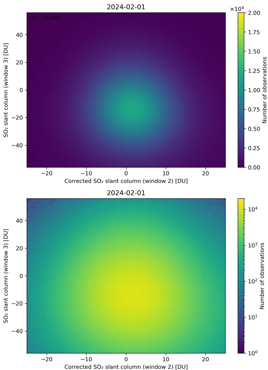
Figure 201: Scatter density plot of “Corrected SO 2 slant column (window 2)” against “SO 2 slant column (window 3)” for 2024-01-31 to 2024-02-02.
