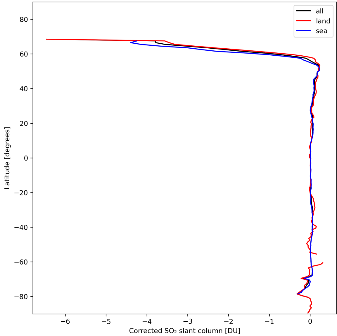
Figure 32: Zonal average of "Corrected SO 2 slant column" for 2024-01-31 to 2024-02-02.
