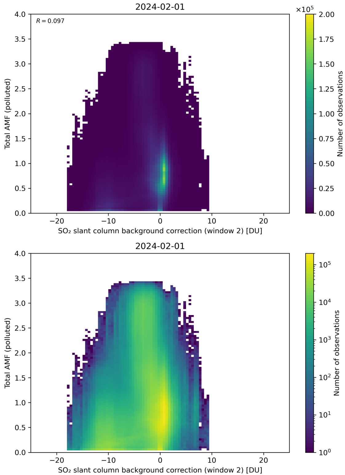
Figure 119: Scatter density plot of “SO 2 slant column background correction (window 2)” against “Total AMF (polluted)” for 2024-01-31 to 2024-02-02.
