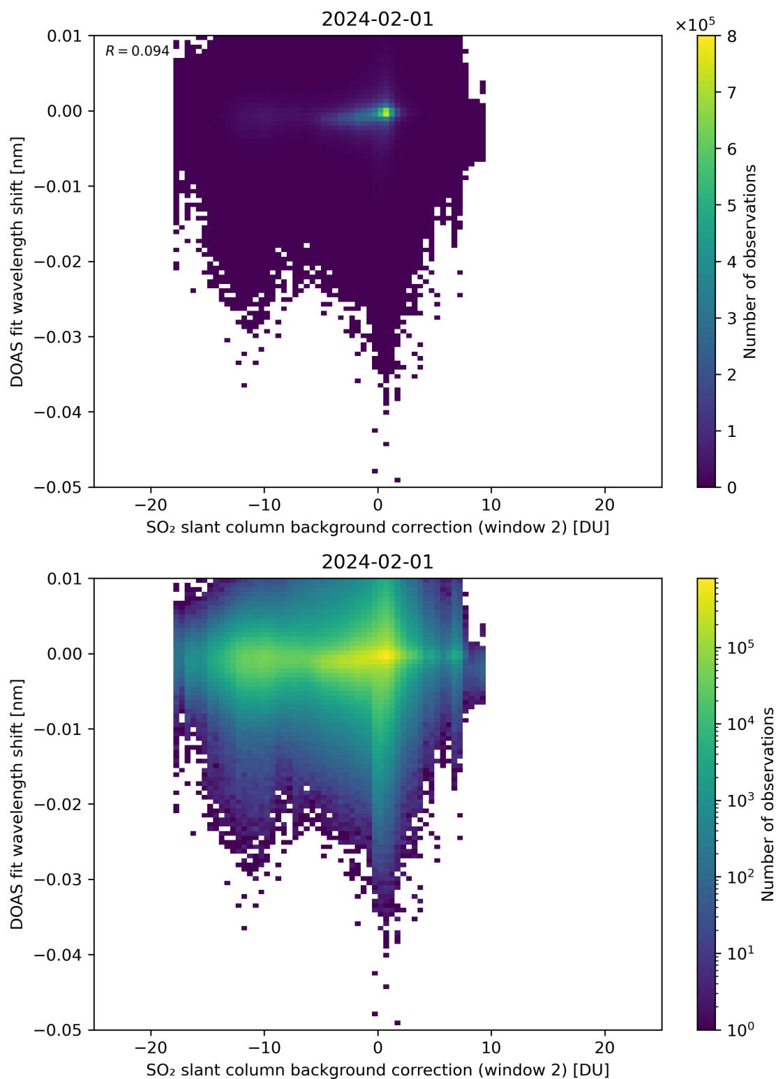
Figure 112: Scatter density plot of “SO 2 slant column background correction (window 2)” against “DOAS fit wavelength shift” for 2024-01-31 to 2024-02-02.
