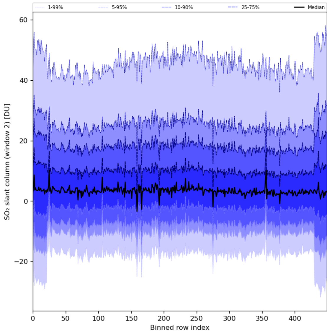
Figure 83: Along track statistics of “SO 2 slant column (window 2)” for 2024-01-31 to 2024-02-02
