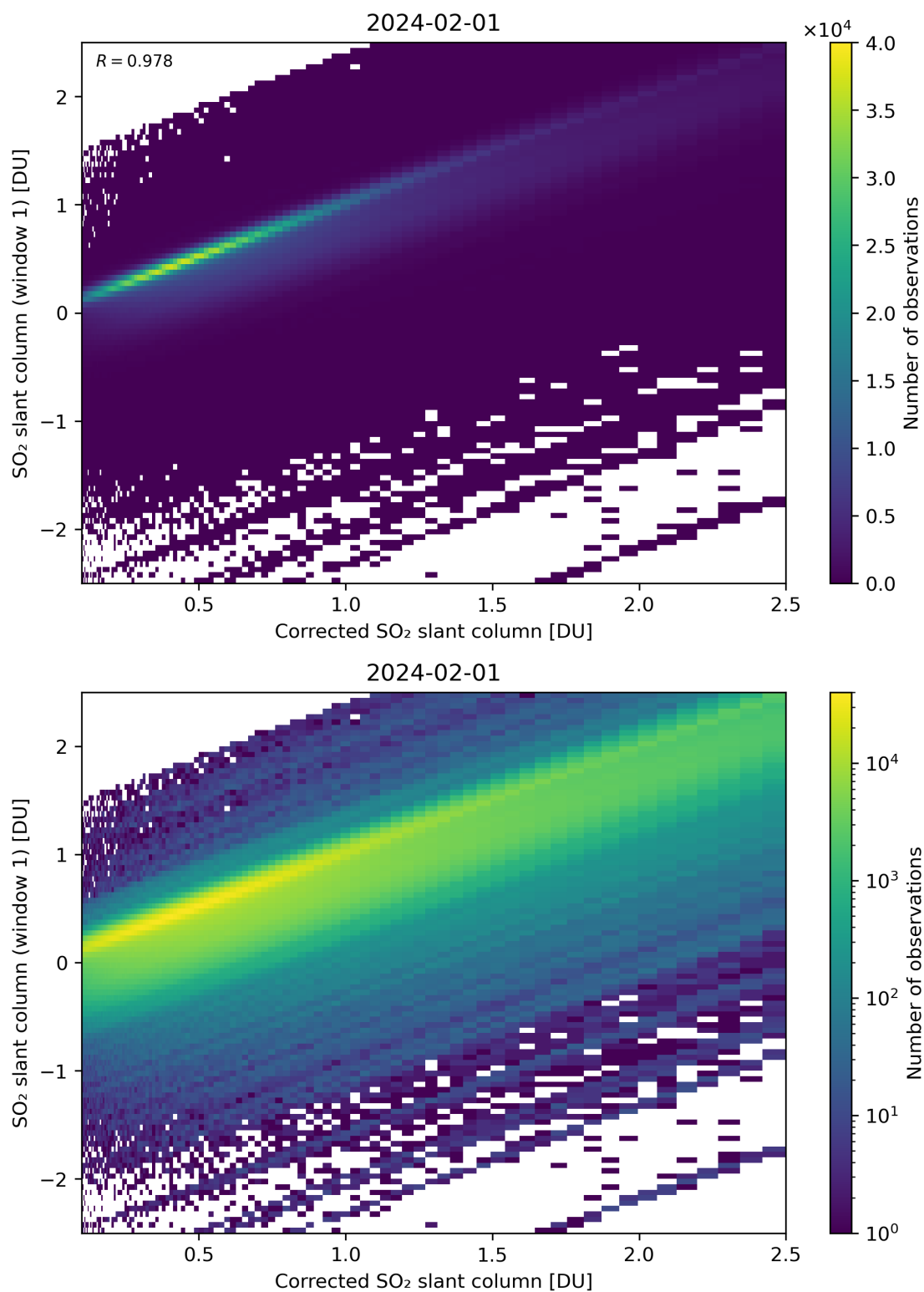
Figure 187: Scatter density plot of “Corrected SO 2 slant column” against “SO 2 slant column (window 1)” for 2024-01-31 to 2024-02-02.
