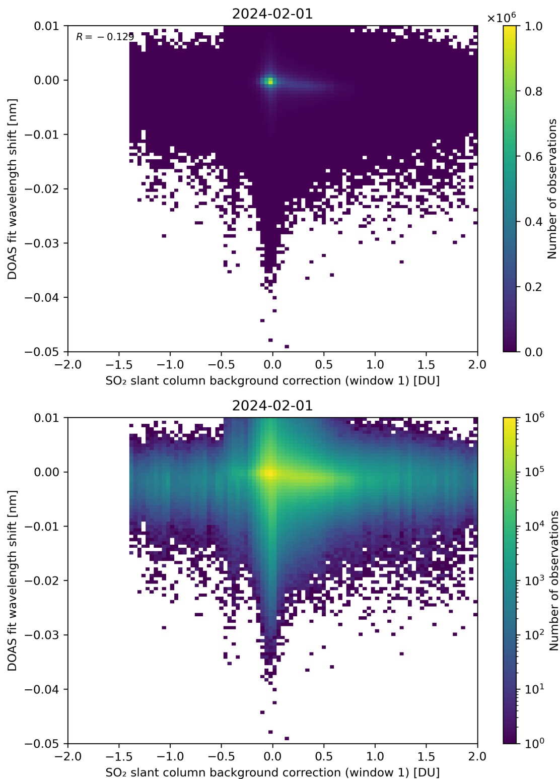
Figure 100: Scatter density plot of “SO 2 slant column background correction (window 1)” against “DOAS fit wavelength shift” for 2024-01-31 to 2024-02-02.
