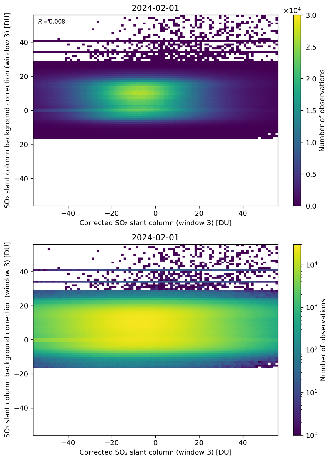
Figure 205: Scatter density plot of “Corrected SO 2 slant column (window 3)” against “SO 2 slant column background correction (window 3)” for 2024-01-31 to 2024-02-02.
