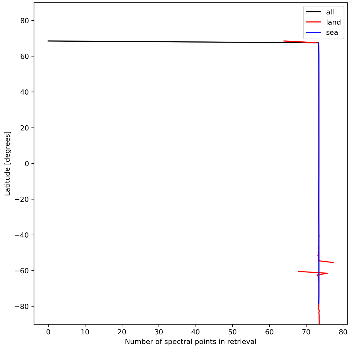
Figure 51: Zonal average of “Number of spectral points in retrieval” for 2024-01-31 to 2024-02-02.
