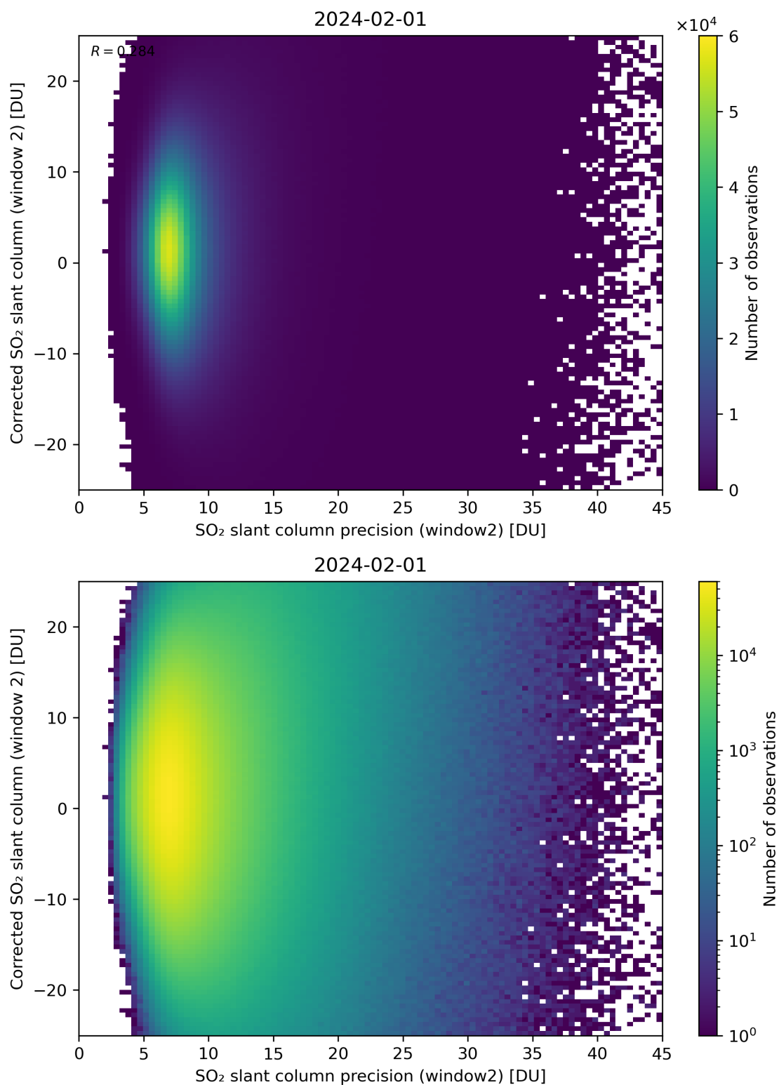
Figure 247: Scatter density plot of “SO 2 slant column precision (window2)” against “Corrected SO 2 slant column (window 2)” for 2024-01-31 to 2024-02-02.
