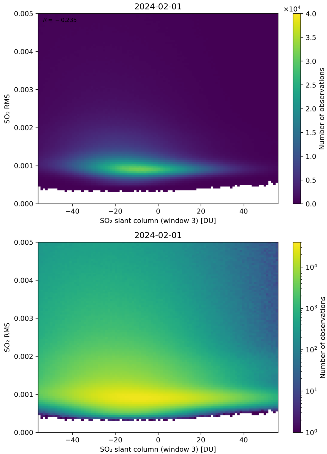
Figure 256: Scatter density plot of “SO 2 slant column (window 3)” against “SO 2 RMS” for 2024-01-31 to 2024-02-02.
