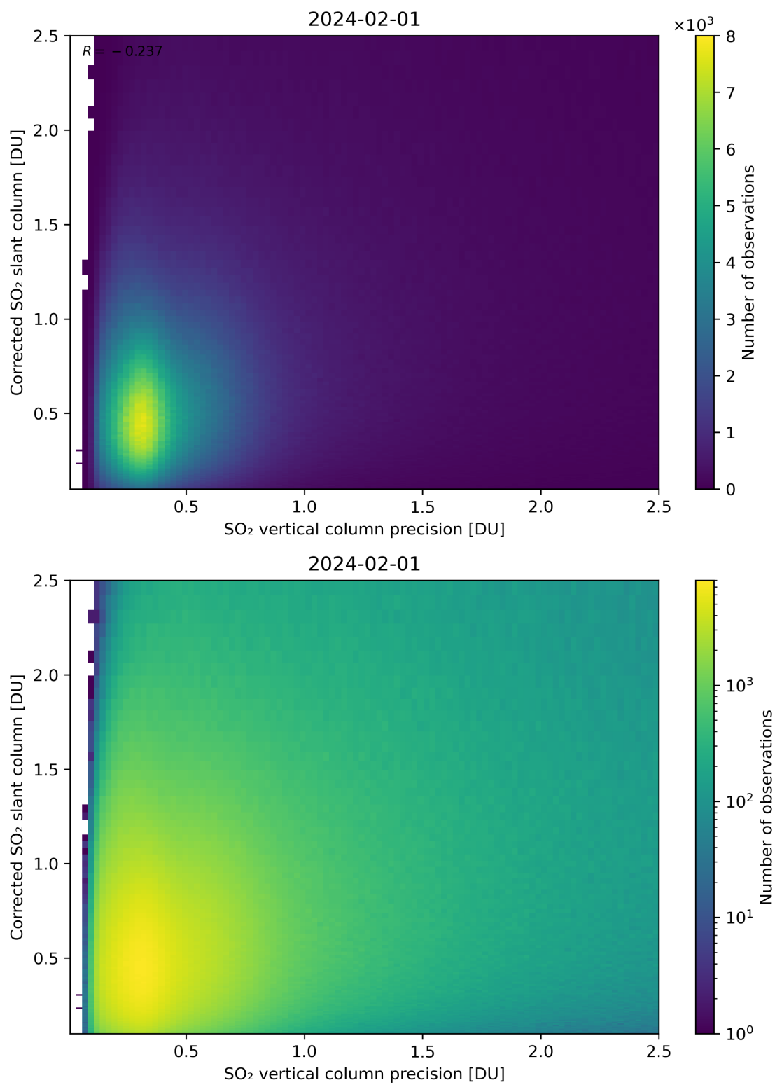
Figure 286: Scatter density plot of “SO 2 vertical column precision” against “Corrected SO 2 slant column” for 2024-01-31 to 2024-02-02.
