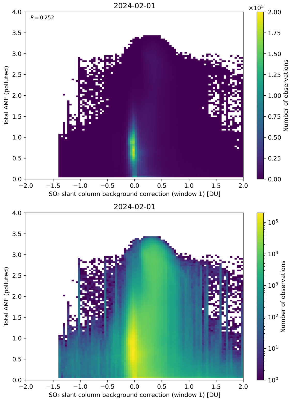
Figure 109: Scatter density plot of “SO 2 slant column background correction (window 1)” against “Total AMF (polluted)” for 2024-01-31 to 2024-02-02.
