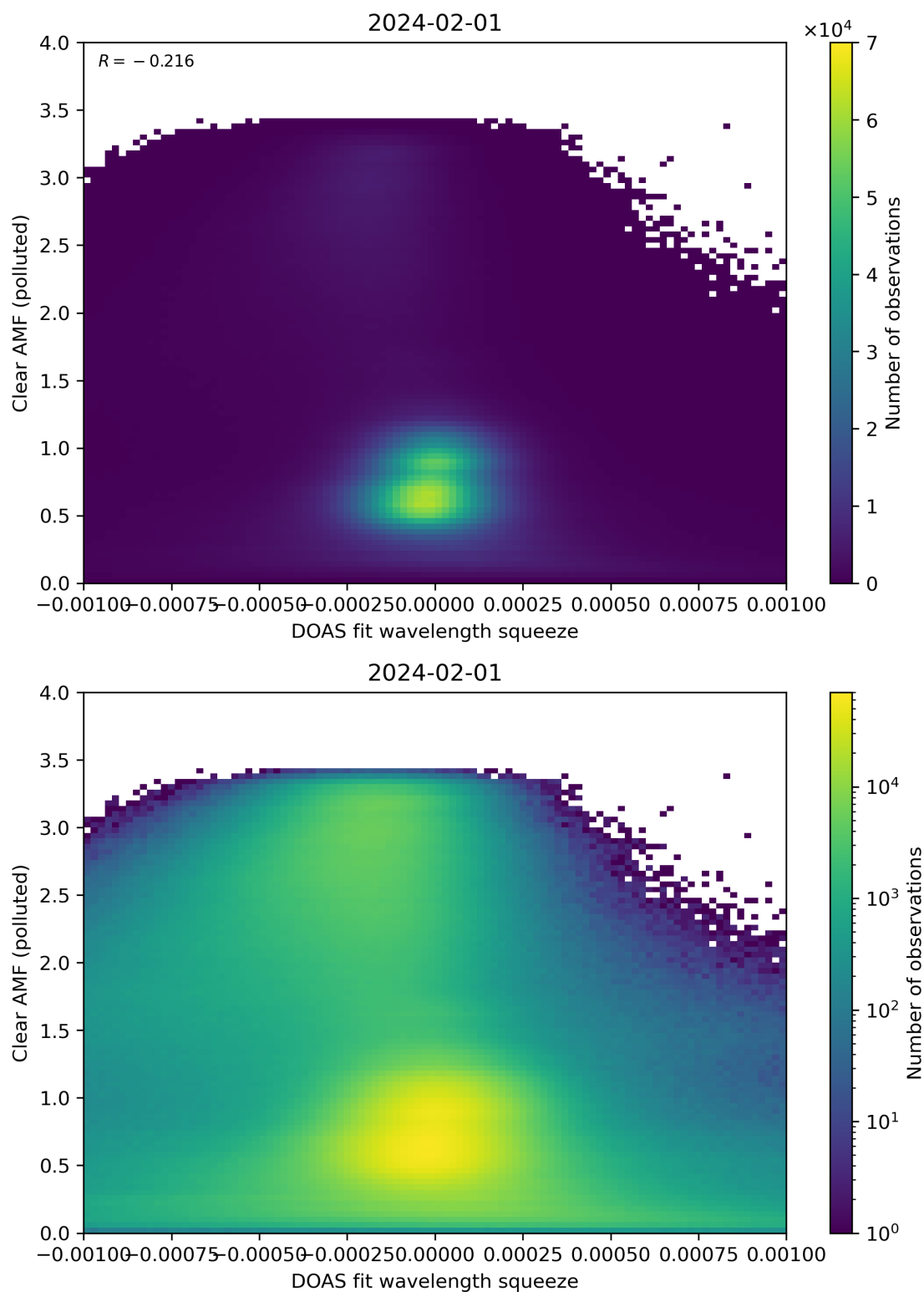
Figure 133: Scatter density plot of “DOAS fit wavelength squeeze” against “Clear AMF (polluted)” for 2024-01-31 to 2024-02-02.
