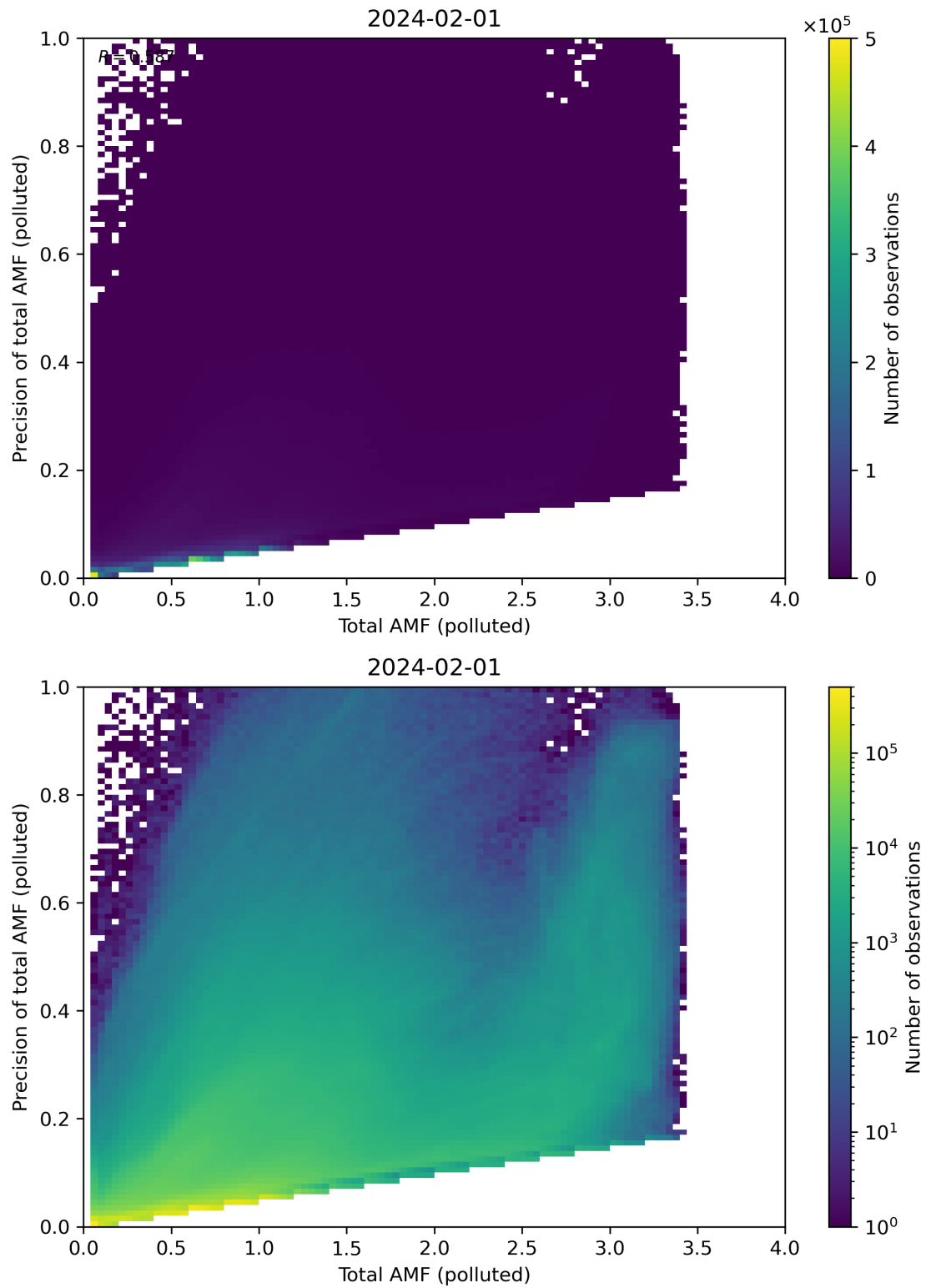
Figure 272: Scatter density plot of “Total AMF (polluted)” against “Precision of total AMF (polluted)” for 2024-01-31 to 2024-02-02.
