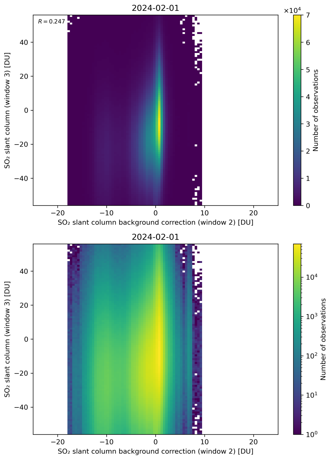
Figure 117: Scatter density plot of “SO 2 slant column background correction (window 2)” against “SO 2 slant column (window 3)” for 2024-01-31 to 2024-02-02.
