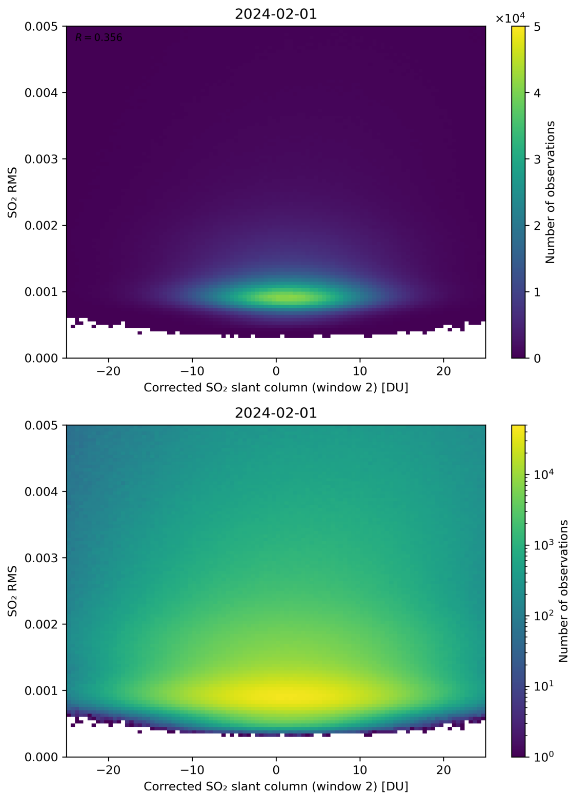
Figure 198: Scatter density plot of “Corrected SO 2 slant column (window 2)” against “SO 2 RMS” for 2024-01-31 to 2024-02-02.
