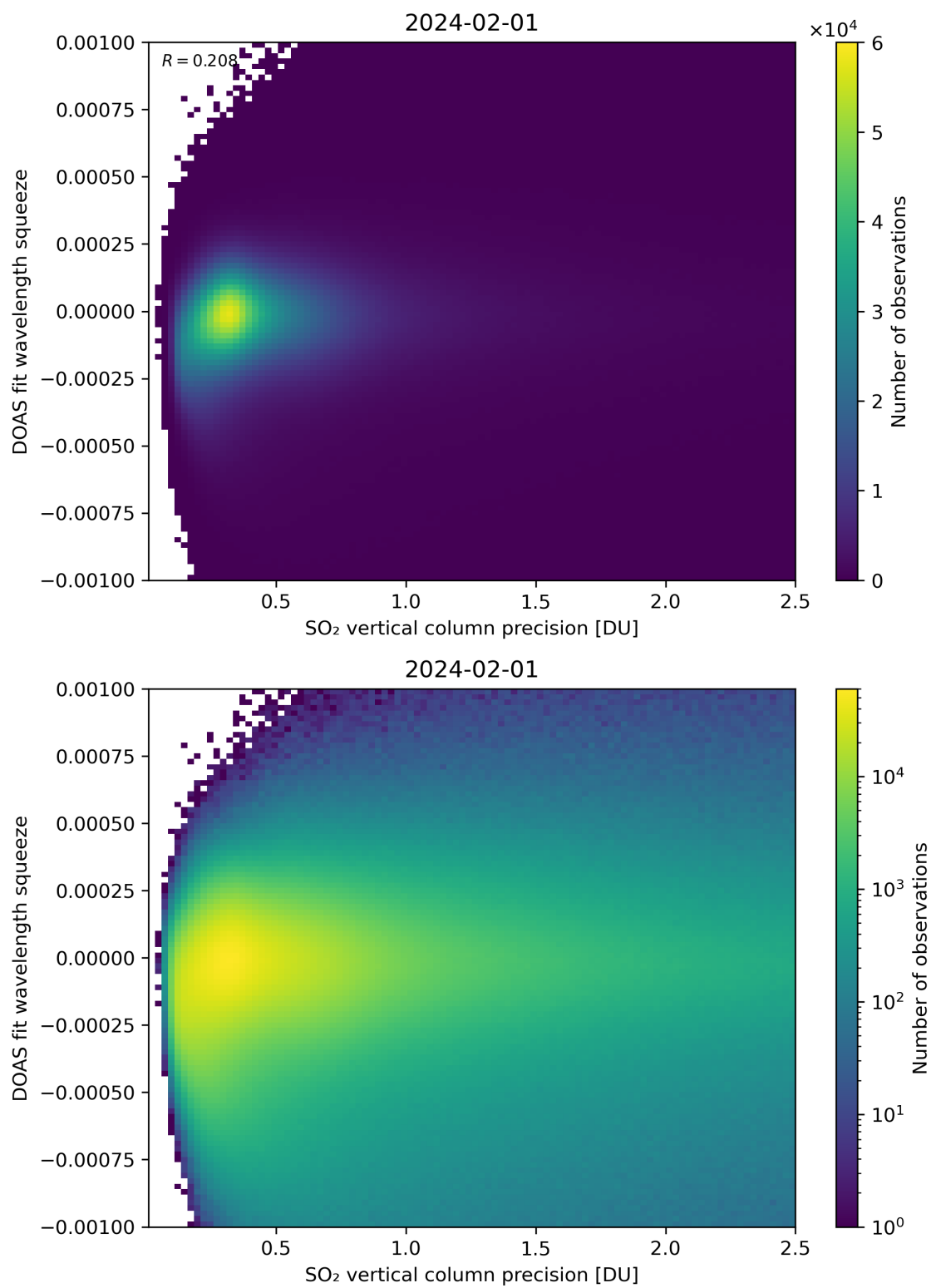
Figure 283: Scatter density plot of “SO 2 vertical column precision” against “DOAS fit wavelength squeeze” for 2024-01-31 to 2024-02-02.
