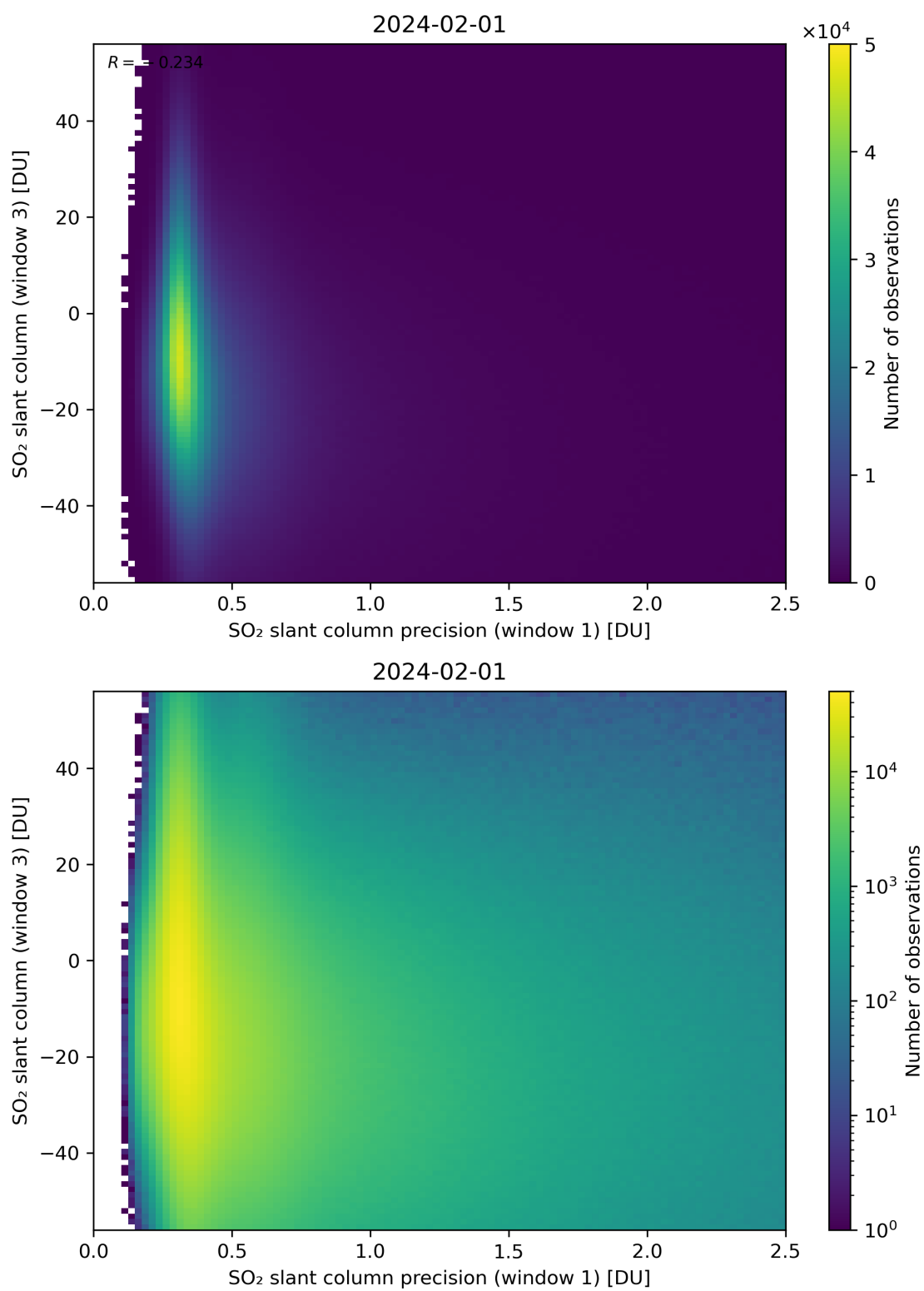
Figure 228: Scatter density plot of “SO 2 slant column precision (window 1)” against “SO 2 slant column (window 3)” for 2024-01-31 to 2024-02-02.
