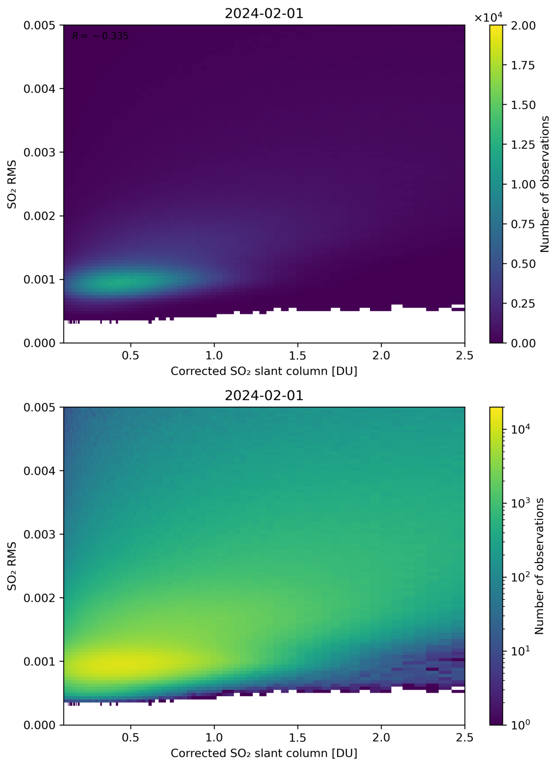
Figure 183: Scatter density plot of “Corrected SO 2 slant column” against “SO 2 RMS” for 2024-01-31 to 2024-02-02.
