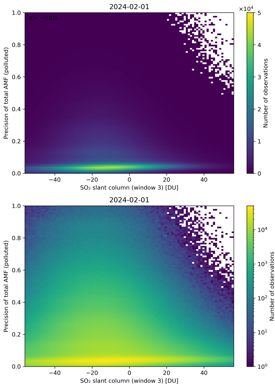
Figure 269: Scatter density plot of “SO 2 slant column (window 3)” against “Precision of total AMF (polluted)” for 2024-01-31 to 2024-02-02.
