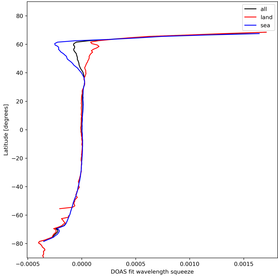
Figure 46: Zonal average of "DOAS fit wavelength squeeze" for 2024-01-31 to 2024-02-02.
