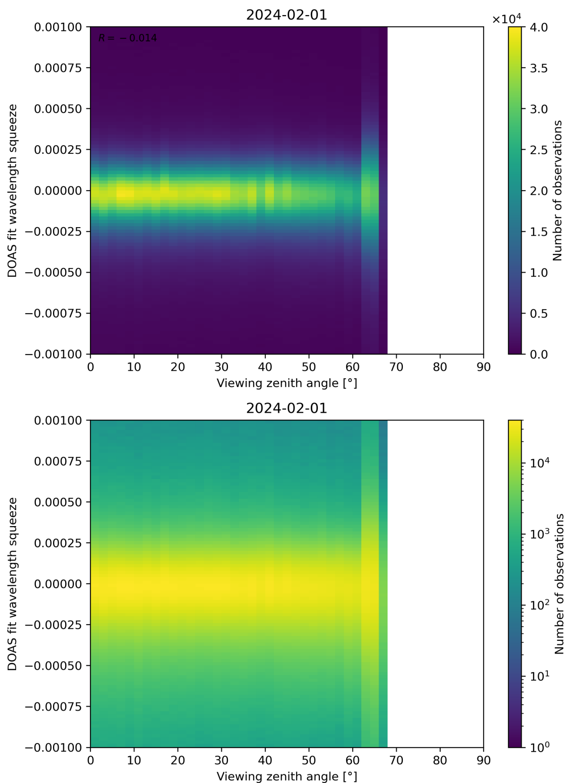
Figure 312: Scatter density plot of “Viewing zenith angle” against “DOAS fit wavelength squeeze” for 2024-01-31 to 2024-02-02.
