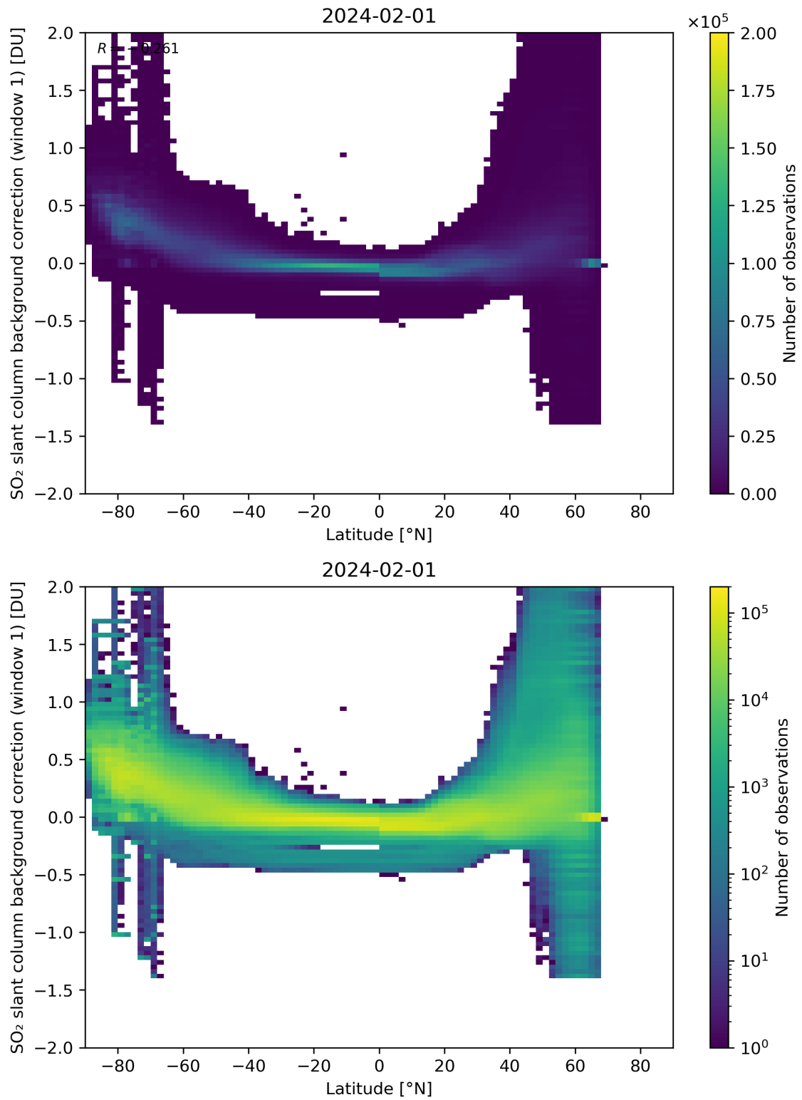
Figure 139: Scatter density plot of “Latitude” against “SO 2 slant column background correction (window 1)” for 2024-01-31 to 2024-02-02.
