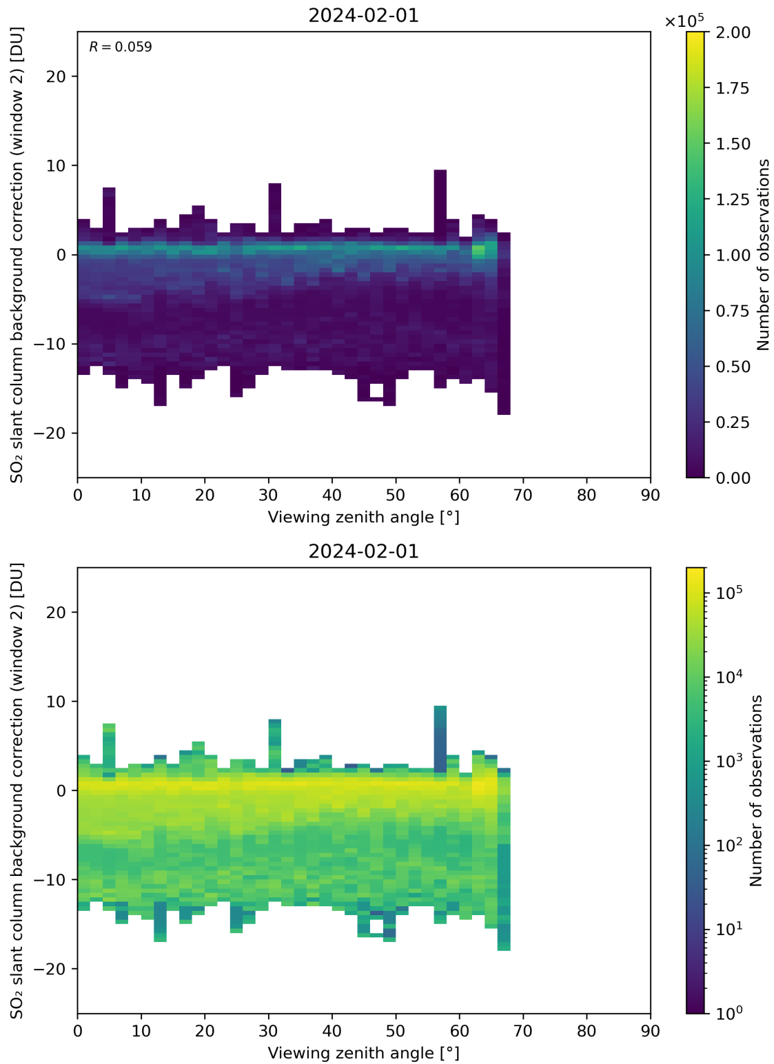
Figure 309: Scatter density plot of “Viewing zenith angle” against “SO 2 slant column background correction (window 2)” for 2024-01-31 to 2024-02-02.
