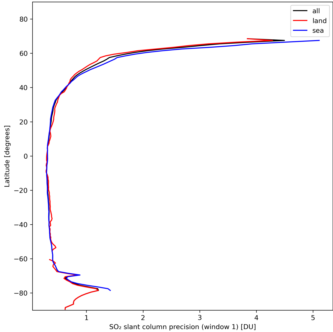
Figure 34: Zonal average of “SO 2 slant column precision (window 1)” for 2024-01-31 to 2024-02-02.
