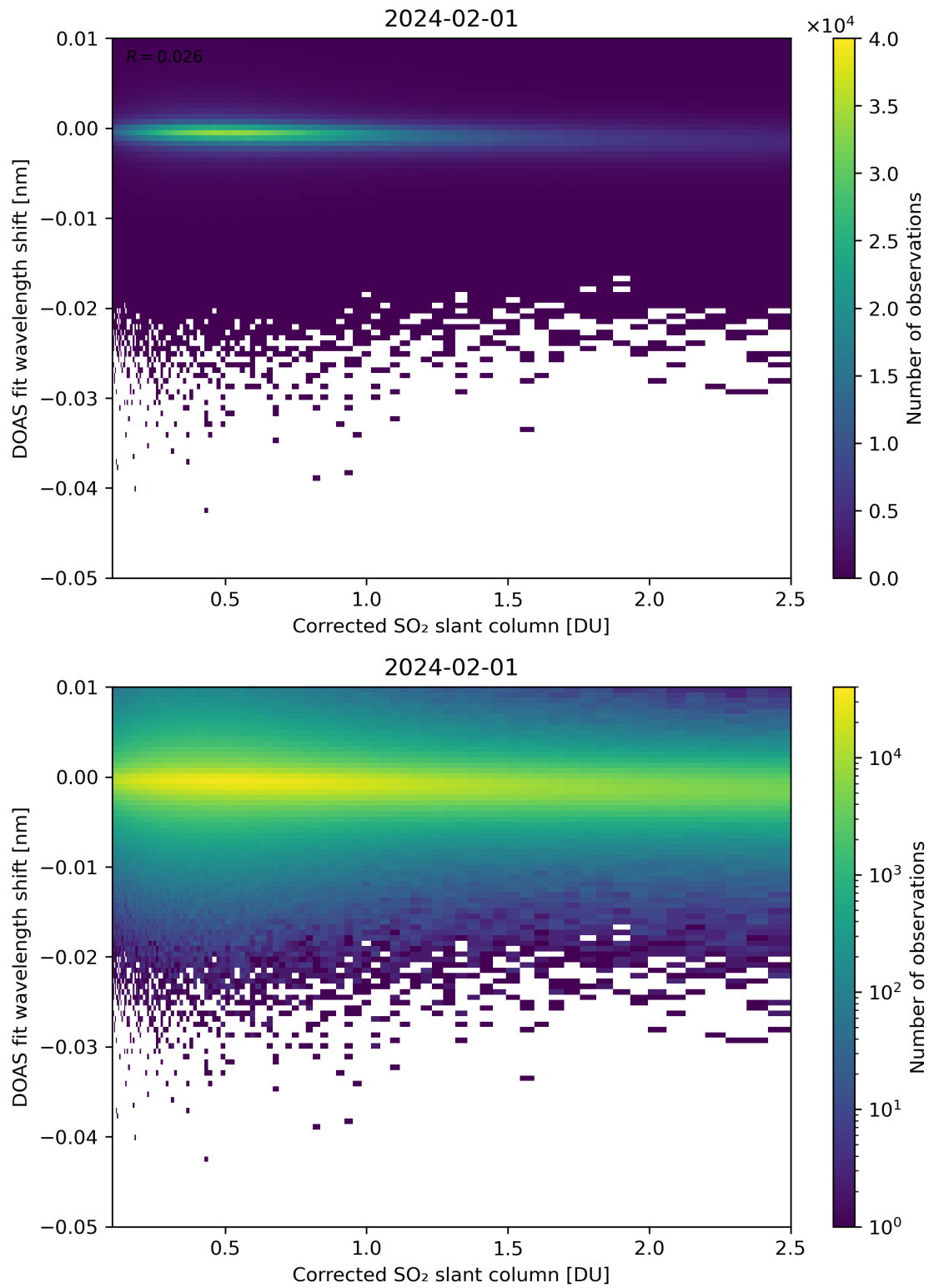
Figure 181: Scatter density plot of “Corrected SO 2 slant column” against “DOAS fit wavelength shift” for 2024-01-31 to 2024-02-02.
