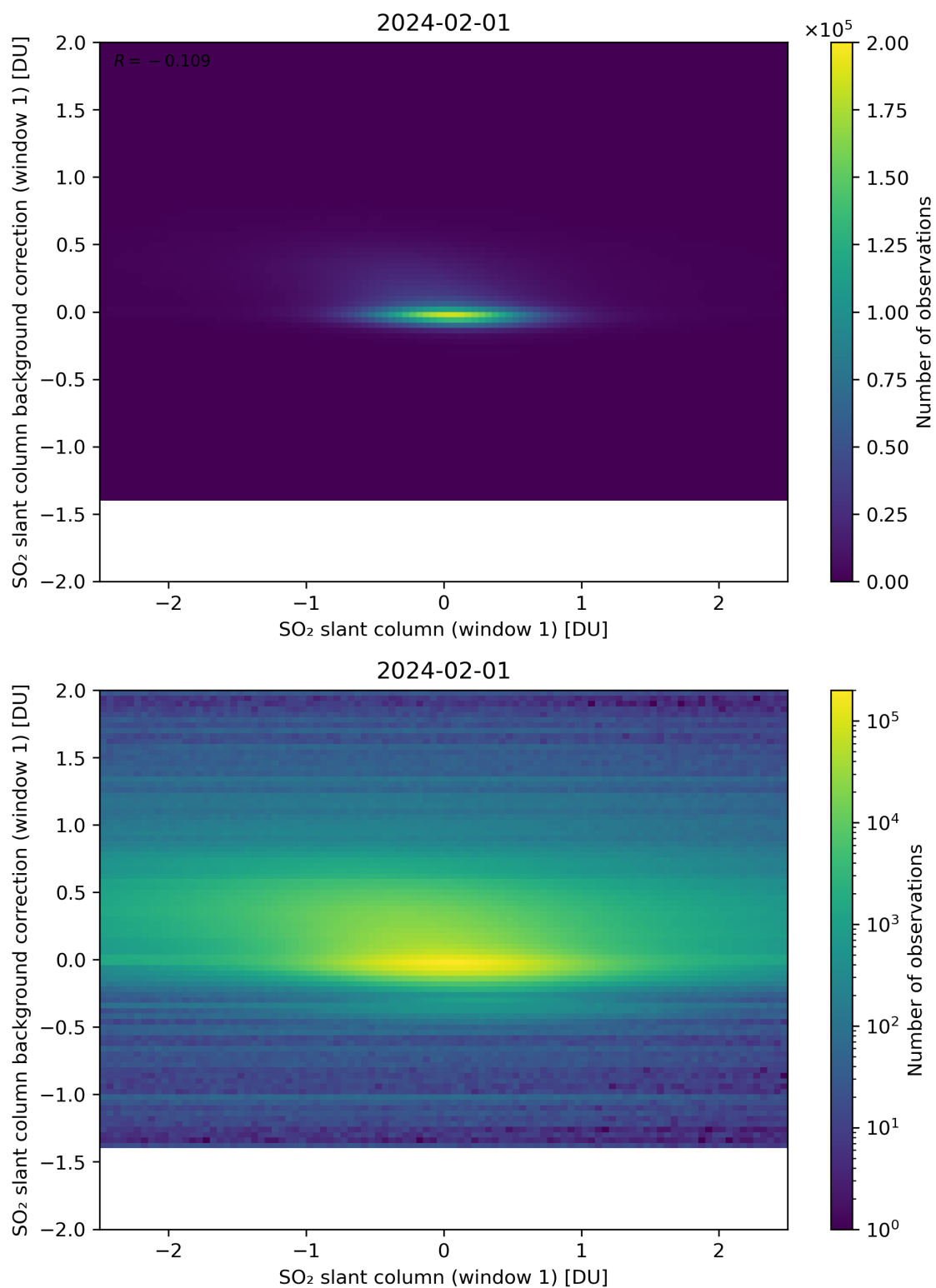
Figure 212: Scatter density plot of “SO 2 slant column (window 1)” against “SO 2 slant column background correction (window 1)” for 2024-01-31 to 2024-02-02.
