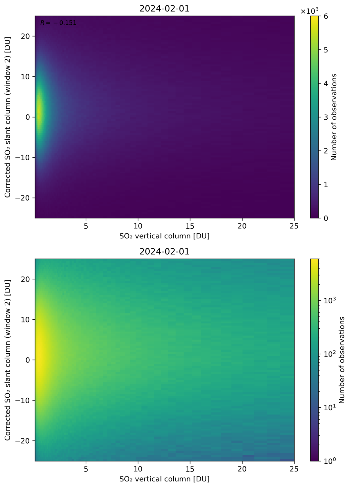
Figure 298: Scatter density plot of “SO 2 vertical column” against “Corrected SO 2 slant column (window 2)” for 2024-01-31 to 2024-02-02.
