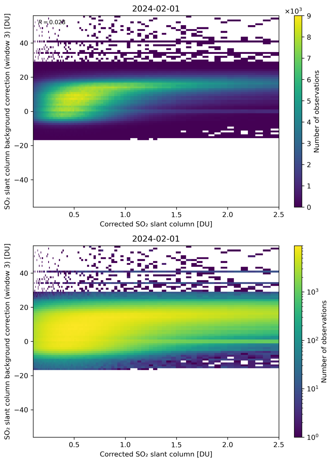
Figure 180: Scatter density plot of “Corrected SO 2 slant column” against “SO 2 slant column background correction (window 3)” for 2024-01-31 to 2024-02-02.
