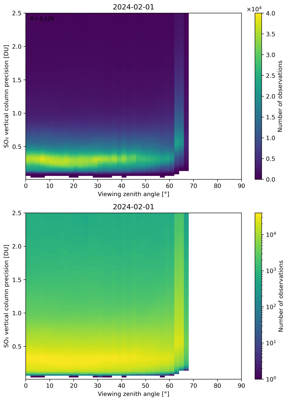
Figure 328: Scatter density plot of “Viewing zenith angle” against “SO 2 vertical column precision” for 2024-01-31 to 2024-02-02.
