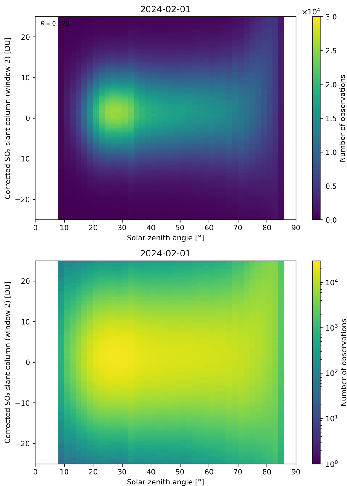
Figure 167: Scatter density plot of “Solar zenith angle” against “Corrected SO 2 slant column (window 2)” for 2024-01-31 to 2024-02-02.
