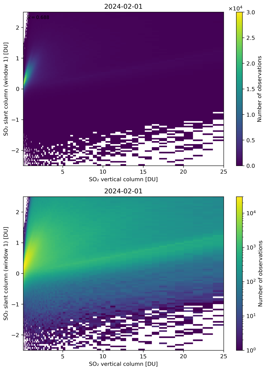
Figure 300: Scatter density plot of “SO 2 vertical column” against “SO 2 slant column (window 1)” for 2024-01-31 to 2024-02-02.
