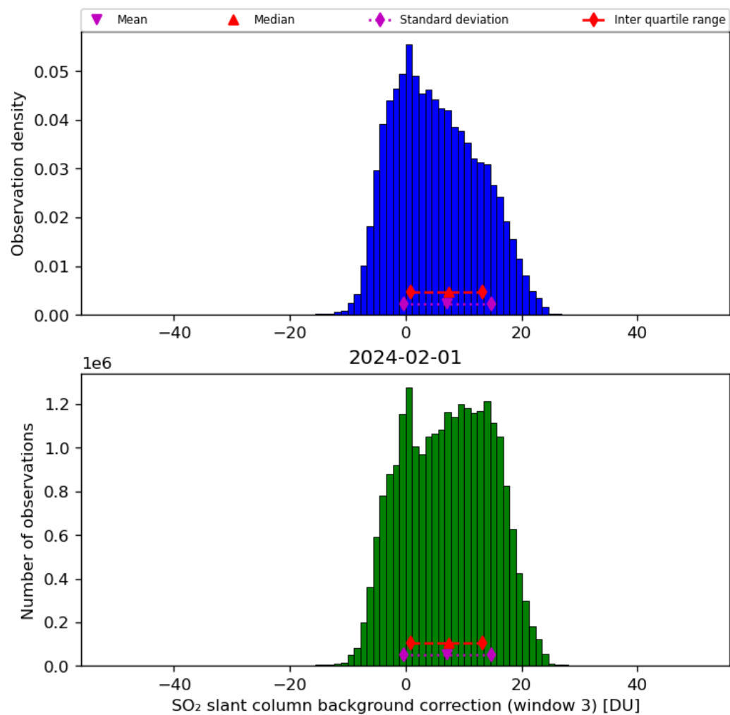
Figure 67: Histogram of “SO 2 slant column background correction (window 3)” for 2024-01-31 to 2024-02-02
