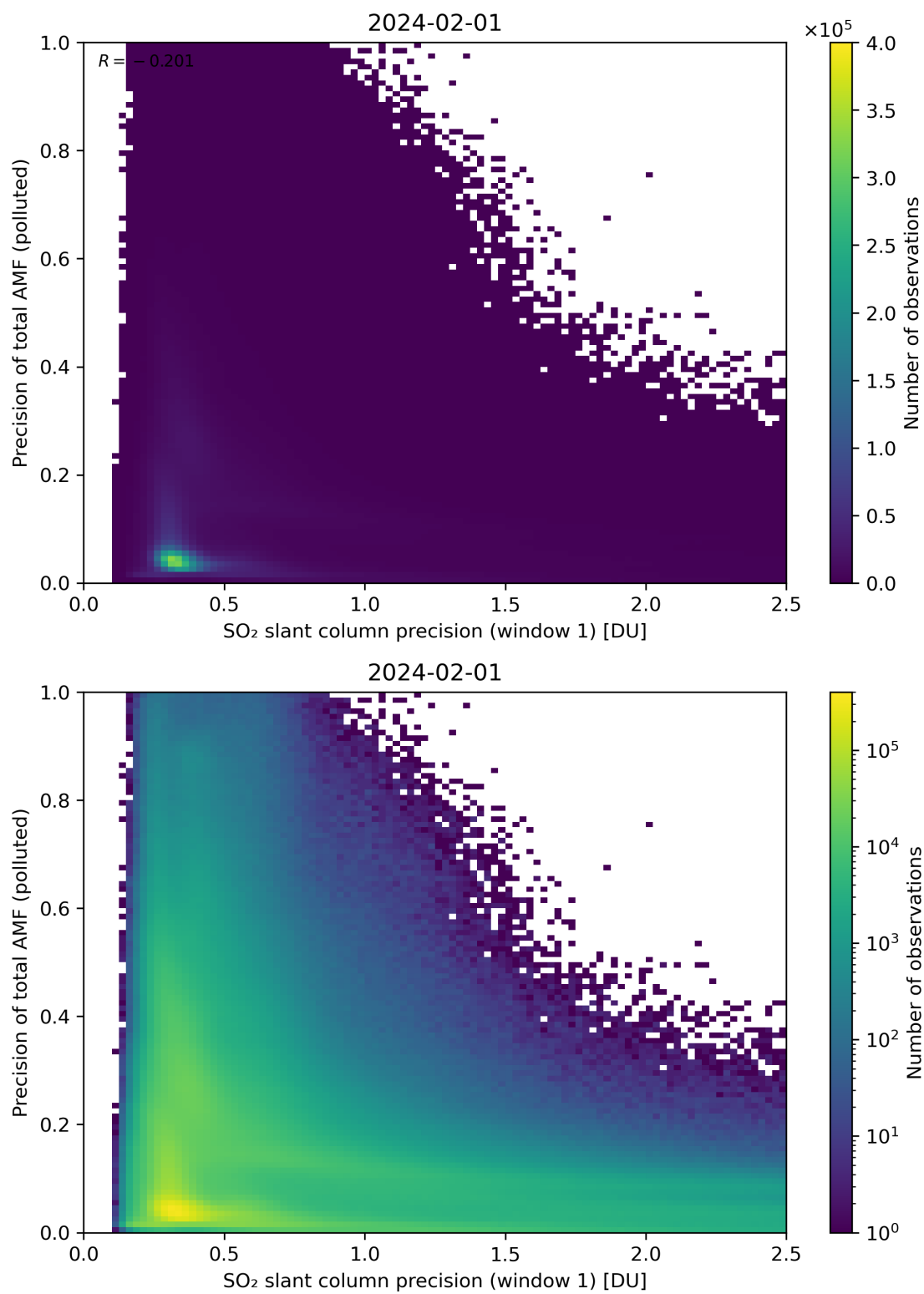
Figure 231: Scatter density plot of “SO 2 slant column precision (window 1)” against “Precision of total AMF (polluted)” for 2024-01-31 to 2024-02-02.
