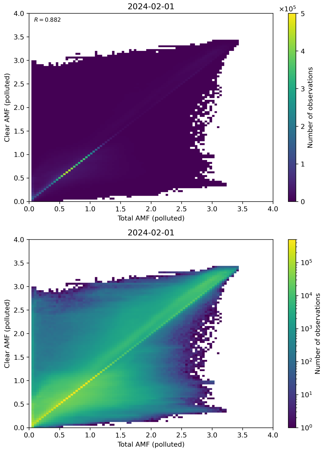
Figure 271: Scatter density plot of “Total AMF (polluted)” against “Clear AMF (polluted)” for 2024-01-31 to 2024-02-02.
