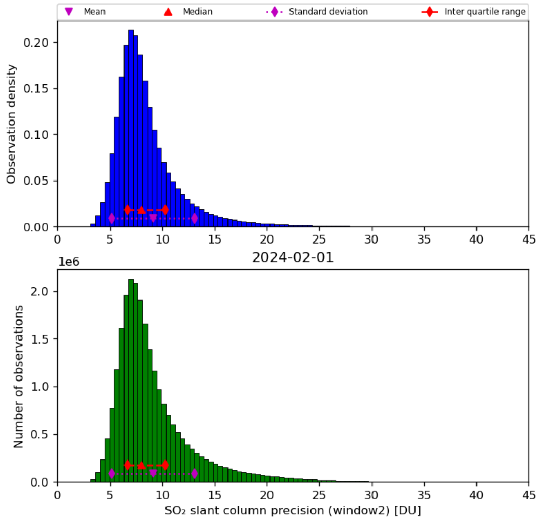
Figure 61: Histogram of “SO 2 slant column precision (window2)” for 2024-01-31 to 2024-02-02
