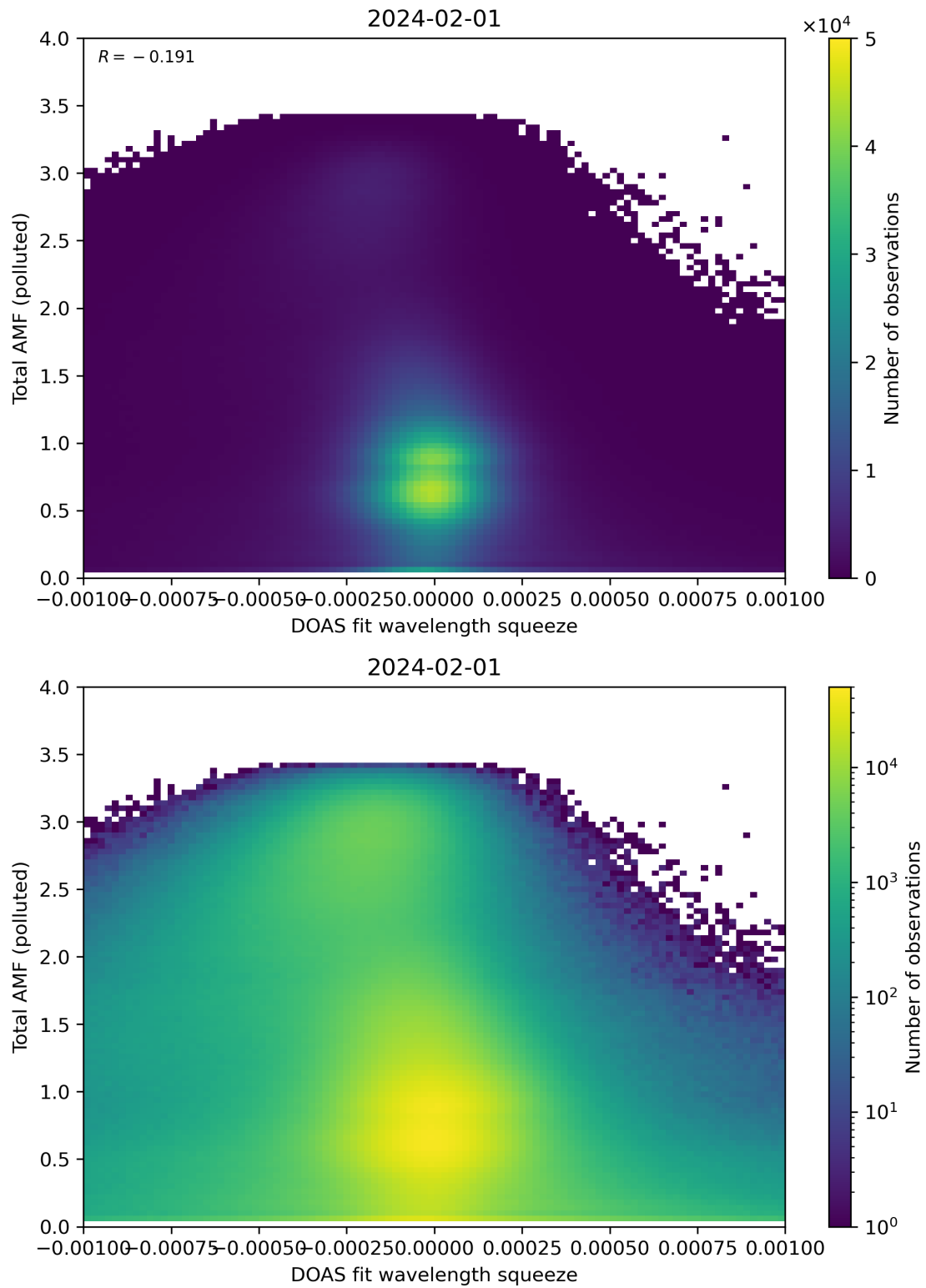
Figure 134: Scatter density plot of “DOAS fit wavelength squeeze” against “Total AMF (polluted)” for 2024-01-31 to 2024-02-02.
