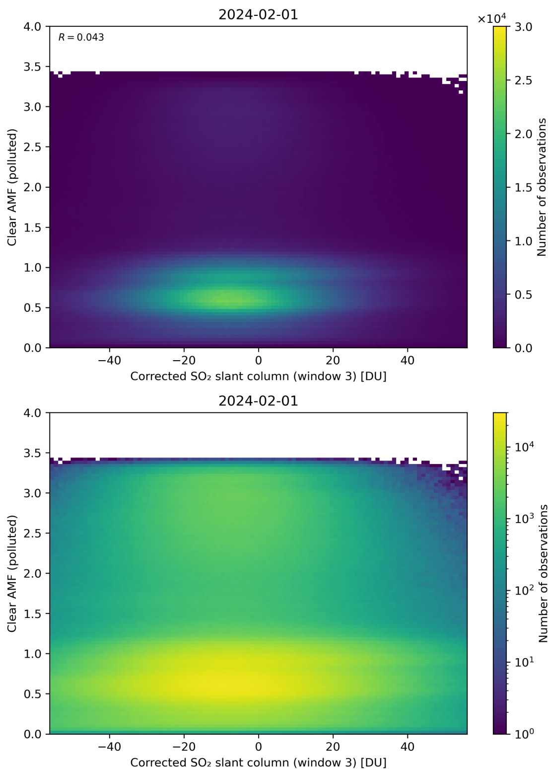
Figure 209: Scatter density plot of “Corrected SO 2 slant column (window 3)” against “Clear AMF (polluted)” for 2024-01-31 to 2024-02-02.
