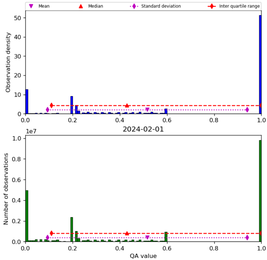
Figure 52: Histogram of “QA value” for 2024-01-31 to 2024-02-02
