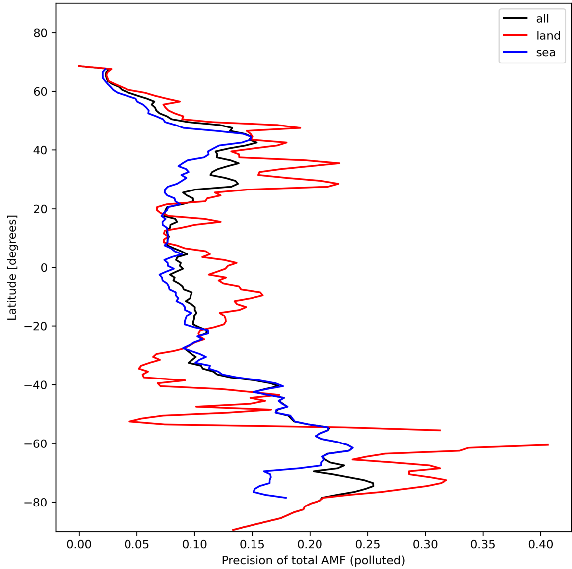
Figure 49: Zonal average of “Precision of total AMF (polluted)” for 2024-01-31 to 2024-02-02.
