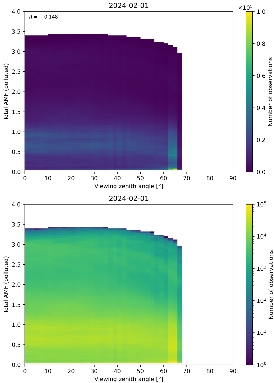
Figure 325: Scatter density plot of “Viewing zenith angle” against “Total AMF (polluted)” for 2024-01-31 to 2024-02-02.
