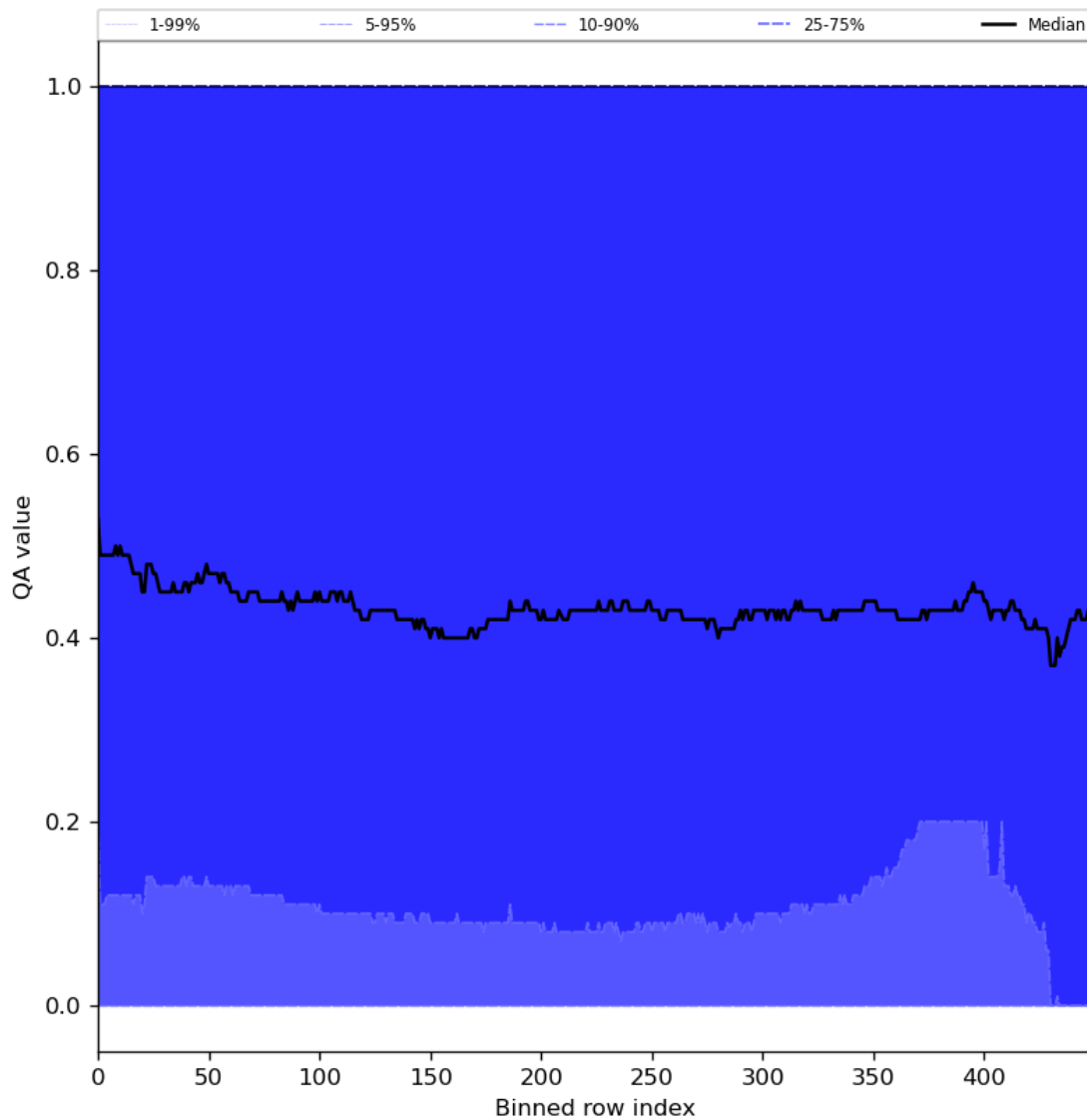
Figure 75: Along track statistics of “QA value” for 2024-01-31 to 2024-02-02
