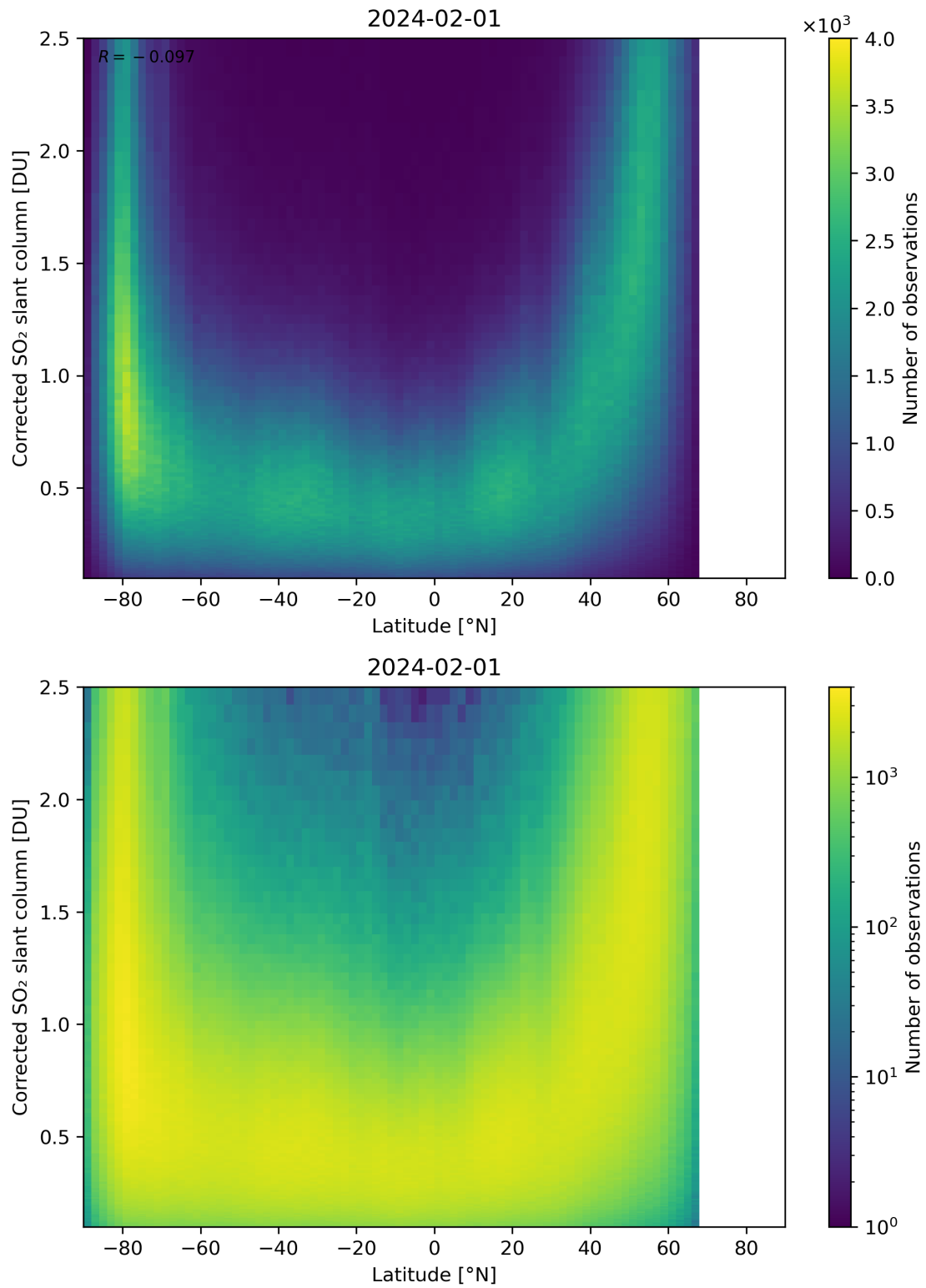
Figure 146: Scatter density plot of “Latitude” against “Corrected SO 2 slant column” for 2024-01-31 to 2024-02-02.
