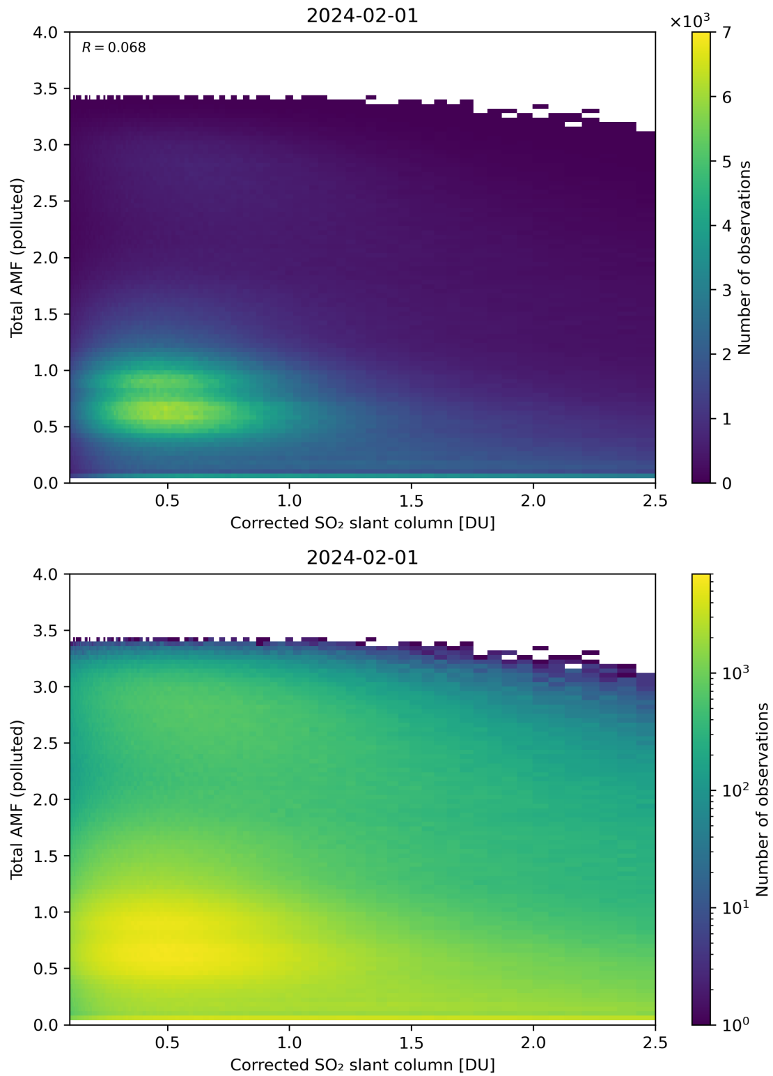
Figure 192: Scatter density plot of “Corrected SO 2 slant column” against “Total AMF (polluted)” for 2024-01-31 to 2024-02-02.
