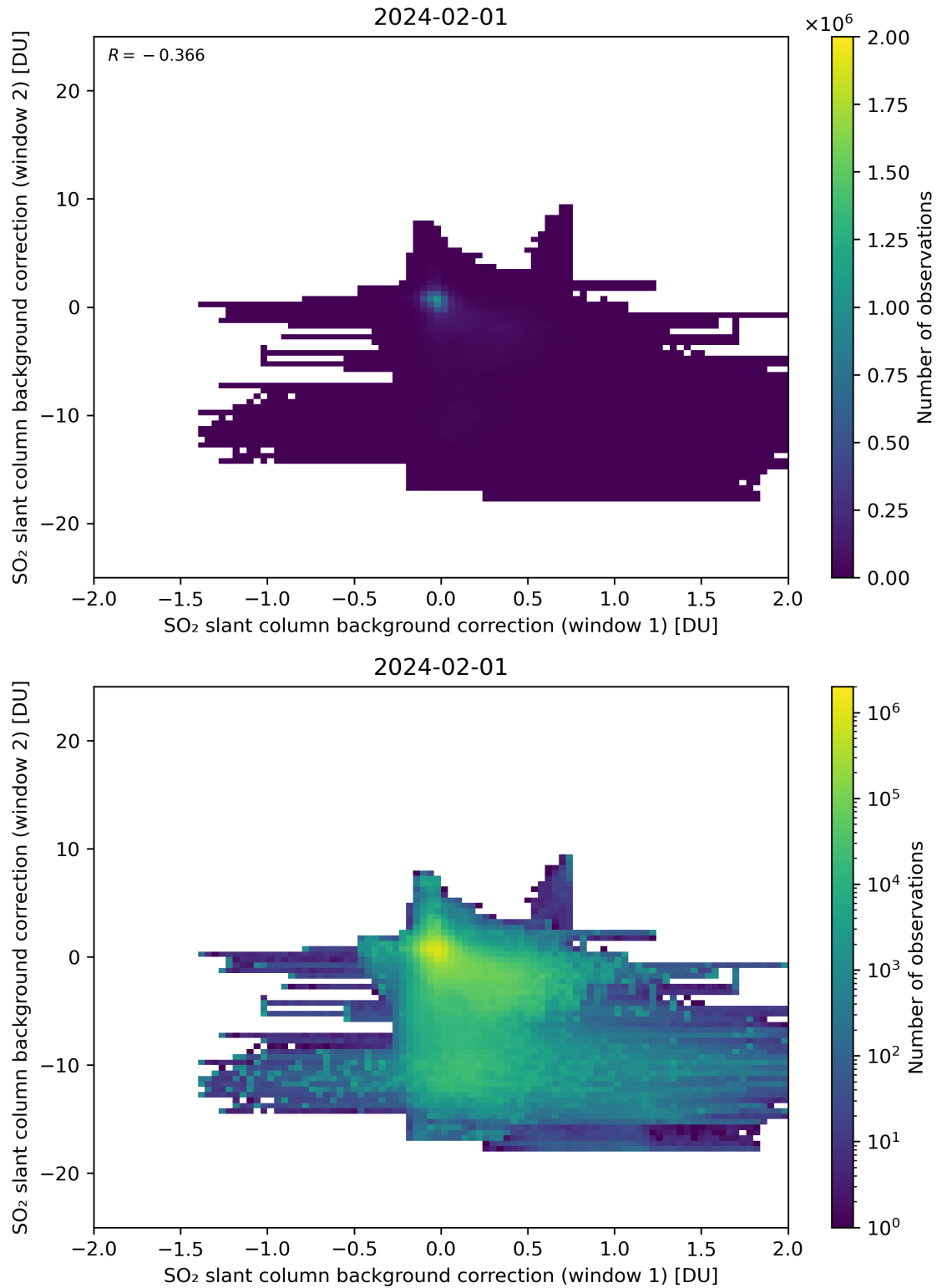
Figure 98: Scatter density plot of “SO 2 slant column background correction (window 1)” against “SO 2 slant column background correction (window 2)” for 2024-01-31 to 2024-02-02.
