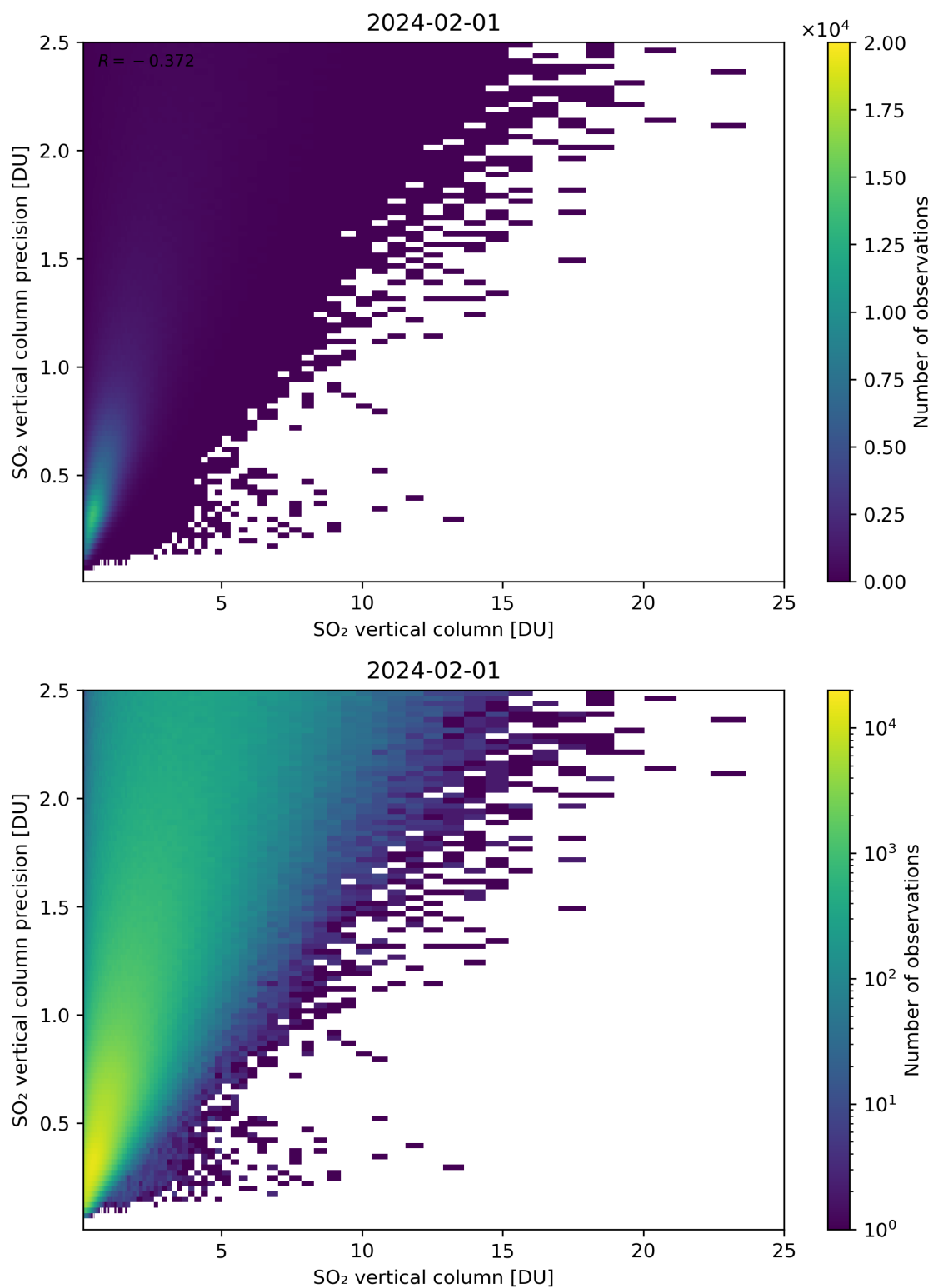
Figure 307: Scatter density plot of “SO 2 vertical column” against “SO 2 vertical column precision” for 2024-01-31 to 2024-02-02.
