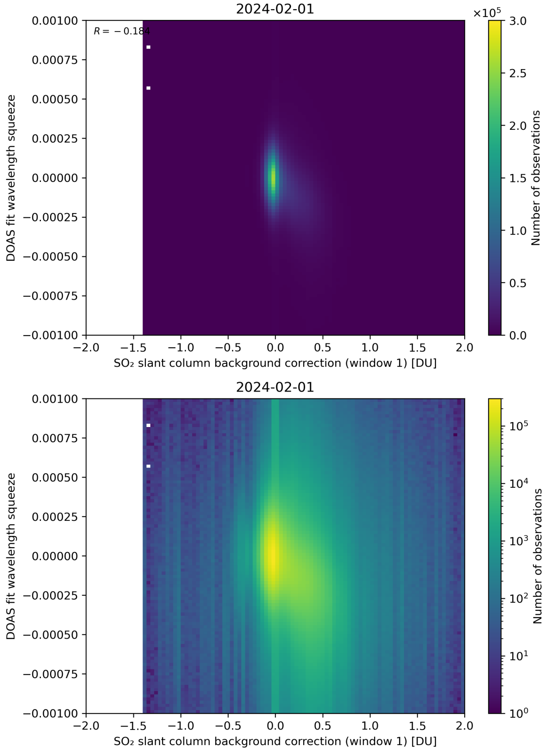
Figure 101: Scatter density plot of “SO 2 slant column background correction (window 1)” against “DOAS fit wavelength squeeze” for 2024-01-31 to 2024-02-02.
