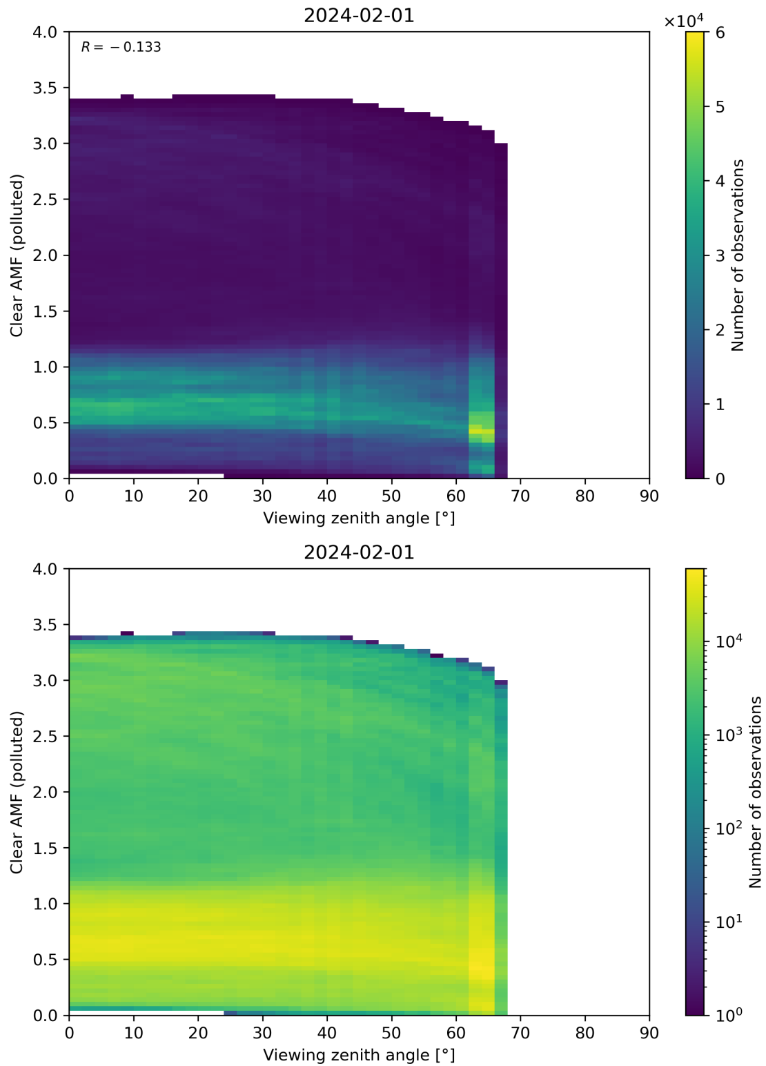
Figure 316: Scatter density plot of “Viewing zenith angle” against “Clear AMF (polluted)” for 2024-01-31 to 2024-02-02.
