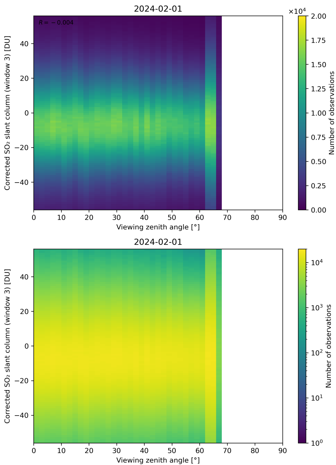
Figure 319: Scatter density plot of “Viewing zenith angle” against “Corrected SO 2 slant column (window 3)” for 2024-01-31 to 2024-02-02.
