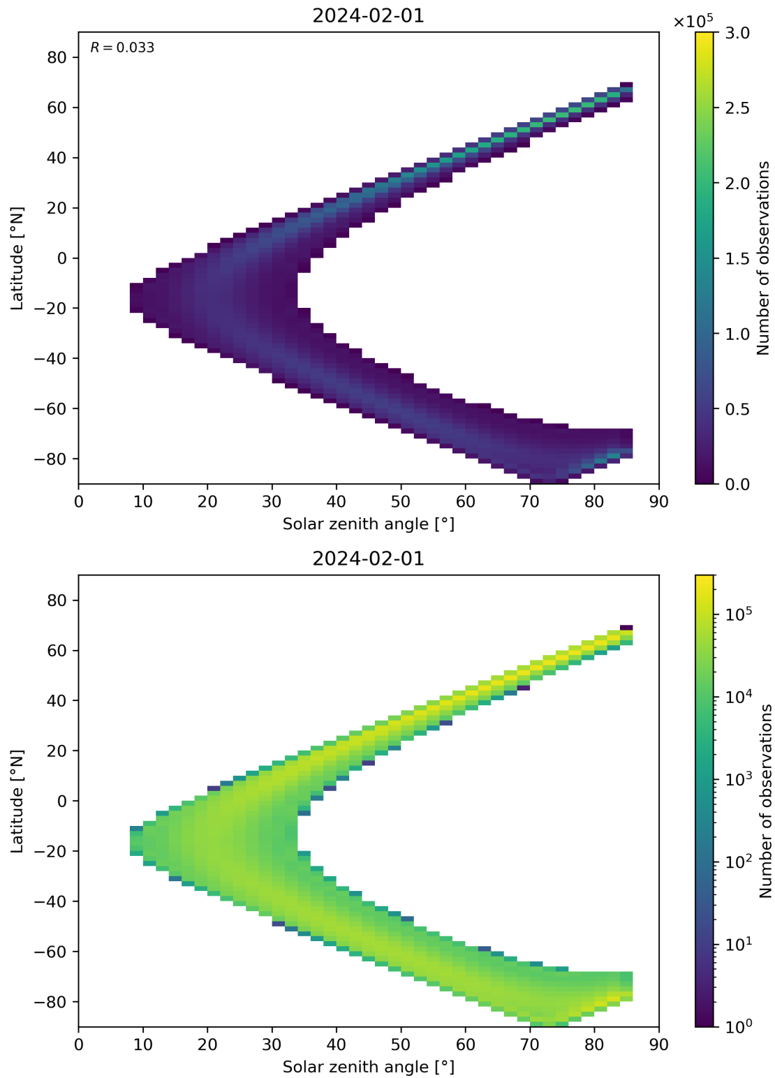
Figure 164: Scatter density plot of “Solar zenith angle” against “Latitude” for 2024-01-31 to 2024-02-02.
