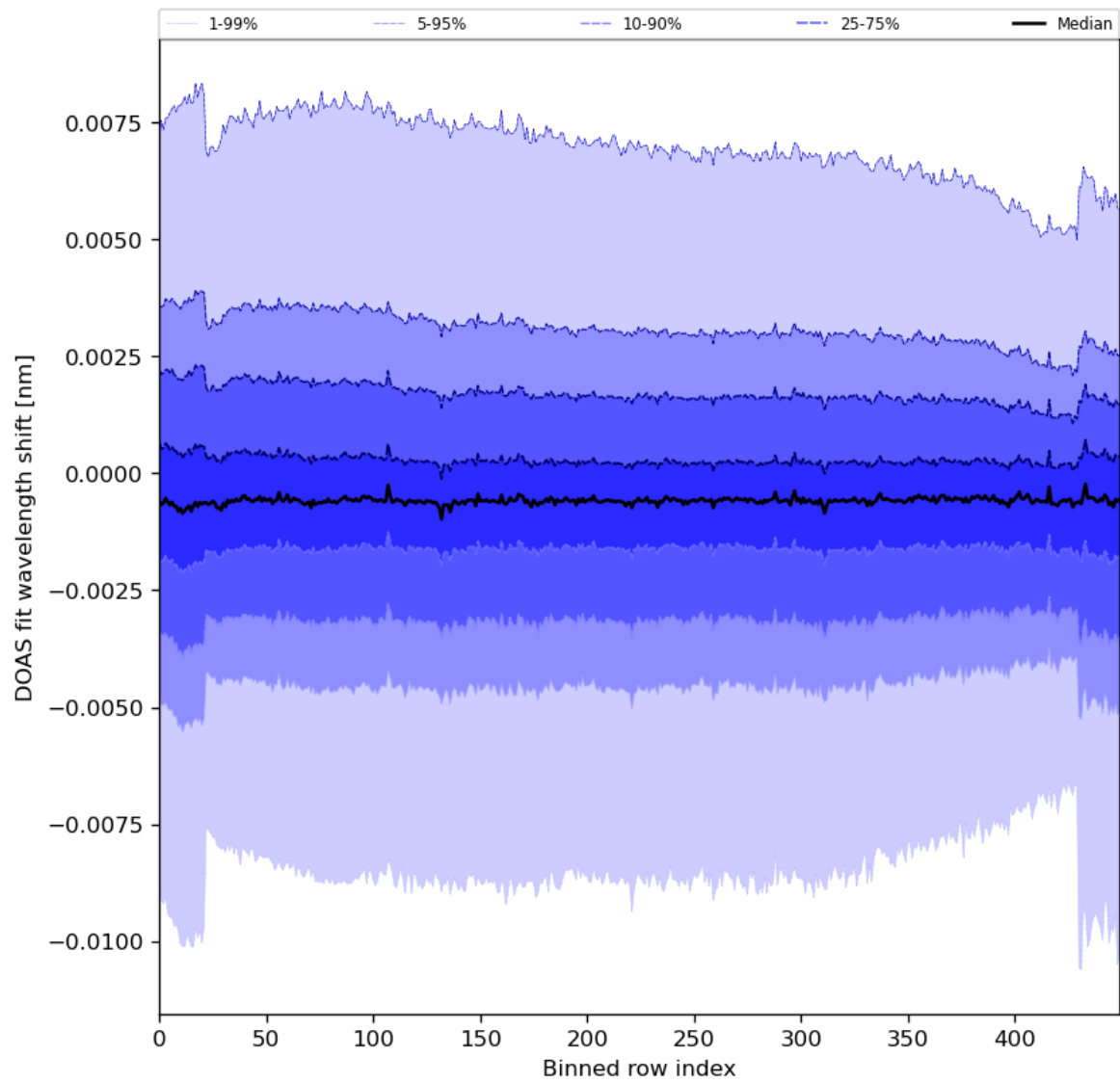
Figure 91: Along track statistics of “DOAS fit wavelength shift” for 2024-01-31 to 2024-02-02
