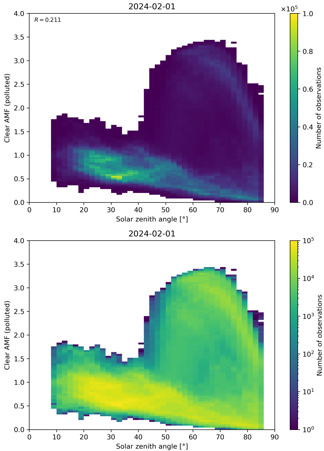
Figure 165: Scatter density plot of “Solar zenith angle” against “Clear AMF (polluted)” for 2024-01-31 to 2024-02-02.
