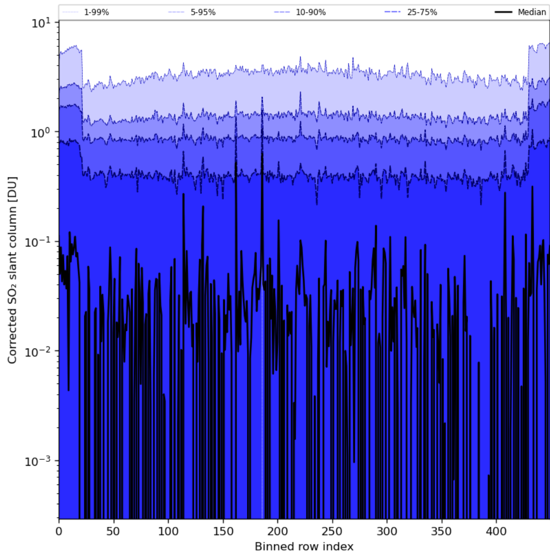
Figure 78: Along track statistics of “Corrected SO 2 slant column” for 2024-01-31 to 2024-02-02
