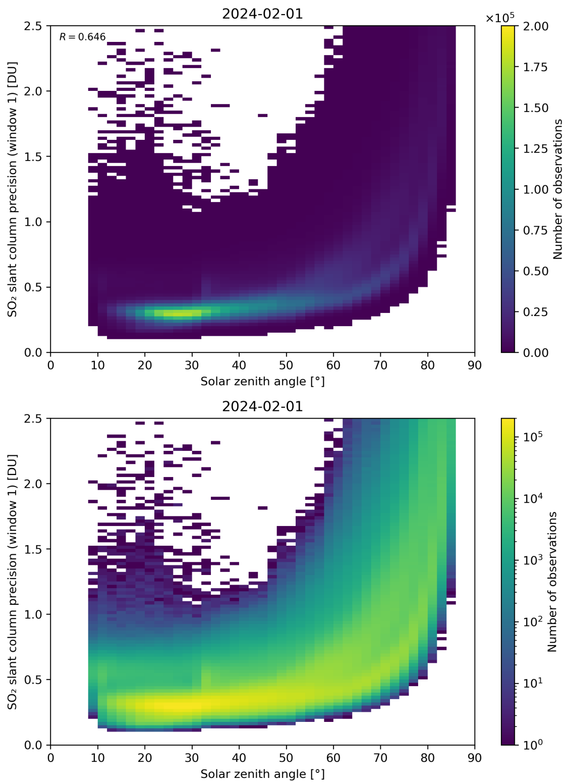
Figure 170: Scatter density plot of “Solar zenith angle” against “SO 2 slant column precision (window 1)” for 2024-01-31 to 2024-02-02.
