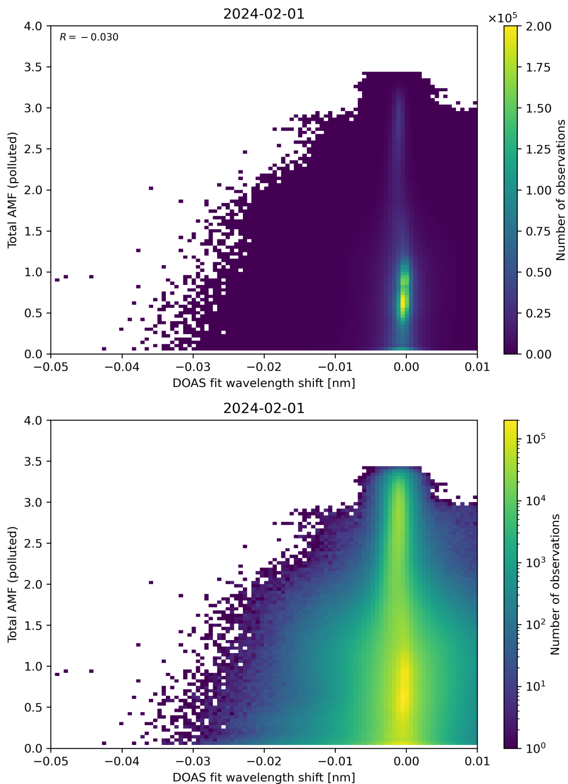
Figure 130: Scatter density plot of “DOAS fit wavelength shift” against “Total AMF (polluted)” for 2024-01-31 to 2024-02-02.
