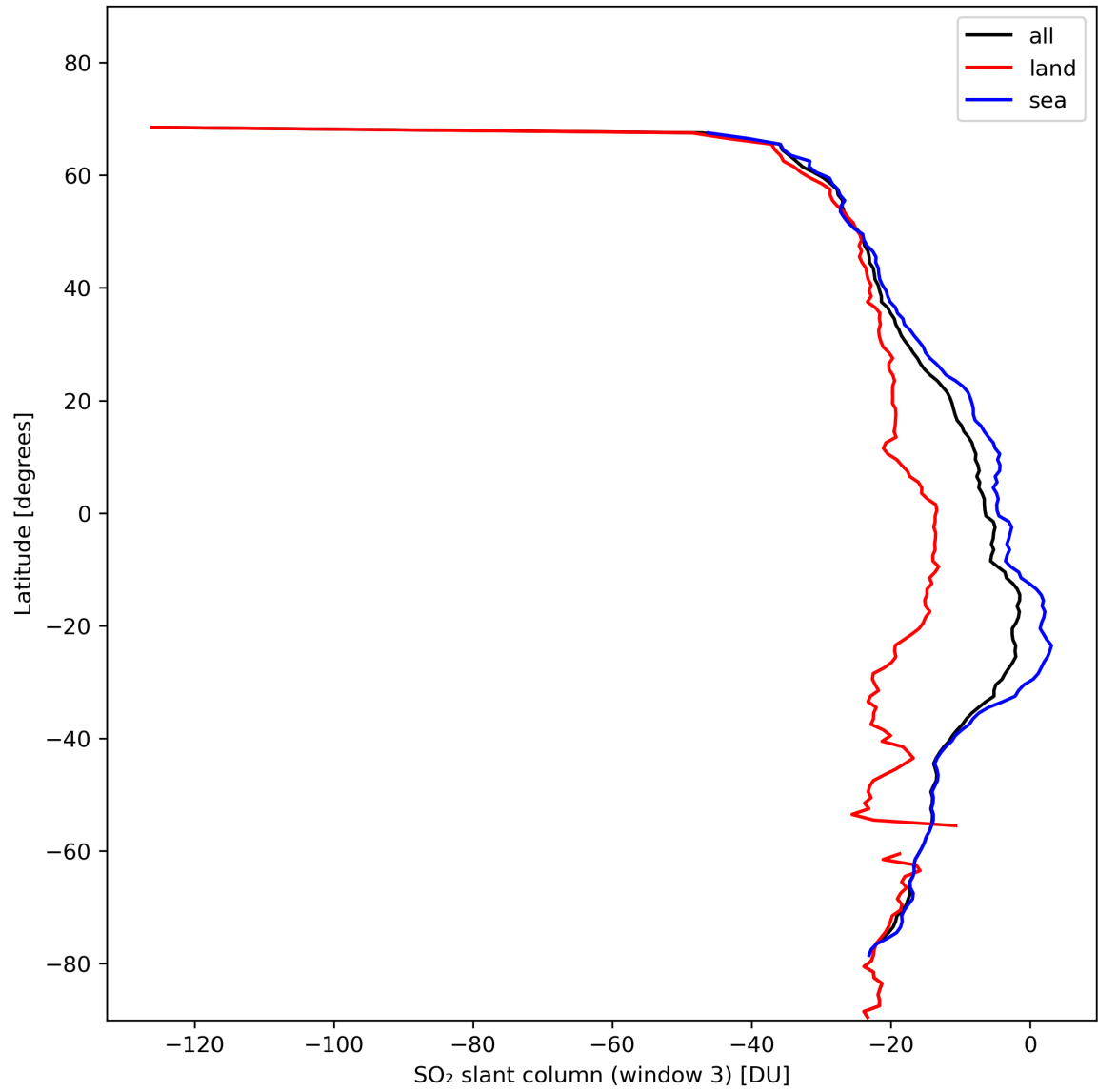
Figure 41: Zonal average of “SO 2 slant column (window 3)” for 2024-01-31 to 2024-02-02.
