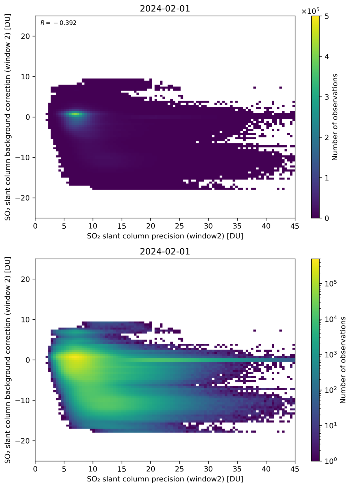
Figure 241: Scatter density plot of “SO 2 slant column precision (window2)” against “SO 2 slant column background correction (window 2)” for 2024-01-31 to 2024-02-02.
