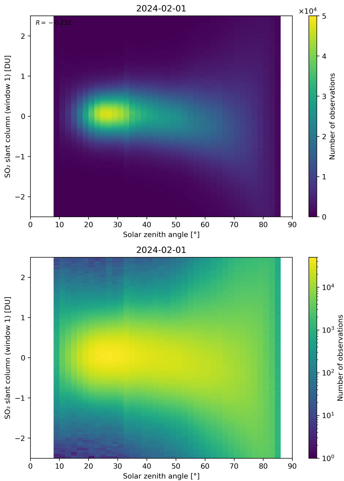
Figure 169: Scatter density plot of “Solar zenith angle” against “SO 2 slant column (window 1)” for 2024-01-31 to 2024-02-02.
