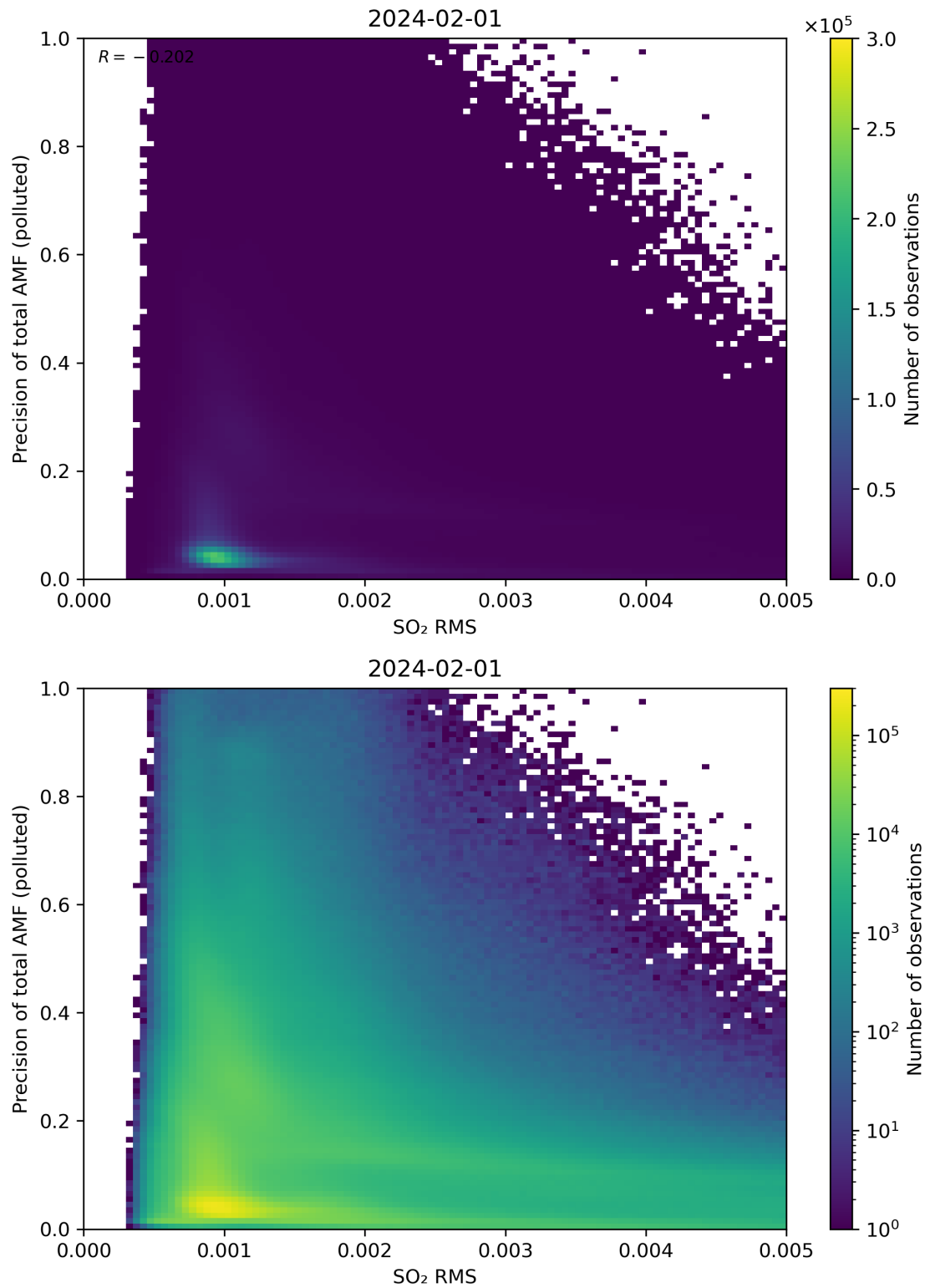
Figure 138: Scatter density plot of “SO 2 RMS” against “Precision of total AMF (polluted)” for 2024-01-31 to 2024-02-02.
