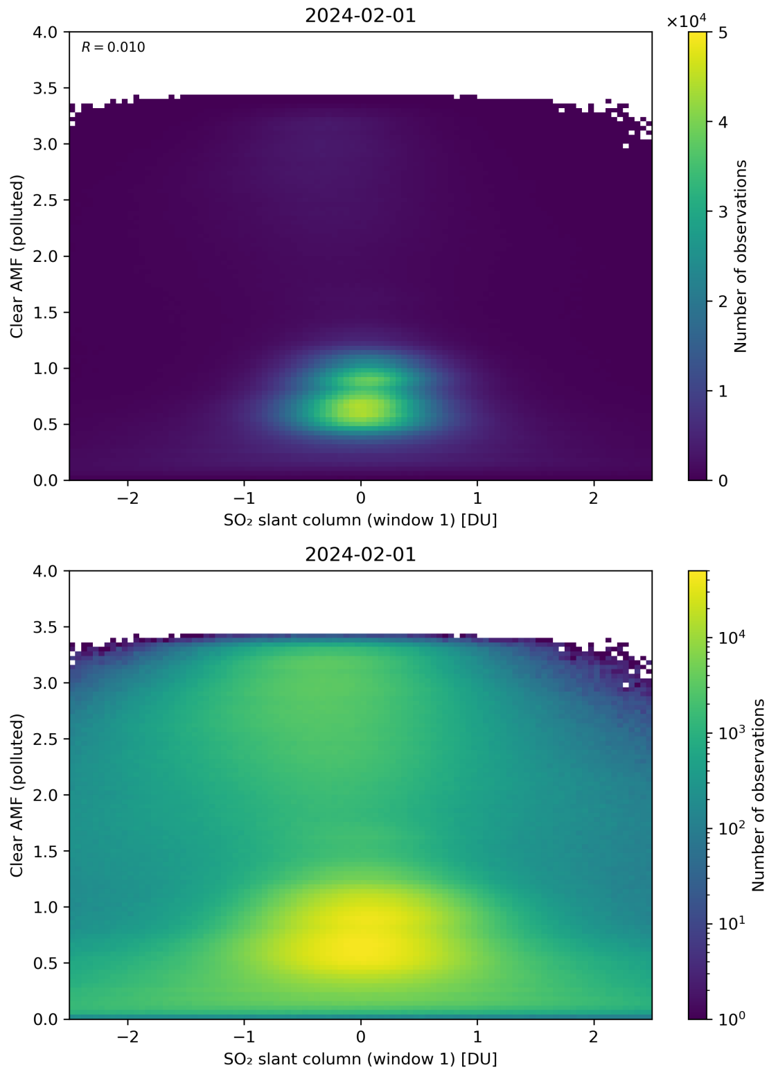
Figure 232: Scatter density plot of “SO 2 slant column (window 1)” against “Clear AMF (polluted)” for 2024-01-31 to 2024-02-02.
