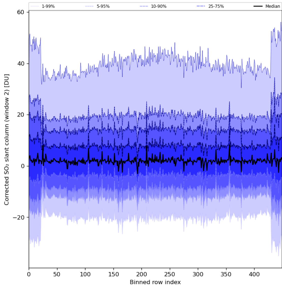
Figure 85: Along track statistics of “Corrected SO 2 slant column (window 2)” for 2024-01-31 to 2024-02-02
