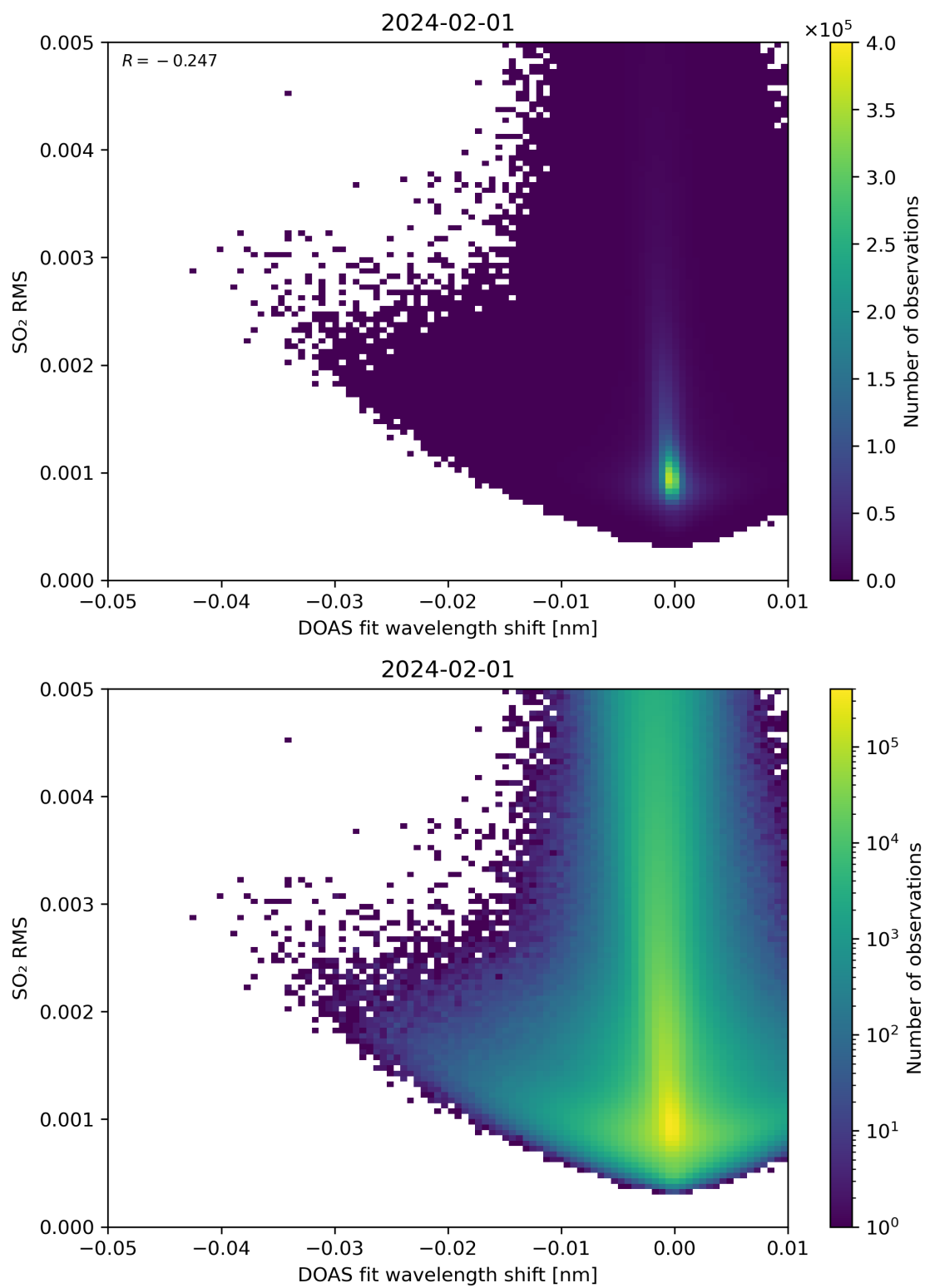
Figure 128: Scatter density plot of “DOAS fit wavelength shift” against “SO 2 RMS” for 2024-01-31 to 2024-02-02.
