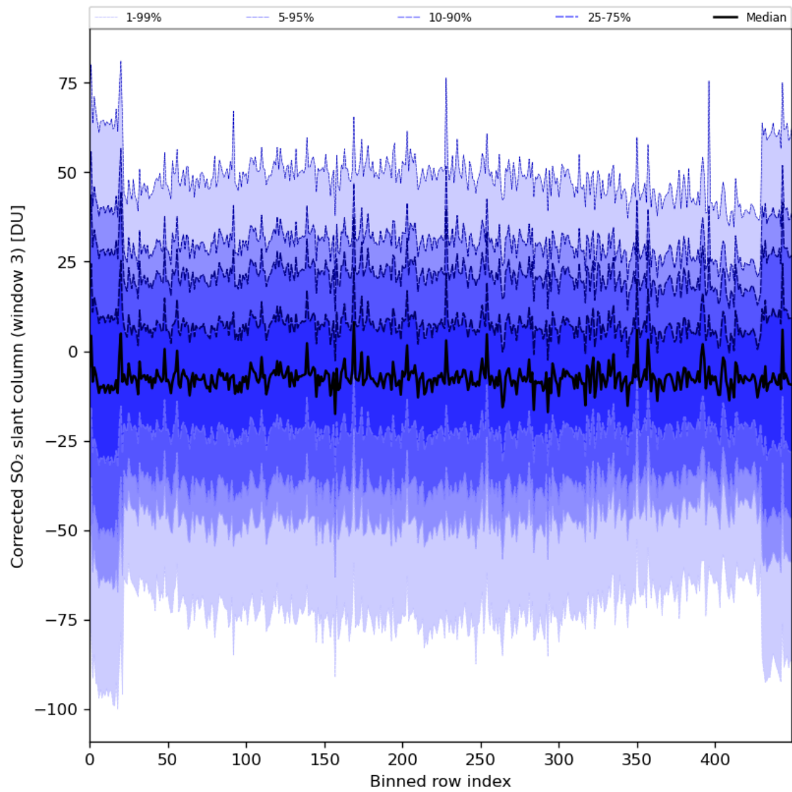
Figure 89: Along track statistics of “Corrected SO 2 slant column (window 3)” for 2024-01-31 to 2024-02-02
