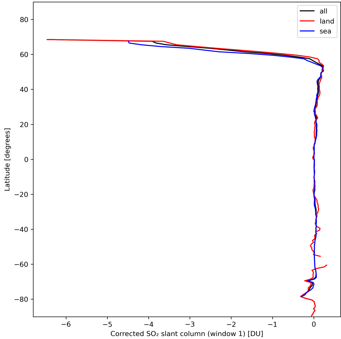
Figure 35: Zonal average of “Corrected SO 2 slant column (window 1)” for 2024-01-31 to 2024-02-02.
