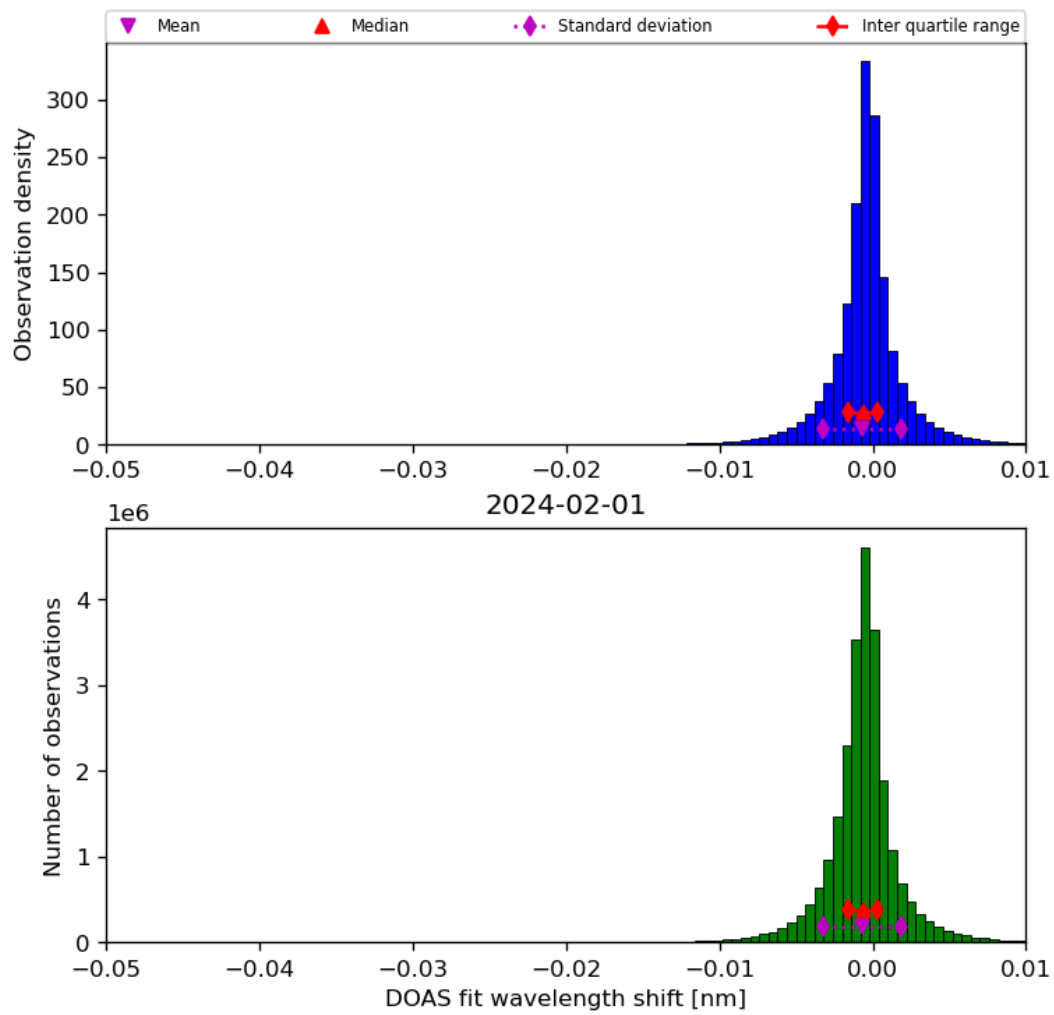
Figure 68: Histogram of “DOAS fit wavelength shift” for 2024-01-31 to 2024-02-02
