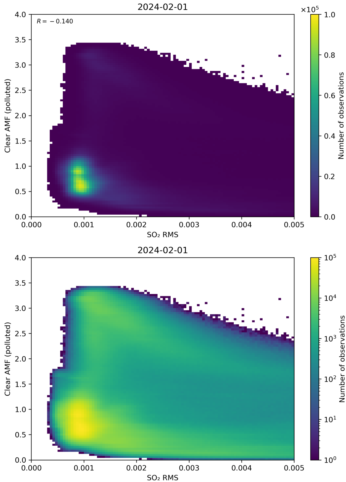
Figure 136: Scatter density plot of “SO 2 RMS” against “Clear AMF (polluted)” for 2024-01-31 to 2024-02-02.
