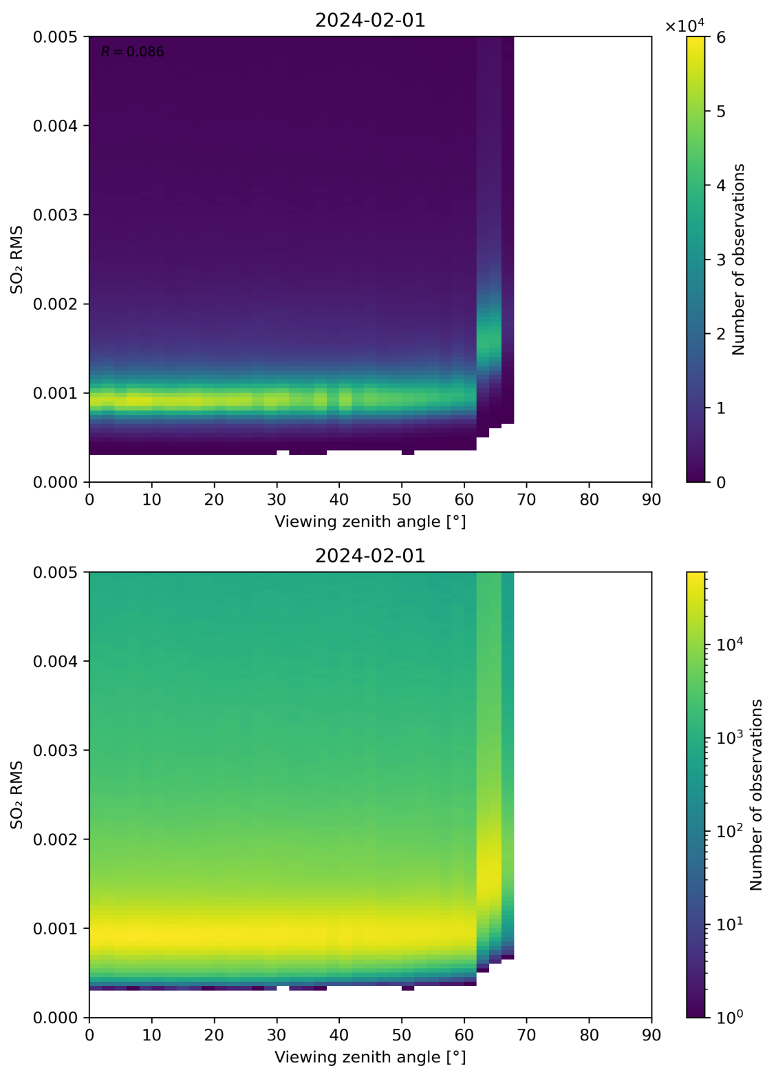
Figure 313: Scatter density plot of “Viewing zenith angle” against “SO 2 RMS” for 2024-01-31 to 2024-02-02.
