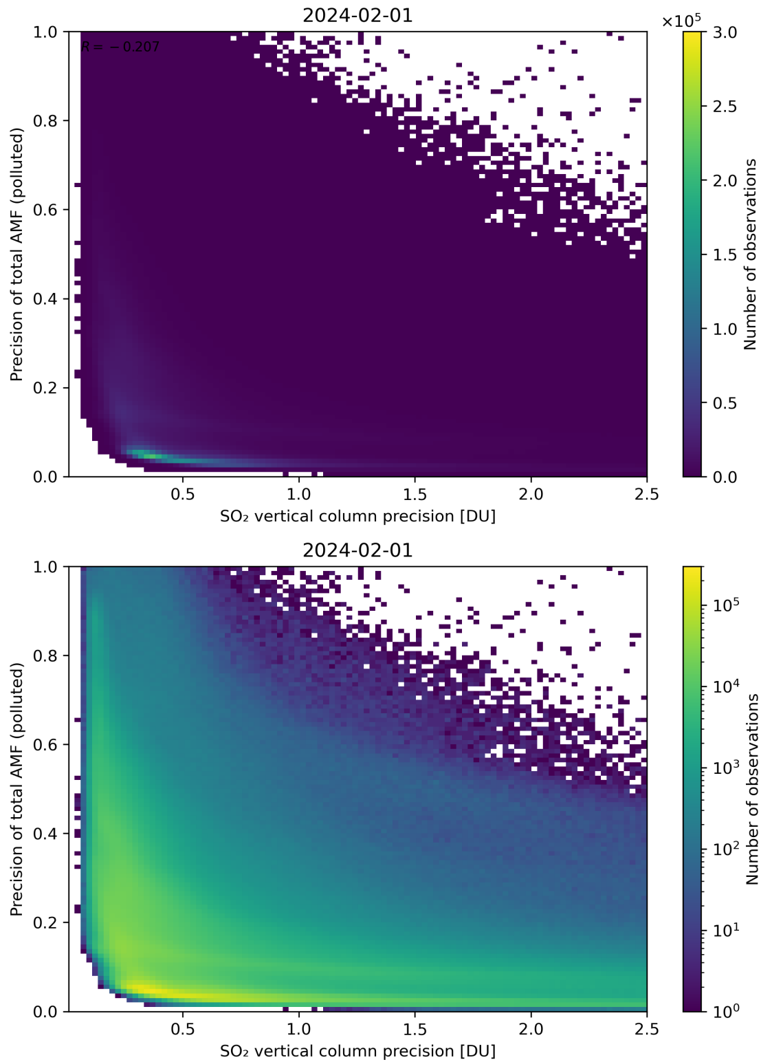
Figure 295: Scatter density plot of “SO 2 vertical column precision” against “Precision of total AMF (polluted)” for 2024-01-31 to 2024-02-02.
