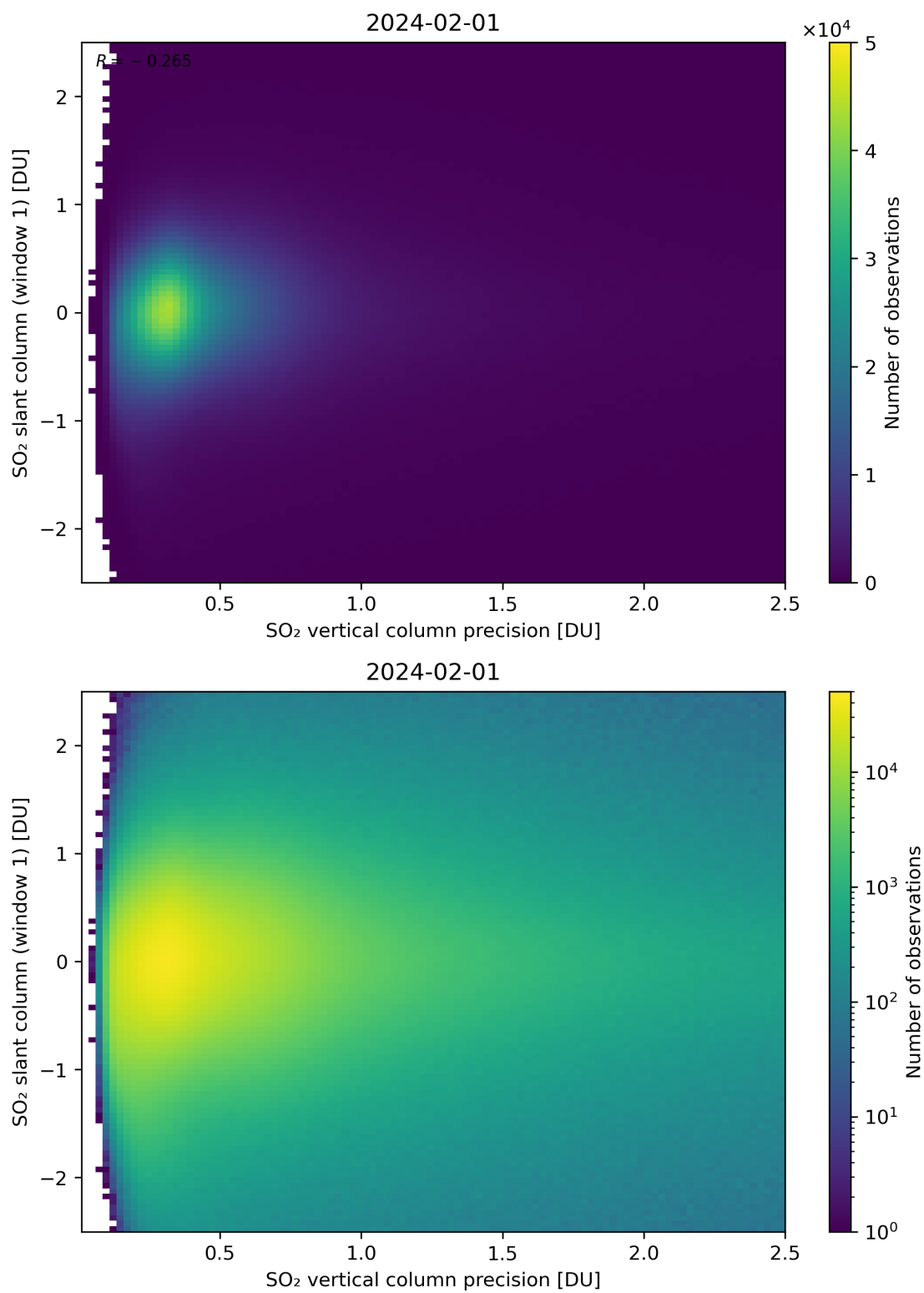
Figure 289: Scatter density plot of “SO 2 vertical column precision” against “SO 2 slant column (window 1)” for 2024-01-31 to 2024-02-02.
