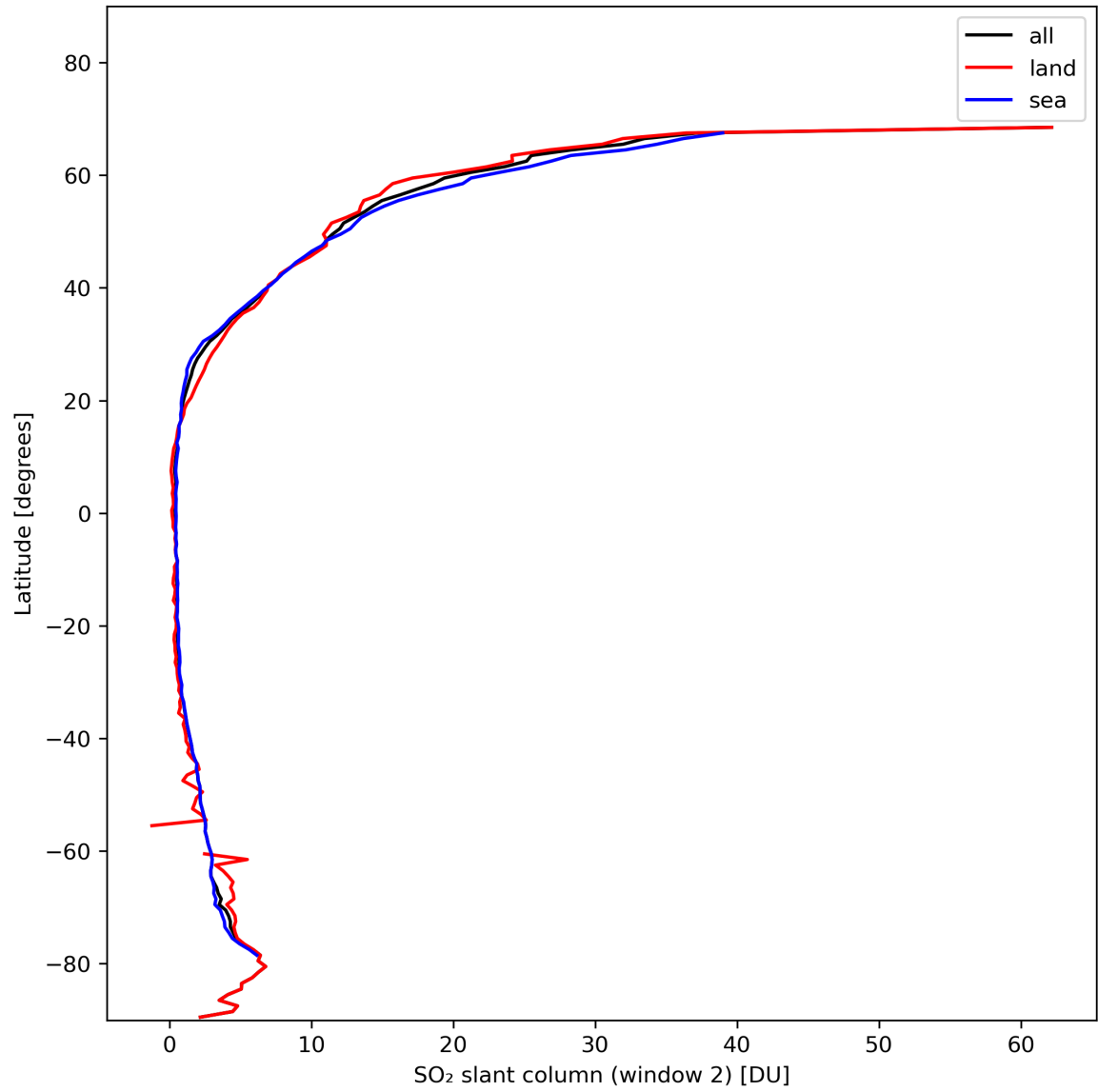
Figure 37: Zonal average of “SO 2 slant column (window 2)” for 2024-01-31 to 2024-02-02.
