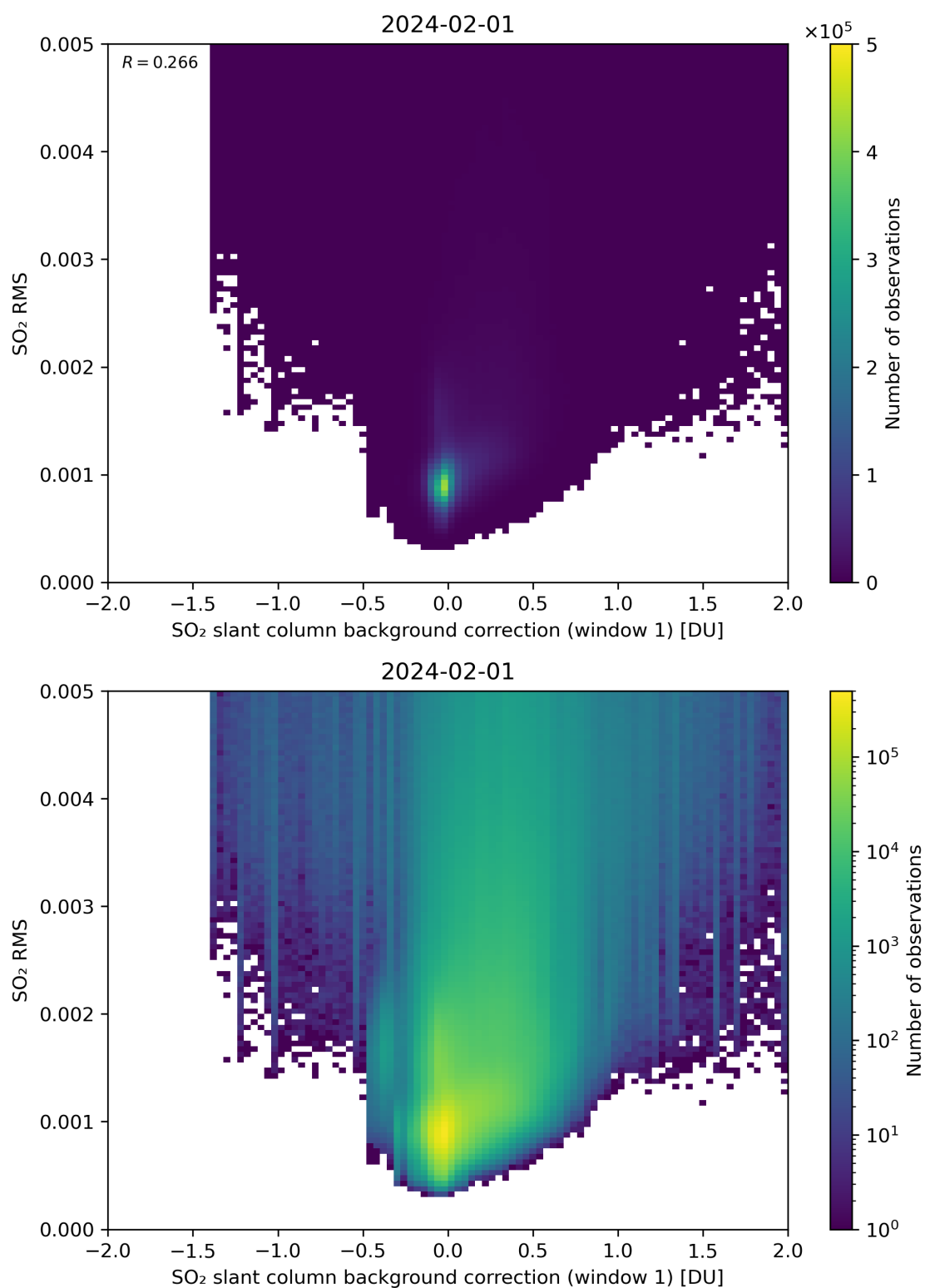
Figure 102: Scatter density plot of “SO 2 slant column background correction (window 1)” against “SO 2 RMS” for 2024-01-31 to 2024-02-02.
