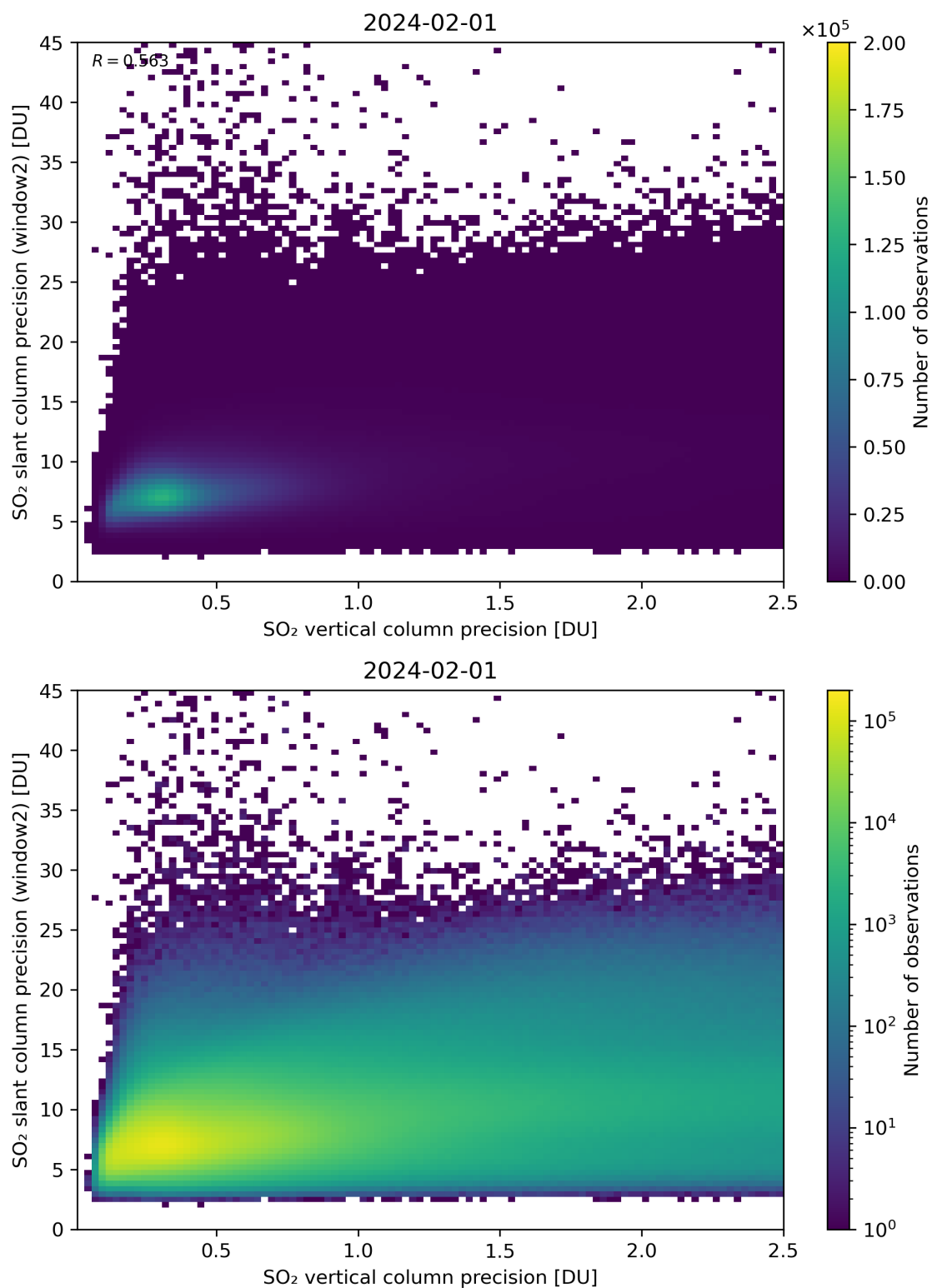
Figure 291: Scatter density plot of “SO 2 vertical column precision” against “SO 2 slant column precision (window2)” for 2024-01-31 to 2024-02-02.
