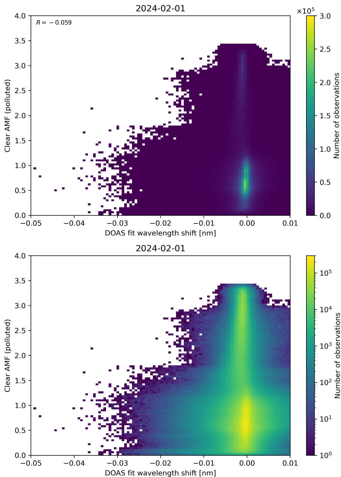
Figure 129: Scatter density plot of “DOAS fit wavelength shift” against “Clear AMF (polluted)” for 2024-01-31 to 2024-02-02.
