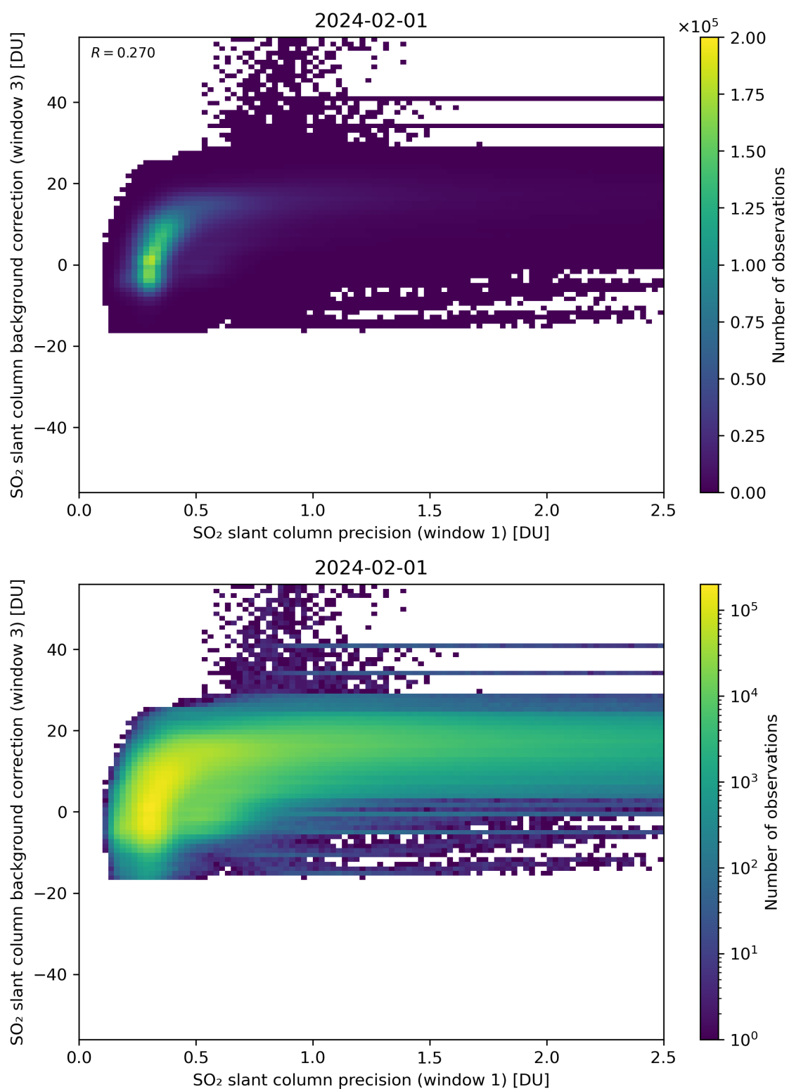
Figure 220: Scatter density plot of “SO 2 slant column precision (window 1)” against “SO 2 slant column background correction (window 3)” for 2024-01-31 to 2024-02-02.
