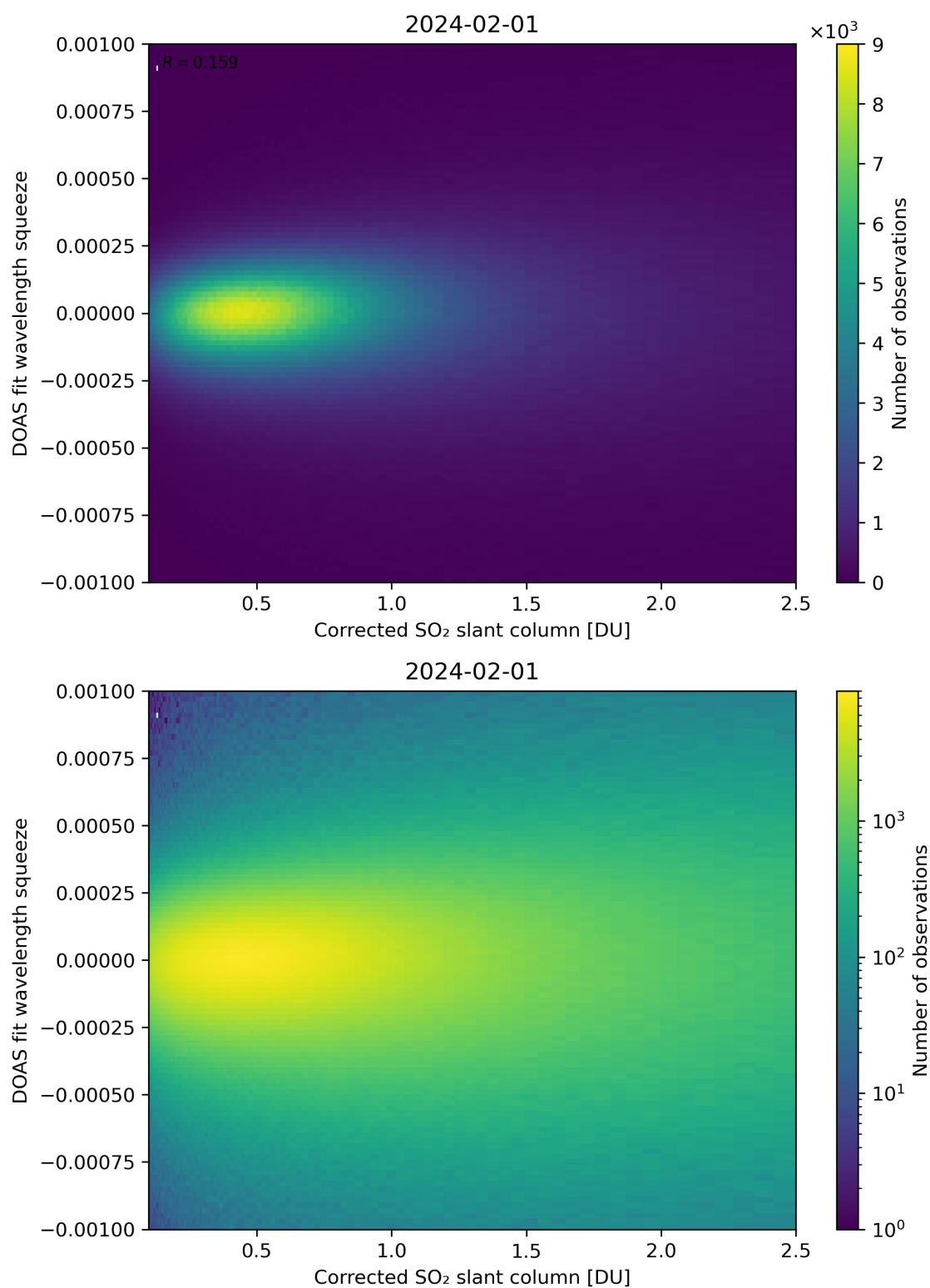
Figure 182: Scatter density plot of “Corrected SO 2 slant column” against “DOAS fit wavelength squeeze” for 2024-01-31 to 2024-02-02.
