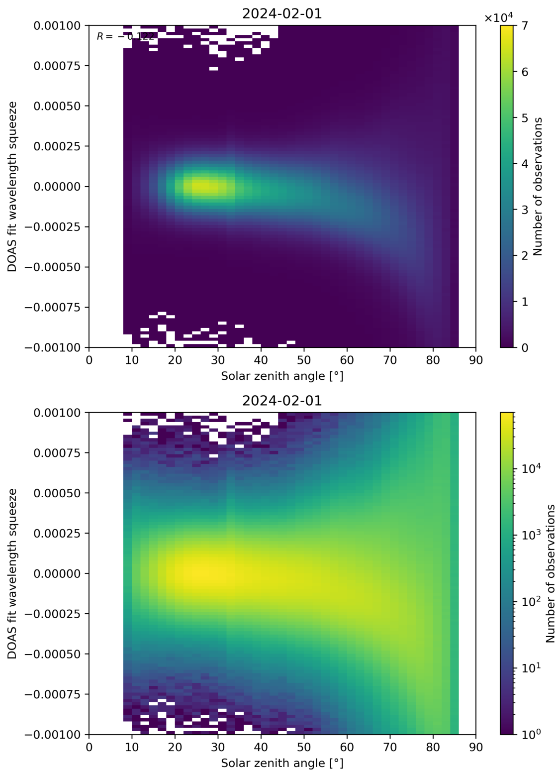
Figure 162: Scatter density plot of “Solar zenith angle” against “DOAS fit wavelength squeeze” for 2024-01-31 to 2024-02-02.
