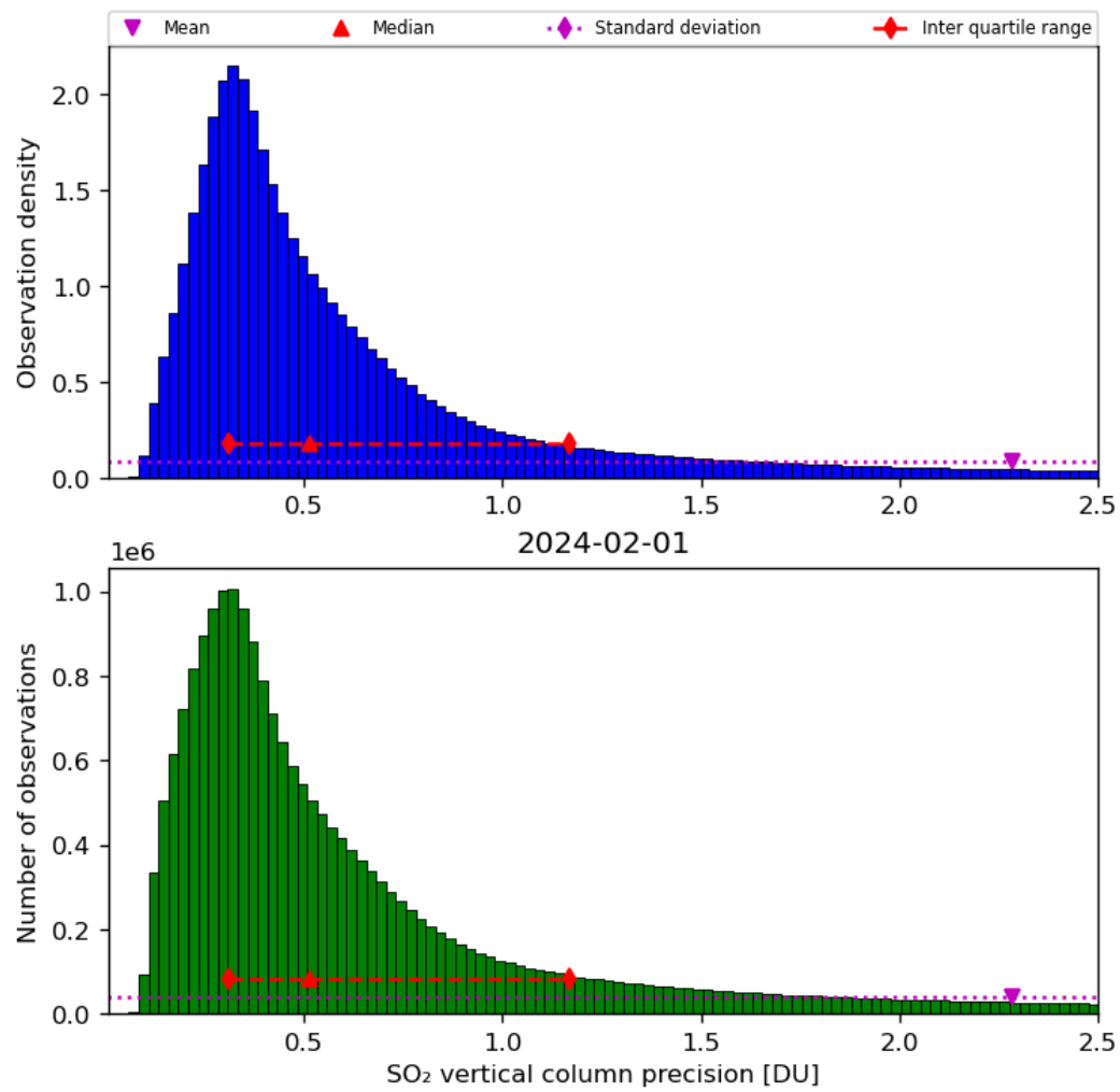
Figure 54: Histogram of “SO 2 vertical column precision” for 2024-01-31 to 2024-02-02
