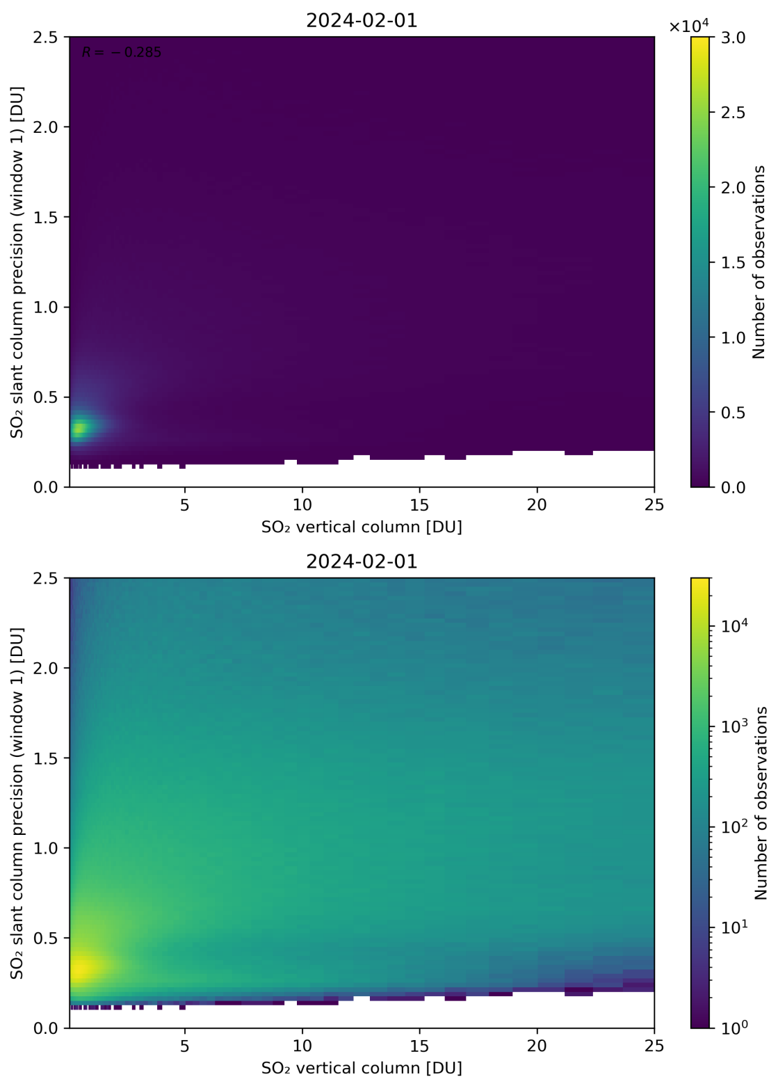
Figure 301: Scatter density plot of “SO 2 vertical column” against “SO 2 slant column precision (window 1)” for 2024-01-31 to 2024-02-02.
