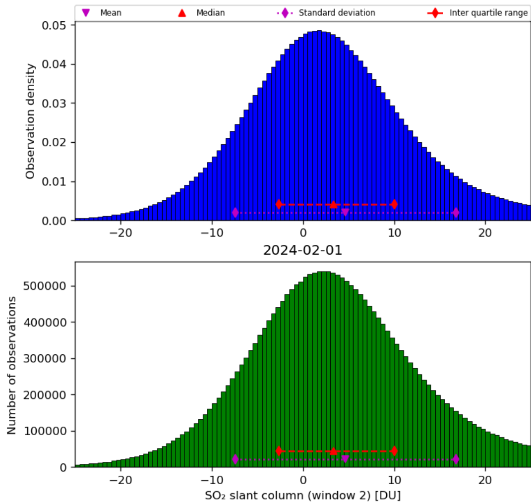
Figure 60: Histogram of “SO 2 slant column (window 2)” for 2024-01-31 to 2024-02-02
