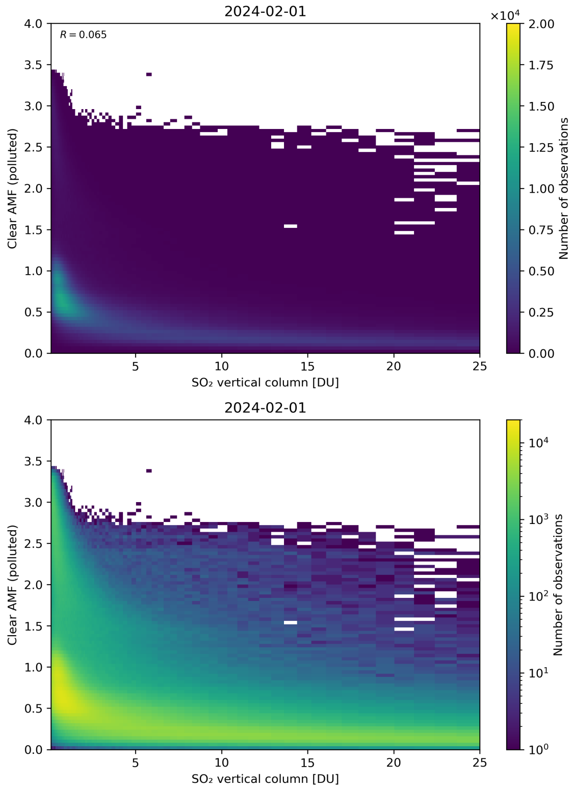
Figure 296: Scatter density plot of “SO 2 vertical column” against “Clear AMF (polluted)” for 2024-01-31 to 2024-02-02.
