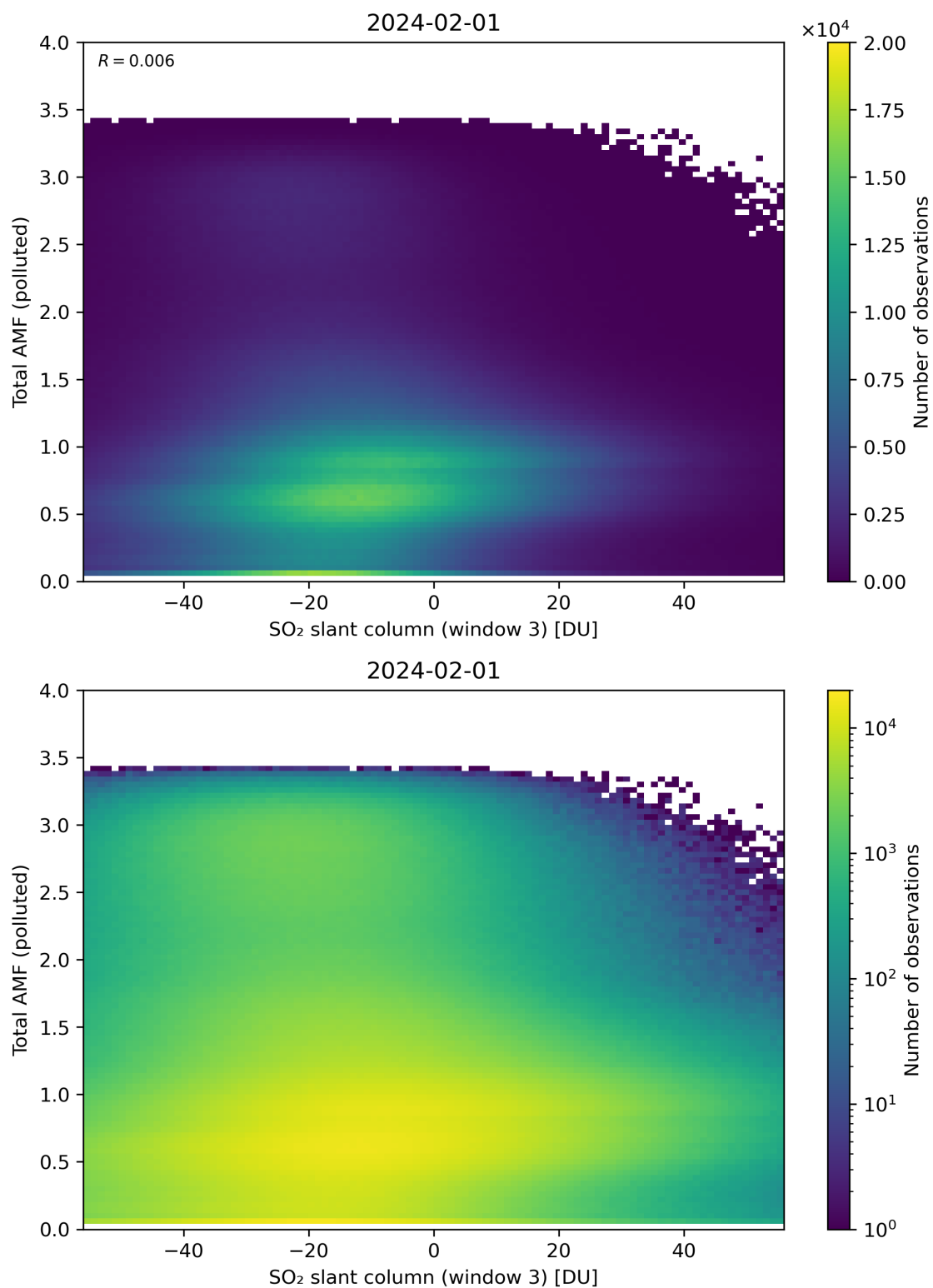
Figure 268: Scatter density plot of “SO 2 slant column (window 3)” against “Total AMF (polluted)” for 2024-01-31 to 2024-02-02.
