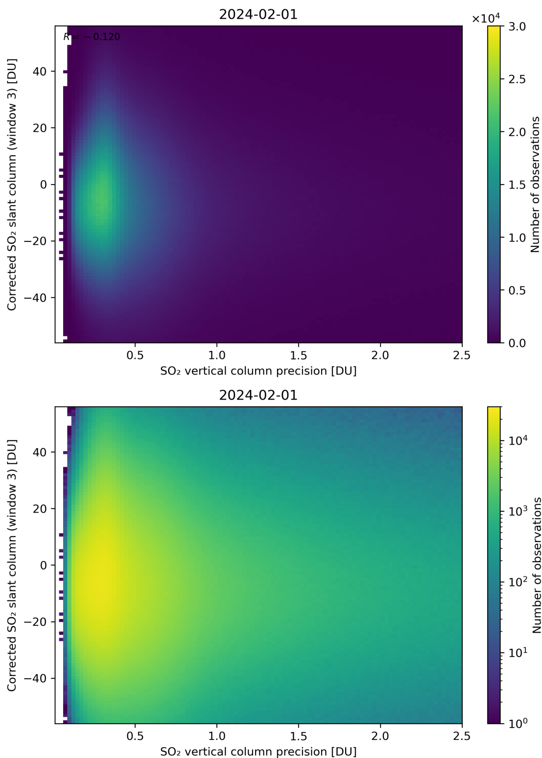
Figure 288: Scatter density plot of “SO 2 vertical column precision” against “Corrected SO 2 slant column (window 3)” for 2024-01-31 to 2024-02-02.
