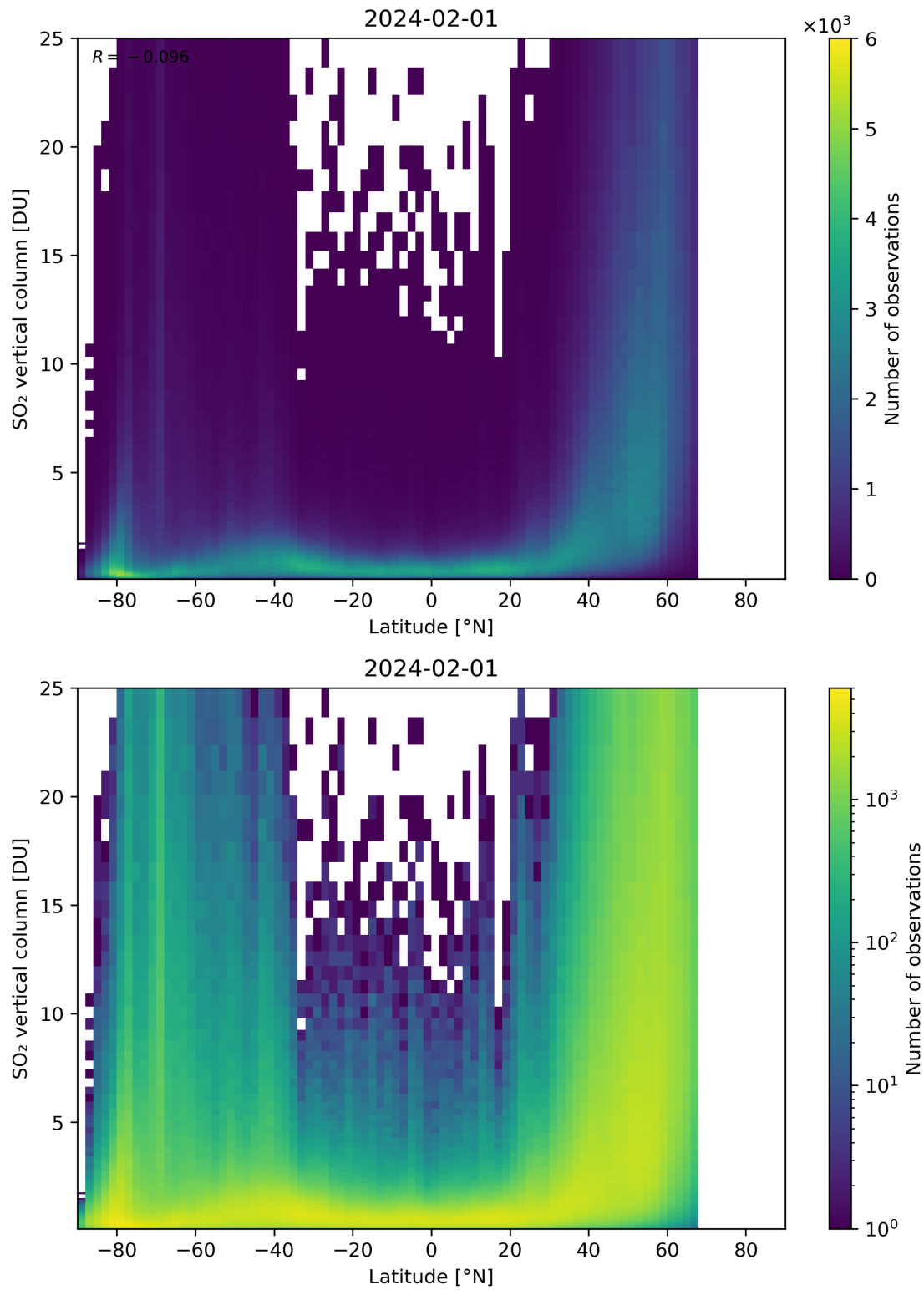
Figure 156: Scatter density plot of “Latitude” against “SO 2 vertical column” for 2024-01-31 to 2024-02-02.
