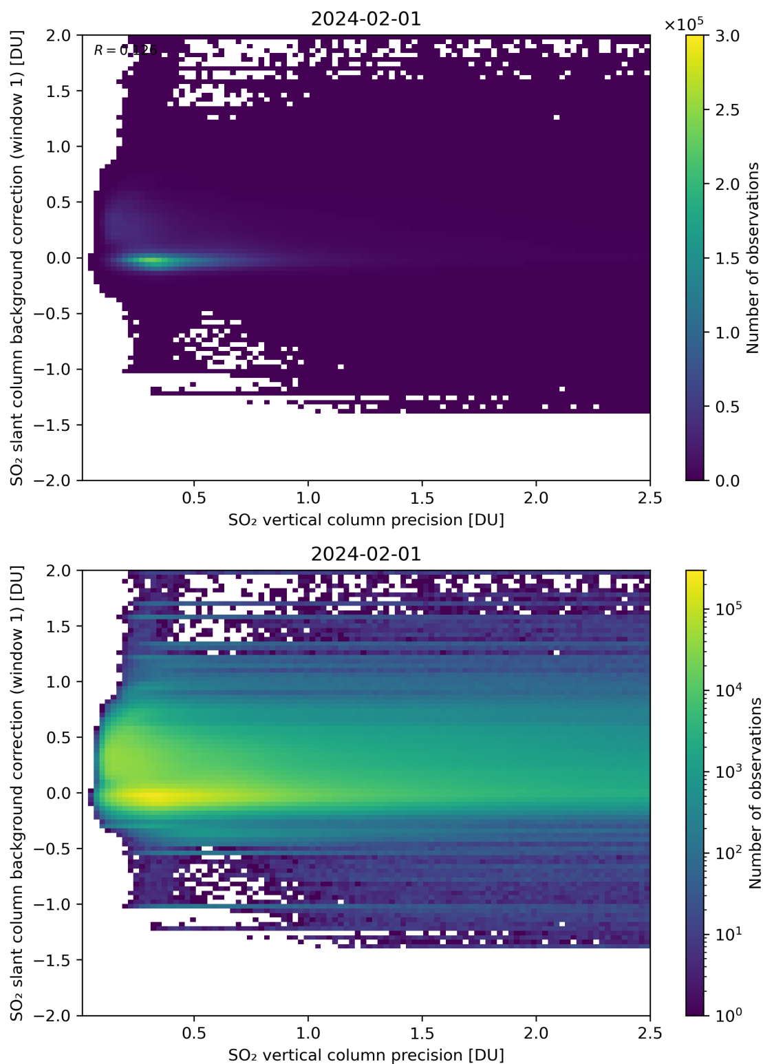
Figure 279: Scatter density plot of “SO 2 vertical column precision” against “SO 2 slant column background correction (window 1)” for 2024-01-31 to 2024-02-02.
