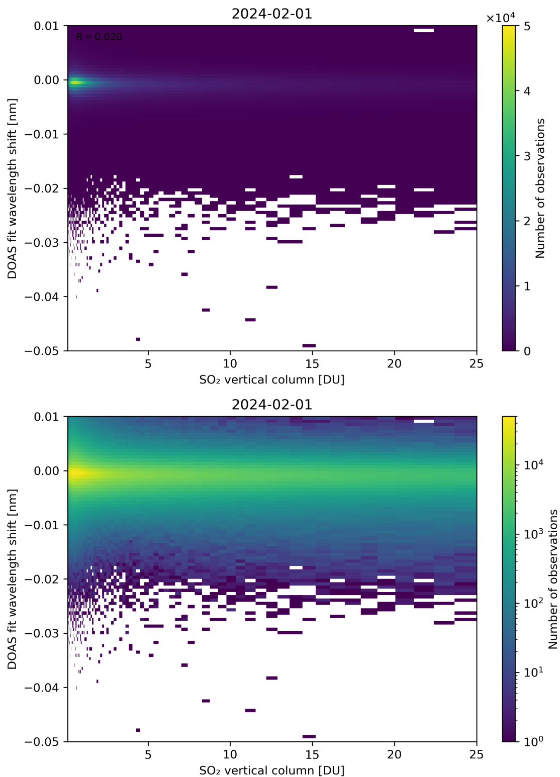
Figure 276: Scatter density plot of “SO 2 vertical column” against “DOAS fit wavelength shift” for 2024-01-31 to 2024-02-02.
