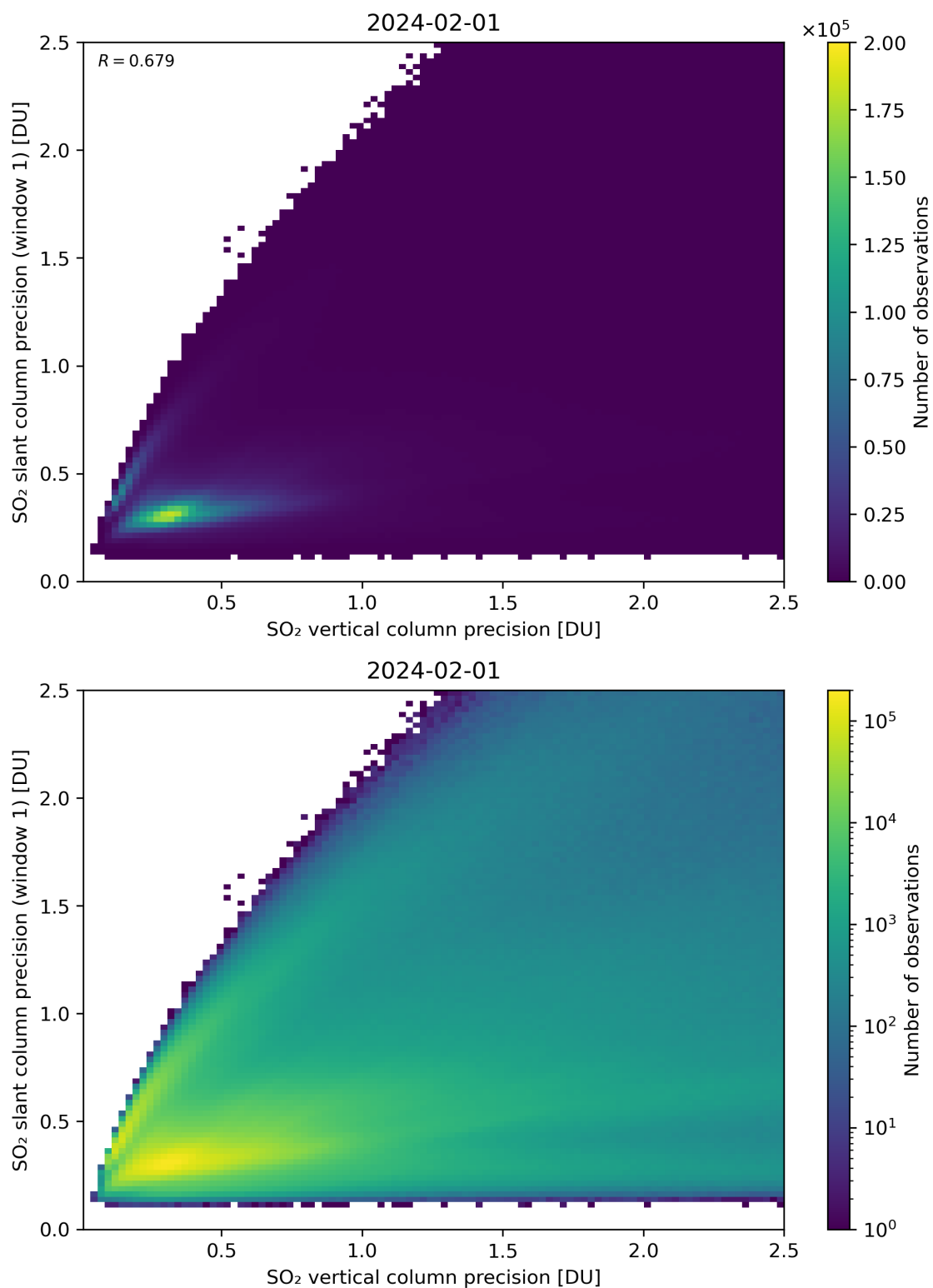
Figure 290: Scatter density plot of “SO 2 vertical column precision” against “SO 2 slant column precision (window 1)” for 2024-01-31 to 2024-02-02.
