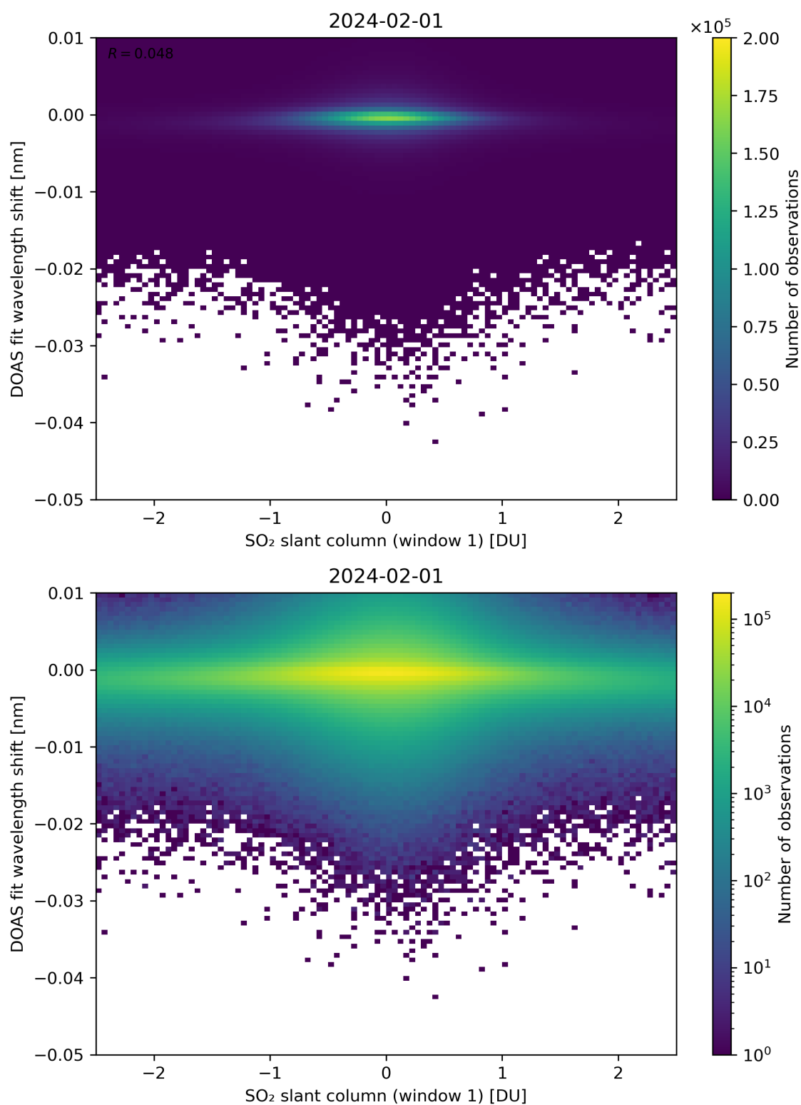
Figure 215: Scatter density plot of “SO 2 slant column (window 1)” against “DOAS fit wavelength shift” for 2024-01-31 to 2024-02-02.
