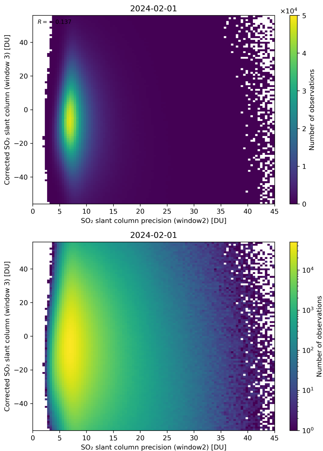
Figure 248: Scatter density plot of “SO 2 slant column precision (window2)” against “Corrected SO 2 slant column (window 3)” for 2024-01-31 to 2024-02-02.
