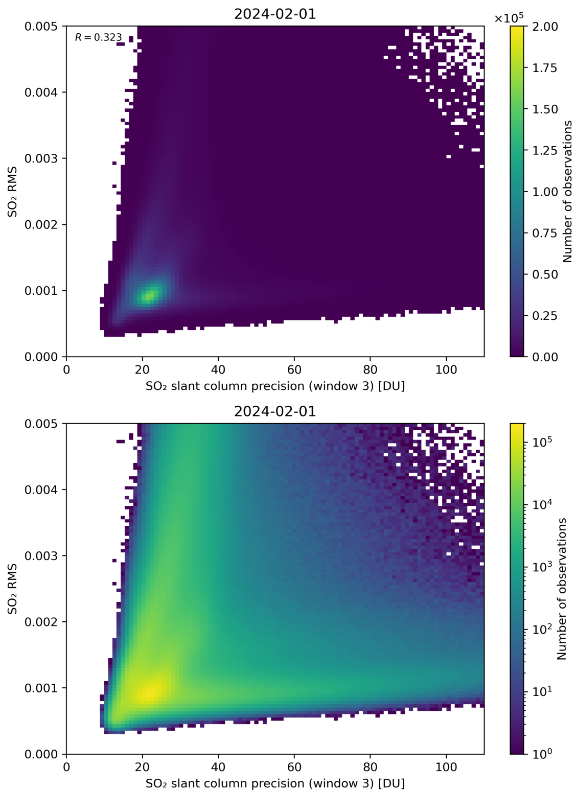
Figure 260: Scatter density plot of “SO 2 slant column precision (window 3)” against “SO 2 RMS” for 2024-01-31 to 2024-02-02.
