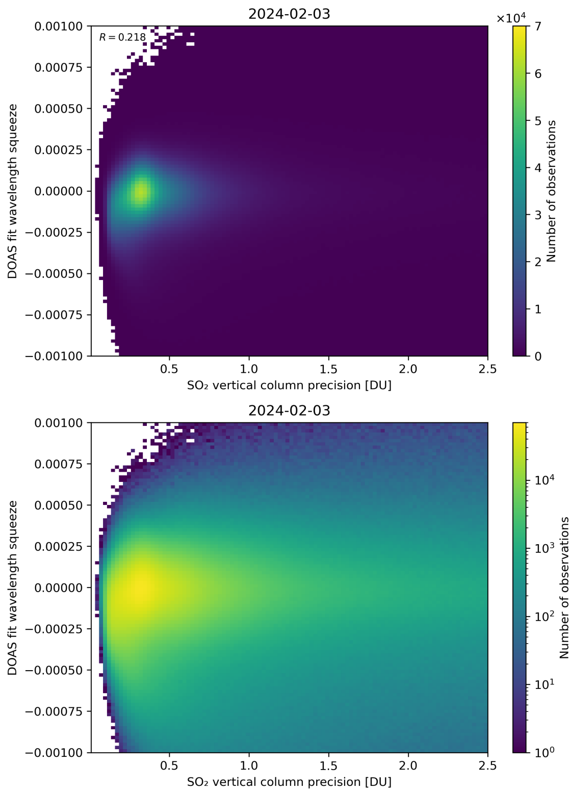
Figure 283: Scatter density plot of “SO 2 vertical column precision” against “DOAS fit wavelength squeeze” for 2024-02-02 to 2024-02-04.
