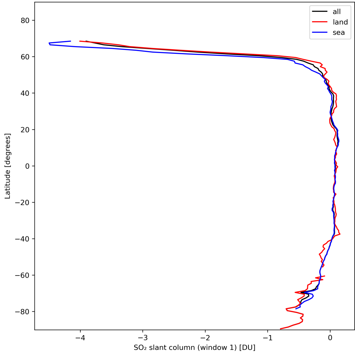
Figure 33: Zonal average of “SO 2 slant column (window 1)” for 2024-02-02 to 2024-02-04.
