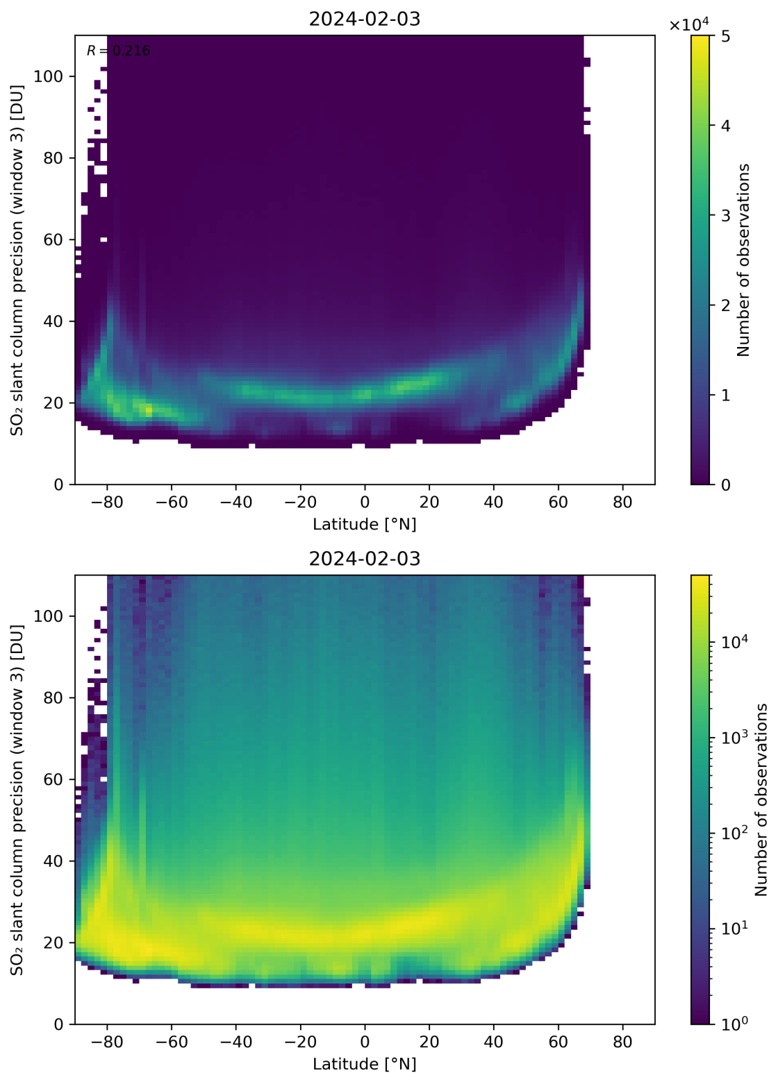
Figure 153: Scatter density plot of “Latitude” against “SO 2 slant column precision (window 3)” for 2024-02-02 to 2024-02-04.
