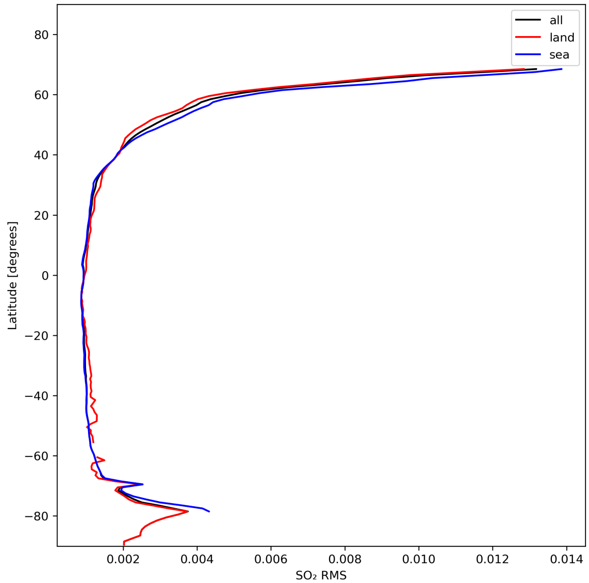
Figure 47: Zonal average of “SO 2 RMS” for 2024-02-02 to 2024-02-04.
