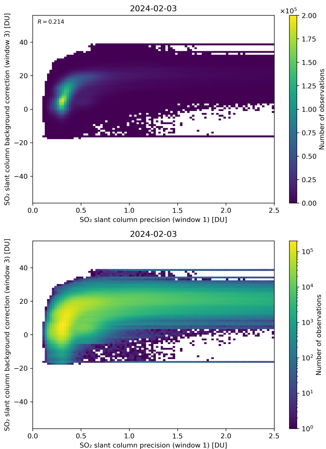
Figure 220: Scatter density plot of “SO 2 slant column precision (window 1)” against “SO 2 slant column background correction (window 3)” for 2024-02-02 to 2024-02-04.
