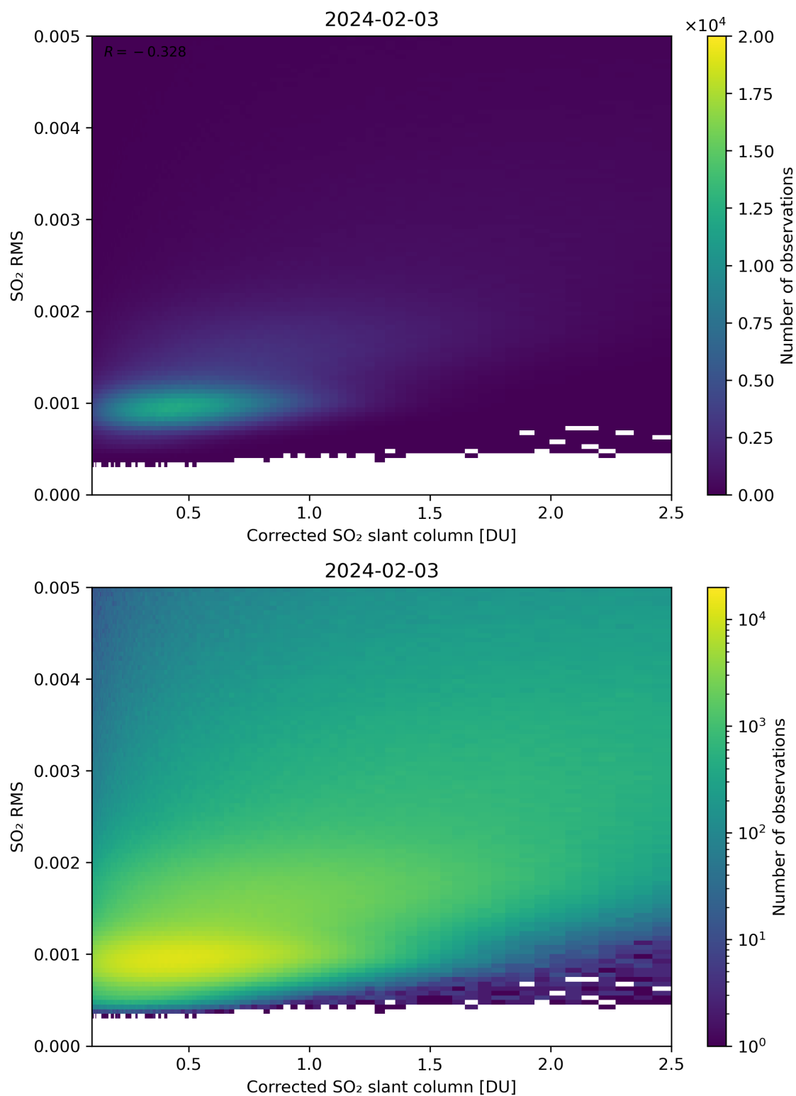
Figure 183: Scatter density plot of “Corrected SO 2 slant column” against “SO 2 RMS” for 2024-02-02 to 2024-02-04.
