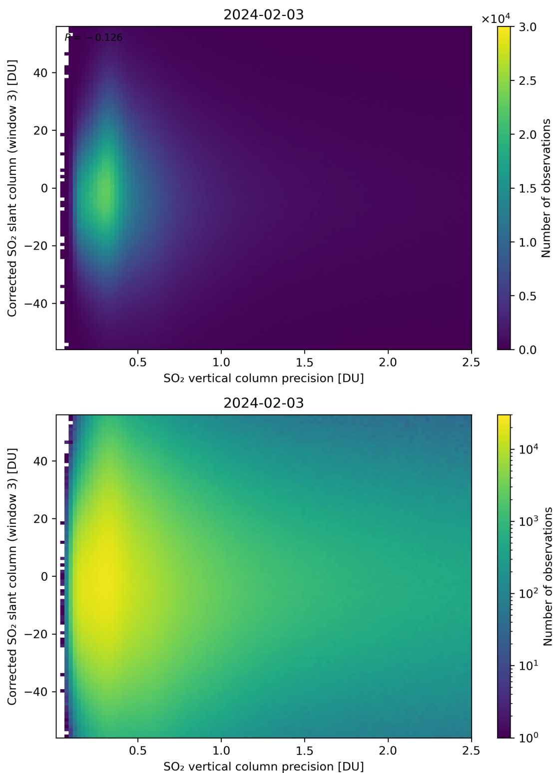
Figure 288: Scatter density plot of “SO 2 vertical column precision” against “Corrected SO 2 slant column (window 3)” for 2024-02-02 to 2024-02-04.
