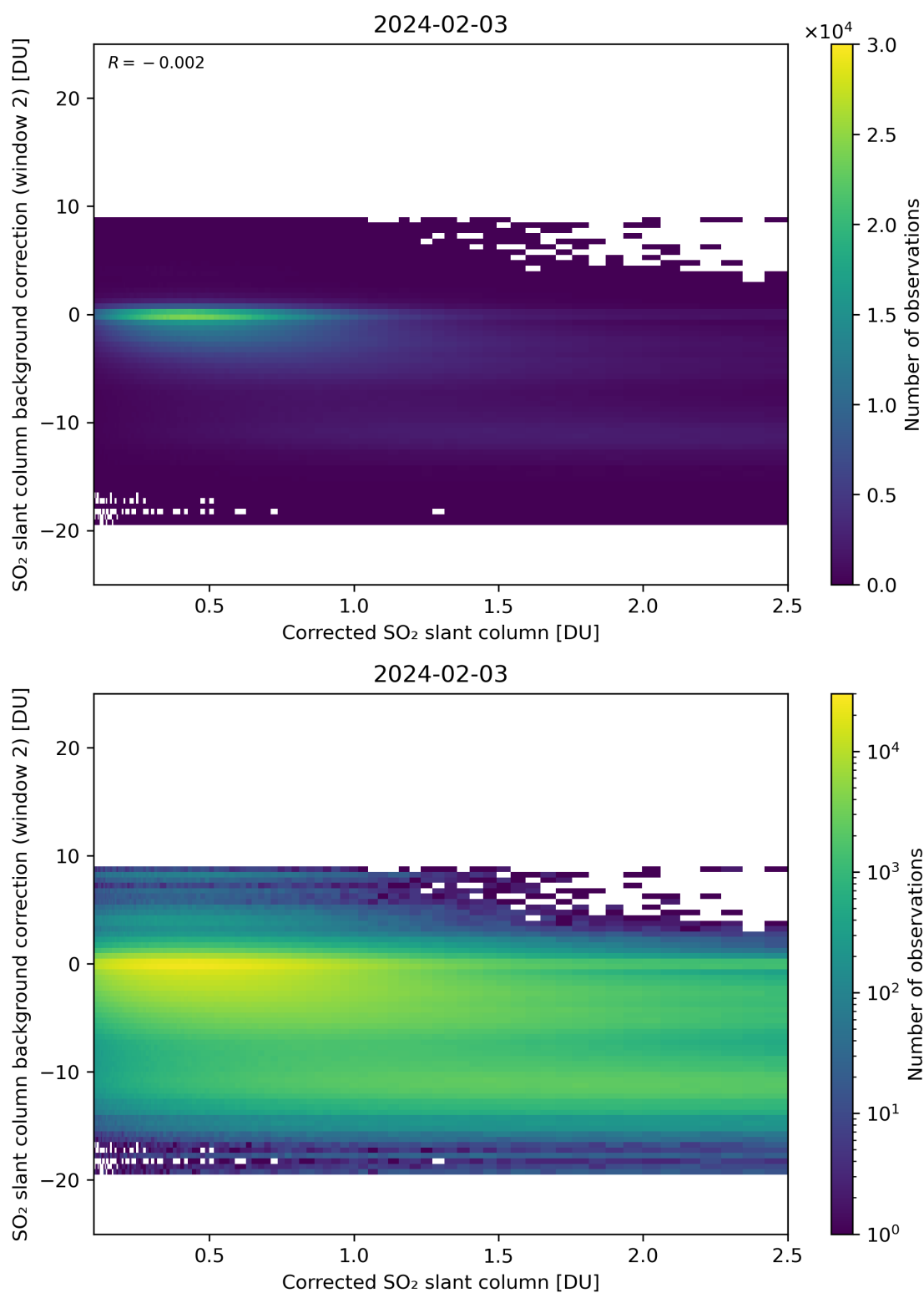
Figure 179: Scatter density plot of “Corrected SO 2 slant column” against “SO 2 slant column background correction (window 2)” for 2024-02-02 to 2024-02-04.
