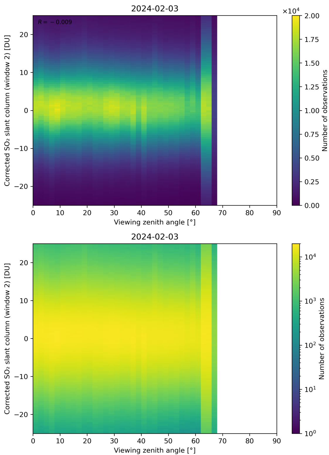
Figure 318: Scatter density plot of “Viewing zenith angle” against “Corrected SO 2 slant column (window 2)” for 2024-02-02 to 2024-02-04.
