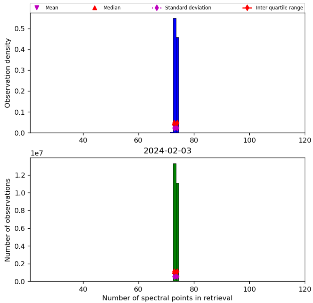
Figure 74: Histogram of “Number of spectral points in retrieval” for 2024-02-02 to 2024-02-04
