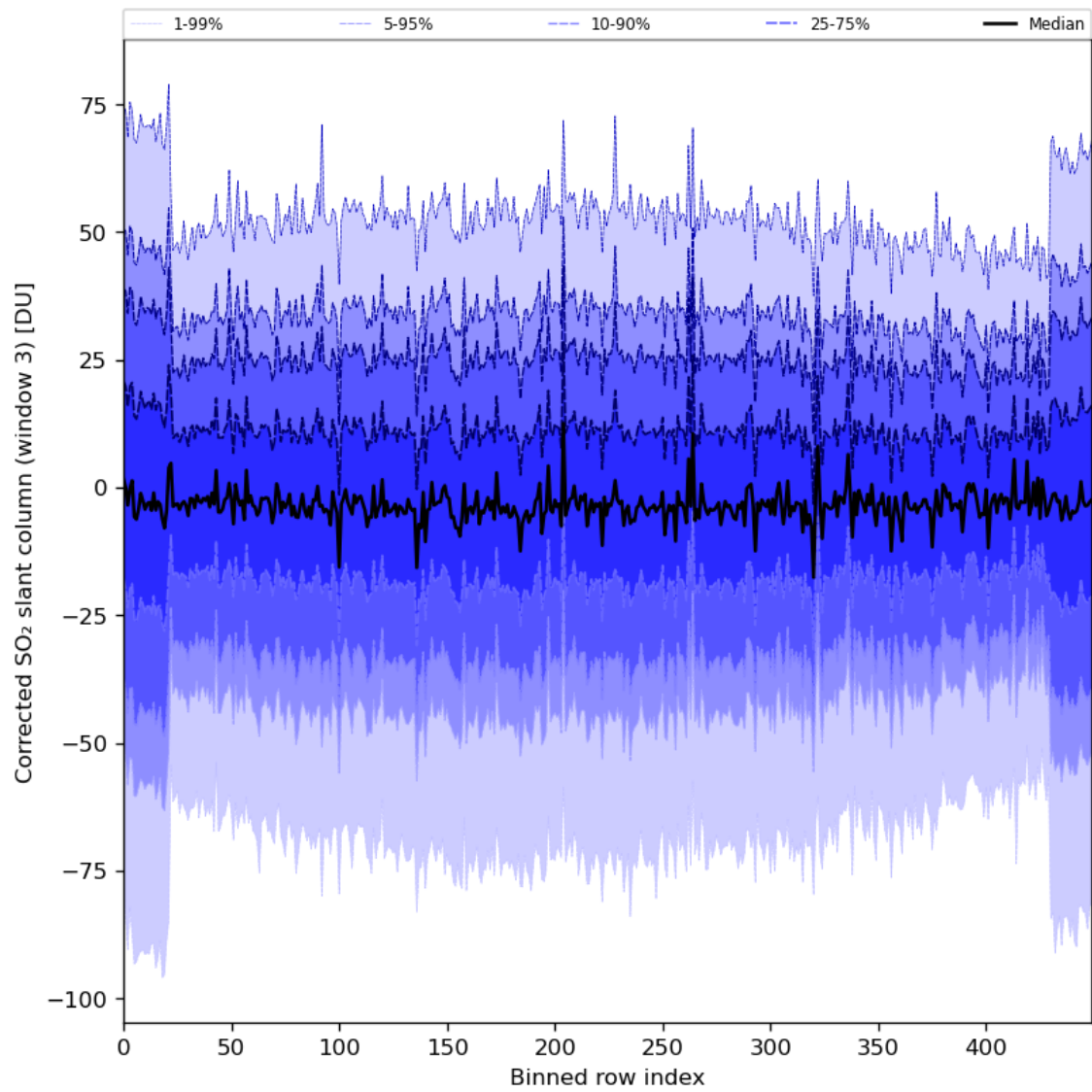
Figure 89: Along track statistics of “Corrected SO 2 slant column (window 3)” for 2024-02-02 to 2024-02-04
