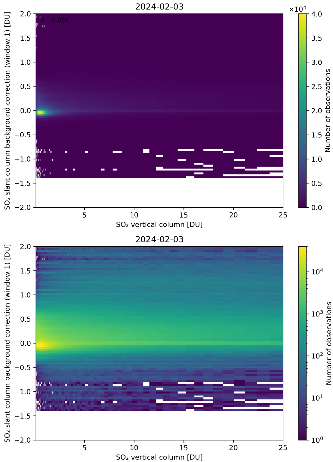
Figure 273: Scatter density plot of “SO 2 vertical column” against “SO 2 slant column background correction (window 1)” for 2024-02-02 to 2024-02-04.
