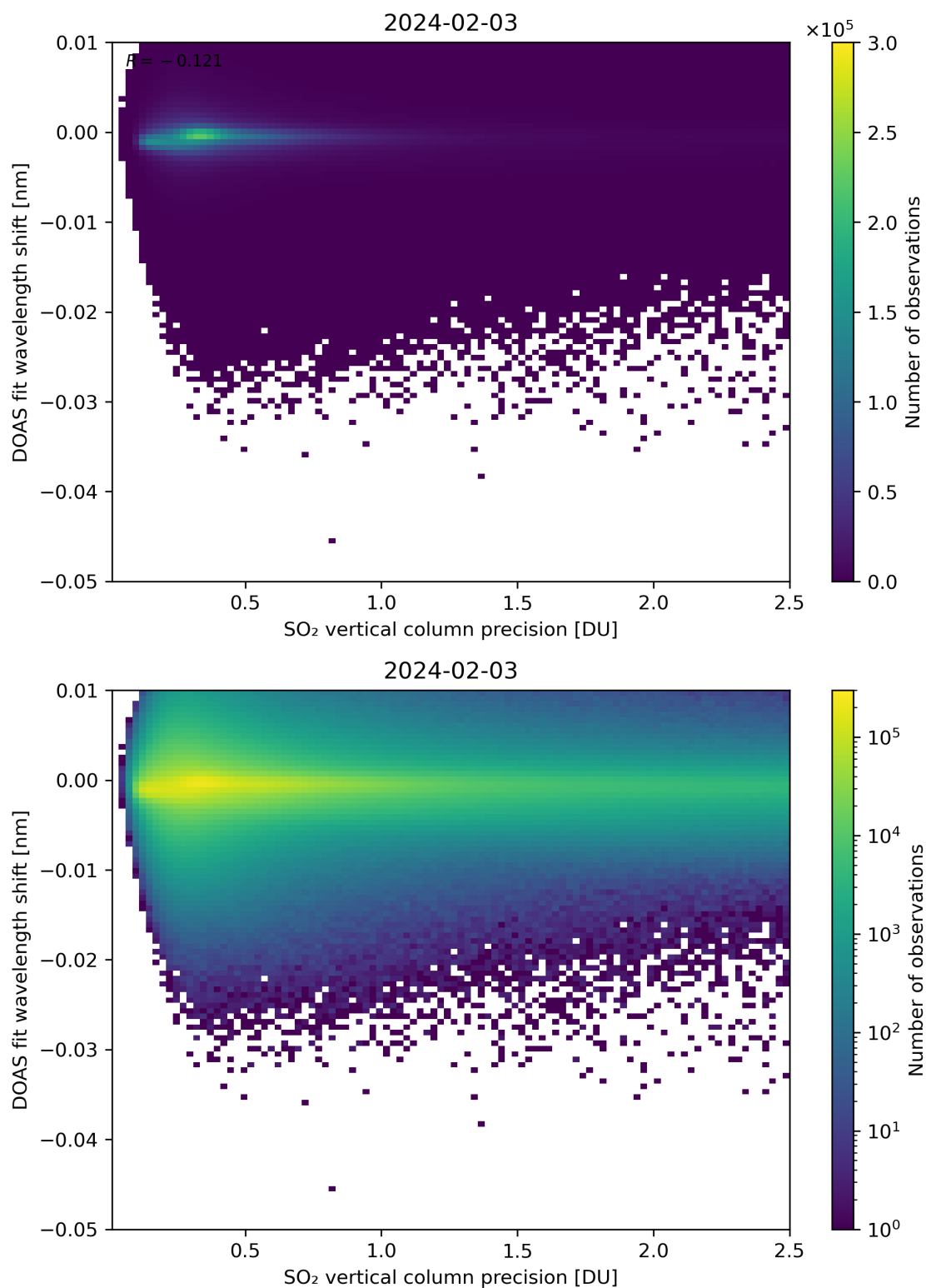
Figure 282: Scatter density plot of “SO 2 vertical column precision” against “DOAS fit wavelength shift” for 2024-02-02 to 2024-02-04.
