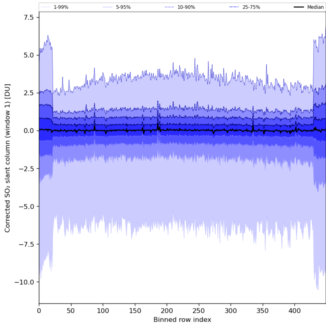
Figure 81: Along track statistics of “Corrected SO 2 slant column (window 1)” for 2024-02-02 to 2024-02-04
