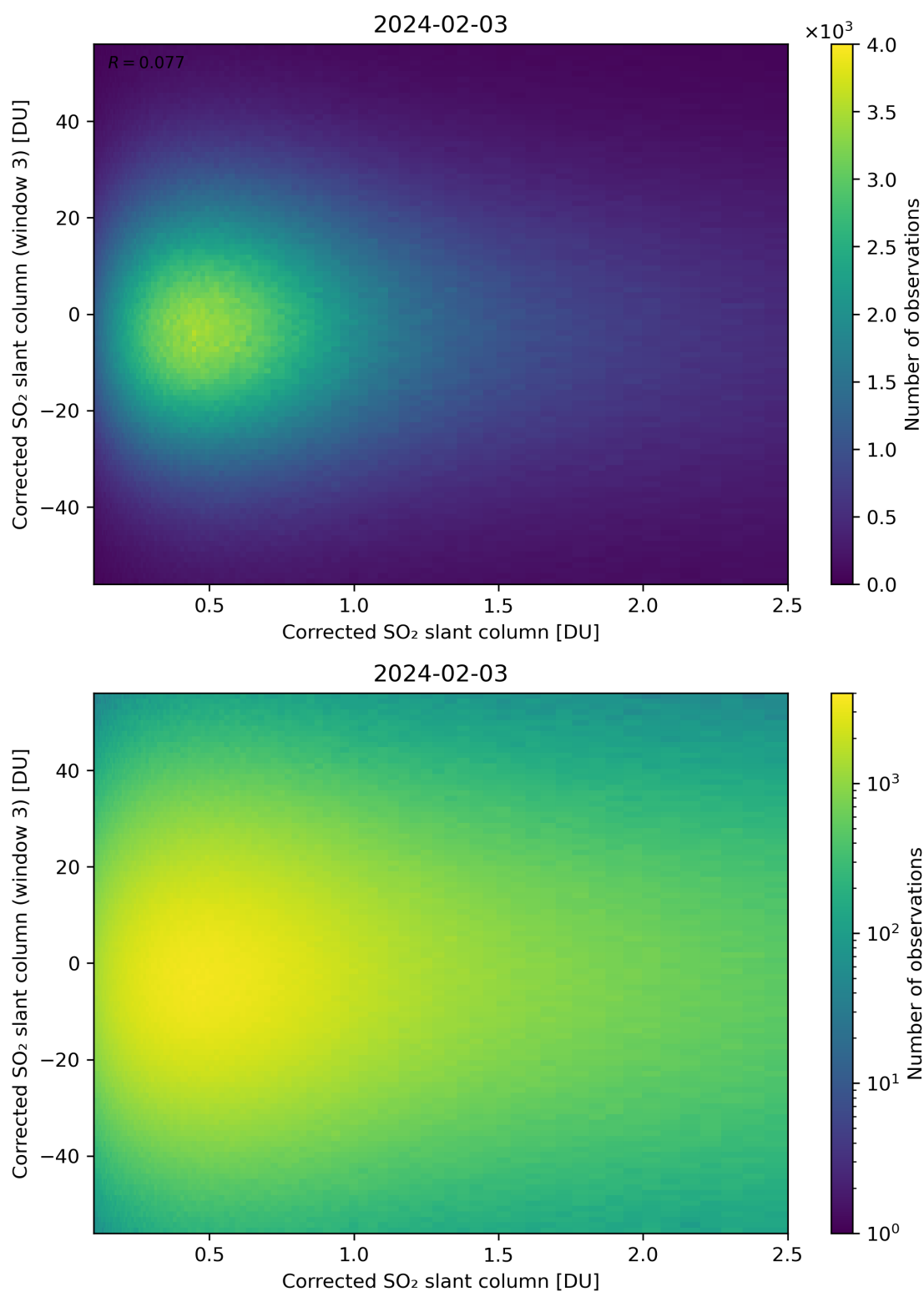
Figure 186: Scatter density plot of “Corrected SO 2 slant column” against “Corrected SO 2 slant column (window 3)” for 2024-02-02 to 2024-02-04.
