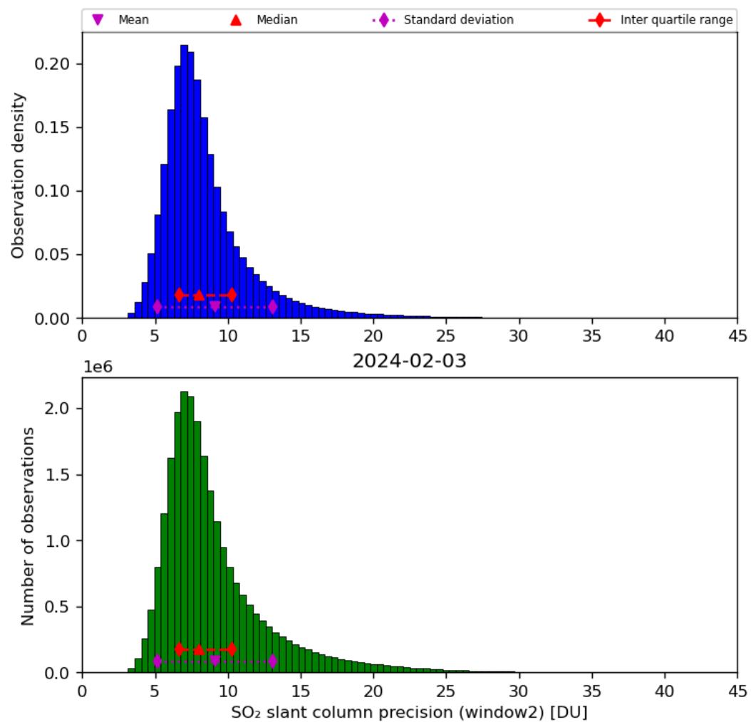
Figure 61: Histogram of “SO 2 slant column precision (window2)” for 2024-02-02 to 2024-02-04
