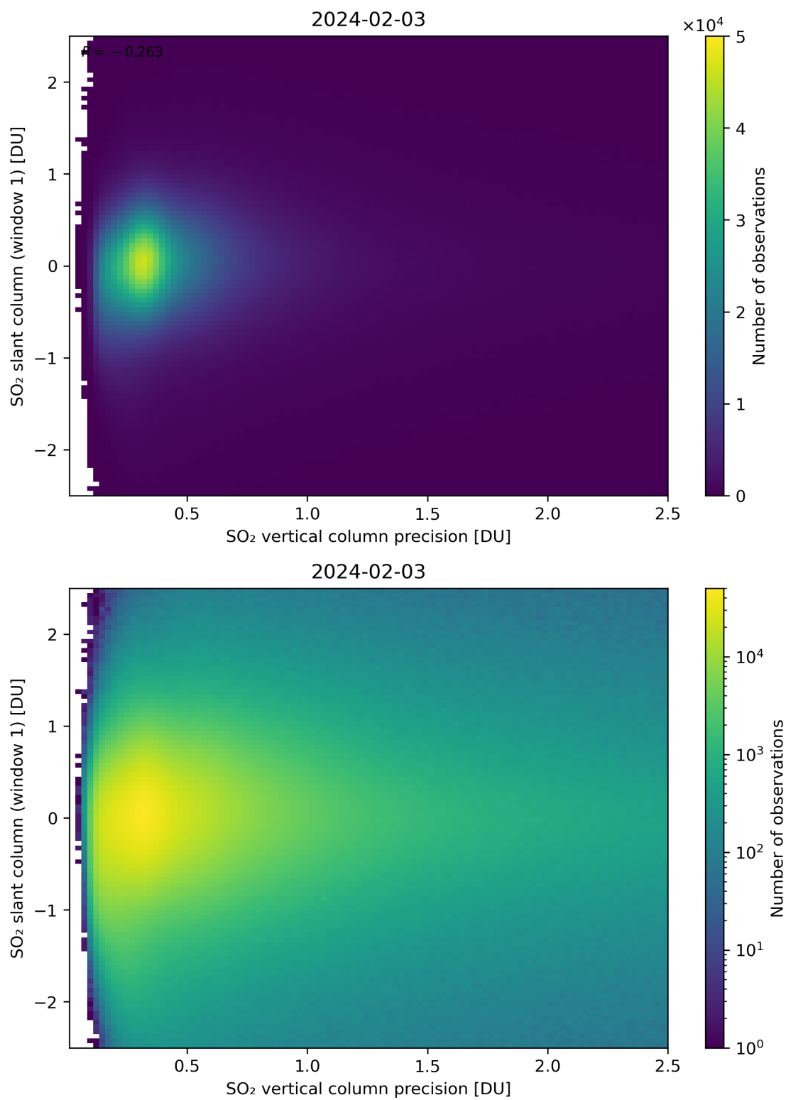
Figure 289: Scatter density plot of “SO 2 vertical column precision” against “SO 2 slant column (window 1)” for 2024-02-02 to 2024-02-04.
