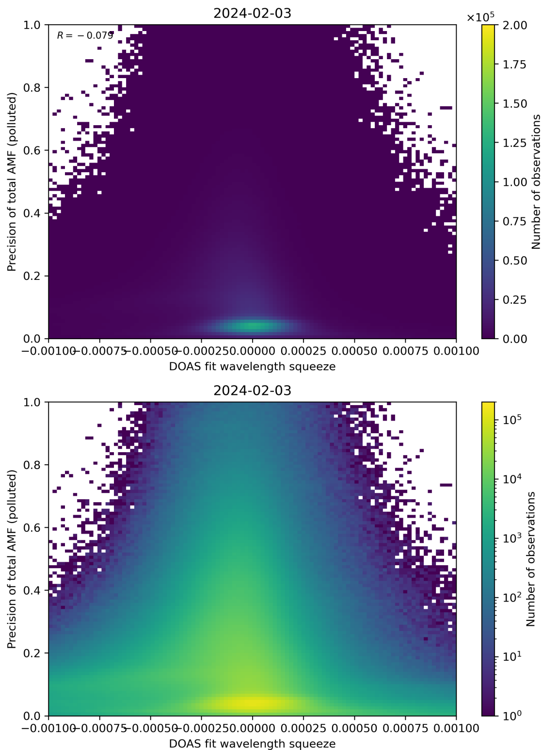
Figure 135: Scatter density plot of “DOAS fit wavelength squeeze” against “Precision of total AMF (polluted)” for 2024-02-02 to 2024-02-04.
