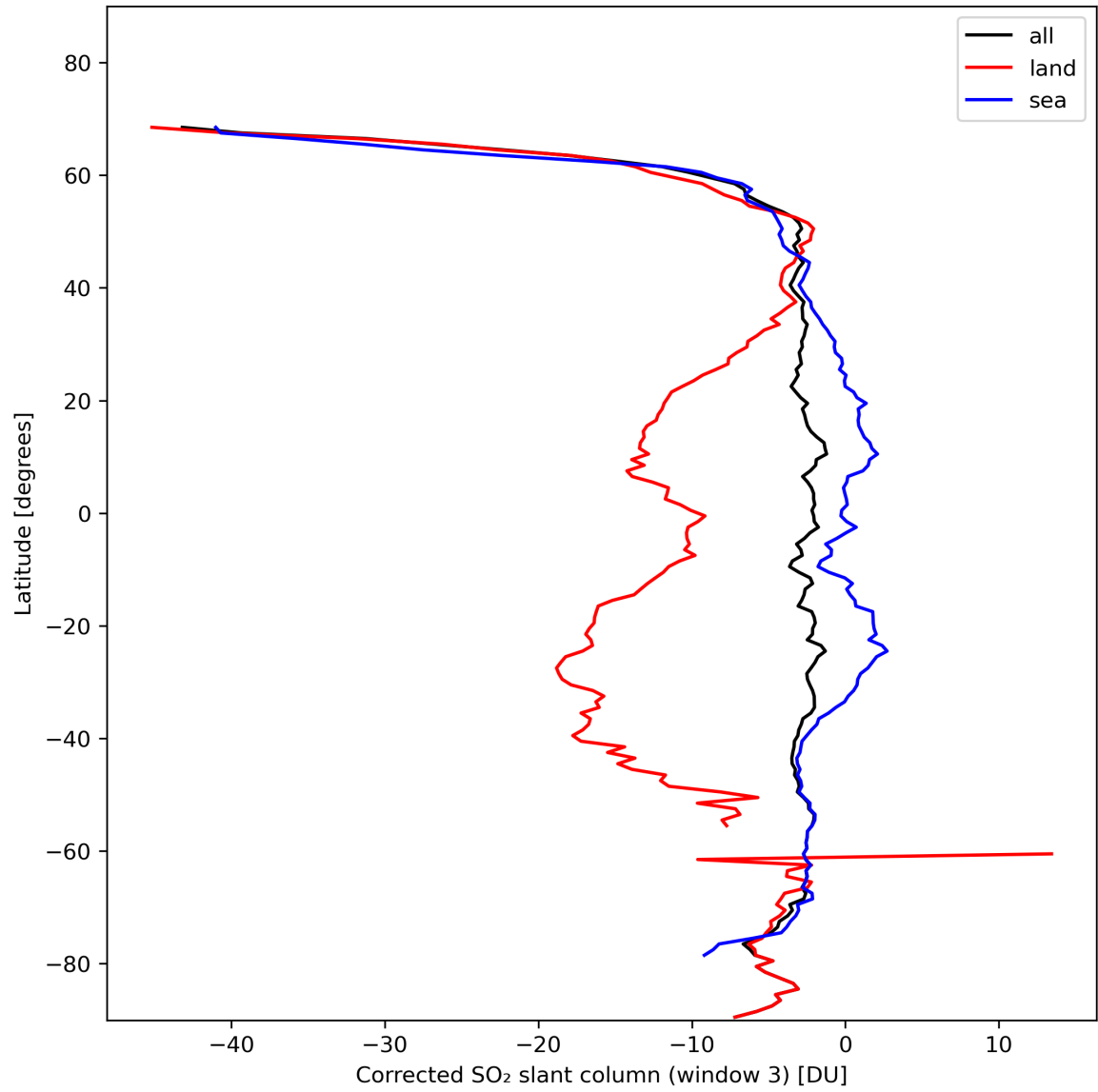
Figure 43: Zonal average of “Corrected SO 2 slant column (window 3)” for 2024-02-02 to 2024-02-04.
