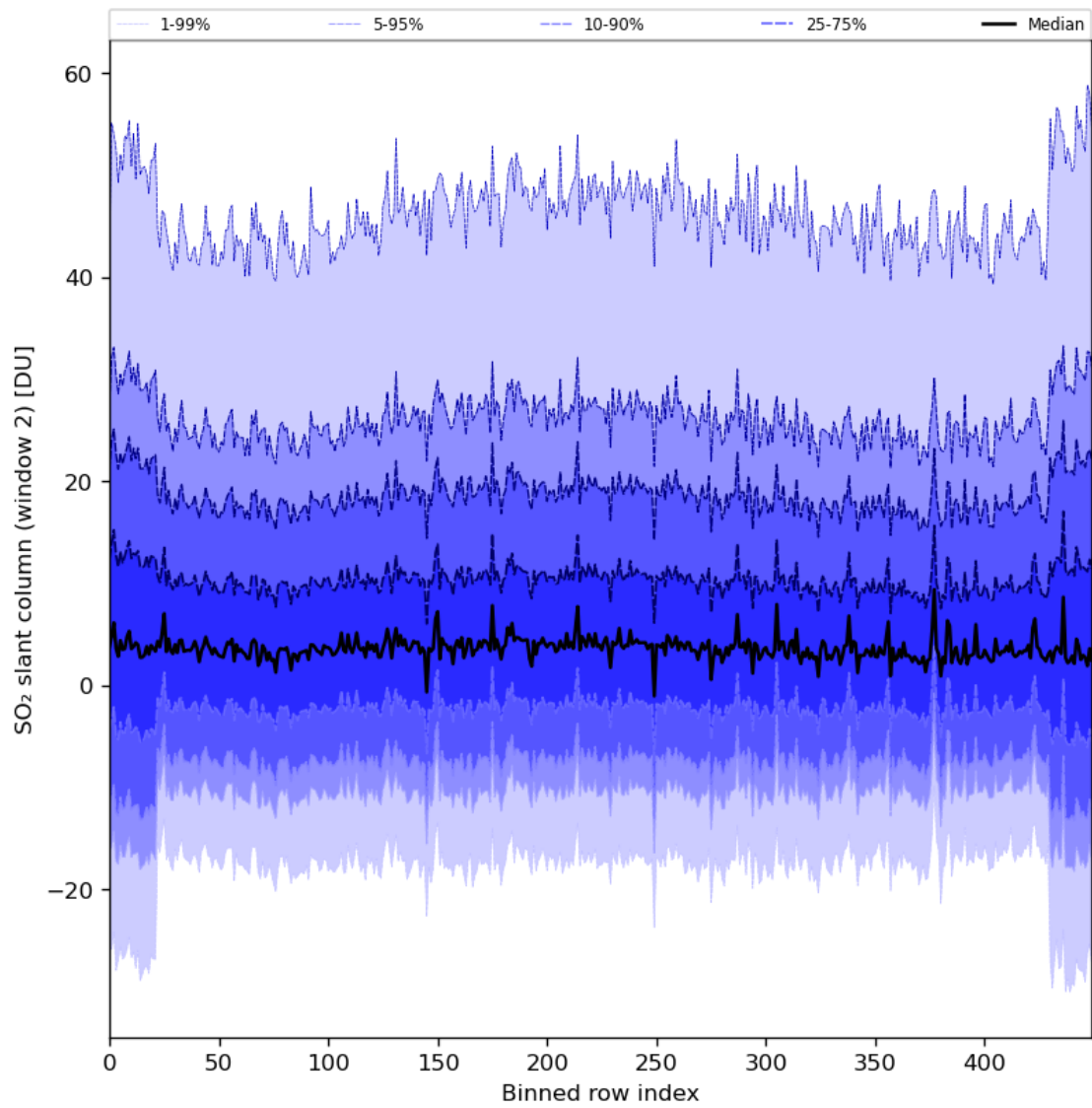
Figure 83: Along track statistics of “SO 2 slant column (window 2)” for 2024-02-02 to 2024-02-04
