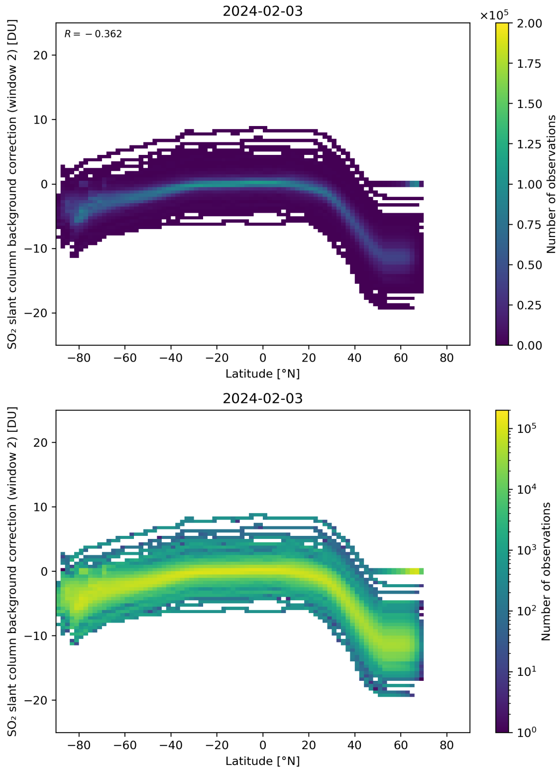
Figure 140: Scatter density plot of “Latitude” against “SO 2 slant column background correction (window 2)” for 2024-02-02 to 2024-02-04.
