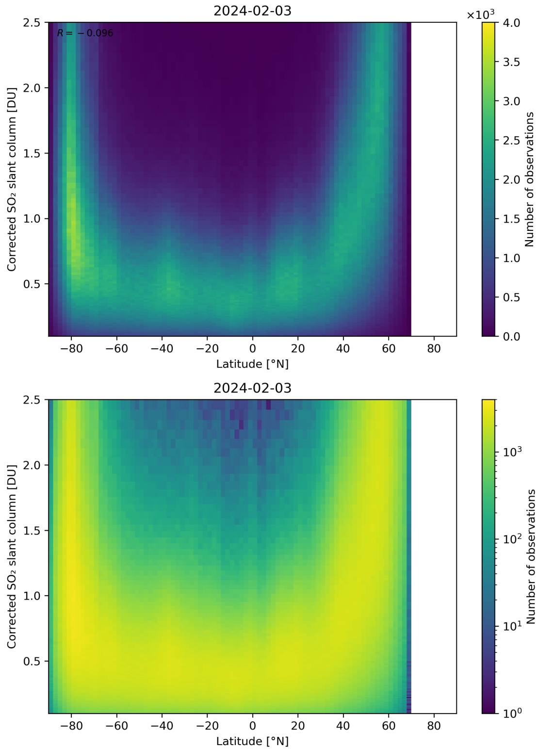
Figure 146: Scatter density plot of “Latitude” against “Corrected SO 2 slant column” for 2024-02-02 to 2024-02-04.
