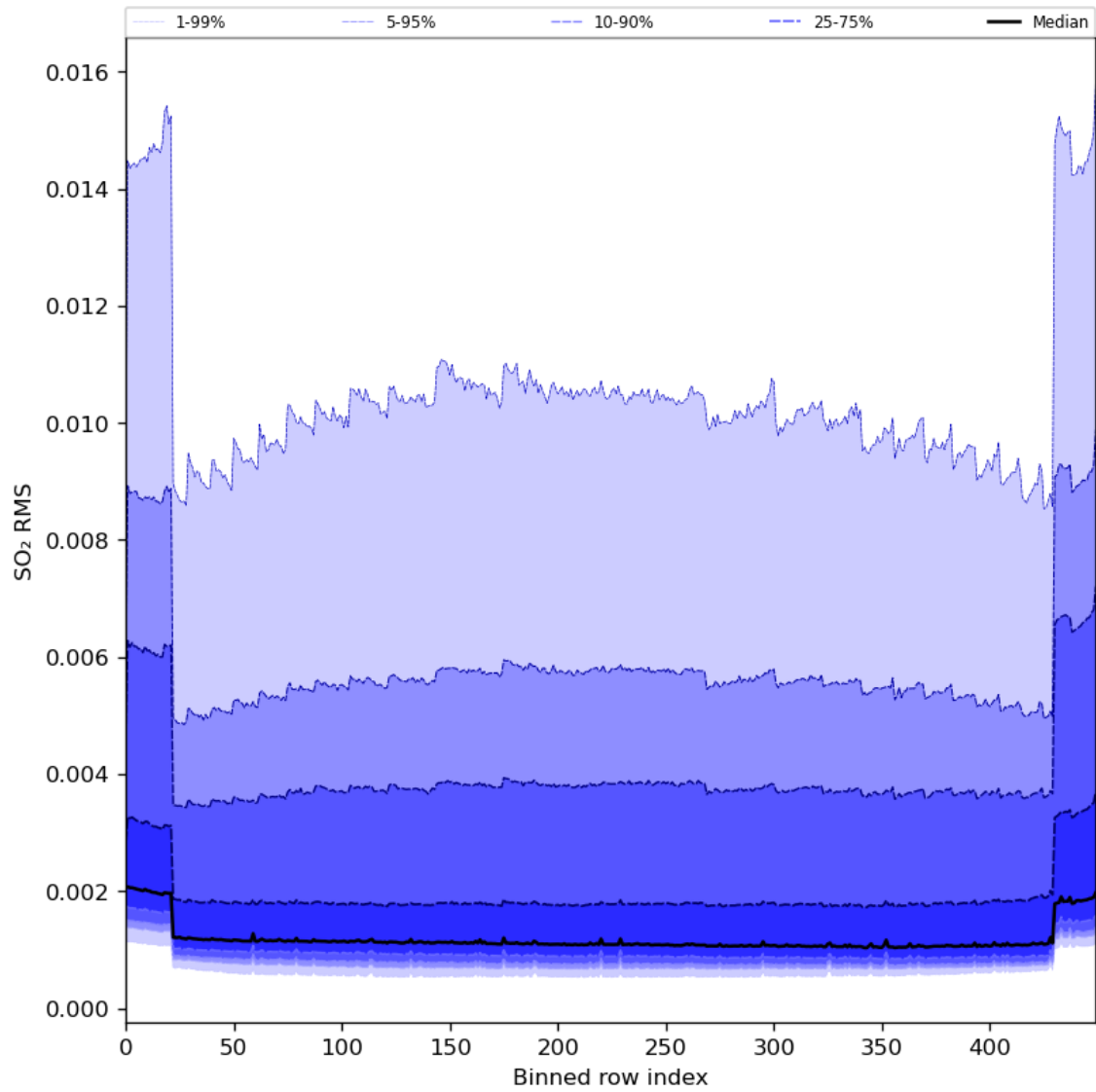
Figure 93: Along track statistics of “SO 2 RMS” for 2024-02-02 to 2024-02-04
