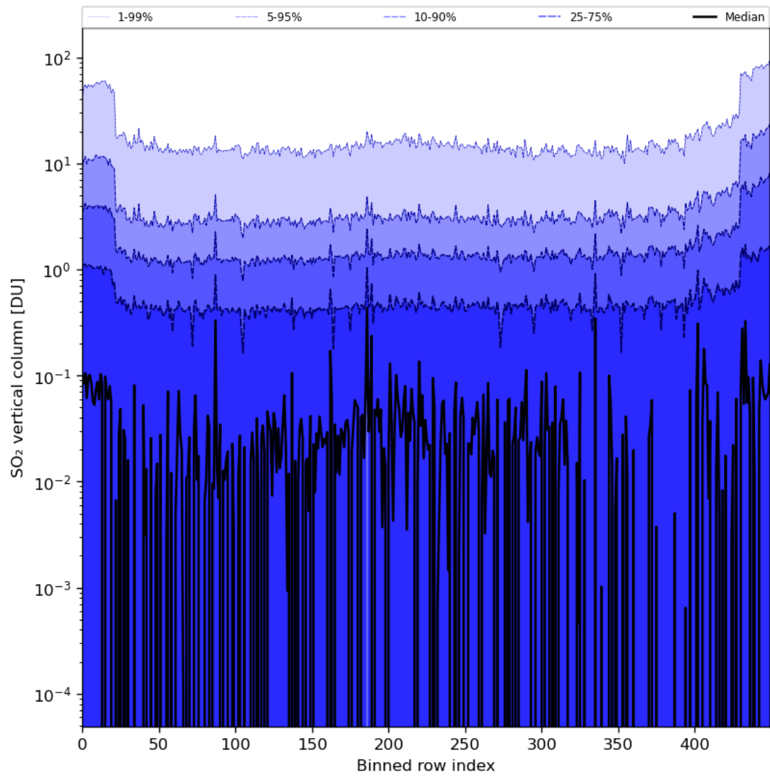
Figure 76: Along track statistics of “SO 2 vertical column” for 2024-02-02 to 2024-02-04
