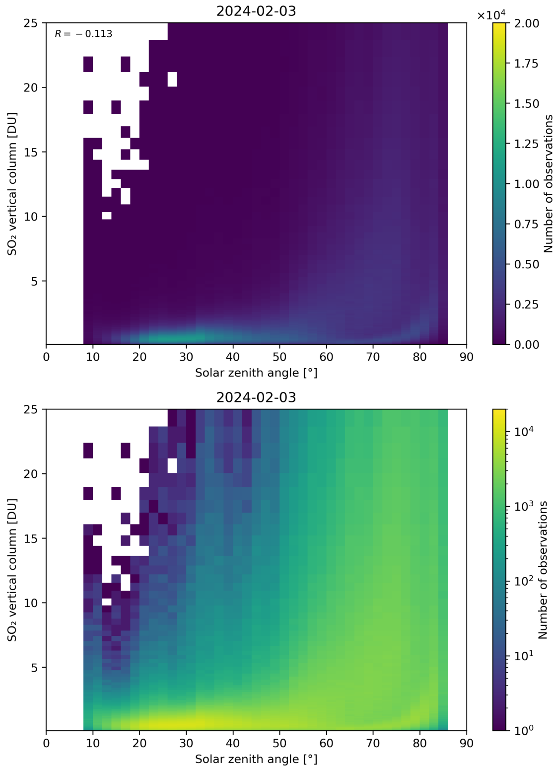
Figure 176: Scatter density plot of “Solar zenith angle” against “SO 2 vertical column” for 2024-02-02 to 2024-02-04.
