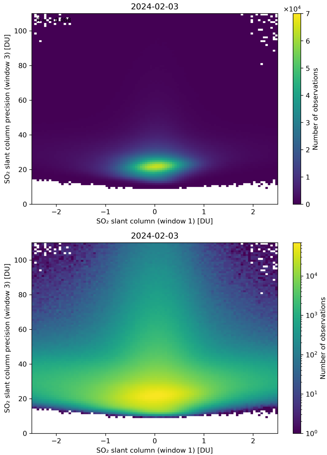
Figure 238: Scatter density plot of “SO 2 slant column (window 1)” against “SO 2 slant column precision (window 3)” for 2024-02-02 to 2024-02-04.
