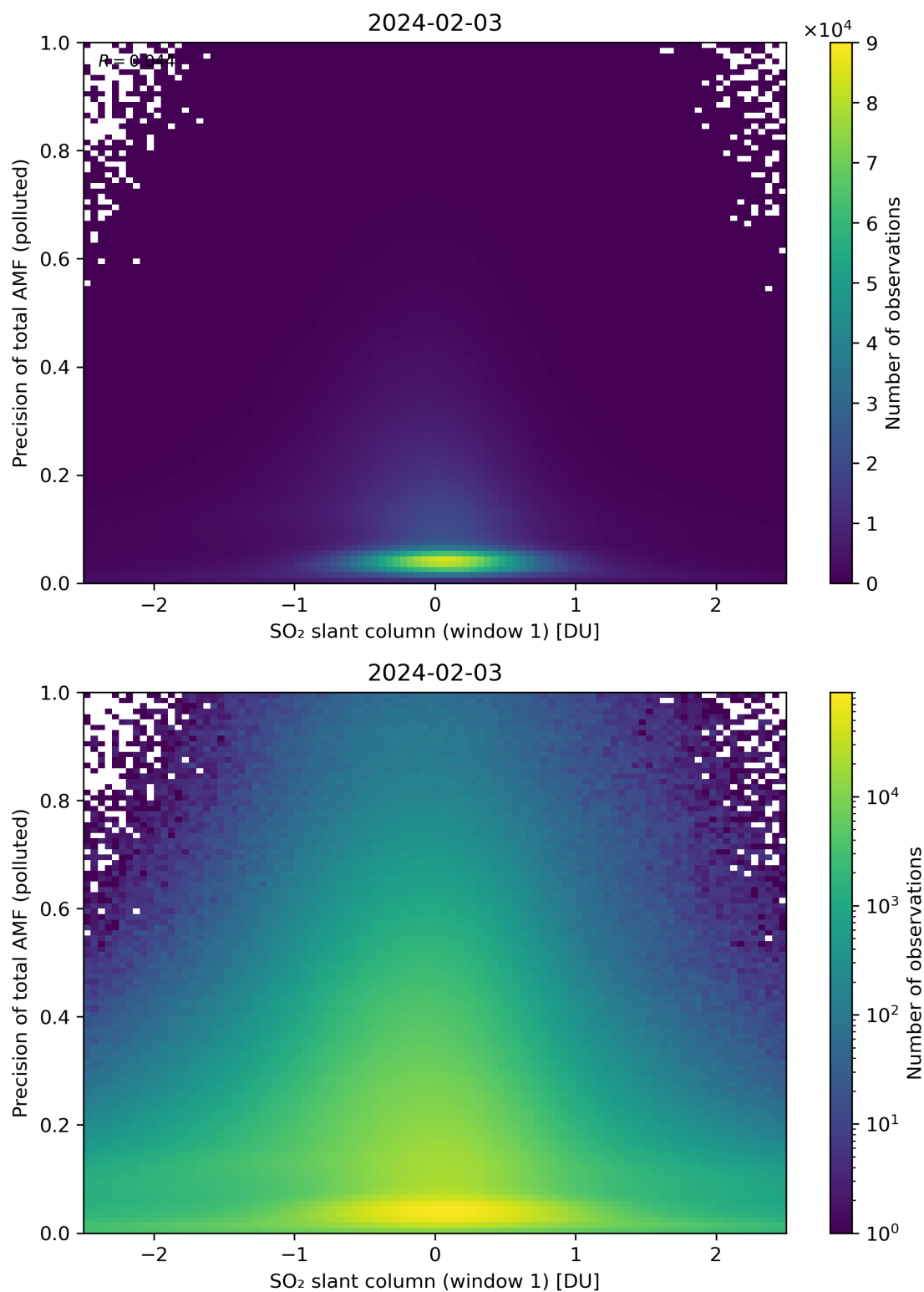
Figure 240: Scatter density plot of “SO 2 slant column (window 1)” against “Precision of total AMF (polluted)” for 2024-02-02 to 2024-02-04.
