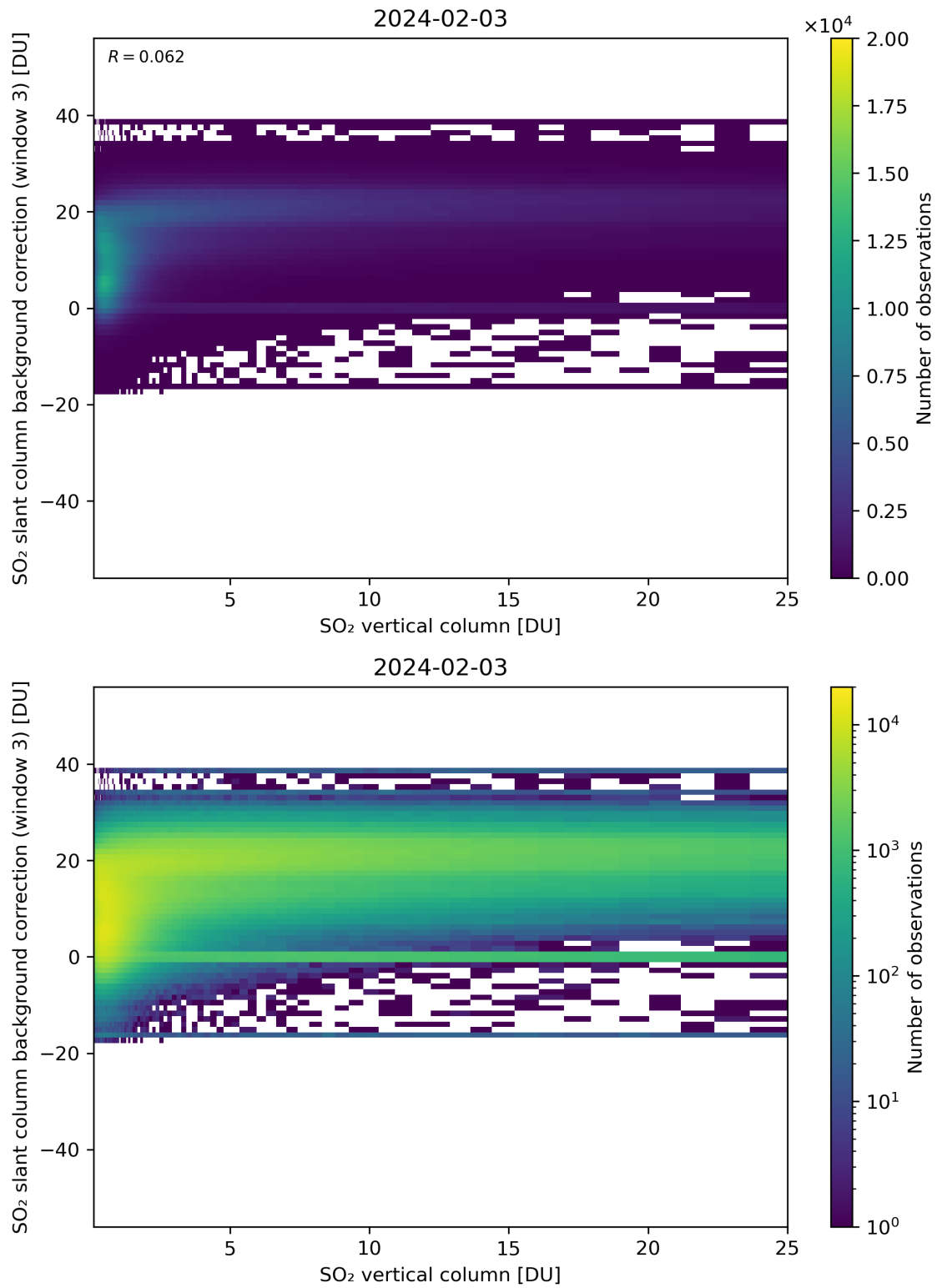
Figure 275: Scatter density plot of “SO 2 vertical column” against “SO 2 slant column background correction (window 3)” for 2024-02-02 to 2024-02-04.
