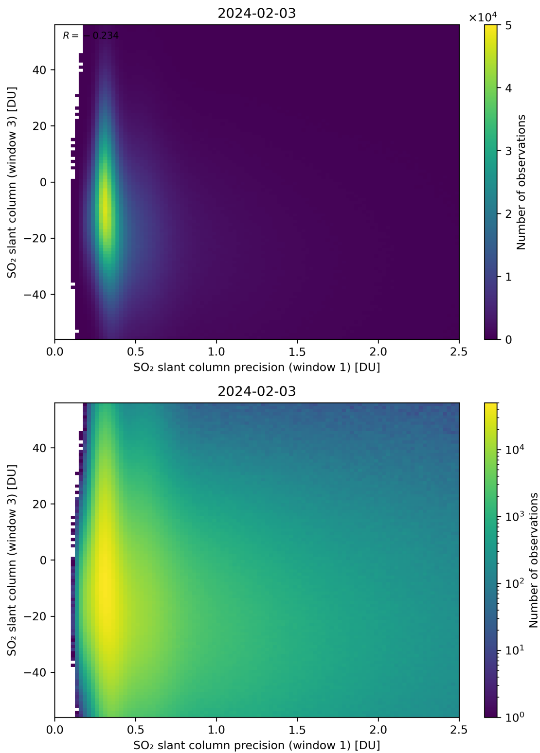
Figure 228: Scatter density plot of “SO 2 slant column precision (window 1)” against “SO 2 slant column (window 3)” for 2024-02-02 to 2024-02-04.
