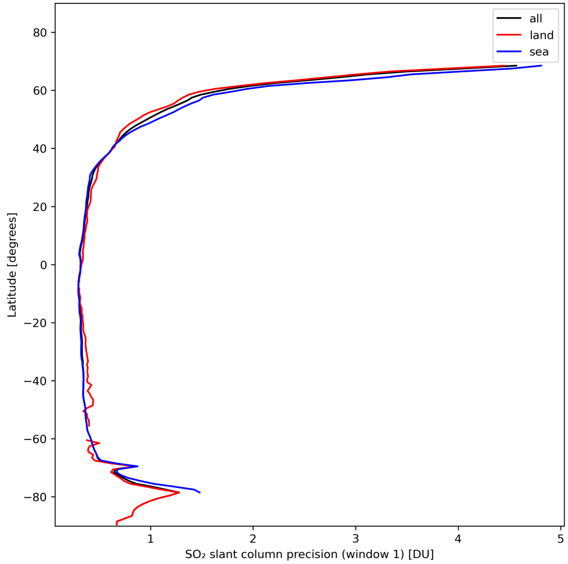
Figure 34: Zonal average of “SO 2 slant column precision (window 1)” for 2024-02-02 to 2024-02-04.
