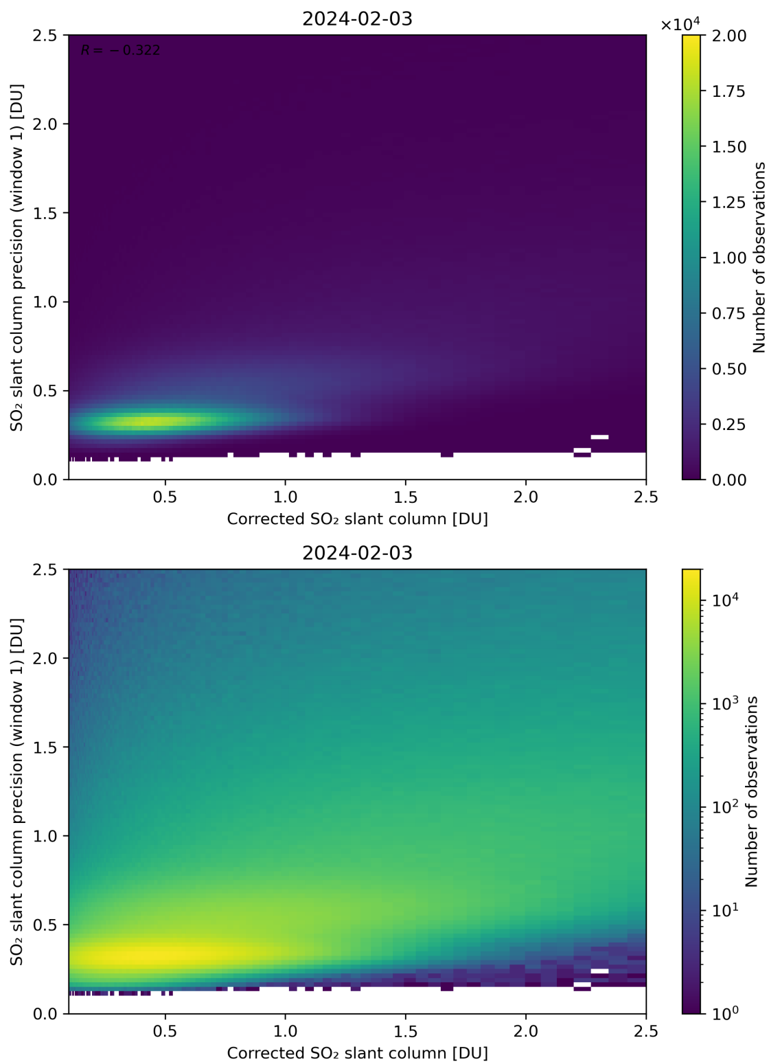
Figure 188: Scatter density plot of “Corrected SO 2 slant column” against “SO 2 slant column precision (window 1)” for 2024-02-02 to 2024-02-04.
