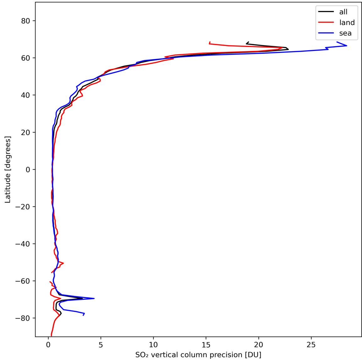
Figure 31: Zonal average of “SO 2 vertical column precision” for 2024-02-02 to 2024-02-04.
