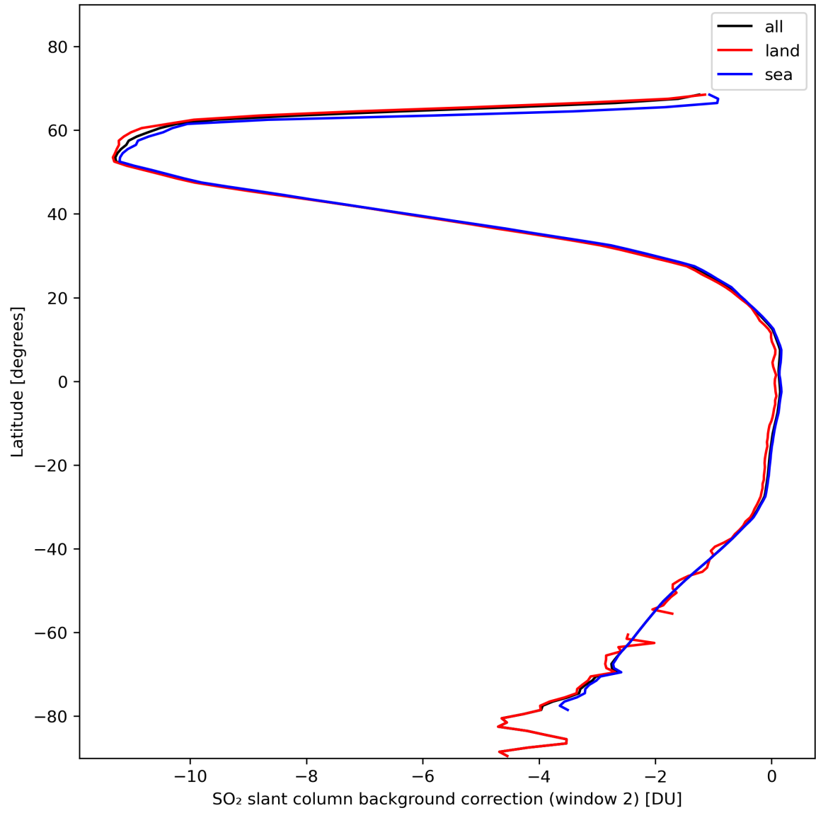
Figure 40: Zonal average of “SO 2 slant column background correction (window 2)” for 2024-02-02 to 2024-02-04.
