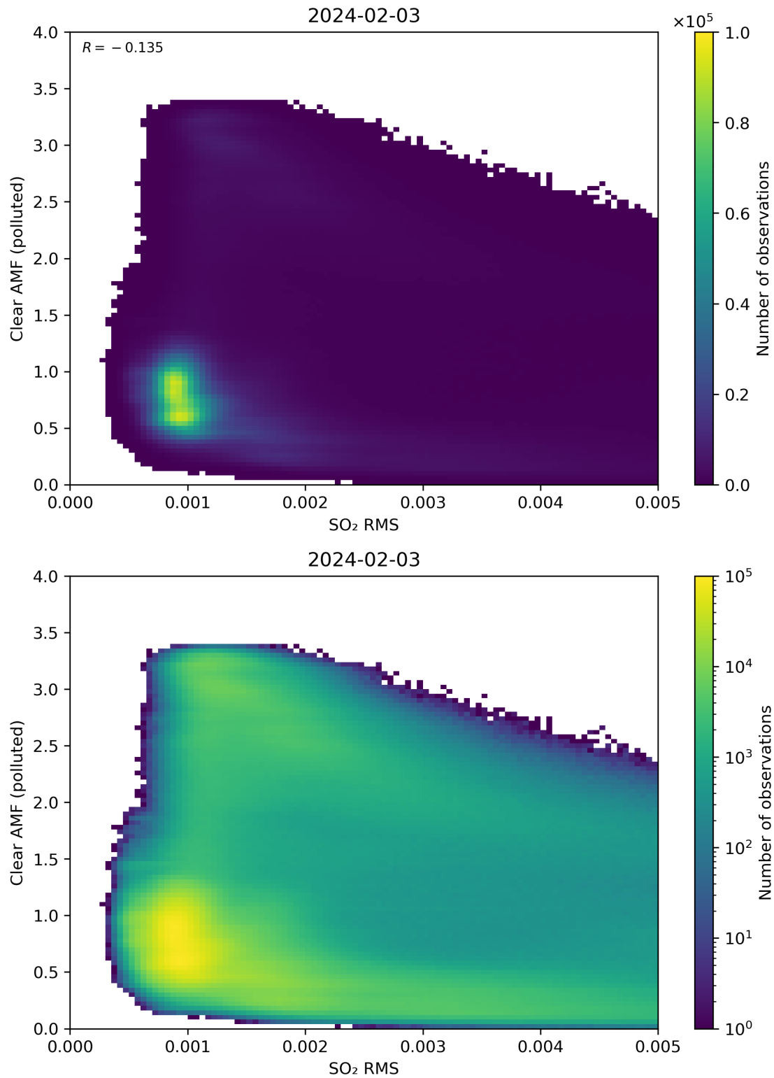
Figure 136: Scatter density plot of “SO 2 RMS” against “Clear AMF (polluted)” for 2024-02-02 to 2024-02-04.
