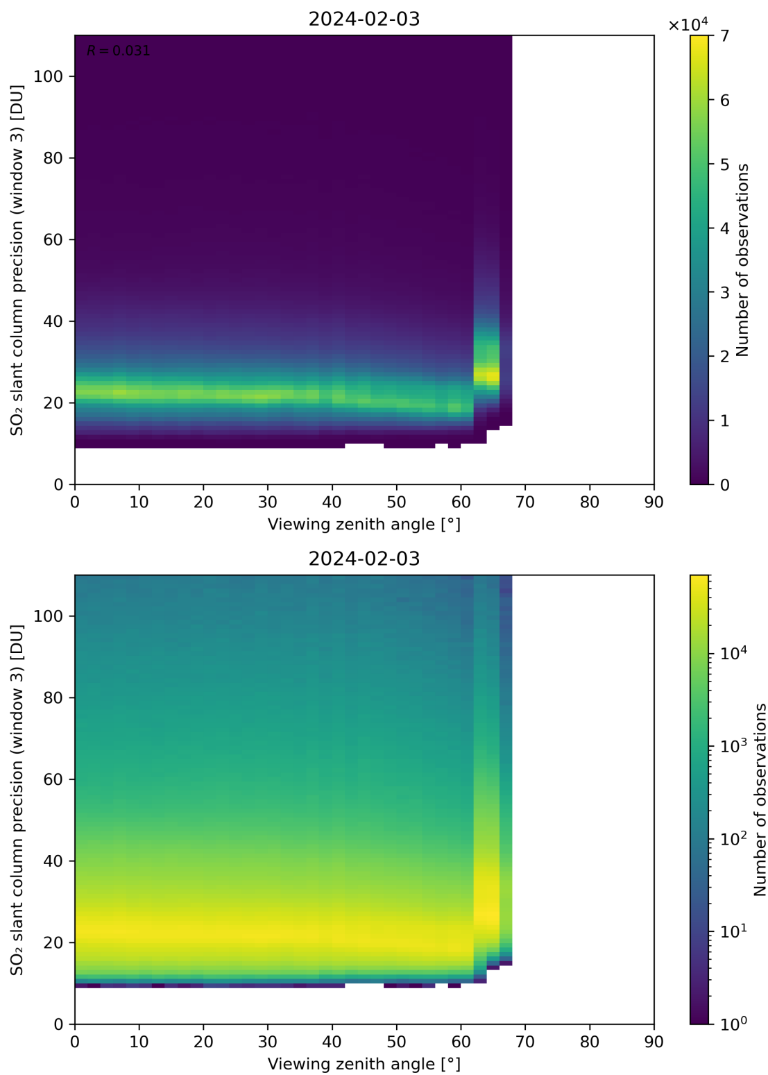
Figure 324: Scatter density plot of “Viewing zenith angle” against “SO 2 slant column precision (window 3)” for 2024-02-02 to 2024-02-04.
