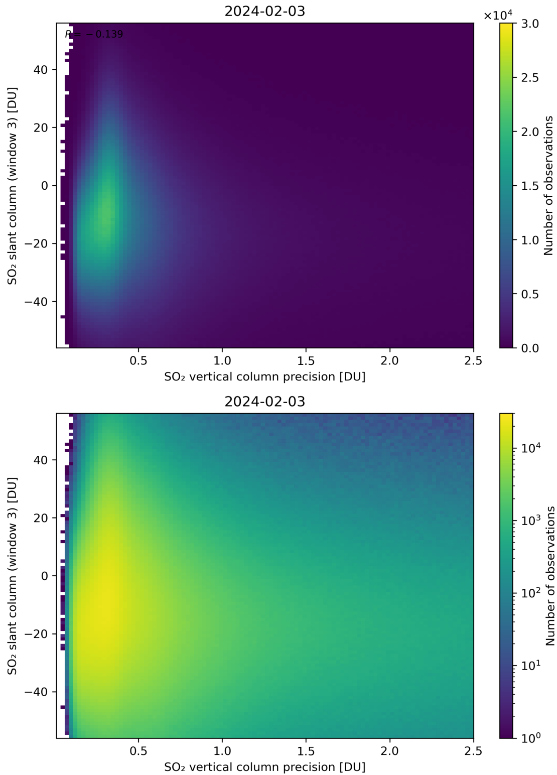
Figure 292: Scatter density plot of “SO 2 vertical column precision” against “SO 2 slant column (window 3)” for 2024-02-02 to 2024-02-04.
