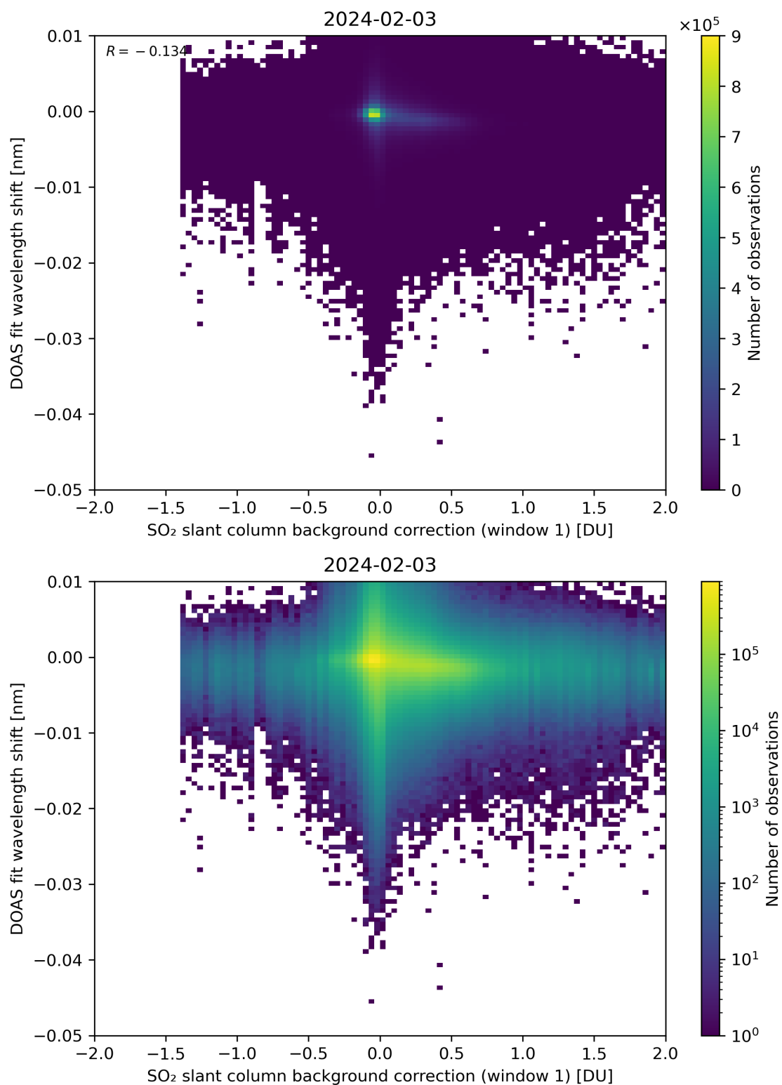
Figure 100: Scatter density plot of “SO 2 slant column background correction (window 1)” against “DOAS fit wavelength shift” for 2024-02-02 to 2024-02-04.
