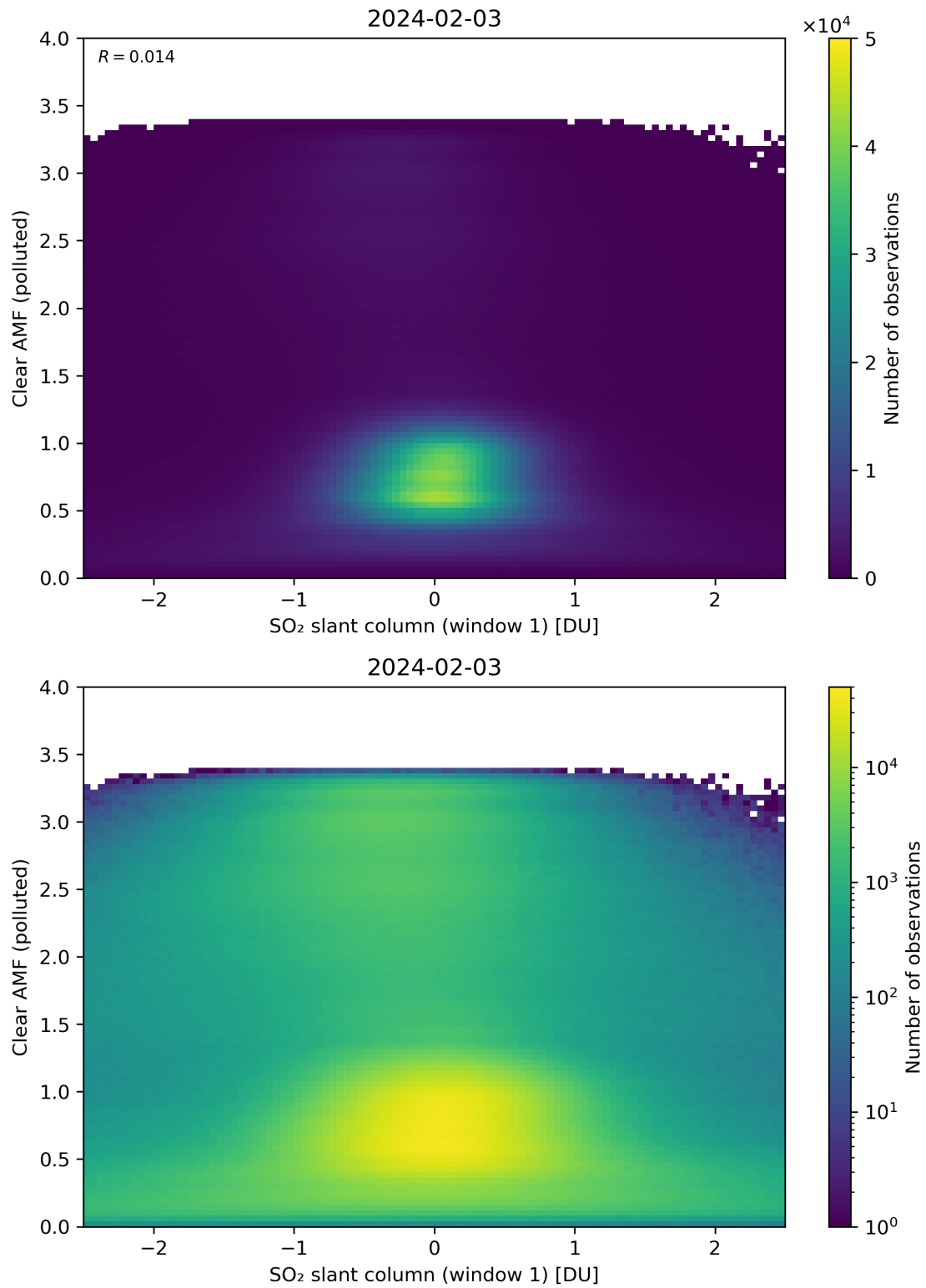
Figure 232: Scatter density plot of “SO 2 slant column (window 1)” against “Clear AMF (polluted)” for 2024-02-02 to 2024-02-04.
