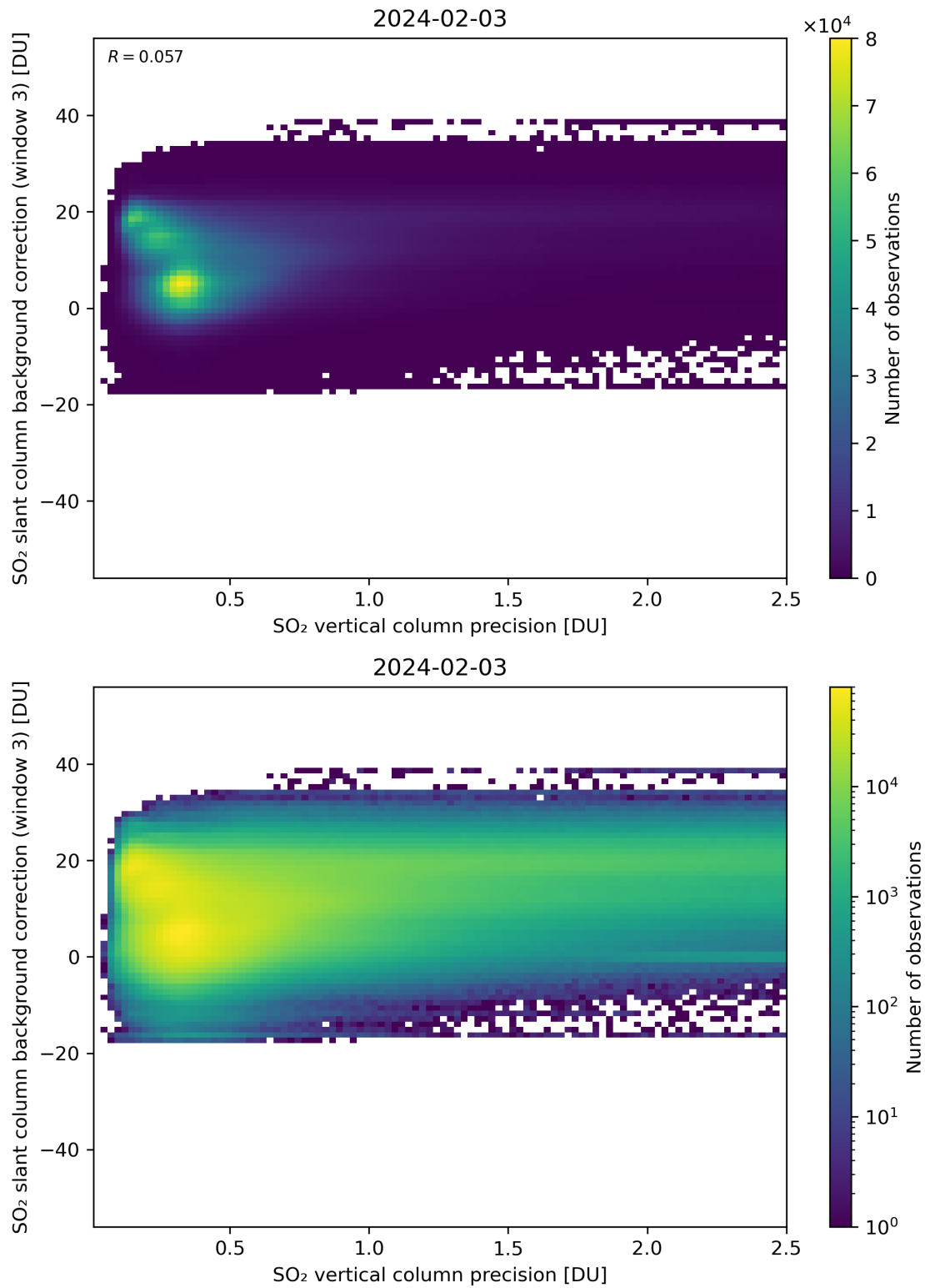
Figure 281: Scatter density plot of “SO 2 vertical column precision” against “SO 2 slant column background correction (window 3)” for 2024-02-02 to 2024-02-04.
