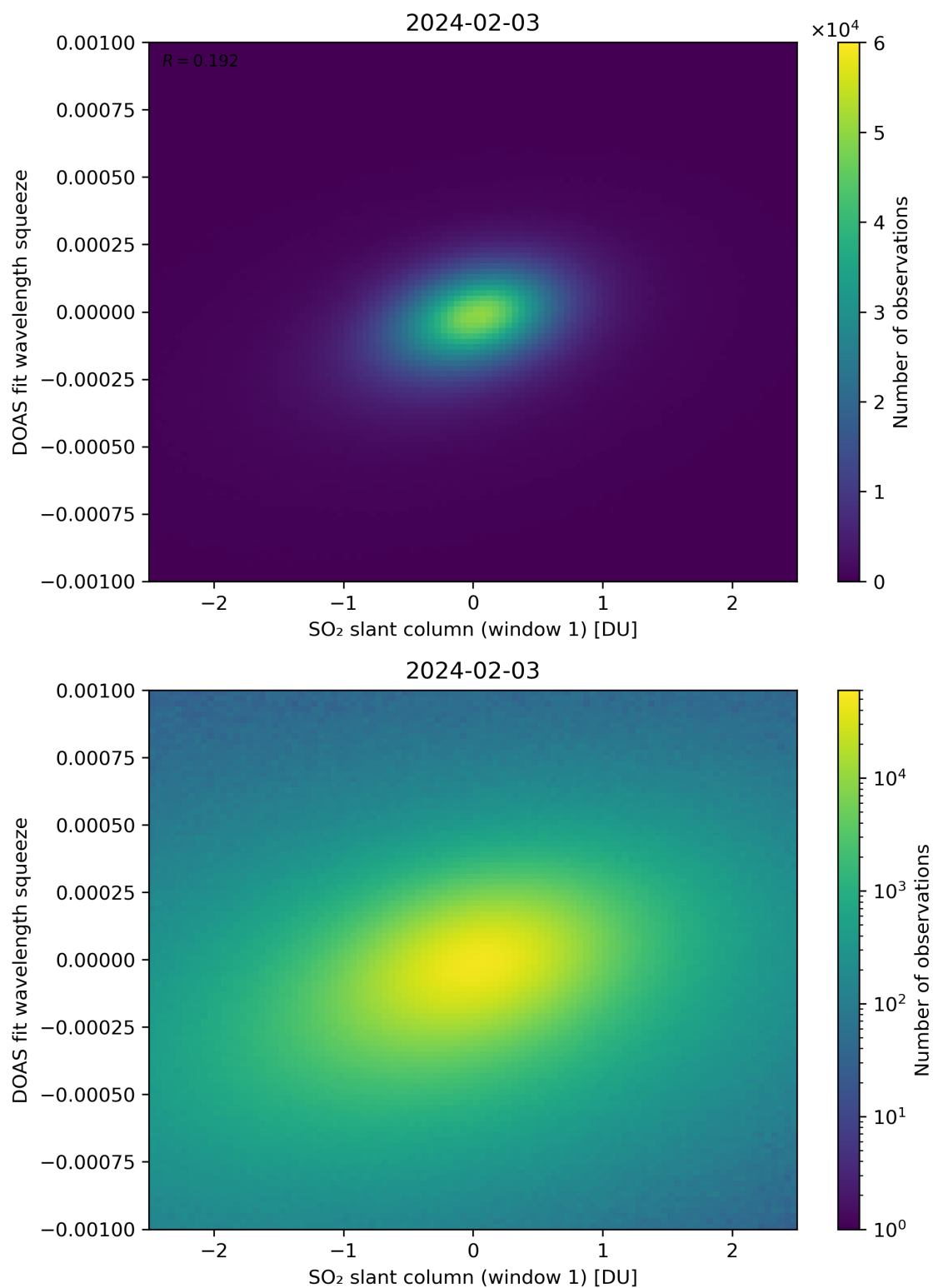
Figure 216: Scatter density plot of “SO 2 slant column (window 1)” against “DOAS fit wavelength squeeze” for 2024-02-02 to 2024-02-04.
