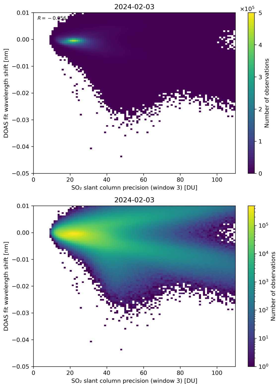
Figure 258: Scatter density plot of “SO 2 slant column precision (window 3)” against “DOAS fit wavelength shift” for 2024-02-02 to 2024-02-04.
