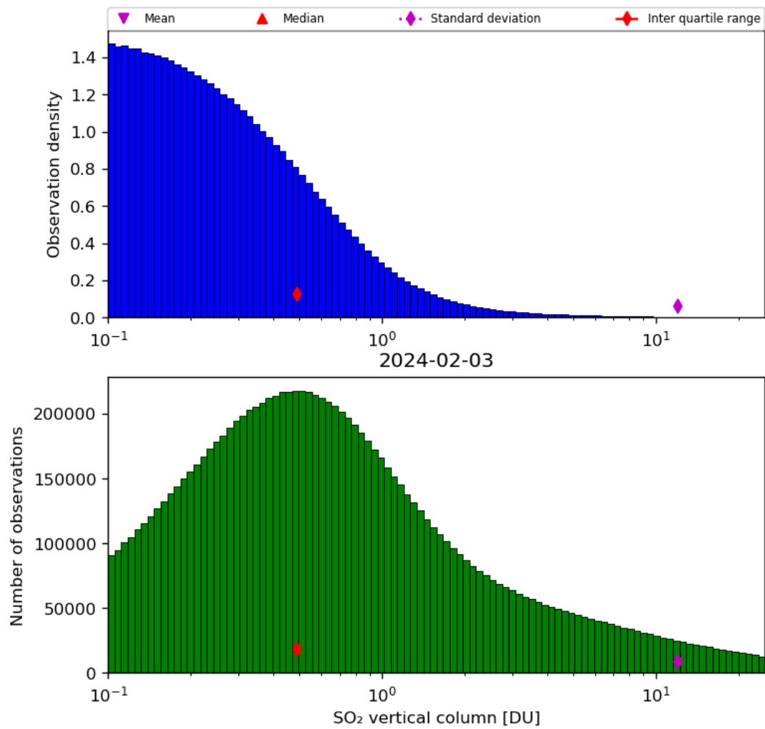
Figure 53: Histogram of “SO 2 vertical column” for 2024-02-02 to 2024-02-04
