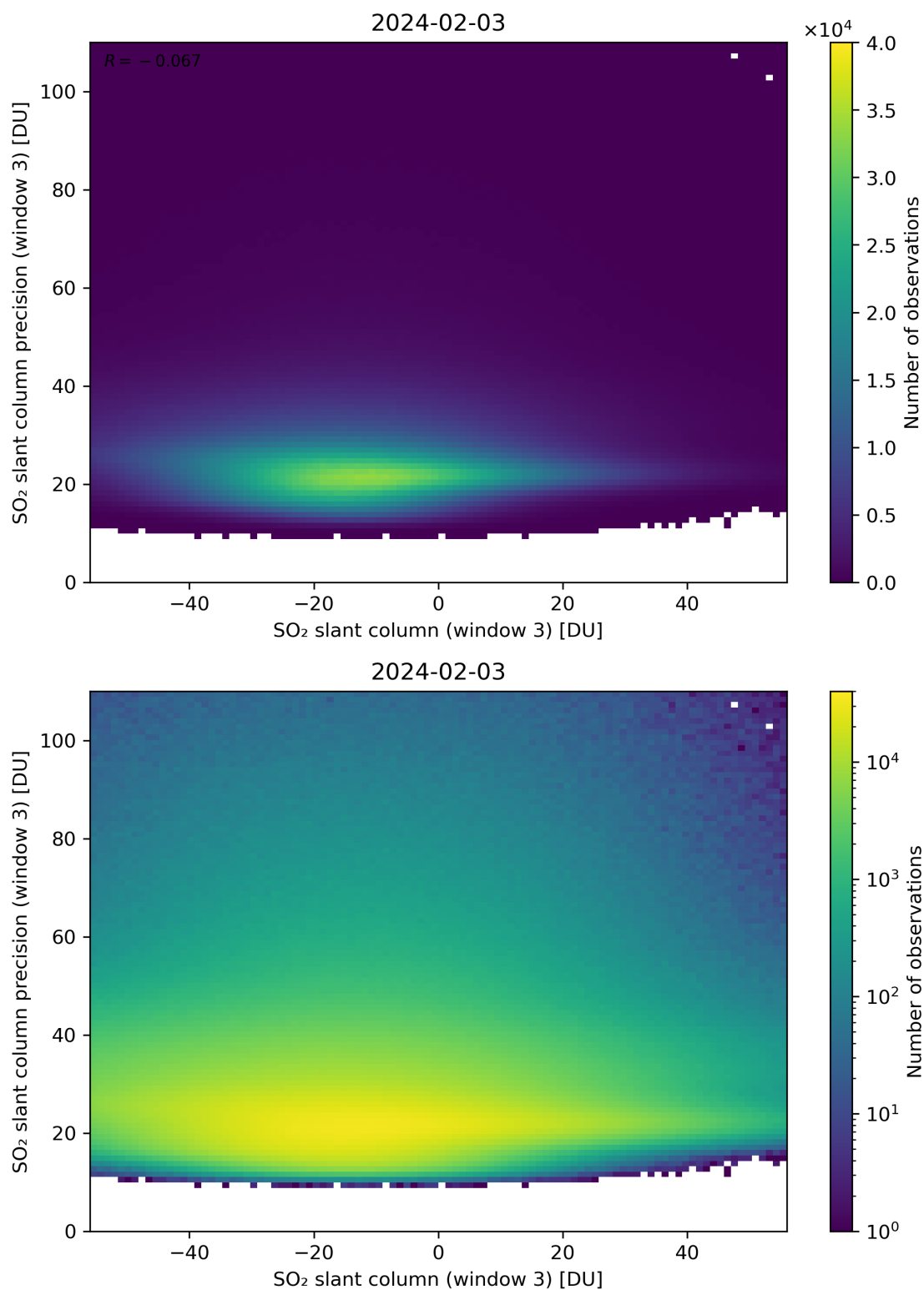
Figure 267: Scatter density plot of “SO 2 slant column (window 3)” against “SO 2 slant column precision (window 3)” for 2024-02-02 to 2024-02-04.
