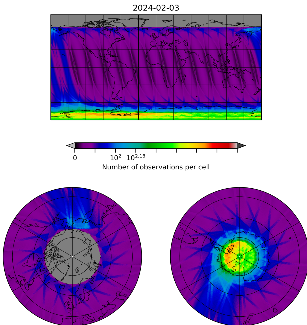
Figure 28: Map of the number of observations for 2024-02-02 to 2024-02-04
