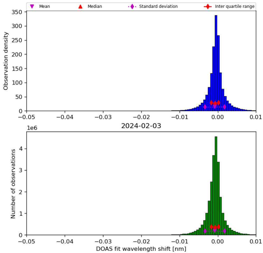
Figure 68: Histogram of “DOAS fit wavelength shift” for 2024-02-02 to 2024-02-04
