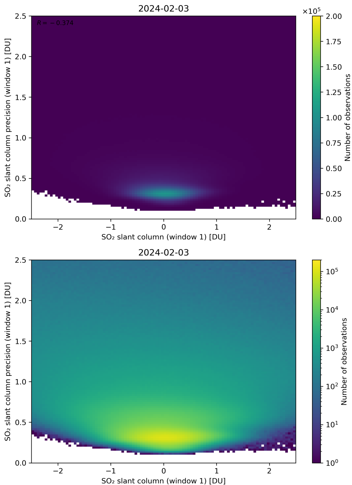
Figure 235: Scatter density plot of “SO 2 slant column (window 1)” against “SO 2 slant column precision (window 1)” for 2024-02-02 to 2024-02-04.
