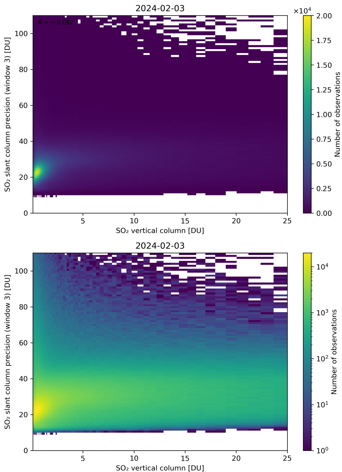
Figure 304: Scatter density plot of “SO 2 vertical column” against “SO 2 slant column precision (window 3)” for 2024-02-02 to 2024-02-04.
