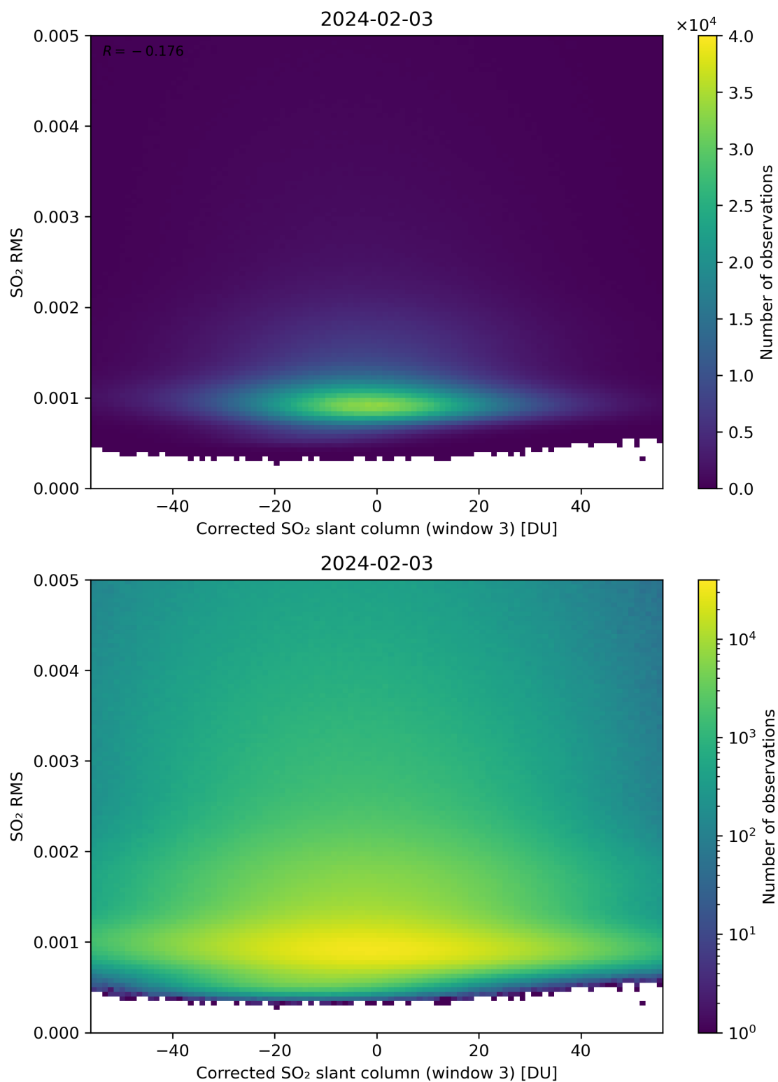
Figure 208: Scatter density plot of “Corrected SO 2 slant column (window 3)” against “SO 2 RMS” for 2024-02-02 to 2024-02-04.
