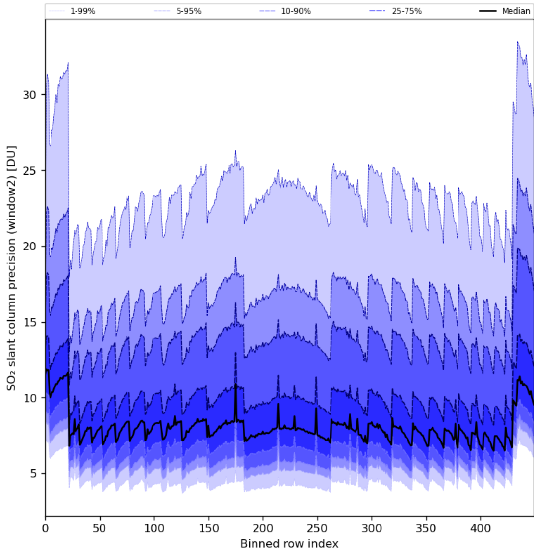
Figure 84: Along track statistics of “SO 2 slant column precision (window2)” for 2024-02-02 to 2024-02-04
