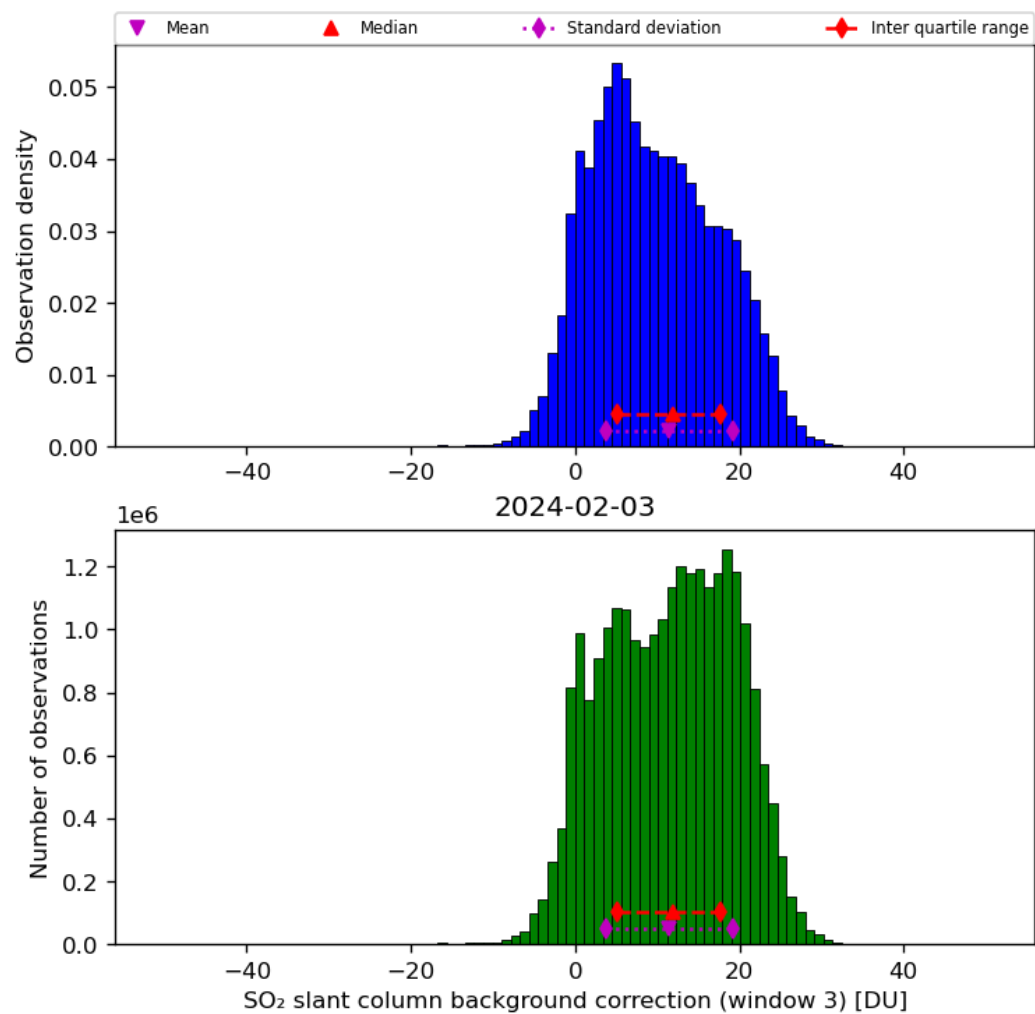
Figure 67: Histogram of “SO 2 slant column background correction (window 3)” for 2024-02-02 to 2024-02-04
