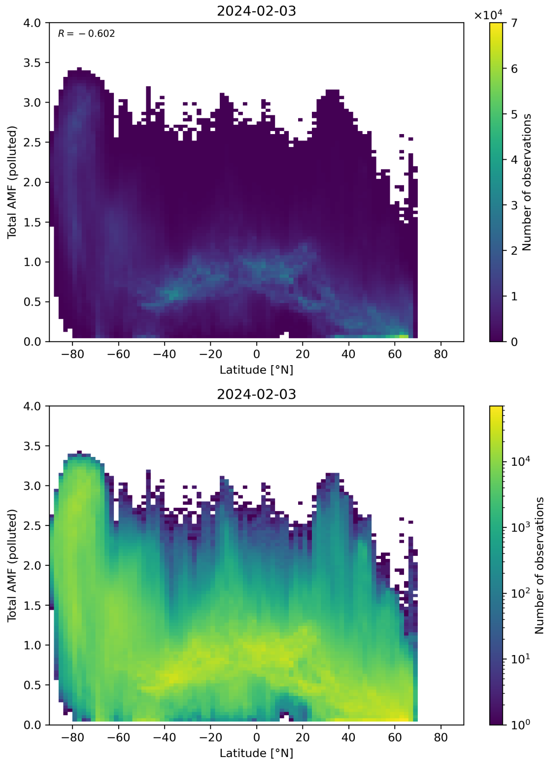
Figure 154: Scatter density plot of “Latitude” against “Total AMF (polluted)” for 2024-02-02 to 2024-02-04.
