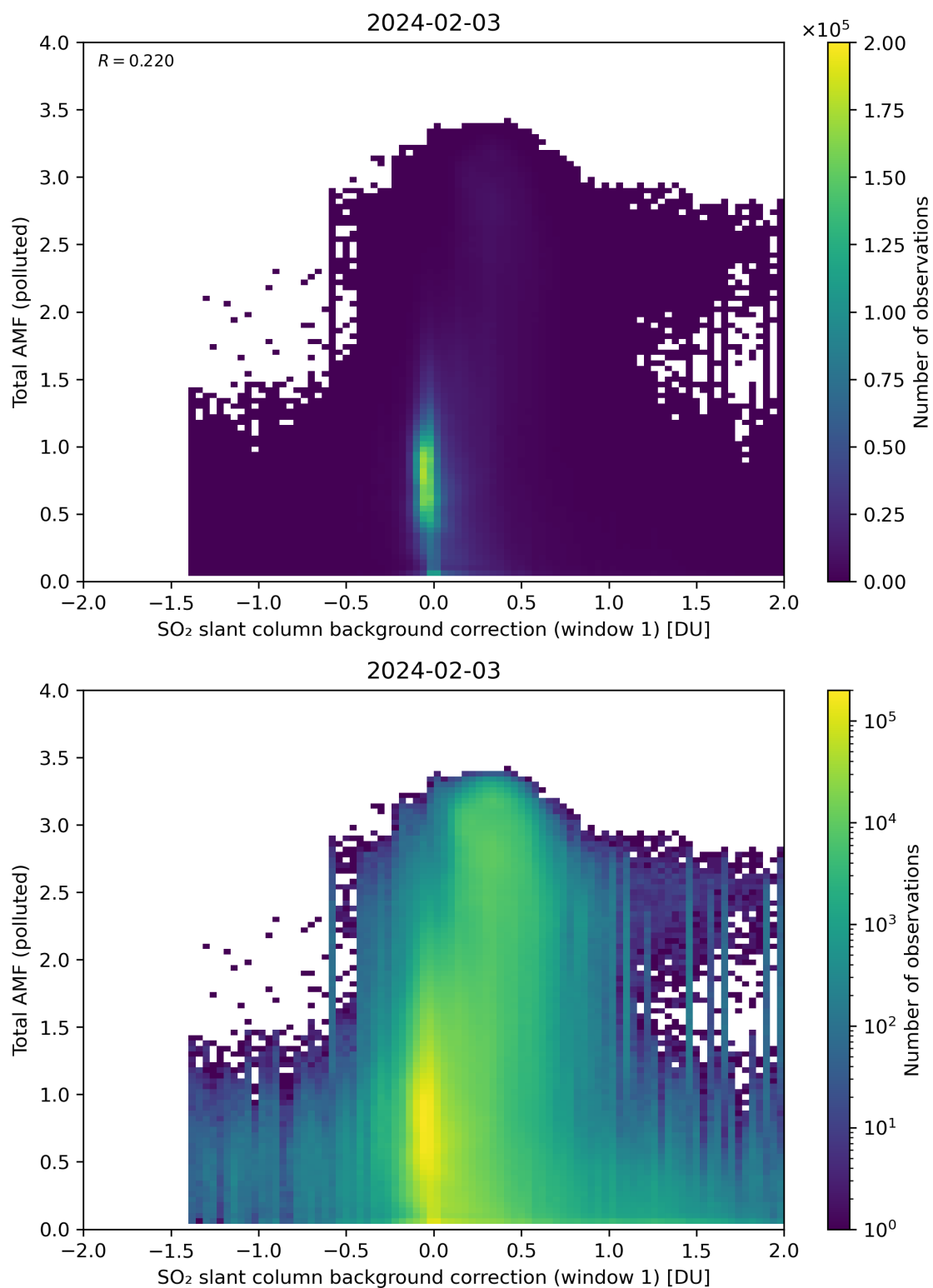
Figure 109: Scatter density plot of “SO 2 slant column background correction (window 1)” against “Total AMF (polluted)” for 2024-02-02 to 2024-02-04.
