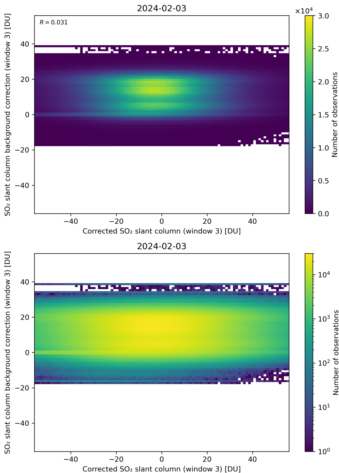
Figure 205: Scatter density plot of “Corrected SO 2 slant column (window 3)” against “SO 2 slant column background correction (window 3)” for 2024-02-02 to 2024-02-04.
