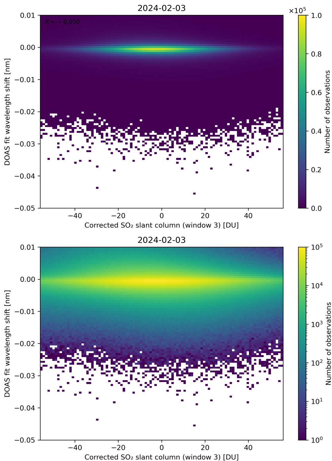
Figure 206: Scatter density plot of “Corrected SO 2 slant column (window 3)” against “DOAS fit wavelength shift” for 2024-02-02 to 2024-02-04.
