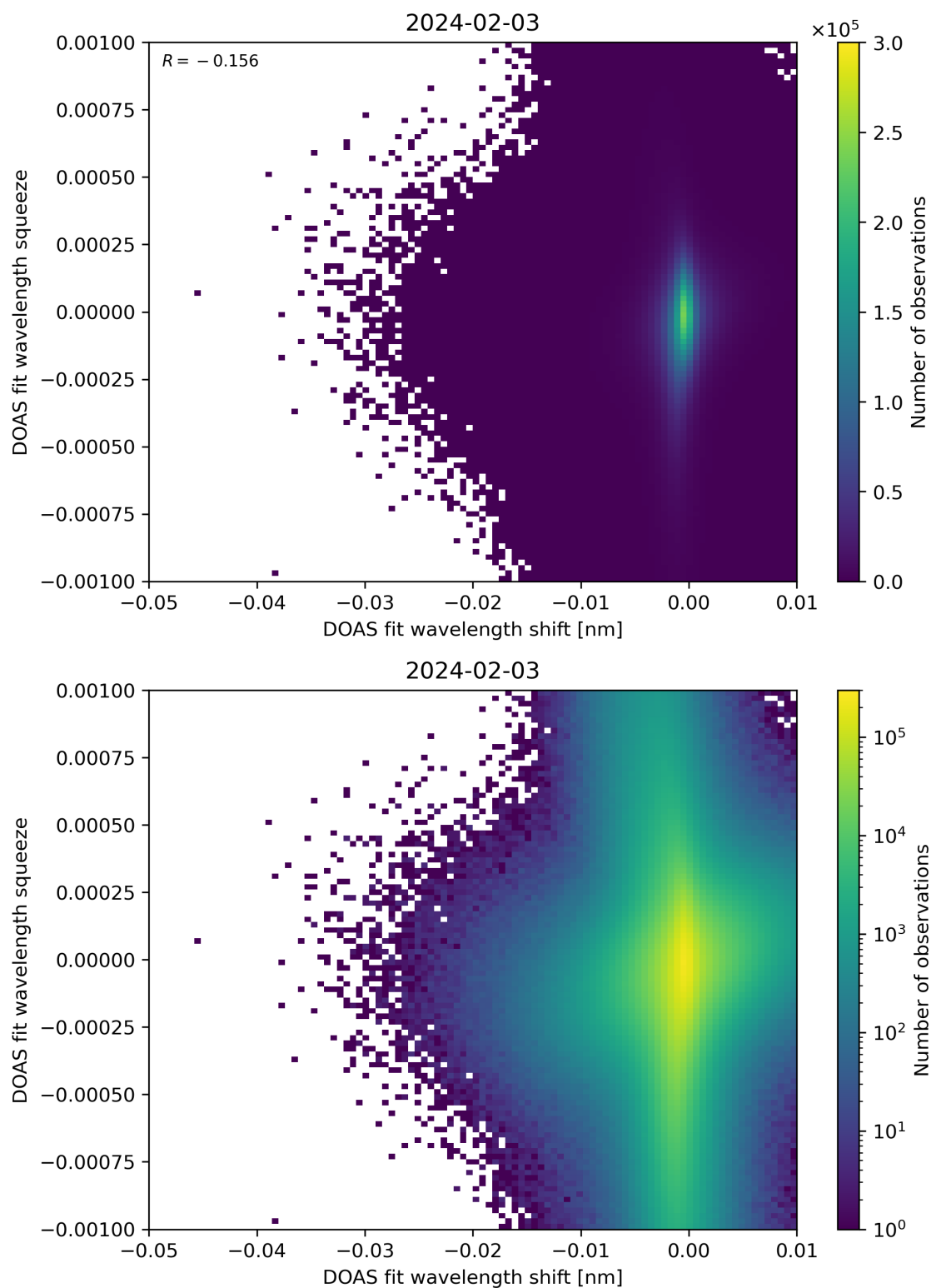
Figure 127: Scatter density plot of “DOAS fit wavelength shift” against “DOAS fit wavelength squeeze” for 2024-02-02 to 2024-02-04.
