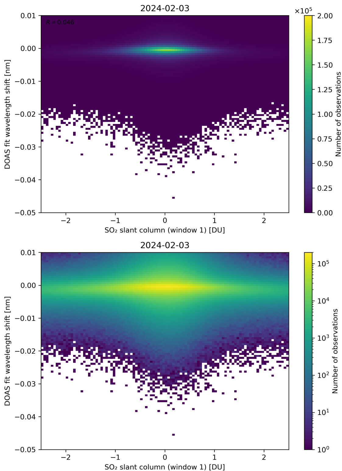
Figure 215: Scatter density plot of “SO 2 slant column (window 1)” against “DOAS fit wavelength shift” for 2024-02-02 to 2024-02-04.
