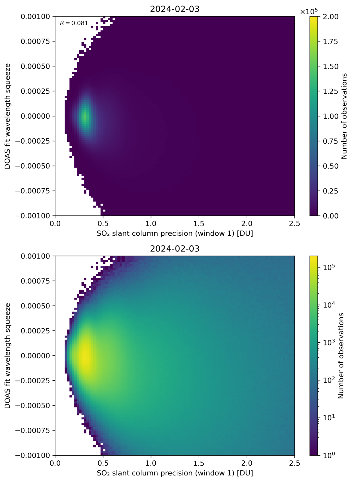
Figure 222: Scatter density plot of “SO 2 slant column precision (window 1)” against “DOAS fit wavelength squeeze” for 2024-02-02 to 2024-02-04.
