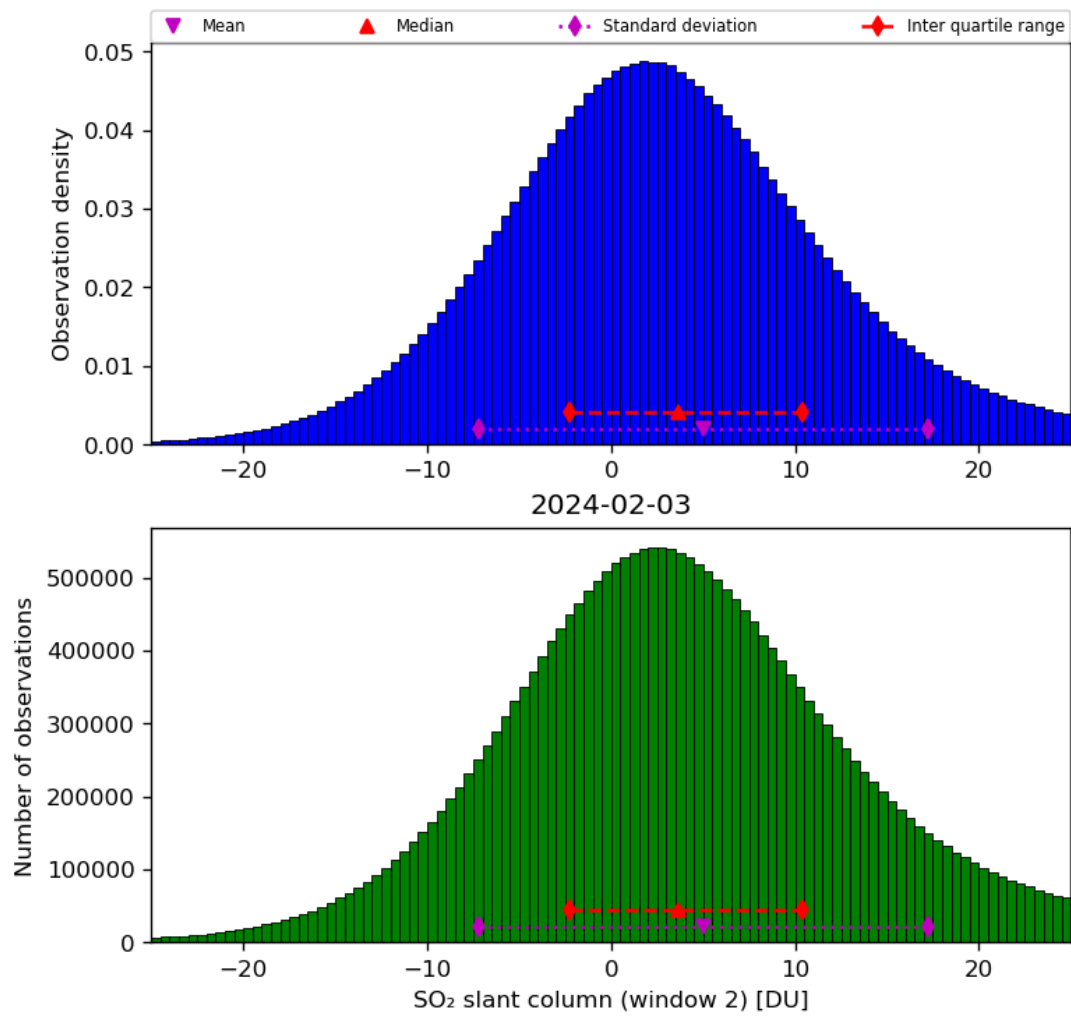
Figure 60: Histogram of “SO 2 slant column (window 2)” for 2024-02-02 to 2024-02-04
