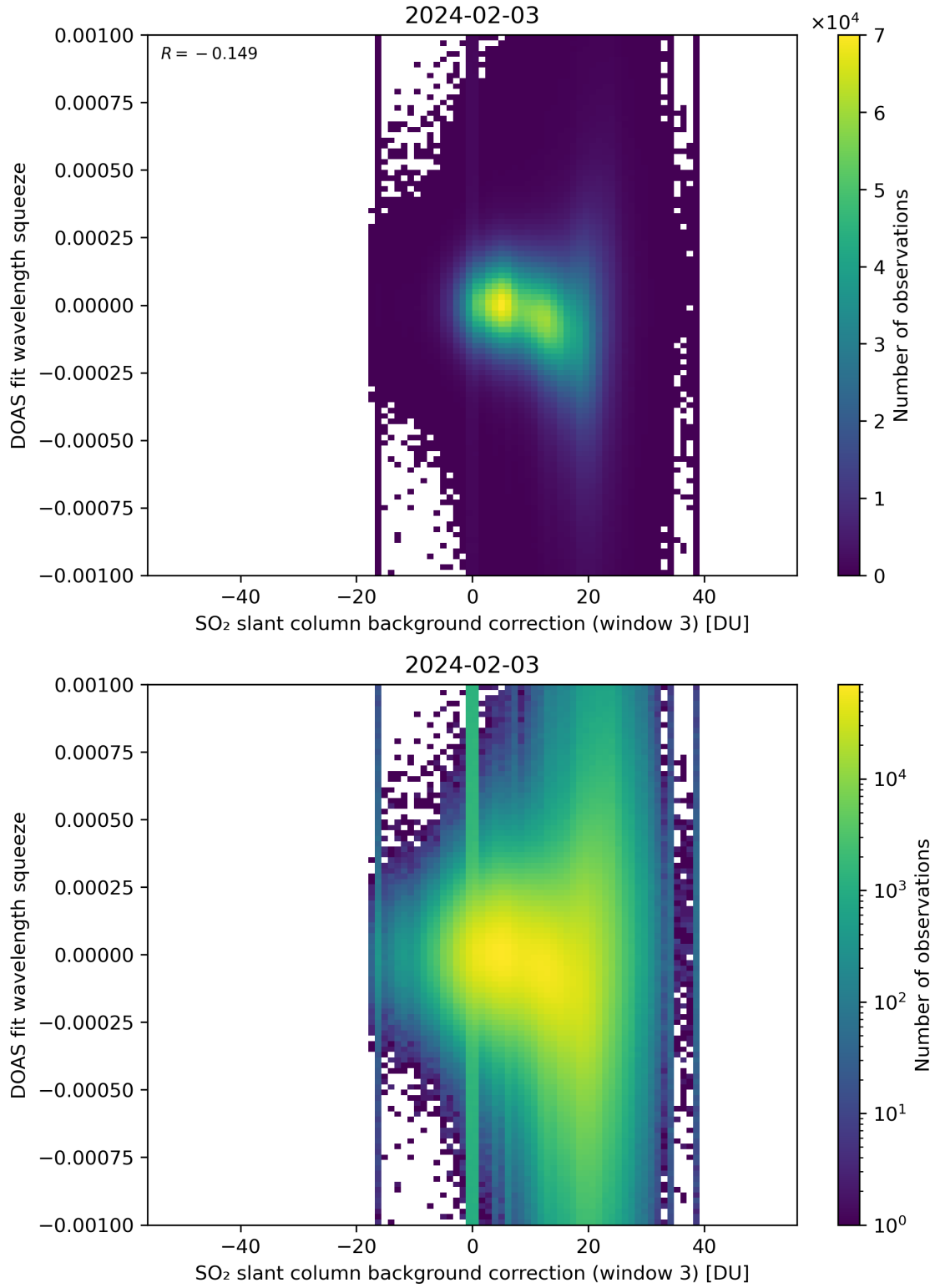
Figure 122: Scatter density plot of “SO 2 slant column background correction (window 3)” against “DOAS fit wavelength squeeze” for 2024-02-02 to 2024-02-04.
