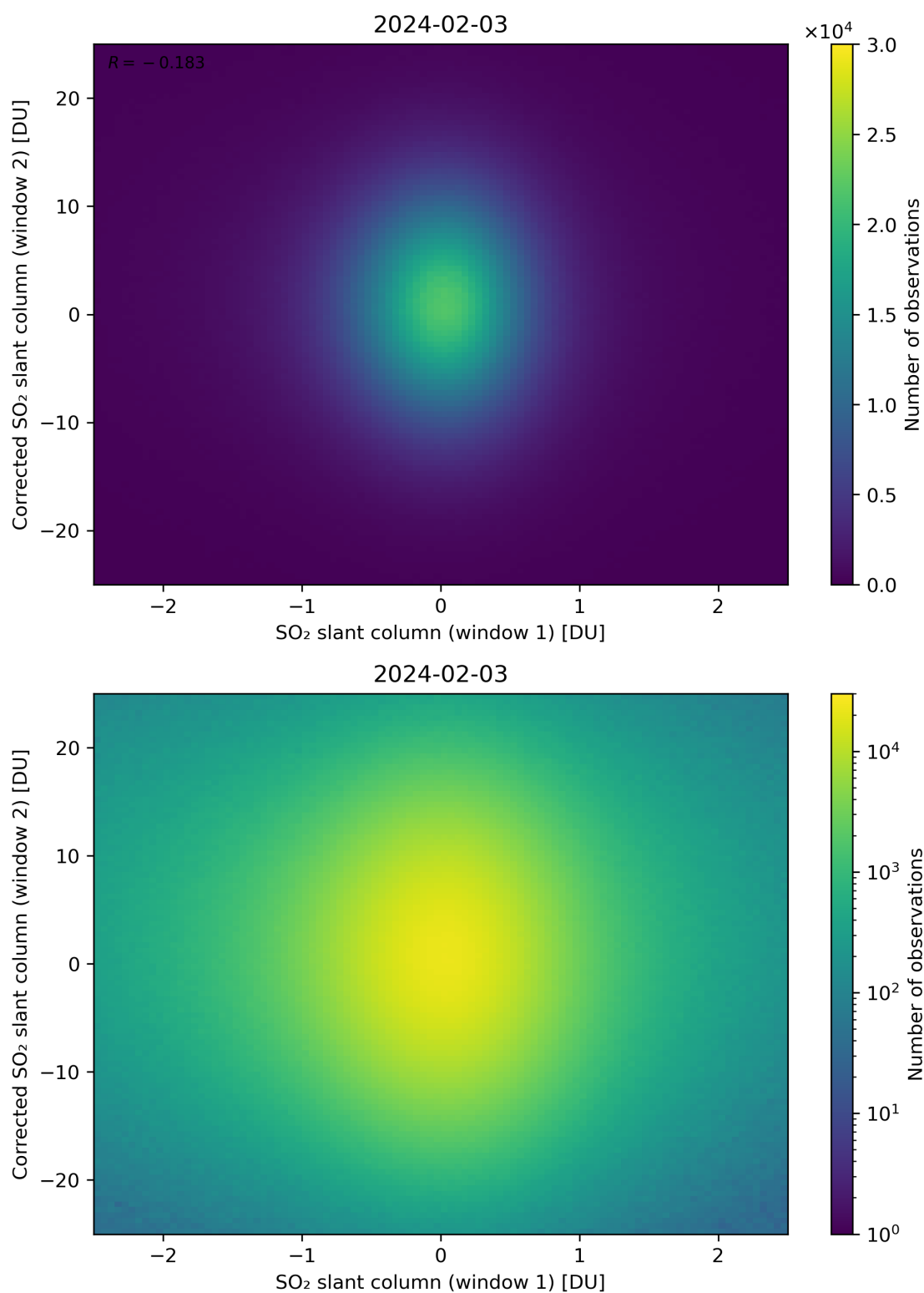
Figure 233: Scatter density plot of “SO 2 slant column (window 1)” against “Corrected SO 2 slant column (window 2)” for 2024-02-02 to 2024-02-04.
