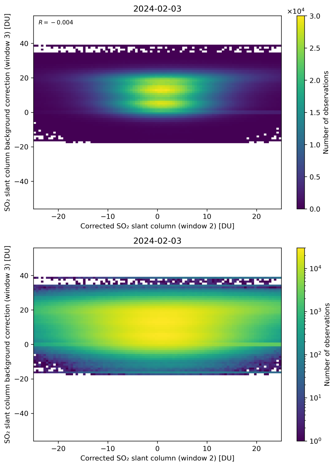
Figure 195: Scatter density plot of “Corrected SO 2 slant column (window 2)” against “SO 2 slant column background correction (window 3)” for 2024-02-02 to 2024-02-04.
