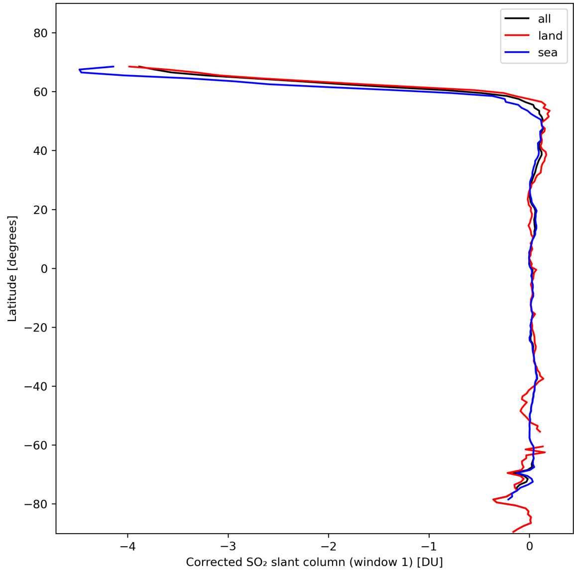
Figure 35: Zonal average of “Corrected SO 2 slant column (window 1)” for 2024-02-02 to 2024-02-04.
