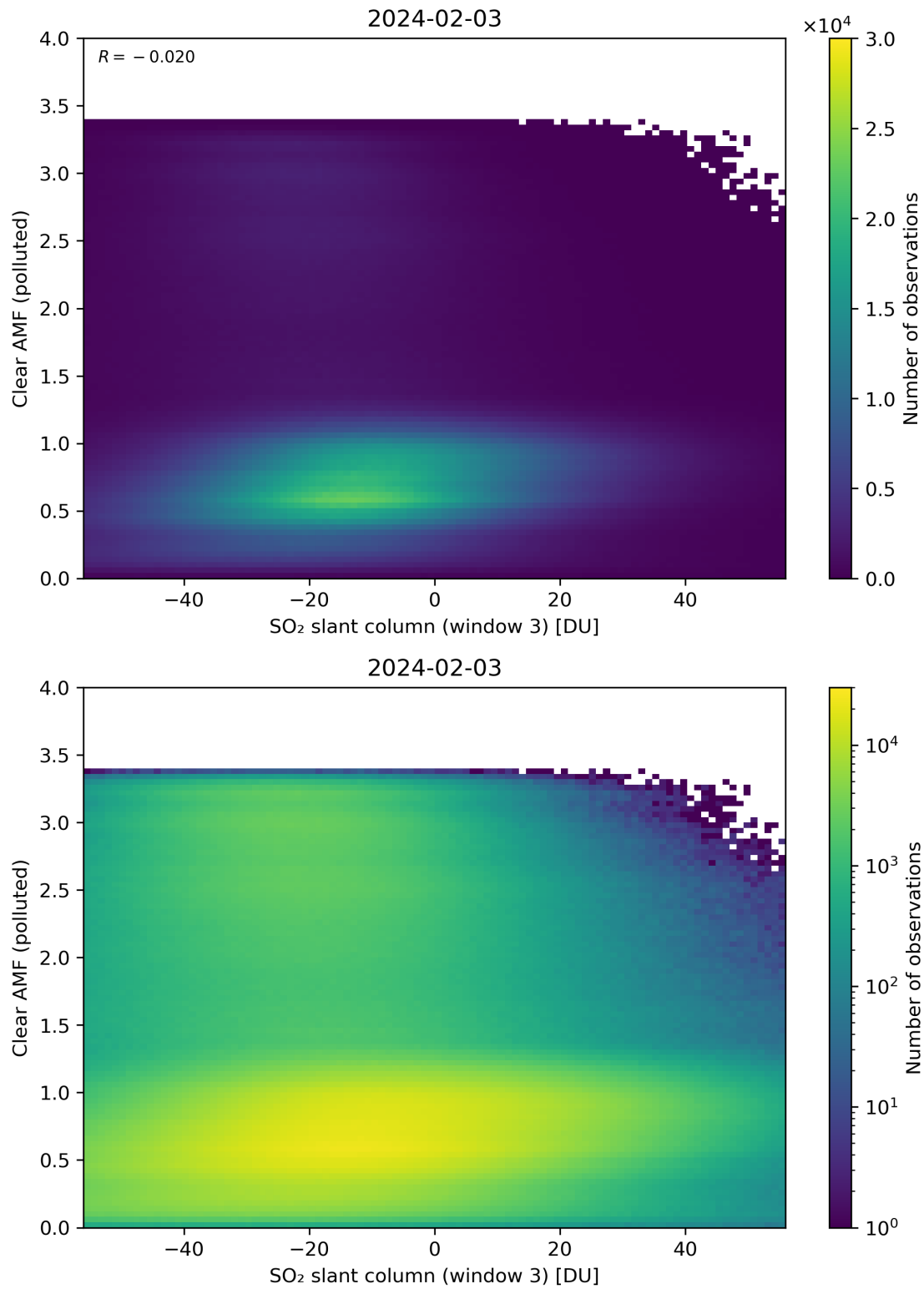
Figure 265: Scatter density plot of “SO 2 slant column (window 3)” against “Clear AMF (polluted)” for 2024-02-02 to 2024-02-04.
