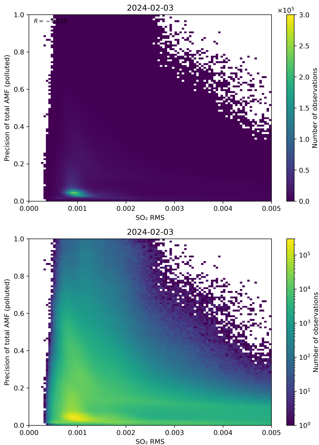
Figure 138: Scatter density plot of “SO 2 RMS” against “Precision of total AMF (polluted)” for 2024-02-02 to 2024-02-04.
