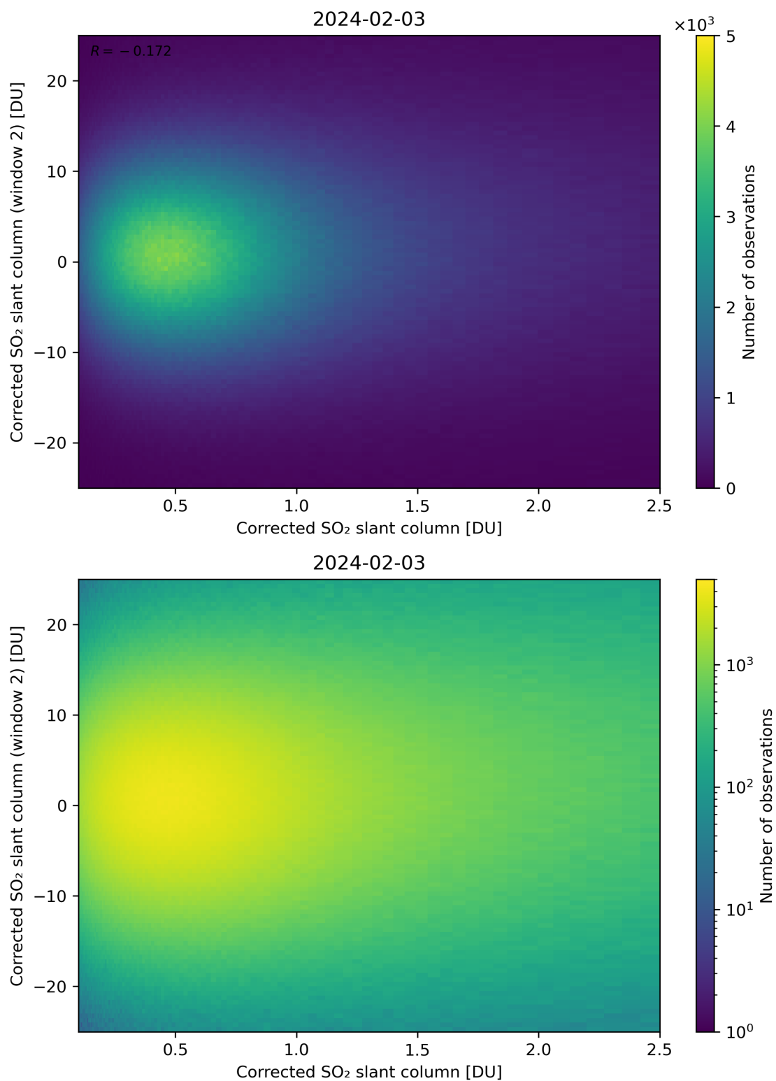
Figure 185: Scatter density plot of “Corrected SO 2 slant column” against “Corrected SO 2 slant column (window 2)” for 2024-02-02 to 2024-02-04.
