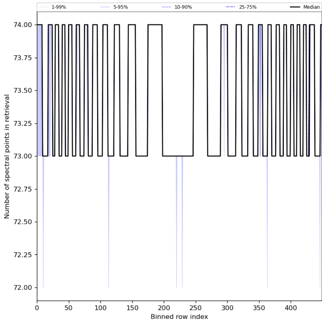
Figure 97: Along track statistics of “Number of spectral points in retrieval” for 2024-02-02 to 2024-02-04
