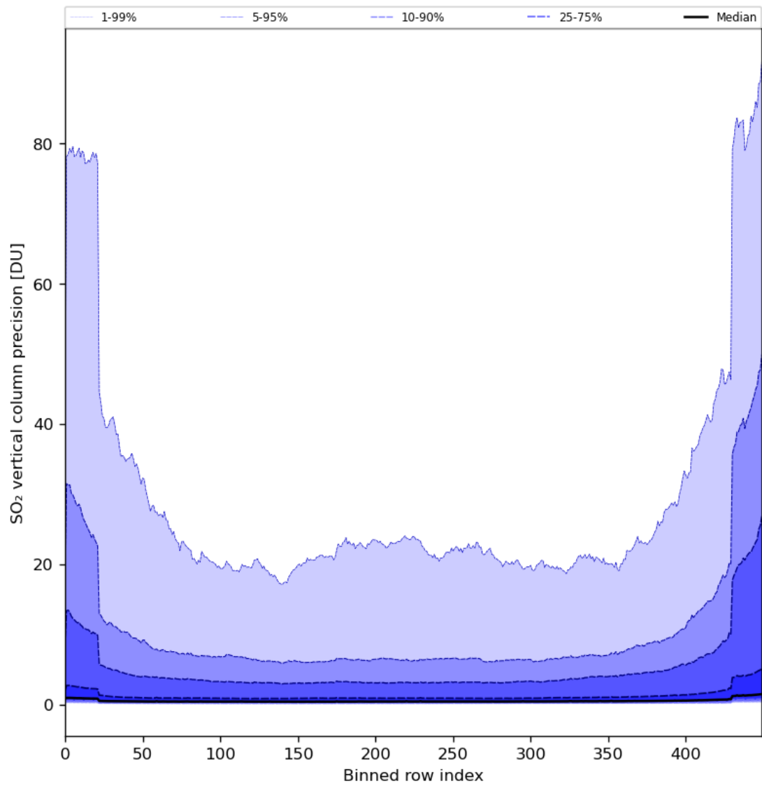
Figure 77: Along track statistics of “SO 2 vertical column precision” for 2024-02-02 to 2024-02-04
