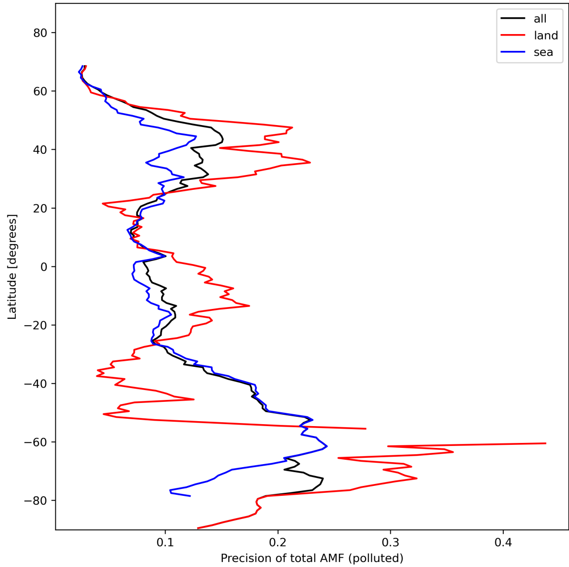
Figure 49: Zonal average of “Precision of total AMF (polluted)” for 2024-02-02 to 2024-02-04.
