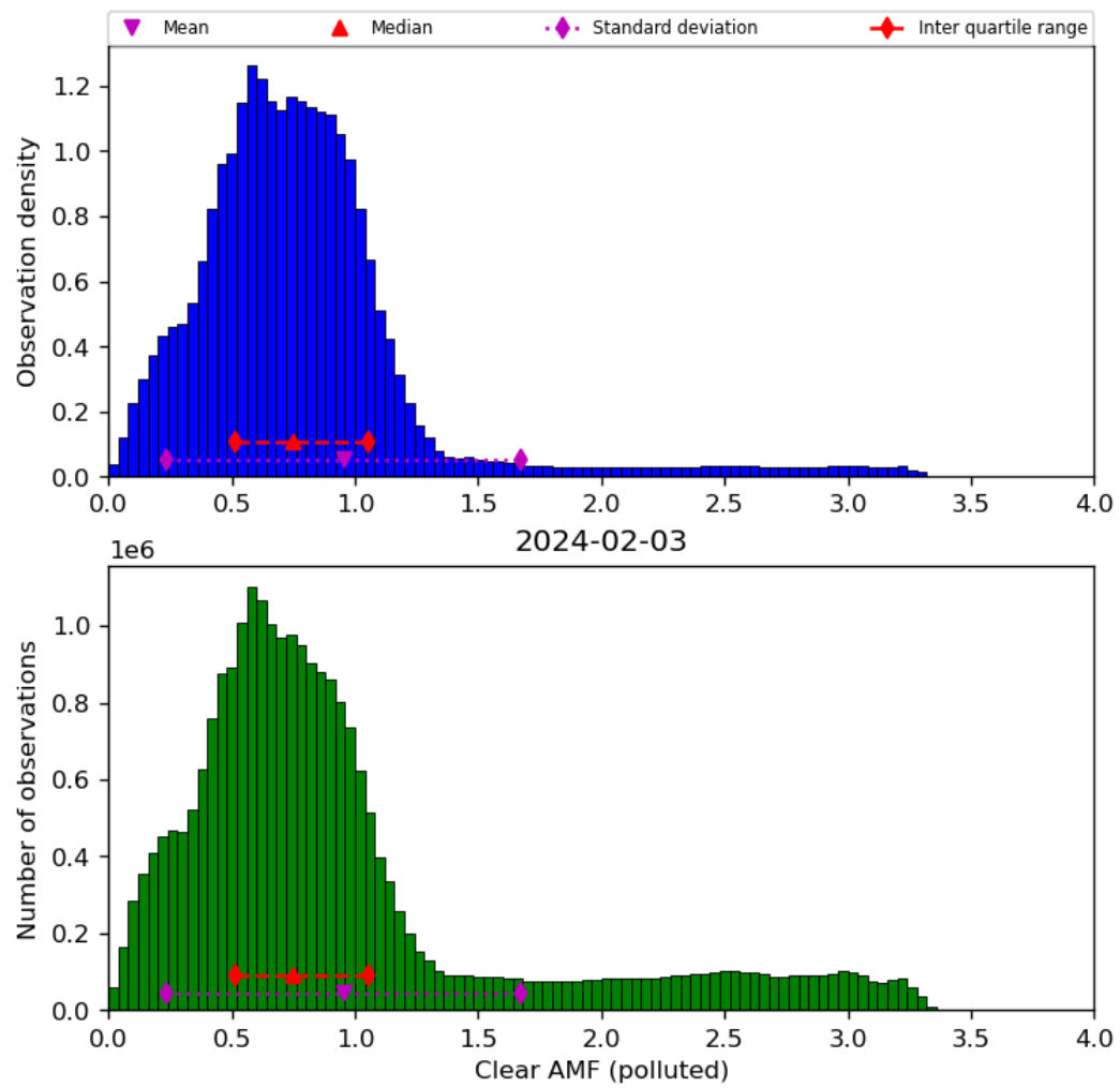
Figure 73: Histogram of “Clear AMF (polluted)” for 2024-02-02 to 2024-02-04
