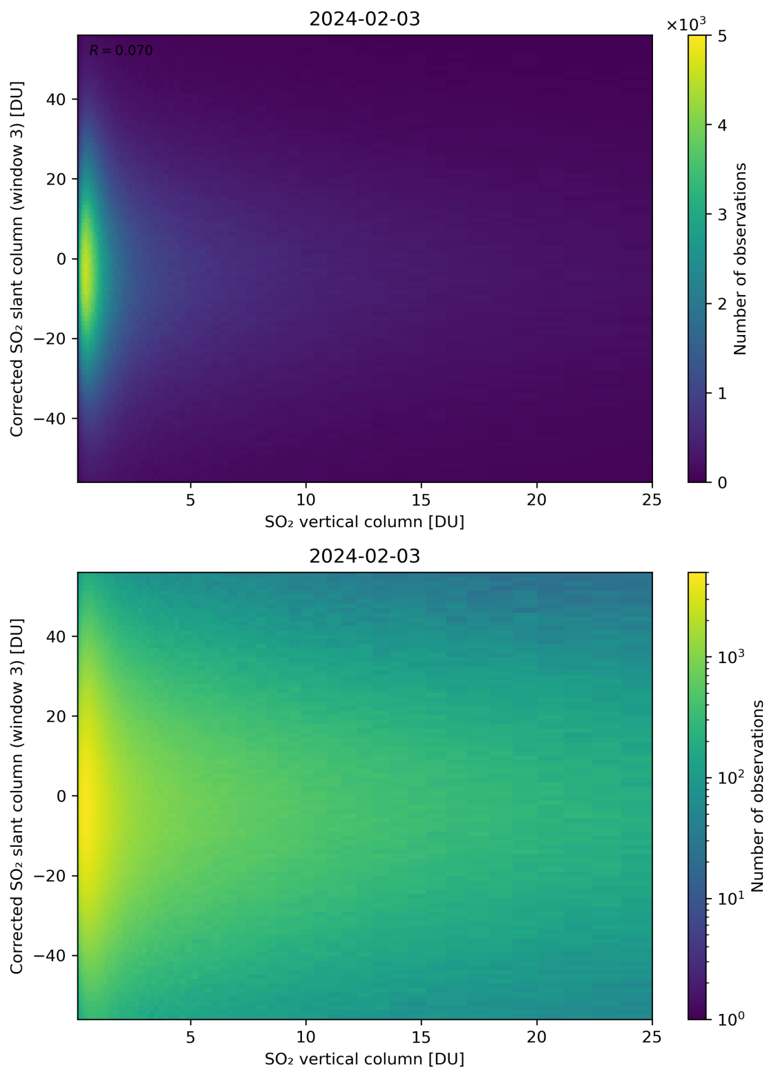
Figure 299: Scatter density plot of “SO 2 vertical column” against “Corrected SO 2 slant column (window 3)” for 2024-02-02 to 2024-02-04.
