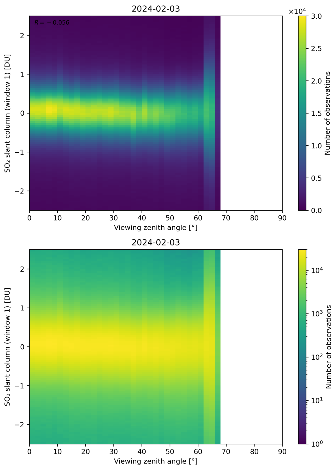
Figure 320: Scatter density plot of “Viewing zenith angle” against “SO 2 slant column (window 1)” for 2024-02-02 to 2024-02-04.
