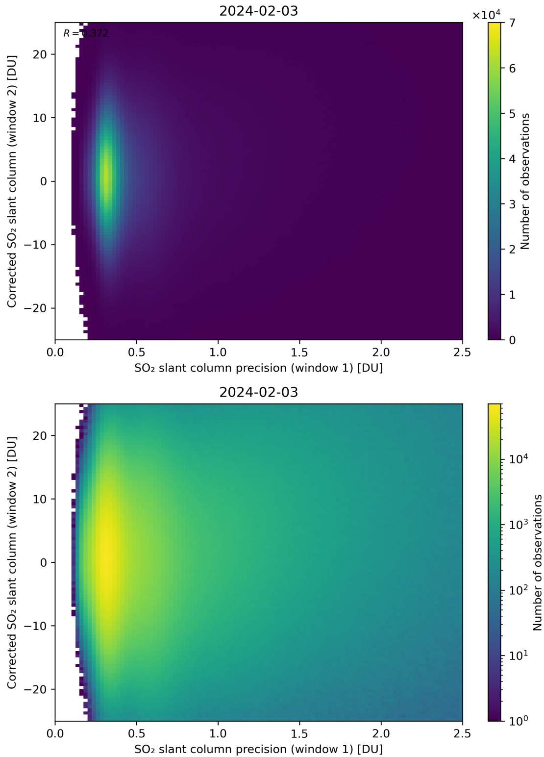
Figure 225: Scatter density plot of “SO 2 slant column precision (window 1)” against “Corrected SO 2 slant column (window 2)” for 2024-02-02 to 2024-02-04.
