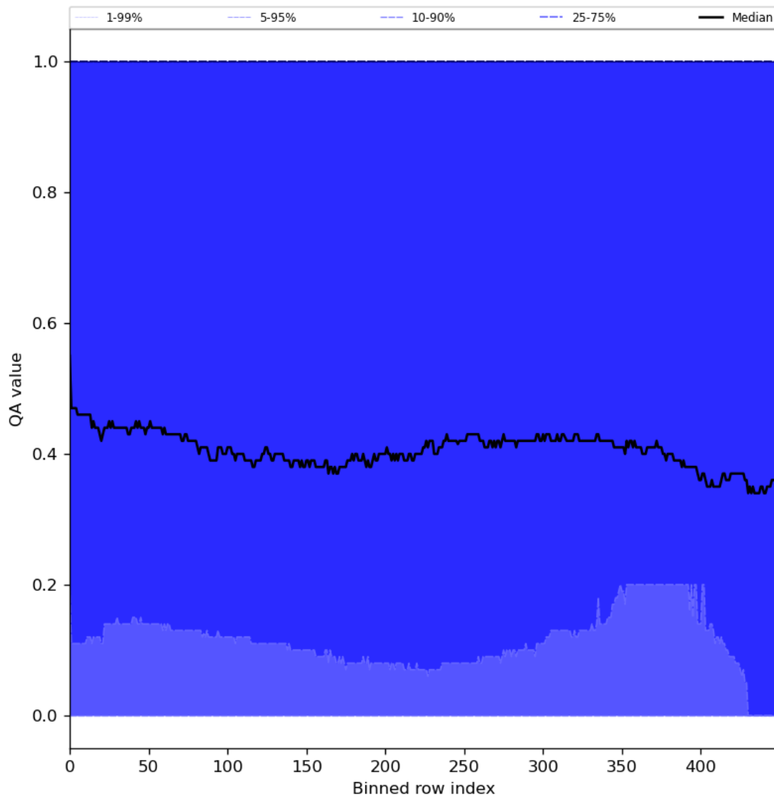
Figure 75: Along track statistics of “QA value” for 2024-02-02 to 2024-02-04
