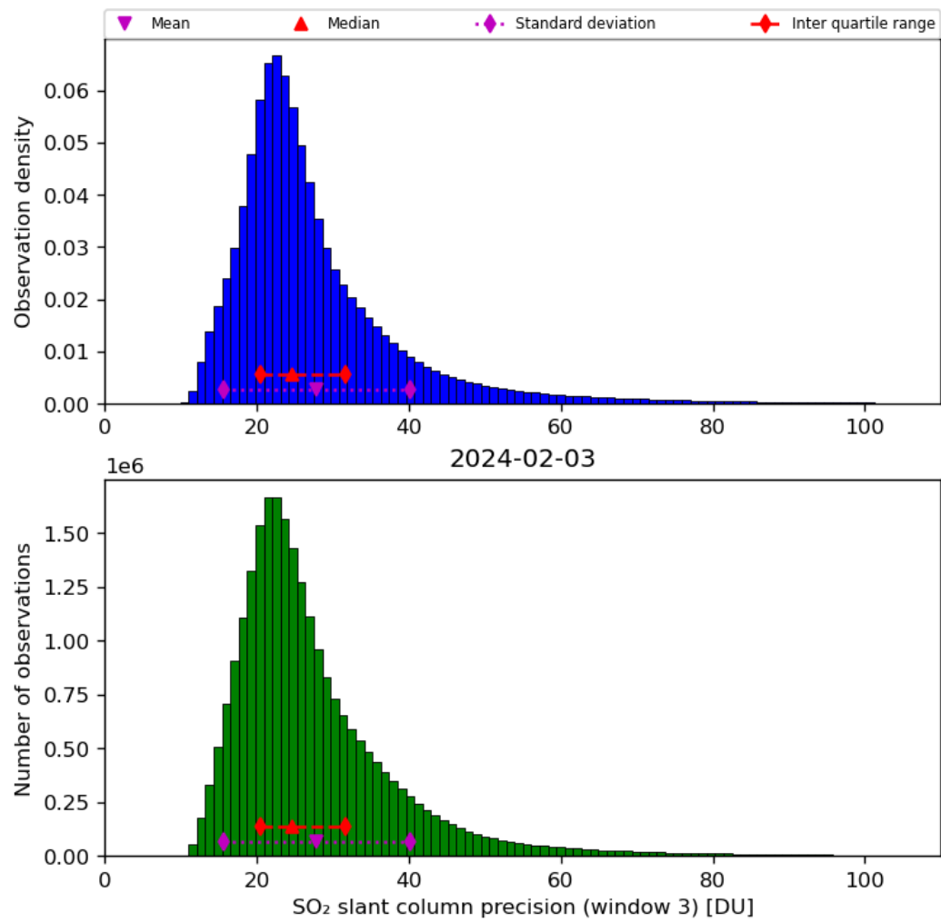
Figure 65: Histogram of “SO 2 slant column precision (window 3)” for 2024-02-02 to 2024-02-04
