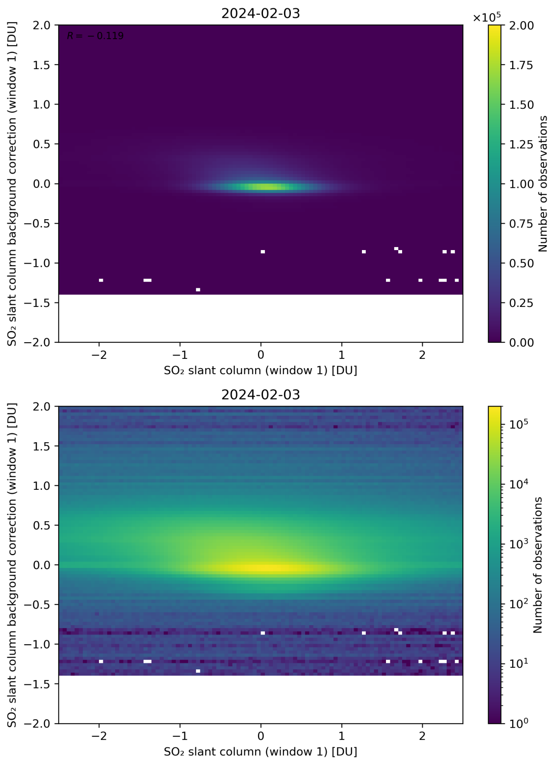
Figure 212: Scatter density plot of “SO 2 slant column (window 1)” against “SO 2 slant column background correction (window 1)” for 2024-02-02 to 2024-02-04.
