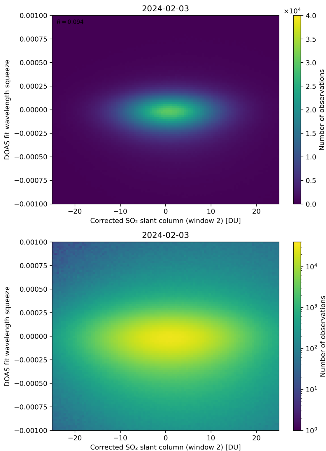
Figure 197: Scatter density plot of “Corrected SO 2 slant column (window 2)” against “DOAS fit wavelength squeeze” for 2024-02-02 to 2024-02-04.
