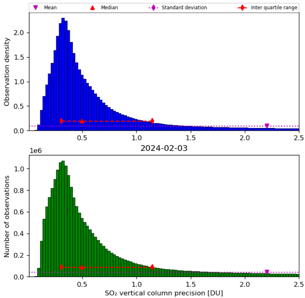
Figure 54: Histogram of “SO 2 vertical column precision” for 2024-02-02 to 2024-02-04
