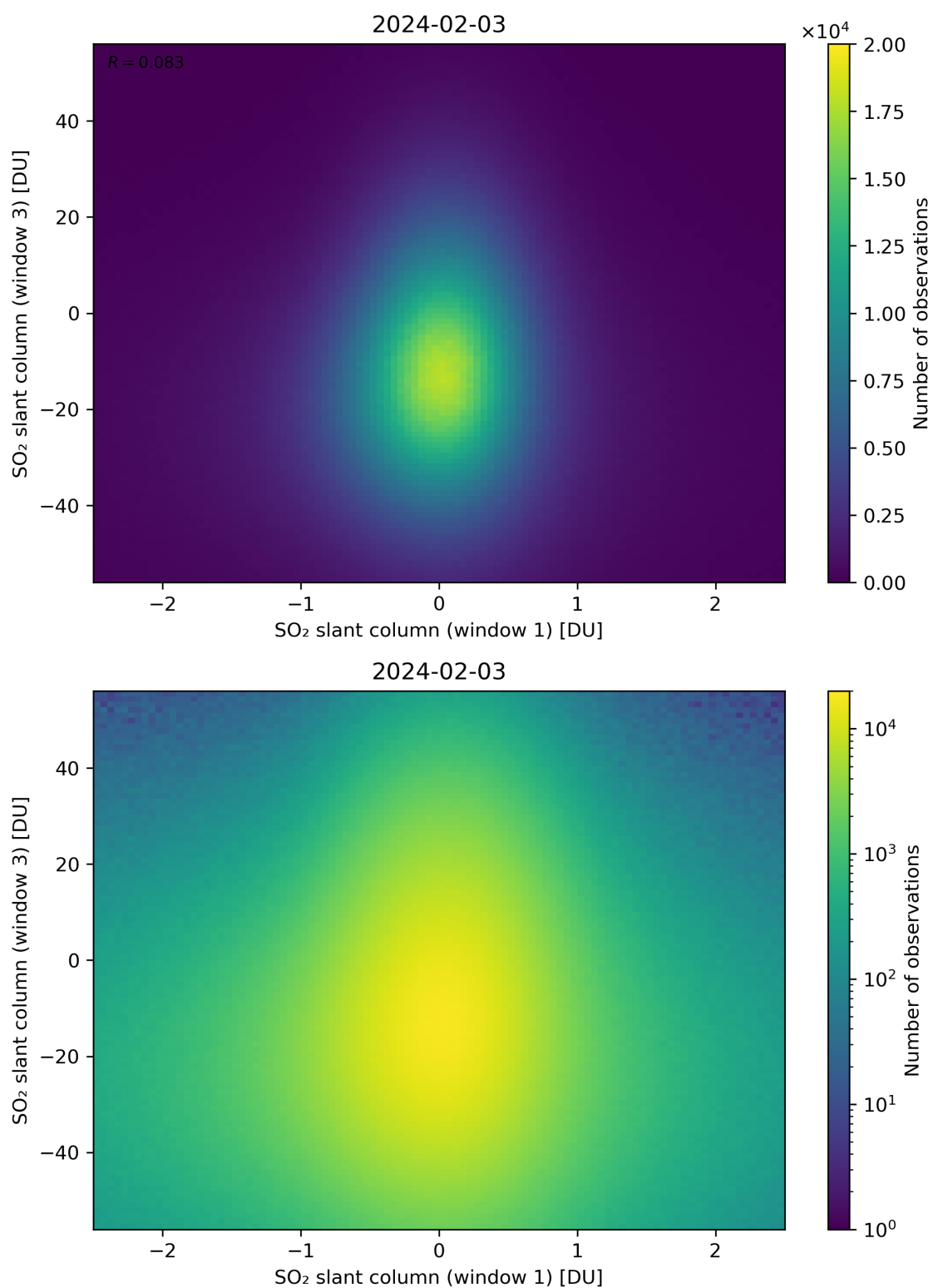
Figure 237: Scatter density plot of “SO 2 slant column (window 1)” against “SO 2 slant column (window 3)” for 2024-02-02 to 2024-02-04.
