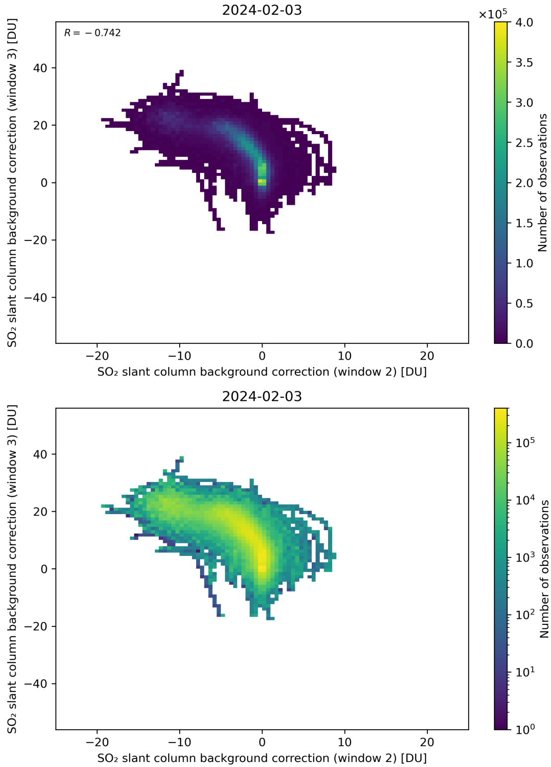
Figure 111: Scatter density plot of “SO 2 slant column background correction (window 2)” against “SO 2 slant column background correction (window 3)” for 2024-02-02 to 2024-02-04.
