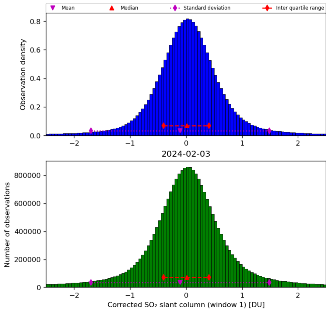
Figure 58: Histogram of “Corrected SO 2 slant column (window 1)” for 2024-02-02 to 2024-02-04
