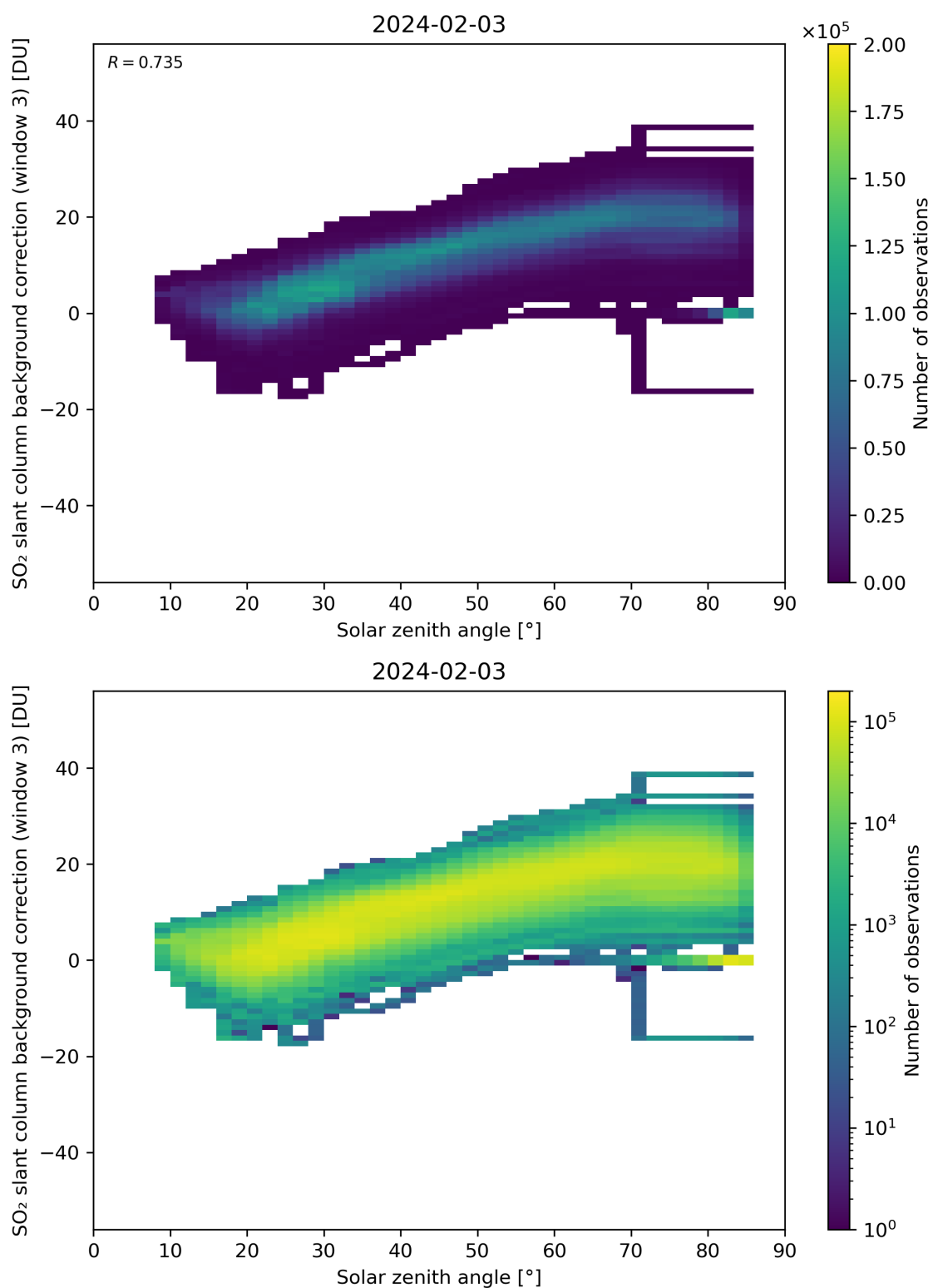
Figure 160: Scatter density plot of “Solar zenith angle” against “SO 2 slant column background correction (window 3)” for 2024-02-02 to 2024-02-04.
