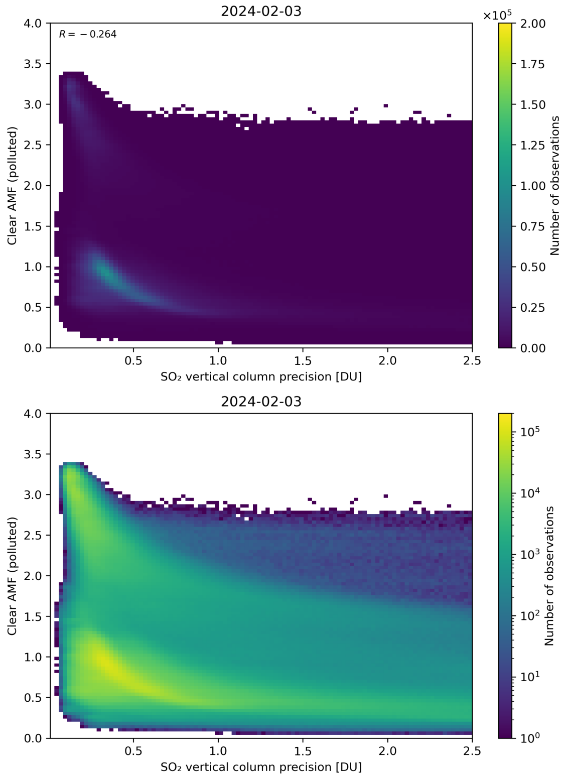
Figure 285: Scatter density plot of “SO 2 vertical column precision” against “Clear AMF (polluted)” for 2024-02-02 to 2024-02-04.
