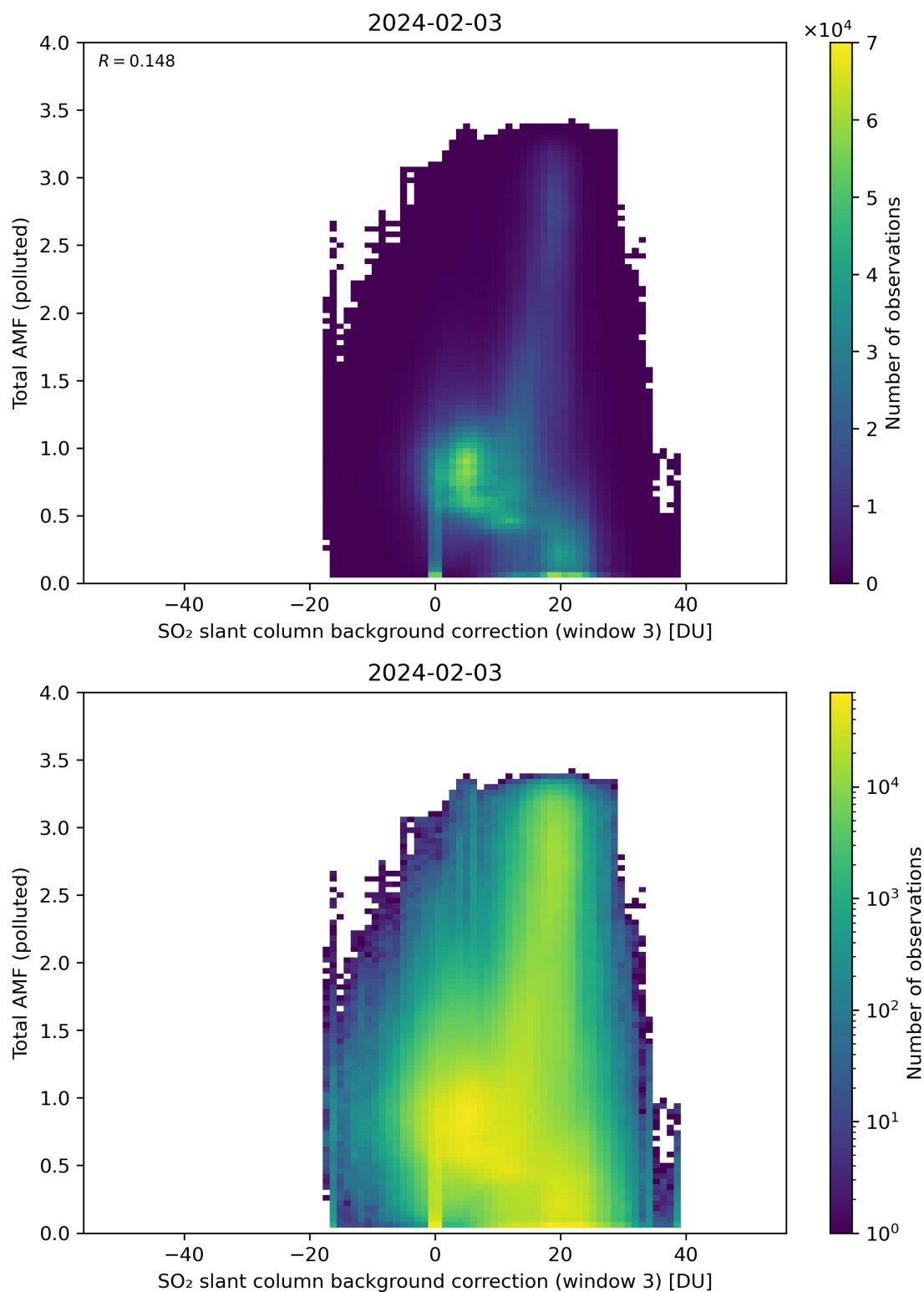
Figure 125: Scatter density plot of “SO 2 slant column background correction (window 3)” against “Total AMF (polluted)” for 2024-02-02 to 2024-02-04.
