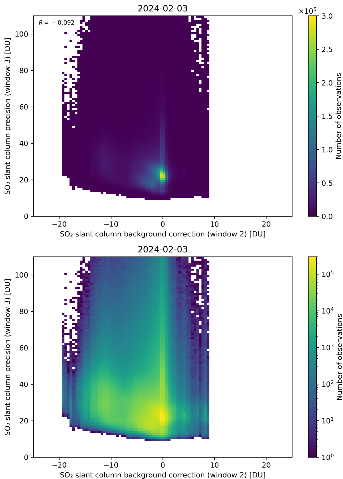
Figure 118: Scatter density plot of “SO 2 slant column background correction (window 2)” against “SO 2 slant column precision (window 3)” for 2024-02-02 to 2024-02-04.
