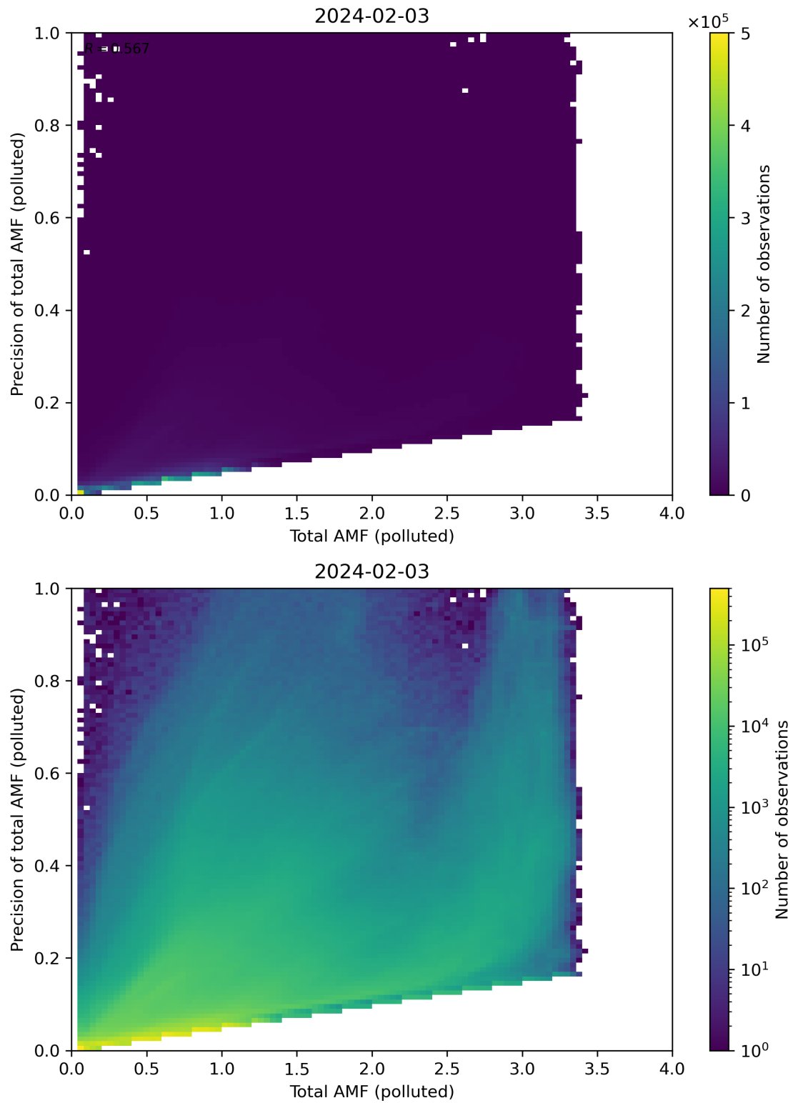
Figure 272: Scatter density plot of “Total AMF (polluted)” against “Precision of total AMF (polluted)” for 2024-02-02 to 2024-02-04.
