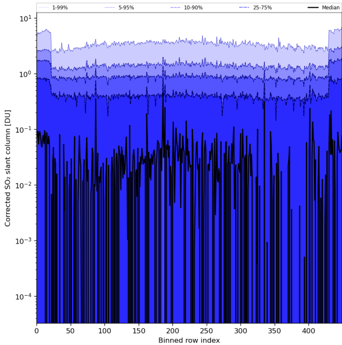
Figure 78: Along track statistics of “Corrected SO 2 slant column” for 2024-02-02 to 2024-02-04
