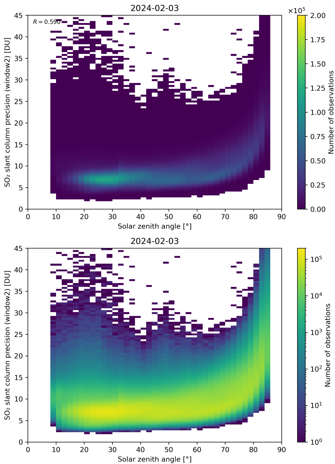
Figure 171: Scatter density plot of “Solar zenith angle” against “SO 2 slant column precision (window2)” for 2024-02-02 to 2024-02-04.
