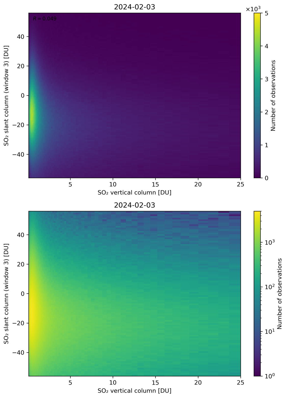
Figure 303: Scatter density plot of “SO 2 vertical column” against “SO 2 slant column (window 3)” for 2024-02-02 to 2024-02-04.
