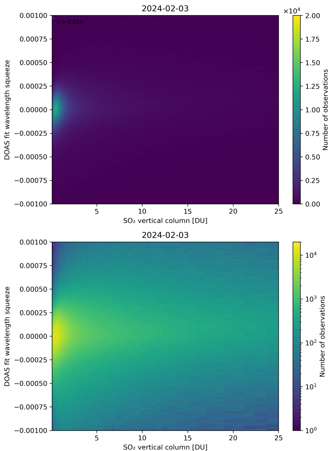
Figure 277: Scatter density plot of “SO 2 vertical column” against “DOAS fit wavelength squeeze” for 2024-02-02 to 2024-02-04.
