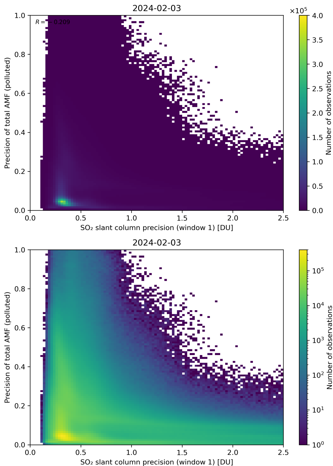
Figure 231: Scatter density plot of “SO 2 slant column precision (window 1)” against “Precision of total AMF (polluted)” for 2024-02-02 to 2024-02-04.
