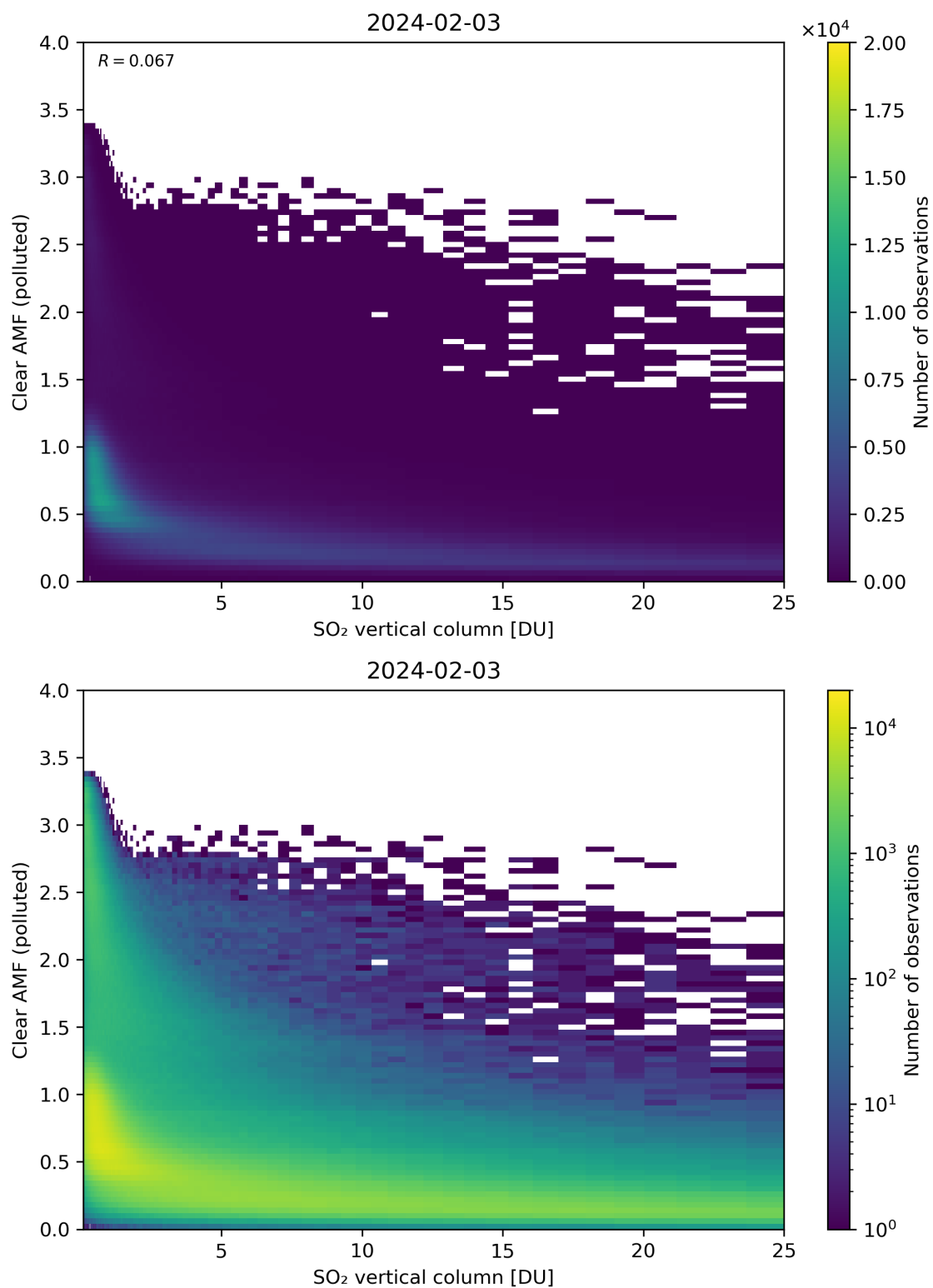
Figure 296: Scatter density plot of “SO 2 vertical column” against “Clear AMF (polluted)” for 2024-02-02 to 2024-02-04.
