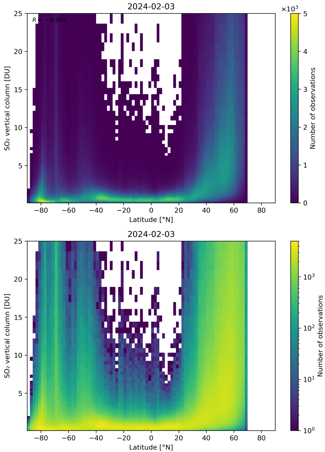
Figure 156: Scatter density plot of “Latitude” against “SO 2 vertical column” for 2024-02-02 to 2024-02-04.
