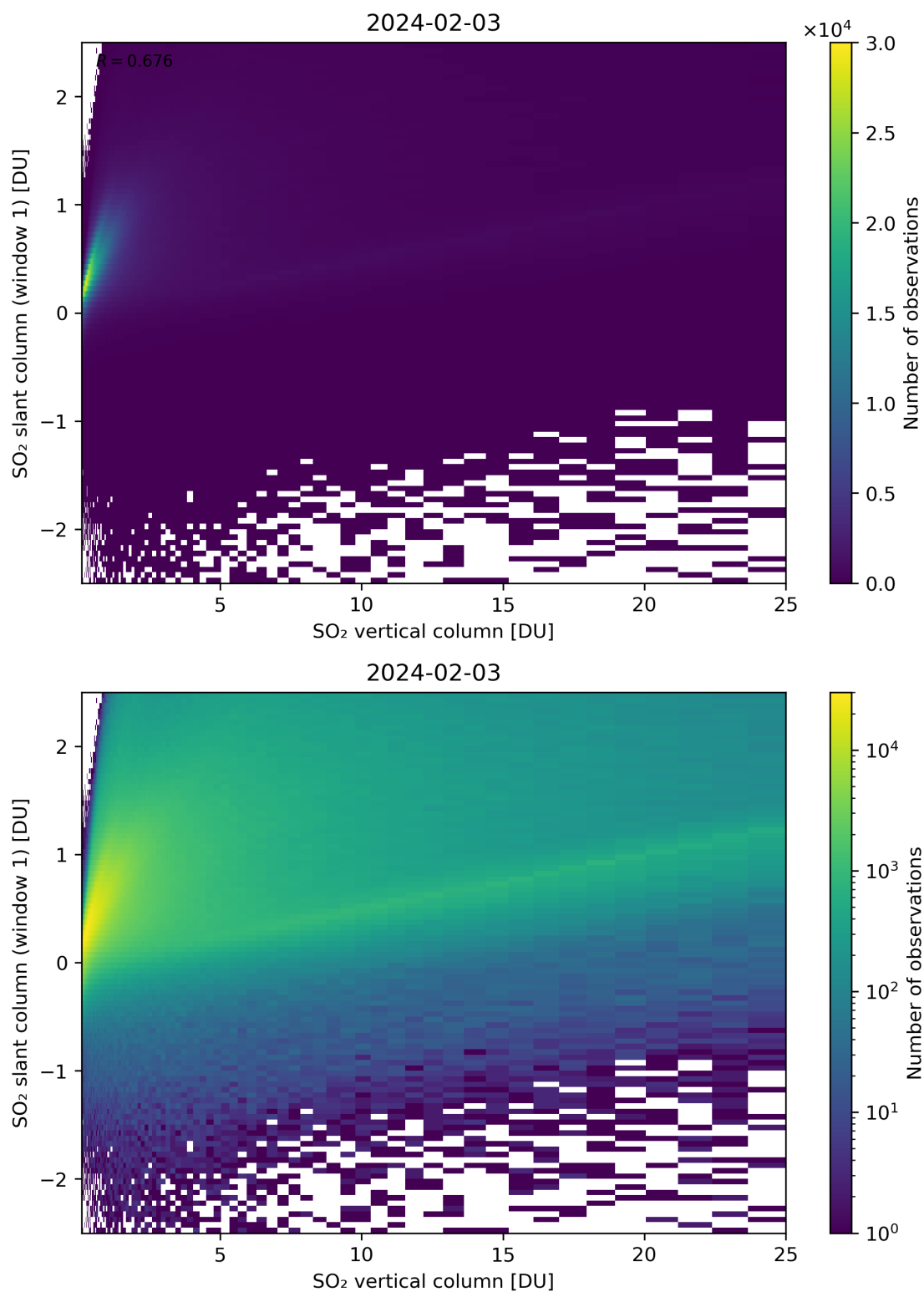
Figure 300: Scatter density plot of “SO 2 vertical column” against “SO 2 slant column (window 1)” for 2024-02-02 to 2024-02-04.
