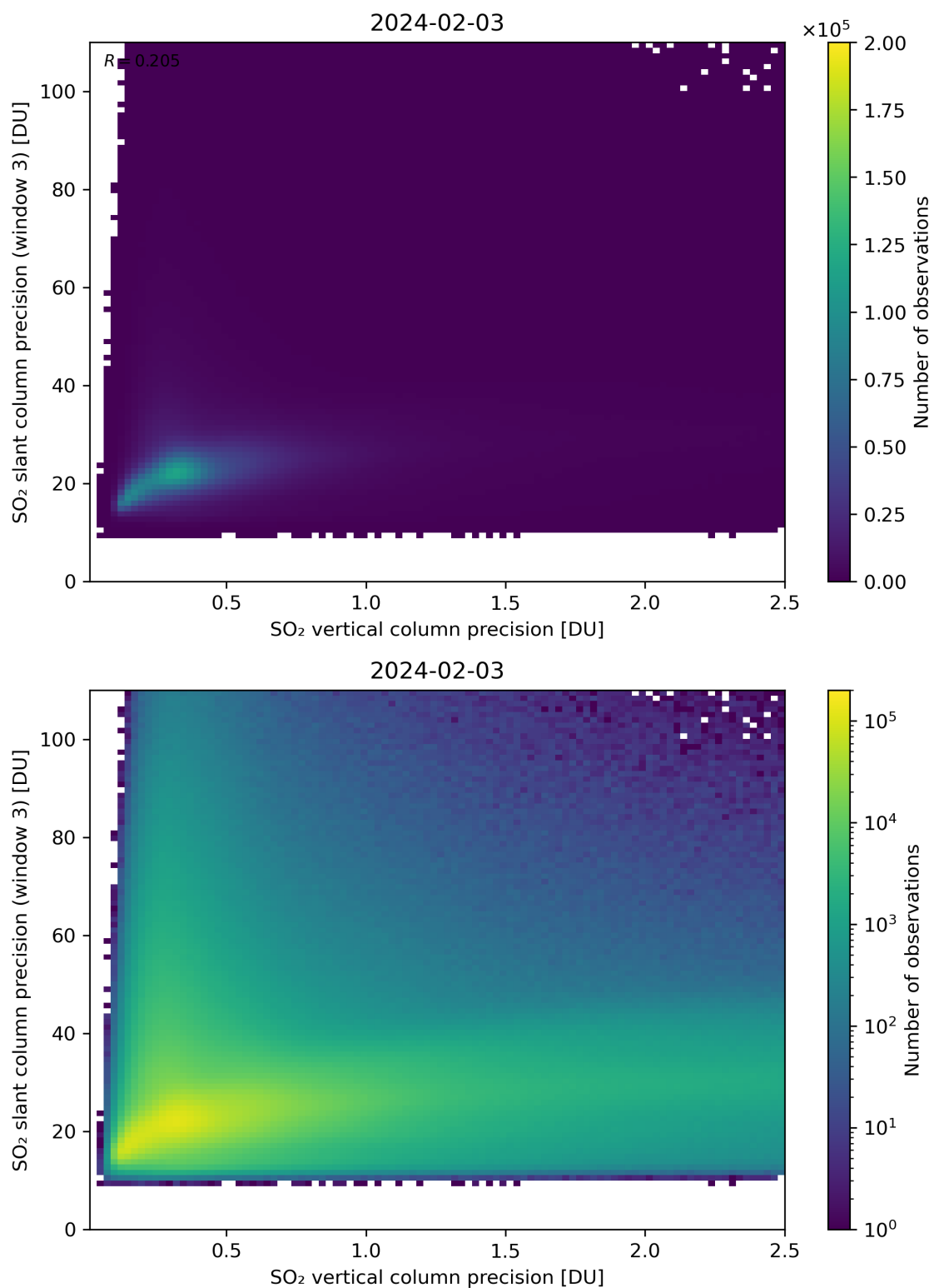
Figure 293: Scatter density plot of “SO 2 vertical column precision” against “SO 2 slant column precision (window 3)” for 2024-02-02 to 2024-02-04.
