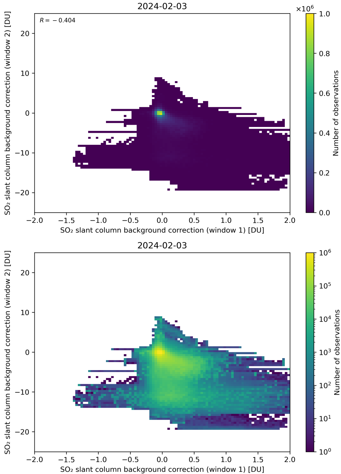
Figure 98: Scatter density plot of “SO 2 slant column background correction (window 1)” against “SO 2 slant column background correction (window 2)” for 2024-02-02 to 2024-02-04.
