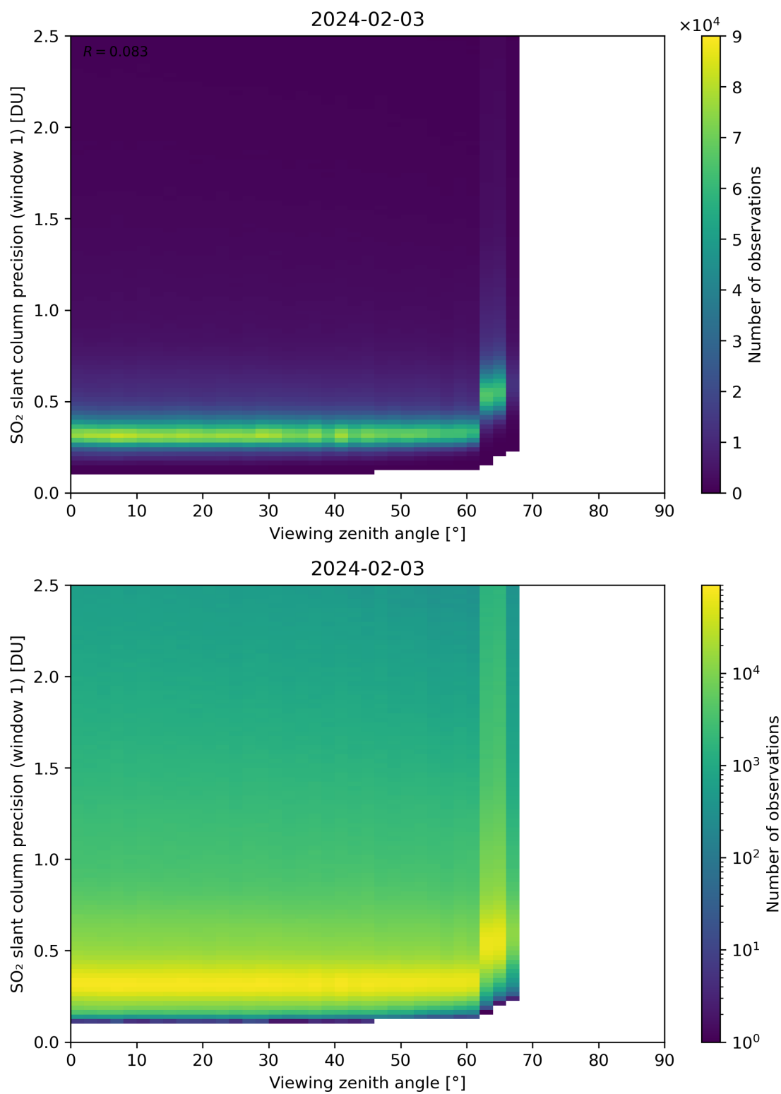
Figure 321: Scatter density plot of “Viewing zenith angle” against “SO 2 slant column precision (window 1)” for 2024-02-02 to 2024-02-04.
