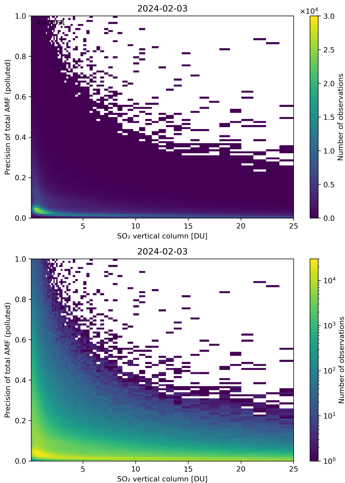
Figure 306: Scatter density plot of “SO 2 vertical column” against “Precision of total AMF (polluted)” for 2024-02-02 to 2024-02-04.
