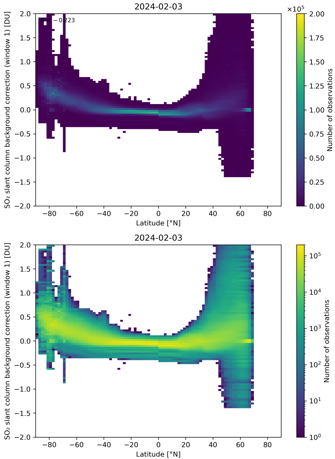
Figure 139: Scatter density plot of “Latitude” against “SO 2 slant column background correction (window 1)” for 2024-02-02 to 2024-02-04.
