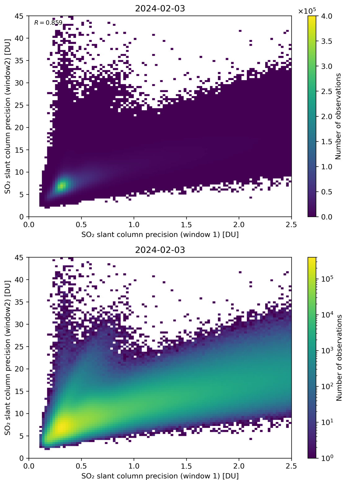
Figure 227: Scatter density plot of “SO 2 slant column precision (window 1)” against “SO 2 slant column precision (window2)” for 2024-02-02 to 2024-02-04.
