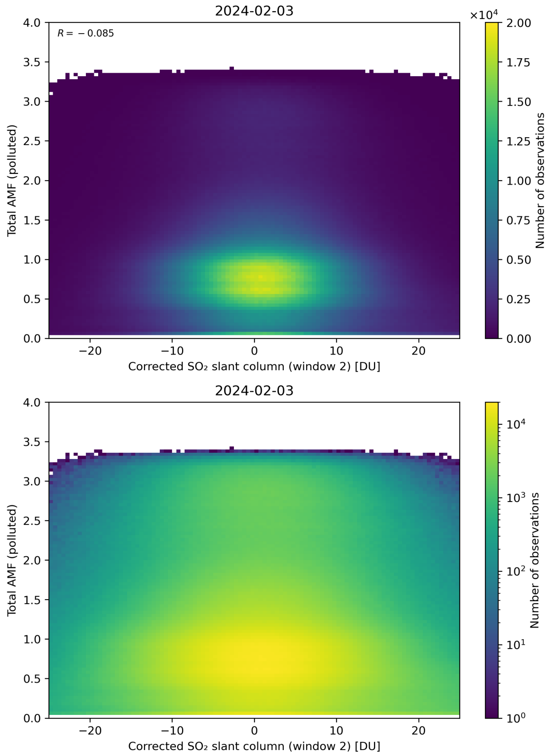
Figure 203: Scatter density plot of “Corrected SO 2 slant column (window 2)” against “Total AMF (polluted)” for 2024-02-02 to 2024-02-04.
