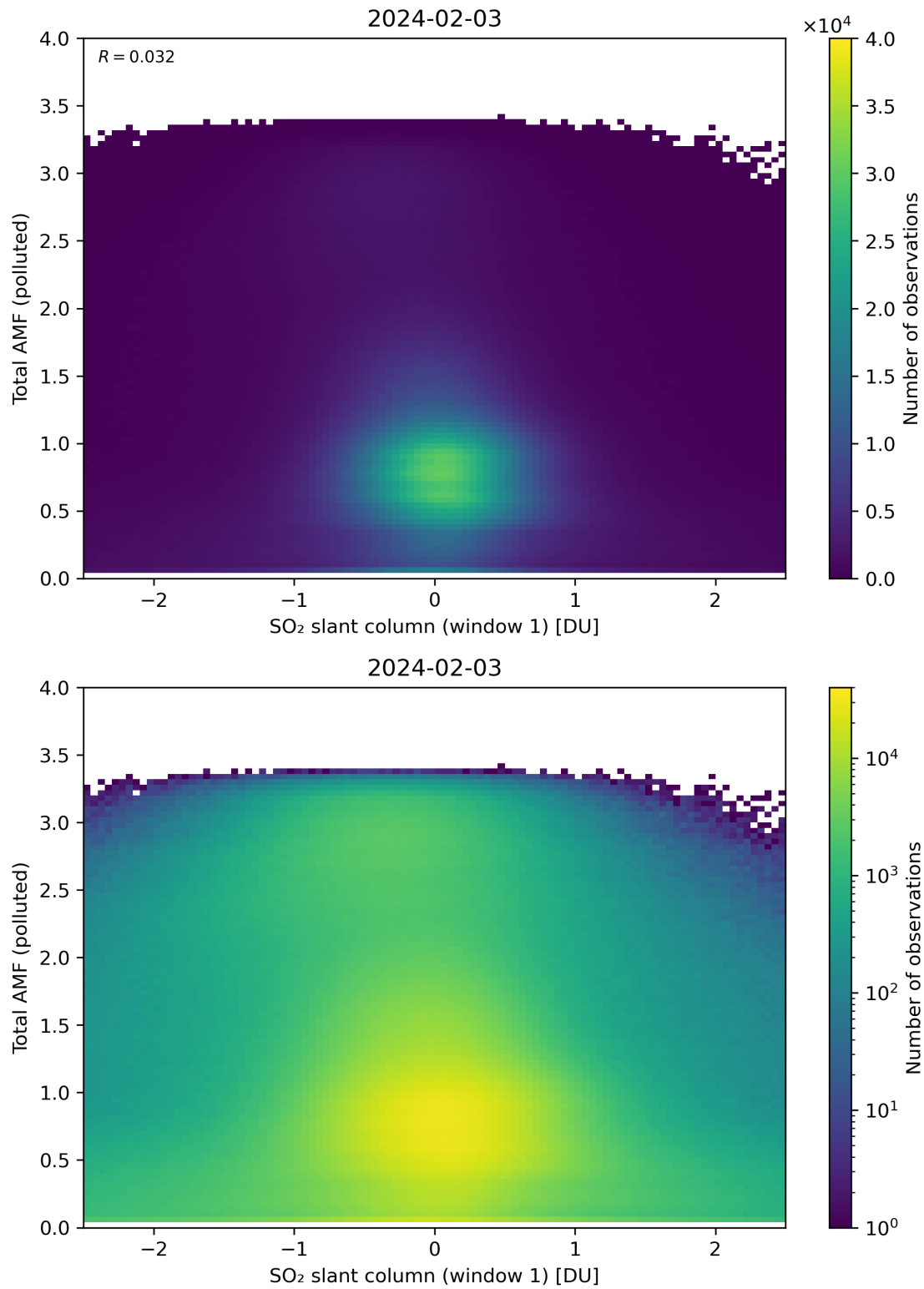
Figure 239: Scatter density plot of “SO 2 slant column (window 1)” against “Total AMF (polluted)” for 2024-02-02 to 2024-02-04.
