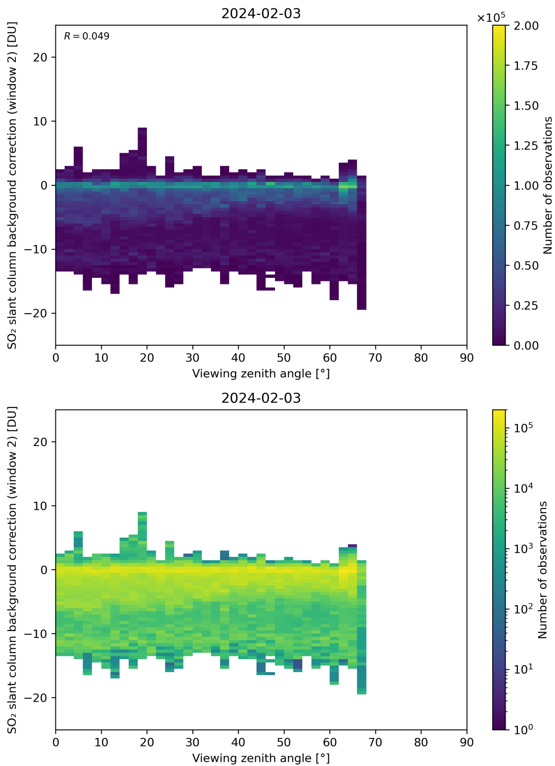
Figure 309: Scatter density plot of “Viewing zenith angle” against “SO 2 slant column background correction (window 2)” for 2024-02-02 to 2024-02-04.
