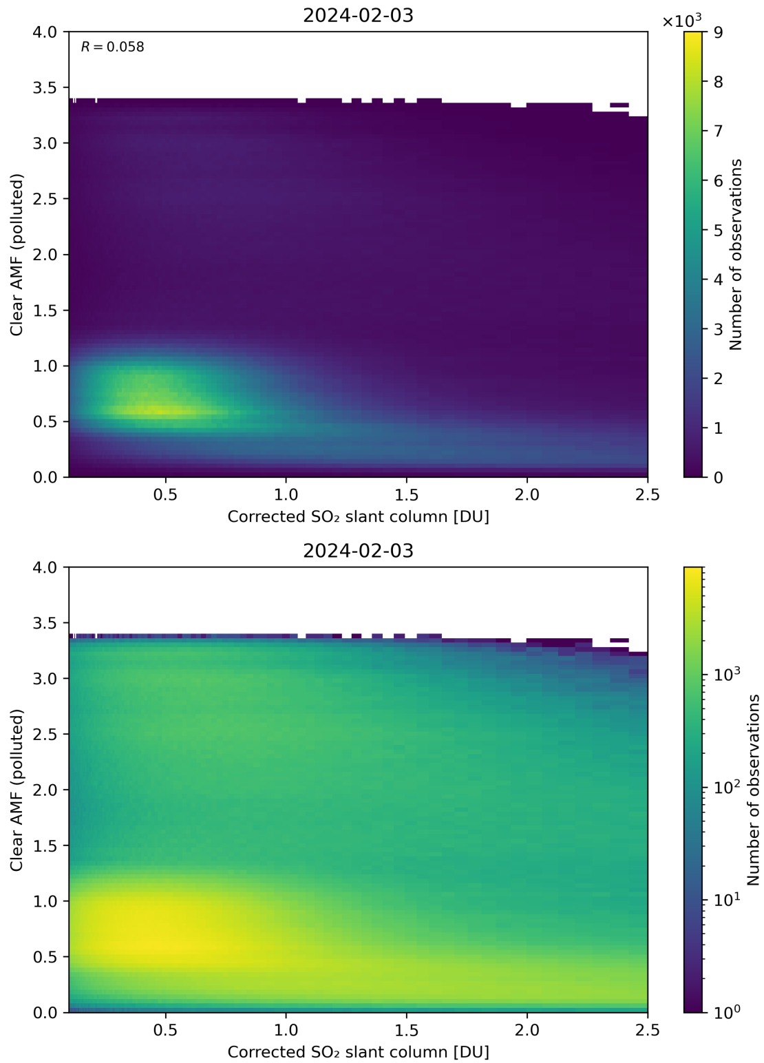
Figure 184: Scatter density plot of “Corrected SO 2 slant column” against “Clear AMF (polluted)” for 2024-02-02 to 2024-02-04.
