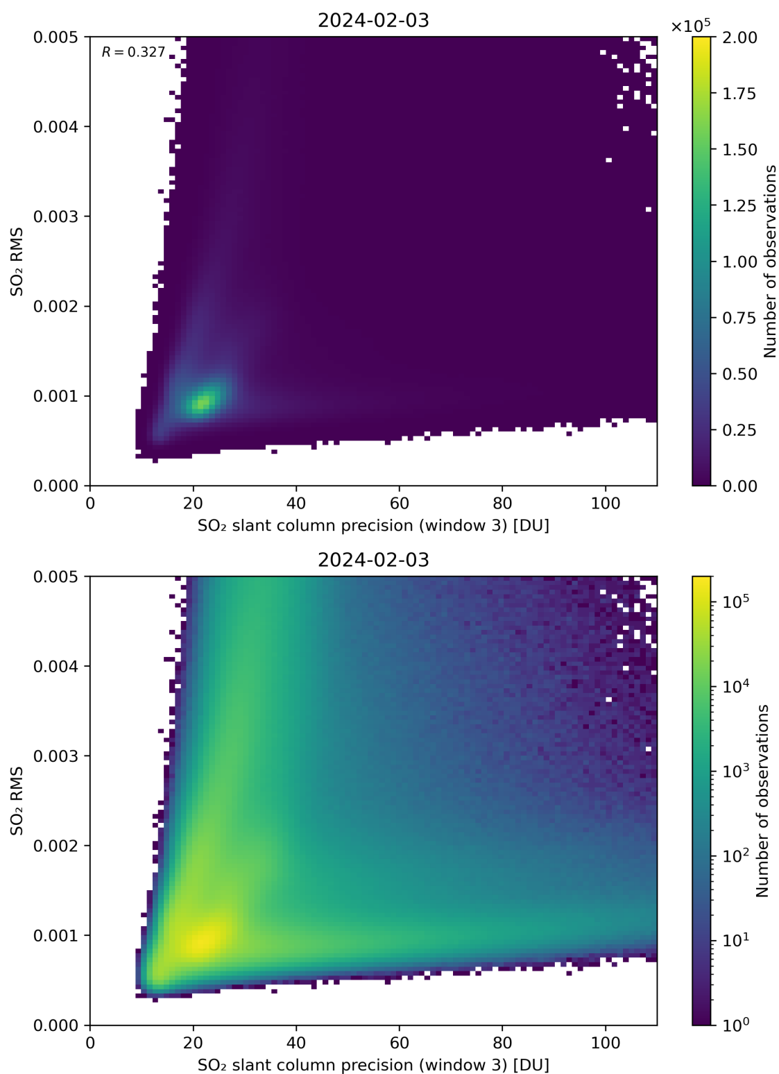
Figure 260: Scatter density plot of “SO 2 slant column precision (window 3)” against “SO 2 RMS” for 2024-02-02 to 2024-02-04.
