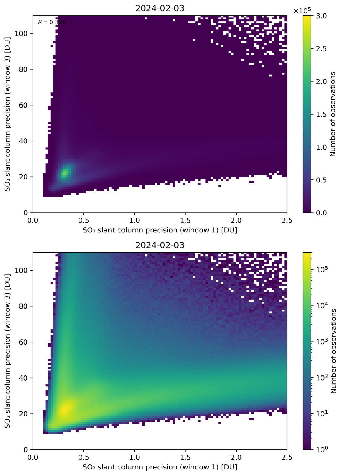
Figure 229: Scatter density plot of “SO 2 slant column precision (window 1)” against “SO 2 slant column precision (window 3)” for 2024-02-02 to 2024-02-04.
