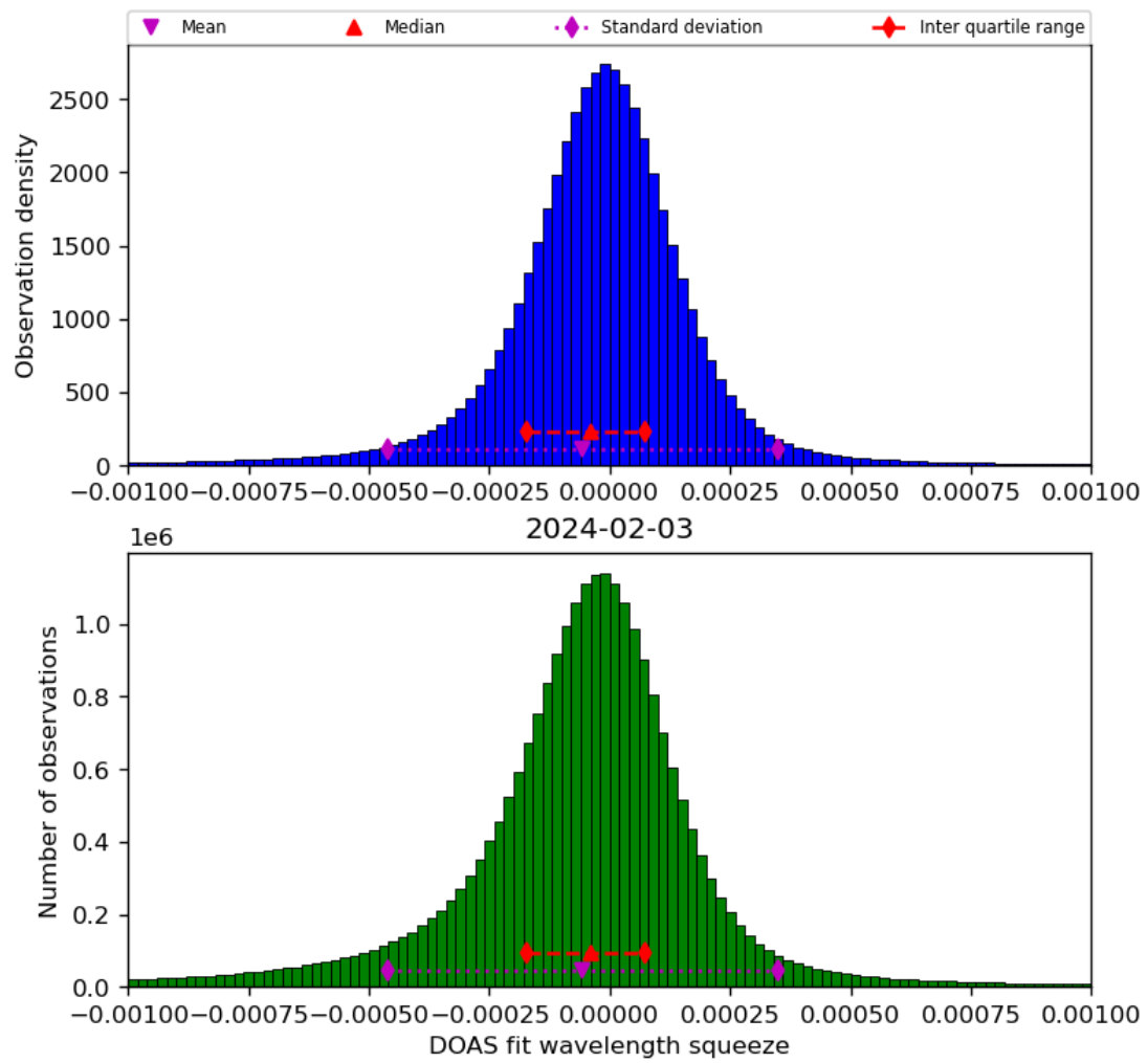
Figure 69: Histogram of “DOAS fit wavelength squeeze” for 2024-02-02 to 2024-02-04
