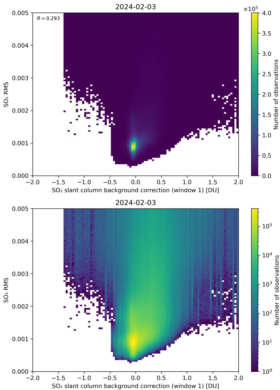
Figure 102: Scatter density plot of “SO 2 slant column background correction (window 1)” against “SO 2 RMS” for 2024-02-02 to 2024-02-04.
