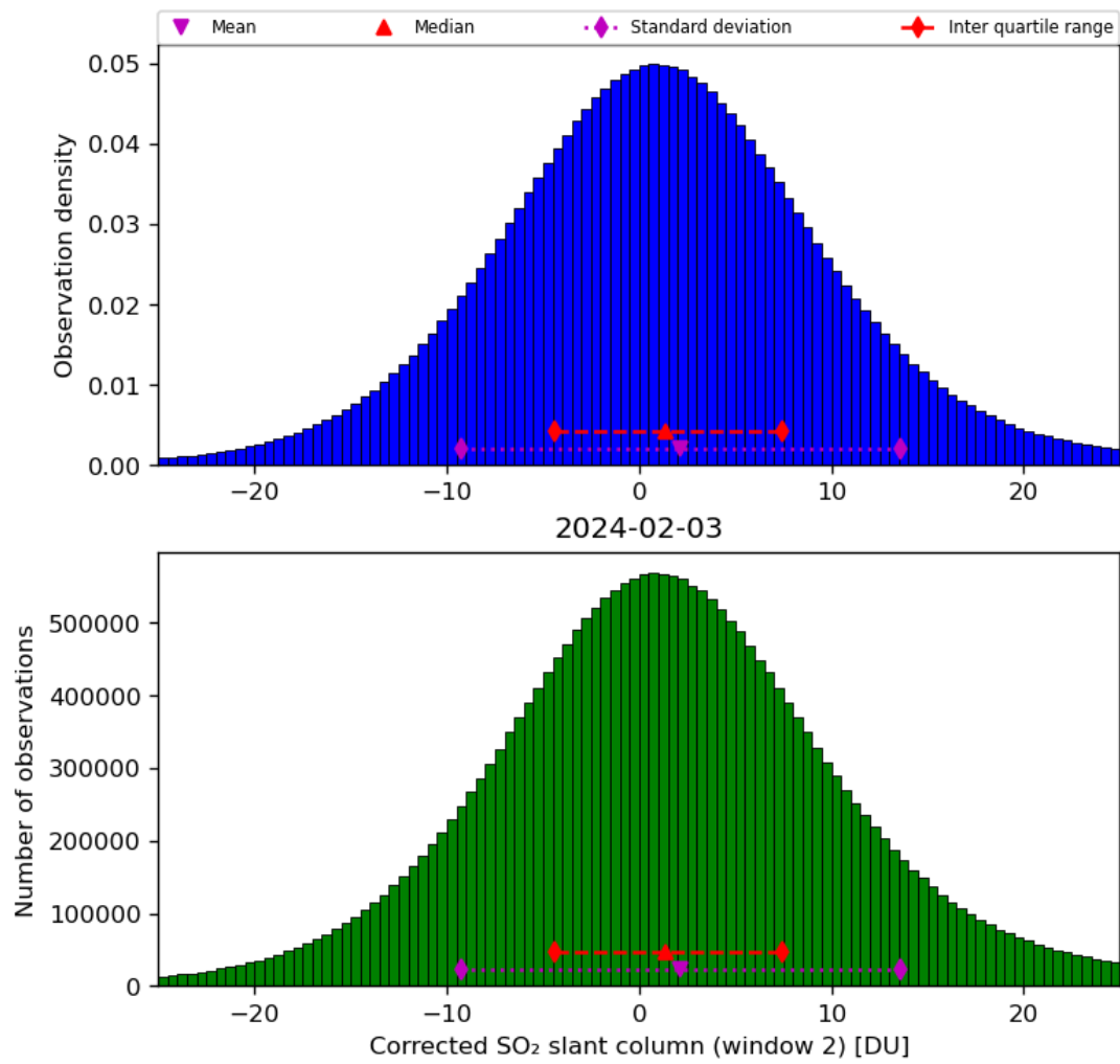
Figure 62: Histogram of “Corrected SO 2 slant column (window 2)” for 2024-02-02 to 2024-02-04
