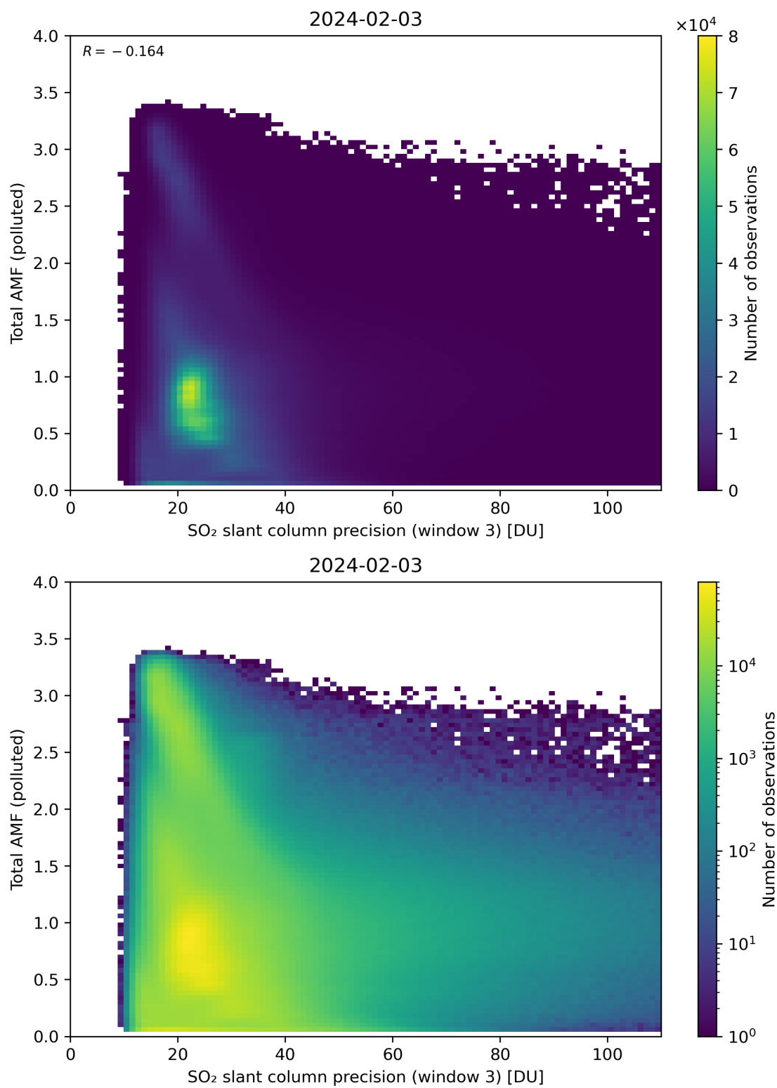
Figure 263: Scatter density plot of “SO 2 slant column precision (window 3)” against “Total AMF (polluted)” for 2024-02-02 to 2024-02-04.
