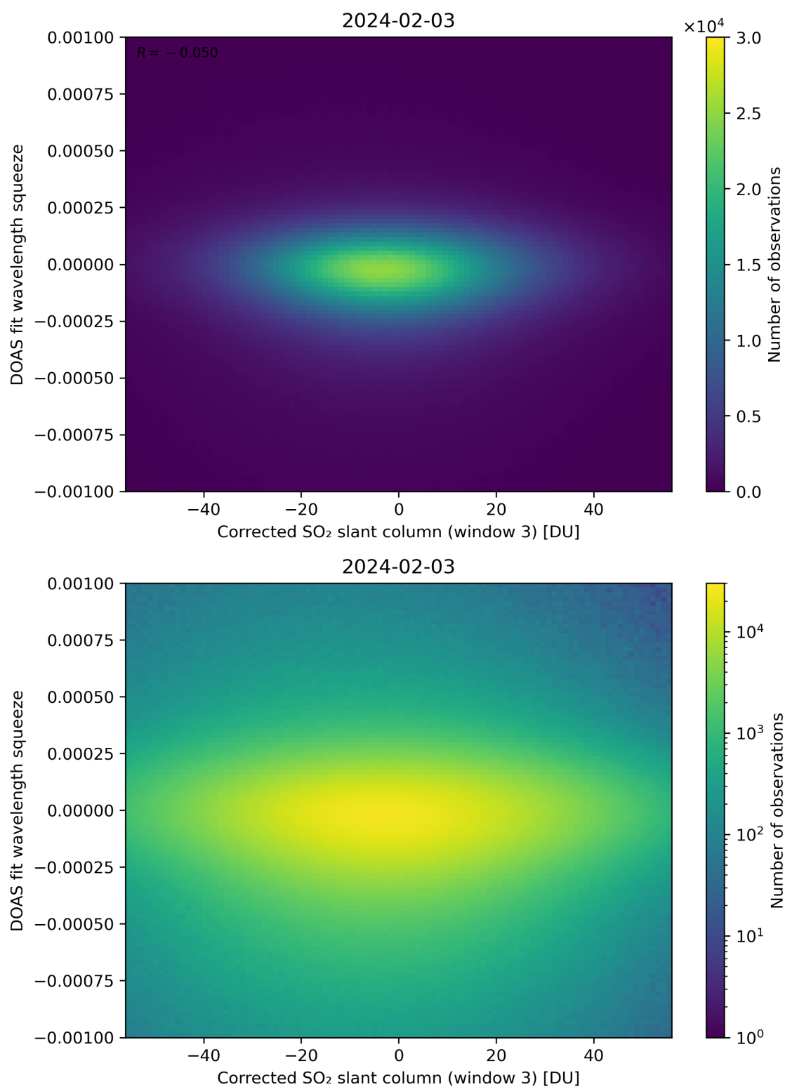
Figure 207: Scatter density plot of “Corrected SO 2 slant column (window 3)” against “DOAS fit wavelength squeeze” for 2024-02-02 to 2024-02-04.
