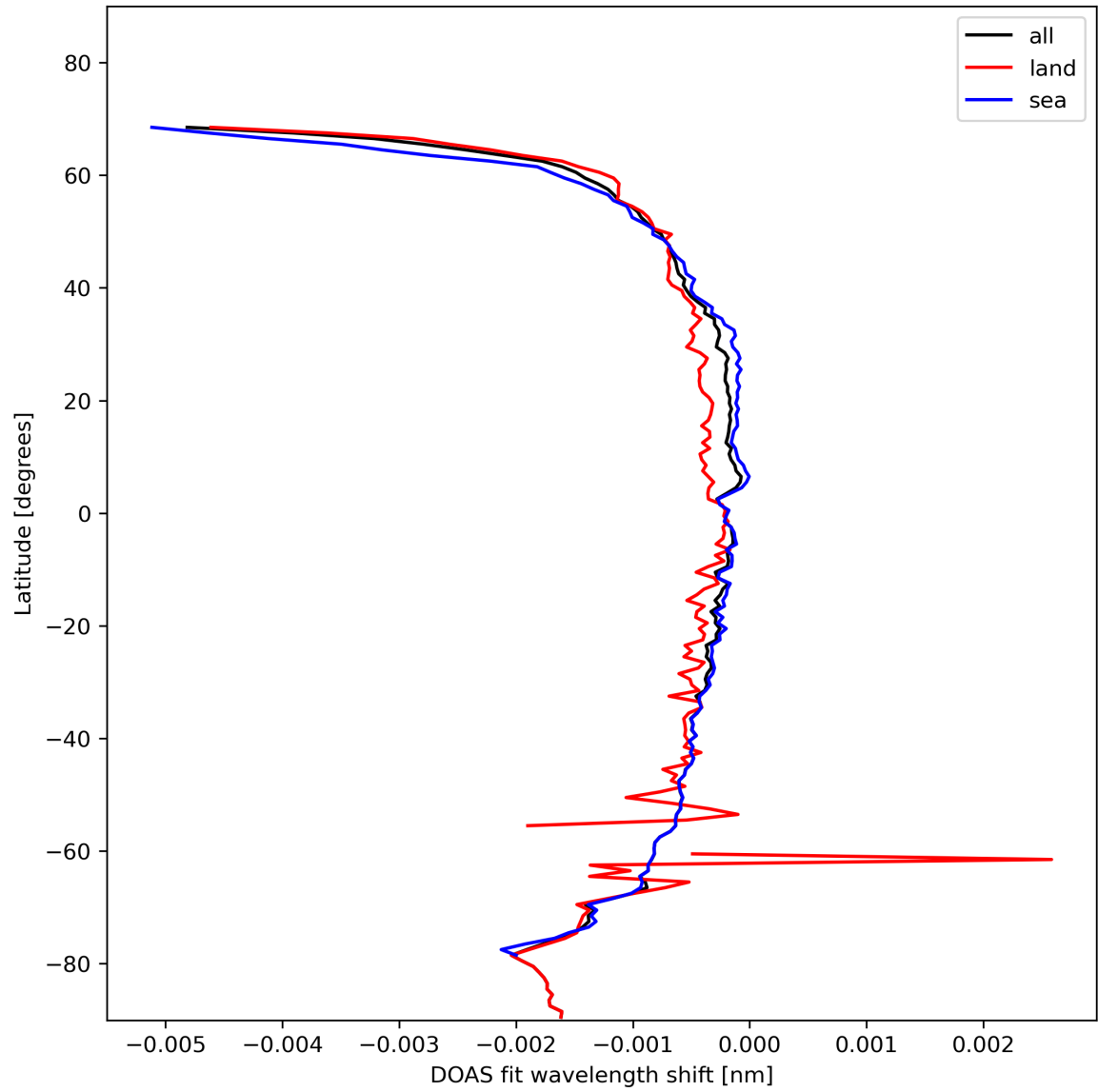
Figure 45: Zonal average of “DOAS fit wavelength shift” for 2024-02-02 to 2024-02-04.
