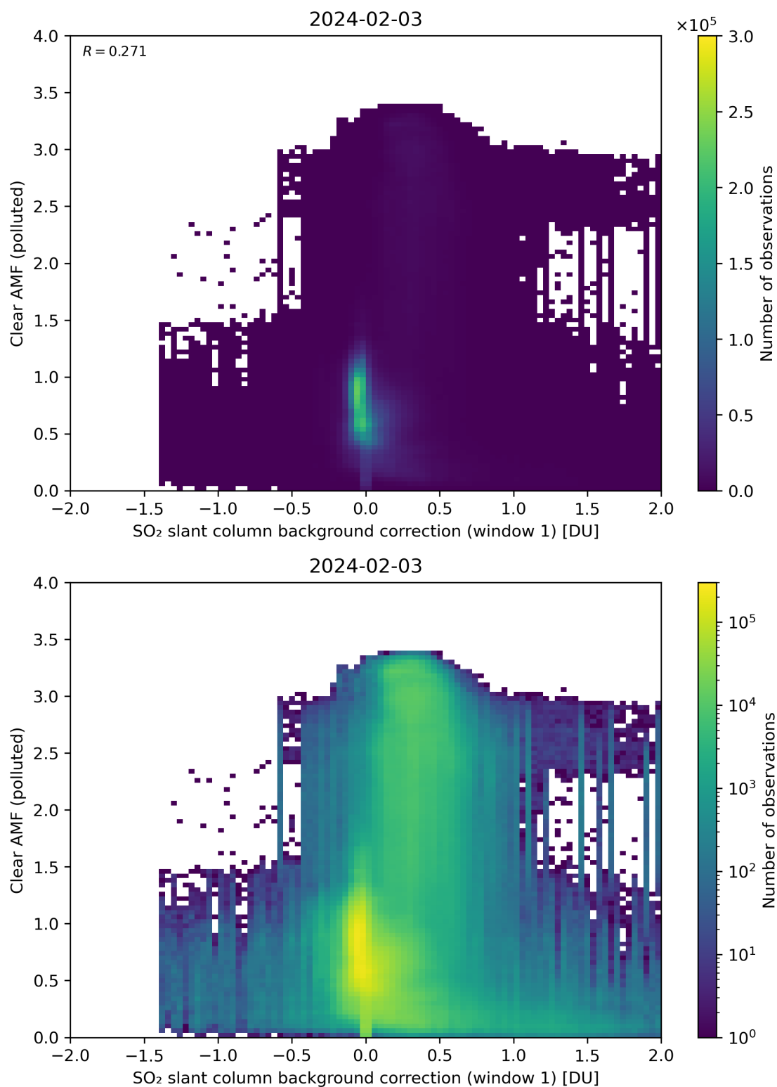
Figure 103: Scatter density plot of “SO 2 slant column background correction (window 1)” against “Clear AMF (polluted)” for 2024-02-02 to 2024-02-04.
