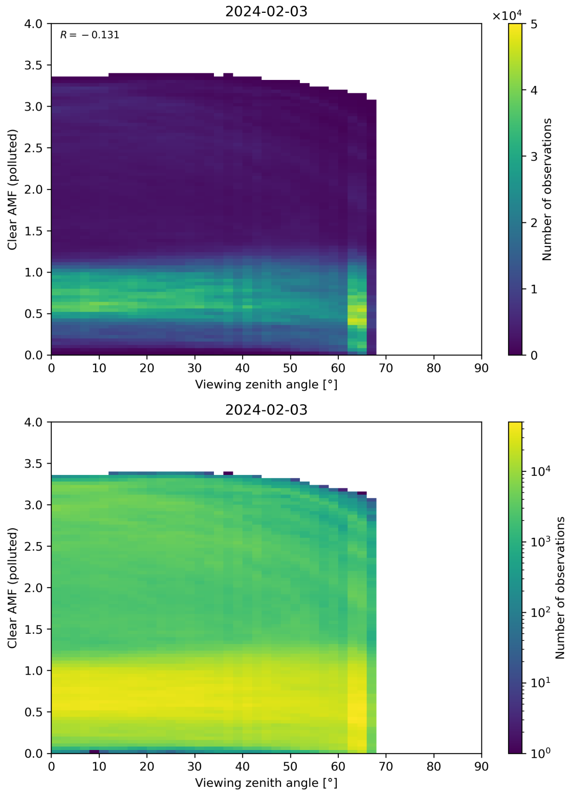
Figure 316: Scatter density plot of “Viewing zenith angle” against “Clear AMF (polluted)” for 2024-02-02 to 2024-02-04.
