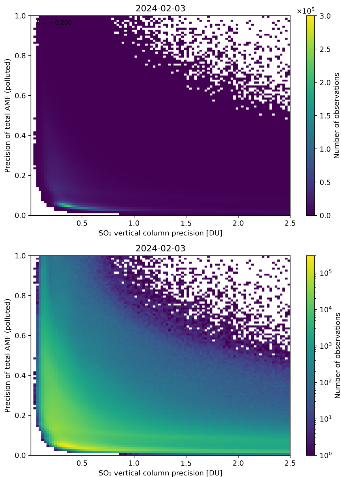
Figure 295: Scatter density plot of “SO 2 vertical column precision” against “Precision of total AMF (polluted)” for 2024-02-02 to 2024-02-04.
