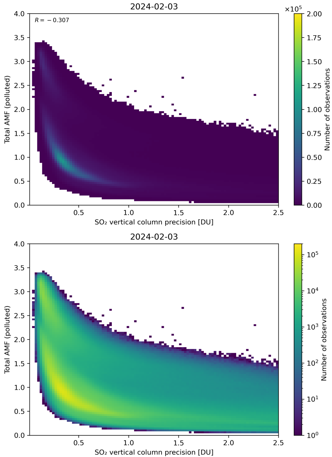
Figure 294: Scatter density plot of “SO 2 vertical column precision” against “Total AMF (polluted)” for 2024-02-02 to 2024-02-04.
