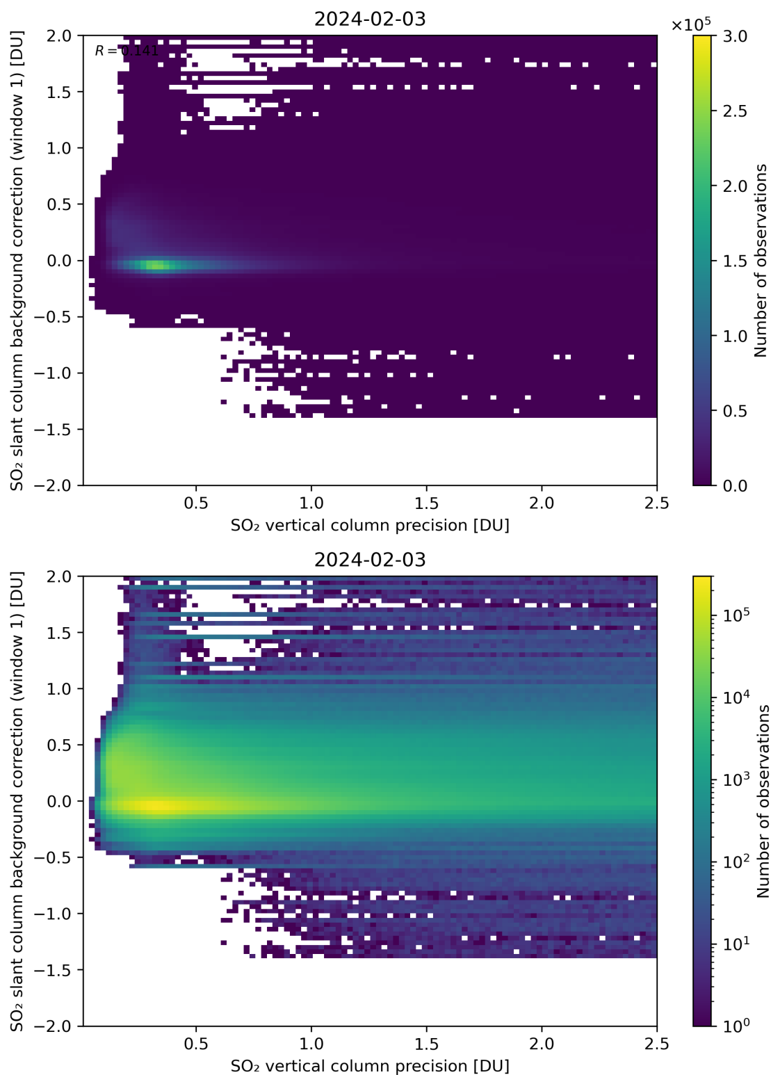
Figure 279: Scatter density plot of “SO 2 vertical column precision” against “SO 2 slant column background correction (window 1)” for 2024-02-02 to 2024-02-04.
