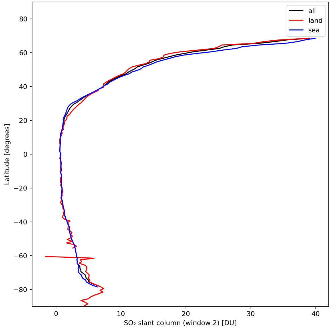
Figure 37: Zonal average of “SO 2 slant column (window 2)” for 2024-02-02 to 2024-02-04.
