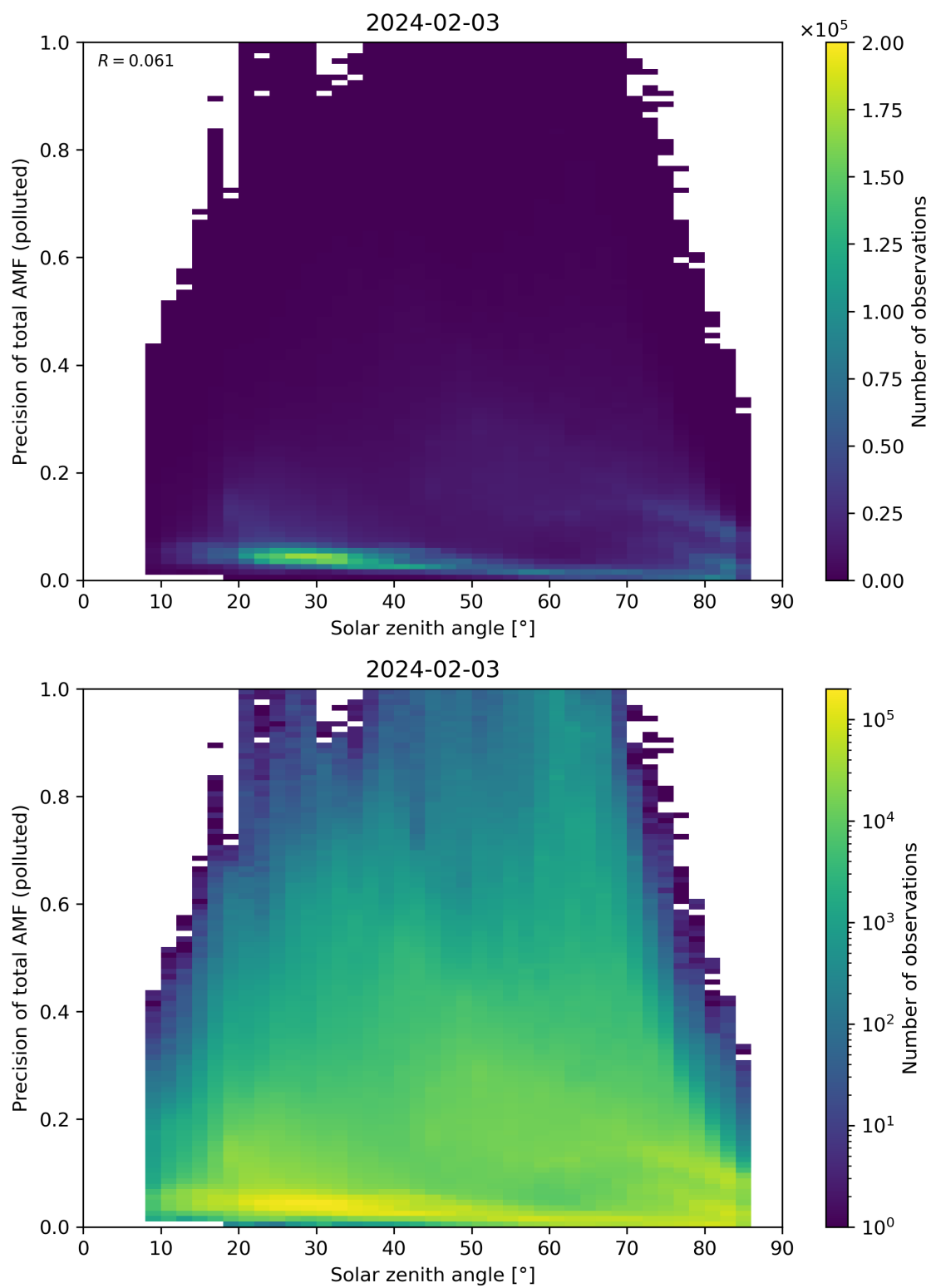
Figure 175: Scatter density plot of “Solar zenith angle” against “Precision of total AMF (polluted)” for 2024-02-02 to 2024-02-04.
