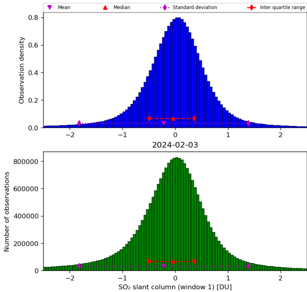
Figure 56: Histogram of “SO 2 slant column (window 1)” for 2024-02-02 to 2024-02-04
