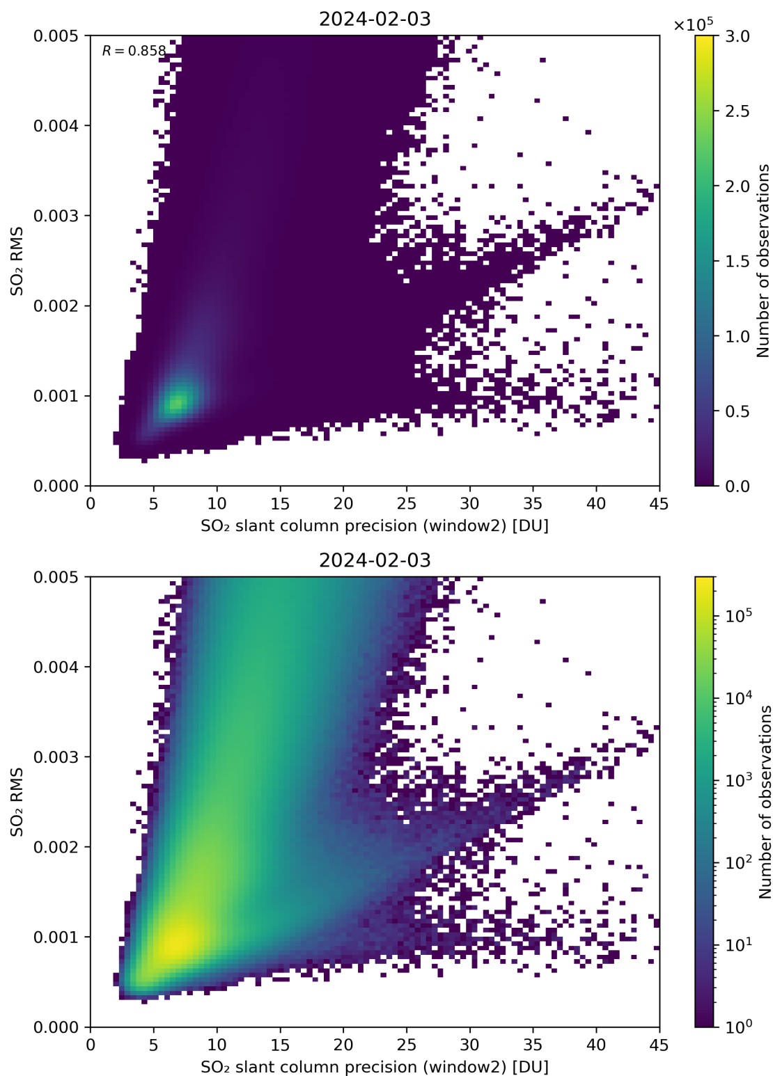
Figure 245: Scatter density plot of “SO 2 slant column precision (window2)” against “SO 2 RMS” for 2024-02-02 to 2024-02-04.
