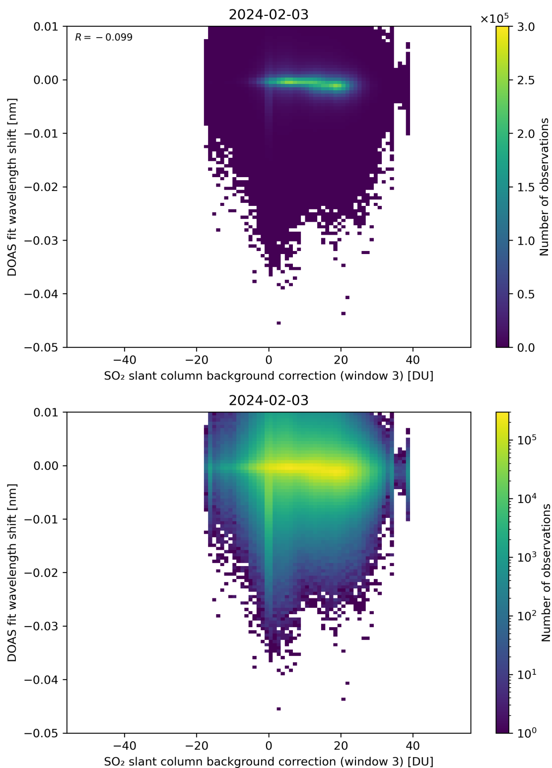
Figure 121: Scatter density plot of “SO 2 slant column background correction (window 3)” against “DOAS fit wavelength shift” for 2024-02-02 to 2024-02-04.
