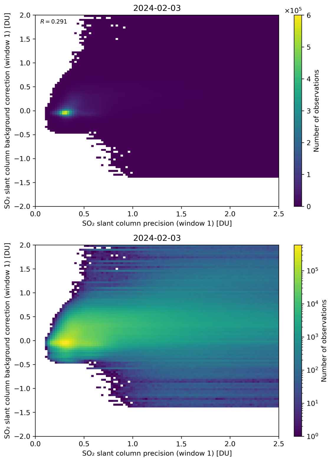
Figure 218: Scatter density plot of “SO 2 slant column precision (window 1)” against “SO 2 slant column background correction (window 1)” for 2024-02-02 to 2024-02-04.
