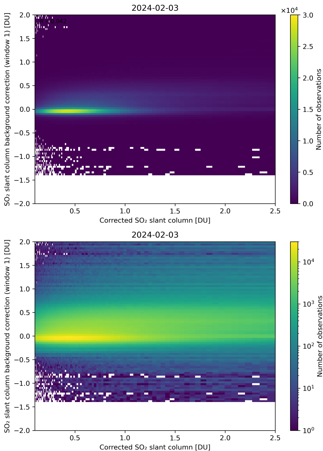
Figure 178: Scatter density plot of “Corrected SO 2 slant column” against “SO 2 slant column background correction (window 1)” for 2024-02-02 to 2024-02-04.
