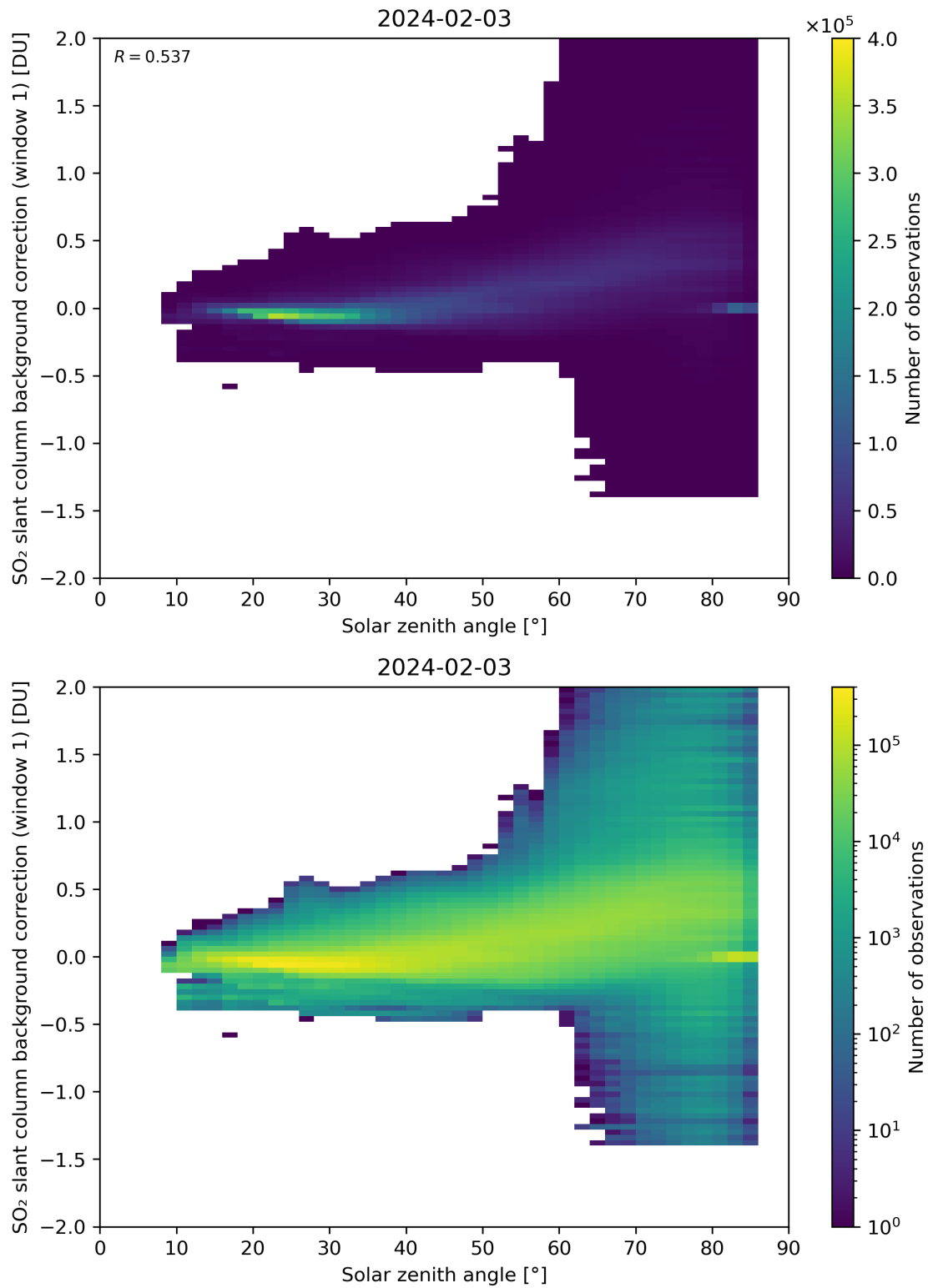
Figure 158: Scatter density plot of “Solar zenith angle” against “SO 2 slant column background correction (window 1)” for 2024-02-02 to 2024-02-04.
