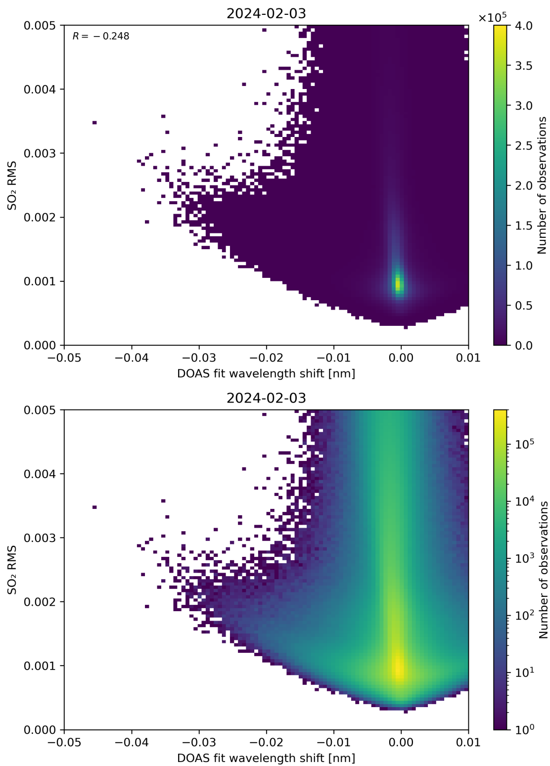
Figure 128: Scatter density plot of “DOAS fit wavelength shift” against “SO 2 RMS” for 2024-02-02 to 2024-02-04.
