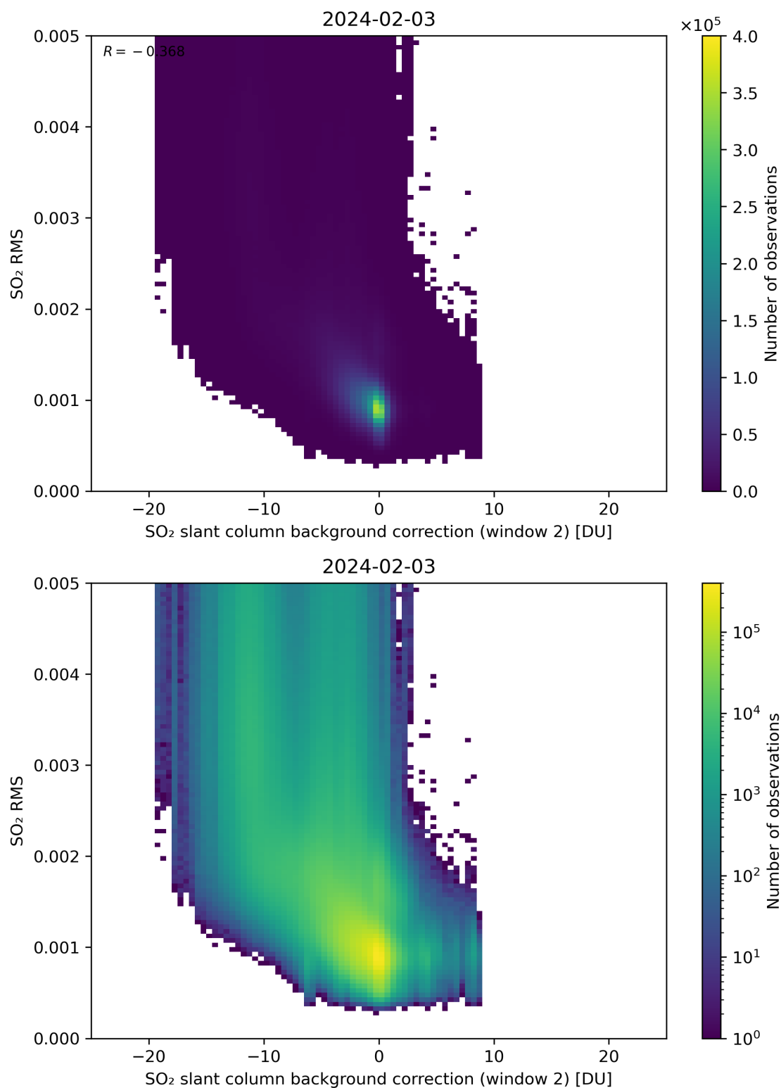
Figure 114: Scatter density plot of “SO 2 slant column background correction (window 2)” against “SO 2 RMS” for 2024-02-02 to 2024-02-04.
