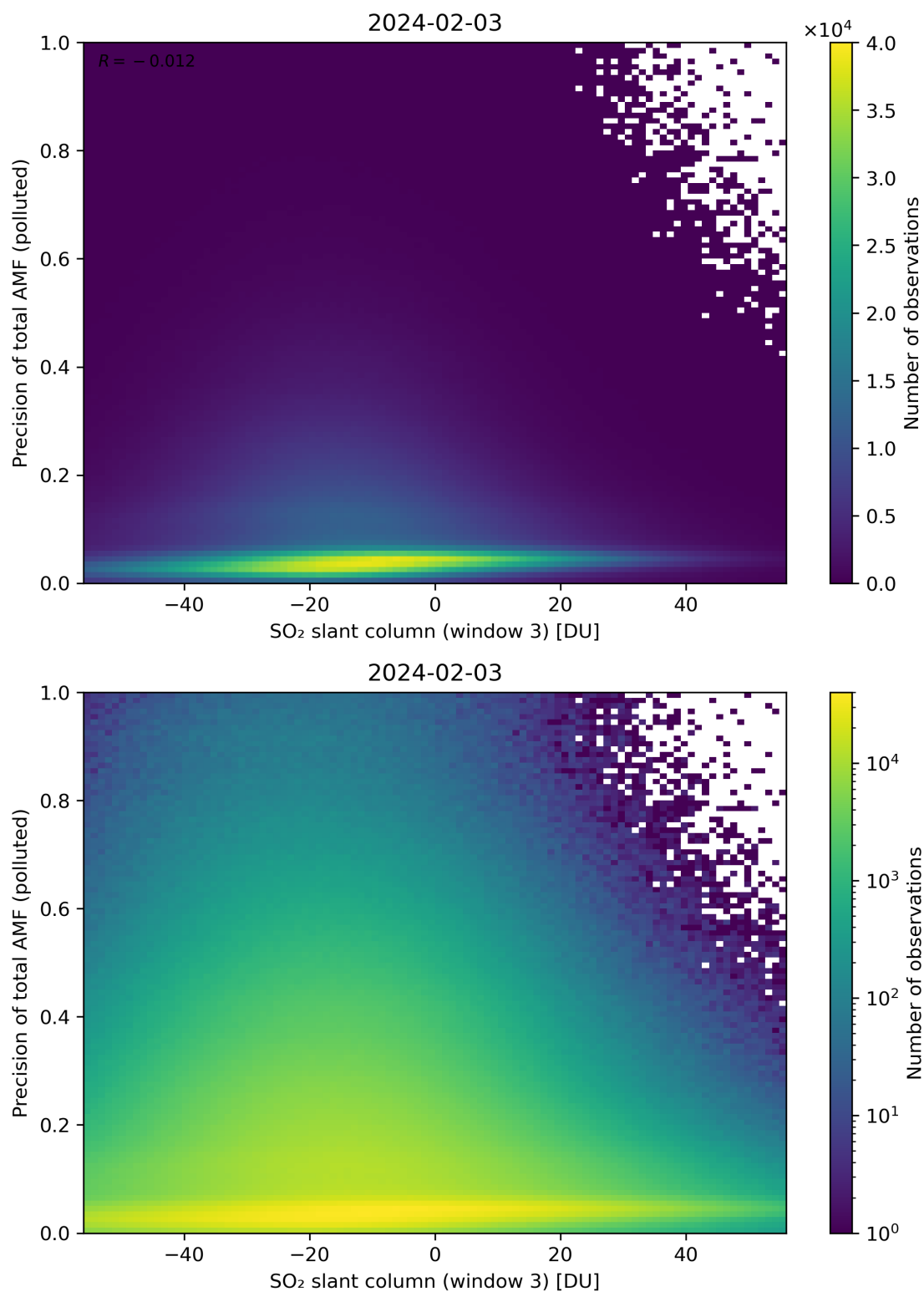
Figure 269: Scatter density plot of “SO 2 slant column (window 3)” against “Precision of total AMF (polluted)” for 2024-02-02 to 2024-02-04.
