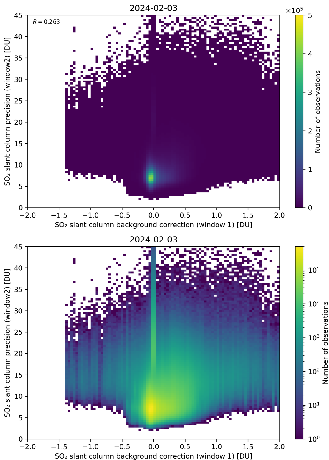
Figure 106: Scatter density plot of “SO 2 slant column background correction (window 1)” against “SO 2 slant column precision (window2)” for 2024-02-02 to 2024-02-04.
