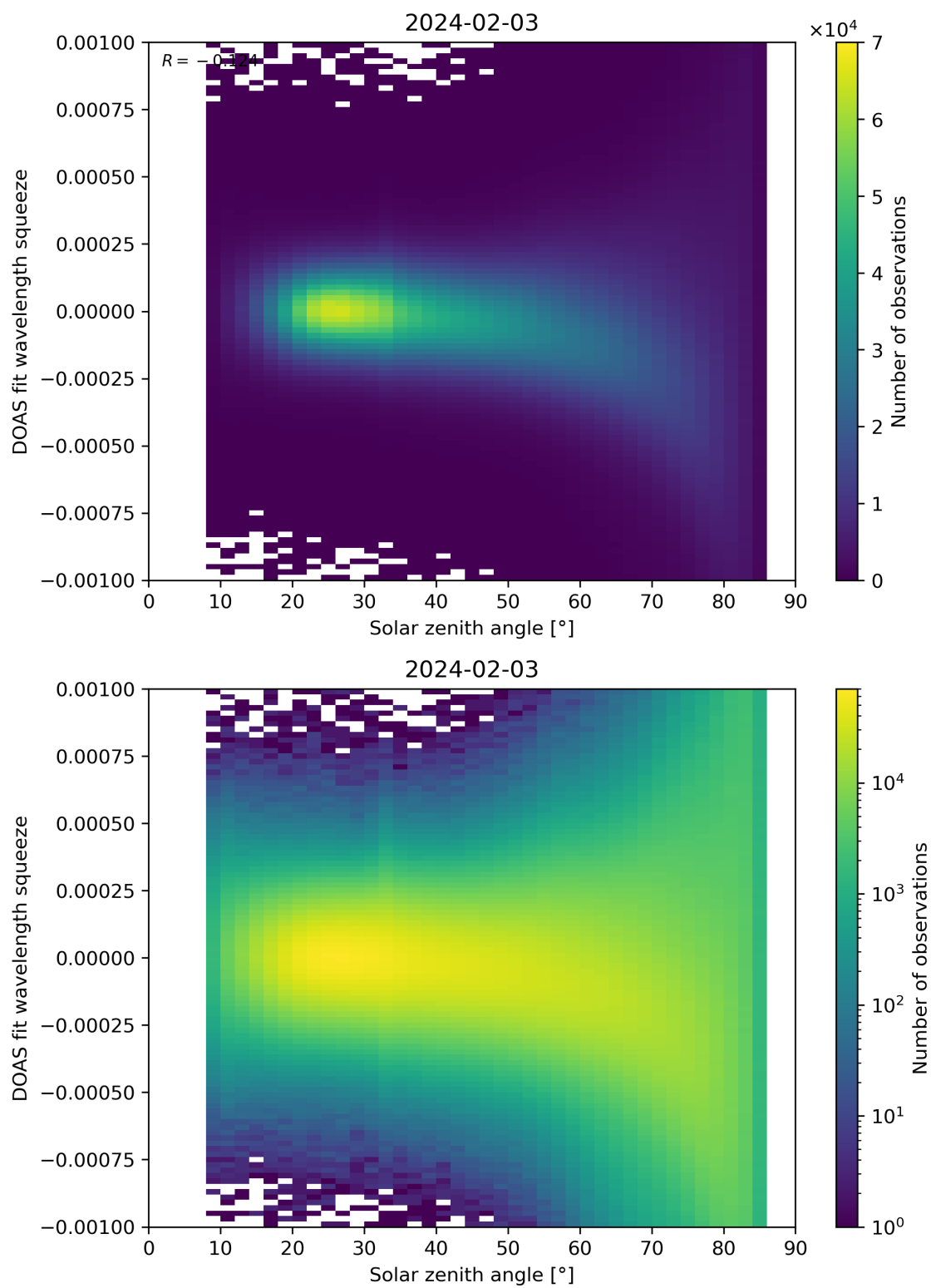
Figure 162: Scatter density plot of “Solar zenith angle” against “DOAS fit wavelength squeeze” for 2024-02-02 to 2024-02-04.
