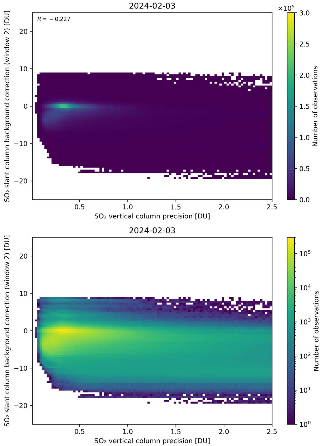
Figure 280: Scatter density plot of “SO 2 vertical column precision” against “SO 2 slant column background correction (window 2)” for 2024-02-02 to 2024-02-04.
