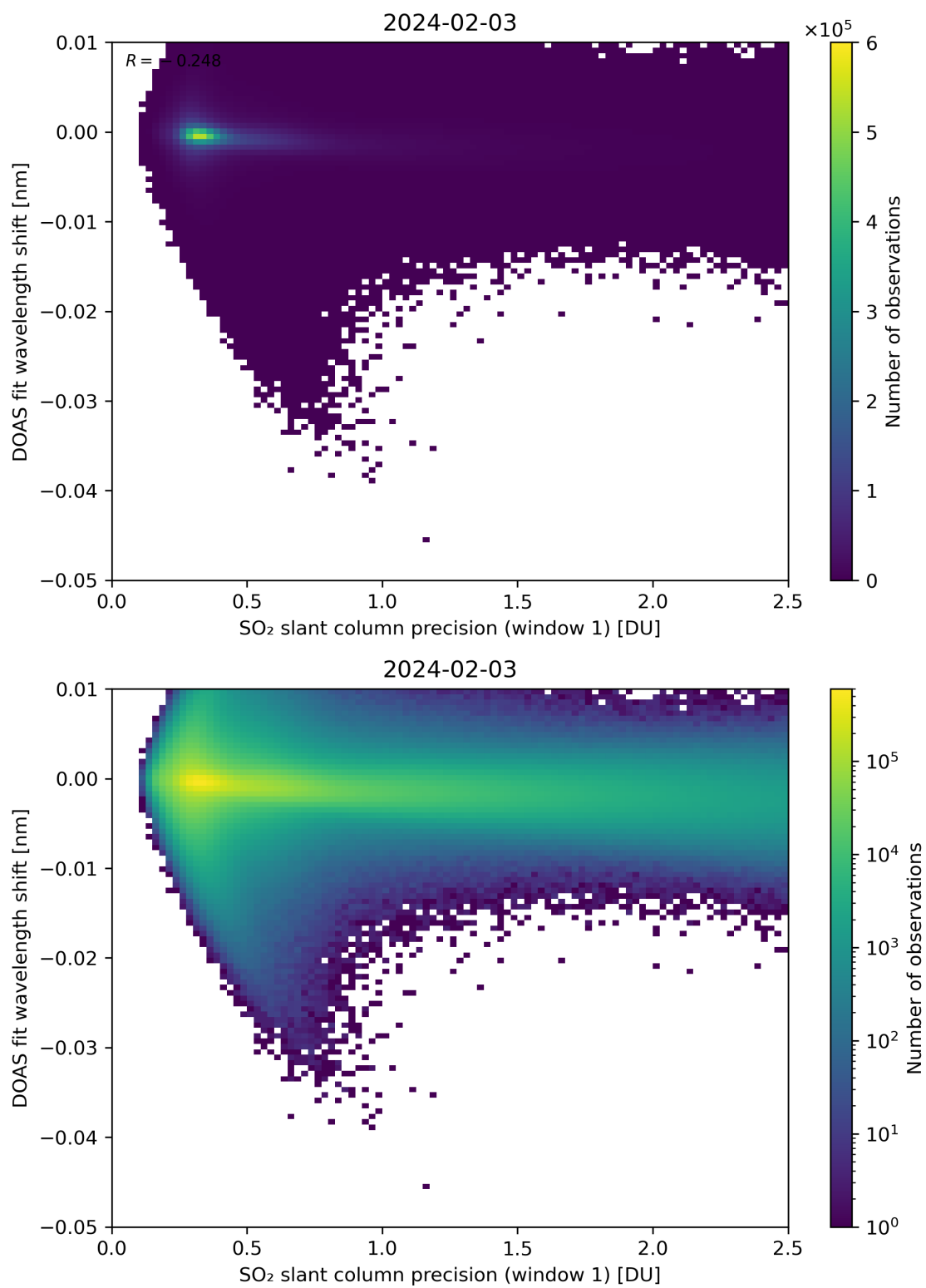
Figure 221: Scatter density plot of “SO 2 slant column precision (window 1)” against “DOAS fit wavelength shift” for 2024-02-02 to 2024-02-04.
