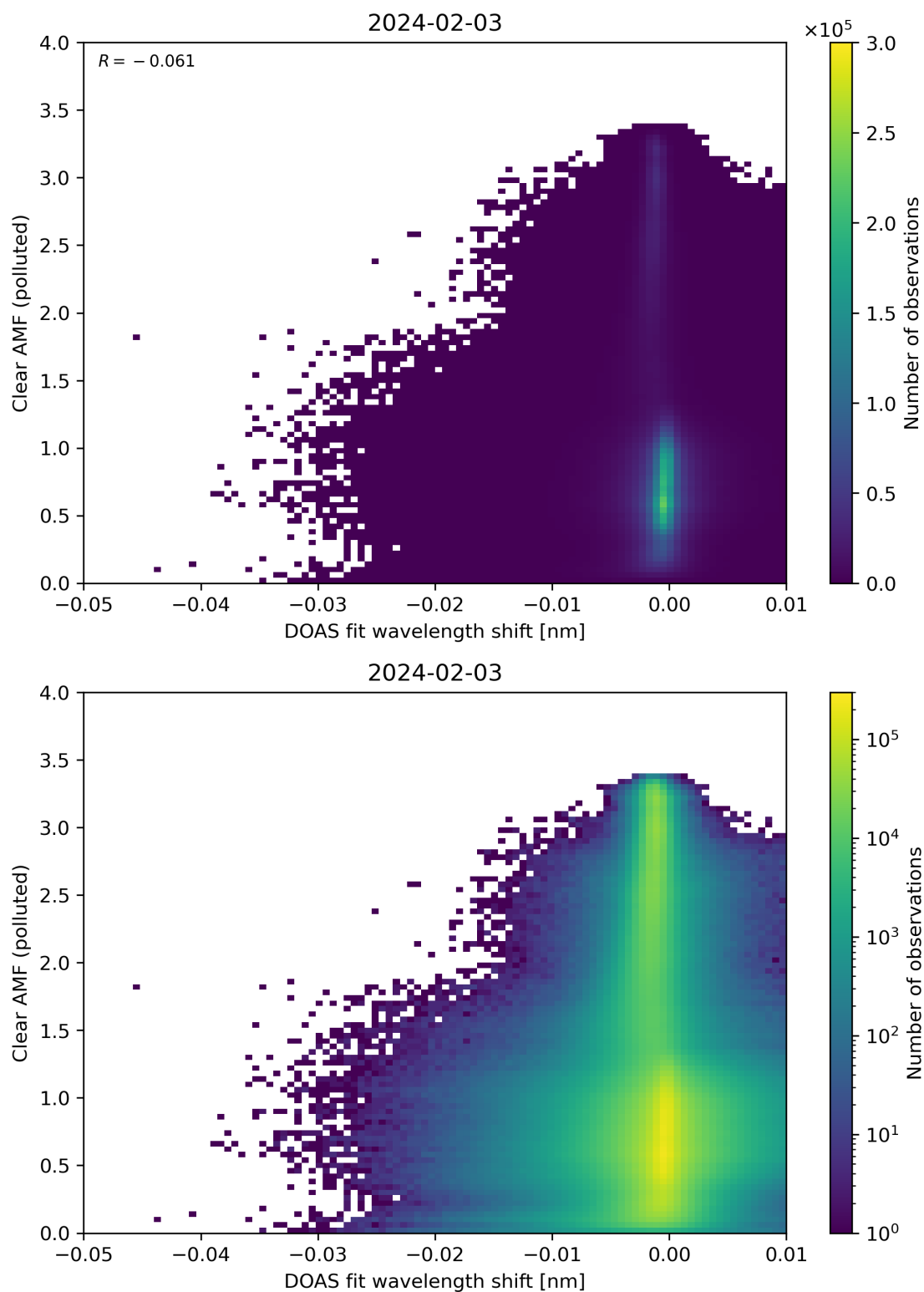
Figure 129: Scatter density plot of “DOAS fit wavelength shift” against “Clear AMF (polluted)” for 2024-02-02 to 2024-02-04.
