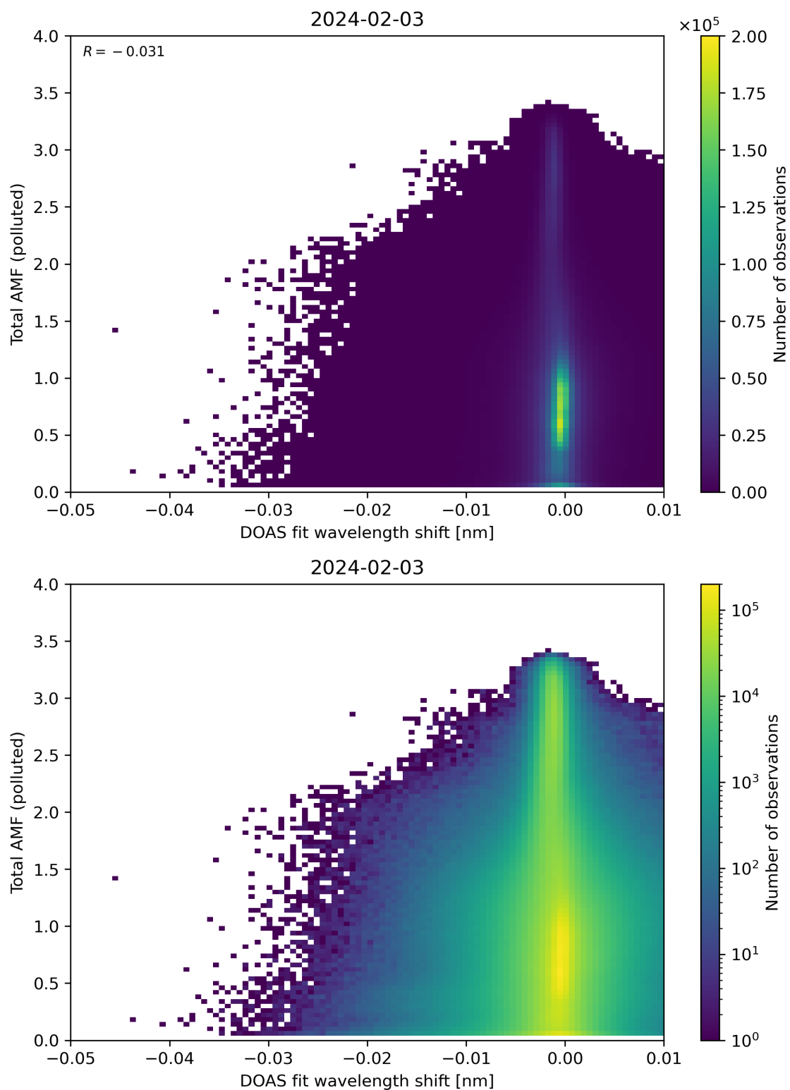
Figure 130: Scatter density plot of “DOAS fit wavelength shift” against “Total AMF (polluted)” for 2024-02-02 to 2024-02-04.
