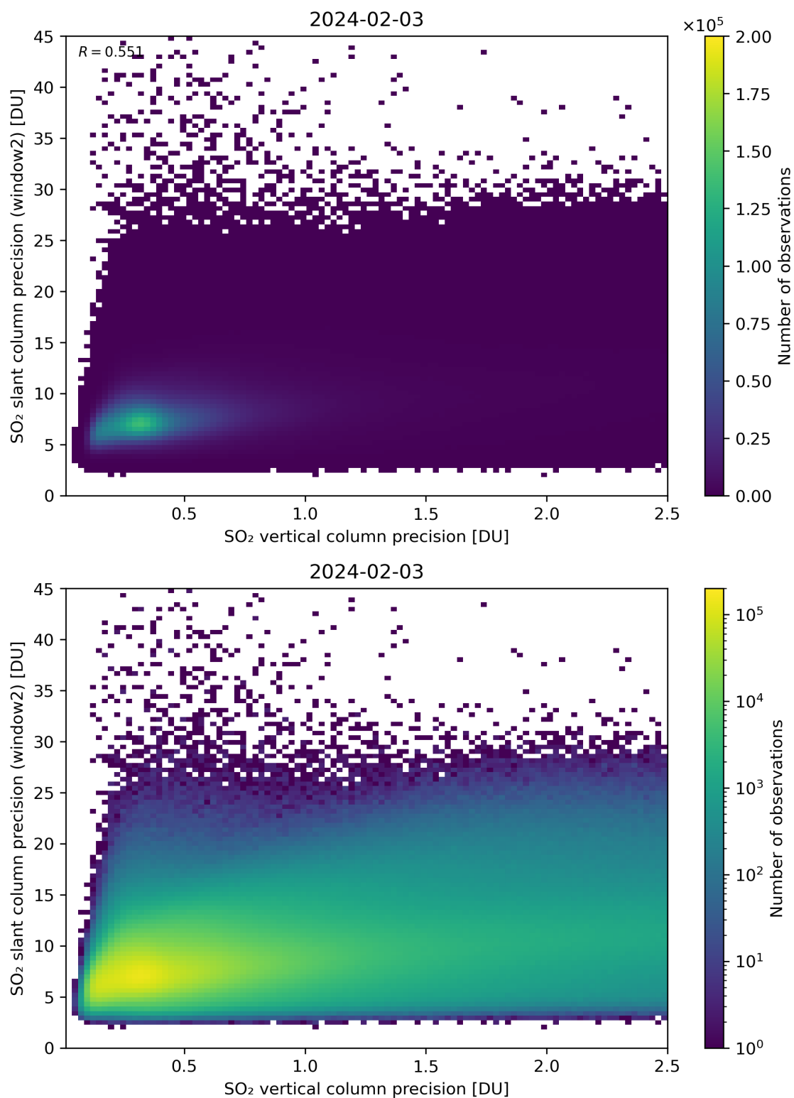
Figure 291: Scatter density plot of “SO 2 vertical column precision” against “SO 2 slant column precision (window2)” for 2024-02-02 to 2024-02-04.
