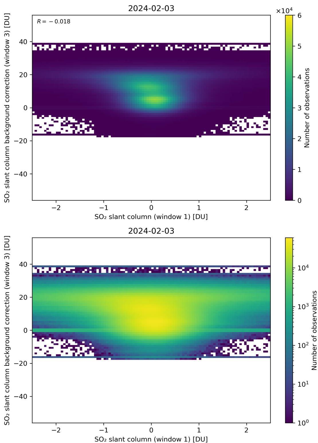
Figure 214: Scatter density plot of “SO 2 slant column (window 1)” against “SO 2 slant column background correction (window 3)” for 2024-02-02 to 2024-02-04.
