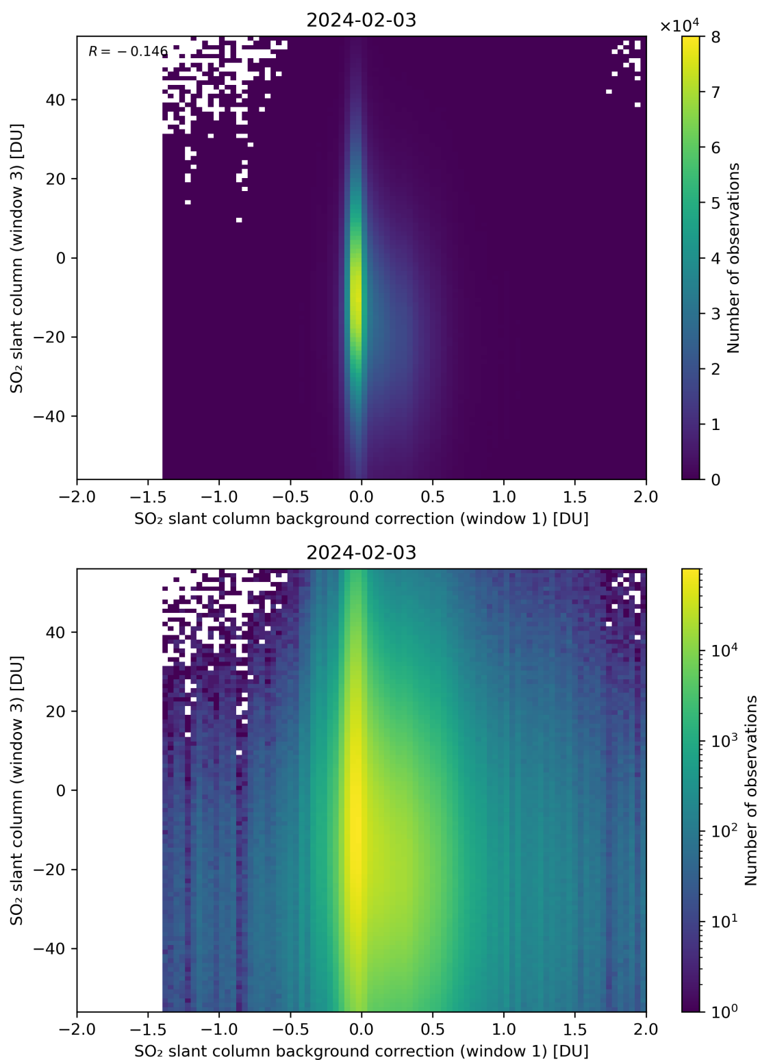
Figure 107: Scatter density plot of “SO 2 slant column background correction (window 1)” against “SO 2 slant column (window 3)” for 2024-02-02 to 2024-02-04.
