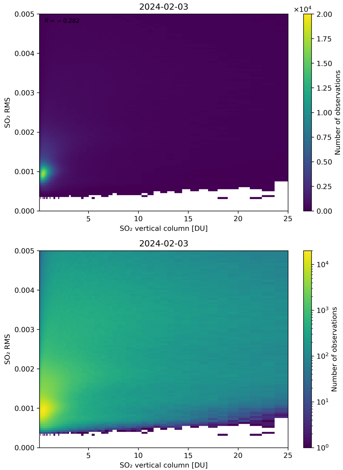
Figure 278: Scatter density plot of “SO 2 vertical column” against “SO 2 RMS” for 2024-02-02 to 2024-02-04.
