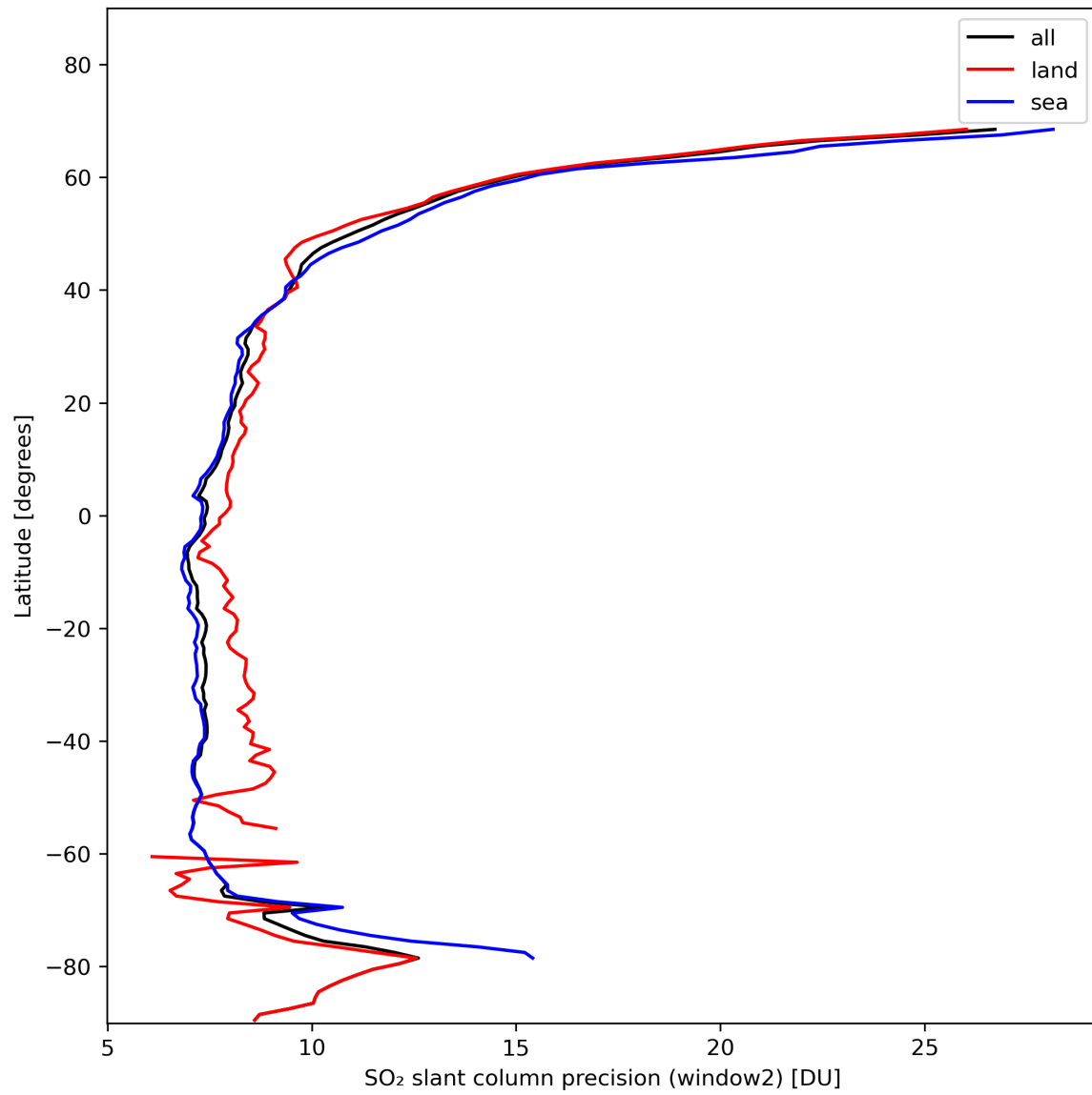
Figure 38: Zonal average of “SO 2 slant column precision (window2)” for 2024-02-02 to 2024-02-04.
