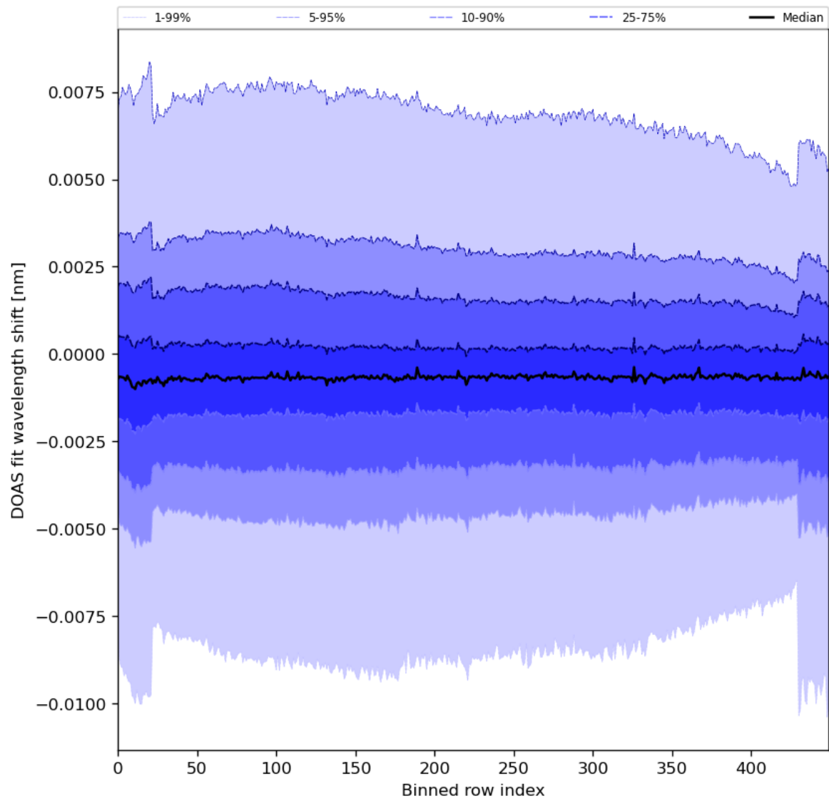
Figure 91: Along track statistics of “DOAS fit wavelength shift” for 2024-02-02 to 2024-02-04
