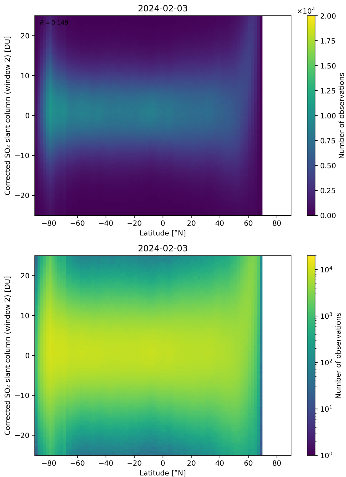
Figure 147: Scatter density plot of “Latitude” against “Corrected SO 2 slant column (window 2)” for 2024-02-02 to 2024-02-04.
