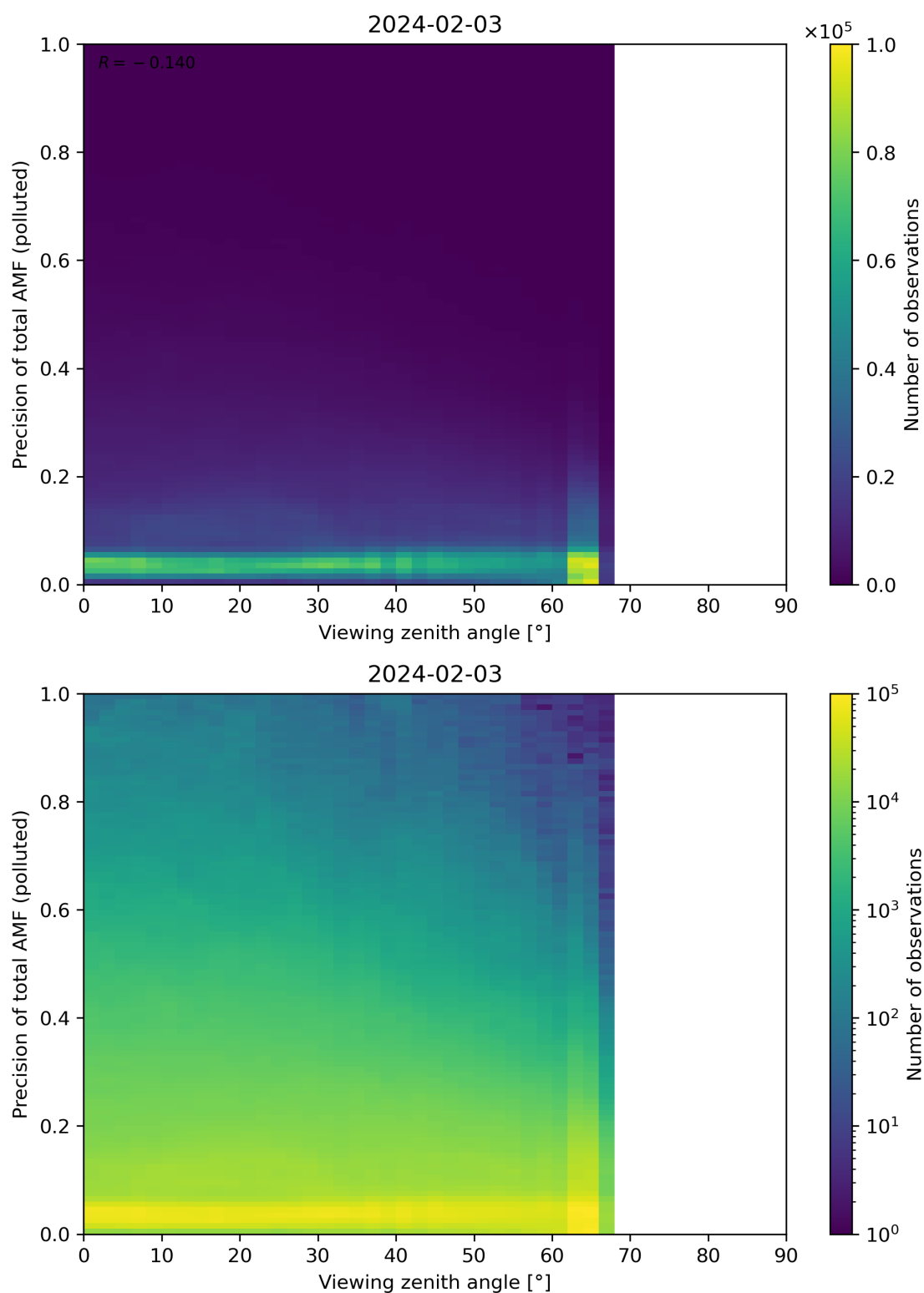
Figure 326: Scatter density plot of “Viewing zenith angle” against “Precision of total AMF (polluted)” for 2024-02-02 to 2024-02-04.
