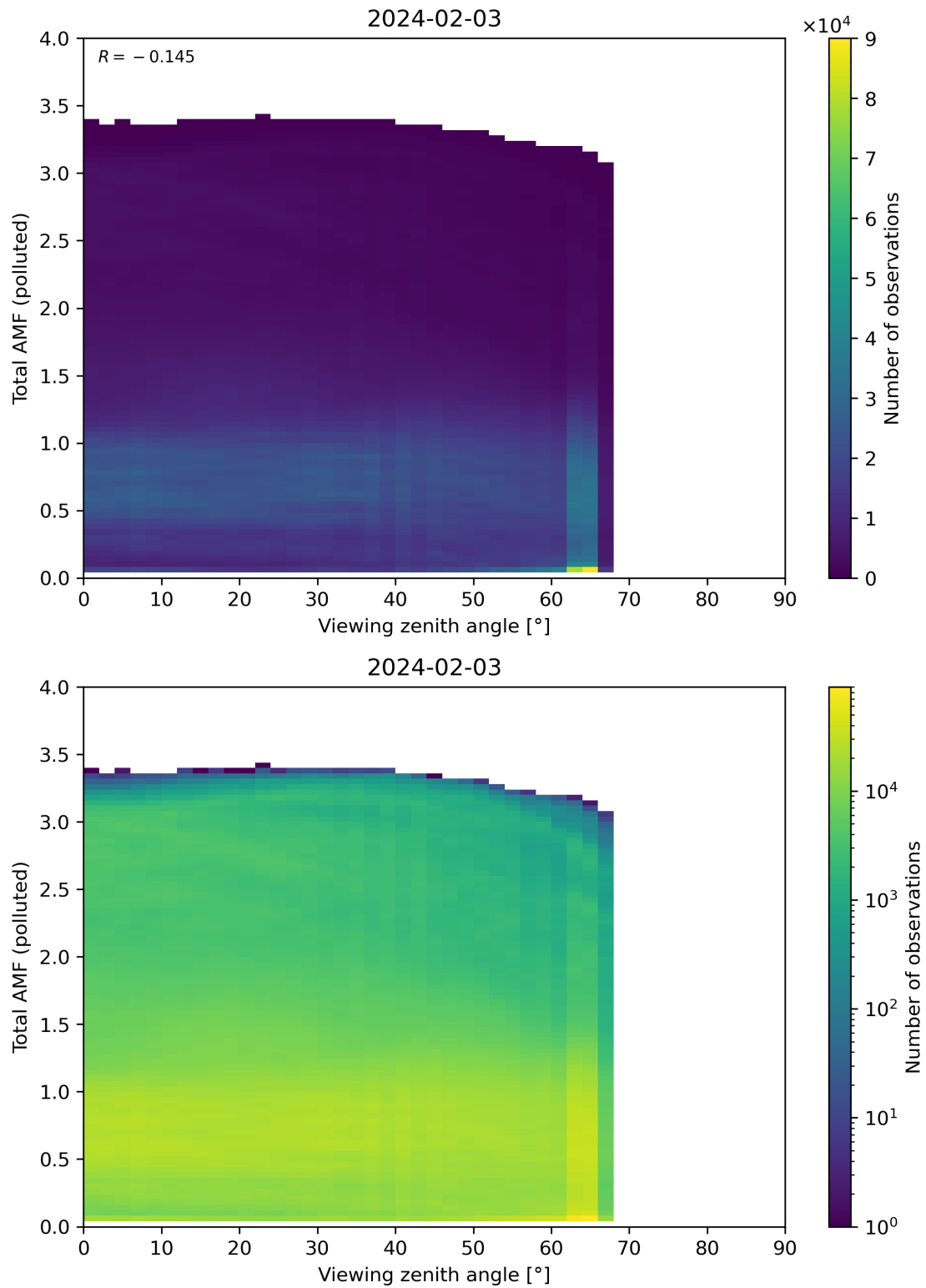
Figure 325: Scatter density plot of “Viewing zenith angle” against “Total AMF (polluted)” for 2024-02-02 to 2024-02-04.
