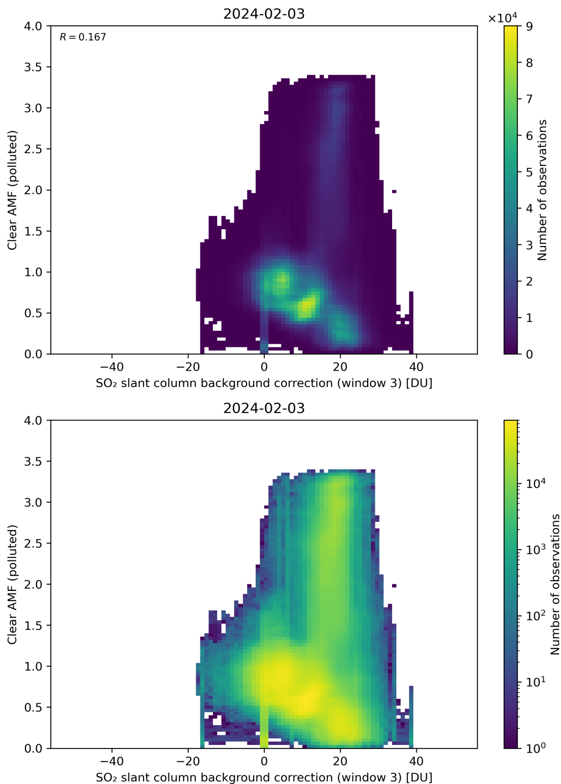
Figure 124: Scatter density plot of “SO 2 slant column background correction (window 3)” against “Clear AMF (polluted)” for 2024-02-02 to 2024-02-04.
