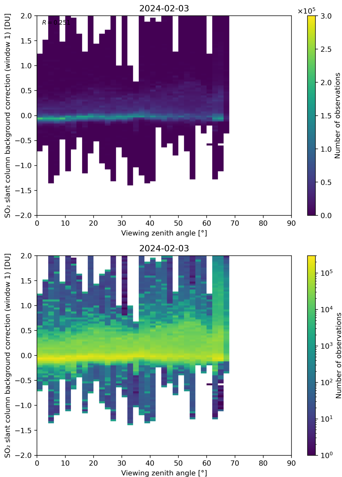
Figure 308: Scatter density plot of “Viewing zenith angle” against “SO 2 slant column background correction (window 1)” for 2024-02-02 to 2024-02-04.
