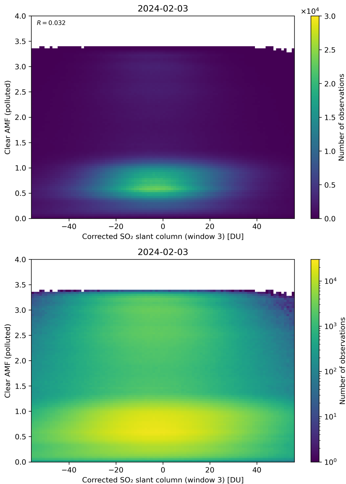
Figure 209: Scatter density plot of “Corrected SO 2 slant column (window 3)” against “Clear AMF (polluted)” for 2024-02-02 to 2024-02-04.
