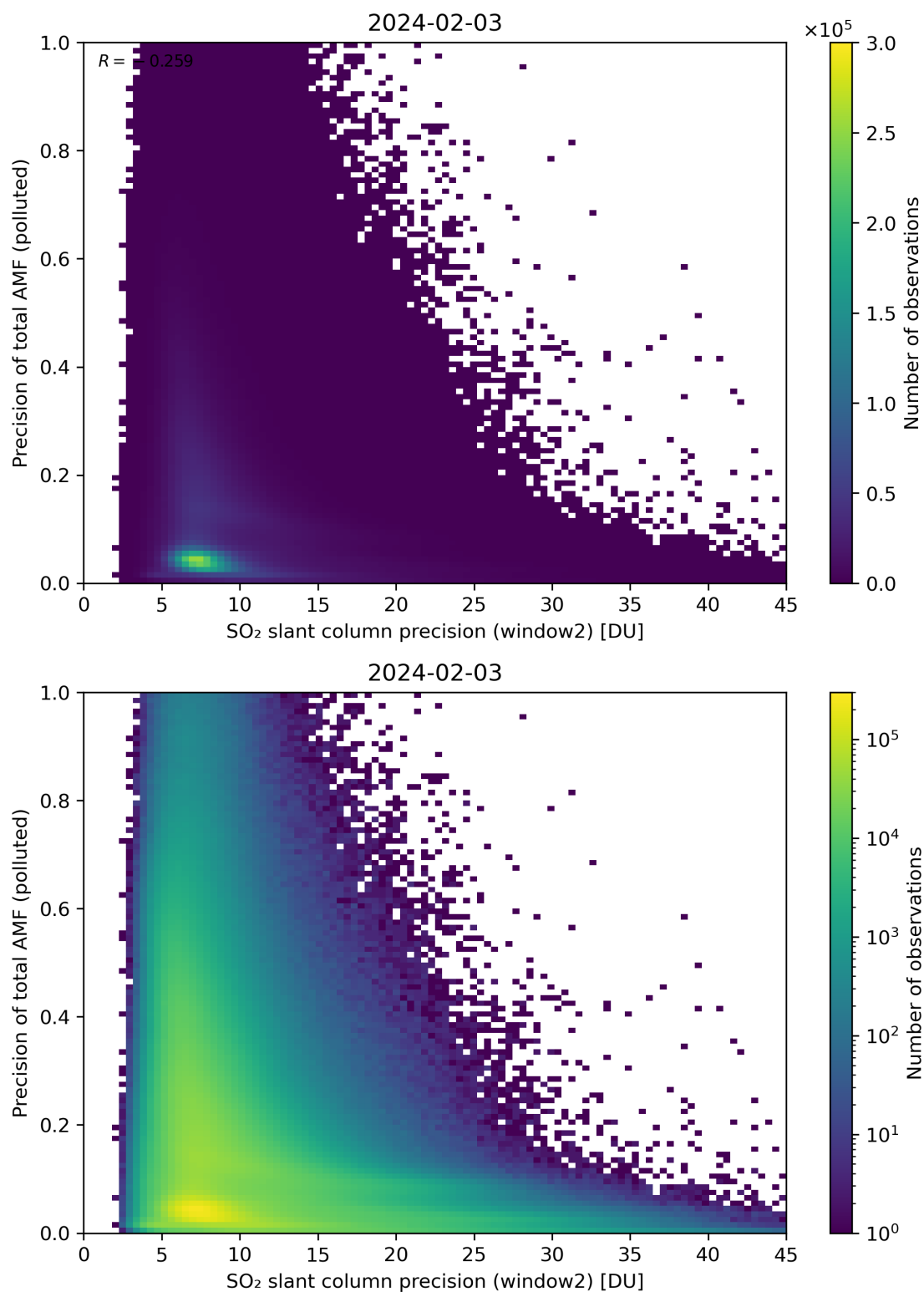
Figure 252: Scatter density plot of “SO 2 slant column precision (window2)” against “Precision of total AMF (polluted)” for 2024-02-02 to 2024-02-04.
