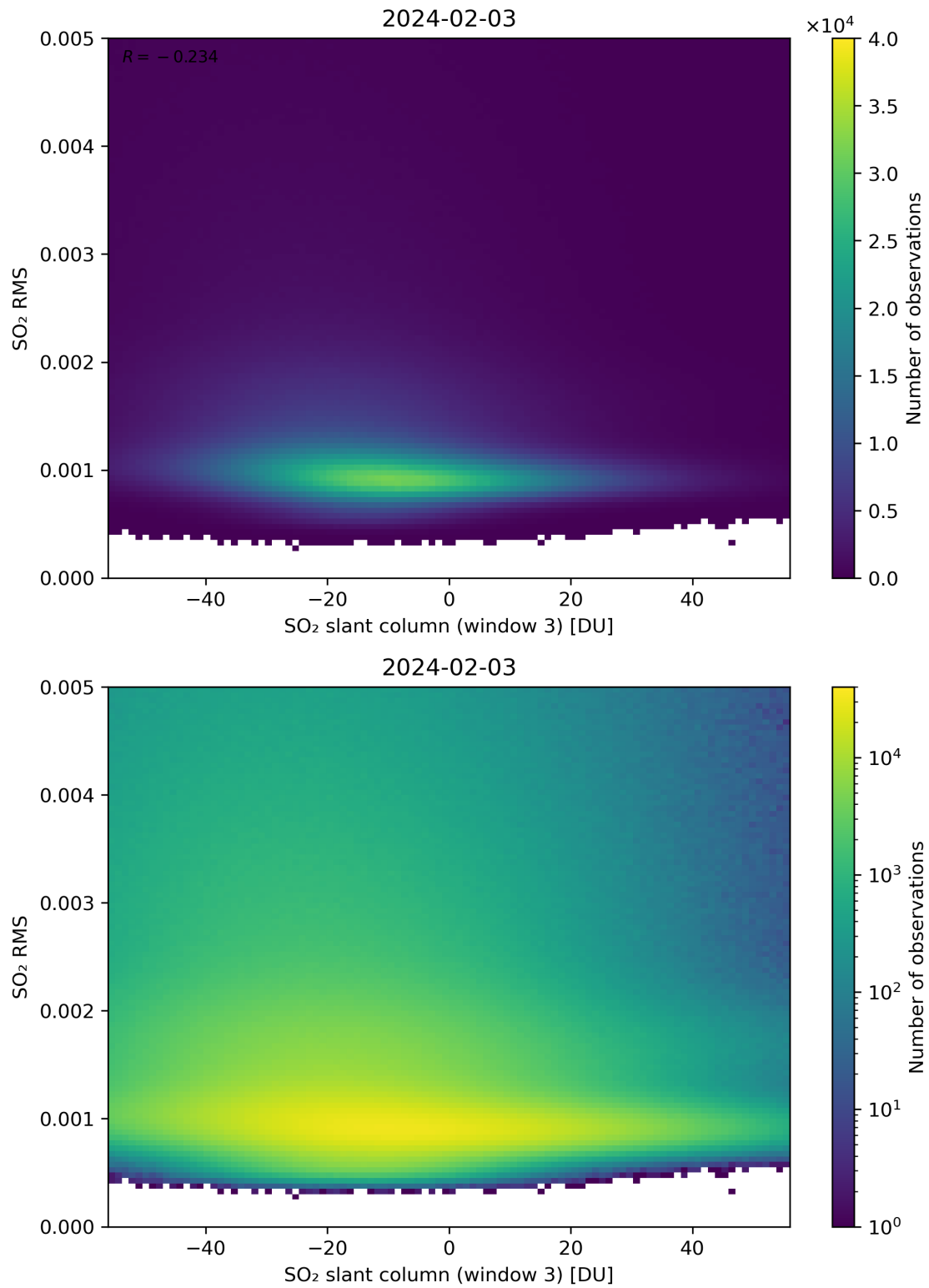
Figure 256: Scatter density plot of “SO 2 slant column (window 3)” against “SO 2 RMS” for 2024-02-02 to 2024-02-04.
