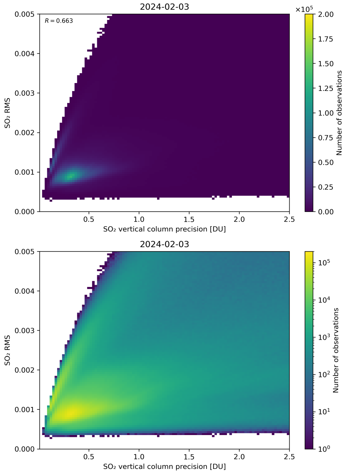
Figure 284: Scatter density plot of “SO 2 vertical column precision” against “SO 2 RMS” for 2024-02-02 to 2024-02-04.
