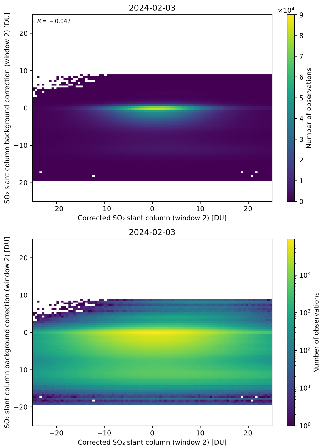
Figure 194: Scatter density plot of “Corrected SO 2 slant column (window 2)” against “SO 2 slant column background correction (window 2)” for 2024-02-02 to 2024-02-04.
