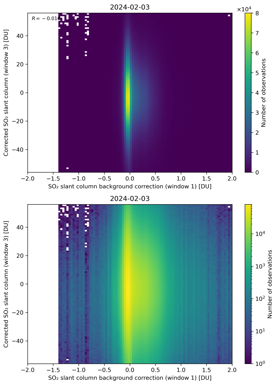
Figure 105: Scatter density plot of “SO 2 slant column background correction (window 1)” against “Corrected SO 2 slant column (window 3)” for 2024-02-02 to 2024-02-04.
