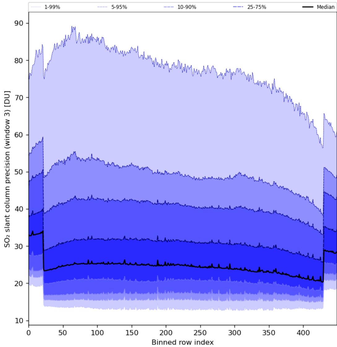
Figure 88: Along track statistics of “SO 2 slant column precision (window 3)” for 2024-02-02 to 2024-02-04
