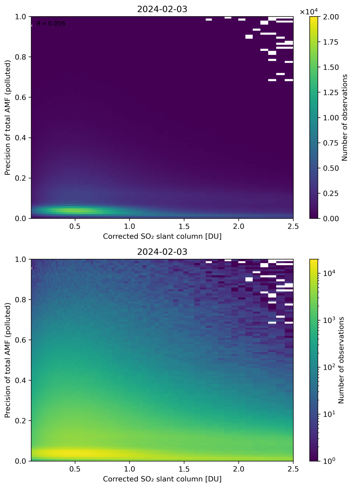
Figure 193: Scatter density plot of “Corrected SO 2 slant column” against “Precision of total AMF (polluted)” for 2024-02-02 to 2024-02-04.
