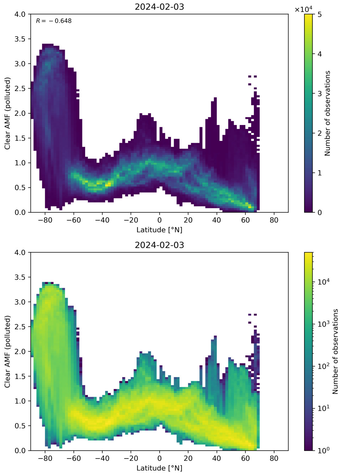
Figure 145: Scatter density plot of “Latitude” against “Clear AMF (polluted)” for 2024-02-02 to 2024-02-04.
