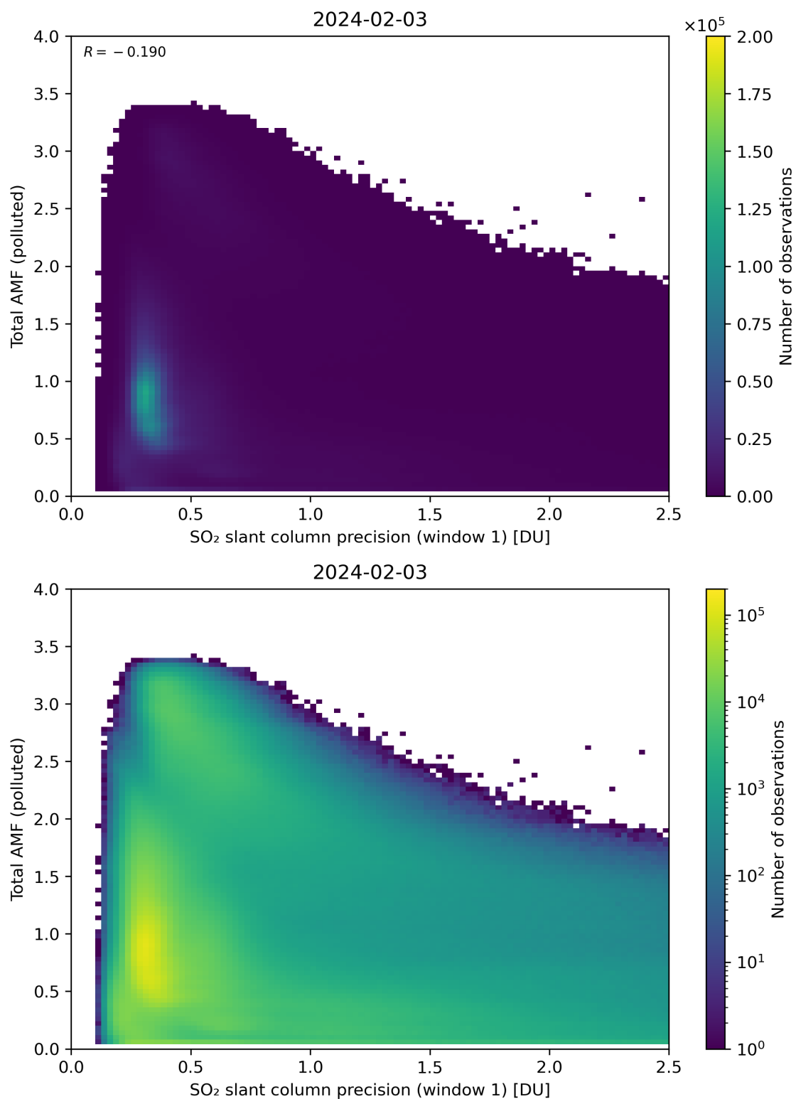
Figure 230: Scatter density plot of “SO 2 slant column precision (window 1)” against “Total AMF (polluted)” for 2024-02-02 to 2024-02-04.
