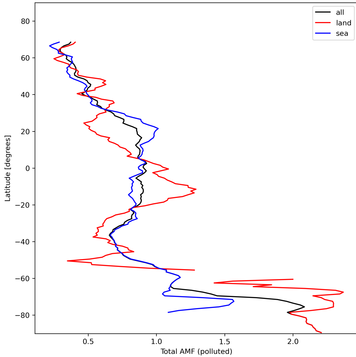
Figure 48: Zonal average of “Total AMF (polluted)” for 2024-02-02 to 2024-02-04.
