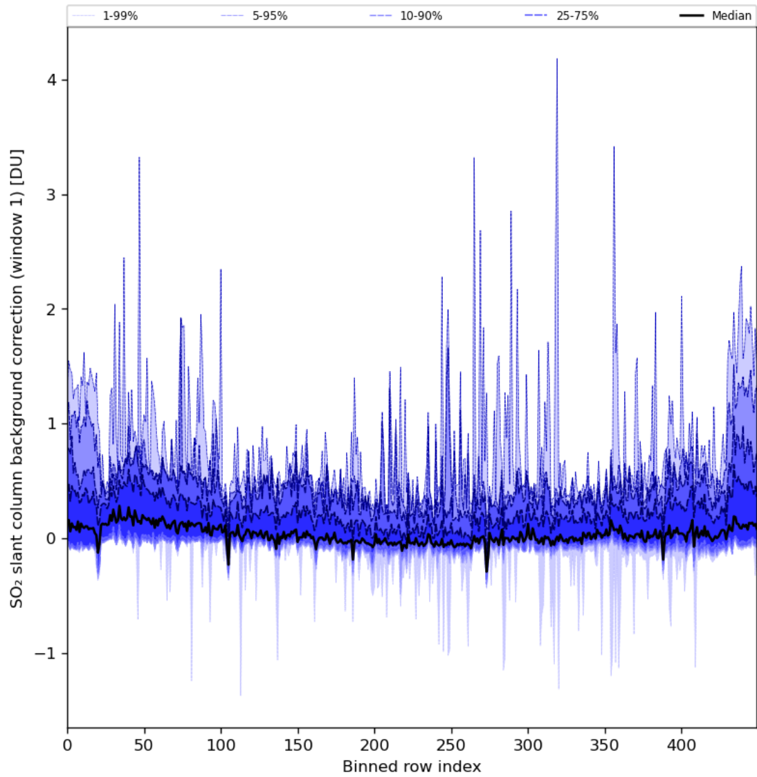
Figure 82: Along track statistics of “SO 2 slant column background correction (window 1)” for 2024-02-02 to 2024-02-04
