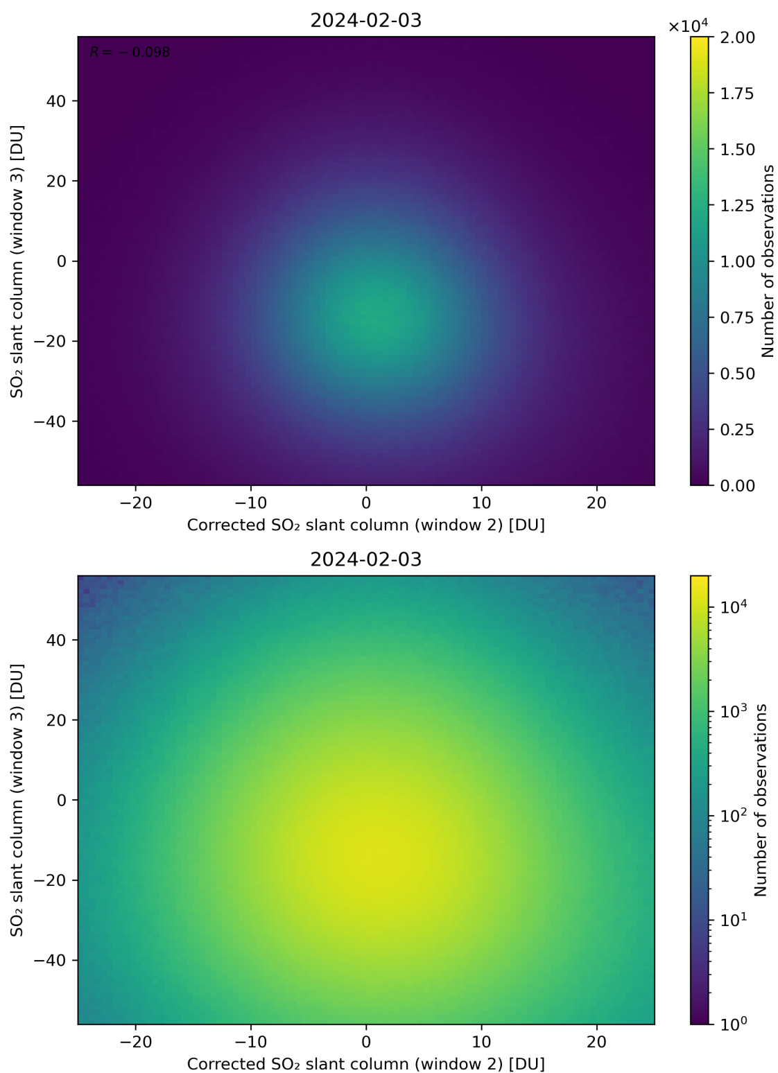
Figure 201: Scatter density plot of “Corrected SO 2 slant column (window 2)” against “SO 2 slant column (window 3)” for 2024-02-02 to 2024-02-04.
