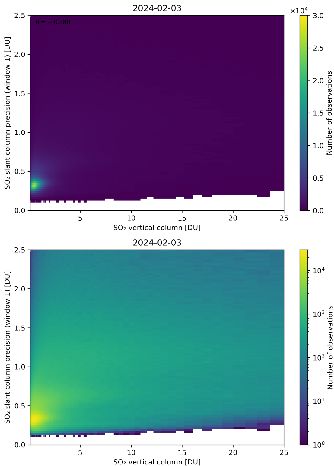
Figure 301: Scatter density plot of “SO 2 vertical column” against “SO 2 slant column precision (window 1)” for 2024-02-02 to 2024-02-04.
