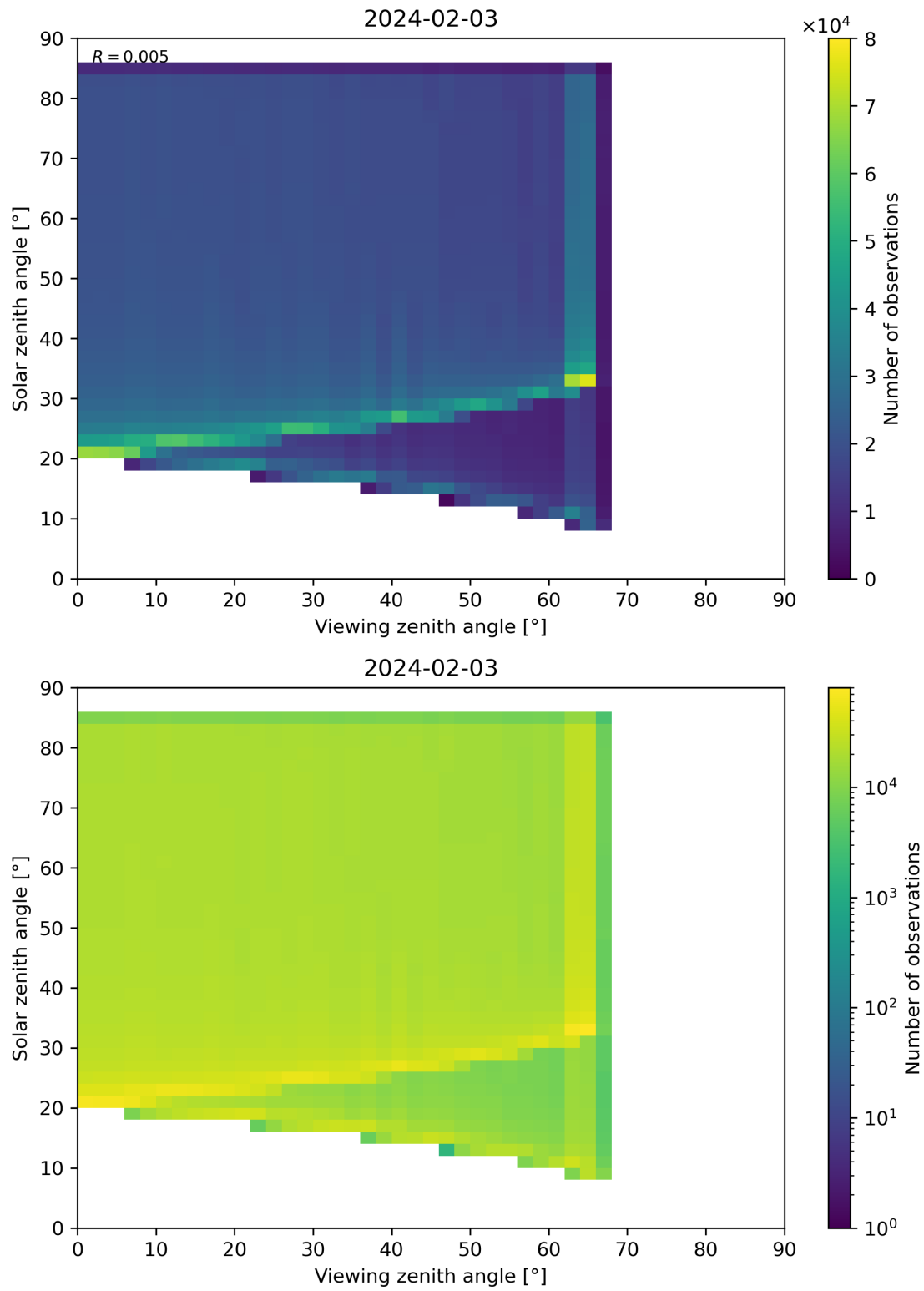
Figure 315: Scatter density plot of “Viewing zenith angle” against “Solar zenith angle” for 2024-02-02 to 2024-02-04.
