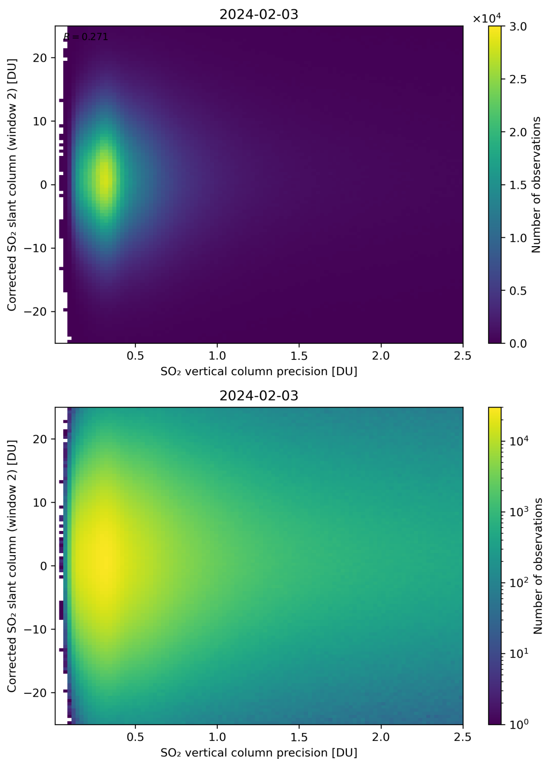
Figure 287: Scatter density plot of “SO 2 vertical column precision” against “Corrected SO 2 slant column (window 2)” for 2024-02-02 to 2024-02-04.
