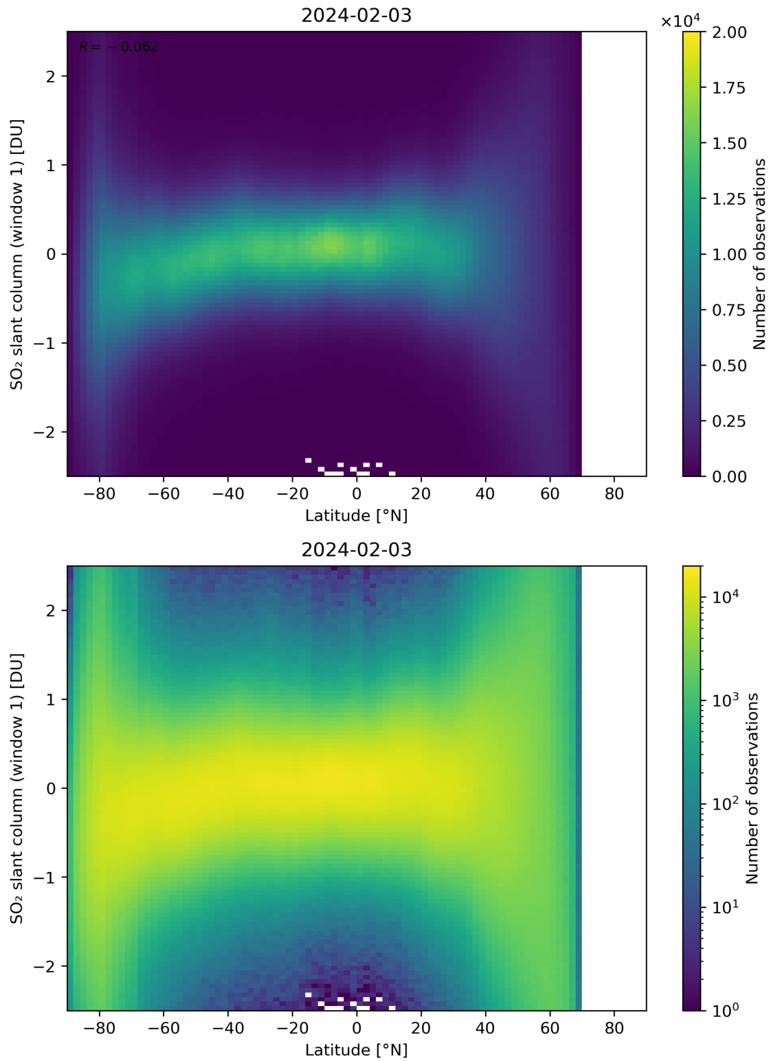
Figure 149: Scatter density plot of “Latitude” against “SO 2 slant column (window 1)” for 2024-02-02 to 2024-02-04.
