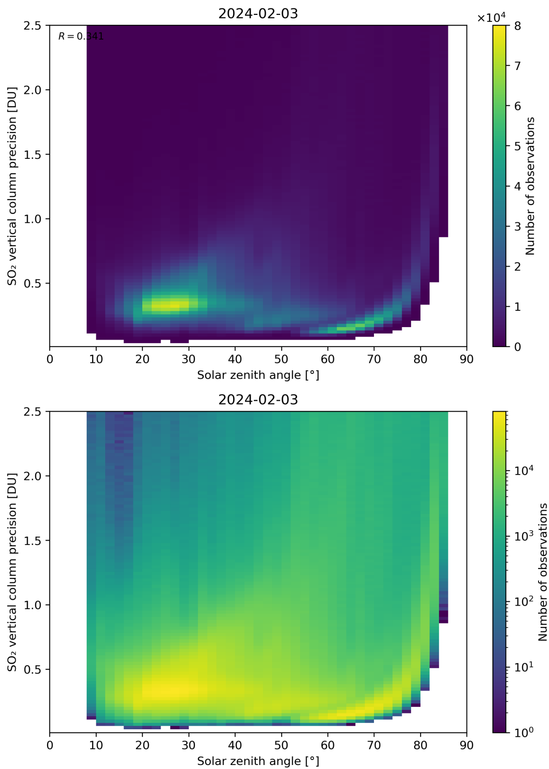
Figure 177: Scatter density plot of “Solar zenith angle” against “SO 2 vertical column precision” for 2024-02-02 to 2024-02-04.
