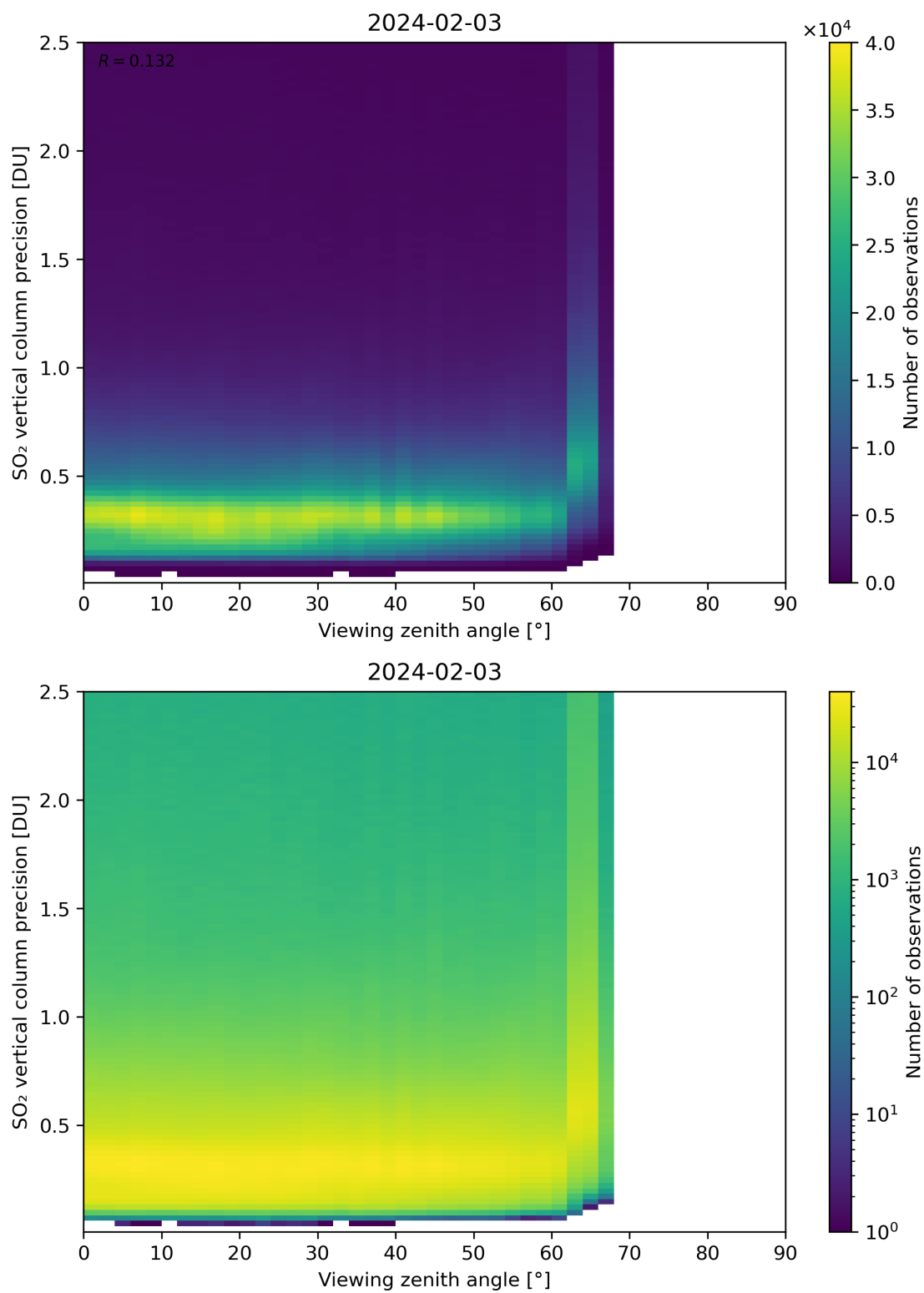
Figure 328: Scatter density plot of “Viewing zenith angle” against “SO 2 vertical column precision” for 2024-02-02 to 2024-02-04.
