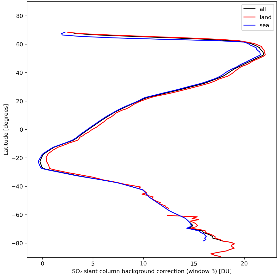
Figure 44: Zonal average of “SO 2 slant column background correction (window 3)” for 2024-02-02 to 2024-02-04.
