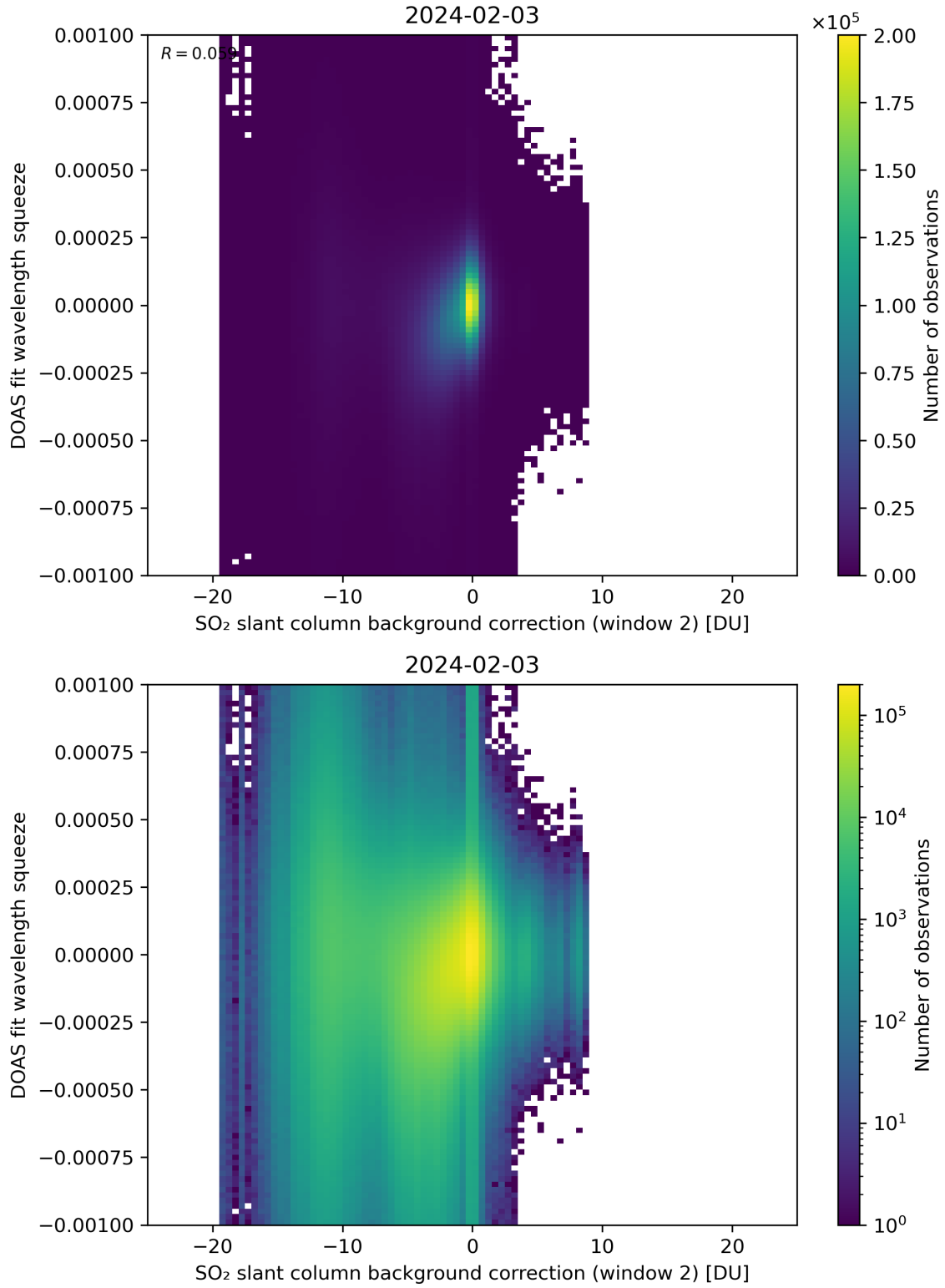
Figure 113: Scatter density plot of “SO 2 slant column background correction (window 2)” against “DOAS fit wavelength squeeze” for 2024-02-02 to 2024-02-04.
