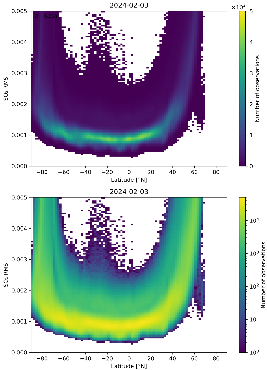
Figure 144: Scatter density plot of “Latitude” against “SO 2 RMS” for 2024-02-02 to 2024-02-04.
