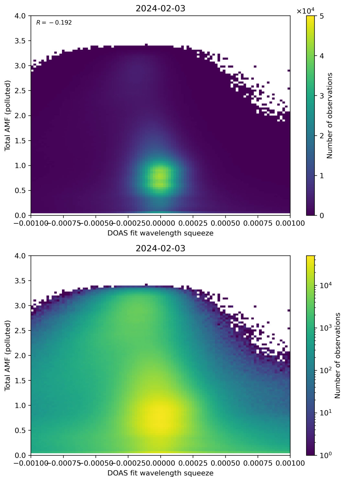
Figure 134: Scatter density plot of “DOAS fit wavelength squeeze” against “Total AMF (polluted)” for 2024-02-02 to 2024-02-04.
