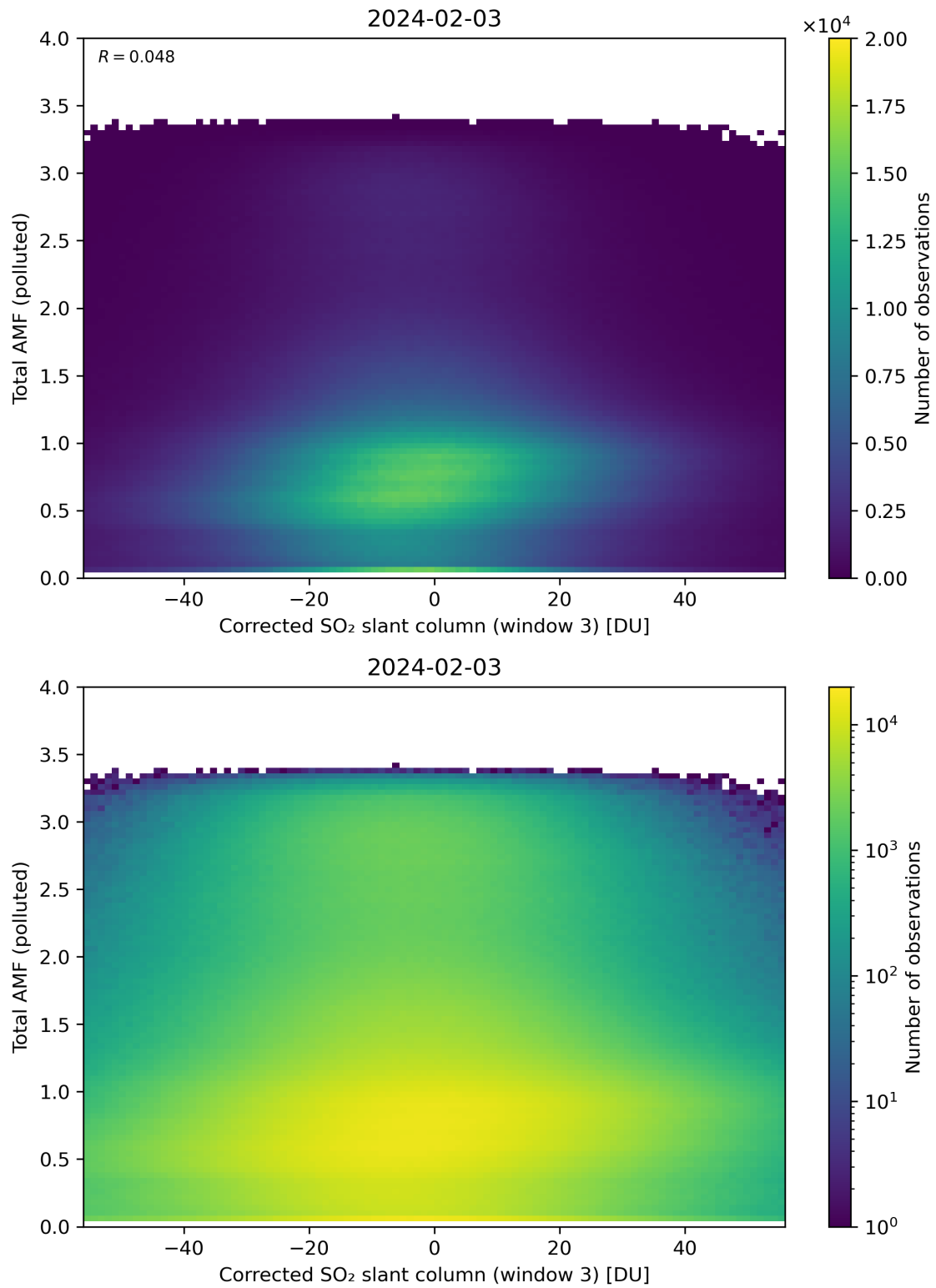
Figure 210: Scatter density plot of “Corrected SO 2 slant column (window 3)” against “Total AMF (polluted)” for 2024-02-02 to 2024-02-04.
