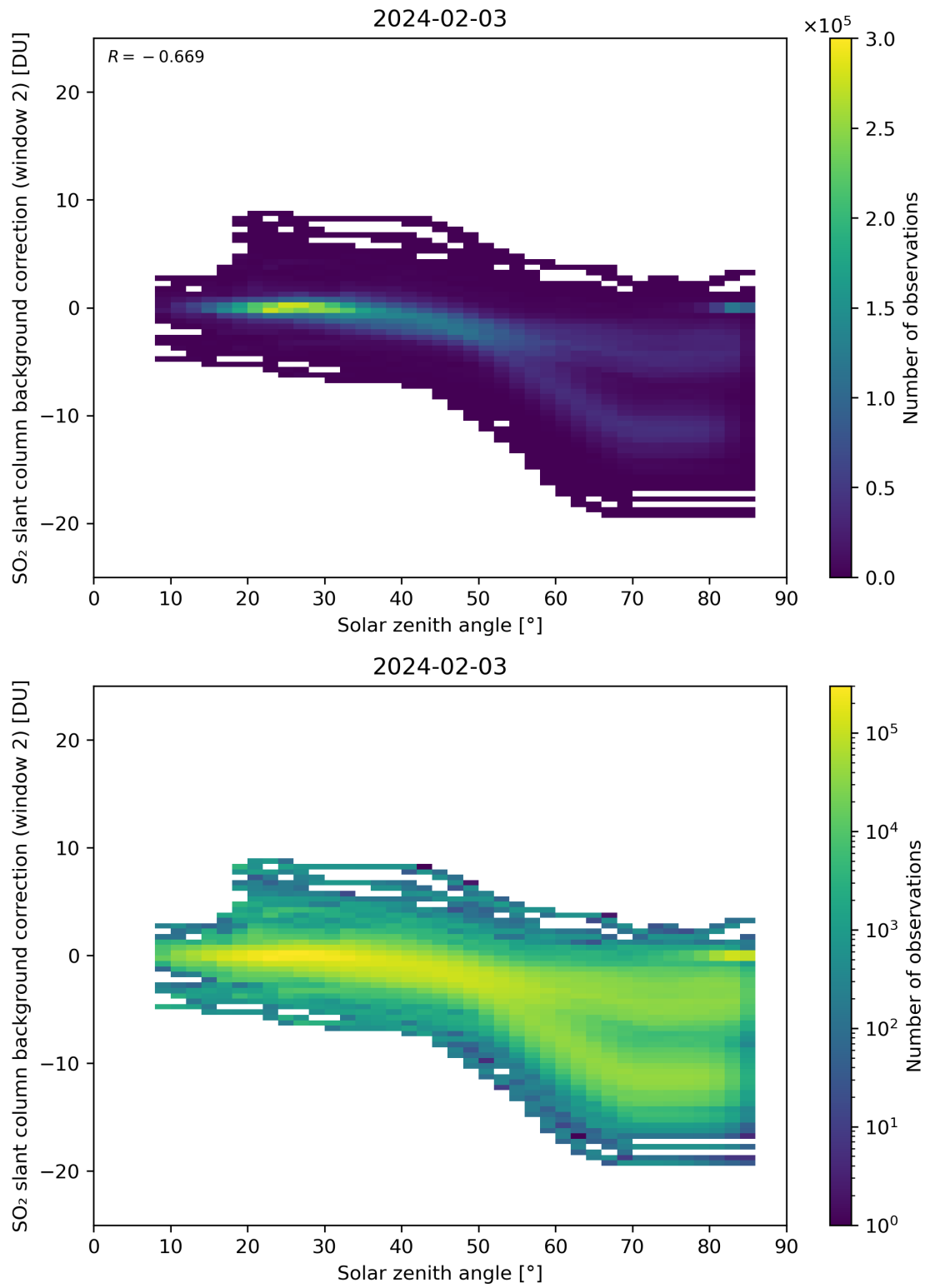
Figure 159: Scatter density plot of “Solar zenith angle” against “SO 2 slant column background correction (window 2)” for 2024-02-02 to 2024-02-04.
