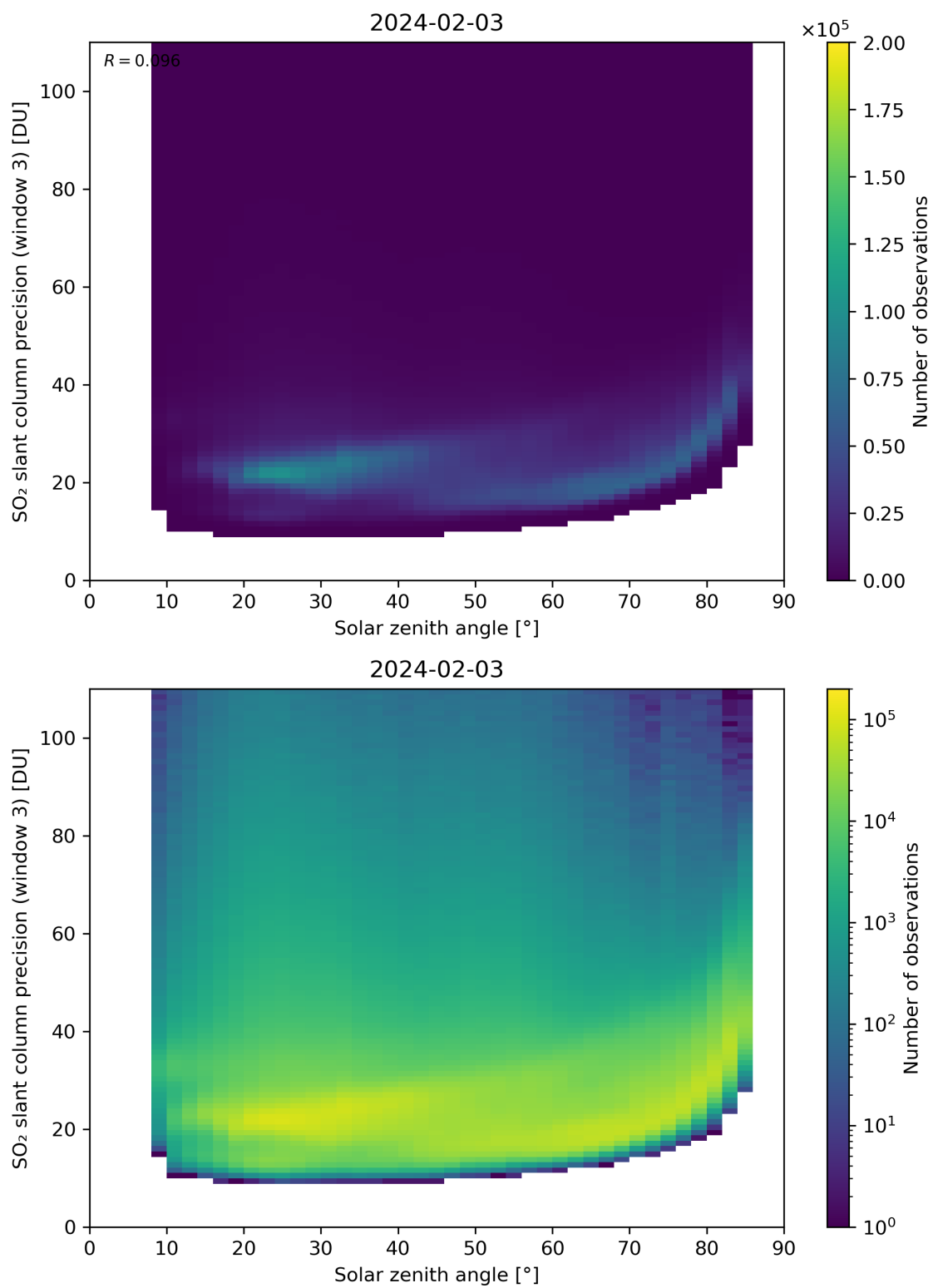
Figure 173: Scatter density plot of “Solar zenith angle” against “SO 2 slant column precision (window 3)” for 2024-02-02 to 2024-02-04.
