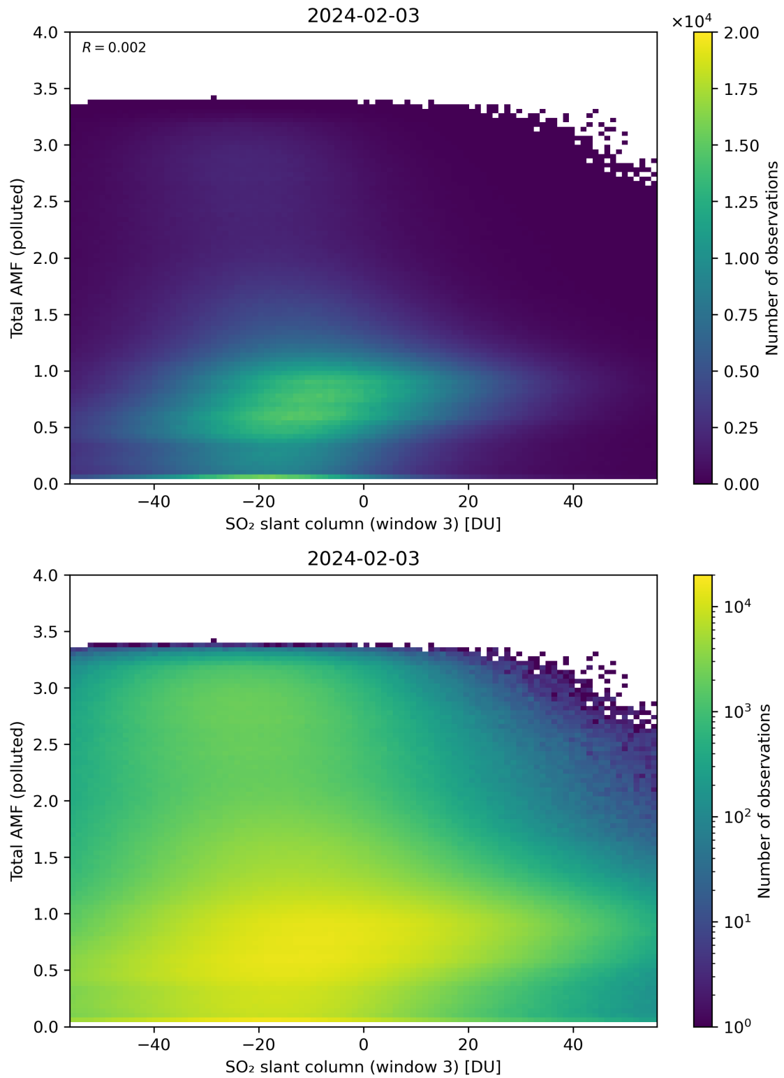
Figure 268: Scatter density plot of “SO 2 slant column (window 3)” against “Total AMF (polluted)” for 2024-02-02 to 2024-02-04.
