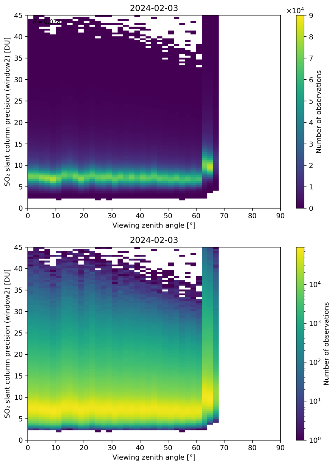
Figure 322: Scatter density plot of “Viewing zenith angle” against “SO 2 slant column precision (window2)” for 2024-02-02 to 2024-02-04.
