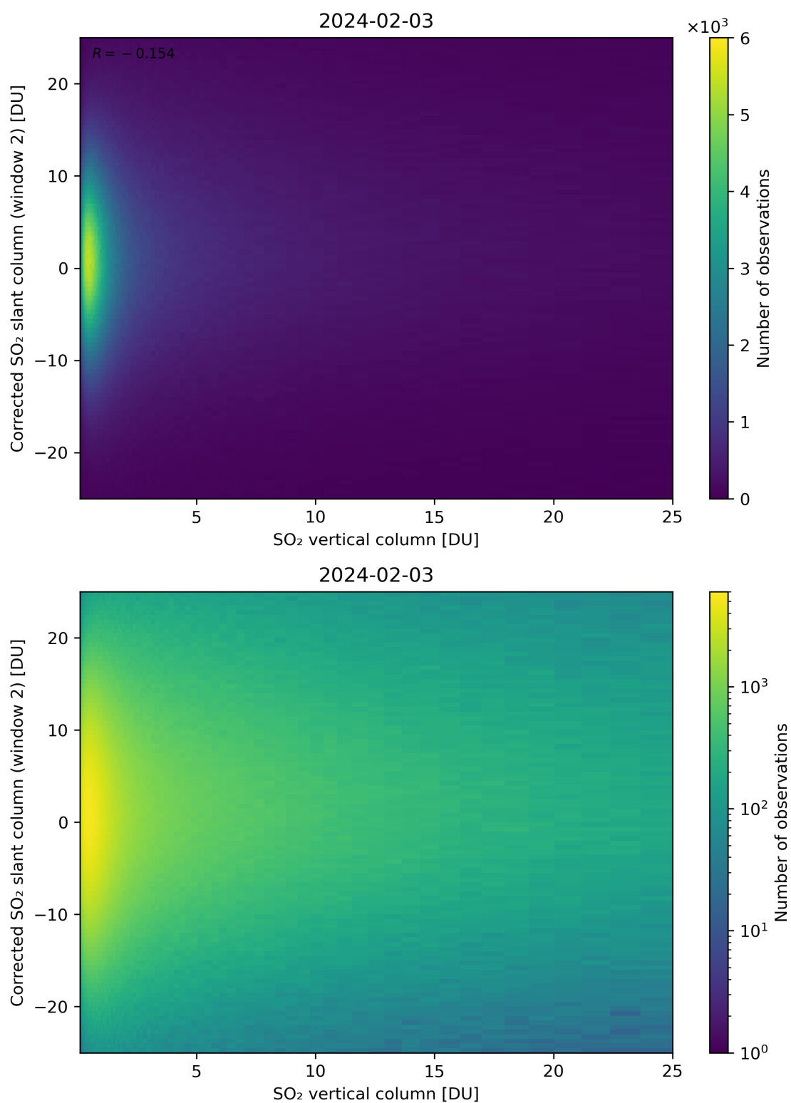
Figure 298: Scatter density plot of “SO 2 vertical column” against “Corrected SO 2 slant column (window 2)” for 2024-02-02 to 2024-02-04.
