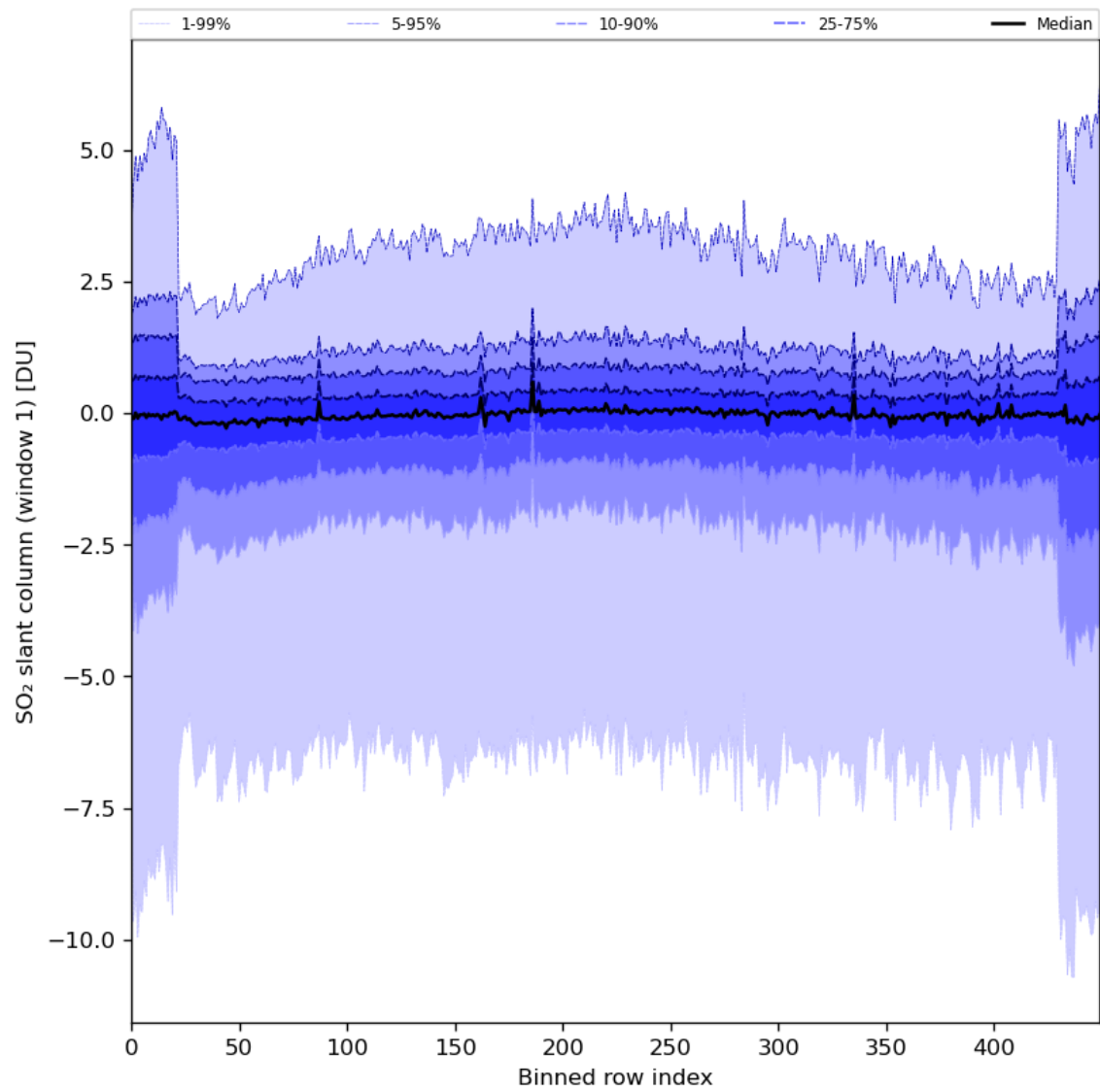
Figure 79: Along track statistics of “SO 2 slant column (window 1)” for 2024-02-02 to 2024-02-04
