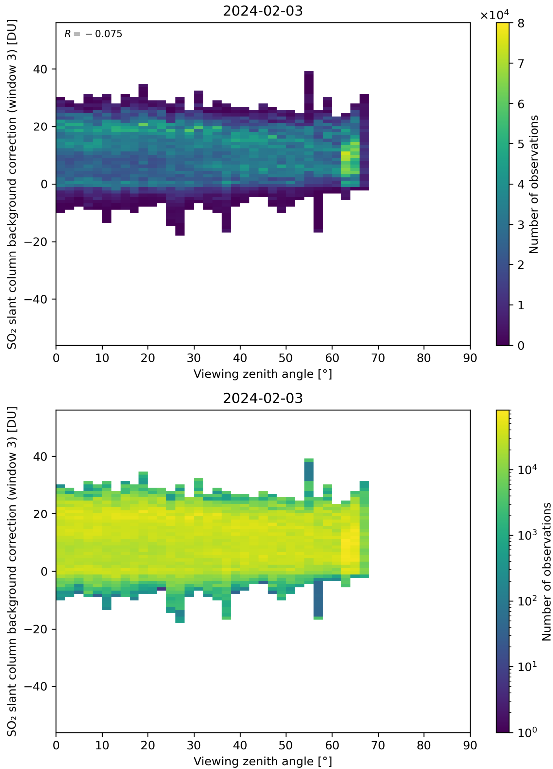
Figure 310: Scatter density plot of “Viewing zenith angle” against “SO 2 slant column background correction (window 3)” for 2024-02-02 to 2024-02-04.
