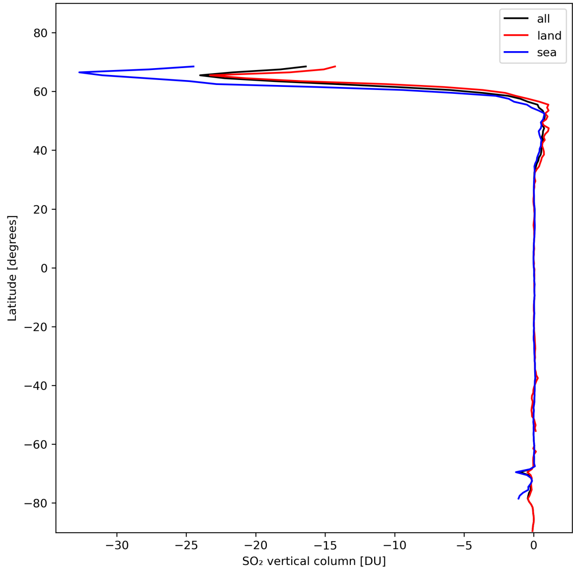
Figure 30: Zonal average of “SO 2 vertical column” for 2024-02-02 to 2024-02-04.
