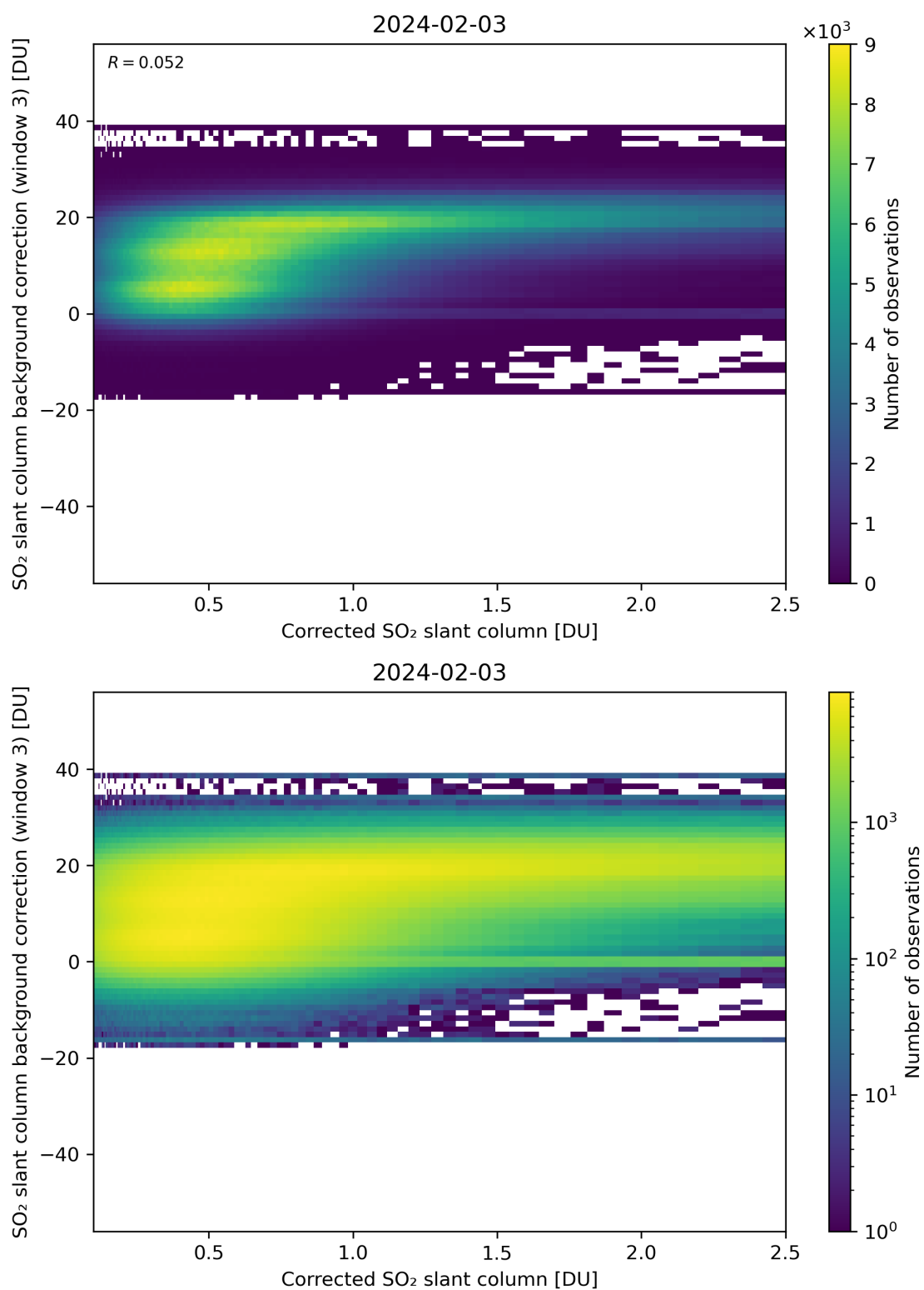
Figure 180: Scatter density plot of “Corrected SO 2 slant column” against “SO 2 slant column background correction (window 3)” for 2024-02-02 to 2024-02-04.
