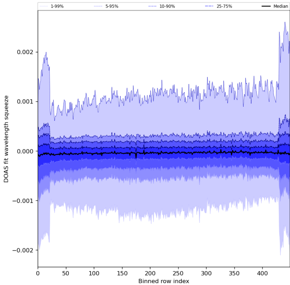
Figure 92: Along track statistics of “DOAS fit wavelength squeeze” for 2024-02-02 to 2024-02-04
