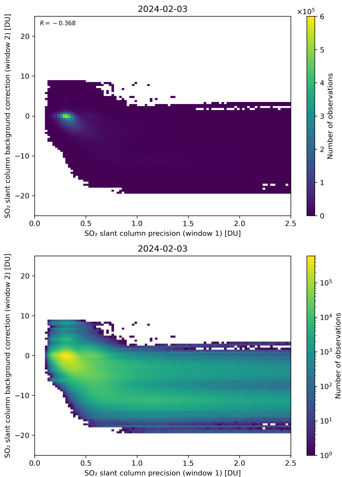
Figure 219: Scatter density plot of “SO 2 slant column precision (window 1)” against “SO 2 slant column background correction (window 2)” for 2024-02-02 to 2024-02-04.
