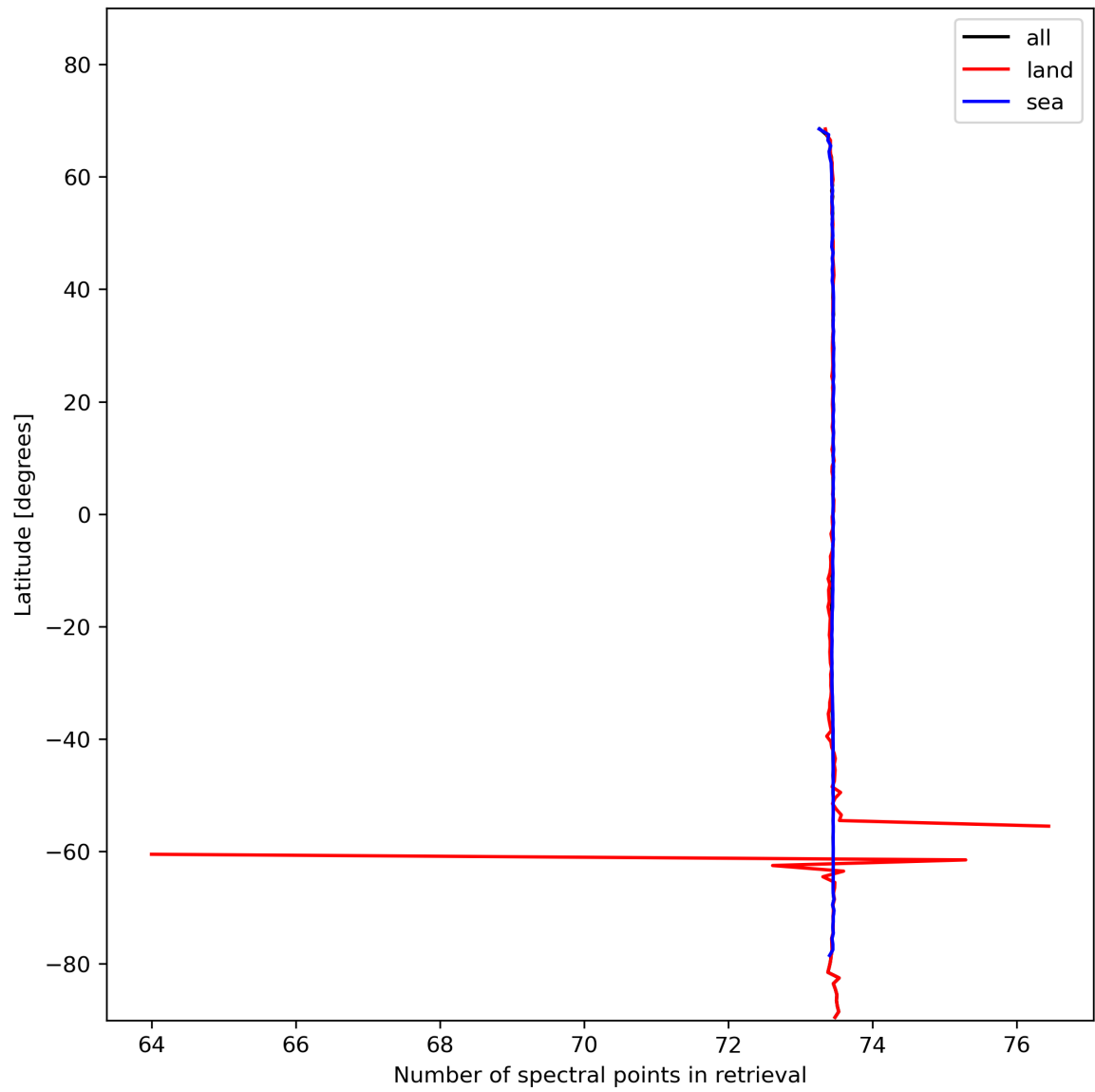
Figure 51: Zonal average of “Number of spectral points in retrieval” for 2024-02-02 to 2024-02-04.
