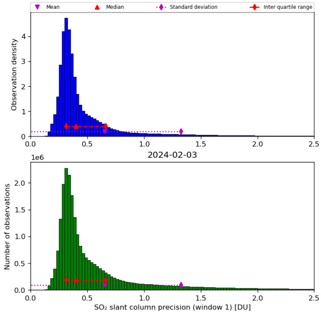
Figure 57: Histogram of “SO 2 slant column precision (window 1)” for 2024-02-02 to 2024-02-04
