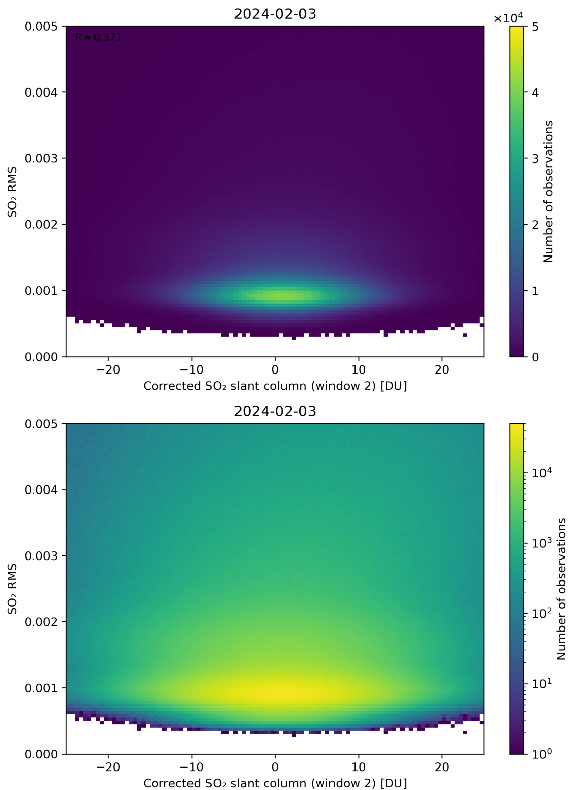
Figure 198: Scatter density plot of “Corrected SO 2 slant column (window 2)” against “SO 2 RMS” for 2024-02-02 to 2024-02-04.
