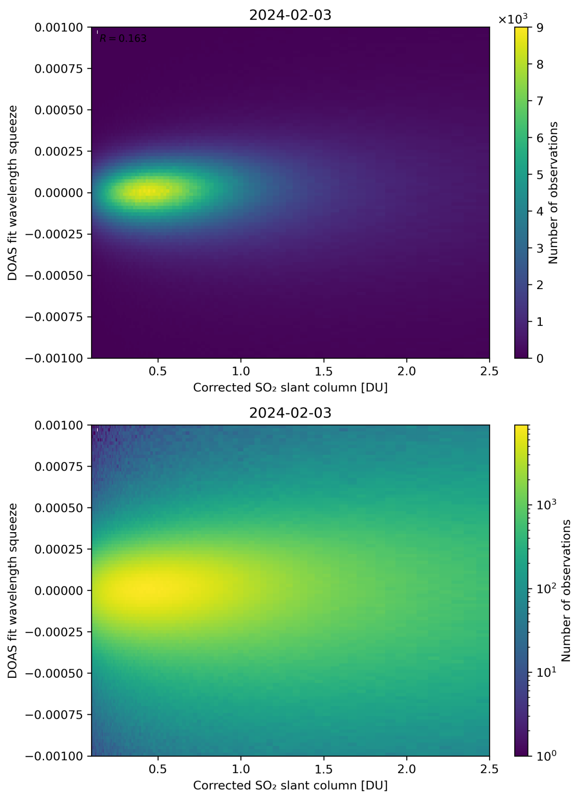
Figure 182: Scatter density plot of “Corrected SO 2 slant column” against “DOAS fit wavelength squeeze” for 2024-02-02 to 2024-02-04.
