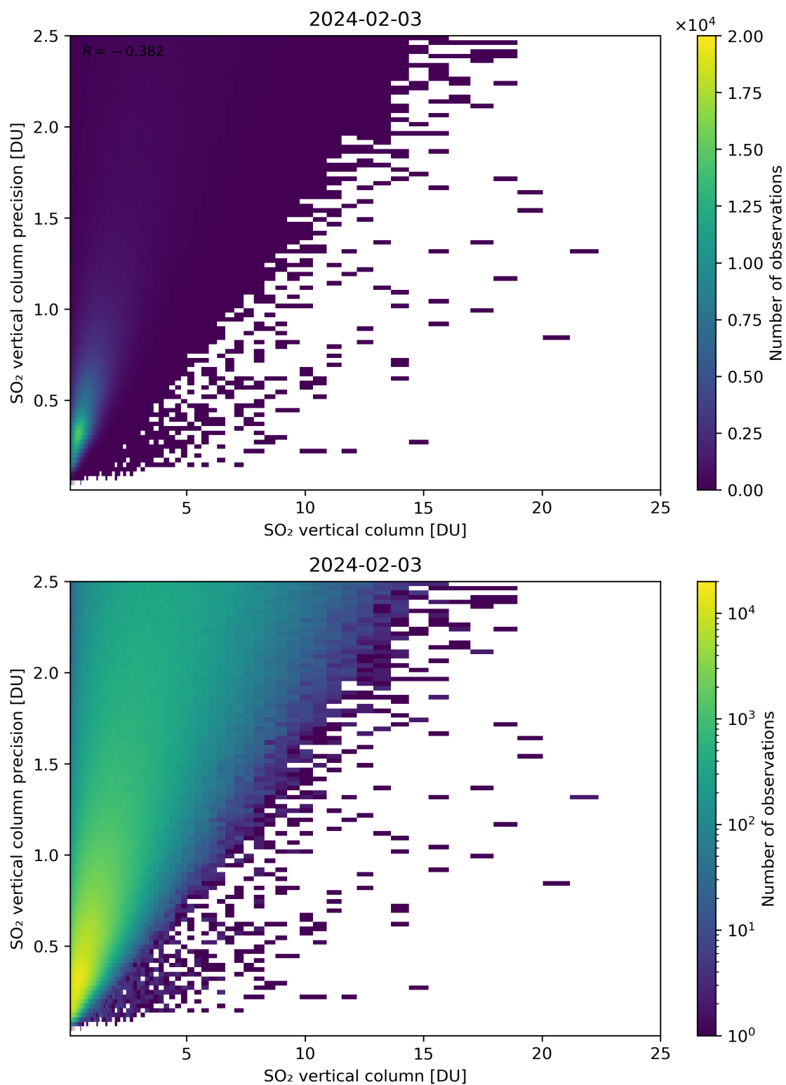
Figure 307: Scatter density plot of “SO 2 vertical column” against “SO 2 vertical column precision” for 2024-02-02 to 2024-02-04.
