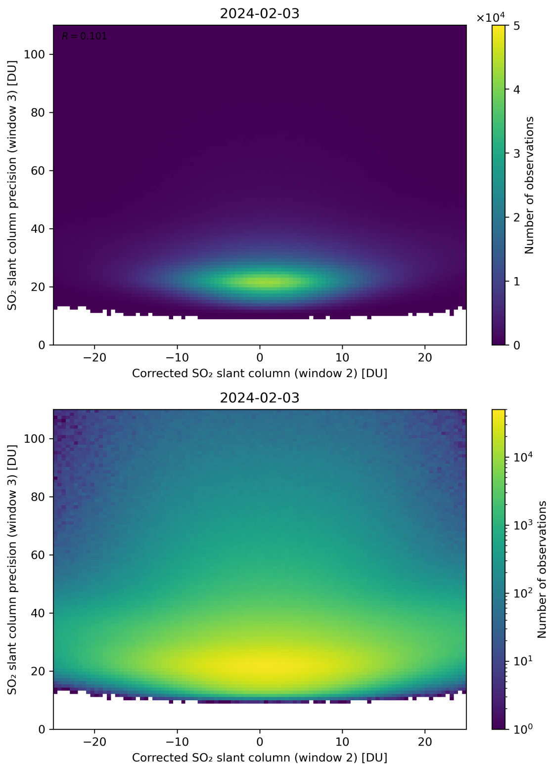
Figure 202: Scatter density plot of “Corrected SO 2 slant column (window 2)” against “SO 2 slant column precision (window 3)” for 2024-02-02 to 2024-02-04.
