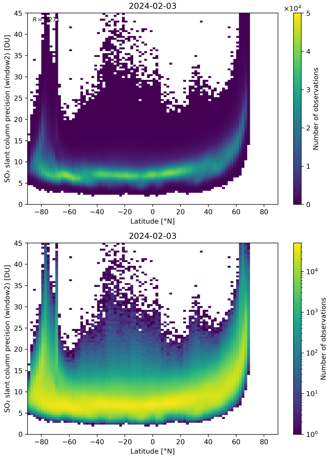
Figure 151: Scatter density plot of “Latitude” against “SO 2 slant column precision (window2)” for 2024-02-02 to 2024-02-04.
