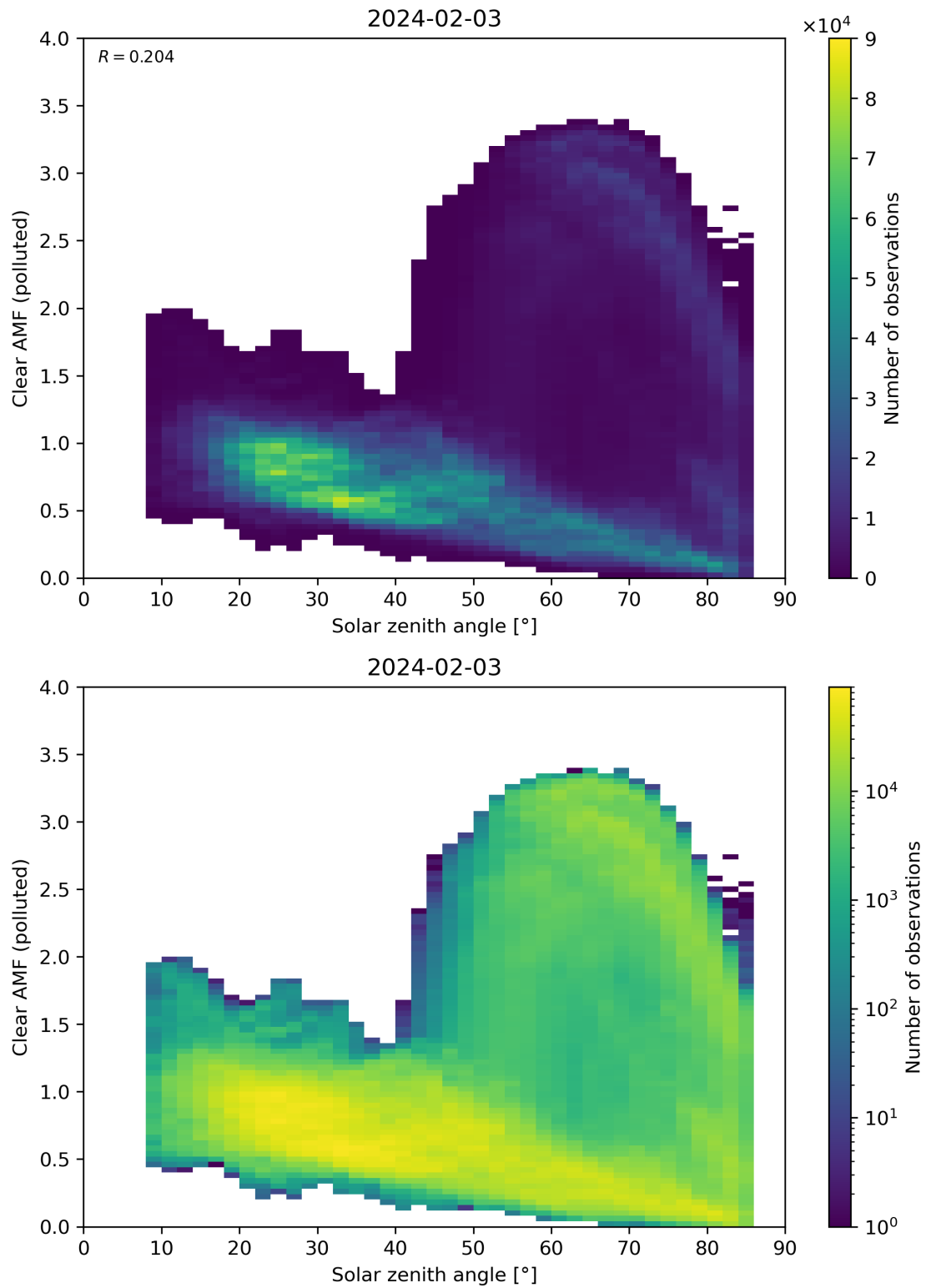
Figure 165: Scatter density plot of “Solar zenith angle” against “Clear AMF (polluted)” for 2024-02-02 to 2024-02-04.
