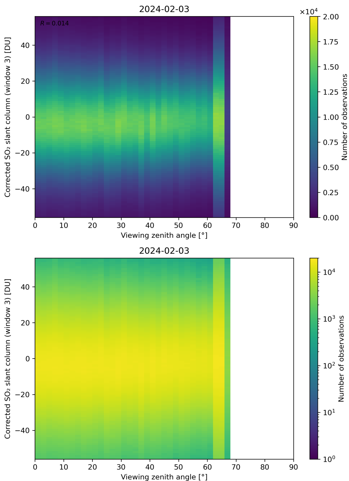
Figure 319: Scatter density plot of “Viewing zenith angle” against “Corrected SO 2 slant column (window 3)” for 2024-02-02 to 2024-02-04.
