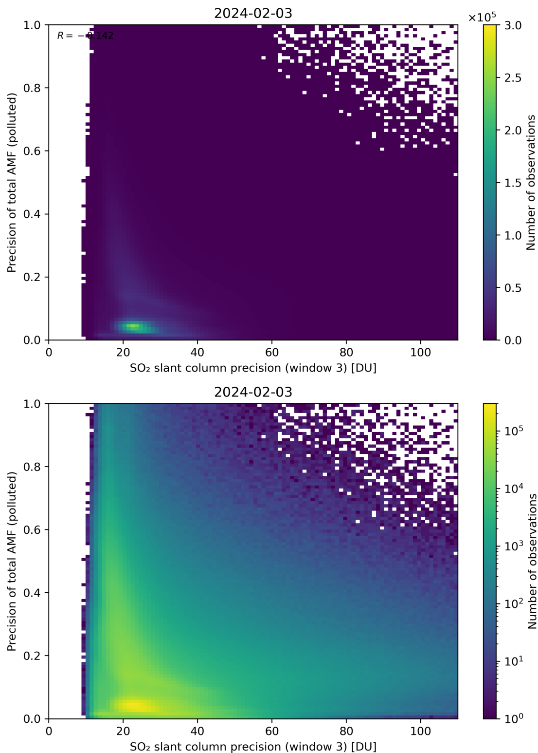
Figure 264: Scatter density plot of “SO 2 slant column precision (window 3)” against “Precision of total AMF (polluted)” for 2024-02-02 to 2024-02-04.
