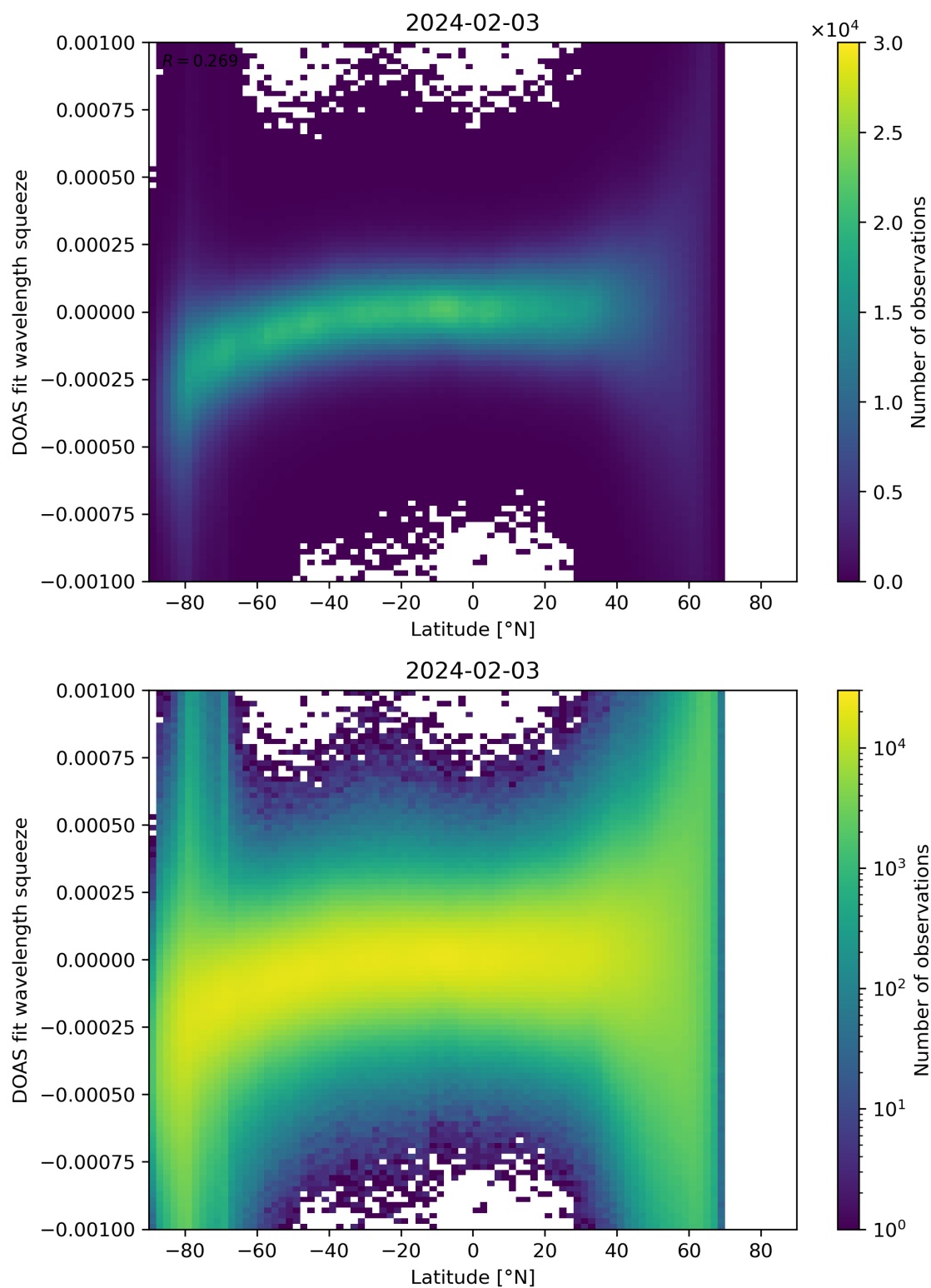
Figure 143: Scatter density plot of “Latitude” against “DOAS fit wavelength squeeze” for 2024-02-02 to 2024-02-04.
