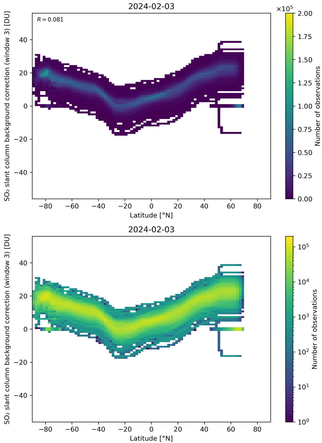
Figure 141: Scatter density plot of “Latitude” against “SO 2 slant column background correction (window 3)” for 2024-02-02 to 2024-02-04.
