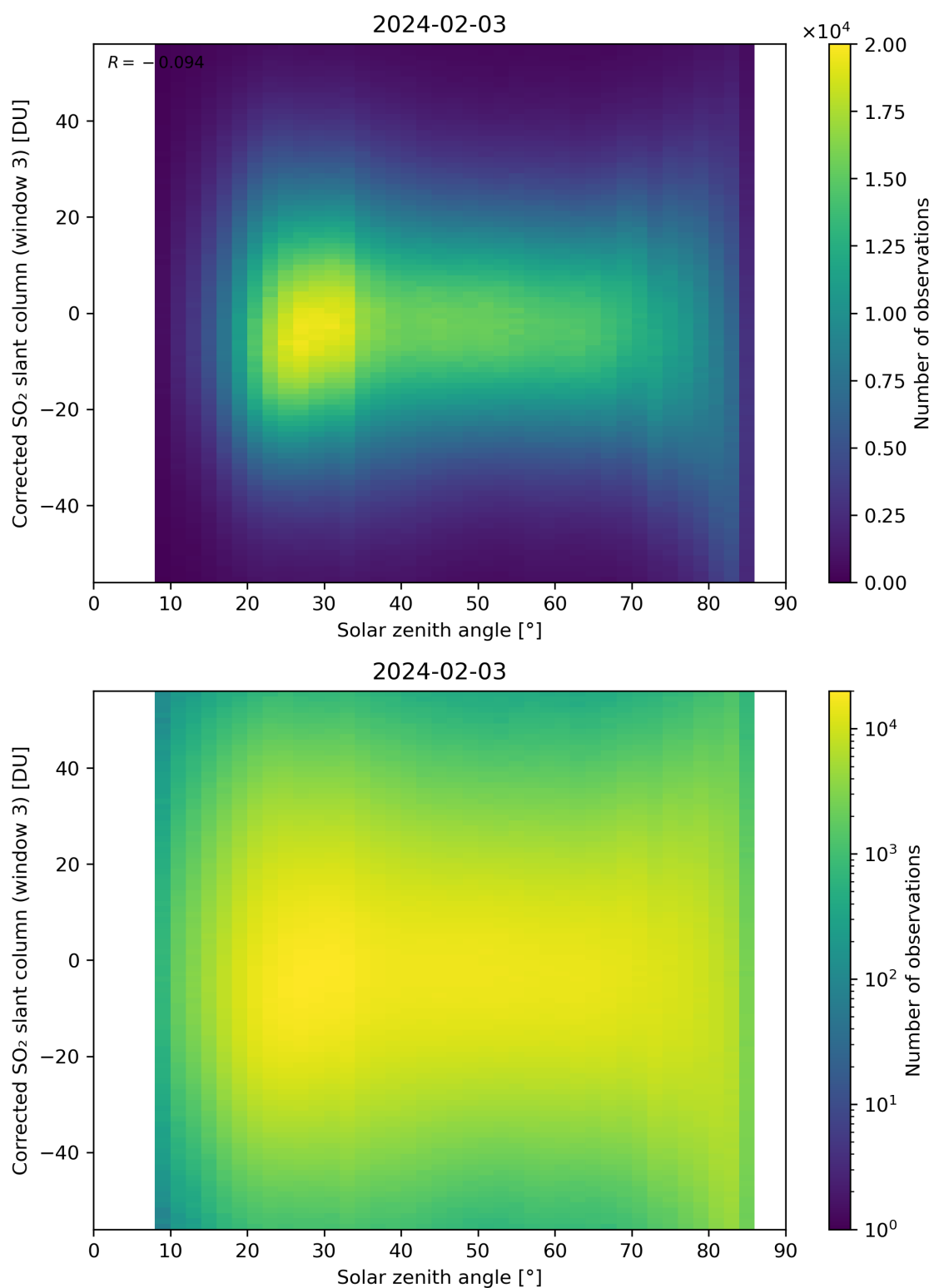
Figure 168: Scatter density plot of “Solar zenith angle” against “Corrected SO 2 slant column (window 3)” for 2024-02-02 to 2024-02-04.
