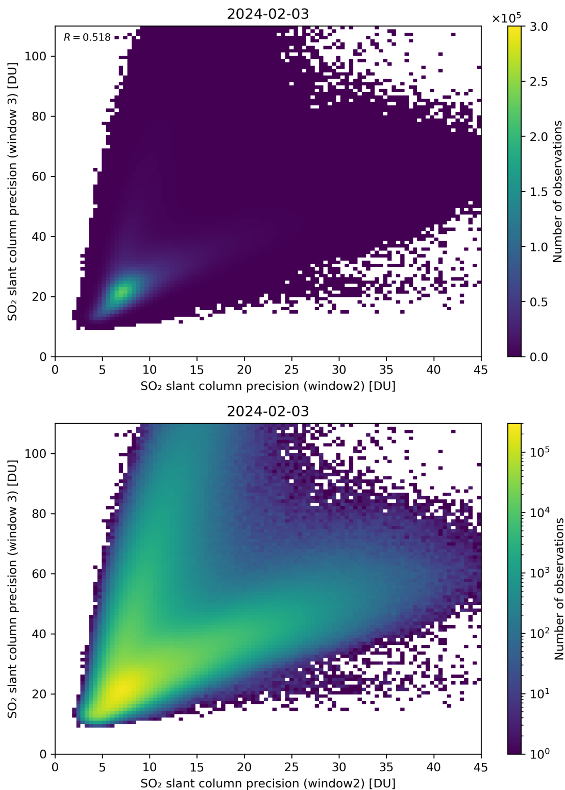
Figure 250: Scatter density plot of “SO 2 slant column precision (window2)” against “SO 2 slant column precision (window 3)” for 2024-02-02 to 2024-02-04.
