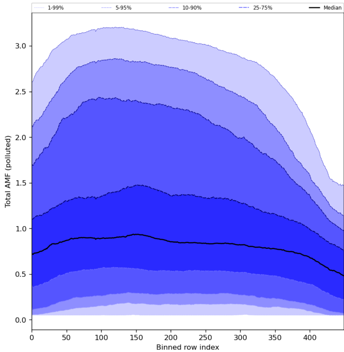
Figure 94: Along track statistics of “Total AMF (polluted)” for 2024-02-02 to 2024-02-04
