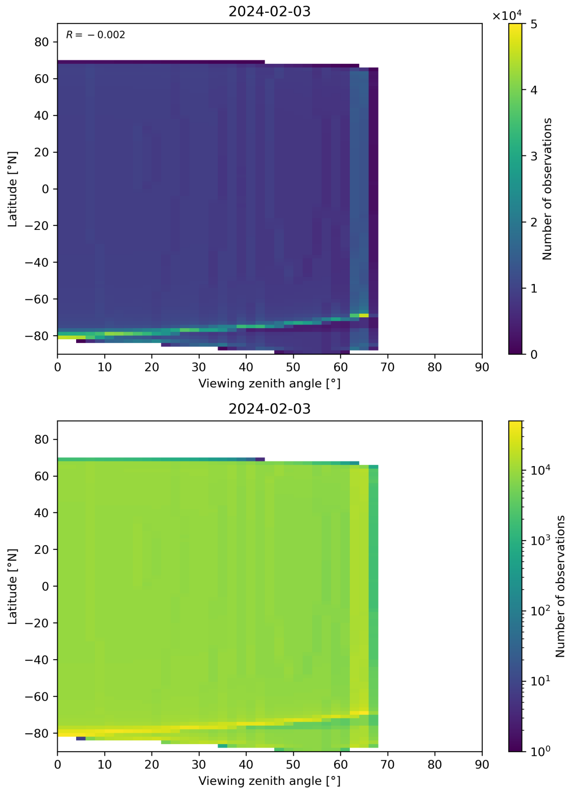
Figure 314: Scatter density plot of “Viewing zenith angle” against “Latitude” for 2024-02-02 to 2024-02-04.
