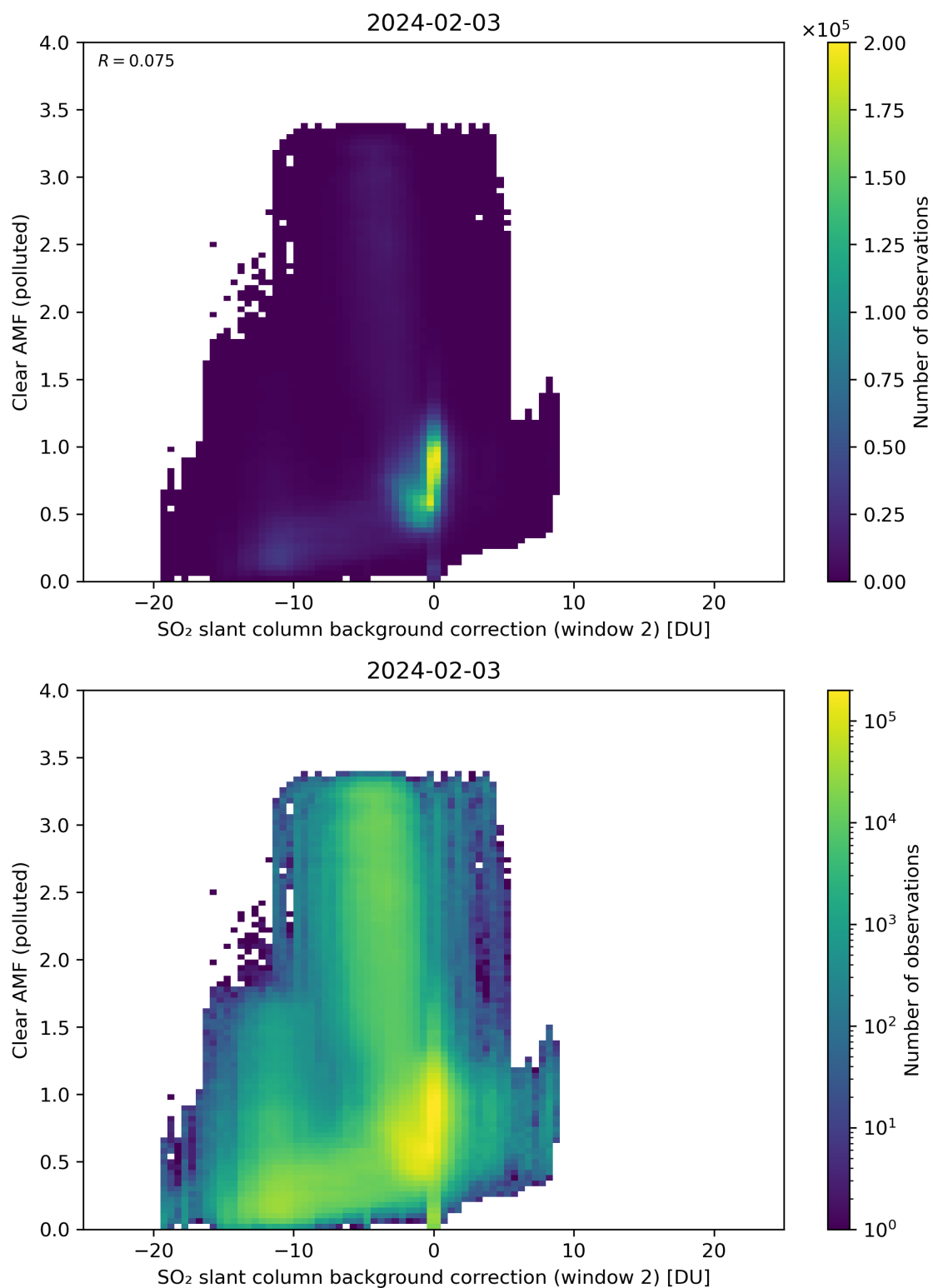
Figure 115: Scatter density plot of “SO 2 slant column background correction (window 2)” against “Clear AMF (polluted)” for 2024-02-02 to 2024-02-04.
