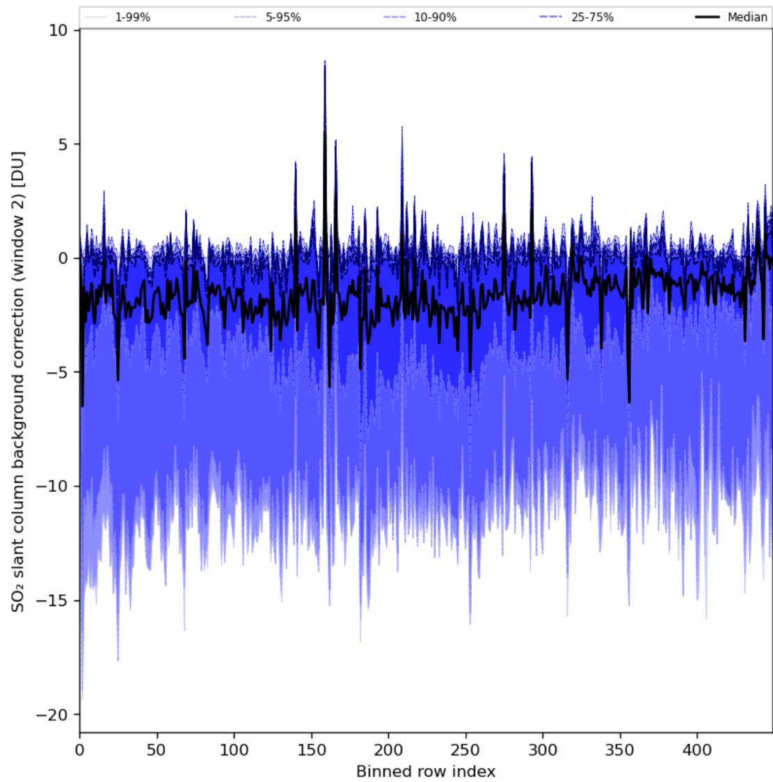
Figure 86: Along track statistics of “SO 2 slant column background correction (window 2)” for 2024-02-02 to 2024-02-04
