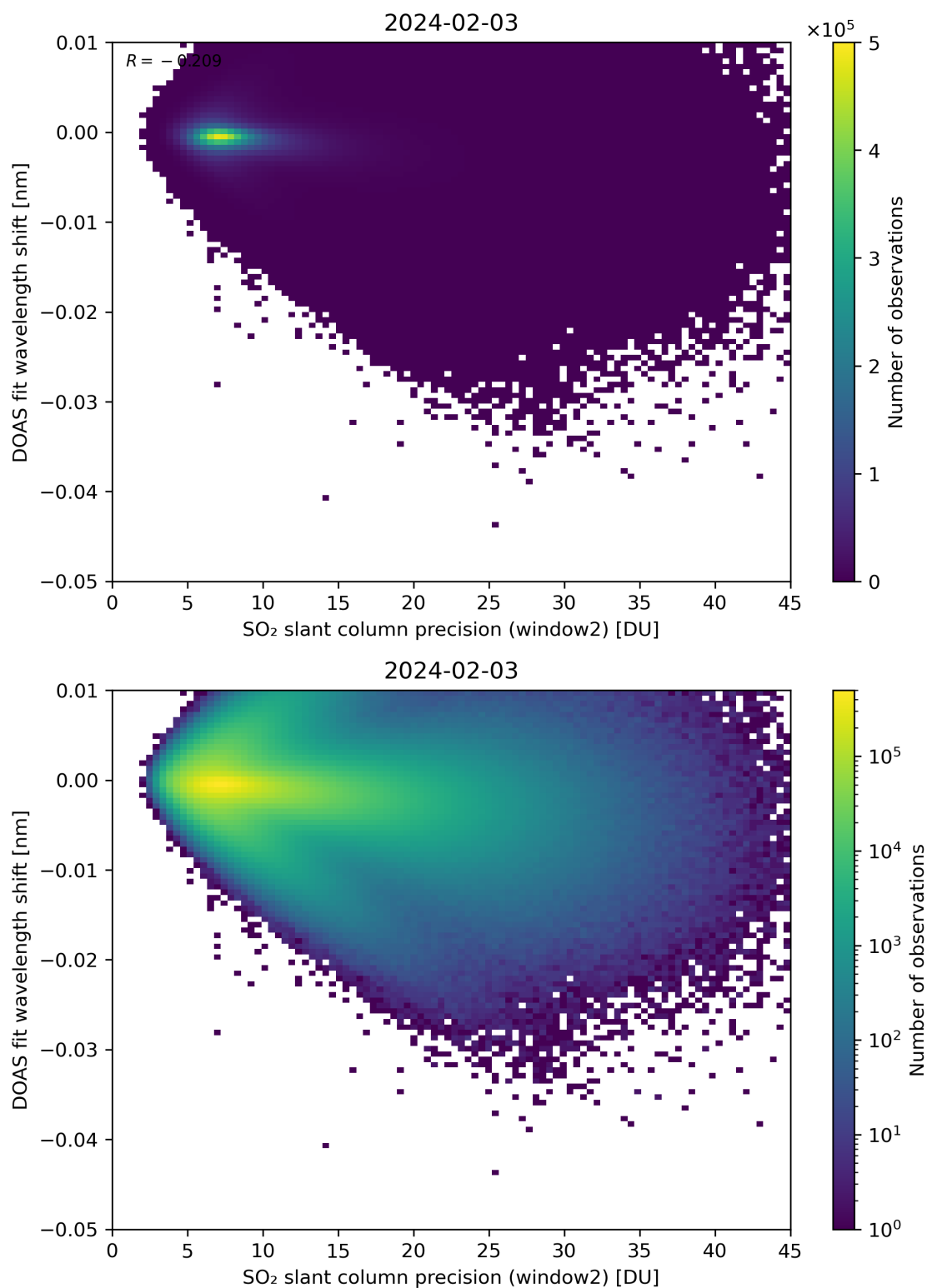
Figure 243: Scatter density plot of “SO 2 slant column precision (window2)” against “DOAS fit wavelength shift” for 2024-02-02 to 2024-02-04.
