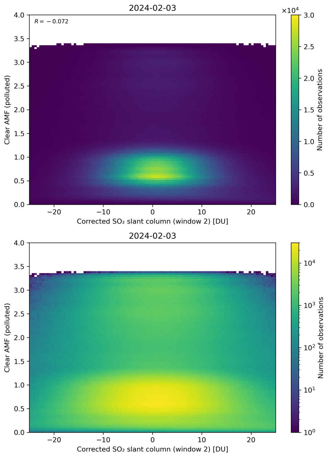
Figure 199: Scatter density plot of “Corrected SO 2 slant column (window 2)” against “Clear AMF (polluted)” for 2024-02-02 to 2024-02-04.
