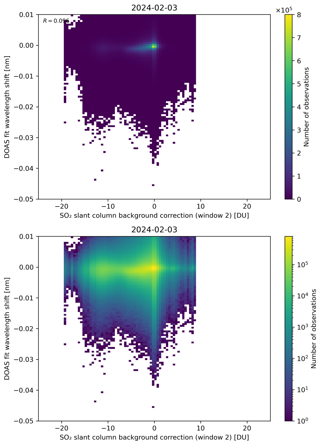
Figure 112: Scatter density plot of “SO 2 slant column background correction (window 2)” against “DOAS fit wavelength shift” for 2024-02-02 to 2024-02-04.
