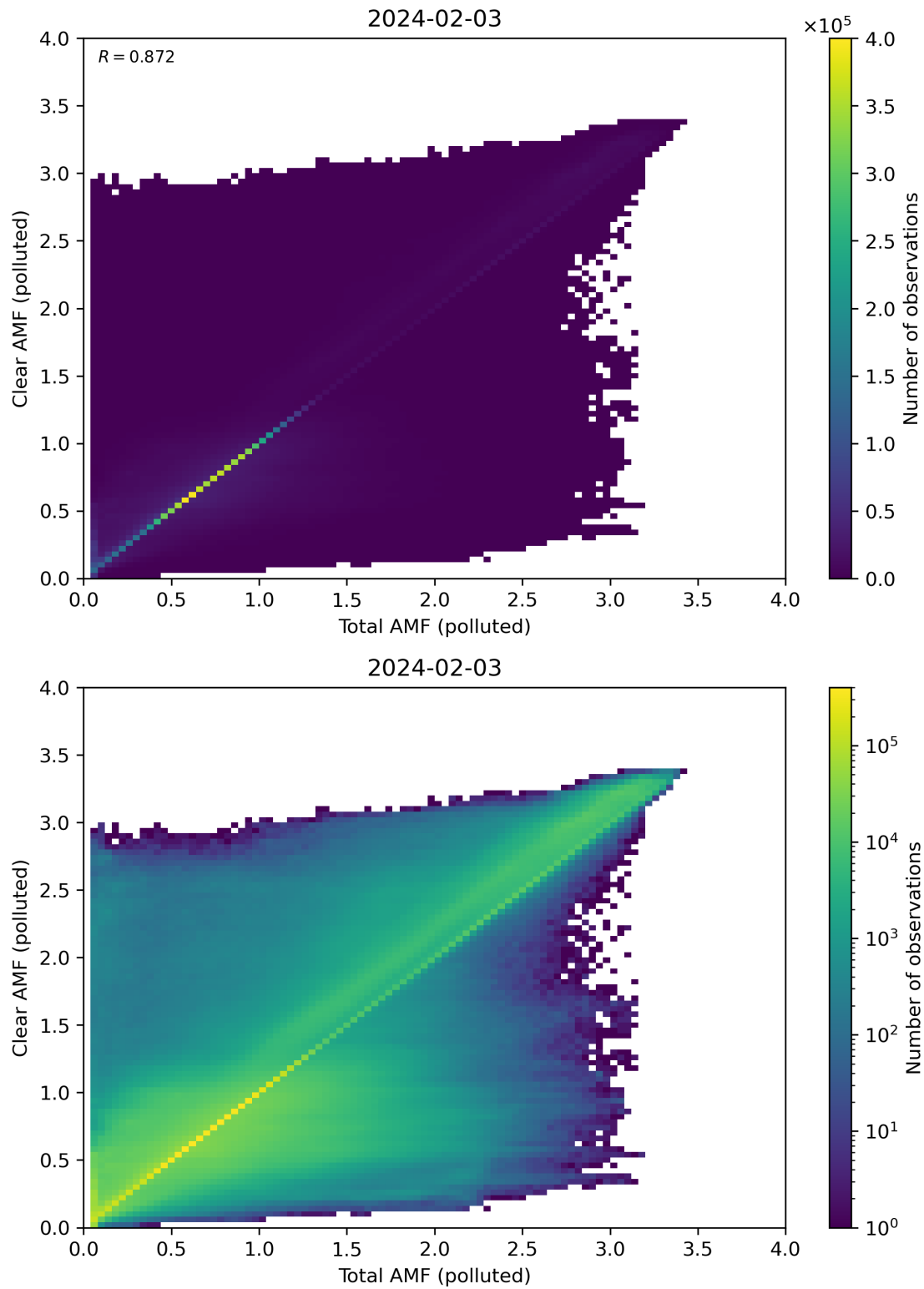
Figure 271: Scatter density plot of “Total AMF (polluted)” against “Clear AMF (polluted)” for 2024-02-02 to 2024-02-04.
