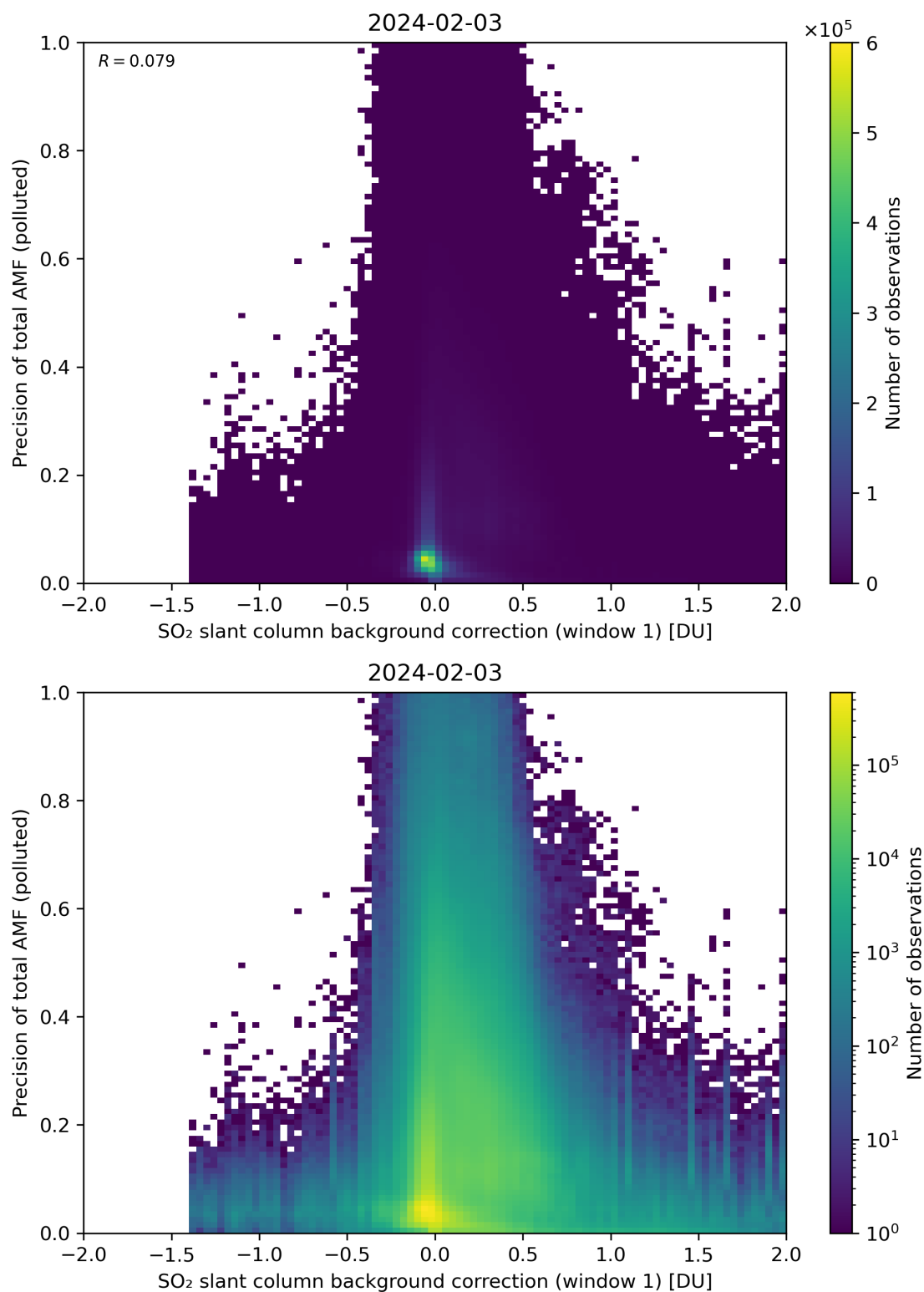
Figure 110: Scatter density plot of “SO 2 slant column background correction (window 1)” against “Precision of total AMF (polluted)” for 2024-02-02 to 2024-02-04.
