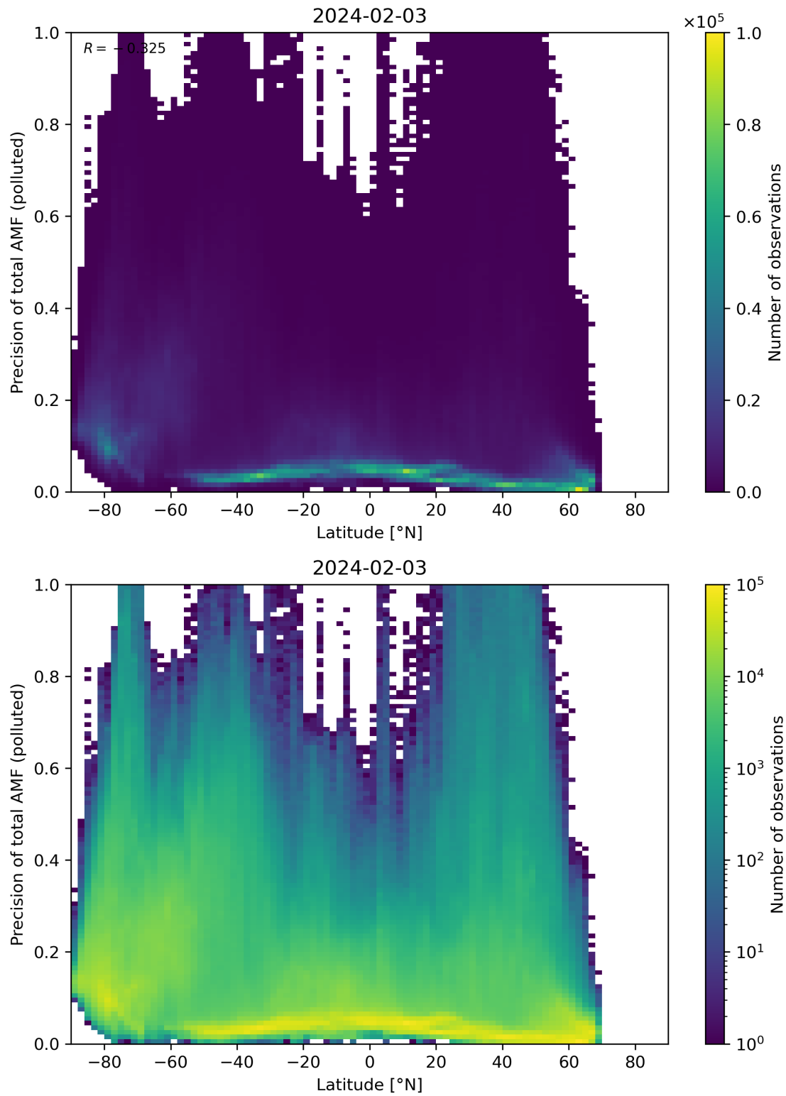
Figure 155: Scatter density plot of “Latitude” against “Precision of total AMF (polluted)” for 2024-02-02 to 2024-02-04.
