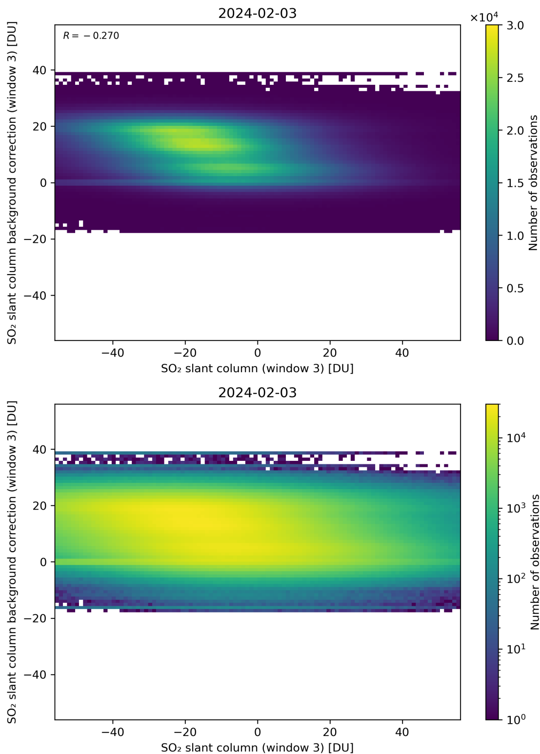
Figure 253: Scatter density plot of “SO 2 slant column (window 3)” against “SO 2 slant column background correction (window 3)” for 2024-02-02 to 2024-02-04.
