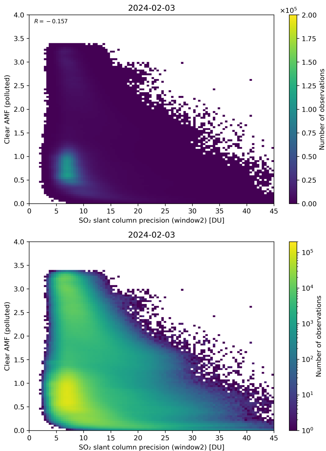
Figure 246: Scatter density plot of “SO 2 slant column precision (window2)” against “Clear AMF (polluted)” for 2024-02-02 to 2024-02-04.
