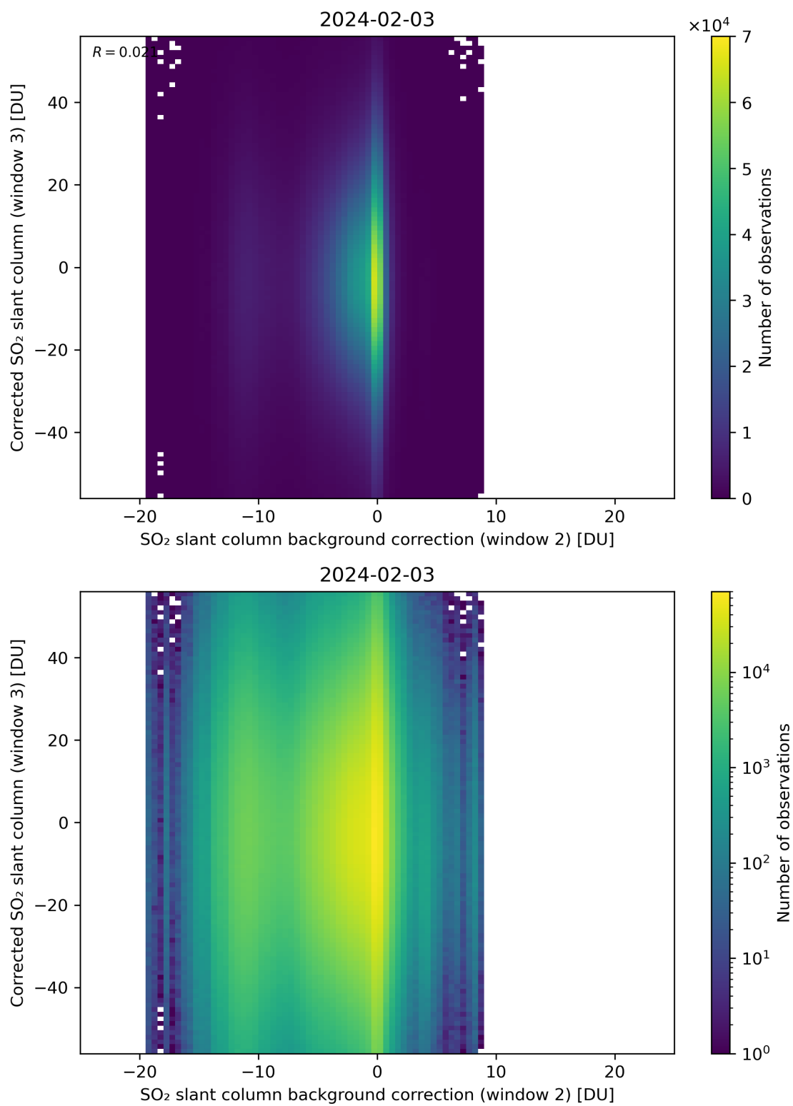
Figure 116: Scatter density plot of “SO 2 slant column background correction (window 2)” against “Corrected SO 2 slant column (window 3)” for 2024-02-02 to 2024-02-04.
