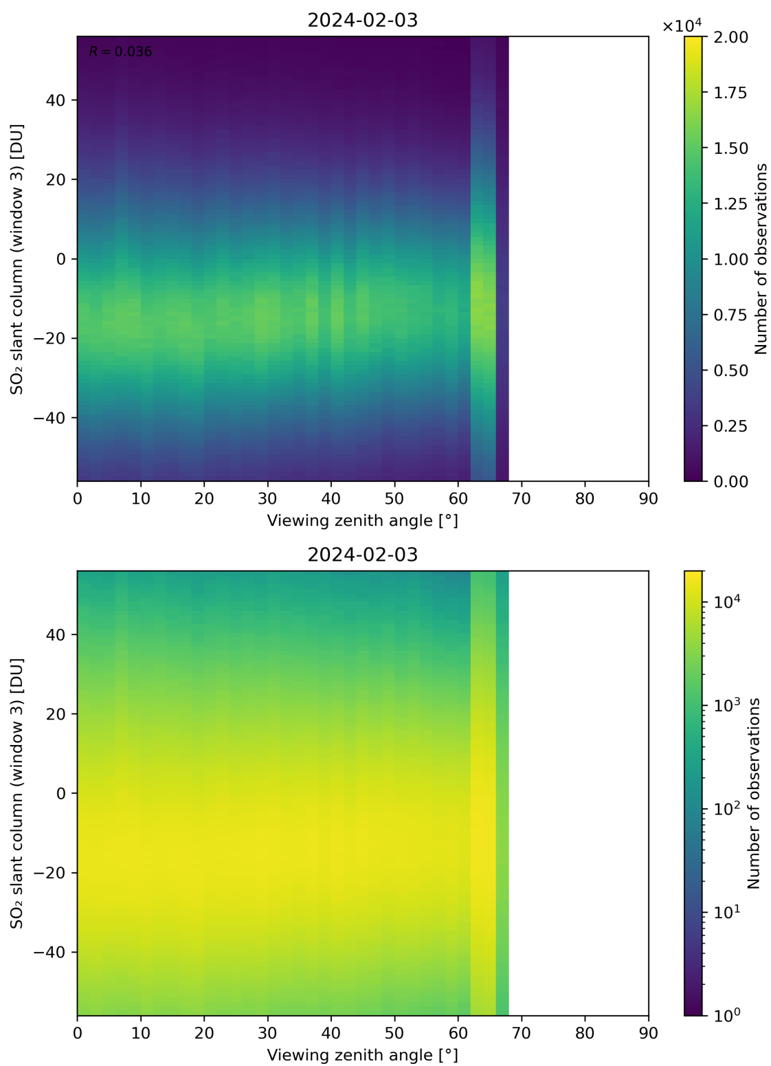
Figure 323: Scatter density plot of “Viewing zenith angle” against “SO 2 slant column (window 3)” for 2024-02-02 to 2024-02-04.
