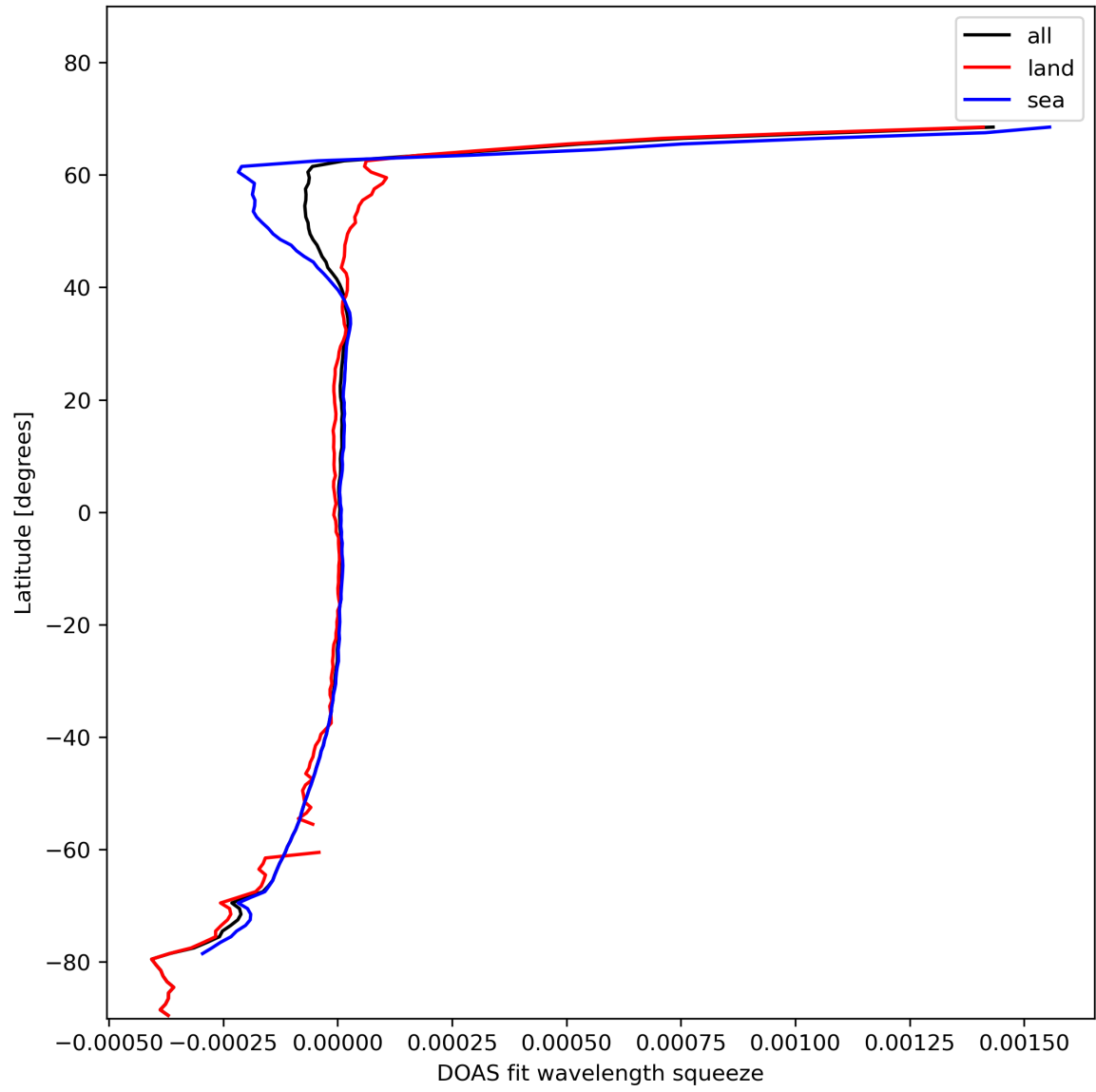
Figure 46: Zonal average of “DOAS fit wavelength squeeze” for 2024-02-02 to 2024-02-04.
