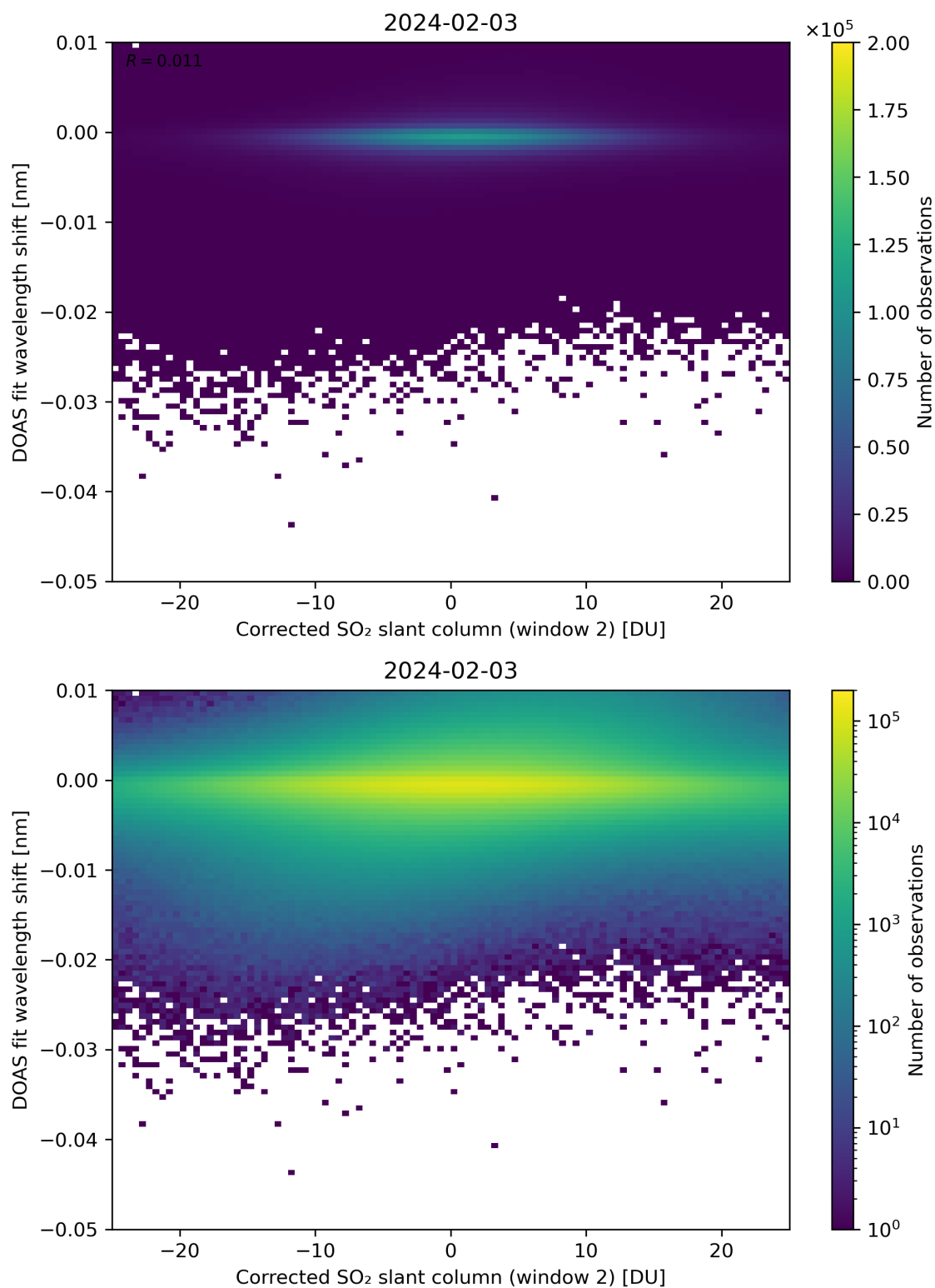
Figure 196: Scatter density plot of “Corrected SO 2 slant column (window 2)” against “DOAS fit wavelength shift” for 2024-02-02 to 2024-02-04.
