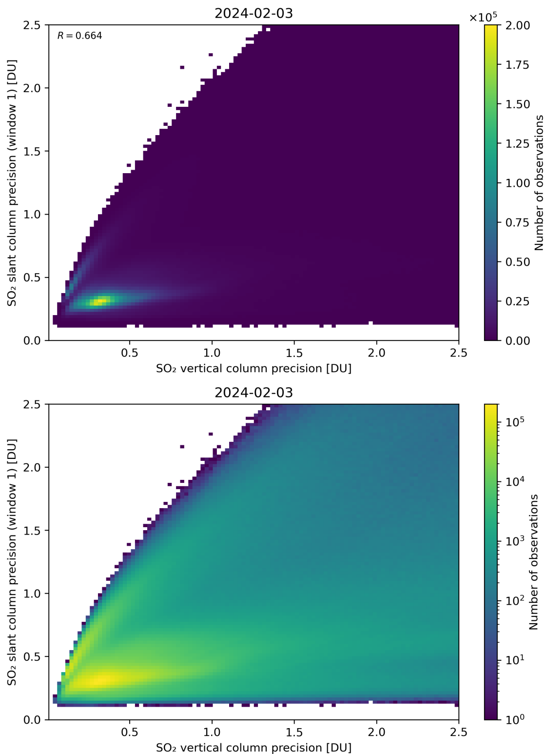
Figure 290: Scatter density plot of “SO 2 vertical column precision” against “SO 2 slant column precision (window 1)” for 2024-02-02 to 2024-02-04.
