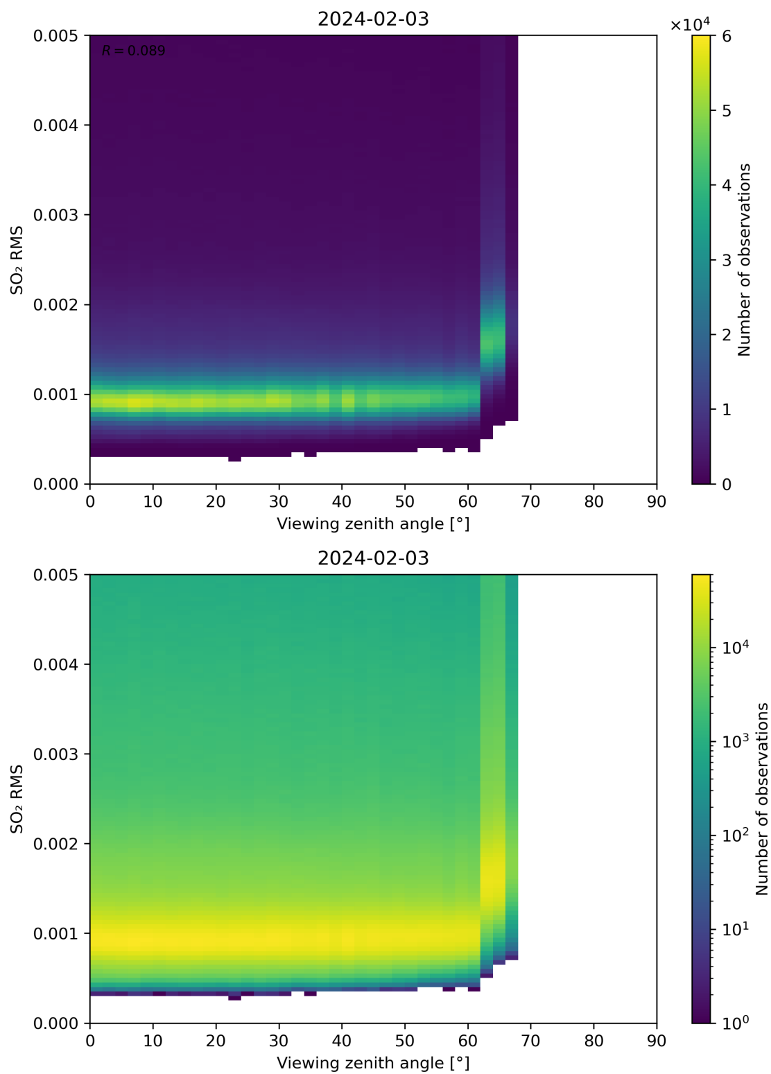
Figure 313: Scatter density plot of “Viewing zenith angle” against “SO 2 RMS” for 2024-02-02 to 2024-02-04.
