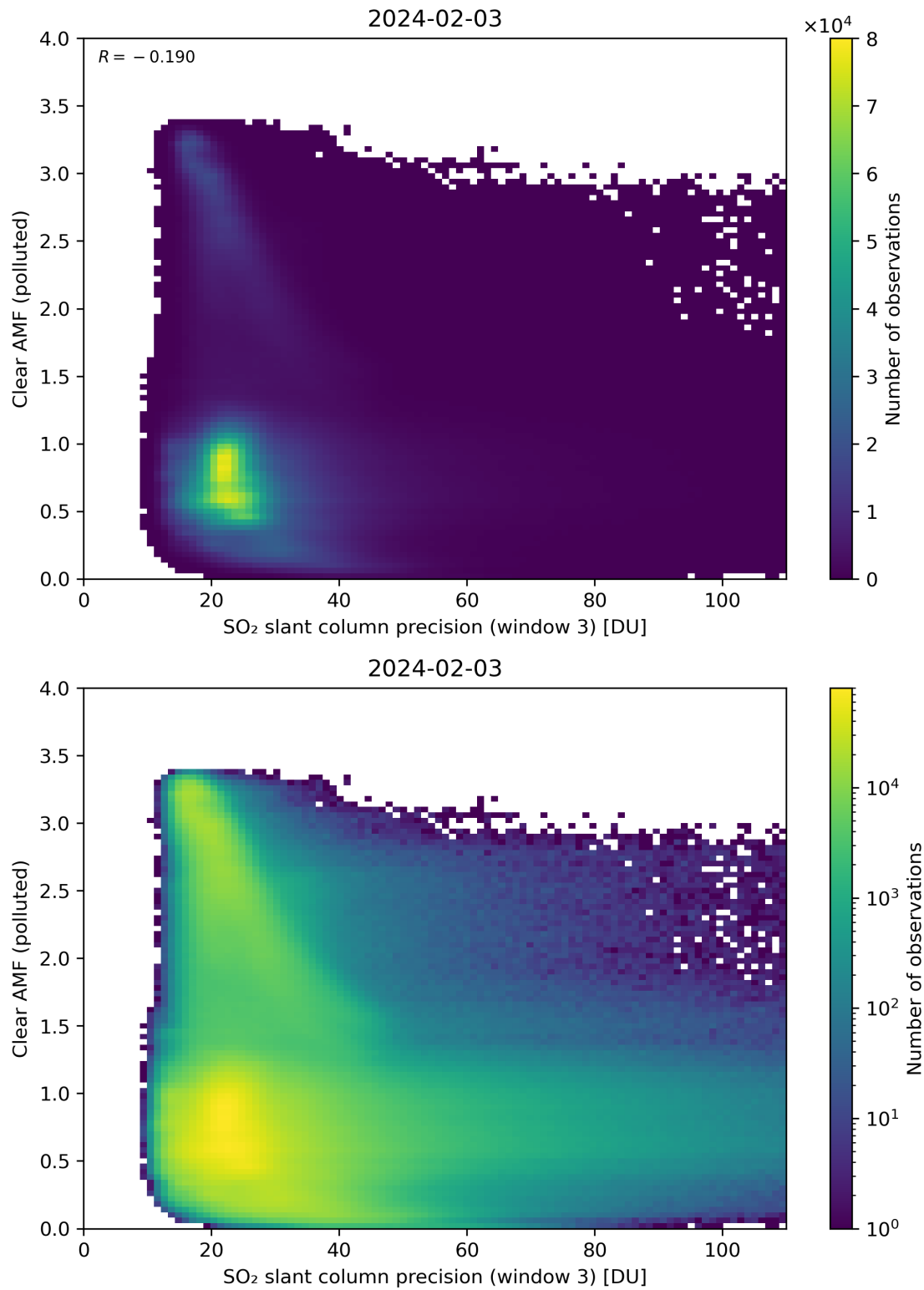
Figure 261: Scatter density plot of “SO 2 slant column precision (window 3)” against “Clear AMF (polluted)” for 2024-02-02 to 2024-02-04.
