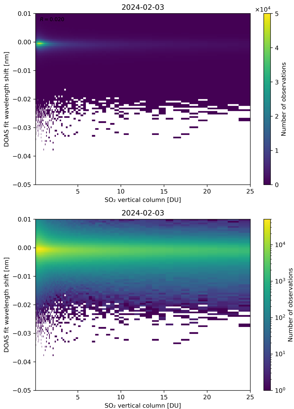
Figure 276: Scatter density plot of “SO 2 vertical column” against “DOAS fit wavelength shift” for 2024-02-02 to 2024-02-04.
