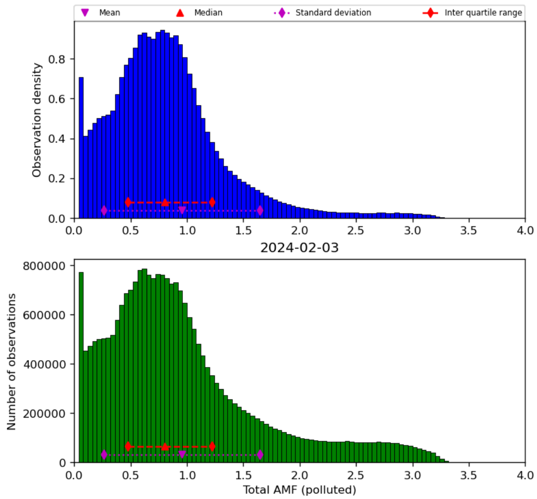
Figure 71: Histogram of “Total AMF (polluted)” for 2024-02-02 to 2024-02-04
