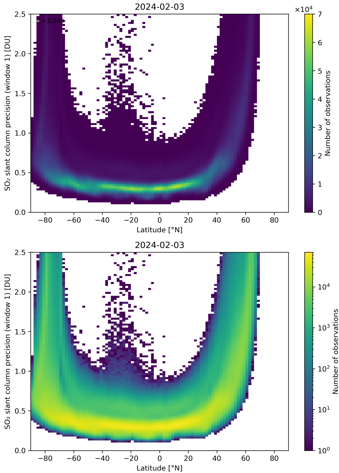
Figure 150: Scatter density plot of “Latitude” against “SO 2 slant column precision (window 1)” for 2024-02-02 to 2024-02-04.
