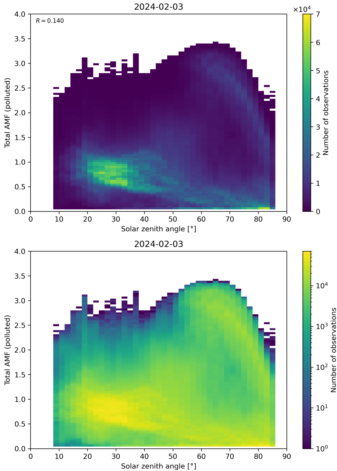
Figure 174: Scatter density plot of “Solar zenith angle” against “Total AMF (polluted)” for 2024-02-02 to 2024-02-04.
