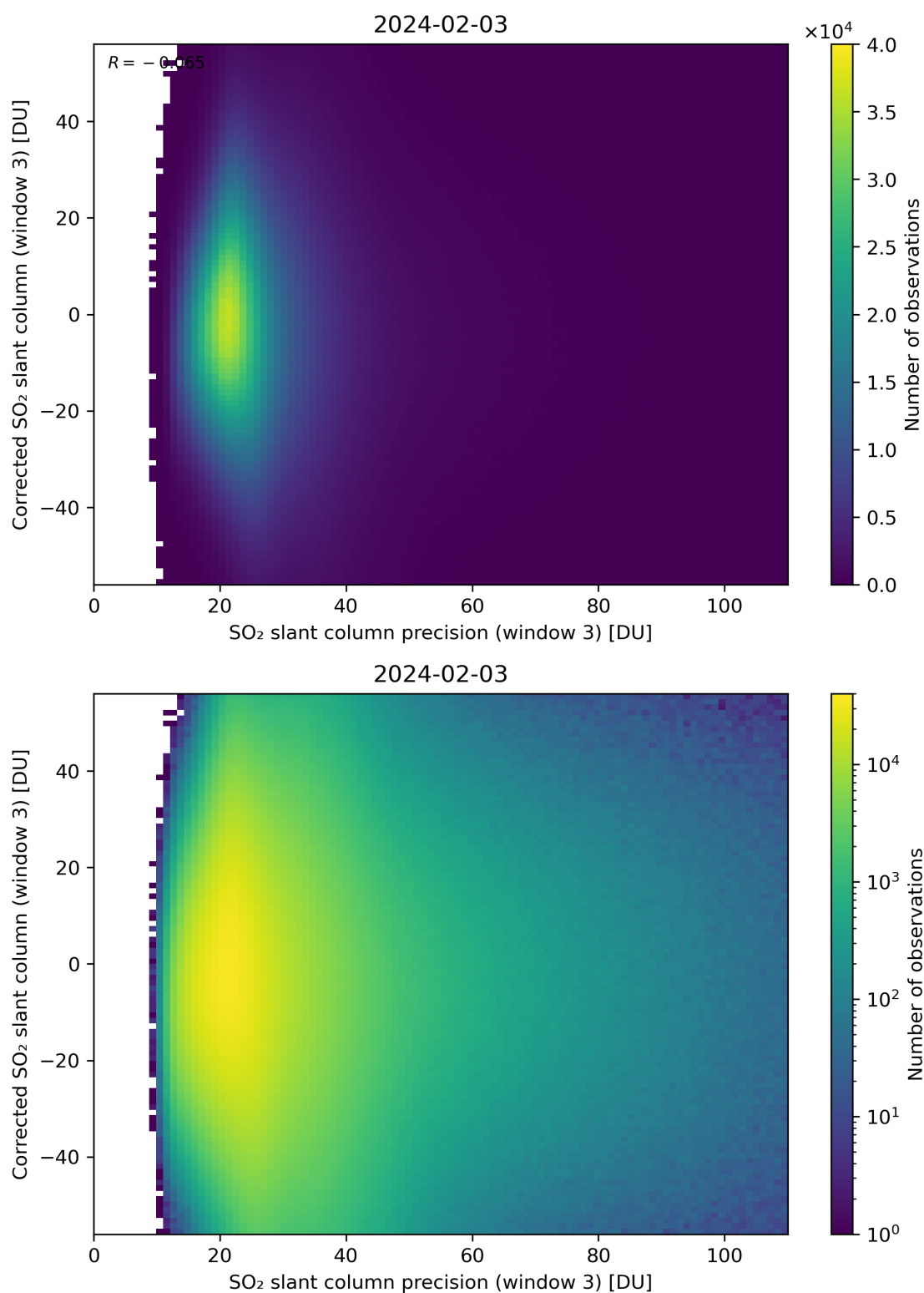
Figure 262: Scatter density plot of “SO 2 slant column precision (window 3)” against “Corrected SO 2 slant column (window 3)” for 2024-02-02 to 2024-02-04.
