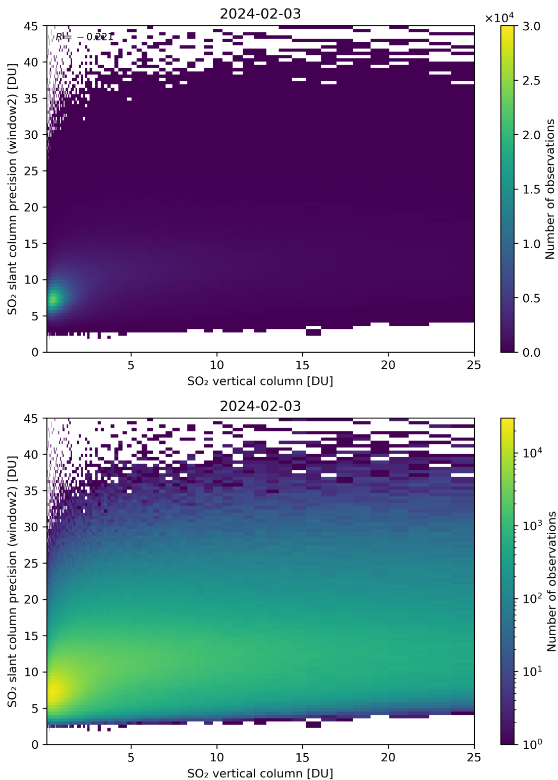
Figure 302: Scatter density plot of “SO 2 vertical column” against “SO 2 slant column precision (window2)” for 2024-02-02 to 2024-02-04.
