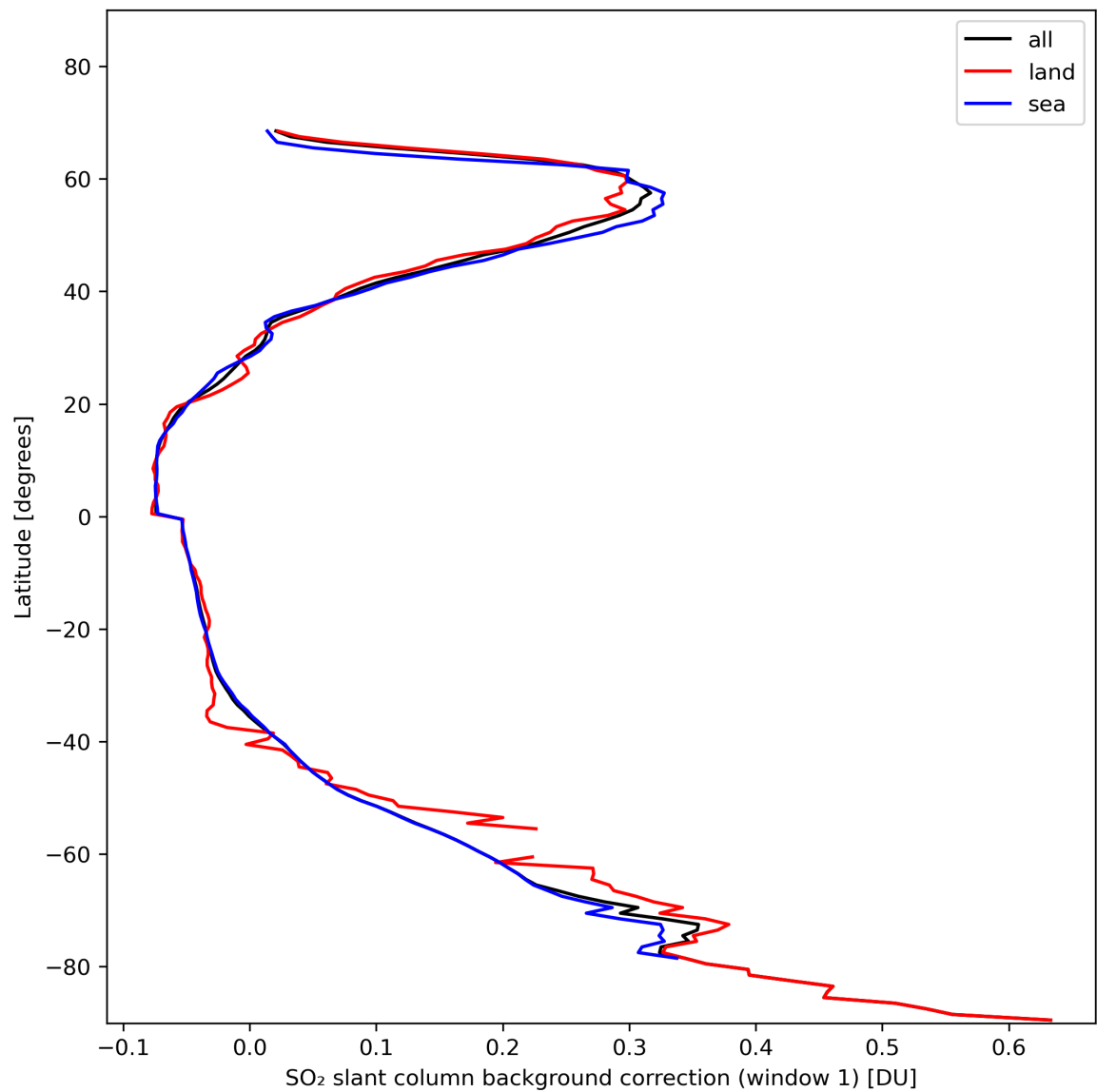
Figure 36: Zonal average of “SO 2 slant column background correction (window 1)” for 2024-02-02 to 2024-02-04.
