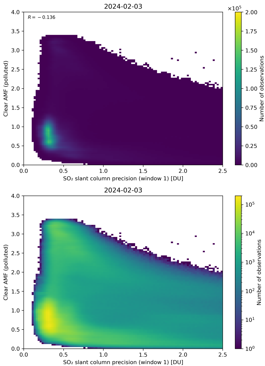
Figure 224: Scatter density plot of “SO 2 slant column precision (window 1)” against “Clear AMF (polluted)” for 2024-02-02 to 2024-02-04.
