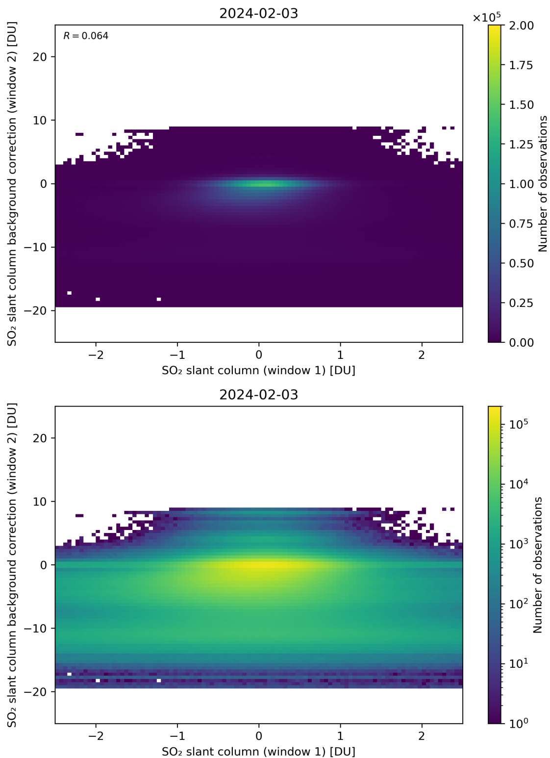
Figure 213: Scatter density plot of “SO 2 slant column (window 1)” against “SO 2 slant column background correction (window 2)” for 2024-02-02 to 2024-02-04.
