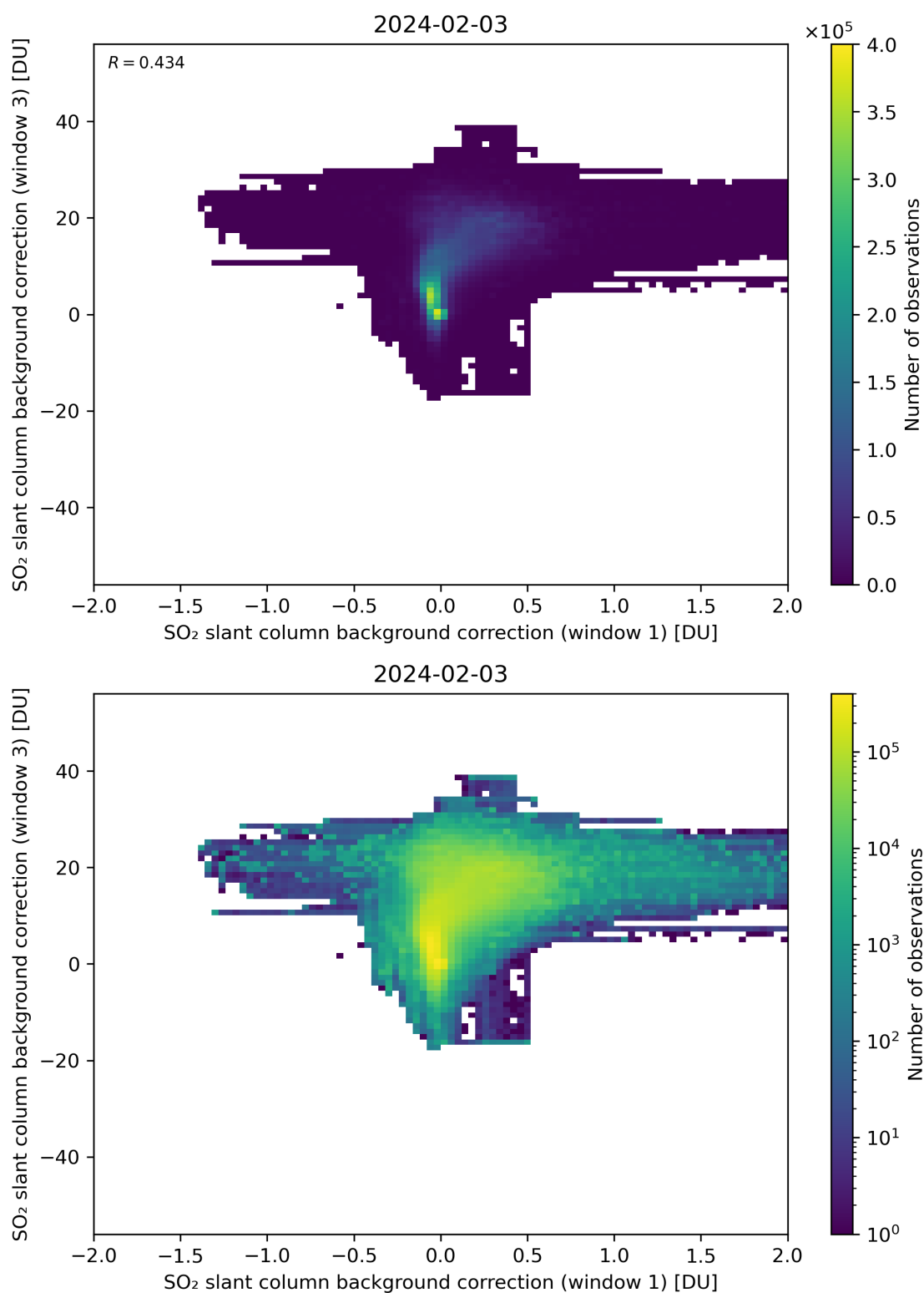
Figure 99: Scatter density plot of “SO 2 slant column background correction (window 1)” against “SO 2 slant column background correction (window 3)” for 2024-02-02 to 2024-02-04.
