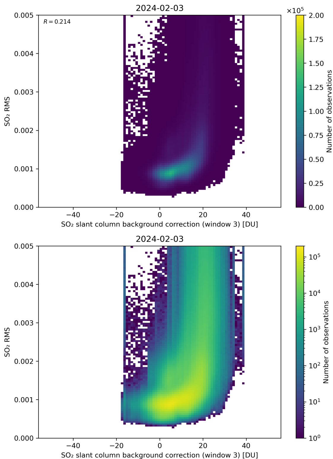
Figure 123: Scatter density plot of “SO 2 slant column background correction (window 3)” against “SO 2 RMS” for 2024-02-02 to 2024-02-04.
