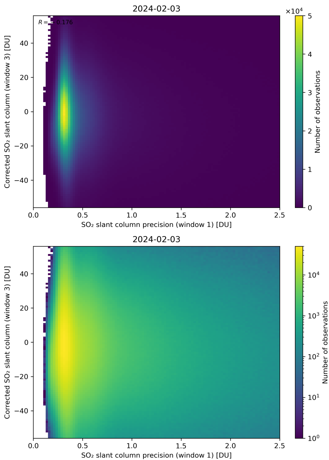
Figure 226: Scatter density plot of “SO 2 slant column precision (window 1)” against “Corrected SO 2 slant column (window 3)” for 2024-02-02 to 2024-02-04.
