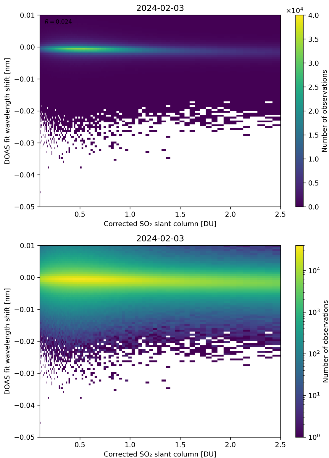
Figure 181: Scatter density plot of “Corrected SO 2 slant column” against “DOAS fit wavelength shift” for 2024-02-02 to 2024-02-04.
