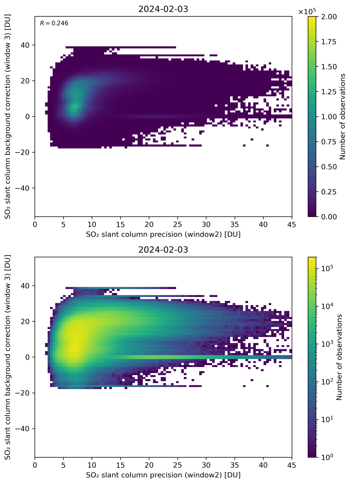
Figure 242: Scatter density plot of “SO 2 slant column precision (window2)” against “SO 2 slant column background correction (window 3)” for 2024-02-02 to 2024-02-04.
