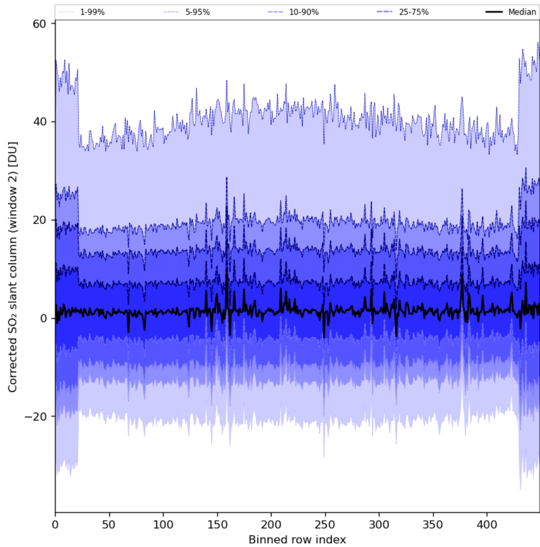
Figure 85: Along track statistics of “Corrected SO 2 slant column (window 2)” for 2024-02-02 to 2024-02-04
