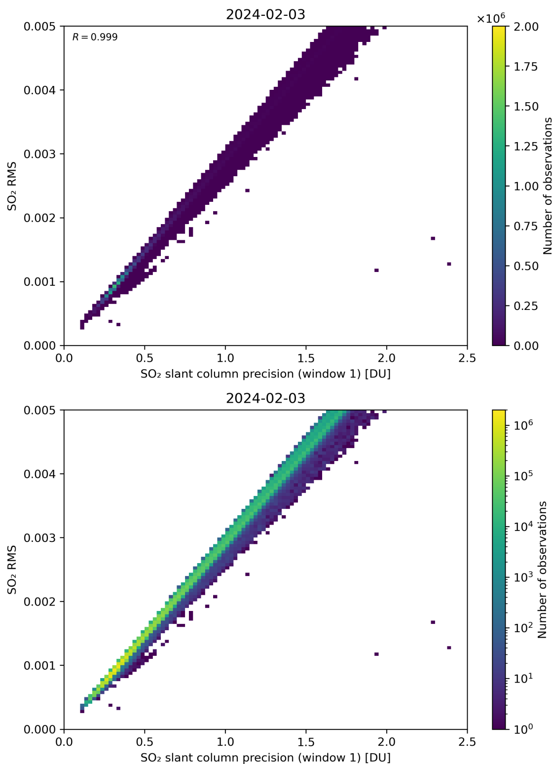
Figure 223: Scatter density plot of “SO 2 slant column precision (window 1)” against “SO 2 RMS” for 2024-02-02 to 2024-02-04.
