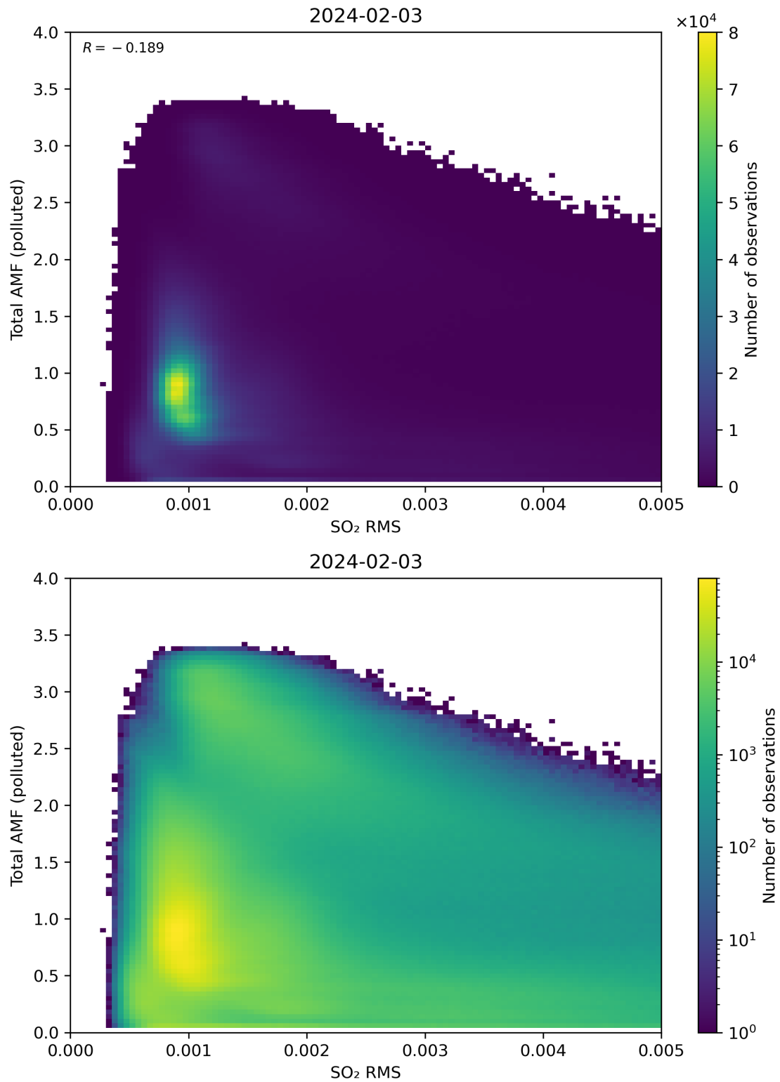
Figure 137: Scatter density plot of “SO 2 RMS” against “Total AMF (polluted)” for 2024-02-02 to 2024-02-04.
