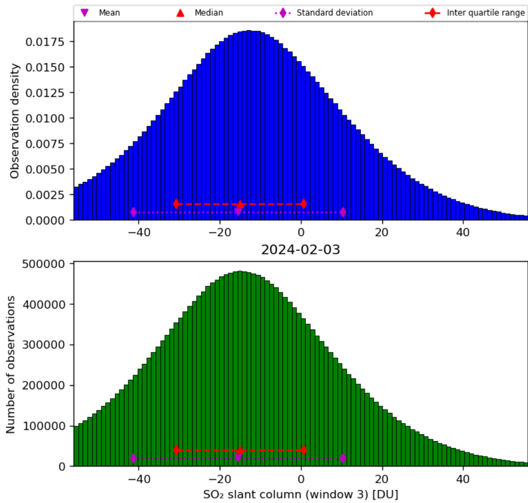
Figure 64: Histogram of “SO 2 slant column (window 3)” for 2024-02-02 to 2024-02-04
