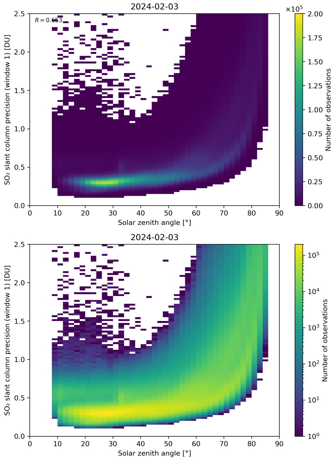
Figure 170: Scatter density plot of “Solar zenith angle” against “SO 2 slant column precision (window 1)” for 2024-02-02 to 2024-02-04.
