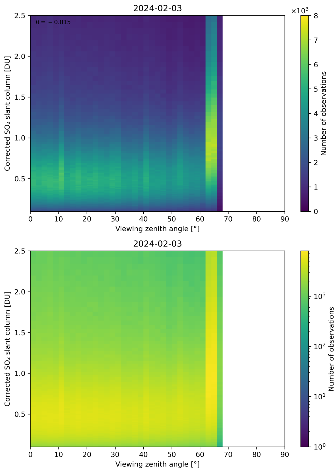
Figure 317: Scatter density plot of “Viewing zenith angle” against “Corrected SO 2 slant column” for 2024-02-02 to 2024-02-04.
