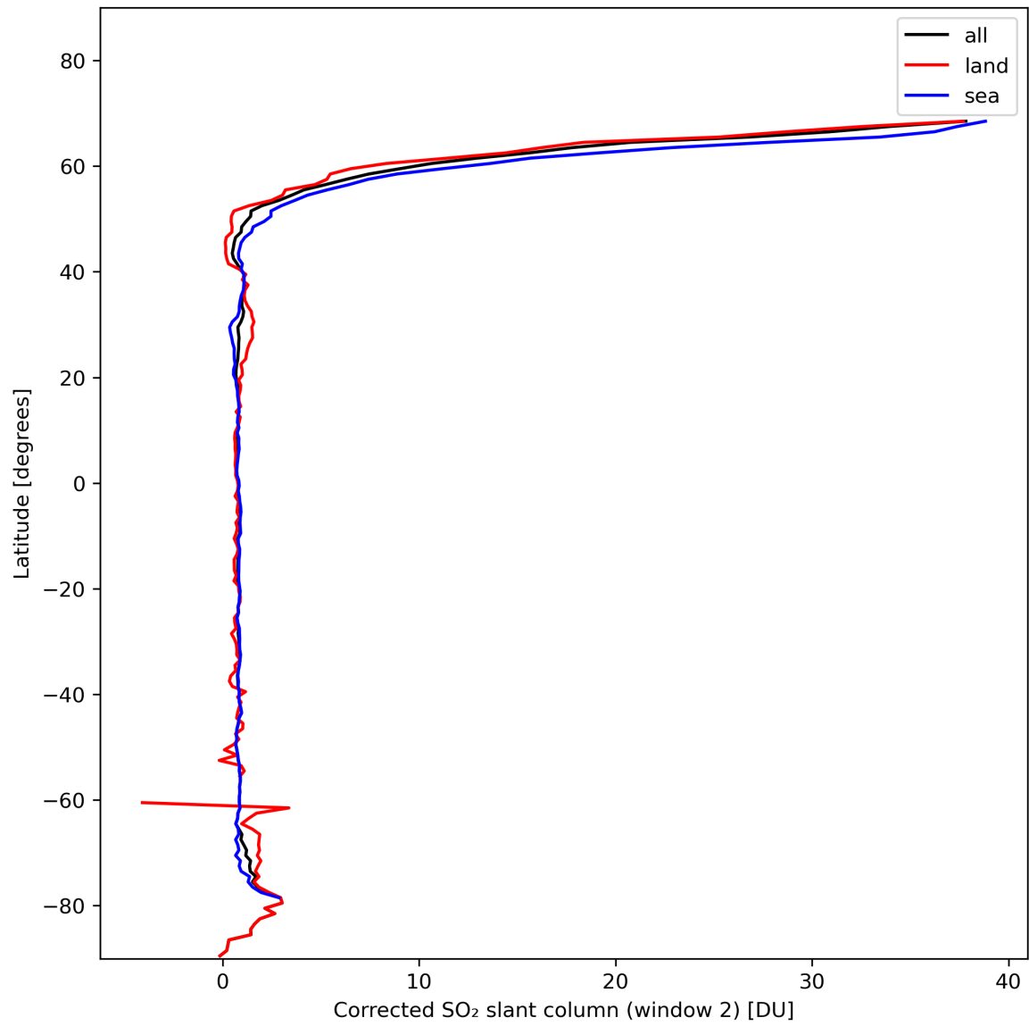
Figure 39: Zonal average of “Corrected SO 2 slant column (window 2)” for 2024-02-02 to 2024-02-04.
