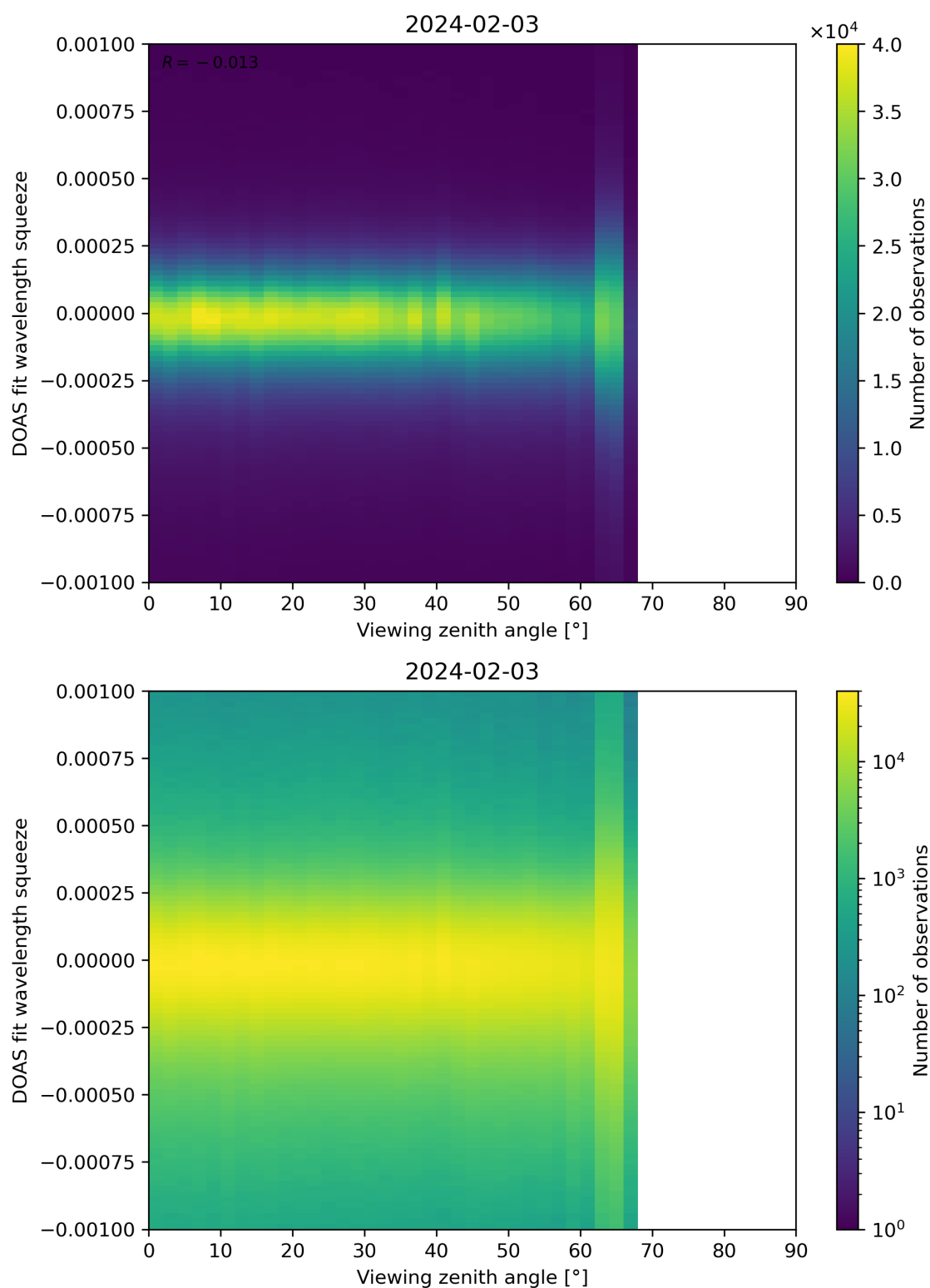
Figure 312: Scatter density plot of “Viewing zenith angle” against “DOAS fit wavelength squeeze” for 2024-02-02 to 2024-02-04.
