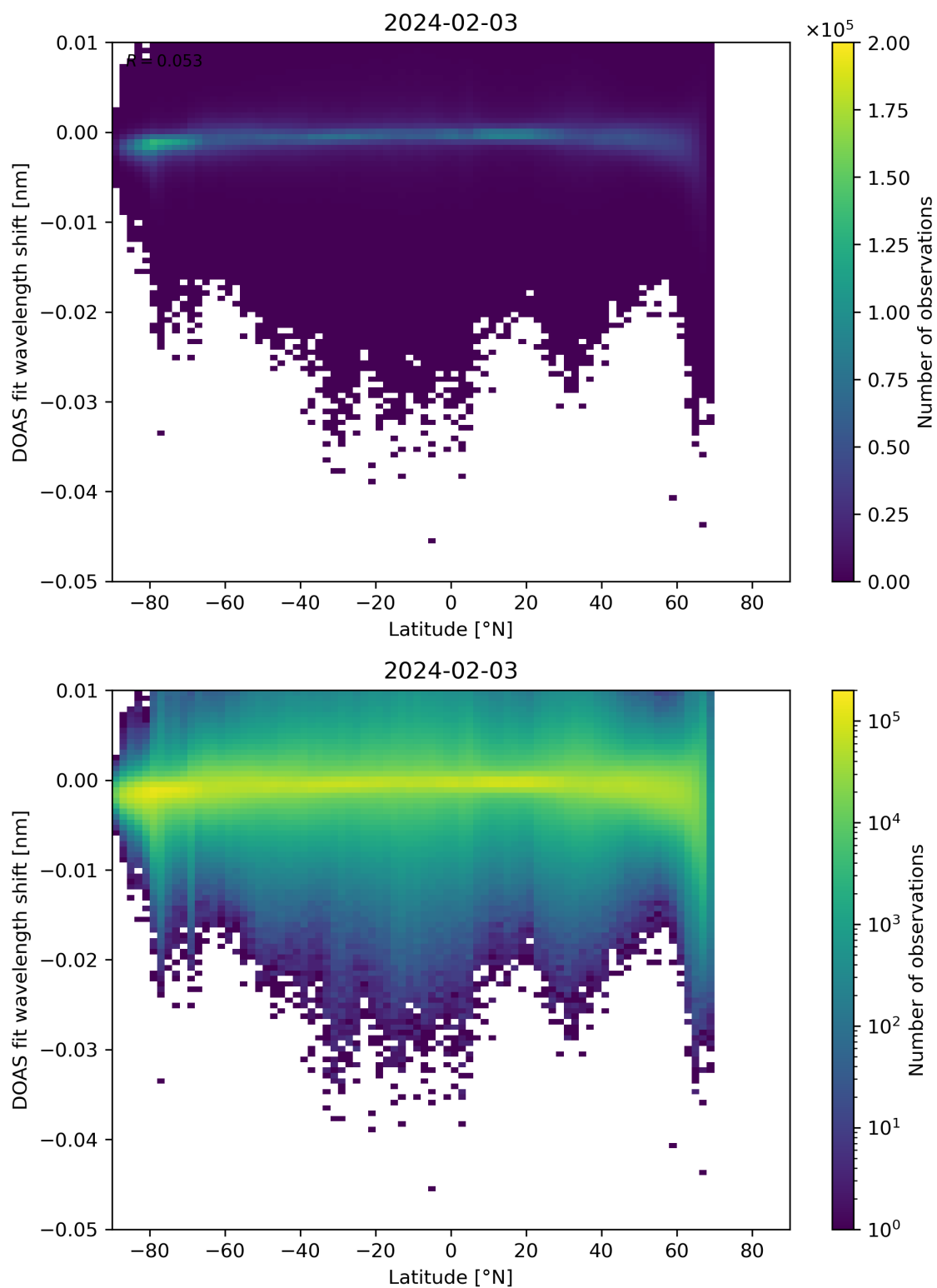
Figure 142: Scatter density plot of “Latitude” against “DOAS fit wavelength shift” for 2024-02-02 to 2024-02-04.
