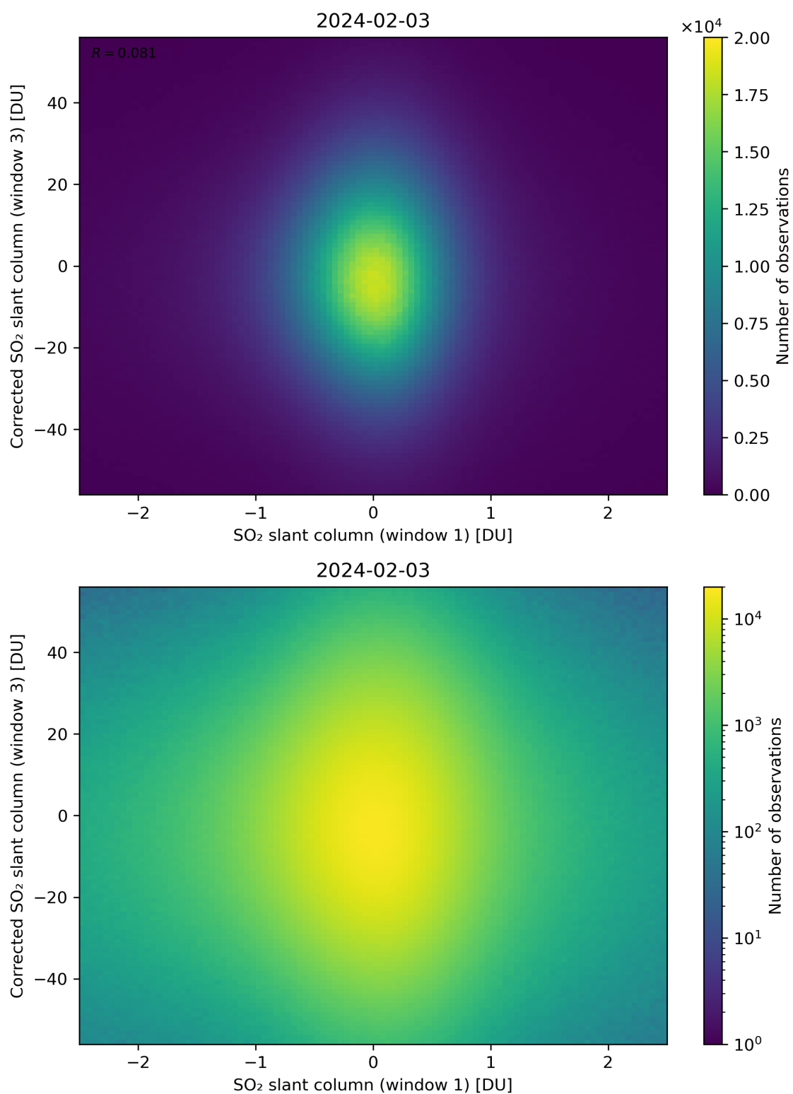
Figure 234: Scatter density plot of “SO 2 slant column (window 1)” against “Corrected SO 2 slant column (window 3)” for 2024-02-02 to 2024-02-04.
