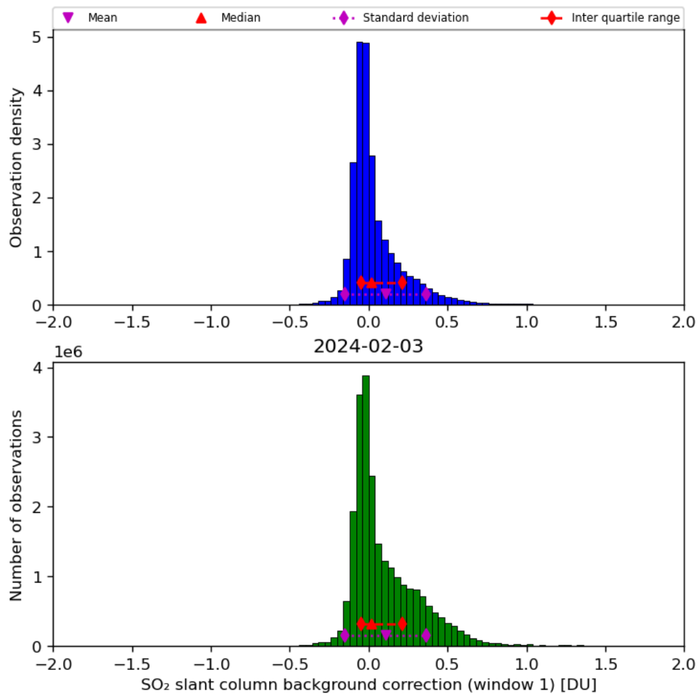
Figure 59: Histogram of “SO 2 slant column background correction (window 1)” for 2024-02-02 to 2024-02-04
