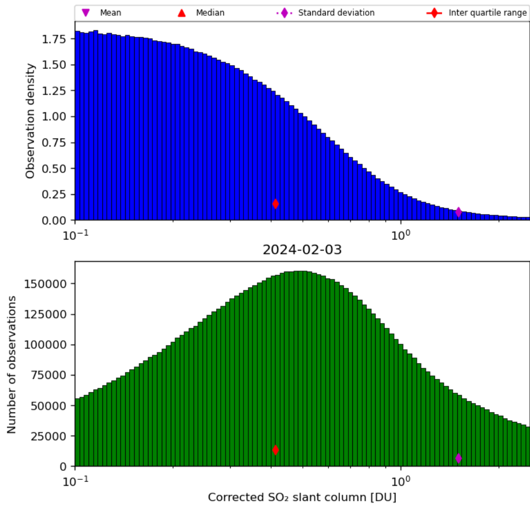
Figure 55: Histogram of “Corrected SO 2 slant column” for 2024-02-02 to 2024-02-04
