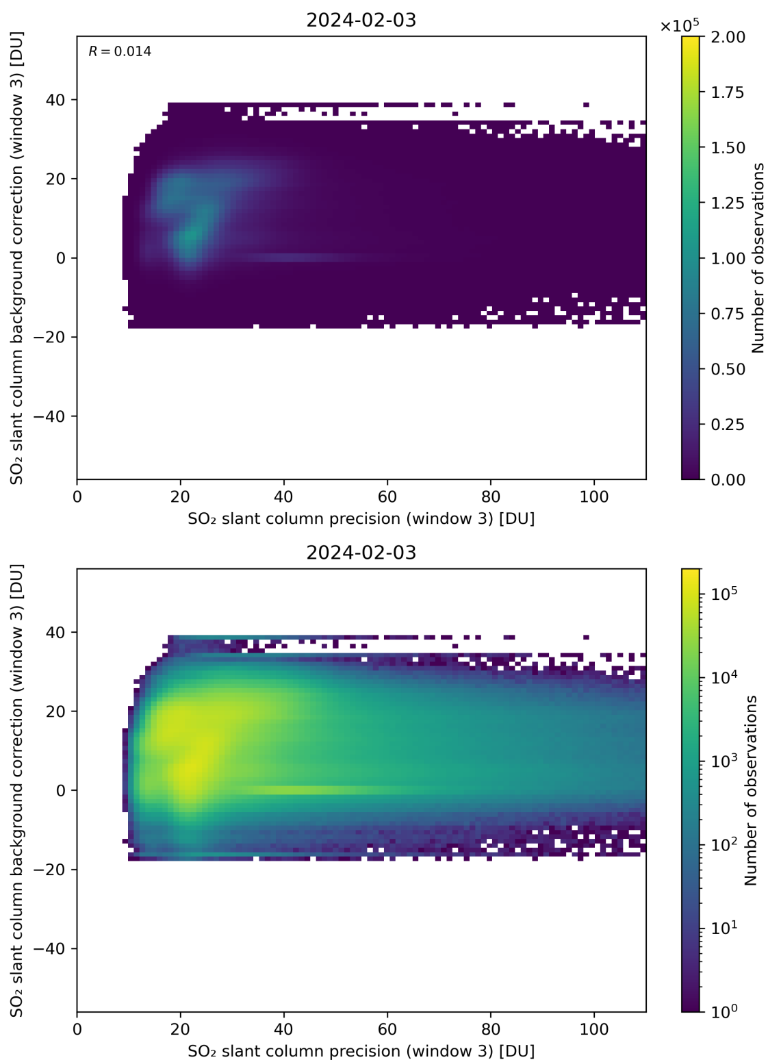
Figure 257: Scatter density plot of “SO 2 slant column precision (window 3)” against “SO 2 slant column background correction (window 3)” for 2024-02-02 to 2024-02-04.
