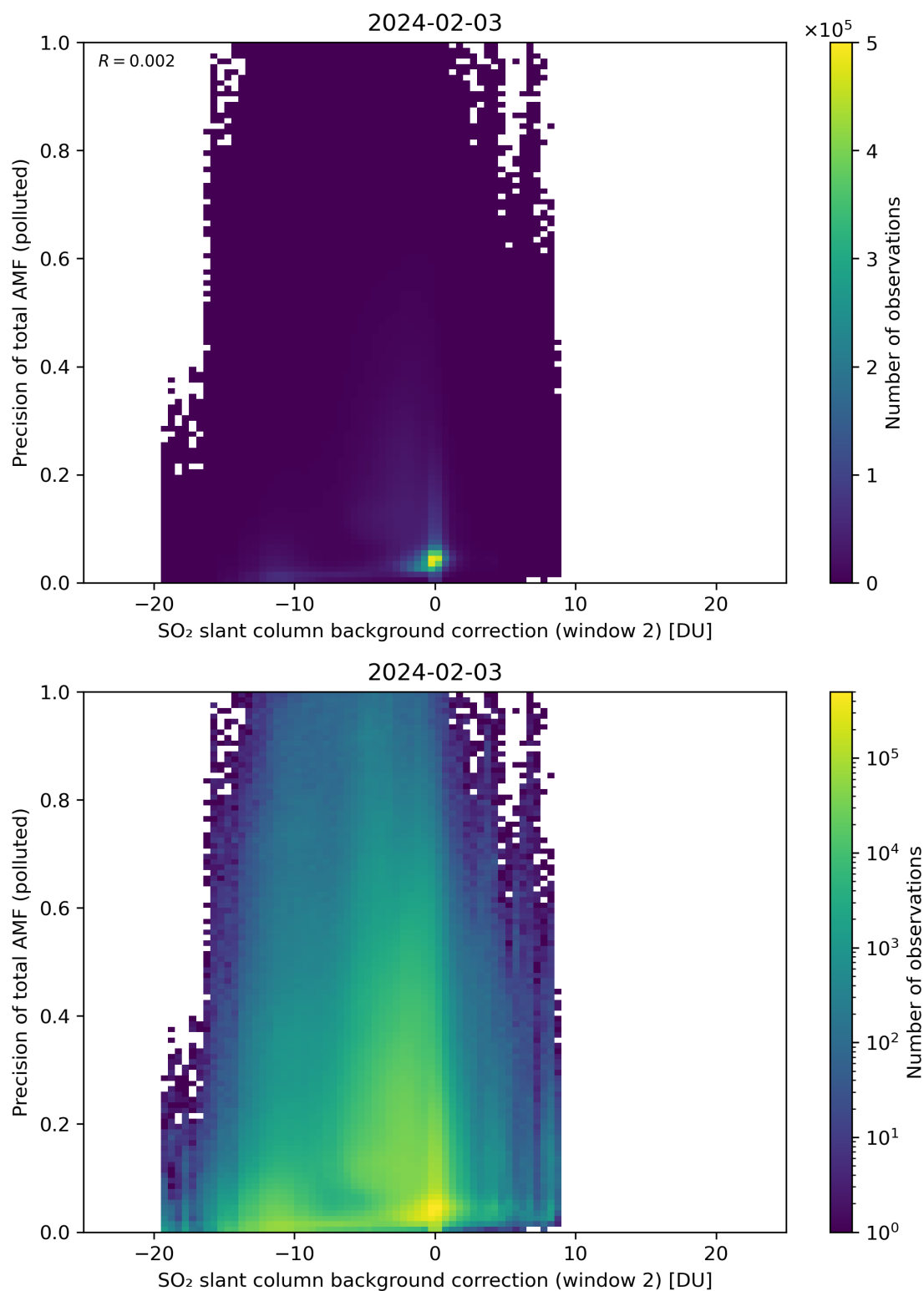
Figure 120: Scatter density plot of “SO 2 slant column background correction (window 2)” against “Precision of total AMF (polluted)” for 2024-02-02 to 2024-02-04.
