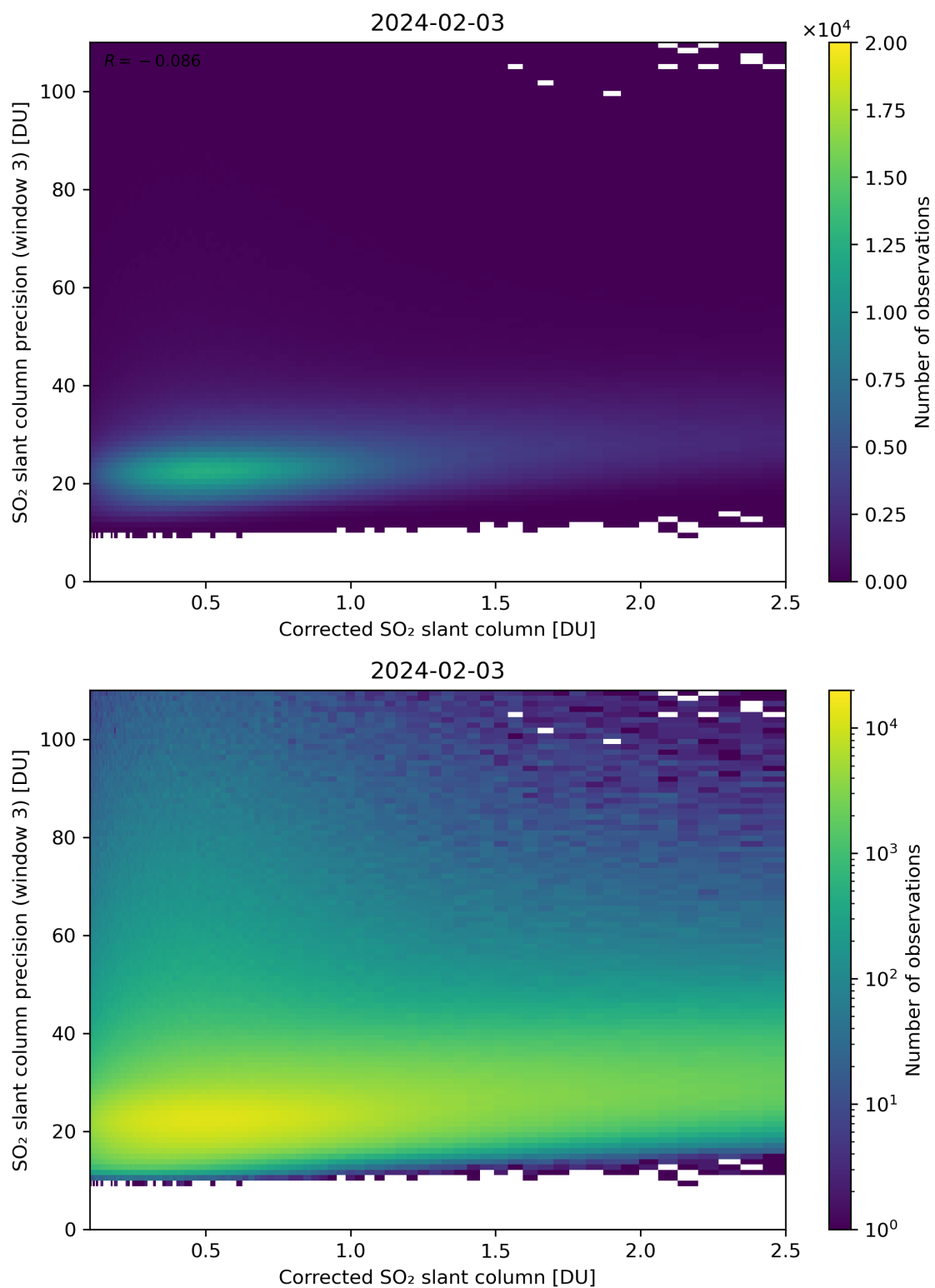
Figure 191: Scatter density plot of “Corrected SO 2 slant column” against “SO 2 slant column precision (window 3)” for 2024-02-02 to 2024-02-04.
