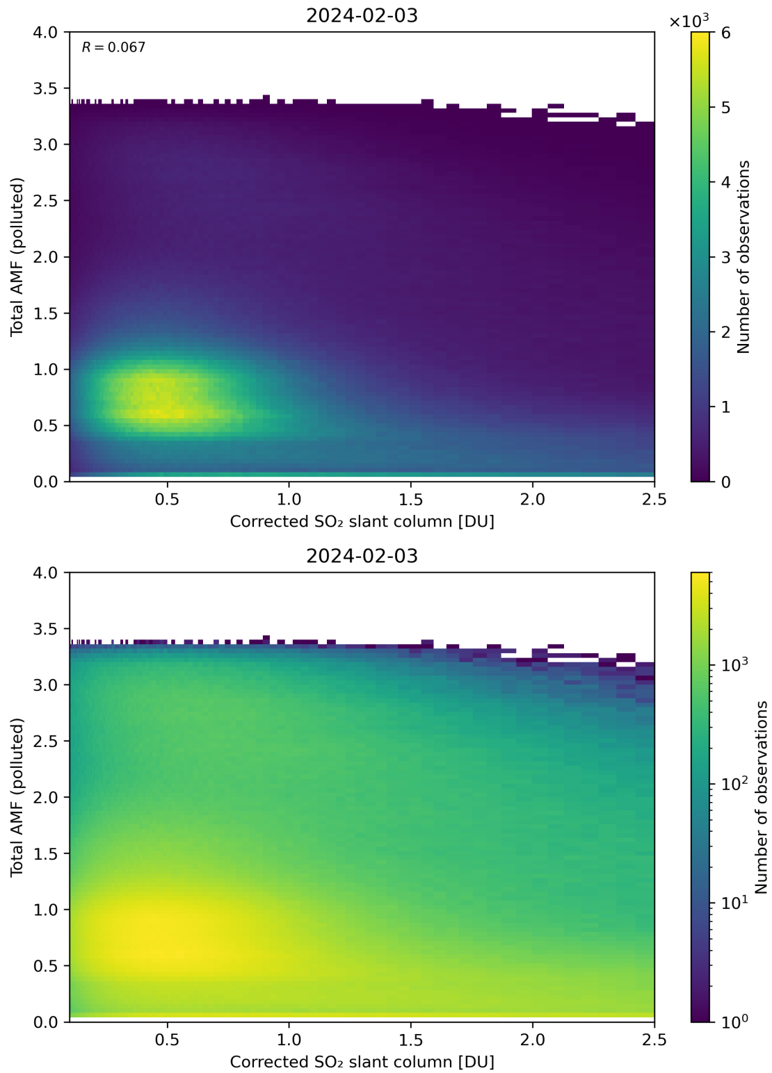
Figure 192: Scatter density plot of “Corrected SO 2 slant column” against “Total AMF (polluted)” for 2024-02-02 to 2024-02-04.
