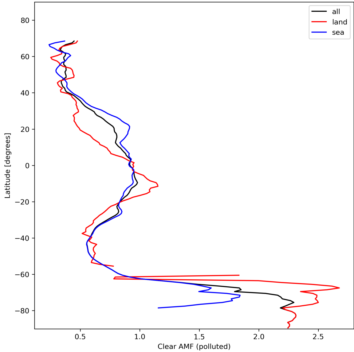
Figure 50: Zonal average of “Clear AMF (polluted)” for 2024-02-02 to 2024-02-04.
