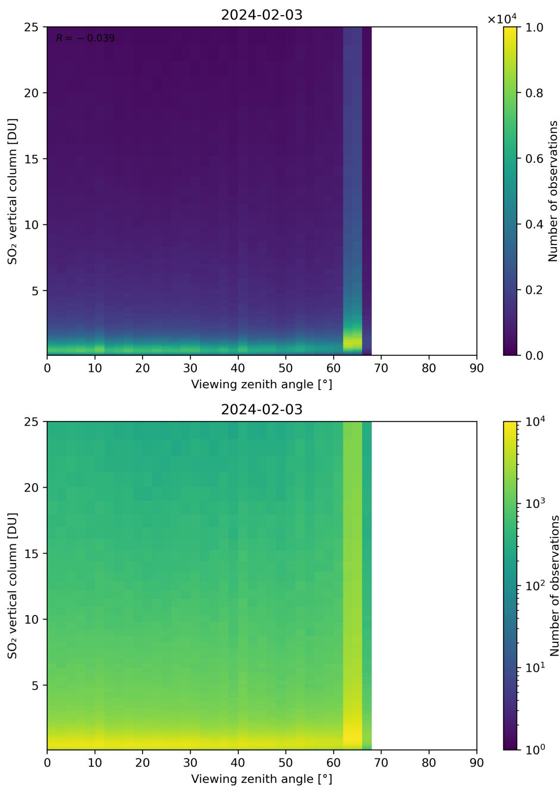
Figure 327: Scatter density plot of “Viewing zenith angle” against “SO 2 vertical column” for 2024-02-02 to 2024-02-04.
