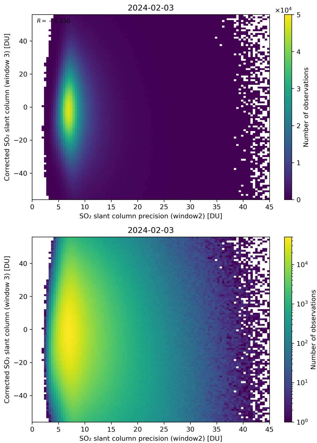
Figure 248: Scatter density plot of “SO 2 slant column precision (window2)” against “Corrected SO 2 slant column (window 3)” for 2024-02-02 to 2024-02-04.
