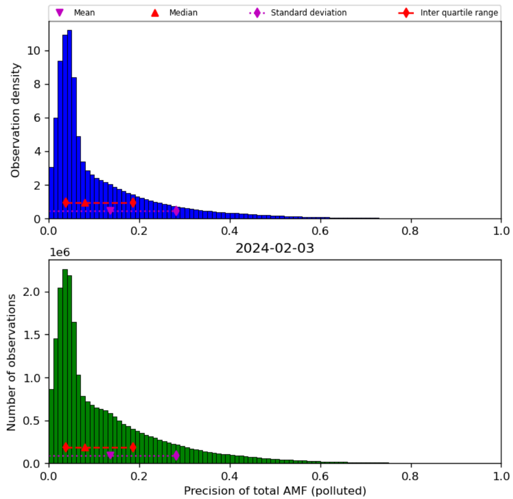
Figure 72: Histogram of “Precision of total AMF (polluted)” for 2024-02-02 to 2024-02-04
