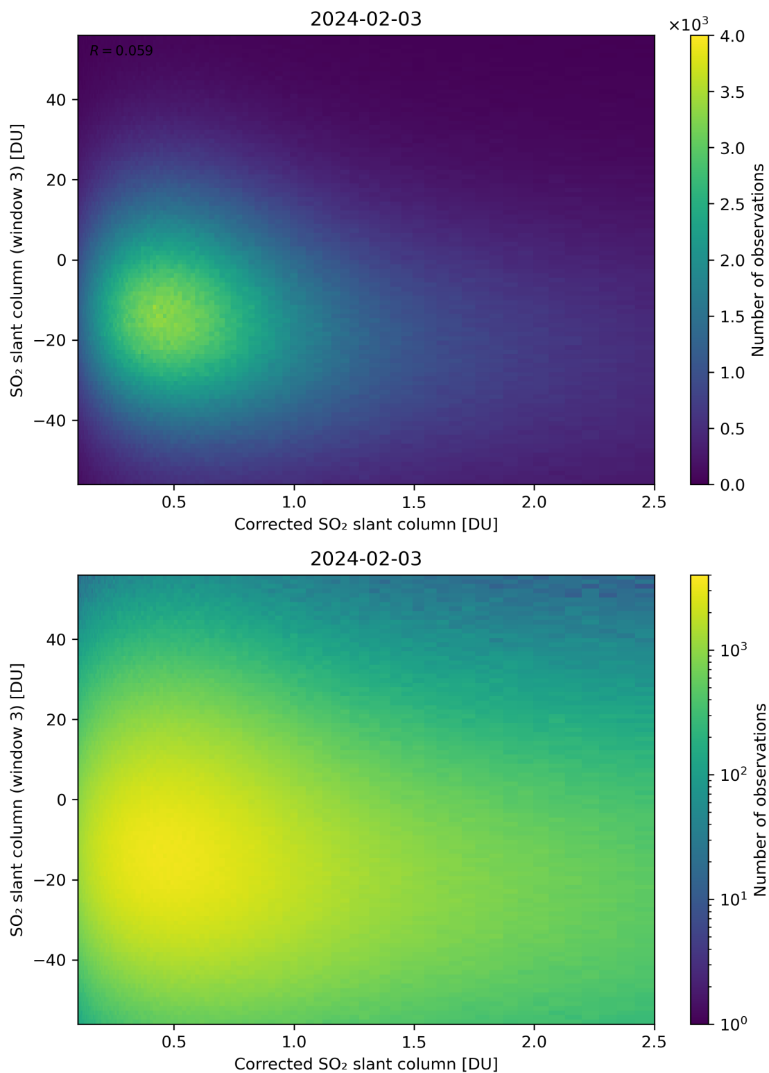
Figure 190: Scatter density plot of “Corrected SO 2 slant column” against “SO 2 slant column (window 3)” for 2024-02-02 to 2024-02-04.
