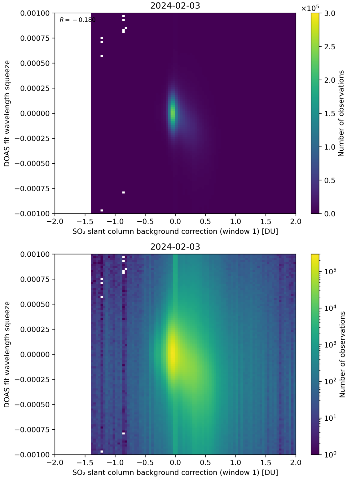
Figure 101: Scatter density plot of “SO 2 slant column background correction (window 1)” against “DOAS fit wavelength squeeze” for 2024-02-02 to 2024-02-04.
