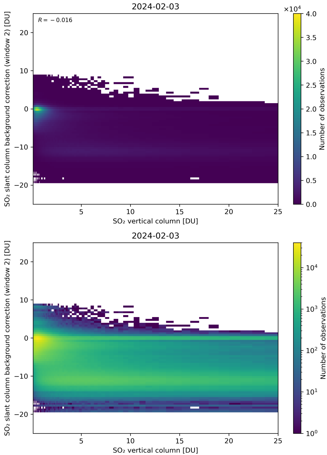
Figure 274: Scatter density plot of “SO 2 vertical column” against “SO 2 slant column background correction (window 2)” for 2024-02-02 to 2024-02-04.
