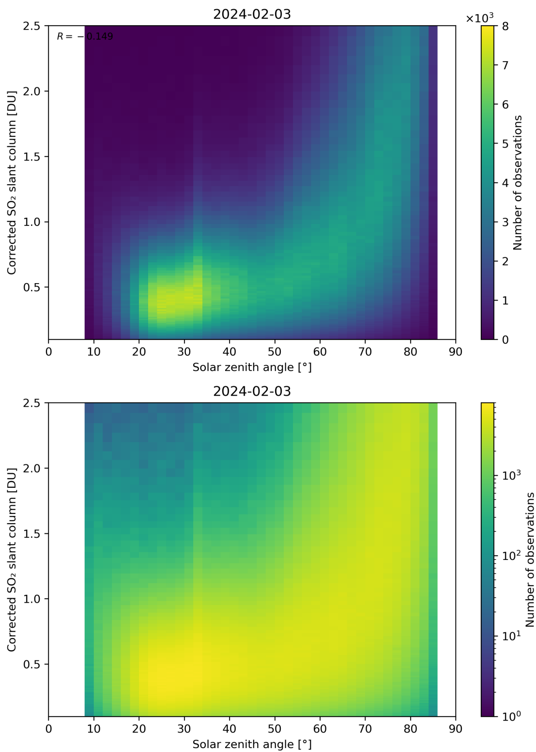
Figure 166: Scatter density plot of “Solar zenith angle” against “Corrected SO 2 slant column” for 2024-02-02 to 2024-02-04.
