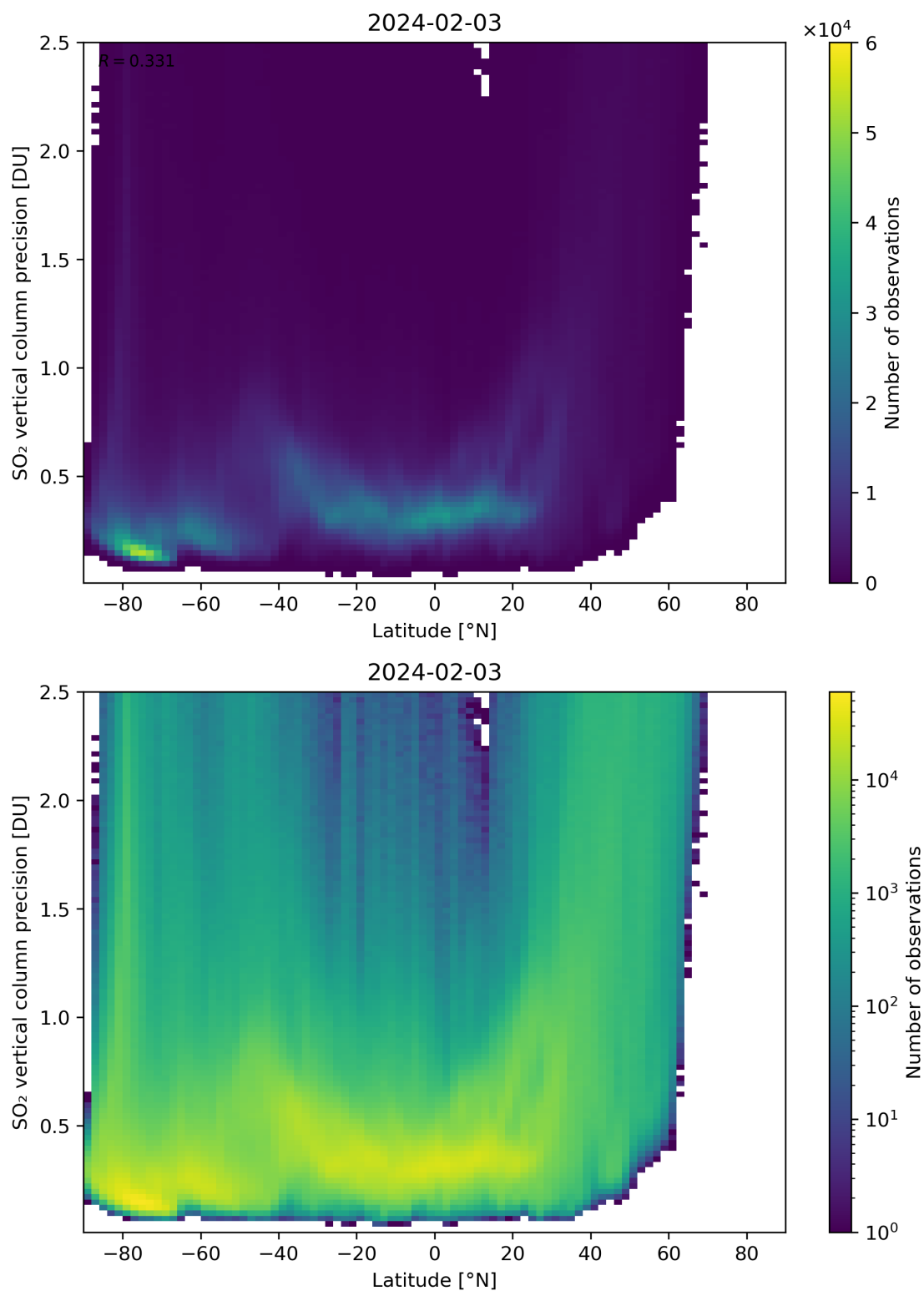
Figure 157: Scatter density plot of “Latitude” against “SO 2 vertical column precision” for 2024-02-02 to 2024-02-04.
