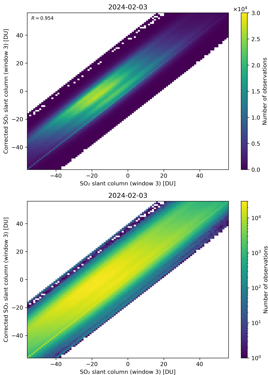
Figure 266: Scatter density plot of “SO 2 slant column (window 3)” against “Corrected SO 2 slant column (window 3)” for 2024-02-02 to 2024-02-04.
