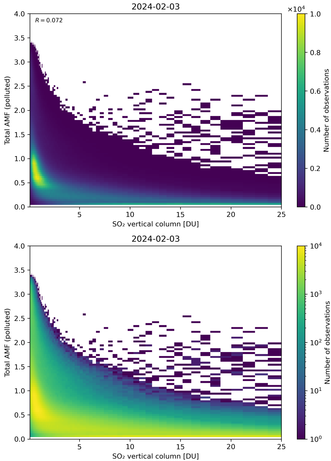
Figure 305: Scatter density plot of “SO 2 vertical column” against “Total AMF (polluted)” for 2024-02-02 to 2024-02-04.
