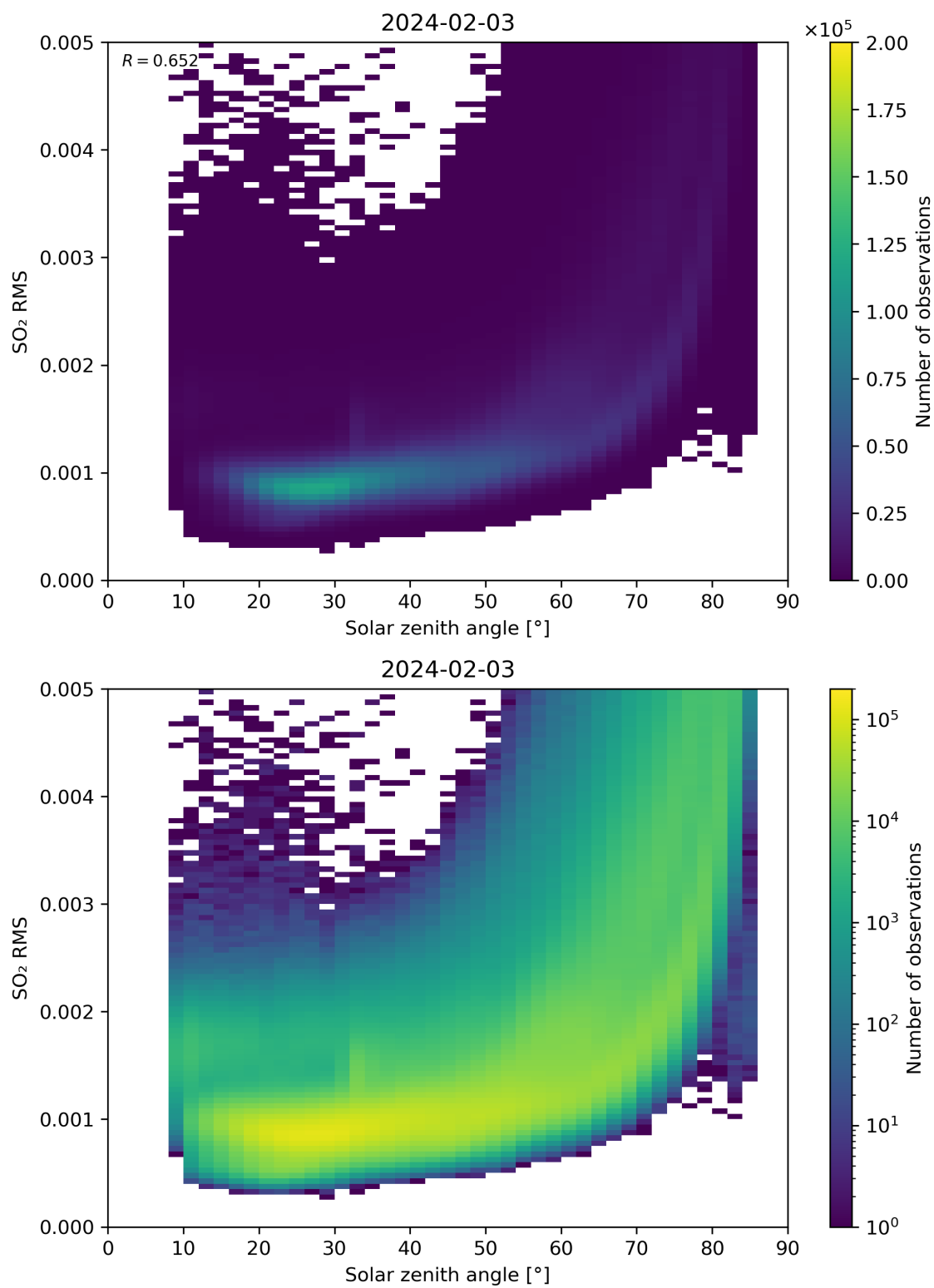
Figure 163: Scatter density plot of “Solar zenith angle” against “SO 2 RMS” for 2024-02-02 to 2024-02-04.
