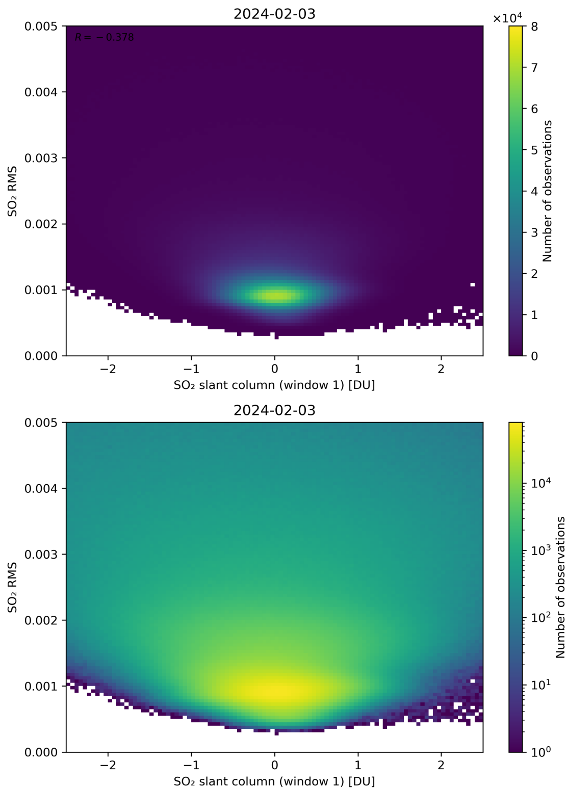
Figure 217: Scatter density plot of “SO 2 slant column (window 1)” against “SO 2 RMS” for 2024-02-02 to 2024-02-04.
