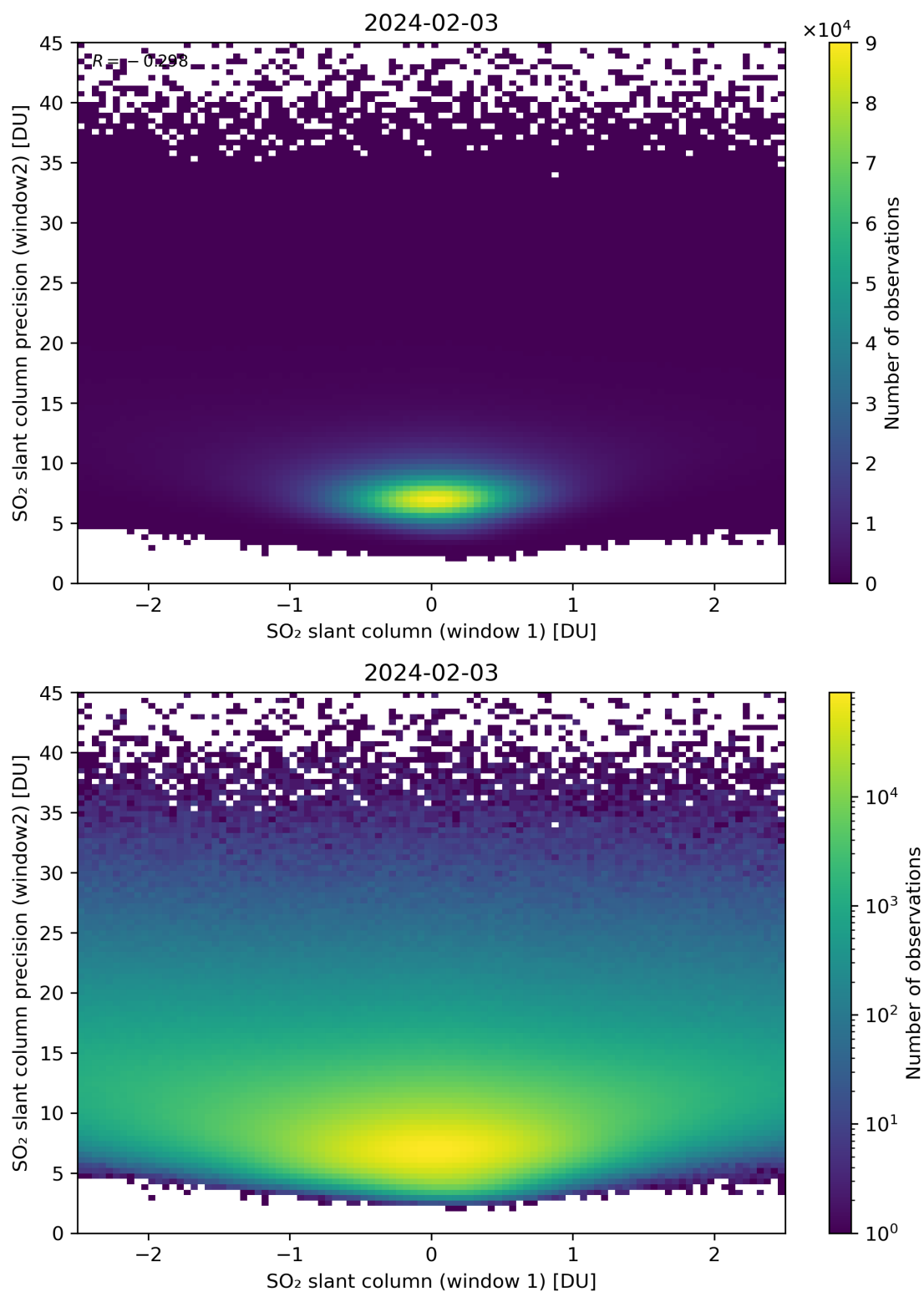
Figure 236: Scatter density plot of “SO 2 slant column (window 1)” against “SO 2 slant column precision (window2)” for 2024-02-02 to 2024-02-04.
