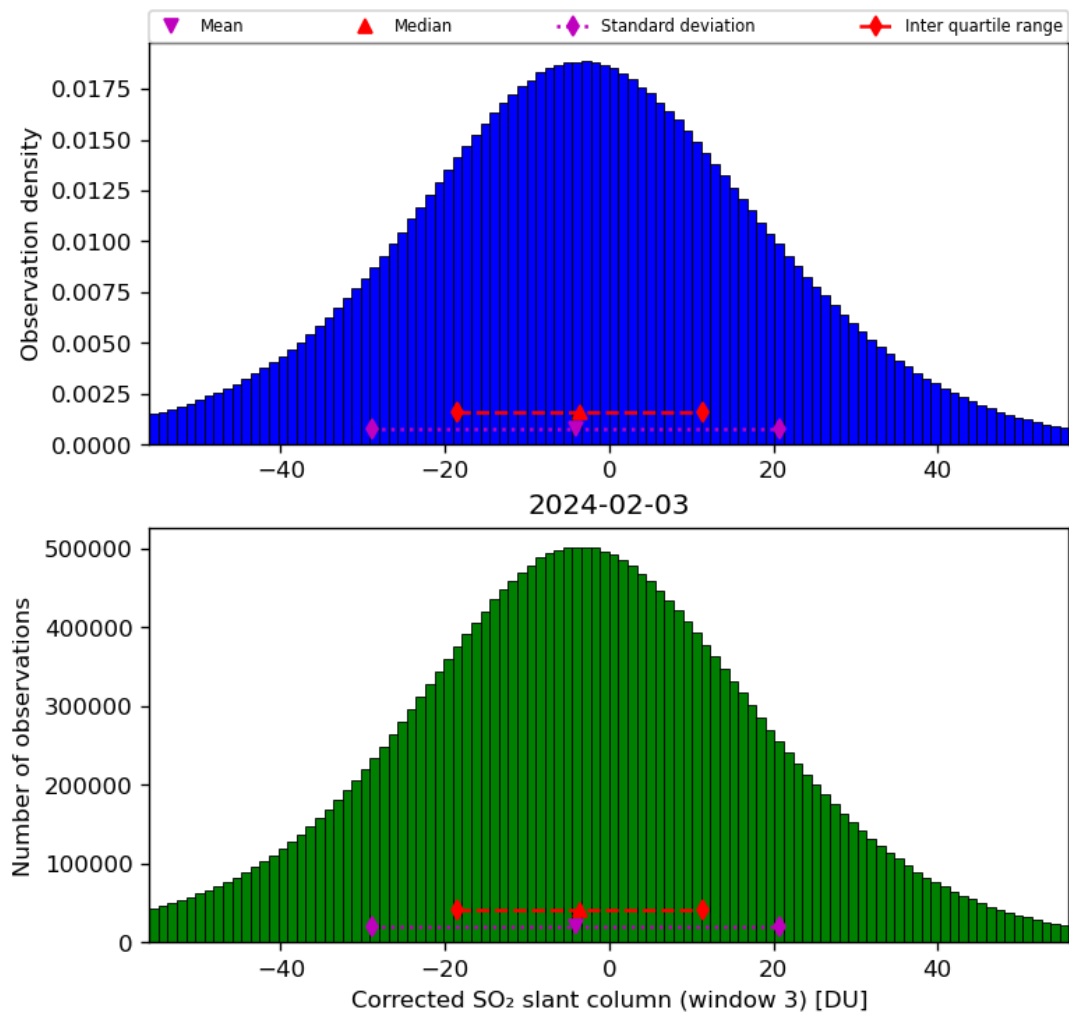
Figure 66: Histogram of “Corrected SO 2 slant column (window 3)” for 2024-02-02 to 2024-02-04
