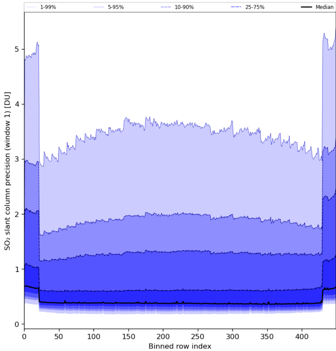
Figure 80: Along track statistics of “SO 2 slant column precision (window 1)” for 2024-02-02 to 2024-02-04
