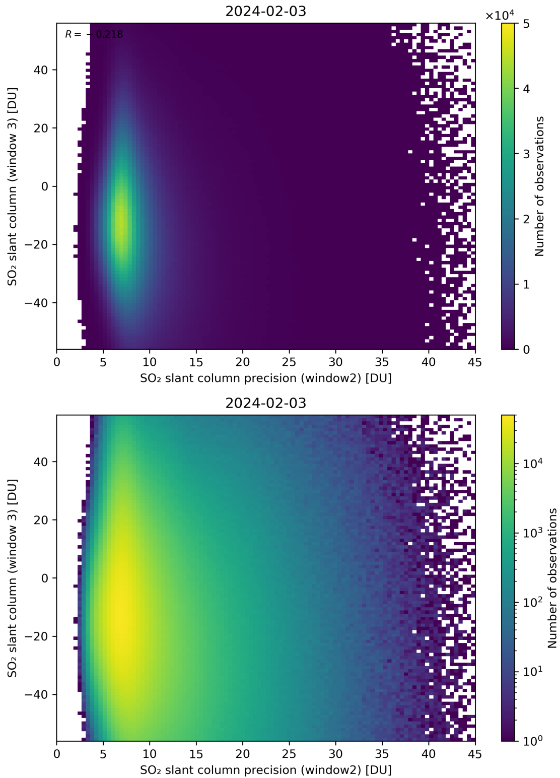
Figure 249: Scatter density plot of “SO 2 slant column precision (window2)” against “SO 2 slant column (window 3)” for 2024-02-02 to 2024-02-04.
