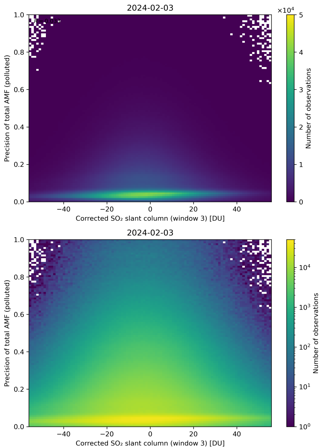
Figure 211: Scatter density plot of “Corrected SO 2 slant column (window 3)” against “Precision of total AMF (polluted)” for 2024-02-02 to 2024-02-04.
