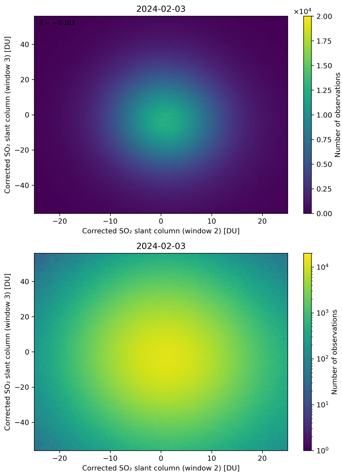
Figure 200: Scatter density plot of “Corrected SO 2 slant column (window 2)” against “Corrected SO 2 slant column (window 3)” for 2024-02-02 to 2024-02-04.
