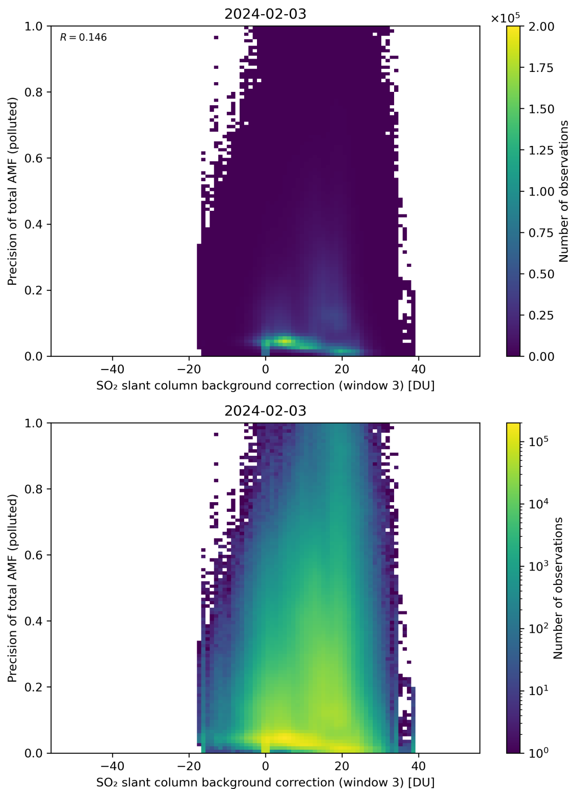
Figure 126: Scatter density plot of “SO 2 slant column background correction (window 3)” against “Precision of total AMF (polluted)” for 2024-02-02 to 2024-02-04.
