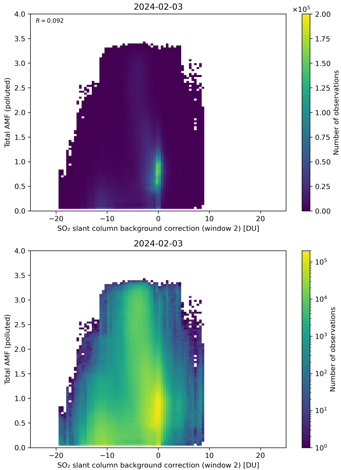
Figure 119: Scatter density plot of “SO 2 slant column background correction (window 2)” against “Total AMF (polluted)” for 2024-02-02 to 2024-02-04.
