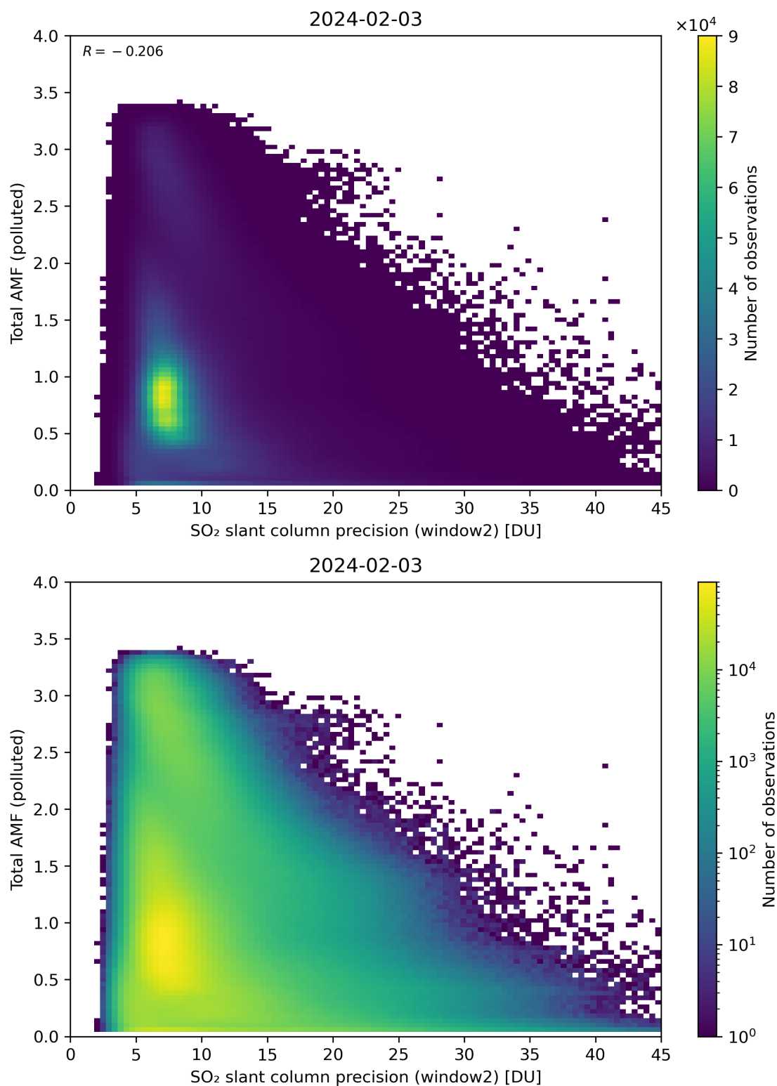
Figure 251: Scatter density plot of “SO 2 slant column precision (window2)” against “Total AMF (polluted)” for 2024-02-02 to 2024-02-04.
