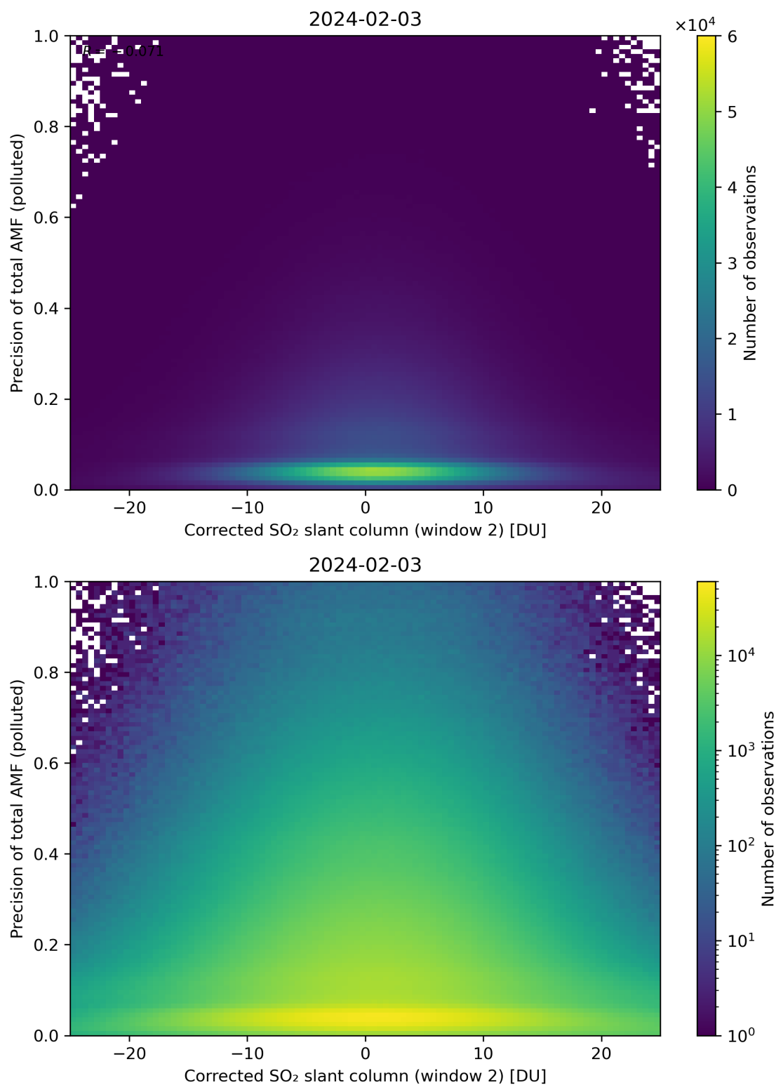
Figure 204: Scatter density plot of “Corrected SO 2 slant column (window 2)” against “Precision of total AMF (polluted)” for 2024-02-02 to 2024-02-04.
