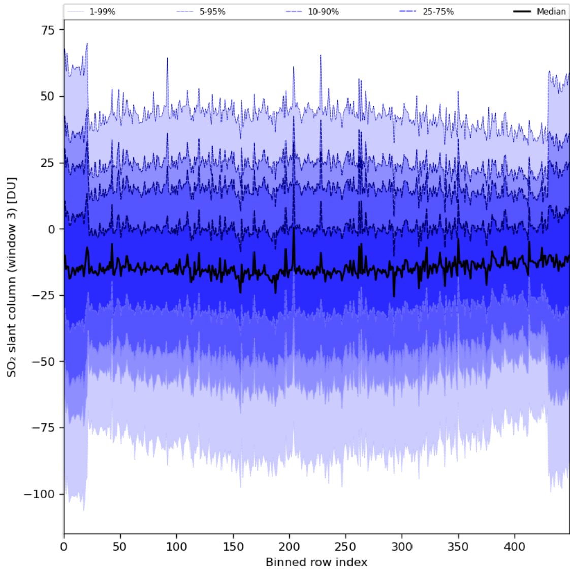
Figure 87: Along track statistics of “SO 2 slant column (window 3)” for 2024-02-02 to 2024-02-04
