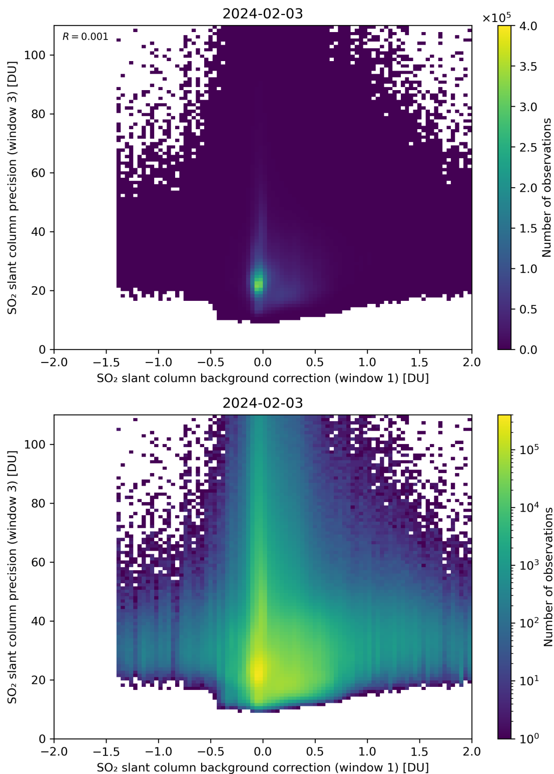
Figure 108: Scatter density plot of “SO 2 slant column background correction (window 1)” against “SO 2 slant column precision (window 3)” for 2024-02-02 to 2024-02-04.
