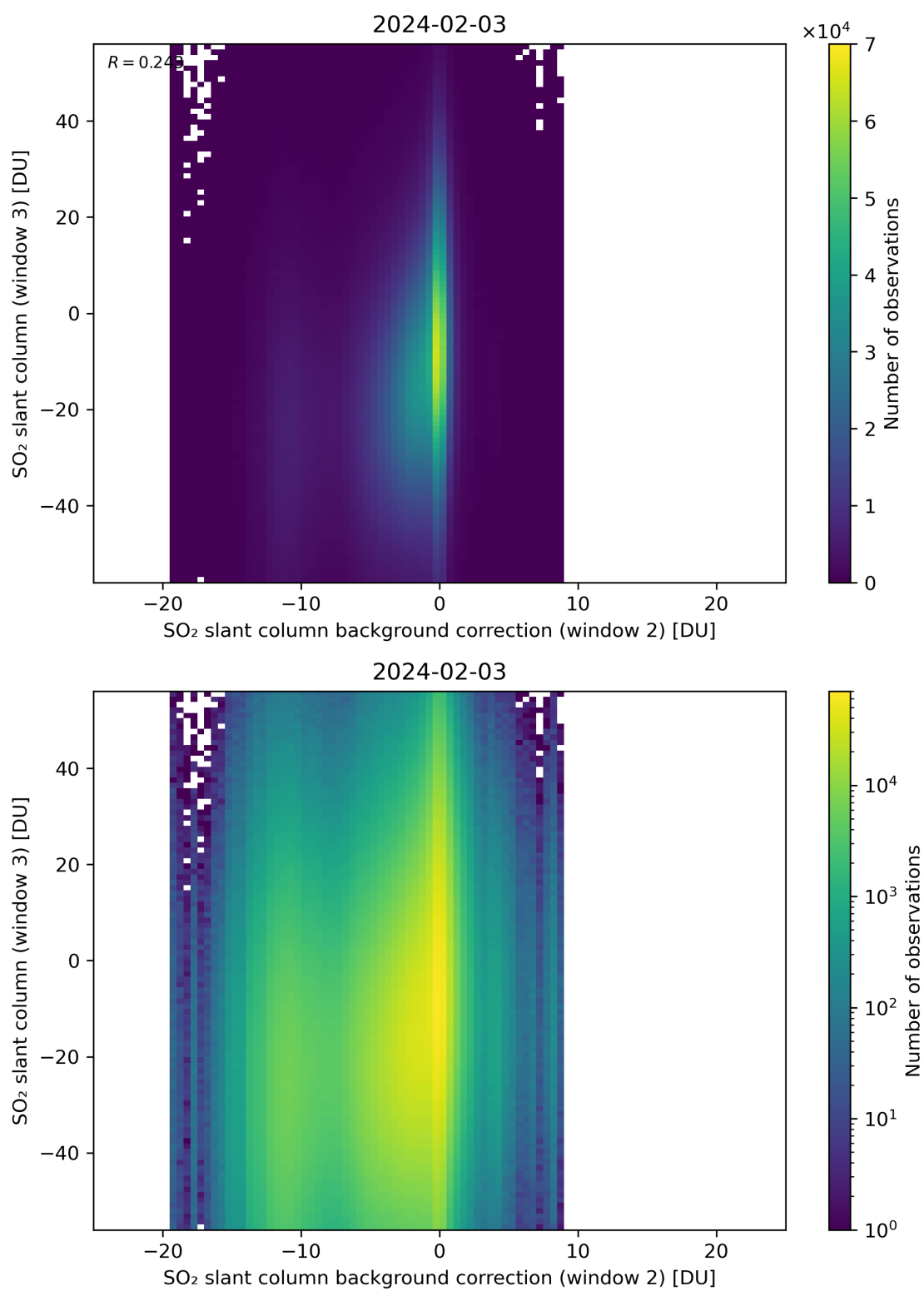
Figure 117: Scatter density plot of “SO 2 slant column background correction (window 2)” against “SO 2 slant column (window 3)” for 2024-02-02 to 2024-02-04.
