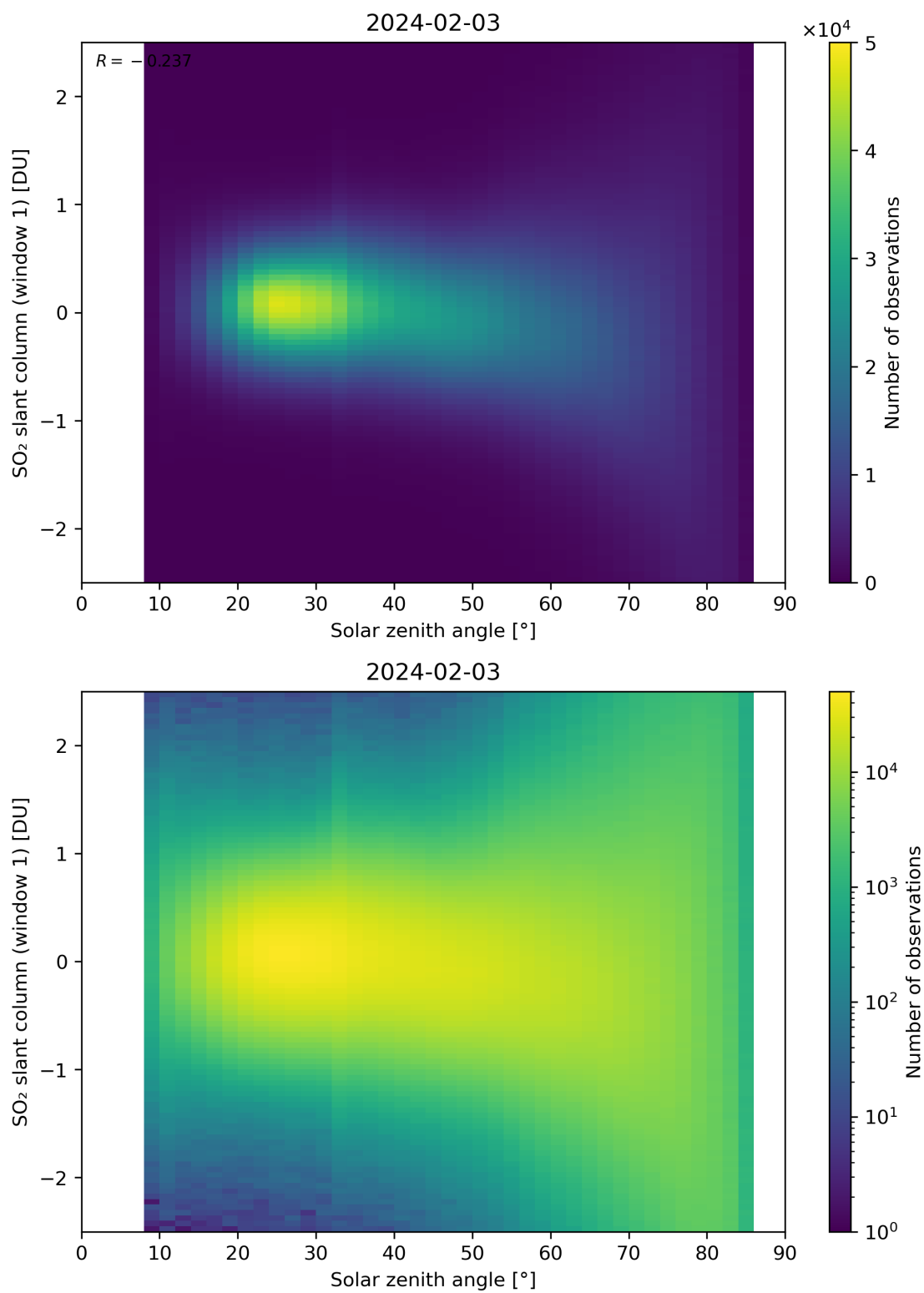
Figure 169: Scatter density plot of “Solar zenith angle” against “SO 2 slant column (window 1)” for 2024-02-02 to 2024-02-04.
