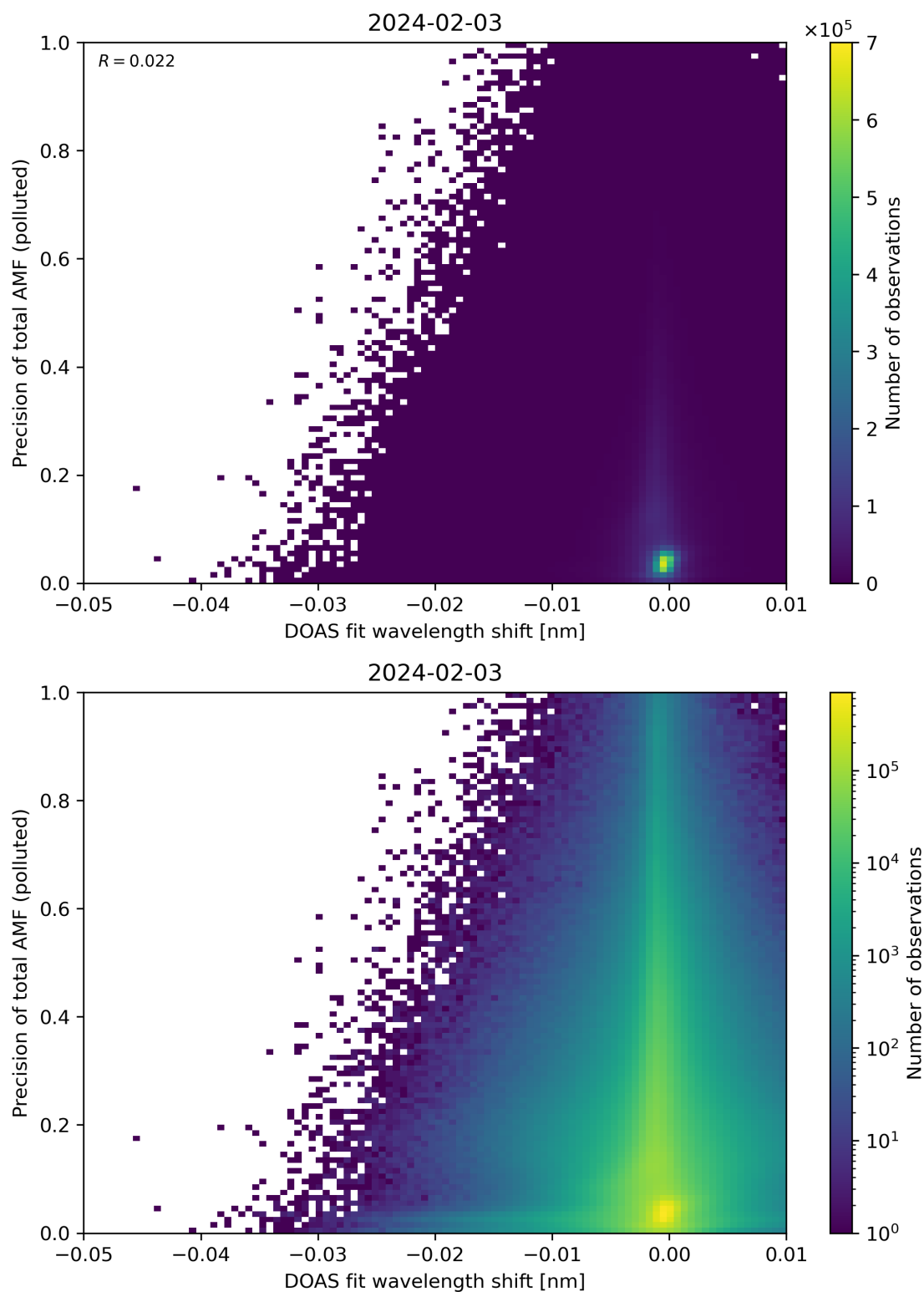
Figure 131: Scatter density plot of “DOAS fit wavelength shift” against “Precision of total AMF (polluted)” for 2024-02-02 to 2024-02-04.
