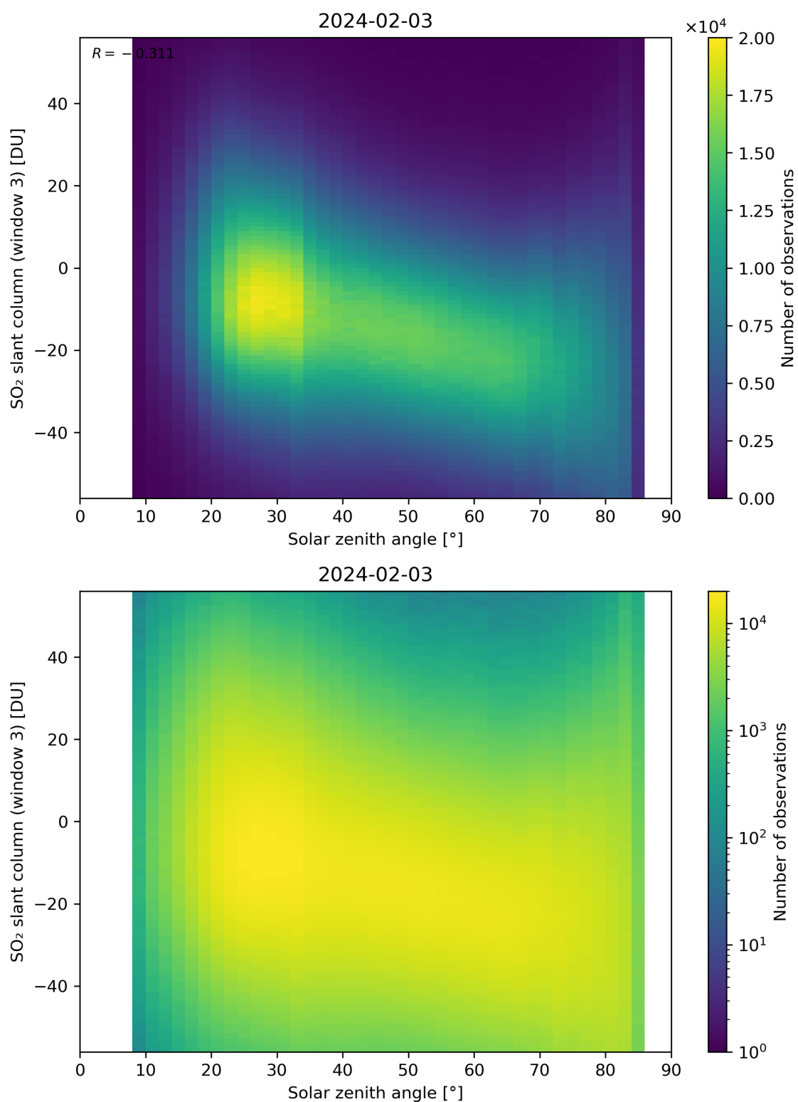
Figure 172: Scatter density plot of “Solar zenith angle” against “SO 2 slant column (window 3)” for 2024-02-02 to 2024-02-04.
