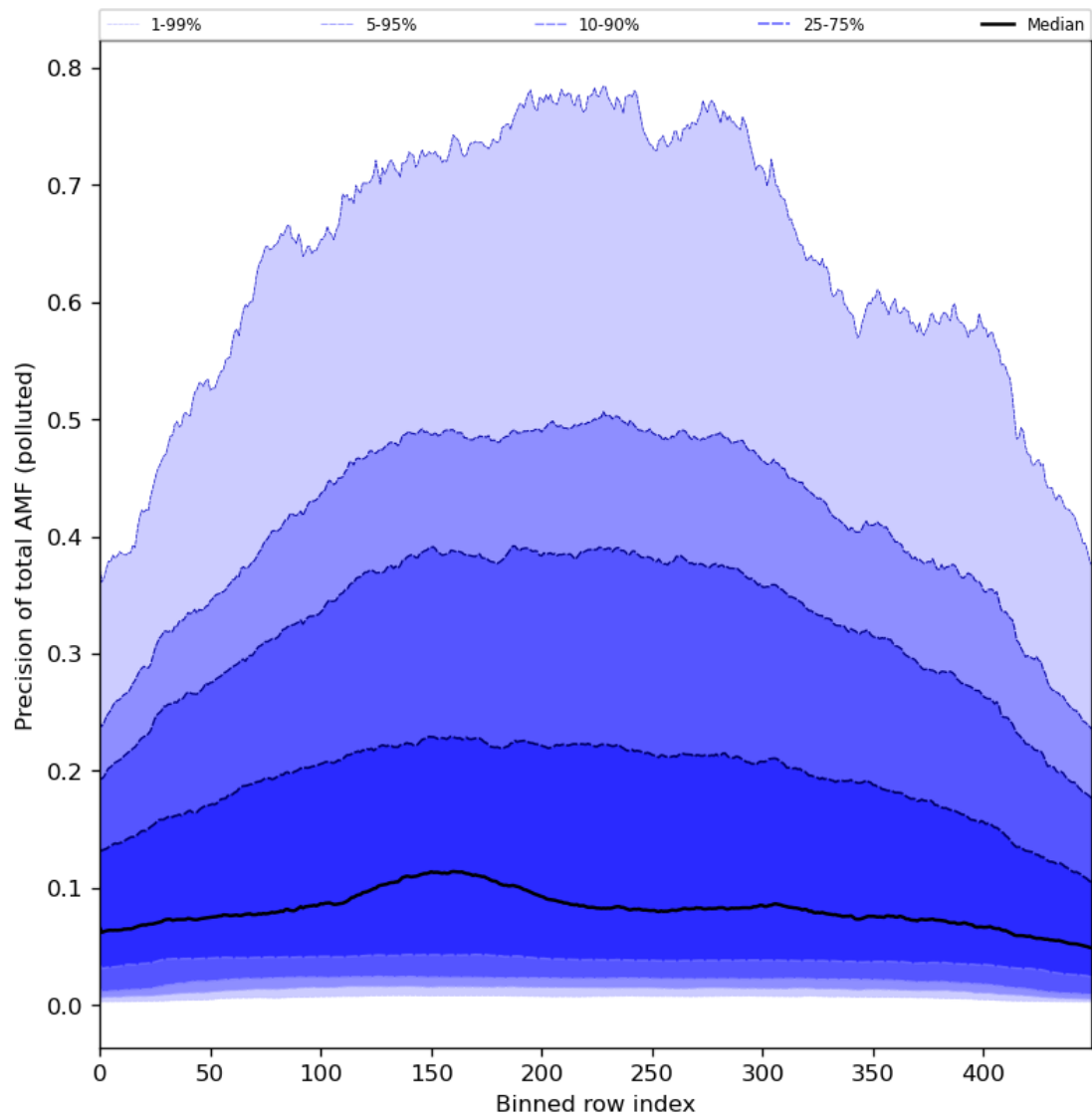
Figure 95: Along track statistics of “Precision of total AMF (polluted)” for 2024-02-02 to 2024-02-04
