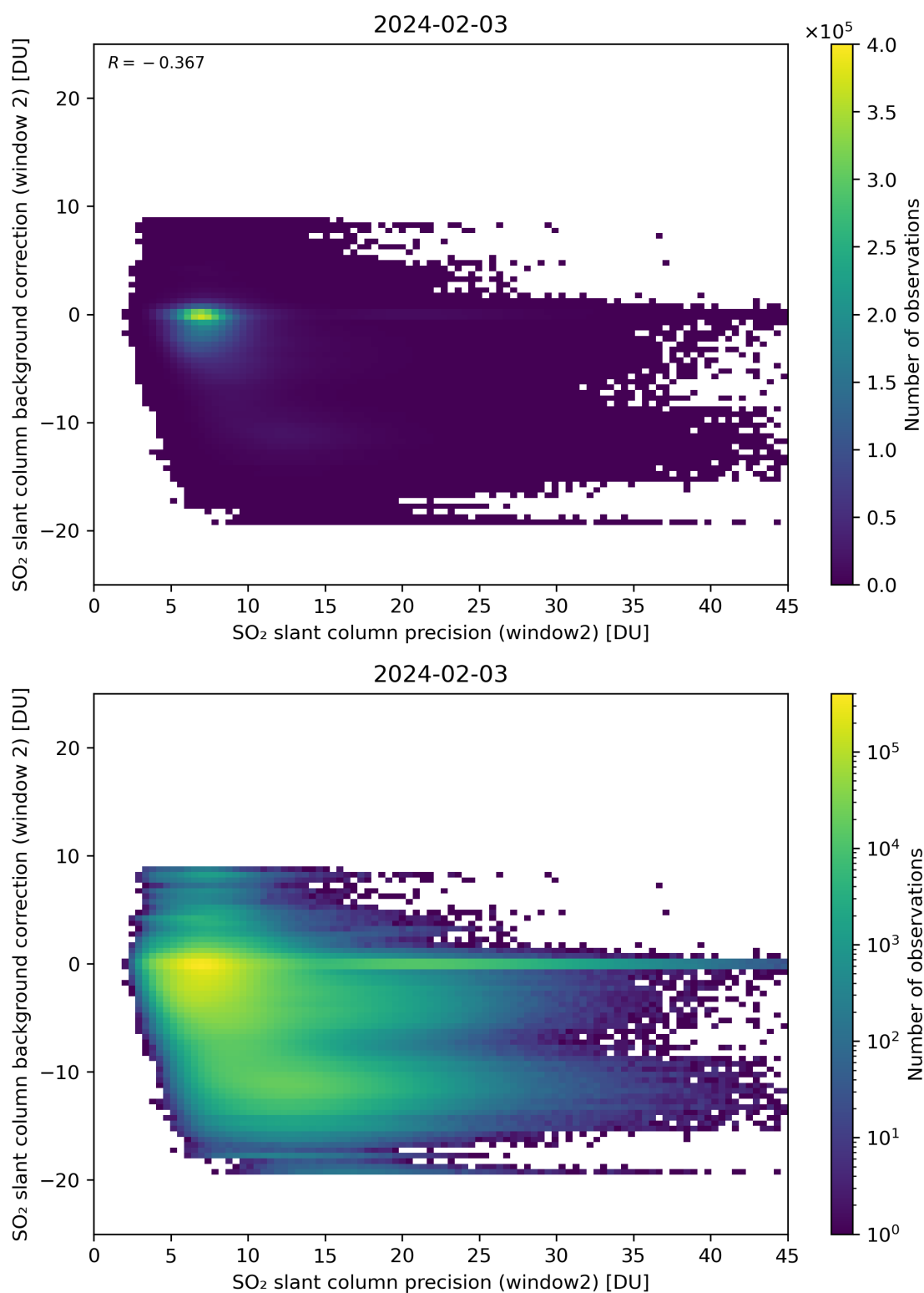
Figure 241: Scatter density plot of “SO 2 slant column precision (window2)” against “SO 2 slant column background correction (window 2)” for 2024-02-02 to 2024-02-04.
