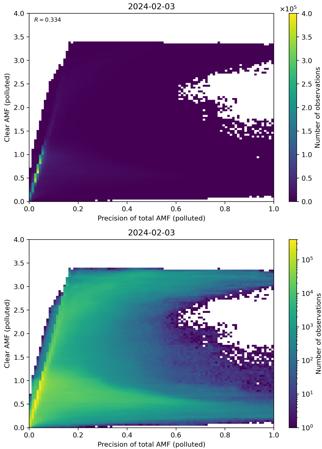
Figure 270: Scatter density plot of “Precision of total AMF (polluted)” against “Clear AMF (polluted)” for 2024-02-02 to 2024-02-04.
