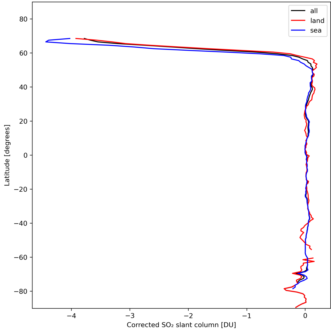
Figure 32: Zonal average of “Corrected SO 2 slant column” for 2024-02-02 to 2024-02-04.
