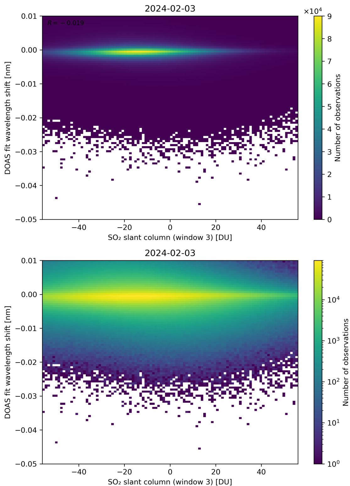
Figure 254: Scatter density plot of “SO 2 slant column (window 3)” against “DOAS fit wavelength shift” for 2024-02-02 to 2024-02-04.
