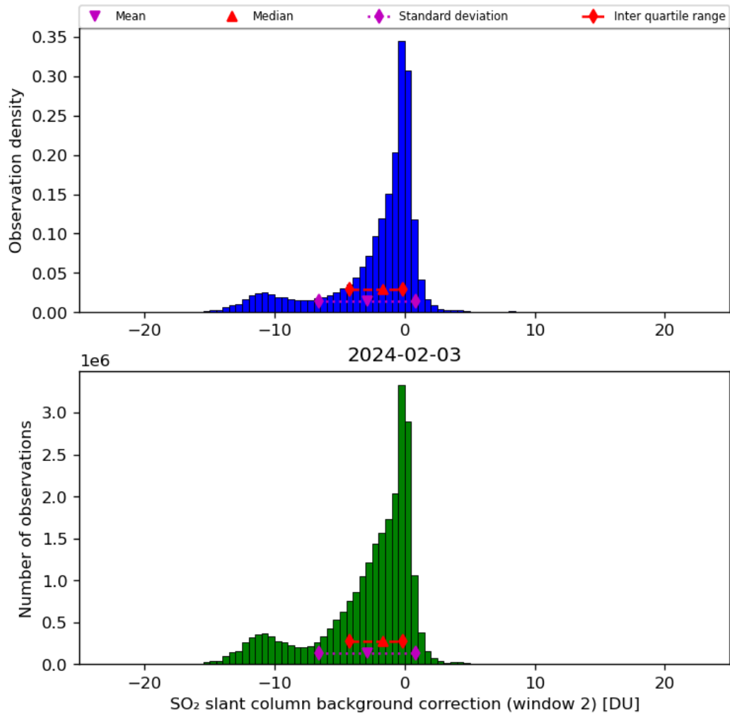
Figure 63: Histogram of “SO 2 slant column background correction (window 2)” for 2024-02-02 to 2024-02-04
