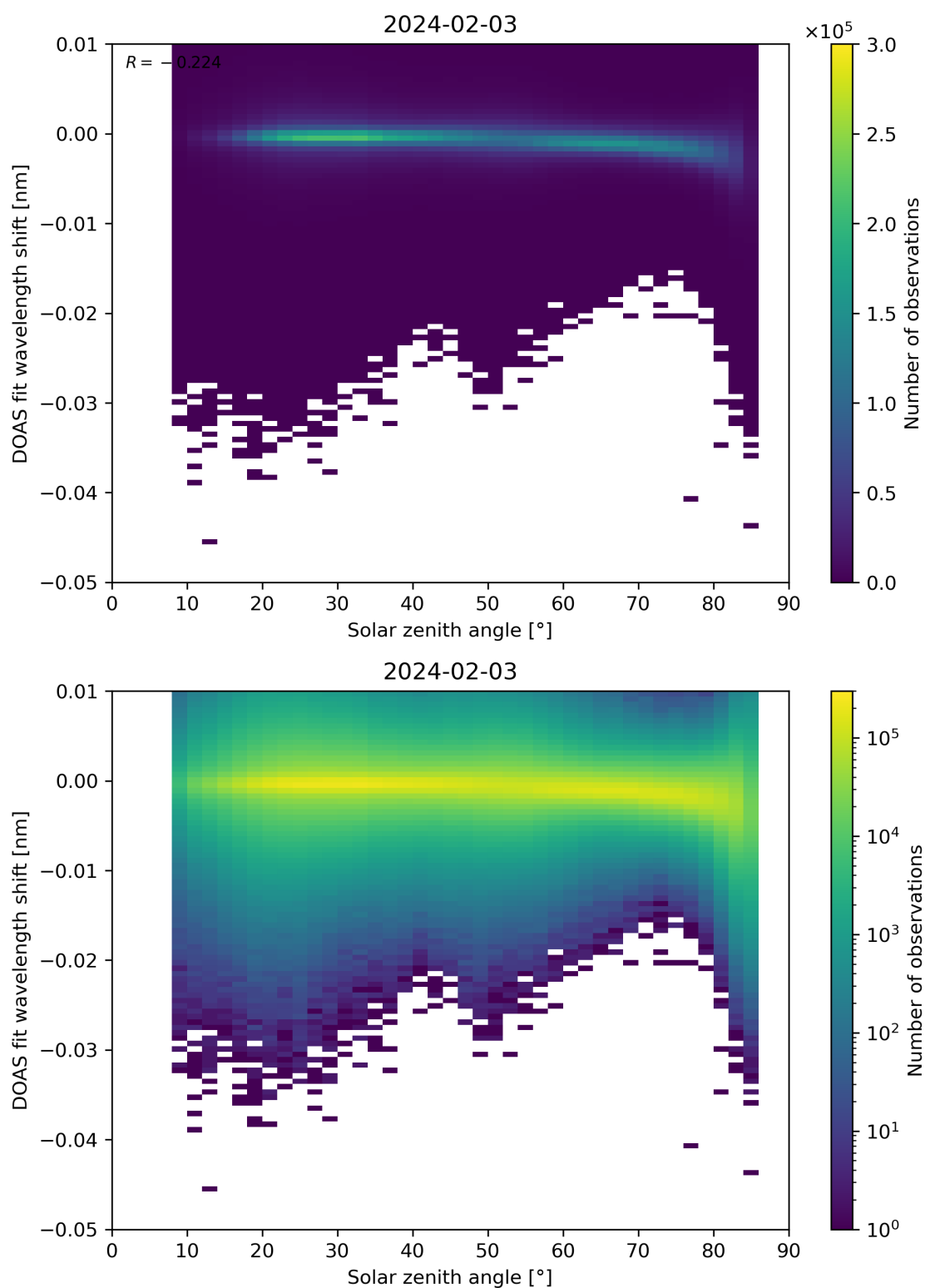
Figure 161: Scatter density plot of “Solar zenith angle” against “DOAS fit wavelength shift” for 2024-02-02 to 2024-02-04.
