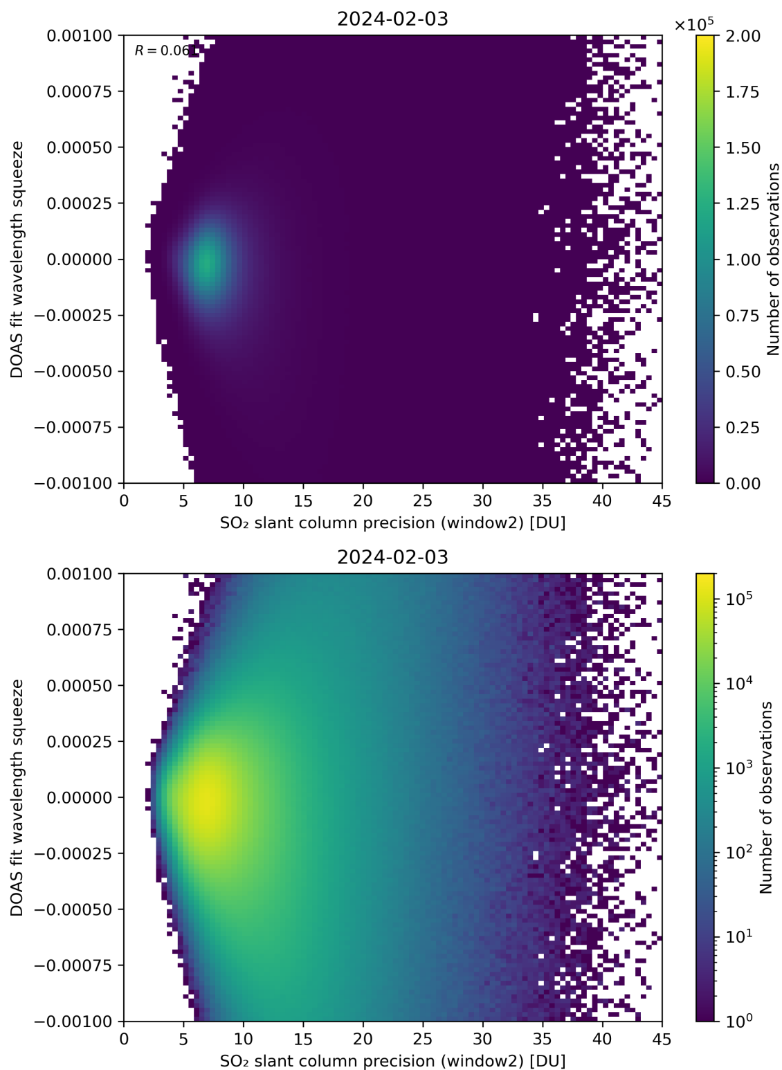
Figure 244: Scatter density plot of “SO 2 slant column precision (window2)” against “DOAS fit wavelength squeeze” for 2024-02-02 to 2024-02-04.
