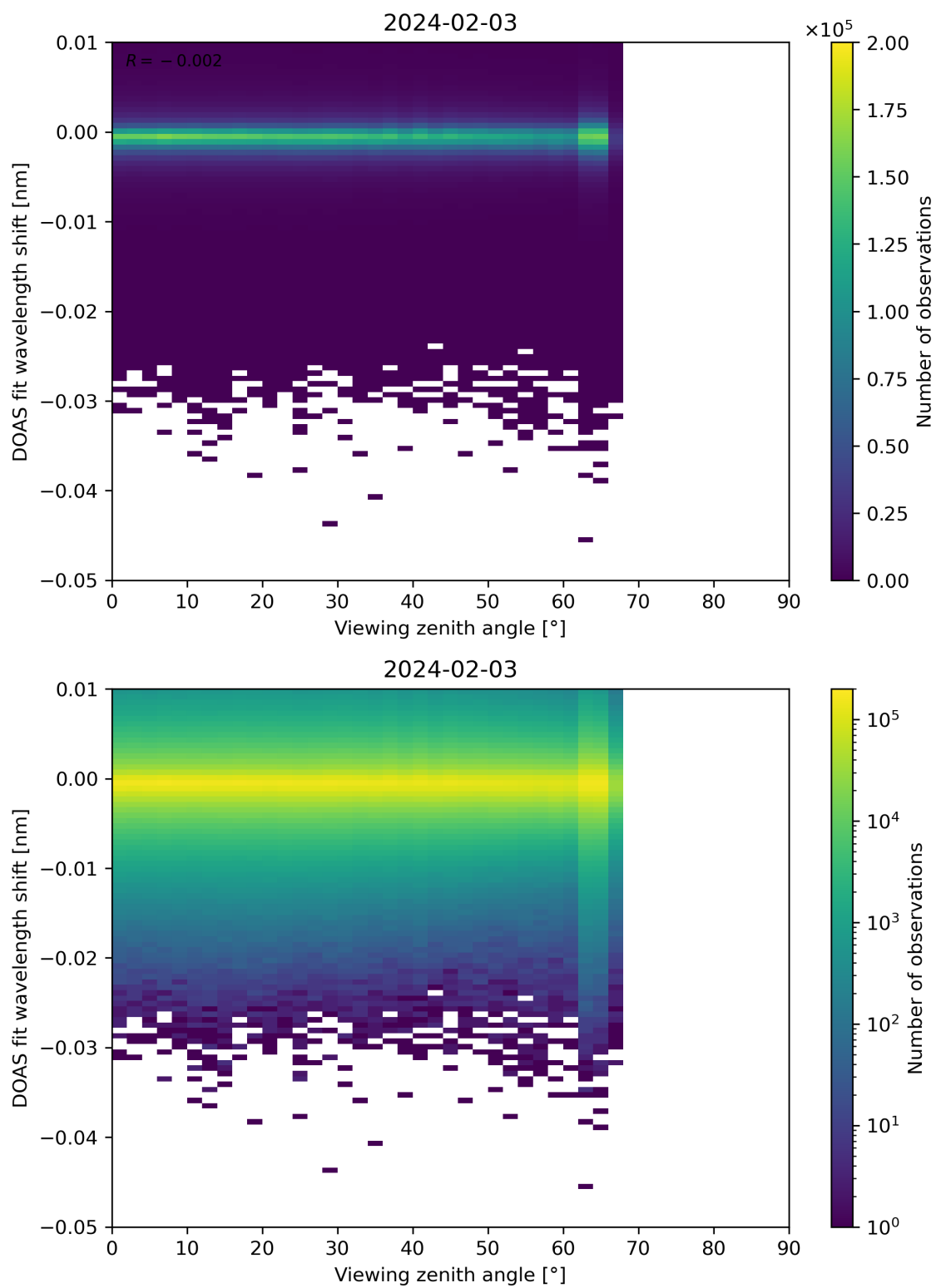
Figure 311: Scatter density plot of “Viewing zenith angle” against “DOAS fit wavelength shift” for 2024-02-02 to 2024-02-04.
