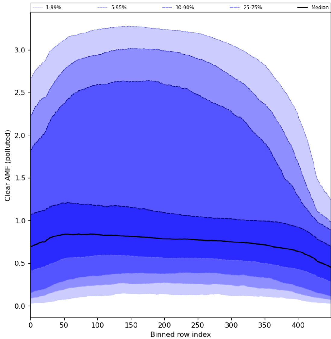
Figure 96: Along track statistics of “Clear AMF (polluted)” for 2024-02-02 to 2024-02-04
