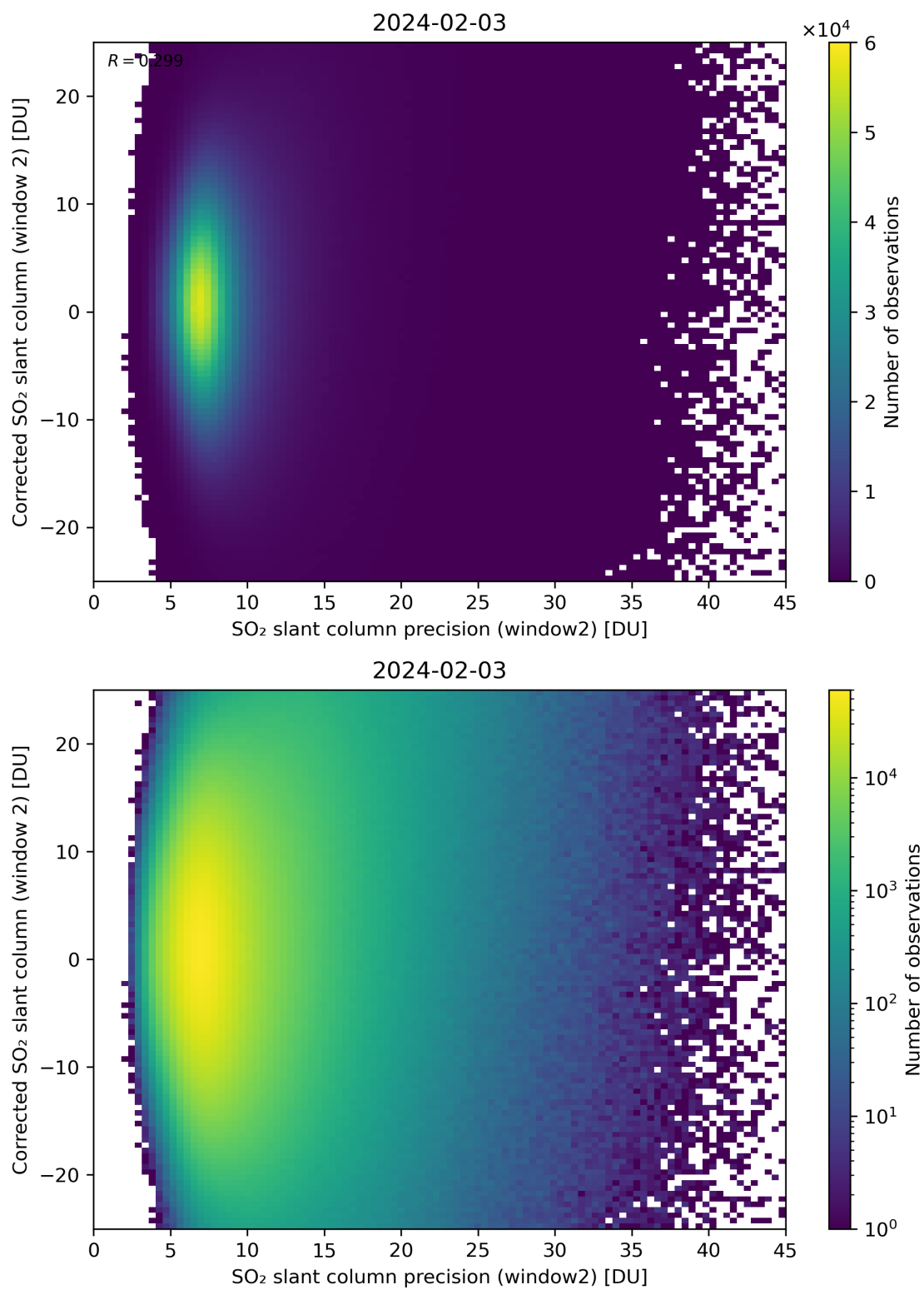
Figure 247: Scatter density plot of “SO 2 slant column precision (window2)” against “Corrected SO 2 slant column (window 2)” for 2024-02-02 to 2024-02-04.
