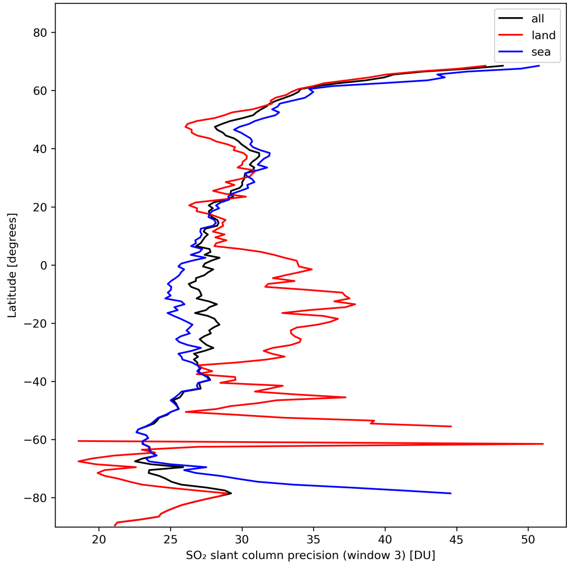
Figure 42: Zonal average of “SO 2 slant column precision (window 3)” for 2024-02-02 to 2024-02-04.
