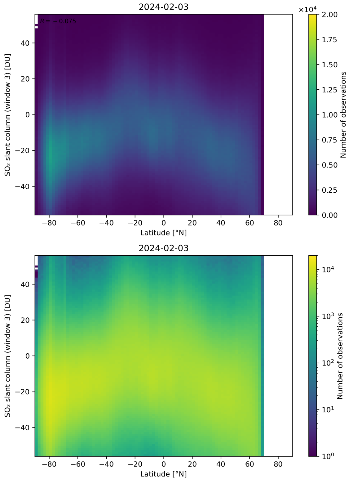
Figure 152: Scatter density plot of “Latitude” against “SO 2 slant column (window 3)” for 2024-02-02 to 2024-02-04.
