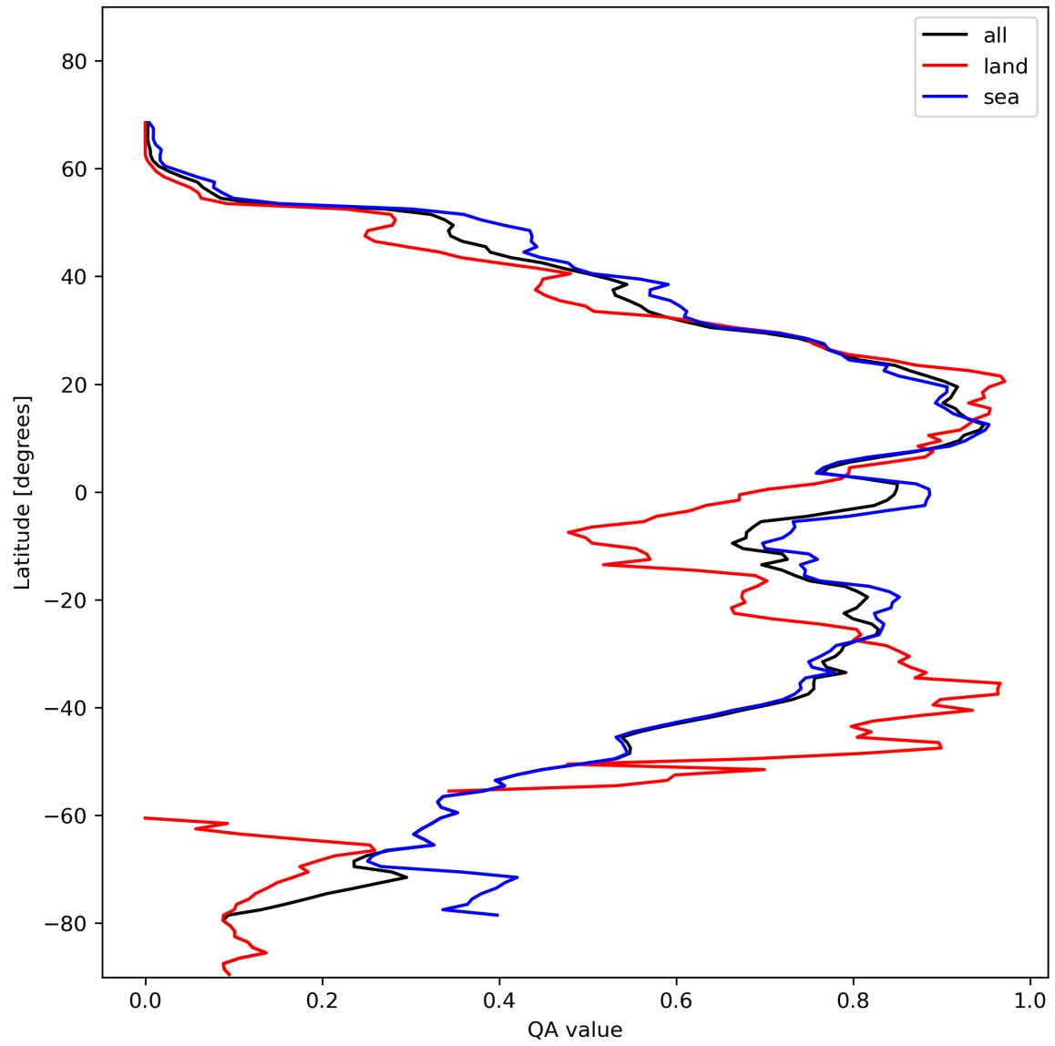
Figure 29: Zonal average of “QA value” for 2024-02-02 to 2024-02-04.
