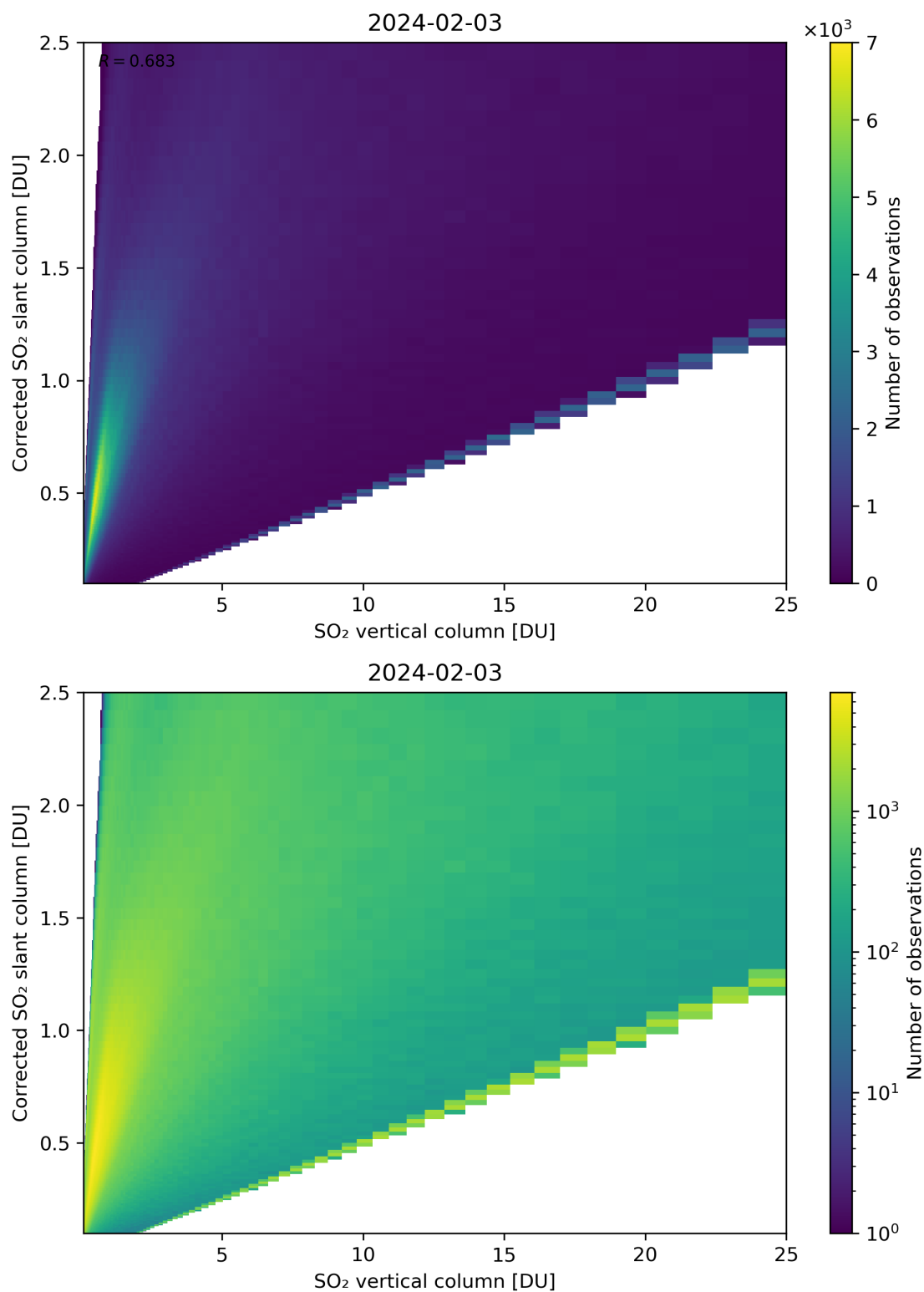
Figure 297: Scatter density plot of “SO 2 vertical column” against “Corrected SO 2 slant column” for 2024-02-02 to 2024-02-04.
