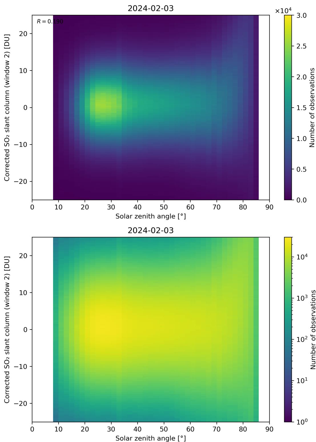
Figure 167: Scatter density plot of “Solar zenith angle” against “Corrected SO 2 slant column (window 2)” for 2024-02-02 to 2024-02-04.
