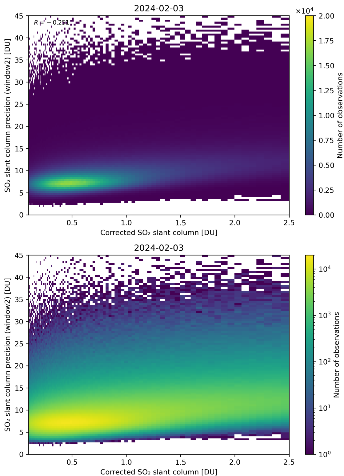
Figure 189: Scatter density plot of “Corrected SO 2 slant column” against “SO 2 slant column precision (window2)” for 2024-02-02 to 2024-02-04.
