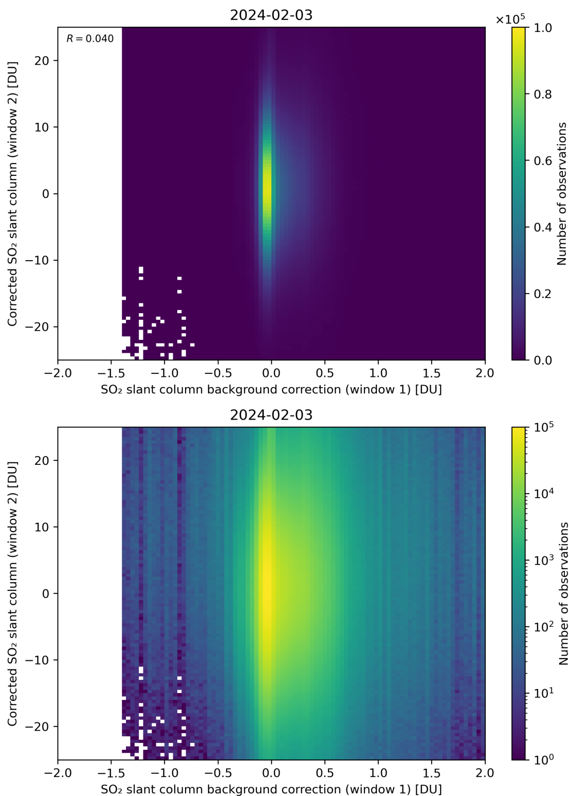
Figure 104: Scatter density plot of “SO 2 slant column background correction (window 1)” against “Corrected SO 2 slant column (window 2)” for 2024-02-02 to 2024-02-04.
