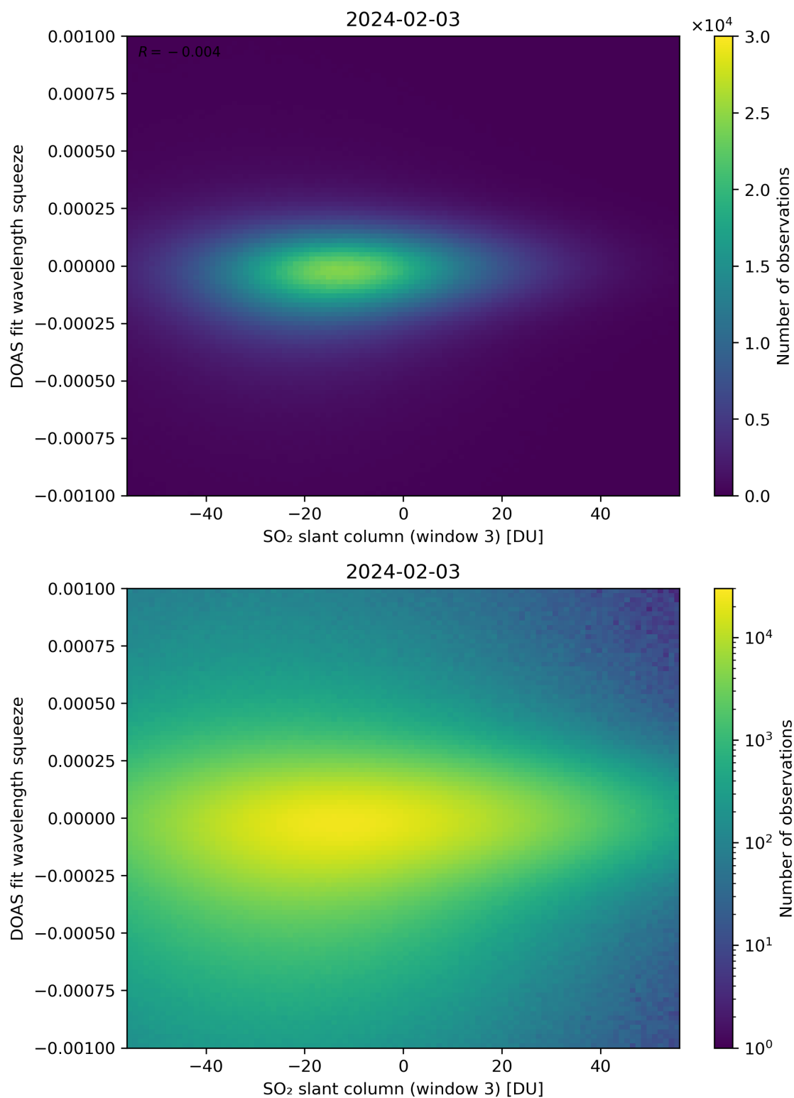
Figure 255: Scatter density plot of “SO 2 slant column (window 3)” against “DOAS fit wavelength squeeze” for 2024-02-02 to 2024-02-04.
