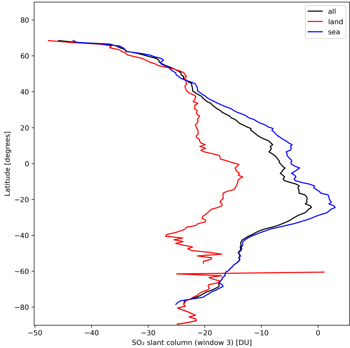
Figure 41: Zonal average of “SO 2 slant column (window 3)” for 2024-02-02 to 2024-02-04.
