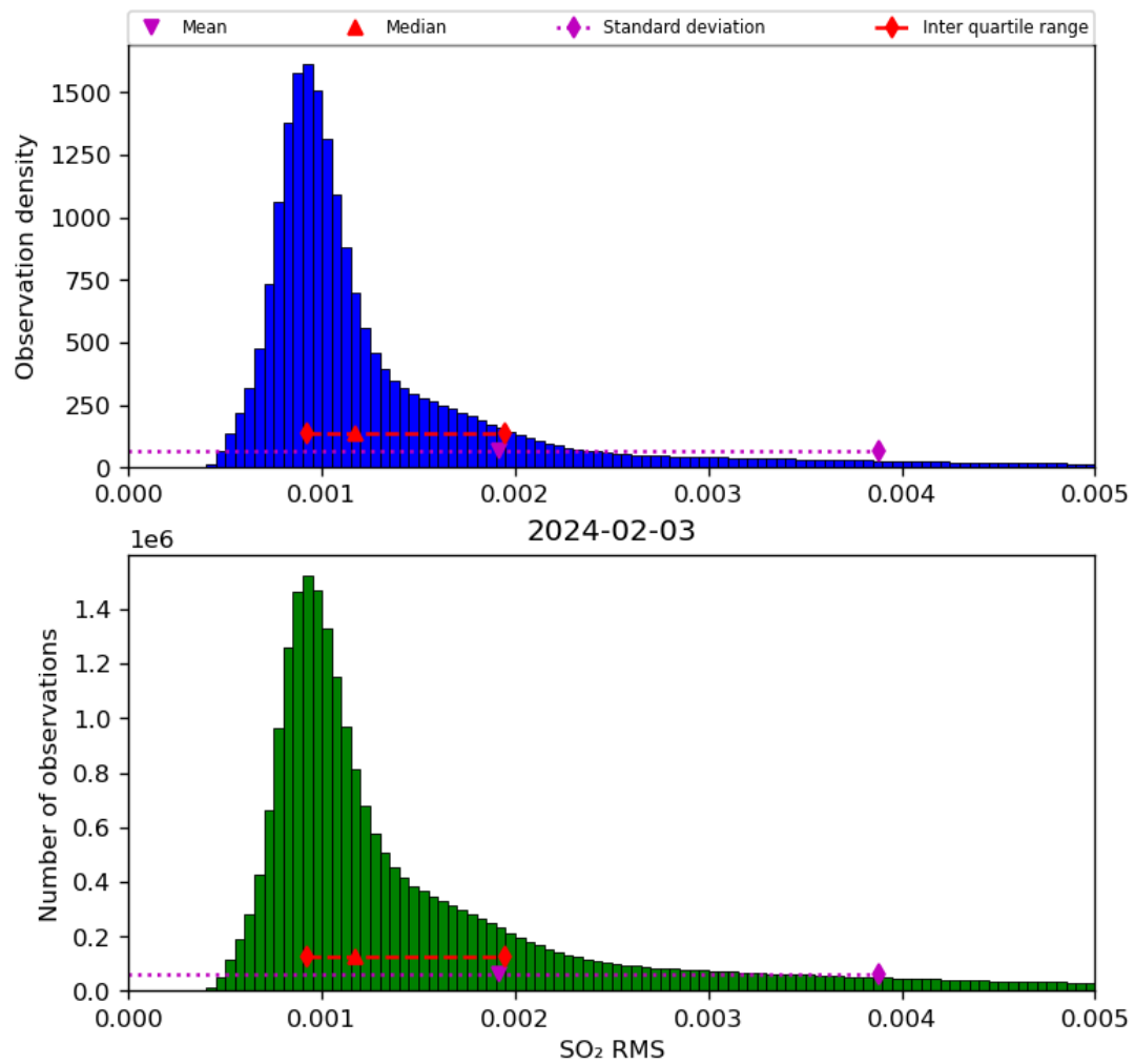
Figure 70: Histogram of “SO 2 RMS” for 2024-02-02 to 2024-02-04
