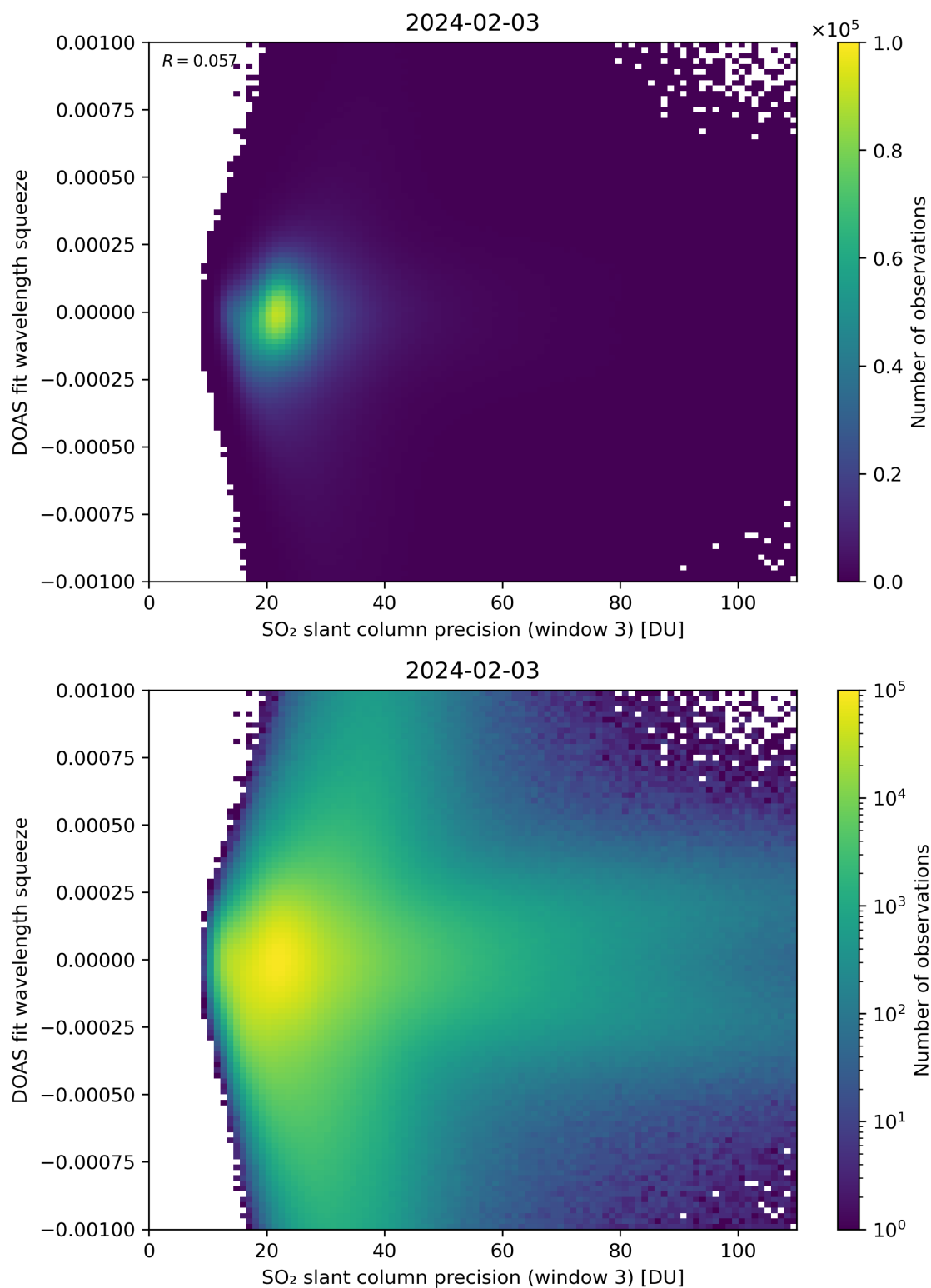
Figure 259: Scatter density plot of “SO 2 slant column precision (window 3)” against “DOAS fit wavelength squeeze” for 2024-02-02 to 2024-02-04.
