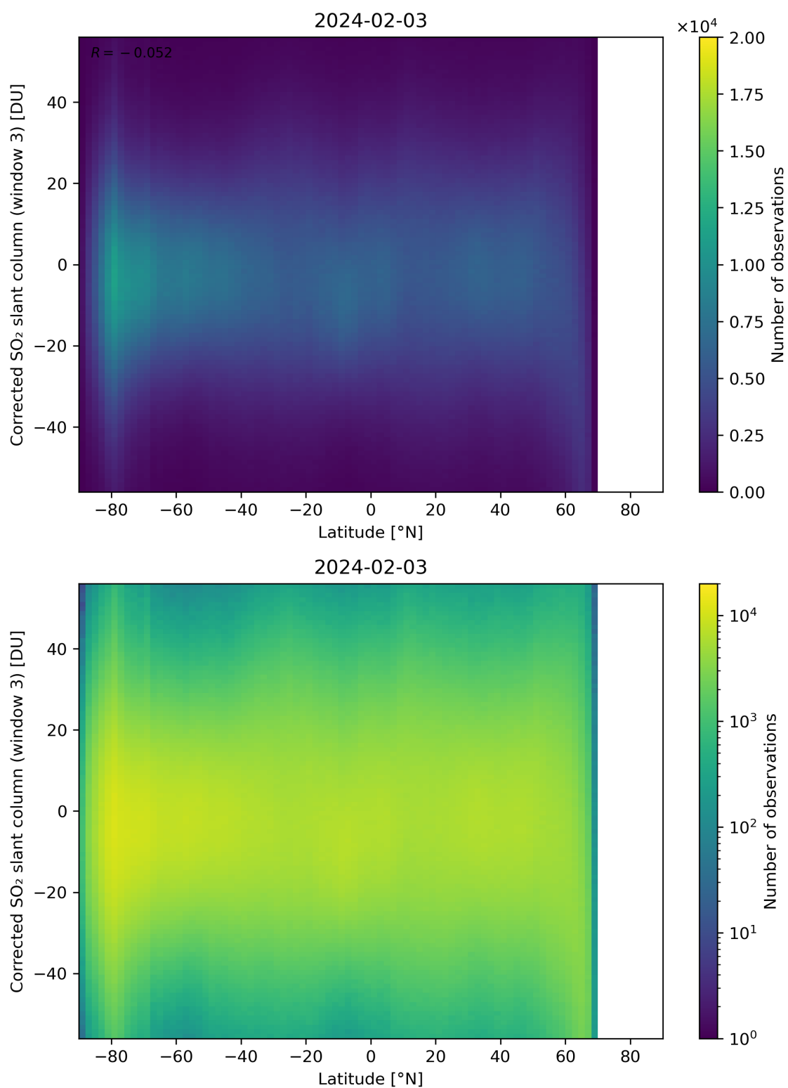
Figure 148: Scatter density plot of “Latitude” against “Corrected SO 2 slant column (window 3)” for 2024-02-02 to 2024-02-04.
