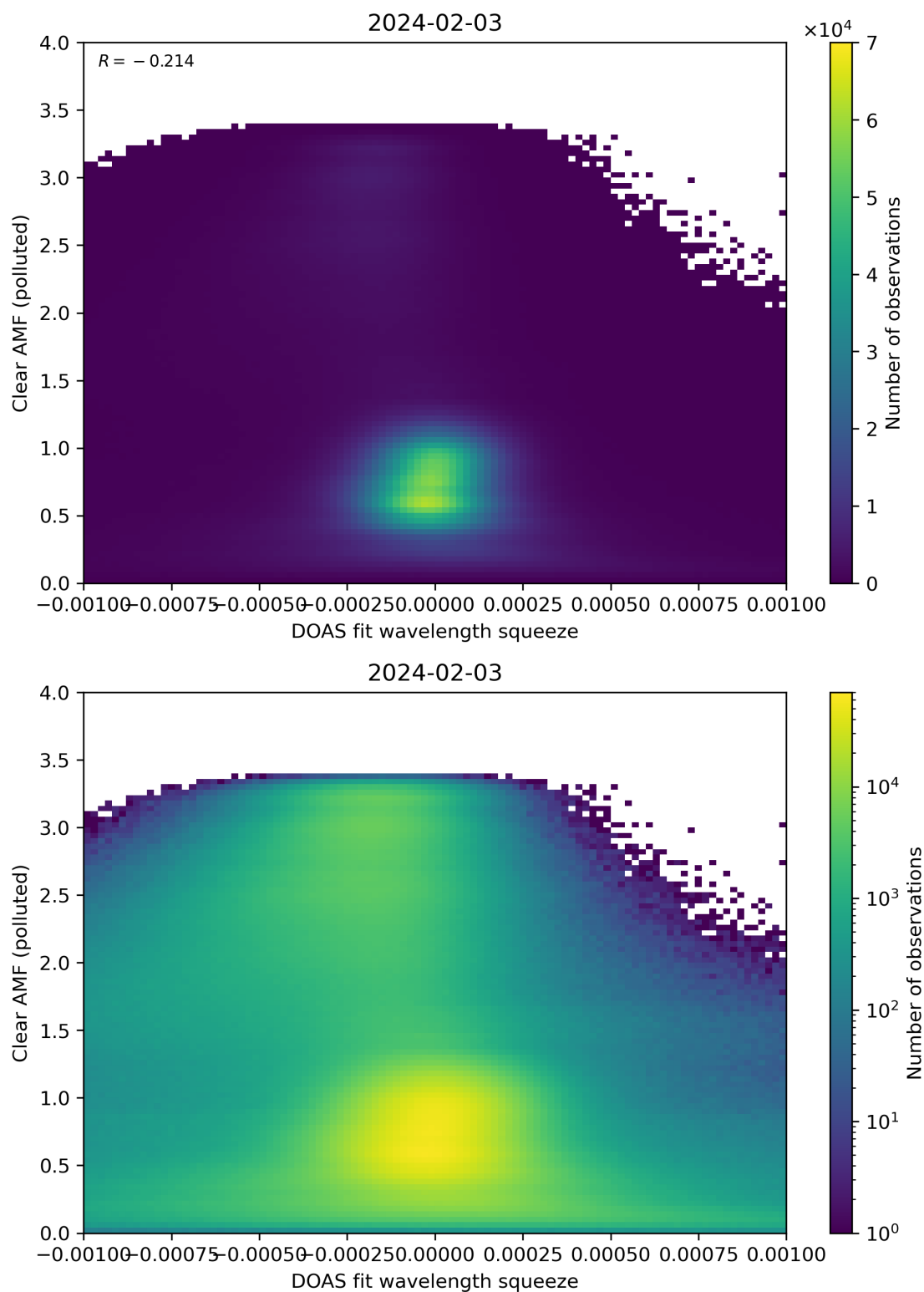
Figure 133: Scatter density plot of “DOAS fit wavelength squeeze” against “Clear AMF (polluted)” for 2024-02-02 to 2024-02-04.
