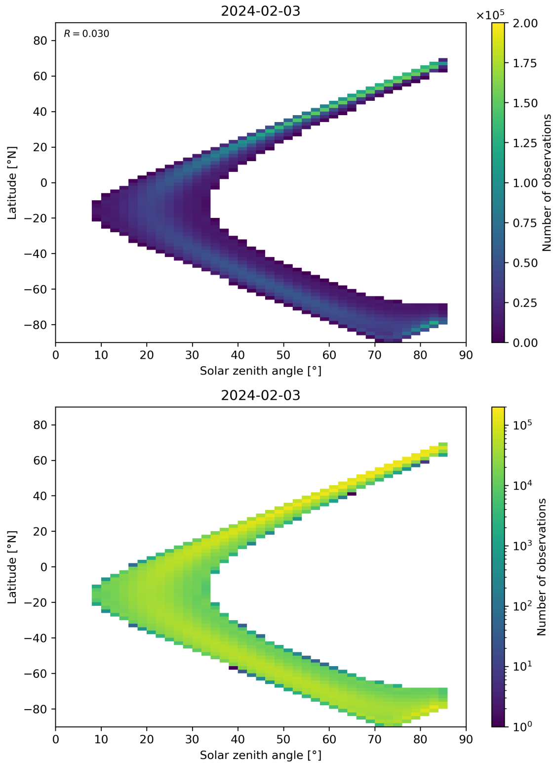
Figure 164: Scatter density plot of “Solar zenith angle” against “Latitude” for 2024-02-02 to 2024-02-04.
