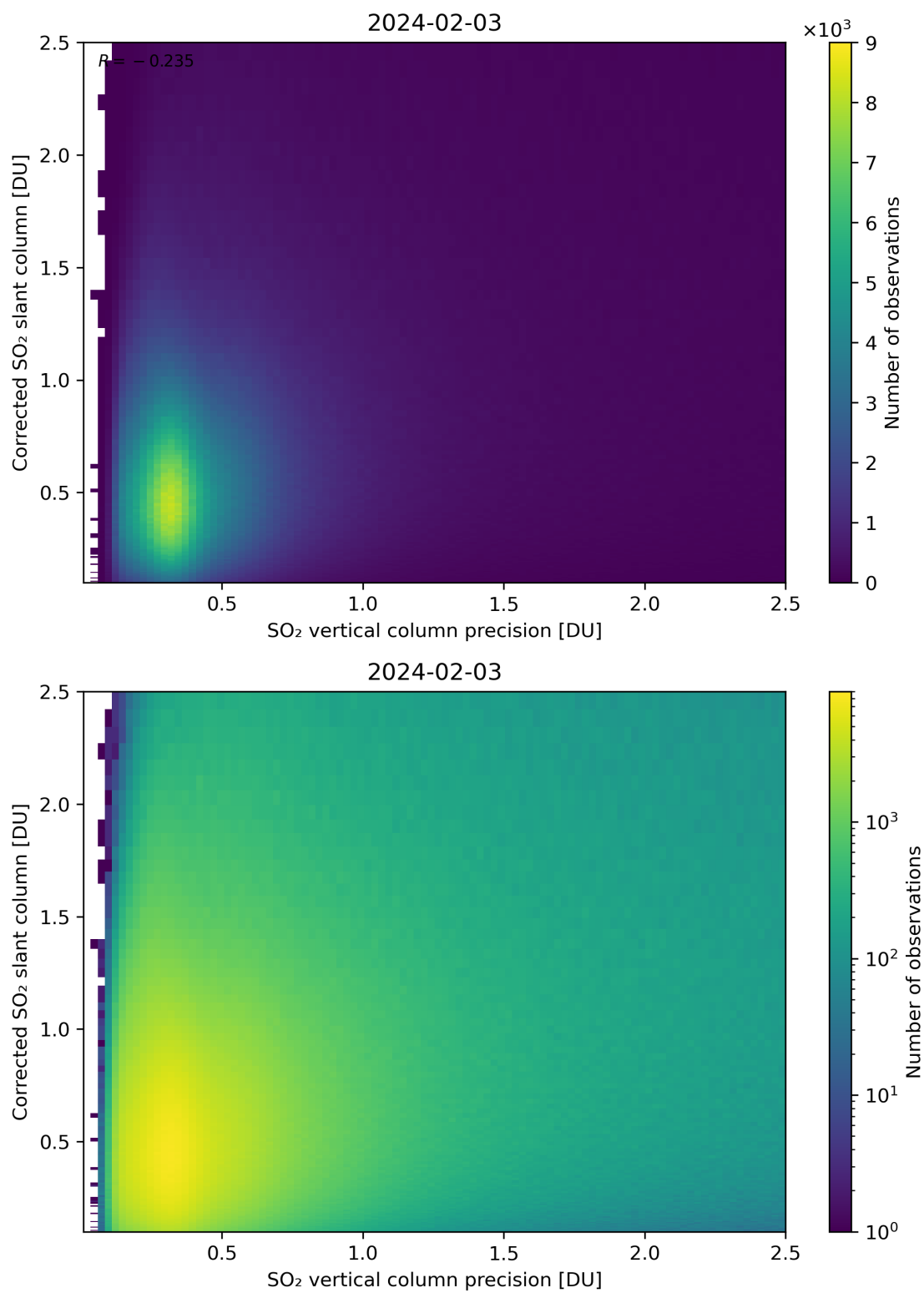
Figure 286: Scatter density plot of “SO 2 vertical column precision” against “Corrected SO 2 slant column” for 2024-02-02 to 2024-02-04.
