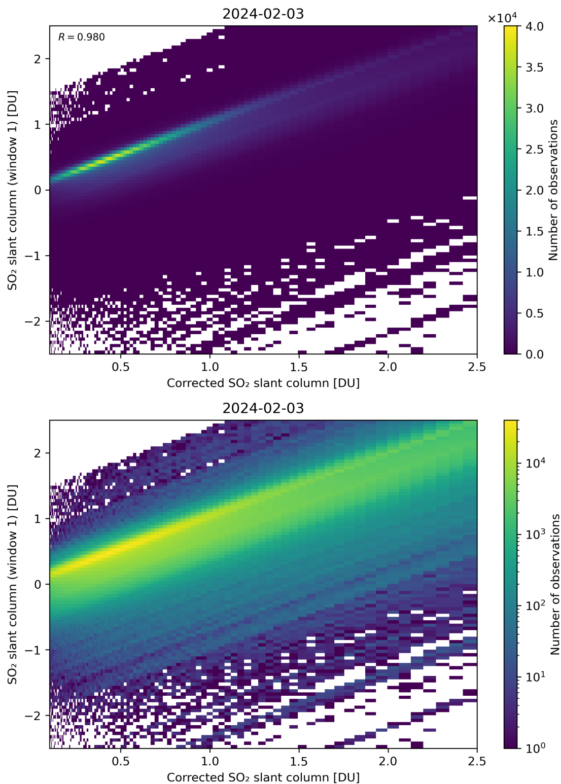
Figure 187: Scatter density plot of “Corrected SO 2 slant column” against “SO 2 slant column (window 1)” for 2024-02-02 to 2024-02-04.
