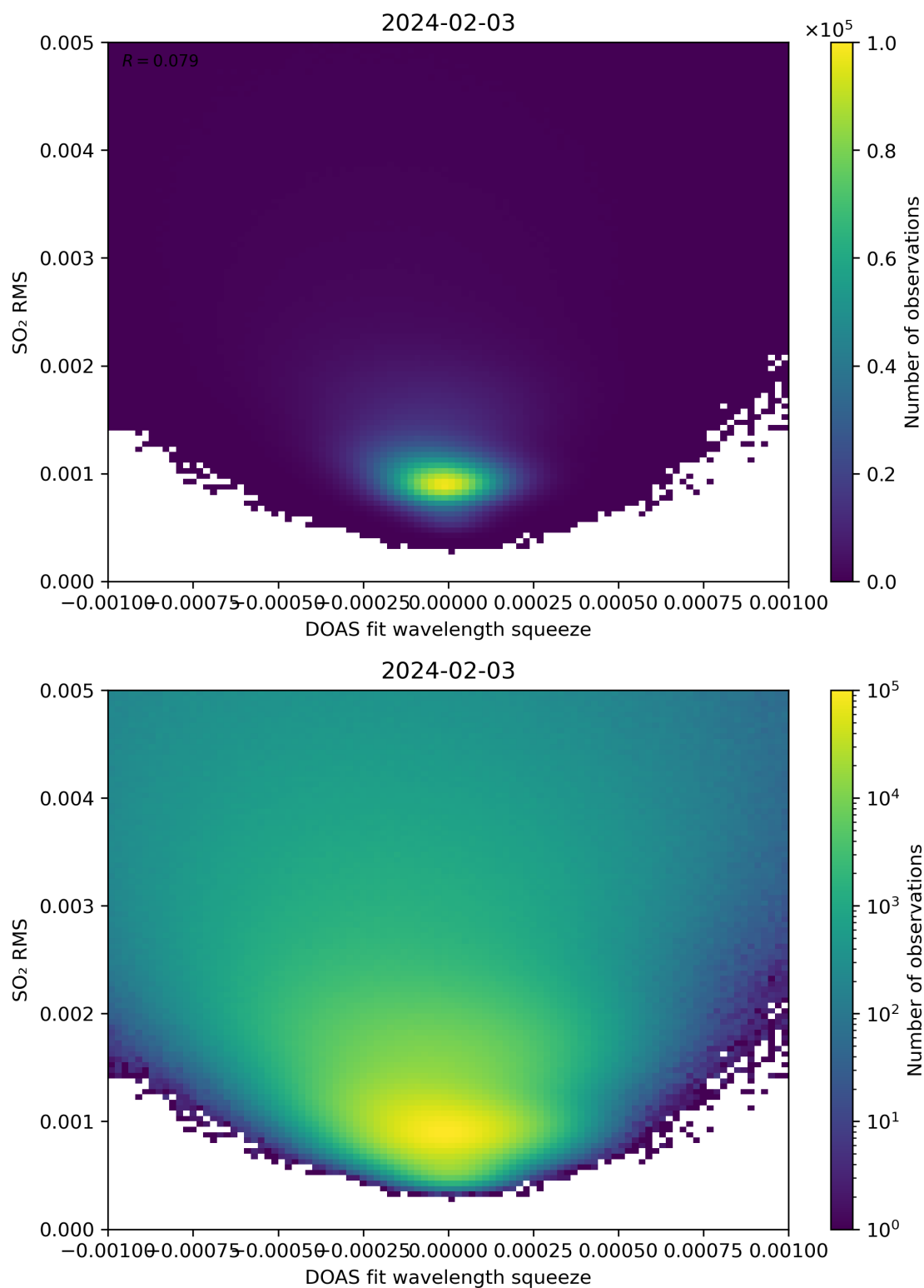
Figure 132: Scatter density plot of “DOAS fit wavelength squeeze” against “SO 2 RMS” for 2024-02-02 to 2024-02-04.
