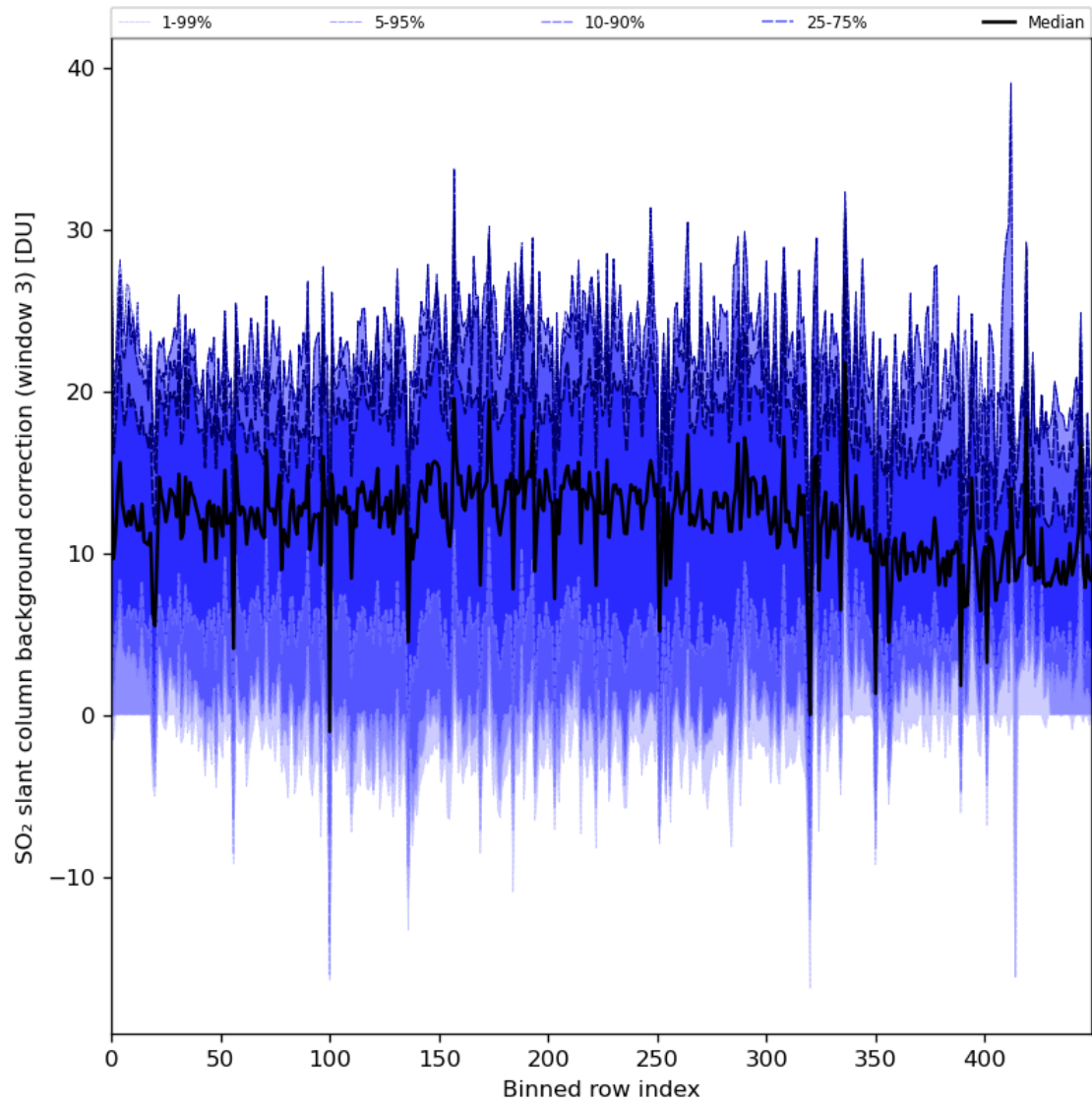
Figure 90: Along track statistics of “SO 2 slant column background correction (window 3)” for 2024-02-02 to 2024-02-04
