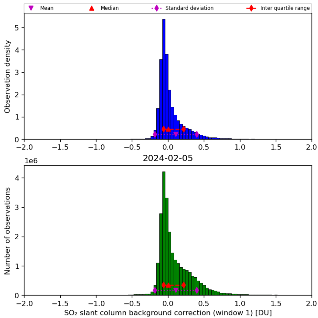
Figure 59: Histogram of “SO 2 slant column background correction (window 1)” for 2024-02-04 to 2024-02-06
