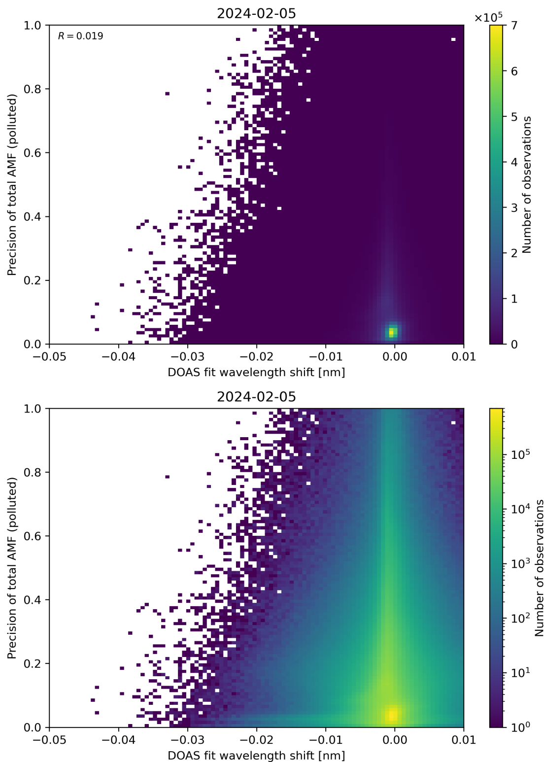
Figure 131: Scatter density plot of “DOAS fit wavelength shift” against “Precision of total AMF (polluted)” for 2024-02-04 to 2024-02-06.
