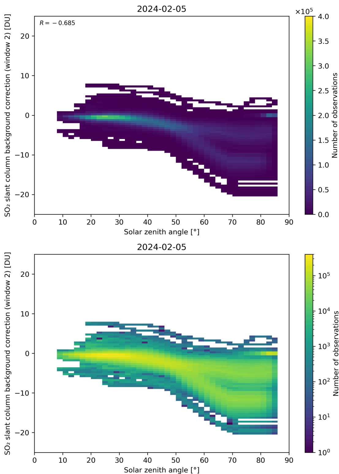
Figure 159: Scatter density plot of “Solar zenith angle” against “SO 2 slant column background correction (window 2)” for 2024-02-04 to 2024-02-06.
