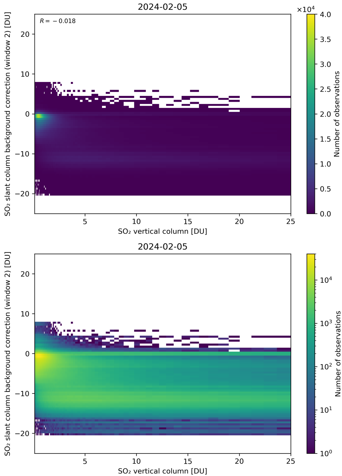
Figure 274: Scatter density plot of “SO 2 vertical column” against “SO 2 slant column background correction (window 2)” for 2024-02-04 to 2024-02-06.
