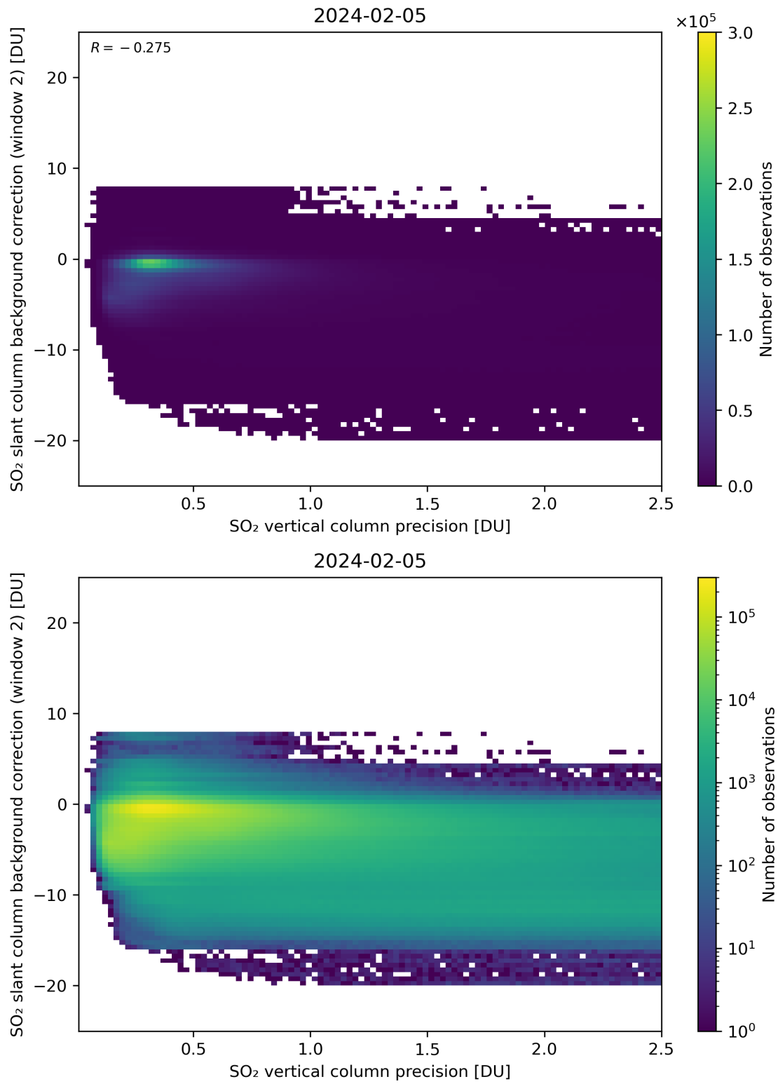
Figure 280: Scatter density plot of “SO 2 vertical column precision” against “SO 2 slant column background correction (window 2)” for 2024-02-04 to 2024-02-06.
