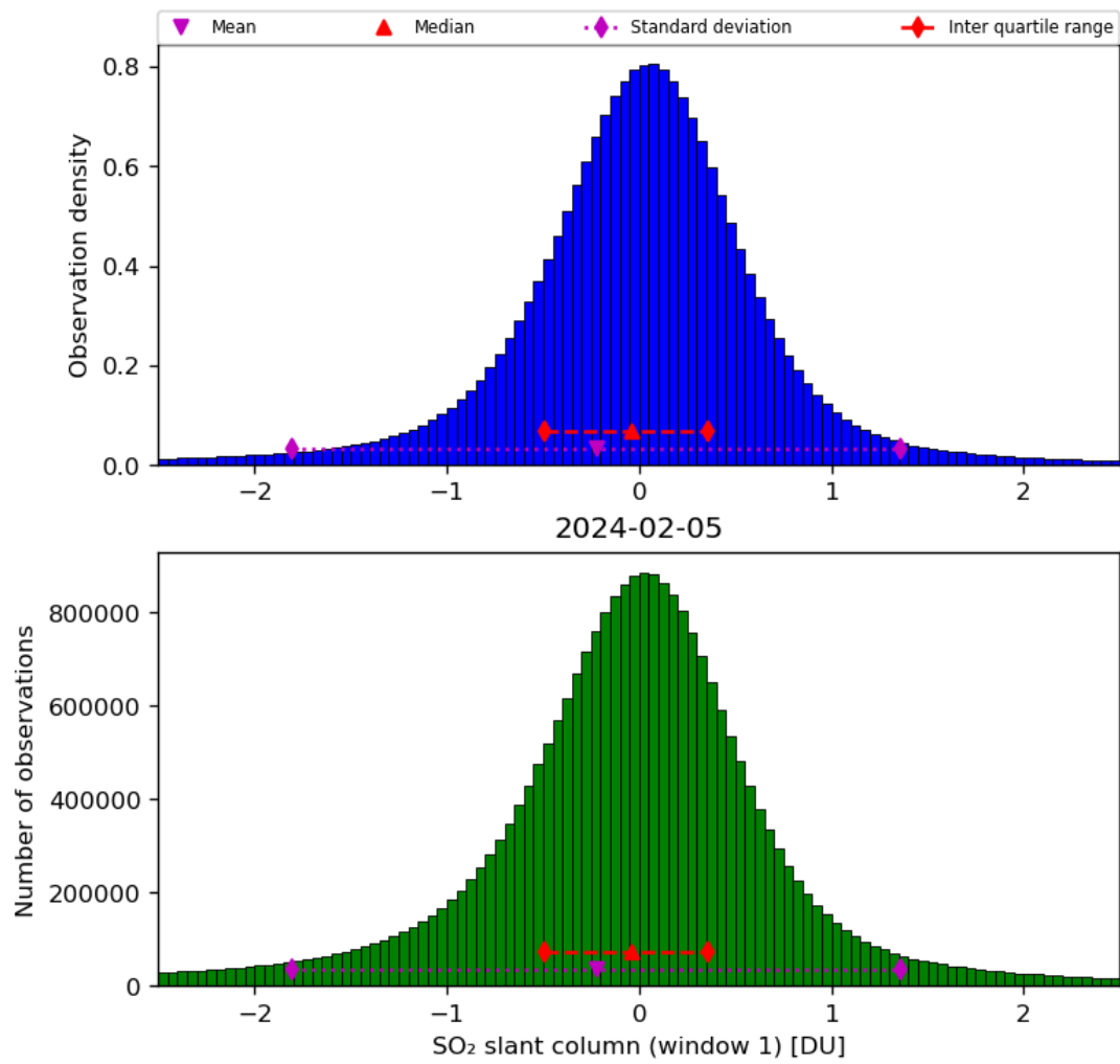
Figure 56: Histogram of “SO 2 slant column (window 1)” for 2024-02-04 to 2024-02-06
