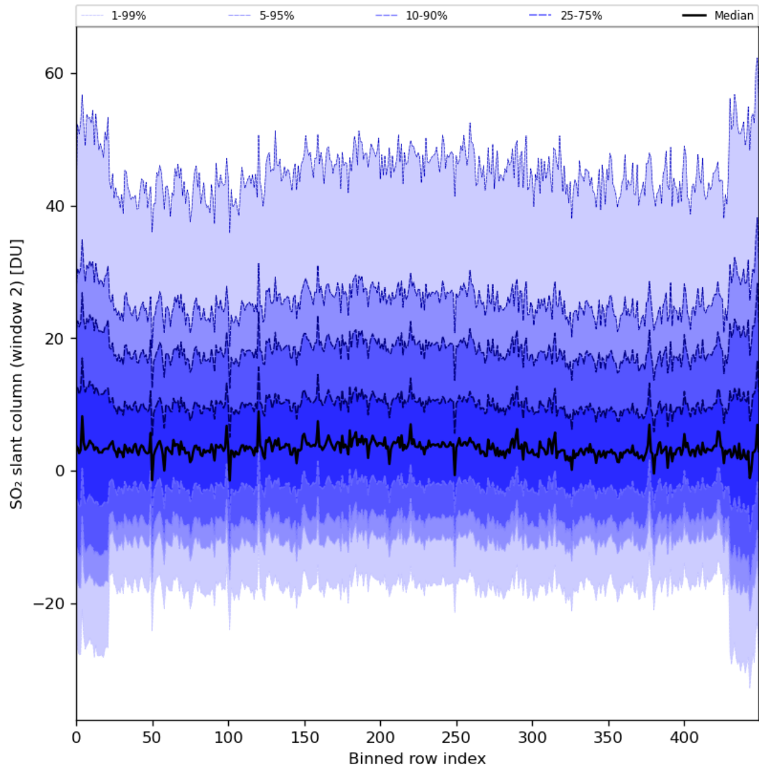
Figure 83: Along track statistics of “SO 2 slant column (window 2)” for 2024-02-04 to 2024-02-06
