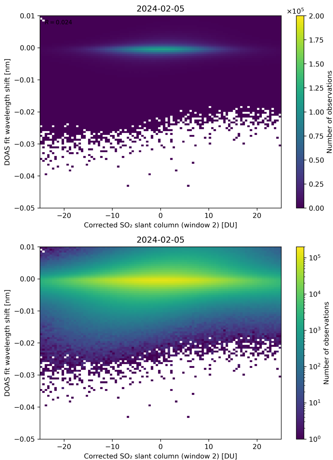
Figure 196: Scatter density plot of “Corrected SO 2 slant column (window 2)” against “DOAS fit wavelength shift” for 2024-02-04 to 2024-02-06.
