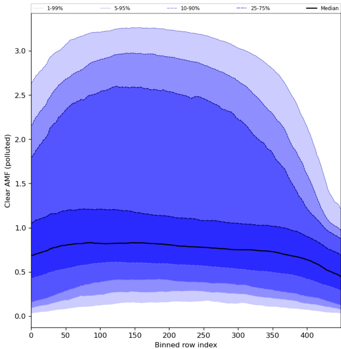
Figure 96: Along track statistics of “Clear AMF (polluted)” for 2024-02-04 to 2024-02-06
