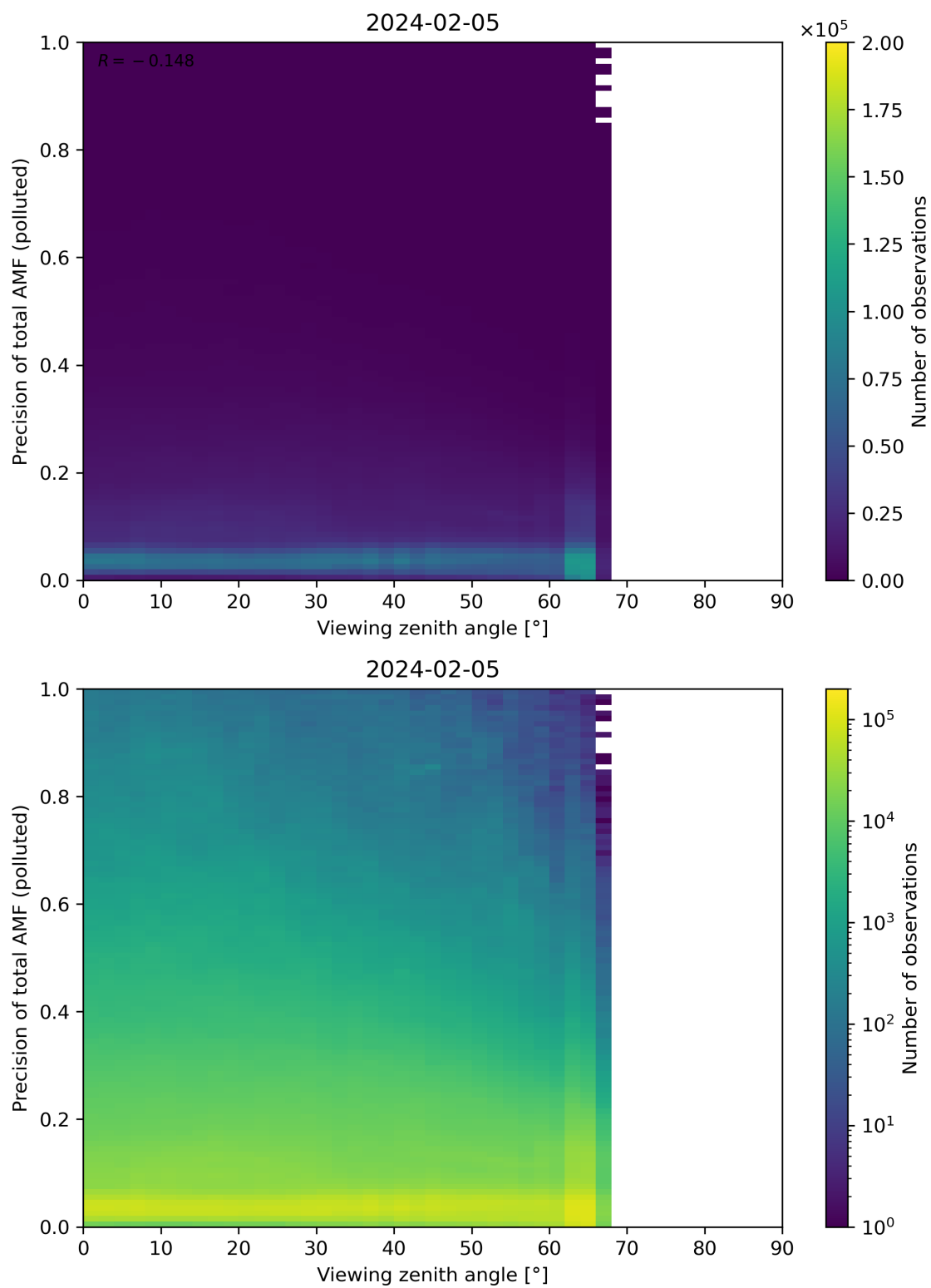
Figure 326: Scatter density plot of “Viewing zenith angle” against “Precision of total AMF (polluted)” for 2024-02-04 to 2024-02-06.
