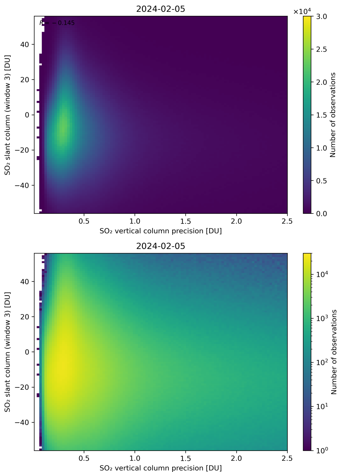
Figure 292: Scatter density plot of “SO 2 vertical column precision” against “SO 2 slant column (window 3)” for 2024-02-04 to 2024-02-06.
