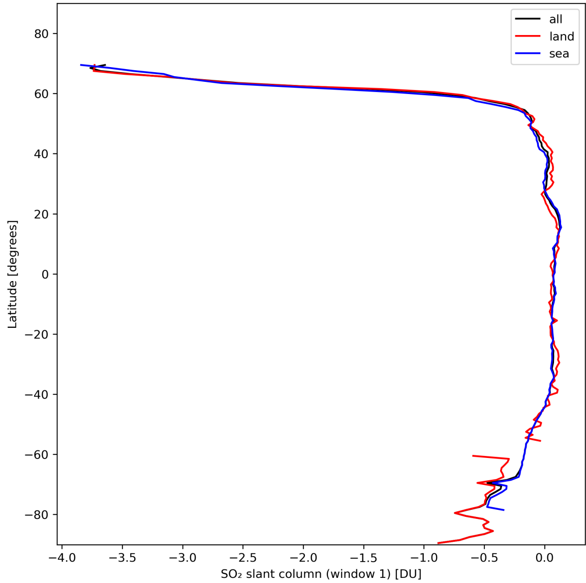
Figure 33: Zonal average of “SO 2 slant column (window 1)” for 2024-02-04 to 2024-02-06.
