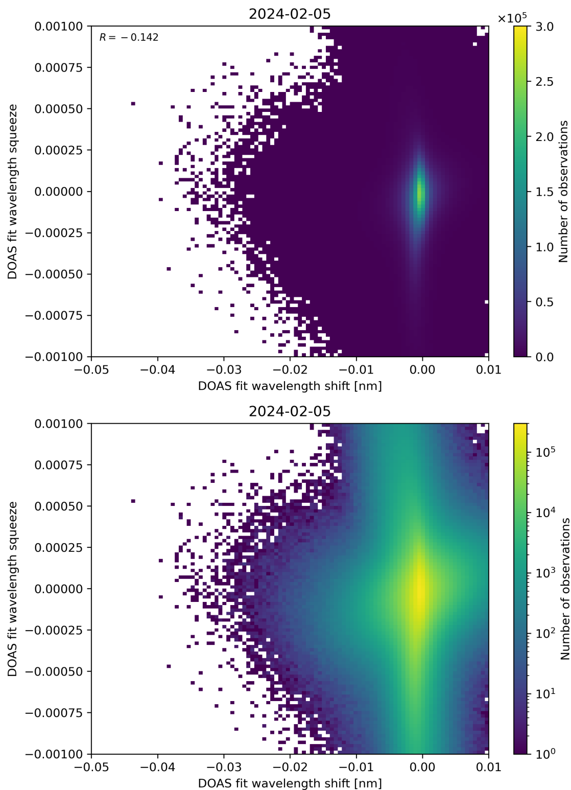
Figure 127: Scatter density plot of “DOAS fit wavelength shift” against “DOAS fit wavelength squeeze” for 2024-02-04 to 2024-02-06.
