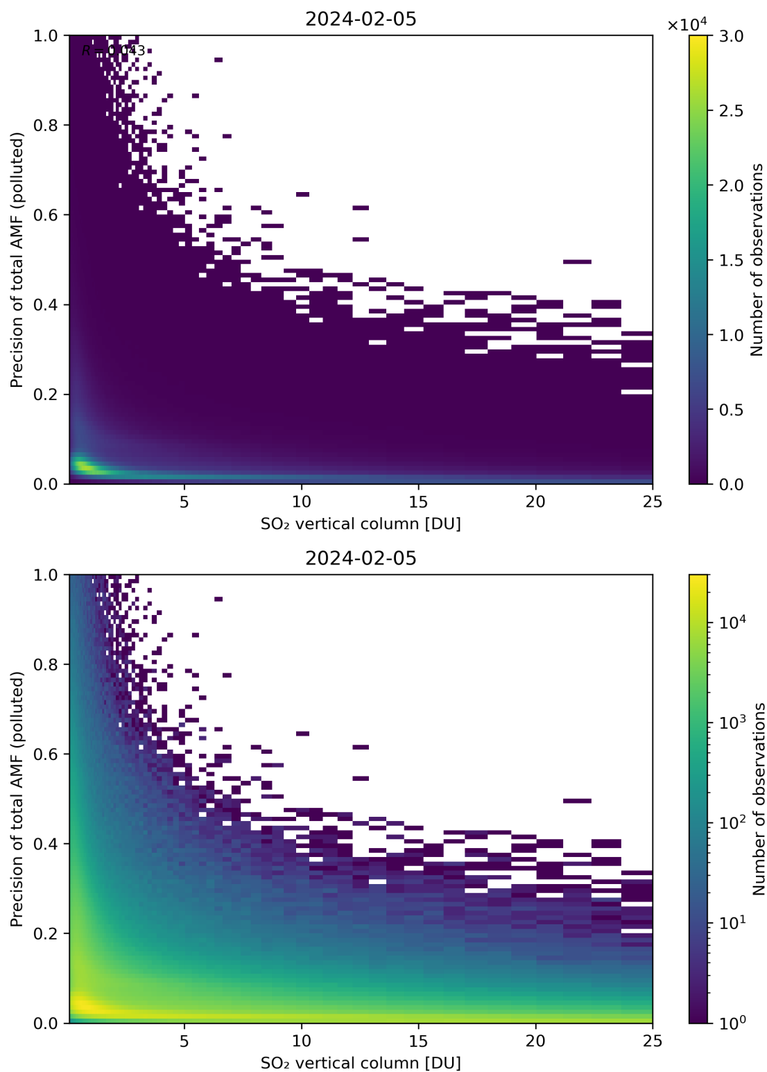
Figure 306: Scatter density plot of “SO 2 vertical column” against “Precision of total AMF (polluted)” for 2024-02-04 to 2024-02-06.
