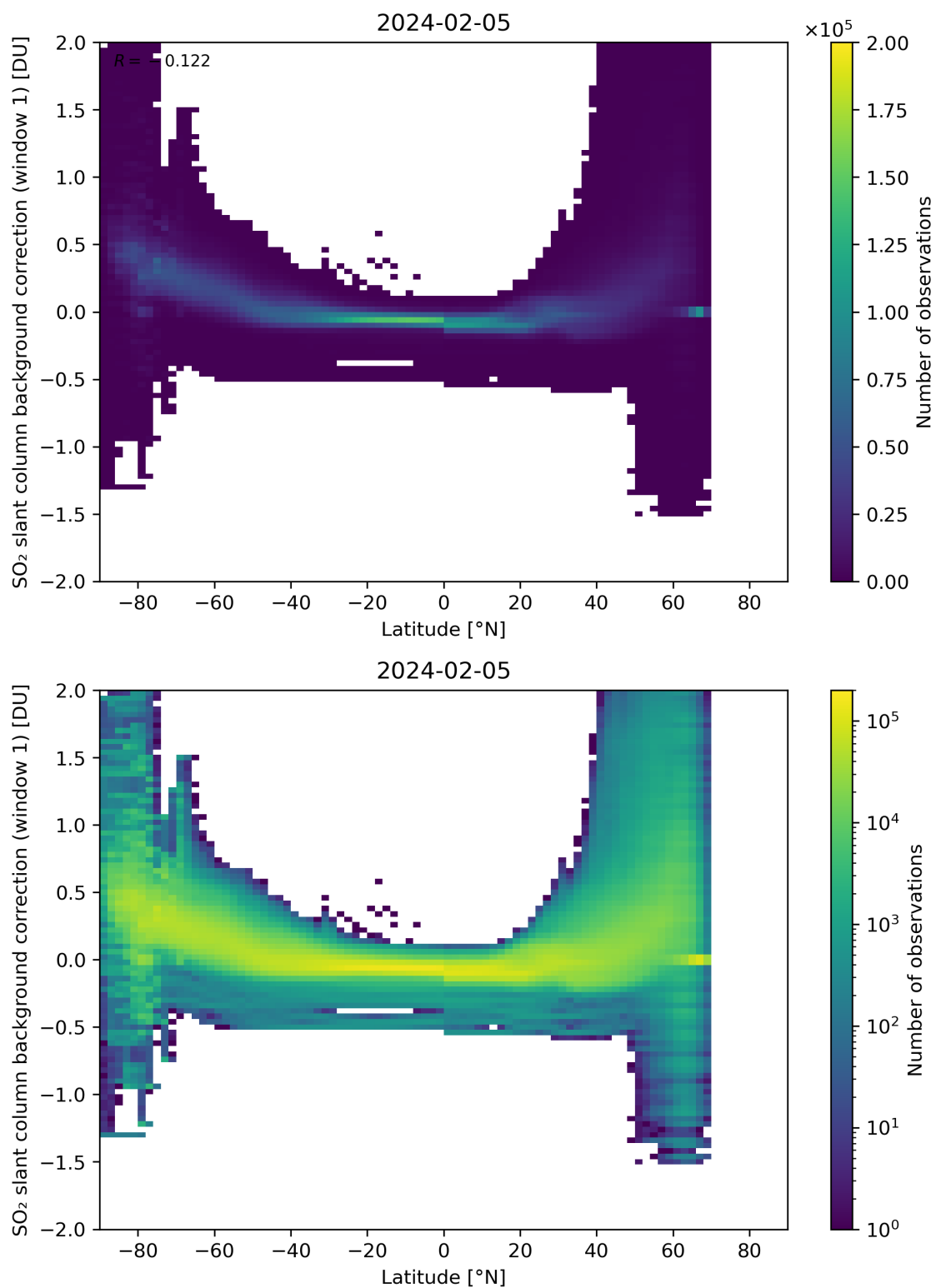
Figure 139: Scatter density plot of “Latitude” against “SO 2 slant column background correction (window 1)” for 2024-02-04 to 2024-02-06.
