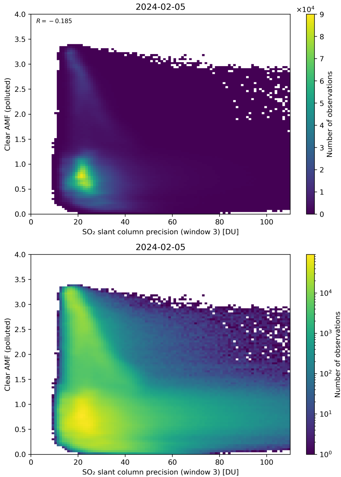
Figure 261: Scatter density plot of “SO 2 slant column precision (window 3)” against “Clear AMF (polluted)” for 2024-02-04 to 2024-02-06.
