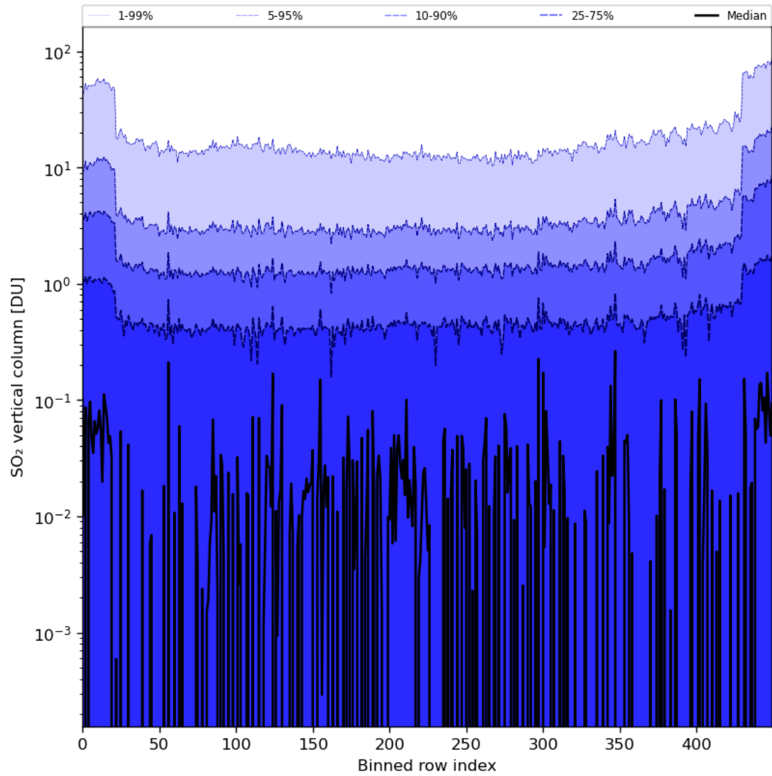
Figure 76: Along track statistics of “SO 2 vertical column” for 2024-02-04 to 2024-02-06
