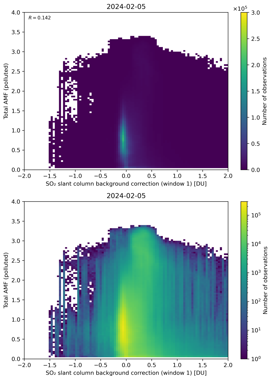
Figure 109: Scatter density plot of “SO 2 slant column background correction (window 1)” against “Total AMF (polluted)” for 2024-02-04 to 2024-02-06.
