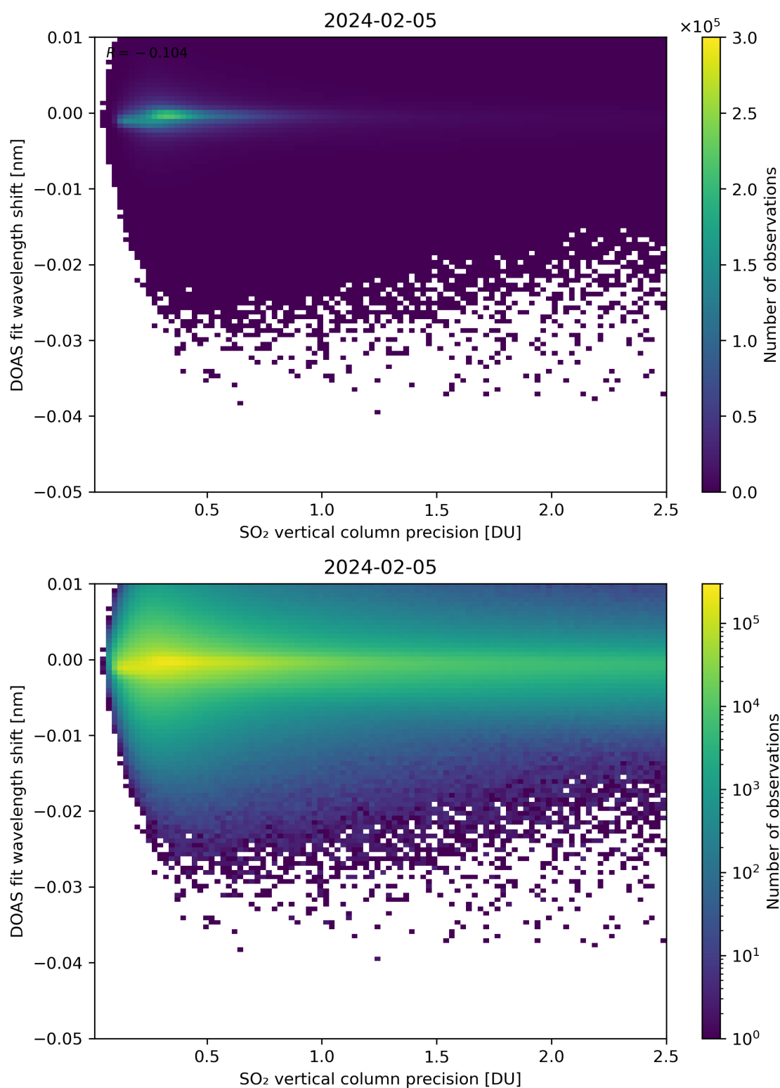
Figure 282: Scatter density plot of “SO 2 vertical column precision” against “DOAS fit wavelength shift” for 2024-02-04 to 2024-02-06.
