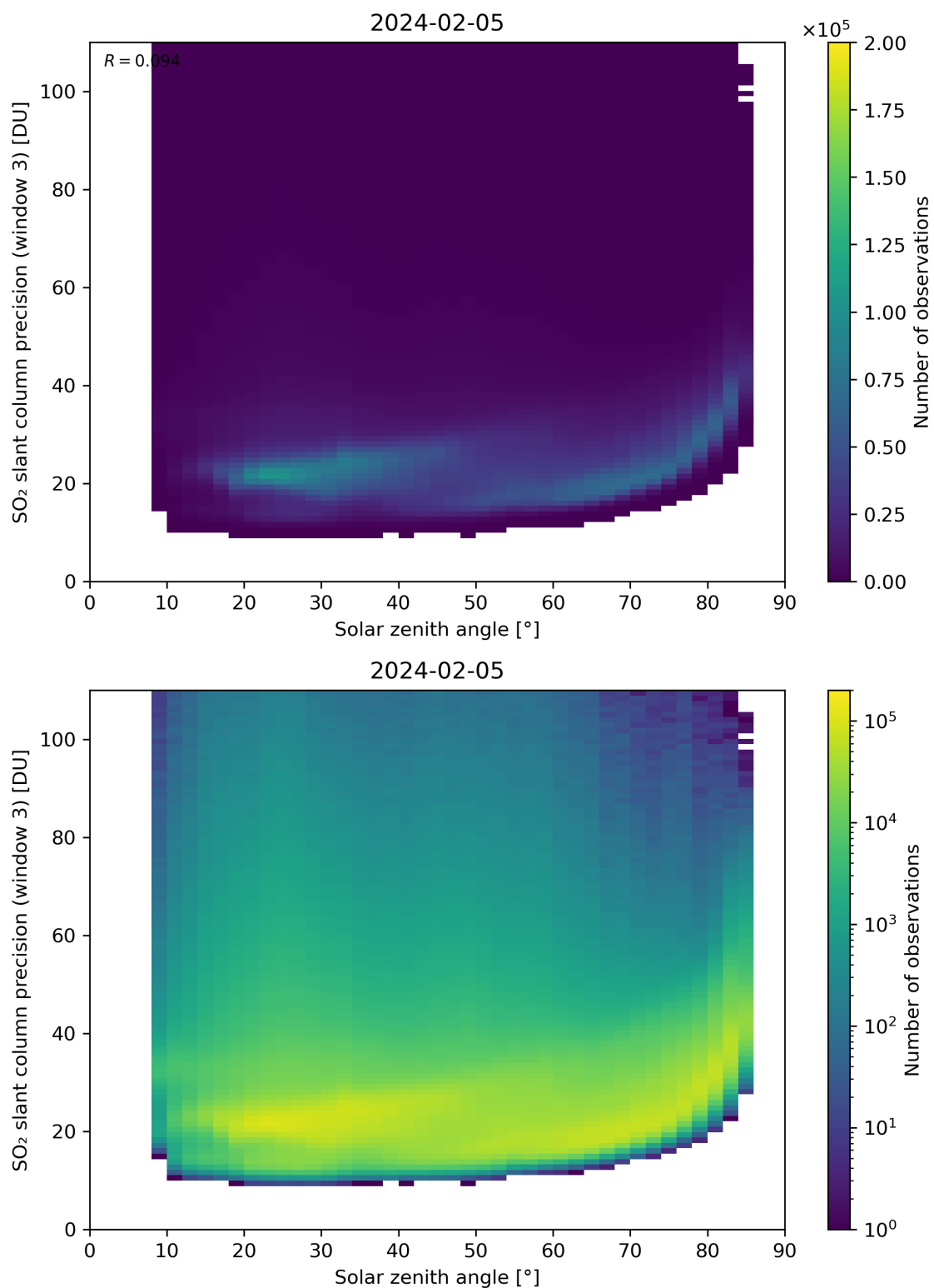
Figure 173: Scatter density plot of “Solar zenith angle” against “SO 2 slant column precision (window 3)” for 2024-02-04 to 2024-02-06.
