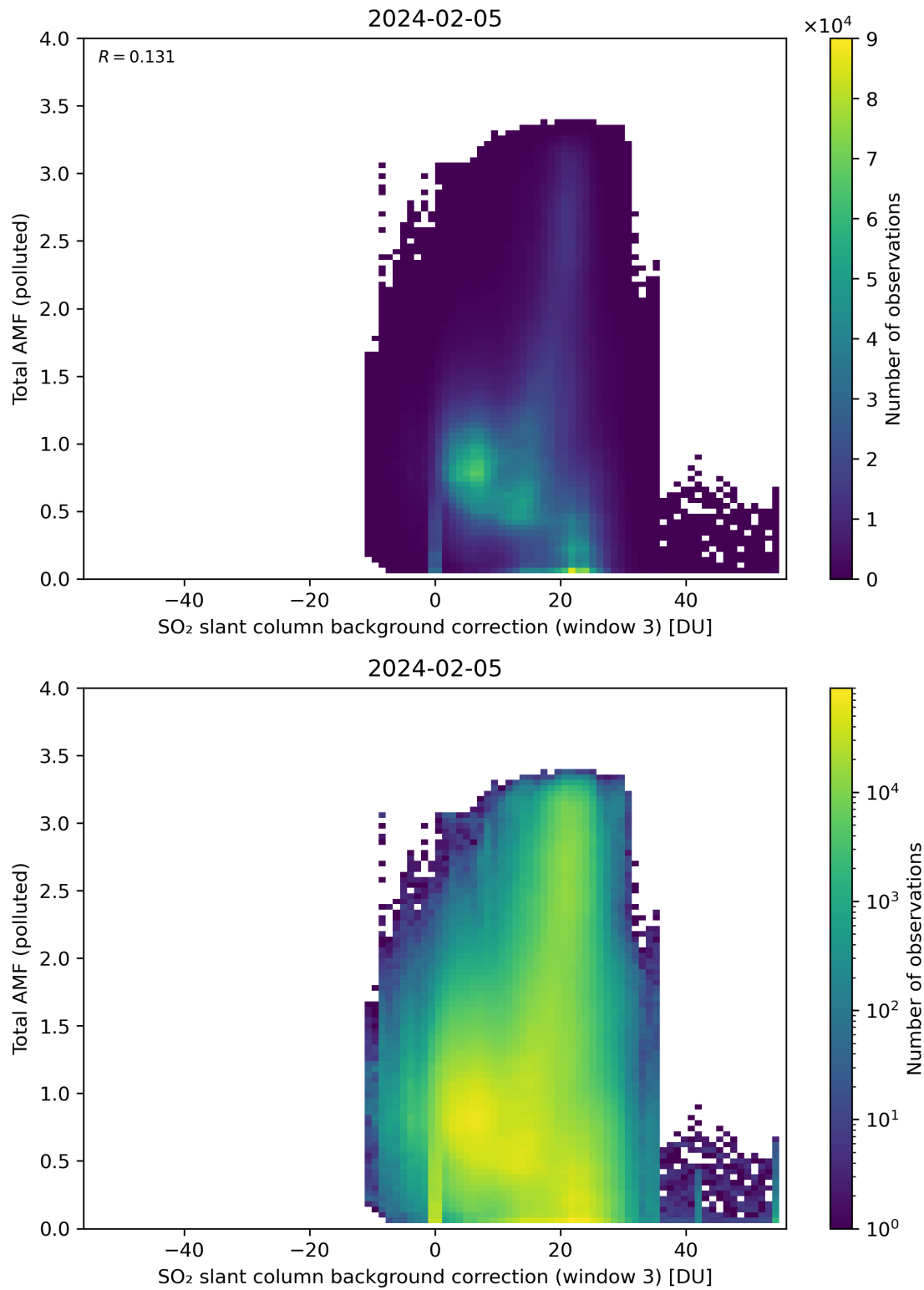
Figure 125: Scatter density plot of “SO 2 slant column background correction (window 3)” against “Total AMF (polluted)” for 2024-02-04 to 2024-02-06.
