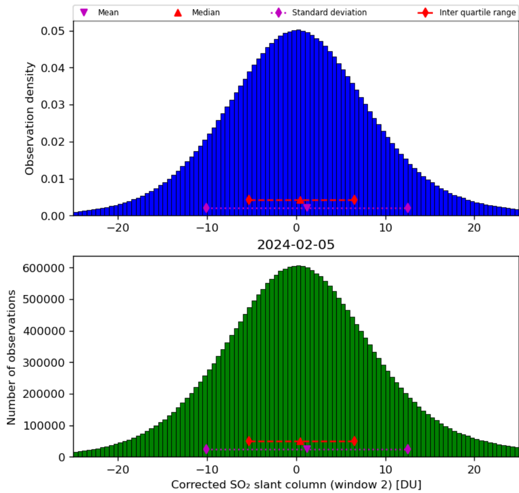
Figure 62: Histogram of “Corrected SO 2 slant column (window 2)” for 2024-02-04 to 2024-02-06
