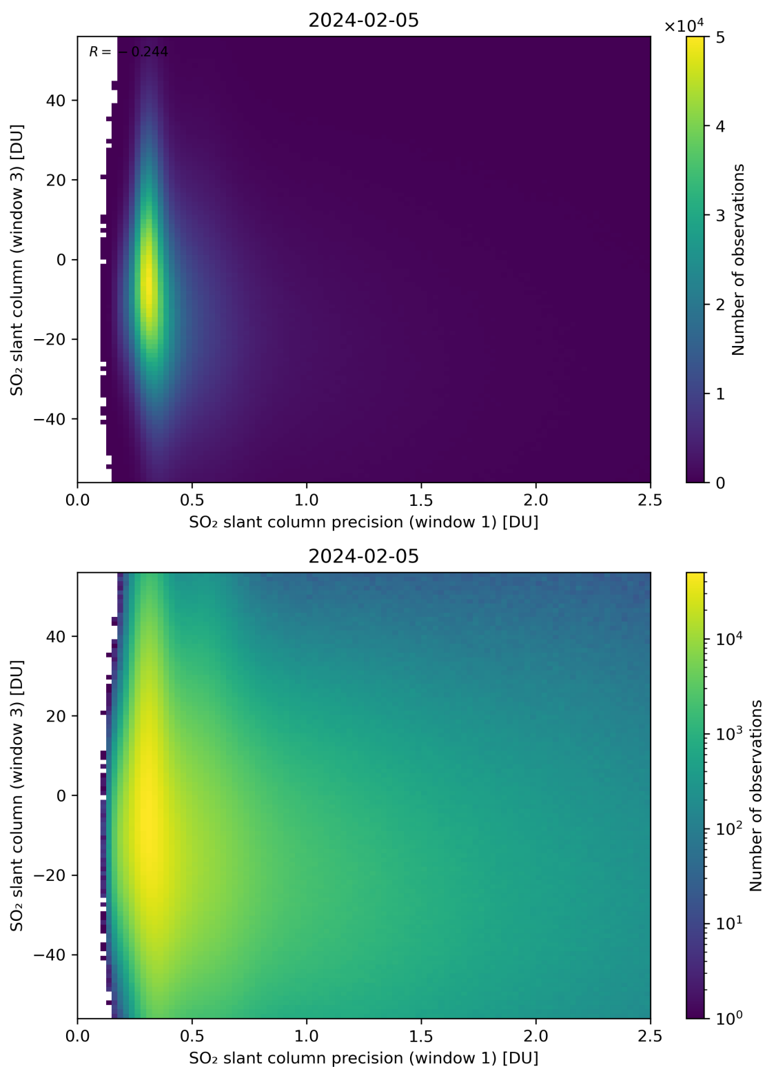
Figure 228: Scatter density plot of “SO 2 slant column precision (window 1)” against “SO 2 slant column (window 3)” for 2024-02-04 to 2024-02-06.
