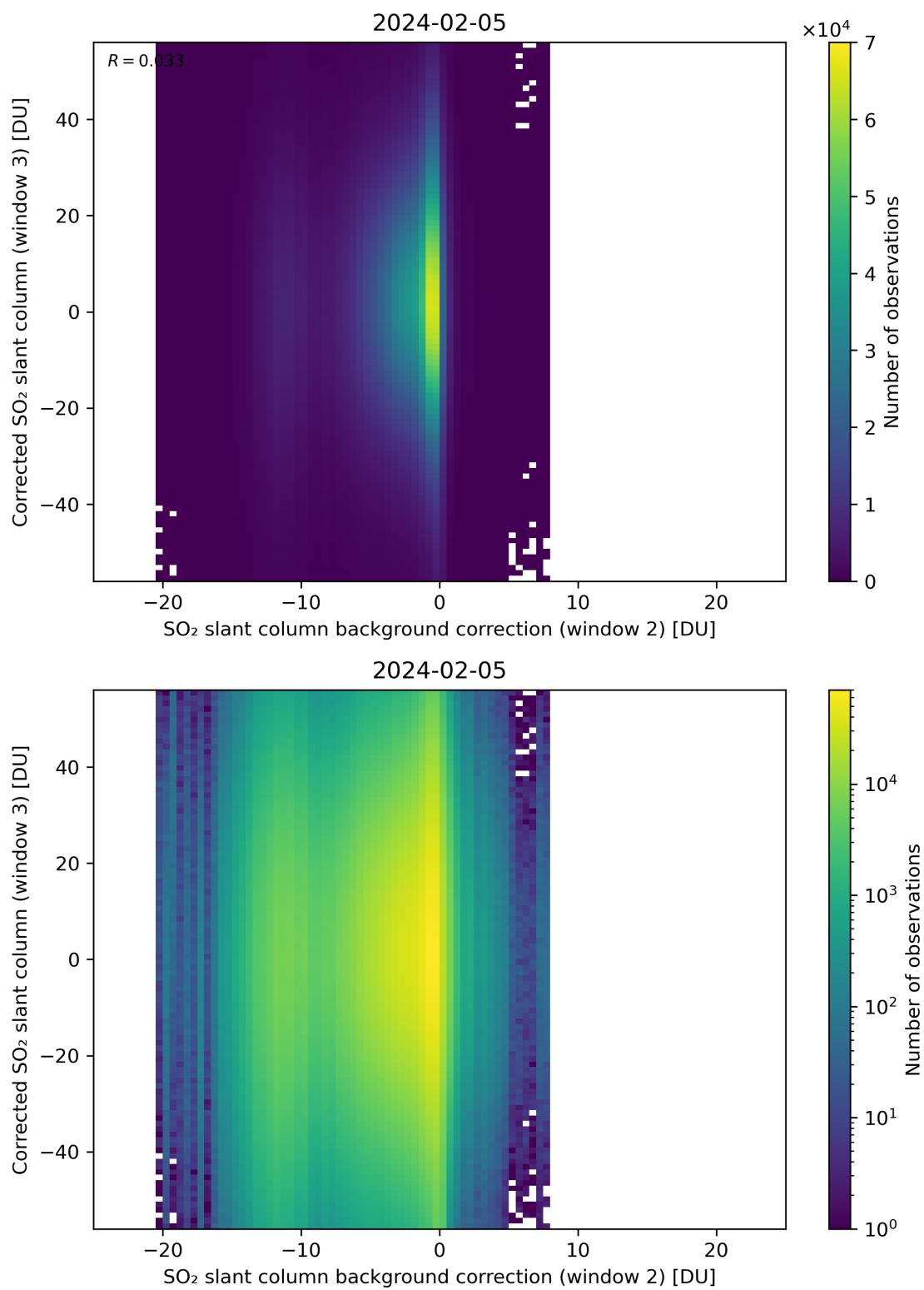
Figure 116: Scatter density plot of “SO 2 slant column background correction (window 2)” against “Corrected SO 2 slant column (window 3)” for 2024-02-04 to 2024-02-06.
