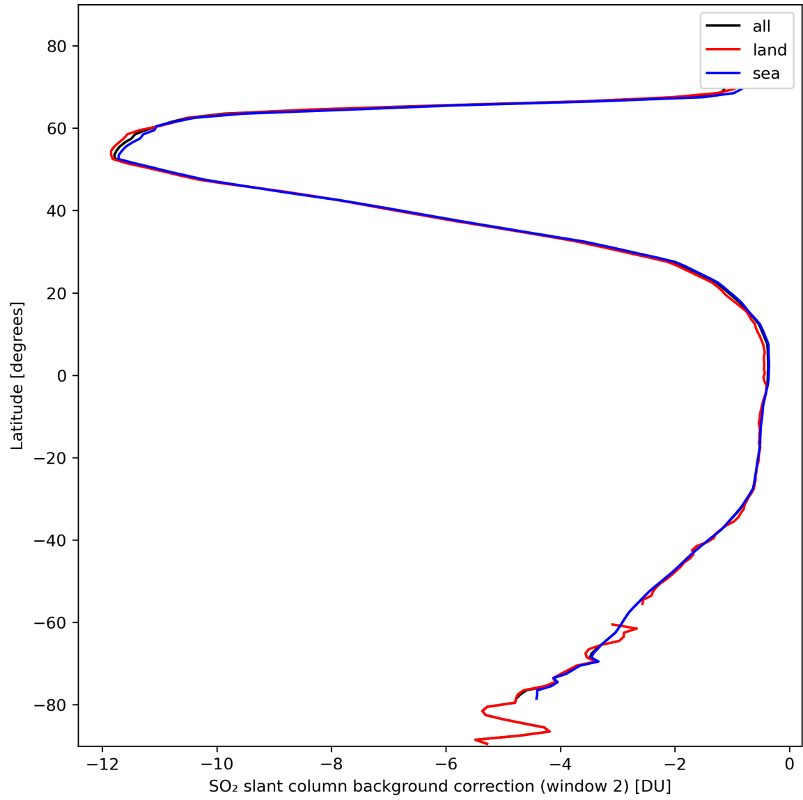
Figure 40: Zonal average of “SO 2 slant column background correction (window 2)” for 2024-02-04 to 2024-02-06.
