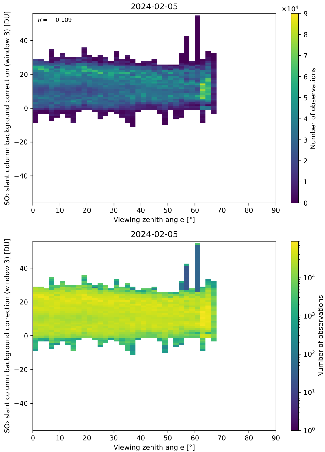
Figure 310: Scatter density plot of “Viewing zenith angle” against “SO 2 slant column background correction (window 3)” for 2024-02-04 to 2024-02-06.
