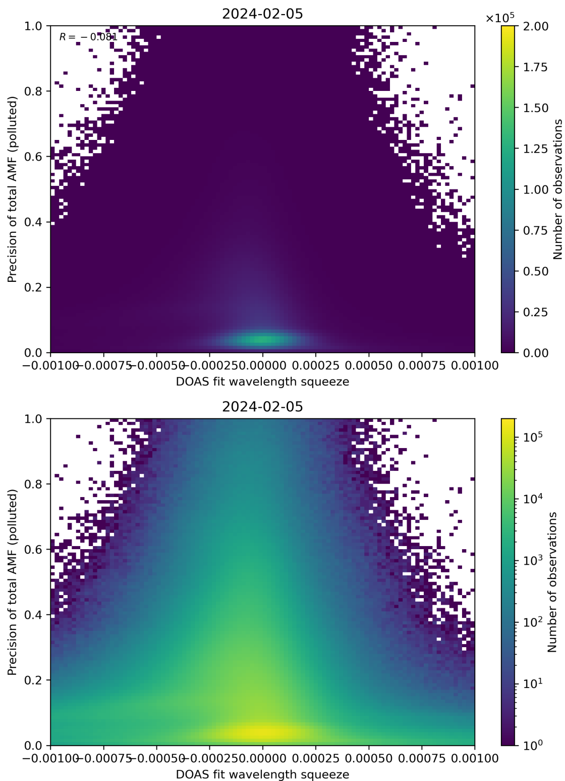
Figure 135: Scatter density plot of “DOAS fit wavelength squeeze” against “Precision of total AMF (polluted)” for 2024-02-04 to 2024-02-06.
