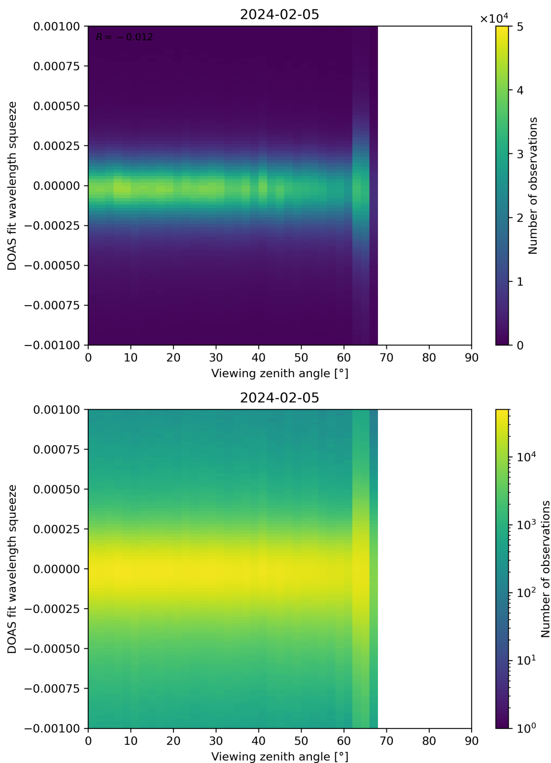
Figure 312: Scatter density plot of “Viewing zenith angle” against “DOAS fit wavelength squeeze” for 2024-02-04 to 2024-02-06.
