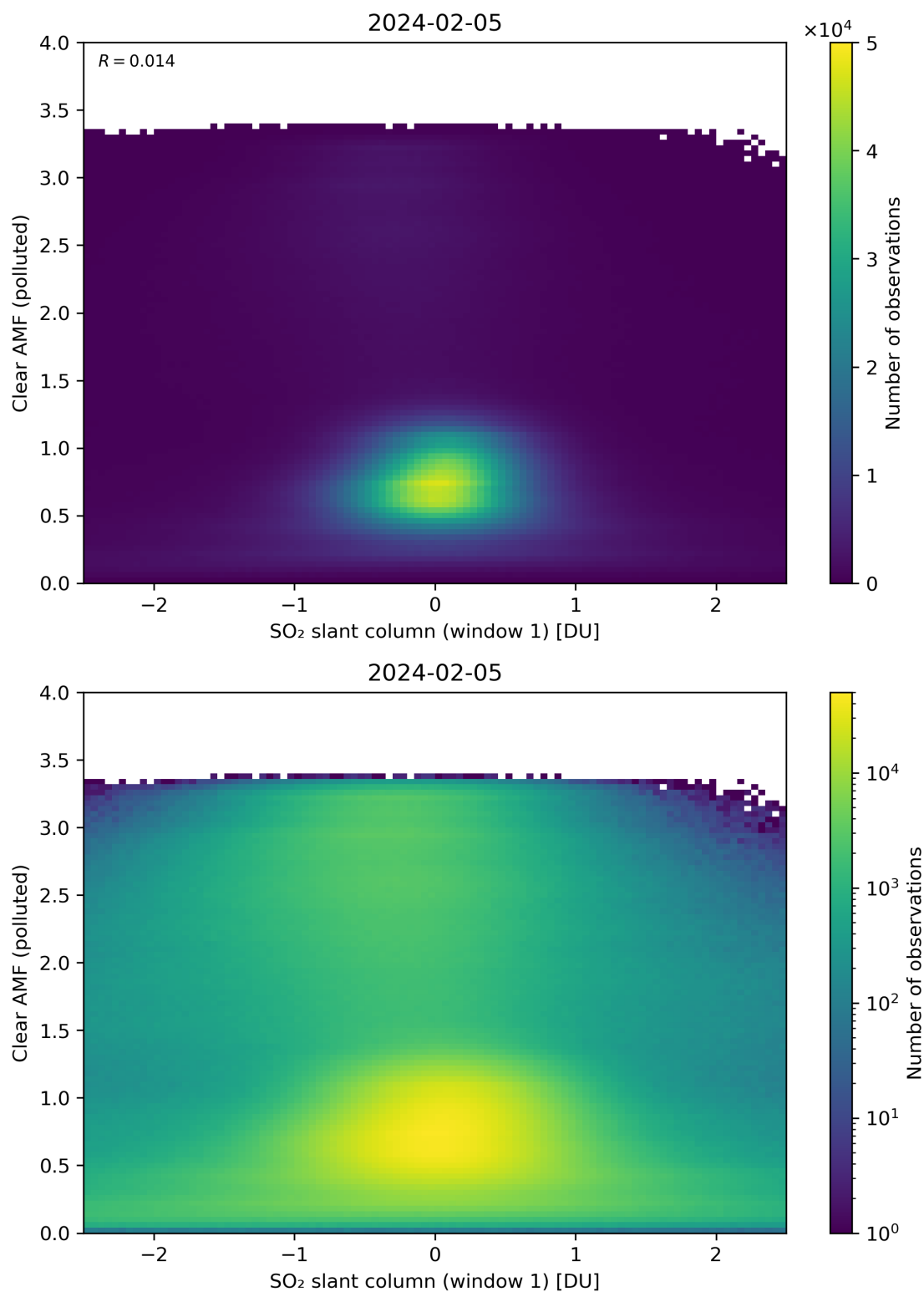
Figure 232: Scatter density plot of “SO 2 slant column (window 1)” against “Clear AMF (polluted)” for 2024-02-04 to 2024-02-06.
