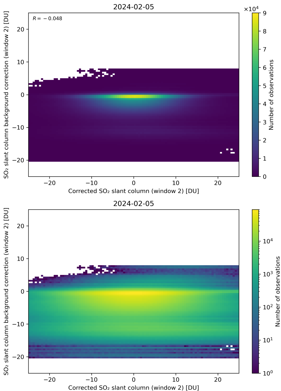
Figure 194: Scatter density plot of “Corrected SO 2 slant column (window 2)” against “SO 2 slant column background correction (window 2)” for 2024-02-04 to 2024-02-06.
