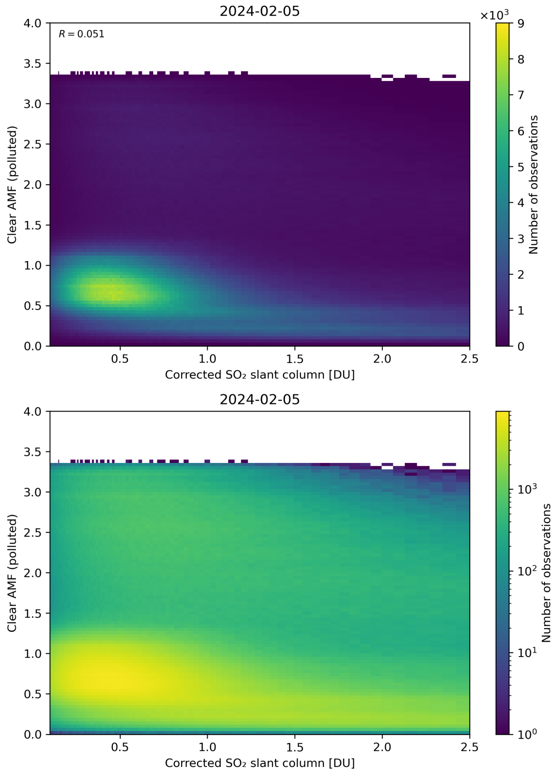
Figure 184: Scatter density plot of “Corrected SO 2 slant column” against “Clear AMF (polluted)” for 2024-02-04 to 2024-02-06.
