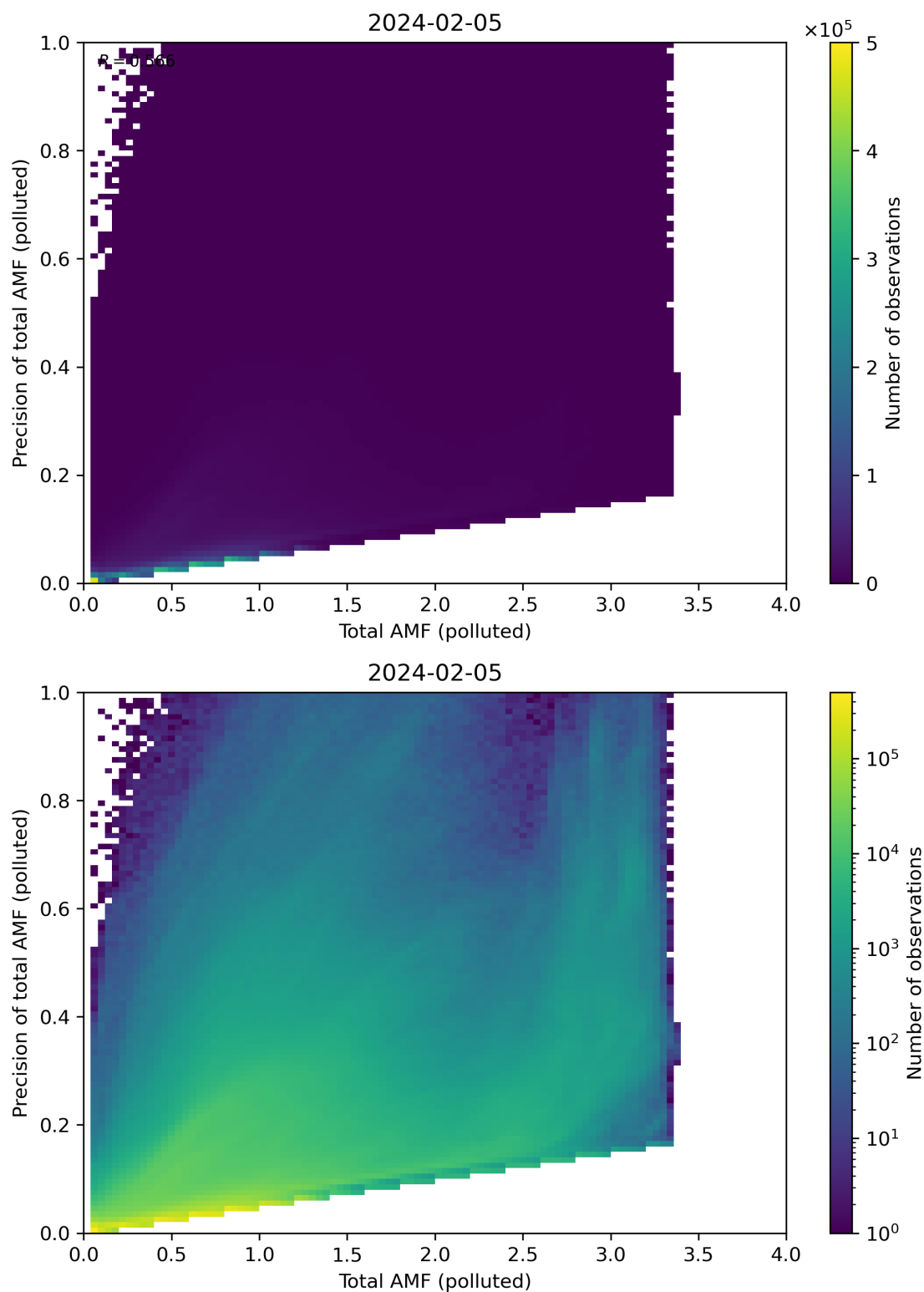
Figure 272: Scatter density plot of “Total AMF (polluted)” against “Precision of total AMF (polluted)” for 2024-02-04 to 2024-02-06.
