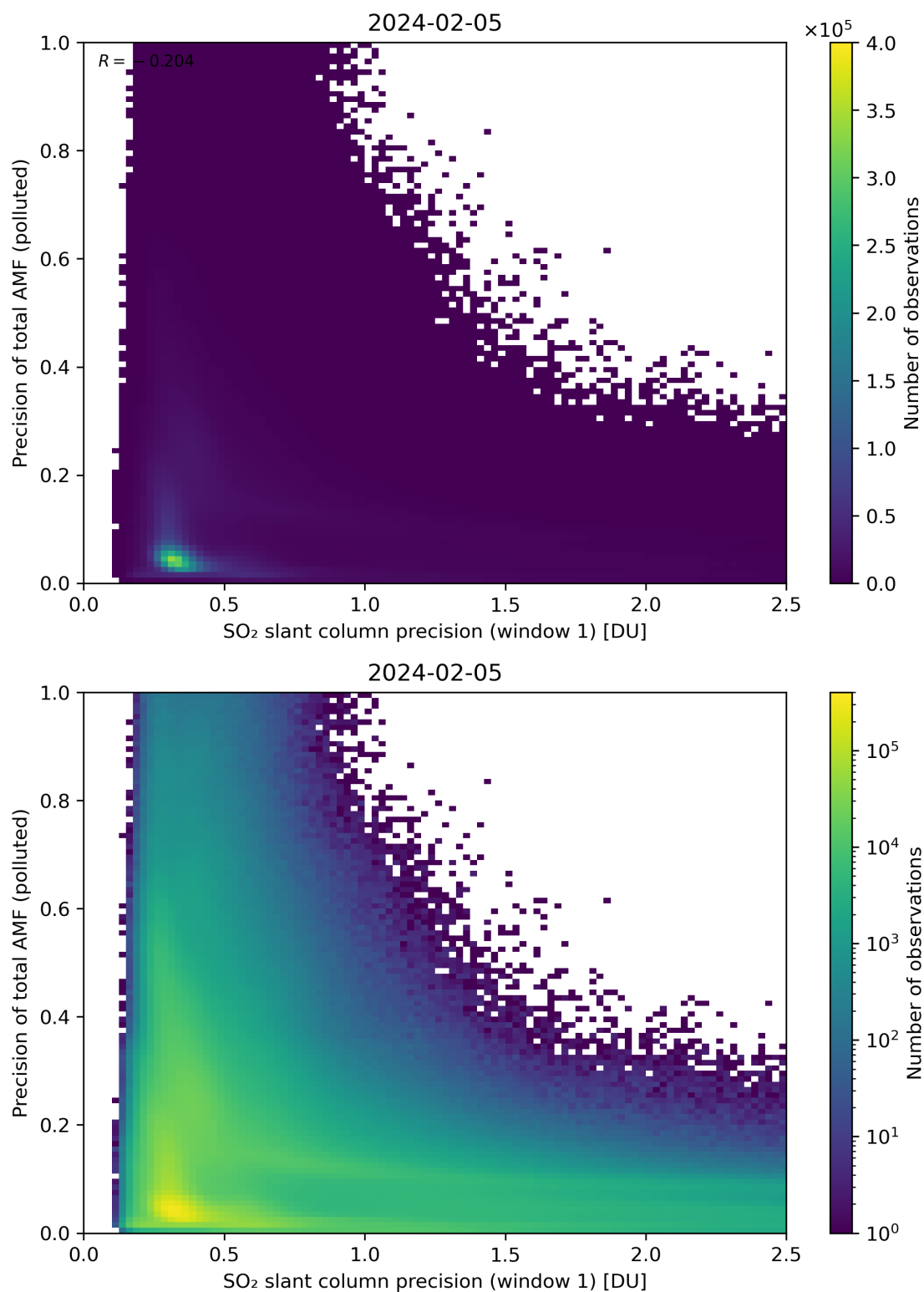
Figure 231: Scatter density plot of “SO 2 slant column precision (window 1)” against “Precision of total AMF (polluted)” for 2024-02-04 to 2024-02-06.
