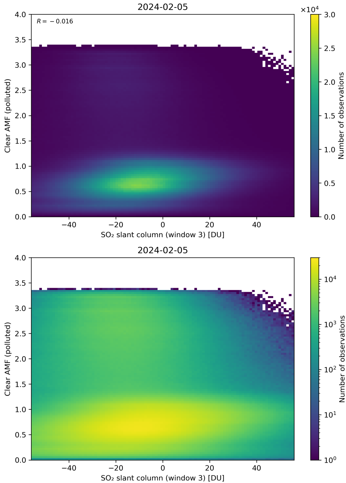
Figure 265: Scatter density plot of “SO 2 slant column (window 3)” against “Clear AMF (polluted)” for 2024-02-04 to 2024-02-06.
