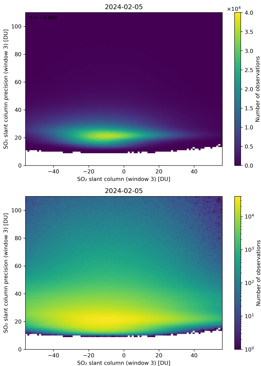
Figure 267: Scatter density plot of “SO 2 slant column (window 3)” against “SO 2 slant column precision (window 3)” for 2024-02-04 to 2024-02-06.
