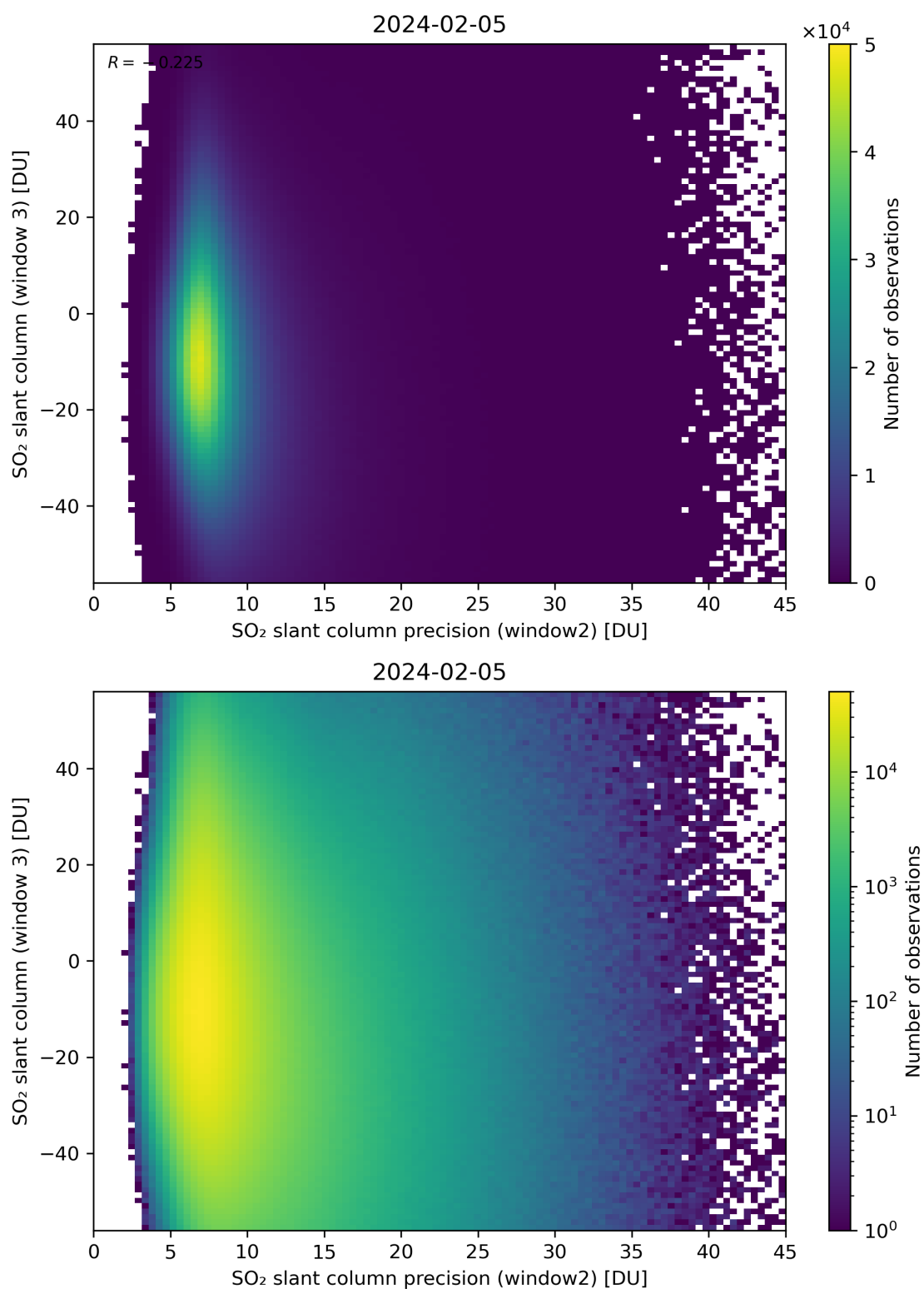
Figure 249: Scatter density plot of “SO 2 slant column precision (window2)” against “SO 2 slant column (window 3)” for 2024-02-04 to 2024-02-06.
