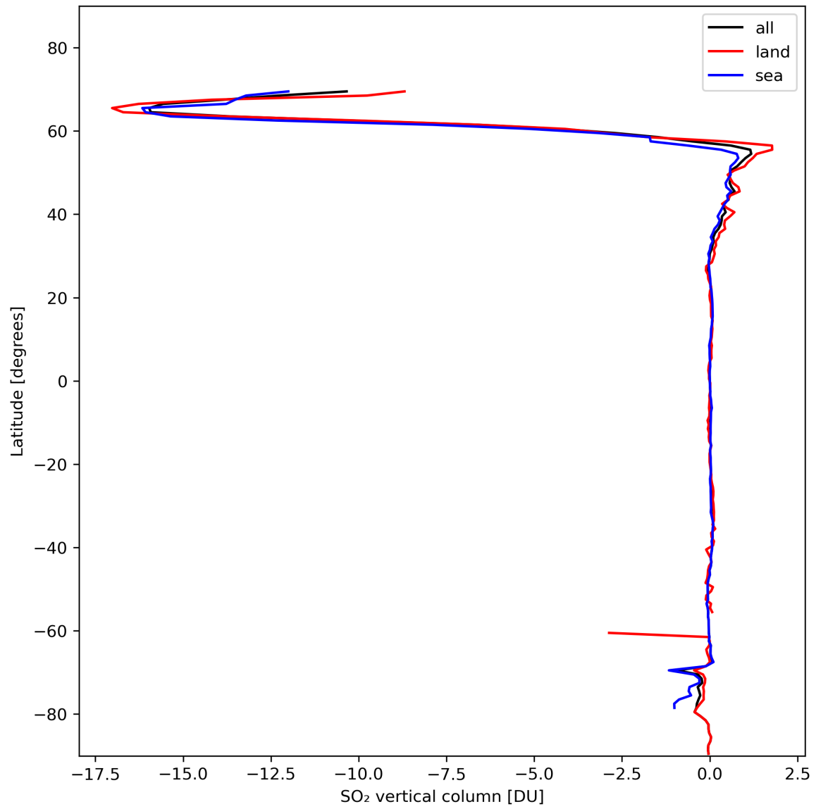
Figure 30: Zonal average of “SO 2 vertical column” for 2024-02-04 to 2024-02-06.
