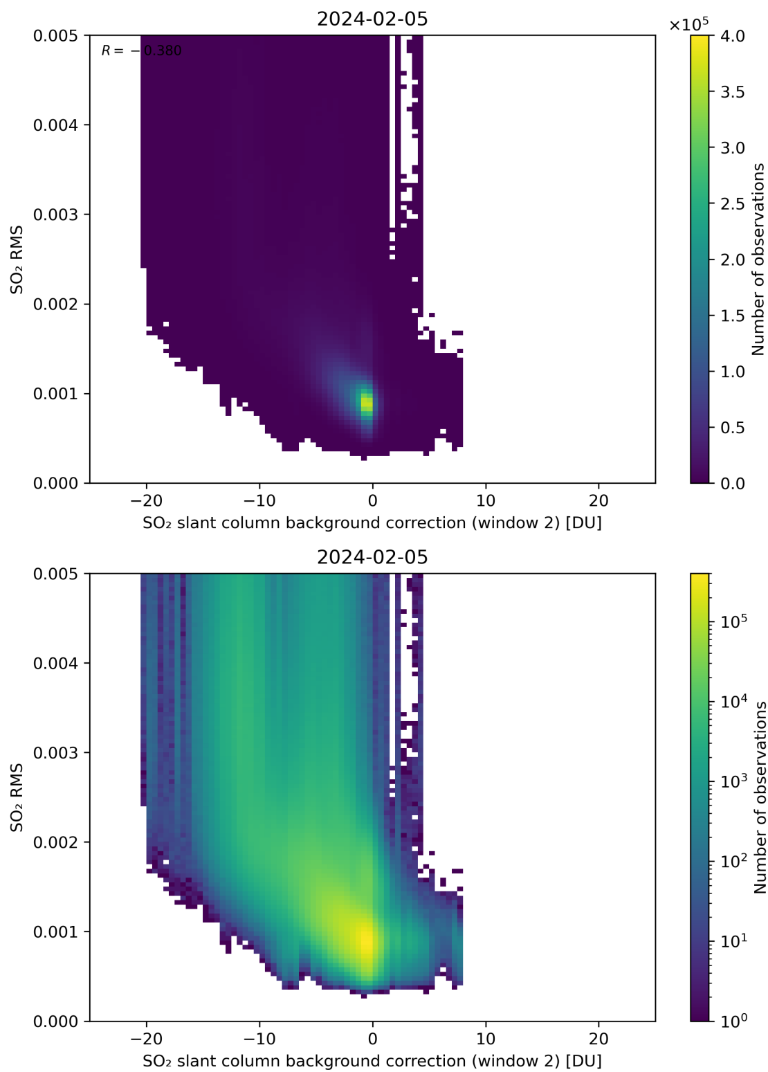
Figure 114: Scatter density plot of “SO 2 slant column background correction (window 2)” against “SO 2 RMS” for 2024-02-04 to 2024-02-06.
