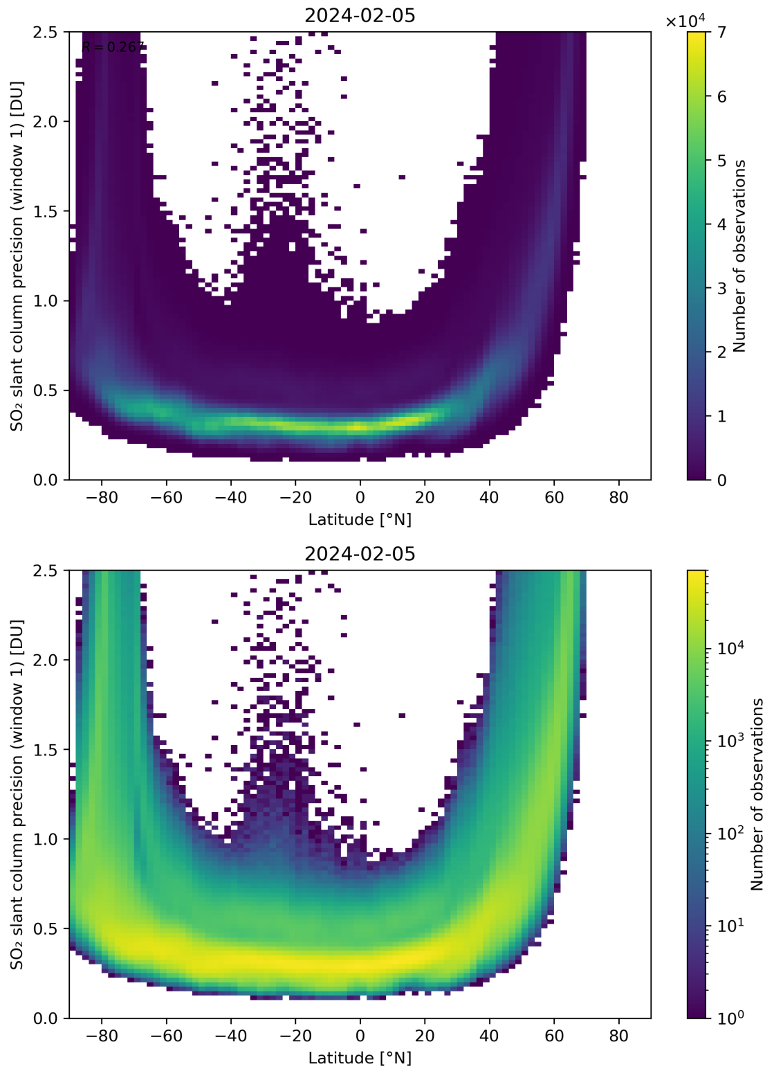
Figure 150: Scatter density plot of “Latitude” against “SO 2 slant column precision (window 1)” for 2024-02-04 to 2024-02-06.
