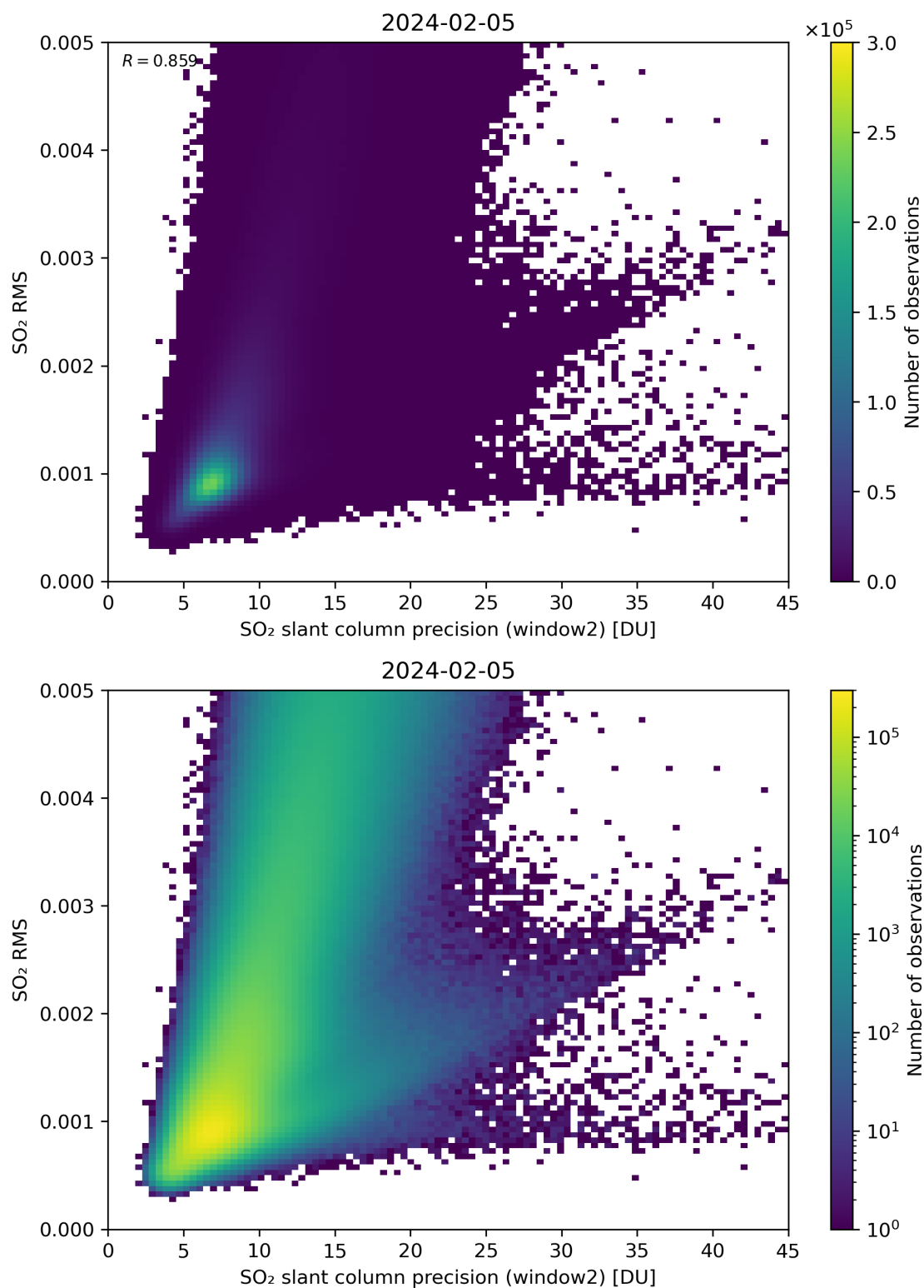
Figure 245: Scatter density plot of “SO 2 slant column precision (window2)” against “SO 2 RMS” for 2024-02-04 to 2024-02-06.
