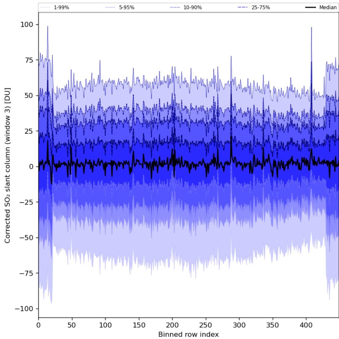
Figure 89: Along track statistics of “Corrected SO 2 slant column (window 3)” for 2024-02-04 to 2024-02-06
