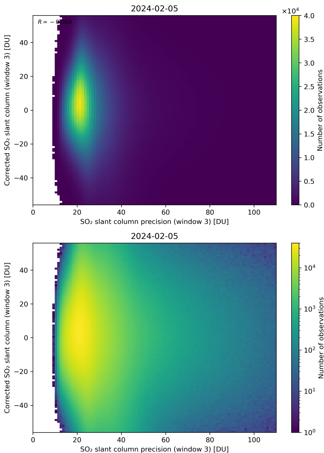
Figure 262: Scatter density plot of “SO 2 slant column precision (window 3)” against “Corrected SO 2 slant column (window 3)” for 2024-02-04 to 2024-02-06.
