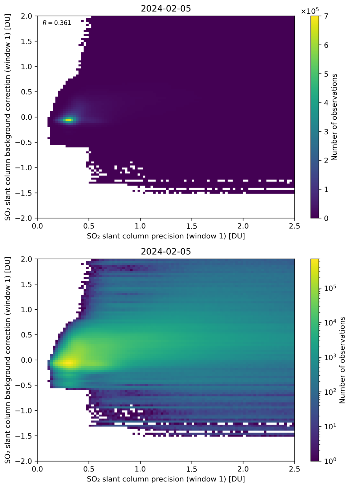
Figure 218: Scatter density plot of “SO 2 slant column precision (window 1)” against “SO 2 slant column background correction (window 1)” for 2024-02-04 to 2024-02-06.
