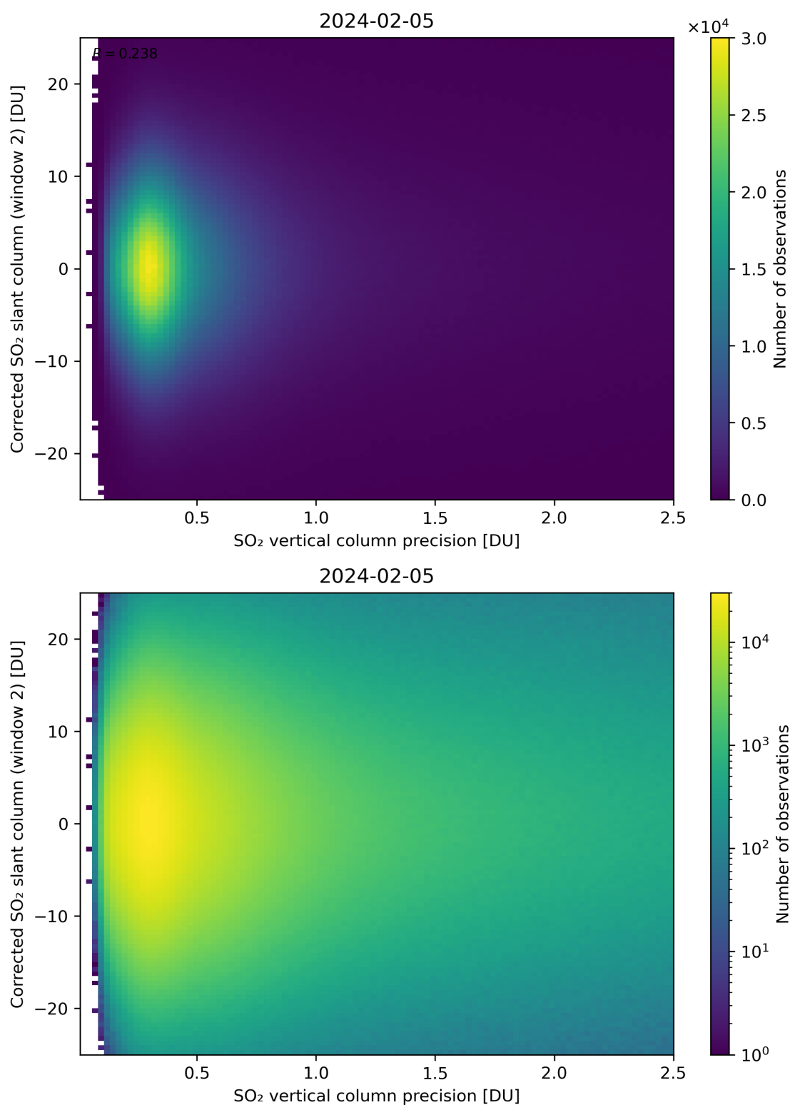
Figure 287: Scatter density plot of “SO 2 vertical column precision” against “Corrected SO 2 slant column (window 2)” for 2024-02-04 to 2024-02-06.
