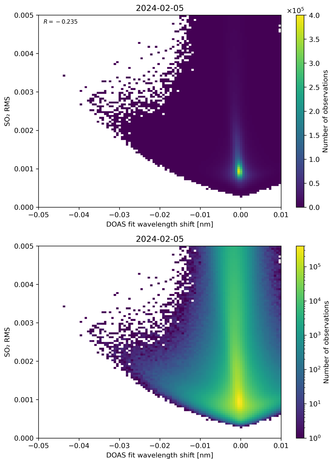
Figure 128: Scatter density plot of “DOAS fit wavelength shift” against “SO 2 RMS” for 2024-02-04 to 2024-02-06.
