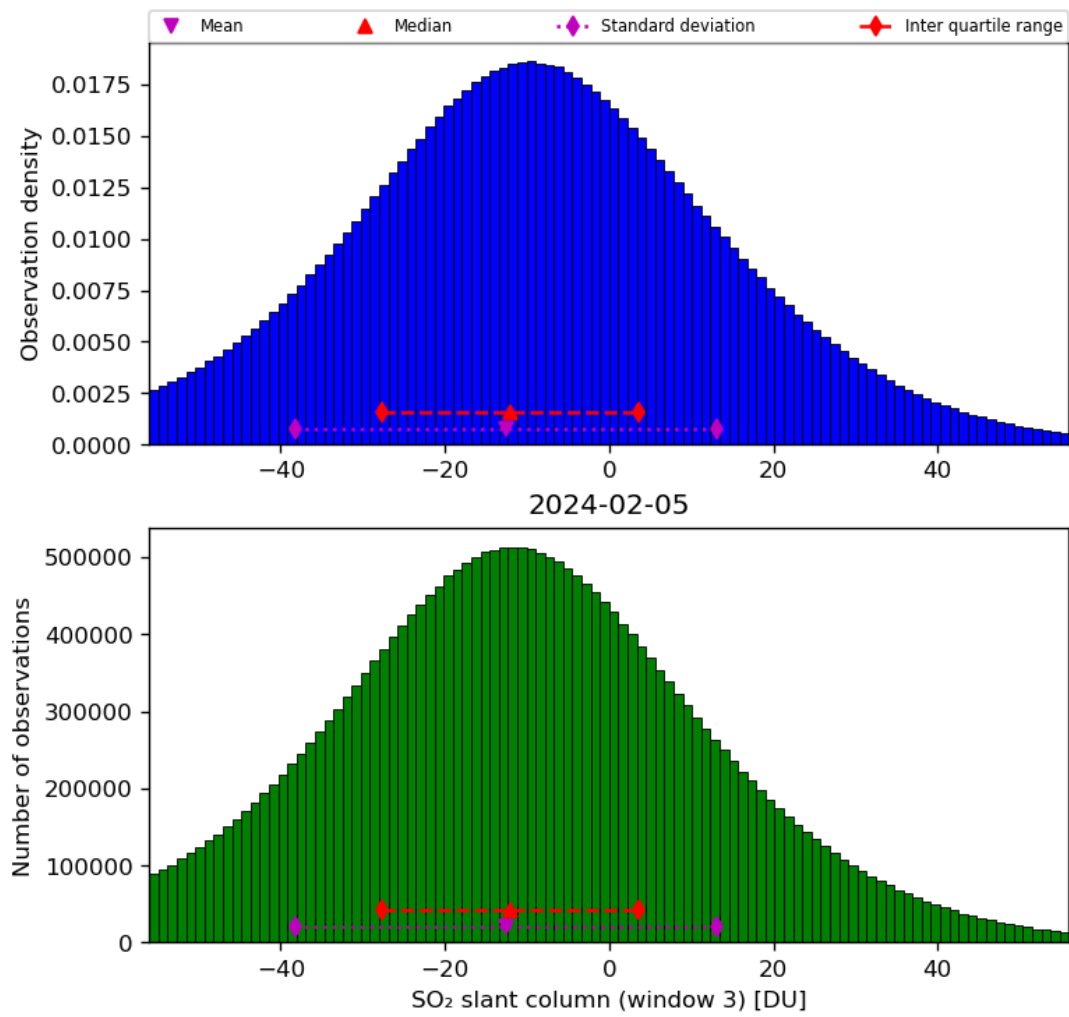
Figure 64: Histogram of “SO 2 slant column (window 3)” for 2024-02-04 to 2024-02-06
