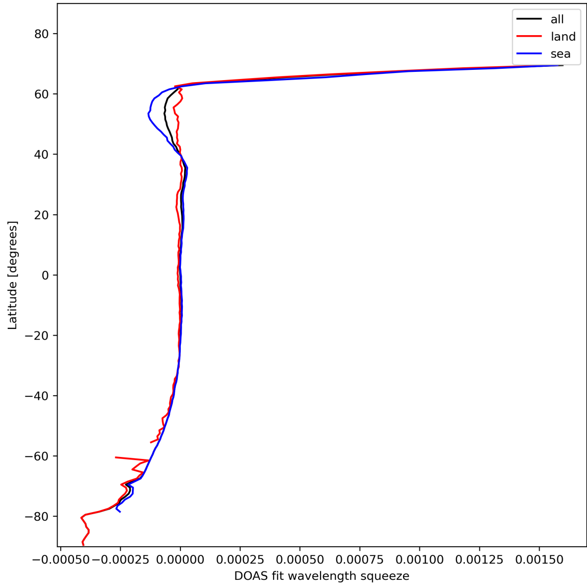
Figure 46: Zonal average of “DOAS fit wavelength squeeze” for 2024-02-04 to 2024-02-06.
