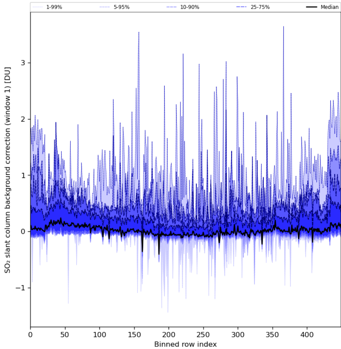
Figure 82: Along track statistics of “SO 2 slant column background correction (window 1)” for 2024-02-04 to 2024-02-06
