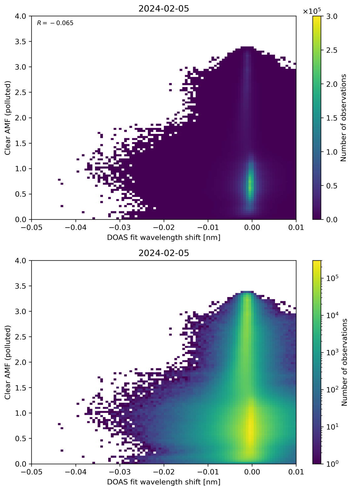
Figure 129: Scatter density plot of “DOAS fit wavelength shift” against “Clear AMF (polluted)” for 2024-02-04 to 2024-02-06.
