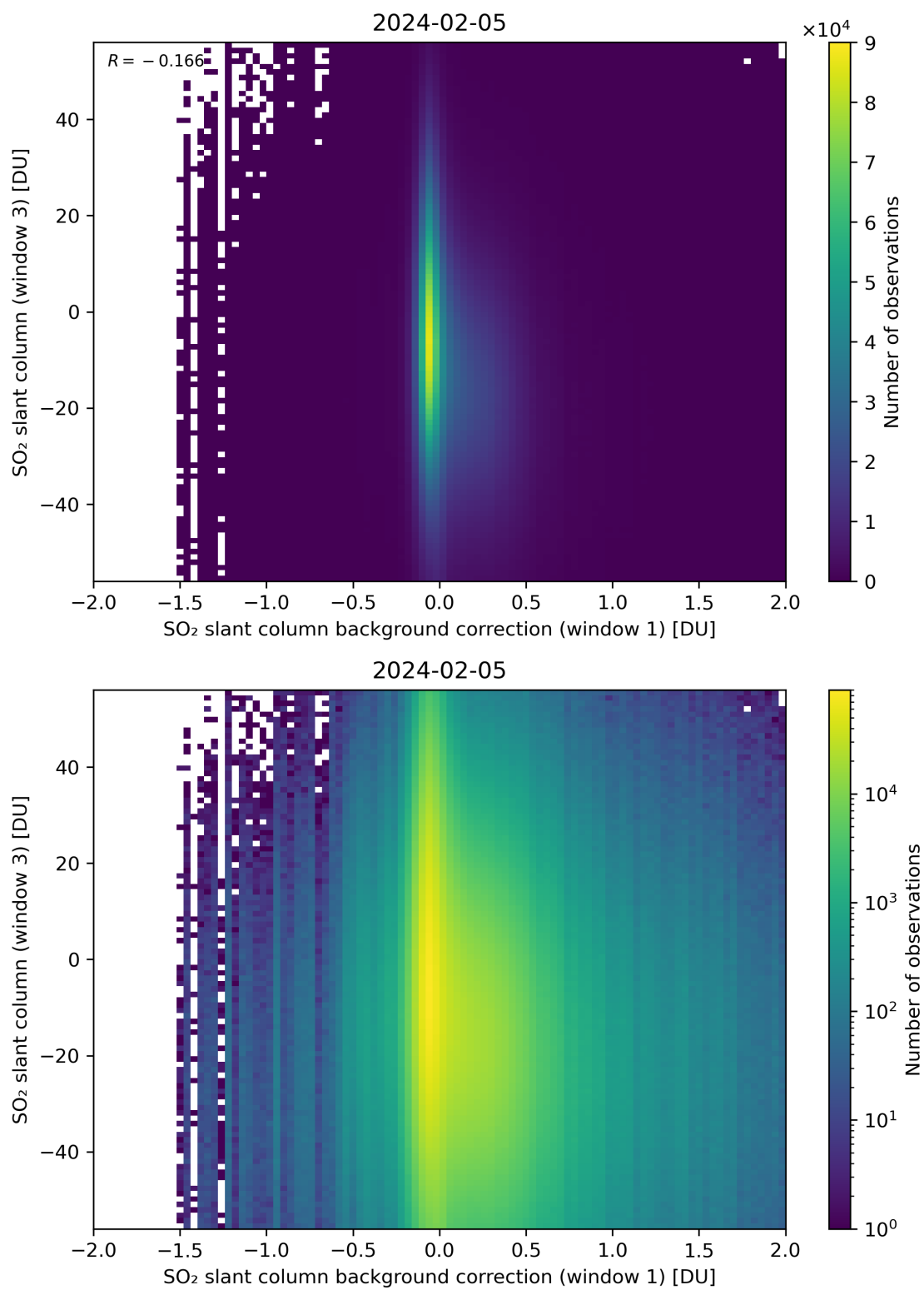
Figure 107: Scatter density plot of “SO 2 slant column background correction (window 1)” against “SO 2 slant column (window 3)” for 2024-02-04 to 2024-02-06.
