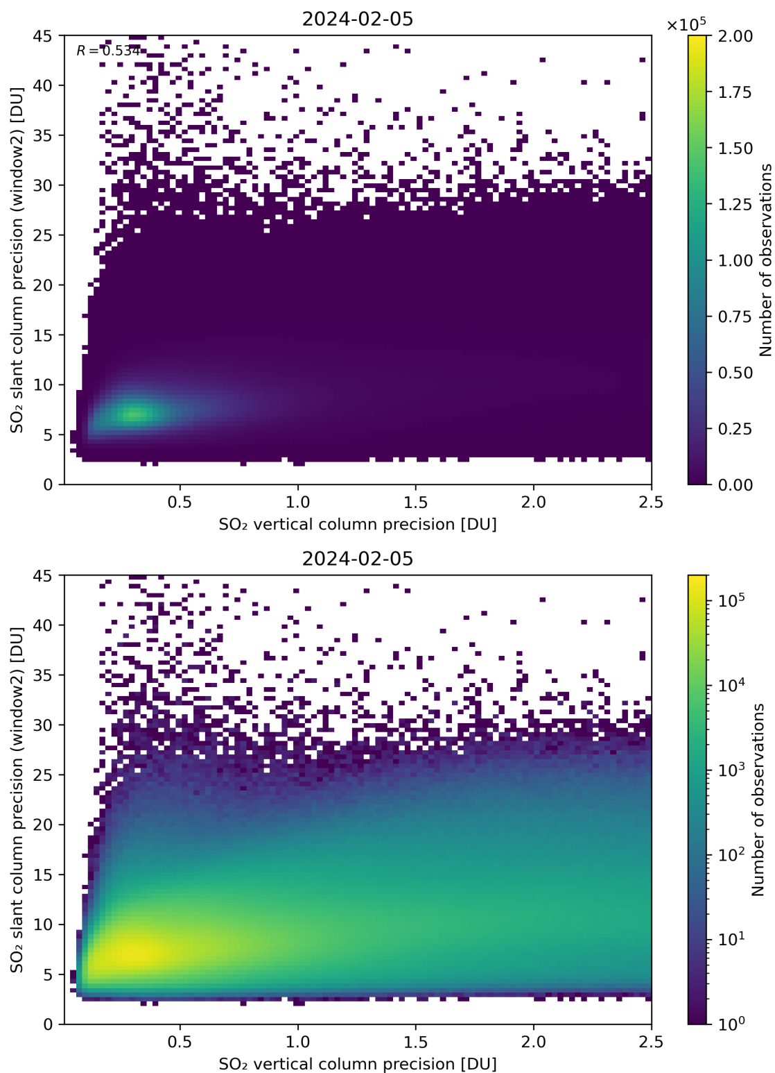
Figure 291: Scatter density plot of “SO 2 vertical column precision” against “SO 2 slant column precision (window2)” for 2024-02-04 to 2024-02-06.
