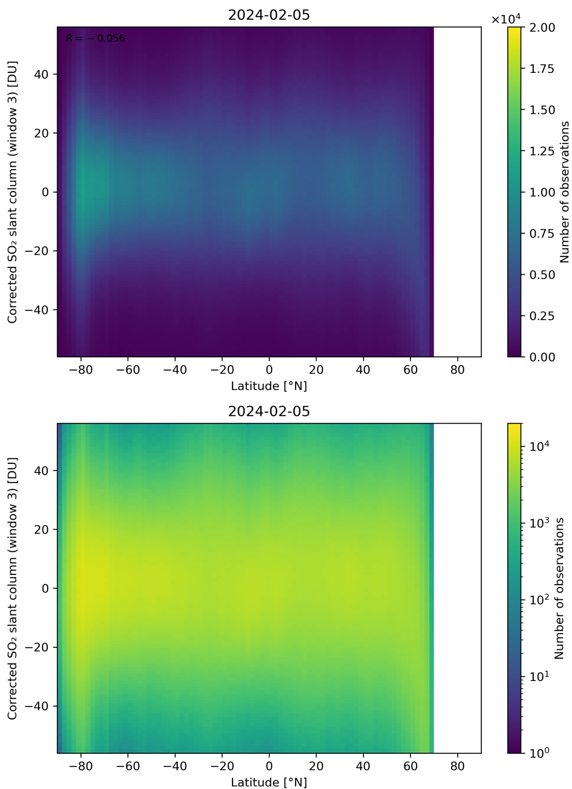
Figure 148: Scatter density plot of “Latitude” against “Corrected SO 2 slant column (window 3)” for 2024-02-04 to 2024-02-06.
