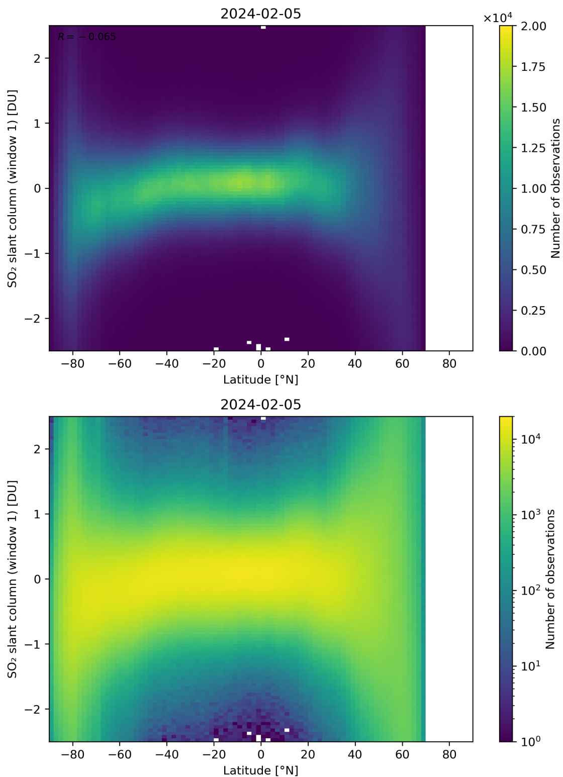
Figure 149: Scatter density plot of “Latitude” against “SO 2 slant column (window 1)” for 2024-02-04 to 2024-02-06.
