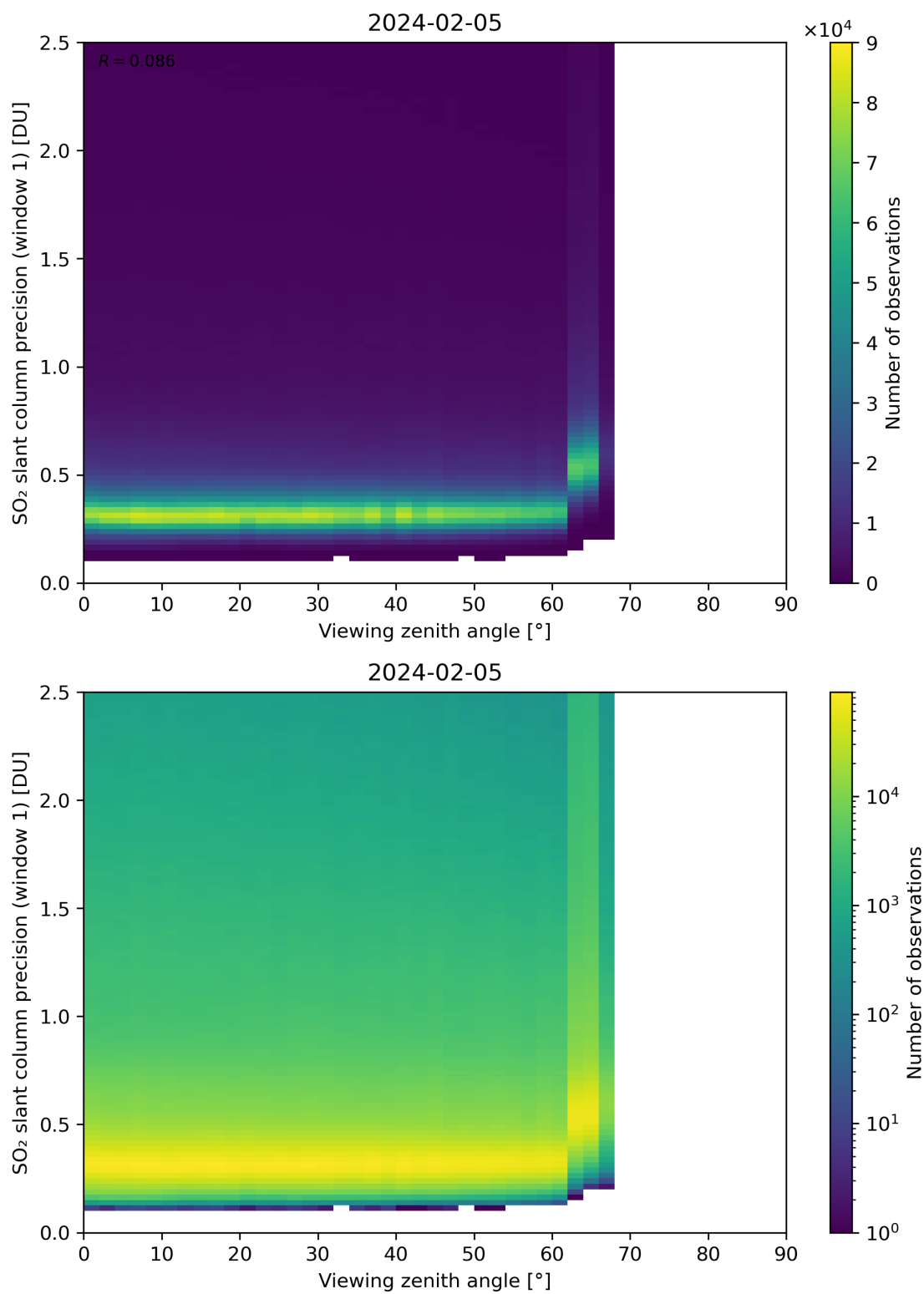
Figure 321: Scatter density plot of “Viewing zenith angle” against “SO 2 slant column precision (window 1)” for 2024-02-04 to 2024-02-06.
