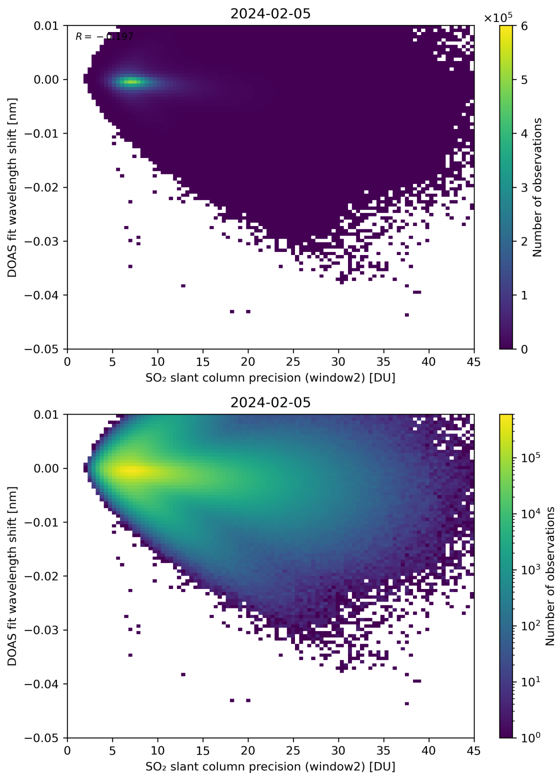
Figure 243: Scatter density plot of “SO 2 slant column precision (window2)” against “DOAS fit wavelength shift” for 2024-02-04 to 2024-02-06.
