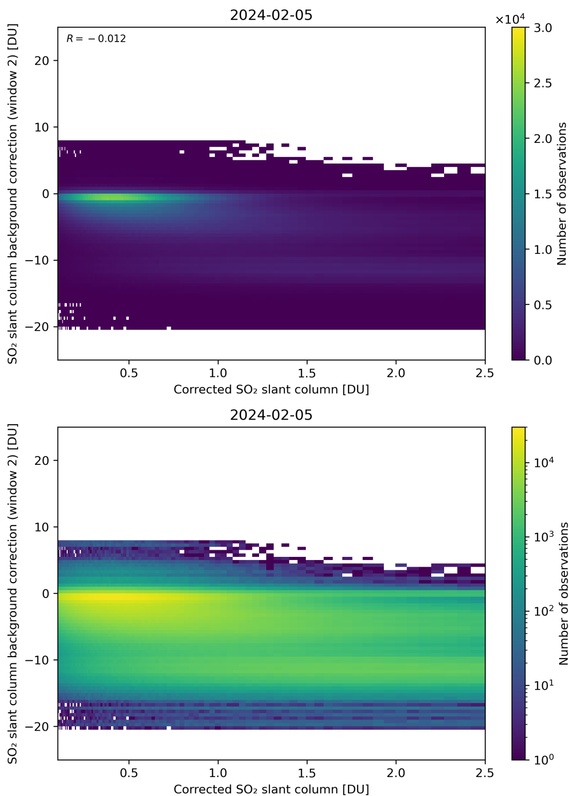
Figure 179: Scatter density plot of “Corrected SO 2 slant column” against “SO 2 slant column background correction (window 2)” for 2024-02-04 to 2024-02-06.
