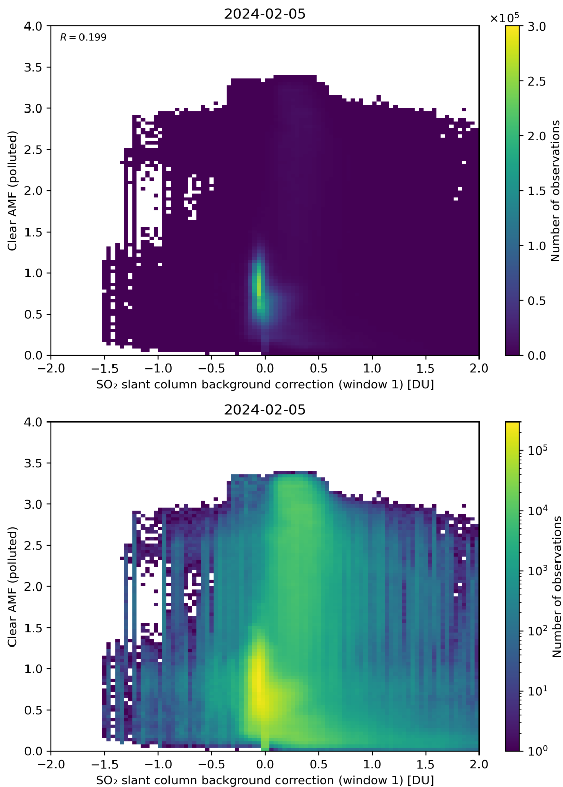
Figure 103: Scatter density plot of “SO 2 slant column background correction (window 1)” against “Clear AMF (polluted)” for 2024-02-04 to 2024-02-06.
