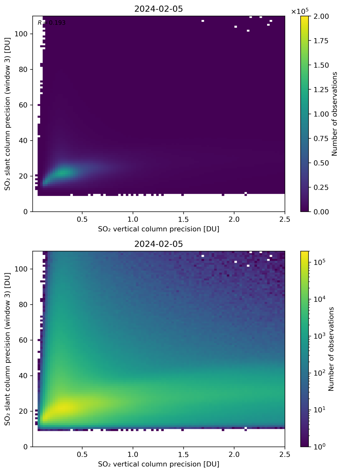
Figure 293: Scatter density plot of “SO 2 vertical column precision” against “SO 2 slant column precision (window 3)” for 2024-02-04 to 2024-02-06.
