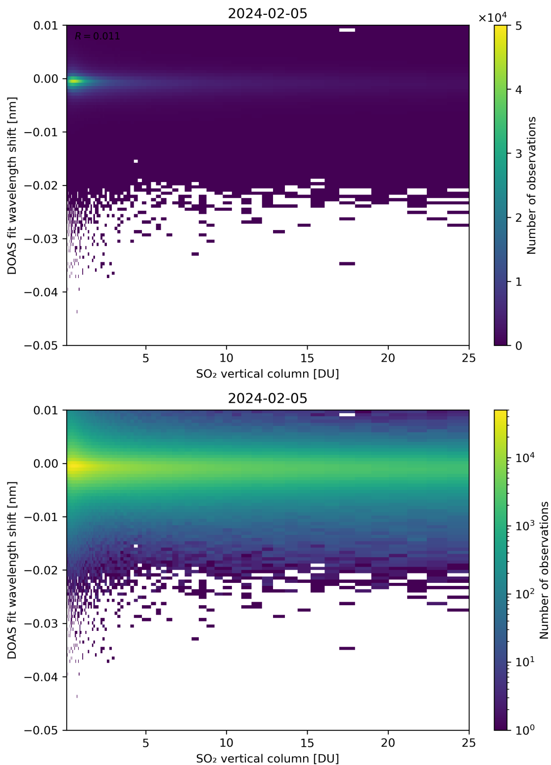
Figure 276: Scatter density plot of “SO 2 vertical column” against “DOAS fit wavelength shift” for 2024-02-04 to 2024-02-06.
