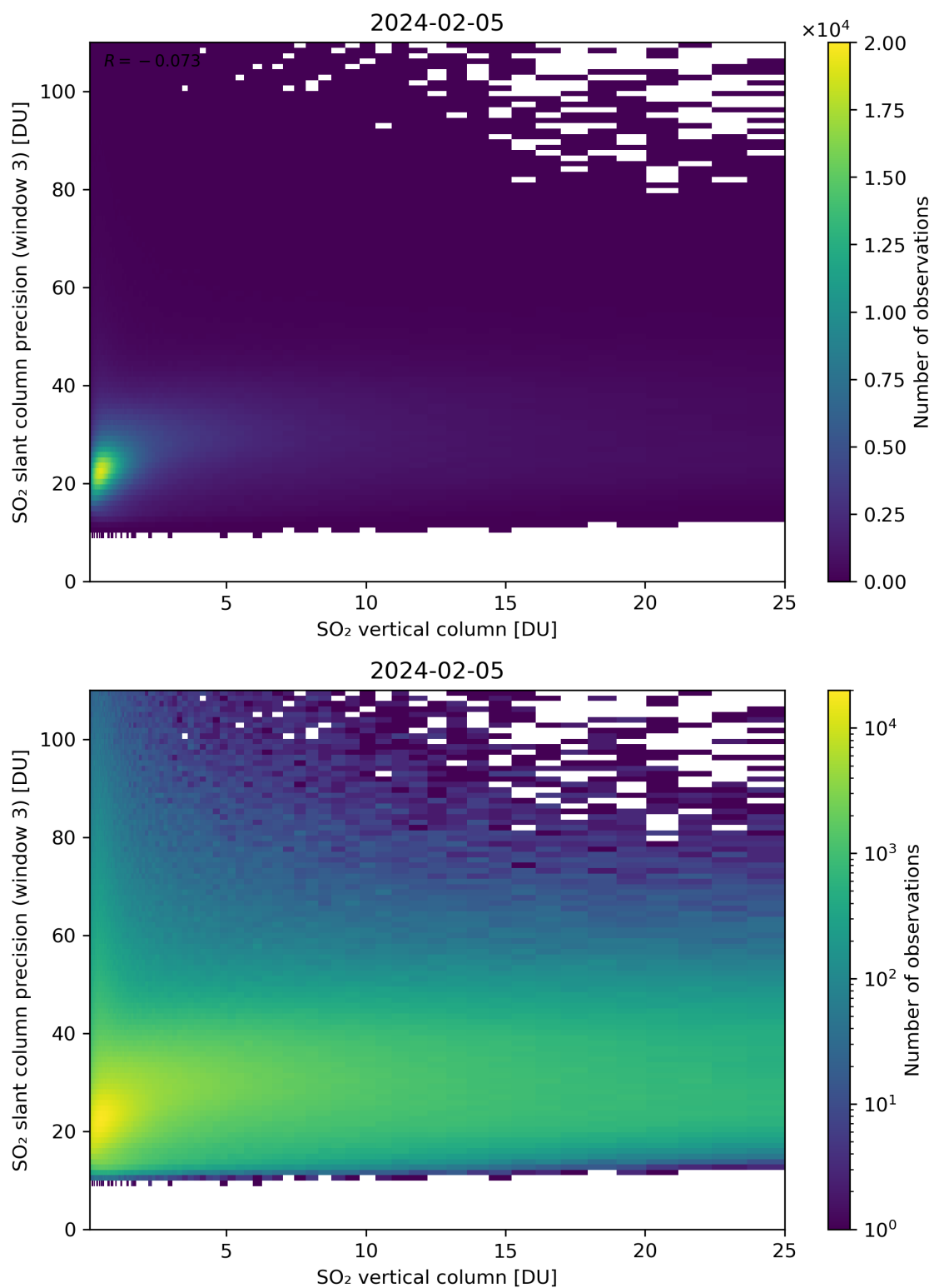
Figure 304: Scatter density plot of “SO 2 vertical column” against “SO 2 slant column precision (window 3)” for 2024-02-04 to 2024-02-06.
