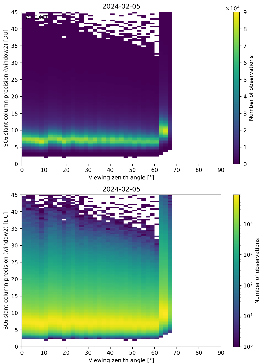
Figure 322: Scatter density plot of “Viewing zenith angle” against “SO 2 slant column precision (window2)” for 2024-02-04 to 2024-02-06.
