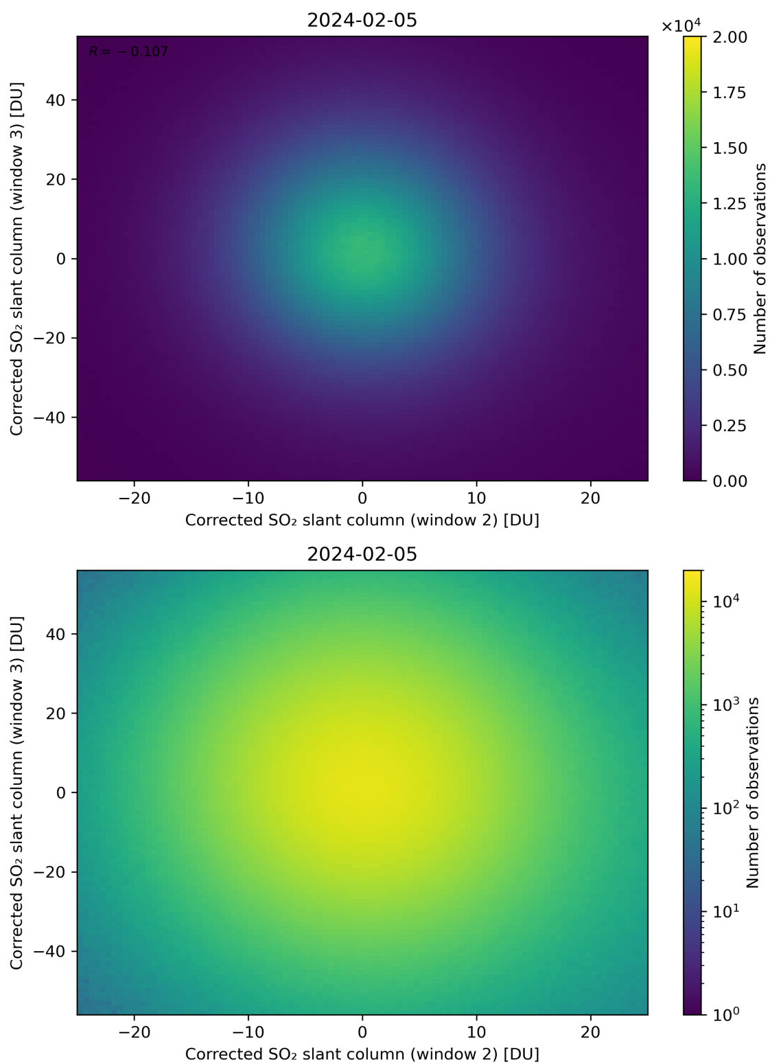
Figure 200: Scatter density plot of “Corrected SO 2 slant column (window 2)” against “Corrected SO 2 slant column (window 3)” for 2024-02-04 to 2024-02-06.
