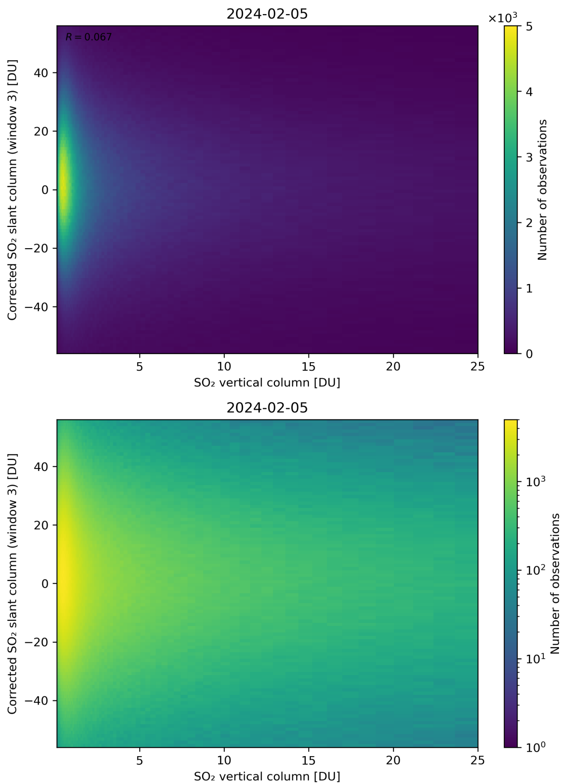
Figure 299: Scatter density plot of “SO 2 vertical column” against “Corrected SO 2 slant column (window 3)” for 2024-02-04 to 2024-02-06.
