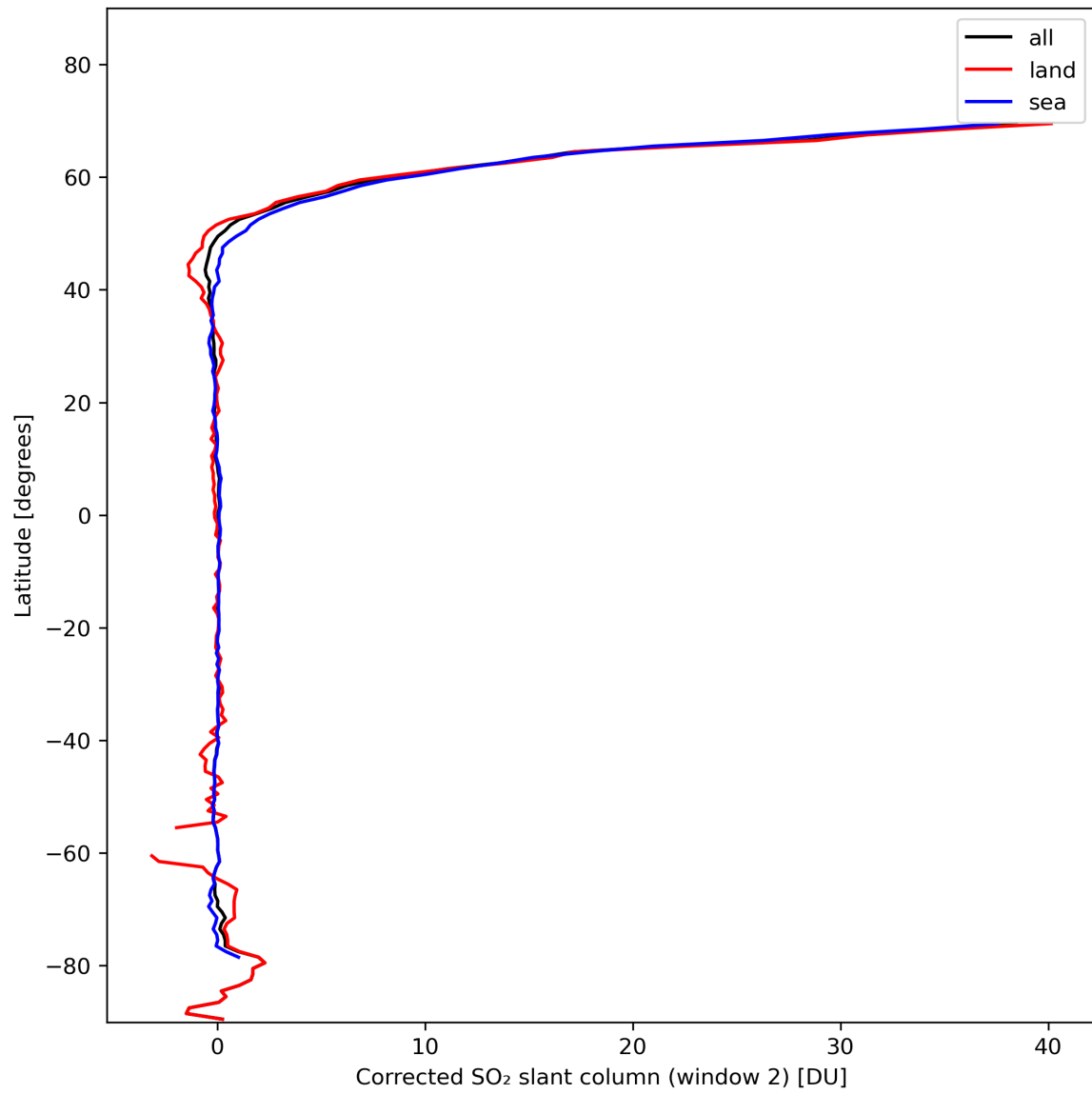
Figure 39: Zonal average of “Corrected SO 2 slant column (window 2)” for 2024-02-04 to 2024-02-06.
