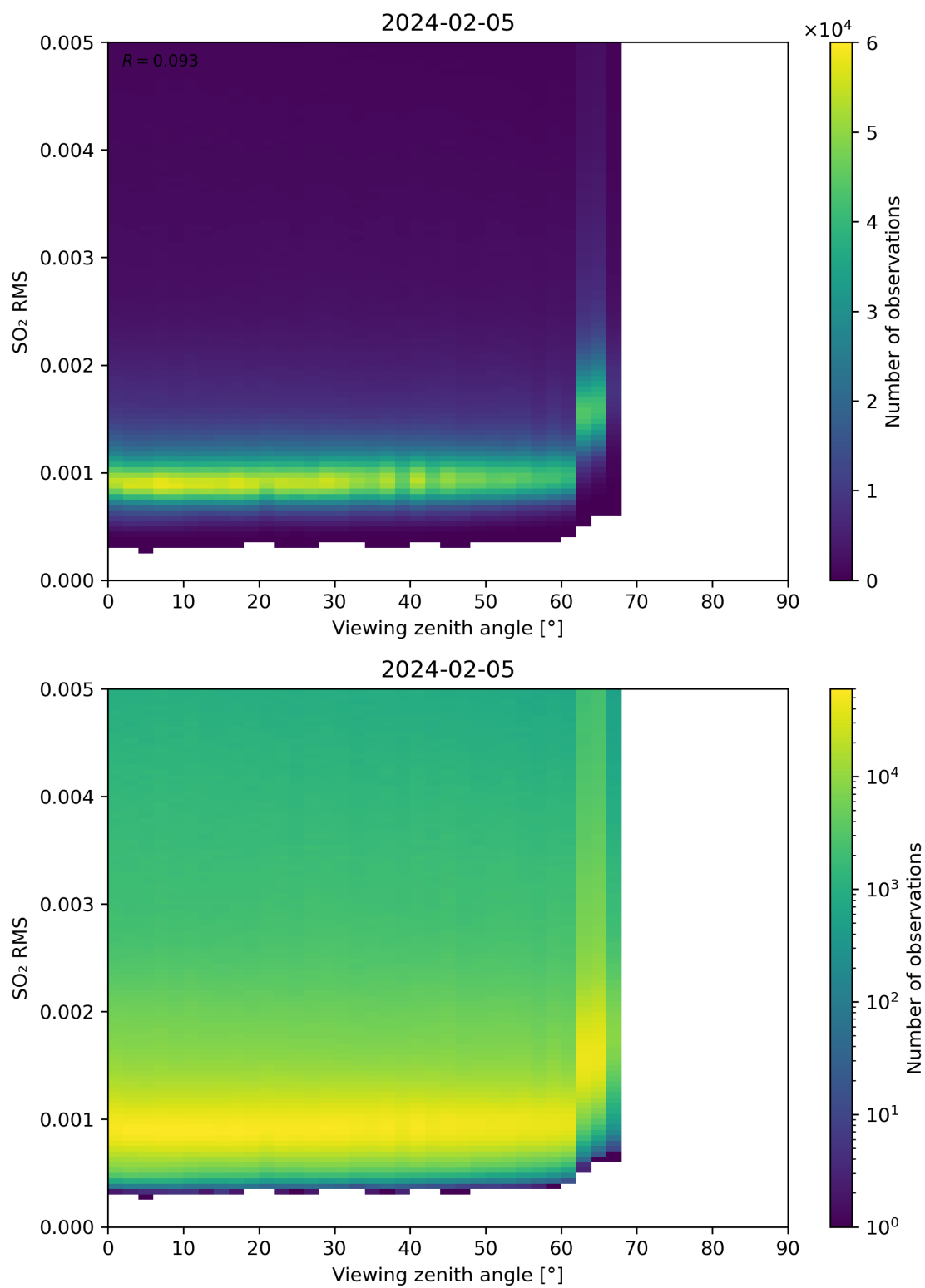
Figure 313: Scatter density plot of “Viewing zenith angle” against “SO 2 RMS” for 2024-02-04 to 2024-02-06.
