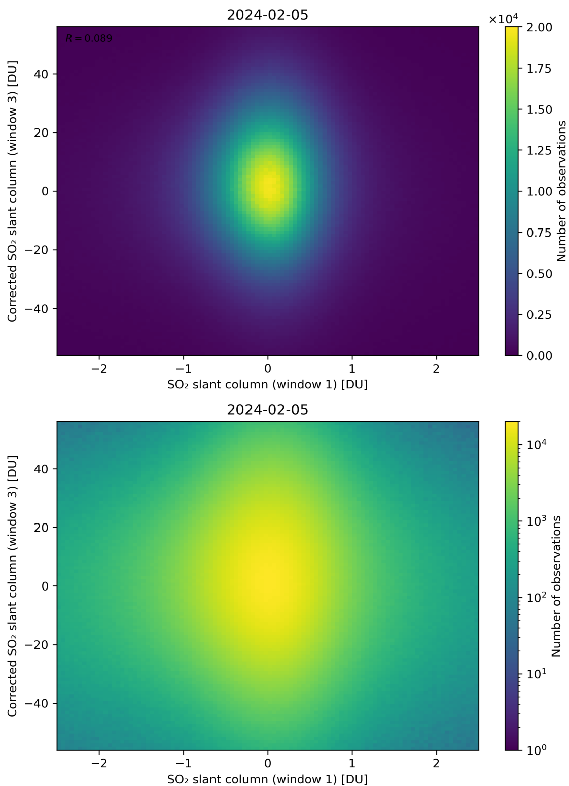
Figure 234: Scatter density plot of “SO 2 slant column (window 1)” against “Corrected SO 2 slant column (window 3)” for 2024-02-04 to 2024-02-06.
