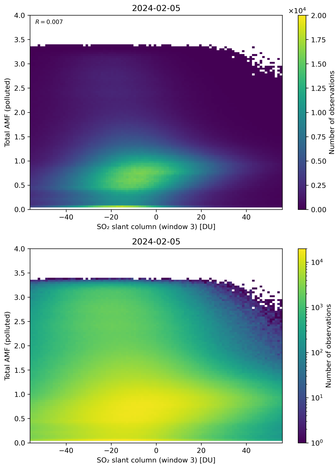
Figure 268: Scatter density plot of “SO 2 slant column (window 3)” against “Total AMF (polluted)” for 2024-02-04 to 2024-02-06.
