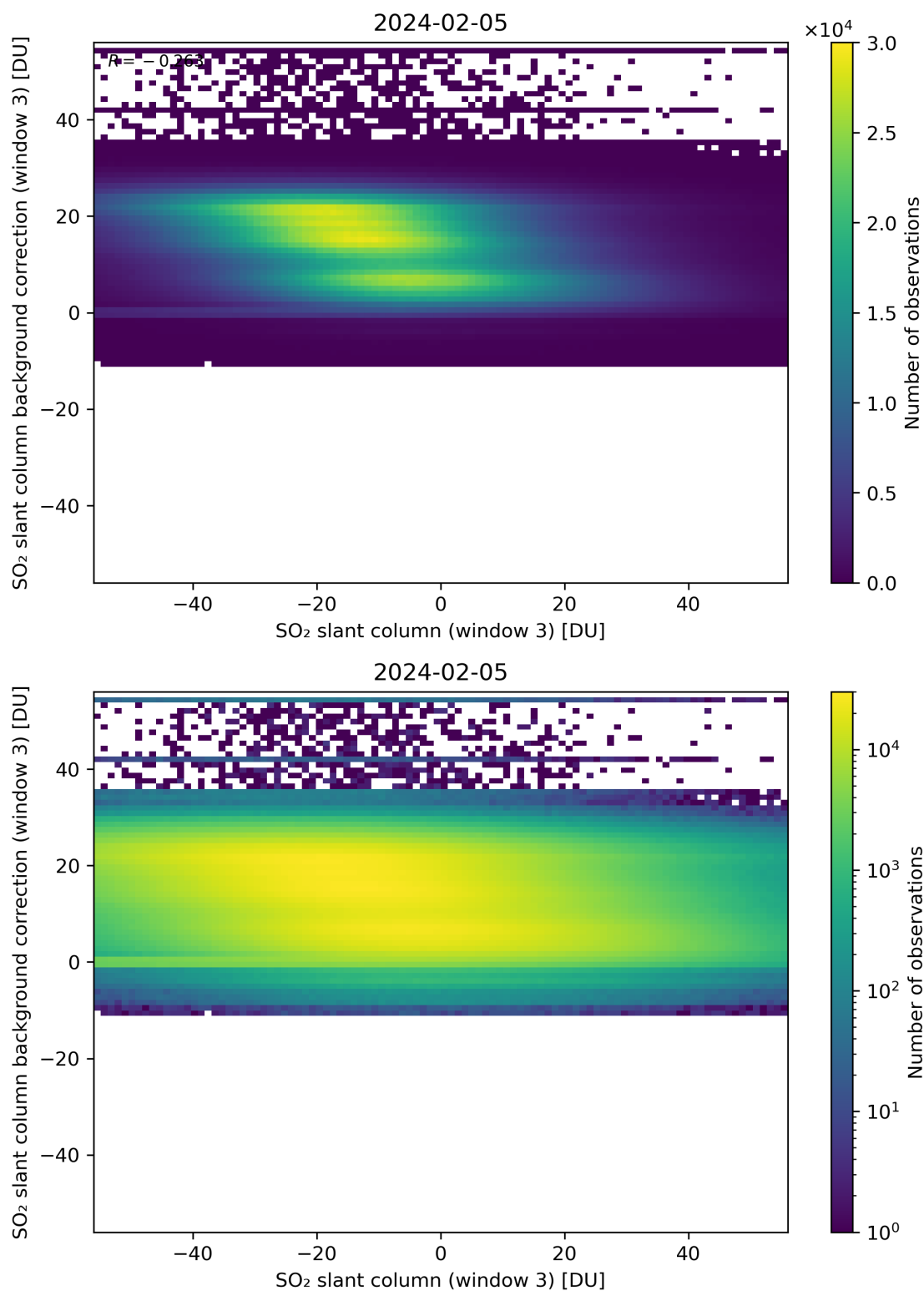
Figure 253: Scatter density plot of “SO 2 slant column (window 3)” against “SO 2 slant column background correction (window 3)” for 2024-02-04 to 2024-02-06.
