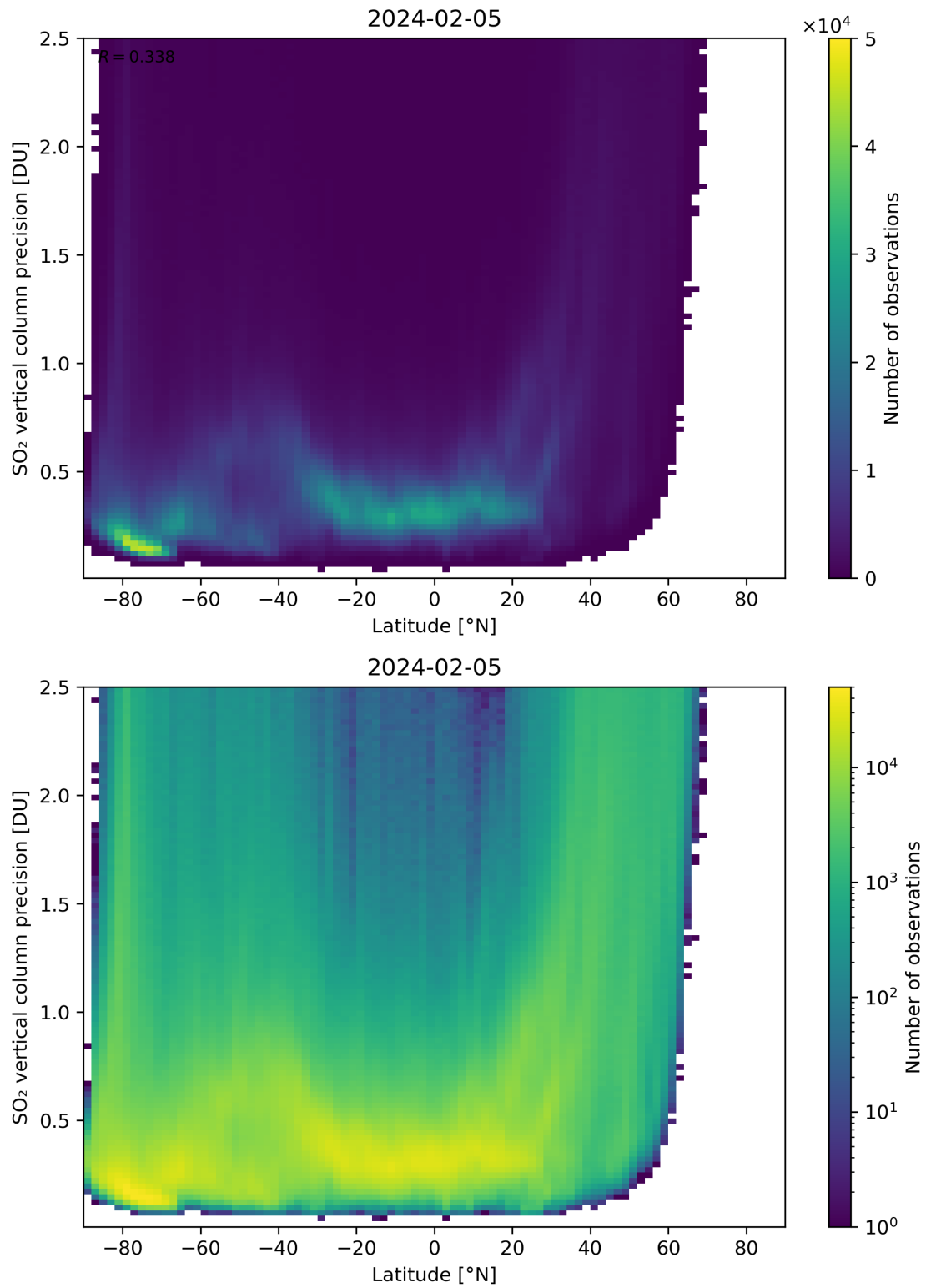
Figure 157: Scatter density plot of “Latitude” against “SO 2 vertical column precision” for 2024-02-04 to 2024-02-06.
