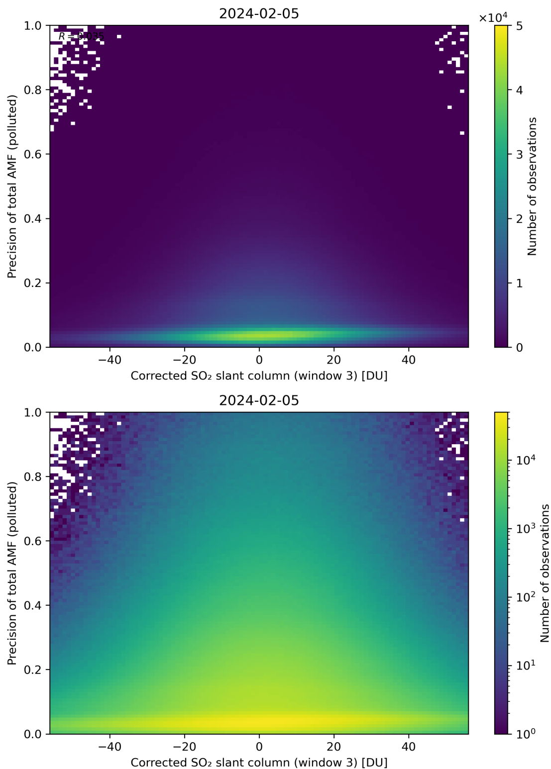
Figure 211: Scatter density plot of “Corrected SO 2 slant column (window 3)” against “Precision of total AMF (polluted)” for 2024-02-04 to 2024-02-06.
