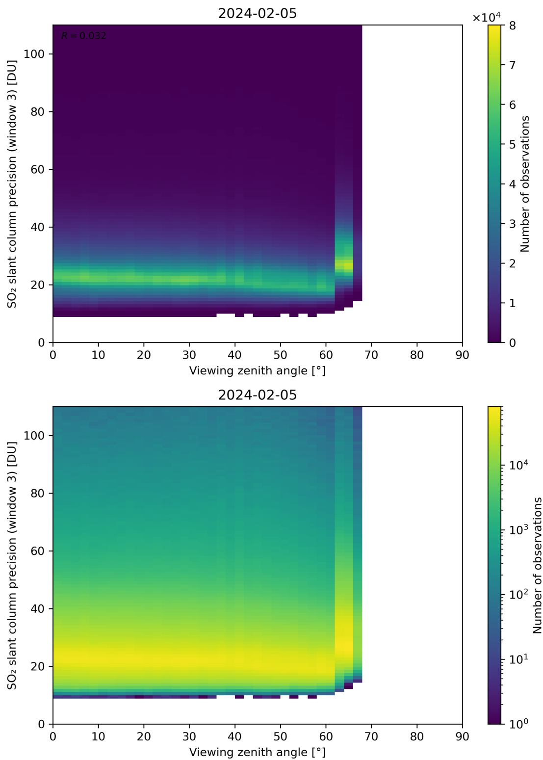
Figure 324: Scatter density plot of “Viewing zenith angle” against “SO 2 slant column precision (window 3)” for 2024-02-04 to 2024-02-06.
