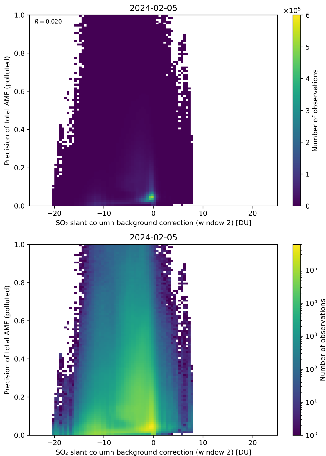
Figure 120: Scatter density plot of “SO 2 slant column background correction (window 2)” against “Precision of total AMF (polluted)” for 2024-02-04 to 2024-02-06.
