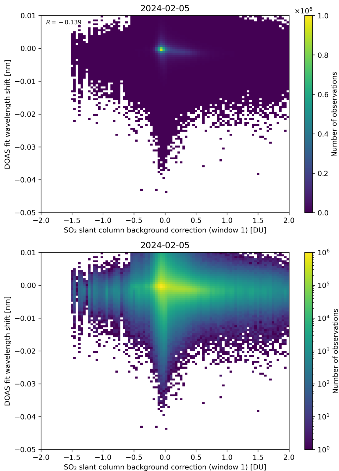
Figure 100: Scatter density plot of “SO 2 slant column background correction (window 1)” against “DOAS fit wavelength shift” for 2024-02-04 to 2024-02-06.
