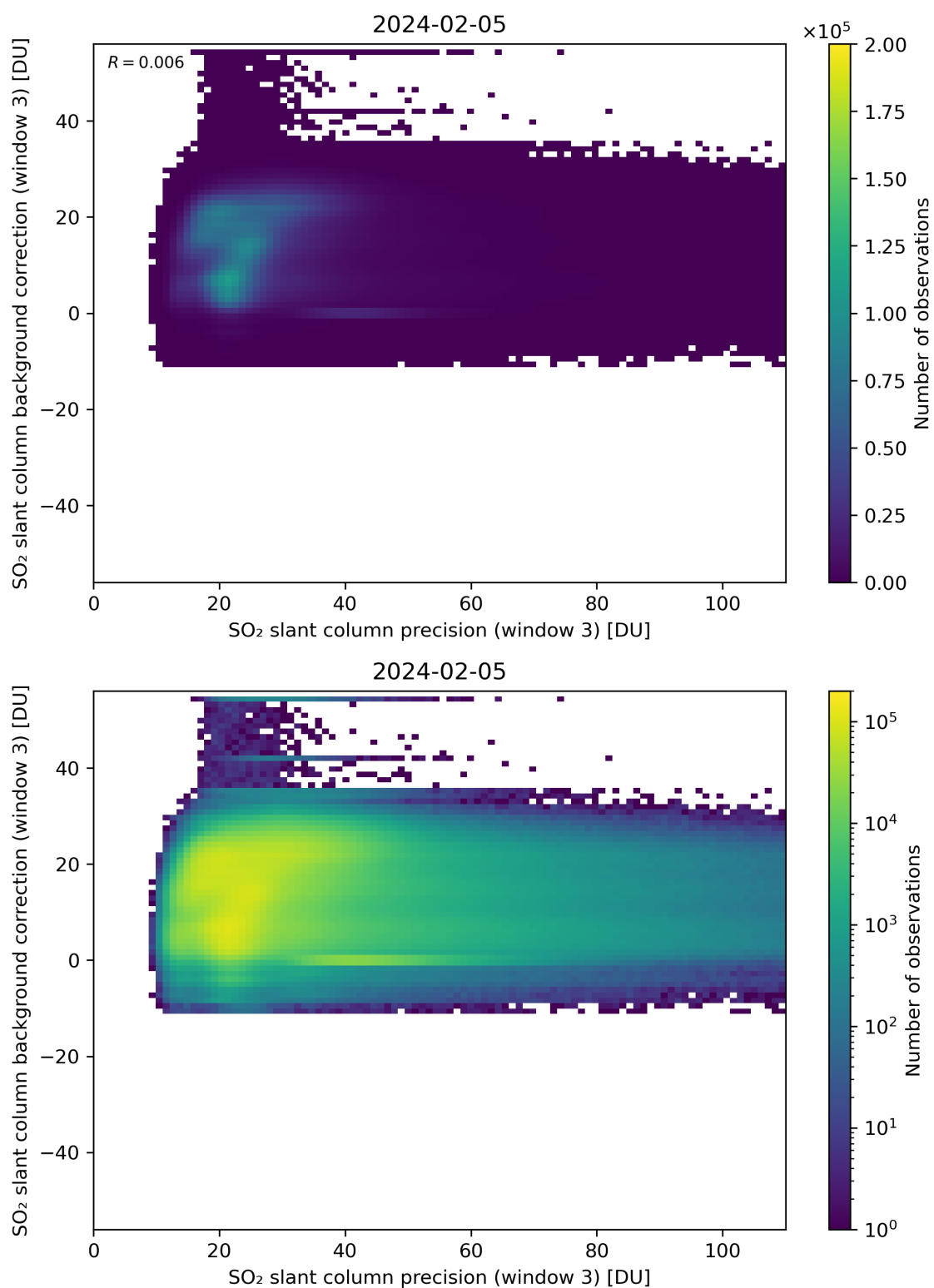
Figure 257: Scatter density plot of “SO 2 slant column precision (window 3)” against “SO 2 slant column background correction (window 3)” for 2024-02-04 to 2024-02-06.
