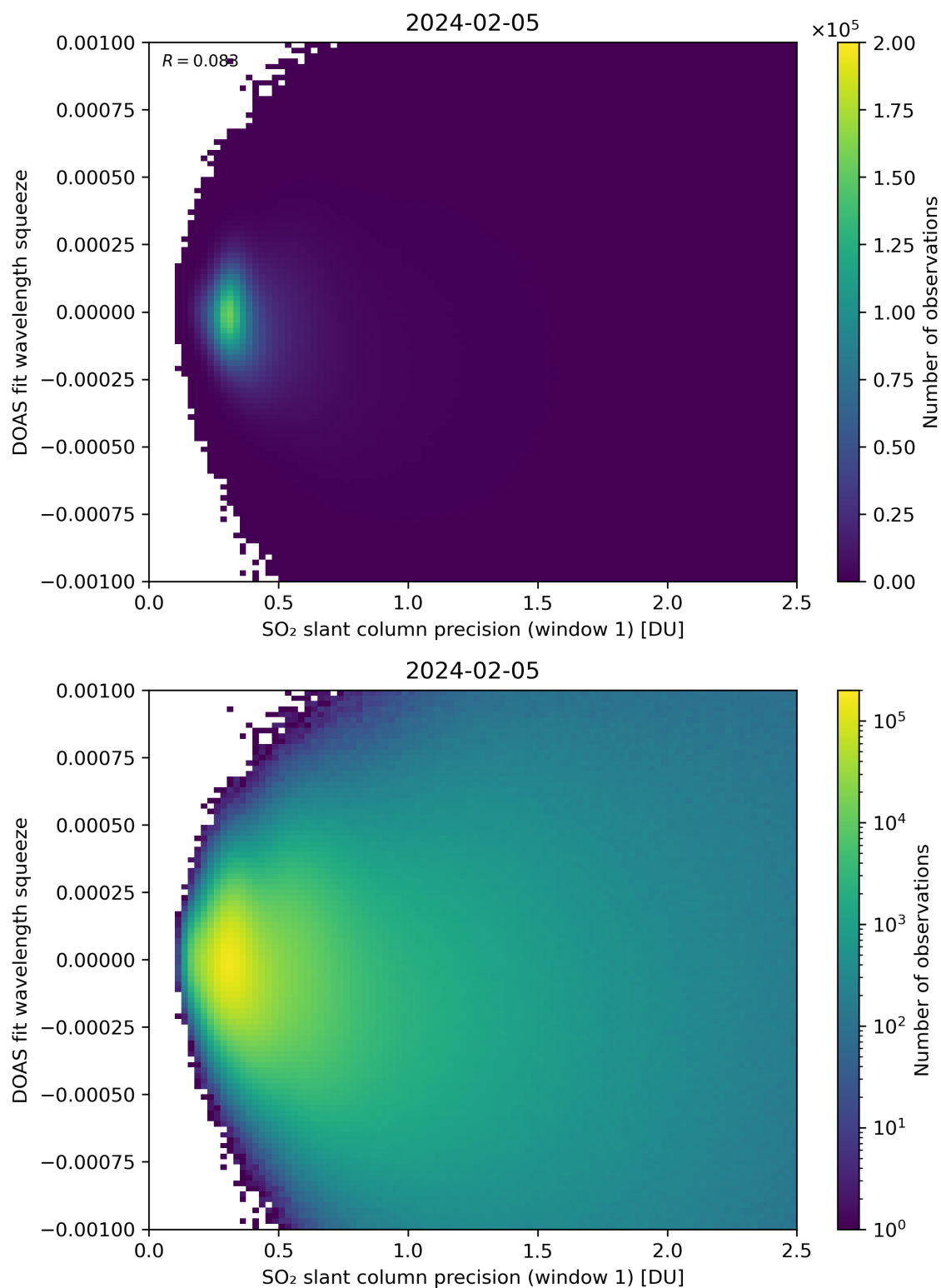
Figure 222: Scatter density plot of “SO 2 slant column precision (window 1)” against “DOAS fit wavelength squeeze” for 2024-02-04 to 2024-02-06.
