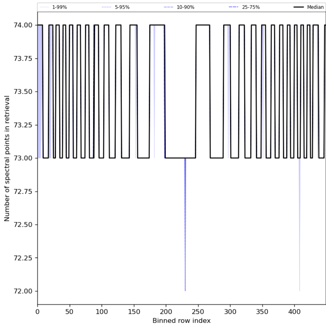
Figure 97: Along track statistics of “Number of spectral points in retrieval” for 2024-02-04 to 2024-02-06
