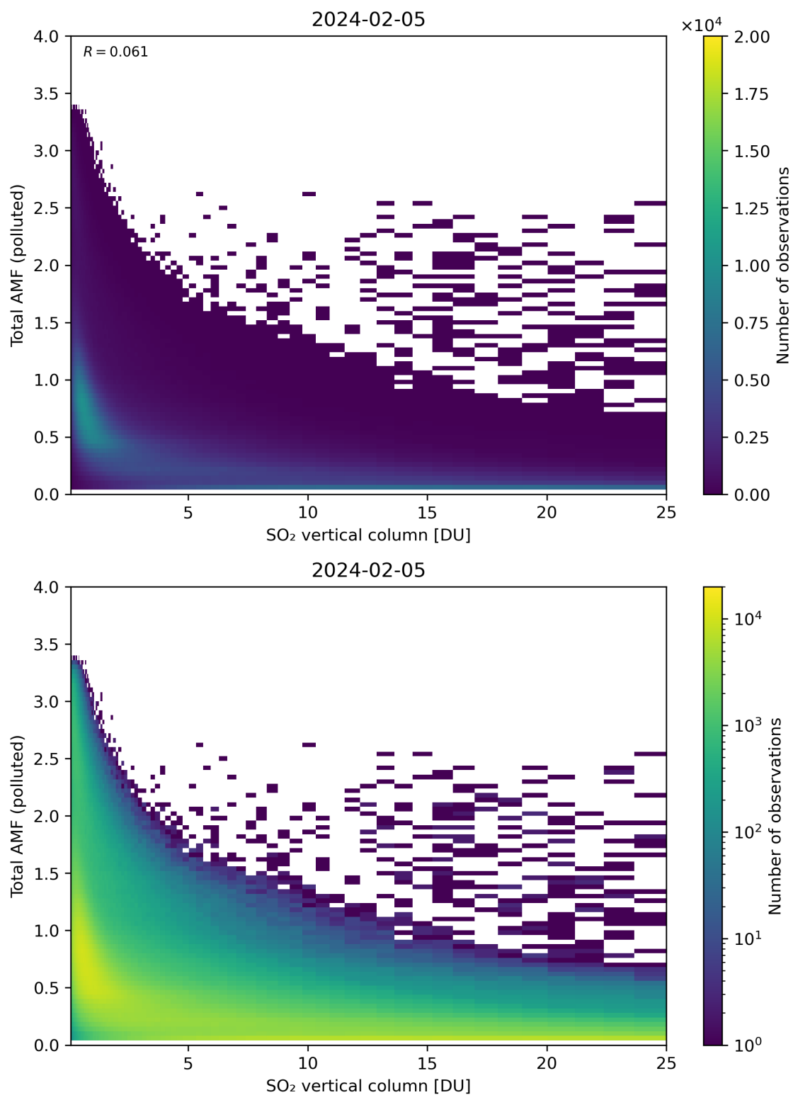
Figure 305: Scatter density plot of “SO 2 vertical column” against “Total AMF (polluted)” for 2024-02-04 to 2024-02-06.
