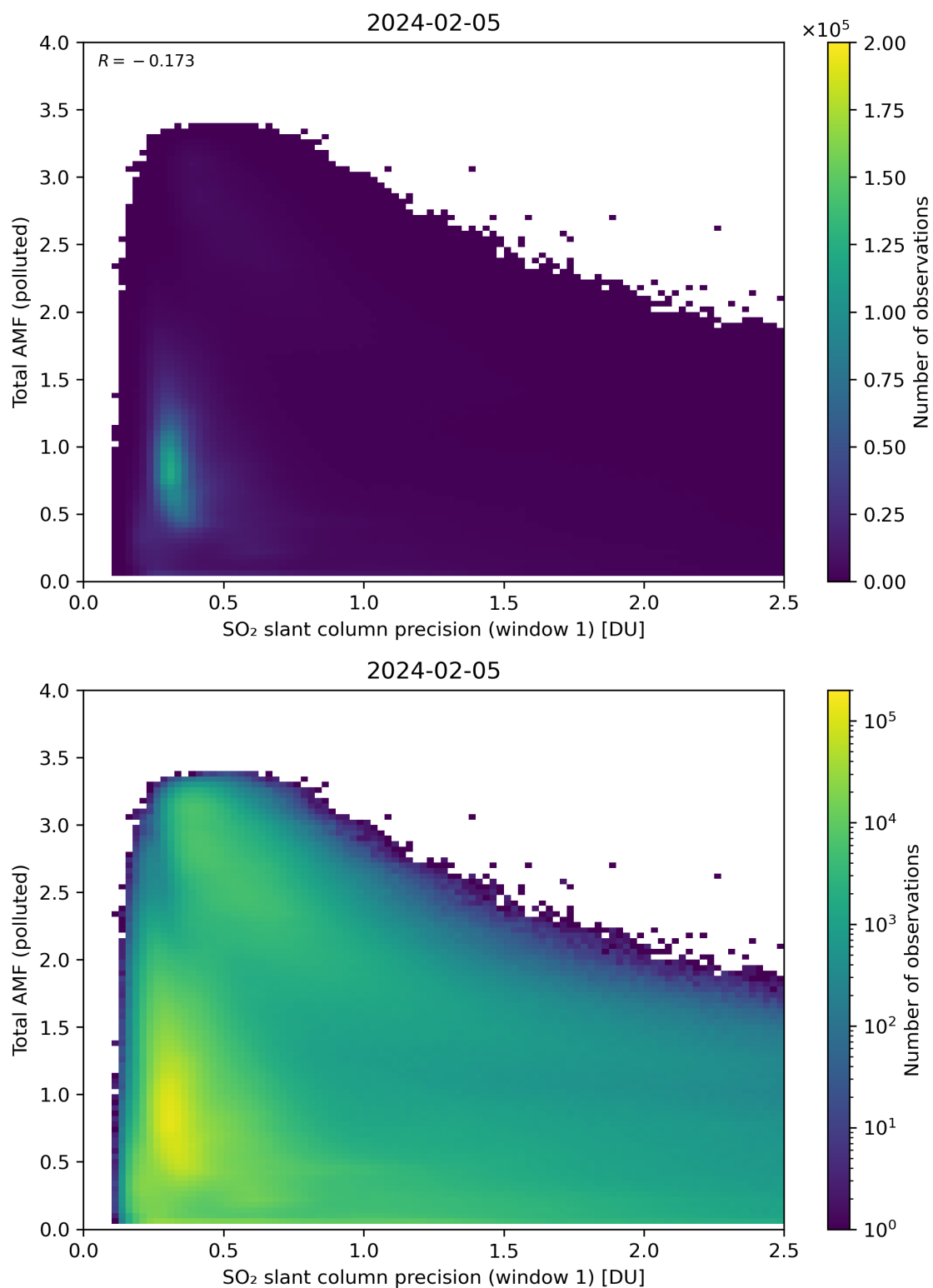
Figure 230: Scatter density plot of “SO 2 slant column precision (window 1)” against “Total AMF (polluted)” for 2024-02-04 to 2024-02-06.
