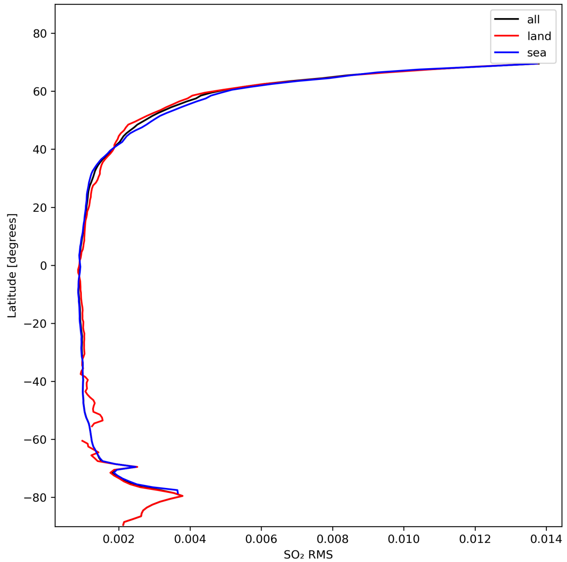
Figure 47: Zonal average of “SO 2 RMS” for 2024-02-04 to 2024-02-06.
