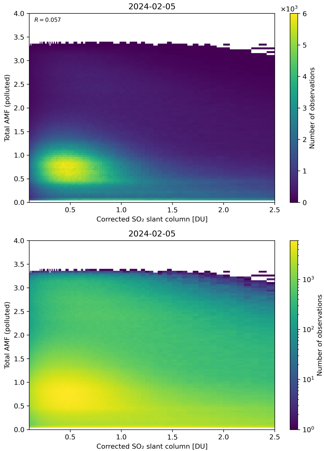
Figure 192: Scatter density plot of “Corrected SO 2 slant column” against “Total AMF (polluted)” for 2024-02-04 to 2024-02-06.
