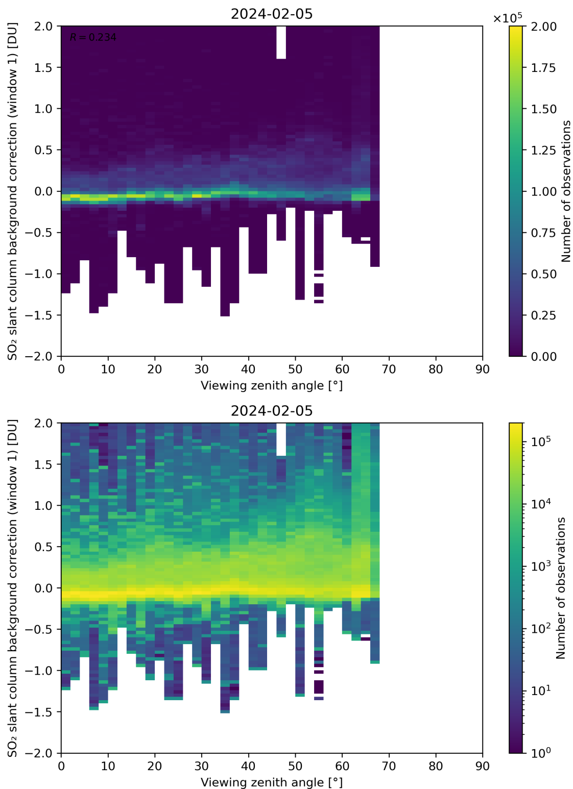
Figure 308: Scatter density plot of “Viewing zenith angle” against “SO 2 slant column background correction (window 1)” for 2024-02-04 to 2024-02-06.
