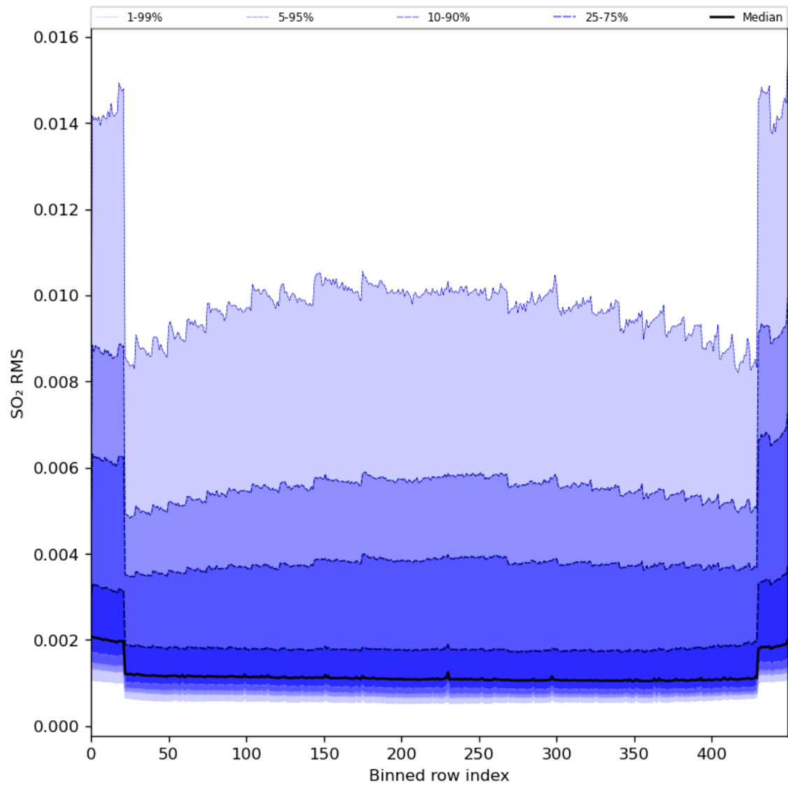
Figure 93: Along track statistics of “SO 2 RMS” for 2024-02-04 to 2024-02-06
