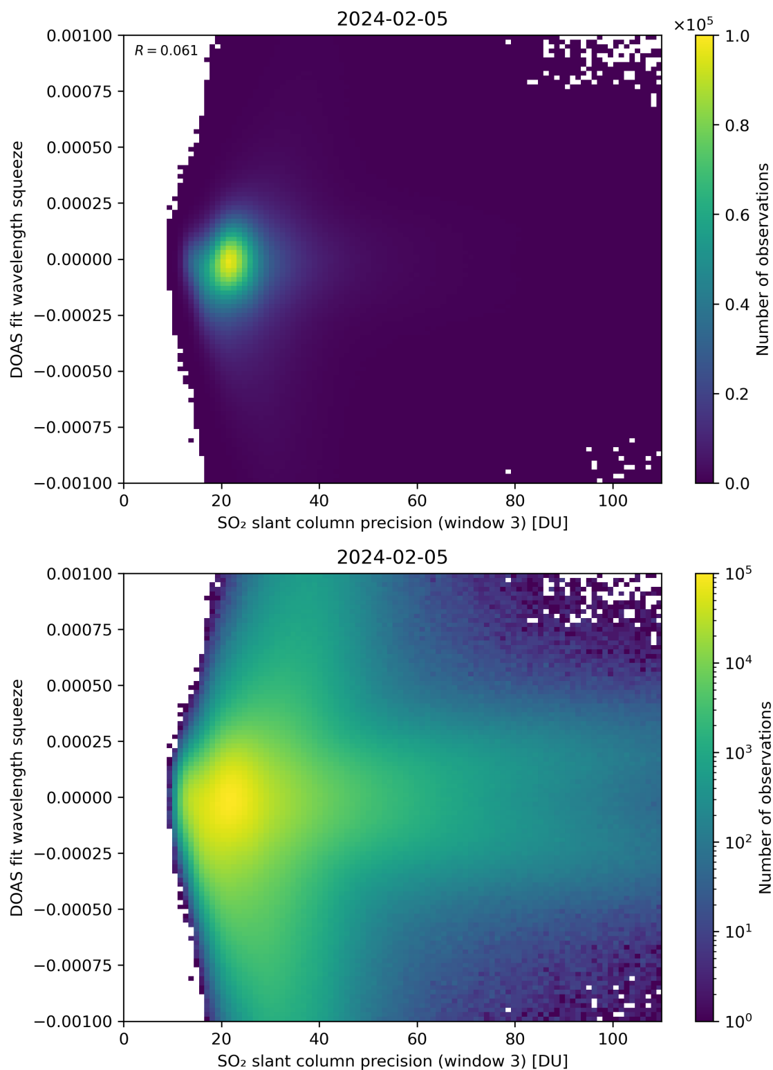
Figure 259: Scatter density plot of “SO 2 slant column precision (window 3)” against “DOAS fit wavelength squeeze” for 2024-02-04 to 2024-02-06.
