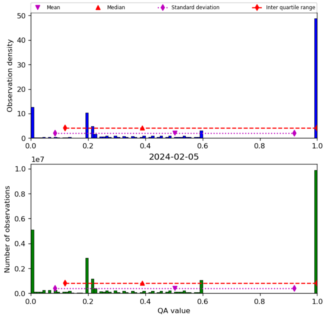
Figure 52: Histogram of “QA value” for 2024-02-04 to 2024-02-06
