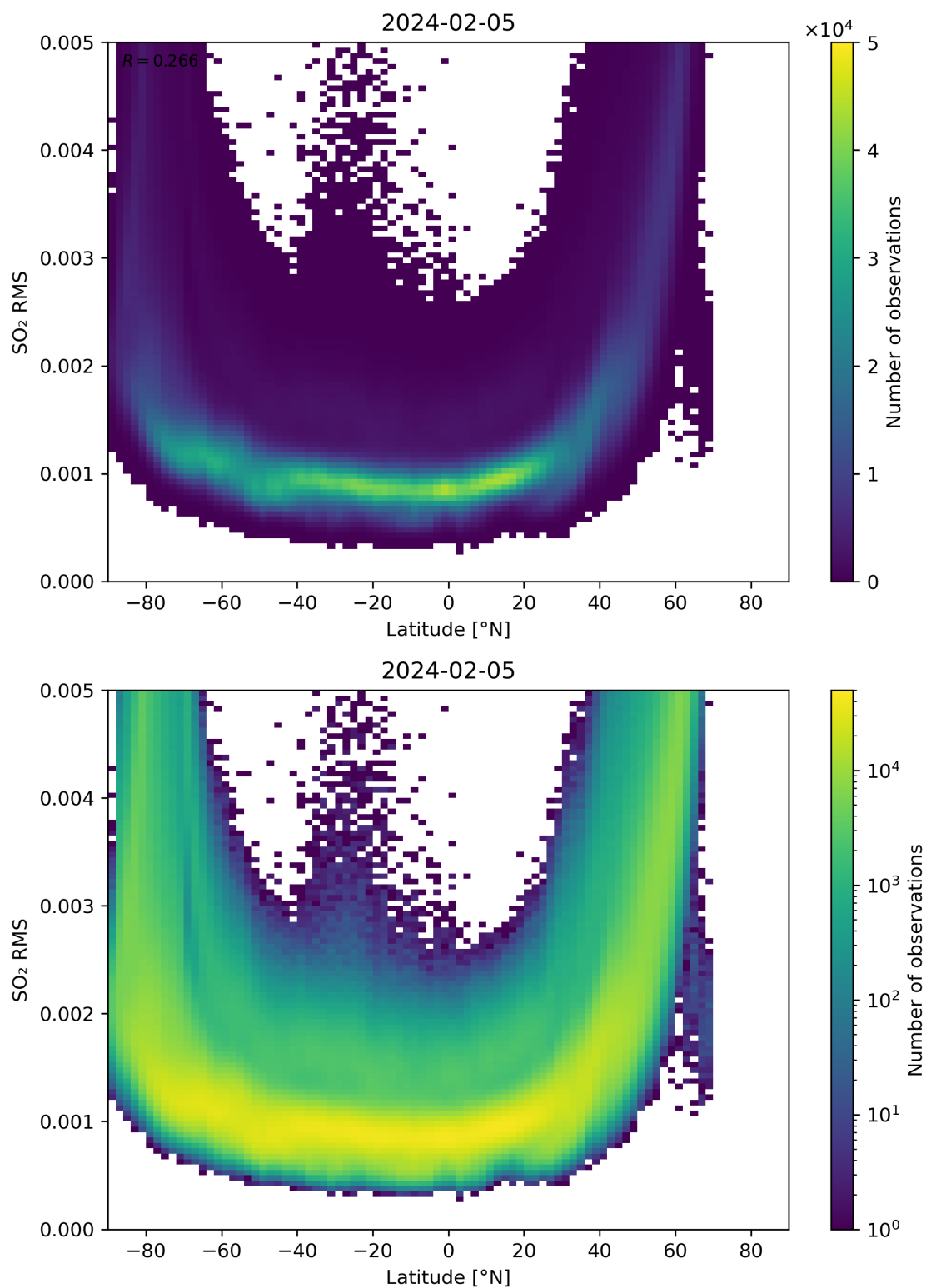
Figure 144: Scatter density plot of “Latitude” against “SO 2 RMS” for 2024-02-04 to 2024-02-06.
