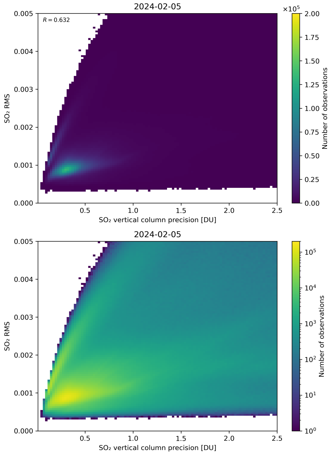
Figure 284: Scatter density plot of “SO 2 vertical column precision” against “SO 2 RMS” for 2024-02-04 to 2024-02-06.
