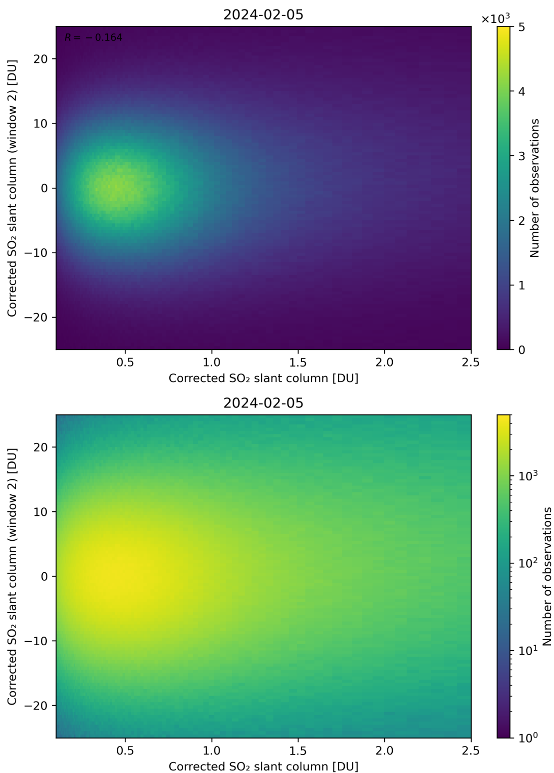
Figure 185: Scatter density plot of “Corrected SO 2 slant column” against “Corrected SO 2 slant column (window 2)” for 2024-02-04 to 2024-02-06.
