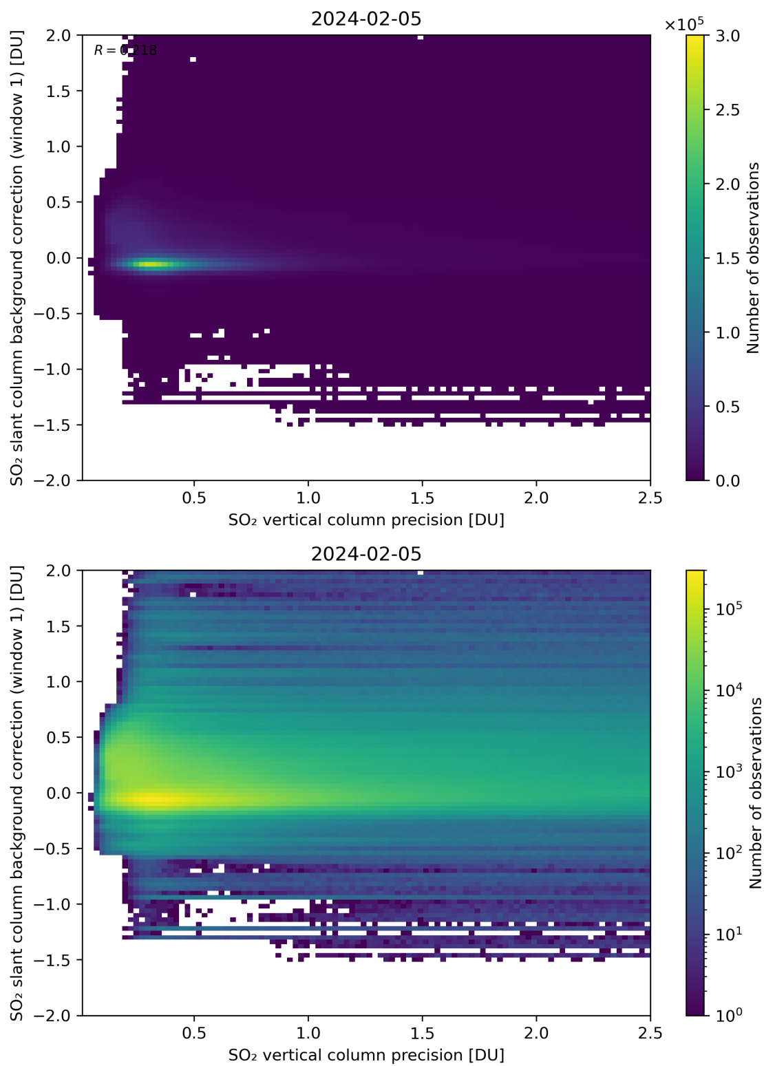
Figure 279: Scatter density plot of “SO 2 vertical column precision” against “SO 2 slant column background correction (window 1)” for 2024-02-04 to 2024-02-06.
