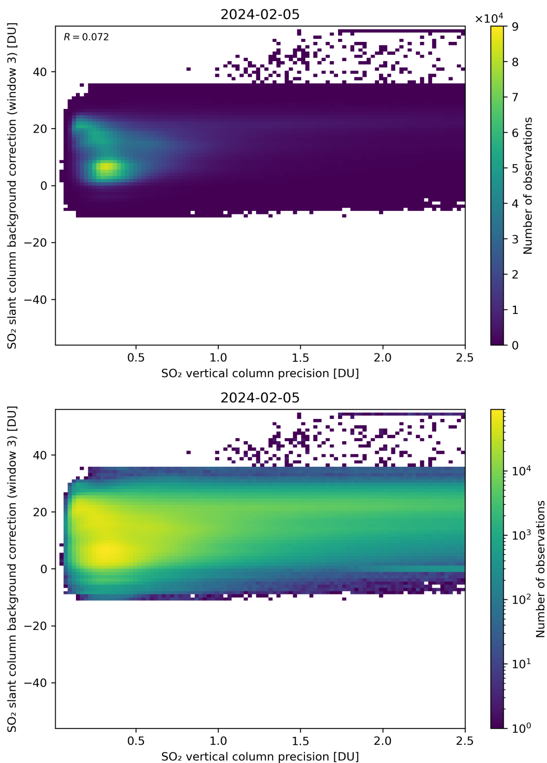
Figure 281: Scatter density plot of “SO 2 vertical column precision” against “SO 2 slant column background correction (window 3)” for 2024-02-04 to 2024-02-06.
