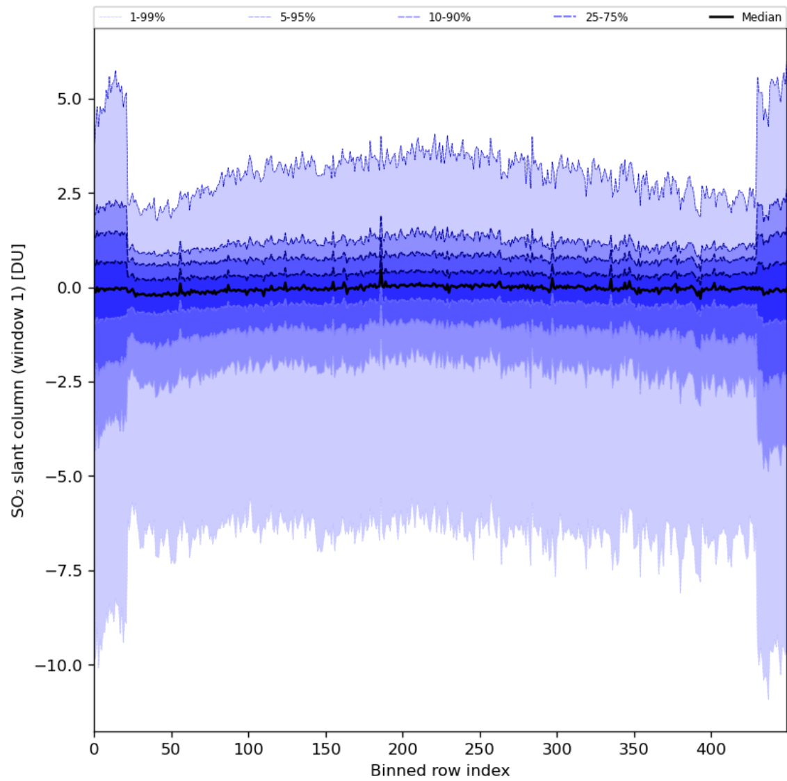
Figure 79: Along track statistics of “SO 2 slant column (window 1)” for 2024-02-04 to 2024-02-06
