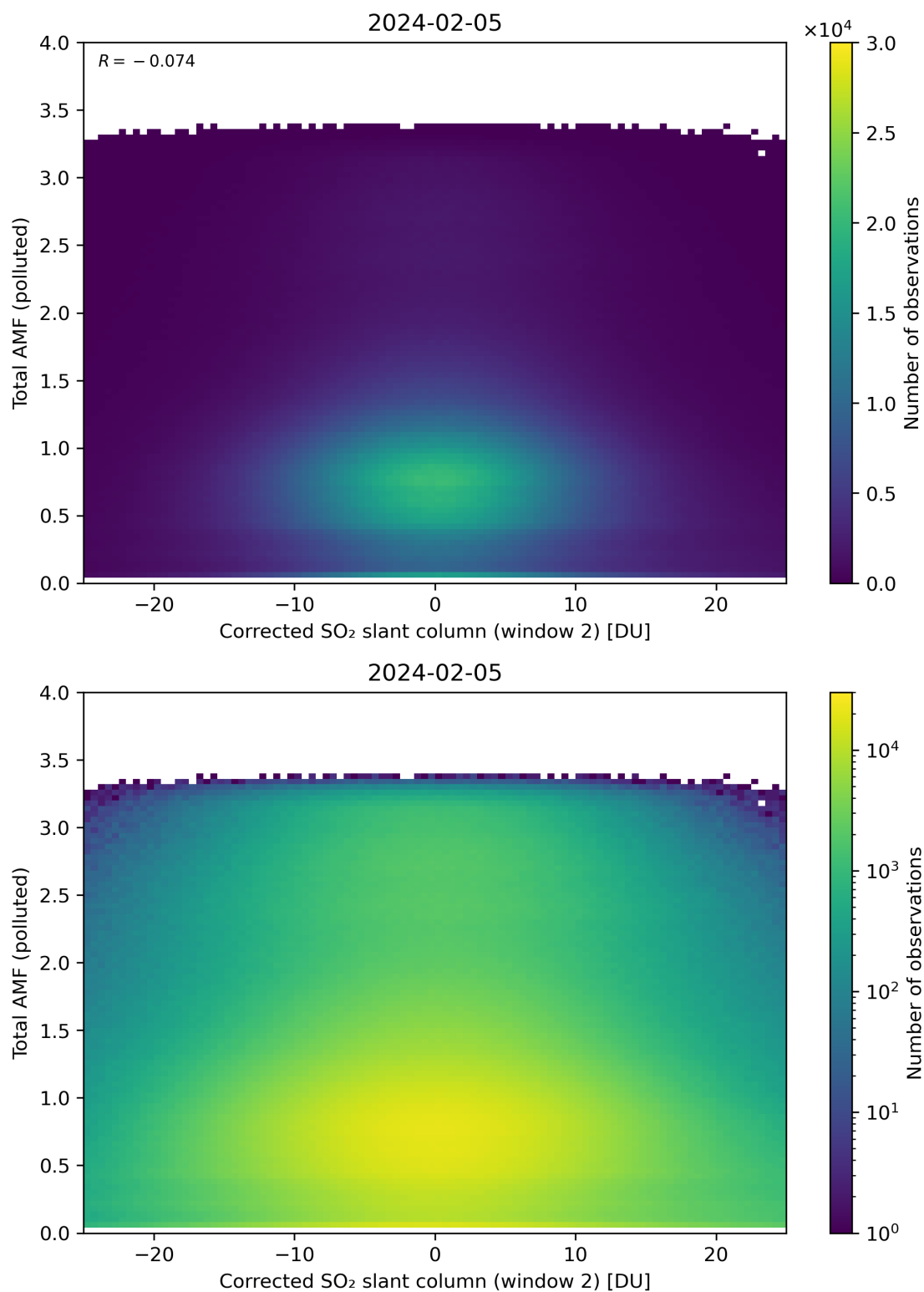
Figure 203: Scatter density plot of “Corrected SO 2 slant column (window 2)” against “Total AMF (polluted)” for 2024-02-04 to 2024-02-06.
