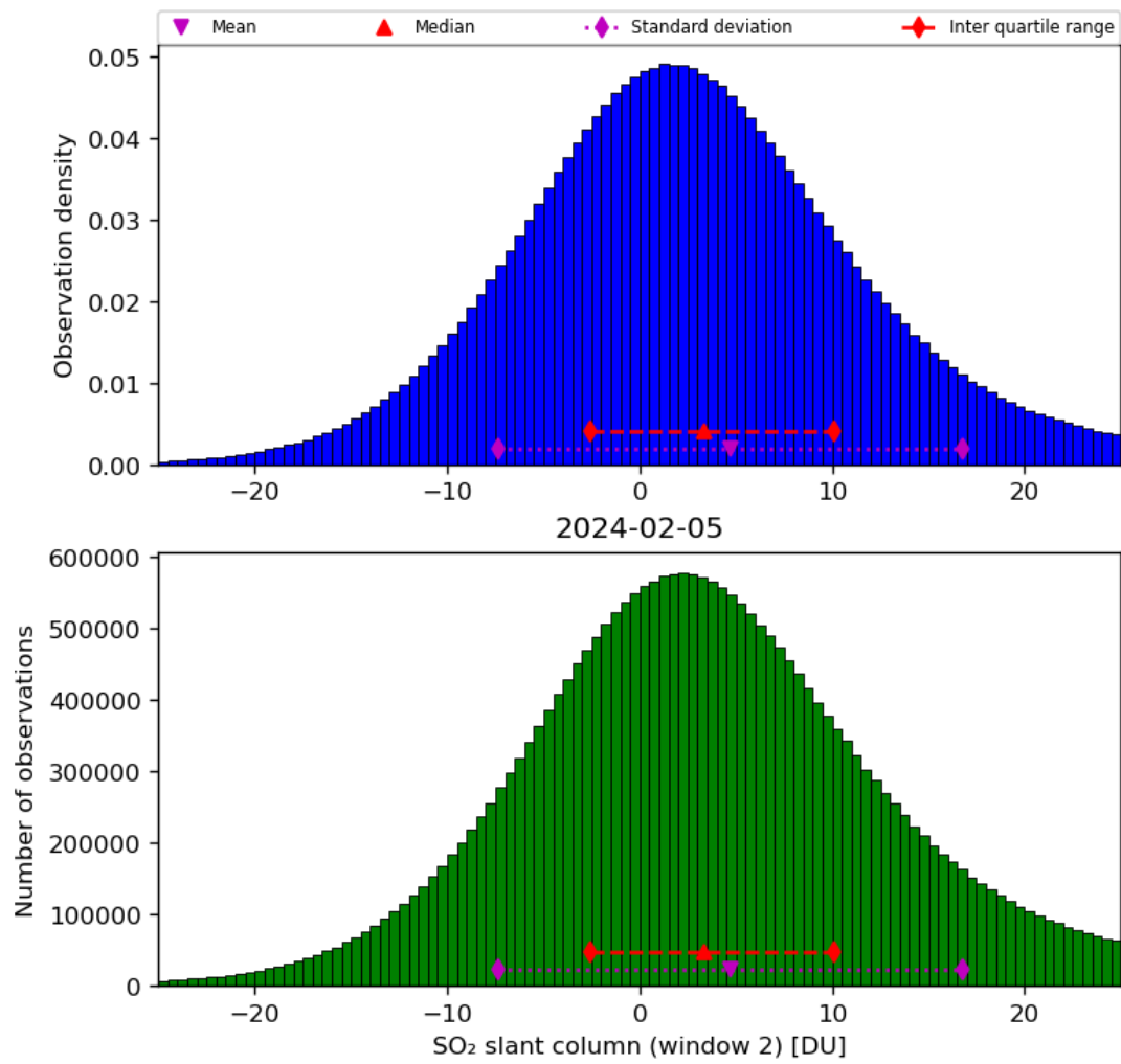
Figure 60: Histogram of “SO 2 slant column (window 2)” for 2024-02-04 to 2024-02-06
