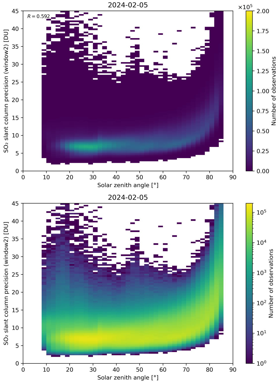
Figure 171: Scatter density plot of “Solar zenith angle” against “SO 2 slant column precision (window2)” for 2024-02-04 to 2024-02-06.
