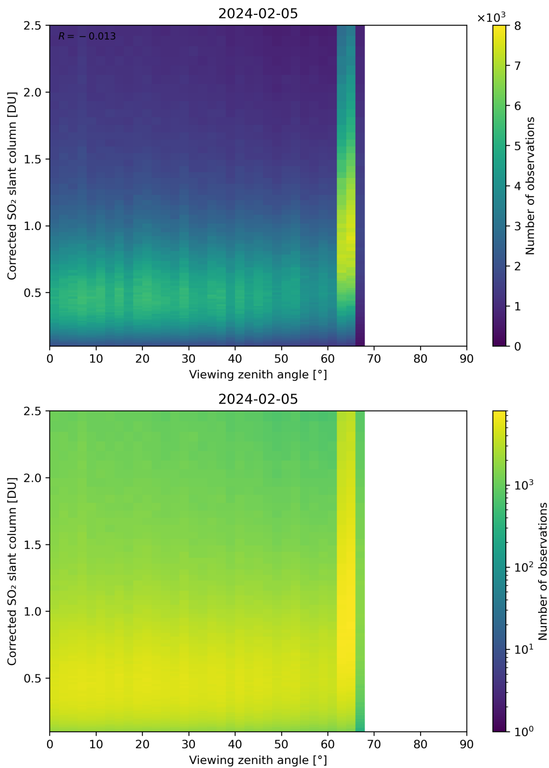
Figure 317: Scatter density plot of “Viewing zenith angle” against “Corrected SO 2 slant column” for 2024-02-04 to 2024-02-06.
