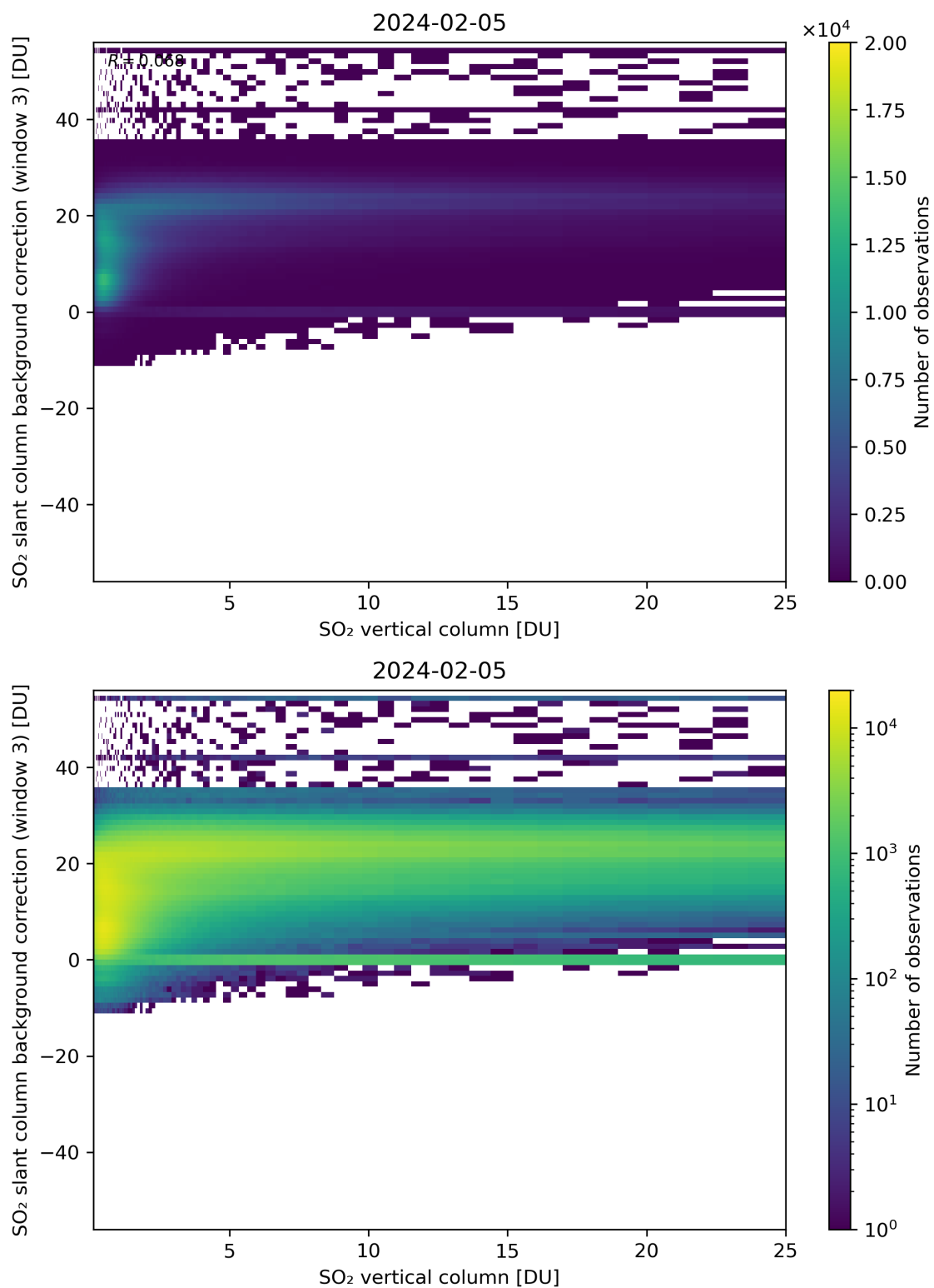
Figure 275: Scatter density plot of “SO 2 vertical column” against “SO 2 slant column background correction (window 3)” for 2024-02-04 to 2024-02-06.
