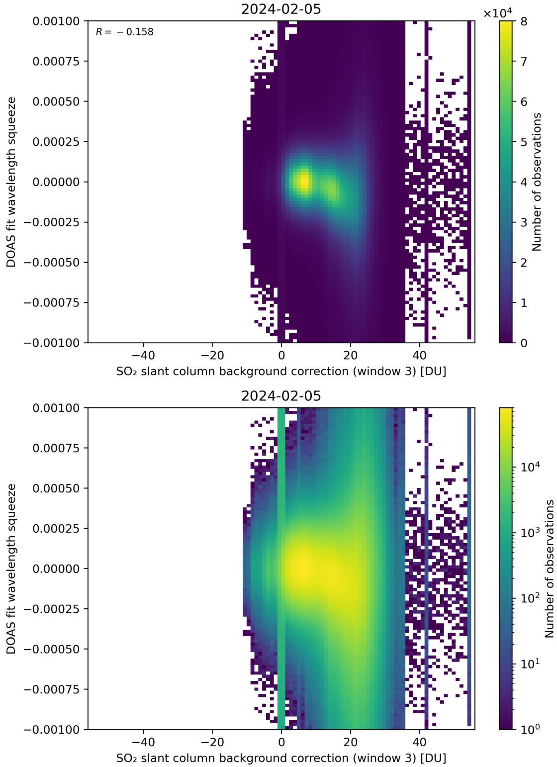
Figure 122: Scatter density plot of “SO 2 slant column background correction (window 3)” against “DOAS fit wavelength squeeze” for 2024-02-04 to 2024-02-06.
