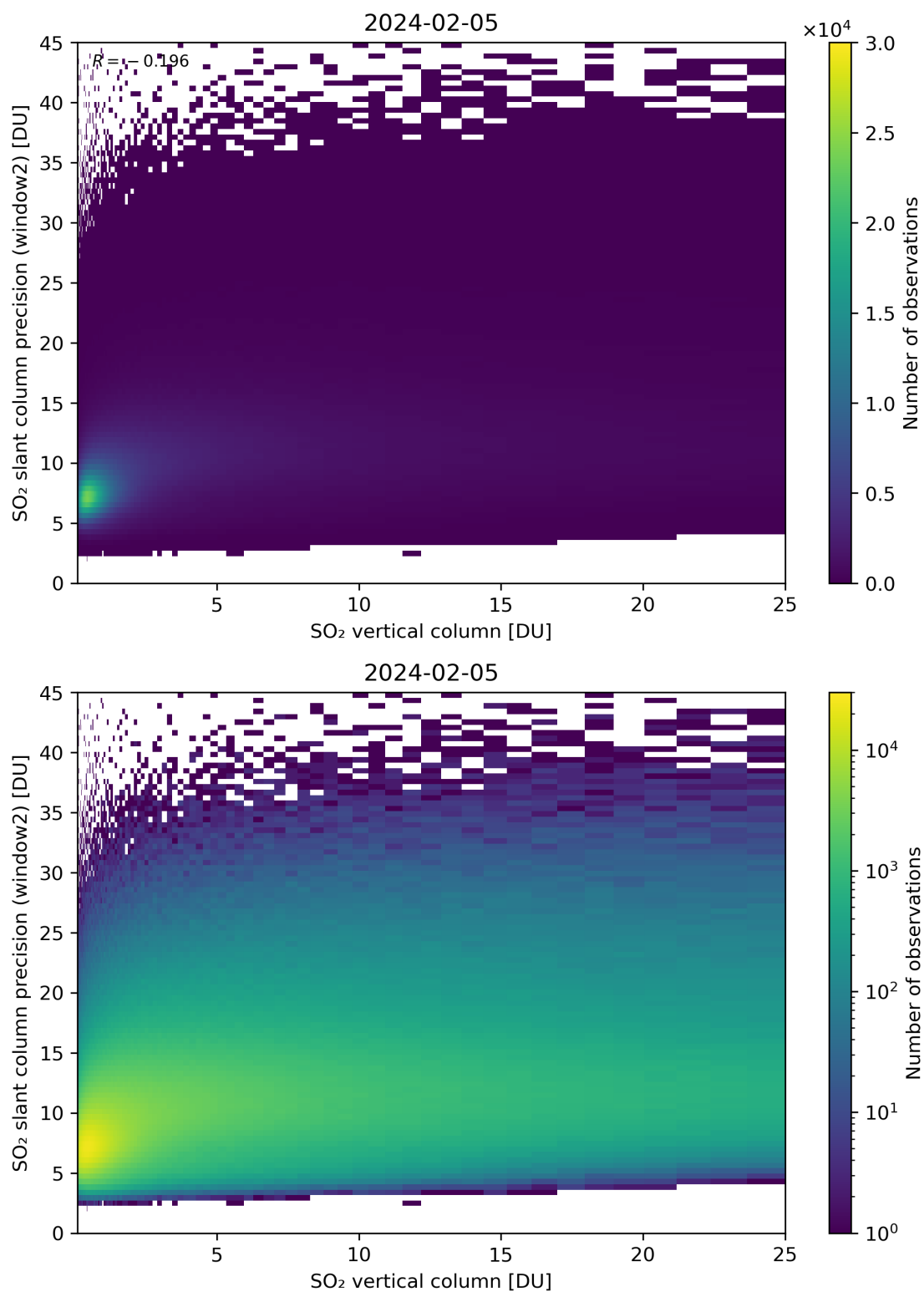
Figure 302: Scatter density plot of “SO 2 vertical column” against “SO 2 slant column precision (window2)” for 2024-02-04 to 2024-02-06.
