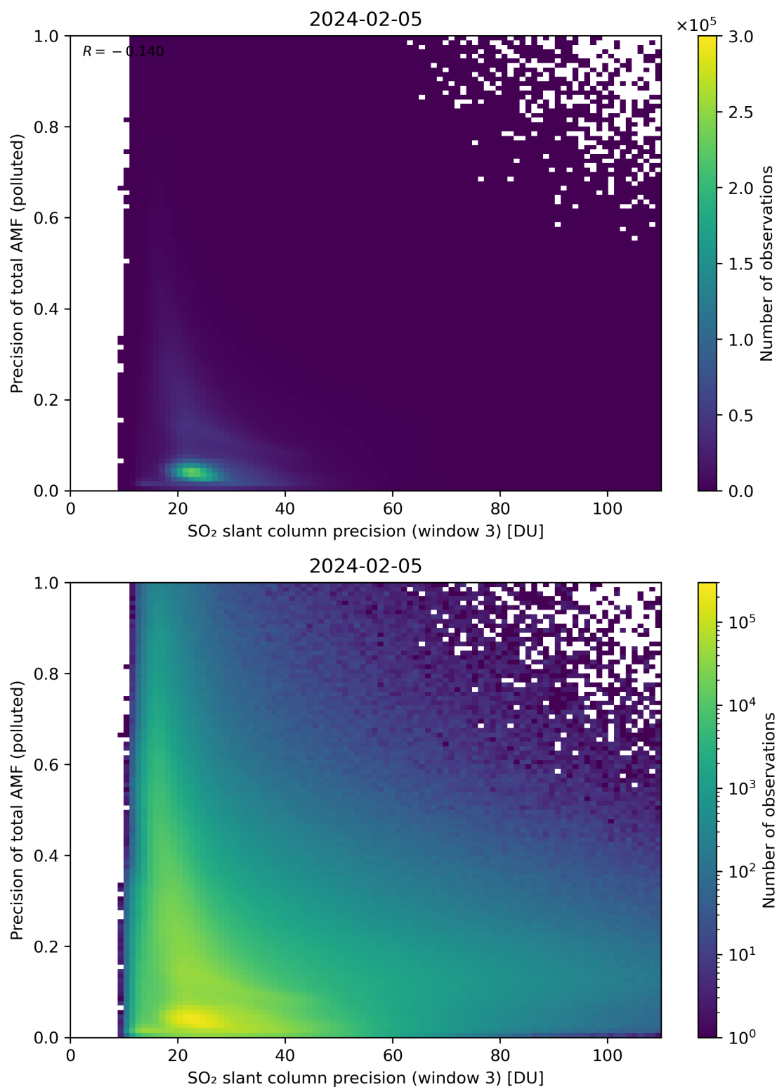
Figure 264: Scatter density plot of “SO 2 slant column precision (window 3)” against “Precision of total AMF (polluted)” for 2024-02-04 to 2024-02-06.
