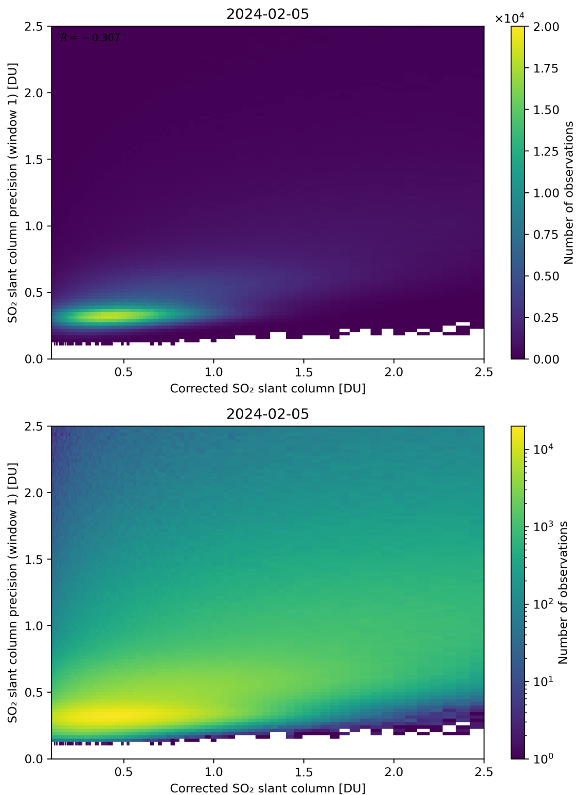
Figure 188: Scatter density plot of “Corrected SO 2 slant column” against “SO 2 slant column precision (window 1)” for 2024-02-04 to 2024-02-06.
