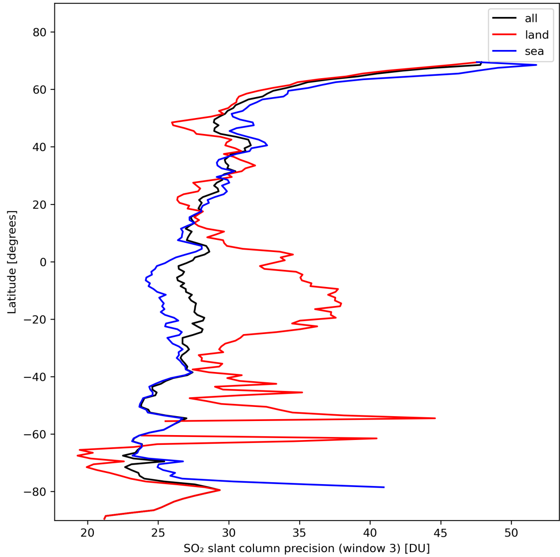
Figure 42: Zonal average of “SO 2 slant column precision (window 3)” for 2024-02-04 to 2024-02-06.
