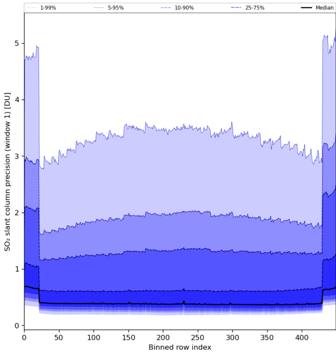
Figure 80: Along track statistics of “SO 2 slant column precision (window 1)” for 2024-02-04 to 2024-02-06
