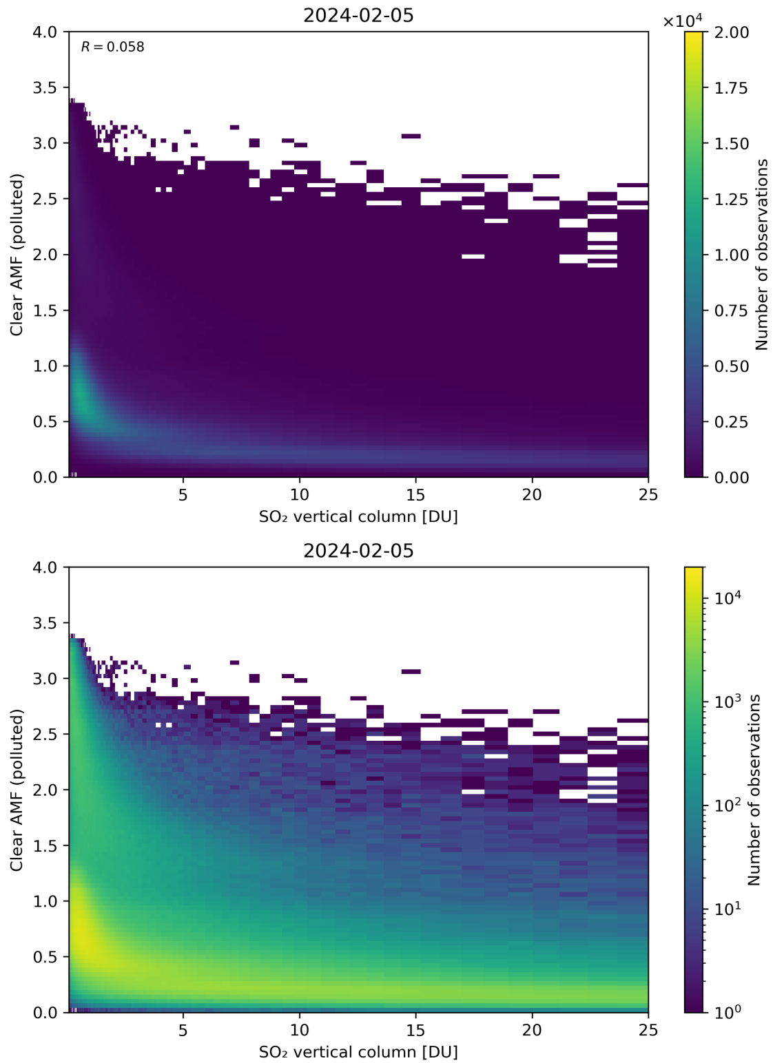
Figure 296: Scatter density plot of “SO 2 vertical column” against “Clear AMF (polluted)” for 2024-02-04 to 2024-02-06.
