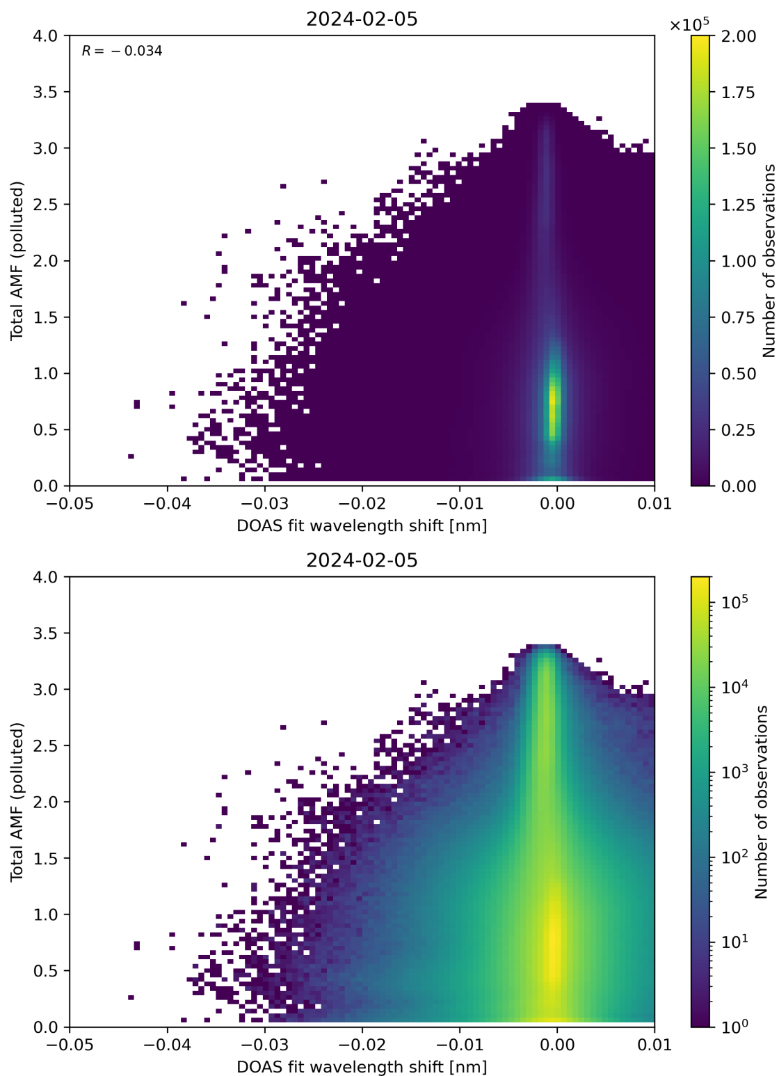
Figure 130: Scatter density plot of “DOAS fit wavelength shift” against “Total AMF (polluted)” for 2024-02-04 to 2024-02-06.
