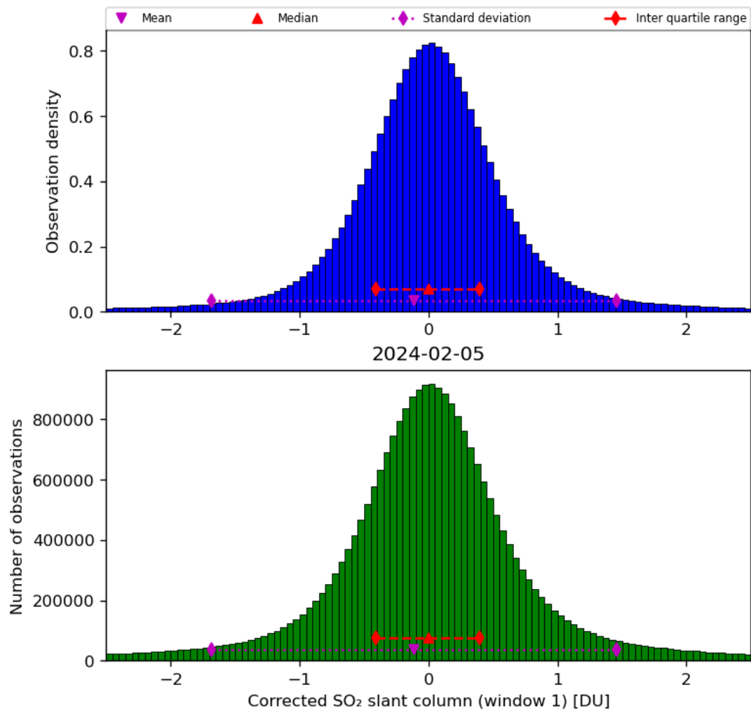
Figure 58: Histogram of “Corrected SO 2 slant column (window 1)” for 2024-02-04 to 2024-02-06
