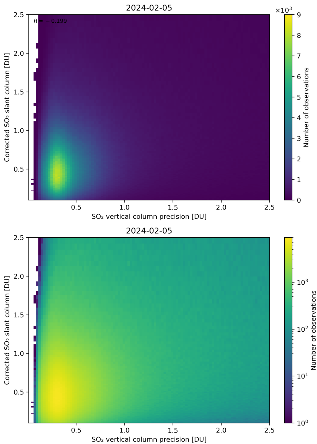
Figure 286: Scatter density plot of “SO 2 vertical column precision” against “Corrected SO 2 slant column” for 2024-02-04 to 2024-02-06.
