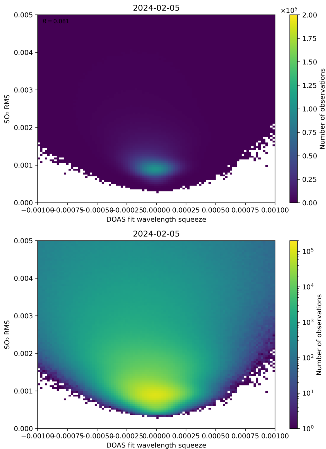
Figure 132: Scatter density plot of “DOAS fit wavelength squeeze” against “SO 2 RMS” for 2024-02-04 to 2024-02-06.
