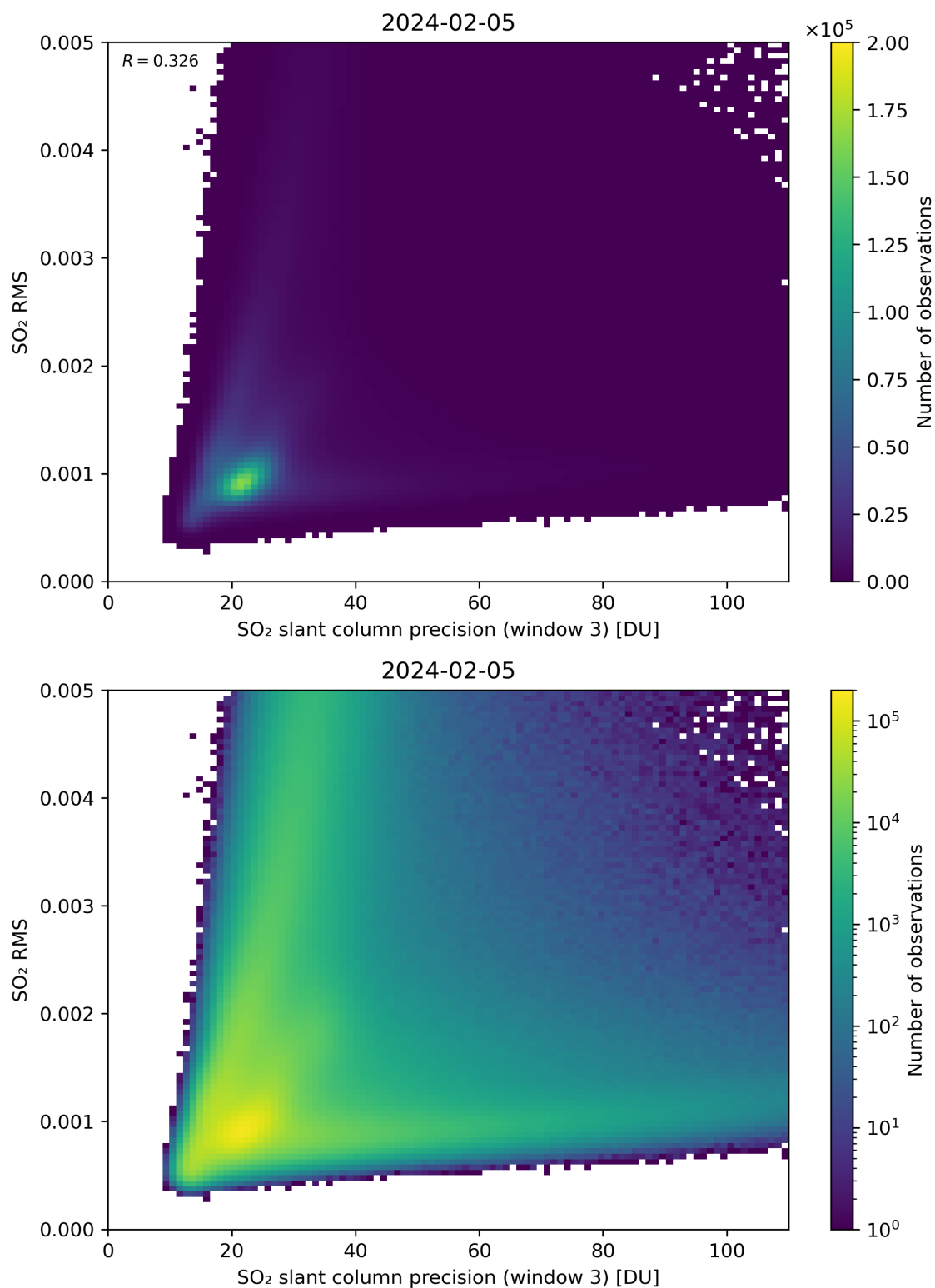
Figure 260: Scatter density plot of “SO 2 slant column precision (window 3)” against “SO 2 RMS” for 2024-02-04 to 2024-02-06.
