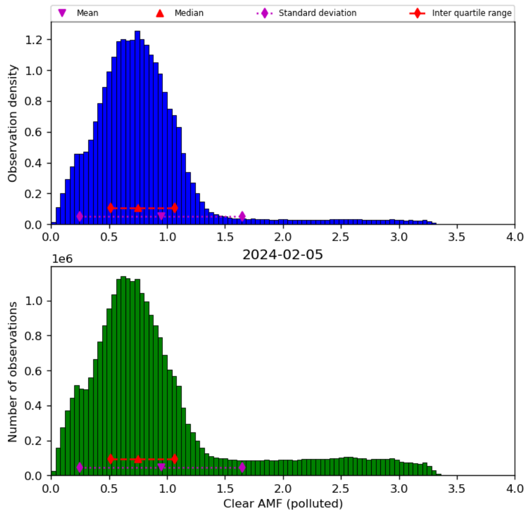
Figure 73: Histogram of “Clear AMF (polluted)” for 2024-02-04 to 2024-02-06
