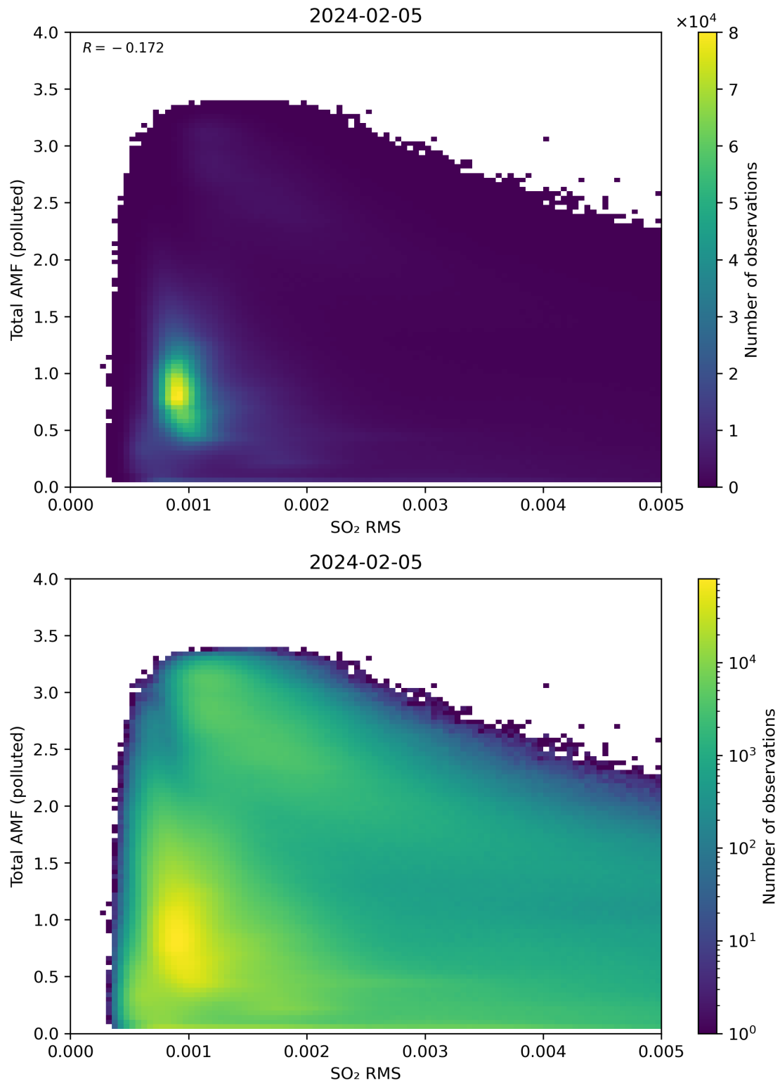
Figure 137: Scatter density plot of “SO 2 RMS” against “Total AMF (polluted)” for 2024-02-04 to 2024-02-06.
