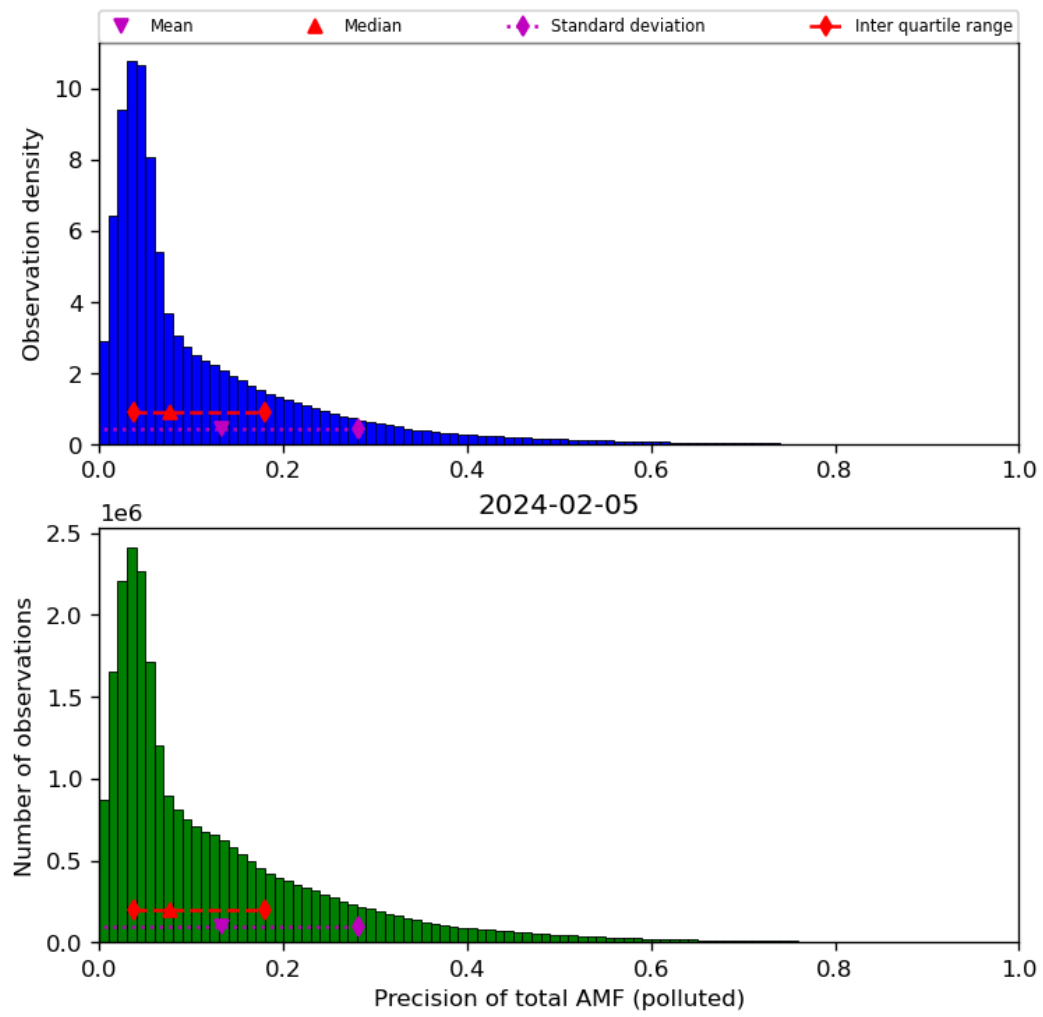
Figure 72: Histogram of “Precision of total AMF (polluted)” for 2024-02-04 to 2024-02-06
