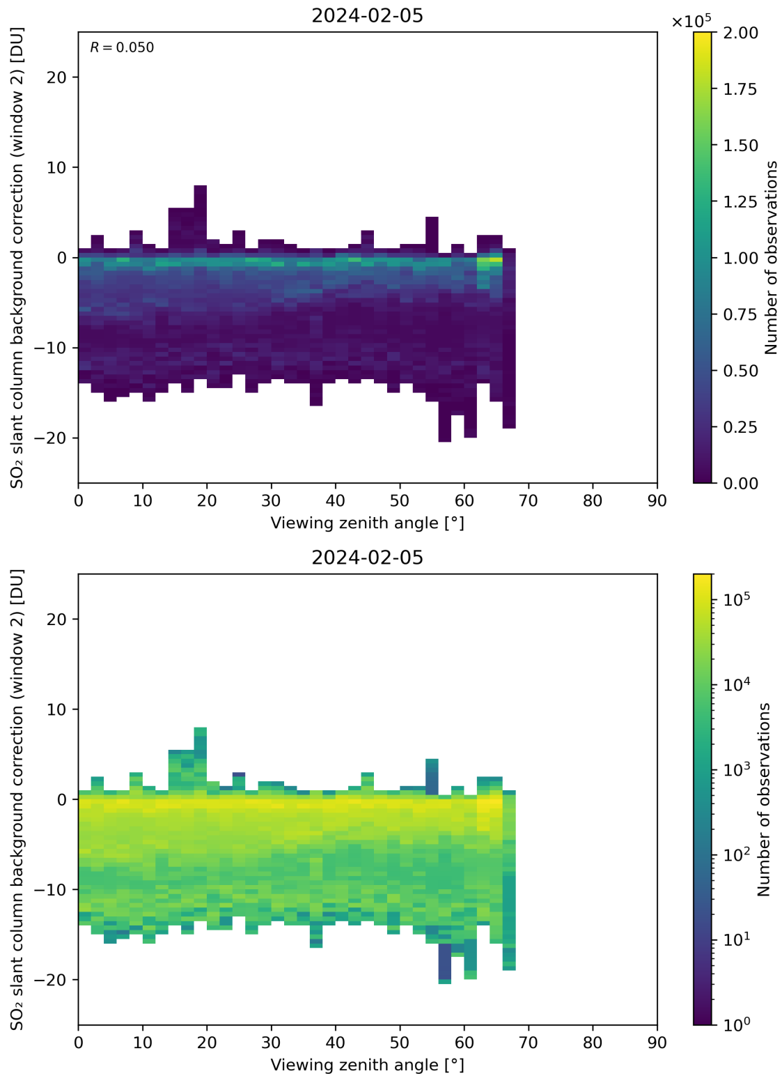
Figure 309: Scatter density plot of “Viewing zenith angle” against “SO 2 slant column background correction (window 2)” for 2024-02-04 to 2024-02-06.
