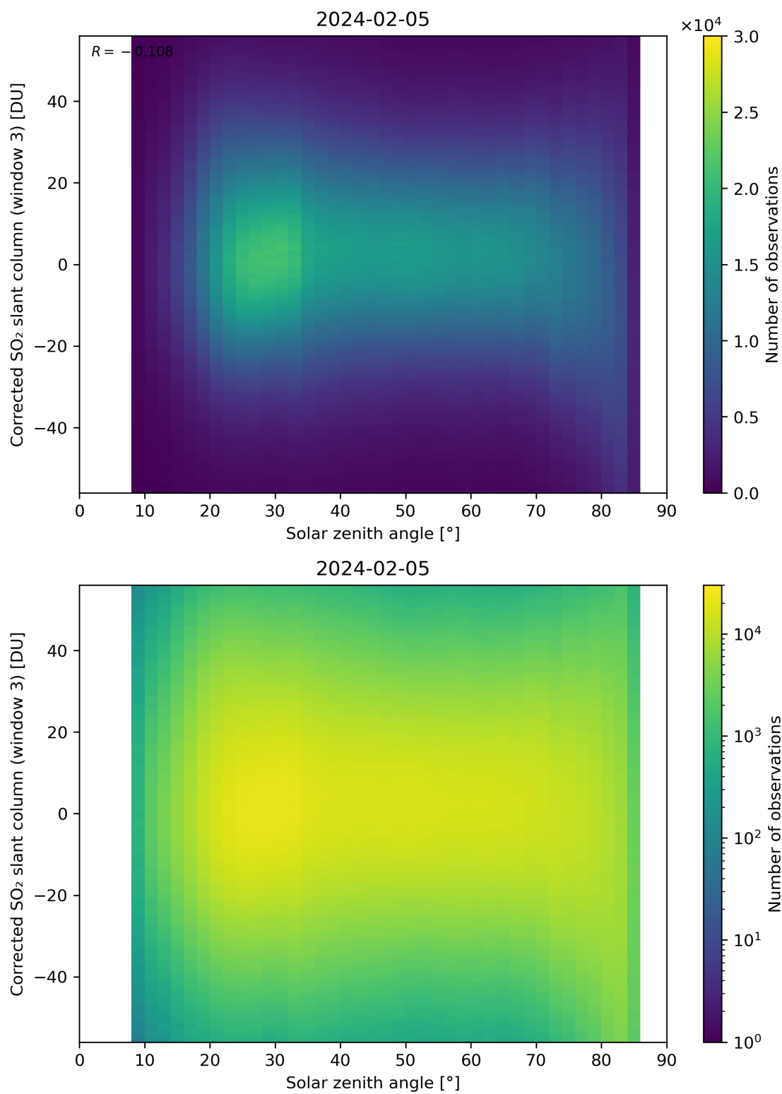
Figure 168: Scatter density plot of “Solar zenith angle” against “Corrected SO 2 slant column (window 3)” for 2024-02-04 to 2024-02-06.
