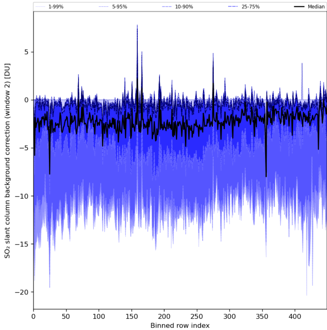
Figure 86: Along track statistics of “SO 2 slant column background correction (window 2)” for 2024-02-04 to 2024-02-06
