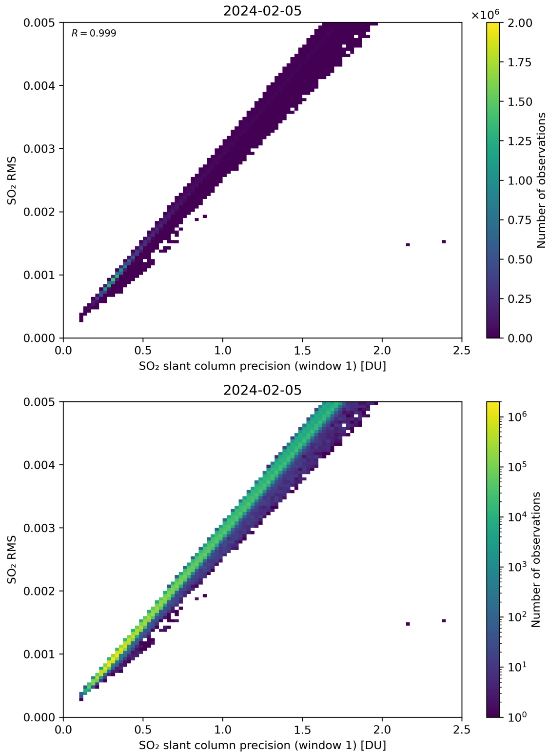
Figure 223: Scatter density plot of “SO 2 slant column precision (window 1)” against “SO 2 RMS” for 2024-02-04 to 2024-02-06.
