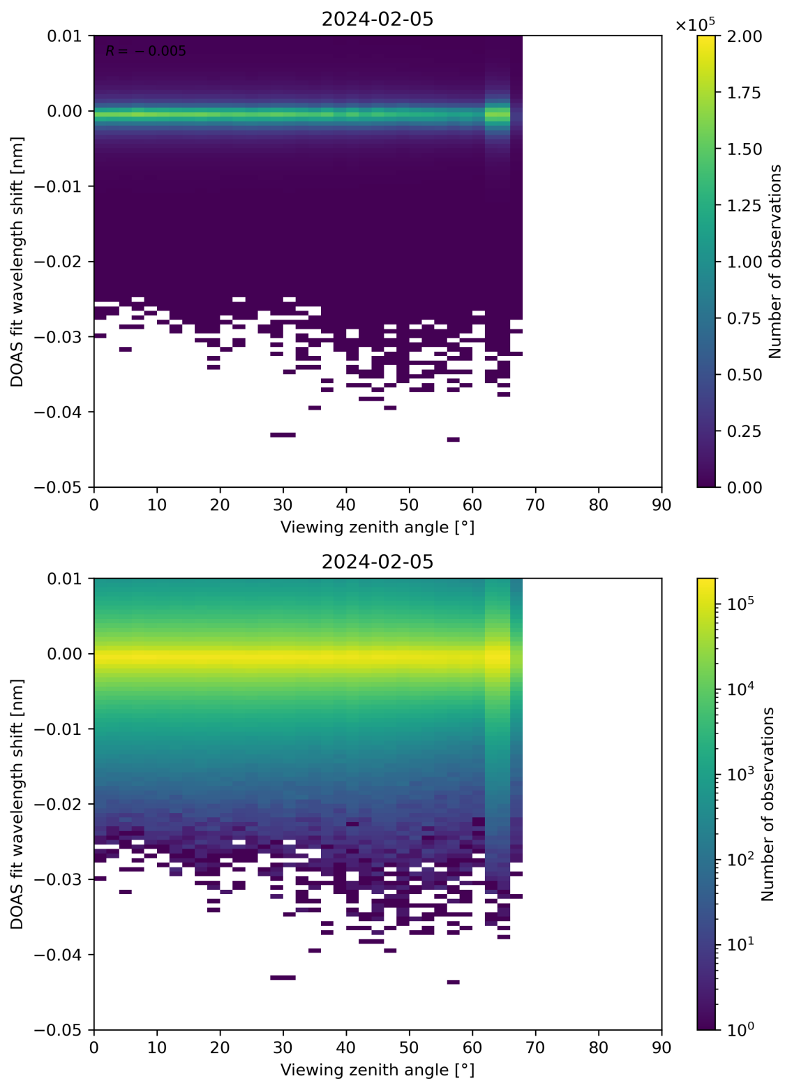
Figure 311: Scatter density plot of “Viewing zenith angle” against “DOAS fit wavelength shift” for 2024-02-04 to 2024-02-06.
