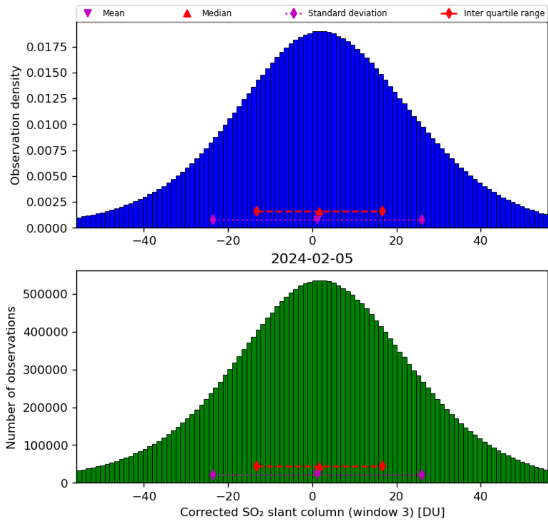
Figure 66: Histogram of “Corrected SO 2 slant column (window 3)” for 2024-02-04 to 2024-02-06
