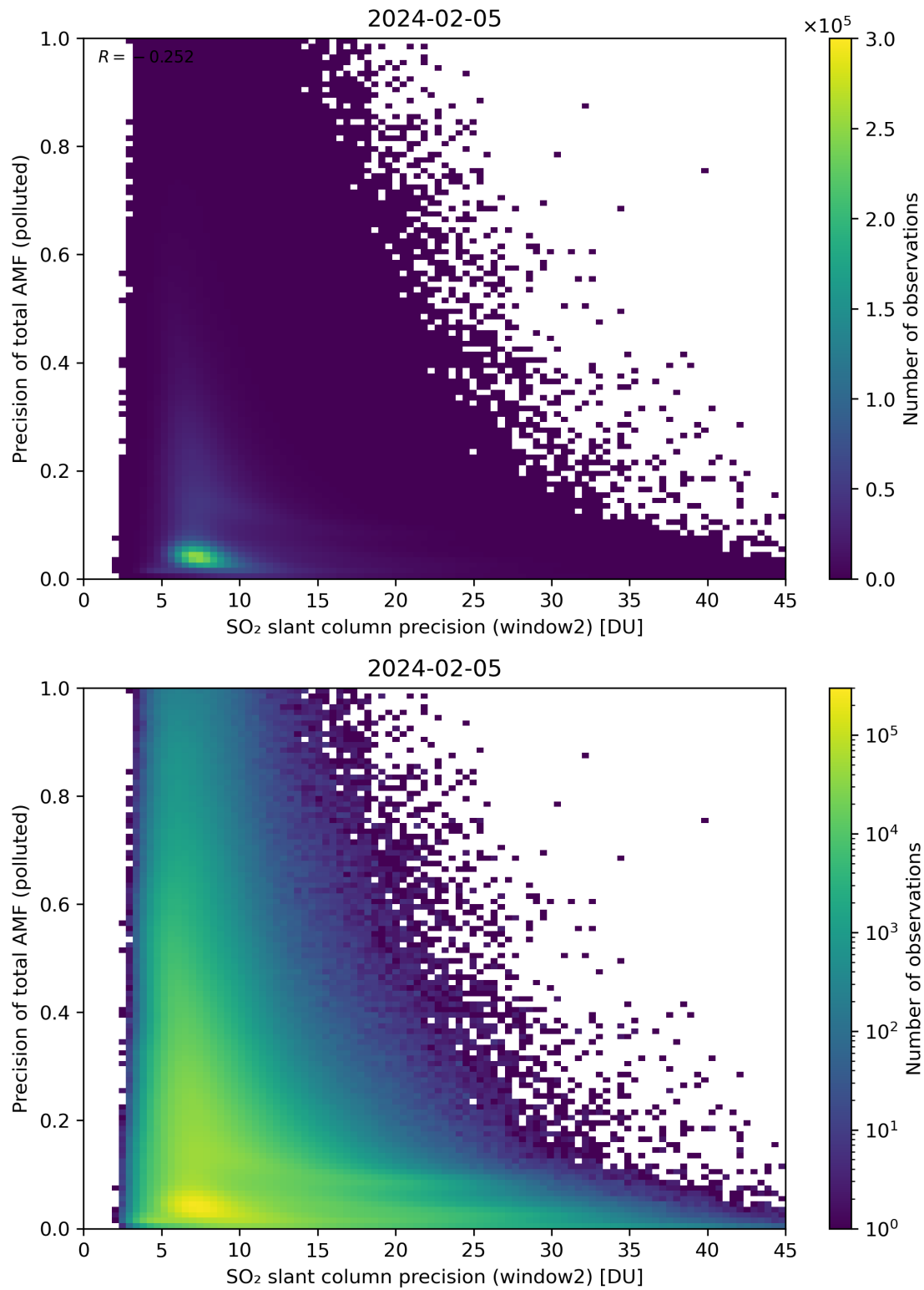
Figure 252: Scatter density plot of “SO 2 slant column precision (window2)” against “Precision of total AMF (polluted)” for 2024-02-04 to 2024-02-06.
