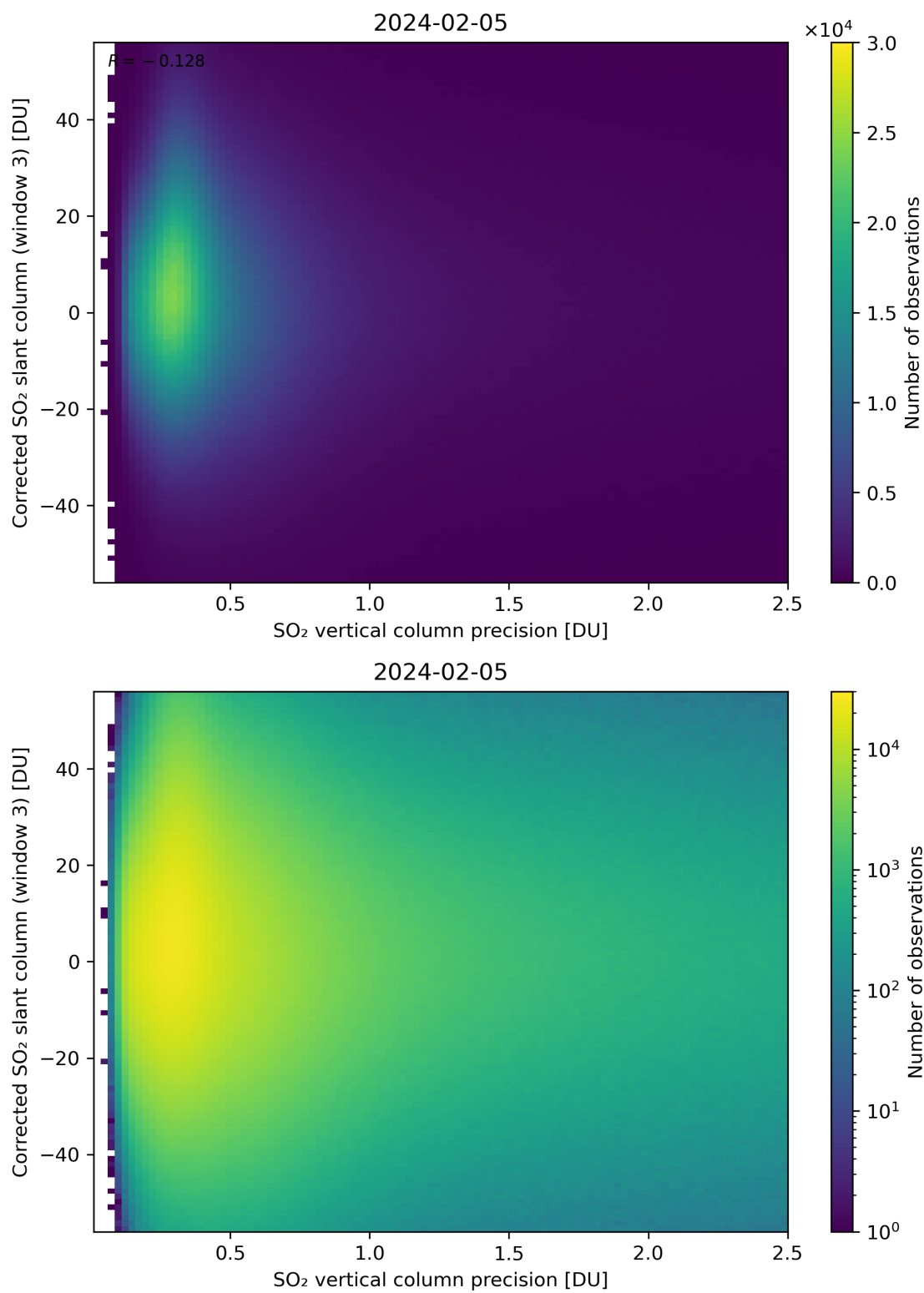
Figure 288: Scatter density plot of “SO 2 vertical column precision” against “Corrected SO 2 slant column (window 3)” for 2024-02-04 to 2024-02-06.
