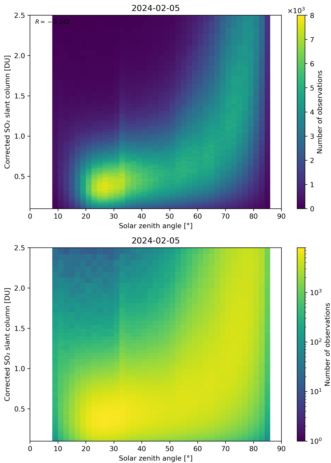
Figure 166: Scatter density plot of “Solar zenith angle” against “Corrected SO 2 slant column” for 2024-02-04 to 2024-02-06.
