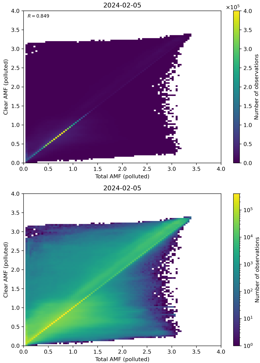
Figure 271: Scatter density plot of “Total AMF (polluted)” against “Clear AMF (polluted)” for 2024-02-04 to 2024-02-06.
