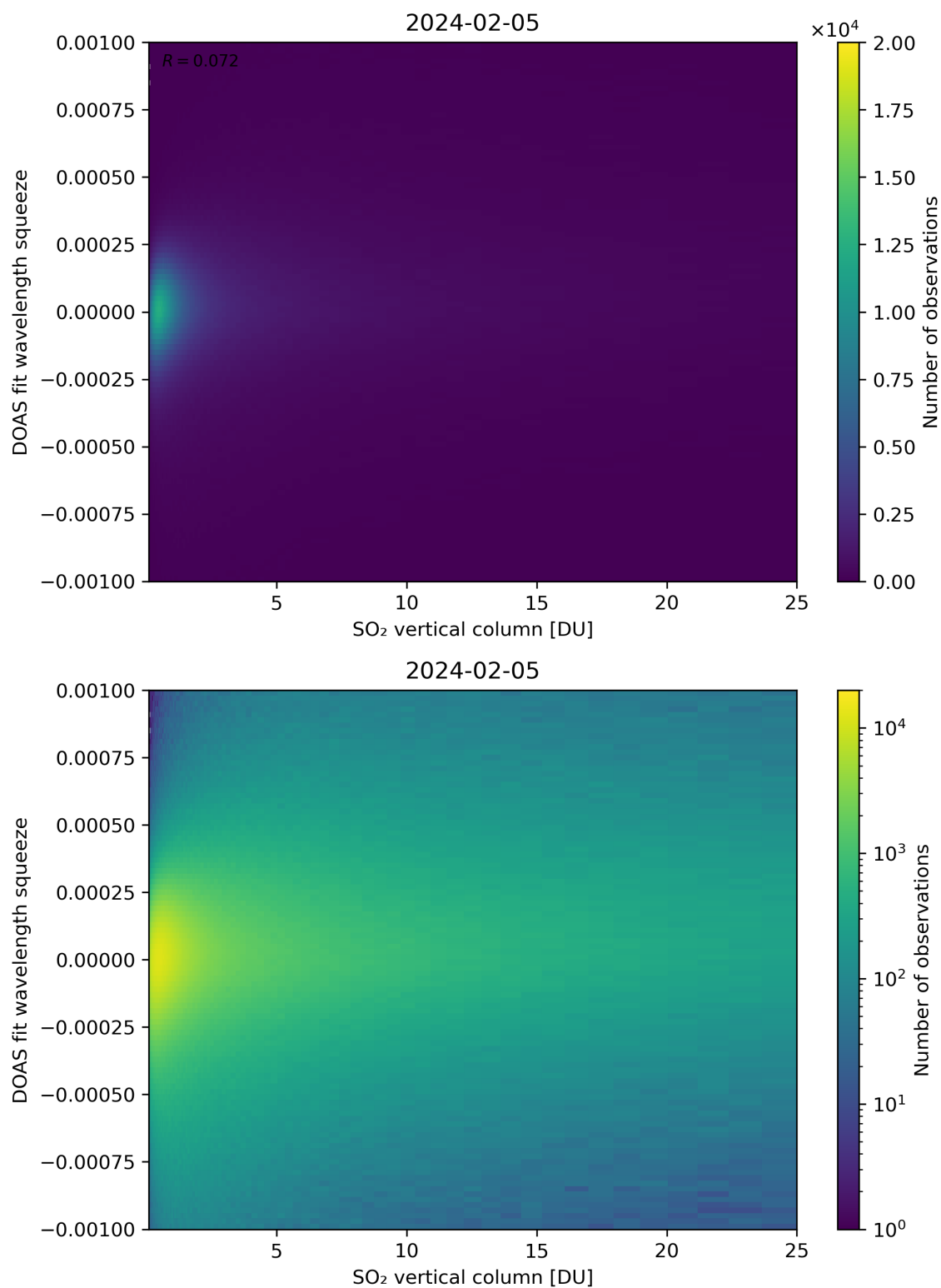
Figure 277: Scatter density plot of “SO 2 vertical column” against “DOAS fit wavelength squeeze” for 2024-02-04 to 2024-02-06.
