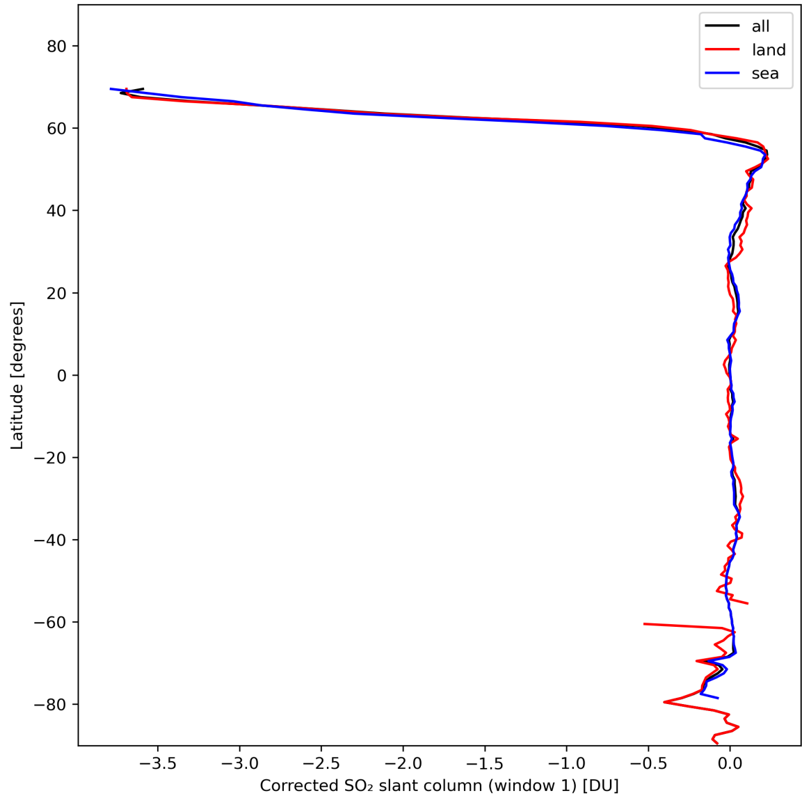
Figure 35: Zonal average of “Corrected SO 2 slant column (window 1)” for 2024-02-04 to 2024-02-06.
