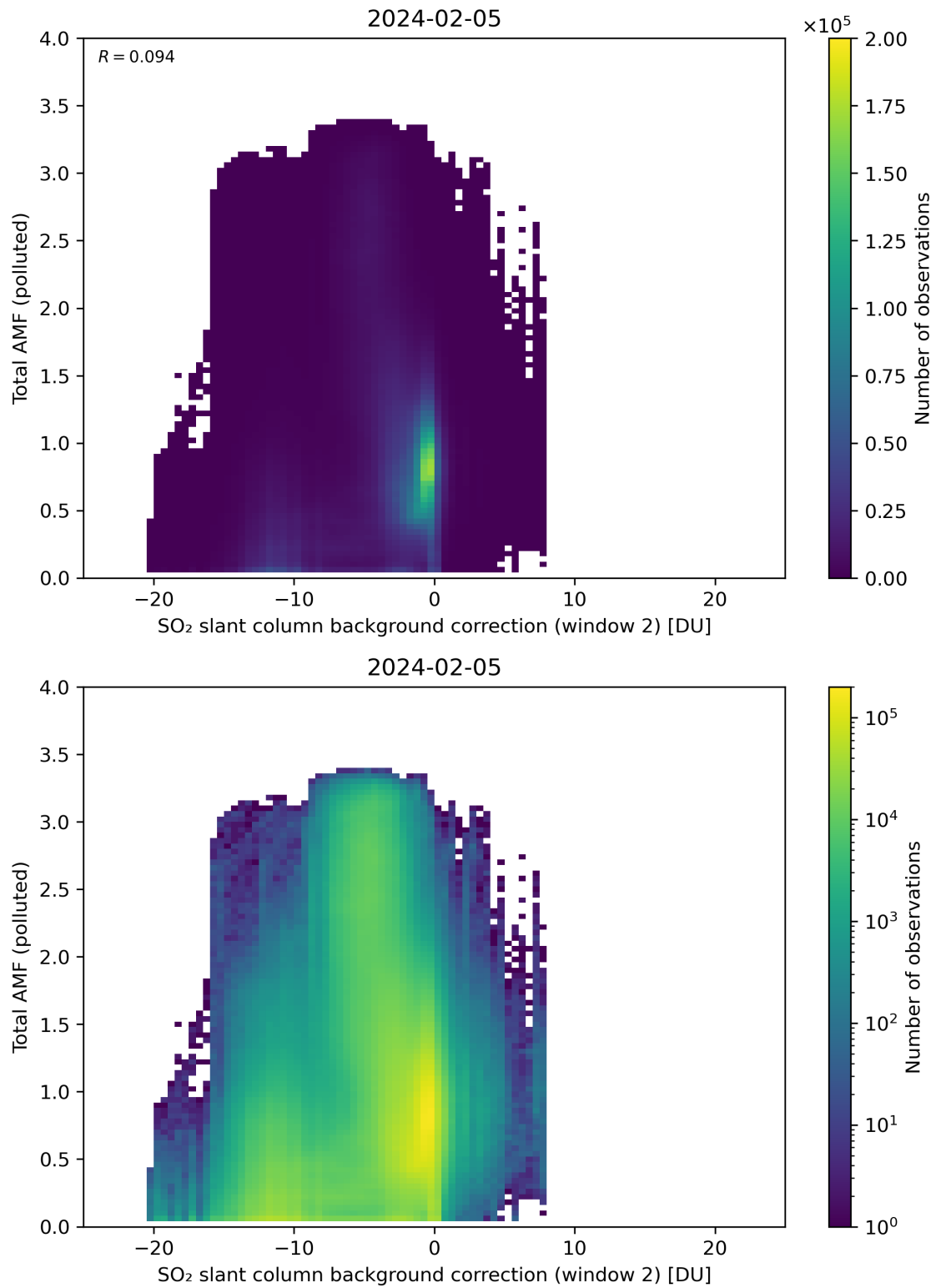
Figure 119: Scatter density plot of “SO 2 slant column background correction (window 2)” against “Total AMF (polluted)” for 2024-02-04 to 2024-02-06.
