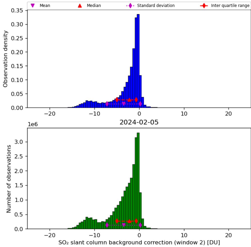
Figure 63: Histogram of “SO 2 slant column background correction (window 2)” for 2024-02-04 to 2024-02-06
