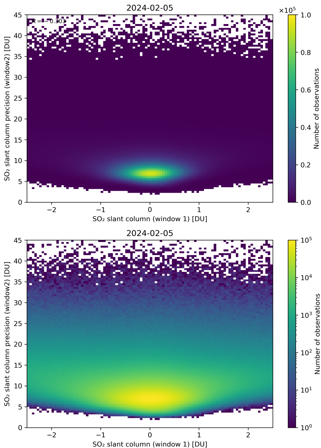
Figure 236: Scatter density plot of “SO 2 slant column (window 1)” against “SO 2 slant column precision (window2)” for 2024-02-04 to 2024-02-06.
