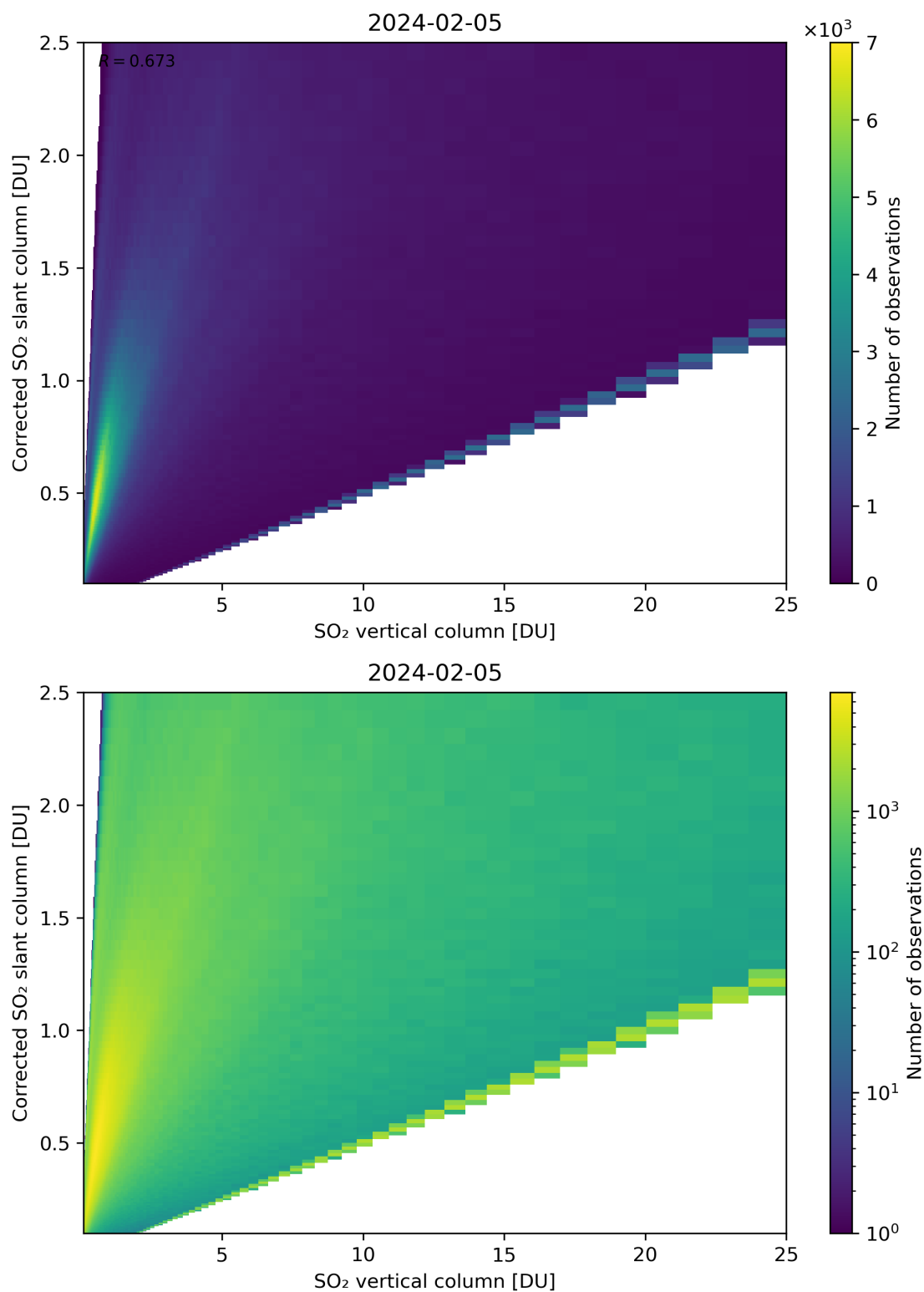
Figure 297: Scatter density plot of “SO 2 vertical column” against “Corrected SO 2 slant column” for 2024-02-04 to 2024-02-06.
