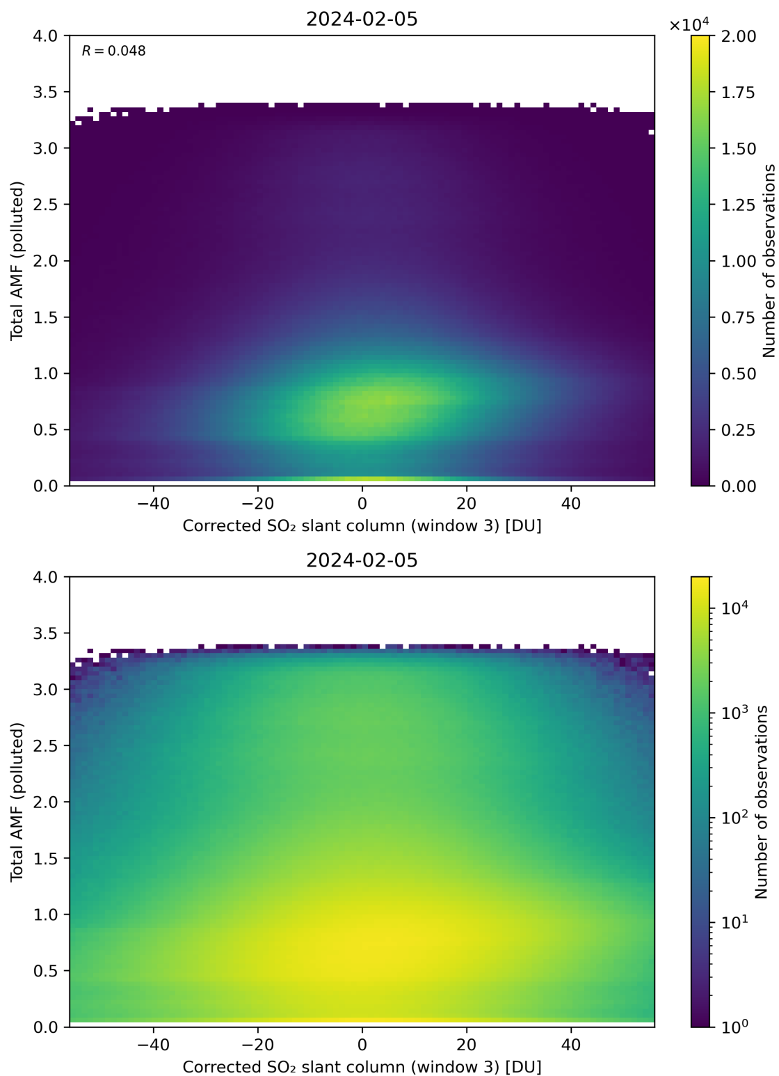
Figure 210: Scatter density plot of “Corrected SO 2 slant column (window 3)” against “Total AMF (polluted)” for 2024-02-04 to 2024-02-06.
