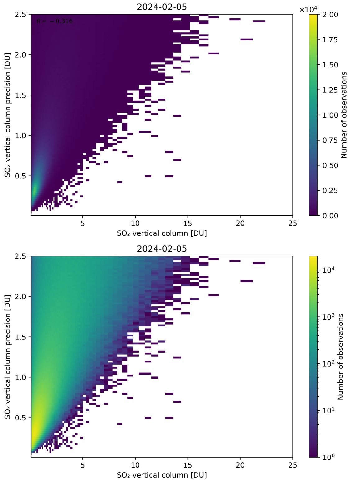
Figure 307: Scatter density plot of “SO 2 vertical column” against “SO 2 vertical column precision” for 2024-02-04 to 2024-02-06.
