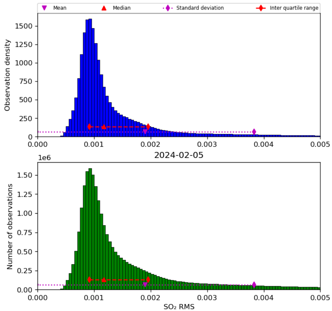
Figure 70: Histogram of “SO 2 RMS” for 2024-02-04 to 2024-02-06
