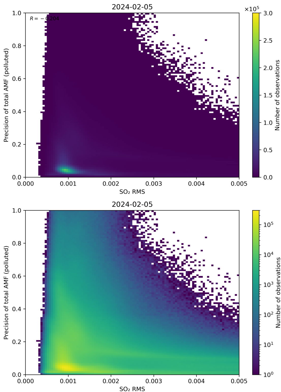
Figure 138: Scatter density plot of “SO 2 RMS” against “Precision of total AMF (polluted)” for 2024-02-04 to 2024-02-06.
