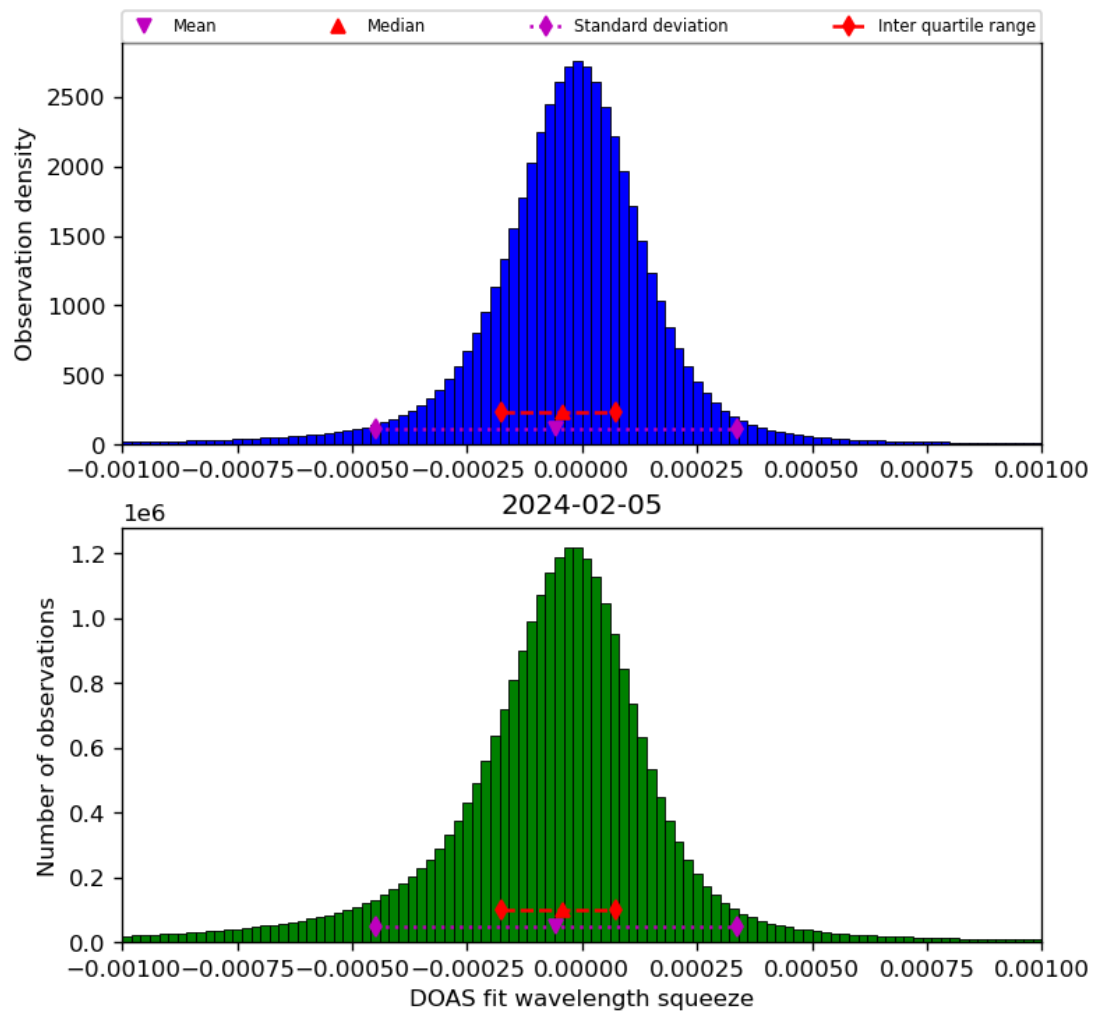
Figure 69: Histogram of “DOAS fit wavelength squeeze” for 2024-02-04 to 2024-02-06
