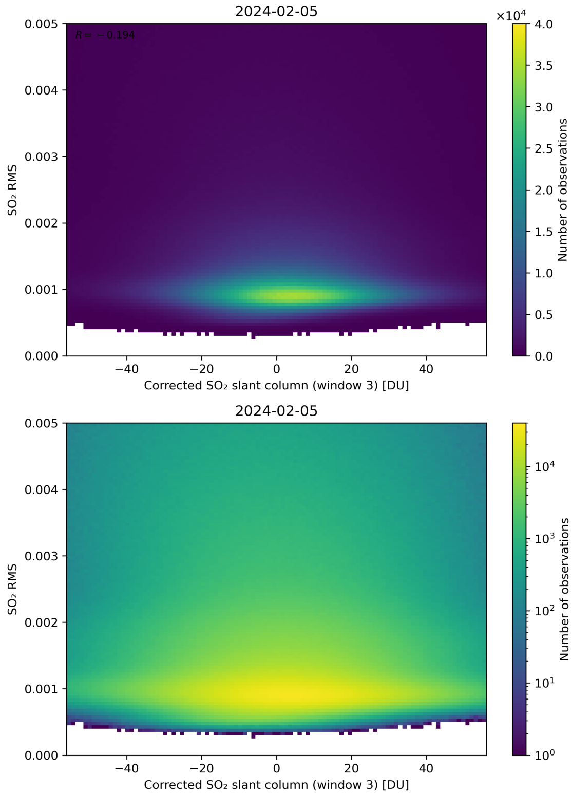
Figure 208: Scatter density plot of “Corrected SO 2 slant column (window 3)” against “SO 2 RMS” for 2024-02-04 to 2024-02-06.
