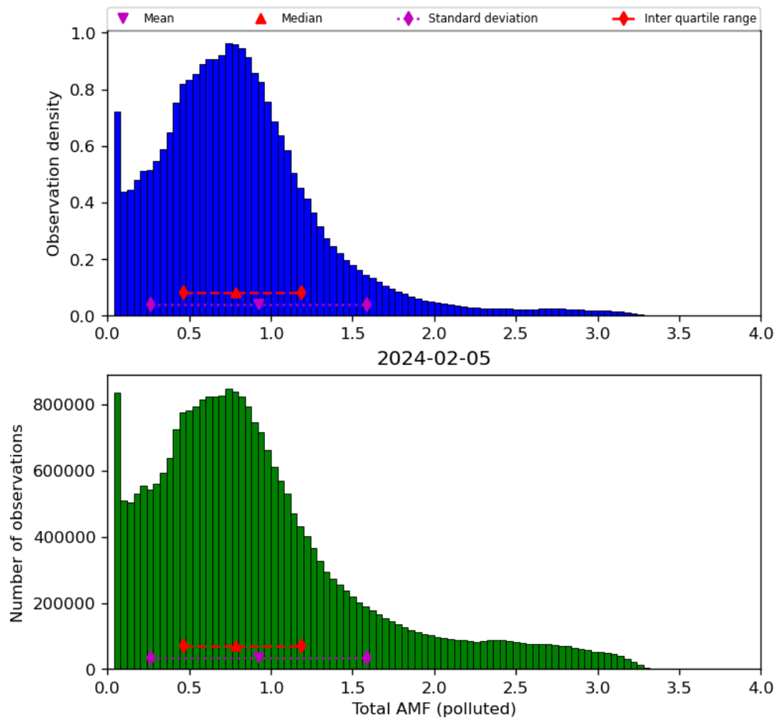
Figure 71: Histogram of “Total AMF (polluted)” for 2024-02-04 to 2024-02-06
