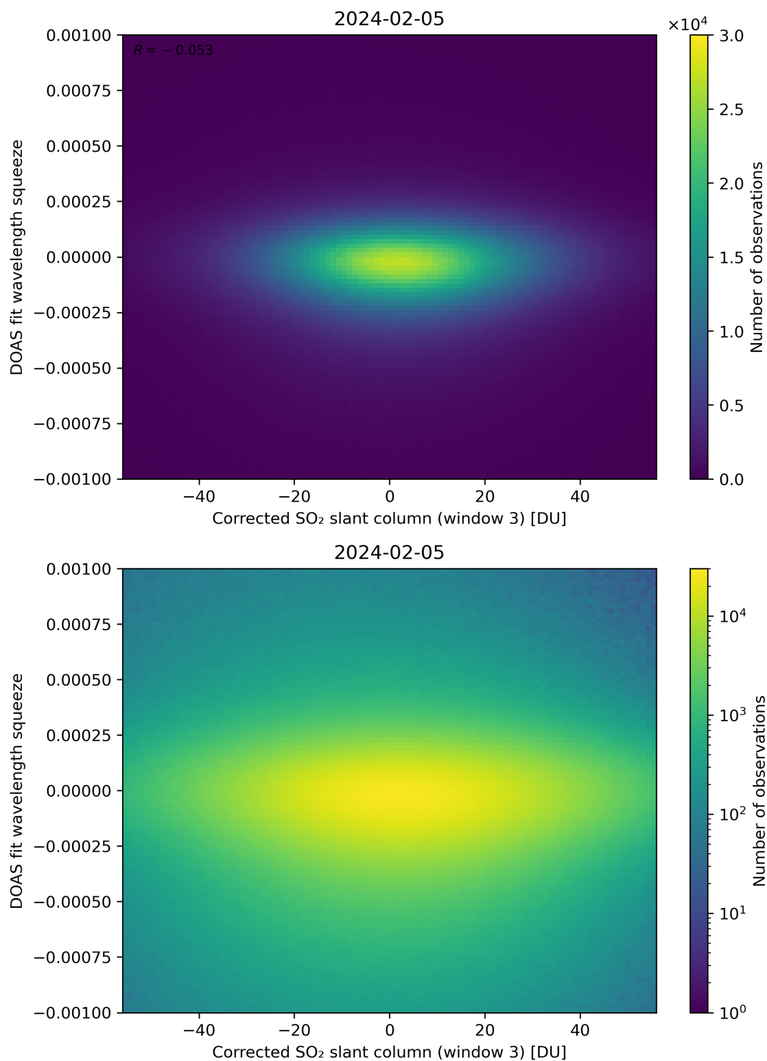
Figure 207: Scatter density plot of “Corrected SO 2 slant column (window 3)” against “DOAS fit wavelength squeeze” for 2024-02-04 to 2024-02-06.
