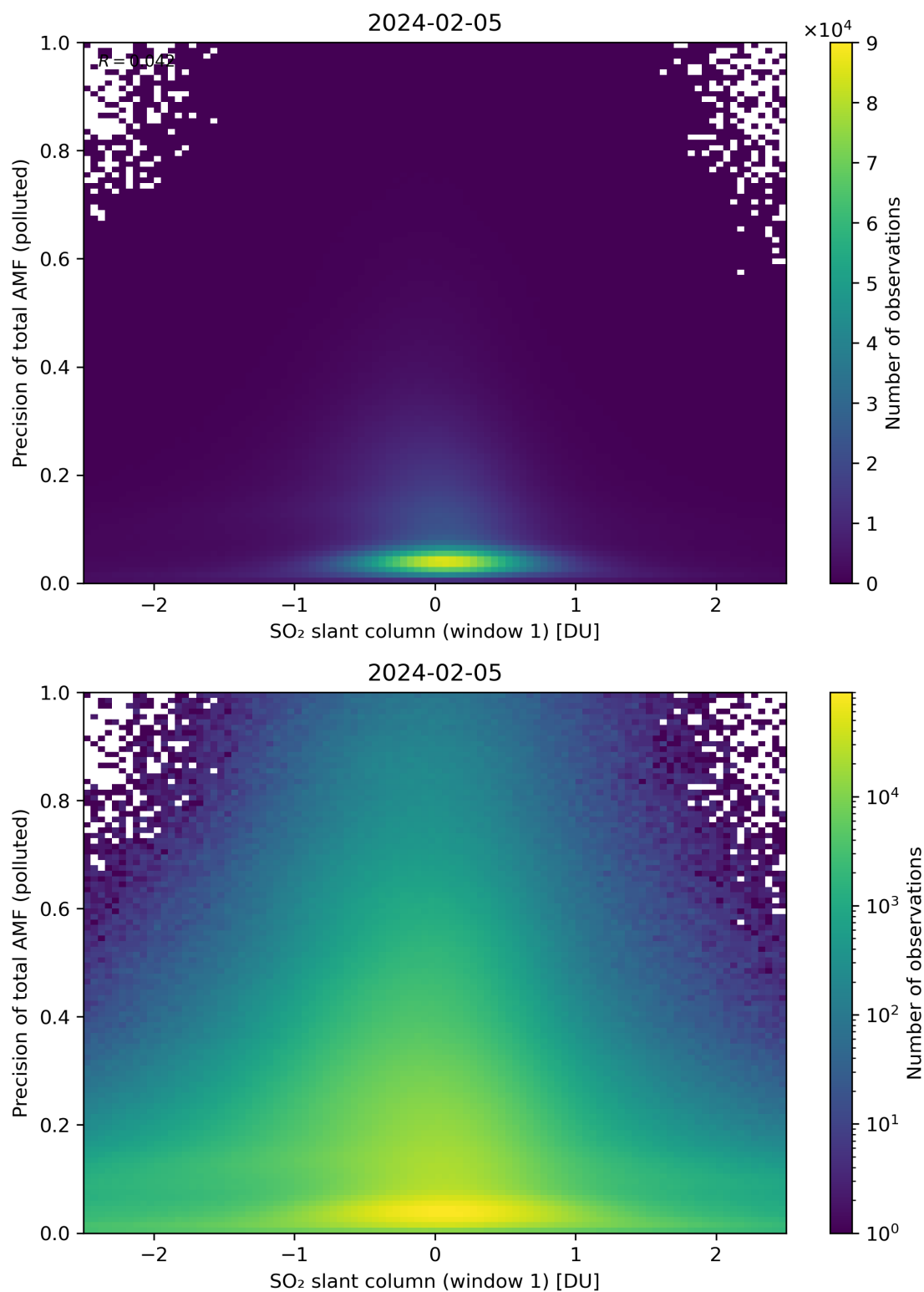
Figure 240: Scatter density plot of “SO 2 slant column (window 1)” against “Precision of total AMF (polluted)” for 2024-02-04 to 2024-02-06.
