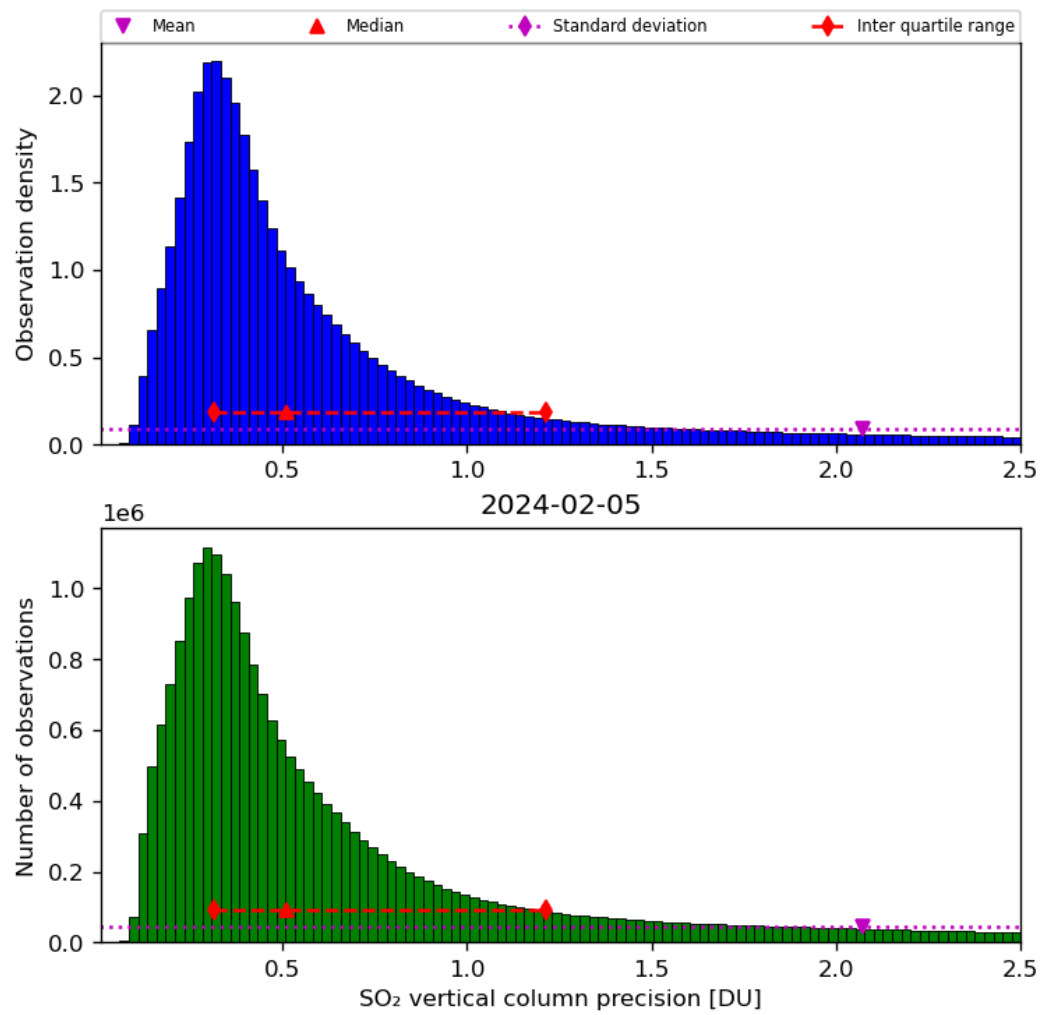
Figure 54: Histogram of “SO 2 vertical column precision” for 2024-02-04 to 2024-02-06
