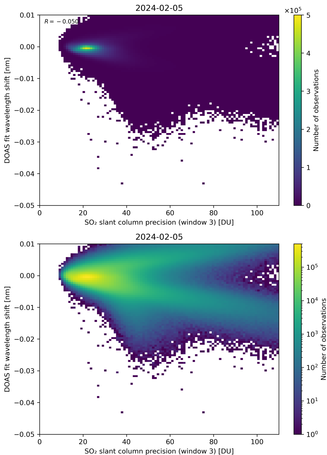
Figure 258: Scatter density plot of “SO 2 slant column precision (window 3)” against “DOAS fit wavelength shift” for 2024-02-04 to 2024-02-06.
