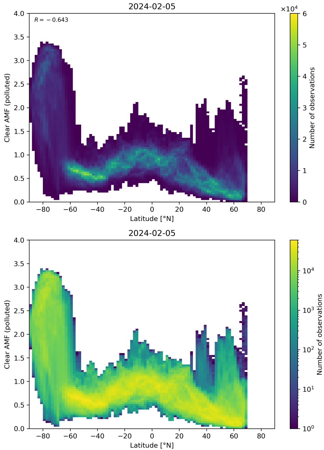
Figure 145: Scatter density plot of “Latitude” against “Clear AMF (polluted)” for 2024-02-04 to 2024-02-06.
