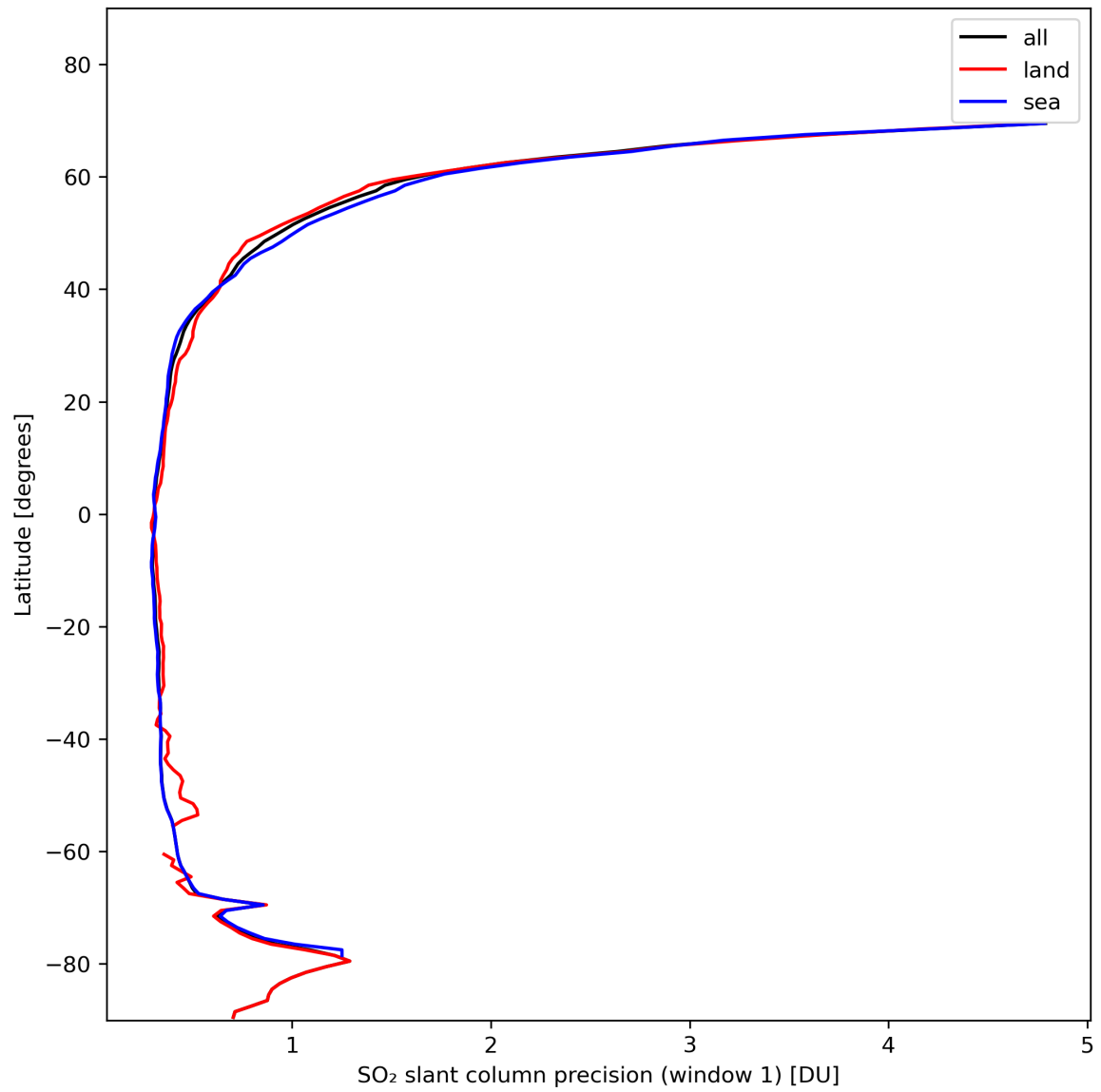
Figure 34: Zonal average of “SO 2 slant column precision (window 1)” for 2024-02-04 to 2024-02-06.
