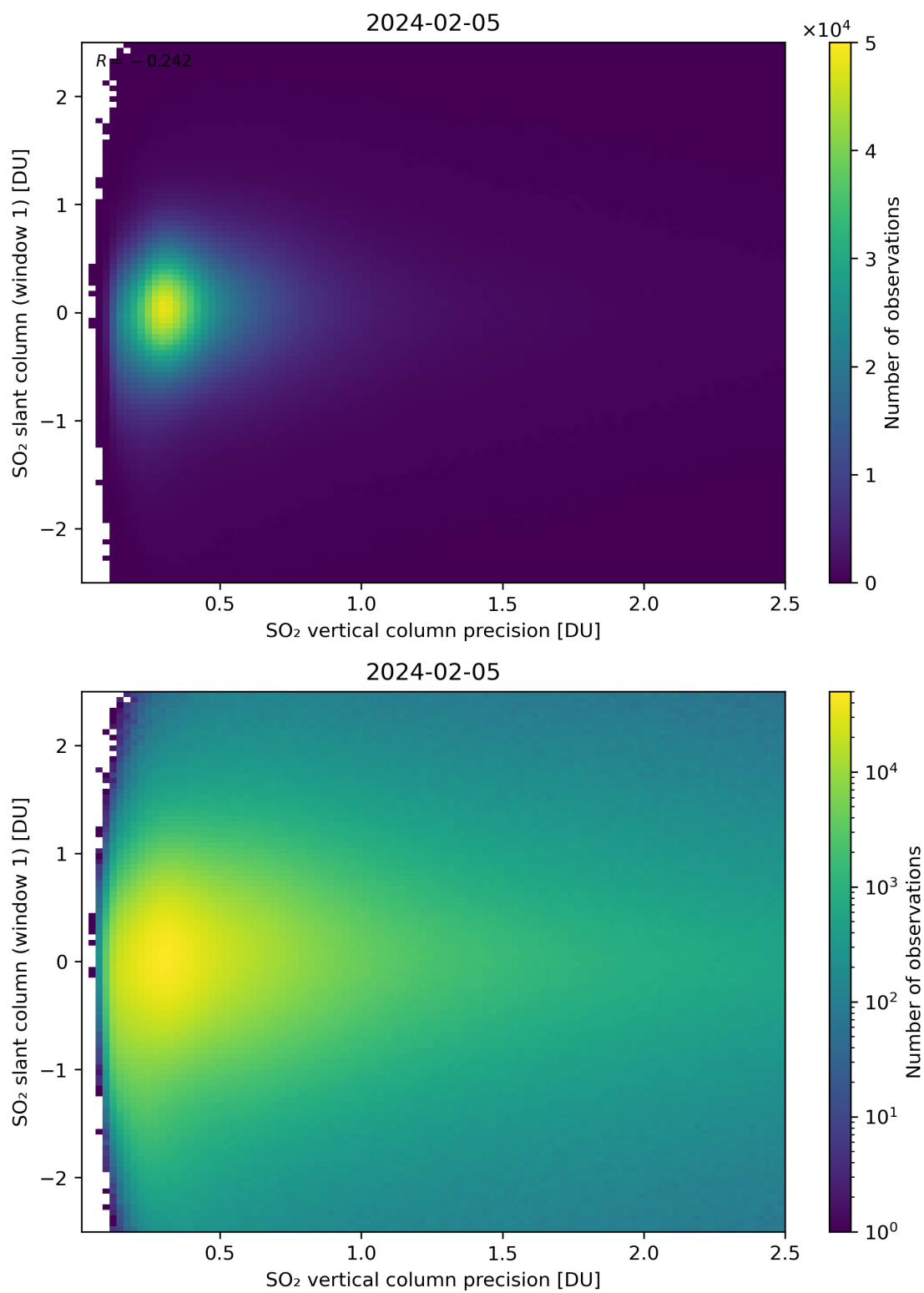
Figure 289: Scatter density plot of “SO 2 vertical column precision” against “SO 2 slant column (window 1)” for 2024-02-04 to 2024-02-06.
