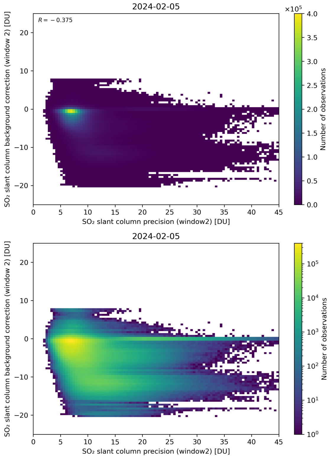
Figure 241: Scatter density plot of “SO 2 slant column precision (window2)” against “SO 2 slant column background correction (window 2)” for 2024-02-04 to 2024-02-06.
