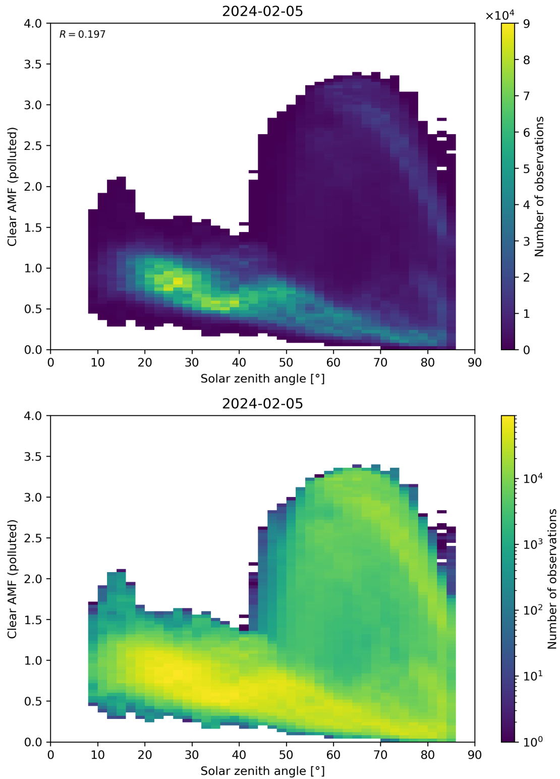
Figure 165: Scatter density plot of “Solar zenith angle” against “Clear AMF (polluted)” for 2024-02-04 to 2024-02-06.
