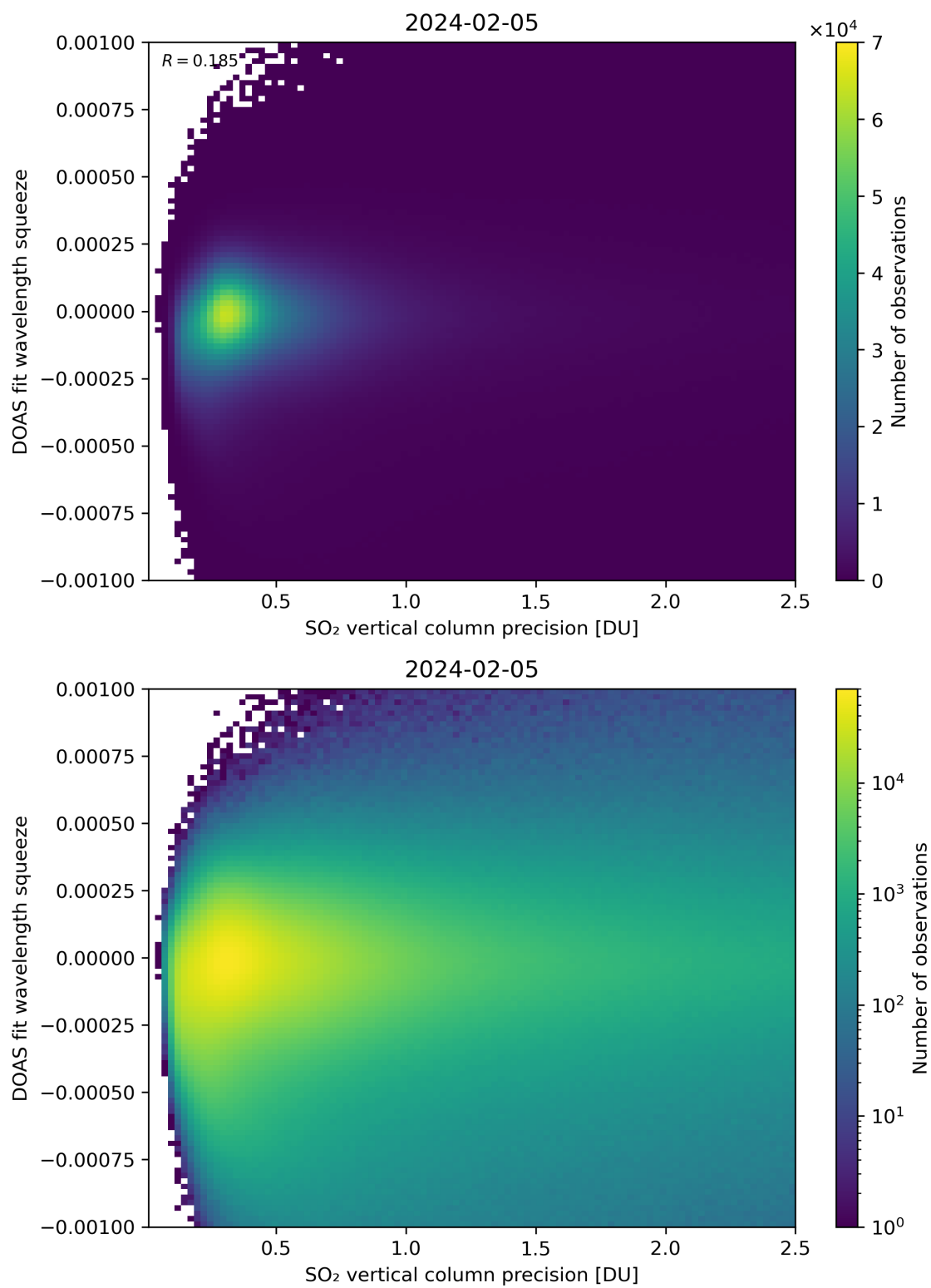
Figure 283: Scatter density plot of “SO 2 vertical column precision” against “DOAS fit wavelength squeeze” for 2024-02-04 to 2024-02-06.
