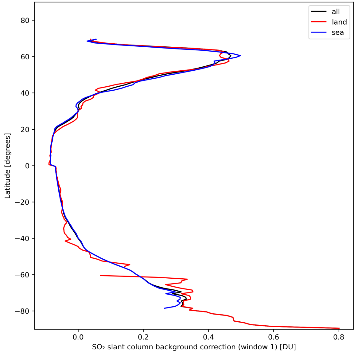
Figure 36: Zonal average of “SO 2 slant column background correction (window 1)” for 2024-02-04 to 2024-02-06.
