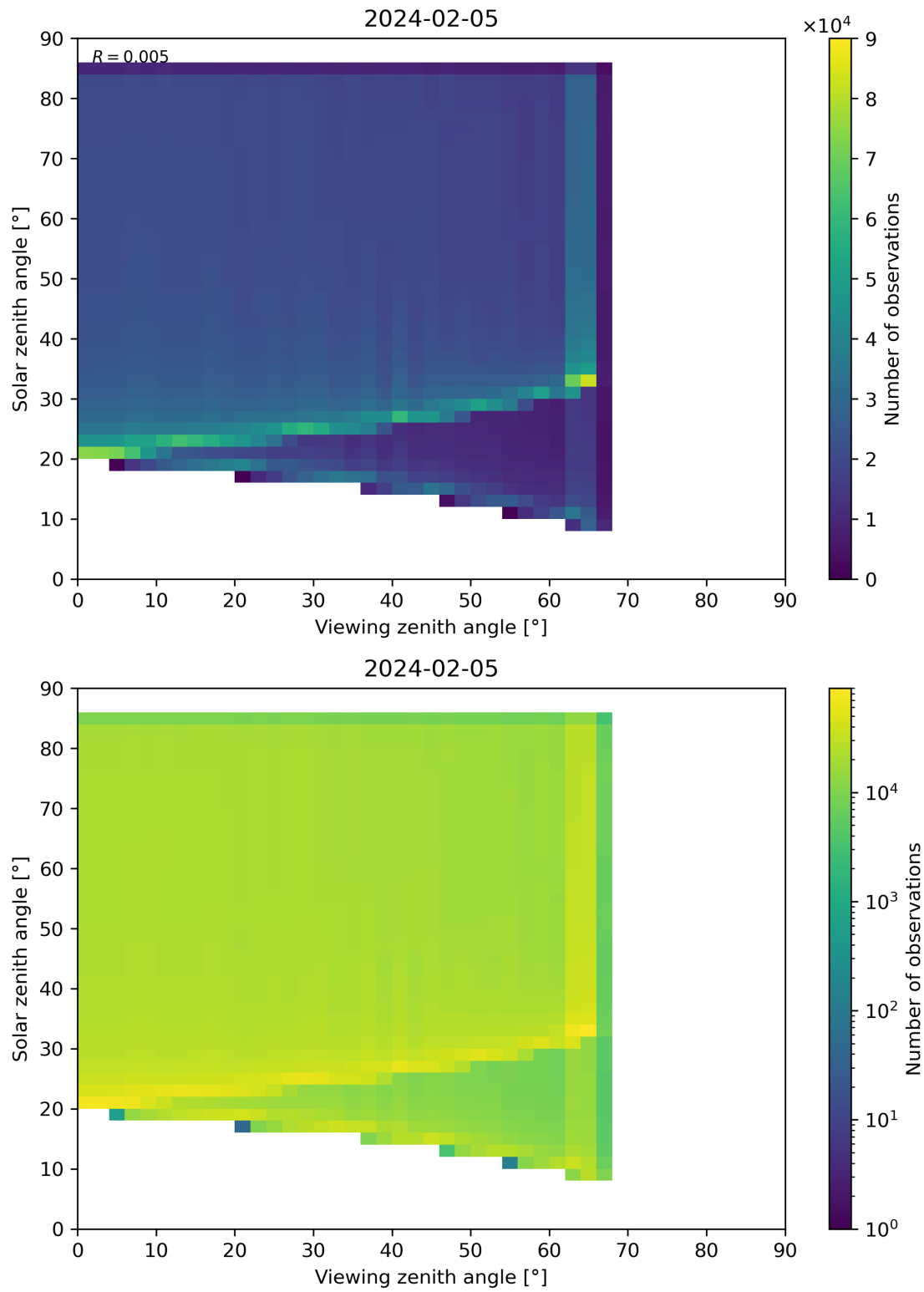
Figure 315: Scatter density plot of “Viewing zenith angle” against “Solar zenith angle” for 2024-02-04 to 2024-02-06.
