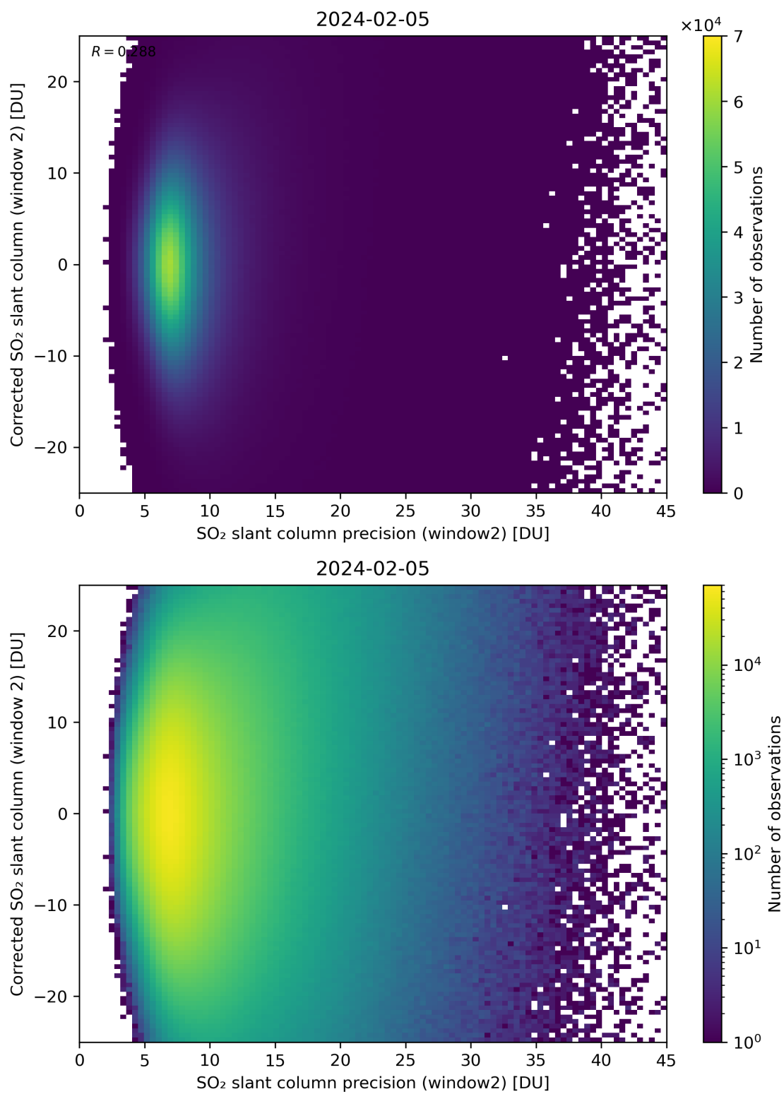
Figure 247: Scatter density plot of “SO 2 slant column precision (window2)” against “Corrected SO 2 slant column (window 2)” for 2024-02-04 to 2024-02-06.
