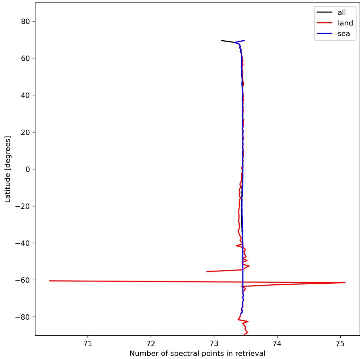
Figure 51: Zonal average of “Number of spectral points in retrieval” for 2024-02-04 to 2024-02-06.
