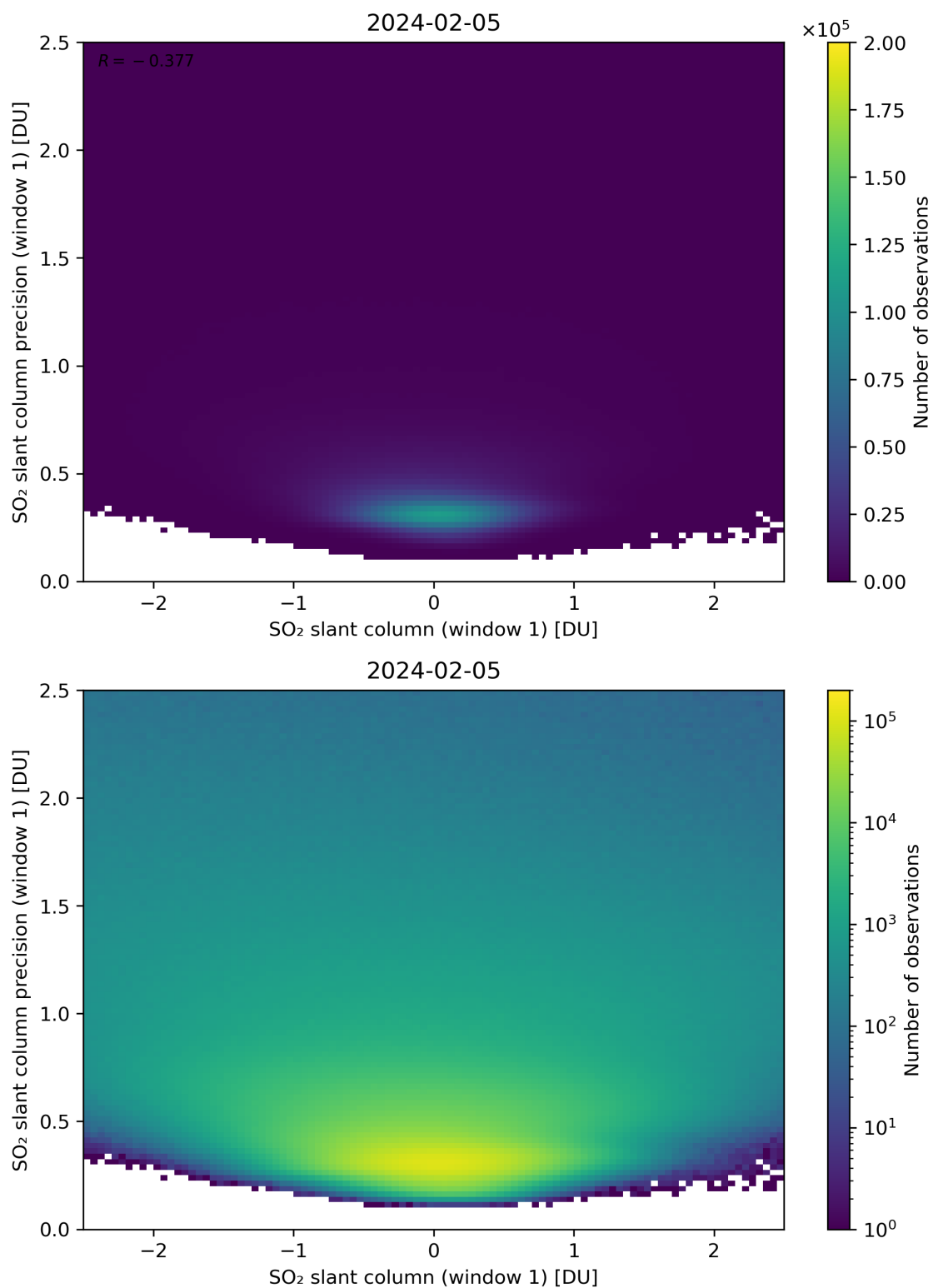
Figure 235: Scatter density plot of “SO 2 slant column (window 1)” against “SO 2 slant column precision (window 1)” for 2024-02-04 to 2024-02-06.
