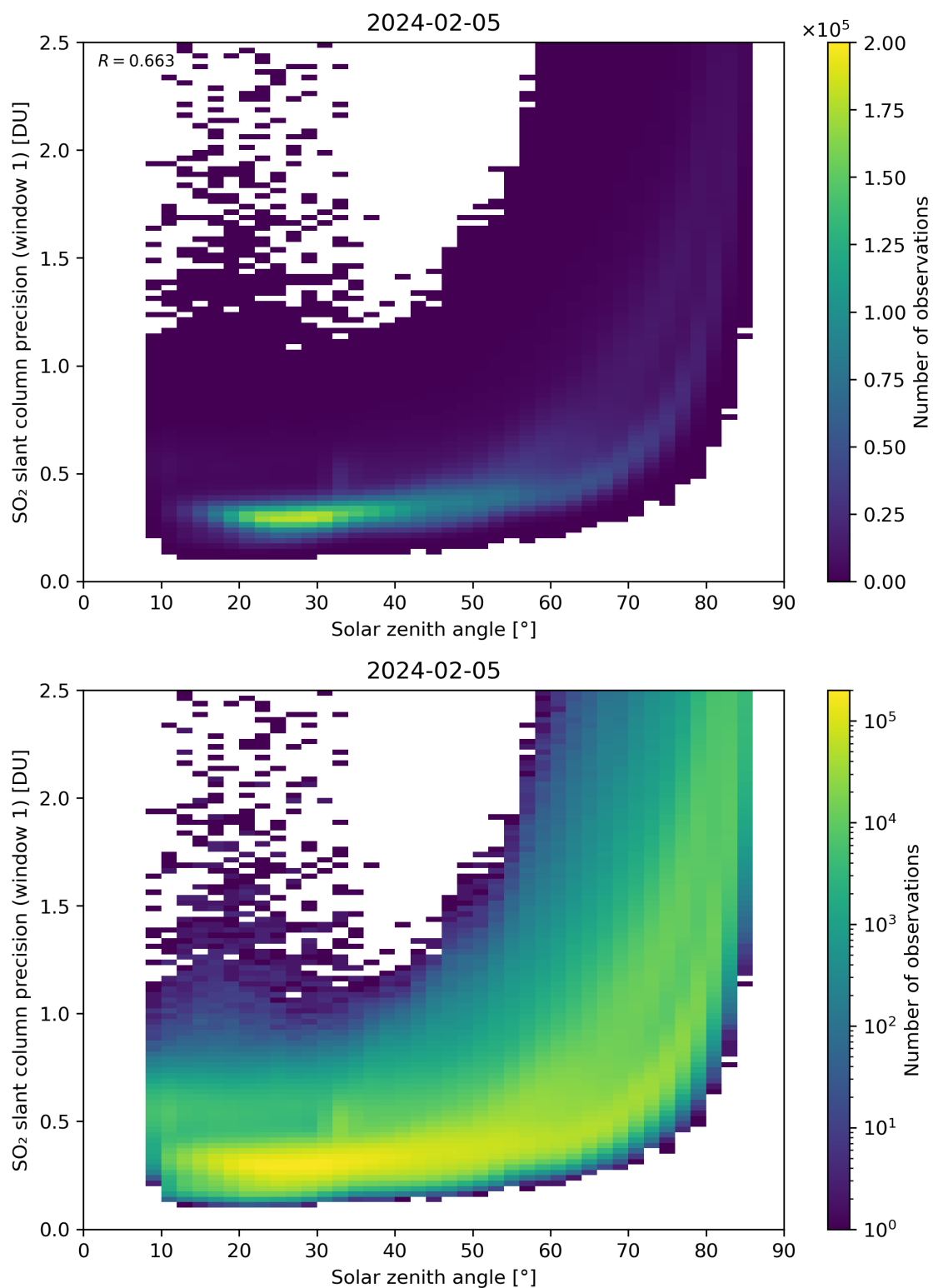
Figure 170: Scatter density plot of “Solar zenith angle” against “SO 2 slant column precision (window 1)” for 2024-02-04 to 2024-02-06.
