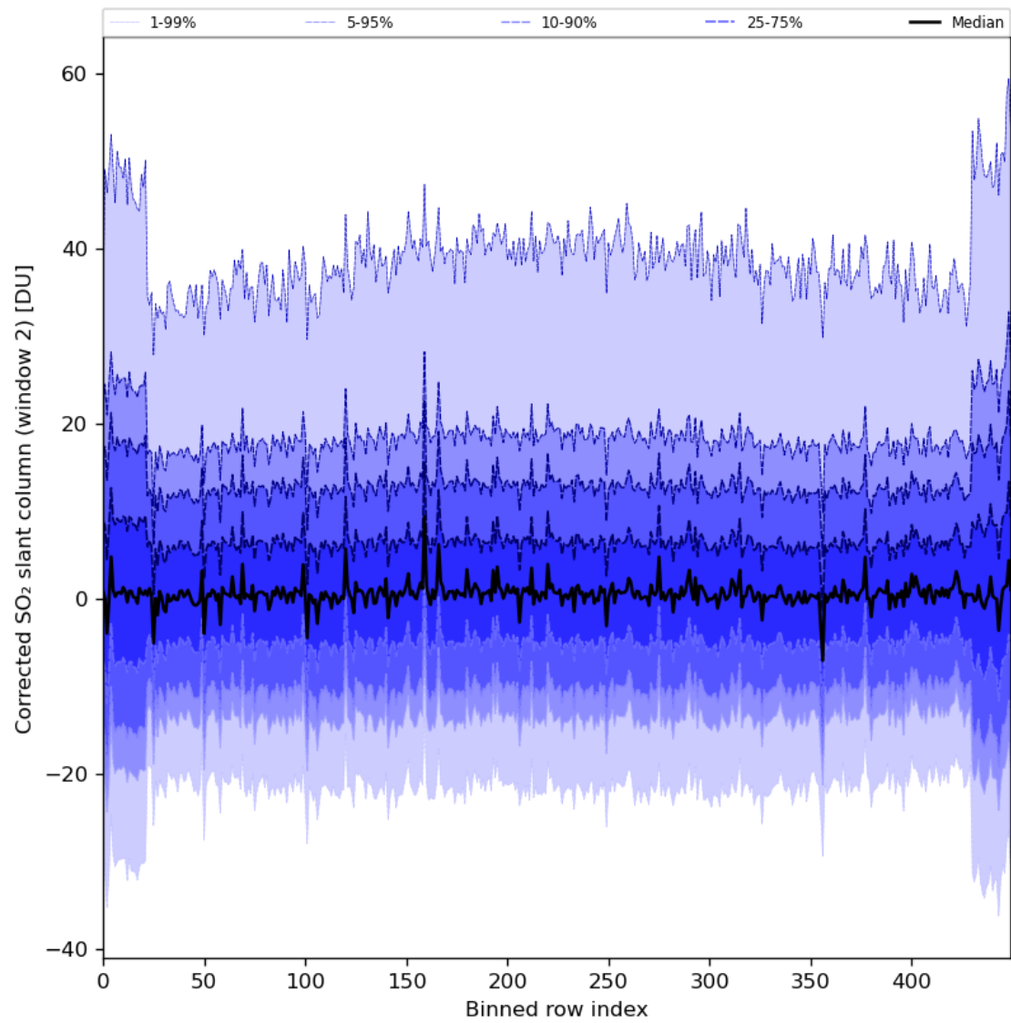
Figure 85: Along track statistics of “Corrected SO 2 slant column (window 2)” for 2024-02-04 to 2024-02-06
