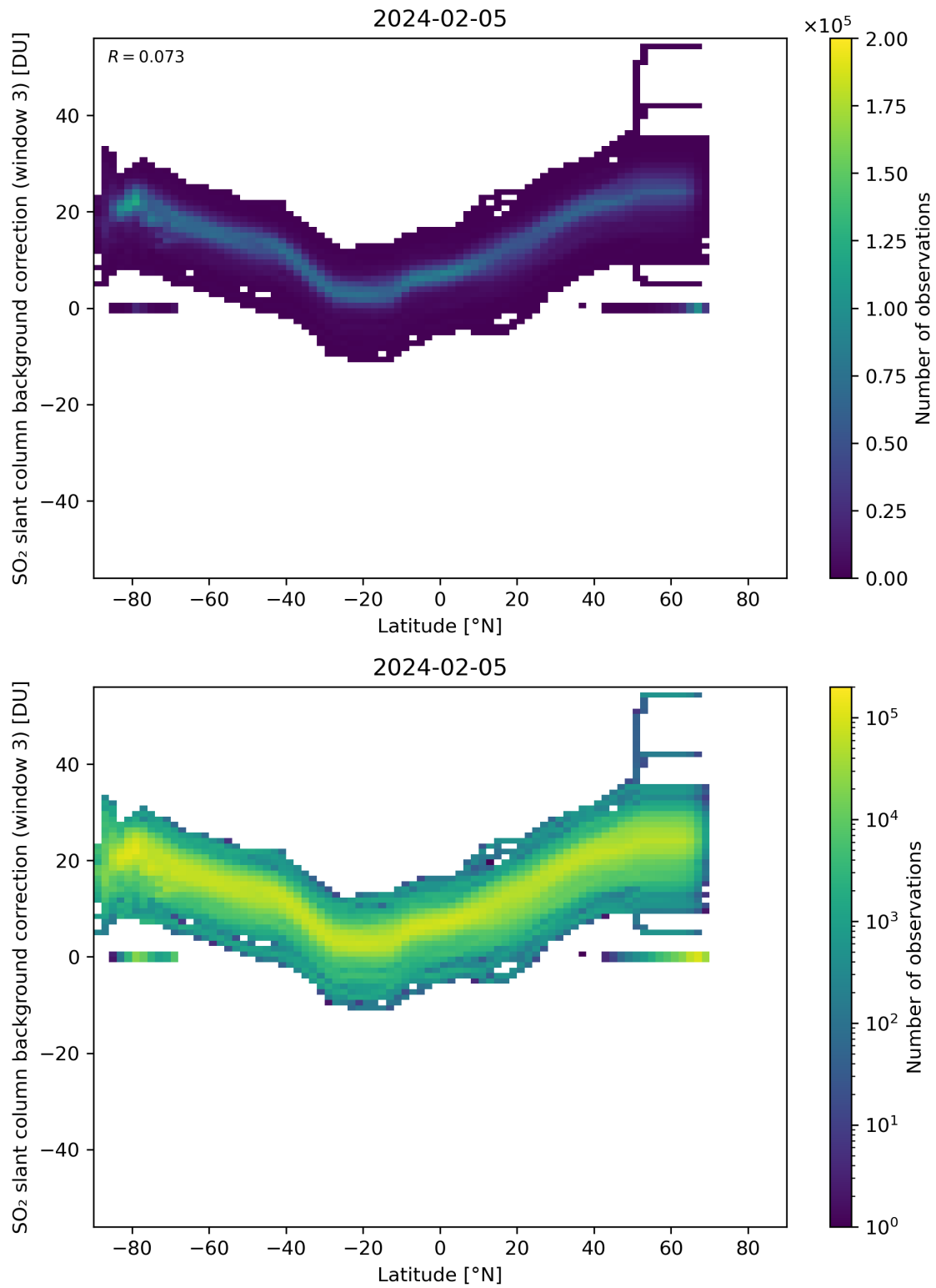
Figure 141: Scatter density plot of “Latitude” against “SO 2 slant column background correction (window 3)” for 2024-02-04 to 2024-02-06.
