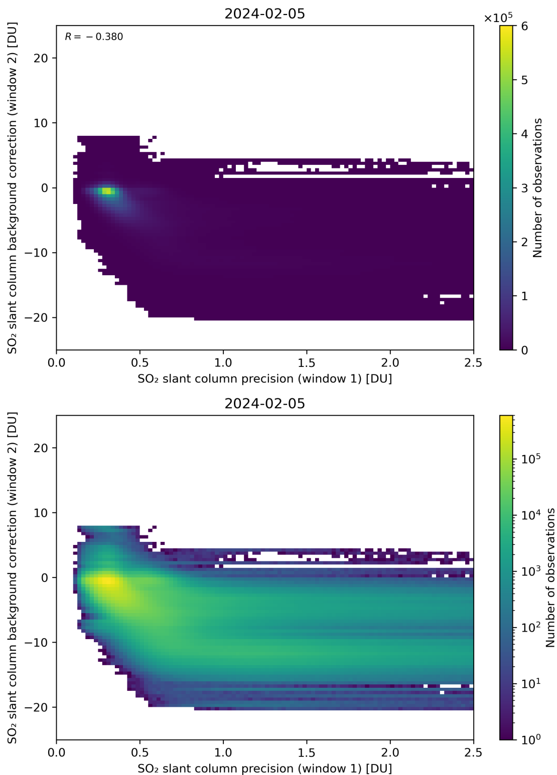
Figure 219: Scatter density plot of “SO 2 slant column precision (window 1)” against “SO 2 slant column background correction (window 2)” for 2024-02-04 to 2024-02-06.
