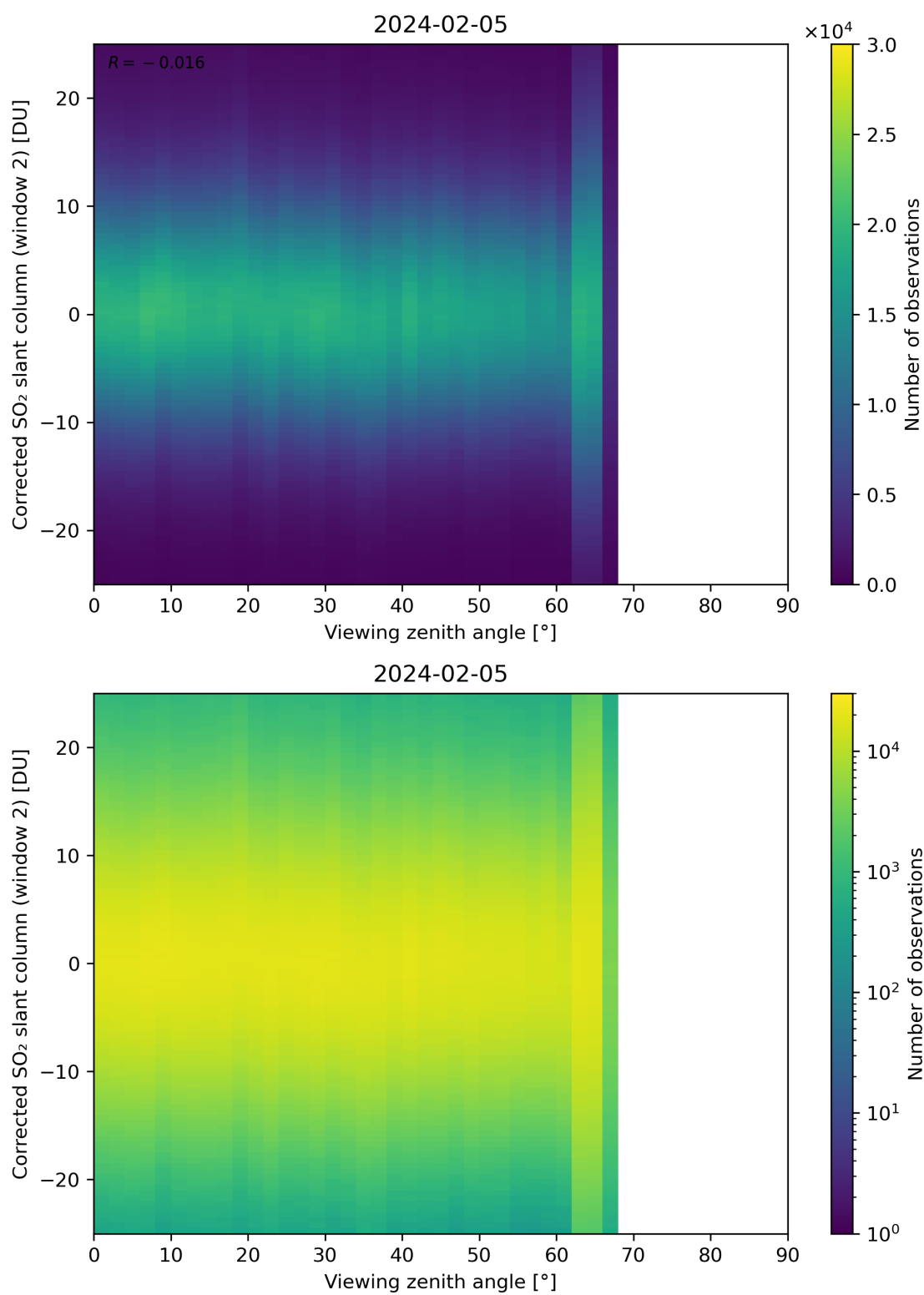
Figure 318: Scatter density plot of “Viewing zenith angle” against “Corrected SO 2 slant column (window 2)” for 2024-02-04 to 2024-02-06.
