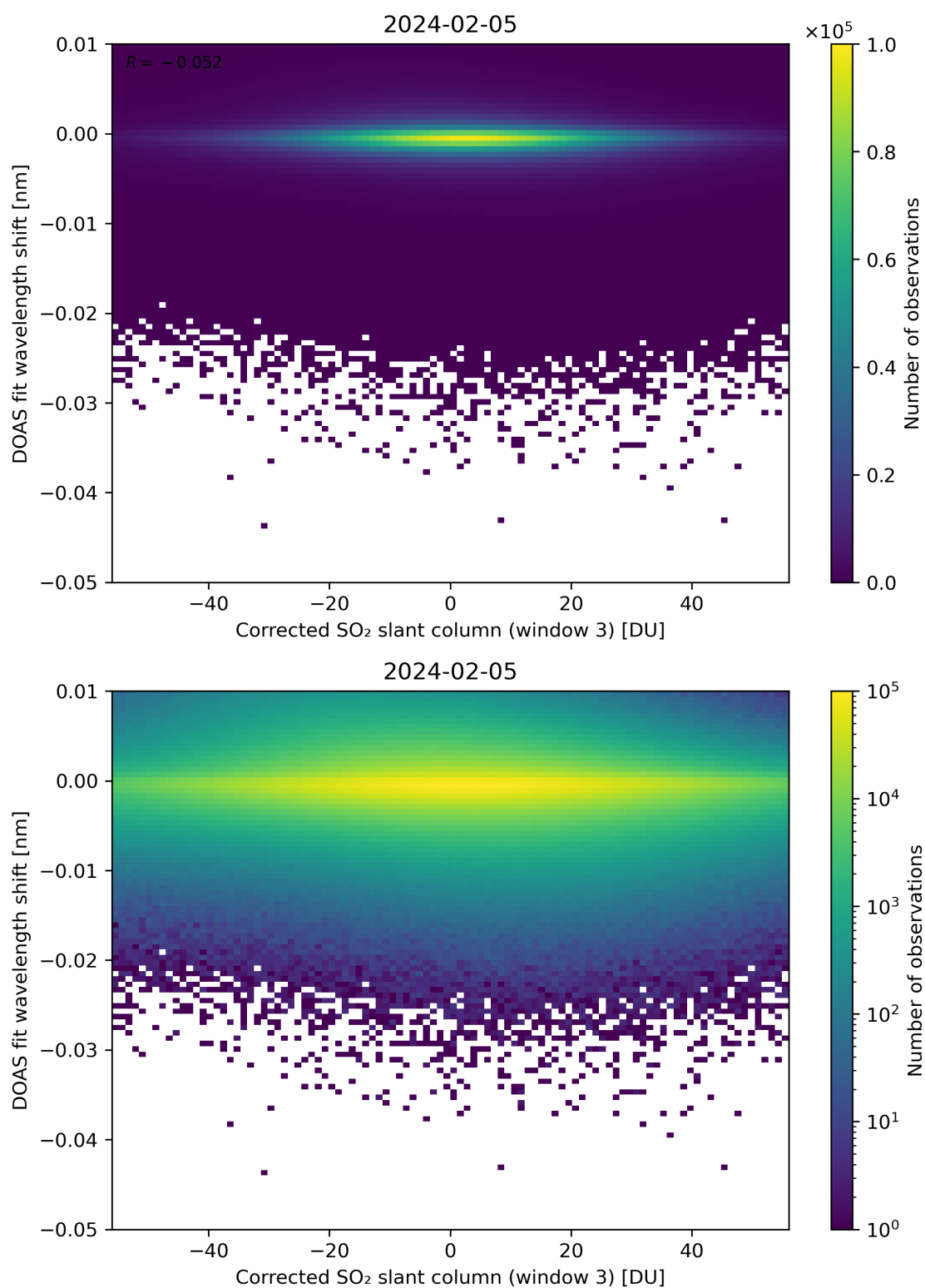
Figure 206: Scatter density plot of “Corrected SO 2 slant column (window 3)” against “DOAS fit wavelength shift” for 2024-02-04 to 2024-02-06.
