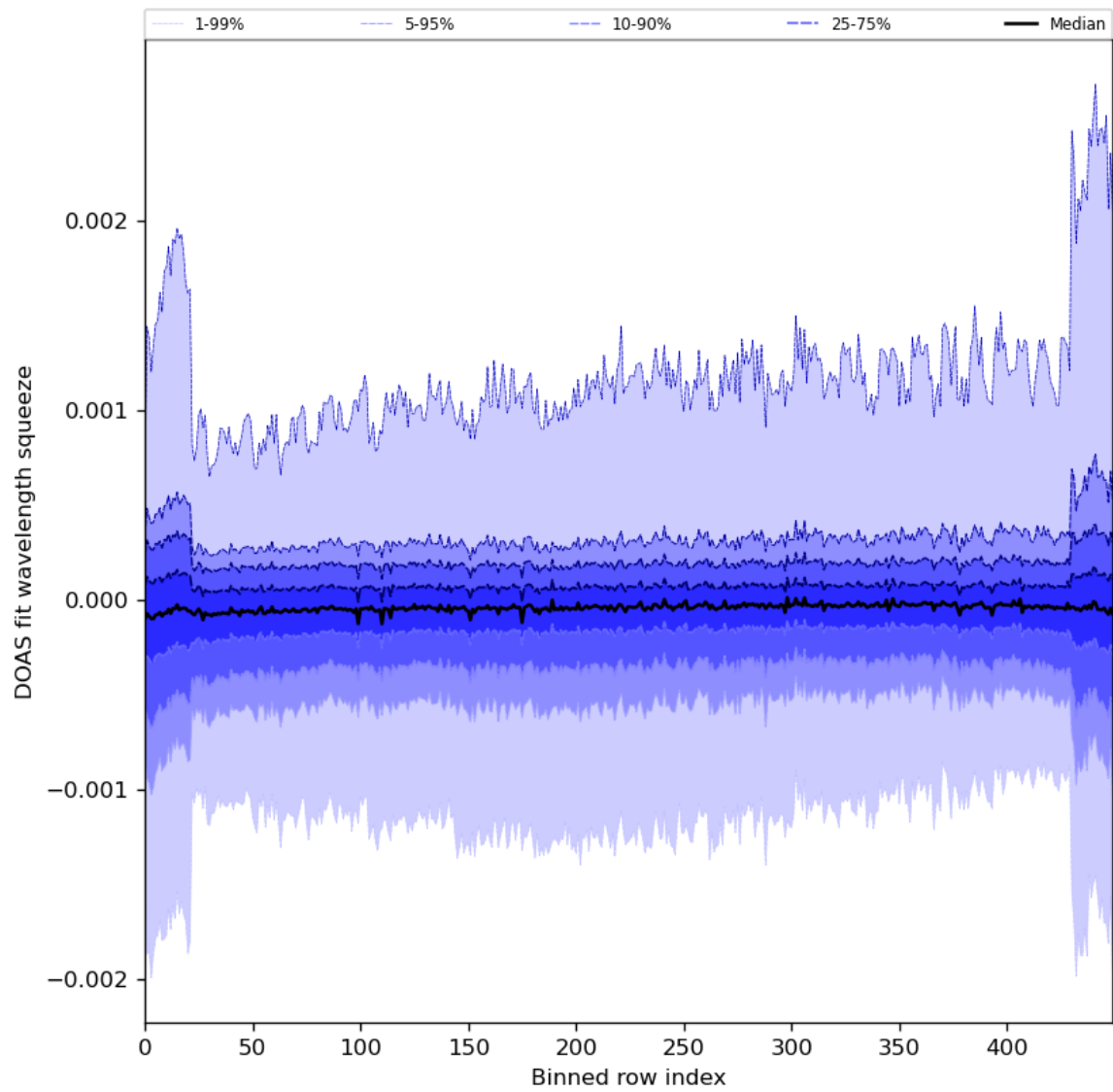
Figure 92: Along track statistics of “DOAS fit wavelength squeeze” for 2024-02-04 to 2024-02-06
