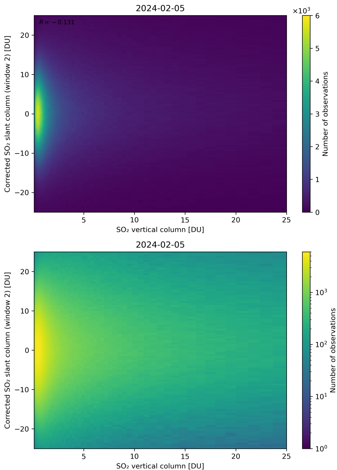
Figure 298: Scatter density plot of “SO 2 vertical column” against “Corrected SO 2 slant column (window 2)” for 2024-02-04 to 2024-02-06.
