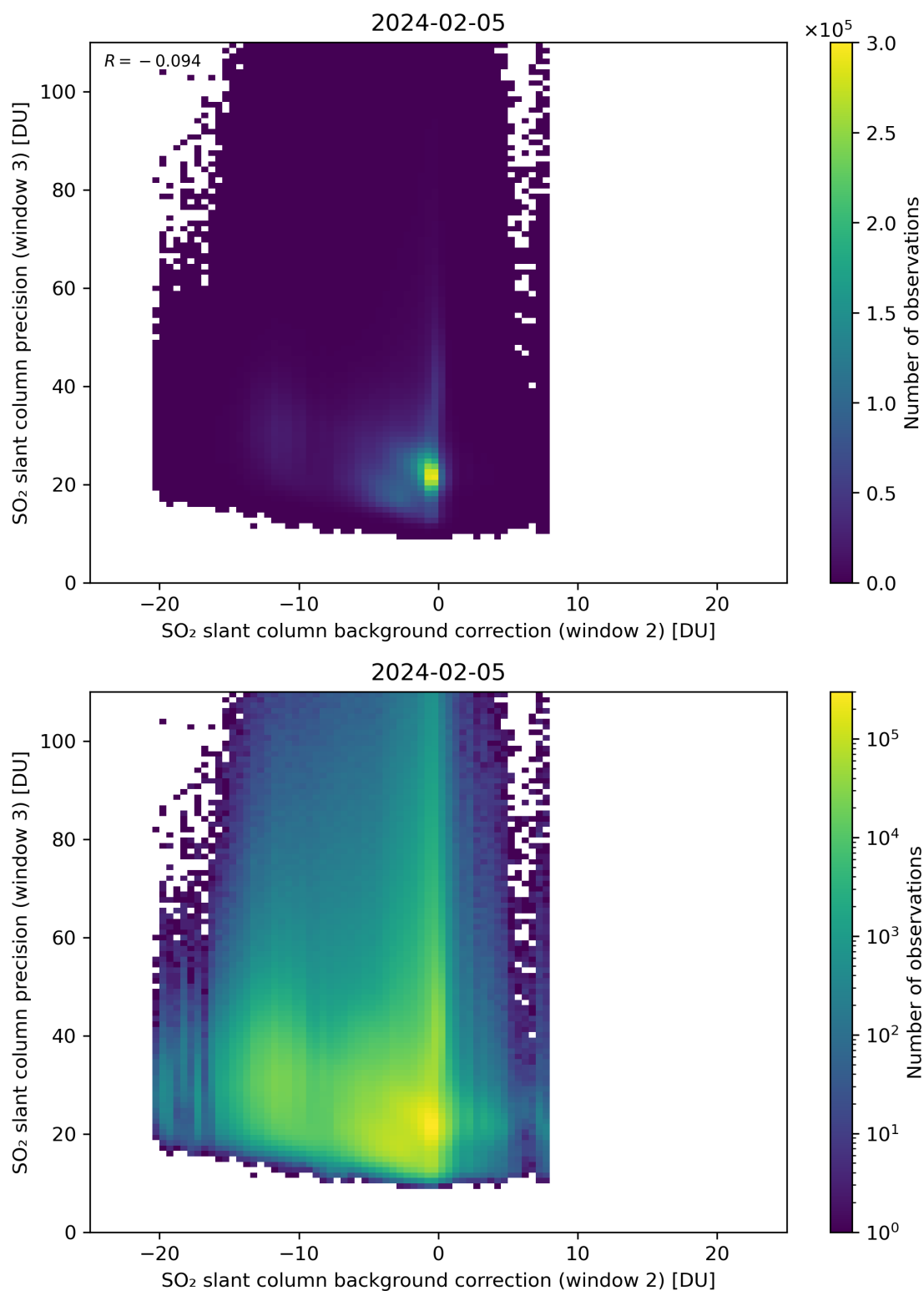
Figure 118: Scatter density plot of “SO 2 slant column background correction (window 2)” against “SO 2 slant column precision (window 3)” for 2024-02-04 to 2024-02-06.
