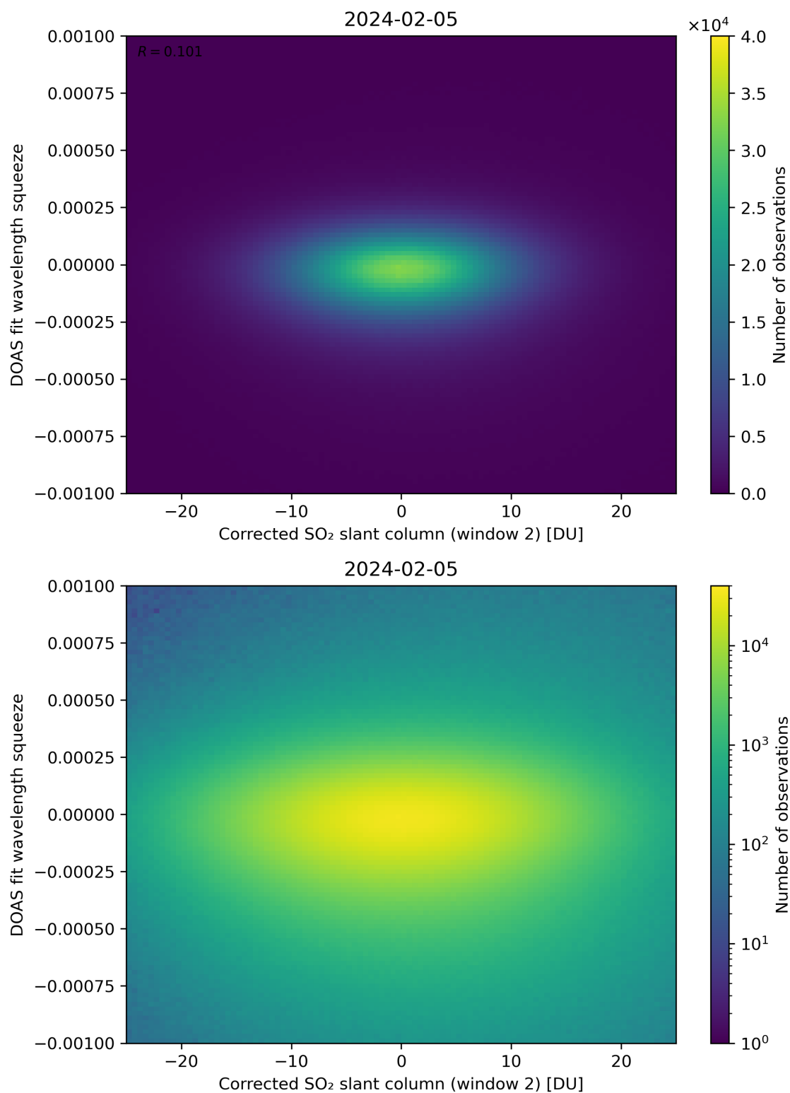
Figure 197: Scatter density plot of “Corrected SO 2 slant column (window 2)” against “DOAS fit wavelength squeeze” for 2024-02-04 to 2024-02-06.
