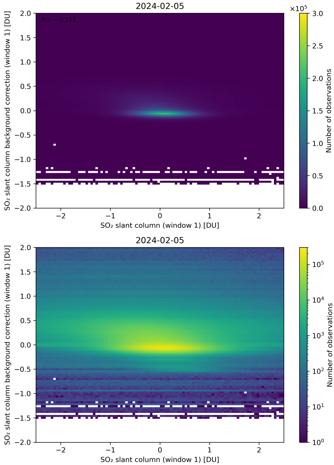
Figure 212: Scatter density plot of “SO 2 slant column (window 1)” against “SO 2 slant column background correction (window 1)” for 2024-02-04 to 2024-02-06.
