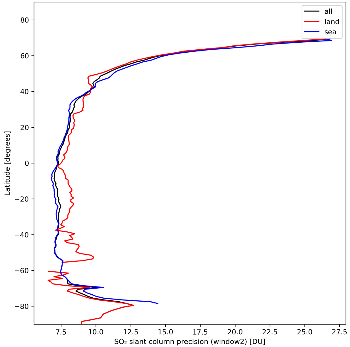
Figure 38: Zonal average of “SO 2 slant column precision (window2)” for 2024-02-04 to 2024-02-06.
