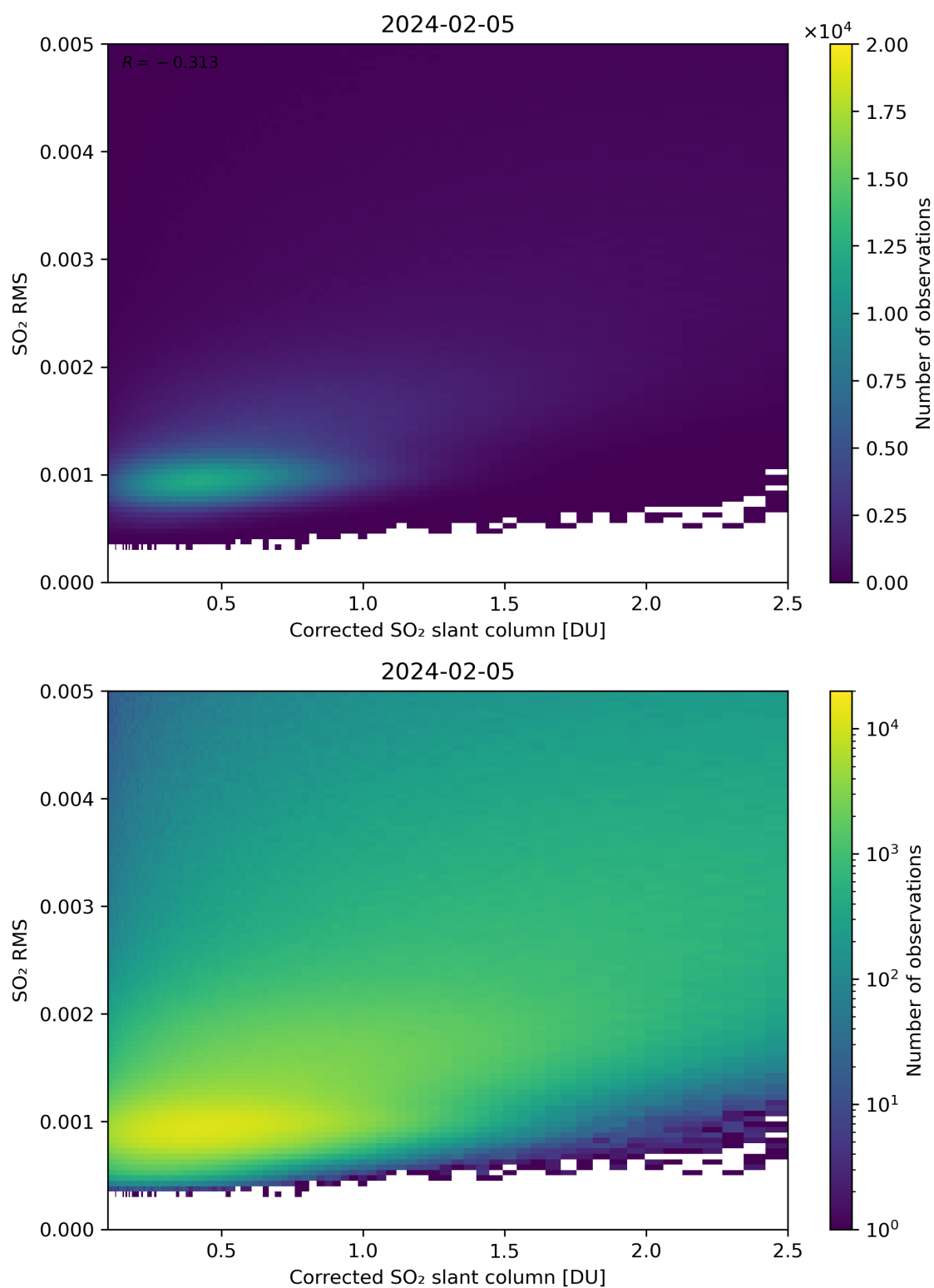
Figure 183: Scatter density plot of “Corrected SO 2 slant column” against “SO 2 RMS” for 2024-02-04 to 2024-02-06.
