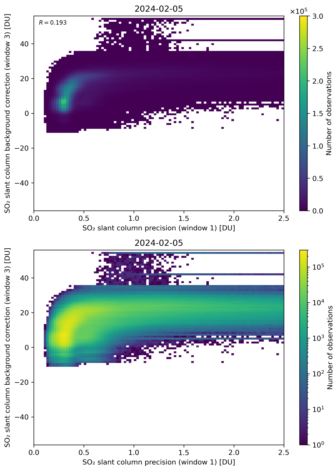
Figure 220: Scatter density plot of “SO 2 slant column precision (window 1)” against “SO 2 slant column background correction (window 3)” for 2024-02-04 to 2024-02-06.
