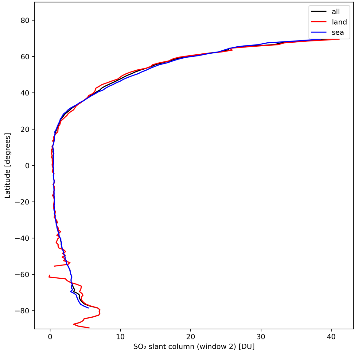
Figure 37: Zonal average of “SO 2 slant column (window 2)” for 2024-02-04 to 2024-02-06.
