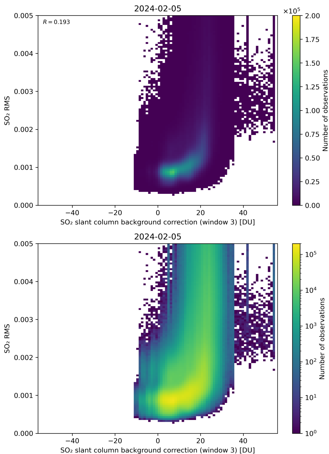
Figure 123: Scatter density plot of “SO 2 slant column background correction (window 3)” against “SO 2 RMS” for 2024-02-04 to 2024-02-06.
