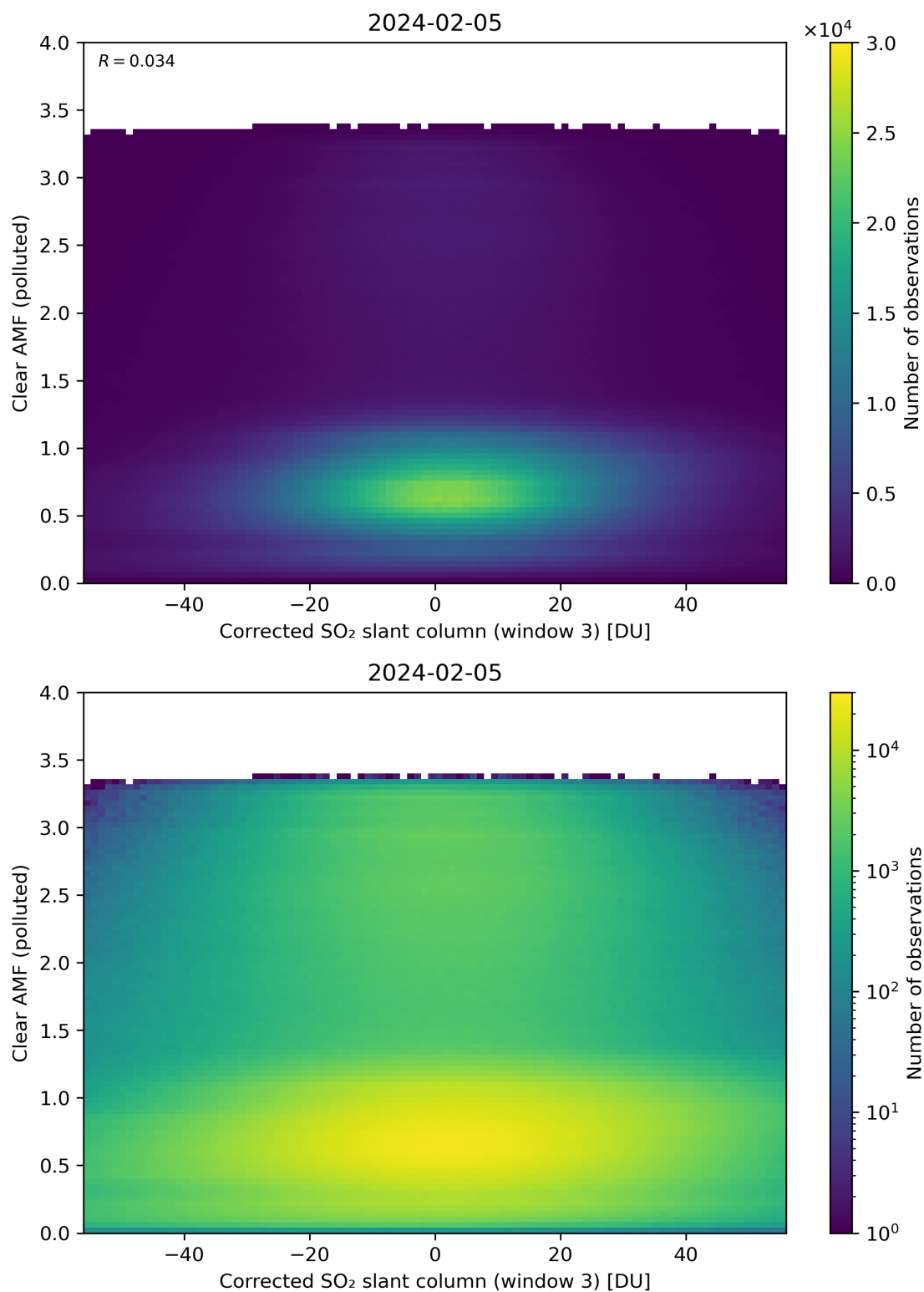
Figure 209: Scatter density plot of “Corrected SO 2 slant column (window 3)” against “Clear AMF (polluted)” for 2024-02-04 to 2024-02-06.
