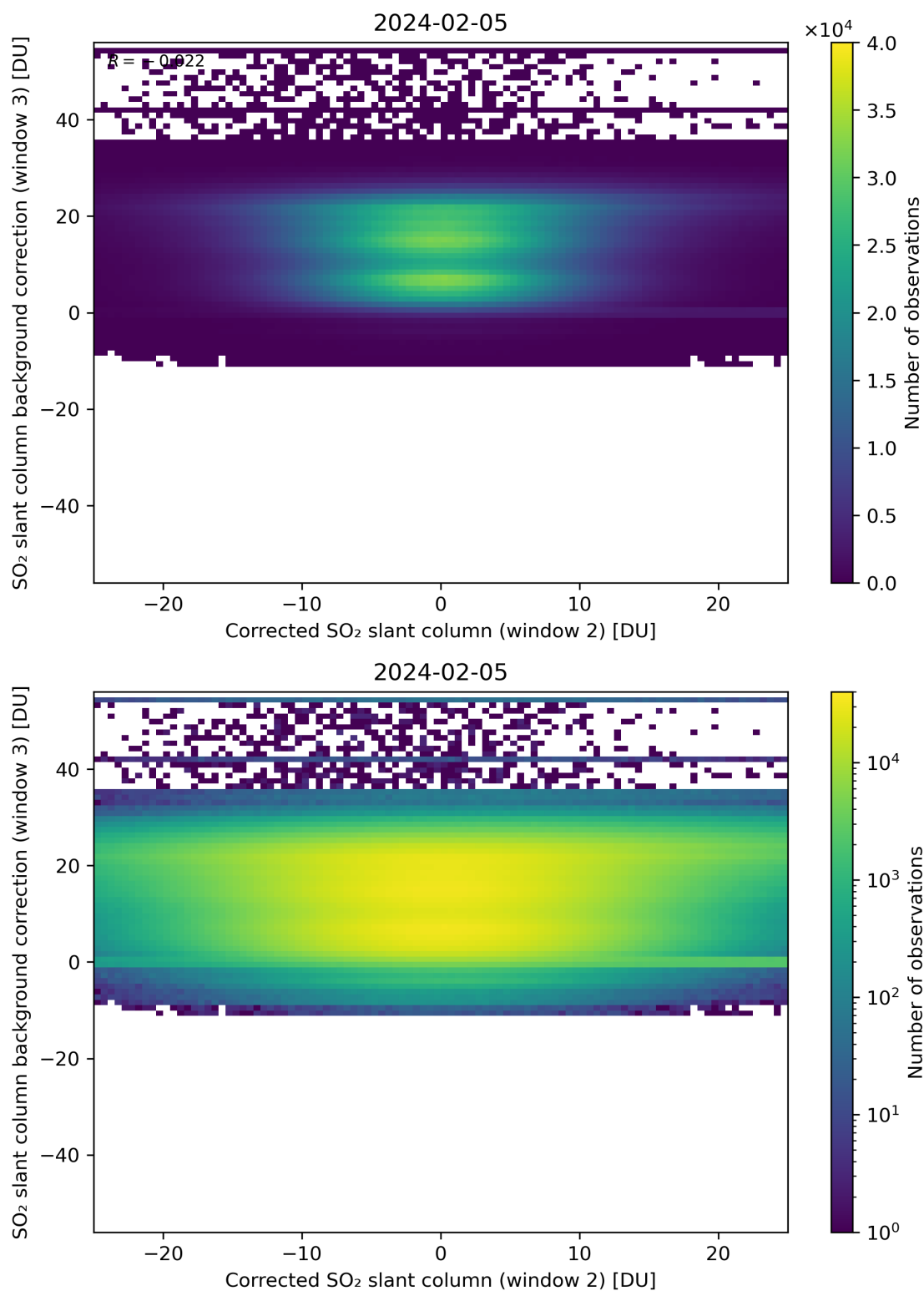
Figure 195: Scatter density plot of “Corrected SO 2 slant column (window 2)” against “SO 2 slant column background correction (window 3)” for 2024-02-04 to 2024-02-06.
