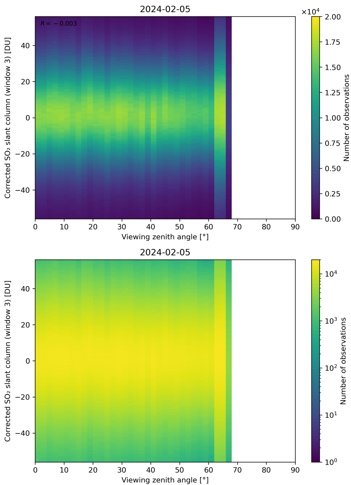
Figure 319: Scatter density plot of “Viewing zenith angle” against “Corrected SO 2 slant column (window 3)” for 2024-02-04 to 2024-02-06.
