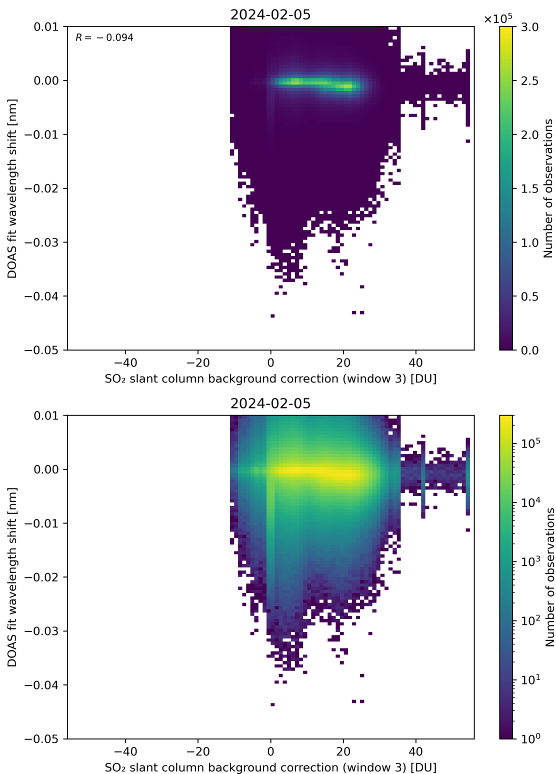
Figure 121: Scatter density plot of “SO 2 slant column background correction (window 3)” against “DOAS fit wavelength shift” for 2024-02-04 to 2024-02-06.
