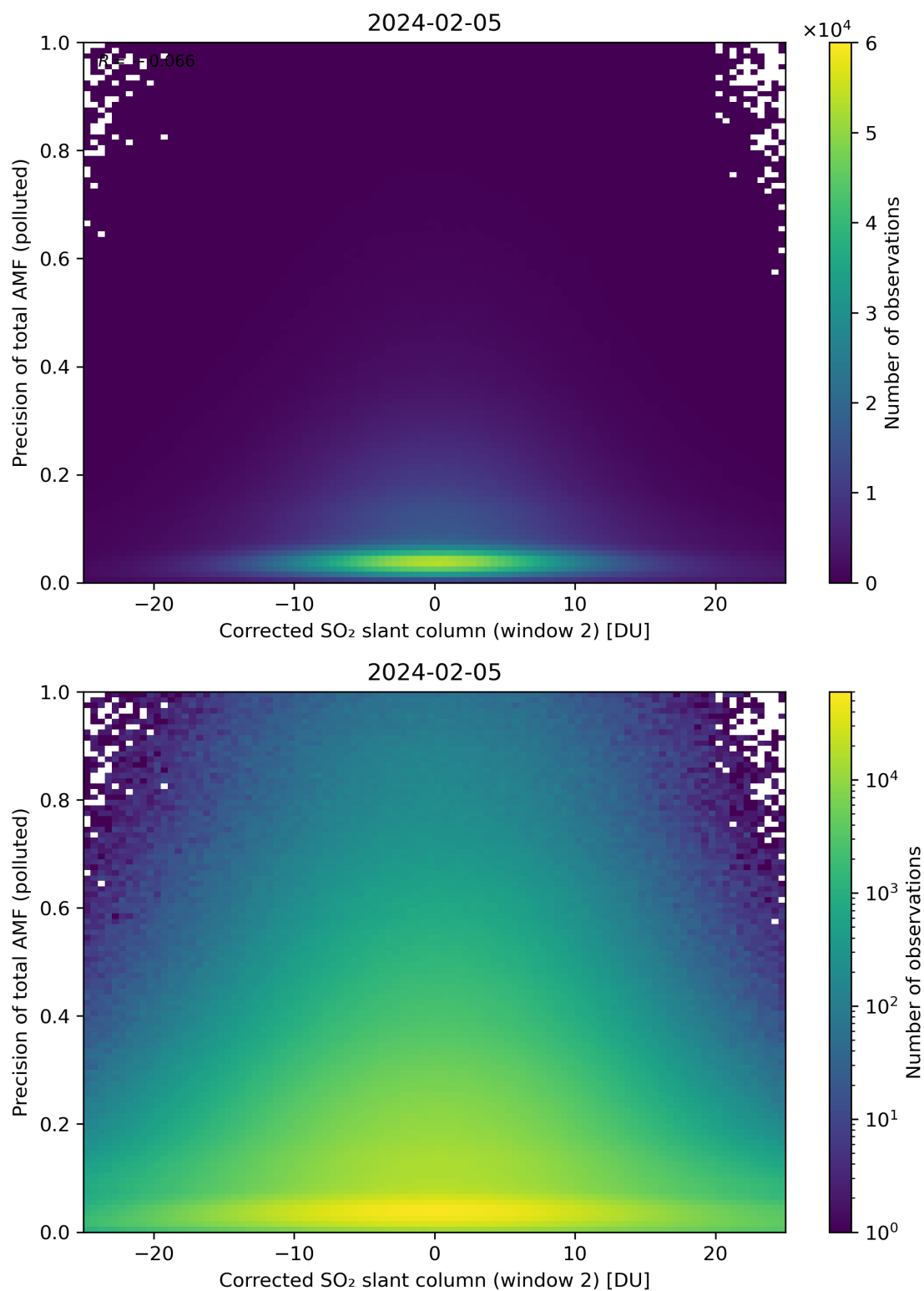
Figure 204: Scatter density plot of “Corrected SO 2 slant column (window 2)” against “Precision of total AMF (polluted)” for 2024-02-04 to 2024-02-06.
