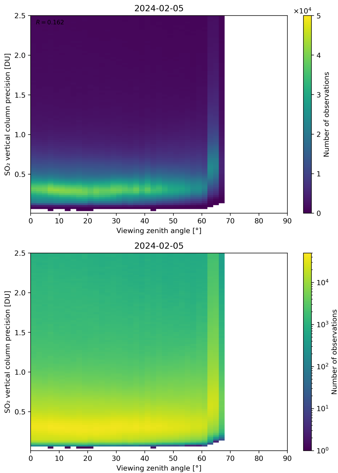
Figure 328: Scatter density plot of “Viewing zenith angle” against “SO 2 vertical column precision” for 2024-02-04 to 2024-02-06.
