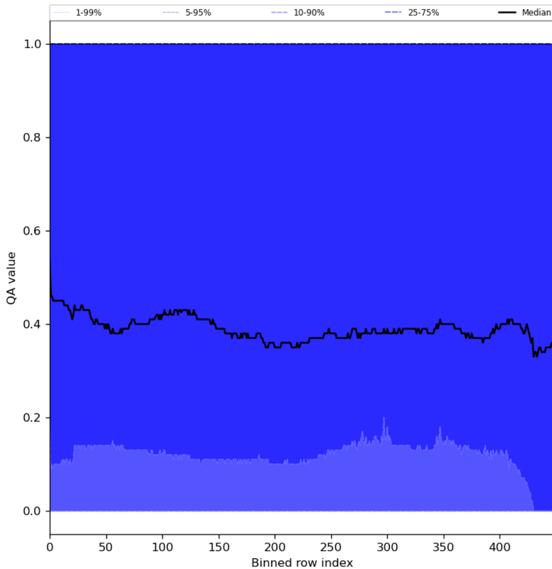
Figure 75: Along track statistics of “QA value” for 2024-02-04 to 2024-02-06
