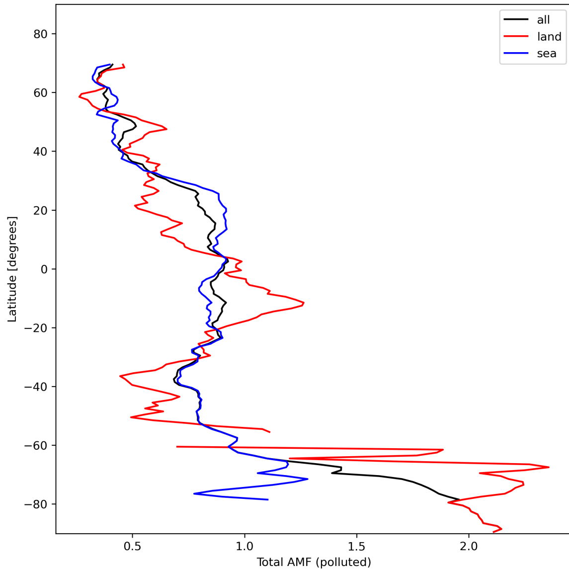
Figure 48: Zonal average of “Total AMF (polluted)” for 2024-02-04 to 2024-02-06.
