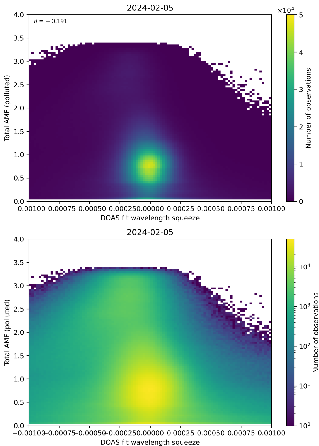
Figure 134: Scatter density plot of “DOAS fit wavelength squeeze” against “Total AMF (polluted)” for 2024-02-04 to 2024-02-06.
