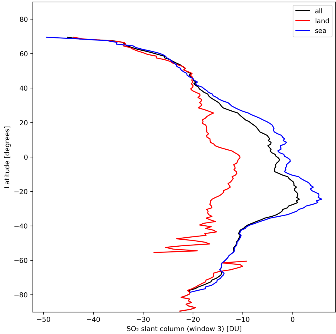
Figure 41: Zonal average of “SO 2 slant column (window 3)” for 2024-02-04 to 2024-02-06.
