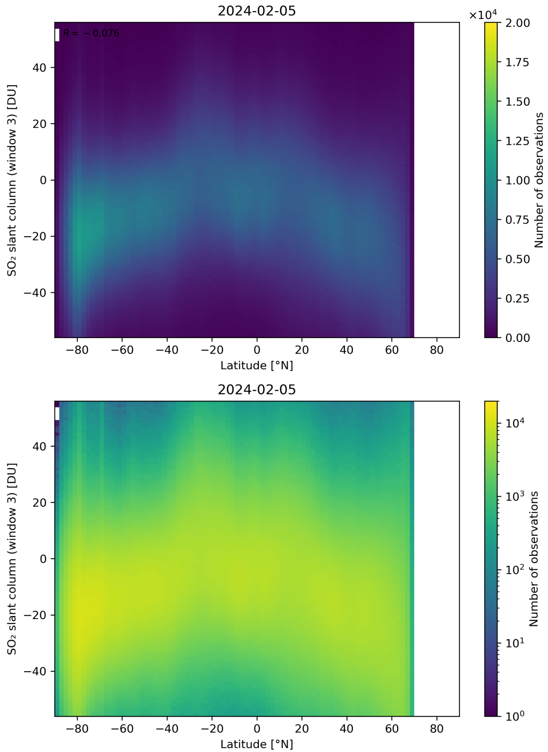
Figure 152: Scatter density plot of “Latitude” against “SO 2 slant column (window 3)” for 2024-02-04 to 2024-02-06.
