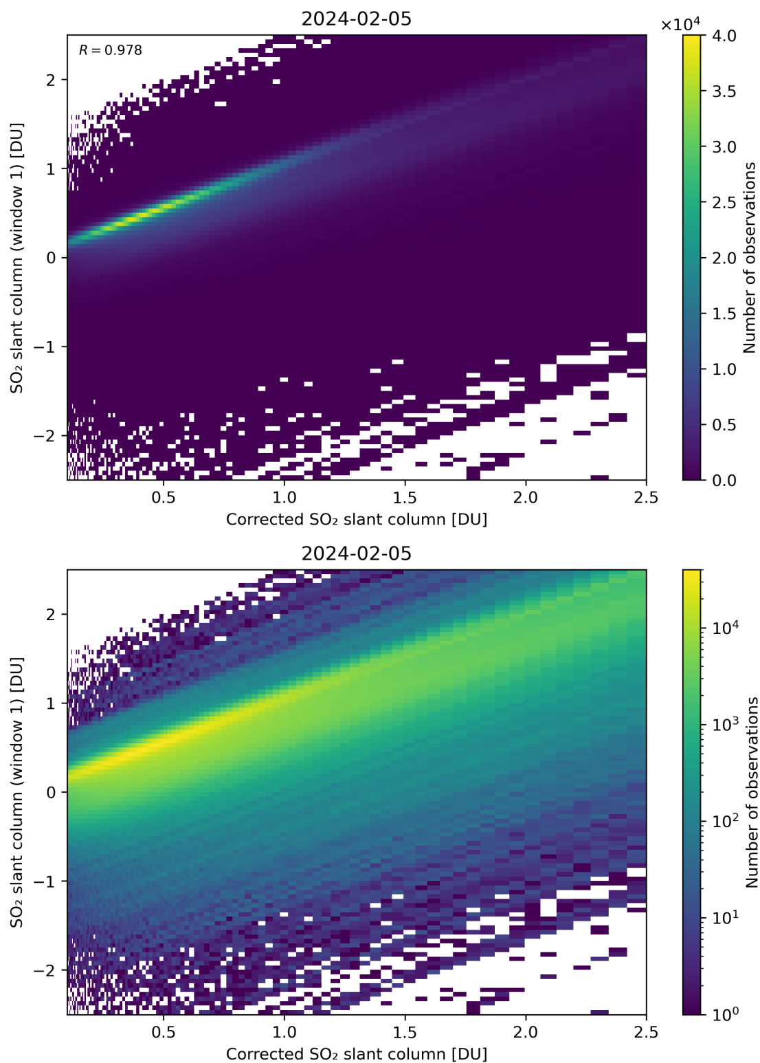
Figure 187: Scatter density plot of “Corrected SO 2 slant column” against “SO 2 slant column (window 1)” for 2024-02-04 to 2024-02-06.
