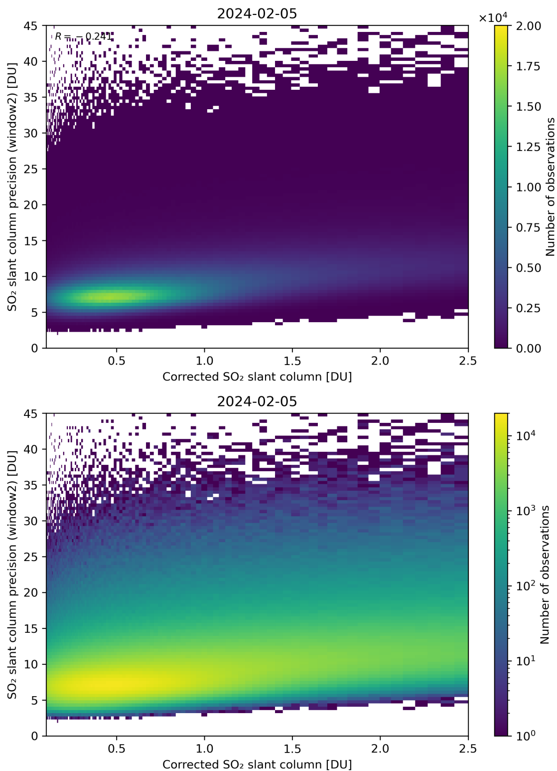
Figure 189: Scatter density plot of “Corrected SO 2 slant column” against “SO 2 slant column precision (window2)” for 2024-02-04 to 2024-02-06.
