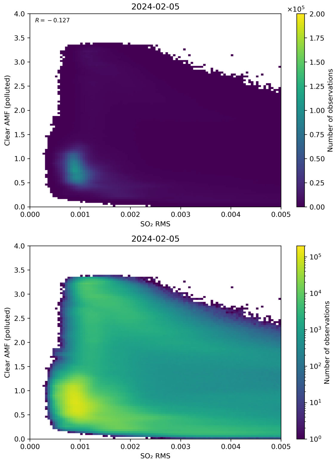
Figure 136: Scatter density plot of “SO 2 RMS” against “Clear AMF (polluted)” for 2024-02-04 to 2024-02-06.
