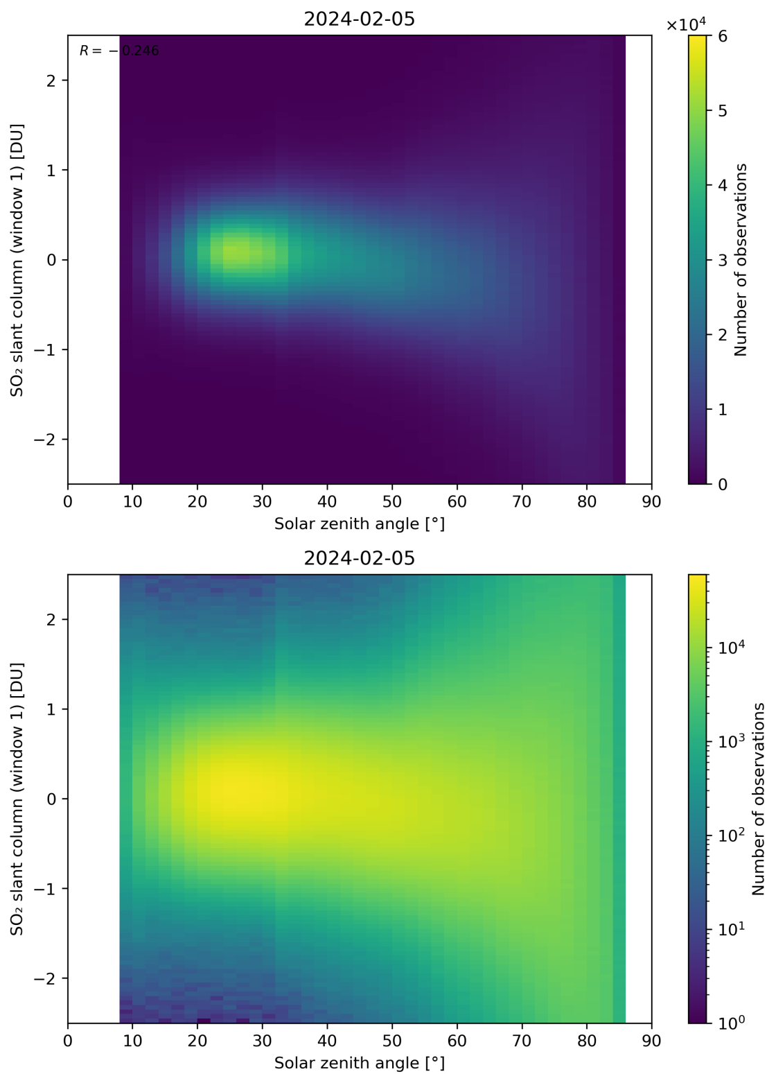
Figure 169: Scatter density plot of “Solar zenith angle” against “SO 2 slant column (window 1)” for 2024-02-04 to 2024-02-06.
