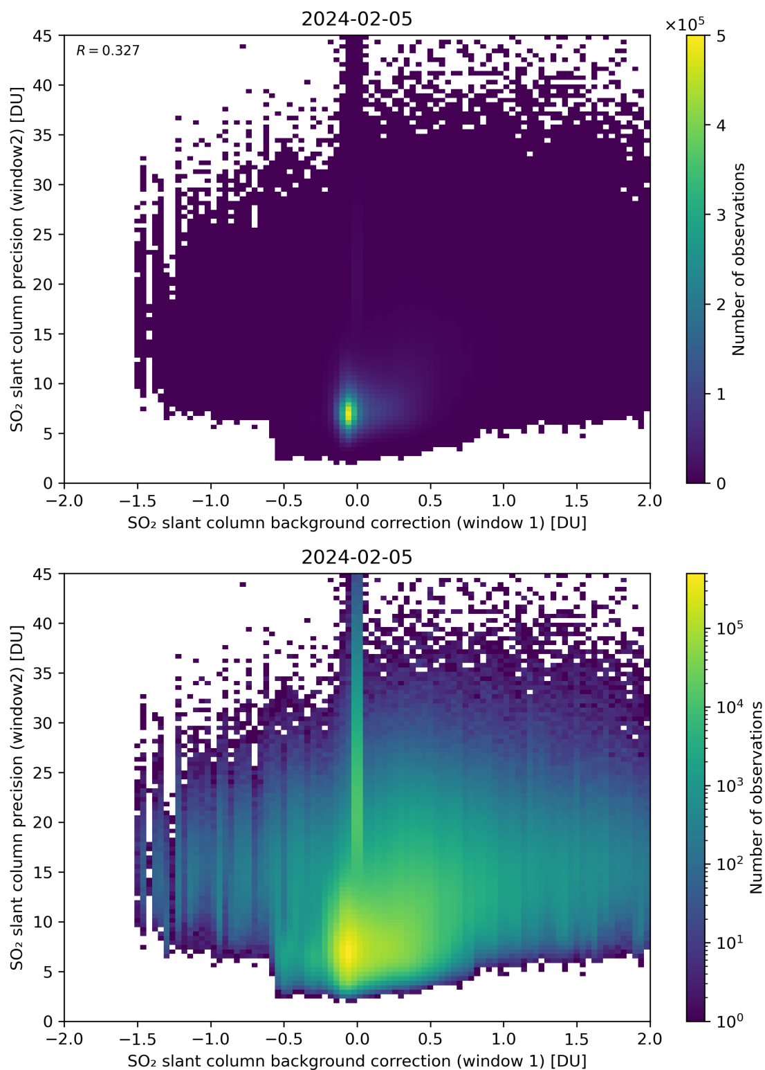
Figure 106: Scatter density plot of “SO 2 slant column background correction (window 1)” against “SO 2 slant column precision (window2)” for 2024-02-04 to 2024-02-06.
