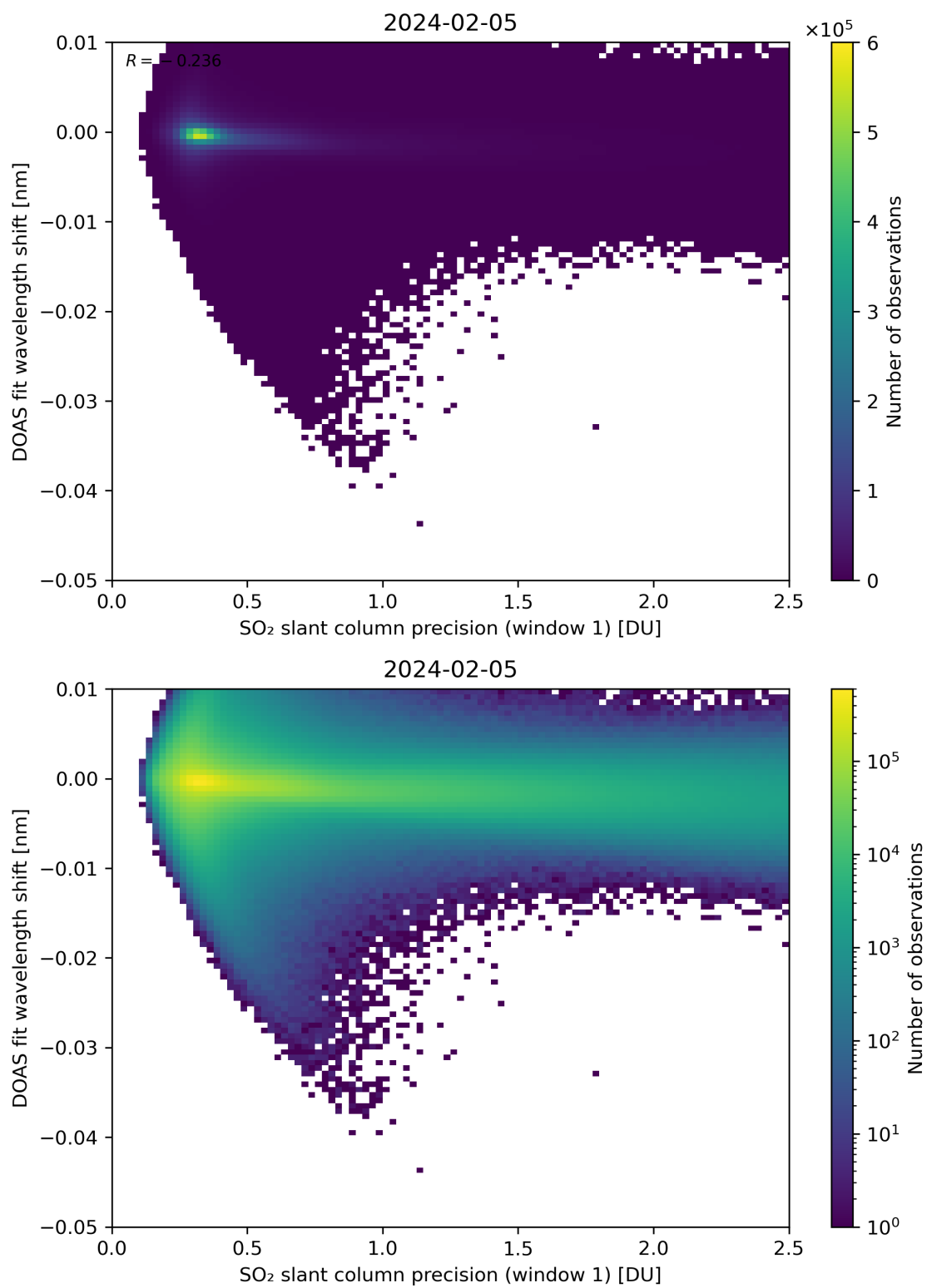
Figure 221: Scatter density plot of “SO 2 slant column precision (window 1)” against “DOAS fit wavelength shift” for 2024-02-04 to 2024-02-06.
