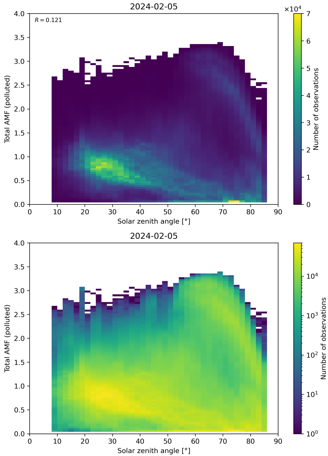
Figure 174: Scatter density plot of “Solar zenith angle” against “Total AMF (polluted)” for 2024-02-04 to 2024-02-06.
