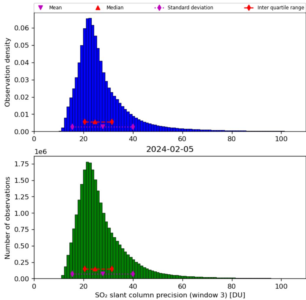
Figure 65: Histogram of “SO 2 slant column precision (window 3)” for 2024-02-04 to 2024-02-06
