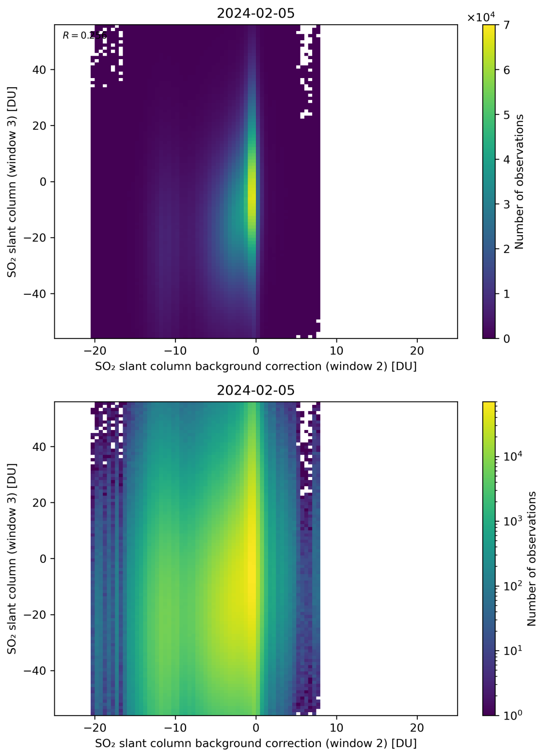
Figure 117: Scatter density plot of “SO 2 slant column background correction (window 2)” against “SO 2 slant column (window 3)” for 2024-02-04 to 2024-02-06.
