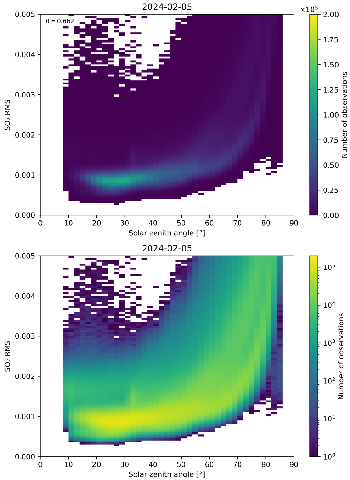
Figure 163: Scatter density plot of “Solar zenith angle” against “SO 2 RMS” for 2024-02-04 to 2024-02-06.
