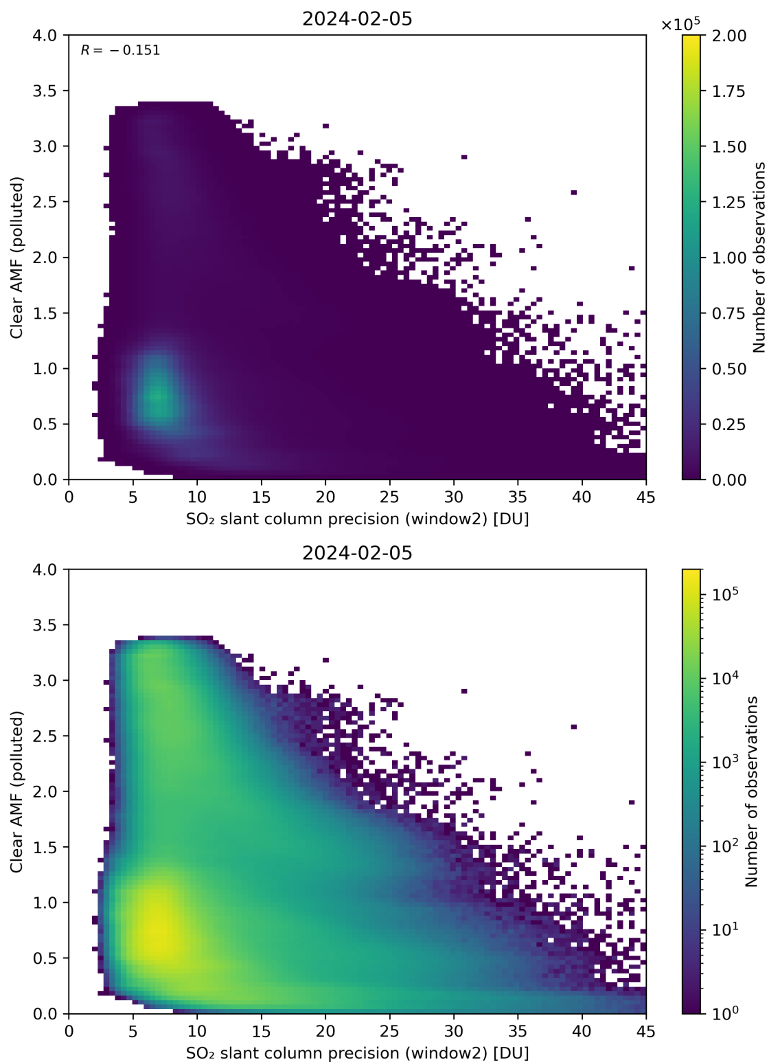
Figure 246: Scatter density plot of “SO 2 slant column precision (window2)” against “Clear AMF (polluted)” for 2024-02-04 to 2024-02-06.
