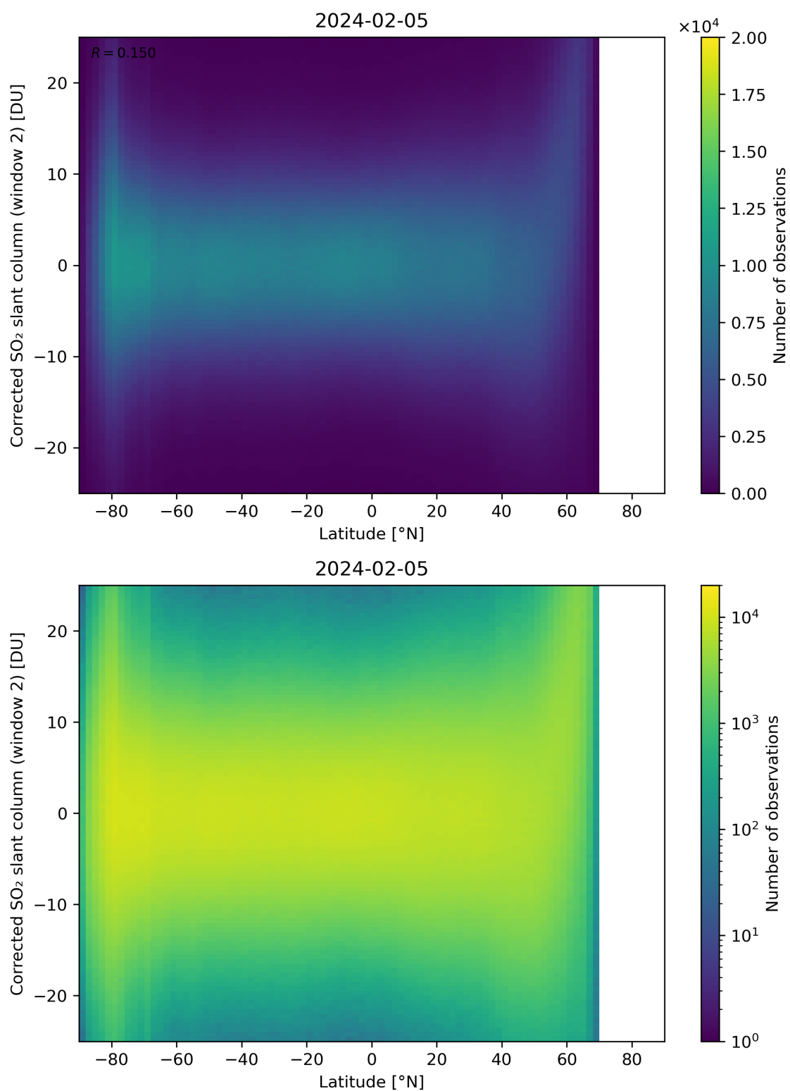
Figure 147: Scatter density plot of “Latitude” against “Corrected SO 2 slant column (window 2)” for 2024-02-04 to 2024-02-06.
