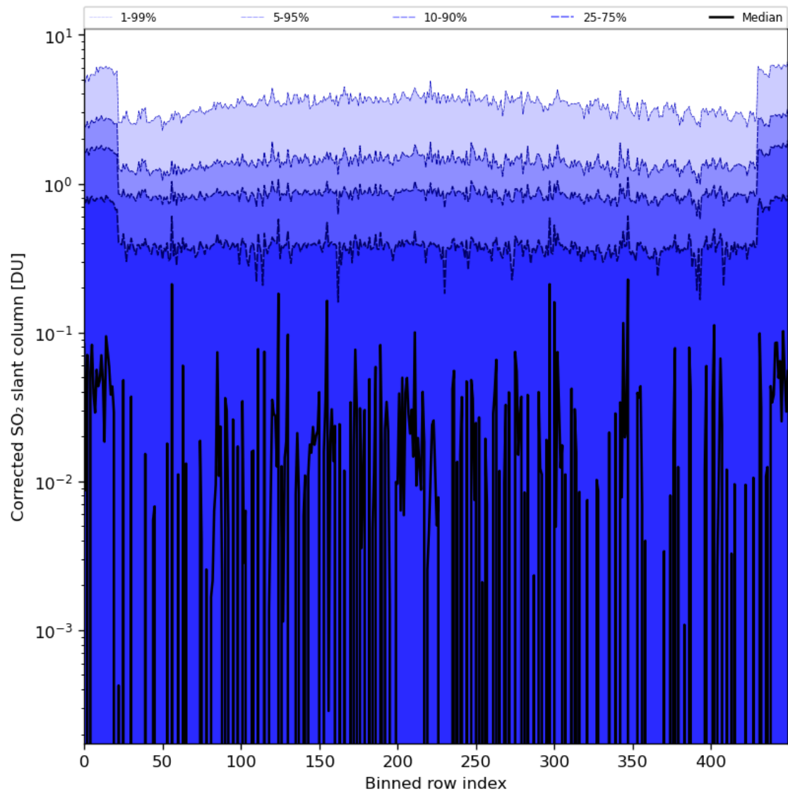
Figure 78: Along track statistics of “Corrected SO 2 slant column” for 2024-02-04 to 2024-02-06
