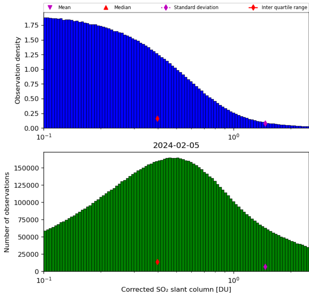
Figure 55: Histogram of “Corrected SO 2 slant column” for 2024-02-04 to 2024-02-06
