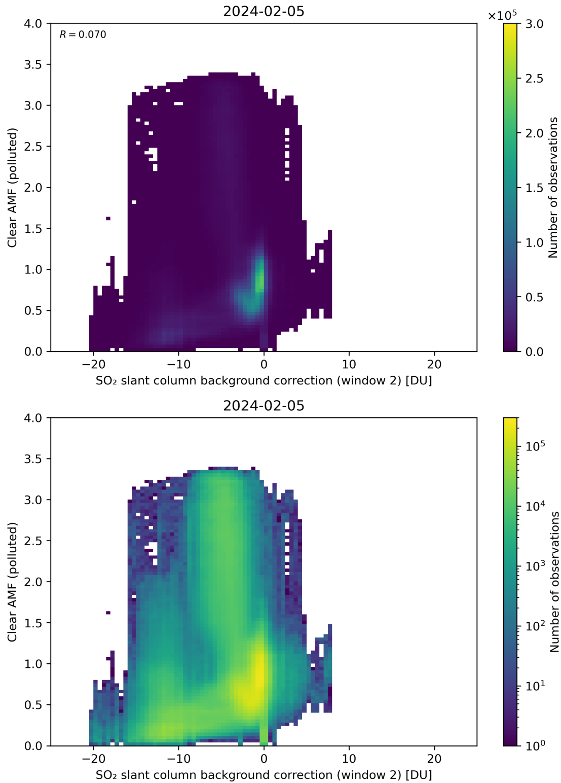
Figure 115: Scatter density plot of “SO 2 slant column background correction (window 2)” against “Clear AMF (polluted)” for 2024-02-04 to 2024-02-06.
