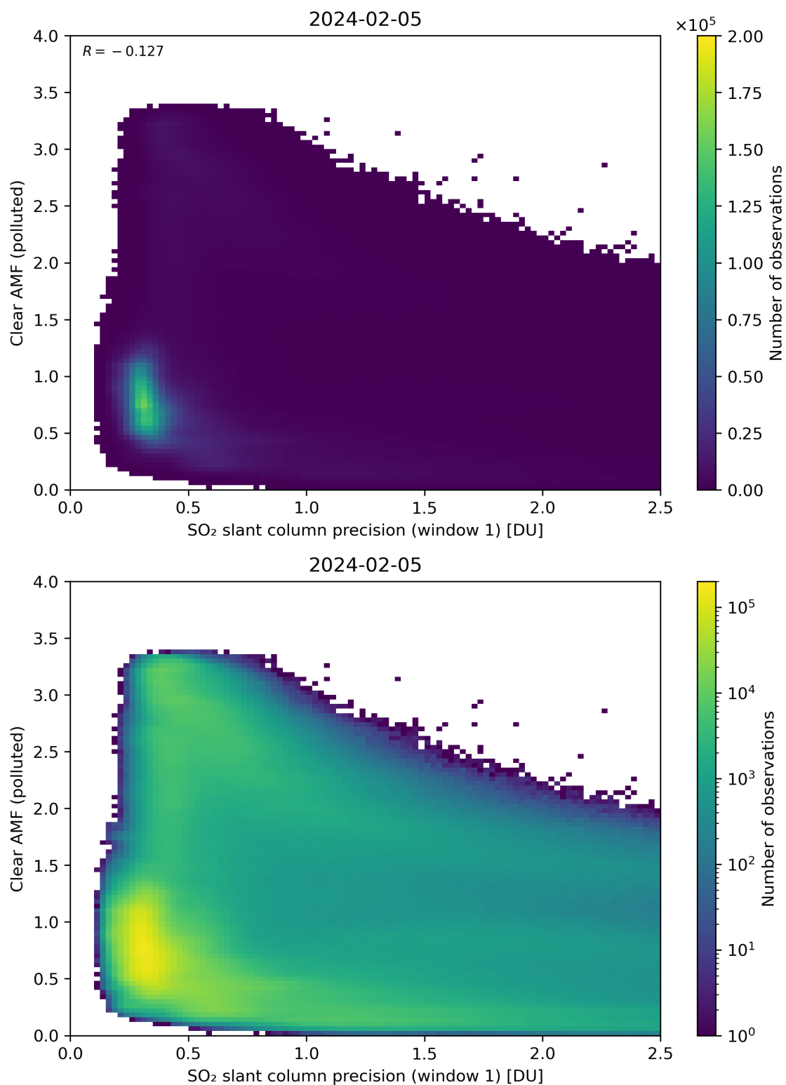
Figure 224: Scatter density plot of “SO 2 slant column precision (window 1)” against “Clear AMF (polluted)” for 2024-02-04 to 2024-02-06.
