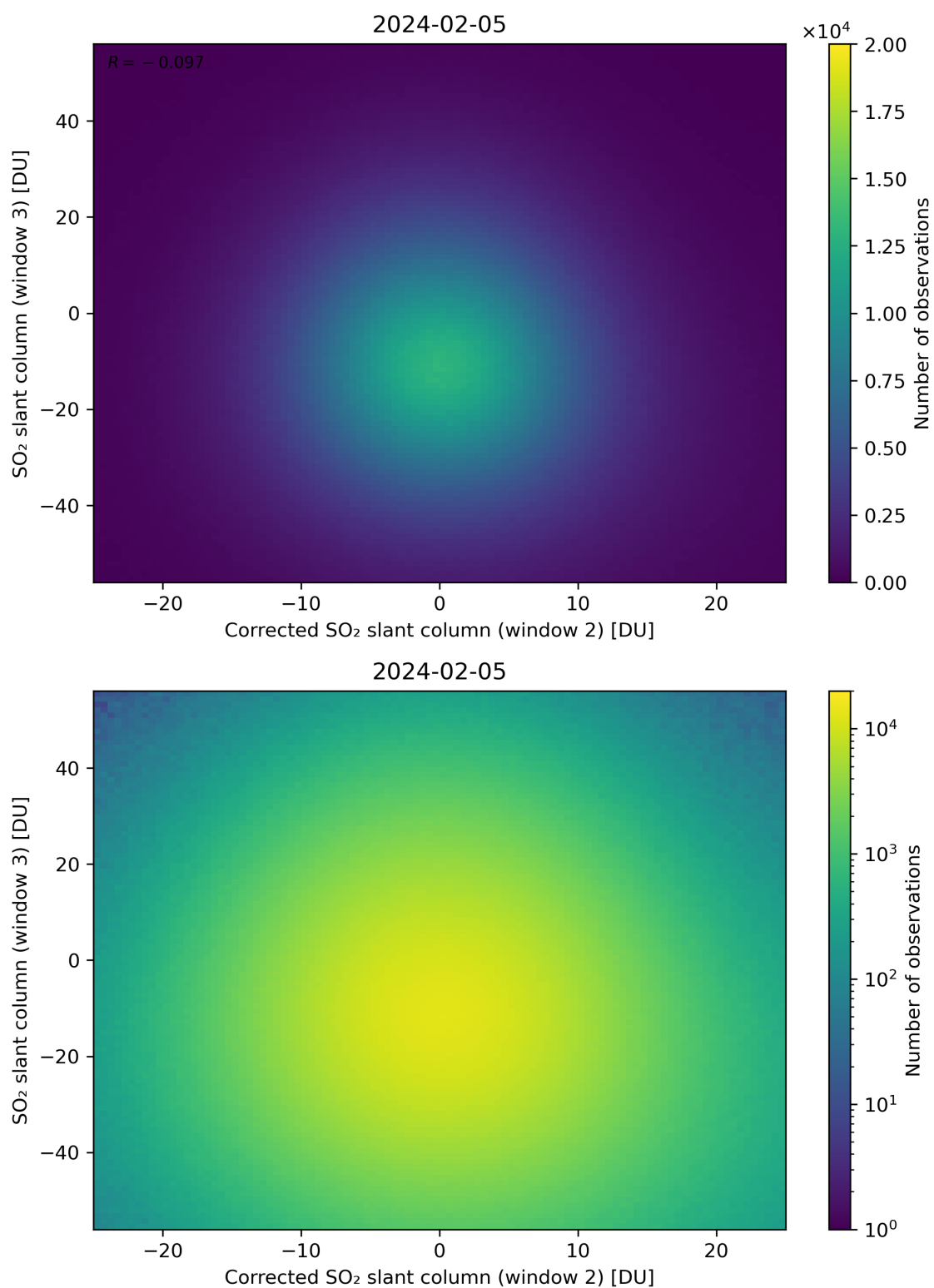
Figure 201: Scatter density plot of “Corrected SO 2 slant column (window 2)” against “SO 2 slant column (window 3)” for 2024-02-04 to 2024-02-06.
