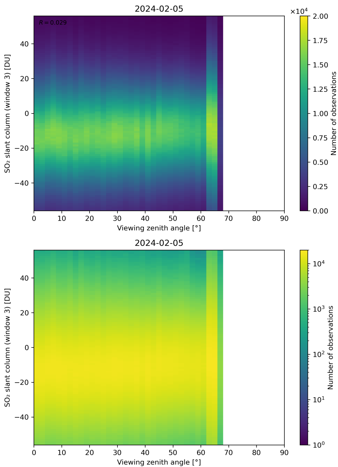
Figure 323: Scatter density plot of “Viewing zenith angle” against “SO 2 slant column (window 3)” for 2024-02-04 to 2024-02-06.
