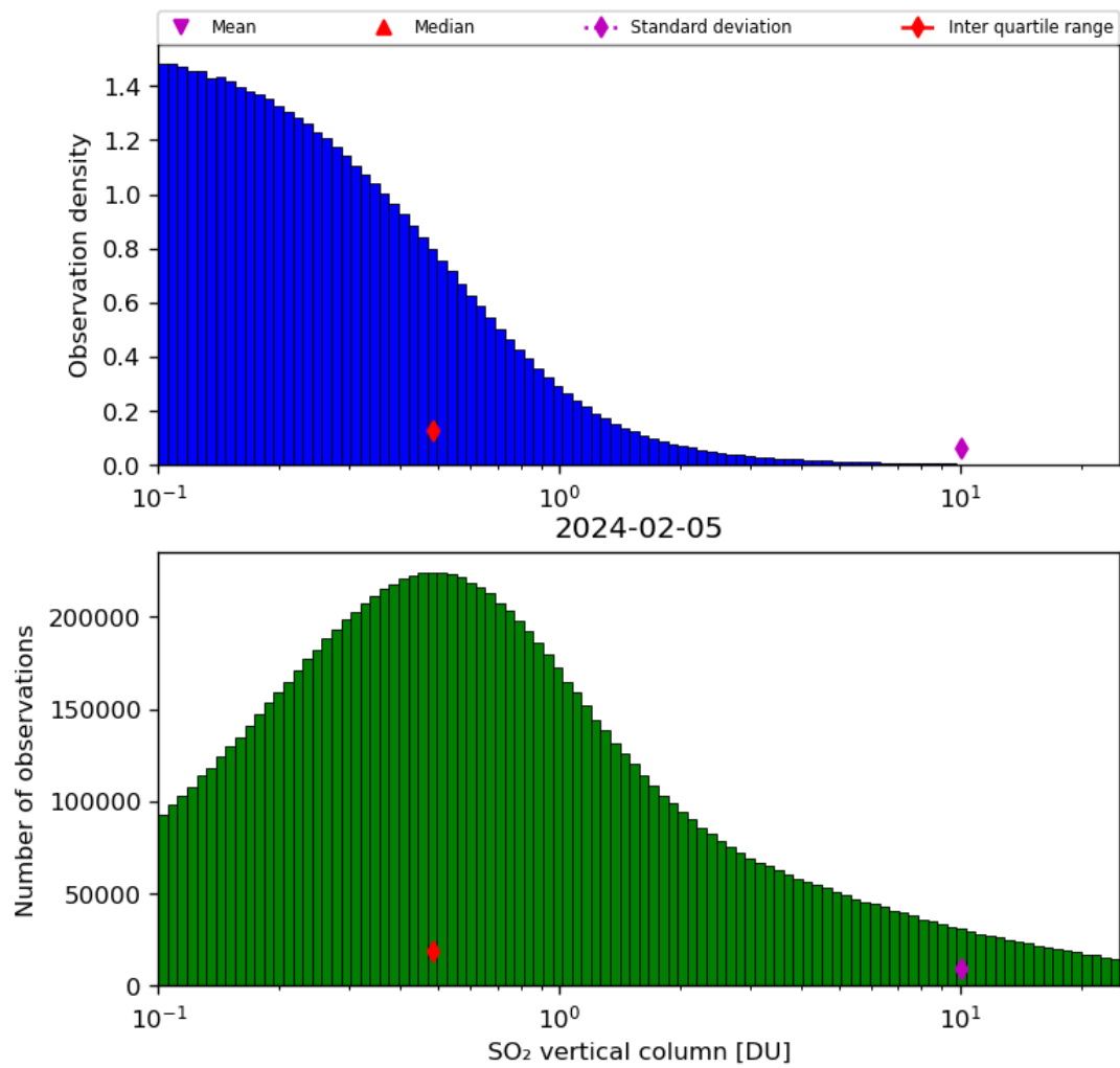
Figure 53: Histogram of “SO 2 vertical column” for 2024-02-04 to 2024-02-06
