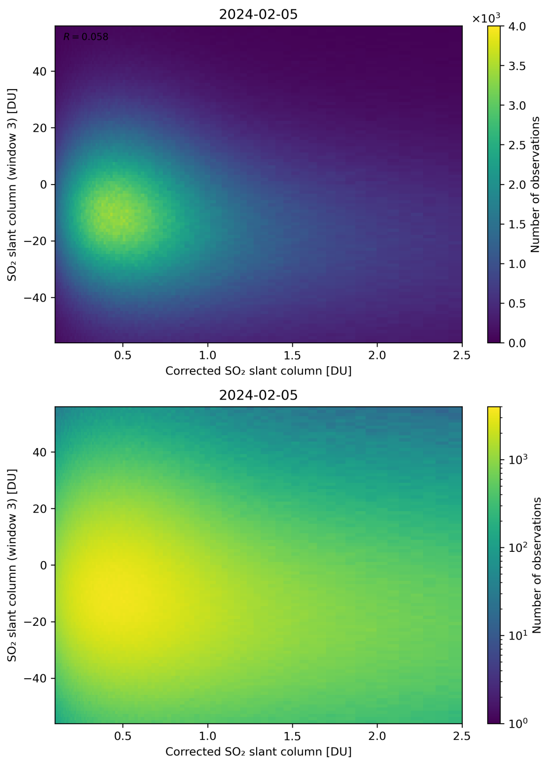
Figure 190: Scatter density plot of “Corrected SO 2 slant column” against “SO 2 slant column (window 3)” for 2024-02-04 to 2024-02-06.
