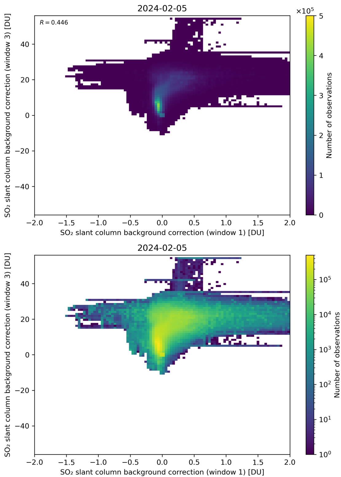
Figure 99: Scatter density plot of “SO 2 slant column background correction (window 1)” against “SO 2 slant column background correction (window 3)” for 2024-02-04 to 2024-02-06.
