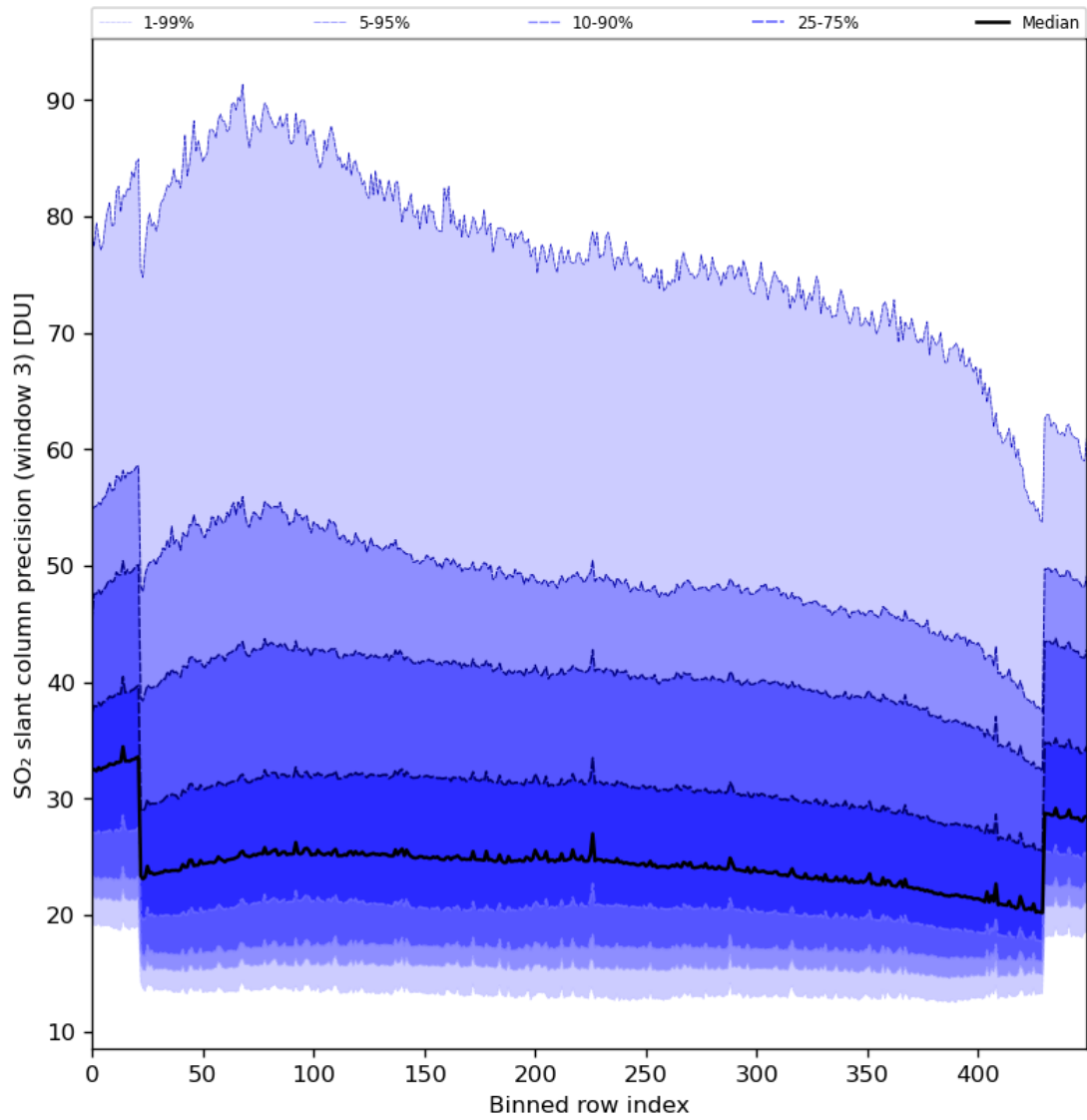
Figure 88: Along track statistics of “SO 2 slant column precision (window 3)” for 2024-02-04 to 2024-02-06
