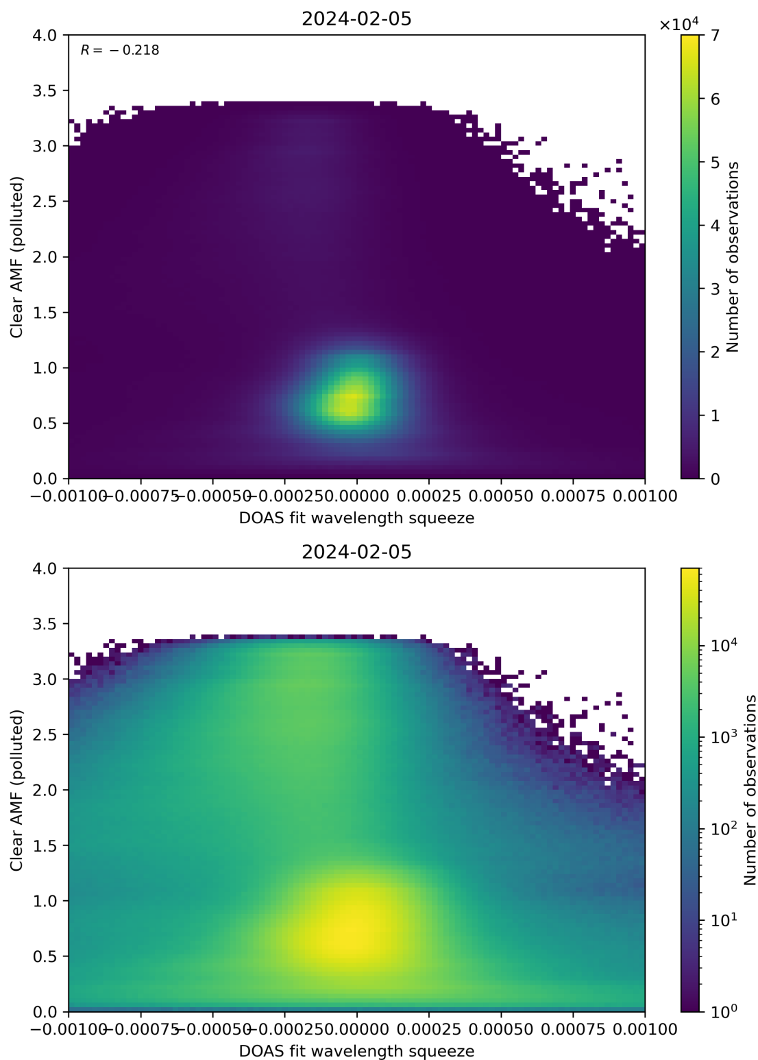
Figure 133: Scatter density plot of “DOAS fit wavelength squeeze” against “Clear AMF (polluted)” for 2024-02-04 to 2024-02-06.
