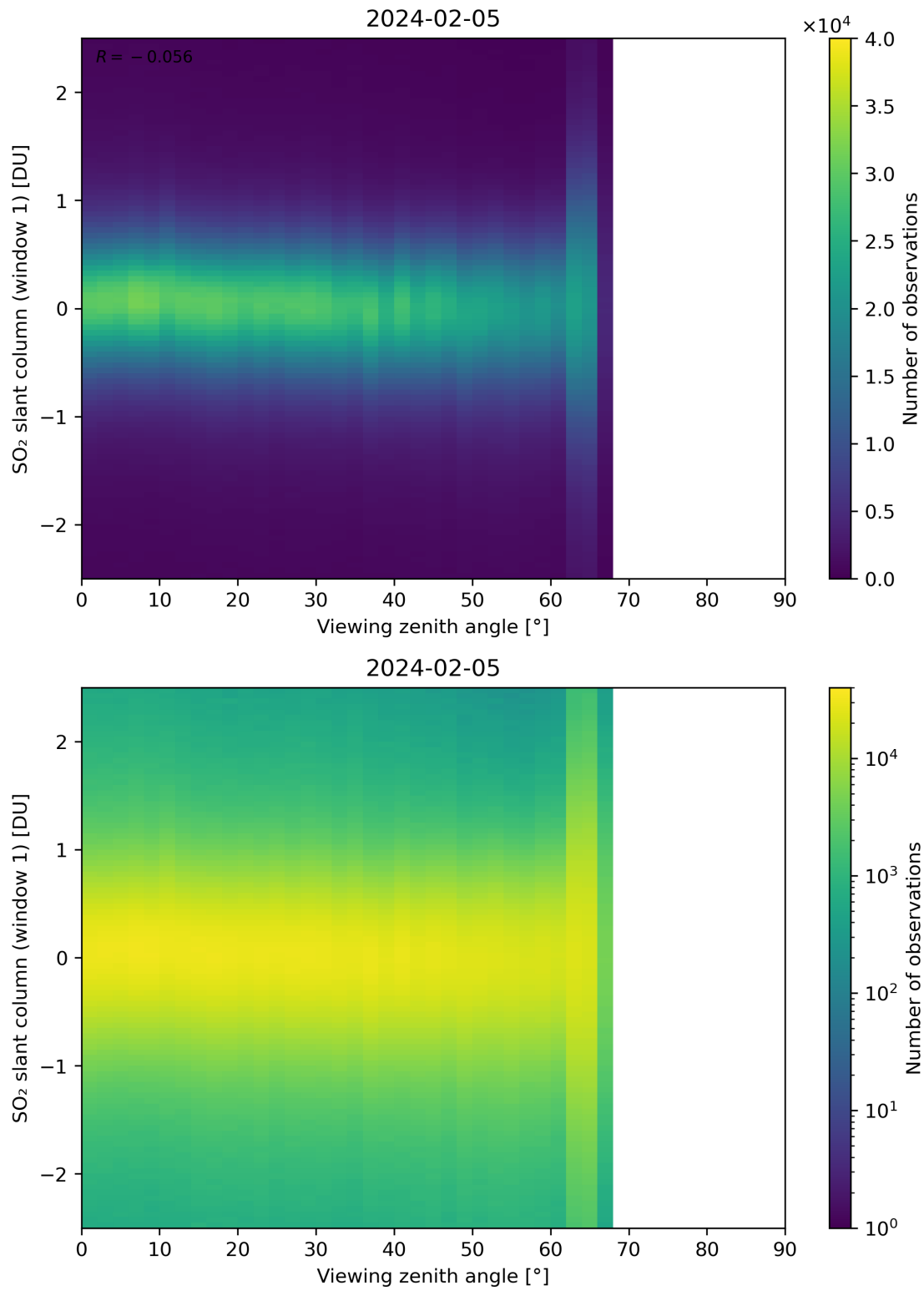
Figure 320: Scatter density plot of “Viewing zenith angle” against “SO 2 slant column (window 1)” for 2024-02-04 to 2024-02-06.
