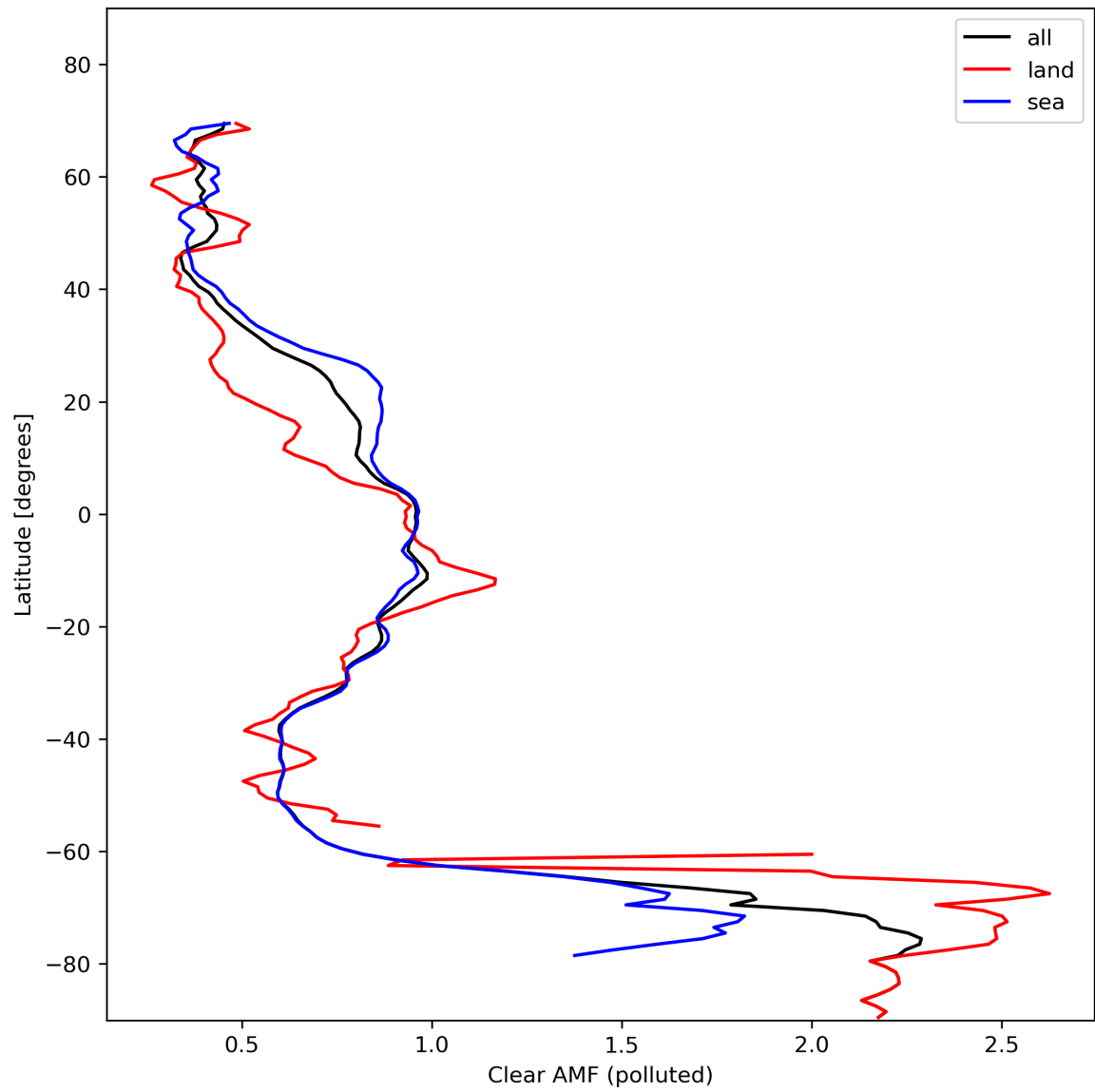
Figure 50: Zonal average of “Clear AMF (polluted)” for 2024-02-04 to 2024-02-06.
