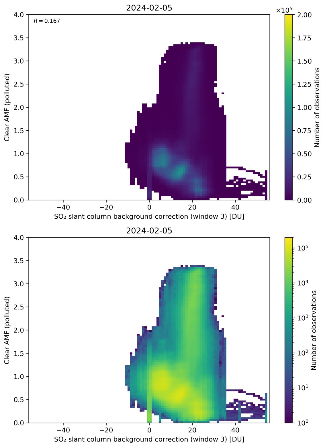
Figure 124: Scatter density plot of “SO 2 slant column background correction (window 3)” against “Clear AMF (polluted)” for 2024-02-04 to 2024-02-06.
