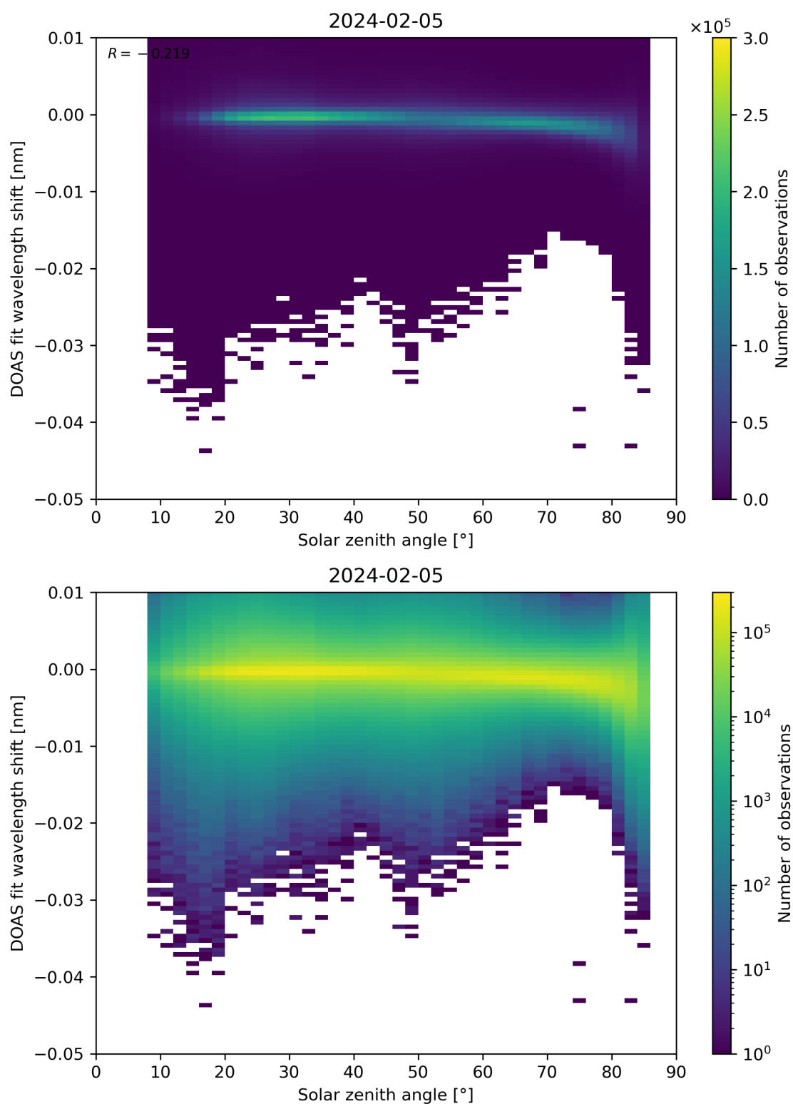
Figure 161: Scatter density plot of “Solar zenith angle” against “DOAS fit wavelength shift” for 2024-02-04 to 2024-02-06.
