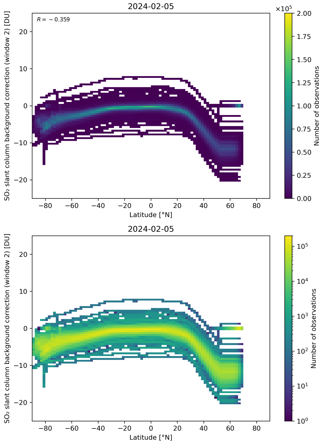
Figure 140: Scatter density plot of “Latitude” against “SO 2 slant column background correction (window 2)” for 2024-02-04 to 2024-02-06.
