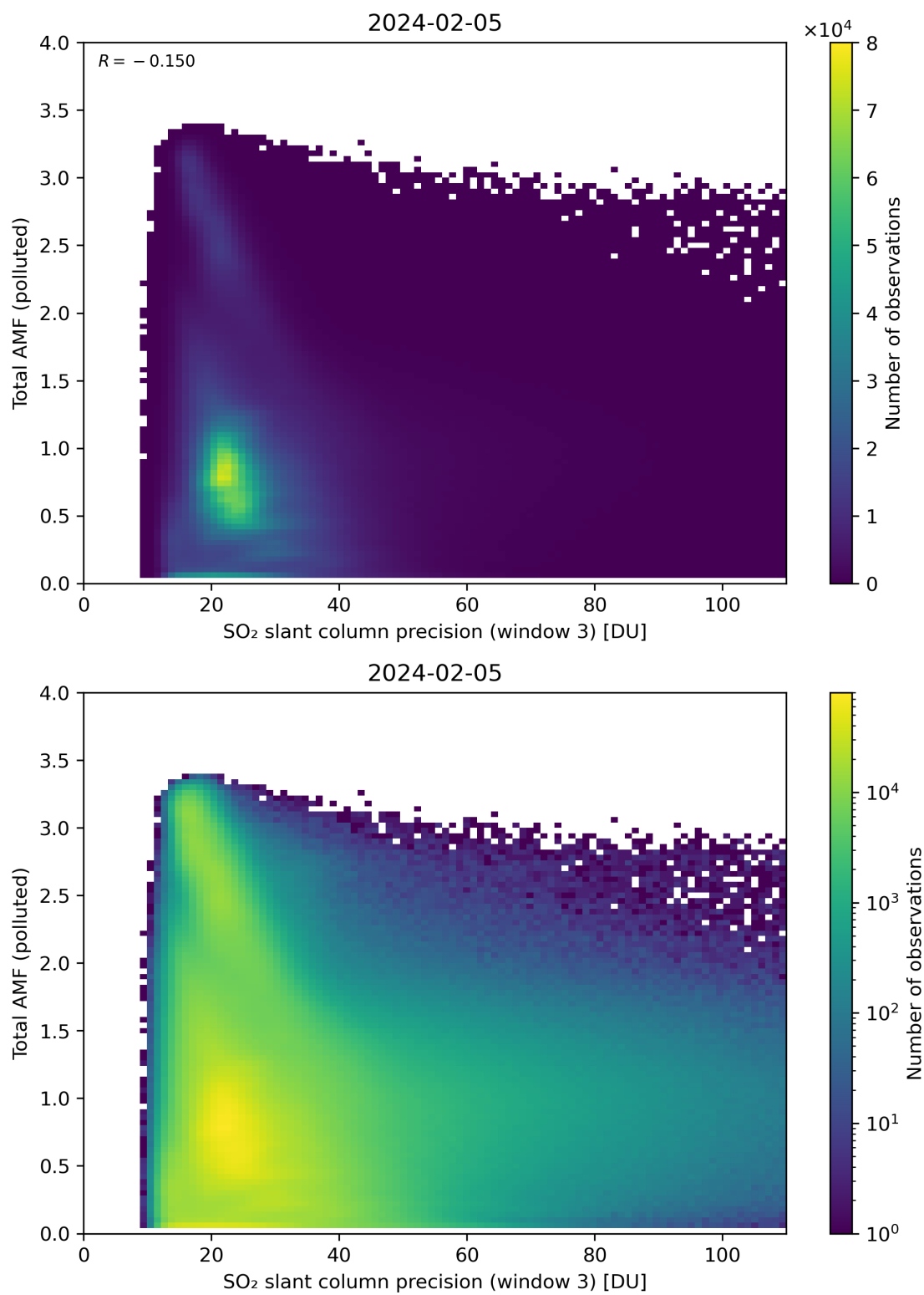
Figure 263: Scatter density plot of “SO 2 slant column precision (window 3)” against “Total AMF (polluted)” for 2024-02-04 to 2024-02-06.
