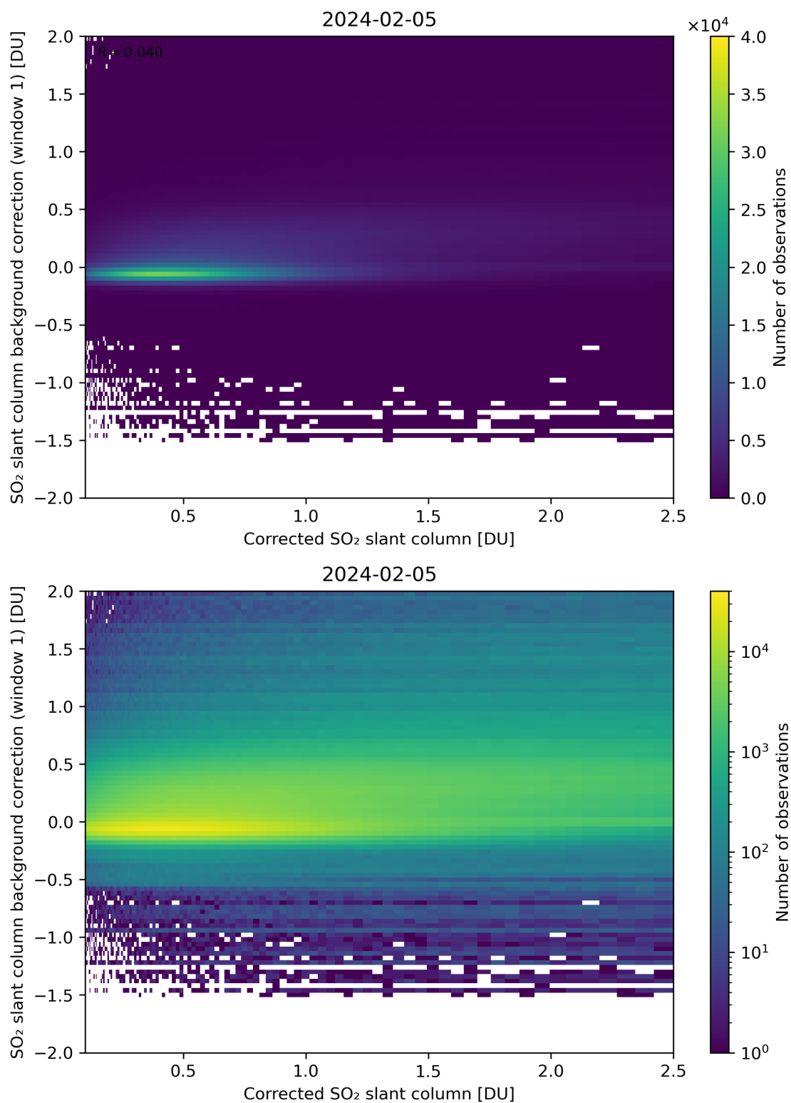
Figure 178: Scatter density plot of “Corrected SO 2 slant column” against “SO 2 slant column background correction (window 1)” for 2024-02-04 to 2024-02-06.
