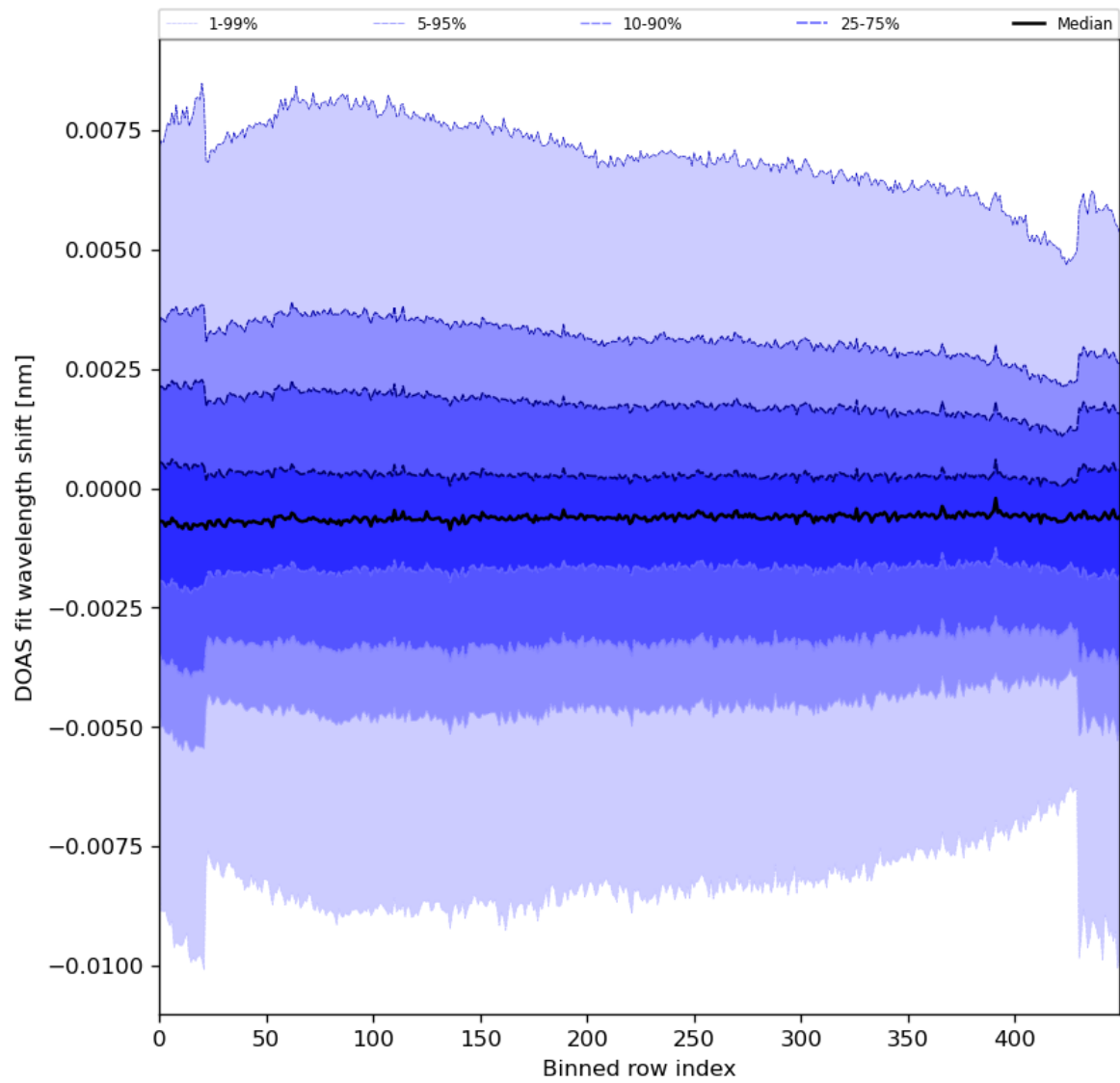
Figure 91: Along track statistics of “DOAS fit wavelength shift” for 2024-02-04 to 2024-02-06
