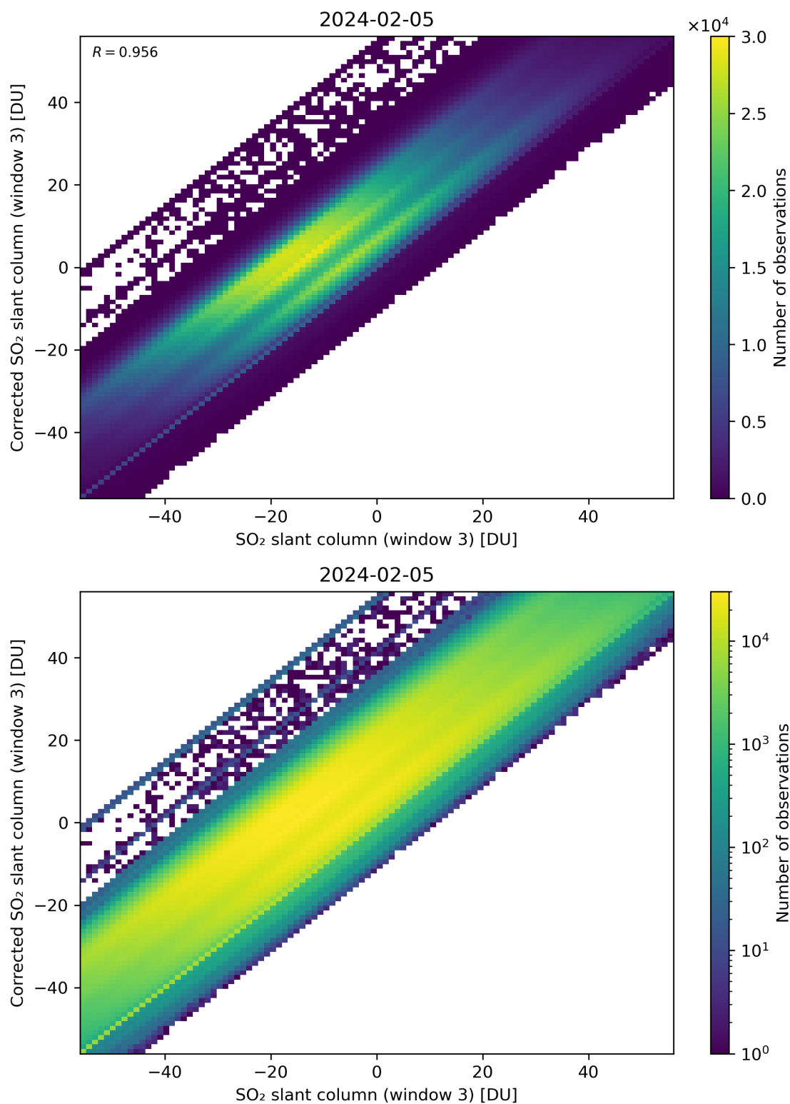
Figure 266: Scatter density plot of “SO 2 slant column (window 3)” against “Corrected SO 2 slant column (window 3)” for 2024-02-04 to 2024-02-06.
