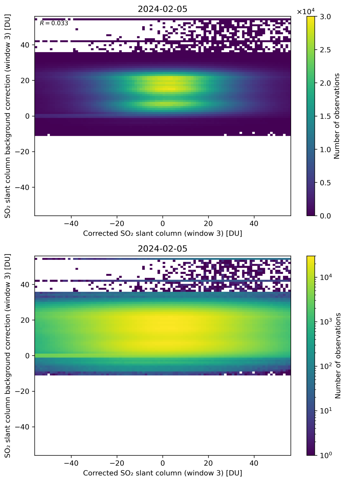
Figure 205: Scatter density plot of “Corrected SO 2 slant column (window 3)” against “SO 2 slant column background correction (window 3)” for 2024-02-04 to 2024-02-06.
