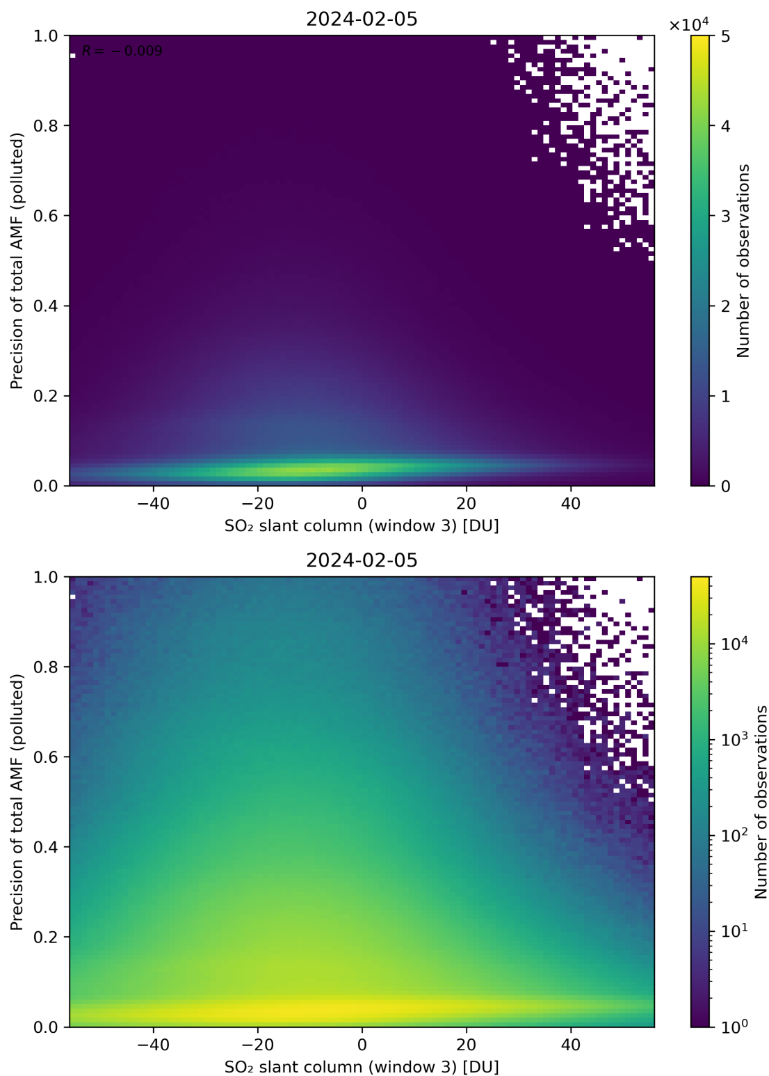
Figure 269: Scatter density plot of “SO 2 slant column (window 3)” against “Precision of total AMF (polluted)” for 2024-02-04 to 2024-02-06.
