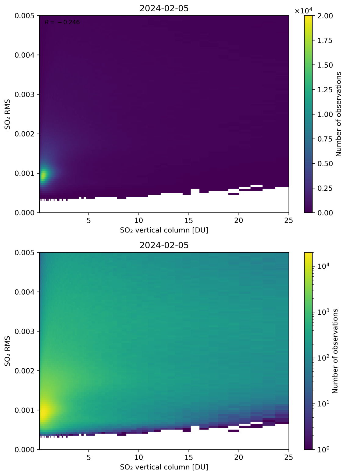
Figure 278: Scatter density plot of “SO 2 vertical column” against “SO 2 RMS” for 2024-02-04 to 2024-02-06.
