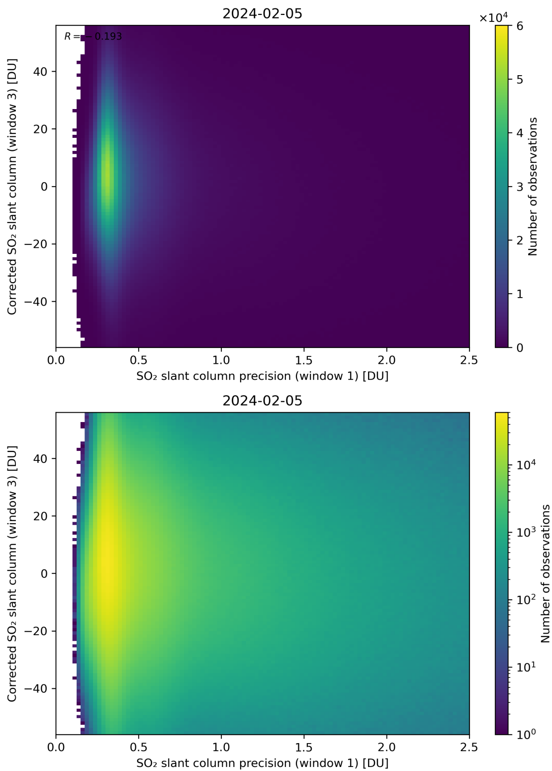
Figure 226: Scatter density plot of “SO 2 slant column precision (window 1)” against “Corrected SO 2 slant column (window 3)” for 2024-02-04 to 2024-02-06.
