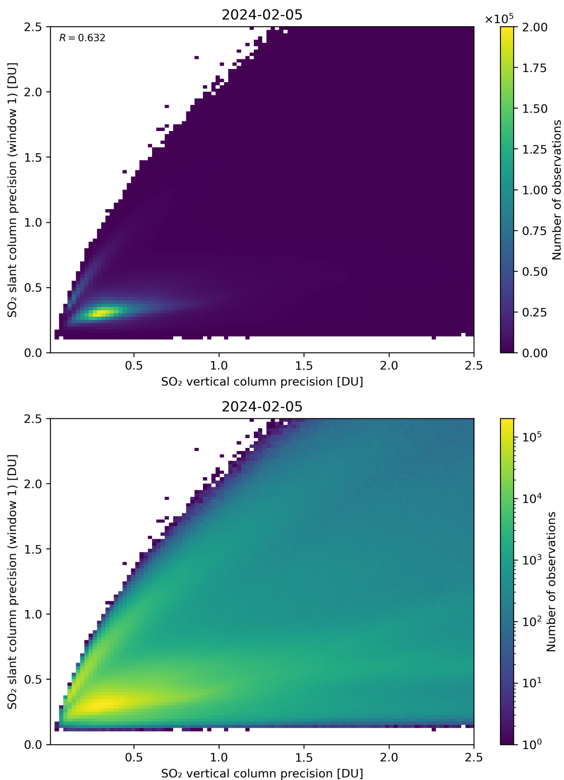
Figure 290: Scatter density plot of “SO 2 vertical column precision” against “SO 2 slant column precision (window 1)” for 2024-02-04 to 2024-02-06.
