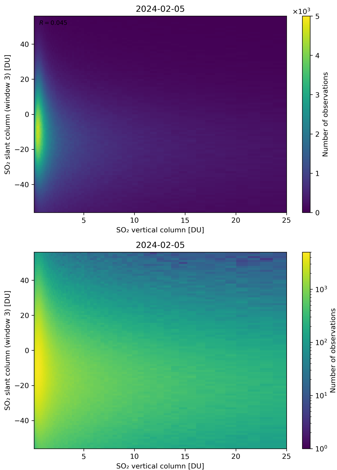
Figure 303: Scatter density plot of “SO 2 vertical column” against “SO 2 slant column (window 3)” for 2024-02-04 to 2024-02-06.
