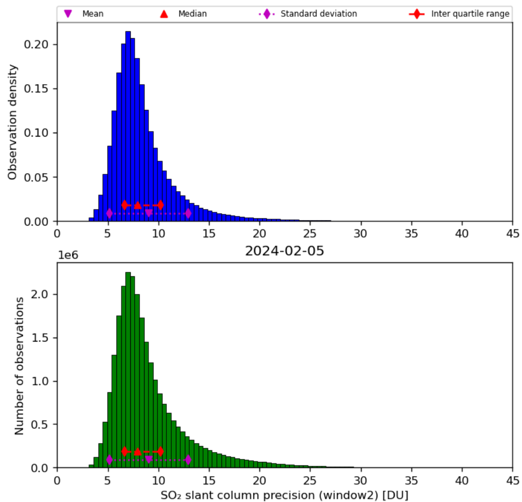
Figure 61: Histogram of “SO 2 slant column precision (window2)” for 2024-02-04 to 2024-02-06
