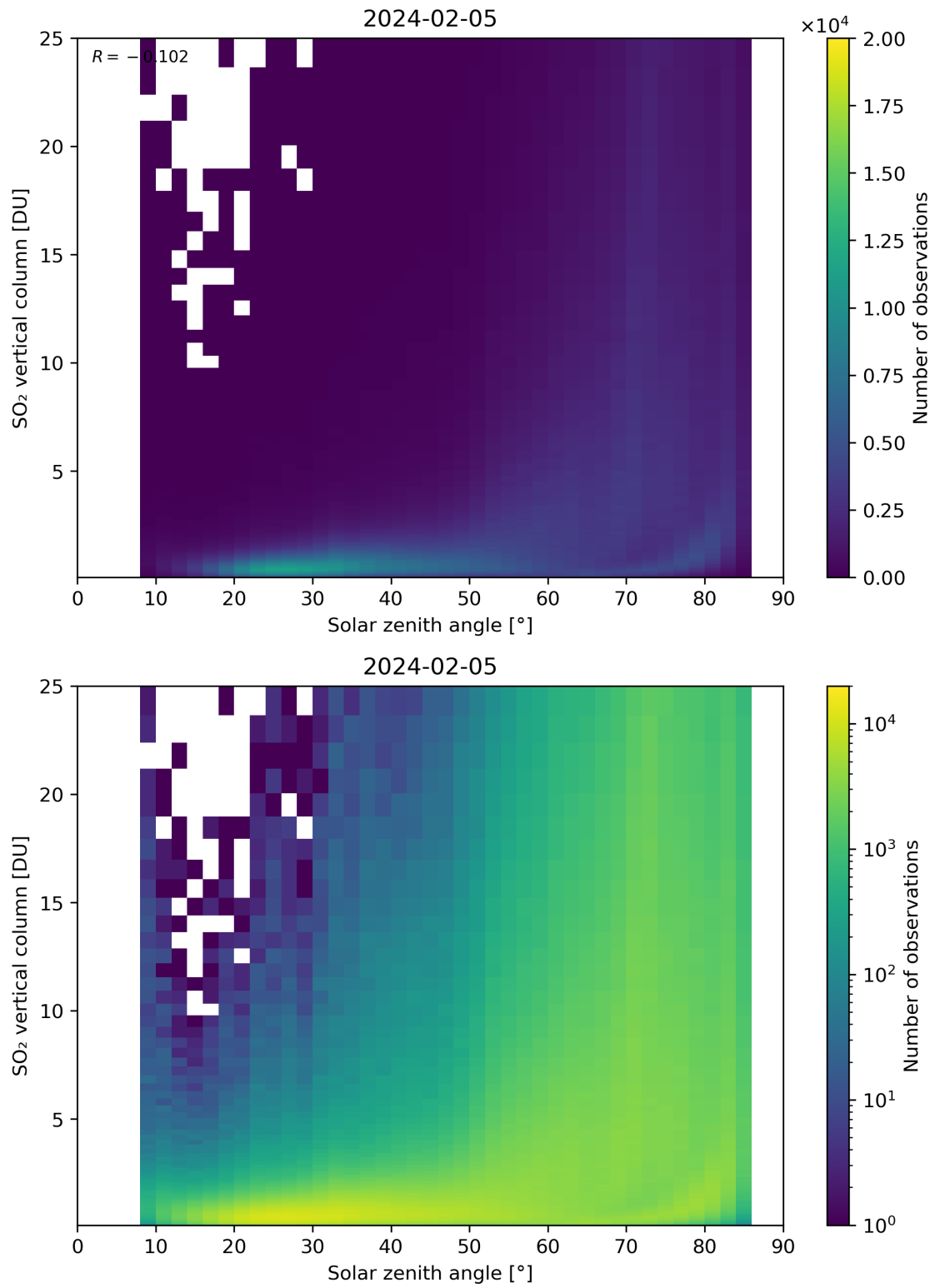
Figure 176: Scatter density plot of “Solar zenith angle” against “SO 2 vertical column” for 2024-02-04 to 2024-02-06.
