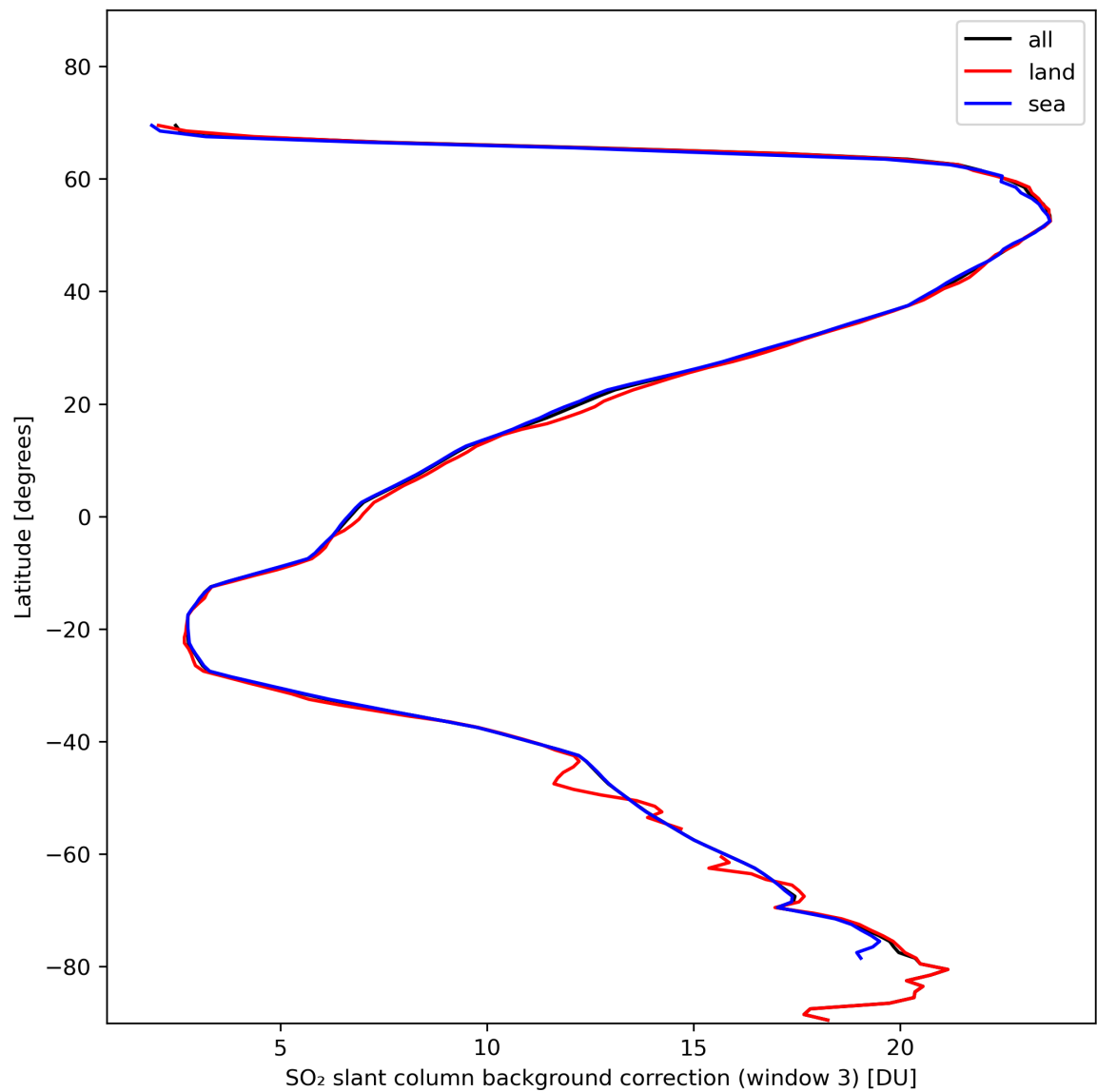
Figure 44: Zonal average of “SO 2 slant column background correction (window 3)” for 2024-02-04 to 2024-02-06.
