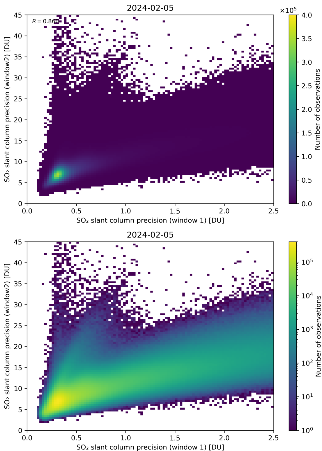
Figure 227: Scatter density plot of “SO 2 slant column precision (window 1)” against “SO 2 slant column precision (window2)” for 2024-02-04 to 2024-02-06.
