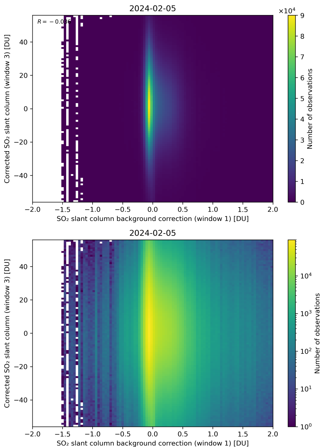
Figure 105: Scatter density plot of “SO 2 slant column background correction (window 1)” against “Corrected SO 2 slant column (window 3)” for 2024-02-04 to 2024-02-06.
