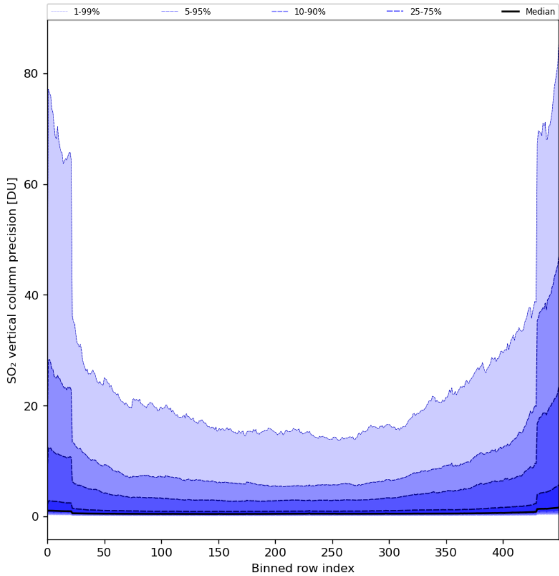
Figure 77: Along track statistics of “SO 2 vertical column precision” for 2024-02-04 to 2024-02-06
