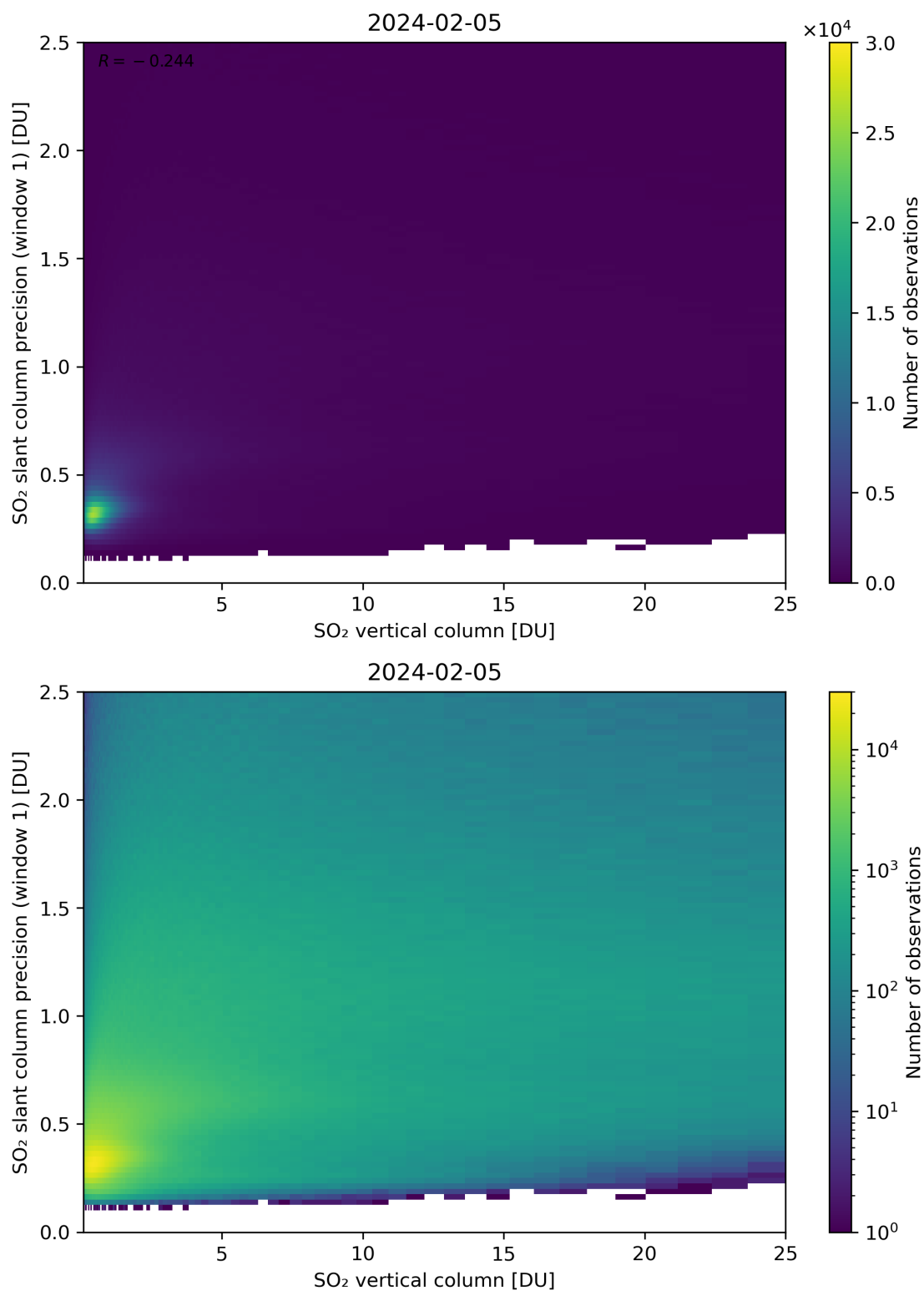
Figure 301: Scatter density plot of “SO 2 vertical column” against “SO 2 slant column precision (window 1)” for 2024-02-04 to 2024-02-06.
