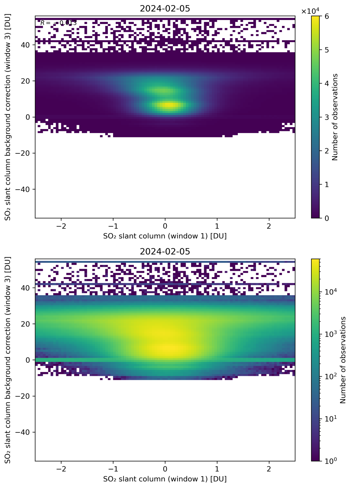
Figure 214: Scatter density plot of “SO 2 slant column (window 1)” against “SO 2 slant column background correction (window 3)” for 2024-02-04 to 2024-02-06.
