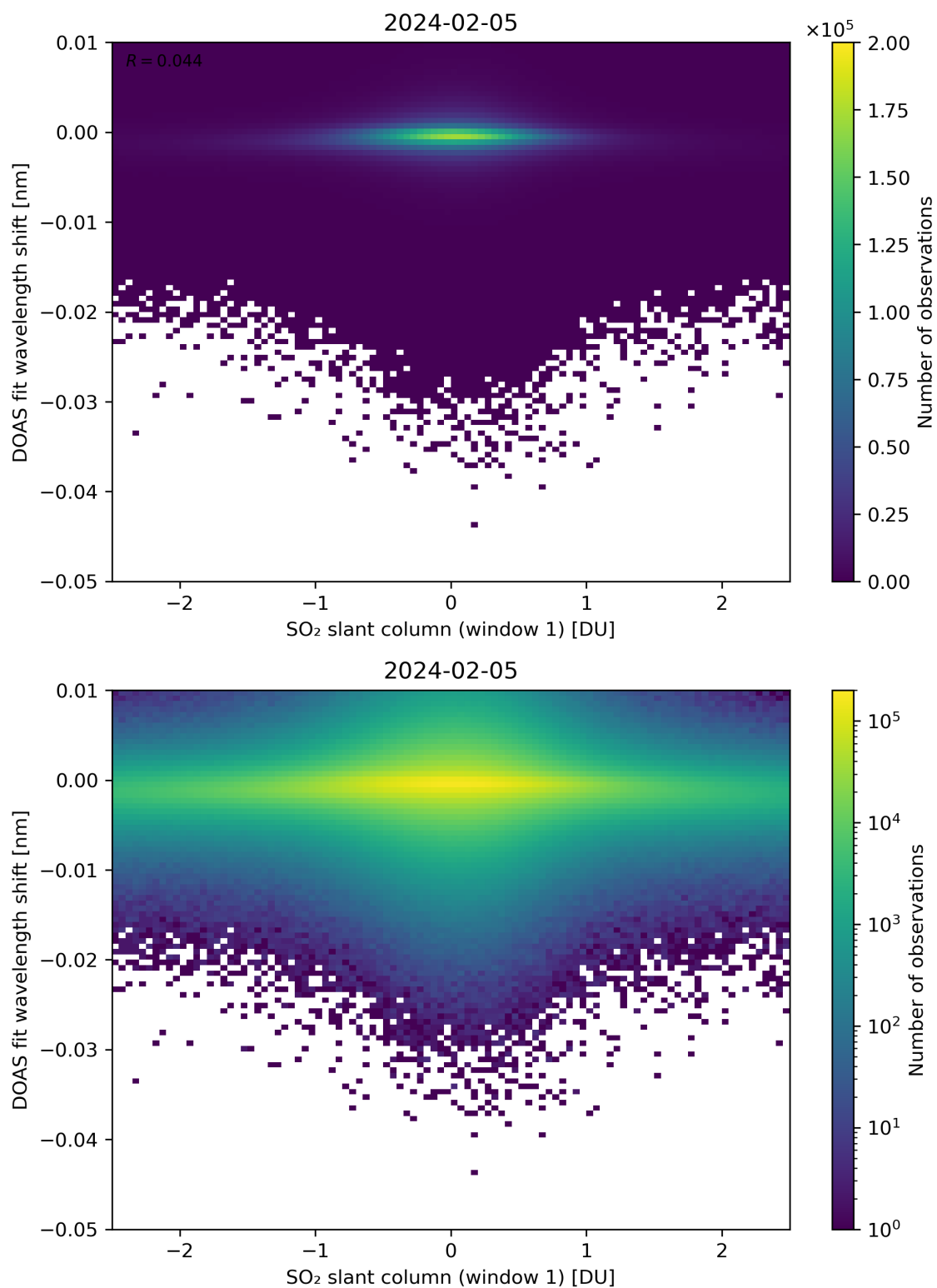
Figure 215: Scatter density plot of “SO 2 slant column (window 1)” against “DOAS fit wavelength shift” for 2024-02-04 to 2024-02-06.
