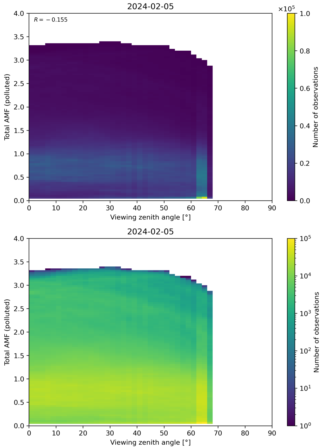
Figure 325: Scatter density plot of “Viewing zenith angle” against “Total AMF (polluted)” for 2024-02-04 to 2024-02-06.
