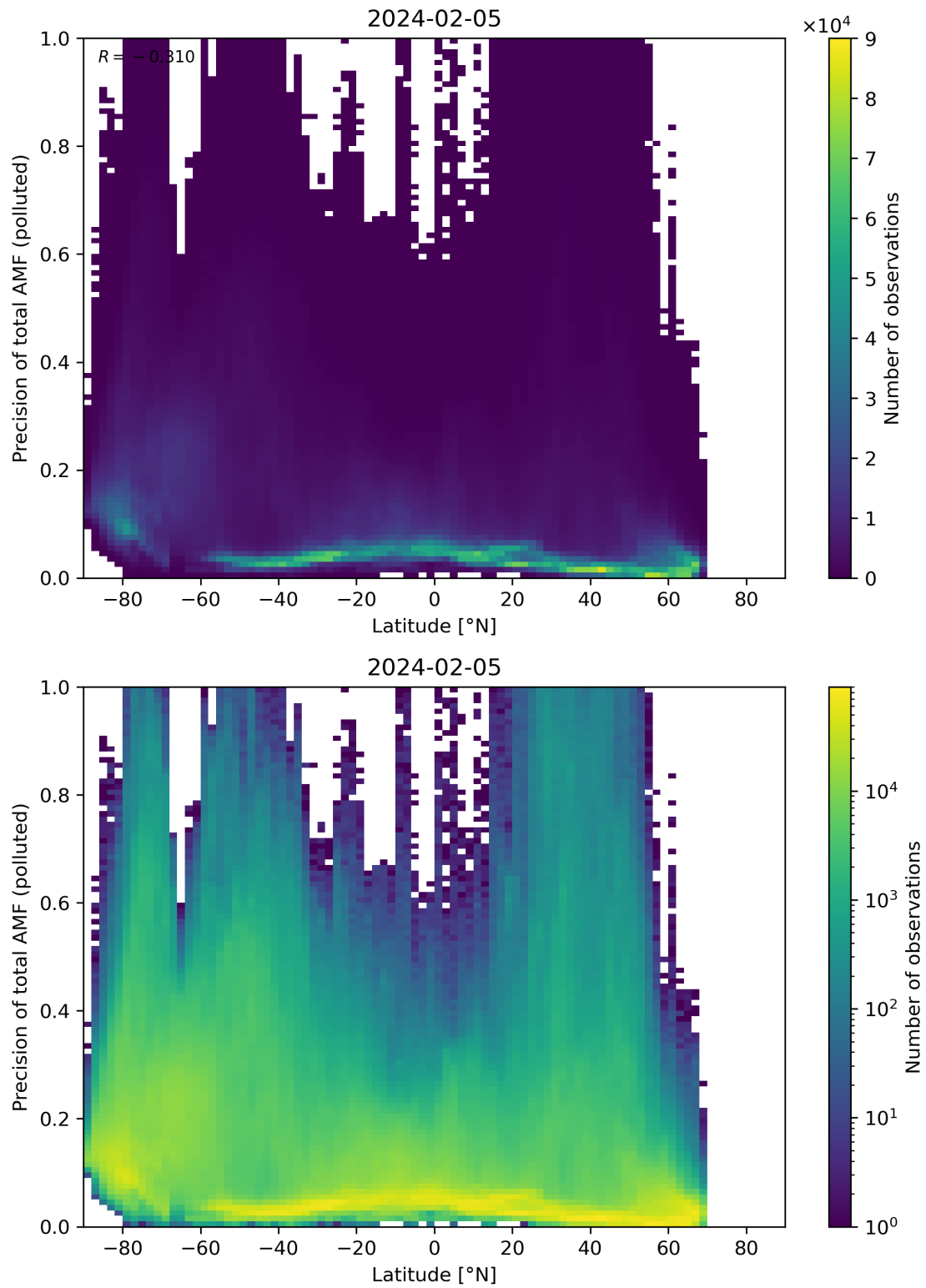
Figure 155: Scatter density plot of “Latitude” against “Precision of total AMF (polluted)” for 2024-02-04 to 2024-02-06.
