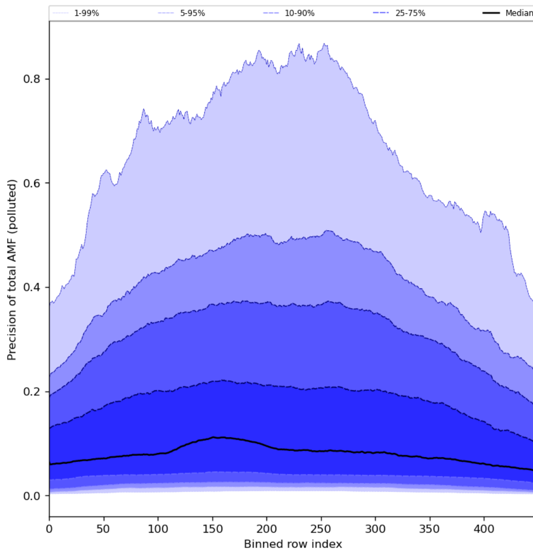
Figure 95: Along track statistics of “Precision of total AMF (polluted)” for 2024-02-04 to 2024-02-06
