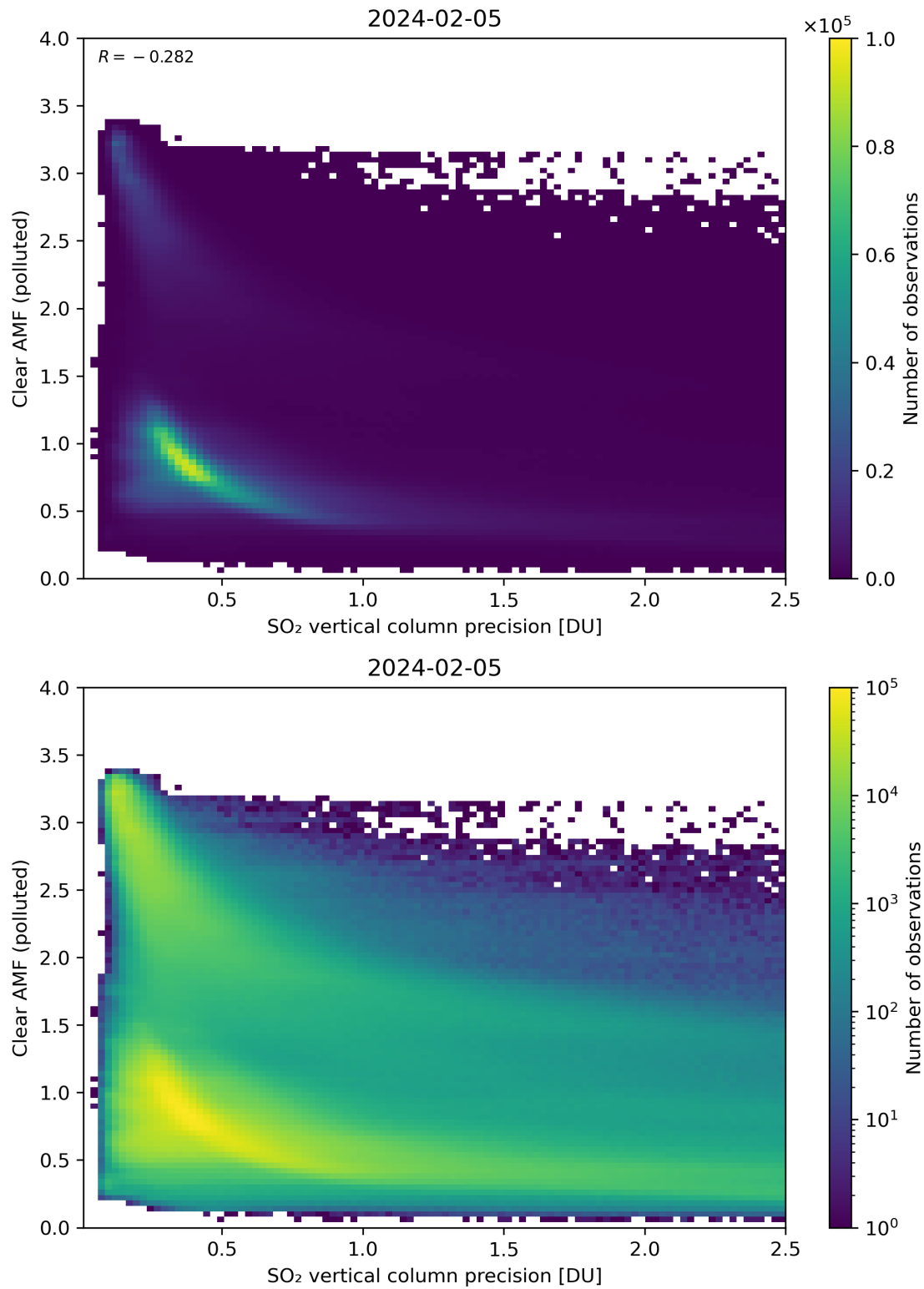
Figure 285: Scatter density plot of “SO 2 vertical column precision” against “Clear AMF (polluted)” for 2024-02-04 to 2024-02-06.
