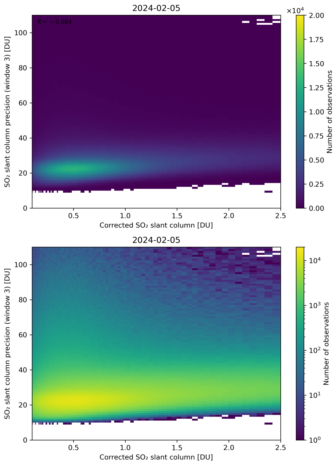
Figure 191: Scatter density plot of “Corrected SO 2 slant column” against “SO 2 slant column precision (window 3)” for 2024-02-04 to 2024-02-06.
