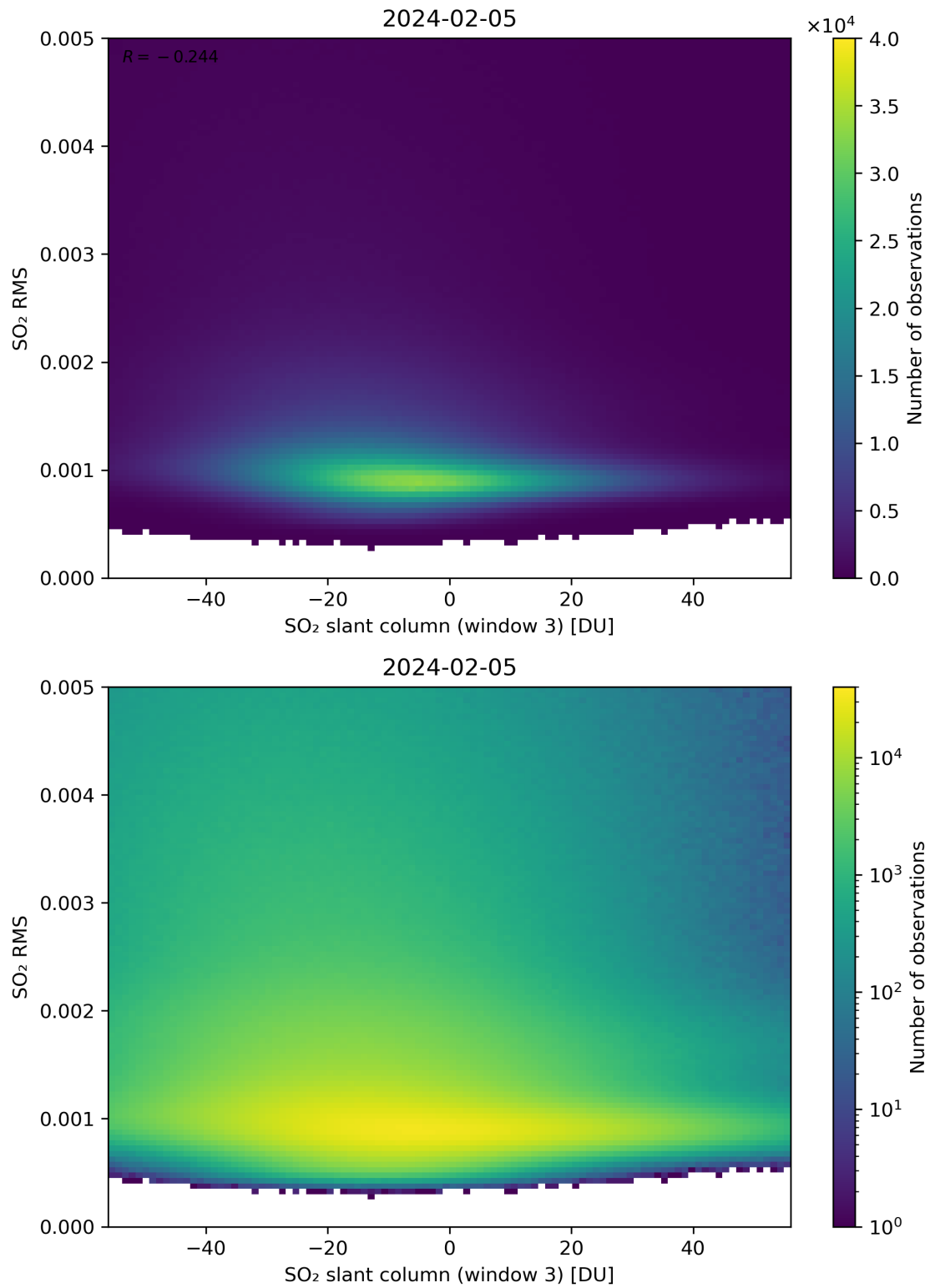
Figure 256: Scatter density plot of “SO 2 slant column (window 3)” against “SO 2 RMS” for 2024-02-04 to 2024-02-06.
