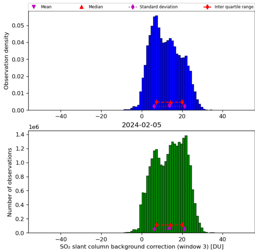
Figure 67: Histogram of “SO 2 slant column background correction (window 3)” for 2024-02-04 to 2024-02-06
