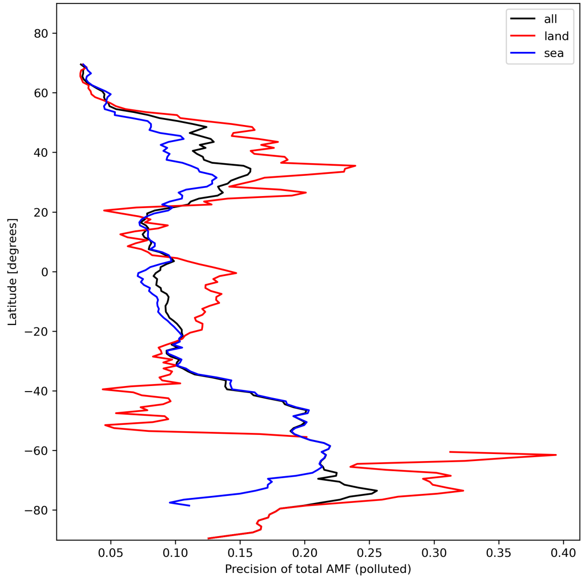
Figure 49: Zonal average of “Precision of total AMF (polluted)” for 2024-02-04 to 2024-02-06.
