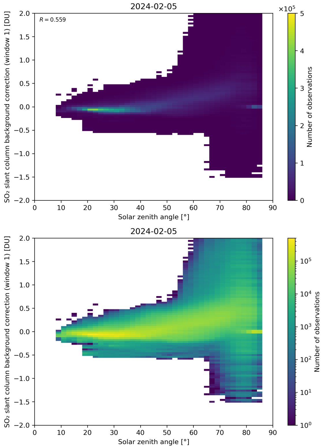
Figure 158: Scatter density plot of “Solar zenith angle” against “SO 2 slant column background correction (window 1)” for 2024-02-04 to 2024-02-06.
