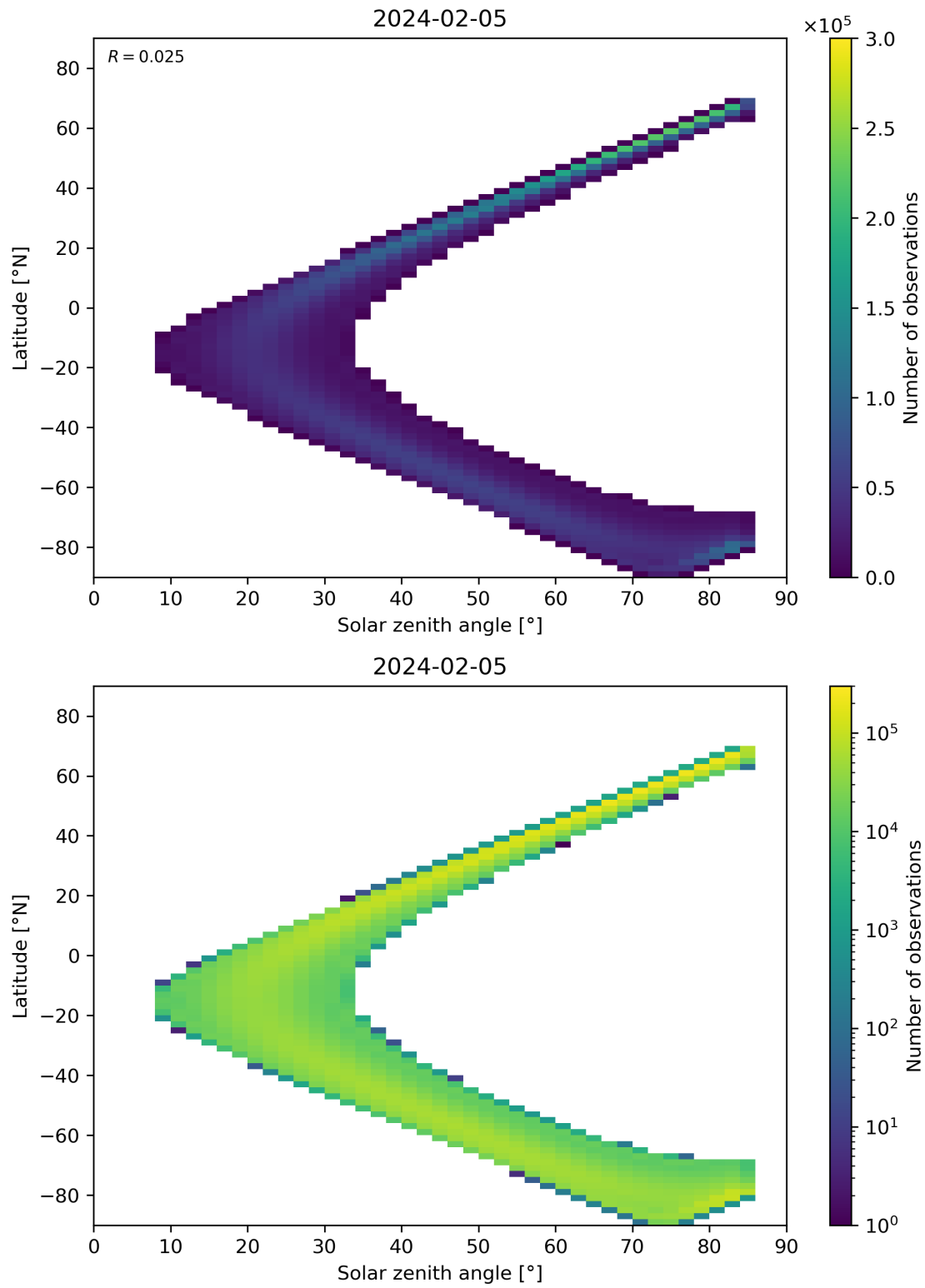
Figure 164: Scatter density plot of “Solar zenith angle” against “Latitude” for 2024-02-04 to 2024-02-06.
