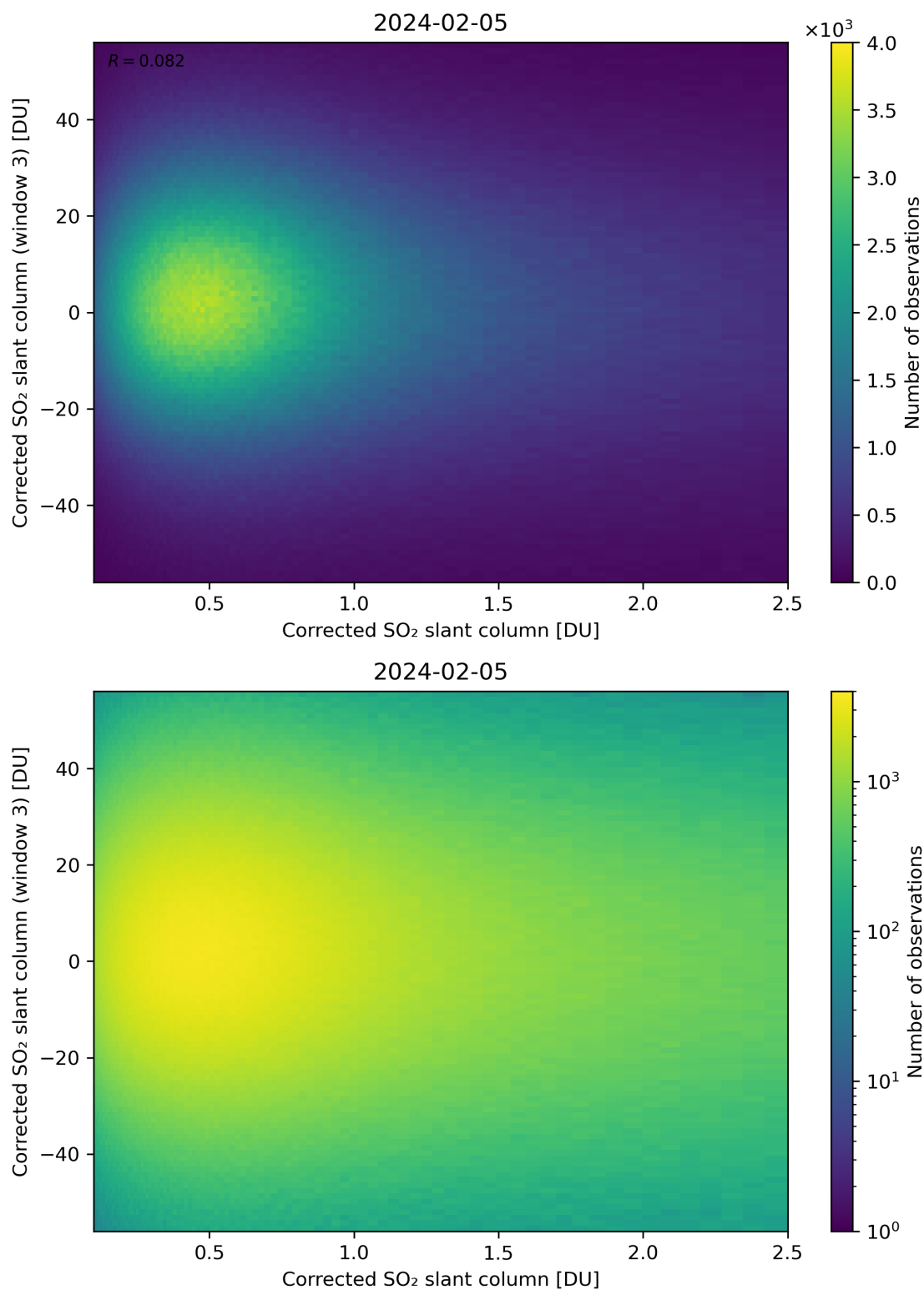
Figure 186: Scatter density plot of “Corrected SO 2 slant column” against “Corrected SO 2 slant column (window 3)” for 2024-02-04 to 2024-02-06.
