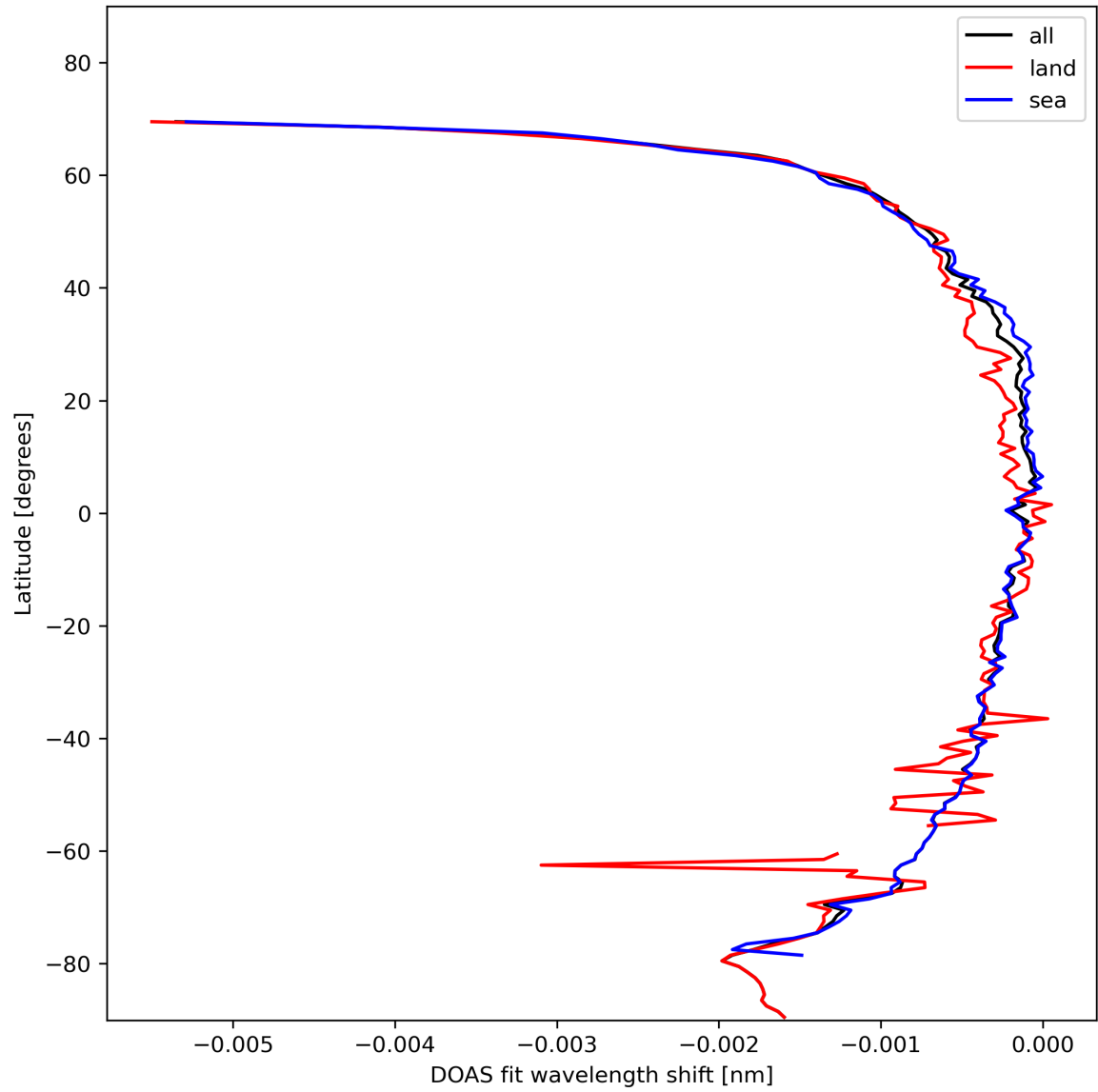
Figure 45: Zonal average of “DOAS fit wavelength shift” for 2024-02-04 to 2024-02-06.
