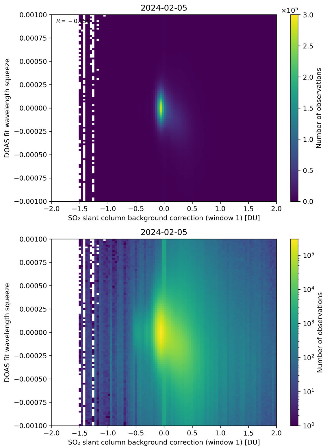
Figure 101: Scatter density plot of “SO 2 slant column background correction (window 1)” against “DOAS fit wavelength squeeze” for 2024-02-04 to 2024-02-06.
