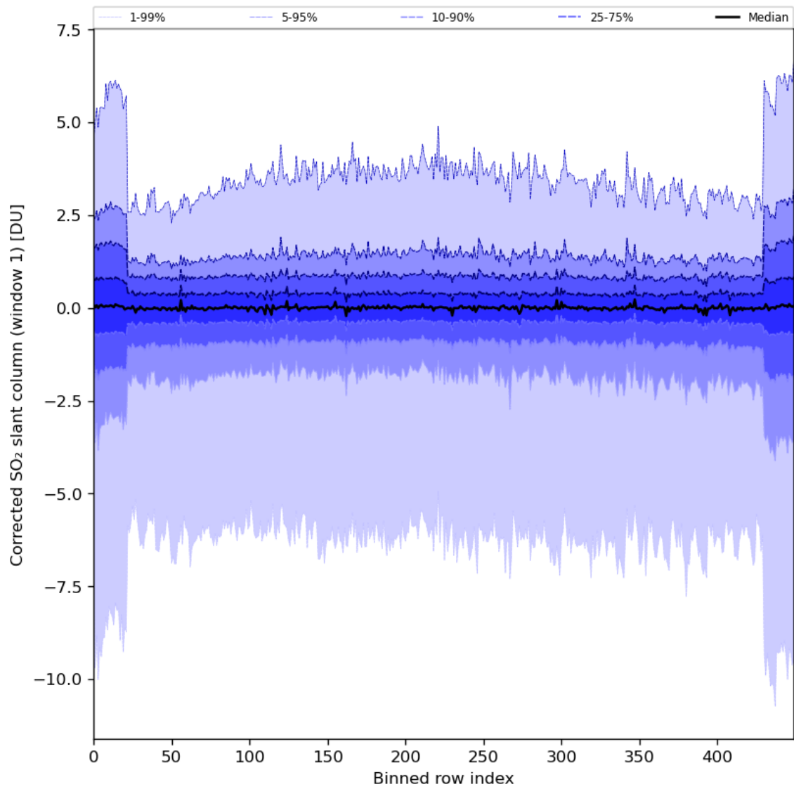
Figure 81: Along track statistics of “Corrected SO 2 slant column (window 1)” for 2024-02-04 to 2024-02-06
