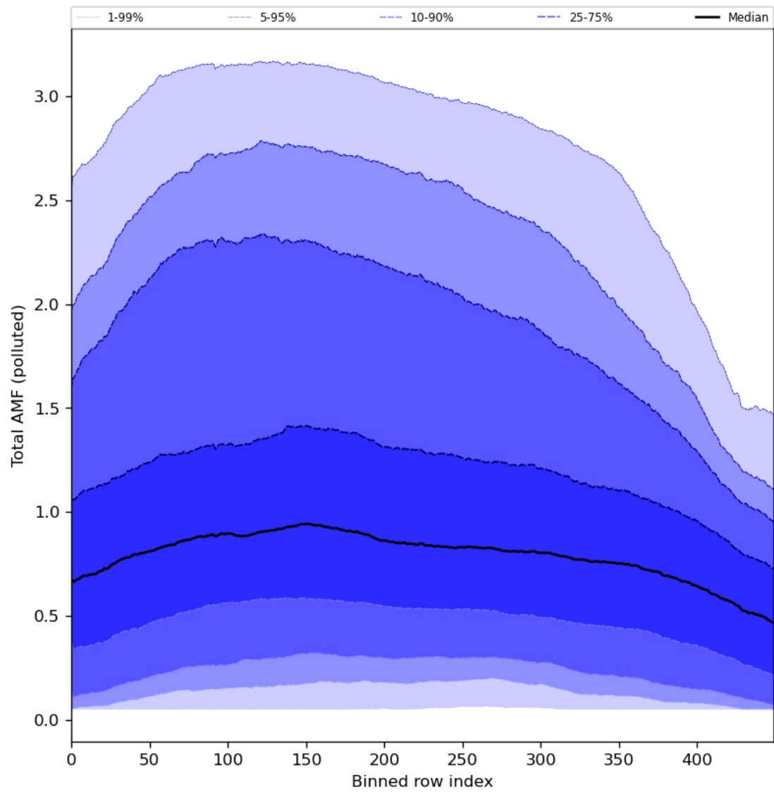
Figure 94: Along track statistics of “Total AMF (polluted)” for 2024-02-04 to 2024-02-06
