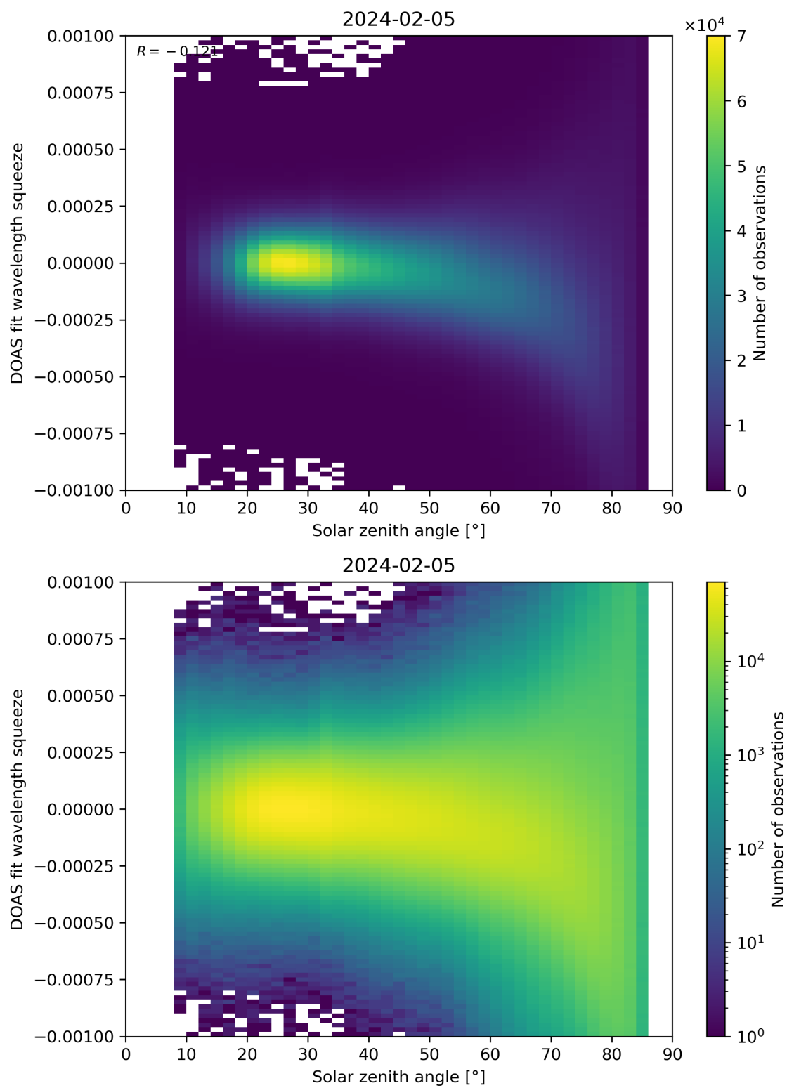
Figure 162: Scatter density plot of “Solar zenith angle” against “DOAS fit wavelength squeeze” for 2024-02-04 to 2024-02-06.
