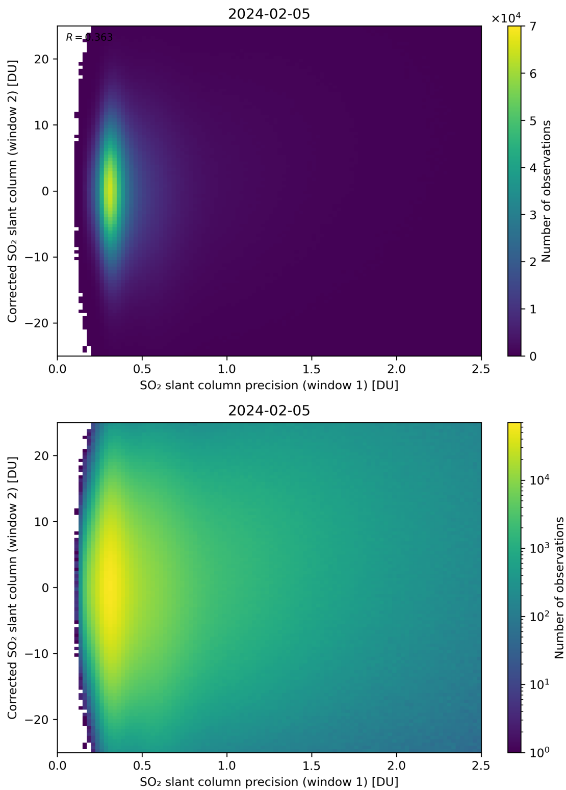
Figure 225: Scatter density plot of “SO 2 slant column precision (window 1)” against “Corrected SO 2 slant column (window 2)” for 2024-02-04 to 2024-02-06.
