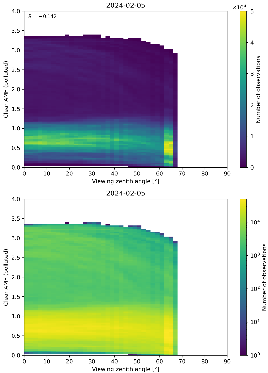
Figure 316: Scatter density plot of “Viewing zenith angle” against “Clear AMF (polluted)” for 2024-02-04 to 2024-02-06.
