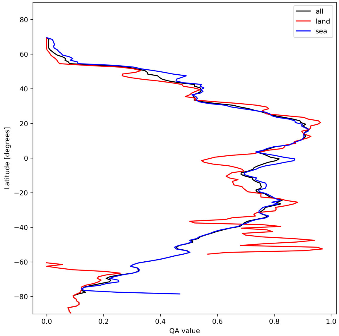
Figure 29: Zonal average of “QA value” for 2024-02-04 to 2024-02-06.
