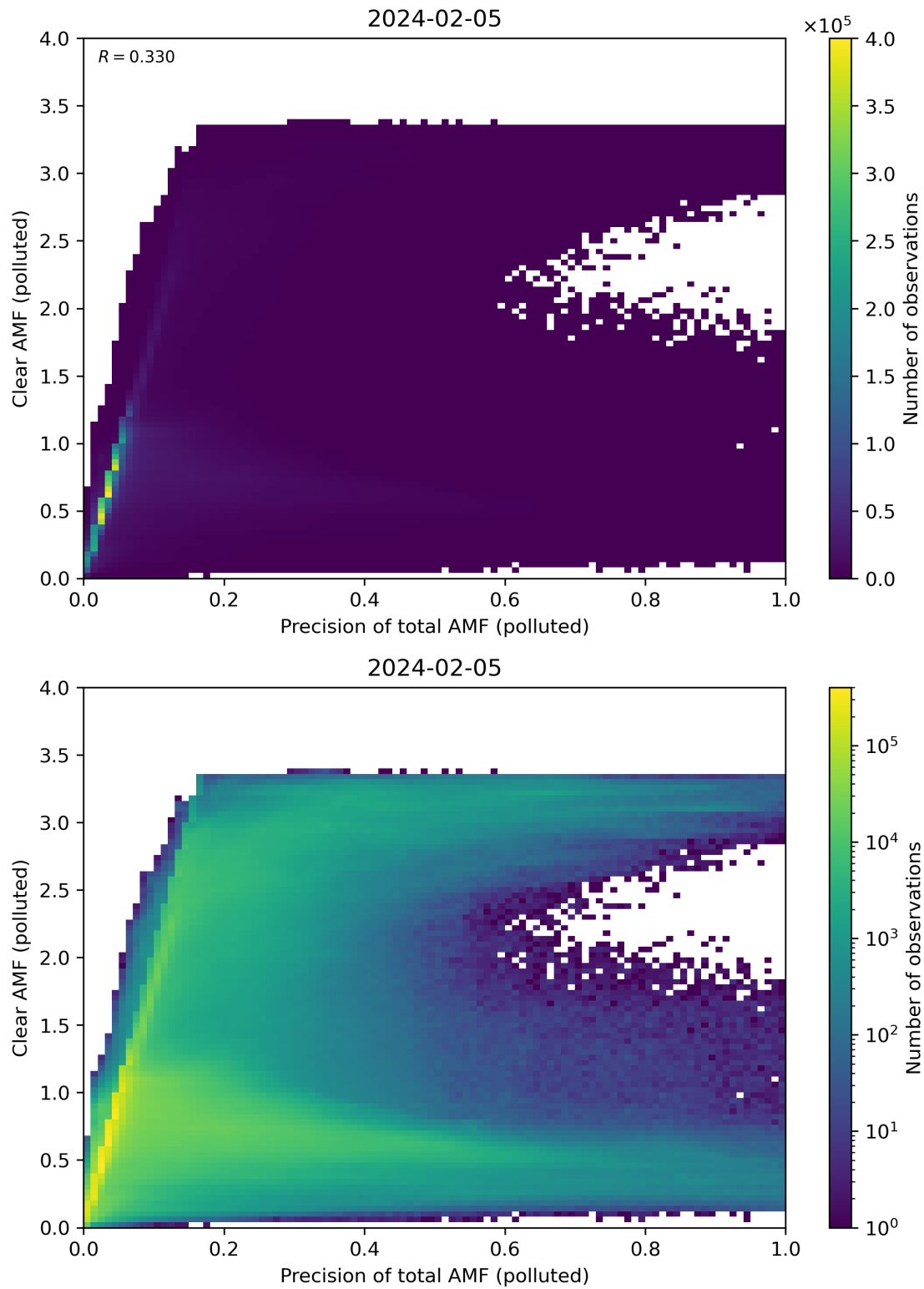
Figure 270: Scatter density plot of “Precision of total AMF (polluted)” against “Clear AMF (polluted)” for 2024-02-04 to 2024-02-06.
