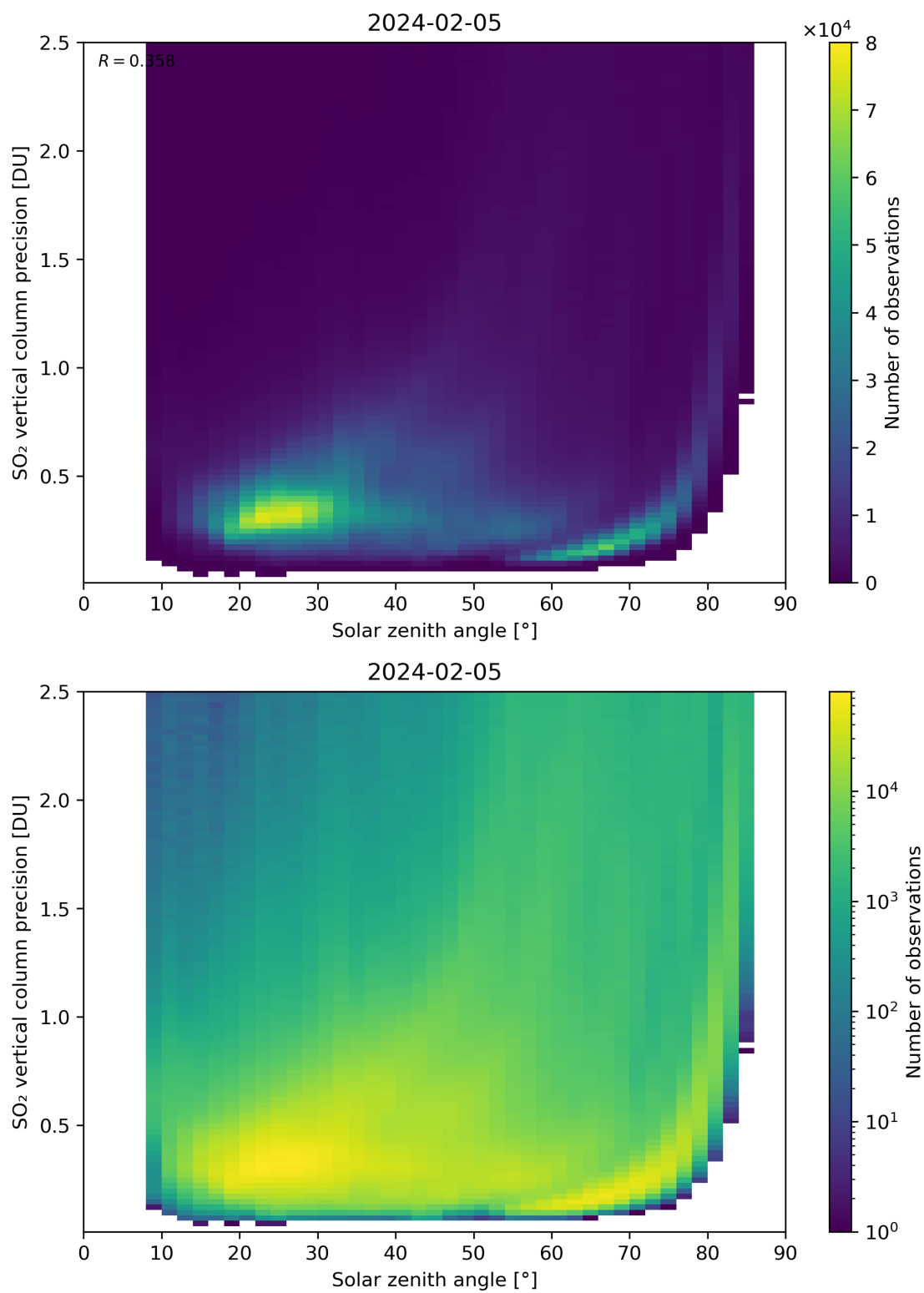
Figure 177: Scatter density plot of “Solar zenith angle” against “SO 2 vertical column precision” for 2024-02-04 to 2024-02-06.
