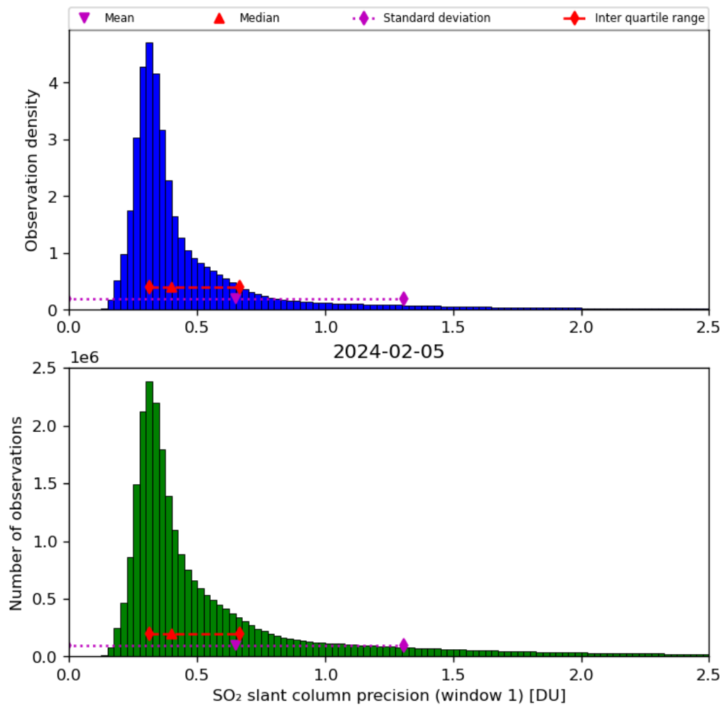
Figure 57: Histogram of “SO 2 slant column precision (window 1)” for 2024-02-04 to 2024-02-06
