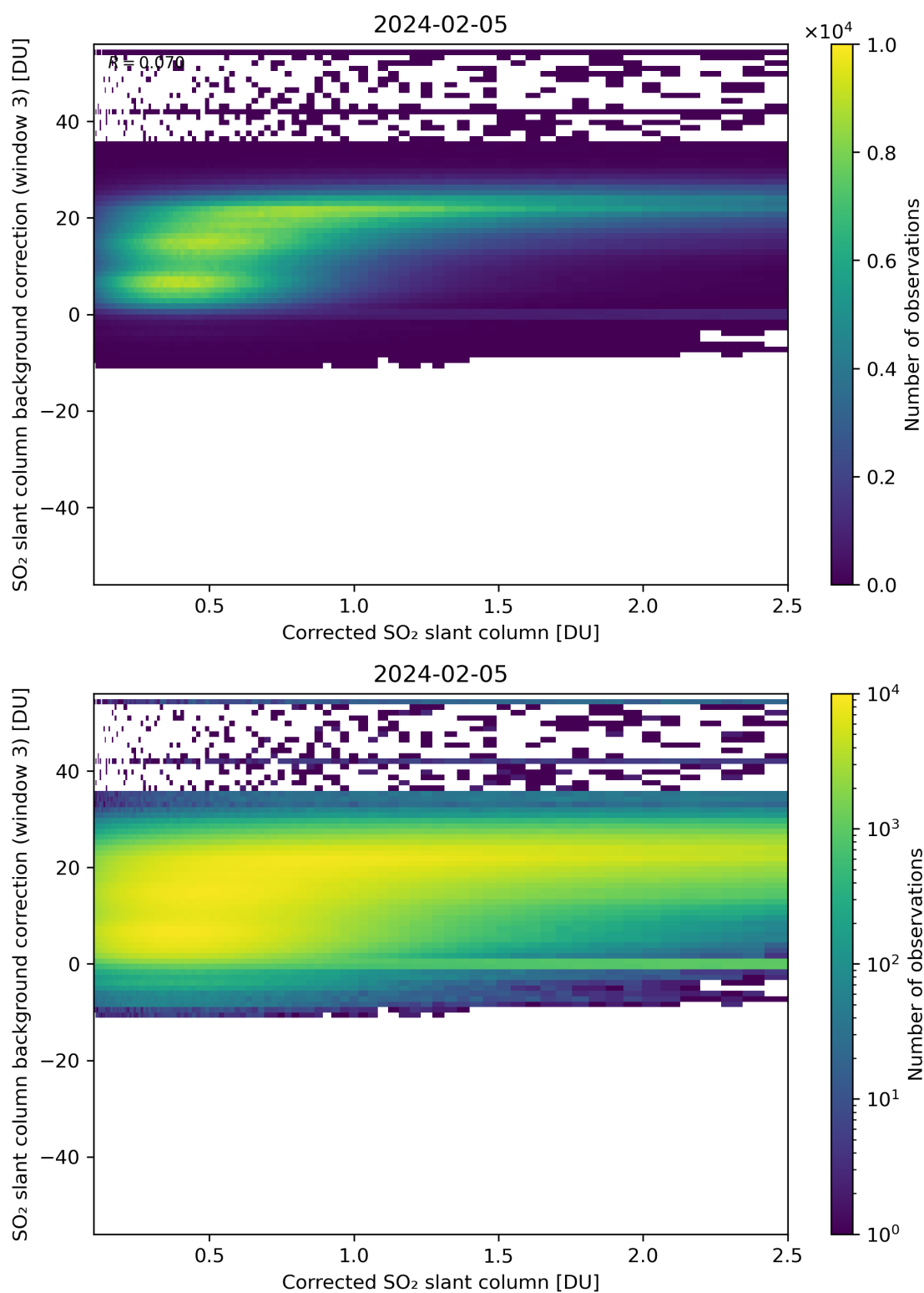
Figure 180: Scatter density plot of “Corrected SO 2 slant column” against “SO 2 slant column background correction (window 3)” for 2024-02-04 to 2024-02-06.
