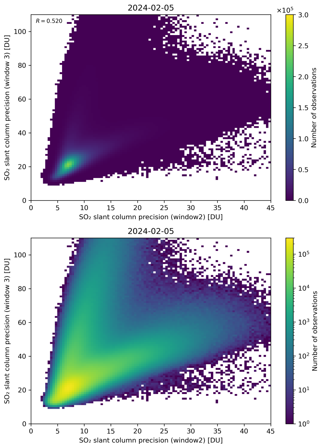
Figure 250: Scatter density plot of “SO 2 slant column precision (window2)” against “SO 2 slant column precision (window 3)” for 2024-02-04 to 2024-02-06.
