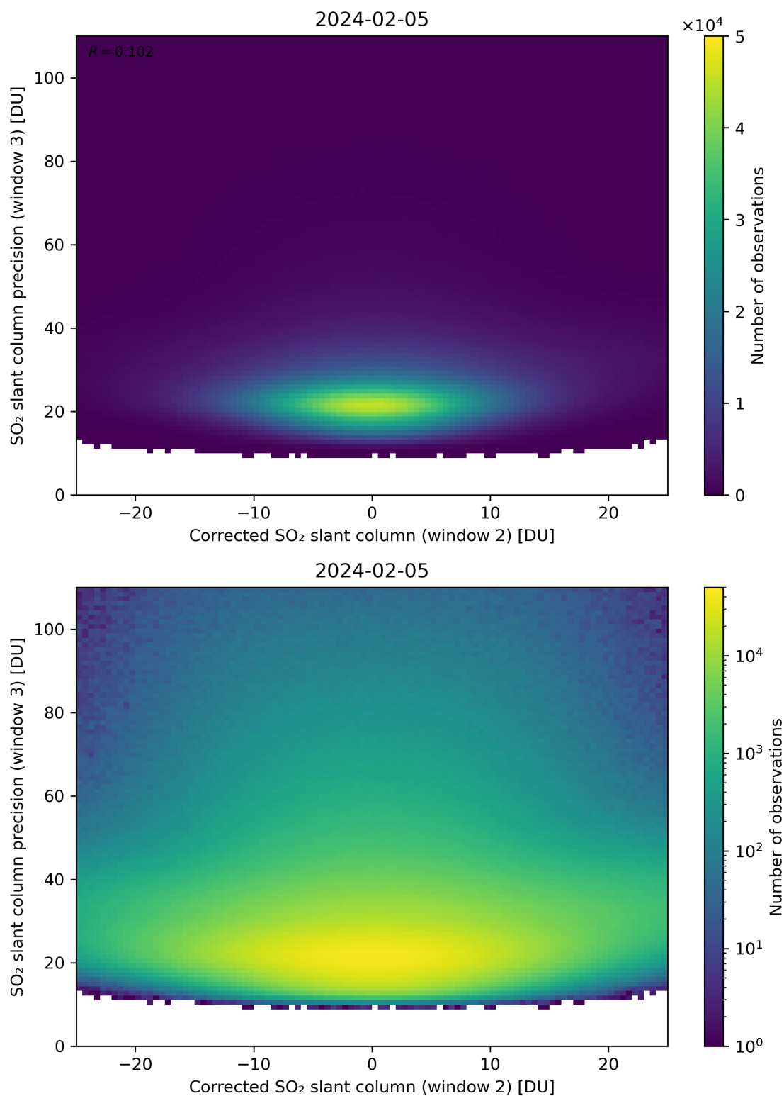
Figure 202: Scatter density plot of “Corrected SO 2 slant column (window 2)” against “SO 2 slant column precision (window 3)” for 2024-02-04 to 2024-02-06.
