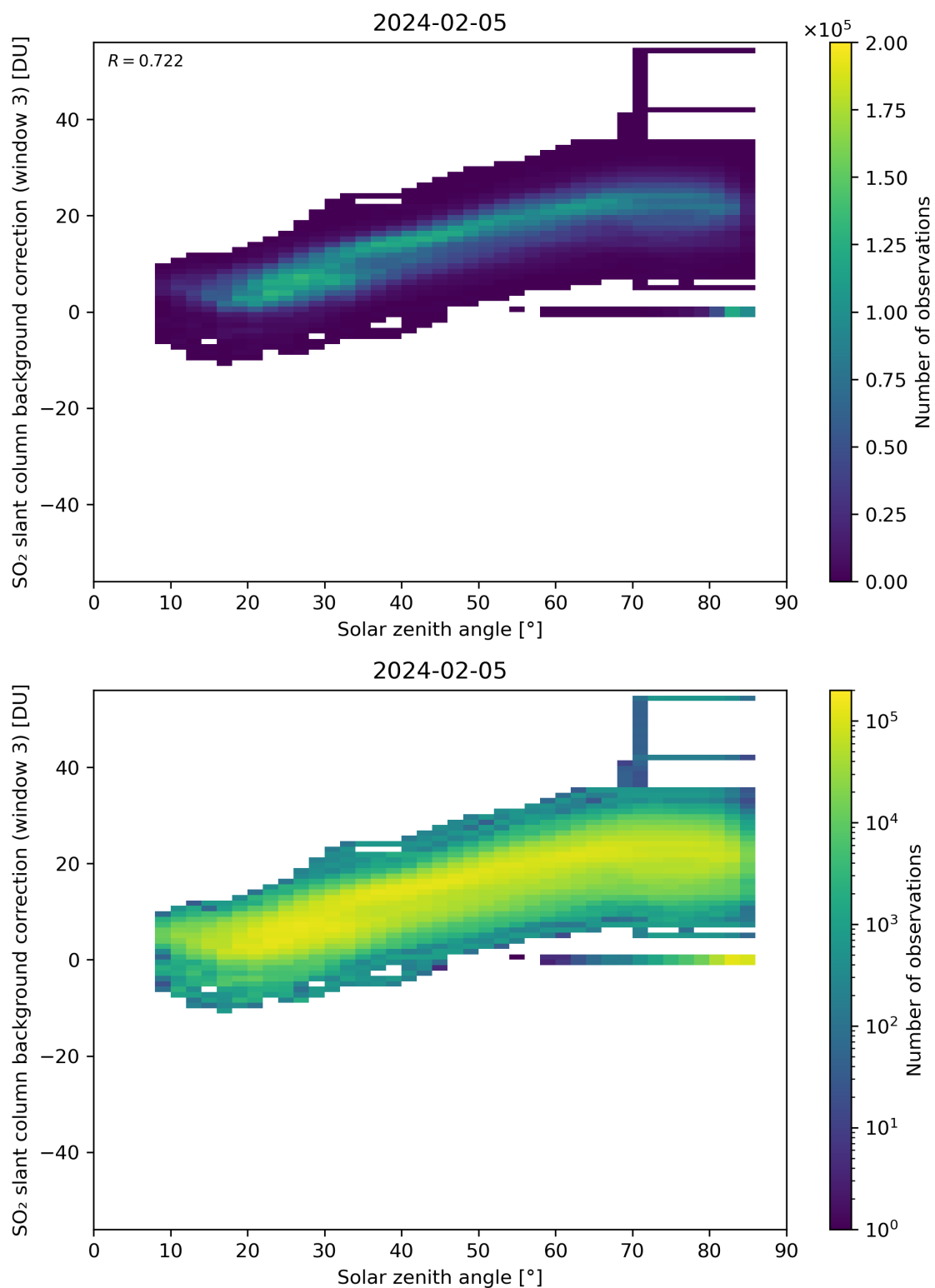
Figure 160: Scatter density plot of “Solar zenith angle” against “SO 2 slant column background correction (window 3)” for 2024-02-04 to 2024-02-06.
