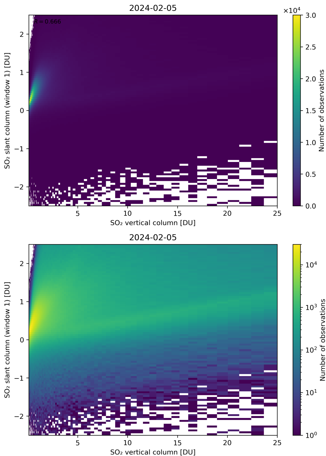
Figure 300: Scatter density plot of “SO 2 vertical column” against “SO 2 slant column (window 1)” for 2024-02-04 to 2024-02-06.
