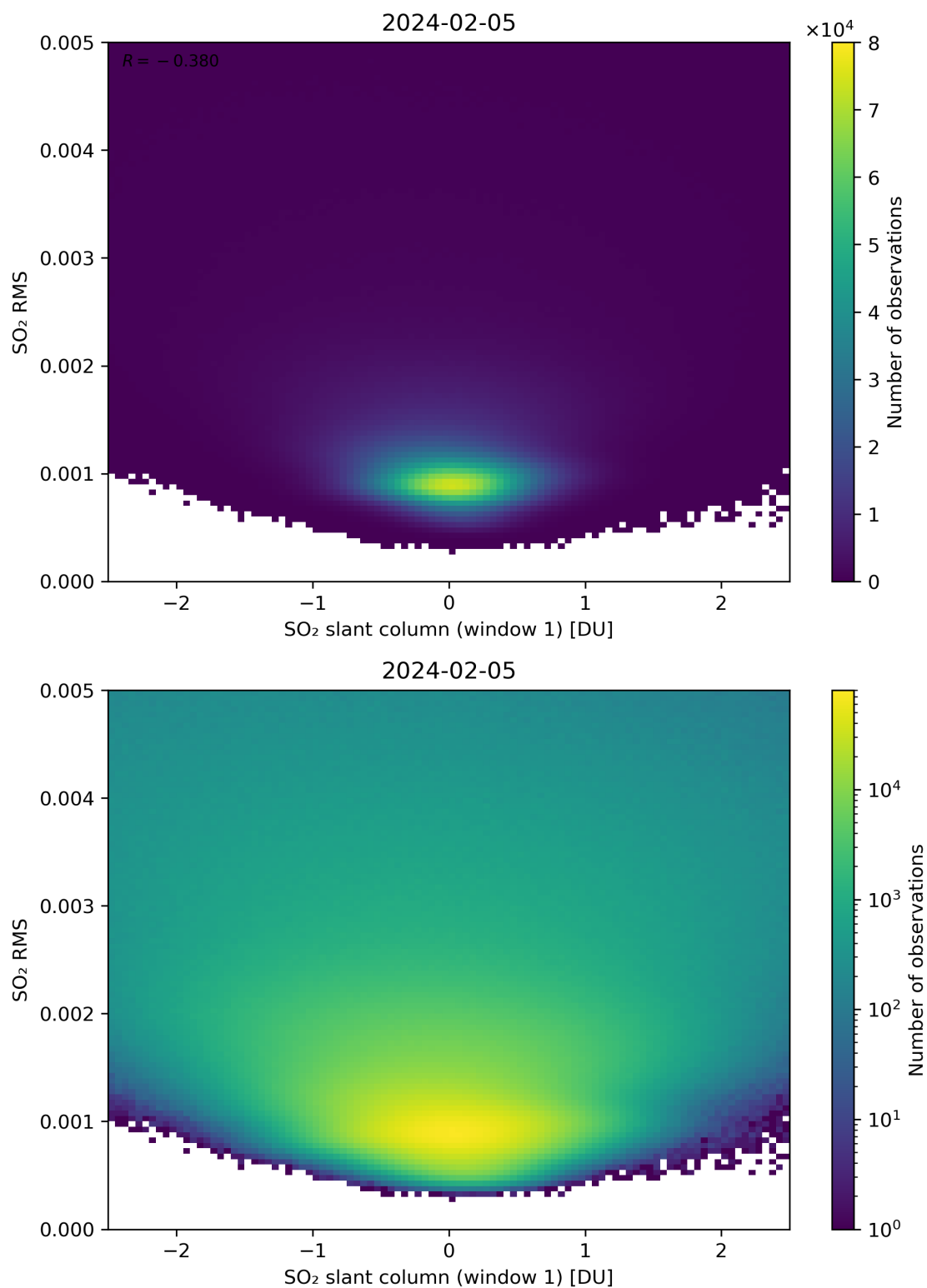
Figure 217: Scatter density plot of “SO 2 slant column (window 1)” against “SO 2 RMS” for 2024-02-04 to 2024-02-06.
