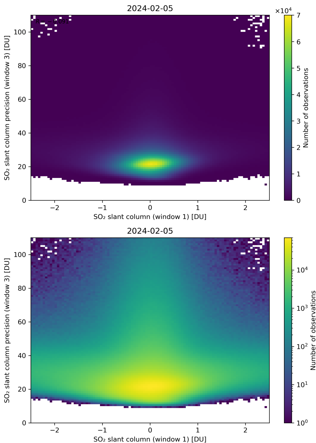
Figure 238: Scatter density plot of “SO 2 slant column (window 1)” against “SO 2 slant column precision (window 3)” for 2024-02-04 to 2024-02-06.
