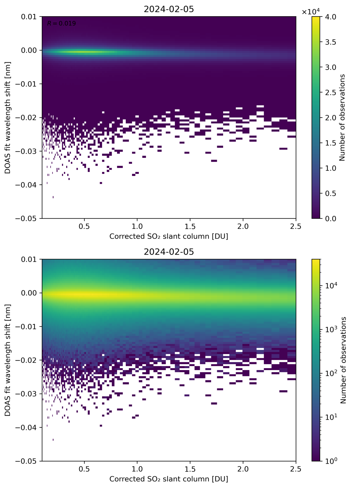
Figure 181: Scatter density plot of “Corrected SO 2 slant column” against “DOAS fit wavelength shift” for 2024-02-04 to 2024-02-06.
