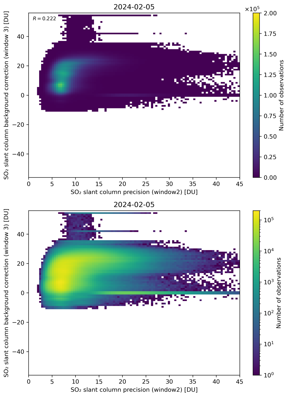
Figure 242: Scatter density plot of “SO 2 slant column precision (window2)” against “SO 2 slant column background correction (window 3)” for 2024-02-04 to 2024-02-06.
