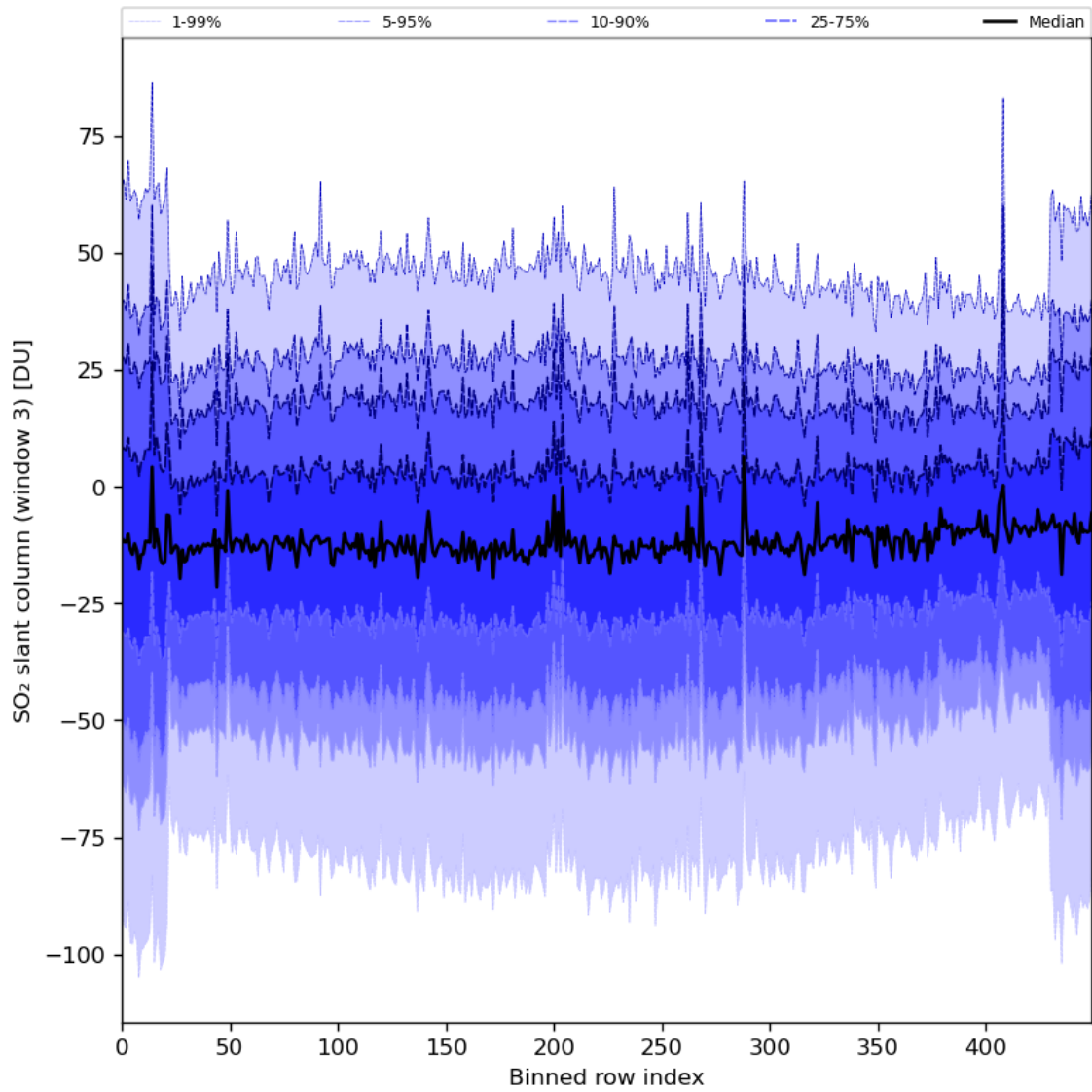
Figure 87: Along track statistics of “SO 2 slant column (window 3)” for 2024-02-04 to 2024-02-06
