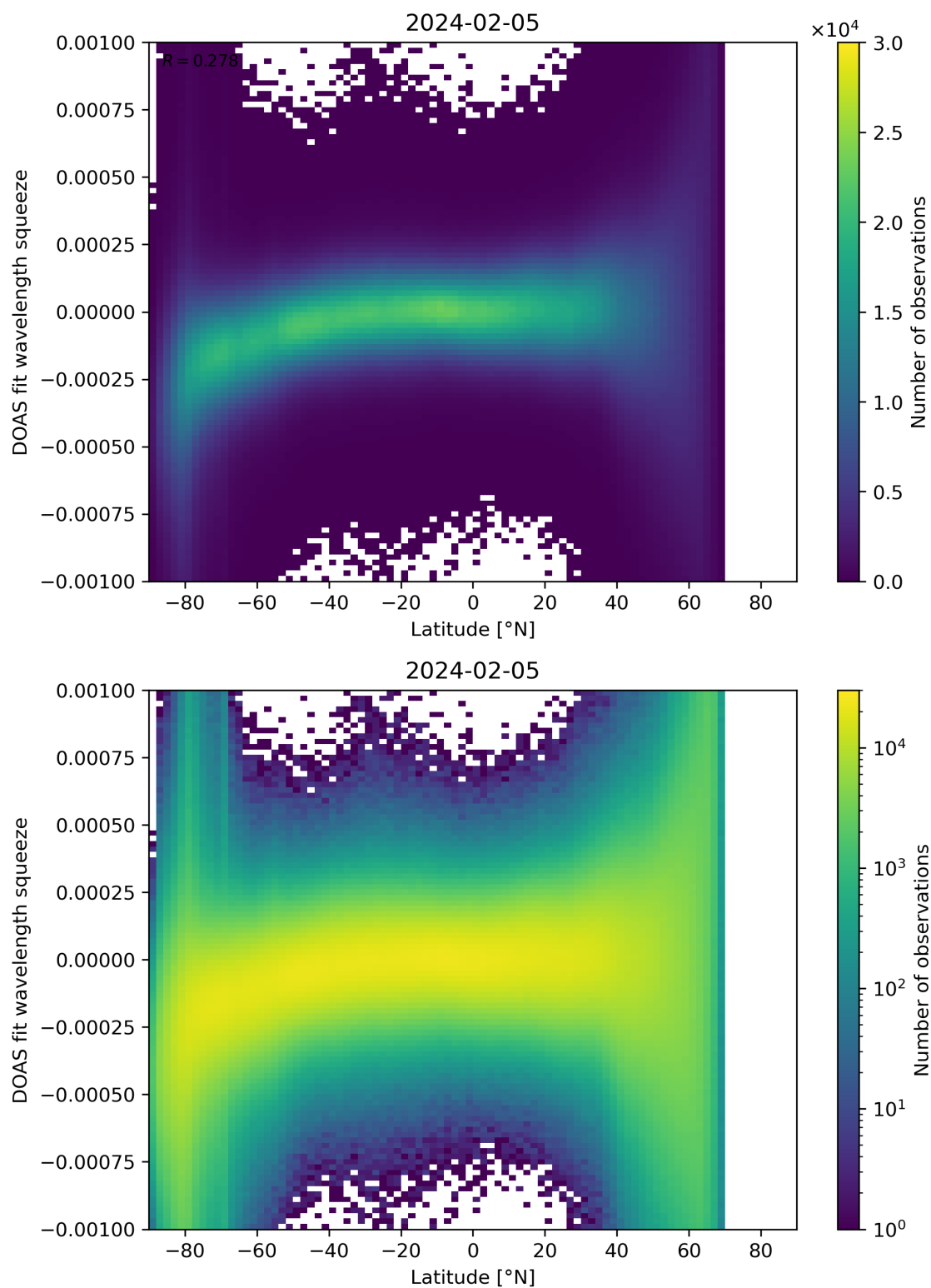
Figure 143: Scatter density plot of “Latitude” against “DOAS fit wavelength squeeze” for 2024-02-04 to 2024-02-06.
