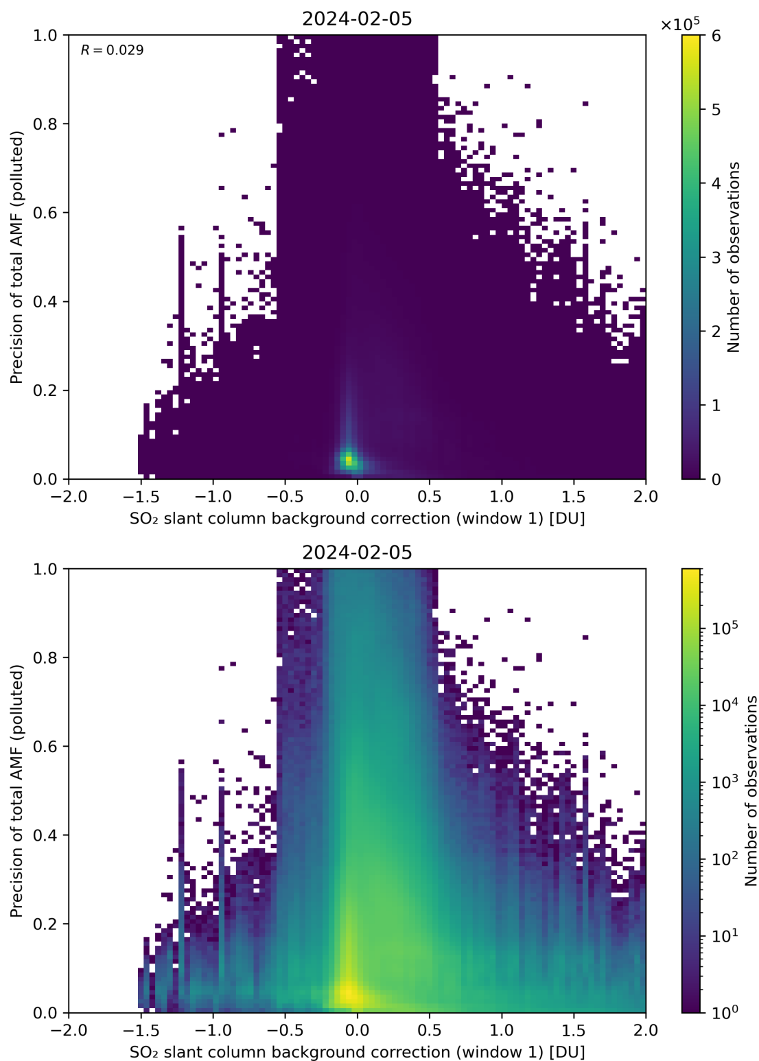
Figure 110: Scatter density plot of “SO 2 slant column background correction (window 1)” against “Precision of total AMF (polluted)” for 2024-02-04 to 2024-02-06.
