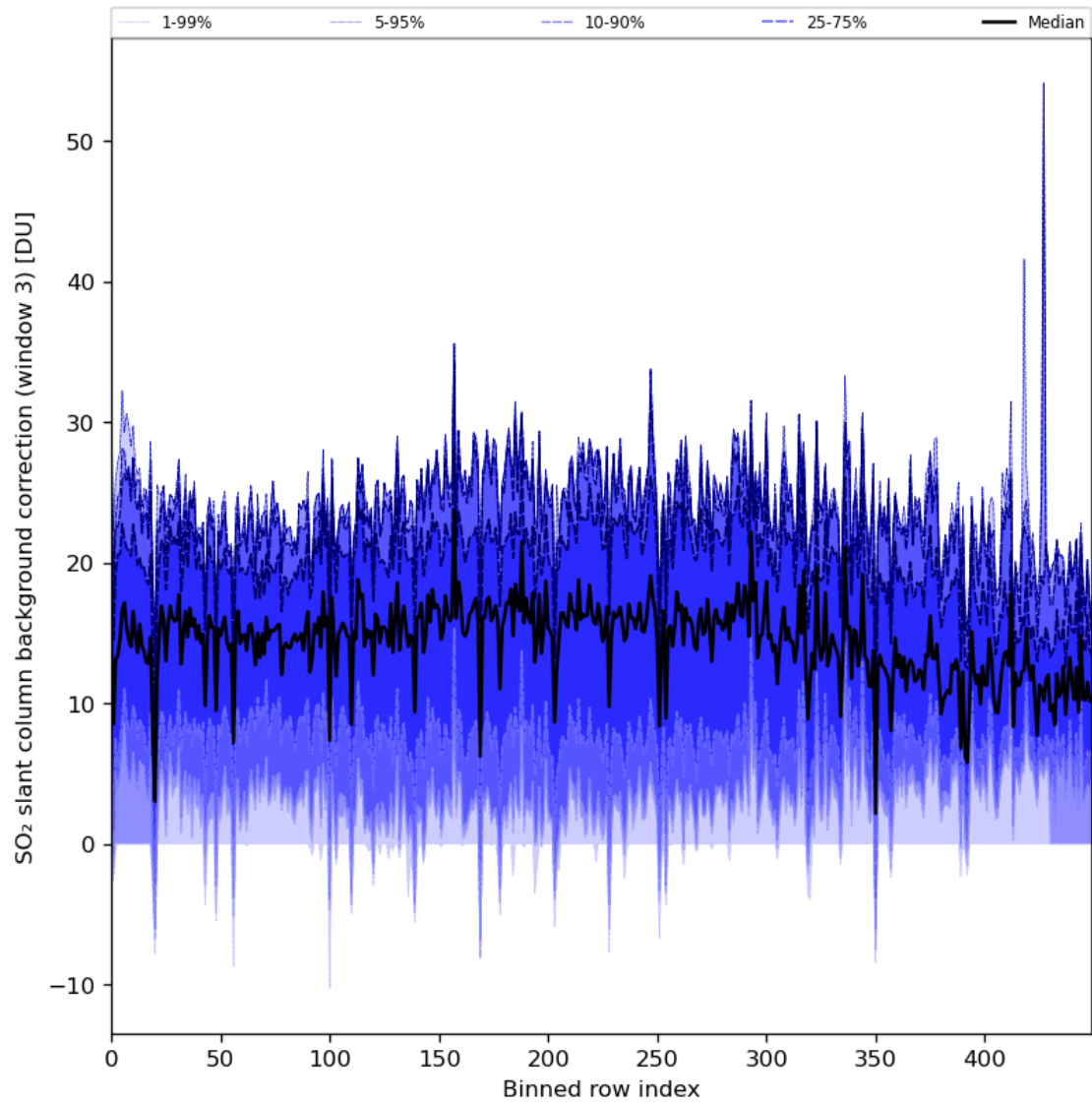
Figure 90: Along track statistics of “SO 2 slant column background correction (window 3)” for 2024-02-04 to 2024-02-06
