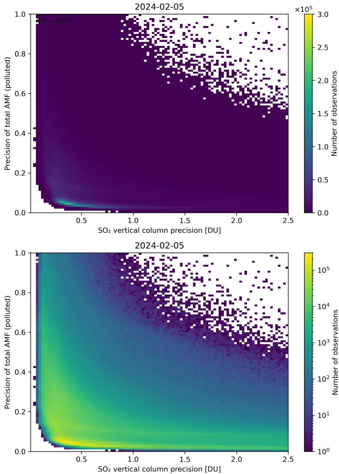
Figure 295: Scatter density plot of “SO 2 vertical column precision” against “Precision of total AMF (polluted)” for 2024-02-04 to 2024-02-06.
