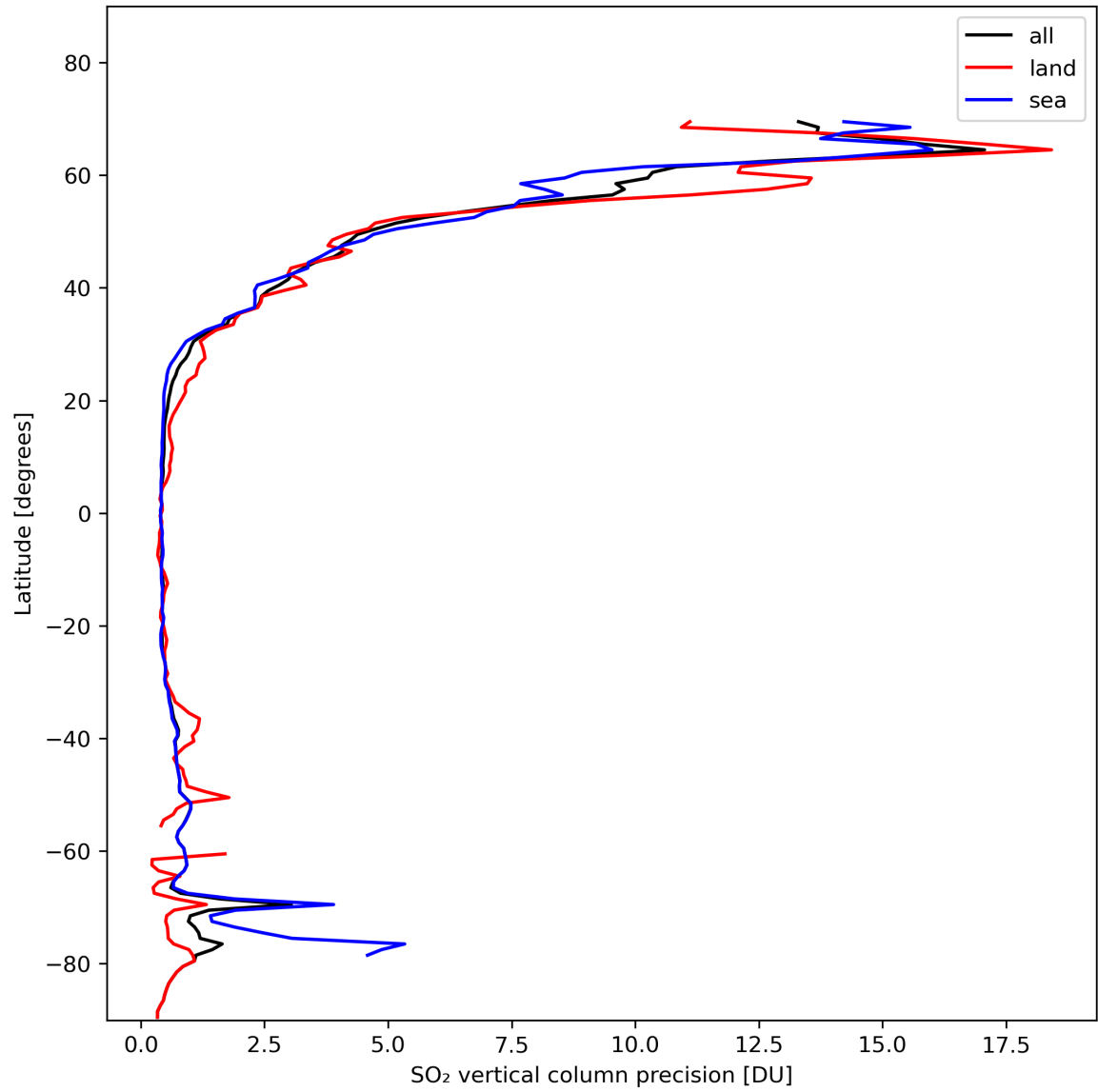
Figure 31: Zonal average of “SO 2 vertical column precision” for 2024-02-04 to 2024-02-06.
