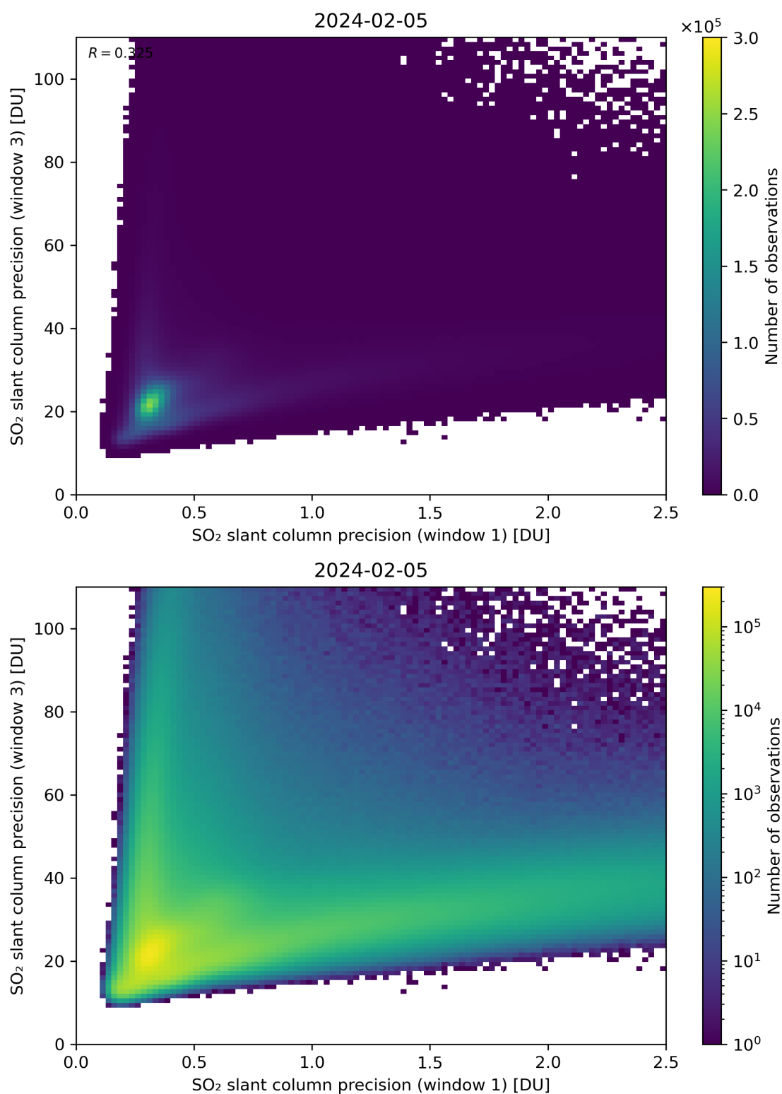
Figure 229: Scatter density plot of “SO 2 slant column precision (window 1)” against “SO 2 slant column precision (window 3)” for 2024-02-04 to 2024-02-06.
