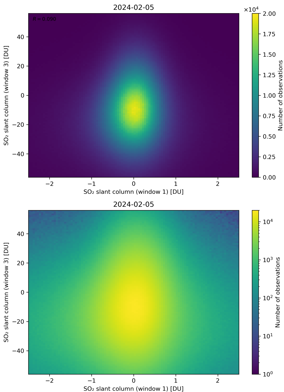
Figure 237: Scatter density plot of “SO 2 slant column (window 1)” against “SO 2 slant column (window 3)” for 2024-02-04 to 2024-02-06.
