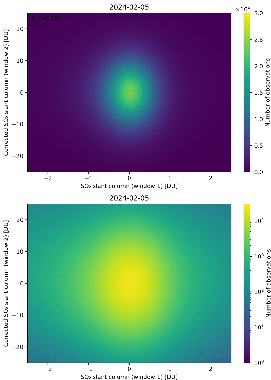
Figure 233: Scatter density plot of “SO 2 slant column (window 1)” against “Corrected SO 2 slant column (window 2)” for 2024-02-04 to 2024-02-06.
