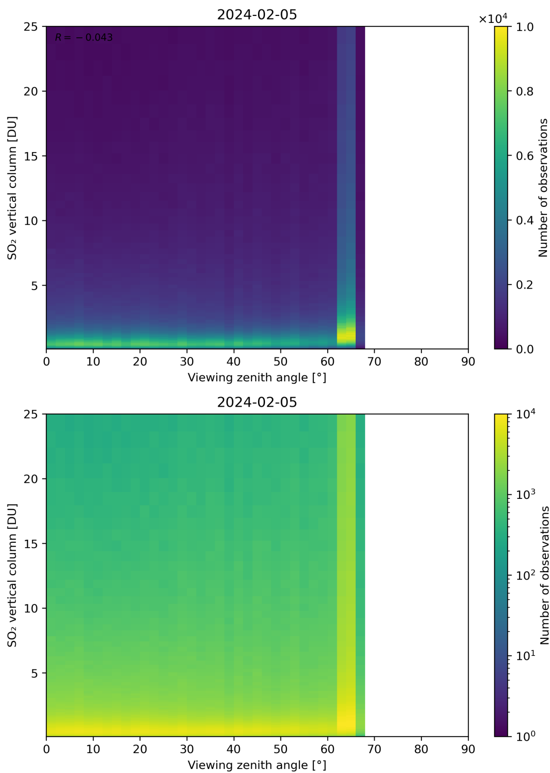
Figure 327: Scatter density plot of “Viewing zenith angle” against “SO 2 vertical column” for 2024-02-04 to 2024-02-06.
