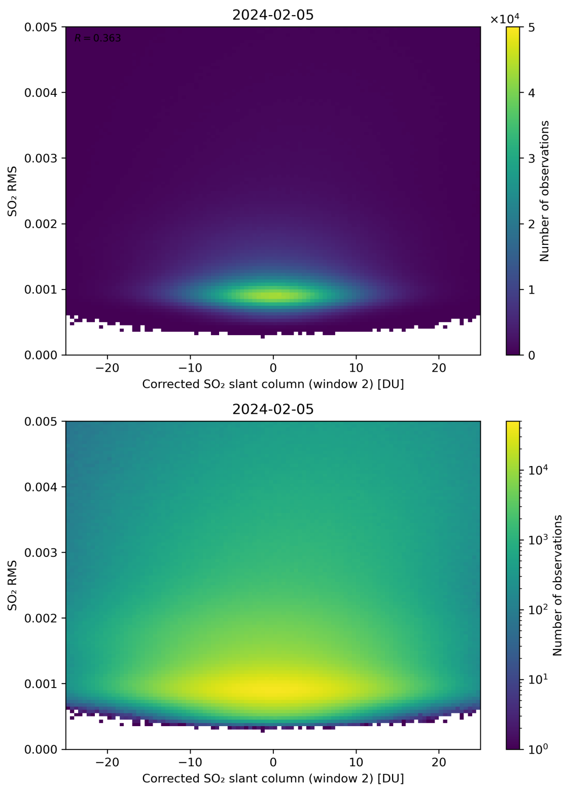
Figure 198: Scatter density plot of “Corrected SO 2 slant column (window 2)” against “SO 2 RMS” for 2024-02-04 to 2024-02-06.
