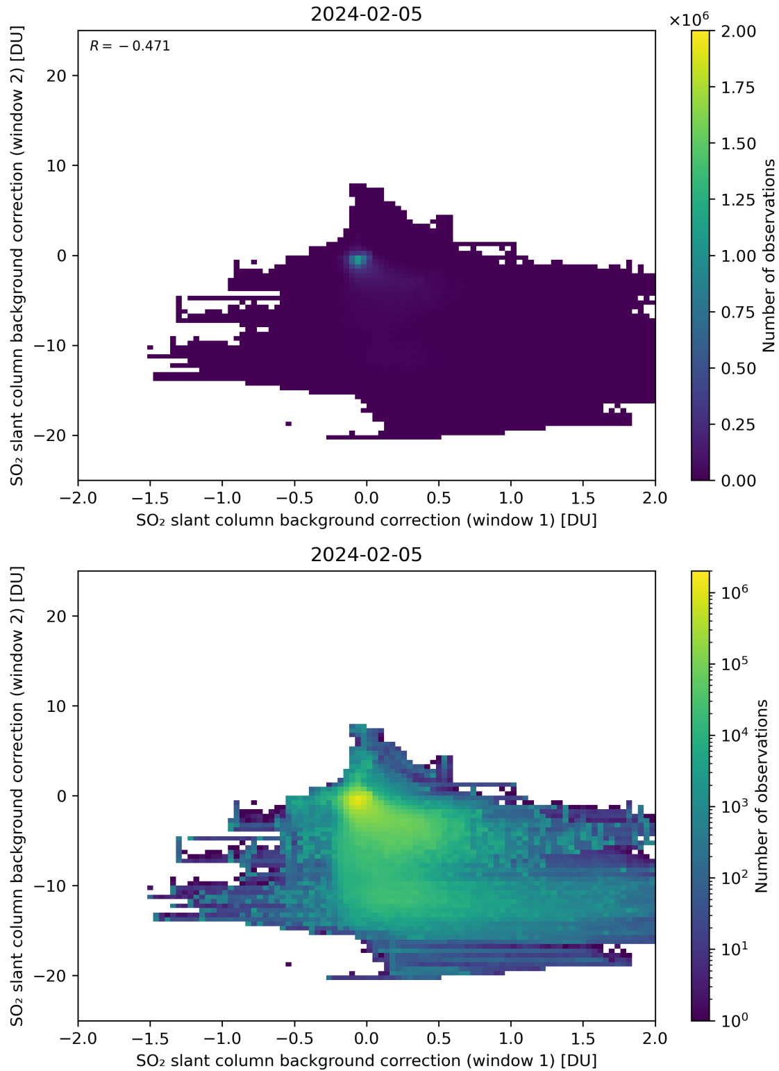
Figure 98: Scatter density plot of “SO 2 slant column background correction (window 1)” against “SO 2 slant column background correction (window 2)” for 2024-02-04 to 2024-02-06.
