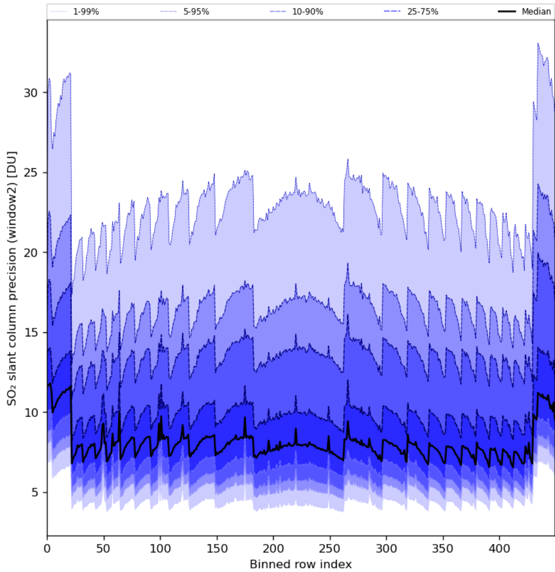
Figure 84: Along track statistics of “SO 2 slant column precision (window2)” for 2024-02-04 to 2024-02-06
