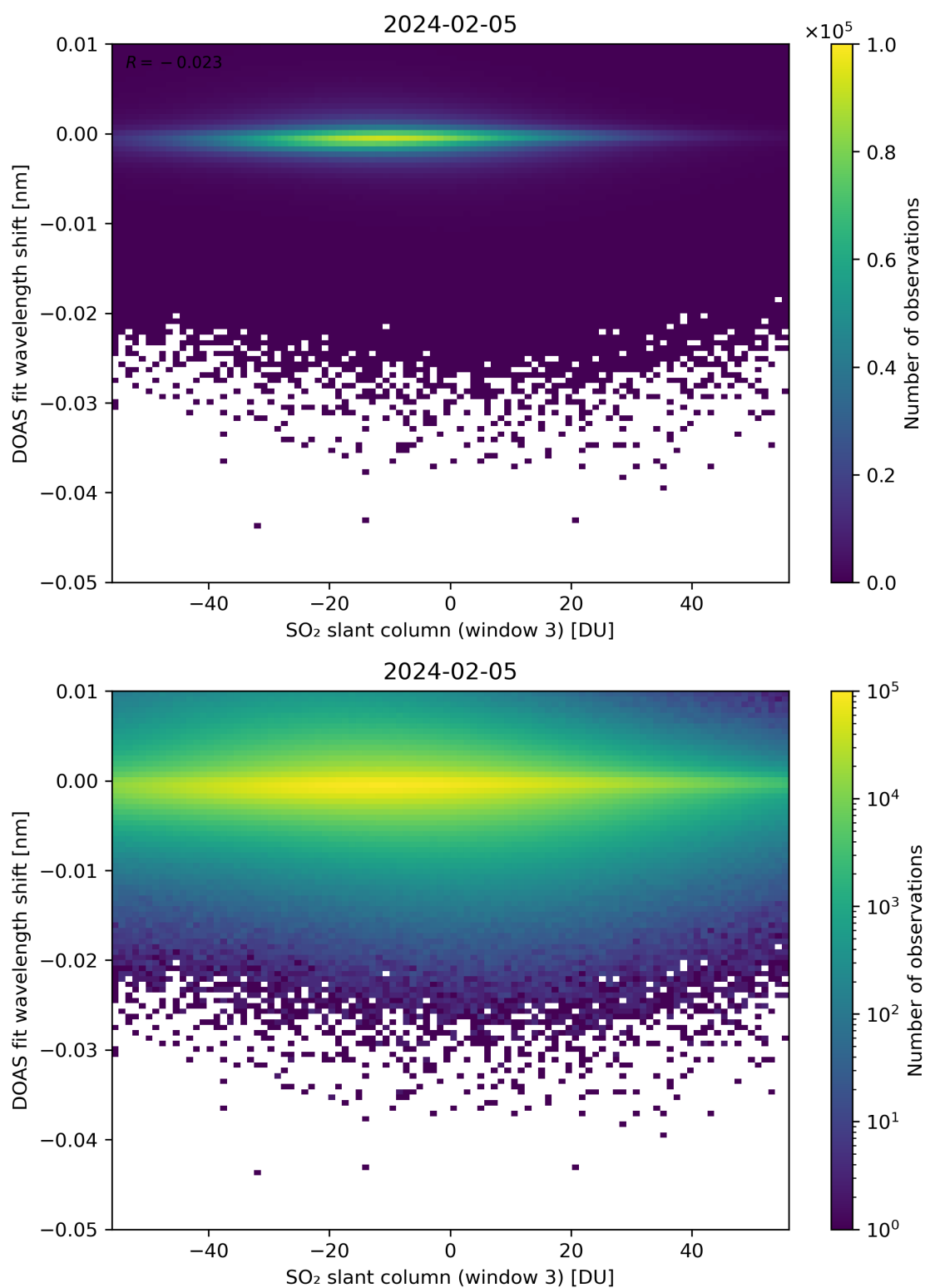
Figure 254: Scatter density plot of “SO 2 slant column (window 3)” against “DOAS fit wavelength shift” for 2024-02-04 to 2024-02-06.
