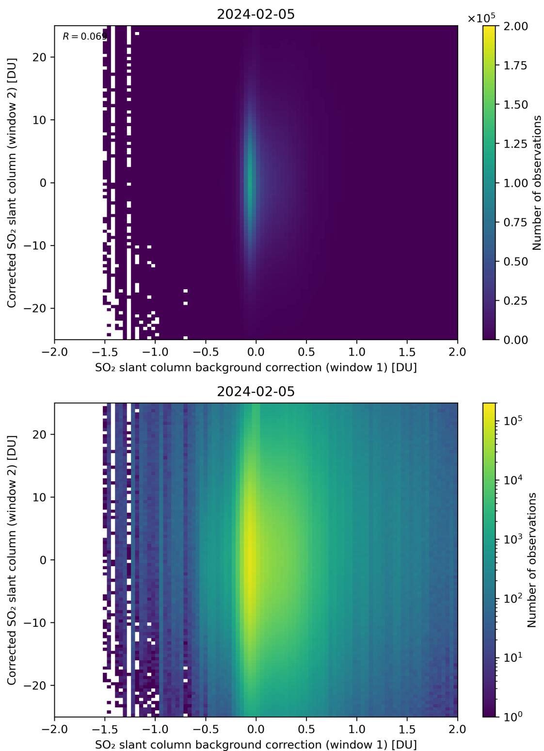
Figure 104: Scatter density plot of “SO 2 slant column background correction (window 1)” against “Corrected SO 2 slant column (window 2)” for 2024-02-04 to 2024-02-06.
