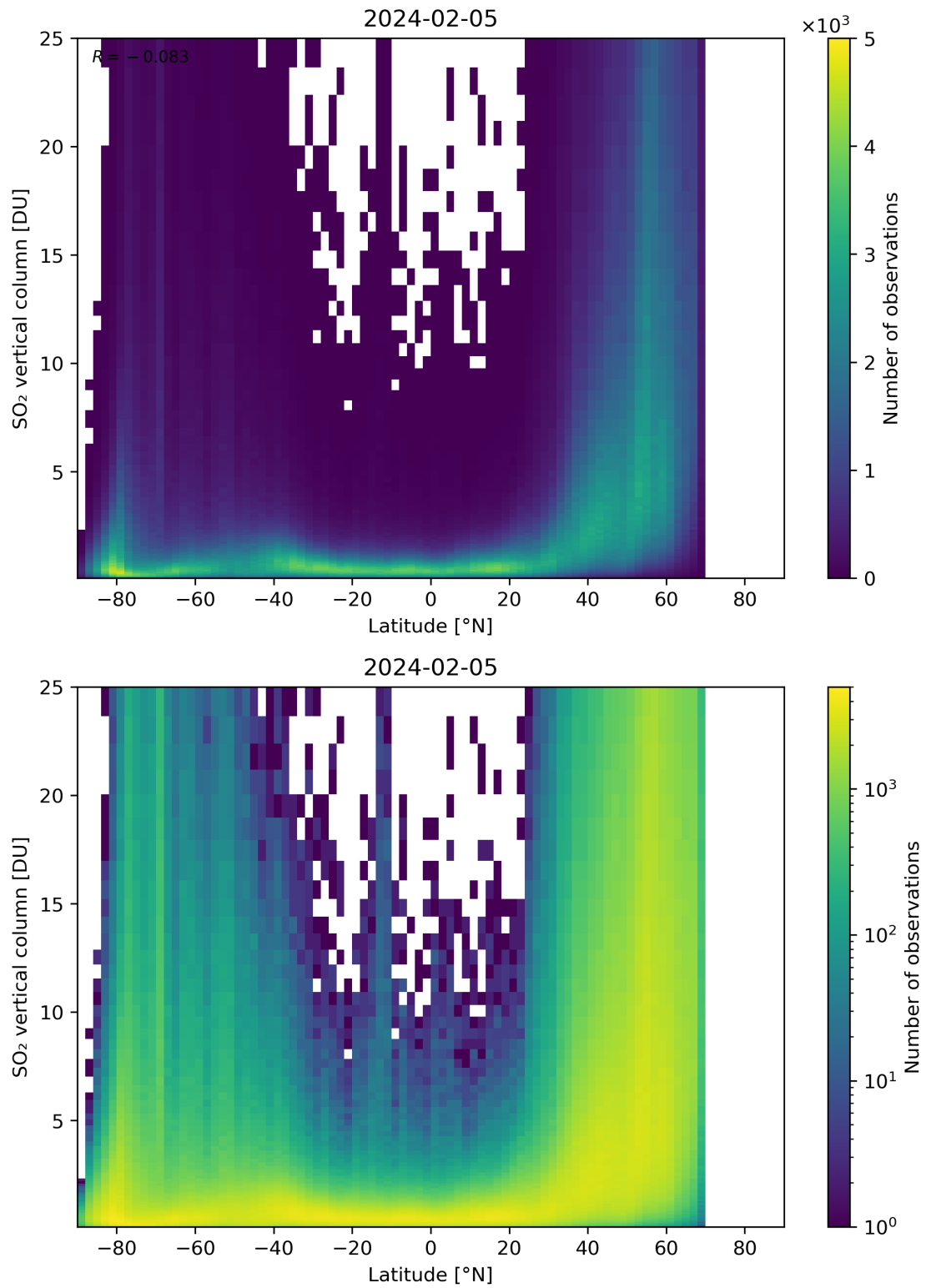
Figure 156: Scatter density plot of “Latitude” against “SO 2 vertical column” for 2024-02-04 to 2024-02-06.
