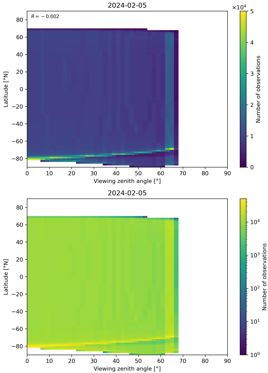
Figure 314: Scatter density plot of “Viewing zenith angle” against “Latitude” for 2024-02-04 to 2024-02-06.
