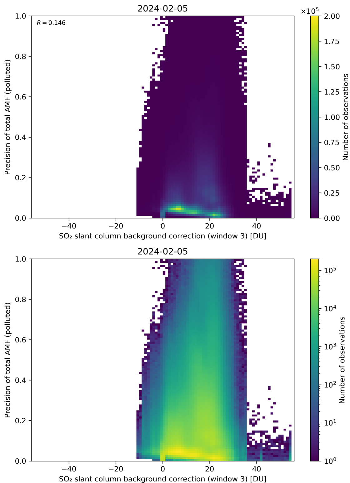
Figure 126: Scatter density plot of “SO 2 slant column background correction (window 3)” against “Precision of total AMF (polluted)” for 2024-02-04 to 2024-02-06.
