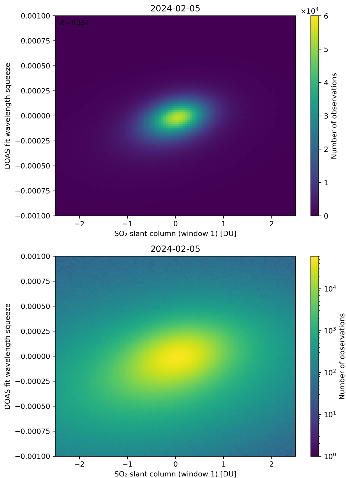
Figure 216: Scatter density plot of “SO 2 slant column (window 1)” against “DOAS fit wavelength squeeze” for 2024-02-04 to 2024-02-06.
