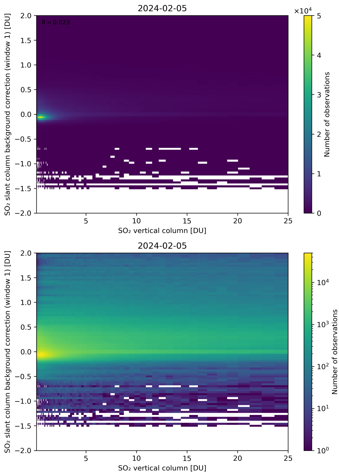
Figure 273: Scatter density plot of “SO 2 vertical column” against “SO 2 slant column background correction (window 1)” for 2024-02-04 to 2024-02-06.
