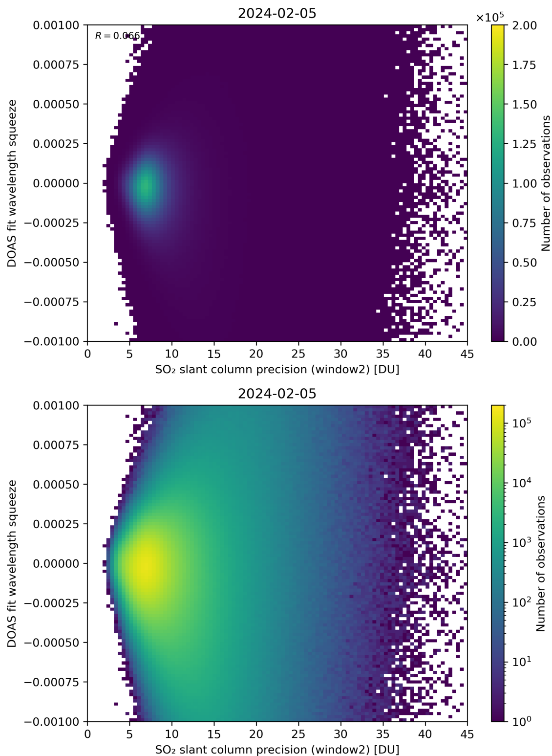
Figure 244: Scatter density plot of “SO 2 slant column precision (window2)” against “DOAS fit wavelength squeeze” for 2024-02-04 to 2024-02-06.
