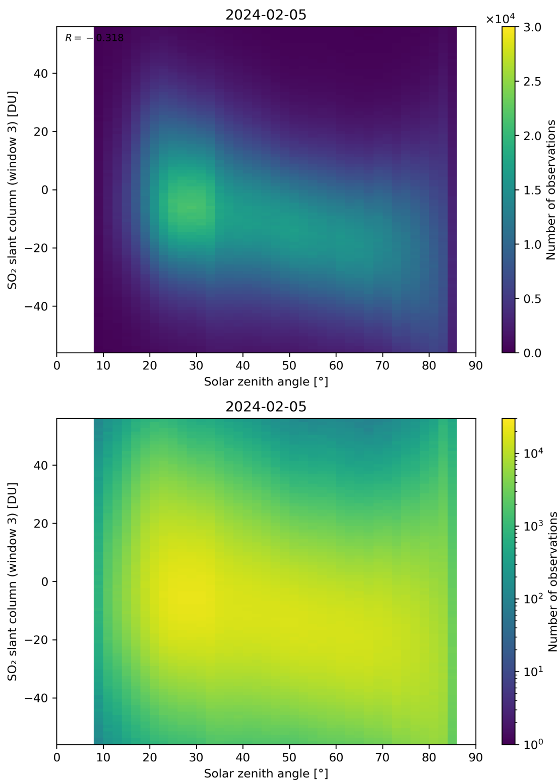
Figure 172: Scatter density plot of “Solar zenith angle” against “SO 2 slant column (window 3)” for 2024-02-04 to 2024-02-06.
