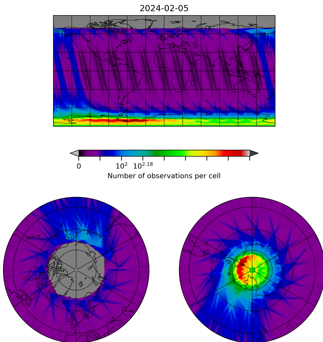
Figure 28: Map of the number of observations for 2024-02-04 to 2024-02-06
