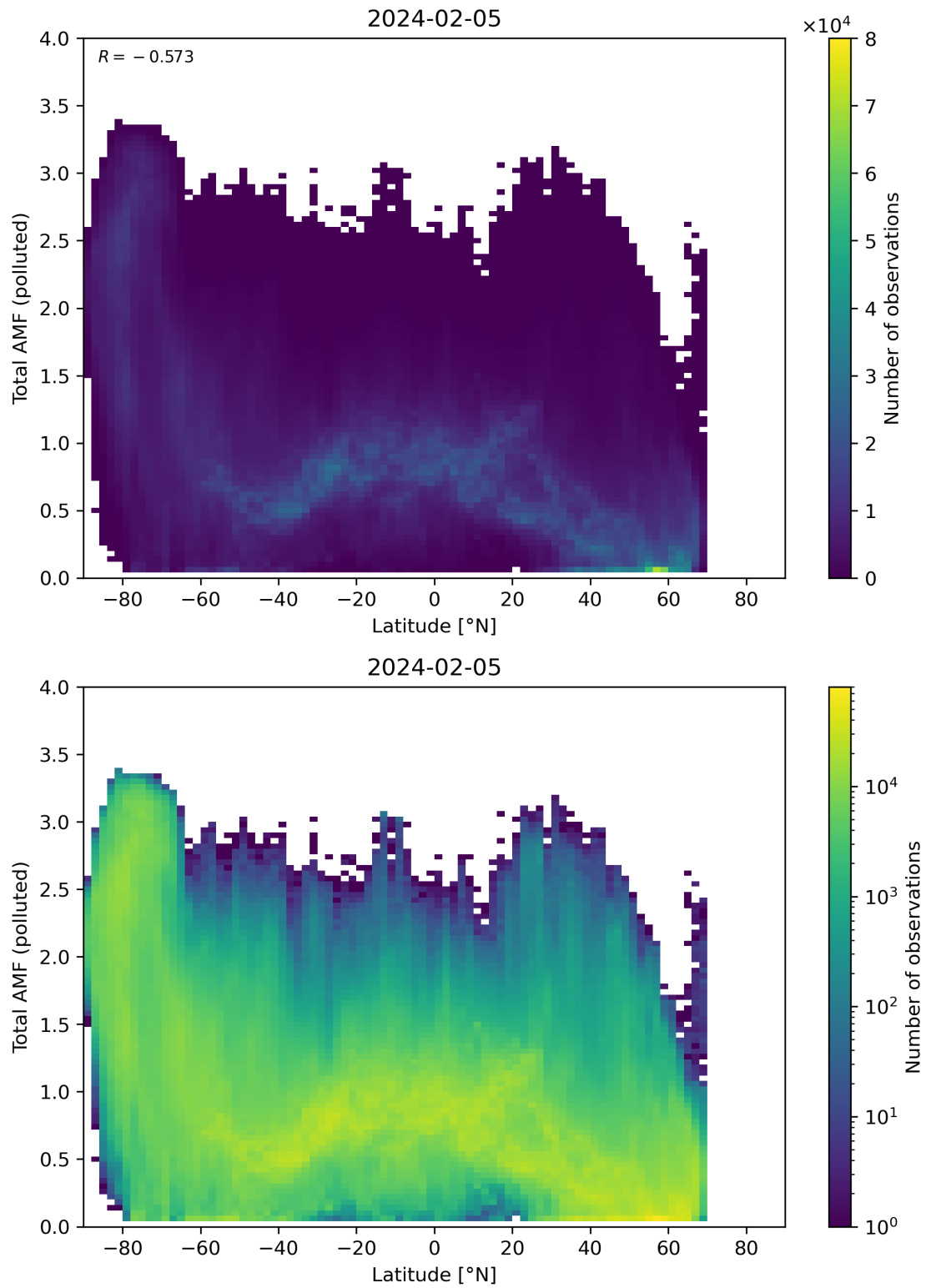
Figure 154: Scatter density plot of “Latitude” against “Total AMF (polluted)” for 2024-02-04 to 2024-02-06.
