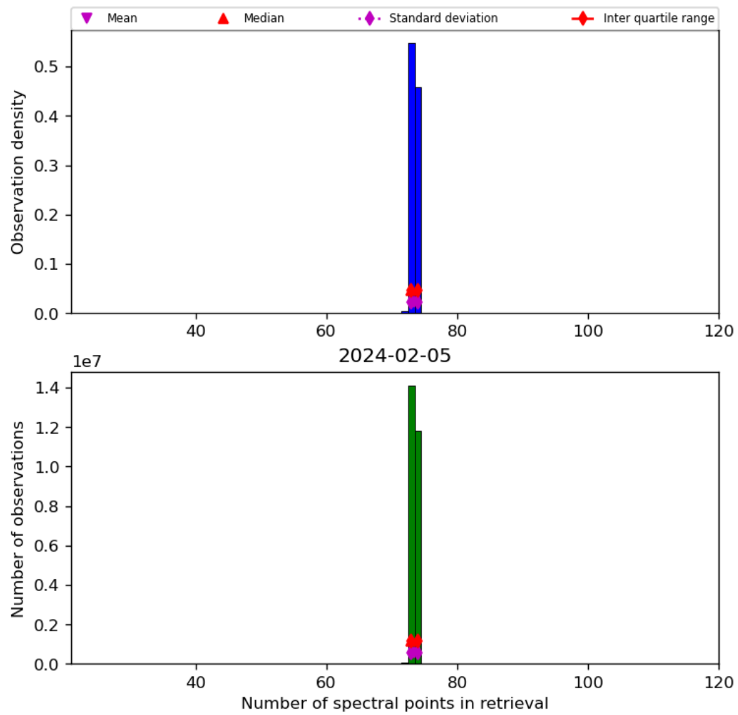
Figure 74: Histogram of “Number of spectral points in retrieval” for 2024-02-04 to 2024-02-06
