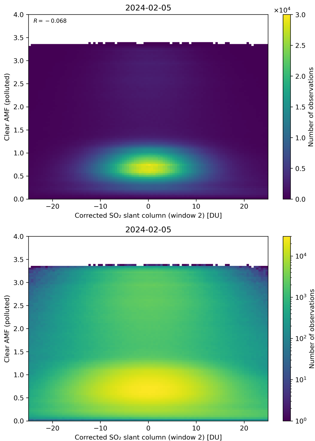
Figure 199: Scatter density plot of “Corrected SO 2 slant column (window 2)” against “Clear AMF (polluted)” for 2024-02-04 to 2024-02-06.
