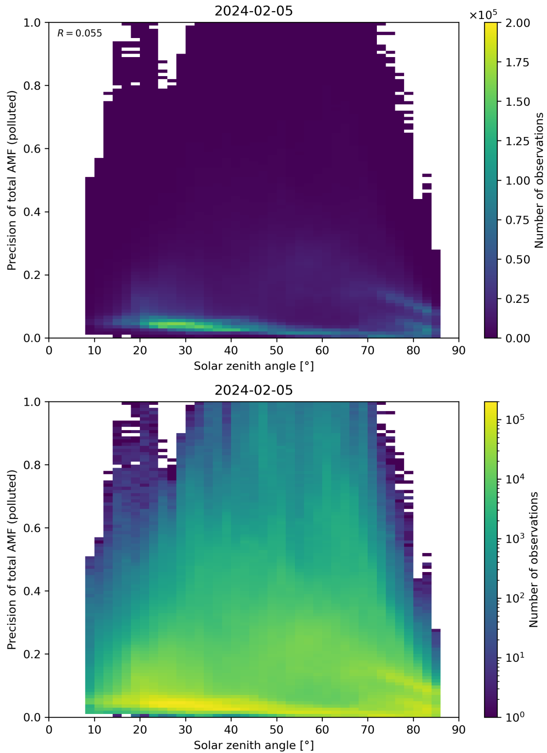
Figure 175: Scatter density plot of “Solar zenith angle” against “Precision of total AMF (polluted)” for 2024-02-04 to 2024-02-06.
