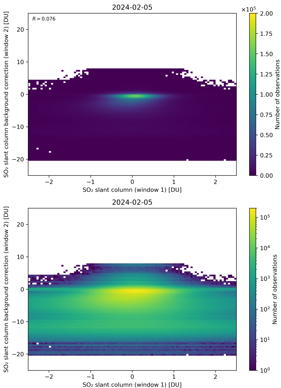
Figure 213: Scatter density plot of “SO 2 slant column (window 1)” against “SO 2 slant column background correction (window 2)” for 2024-02-04 to 2024-02-06.
