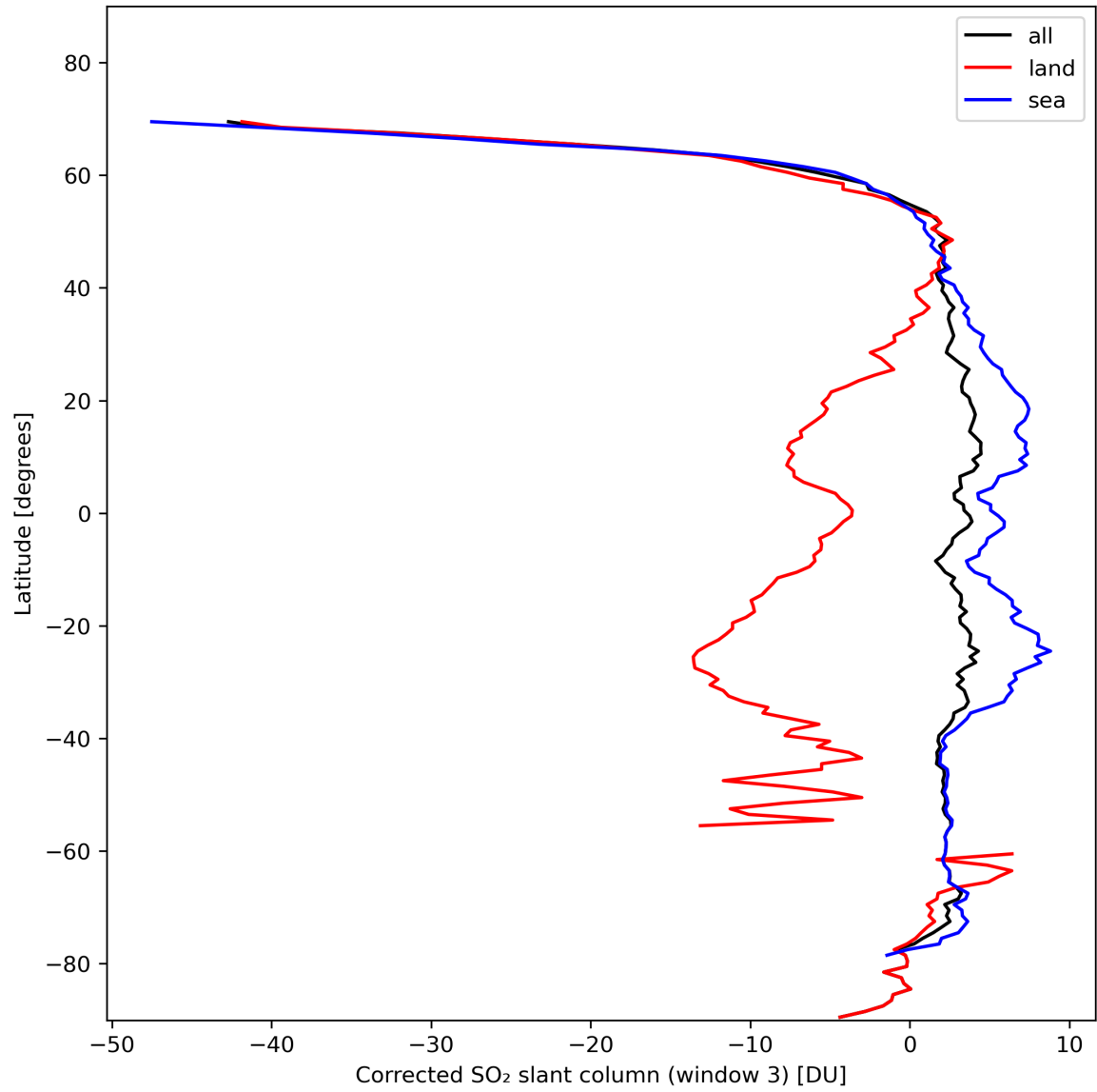
Figure 43: Zonal average of “Corrected SO 2 slant column (window 3)” for 2024-02-04 to 2024-02-06.
