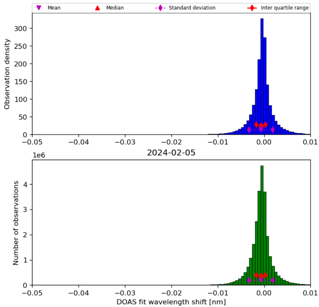
Figure 68: Histogram of “DOAS fit wavelength shift” for 2024-02-04 to 2024-02-06
