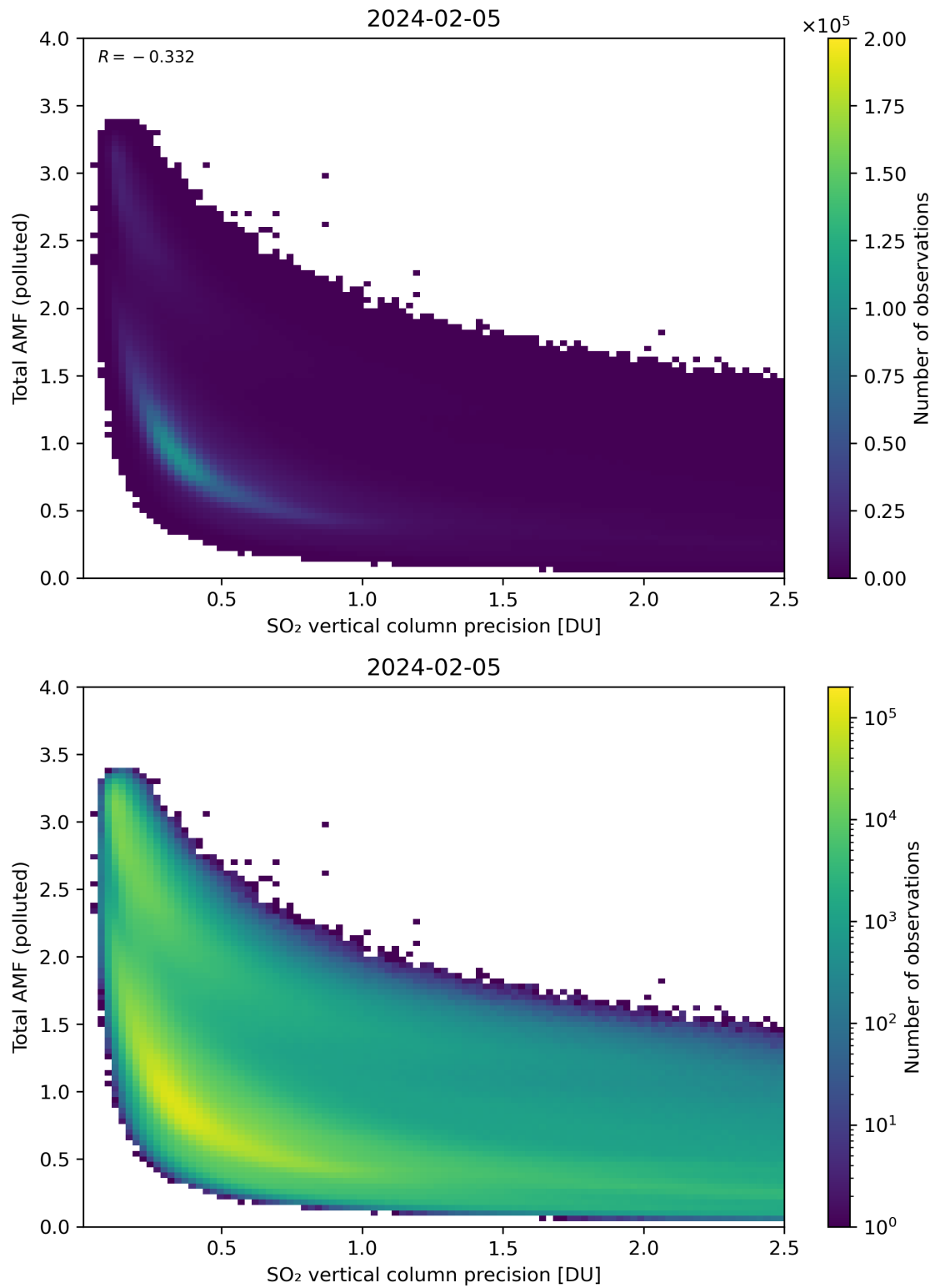
Figure 294: Scatter density plot of “SO 2 vertical column precision” against “Total AMF (polluted)” for 2024-02-04 to 2024-02-06.
