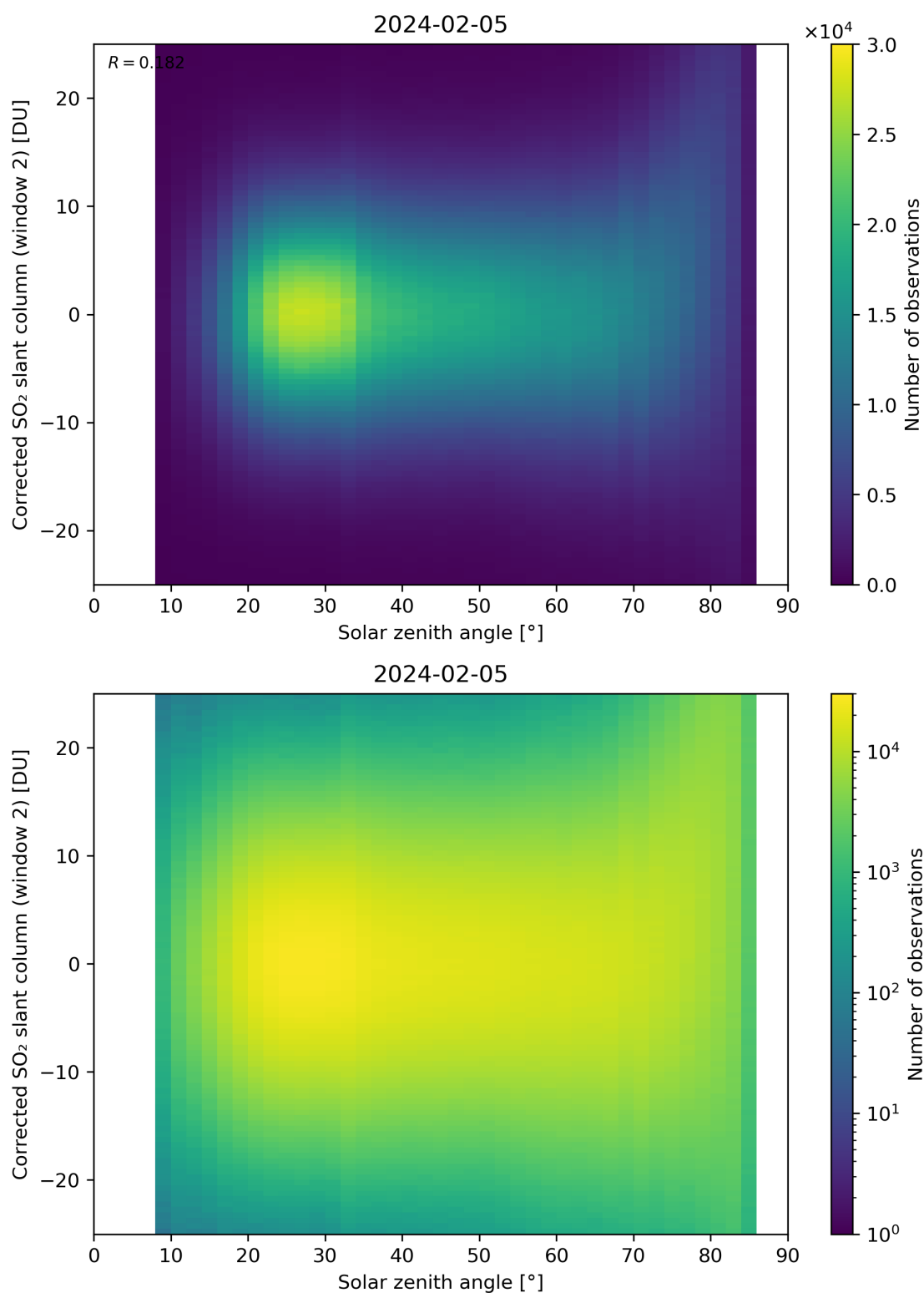
Figure 167: Scatter density plot of “Solar zenith angle” against “Corrected SO 2 slant column (window 2)” for 2024-02-04 to 2024-02-06.
