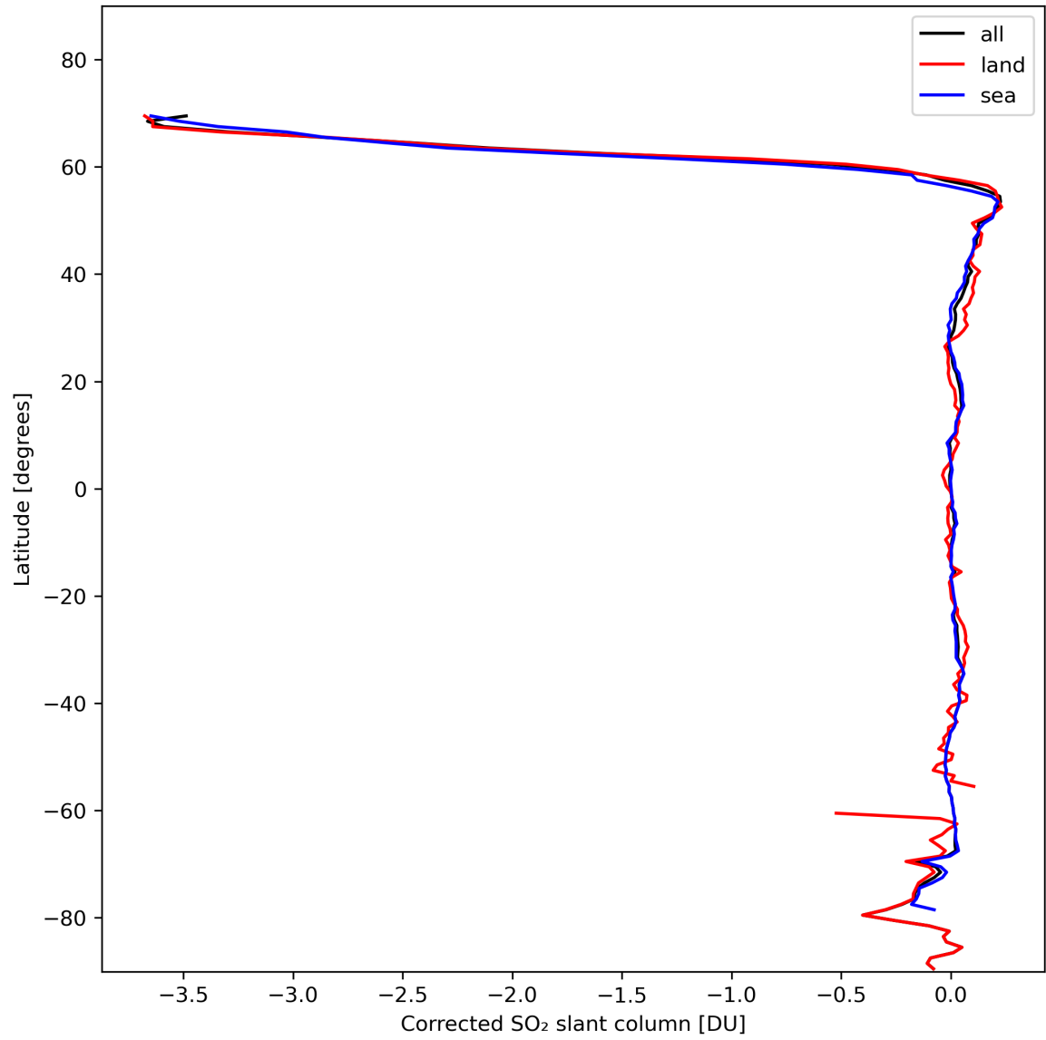
Figure 32: Zonal average of “Corrected SO 2 slant column” for 2024-02-04 to 2024-02-06.
