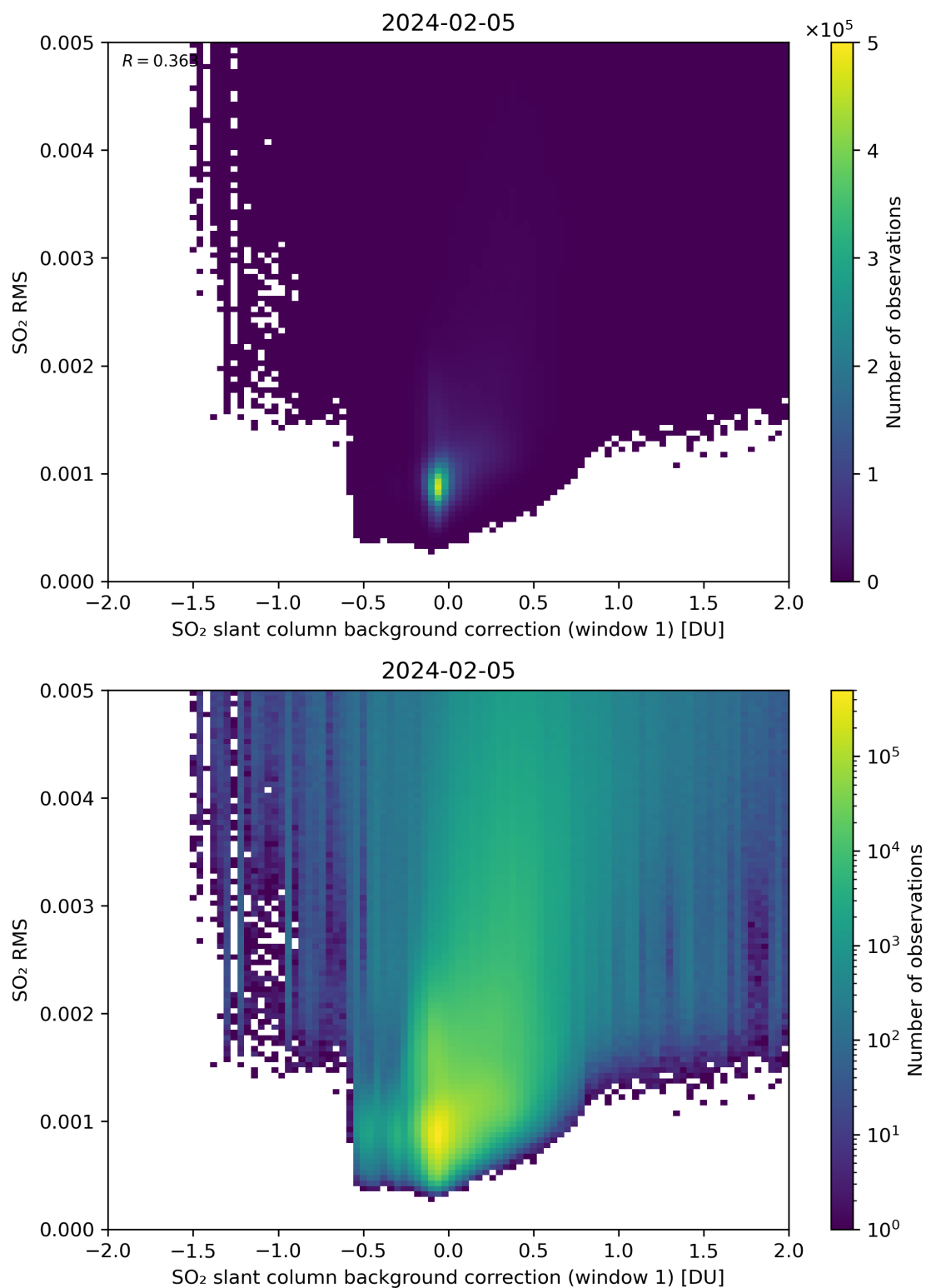
Figure 102: Scatter density plot of “SO 2 slant column background correction (window 1)” against “SO 2 RMS” for 2024-02-04 to 2024-02-06.
