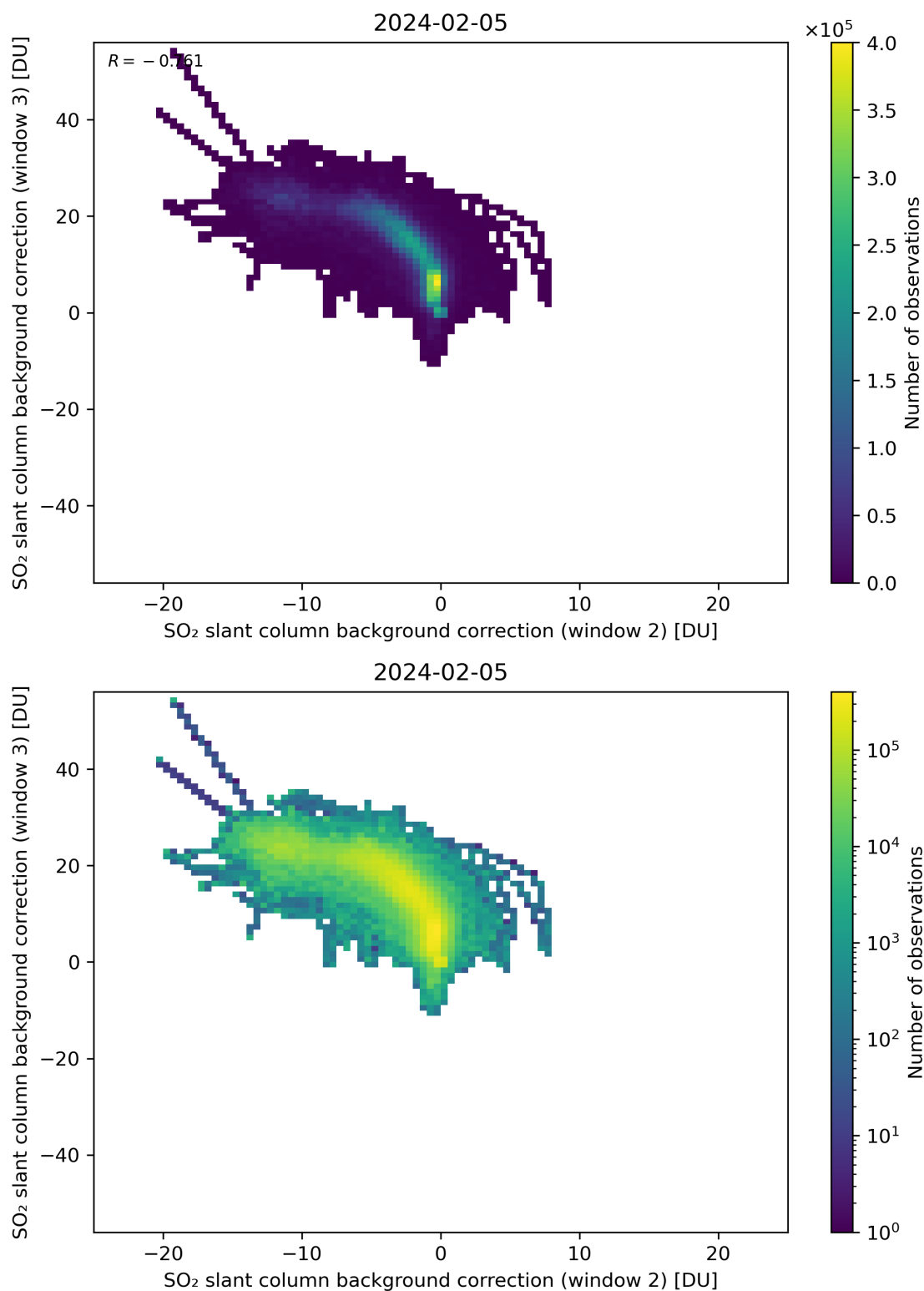
Figure 111: Scatter density plot of “SO 2 slant column background correction (window 2)” against “SO 2 slant column background correction (window 3)” for 2024-02-04 to 2024-02-06.
