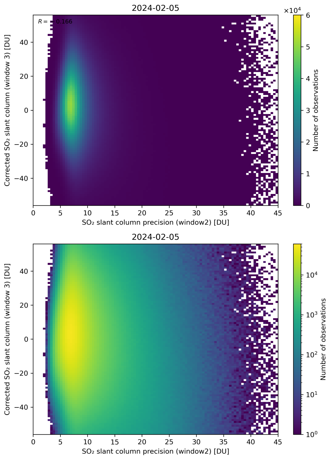
Figure 248: Scatter density plot of “SO 2 slant column precision (window2)” against “Corrected SO 2 slant column (window 3)” for 2024-02-04 to 2024-02-06.
