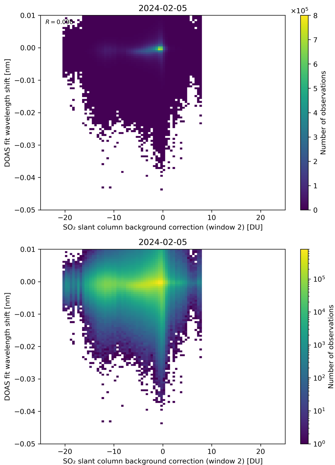
Figure 112: Scatter density plot of “SO 2 slant column background correction (window 2)” against “DOAS fit wavelength shift” for 2024-02-04 to 2024-02-06.
