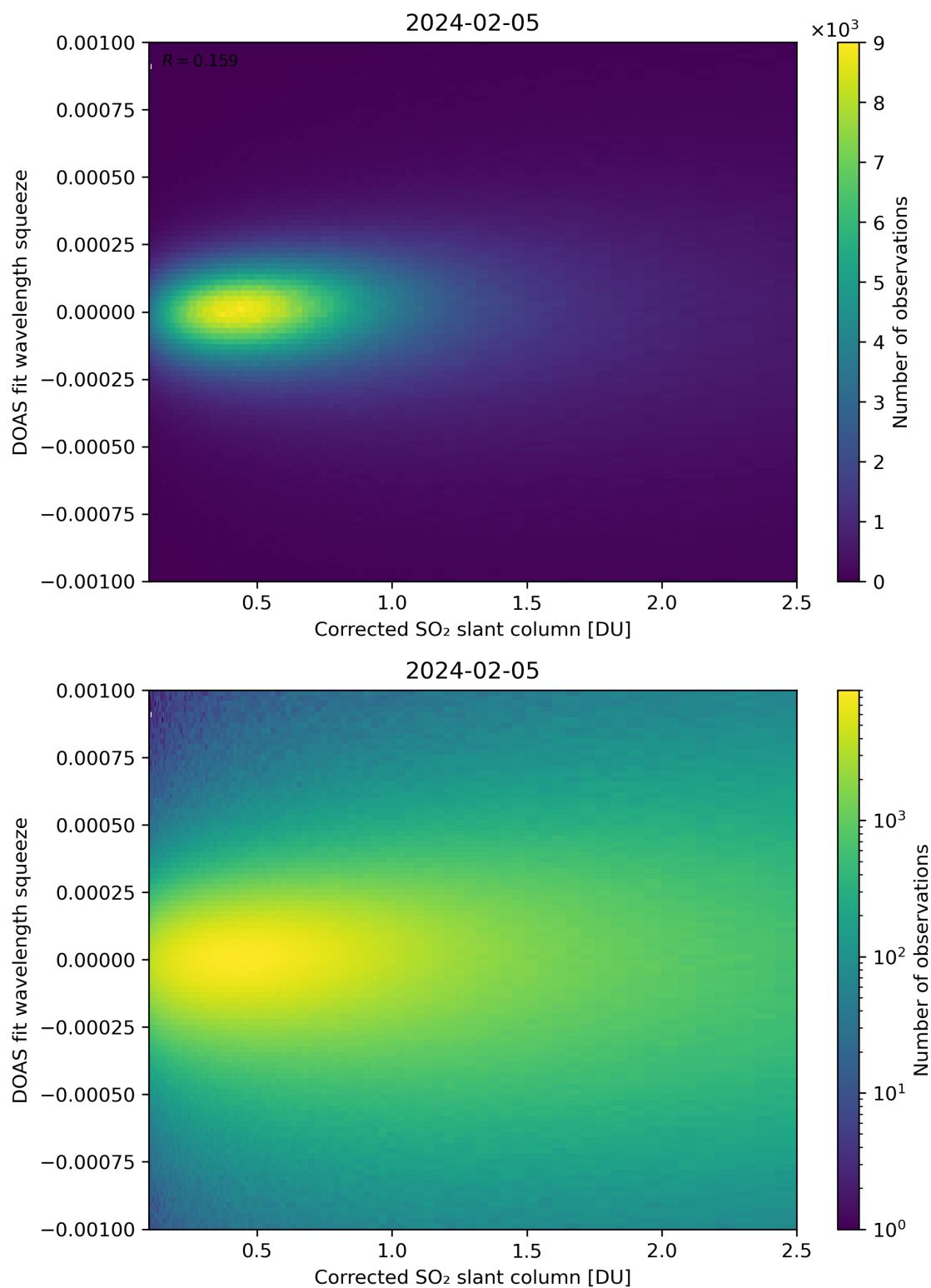
Figure 182: Scatter density plot of “Corrected SO 2 slant column” against “DOAS fit wavelength squeeze” for 2024-02-04 to 2024-02-06.
