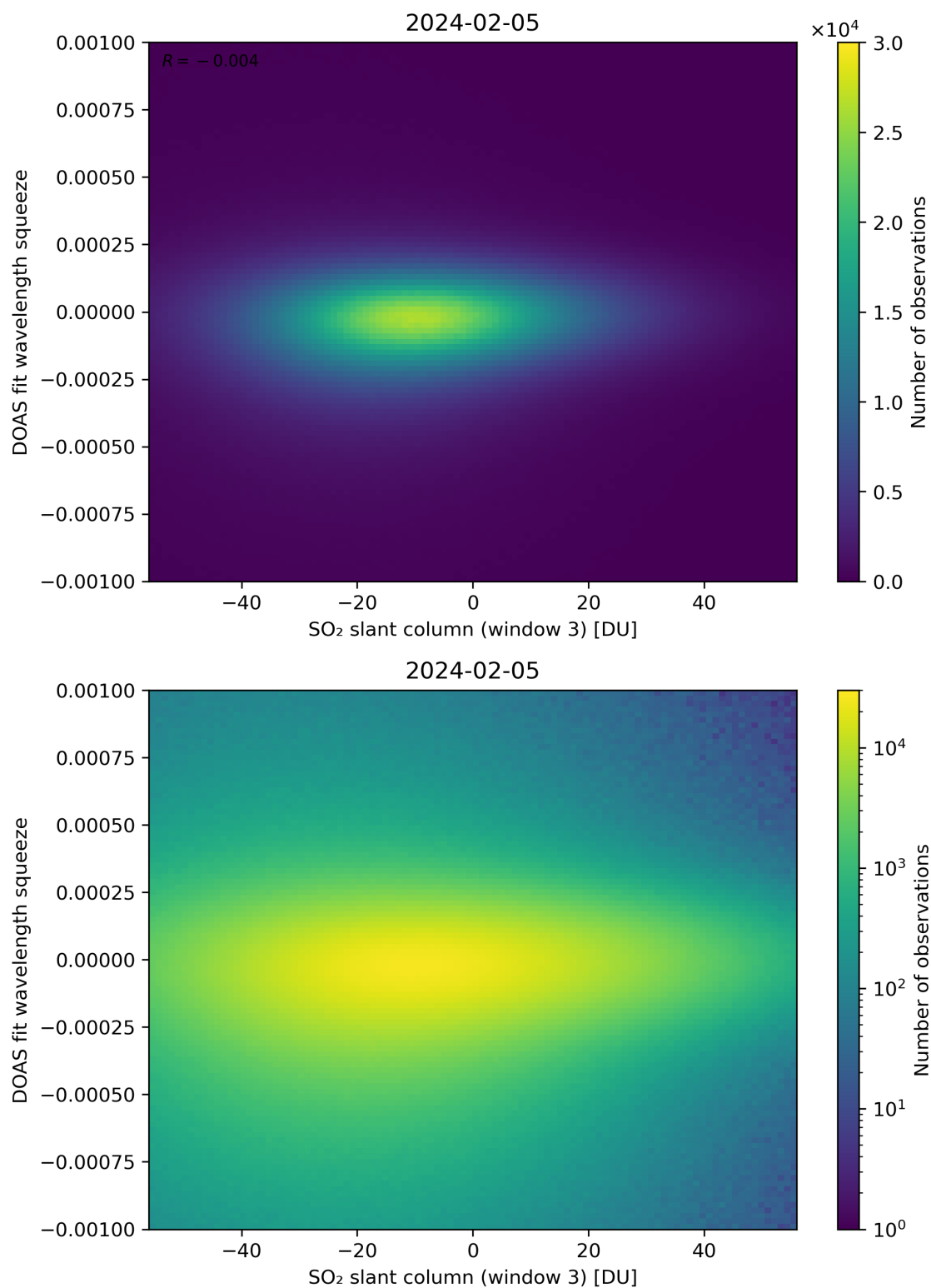
Figure 255: Scatter density plot of “SO 2 slant column (window 3)” against “DOAS fit wavelength squeeze” for 2024-02-04 to 2024-02-06.
