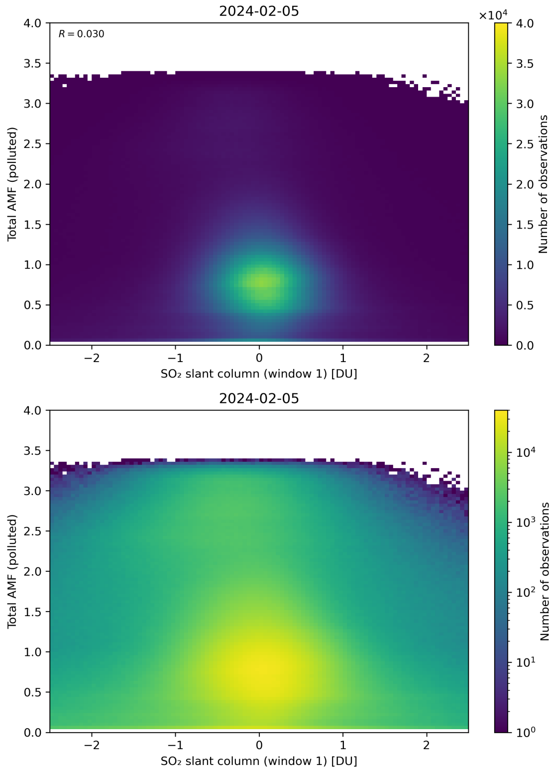
Figure 239: Scatter density plot of “SO 2 slant column (window 1)” against “Total AMF (polluted)” for 2024-02-04 to 2024-02-06.
