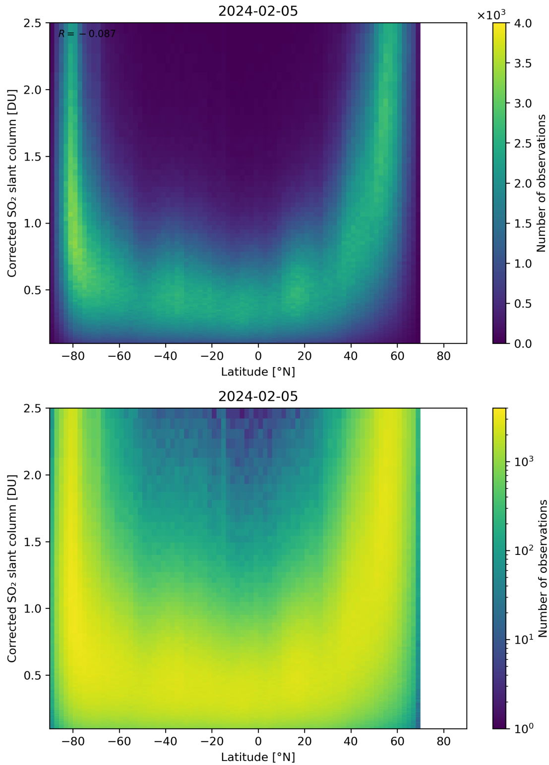
Figure 146: Scatter density plot of “Latitude” against “Corrected SO 2 slant column” for 2024-02-04 to 2024-02-06.
