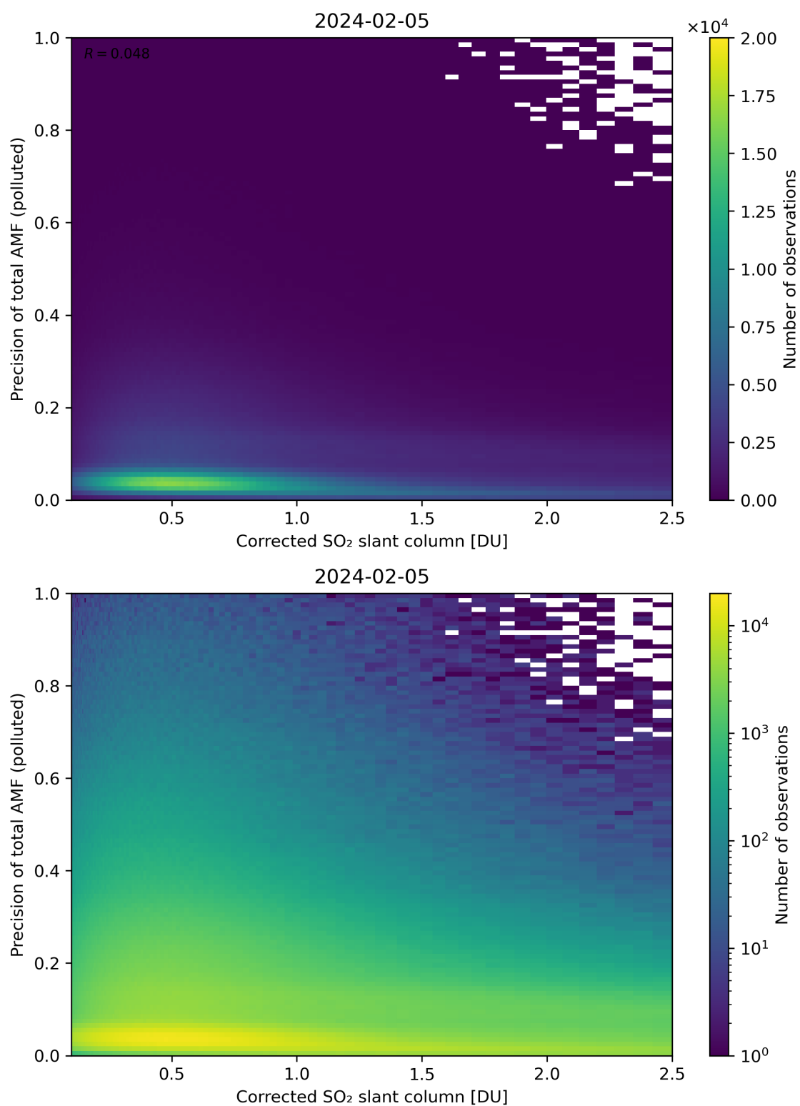
Figure 193: Scatter density plot of “Corrected SO 2 slant column” against “Precision of total AMF (polluted)” for 2024-02-04 to 2024-02-06.
