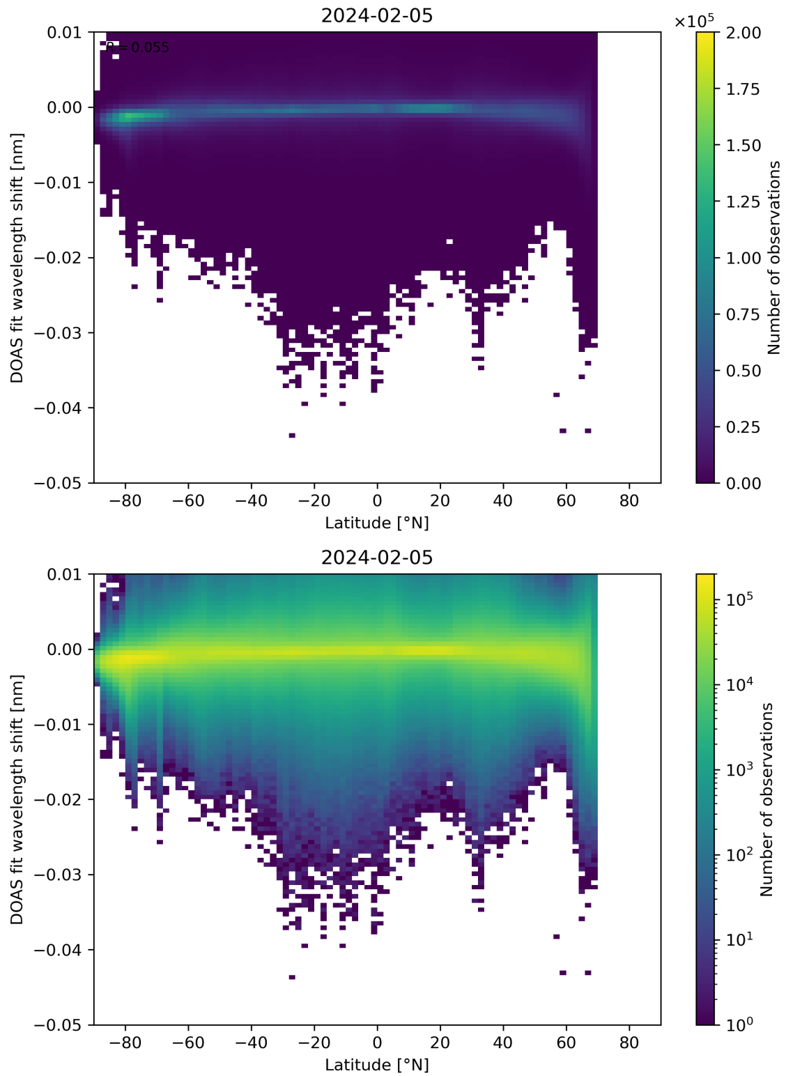
Figure 142: Scatter density plot of “Latitude” against “DOAS fit wavelength shift” for 2024-02-04 to 2024-02-06.
