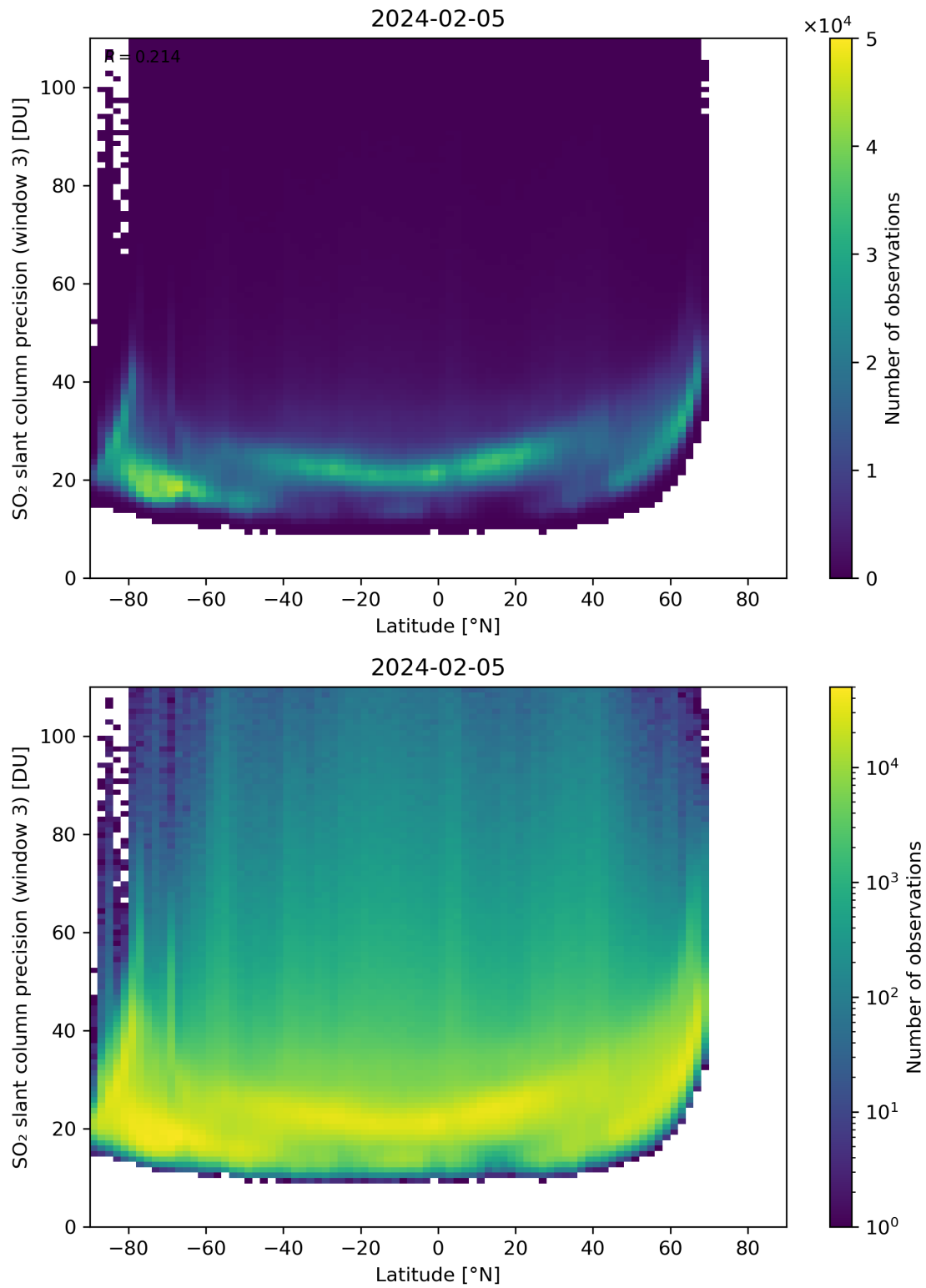
Figure 153: Scatter density plot of “Latitude” against “SO 2 slant column precision (window 3)” for 2024-02-04 to 2024-02-06.
