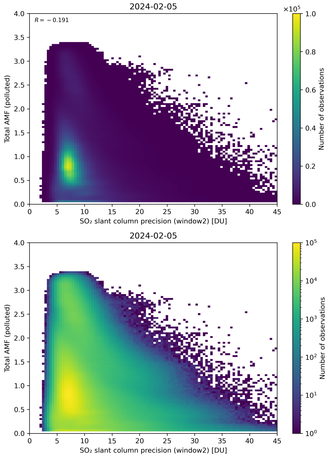
Figure 251: Scatter density plot of “SO 2 slant column precision (window2)” against “Total AMF (polluted)” for 2024-02-04 to 2024-02-06.
