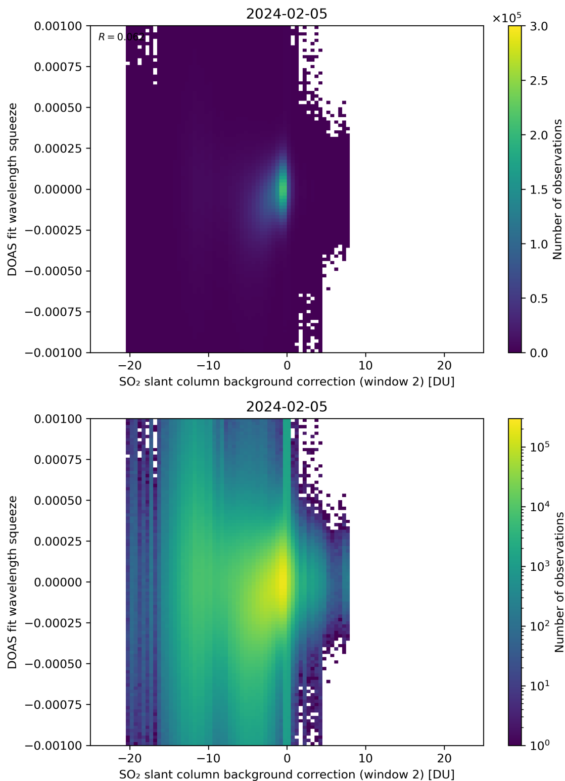
Figure 113: Scatter density plot of “SO 2 slant column background correction (window 2)” against “DOAS fit wavelength squeeze” for 2024-02-04 to 2024-02-06.
