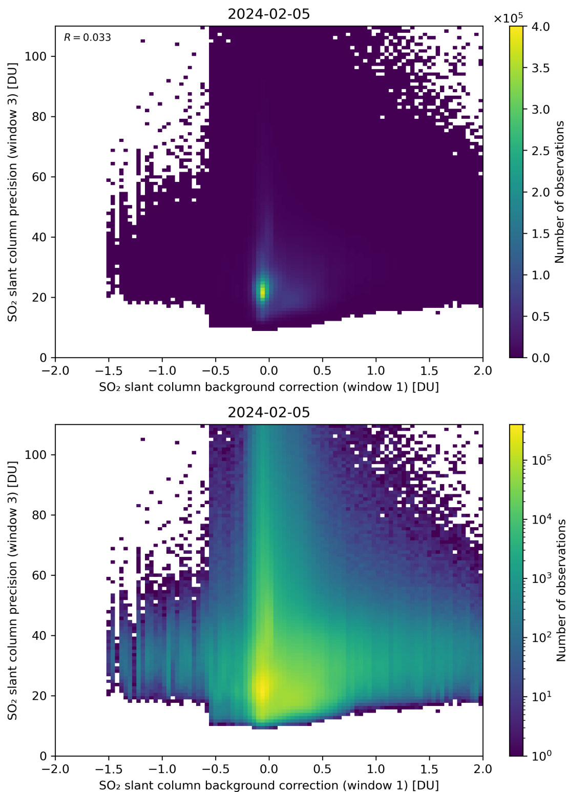
Figure 108: Scatter density plot of “SO 2 slant column background correction (window 1)” against “SO 2 slant column precision (window 3)” for 2024-02-04 to 2024-02-06.
