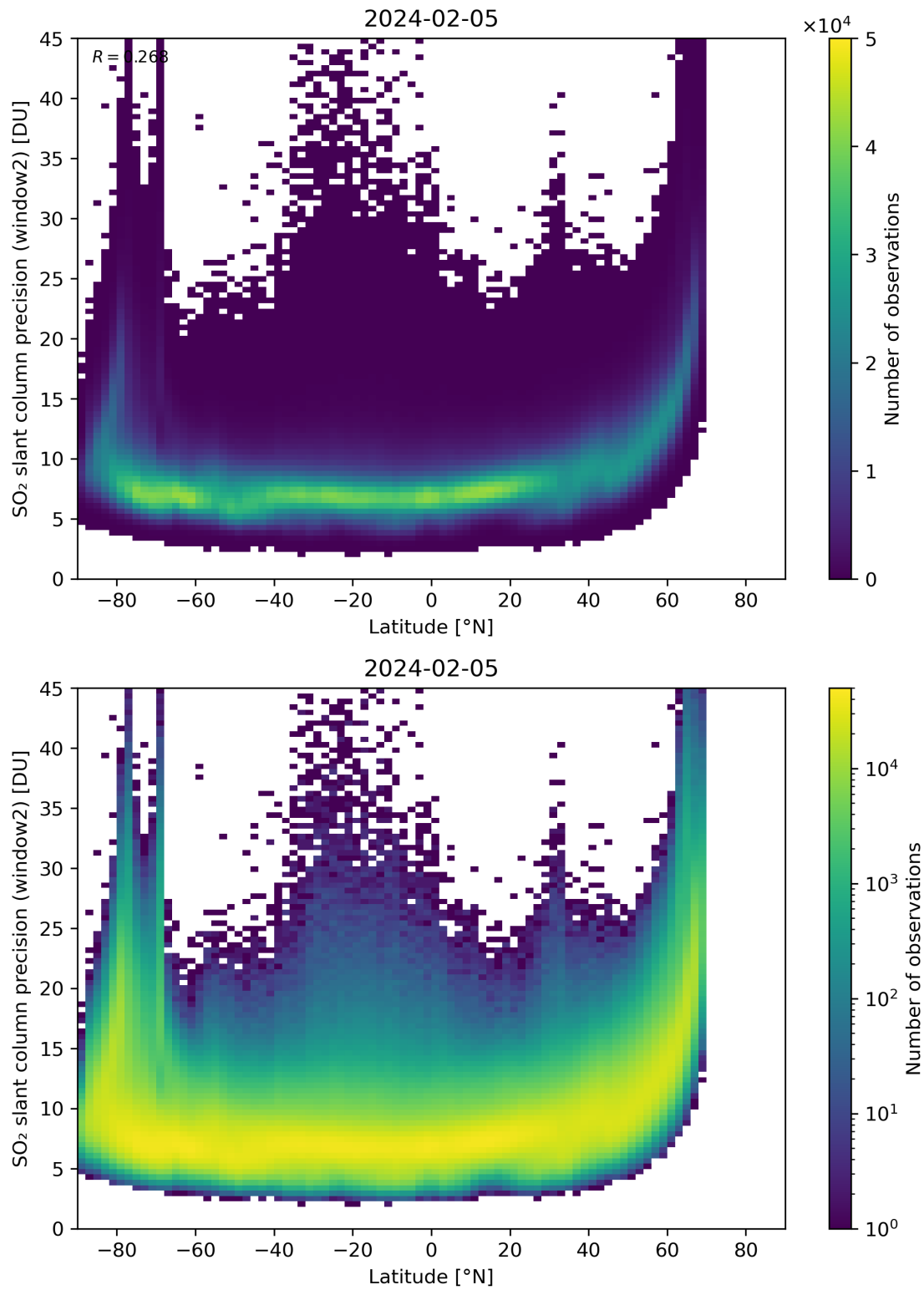
Figure 151: Scatter density plot of “Latitude” against “SO 2 slant column precision (window2)” for 2024-02-04 to 2024-02-06.
