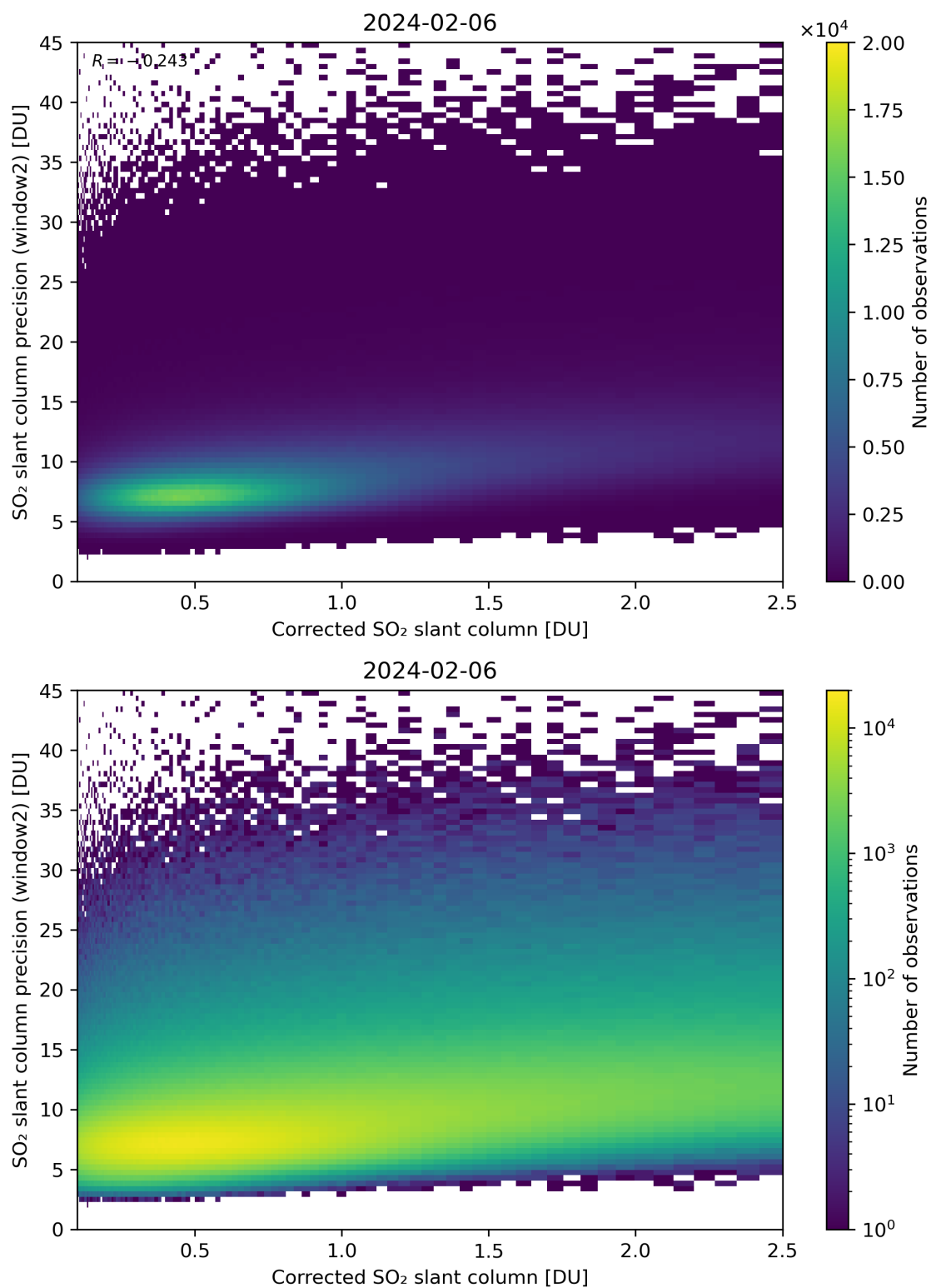
Figure 189: Scatter density plot of “Corrected SO 2 slant column” against “SO 2 slant column precision (window2)” for 2024-02-06 to 2024-02-07.
