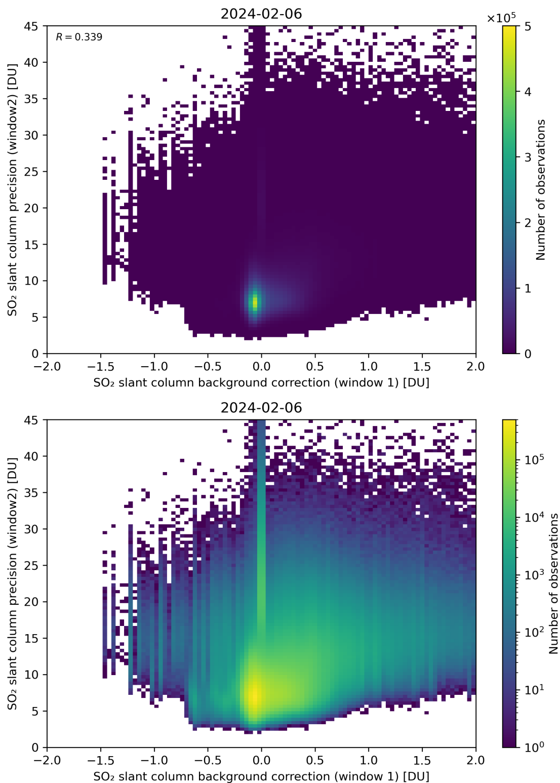
Figure 106: Scatter density plot of “SO 2 slant column background correction (window 1)” against “SO 2 slant column precision (window2)” for 2024-02-06 to 2024-02-07.
