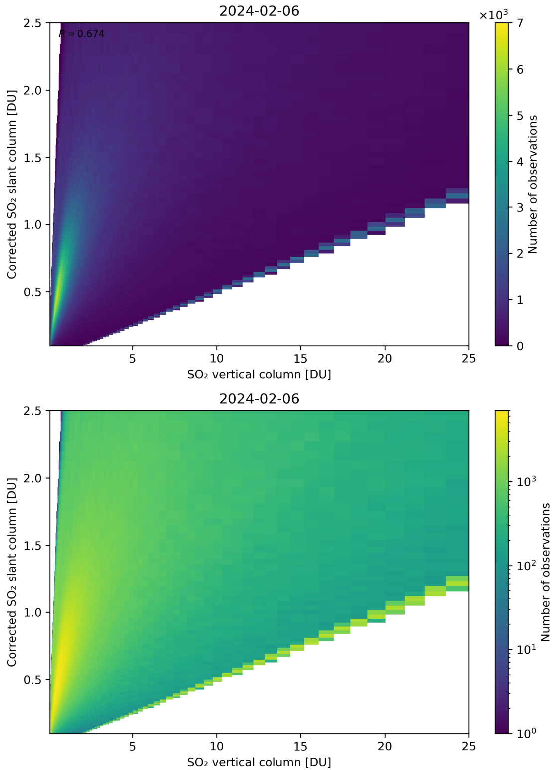
Figure 297: Scatter density plot of “SO 2 vertical column” against “Corrected SO 2 slant column” for 2024-02-06 to 2024-02-07.
