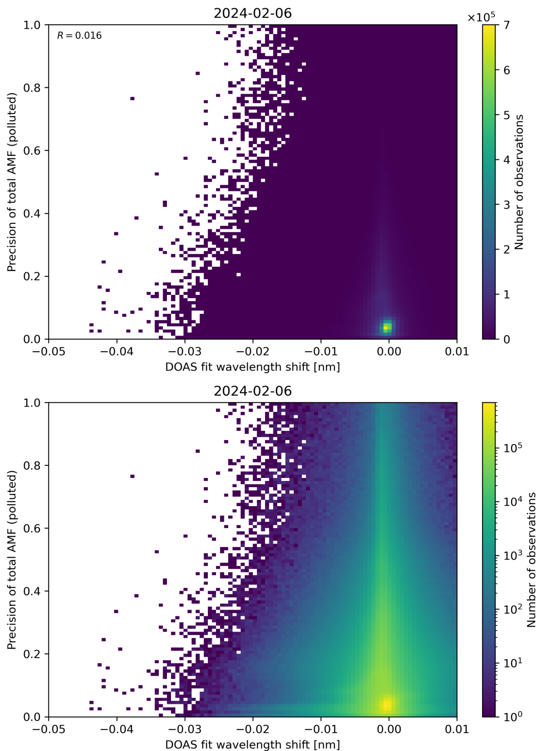
Figure 131: Scatter density plot of “DOAS fit wavelength shift” against “Precision of total AMF (polluted)” for 2024-02-06 to 2024-02-07.
