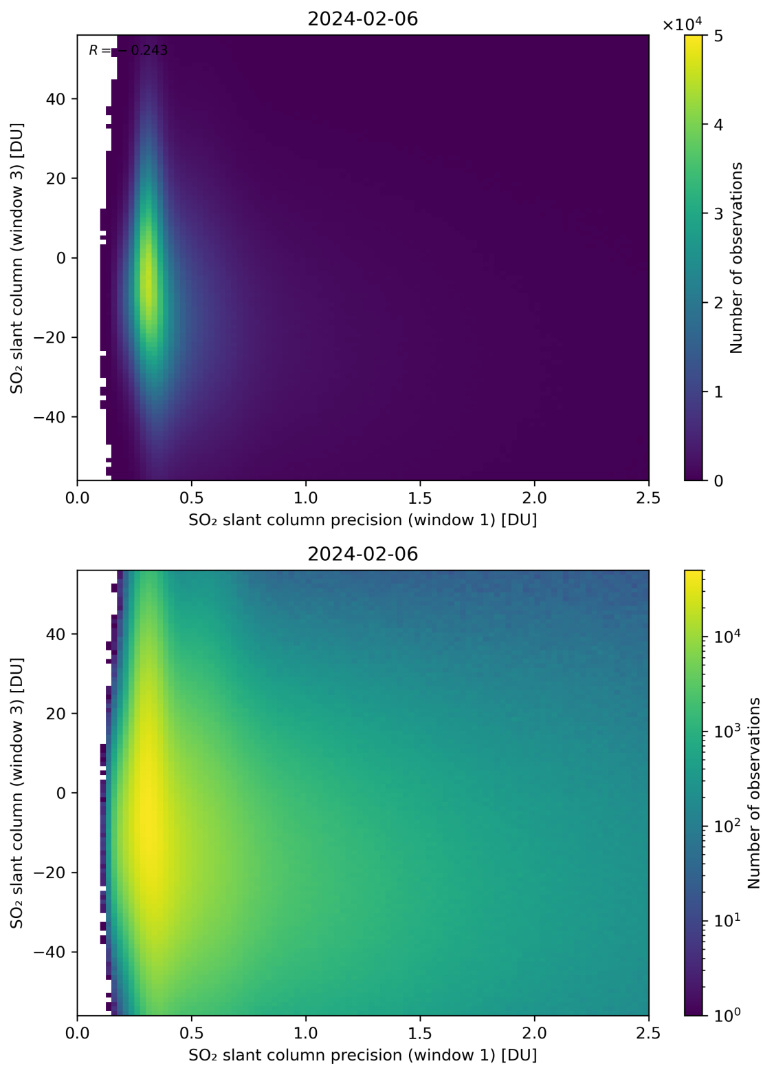
Figure 228: Scatter density plot of “SO 2 slant column precision (window 1)” against “SO 2 slant column (window 3)” for 2024-02-06 to 2024-02-07.
