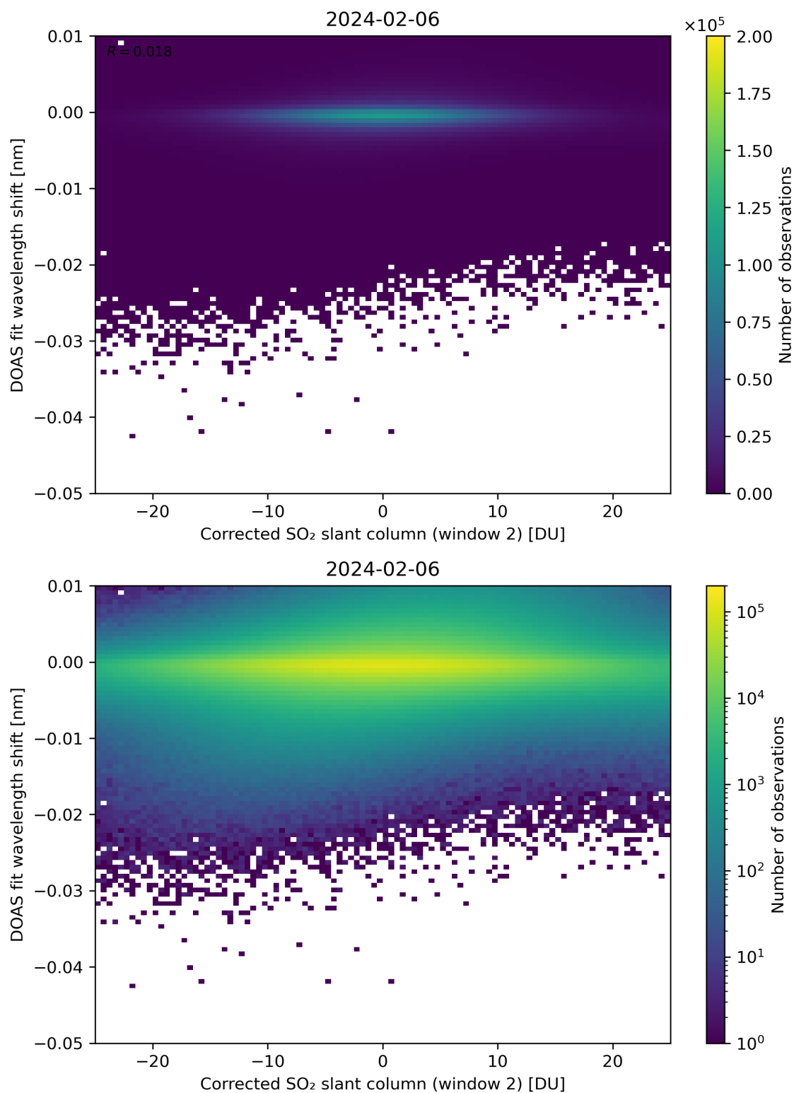
Figure 196: Scatter density plot of “Corrected SO 2 slant column (window 2)” against “DOAS fit wavelength shift” for 2024-02-06 to 2024-02-07.
