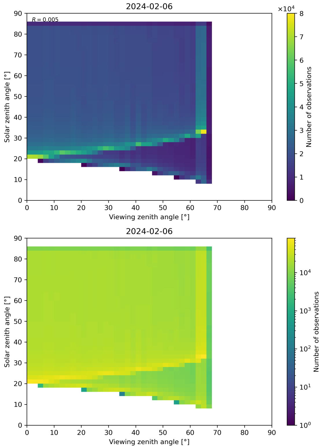
Figure 315: Scatter density plot of “Viewing zenith angle” against “Solar zenith angle” for 2024-02-06 to 2024-02-07.
