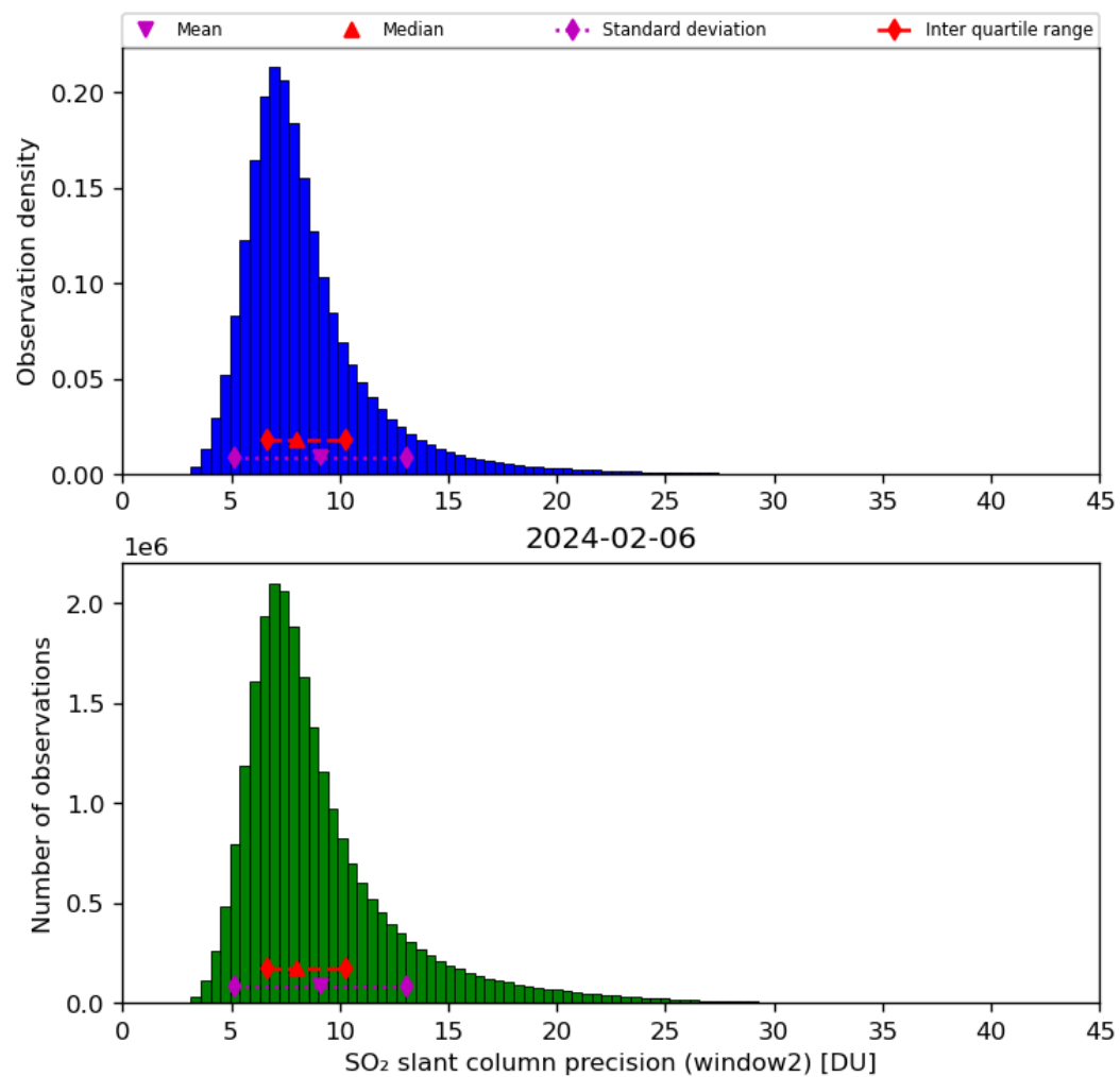
Figure 61: Histogram of “SO 2 slant column precision (window2)” for 2024-02-06 to 2024-02-07
