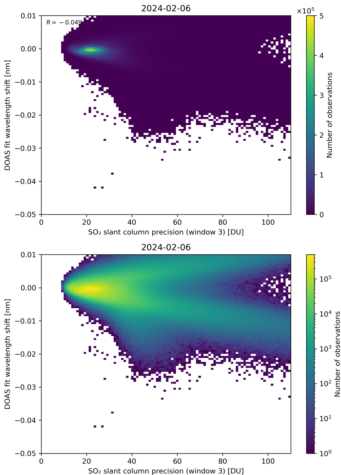
Figure 258: Scatter density plot of “SO 2 slant column precision (window 3)” against “DOAS fit wavelength shift” for 2024-02-06 to 2024-02-07.
