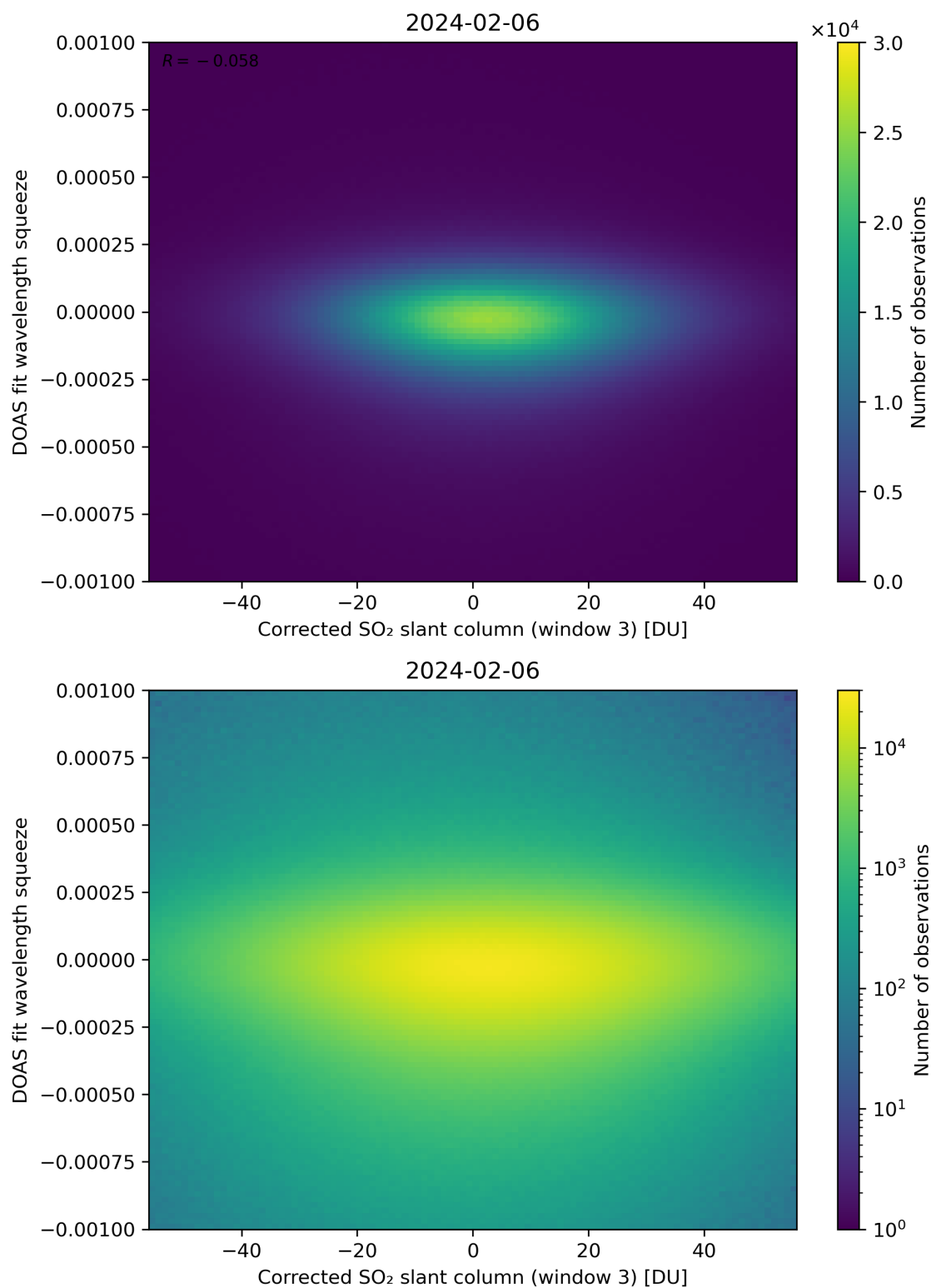
Figure 207: Scatter density plot of “Corrected SO 2 slant column (window 3)” against “DOAS fit wavelength squeeze” for 2024-02-06 to 2024-02-07.
