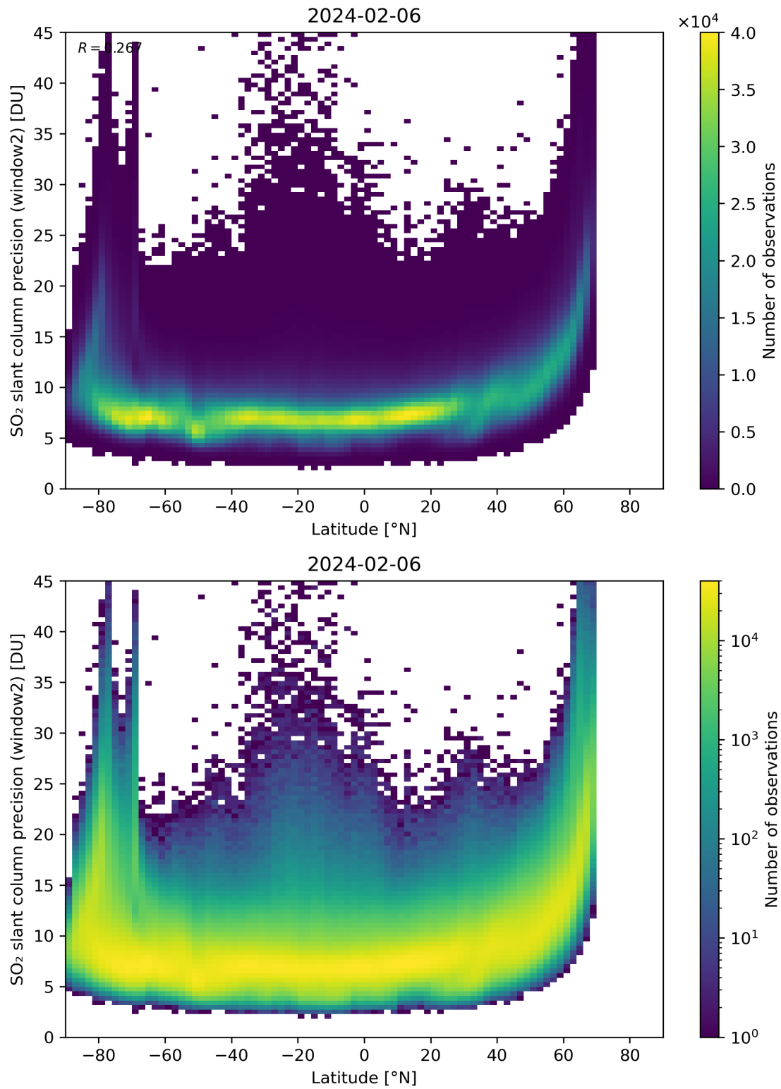
Figure 151: Scatter density plot of “Latitude” against “SO 2 slant column precision (window2)” for 2024-02-06 to 2024-02-07.
