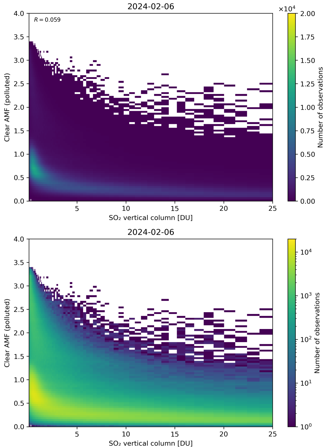
Figure 296: Scatter density plot of “SO 2 vertical column” against “Clear AMF (polluted)” for 2024-02-06 to 2024-02-07.
