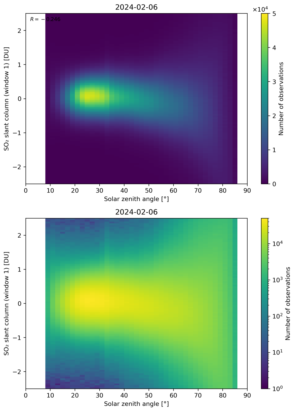
Figure 169: Scatter density plot of “Solar zenith angle” against “SO 2 slant column (window 1)” for 2024-02-06 to 2024-02-07.
