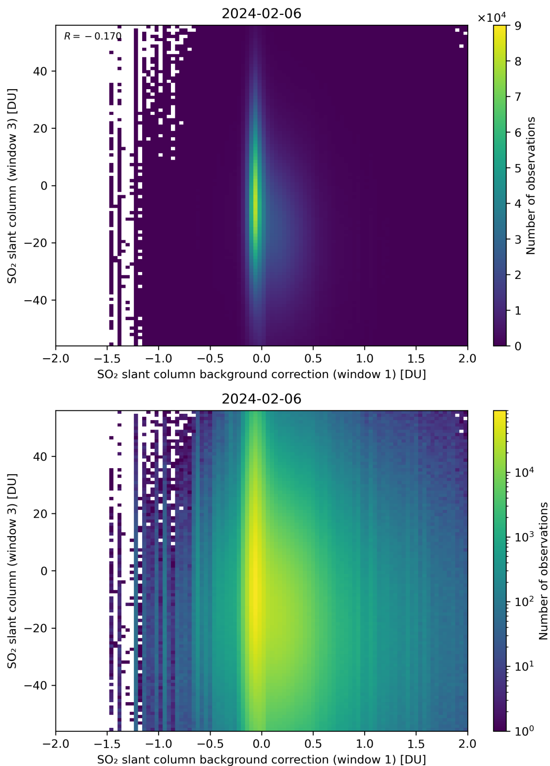
Figure 107: Scatter density plot of “SO 2 slant column background correction (window 1)” against “SO 2 slant column (window 3)” for 2024-02-06 to 2024-02-07.
