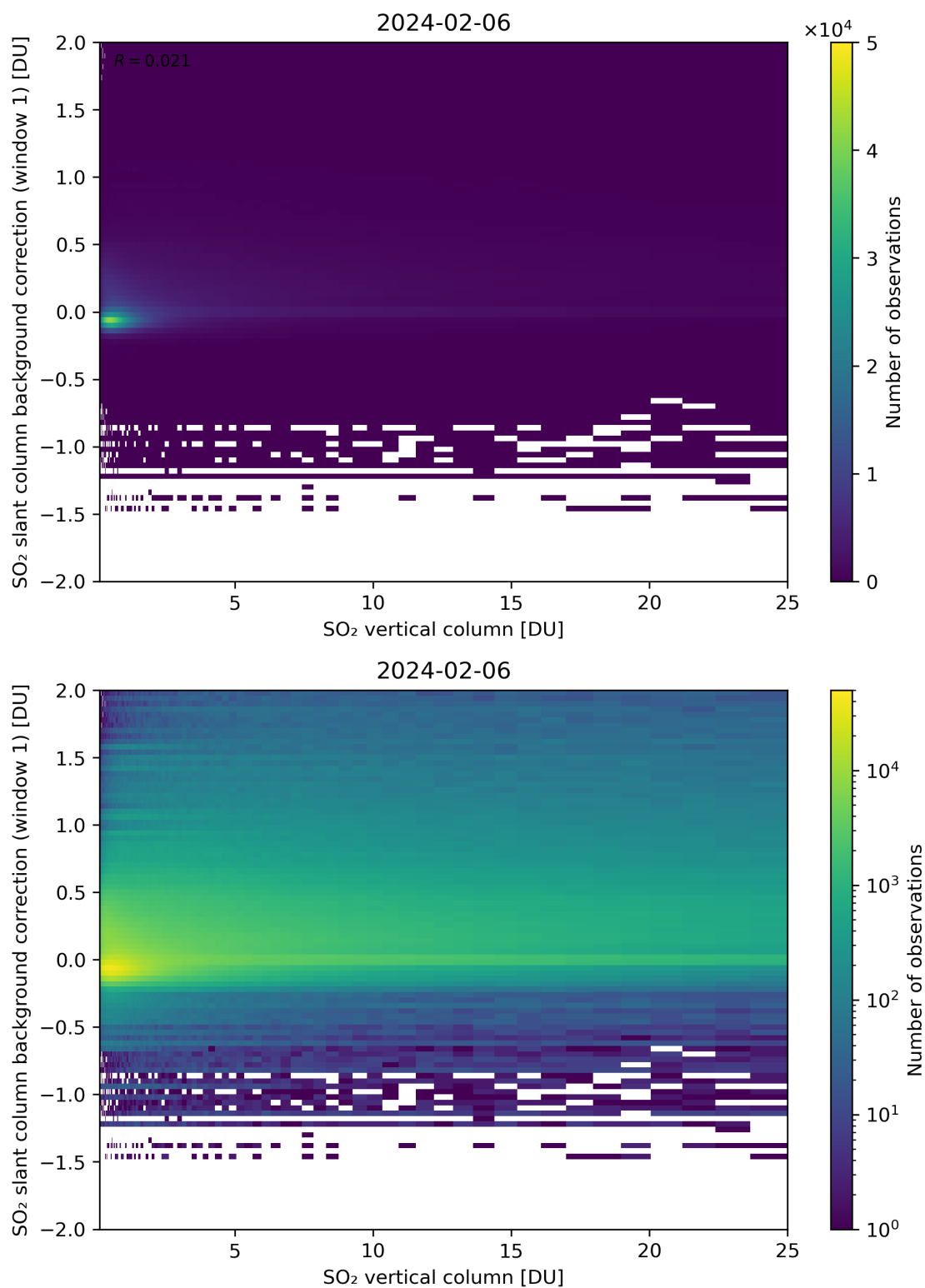
Figure 273: Scatter density plot of “SO 2 vertical column” against “SO 2 slant column background correction (window 1)” for 2024-02-06 to 2024-02-07.
