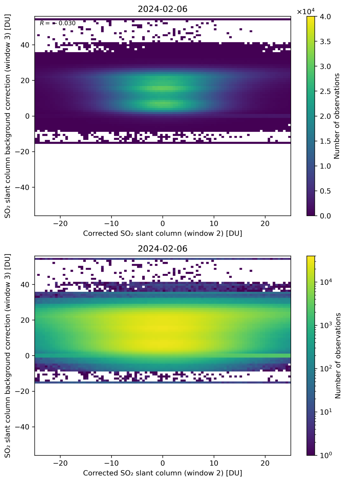
Figure 195: Scatter density plot of “Corrected SO 2 slant column (window 2)” against “SO 2 slant column background correction (window 3)” for 2024-02-06 to 2024-02-07.
