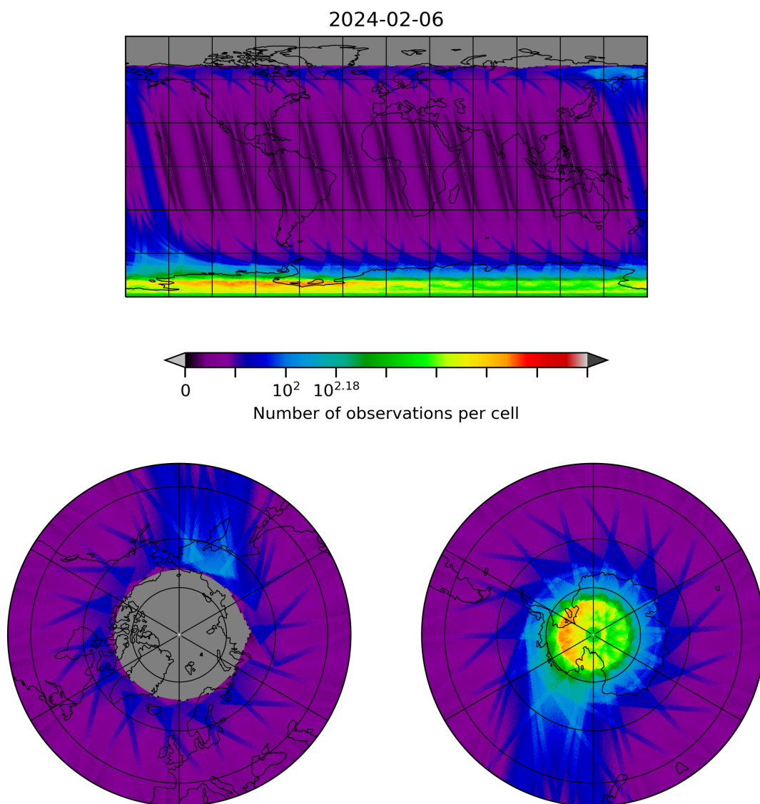
Figure 28: Map of the number of observations for 2024-02-06 to 2024-02-07
