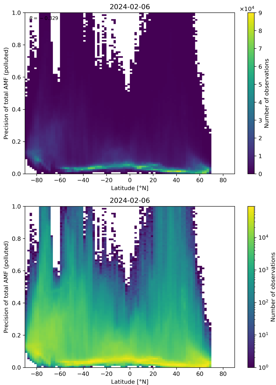
Figure 155: Scatter density plot of “Latitude” against “Precision of total AMF (polluted)” for 2024-02-06 to 2024-02-07.
