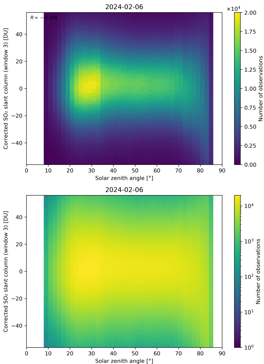
Figure 168: Scatter density plot of “Solar zenith angle” against “Corrected SO 2 slant column (window 3)” for 2024-02-06 to 2024-02-07.
