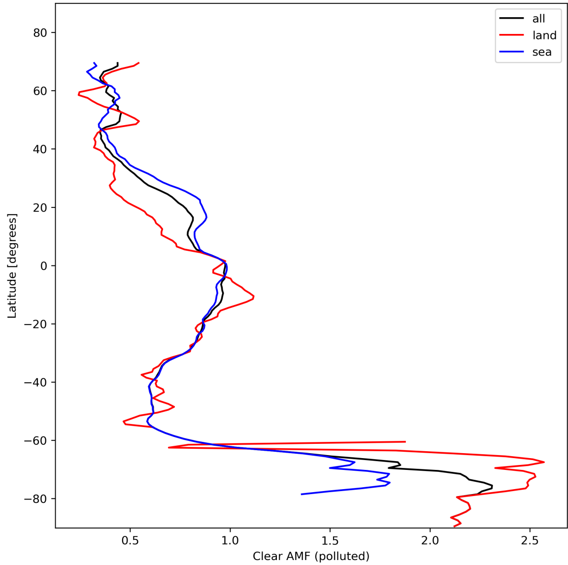
Figure 50: Zonal average of “Clear AMF (polluted)” for 2024-02-06 to 2024-02-07.
