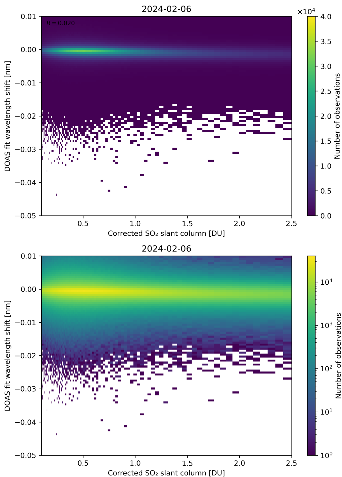
Figure 181: Scatter density plot of “Corrected SO 2 slant column” against “DOAS fit wavelength shift” for 2024-02-06 to 2024-02-07.
