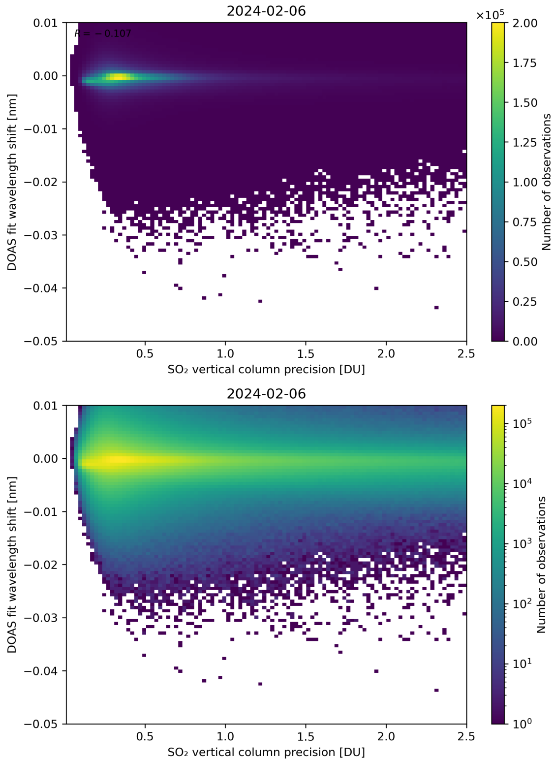
Figure 282: Scatter density plot of “SO 2 vertical column precision” against “DOAS fit wavelength shift” for 2024-02-06 to 2024-02-07.
