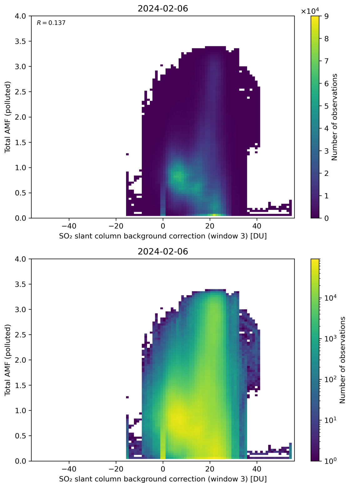
Figure 125: Scatter density plot of “SO 2 slant column background correction (window 3)” against “Total AMF (polluted)” for 2024-02-06 to 2024-02-07.
