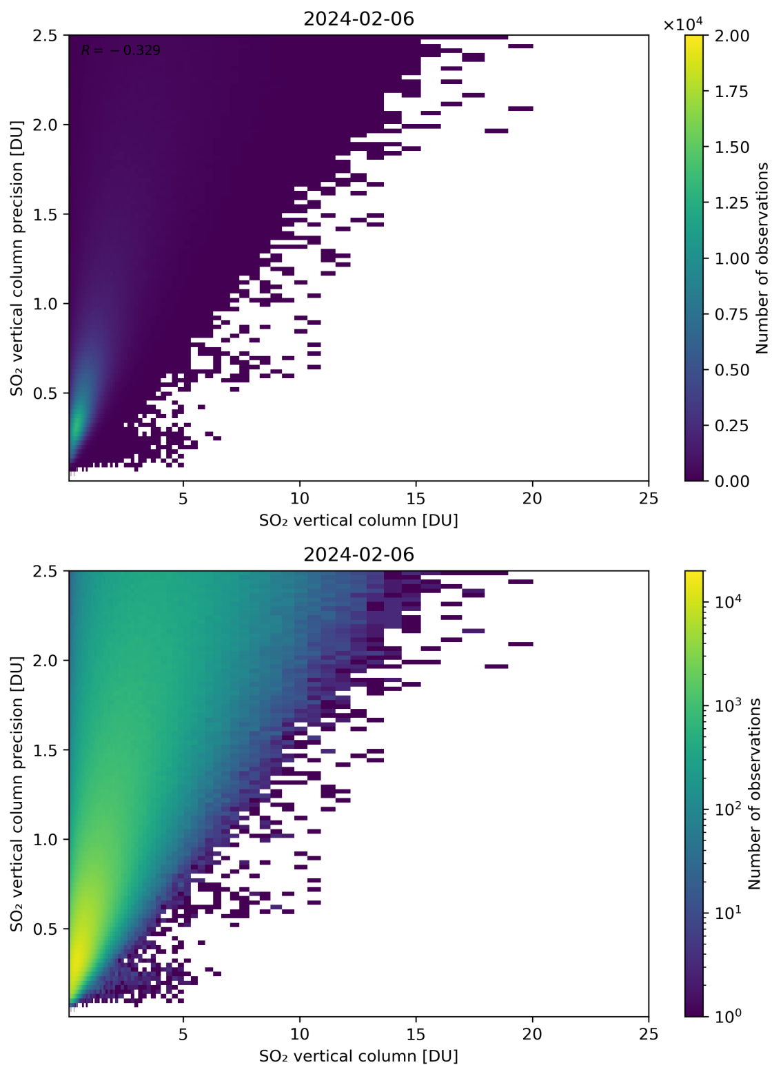
Figure 307: Scatter density plot of “SO 2 vertical column” against “SO 2 vertical column precision” for 2024-02-06 to 2024-02-07.
