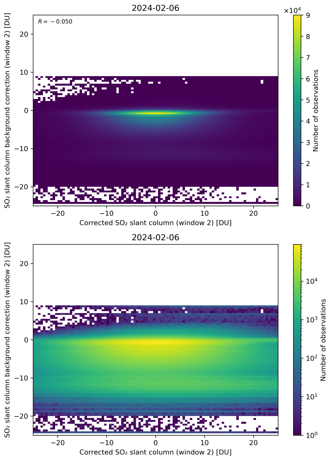
Figure 194: Scatter density plot of “Corrected SO 2 slant column (window 2)” against “SO 2 slant column background correction (window 2)” for 2024-02-06 to 2024-02-07.
