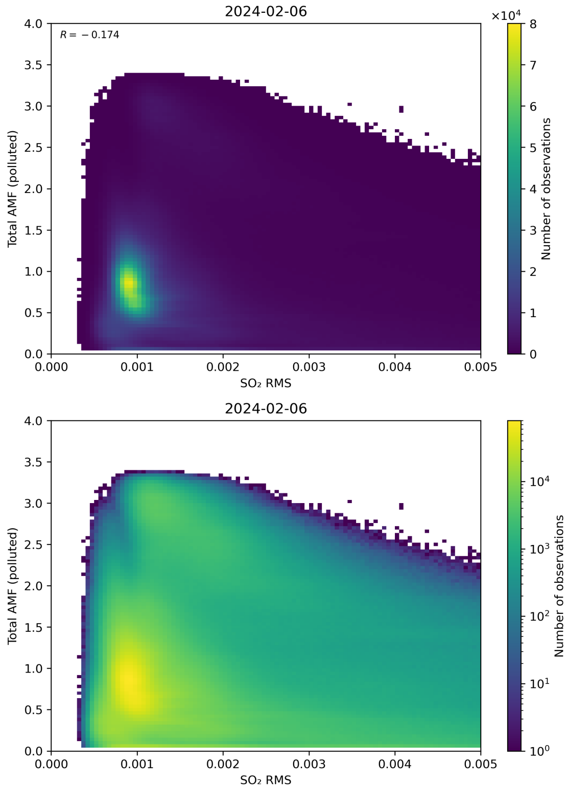
Figure 137: Scatter density plot of “SO 2 RMS” against “Total AMF (polluted)” for 2024-02-06 to 2024-02-07.
