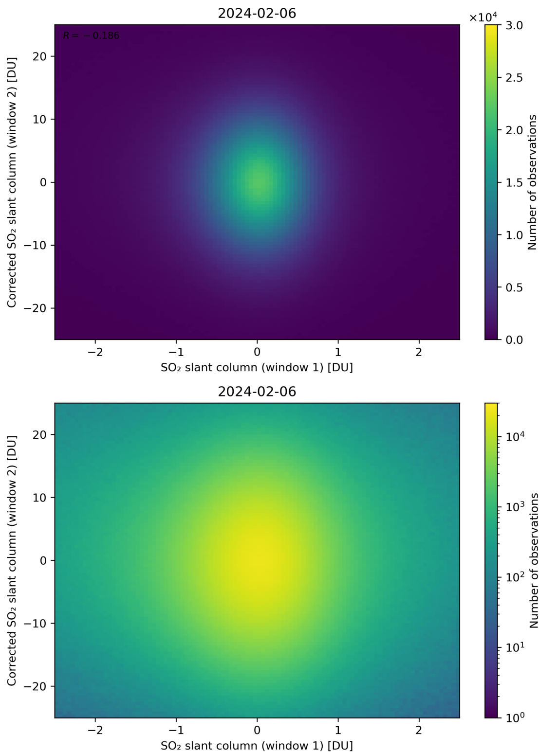
Figure 233: Scatter density plot of “SO 2 slant column (window 1)” against “Corrected SO 2 slant column (window 2)” for 2024-02-06 to 2024-02-07.
