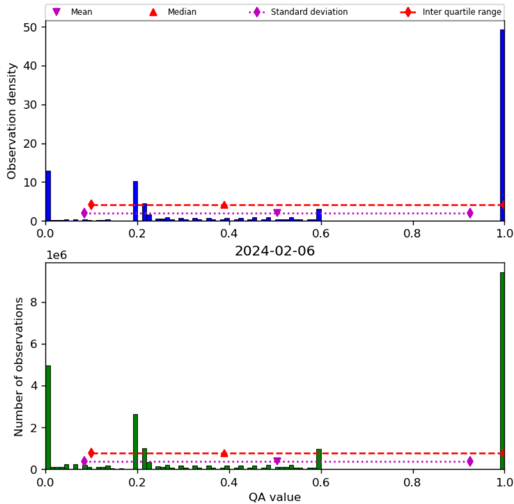
Figure 52: Histogram of “QA value” for 2024-02-06 to 2024-02-07
