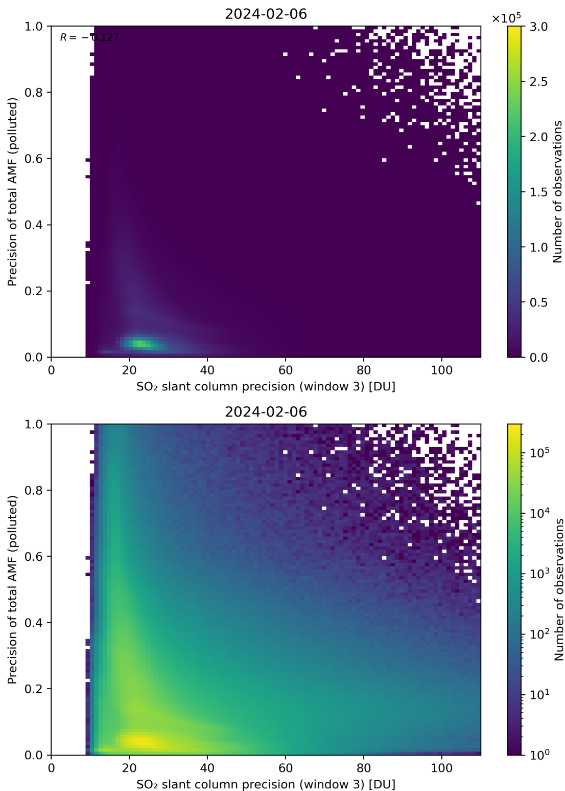
Figure 264: Scatter density plot of “SO 2 slant column precision (window 3)” against “Precision of total AMF (polluted)” for 2024-02-06 to 2024-02-07.
