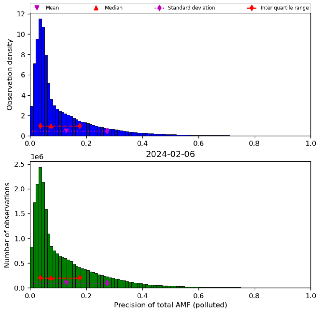
Figure 72: Histogram of “Precision of total AMF (polluted)” for 2024-02-06 to 2024-02-07
