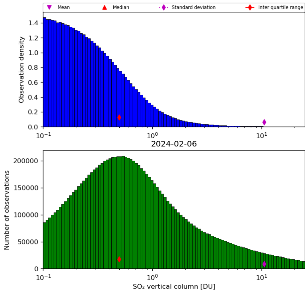
Figure 53: Histogram of “SO 2 vertical column” for 2024-02-06 to 2024-02-07
