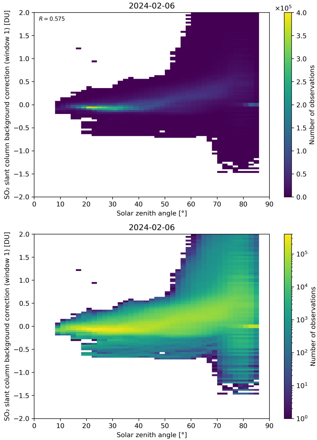
Figure 158: Scatter density plot of “Solar zenith angle” against “SO 2 slant column background correction (window 1)” for 2024-02-06 to 2024-02-07.
