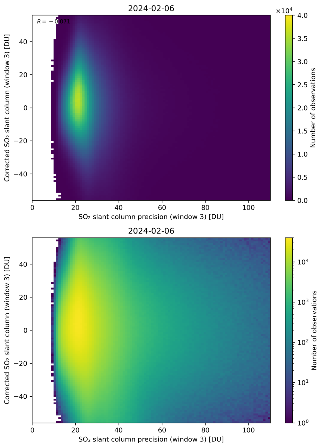
Figure 262: Scatter density plot of “SO 2 slant column precision (window 3)” against “Corrected SO 2 slant column (window 3)” for 2024-02-06 to 2024-02-07.
