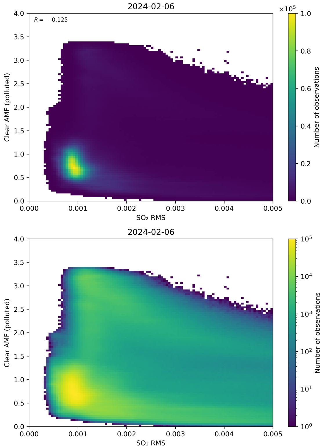
Figure 136: Scatter density plot of “SO 2 RMS” against “Clear AMF (polluted)” for 2024-02-06 to 2024-02-07.
