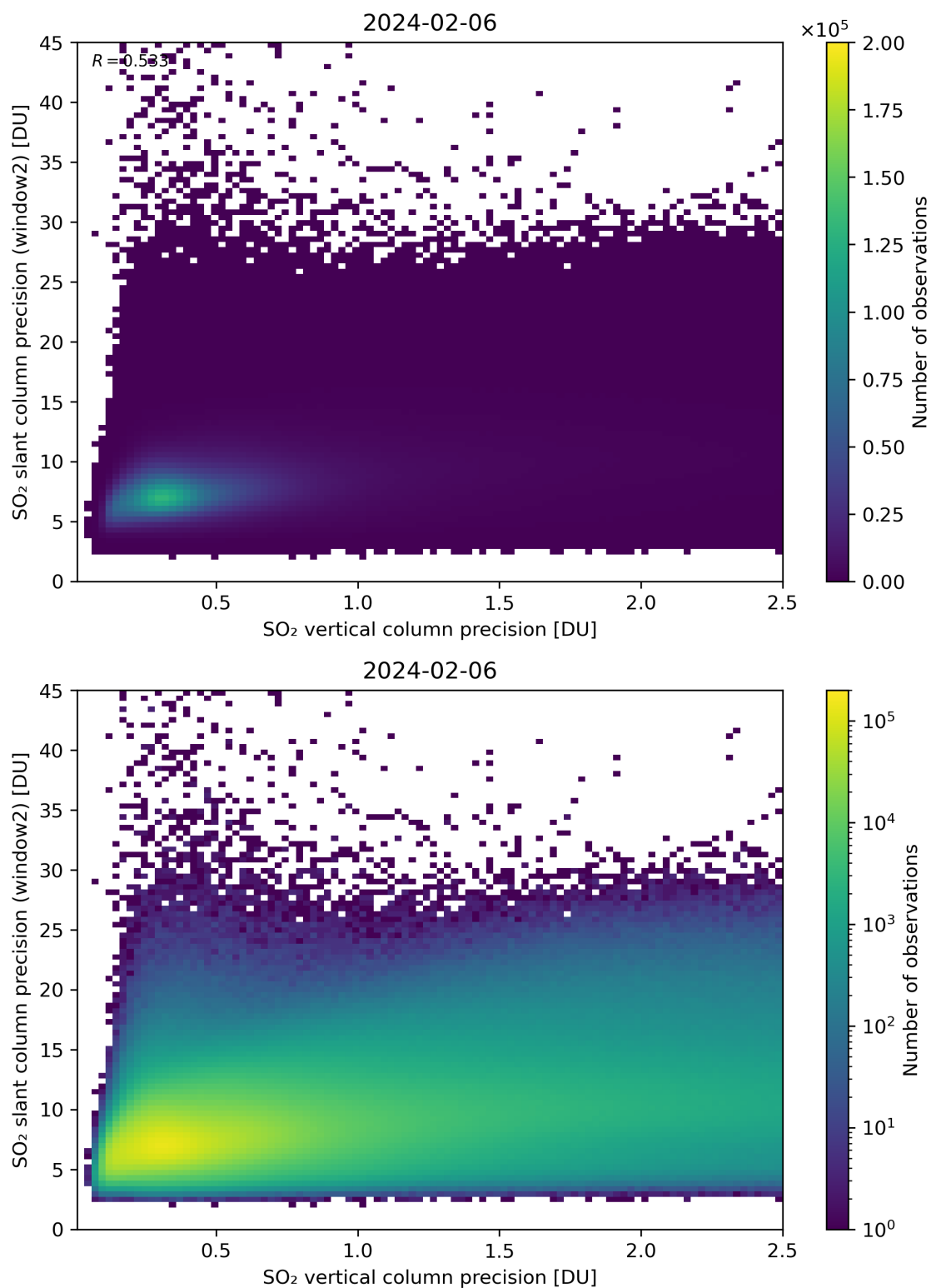
Figure 291: Scatter density plot of “SO 2 vertical column precision” against “SO 2 slant column precision (window2)” for 2024-02-06 to 2024-02-07.
