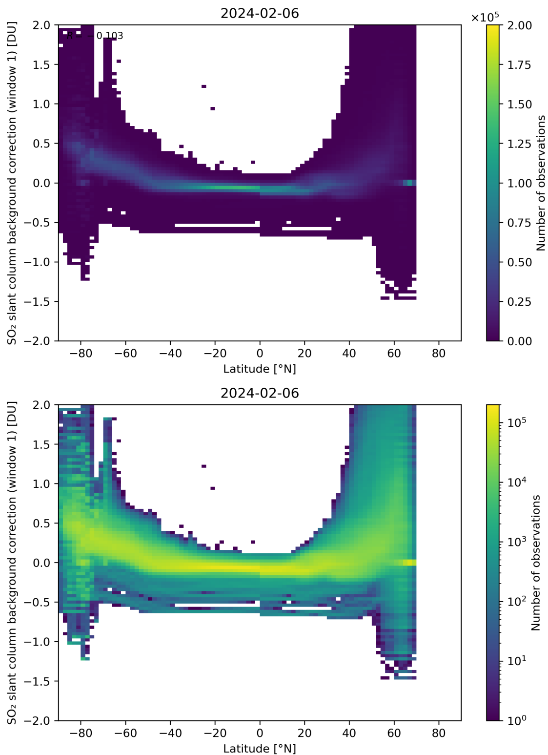
Figure 139: Scatter density plot of “Latitude” against “SO 2 slant column background correction (window 1)” for 2024-02-06 to 2024-02-07.
