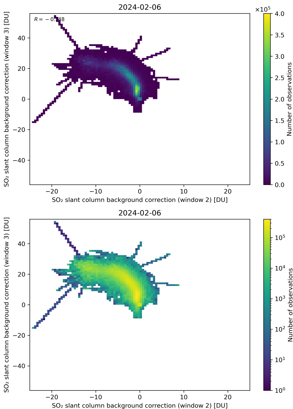
Figure 111: Scatter density plot of “SO 2 slant column background correction (window 2)” against “SO 2 slant column background correction (window 3)” for 2024-02-06 to 2024-02-07.
