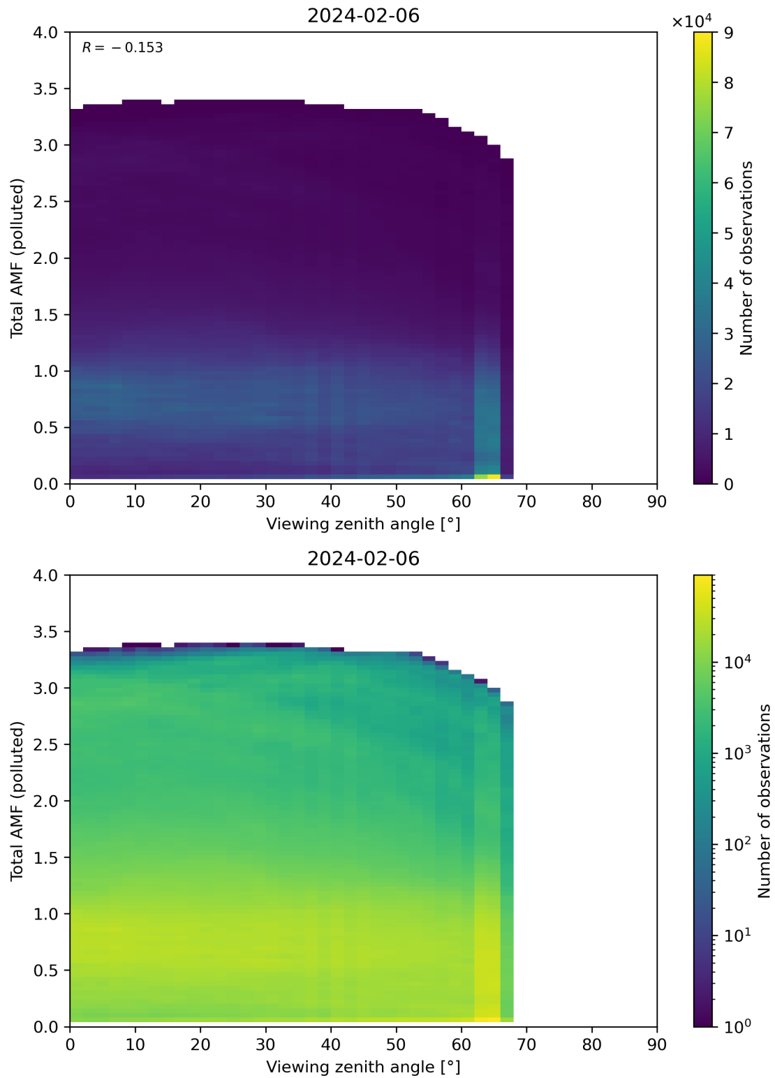
Figure 325: Scatter density plot of “Viewing zenith angle” against “Total AMF (polluted)” for 2024-02-06 to 2024-02-07.
