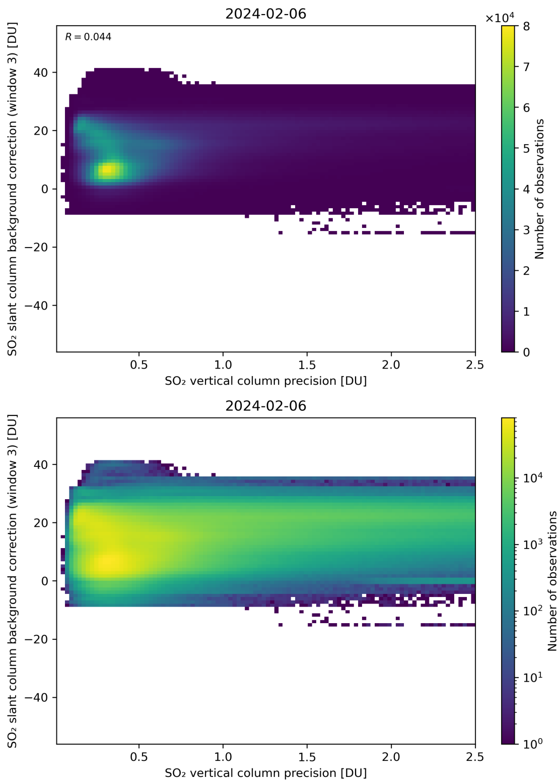
Figure 281: Scatter density plot of “SO 2 vertical column precision” against “SO 2 slant column background correction (window 3)” for 2024-02-06 to 2024-02-07.
