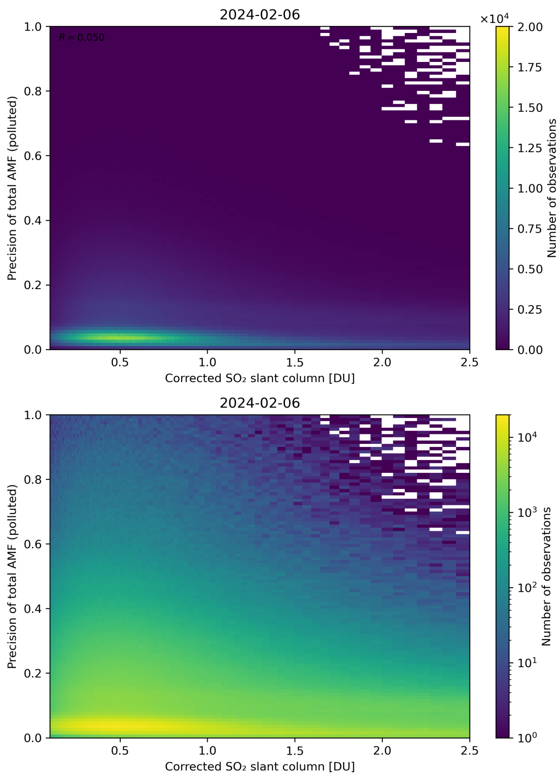
Figure 193: Scatter density plot of “Corrected SO 2 slant column” against “Precision of total AMF (polluted)” for 2024-02-06 to 2024-02-07.
