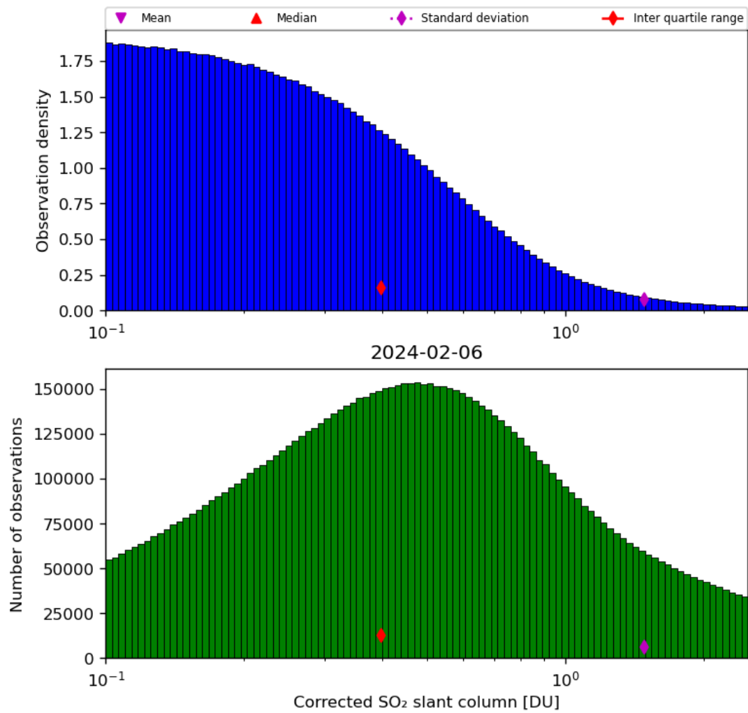
Figure 55: Histogram of “Corrected SO 2 slant column” for 2024-02-06 to 2024-02-07
