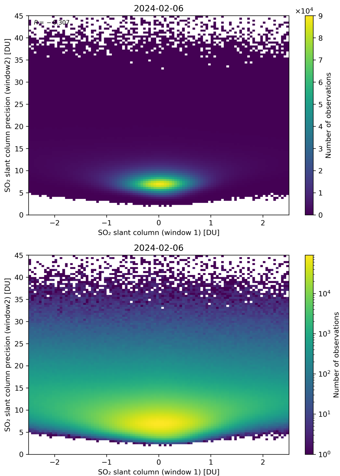
Figure 236: Scatter density plot of “SO 2 slant column (window 1)” against “SO 2 slant column precision (window2)” for 2024-02-06 to 2024-02-07.
