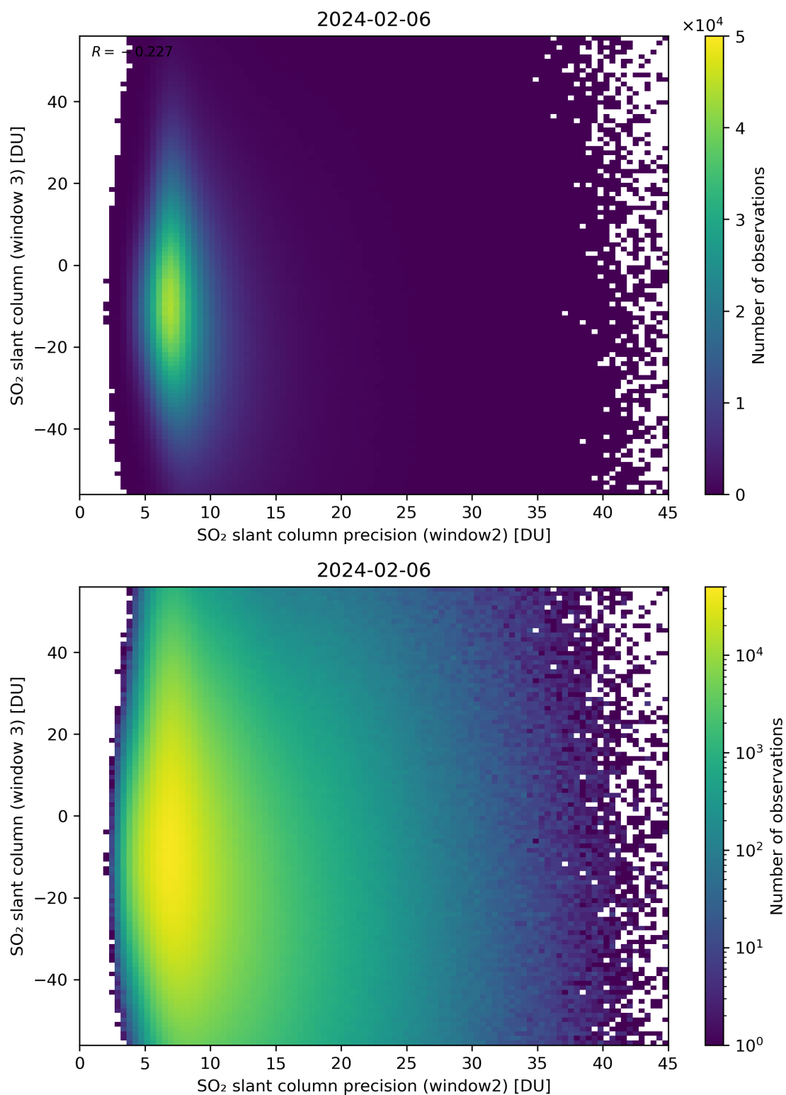
Figure 249: Scatter density plot of “SO 2 slant column precision (window2)” against “SO 2 slant column (window 3)” for 2024-02-06 to 2024-02-07.
