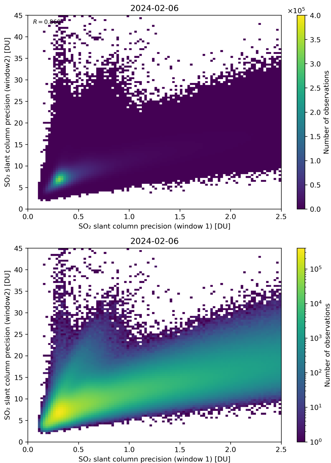
Figure 227: Scatter density plot of “SO 2 slant column precision (window 1)” against “SO 2 slant column precision (window2)” for 2024-02-06 to 2024-02-07.
