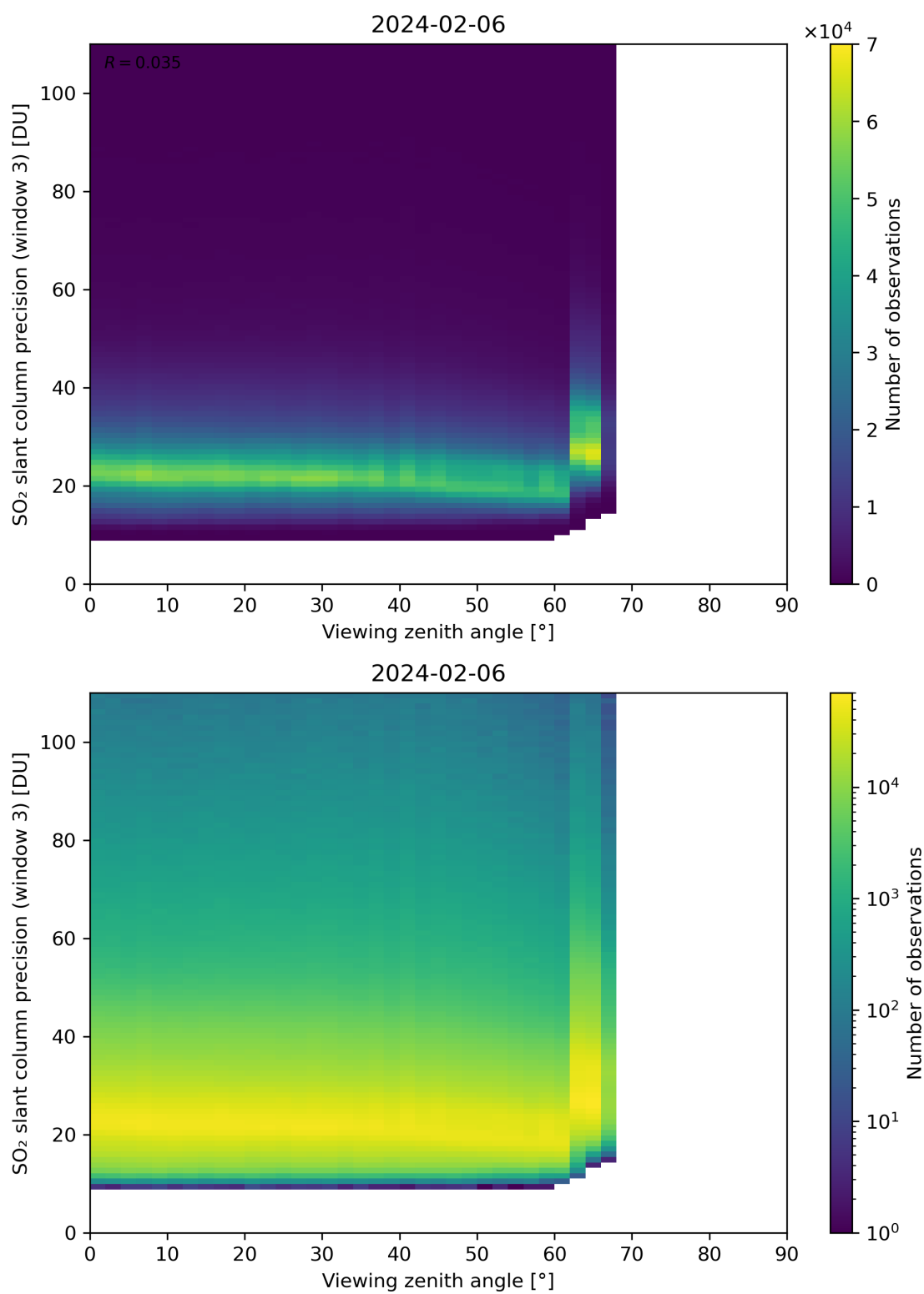
Figure 324: Scatter density plot of “Viewing zenith angle” against “SO 2 slant column precision (window 3)” for 2024-02-06 to 2024-02-07.
