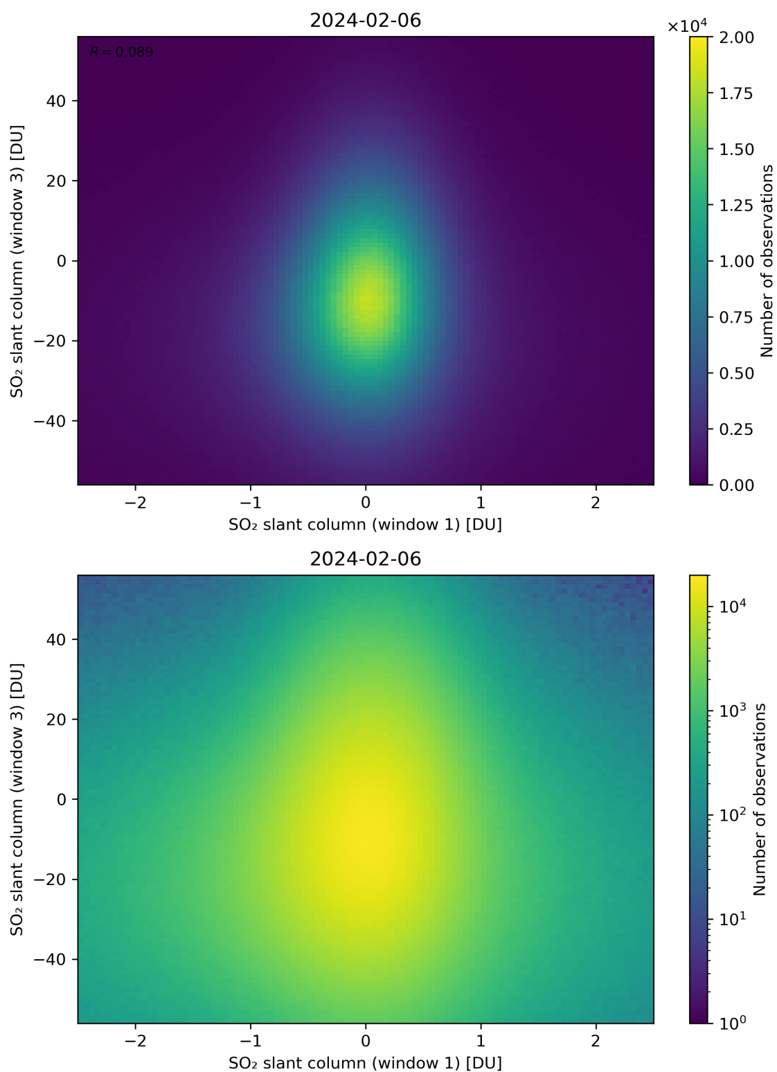
Figure 237: Scatter density plot of “SO 2 slant column (window 1)” against “SO 2 slant column (window 3)” for 2024-02-06 to 2024-02-07.
