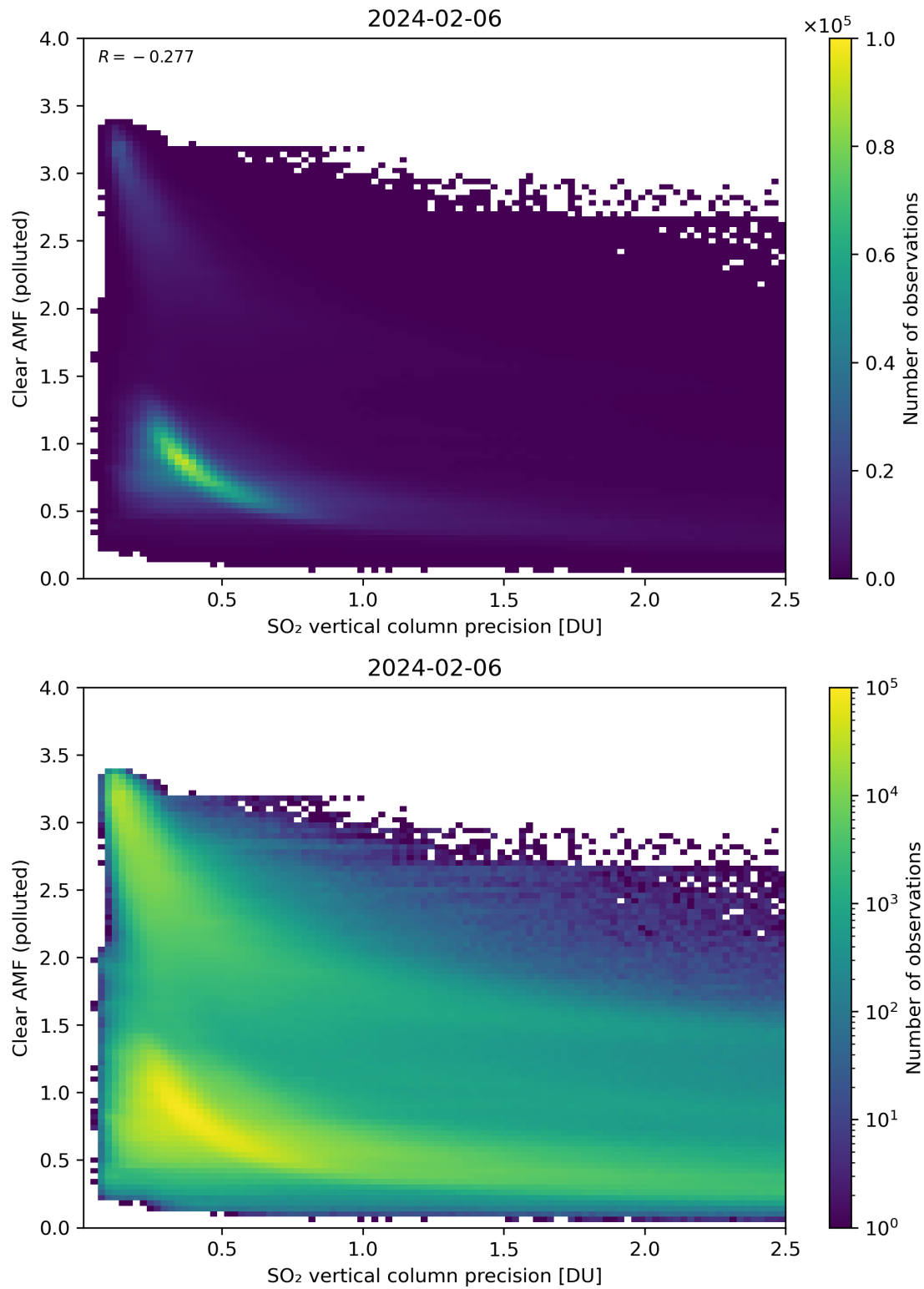
Figure 285: Scatter density plot of “SO 2 vertical column precision” against “Clear AMF (polluted)” for 2024-02-06 to 2024-02-07.
