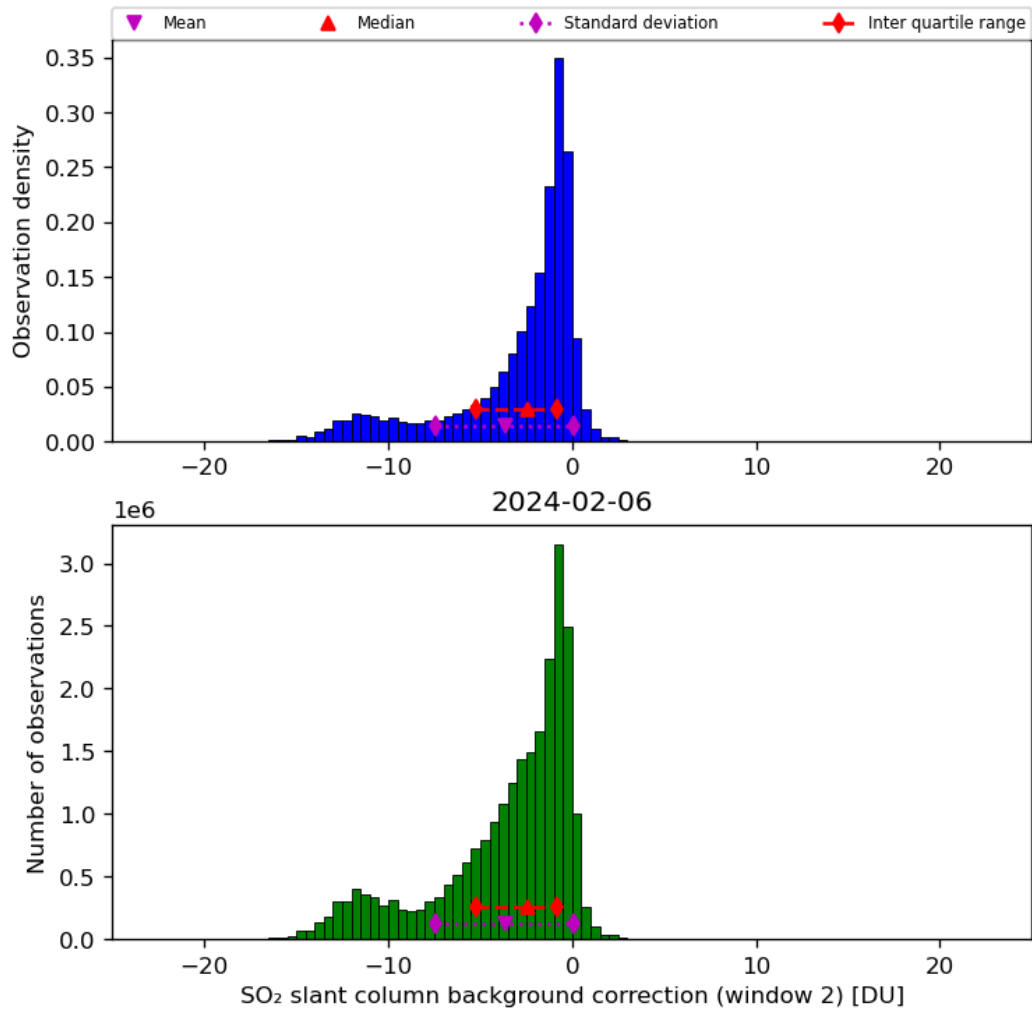
Figure 63: Histogram of “SO 2 slant column background correction (window 2)” for 2024-02-06 to 2024-02-07
