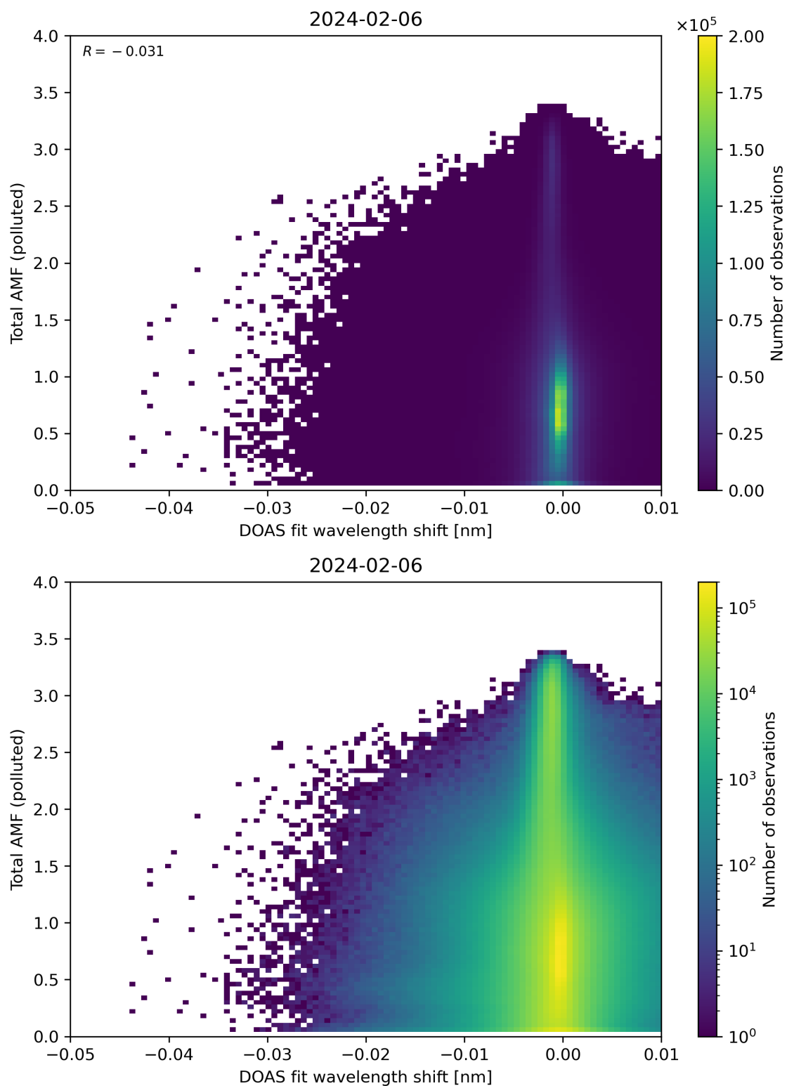
Figure 130: Scatter density plot of “DOAS fit wavelength shift” against “Total AMF (polluted)” for 2024-02-06 to 2024-02-07.
