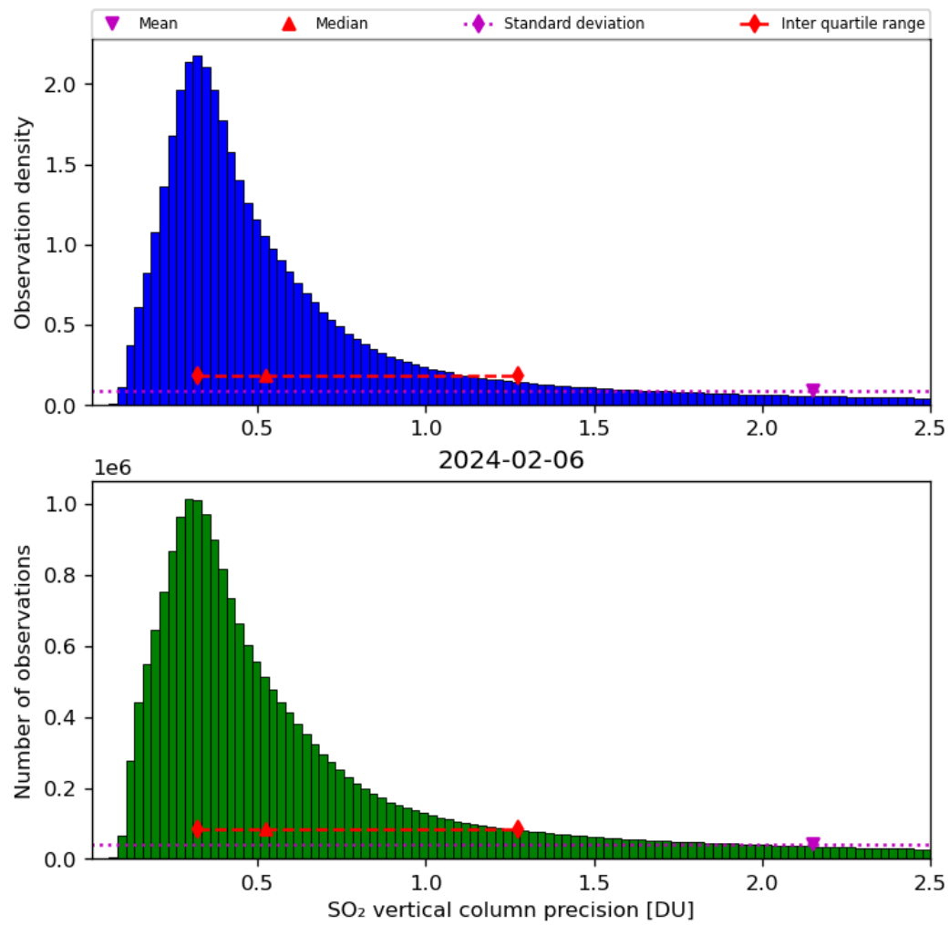
Figure 54: Histogram of “SO 2 vertical column precision” for 2024-02-06 to 2024-02-07
