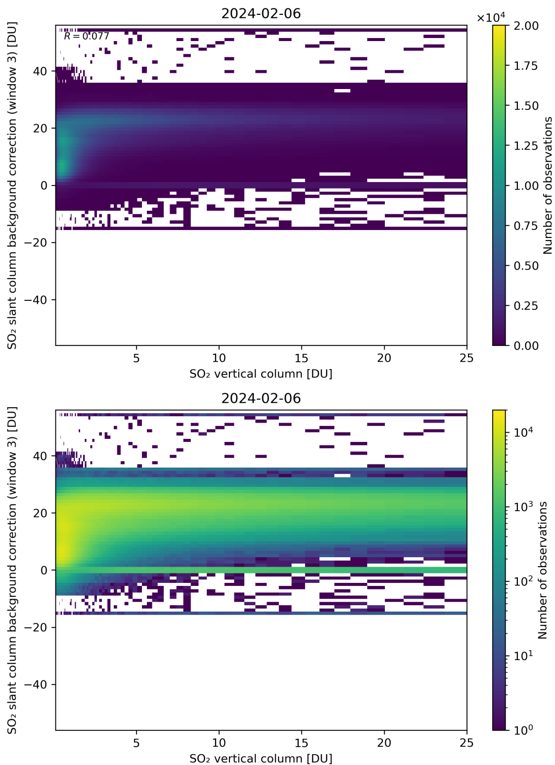
Figure 275: Scatter density plot of “SO 2 vertical column” against “SO 2 slant column background correction (window 3)” for 2024-02-06 to 2024-02-07.
