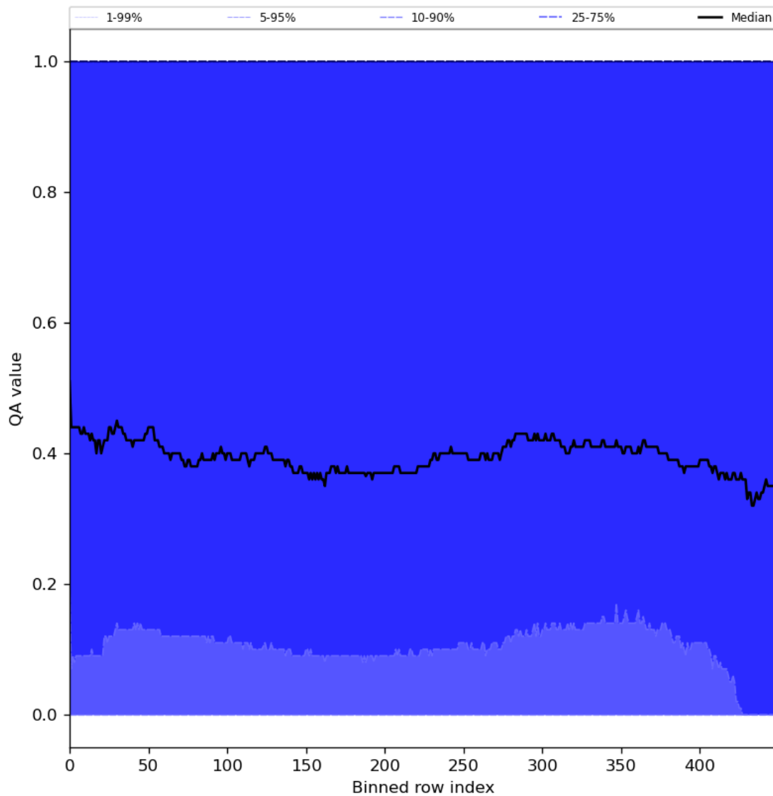
Figure 75: Along track statistics of “QA value” for 2024-02-06 to 2024-02-07
