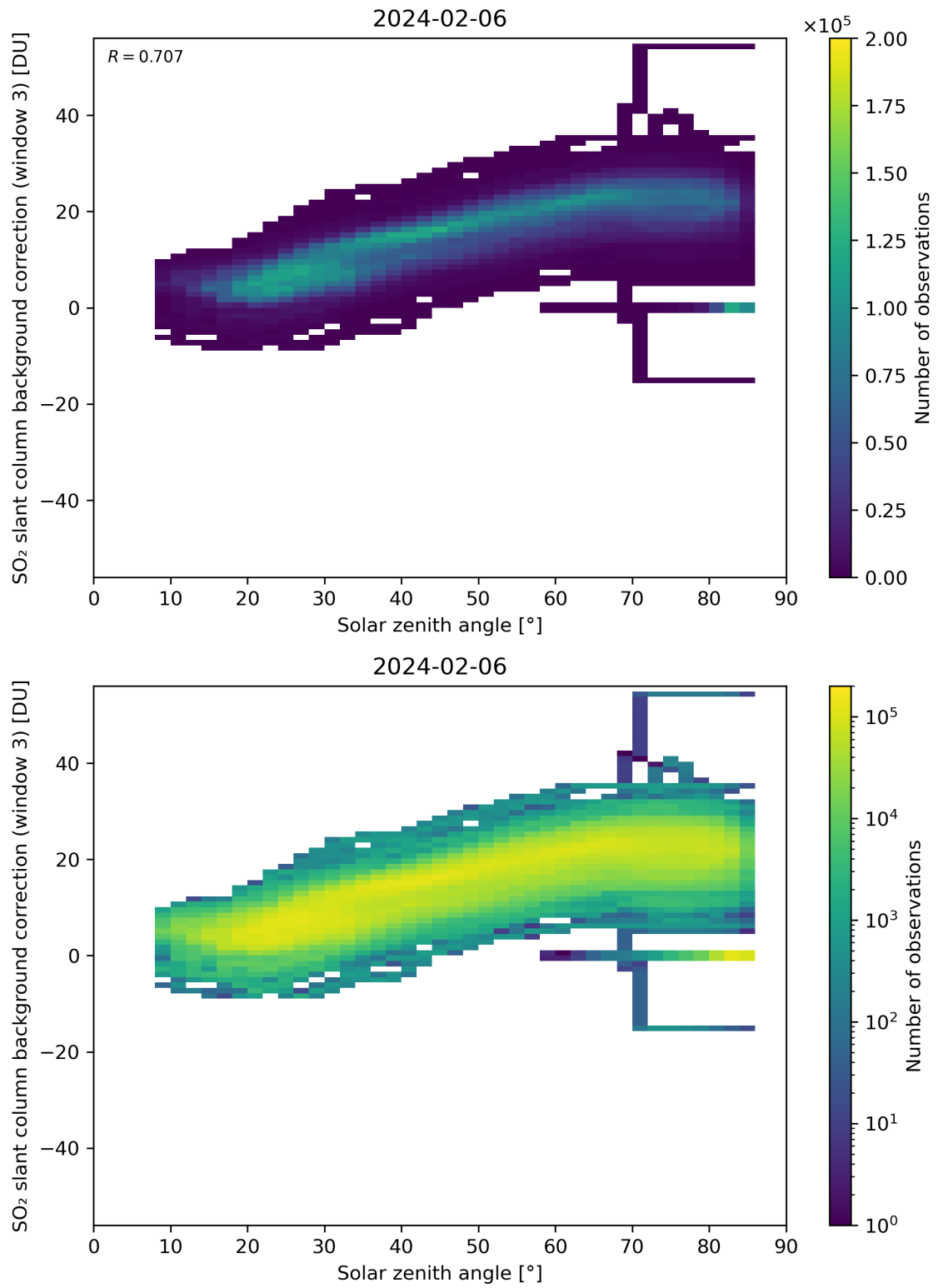
Figure 160: Scatter density plot of “Solar zenith angle” against “SO 2 slant column background correction (window 3)” for 2024-02-06 to 2024-02-07.
