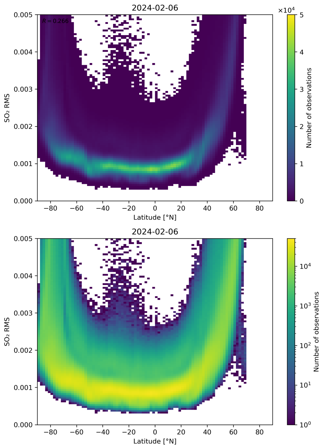
Figure 144: Scatter density plot of “Latitude” against “SO 2 RMS” for 2024-02-06 to 2024-02-07.
