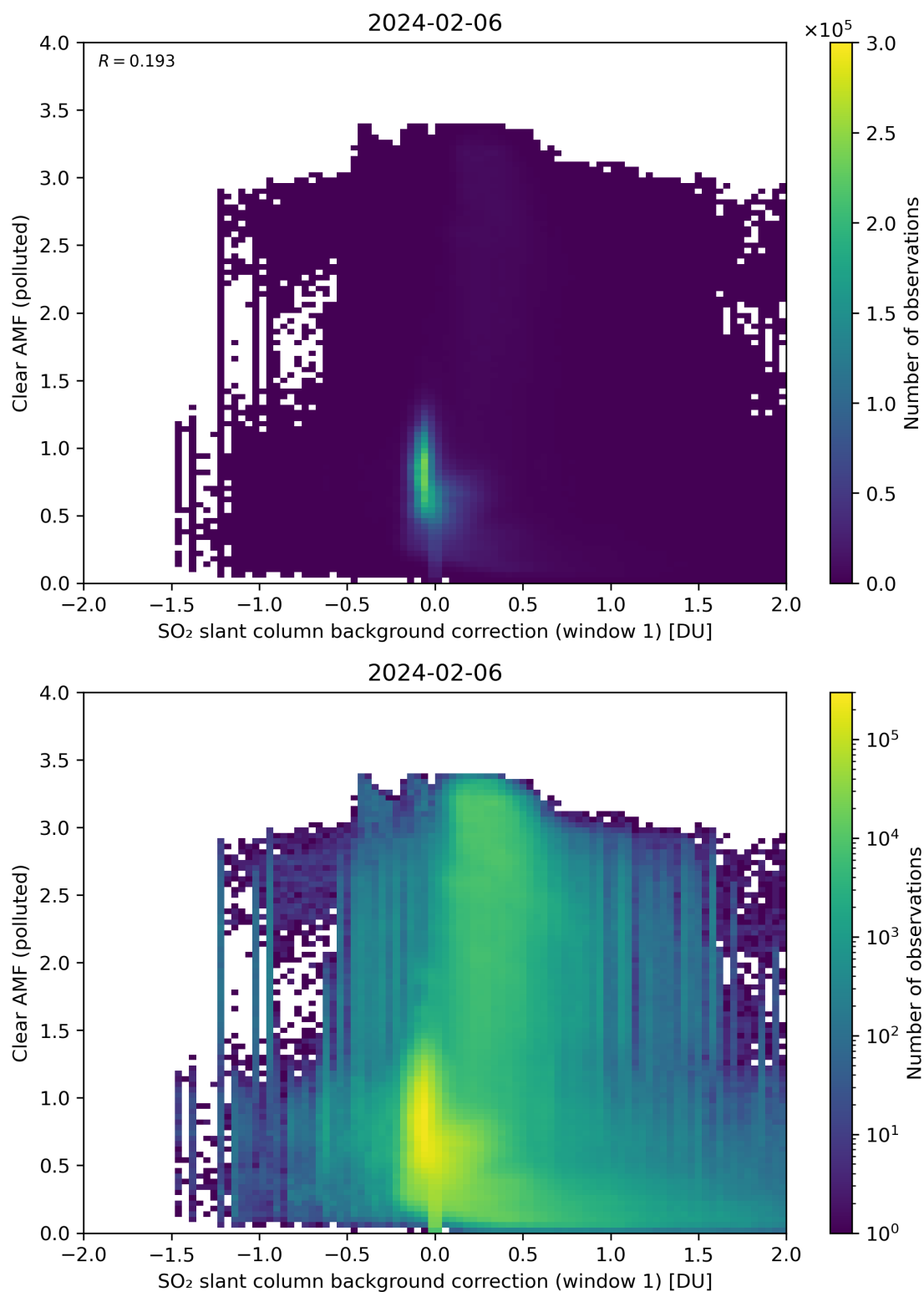
Figure 103: Scatter density plot of “SO 2 slant column background correction (window 1)” against “Clear AMF (polluted)” for 2024-02-06 to 2024-02-07.
