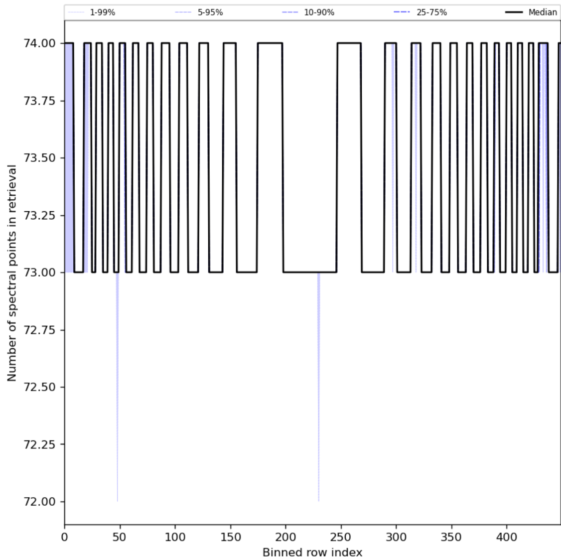
Figure 97: Along track statistics of “Number of spectral points in retrieval” for 2024-02-06 to 2024-02-07
