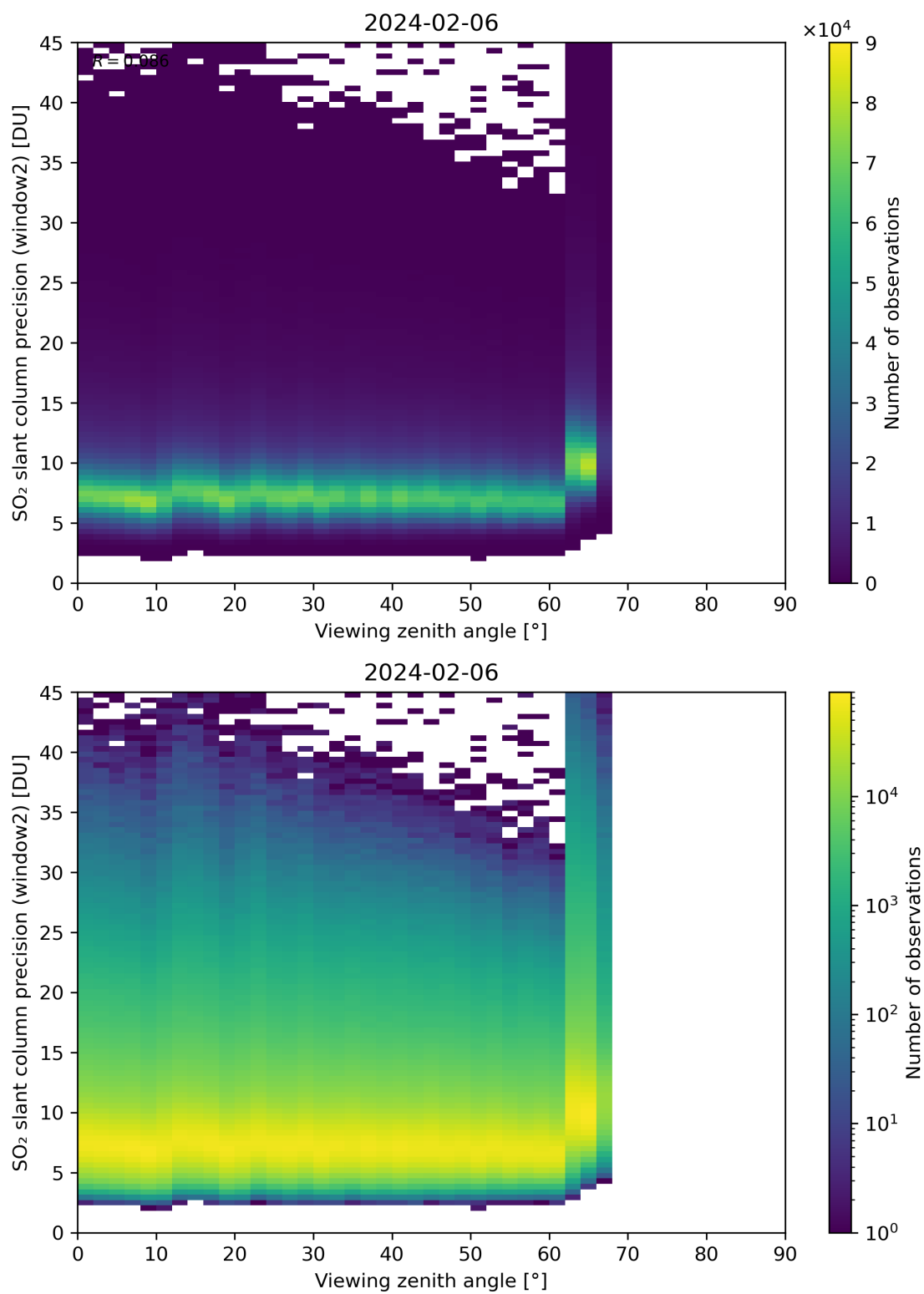
Figure 322: Scatter density plot of “Viewing zenith angle” against “SO 2 slant column precision (window2)” for 2024-02-06 to 2024-02-07.
