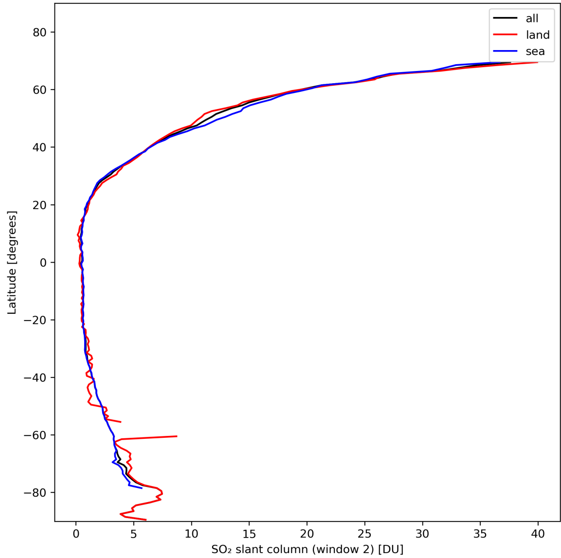
Figure 37: Zonal average of “SO 2 slant column (window 2)” for 2024-02-06 to 2024-02-07.
