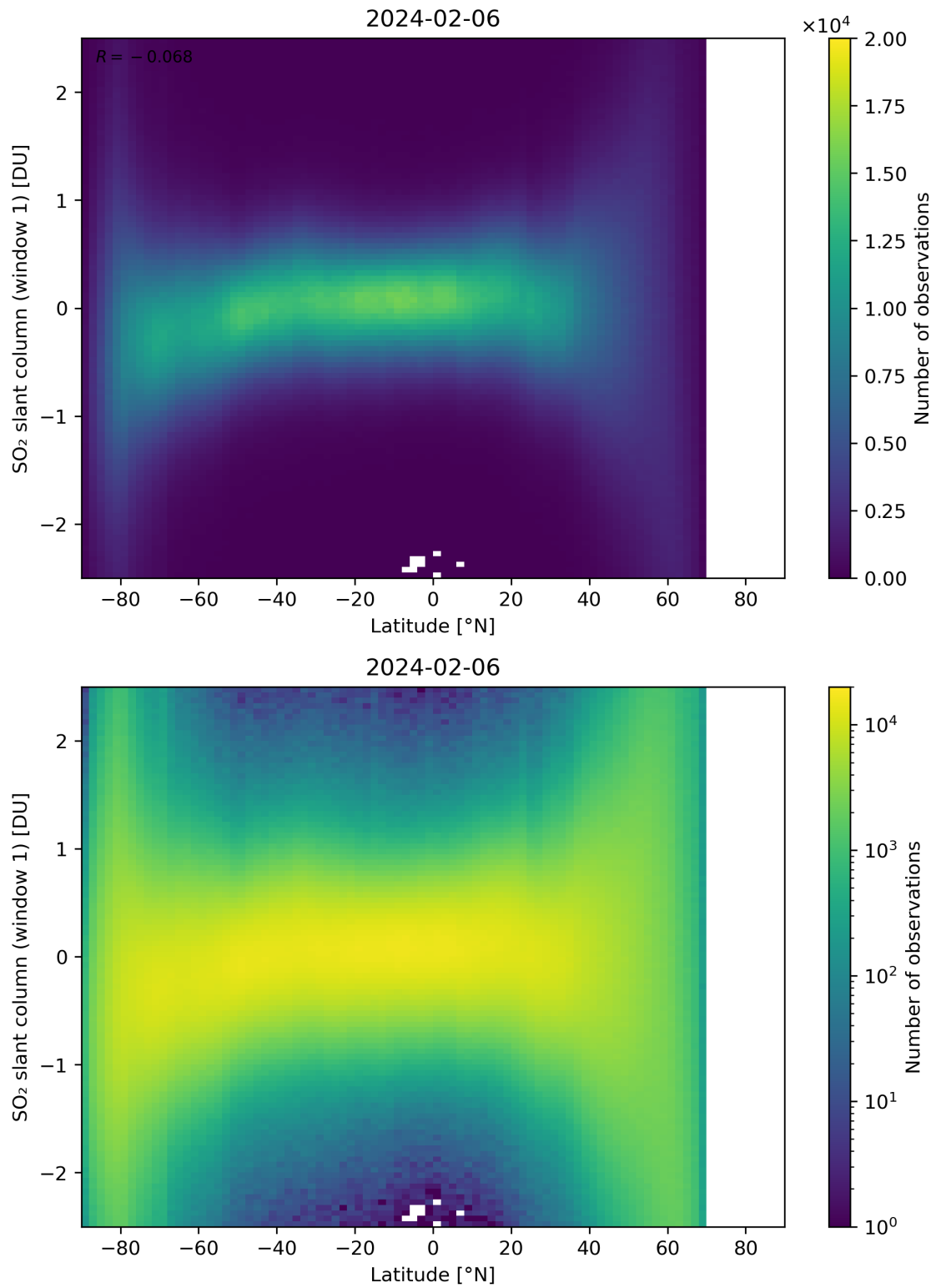
Figure 149: Scatter density plot of “Latitude” against “SO 2 slant column (window 1)” for 2024-02-06 to 2024-02-07.
