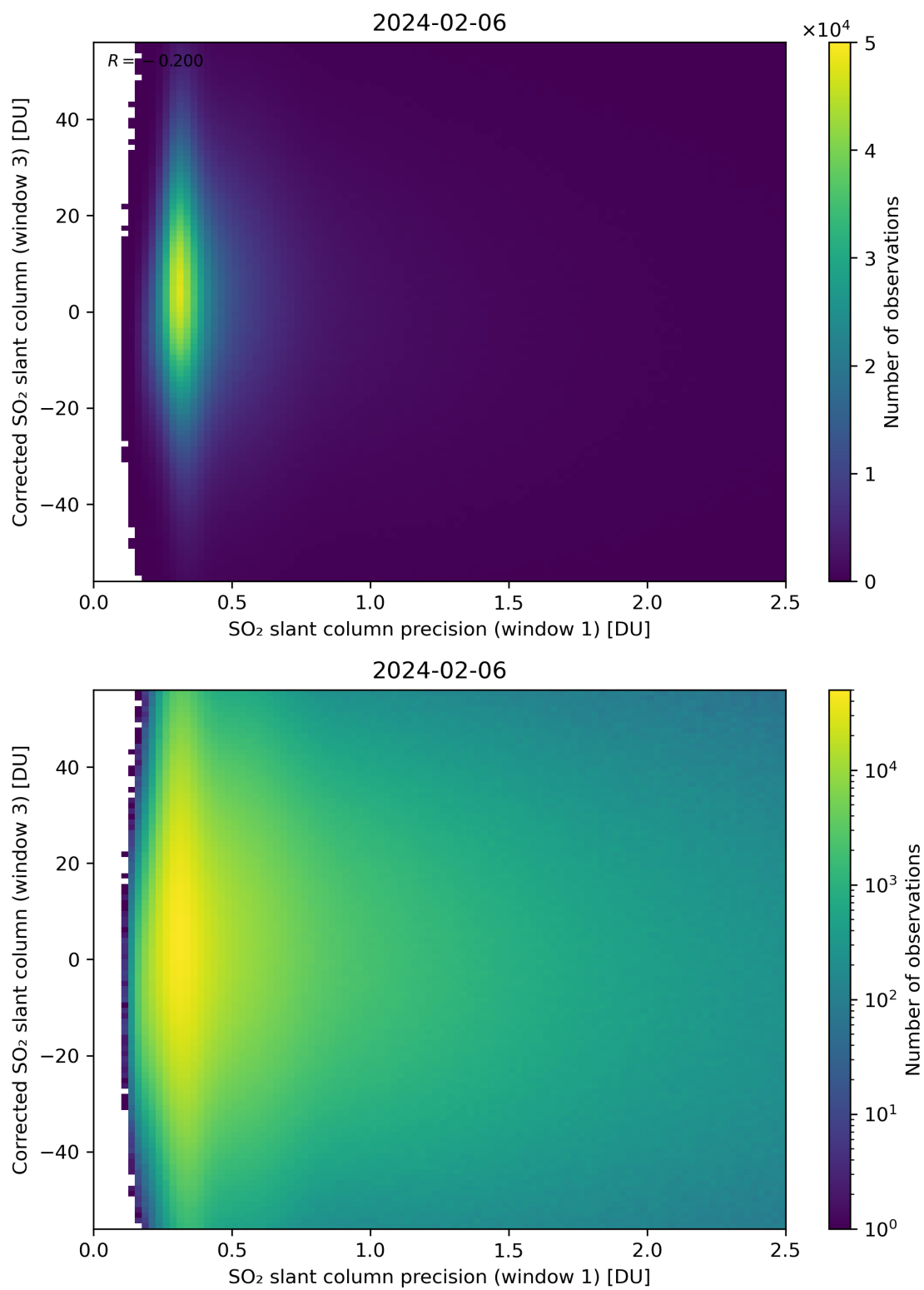
Figure 226: Scatter density plot of “SO 2 slant column precision (window 1)” against “Corrected SO 2 slant column (window 3)” for 2024-02-06 to 2024-02-07.
