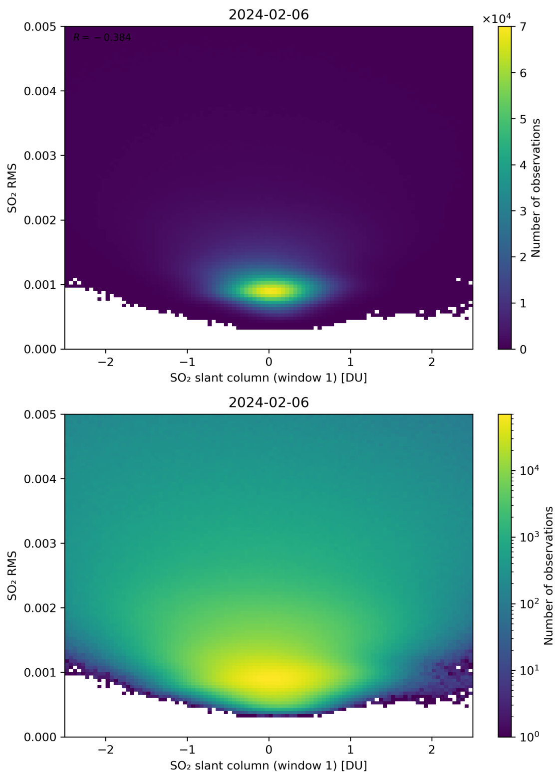
Figure 217: Scatter density plot of “SO 2 slant column (window 1)” against “SO 2 RMS” for 2024-02-06 to 2024-02-07.
