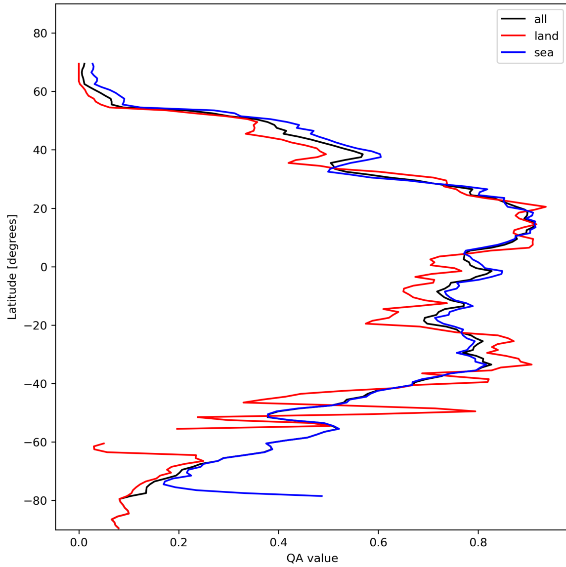
Figure 29: Zonal average of “QA value” for 2024-02-06 to 2024-02-07.
