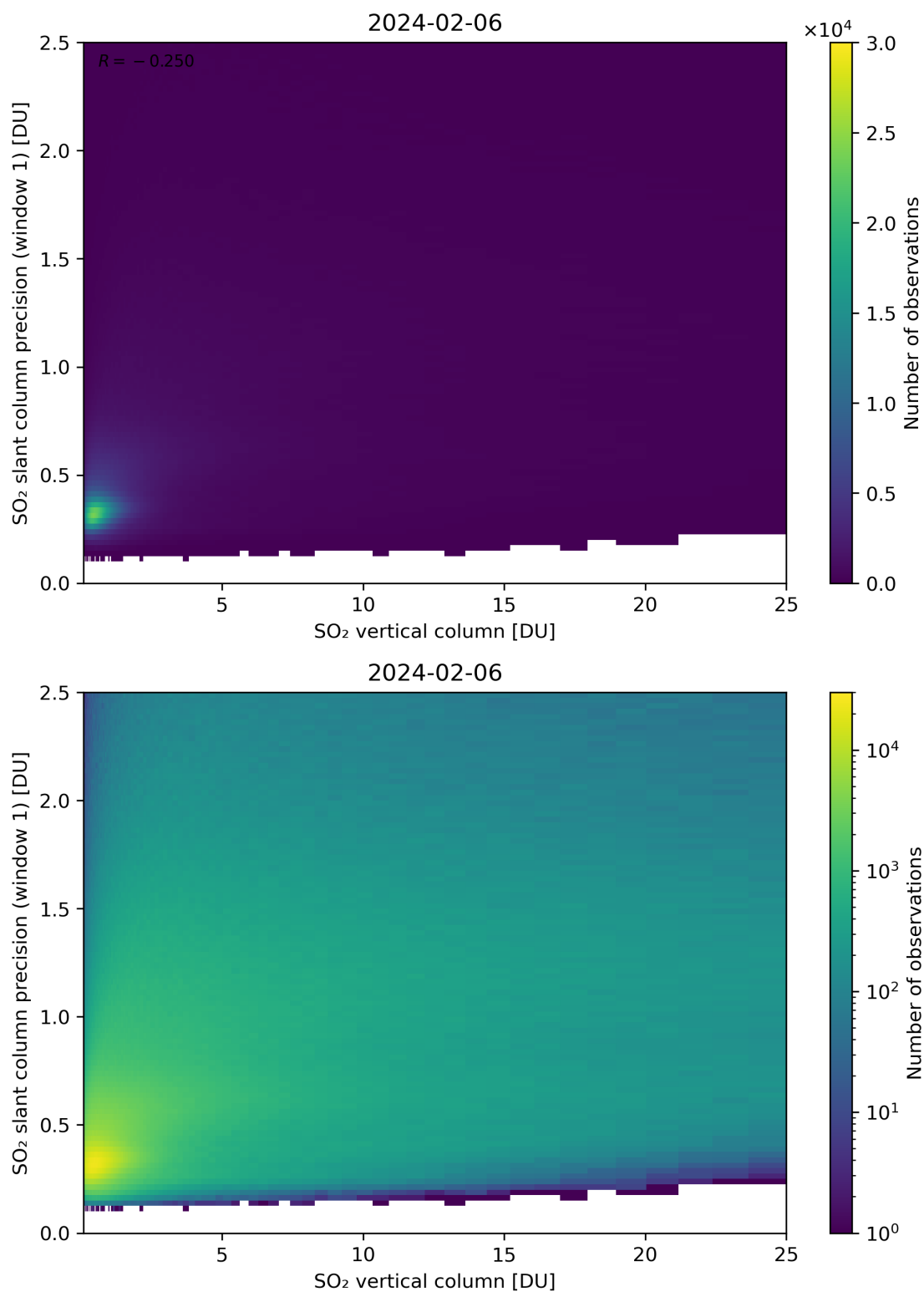
Figure 301: Scatter density plot of “SO 2 vertical column” against “SO 2 slant column precision (window 1)” for 2024-02-06 to 2024-02-07.
