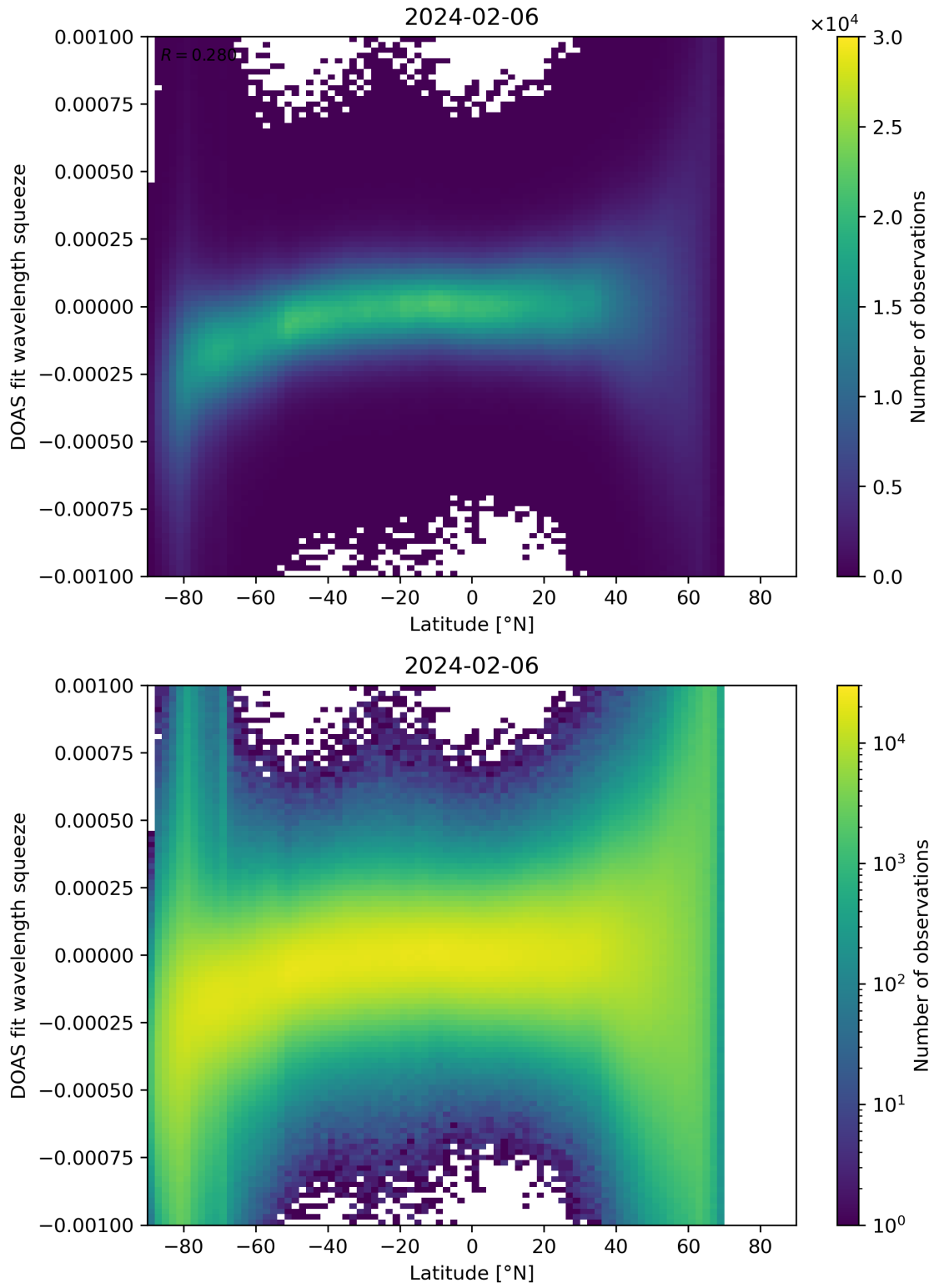
Figure 143: Scatter density plot of “Latitude” against “DOAS fit wavelength squeeze” for 2024-02-06 to 2024-02-07.
