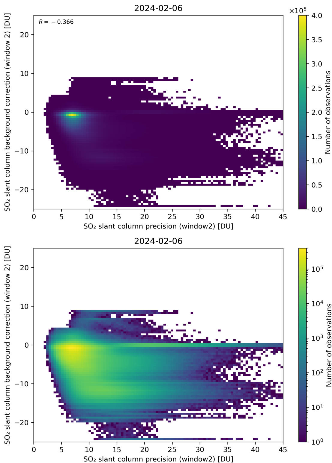
Figure 241: Scatter density plot of “SO 2 slant column precision (window2)” against “SO 2 slant column background correction (window 2)” for 2024-02-06 to 2024-02-07.
