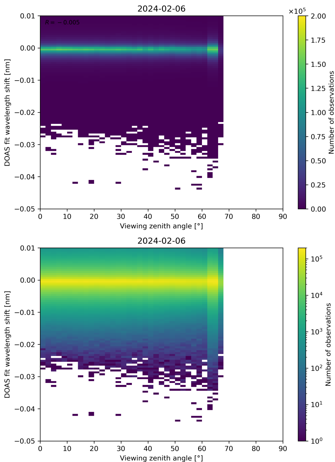
Figure 311: Scatter density plot of “Viewing zenith angle” against “DOAS fit wavelength shift” for 2024-02-06 to 2024-02-07.
