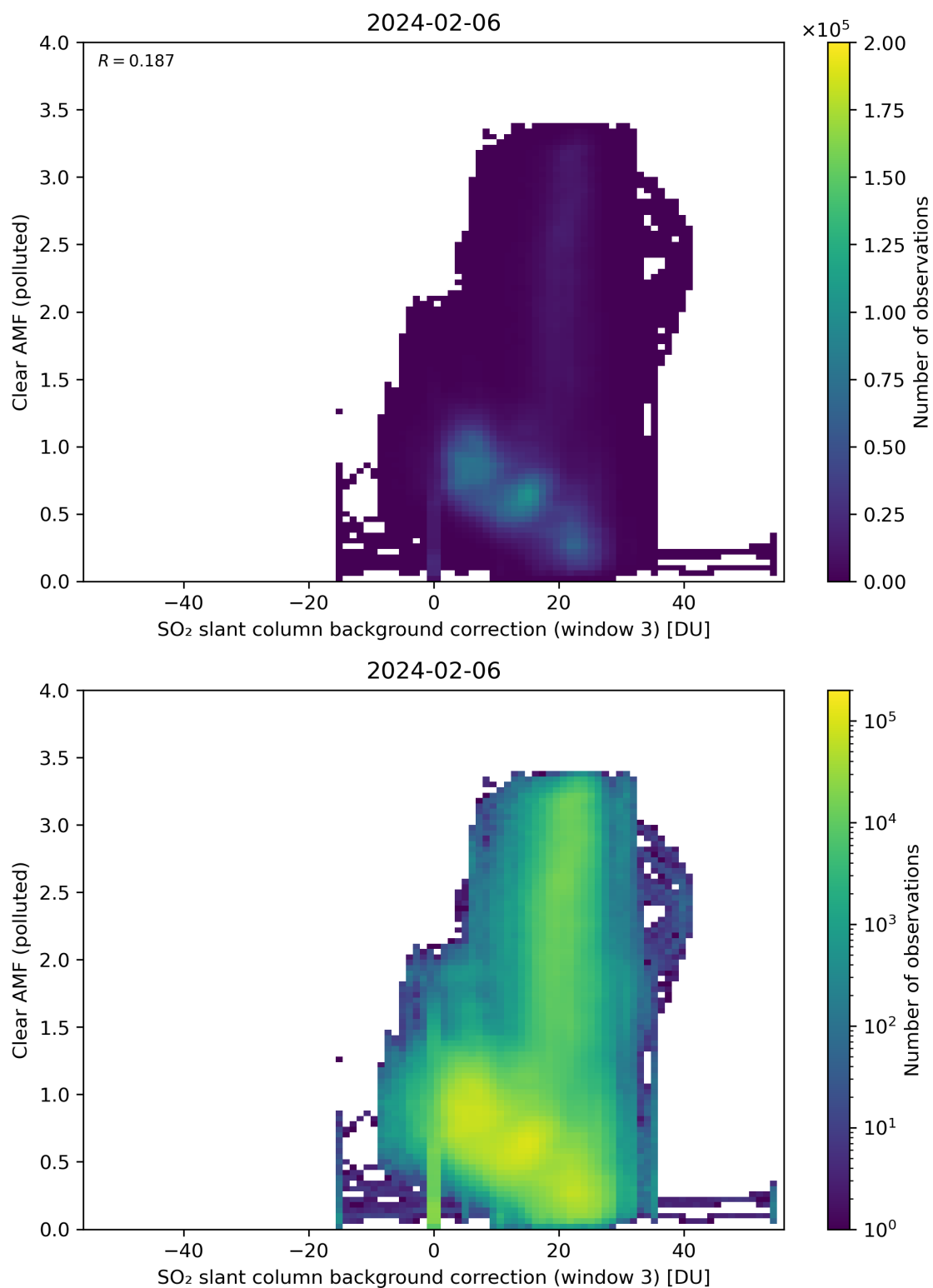
Figure 124: Scatter density plot of “SO 2 slant column background correction (window 3)” against “Clear AMF (polluted)” for 2024-02-06 to 2024-02-07.
