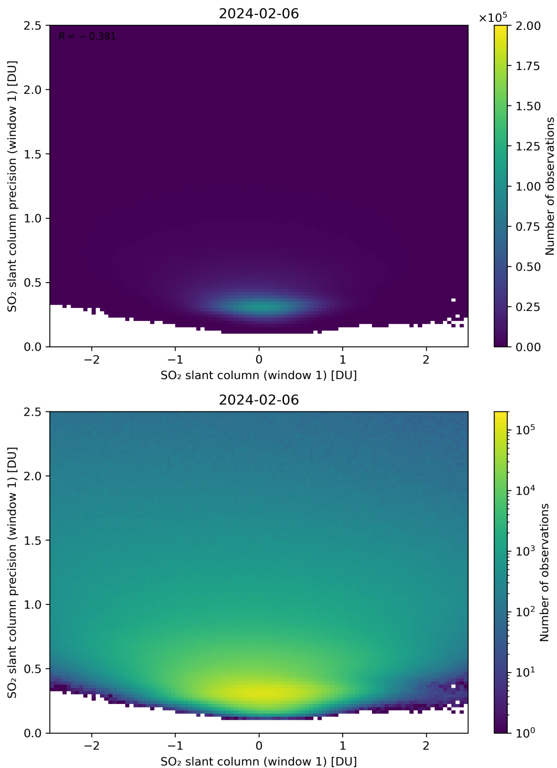
Figure 235: Scatter density plot of “SO 2 slant column (window 1)” against “SO 2 slant column precision (window 1)” for 2024-02-06 to 2024-02-07.
