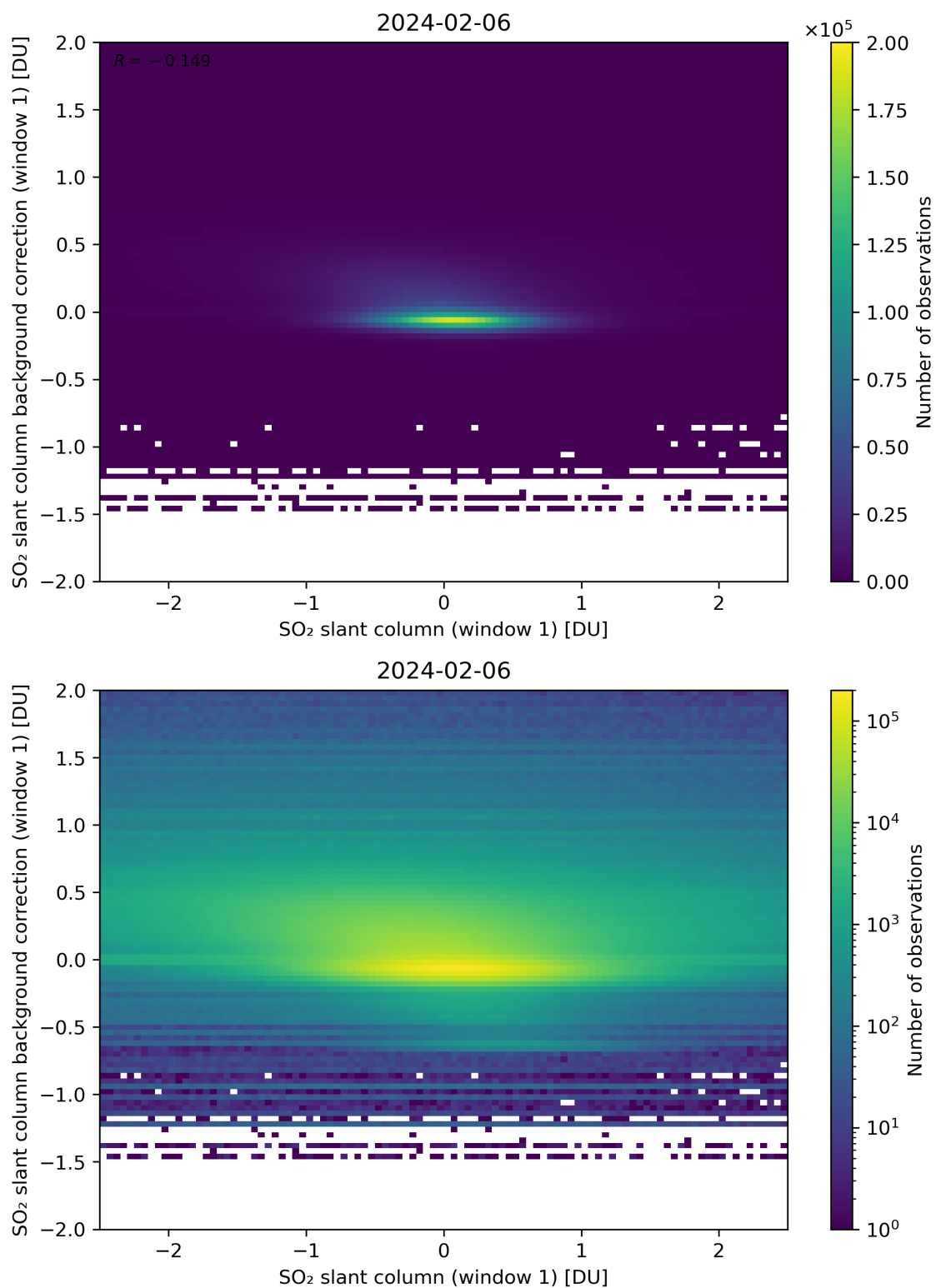
Figure 212: Scatter density plot of “SO 2 slant column (window 1)” against “SO 2 slant column background correction (window 1)” for 2024-02-06 to 2024-02-07.
