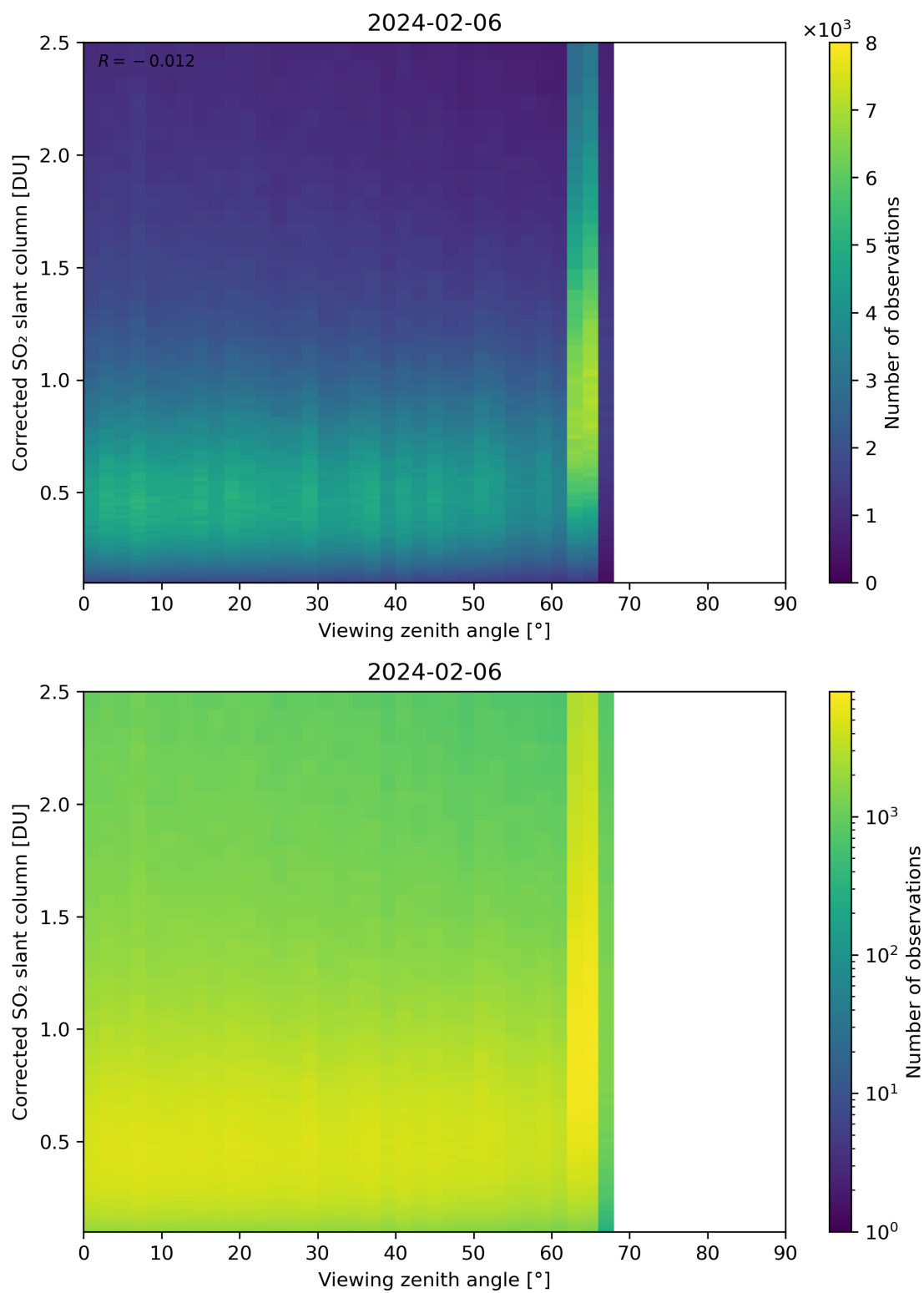
Figure 317: Scatter density plot of “Viewing zenith angle” against “Corrected SO 2 slant column” for 2024-02-06 to 2024-02-07.
