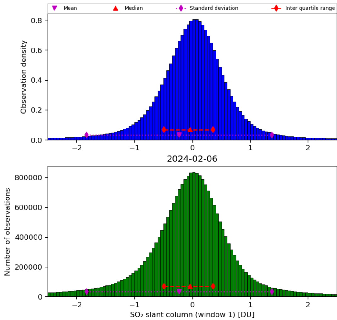
Figure 56: Histogram of “SO 2 slant column (window 1)” for 2024-02-06 to 2024-02-07
