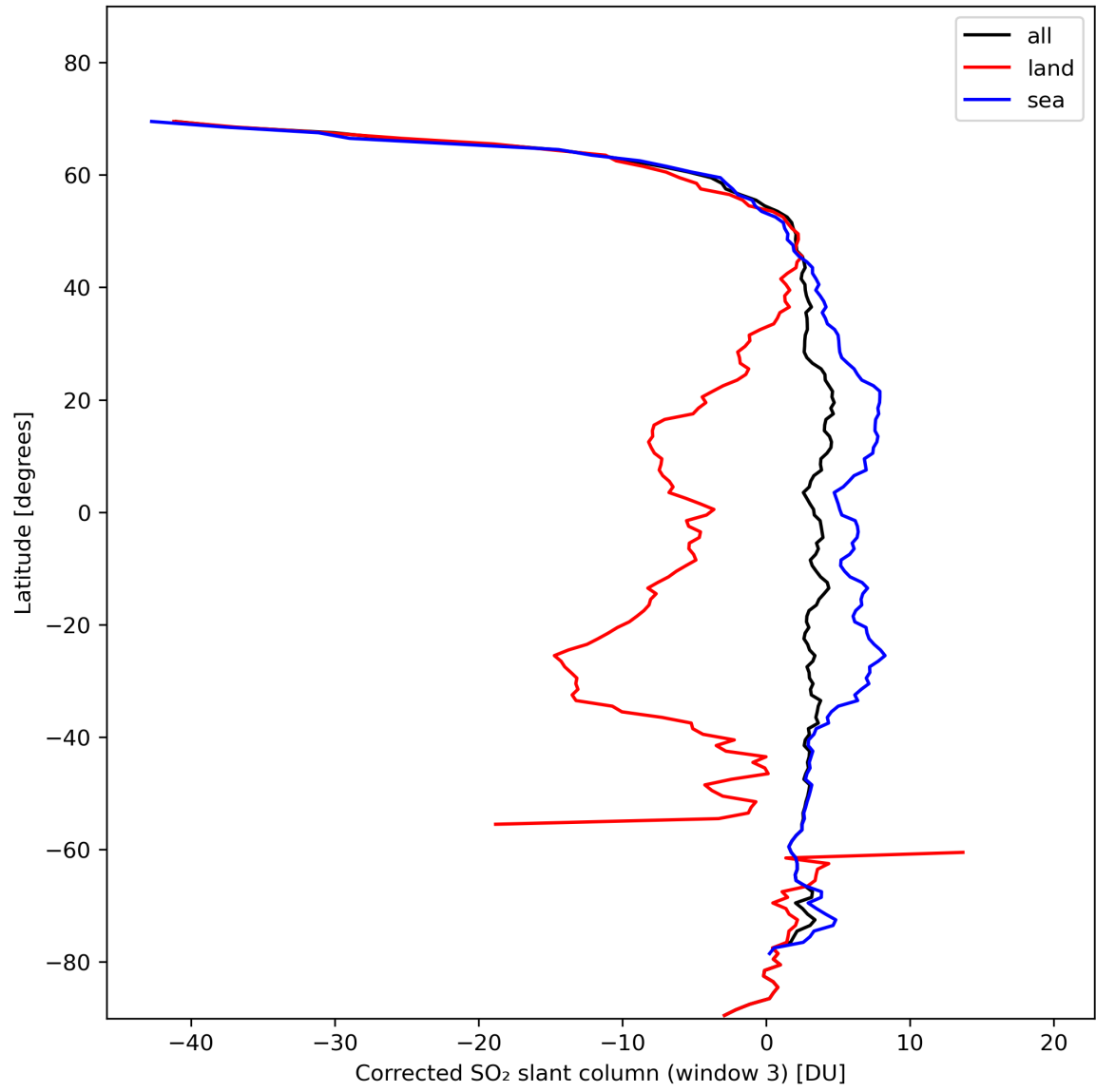
Figure 43: Zonal average of “Corrected SO 2 slant column (window 3)” for 2024-02-06 to 2024-02-07.
