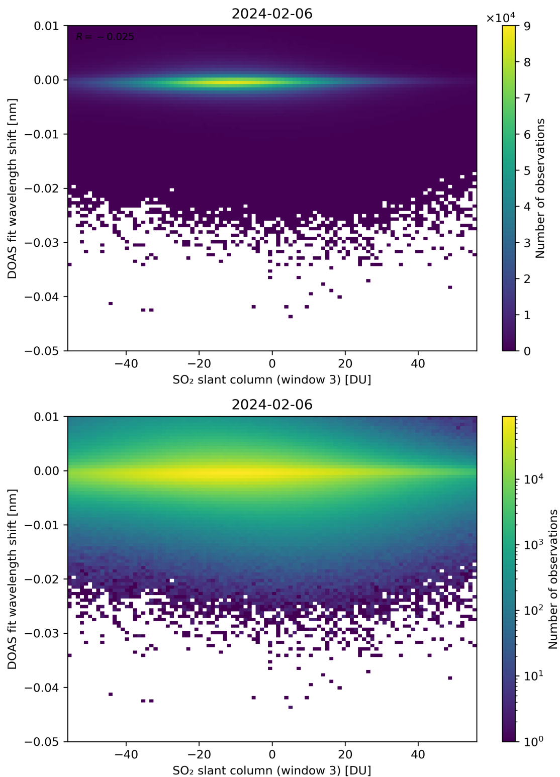
Figure 254: Scatter density plot of “SO 2 slant column (window 3)” against “DOAS fit wavelength shift” for 2024-02-06 to 2024-02-07.
