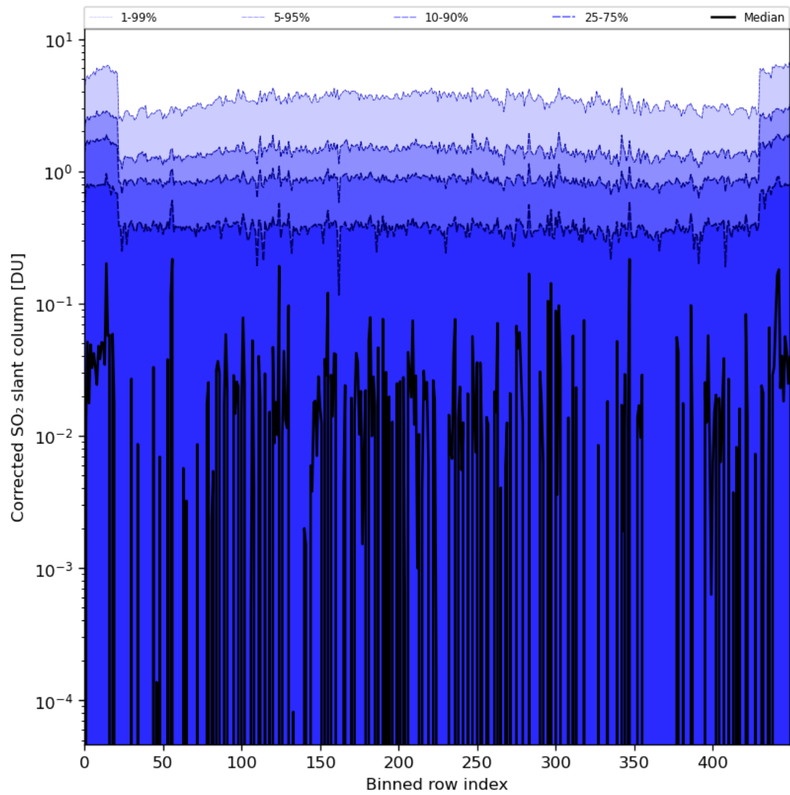
Figure 78: Along track statistics of “Corrected SO 2 slant column” for 2024-02-06 to 2024-02-07
