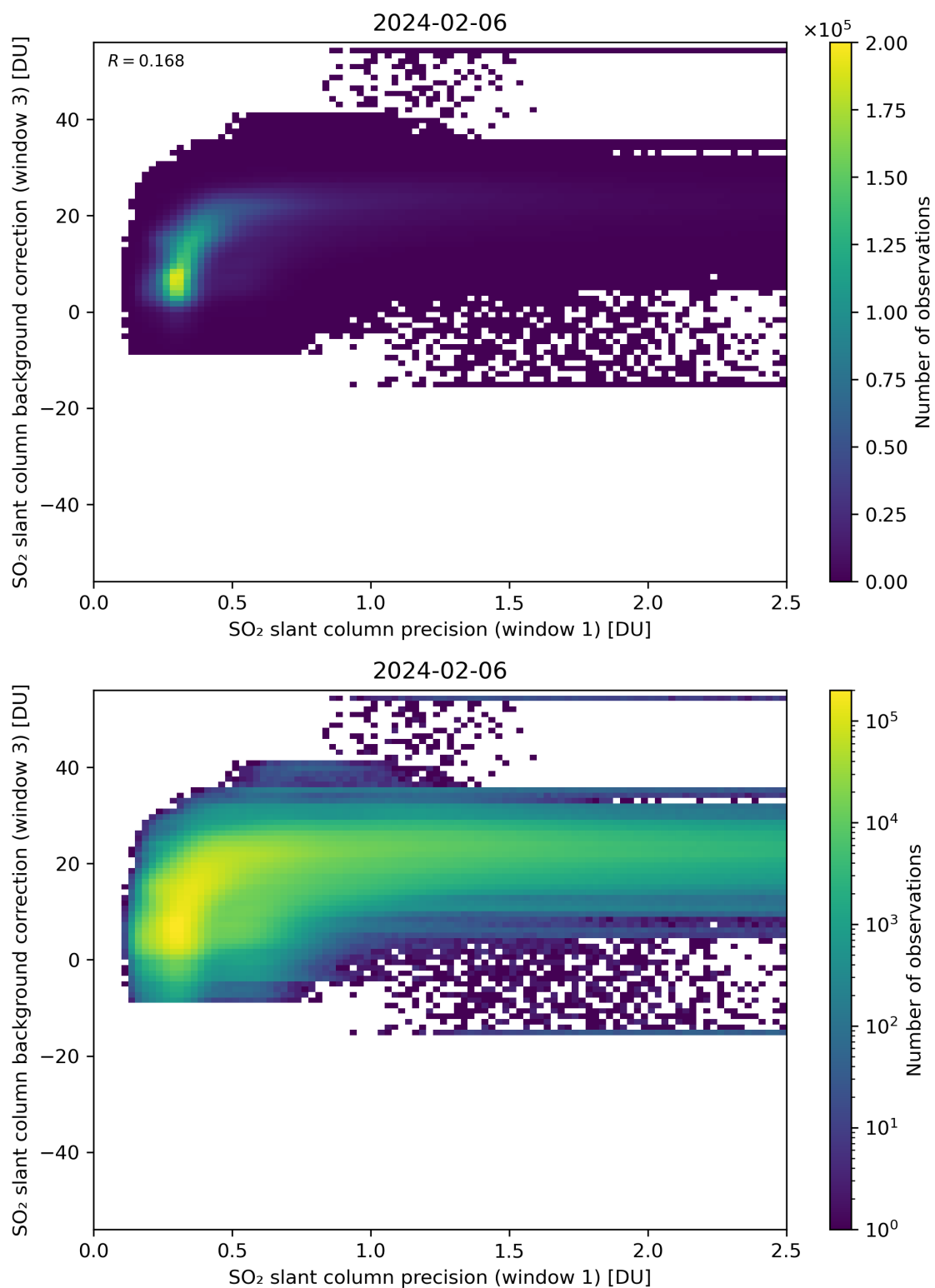
Figure 220: Scatter density plot of “SO 2 slant column precision (window 1)” against “SO 2 slant column background correction (window 3)” for 2024-02-06 to 2024-02-07.
