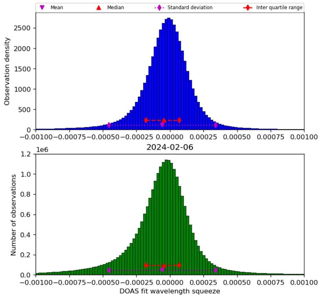
Figure 69: Histogram of “DOAS fit wavelength squeeze” for 2024-02-06 to 2024-02-07
