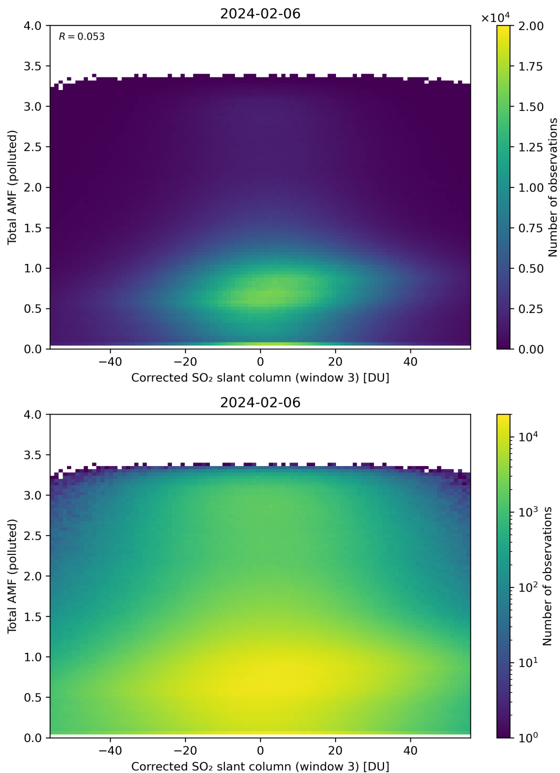
Figure 210: Scatter density plot of “Corrected SO 2 slant column (window 3)” against “Total AMF (polluted)” for 2024-02-06 to 2024-02-07.
