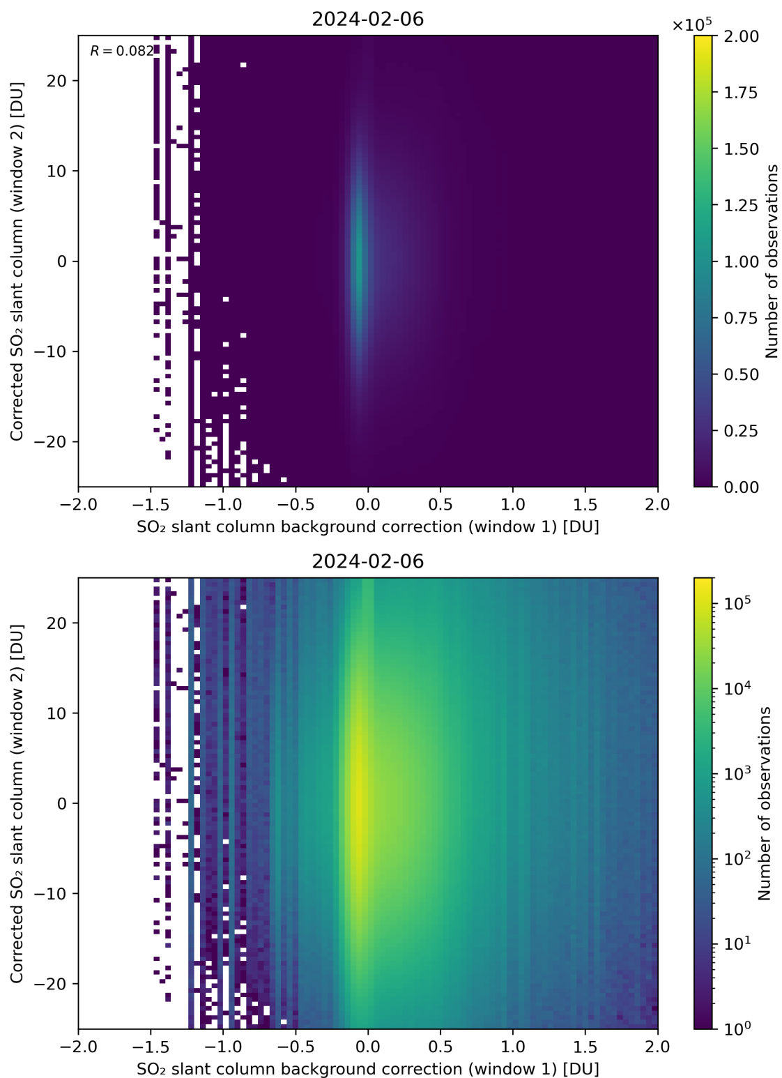
Figure 104: Scatter density plot of “SO 2 slant column background correction (window 1)” against “Corrected SO 2 slant column (window 2)” for 2024-02-06 to 2024-02-07.
