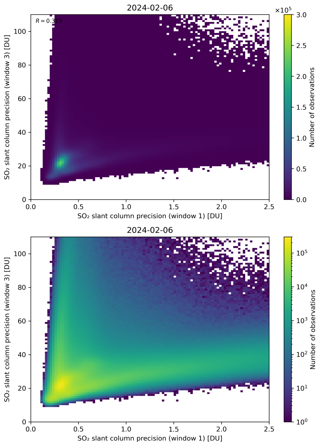
Figure 229: Scatter density plot of “SO 2 slant column precision (window 1)” against “SO 2 slant column precision (window 3)” for 2024-02-06 to 2024-02-07.
