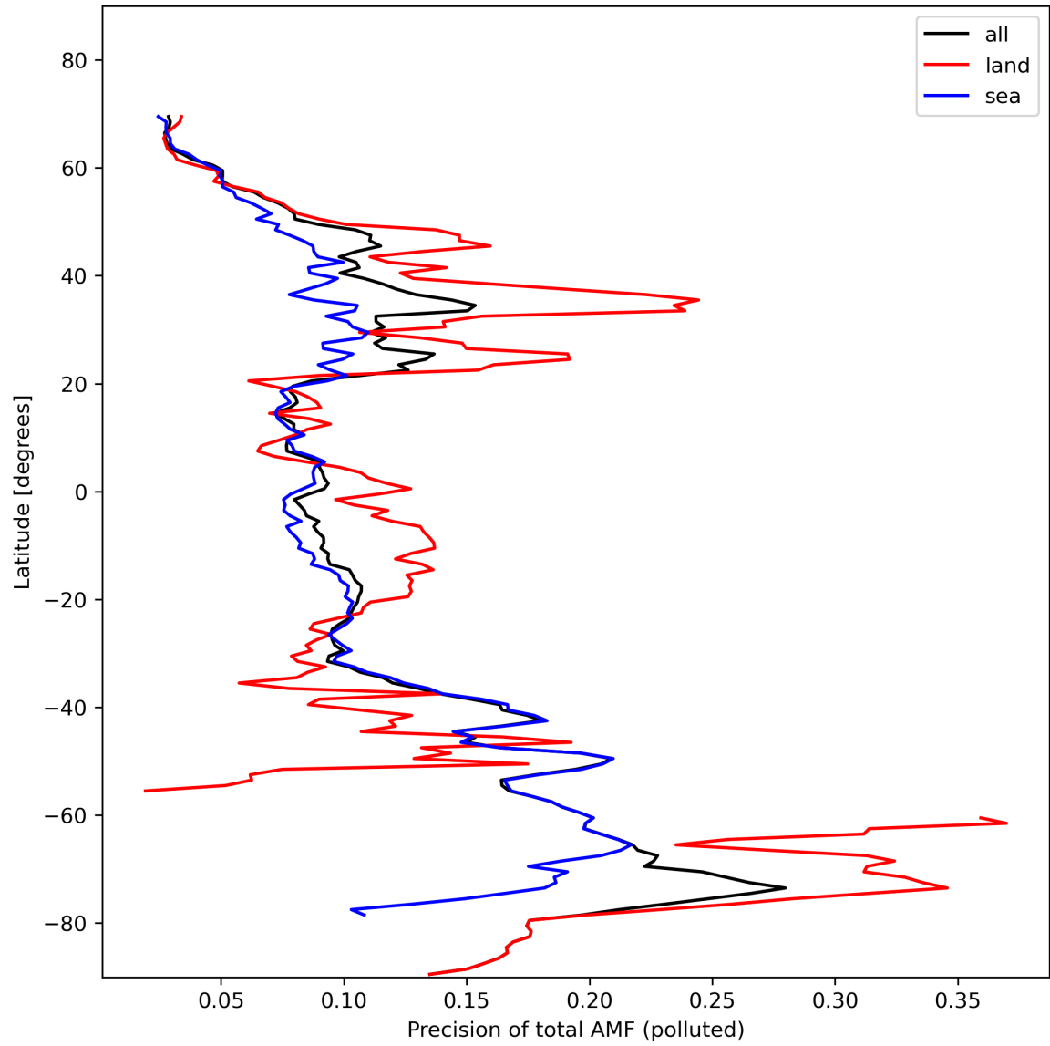
Figure 49: Zonal average of “Precision of total AMF (polluted)” for 2024-02-06 to 2024-02-07.
