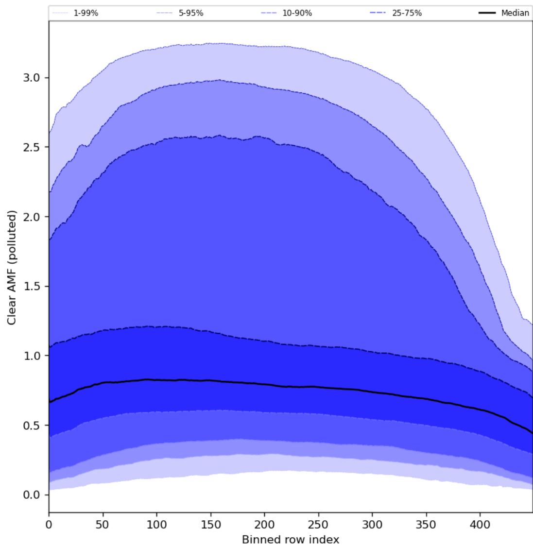
Figure 96: Along track statistics of “Clear AMF (polluted)” for 2024-02-06 to 2024-02-07
