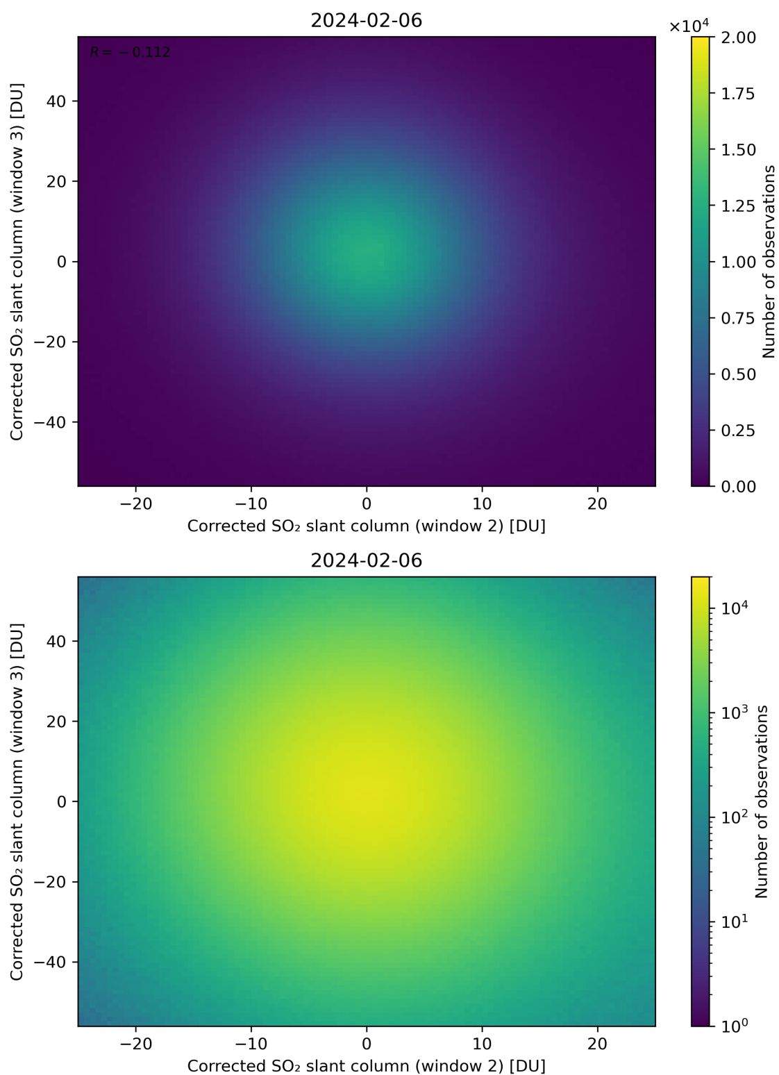
Figure 200: Scatter density plot of “Corrected SO 2 slant column (window 2)” against “Corrected SO 2 slant column (window 3)” for 2024-02-06 to 2024-02-07.
