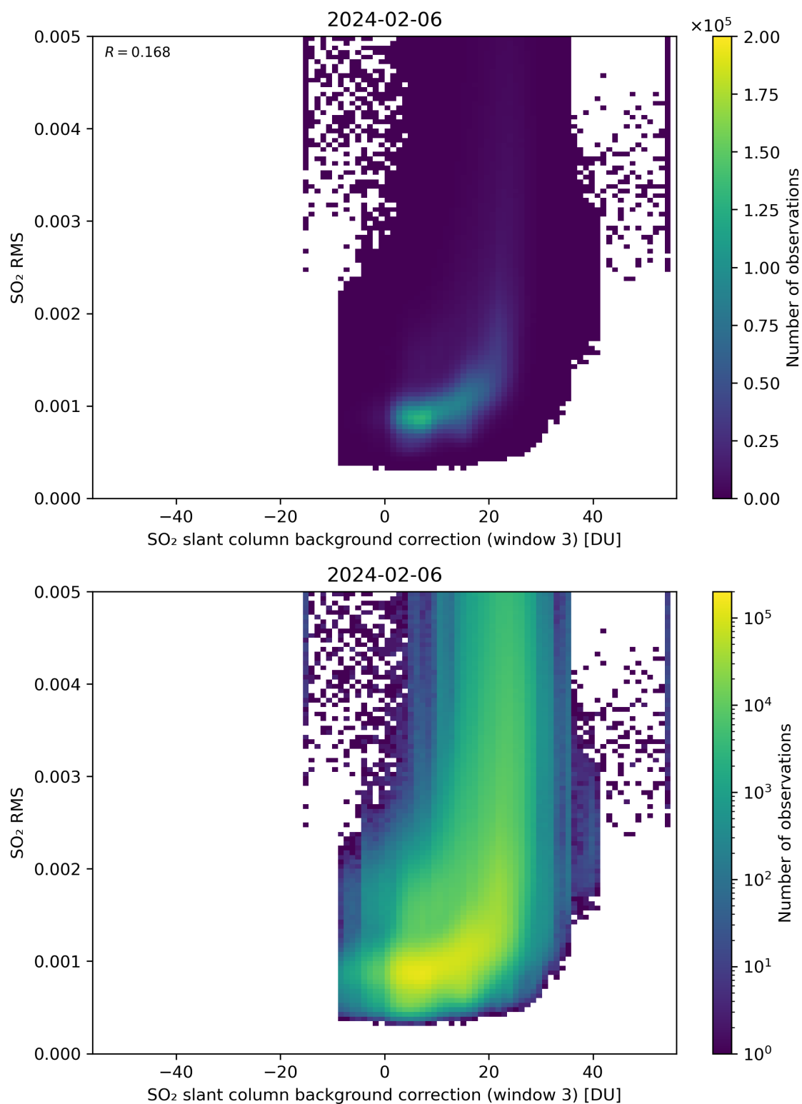
Figure 123: Scatter density plot of “SO 2 slant column background correction (window 3)” against “SO 2 RMS” for 2024-02-06 to 2024-02-07.
