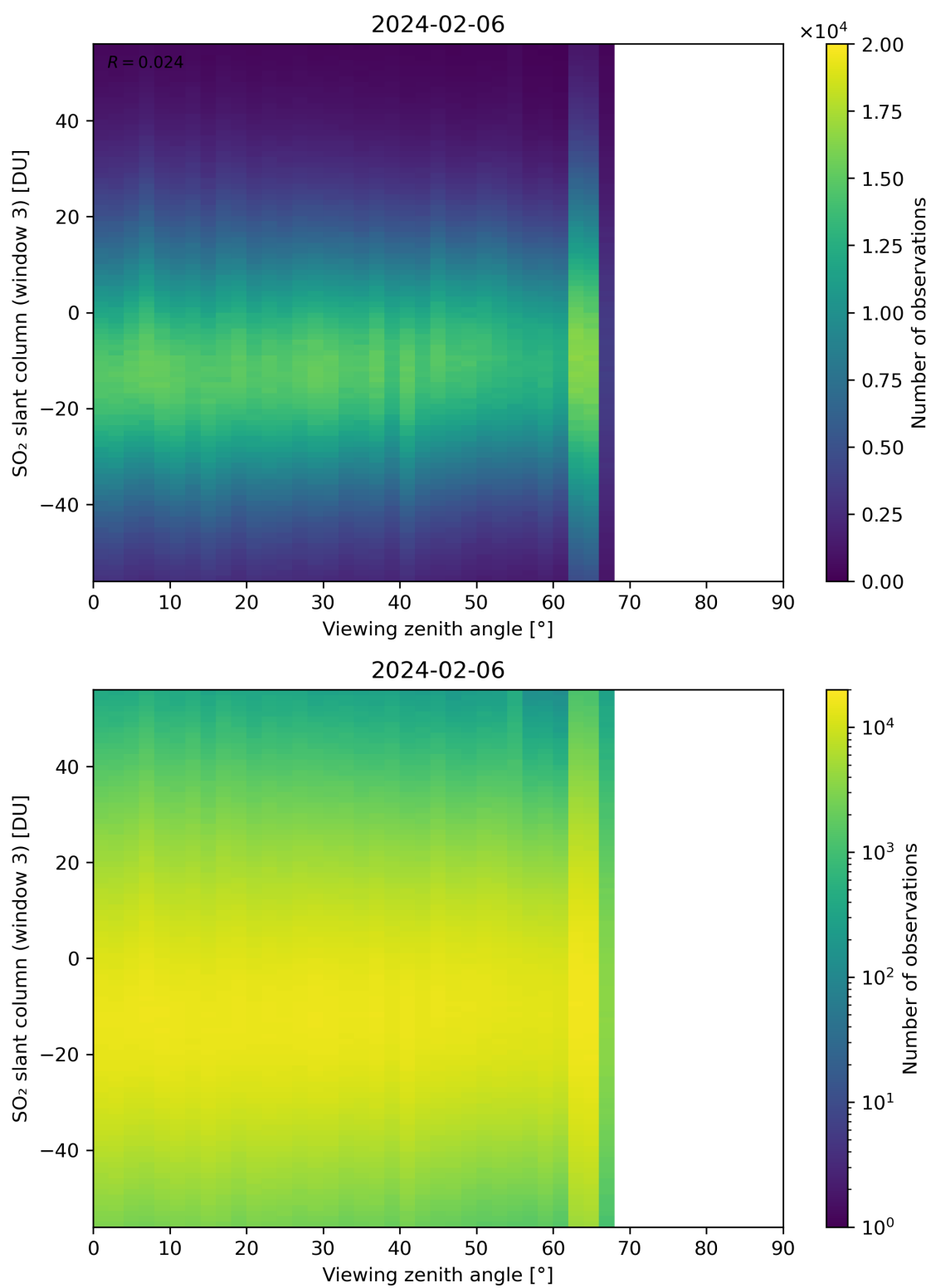
Figure 323: Scatter density plot of “Viewing zenith angle” against “SO 2 slant column (window 3)” for 2024-02-06 to 2024-02-07.
