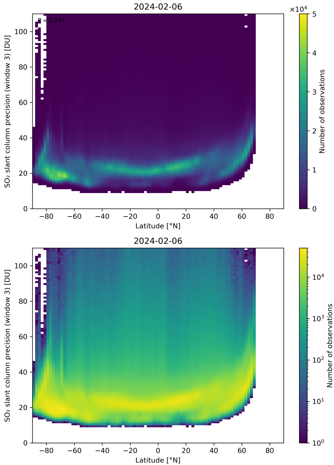
Figure 153: Scatter density plot of “Latitude” against “SO 2 slant column precision (window 3)” for 2024-02-06 to 2024-02-07.
