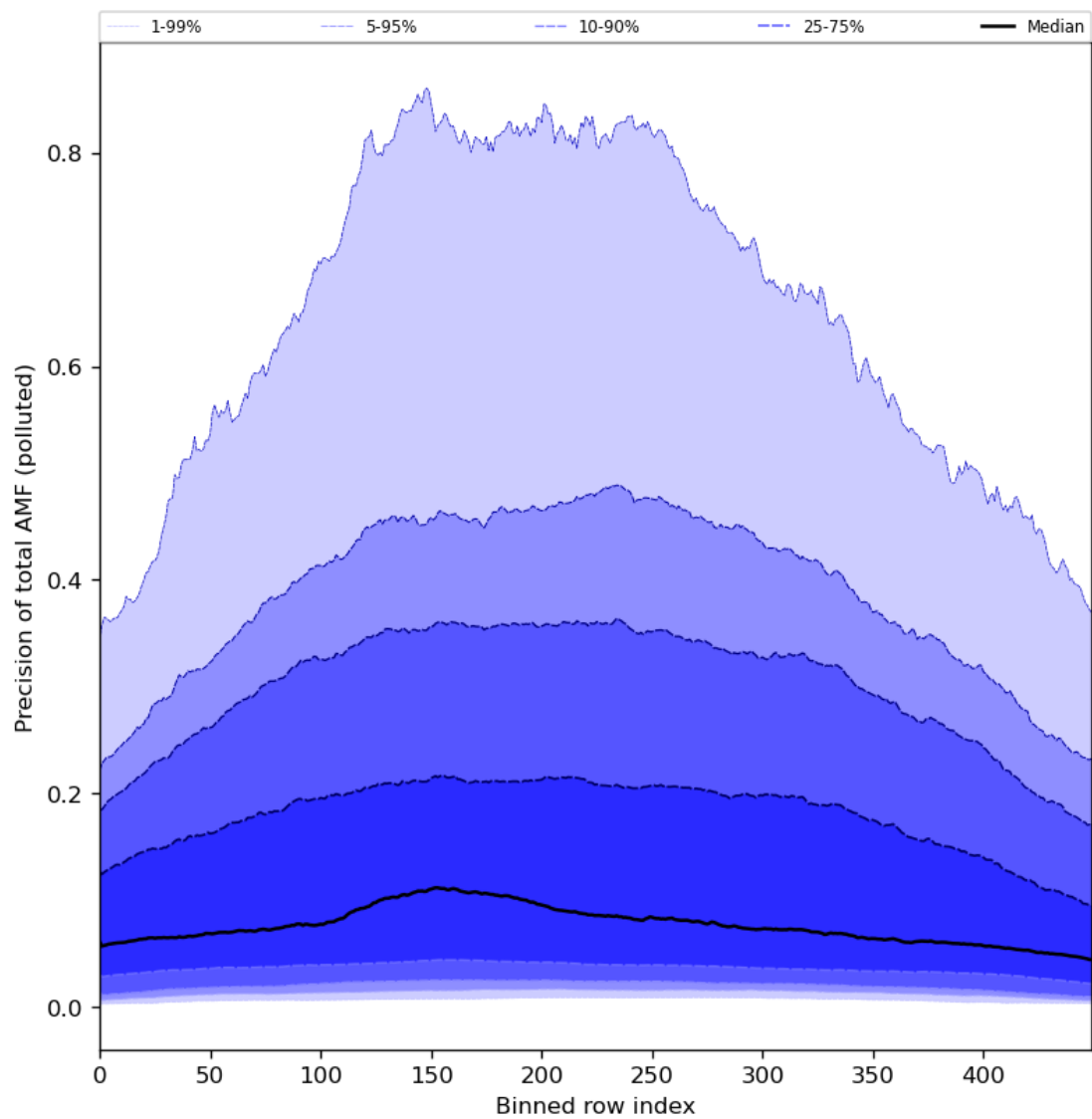
Figure 95: Along track statistics of “Precision of total AMF (polluted)” for 2024-02-06 to 2024-02-07
