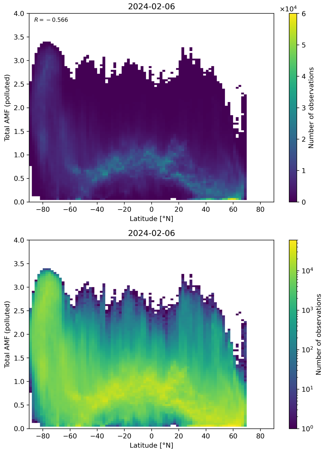
Figure 154: Scatter density plot of “Latitude” against “Total AMF (polluted)” for 2024-02-06 to 2024-02-07.
