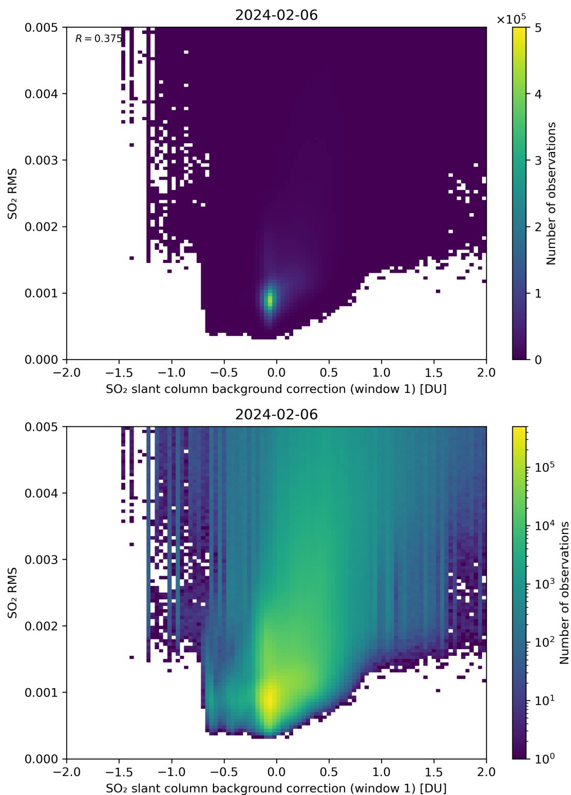
Figure 102: Scatter density plot of “SO 2 slant column background correction (window 1)” against “SO 2 RMS” for 2024-02-06 to 2024-02-07.
