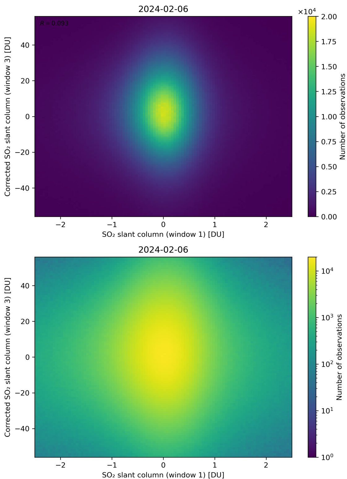
Figure 234: Scatter density plot of “SO 2 slant column (window 1)” against “Corrected SO 2 slant column (window 3)” for 2024-02-06 to 2024-02-07.
