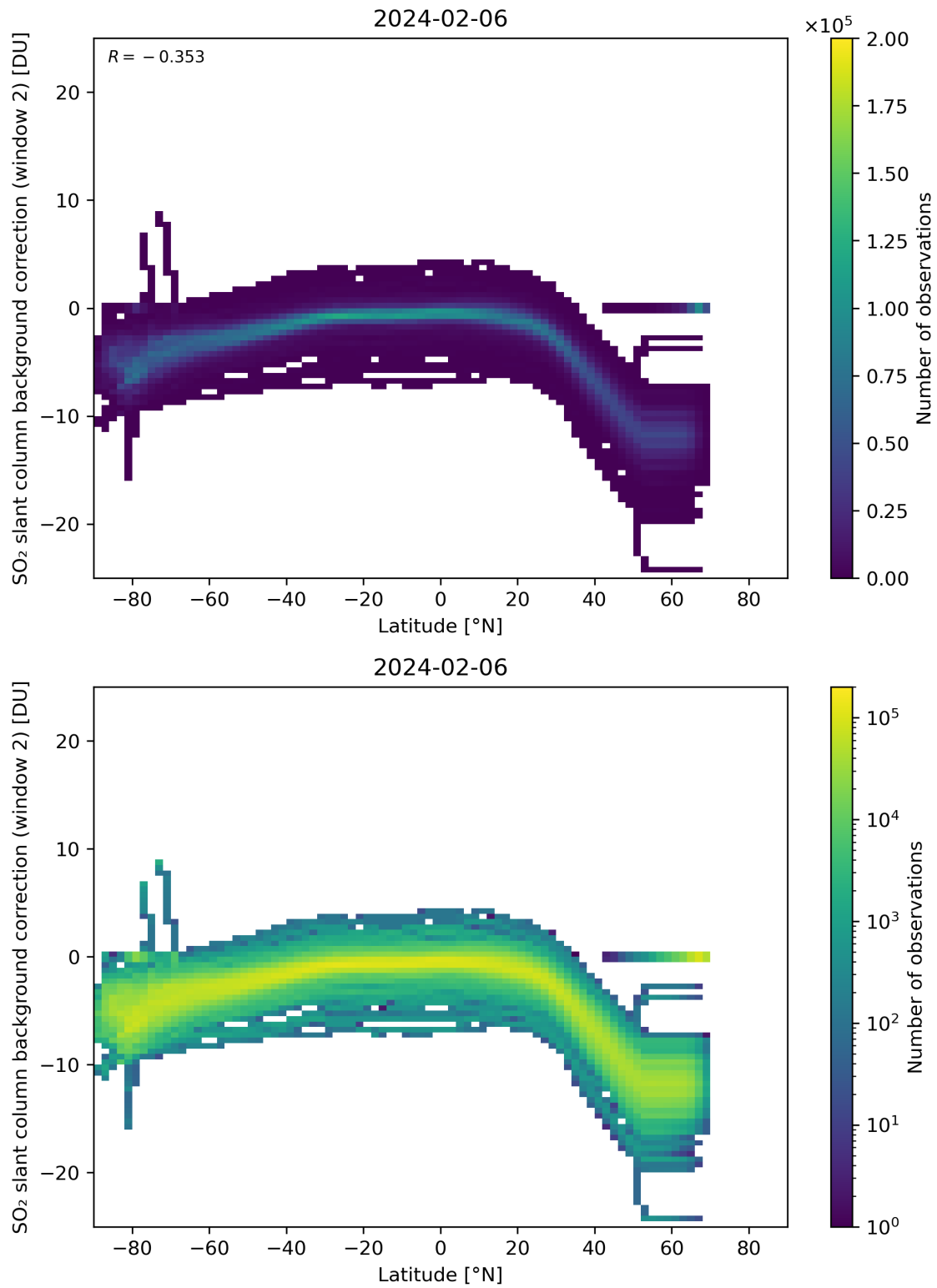
Figure 140: Scatter density plot of “Latitude” against “SO 2 slant column background correction (window 2)” for 2024-02-06 to 2024-02-07.
