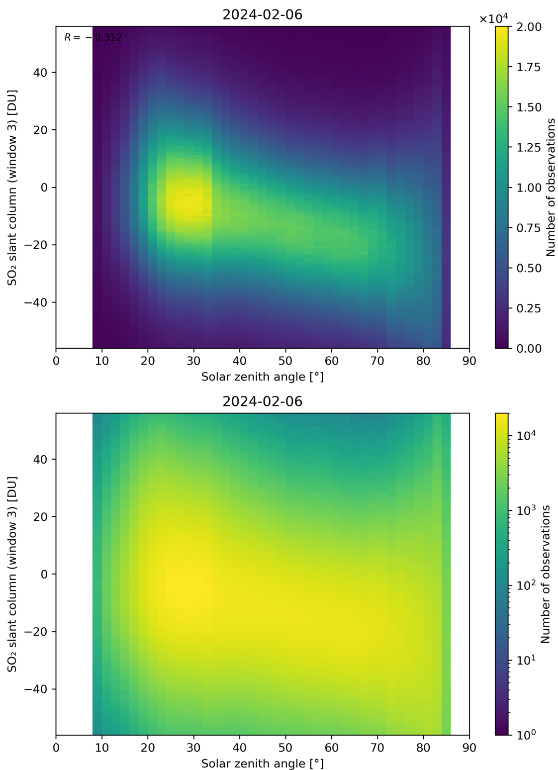
Figure 172: Scatter density plot of “Solar zenith angle” against “SO 2 slant column (window 3)” for 2024-02-06 to 2024-02-07.
