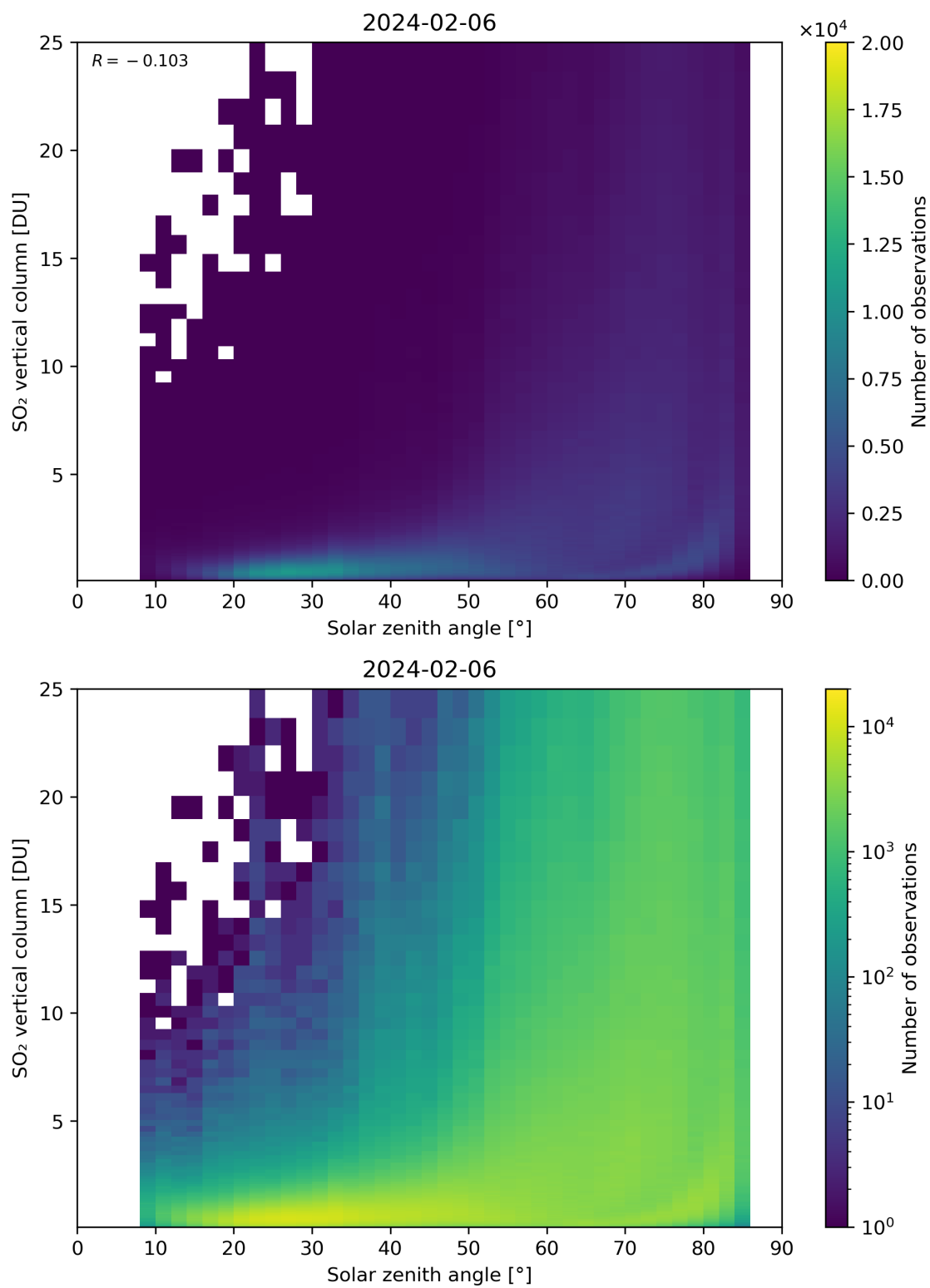
Figure 176: Scatter density plot of “Solar zenith angle” against “SO 2 vertical column” for 2024-02-06 to 2024-02-07.
