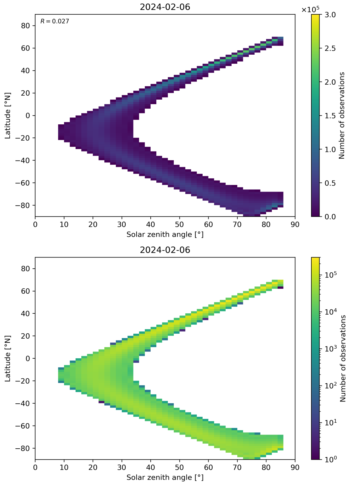
Figure 164: Scatter density plot of “Solar zenith angle” against “Latitude” for 2024-02-06 to 2024-02-07.
