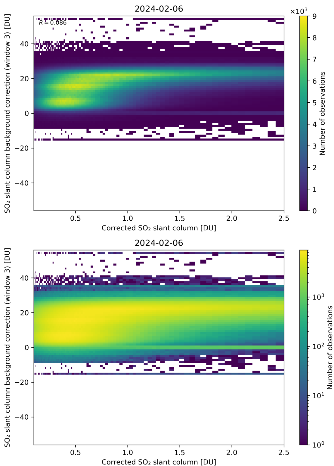
Figure 180: Scatter density plot of “Corrected SO 2 slant column” against “SO 2 slant column background correction (window 3)” for 2024-02-06 to 2024-02-07.
