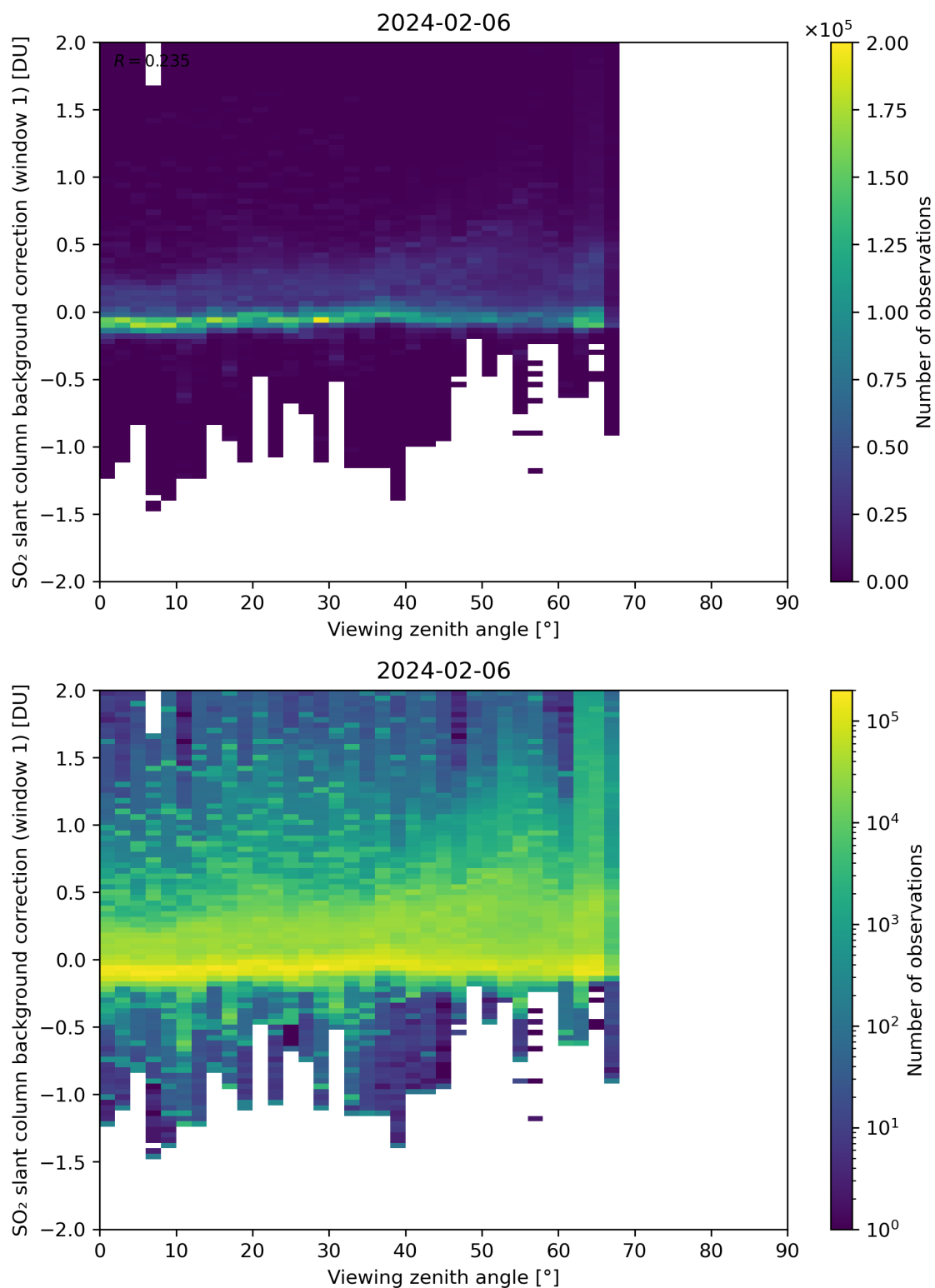
Figure 308: Scatter density plot of “Viewing zenith angle” against “SO 2 slant column background correction (window 1)” for 2024-02-06 to 2024-02-07.
