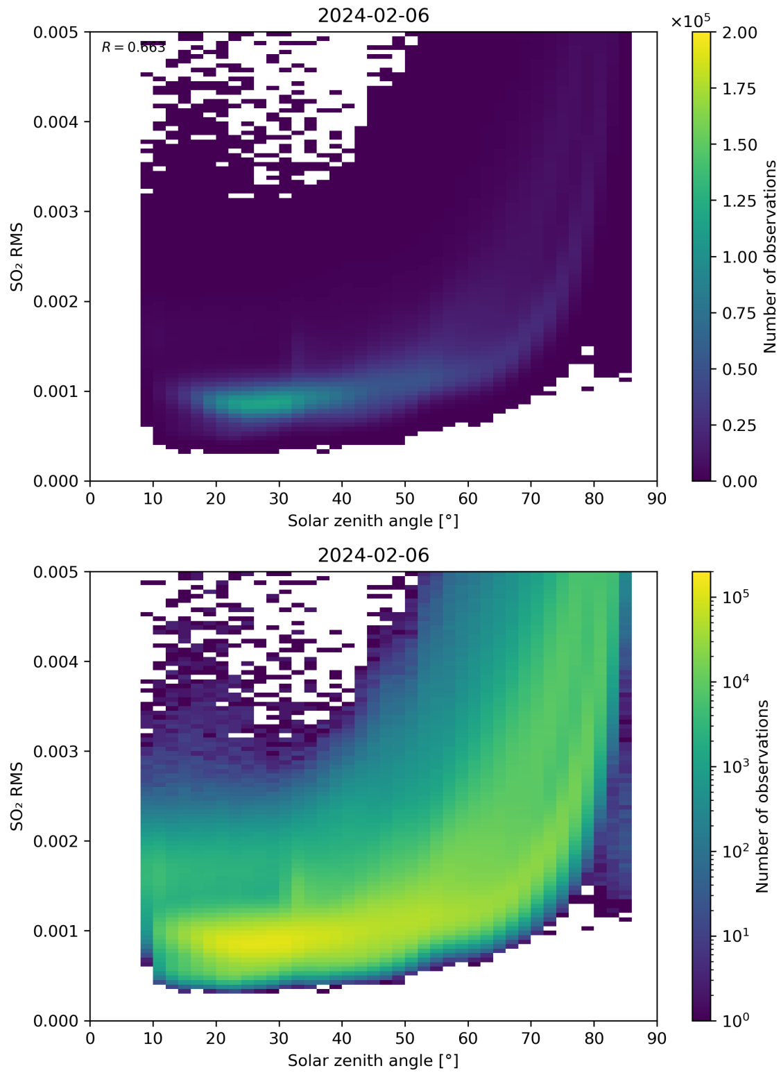
Figure 163: Scatter density plot of “Solar zenith angle” against “SO 2 RMS” for 2024-02-06 to 2024-02-07.
