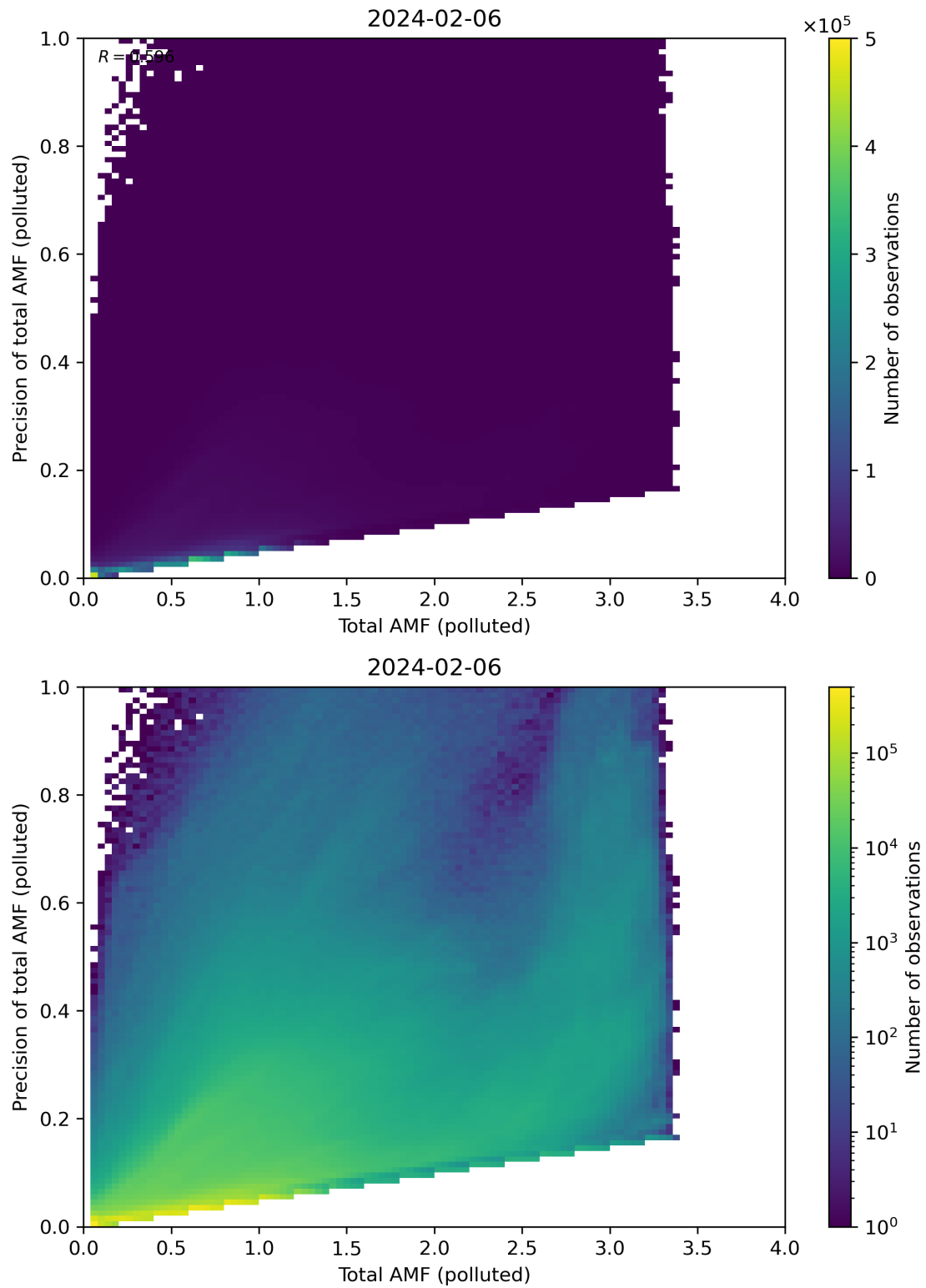
Figure 272: Scatter density plot of “Total AMF (polluted)” against “Precision of total AMF (polluted)” for 2024-02-06 to 2024-02-07.
