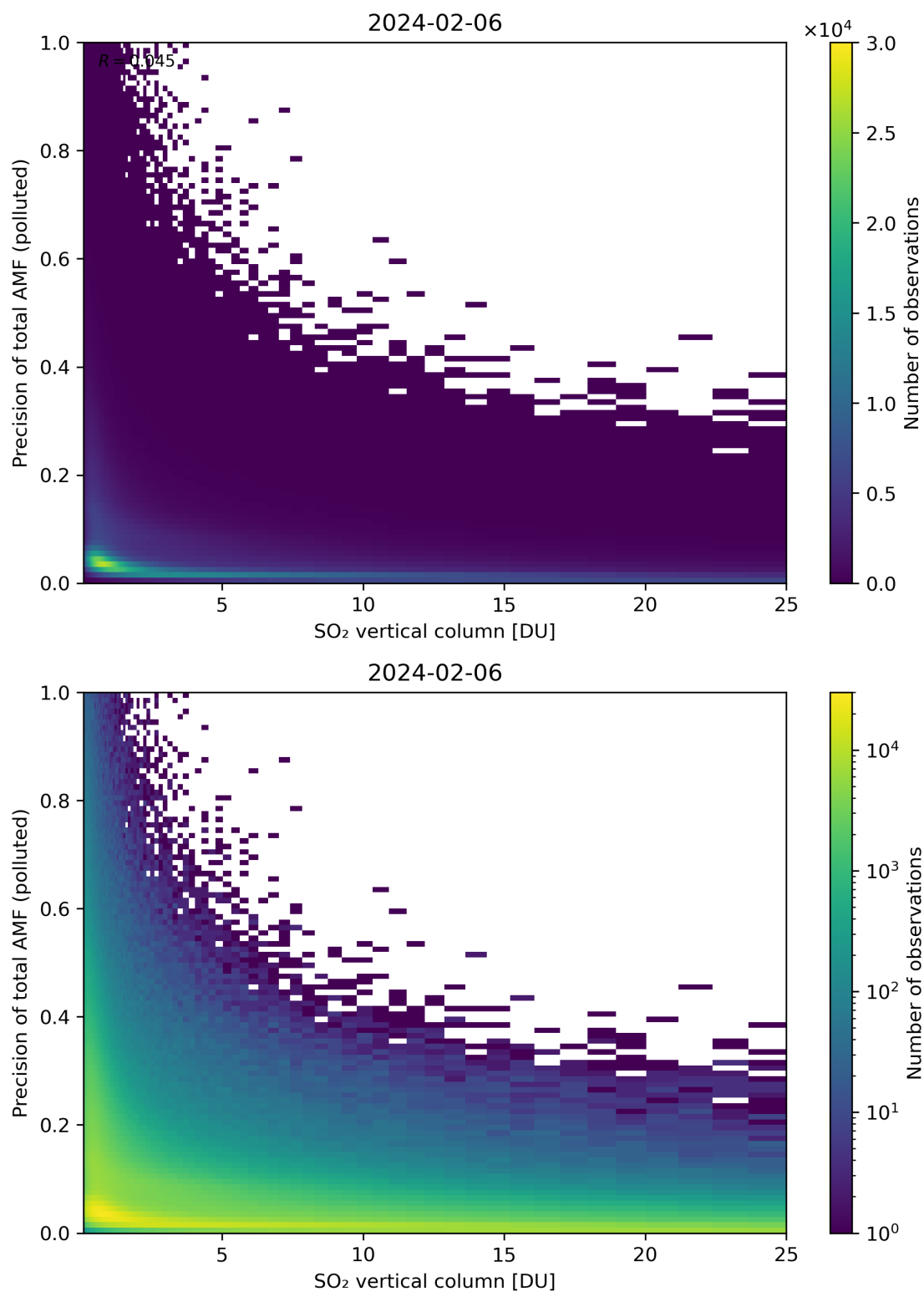
Figure 306: Scatter density plot of “SO 2 vertical column” against “Precision of total AMF (polluted)” for 2024-02-06 to 2024-02-07.
