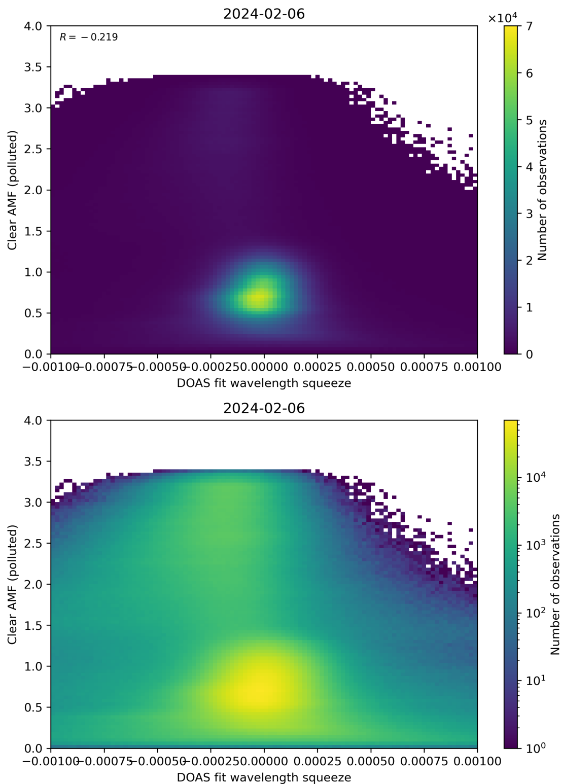
Figure 133: Scatter density plot of “DOAS fit wavelength squeeze” against “Clear AMF (polluted)” for 2024-02-06 to 2024-02-07.
