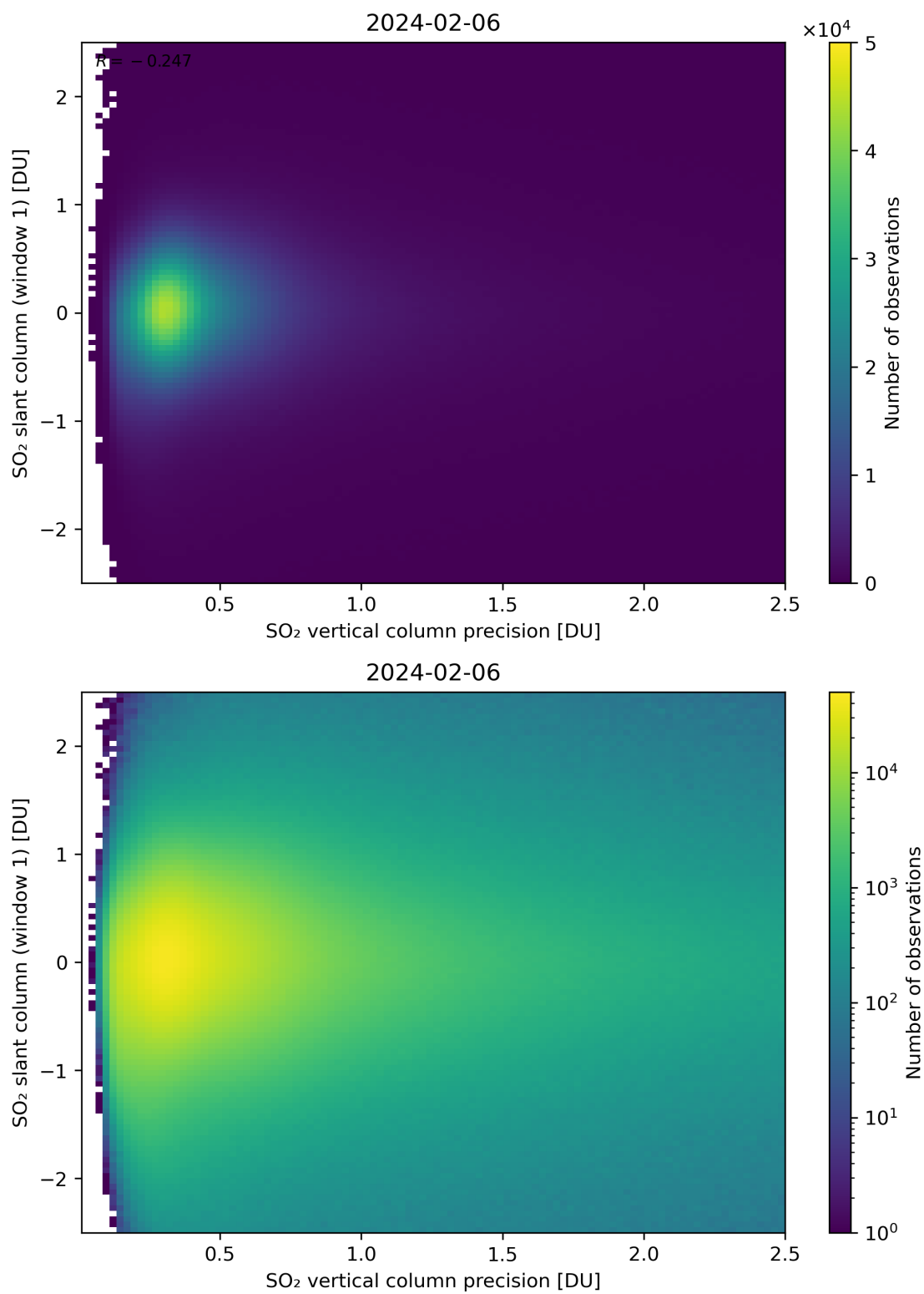
Figure 289: Scatter density plot of “SO 2 vertical column precision” against “SO 2 slant column (window 1)” for 2024-02-06 to 2024-02-07.
