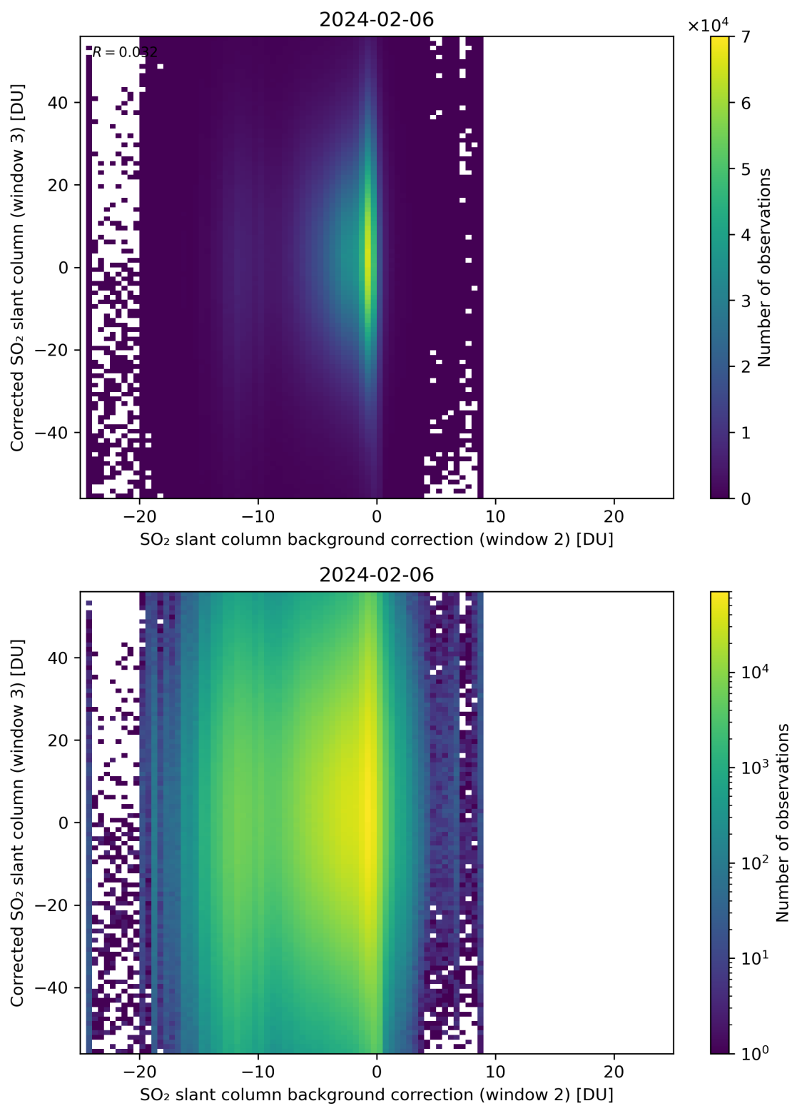
Figure 116: Scatter density plot of “SO 2 slant column background correction (window 2)” against “Corrected SO 2 slant column (window 3)” for 2024-02-06 to 2024-02-07.
