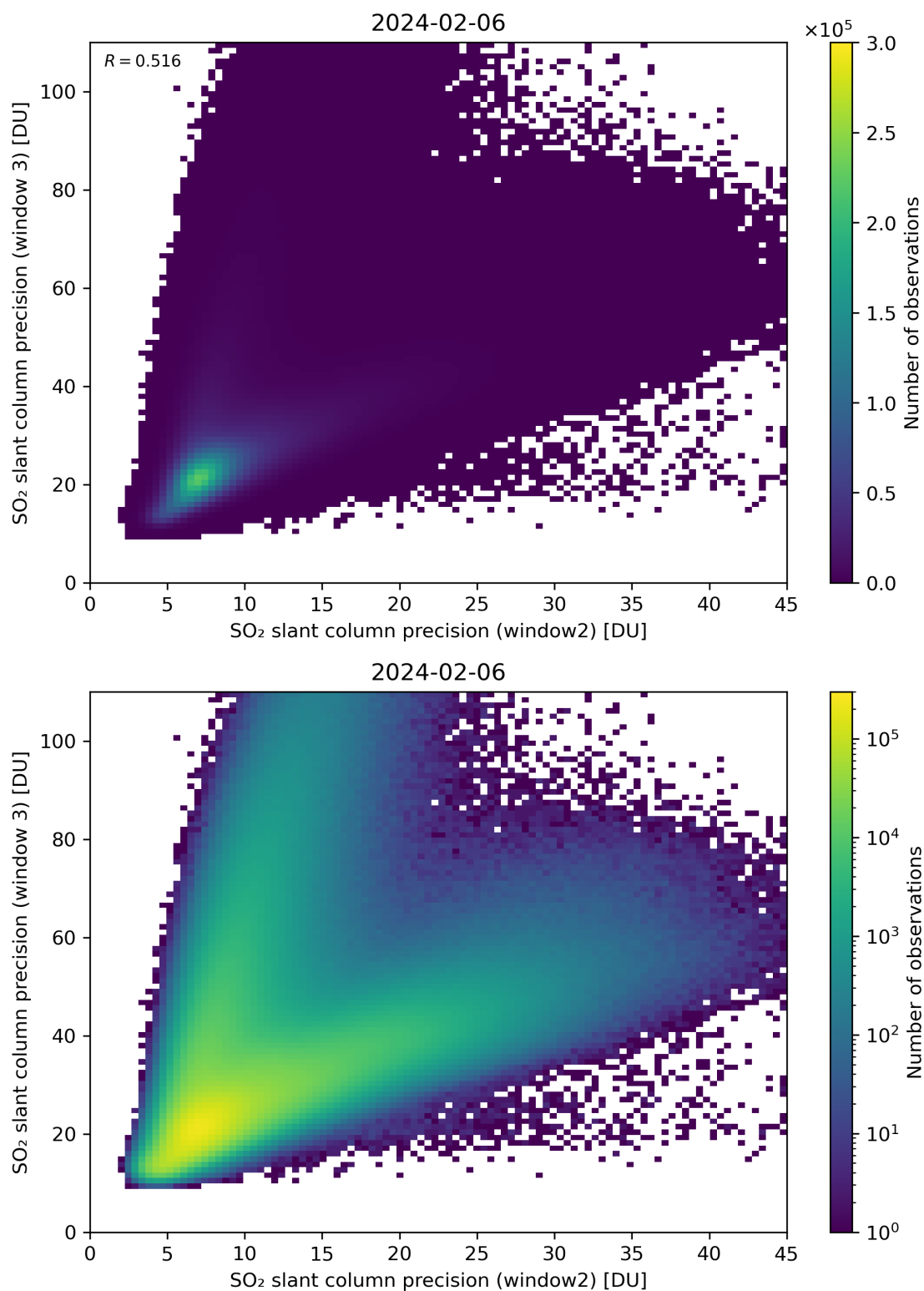
Figure 250: Scatter density plot of “SO 2 slant column precision (window2)” against “SO 2 slant column precision (window 3)” for 2024-02-06 to 2024-02-07.
