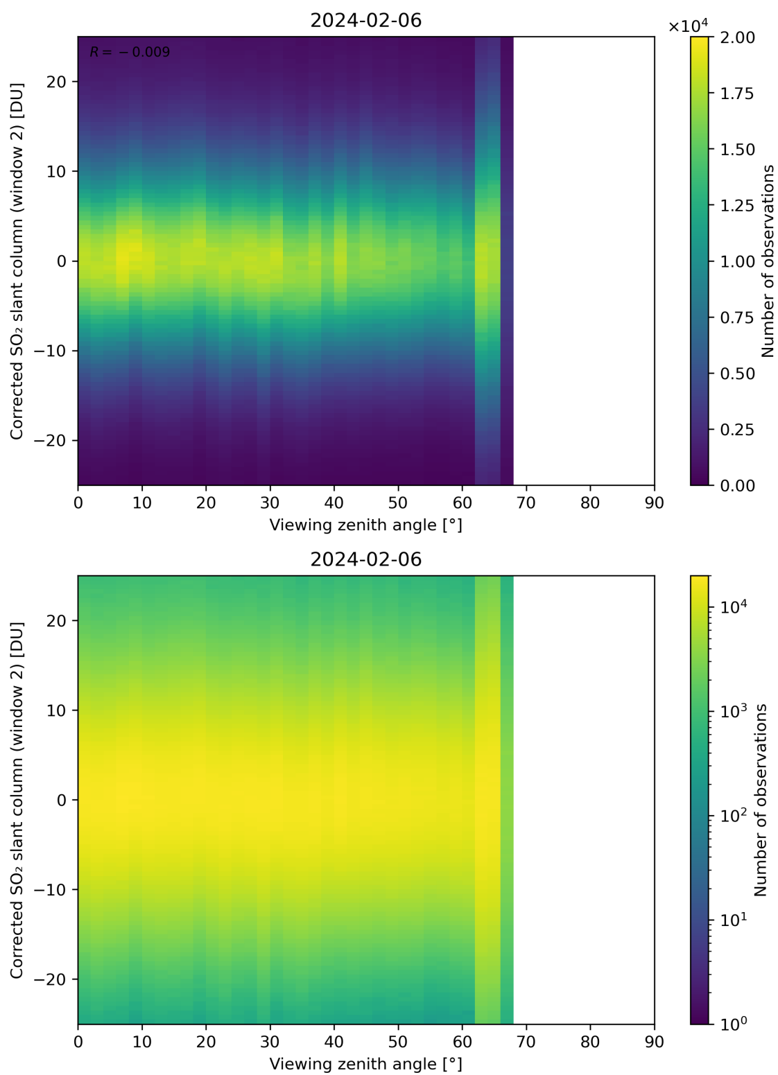
Figure 318: Scatter density plot of “Viewing zenith angle” against “Corrected SO 2 slant column (window 2)” for 2024-02-06 to 2024-02-07.
