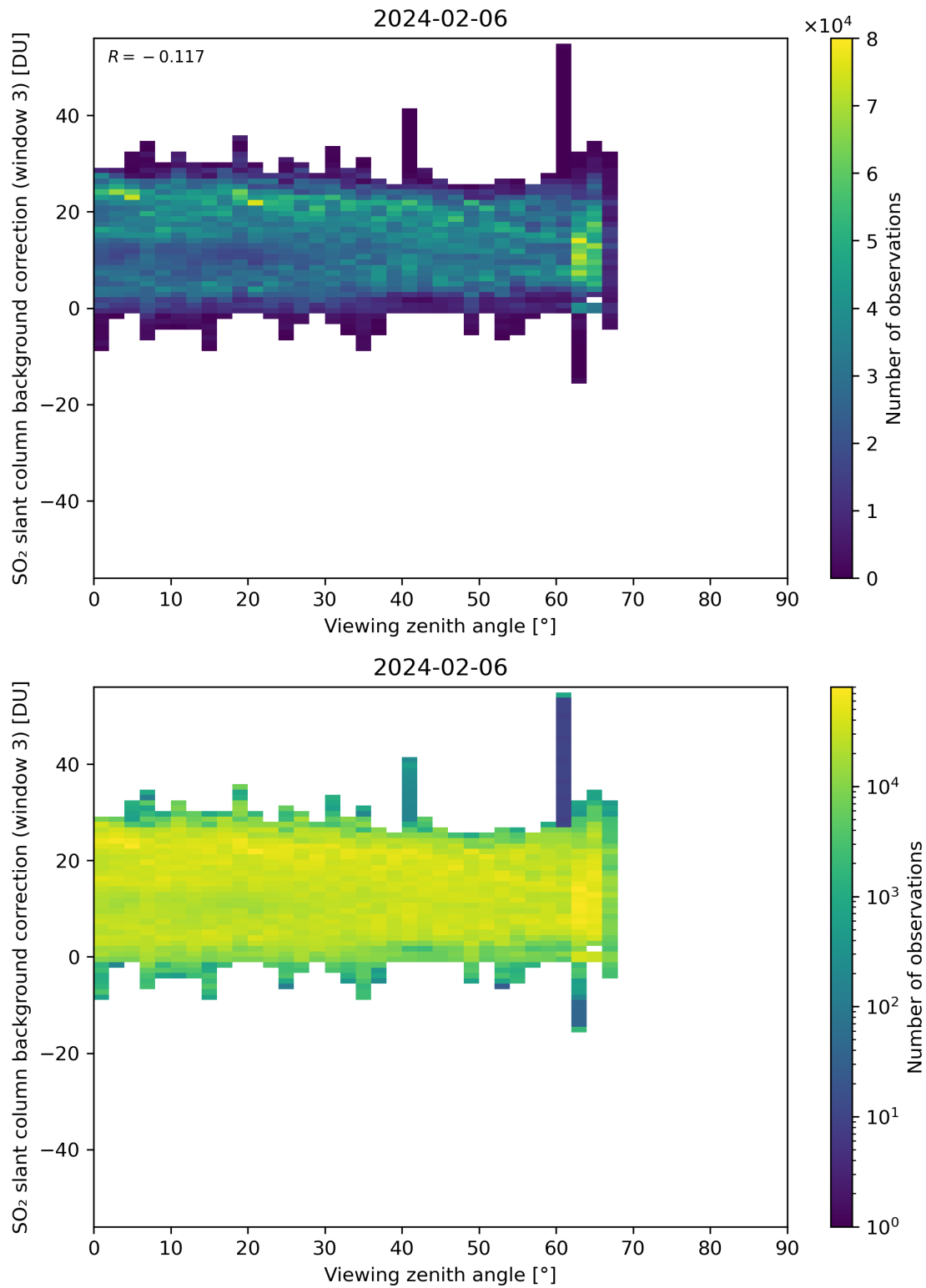
Figure 310: Scatter density plot of “Viewing zenith angle” against “SO 2 slant column background correction (window 3)” for 2024-02-06 to 2024-02-07.
