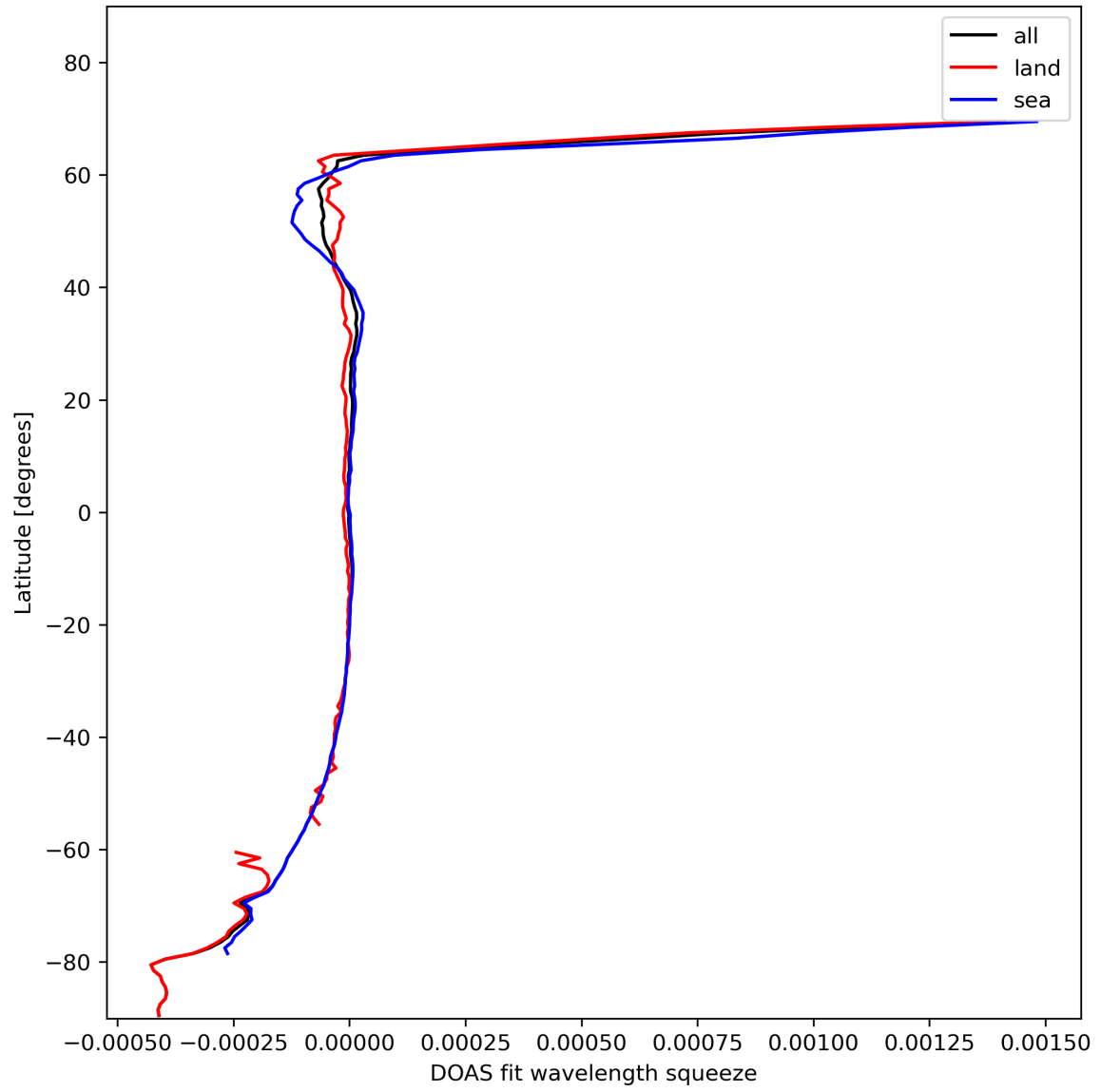
Figure 46: Zonal average of “DOAS fit wavelength squeeze” for 2024-02-06 to 2024-02-07.
