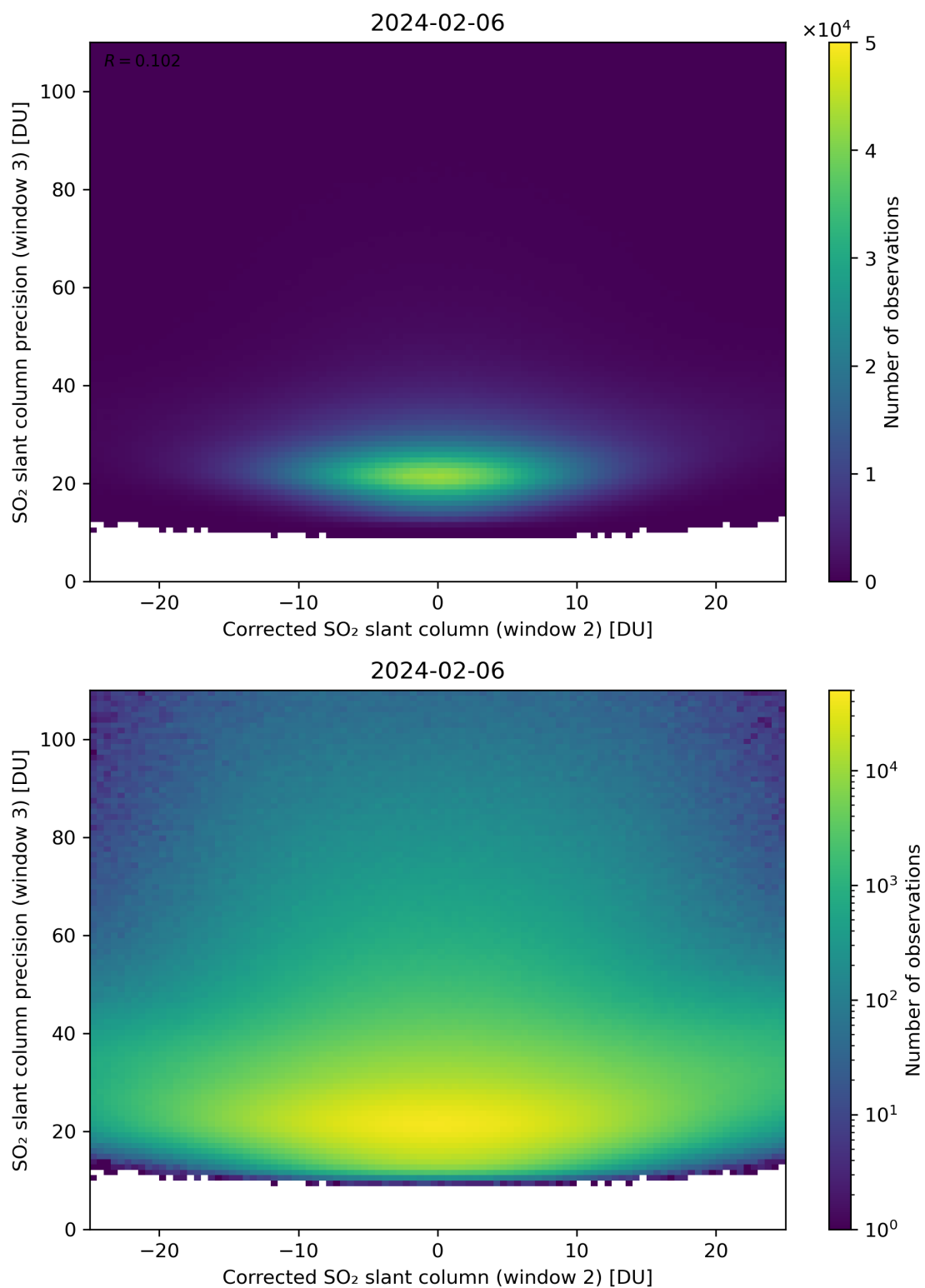
Figure 202: Scatter density plot of “Corrected SO 2 slant column (window 2)” against “SO 2 slant column precision (window 3)” for 2024-02-06 to 2024-02-07.
