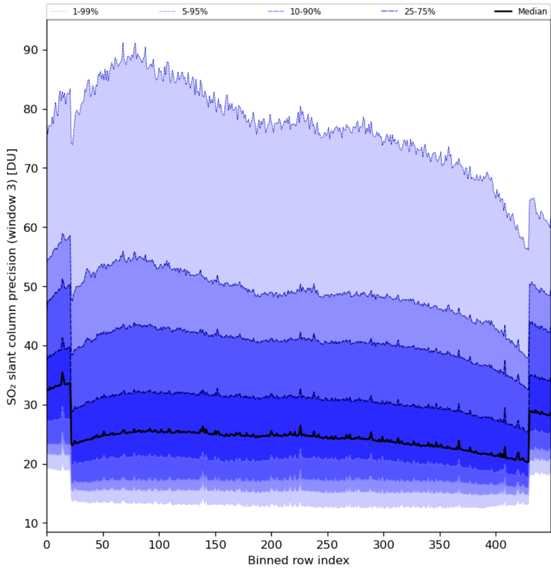
Figure 88: Along track statistics of “SO 2 slant column precision (window 3)” for 2024-02-06 to 2024-02-07
