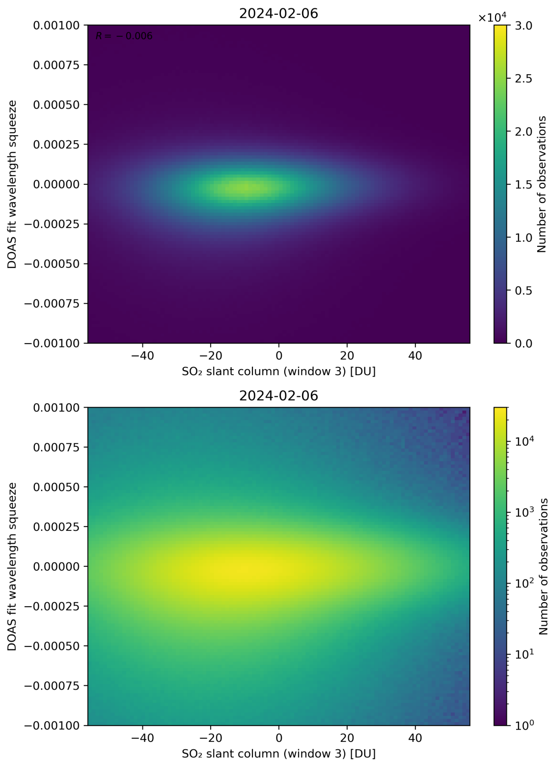
Figure 255: Scatter density plot of “SO 2 slant column (window 3)” against “DOAS fit wavelength squeeze” for 2024-02-06 to 2024-02-07.
