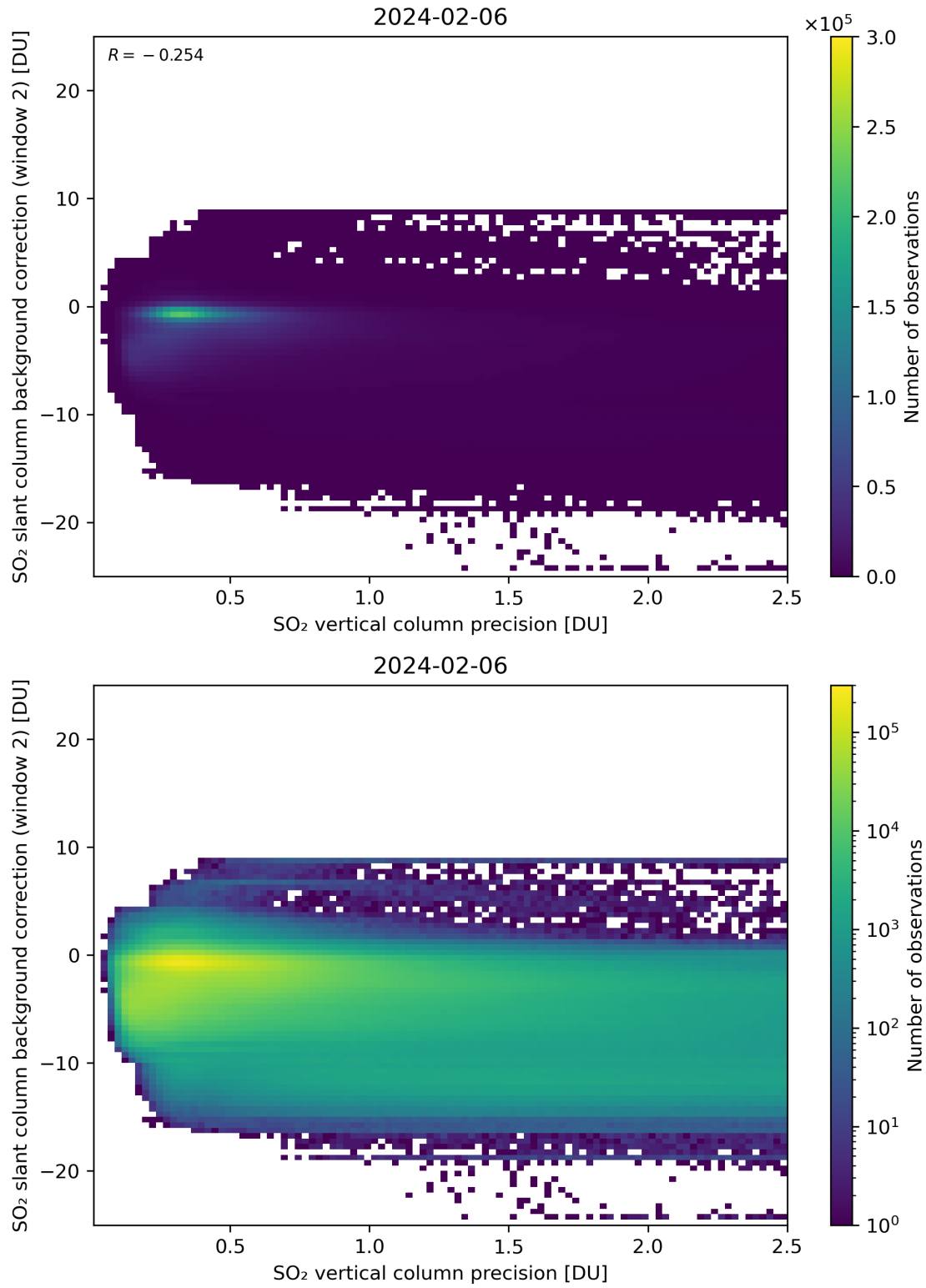
Figure 280: Scatter density plot of “SO 2 vertical column precision” against “SO 2 slant column background correction (window 2)” for 2024-02-06 to 2024-02-07.
