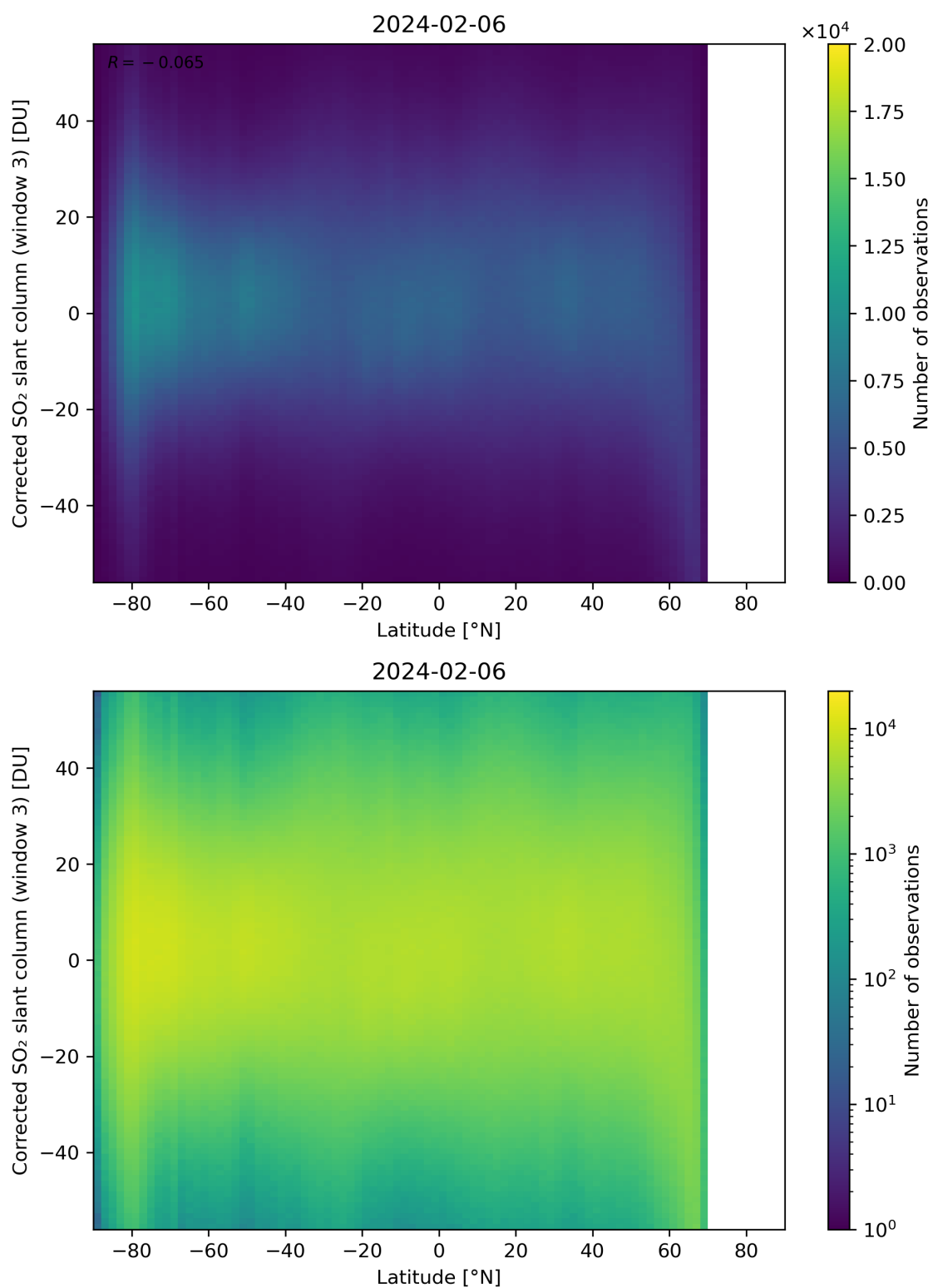
Figure 148: Scatter density plot of “Latitude” against “Corrected SO 2 slant column (window 3)” for 2024-02-06 to 2024-02-07.
