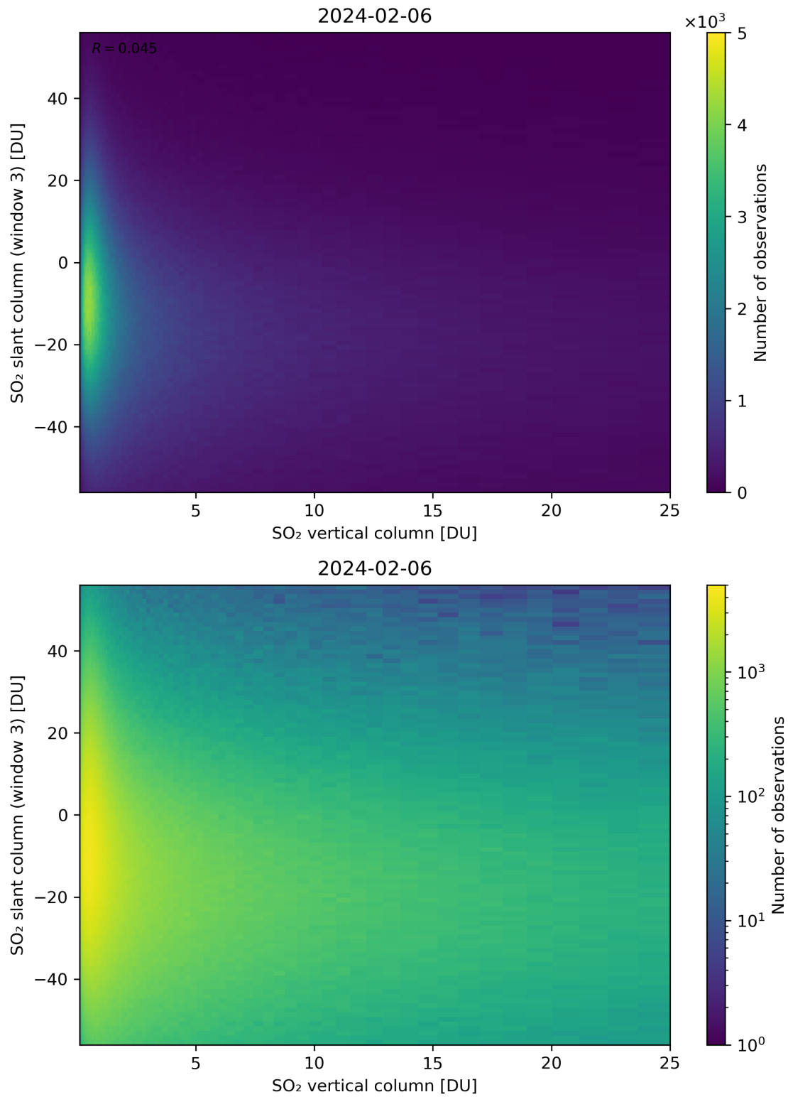
Figure 303: Scatter density plot of “SO 2 vertical column” against “SO 2 slant column (window 3)” for 2024-02-06 to 2024-02-07.
