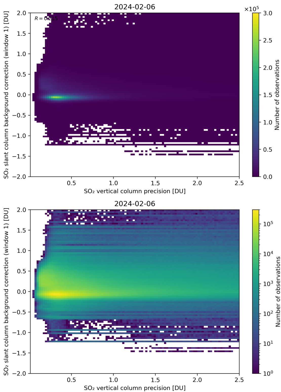
Figure 279: Scatter density plot of “SO 2 vertical column precision” against “SO 2 slant column background correction (window 1)” for 2024-02-06 to 2024-02-07.
