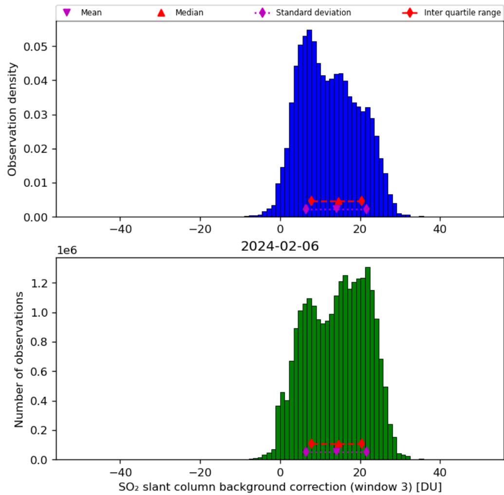
Figure 67: Histogram of “SO 2 slant column background correction (window 3)” for 2024-02-06 to 2024-02-07
