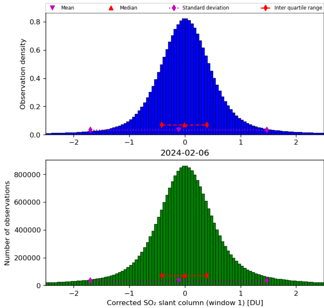
Figure 58: Histogram of “Corrected SO 2 slant column (window 1)” for 2024-02-06 to 2024-02-07
