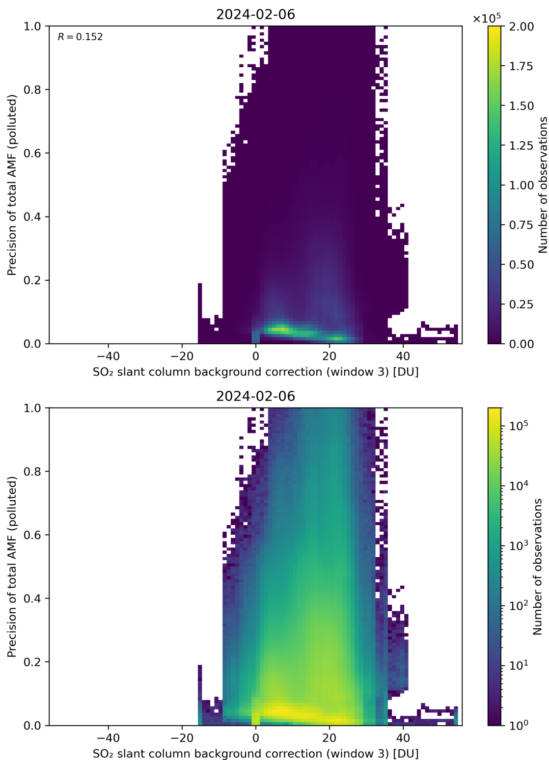
Figure 126: Scatter density plot of “SO 2 slant column background correction (window 3)” against “Precision of total AMF (polluted)” for 2024-02-06 to 2024-02-07.
