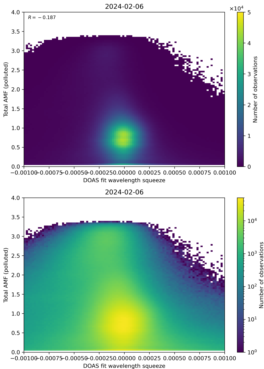
Figure 134: Scatter density plot of “DOAS fit wavelength squeeze” against “Total AMF (polluted)” for 2024-02-06 to 2024-02-07.
