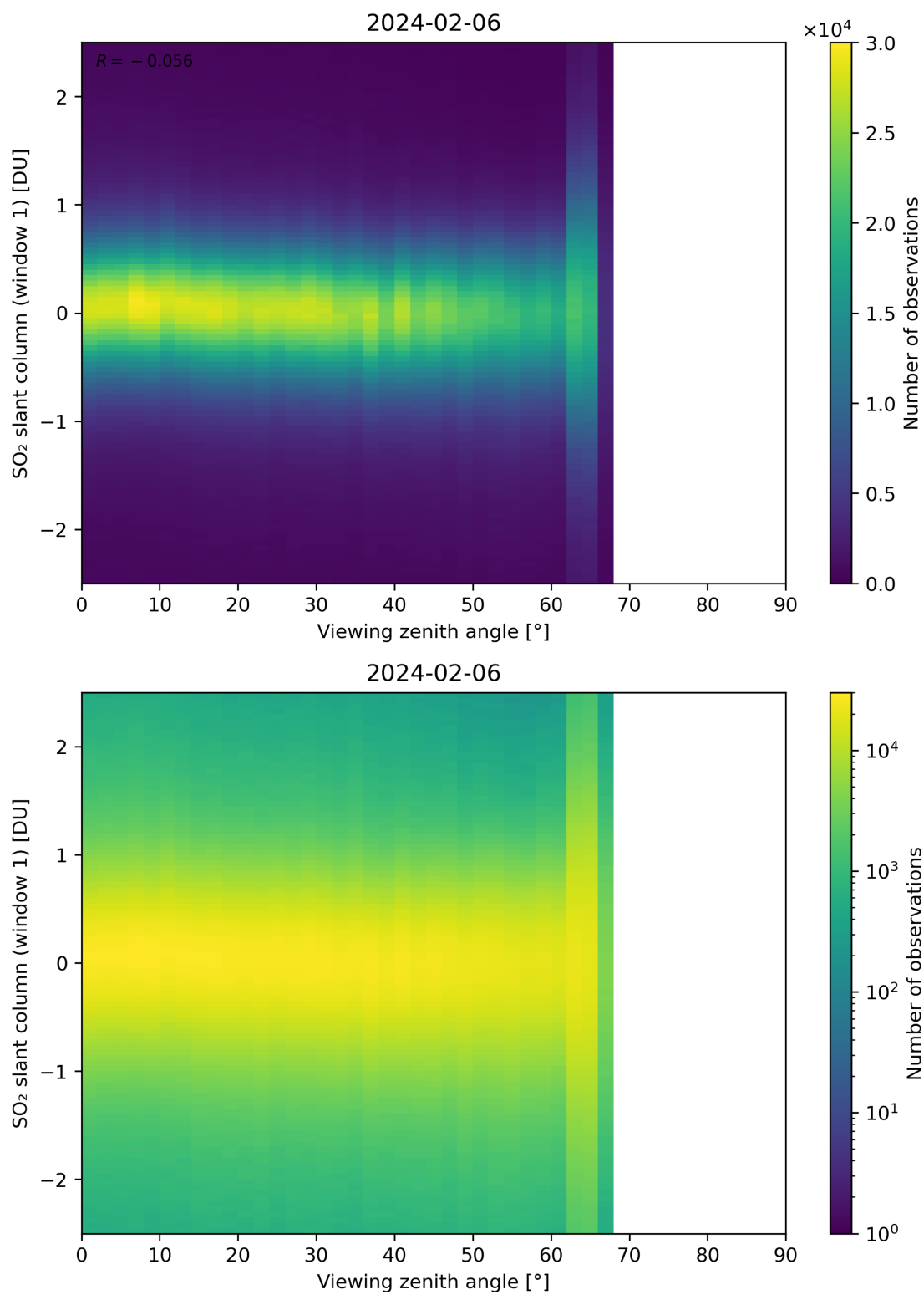
Figure 320: Scatter density plot of “Viewing zenith angle” against “SO 2 slant column (window 1)” for 2024-02-06 to 2024-02-07.
