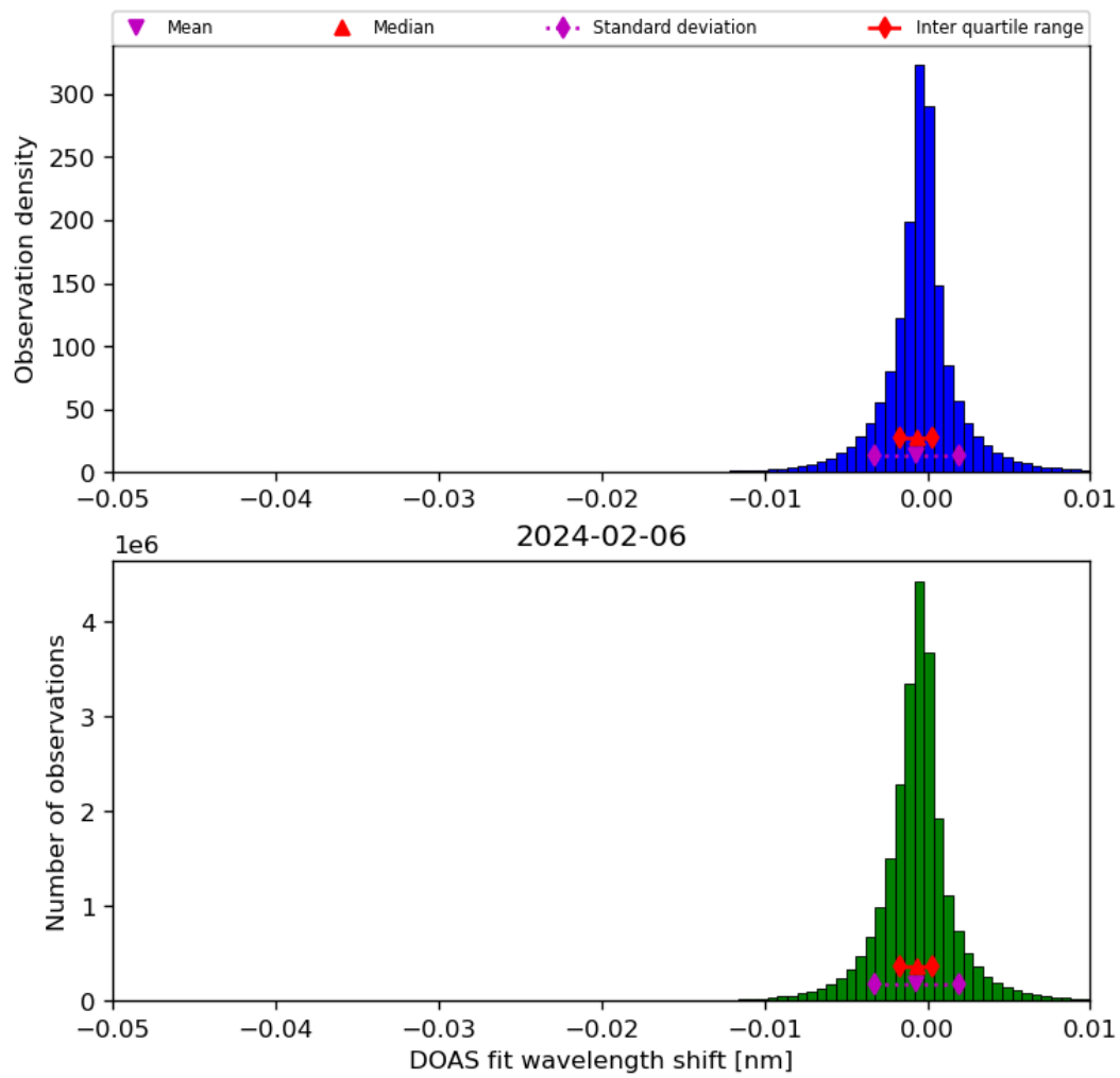
Figure 68: Histogram of “DOAS fit wavelength shift” for 2024-02-06 to 2024-02-07
