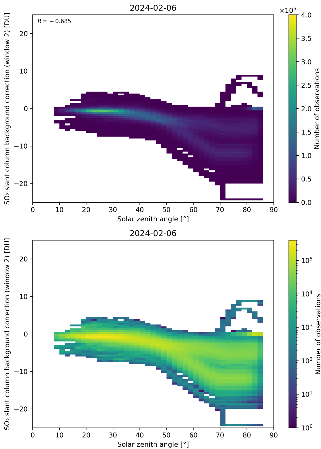
Figure 159: Scatter density plot of “Solar zenith angle” against “SO 2 slant column background correction (window 2)” for 2024-02-06 to 2024-02-07.
