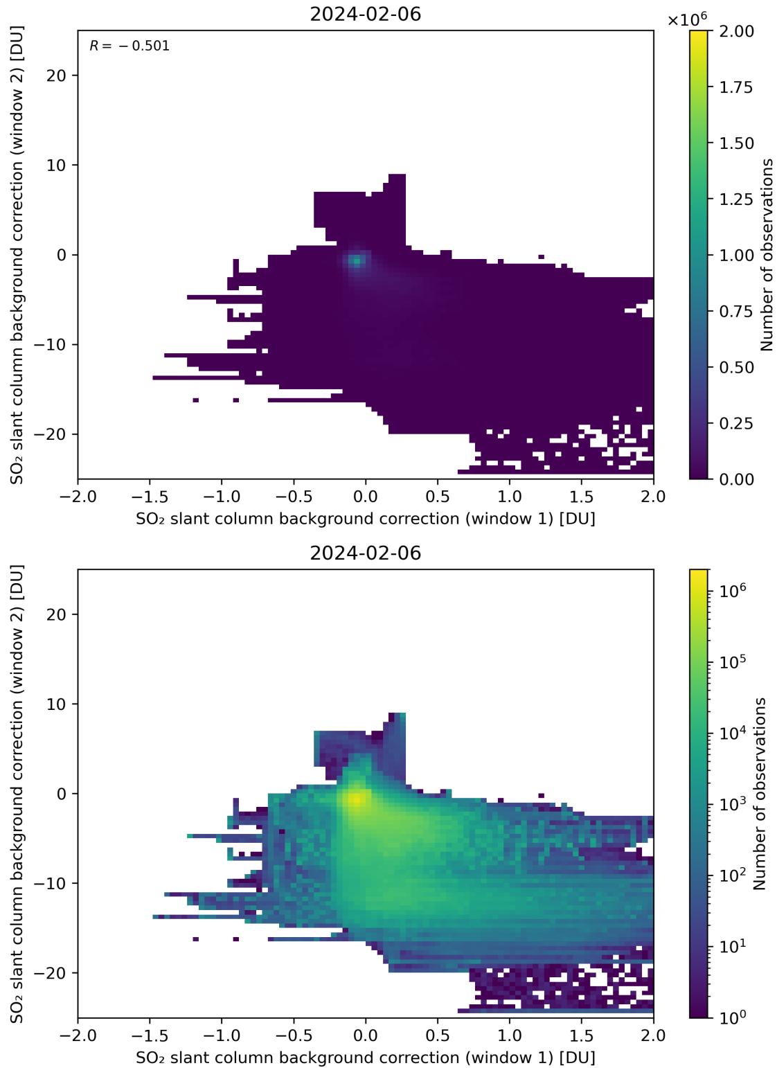
Figure 98: Scatter density plot of “SO 2 slant column background correction (window 1)” against “SO 2 slant column background correction (window 2)” for 2024-02-06 to 2024-02-07.
