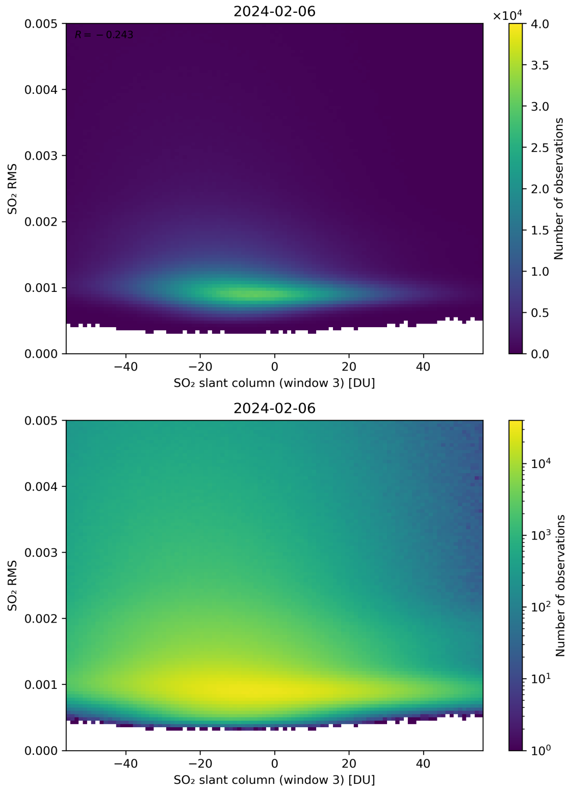
Figure 256: Scatter density plot of “SO 2 slant column (window 3)” against “SO 2 RMS” for 2024-02-06 to 2024-02-07.
