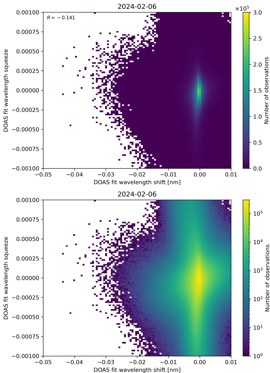
Figure 127: Scatter density plot of “DOAS fit wavelength shift” against “DOAS fit wavelength squeeze” for 2024-02-06 to 2024-02-07.
