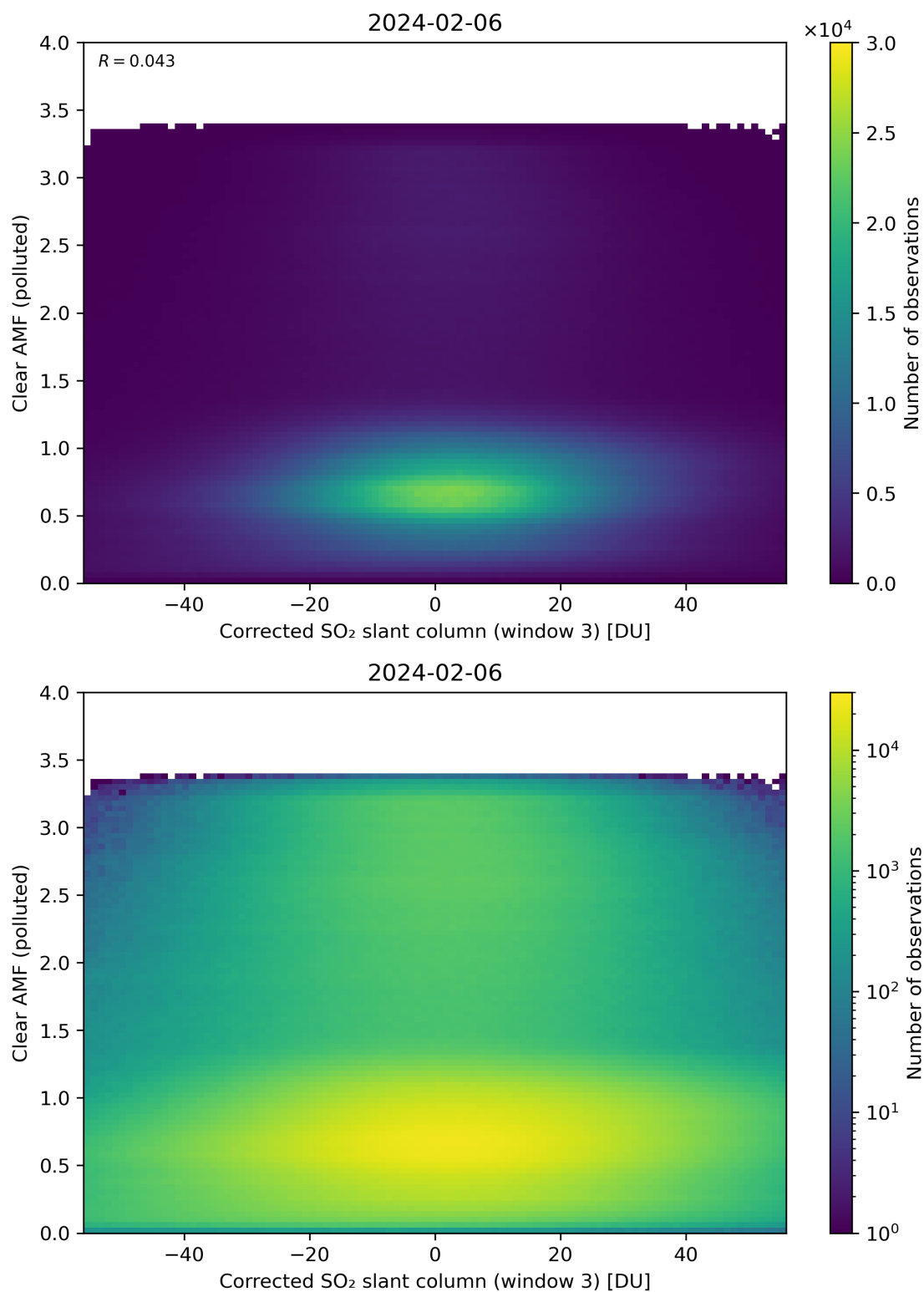
Figure 209: Scatter density plot of “Corrected SO 2 slant column (window 3)” against “Clear AMF (polluted)” for 2024-02-06 to 2024-02-07.
