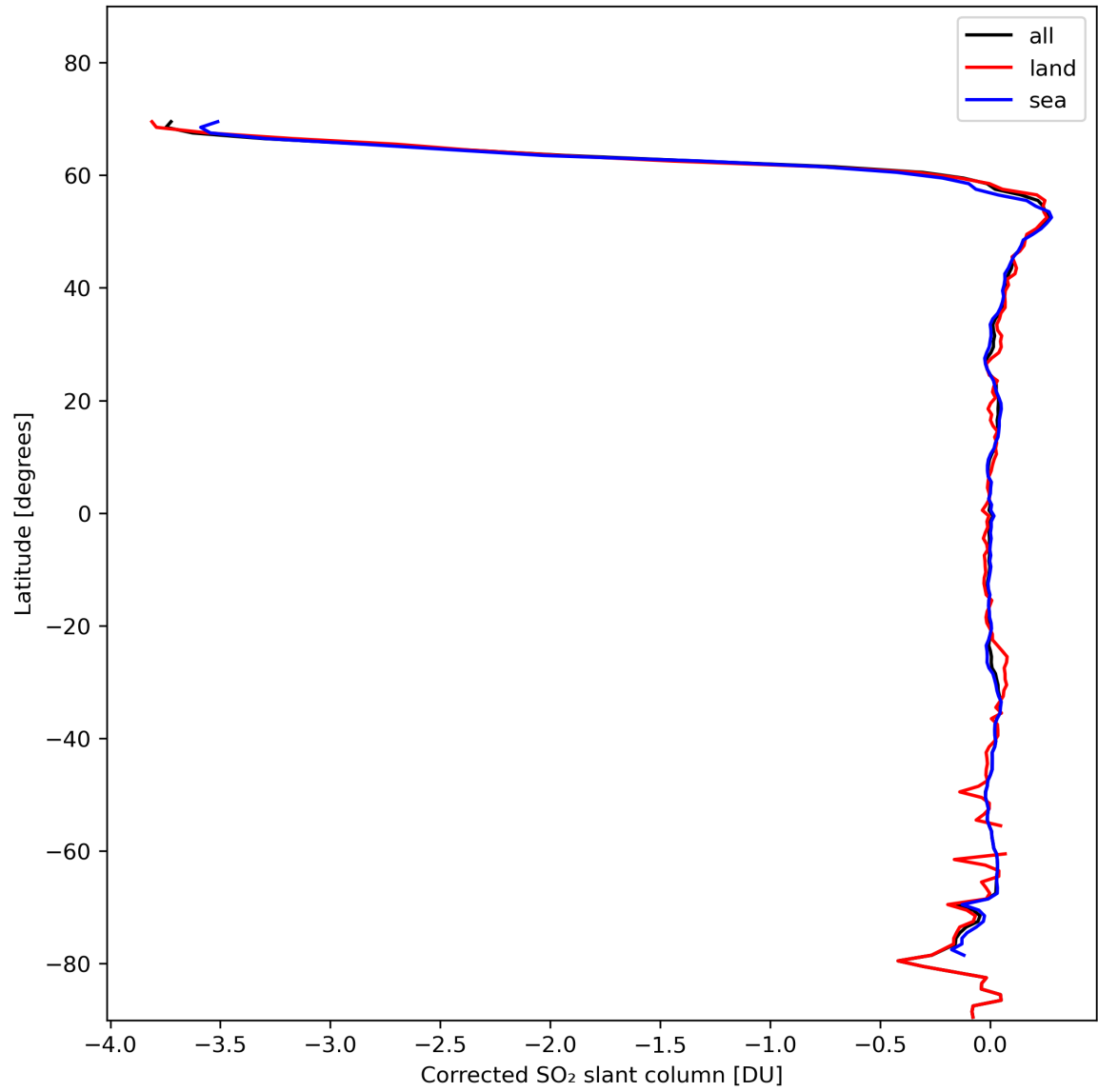
Figure 32: Zonal average of “Corrected SO 2 slant column” for 2024-02-06 to 2024-02-07.
