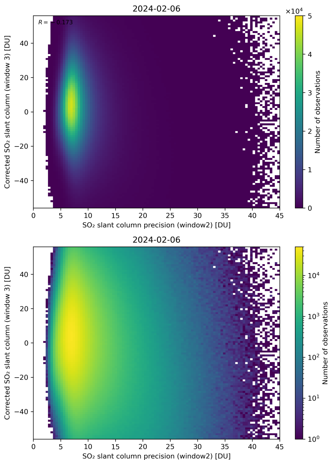
Figure 248: Scatter density plot of “SO 2 slant column precision (window2)” against “Corrected SO 2 slant column (window 3)” for 2024-02-06 to 2024-02-07.
