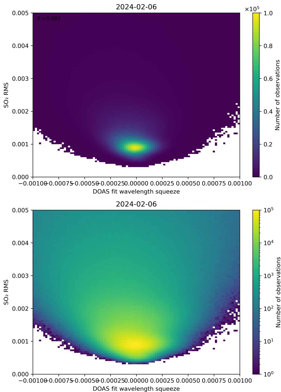
Figure 132: Scatter density plot of “DOAS fit wavelength squeeze” against “SO 2 RMS” for 2024-02-06 to 2024-02-07.
