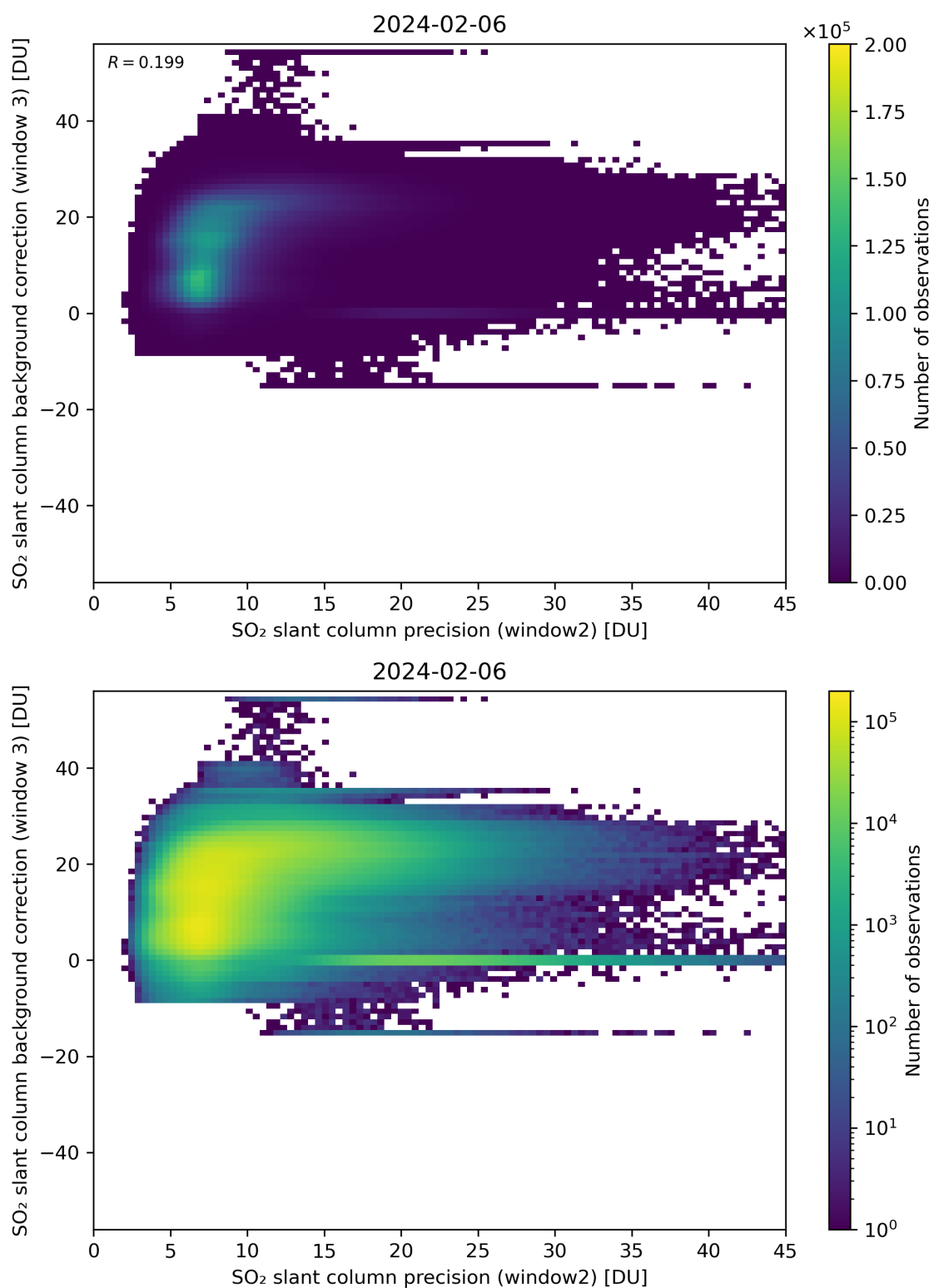
Figure 242: Scatter density plot of “SO 2 slant column precision (window2)” against “SO 2 slant column background correction (window 3)” for 2024-02-06 to 2024-02-07.
