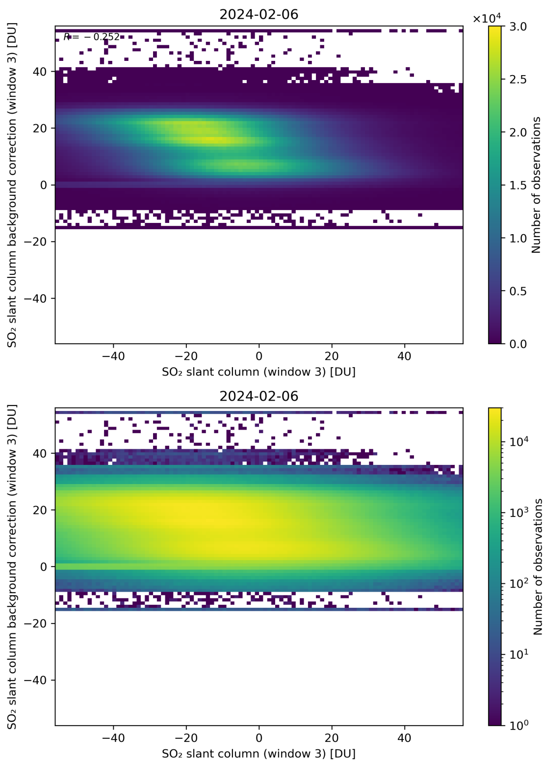
Figure 253: Scatter density plot of “SO 2 slant column (window 3)” against “SO 2 slant column background correction (window 3)” for 2024-02-06 to 2024-02-07.
