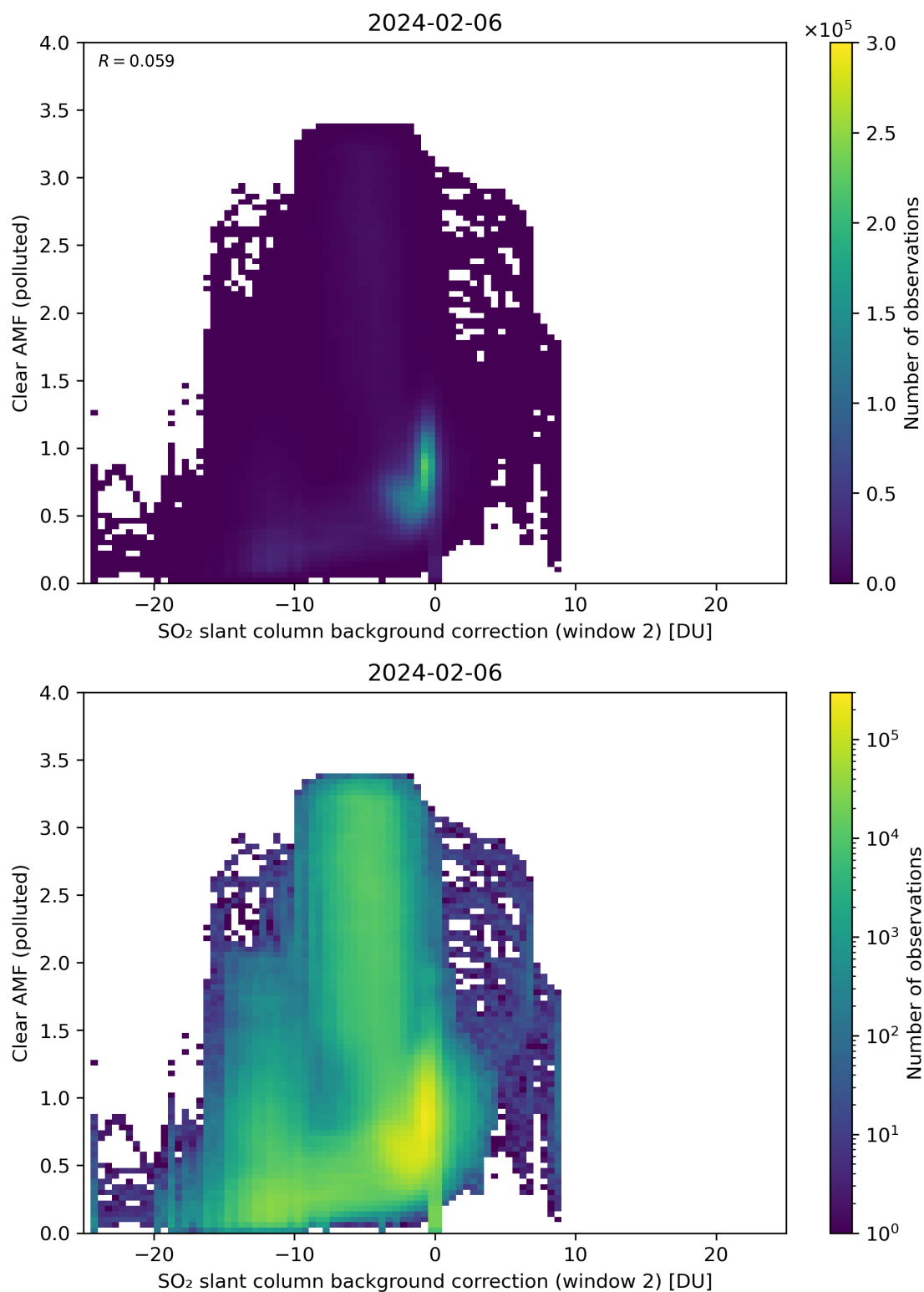
Figure 115: Scatter density plot of “SO 2 slant column background correction (window 2)” against “Clear AMF (polluted)” for 2024-02-06 to 2024-02-07.
