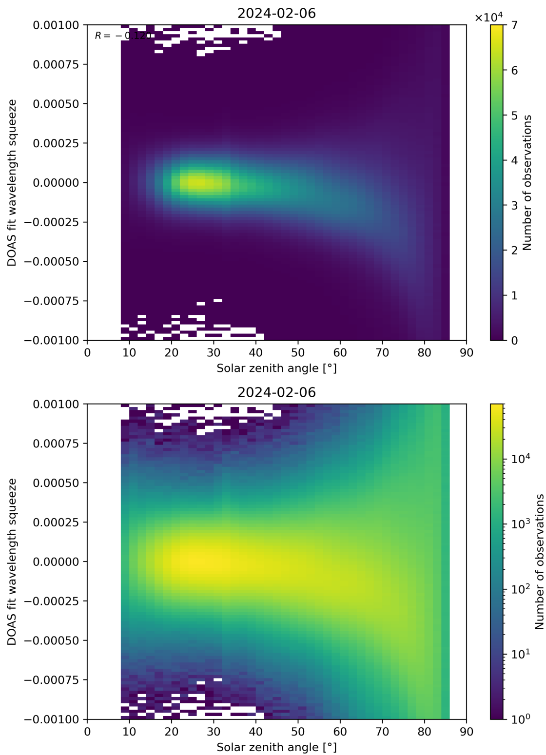
Figure 162: Scatter density plot of “Solar zenith angle” against “DOAS fit wavelength squeeze” for 2024-02-06 to 2024-02-07.
