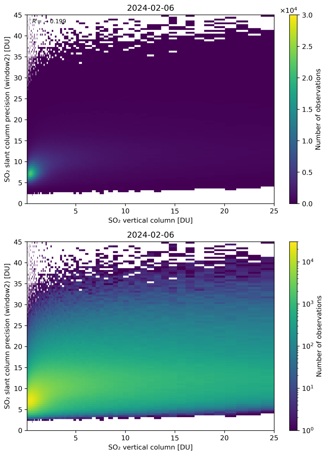
Figure 302: Scatter density plot of “SO 2 vertical column” against “SO 2 slant column precision (window2)” for 2024-02-06 to 2024-02-07.
