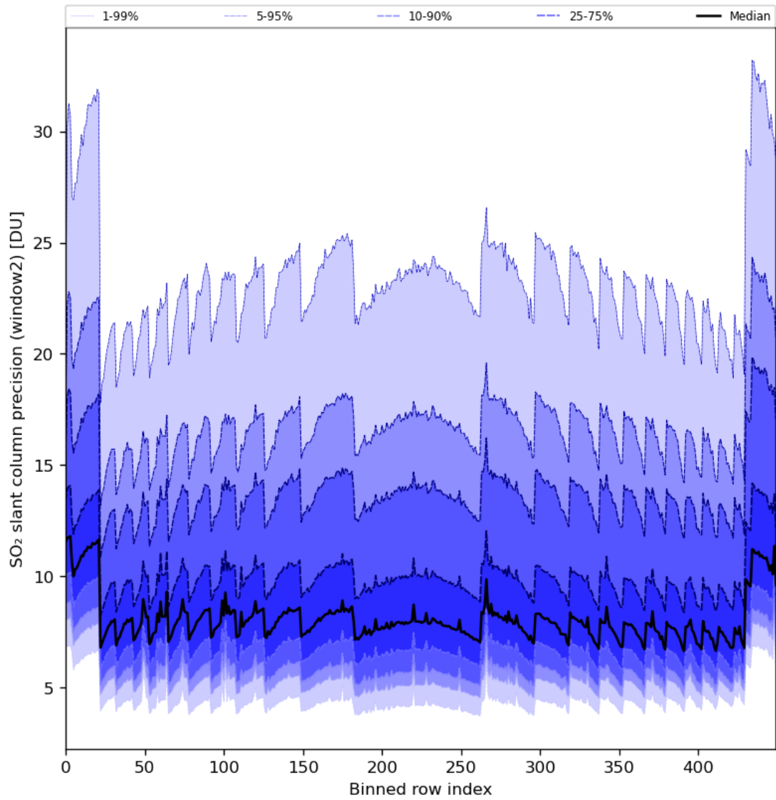
Figure 84: Along track statistics of “SO 2 slant column precision (window2)” for 2024-02-06 to 2024-02-07
