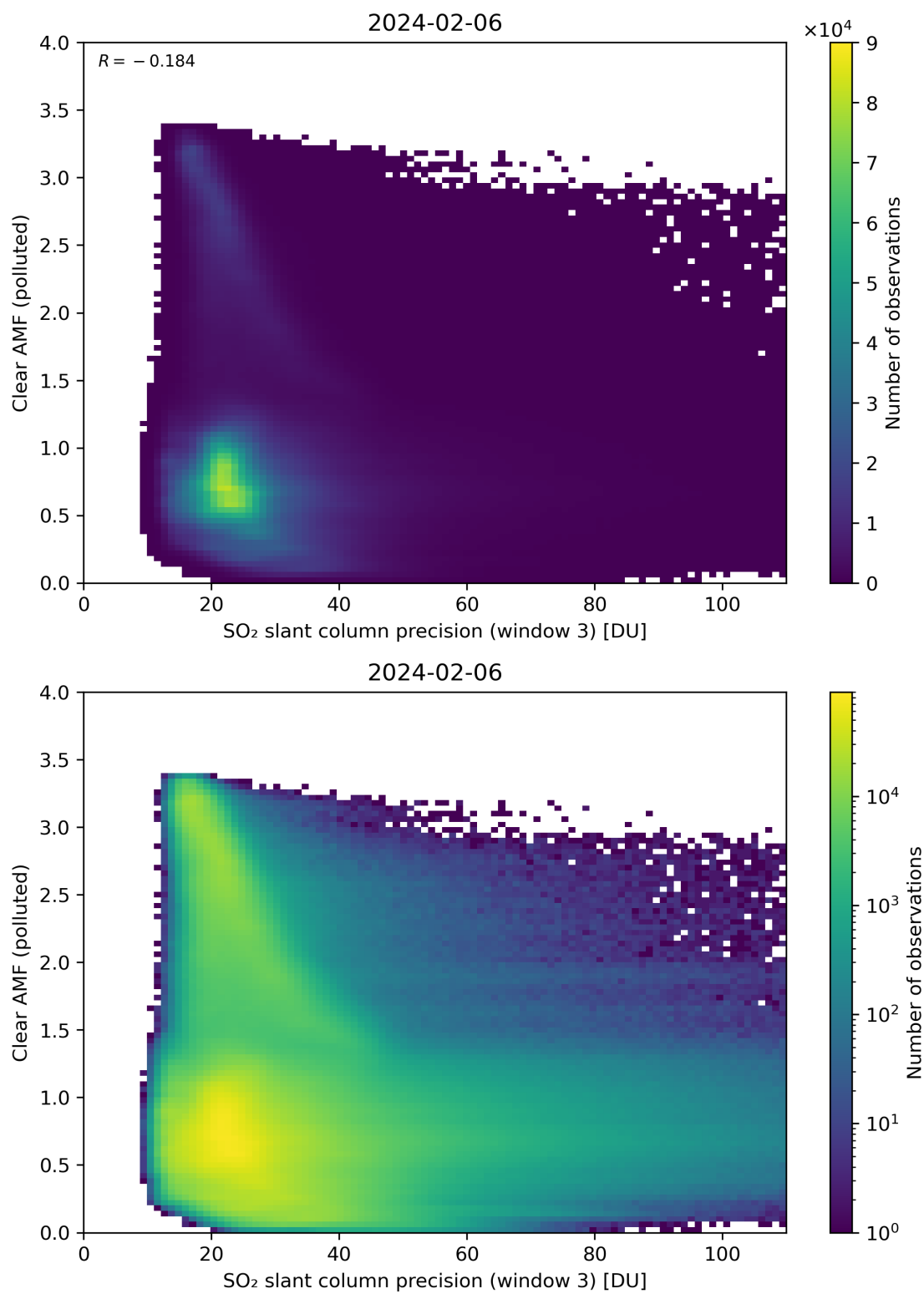
Figure 261: Scatter density plot of “SO 2 slant column precision (window 3)” against “Clear AMF (polluted)” for 2024-02-06 to 2024-02-07.
