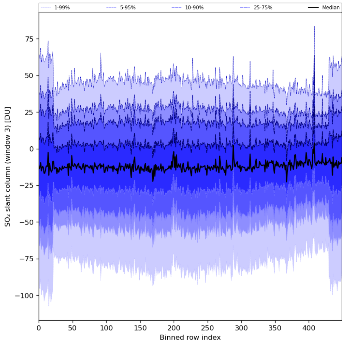
Figure 87: Along track statistics of “SO 2 slant column (window 3)” for 2024-02-06 to 2024-02-07
