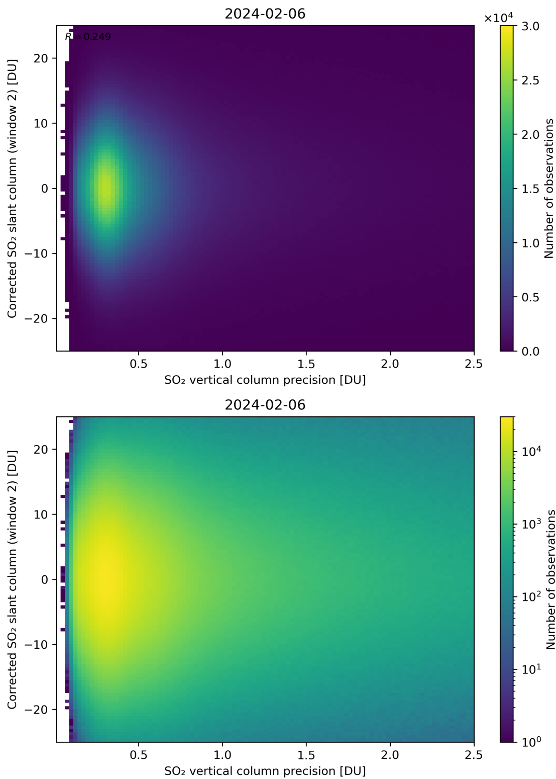
Figure 287: Scatter density plot of “SO 2 vertical column precision” against “Corrected SO 2 slant column (window 2)” for 2024-02-06 to 2024-02-07.
