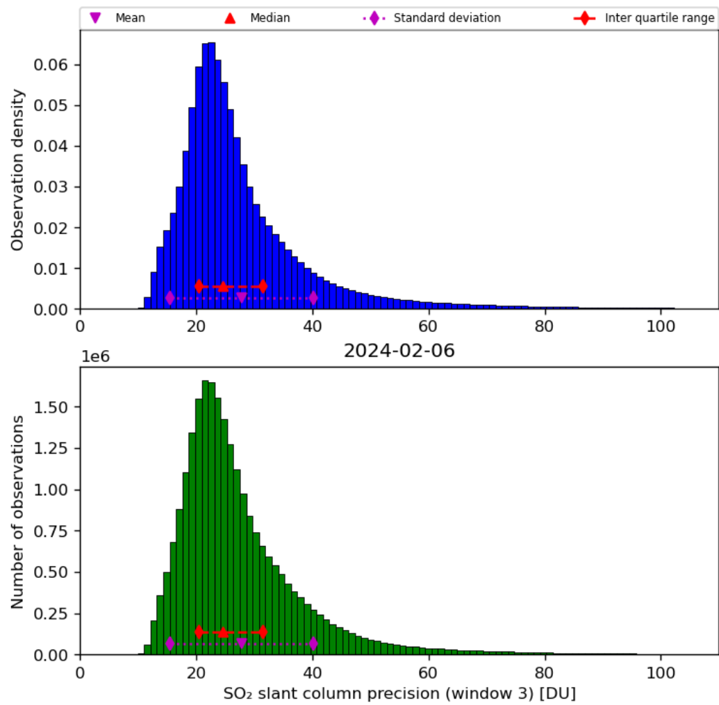
Figure 65: Histogram of “SO 2 slant column precision (window 3)” for 2024-02-06 to 2024-02-07
