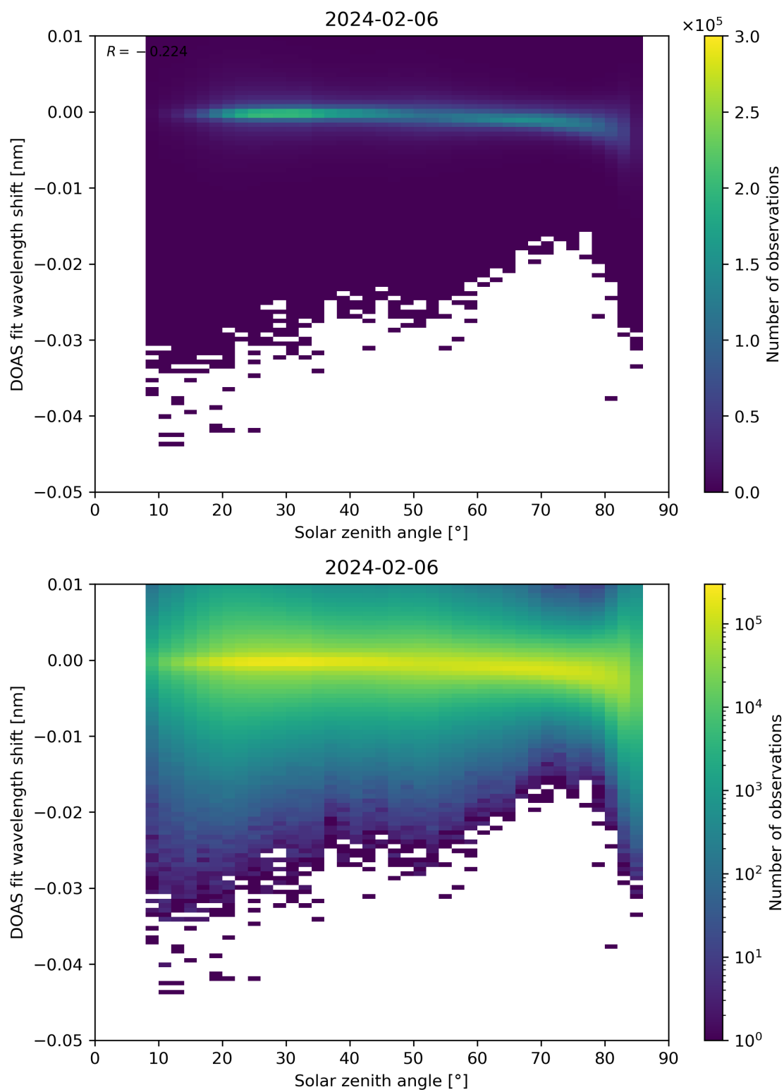
Figure 161: Scatter density plot of “Solar zenith angle” against “DOAS fit wavelength shift” for 2024-02-06 to 2024-02-07.
