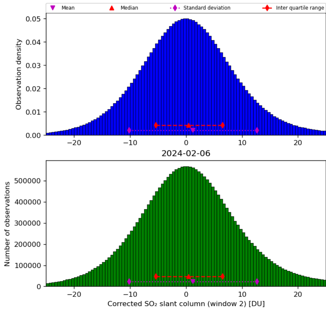
Figure 62: Histogram of “Corrected SO 2 slant column (window 2)” for 2024-02-06 to 2024-02-07
