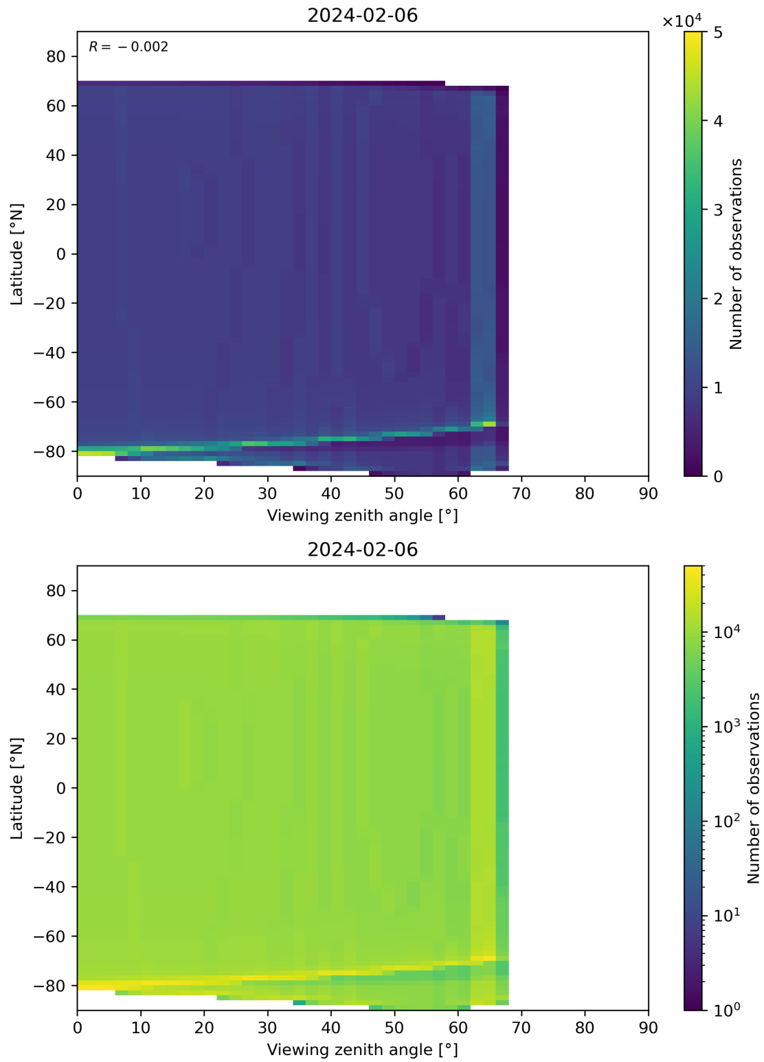
Figure 314: Scatter density plot of “Viewing zenith angle” against “Latitude” for 2024-02-06 to 2024-02-07.
