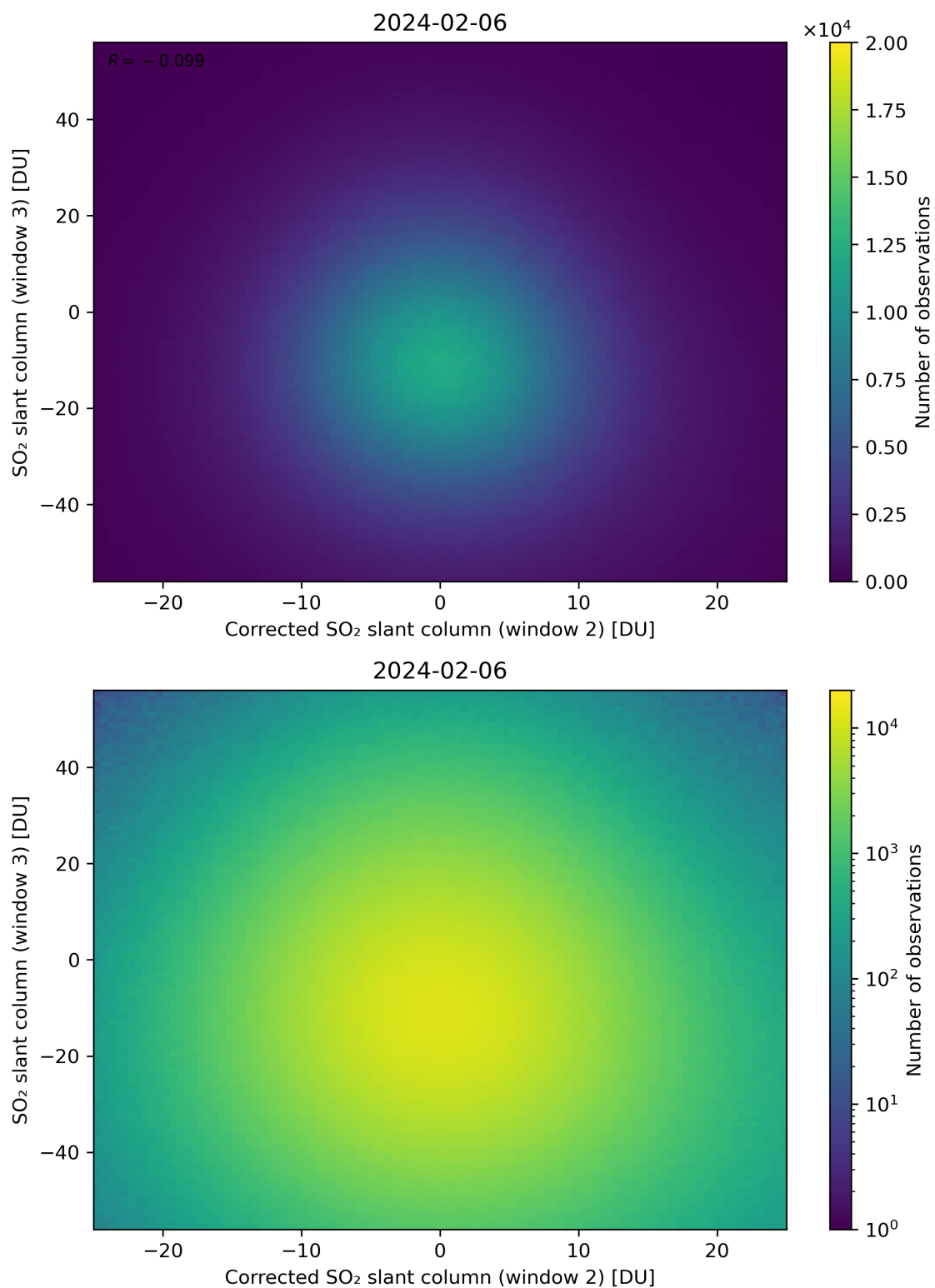
Figure 201: Scatter density plot of “Corrected SO 2 slant column (window 2)” against “SO 2 slant column (window 3)” for 2024-02-06 to 2024-02-07.
