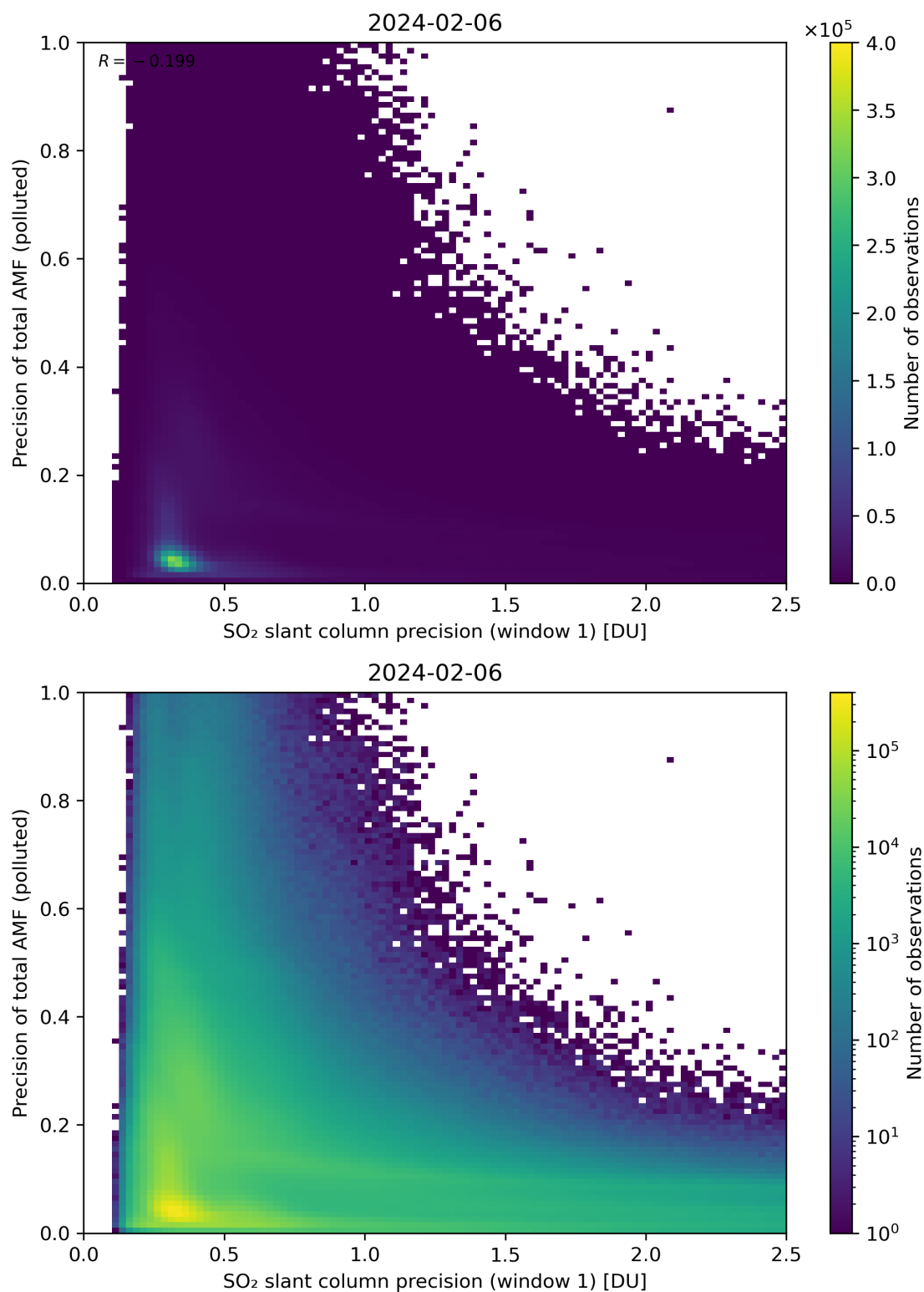
Figure 231: Scatter density plot of “SO 2 slant column precision (window 1)” against “Precision of total AMF (polluted)” for 2024-02-06 to 2024-02-07.
