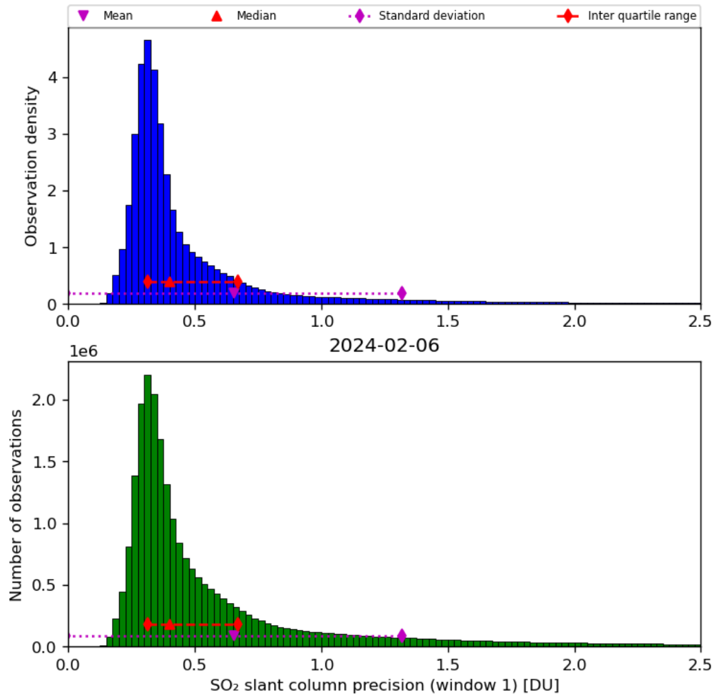
Figure 57: Histogram of “SO 2 slant column precision (window 1)” for 2024-02-06 to 2024-02-07
