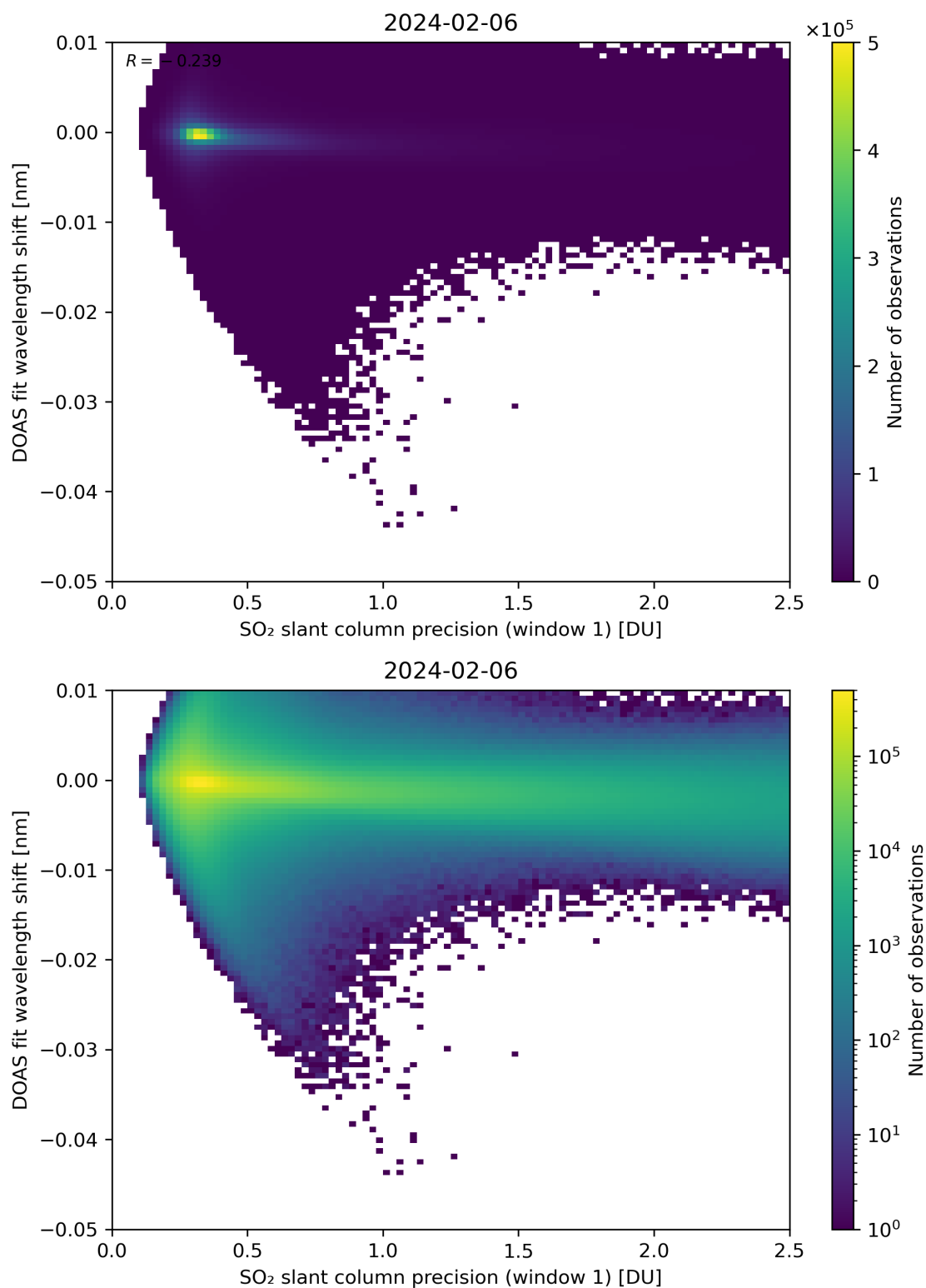
Figure 221: Scatter density plot of “SO 2 slant column precision (window 1)” against “DOAS fit wavelength shift” for 2024-02-06 to 2024-02-07.
