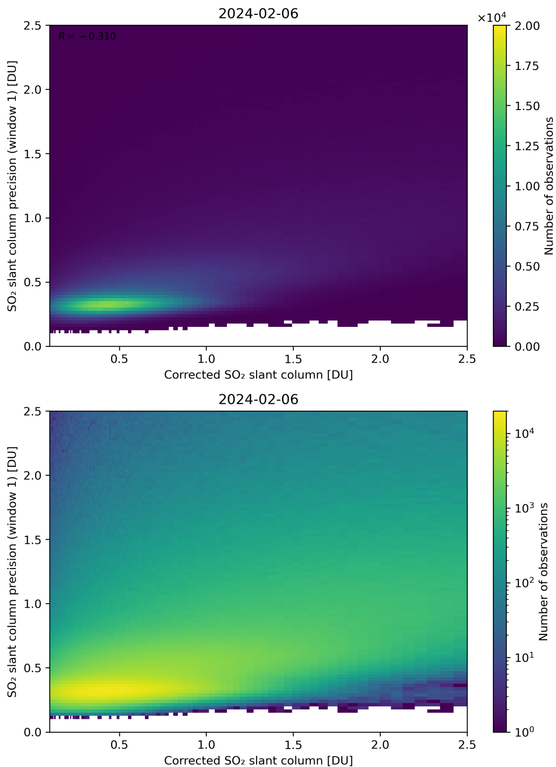
Figure 188: Scatter density plot of “Corrected SO 2 slant column” against “SO 2 slant column precision (window 1)” for 2024-02-06 to 2024-02-07.
