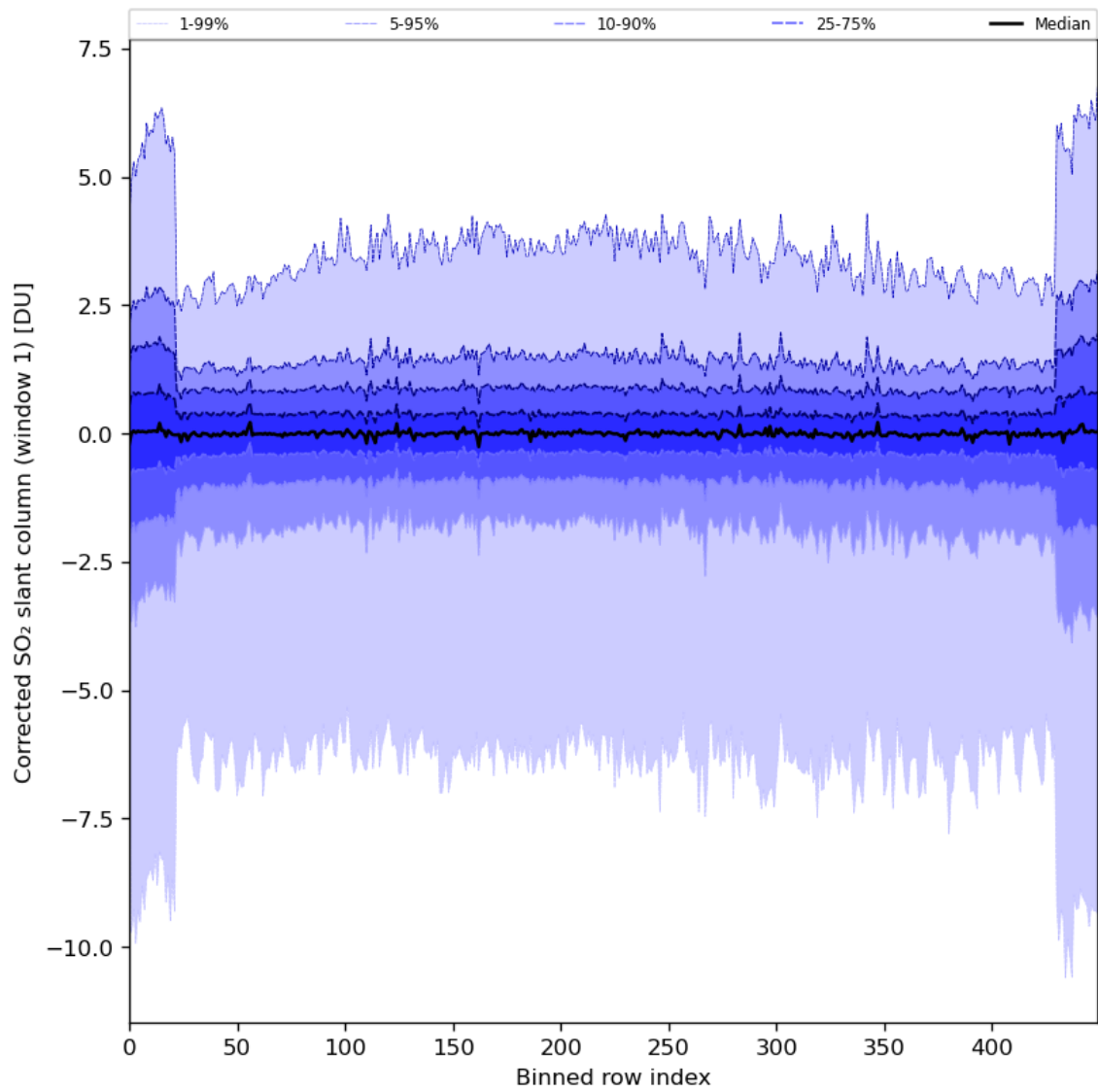
Figure 81: Along track statistics of “Corrected SO 2 slant column (window 1)” for 2024-02-06 to 2024-02-07
