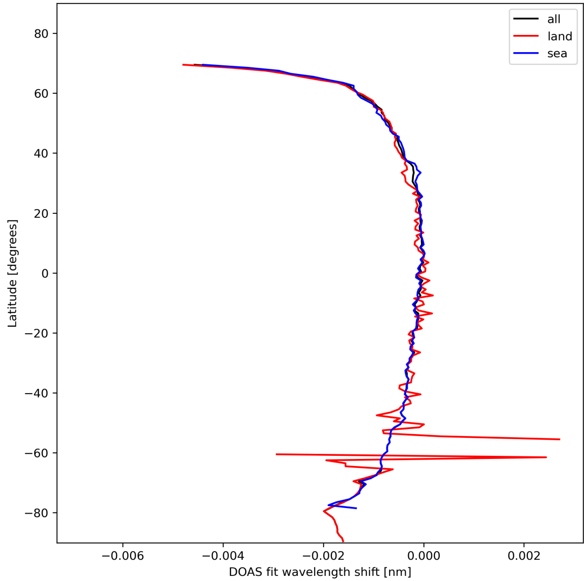
Figure 45: Zonal average of “DOAS fit wavelength shift” for 2024-02-06 to 2024-02-07.
