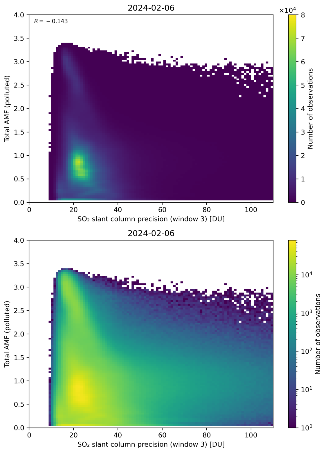
Figure 263: Scatter density plot of “SO 2 slant column precision (window 3)” against “Total AMF (polluted)” for 2024-02-06 to 2024-02-07.
