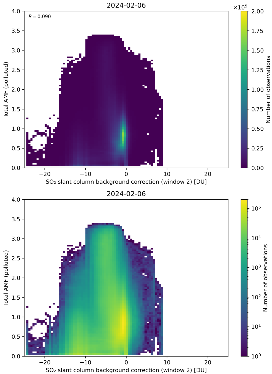
Figure 119: Scatter density plot of “SO 2 slant column background correction (window 2)” against “Total AMF (polluted)” for 2024-02-06 to 2024-02-07.
