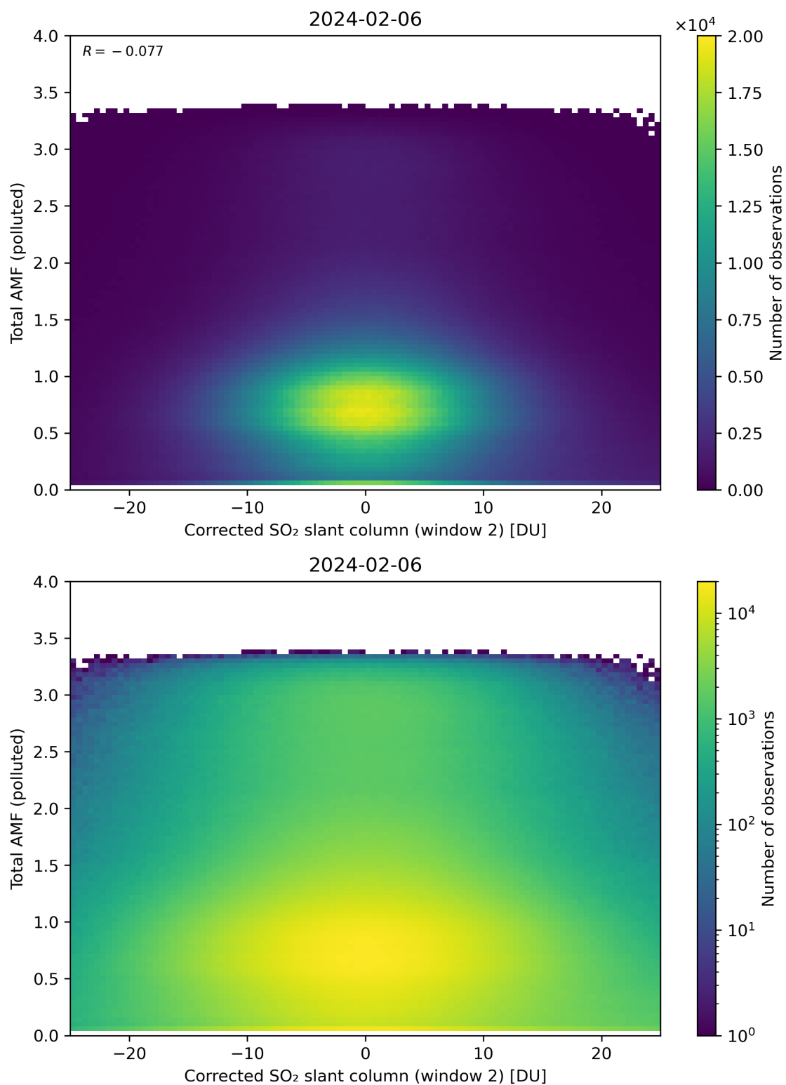
Figure 203: Scatter density plot of “Corrected SO 2 slant column (window 2)” against “Total AMF (polluted)” for 2024-02-06 to 2024-02-07.
