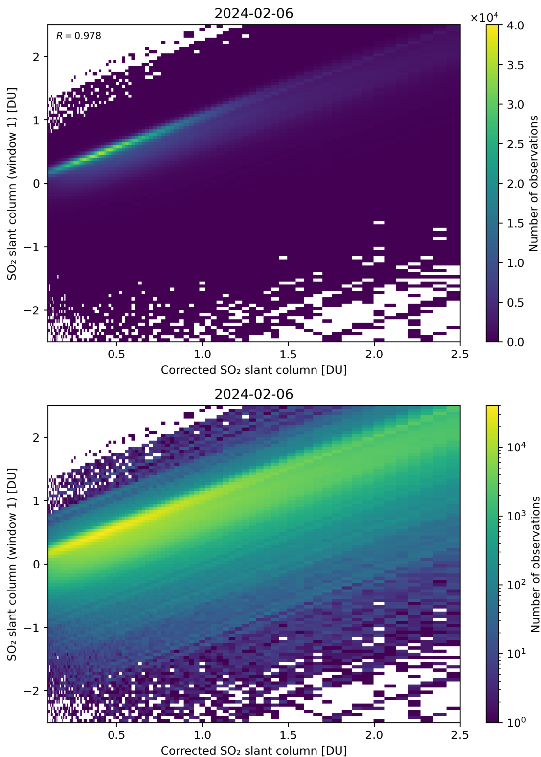
Figure 187: Scatter density plot of “Corrected SO 2 slant column” against “SO 2 slant column (window 1)” for 2024-02-06 to 2024-02-07.
