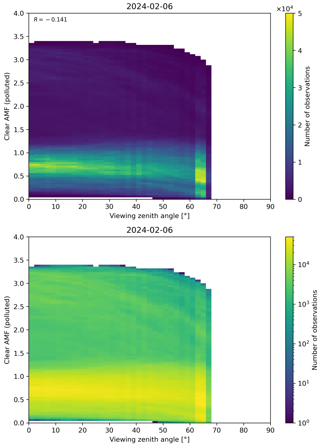
Figure 316: Scatter density plot of “Viewing zenith angle” against “Clear AMF (polluted)” for 2024-02-06 to 2024-02-07.
