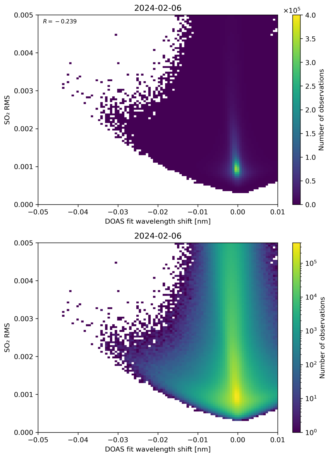
Figure 128: Scatter density plot of “DOAS fit wavelength shift” against “SO 2 RMS” for 2024-02-06 to 2024-02-07.
