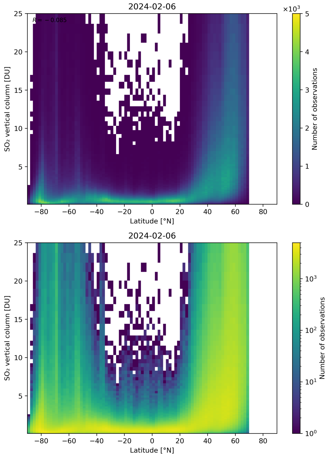
Figure 156: Scatter density plot of “Latitude” against “SO 2 vertical column” for 2024-02-06 to 2024-02-07.
