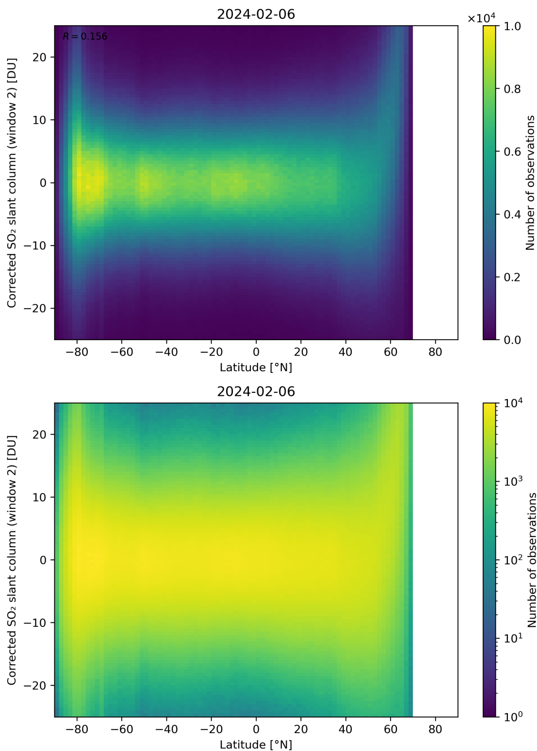
Figure 147: Scatter density plot of “Latitude” against “Corrected SO 2 slant column (window 2)” for 2024-02-06 to 2024-02-07.
