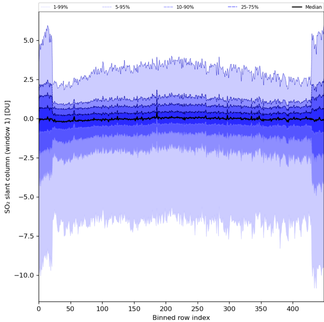
Figure 79: Along track statistics of “SO 2 slant column (window 1)” for 2024-02-06 to 2024-02-07
