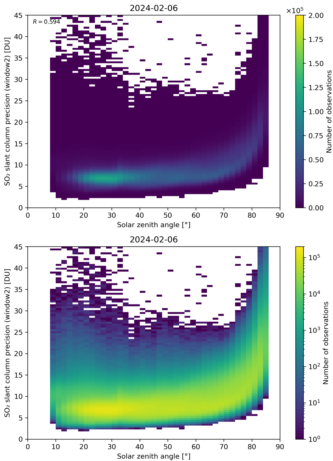
Figure 171: Scatter density plot of “Solar zenith angle” against “SO 2 slant column precision (window2)” for 2024-02-06 to 2024-02-07.
