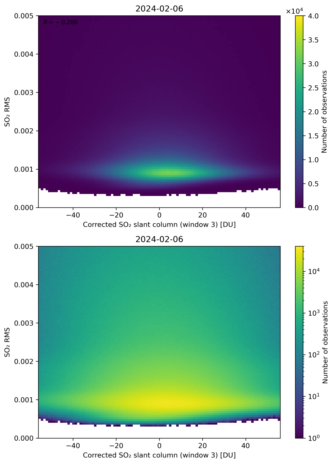
Figure 208: Scatter density plot of “Corrected SO 2 slant column (window 3)” against “SO 2 RMS” for 2024-02-06 to 2024-02-07.
