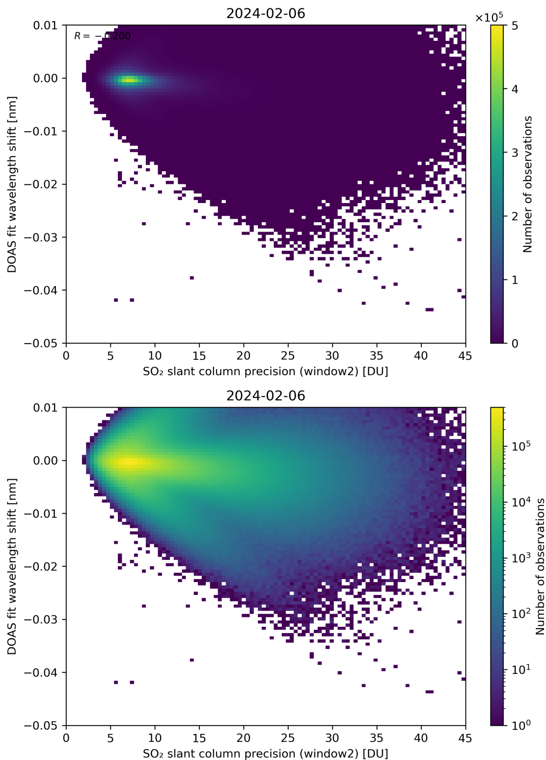
Figure 243: Scatter density plot of “SO 2 slant column precision (window2)” against “DOAS fit wavelength shift” for 2024-02-06 to 2024-02-07.
