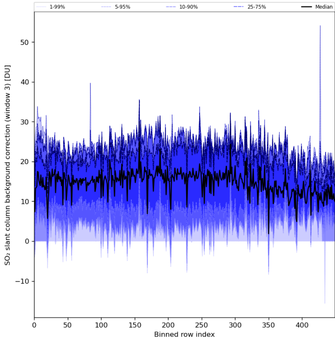
Figure 90: Along track statistics of “SO 2 slant column background correction (window 3)” for 2024-02-06 to 2024-02-07
