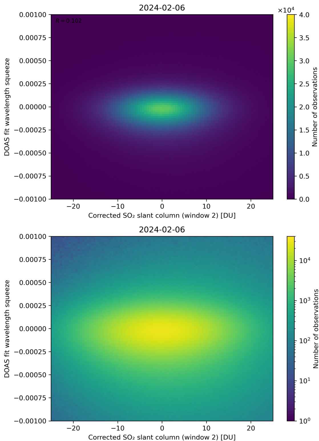
Figure 197: Scatter density plot of “Corrected SO 2 slant column (window 2)” against “DOAS fit wavelength squeeze” for 2024-02-06 to 2024-02-07.
