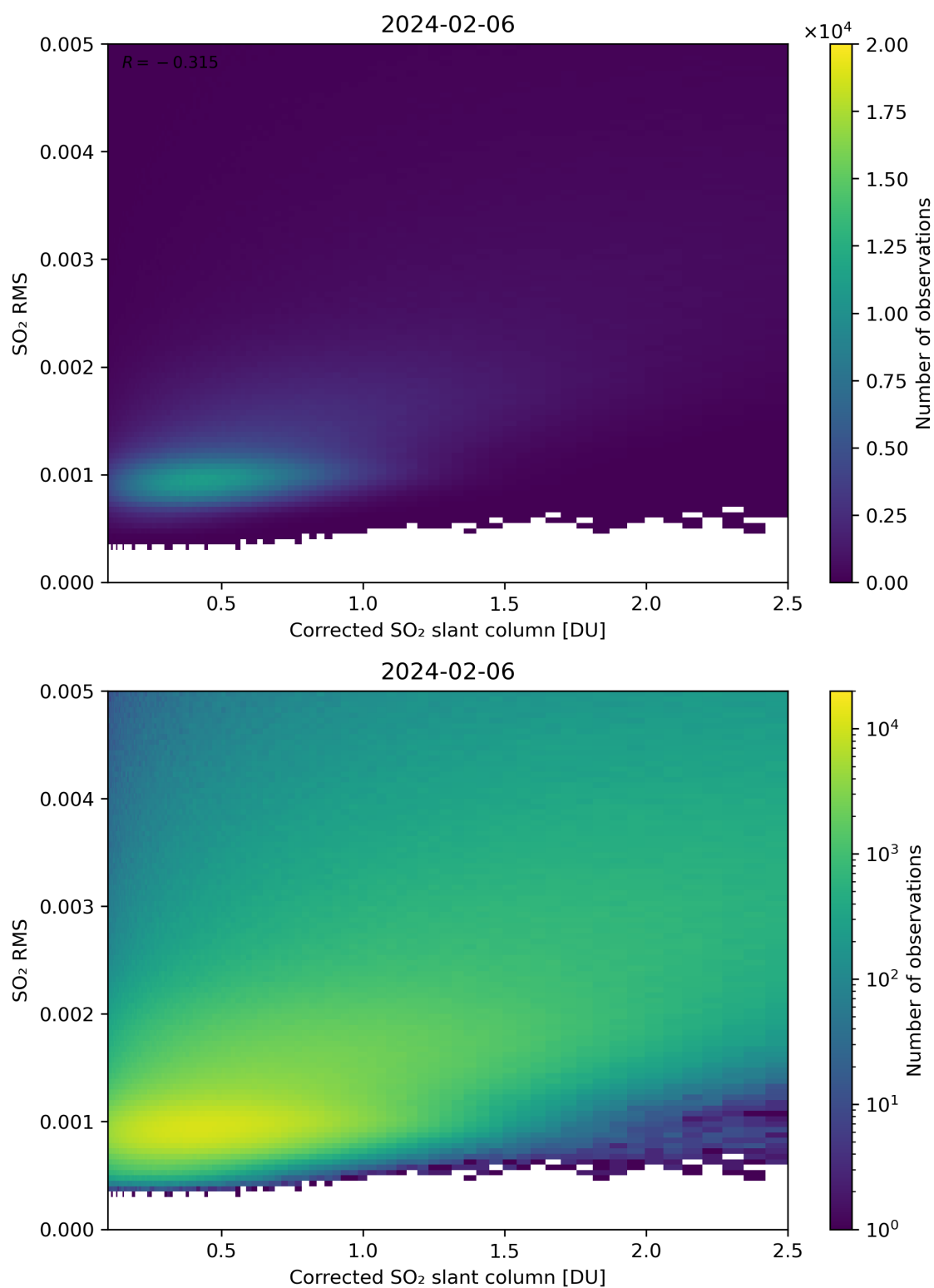
Figure 183: Scatter density plot of “Corrected SO 2 slant column” against “SO 2 RMS” for 2024-02-06 to 2024-02-07.
