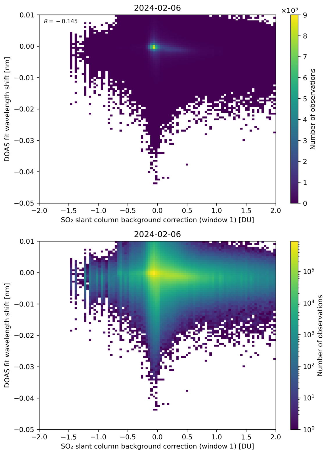
Figure 100: Scatter density plot of “SO 2 slant column background correction (window 1)” against “DOAS fit wavelength shift” for 2024-02-06 to 2024-02-07.
