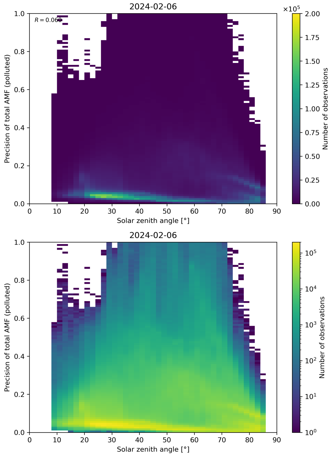
Figure 175: Scatter density plot of “Solar zenith angle” against “Precision of total AMF (polluted)” for 2024-02-06 to 2024-02-07.
