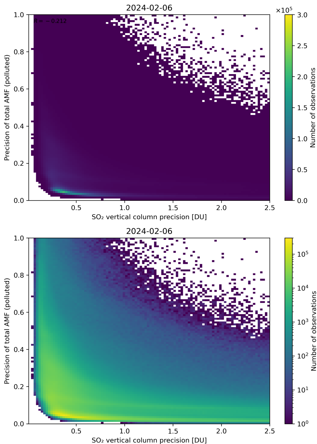
Figure 295: Scatter density plot of “SO 2 vertical column precision” against “Precision of total AMF (polluted)” for 2024-02-06 to 2024-02-07.
