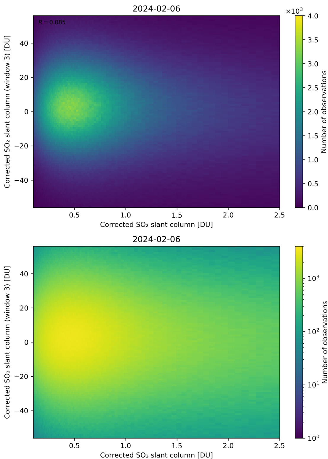
Figure 186: Scatter density plot of “Corrected SO 2 slant column” against “Corrected SO 2 slant column (window 3)” for 2024-02-06 to 2024-02-07.
