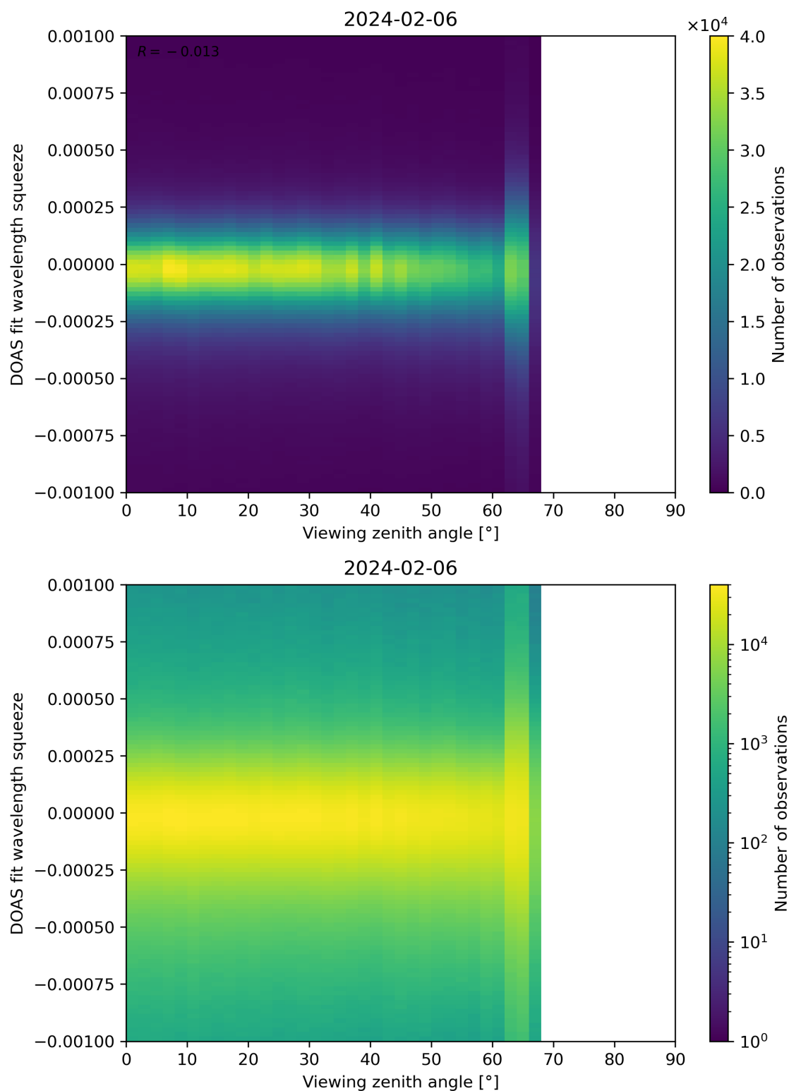
Figure 312: Scatter density plot of “Viewing zenith angle” against “DOAS fit wavelength squeeze” for 2024-02-06 to 2024-02-07.
