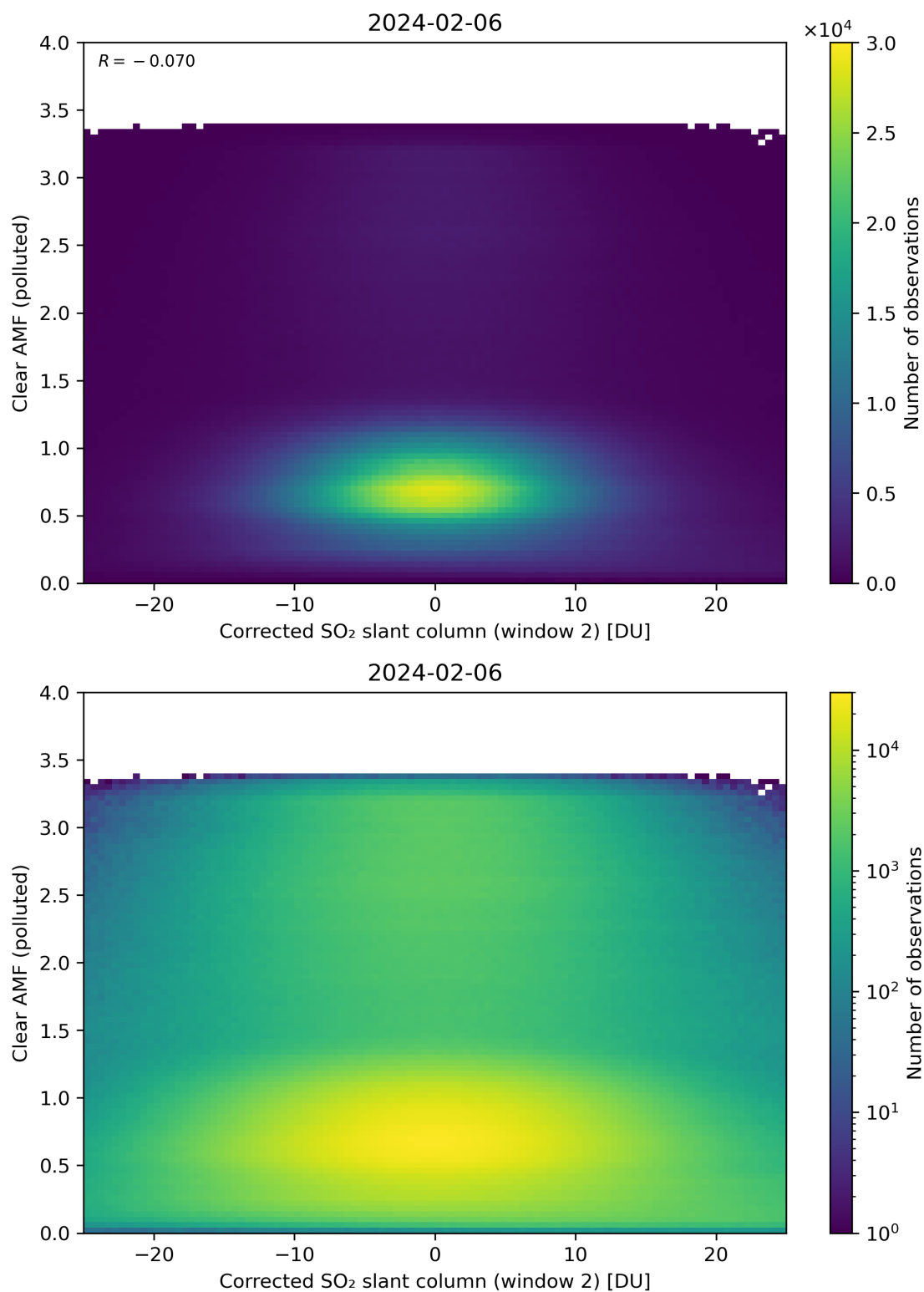
Figure 199: Scatter density plot of “Corrected SO 2 slant column (window 2)” against “Clear AMF (polluted)” for 2024-02-06 to 2024-02-07.
