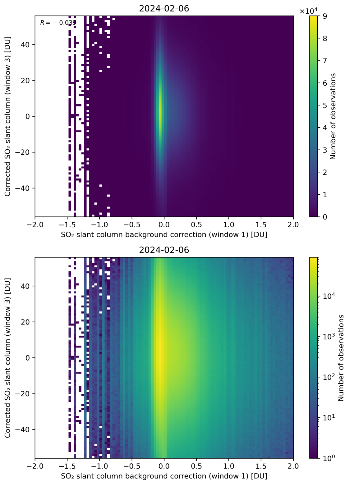
Figure 105: Scatter density plot of “SO 2 slant column background correction (window 1)” against “Corrected SO 2 slant column (window 3)” for 2024-02-06 to 2024-02-07.
