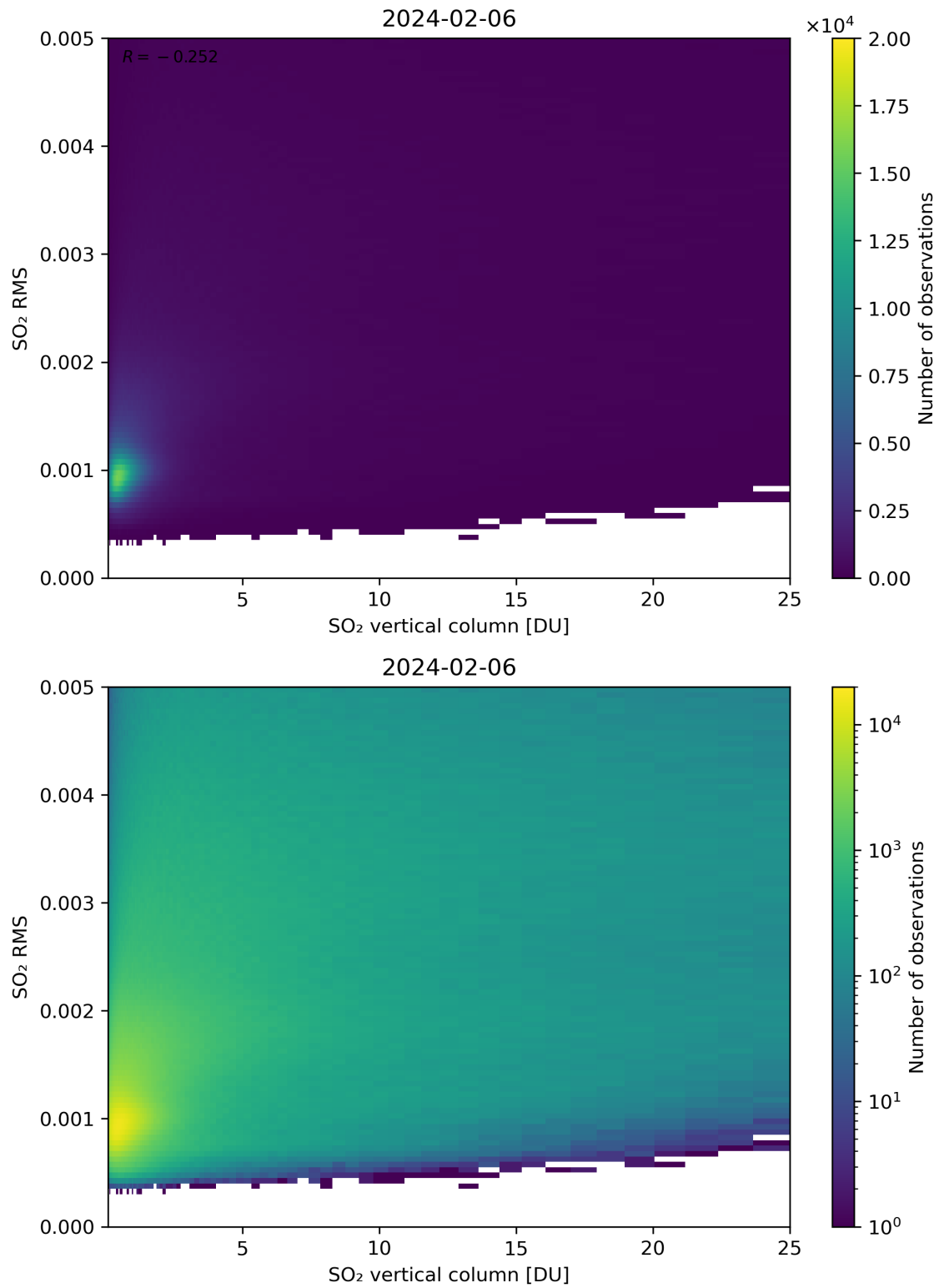
Figure 278: Scatter density plot of “SO 2 vertical column” against “SO 2 RMS” for 2024-02-06 to 2024-02-07.
