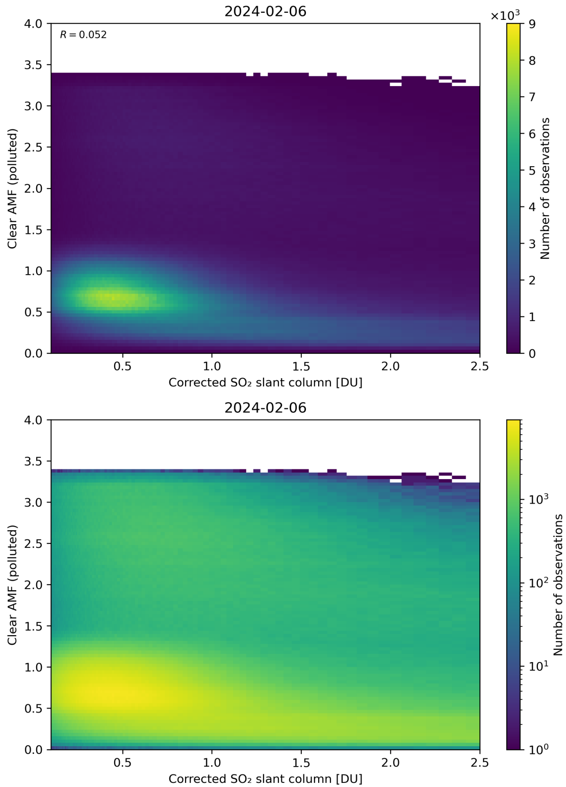
Figure 184: Scatter density plot of “Corrected SO 2 slant column” against “Clear AMF (polluted)” for 2024-02-06 to 2024-02-07.
