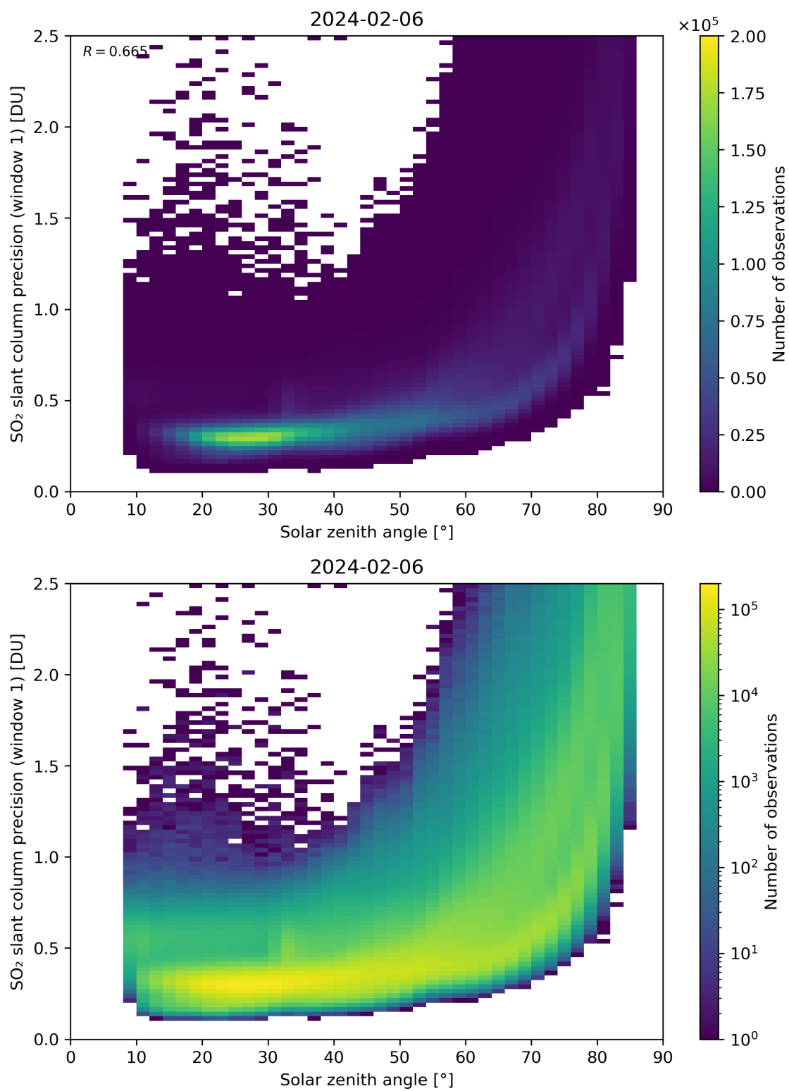
Figure 170: Scatter density plot of “Solar zenith angle” against “SO 2 slant column precision (window 1)” for 2024-02-06 to 2024-02-07.
