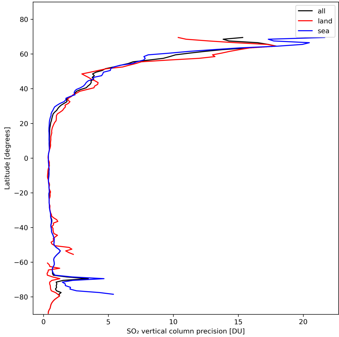
Figure 31: Zonal average of “SO 2 vertical column precision” for 2024-02-06 to 2024-02-07.
