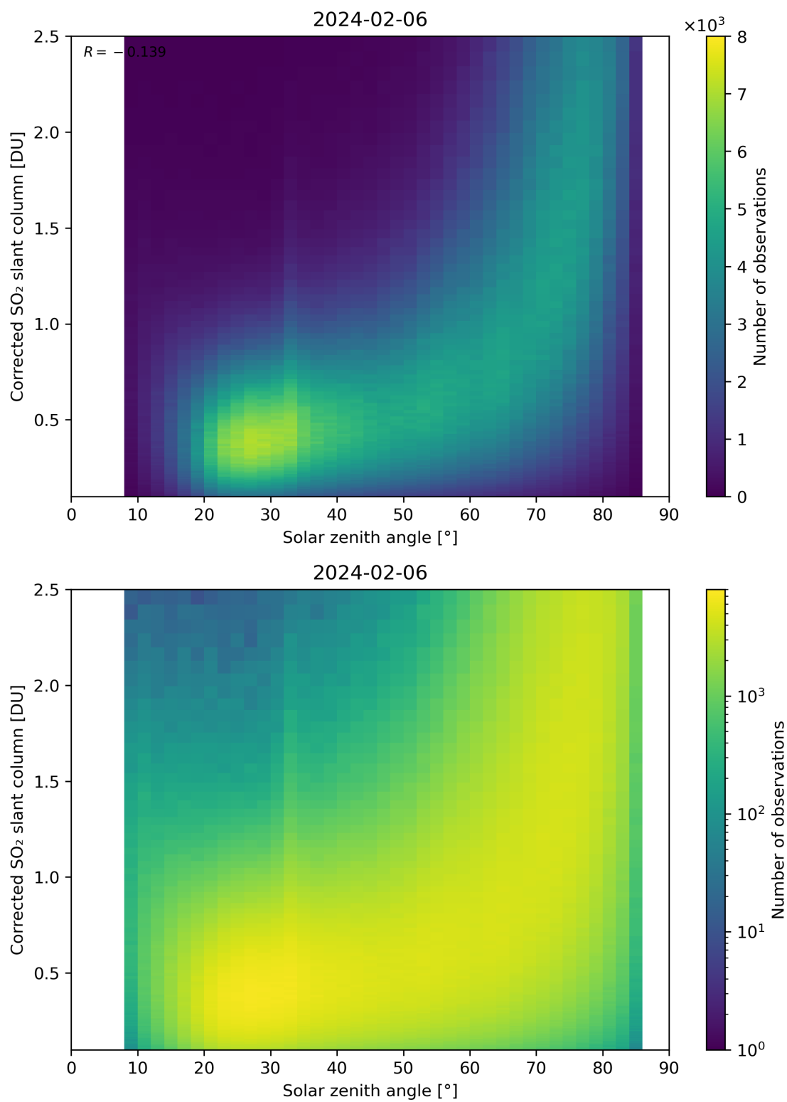
Figure 166: Scatter density plot of “Solar zenith angle” against “Corrected SO 2 slant column” for 2024-02-06 to 2024-02-07.
