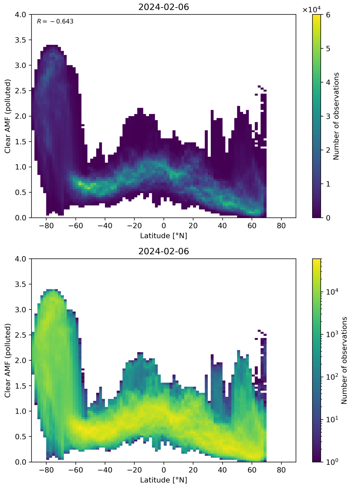
Figure 145: Scatter density plot of “Latitude” against “Clear AMF (polluted)” for 2024-02-06 to 2024-02-07.
