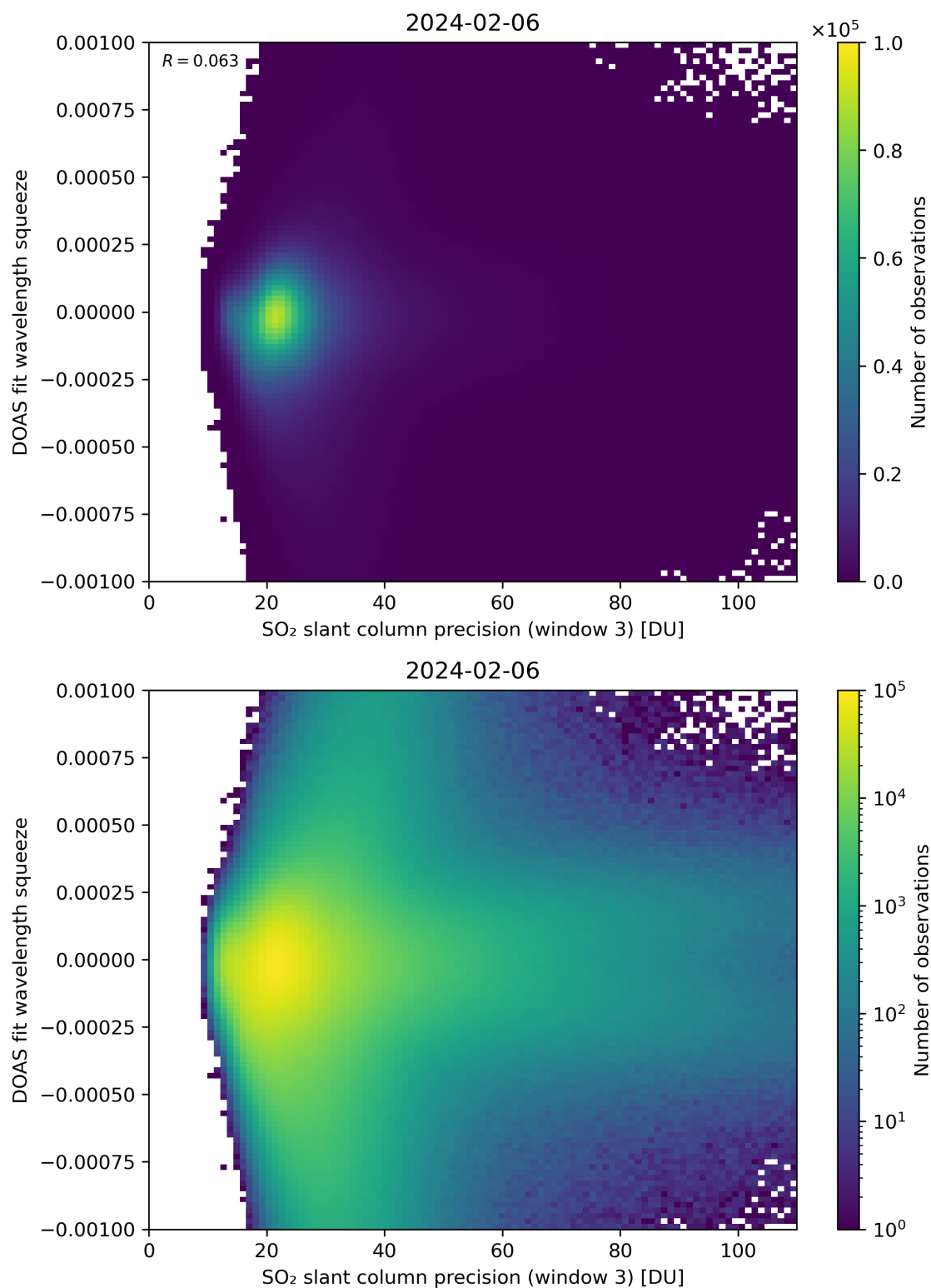
Figure 259: Scatter density plot of “SO 2 slant column precision (window 3)” against “DOAS fit wavelength squeeze” for 2024-02-06 to 2024-02-07.
