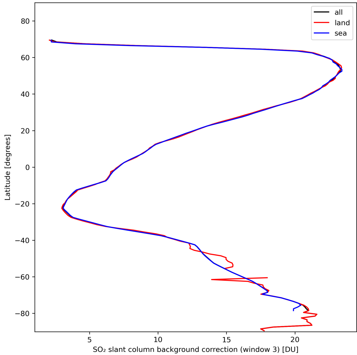
Figure 44: Zonal average of “SO 2 slant column background correction (window 3)” for 2024-02-06 to 2024-02-07.
