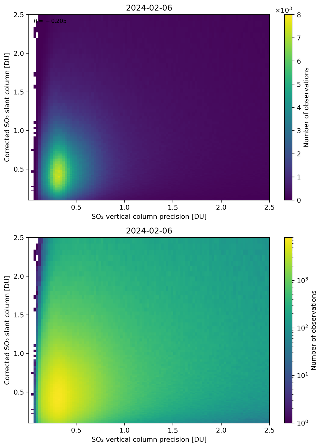
Figure 286: Scatter density plot of “SO 2 vertical column precision” against “Corrected SO 2 slant column” for 2024-02-06 to 2024-02-07.
