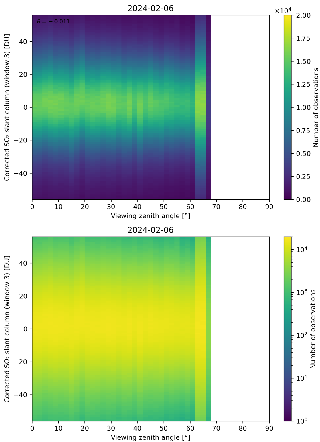
Figure 319: Scatter density plot of “Viewing zenith angle” against “Corrected SO 2 slant column (window 3)” for 2024-02-06 to 2024-02-07.
