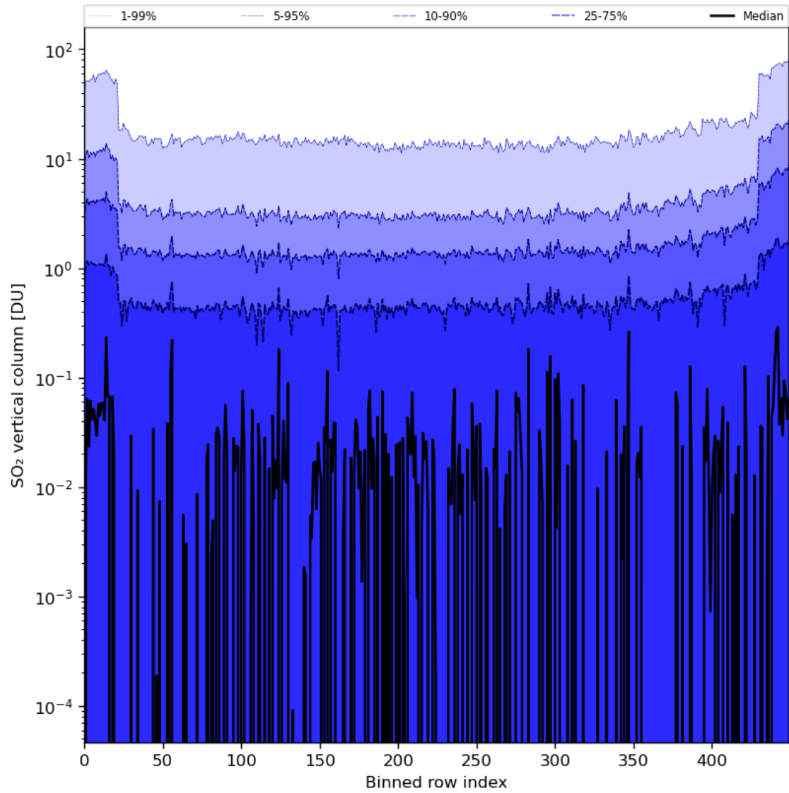
Figure 76: Along track statistics of “SO 2 vertical column” for 2024-02-06 to 2024-02-07
