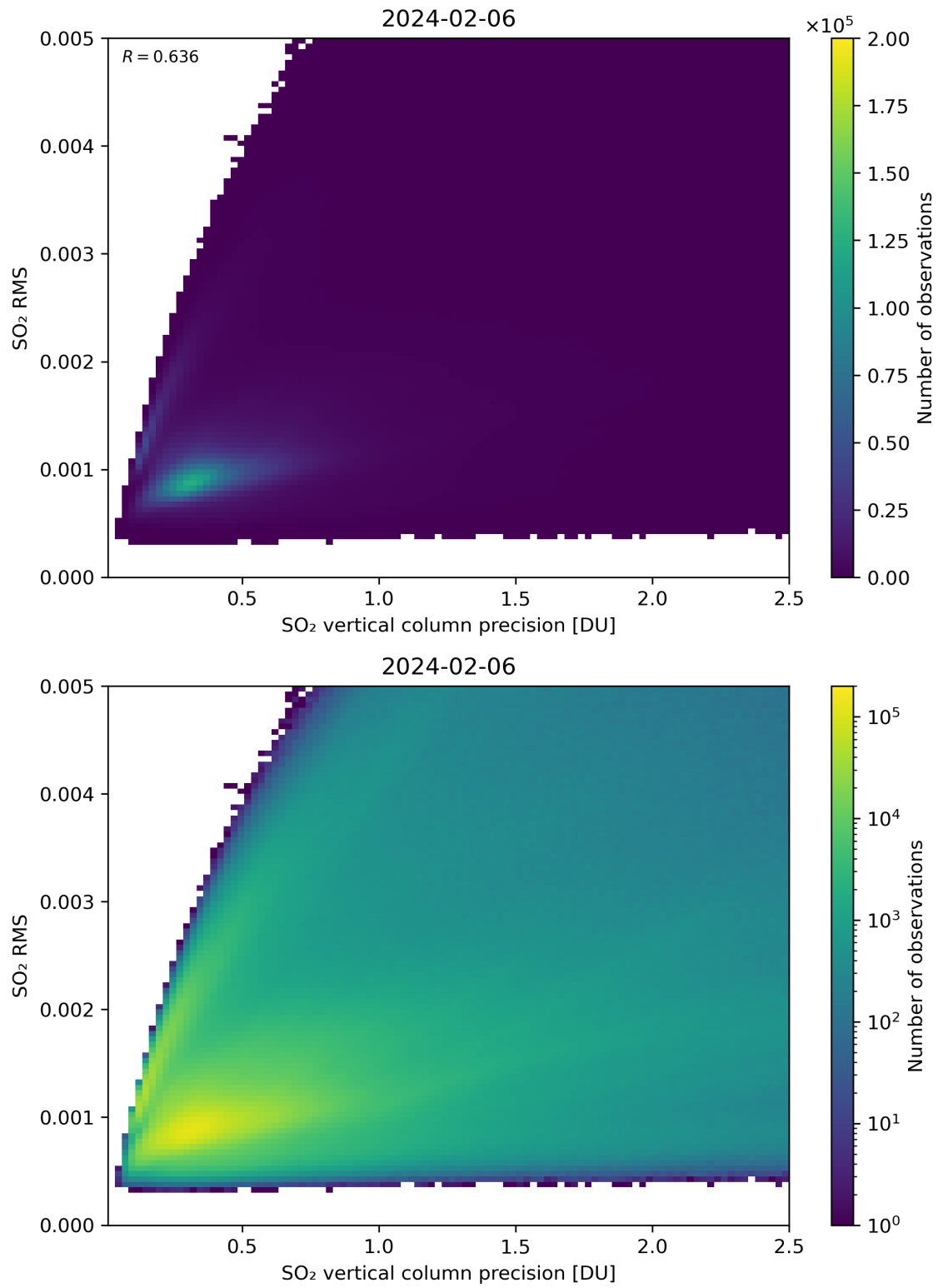
Figure 284: Scatter density plot of “SO 2 vertical column precision” against “SO 2 RMS” for 2024-02-06 to 2024-02-07.
