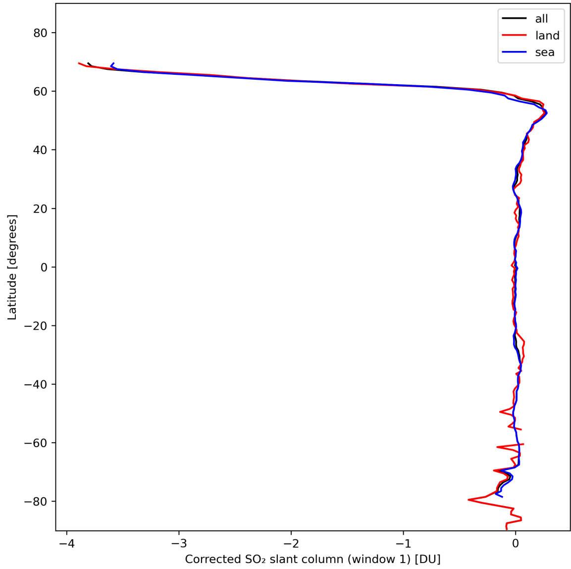
Figure 35: Zonal average of “Corrected SO 2 slant column (window 1)” for 2024-02-06 to 2024-02-07.
