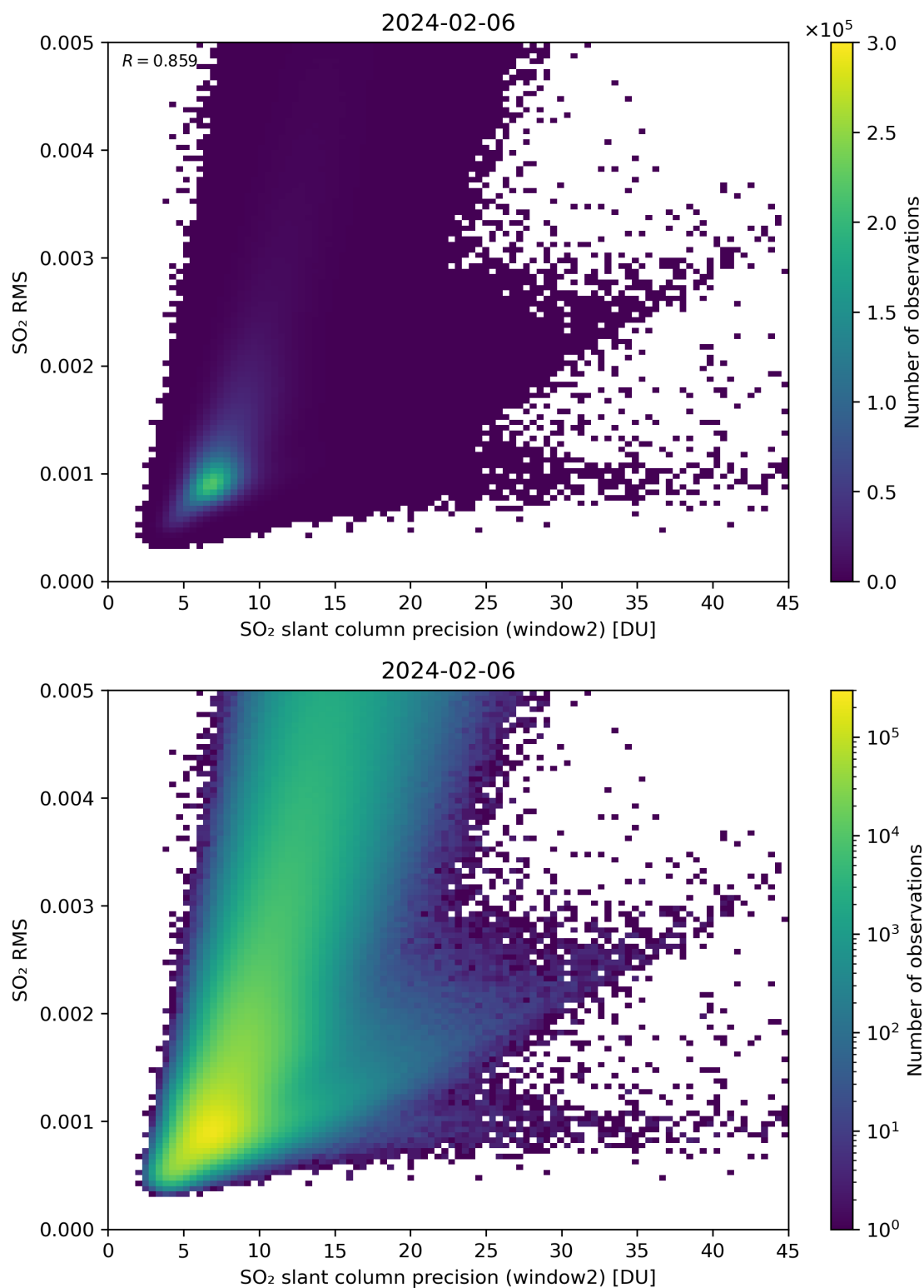
Figure 245: Scatter density plot of “SO 2 slant column precision (window2)” against “SO 2 RMS” for 2024-02-06 to 2024-02-07.
