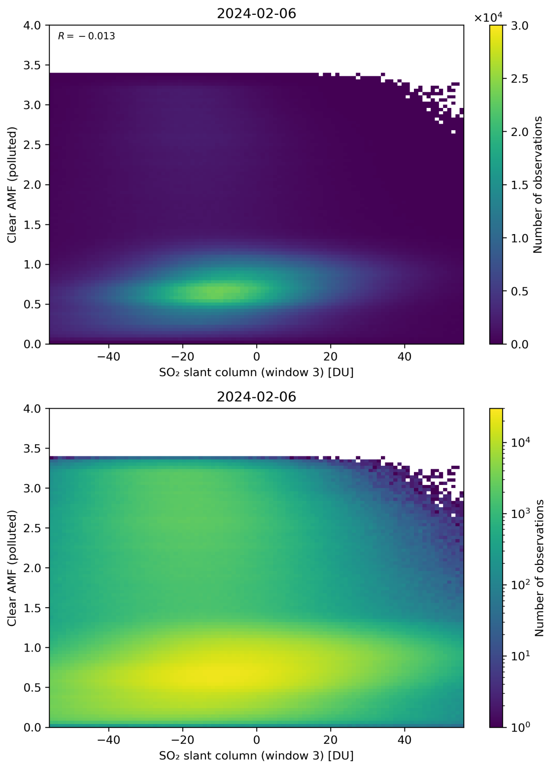
Figure 265: Scatter density plot of “SO 2 slant column (window 3)” against “Clear AMF (polluted)” for 2024-02-06 to 2024-02-07.
