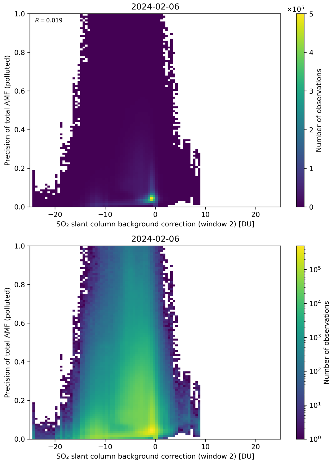
Figure 120: Scatter density plot of “SO 2 slant column background correction (window 2)” against “Precision of total AMF (polluted)” for 2024-02-06 to 2024-02-07.
