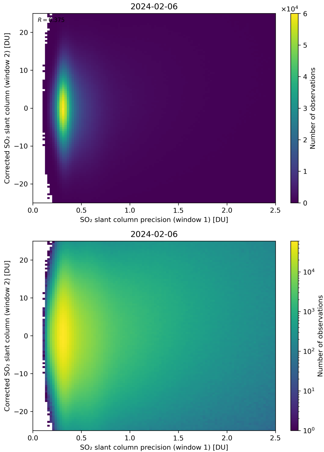
Figure 225: Scatter density plot of “SO 2 slant column precision (window 1)” against “Corrected SO 2 slant column (window 2)” for 2024-02-06 to 2024-02-07.
