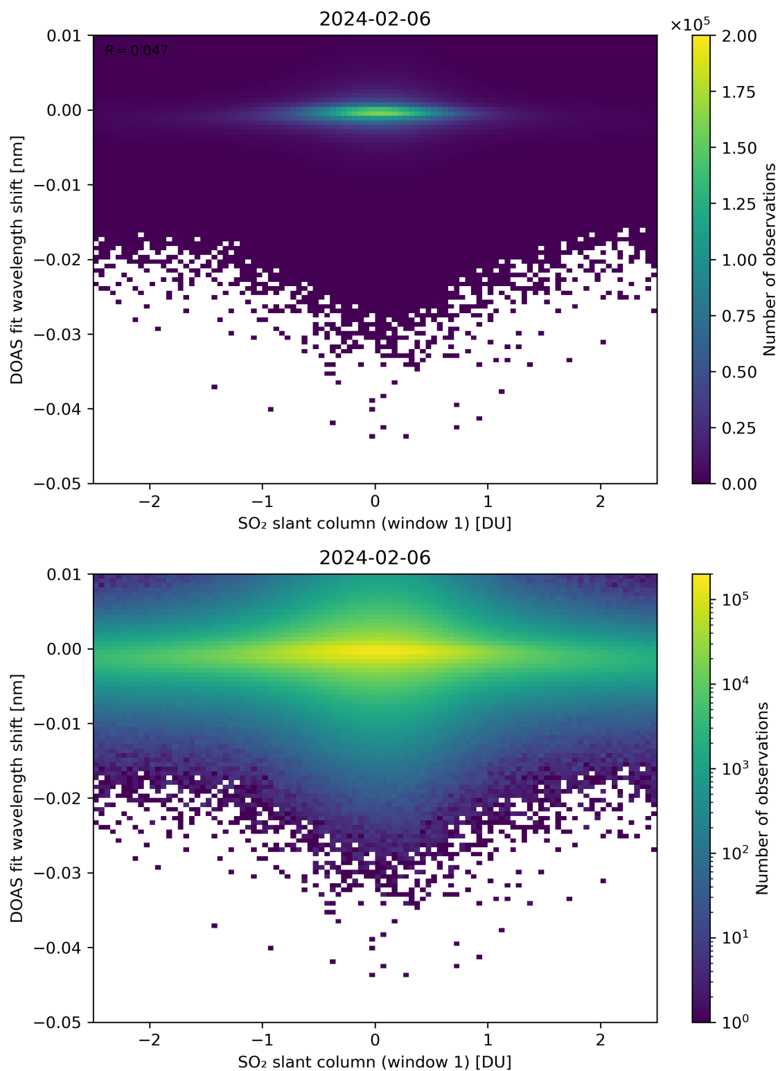
Figure 215: Scatter density plot of “SO 2 slant column (window 1)” against “DOAS fit wavelength shift” for 2024-02-06 to 2024-02-07.
