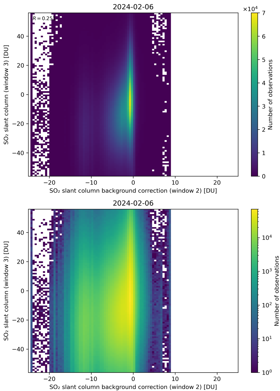
Figure 117: Scatter density plot of “SO 2 slant column background correction (window 2)” against “SO 2 slant column (window 3)” for 2024-02-06 to 2024-02-07.
