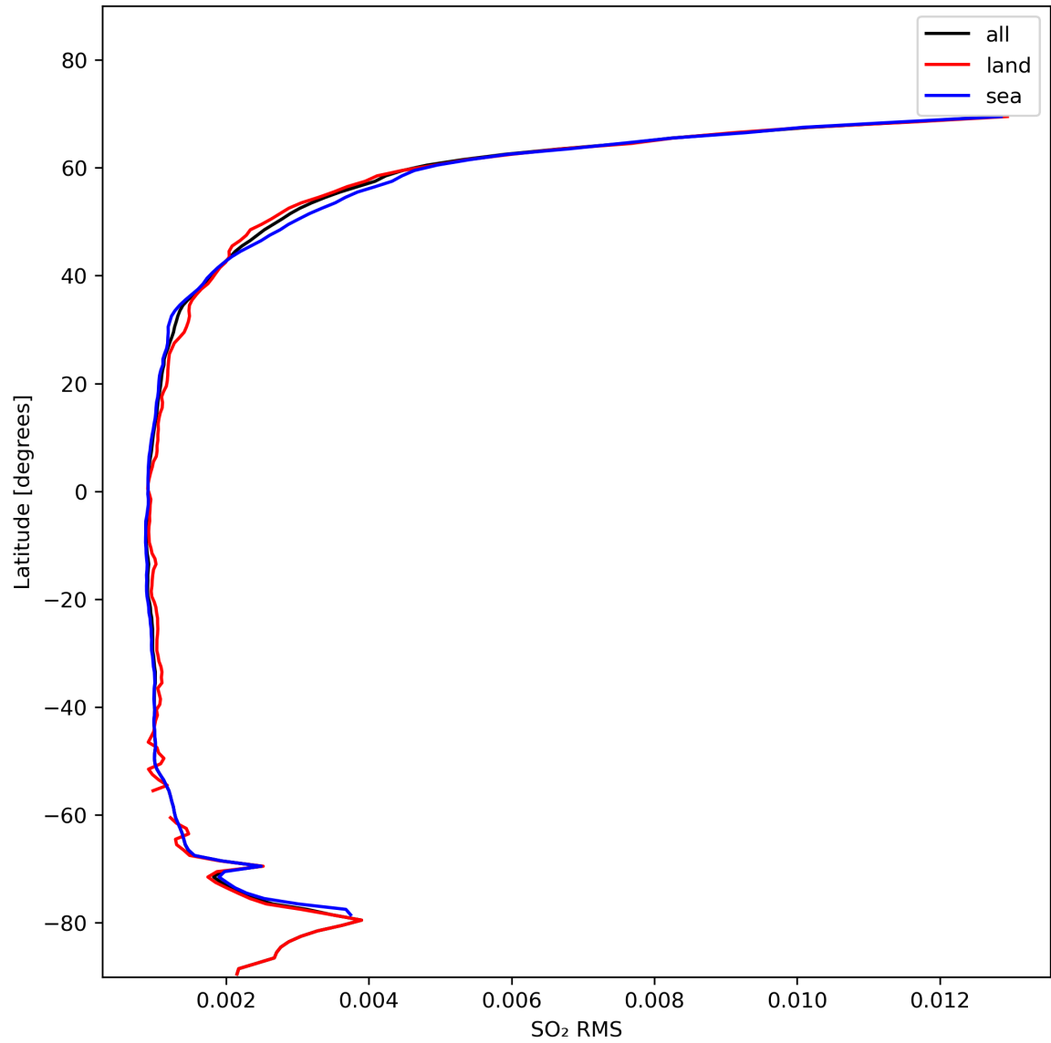
Figure 47: Zonal average of “SO 2 RMS” for 2024-02-06 to 2024-02-07.
