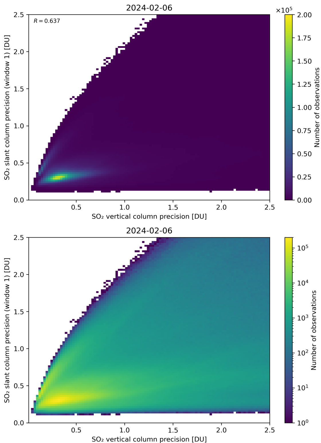
Figure 290: Scatter density plot of “SO 2 vertical column precision” against “SO 2 slant column precision (window 1)” for 2024-02-06 to 2024-02-07.
