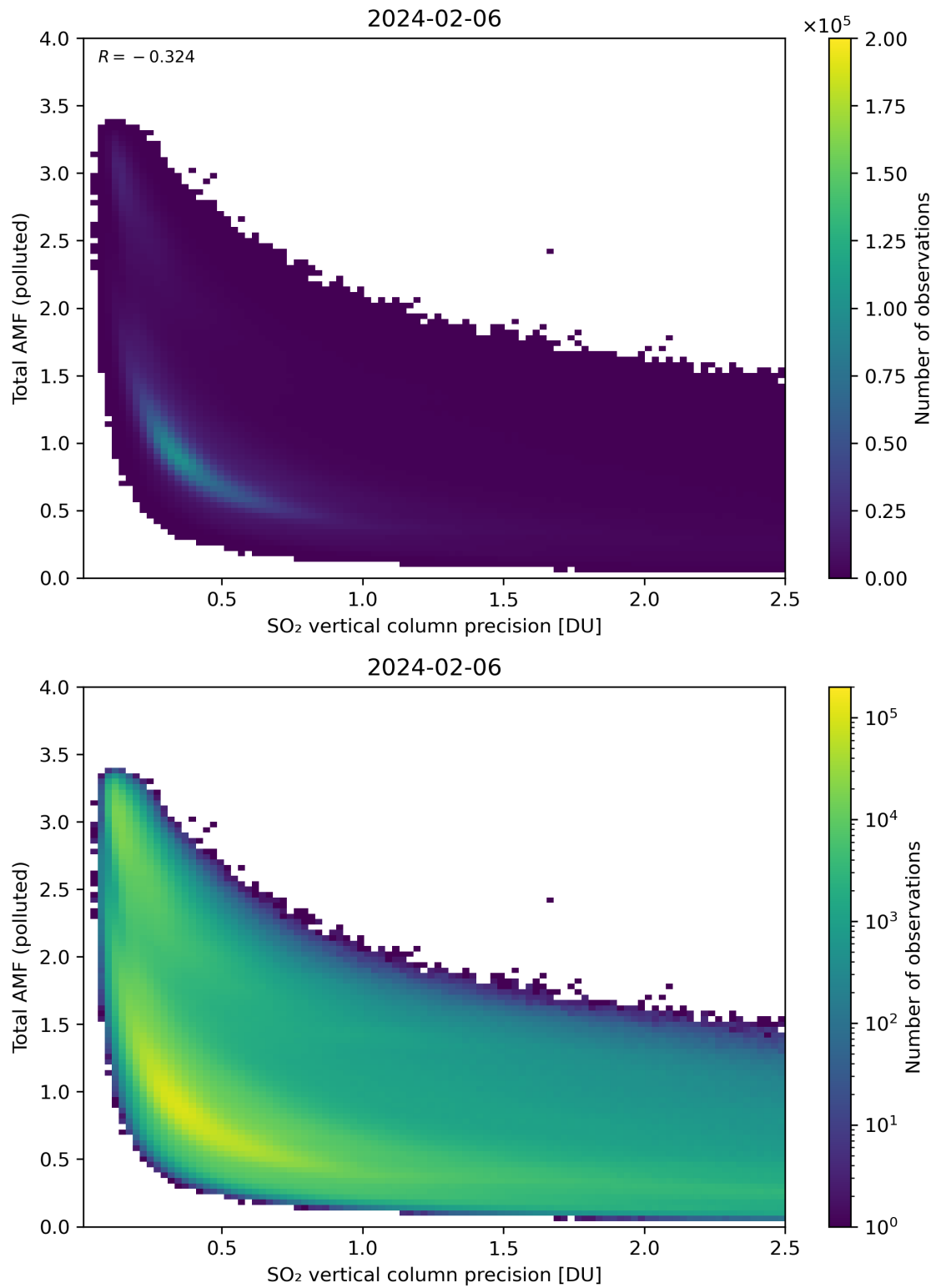
Figure 294: Scatter density plot of “SO 2 vertical column precision” against “Total AMF (polluted)” for 2024-02-06 to 2024-02-07.
