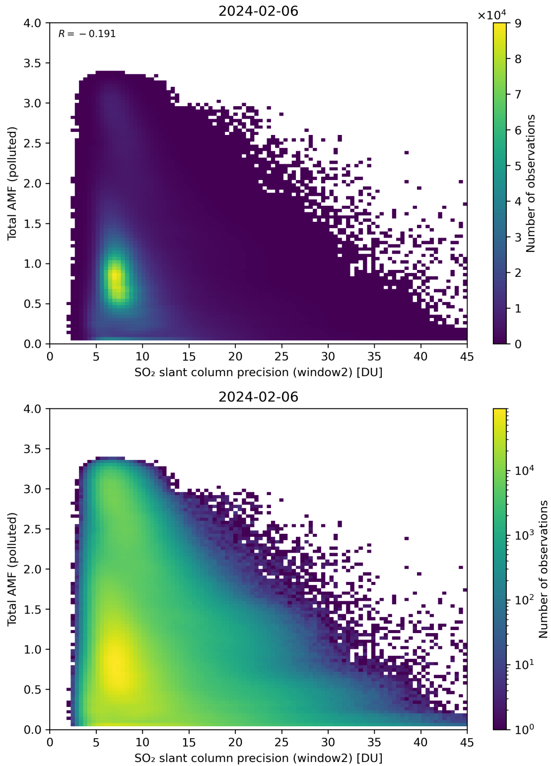
Figure 251: Scatter density plot of “SO 2 slant column precision (window2)” against “Total AMF (polluted)” for 2024-02-06 to 2024-02-07.
