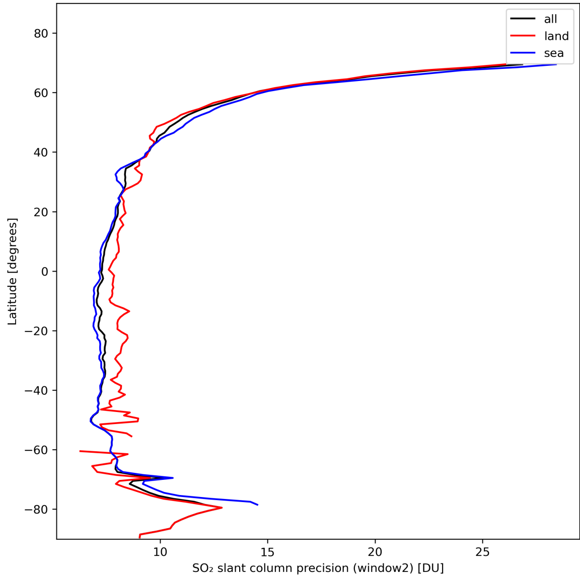
Figure 38: Zonal average of “SO 2 slant column precision (window2)” for 2024-02-06 to 2024-02-07.
