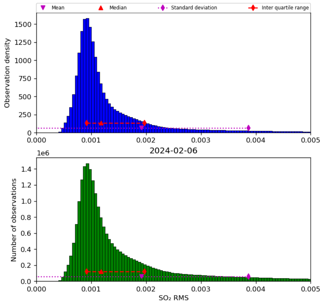
Figure 70: Histogram of “SO 2 RMS” for 2024-02-06 to 2024-02-07
