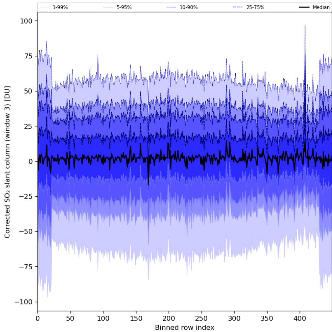
Figure 89: Along track statistics of “Corrected SO 2 slant column (window 3)” for 2024-02-06 to 2024-02-07
