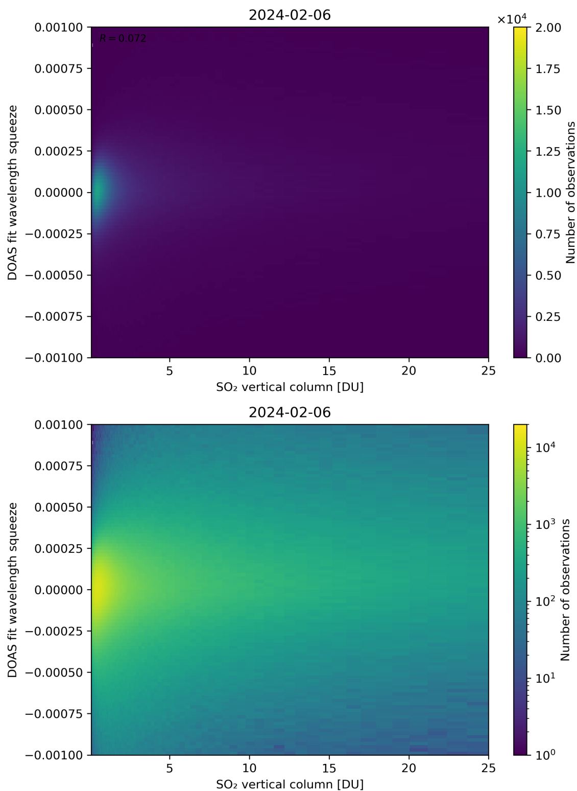
Figure 277: Scatter density plot of “SO 2 vertical column” against “DOAS fit wavelength squeeze” for 2024-02-06 to 2024-02-07.
