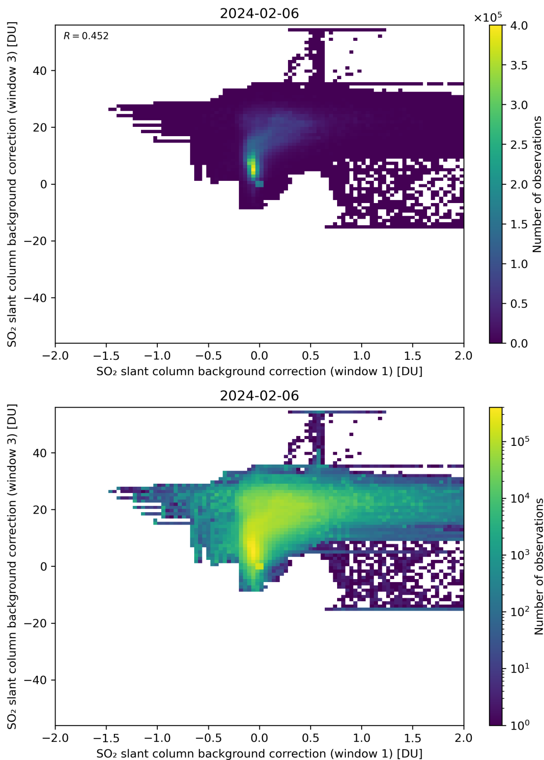
Figure 99: Scatter density plot of “SO 2 slant column background correction (window 1)” against “SO 2 slant column background correction (window 3)” for 2024-02-06 to 2024-02-07.
