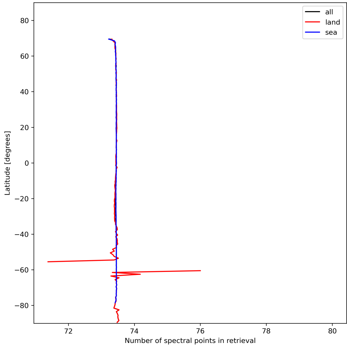
Figure 51: Zonal average of “Number of spectral points in retrieval” for 2024-02-06 to 2024-02-07.
