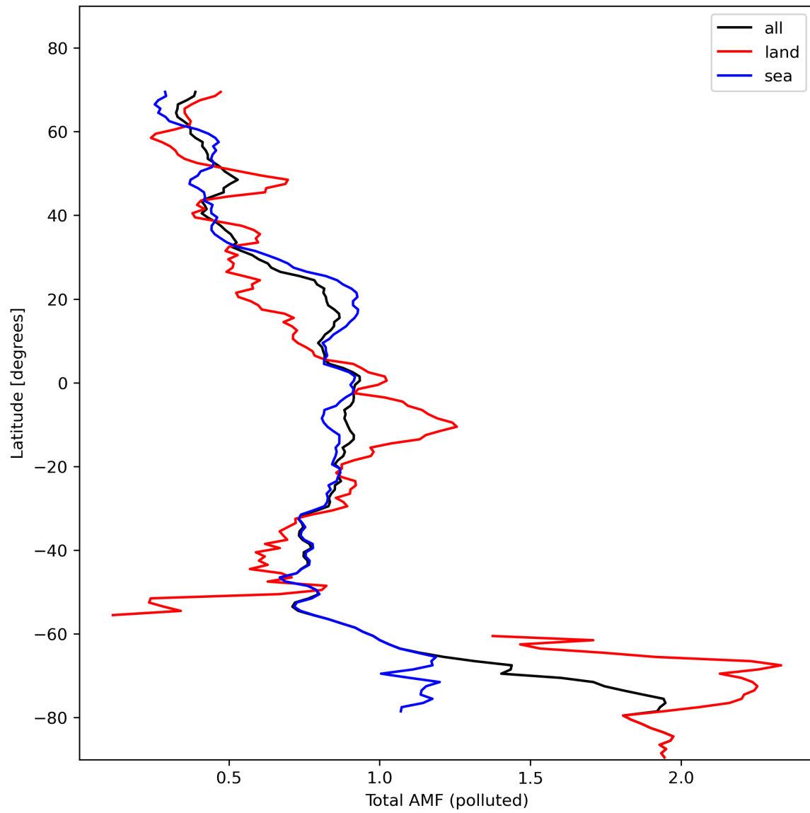
Figure 48: Zonal average of “Total AMF (polluted)” for 2024-02-06 to 2024-02-07.
