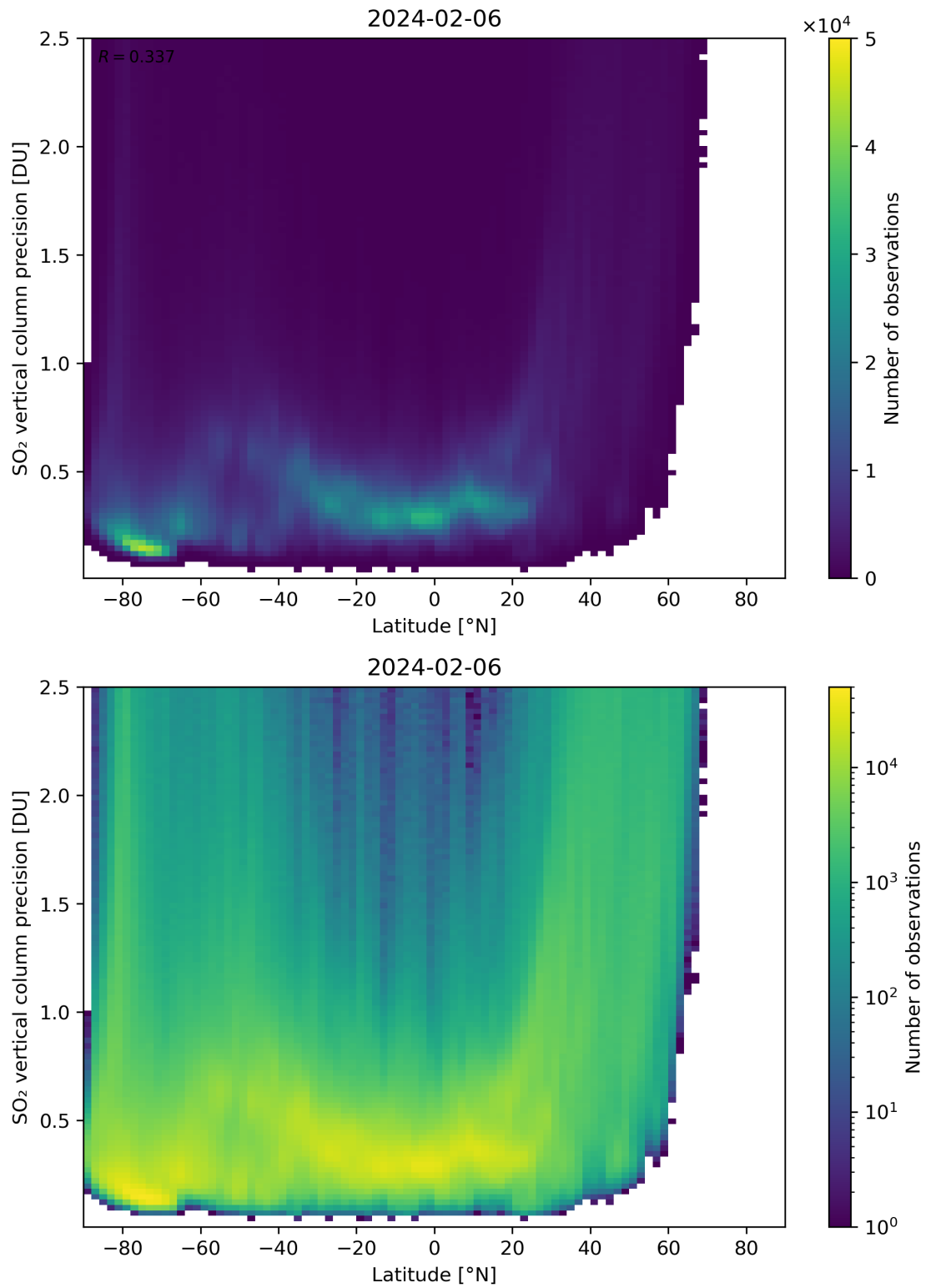
Figure 157: Scatter density plot of “Latitude” against “SO 2 vertical column precision” for 2024-02-06 to 2024-02-07.
