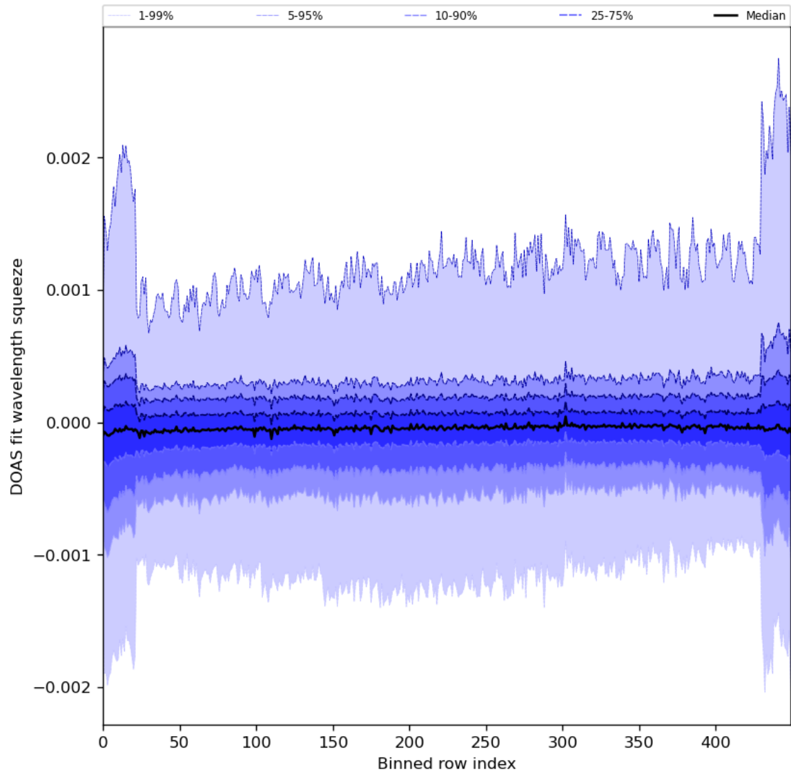
Figure 92: Along track statistics of “DOAS fit wavelength squeeze” for 2024-02-06 to 2024-02-07
