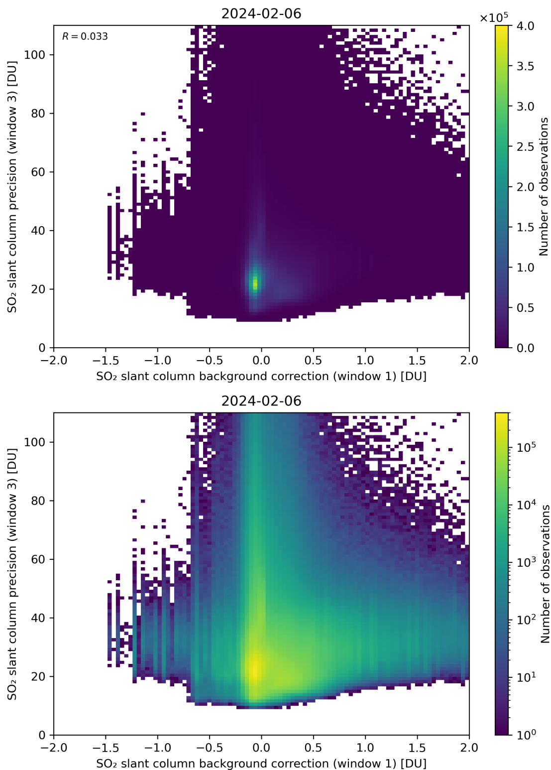
Figure 108: Scatter density plot of “SO 2 slant column background correction (window 1)” against “SO 2 slant column precision (window 3)” for 2024-02-06 to 2024-02-07.
