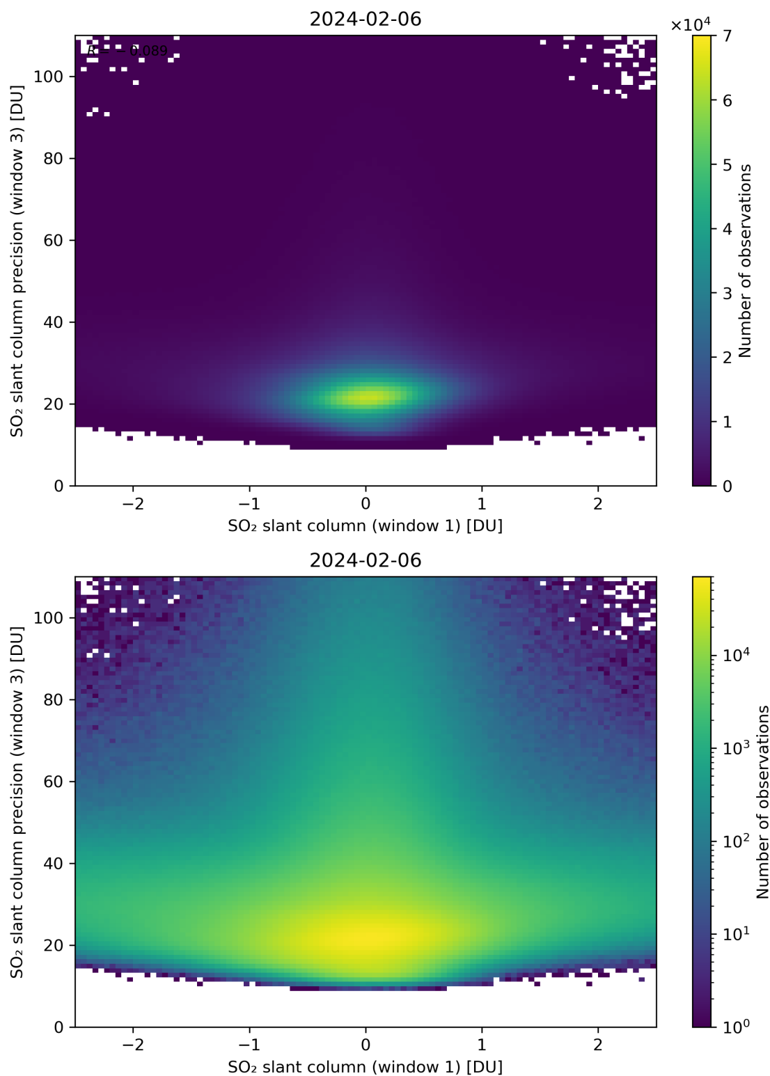
Figure 238: Scatter density plot of “SO 2 slant column (window 1)” against “SO 2 slant column precision (window 3)” for 2024-02-06 to 2024-02-07.
