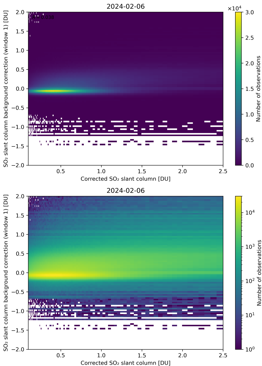
Figure 178: Scatter density plot of “Corrected SO 2 slant column” against “SO 2 slant column background correction (window 1)” for 2024-02-06 to 2024-02-07.
