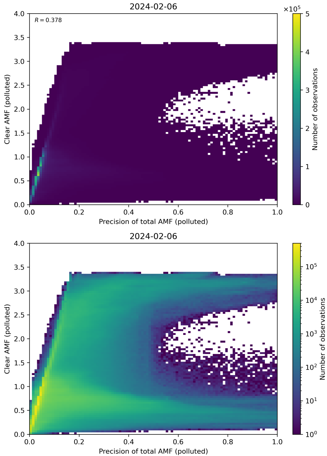
Figure 270: Scatter density plot of “Precision of total AMF (polluted)” against “Clear AMF (polluted)” for 2024-02-06 to 2024-02-07.
