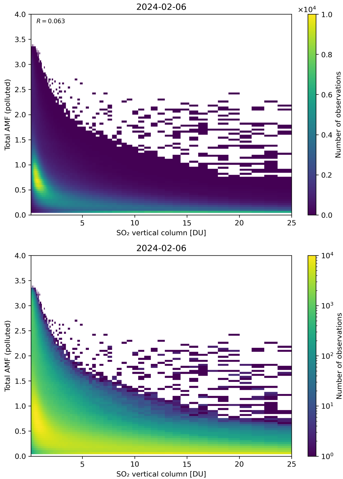
Figure 305: Scatter density plot of “SO 2 vertical column” against “Total AMF (polluted)” for 2024-02-06 to 2024-02-07.
