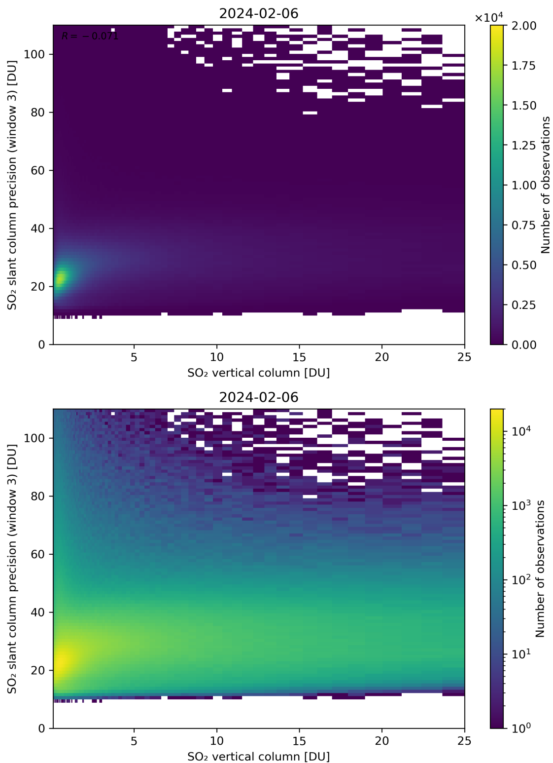
Figure 304: Scatter density plot of “SO 2 vertical column” against “SO 2 slant column precision (window 3)” for 2024-02-06 to 2024-02-07.
