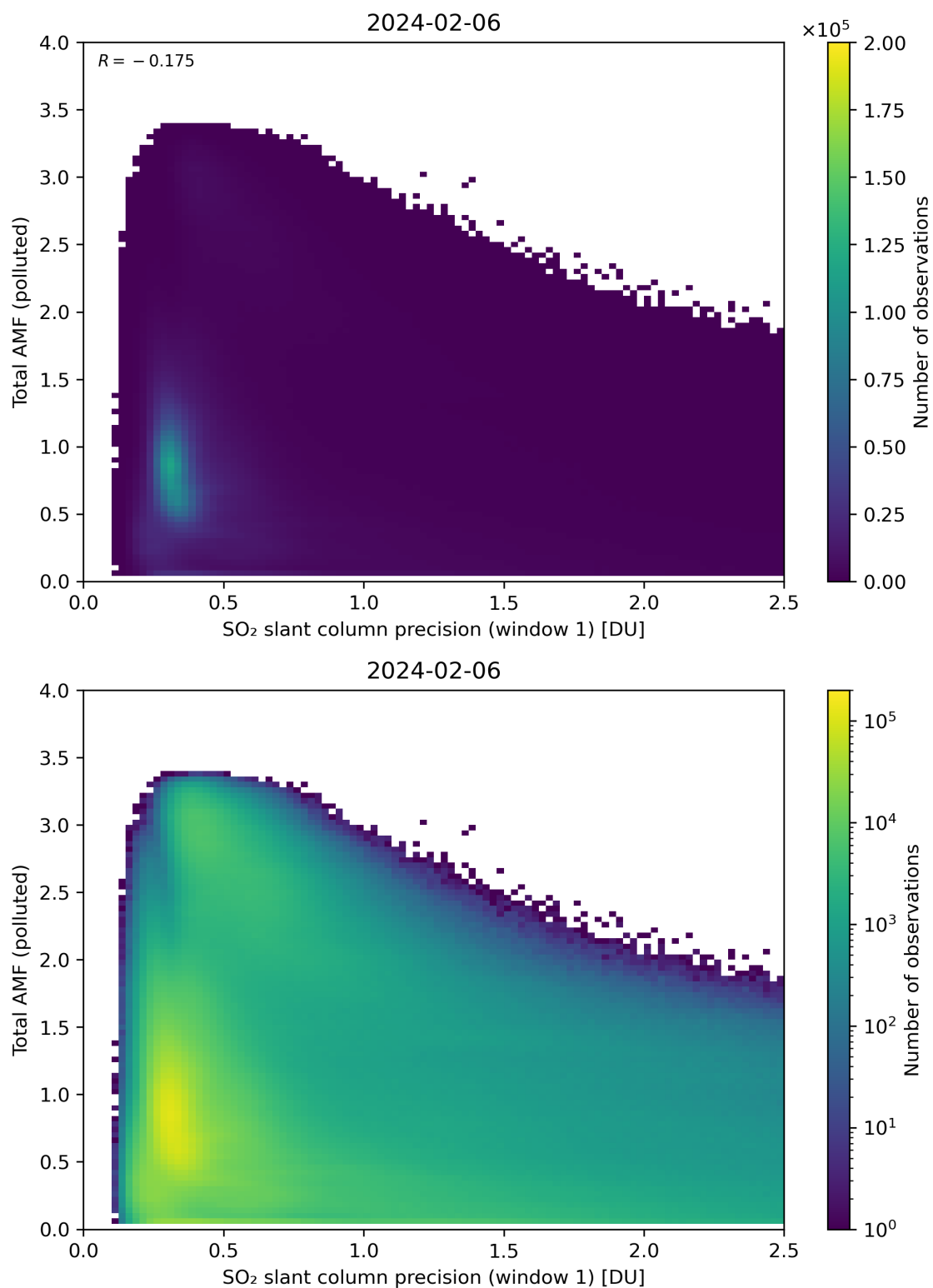
Figure 230: Scatter density plot of “SO 2 slant column precision (window 1)” against “Total AMF (polluted)” for 2024-02-06 to 2024-02-07.
