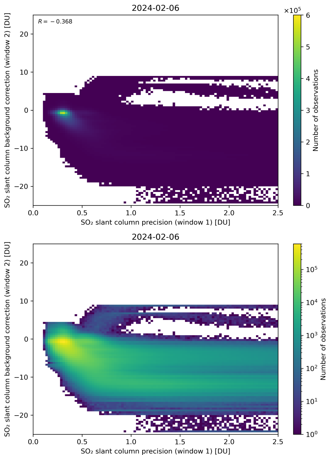
Figure 219: Scatter density plot of “SO 2 slant column precision (window 1)” against “SO 2 slant column background correction (window 2)” for 2024-02-06 to 2024-02-07.
