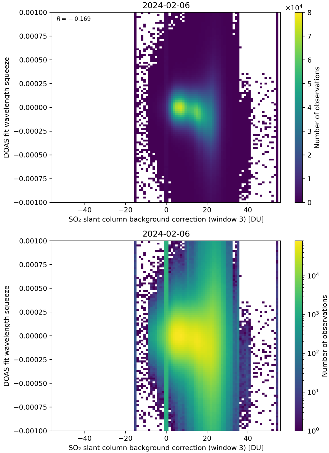
Figure 122: Scatter density plot of “SO 2 slant column background correction (window 3)” against “DOAS fit wavelength squeeze” for 2024-02-06 to 2024-02-07.
