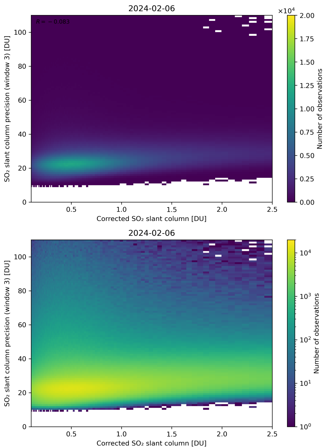
Figure 191: Scatter density plot of “Corrected SO 2 slant column” against “SO 2 slant column precision (window 3)” for 2024-02-06 to 2024-02-07.
