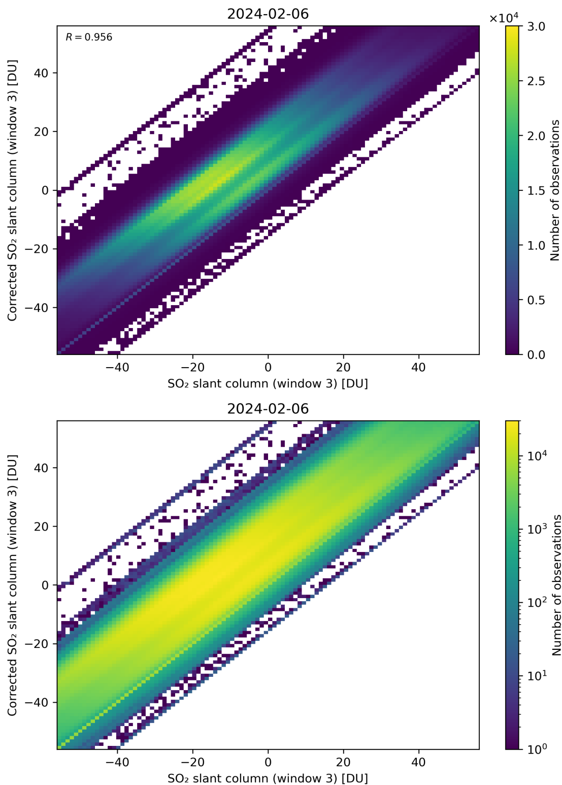
Figure 266: Scatter density plot of “SO 2 slant column (window 3)” against “Corrected SO 2 slant column (window 3)” for 2024-02-06 to 2024-02-07.
