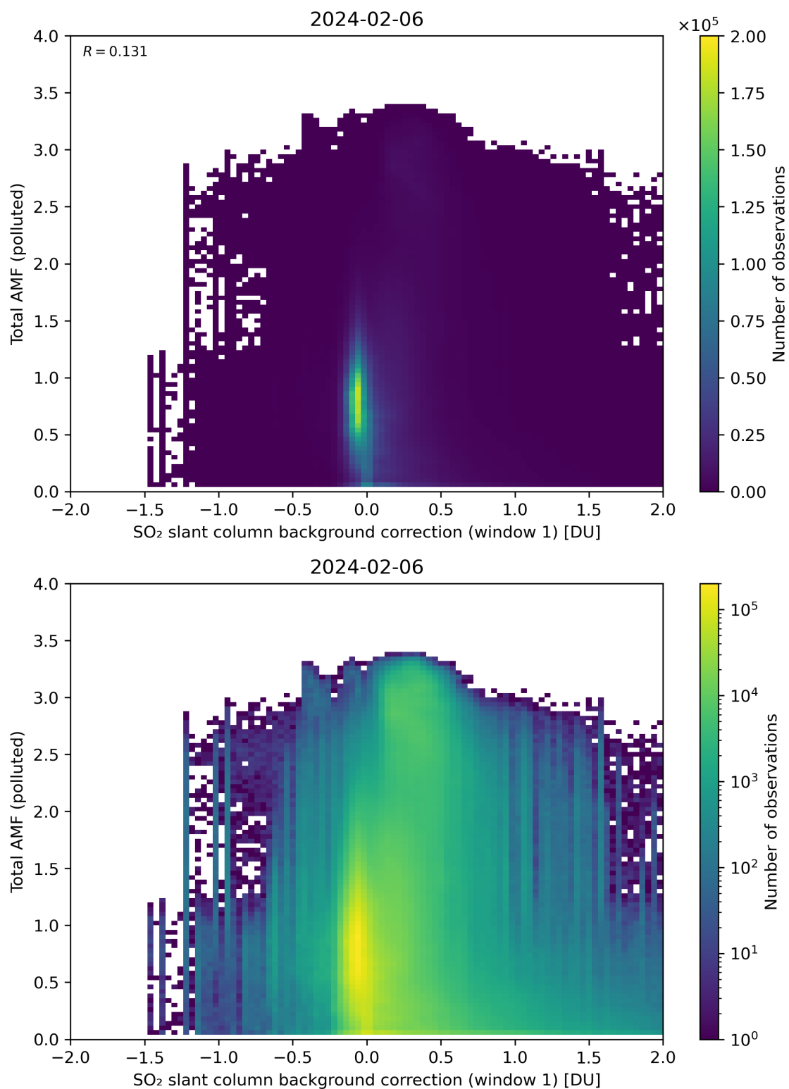
Figure 109: Scatter density plot of “SO 2 slant column background correction (window 1)” against “Total AMF (polluted)” for 2024-02-06 to 2024-02-07.
