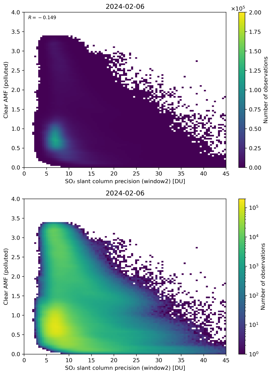
Figure 246: Scatter density plot of “SO 2 slant column precision (window2)” against “Clear AMF (polluted)” for 2024-02-06 to 2024-02-07.
