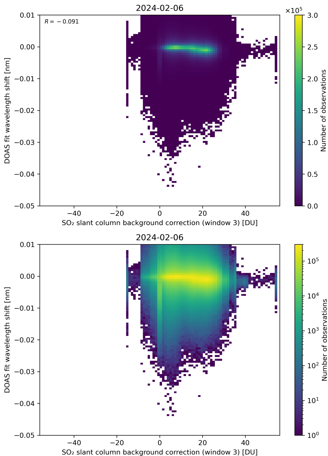
Figure 121: Scatter density plot of “SO 2 slant column background correction (window 3)” against “DOAS fit wavelength shift” for 2024-02-06 to 2024-02-07.
