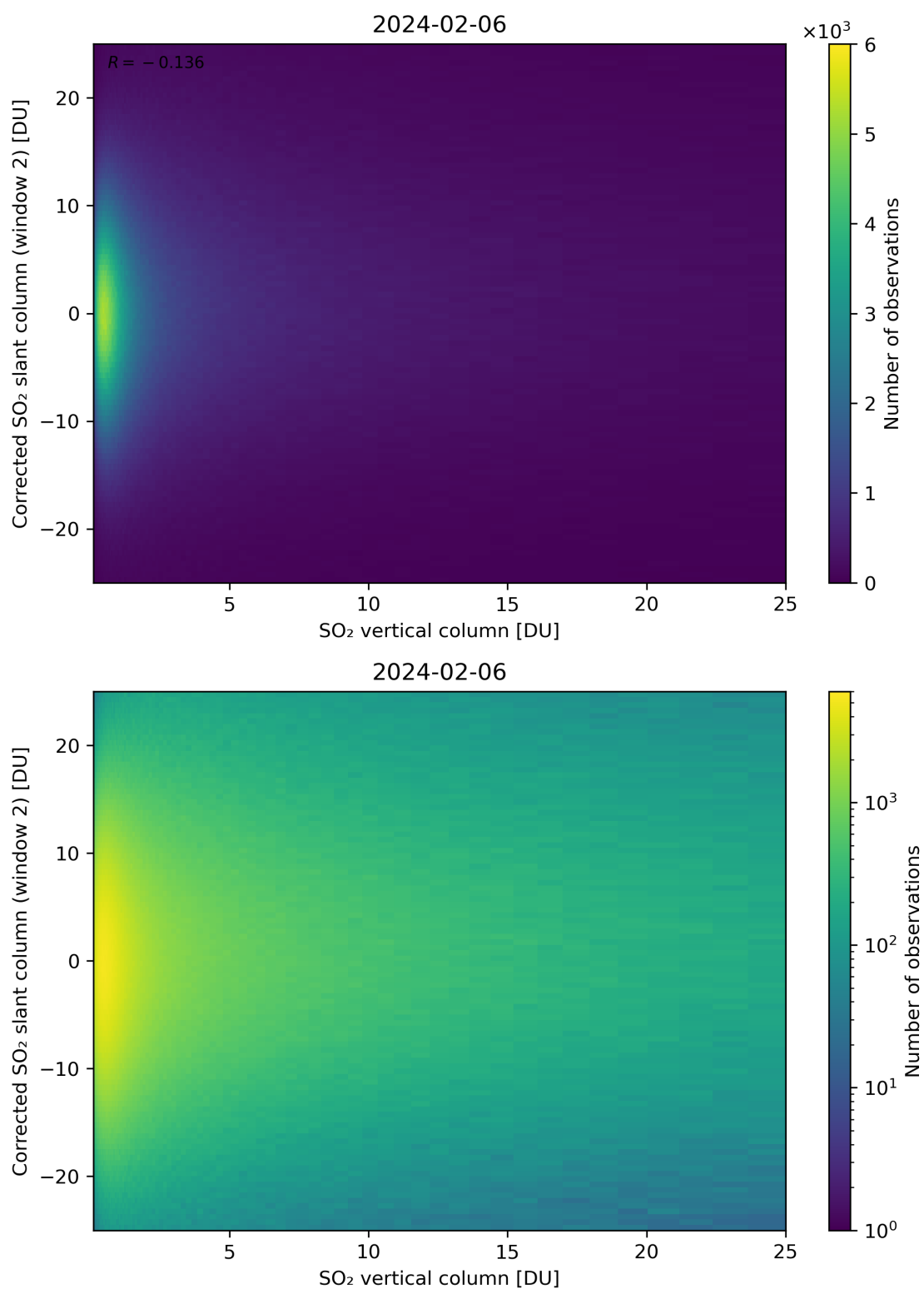
Figure 298: Scatter density plot of “SO 2 vertical column” against “Corrected SO 2 slant column (window 2)” for 2024-02-06 to 2024-02-07.
