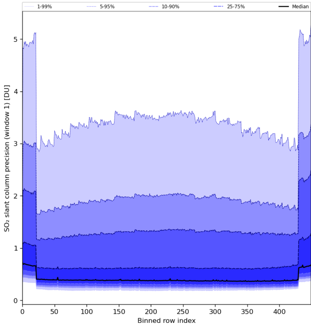
Figure 80: Along track statistics of “SO 2 slant column precision (window 1)” for 2024-02-06 to 2024-02-07
