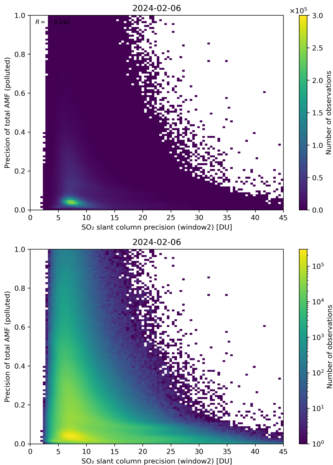
Figure 252: Scatter density plot of “SO 2 slant column precision (window2)” against “Precision of total AMF (polluted)” for 2024-02-06 to 2024-02-07.
