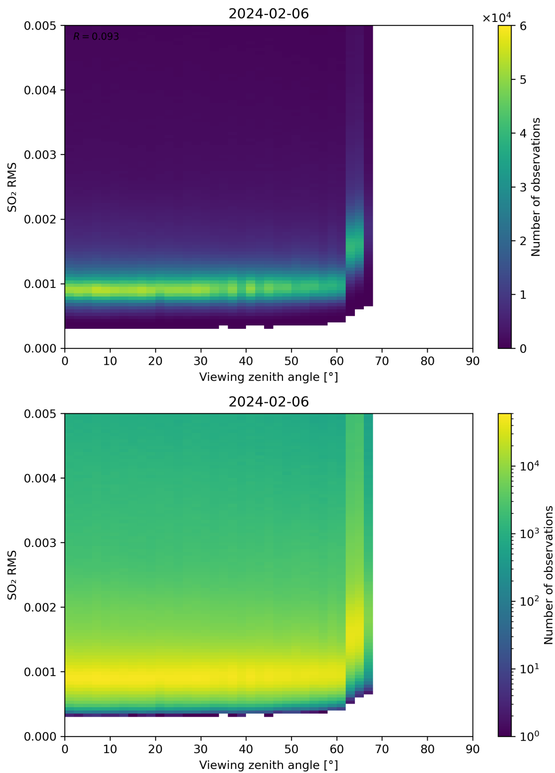
Figure 313: Scatter density plot of “Viewing zenith angle” against “SO 2 RMS” for 2024-02-06 to 2024-02-07.
