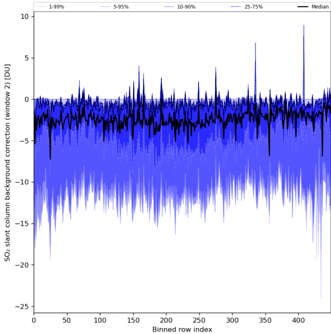
Figure 86: Along track statistics of “SO 2 slant column background correction (window 2)” for 2024-02-06 to 2024-02-07
