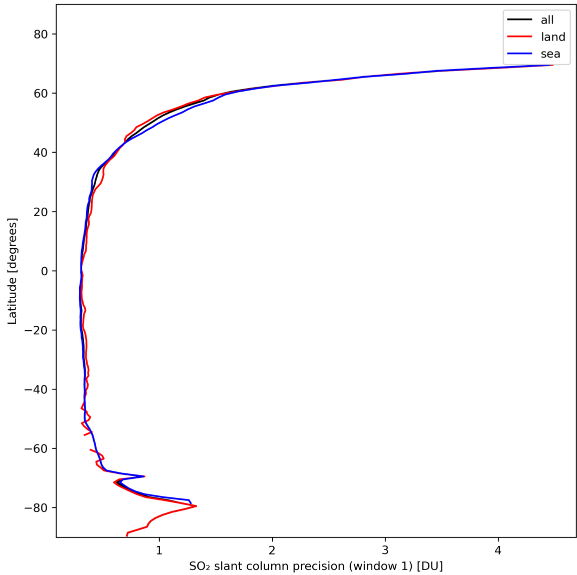
Figure 34: Zonal average of “SO 2 slant column precision (window 1)” for 2024-02-06 to 2024-02-07.
