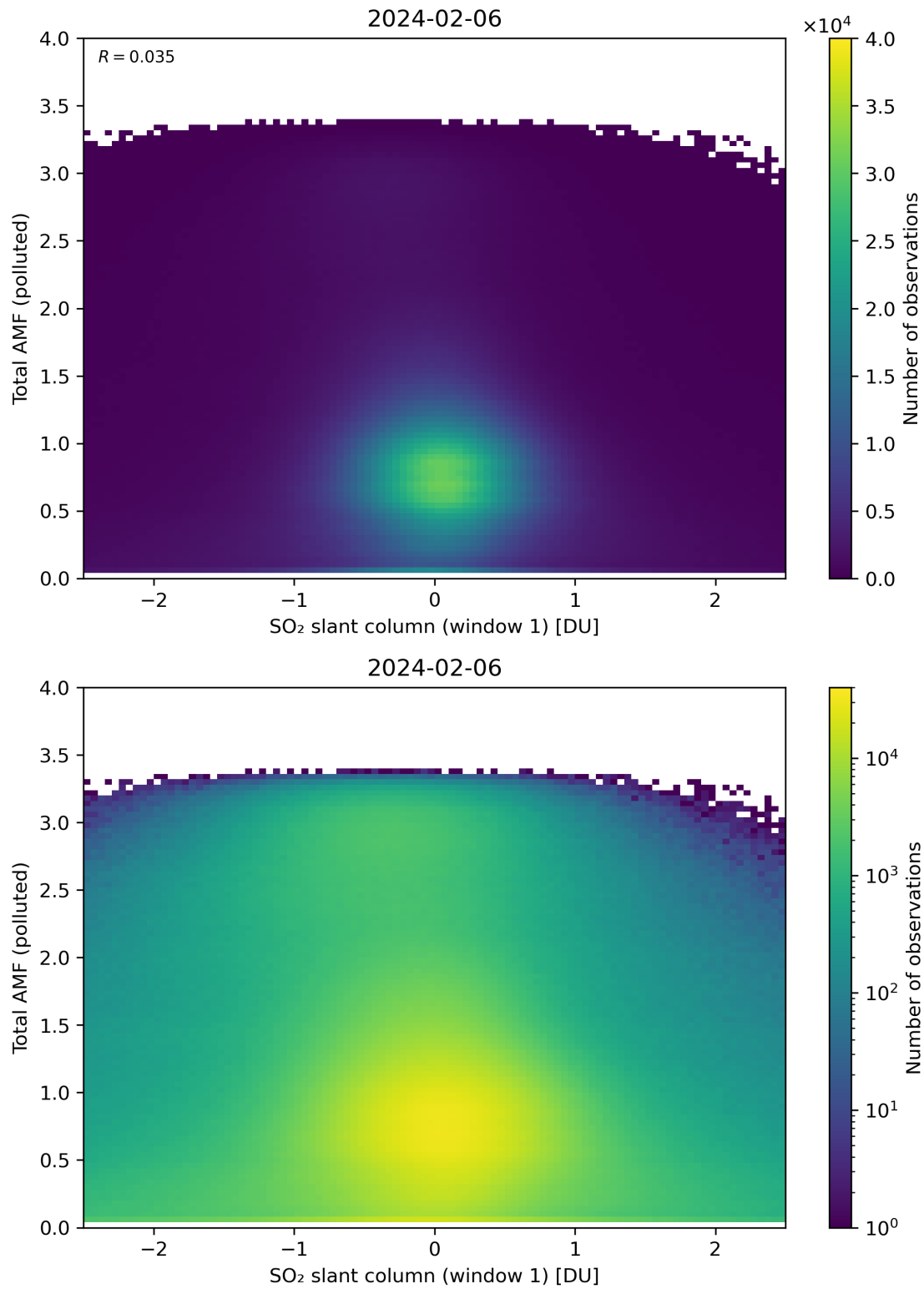
Figure 239: Scatter density plot of “SO 2 slant column (window 1)” against “Total AMF (polluted)” for 2024-02-06 to 2024-02-07.
