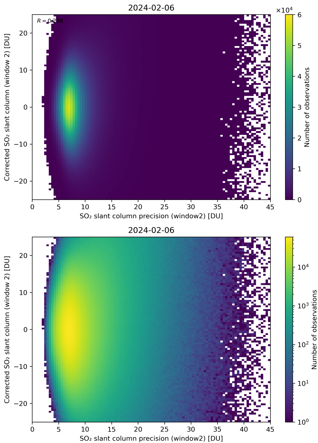
Figure 247: Scatter density plot of “SO 2 slant column precision (window2)” against “Corrected SO 2 slant column (window 2)” for 2024-02-06 to 2024-02-07.
