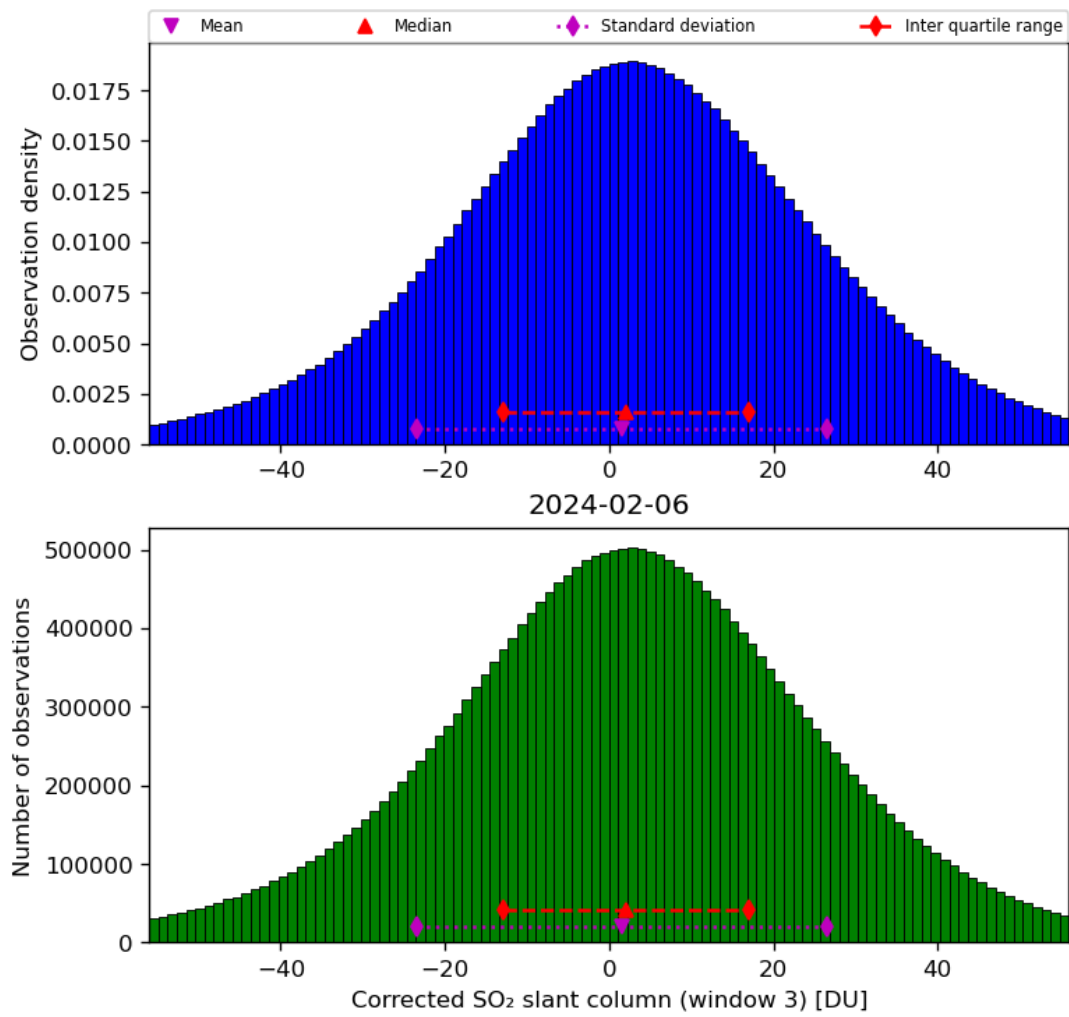
Figure 66: Histogram of “Corrected SO 2 slant column (window 3)” for 2024-02-06 to 2024-02-07
