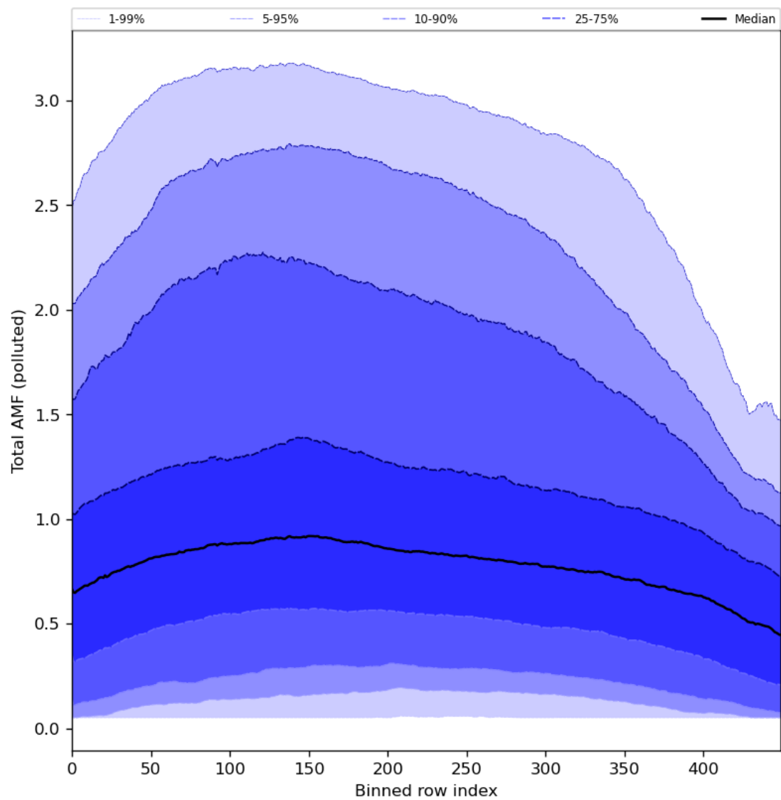
Figure 94: Along track statistics of “Total AMF (polluted)” for 2024-02-06 to 2024-02-07
