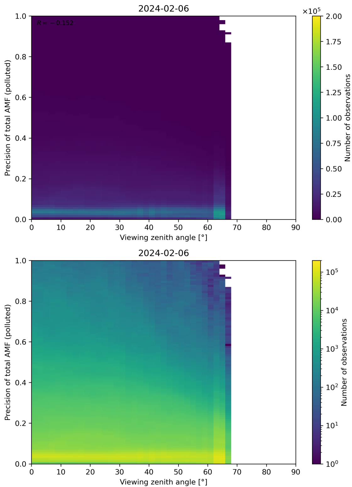
Figure 326: Scatter density plot of “Viewing zenith angle” against “Precision of total AMF (polluted)” for 2024-02-06 to 2024-02-07.
