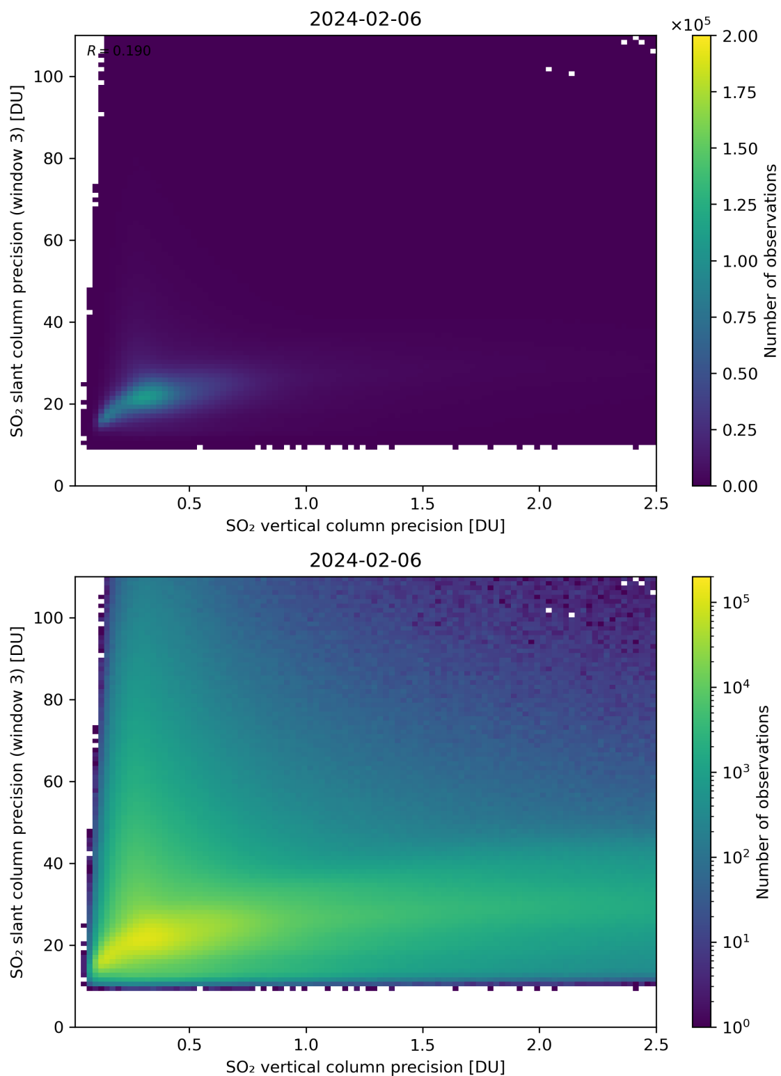
Figure 293: Scatter density plot of “SO 2 vertical column precision” against “SO 2 slant column precision (window 3)” for 2024-02-06 to 2024-02-07.
