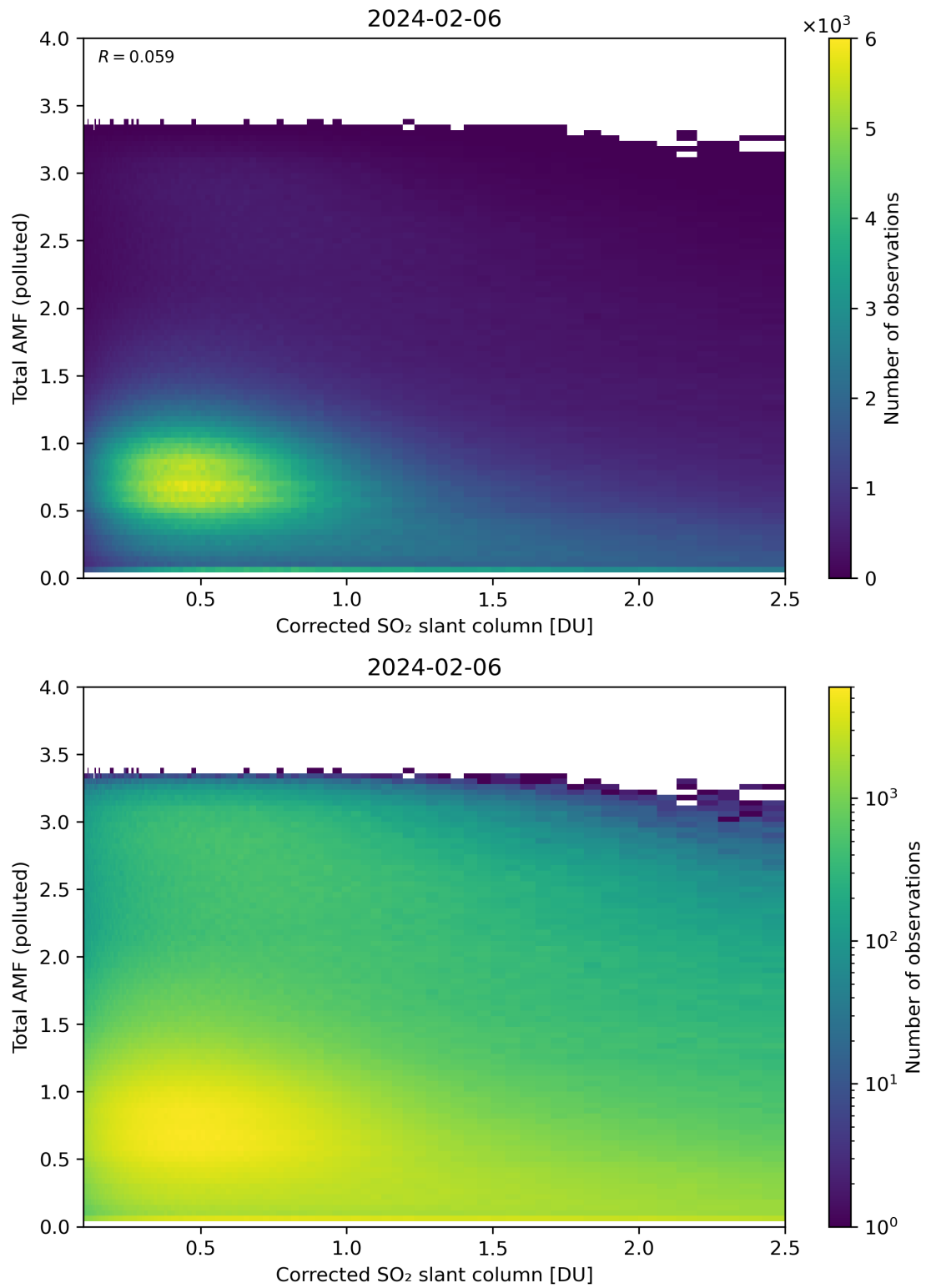
Figure 192: Scatter density plot of “Corrected SO 2 slant column” against “Total AMF (polluted)” for 2024-02-06 to 2024-02-07.
