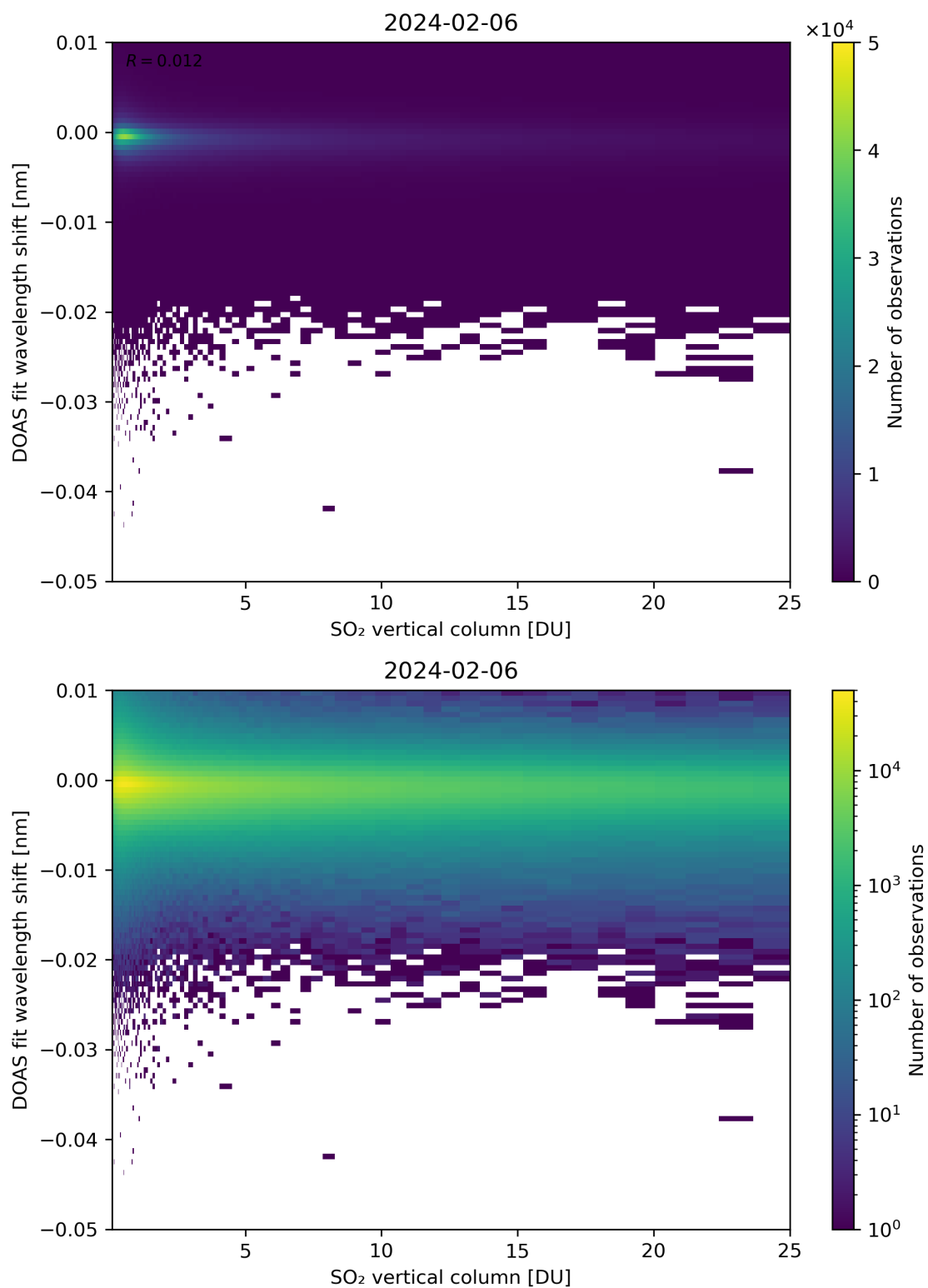
Figure 276: Scatter density plot of “SO 2 vertical column” against “DOAS fit wavelength shift” for 2024-02-06 to 2024-02-07.
