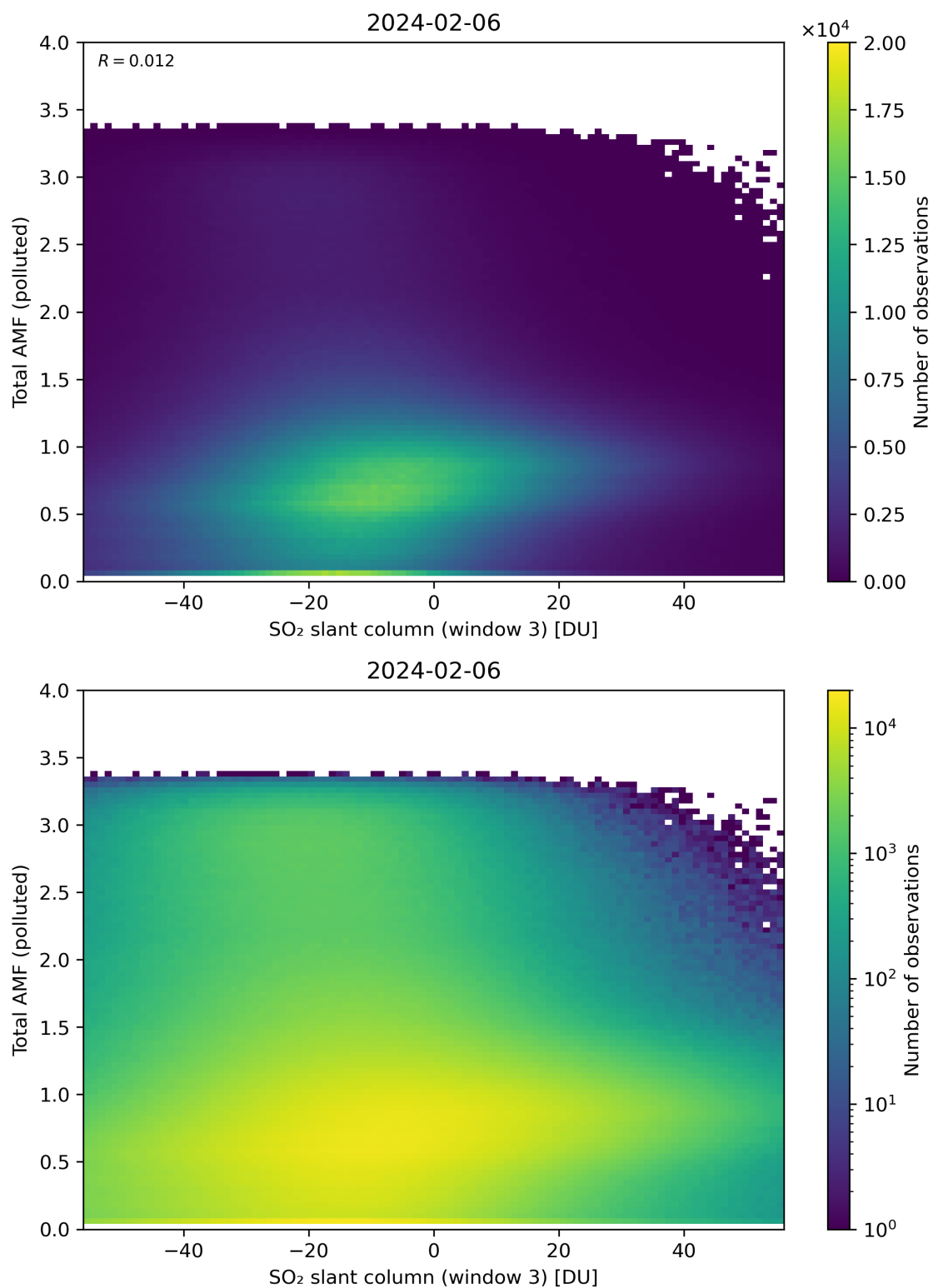
Figure 268: Scatter density plot of “SO 2 slant column (window 3)” against “Total AMF (polluted)” for 2024-02-06 to 2024-02-07.
