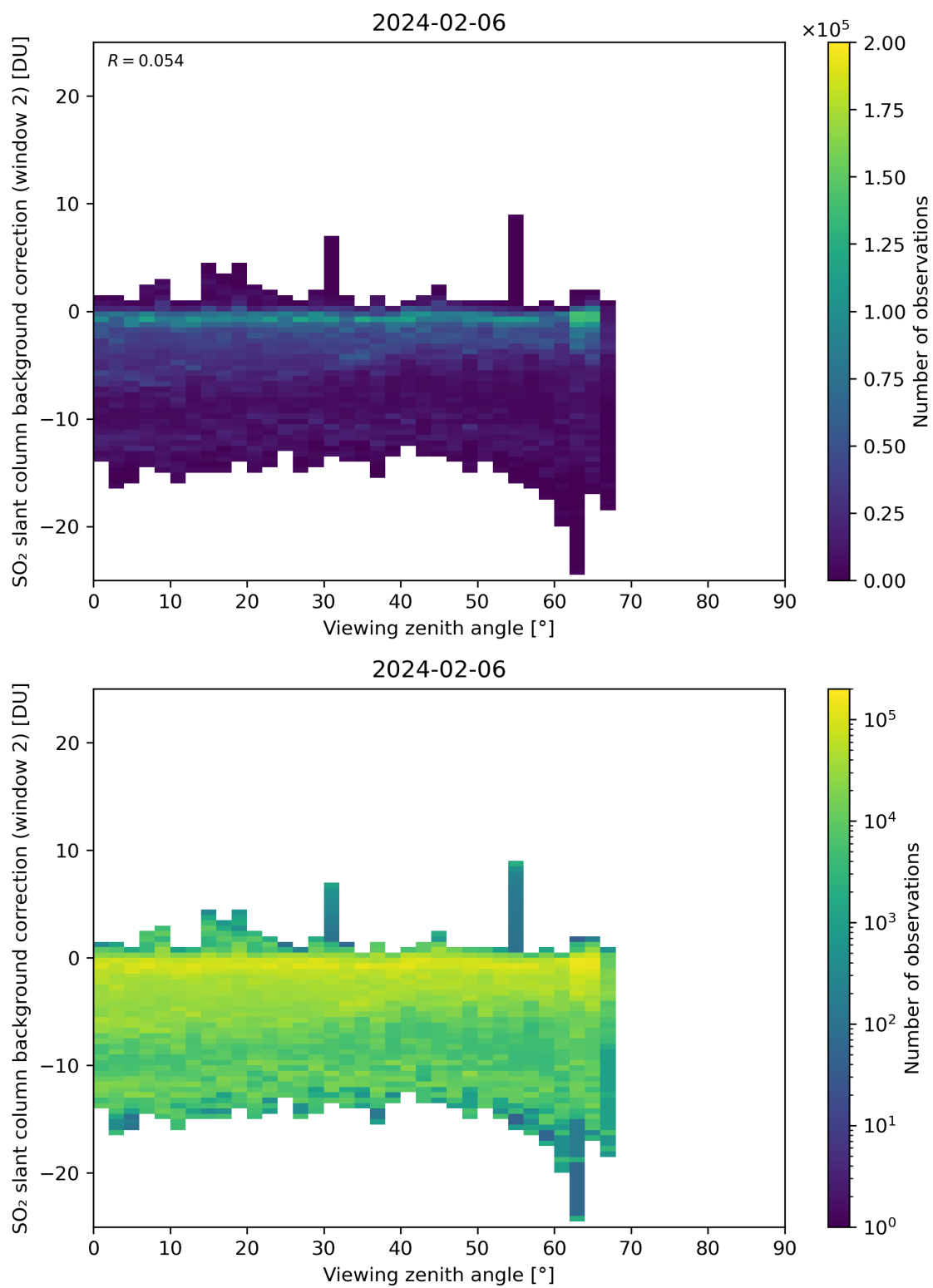
Figure 309: Scatter density plot of “Viewing zenith angle” against “SO 2 slant column background correction (window 2)” for 2024-02-06 to 2024-02-07.
