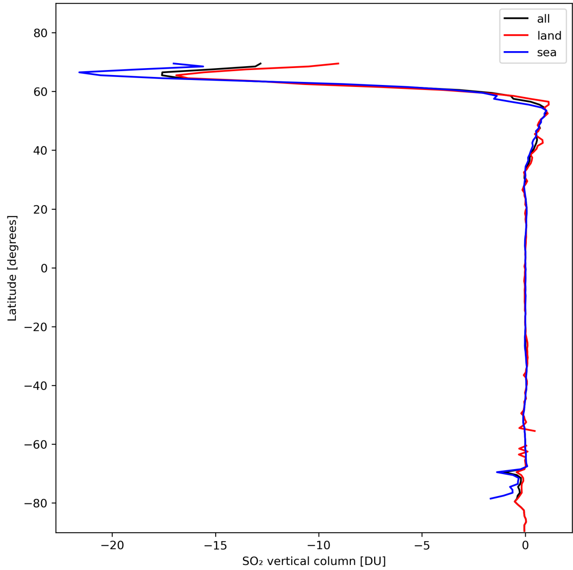
Figure 30: Zonal average of “SO 2 vertical column” for 2024-02-06 to 2024-02-07.
