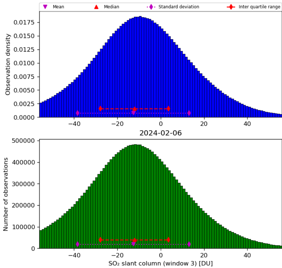
Figure 64: Histogram of “SO 2 slant column (window 3)” for 2024-02-06 to 2024-02-07
