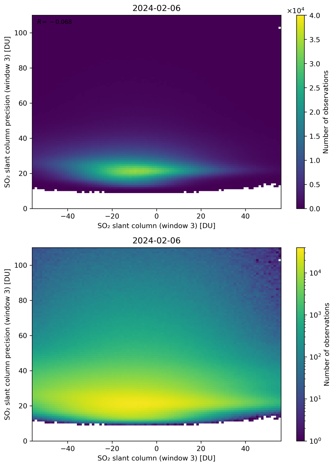
Figure 267: Scatter density plot of “SO 2 slant column (window 3)” against “SO 2 slant column precision (window 3)” for 2024-02-06 to 2024-02-07.
