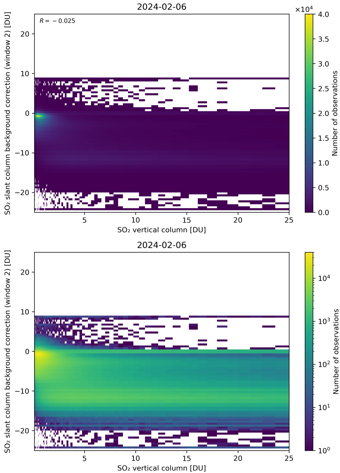
Figure 274: Scatter density plot of “SO 2 vertical column” against “SO 2 slant column background correction (window 2)” for 2024-02-06 to 2024-02-07.
