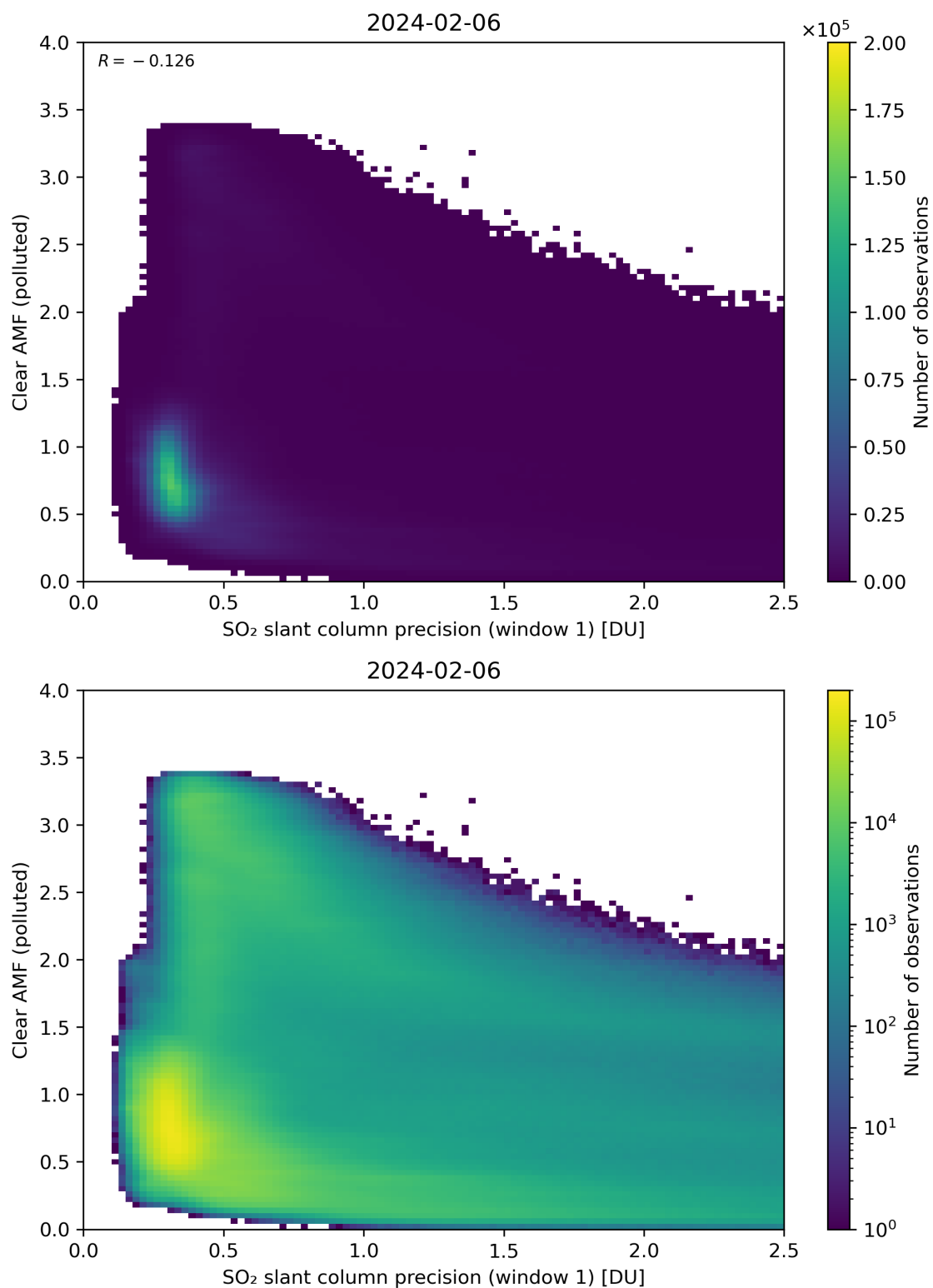
Figure 224: Scatter density plot of “SO 2 slant column precision (window 1)” against “Clear AMF (polluted)” for 2024-02-06 to 2024-02-07.
