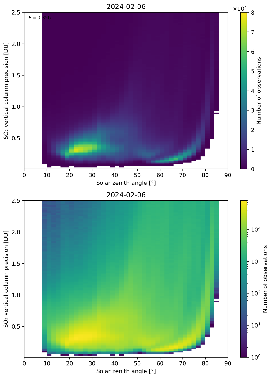
Figure 177: Scatter density plot of “Solar zenith angle” against “SO 2 vertical column precision” for 2024-02-06 to 2024-02-07.
