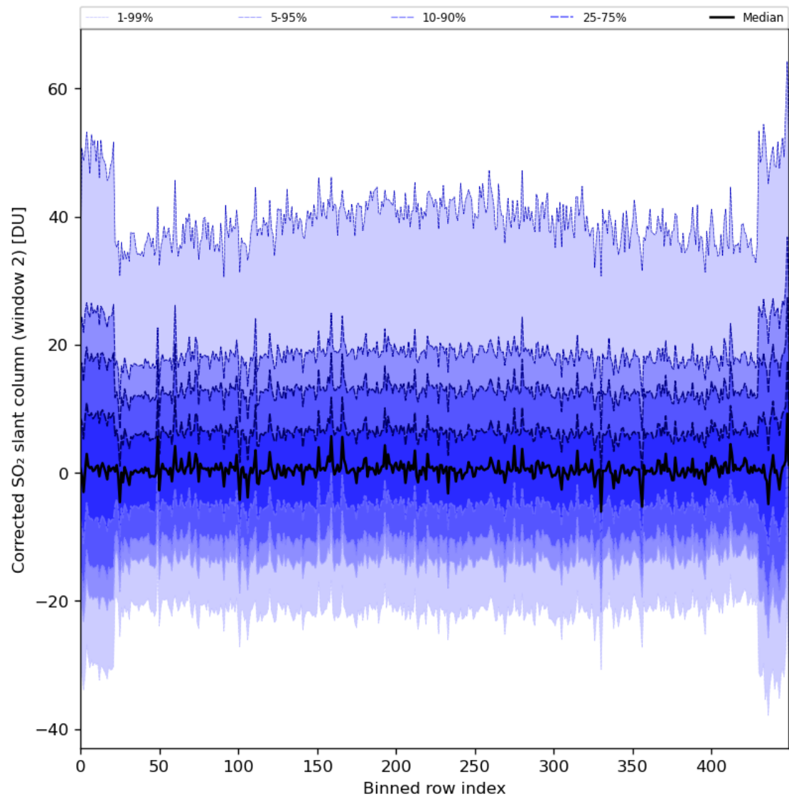
Figure 85: Along track statistics of “Corrected SO 2 slant column (window 2)” for 2024-02-06 to 2024-02-07
