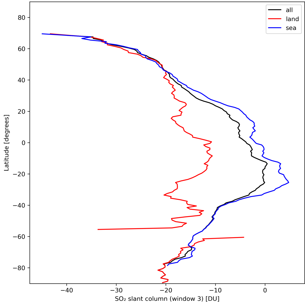
Figure 41: Zonal average of “SO 2 slant column (window 3)” for 2024-02-06 to 2024-02-07.
