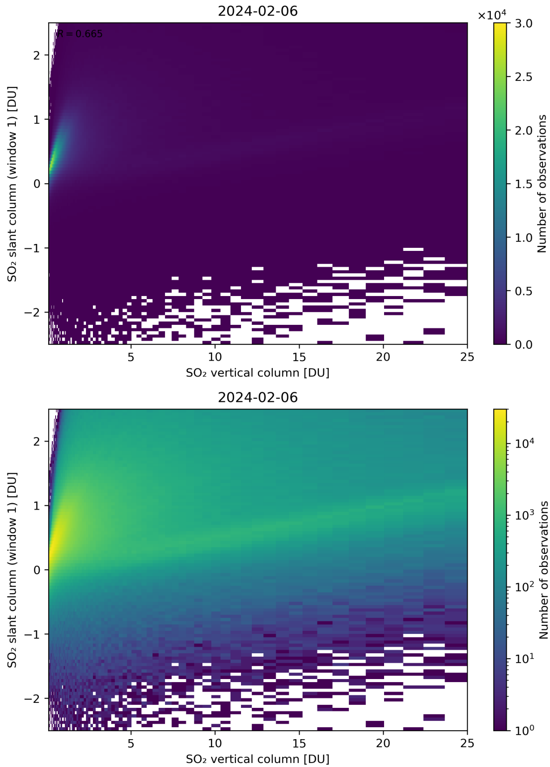
Figure 300: Scatter density plot of “SO 2 vertical column” against “SO 2 slant column (window 1)” for 2024-02-06 to 2024-02-07.
