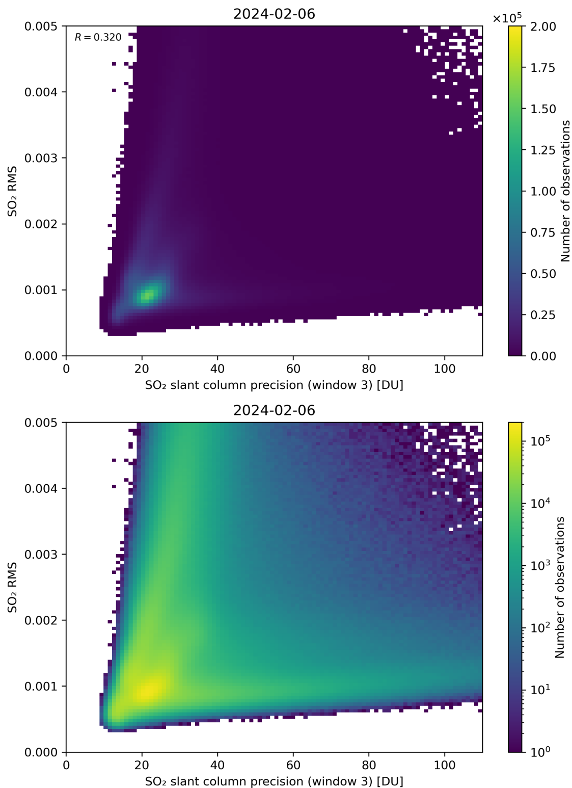
Figure 260: Scatter density plot of “SO 2 slant column precision (window 3)” against “SO 2 RMS” for 2024-02-06 to 2024-02-07.
