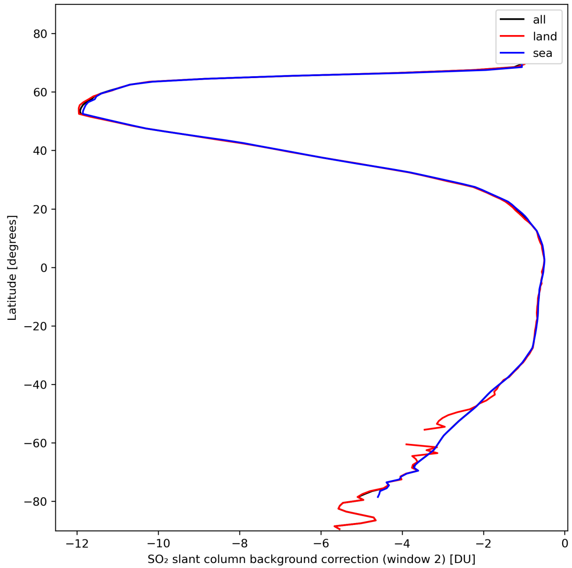
Figure 40: Zonal average of “SO 2 slant column background correction (window 2)” for 2024-02-06 to 2024-02-07.
