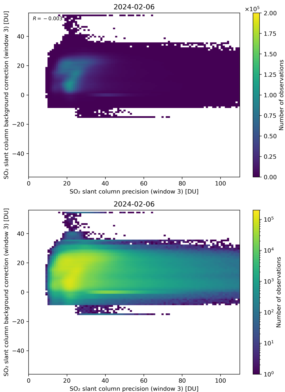
Figure 257: Scatter density plot of “SO 2 slant column precision (window 3)” against “SO 2 slant column background correction (window 3)” for 2024-02-06 to 2024-02-07.
