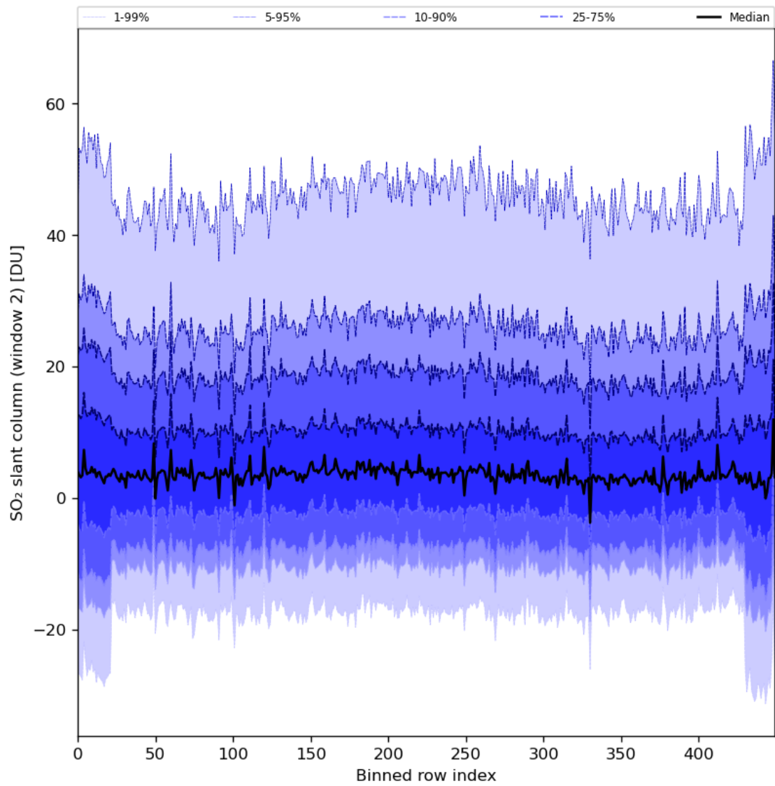
Figure 83: Along track statistics of “SO 2 slant column (window 2)” for 2024-02-06 to 2024-02-07
