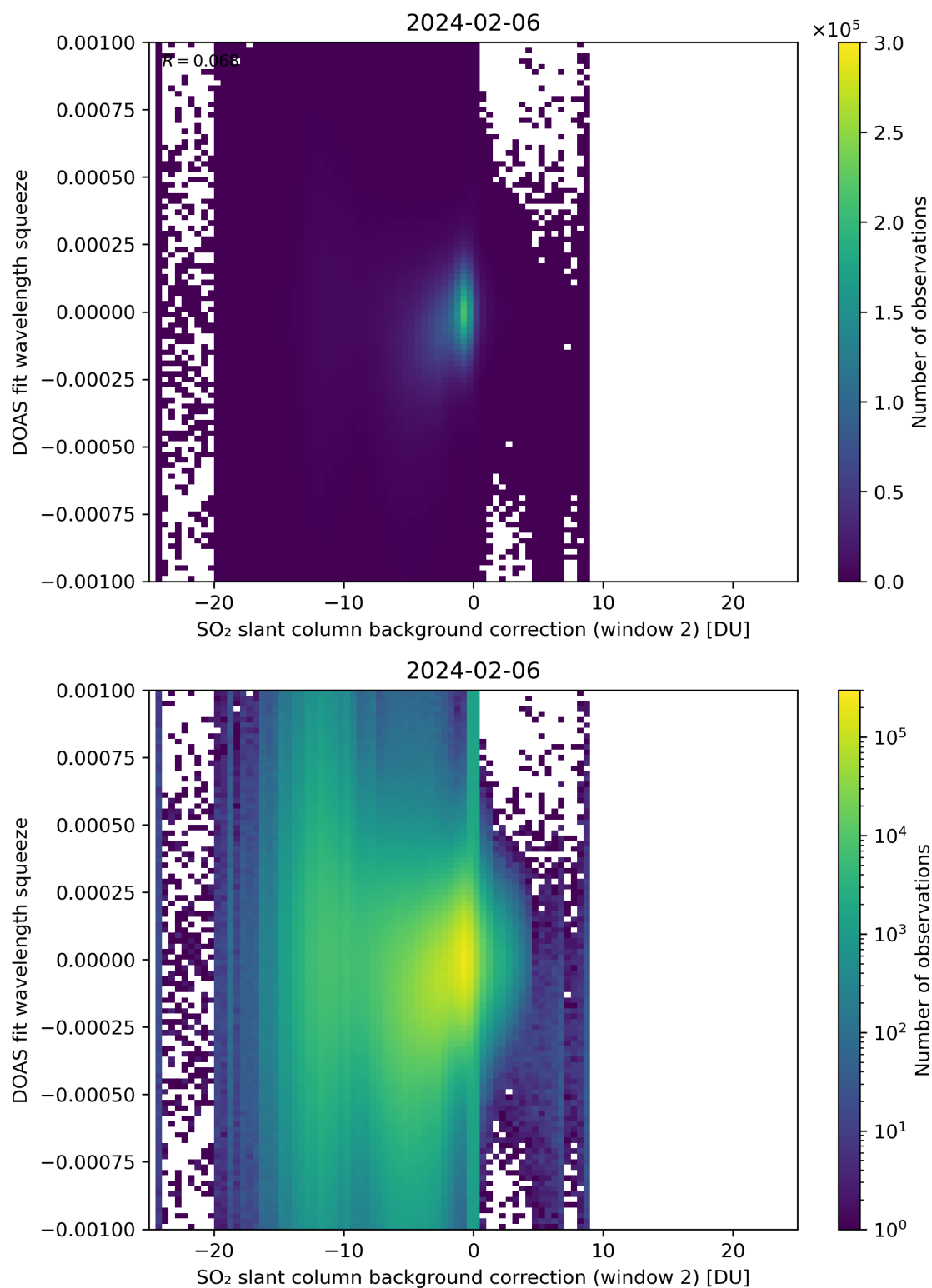
Figure 113: Scatter density plot of “SO 2 slant column background correction (window 2)” against “DOAS fit wavelength squeeze” for 2024-02-06 to 2024-02-07.
