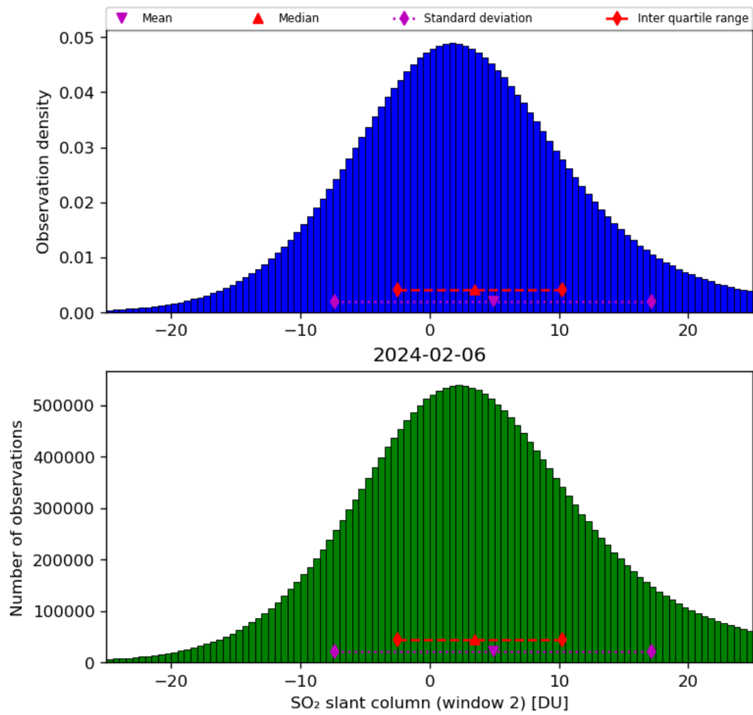
Figure 60: Histogram of “SO 2 slant column (window 2)” for 2024-02-06 to 2024-02-07
