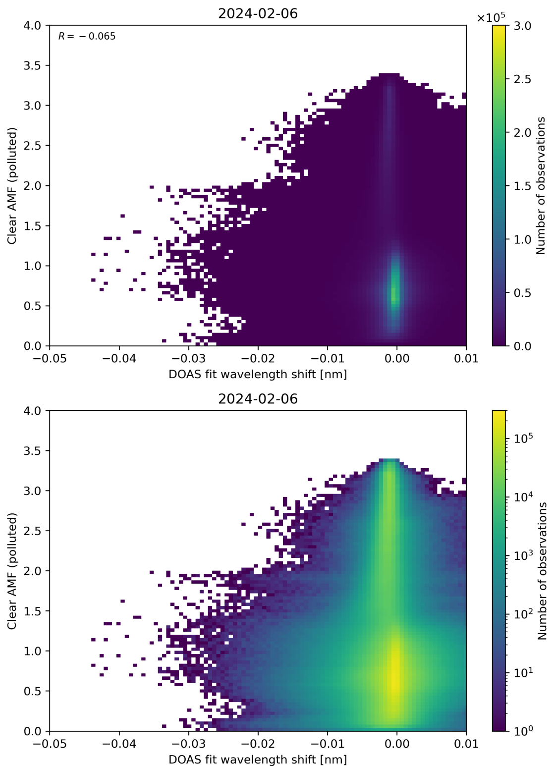
Figure 129: Scatter density plot of “DOAS fit wavelength shift” against “Clear AMF (polluted)” for 2024-02-06 to 2024-02-07.
