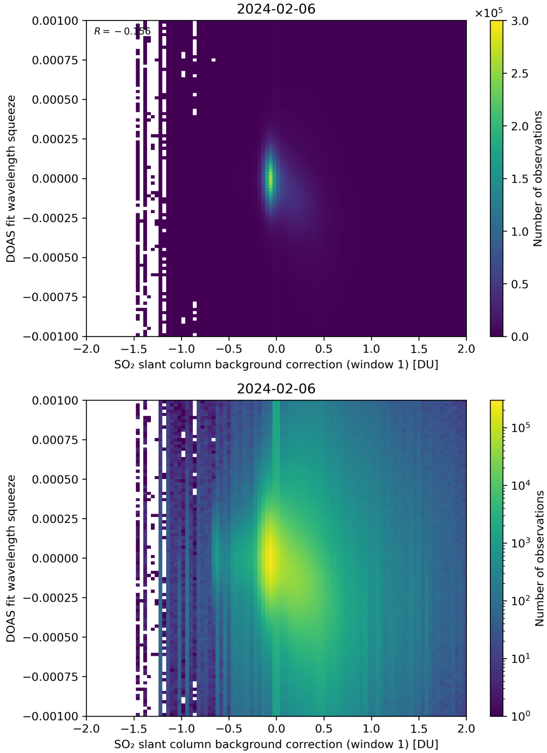
Figure 101: Scatter density plot of “SO 2 slant column background correction (window 1)” against “DOAS fit wavelength squeeze” for 2024-02-06 to 2024-02-07.
