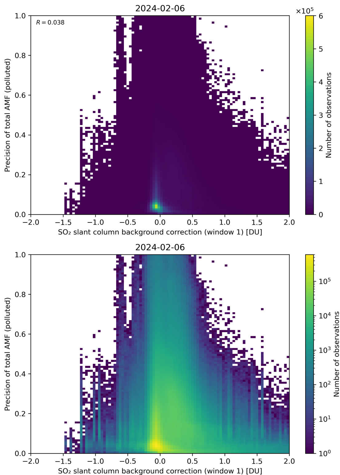
Figure 110: Scatter density plot of “SO 2 slant column background correction (window 1)” against “Precision of total AMF (polluted)” for 2024-02-06 to 2024-02-07.
