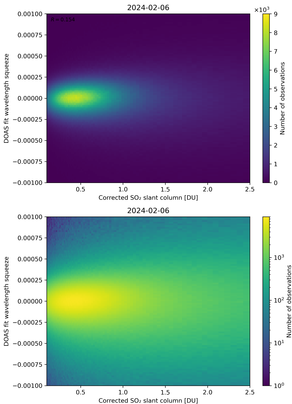
Figure 182: Scatter density plot of “Corrected SO 2 slant column” against “DOAS fit wavelength squeeze” for 2024-02-06 to 2024-02-07.
