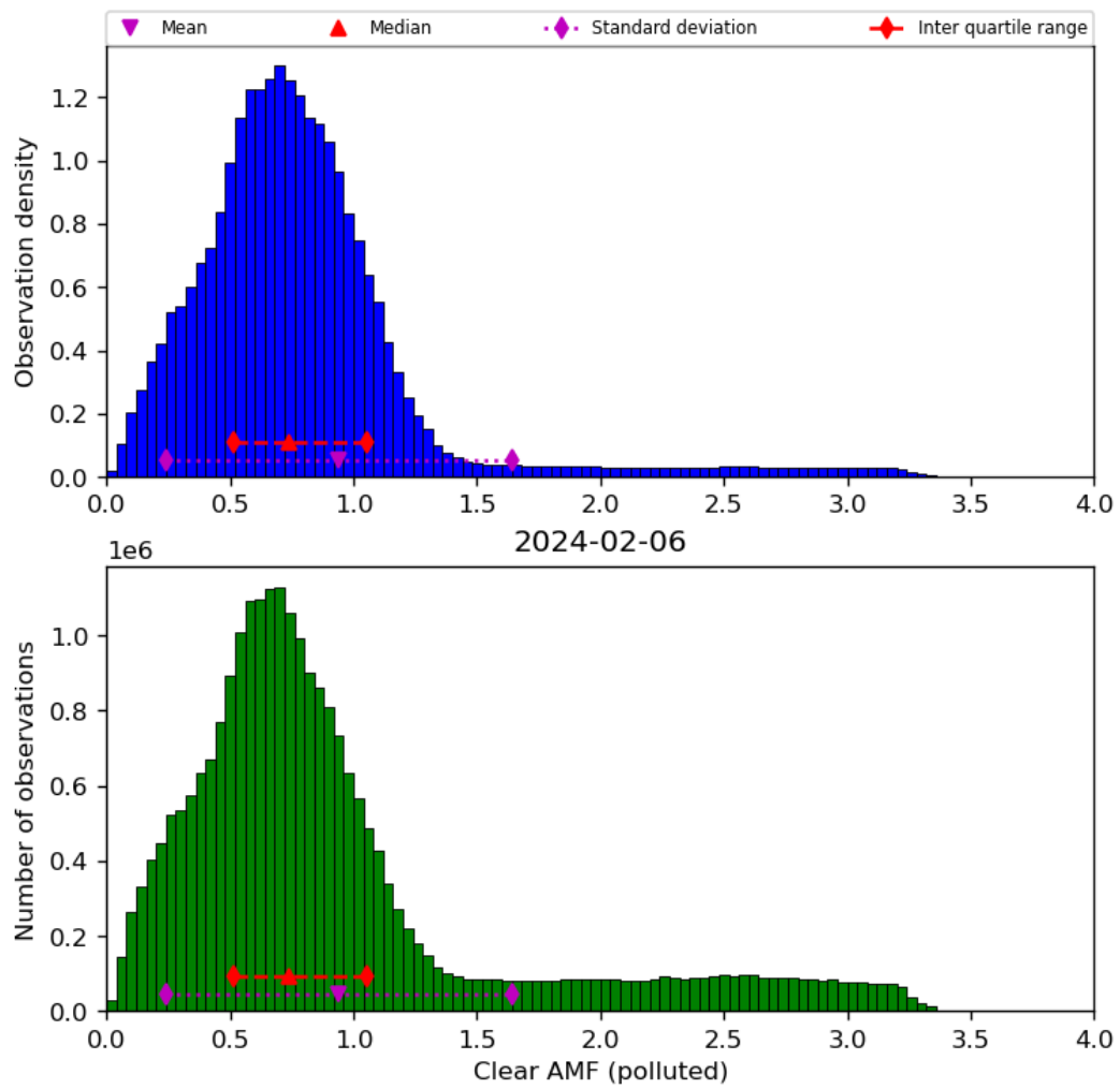
Figure 73: Histogram of “Clear AMF (polluted)” for 2024-02-06 to 2024-02-07
