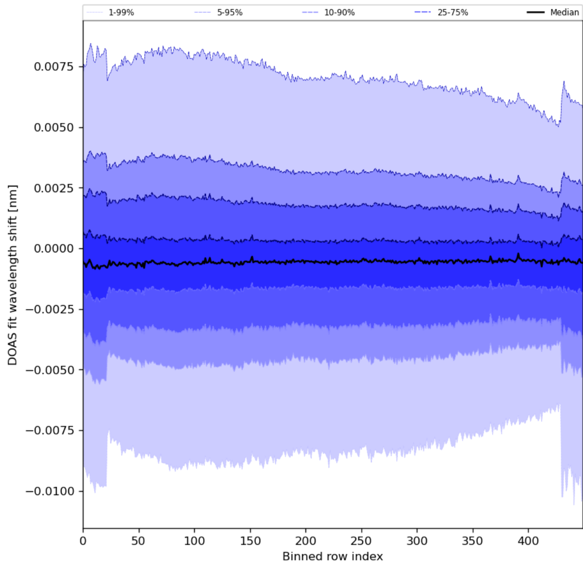
Figure 91: Along track statistics of “DOAS fit wavelength shift” for 2024-02-06 to 2024-02-07
