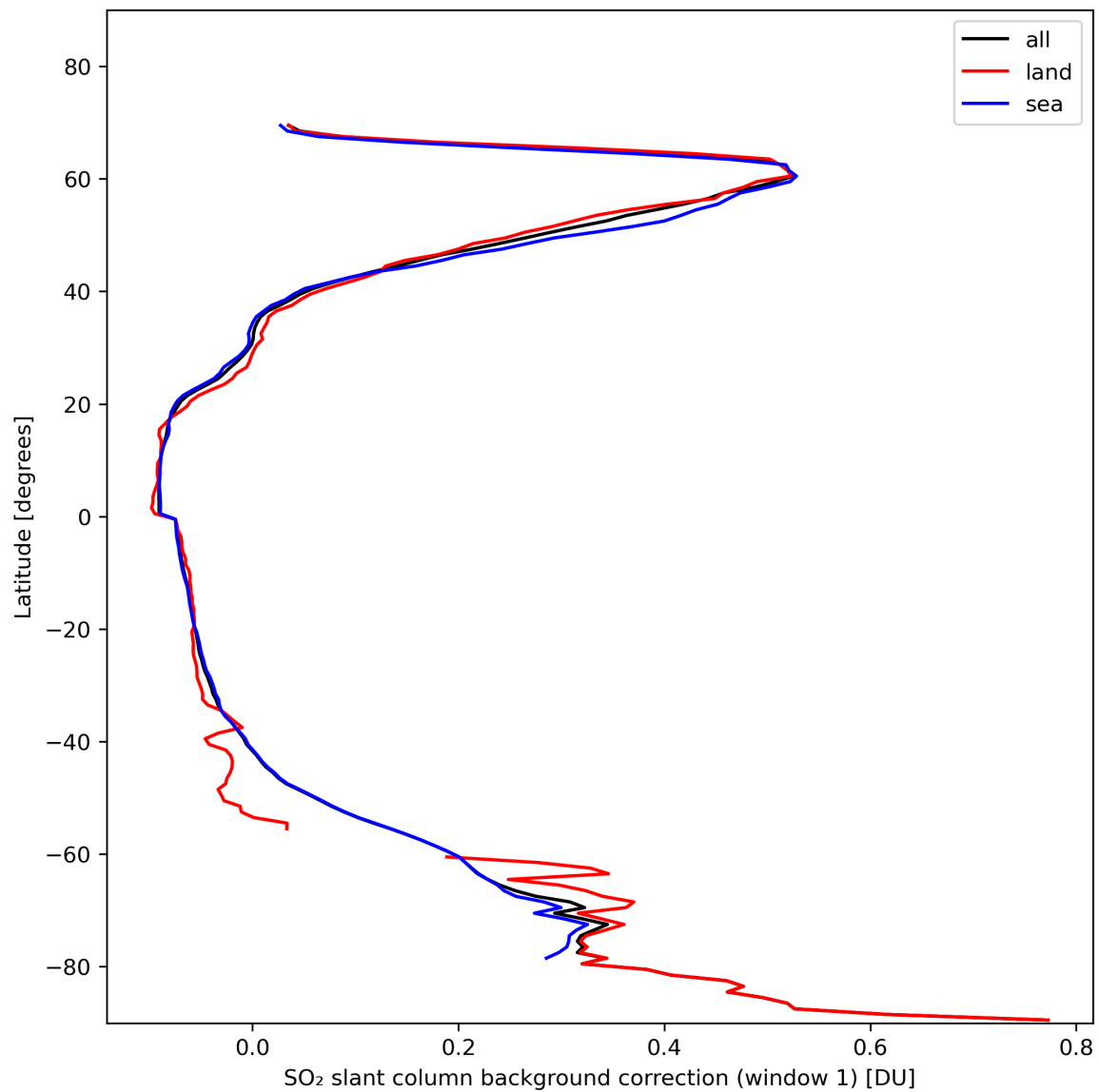
Figure 36: Zonal average of “SO 2 slant column background correction (window 1)” for 2024-02-06 to 2024-02-07.
