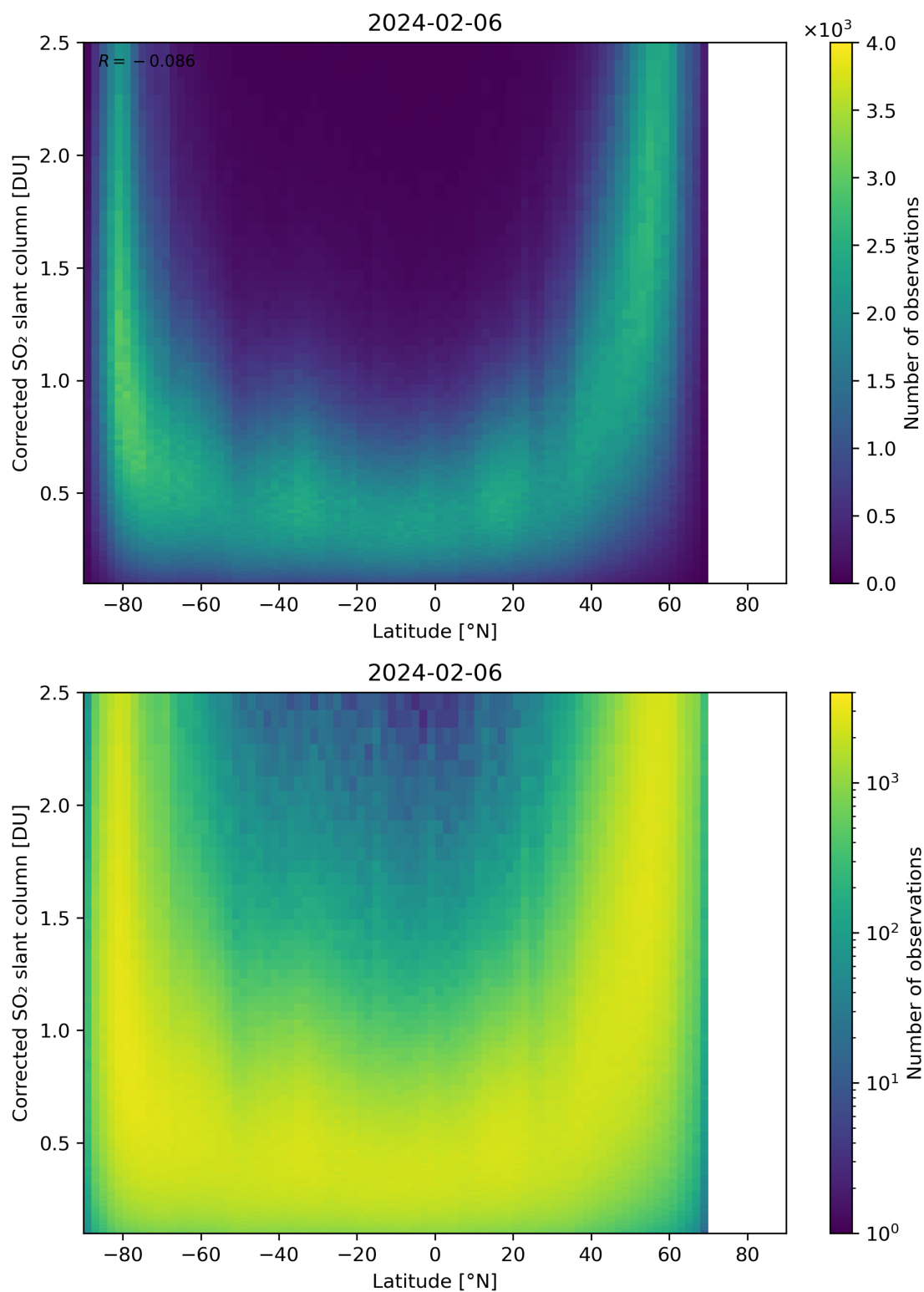
Figure 146: Scatter density plot of “Latitude” against “Corrected SO 2 slant column” for 2024-02-06 to 2024-02-07.
