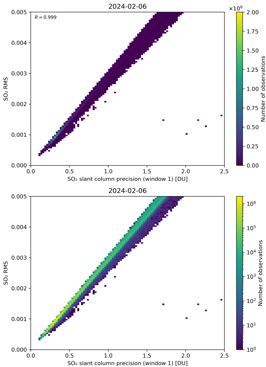
Figure 223: Scatter density plot of “SO 2 slant column precision (window 1)” against “SO 2 RMS” for 2024-02-06 to 2024-02-07.
