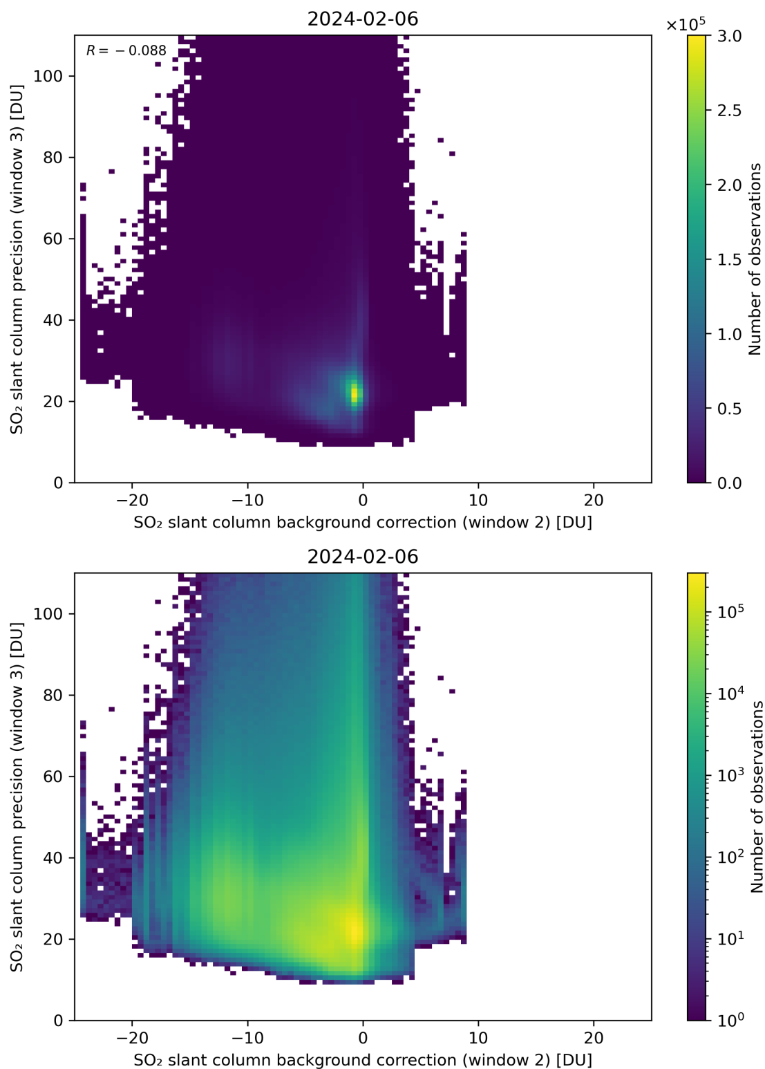
Figure 118: Scatter density plot of “SO 2 slant column background correction (window 2)” against “SO 2 slant column precision (window 3)” for 2024-02-06 to 2024-02-07.
