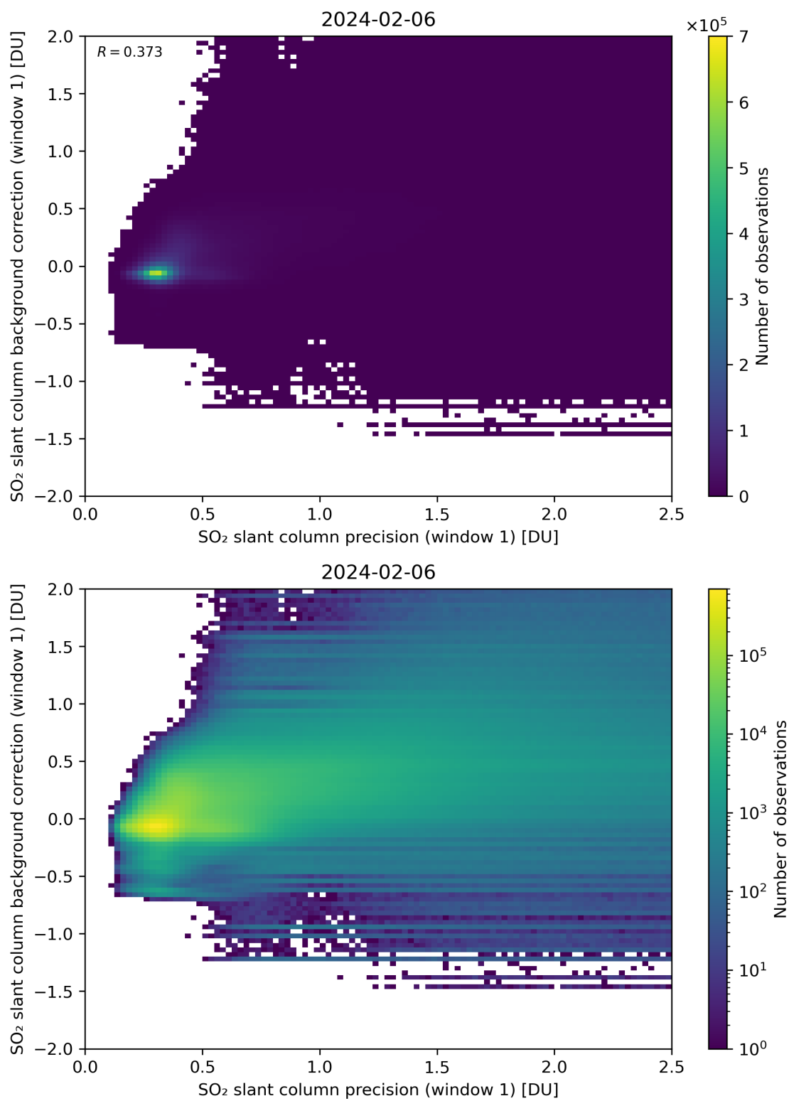
Figure 218: Scatter density plot of “SO 2 slant column precision (window 1)” against “SO 2 slant column background correction (window 1)” for 2024-02-06 to 2024-02-07.
