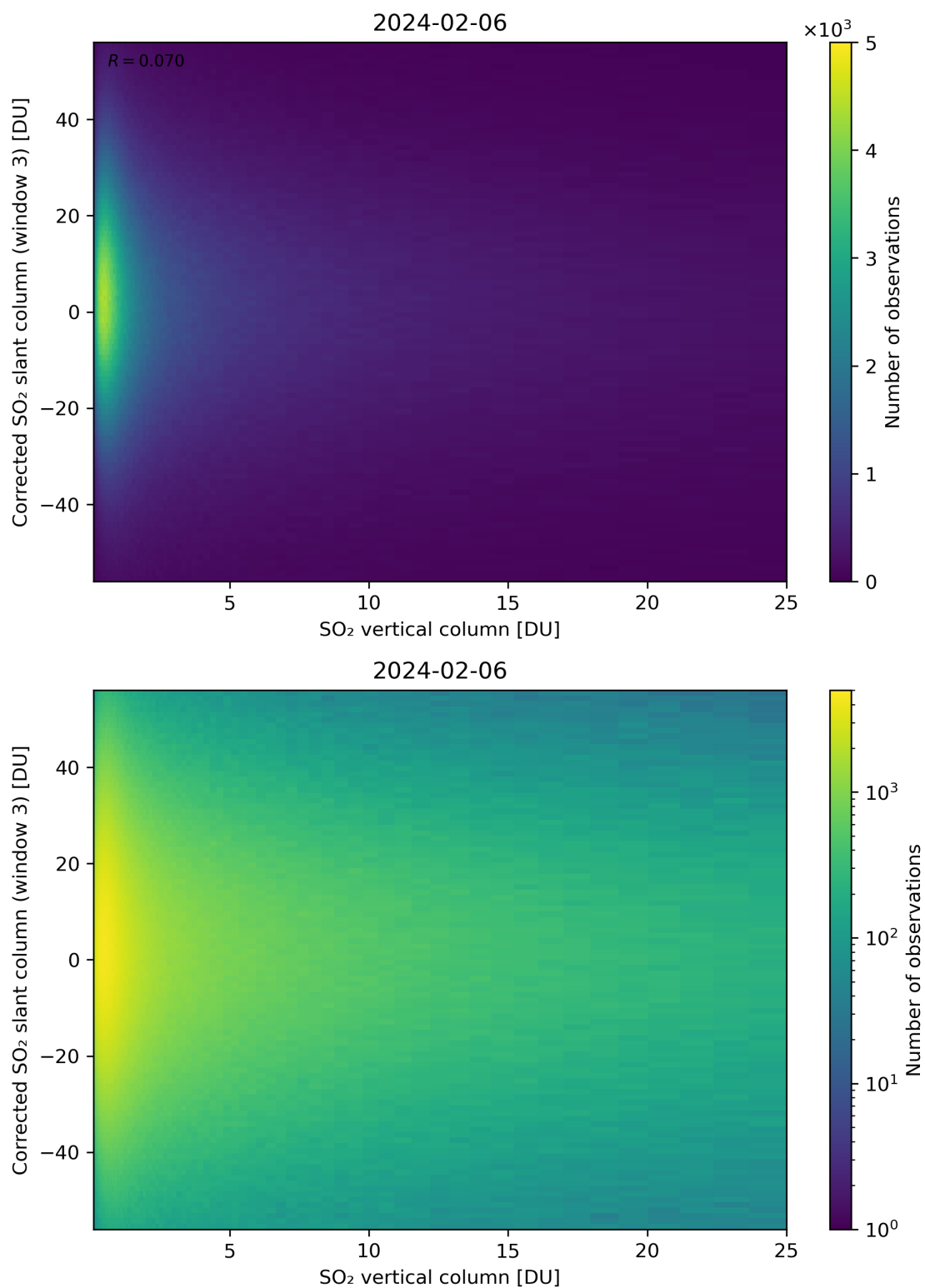
Figure 299: Scatter density plot of “SO 2 vertical column” against “Corrected SO 2 slant column (window 3)” for 2024-02-06 to 2024-02-07.
