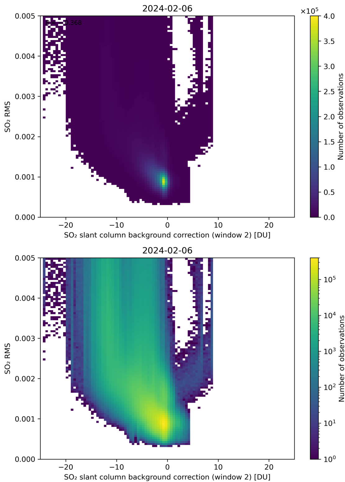
Figure 114: Scatter density plot of “SO 2 slant column background correction (window 2)” against “SO 2 RMS” for 2024-02-06 to 2024-02-07.
