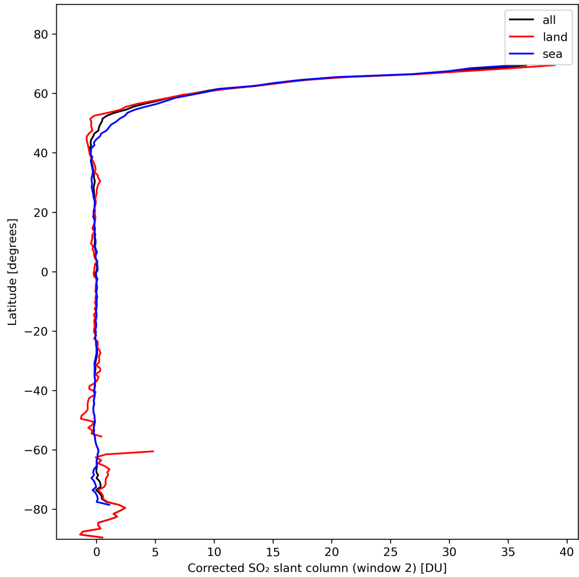
Figure 39: Zonal average of “Corrected SO 2 slant column (window 2)” for 2024-02-06 to 2024-02-07.
