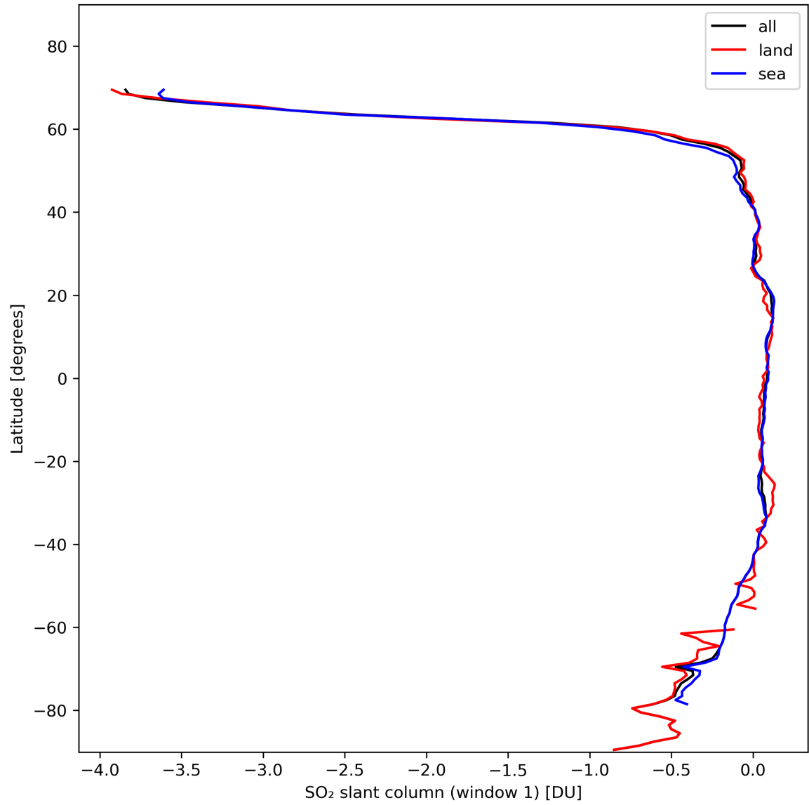
Figure 33: Zonal average of “SO 2 slant column (window 1)” for 2024-02-06 to 2024-02-07.
