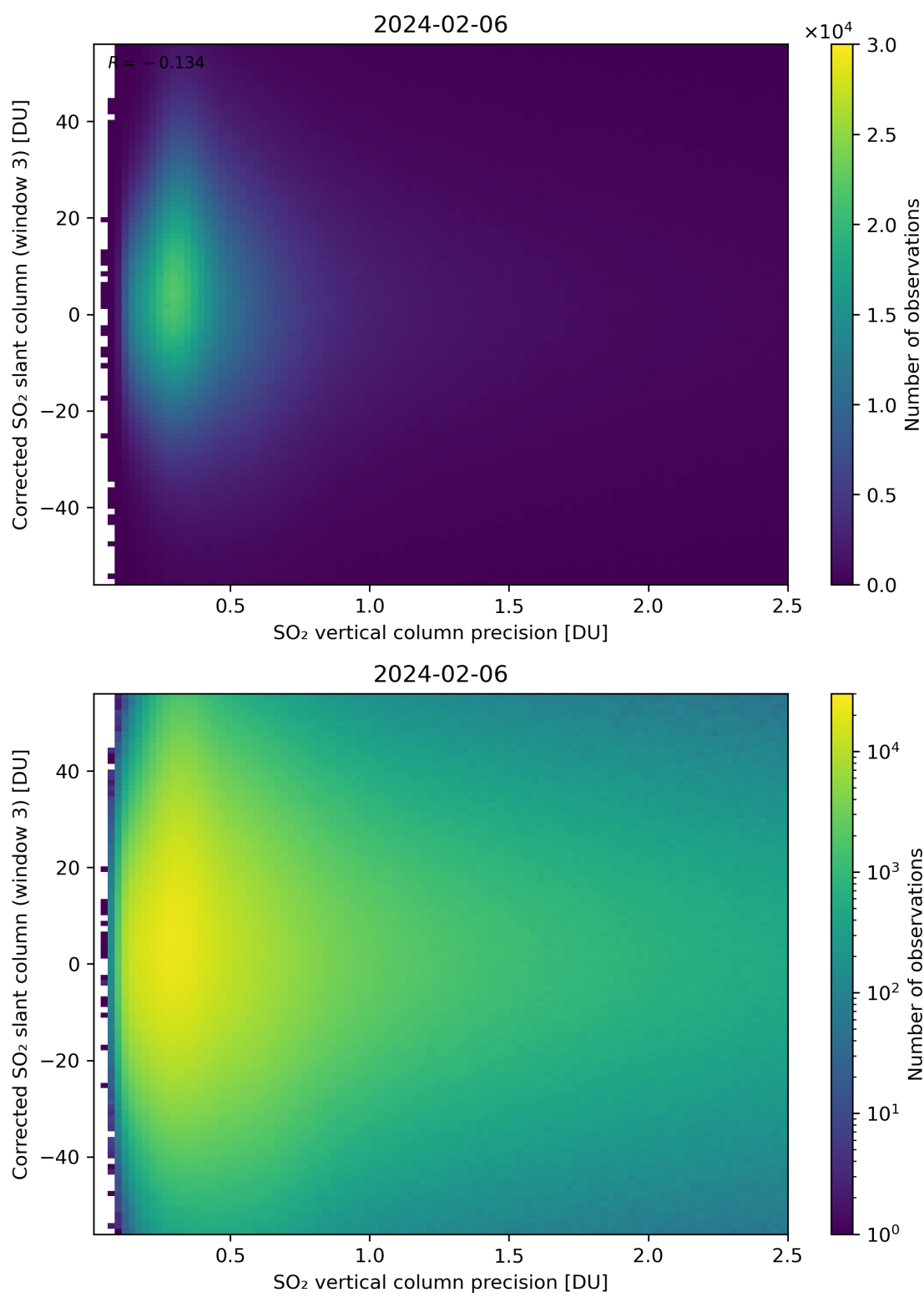
Figure 288: Scatter density plot of “SO 2 vertical column precision” against “Corrected SO 2 slant column (window 3)” for 2024-02-06 to 2024-02-07.
