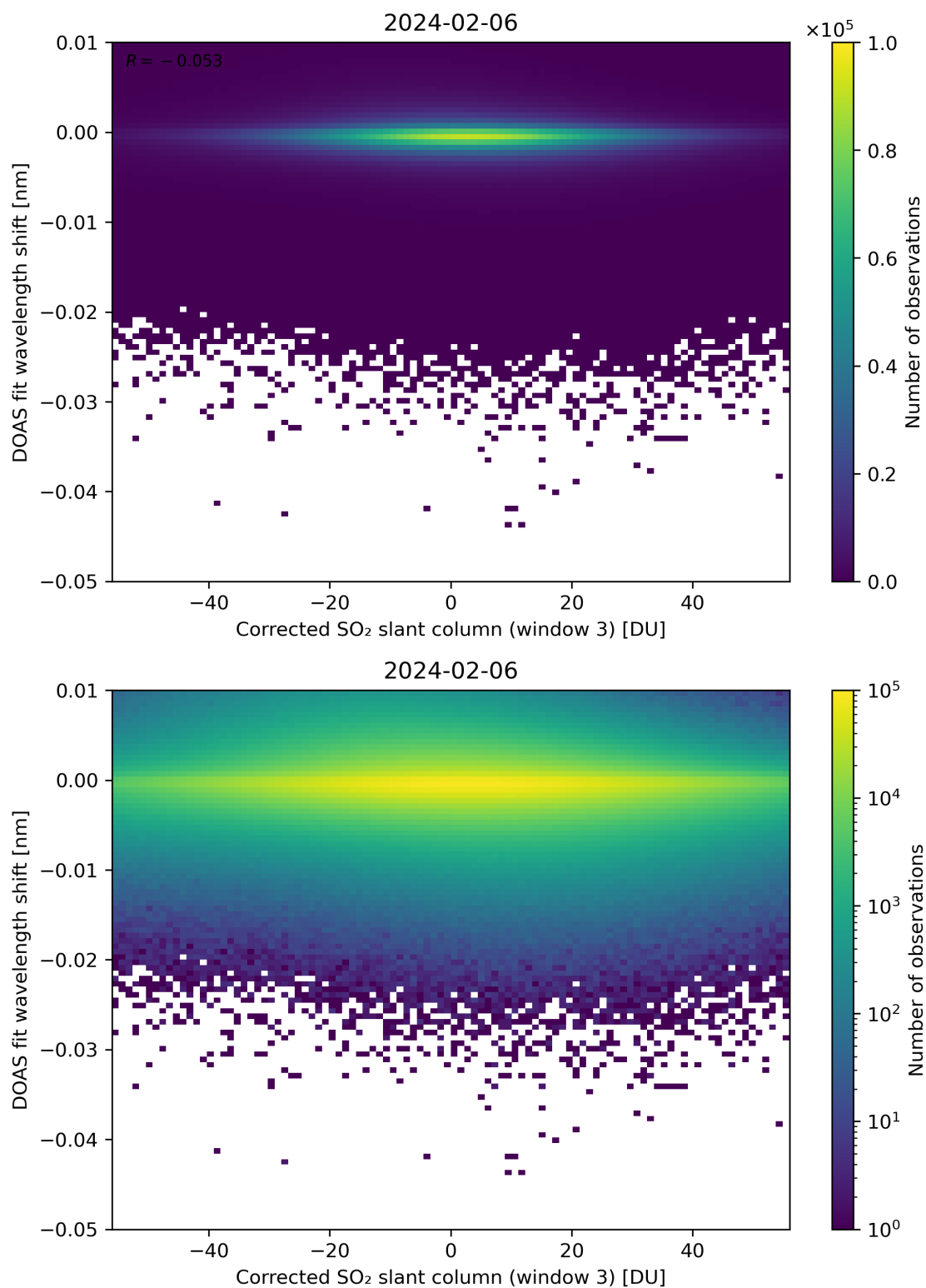
Figure 206: Scatter density plot of “Corrected SO 2 slant column (window 3)” against “DOAS fit wavelength shift” for 2024-02-06 to 2024-02-07.
