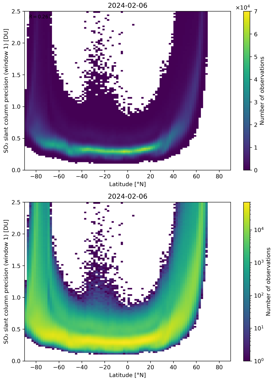
Figure 150: Scatter density plot of “Latitude” against “SO 2 slant column precision (window 1)” for 2024-02-06 to 2024-02-07.
