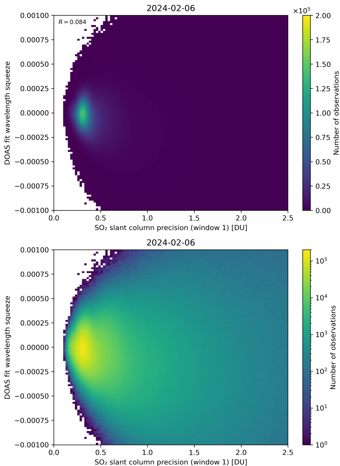
Figure 222: Scatter density plot of “SO 2 slant column precision (window 1)” against “DOAS fit wavelength squeeze” for 2024-02-06 to 2024-02-07.
