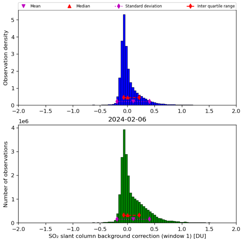
Figure 59: Histogram of “SO 2 slant column background correction (window 1)” for 2024-02-06 to 2024-02-07
