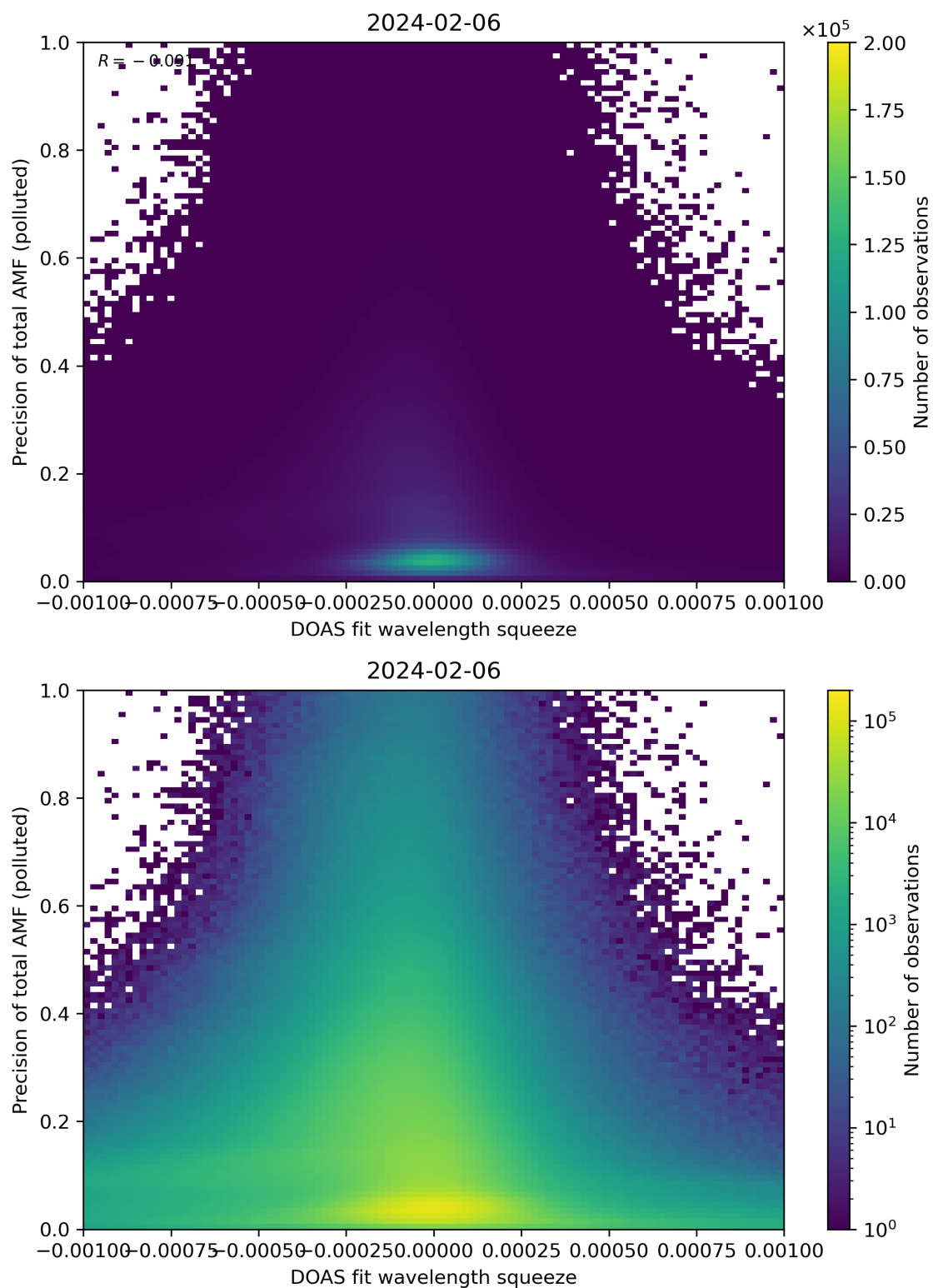
Figure 135: Scatter density plot of “DOAS fit wavelength squeeze” against “Precision of total AMF (polluted)” for 2024-02-06 to 2024-02-07.
