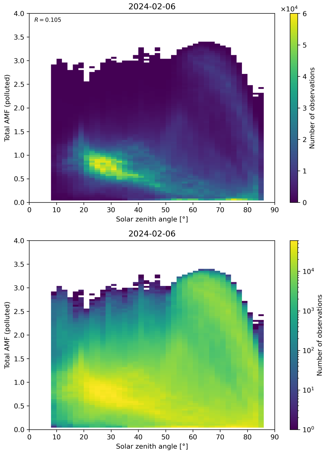
Figure 174: Scatter density plot of “Solar zenith angle” against “Total AMF (polluted)” for 2024-02-06 to 2024-02-07.
