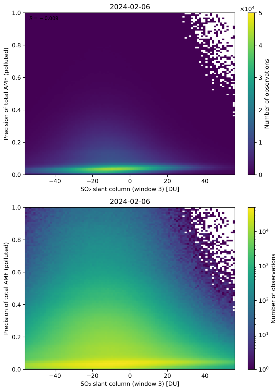
Figure 269: Scatter density plot of “SO 2 slant column (window 3)” against “Precision of total AMF (polluted)” for 2024-02-06 to 2024-02-07.
