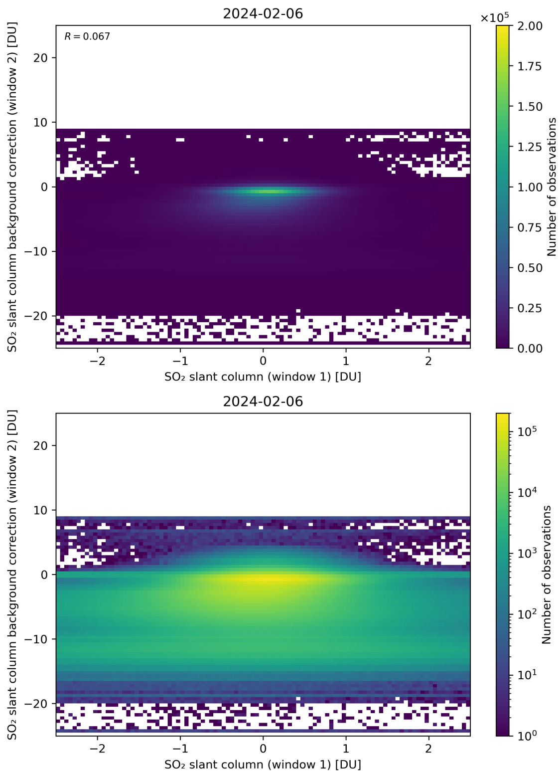
Figure 213: Scatter density plot of “SO 2 slant column (window 1)” against “SO 2 slant column background correction (window 2)” for 2024-02-06 to 2024-02-07.
