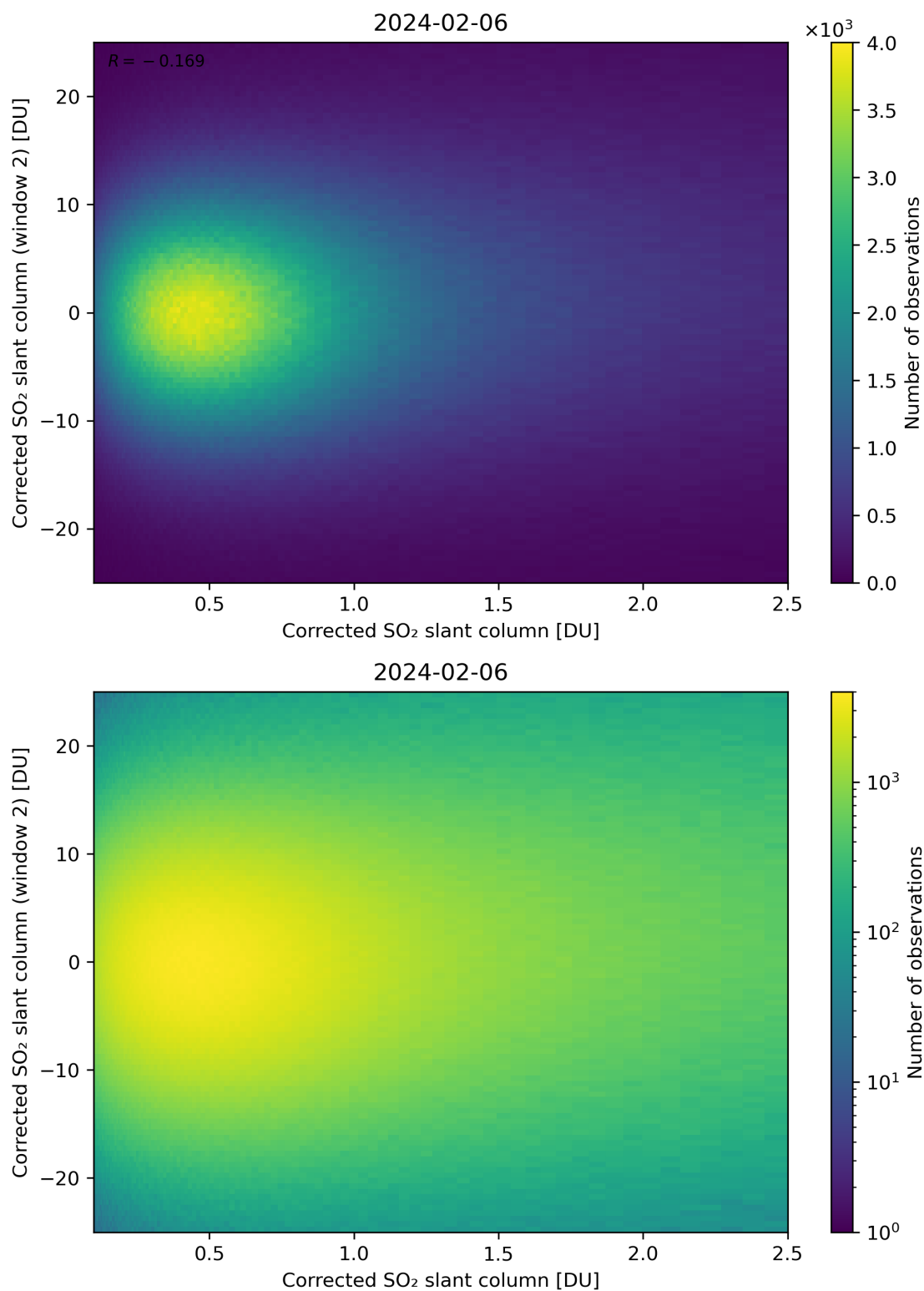
Figure 185: Scatter density plot of “Corrected SO 2 slant column” against “Corrected SO 2 slant column (window 2)” for 2024-02-06 to 2024-02-07.
