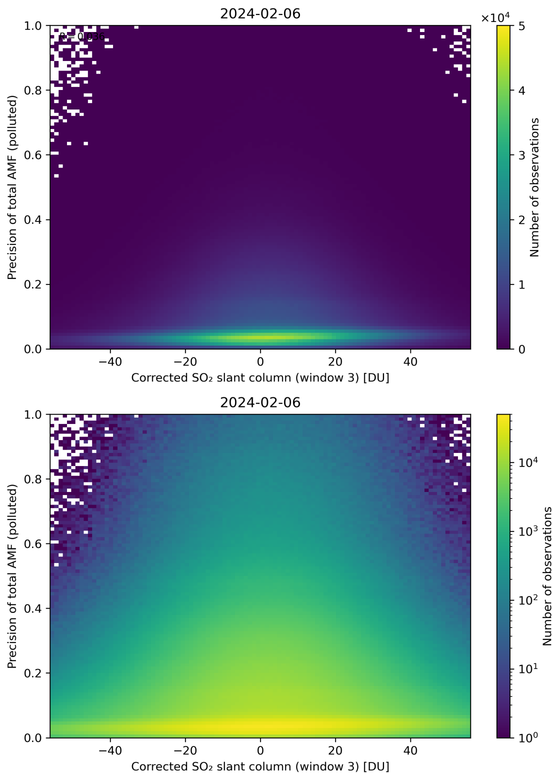
Figure 211: Scatter density plot of “Corrected SO 2 slant column (window 3)” against “Precision of total AMF (polluted)” for 2024-02-06 to 2024-02-07.
