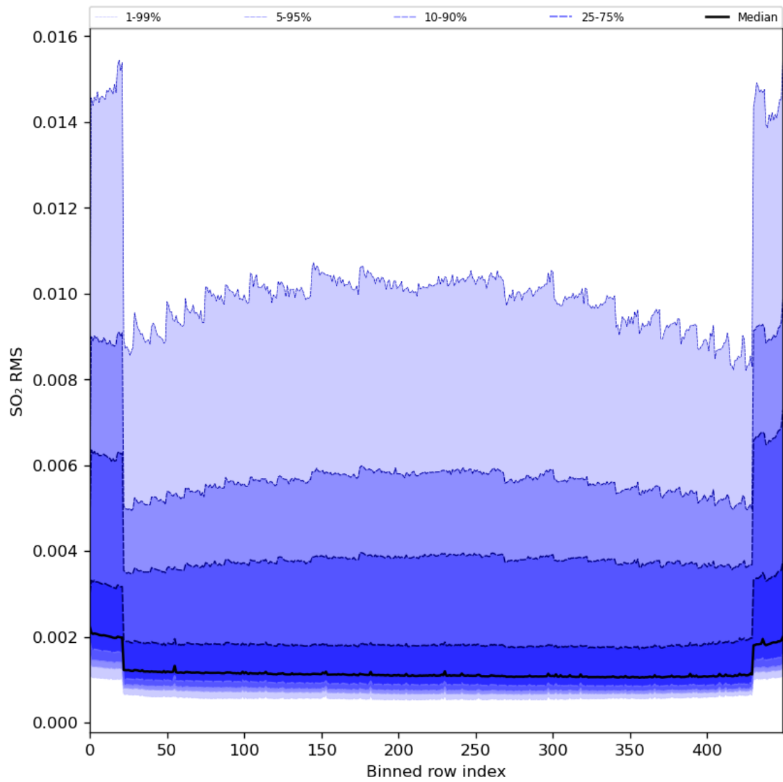
Figure 93: Along track statistics of “SO 2 RMS” for 2024-02-06 to 2024-02-07
