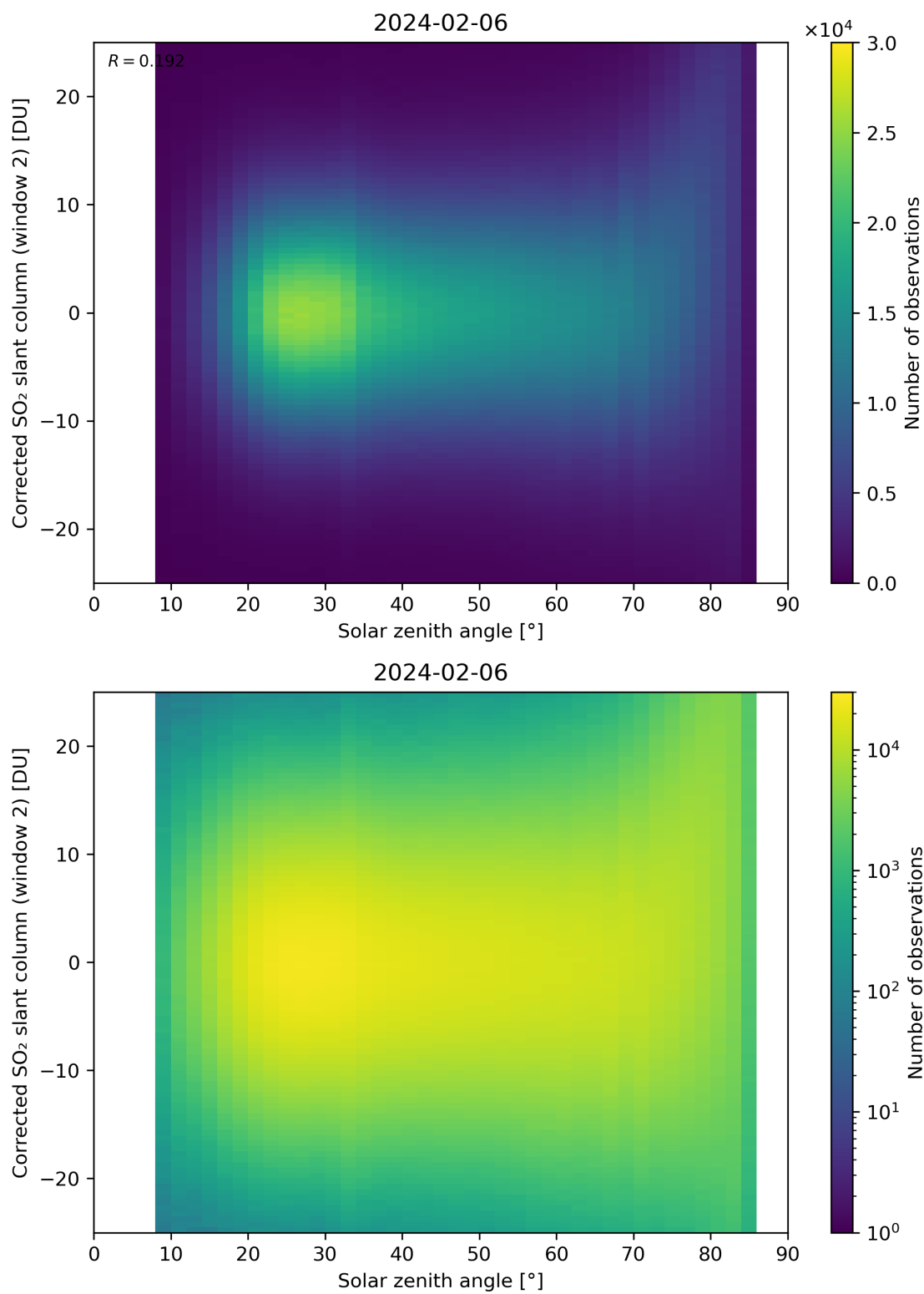
Figure 167: Scatter density plot of “Solar zenith angle” against “Corrected SO 2 slant column (window 2)” for 2024-02-06 to 2024-02-07.
