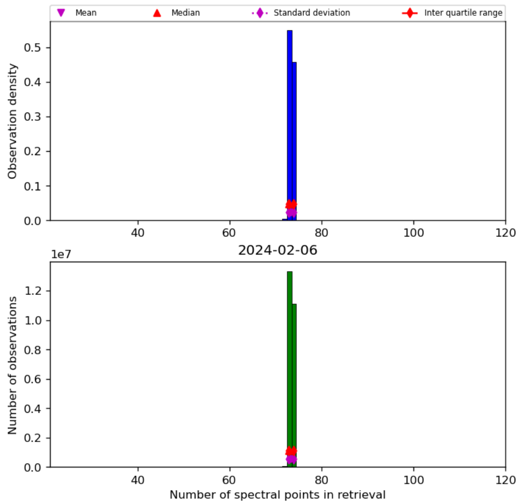
Figure 74: Histogram of “Number of spectral points in retrieval” for 2024-02-06 to 2024-02-07
