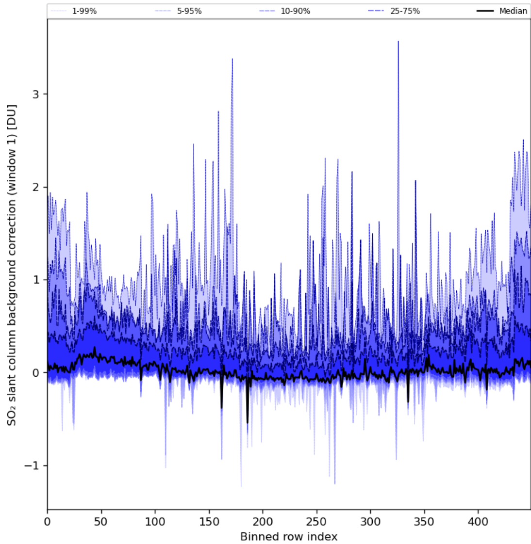
Figure 82: Along track statistics of “SO 2 slant column background correction (window 1)” for 2024-02-06 to 2024-02-07
