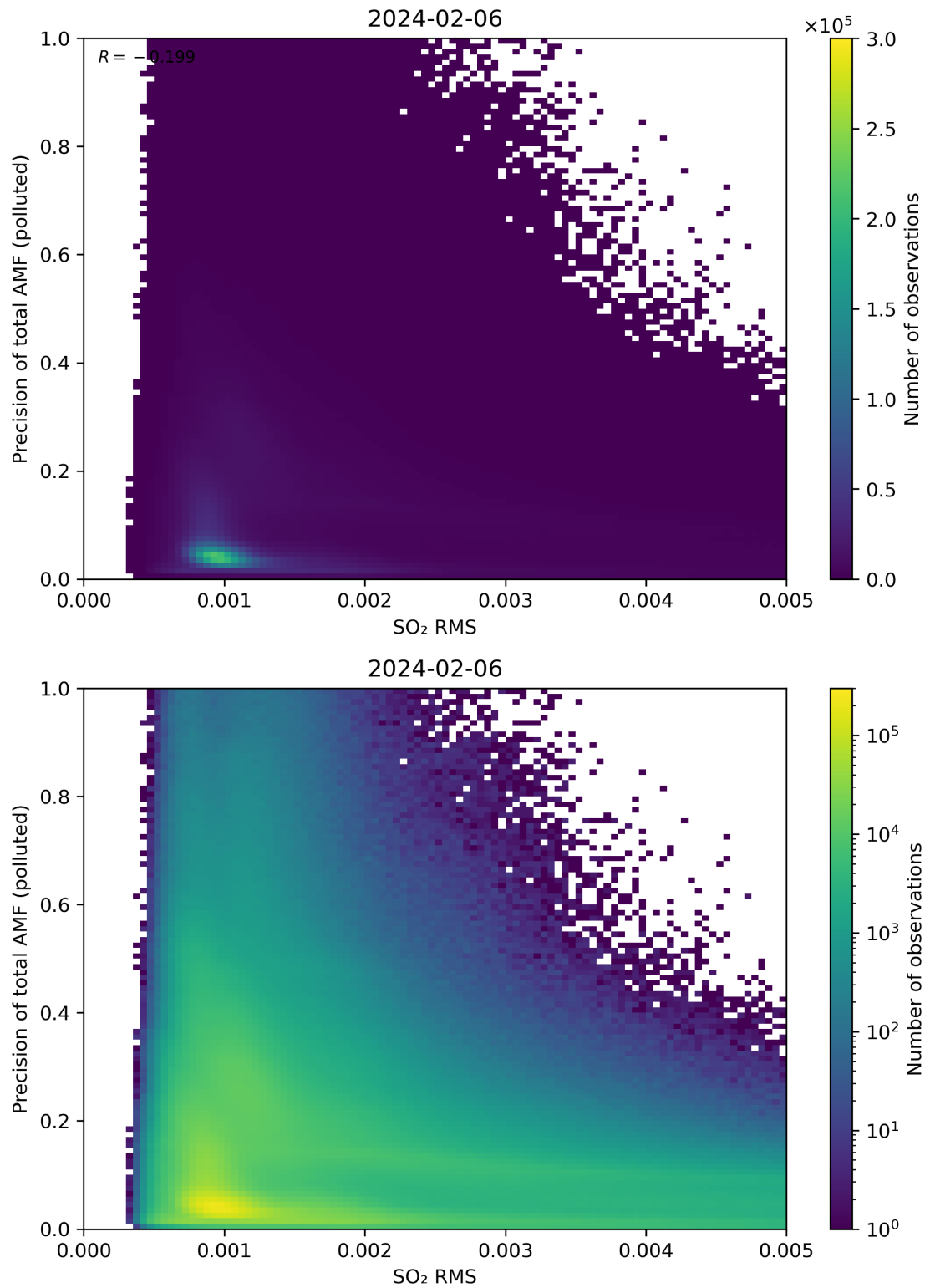
Figure 138: Scatter density plot of “SO 2 RMS” against “Precision of total AMF (polluted)” for 2024-02-06 to 2024-02-07.
