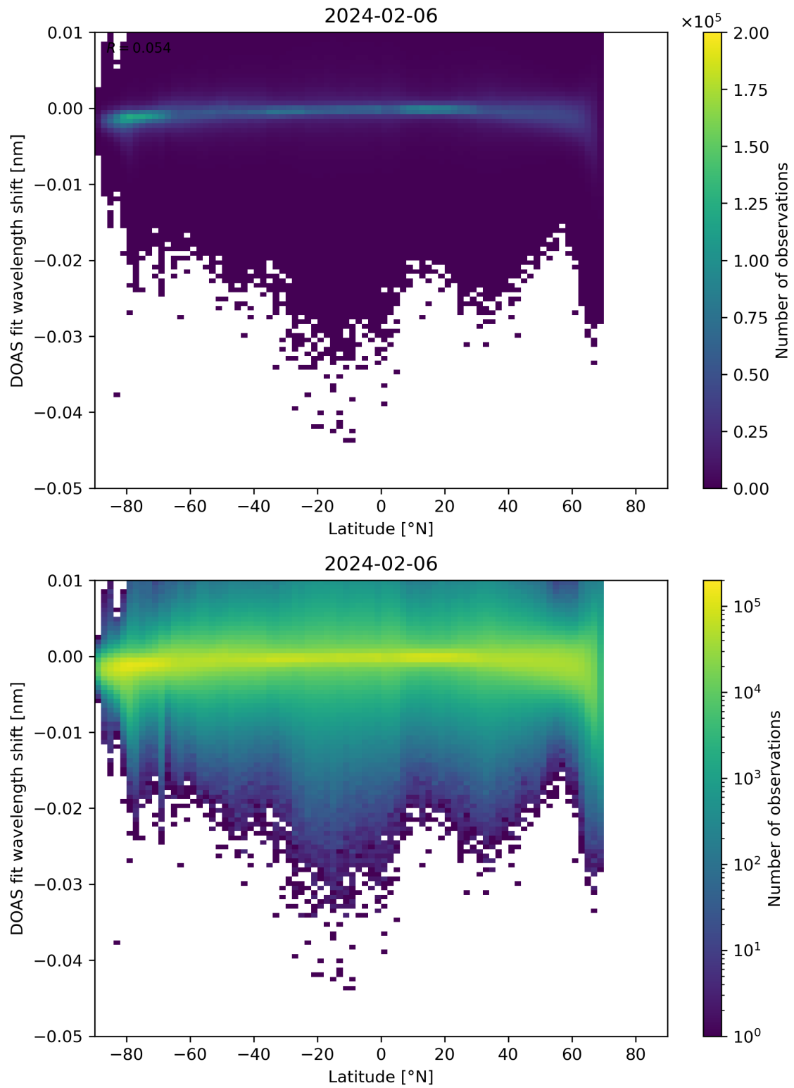
Figure 142: Scatter density plot of “Latitude” against “DOAS fit wavelength shift” for 2024-02-06 to 2024-02-07.
