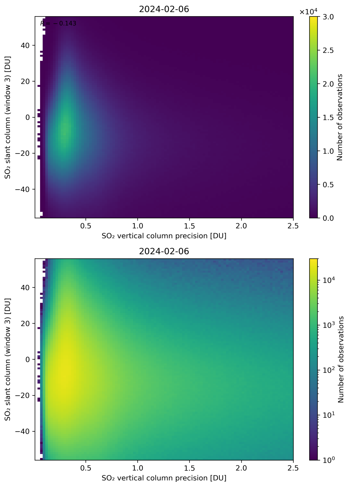
Figure 292: Scatter density plot of “SO 2 vertical column precision” against “SO 2 slant column (window 3)” for 2024-02-06 to 2024-02-07.
