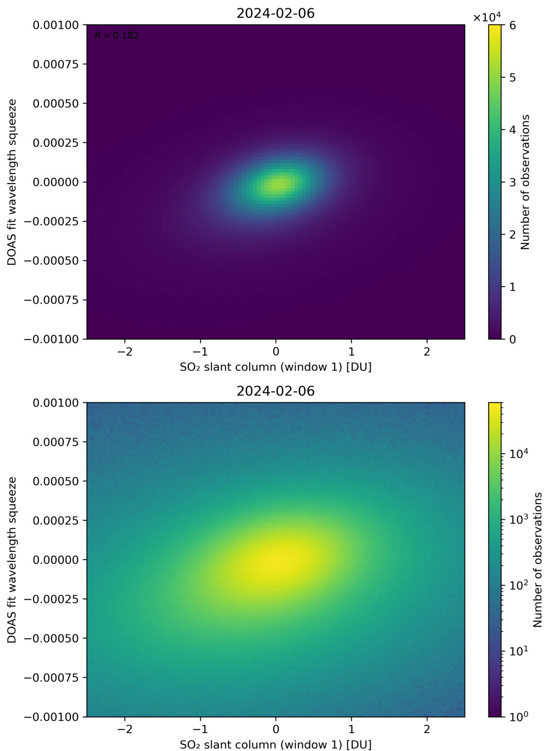
Figure 216: Scatter density plot of “SO 2 slant column (window 1)” against “DOAS fit wavelength squeeze” for 2024-02-06 to 2024-02-07.
