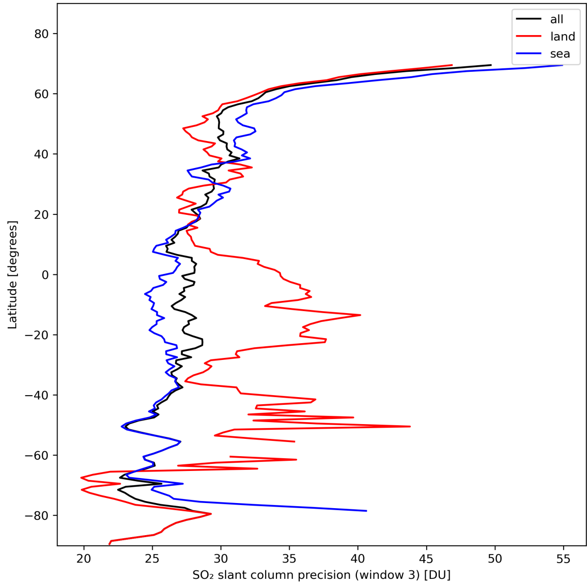
Figure 42: Zonal average of “SO 2 slant column precision (window 3)” for 2024-02-06 to 2024-02-07.
