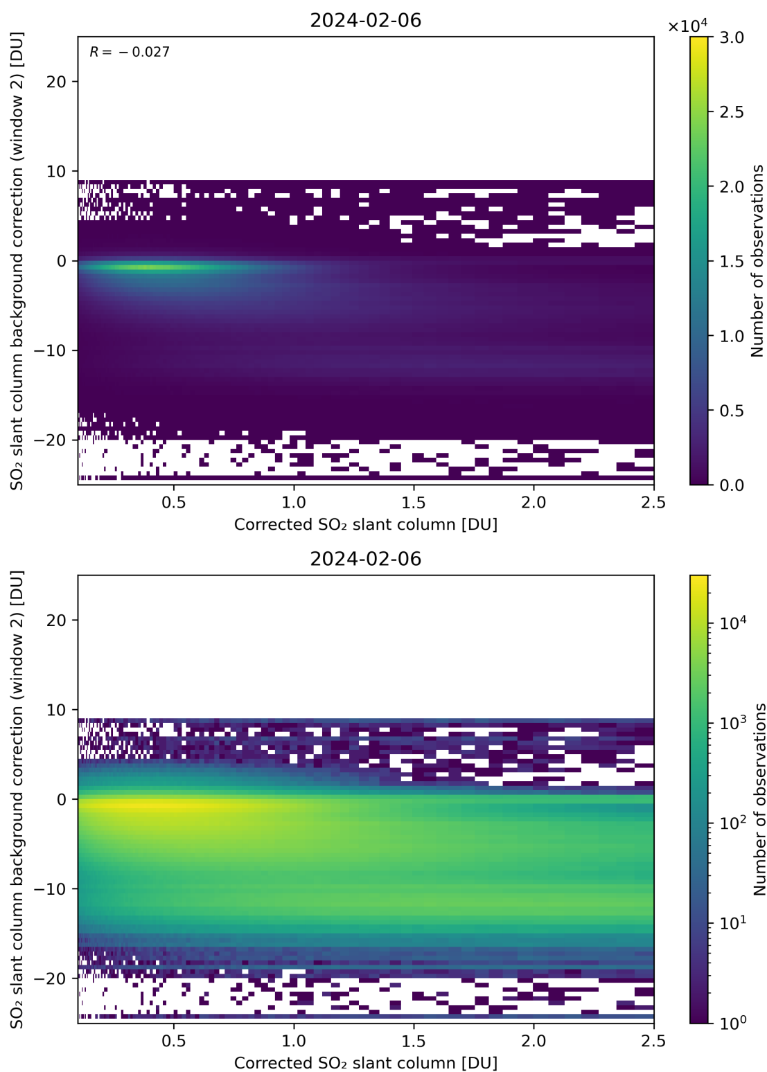
Figure 179: Scatter density plot of “Corrected SO 2 slant column” against “SO 2 slant column background correction (window 2)” for 2024-02-06 to 2024-02-07.
