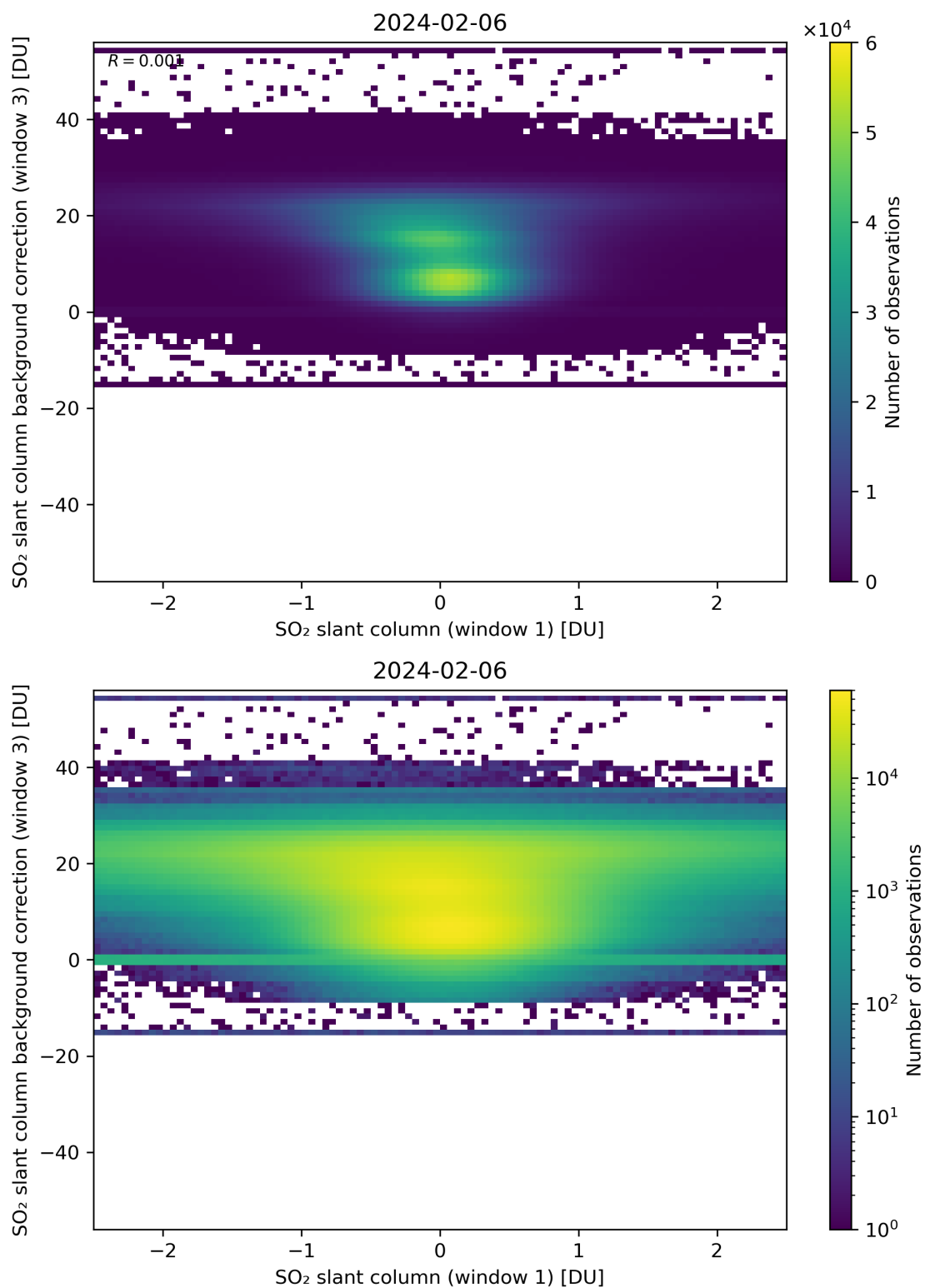
Figure 214: Scatter density plot of “SO 2 slant column (window 1)” against “SO 2 slant column background correction (window 3)” for 2024-02-06 to 2024-02-07.
