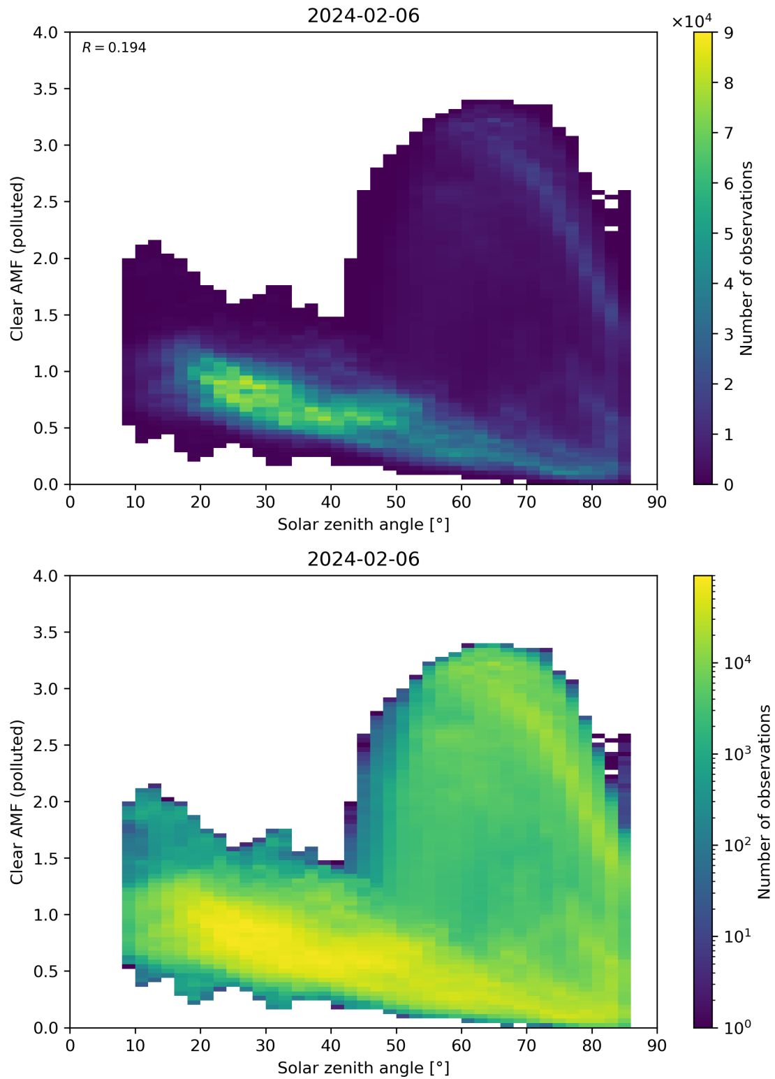
Figure 165: Scatter density plot of “Solar zenith angle” against “Clear AMF (polluted)” for 2024-02-06 to 2024-02-07.
