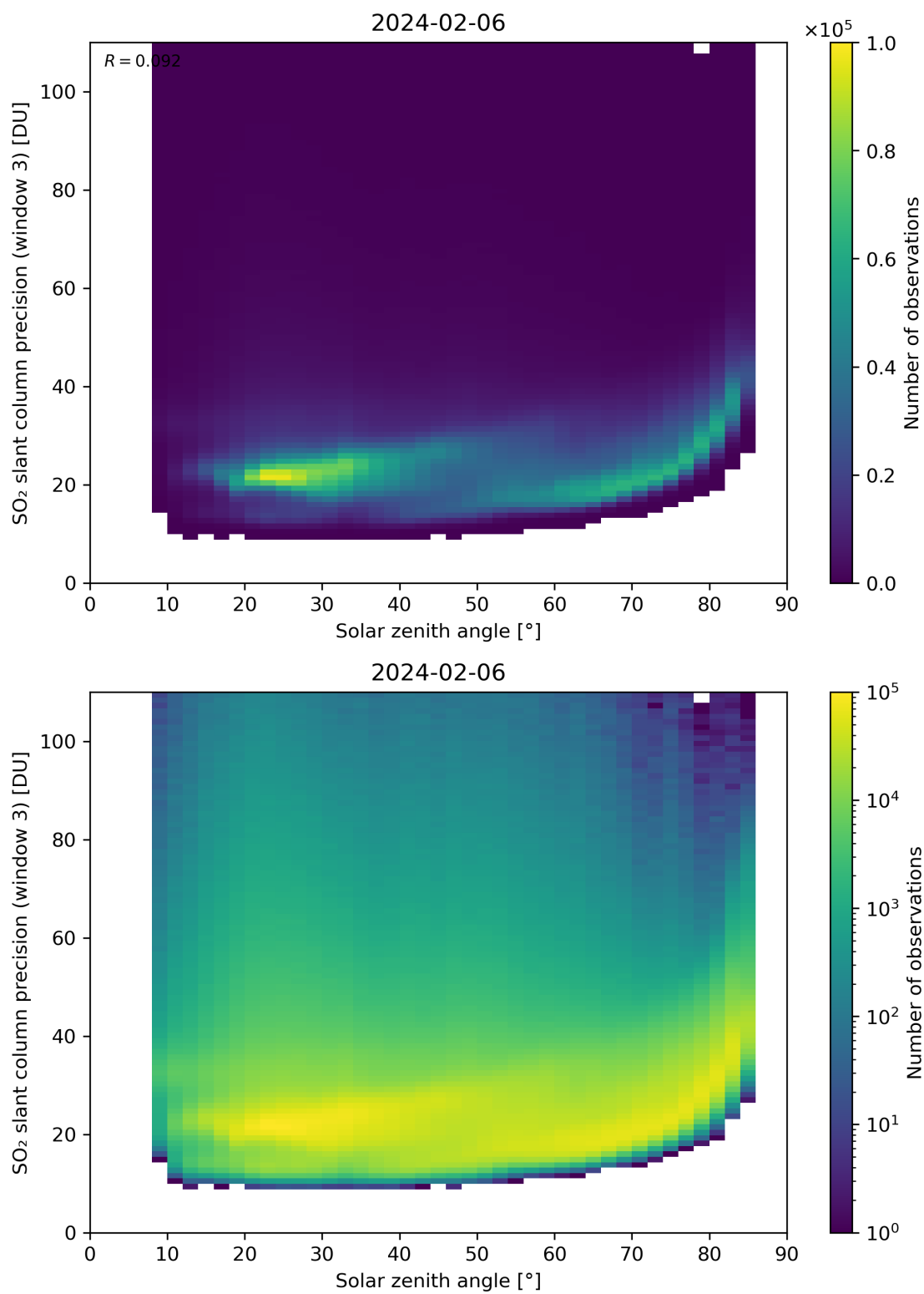
Figure 173: Scatter density plot of “Solar zenith angle” against “SO 2 slant column precision (window 3)” for 2024-02-06 to 2024-02-07.
