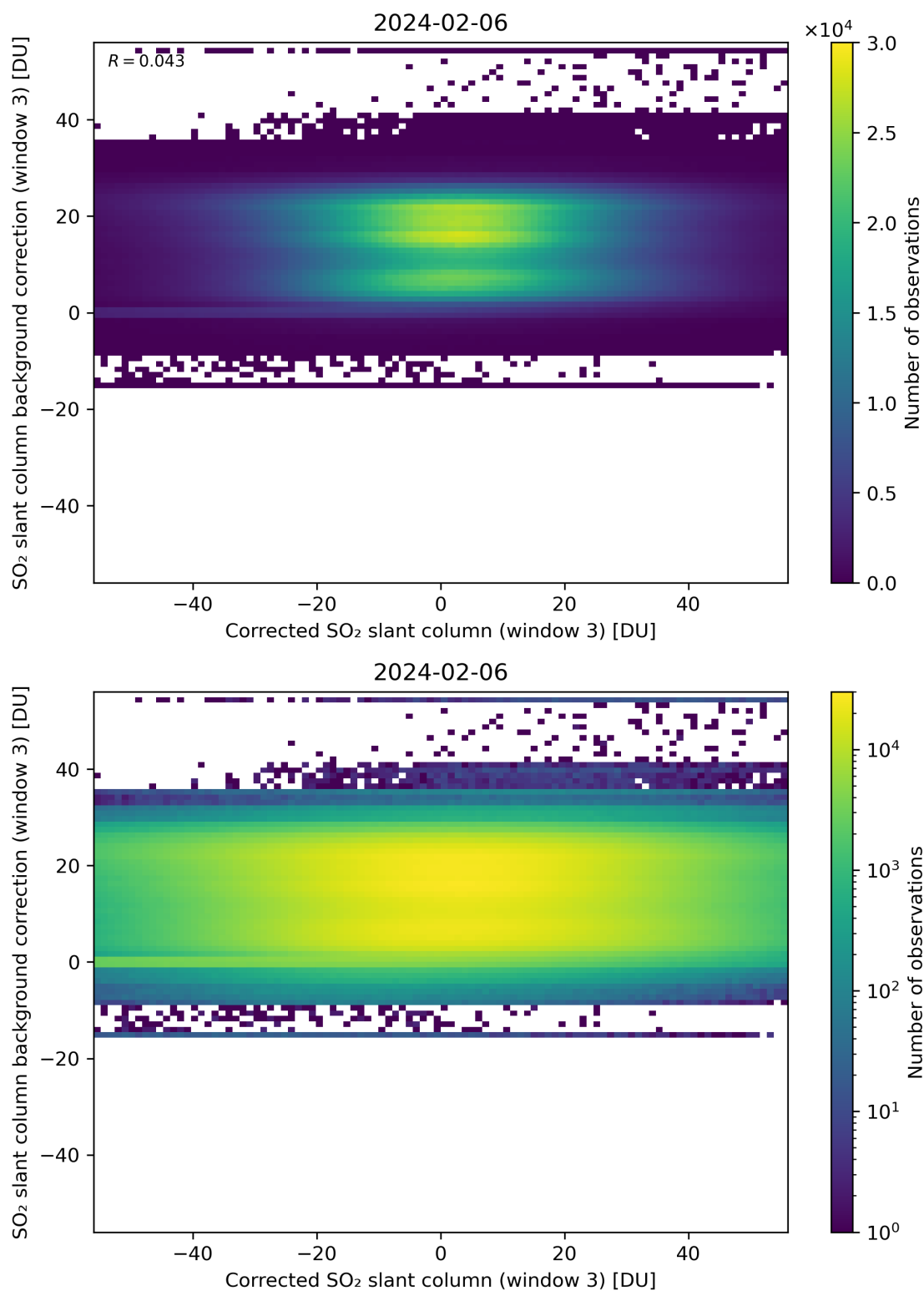
Figure 205: Scatter density plot of “Corrected SO 2 slant column (window 3)” against “SO 2 slant column background correction (window 3)” for 2024-02-06 to 2024-02-07.
