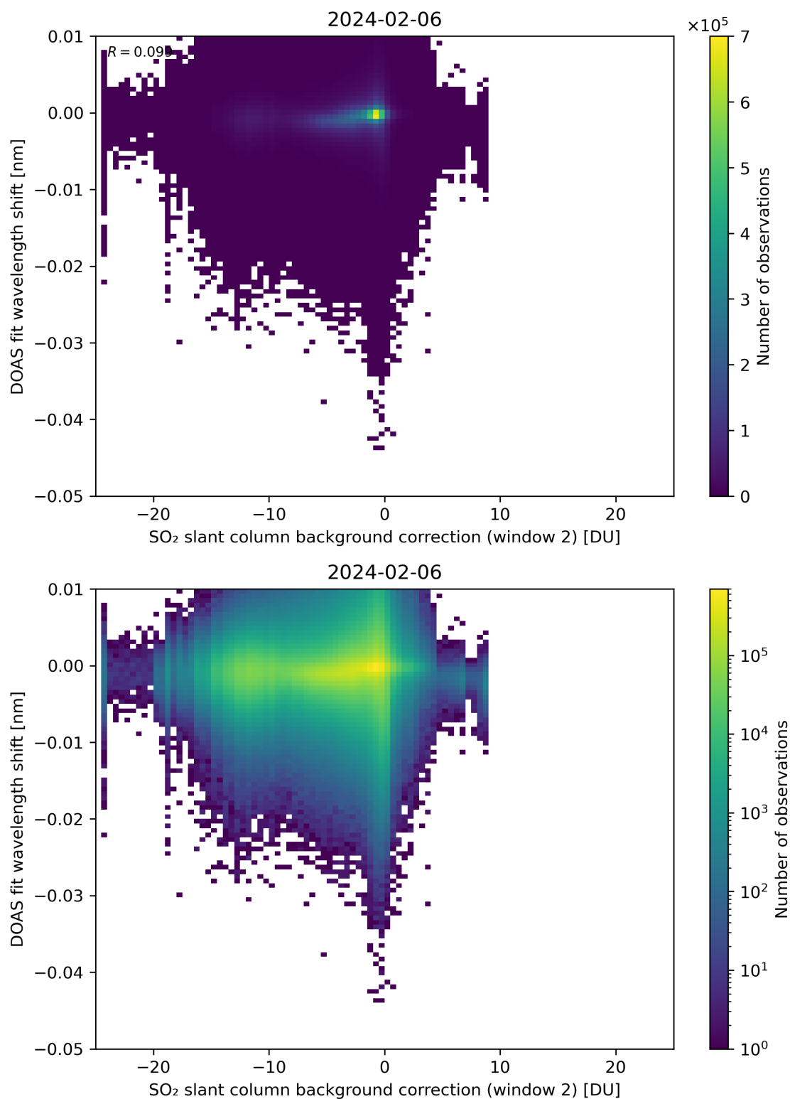
Figure 112: Scatter density plot of “SO 2 slant column background correction (window 2)” against “DOAS fit wavelength shift” for 2024-02-06 to 2024-02-07.
