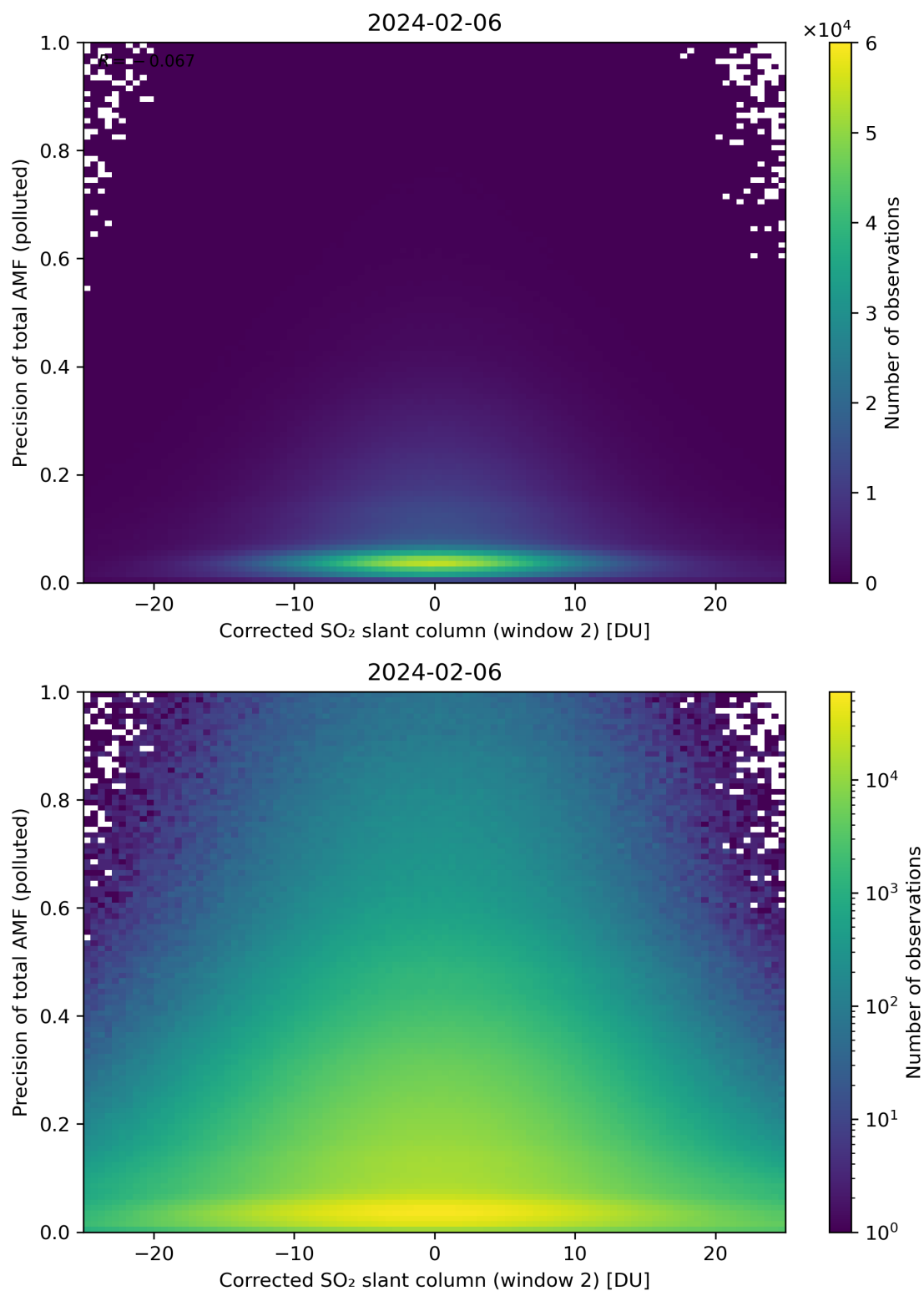
Figure 204: Scatter density plot of “Corrected SO 2 slant column (window 2)” against “Precision of total AMF (polluted)” for 2024-02-06 to 2024-02-07.
