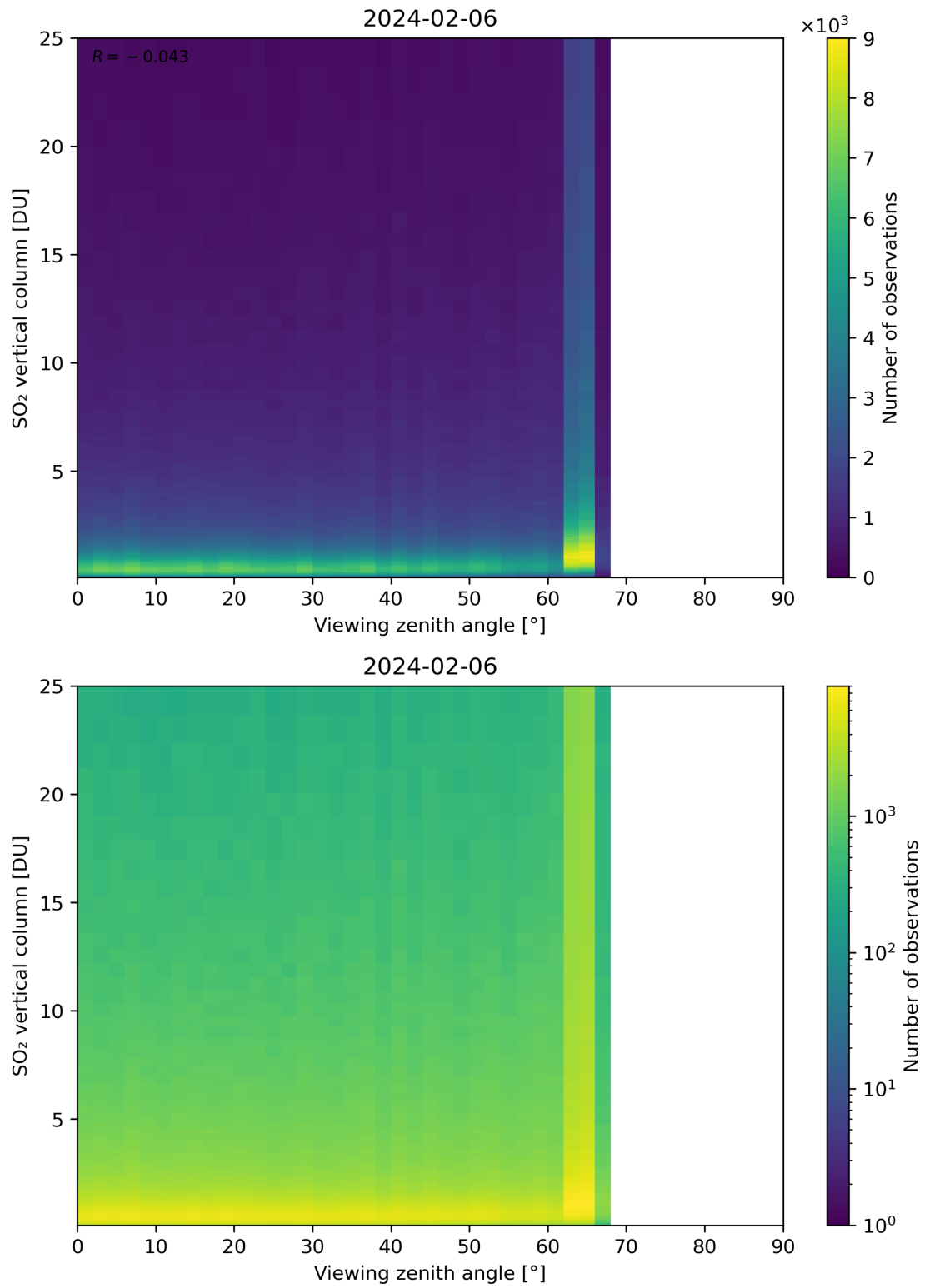
Figure 327: Scatter density plot of “Viewing zenith angle” against “SO 2 vertical column” for 2024-02-06 to 2024-02-07.
