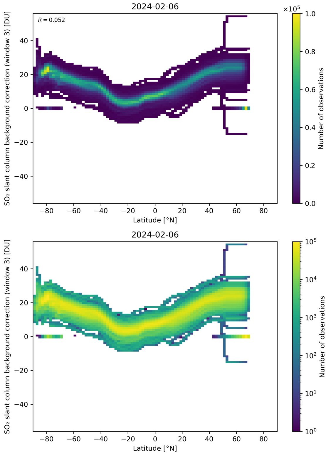
Figure 141: Scatter density plot of “Latitude” against “SO 2 slant column background correction (window 3)” for 2024-02-06 to 2024-02-07.
