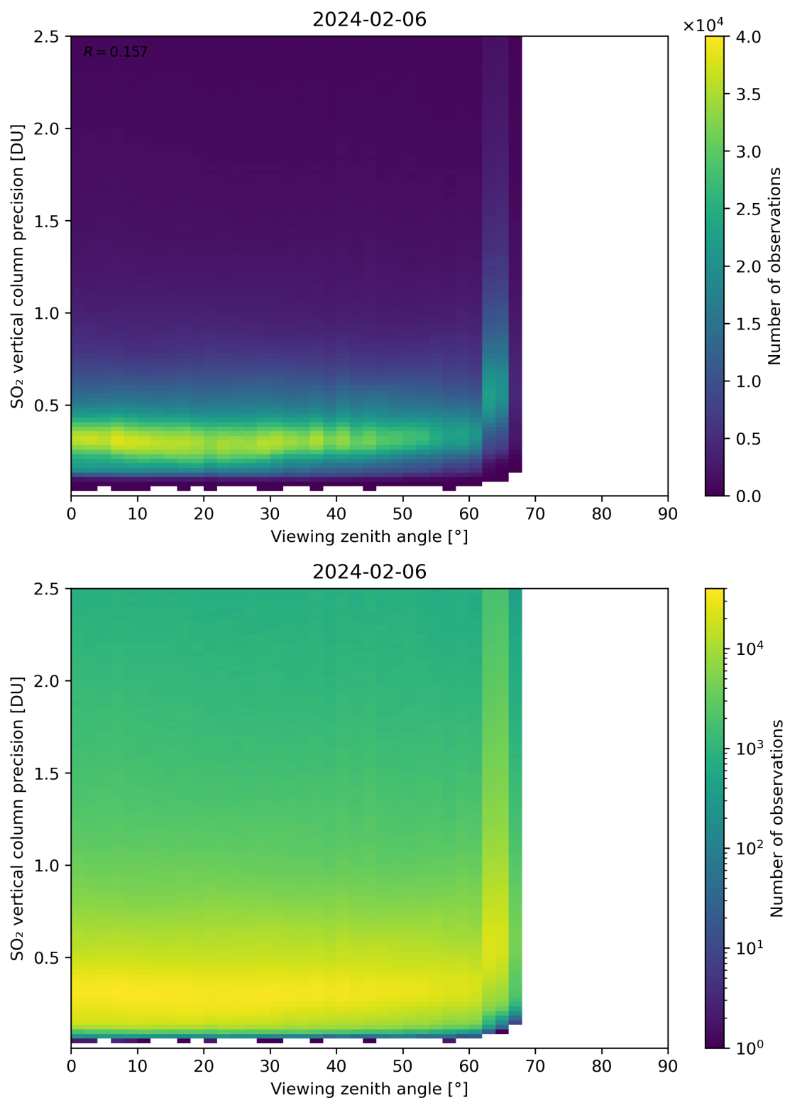
Figure 328: Scatter density plot of “Viewing zenith angle” against “SO 2 vertical column precision” for 2024-02-06 to 2024-02-07.
