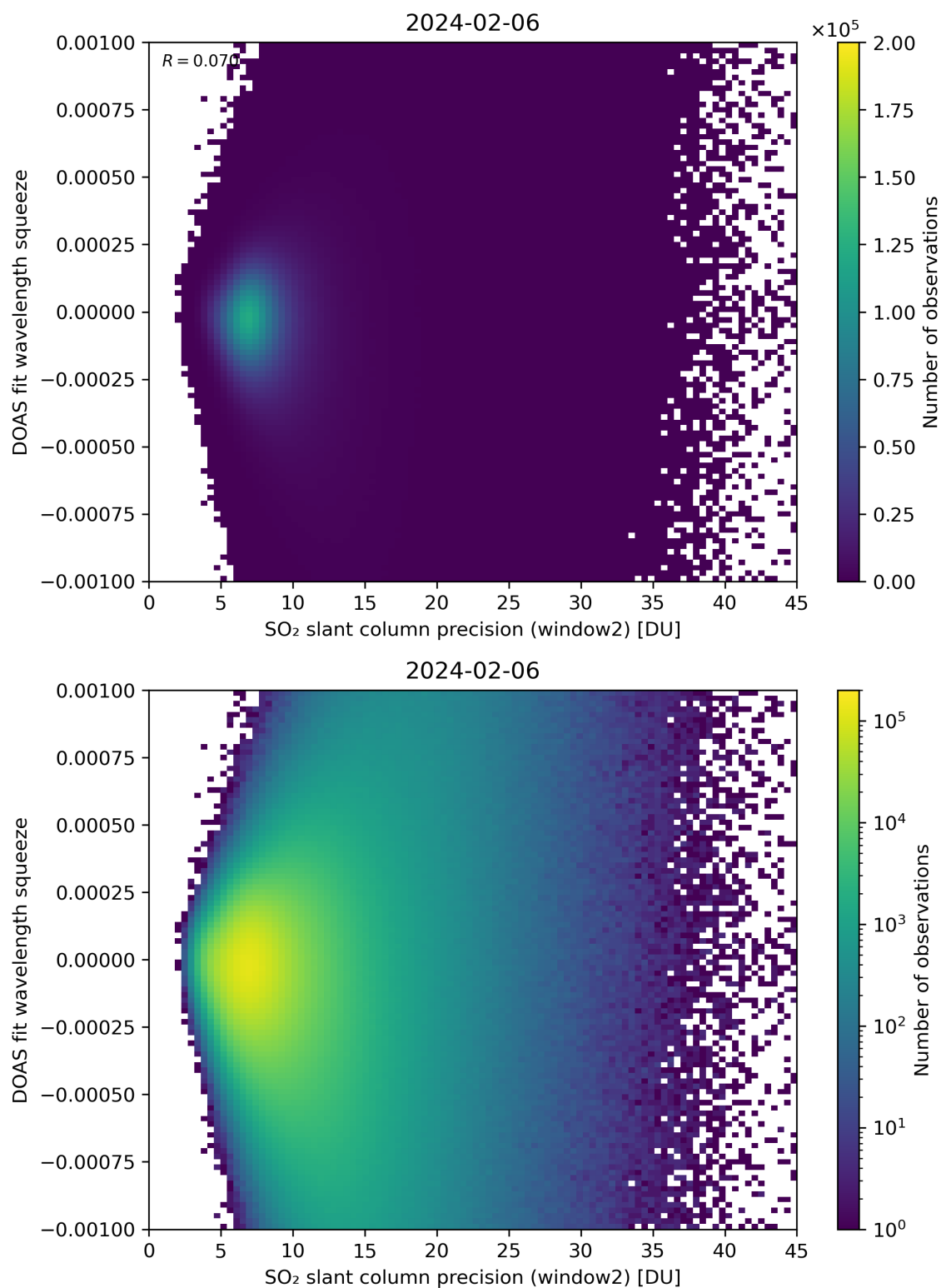
Figure 244: Scatter density plot of “SO 2 slant column precision (window2)” against “DOAS fit wavelength squeeze” for 2024-02-06 to 2024-02-07.
