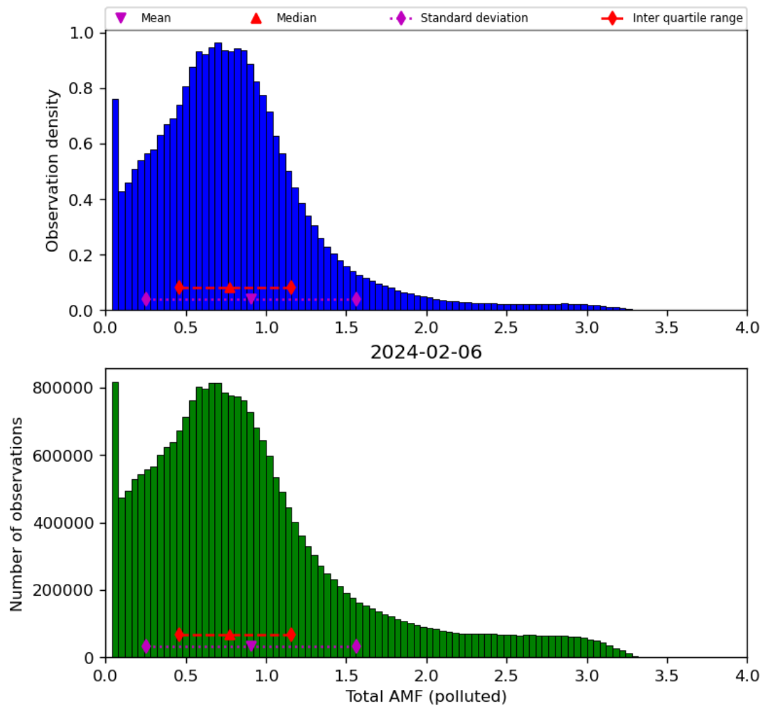
Figure 71: Histogram of “Total AMF (polluted)” for 2024-02-06 to 2024-02-07
