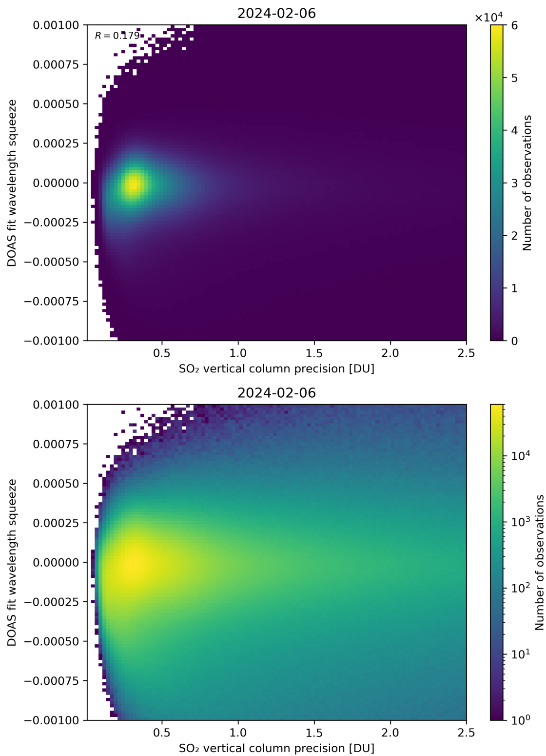
Figure 283: Scatter density plot of “SO 2 vertical column precision” against “DOAS fit wavelength squeeze” for 2024-02-06 to 2024-02-07.
