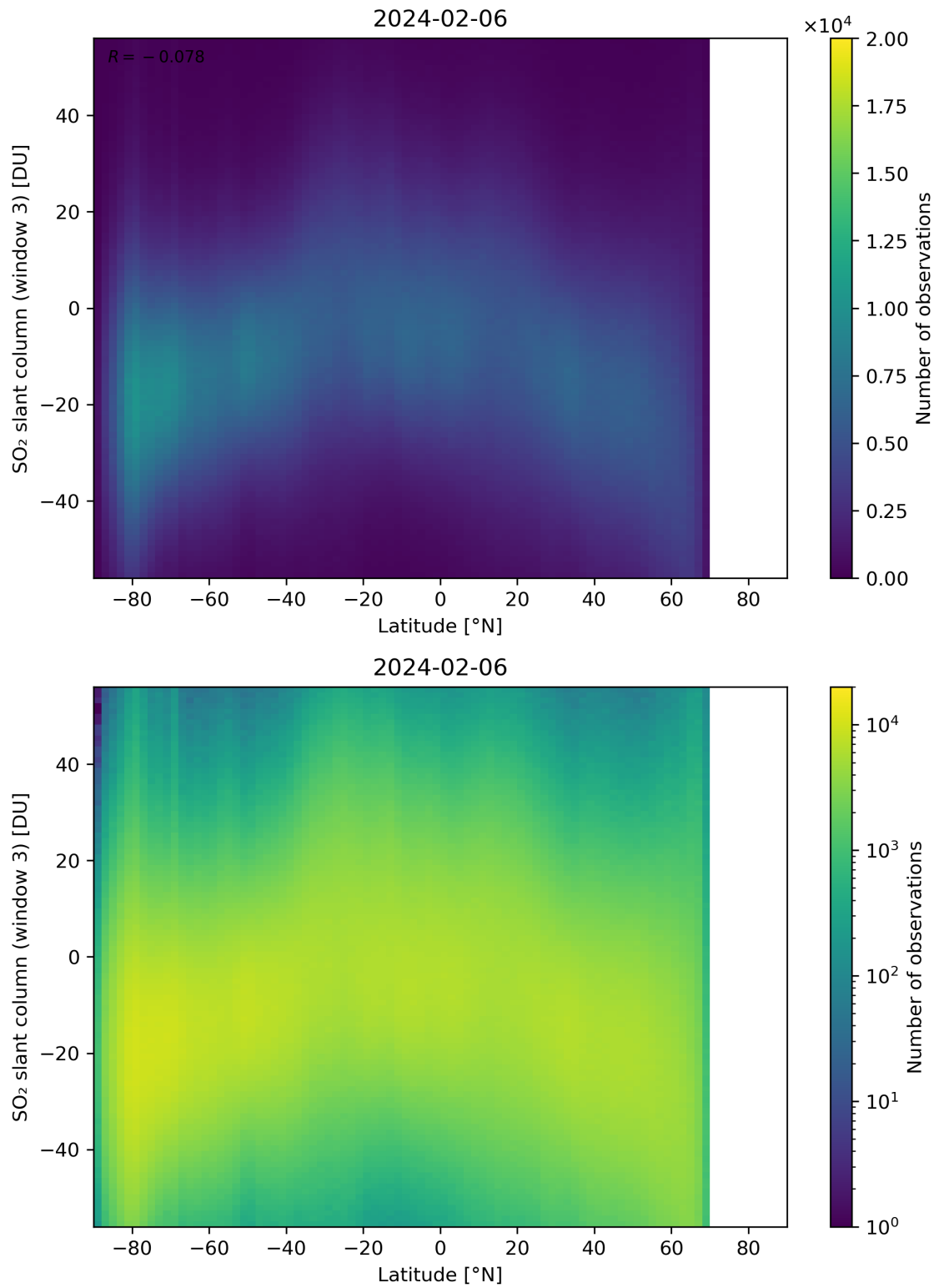
Figure 152: Scatter density plot of “Latitude” against “SO 2 slant column (window 3)” for 2024-02-06 to 2024-02-07.
