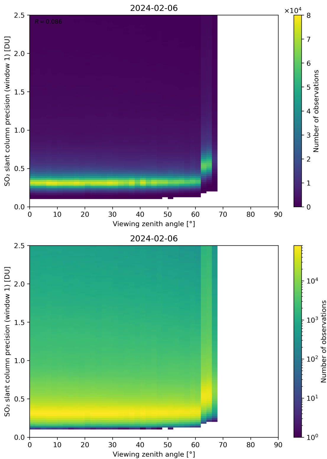
Figure 321: Scatter density plot of “Viewing zenith angle” against “SO 2 slant column precision (window 1)” for 2024-02-06 to 2024-02-07.
