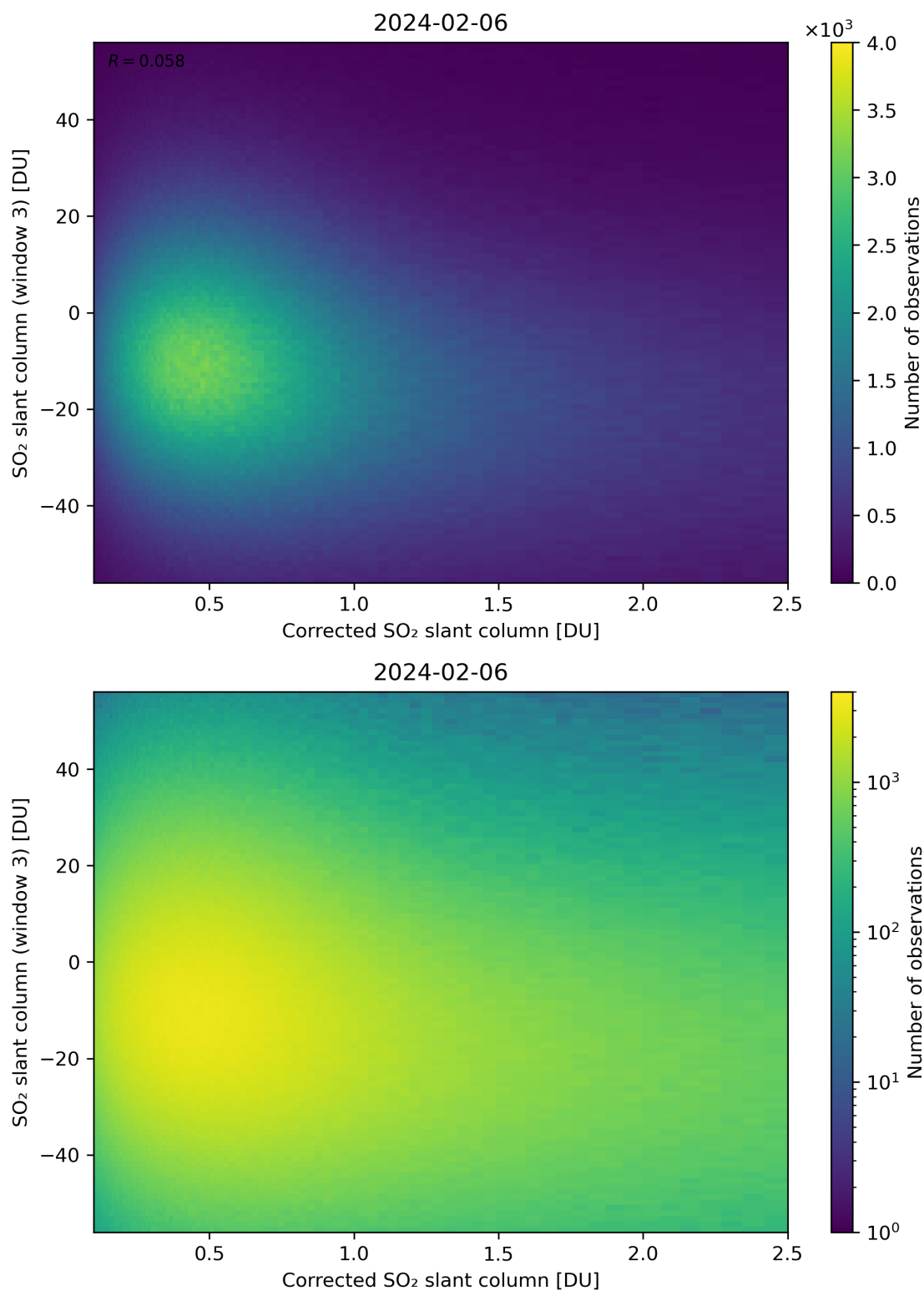
Figure 190: Scatter density plot of “Corrected SO 2 slant column” against “SO 2 slant column (window 3)” for 2024-02-06 to 2024-02-07.
