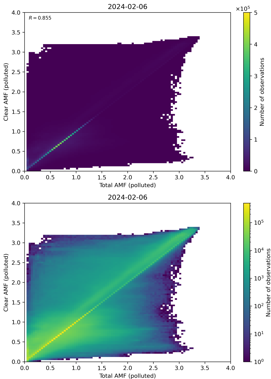
Figure 271: Scatter density plot of “Total AMF (polluted)” against “Clear AMF (polluted)” for 2024-02-06 to 2024-02-07.
