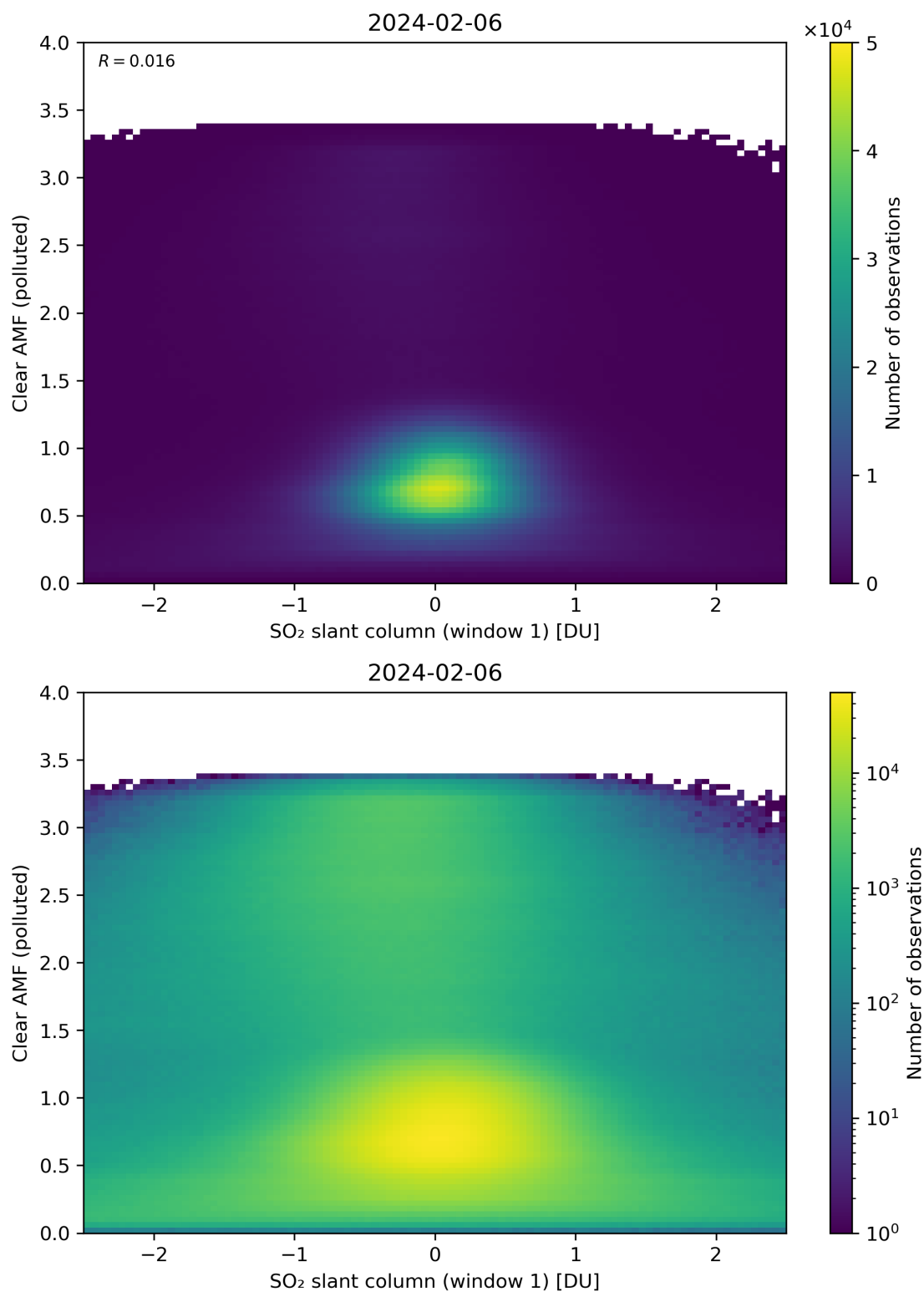
Figure 232: Scatter density plot of “SO 2 slant column (window 1)” against “Clear AMF (polluted)” for 2024-02-06 to 2024-02-07.
