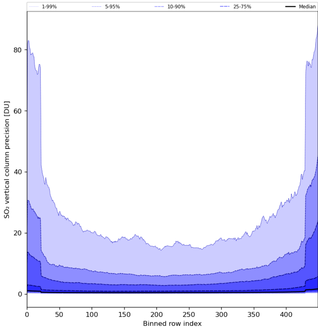
Figure 77: Along track statistics of “SO 2 vertical column precision” for 2024-02-06 to 2024-02-07
