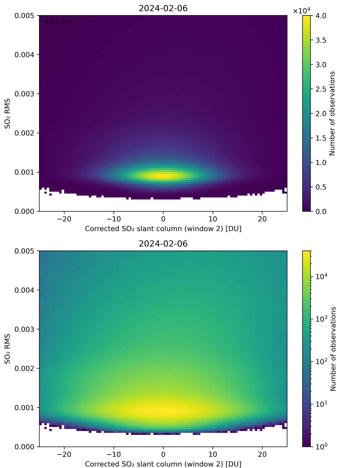
Figure 198: Scatter density plot of “Corrected SO 2 slant column (window 2)” against “SO 2 RMS” for 2024-02-06 to 2024-02-07.
