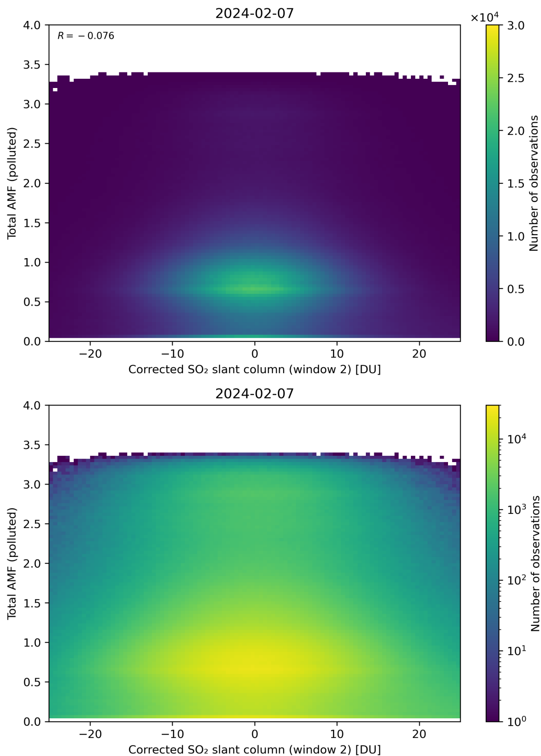
Figure 203: Scatter density plot of “Corrected SO 2 slant column (window 2)” against “Total AMF (polluted)” for 2024-02-06 to 2024-02-08.
