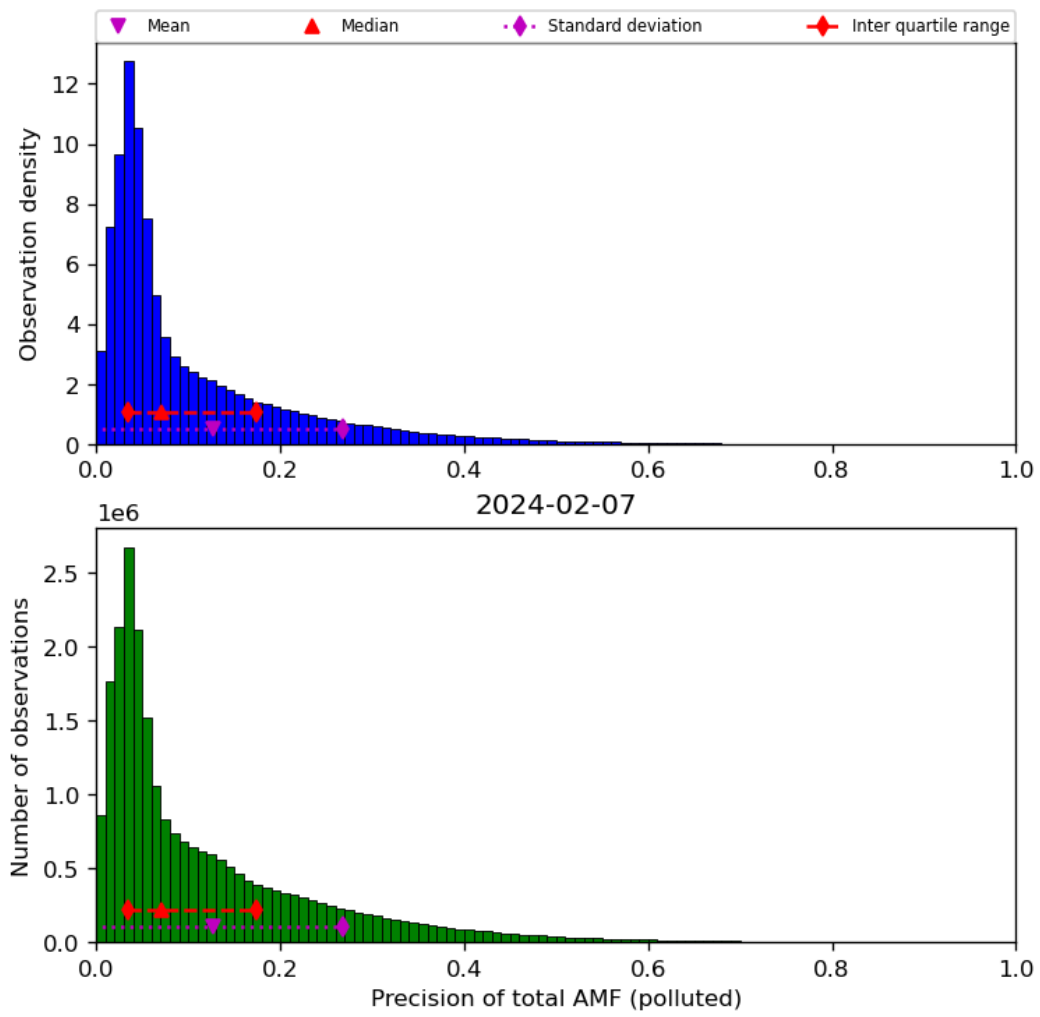
Figure 72: Histogram of “Precision of total AMF (polluted)” for 2024-02-06 to 2024-02-08
