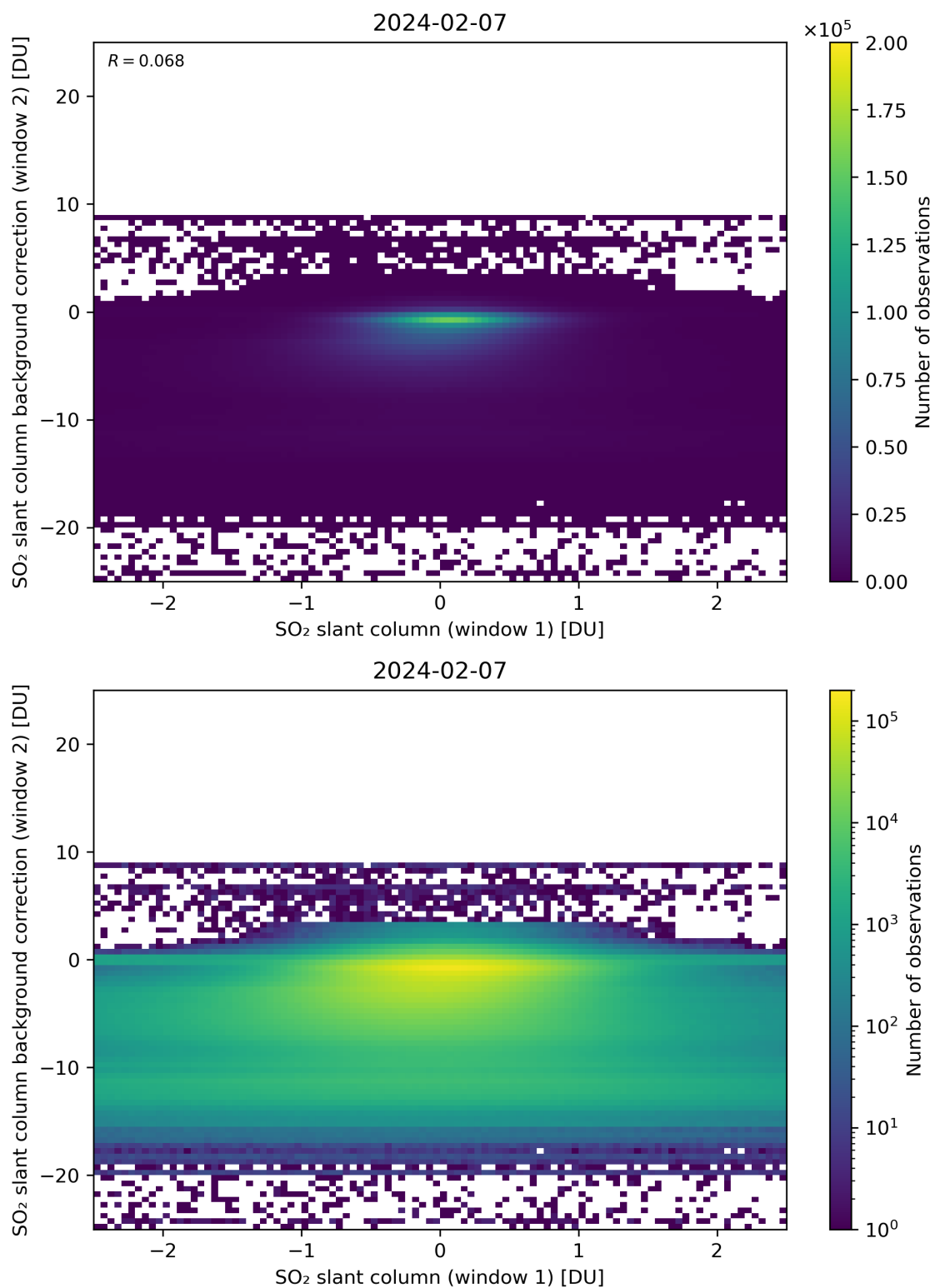
Figure 213: Scatter density plot of “SO 2 slant column (window 1)” against “SO 2 slant column background correction (window 2)” for 2024-02-06 to 2024-02-08.
