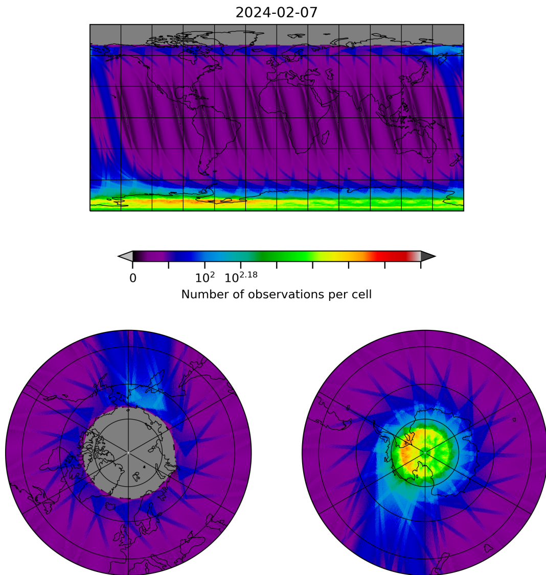
Figure 28: Map of the number of observations for 2024-02-06 to 2024-02-08
