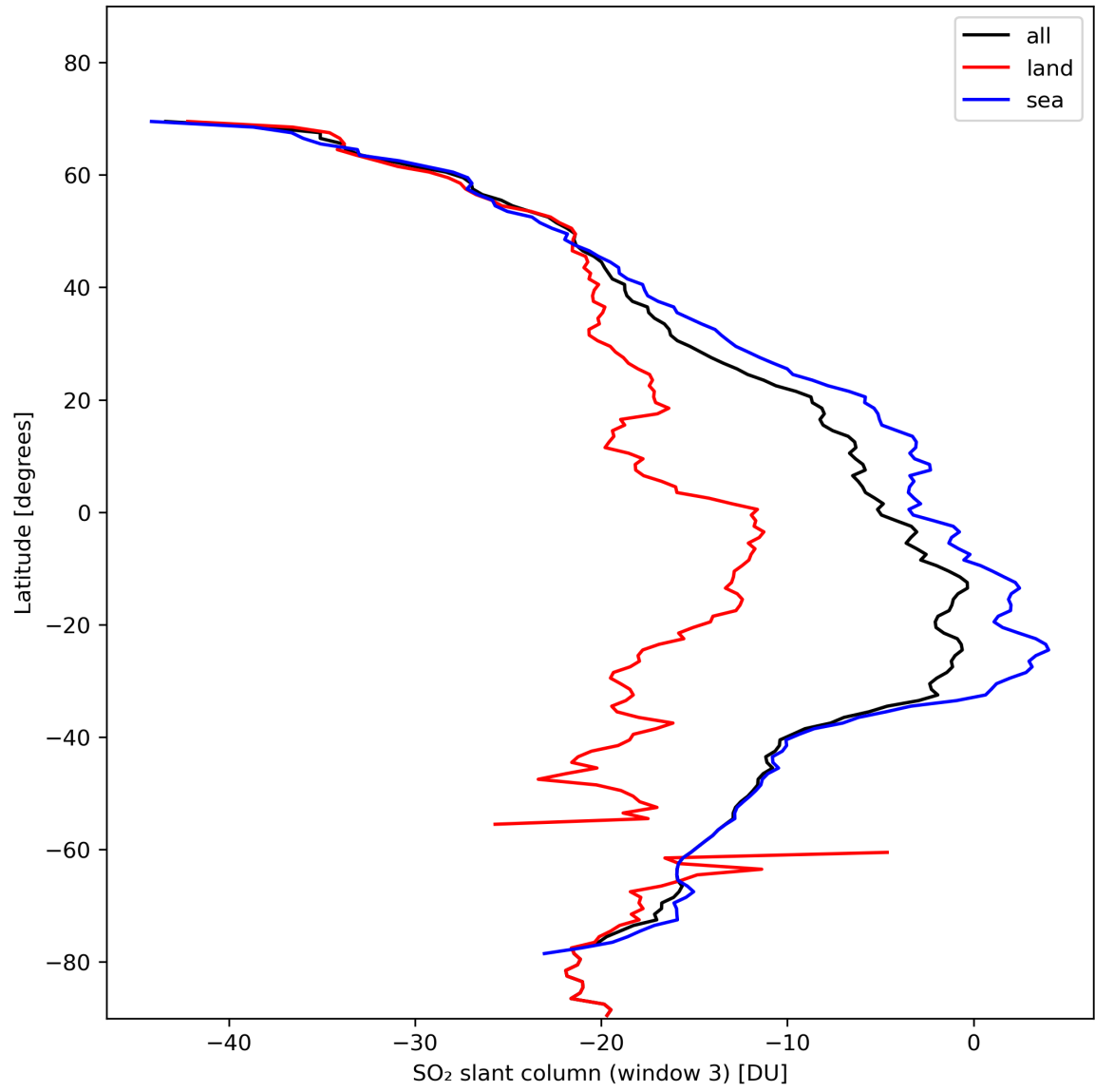
Figure 41: Zonal average of “SO 2 slant column (window 3)” for 2024-02-06 to 2024-02-08.
