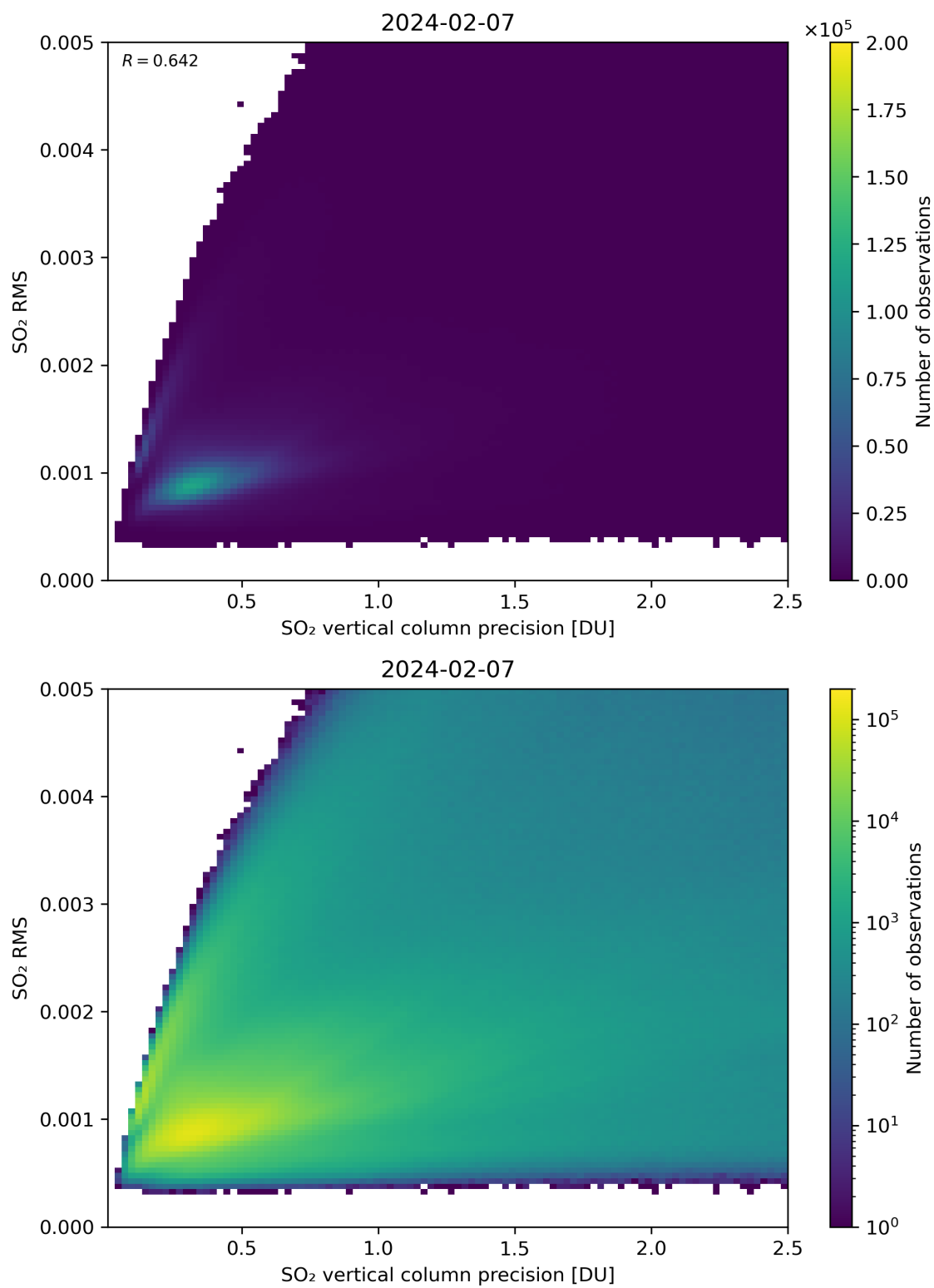
Figure 284: Scatter density plot of “SO 2 vertical column precision” against “SO 2 RMS” for 2024-02-06 to 2024-02-08.
