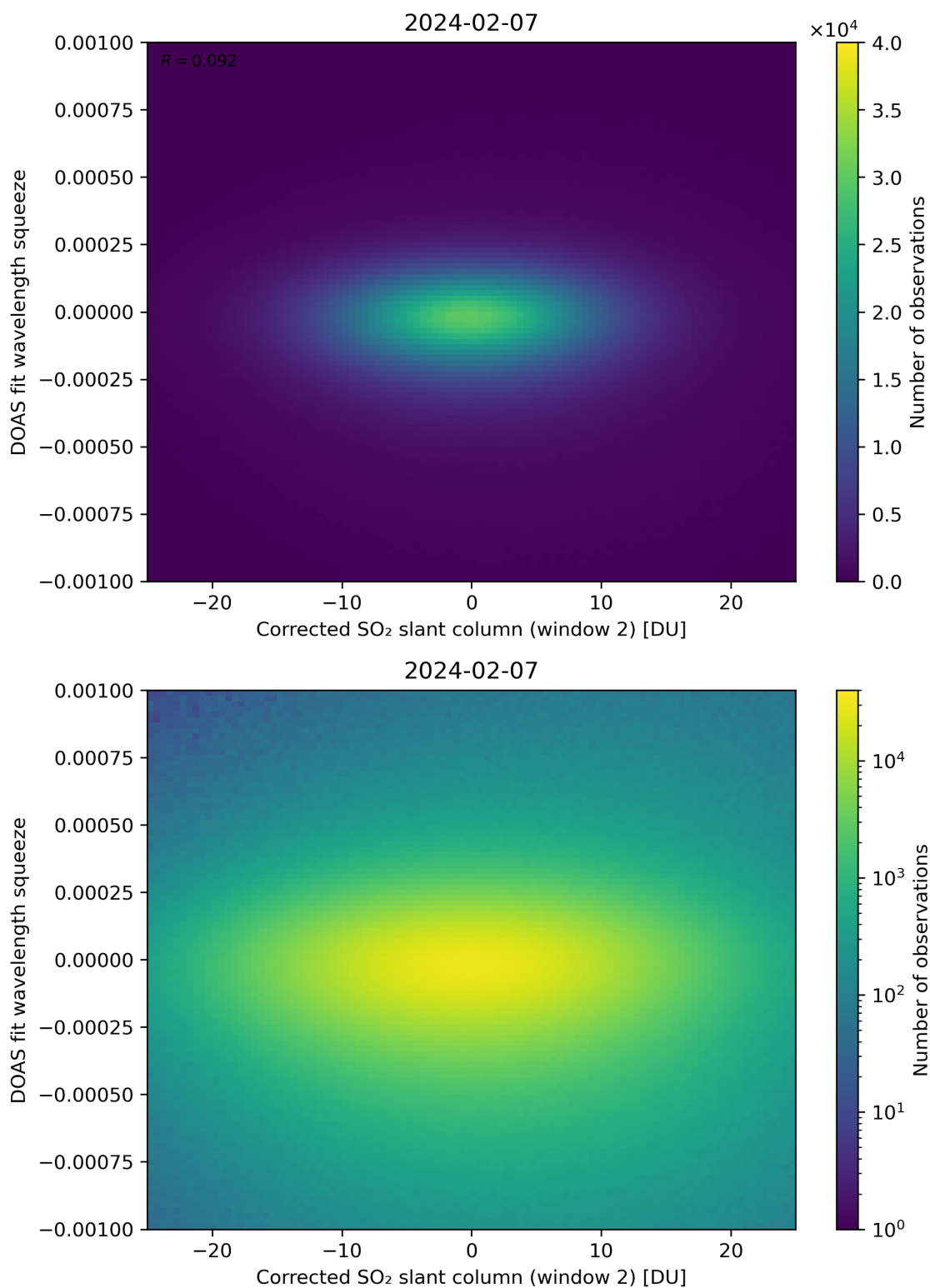
Figure 197: Scatter density plot of “Corrected SO 2 slant column (window 2)” against “DOAS fit wavelength squeeze” for 2024-02-06 to 2024-02-08.
