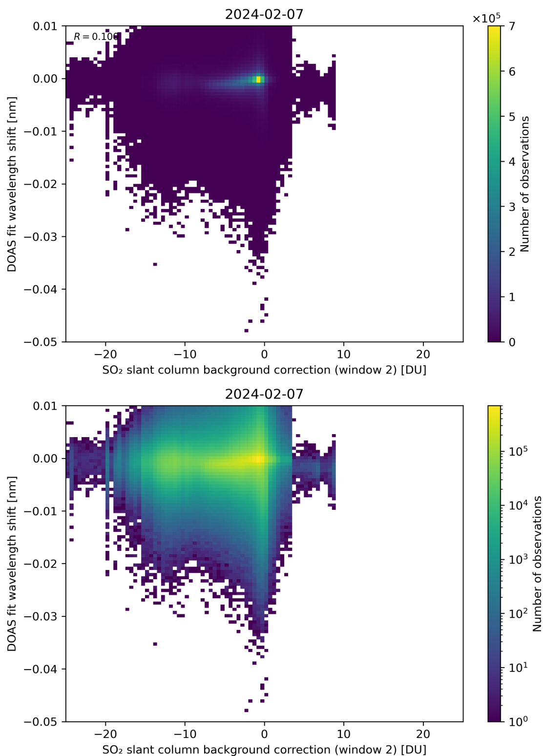
Figure 112: Scatter density plot of “SO 2 slant column background correction (window 2)” against “DOAS fit wavelength shift” for 2024-02-06 to 2024-02-08.
