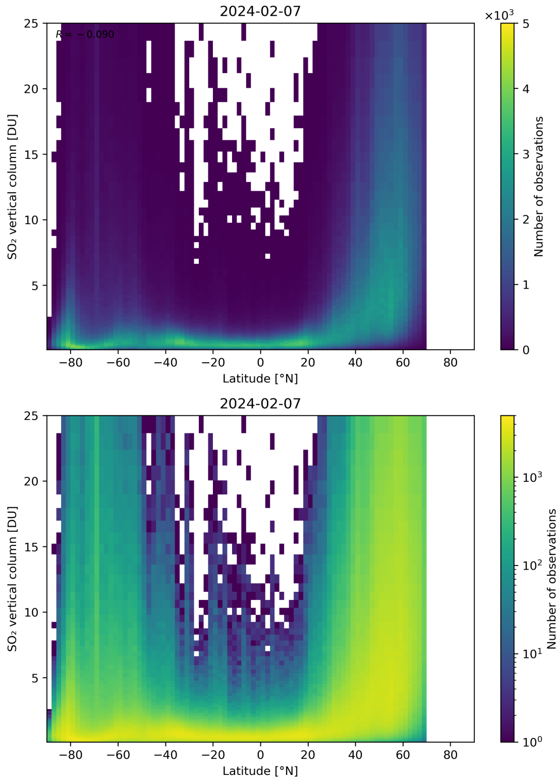
Figure 156: Scatter density plot of “Latitude” against “SO 2 vertical column” for 2024-02-06 to 2024-02-08.
