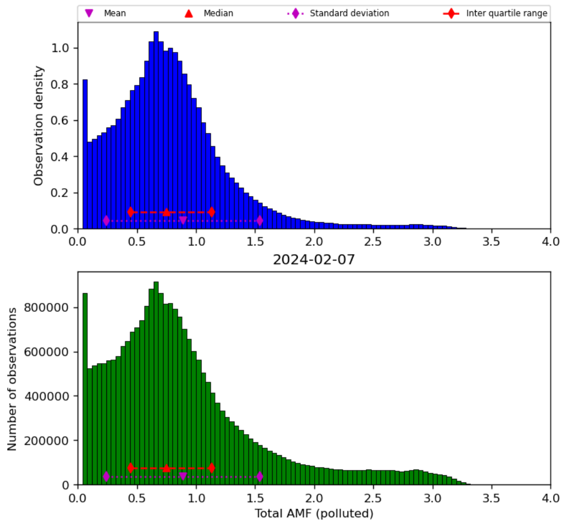
Figure 71: Histogram of “Total AMF (polluted)” for 2024-02-06 to 2024-02-08
