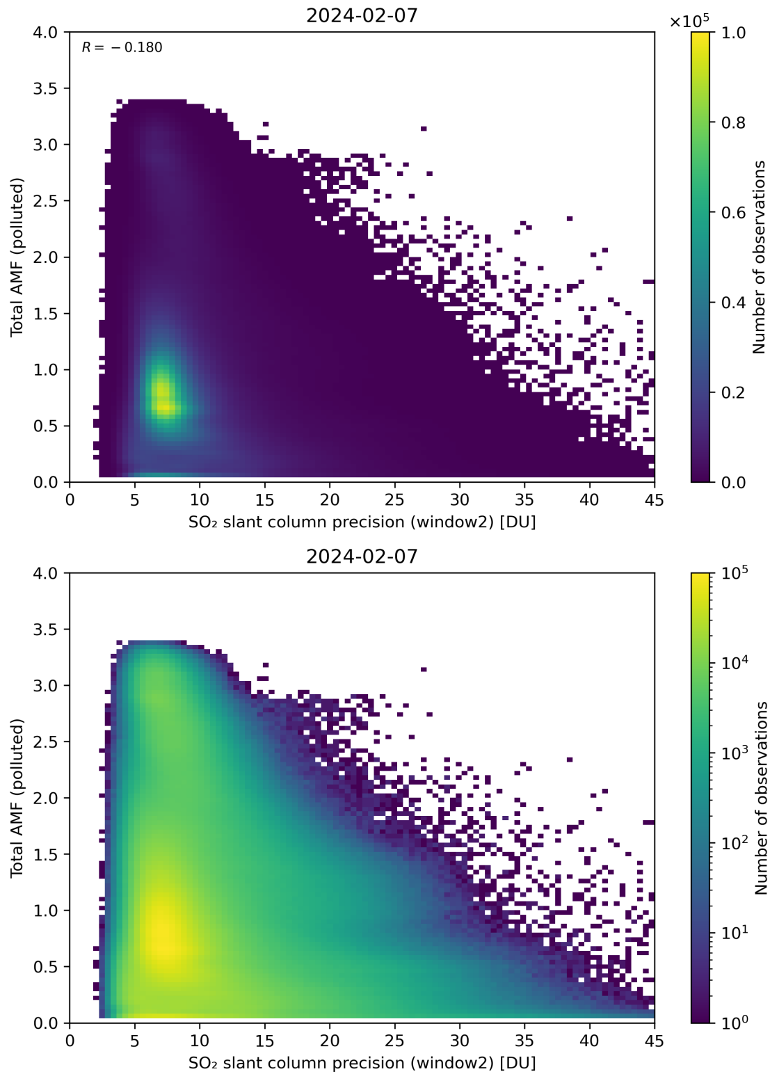
Figure 251: Scatter density plot of “SO 2 slant column precision (window2)” against “Total AMF (polluted)” for 2024-02-06 to 2024-02-08.
