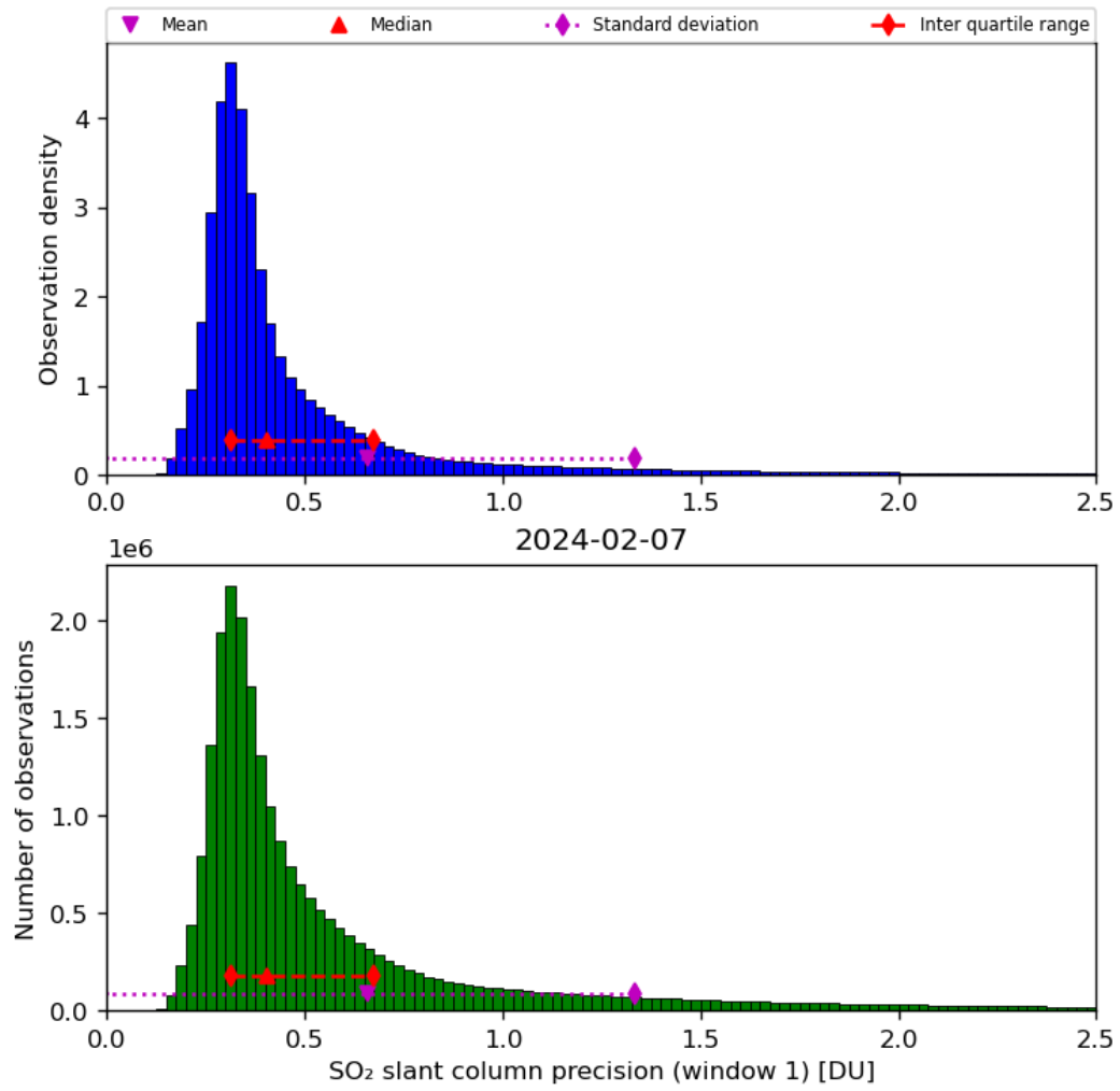
Figure 57: Histogram of “SO 2 slant column precision (window 1)” for 2024-02-06 to 2024-02-08
