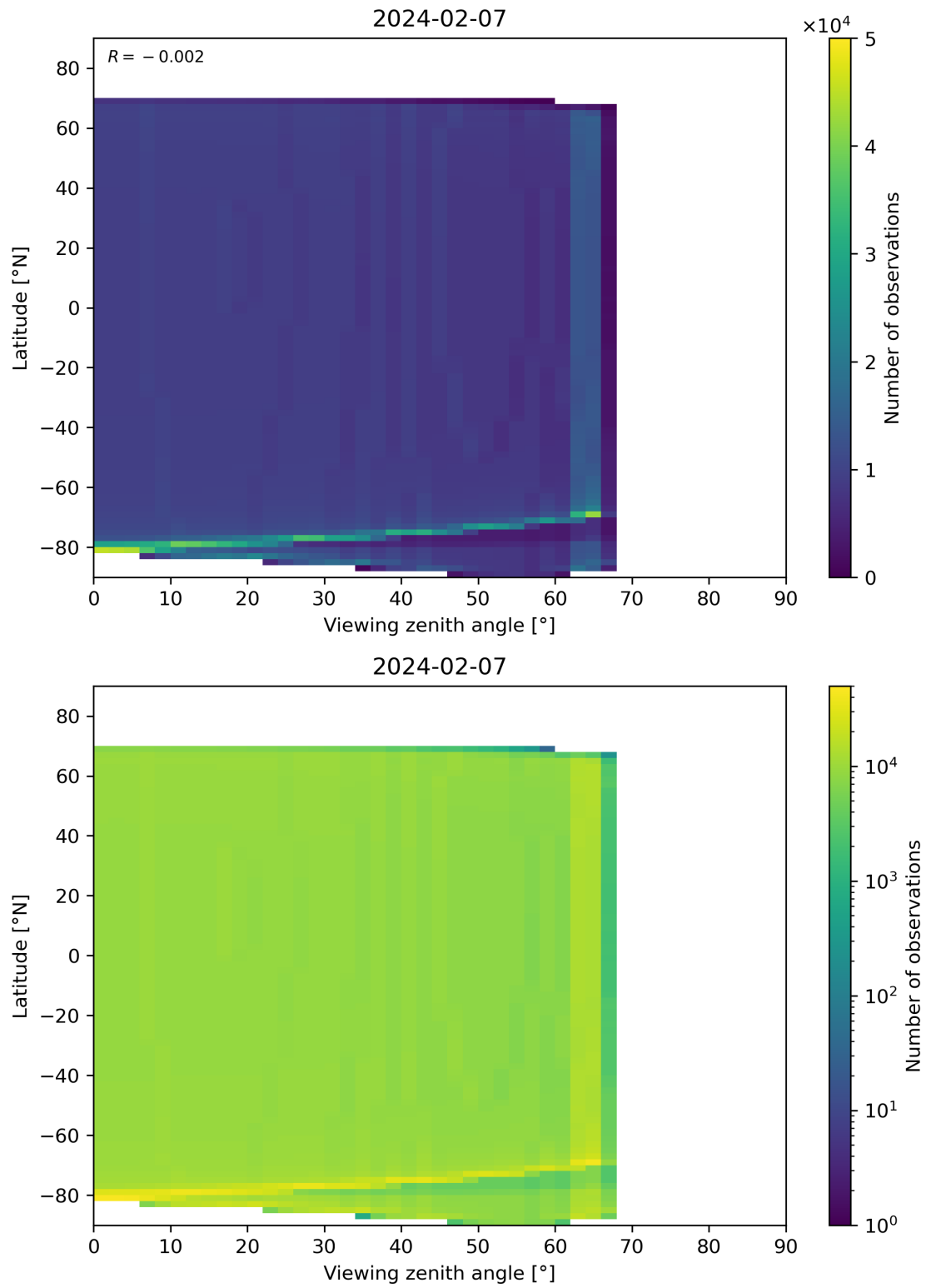
Figure 314: Scatter density plot of “Viewing zenith angle” against “Latitude” for 2024-02-06 to 2024-02-08.
