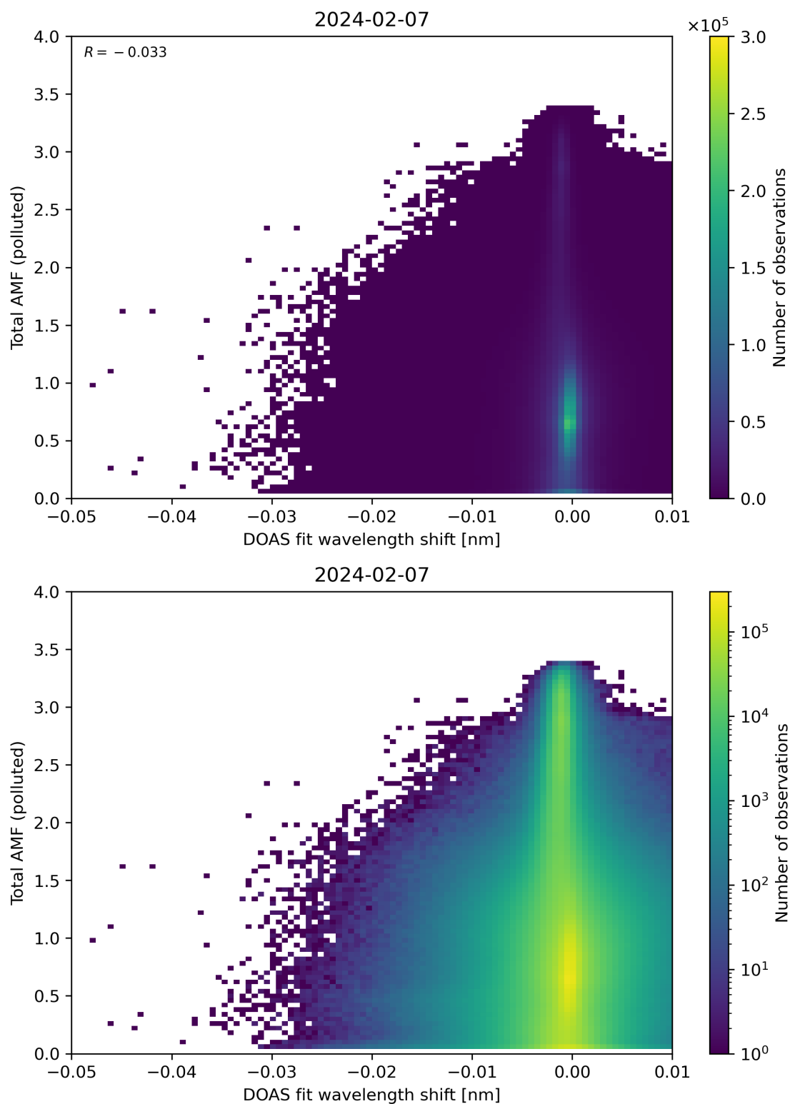
Figure 130: Scatter density plot of “DOAS fit wavelength shift” against “Total AMF (polluted)” for 2024-02-06 to 2024-02-08.
