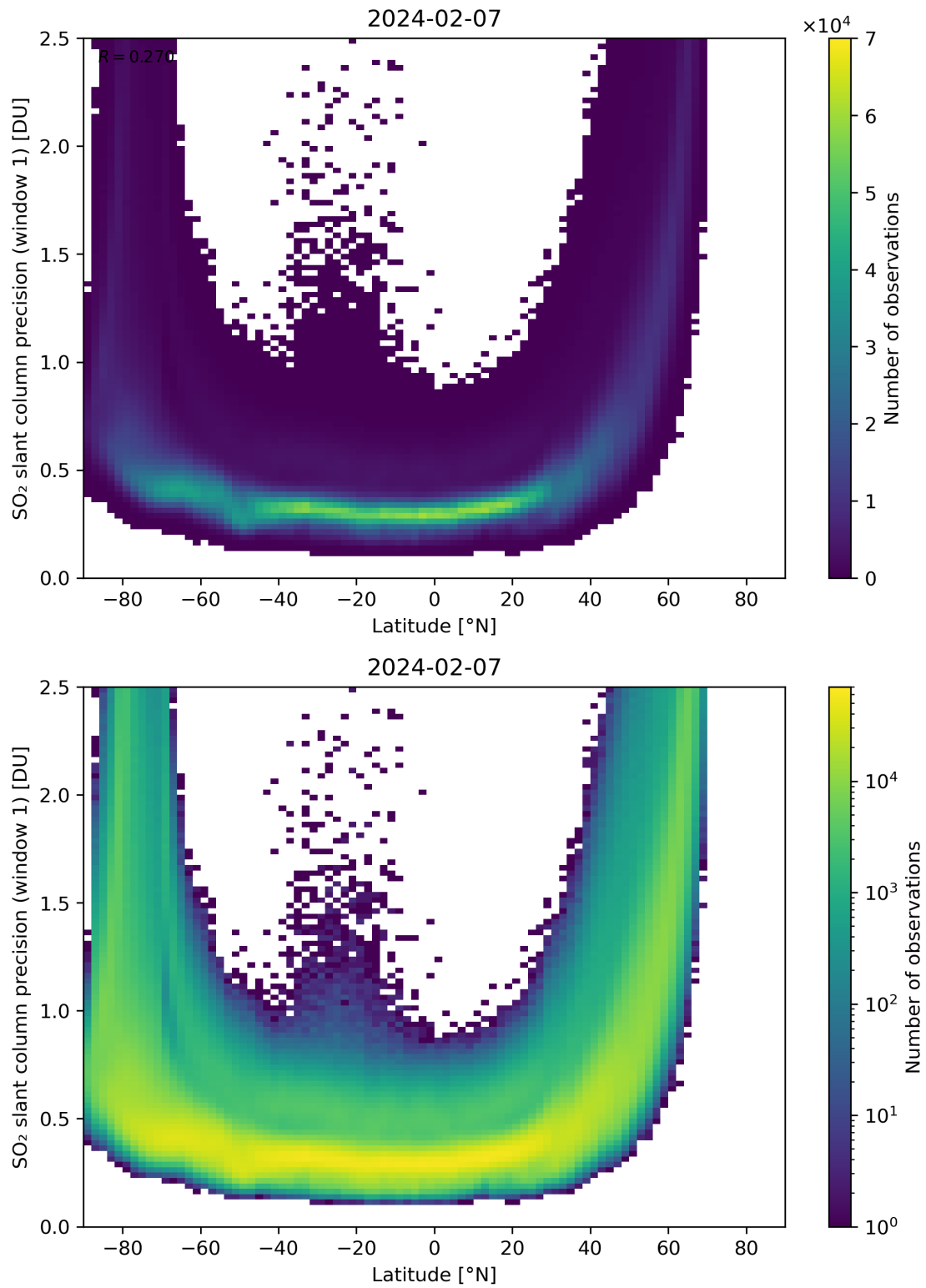
Figure 150: Scatter density plot of “Latitude” against “SO 2 slant column precision (window 1)” for 2024-02-06 to 2024-02-08.
