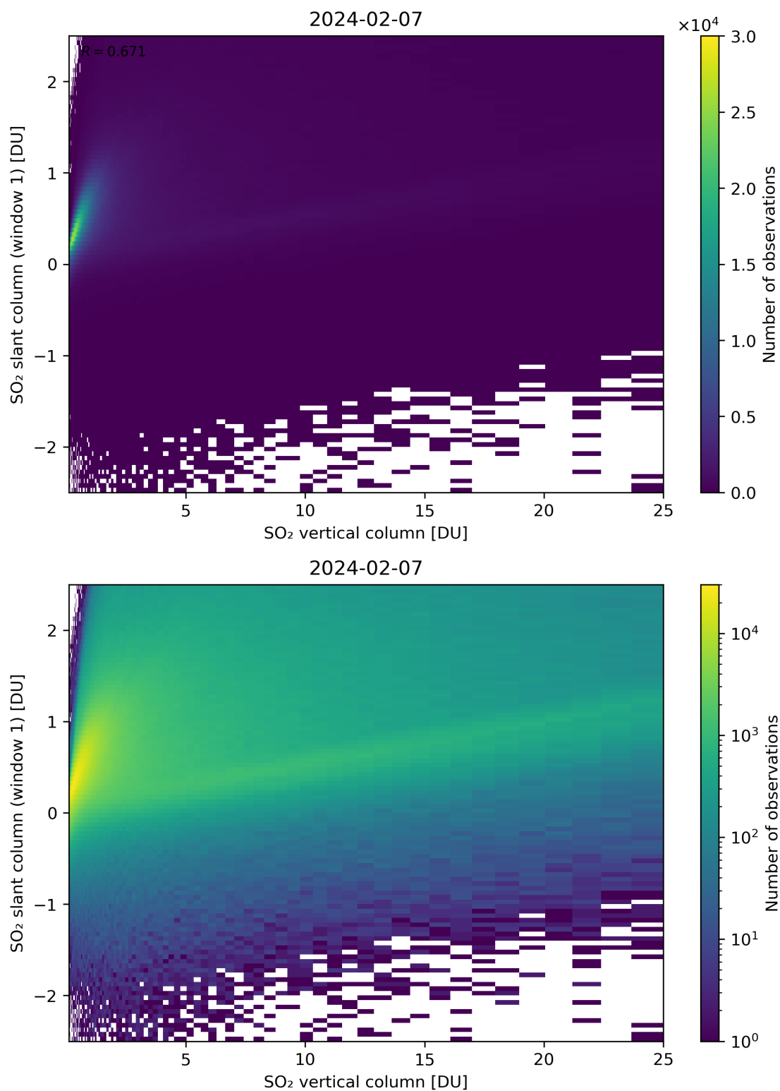
Figure 300: Scatter density plot of “SO 2 vertical column” against “SO 2 slant column (window 1)” for 2024-02-06 to 2024-02-08.
