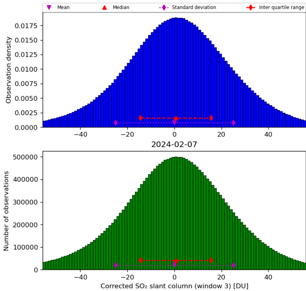
Figure 66: Histogram of “Corrected SO 2 slant column (window 3)” for 2024-02-06 to 2024-02-08
