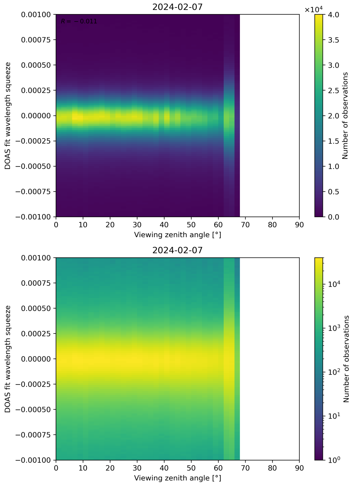
Figure 312: Scatter density plot of “Viewing zenith angle” against “DOAS fit wavelength squeeze” for 2024-02-06 to 2024-02-08.
