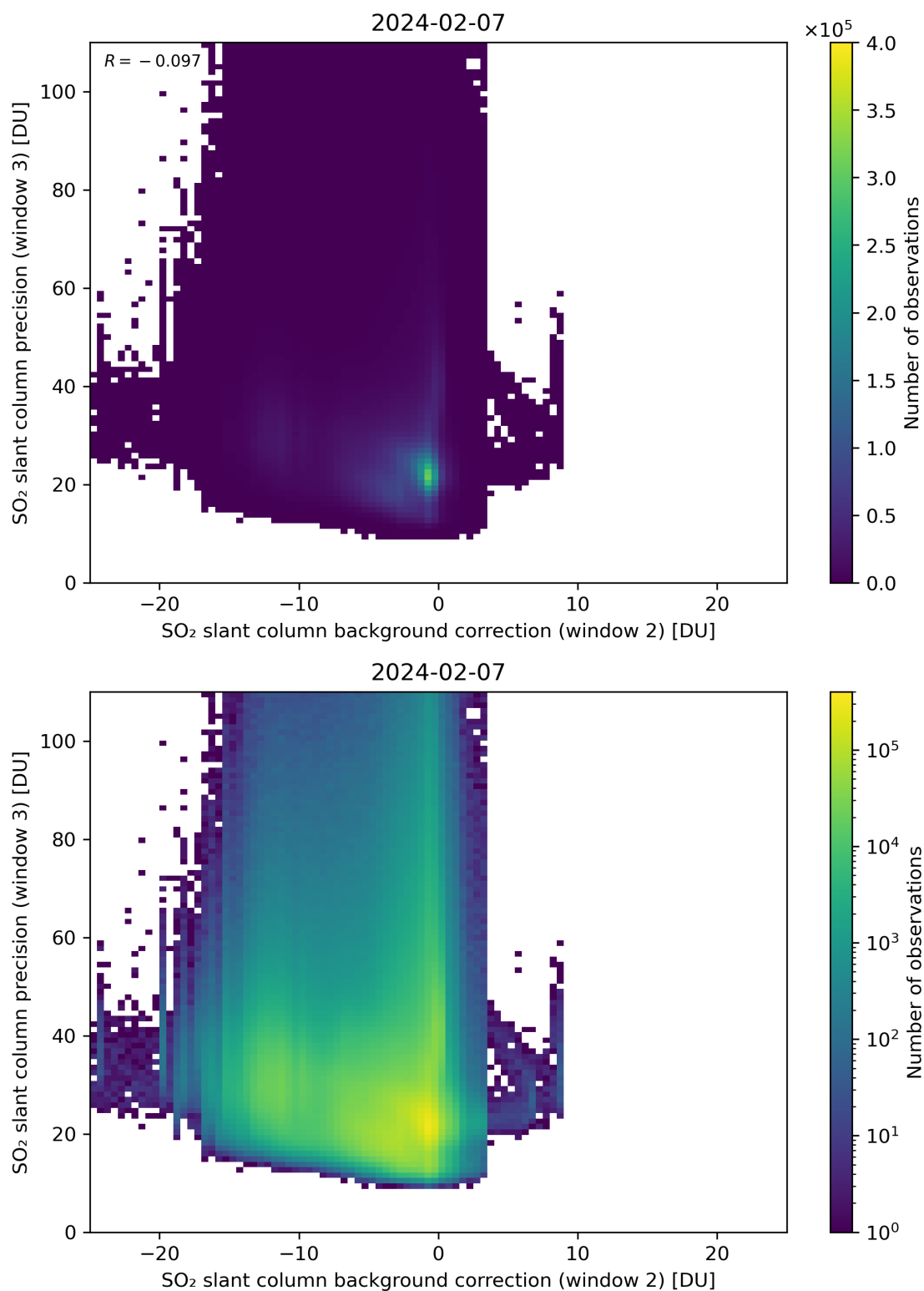
Figure 118: Scatter density plot of “SO 2 slant column background correction (window 2)” against “SO 2 slant column precision (window 3)” for 2024-02-06 to 2024-02-08.
