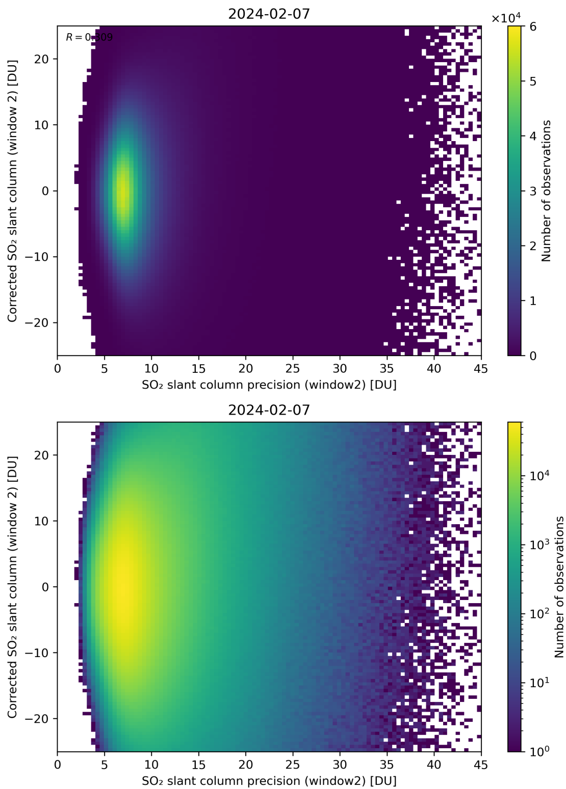
Figure 247: Scatter density plot of “SO 2 slant column precision (window2)” against “Corrected SO 2 slant column (window 2)” for 2024-02-06 to 2024-02-08.
