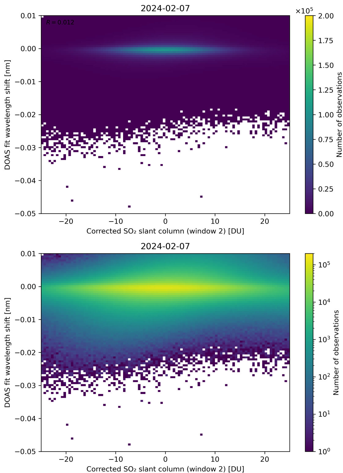
Figure 196: Scatter density plot of “Corrected SO 2 slant column (window 2)” against “DOAS fit wavelength shift” for 2024-02-06 to 2024-02-08.
