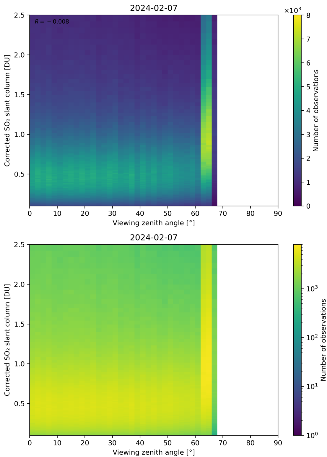
Figure 317: Scatter density plot of “Viewing zenith angle” against “Corrected SO 2 slant column” for 2024-02-06 to 2024-02-08.
