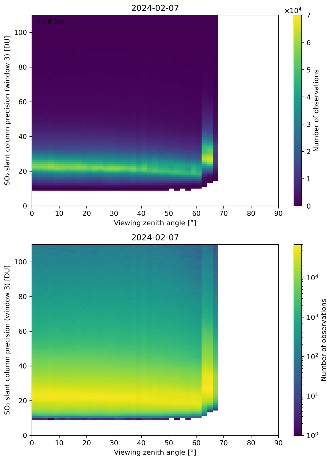
Figure 324: Scatter density plot of “Viewing zenith angle” against “SO 2 slant column precision (window 3)” for 2024-02-06 to 2024-02-08.
