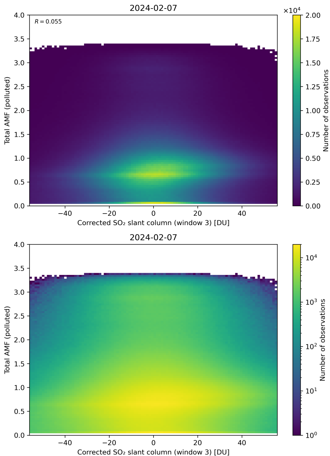
Figure 210: Scatter density plot of “Corrected SO 2 slant column (window 3)” against “Total AMF (polluted)” for 2024-02-06 to 2024-02-08.
