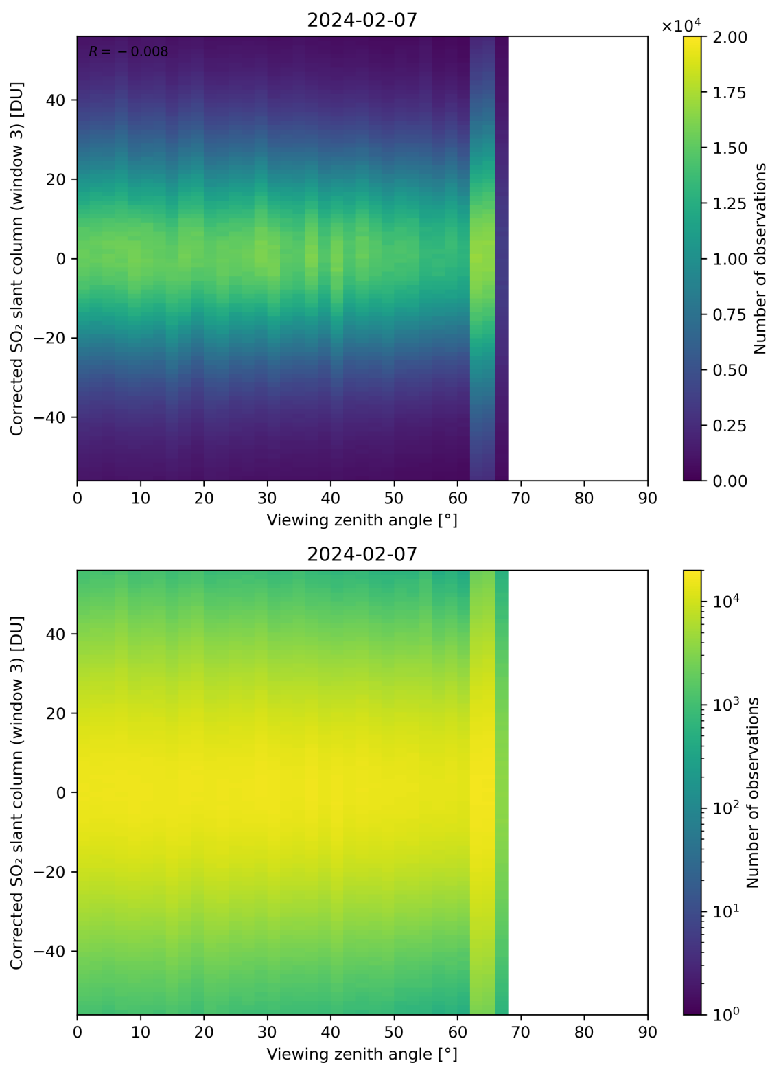
Figure 319: Scatter density plot of “Viewing zenith angle” against “Corrected SO 2 slant column (window 3)” for 2024-02-06 to 2024-02-08.
