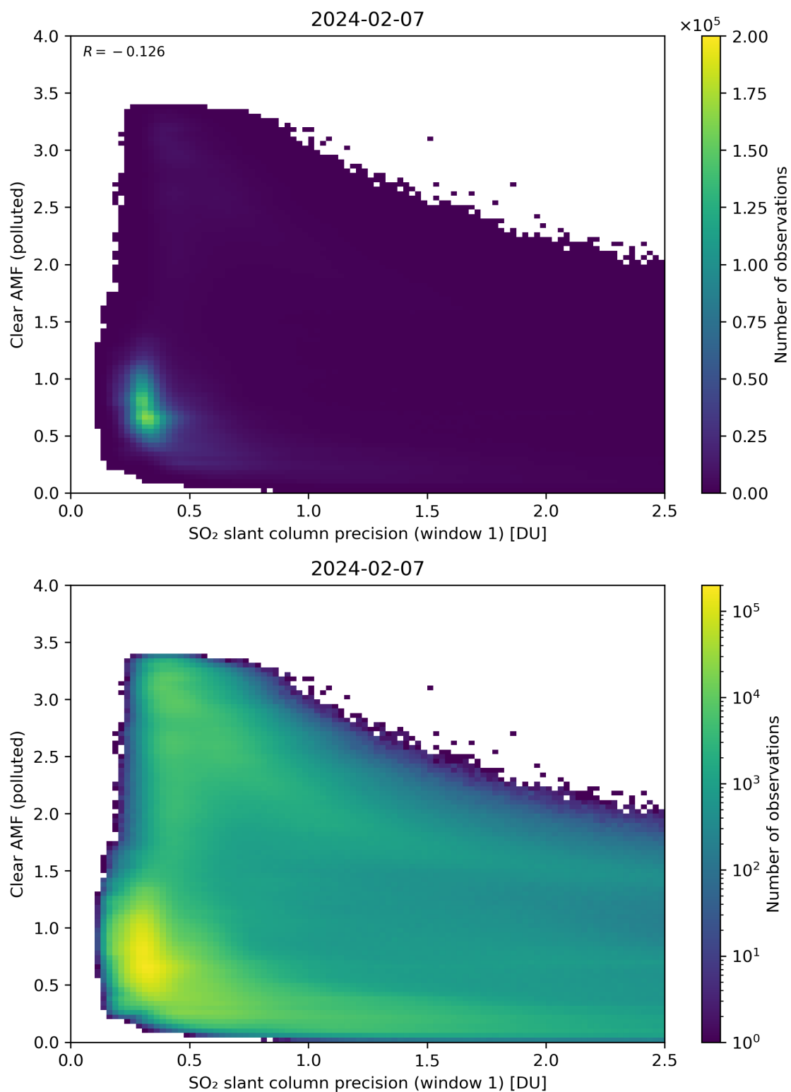
Figure 224: Scatter density plot of “SO 2 slant column precision (window 1)” against “Clear AMF (polluted)” for 2024-02-06 to 2024-02-08.
