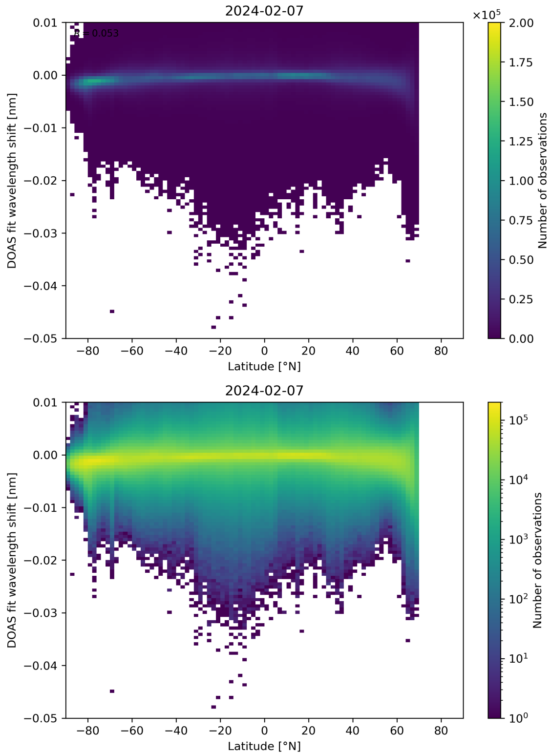
Figure 142: Scatter density plot of “Latitude” against “DOAS fit wavelength shift” for 2024-02-06 to 2024-02-08.
