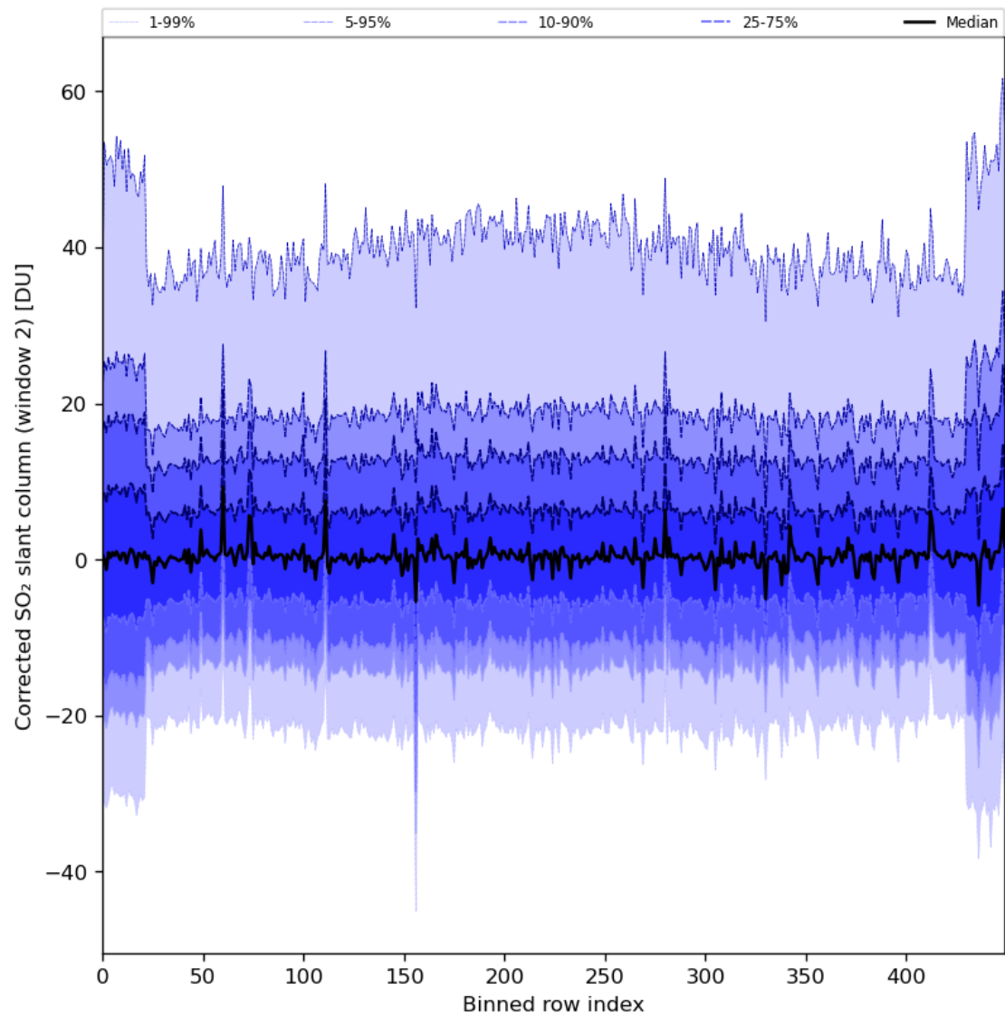
Figure 85: Along track statistics of “Corrected SO 2 slant column (window 2)” for 2024-02-06 to 2024-02-08
