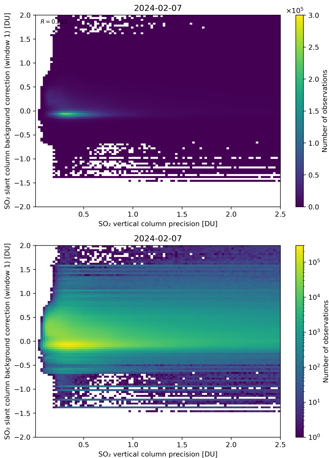
Figure 279: Scatter density plot of “SO 2 vertical column precision” against “SO 2 slant column background correction (window 1)” for 2024-02-06 to 2024-02-08.
