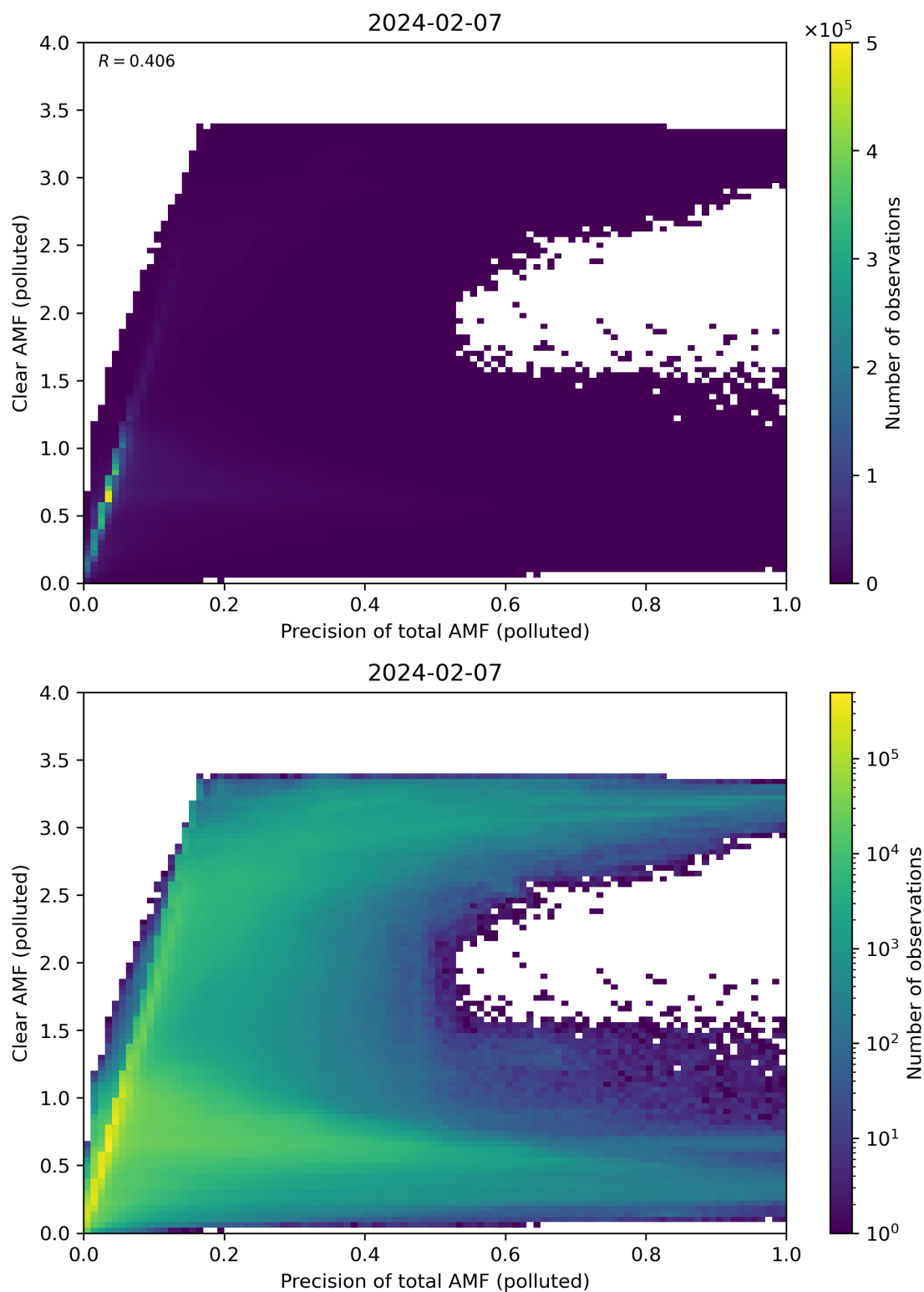
Figure 270: Scatter density plot of “Precision of total AMF (polluted)” against “Clear AMF (polluted)” for 2024-02-06 to 2024-02-08.
