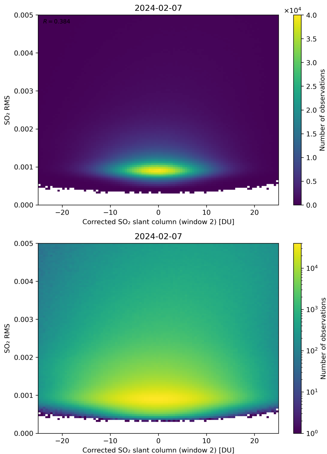
Figure 198: Scatter density plot of “Corrected SO 2 slant column (window 2)” against “SO 2 RMS” for 2024-02-06 to 2024-02-08.
