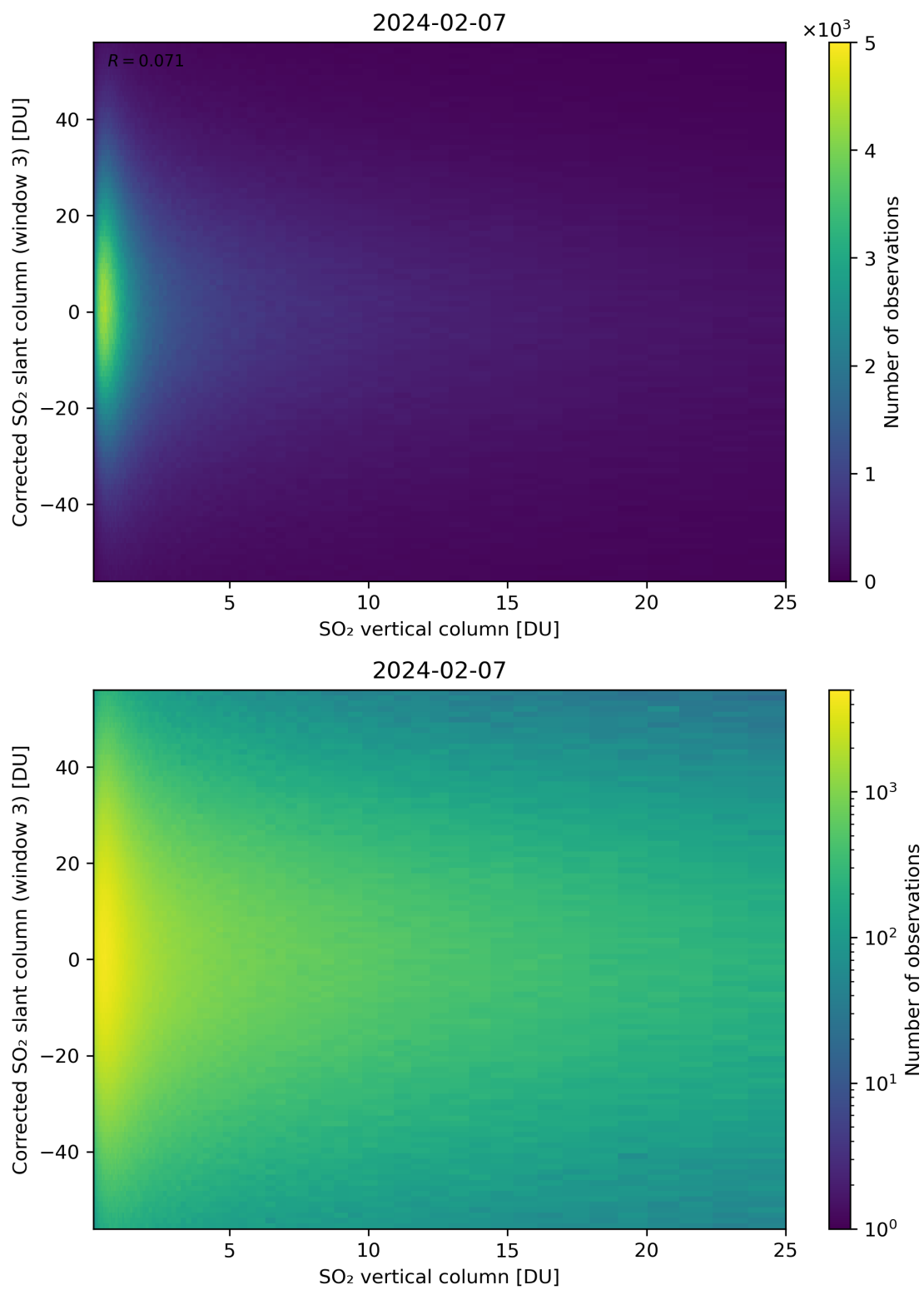
Figure 299: Scatter density plot of “SO 2 vertical column” against “Corrected SO 2 slant column (window 3)” for 2024-02-06 to 2024-02-08.
