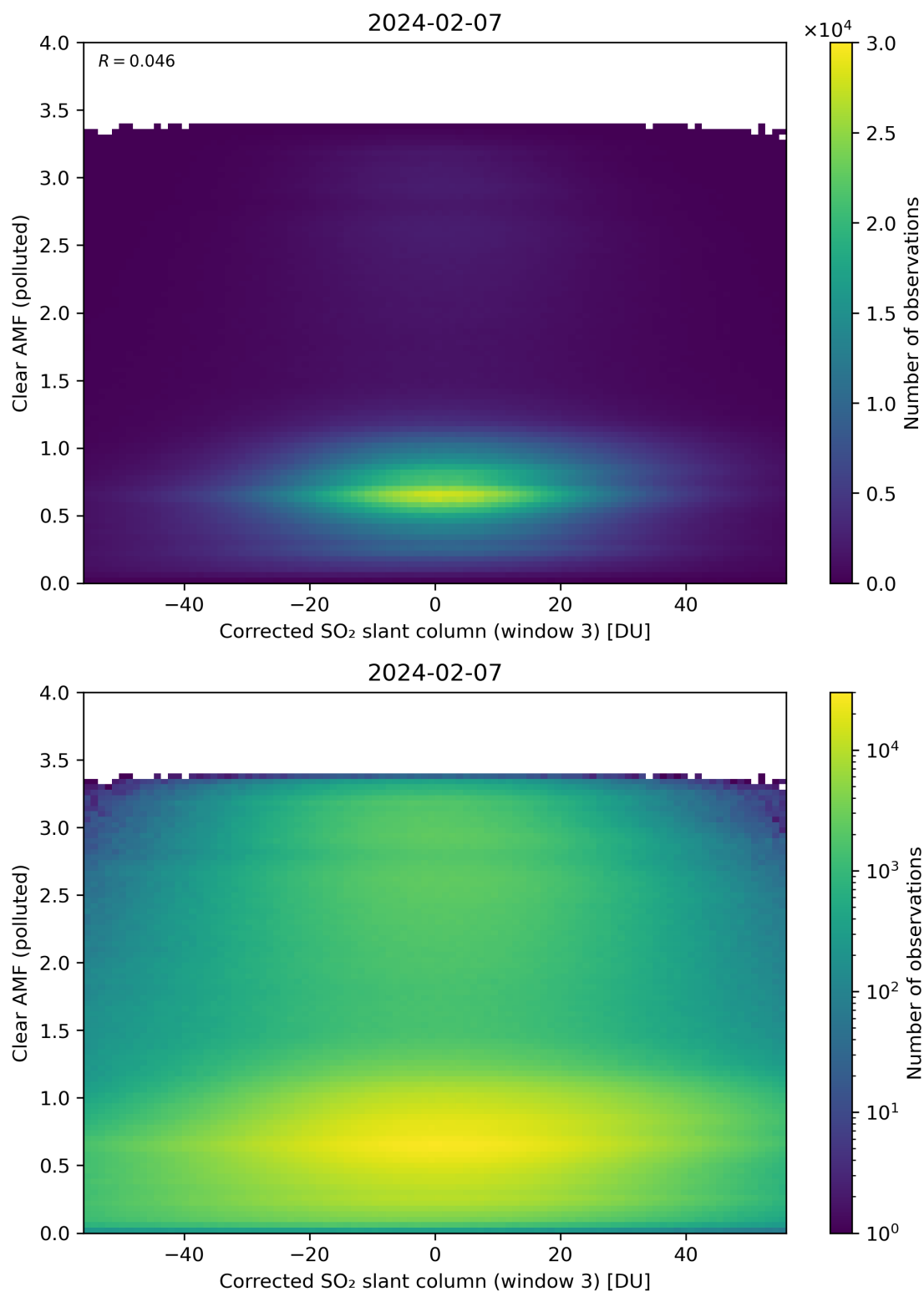
Figure 209: Scatter density plot of “Corrected SO 2 slant column (window 3)” against “Clear AMF (polluted)” for 2024-02-06 to 2024-02-08.
