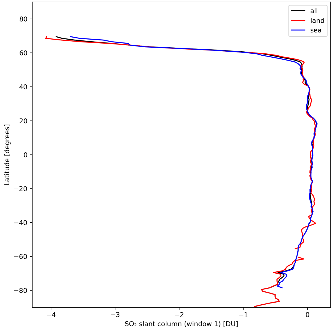
Figure 33: Zonal average of “SO 2 slant column (window 1)” for 2024-02-06 to 2024-02-08.
