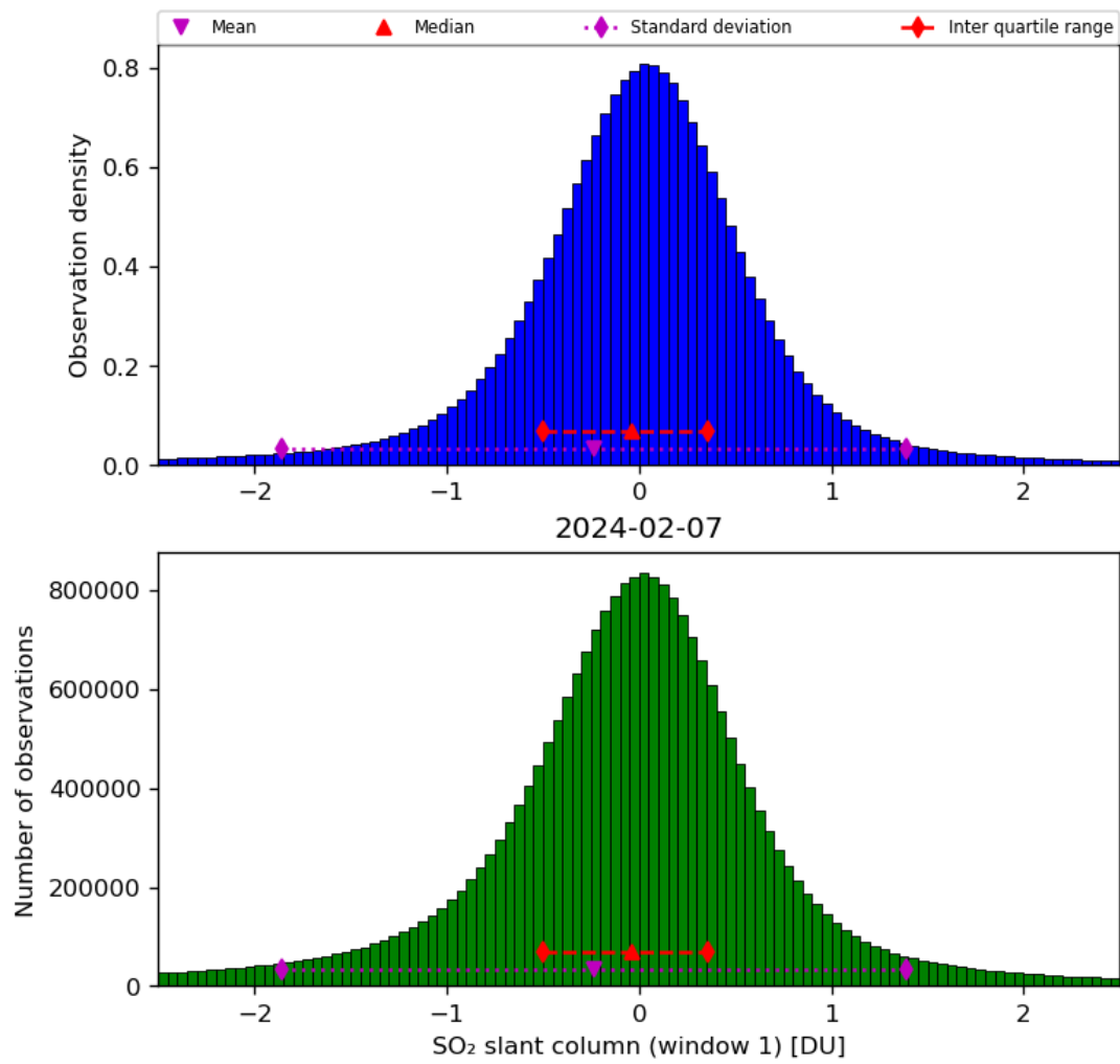
Figure 56: Histogram of “SO 2 slant column (window 1)” for 2024-02-06 to 2024-02-08
