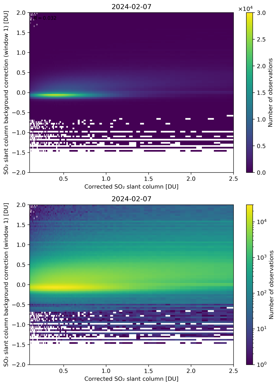
Figure 178: Scatter density plot of “Corrected SO 2 slant column” against “SO 2 slant column background correction (window 1)” for 2024-02-06 to 2024-02-08.
