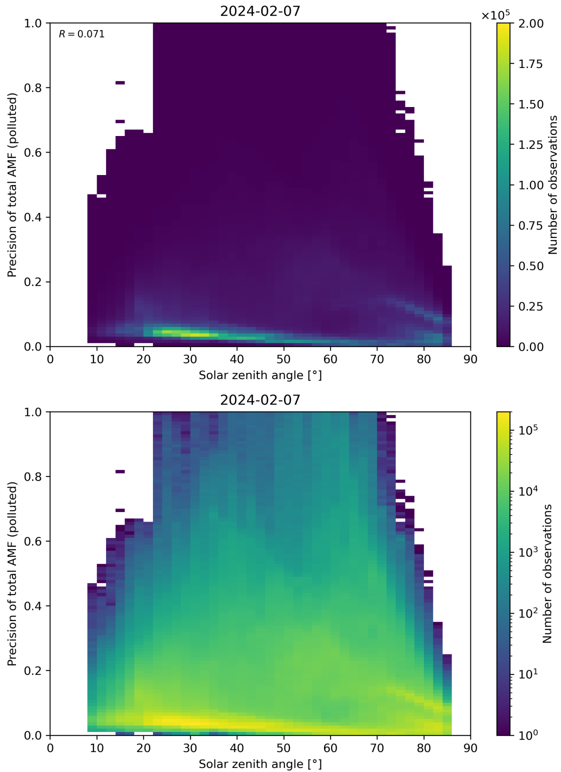
Figure 175: Scatter density plot of “Solar zenith angle” against “Precision of total AMF (polluted)” for 2024-02-06 to 2024-02-08.
