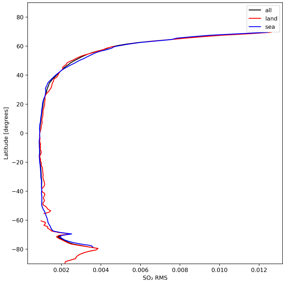
Figure 47: Zonal average of “SO 2 RMS” for 2024-02-06 to 2024-02-08.
