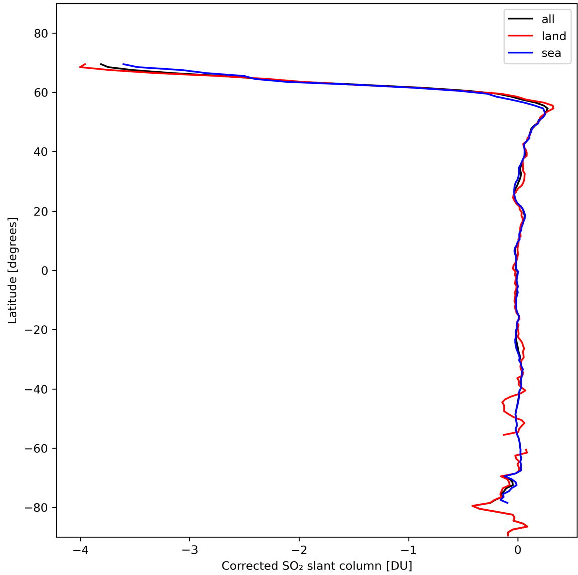
Figure 32: Zonal average of “Corrected SO 2 slant column” for 2024-02-06 to 2024-02-08.
