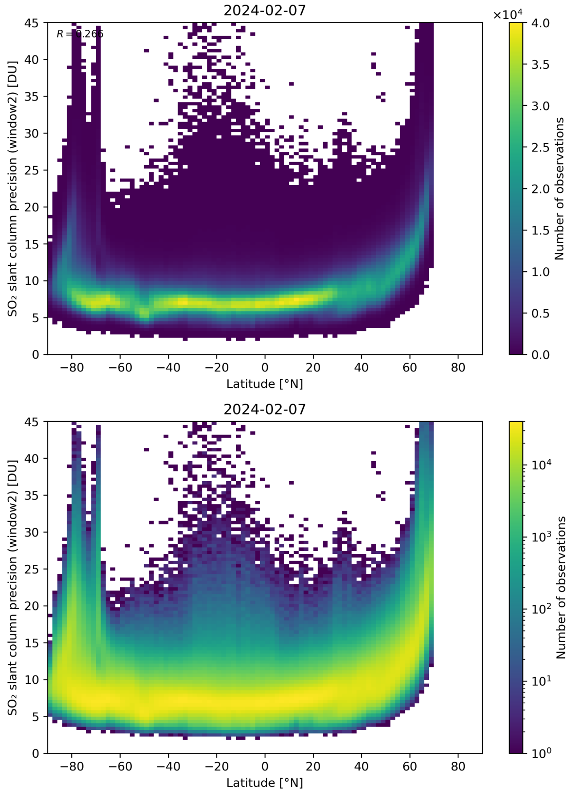
Figure 151: Scatter density plot of “Latitude” against “SO 2 slant column precision (window2)” for 2024-02-06 to 2024-02-08.
