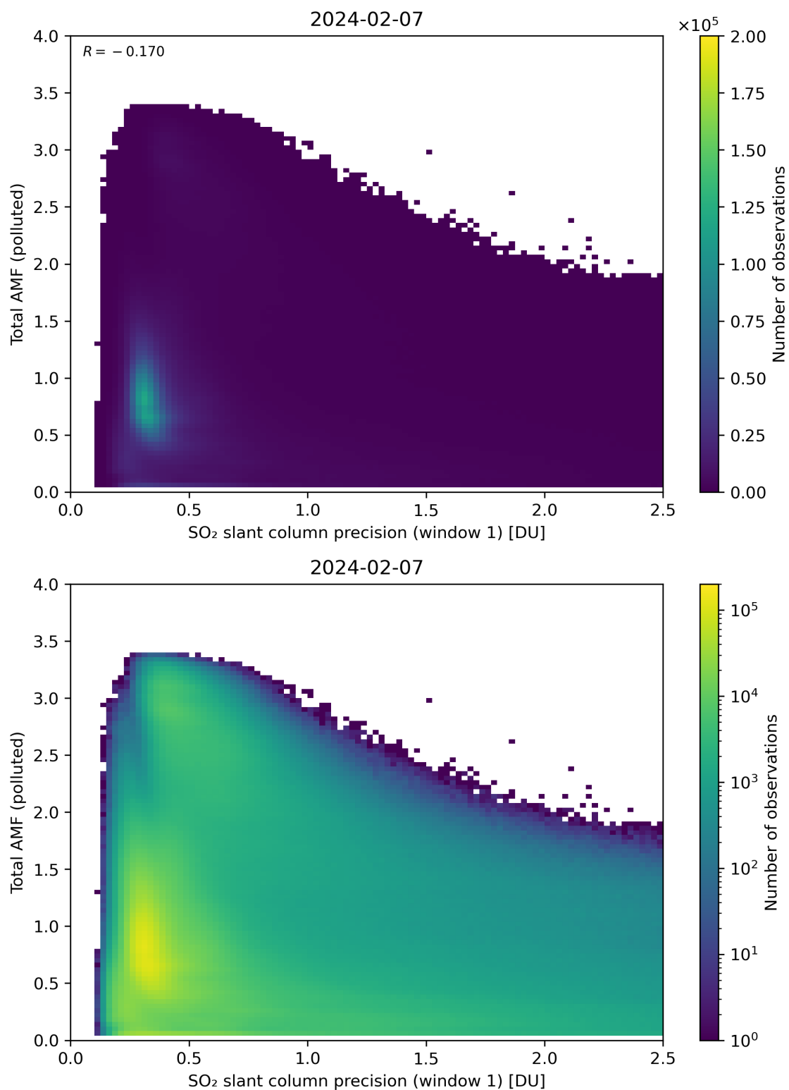
Figure 230: Scatter density plot of “SO 2 slant column precision (window 1)” against “Total AMF (polluted)” for 2024-02-06 to 2024-02-08.
