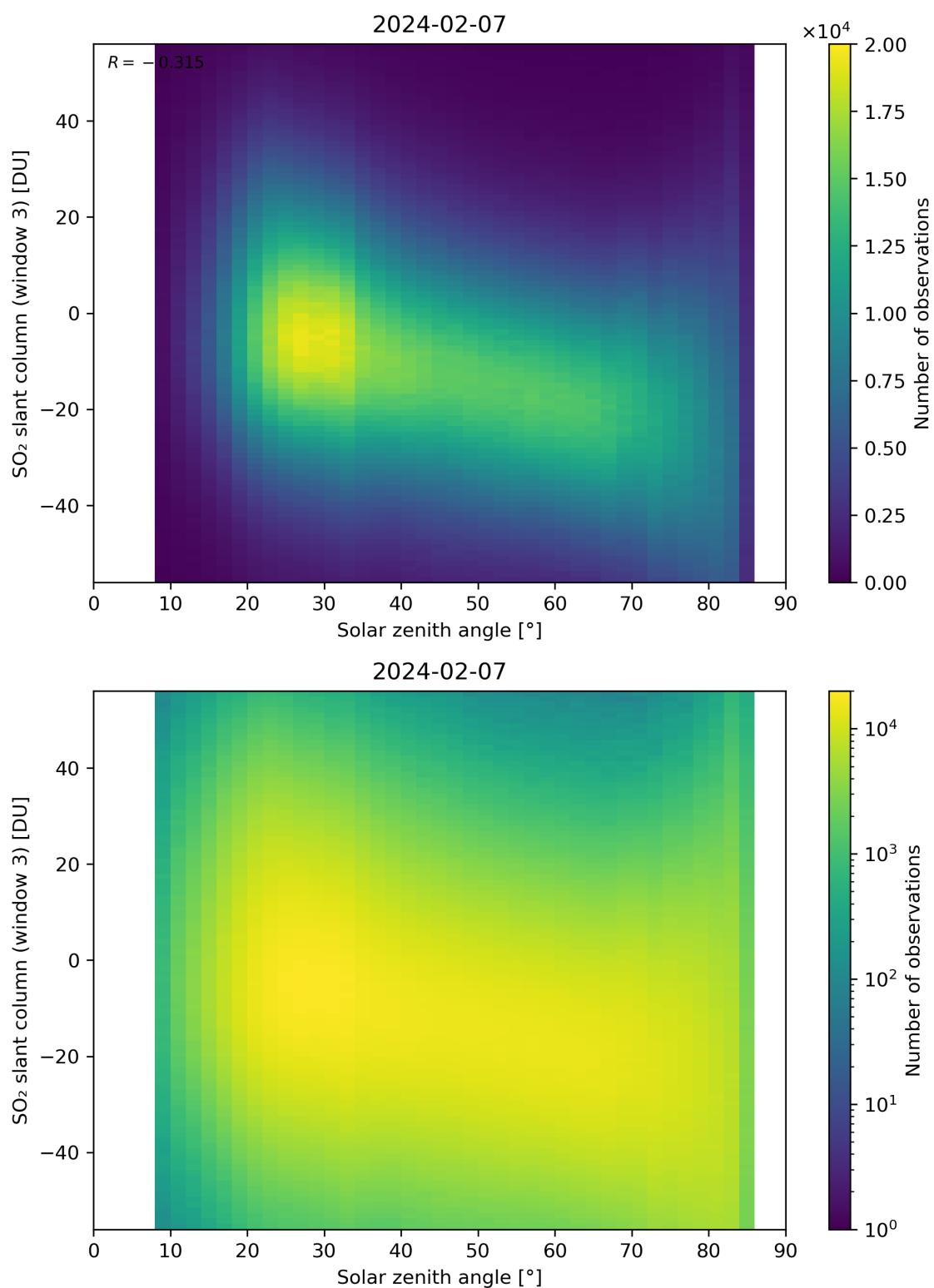
Figure 172: Scatter density plot of “Solar zenith angle” against “SO 2 slant column (window 3)” for 2024-02-06 to 2024-02-08.
