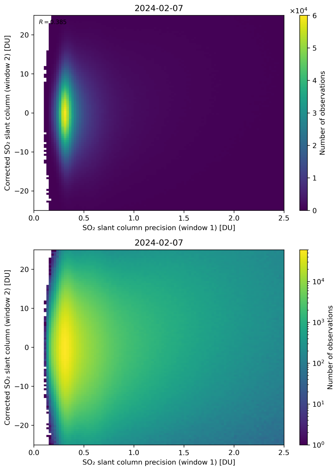
Figure 225: Scatter density plot of “SO 2 slant column precision (window 1)” against “Corrected SO 2 slant column (window 2)” for 2024-02-06 to 2024-02-08.
