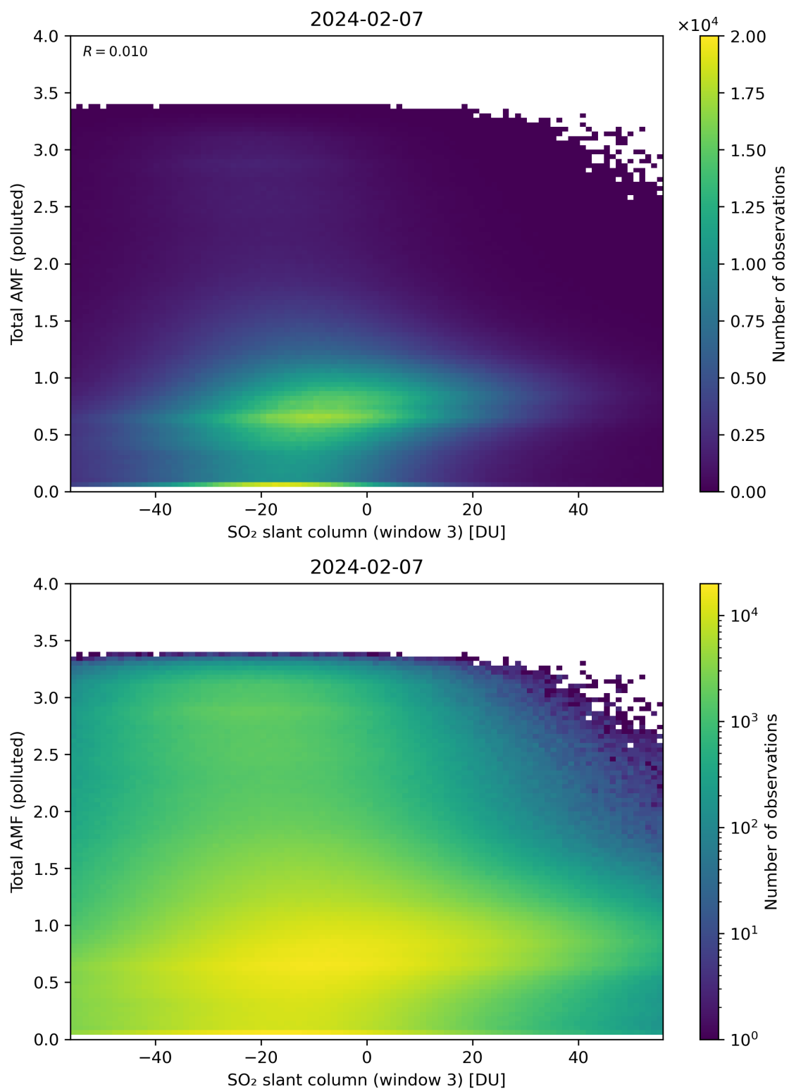
Figure 268: Scatter density plot of “SO 2 slant column (window 3)” against “Total AMF (polluted)” for 2024-02-06 to 2024-02-08.
