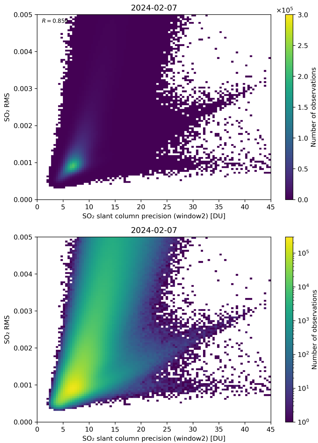
Figure 245: Scatter density plot of “SO 2 slant column precision (window2)” against “SO 2 RMS” for 2024-02-06 to 2024-02-08.
