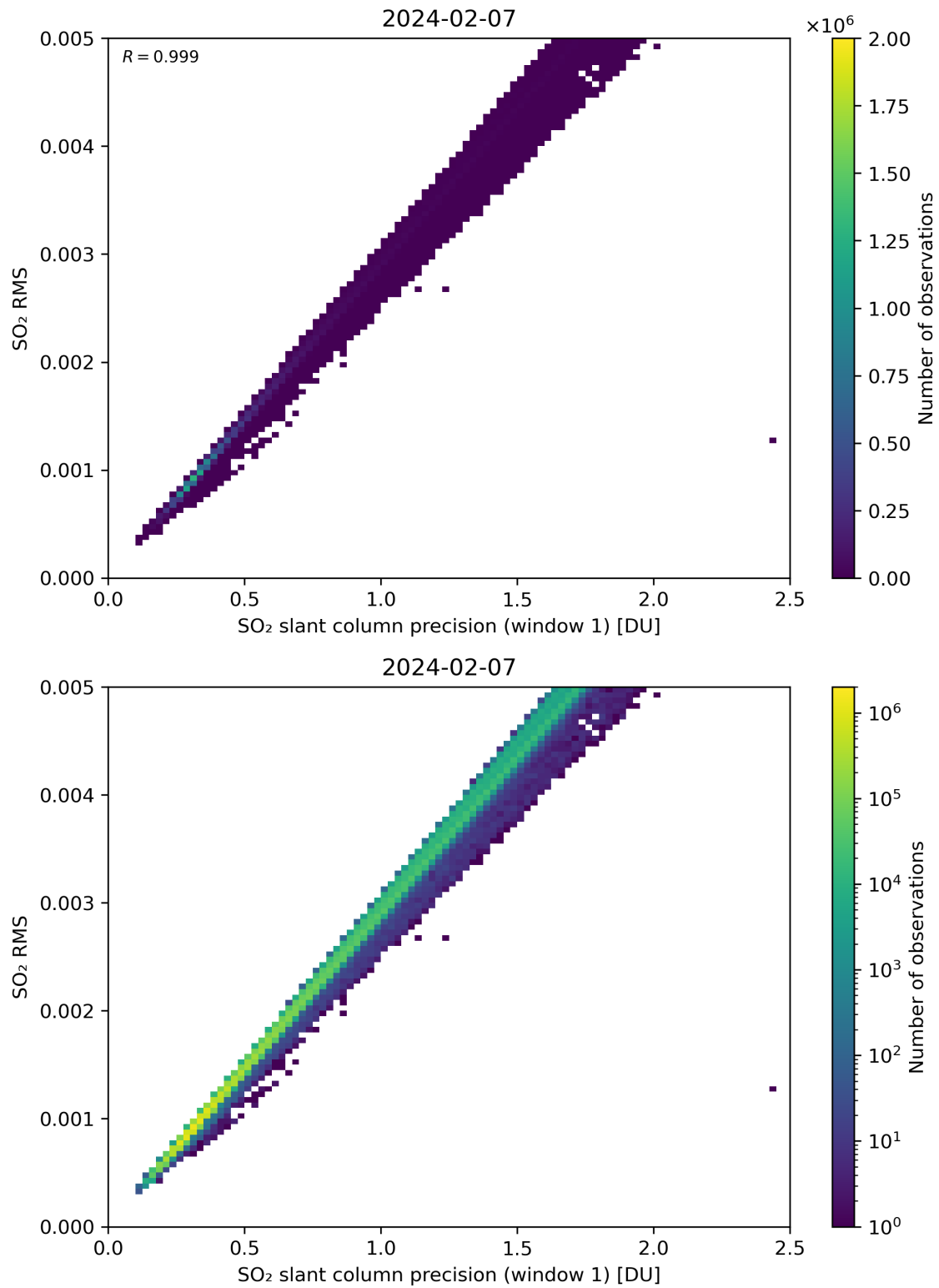
Figure 223: Scatter density plot of “SO 2 slant column precision (window 1)” against “SO 2 RMS” for 2024-02-06 to 2024-02-08.
