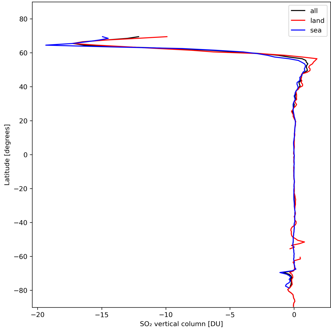
Figure 30: Zonal average of “SO 2 vertical column” for 2024-02-06 to 2024-02-08.
