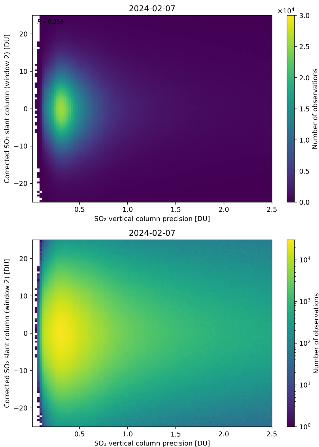
Figure 287: Scatter density plot of “SO 2 vertical column precision” against “Corrected SO 2 slant column (window 2)” for 2024-02-06 to 2024-02-08.
