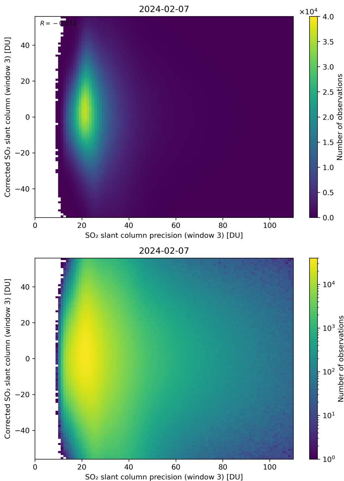
Figure 262: Scatter density plot of “SO 2 slant column precision (window 3)” against “Corrected SO 2 slant column (window 3)” for 2024-02-06 to 2024-02-08.
