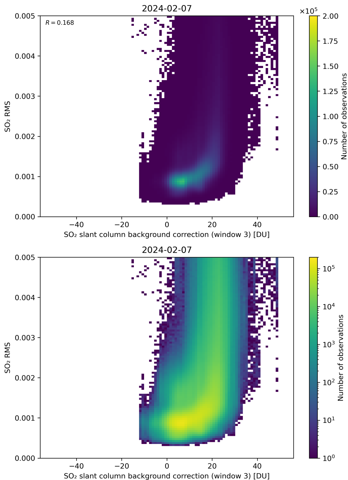
Figure 123: Scatter density plot of “SO 2 slant column background correction (window 3)” against “SO 2 RMS” for 2024-02-06 to 2024-02-08.
