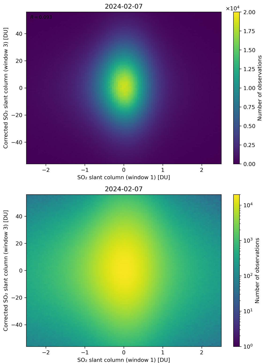
Figure 234: Scatter density plot of “SO 2 slant column (window 1)” against “Corrected SO 2 slant column (window 3)” for 2024-02-06 to 2024-02-08.
