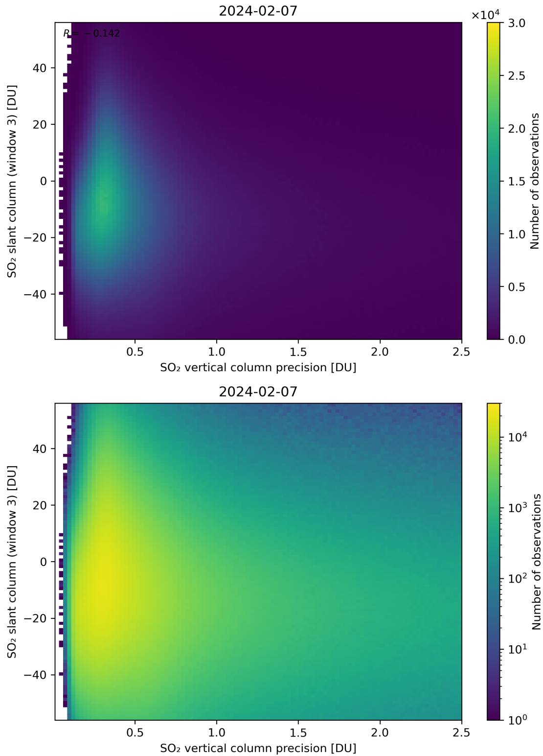
Figure 292: Scatter density plot of “SO 2 vertical column precision” against “SO 2 slant column (window 3)” for 2024-02-06 to 2024-02-08.
