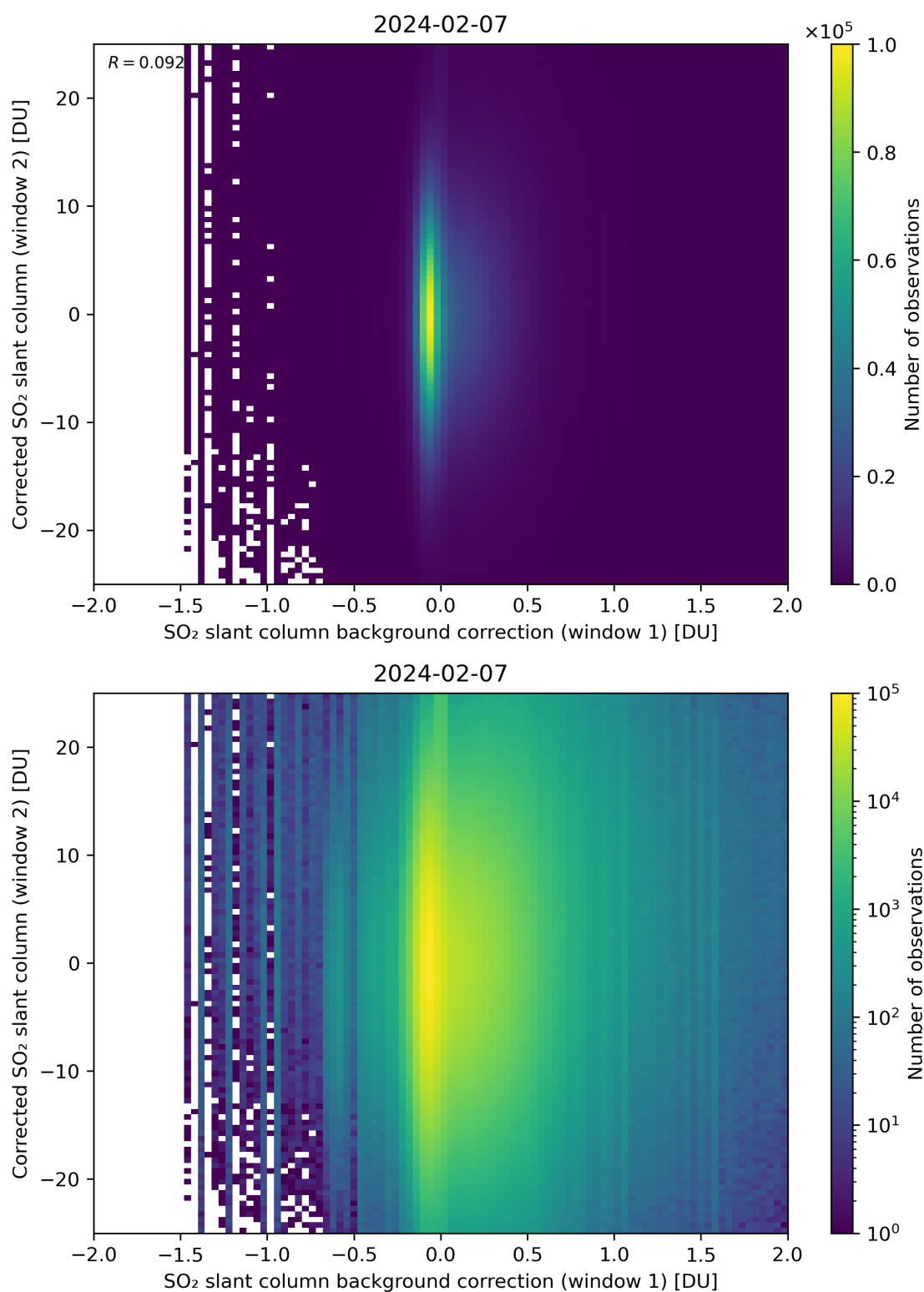
Figure 104: Scatter density plot of “SO 2 slant column background correction (window 1)” against “Corrected SO 2 slant column (window 2)” for 2024-02-06 to 2024-02-08.
