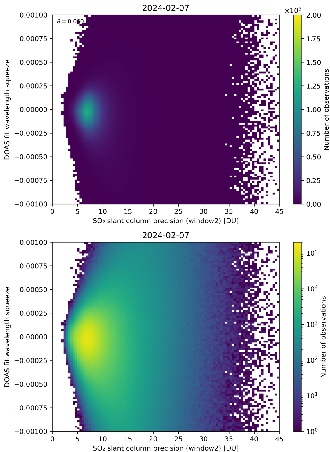
Figure 244: Scatter density plot of “SO 2 slant column precision (window2)” against “DOAS fit wavelength squeeze” for 2024-02-06 to 2024-02-08.
