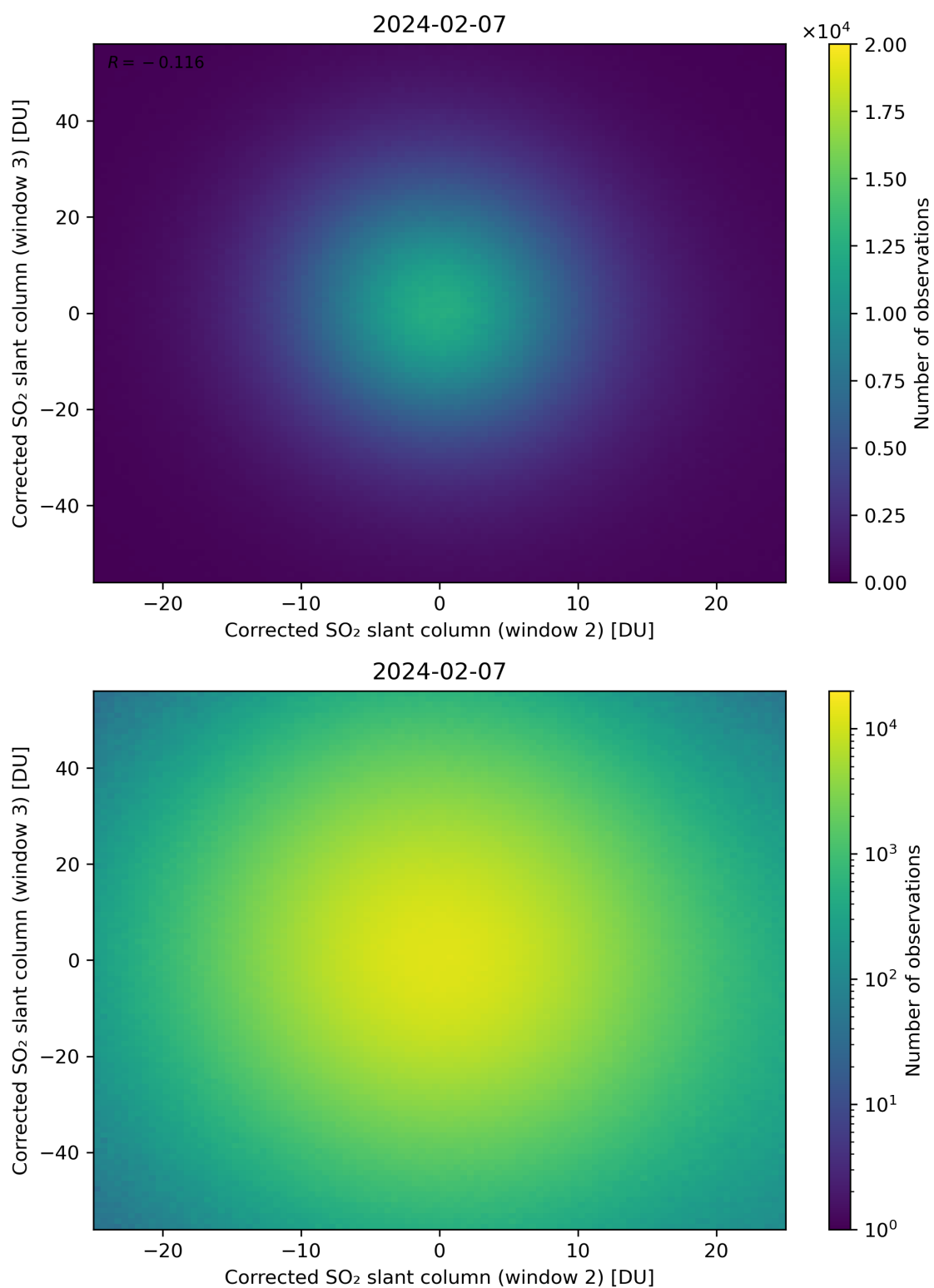
Figure 200: Scatter density plot of “Corrected SO 2 slant column (window 2)” against “Corrected SO 2 slant column (window 3)” for 2024-02-06 to 2024-02-08.
