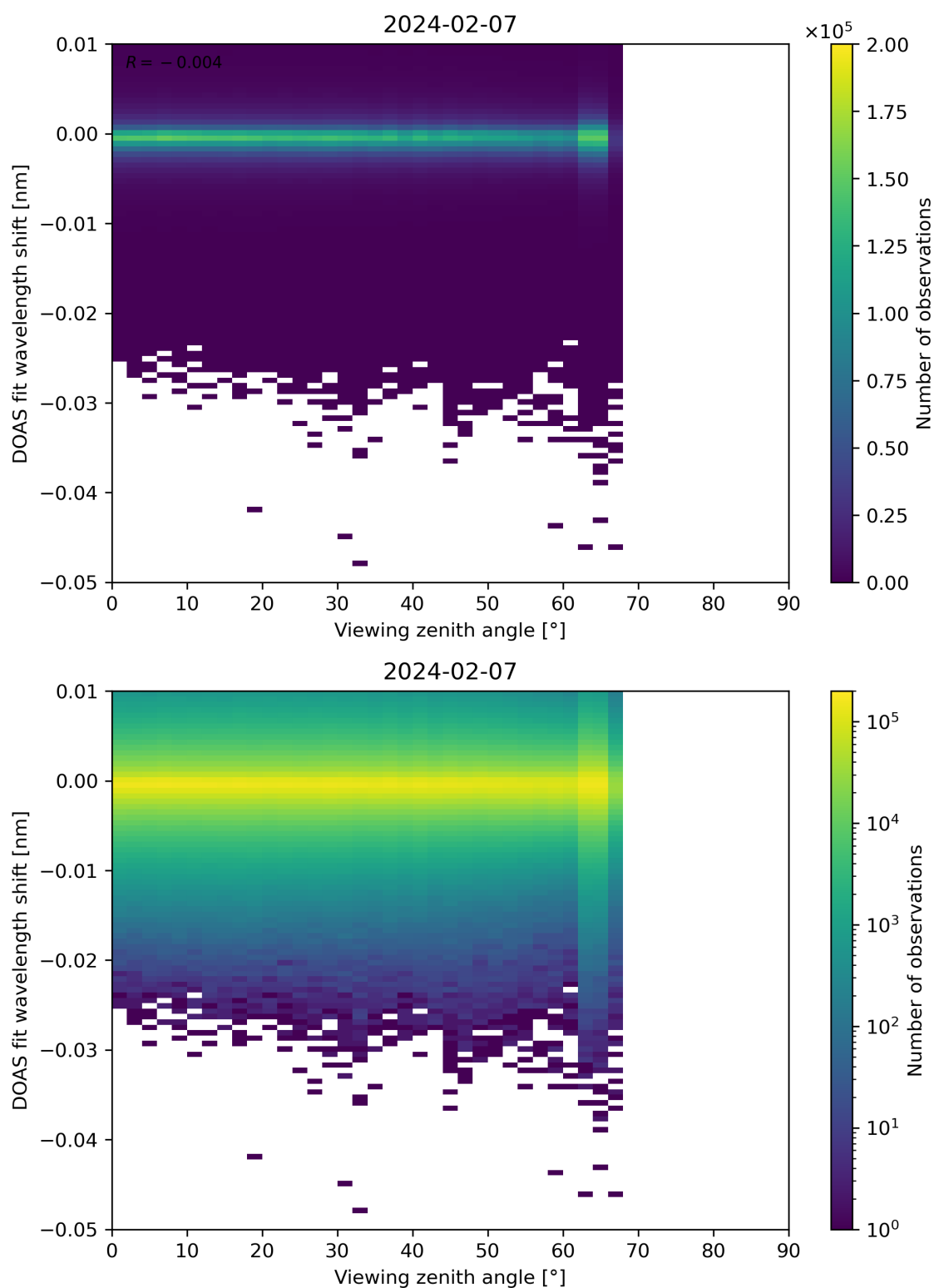
Figure 311: Scatter density plot of “Viewing zenith angle” against “DOAS fit wavelength shift” for 2024-02-06 to 2024-02-08.
