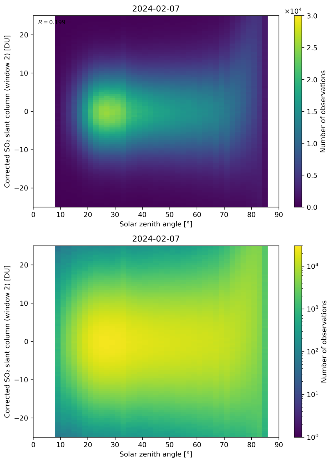
Figure 167: Scatter density plot of “Solar zenith angle” against “Corrected SO 2 slant column (window 2)” for 2024-02-06 to 2024-02-08.
