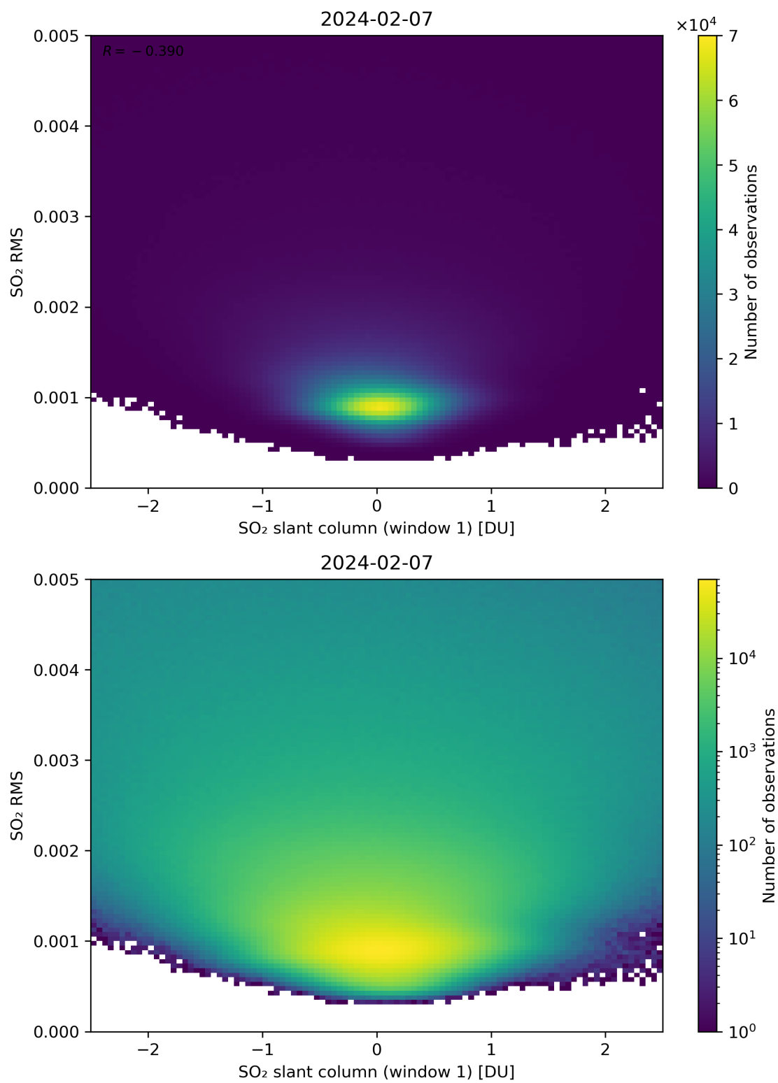
Figure 217: Scatter density plot of “SO 2 slant column (window 1)” against “SO 2 RMS” for 2024-02-06 to 2024-02-08.
