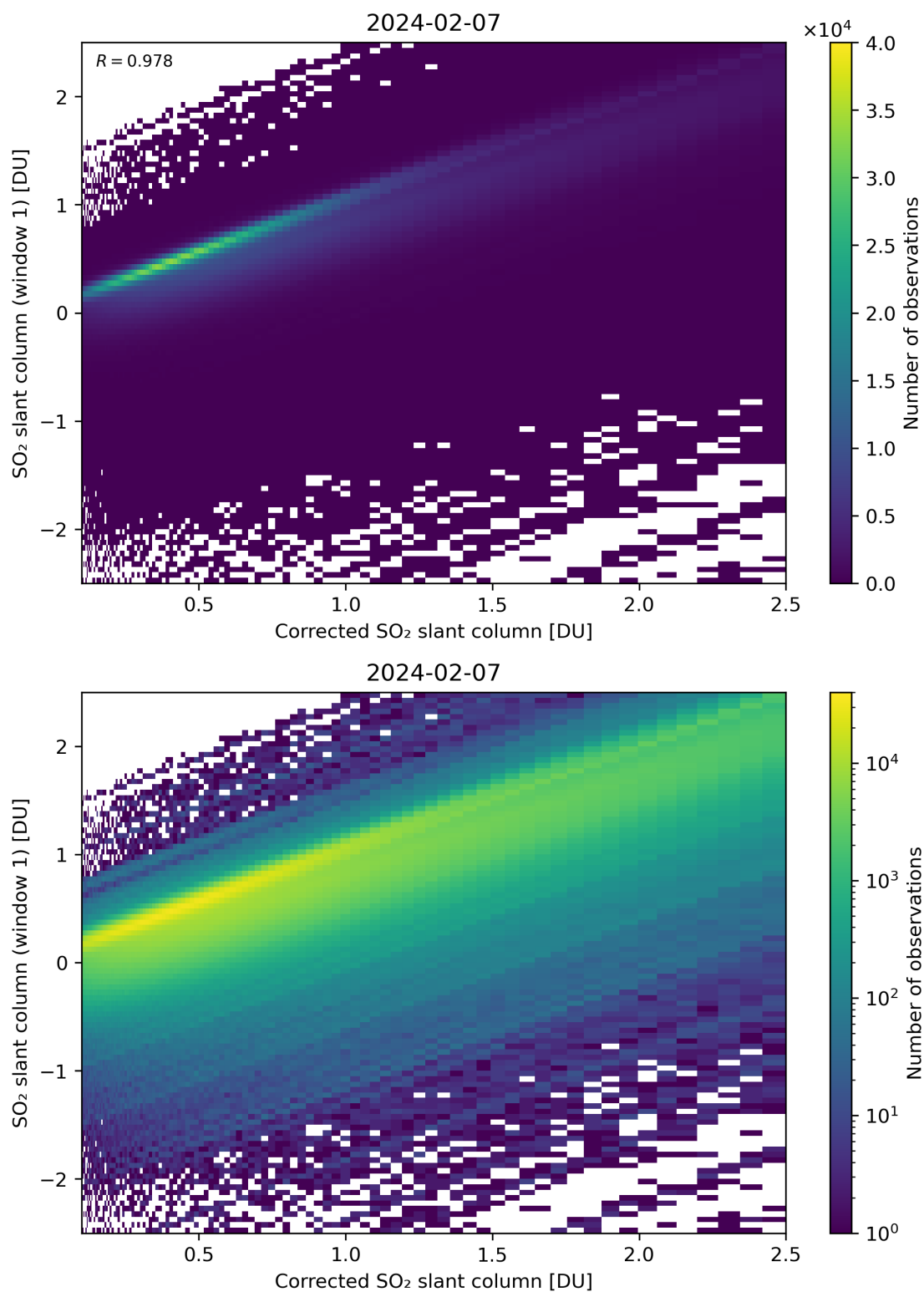
Figure 187: Scatter density plot of “Corrected SO 2 slant column” against “SO 2 slant column (window 1)” for 2024-02-06 to 2024-02-08.
