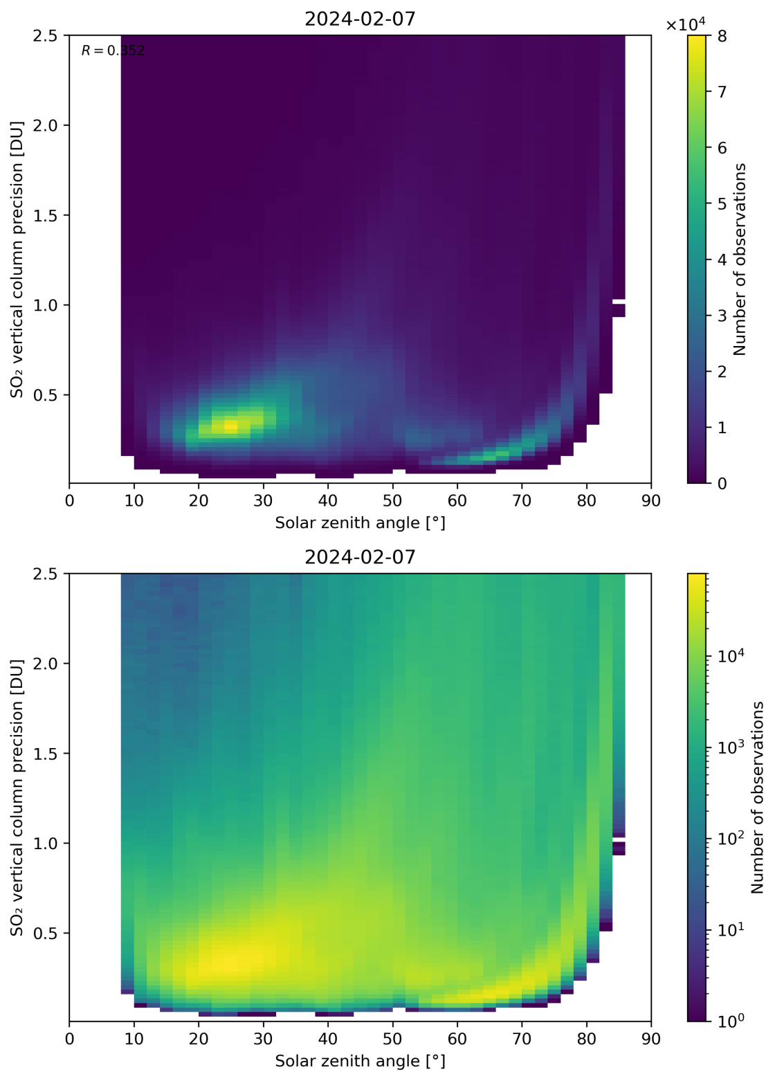
Figure 177: Scatter density plot of “Solar zenith angle” against “SO 2 vertical column precision” for 2024-02-06 to 2024-02-08.
