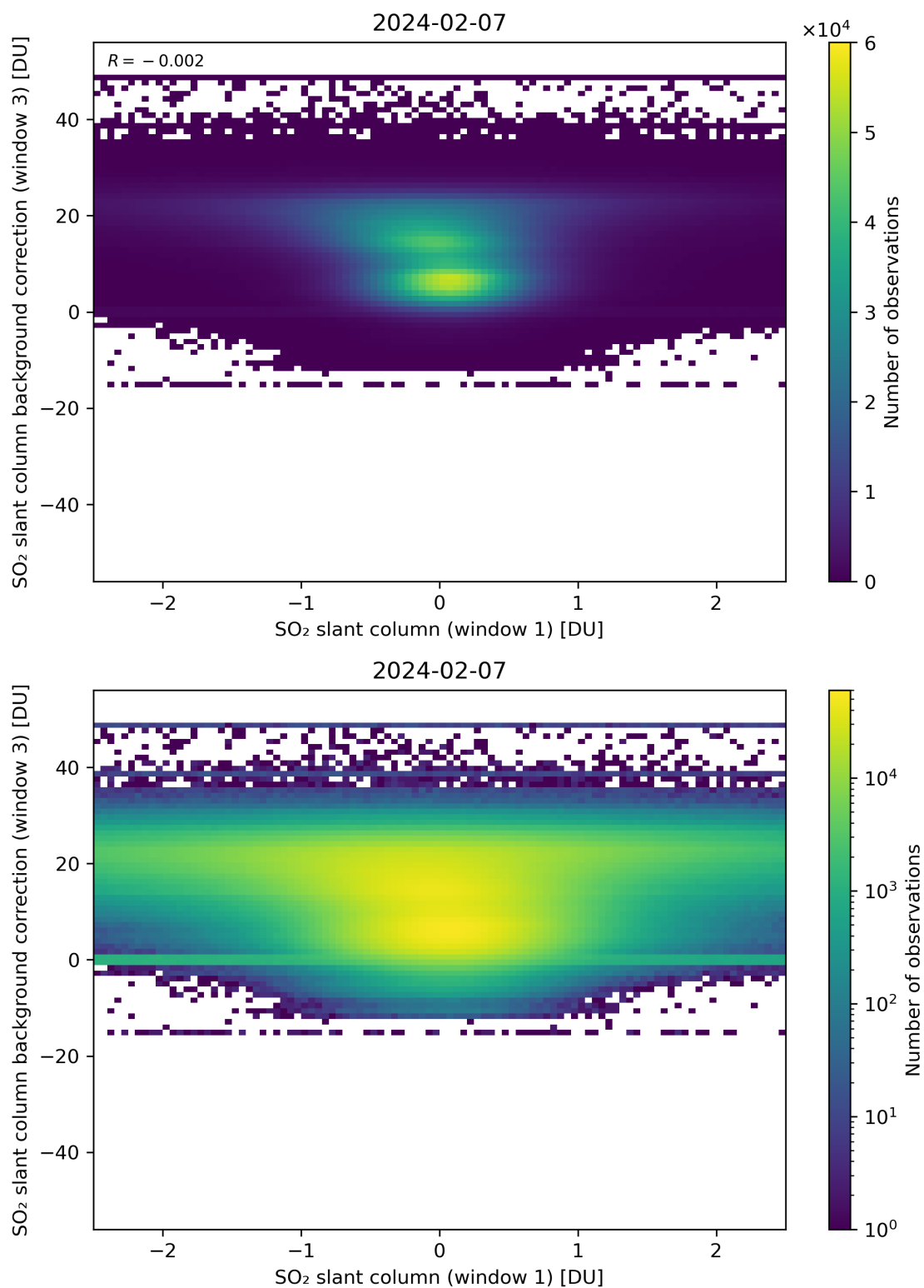
Figure 214: Scatter density plot of “SO 2 slant column (window 1)” against “SO 2 slant column background correction (window 3)” for 2024-02-06 to 2024-02-08.
