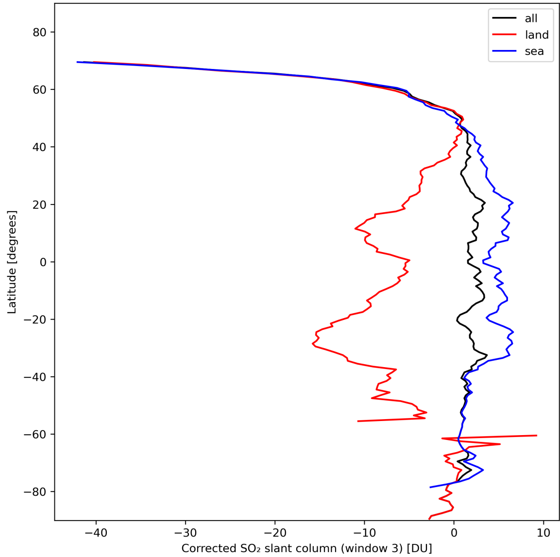
Figure 43: Zonal average of “Corrected SO 2 slant column (window 3)” for 2024-02-06 to 2024-02-08.
