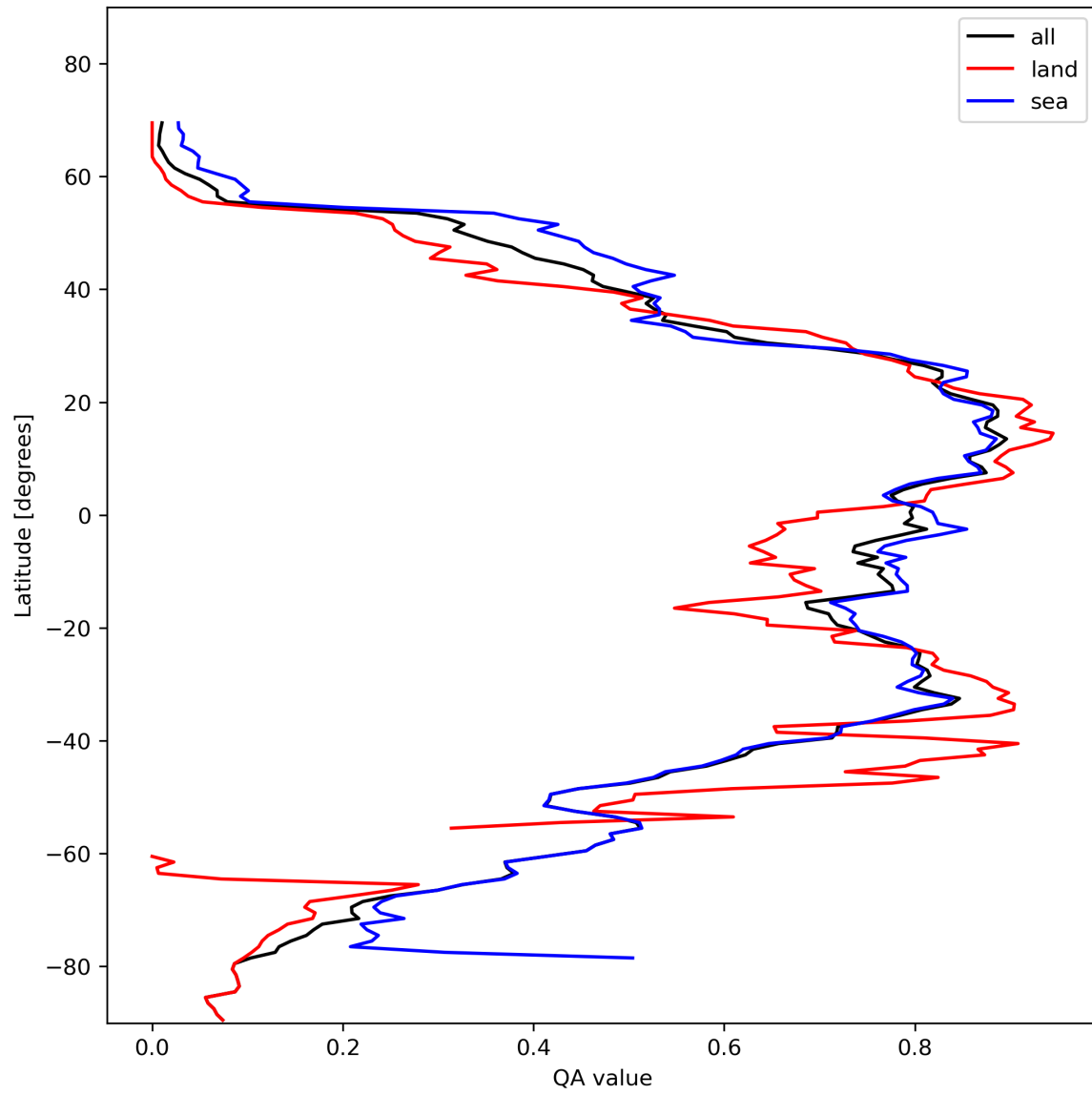
Figure 29: Zonal average of “QA value” for 2024-02-06 to 2024-02-08.
