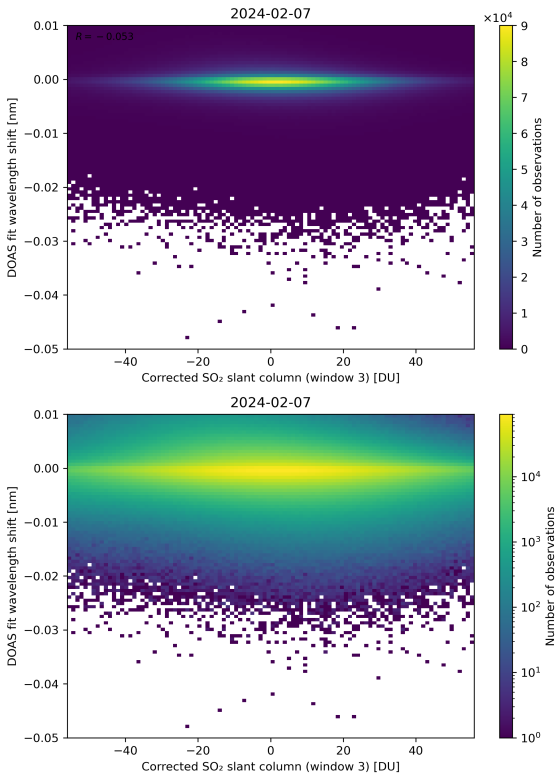
Figure 206: Scatter density plot of “Corrected SO 2 slant column (window 3)” against “DOAS fit wavelength shift” for 2024-02-06 to 2024-02-08.
