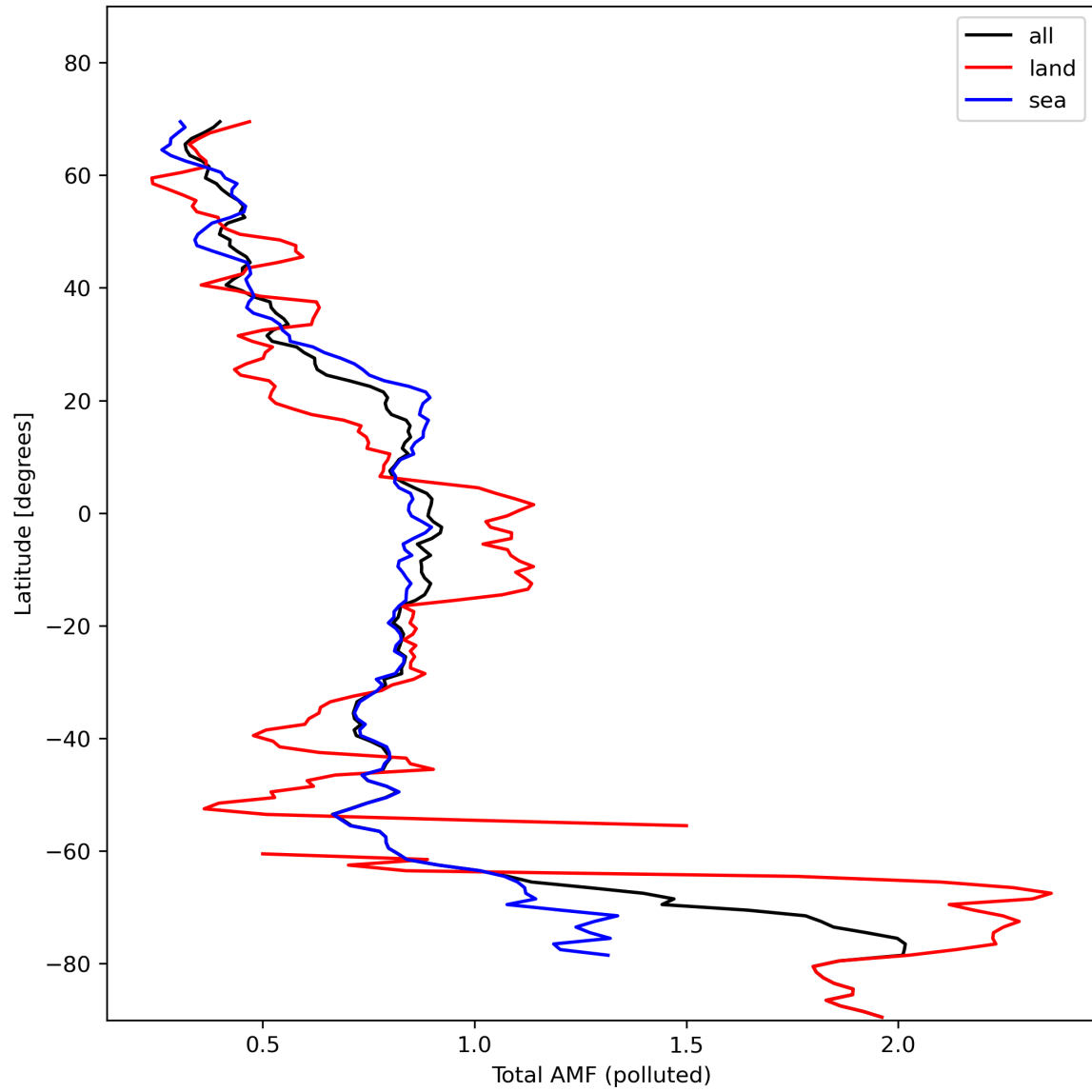
Figure 48: Zonal average of “Total AMF (polluted)” for 2024-02-06 to 2024-02-08.
