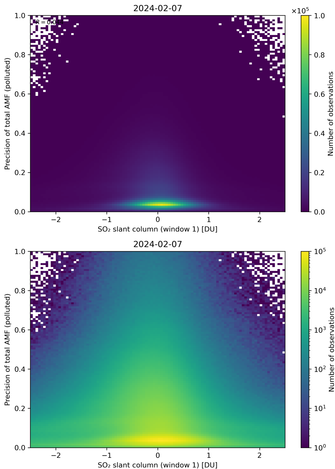
Figure 240: Scatter density plot of “SO 2 slant column (window 1)” against “Precision of total AMF (polluted)” for 2024-02-06 to 2024-02-08.
