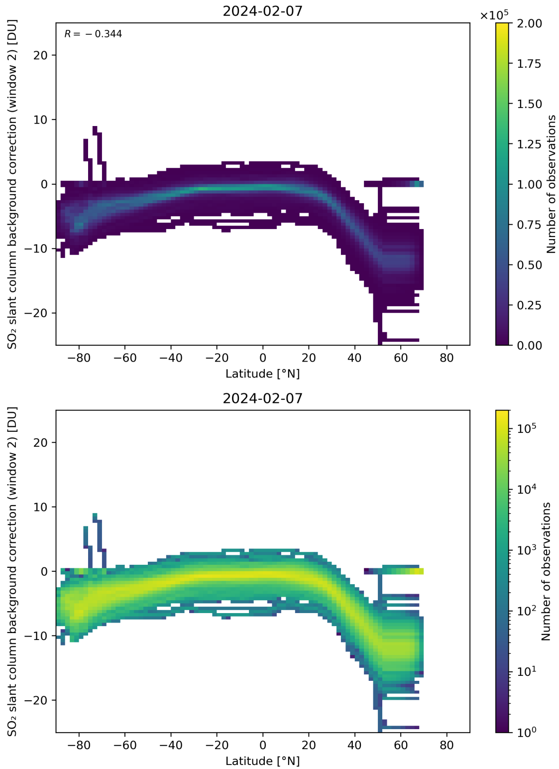
Figure 140: Scatter density plot of “Latitude” against “SO 2 slant column background correction (window 2)” for 2024-02-06 to 2024-02-08.
