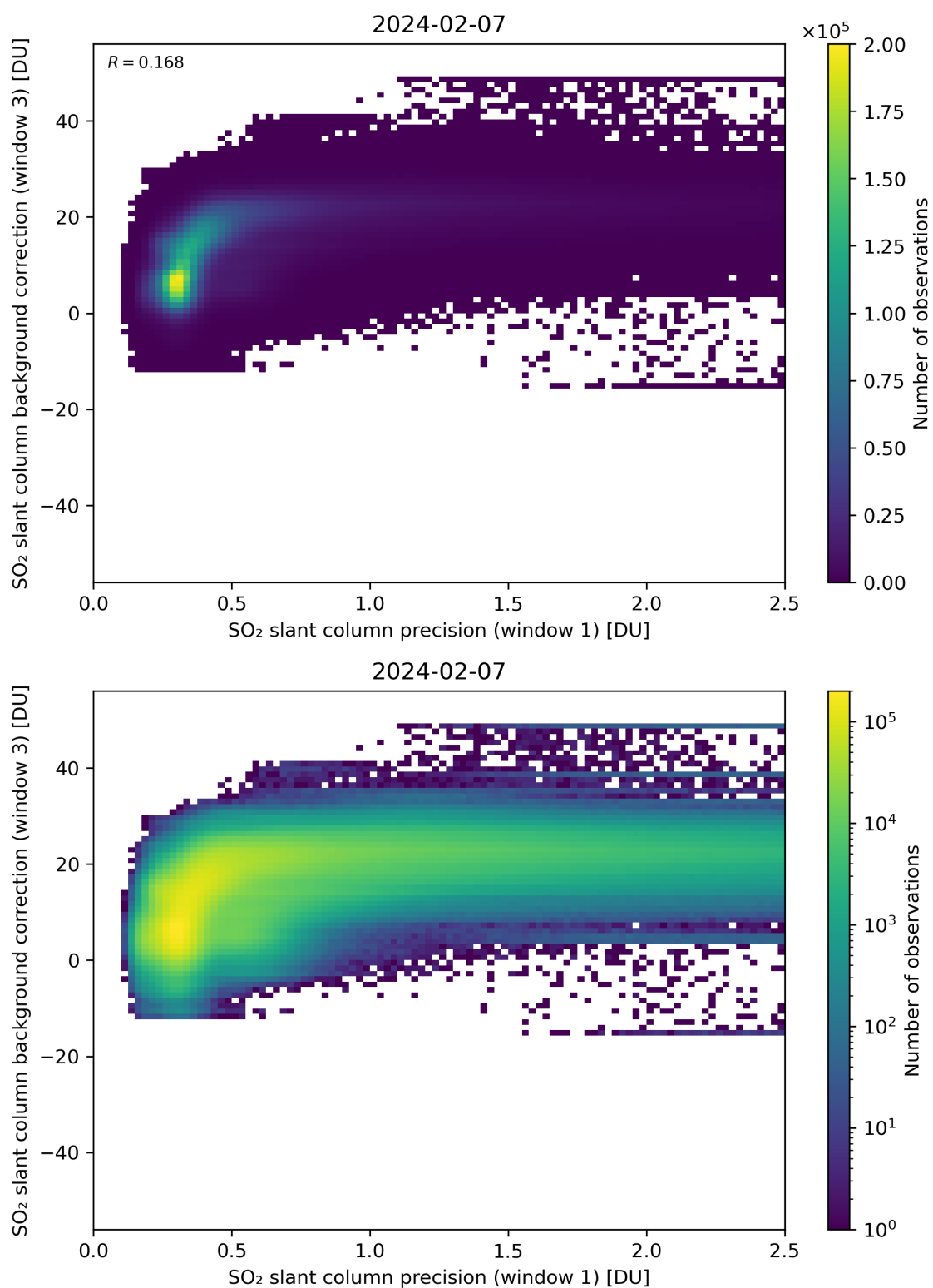
Figure 220: Scatter density plot of “SO 2 slant column precision (window 1)” against “SO 2 slant column background correction (window 3)” for 2024-02-06 to 2024-02-08.
