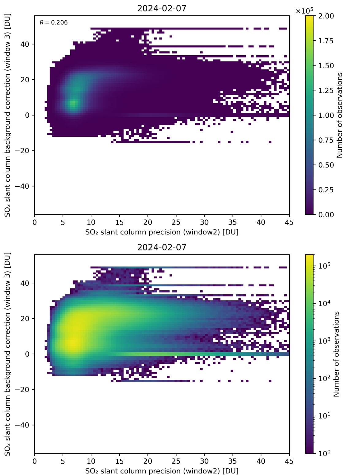
Figure 242: Scatter density plot of “SO 2 slant column precision (window2)” against “SO 2 slant column background correction (window 3)” for 2024-02-06 to 2024-02-08.
