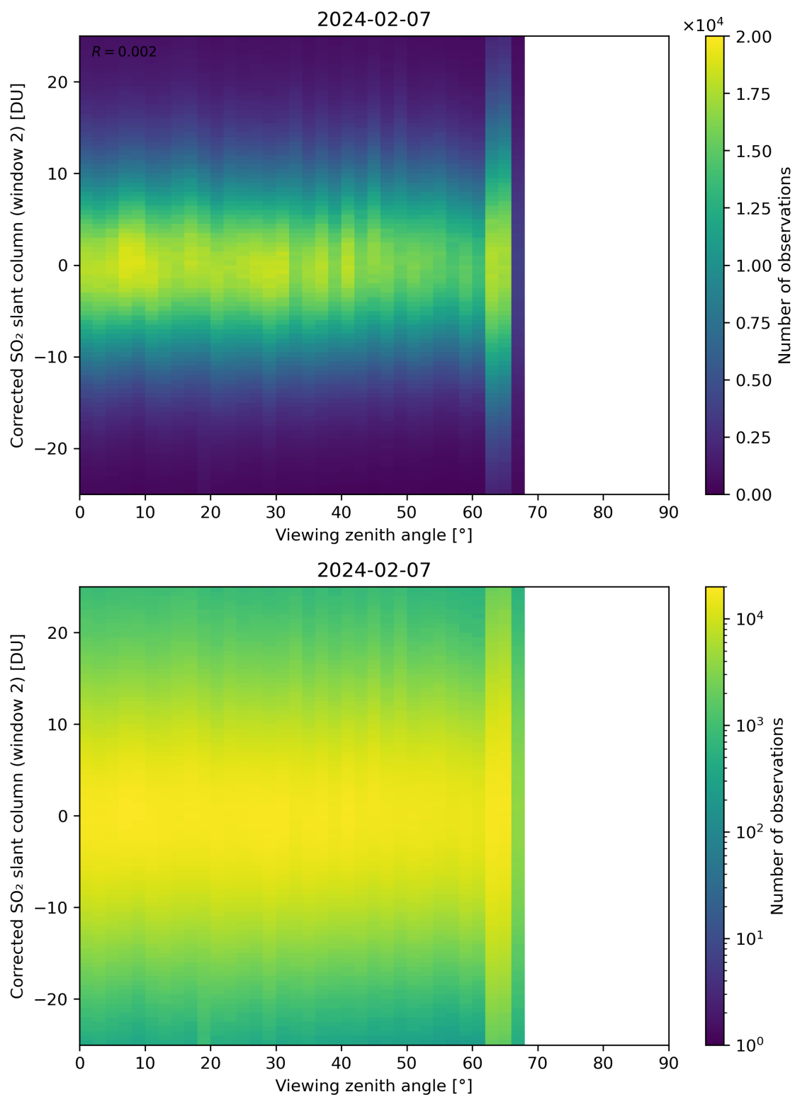
Figure 318: Scatter density plot of “Viewing zenith angle” against “Corrected SO 2 slant column (window 2)” for 2024-02-06 to 2024-02-08.
