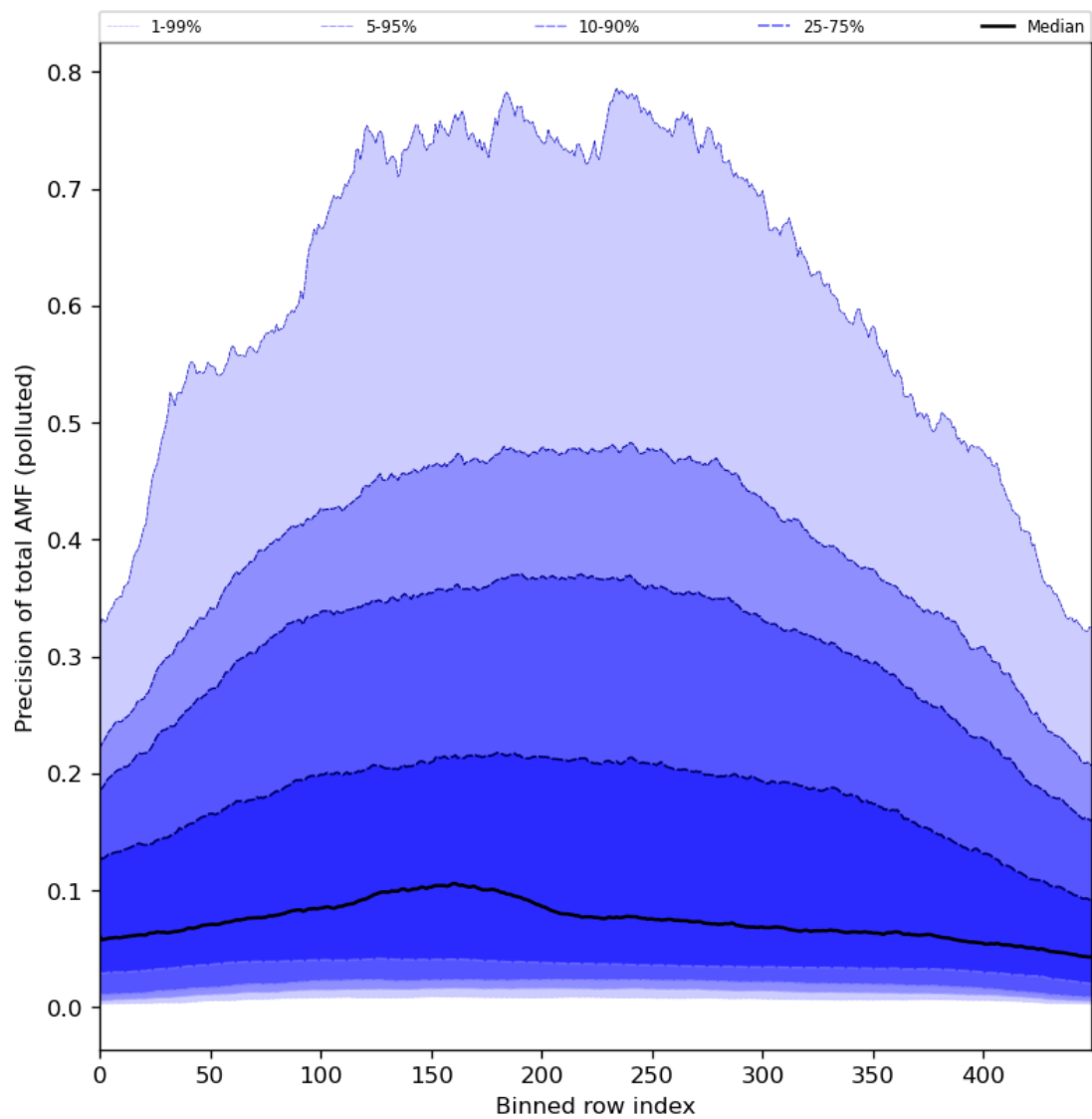
Figure 95: Along track statistics of “Precision of total AMF (polluted)” for 2024-02-06 to 2024-02-08
