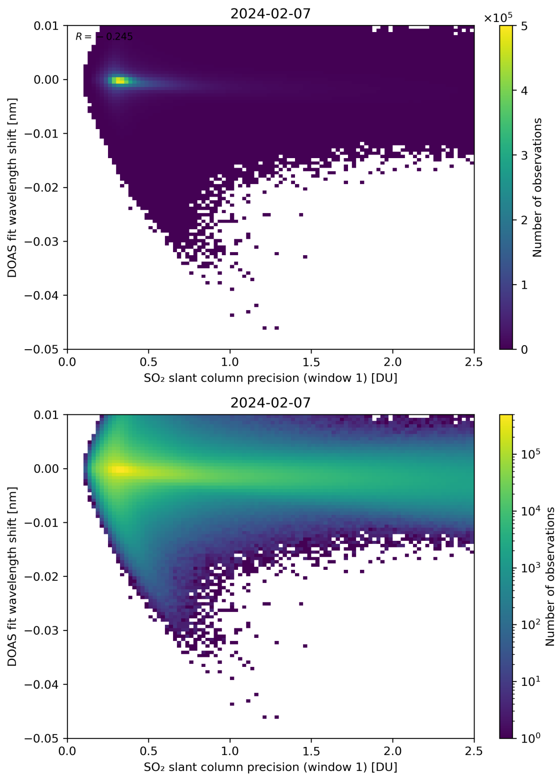
Figure 221: Scatter density plot of “SO 2 slant column precision (window 1)” against “DOAS fit wavelength shift” for 2024-02-06 to 2024-02-08.
