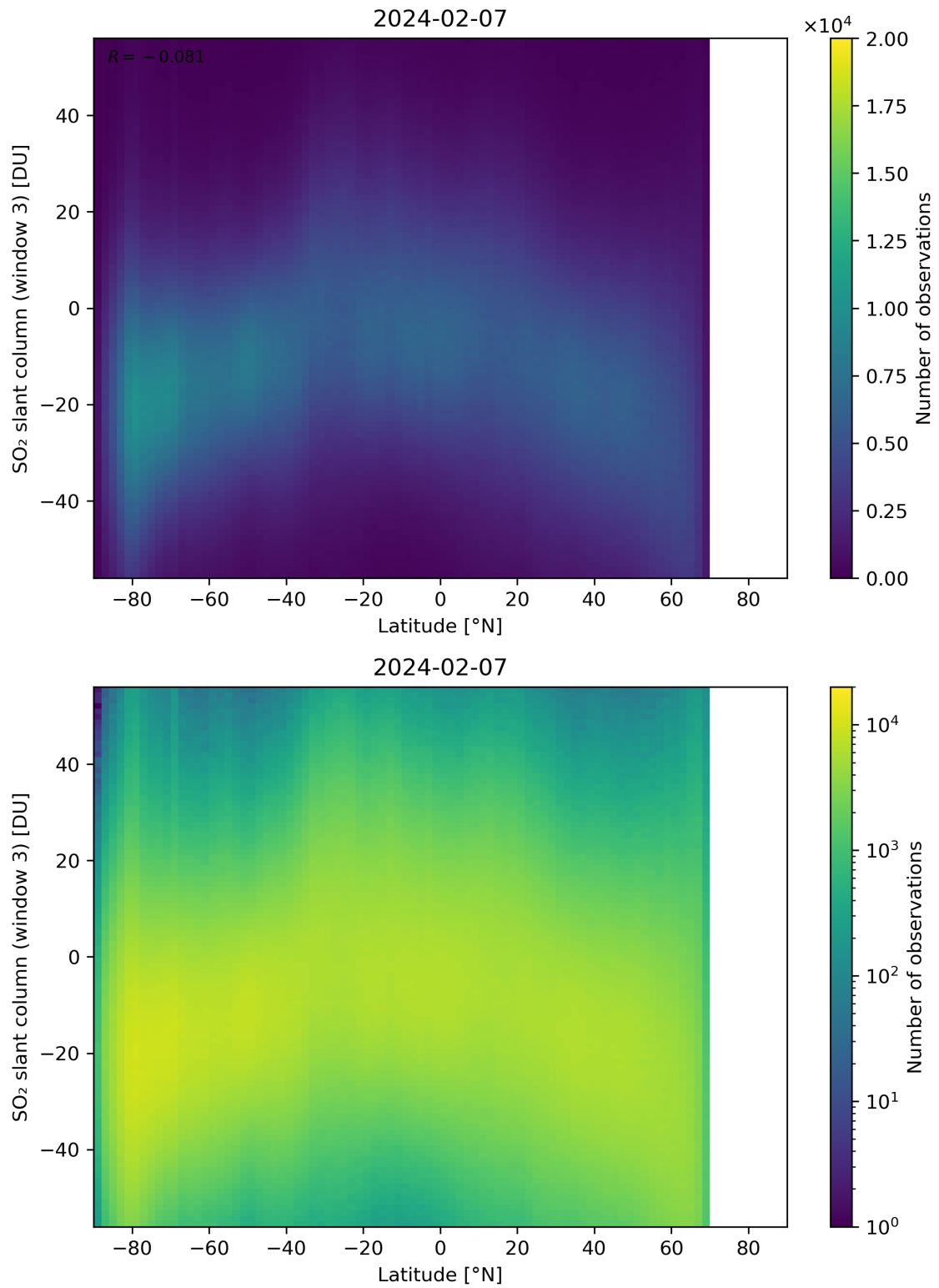
Figure 152: Scatter density plot of “Latitude” against “SO 2 slant column (window 3)” for 2024-02-06 to 2024-02-08.
