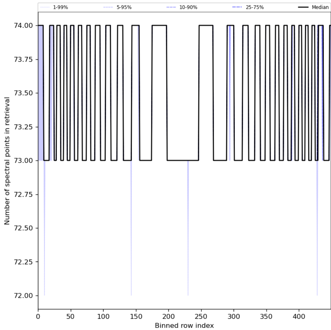
Figure 97: Along track statistics of “Number of spectral points in retrieval” for 2024-02-06 to 2024-02-08
