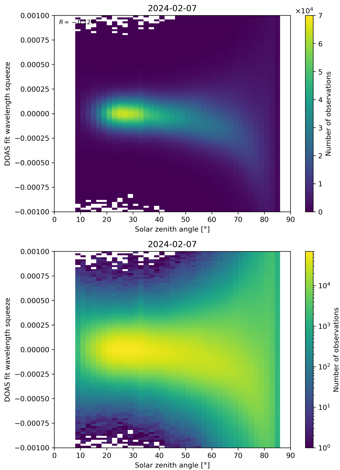
Figure 162: Scatter density plot of “Solar zenith angle” against “DOAS fit wavelength squeeze” for 2024-02-06 to 2024-02-08.
