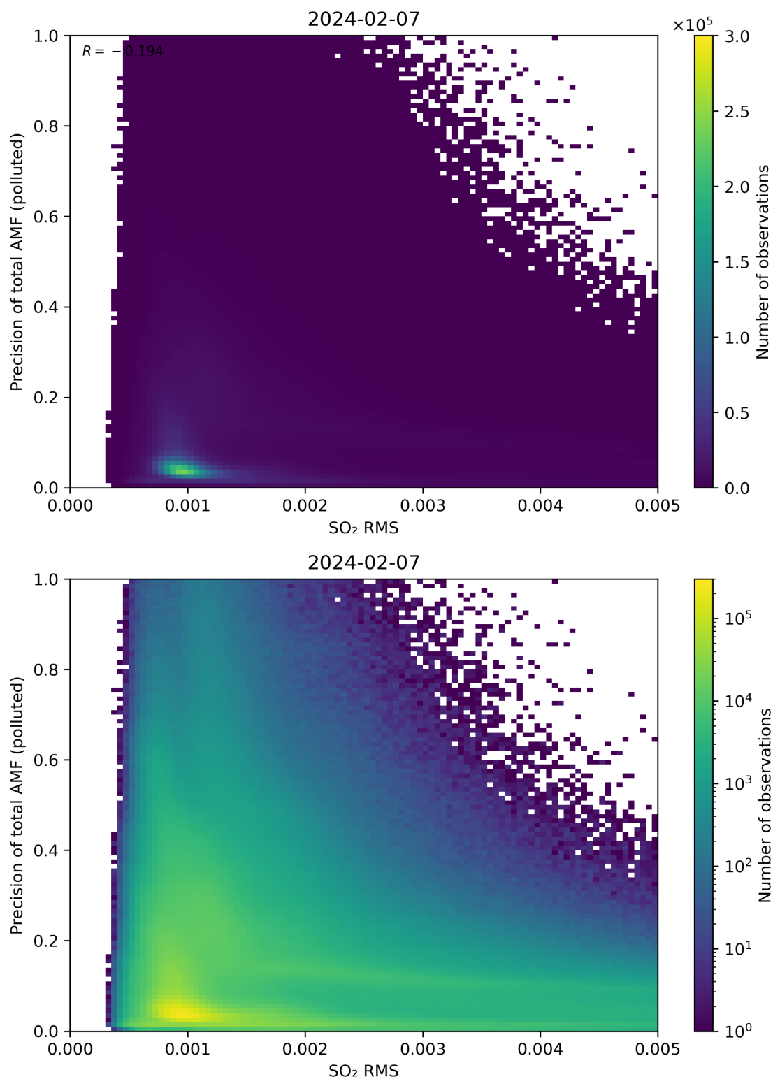
Figure 138: Scatter density plot of “SO 2 RMS” against “Precision of total AMF (polluted)” for 2024-02-06 to 2024-02-08.
