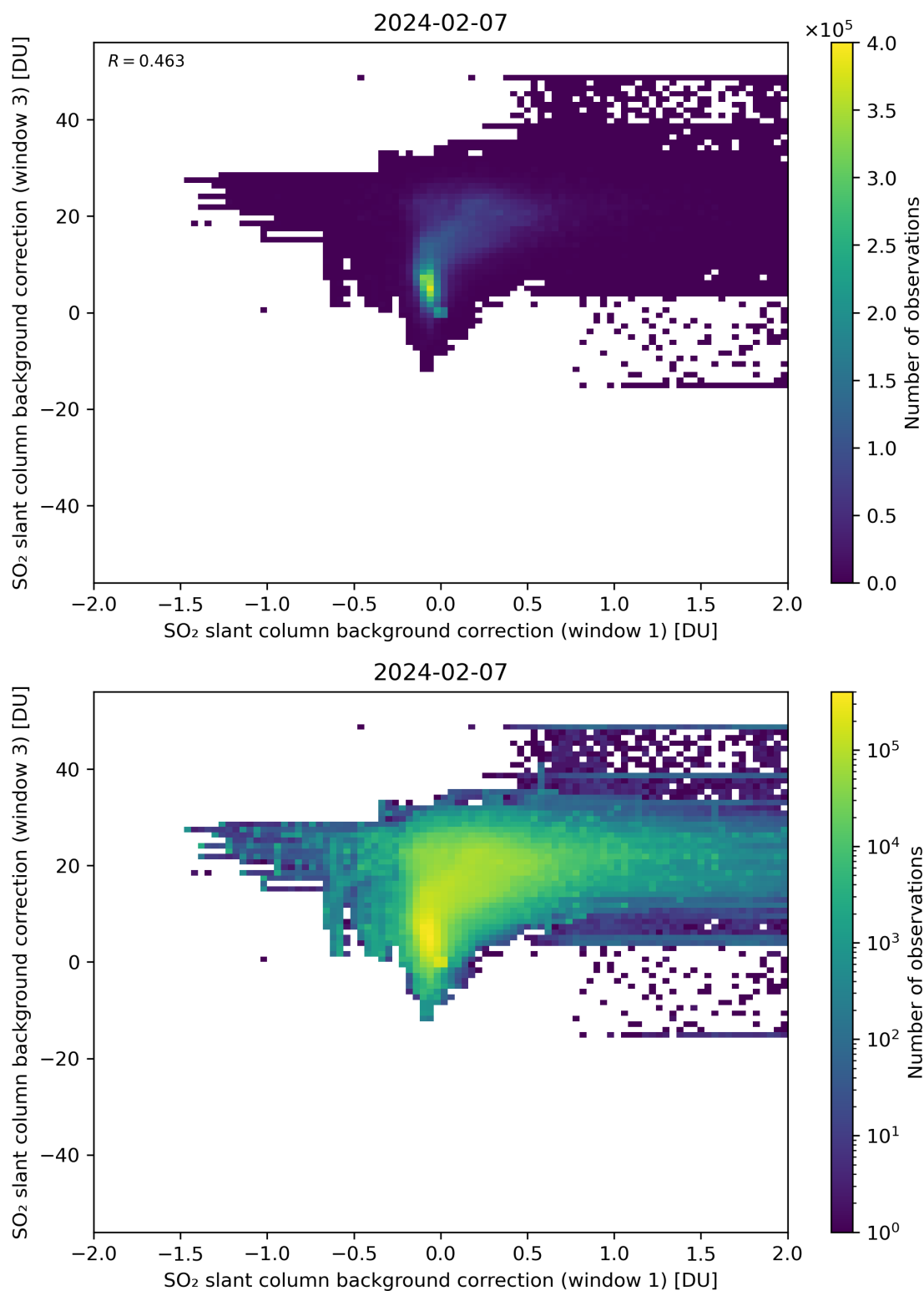
Figure 99: Scatter density plot of “SO 2 slant column background correction (window 1)” against “SO 2 slant column background correction (window 3)” for 2024-02-06 to 2024-02-08.
