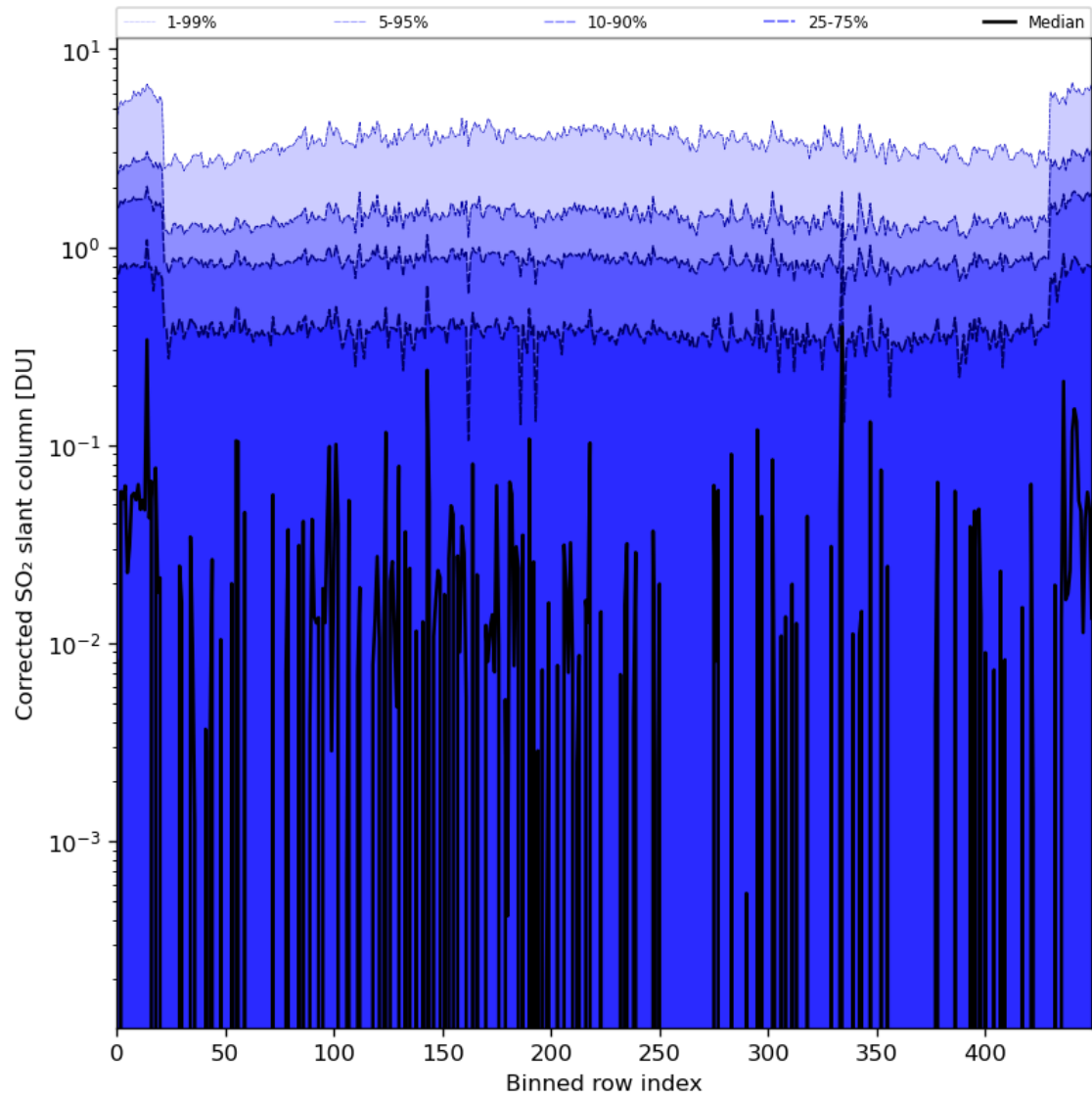
Figure 78: Along track statistics of “Corrected SO 2 slant column” for 2024-02-06 to 2024-02-08
