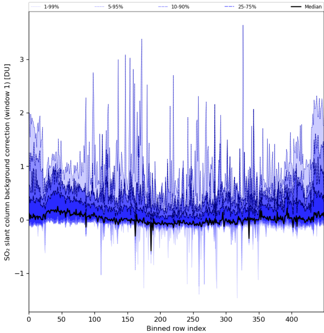
Figure 82: Along track statistics of “SO 2 slant column background correction (window 1)” for 2024-02-06 to 2024-02-08
