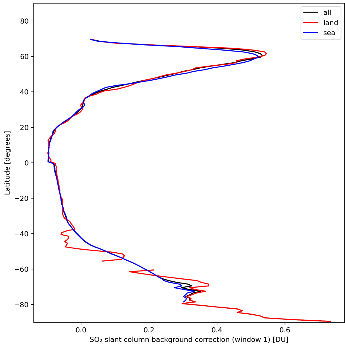
Figure 36: Zonal average of “SO 2 slant column background correction (window 1)” for 2024-02-06 to 2024-02-08.
