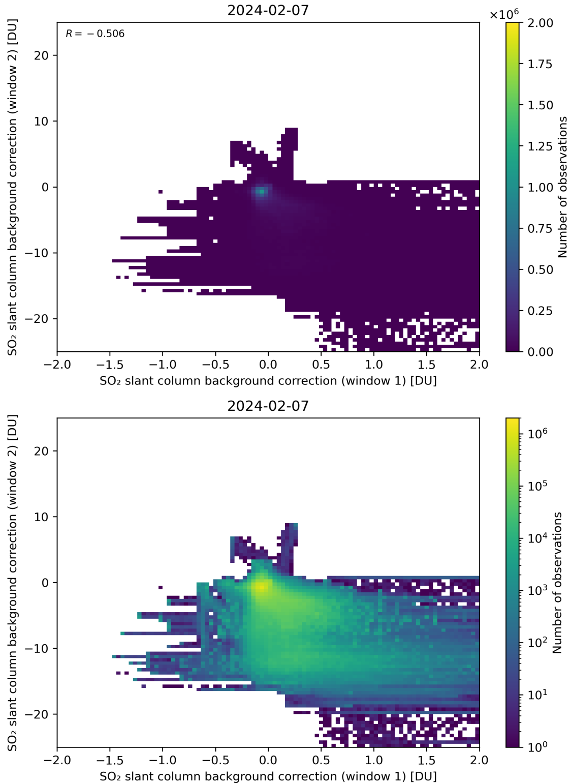
Figure 98: Scatter density plot of “SO 2 slant column background correction (window 1)” against “SO 2 slant column background correction (window 2)” for 2024-02-06 to 2024-02-08.
