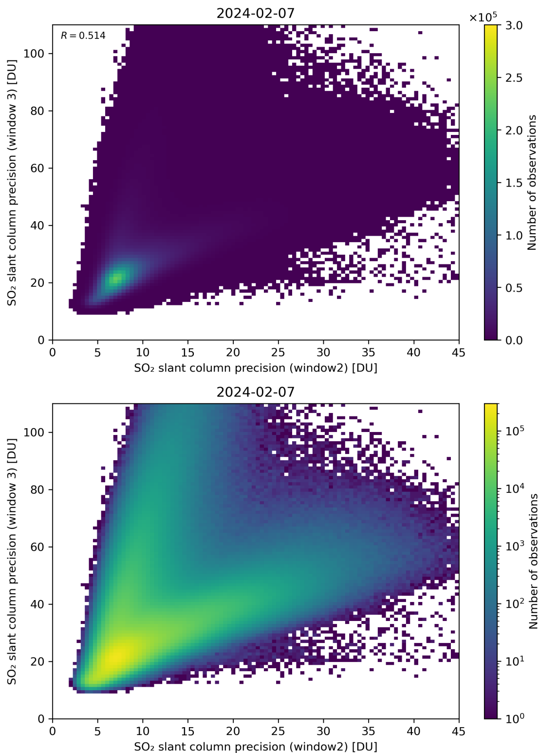
Figure 250: Scatter density plot of “SO 2 slant column precision (window2)” against “SO 2 slant column precision (window 3)” for 2024-02-06 to 2024-02-08.
