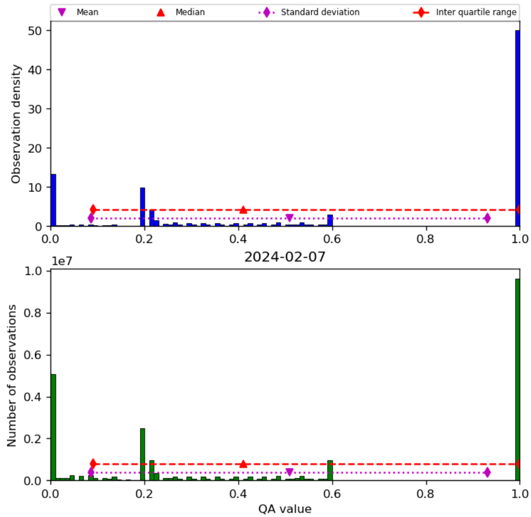
Figure 52: Histogram of “QA value” for 2024-02-06 to 2024-02-08
