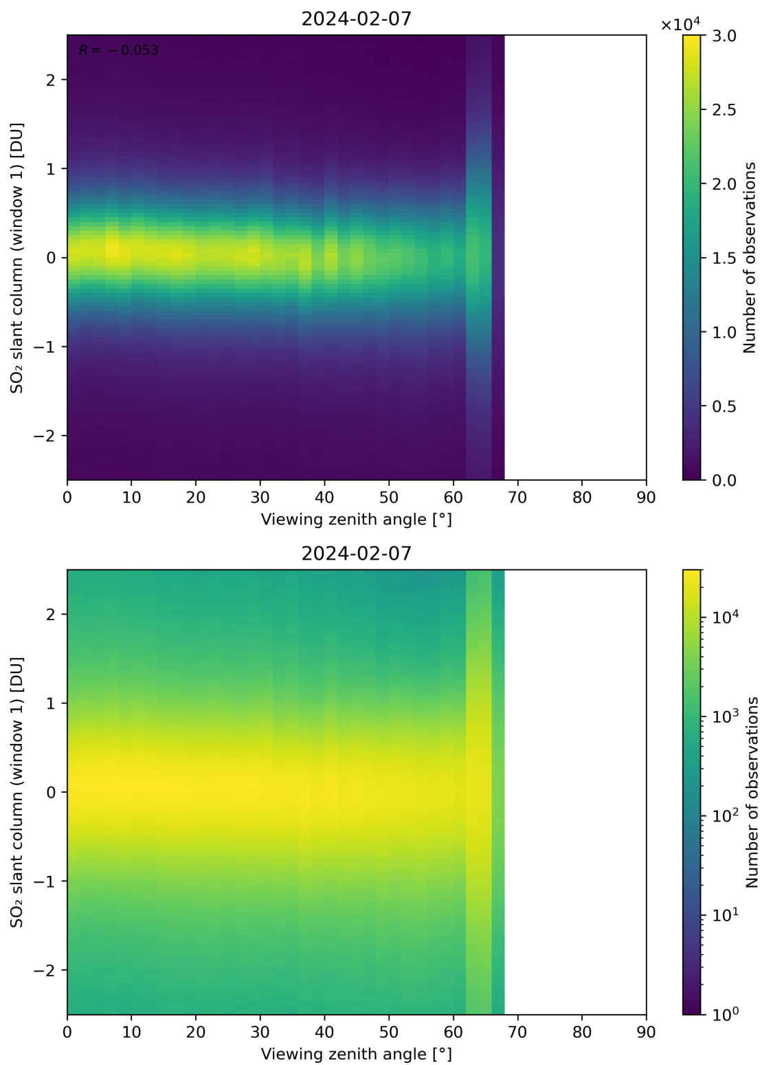
Figure 320: Scatter density plot of “Viewing zenith angle” against “SO 2 slant column (window 1)” for 2024-02-06 to 2024-02-08.
