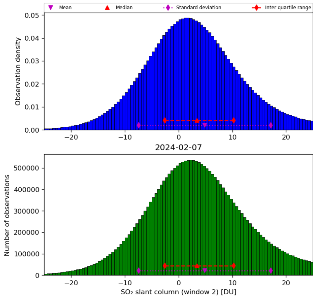
Figure 60: Histogram of “SO 2 slant column (window 2)” for 2024-02-06 to 2024-02-08
