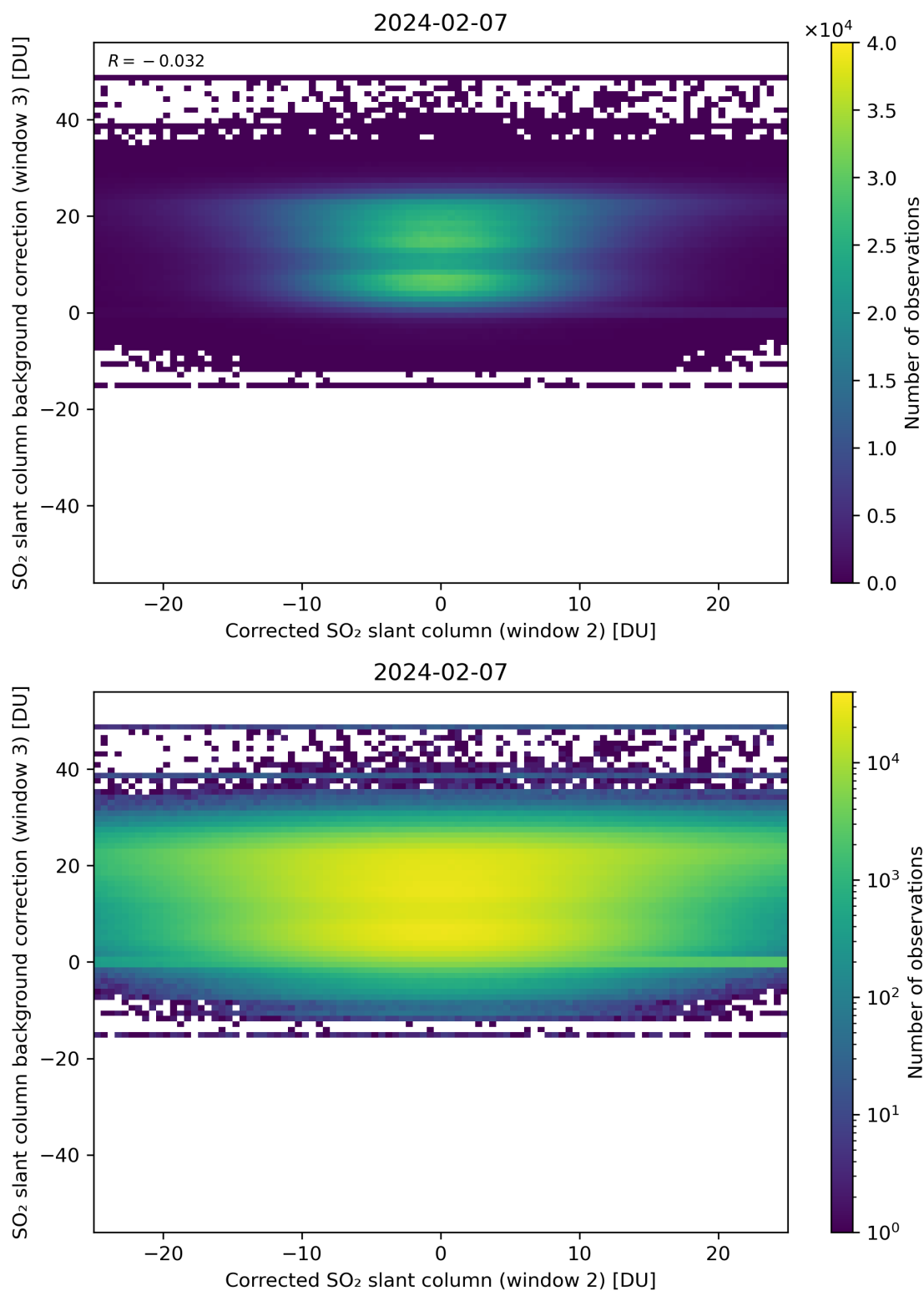
Figure 195: Scatter density plot of “Corrected SO 2 slant column (window 2)” against “SO 2 slant column background correction (window 3)” for 2024-02-06 to 2024-02-08.
