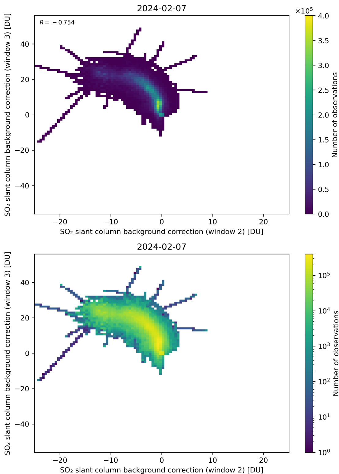
Figure 111: Scatter density plot of “SO 2 slant column background correction (window 2)” against “SO 2 slant column background correction (window 3)” for 2024-02-06 to 2024-02-08.
