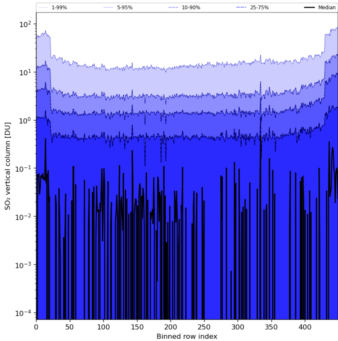
Figure 76: Along track statistics of “SO 2 vertical column” for 2024-02-06 to 2024-02-08
