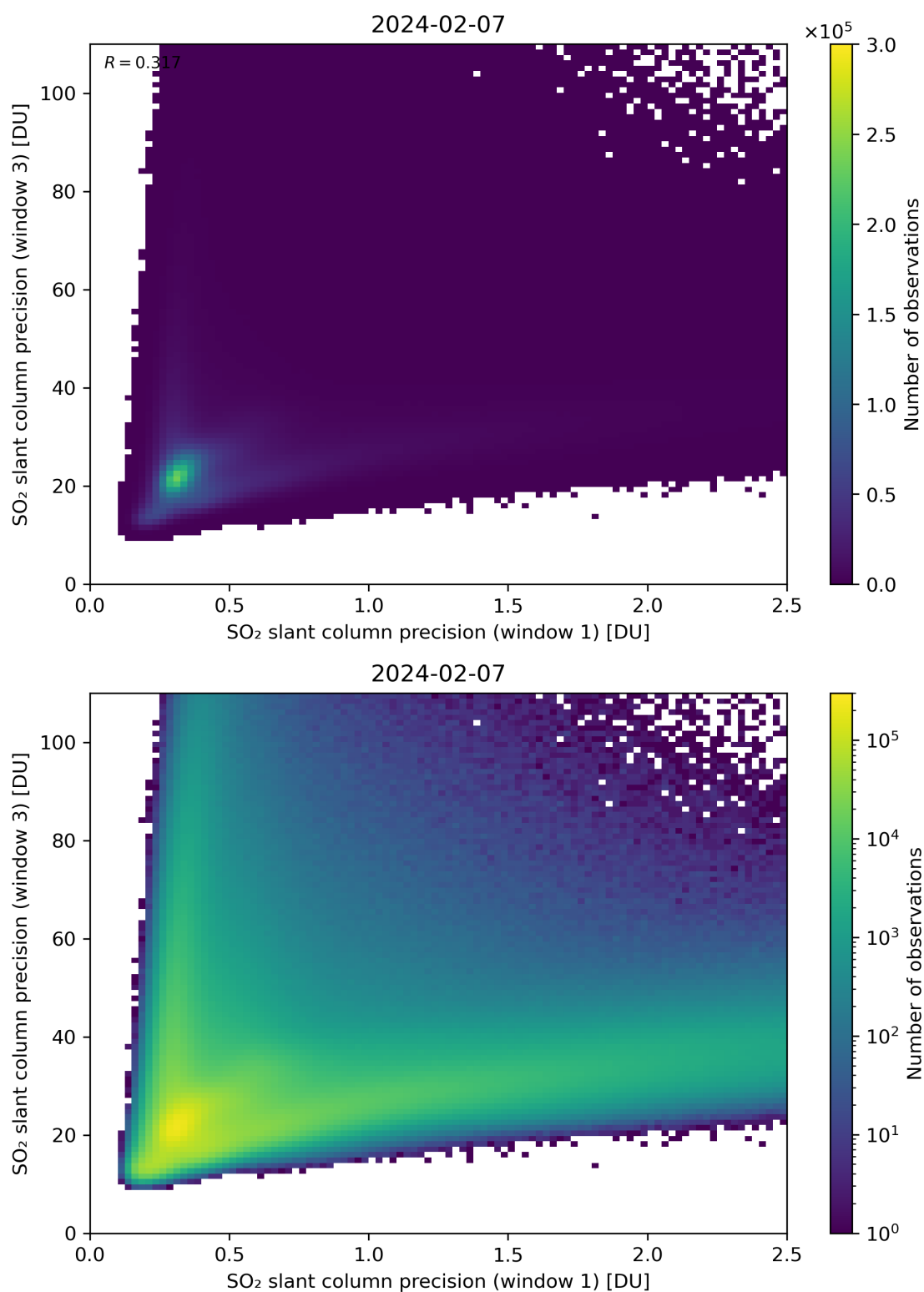
Figure 229: Scatter density plot of “SO 2 slant column precision (window 1)” against “SO 2 slant column precision (window 3)” for 2024-02-06 to 2024-02-08.
