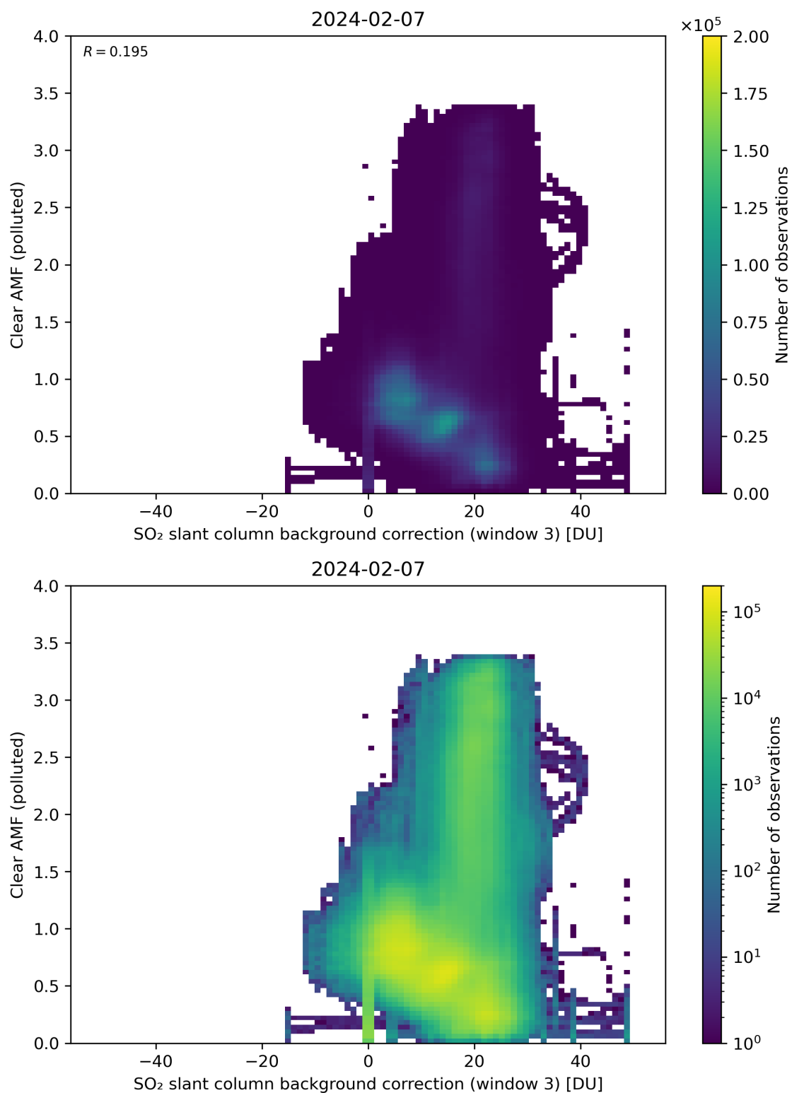
Figure 124: Scatter density plot of “SO 2 slant column background correction (window 3)” against “Clear AMF (polluted)” for 2024-02-06 to 2024-02-08.
