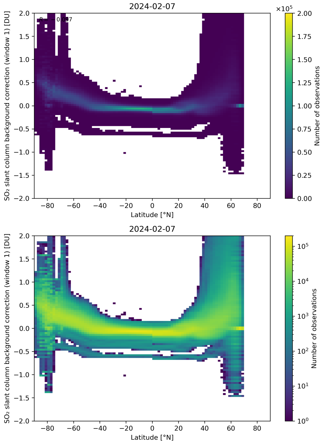
Figure 139: Scatter density plot of “Latitude” against “SO 2 slant column background correction (window 1)” for 2024-02-06 to 2024-02-08.
