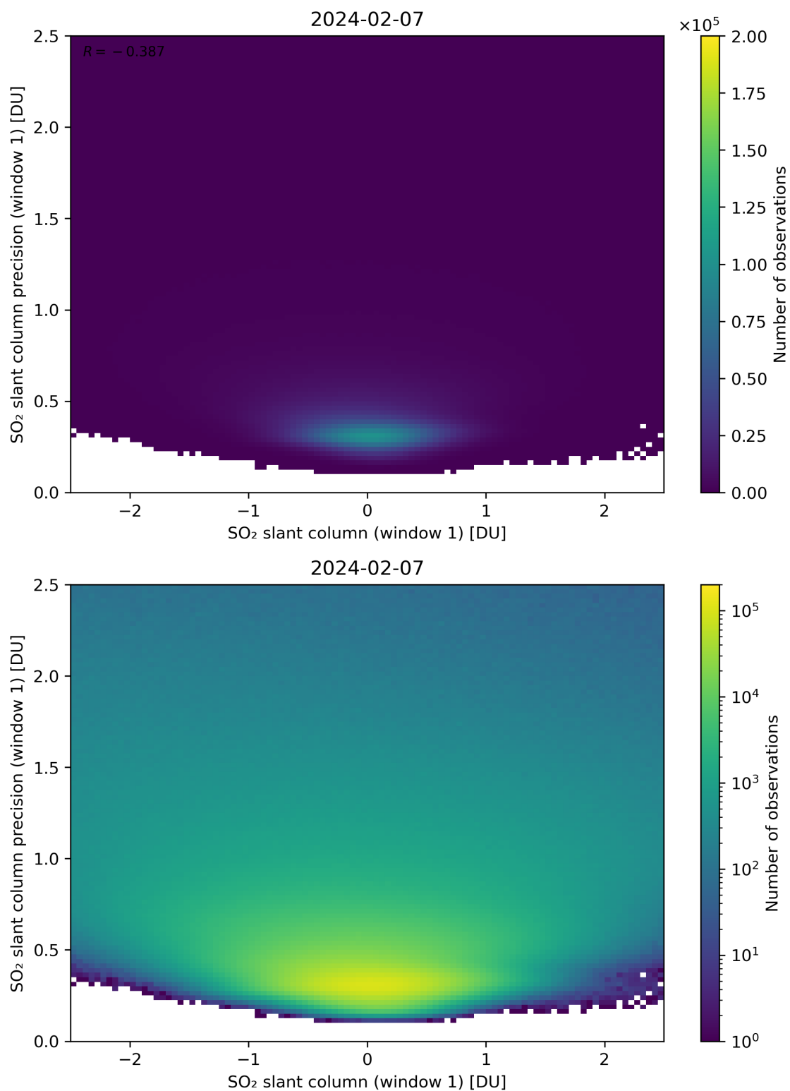
Figure 235: Scatter density plot of “SO 2 slant column (window 1)” against “SO 2 slant column precision (window 1)” for 2024-02-06 to 2024-02-08.
