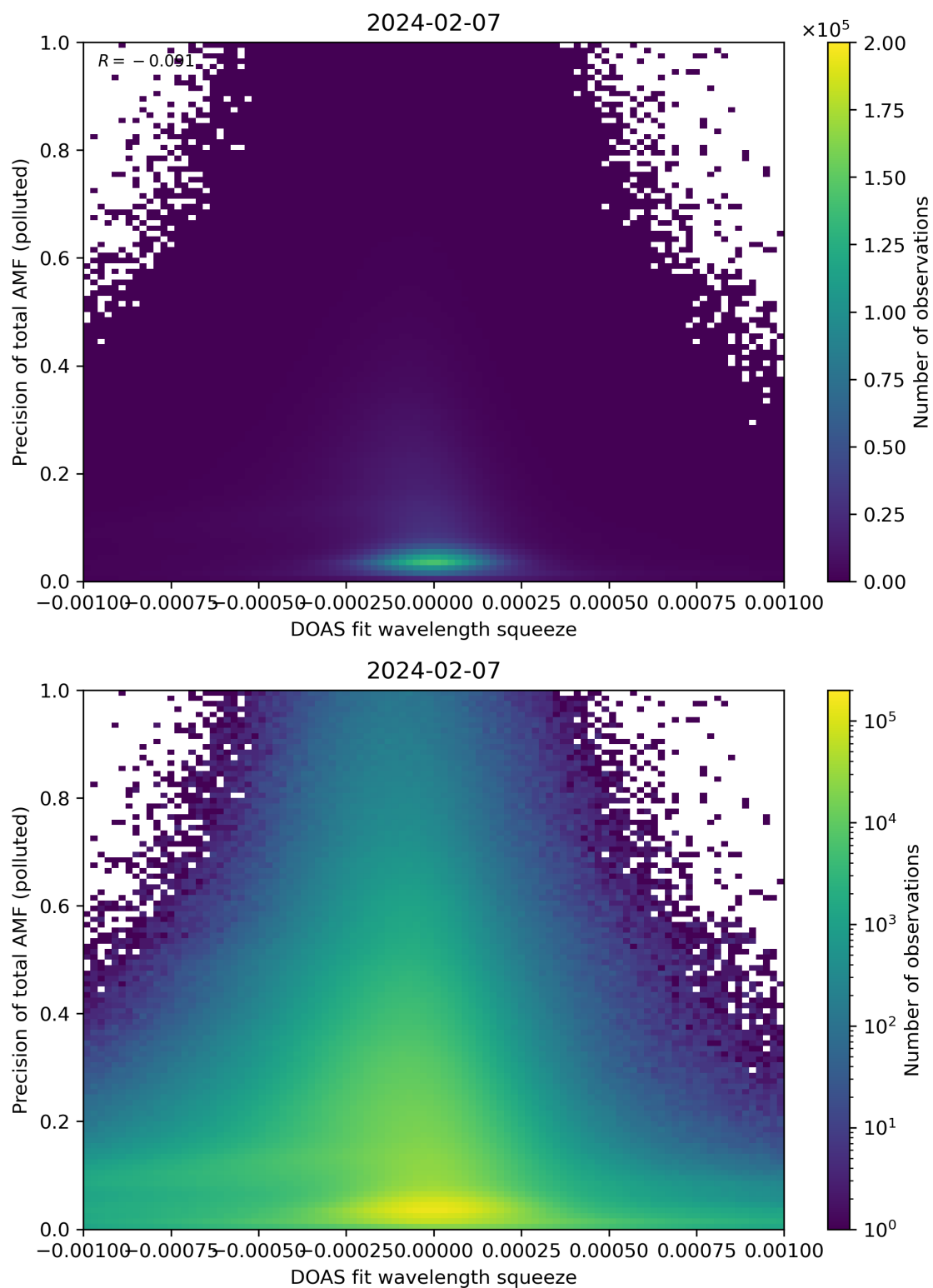
Figure 135: Scatter density plot of “DOAS fit wavelength squeeze” against “Precision of total AMF (polluted)” for 2024-02-06 to 2024-02-08.
