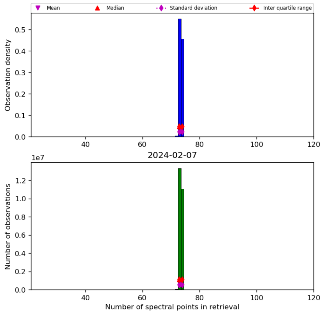
Figure 74: Histogram of “Number of spectral points in retrieval” for 2024-02-06 to 2024-02-08
