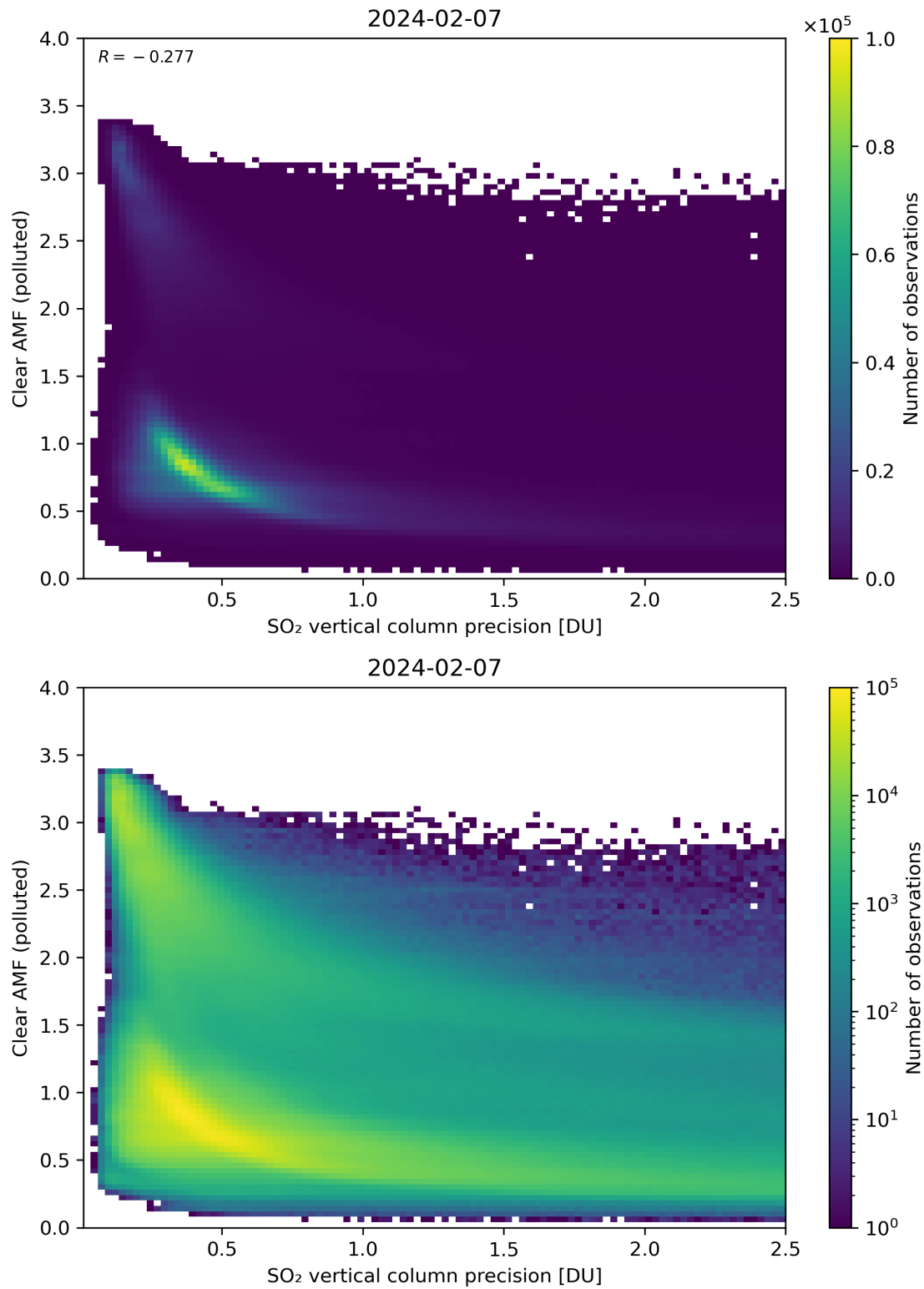
Figure 285: Scatter density plot of “SO 2 vertical column precision” against “Clear AMF (polluted)” for 2024-02-06 to 2024-02-08.
