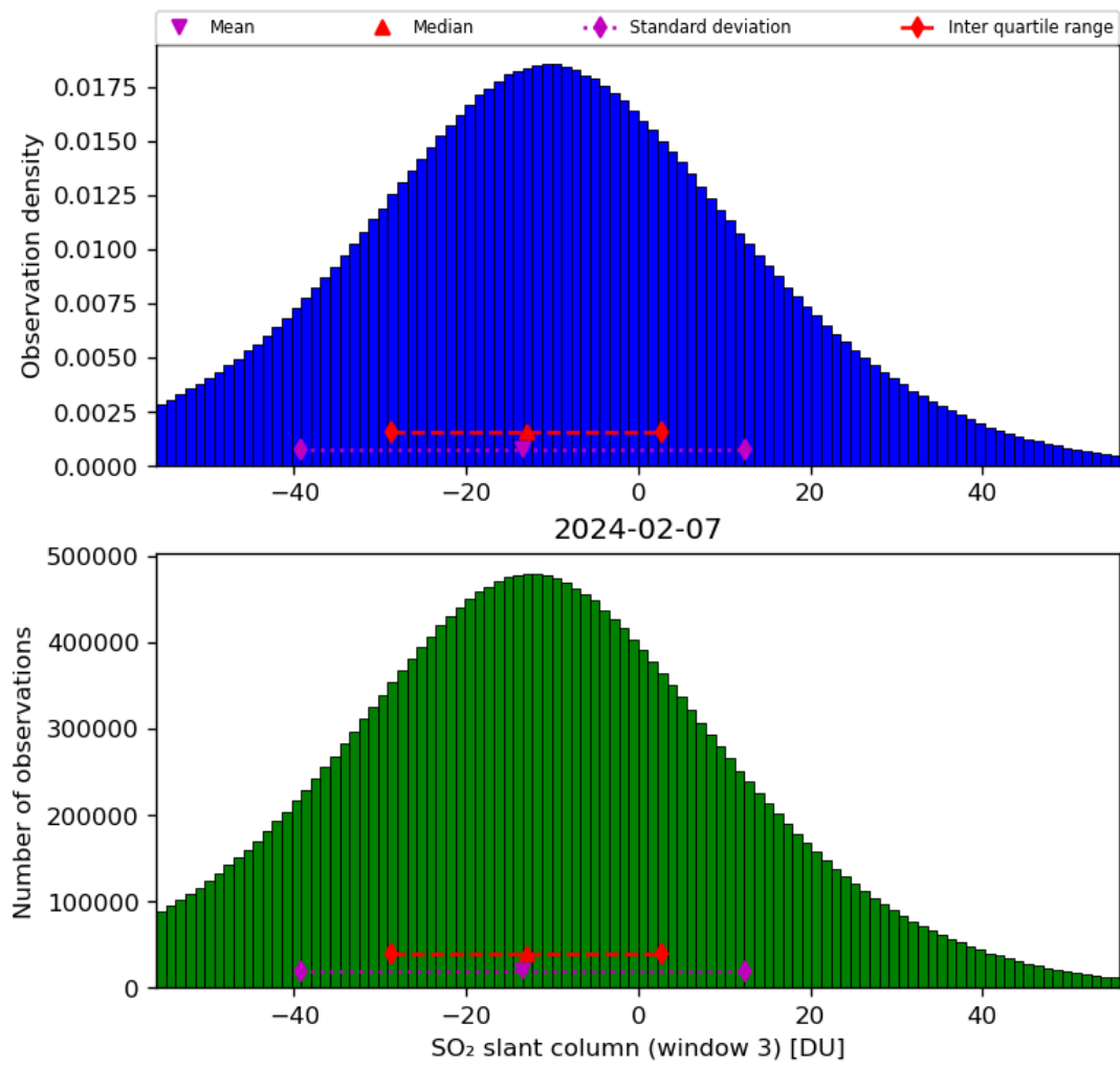
Figure 64: Histogram of “SO 2 slant column (window 3)” for 2024-02-06 to 2024-02-08
