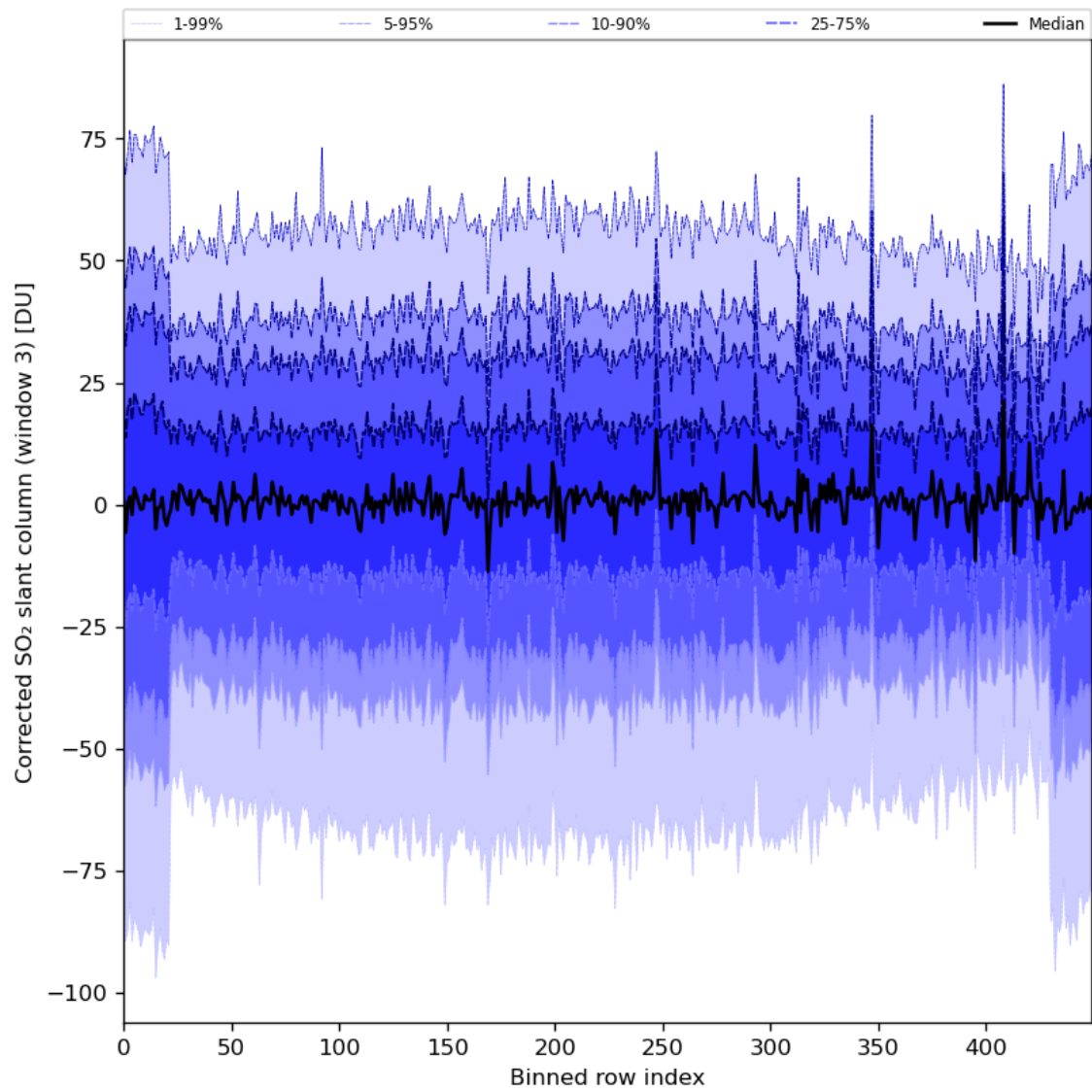
Figure 89: Along track statistics of “Corrected SO 2 slant column (window 3)” for 2024-02-06 to 2024-02-08
