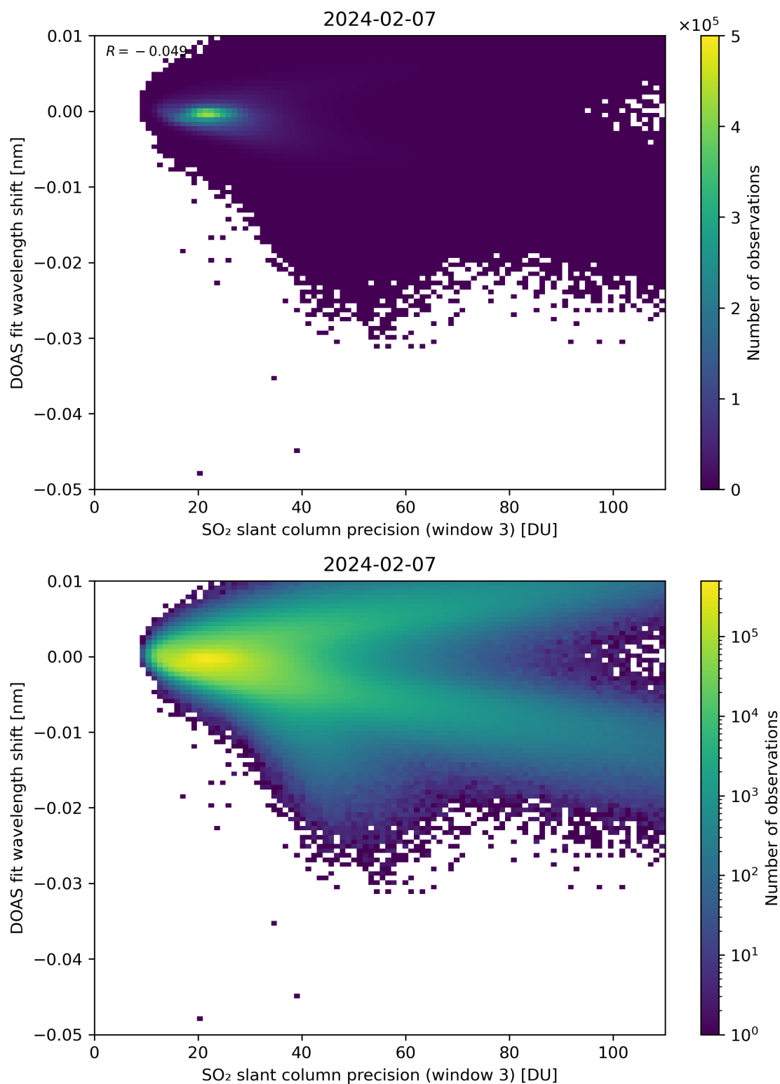
Figure 258: Scatter density plot of “SO 2 slant column precision (window 3)” against “DOAS fit wavelength shift” for 2024-02-06 to 2024-02-08.
