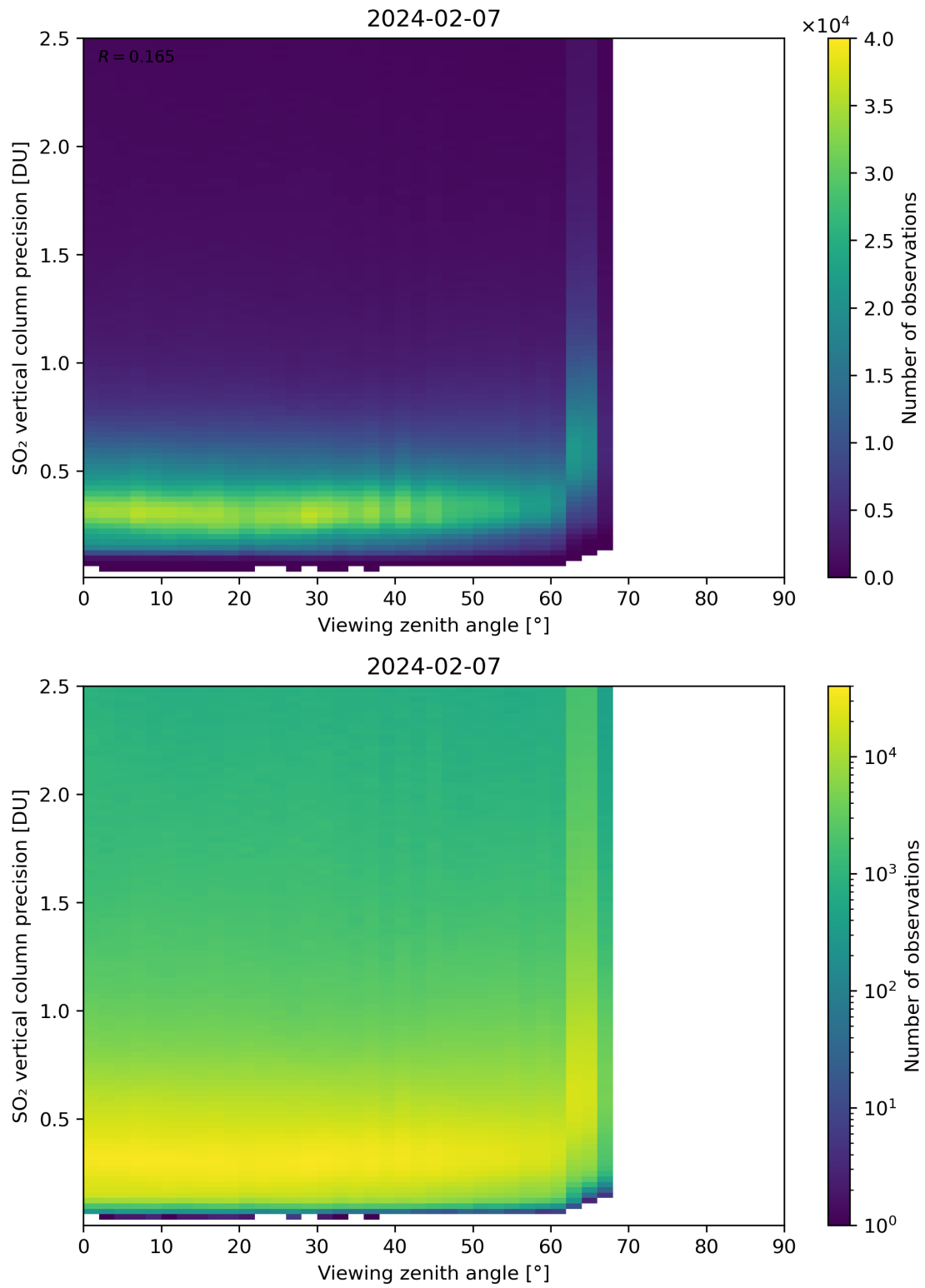
Figure 328: Scatter density plot of “Viewing zenith angle” against “SO 2 vertical column precision” for 2024-02-06 to 2024-02-08.
