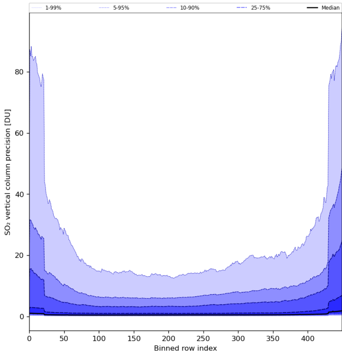
Figure 77: Along track statistics of “SO 2 vertical column precision” for 2024-02-06 to 2024-02-08
