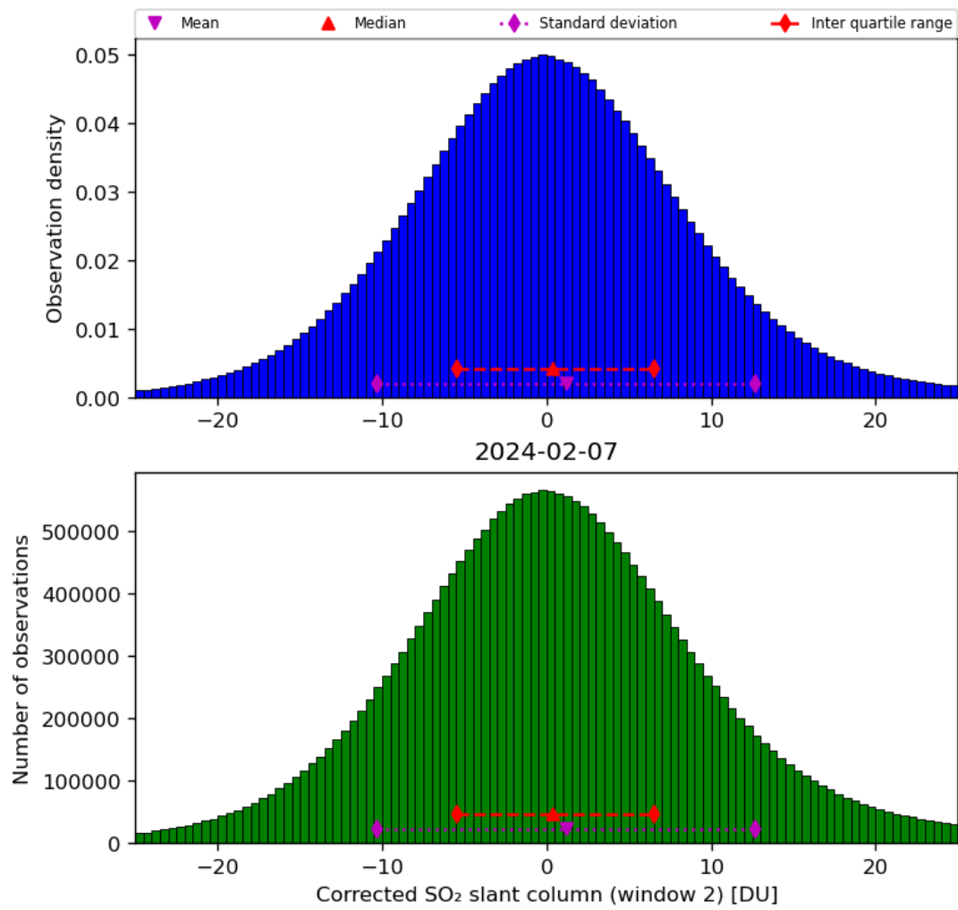
Figure 62: Histogram of “Corrected SO 2 slant column (window 2)” for 2024-02-06 to 2024-02-08
