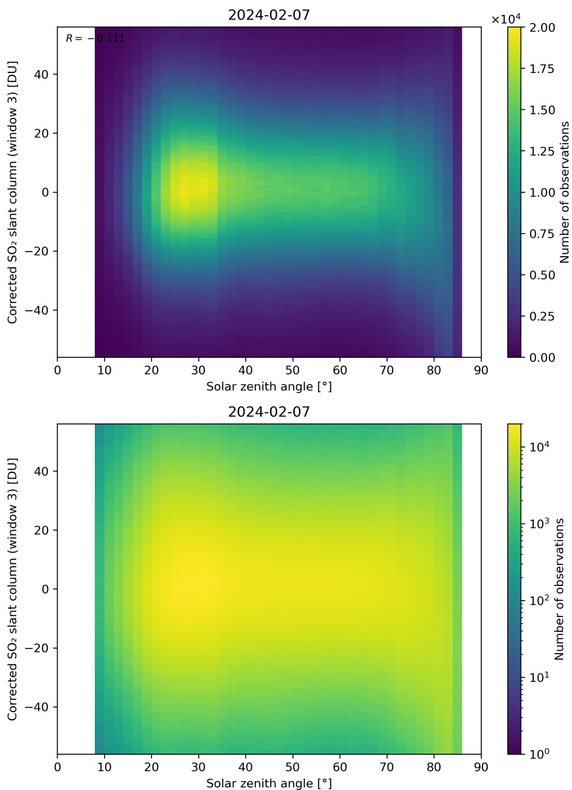
Figure 168: Scatter density plot of “Solar zenith angle” against “Corrected SO 2 slant column (window 3)” for 2024-02-06 to 2024-02-08.
