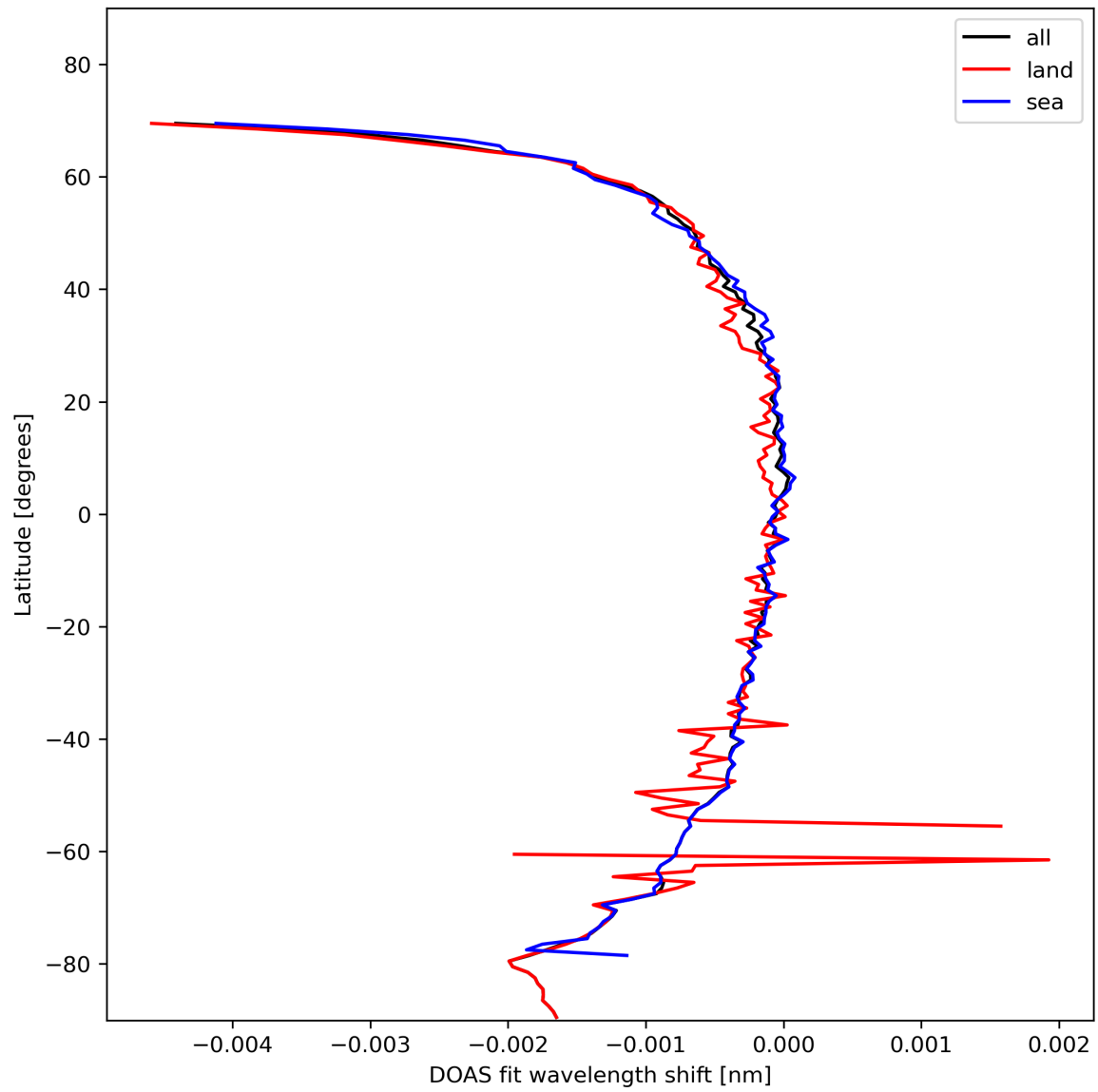
Figure 45: Zonal average of “DOAS fit wavelength shift” for 2024-02-06 to 2024-02-08.
