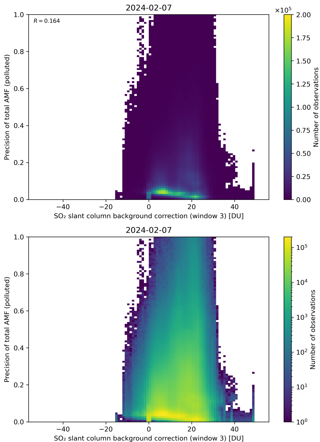
Figure 126: Scatter density plot of “SO 2 slant column background correction (window 3)” against “Precision of total AMF (polluted)” for 2024-02-06 to 2024-02-08.
