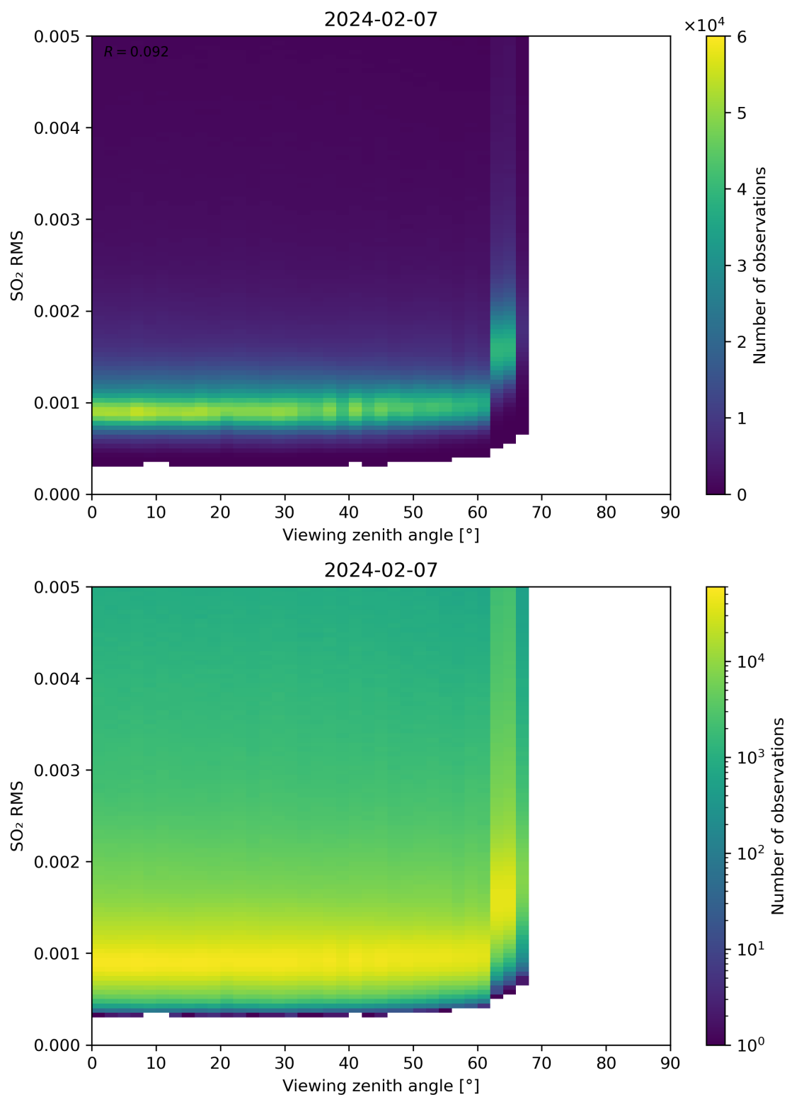
Figure 313: Scatter density plot of “Viewing zenith angle” against “SO 2 RMS” for 2024-02-06 to 2024-02-08.
