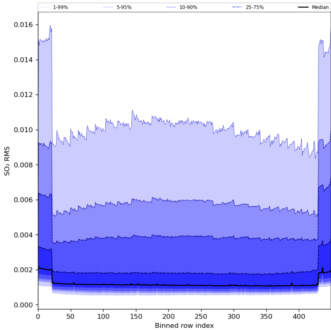
Figure 93: Along track statistics of “SO 2 RMS” for 2024-02-06 to 2024-02-08
