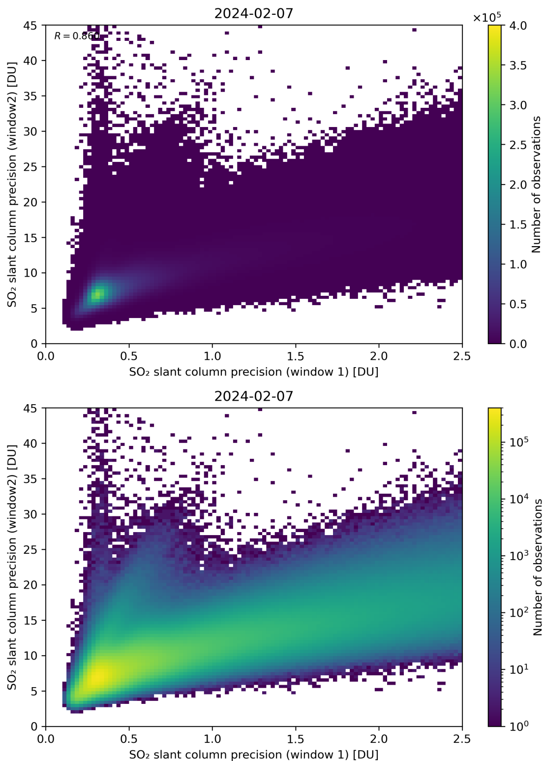
Figure 227: Scatter density plot of “SO 2 slant column precision (window 1)” against “SO 2 slant column precision (window2)” for 2024-02-06 to 2024-02-08.
