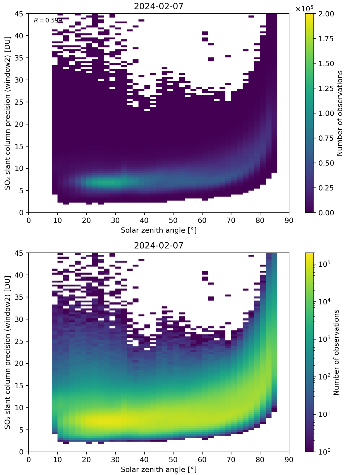
Figure 171: Scatter density plot of “Solar zenith angle” against “SO 2 slant column precision (window2)” for 2024-02-06 to 2024-02-08.
