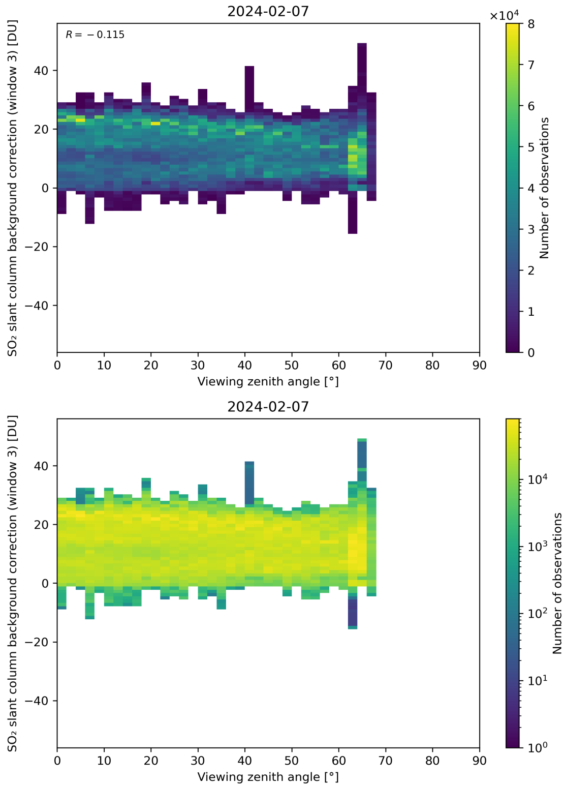
Figure 310: Scatter density plot of “Viewing zenith angle” against “SO 2 slant column background correction (window 3)” for 2024-02-06 to 2024-02-08.
