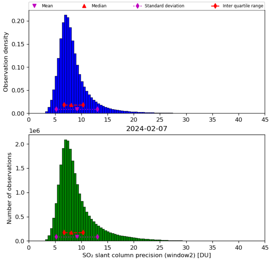
Figure 61: Histogram of “SO 2 slant column precision (window2)” for 2024-02-06 to 2024-02-08
