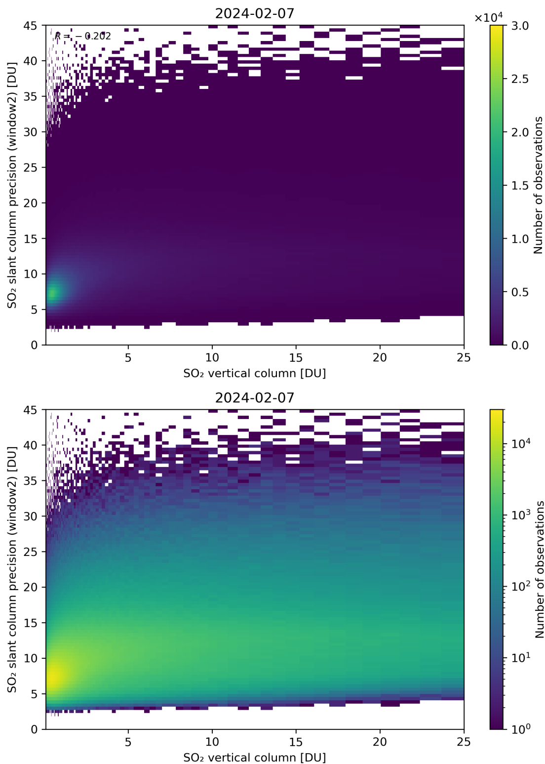
Figure 302: Scatter density plot of “SO 2 vertical column” against “SO 2 slant column precision (window2)” for 2024-02-06 to 2024-02-08.
