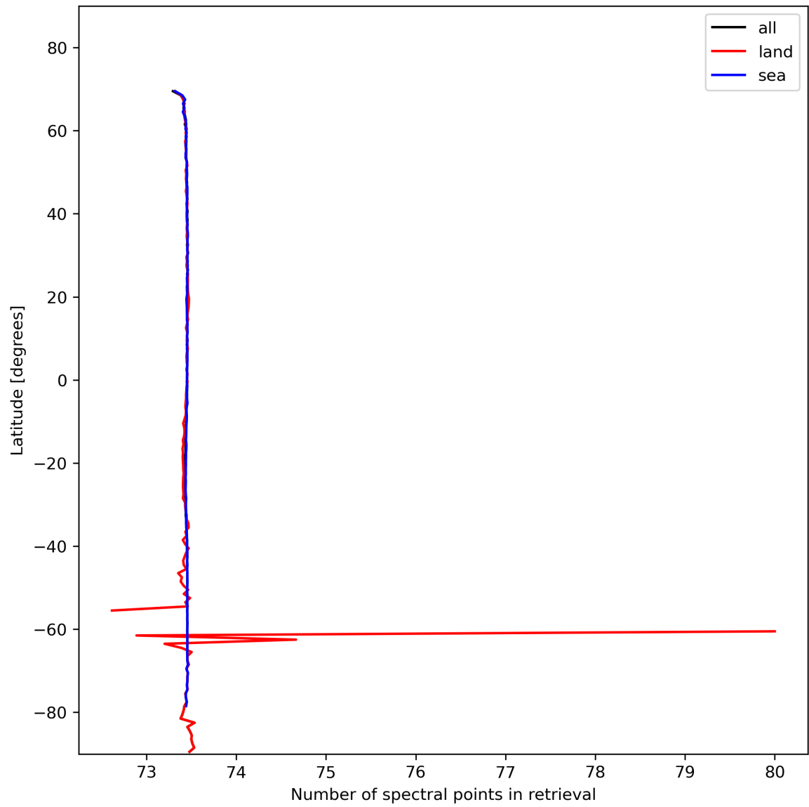
Figure 51: Zonal average of “Number of spectral points in retrieval” for 2024-02-06 to 2024-02-08.
