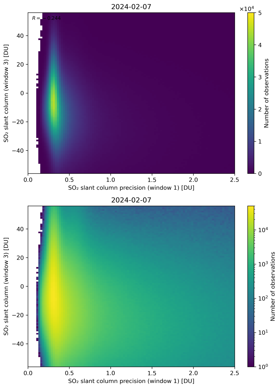
Figure 228: Scatter density plot of “SO 2 slant column precision (window 1)” against “SO 2 slant column (window 3)” for 2024-02-06 to 2024-02-08.
