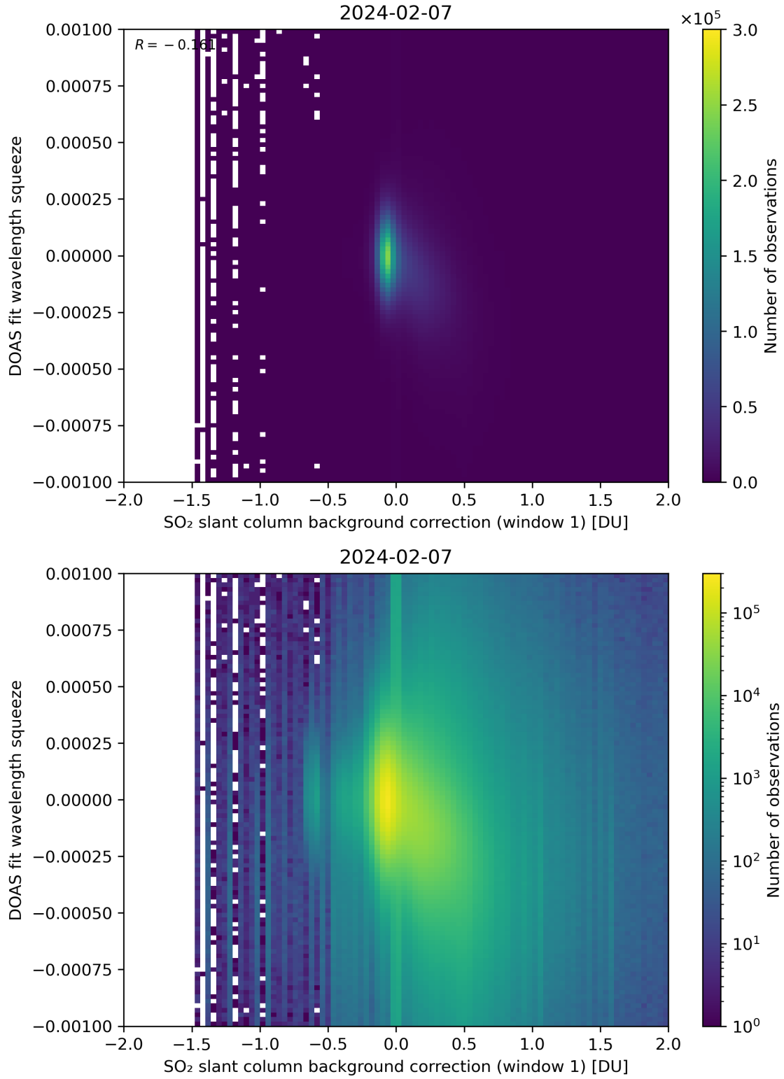
Figure 101: Scatter density plot of “SO 2 slant column background correction (window 1)” against “DOAS fit wavelength squeeze” for 2024-02-06 to 2024-02-08.
