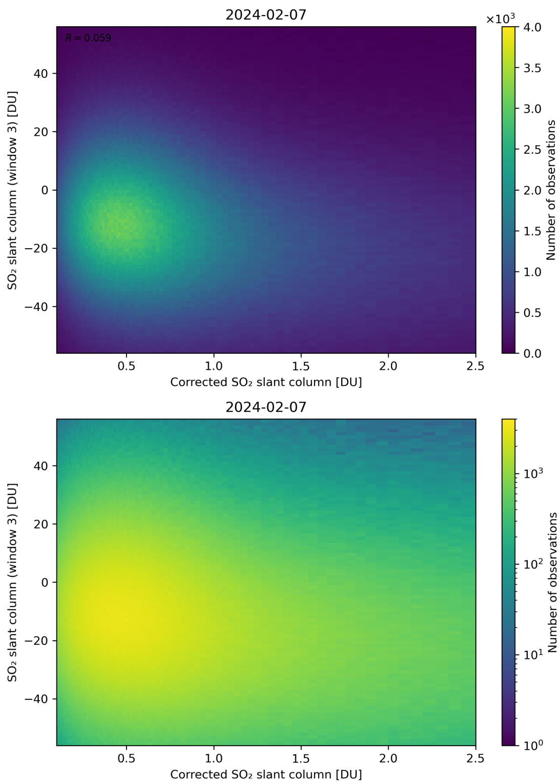
Figure 190: Scatter density plot of “Corrected SO 2 slant column” against “SO 2 slant column (window 3)” for 2024-02-06 to 2024-02-08.
