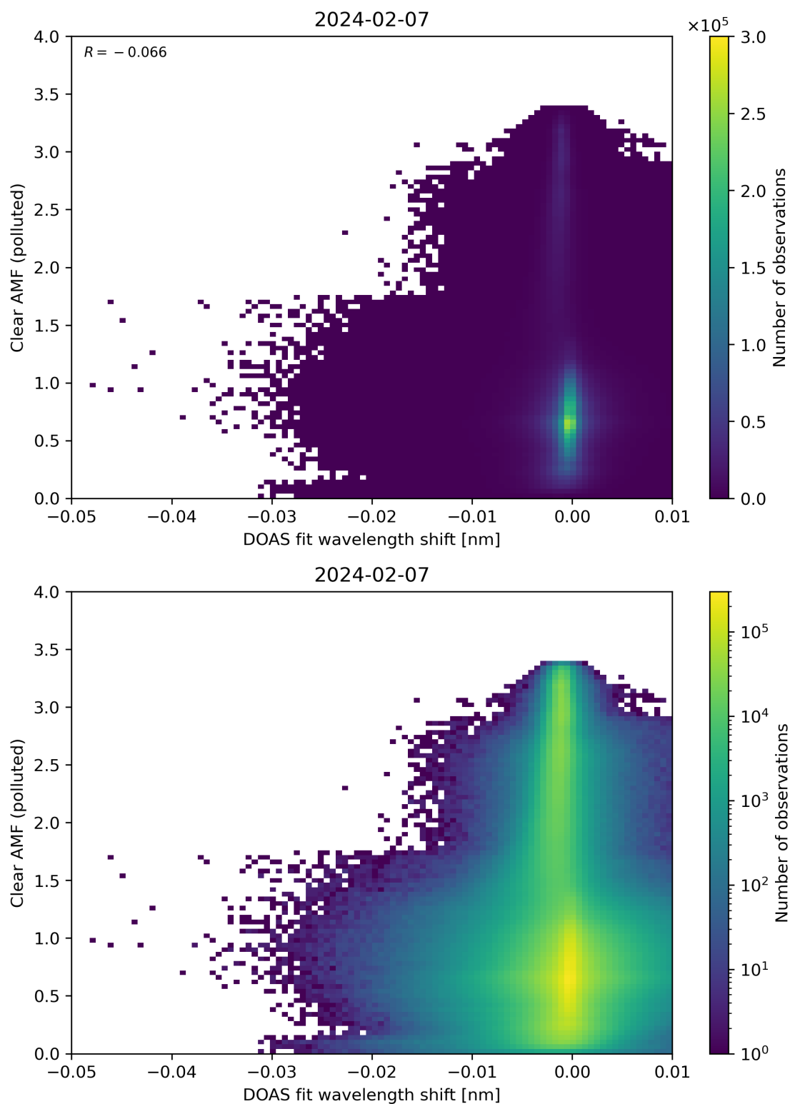
Figure 129: Scatter density plot of “DOAS fit wavelength shift” against “Clear AMF (polluted)” for 2024-02-06 to 2024-02-08.
