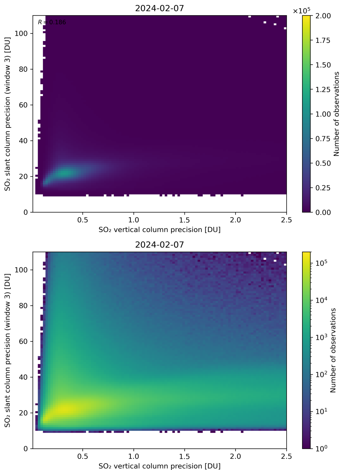
Figure 293: Scatter density plot of “SO 2 vertical column precision” against “SO 2 slant column precision (window 3)” for 2024-02-06 to 2024-02-08.
