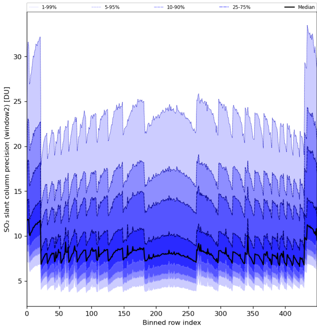
Figure 84: Along track statistics of “SO 2 slant column precision (window2)” for 2024-02-06 to 2024-02-08
