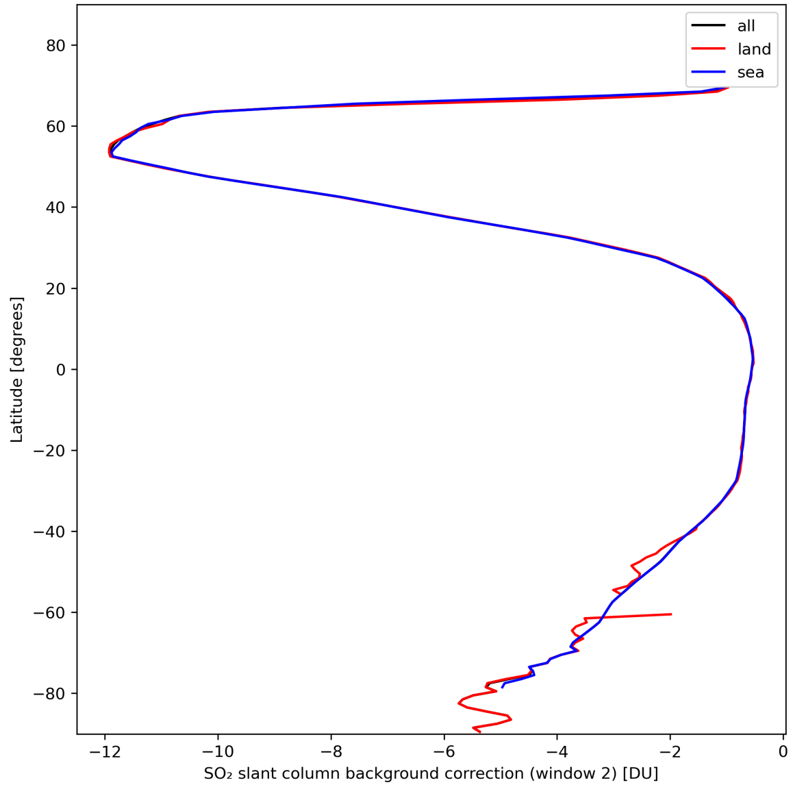
Figure 40: Zonal average of “SO 2 slant column background correction (window 2)” for 2024-02-06 to 2024-02-08.
