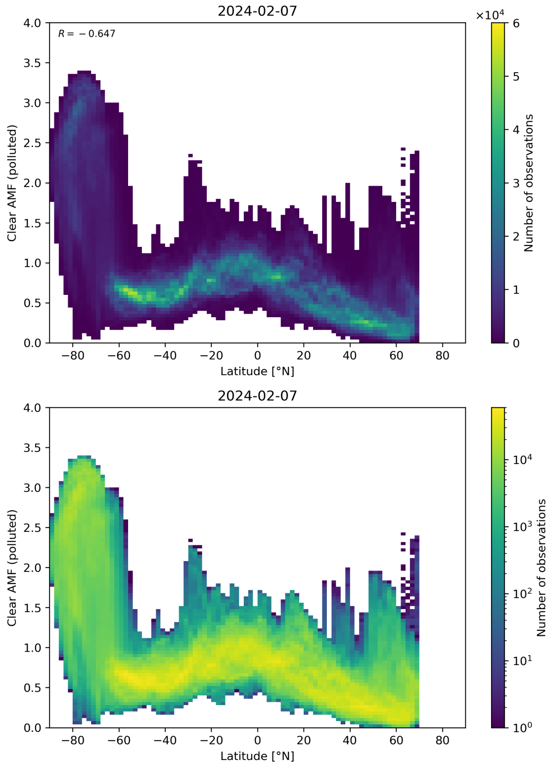
Figure 145: Scatter density plot of “Latitude” against “Clear AMF (polluted)” for 2024-02-06 to 2024-02-08.
