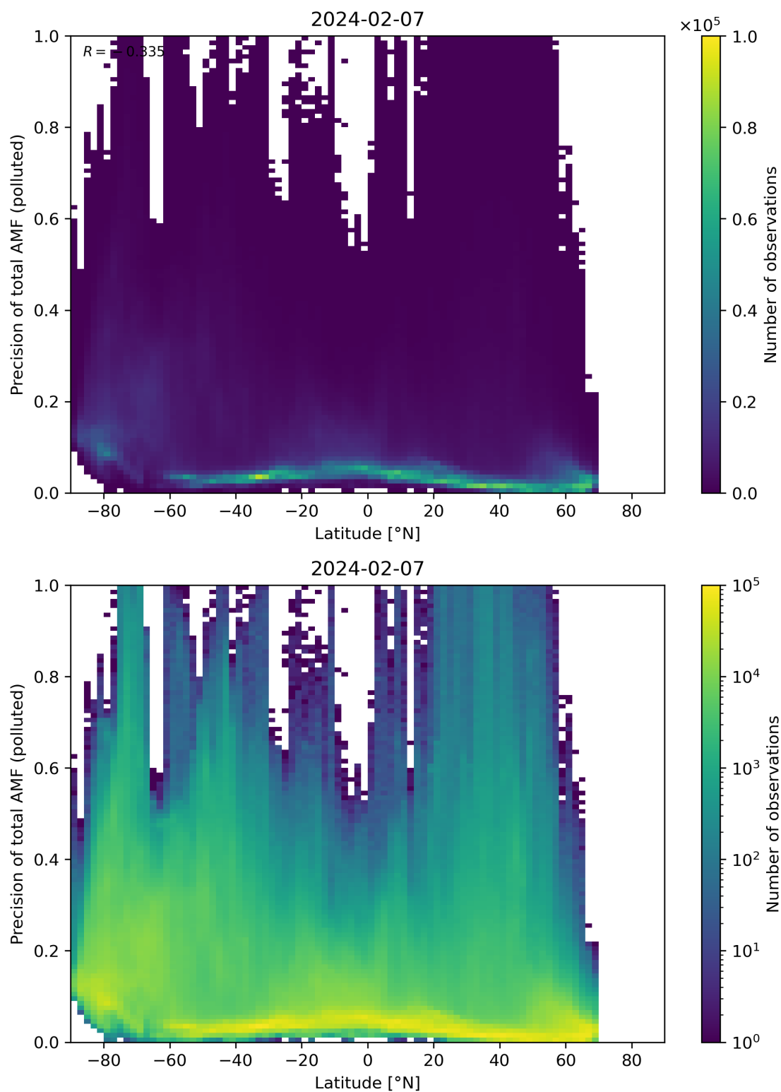
Figure 155: Scatter density plot of “Latitude” against “Precision of total AMF (polluted)” for 2024-02-06 to 2024-02-08.
