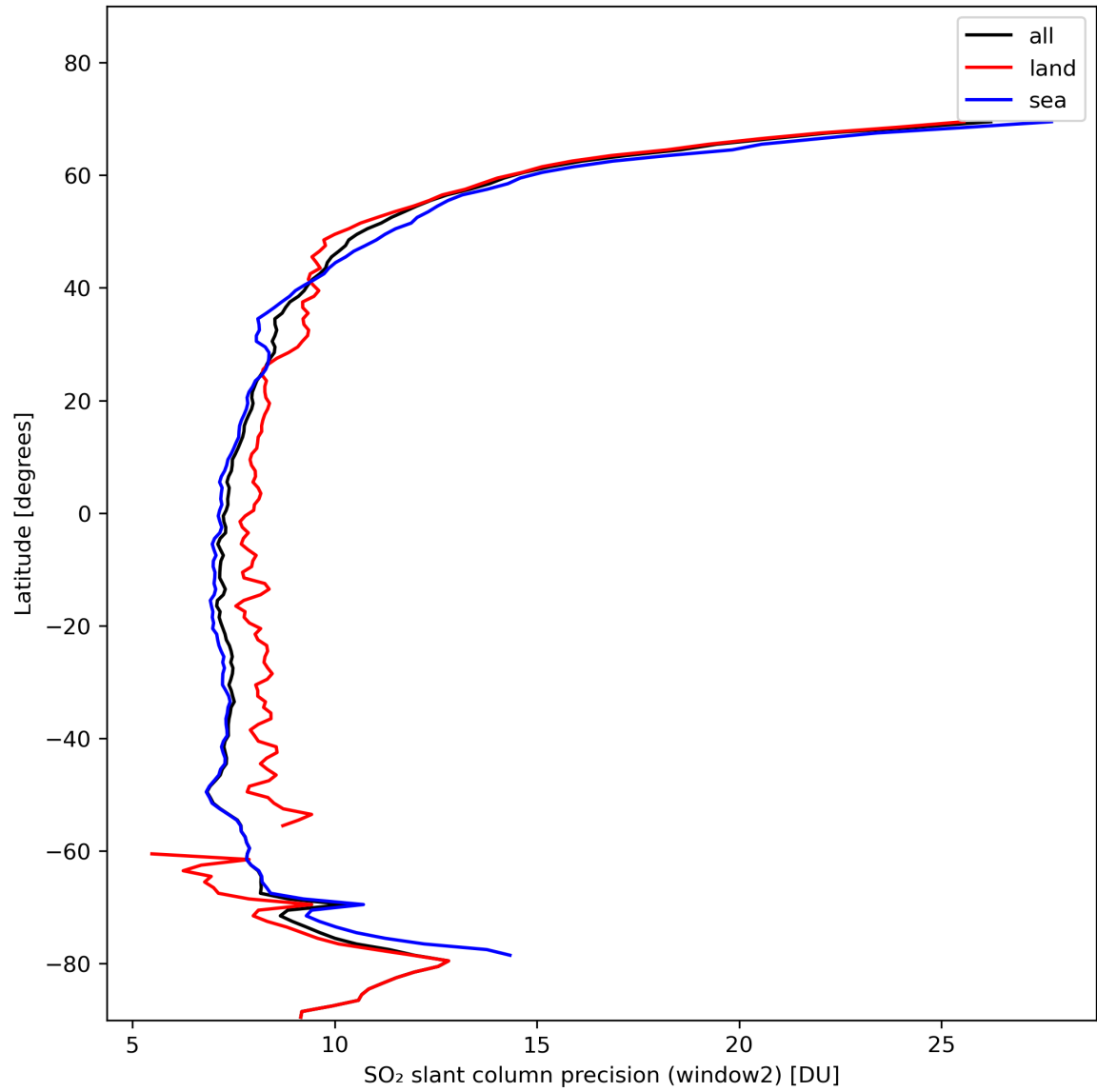
Figure 38: Zonal average of “SO 2 slant column precision (window2)” for 2024-02-06 to 2024-02-08.
