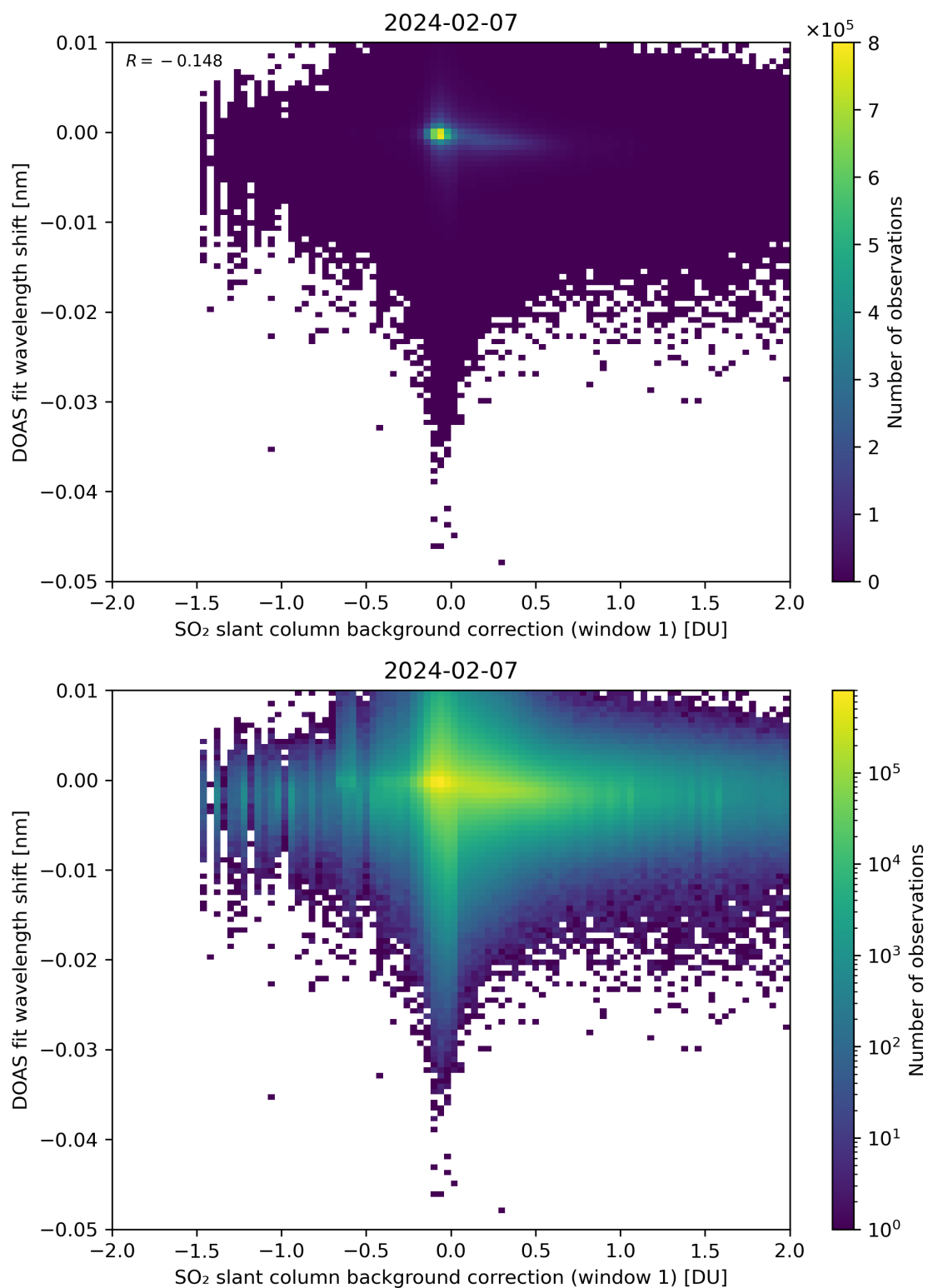
Figure 100: Scatter density plot of “SO 2 slant column background correction (window 1)” against “DOAS fit wavelength shift” for 2024-02-06 to 2024-02-08.
