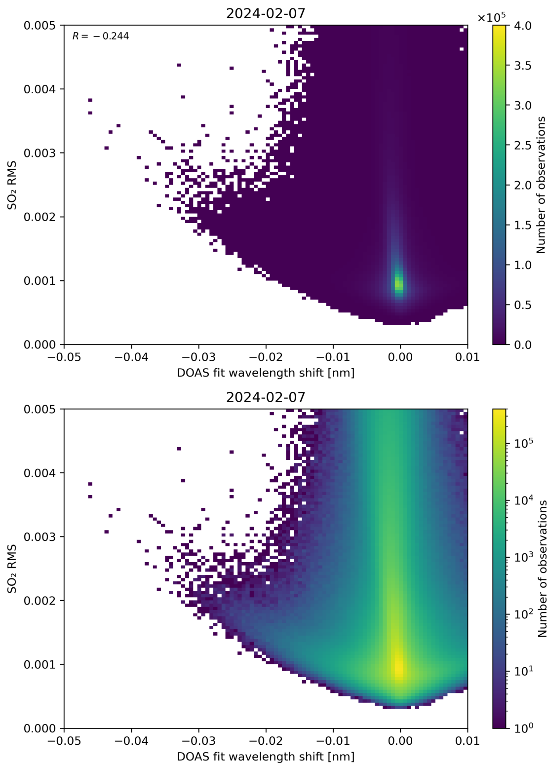
Figure 128: Scatter density plot of “DOAS fit wavelength shift” against “SO 2 RMS” for 2024-02-06 to 2024-02-08.
