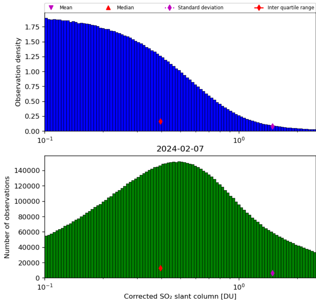
Figure 55: Histogram of “Corrected SO 2 slant column” for 2024-02-06 to 2024-02-08
