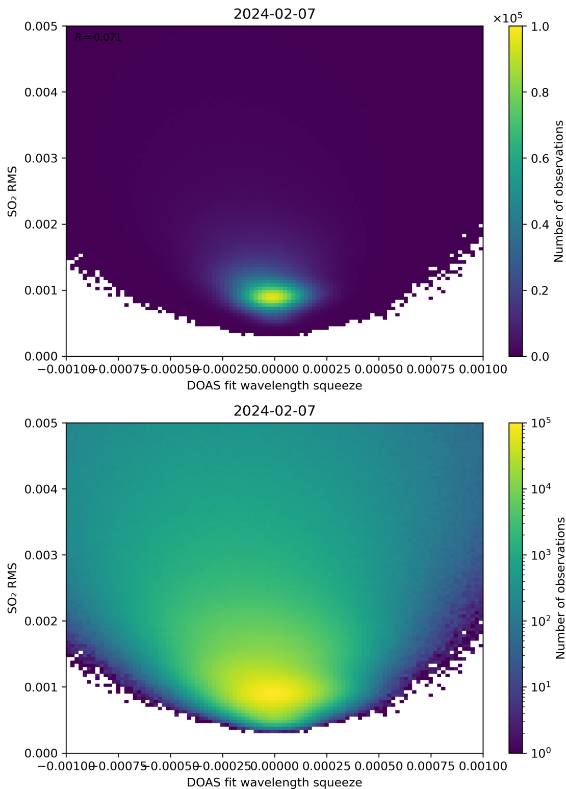
Figure 132: Scatter density plot of “DOAS fit wavelength squeeze” against “SO 2 RMS” for 2024-02-06 to 2024-02-08.
