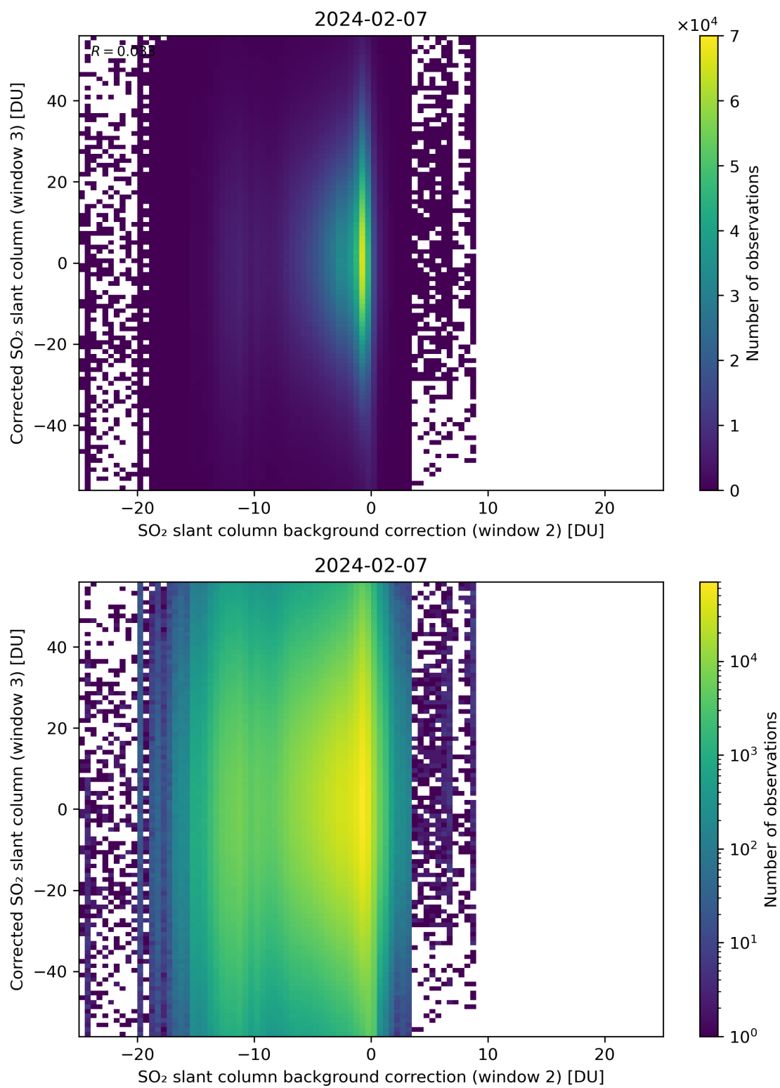
Figure 116: Scatter density plot of “SO 2 slant column background correction (window 2)” against “Corrected SO 2 slant column (window 3)” for 2024-02-06 to 2024-02-08.
