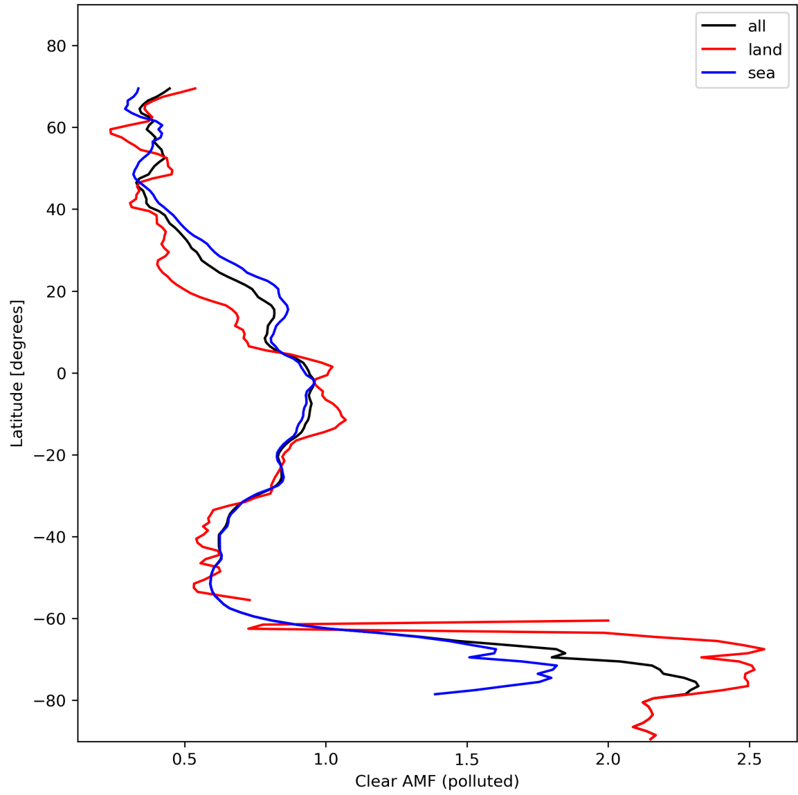
Figure 50: Zonal average of “Clear AMF (polluted)” for 2024-02-06 to 2024-02-08.
