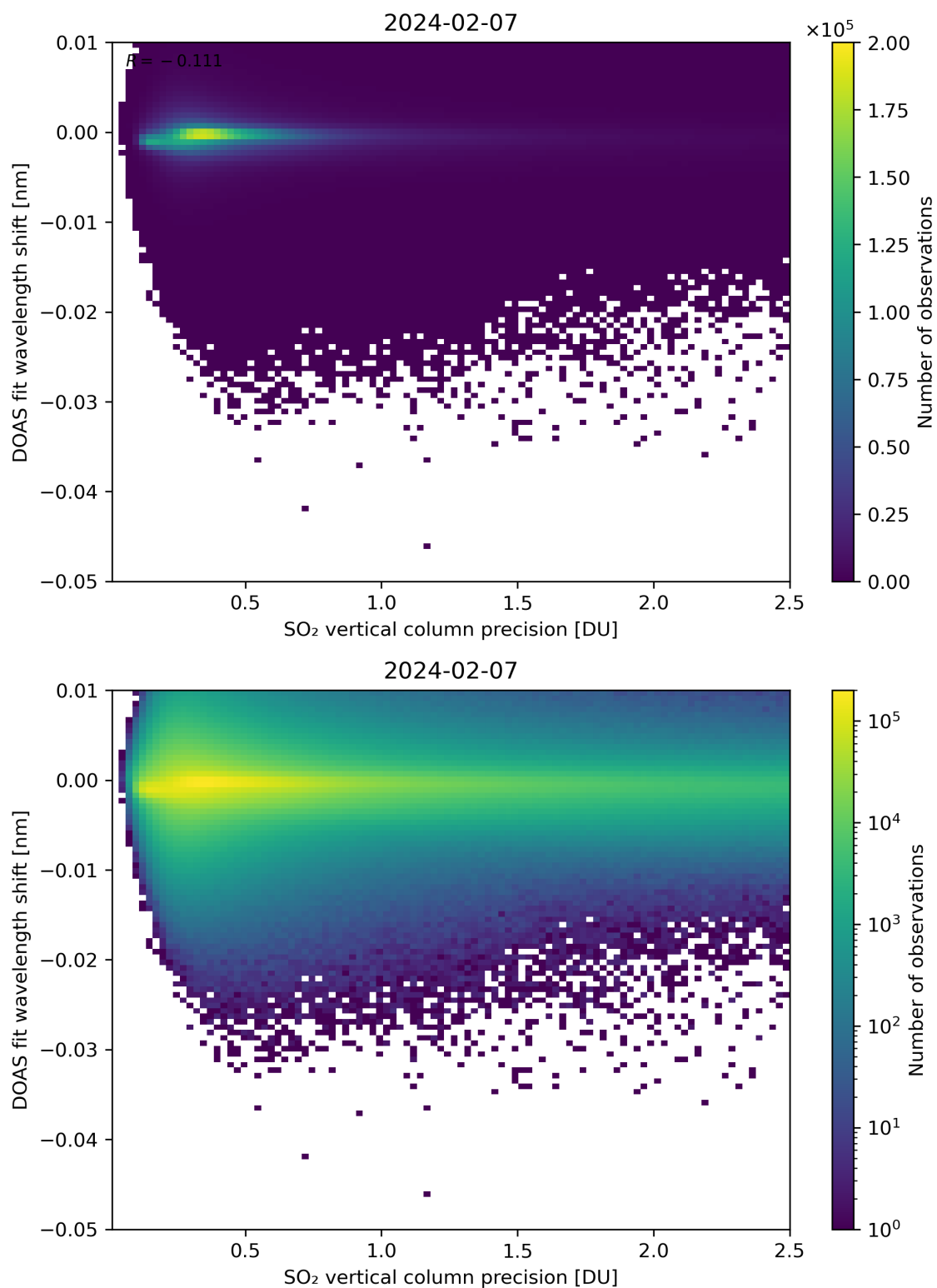
Figure 282: Scatter density plot of “SO 2 vertical column precision” against “DOAS fit wavelength shift” for 2024-02-06 to 2024-02-08.
