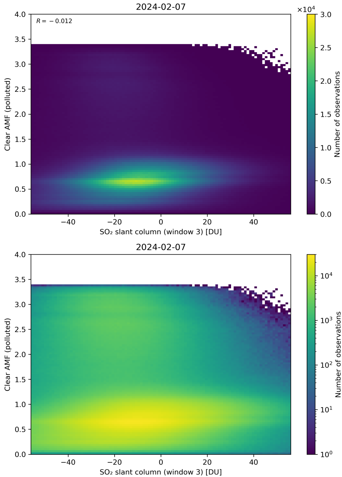
Figure 265: Scatter density plot of “SO 2 slant column (window 3)” against “Clear AMF (polluted)” for 2024-02-06 to 2024-02-08.
