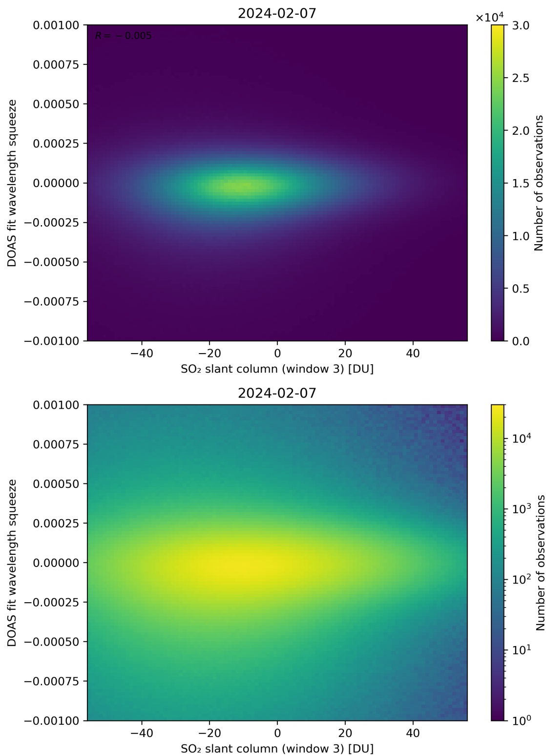
Figure 255: Scatter density plot of “SO 2 slant column (window 3)” against “DOAS fit wavelength squeeze” for 2024-02-06 to 2024-02-08.
