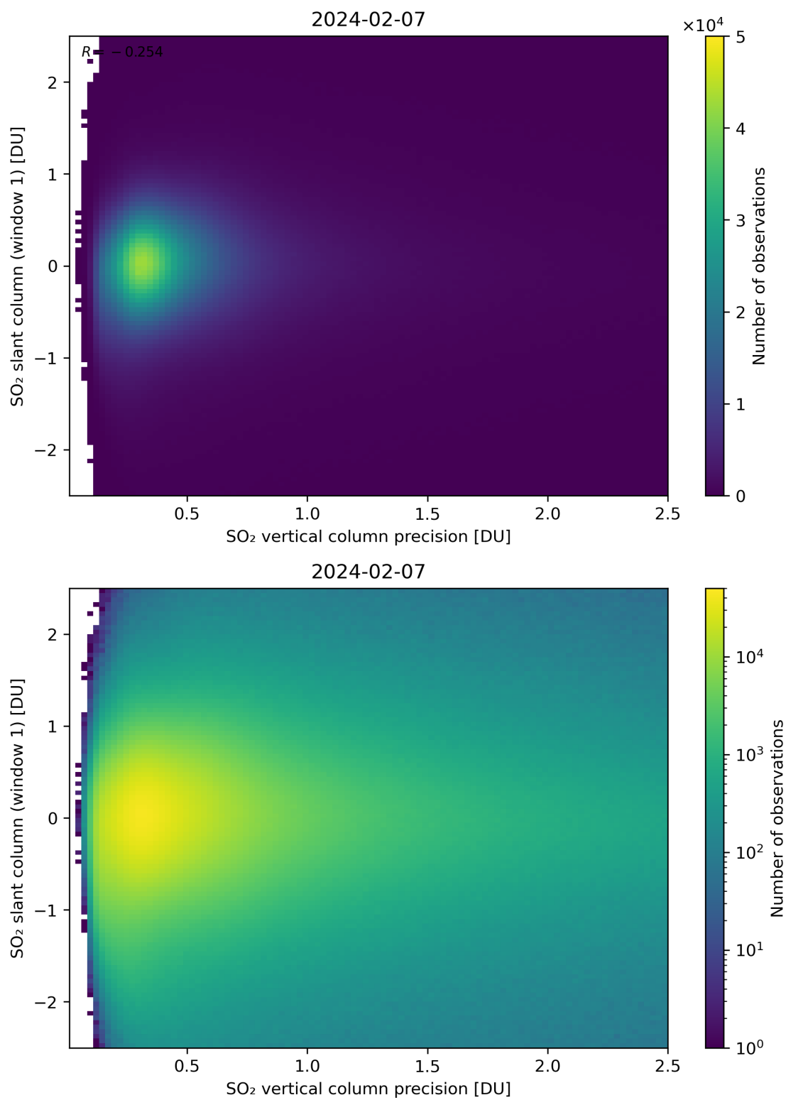
Figure 289: Scatter density plot of “SO 2 vertical column precision” against “SO 2 slant column (window 1)” for 2024-02-06 to 2024-02-08.
