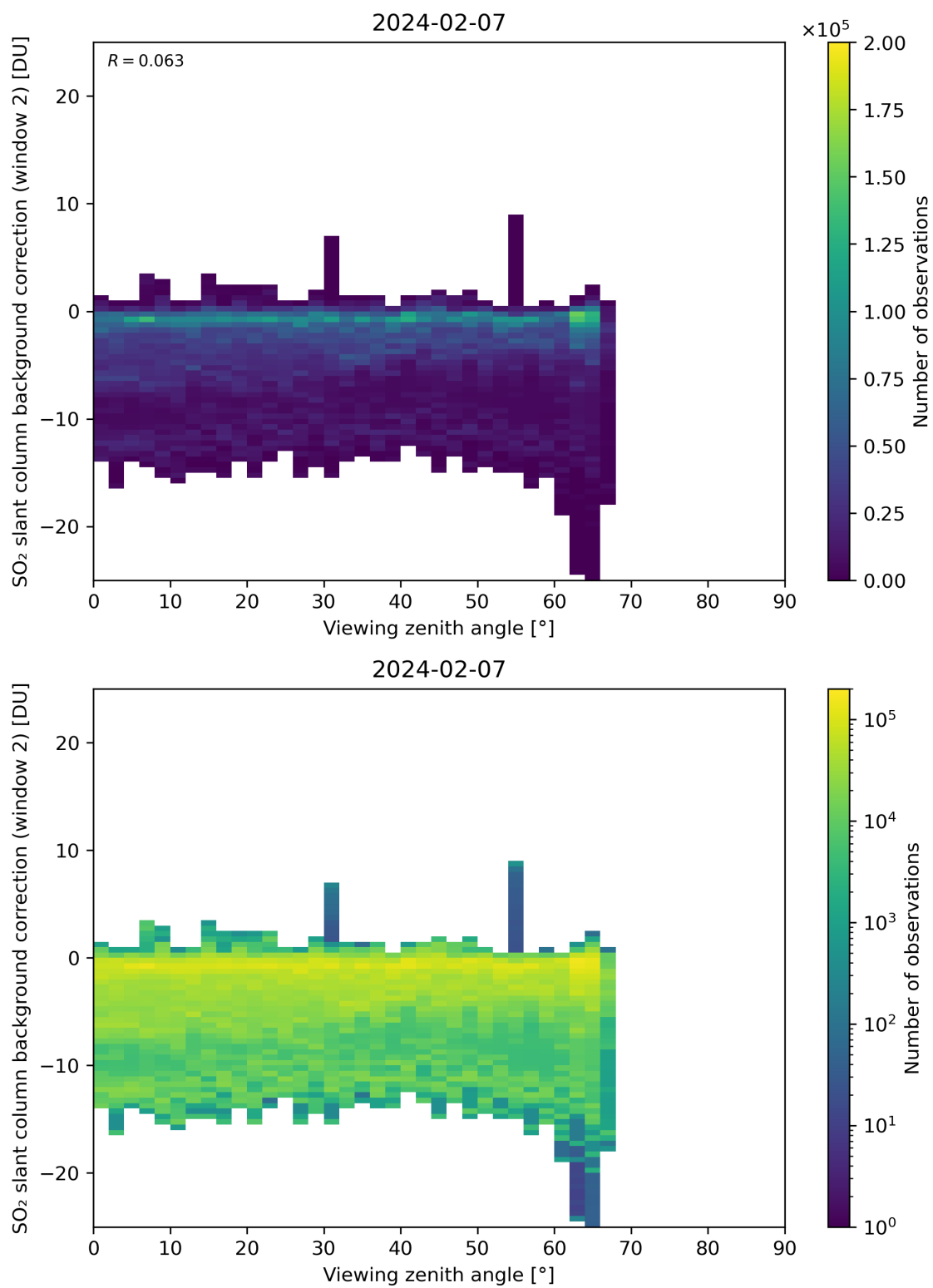
Figure 309: Scatter density plot of “Viewing zenith angle” against “SO 2 slant column background correction (window 2)” for 2024-02-06 to 2024-02-08.
