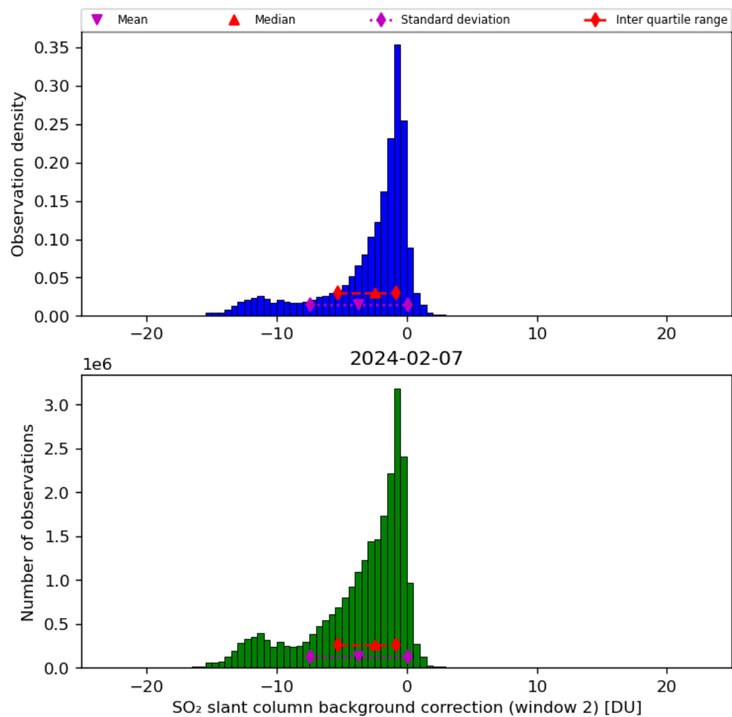
Figure 63: Histogram of “SO 2 slant column background correction (window 2)” for 2024-02-06 to 2024-02-08
