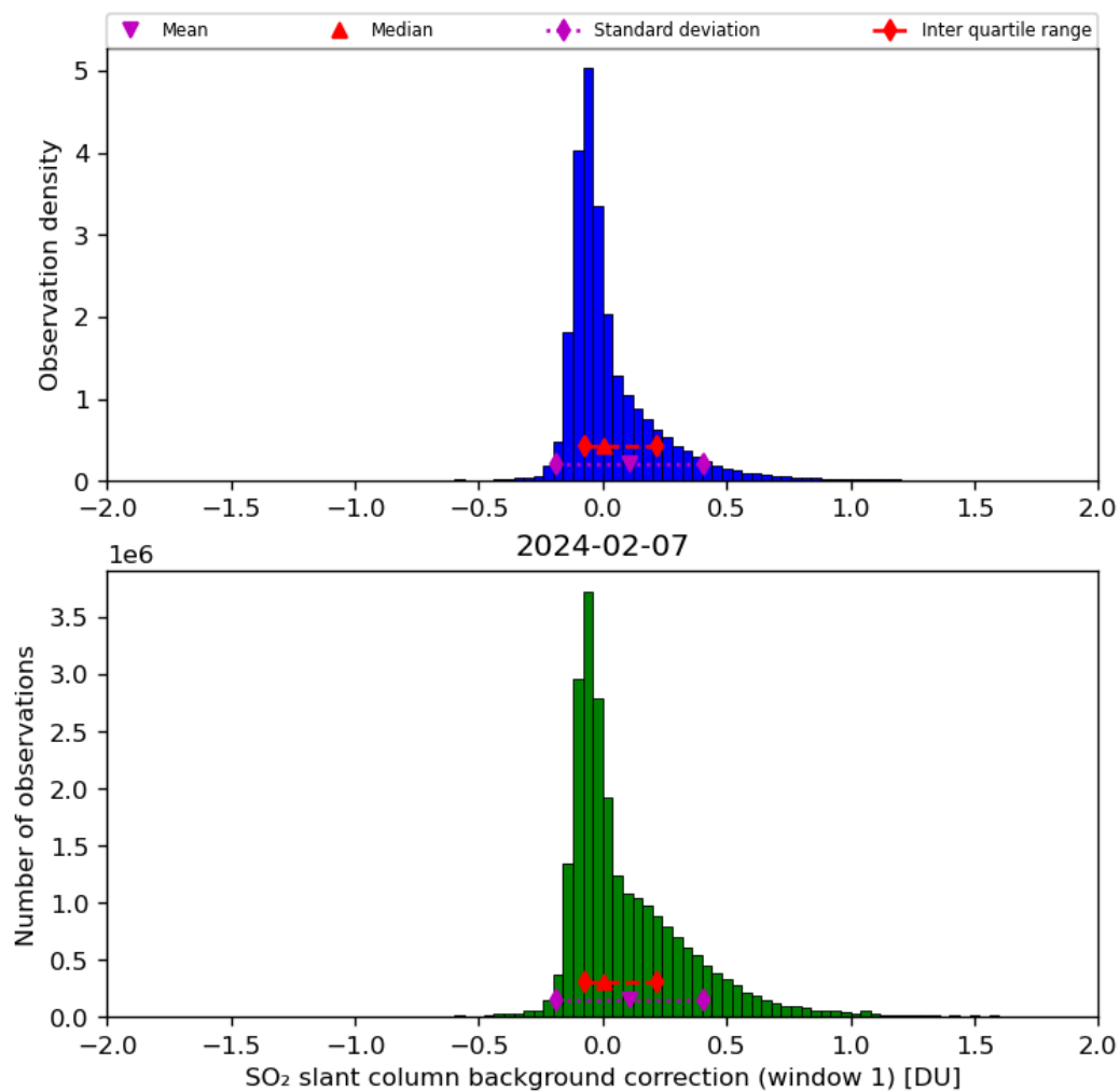
Figure 59: Histogram of “SO 2 slant column background correction (window 1)” for 2024-02-06 to 2024-02-08
