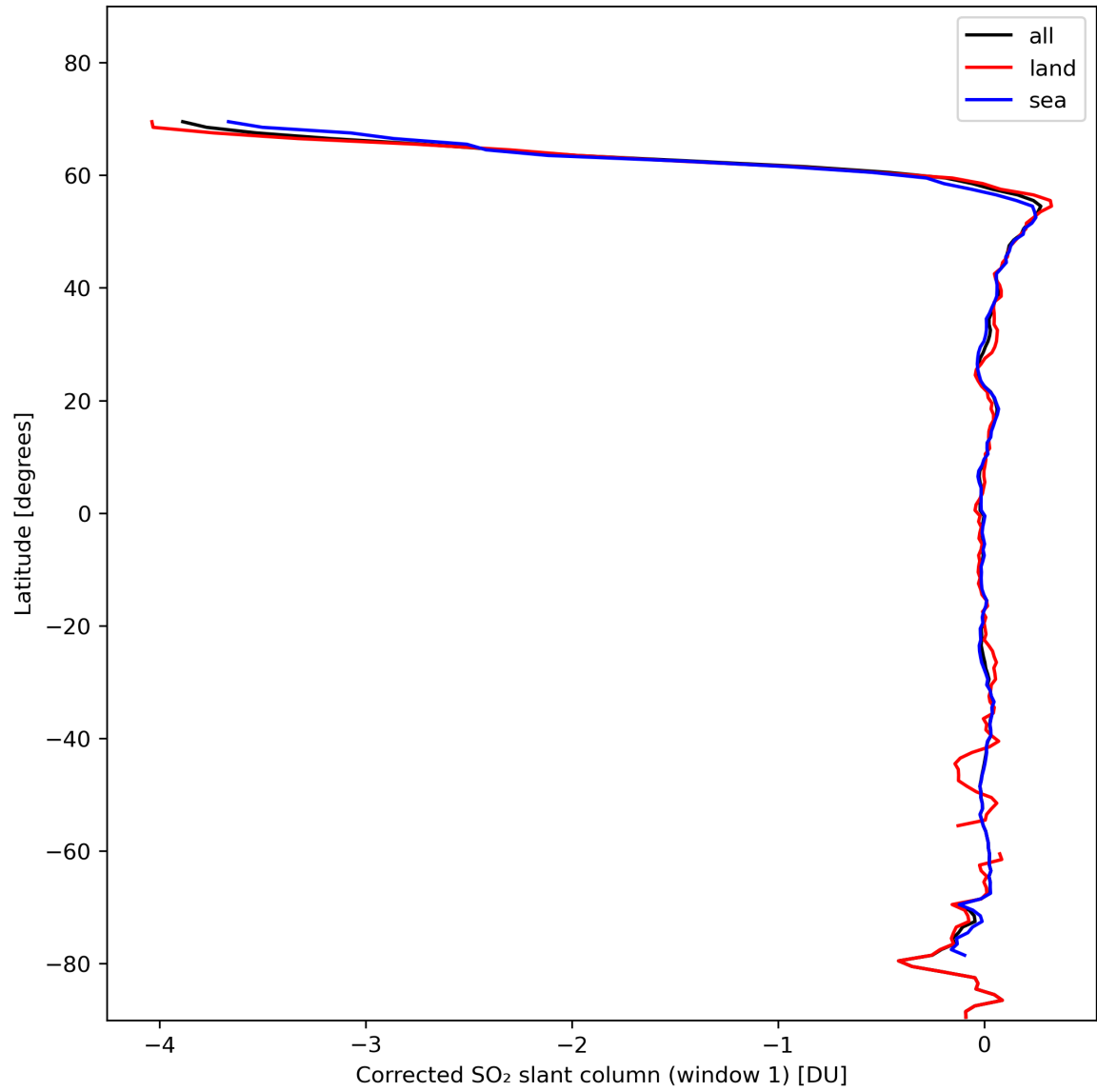
Figure 35: Zonal average of “Corrected SO 2 slant column (window 1)” for 2024-02-06 to 2024-02-08.
