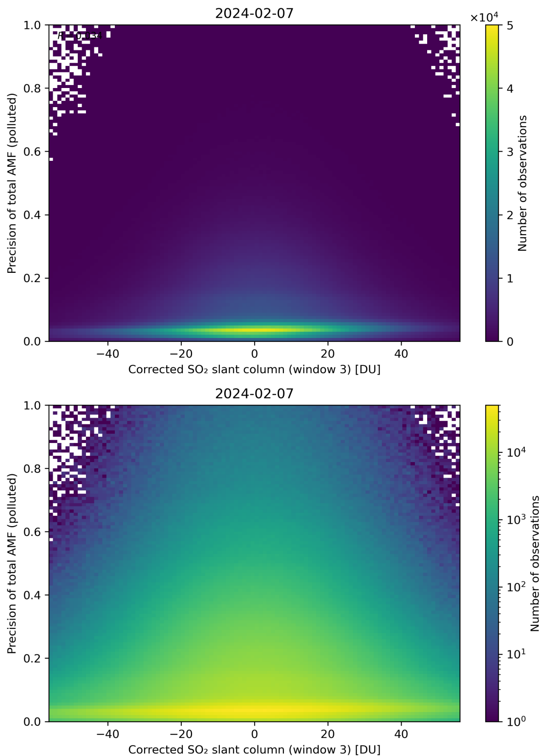
Figure 211: Scatter density plot of “Corrected SO 2 slant column (window 3)” against “Precision of total AMF (polluted)” for 2024-02-06 to 2024-02-08.
