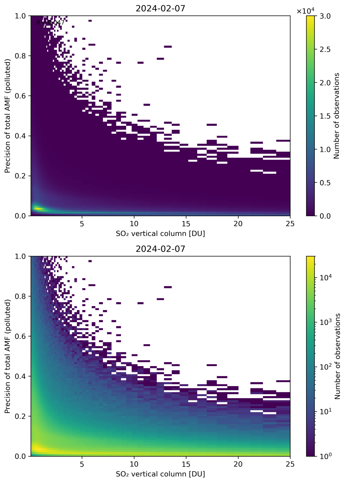
Figure 306: Scatter density plot of “SO 2 vertical column” against “Precision of total AMF (polluted)” for 2024-02-06 to 2024-02-08.
