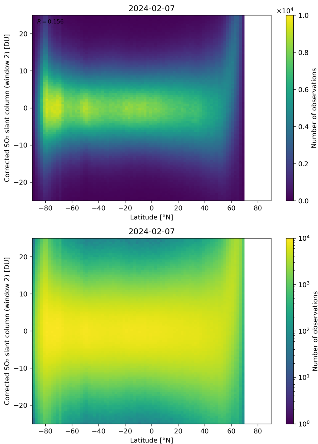
Figure 147: Scatter density plot of “Latitude” against “Corrected SO 2 slant column (window 2)” for 2024-02-06 to 2024-02-08.
