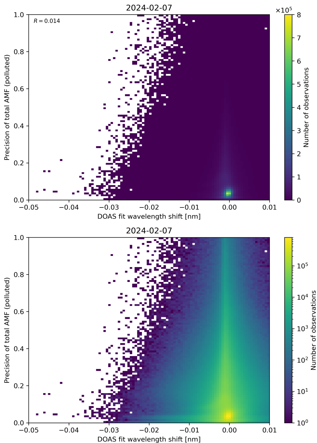
Figure 131: Scatter density plot of “DOAS fit wavelength shift” against “Precision of total AMF (polluted)” for 2024-02-06 to 2024-02-08.
