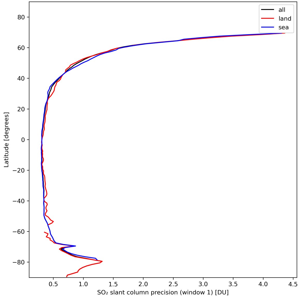
Figure 34: Zonal average of “SO 2 slant column precision (window 1)” for 2024-02-06 to 2024-02-08.
