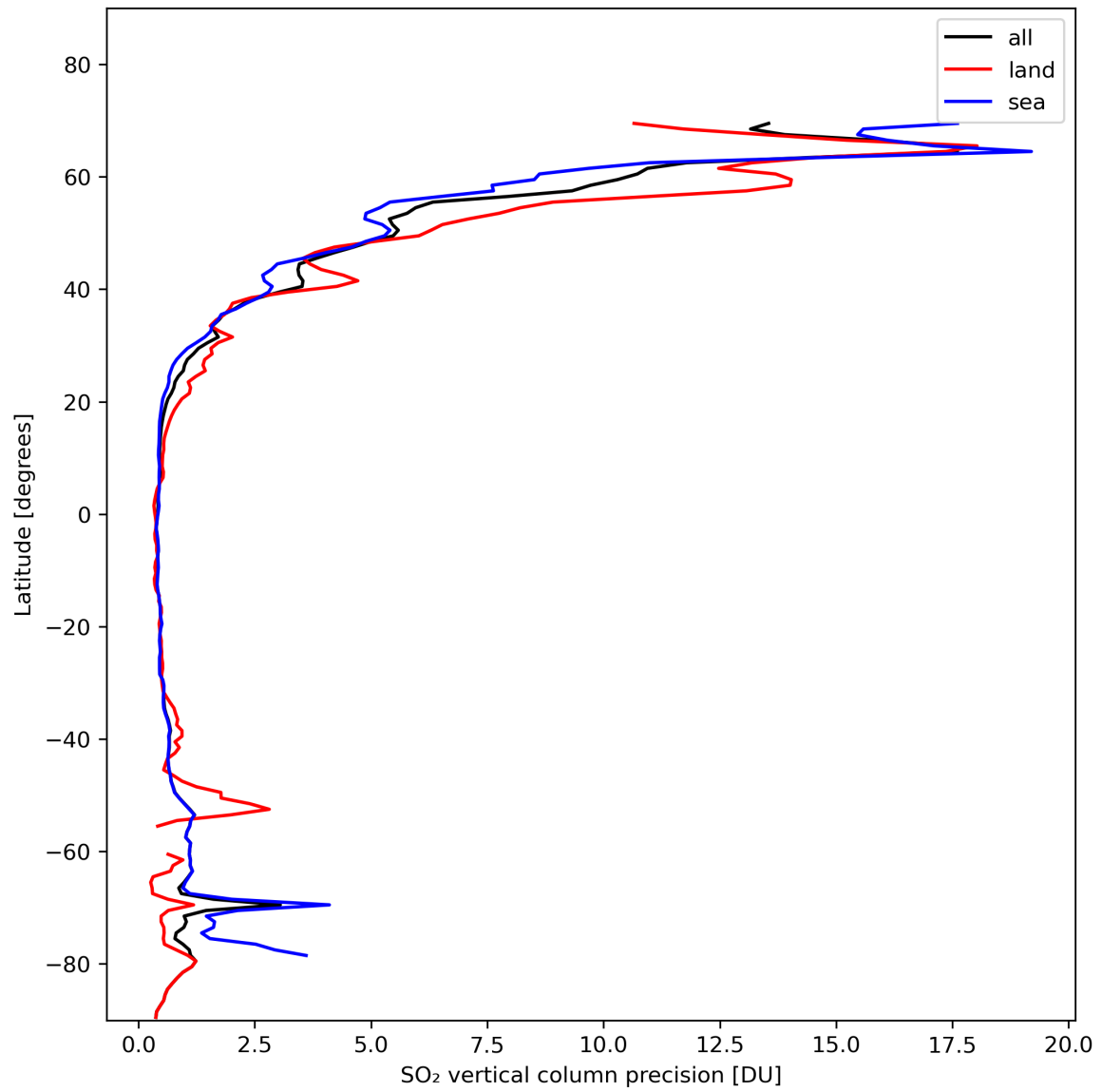
Figure 31: Zonal average of “SO 2 vertical column precision” for 2024-02-06 to 2024-02-08.
