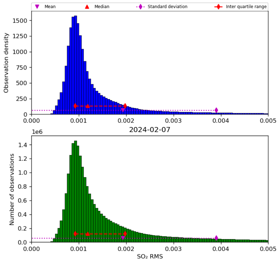
Figure 70: Histogram of “SO 2 RMS” for 2024-02-06 to 2024-02-08
