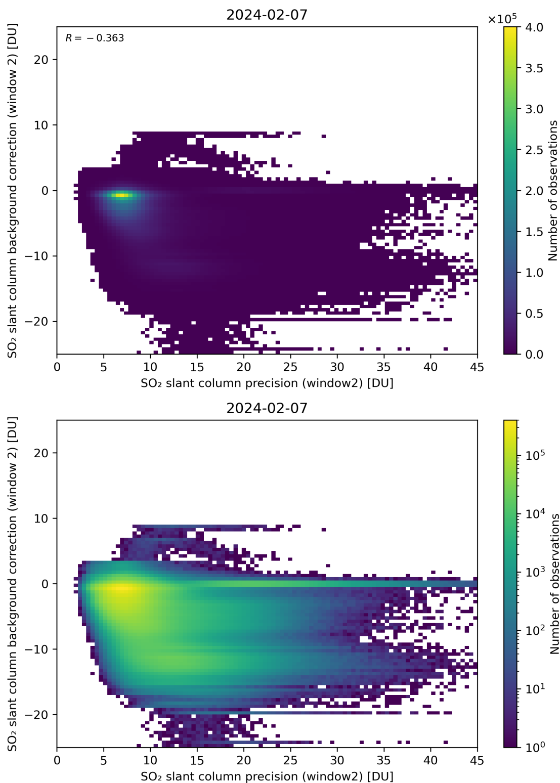
Figure 241: Scatter density plot of “SO 2 slant column precision (window2)” against “SO 2 slant column background correction (window 2)” for 2024-02-06 to 2024-02-08.
