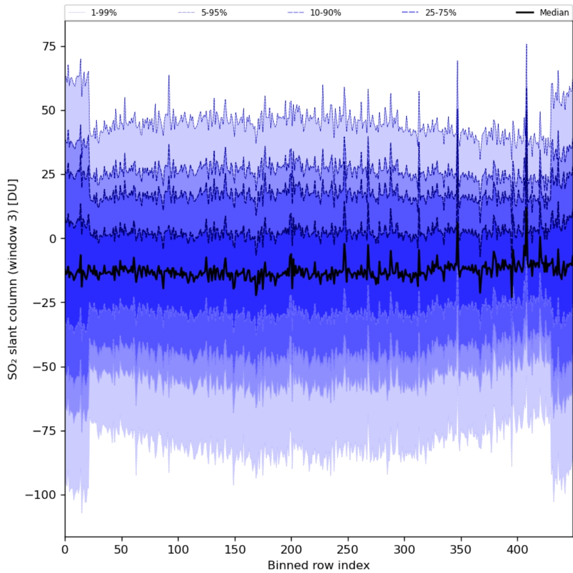
Figure 87: Along track statistics of “SO 2 slant column (window 3)” for 2024-02-06 to 2024-02-08
