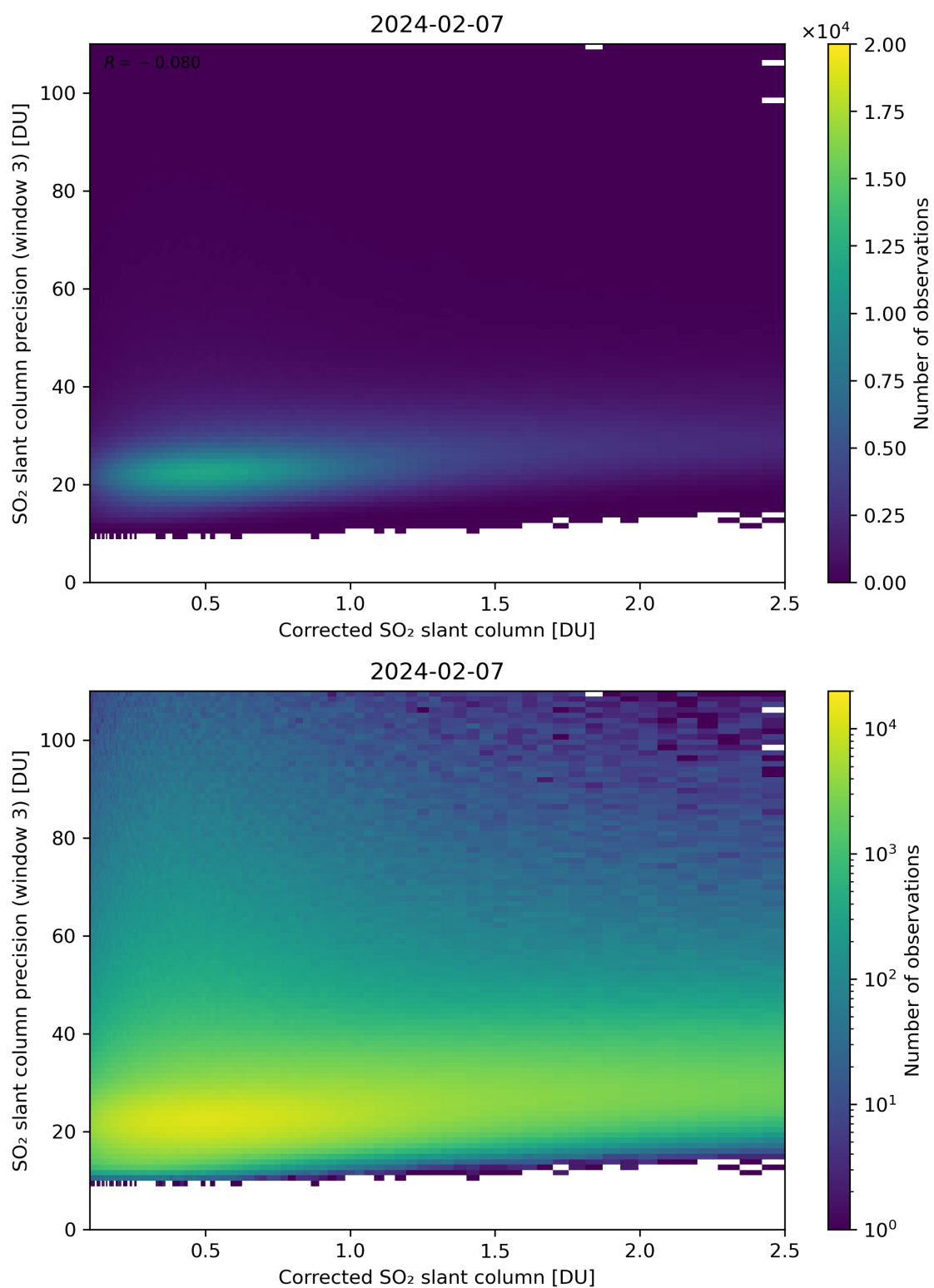
Figure 191: Scatter density plot of “Corrected SO 2 slant column” against “SO 2 slant column precision (window 3)” for 2024-02-06 to 2024-02-08.
