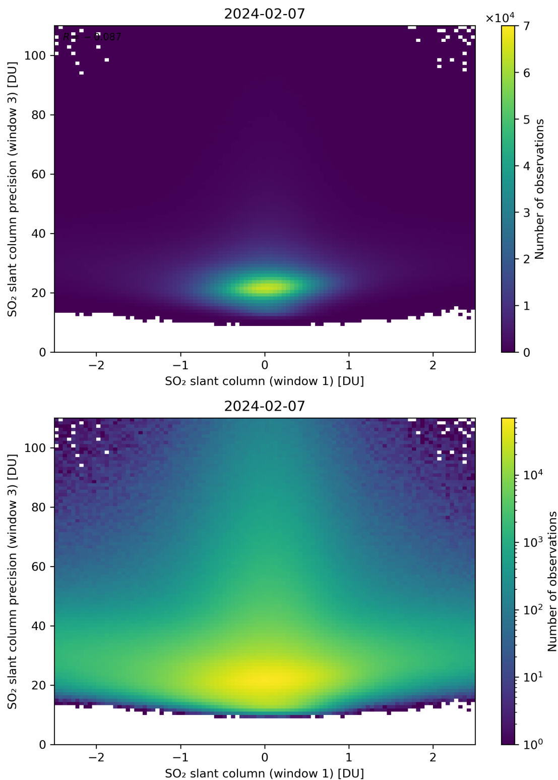
Figure 238: Scatter density plot of “SO 2 slant column (window 1)” against “SO 2 slant column precision (window 3)” for 2024-02-06 to 2024-02-08.
