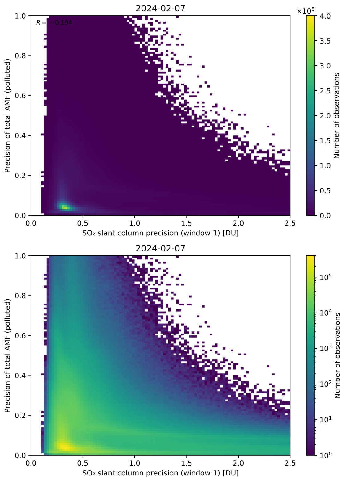
Figure 231: Scatter density plot of “SO 2 slant column precision (window 1)” against “Precision of total AMF (polluted)” for 2024-02-06 to 2024-02-08.
