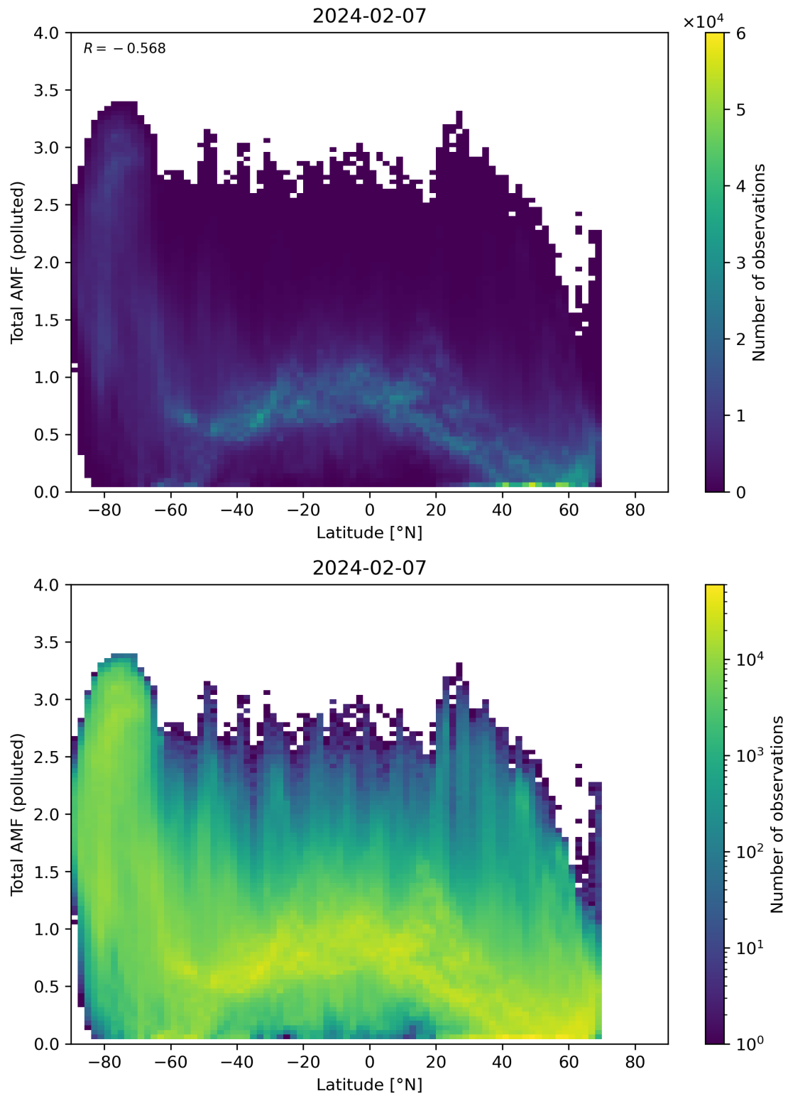
Figure 154: Scatter density plot of “Latitude” against “Total AMF (polluted)” for 2024-02-06 to 2024-02-08.
