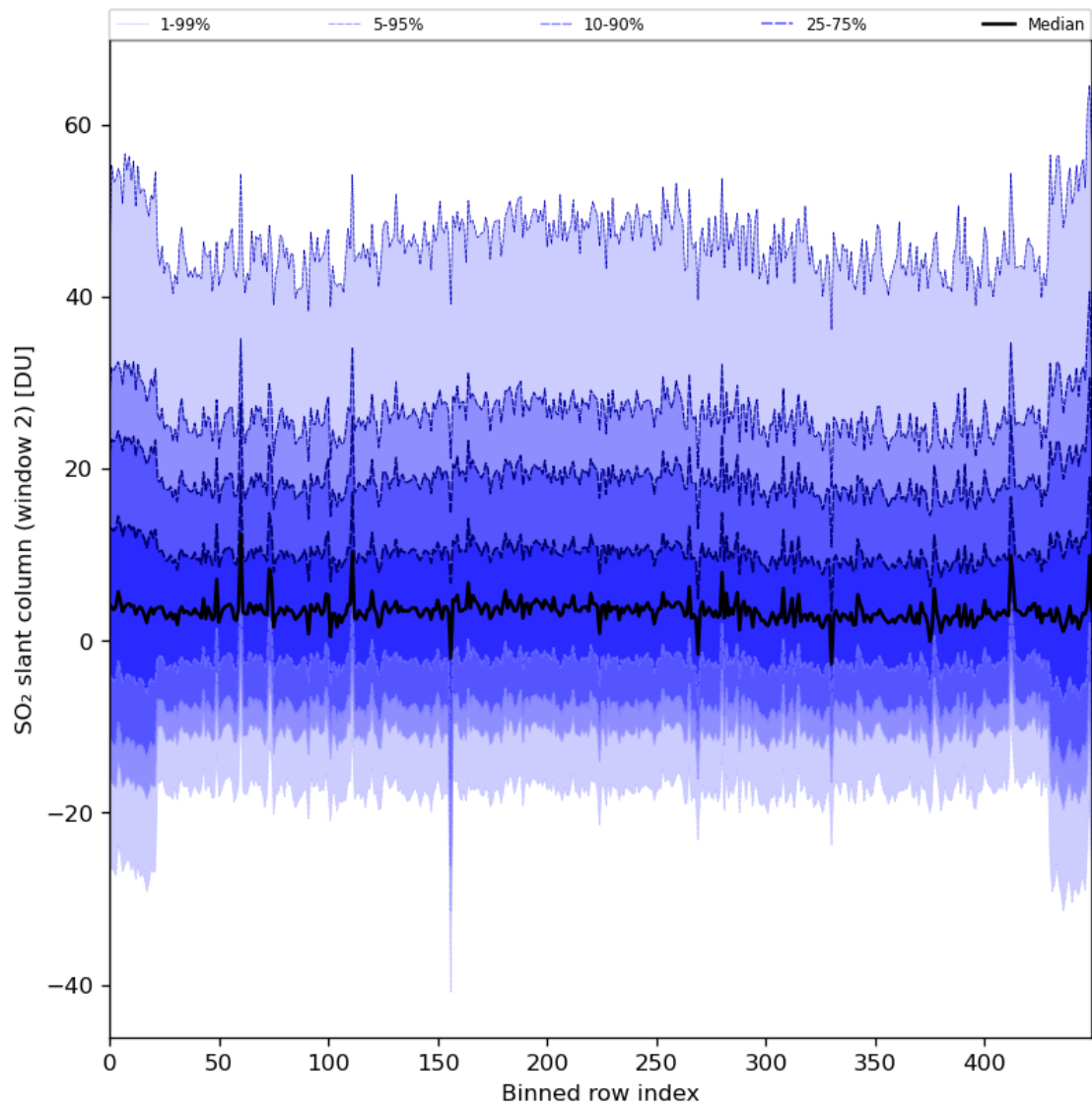
Figure 83: Along track statistics of “SO 2 slant column (window 2)” for 2024-02-06 to 2024-02-08
