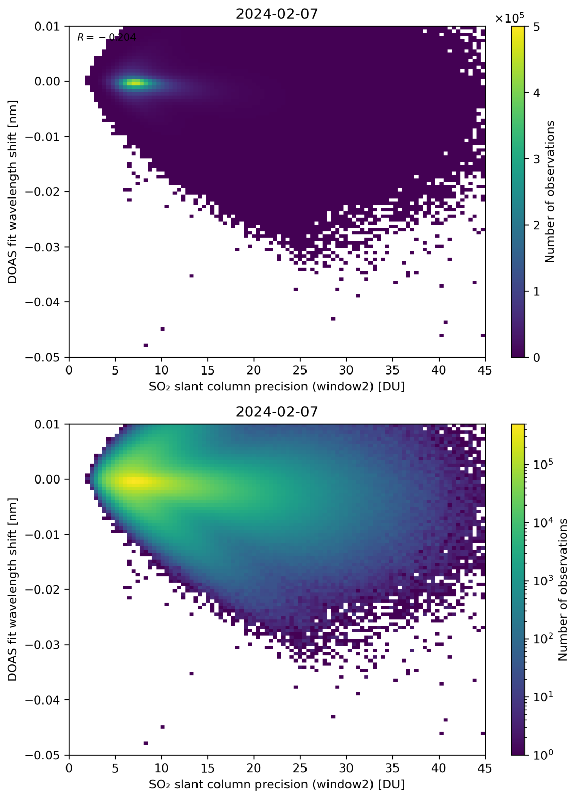
Figure 243: Scatter density plot of “SO 2 slant column precision (window2)” against “DOAS fit wavelength shift” for 2024-02-06 to 2024-02-08.
