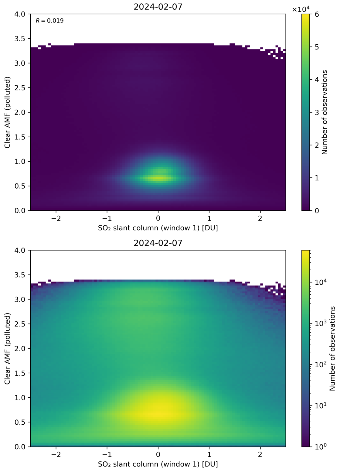
Figure 232: Scatter density plot of “SO 2 slant column (window 1)” against “Clear AMF (polluted)” for 2024-02-06 to 2024-02-08.
