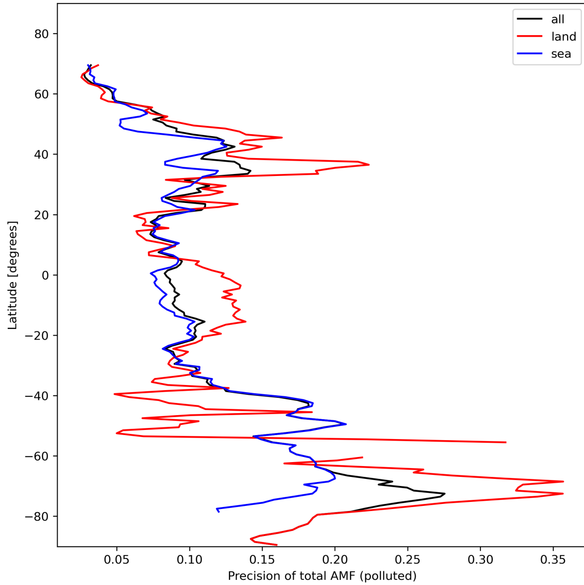
Figure 49: Zonal average of “Precision of total AMF (polluted)” for 2024-02-06 to 2024-02-08.
