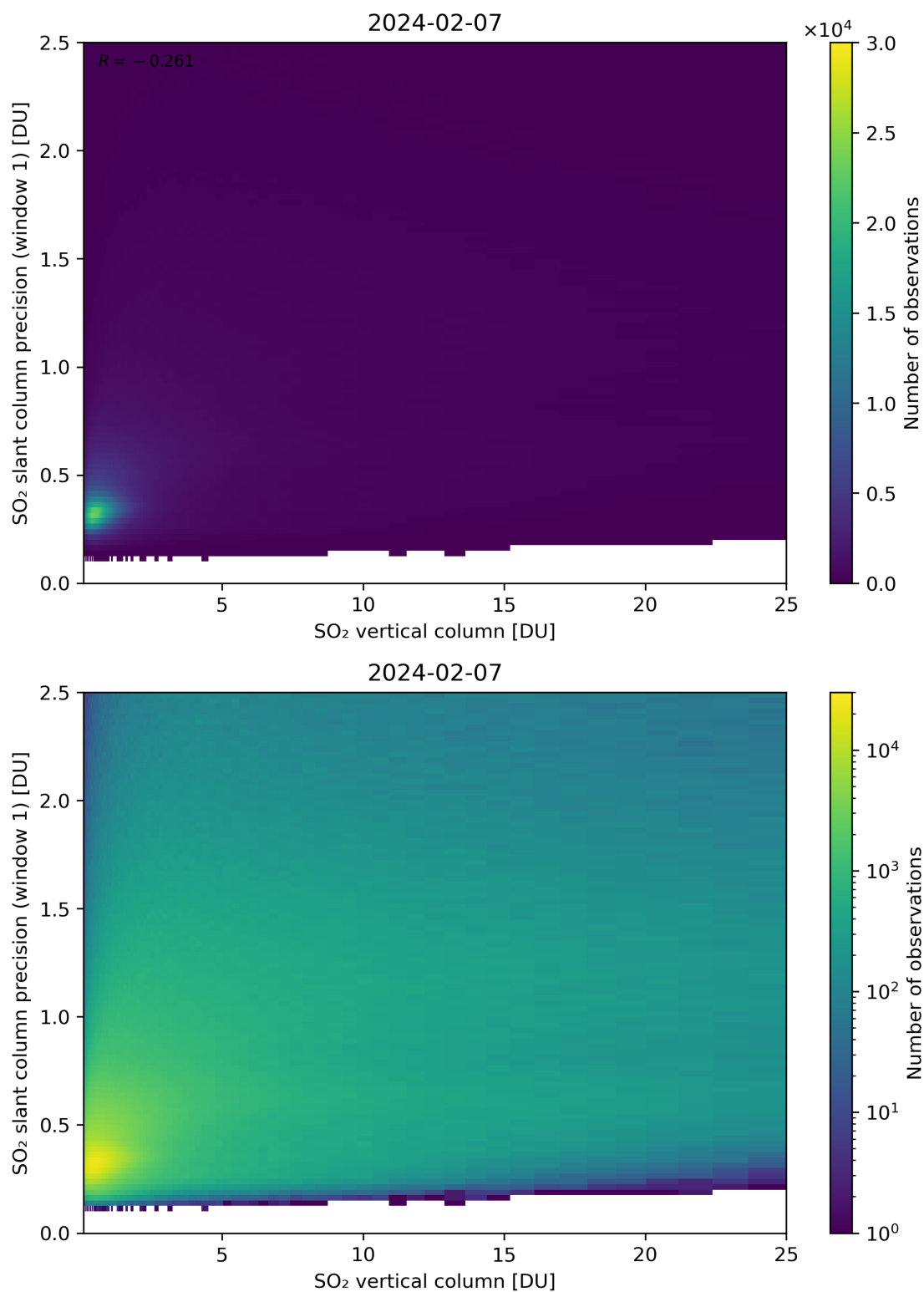
Figure 301: Scatter density plot of “SO 2 vertical column” against “SO 2 slant column precision (window 1)” for 2024-02-06 to 2024-02-08.
