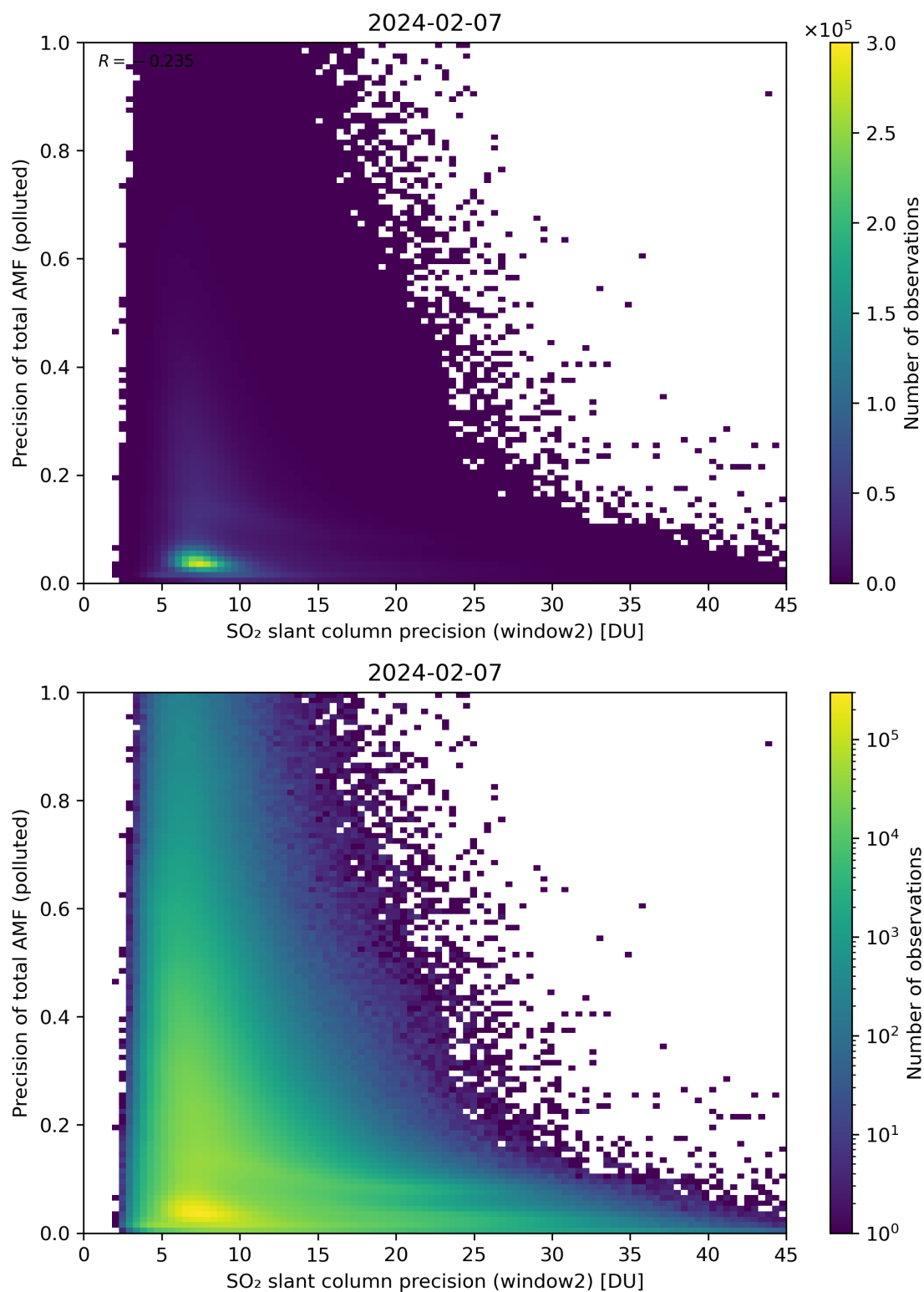
Figure 252: Scatter density plot of “SO 2 slant column precision (window2)” against “Precision of total AMF (polluted)” for 2024-02-06 to 2024-02-08.
