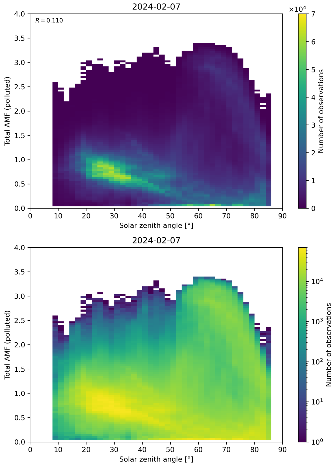
Figure 174: Scatter density plot of “Solar zenith angle” against “Total AMF (polluted)” for 2024-02-06 to 2024-02-08.
