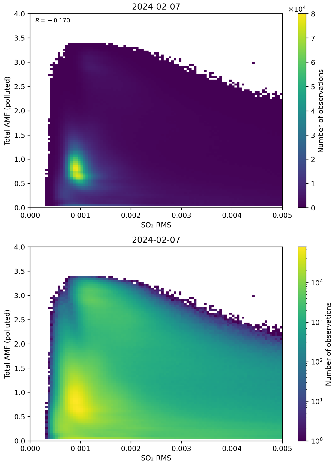
Figure 137: Scatter density plot of “SO 2 RMS” against “Total AMF (polluted)” for 2024-02-06 to 2024-02-08.
