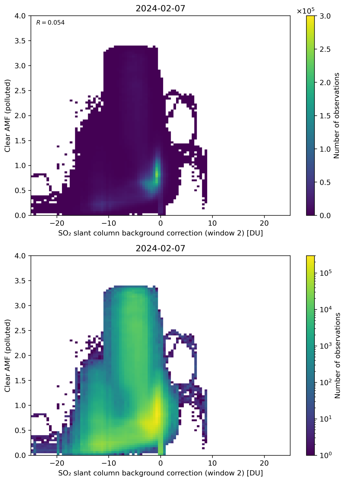
Figure 115: Scatter density plot of “SO 2 slant column background correction (window 2)” against “Clear AMF (polluted)” for 2024-02-06 to 2024-02-08.
