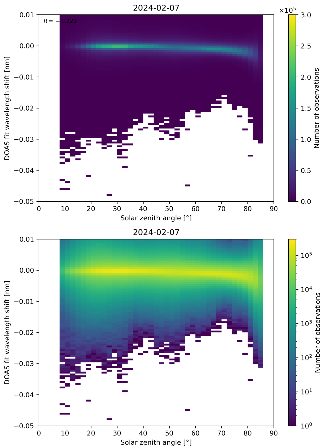
Figure 161: Scatter density plot of “Solar zenith angle” against “DOAS fit wavelength shift” for 2024-02-06 to 2024-02-08.
