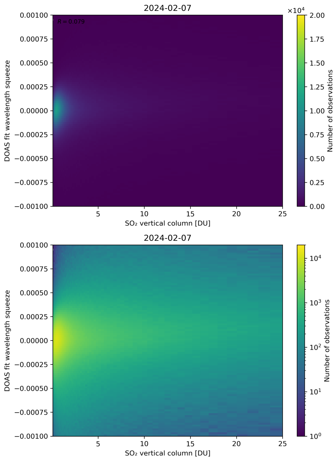
Figure 277: Scatter density plot of “SO 2 vertical column” against “DOAS fit wavelength squeeze” for 2024-02-06 to 2024-02-08.
