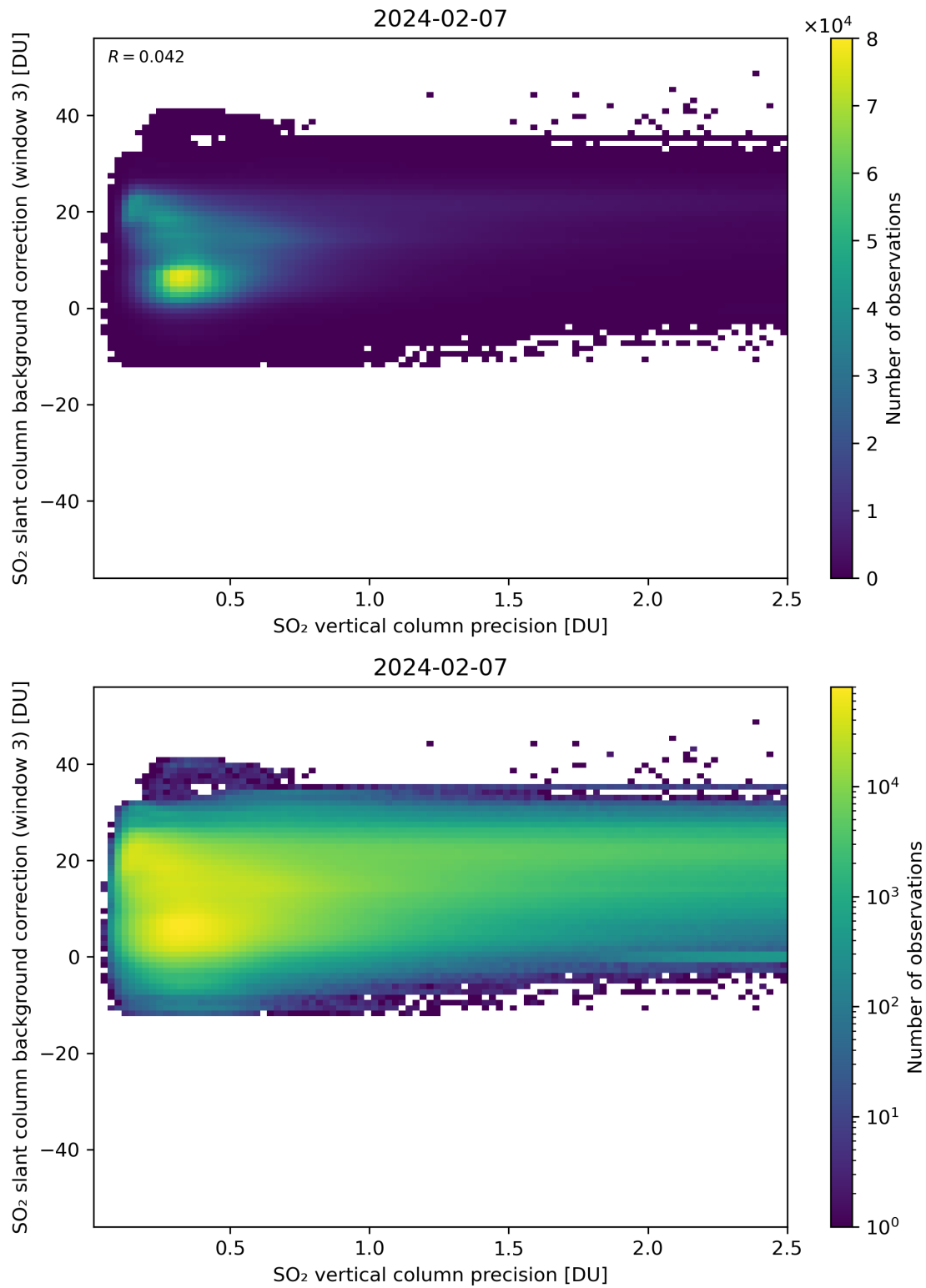
Figure 281: Scatter density plot of “SO 2 vertical column precision” against “SO 2 slant column background correction (window 3)” for 2024-02-06 to 2024-02-08.
