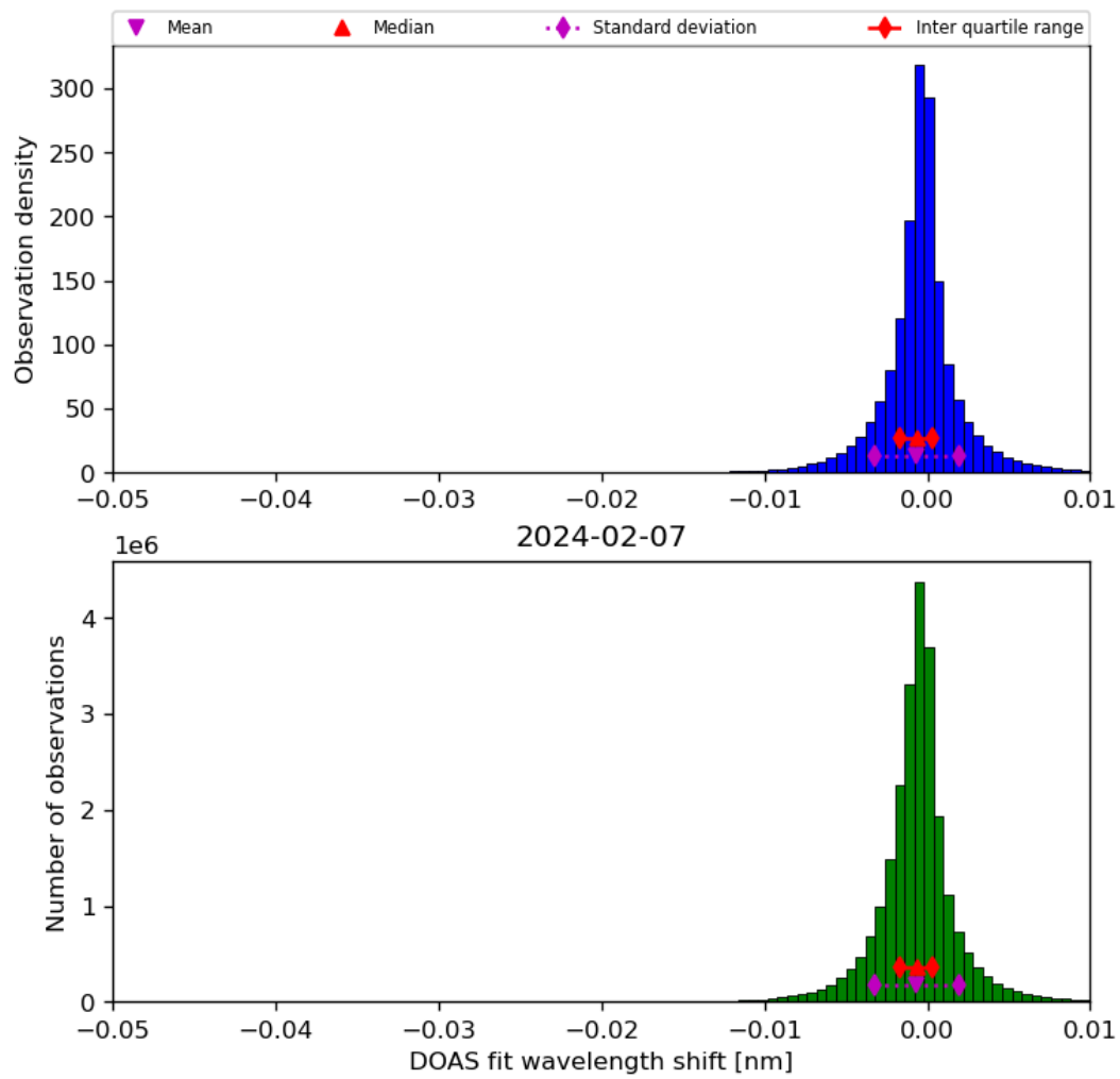
Figure 68: Histogram of “DOAS fit wavelength shift” for 2024-02-06 to 2024-02-08
