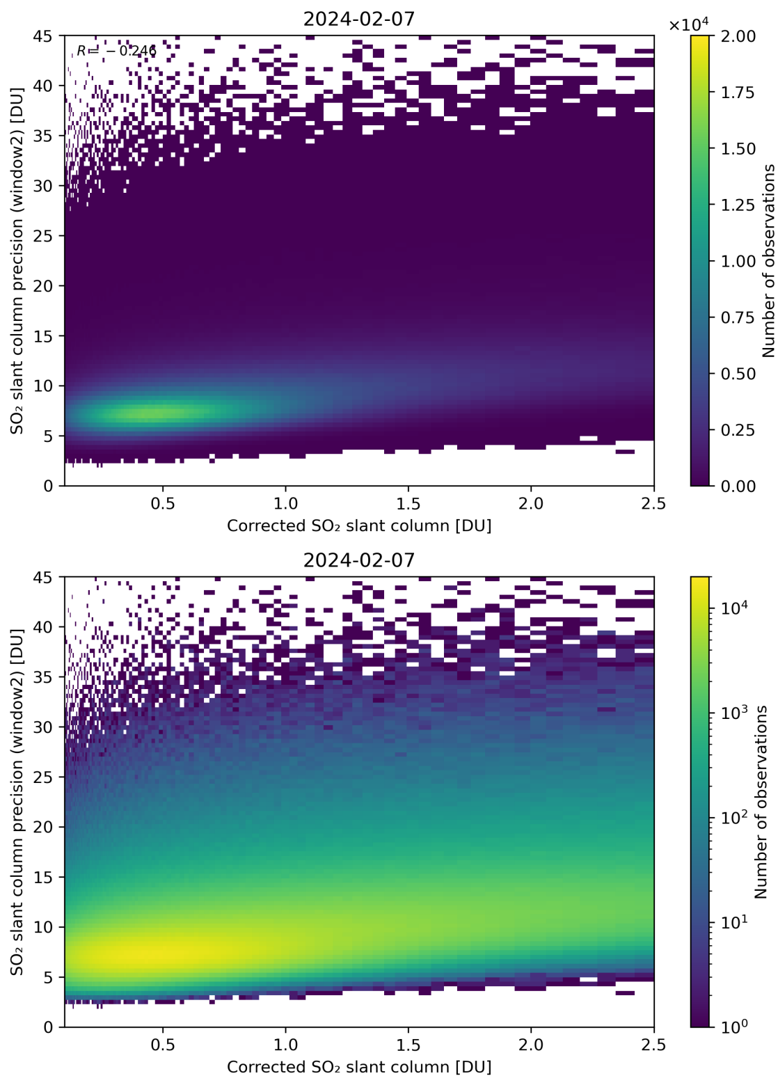
Figure 189: Scatter density plot of “Corrected SO 2 slant column” against “SO 2 slant column precision (window2)” for 2024-02-06 to 2024-02-08.
