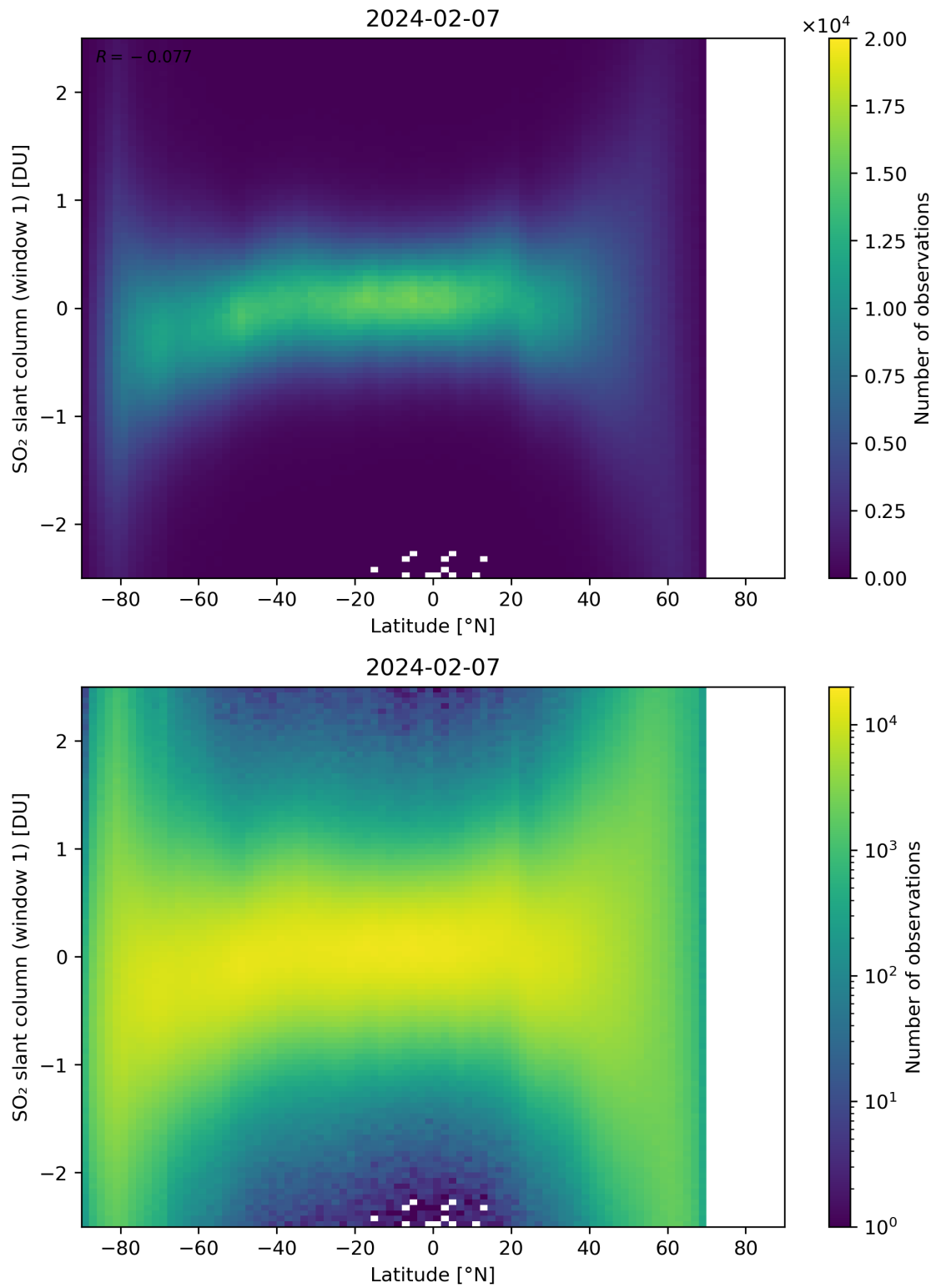
Figure 149: Scatter density plot of “Latitude” against “SO 2 slant column (window 1)” for 2024-02-06 to 2024-02-08.
