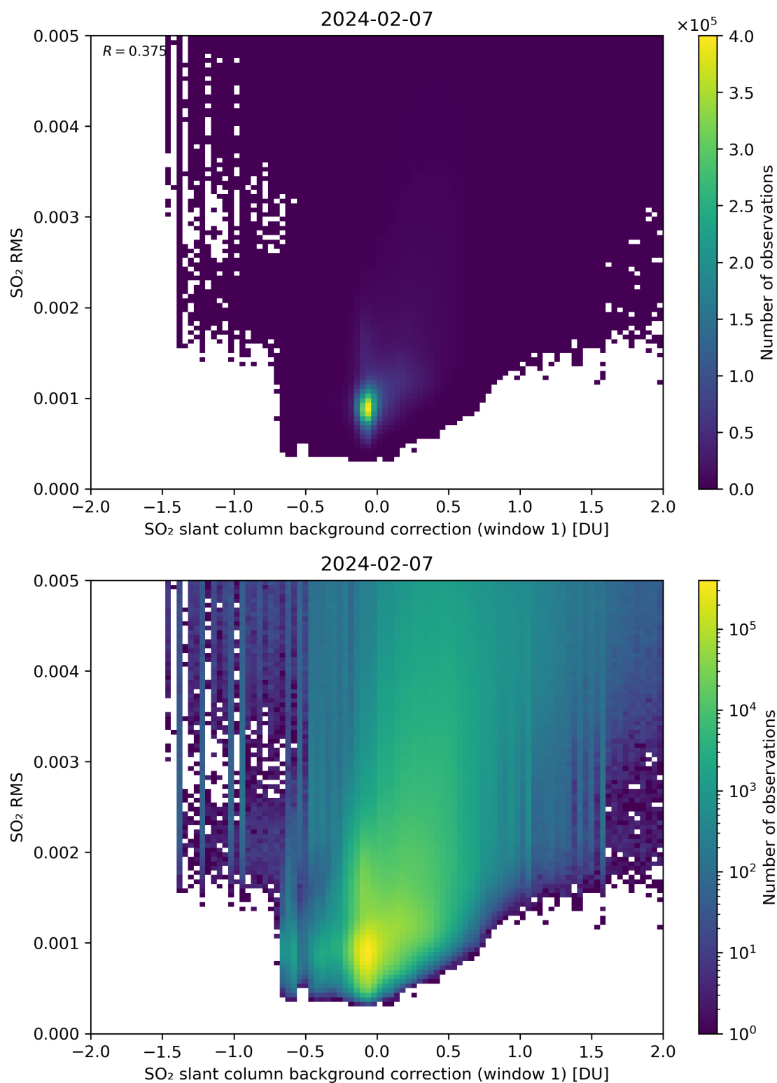
Figure 102: Scatter density plot of “SO 2 slant column background correction (window 1)” against “SO 2 RMS” for 2024-02-06 to 2024-02-08.
