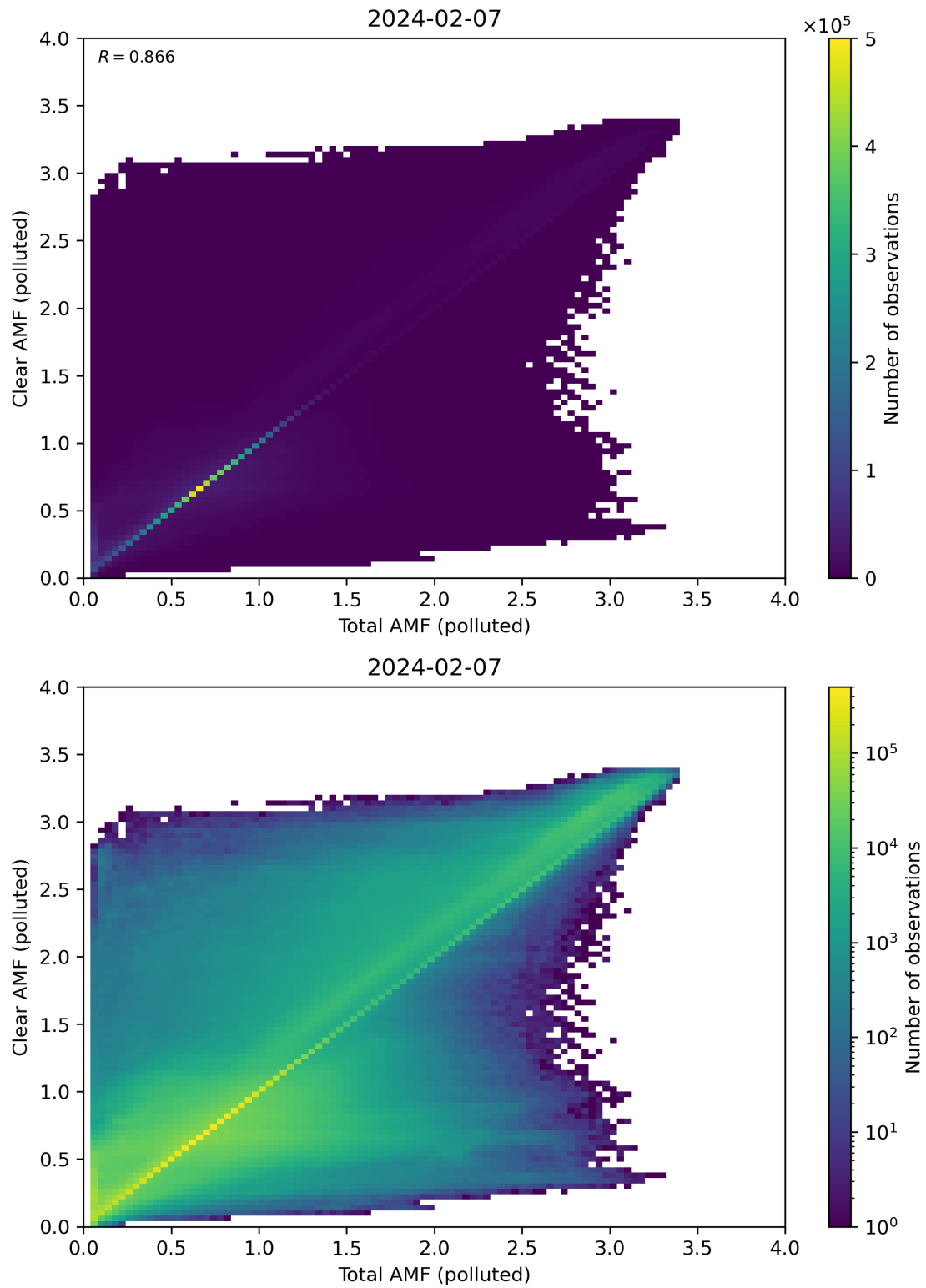
Figure 271: Scatter density plot of “Total AMF (polluted)” against “Clear AMF (polluted)” for 2024-02-06 to 2024-02-08.
