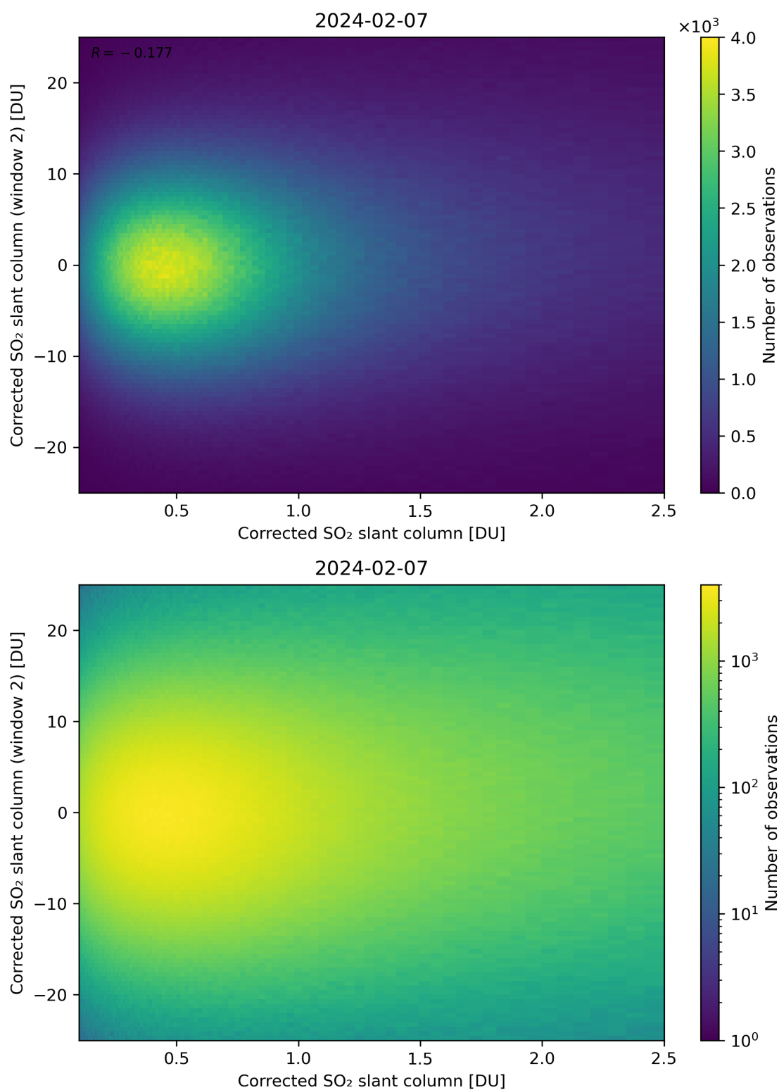
Figure 185: Scatter density plot of “Corrected SO 2 slant column” against “Corrected SO 2 slant column (window 2)” for 2024-02-06 to 2024-02-08.
