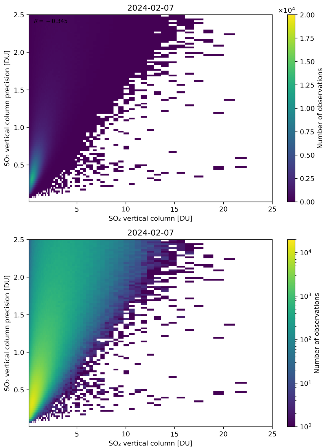
Figure 307: Scatter density plot of “SO 2 vertical column” against “SO 2 vertical column precision” for 2024-02-06 to 2024-02-08.
