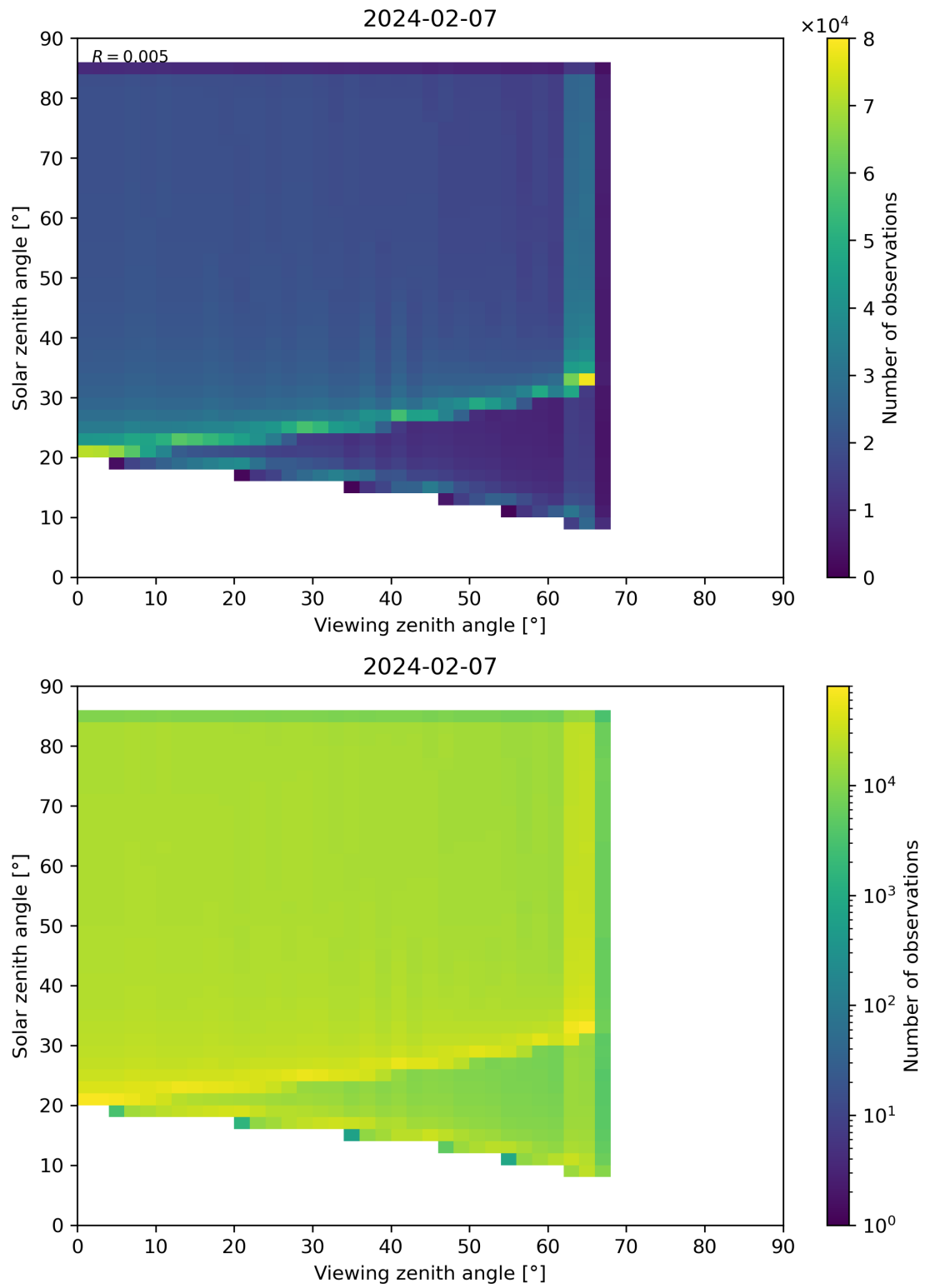
Figure 315: Scatter density plot of “Viewing zenith angle” against “Solar zenith angle” for 2024-02-06 to 2024-02-08.
