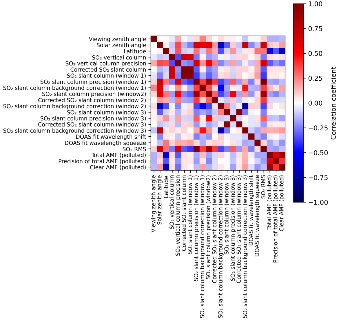
Figure 2: Map of correlation matrix for 2024-02-06 to 2024-02-08.
