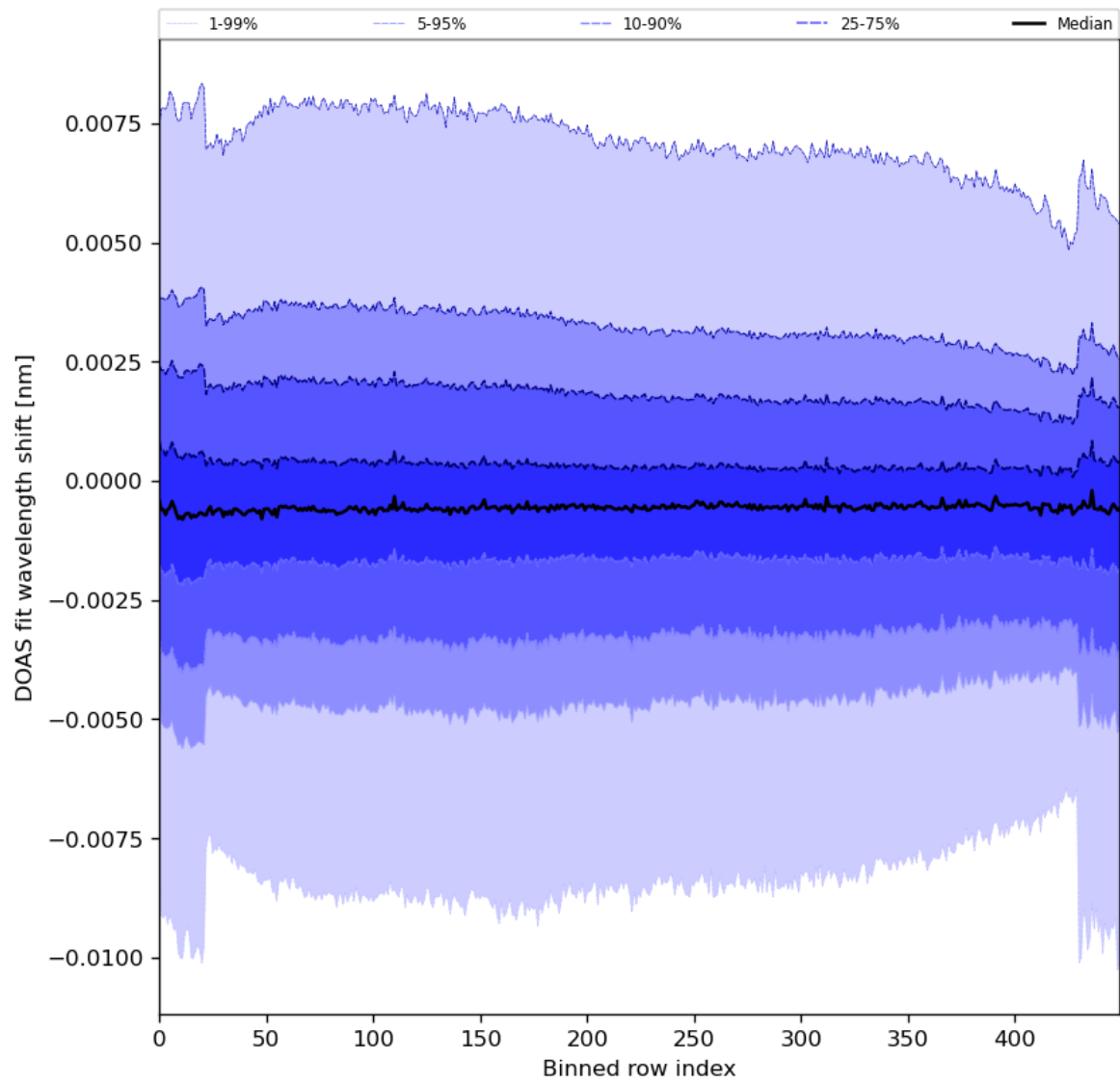
Figure 91: Along track statistics of “DOAS fit wavelength shift” for 2024-02-06 to 2024-02-08
