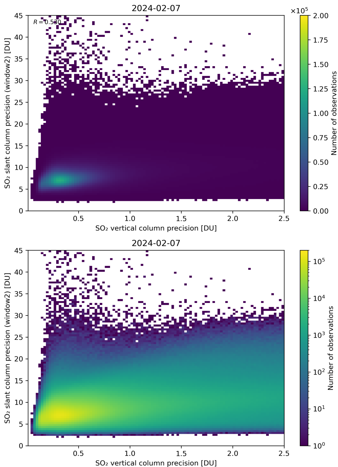
Figure 291: Scatter density plot of “SO 2 vertical column precision” against “SO 2 slant column precision (window2)” for 2024-02-06 to 2024-02-08.
