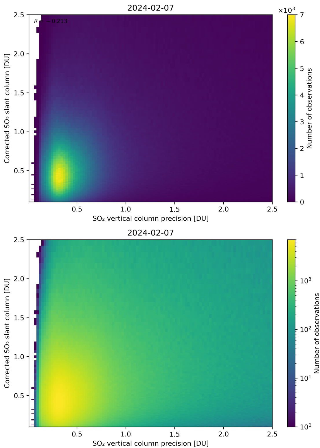
Figure 286: Scatter density plot of “SO 2 vertical column precision” against “Corrected SO 2 slant column” for 2024-02-06 to 2024-02-08.
