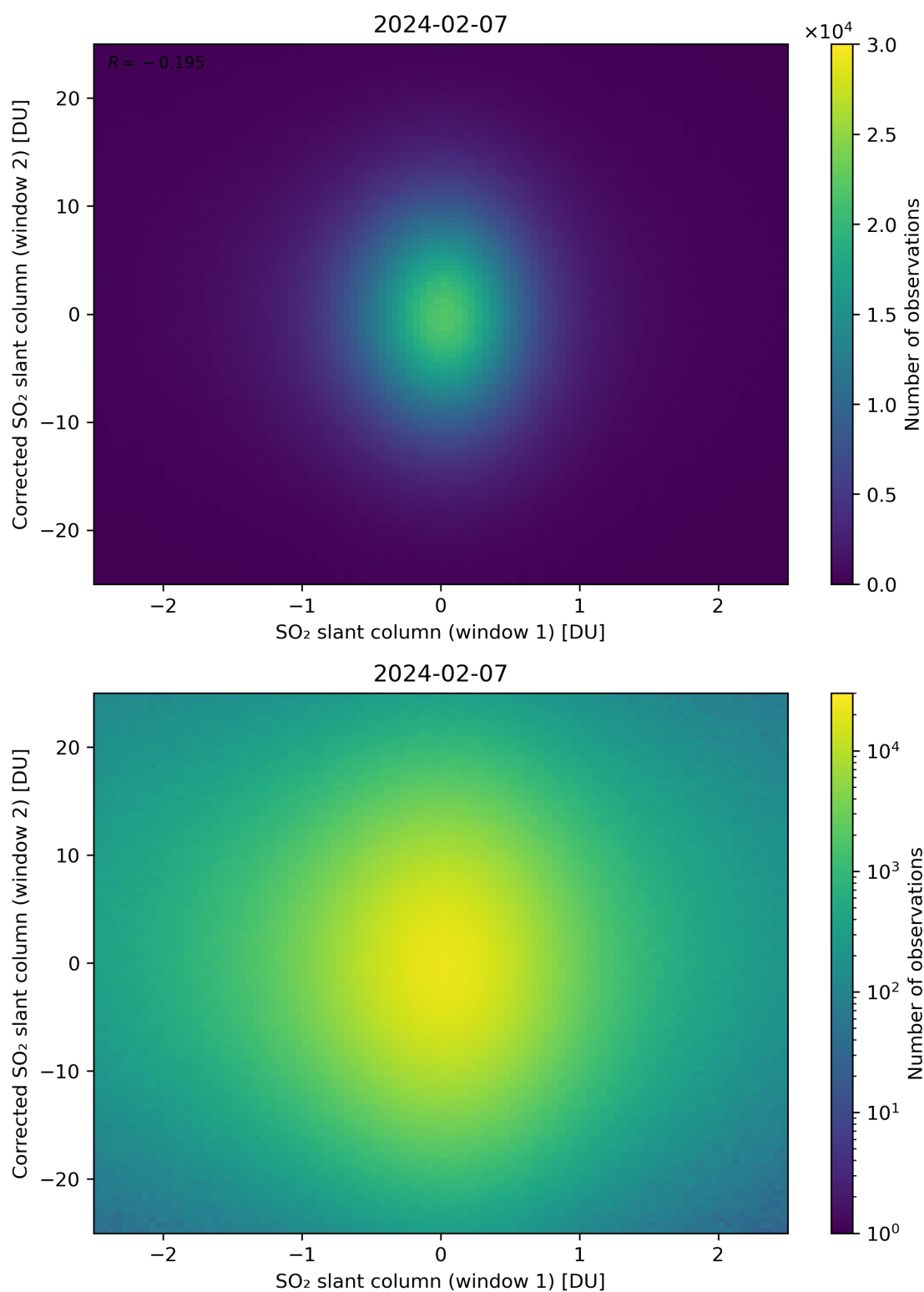
Figure 233: Scatter density plot of “SO 2 slant column (window 1)” against “Corrected SO 2 slant column (window 2)” for 2024-02-06 to 2024-02-08.
