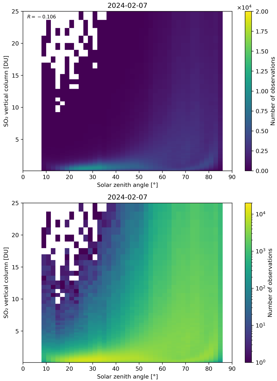
Figure 176: Scatter density plot of “Solar zenith angle” against “SO 2 vertical column” for 2024-02-06 to 2024-02-08.
