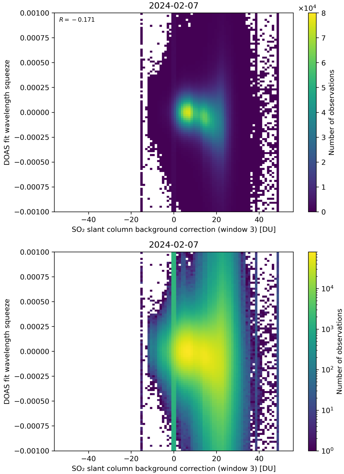
Figure 122: Scatter density plot of “SO 2 slant column background correction (window 3)” against “DOAS fit wavelength squeeze” for 2024-02-06 to 2024-02-08.
