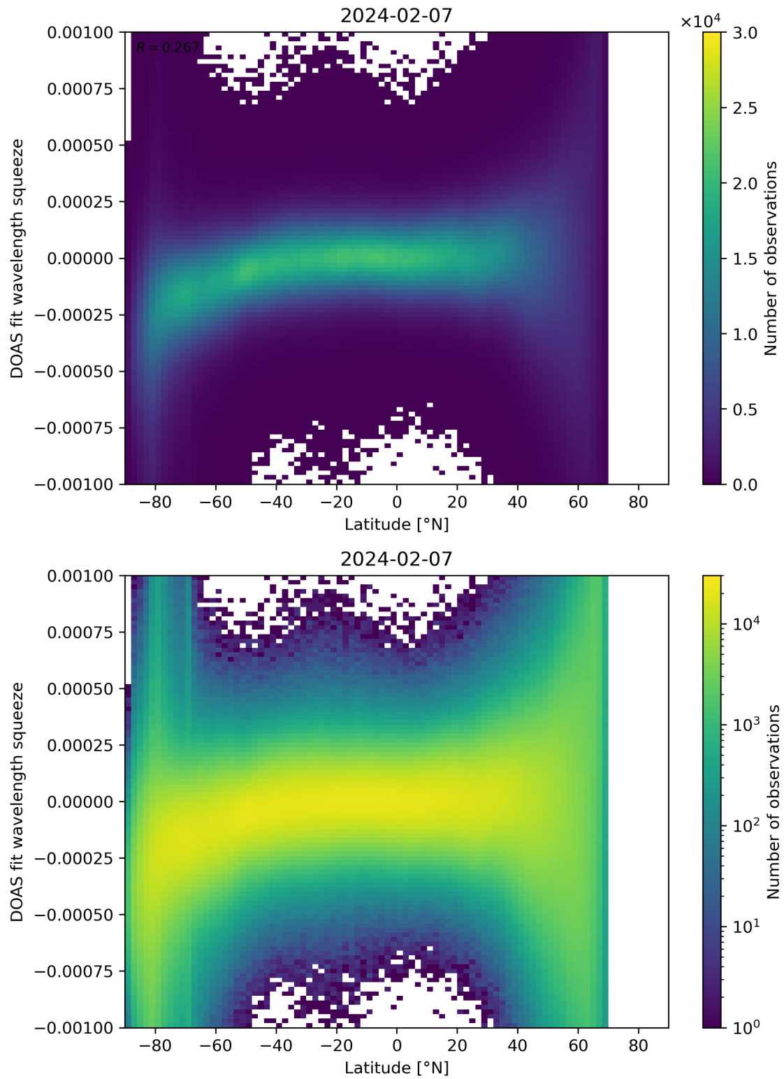
Figure 143: Scatter density plot of “Latitude” against “DOAS fit wavelength squeeze” for 2024-02-06 to 2024-02-08.
