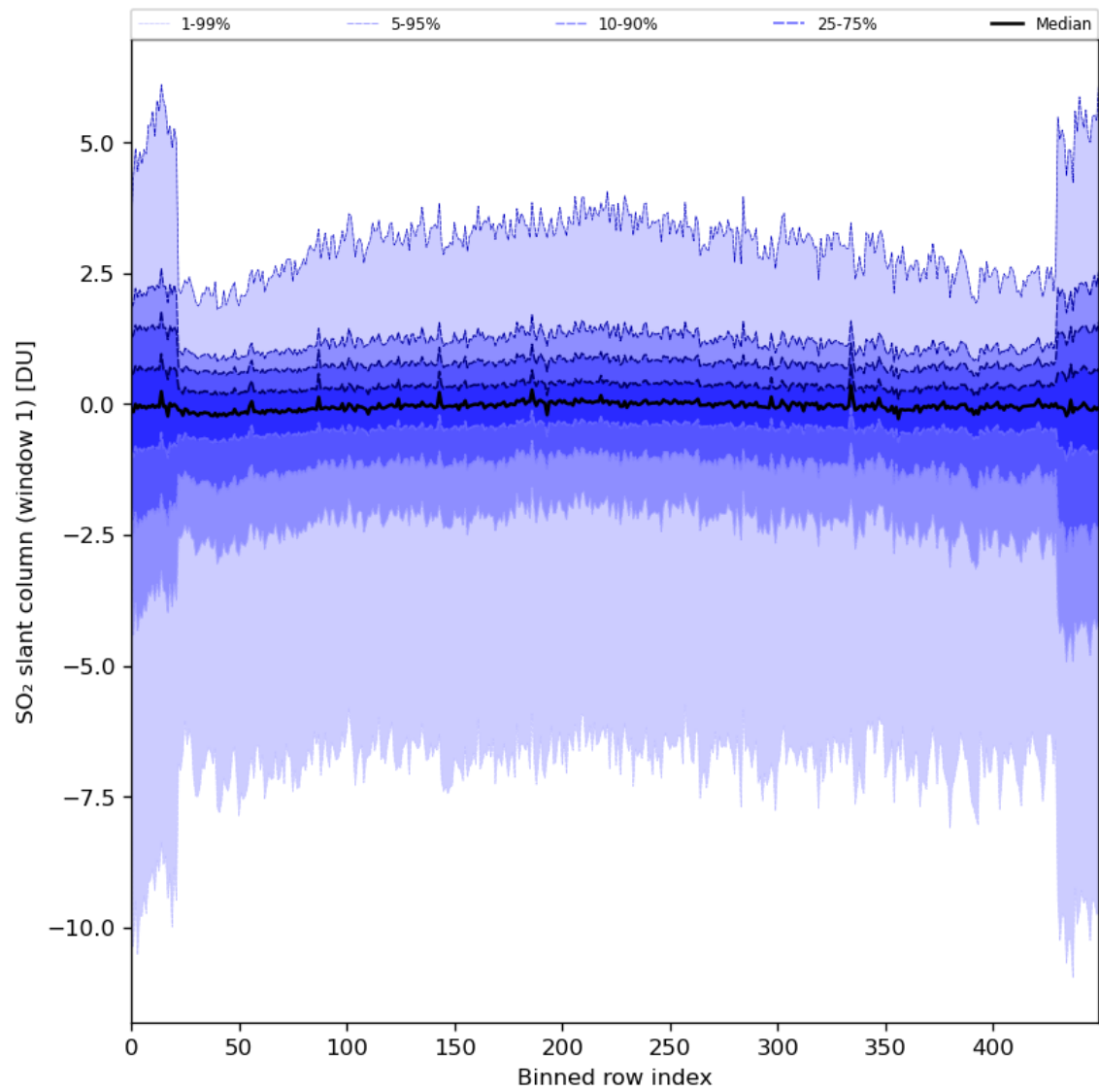
Figure 79: Along track statistics of “SO 2 slant column (window 1)” for 2024-02-06 to 2024-02-08
