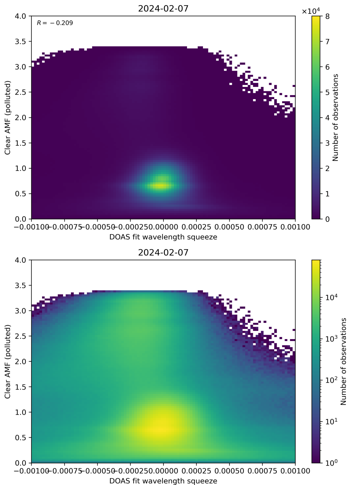
Figure 133: Scatter density plot of “DOAS fit wavelength squeeze” against “Clear AMF (polluted)” for 2024-02-06 to 2024-02-08.
