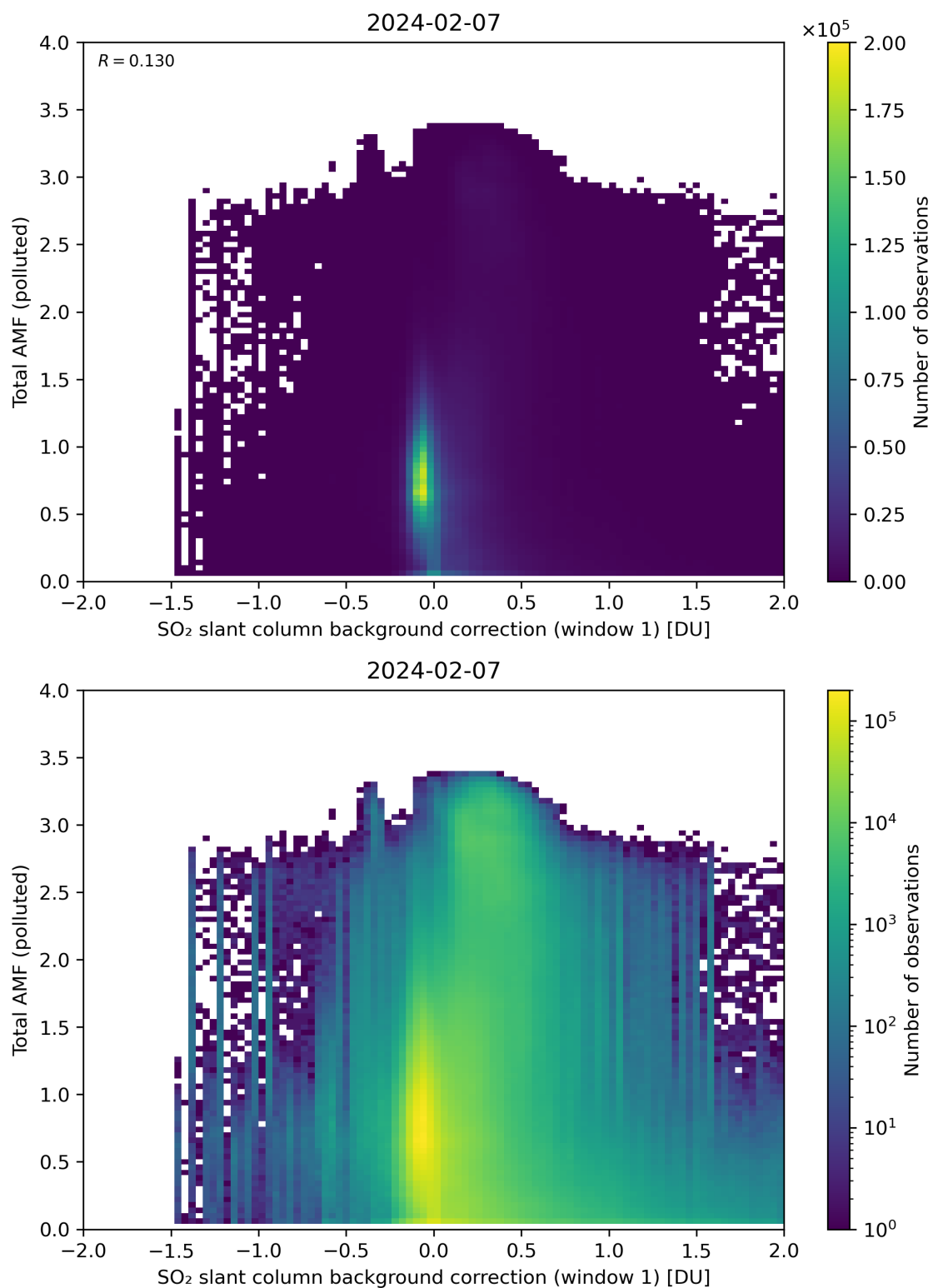
Figure 109: Scatter density plot of “SO 2 slant column background correction (window 1)” against “Total AMF (polluted)” for 2024-02-06 to 2024-02-08.
