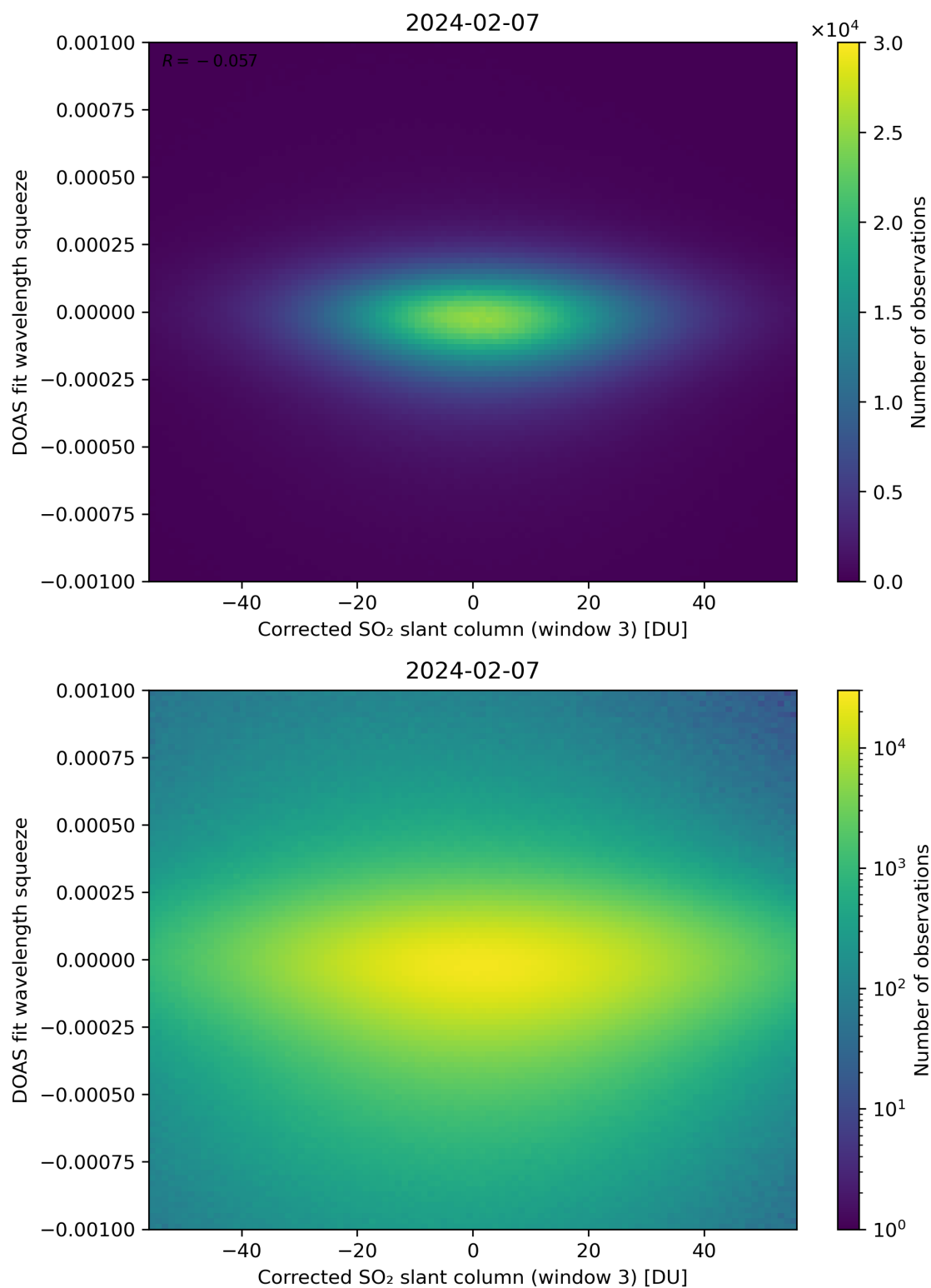
Figure 207: Scatter density plot of “Corrected SO 2 slant column (window 3)” against “DOAS fit wavelength squeeze” for 2024-02-06 to 2024-02-08.
