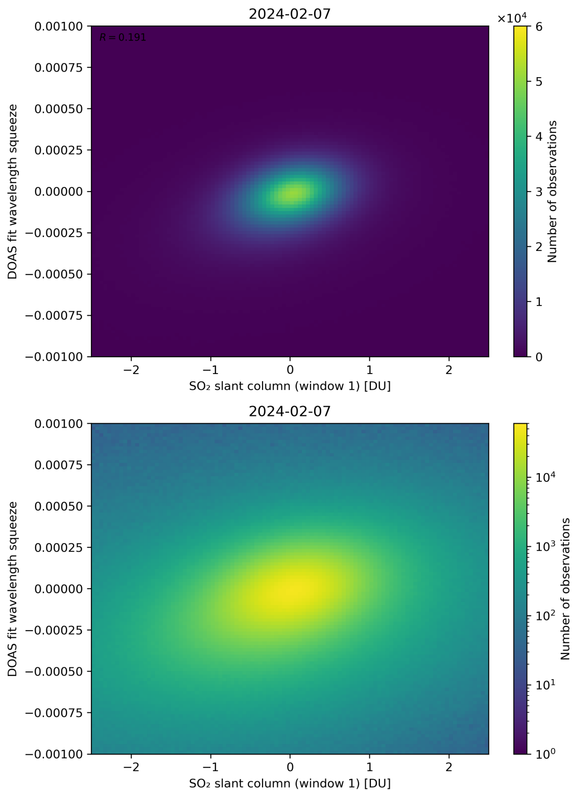
Figure 216: Scatter density plot of “SO 2 slant column (window 1)” against “DOAS fit wavelength squeeze” for 2024-02-06 to 2024-02-08.
