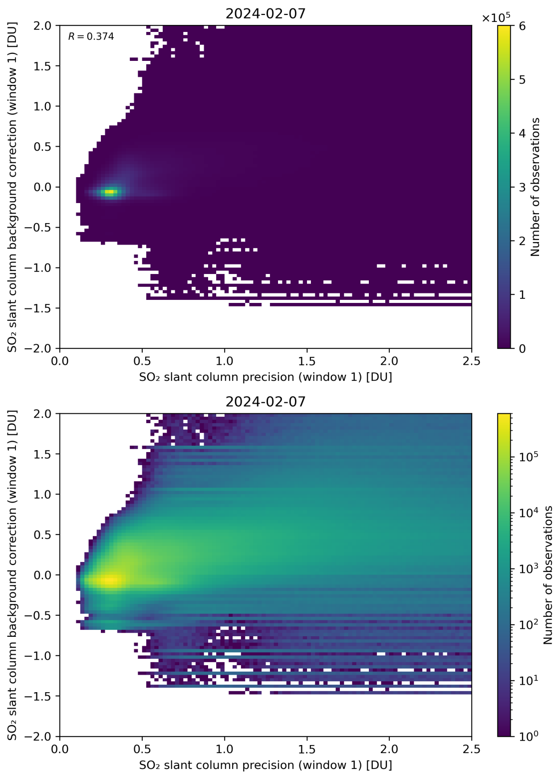
Figure 218: Scatter density plot of “SO 2 slant column precision (window 1)” against “SO 2 slant column background correction (window 1)” for 2024-02-06 to 2024-02-08.
