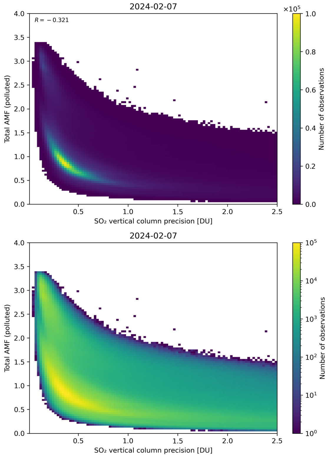
Figure 294: Scatter density plot of “SO 2 vertical column precision” against “Total AMF (polluted)” for 2024-02-06 to 2024-02-08.
