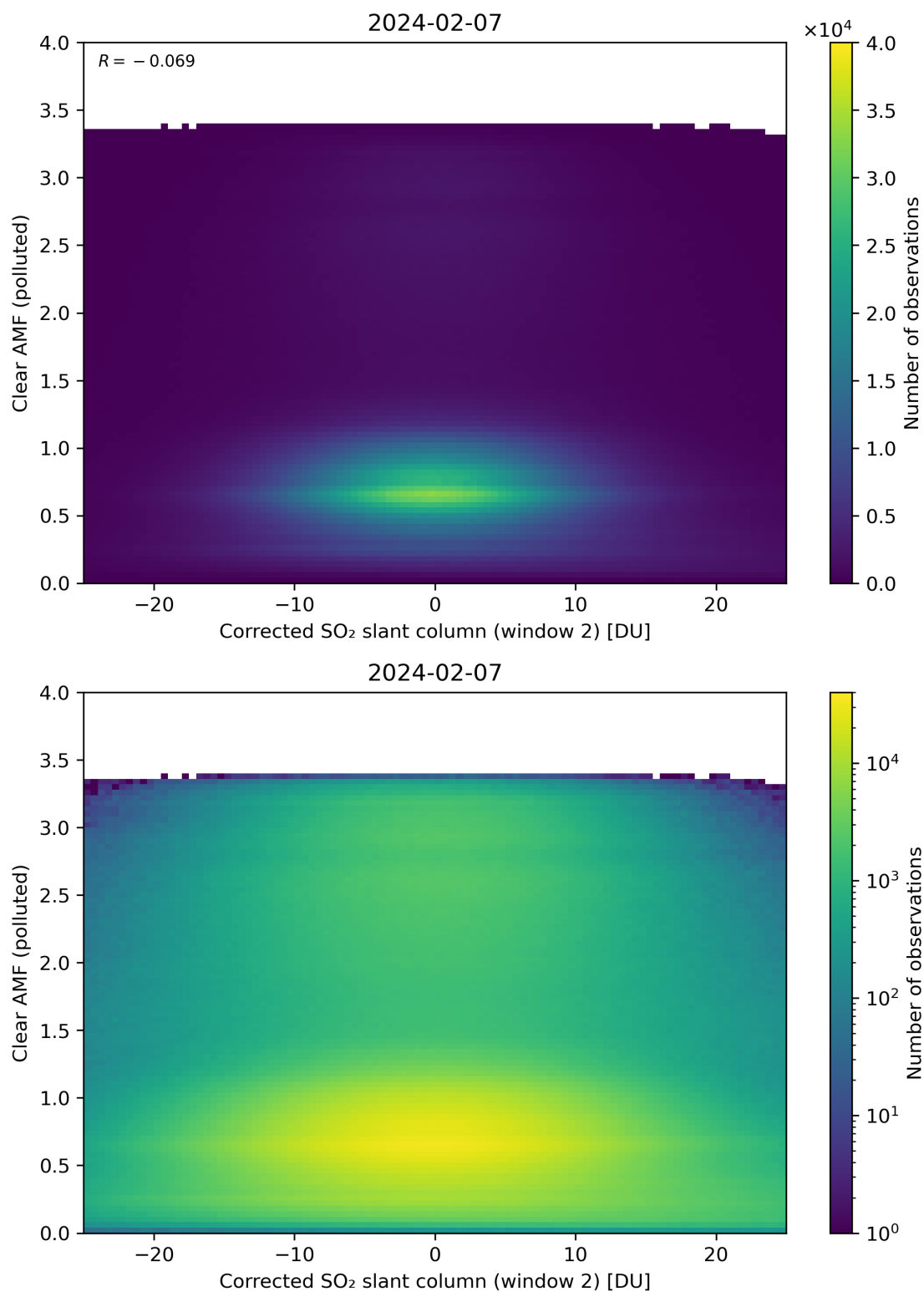
Figure 199: Scatter density plot of “Corrected SO 2 slant column (window 2)” against “Clear AMF (polluted)” for 2024-02-06 to 2024-02-08.
