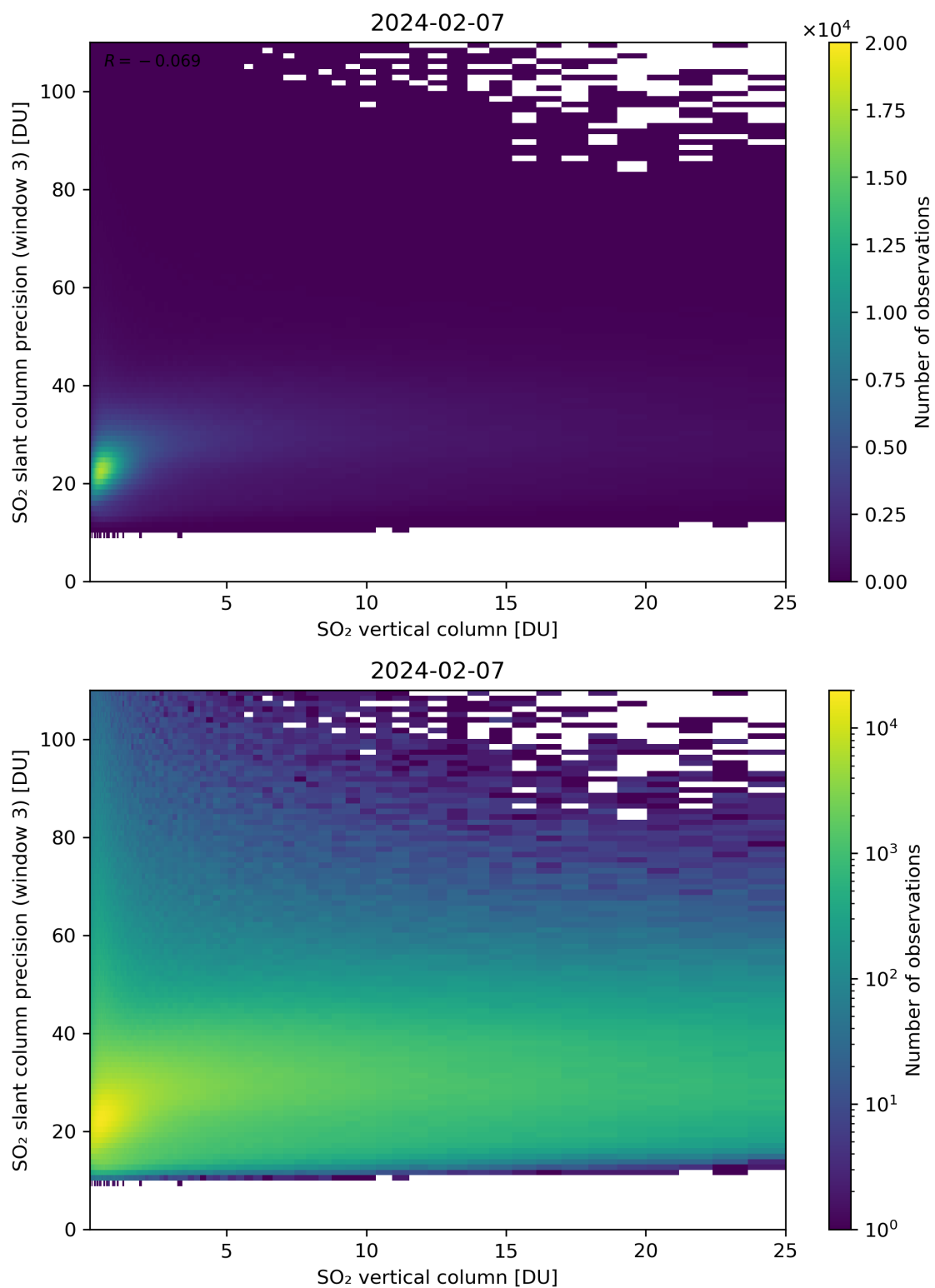
Figure 304: Scatter density plot of “SO 2 vertical column” against “SO 2 slant column precision (window 3)” for 2024-02-06 to 2024-02-08.
