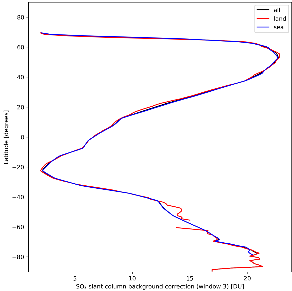
Figure 44: Zonal average of “SO 2 slant column background correction (window 3)” for 2024-02-06 to 2024-02-08.
