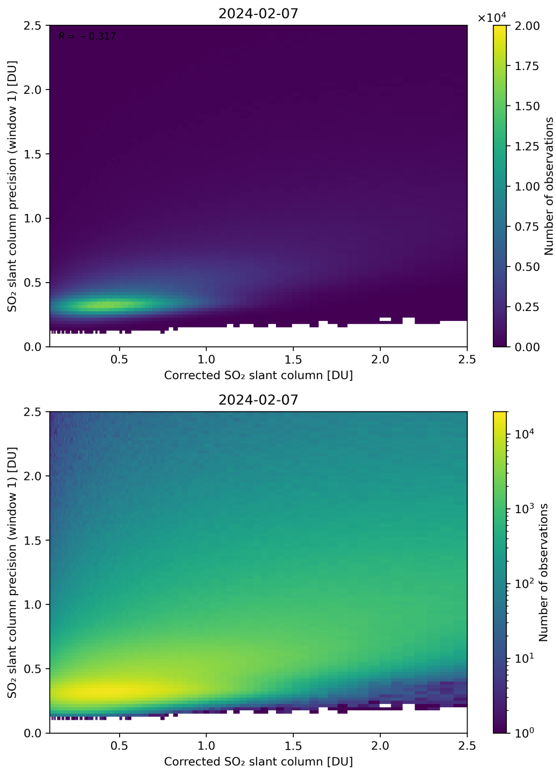
Figure 188: Scatter density plot of “Corrected SO 2 slant column” against “SO 2 slant column precision (window 1)” for 2024-02-06 to 2024-02-08.
