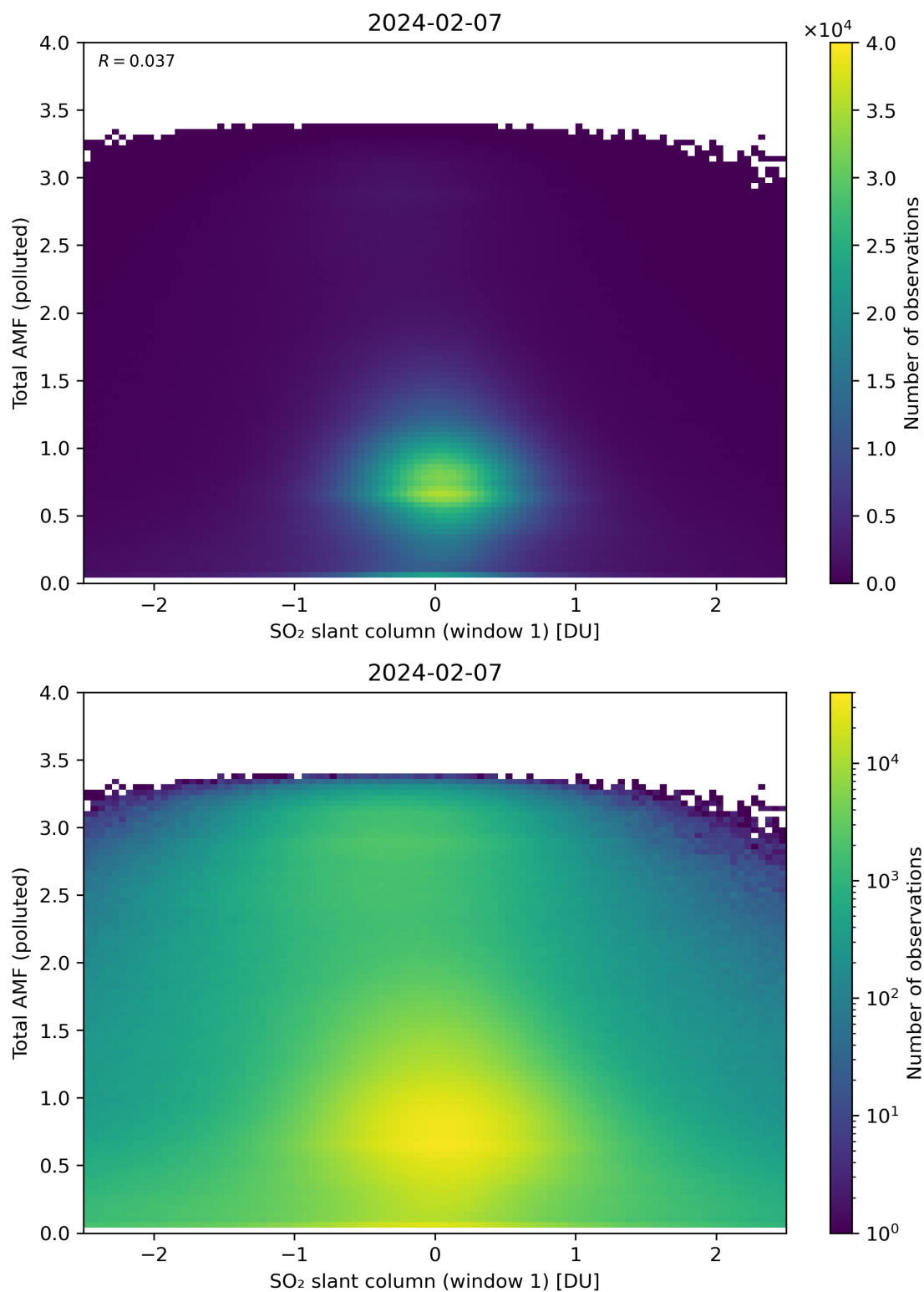
Figure 239: Scatter density plot of “SO 2 slant column (window 1)” against “Total AMF (polluted)” for 2024-02-06 to 2024-02-08.
