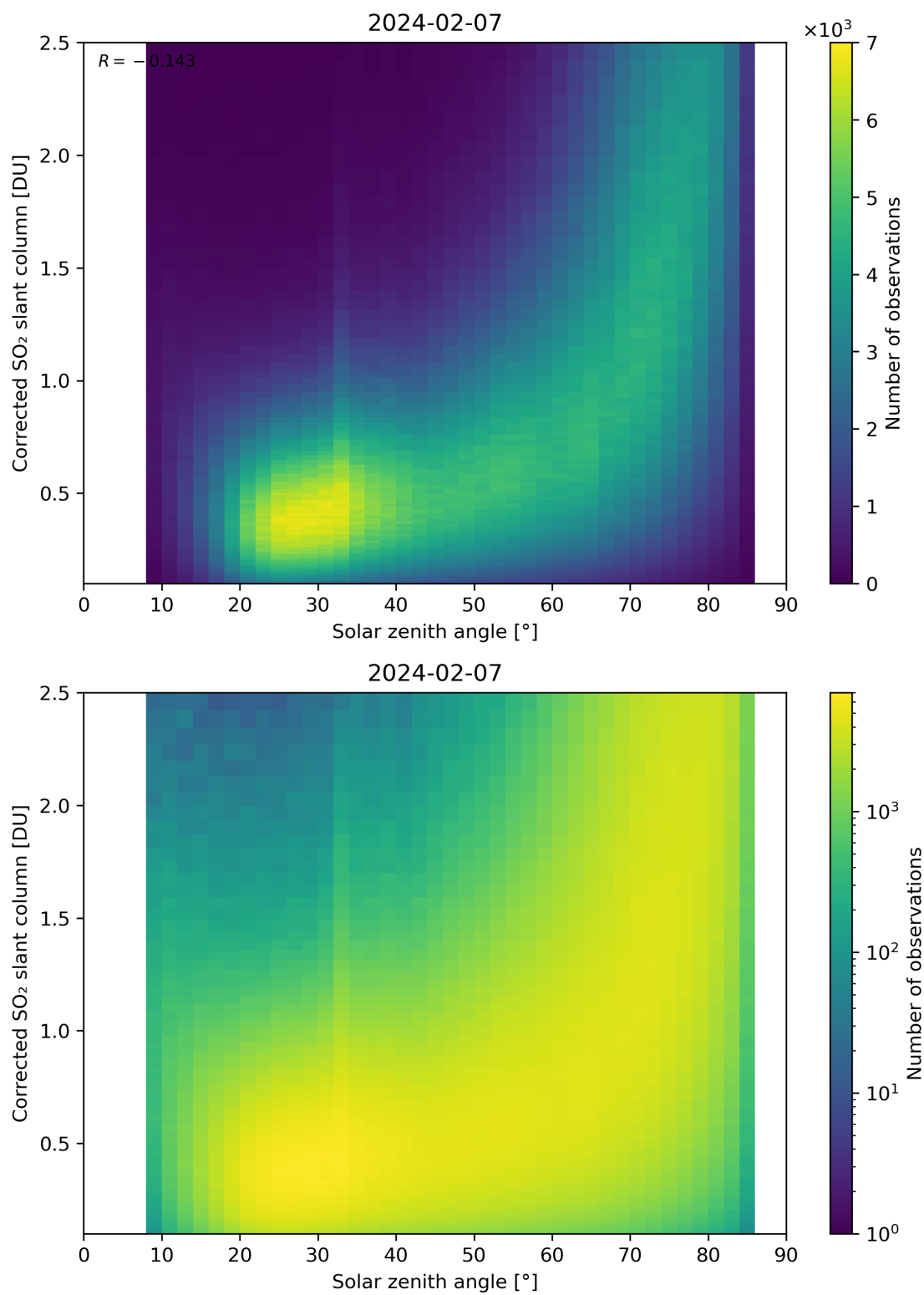
Figure 166: Scatter density plot of “Solar zenith angle” against “Corrected SO 2 slant column” for 2024-02-06 to 2024-02-08.
