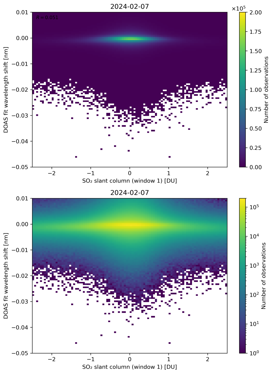
Figure 215: Scatter density plot of “SO 2 slant column (window 1)” against “DOAS fit wavelength shift” for 2024-02-06 to 2024-02-08.
