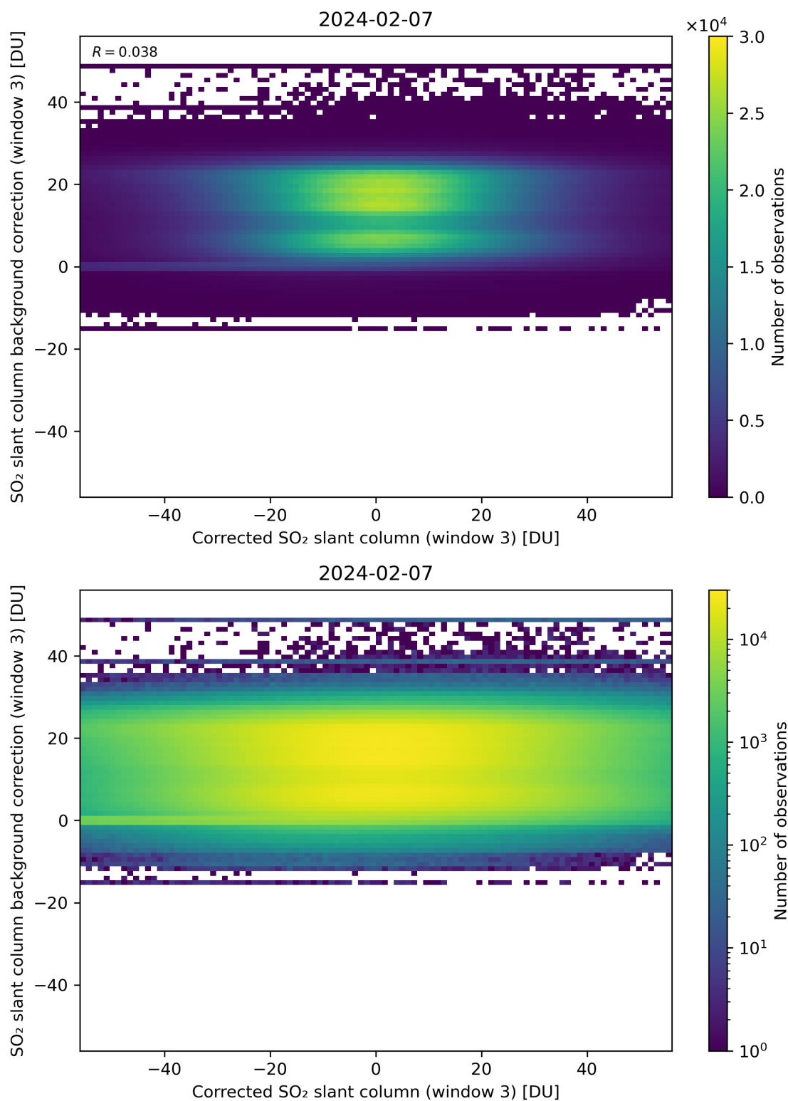
Figure 205: Scatter density plot of “Corrected SO 2 slant column (window 3)” against “SO 2 slant column background correction (window 3)” for 2024-02-06 to 2024-02-08.
