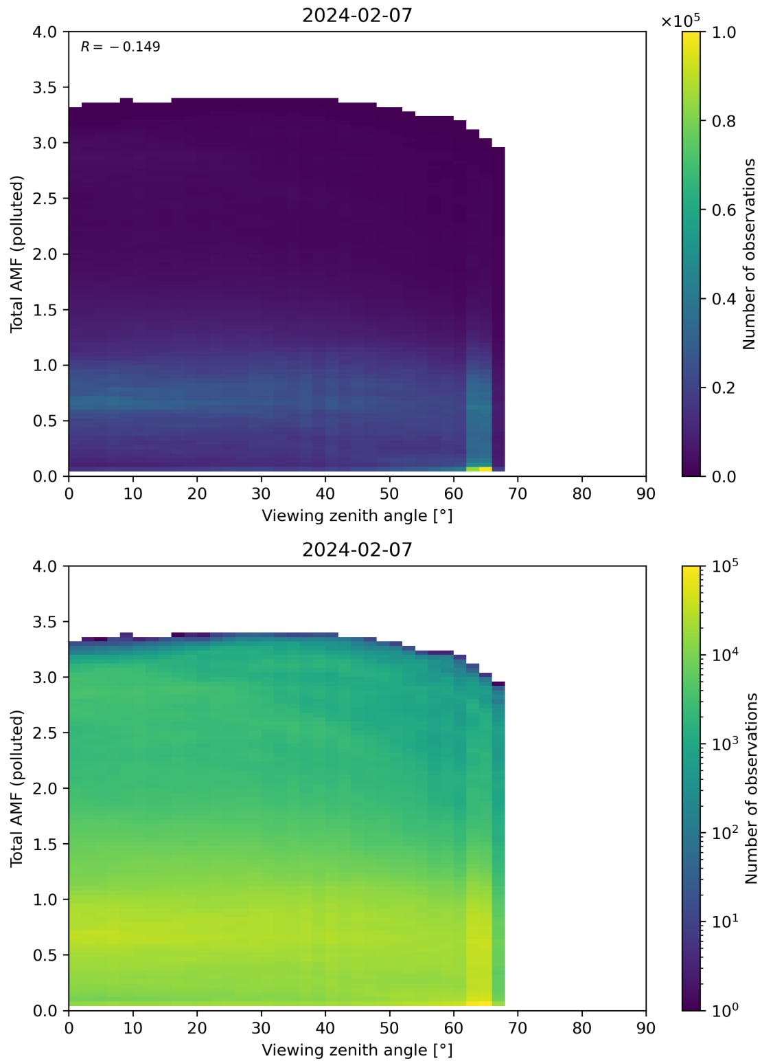
Figure 325: Scatter density plot of “Viewing zenith angle” against “Total AMF (polluted)” for 2024-02-06 to 2024-02-08.
