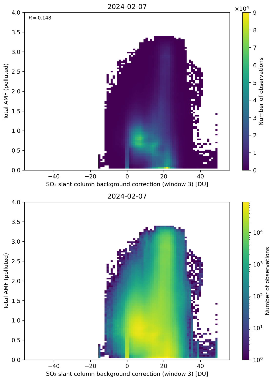
Figure 125: Scatter density plot of “SO 2 slant column background correction (window 3)” against “Total AMF (polluted)” for 2024-02-06 to 2024-02-08.
