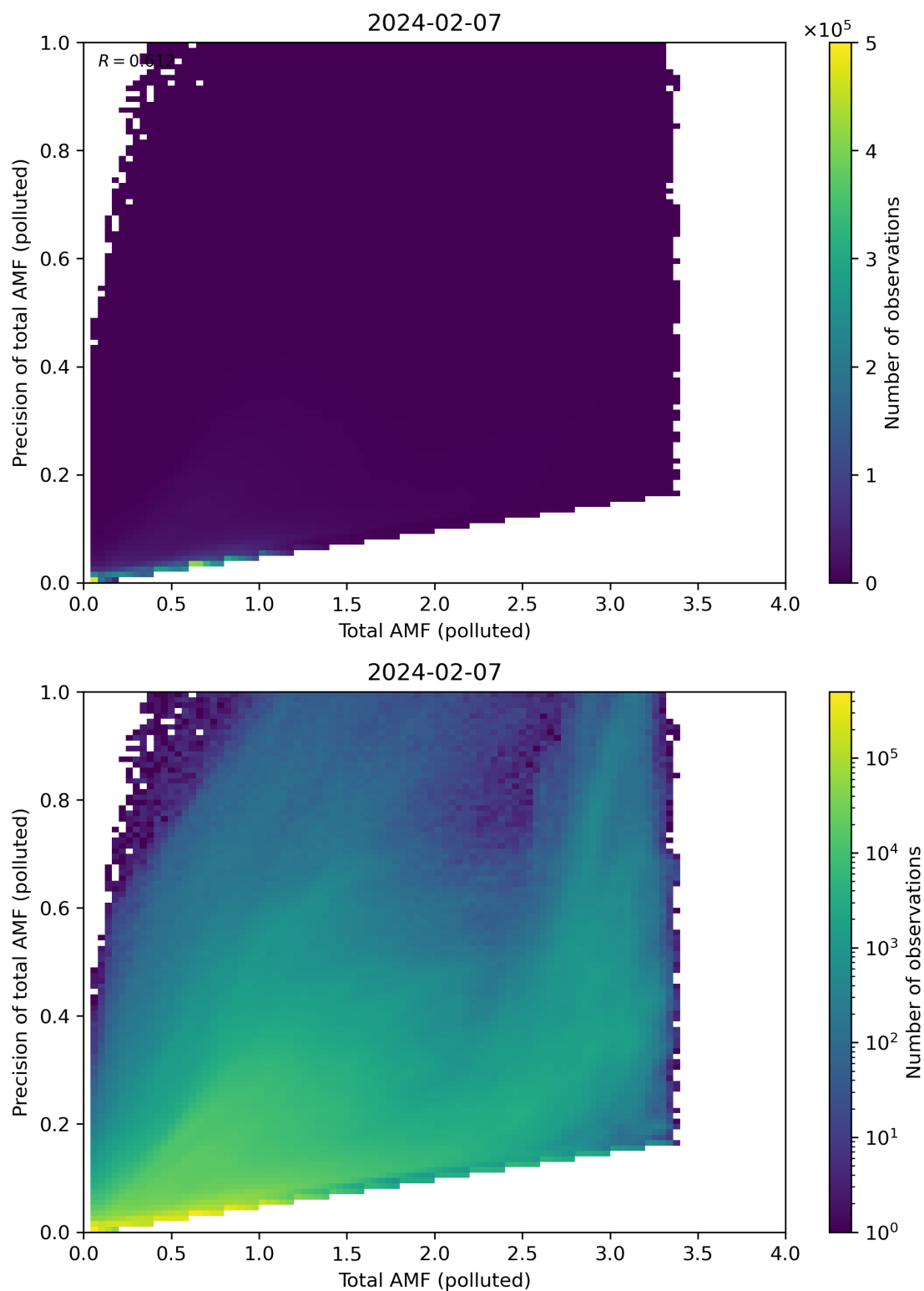
Figure 272: Scatter density plot of “Total AMF (polluted)” against “Precision of total AMF (polluted)” for 2024-02-06 to 2024-02-08.
