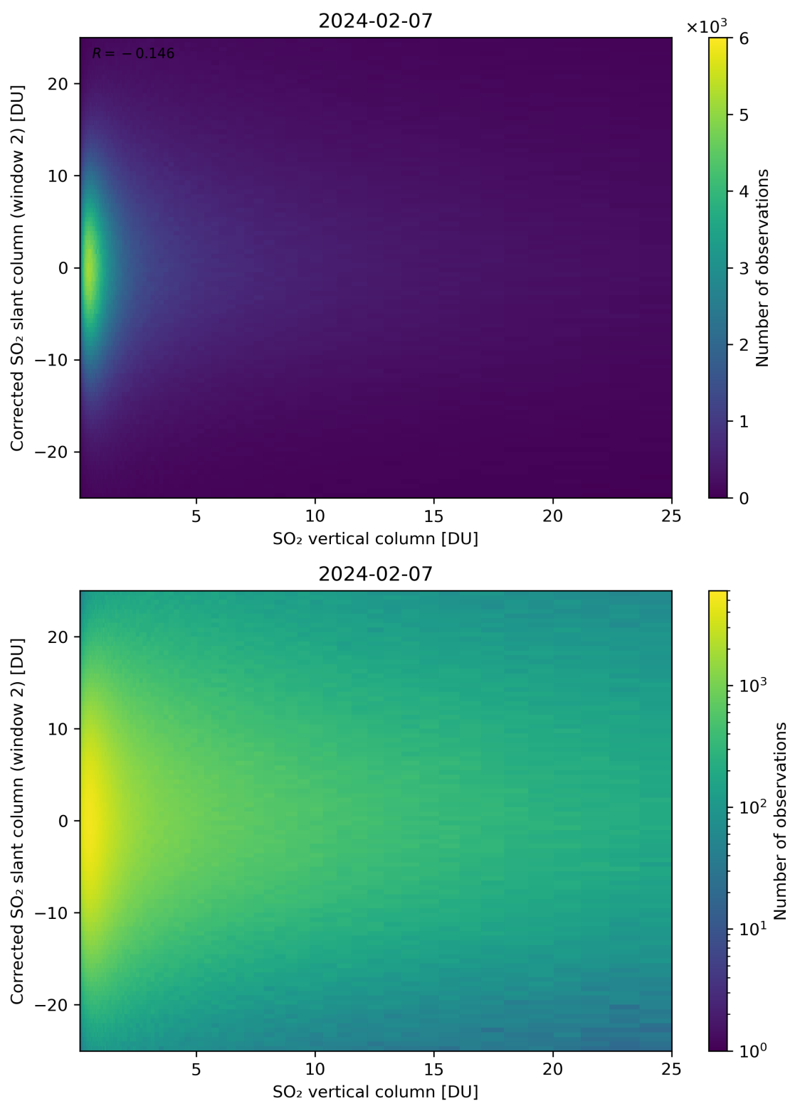
Figure 298: Scatter density plot of “SO 2 vertical column” against “Corrected SO 2 slant column (window 2)” for 2024-02-06 to 2024-02-08.
