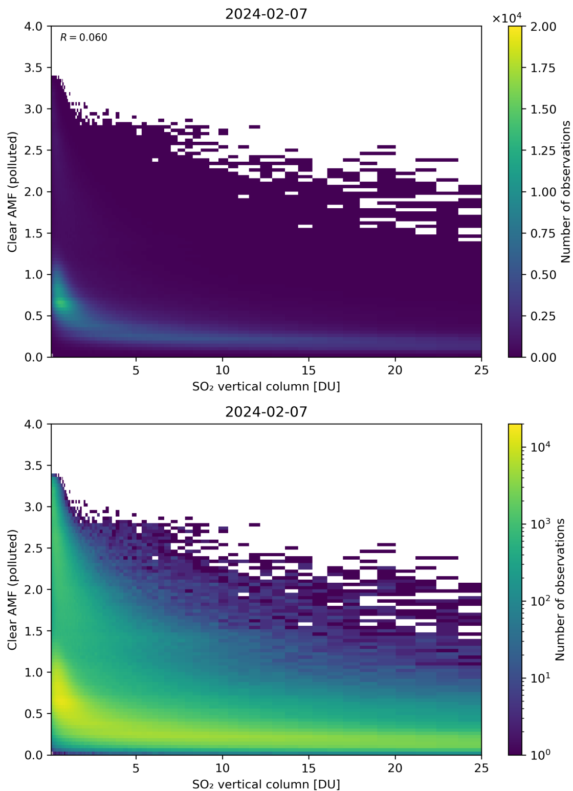
Figure 296: Scatter density plot of “SO 2 vertical column” against “Clear AMF (polluted)” for 2024-02-06 to 2024-02-08.
