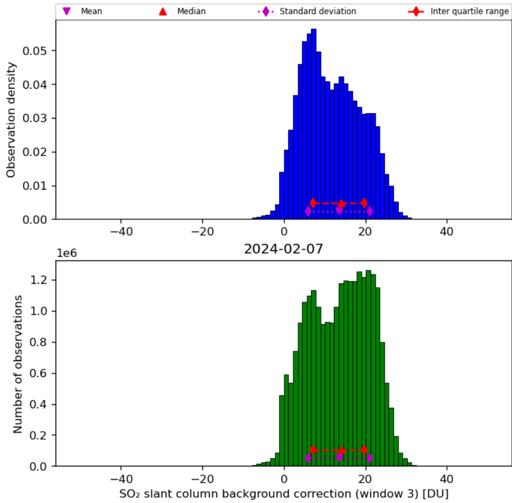
Figure 67: Histogram of “SO 2 slant column background correction (window 3)” for 2024-02-06 to 2024-02-08
