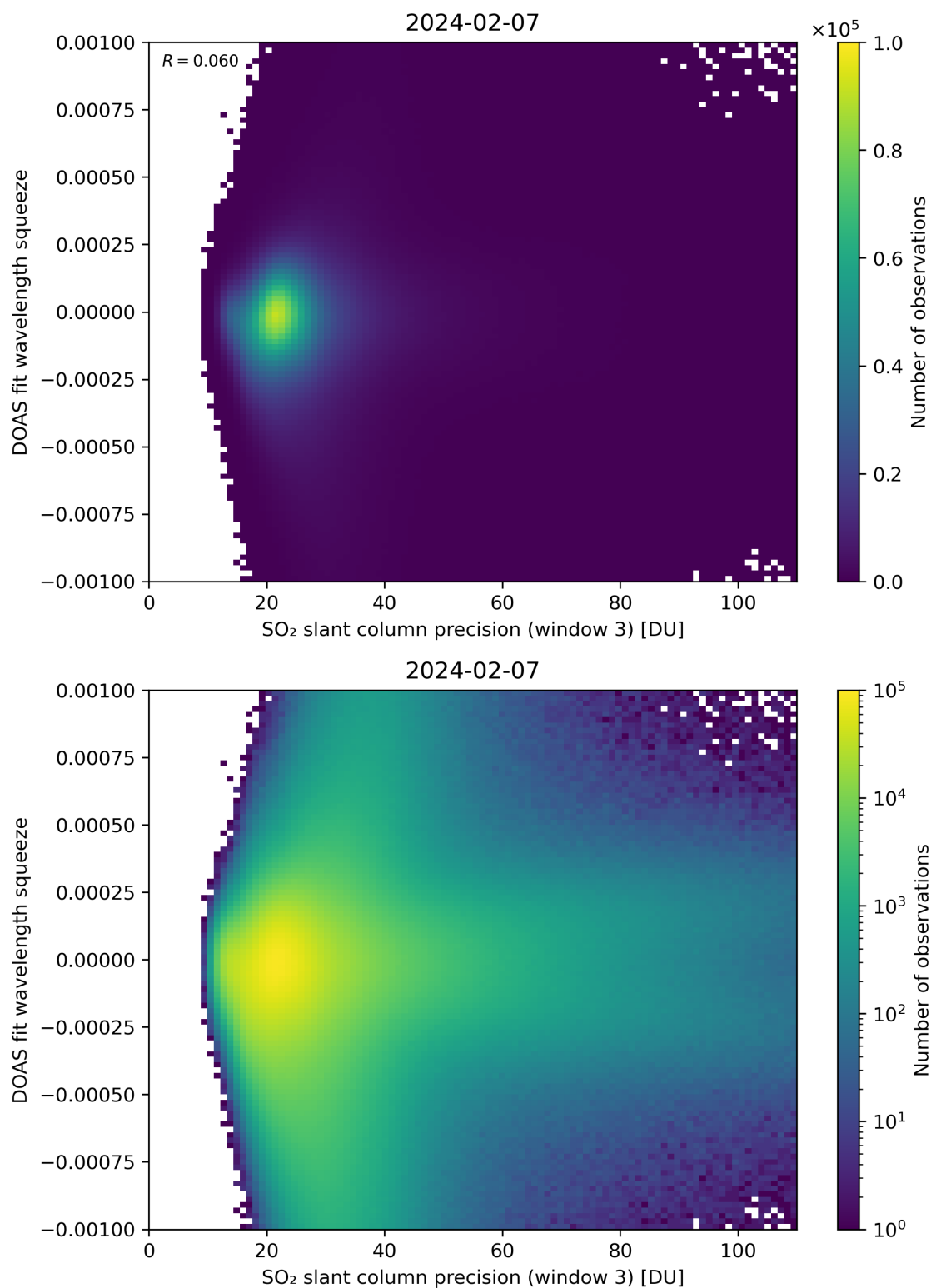
Figure 259: Scatter density plot of “SO 2 slant column precision (window 3)” against “DOAS fit wavelength squeeze” for 2024-02-06 to 2024-02-08.
