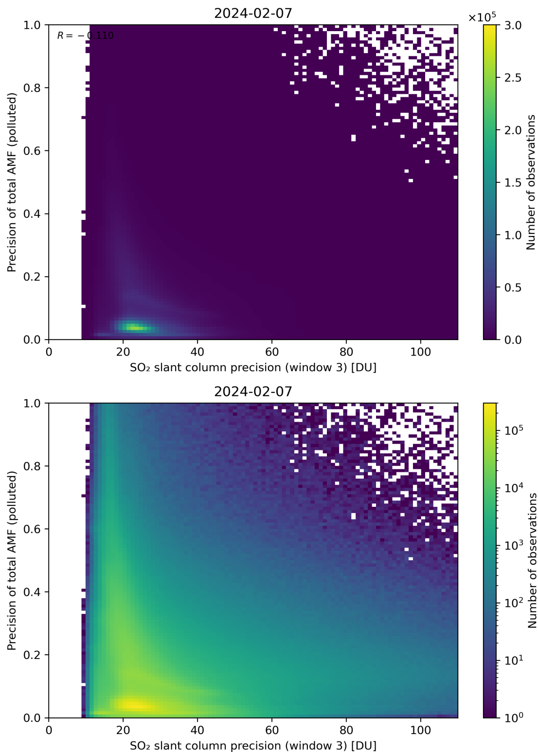
Figure 264: Scatter density plot of “SO 2 slant column precision (window 3)” against “Precision of total AMF (polluted)” for 2024-02-06 to 2024-02-08.
