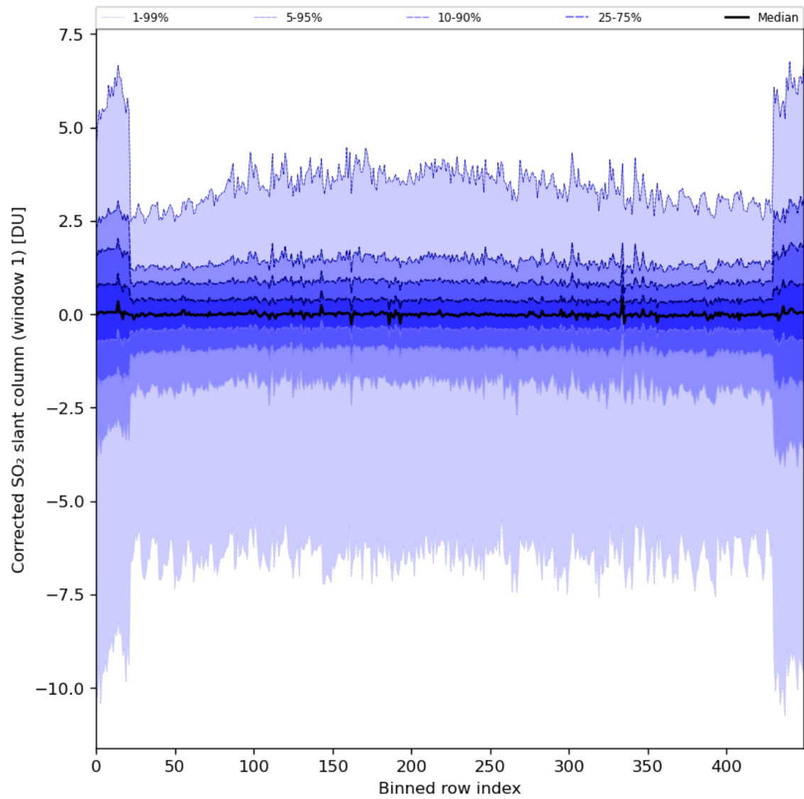
Figure 81: Along track statistics of “Corrected SO 2 slant column (window 1)” for 2024-02-06 to 2024-02-08
