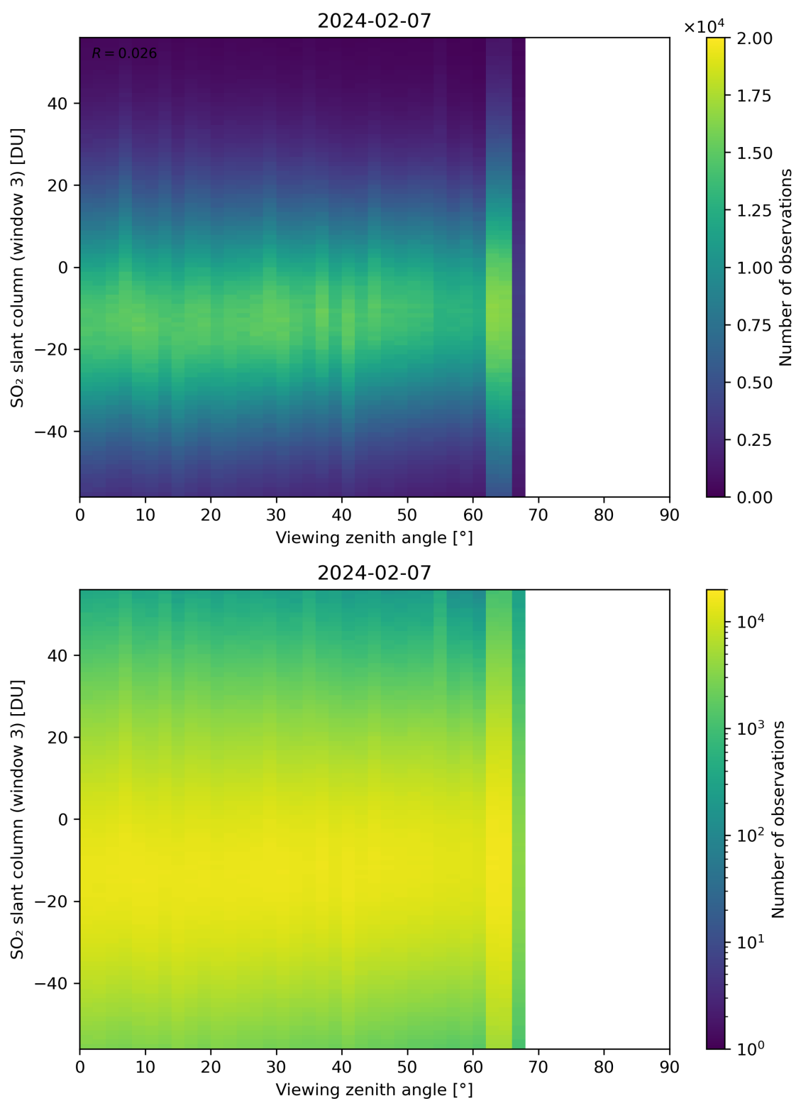
Figure 323: Scatter density plot of “Viewing zenith angle” against “SO 2 slant column (window 3)” for 2024-02-06 to 2024-02-08.
