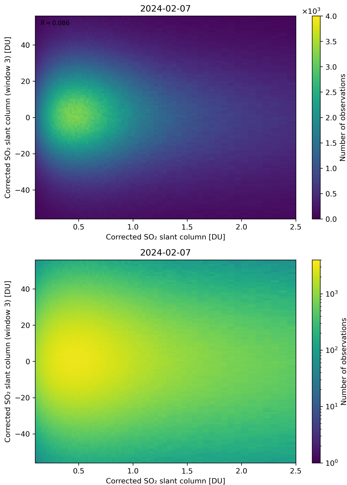
Figure 186: Scatter density plot of “Corrected SO 2 slant column” against “Corrected SO 2 slant column (window 3)” for 2024-02-06 to 2024-02-08.
