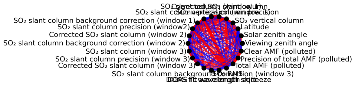
Figure 1: Map of correlation graph for 2024-02-06 to 2024-02-08.
