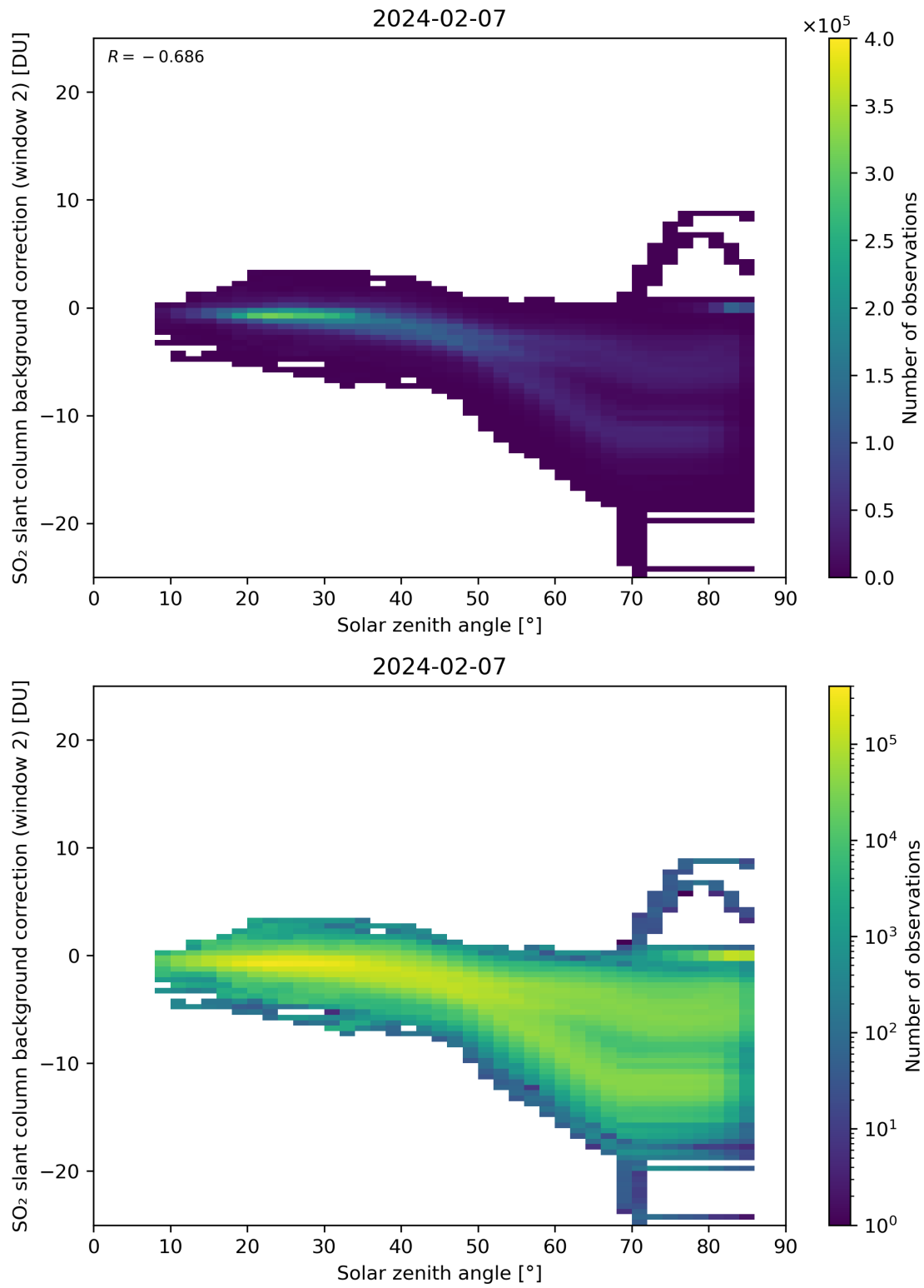
Figure 159: Scatter density plot of “Solar zenith angle” against “SO 2 slant column background correction (window 2)” for 2024-02-06 to 2024-02-08.
