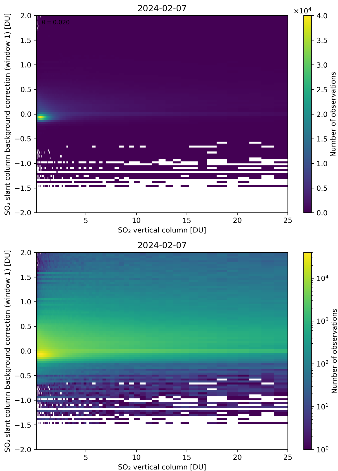
Figure 273: Scatter density plot of “SO 2 vertical column” against “SO 2 slant column background correction (window 1)” for 2024-02-06 to 2024-02-08.
