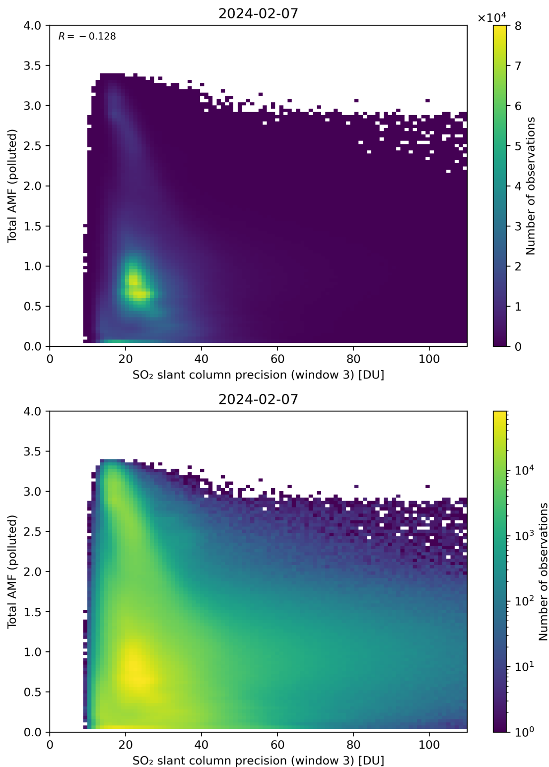
Figure 263: Scatter density plot of “SO 2 slant column precision (window 3)” against “Total AMF (polluted)” for 2024-02-06 to 2024-02-08.
