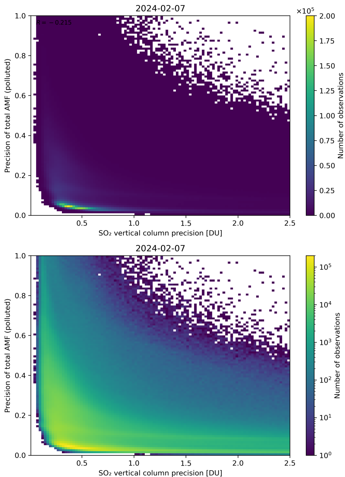
Figure 295: Scatter density plot of “SO 2 vertical column precision” against “Precision of total AMF (polluted)” for 2024-02-06 to 2024-02-08.
