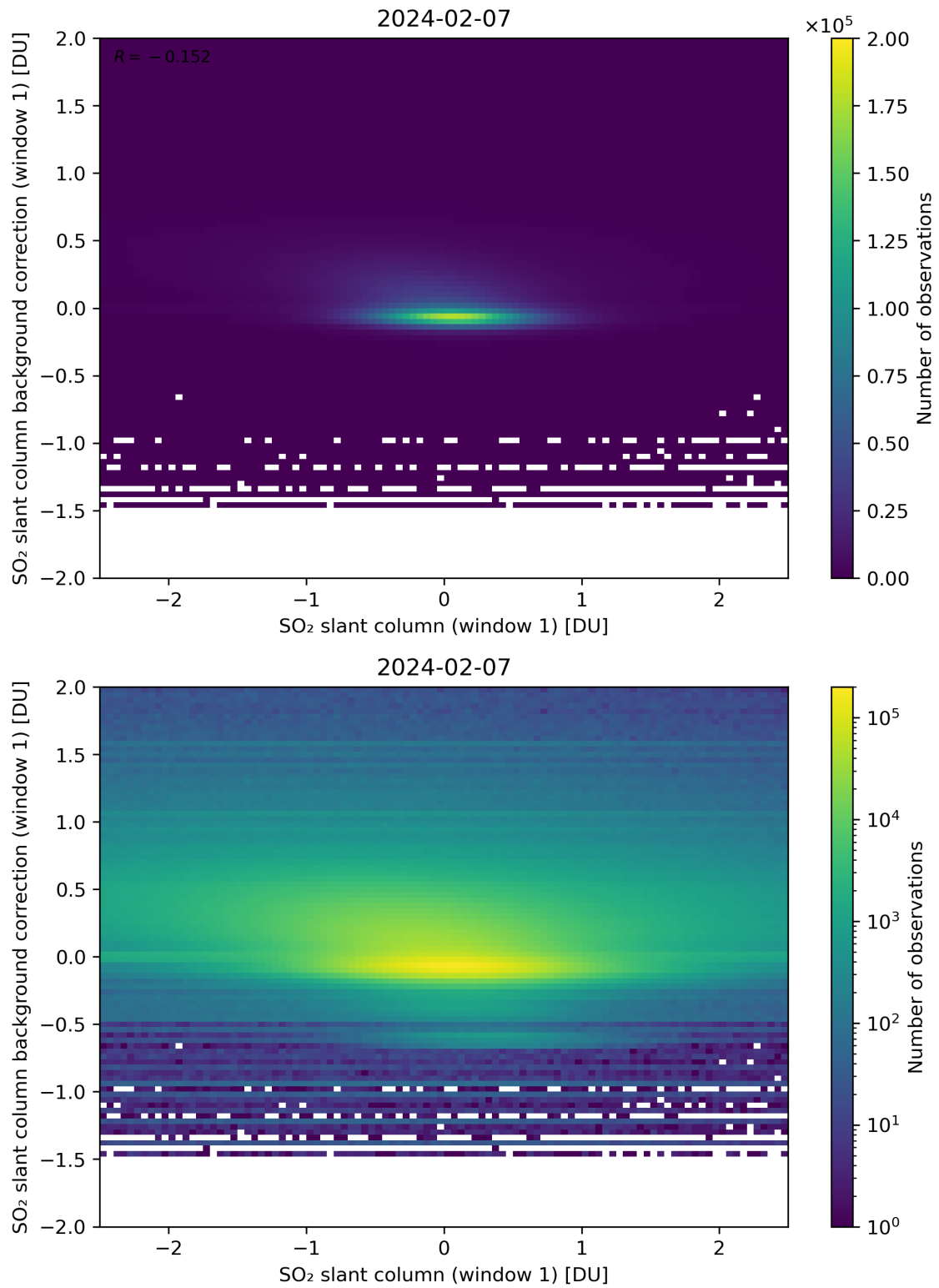
Figure 212: Scatter density plot of “SO 2 slant column (window 1)” against “SO 2 slant column background correction (window 1)” for 2024-02-06 to 2024-02-08.
