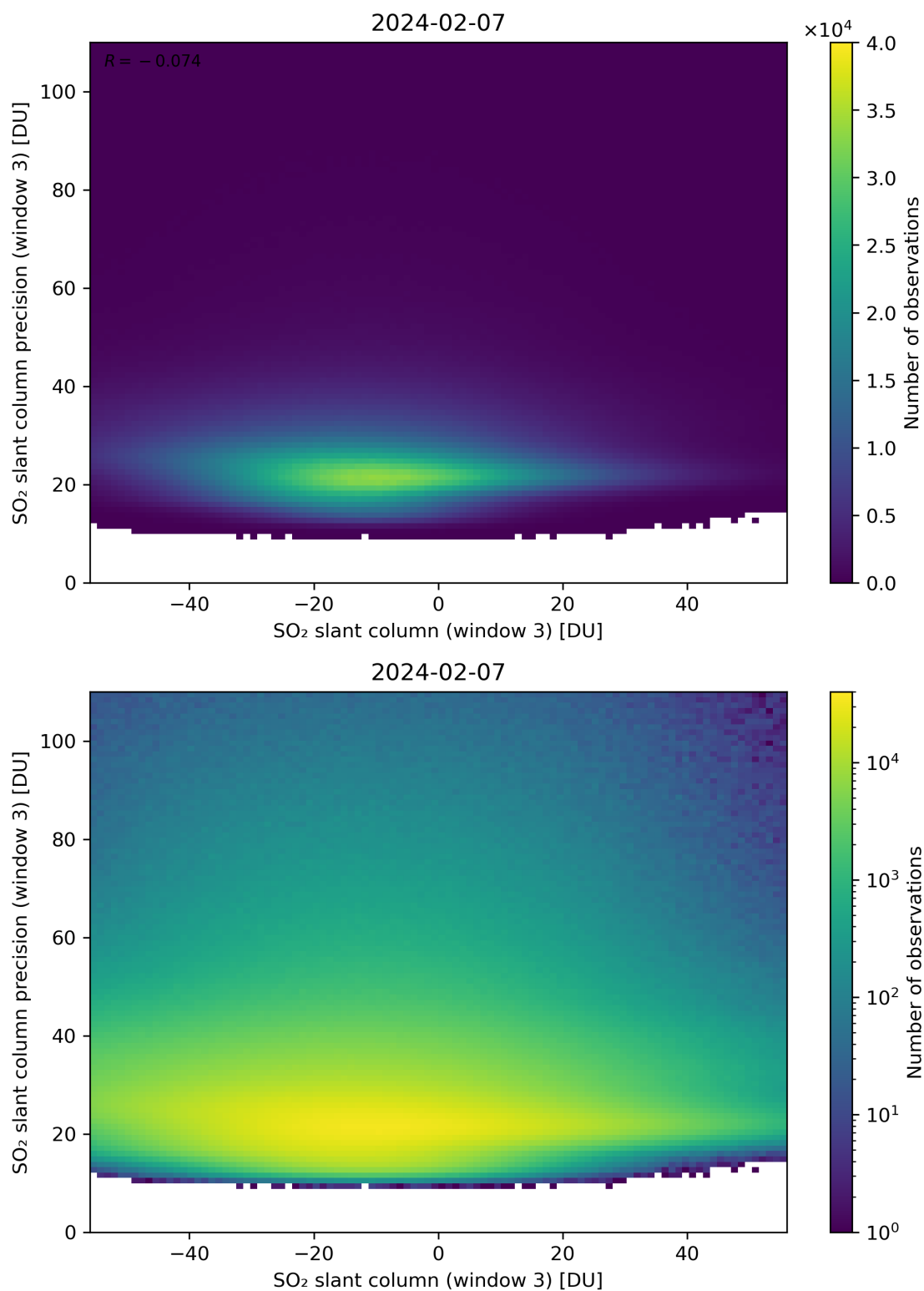
Figure 267: Scatter density plot of “SO 2 slant column (window 3)” against “SO 2 slant column precision (window 3)” for 2024-02-06 to 2024-02-08.
