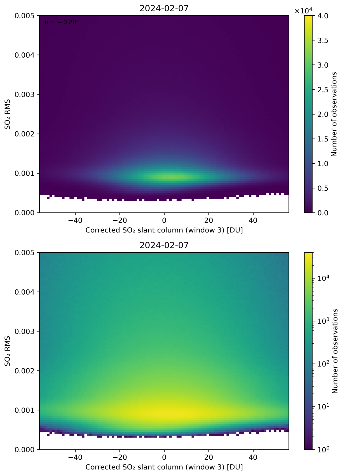
Figure 208: Scatter density plot of “Corrected SO 2 slant column (window 3)” against “SO 2 RMS” for 2024-02-06 to 2024-02-08.
