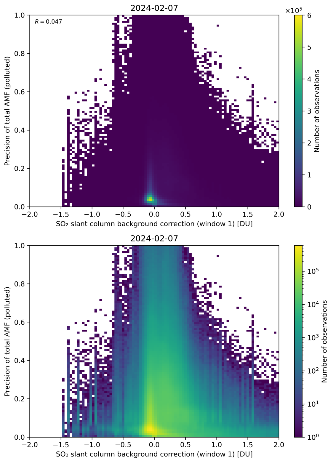
Figure 110: Scatter density plot of “SO 2 slant column background correction (window 1)” against “Precision of total AMF (polluted)” for 2024-02-06 to 2024-02-08.
