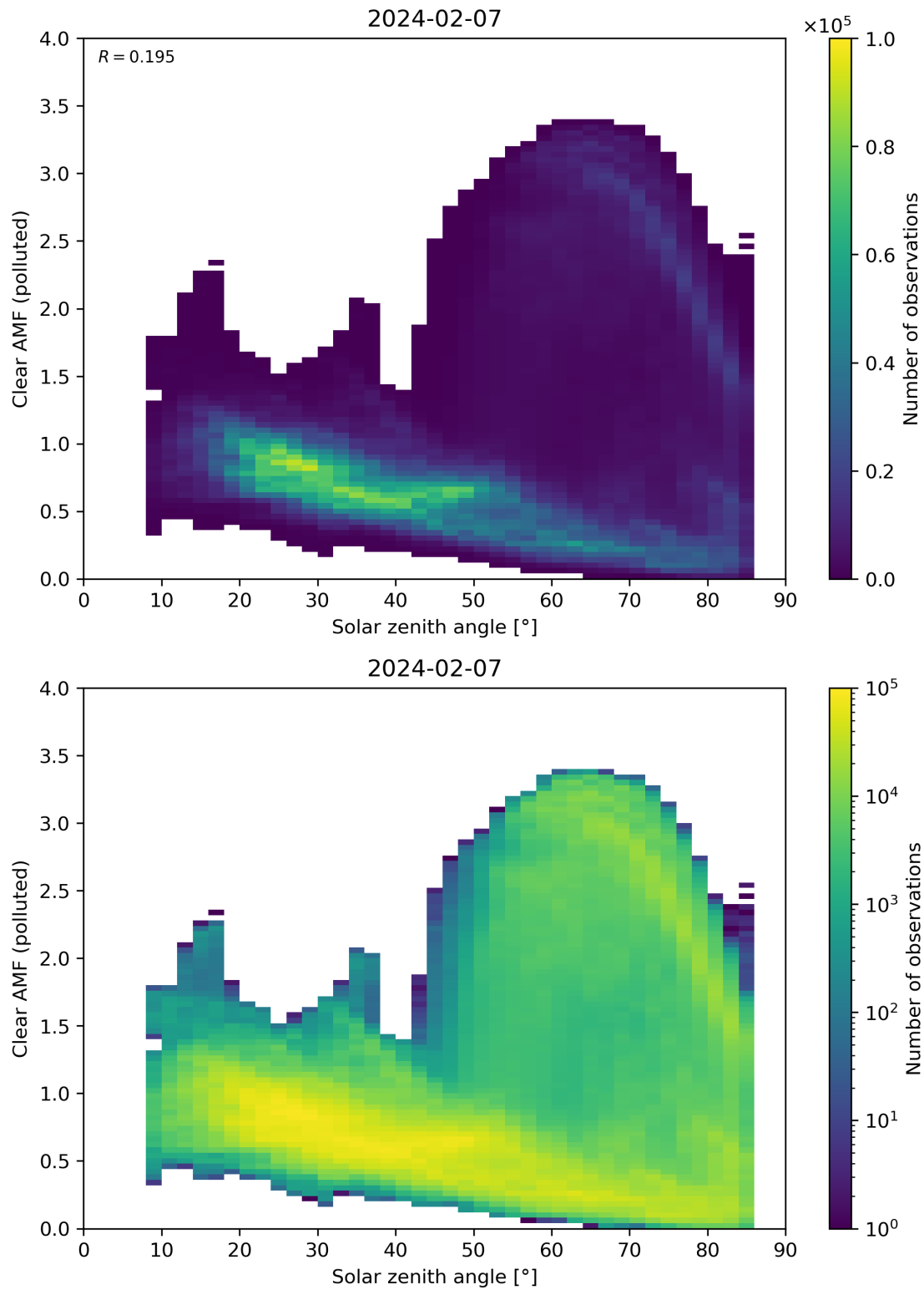
Figure 165: Scatter density plot of “Solar zenith angle” against “Clear AMF (polluted)” for 2024-02-06 to 2024-02-08.
