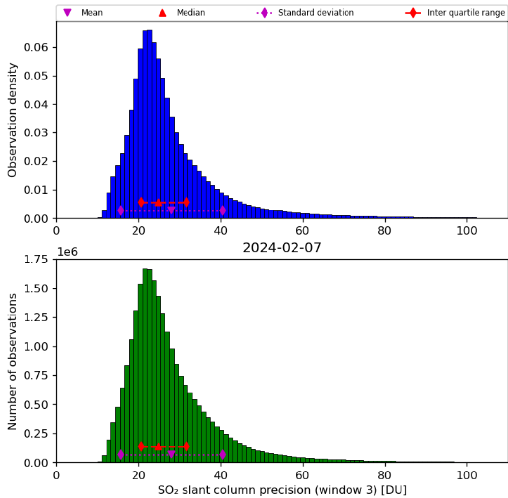
Figure 65: Histogram of “SO 2 slant column precision (window 3)” for 2024-02-06 to 2024-02-08
