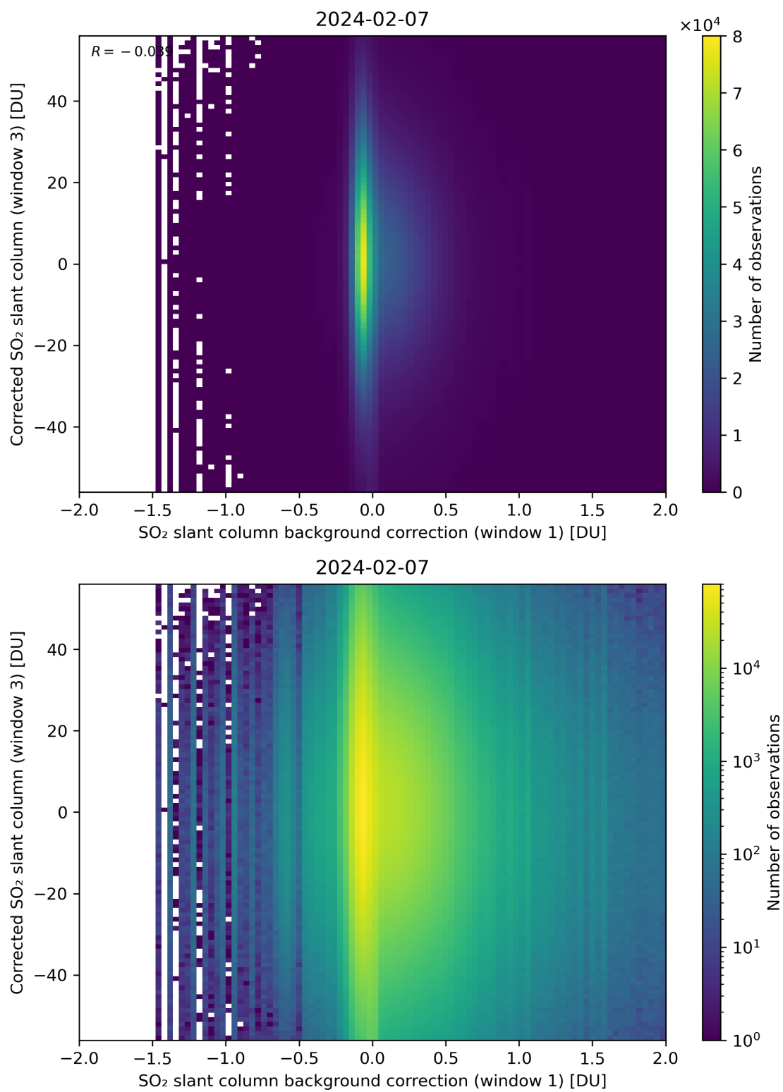
Figure 105: Scatter density plot of “SO 2 slant column background correction (window 1)” against “Corrected SO 2 slant column (window 3)” for 2024-02-06 to 2024-02-08.
