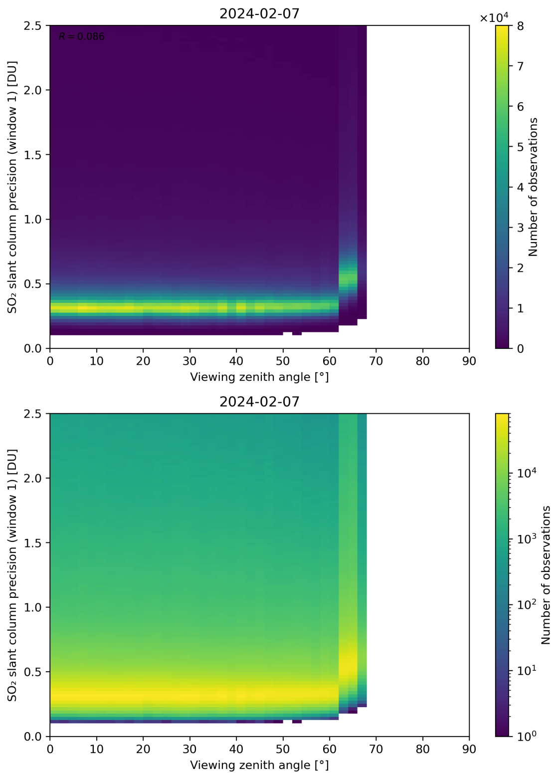
Figure 321: Scatter density plot of “Viewing zenith angle” against “SO 2 slant column precision (window 1)” for 2024-02-06 to 2024-02-08.
