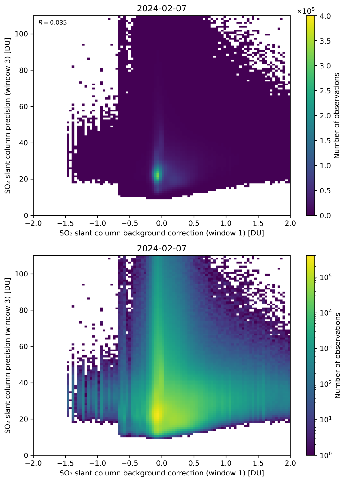
Figure 108: Scatter density plot of “SO 2 slant column background correction (window 1)” against “SO 2 slant column precision (window 3)” for 2024-02-06 to 2024-02-08.
