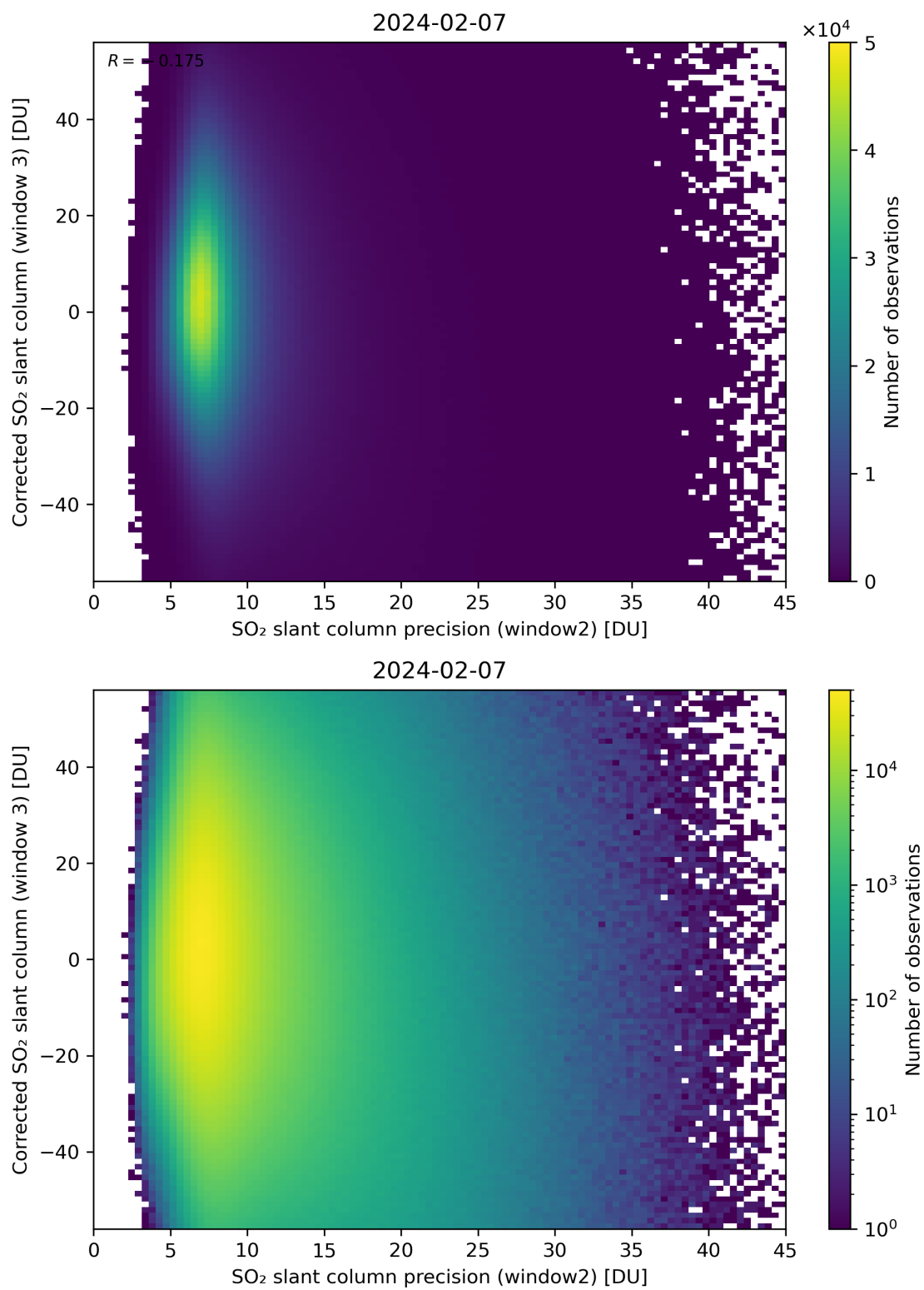
Figure 248: Scatter density plot of “SO 2 slant column precision (window2)” against “Corrected SO 2 slant column (window 3)” for 2024-02-06 to 2024-02-08.
