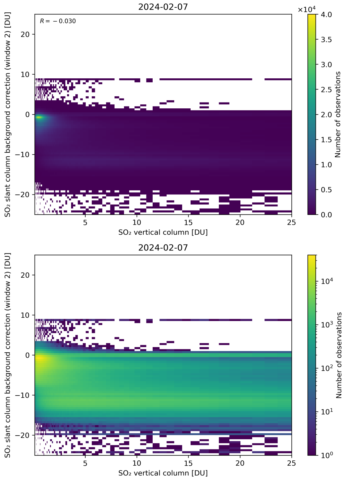
Figure 274: Scatter density plot of “SO 2 vertical column” against “SO 2 slant column background correction (window 2)” for 2024-02-06 to 2024-02-08.
