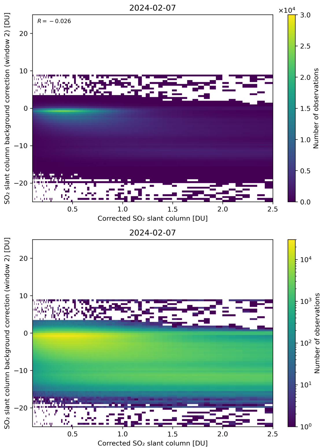
Figure 179: Scatter density plot of “Corrected SO 2 slant column” against “SO 2 slant column background correction (window 2)” for 2024-02-06 to 2024-02-08.
