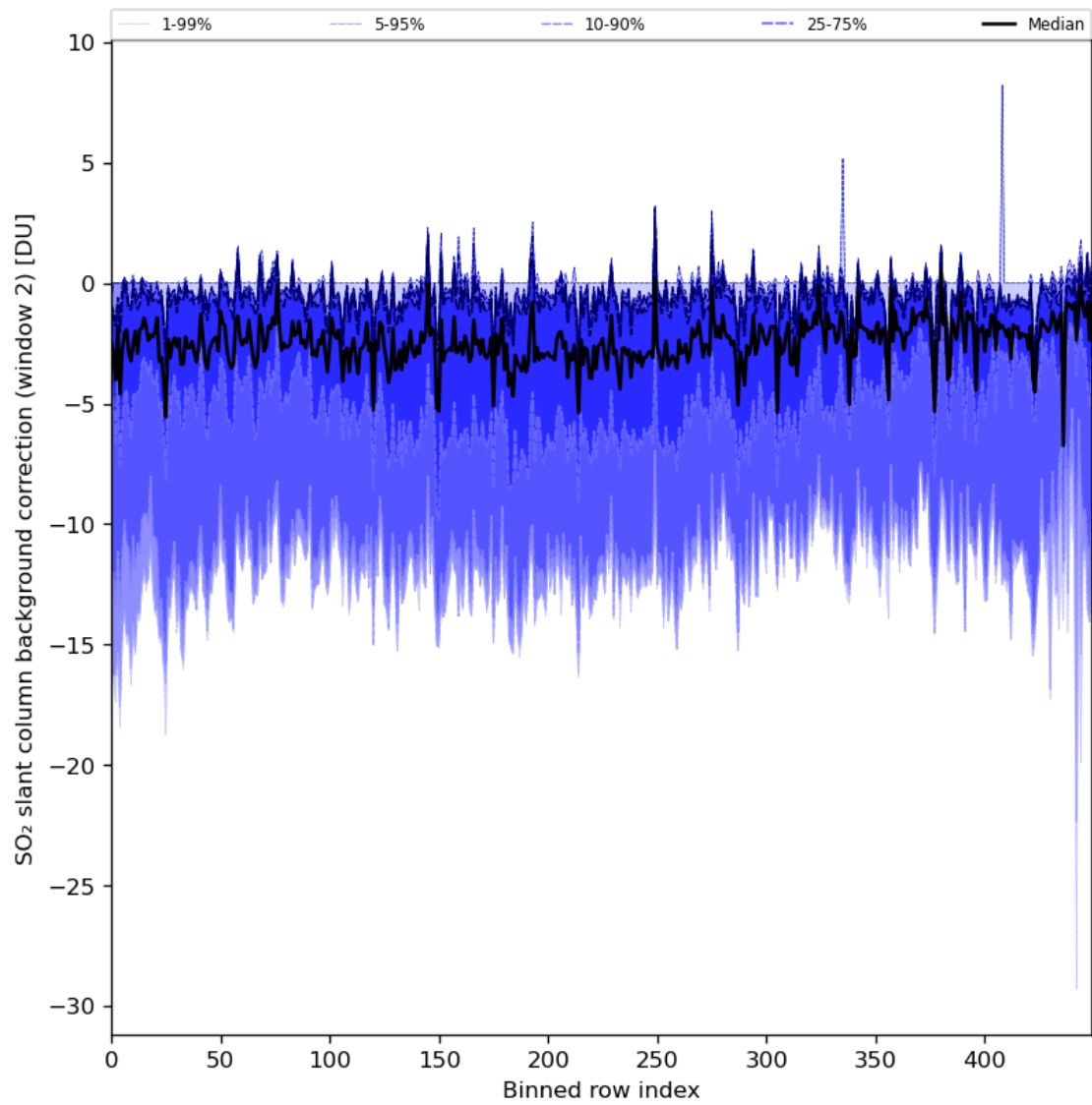
Figure 86: Along track statistics of “SO 2 slant column background correction (window 2)” for 2024-02-06 to 2024-02-08
