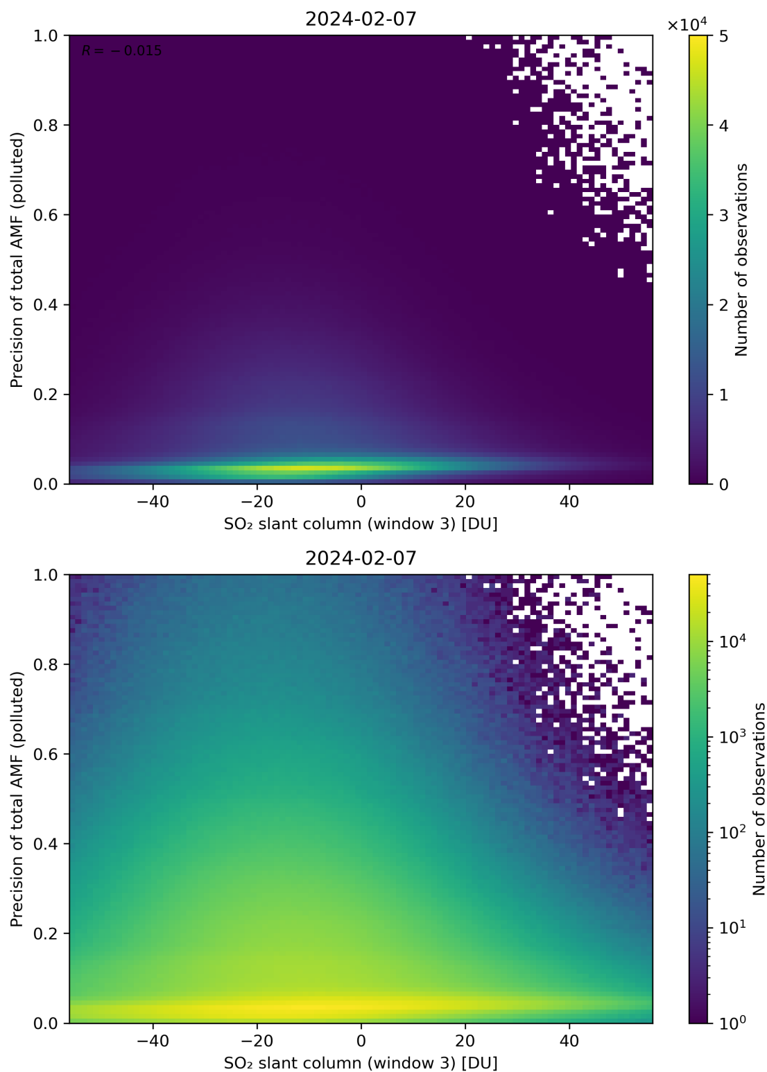
Figure 269: Scatter density plot of “SO 2 slant column (window 3)” against “Precision of total AMF (polluted)” for 2024-02-06 to 2024-02-08.
