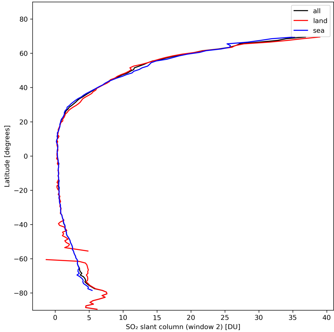
Figure 37: Zonal average of “SO 2 slant column (window 2)” for 2024-02-06 to 2024-02-08.
