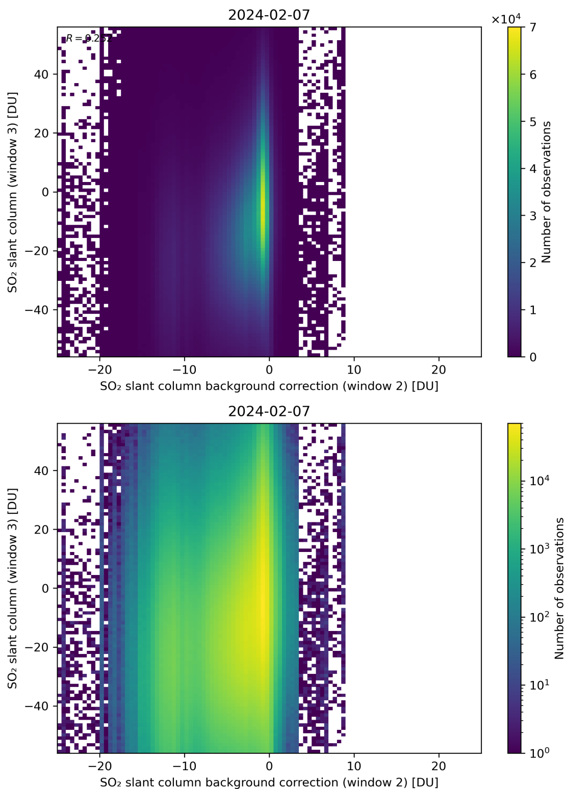
Figure 117: Scatter density plot of “SO 2 slant column background correction (window 2)” against “SO 2 slant column (window 3)” for 2024-02-06 to 2024-02-08.
