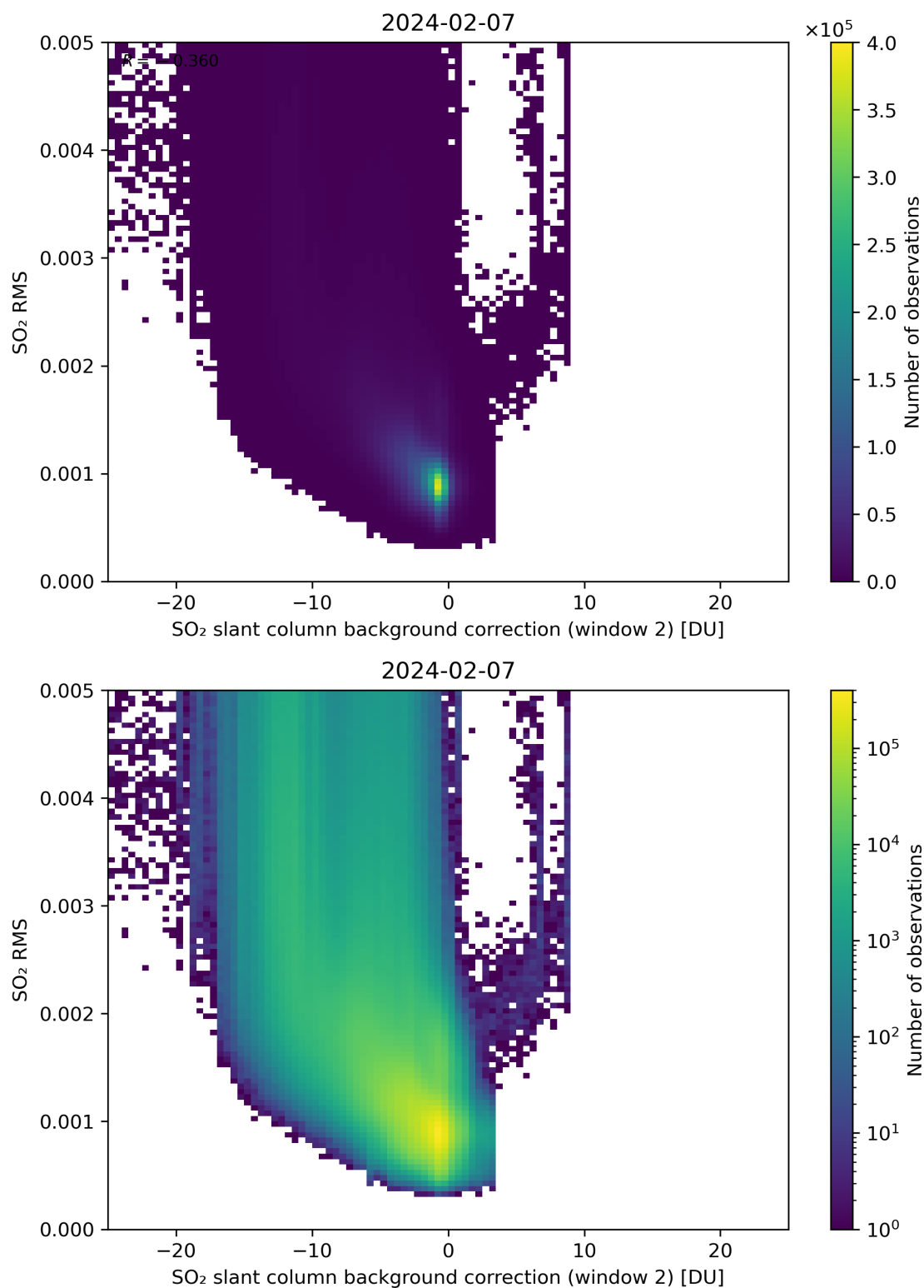
Figure 114: Scatter density plot of “SO 2 slant column background correction (window 2)” against “SO 2 RMS” for 2024-02-06 to 2024-02-08.
