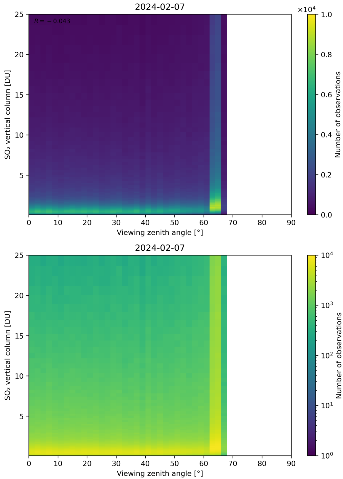
Figure 327: Scatter density plot of “Viewing zenith angle” against “SO 2 vertical column” for 2024-02-06 to 2024-02-08.
