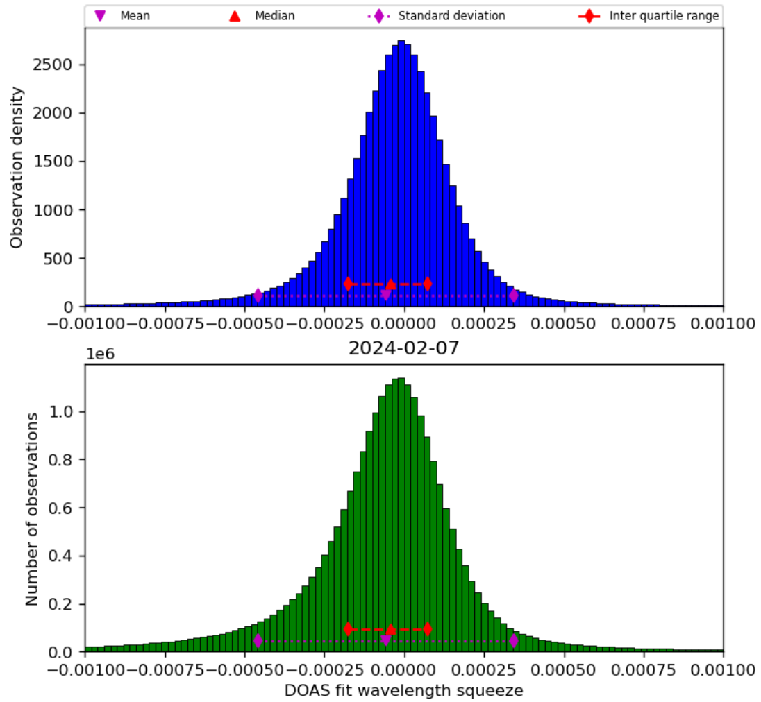
Figure 69: Histogram of “DOAS fit wavelength squeeze” for 2024-02-06 to 2024-02-08
