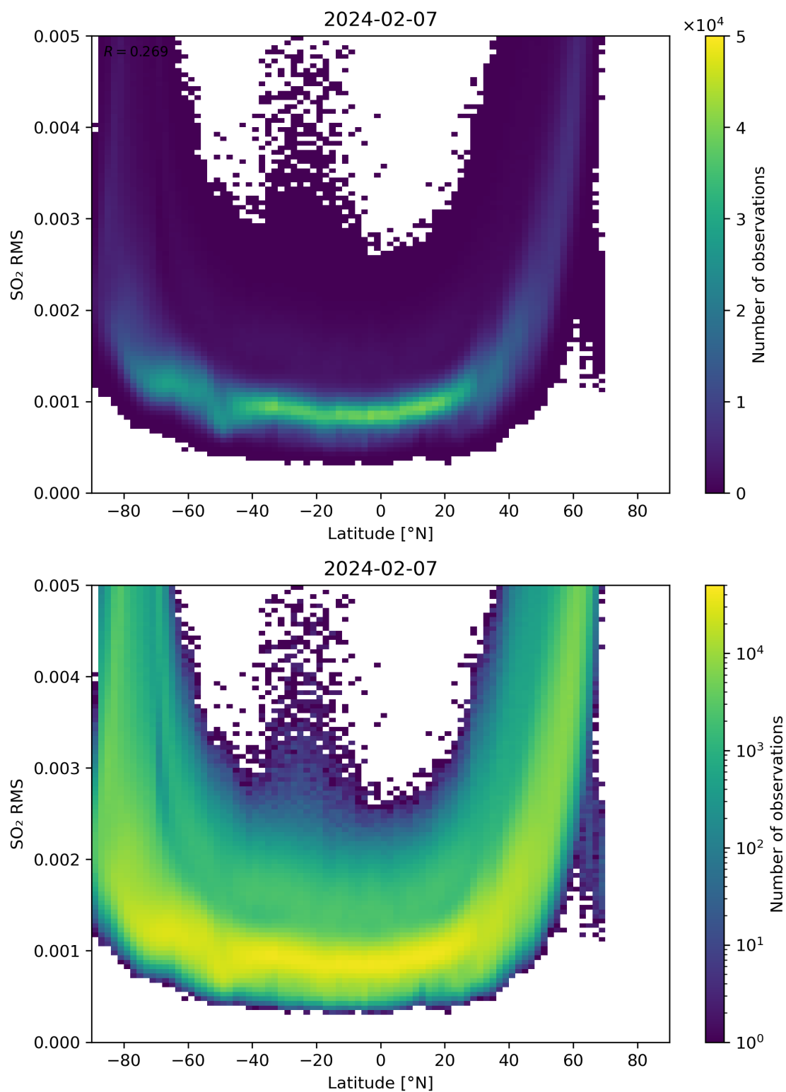
Figure 144: Scatter density plot of “Latitude” against “SO 2 RMS” for 2024-02-06 to 2024-02-08.
