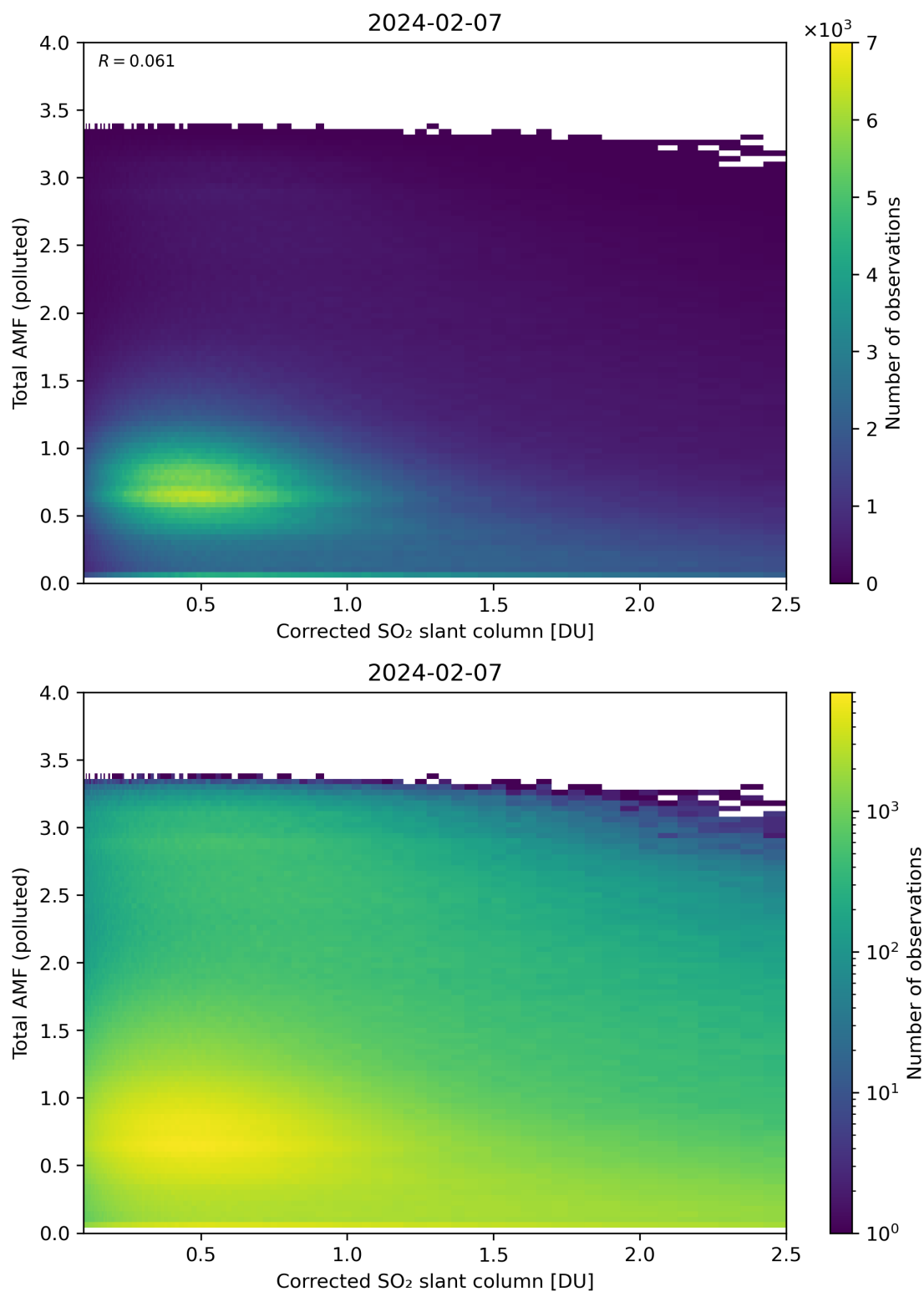
Figure 192: Scatter density plot of “Corrected SO 2 slant column” against “Total AMF (polluted)” for 2024-02-06 to 2024-02-08.
