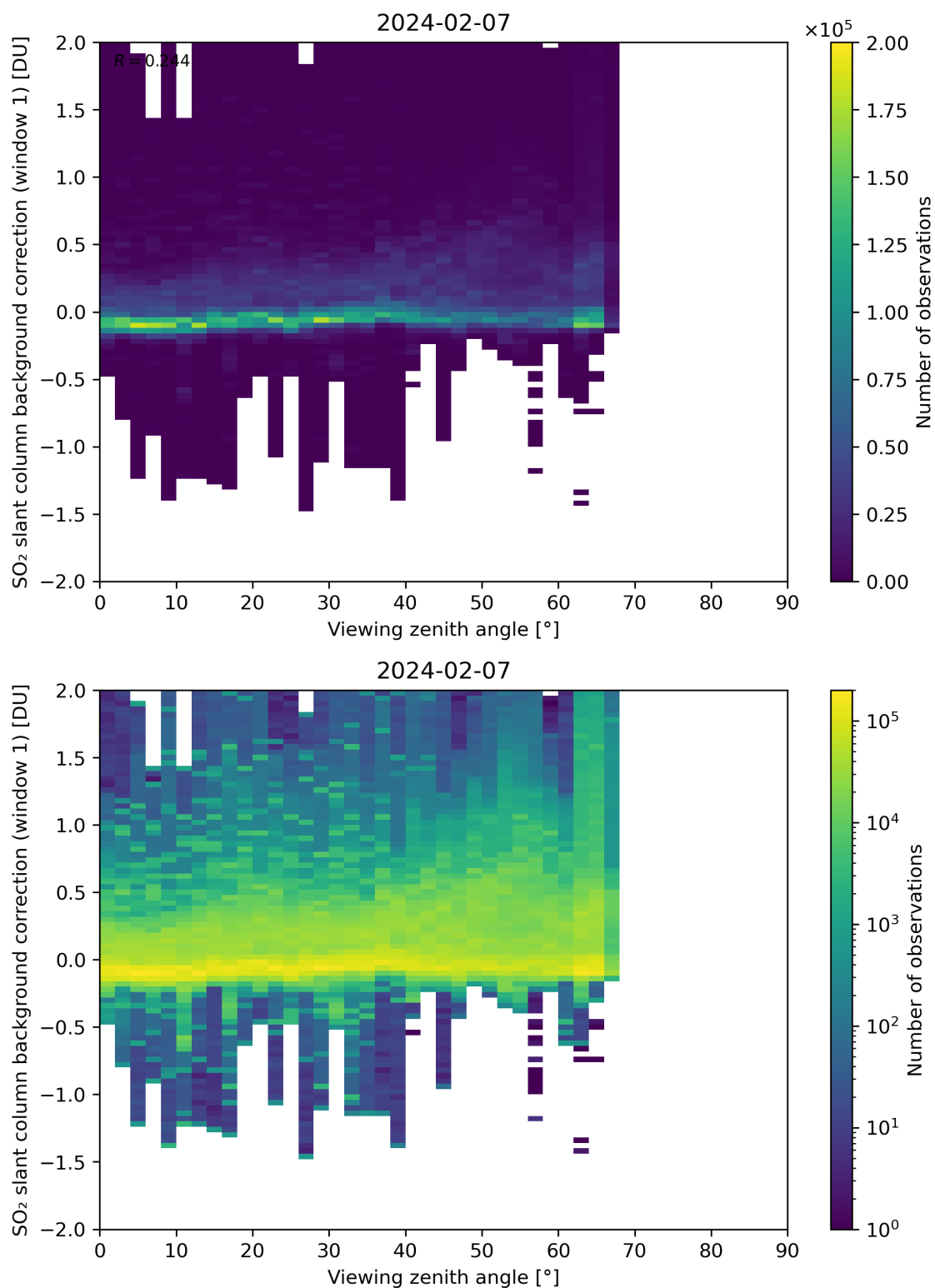
Figure 308: Scatter density plot of “Viewing zenith angle” against “SO 2 slant column background correction (window 1)” for 2024-02-06 to 2024-02-08.
