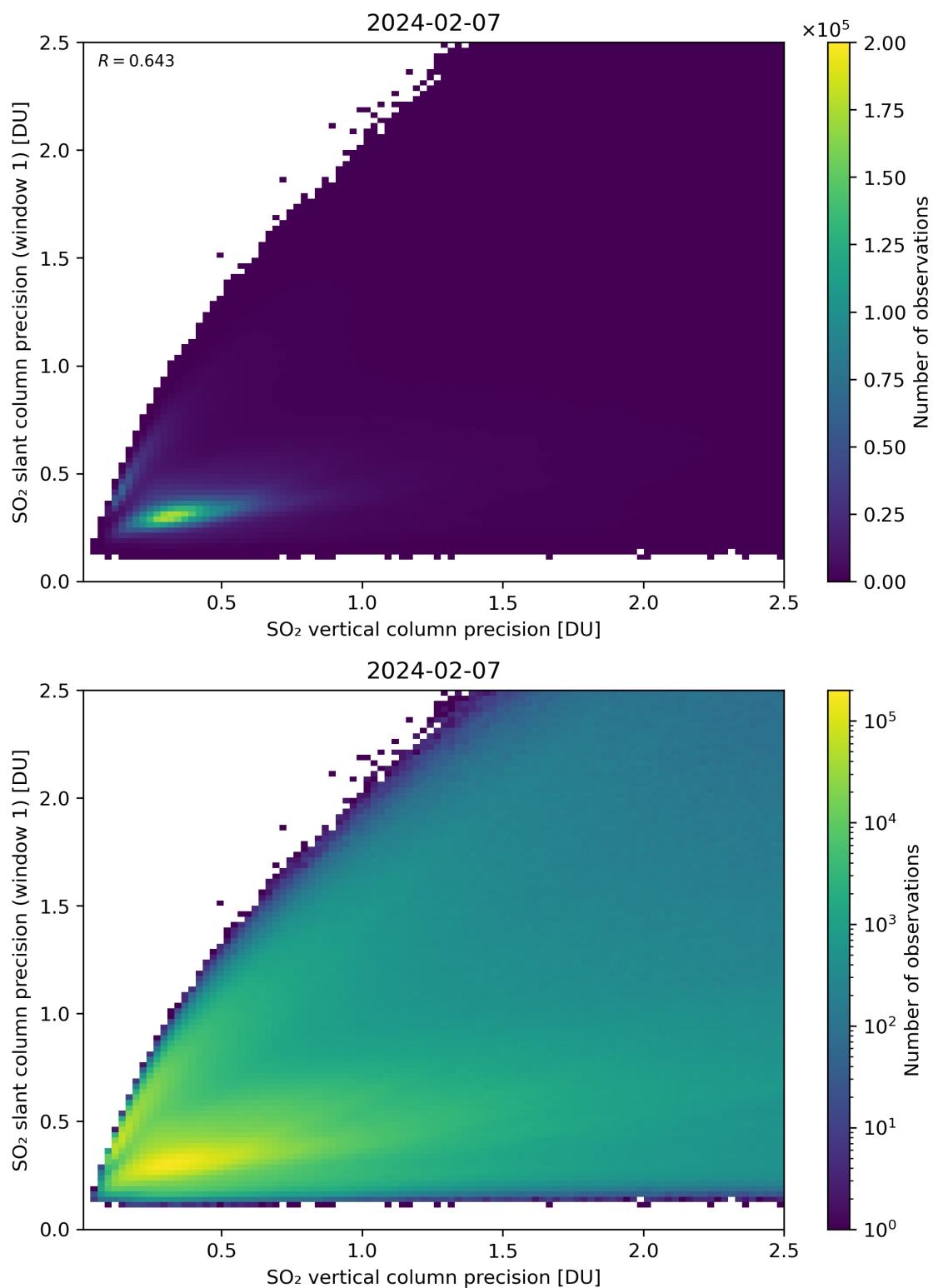
Figure 290: Scatter density plot of “SO 2 vertical column precision” against “SO 2 slant column precision (window 1)” for 2024-02-06 to 2024-02-08.
