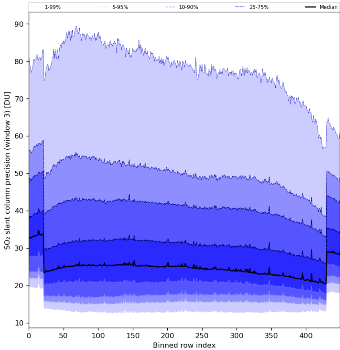
Figure 88: Along track statistics of “SO 2 slant column precision (window 3)” for 2024-02-06 to 2024-02-08
