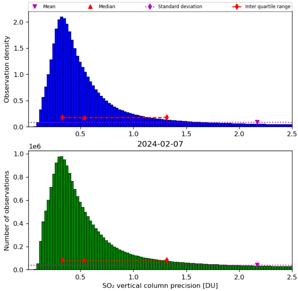
Figure 54: Histogram of “SO 2 vertical column precision” for 2024-02-06 to 2024-02-08
