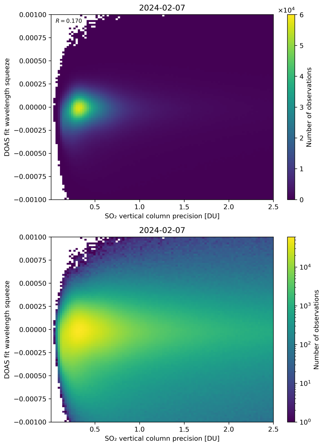
Figure 283: Scatter density plot of “SO 2 vertical column precision” against “DOAS fit wavelength squeeze” for 2024-02-06 to 2024-02-08.
