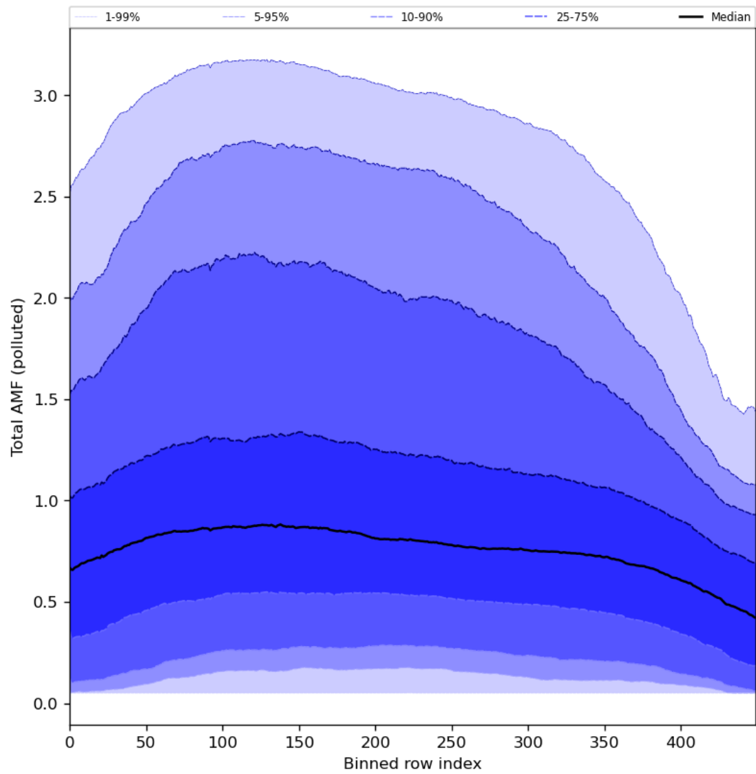
Figure 94: Along track statistics of “Total AMF (polluted)” for 2024-02-06 to 2024-02-08
