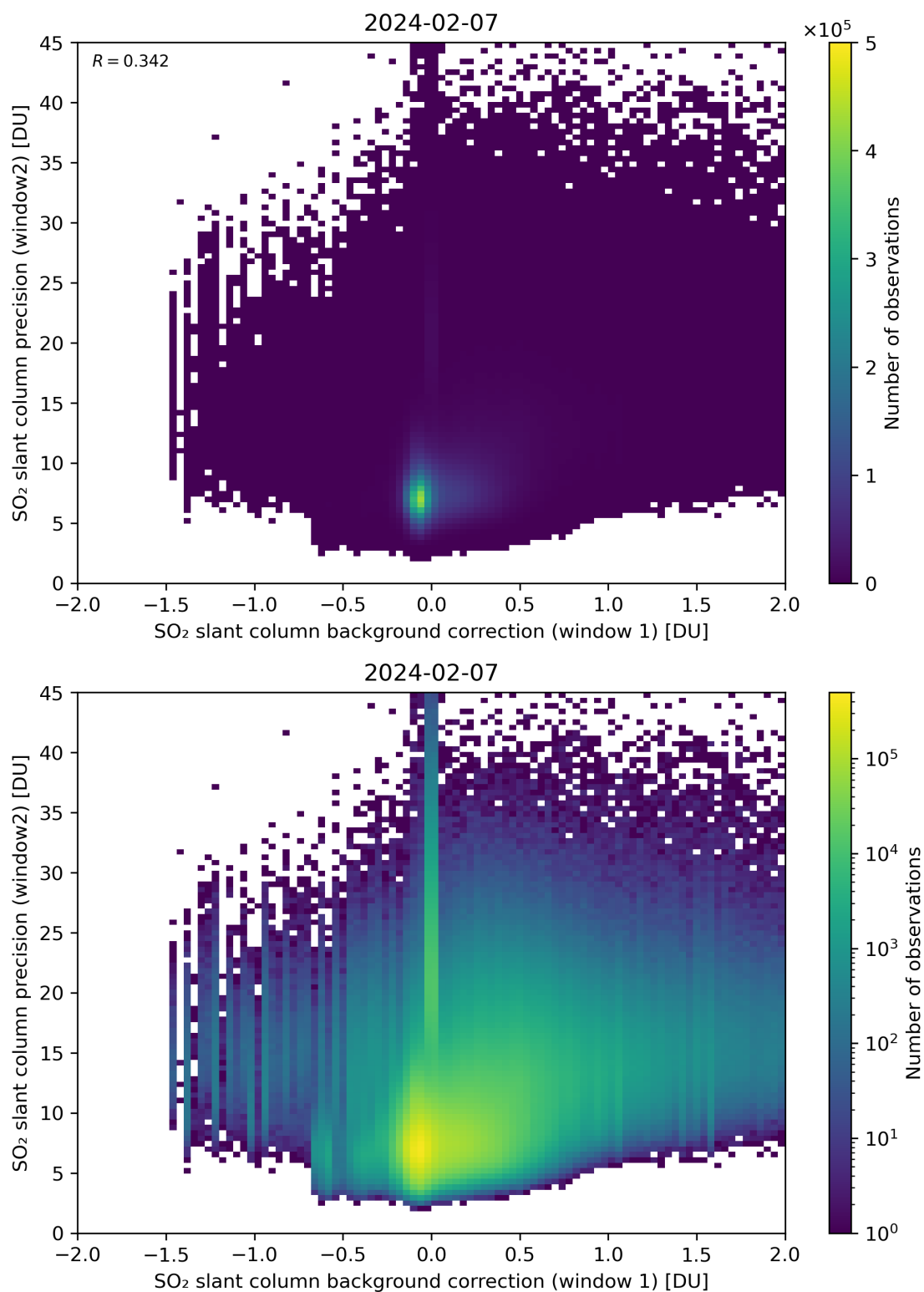
Figure 106: Scatter density plot of “SO 2 slant column background correction (window 1)” against “SO 2 slant column precision (window2)” for 2024-02-06 to 2024-02-08.
