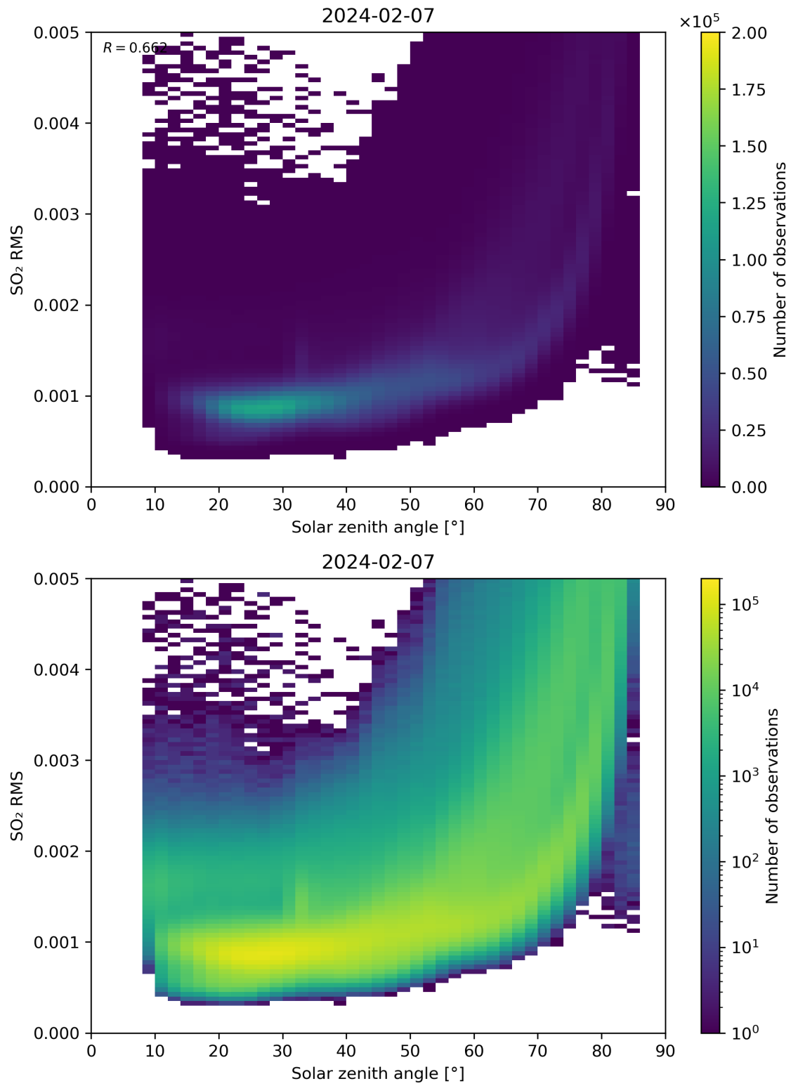
Figure 163: Scatter density plot of “Solar zenith angle” against “SO 2 RMS” for 2024-02-06 to 2024-02-08.
