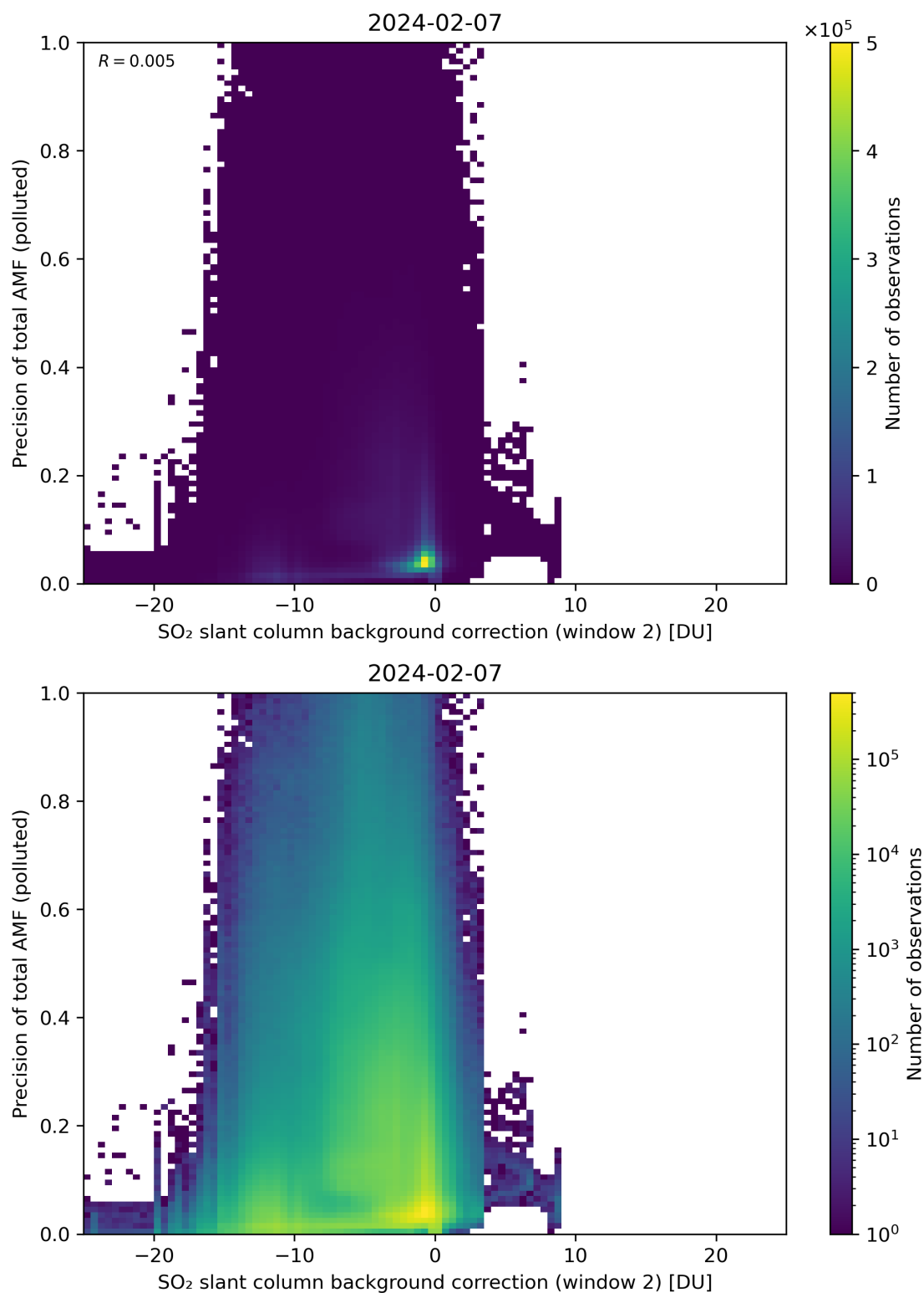
Figure 120: Scatter density plot of “SO 2 slant column background correction (window 2)” against “Precision of total AMF (polluted)” for 2024-02-06 to 2024-02-08.
