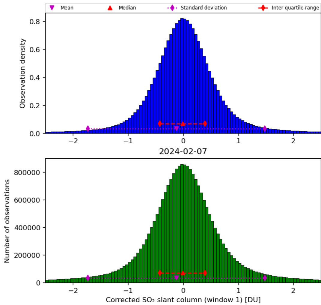
Figure 58: Histogram of “Corrected SO 2 slant column (window 1)” for 2024-02-06 to 2024-02-08
