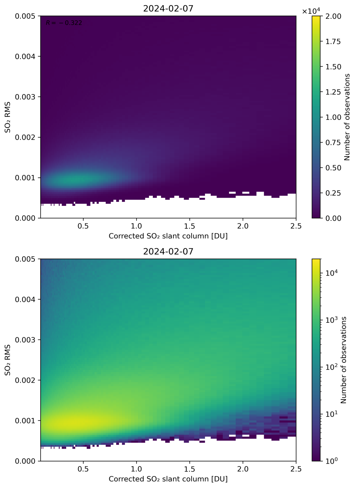
Figure 183: Scatter density plot of “Corrected SO 2 slant column” against “SO 2 RMS” for 2024-02-06 to 2024-02-08.
