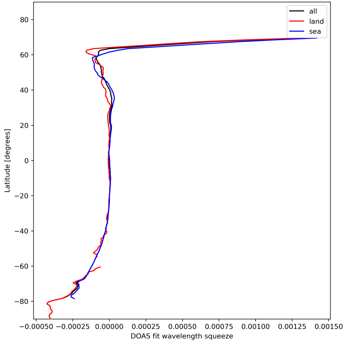
Figure 46: Zonal average of “DOAS fit wavelength squeeze” for 2024-02-06 to 2024-02-08.
