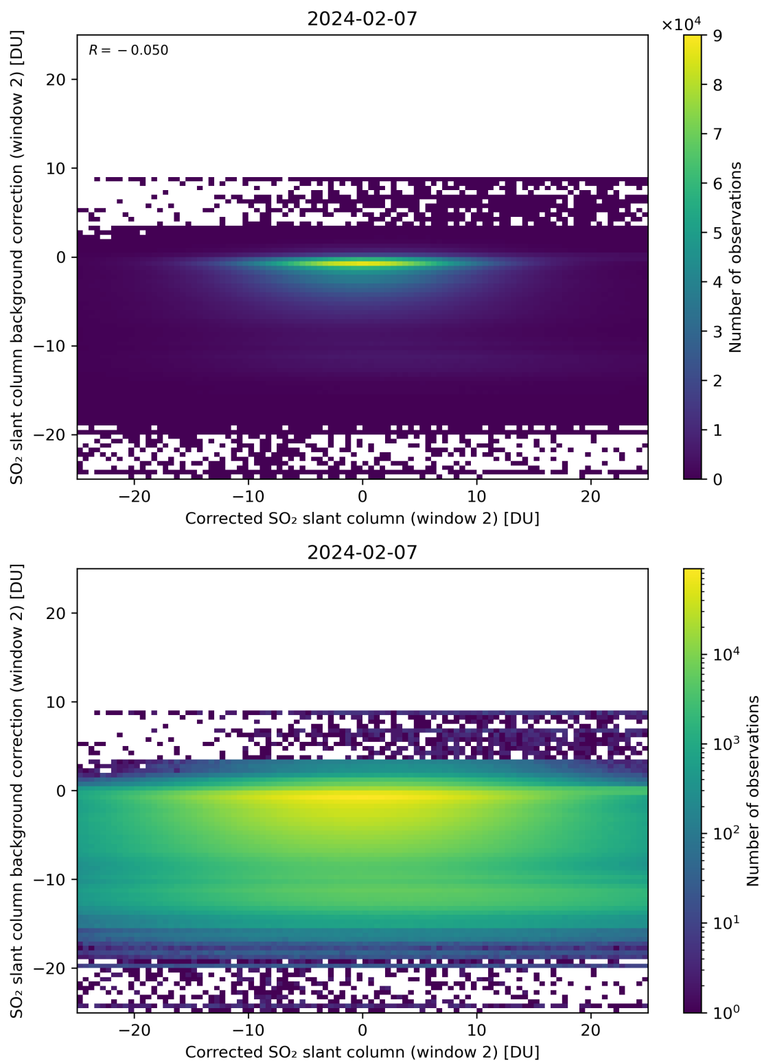
Figure 194: Scatter density plot of “Corrected SO 2 slant column (window 2)” against “SO 2 slant column background correction (window 2)” for 2024-02-06 to 2024-02-08.
