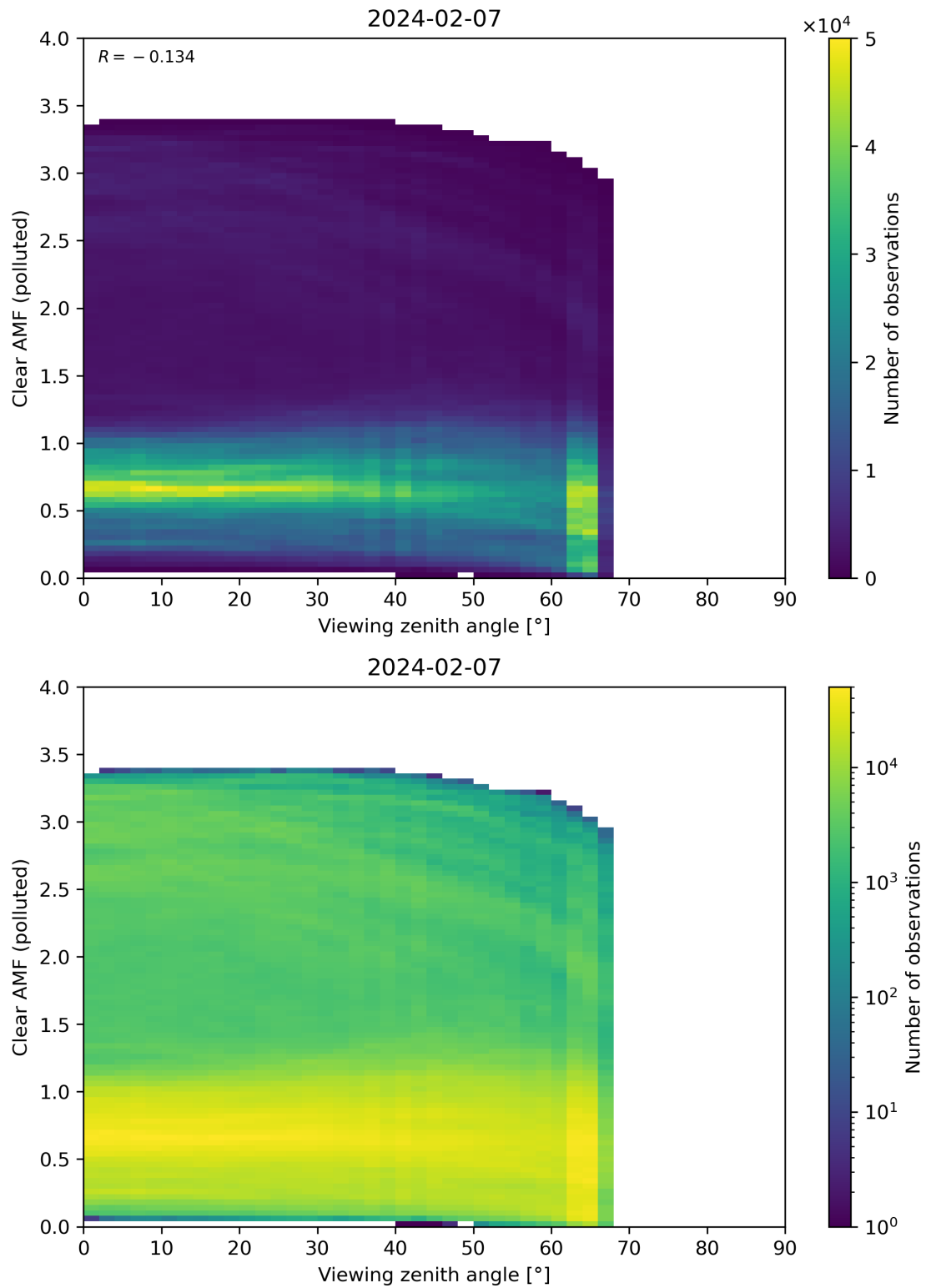
Figure 316: Scatter density plot of “Viewing zenith angle” against “Clear AMF (polluted)” for 2024-02-06 to 2024-02-08.
