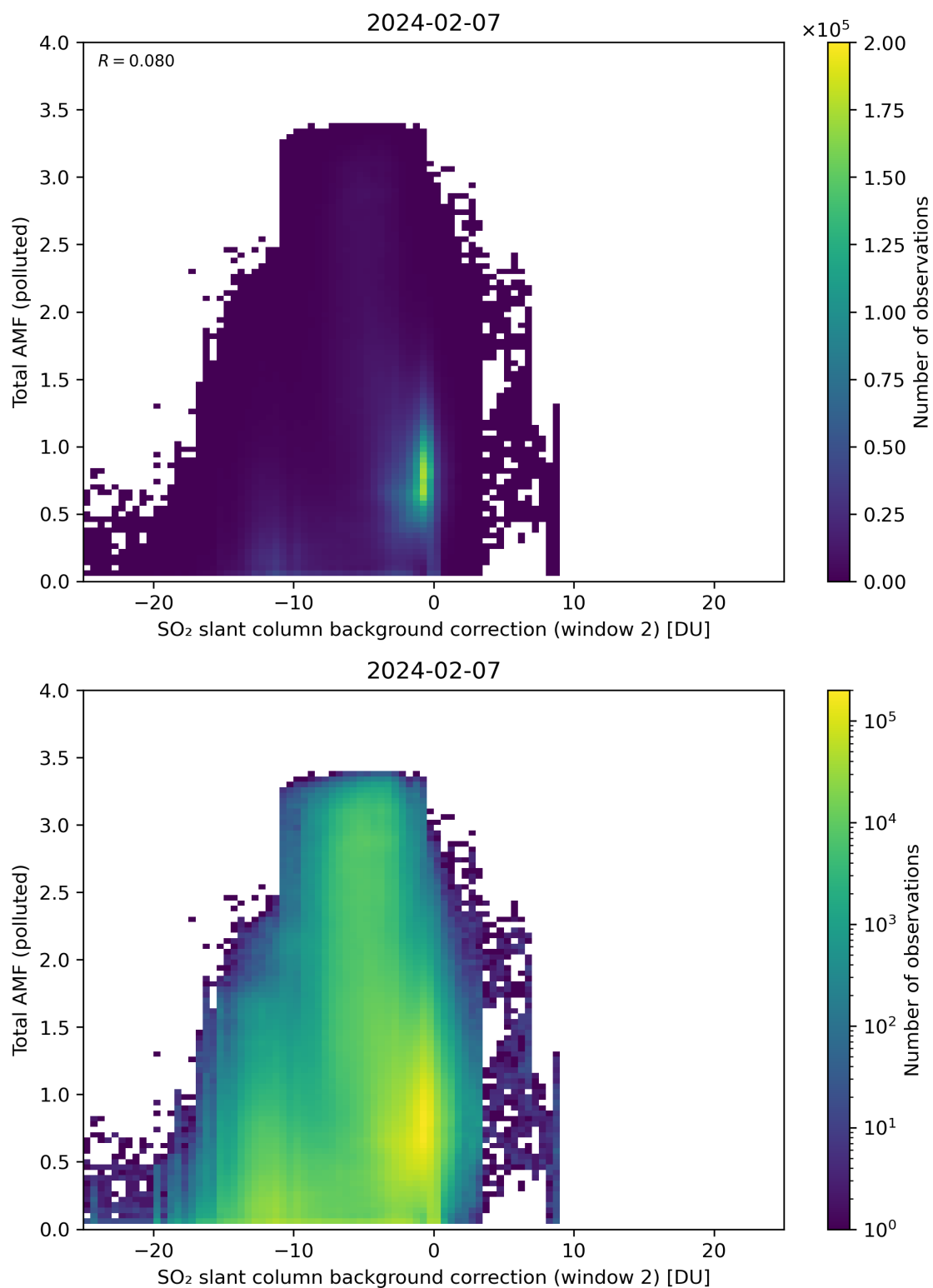
Figure 119: Scatter density plot of “SO 2 slant column background correction (window 2)” against “Total AMF (polluted)” for 2024-02-06 to 2024-02-08.
