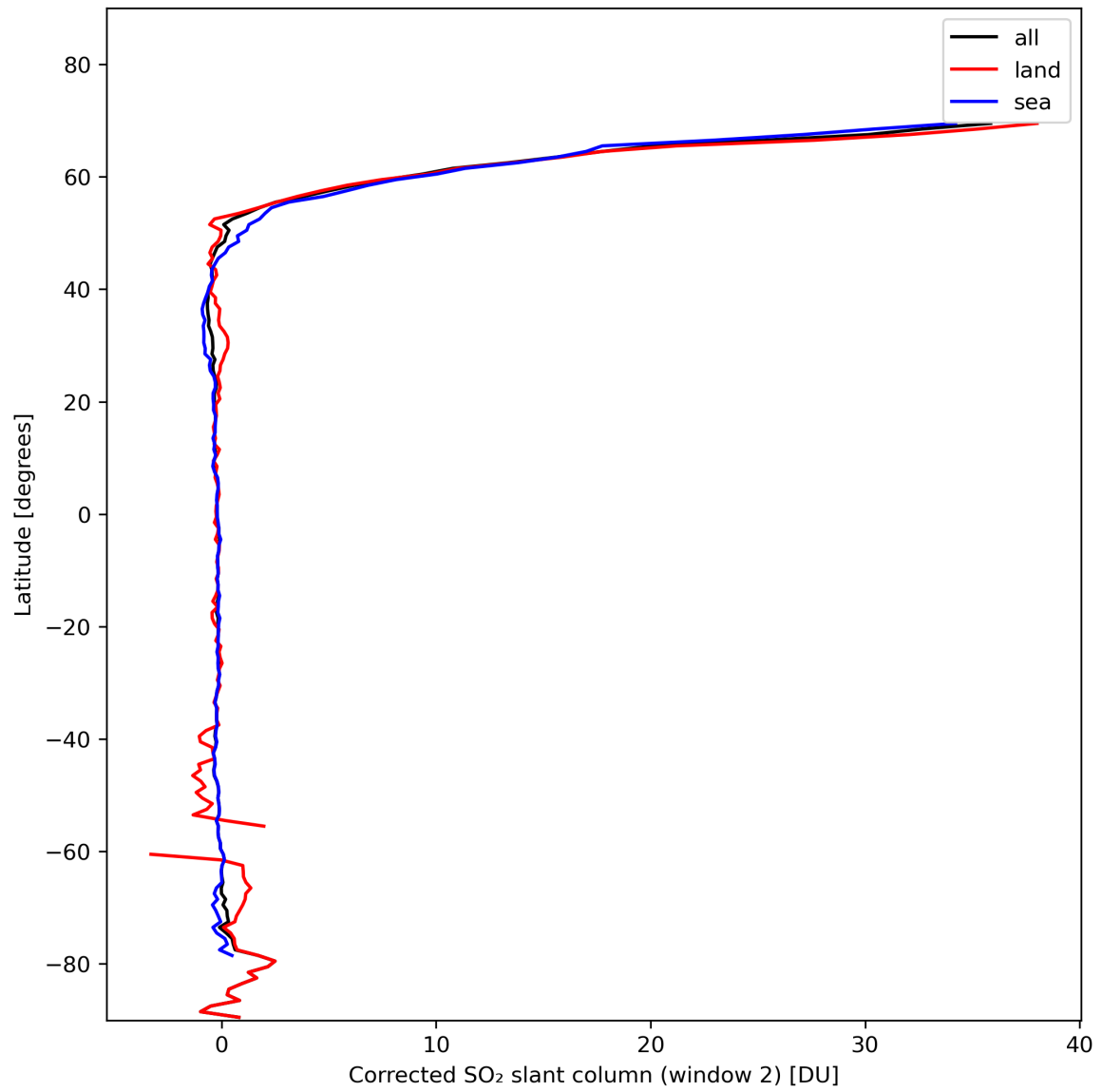
Figure 39: Zonal average of “Corrected SO 2 slant column (window 2)” for 2024-02-06 to 2024-02-08.
