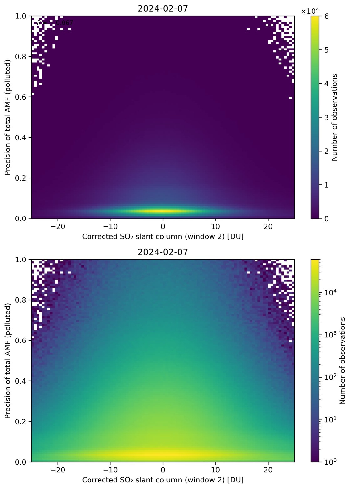
Figure 204: Scatter density plot of “Corrected SO 2 slant column (window 2)” against “Precision of total AMF (polluted)” for 2024-02-06 to 2024-02-08.
