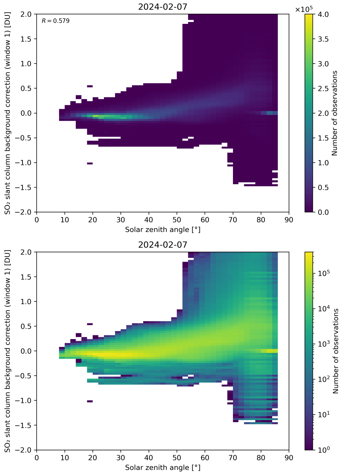
Figure 158: Scatter density plot of “Solar zenith angle” against “SO 2 slant column background correction (window 1)” for 2024-02-06 to 2024-02-08.
