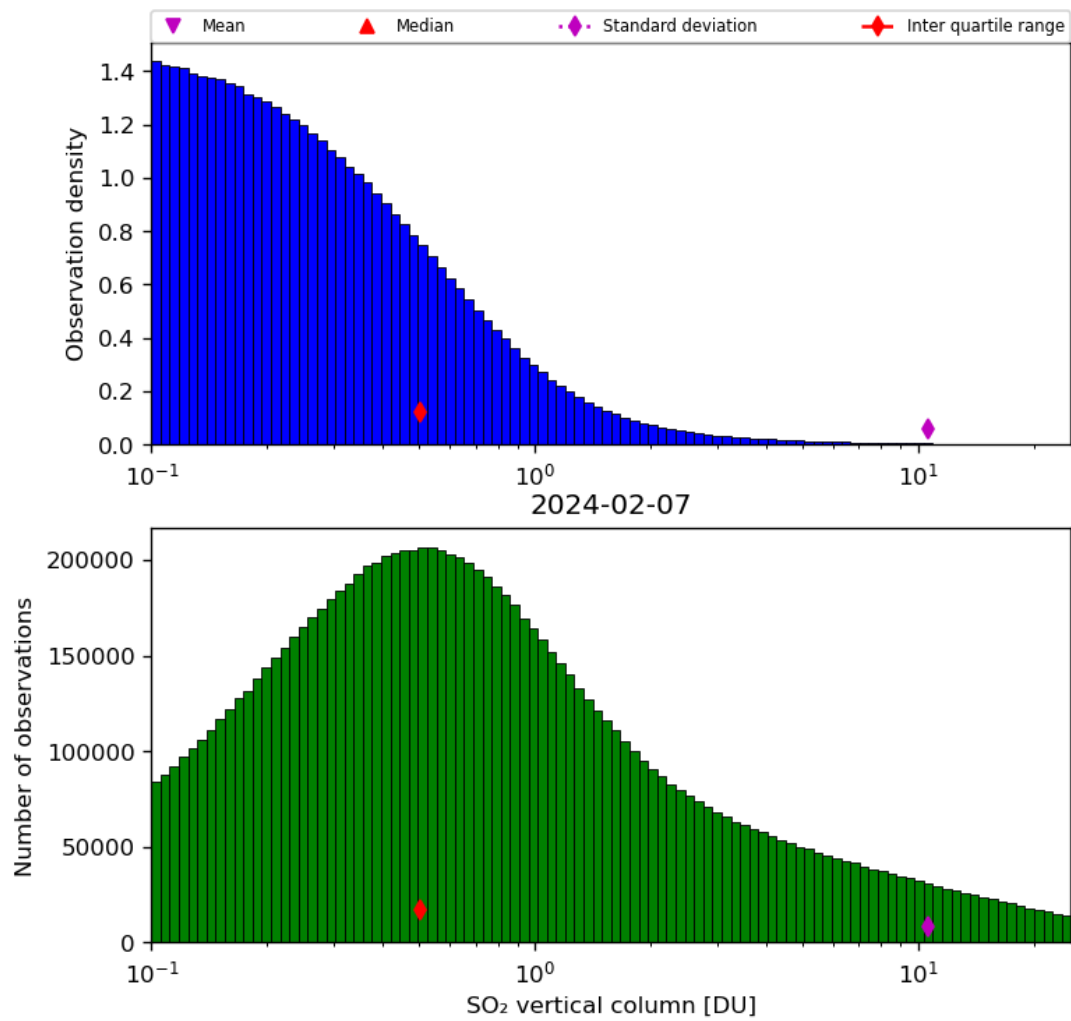
Figure 53: Histogram of “SO 2 vertical column” for 2024-02-06 to 2024-02-08
