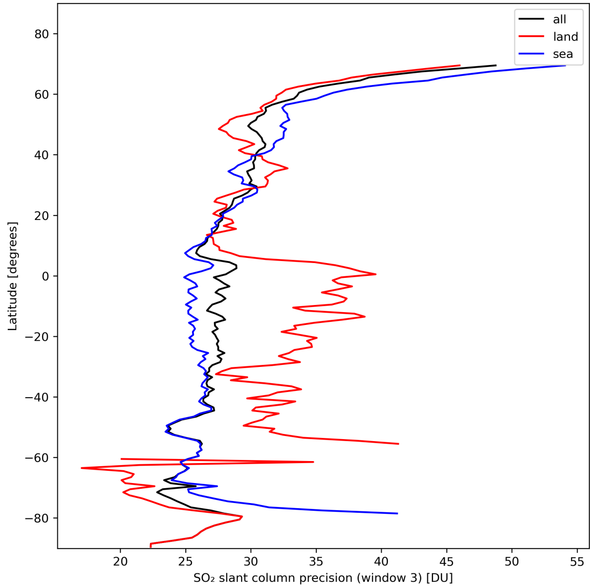
Figure 42: Zonal average of “SO 2 slant column precision (window 3)” for 2024-02-06 to 2024-02-08.
