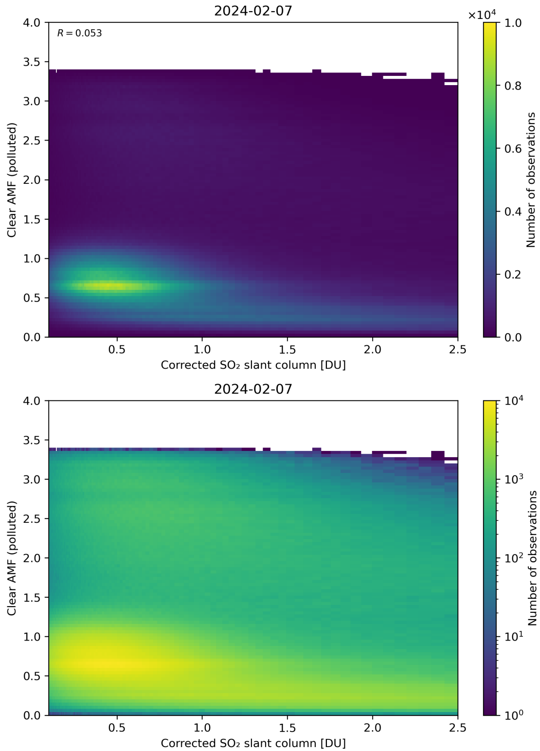
Figure 184: Scatter density plot of “Corrected SO 2 slant column” against “Clear AMF (polluted)” for 2024-02-06 to 2024-02-08.
