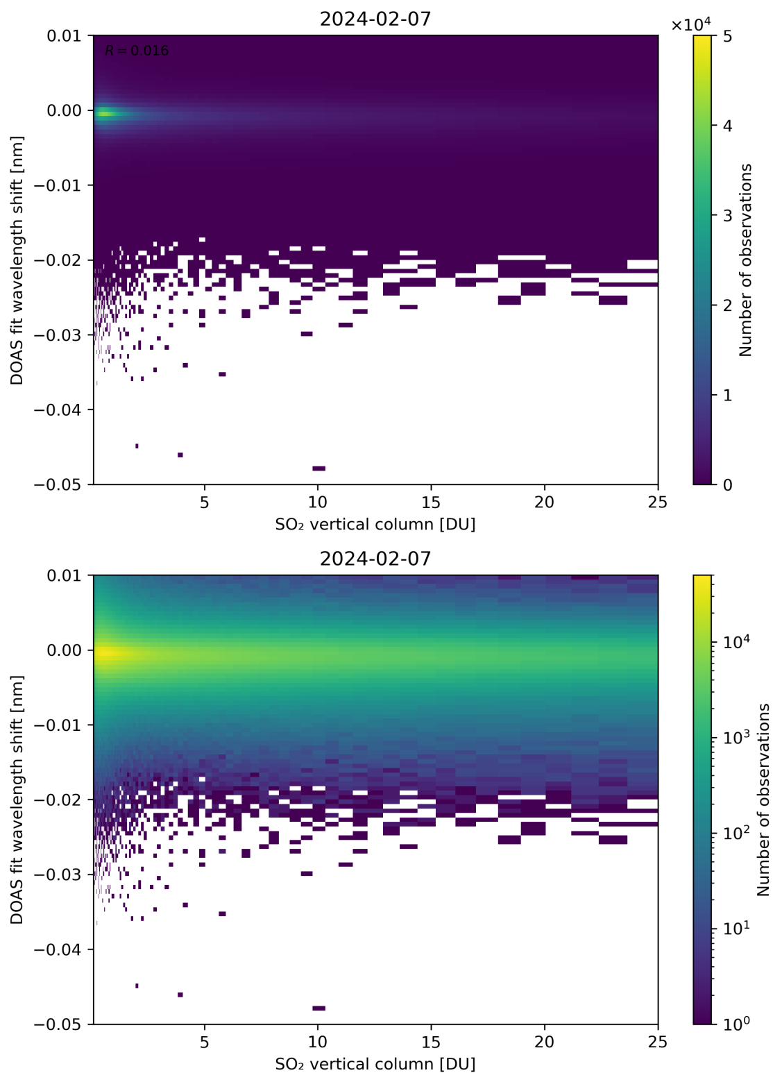
Figure 276: Scatter density plot of “SO 2 vertical column” against “DOAS fit wavelength shift” for 2024-02-06 to 2024-02-08.
