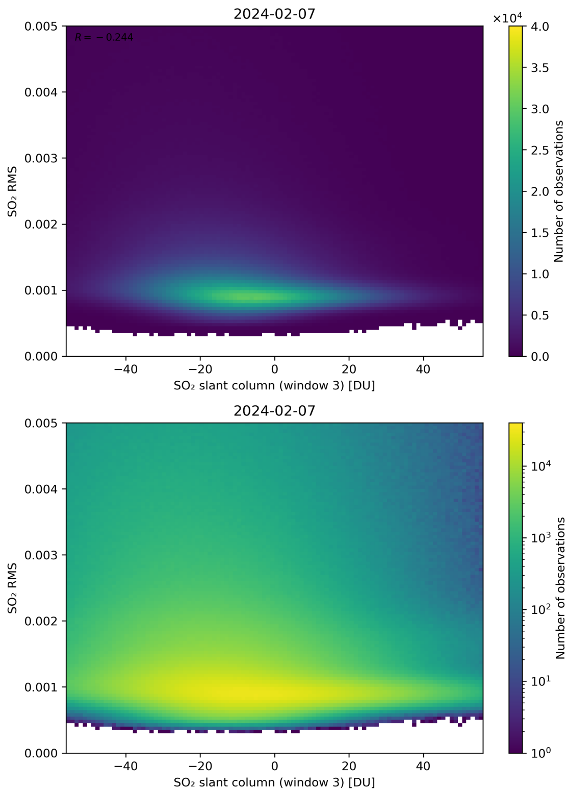
Figure 256: Scatter density plot of “SO 2 slant column (window 3)” against “SO 2 RMS” for 2024-02-06 to 2024-02-08.
