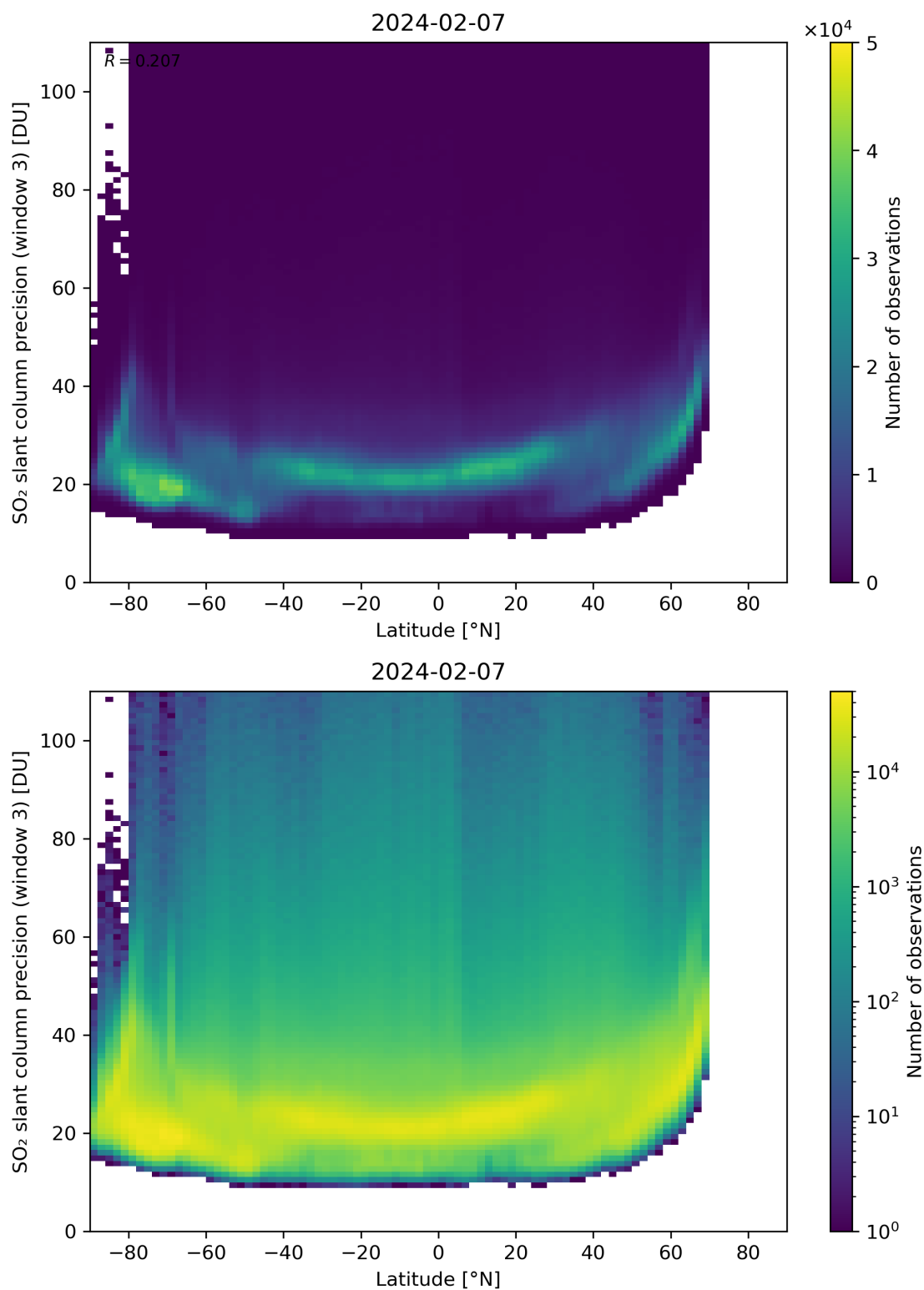
Figure 153: Scatter density plot of “Latitude” against “SO 2 slant column precision (window 3)” for 2024-02-06 to 2024-02-08.
