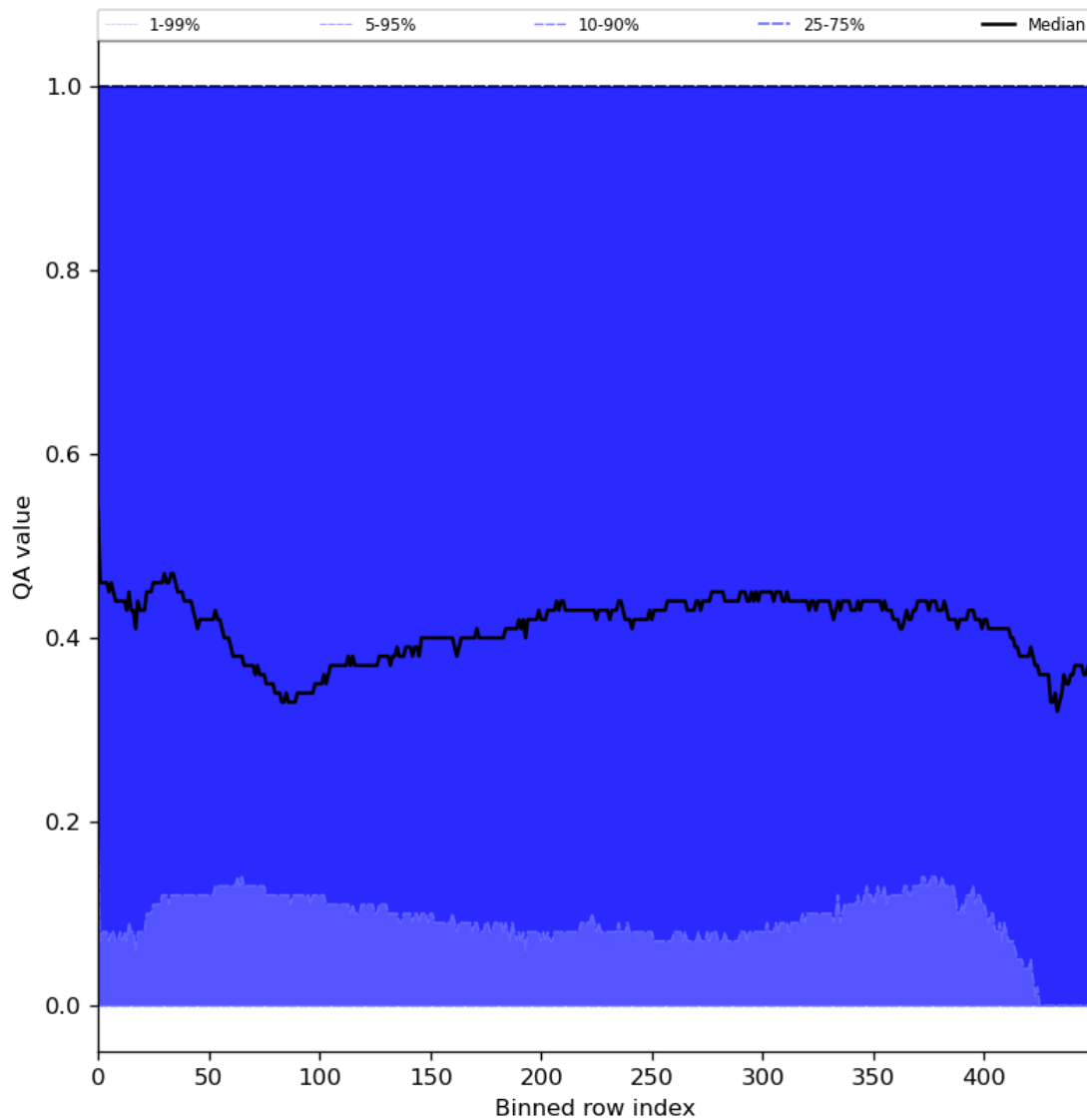
Figure 75: Along track statistics of “QA value” for 2024-02-06 to 2024-02-08
