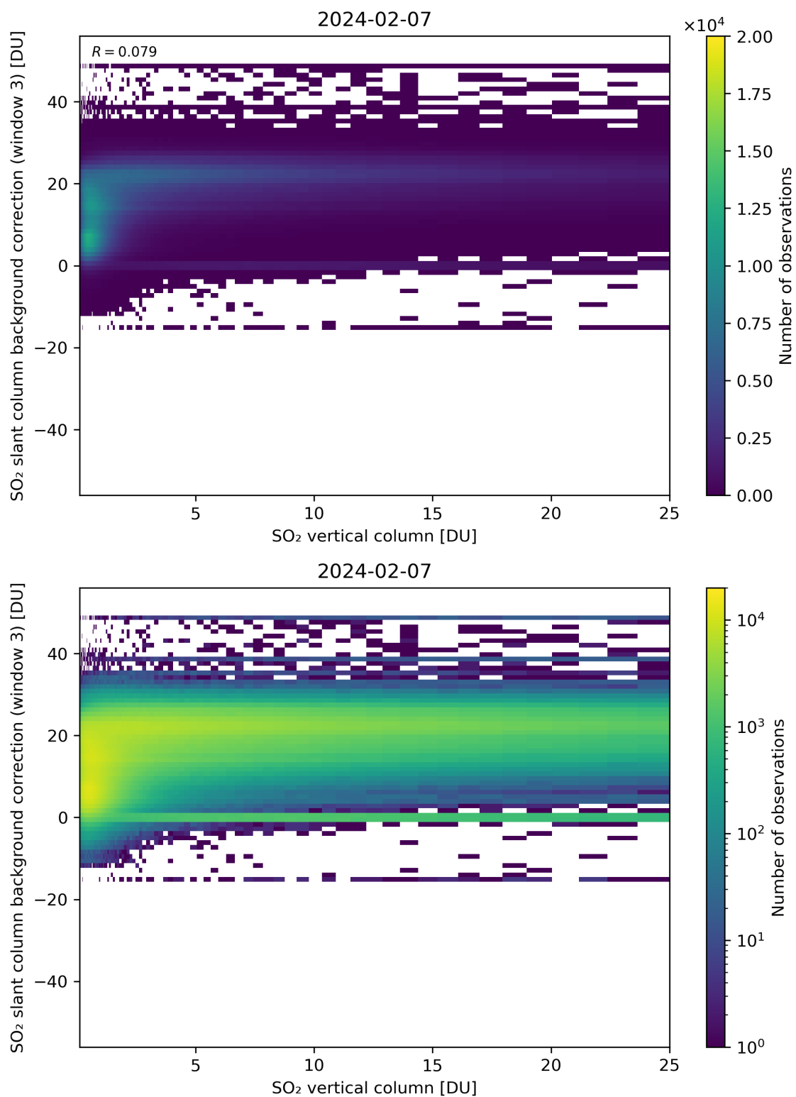
Figure 275: Scatter density plot of “SO 2 vertical column” against “SO 2 slant column background correction (window 3)” for 2024-02-06 to 2024-02-08.
