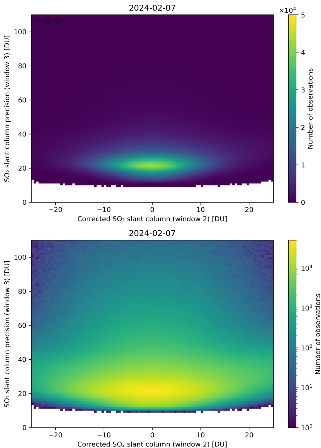
Figure 202: Scatter density plot of “Corrected SO 2 slant column (window 2)” against “SO 2 slant column precision (window 3)” for 2024-02-06 to 2024-02-08.
