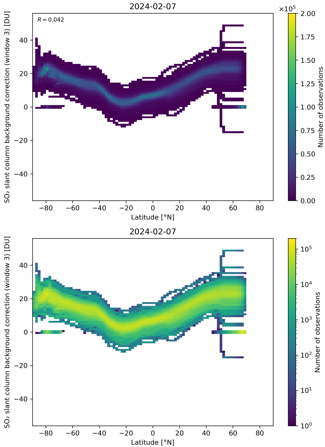
Figure 141: Scatter density plot of “Latitude” against “SO 2 slant column background correction (window 3)” for 2024-02-06 to 2024-02-08.
