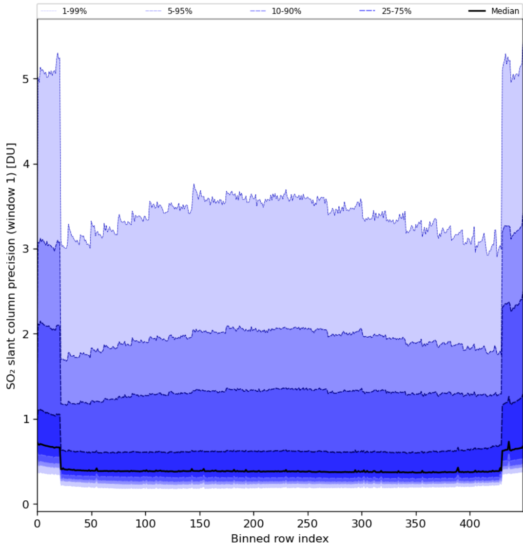
Figure 80: Along track statistics of “SO 2 slant column precision (window 1)” for 2024-02-06 to 2024-02-08
