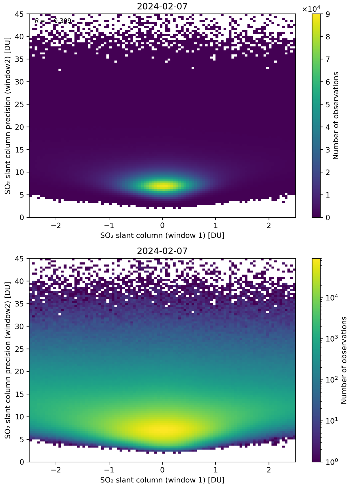
Figure 236: Scatter density plot of “SO 2 slant column (window 1)” against “SO 2 slant column precision (window2)” for 2024-02-06 to 2024-02-08.
