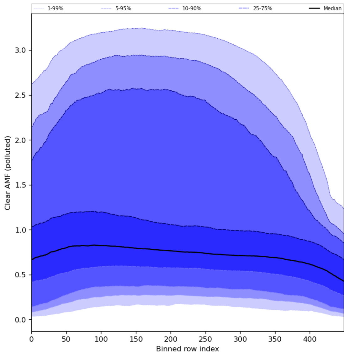
Figure 96: Along track statistics of “Clear AMF (polluted)” for 2024-02-06 to 2024-02-08
