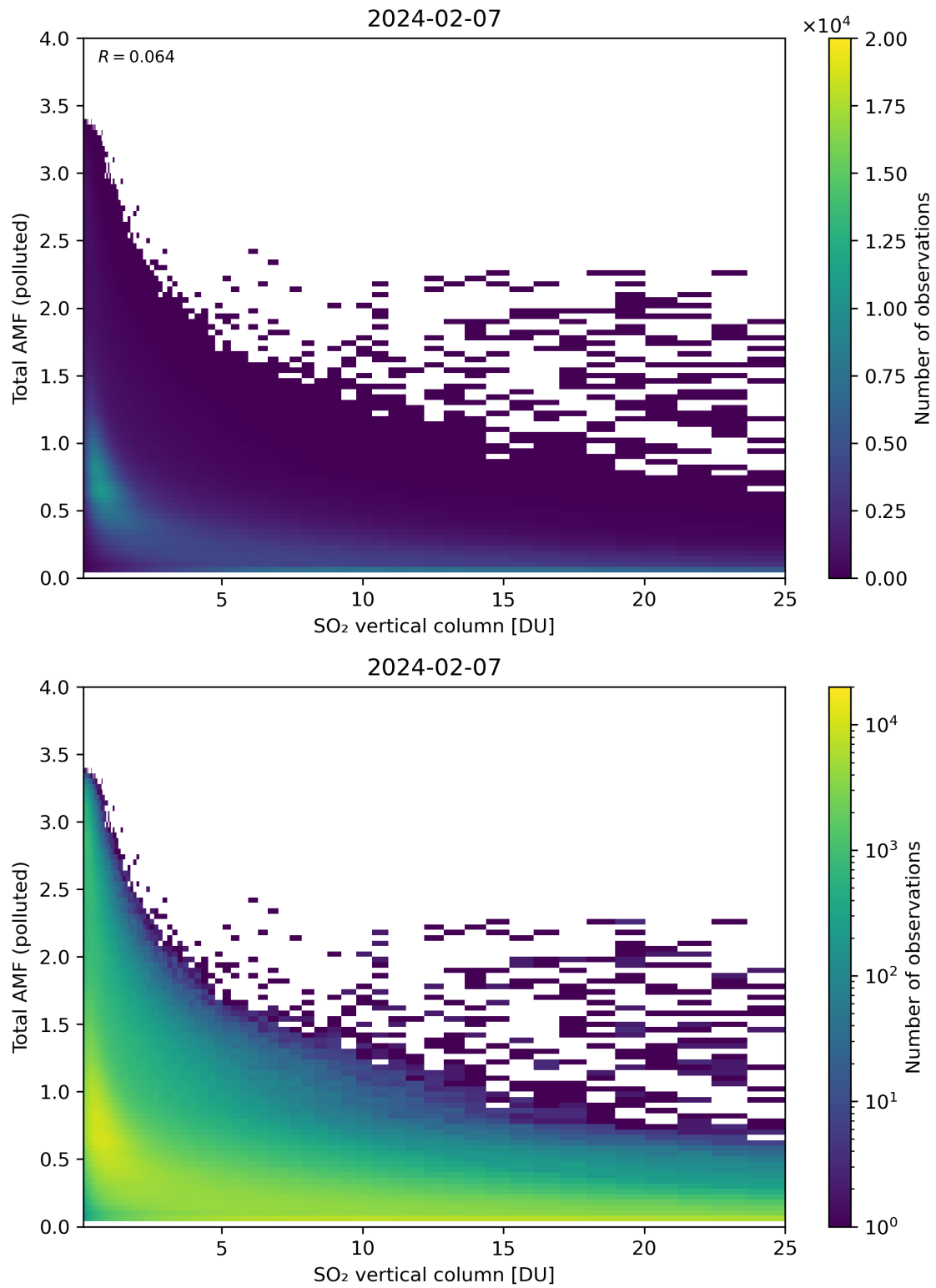
Figure 305: Scatter density plot of “SO 2 vertical column” against “Total AMF (polluted)” for 2024-02-06 to 2024-02-08.
