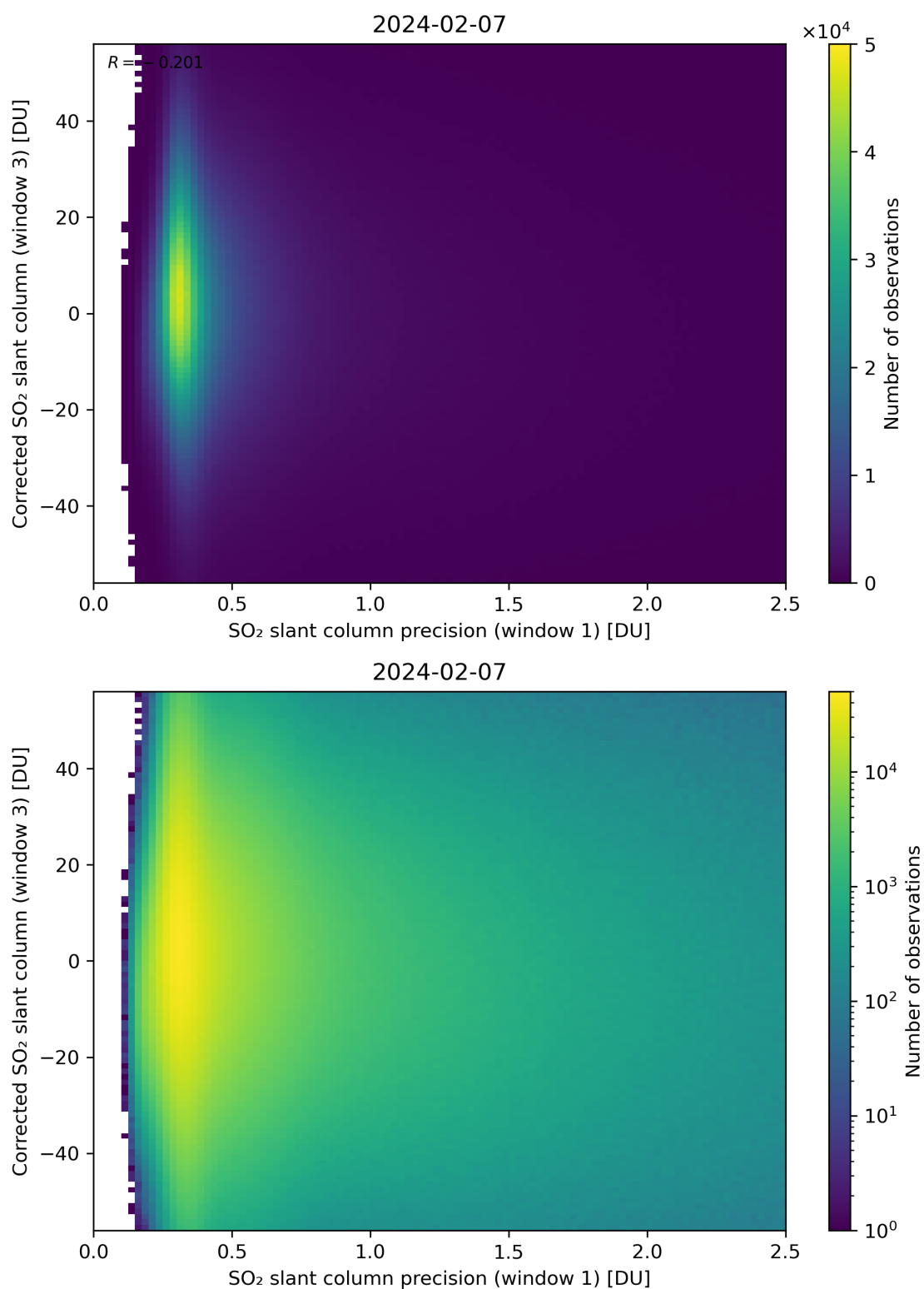
Figure 226: Scatter density plot of “SO 2 slant column precision (window 1)” against “Corrected SO 2 slant column (window 3)” for 2024-02-06 to 2024-02-08.
