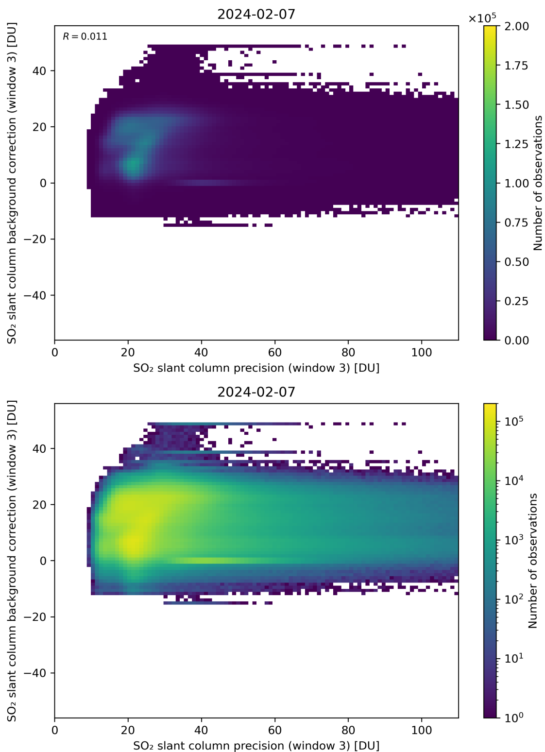
Figure 257: Scatter density plot of “SO 2 slant column precision (window 3)” against “SO 2 slant column background correction (window 3)” for 2024-02-06 to 2024-02-08.
