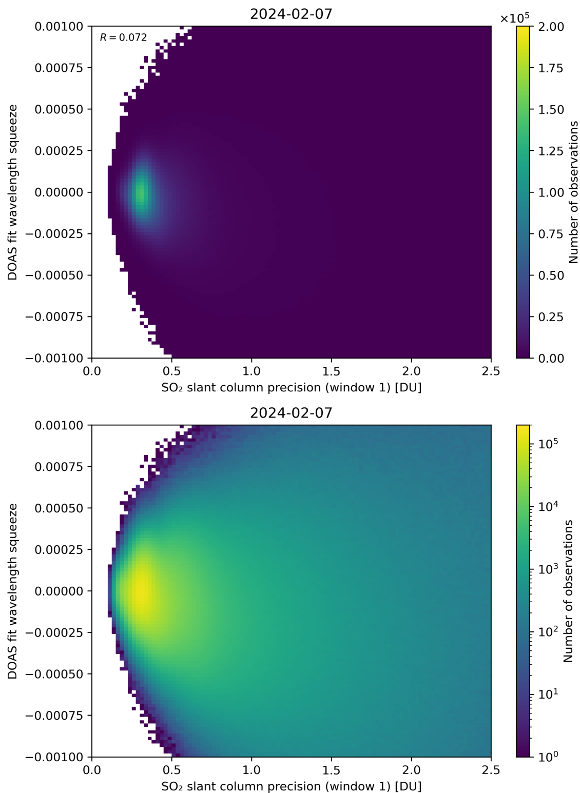
Figure 222: Scatter density plot of “SO 2 slant column precision (window 1)” against “DOAS fit wavelength squeeze” for 2024-02-06 to 2024-02-08.
