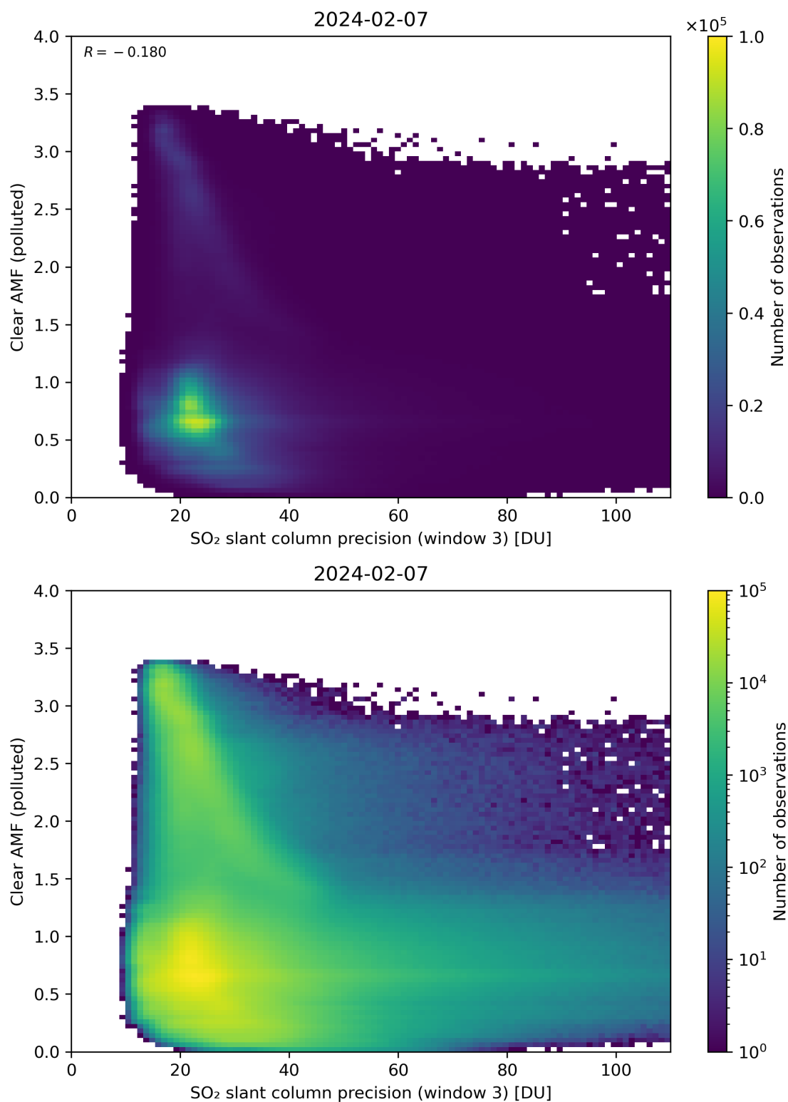
Figure 261: Scatter density plot of “SO 2 slant column precision (window 3)” against “Clear AMF (polluted)” for 2024-02-06 to 2024-02-08.
