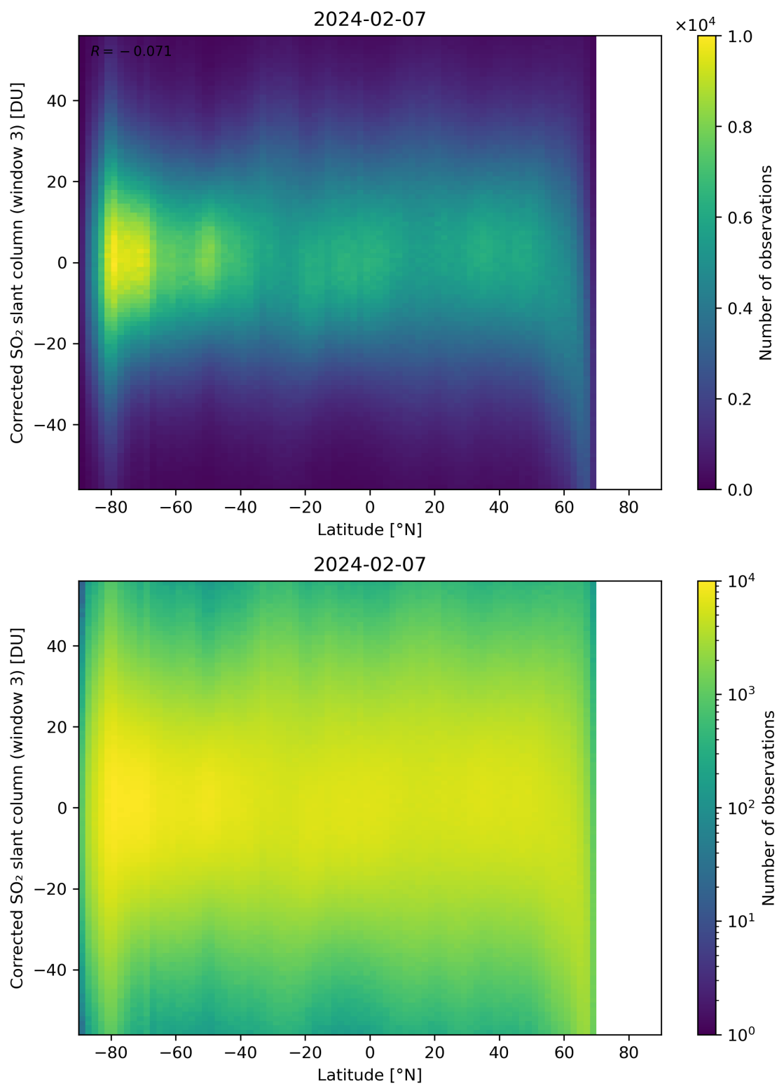
Figure 148: Scatter density plot of “Latitude” against “Corrected SO 2 slant column (window 3)” for 2024-02-06 to 2024-02-08.
