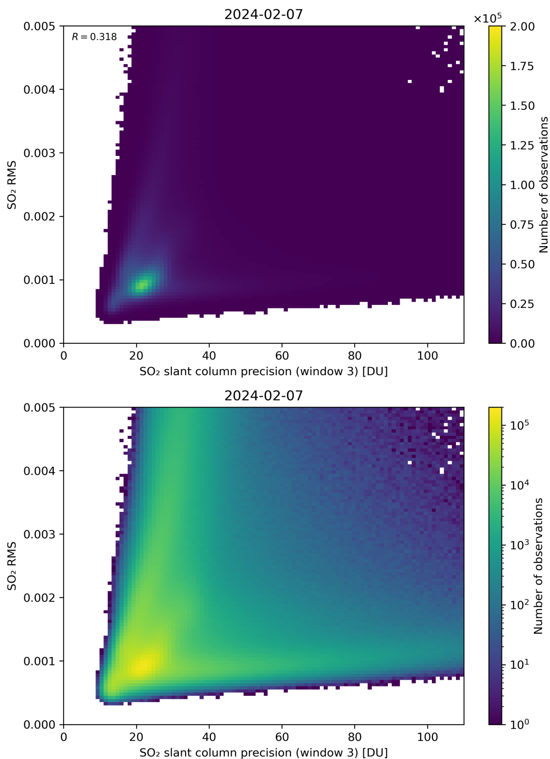
Figure 260: Scatter density plot of “SO 2 slant column precision (window 3)” against “SO 2 RMS” for 2024-02-06 to 2024-02-08.
