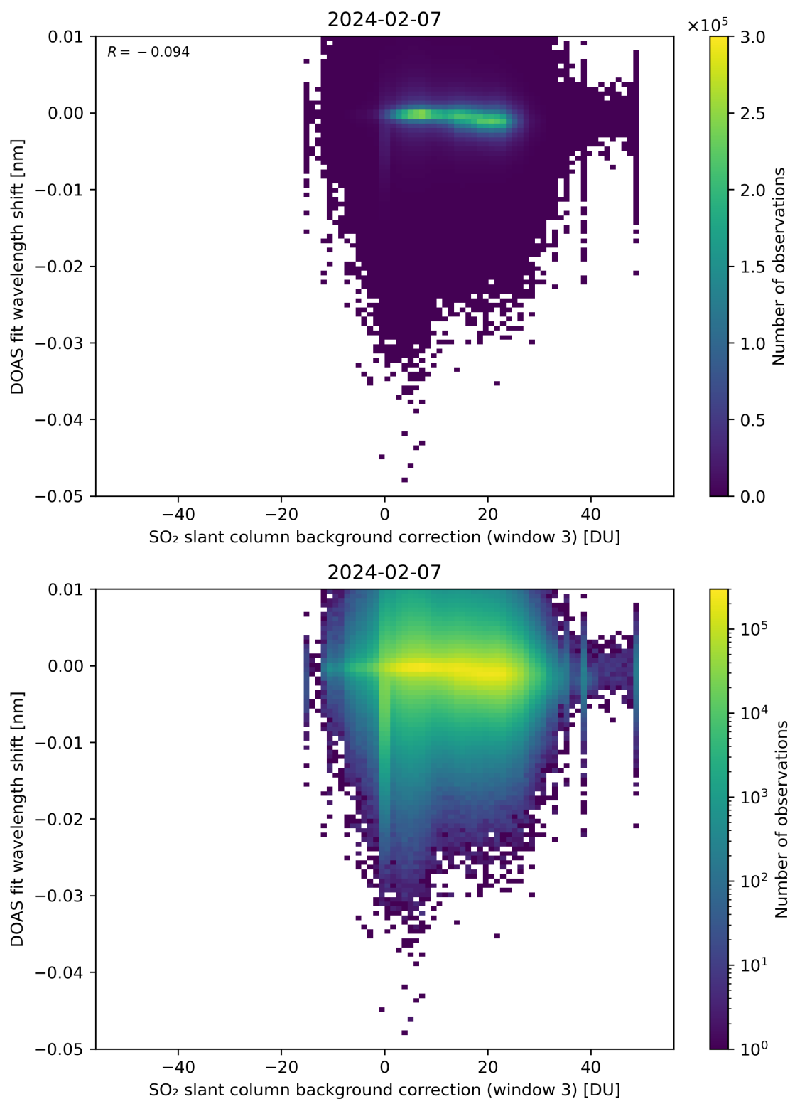
Figure 121: Scatter density plot of “SO 2 slant column background correction (window 3)” against “DOAS fit wavelength shift” for 2024-02-06 to 2024-02-08.
