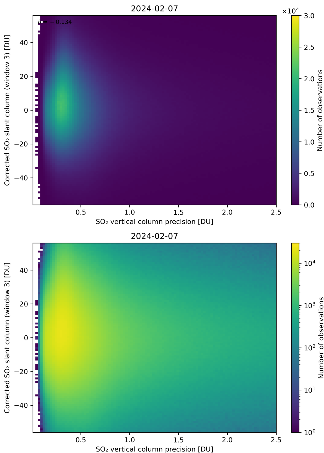
Figure 288: Scatter density plot of “SO 2 vertical column precision” against “Corrected SO 2 slant column (window 3)” for 2024-02-06 to 2024-02-08.
