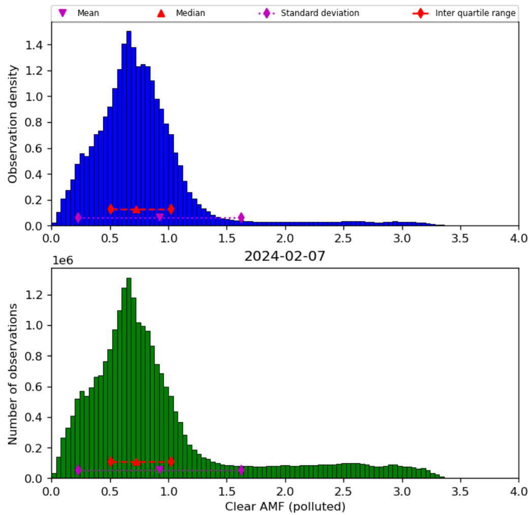
Figure 73: Histogram of “Clear AMF (polluted)” for 2024-02-06 to 2024-02-08
