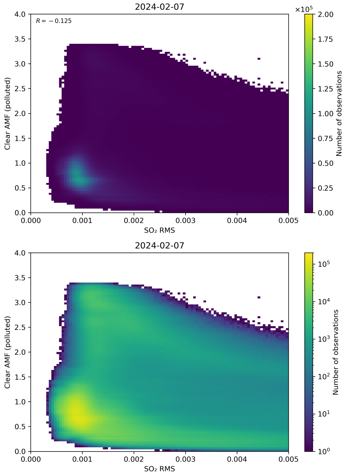
Figure 136: Scatter density plot of “SO 2 RMS” against “Clear AMF (polluted)” for 2024-02-06 to 2024-02-08.
