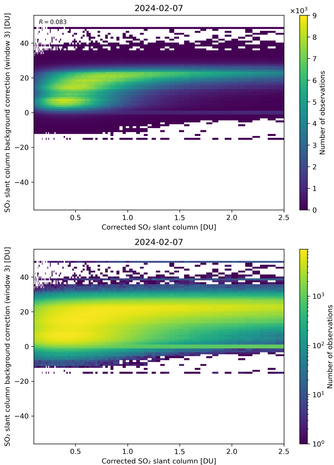
Figure 180: Scatter density plot of “Corrected SO 2 slant column” against “SO 2 slant column background correction (window 3)” for 2024-02-06 to 2024-02-08.
