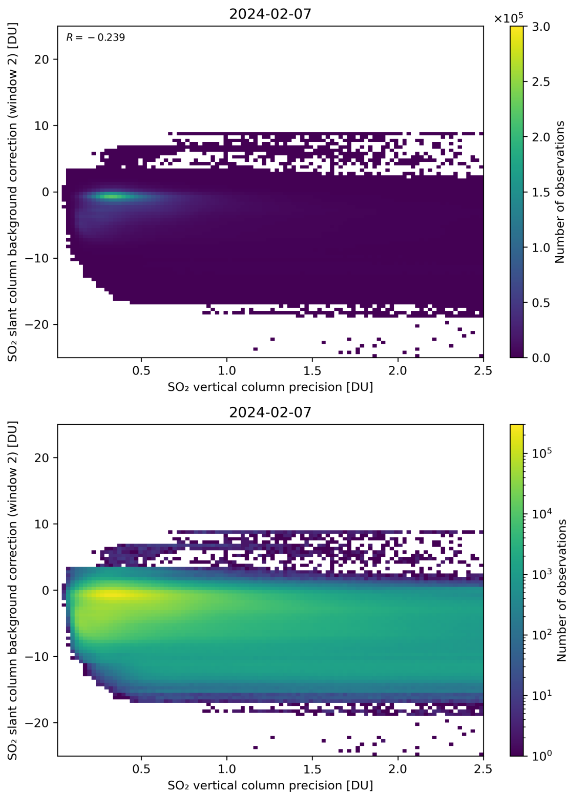
Figure 280: Scatter density plot of “SO 2 vertical column precision” against “SO 2 slant column background correction (window 2)” for 2024-02-06 to 2024-02-08.
