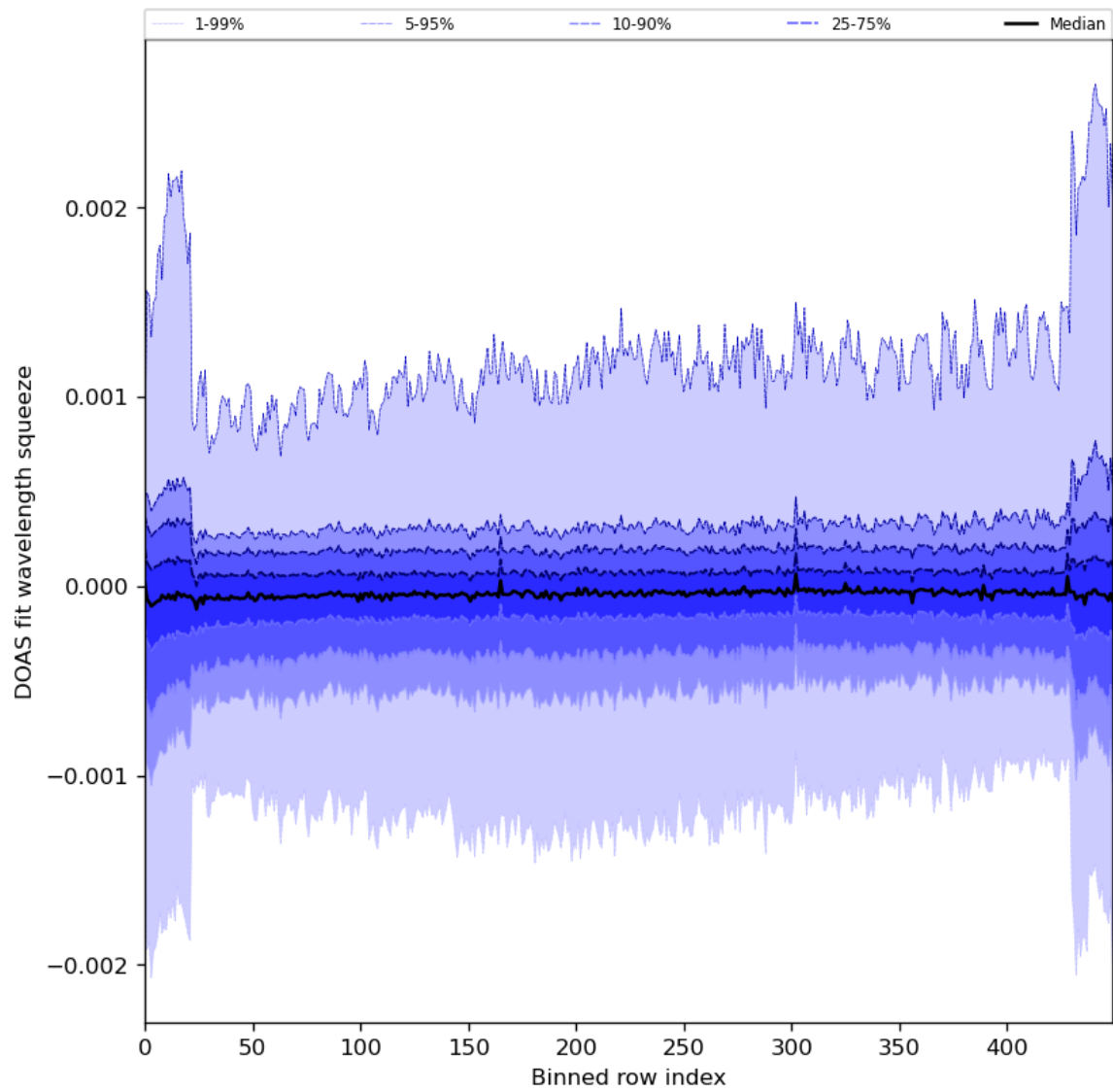
Figure 92: Along track statistics of “DOAS fit wavelength squeeze” for 2024-02-06 to 2024-02-08
