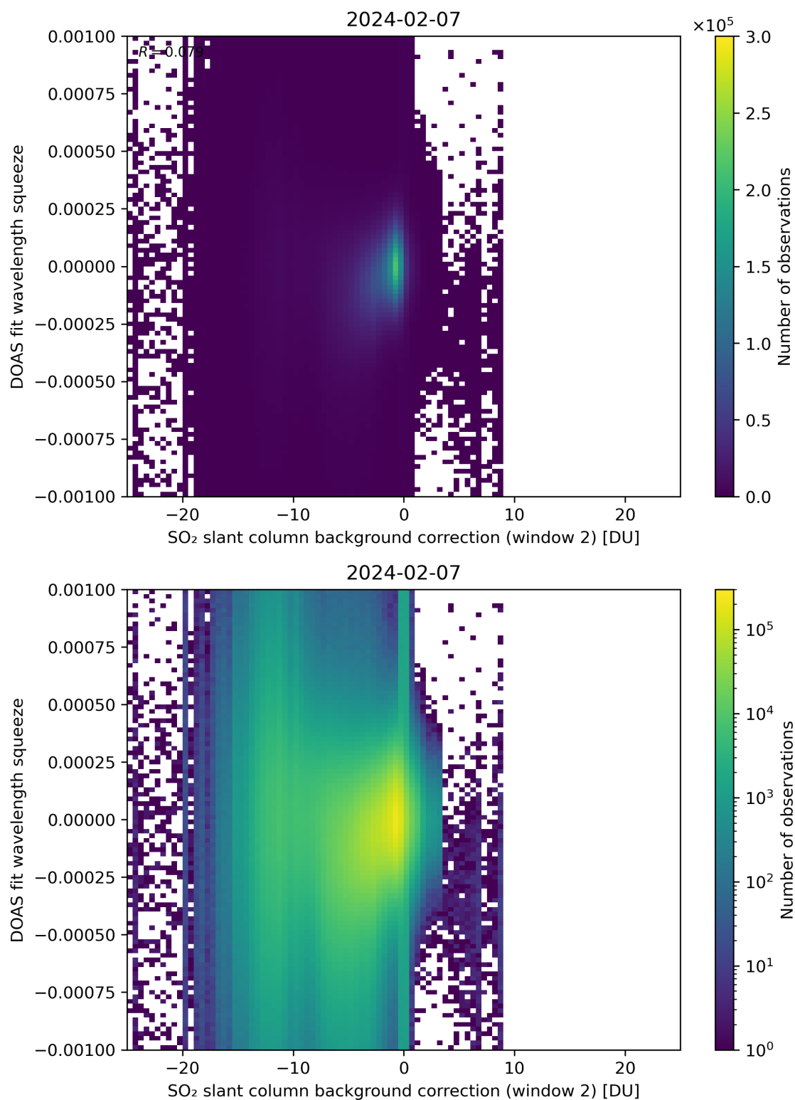
Figure 113: Scatter density plot of “SO 2 slant column background correction (window 2)” against “DOAS fit wavelength squeeze” for 2024-02-06 to 2024-02-08.
