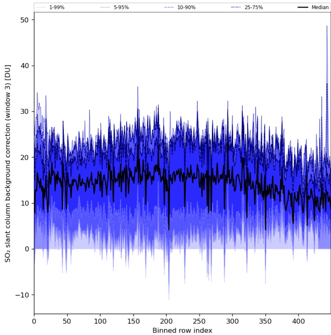
Figure 90: Along track statistics of “SO 2 slant column background correction (window 3)” for 2024-02-06 to 2024-02-08
