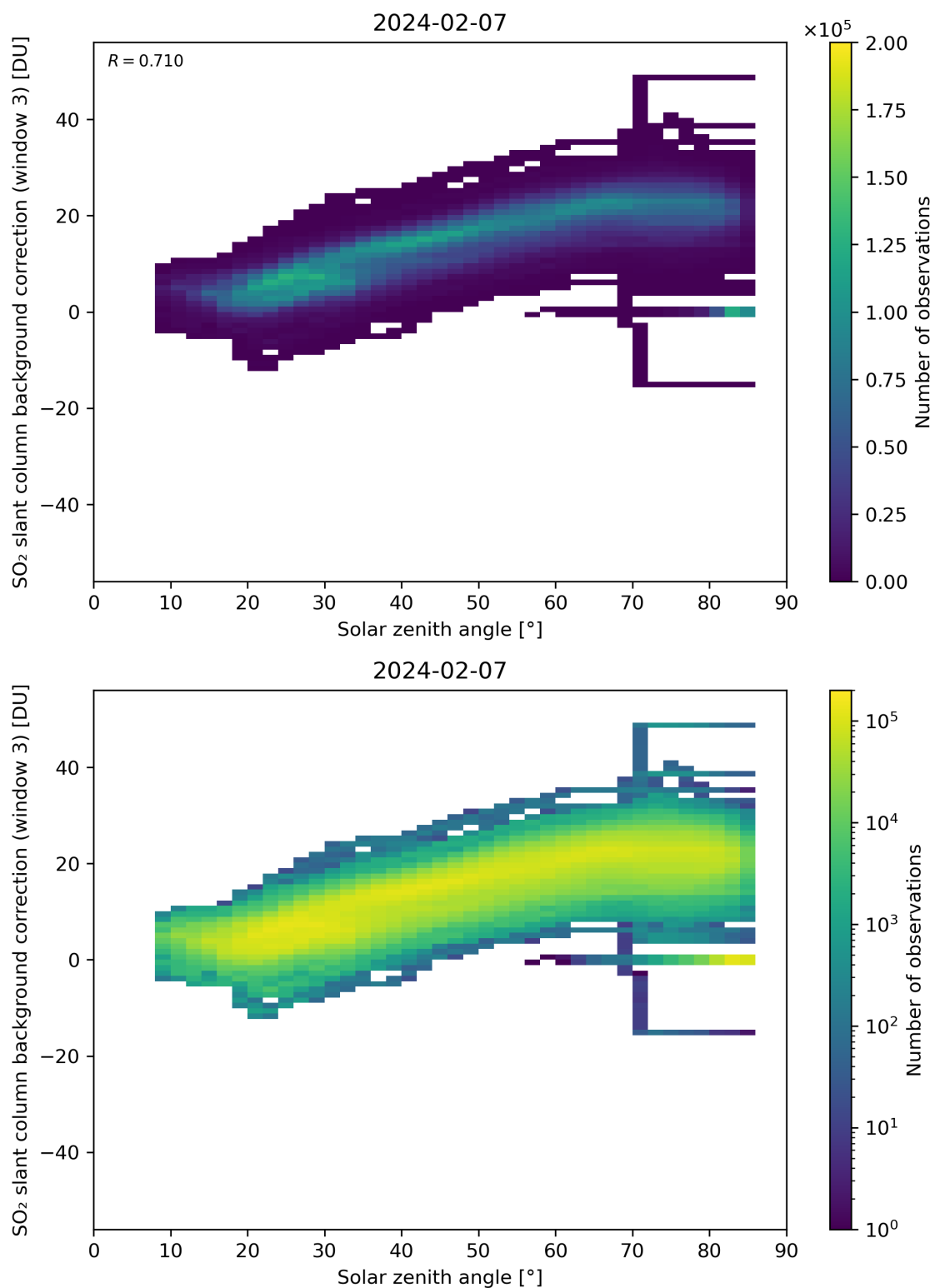
Figure 160: Scatter density plot of “Solar zenith angle” against “SO 2 slant column background correction (window 3)” for 2024-02-06 to 2024-02-08.
