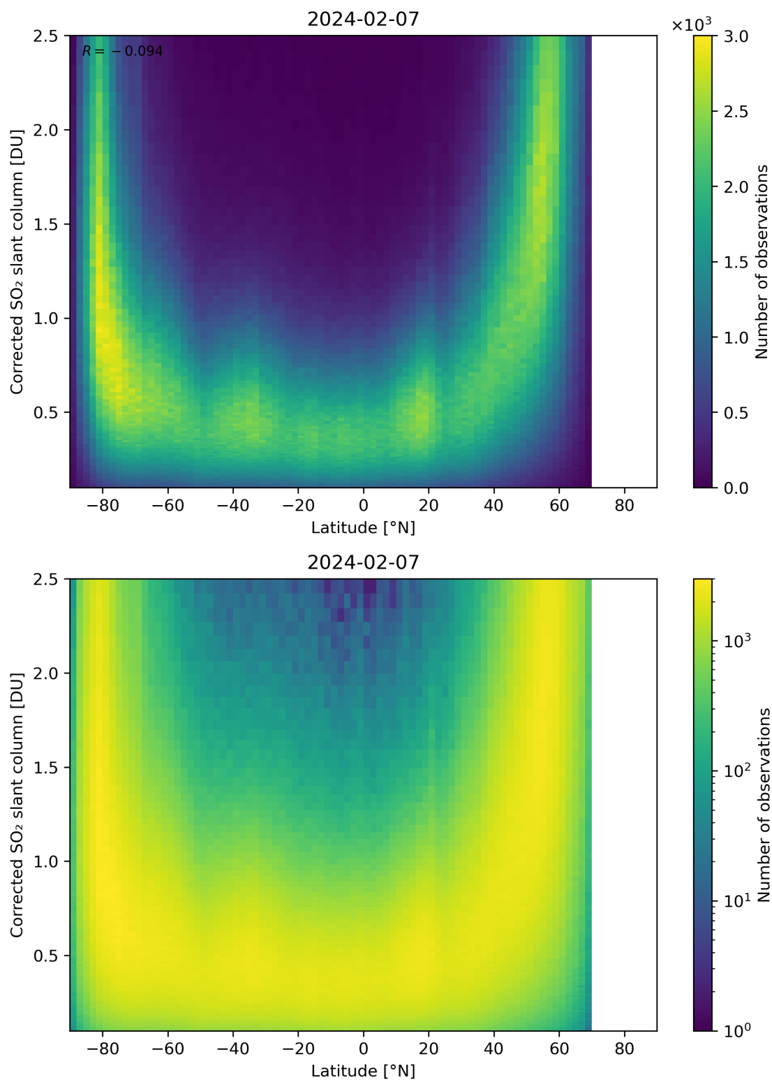
Figure 146: Scatter density plot of “Latitude” against “Corrected SO 2 slant column” for 2024-02-06 to 2024-02-08.
