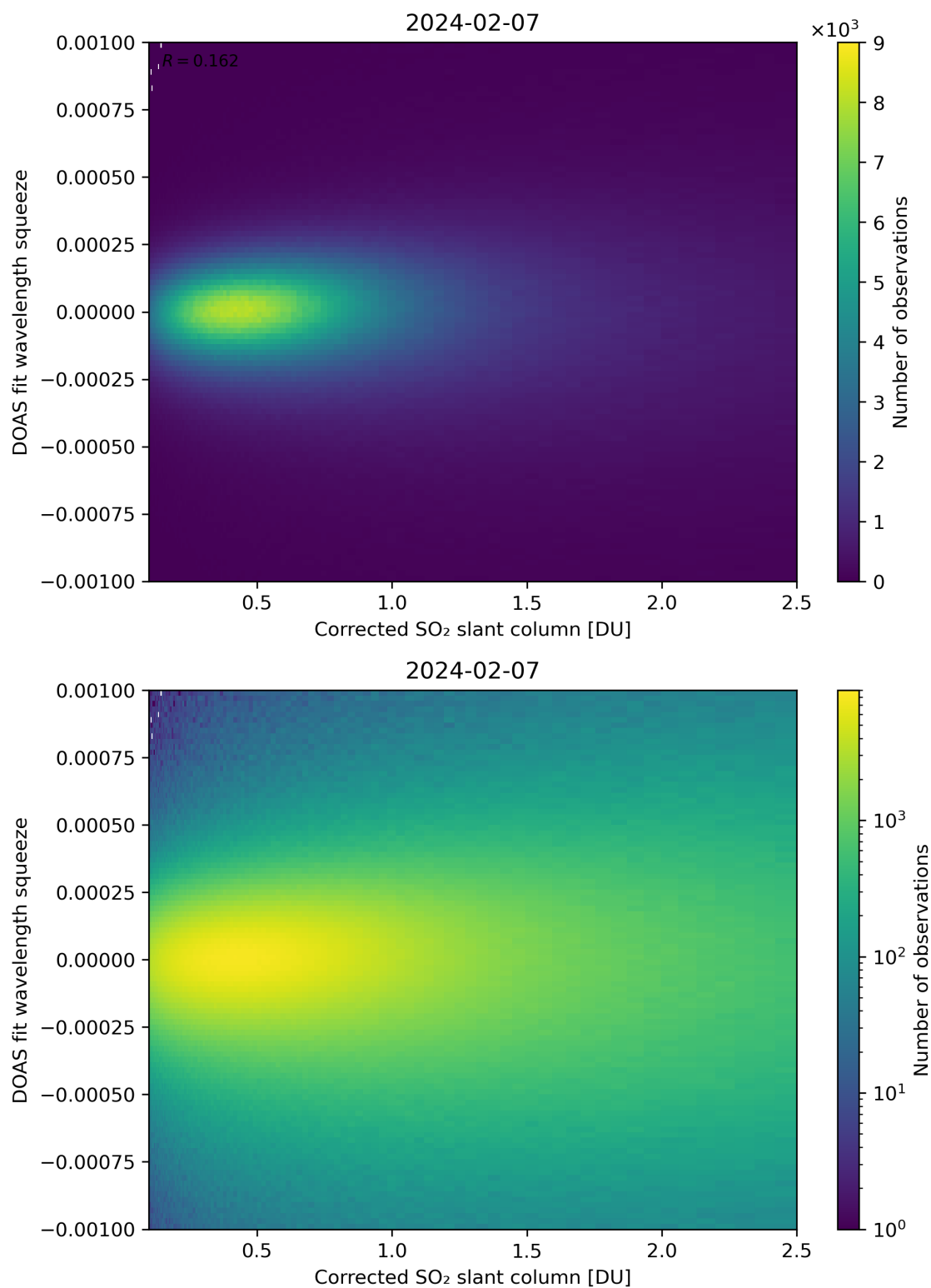
Figure 182: Scatter density plot of “Corrected SO 2 slant column” against “DOAS fit wavelength squeeze” for 2024-02-06 to 2024-02-08.
