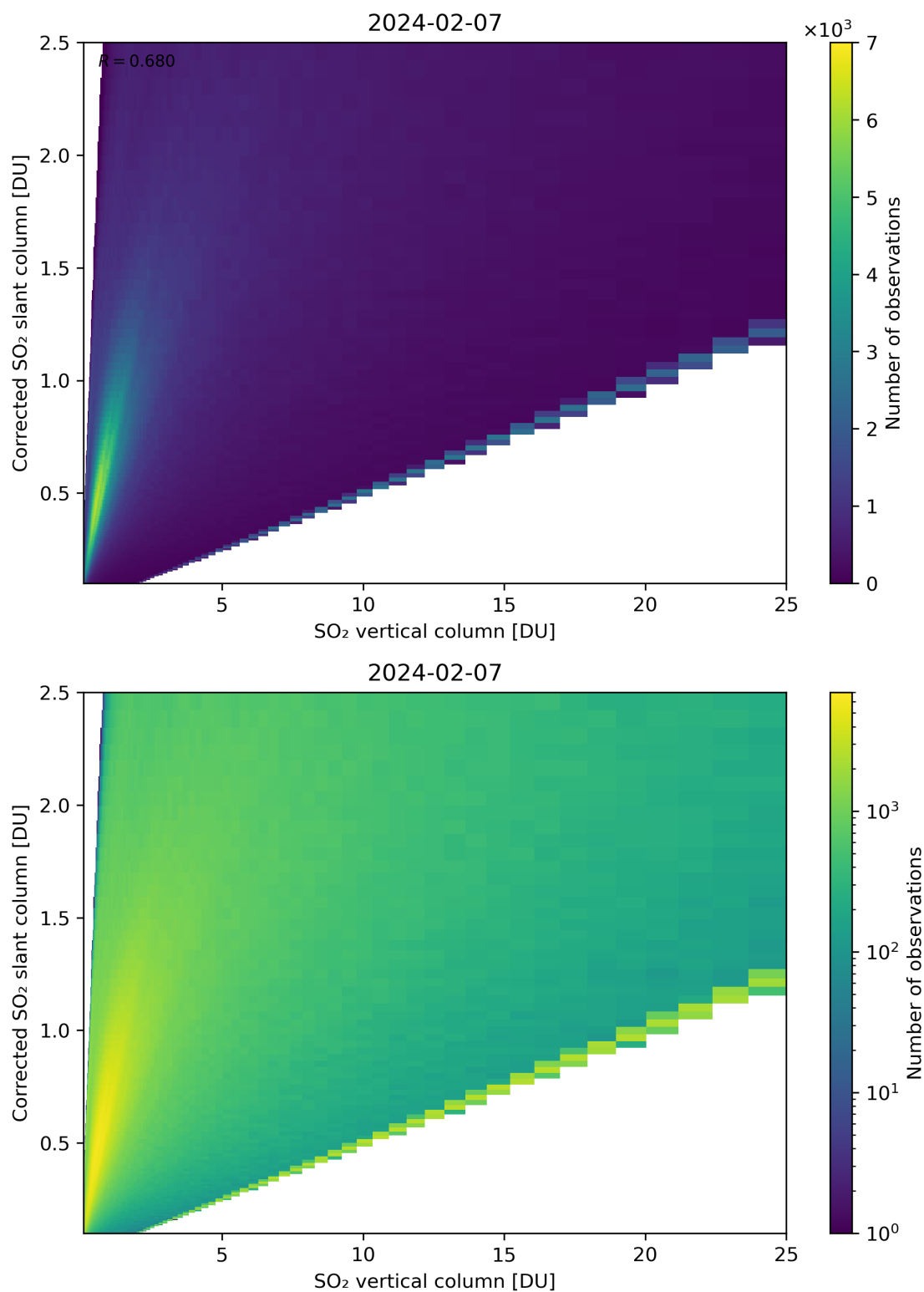
Figure 297: Scatter density plot of “SO 2 vertical column” against “Corrected SO 2 slant column” for 2024-02-06 to 2024-02-08.
