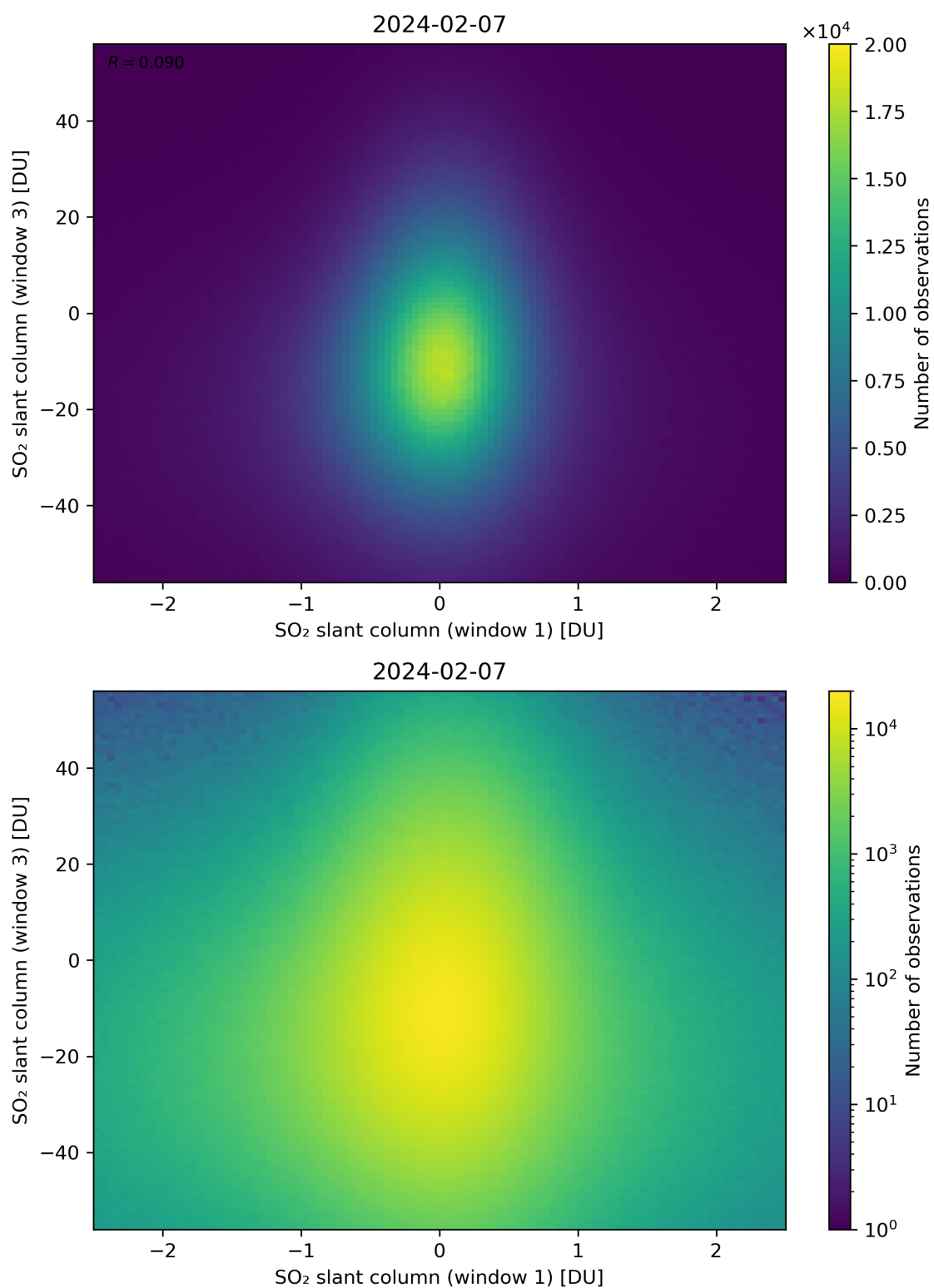
Figure 237: Scatter density plot of “SO 2 slant column (window 1)” against “SO 2 slant column (window 3)” for 2024-02-06 to 2024-02-08.
