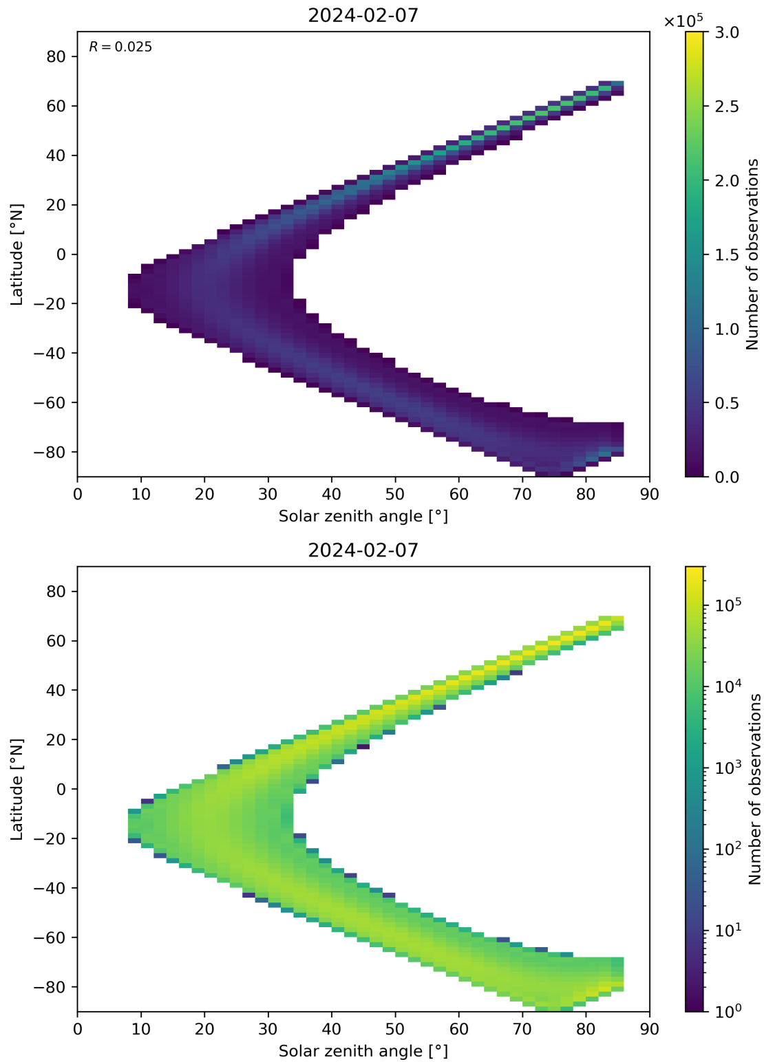
Figure 164: Scatter density plot of “Solar zenith angle” against “Latitude” for 2024-02-06 to 2024-02-08.
