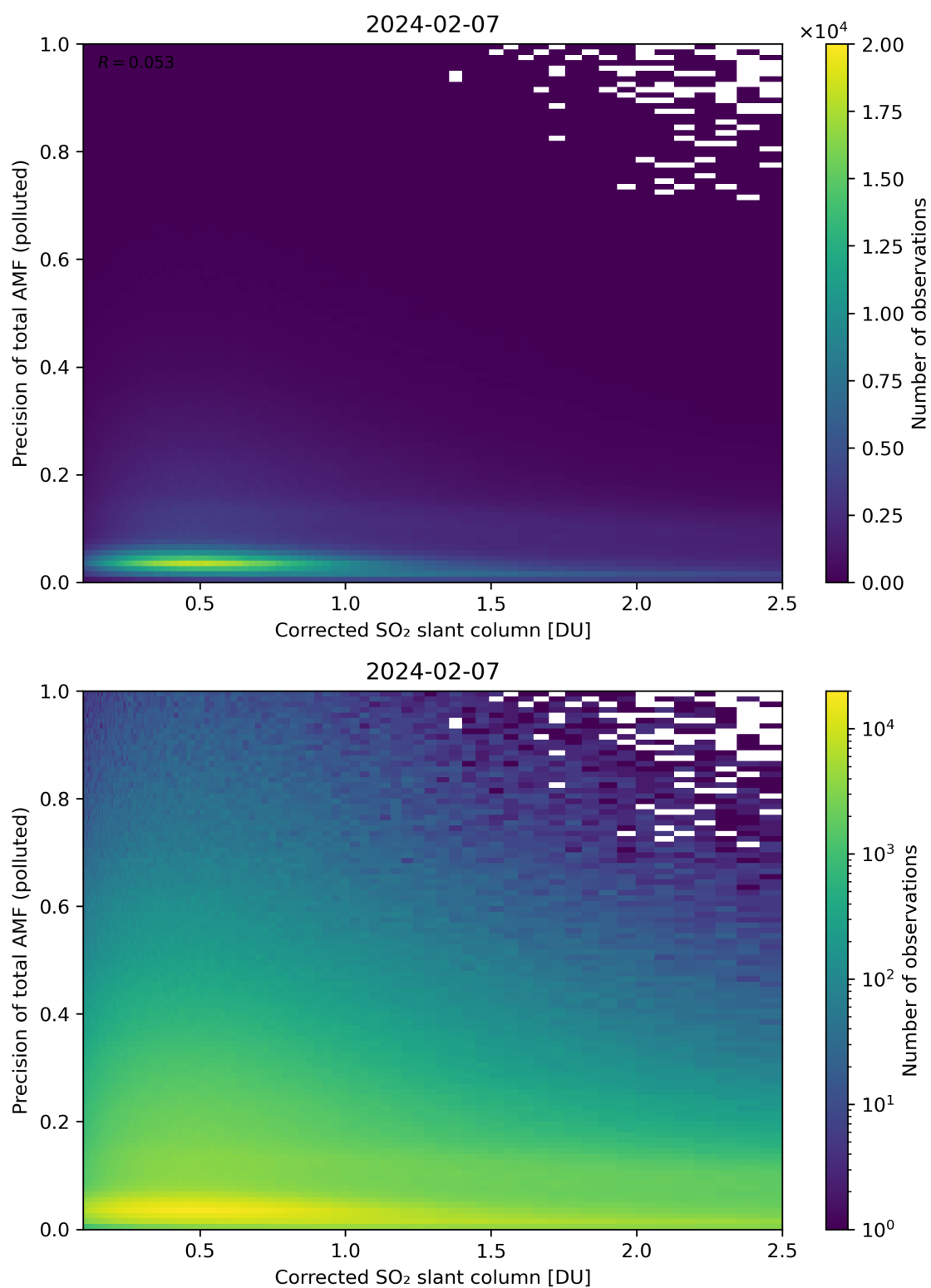
Figure 193: Scatter density plot of “Corrected SO 2 slant column” against “Precision of total AMF (polluted)” for 2024-02-06 to 2024-02-08.
