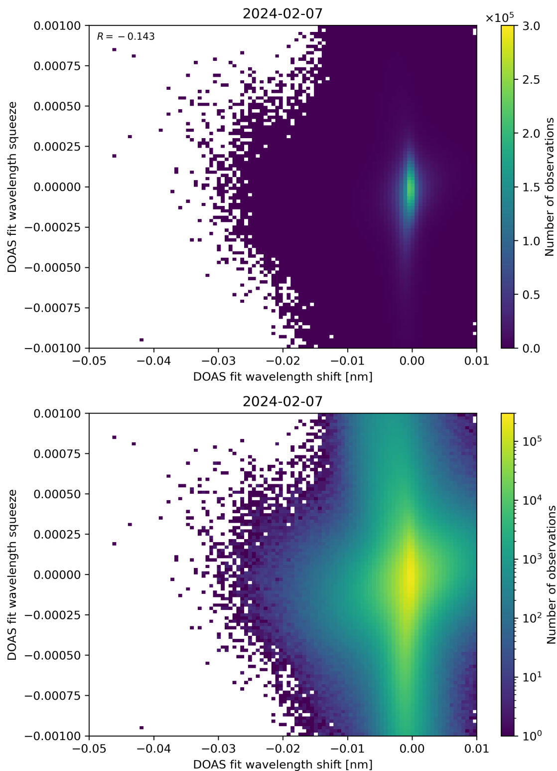
Figure 127: Scatter density plot of “DOAS fit wavelength shift” against “DOAS fit wavelength squeeze” for 2024-02-06 to 2024-02-08.
