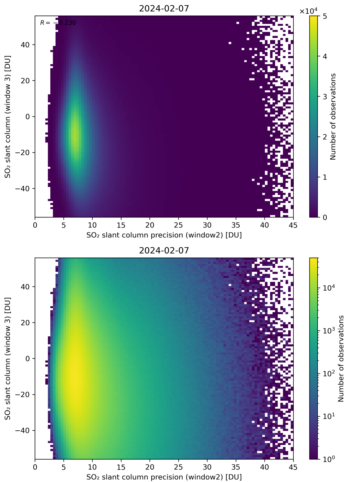
Figure 249: Scatter density plot of “SO 2 slant column precision (window2)” against “SO 2 slant column (window 3)” for 2024-02-06 to 2024-02-08.
