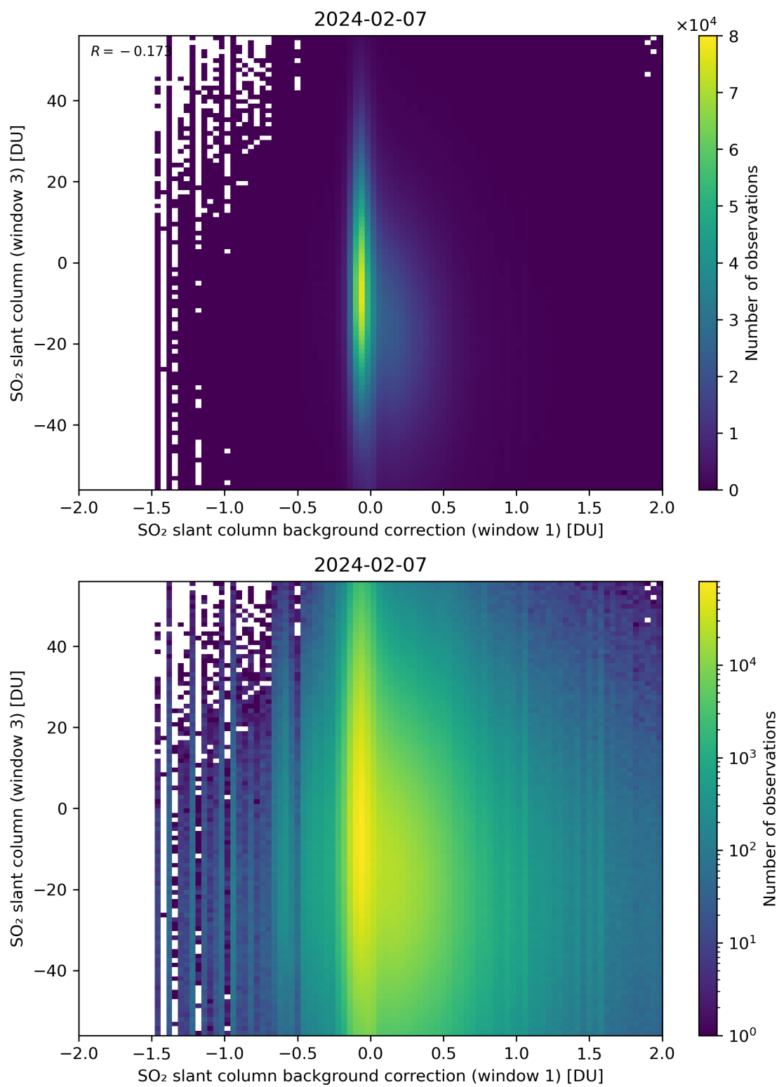
Figure 107: Scatter density plot of “SO 2 slant column background correction (window 1)” against “SO 2 slant column (window 3)” for 2024-02-06 to 2024-02-08.
