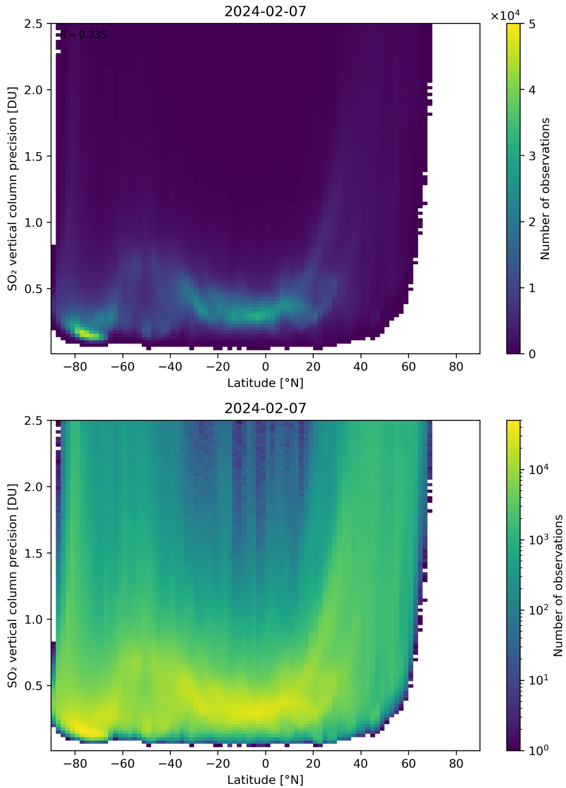
Figure 157: Scatter density plot of “Latitude” against “SO 2 vertical column precision” for 2024-02-06 to 2024-02-08.
