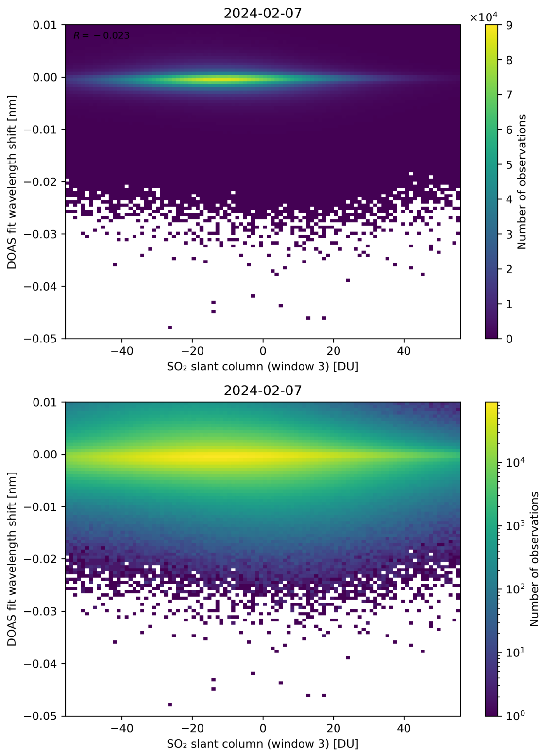
Figure 254: Scatter density plot of “SO 2 slant column (window 3)” against “DOAS fit wavelength shift” for 2024-02-06 to 2024-02-08.
