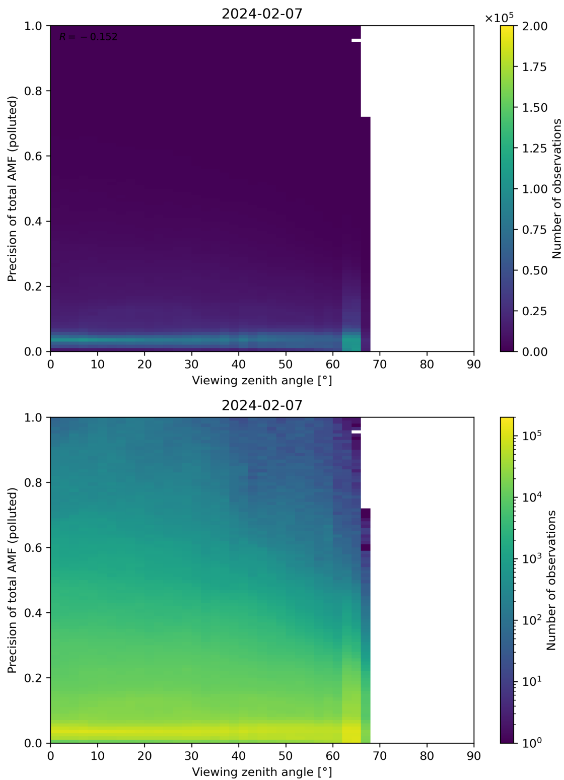
Figure 326: Scatter density plot of “Viewing zenith angle” against “Precision of total AMF (polluted)” for 2024-02-06 to 2024-02-08.
