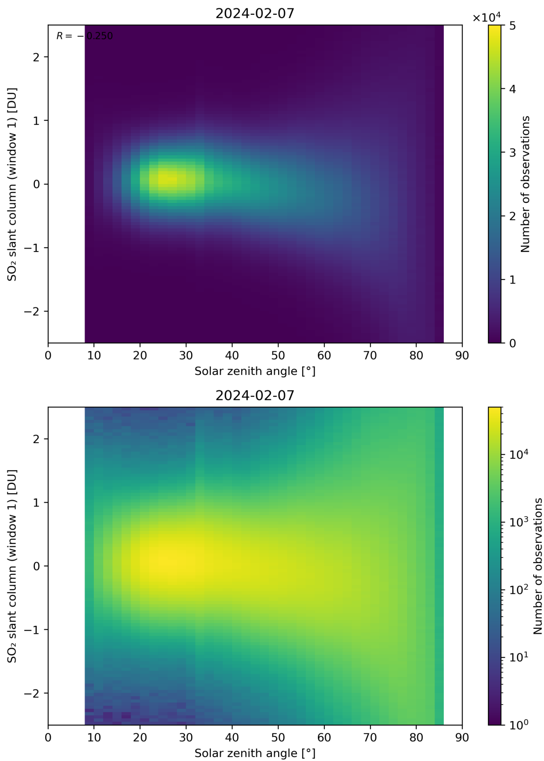
Figure 169: Scatter density plot of “Solar zenith angle” against “SO 2 slant column (window 1)” for 2024-02-06 to 2024-02-08.
