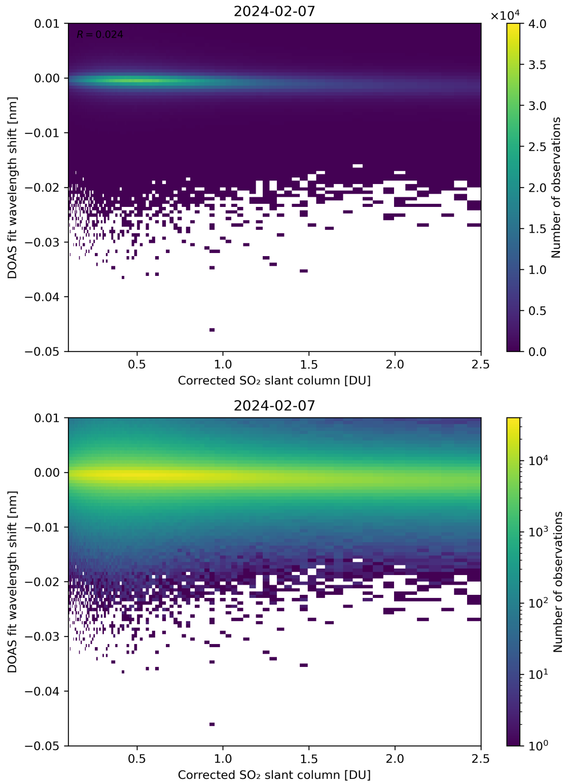
Figure 181: Scatter density plot of “Corrected SO 2 slant column” against “DOAS fit wavelength shift” for 2024-02-06 to 2024-02-08.
