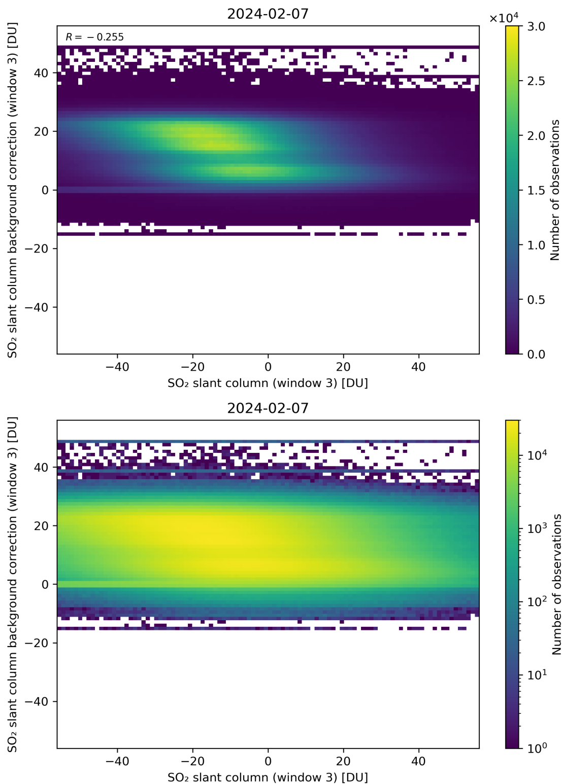
Figure 253: Scatter density plot of “SO 2 slant column (window 3)” against “SO 2 slant column background correction (window 3)” for 2024-02-06 to 2024-02-08.
