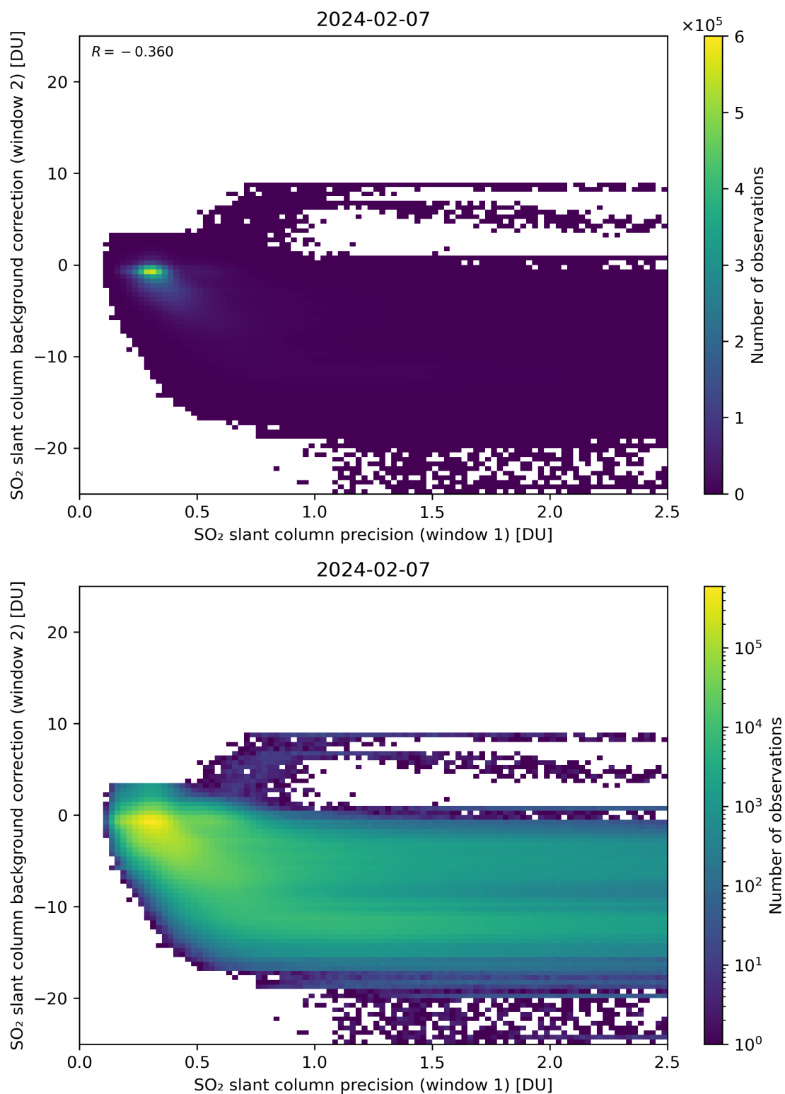
Figure 219: Scatter density plot of “SO 2 slant column precision (window 1)” against “SO 2 slant column background correction (window 2)” for 2024-02-06 to 2024-02-08.
