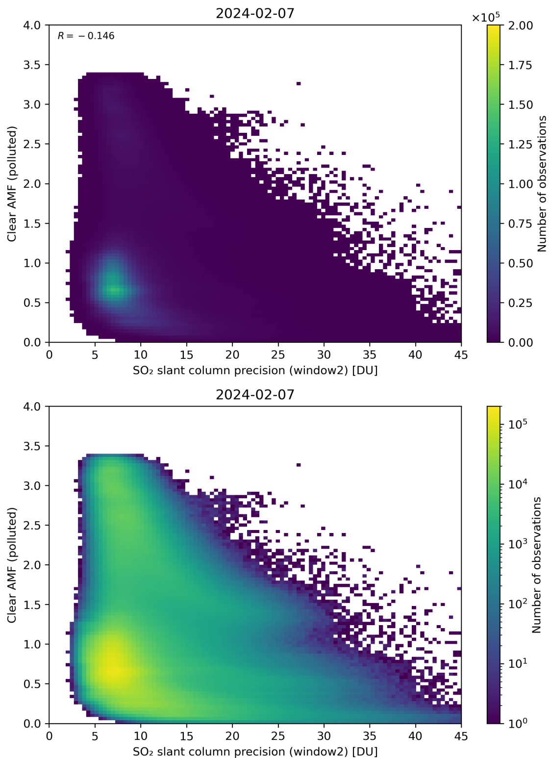
Figure 246: Scatter density plot of “SO 2 slant column precision (window2)” against “Clear AMF (polluted)” for 2024-02-06 to 2024-02-08.
