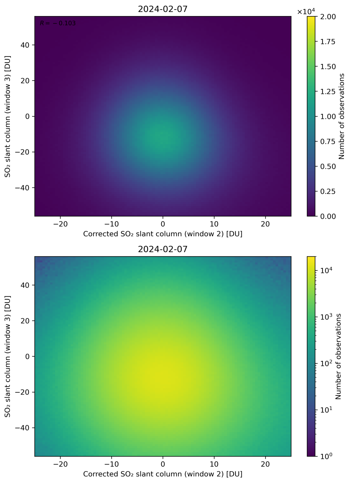
Figure 201: Scatter density plot of “Corrected SO 2 slant column (window 2)” against “SO 2 slant column (window 3)” for 2024-02-06 to 2024-02-08.
