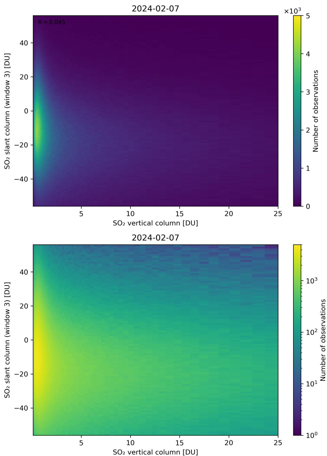
Figure 303: Scatter density plot of “SO 2 vertical column” against “SO 2 slant column (window 3)” for 2024-02-06 to 2024-02-08.
