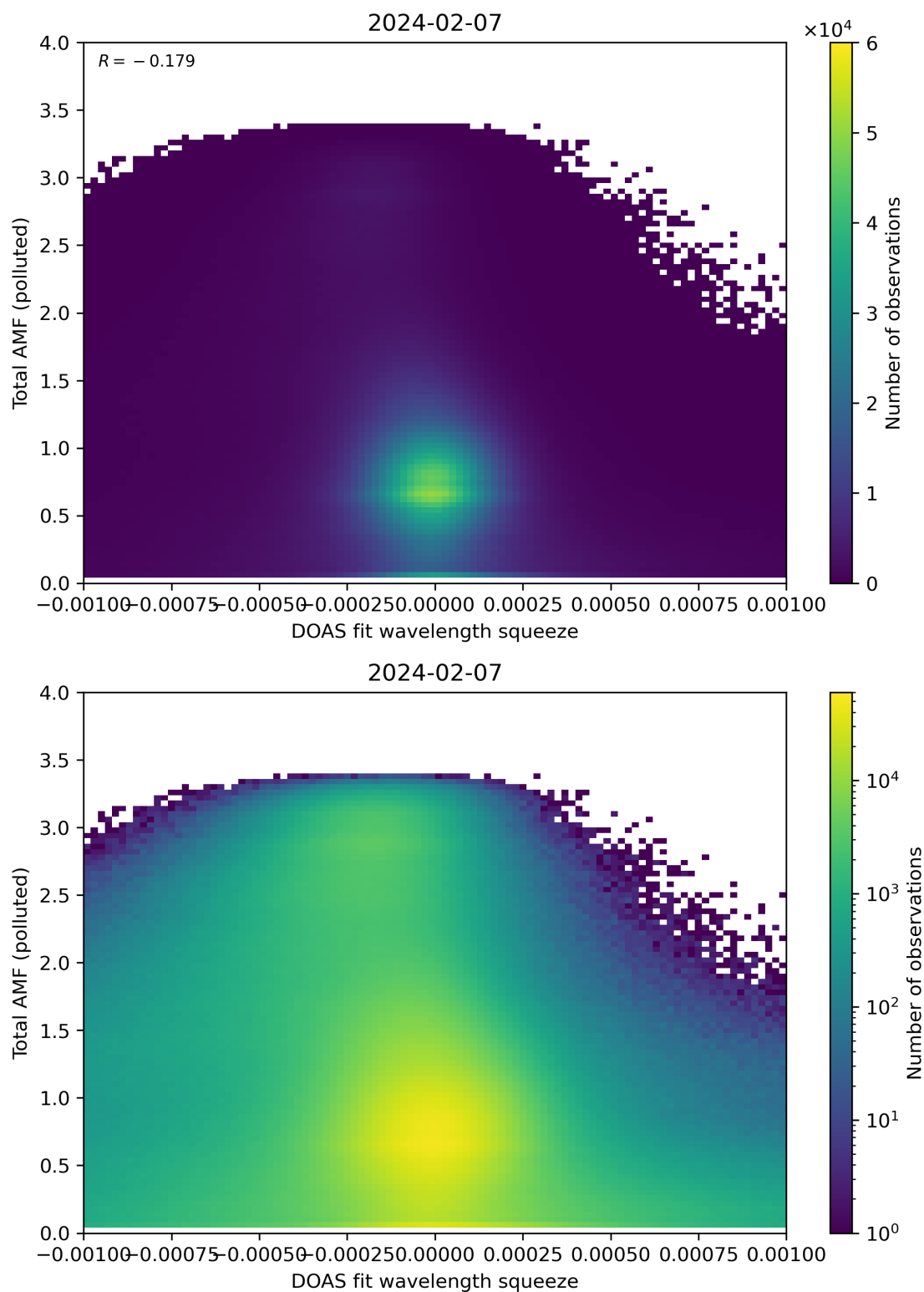
Figure 134: Scatter density plot of “DOAS fit wavelength squeeze” against “Total AMF (polluted)” for 2024-02-06 to 2024-02-08.
