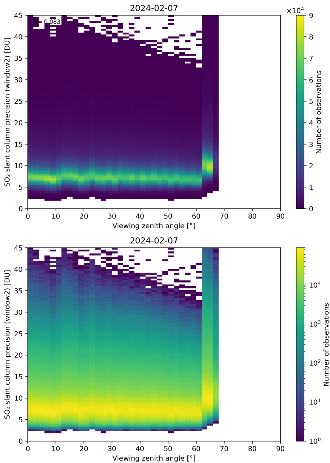
Figure 322: Scatter density plot of “Viewing zenith angle” against “SO 2 slant column precision (window2)” for 2024-02-06 to 2024-02-08.
