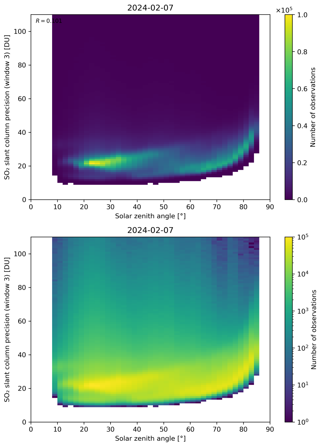
Figure 173: Scatter density plot of “Solar zenith angle” against “SO 2 slant column precision (window 3)” for 2024-02-06 to 2024-02-08.
