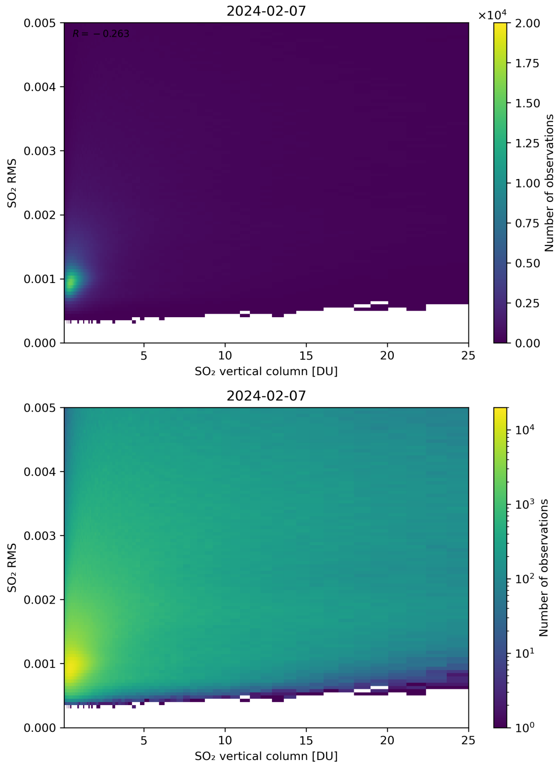
Figure 278: Scatter density plot of “SO 2 vertical column” against “SO 2 RMS” for 2024-02-06 to 2024-02-08.
