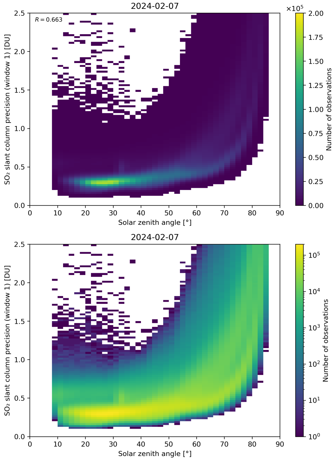
Figure 170: Scatter density plot of “Solar zenith angle” against “SO 2 slant column precision (window 1)” for 2024-02-06 to 2024-02-08.
