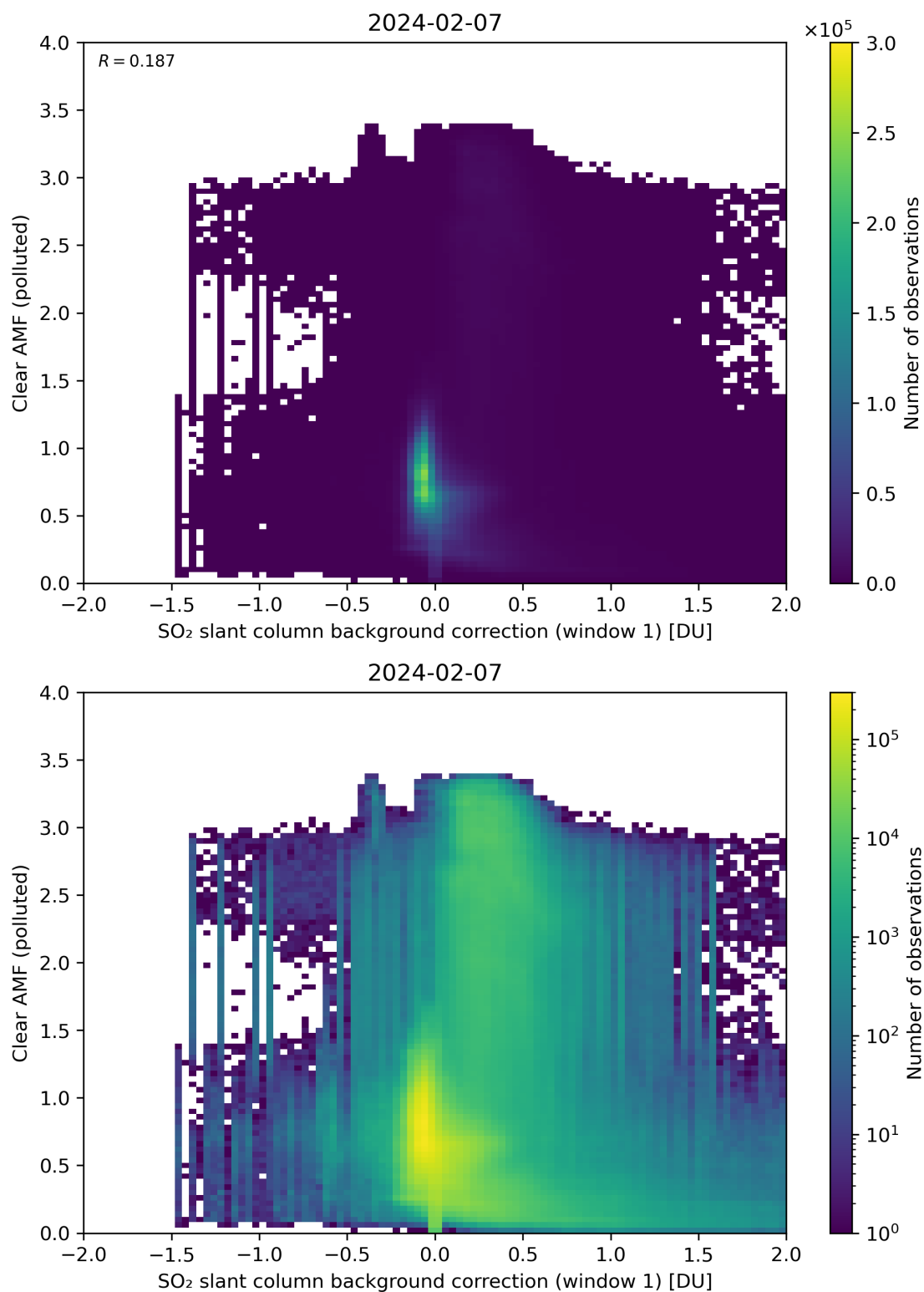
Figure 103: Scatter density plot of “SO 2 slant column background correction (window 1)” against “Clear AMF (polluted)” for 2024-02-06 to 2024-02-08.
