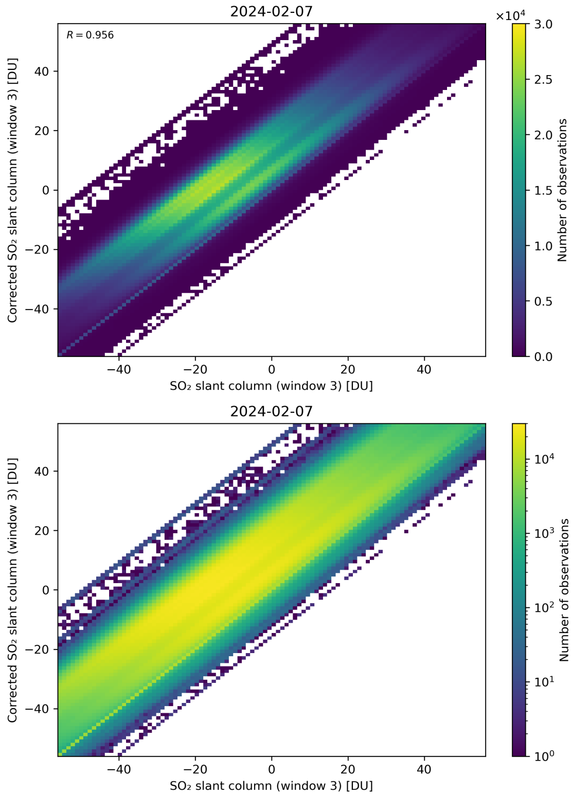
Figure 266: Scatter density plot of “SO 2 slant column (window 3)” against “Corrected SO 2 slant column (window 3)” for 2024-02-06 to 2024-02-08.
