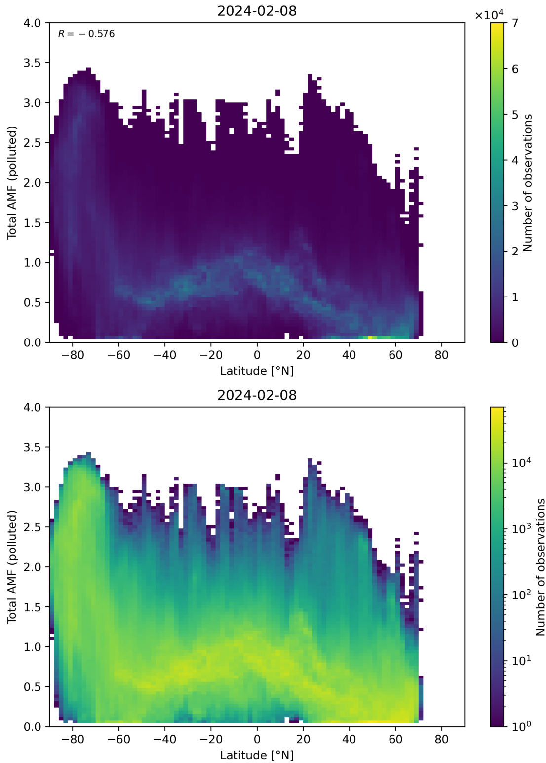
Figure 154: Scatter density plot of “Latitude” against “Total AMF (polluted)” for 2024-02-07 to 2024-02-09.
