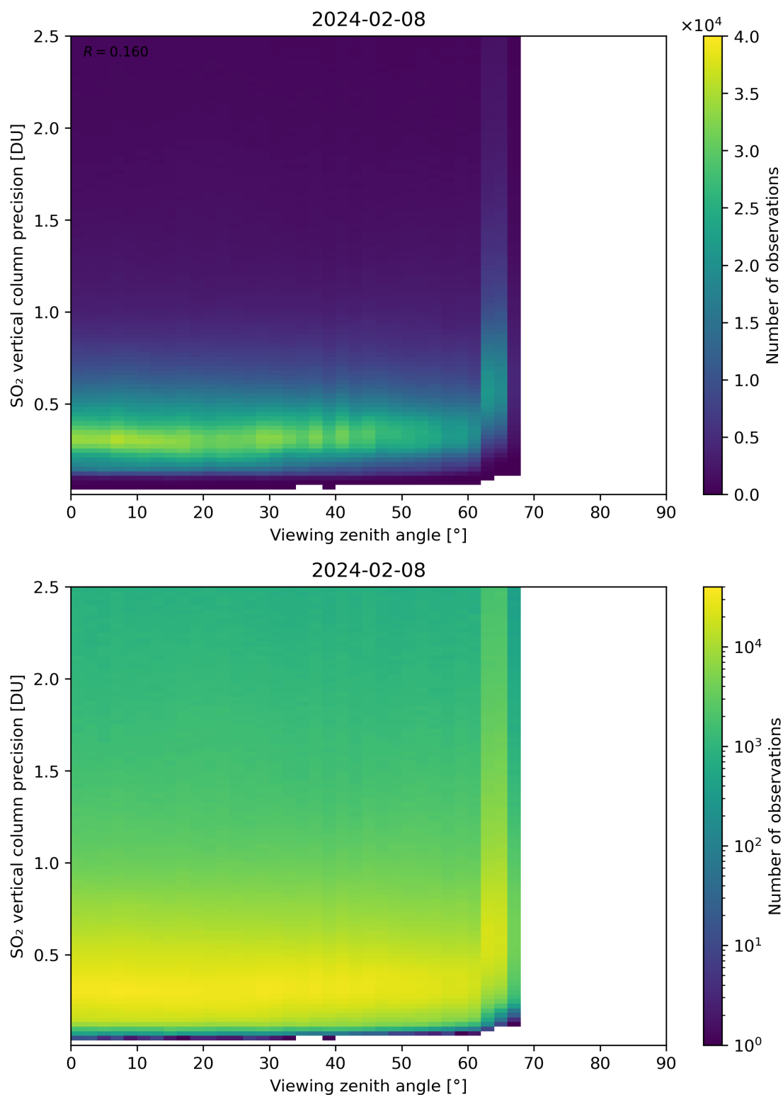
Figure 328: Scatter density plot of “Viewing zenith angle” against “SO 2 vertical column precision” for 2024-02-07 to 2024-02-09.
