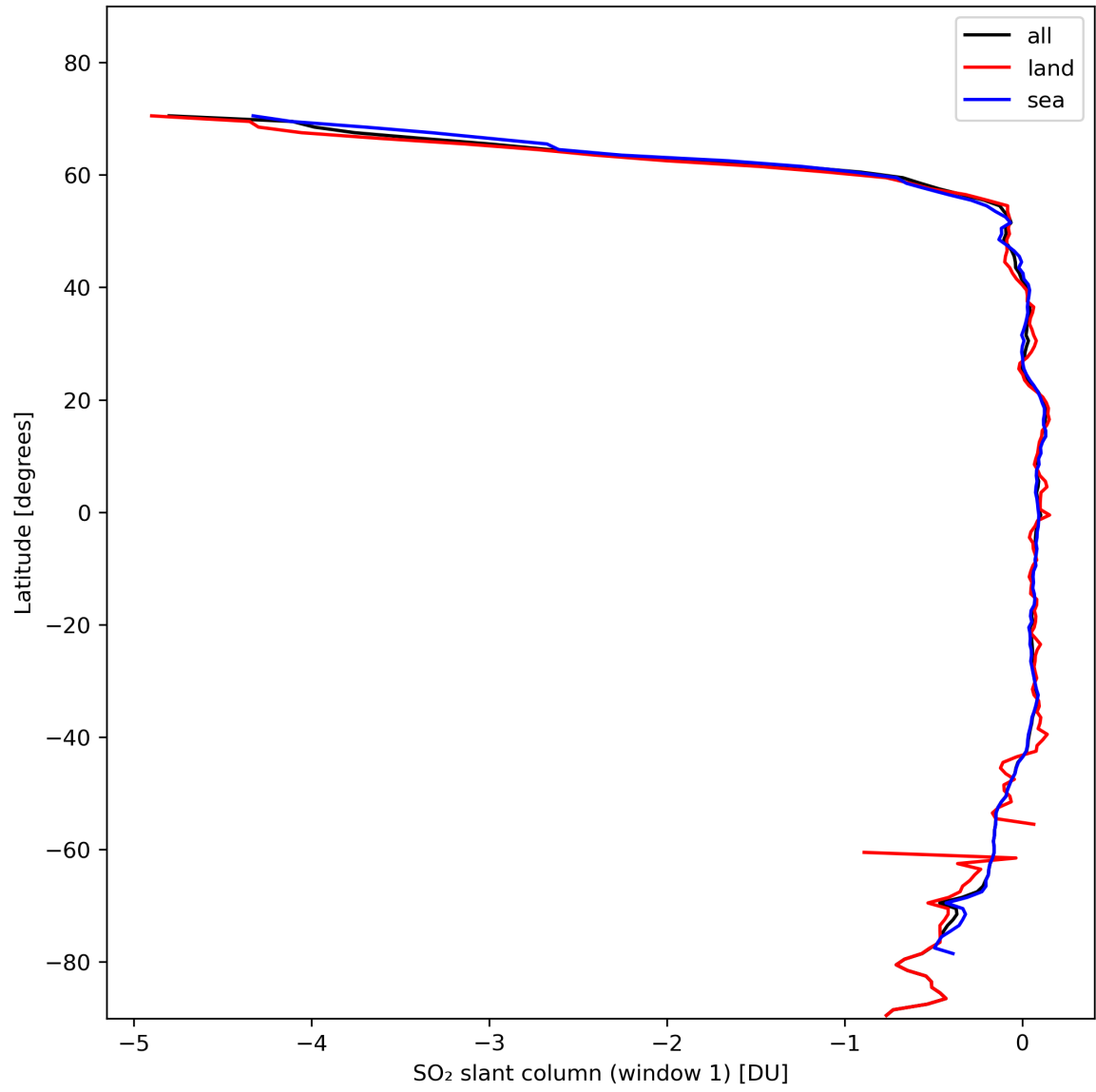
Figure 33: Zonal average of “SO 2 slant column (window 1)” for 2024-02-07 to 2024-02-09.
