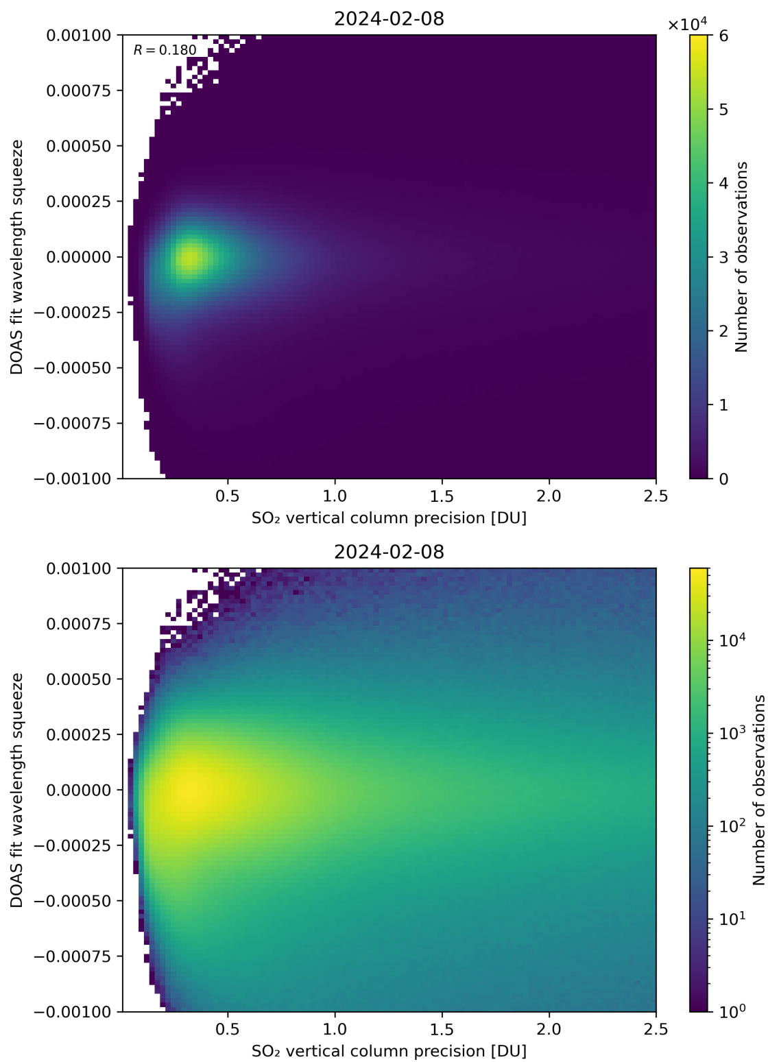
Figure 283: Scatter density plot of “SO 2 vertical column precision” against “DOAS fit wavelength squeeze” for 2024-02-07 to 2024-02-09.
