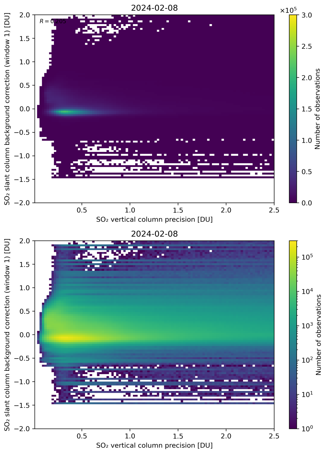
Figure 279: Scatter density plot of “SO 2 vertical column precision” against “SO 2 slant column background correction (window 1)” for 2024-02-07 to 2024-02-09.
