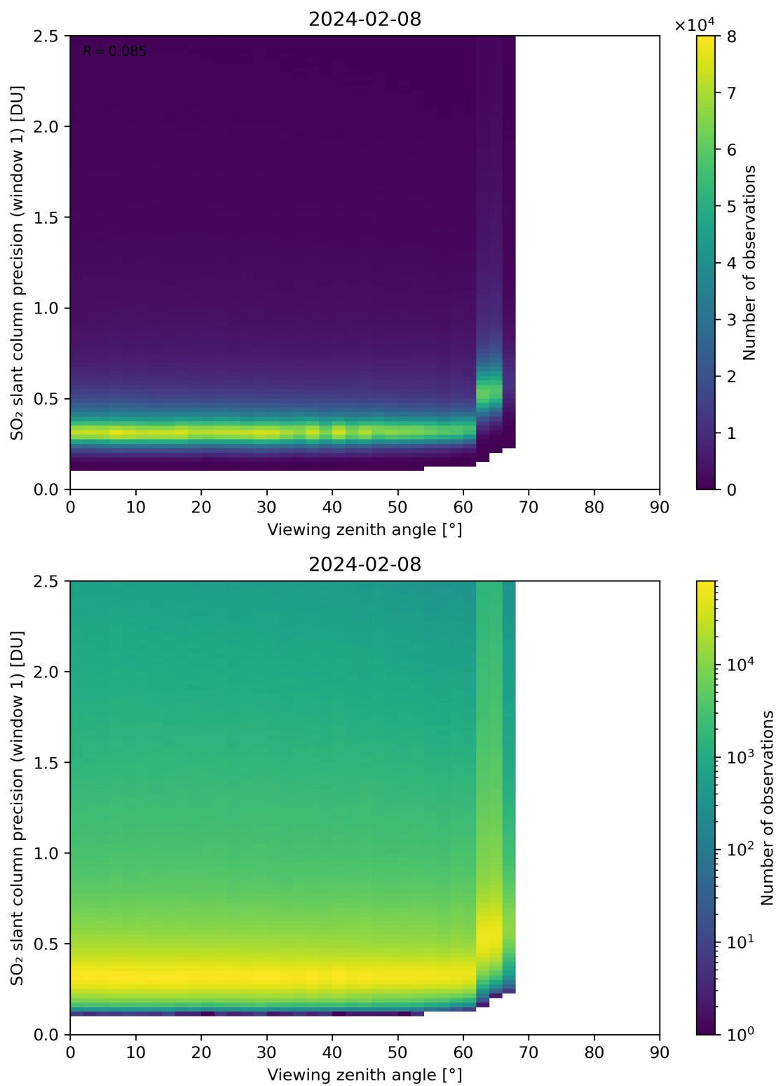
Figure 321: Scatter density plot of “Viewing zenith angle” against “SO 2 slant column precision (window 1)” for 2024-02-07 to 2024-02-09.
