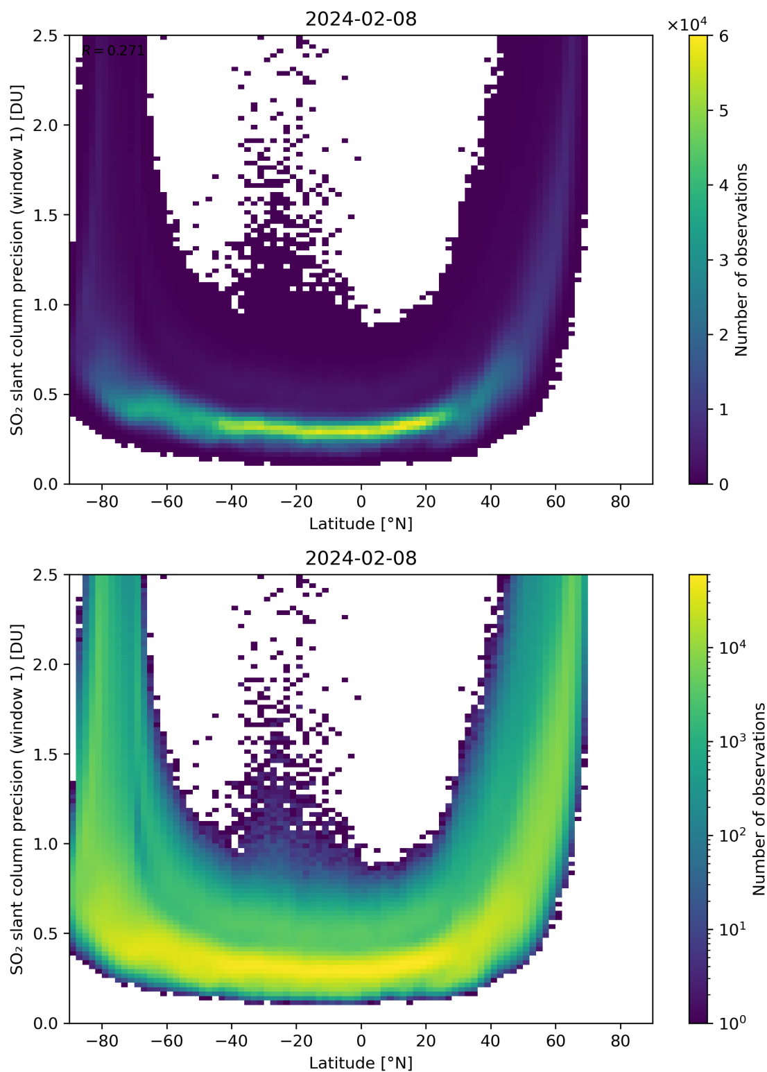
Figure 150: Scatter density plot of “Latitude” against “SO 2 slant column precision (window 1)” for 2024-02-07 to 2024-02-09.
