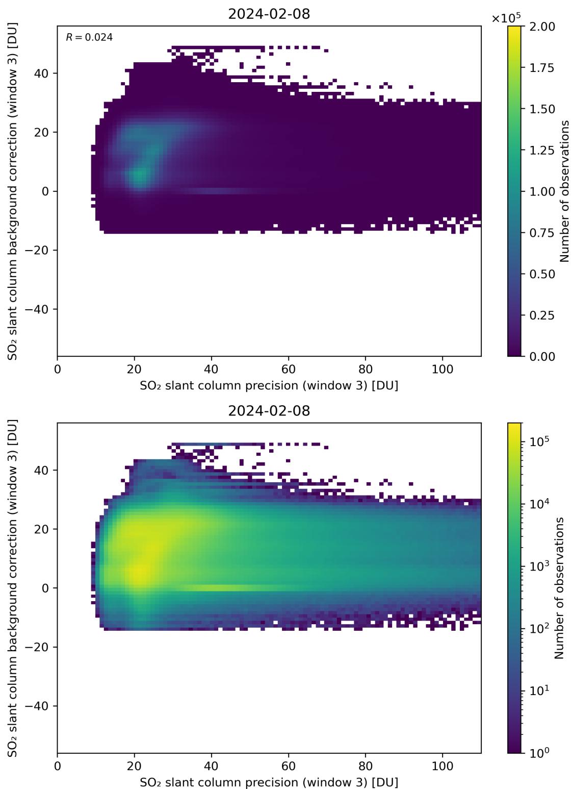
Figure 257: Scatter density plot of “SO 2 slant column precision (window 3)” against “SO 2 slant column background correction (window 3)” for 2024-02-07 to 2024-02-09.
