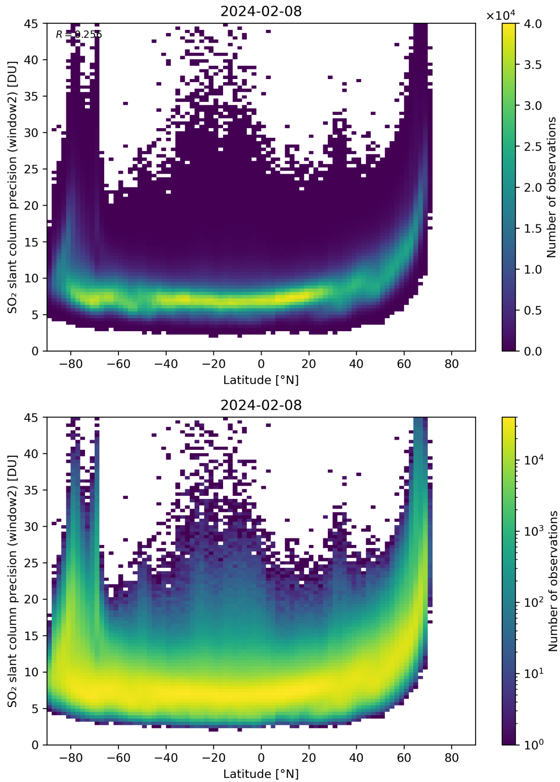
Figure 151: Scatter density plot of “Latitude” against “SO 2 slant column precision (window2)” for 2024-02-07 to 2024-02-09.
