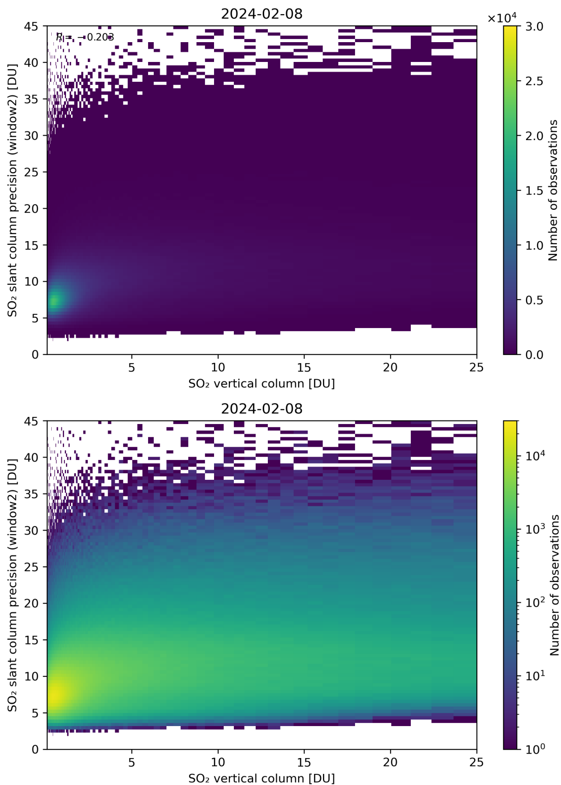
Figure 302: Scatter density plot of “SO 2 vertical column” against “SO 2 slant column precision (window2)” for 2024-02-07 to 2024-02-09.
