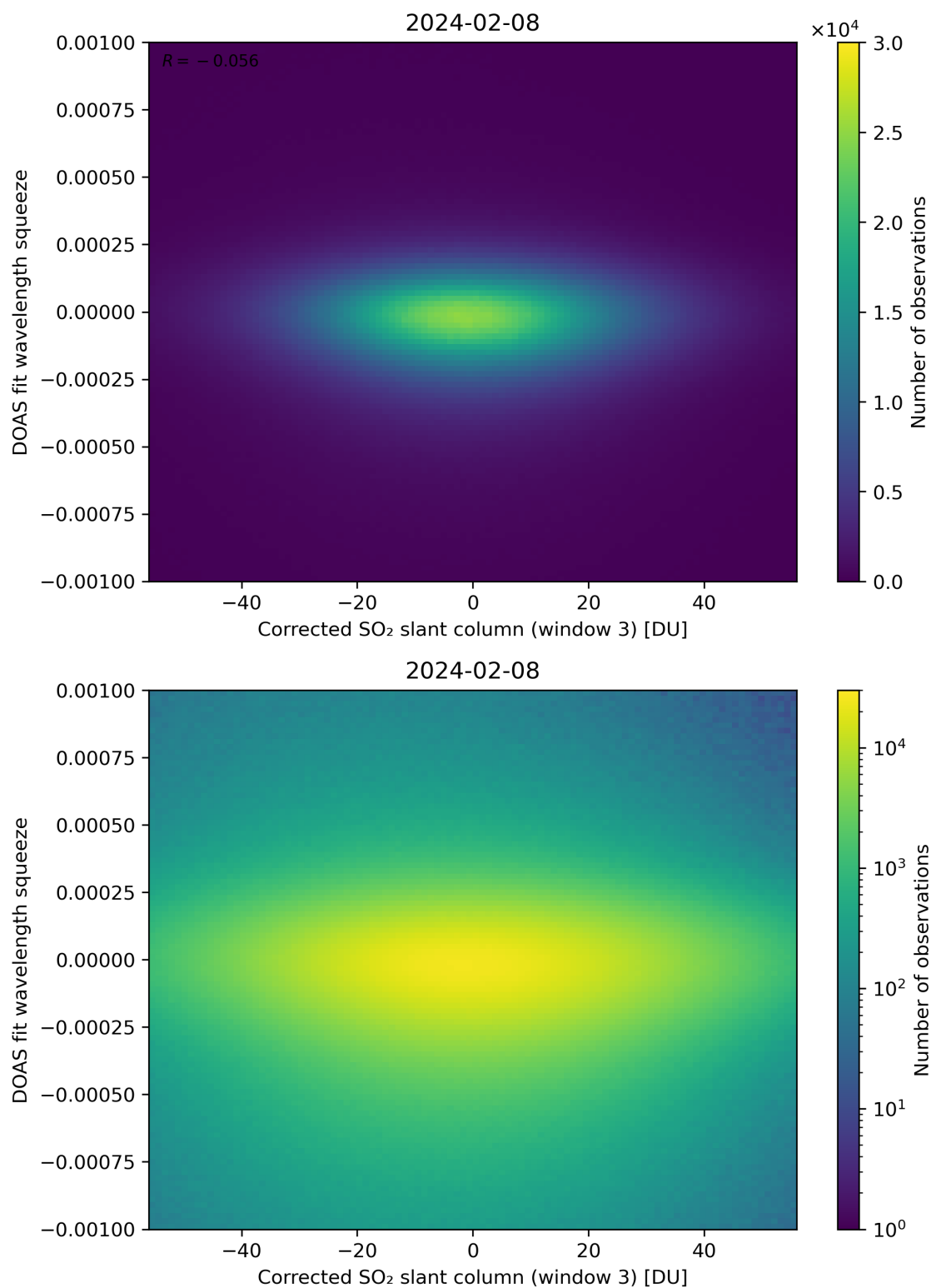
Figure 207: Scatter density plot of “Corrected SO 2 slant column (window 3)” against “DOAS fit wavelength squeeze” for 2024-02-07 to 2024-02-09.
