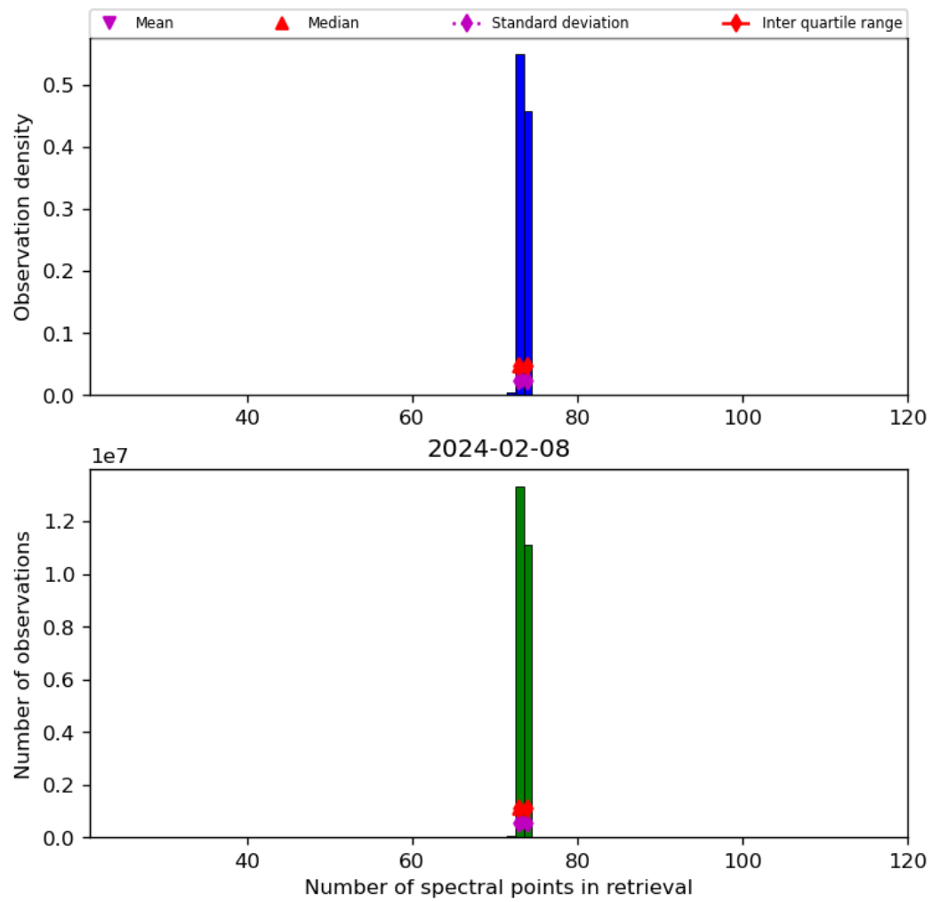
Figure 74: Histogram of “Number of spectral points in retrieval” for 2024-02-07 to 2024-02-09
