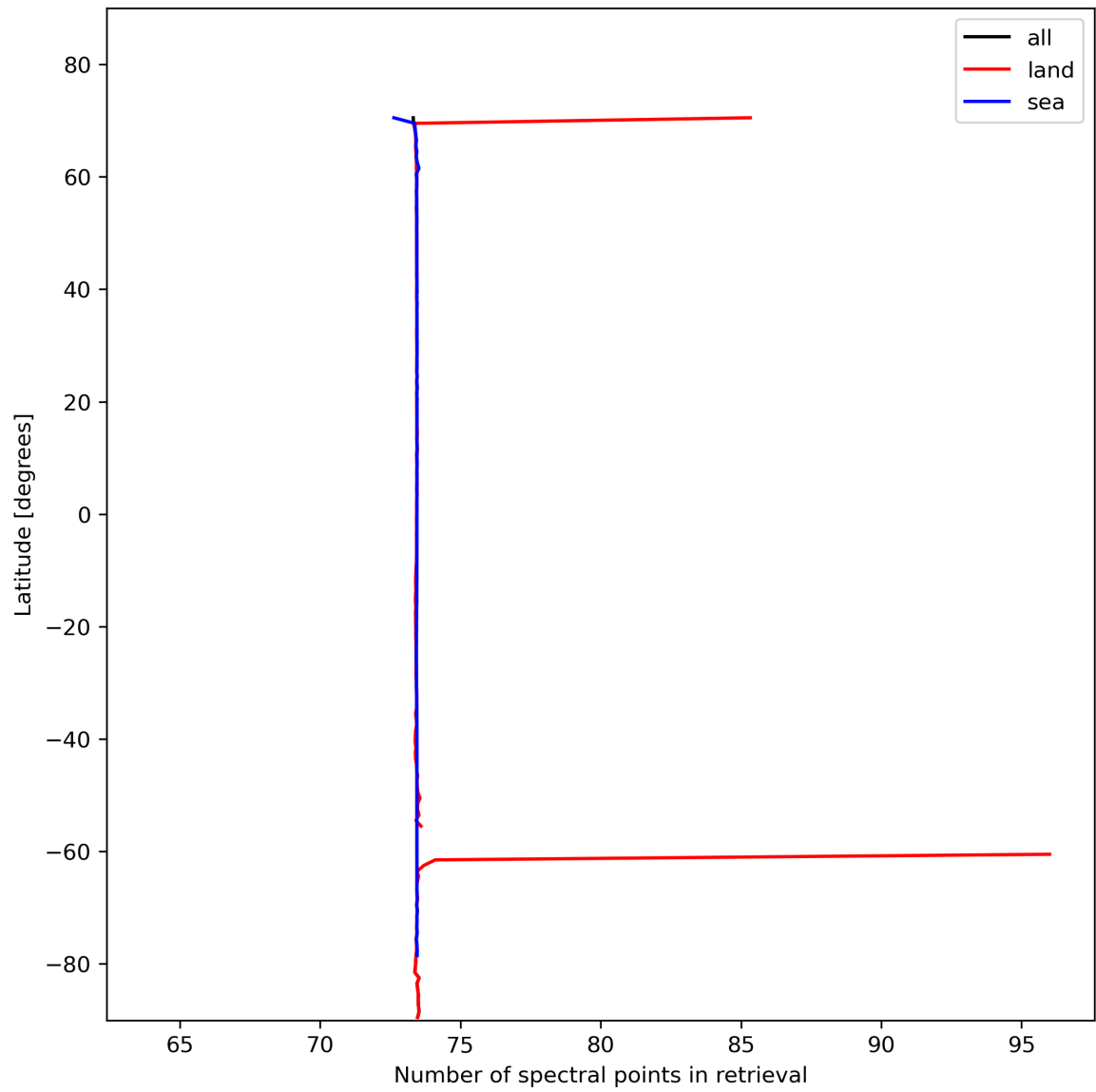
Figure 51: Zonal average of “Number of spectral points in retrieval” for 2024-02-07 to 2024-02-09.
