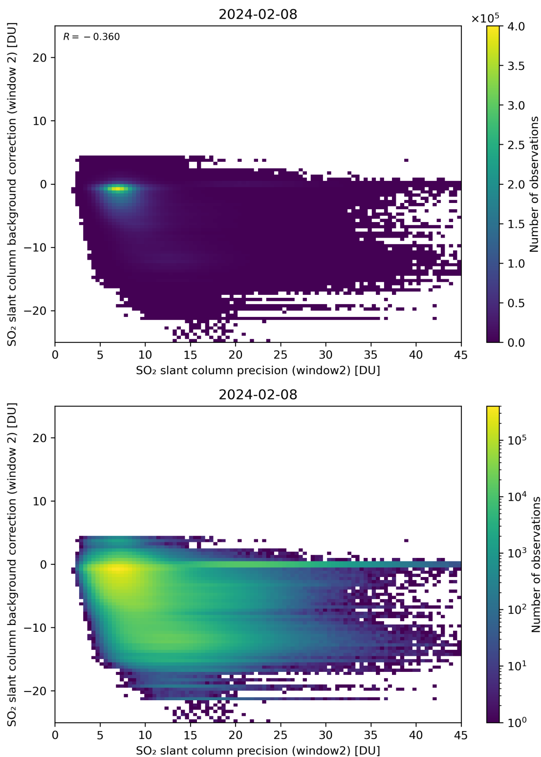
Figure 241: Scatter density plot of “SO 2 slant column precision (window2)” against “SO 2 slant column background correction (window 2)” for 2024-02-07 to 2024-02-09.
