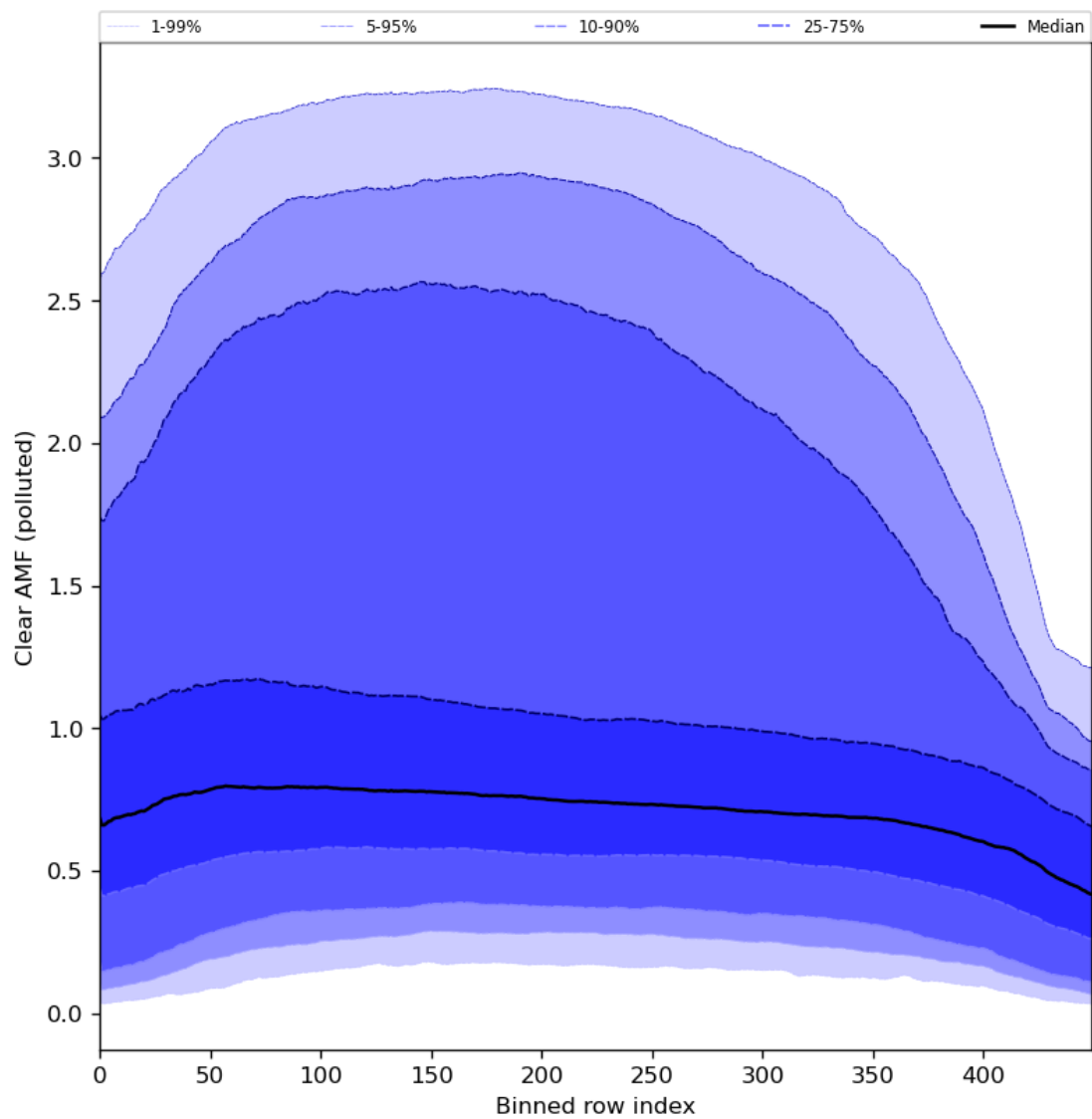
Figure 96: Along track statistics of “Clear AMF (polluted)” for 2024-02-07 to 2024-02-09
