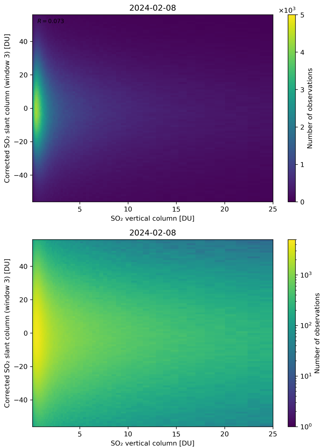
Figure 299: Scatter density plot of “SO 2 vertical column” against “Corrected SO 2 slant column (window 3)” for 2024-02-07 to 2024-02-09.
