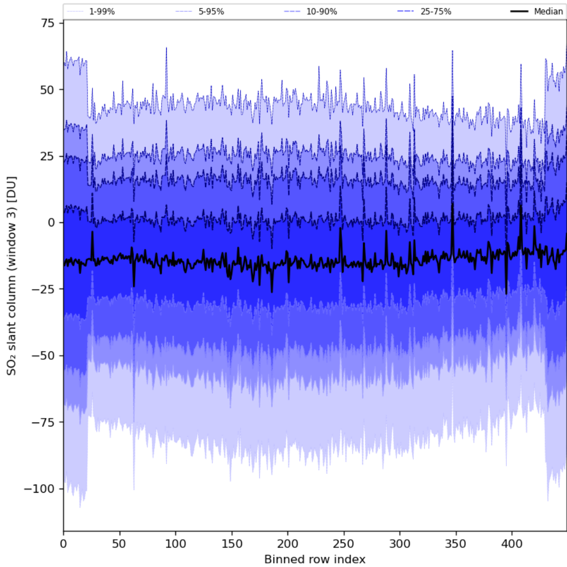
Figure 87: Along track statistics of “SO 2 slant column (window 3)” for 2024-02-07 to 2024-02-09
