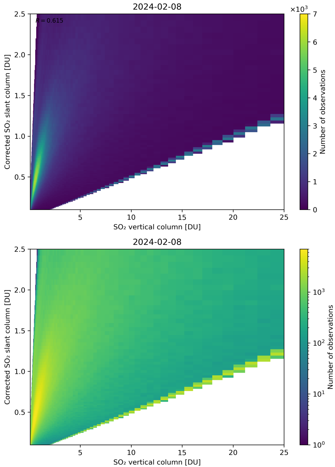
Figure 297: Scatter density plot of “SO 2 vertical column” against “Corrected SO 2 slant column” for 2024-02-07 to 2024-02-09.
