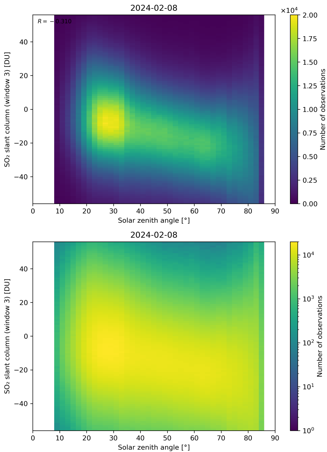
Figure 172: Scatter density plot of “Solar zenith angle” against “SO 2 slant column (window 3)” for 2024-02-07 to 2024-02-09.
