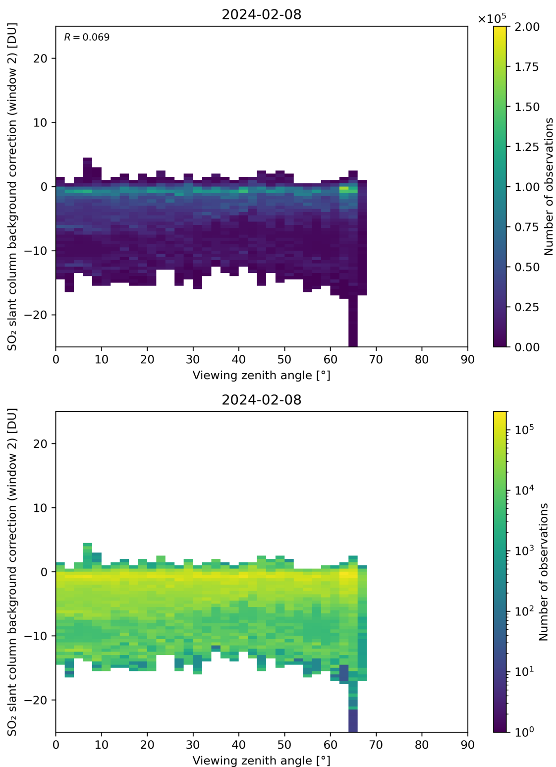
Figure 309: Scatter density plot of “Viewing zenith angle” against “SO 2 slant column background correction (window 2)” for 2024-02-07 to 2024-02-09.
