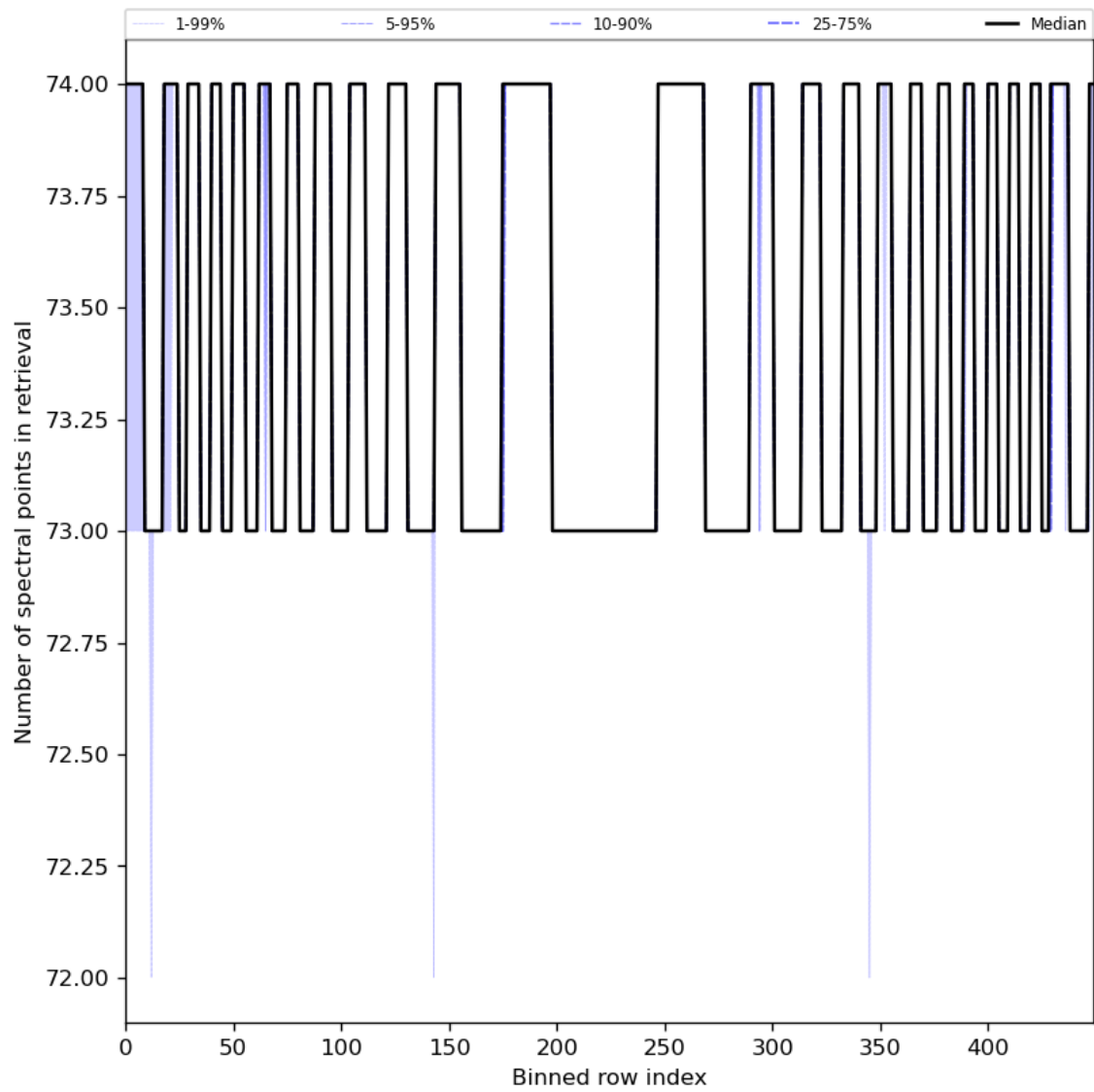
Figure 97: Along track statistics of “Number of spectral points in retrieval” for 2024-02-07 to 2024-02-09
