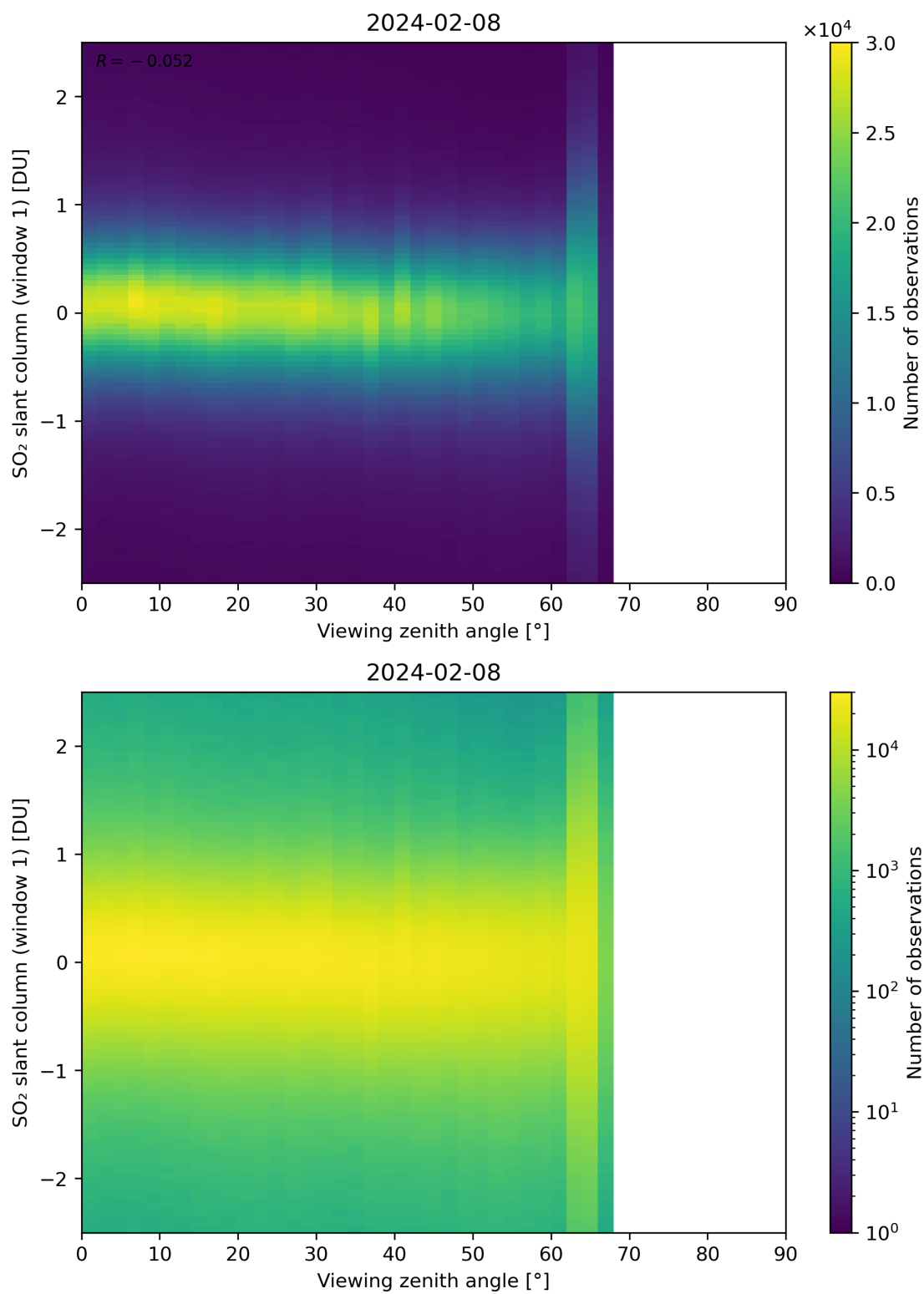
Figure 320: Scatter density plot of “Viewing zenith angle” against “SO 2 slant column (window 1)” for 2024-02-07 to 2024-02-09.
