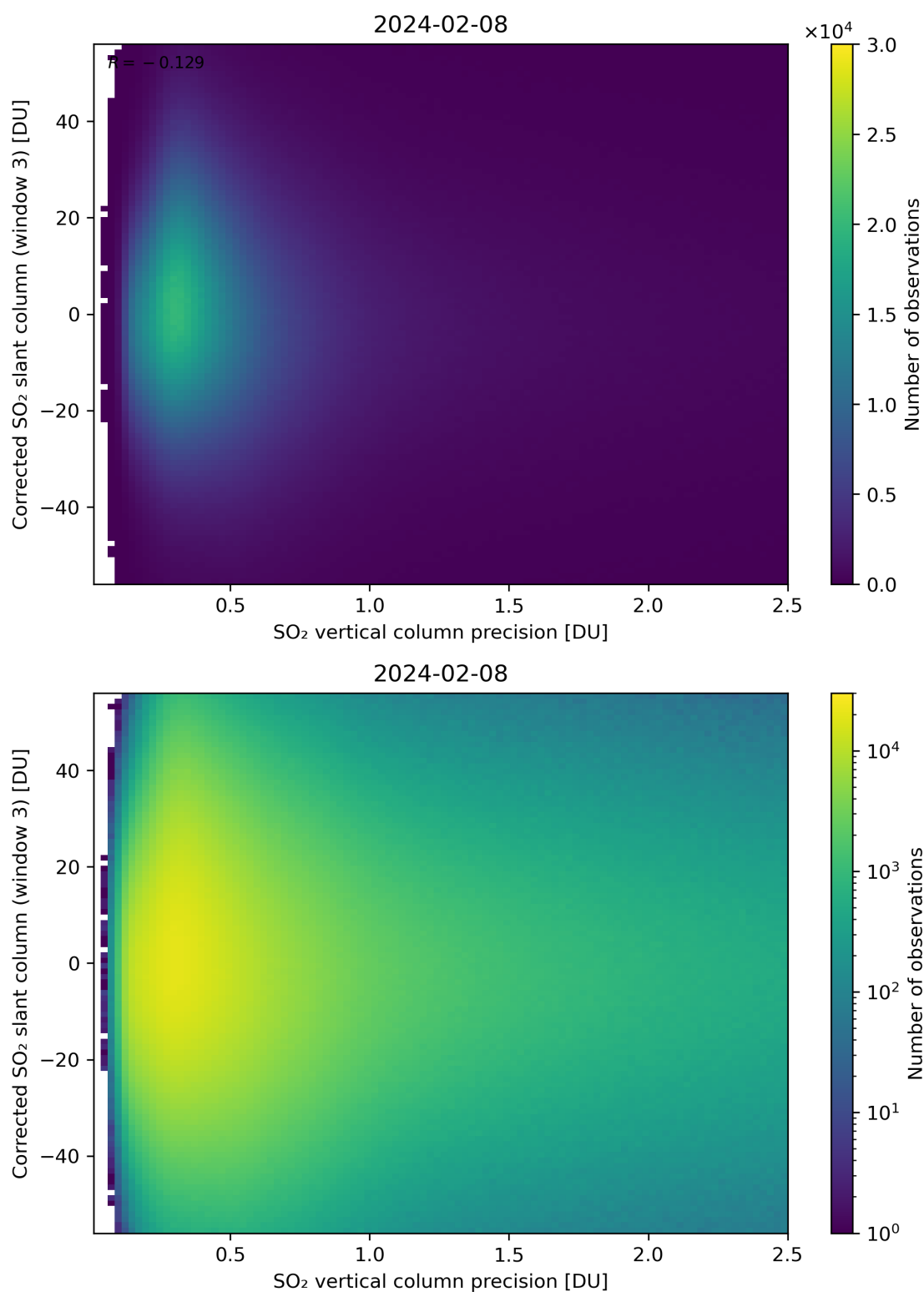
Figure 288: Scatter density plot of “SO 2 vertical column precision” against “Corrected SO 2 slant column (window 3)” for 2024-02-07 to 2024-02-09.
