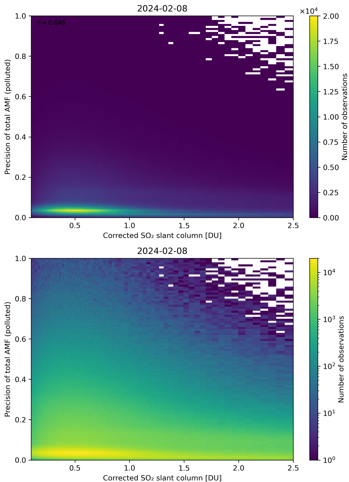
Figure 193: Scatter density plot of “Corrected SO 2 slant column” against “Precision of total AMF (polluted)” for 2024-02-07 to 2024-02-09.
