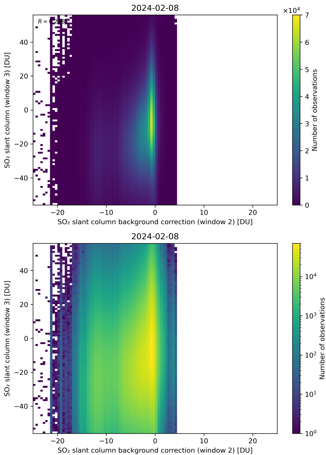
Figure 117: Scatter density plot of “SO 2 slant column background correction (window 2)” against “SO 2 slant column (window 3)” for 2024-02-07 to 2024-02-09.
