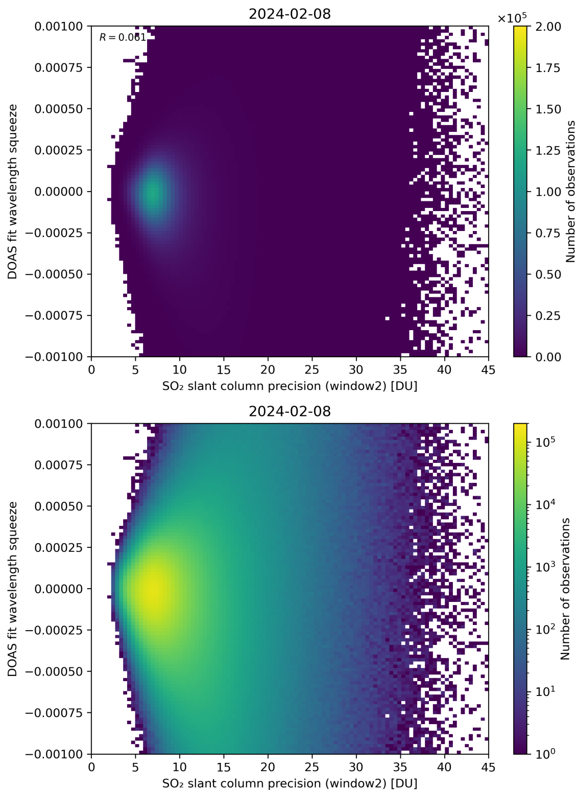
Figure 244: Scatter density plot of “SO 2 slant column precision (window2)” against “DOAS fit wavelength squeeze” for 2024-02-07 to 2024-02-09.
