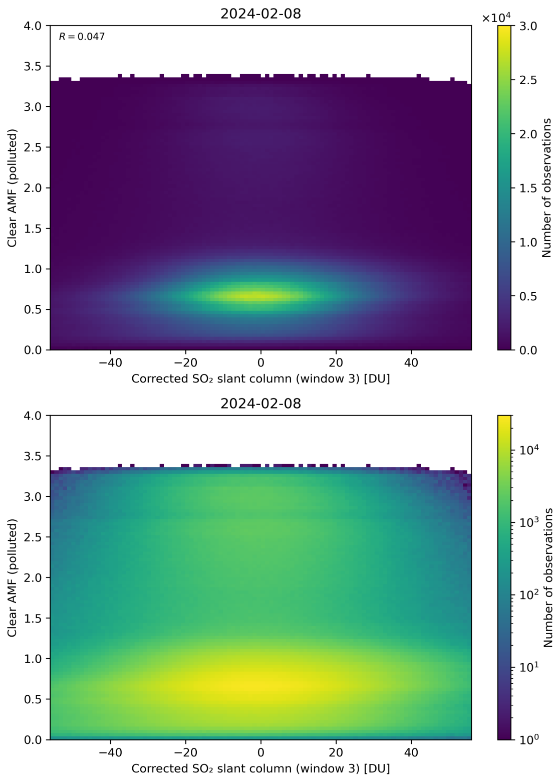
Figure 209: Scatter density plot of “Corrected SO 2 slant column (window 3)” against “Clear AMF (polluted)” for 2024-02-07 to 2024-02-09.
