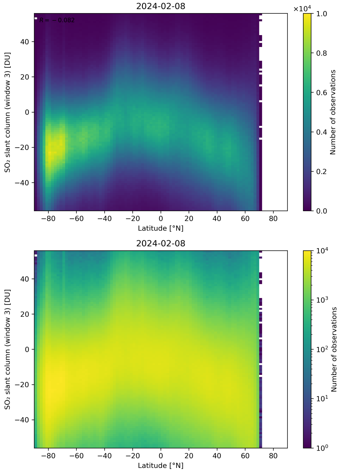
Figure 152: Scatter density plot of “Latitude” against “SO 2 slant column (window 3)” for 2024-02-07 to 2024-02-09.
