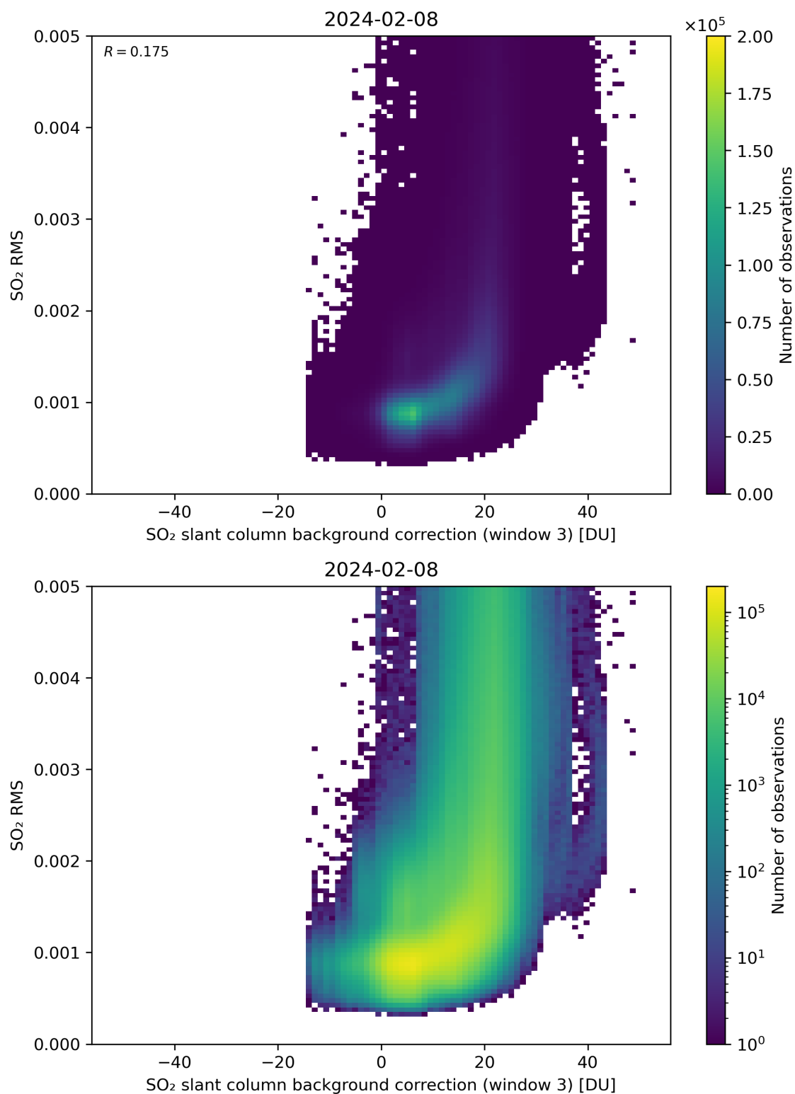
Figure 123: Scatter density plot of “SO 2 slant column background correction (window 3)” against “SO 2 RMS” for 2024-02-07 to 2024-02-09.
