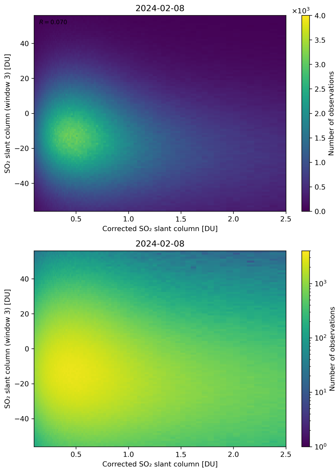
Figure 190: Scatter density plot of “Corrected SO 2 slant column” against “SO 2 slant column (window 3)” for 2024-02-07 to 2024-02-09.
