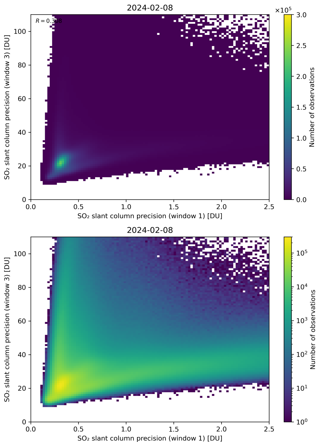
Figure 229: Scatter density plot of “SO 2 slant column precision (window 1)” against “SO 2 slant column precision (window 3)” for 2024-02-07 to 2024-02-09.
