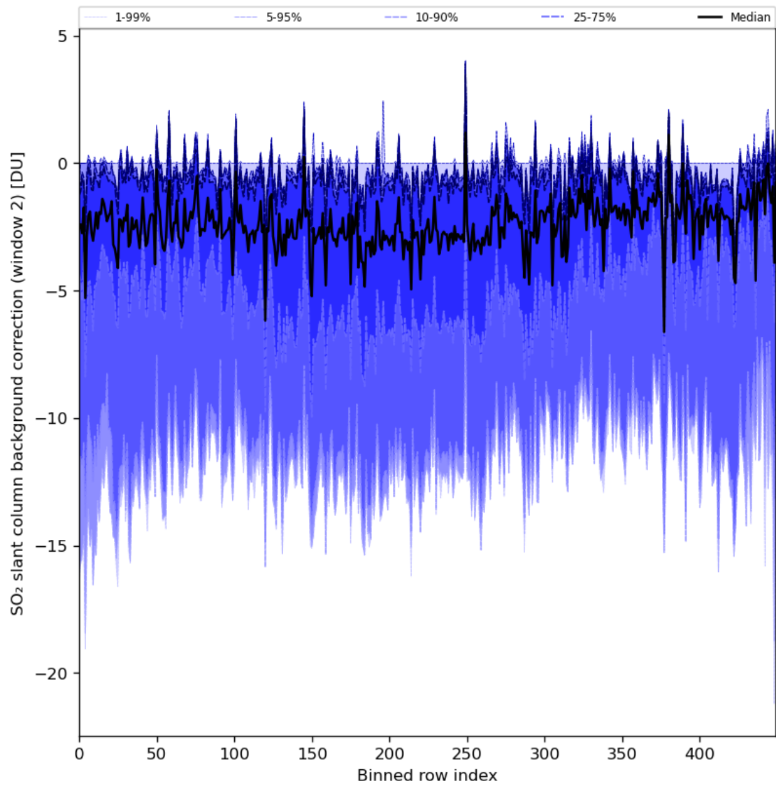
Figure 86: Along track statistics of “SO 2 slant column background correction (window 2)” for 2024-02-07 to 2024-02-09
