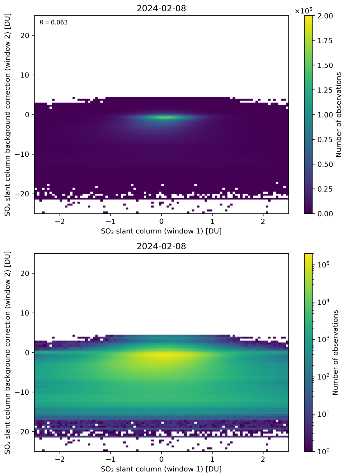
Figure 213: Scatter density plot of “SO 2 slant column (window 1)” against “SO 2 slant column background correction (window 2)” for 2024-02-07 to 2024-02-09.
