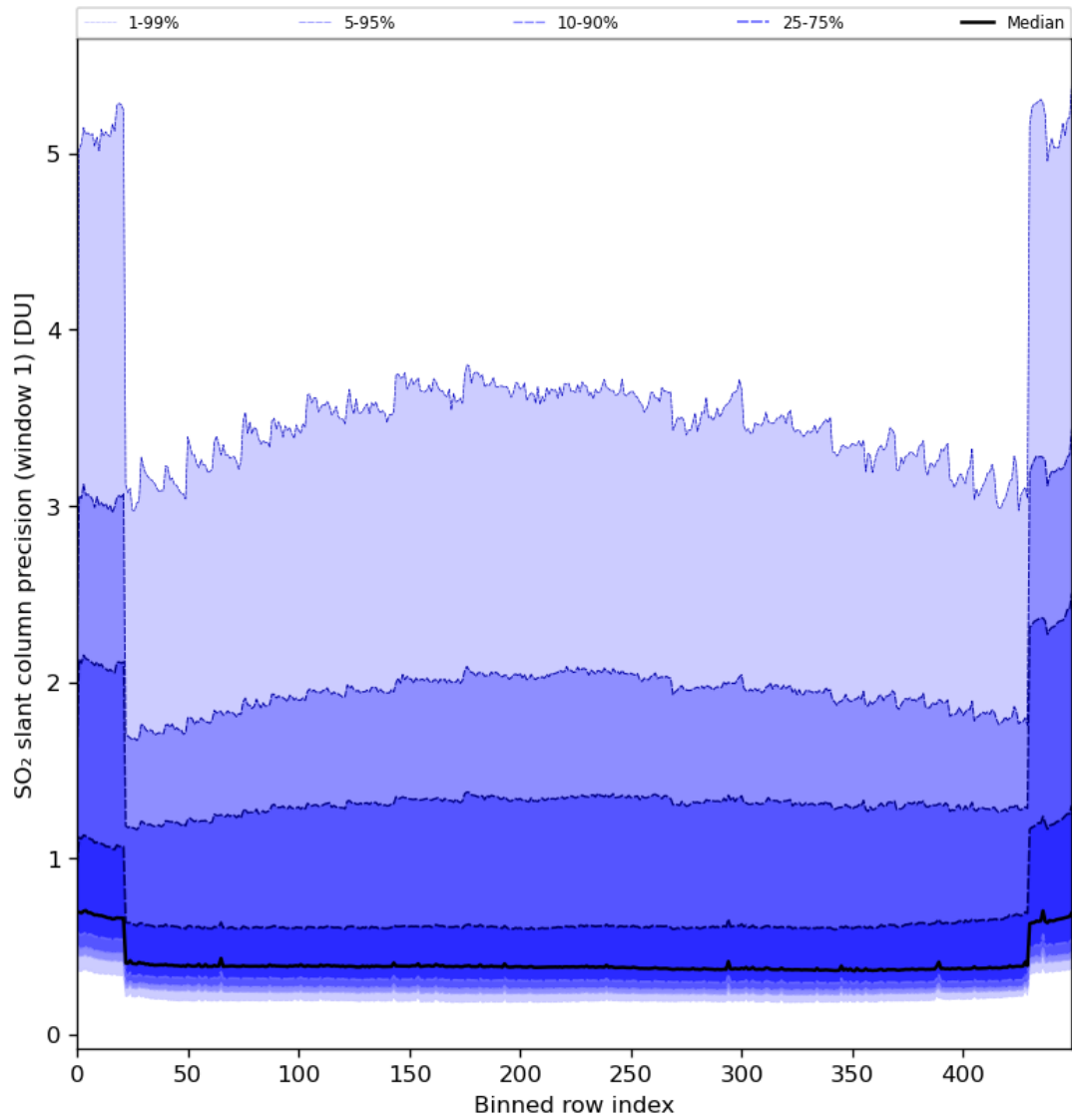
Figure 80: Along track statistics of “SO 2 slant column precision (window 1)” for 2024-02-07 to 2024-02-09
