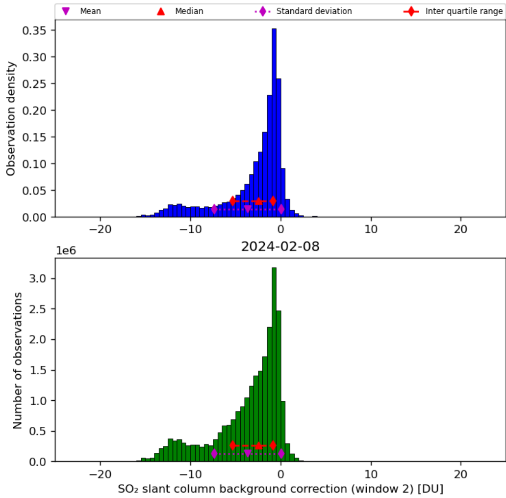
Figure 63: Histogram of “SO 2 slant column background correction (window 2)” for 2024-02-07 to 2024-02-09
