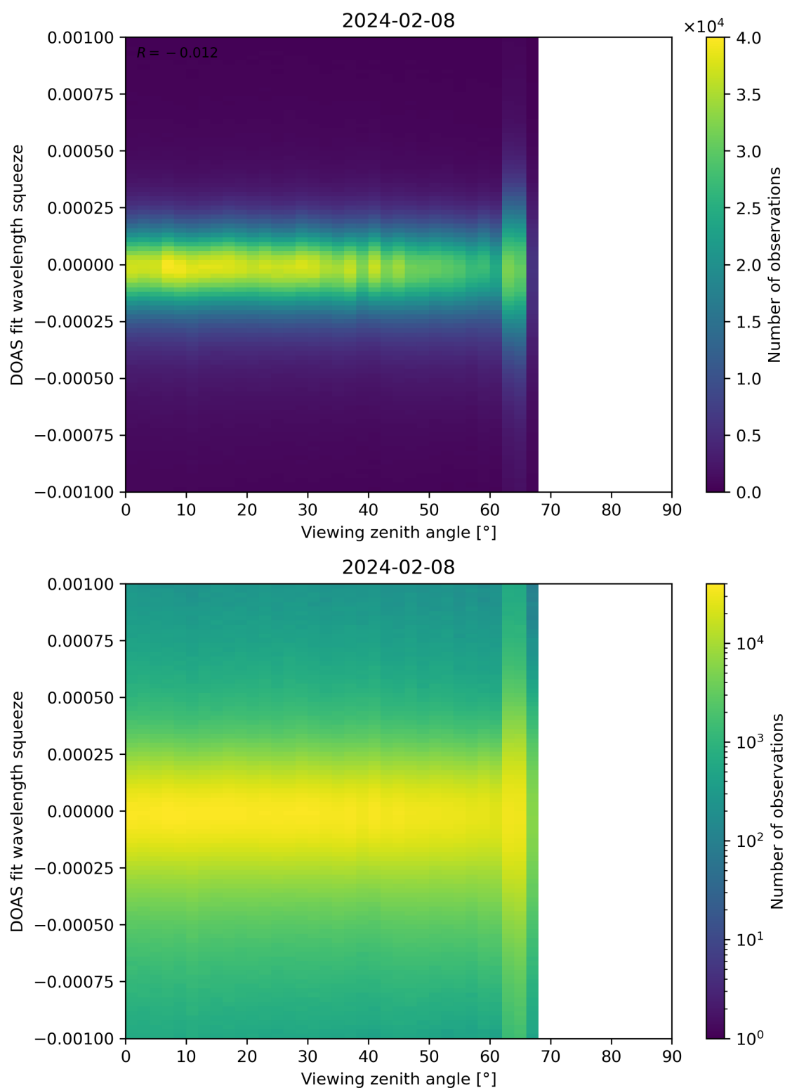
Figure 312: Scatter density plot of “Viewing zenith angle” against “DOAS fit wavelength squeeze” for 2024-02-07 to 2024-02-09.
