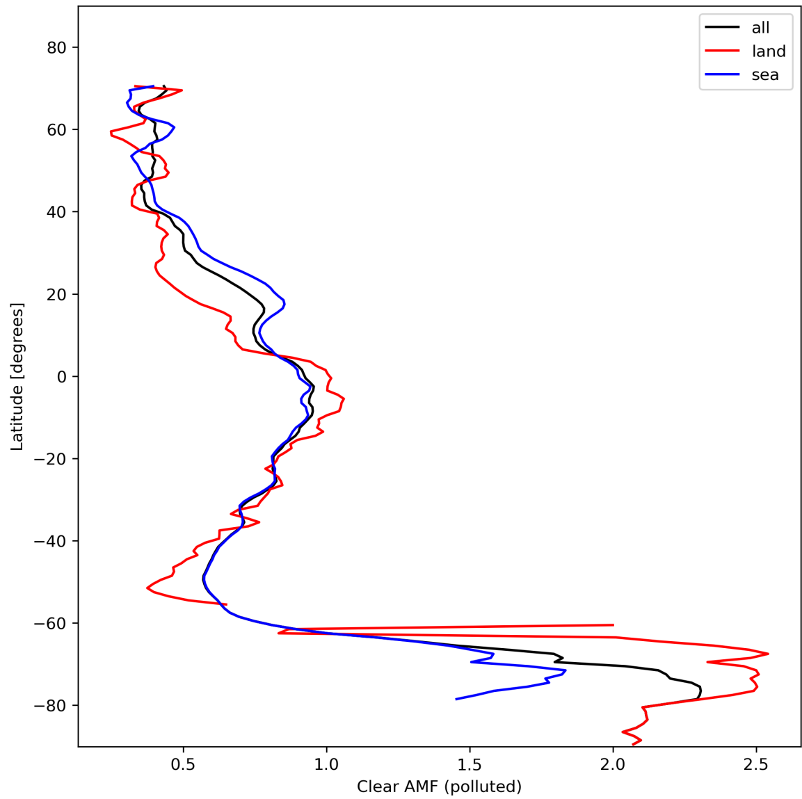
Figure 50: Zonal average of “Clear AMF (polluted)” for 2024-02-07 to 2024-02-09.
