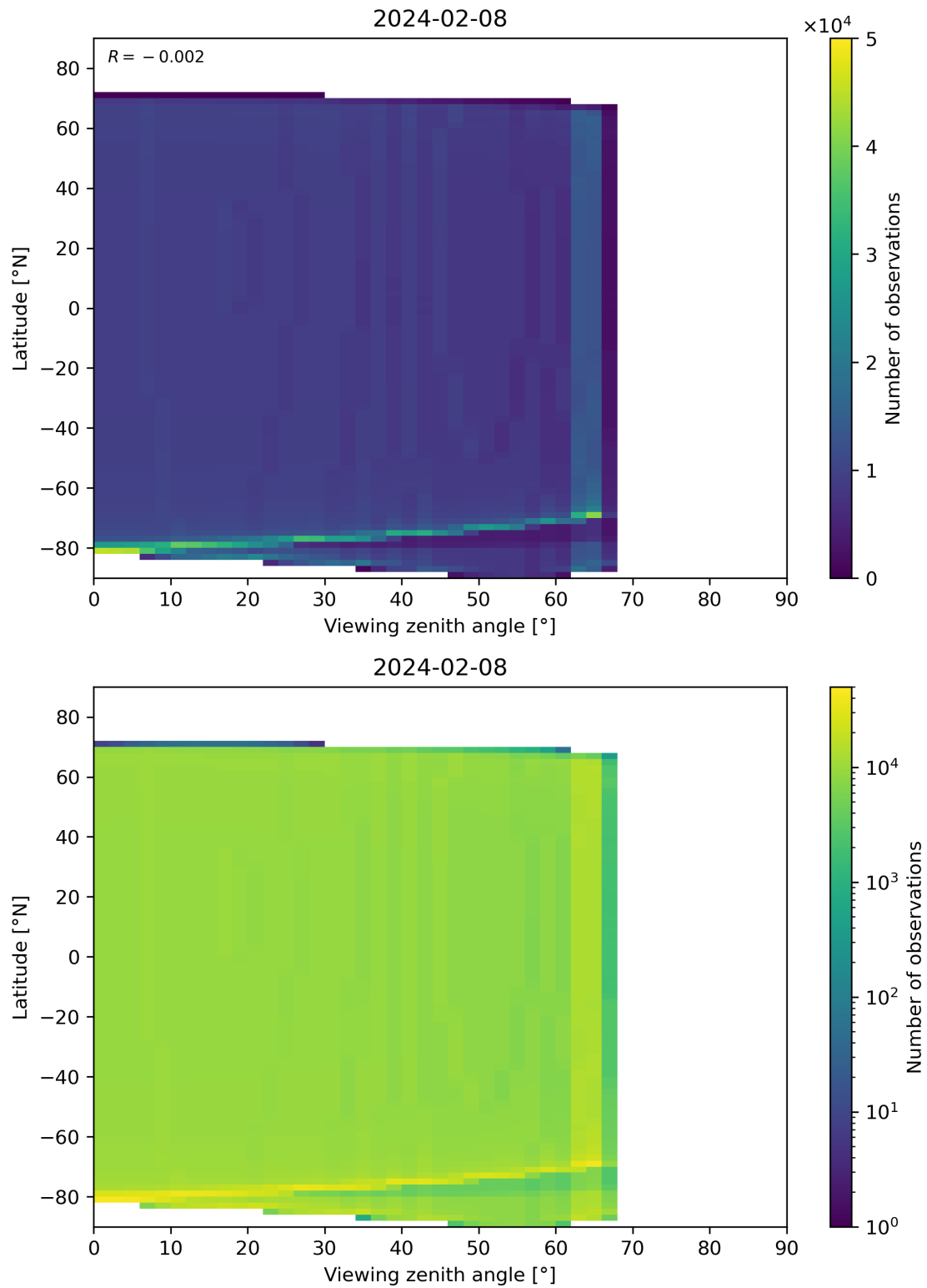
Figure 314: Scatter density plot of “Viewing zenith angle” against “Latitude” for 2024-02-07 to 2024-02-09.
