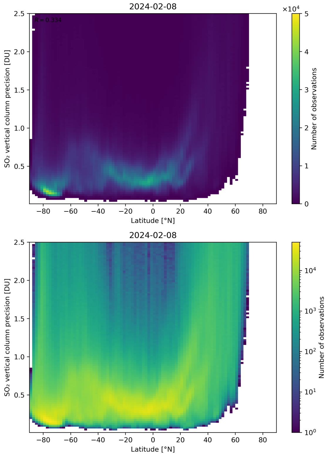
Figure 157: Scatter density plot of “Latitude” against “SO 2 vertical column precision” for 2024-02-07 to 2024-02-09.
