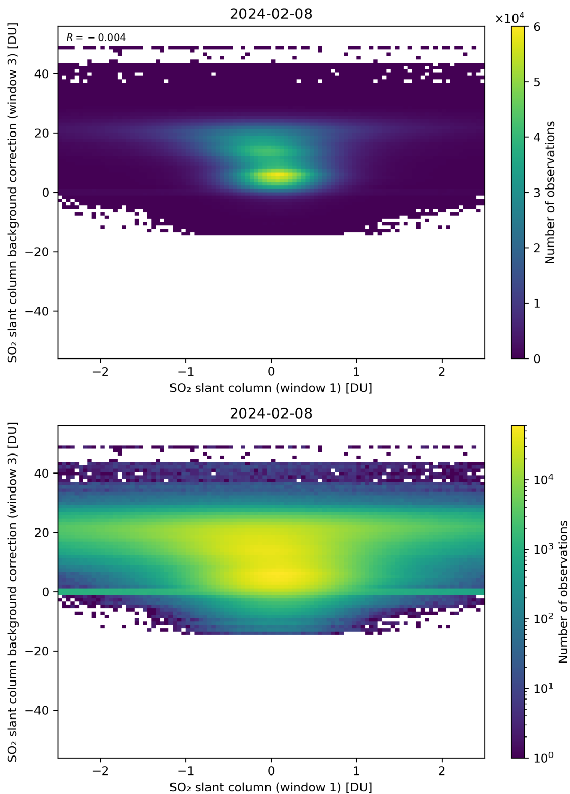
Figure 214: Scatter density plot of “SO 2 slant column (window 1)” against “SO 2 slant column background correction (window 3)” for 2024-02-07 to 2024-02-09.
