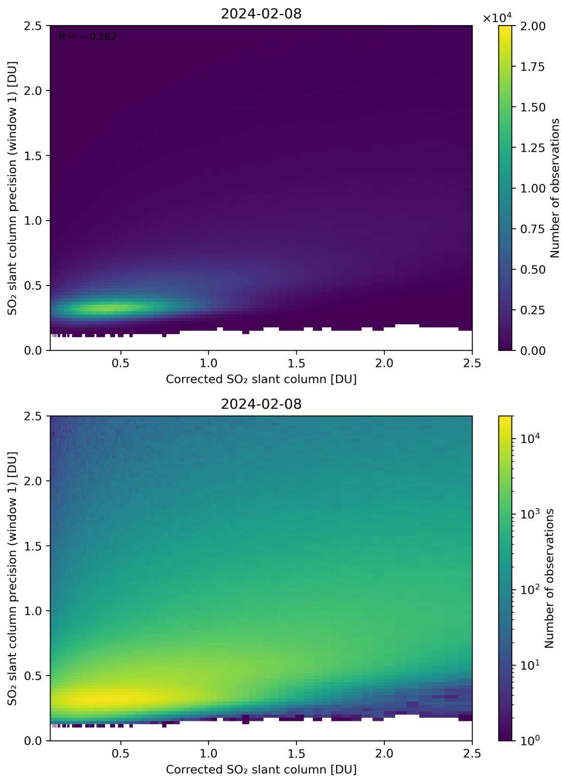
Figure 188: Scatter density plot of “Corrected SO 2 slant column” against “SO 2 slant column precision (window 1)” for 2024-02-07 to 2024-02-09.
