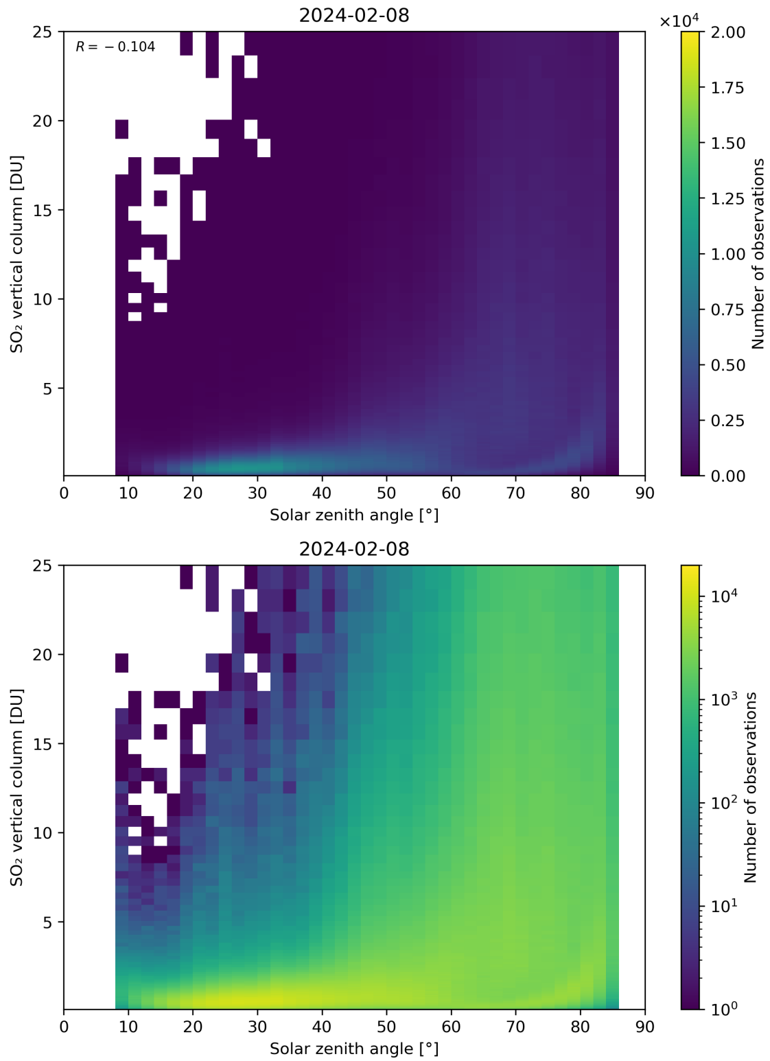
Figure 176: Scatter density plot of “Solar zenith angle” against “SO 2 vertical column” for 2024-02-07 to 2024-02-09.
