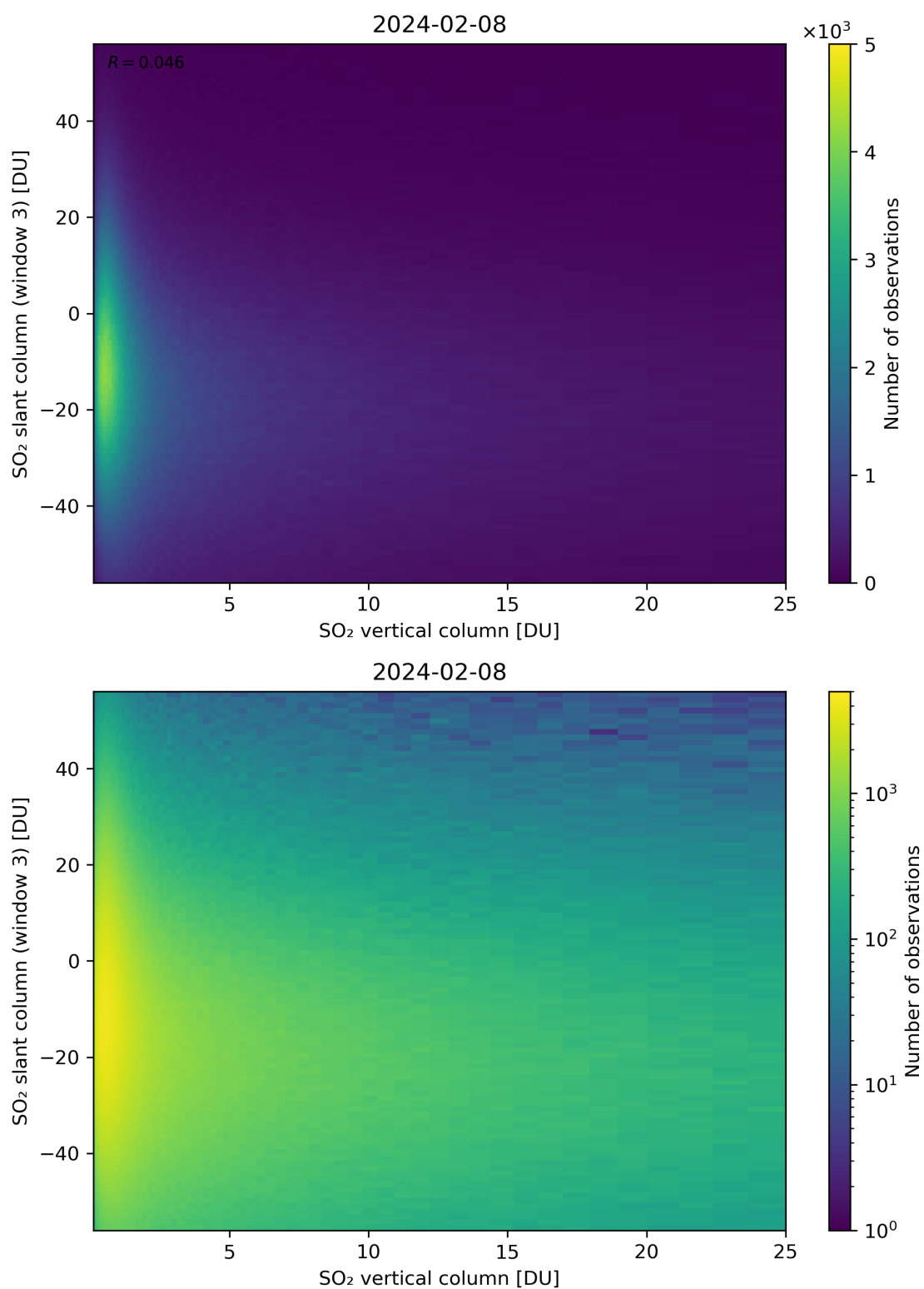
Figure 303: Scatter density plot of “SO 2 vertical column” against “SO 2 slant column (window 3)” for 2024-02-07 to 2024-02-09.
