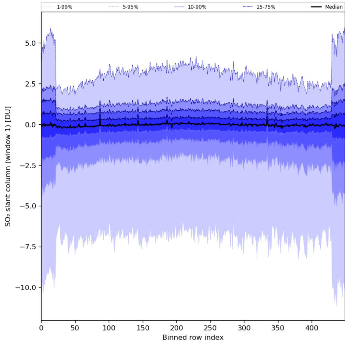
Figure 79: Along track statistics of “SO 2 slant column (window 1)” for 2024-02-07 to 2024-02-09
