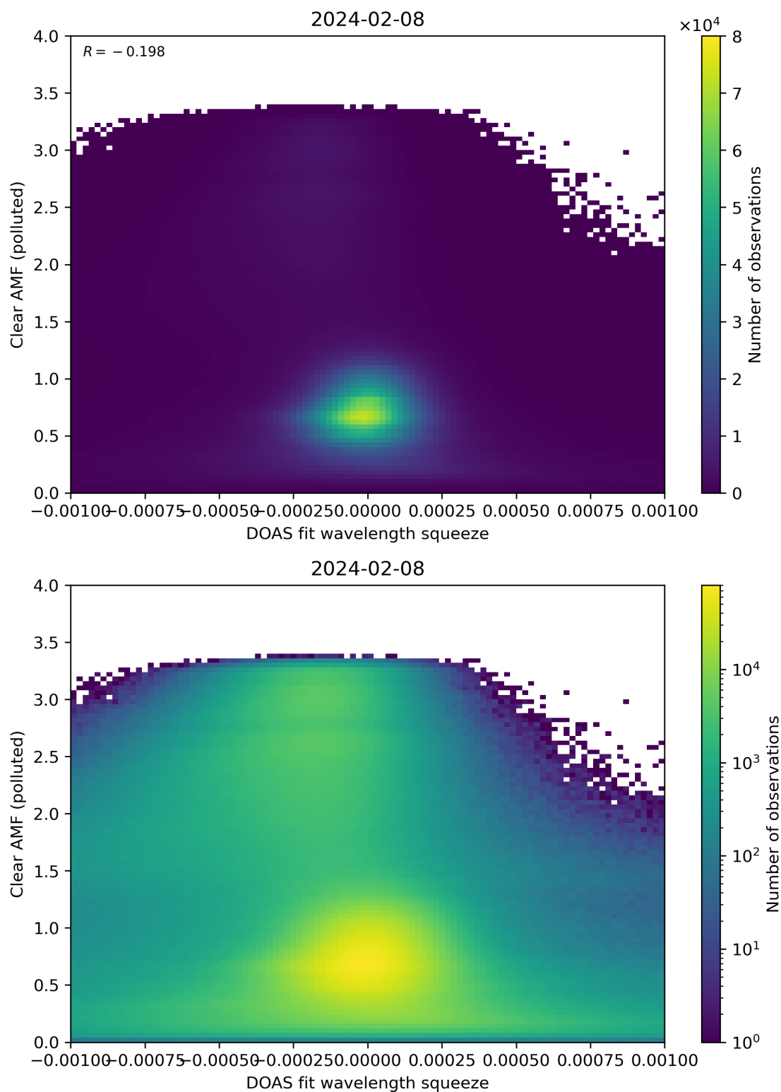
Figure 133: Scatter density plot of “DOAS fit wavelength squeeze” against “Clear AMF (polluted)” for 2024-02-07 to 2024-02-09.
