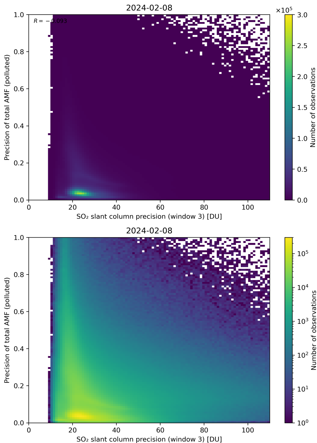
Figure 264: Scatter density plot of “SO 2 slant column precision (window 3)” against “Precision of total AMF (polluted)” for 2024-02-07 to 2024-02-09.
