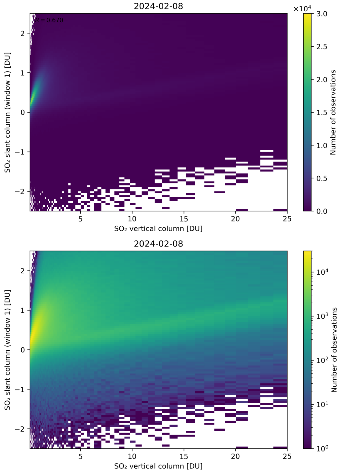
Figure 300: Scatter density plot of “SO 2 vertical column” against “SO 2 slant column (window 1)” for 2024-02-07 to 2024-02-09.
