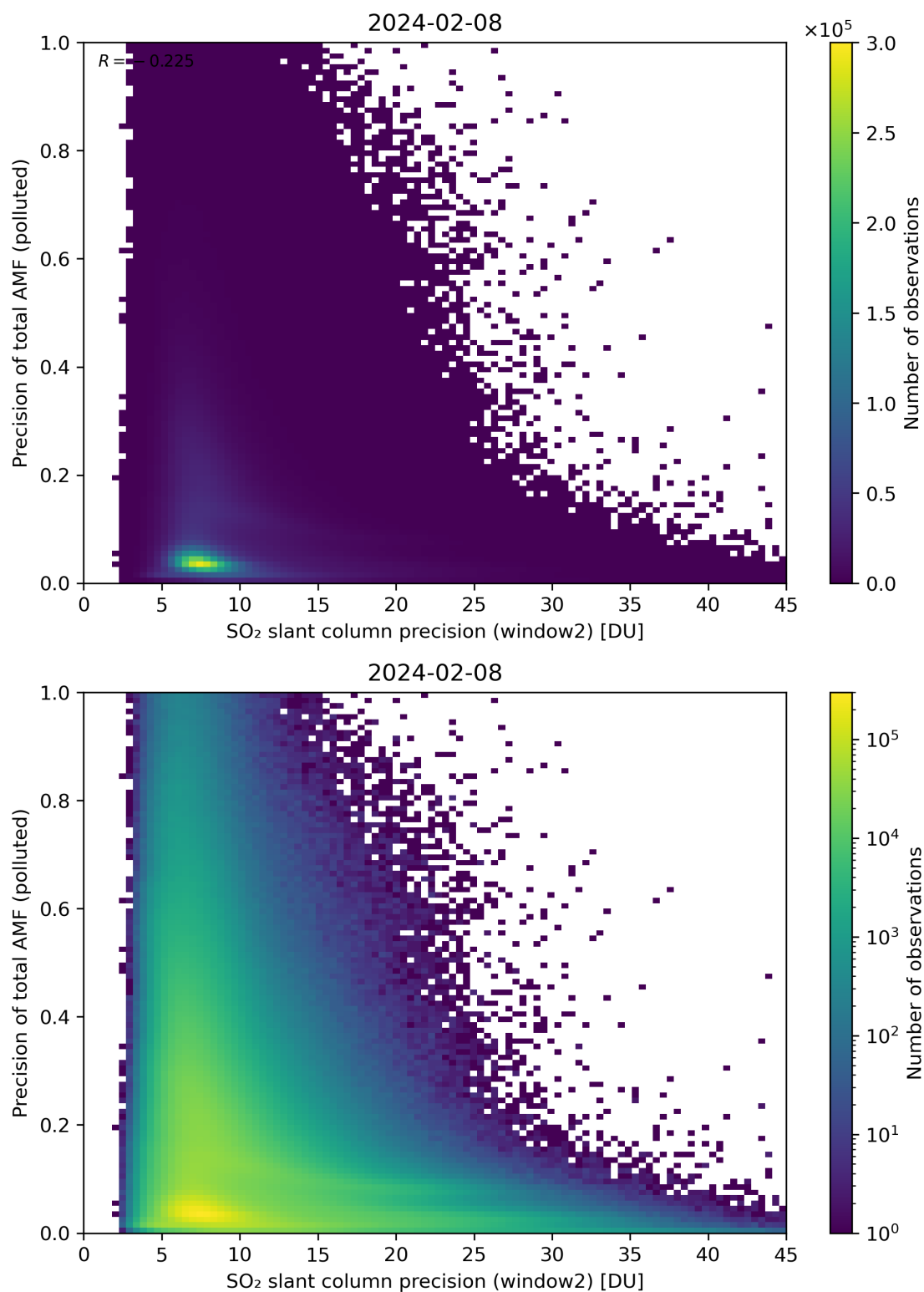
Figure 252: Scatter density plot of “SO 2 slant column precision (window2)” against “Precision of total AMF (polluted)” for 2024-02-07 to 2024-02-09.
