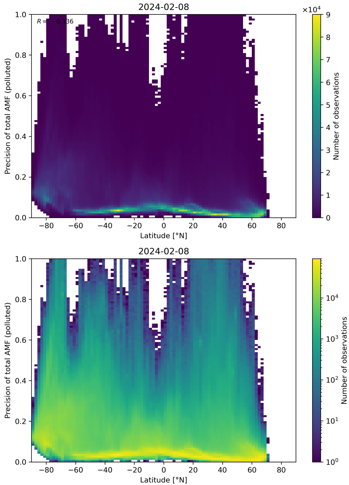
Figure 155: Scatter density plot of “Latitude” against “Precision of total AMF (polluted)” for 2024-02-07 to 2024-02-09.
