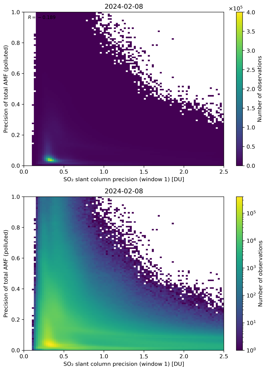
Figure 231: Scatter density plot of “SO 2 slant column precision (window 1)” against “Precision of total AMF (polluted)” for 2024-02-07 to 2024-02-09.
