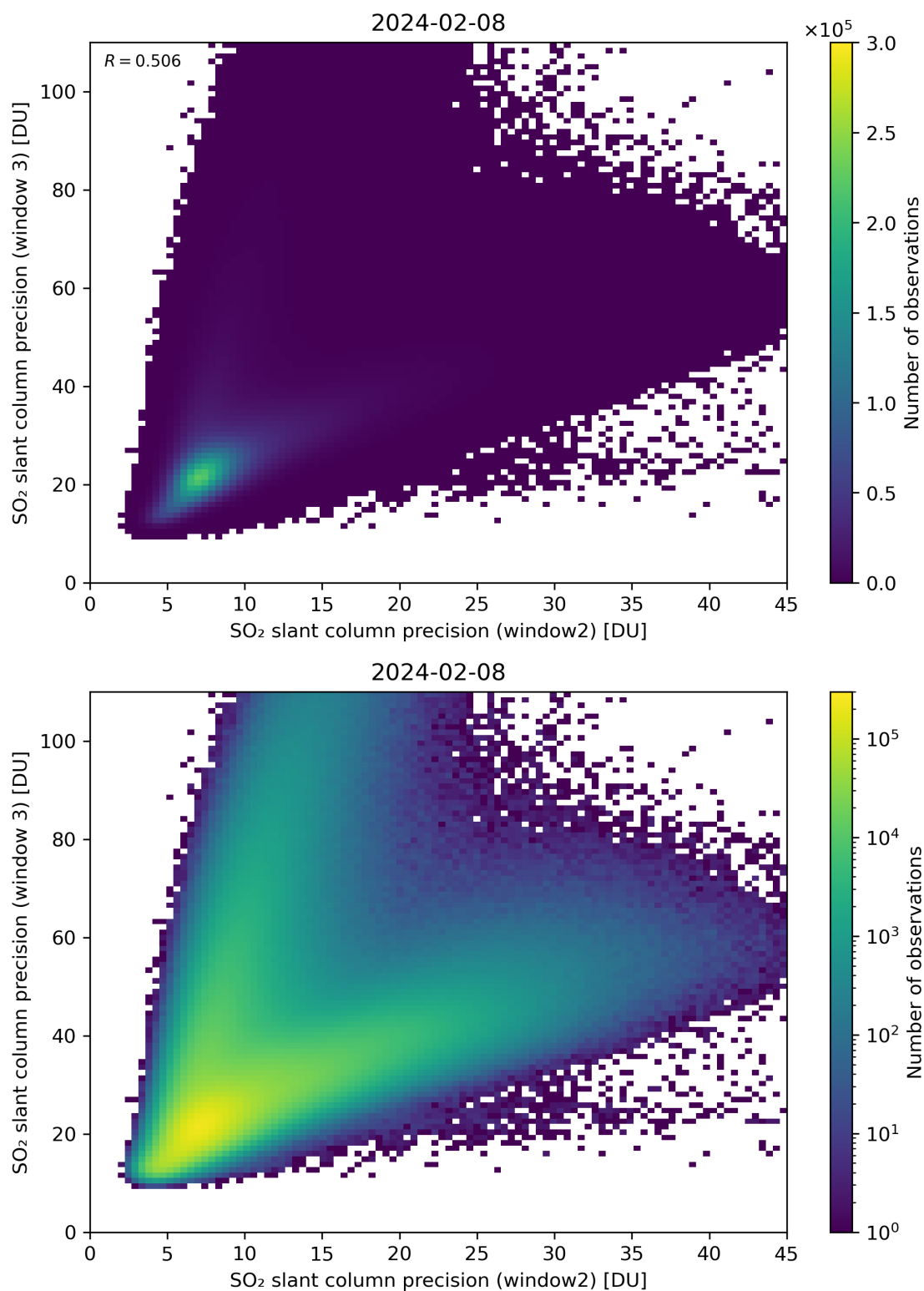
Figure 250: Scatter density plot of “SO 2 slant column precision (window2)” against “SO 2 slant column precision (window 3)” for 2024-02-07 to 2024-02-09.
