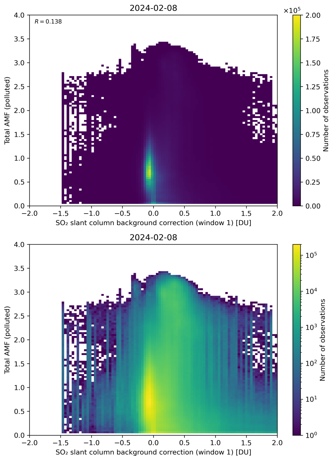
Figure 109: Scatter density plot of “SO 2 slant column background correction (window 1)” against “Total AMF (polluted)” for 2024-02-07 to 2024-02-09.
