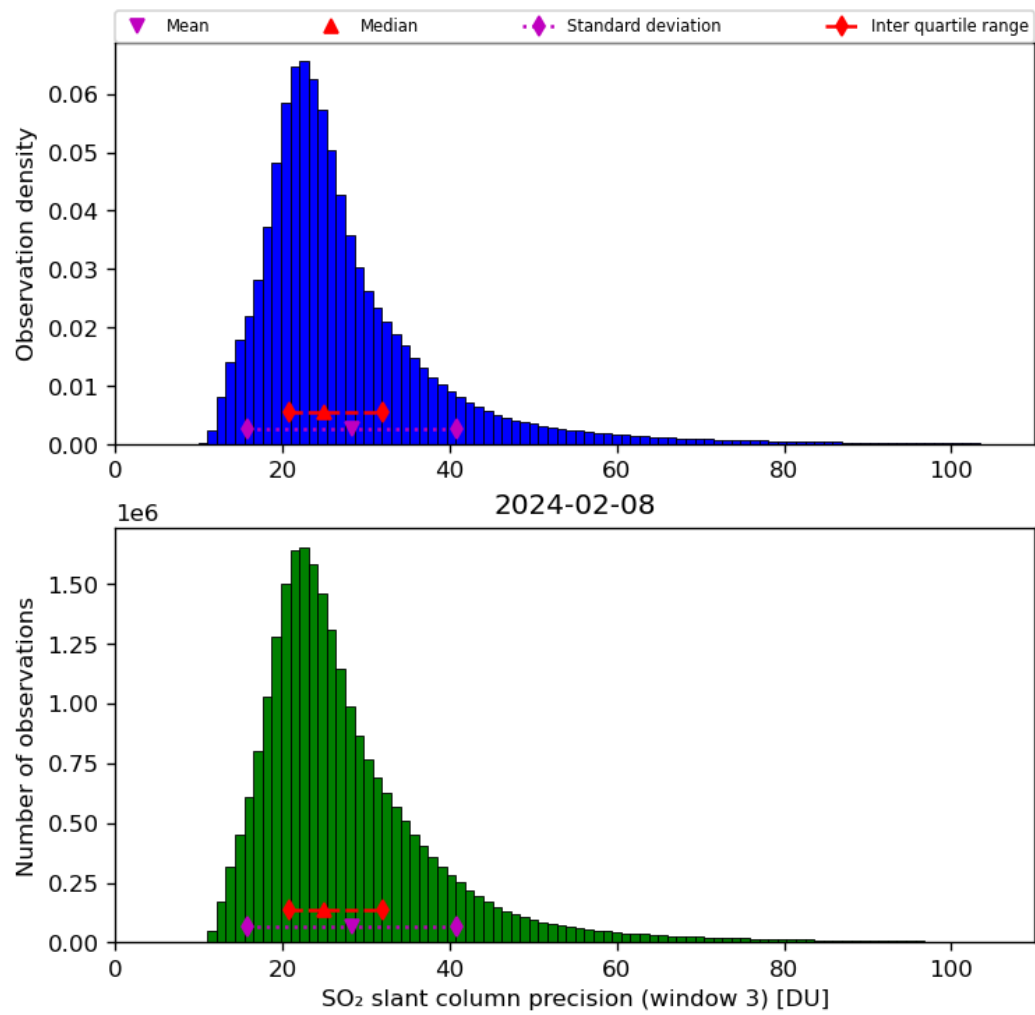
Figure 65: Histogram of “SO 2 slant column precision (window 3)” for 2024-02-07 to 2024-02-09
