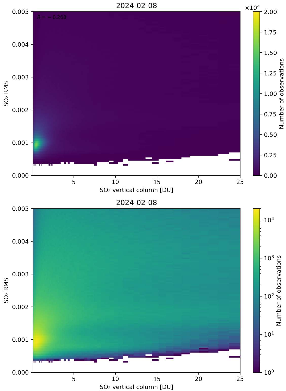
Figure 278: Scatter density plot of “SO 2 vertical column” against “SO 2 RMS” for 2024-02-07 to 2024-02-09.
