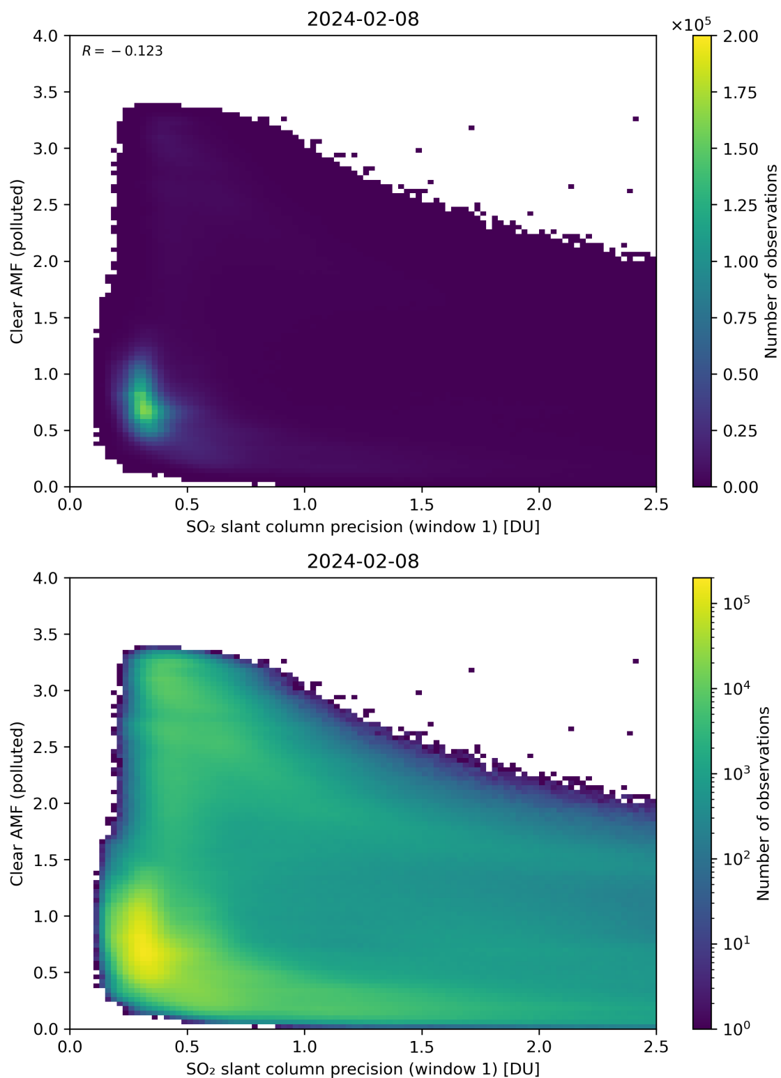
Figure 224: Scatter density plot of “SO 2 slant column precision (window 1)” against “Clear AMF (polluted)” for 2024-02-07 to 2024-02-09.
