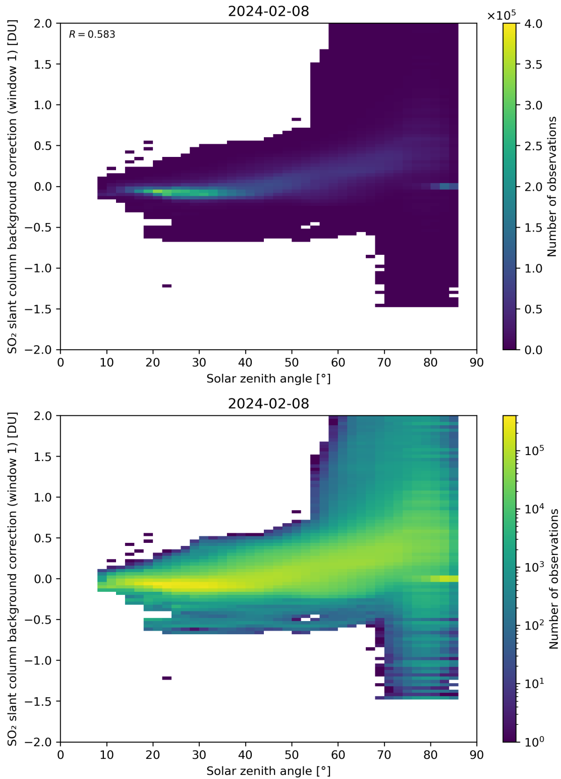
Figure 158: Scatter density plot of “Solar zenith angle” against “SO 2 slant column background correction (window 1)” for 2024-02-07 to 2024-02-09.
