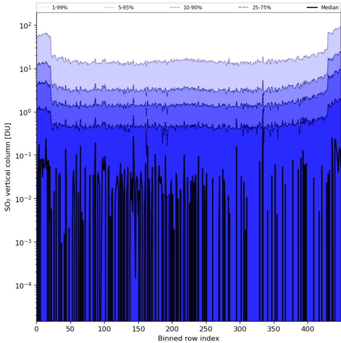
Figure 76: Along track statistics of “SO 2 vertical column” for 2024-02-07 to 2024-02-09
