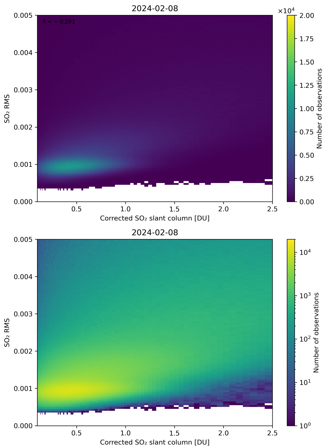
Figure 183: Scatter density plot of “Corrected SO 2 slant column” against “SO 2 RMS” for 2024-02-07 to 2024-02-09.
