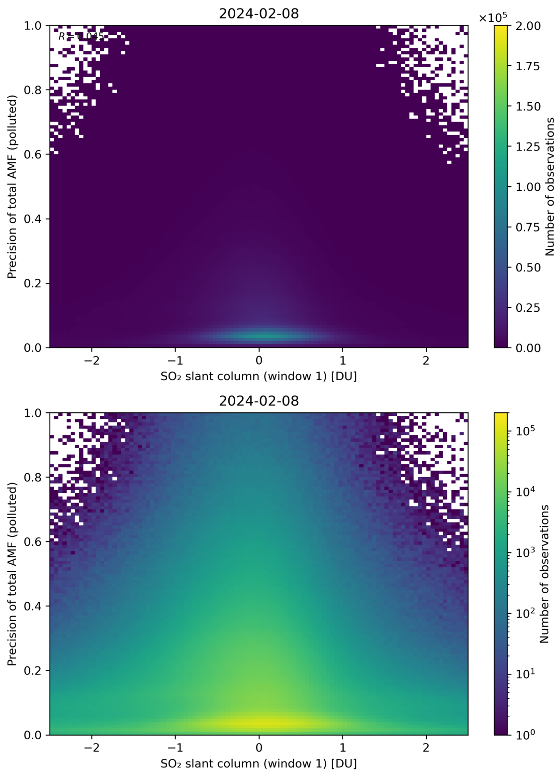
Figure 240: Scatter density plot of “SO 2 slant column (window 1)” against “Precision of total AMF (polluted)” for 2024-02-07 to 2024-02-09.
