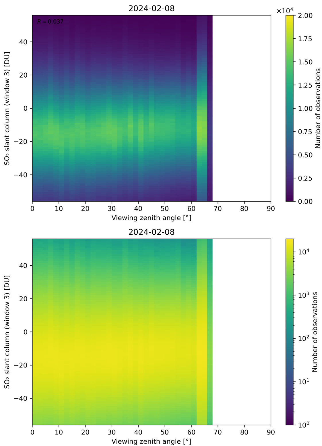
Figure 323: Scatter density plot of “Viewing zenith angle” against “SO 2 slant column (window 3)” for 2024-02-07 to 2024-02-09.
