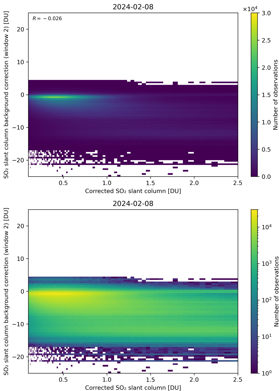
Figure 179: Scatter density plot of “Corrected SO 2 slant column” against “SO 2 slant column background correction (window 2)” for 2024-02-07 to 2024-02-09.
