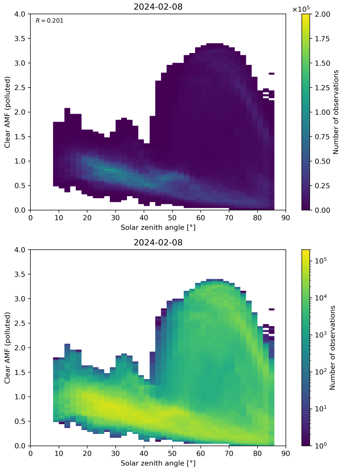
Figure 165: Scatter density plot of “Solar zenith angle” against “Clear AMF (polluted)” for 2024-02-07 to 2024-02-09.
