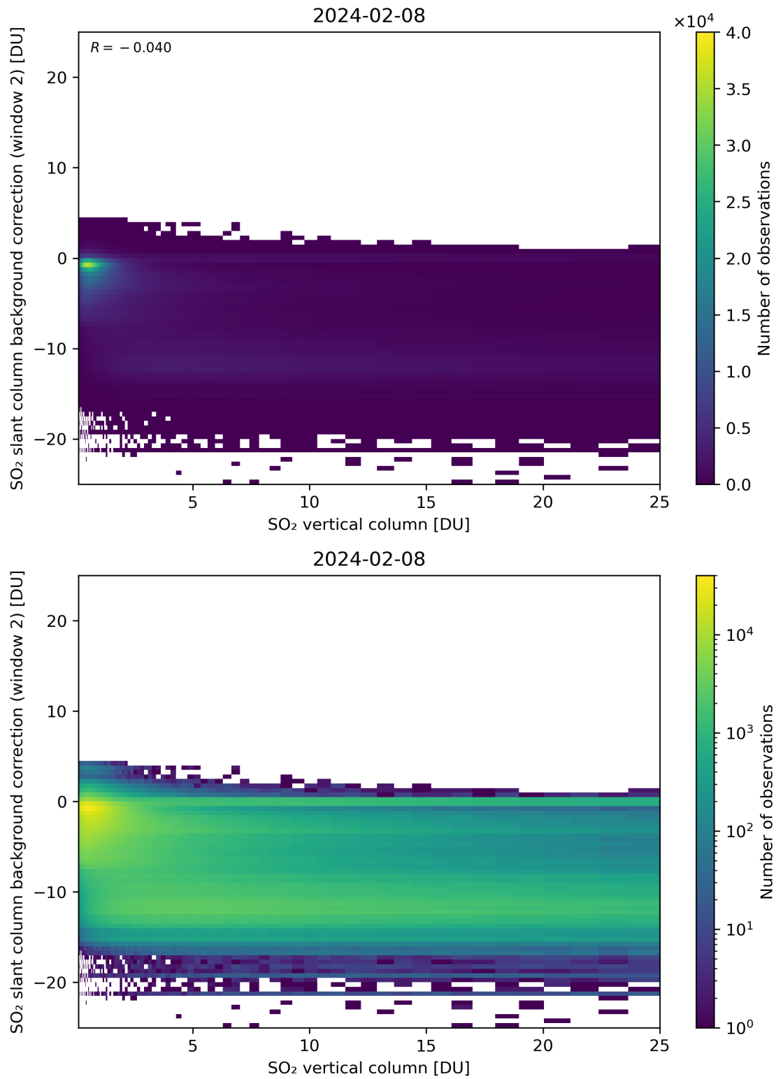
Figure 274: Scatter density plot of “SO 2 vertical column” against “SO 2 slant column background correction (window 2)” for 2024-02-07 to 2024-02-09.
