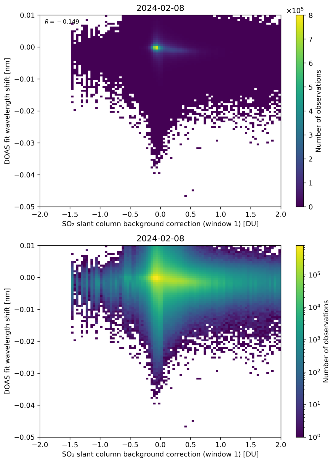
Figure 100: Scatter density plot of “SO 2 slant column background correction (window 1)” against “DOAS fit wavelength shift” for 2024-02-07 to 2024-02-09.
