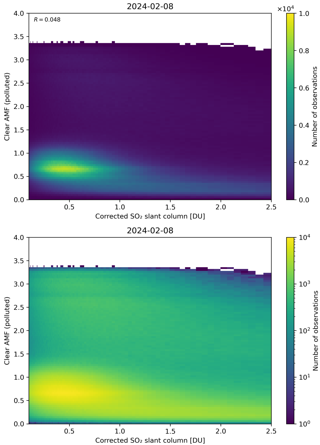
Figure 184: Scatter density plot of “Corrected SO 2 slant column” against “Clear AMF (polluted)” for 2024-02-07 to 2024-02-09.
