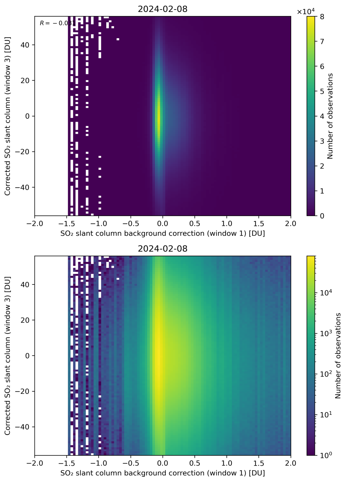
Figure 105: Scatter density plot of “SO 2 slant column background correction (window 1)” against “Corrected SO 2 slant column (window 3)” for 2024-02-07 to 2024-02-09.
