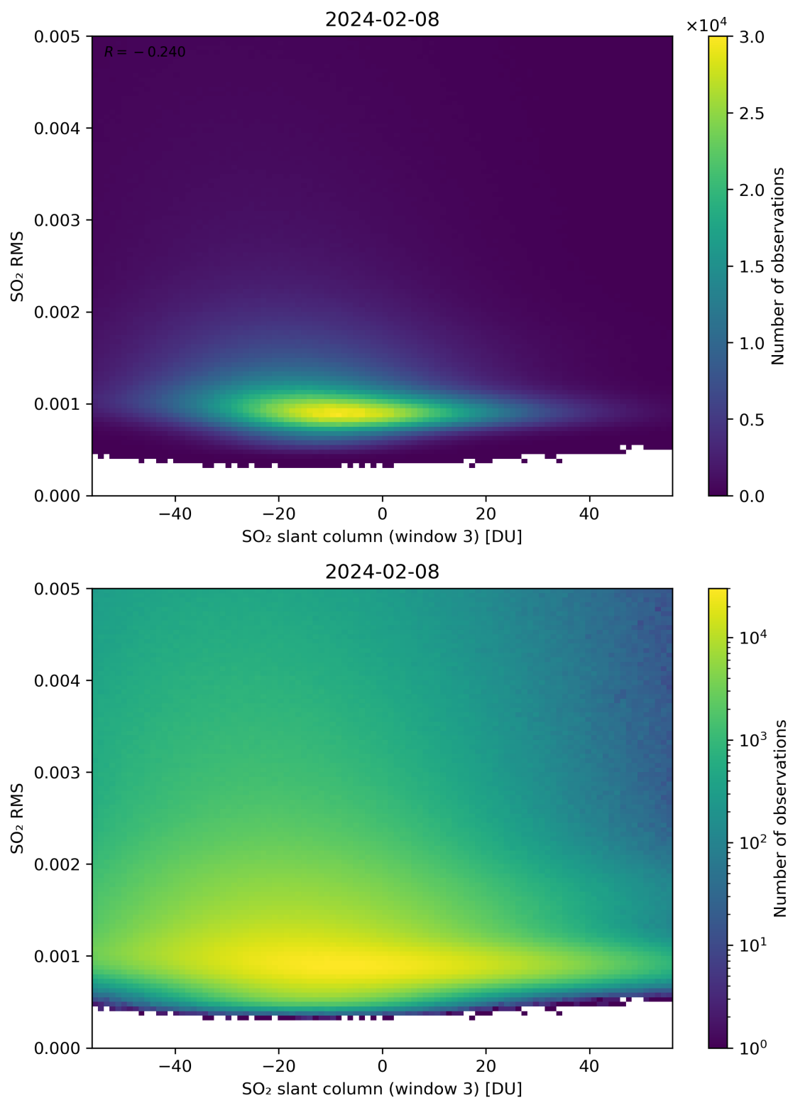
Figure 256: Scatter density plot of “SO 2 slant column (window 3)” against “SO 2 RMS” for 2024-02-07 to 2024-02-09.
