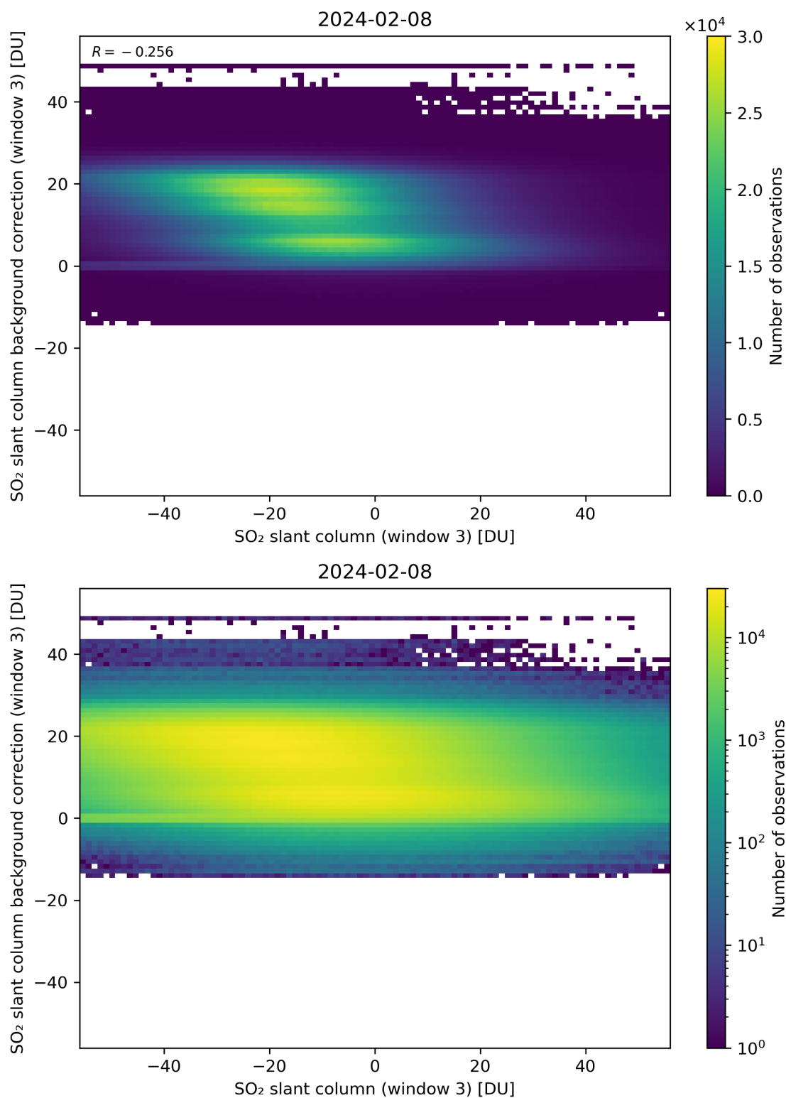
Figure 253: Scatter density plot of “SO 2 slant column (window 3)” against “SO 2 slant column background correction (window 3)” for 2024-02-07 to 2024-02-09.
