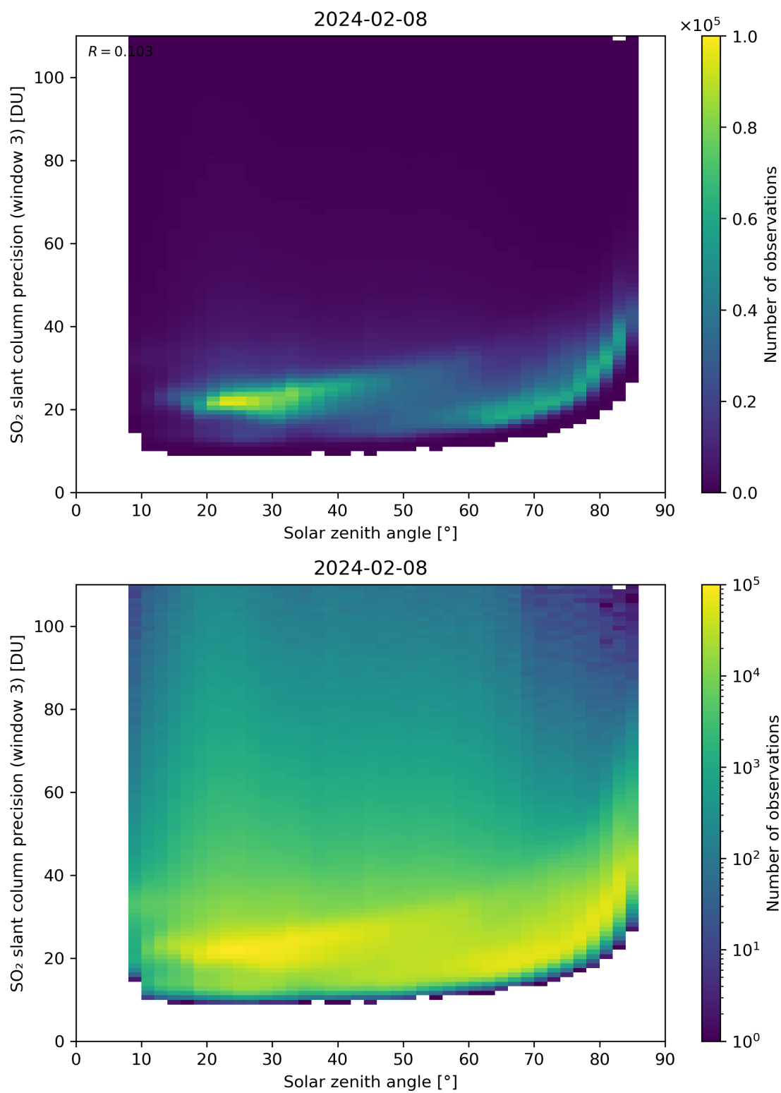
Figure 173: Scatter density plot of “Solar zenith angle” against “SO 2 slant column precision (window 3)” for 2024-02-07 to 2024-02-09.
