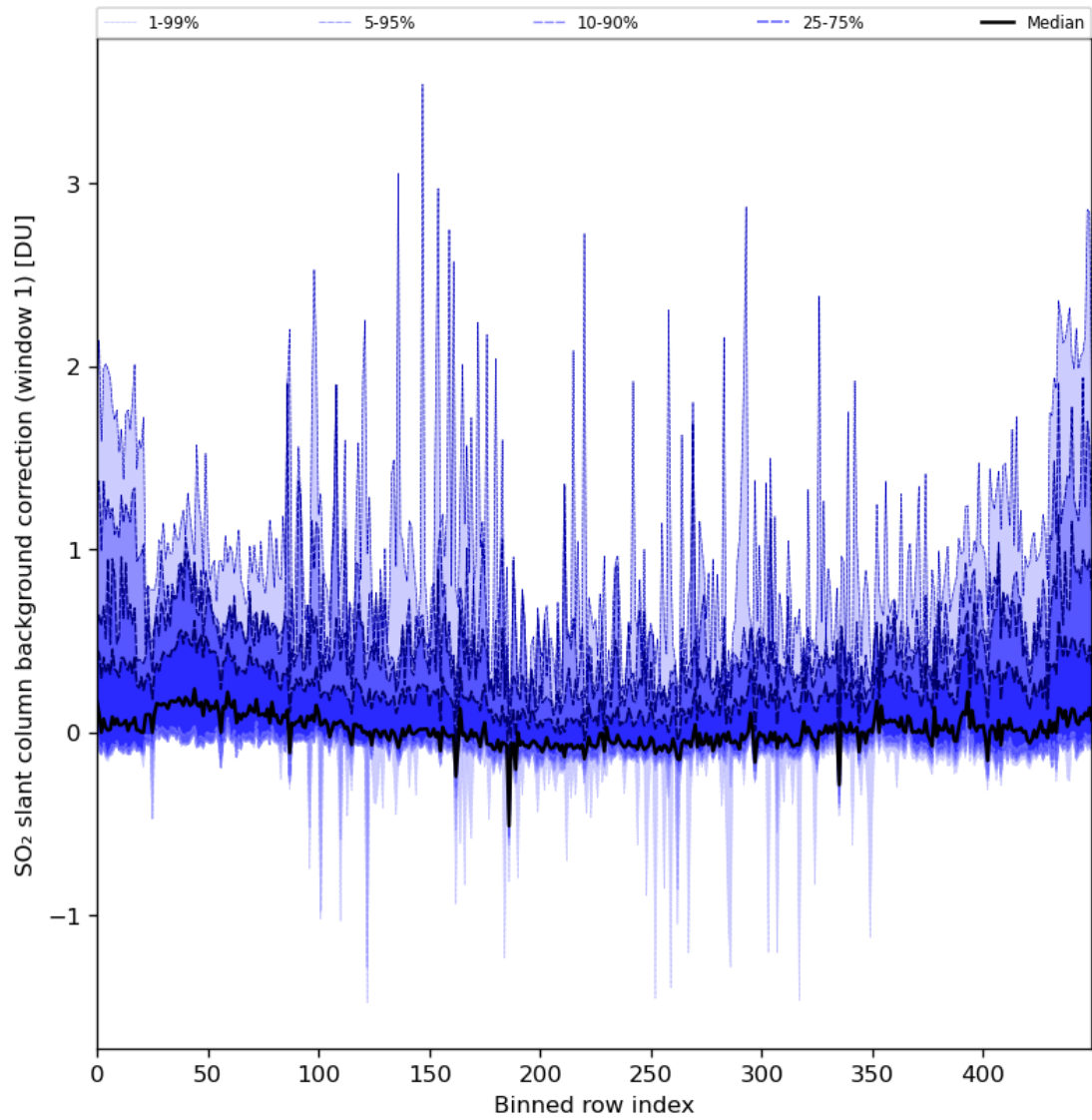
Figure 82: Along track statistics of “SO 2 slant column background correction (window 1)” for 2024-02-07 to 2024-02-09
