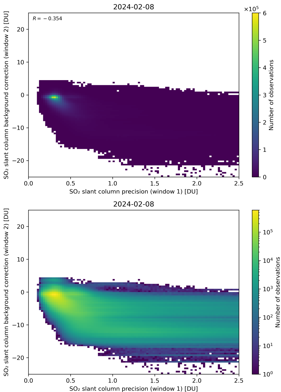
Figure 219: Scatter density plot of “SO 2 slant column precision (window 1)” against “SO 2 slant column background correction (window 2)” for 2024-02-07 to 2024-02-09.
