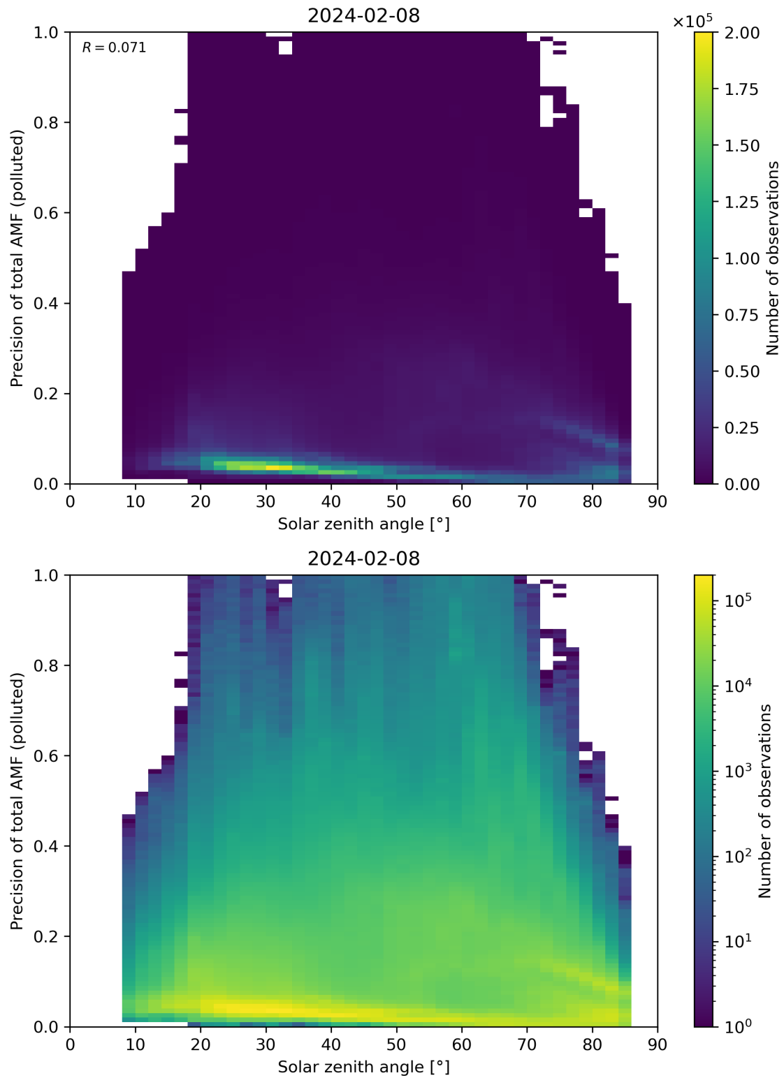
Figure 175: Scatter density plot of “Solar zenith angle” against “Precision of total AMF (polluted)” for 2024-02-07 to 2024-02-09.
