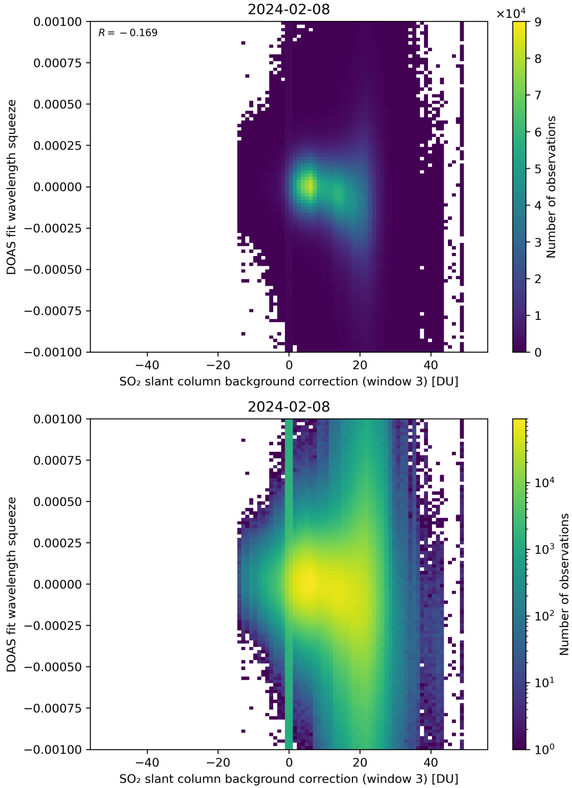
Figure 122: Scatter density plot of “SO 2 slant column background correction (window 3)” against “DOAS fit wavelength squeeze” for 2024-02-07 to 2024-02-09.
