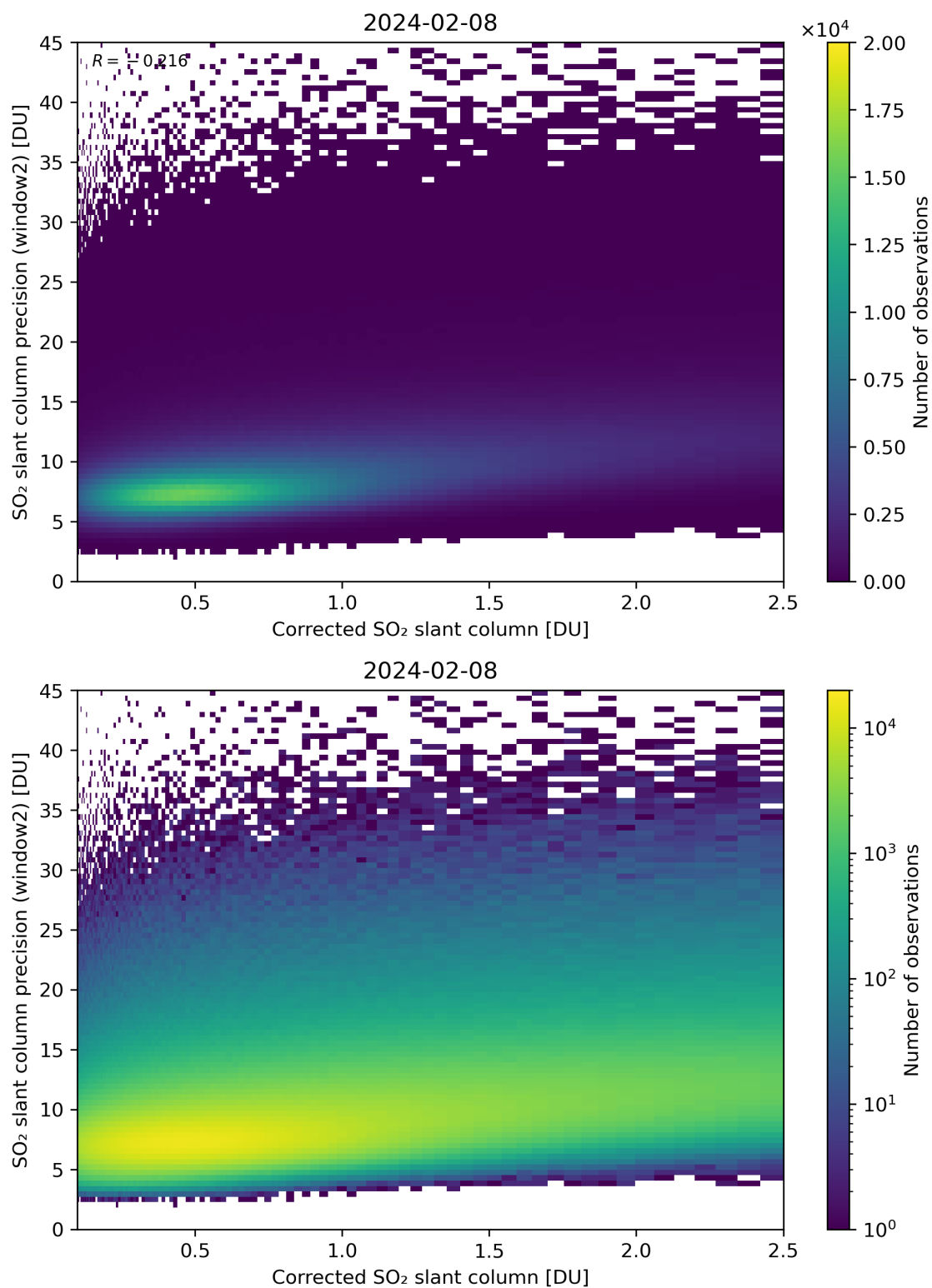
Figure 189: Scatter density plot of “Corrected SO 2 slant column” against “SO 2 slant column precision (window2)” for 2024-02-07 to 2024-02-09.
