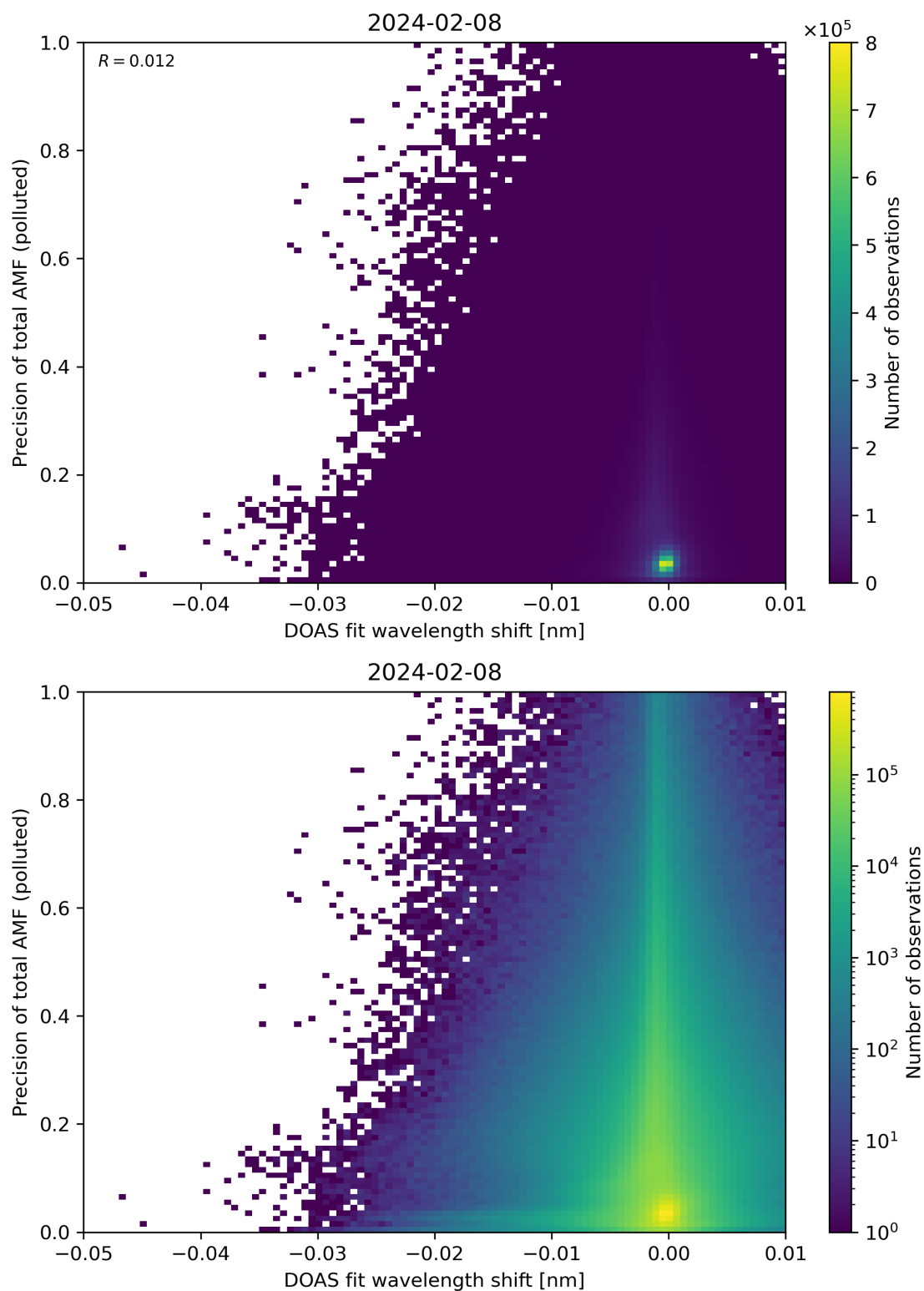
Figure 131: Scatter density plot of “DOAS fit wavelength shift” against “Precision of total AMF (polluted)” for 2024-02-07 to 2024-02-09.
