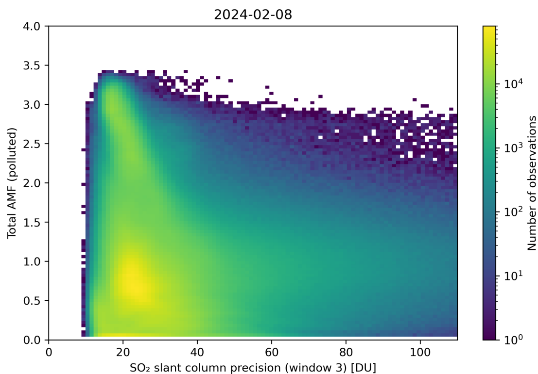
Figure 263: Scatter density plot of “SO 2 slant column precision (window 3)” against “Total AMF (polluted)” for 2024-02-07 to 2024-02-09.
