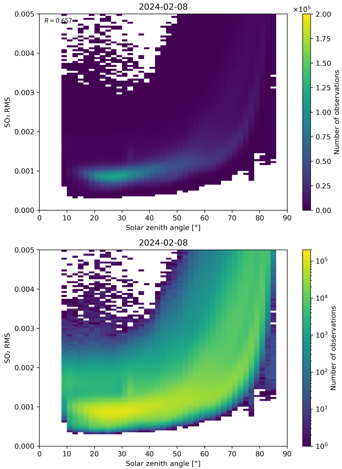
Figure 163: Scatter density plot of “Solar zenith angle” against “SO 2 RMS” for 2024-02-07 to 2024-02-09.
