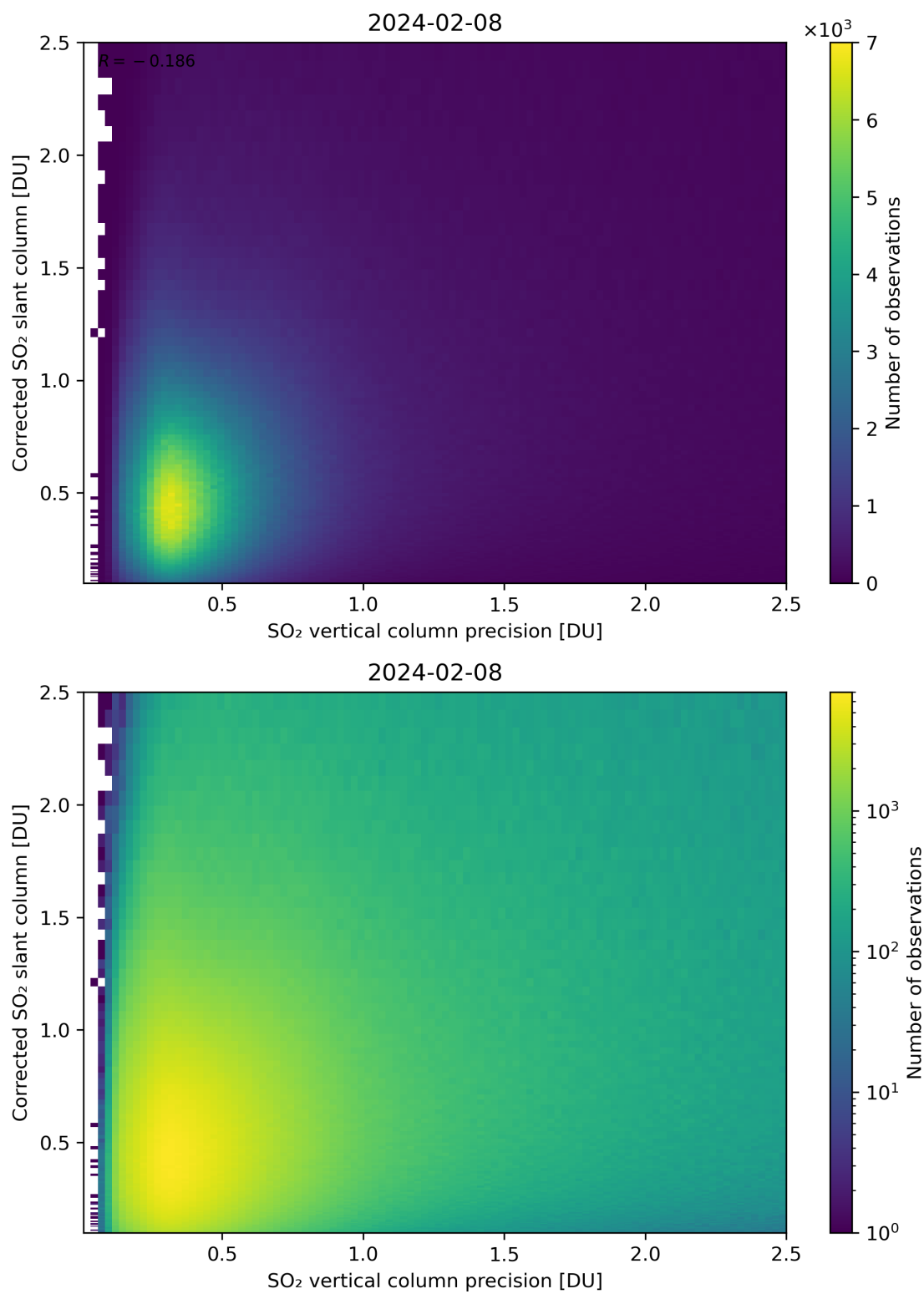
Figure 286: Scatter density plot of “SO 2 vertical column precision” against “Corrected SO 2 slant column” for 2024-02-07 to 2024-02-09.
