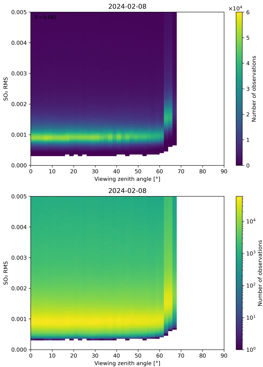
Figure 313: Scatter density plot of “Viewing zenith angle” against “SO 2 RMS” for 2024-02-07 to 2024-02-09.
