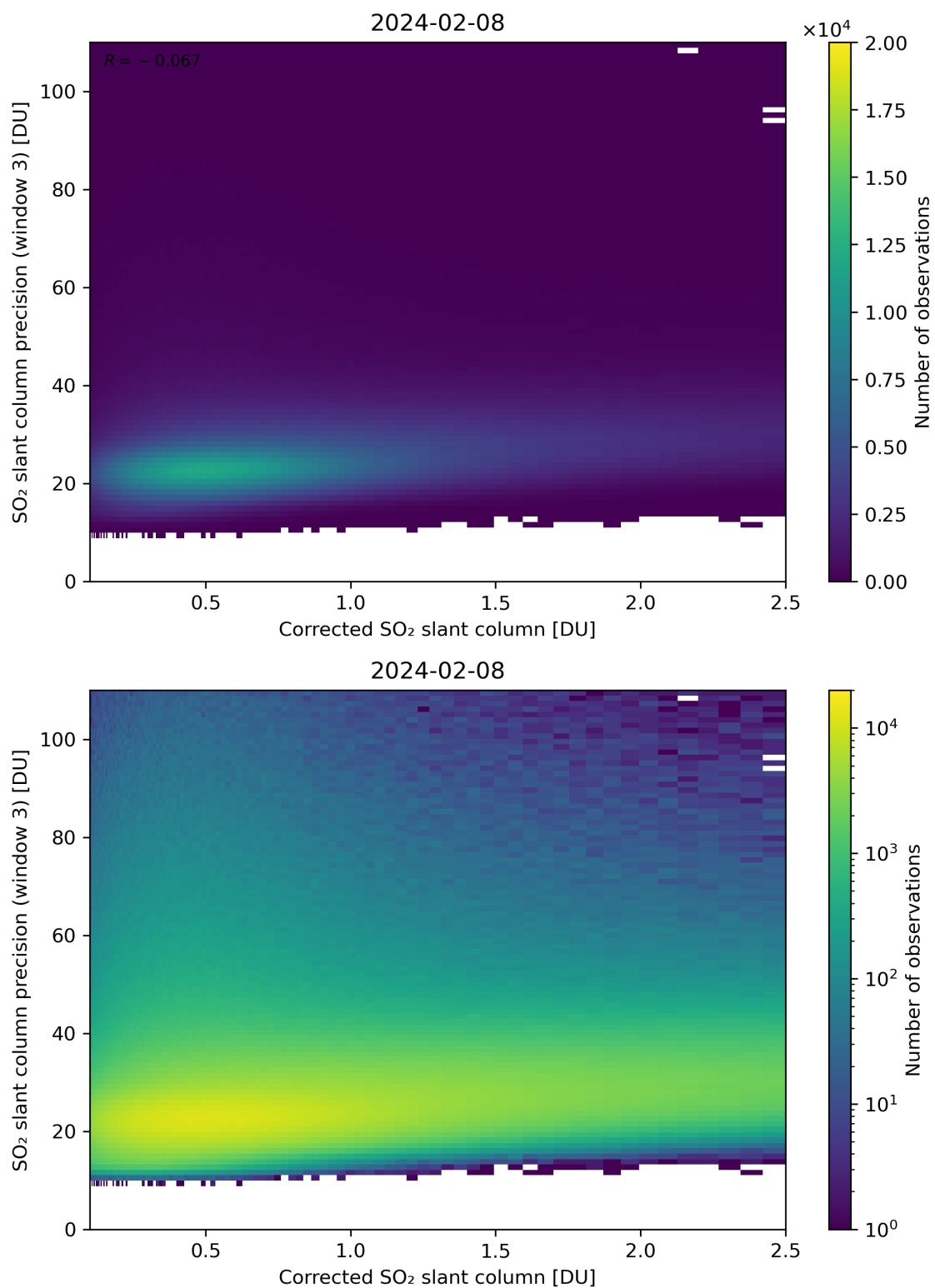
Figure 191: Scatter density plot of “Corrected SO 2 slant column” against “SO 2 slant column precision (window 3)” for 2024-02-07 to 2024-02-09.
