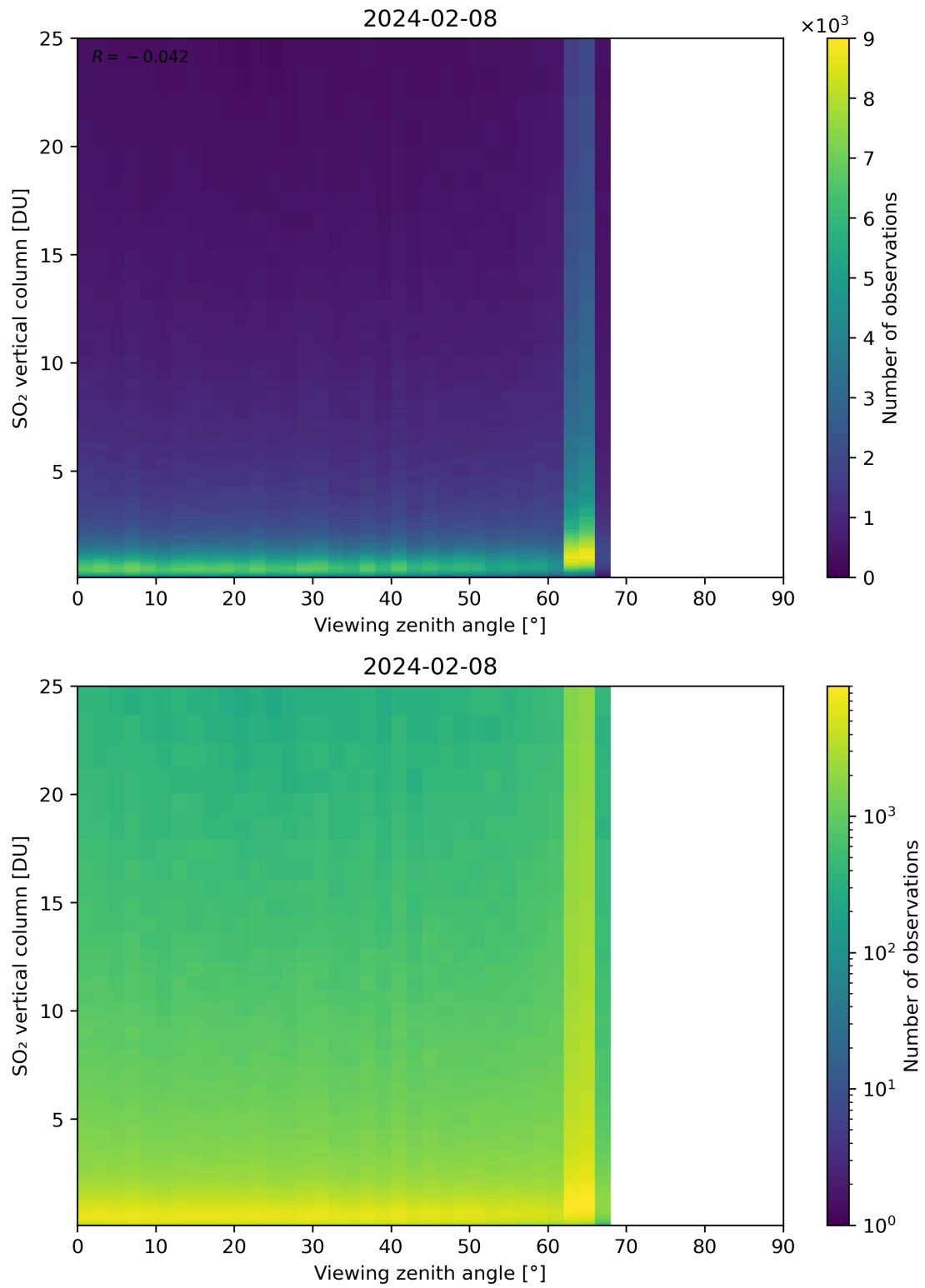
Figure 327: Scatter density plot of “Viewing zenith angle” against “SO 2 vertical column” for 2024-02-07 to 2024-02-09.
