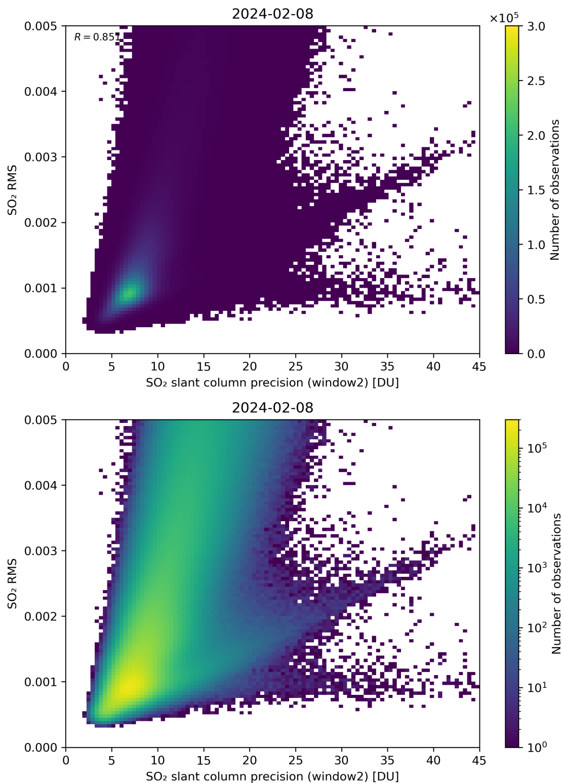
Figure 245: Scatter density plot of “SO 2 slant column precision (window2)” against “SO 2 RMS” for 2024-02-07 to 2024-02-09.
