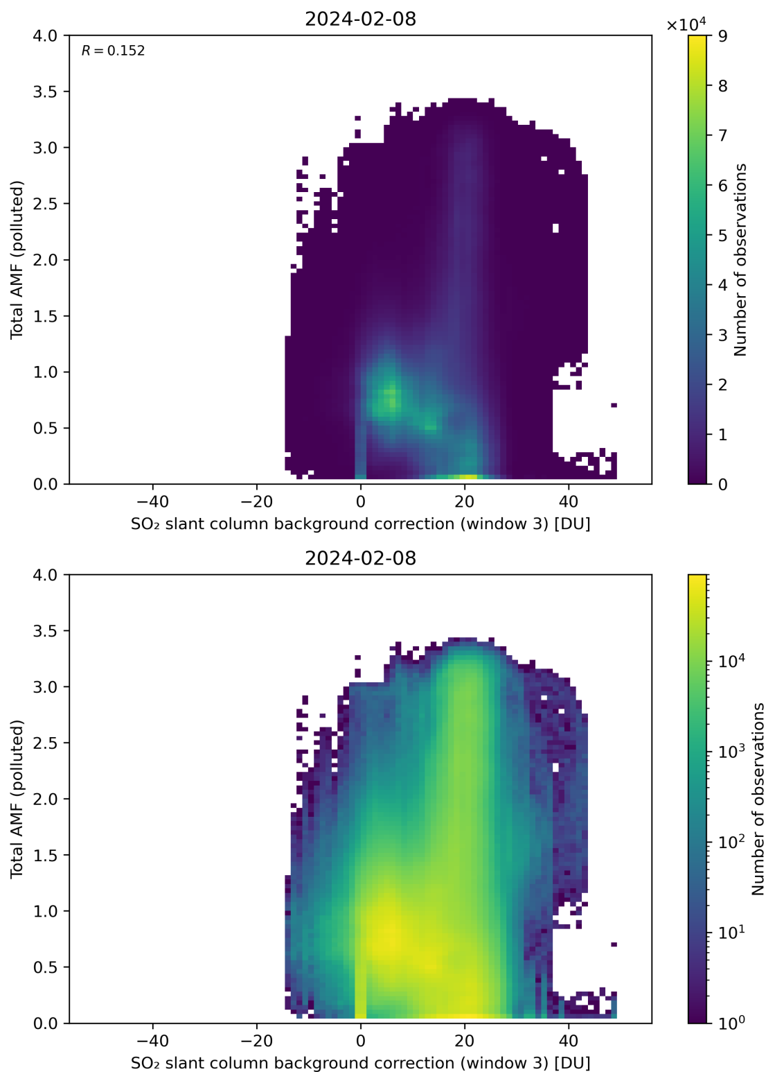
Figure 125: Scatter density plot of “SO 2 slant column background correction (window 3)” against “Total AMF (polluted)” for 2024-02-07 to 2024-02-09.
