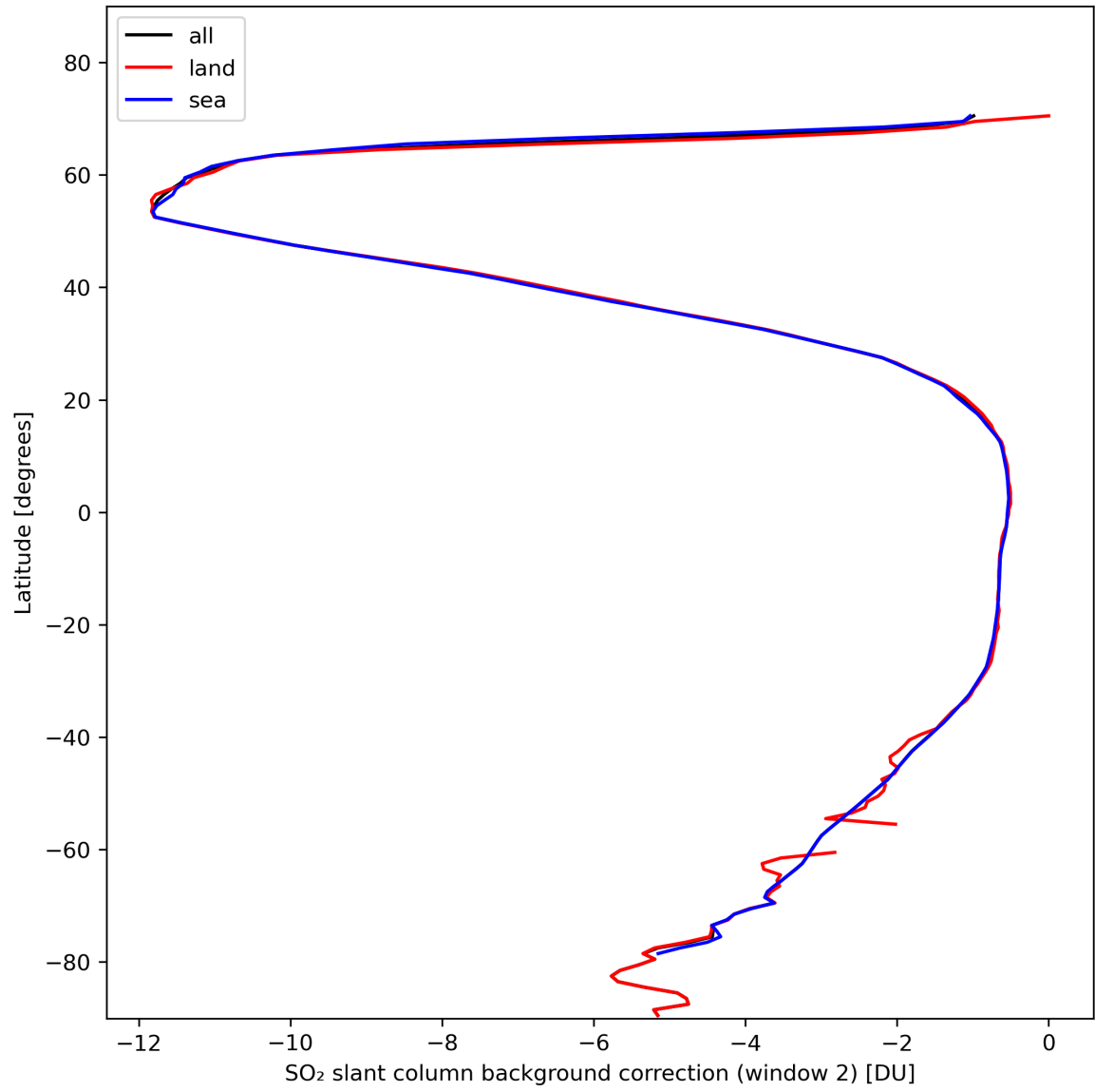
Figure 40: Zonal average of “SO 2 slant column background correction (window 2)” for 2024-02-07 to 2024-02-09.
