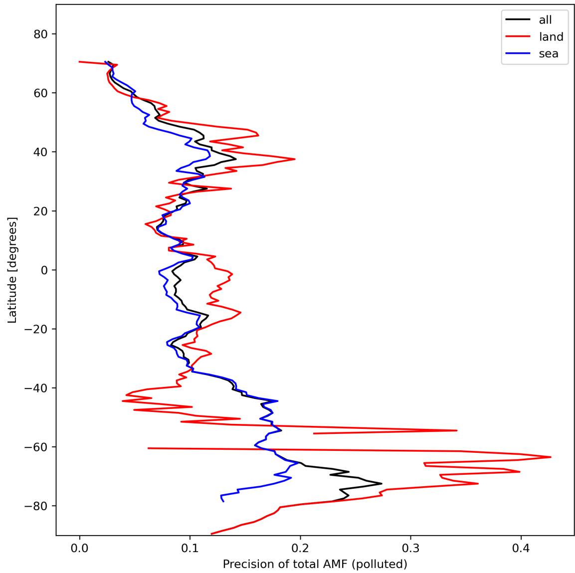
Figure 49: Zonal average of “Precision of total AMF (polluted)” for 2024-02-07 to 2024-02-09.
