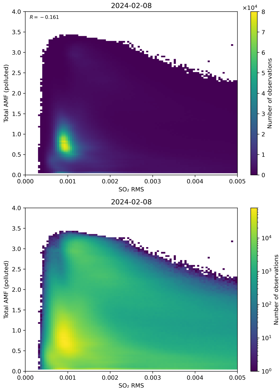
Figure 137: Scatter density plot of “SO 2 RMS” against “Total AMF (polluted)” for 2024-02-07 to 2024-02-09.
