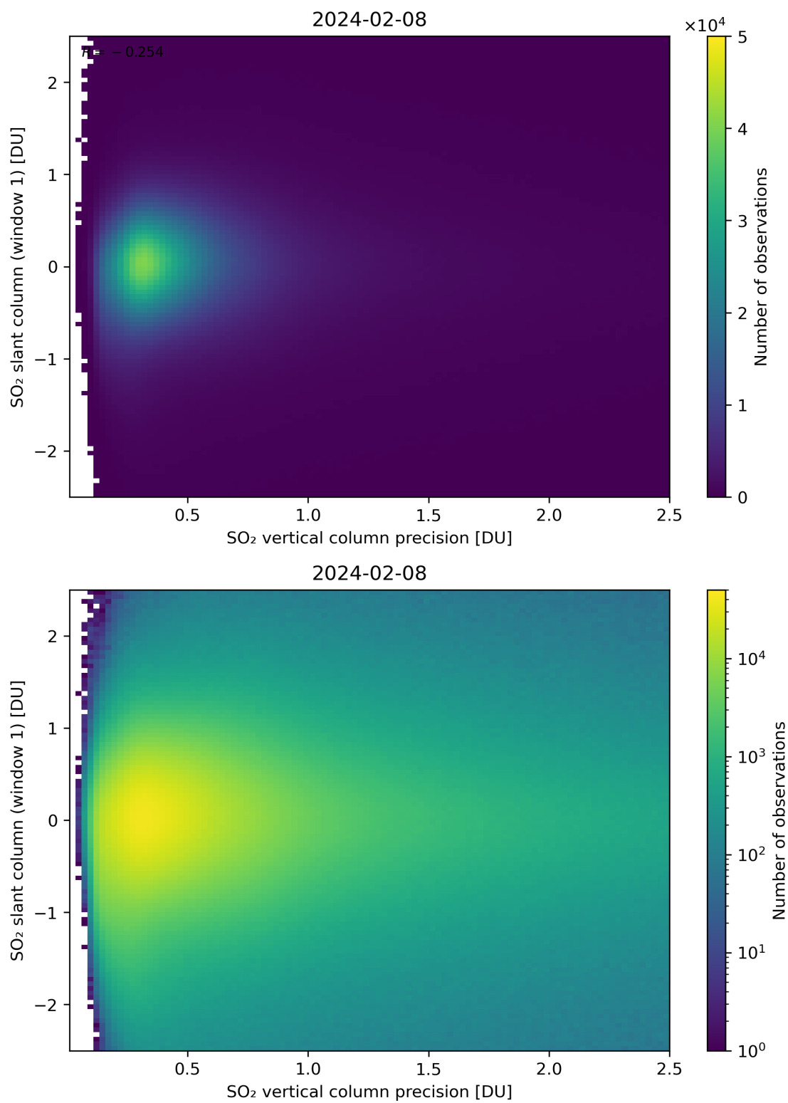
Figure 289: Scatter density plot of “SO 2 vertical column precision” against “SO 2 slant column (window 1)” for 2024-02-07 to 2024-02-09.
