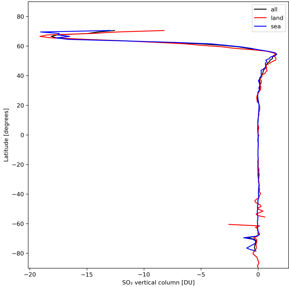
Figure 30: Zonal average of “SO 2 vertical column” for 2024-02-07 to 2024-02-09.
