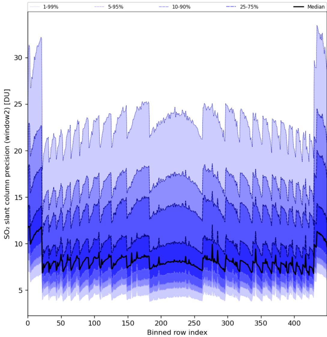
Figure 84: Along track statistics of “SO 2 slant column precision (window2)” for 2024-02-07 to 2024-02-09
