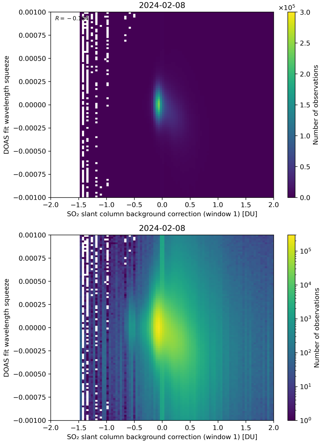
Figure 101: Scatter density plot of “SO 2 slant column background correction (window 1)” against “DOAS fit wavelength squeeze” for 2024-02-07 to 2024-02-09.
