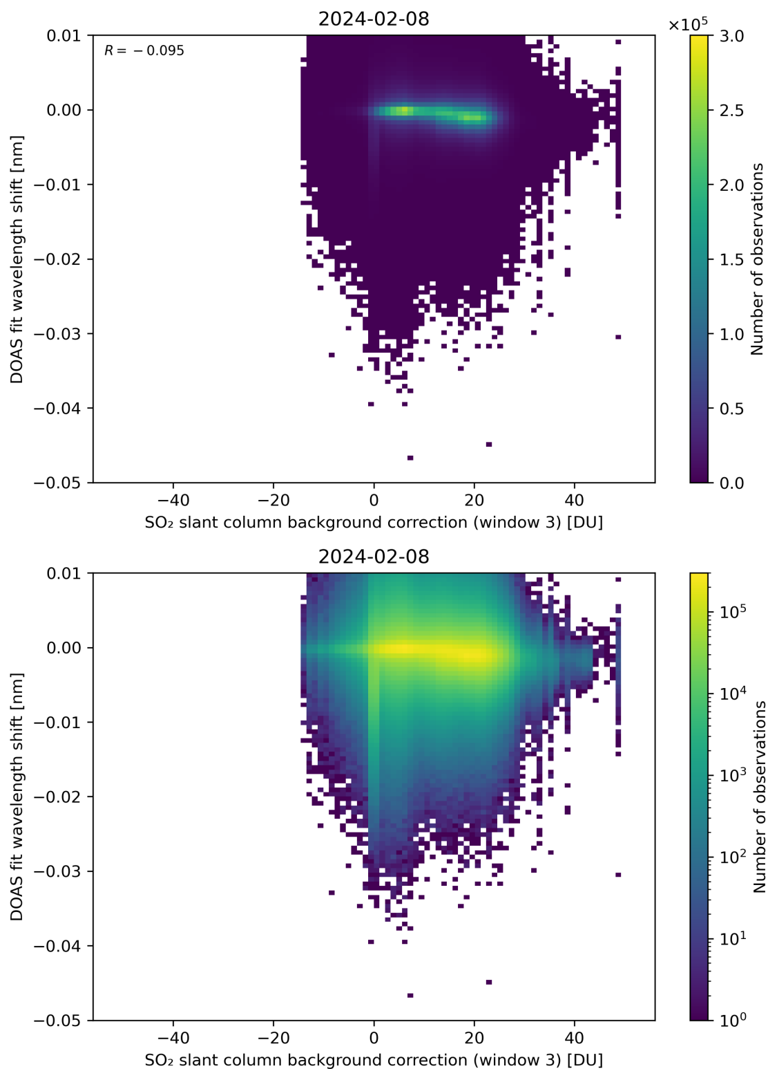
Figure 121: Scatter density plot of “SO 2 slant column background correction (window 3)” against “DOAS fit wavelength shift” for 2024-02-07 to 2024-02-09.
