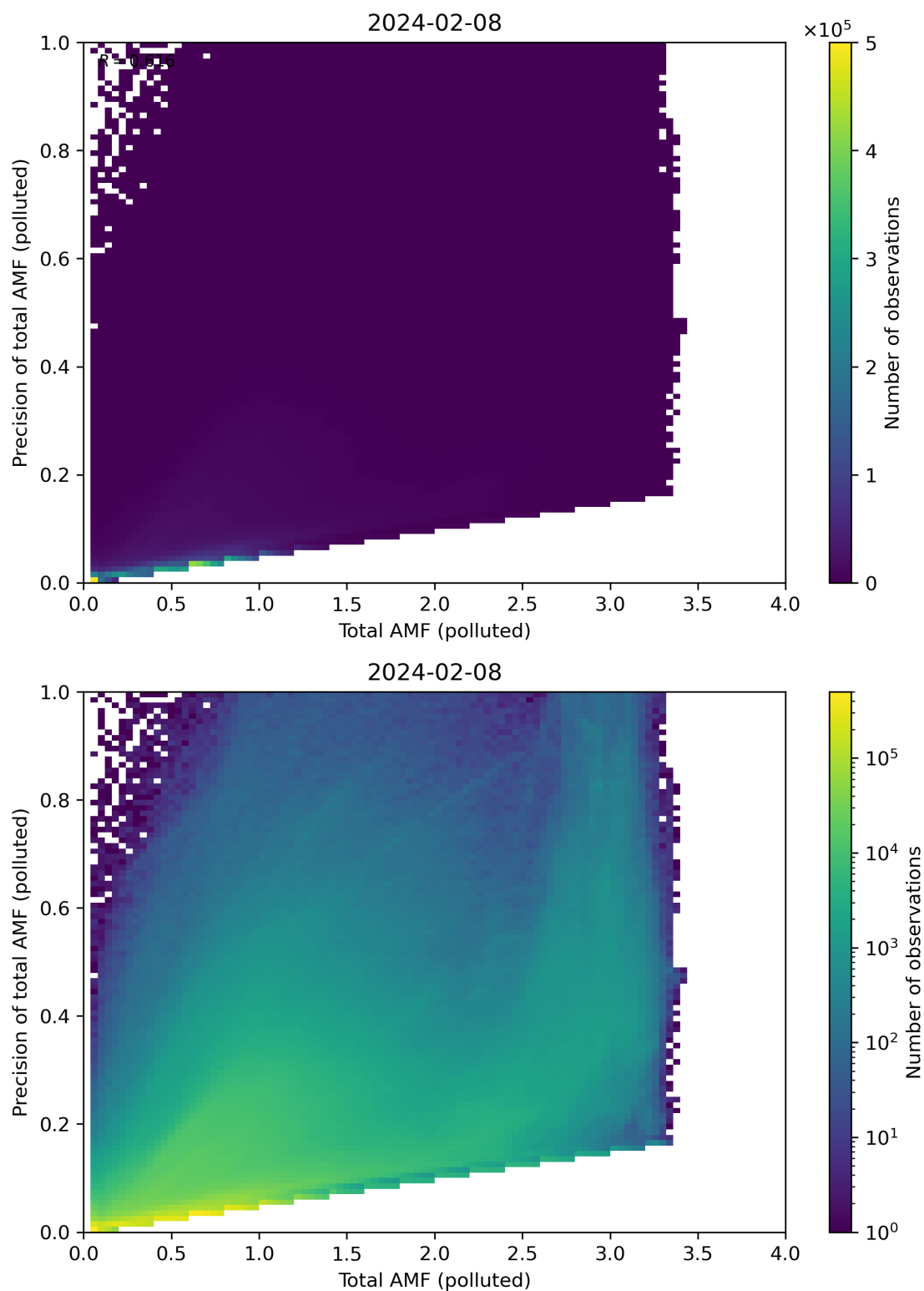
Figure 272: Scatter density plot of “Total AMF (polluted)” against “Precision of total AMF (polluted)” for 2024-02-07 to 2024-02-09.
