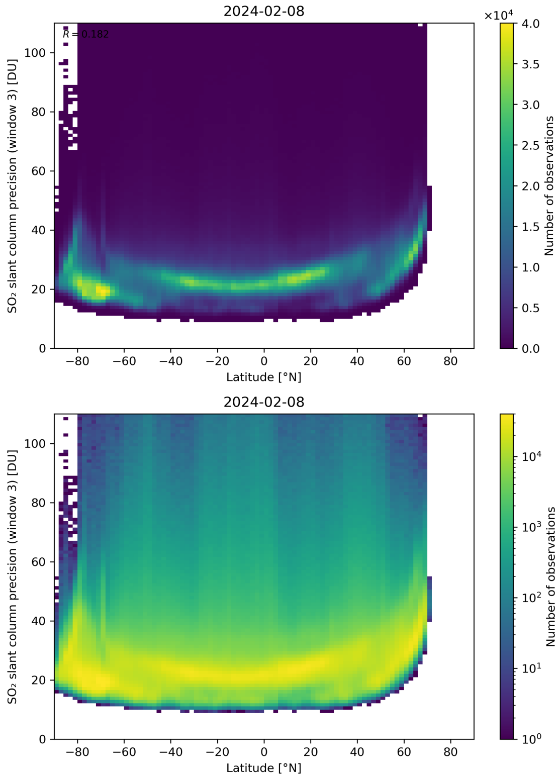
Figure 153: Scatter density plot of “Latitude” against “SO 2 slant column precision (window 3)” for 2024-02-07 to 2024-02-09.
