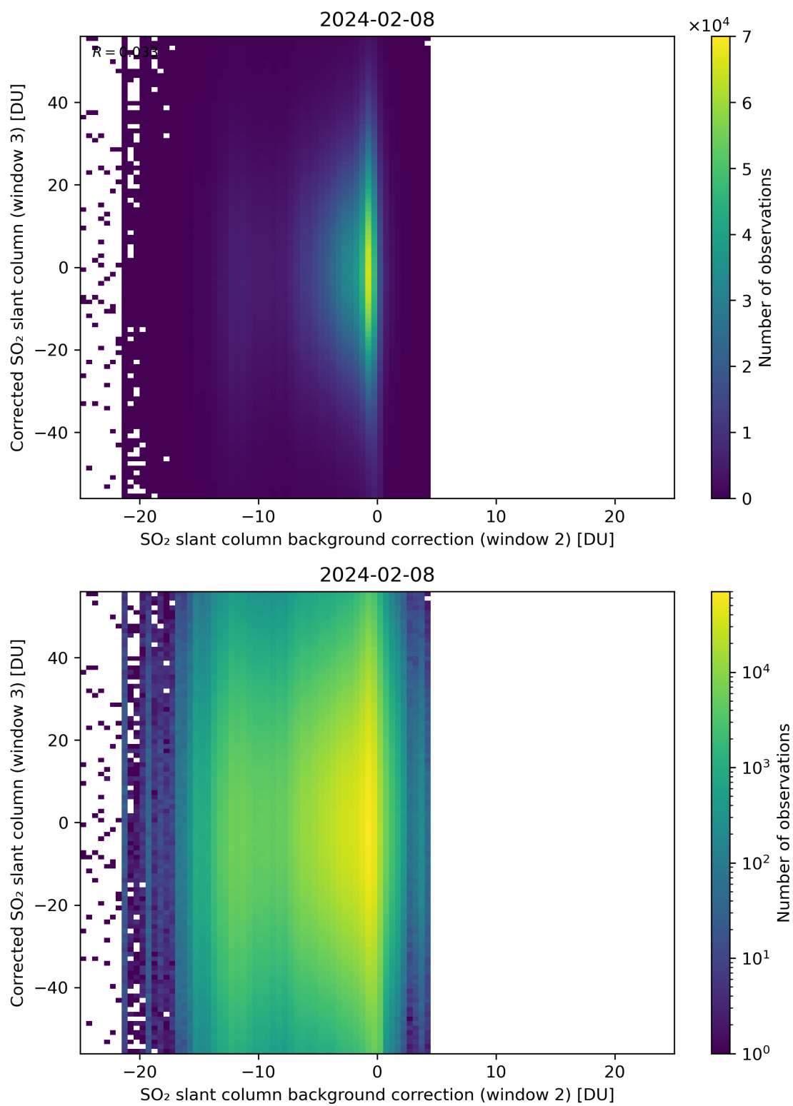
Figure 116: Scatter density plot of “SO 2 slant column background correction (window 2)” against “Corrected SO 2 slant column (window 3)” for 2024-02-07 to 2024-02-09.
