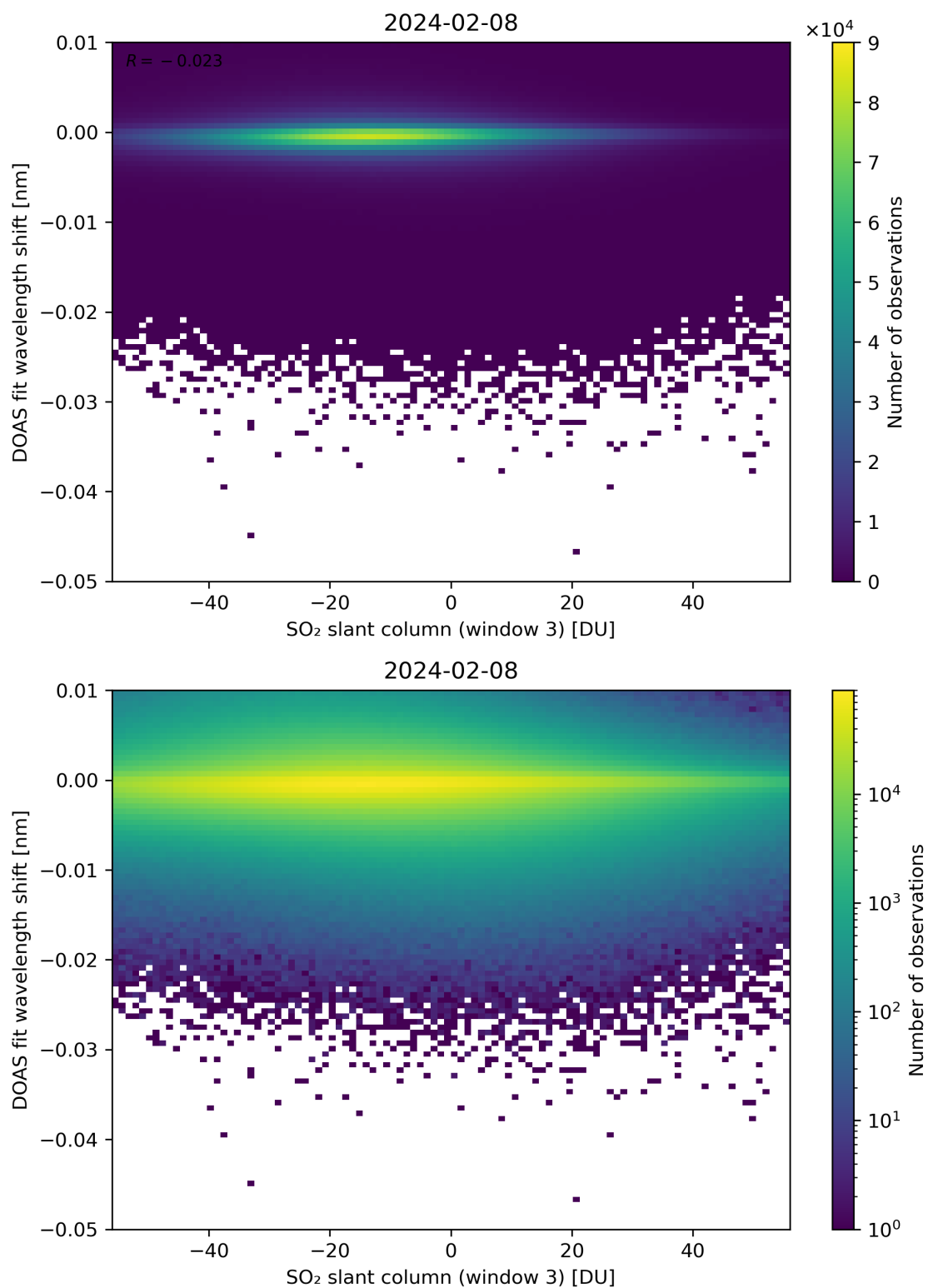
Figure 254: Scatter density plot of “SO 2 slant column (window 3)” against “DOAS fit wavelength shift” for 2024-02-07 to 2024-02-09.
