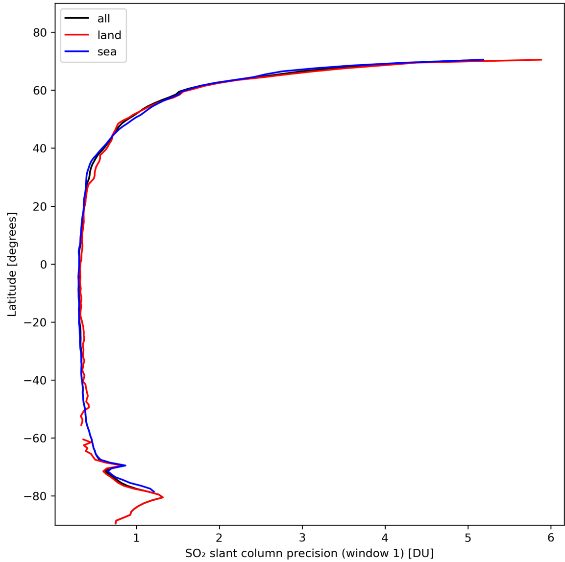
Figure 34: Zonal average of “SO 2 slant column precision (window 1)” for 2024-02-07 to 2024-02-09.
