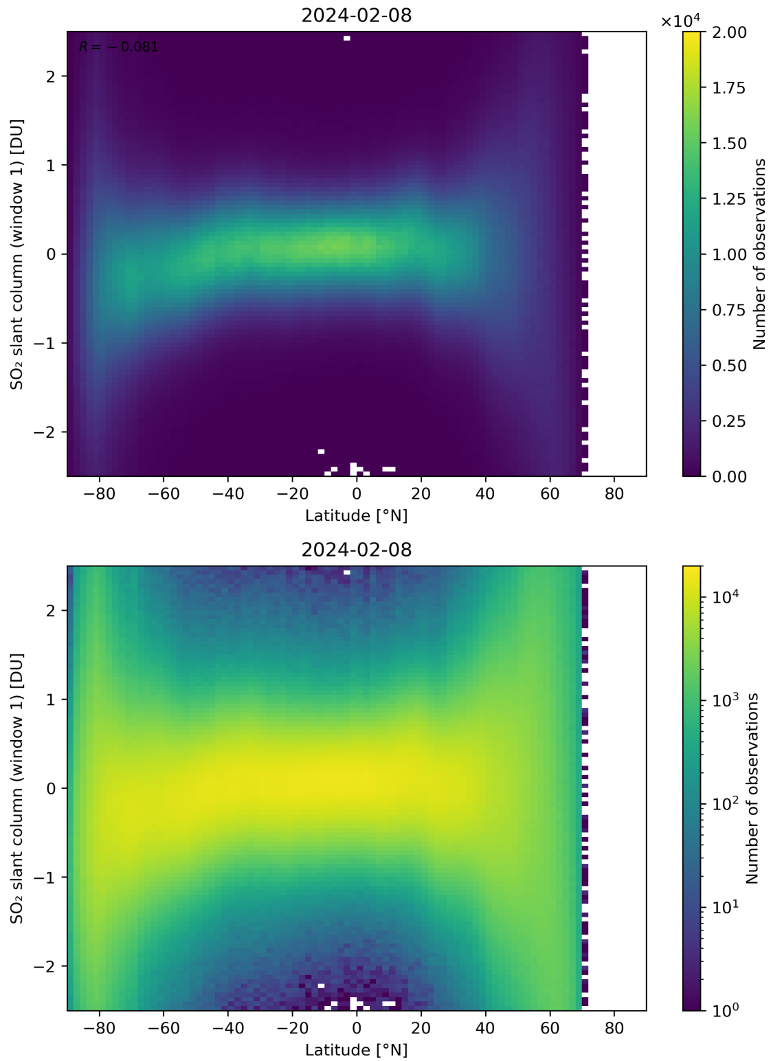
Figure 149: Scatter density plot of “Latitude” against “SO 2 slant column (window 1)” for 2024-02-07 to 2024-02-09.
