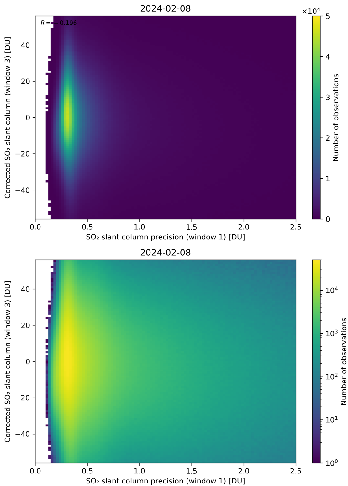
Figure 226: Scatter density plot of “SO 2 slant column precision (window 1)” against “Corrected SO 2 slant column (window 3)” for 2024-02-07 to 2024-02-09.
