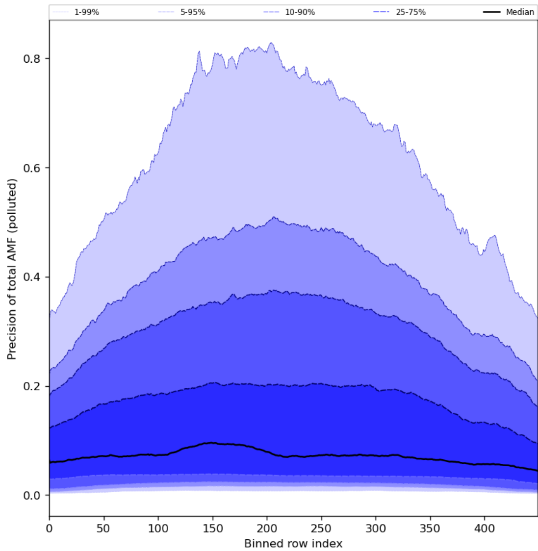
Figure 95: Along track statistics of “Precision of total AMF (polluted)” for 2024-02-07 to 2024-02-09
