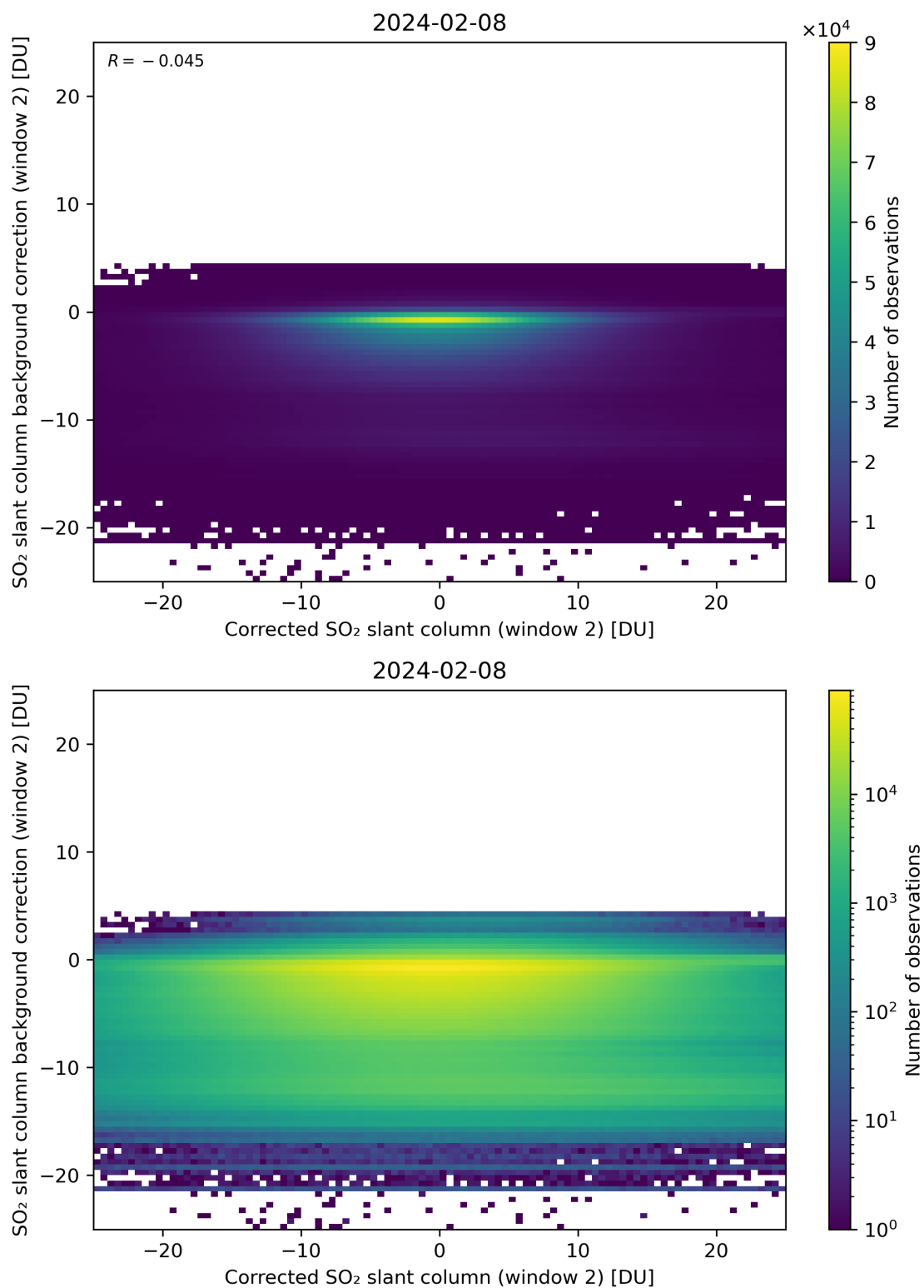
Figure 194: Scatter density plot of “Corrected SO 2 slant column (window 2)” against “SO 2 slant column background correction (window 2)” for 2024-02-07 to 2024-02-09.
