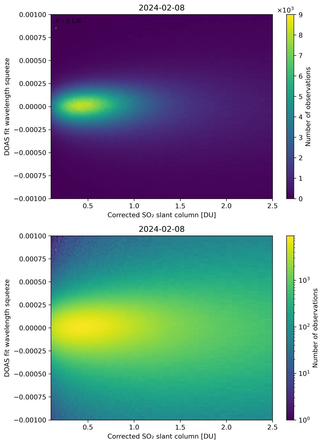
Figure 182: Scatter density plot of “Corrected SO 2 slant column” against “DOAS fit wavelength squeeze” for 2024-02-07 to 2024-02-09.
