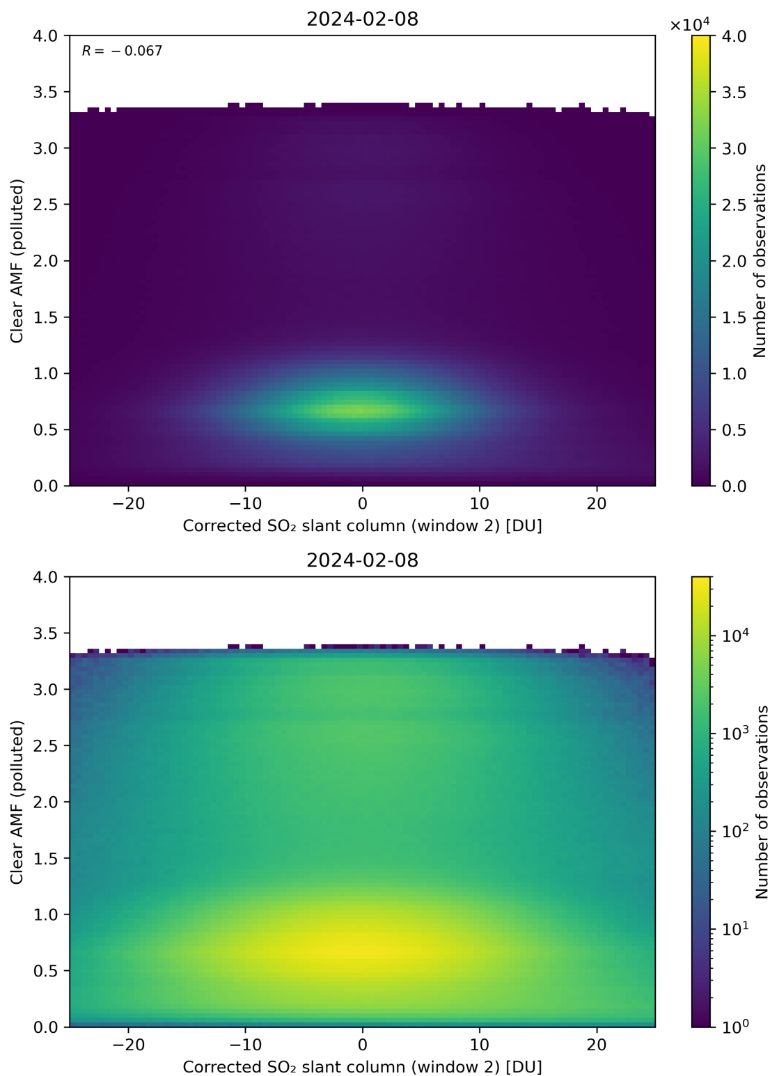
Figure 199: Scatter density plot of “Corrected SO 2 slant column (window 2)” against “Clear AMF (polluted)” for 2024-02-07 to 2024-02-09.
