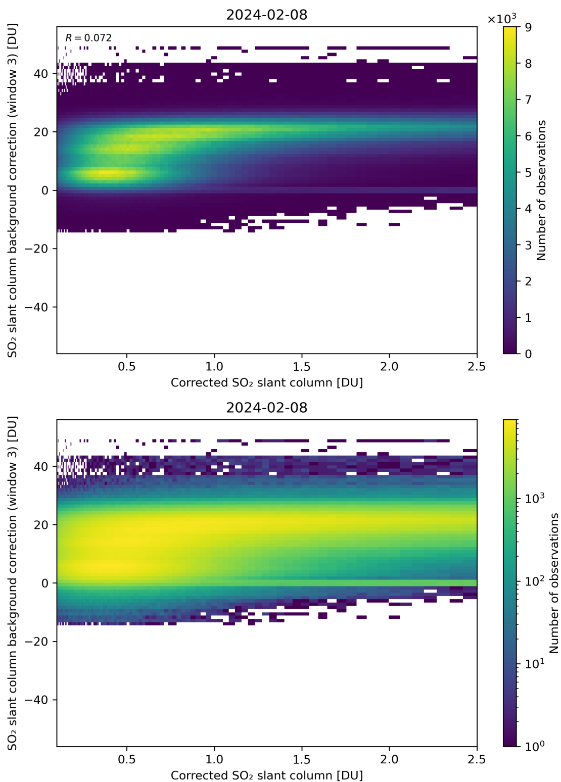
Figure 180: Scatter density plot of “Corrected SO 2 slant column” against “SO 2 slant column background correction (window 3)” for 2024-02-07 to 2024-02-09.
