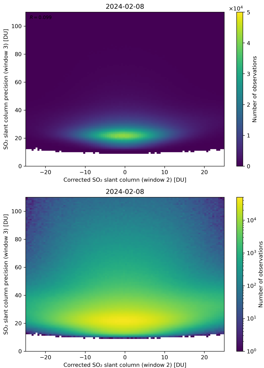
Figure 202: Scatter density plot of “Corrected SO 2 slant column (window 2)” against “SO 2 slant column precision (window 3)” for 2024-02-07 to 2024-02-09.
