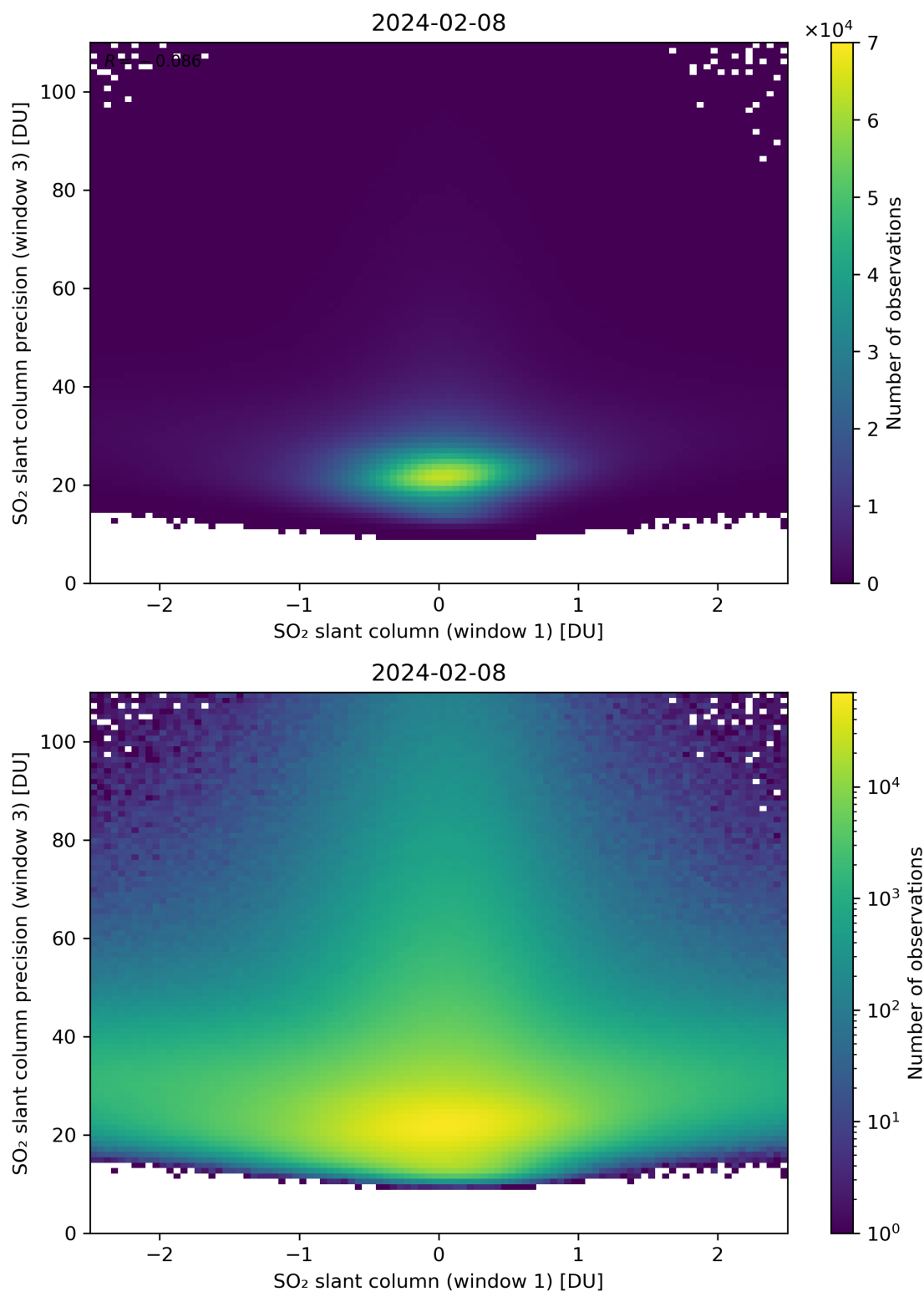
Figure 238: Scatter density plot of “SO 2 slant column (window 1)” against “SO 2 slant column precision (window 3)” for 2024-02-07 to 2024-02-09.
