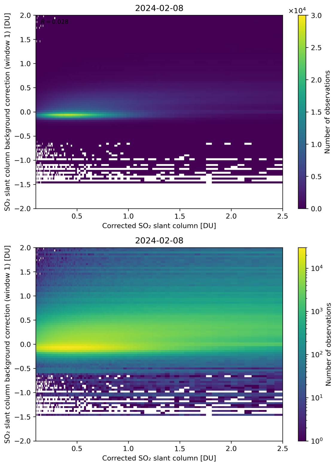
Figure 178: Scatter density plot of “Corrected SO 2 slant column” against “SO 2 slant column background correction (window 1)” for 2024-02-07 to 2024-02-09.
