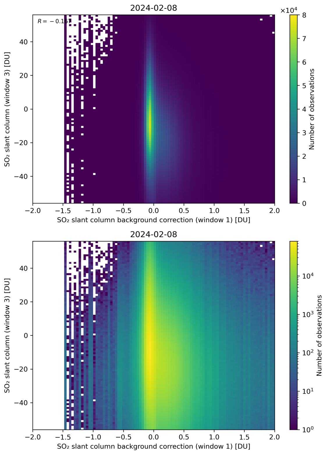
Figure 107: Scatter density plot of “SO 2 slant column background correction (window 1)” against “SO 2 slant column (window 3)” for 2024-02-07 to 2024-02-09.
