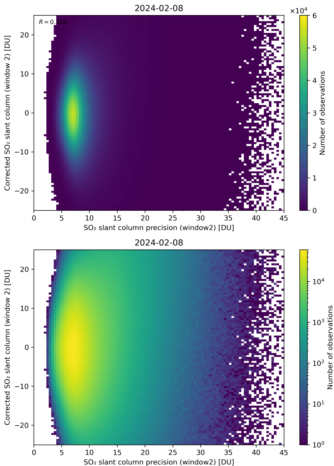
Figure 247: Scatter density plot of “SO 2 slant column precision (window2)” against “Corrected SO 2 slant column (window 2)” for 2024-02-07 to 2024-02-09.
