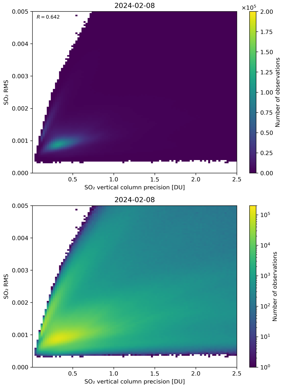
Figure 284: Scatter density plot of “SO 2 vertical column precision” against “SO 2 RMS” for 2024-02-07 to 2024-02-09.
