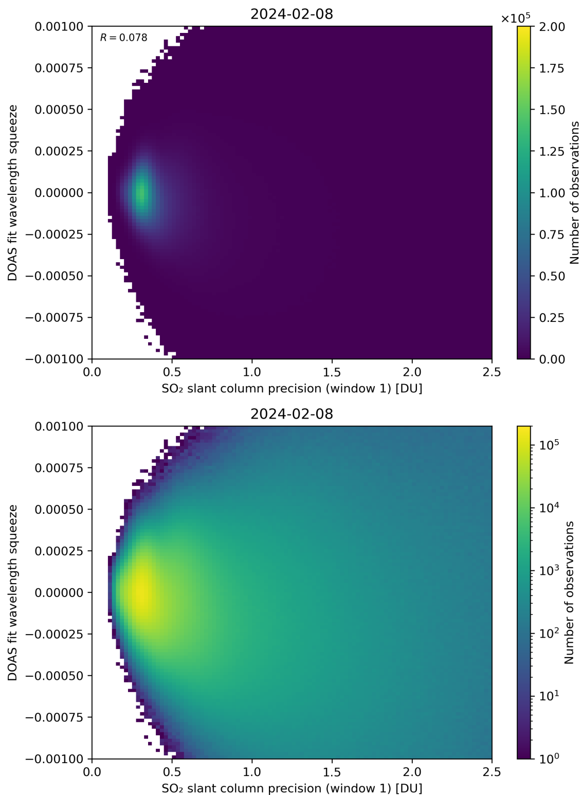
Figure 222: Scatter density plot of “SO 2 slant column precision (window 1)” against “DOAS fit wavelength squeeze” for 2024-02-07 to 2024-02-09.
