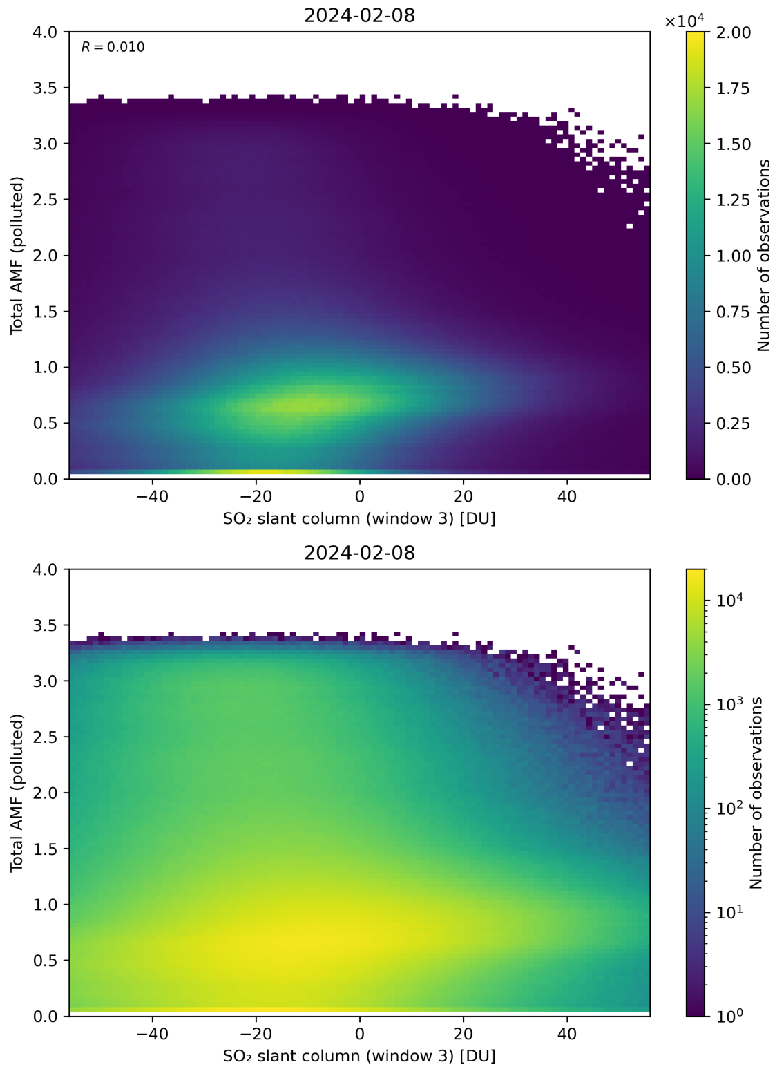
Figure 268: Scatter density plot of “SO 2 slant column (window 3)” against “Total AMF (polluted)” for 2024-02-07 to 2024-02-09.
