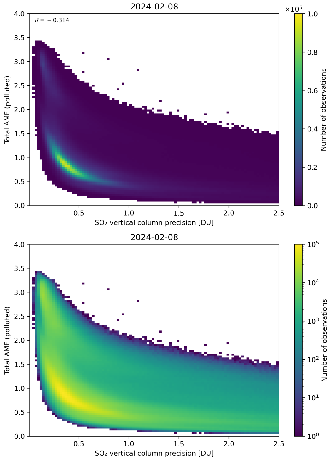
Figure 294: Scatter density plot of “SO 2 vertical column precision” against “Total AMF (polluted)” for 2024-02-07 to 2024-02-09.
