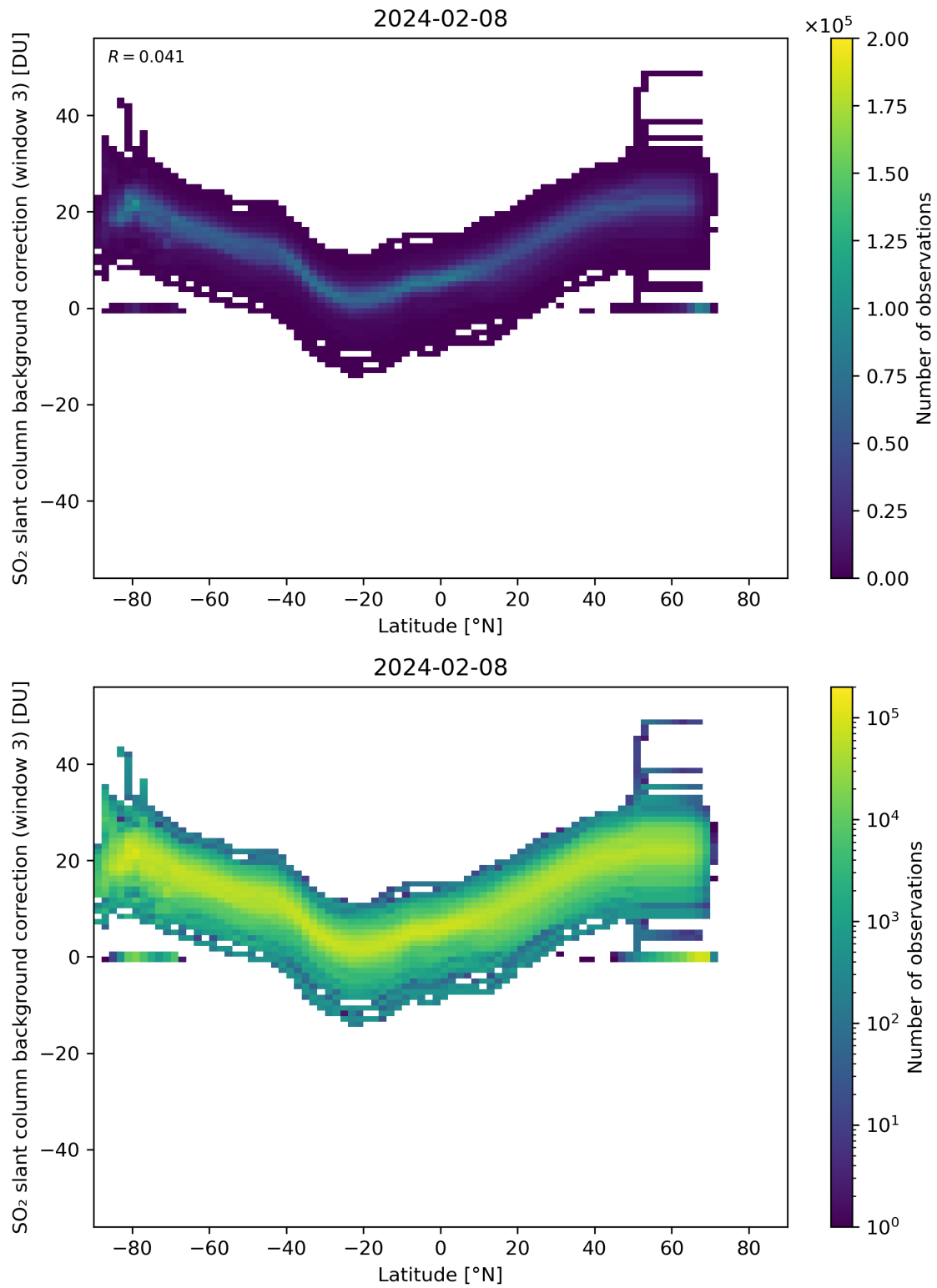
Figure 141: Scatter density plot of “Latitude” against “SO 2 slant column background correction (window 3)” for 2024-02-07 to 2024-02-09.
