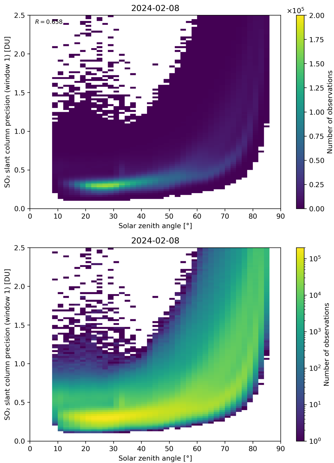
Figure 170: Scatter density plot of “Solar zenith angle” against “SO 2 slant column precision (window 1)” for 2024-02-07 to 2024-02-09.
