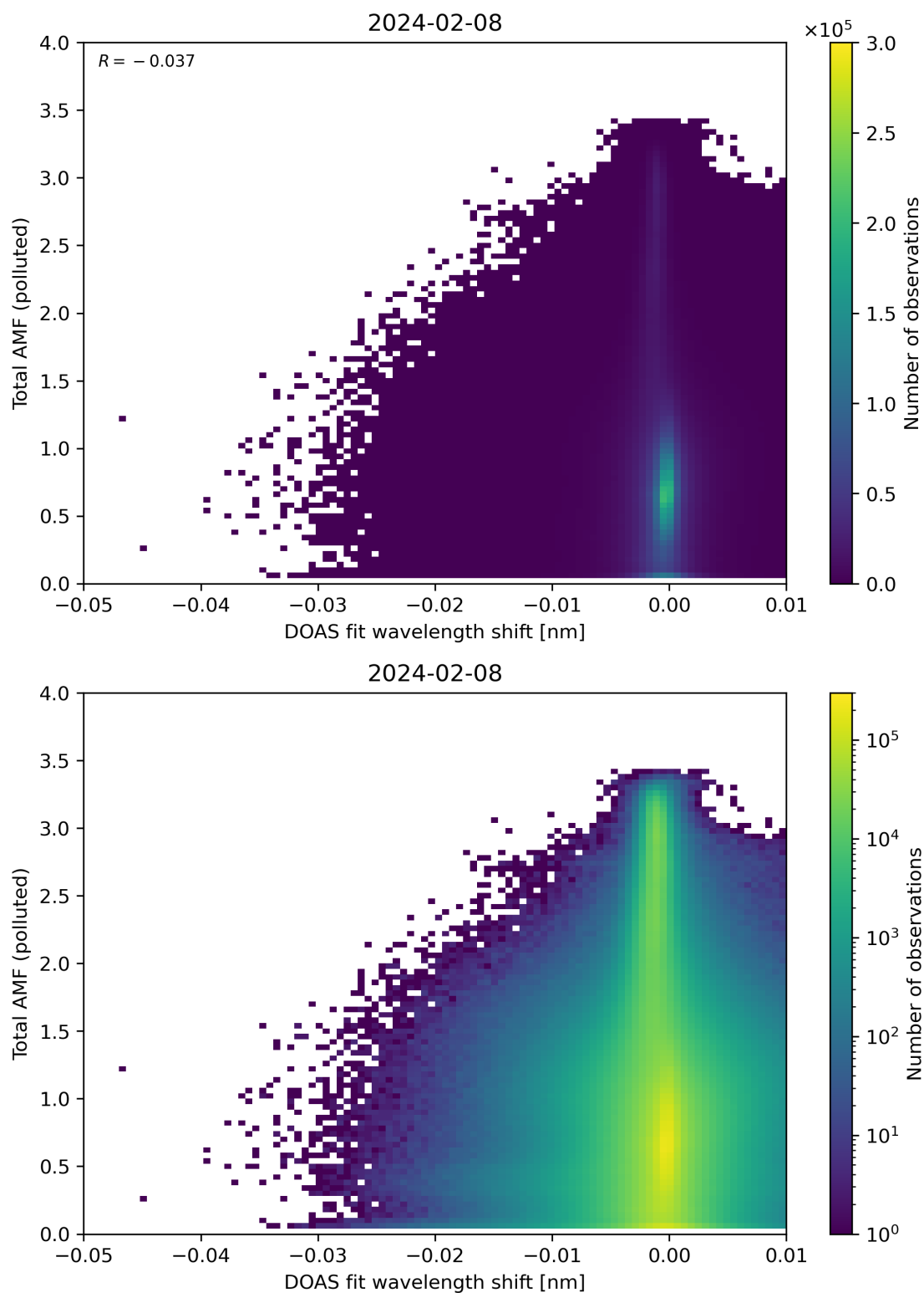
Figure 130: Scatter density plot of “DOAS fit wavelength shift” against “Total AMF (polluted)” for 2024-02-07 to 2024-02-09.
