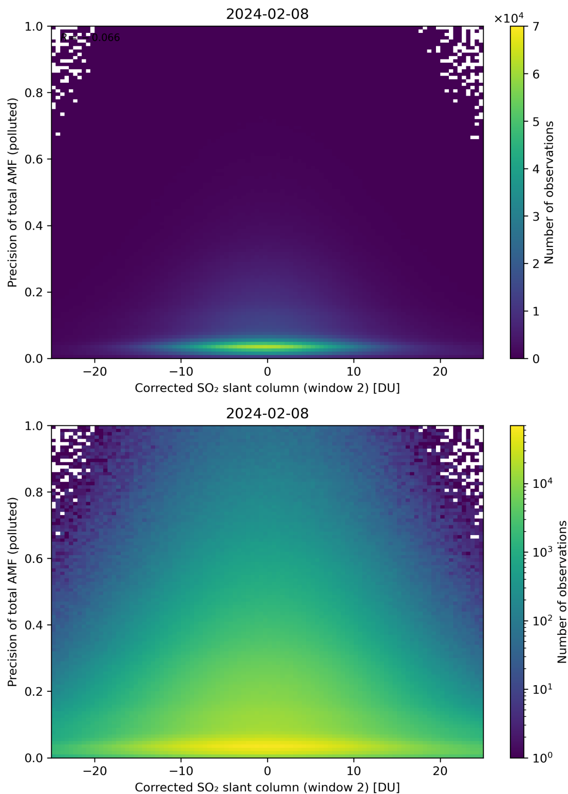
Figure 204: Scatter density plot of “Corrected SO 2 slant column (window 2)” against “Precision of total AMF (polluted)” for 2024-02-07 to 2024-02-09.
