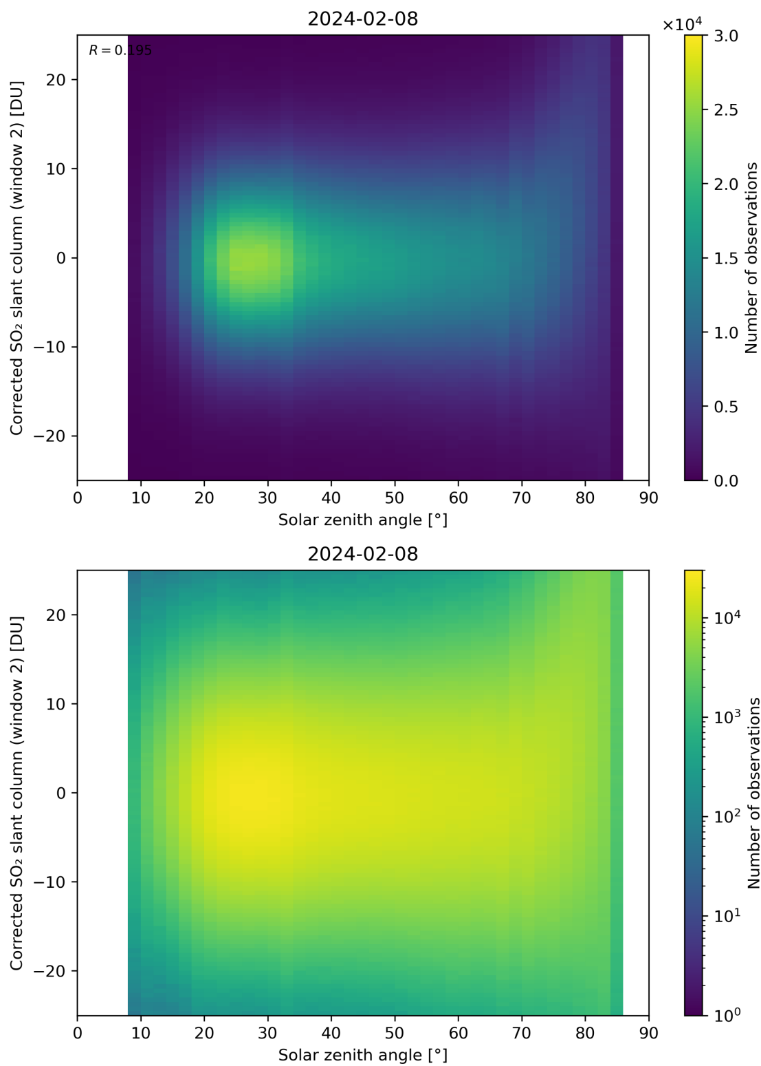
Figure 167: Scatter density plot of “Solar zenith angle” against “Corrected SO 2 slant column (window 2)” for 2024-02-07 to 2024-02-09.
