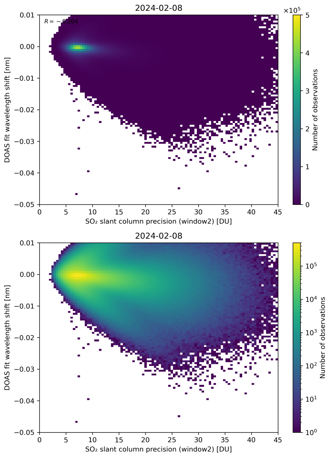
Figure 243: Scatter density plot of “SO 2 slant column precision (window2)” against “DOAS fit wavelength shift” for 2024-02-07 to 2024-02-09.
