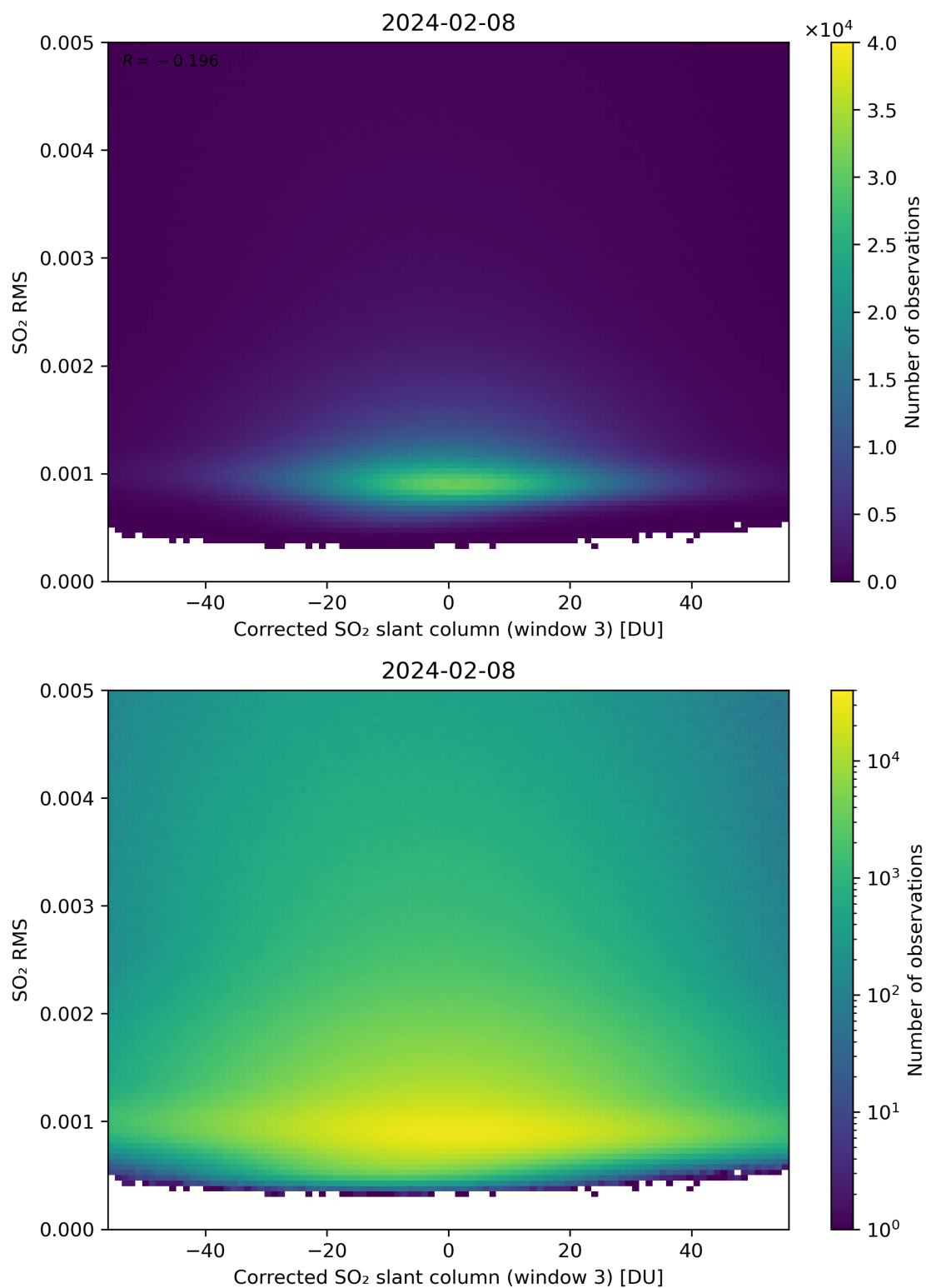
Figure 208: Scatter density plot of “Corrected SO 2 slant column (window 3)” against “SO 2 RMS” for 2024-02-07 to 2024-02-09.
