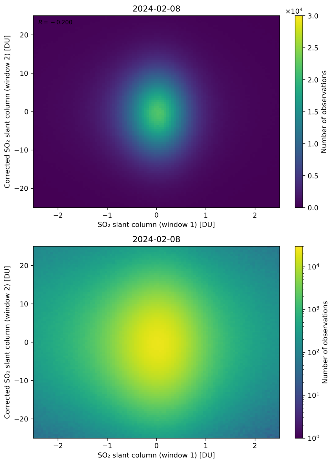
Figure 233: Scatter density plot of “SO 2 slant column (window 1)” against “Corrected SO 2 slant column (window 2)” for 2024-02-07 to 2024-02-09.
