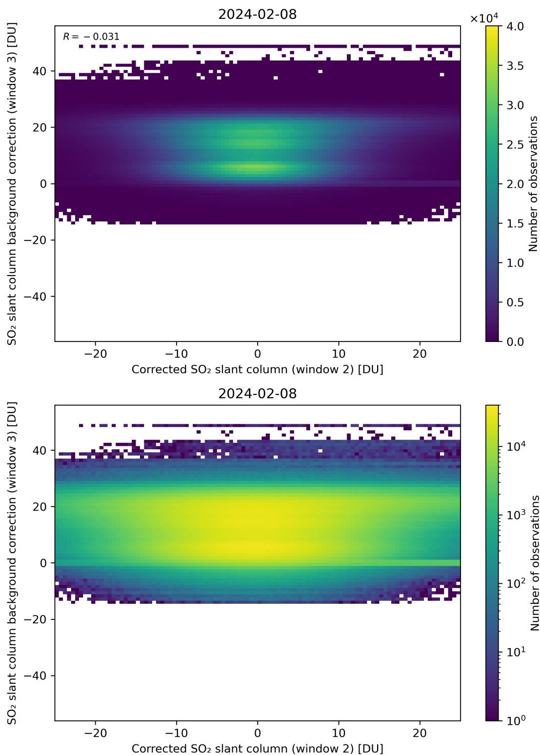
Figure 195: Scatter density plot of “Corrected SO 2 slant column (window 2)” against “SO 2 slant column background correction (window 3)” for 2024-02-07 to 2024-02-09.
