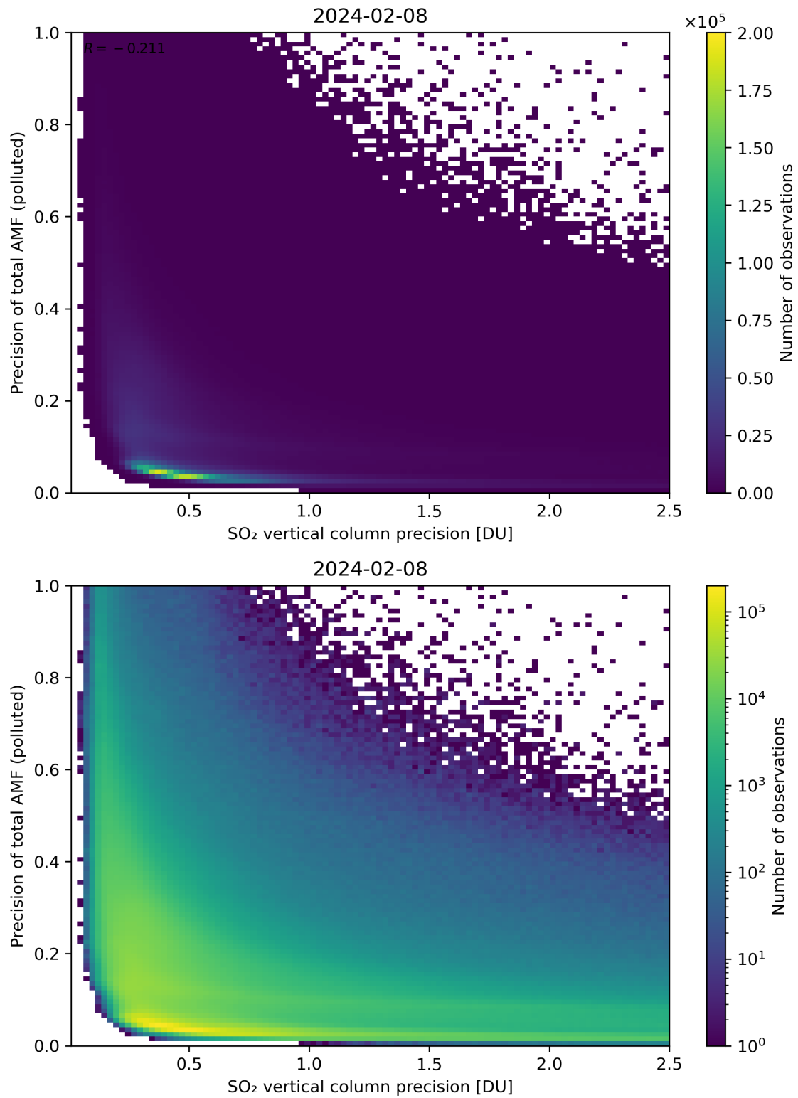
Figure 295: Scatter density plot of “SO 2 vertical column precision” against “Precision of total AMF (polluted)” for 2024-02-07 to 2024-02-09.
