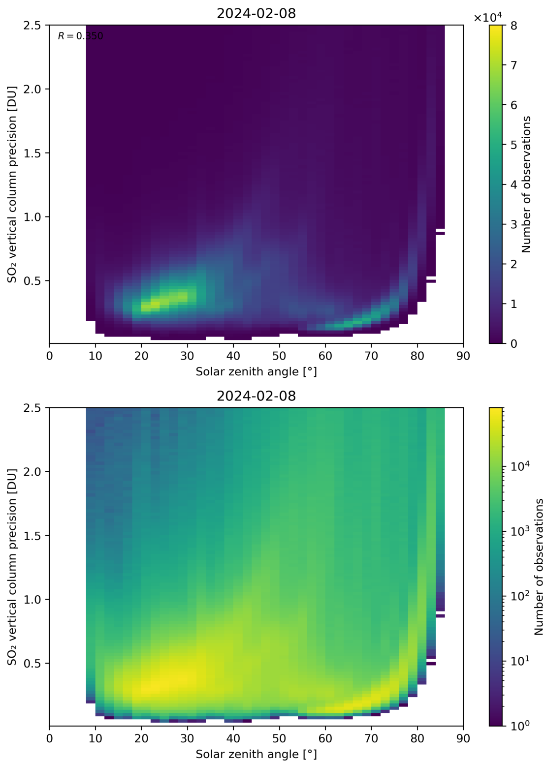
Figure 177: Scatter density plot of “Solar zenith angle” against “SO 2 vertical column precision” for 2024-02-07 to 2024-02-09.
