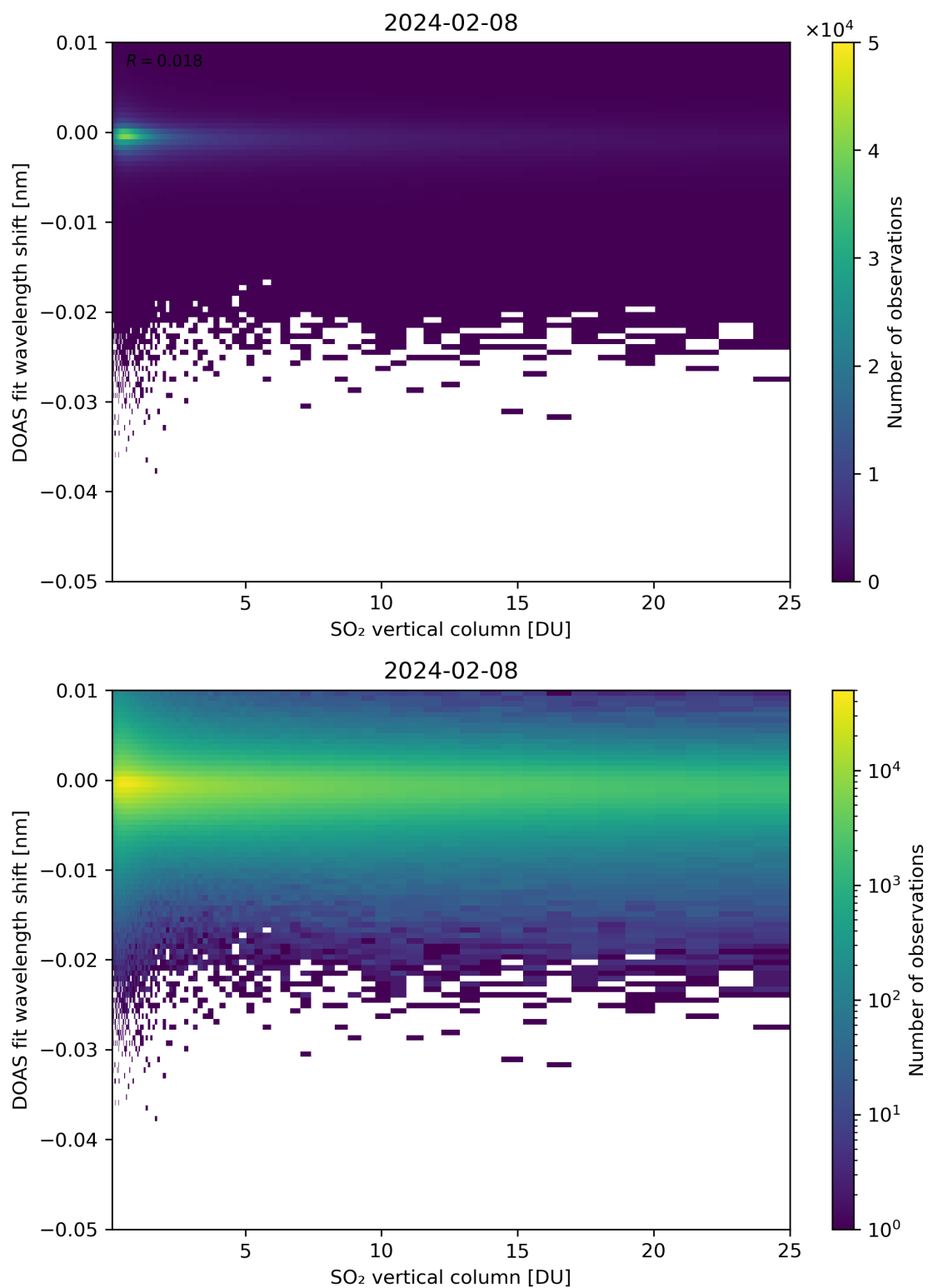
Figure 276: Scatter density plot of “SO 2 vertical column” against “DOAS fit wavelength shift” for 2024-02-07 to 2024-02-09.
