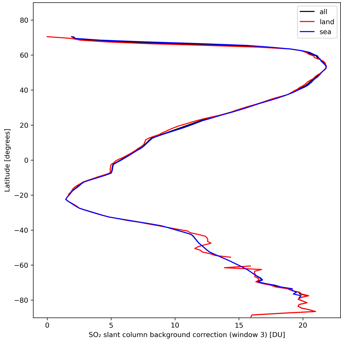
Figure 44: Zonal average of “SO 2 slant column background correction (window 3)” for 2024-02-07 to 2024-02-09.
