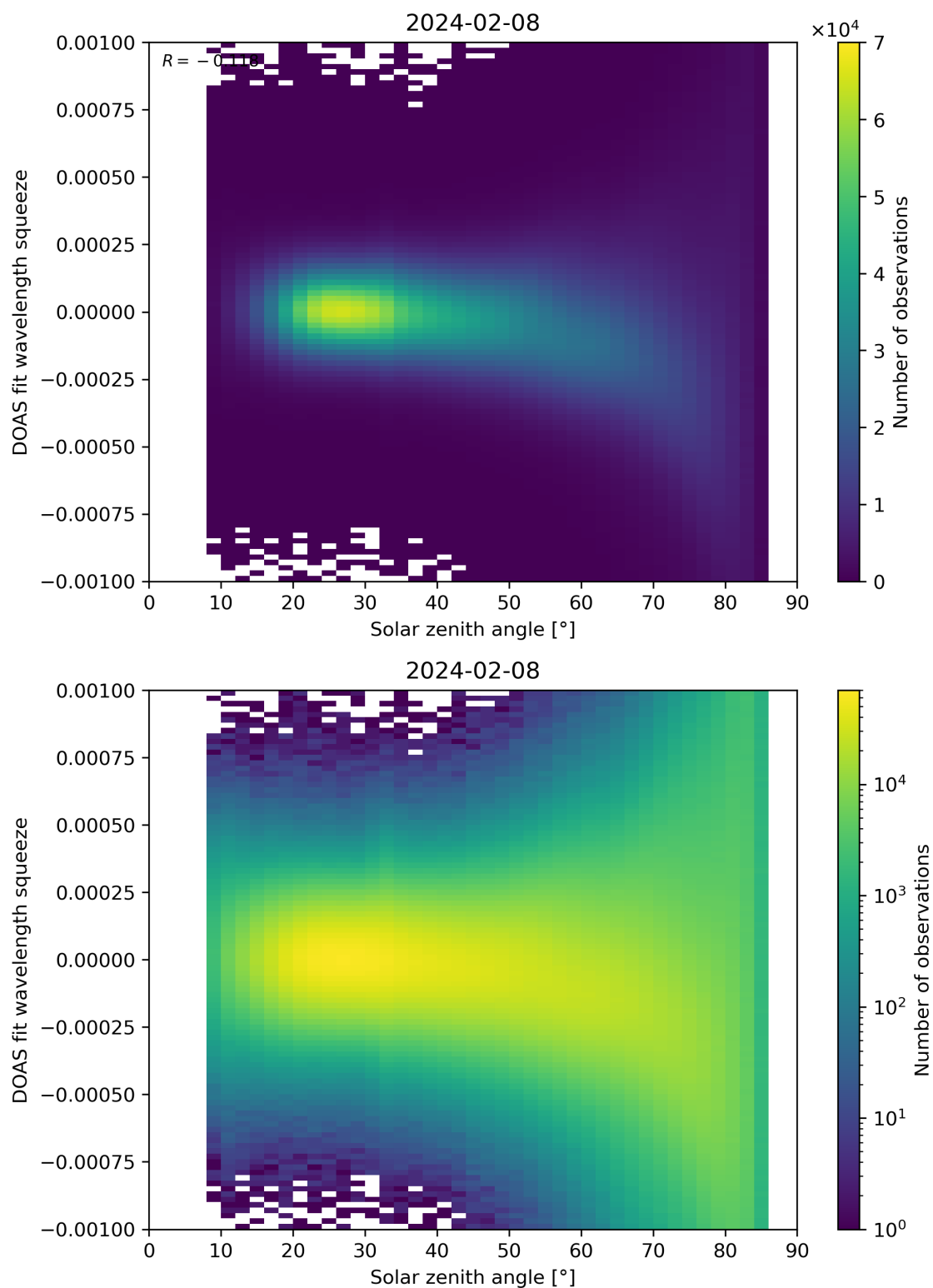
Figure 162: Scatter density plot of “Solar zenith angle” against “DOAS fit wavelength squeeze” for 2024-02-07 to 2024-02-09.
