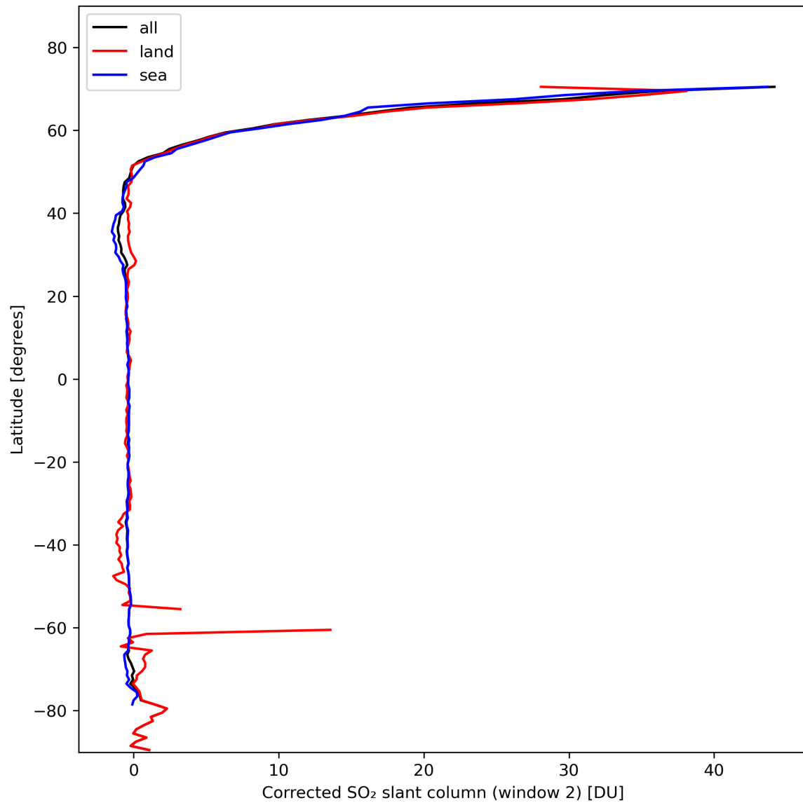
Figure 39: Zonal average of “Corrected SO 2 slant column (window 2)” for 2024-02-07 to 2024-02-09.
