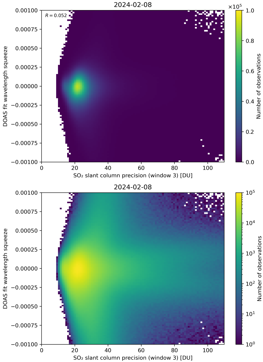
Figure 259: Scatter density plot of “SO 2 slant column precision (window 3)” against “DOAS fit wavelength squeeze” for 2024-02-07 to 2024-02-09.
