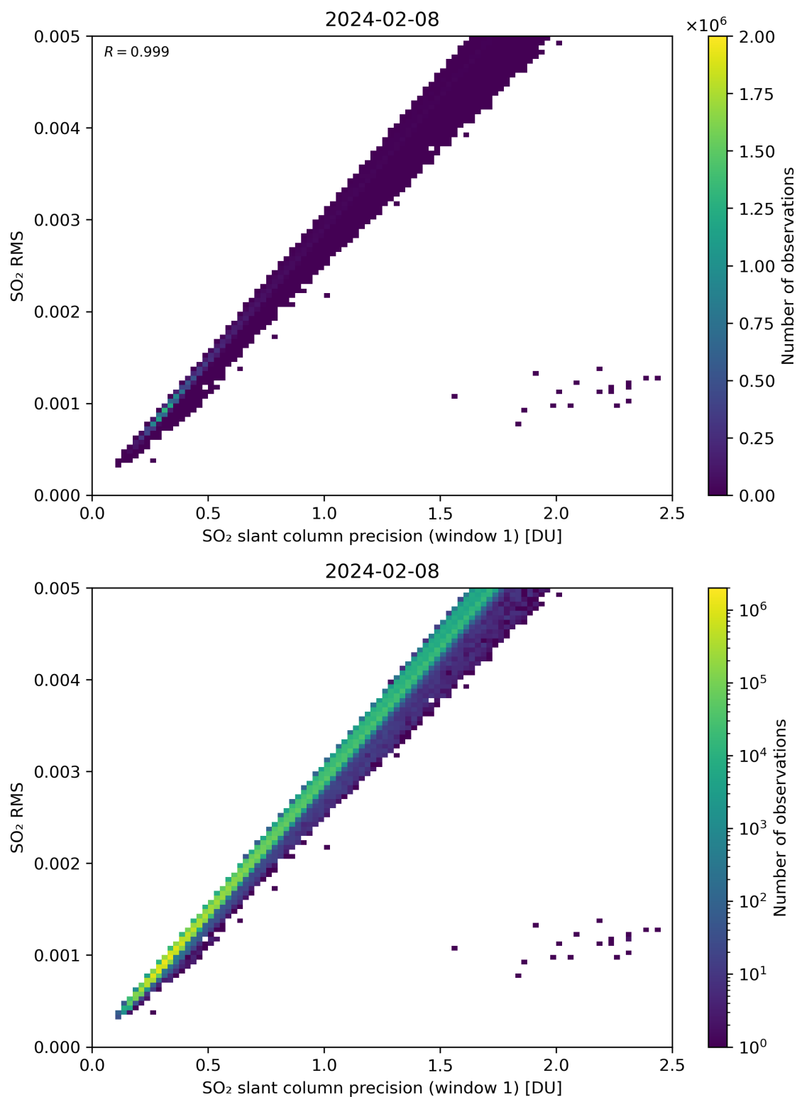
Figure 223: Scatter density plot of “SO 2 slant column precision (window 1)” against “SO 2 RMS” for 2024-02-07 to 2024-02-09.
