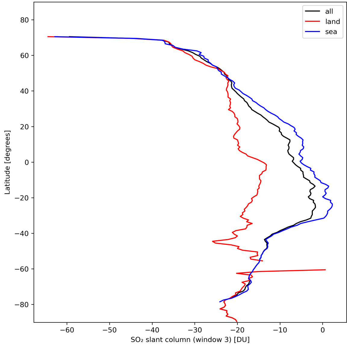
Figure 41: Zonal average of “SO 2 slant column (window 3)” for 2024-02-07 to 2024-02-09.
