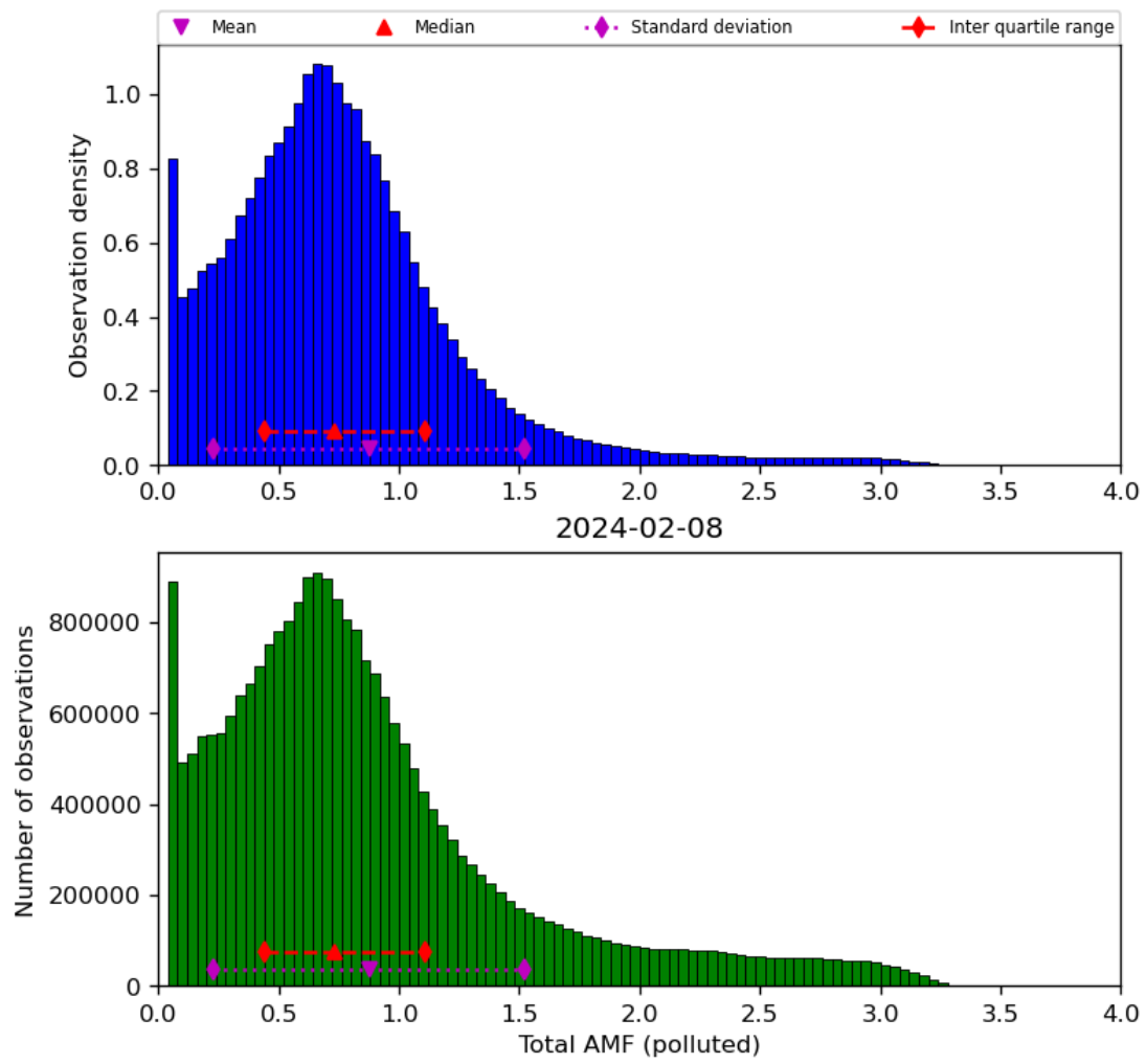
Figure 71: Histogram of “Total AMF (polluted)” for 2024-02-07 to 2024-02-09
