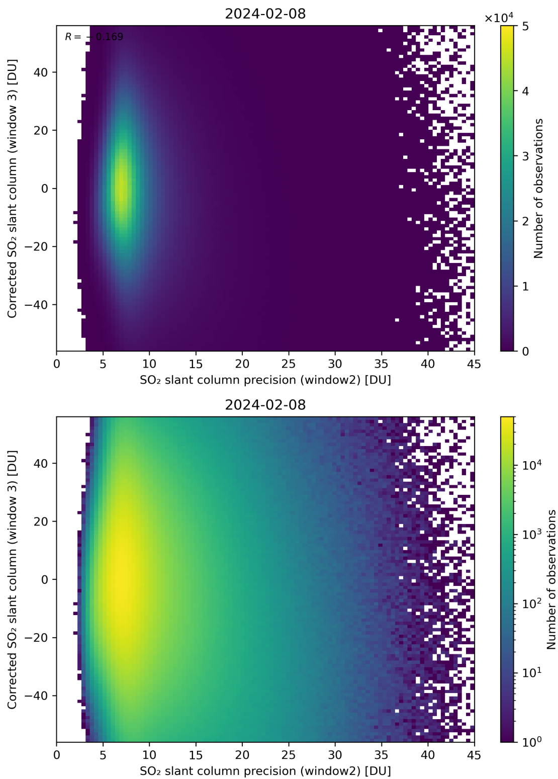
Figure 248: Scatter density plot of “SO 2 slant column precision (window2)” against “Corrected SO 2 slant column (window 3)” for 2024-02-07 to 2024-02-09.
