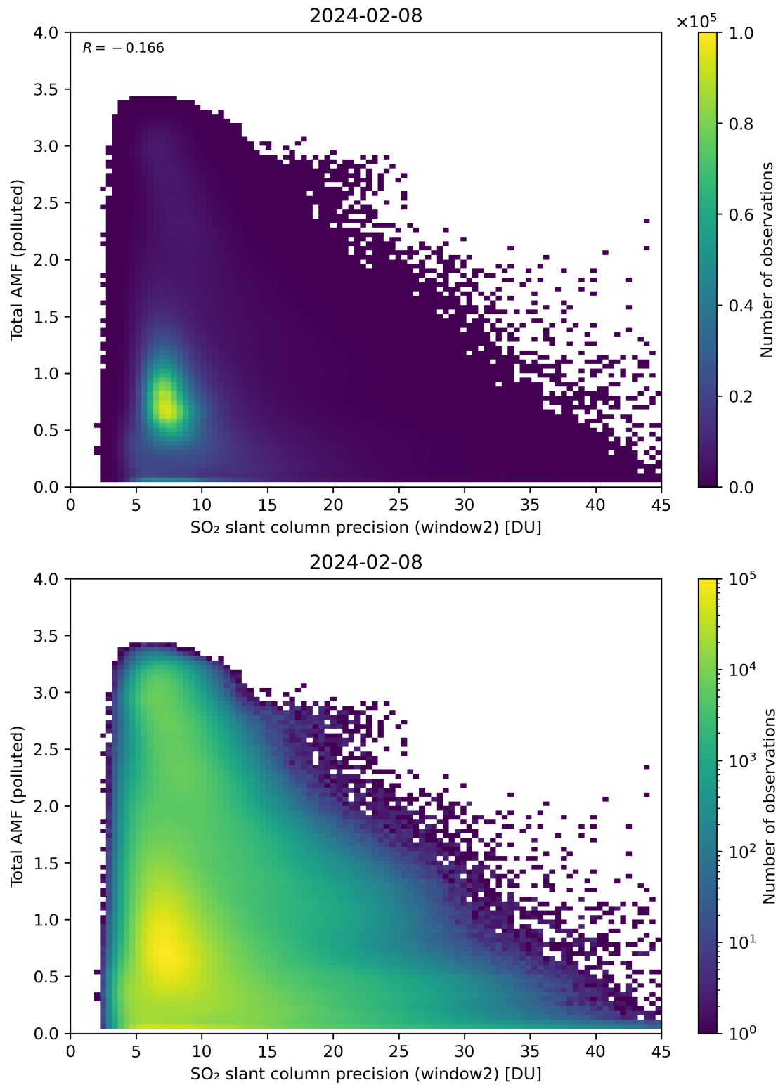
Figure 251: Scatter density plot of “SO 2 slant column precision (window2)” against “Total AMF (polluted)” for 2024-02-07 to 2024-02-09.
