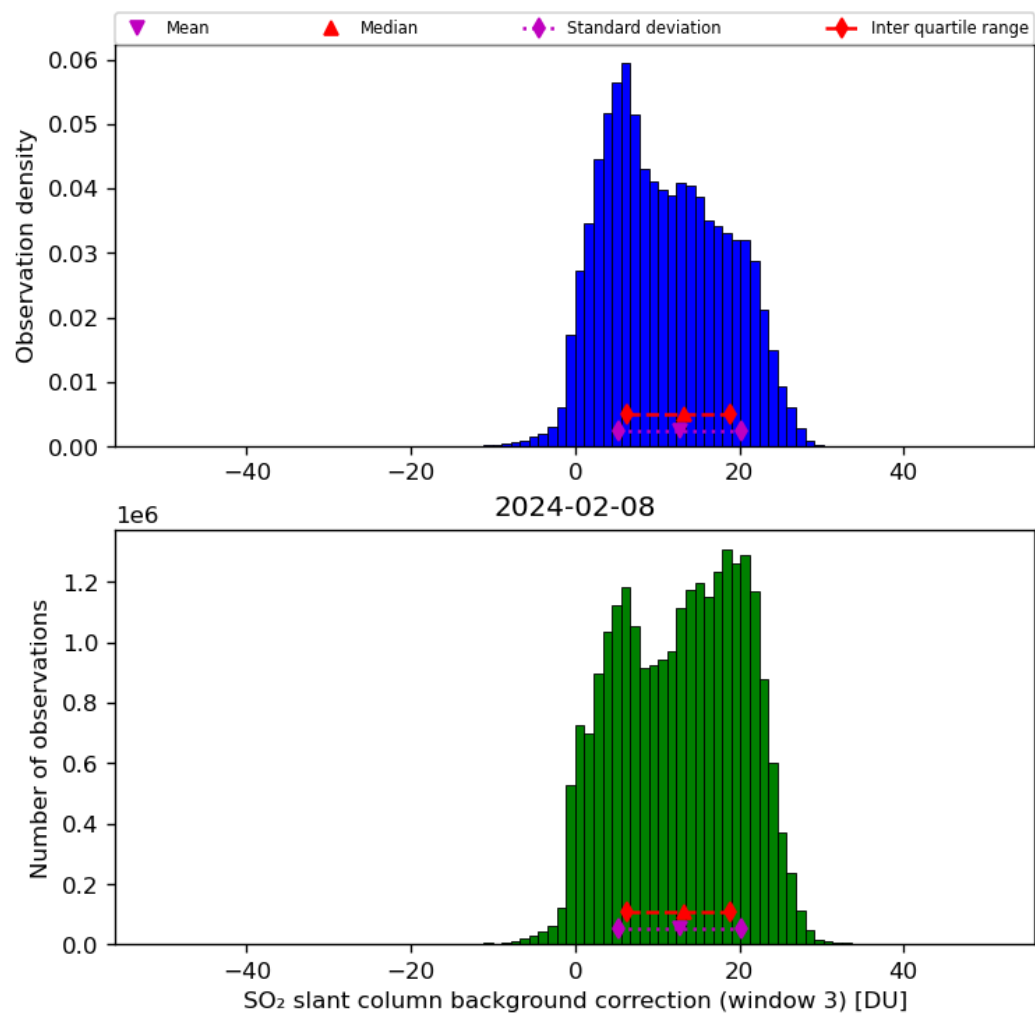
Figure 67: Histogram of “SO 2 slant column background correction (window 3)” for 2024-02-07 to 2024-02-09
