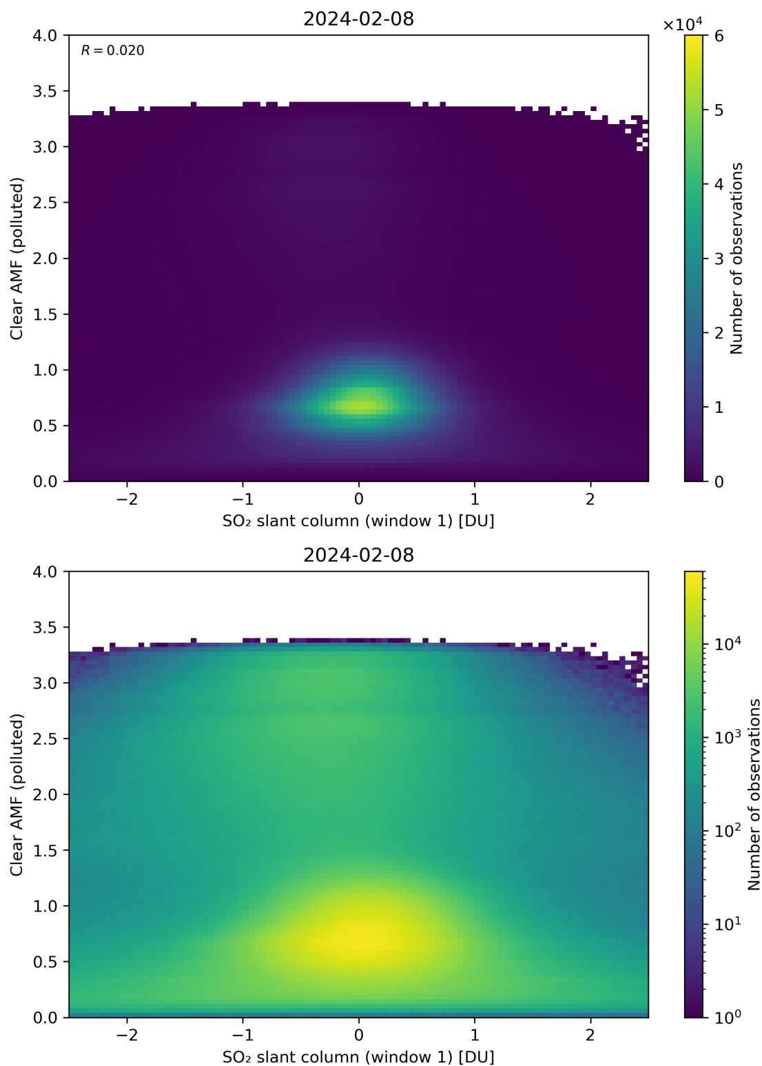
Figure 232: Scatter density plot of “SO 2 slant column (window 1)” against “Clear AMF (polluted)” for 2024-02-07 to 2024-02-09.
