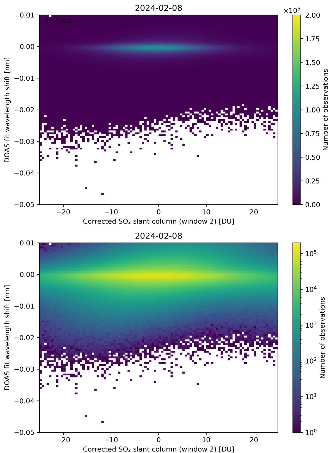
Figure 196: Scatter density plot of “Corrected SO 2 slant column (window 2)” against “DOAS fit wavelength shift” for 2024-02-07 to 2024-02-09.
