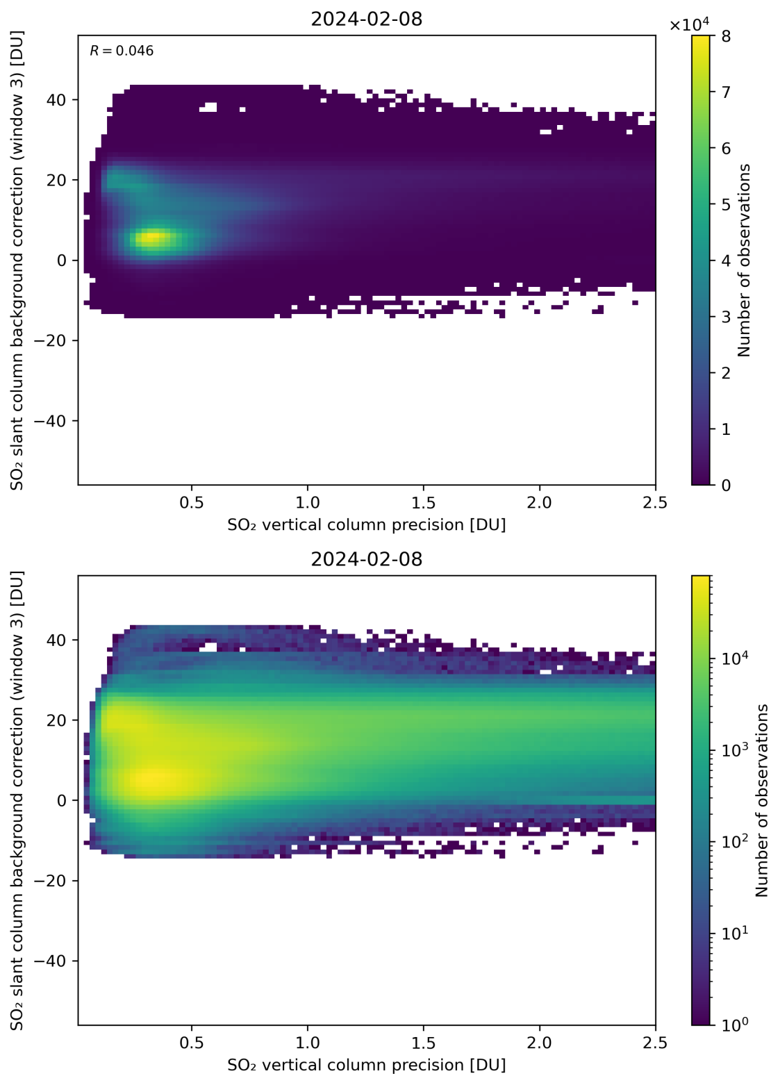
Figure 281: Scatter density plot of “SO 2 vertical column precision” against “SO 2 slant column background correction (window 3)” for 2024-02-07 to 2024-02-09.
