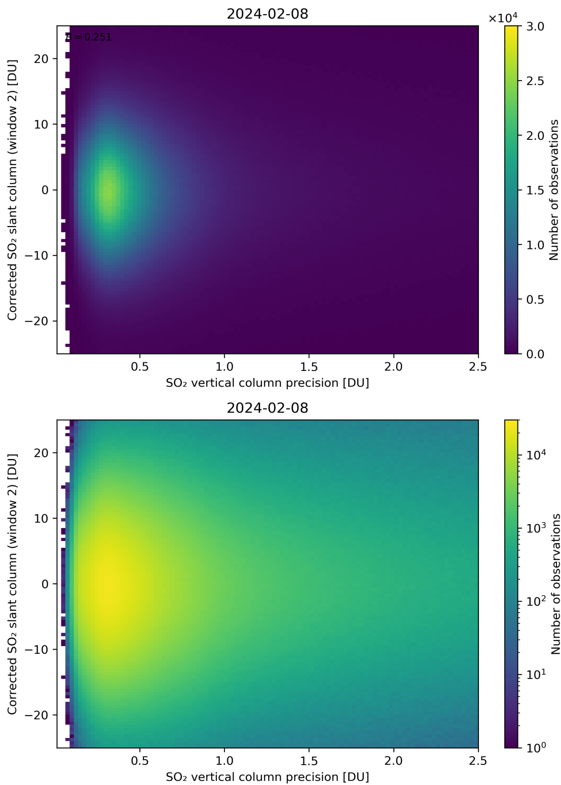
Figure 287: Scatter density plot of “SO 2 vertical column precision” against “Corrected SO 2 slant column (window 2)” for 2024-02-07 to 2024-02-09.
