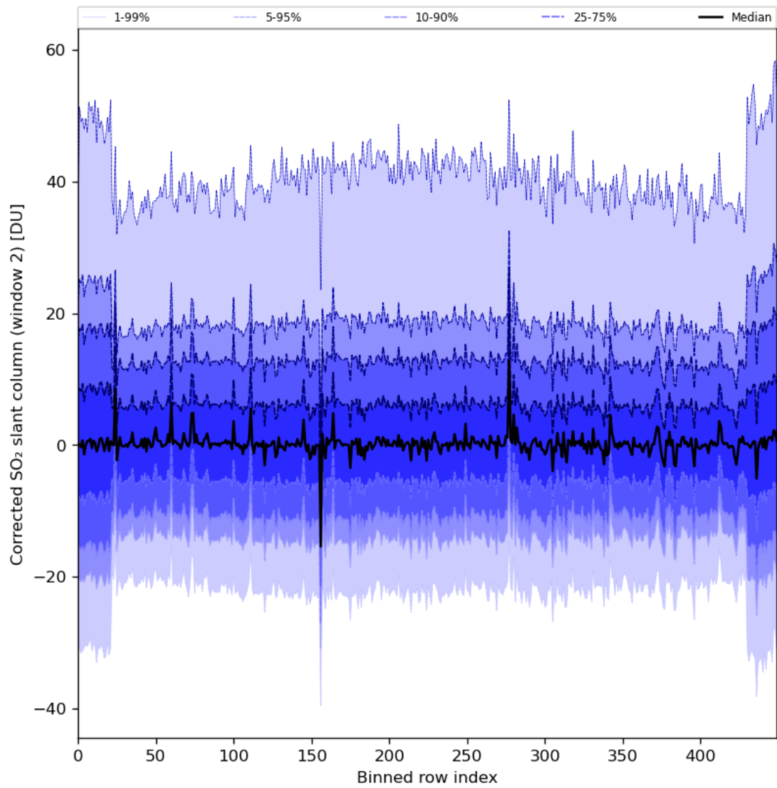
Figure 85: Along track statistics of “Corrected SO 2 slant column (window 2)” for 2024-02-07 to 2024-02-09
