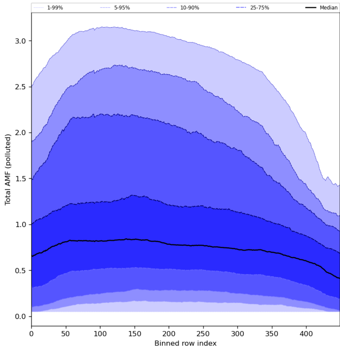
Figure 94: Along track statistics of “Total AMF (polluted)” for 2024-02-07 to 2024-02-09
