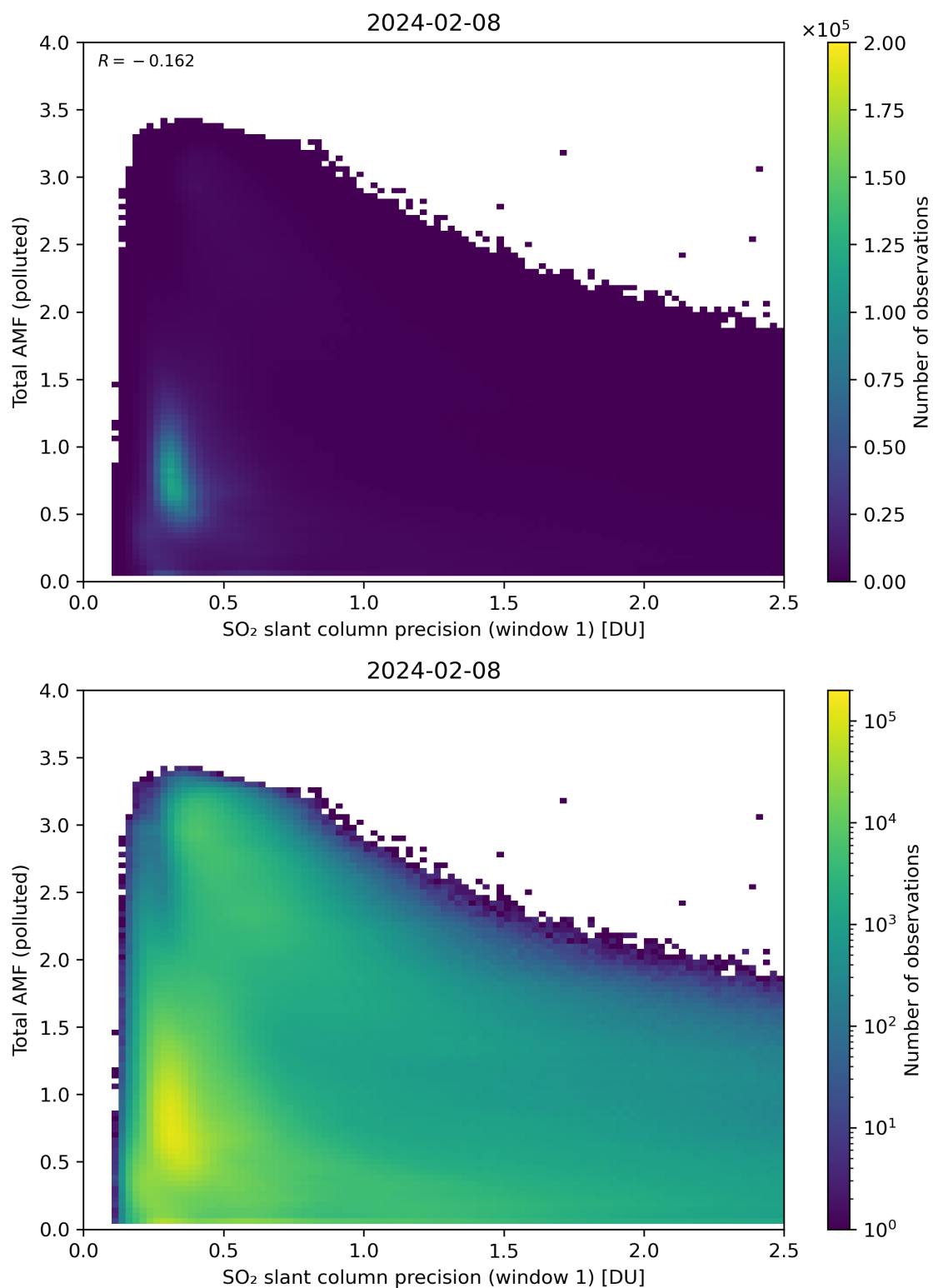
Figure 230: Scatter density plot of “SO 2 slant column precision (window 1)” against “Total AMF (polluted)” for 2024-02-07 to 2024-02-09.
