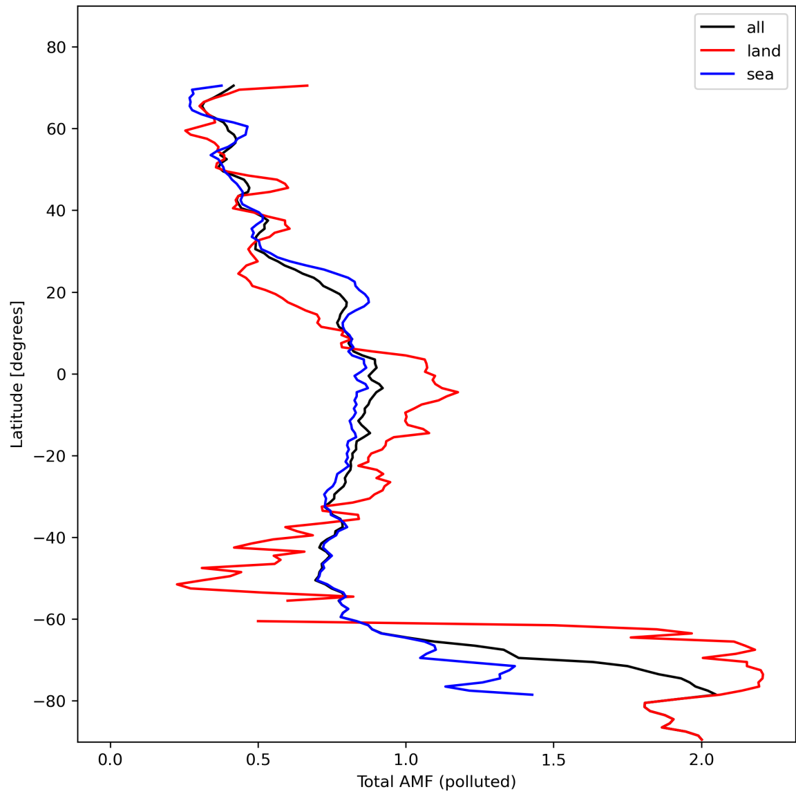
Figure 48: Zonal average of “Total AMF (polluted)” for 2024-02-07 to 2024-02-09.
