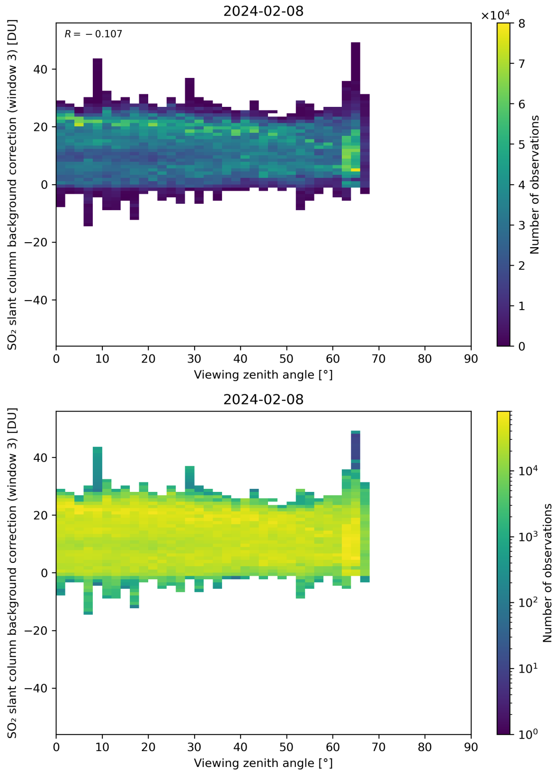
Figure 310: Scatter density plot of “Viewing zenith angle” against “SO 2 slant column background correction (window 3)” for 2024-02-07 to 2024-02-09.
