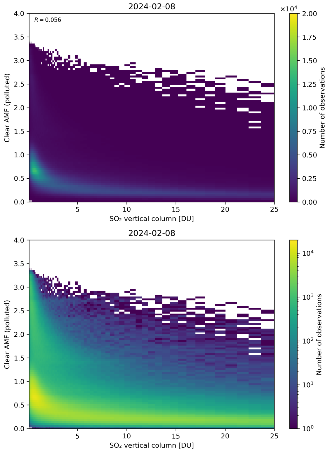
Figure 296: Scatter density plot of “SO 2 vertical column” against “Clear AMF (polluted)” for 2024-02-07 to 2024-02-09.
