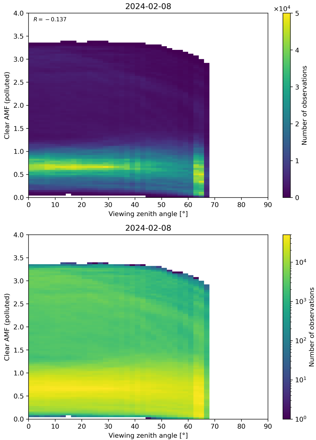
Figure 316: Scatter density plot of “Viewing zenith angle” against “Clear AMF (polluted)” for 2024-02-07 to 2024-02-09.
