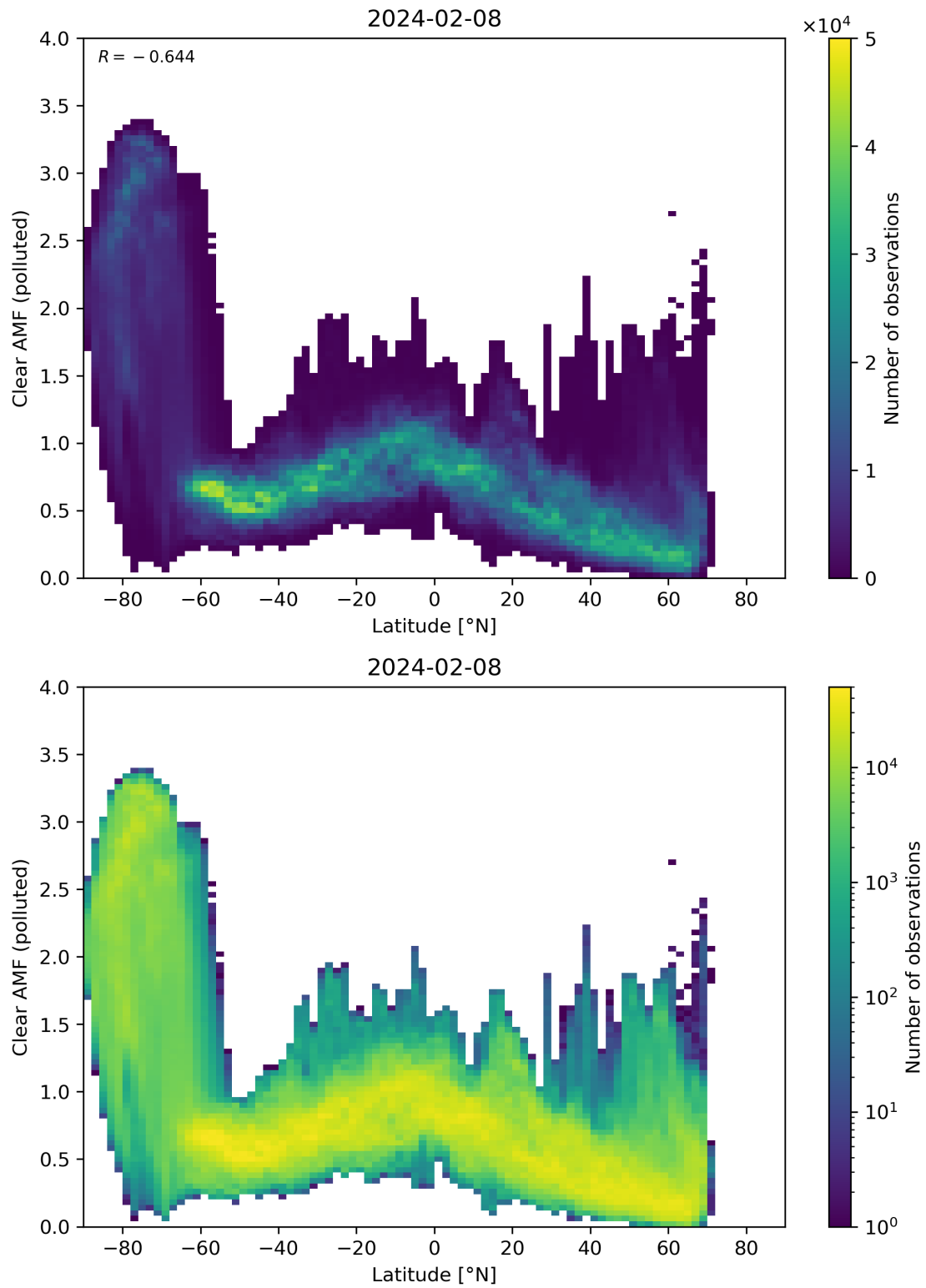
Figure 145: Scatter density plot of “Latitude” against “Clear AMF (polluted)” for 2024-02-07 to 2024-02-09.
