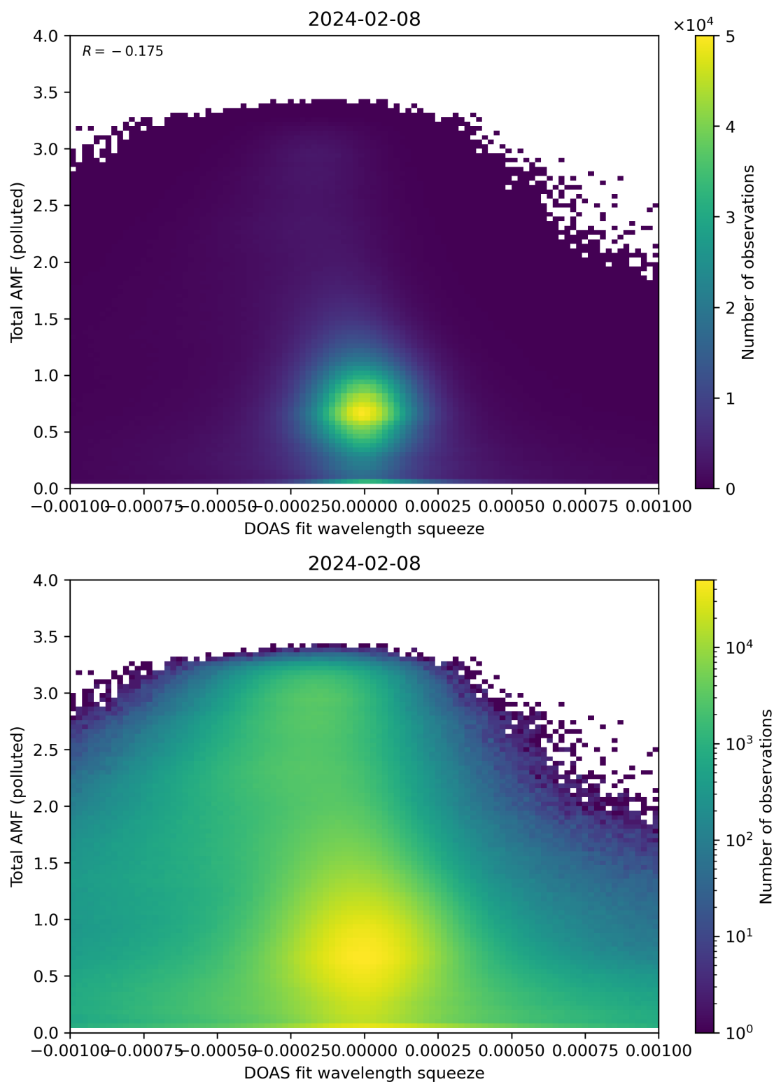
Figure 134: Scatter density plot of “DOAS fit wavelength squeeze” against “Total AMF (polluted)” for 2024-02-07 to 2024-02-09.
