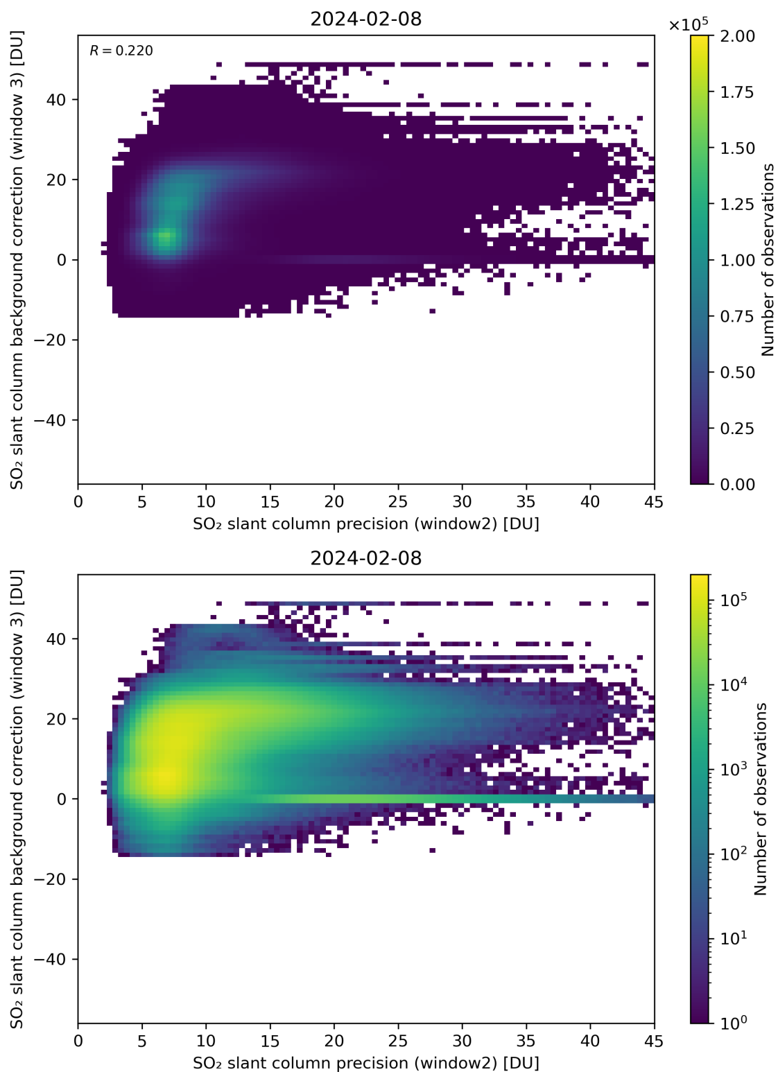
Figure 242: Scatter density plot of “SO 2 slant column precision (window2)” against “SO 2 slant column background correction (window 3)” for 2024-02-07 to 2024-02-09.
