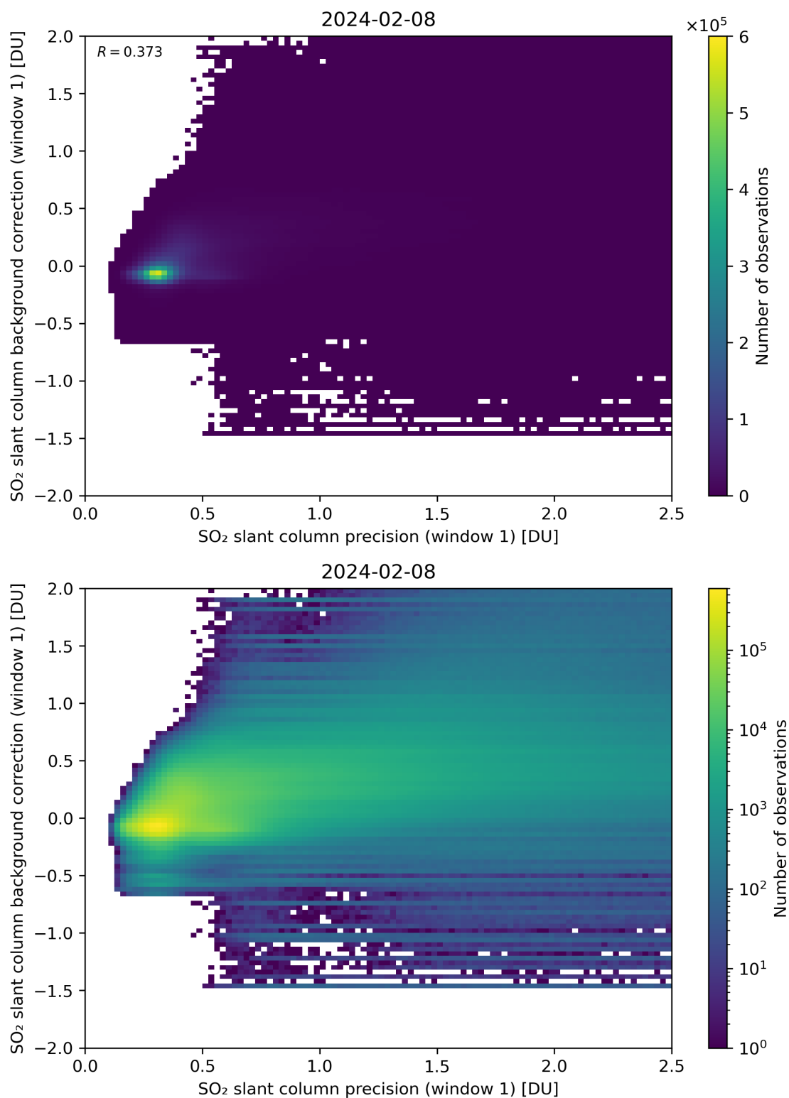
Figure 218: Scatter density plot of “SO 2 slant column precision (window 1)” against “SO 2 slant column background correction (window 1)” for 2024-02-07 to 2024-02-09.
