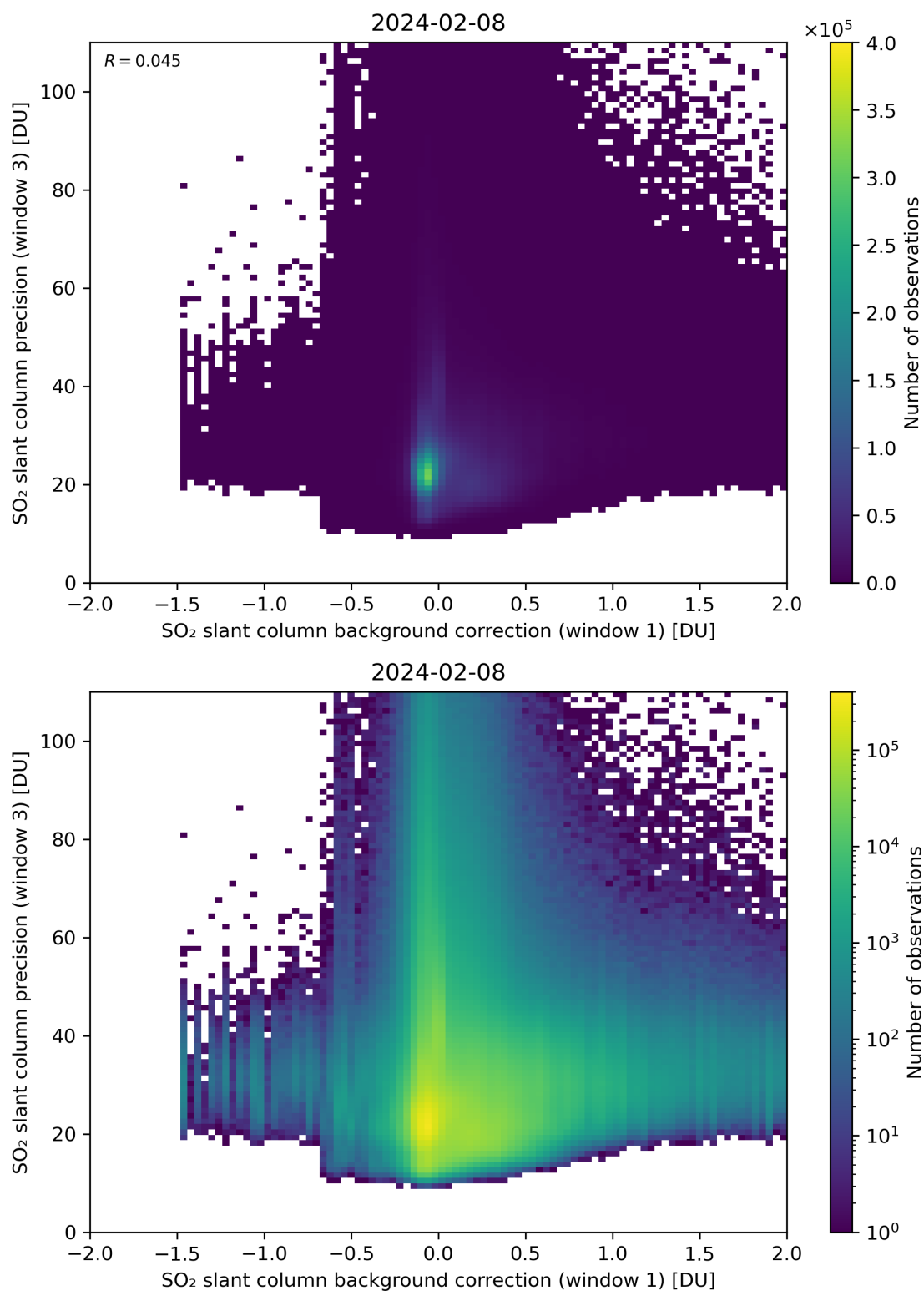
Figure 108: Scatter density plot of “SO 2 slant column background correction (window 1)” against “SO 2 slant column precision (window 3)” for 2024-02-07 to 2024-02-09.
