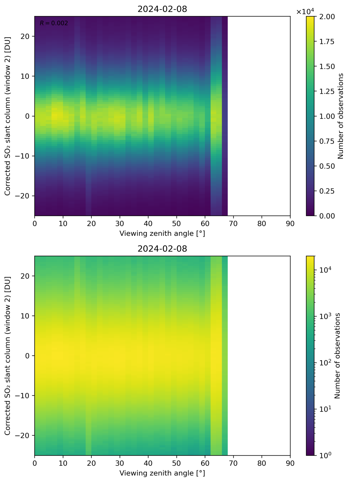
Figure 318: Scatter density plot of “Viewing zenith angle” against “Corrected SO 2 slant column (window 2)” for 2024-02-07 to 2024-02-09.
