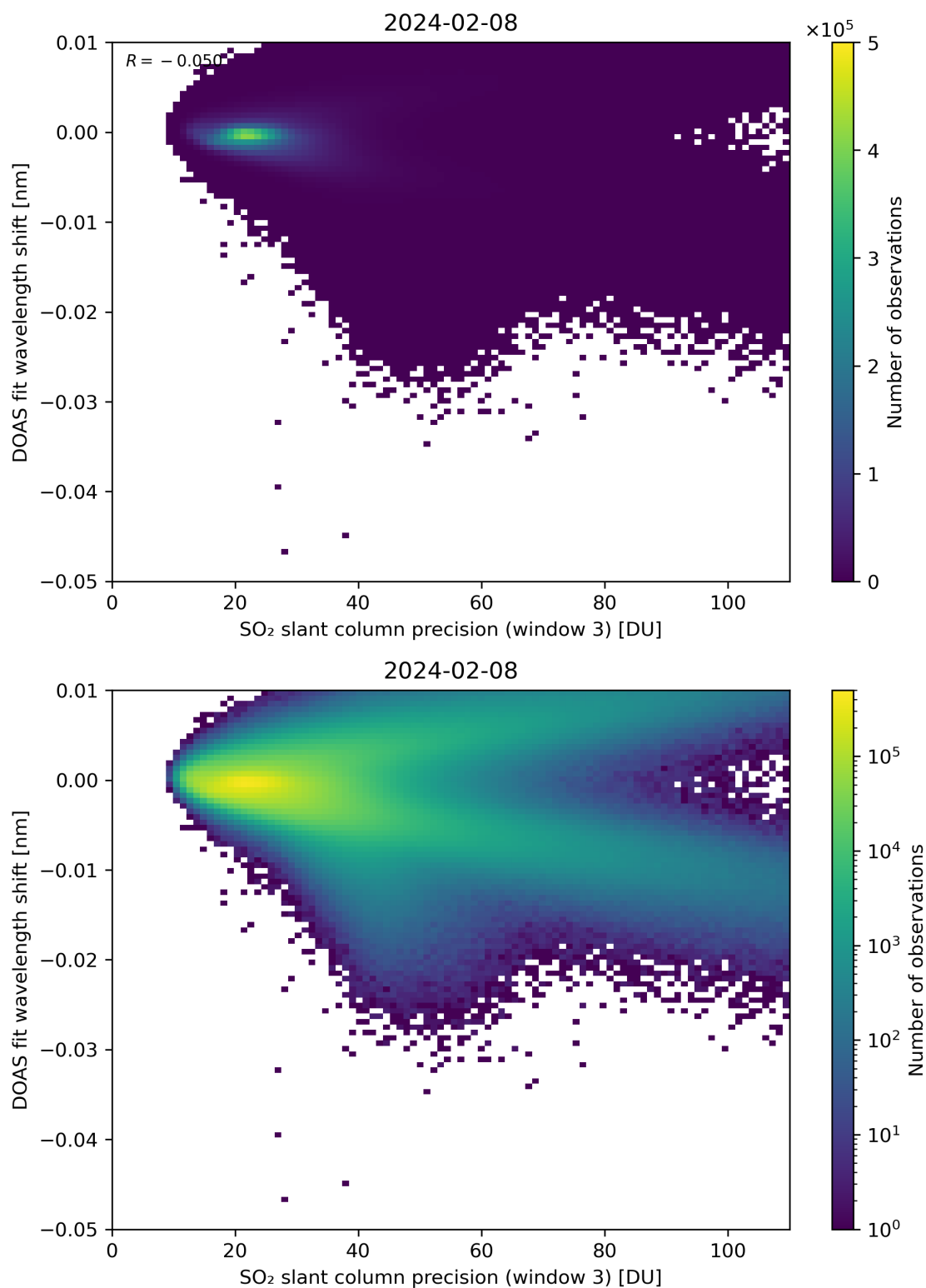
Figure 258: Scatter density plot of “SO 2 slant column precision (window 3)” against “DOAS fit wavelength shift” for 2024-02-07 to 2024-02-09.
