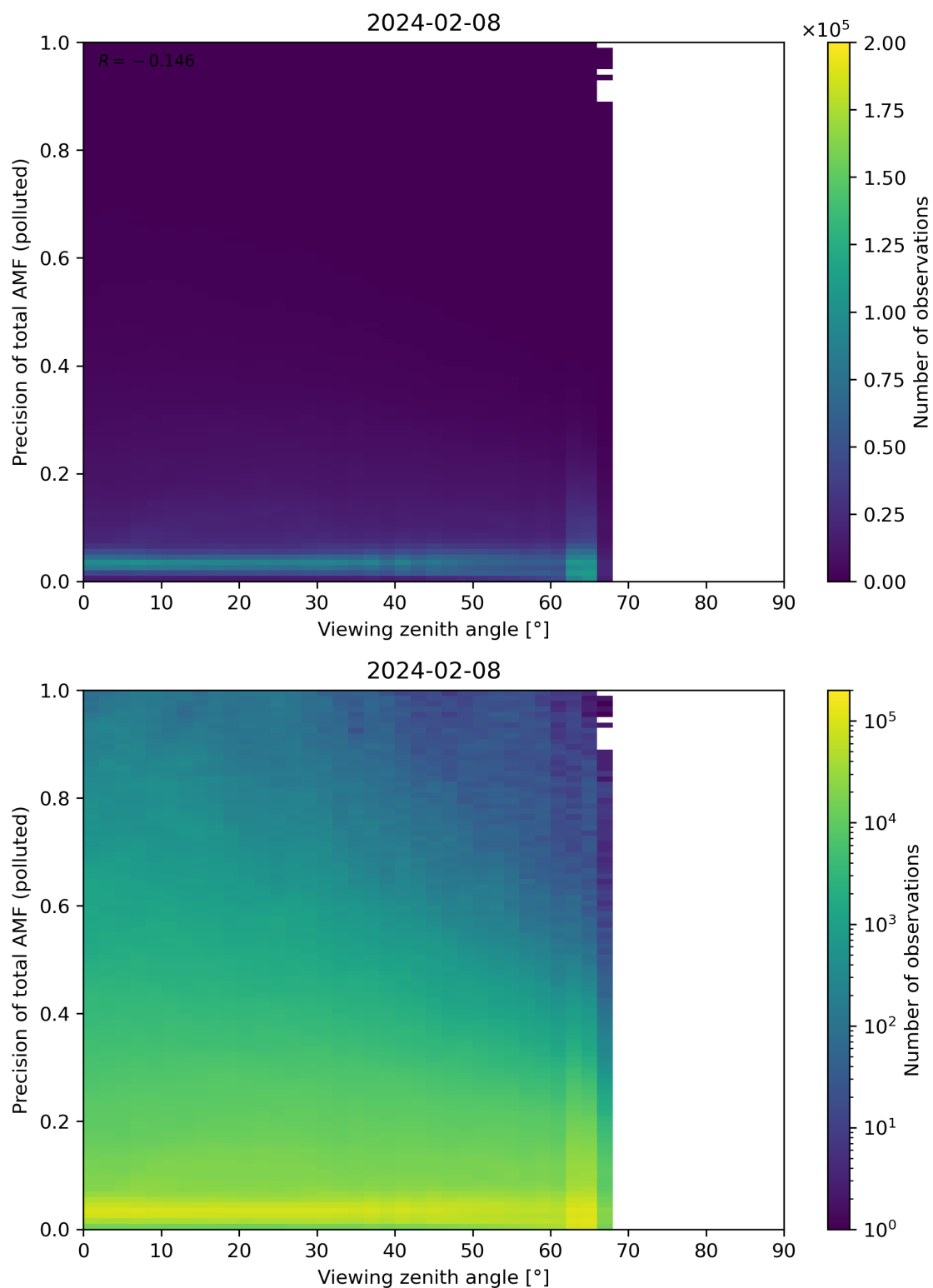
Figure 326: Scatter density plot of “Viewing zenith angle” against “Precision of total AMF (polluted)” for 2024-02-07 to 2024-02-09.
