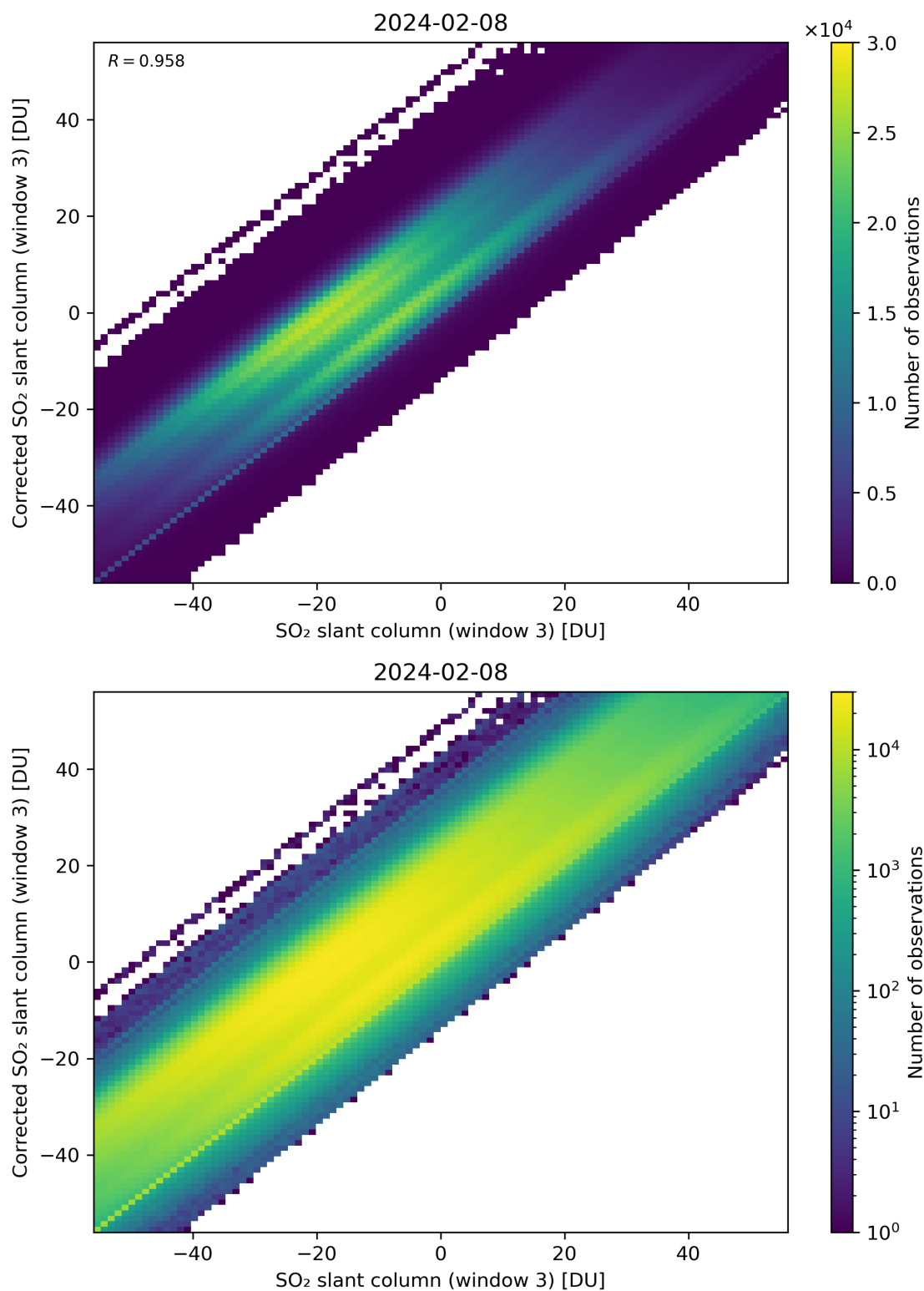
Figure 266: Scatter density plot of “SO 2 slant column (window 3)” against “Corrected SO 2 slant column (window 3)” for 2024-02-07 to 2024-02-09.
