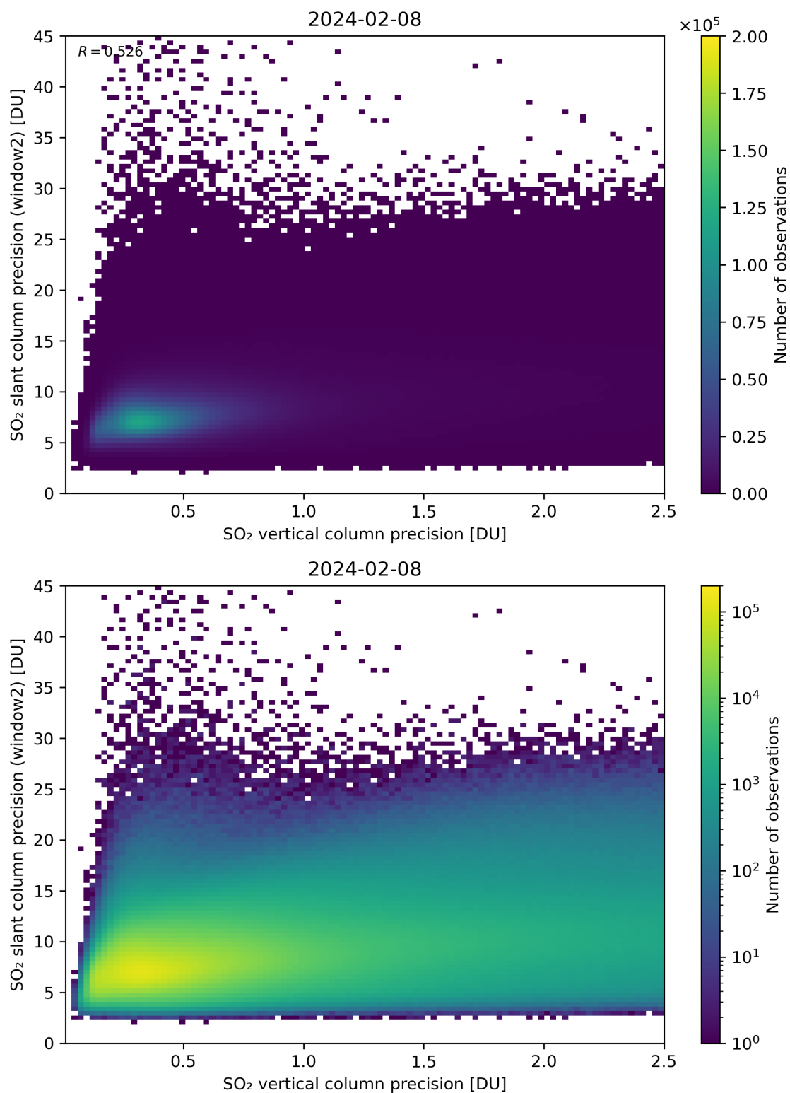
Figure 291: Scatter density plot of “SO 2 vertical column precision” against “SO 2 slant column precision (window2)” for 2024-02-07 to 2024-02-09.
