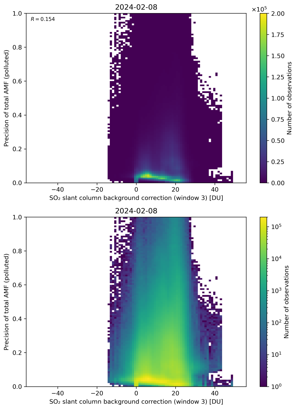
Figure 126: Scatter density plot of “SO 2 slant column background correction (window 3)” against “Precision of total AMF (polluted)” for 2024-02-07 to 2024-02-09.
