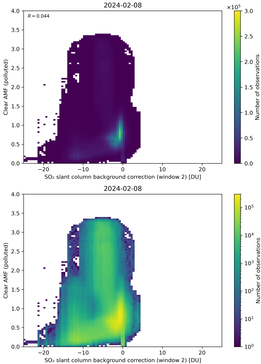
Figure 115: Scatter density plot of “SO 2 slant column background correction (window 2)” against “Clear AMF (polluted)” for 2024-02-07 to 2024-02-09.
