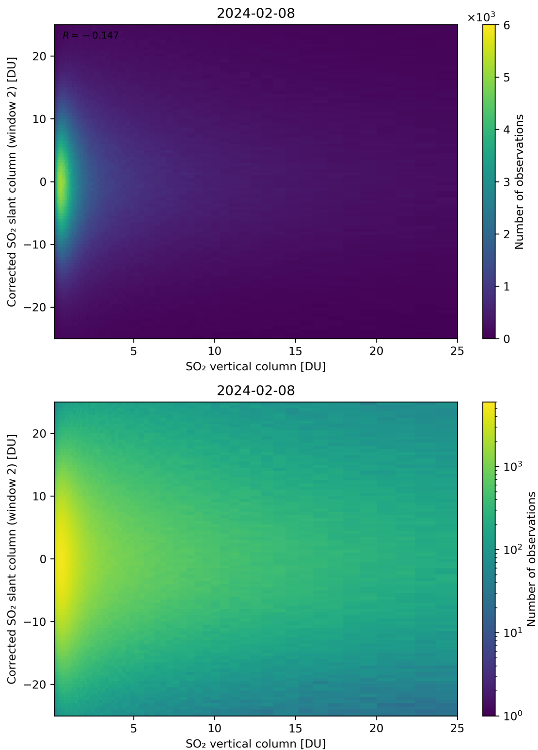
Figure 298: Scatter density plot of “SO 2 vertical column” against “Corrected SO 2 slant column (window 2)” for 2024-02-07 to 2024-02-09.
