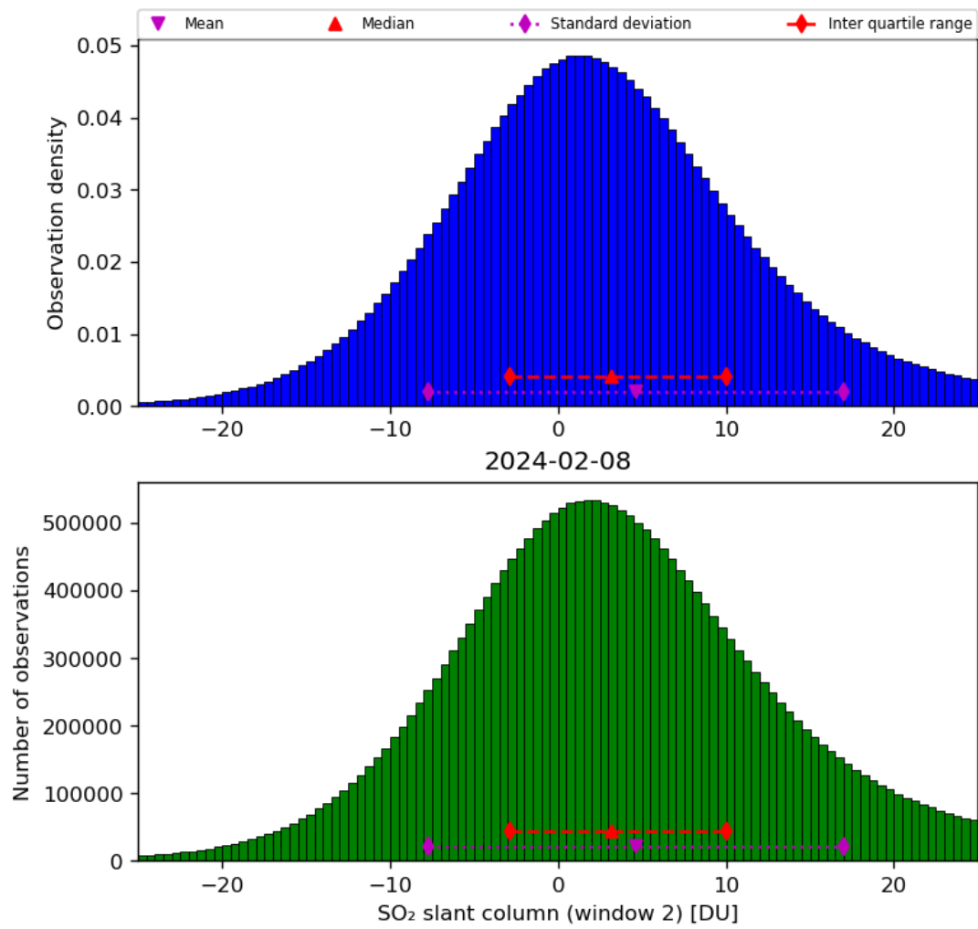
Figure 60: Histogram of “SO 2 slant column (window 2)” for 2024-02-07 to 2024-02-09
