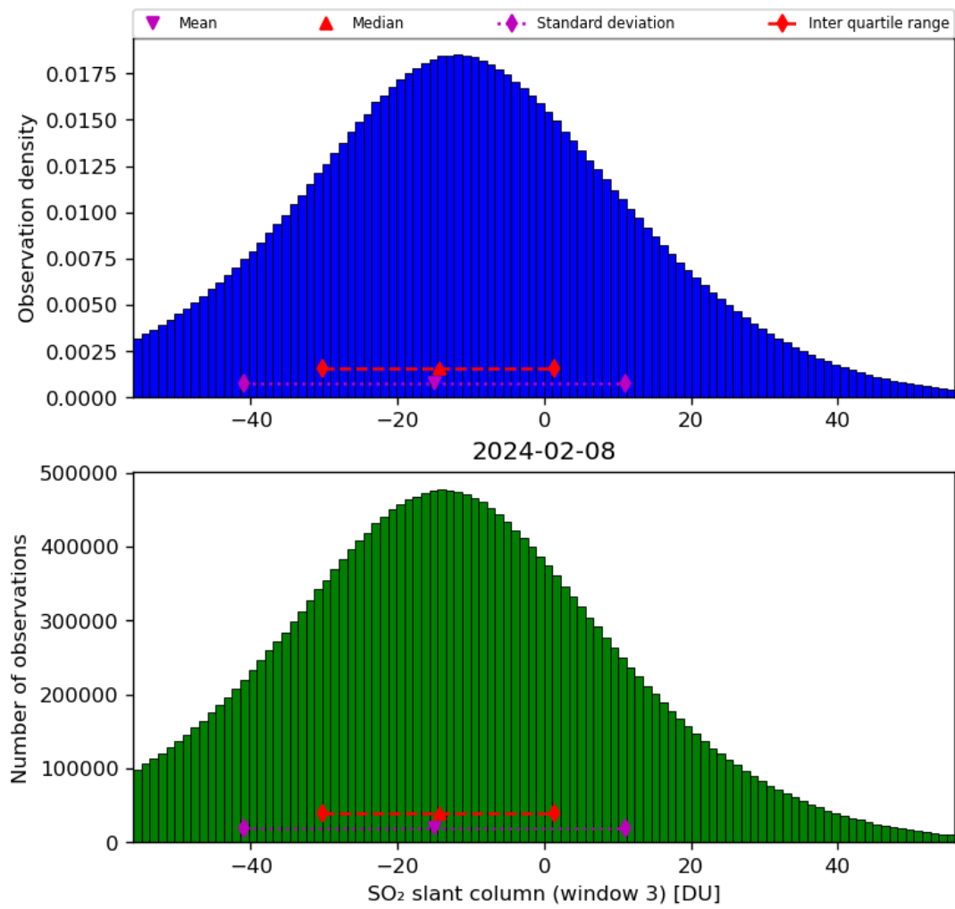
Figure 64: Histogram of “SO 2 slant column (window 3)” for 2024-02-07 to 2024-02-09
