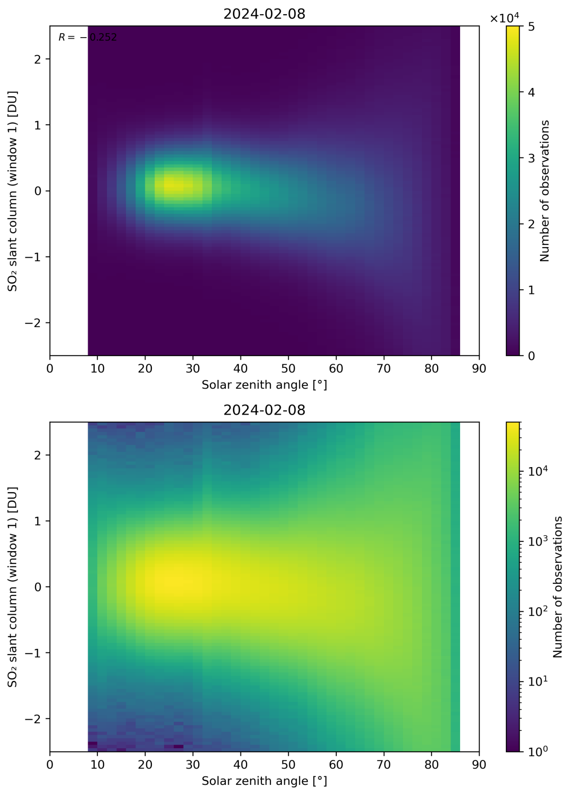
Figure 169: Scatter density plot of “Solar zenith angle” against “SO 2 slant column (window 1)” for 2024-02-07 to 2024-02-09.
