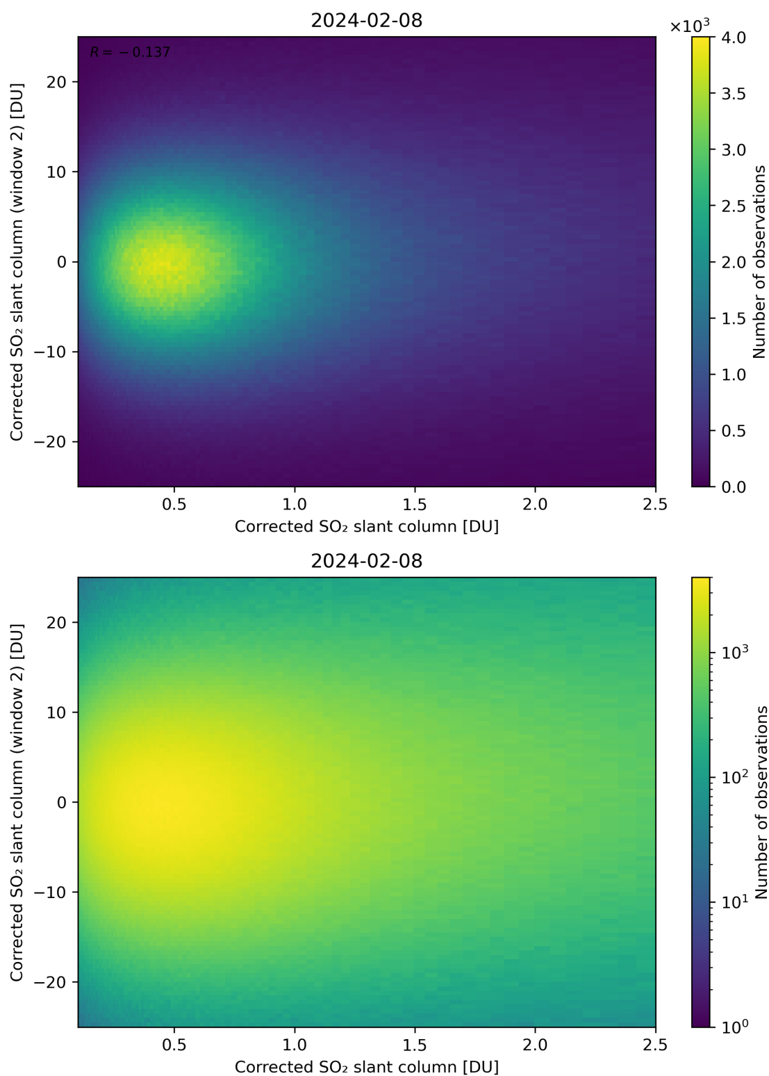
Figure 185: Scatter density plot of “Corrected SO 2 slant column” against “Corrected SO 2 slant column (window 2)” for 2024-02-07 to 2024-02-09.
