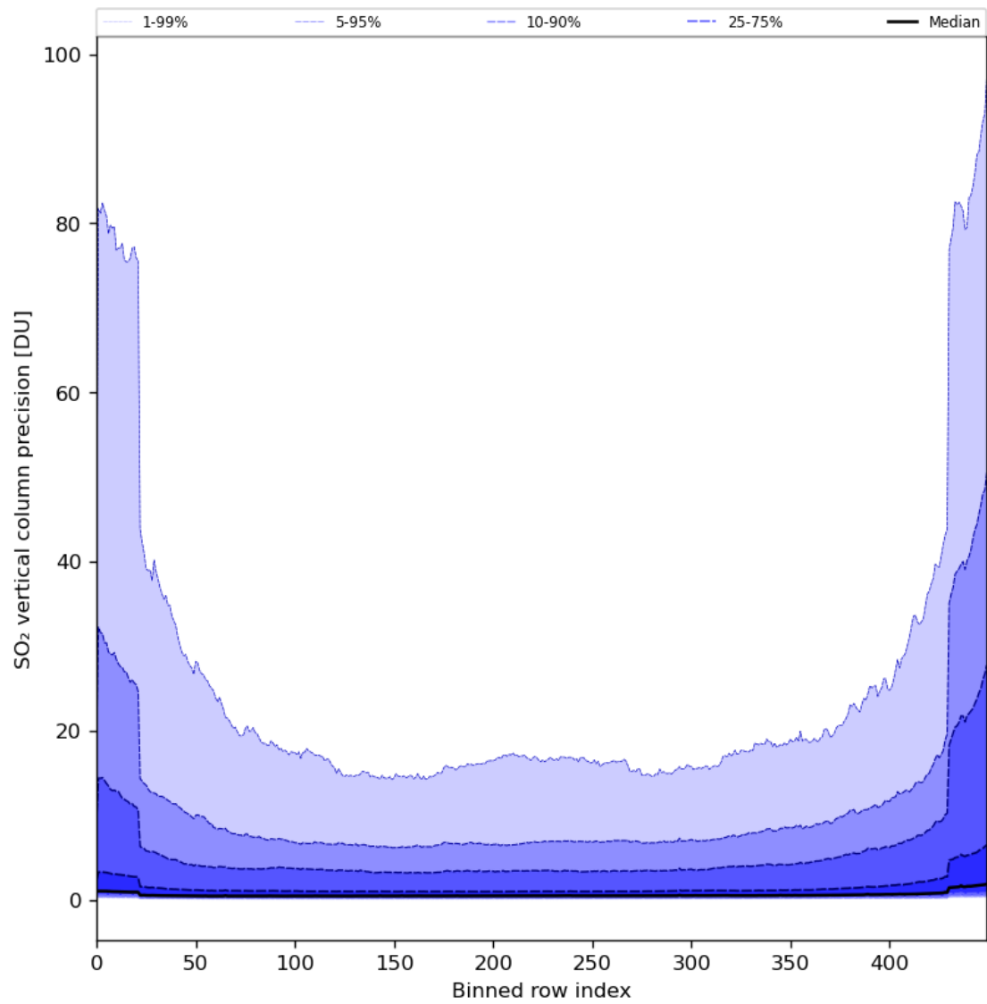
Figure 77: Along track statistics of “SO 2 vertical column precision” for 2024-02-07 to 2024-02-09
