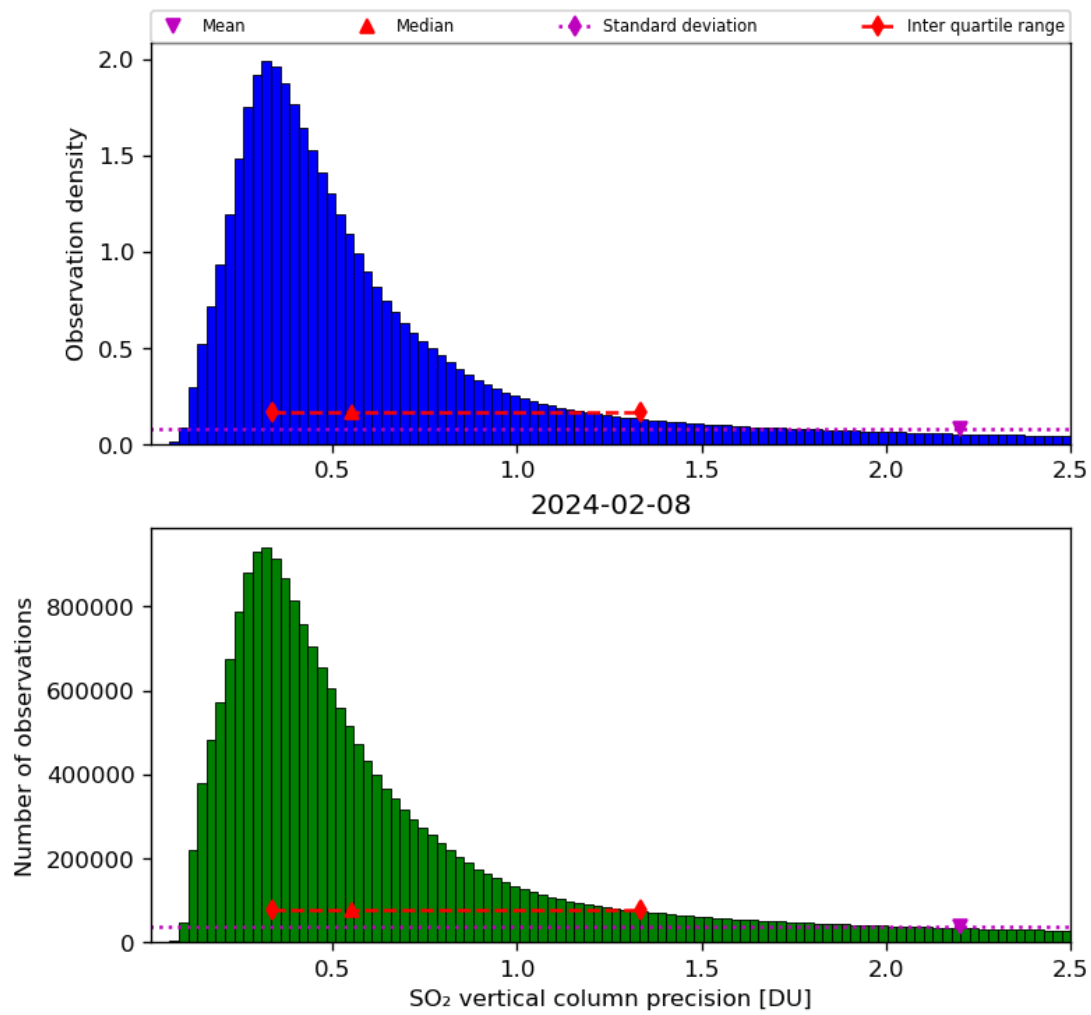
Figure 54: Histogram of “SO 2 vertical column precision” for 2024-02-07 to 2024-02-09
