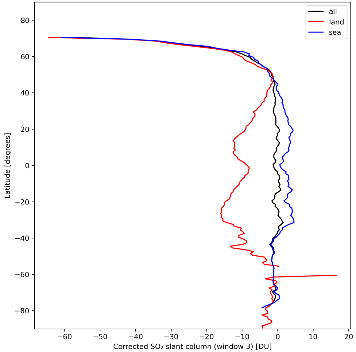
Figure 43: Zonal average of “Corrected SO 2 slant column (window 3)” for 2024-02-07 to 2024-02-09.
