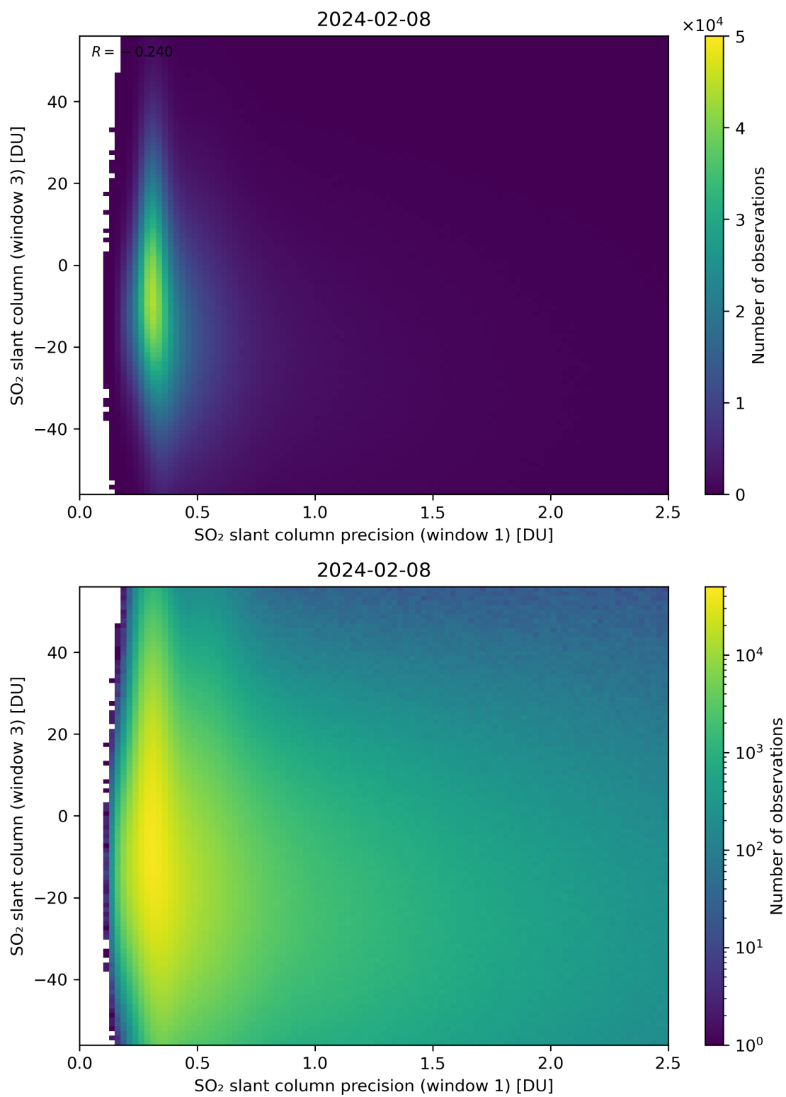
Figure 228: Scatter density plot of “SO 2 slant column precision (window 1)” against “SO 2 slant column (window 3)” for 2024-02-07 to 2024-02-09.
