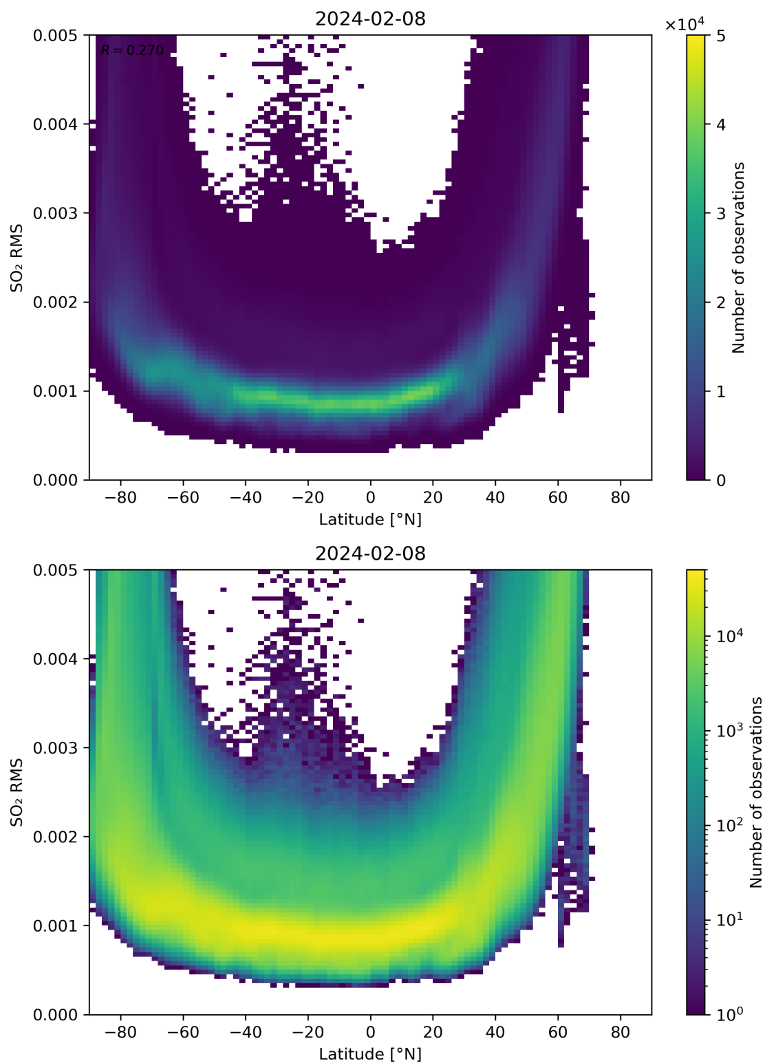
Figure 144: Scatter density plot of “Latitude” against “SO 2 RMS” for 2024-02-07 to 2024-02-09.
