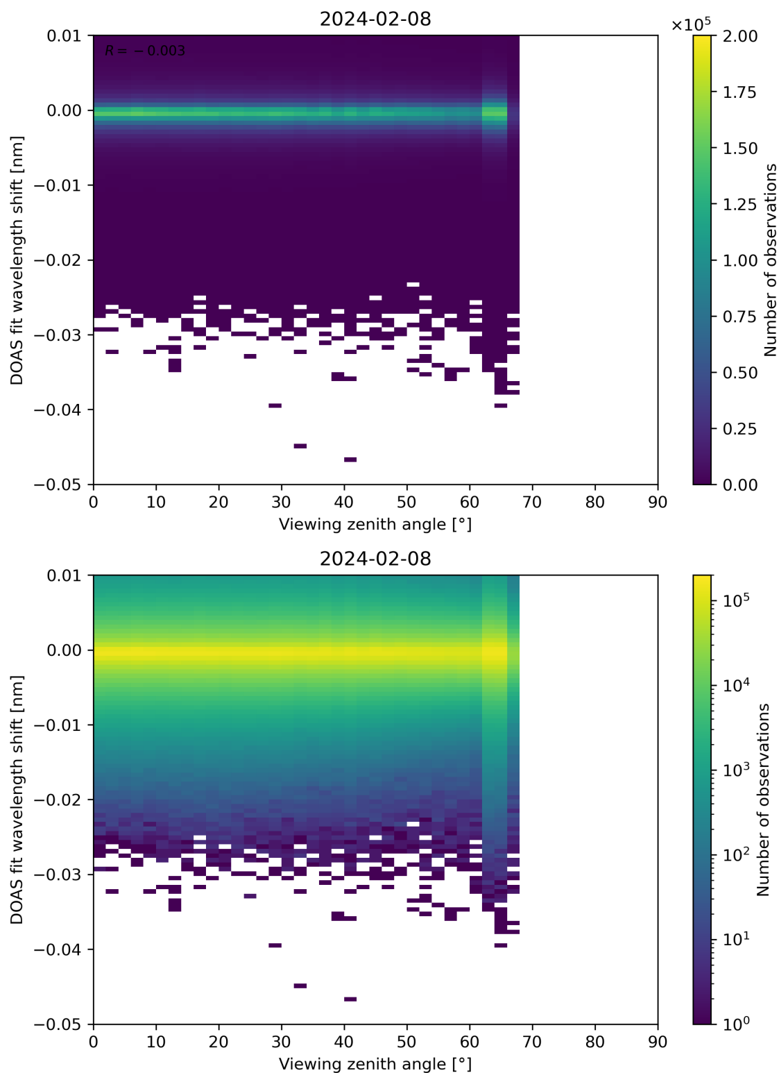
Figure 311: Scatter density plot of “Viewing zenith angle” against “DOAS fit wavelength shift” for 2024-02-07 to 2024-02-09.
