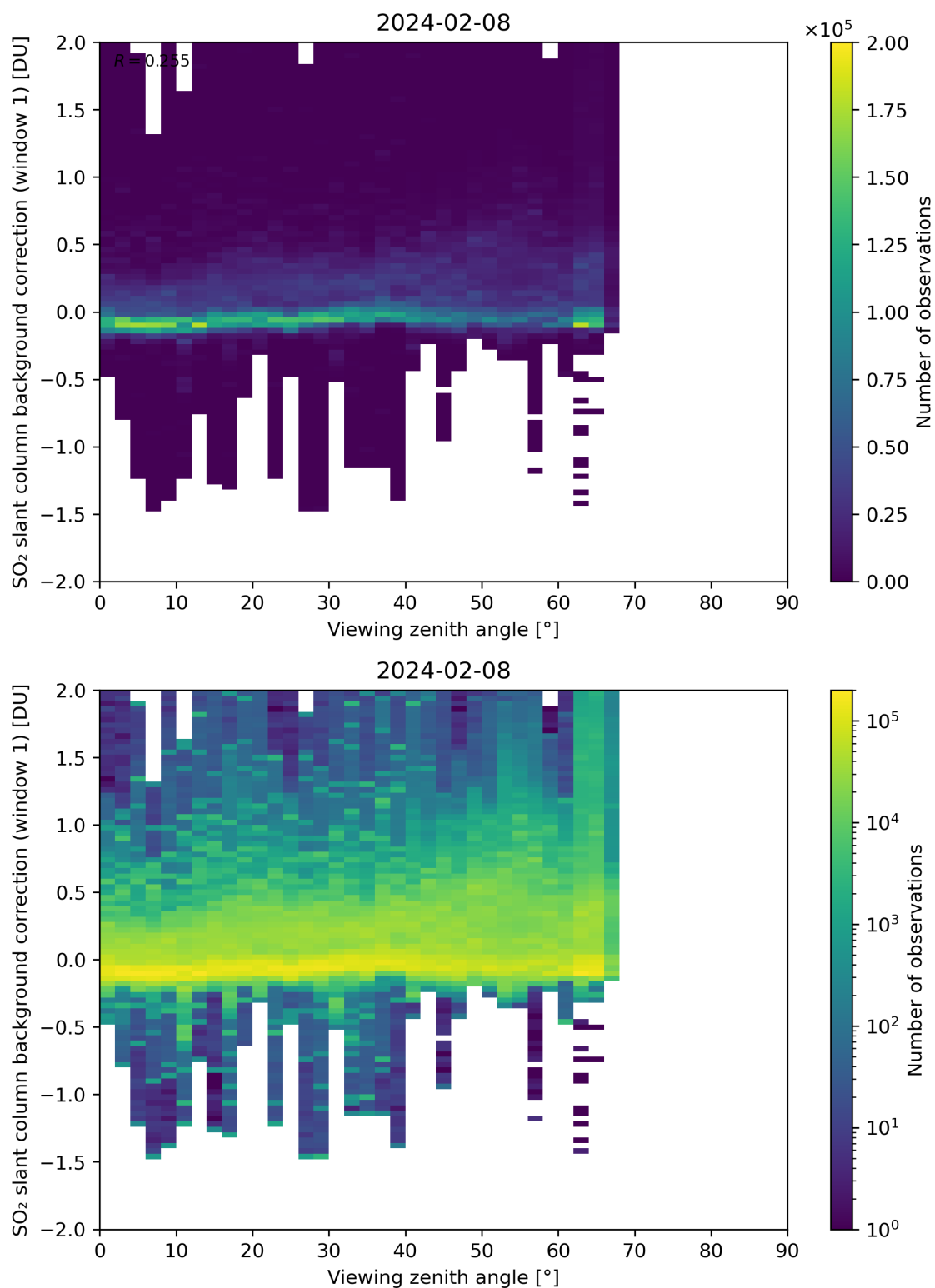
Figure 308: Scatter density plot of “Viewing zenith angle” against “SO 2 slant column background correction (window 1)” for 2024-02-07 to 2024-02-09.
