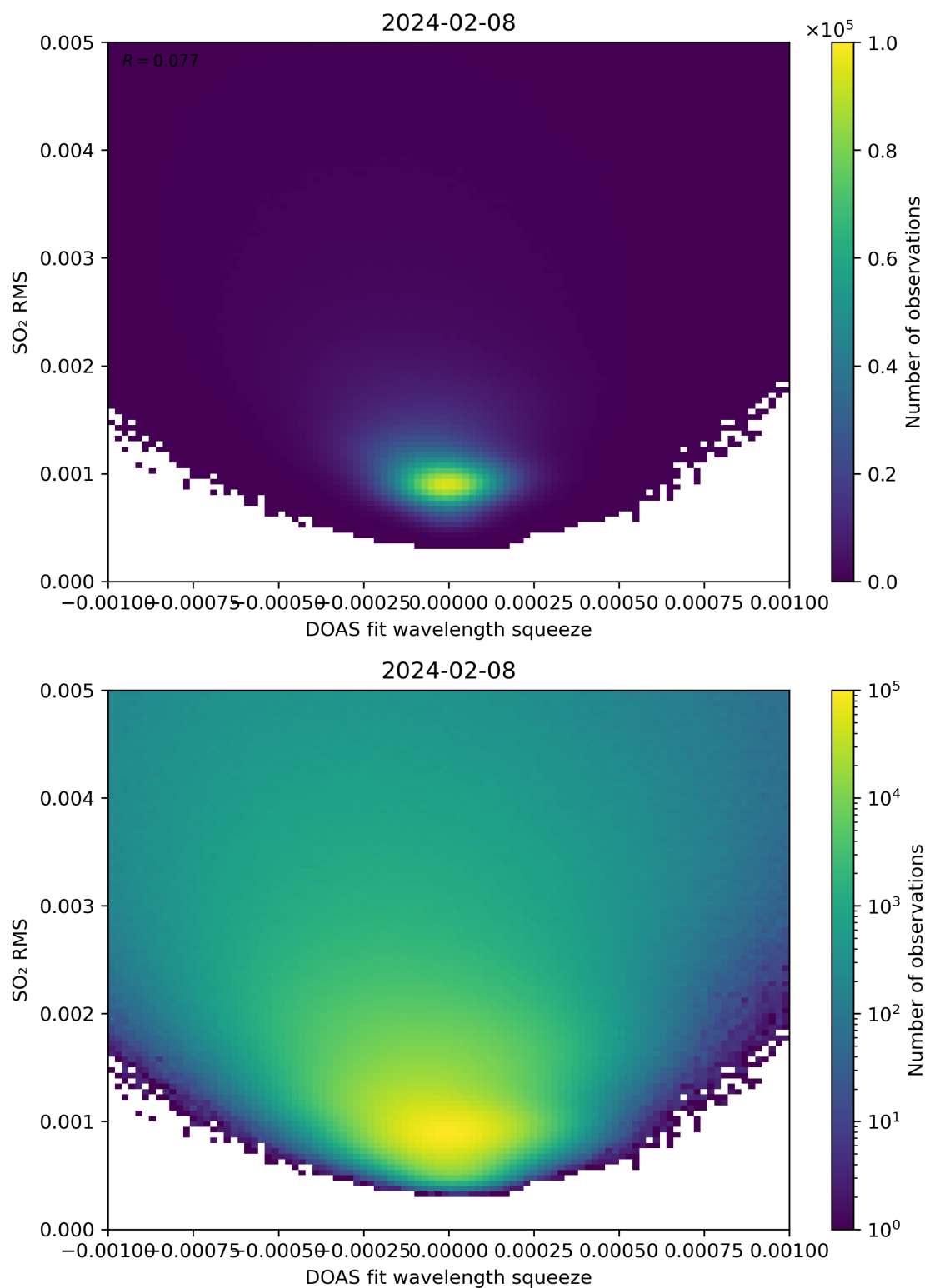
Figure 132: Scatter density plot of “DOAS fit wavelength squeeze” against “SO 2 RMS” for 2024-02-07 to 2024-02-09.
