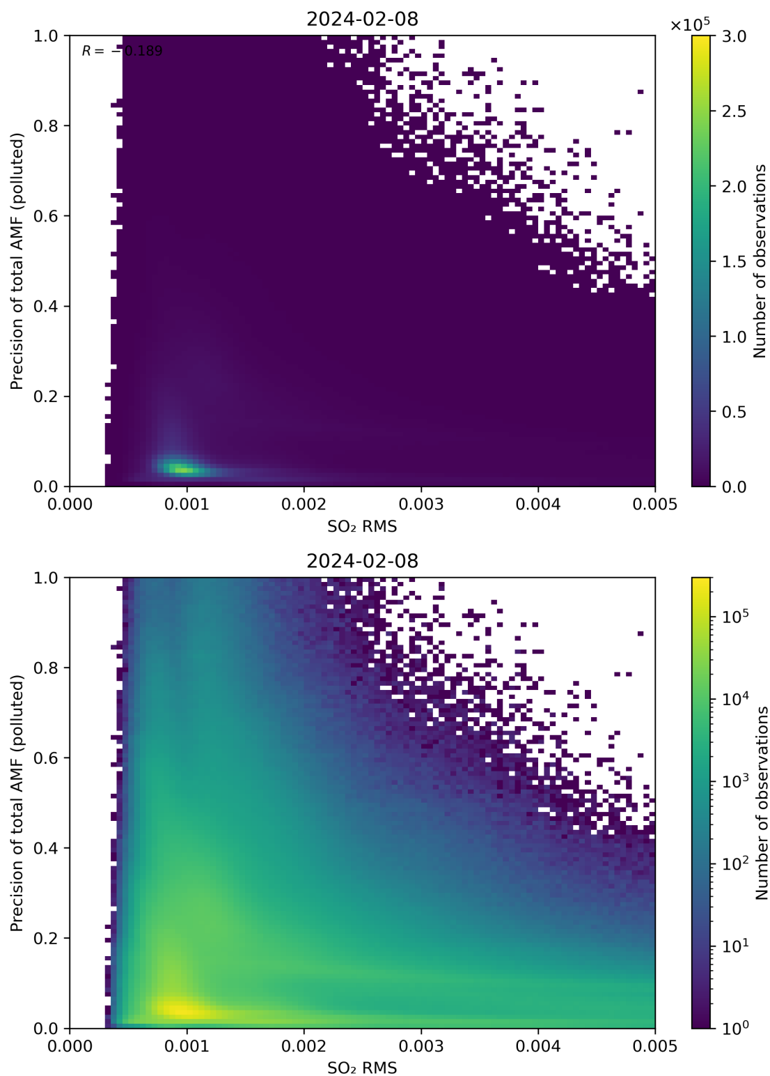
Figure 138: Scatter density plot of “SO 2 RMS” against “Precision of total AMF (polluted)” for 2024-02-07 to 2024-02-09.
