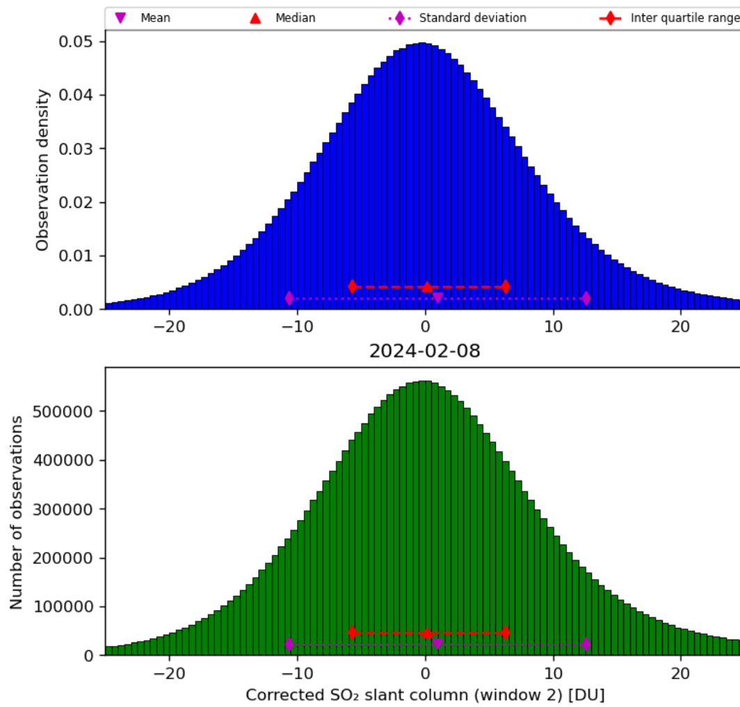
Figure 62: Histogram of “Corrected SO 2 slant column (window 2)” for 2024-02-07 to 2024-02-09
