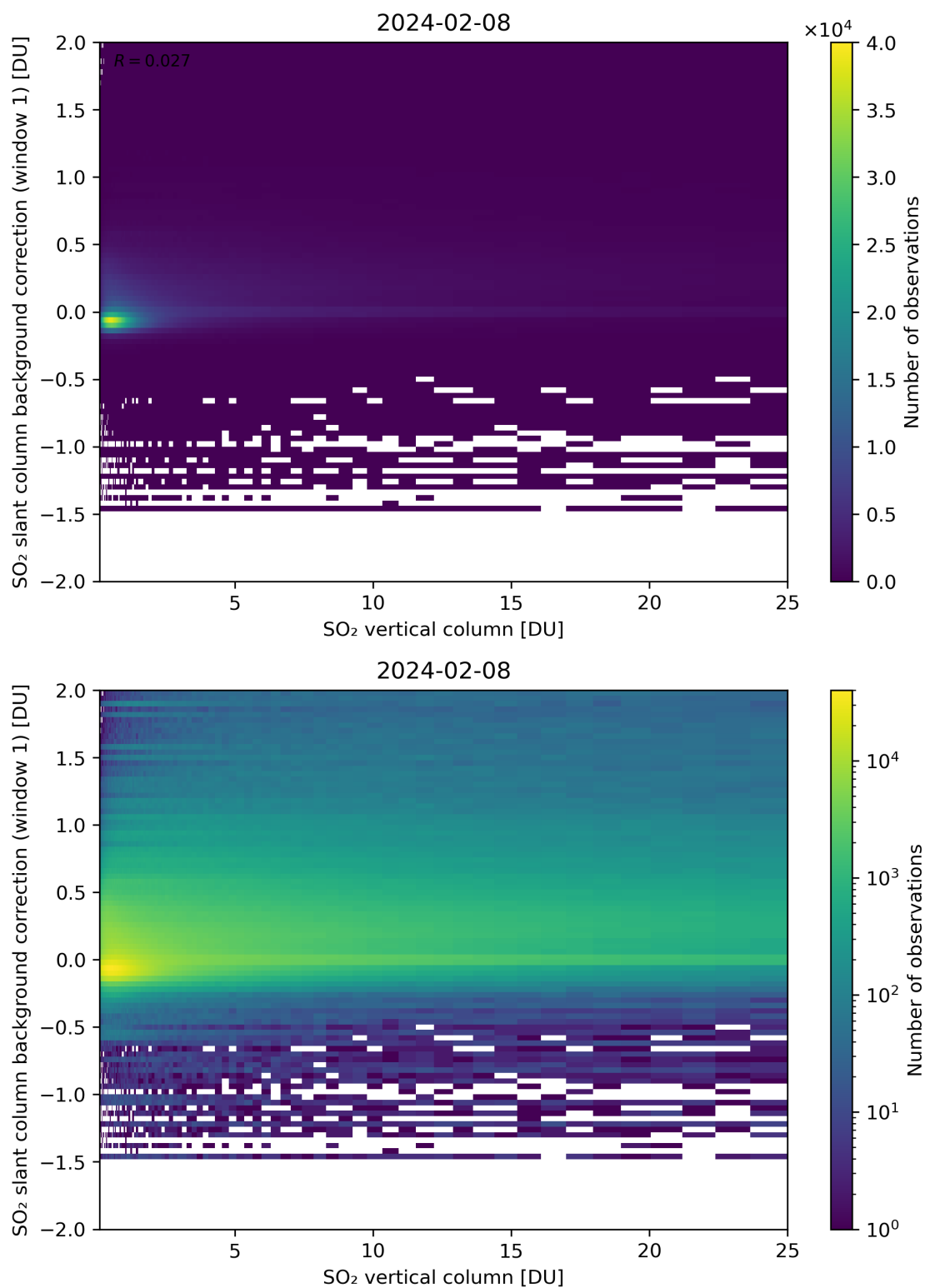
Figure 273: Scatter density plot of “SO 2 vertical column” against “SO 2 slant column background correction (window 1)” for 2024-02-07 to 2024-02-09.
