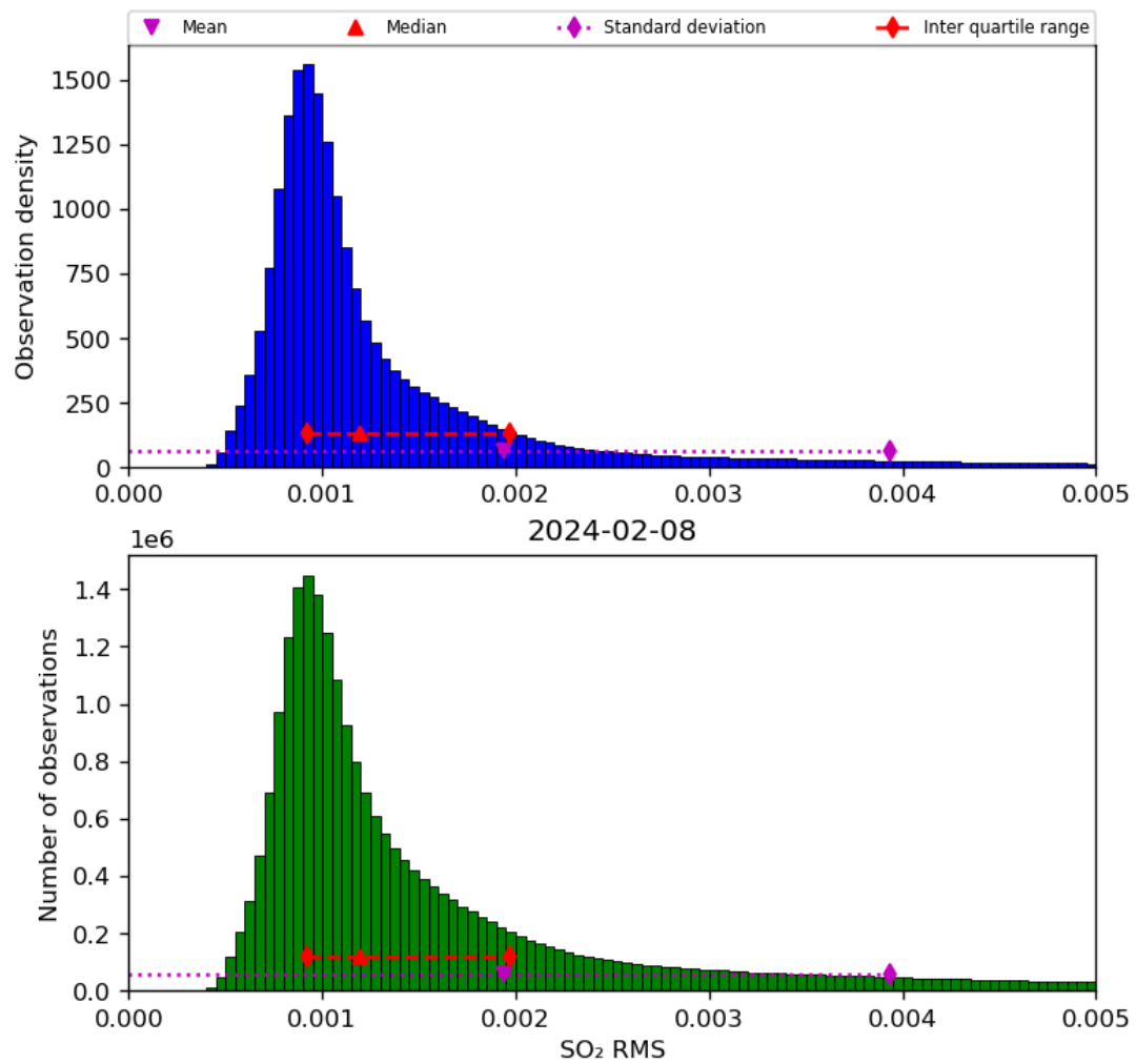
Figure 70: Histogram of “SO 2 RMS” for 2024-02-07 to 2024-02-09
