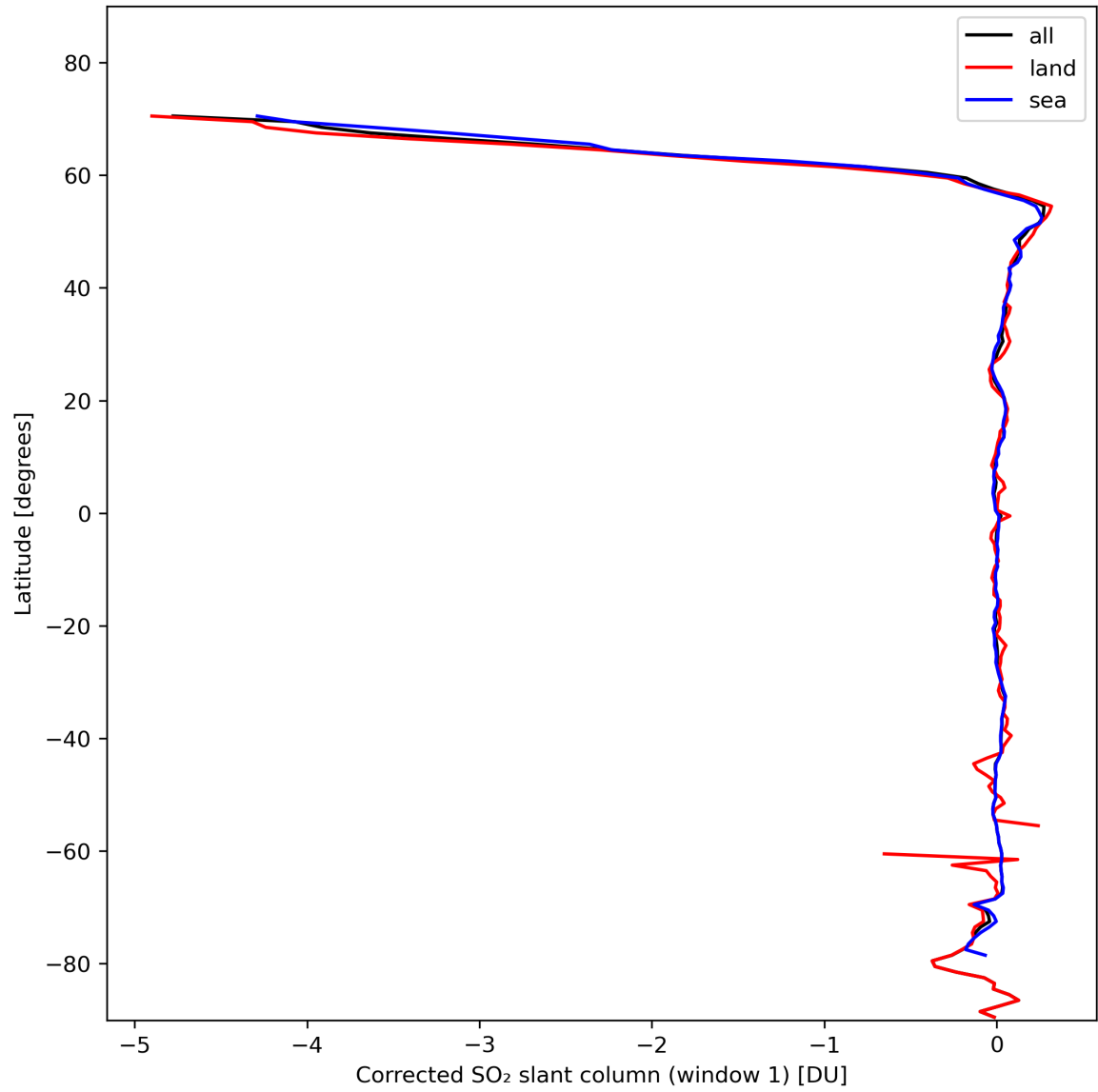
Figure 35: Zonal average of “Corrected SO 2 slant column (window 1)” for 2024-02-07 to 2024-02-09.
