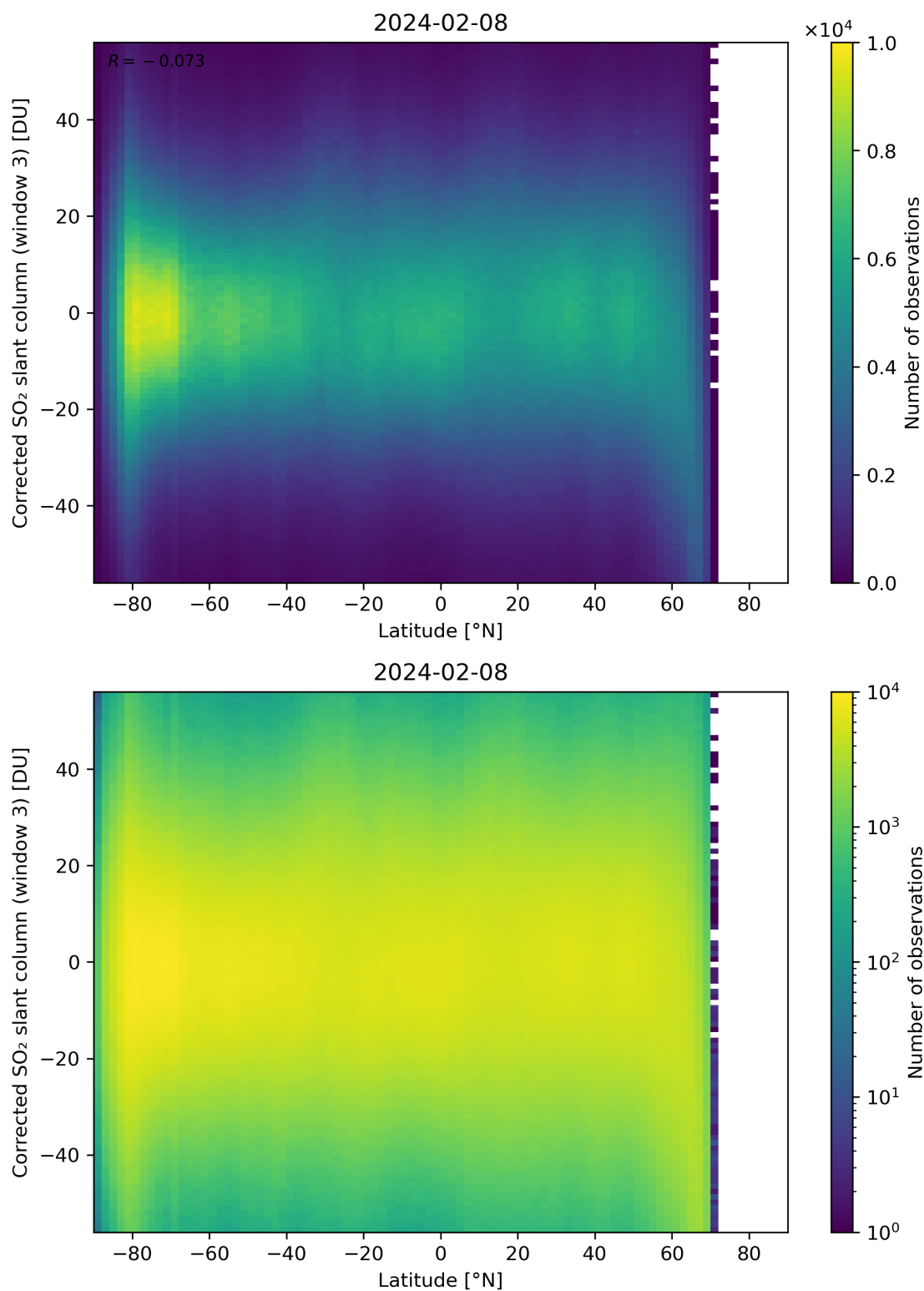
Figure 148: Scatter density plot of “Latitude” against “Corrected SO 2 slant column (window 3)” for 2024-02-07 to 2024-02-09.
