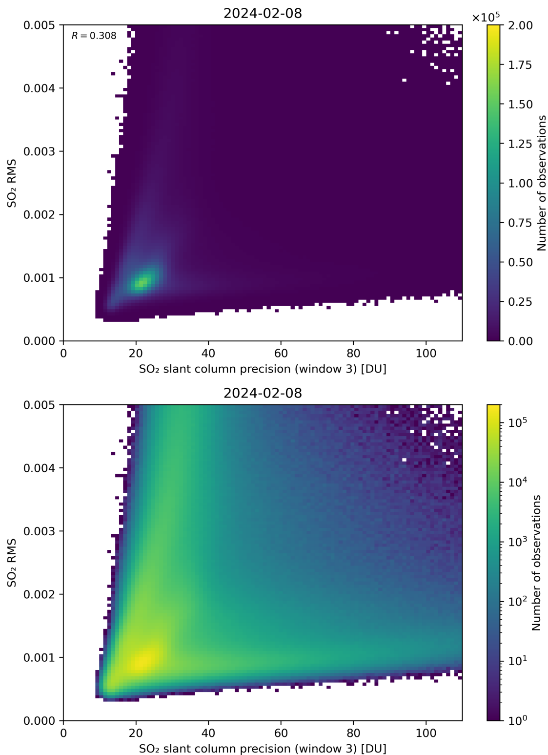
Figure 260: Scatter density plot of “SO 2 slant column precision (window 3)” against “SO 2 RMS” for 2024-02-07 to 2024-02-09.
