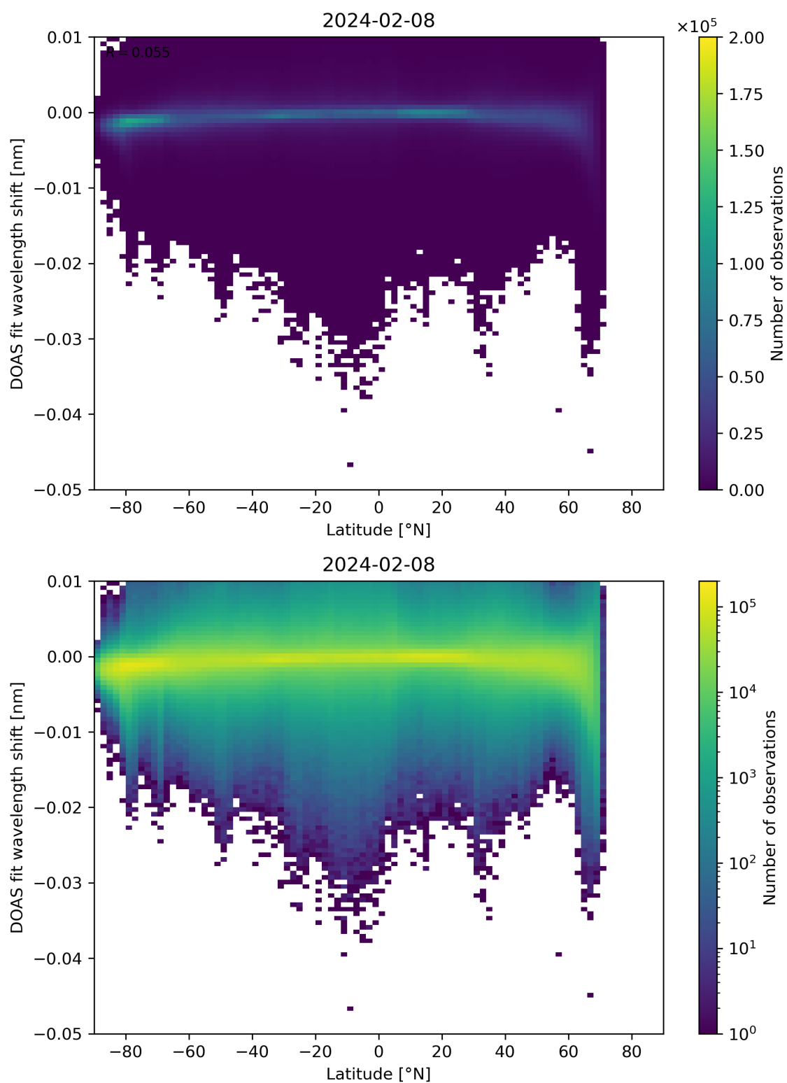
Figure 142: Scatter density plot of “Latitude” against “DOAS fit wavelength shift” for 2024-02-07 to 2024-02-09.
