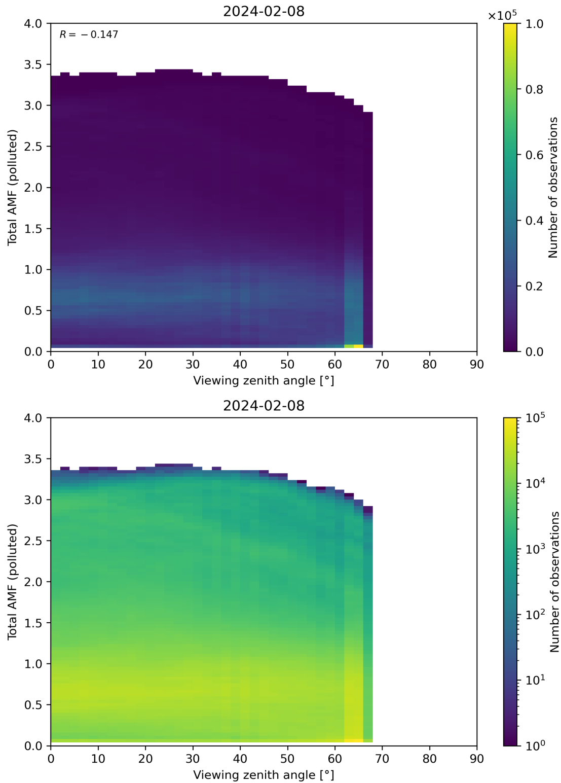
Figure 325: Scatter density plot of “Viewing zenith angle” against “Total AMF (polluted)” for 2024-02-07 to 2024-02-09.
