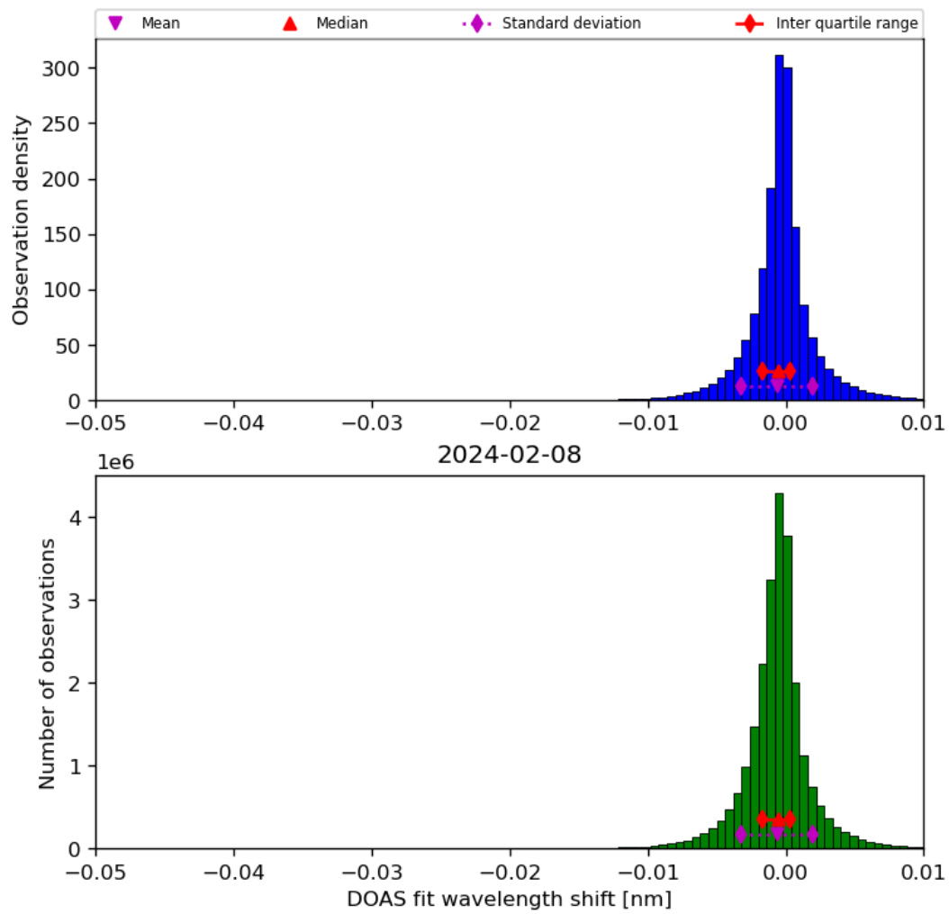
Figure 68: Histogram of “DOAS fit wavelength shift” for 2024-02-07 to 2024-02-09
