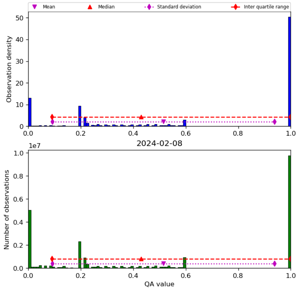
Figure 52: Histogram of “QA value” for 2024-02-07 to 2024-02-09
