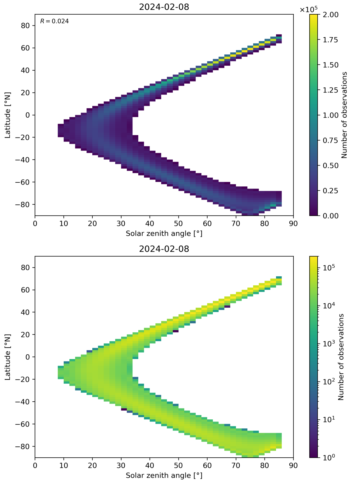
Figure 164: Scatter density plot of “Solar zenith angle” against “Latitude” for 2024-02-07 to 2024-02-09.
