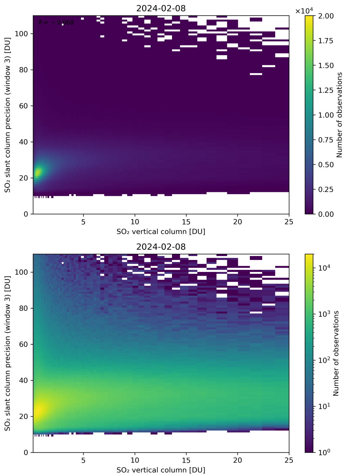
Figure 304: Scatter density plot of “SO 2 vertical column” against “SO 2 slant column precision (window 3)” for 2024-02-07 to 2024-02-09.
