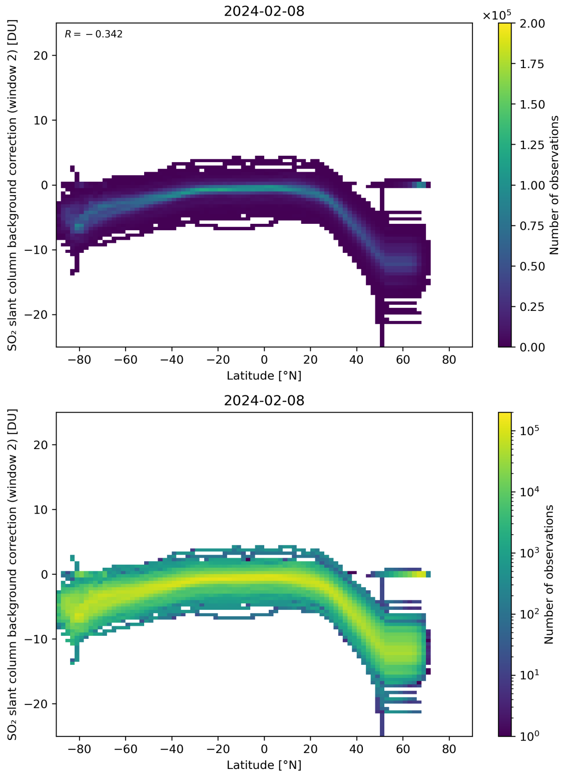
Figure 140: Scatter density plot of “Latitude” against “SO 2 slant column background correction (window 2)” for 2024-02-07 to 2024-02-09.
