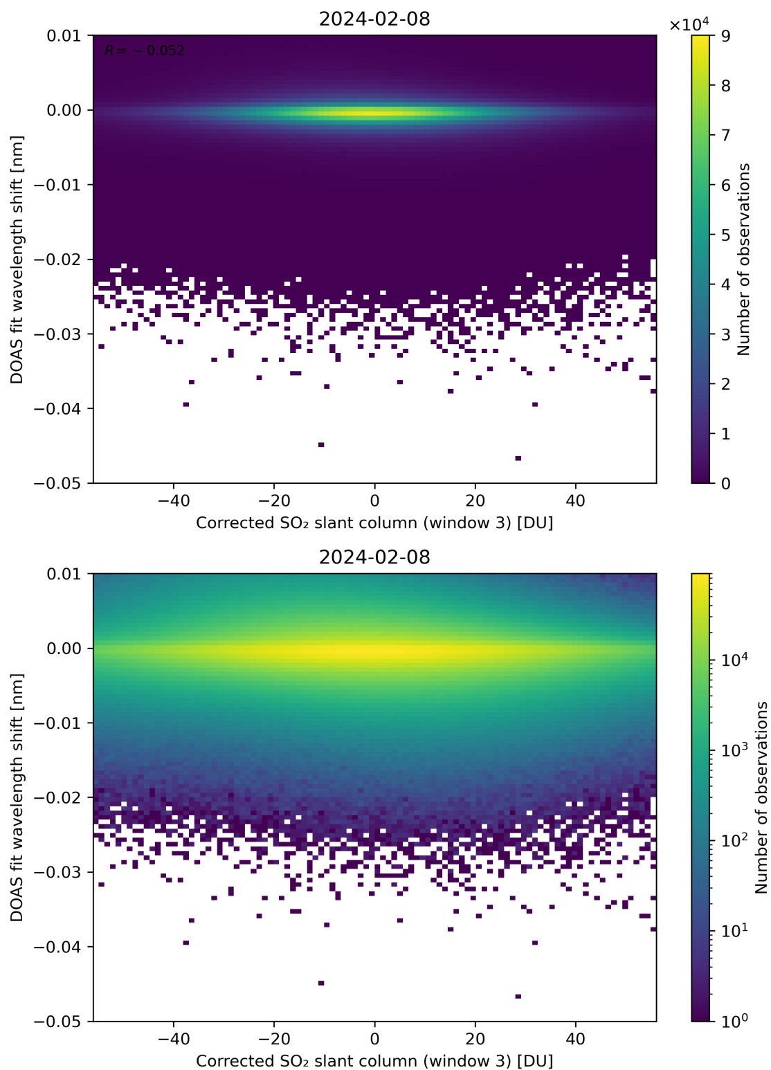
Figure 206: Scatter density plot of “Corrected SO 2 slant column (window 3)” against “DOAS fit wavelength shift” for 2024-02-07 to 2024-02-09.
