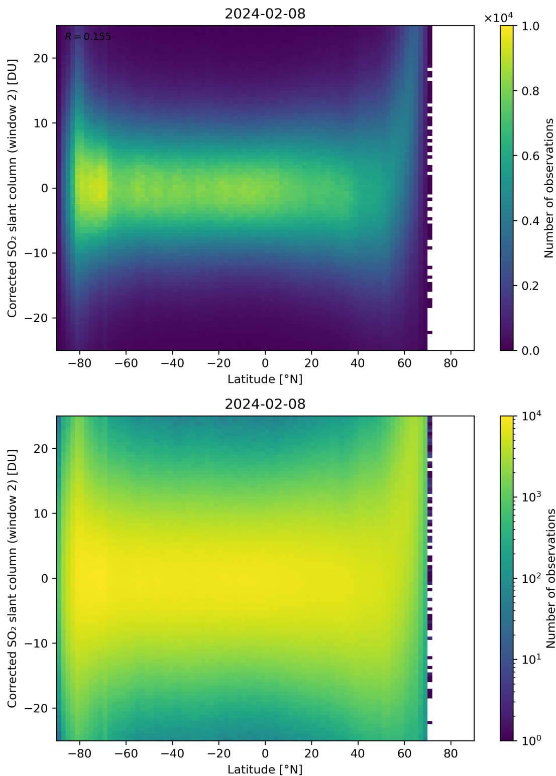
Figure 147: Scatter density plot of “Latitude” against “Corrected SO 2 slant column (window 2)” for 2024-02-07 to 2024-02-09.
