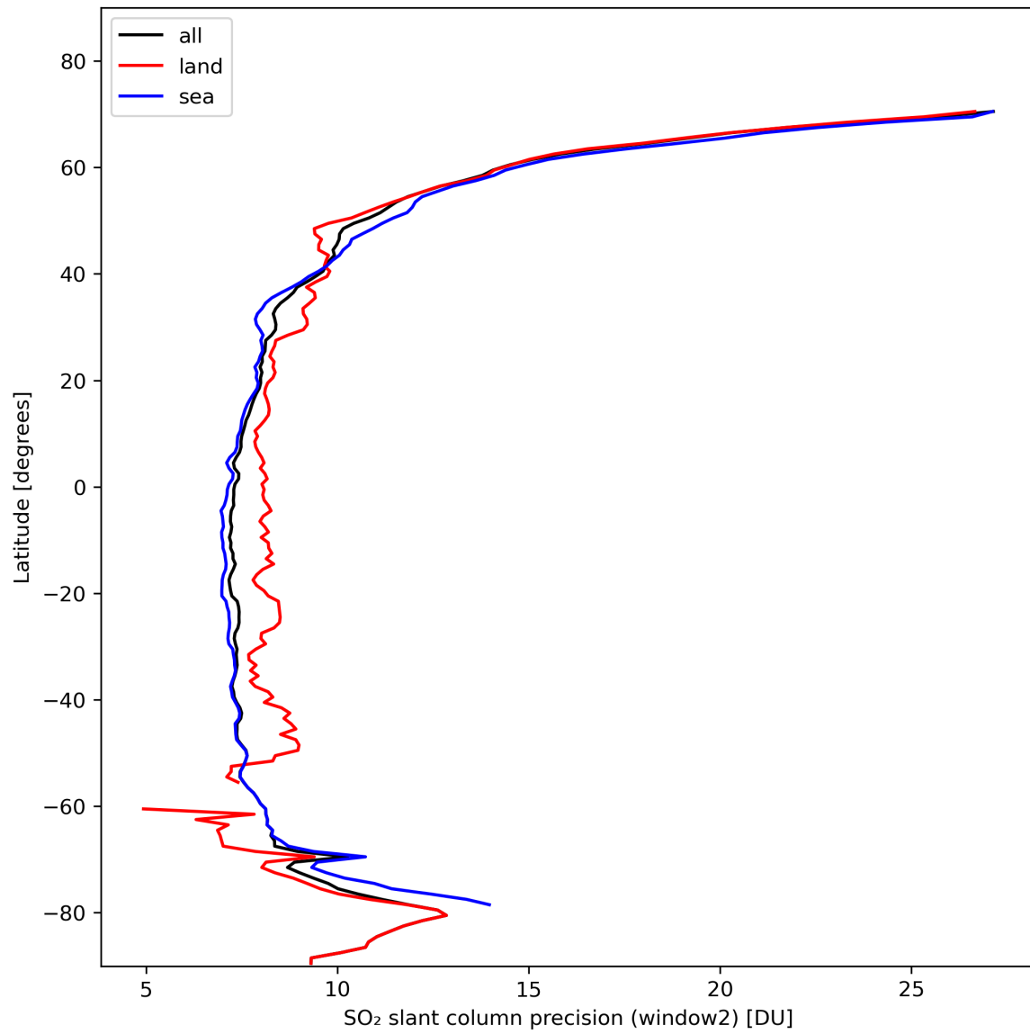
Figure 38: Zonal average of “SO 2 slant column precision (window2)” for 2024-02-07 to 2024-02-09.
