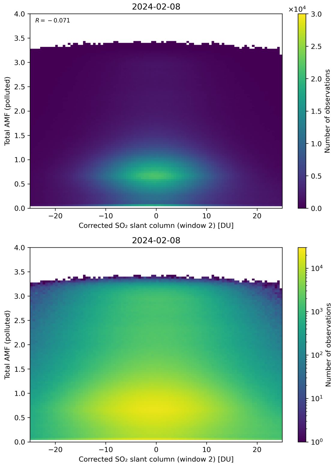
Figure 203: Scatter density plot of “Corrected SO 2 slant column (window 2)” against “Total AMF (polluted)” for 2024-02-07 to 2024-02-09.
