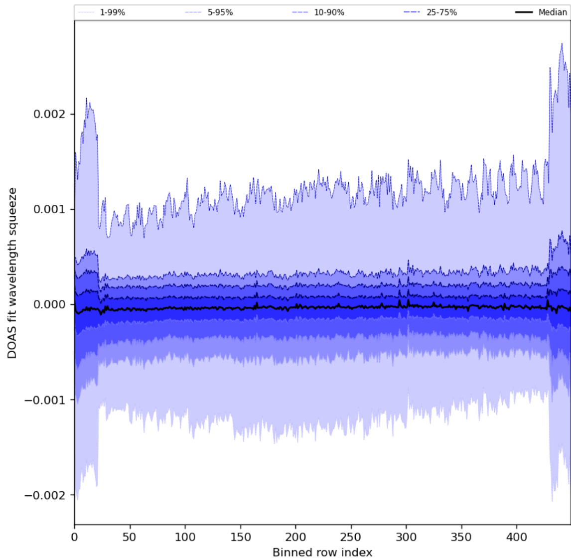
Figure 92: Along track statistics of “DOAS fit wavelength squeeze” for 2024-02-07 to 2024-02-09
