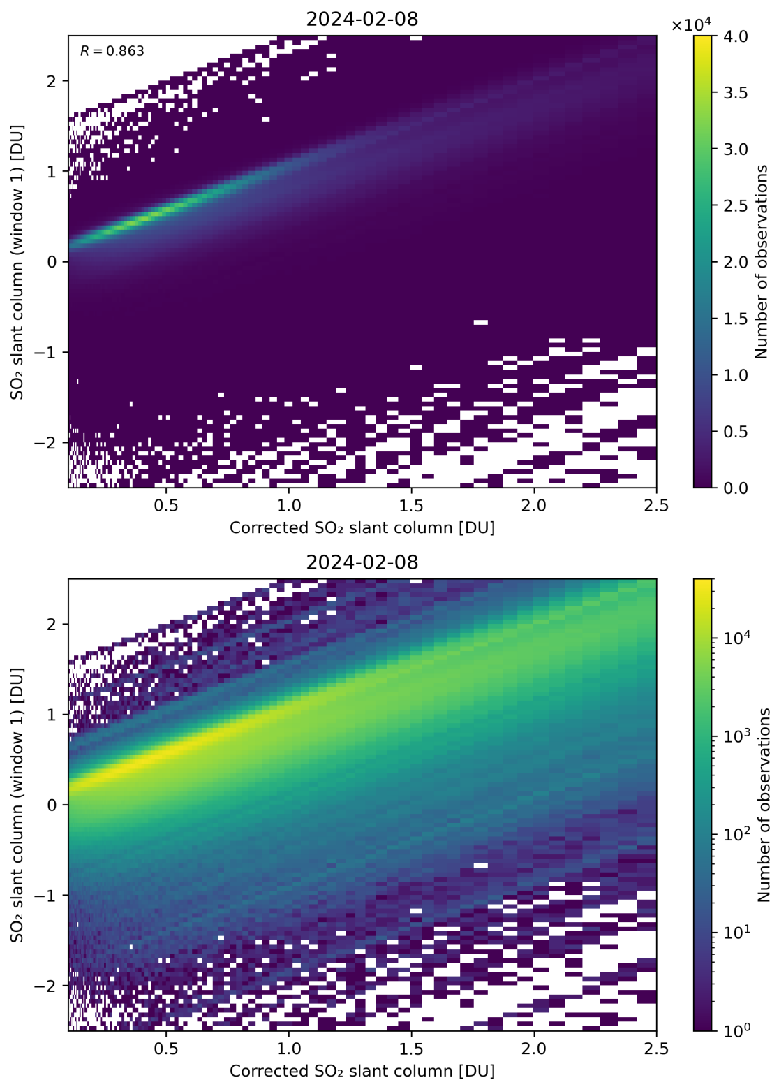
Figure 187: Scatter density plot of “Corrected SO 2 slant column” against “SO 2 slant column (window 1)” for 2024-02-07 to 2024-02-09.
