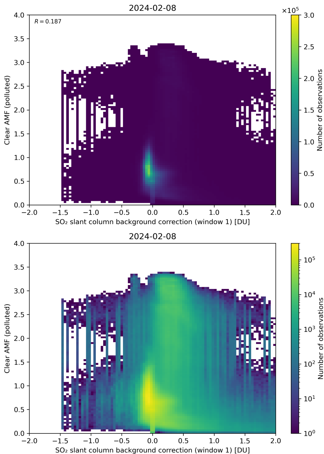
Figure 103: Scatter density plot of “SO 2 slant column background correction (window 1)” against “Clear AMF (polluted)” for 2024-02-07 to 2024-02-09.
