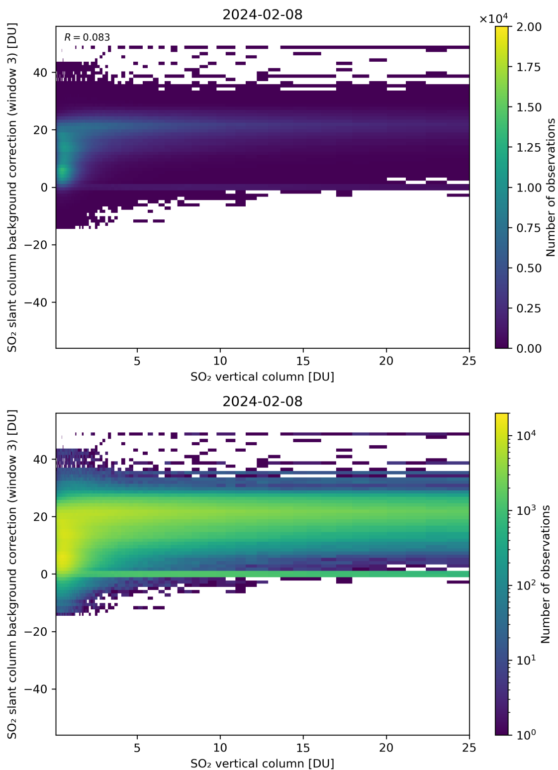
Figure 275: Scatter density plot of “SO 2 vertical column” against “SO 2 slant column background correction (window 3)” for 2024-02-07 to 2024-02-09.
