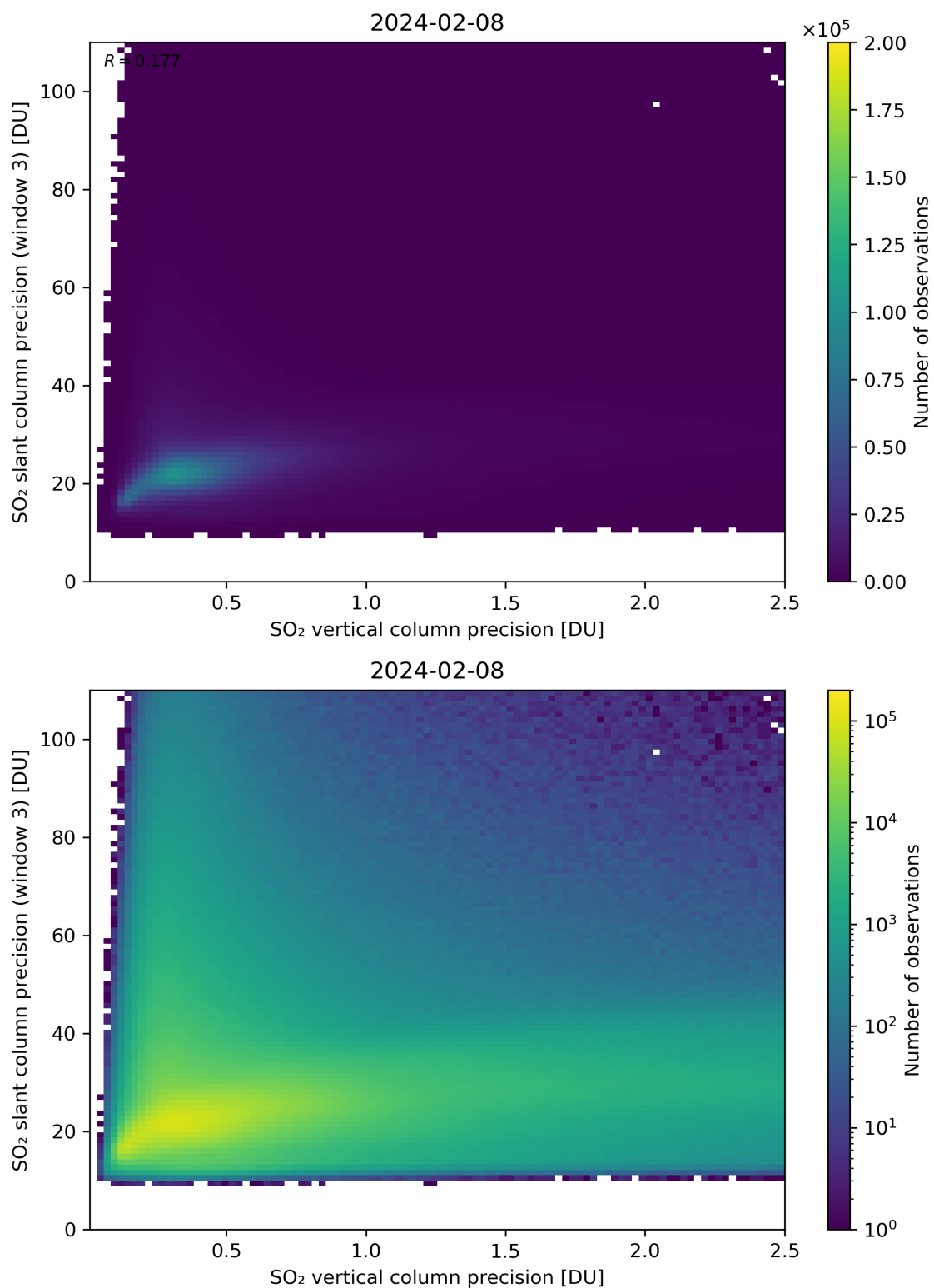
Figure 293: Scatter density plot of “SO 2 vertical column precision” against “SO 2 slant column precision (window 3)” for 2024-02-07 to 2024-02-09.
