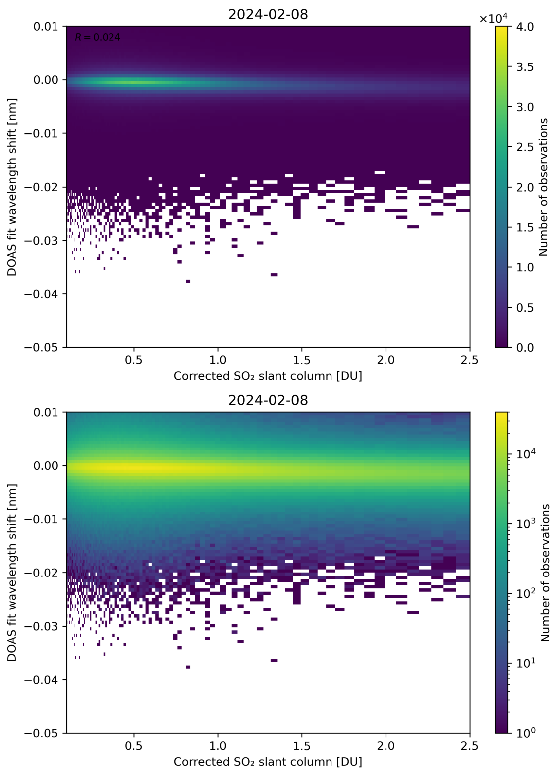
Figure 181: Scatter density plot of “Corrected SO 2 slant column” against “DOAS fit wavelength shift” for 2024-02-07 to 2024-02-09.
