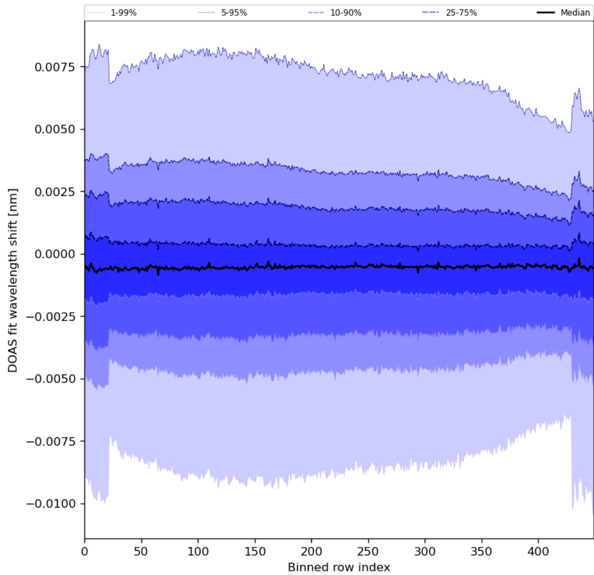
Figure 91: Along track statistics of “DOAS fit wavelength shift” for 2024-02-07 to 2024-02-09
