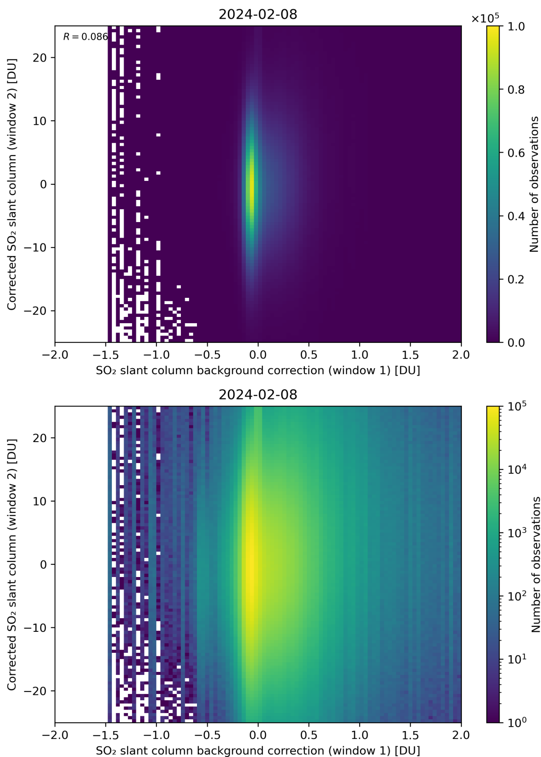
Figure 104: Scatter density plot of “SO 2 slant column background correction (window 1)” against “Corrected SO 2 slant column (window 2)” for 2024-02-07 to 2024-02-09.
