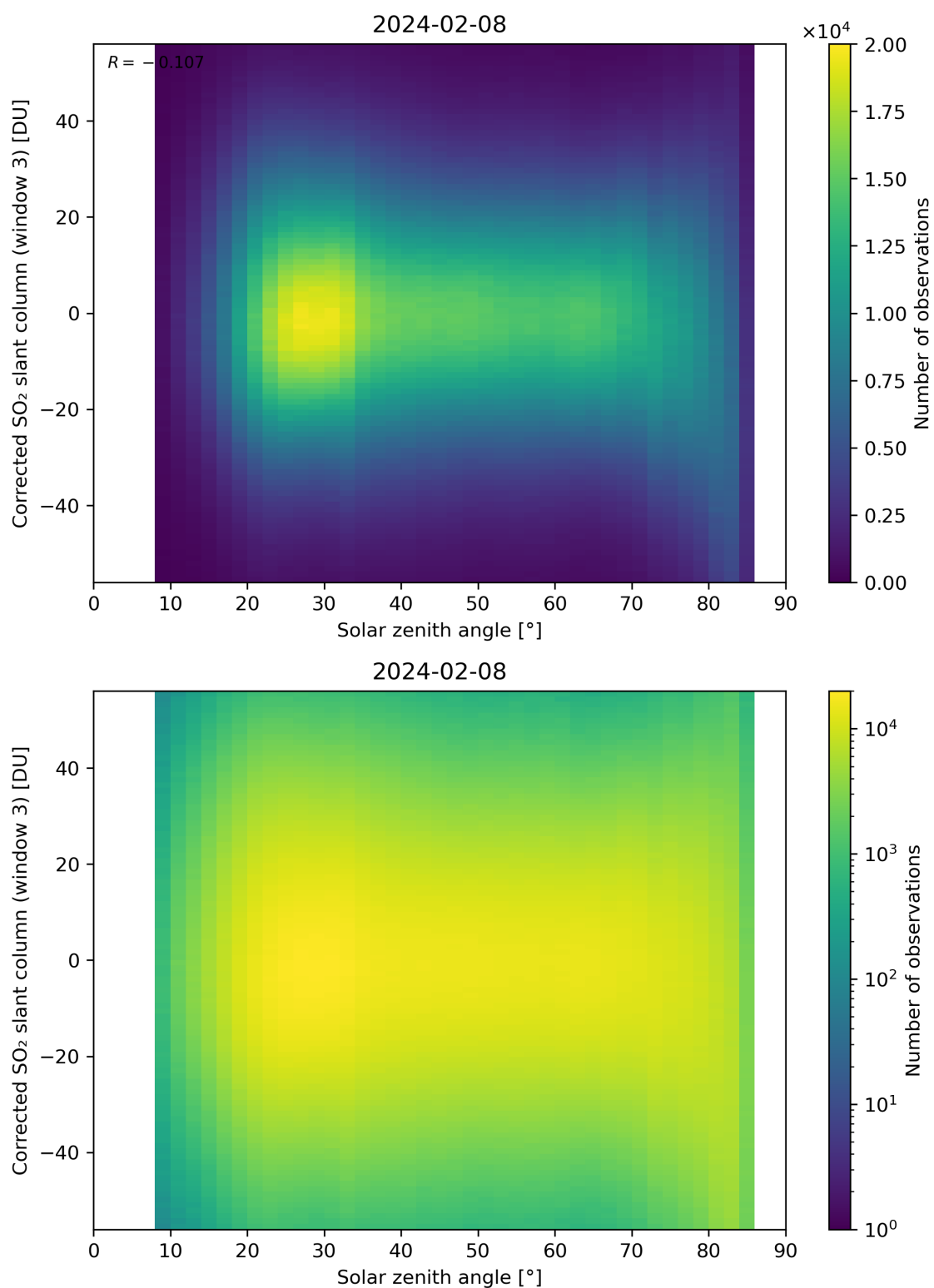
Figure 168: Scatter density plot of “Solar zenith angle” against “Corrected SO 2 slant column (window 3)” for 2024-02-07 to 2024-02-09.
