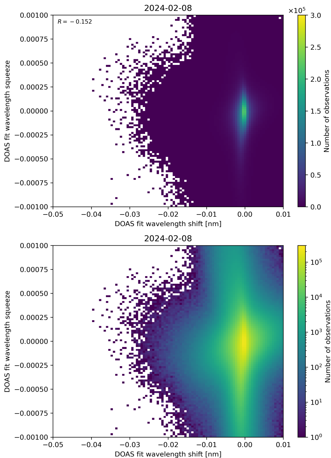
Figure 127: Scatter density plot of “DOAS fit wavelength shift” against “DOAS fit wavelength squeeze” for 2024-02-07 to 2024-02-09.
