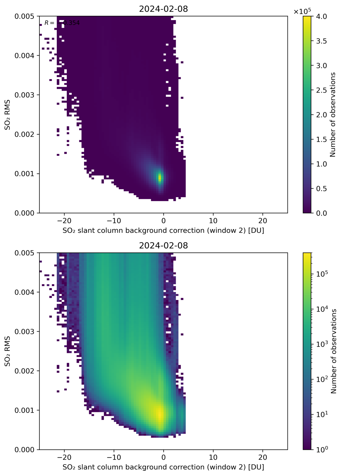
Figure 114: Scatter density plot of “SO 2 slant column background correction (window 2)” against “SO 2 RMS” for 2024-02-07 to 2024-02-09.
