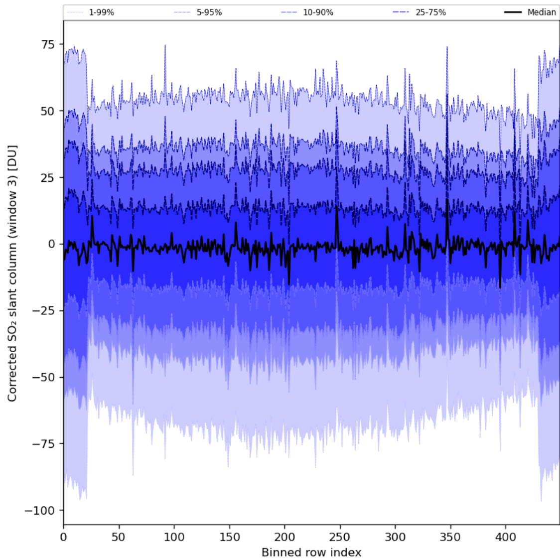
Figure 89: Along track statistics of “Corrected SO 2 slant column (window 3)” for 2024-02-07 to 2024-02-09
