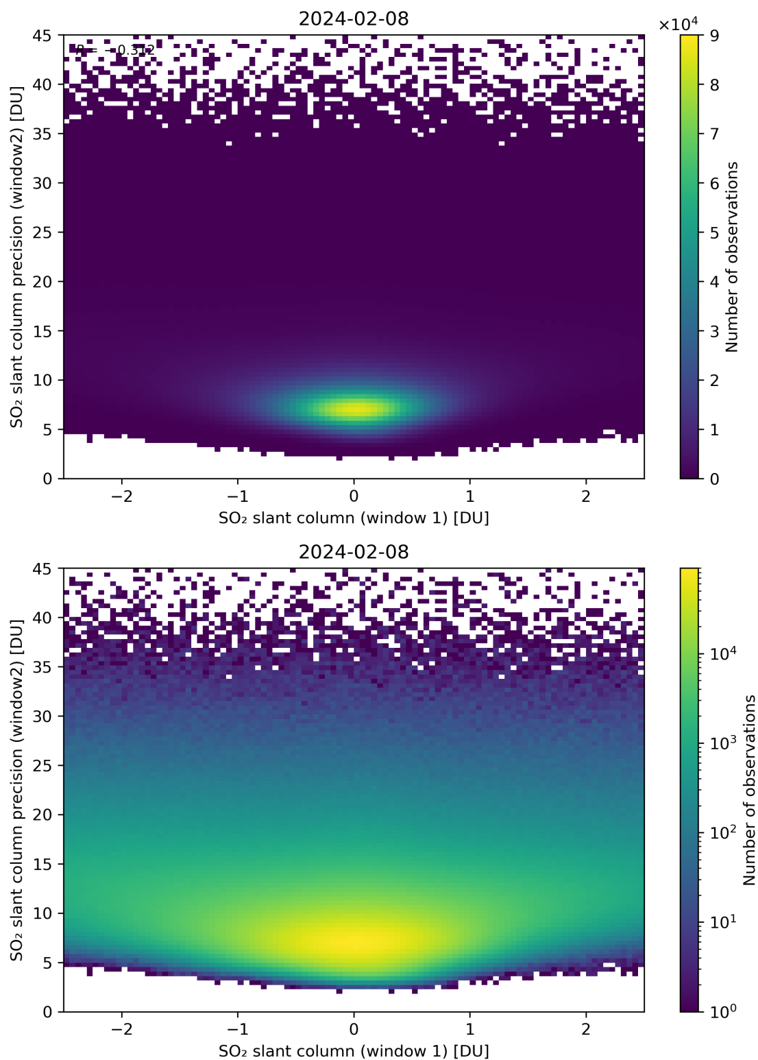
Figure 236: Scatter density plot of “SO 2 slant column (window 1)” against “SO 2 slant column precision (window2)” for 2024-02-07 to 2024-02-09.
