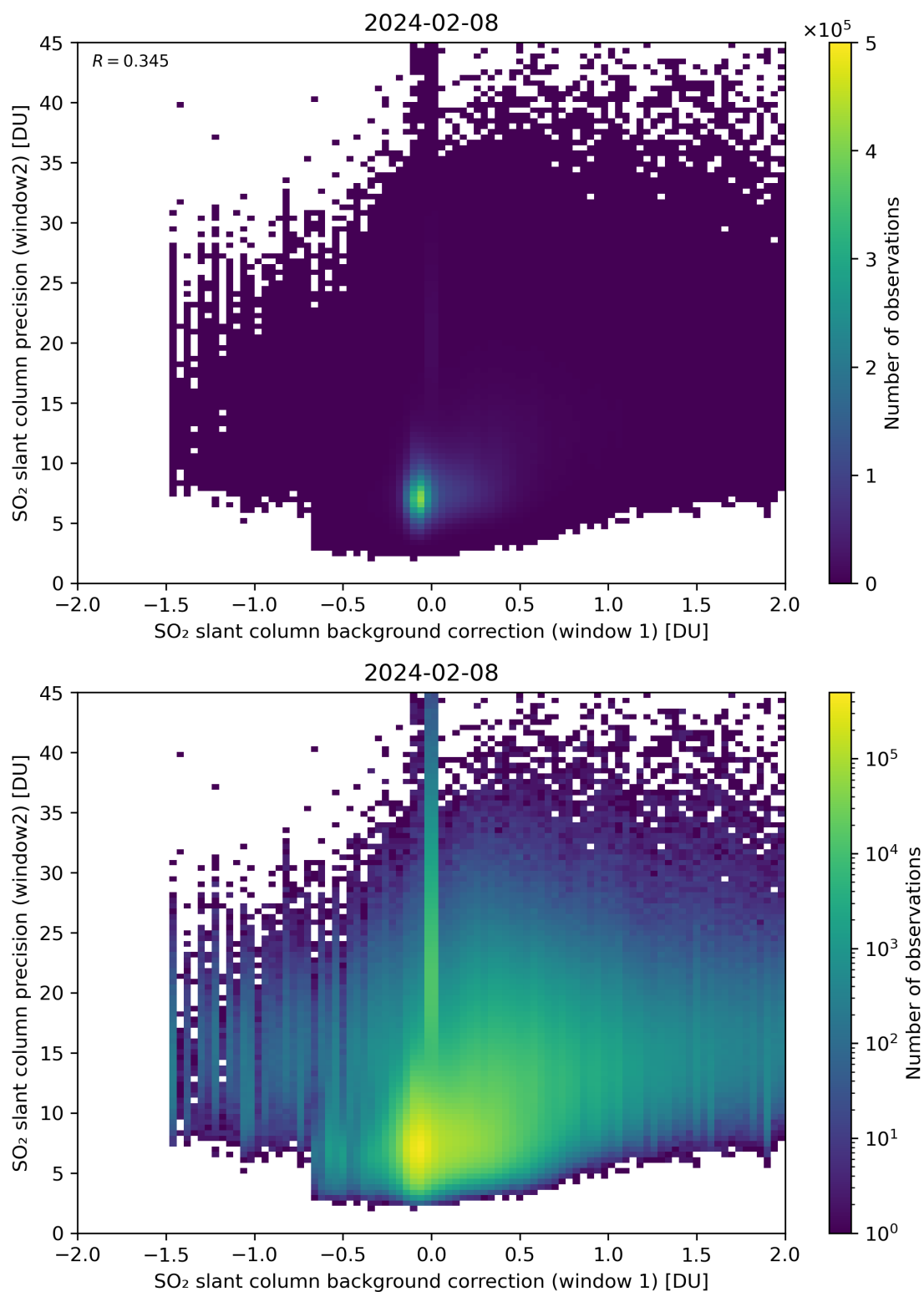
Figure 106: Scatter density plot of “SO 2 slant column background correction (window 1)” against “SO 2 slant column precision (window2)” for 2024-02-07 to 2024-02-09.
