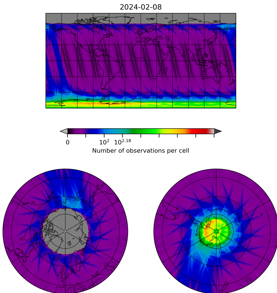
Figure 28: Map of the number of observations for 2024-02-07 to 2024-02-09
