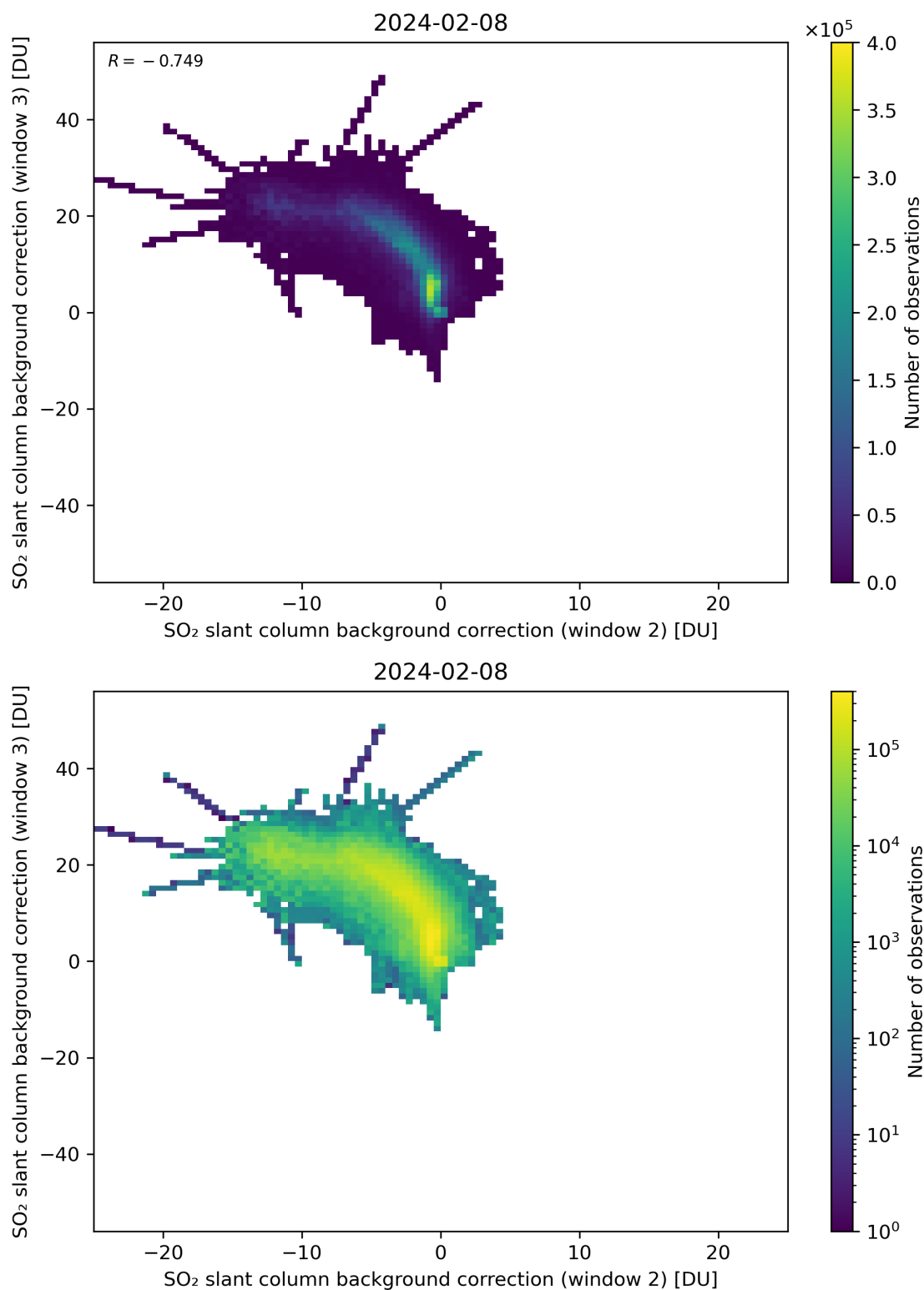
Figure 111: Scatter density plot of “SO 2 slant column background correction (window 2)” against “SO 2 slant column background correction (window 3)” for 2024-02-07 to 2024-02-09.
