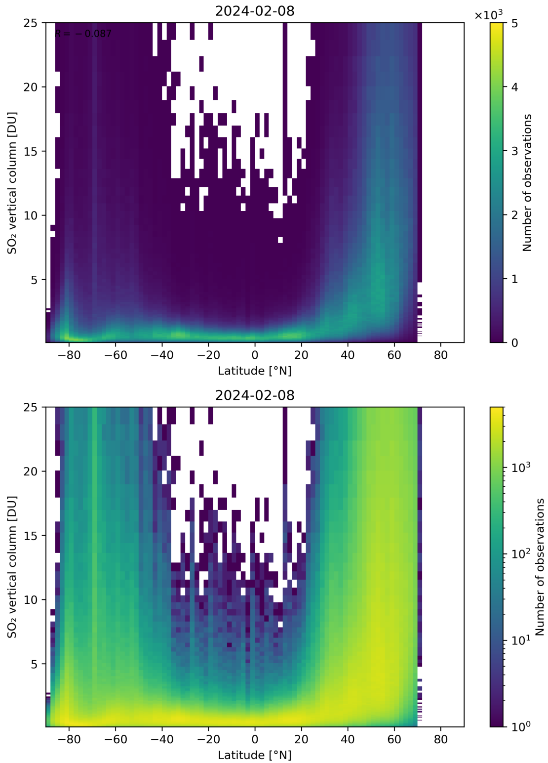
Figure 156: Scatter density plot of “Latitude” against “SO 2 vertical column” for 2024-02-07 to 2024-02-09.
