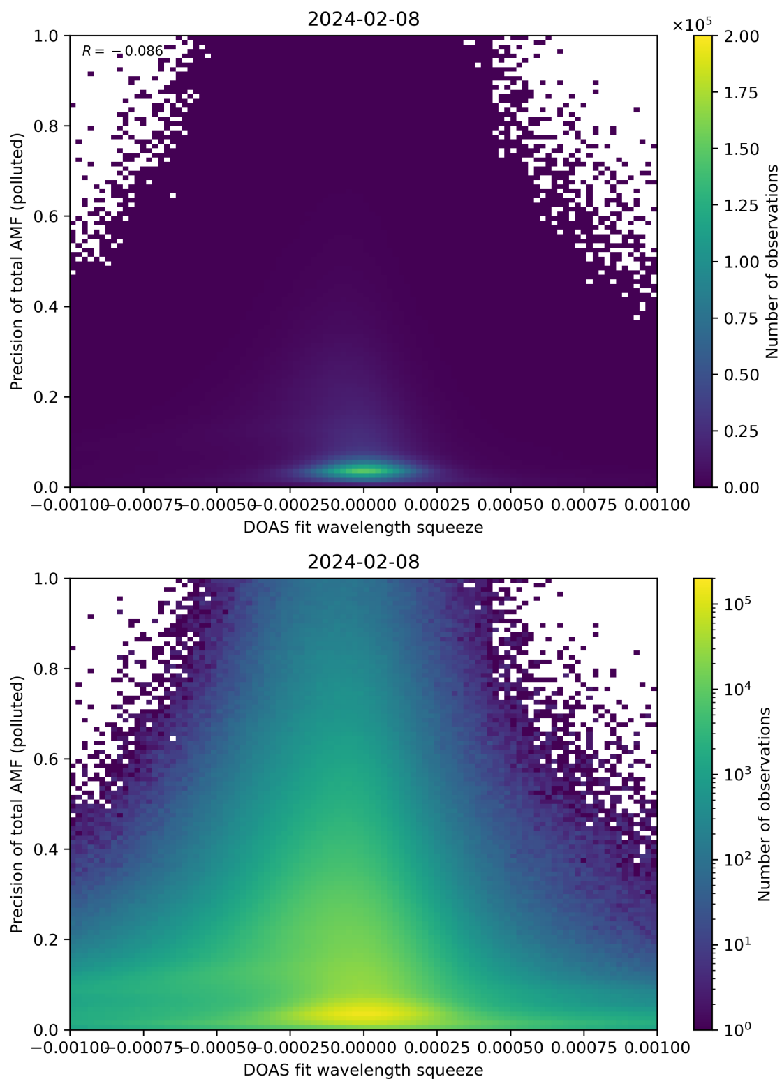
Figure 135: Scatter density plot of “DOAS fit wavelength squeeze” against “Precision of total AMF (polluted)” for 2024-02-07 to 2024-02-09.
