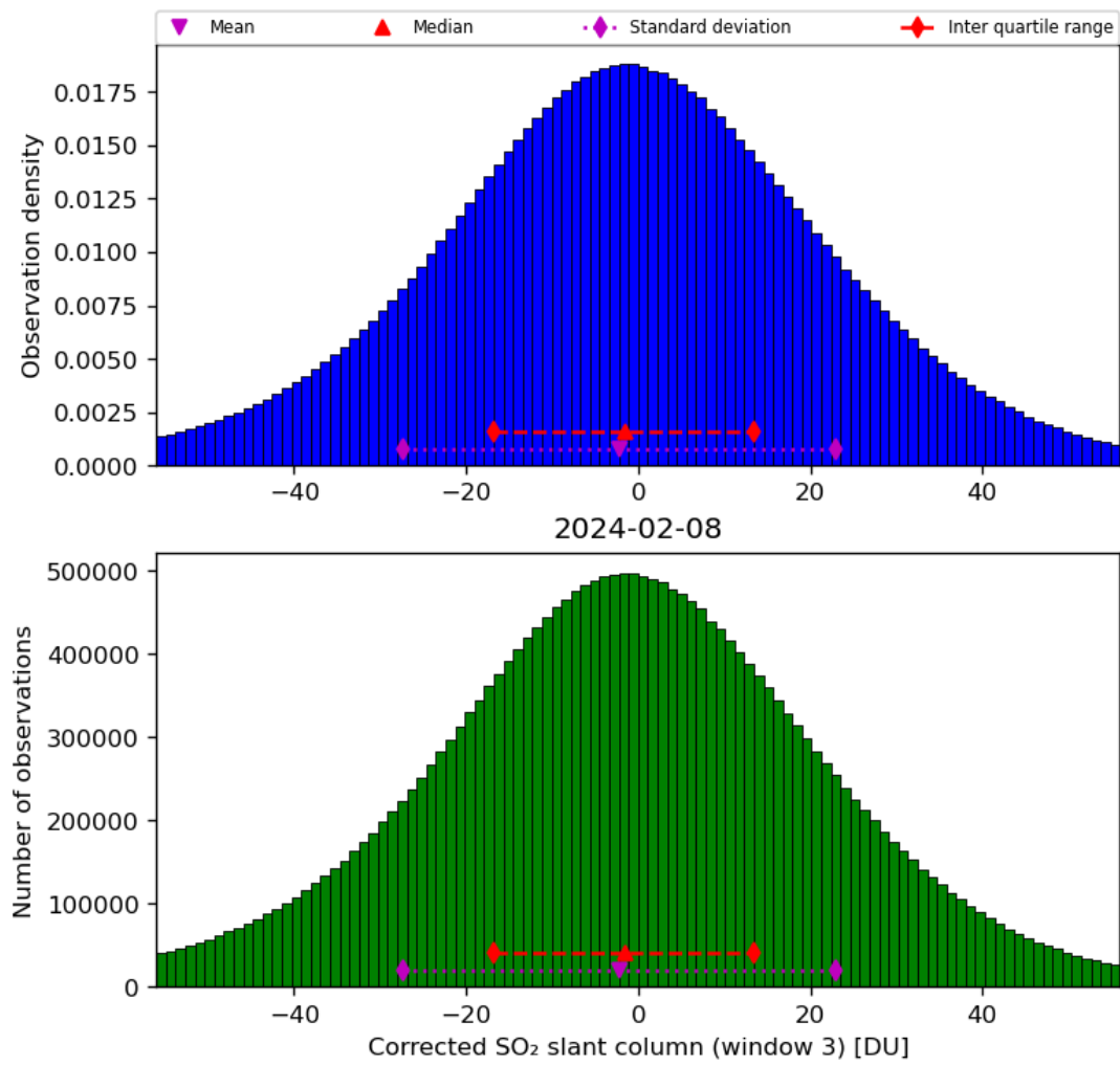
Figure 66: Histogram of “Corrected SO 2 slant column (window 3)” for 2024-02-07 to 2024-02-09
