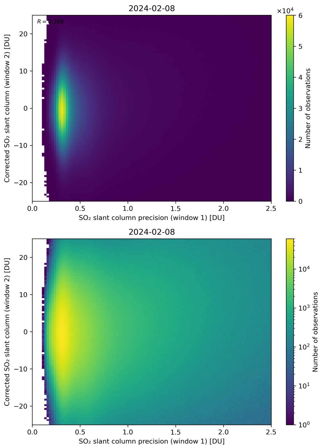
Figure 225: Scatter density plot of “SO 2 slant column precision (window 1)” against “Corrected SO 2 slant column (window 2)” for 2024-02-07 to 2024-02-09.
