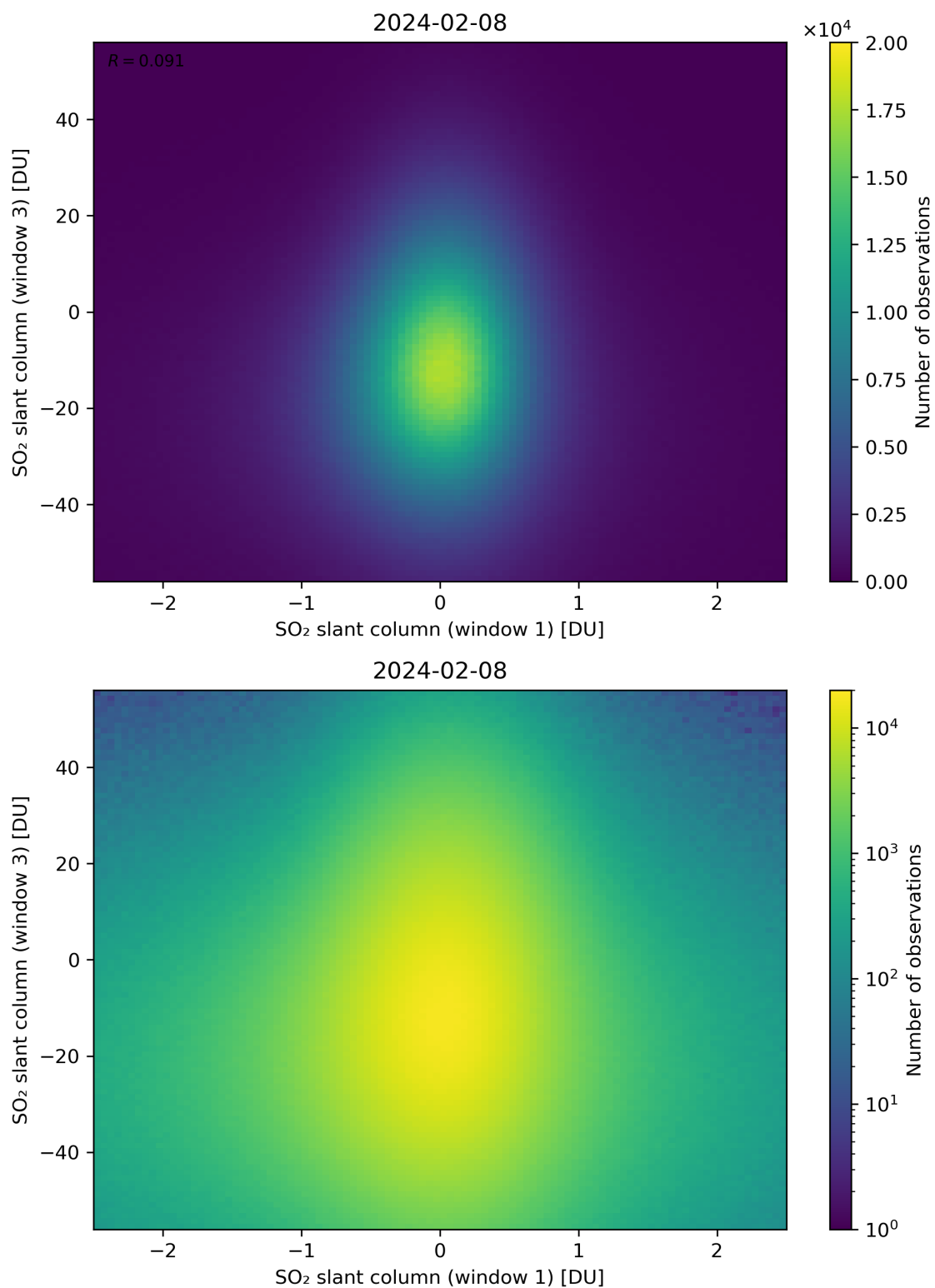
Figure 237: Scatter density plot of “SO 2 slant column (window 1)” against “SO 2 slant column (window 3)” for 2024-02-07 to 2024-02-09.
