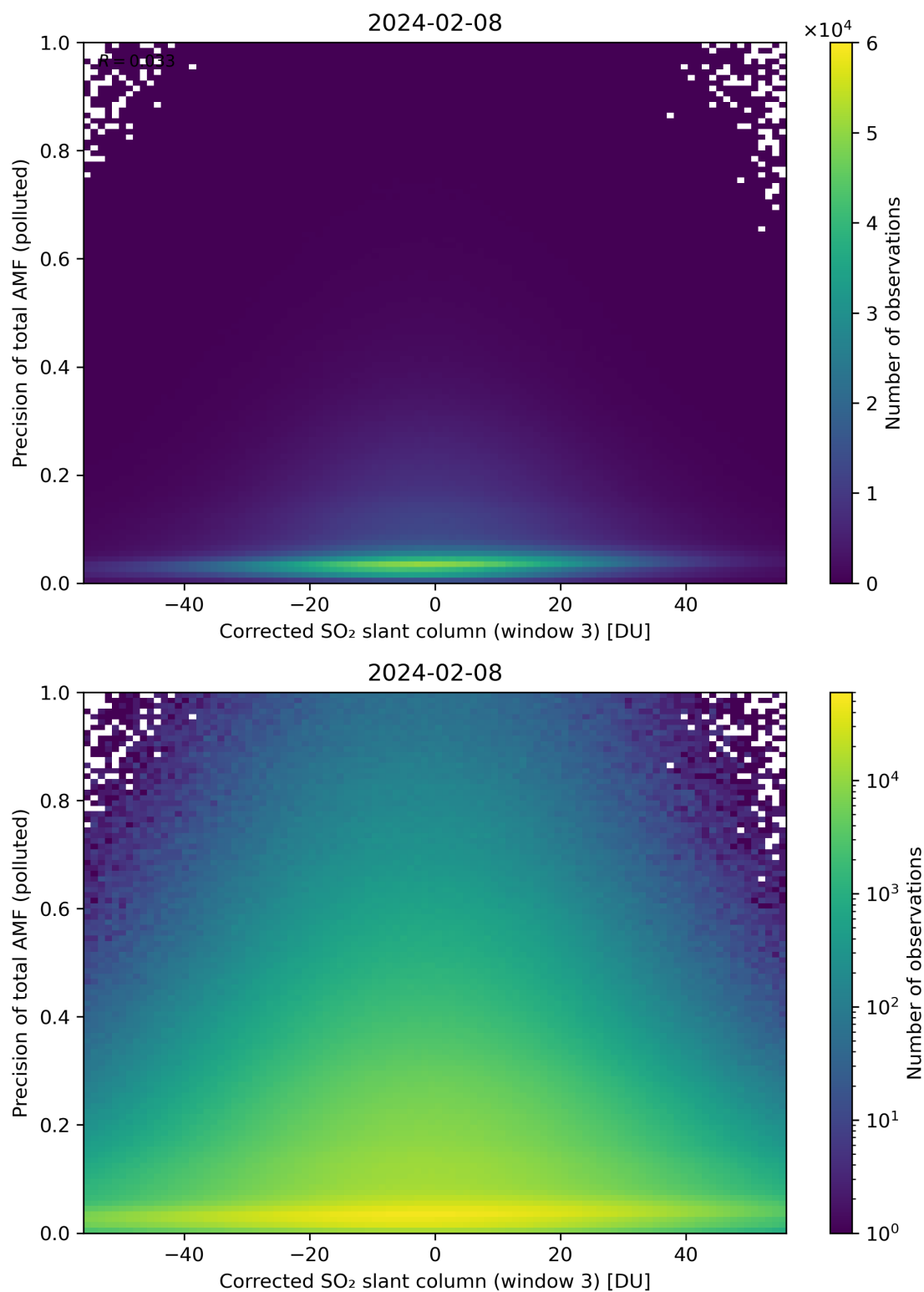
Figure 211: Scatter density plot of “Corrected SO 2 slant column (window 3)” against “Precision of total AMF (polluted)” for 2024-02-07 to 2024-02-09.
