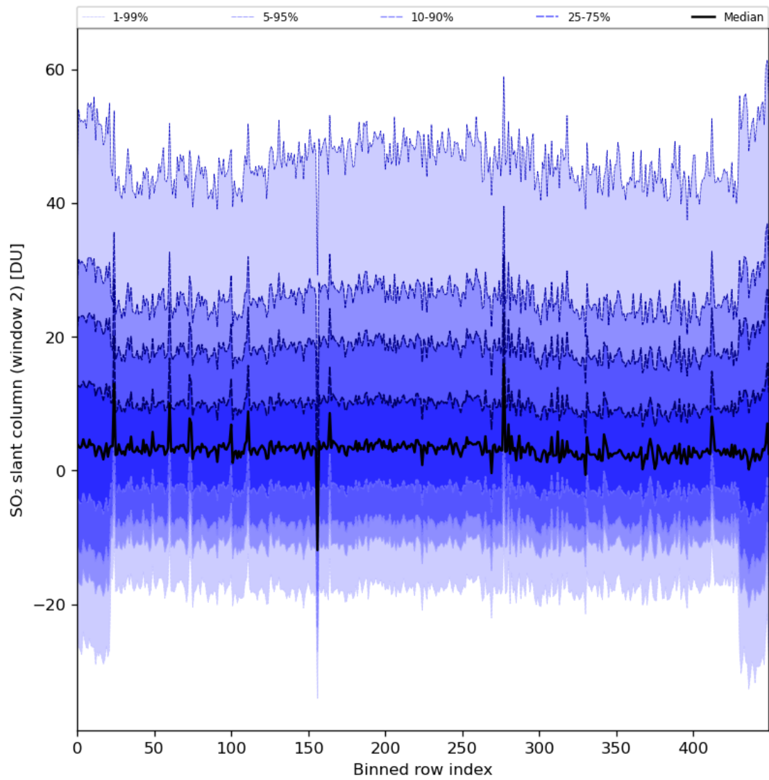
Figure 83: Along track statistics of “SO 2 slant column (window 2)” for 2024-02-07 to 2024-02-09
