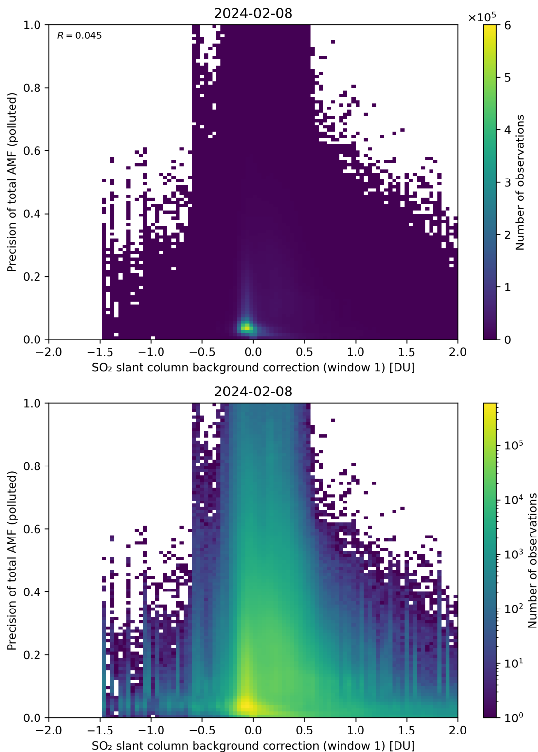
Figure 110: Scatter density plot of “SO 2 slant column background correction (window 1)” against “Precision of total AMF (polluted)” for 2024-02-07 to 2024-02-09.
