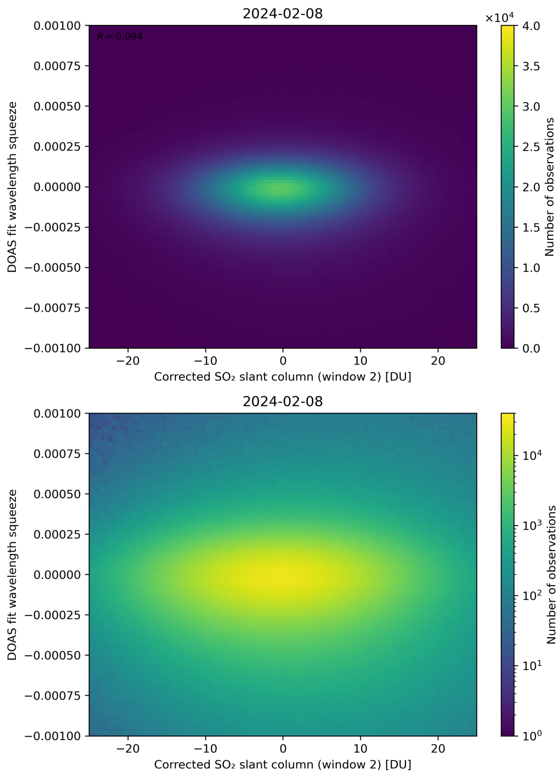
Figure 197: Scatter density plot of “Corrected SO 2 slant column (window 2)” against “DOAS fit wavelength squeeze” for 2024-02-07 to 2024-02-09.
