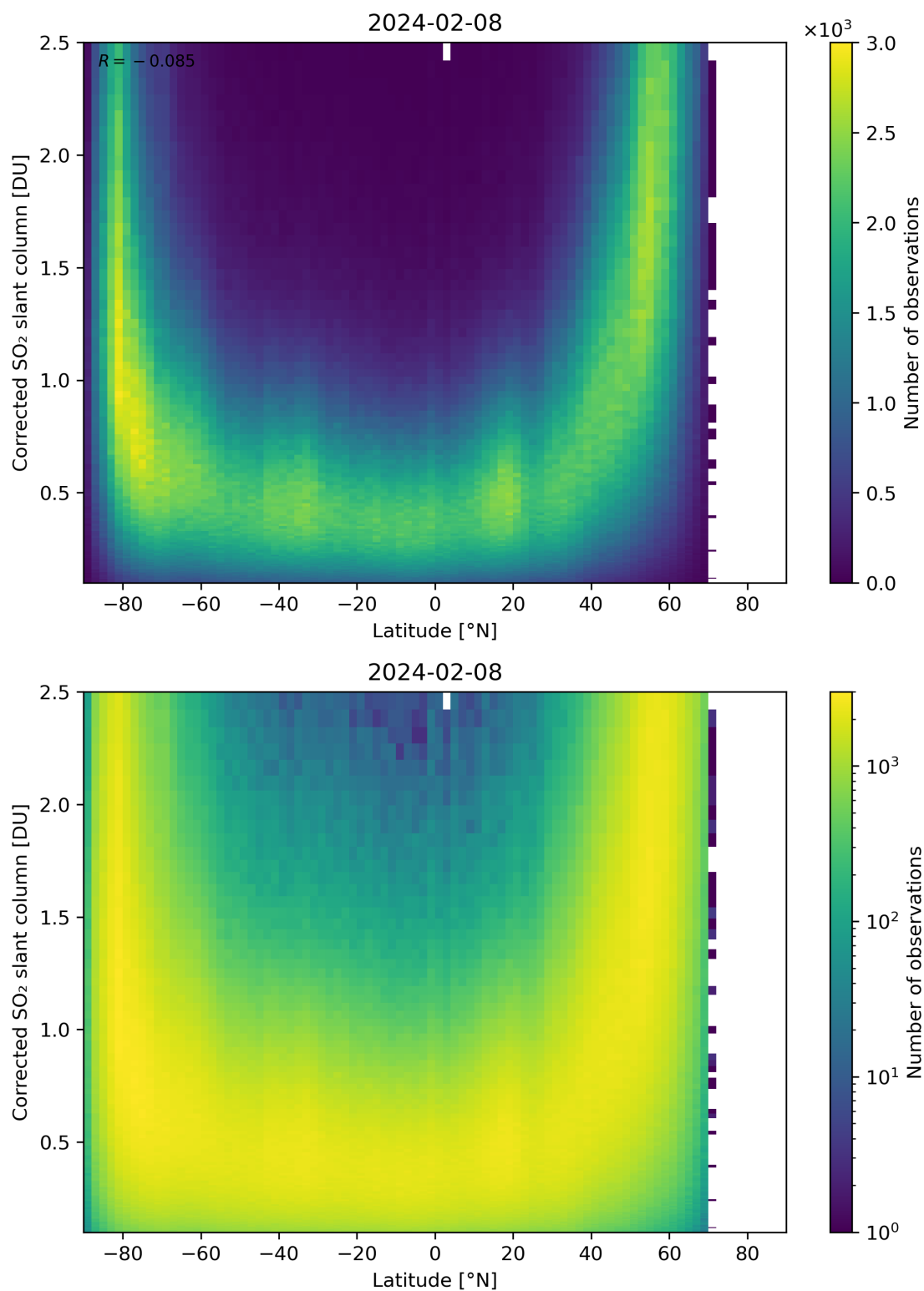
Figure 146: Scatter density plot of “Latitude” against “Corrected SO 2 slant column” for 2024-02-07 to 2024-02-09.
