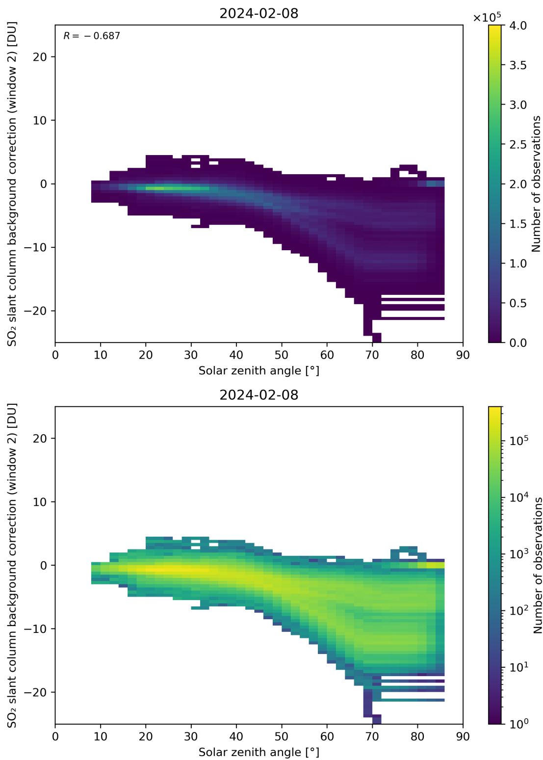
Figure 159: Scatter density plot of “Solar zenith angle” against “SO 2 slant column background correction (window 2)” for 2024-02-07 to 2024-02-09.
