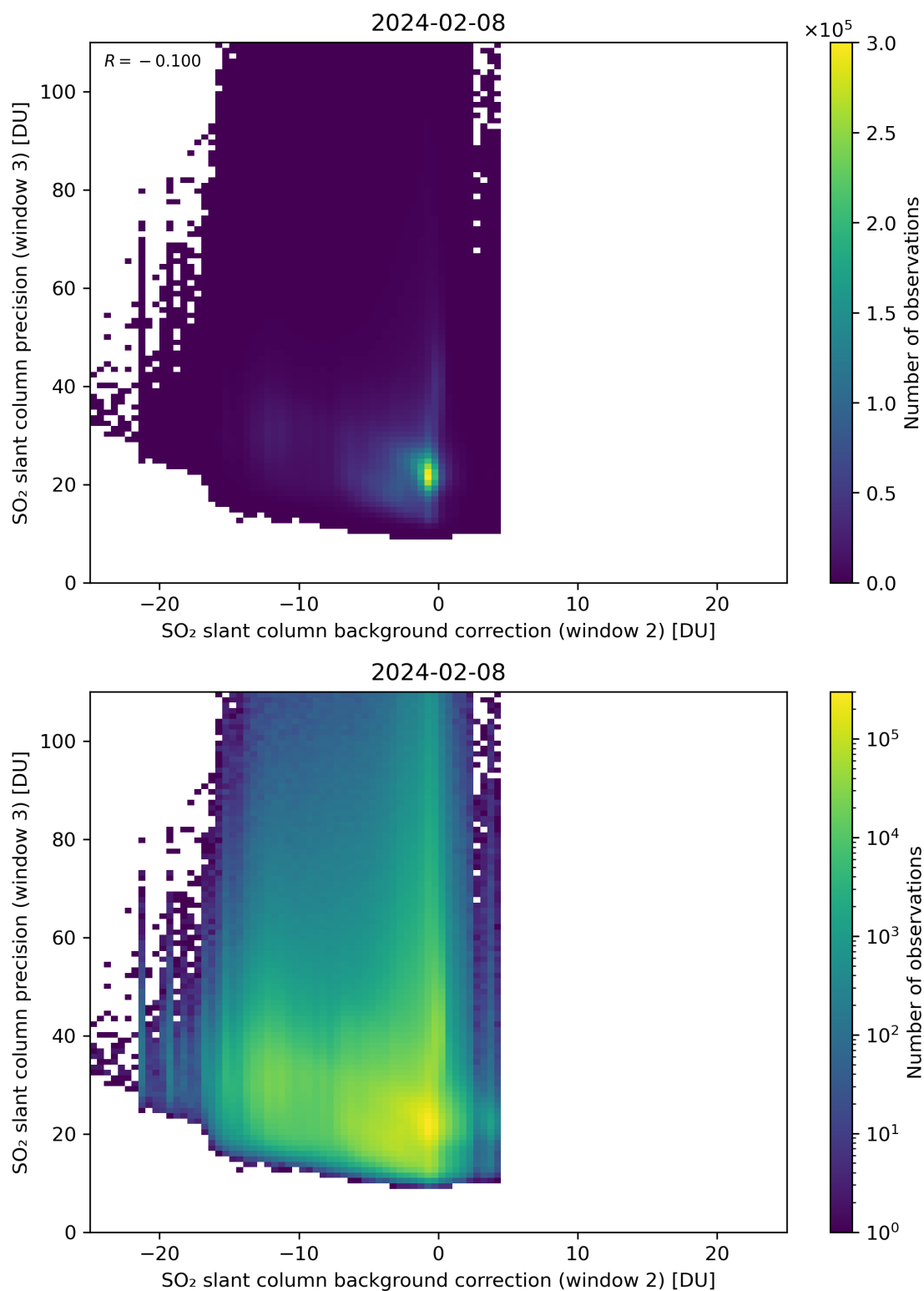
Figure 118: Scatter density plot of “SO 2 slant column background correction (window 2)” against “SO 2 slant column precision (window 3)” for 2024-02-07 to 2024-02-09.
