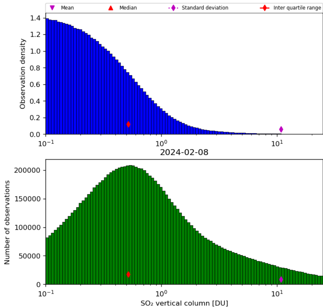
Figure 53: Histogram of “SO 2 vertical column” for 2024-02-07 to 2024-02-09
