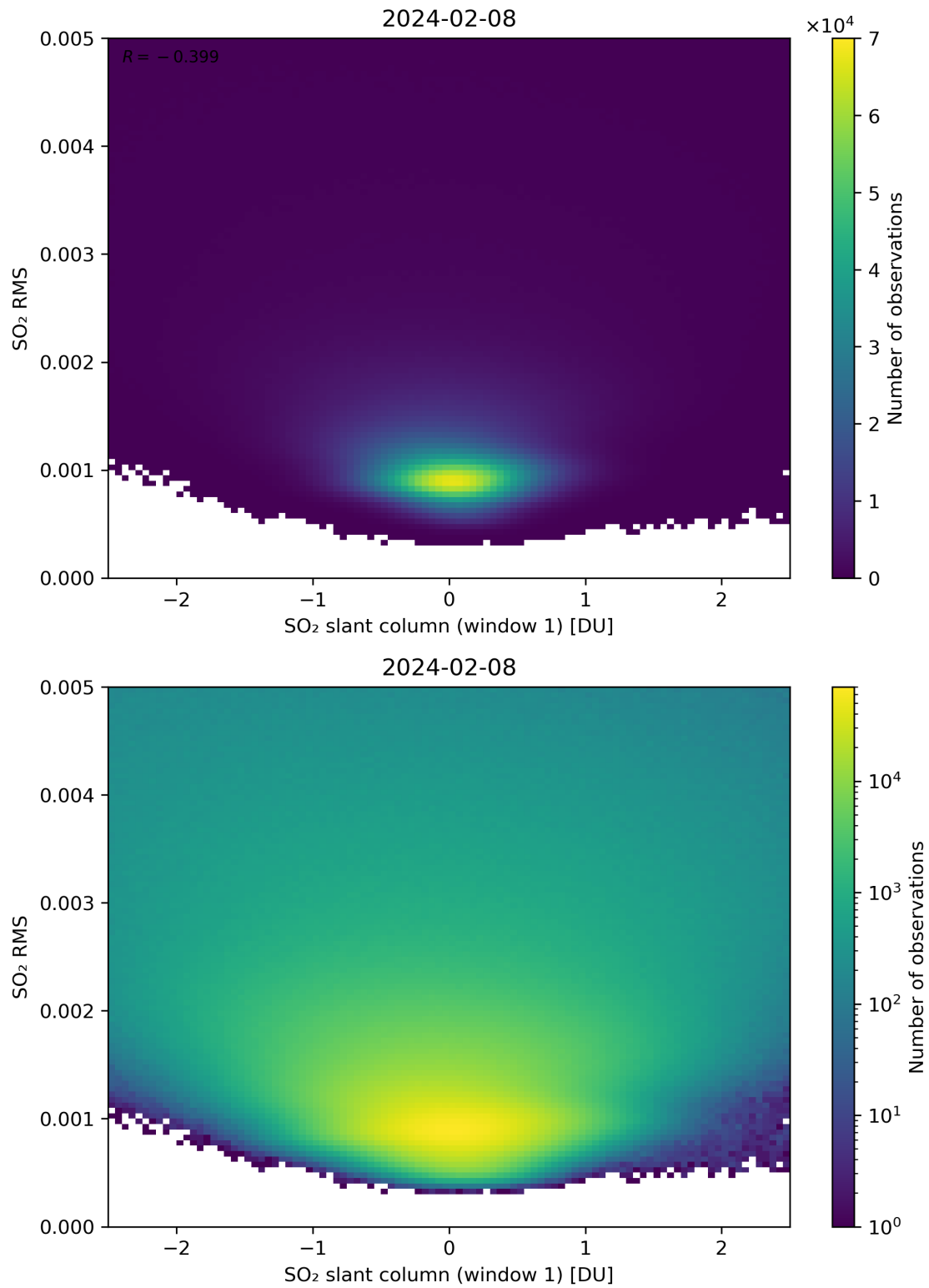
Figure 217: Scatter density plot of “SO 2 slant column (window 1)” against “SO 2 RMS” for 2024-02-07 to 2024-02-09.
