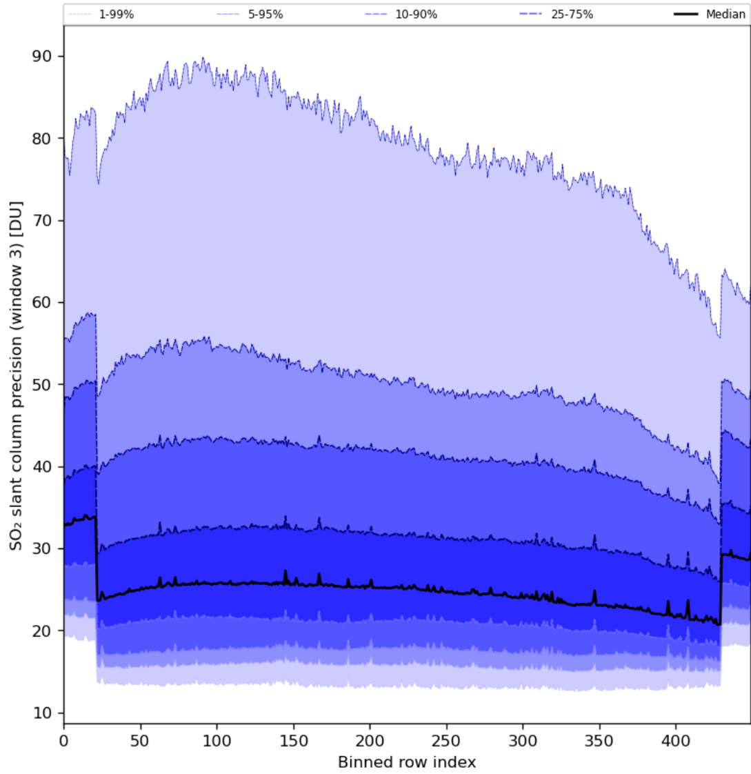
Figure 88: Along track statistics of “SO 2 slant column precision (window 3)” for 2024-02-07 to 2024-02-09
