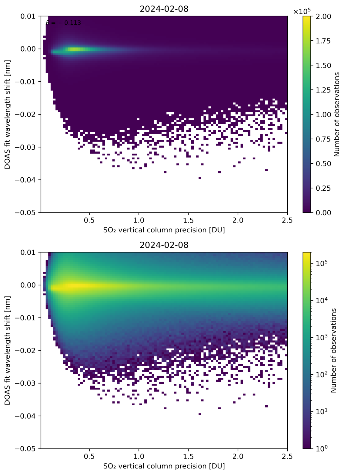
Figure 282: Scatter density plot of “SO 2 vertical column precision” against “DOAS fit wavelength shift” for 2024-02-07 to 2024-02-09.
