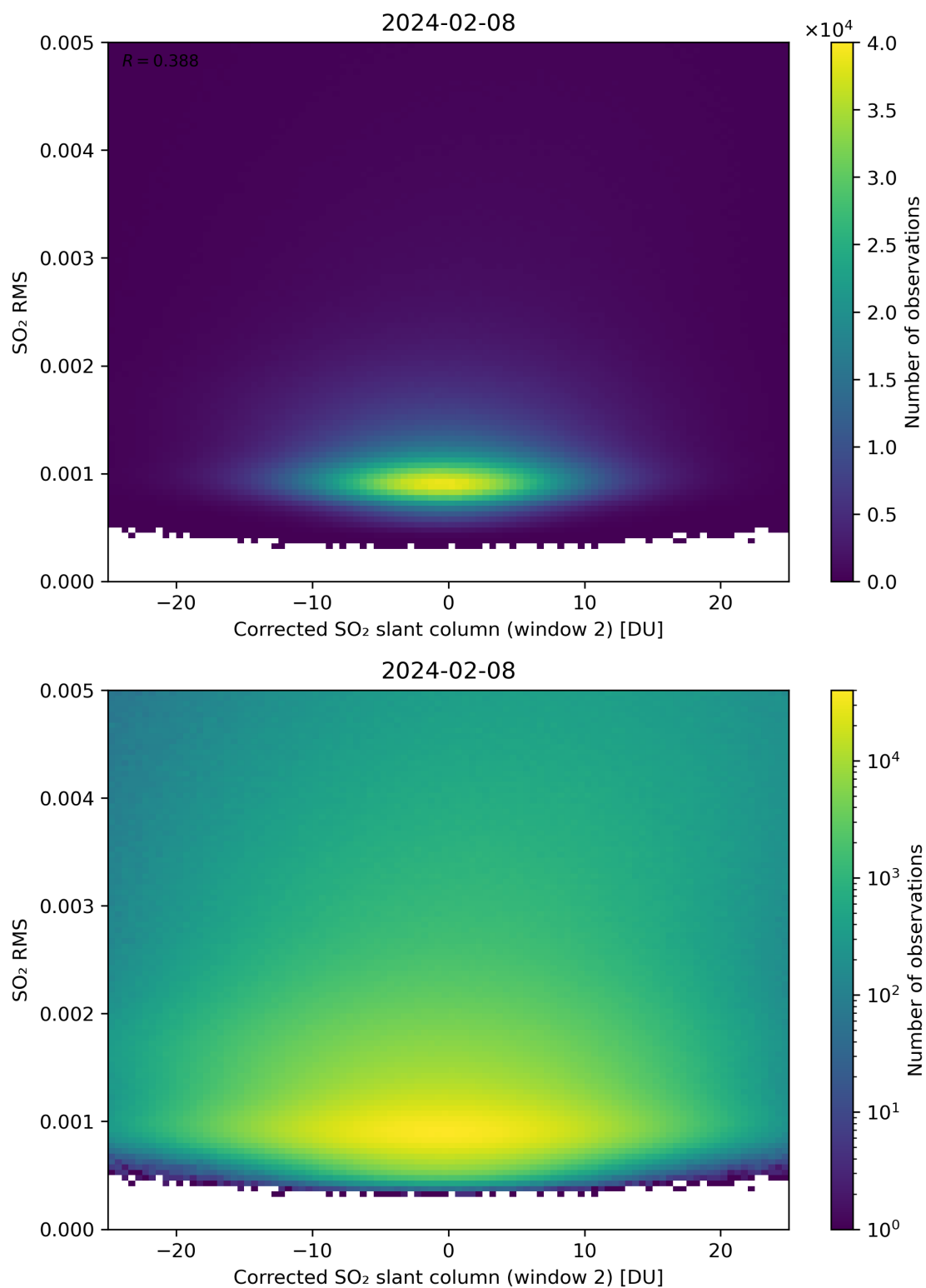
Figure 198: Scatter density plot of “Corrected SO 2 slant column (window 2)” against “SO 2 RMS” for 2024-02-07 to 2024-02-09.
