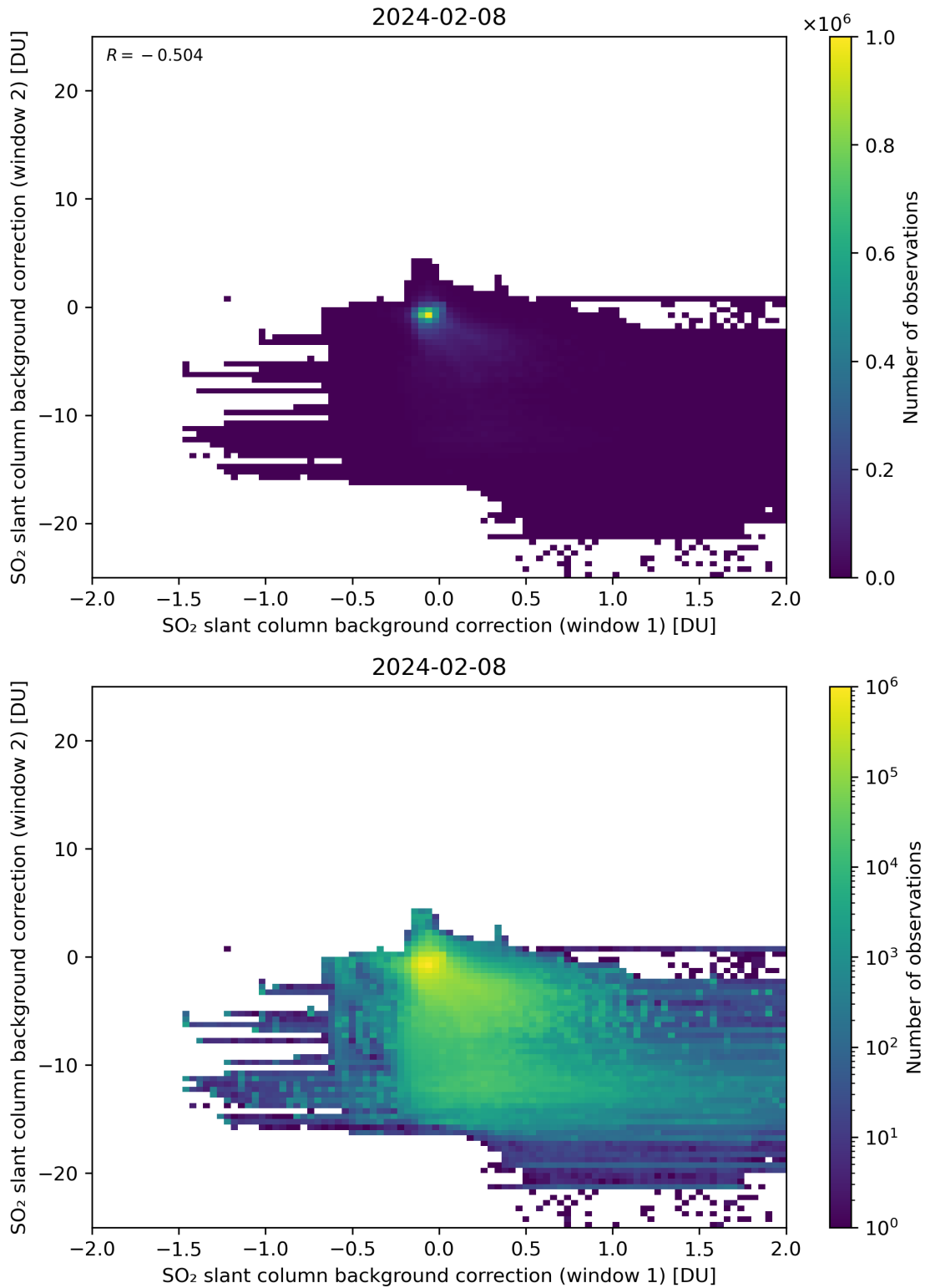
Figure 98: Scatter density plot of “SO 2 slant column background correction (window 1)” against “SO 2 slant column background correction (window 2)” for 2024-02-07 to 2024-02-09.
