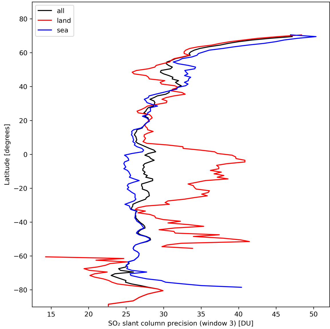
Figure 42: Zonal average of “SO 2 slant column precision (window 3)” for 2024-02-07 to 2024-02-09.
