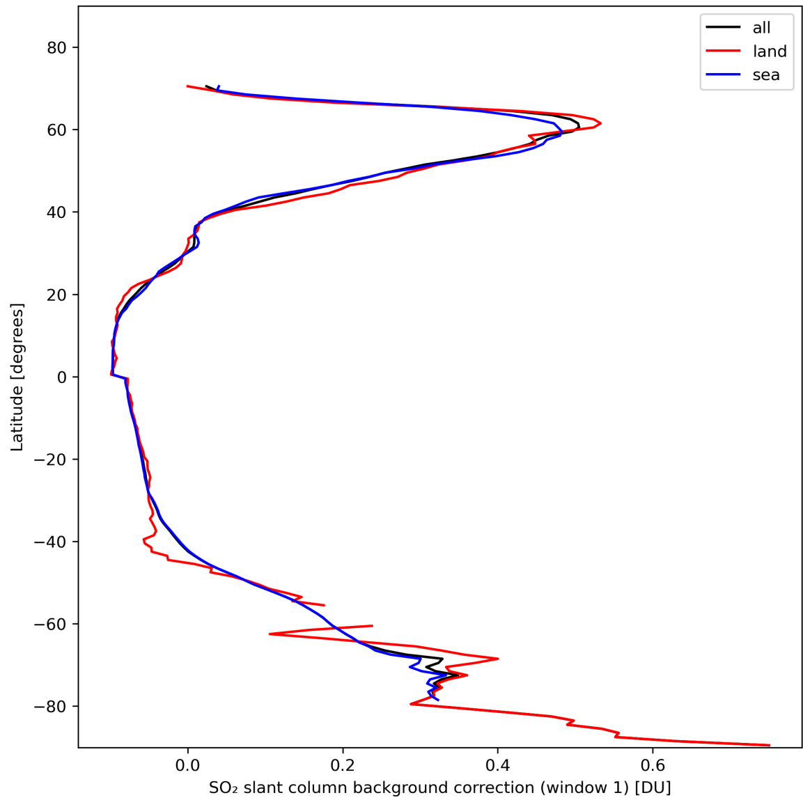
Figure 36: Zonal average of “SO 2 slant column background correction (window 1)” for 2024-02-07 to 2024-02-09.
