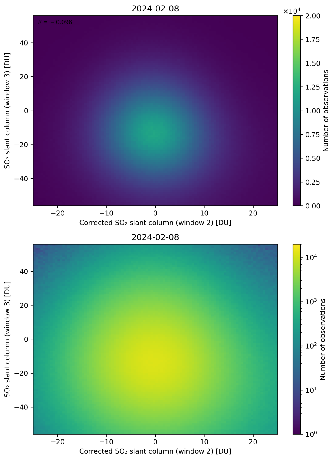
Figure 201: Scatter density plot of “Corrected SO 2 slant column (window 2)” against “SO 2 slant column (window 3)” for 2024-02-07 to 2024-02-09.
