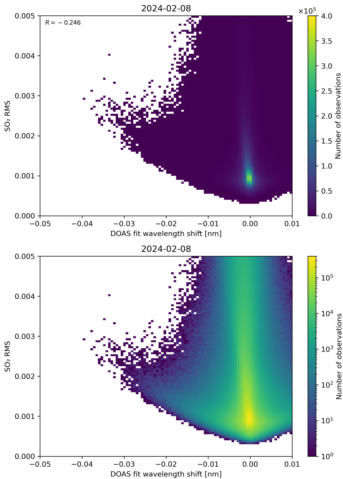
Figure 128: Scatter density plot of “DOAS fit wavelength shift” against “SO 2 RMS” for 2024-02-07 to 2024-02-09.
