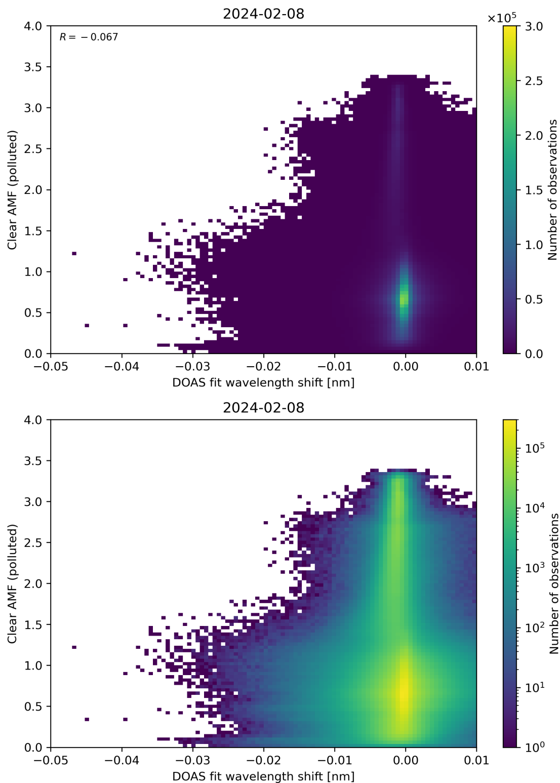
Figure 129: Scatter density plot of “DOAS fit wavelength shift” against “Clear AMF (polluted)” for 2024-02-07 to 2024-02-09.
