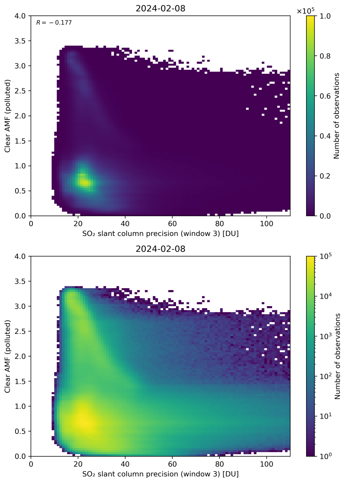
Figure 261: Scatter density plot of “SO 2 slant column precision (window 3)” against “Clear AMF (polluted)” for 2024-02-07 to 2024-02-09.
