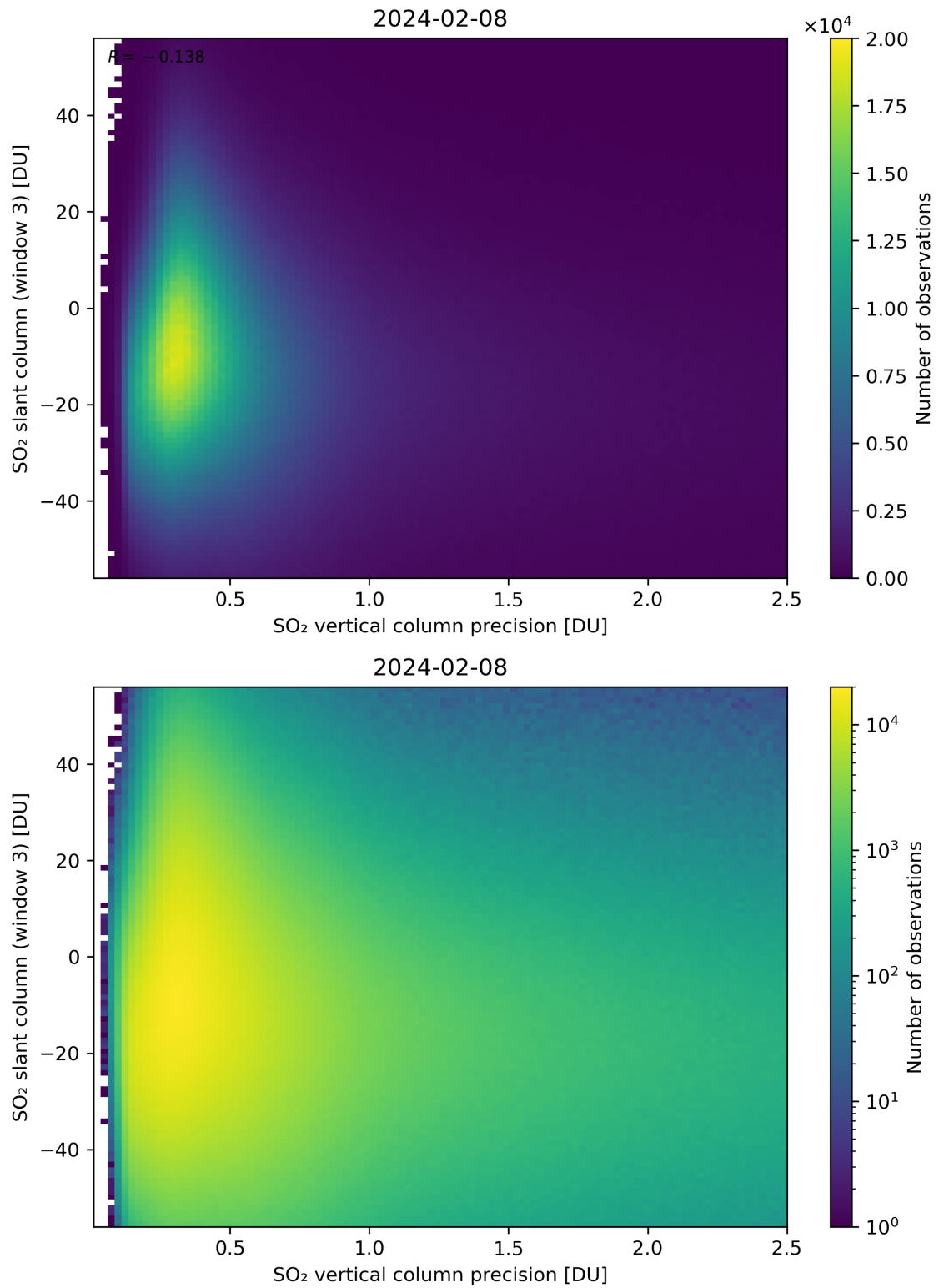
Figure 292: Scatter density plot of “SO 2 vertical column precision” against “SO 2 slant column (window 3)” for 2024-02-07 to 2024-02-09.
