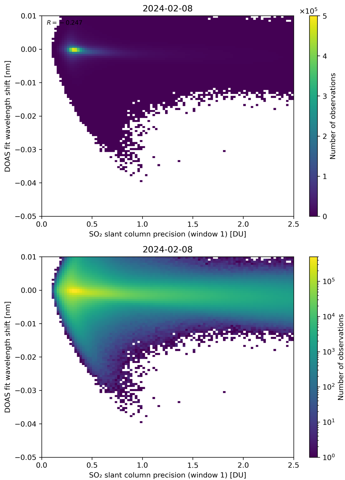
Figure 221: Scatter density plot of “SO 2 slant column precision (window 1)” against “DOAS fit wavelength shift” for 2024-02-07 to 2024-02-09.
