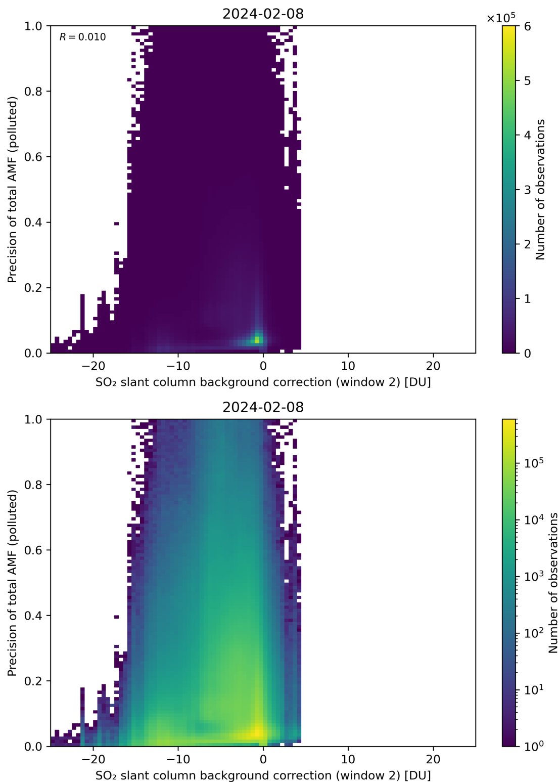
Figure 120: Scatter density plot of “SO 2 slant column background correction (window 2)” against “Precision of total AMF (polluted)” for 2024-02-07 to 2024-02-09.
