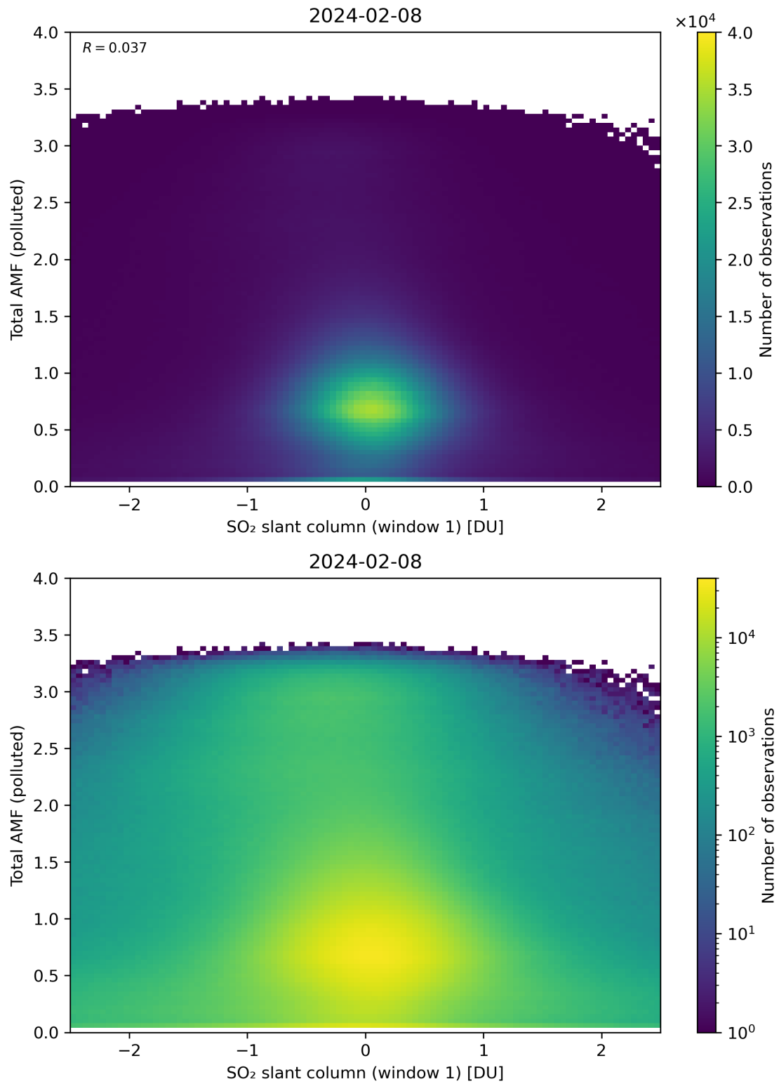
Figure 239: Scatter density plot of “SO 2 slant column (window 1)” against “Total AMF (polluted)” for 2024-02-07 to 2024-02-09.
