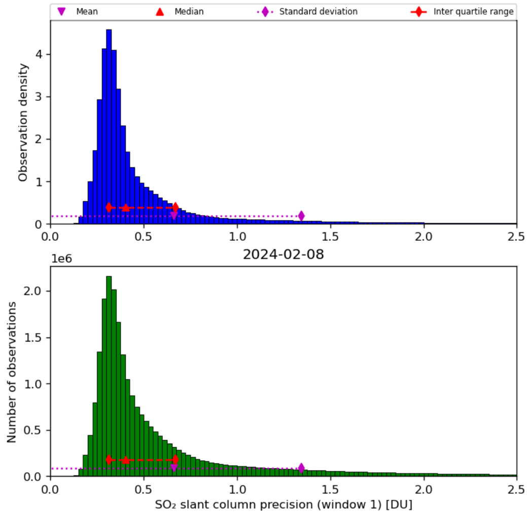
Figure 57: Histogram of “SO 2 slant column precision (window 1)” for 2024-02-07 to 2024-02-09
