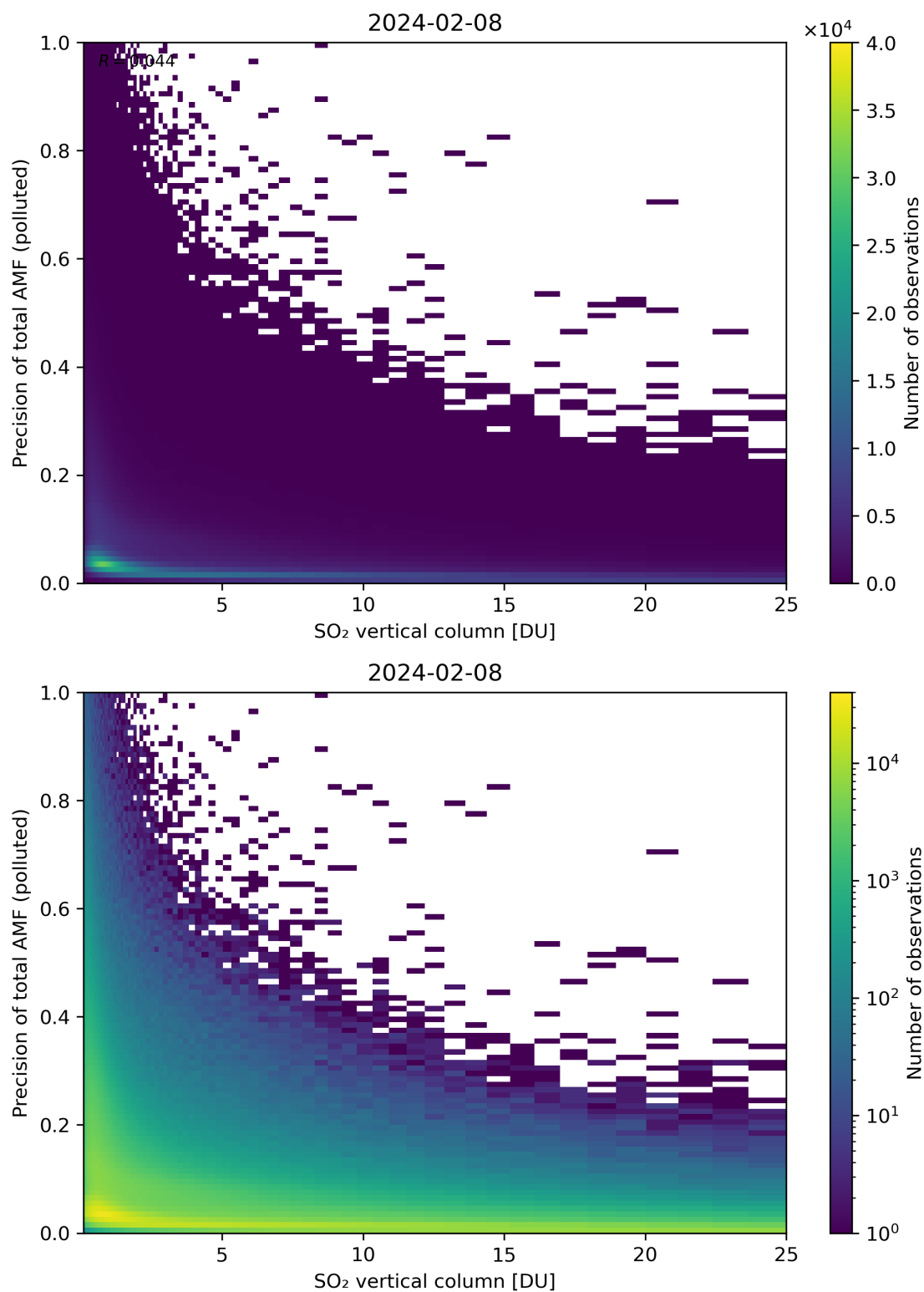
Figure 306: Scatter density plot of “SO 2 vertical column” against “Precision of total AMF (polluted)” for 2024-02-07 to 2024-02-09.
