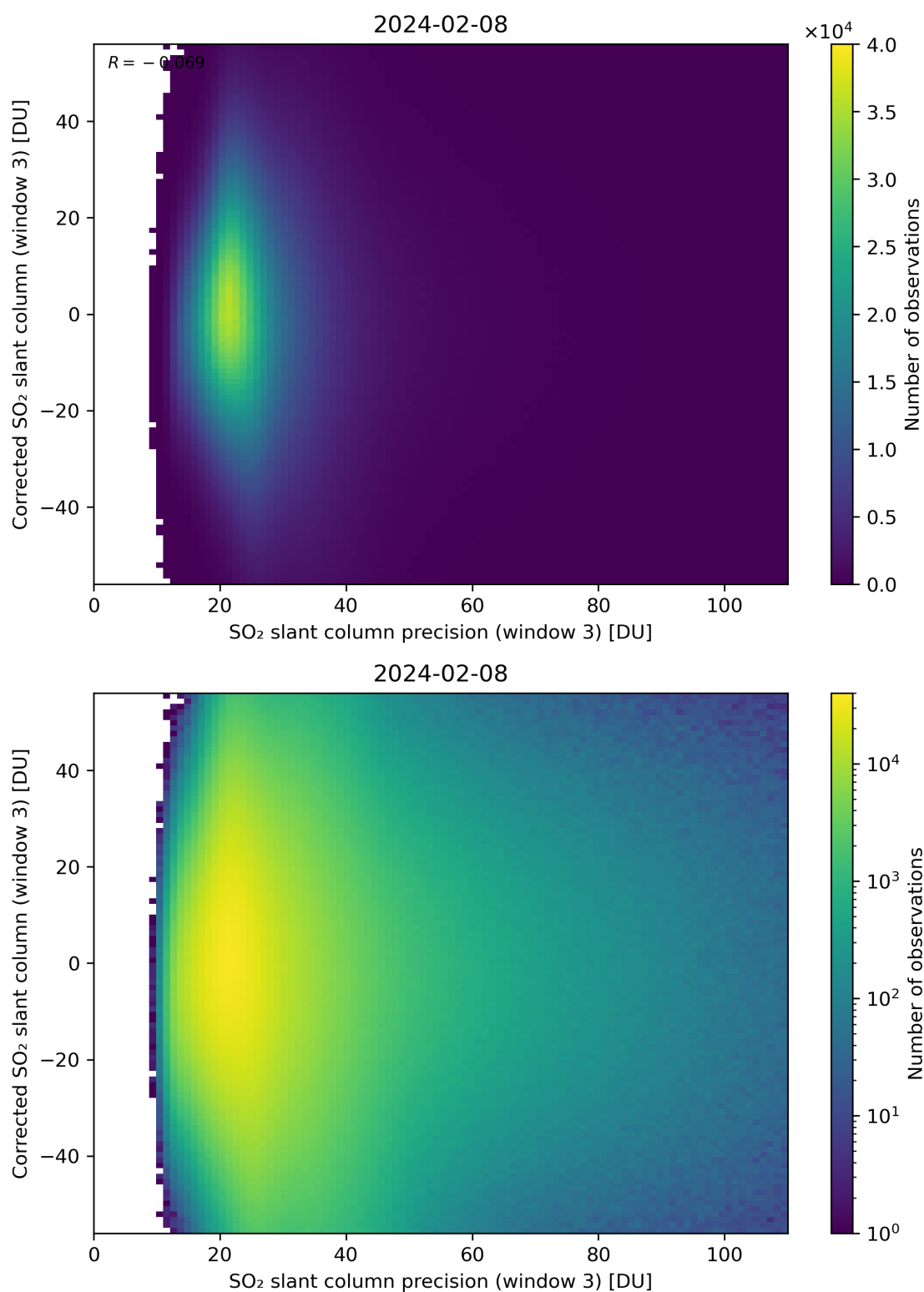
Figure 262: Scatter density plot of “SO 2 slant column precision (window 3)” against “Corrected SO 2 slant column (window 3)” for 2024-02-07 to 2024-02-09.
