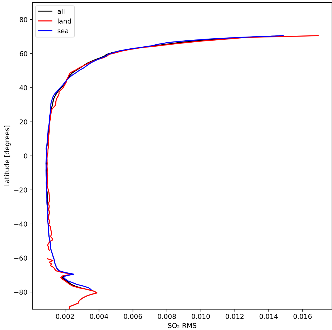
Figure 47: Zonal average of “SO 2 RMS” for 2024-02-07 to 2024-02-09.
