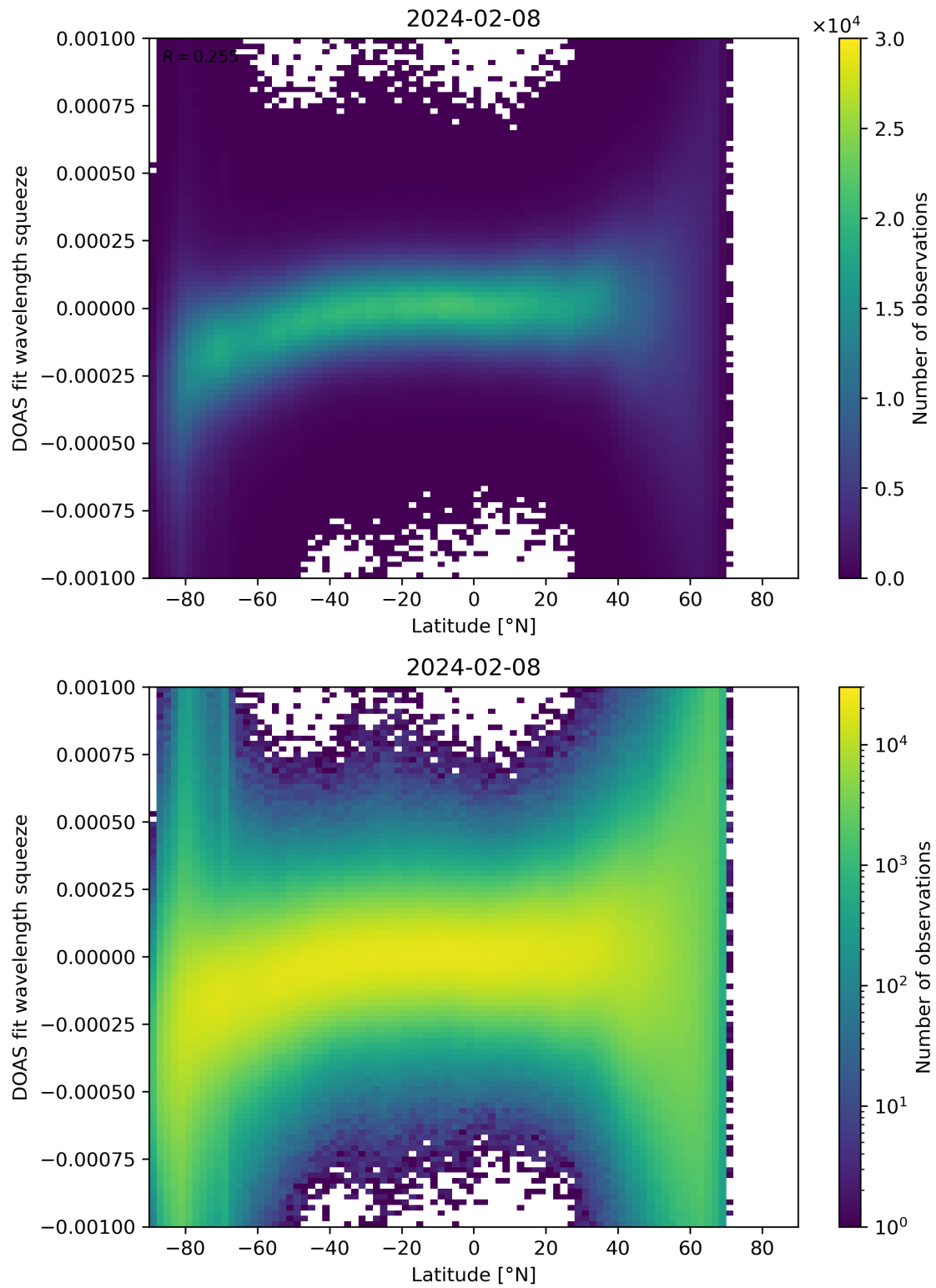
Figure 143: Scatter density plot of “Latitude” against “DOAS fit wavelength squeeze” for 2024-02-07 to 2024-02-09.
