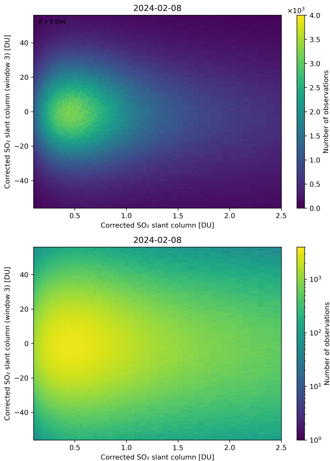
Figure 186: Scatter density plot of “Corrected SO 2 slant column” against “Corrected SO 2 slant column (window 3)” for 2024-02-07 to 2024-02-09.
