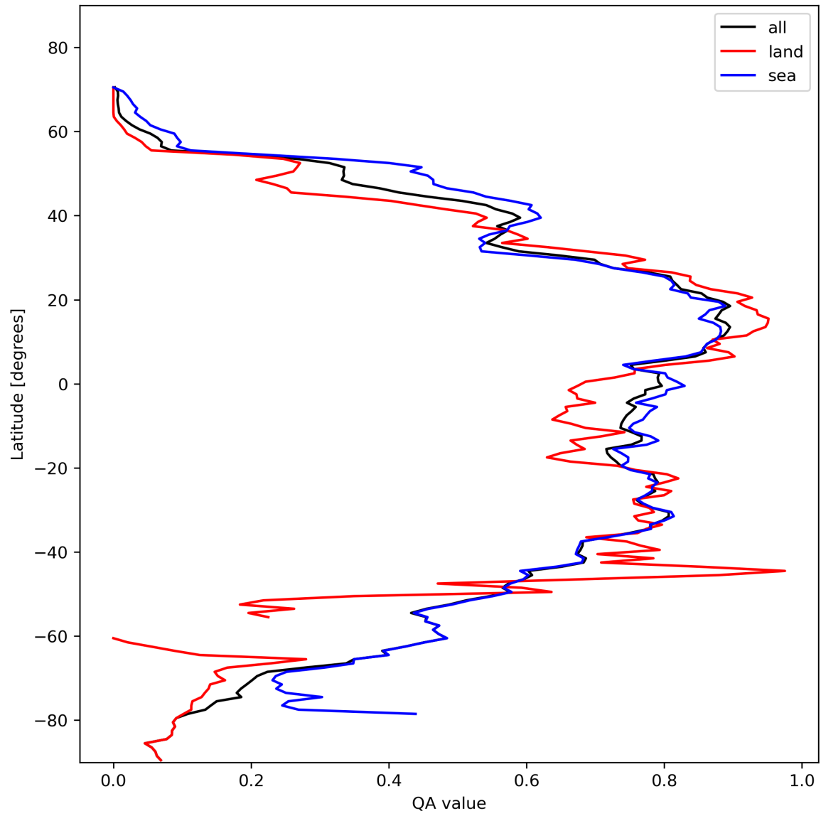
Figure 29: Zonal average of “QA value” for 2024-02-07 to 2024-02-09.
