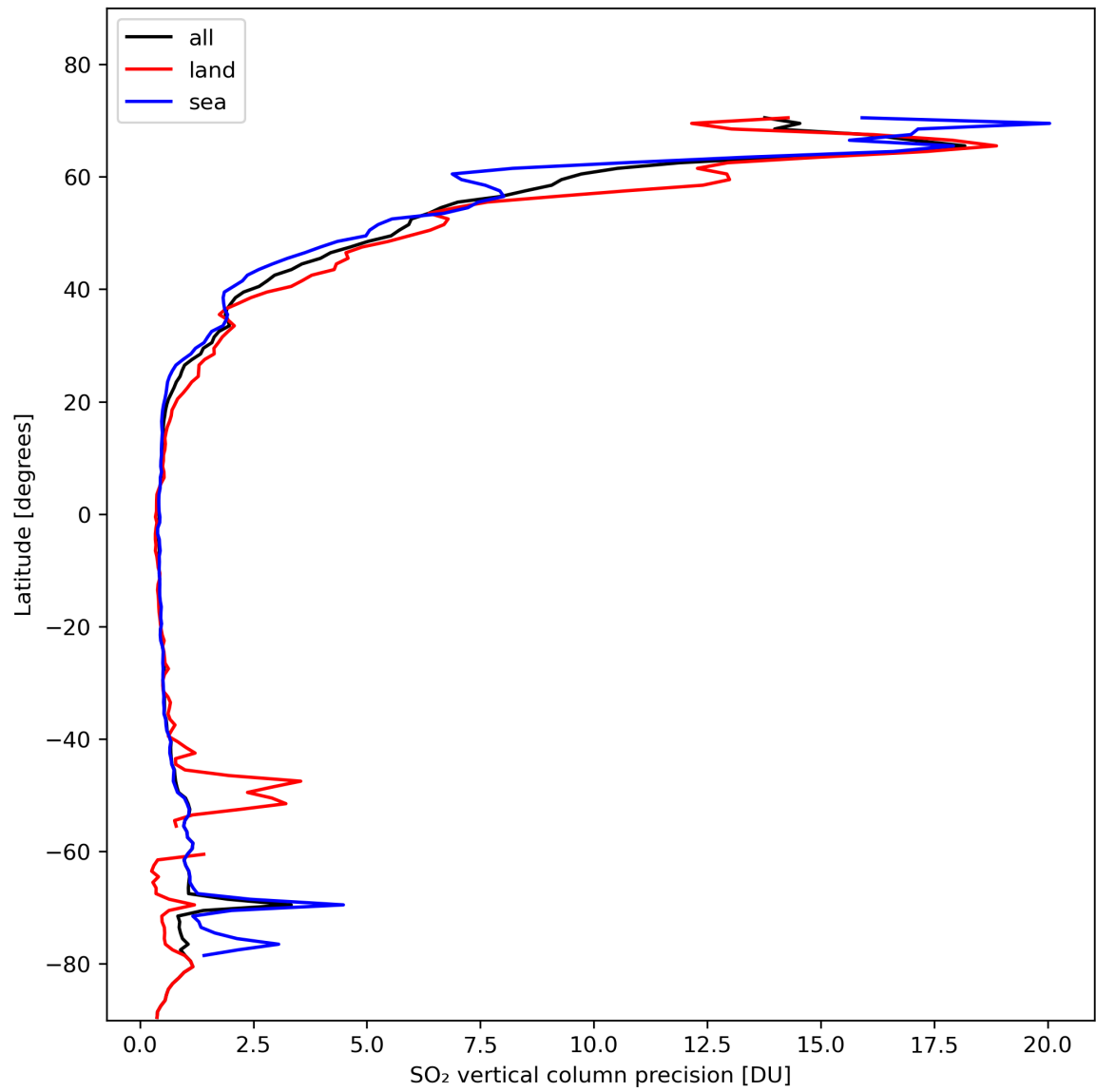
Figure 31: Zonal average of “SO 2 vertical column precision” for 2024-02-07 to 2024-02-09.
