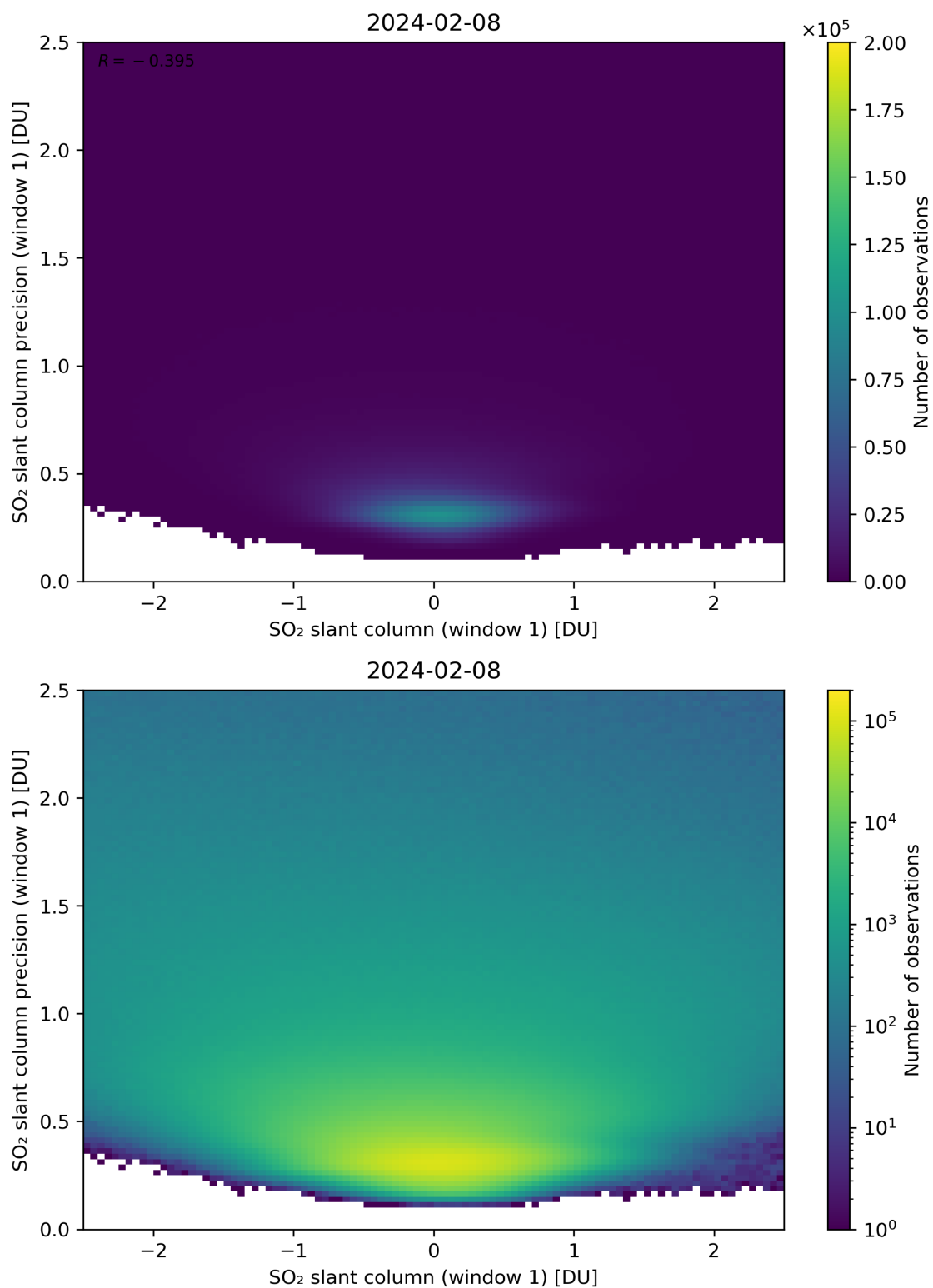
Figure 235: Scatter density plot of “SO 2 slant column (window 1)” against “SO 2 slant column precision (window 1)” for 2024-02-07 to 2024-02-09.
