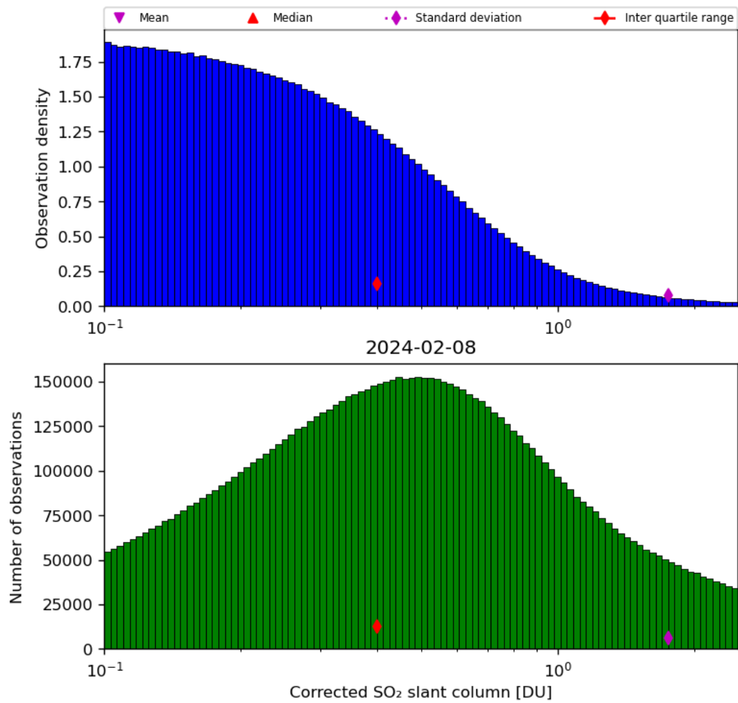
Figure 55: Histogram of “Corrected SO 2 slant column” for 2024-02-07 to 2024-02-09
