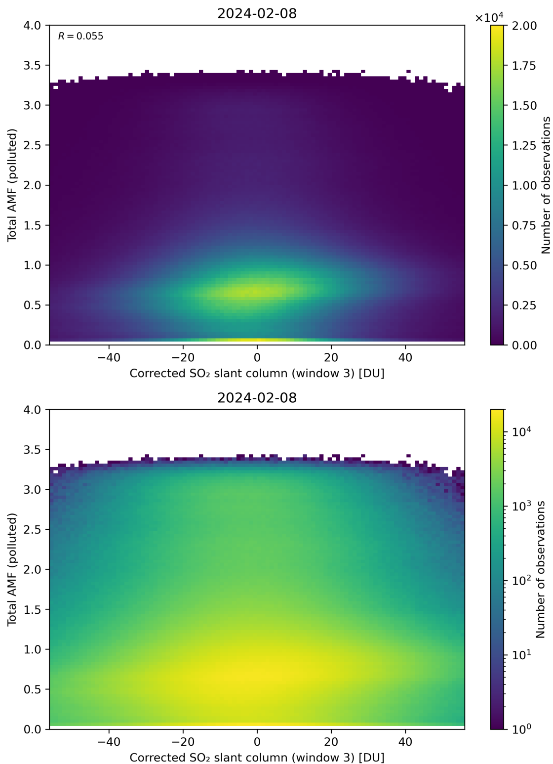
Figure 210: Scatter density plot of “Corrected SO 2 slant column (window 3)” against “Total AMF (polluted)” for 2024-02-07 to 2024-02-09.
