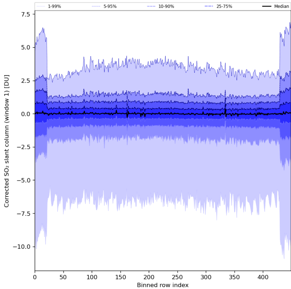
Figure 81: Along track statistics of “Corrected SO 2 slant column (window 1)” for 2024-02-07 to 2024-02-09
