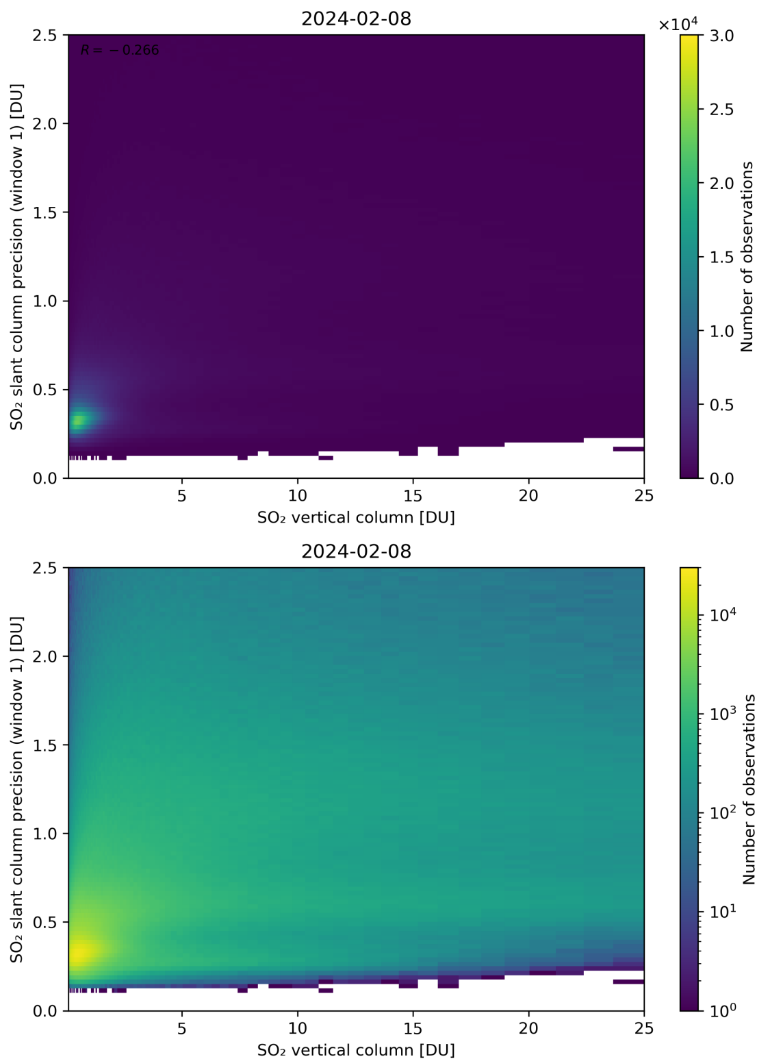
Figure 301: Scatter density plot of “SO 2 vertical column” against “SO 2 slant column precision (window 1)” for 2024-02-07 to 2024-02-09.
