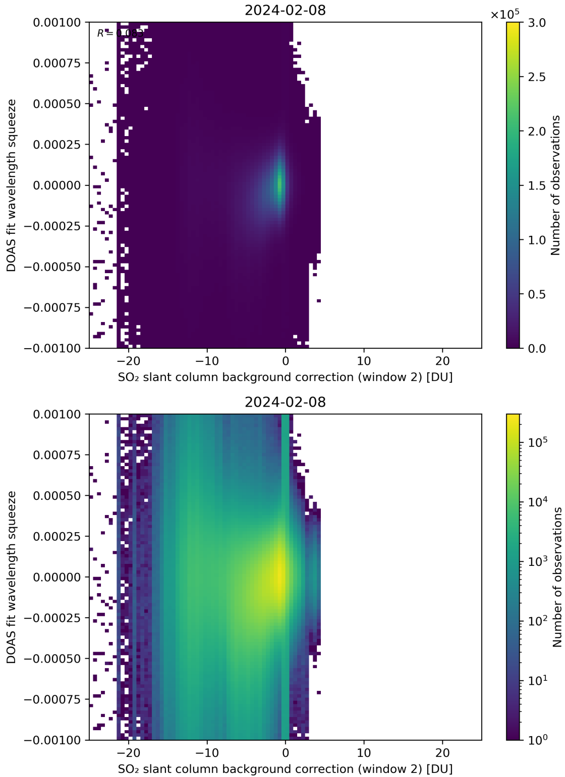
Figure 113: Scatter density plot of “SO 2 slant column background correction (window 2)” against “DOAS fit wavelength squeeze” for 2024-02-07 to 2024-02-09.
