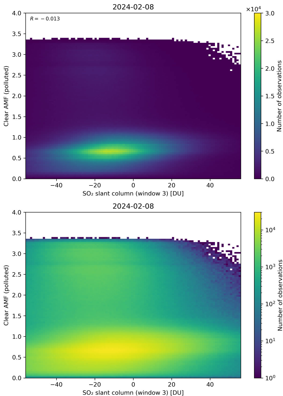
Figure 265: Scatter density plot of “SO 2 slant column (window 3)” against “Clear AMF (polluted)” for 2024-02-07 to 2024-02-09.
