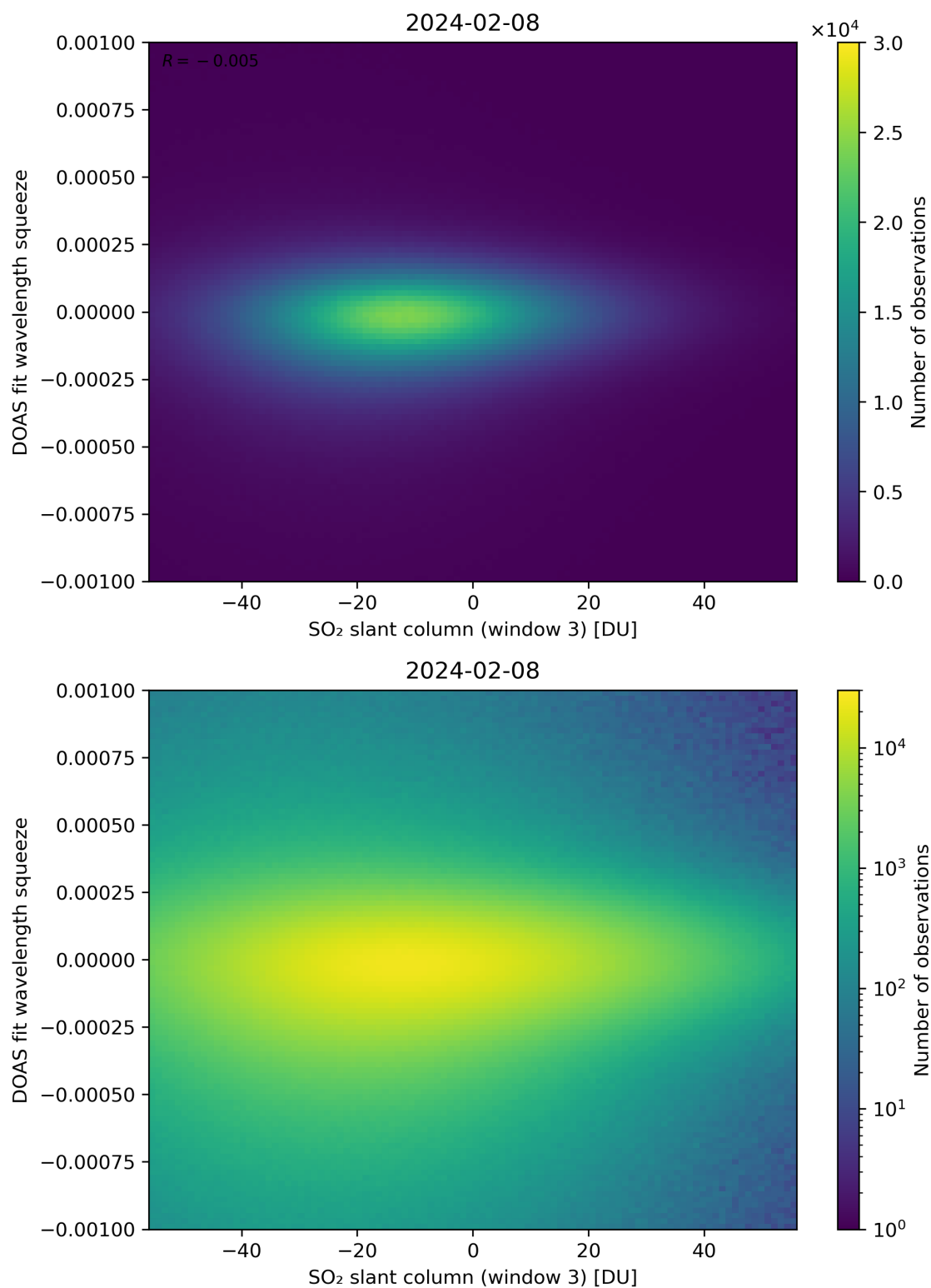
Figure 255: Scatter density plot of “SO 2 slant column (window 3)” against “DOAS fit wavelength squeeze” for 2024-02-07 to 2024-02-09.
