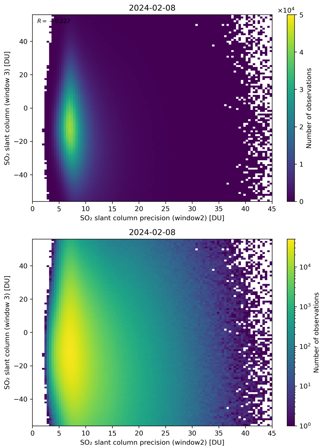
Figure 249: Scatter density plot of “SO 2 slant column precision (window2)” against “SO 2 slant column (window 3)” for 2024-02-07 to 2024-02-09.
