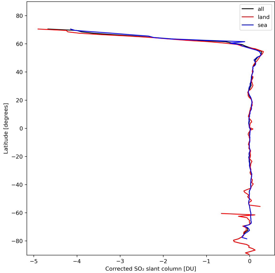
Figure 32: Zonal average of “Corrected SO 2 slant column” for 2024-02-07 to 2024-02-09.
