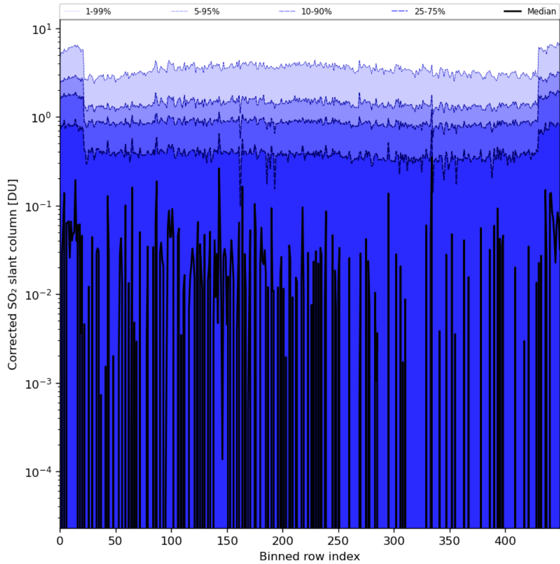
Figure 78: Along track statistics of “Corrected SO 2 slant column” for 2024-02-07 to 2024-02-09
