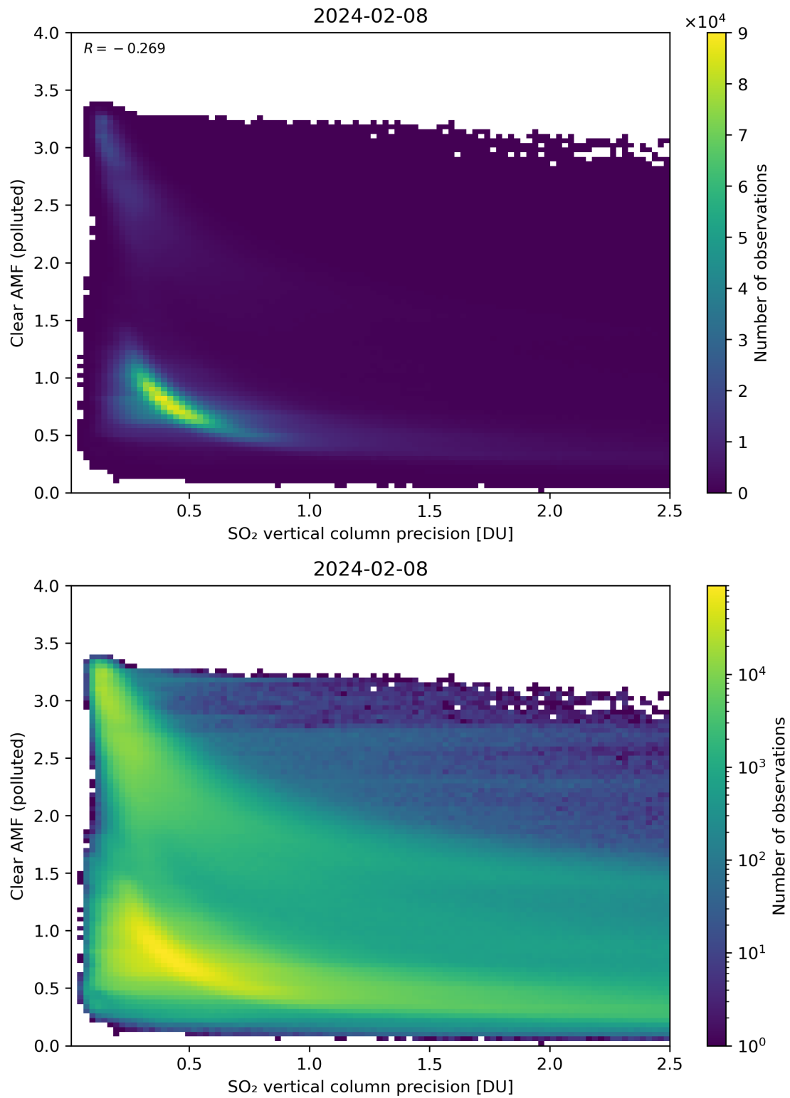
Figure 285: Scatter density plot of “SO 2 vertical column precision” against “Clear AMF (polluted)” for 2024-02-07 to 2024-02-09.
