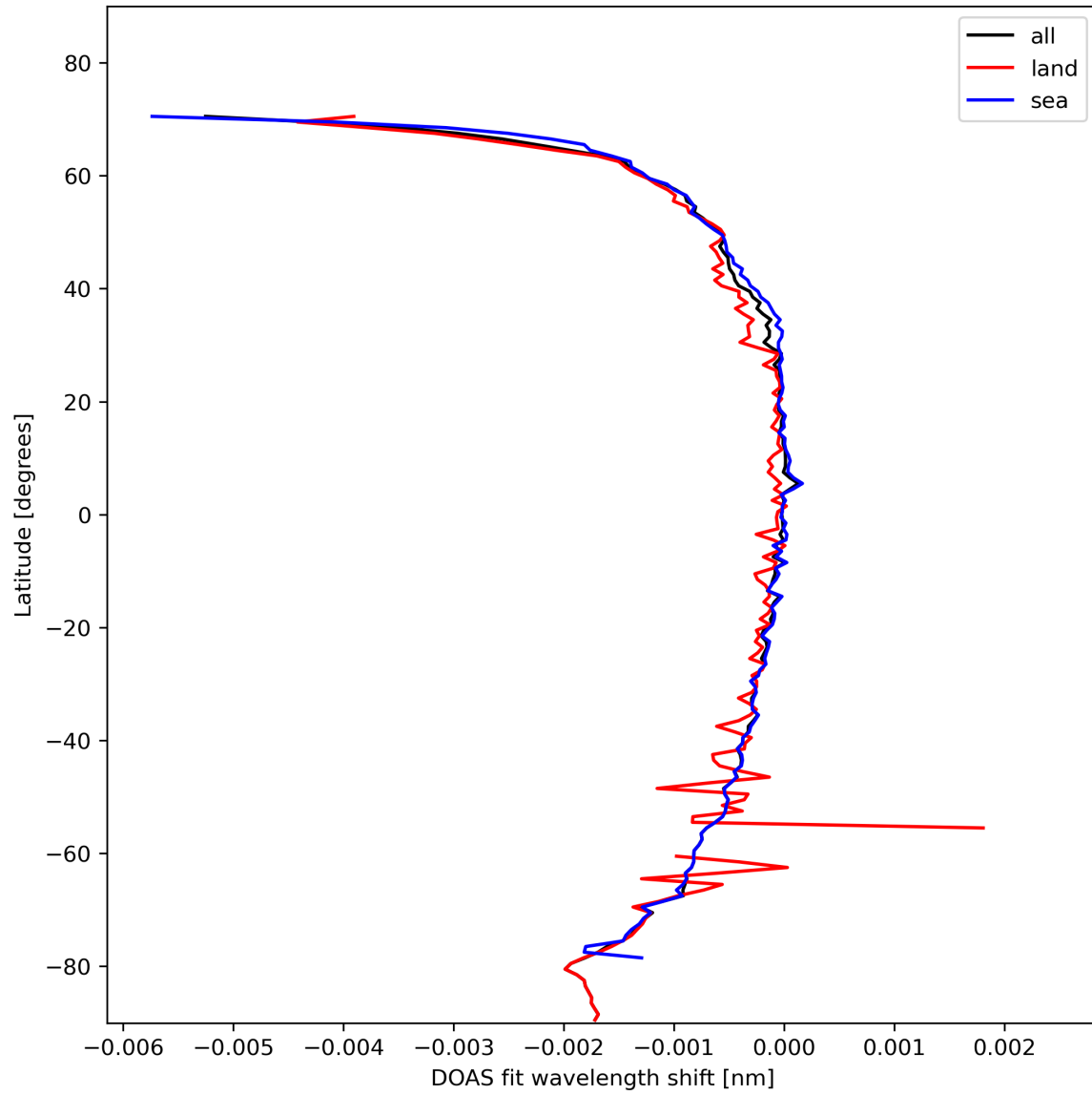
Figure 45: Zonal average of “DOAS fit wavelength shift” for 2024-02-07 to 2024-02-09.
