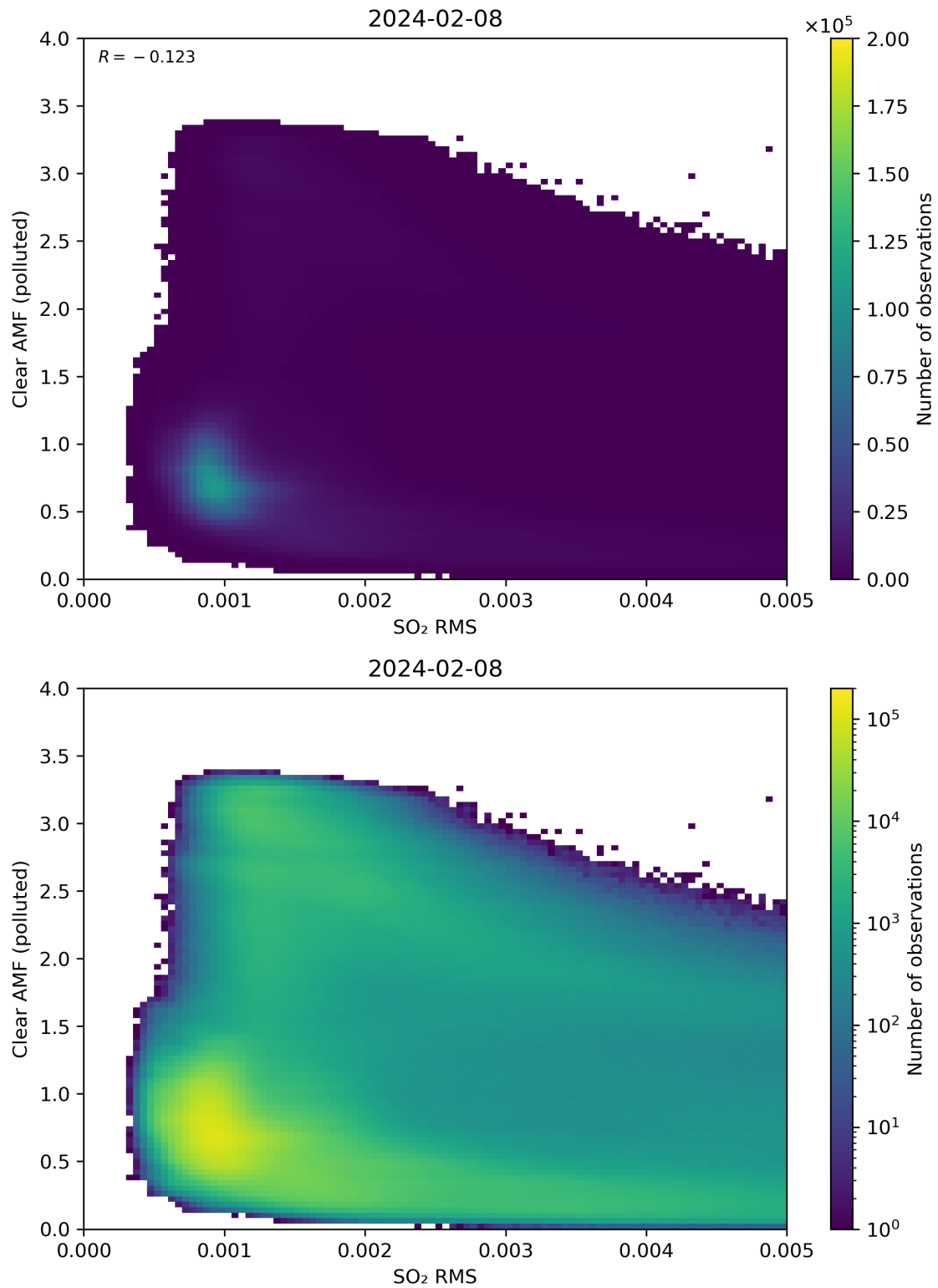
Figure 136: Scatter density plot of “SO 2 RMS” against “Clear AMF (polluted)” for 2024-02-07 to 2024-02-09.
