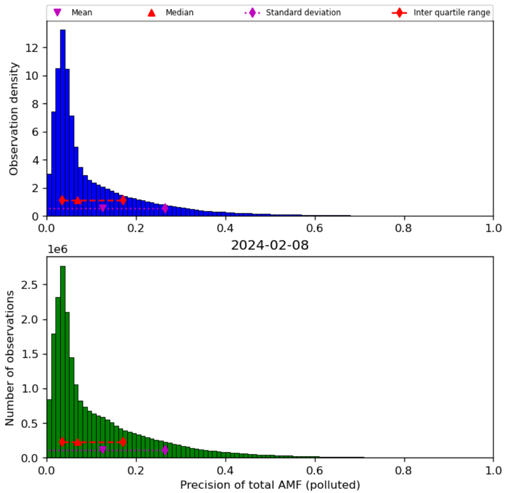
Figure 72: Histogram of “Precision of total AMF (polluted)” for 2024-02-07 to 2024-02-09
