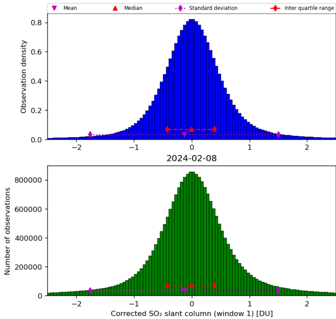
Figure 58: Histogram of “Corrected SO 2 slant column (window 1)” for 2024-02-07 to 2024-02-09
