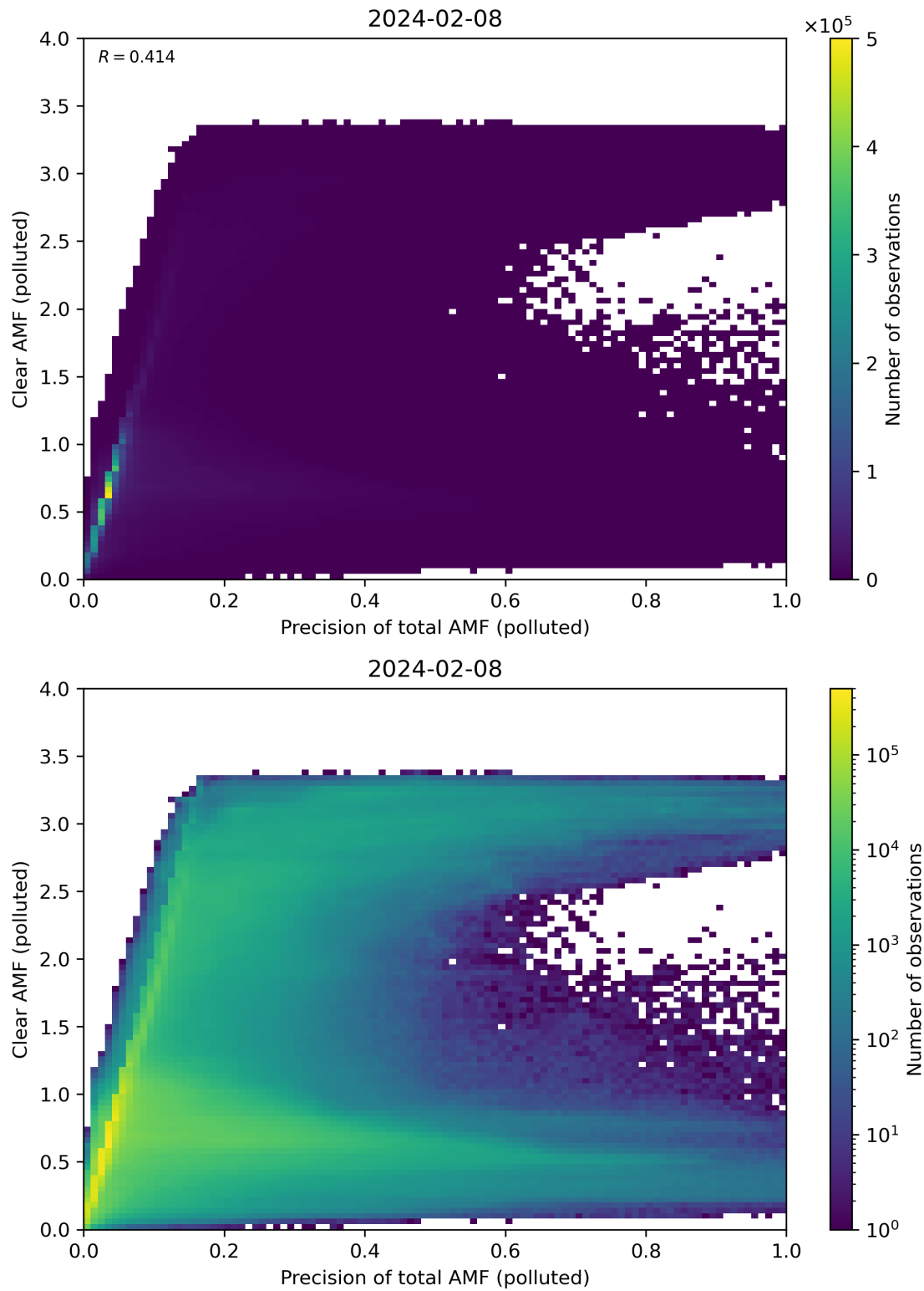
Figure 270: Scatter density plot of “Precision of total AMF (polluted)” against “Clear AMF (polluted)” for 2024-02-07 to 2024-02-09.
