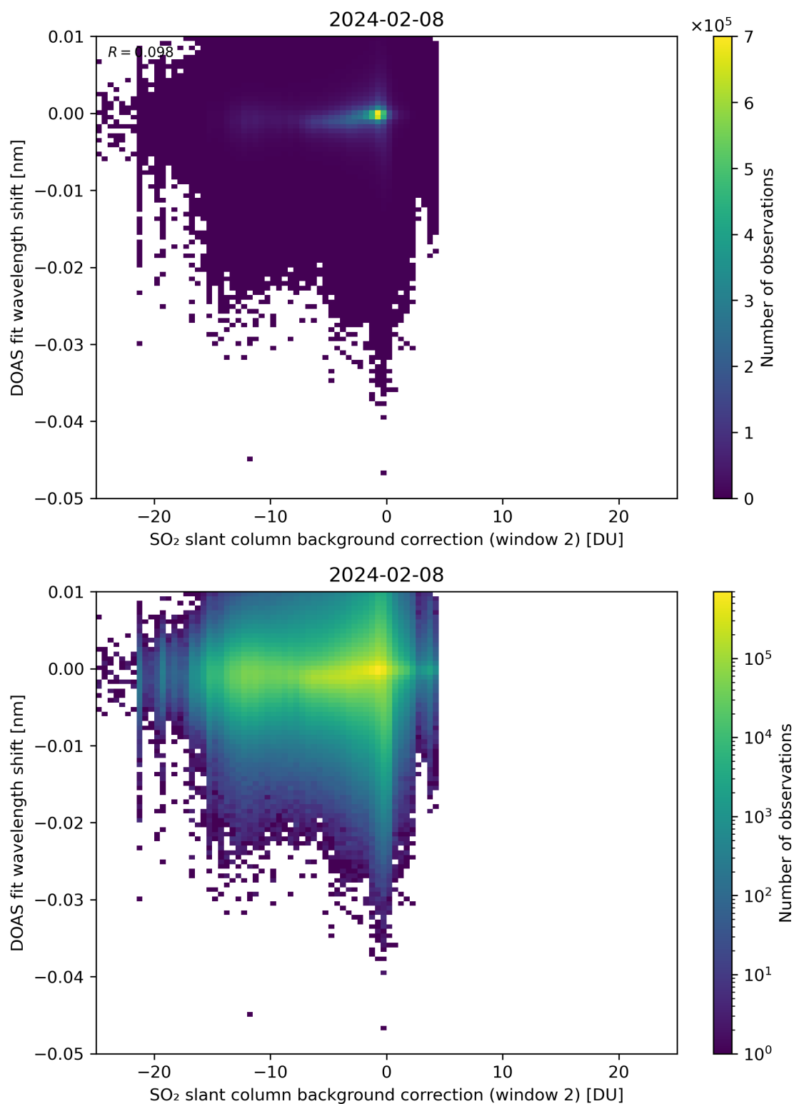
Figure 112: Scatter density plot of “SO 2 slant column background correction (window 2)” against “DOAS fit wavelength shift” for 2024-02-07 to 2024-02-09.
