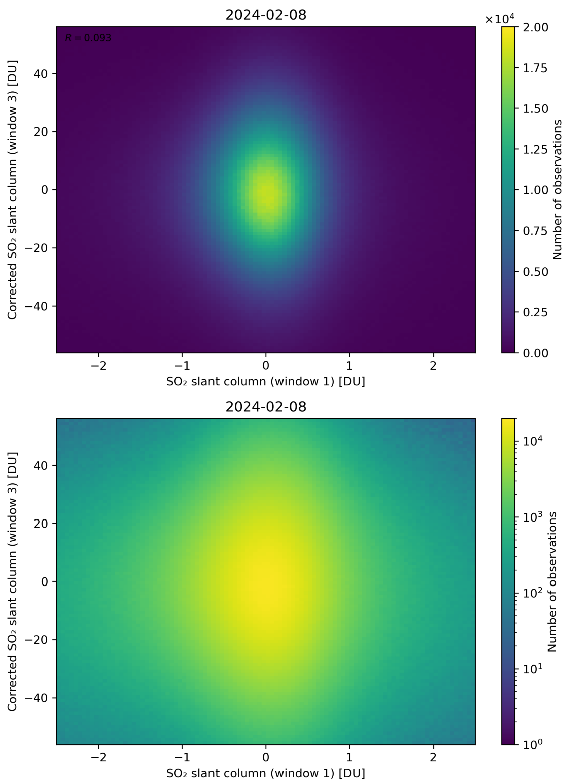
Figure 234: Scatter density plot of “SO 2 slant column (window 1)” against “Corrected SO 2 slant column (window 3)” for 2024-02-07 to 2024-02-09.
