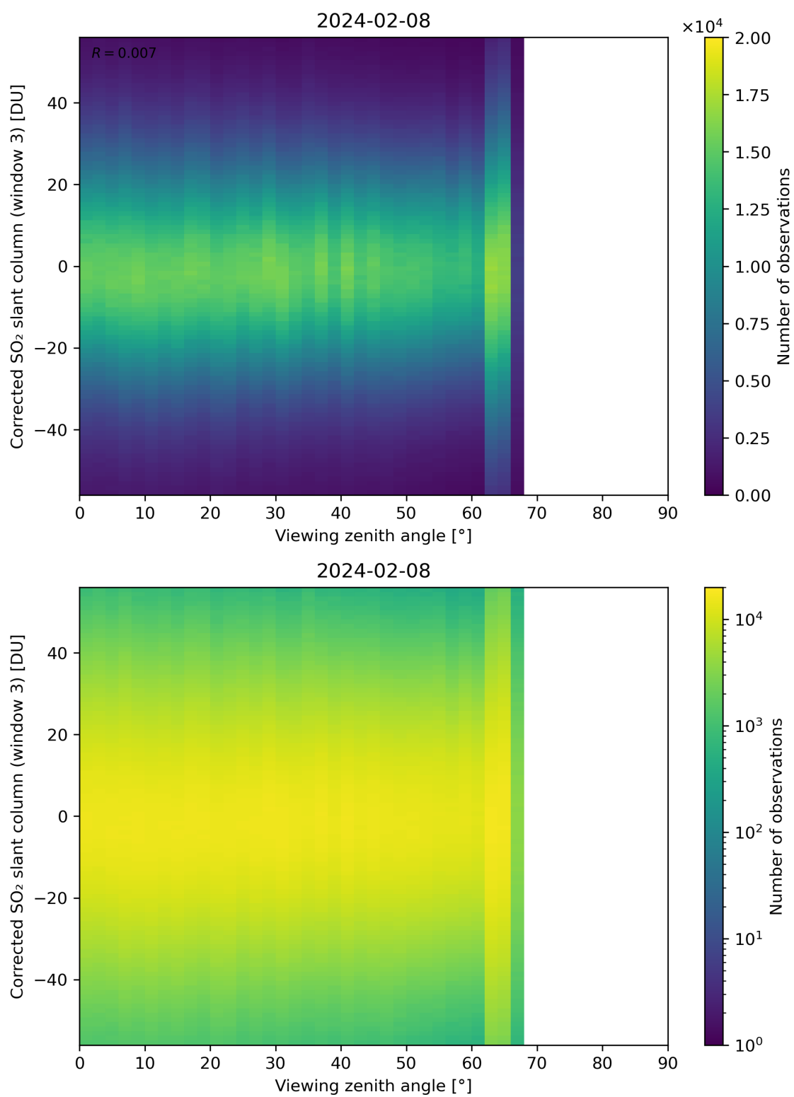
Figure 319: Scatter density plot of “Viewing zenith angle” against “Corrected SO 2 slant column (window 3)” for 2024-02-07 to 2024-02-09.
