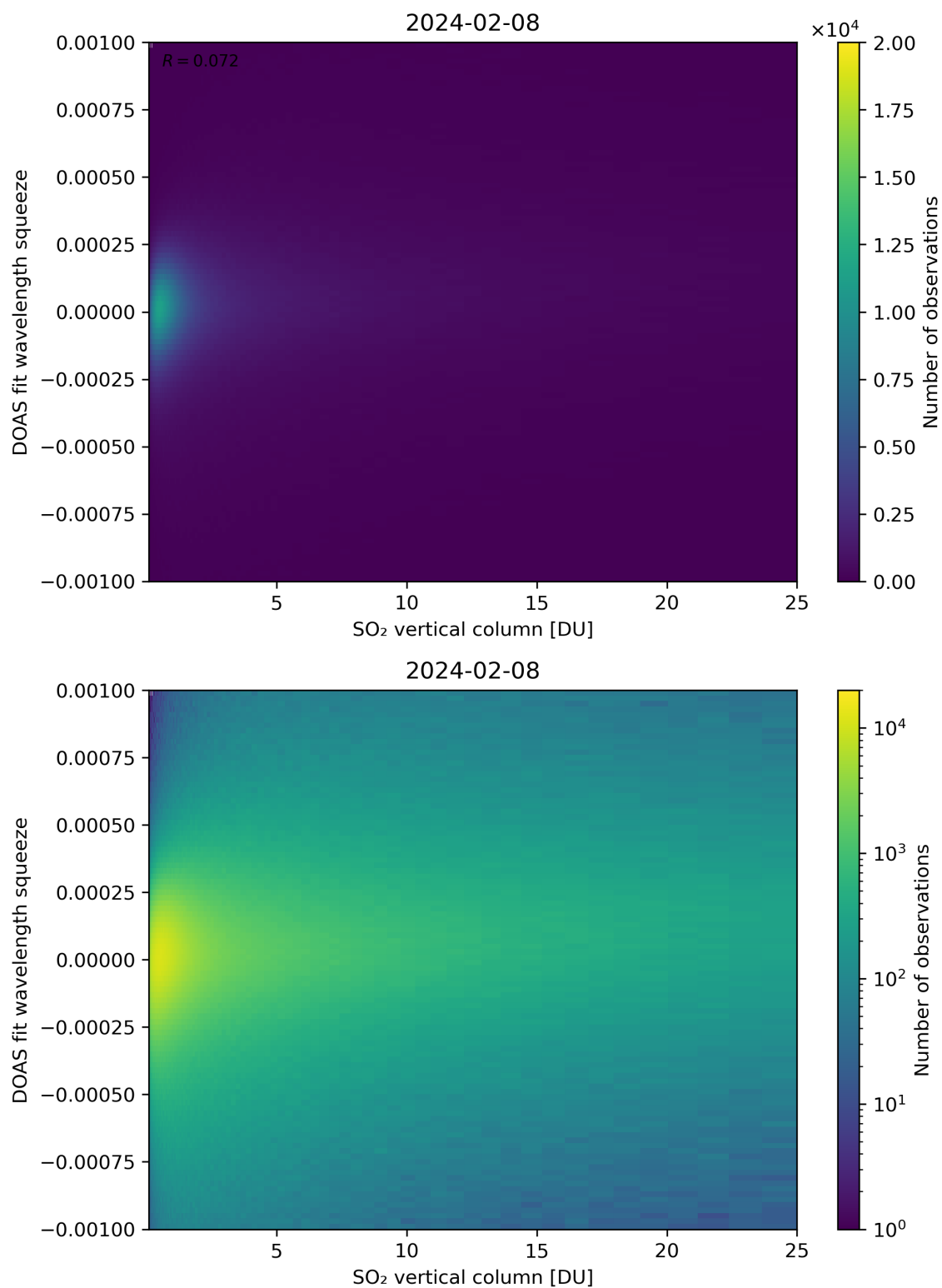
Figure 277: Scatter density plot of “SO 2 vertical column” against “DOAS fit wavelength squeeze” for 2024-02-07 to 2024-02-09.
