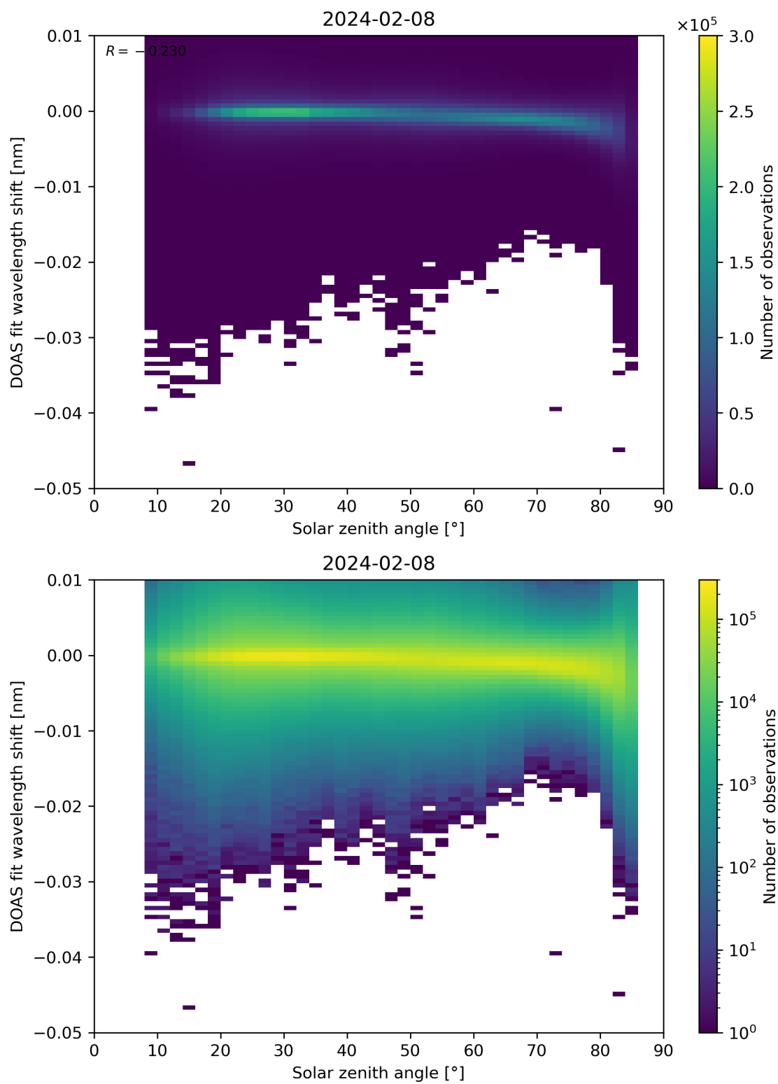
Figure 161: Scatter density plot of “Solar zenith angle” against “DOAS fit wavelength shift” for 2024-02-07 to 2024-02-09.
