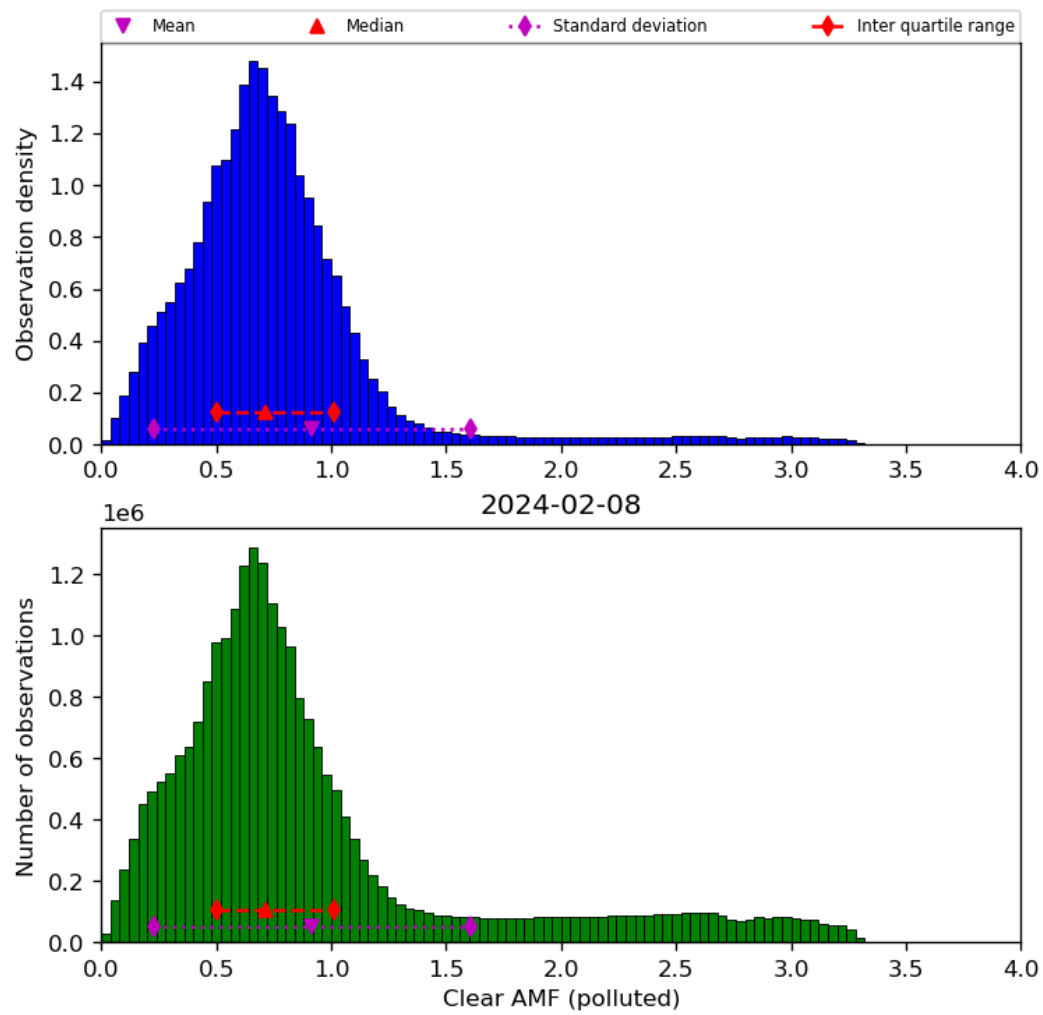
Figure 73: Histogram of “Clear AMF (polluted)” for 2024-02-07 to 2024-02-09
