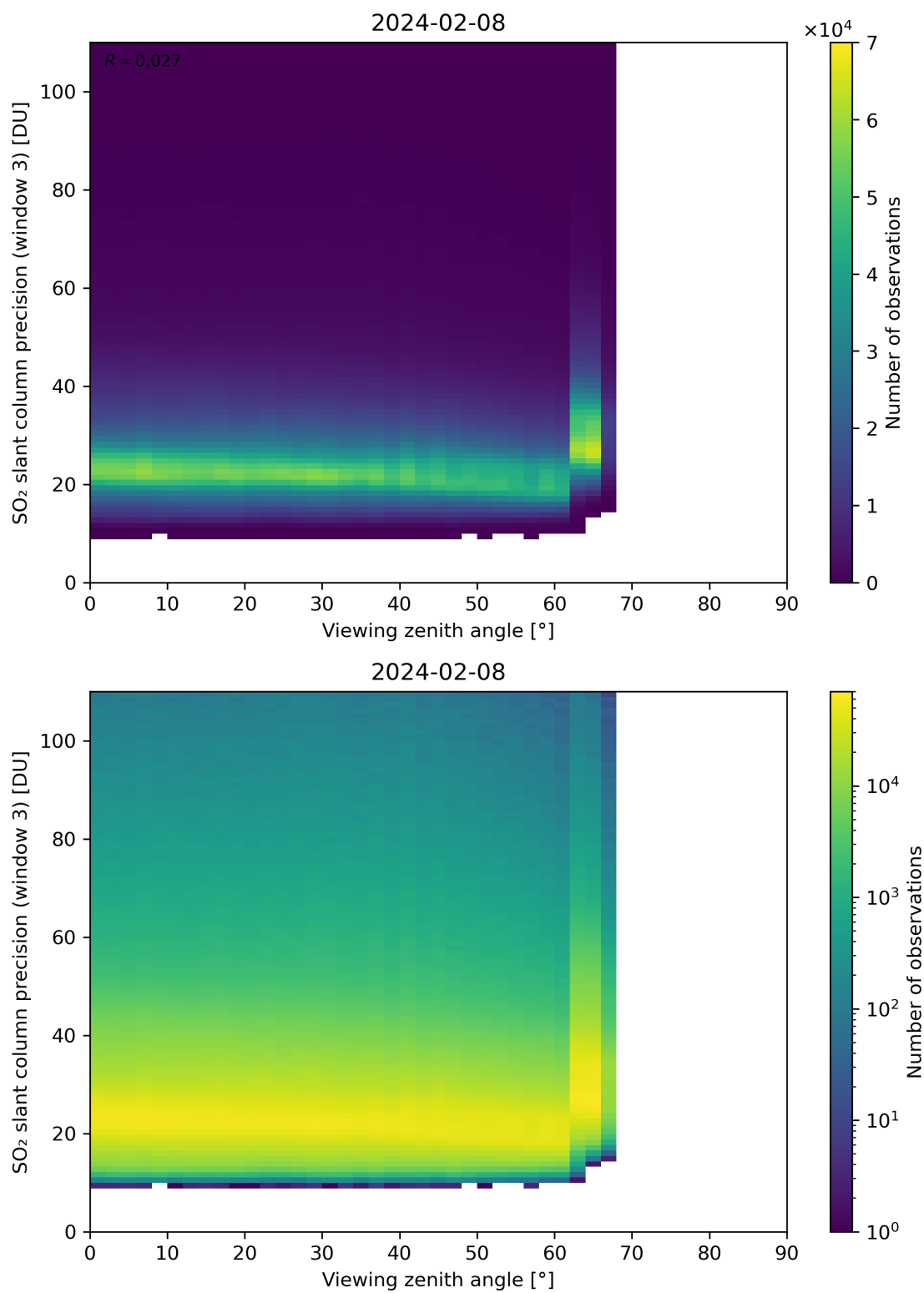
Figure 324: Scatter density plot of “Viewing zenith angle” against “SO 2 slant column precision (window 3)” for 2024-02-07 to 2024-02-09.
