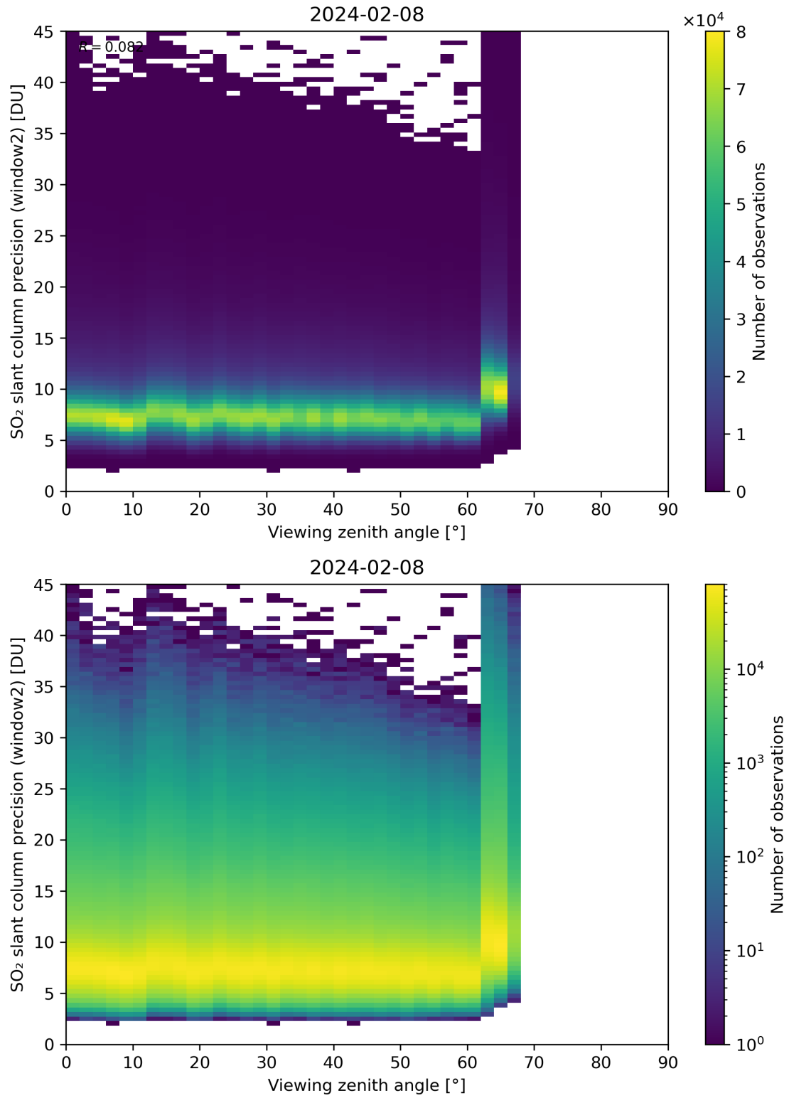
Figure 322: Scatter density plot of “Viewing zenith angle” against “SO 2 slant column precision (window2)” for 2024-02-07 to 2024-02-09.
