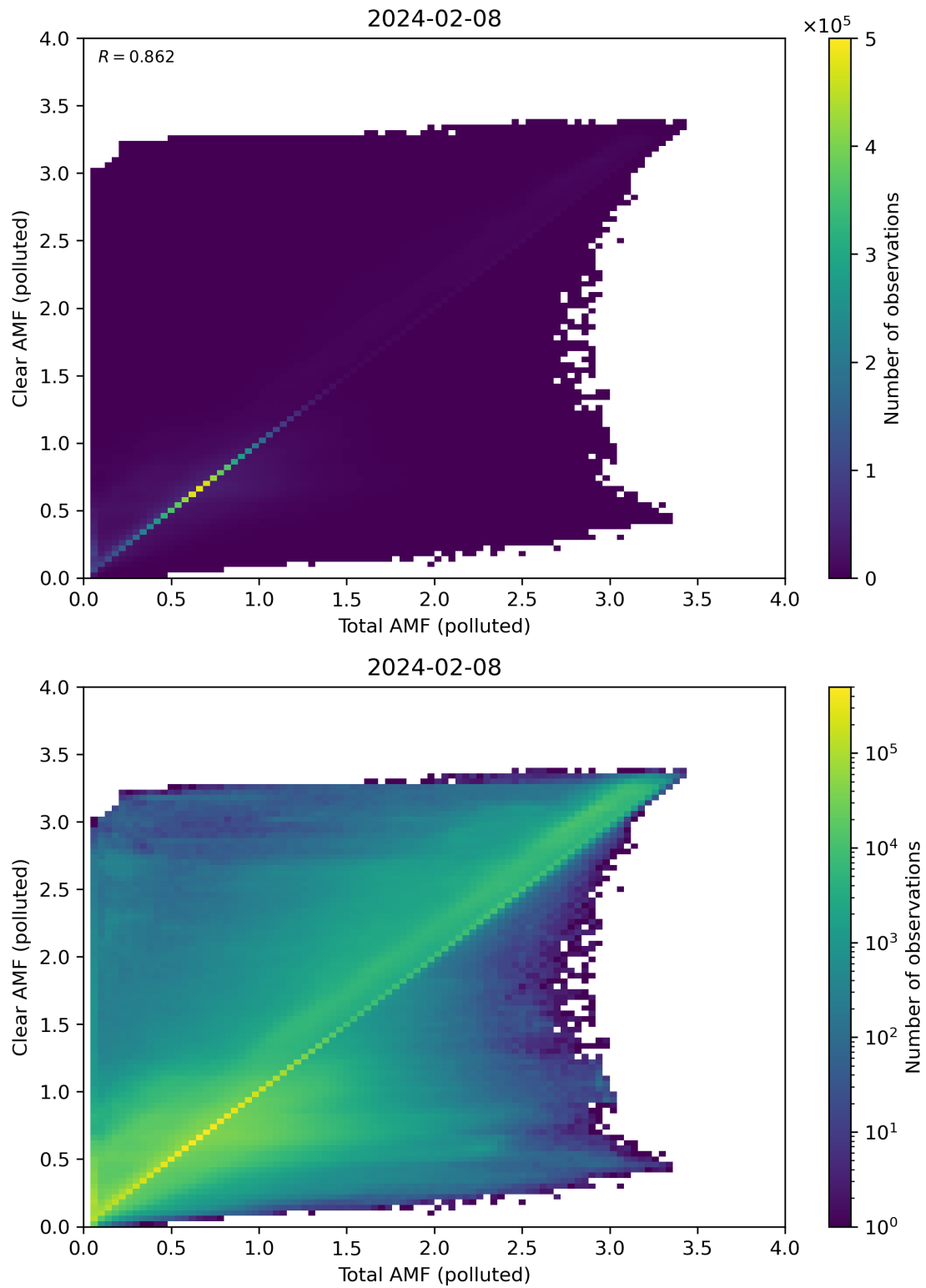
Figure 271: Scatter density plot of “Total AMF (polluted)” against “Clear AMF (polluted)” for 2024-02-07 to 2024-02-09.
