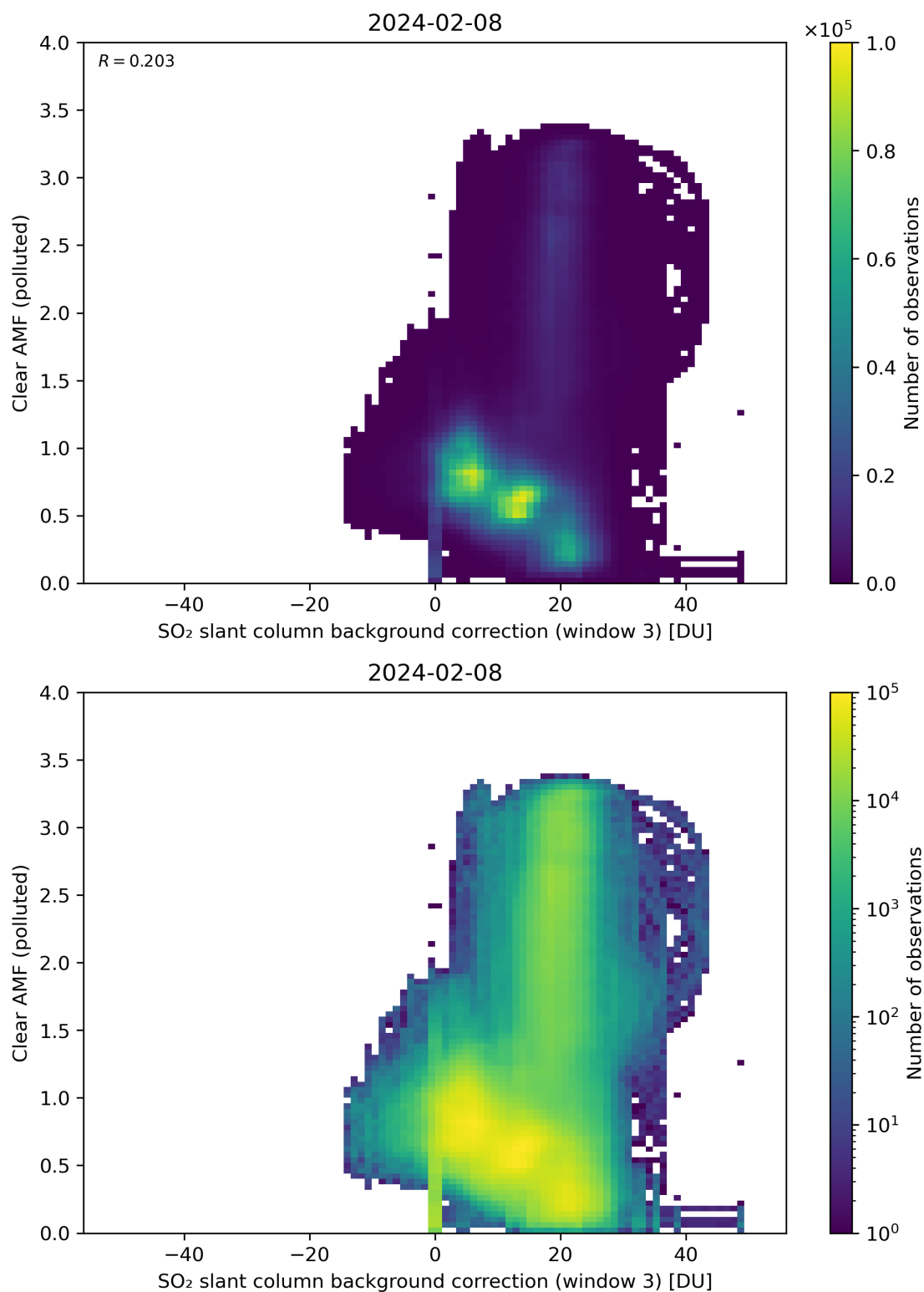
Figure 124: Scatter density plot of “SO 2 slant column background correction (window 3)” against “Clear AMF (polluted)” for 2024-02-07 to 2024-02-09.
