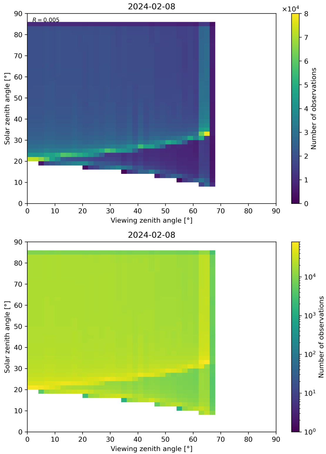
Figure 315: Scatter density plot of “Viewing zenith angle” against “Solar zenith angle” for 2024-02-07 to 2024-02-09.
