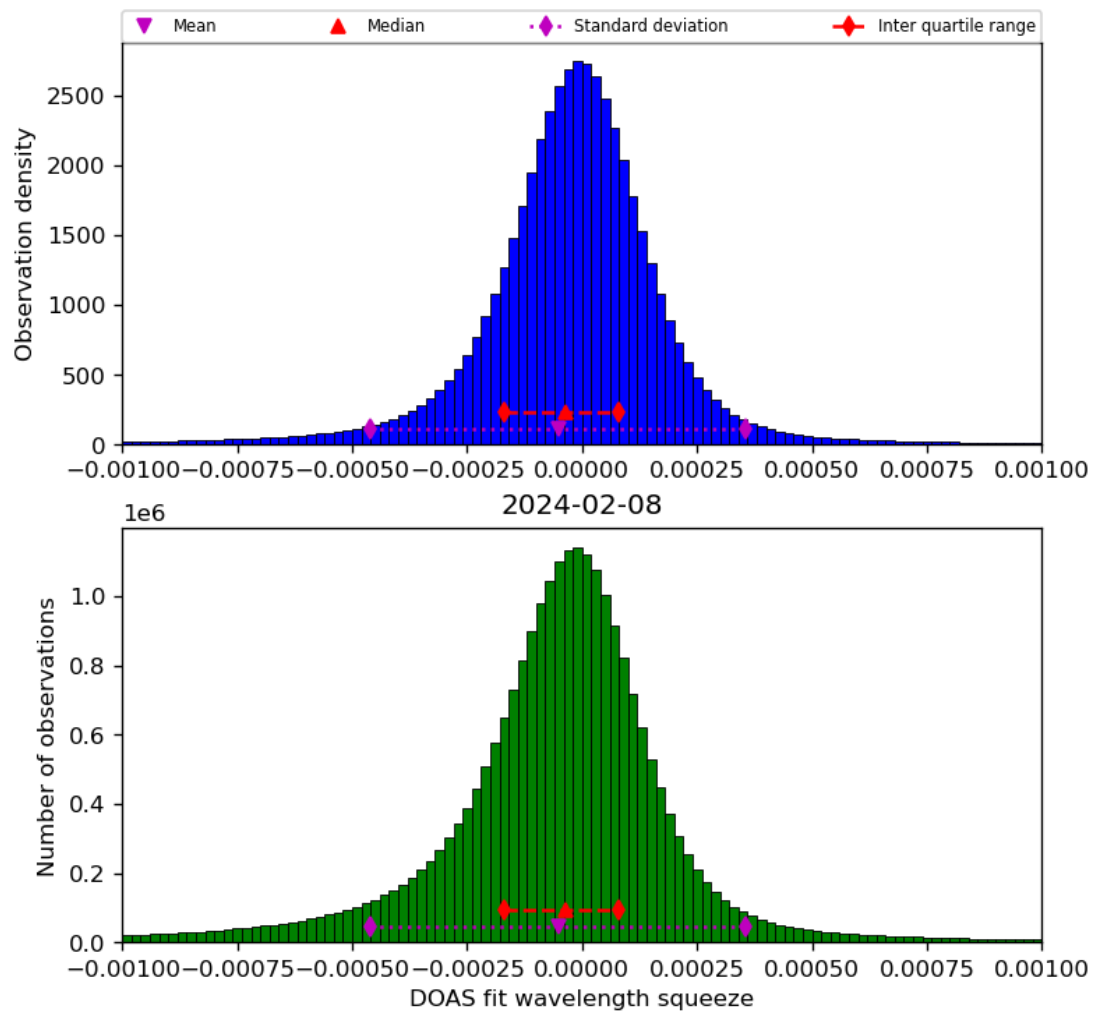
Figure 69: Histogram of “DOAS fit wavelength squeeze” for 2024-02-07 to 2024-02-09
