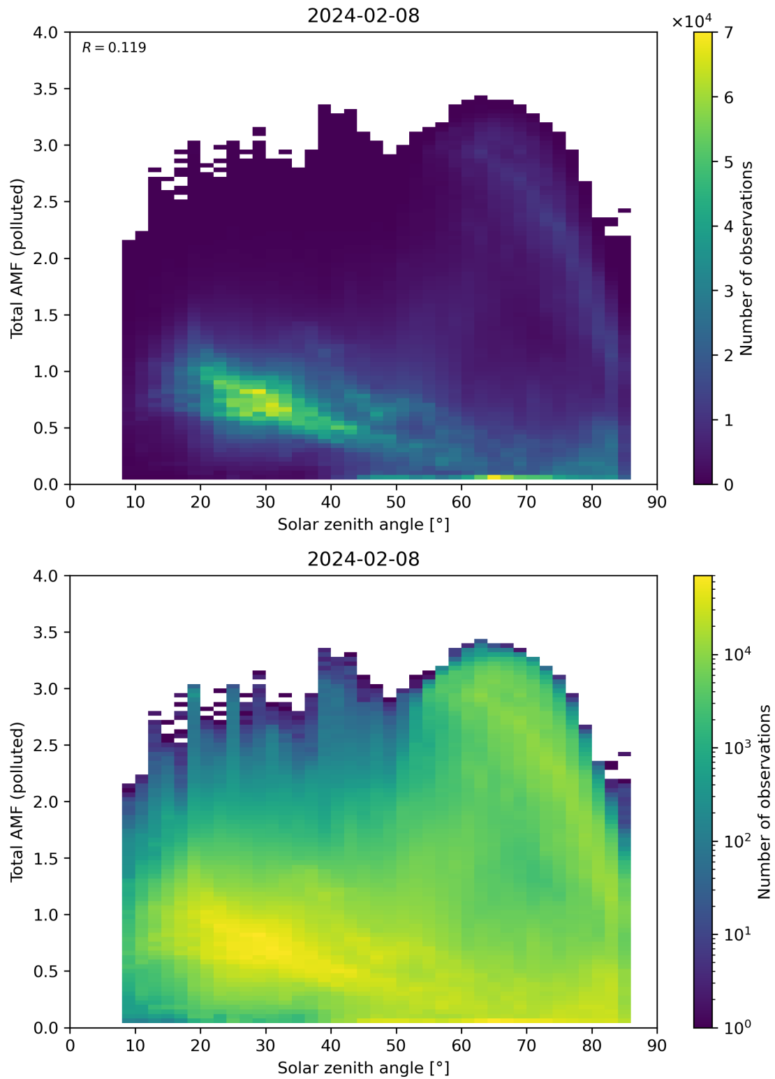
Figure 174: Scatter density plot of “Solar zenith angle” against “Total AMF (polluted)” for 2024-02-07 to 2024-02-09.
