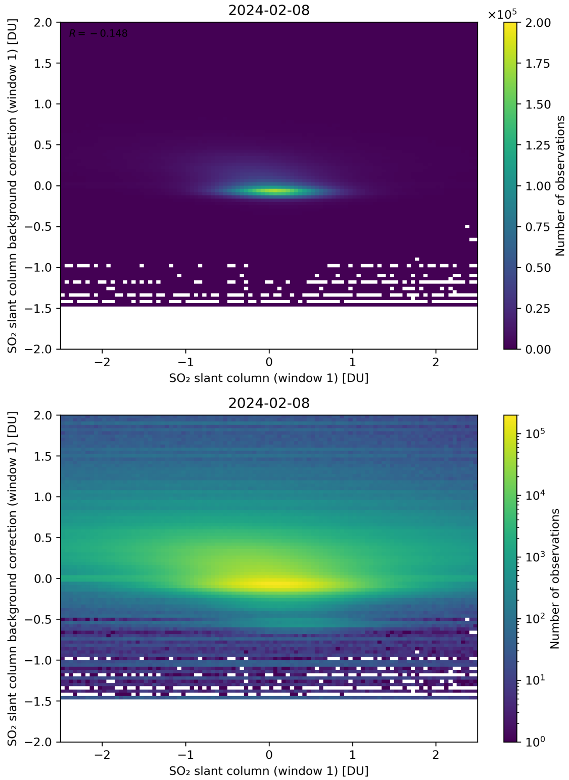
Figure 212: Scatter density plot of “SO 2 slant column (window 1)” against “SO 2 slant column background correction (window 1)” for 2024-02-07 to 2024-02-09.
