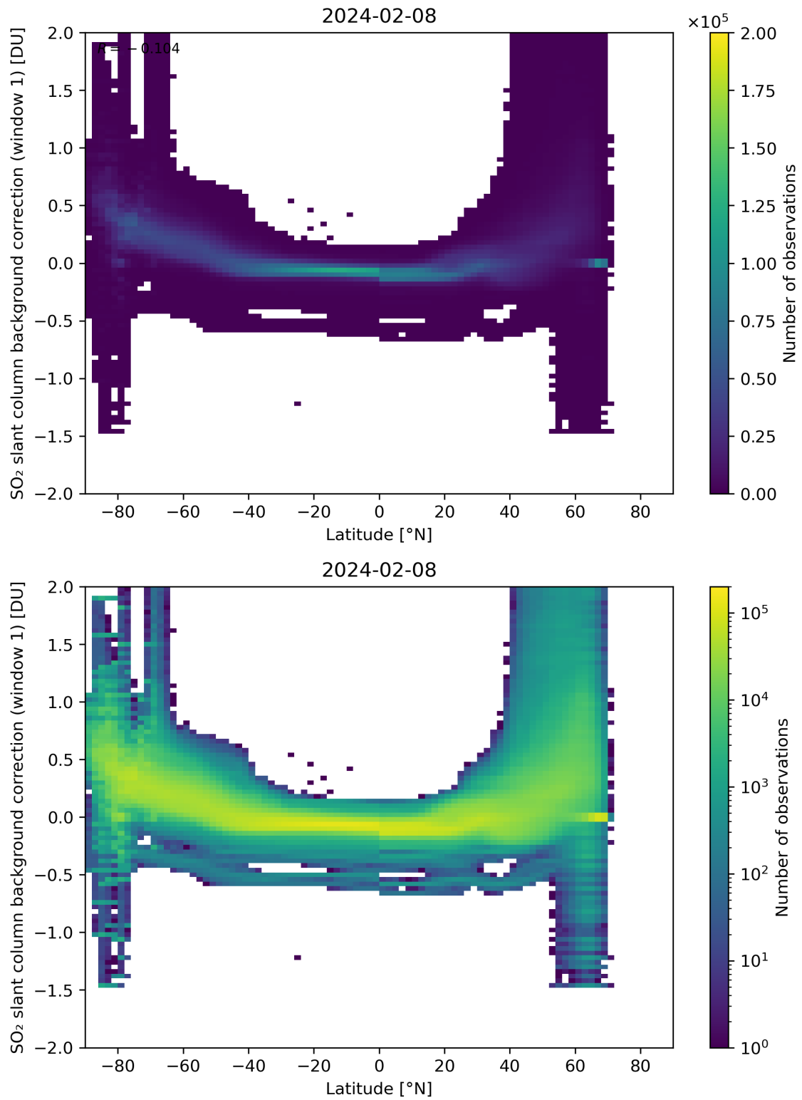
Figure 139: Scatter density plot of “Latitude” against “SO 2 slant column background correction (window 1)” for 2024-02-07 to 2024-02-09.
