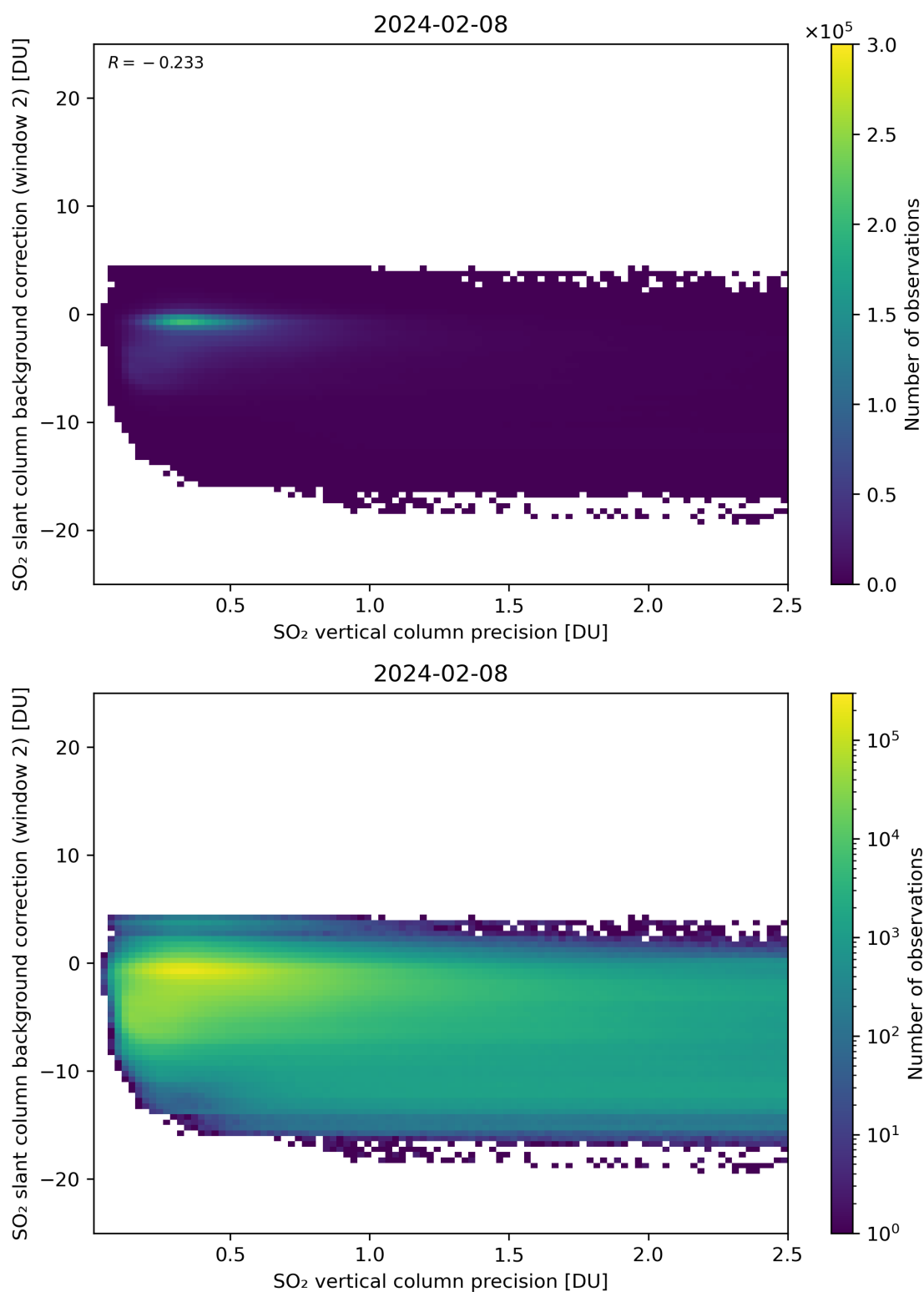
Figure 280: Scatter density plot of “SO 2 vertical column precision” against “SO 2 slant column background correction (window 2)” for 2024-02-07 to 2024-02-09.
