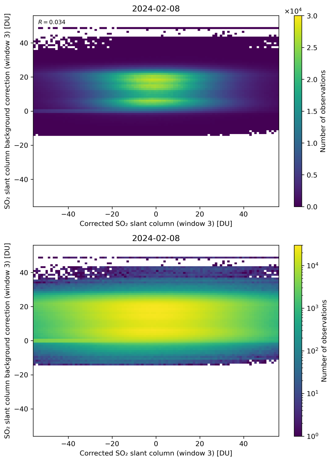
Figure 205: Scatter density plot of “Corrected SO 2 slant column (window 3)” against “SO 2 slant column background correction (window 3)” for 2024-02-07 to 2024-02-09.
