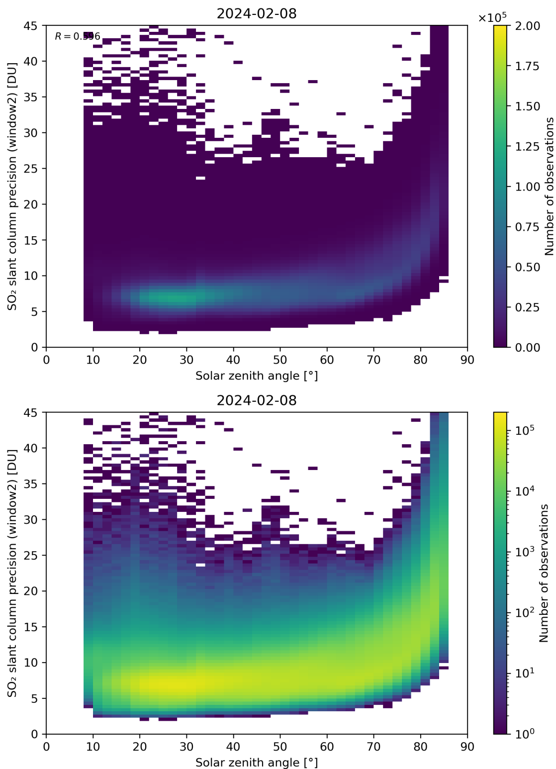
Figure 171: Scatter density plot of “Solar zenith angle” against “SO 2 slant column precision (window2)” for 2024-02-07 to 2024-02-09.
