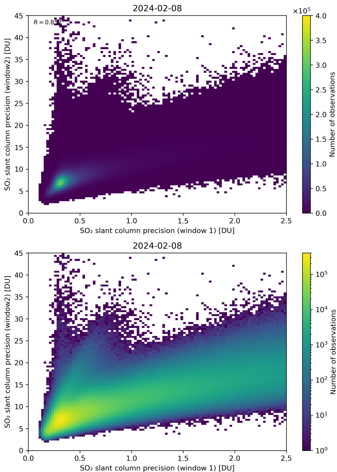
Figure 227: Scatter density plot of “SO 2 slant column precision (window 1)” against “SO 2 slant column precision (window2)” for 2024-02-07 to 2024-02-09.
