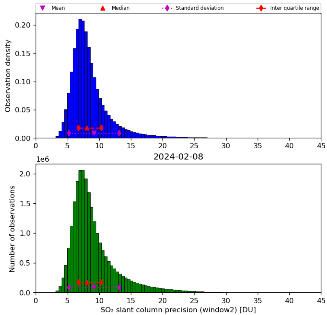
Figure 61: Histogram of “SO 2 slant column precision (window2)” for 2024-02-07 to 2024-02-09
