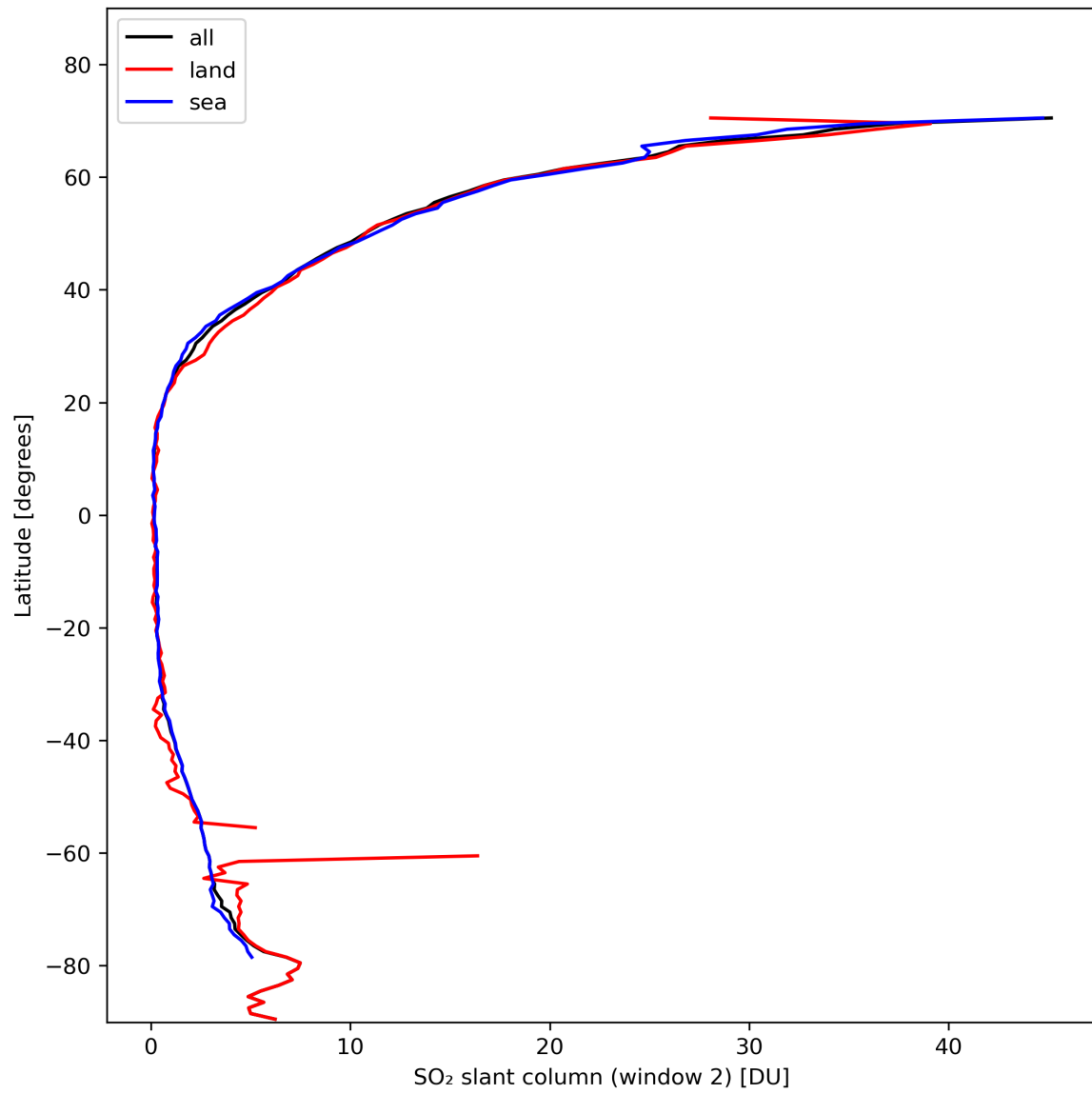
Figure 37: Zonal average of “SO 2 slant column (window 2)” for 2024-02-07 to 2024-02-09.
