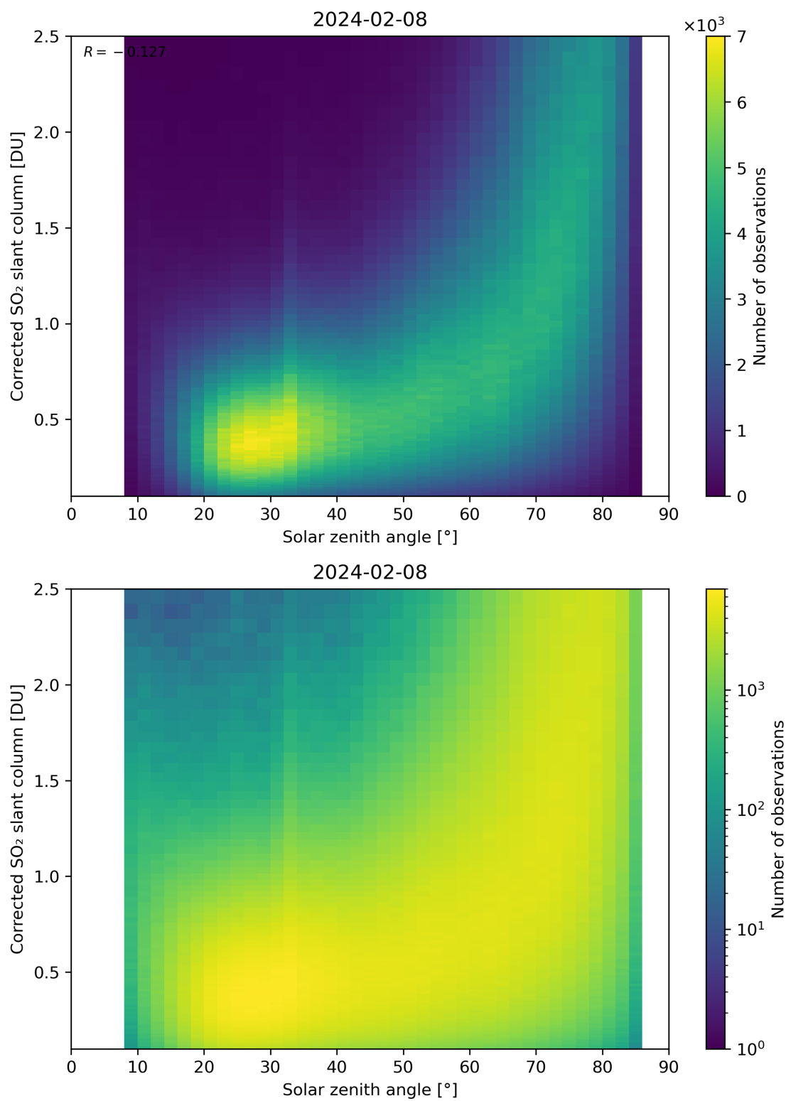
Figure 166: Scatter density plot of “Solar zenith angle” against “Corrected SO 2 slant column” for 2024-02-07 to 2024-02-09.
