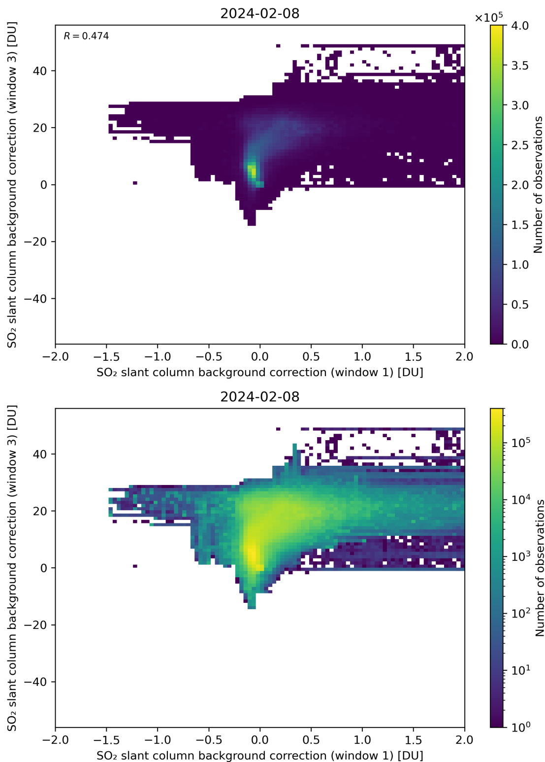
Figure 99: Scatter density plot of “SO 2 slant column background correction (window 1)” against “SO 2 slant column background correction (window 3)” for 2024-02-07 to 2024-02-09.
