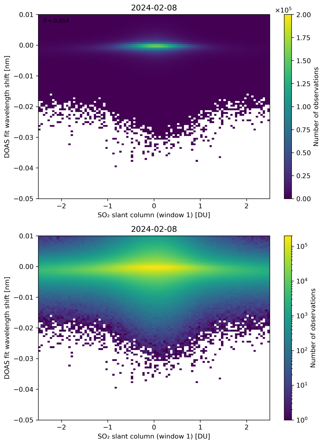
Figure 215: Scatter density plot of “SO 2 slant column (window 1)” against “DOAS fit wavelength shift” for 2024-02-07 to 2024-02-09.
