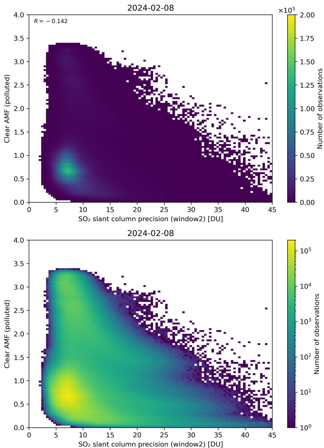
Figure 246: Scatter density plot of “SO 2 slant column precision (window2)” against “Clear AMF (polluted)” for 2024-02-07 to 2024-02-09.
