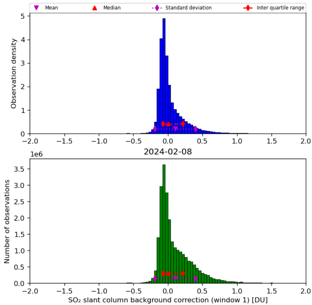
Figure 59: Histogram of “SO 2 slant column background correction (window 1)” for 2024-02-07 to 2024-02-09
