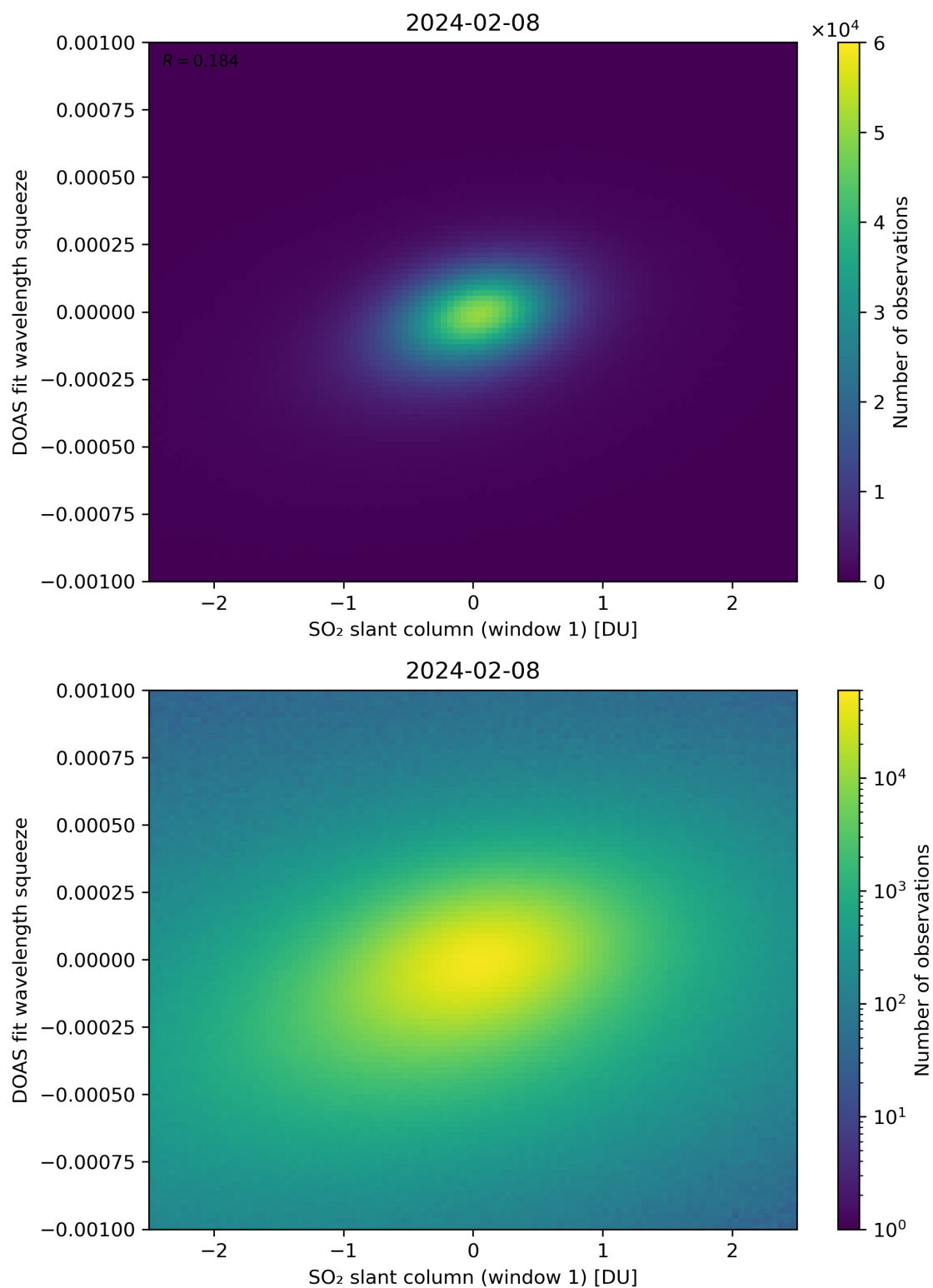
Figure 216: Scatter density plot of “SO 2 slant column (window 1)” against “DOAS fit wavelength squeeze” for 2024-02-07 to 2024-02-09.
