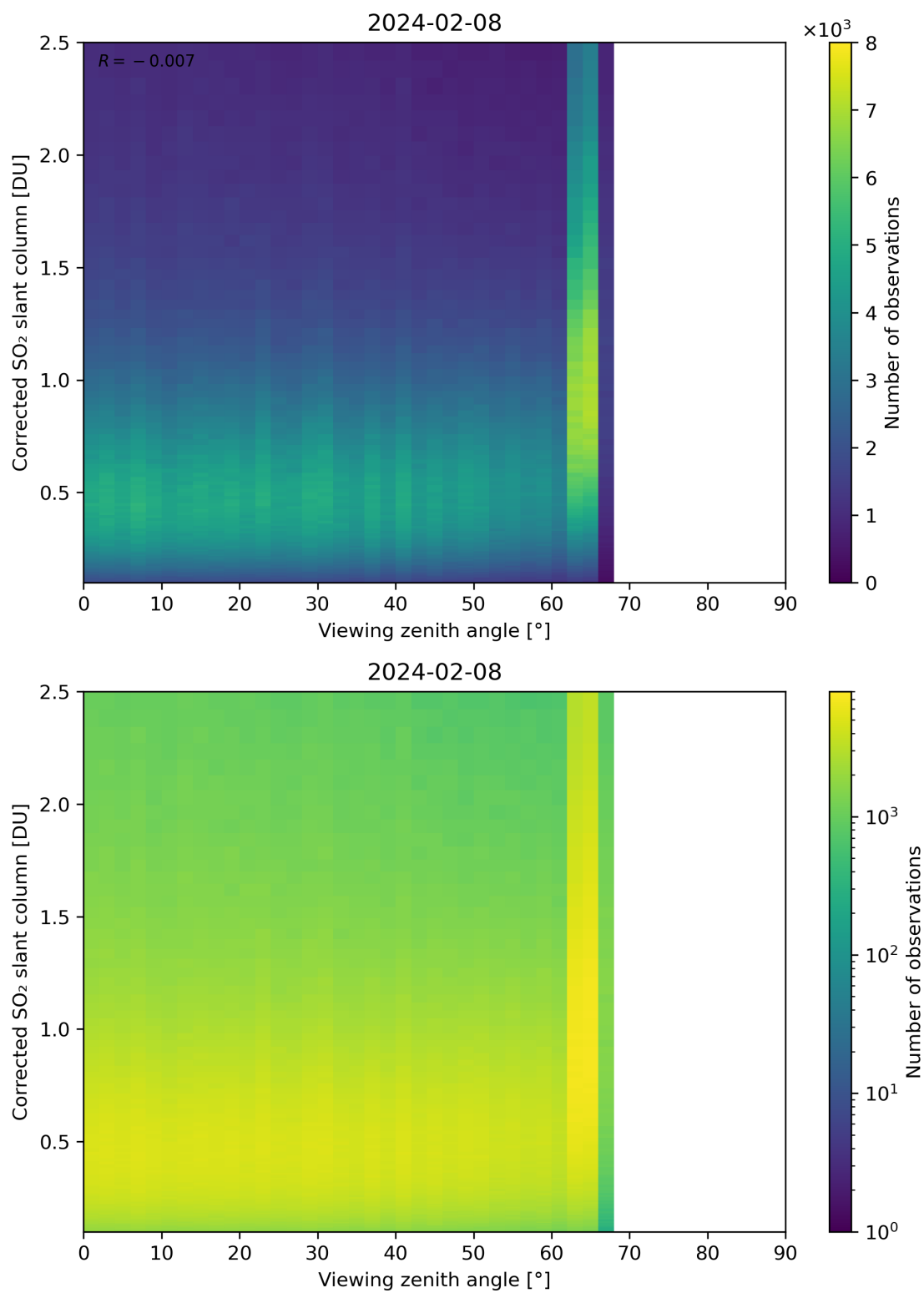
Figure 317: Scatter density plot of “Viewing zenith angle” against “Corrected SO 2 slant column” for 2024-02-07 to 2024-02-09.
