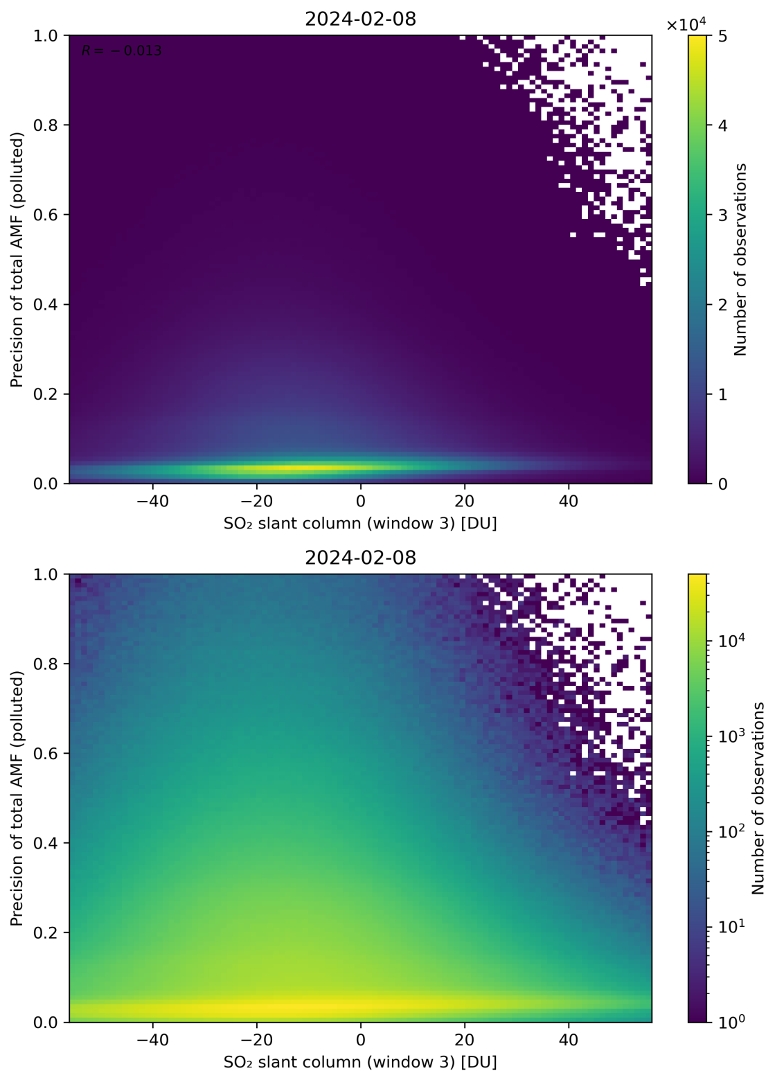
Figure 269: Scatter density plot of “SO 2 slant column (window 3)” against “Precision of total AMF (polluted)” for 2024-02-07 to 2024-02-09.
