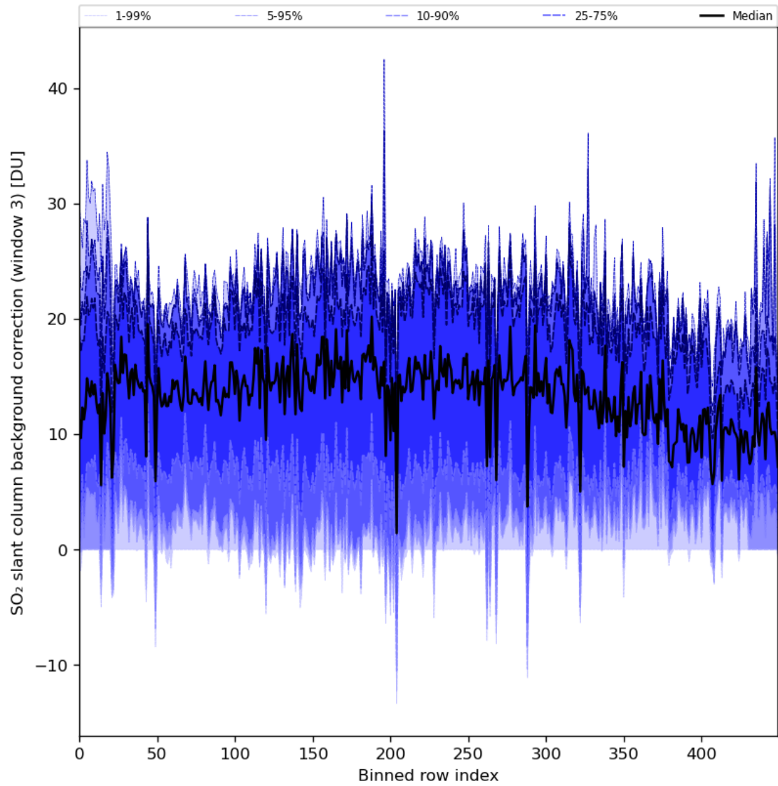
Figure 90: Along track statistics of “SO 2 slant column background correction (window 3)” for 2024-02-07 to 2024-02-09
