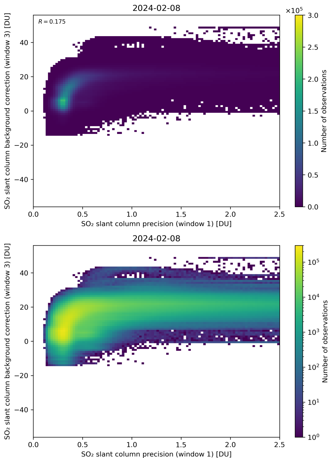
Figure 220: Scatter density plot of “SO 2 slant column precision (window 1)” against “SO 2 slant column background correction (window 3)” for 2024-02-07 to 2024-02-09.
