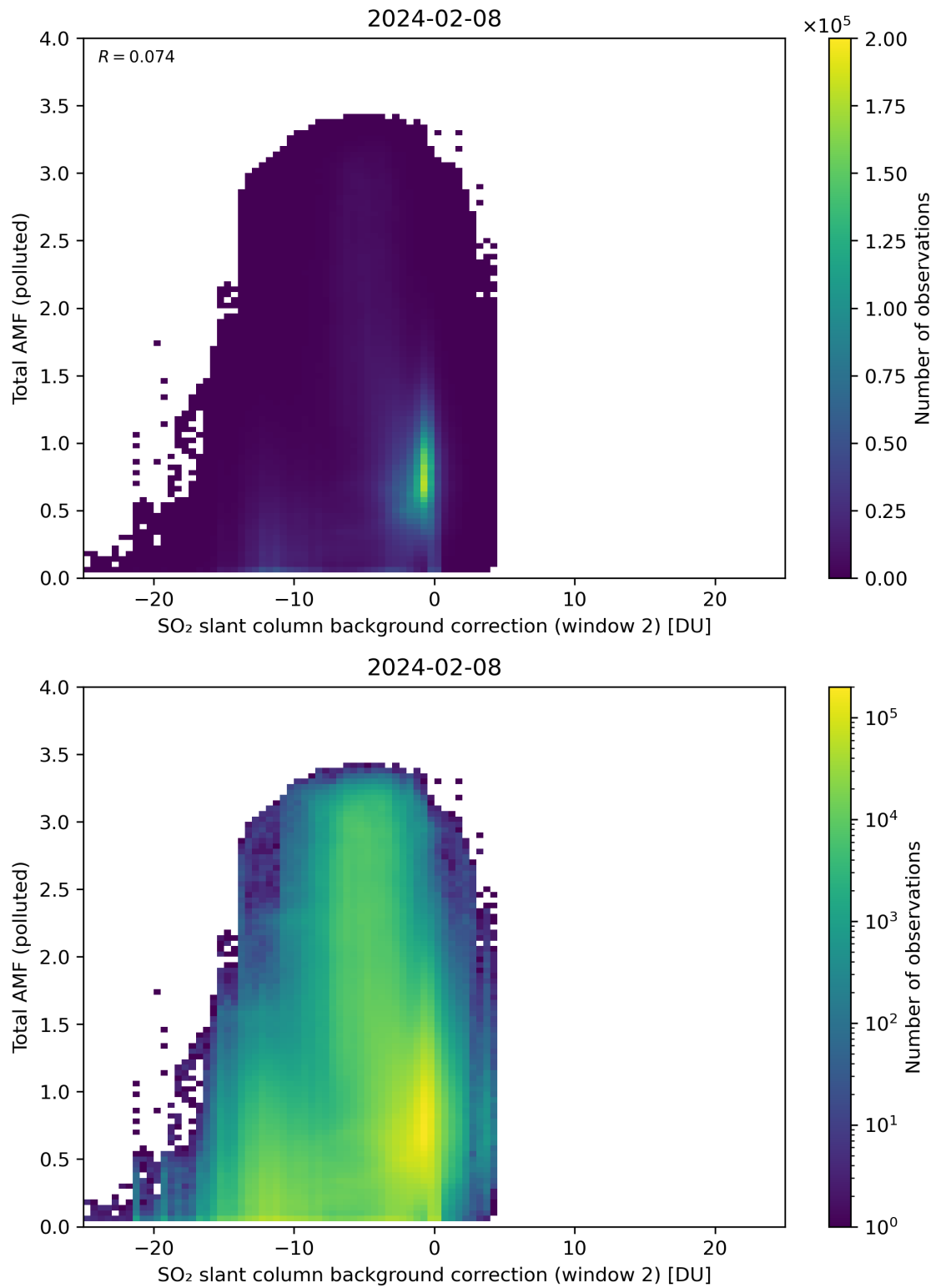
Figure 119: Scatter density plot of “SO 2 slant column background correction (window 2)” against “Total AMF (polluted)” for 2024-02-07 to 2024-02-09.
