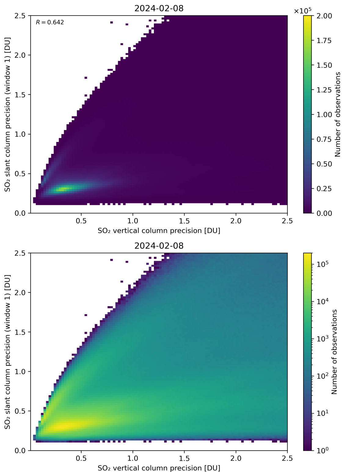
Figure 290: Scatter density plot of “SO 2 vertical column precision” against “SO 2 slant column precision (window 1)” for 2024-02-07 to 2024-02-09.
