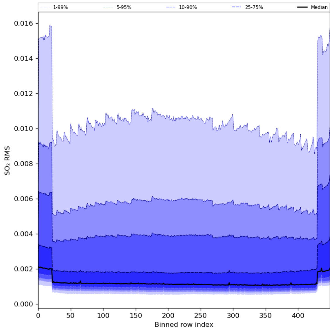
Figure 93: Along track statistics of “SO 2 RMS” for 2024-02-07 to 2024-02-09
