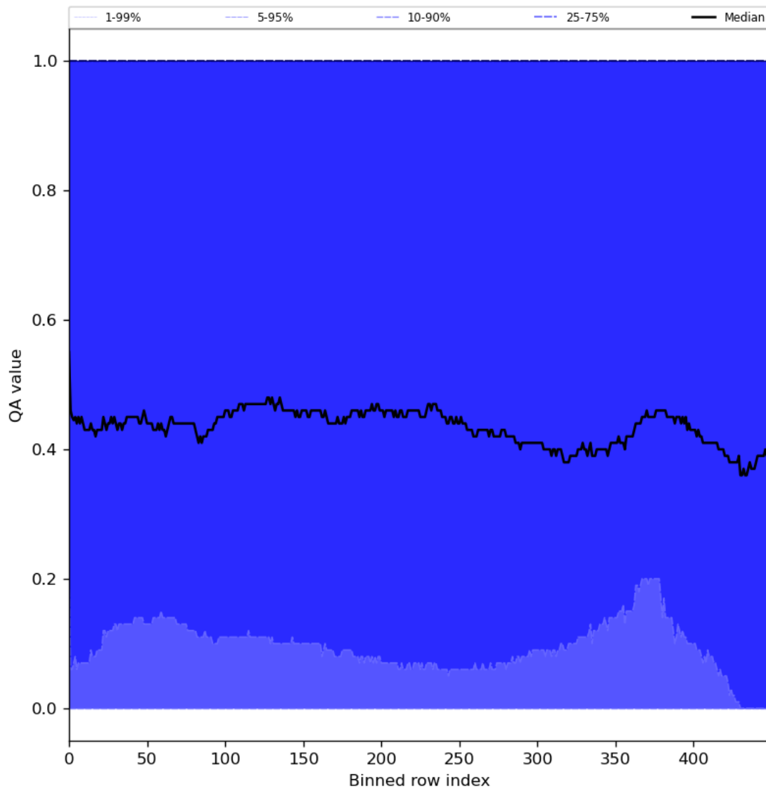
Figure 75: Along track statistics of “QA value” for 2024-02-07 to 2024-02-09
