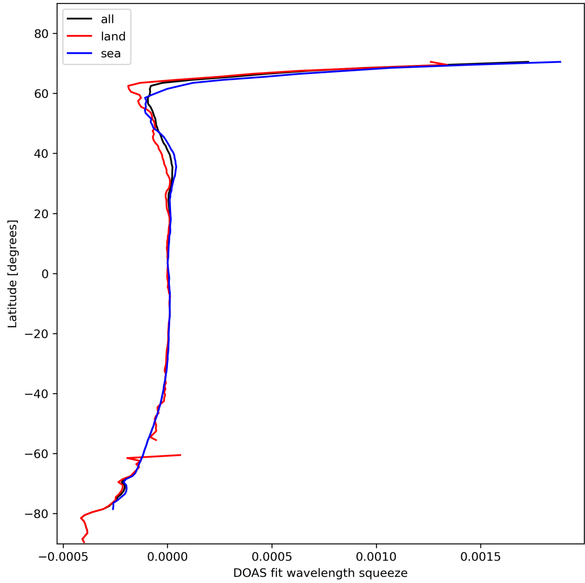
Figure 46: Zonal average of “DOAS fit wavelength squeeze” for 2024-02-07 to 2024-02-09.
