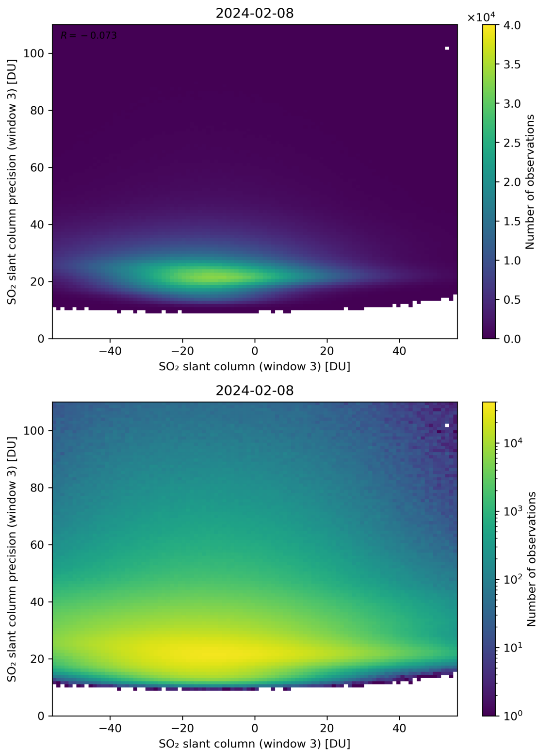
Figure 267: Scatter density plot of “SO 2 slant column (window 3)” against “SO 2 slant column precision (window 3)” for 2024-02-07 to 2024-02-09.
