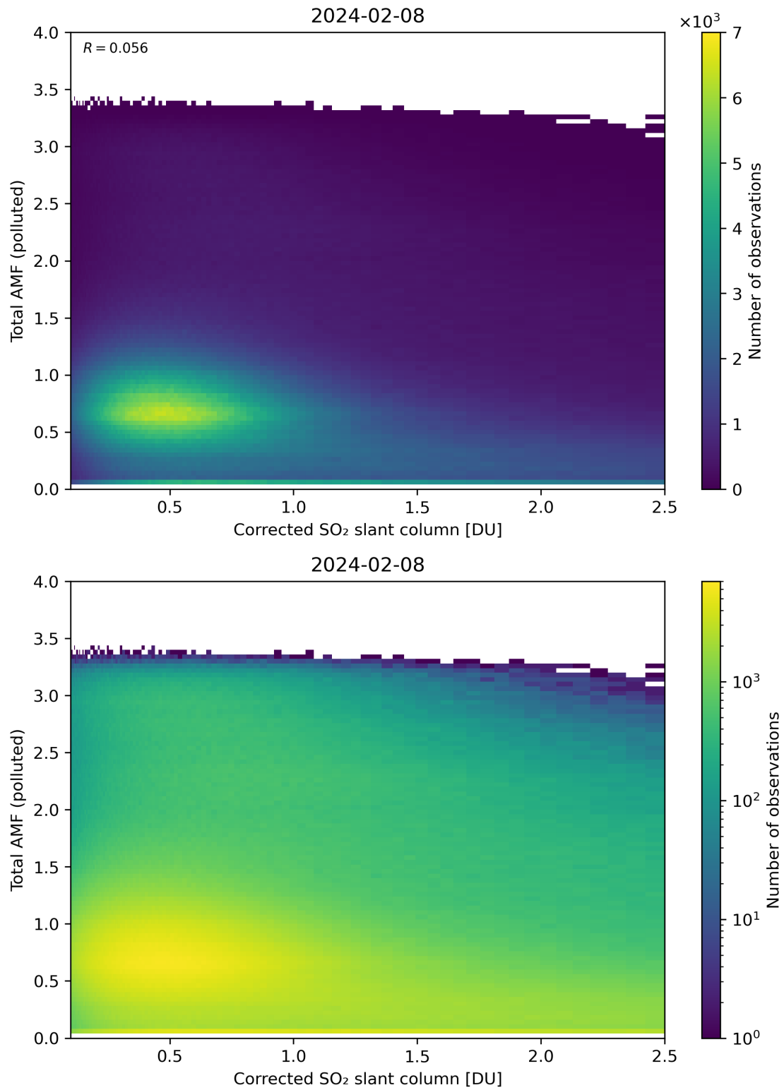
Figure 192: Scatter density plot of “Corrected SO 2 slant column” against “Total AMF (polluted)” for 2024-02-07 to 2024-02-09.
