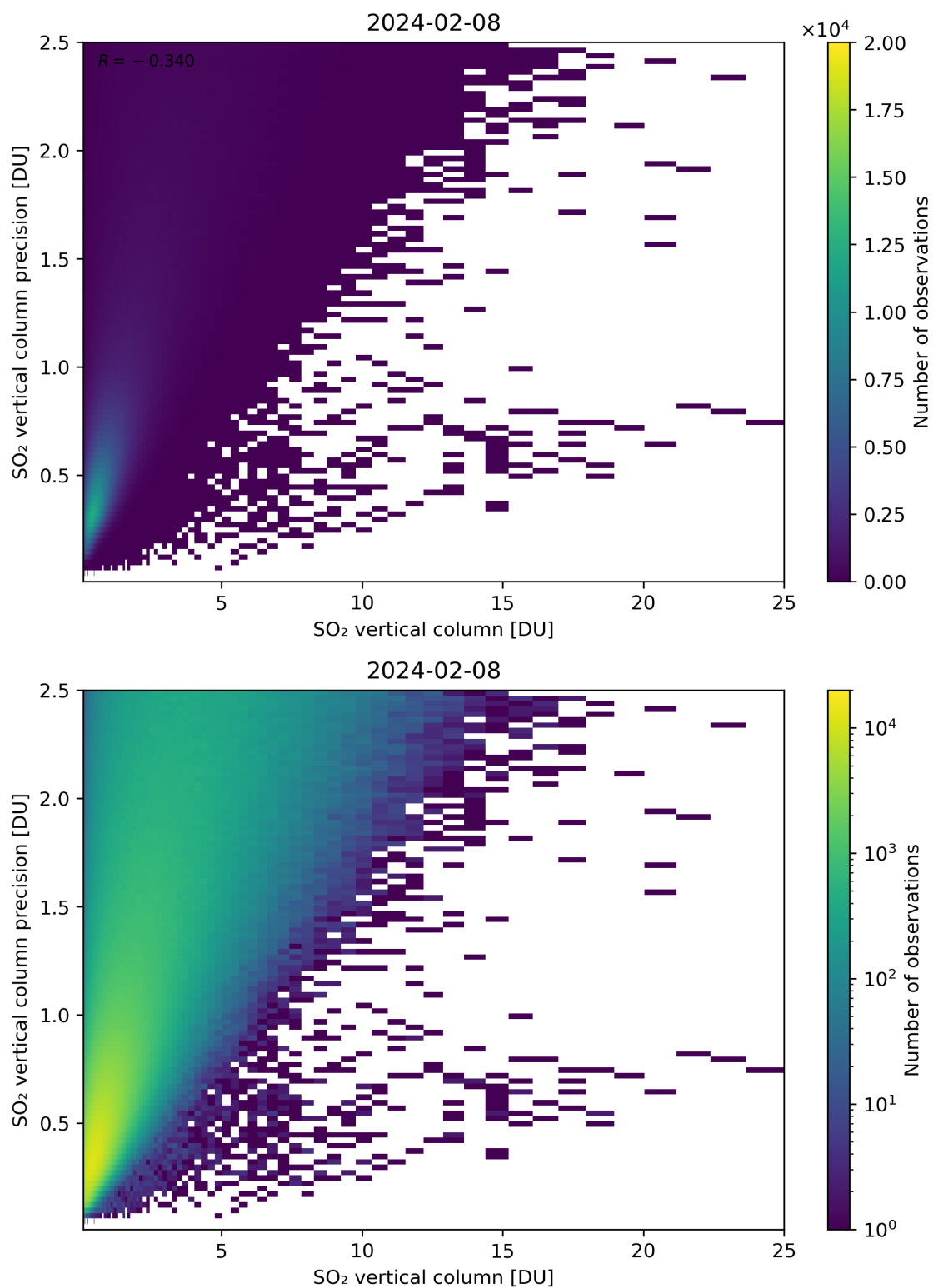
Figure 307: Scatter density plot of “SO 2 vertical column” against “SO 2 vertical column precision” for 2024-02-07 to 2024-02-09.
