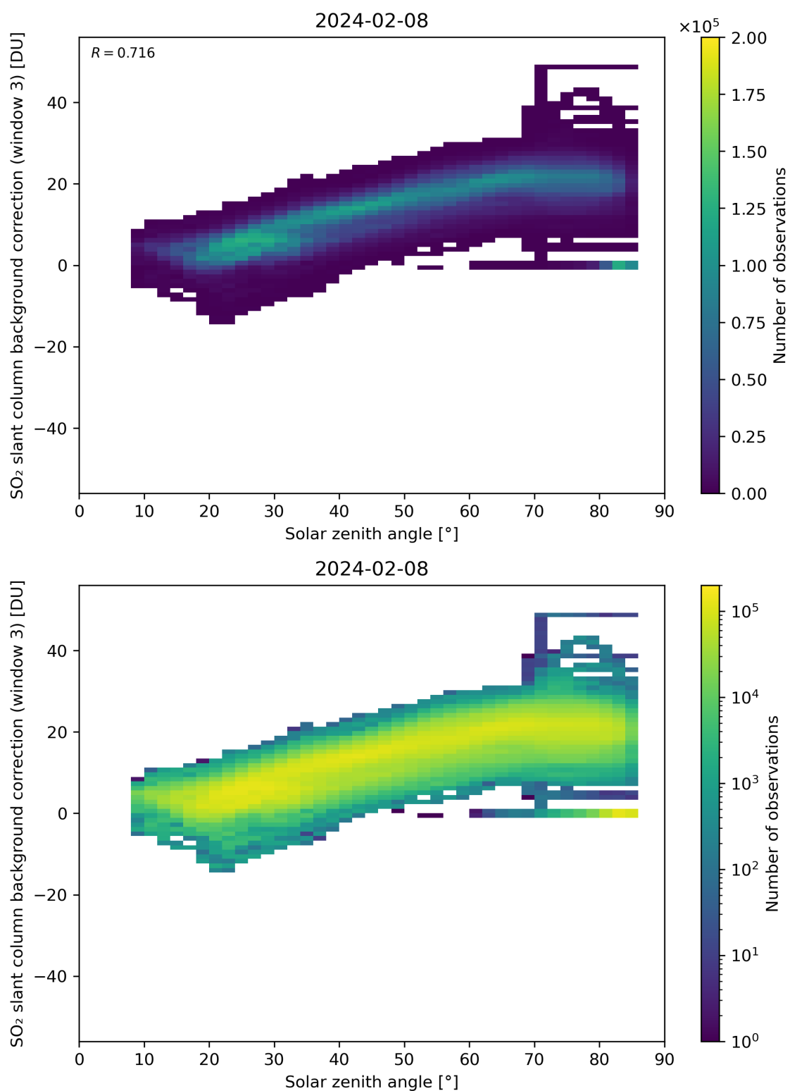
Figure 160: Scatter density plot of “Solar zenith angle” against “SO 2 slant column background correction (window 3)” for 2024-02-07 to 2024-02-09.
