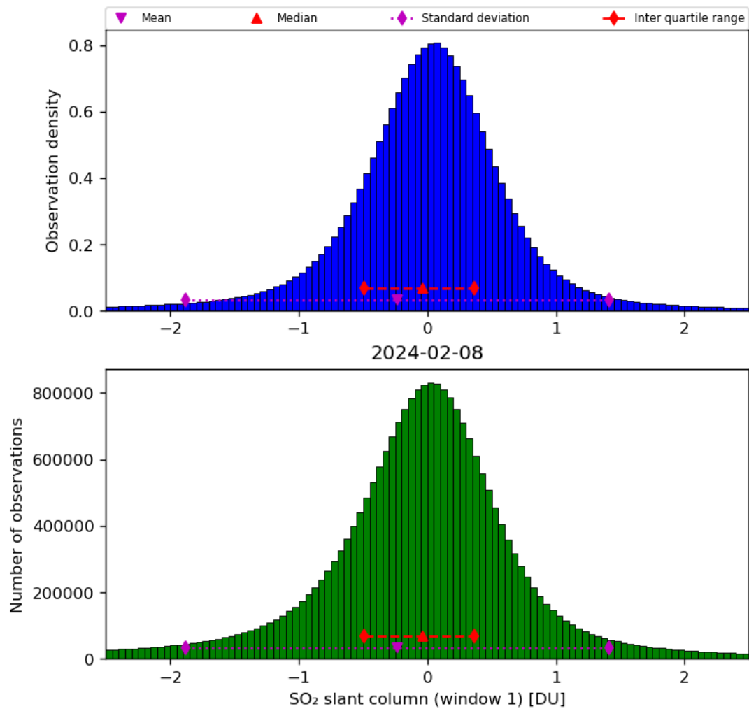
Figure 56: Histogram of “SO 2 slant column (window 1)” for 2024-02-07 to 2024-02-09
