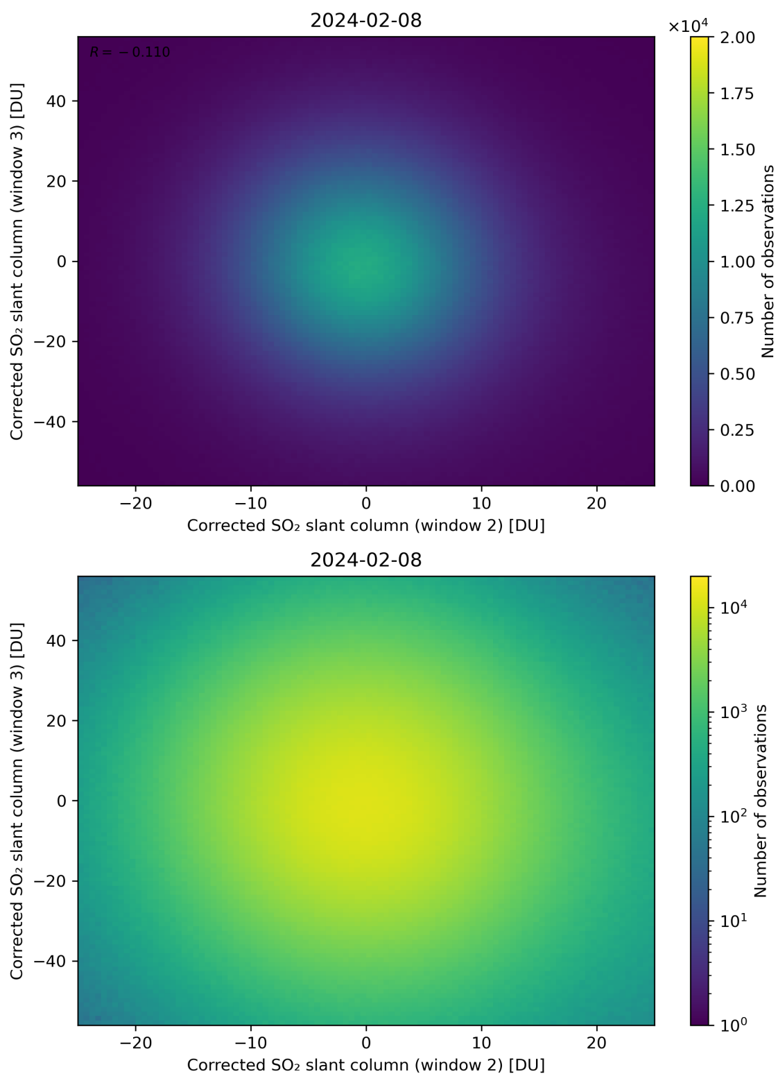
Figure 200: Scatter density plot of “Corrected SO 2 slant column (window 2)” against “Corrected SO 2 slant column (window 3)” for 2024-02-07 to 2024-02-09.
