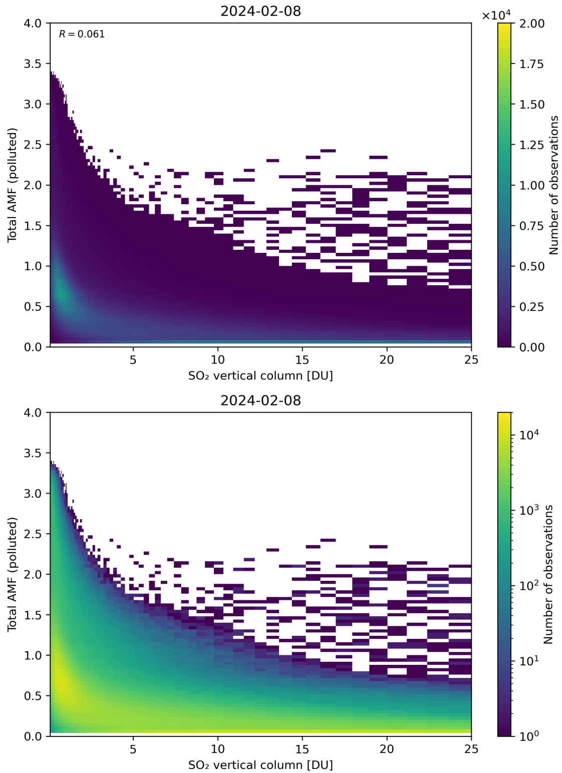
Figure 305: Scatter density plot of “SO 2 vertical column” against “Total AMF (polluted)” for 2024-02-07 to 2024-02-09.
