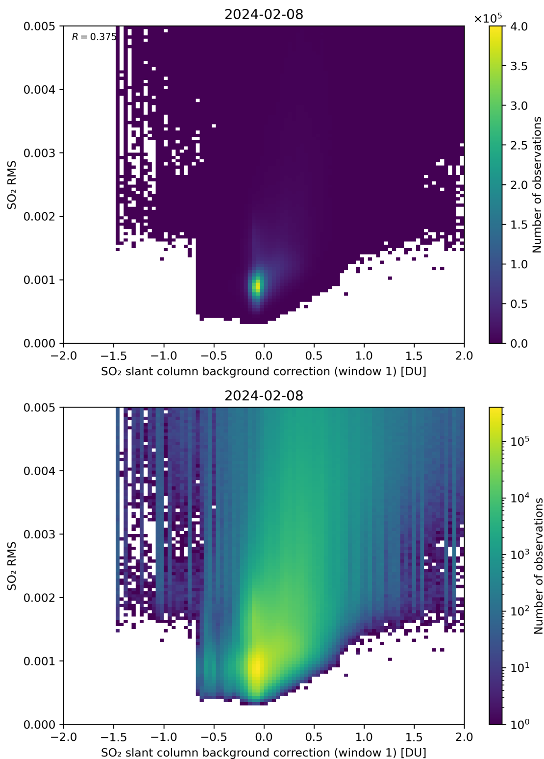
Figure 102: Scatter density plot of “SO 2 slant column background correction (window 1)” against “SO 2 RMS” for 2024-02-07 to 2024-02-09.
