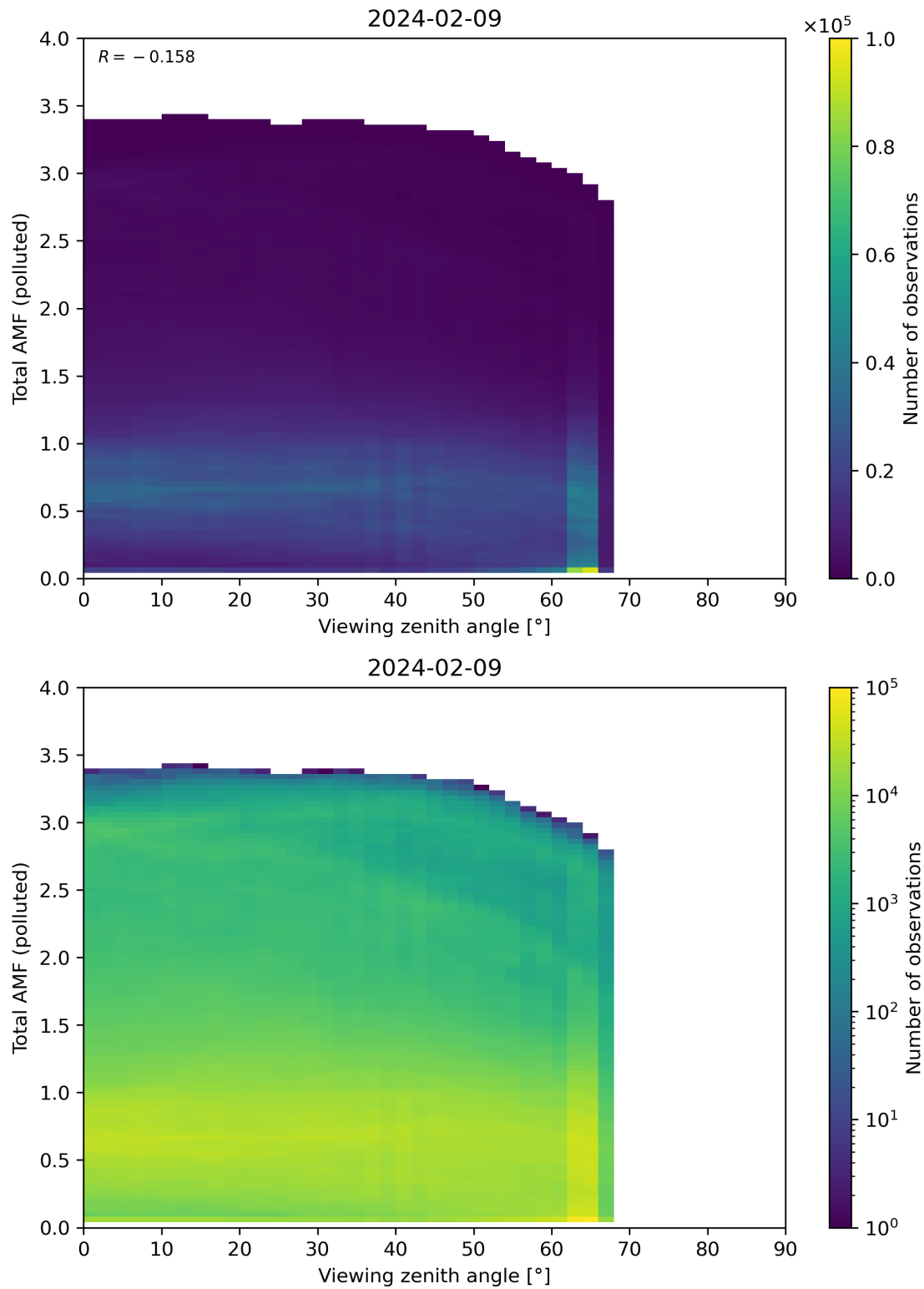
Figure 325: Scatter density plot of “Viewing zenith angle” against “Total AMF (polluted)” for 2024-02-08 to 2024-02-10.
