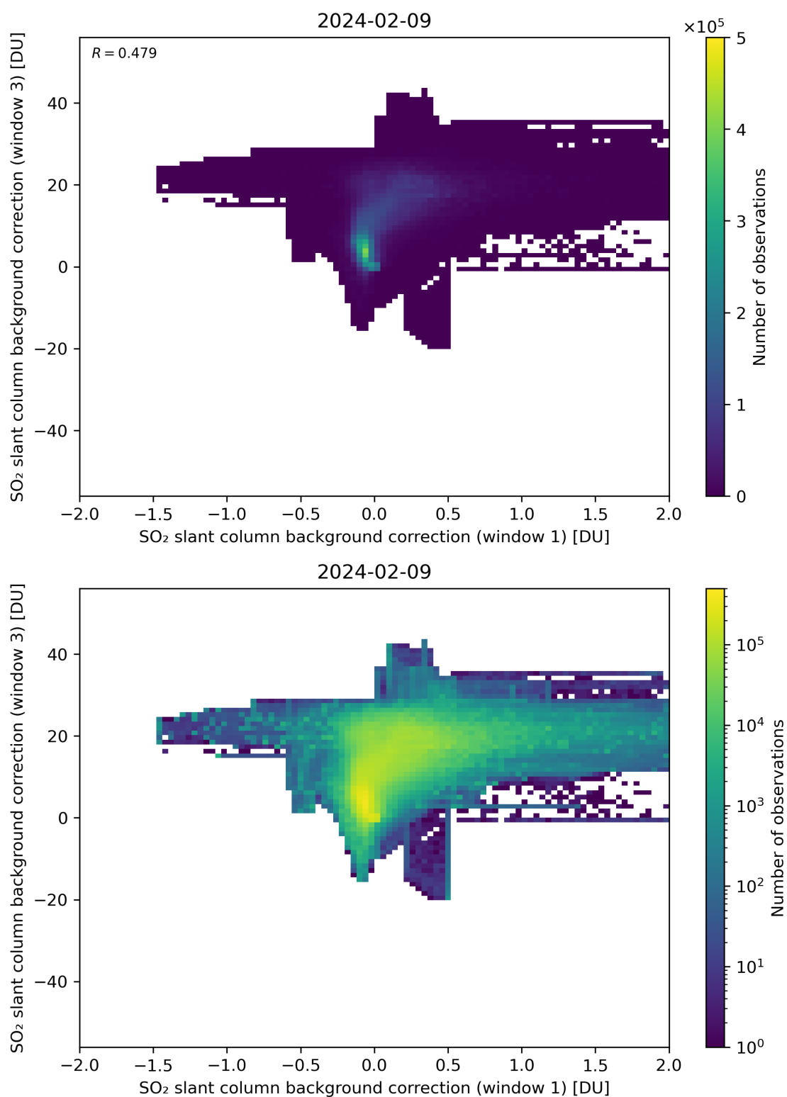
Figure 99: Scatter density plot of “SO 2 slant column background correction (window 1)” against “SO 2 slant column background correction (window 3)” for 2024-02-08 to 2024-02-10.
