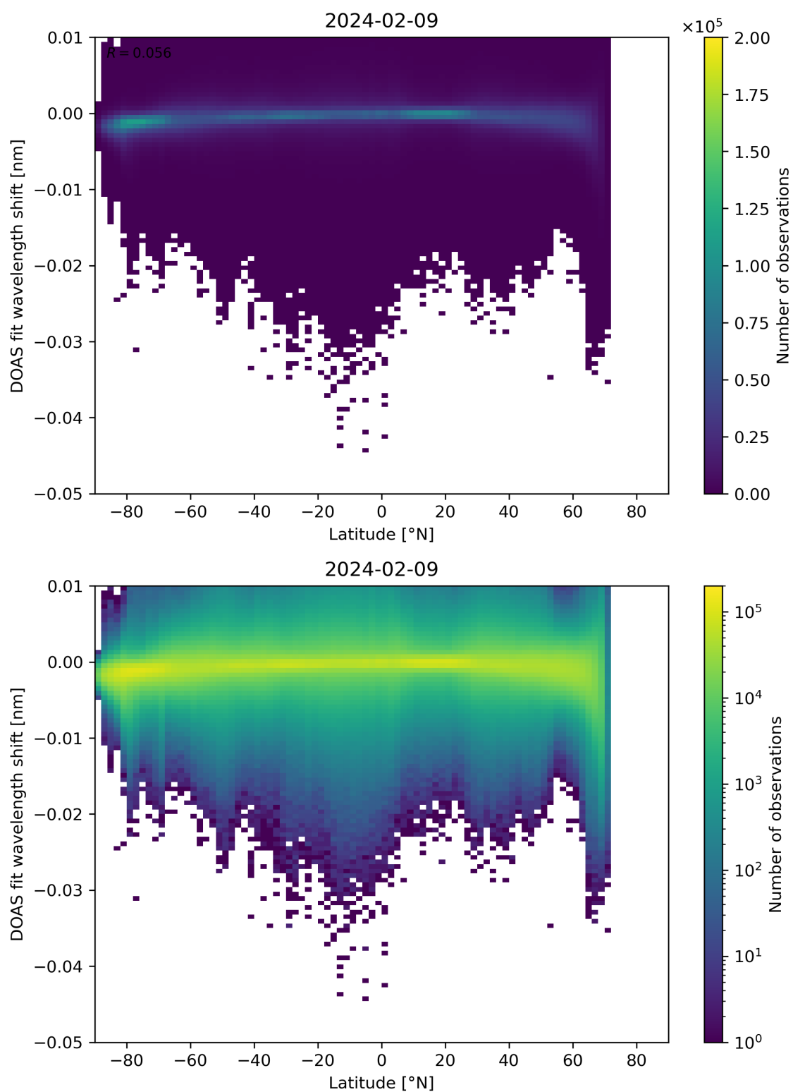
Figure 142: Scatter density plot of “Latitude” against “DOAS fit wavelength shift” for 2024-02-08 to 2024-02-10.
