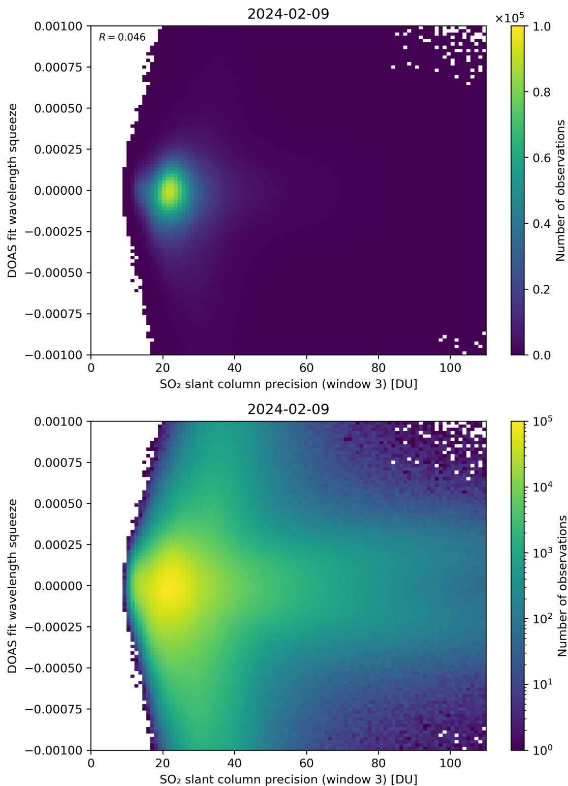
Figure 259: Scatter density plot of “SO 2 slant column precision (window 3)” against “DOAS fit wavelength squeeze” for 2024-02-08 to 2024-02-10.
