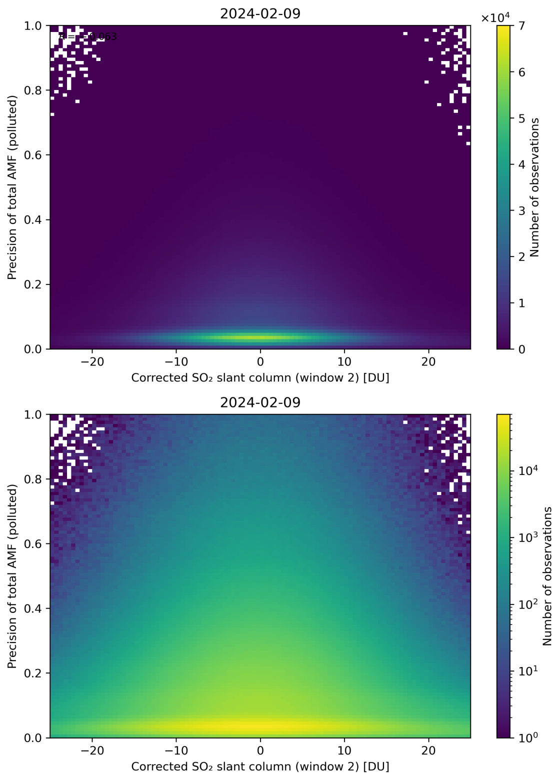
Figure 204: Scatter density plot of “Corrected SO 2 slant column (window 2)” against “Precision of total AMF (polluted)” for 2024-02-08 to 2024-02-10.
