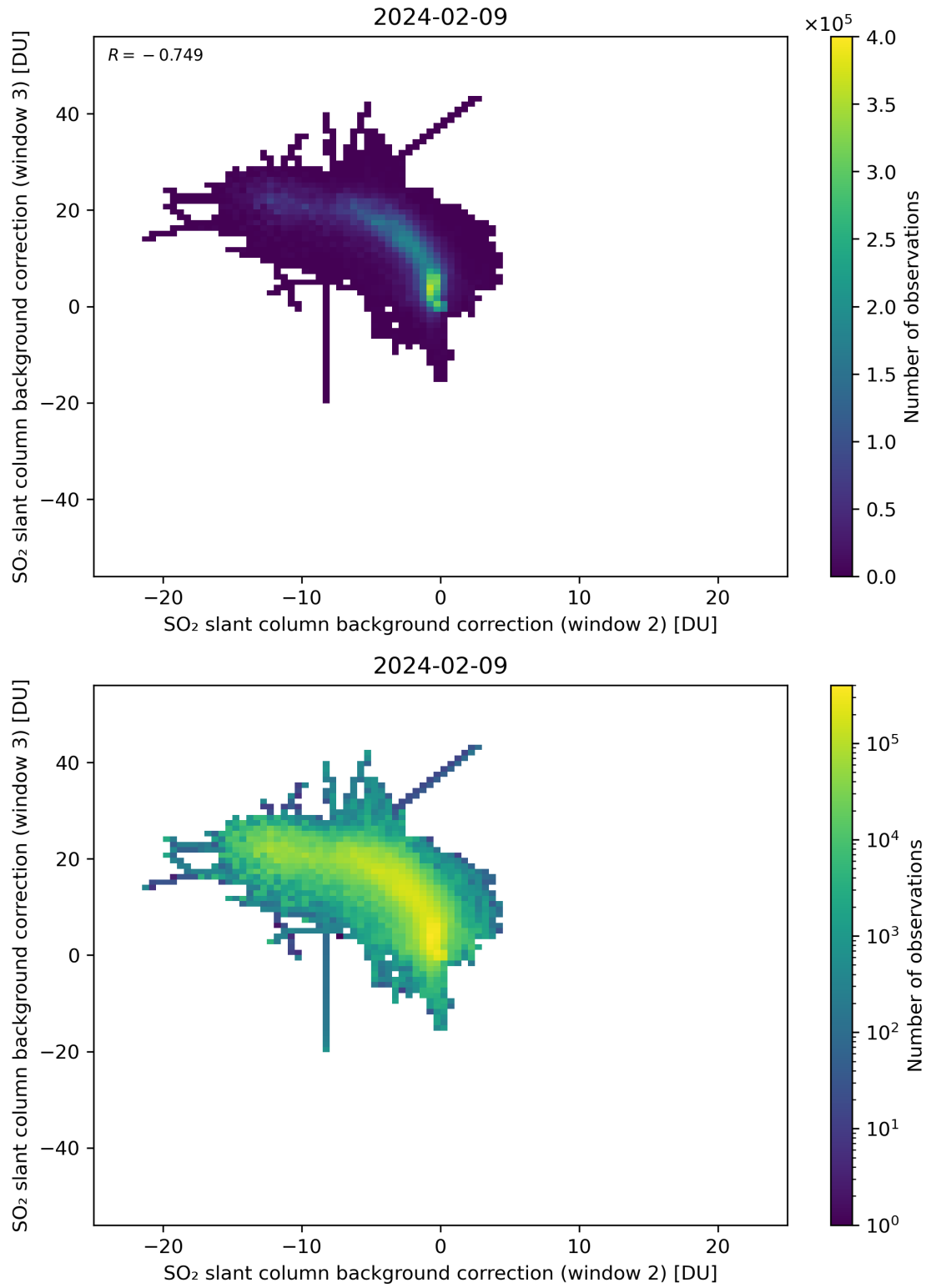
Figure 111: Scatter density plot of “SO 2 slant column background correction (window 2)” against “SO 2 slant column background correction (window 3)” for 2024-02-08 to 2024-02-10.
