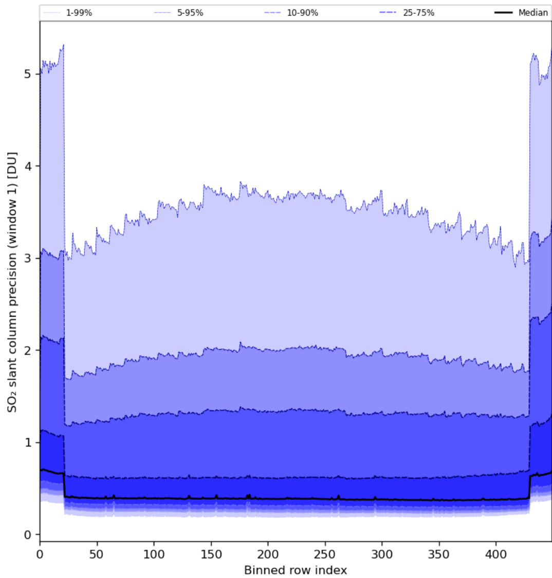
Figure 80: Along track statistics of “SO 2 slant column precision (window 1)” for 2024-02-08 to 2024-02-10
