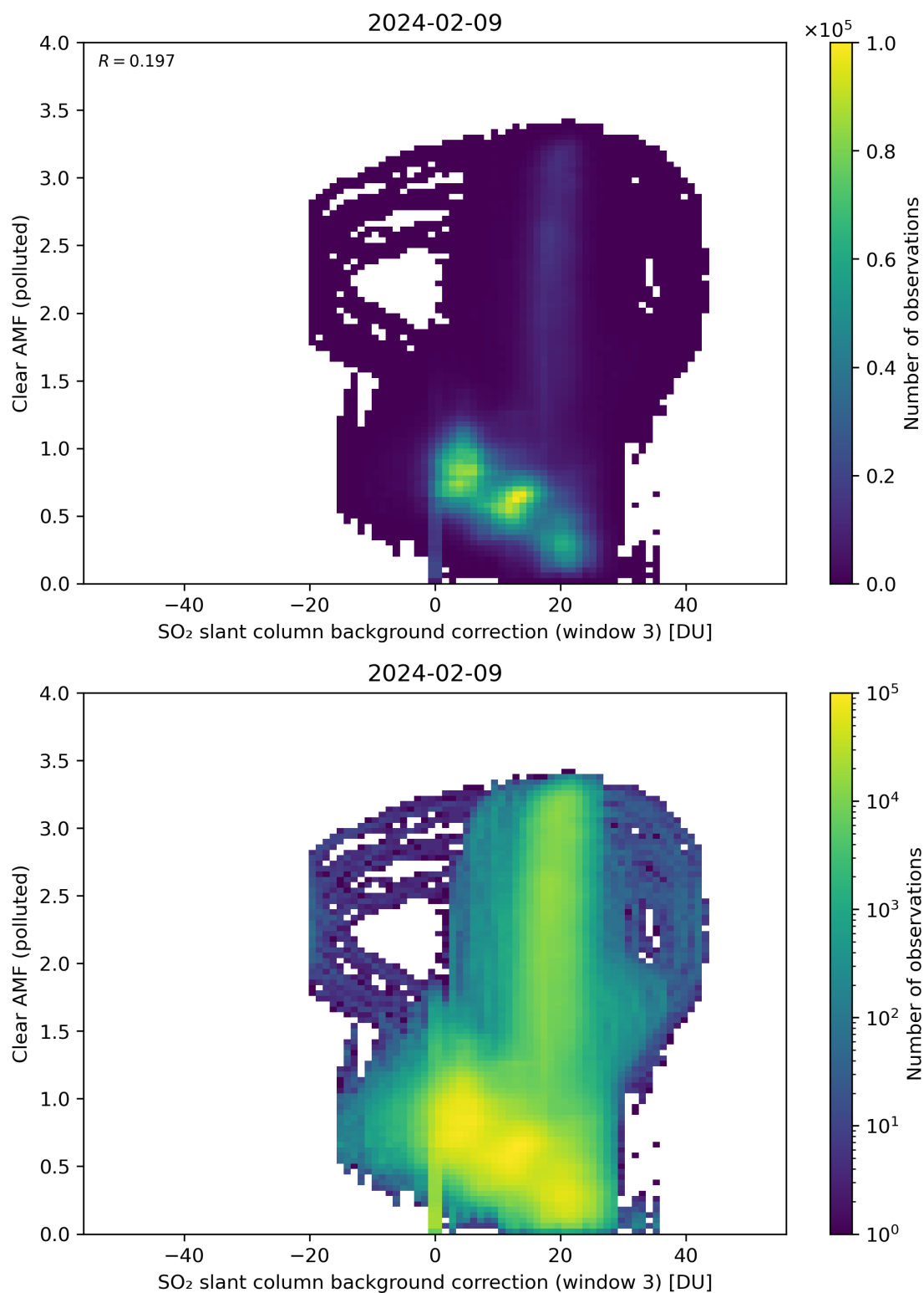
Figure 124: Scatter density plot of “SO 2 slant column background correction (window 3)” against “Clear AMF (polluted)” for 2024-02-08 to 2024-02-10.
