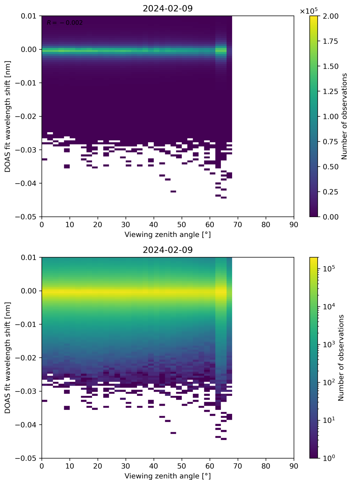
Figure 311: Scatter density plot of “Viewing zenith angle” against “DOAS fit wavelength shift” for 2024-02-08 to 2024-02-10.
