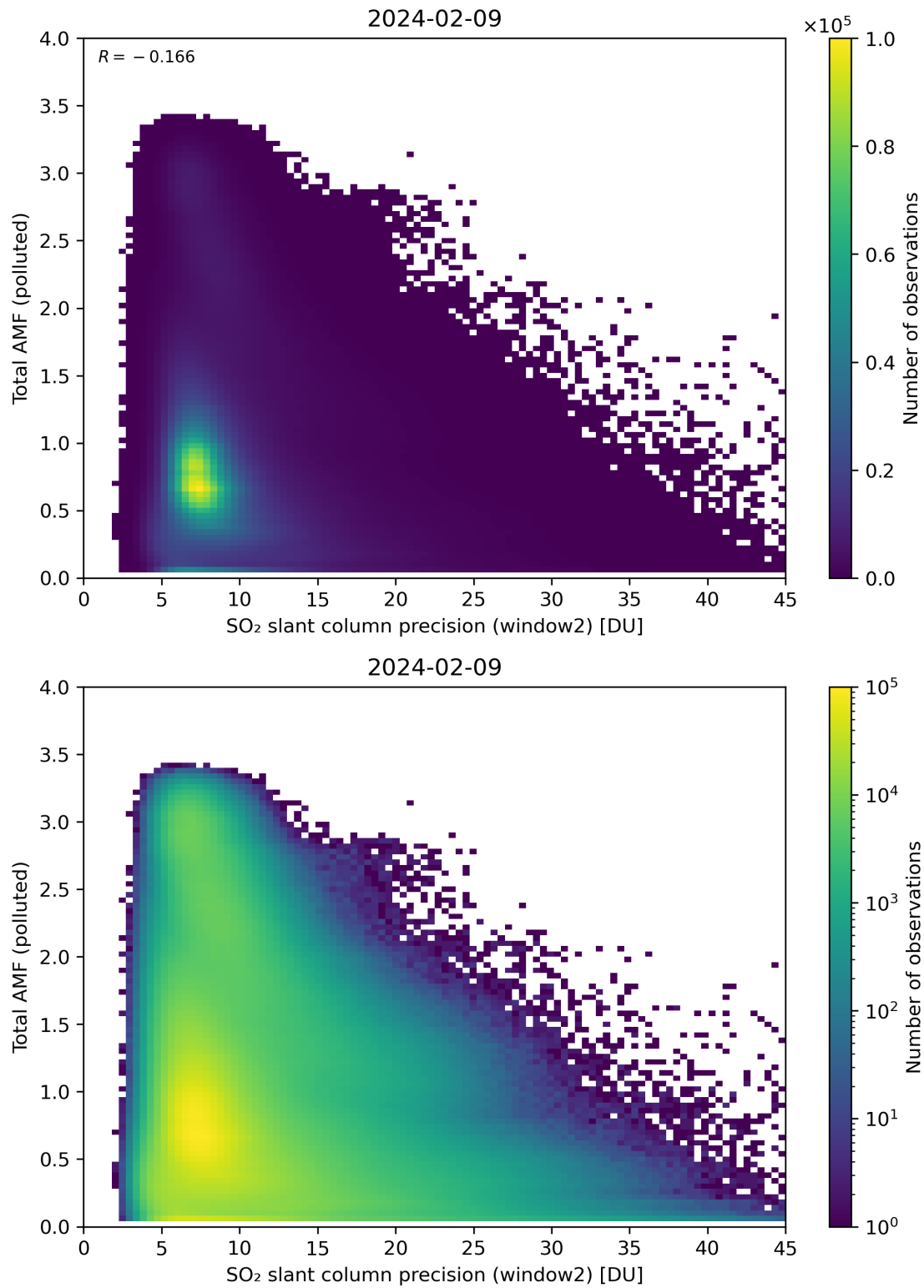
Figure 251: Scatter density plot of “SO 2 slant column precision (window2)” against “Total AMF (polluted)” for 2024-02-08 to 2024-02-10.
