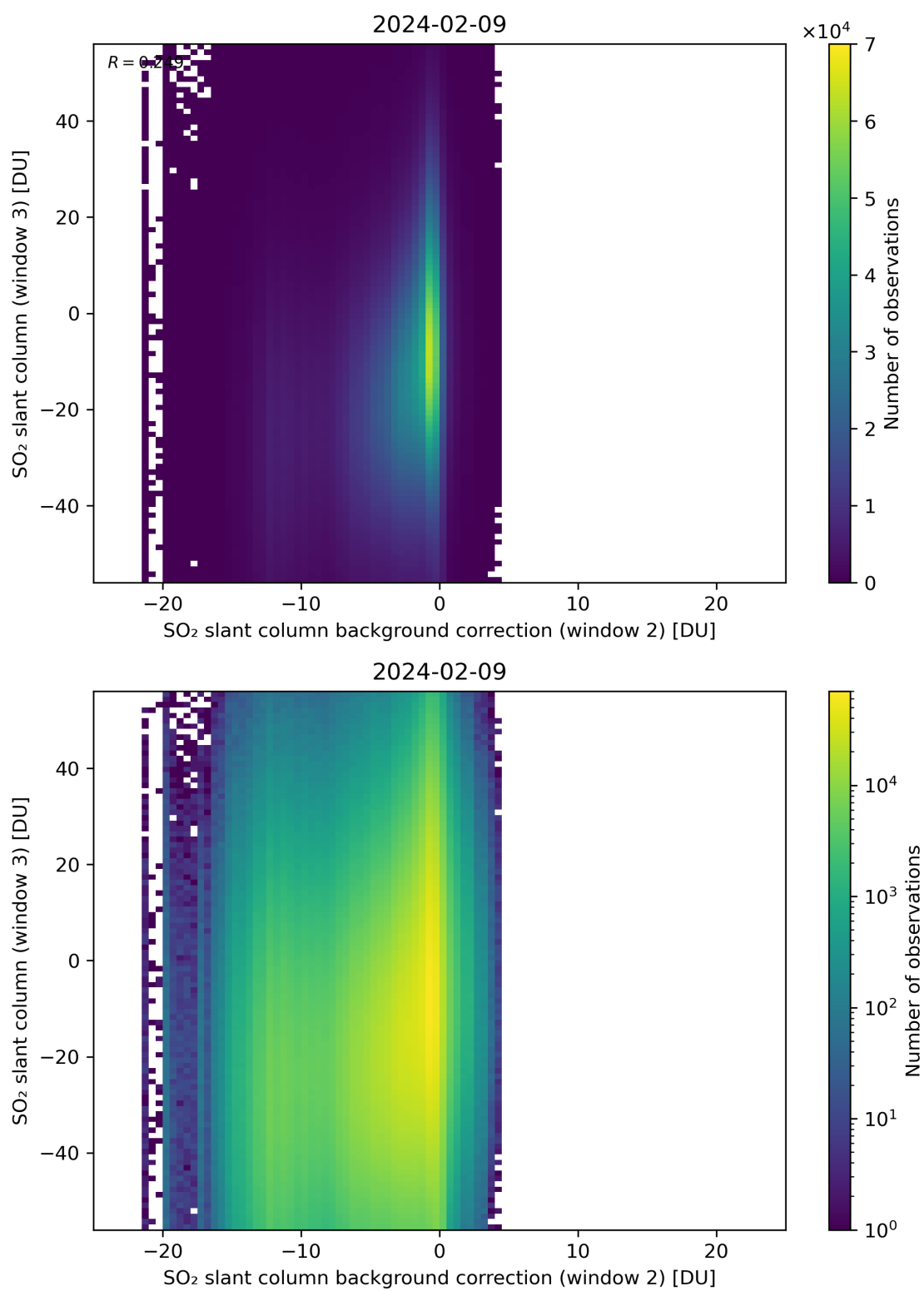
Figure 117: Scatter density plot of “SO 2 slant column background correction (window 2)” against “SO 2 slant column (window 3)” for 2024-02-08 to 2024-02-10.
