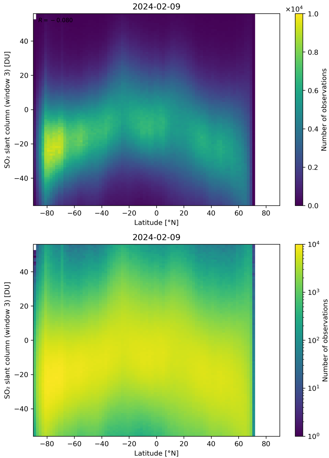
Figure 152: Scatter density plot of “Latitude” against “SO 2 slant column (window 3)” for 2024-02-08 to 2024-02-10.
