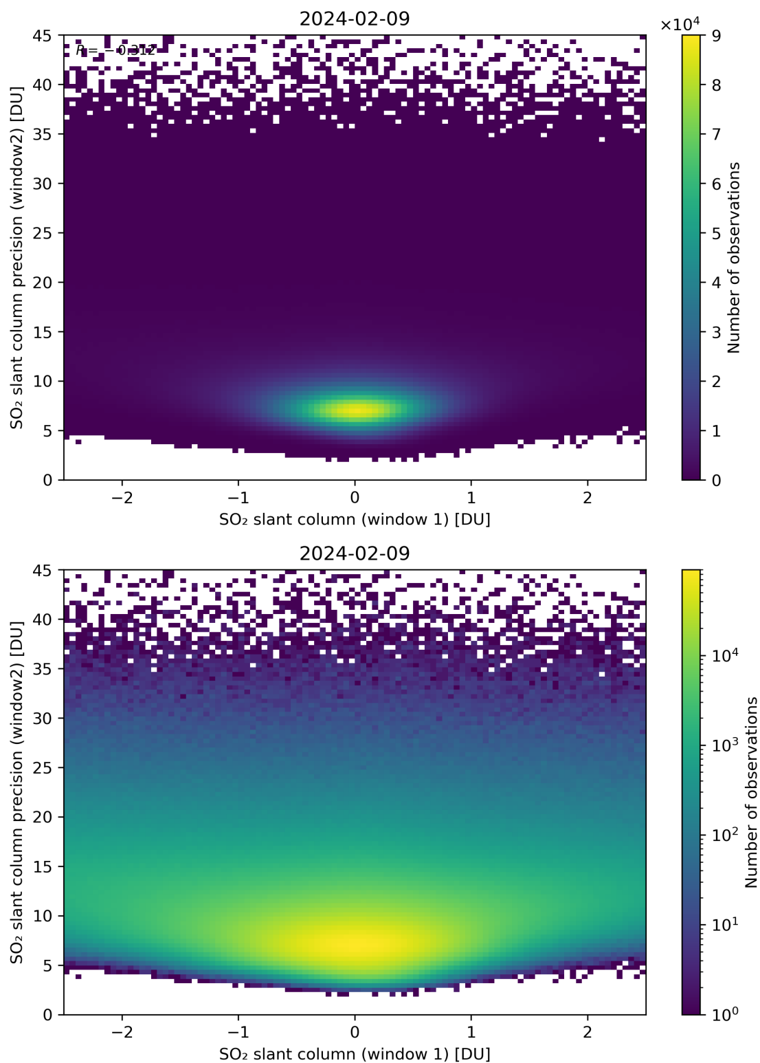
Figure 236: Scatter density plot of “SO 2 slant column (window 1)” against “SO 2 slant column precision (window2)” for 2024-02-08 to 2024-02-10.
