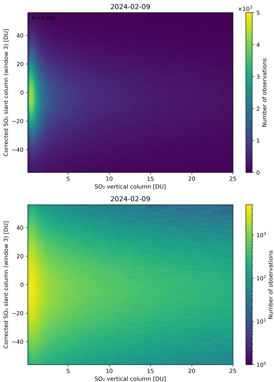
Figure 299: Scatter density plot of “SO 2 vertical column” against “Corrected SO 2 slant column (window 3)” for 2024-02-08 to 2024-02-10.
