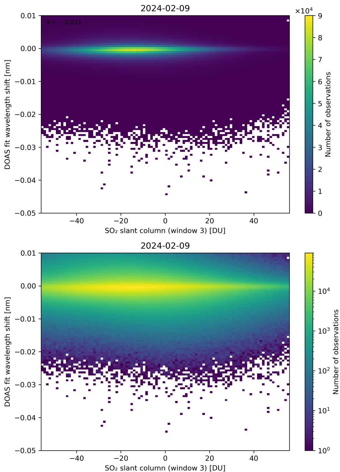
Figure 254: Scatter density plot of “SO 2 slant column (window 3)” against “DOAS fit wavelength shift” for 2024-02-08 to 2024-02-10.
