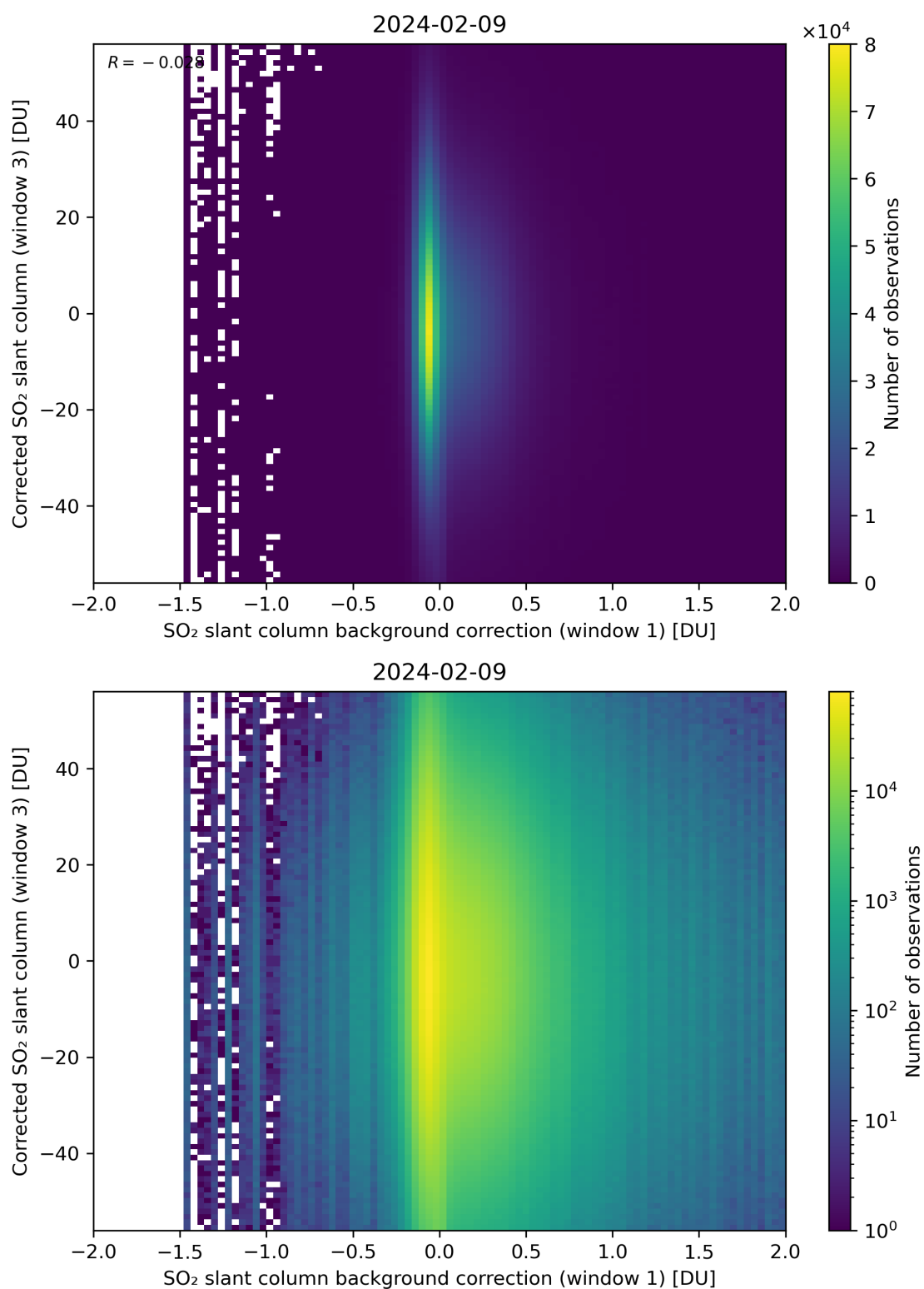
Figure 105: Scatter density plot of “SO 2 slant column background correction (window 1)” against “Corrected SO 2 slant column (window 3)” for 2024-02-08 to 2024-02-10.
