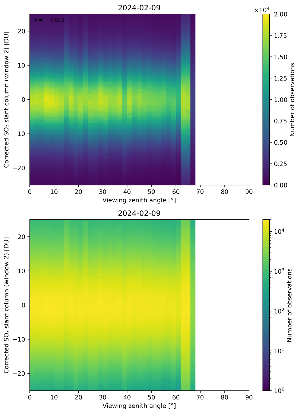
Figure 318: Scatter density plot of “Viewing zenith angle” against “Corrected SO 2 slant column (window 2)” for 2024-02-08 to 2024-02-10.
