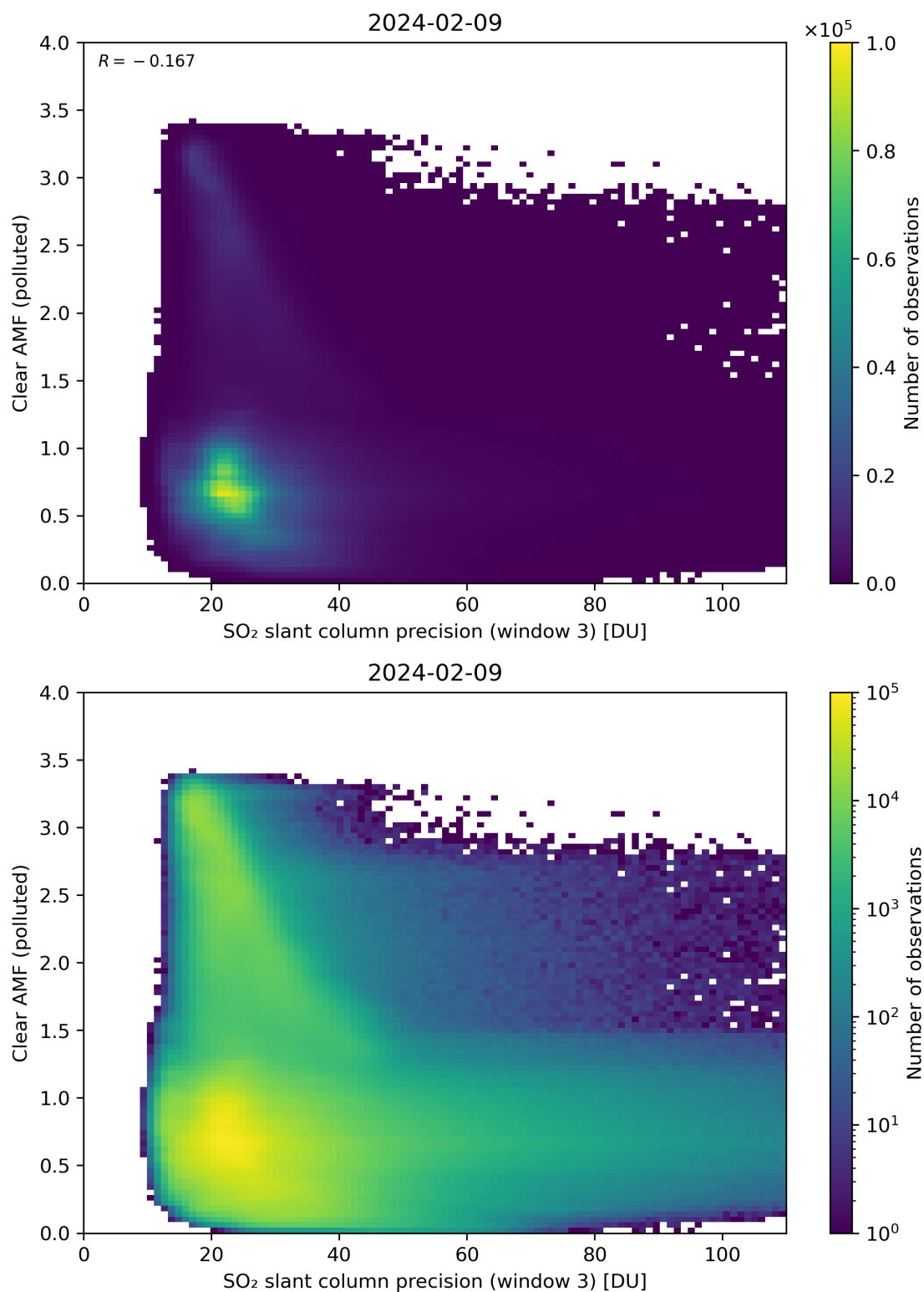
Figure 261: Scatter density plot of “SO 2 slant column precision (window 3)” against “Clear AMF (polluted)” for 2024-02-08 to 2024-02-10.
