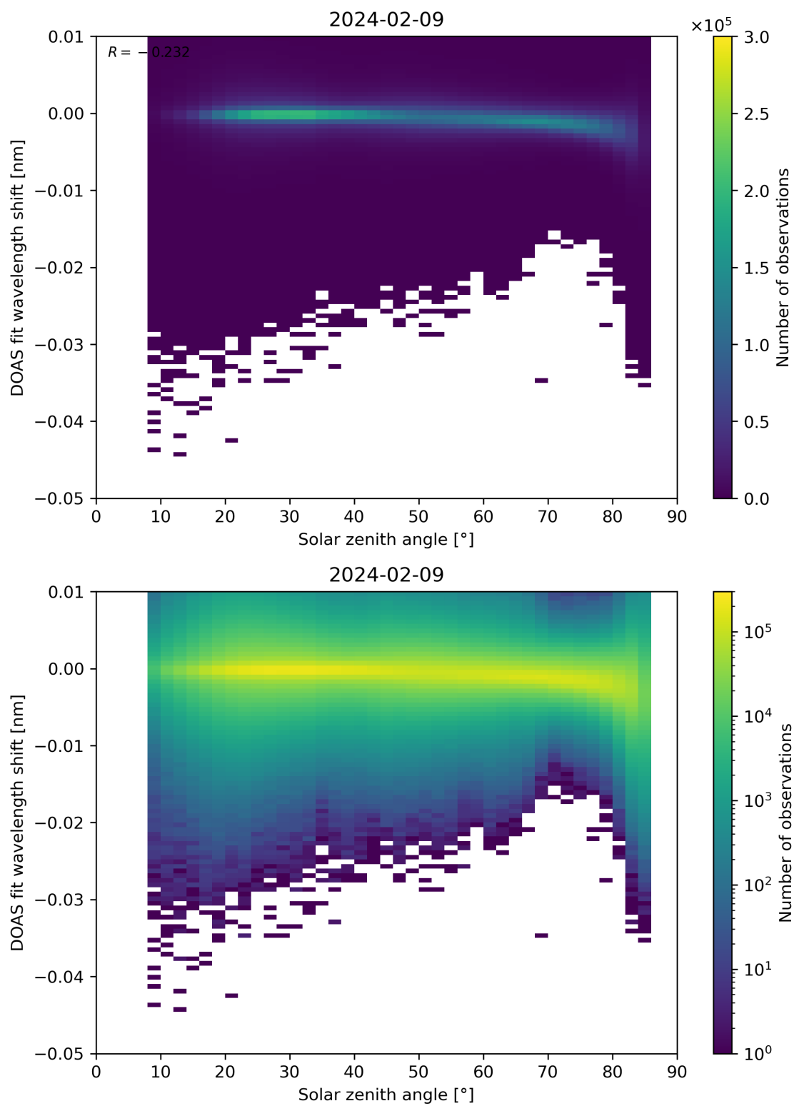
Figure 161: Scatter density plot of “Solar zenith angle” against “DOAS fit wavelength shift” for 2024-02-08 to 2024-02-10.
