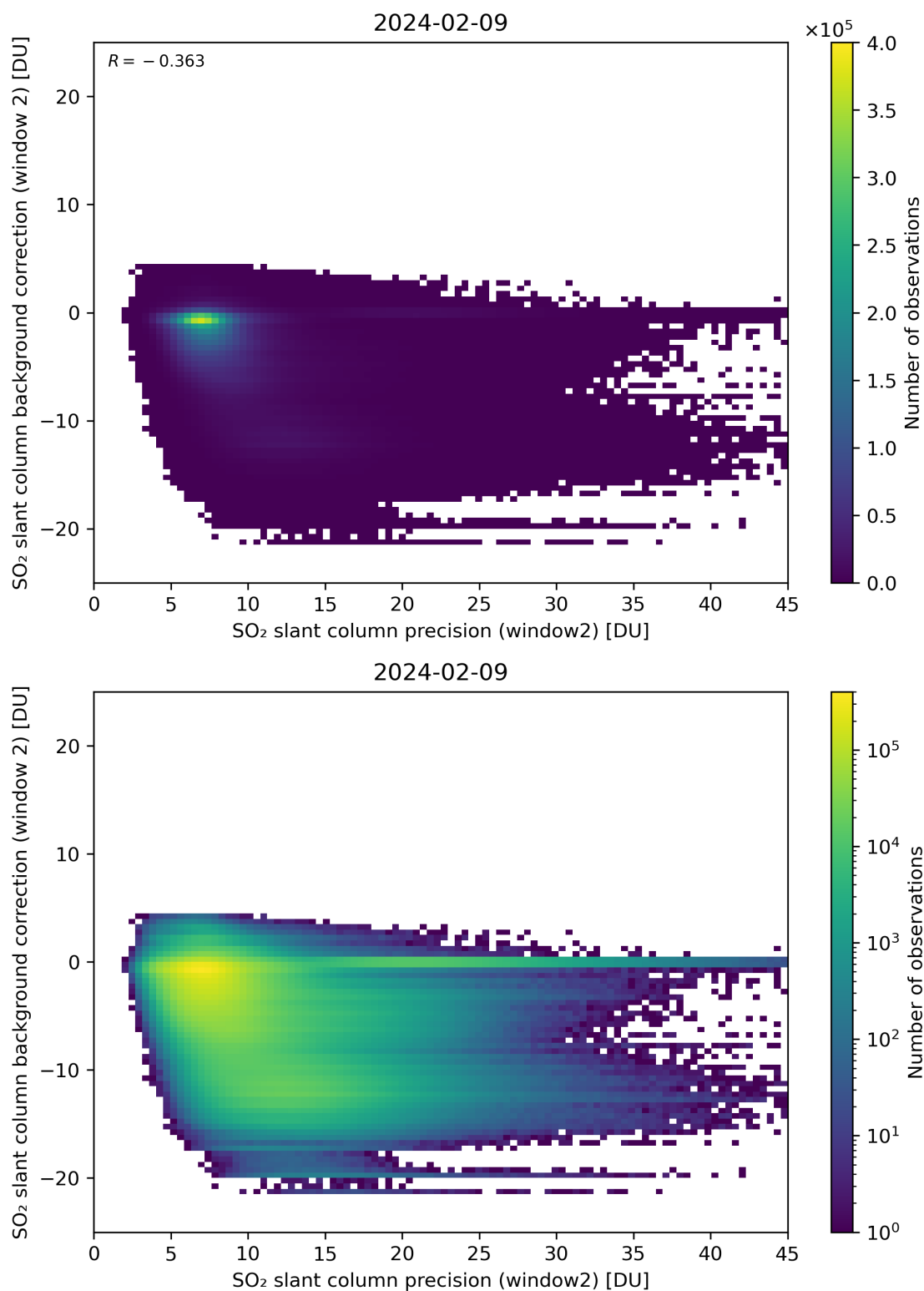
Figure 241: Scatter density plot of “SO 2 slant column precision (window2)” against “SO 2 slant column background correction (window 2)” for 2024-02-08 to 2024-02-10.
