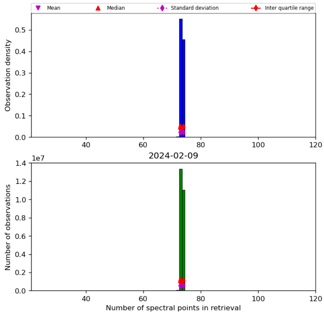
Figure 74: Histogram of “Number of spectral points in retrieval” for 2024-02-08 to 2024-02-10
