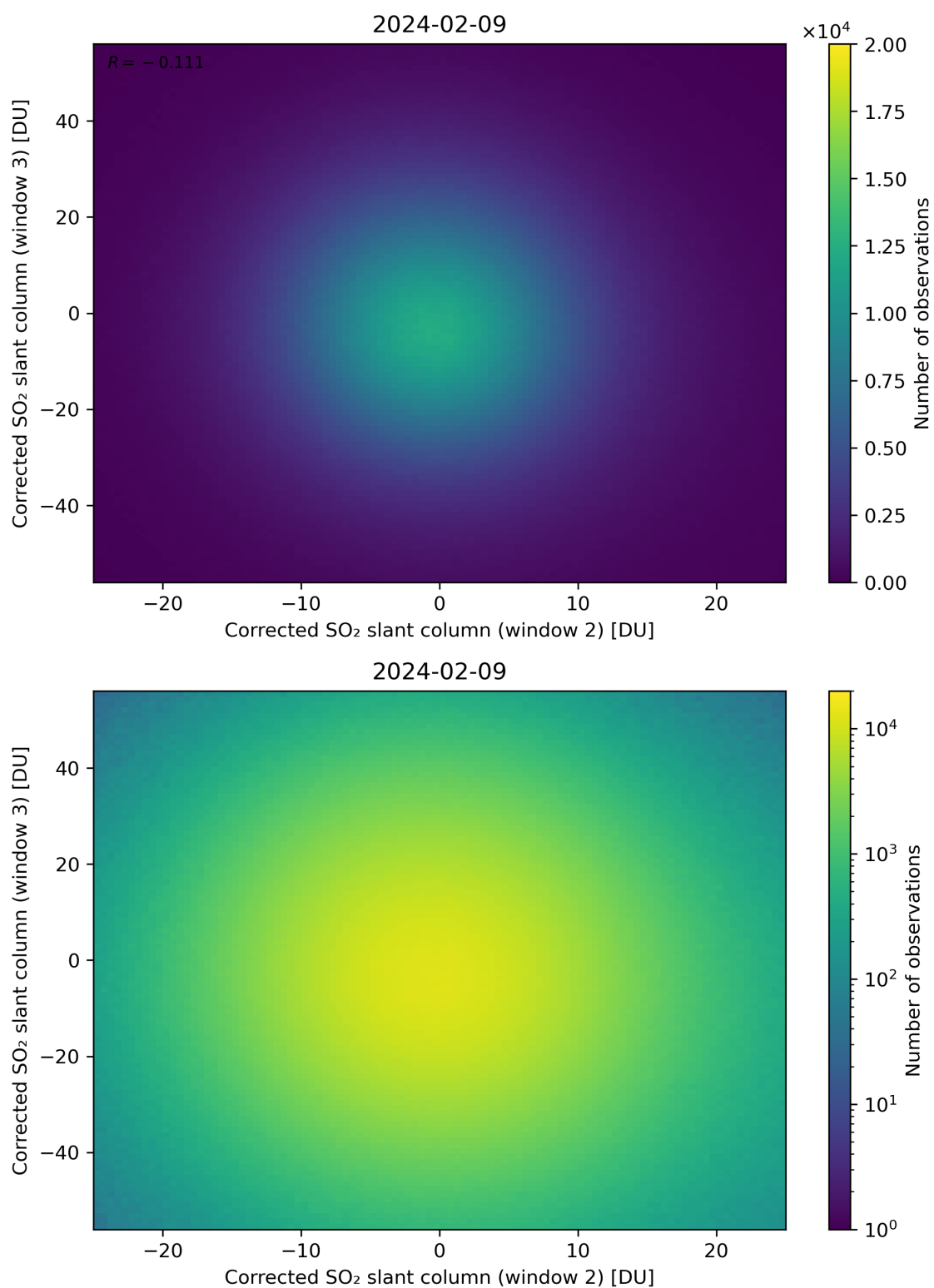
Figure 200: Scatter density plot of “Corrected SO 2 slant column (window 2)” against “Corrected SO 2 slant column (window 3)” for 2024-02-08 to 2024-02-10.
