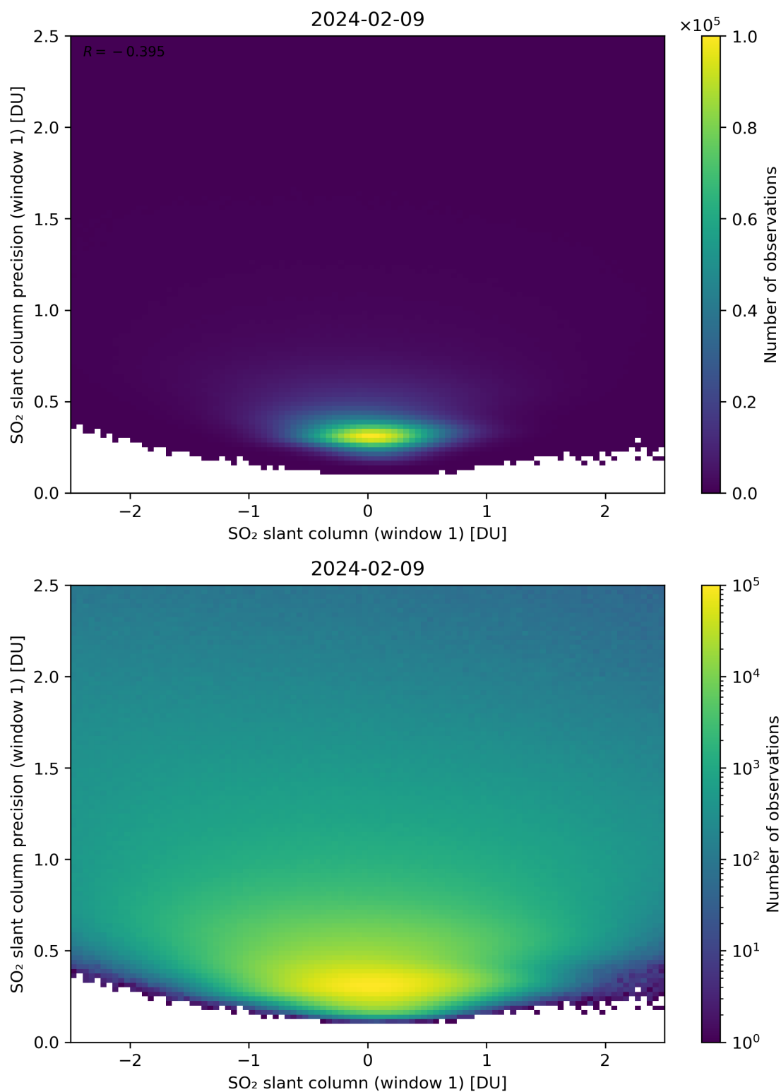
Figure 235: Scatter density plot of “SO 2 slant column (window 1)” against “SO 2 slant column precision (window 1)” for 2024-02-08 to 2024-02-10.
