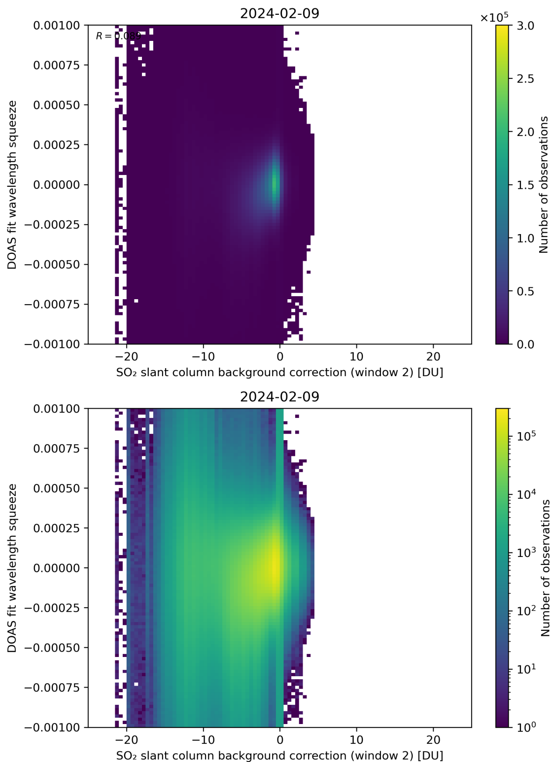
Figure 113: Scatter density plot of “SO 2 slant column background correction (window 2)” against “DOAS fit wavelength squeeze” for 2024-02-08 to 2024-02-10.
