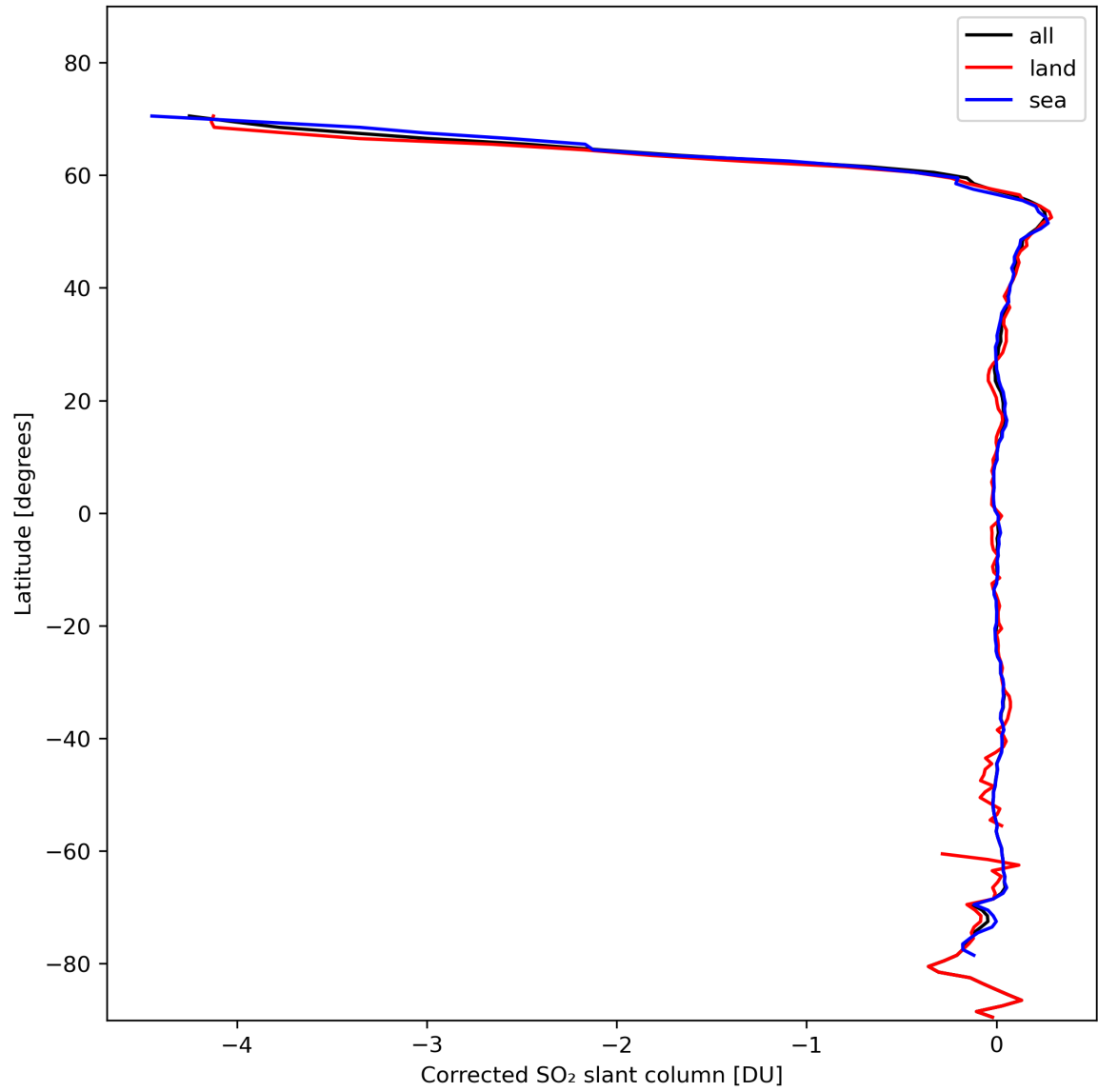
Figure 32: Zonal average of “Corrected SO 2 slant column” for 2024-02-08 to 2024-02-10.
