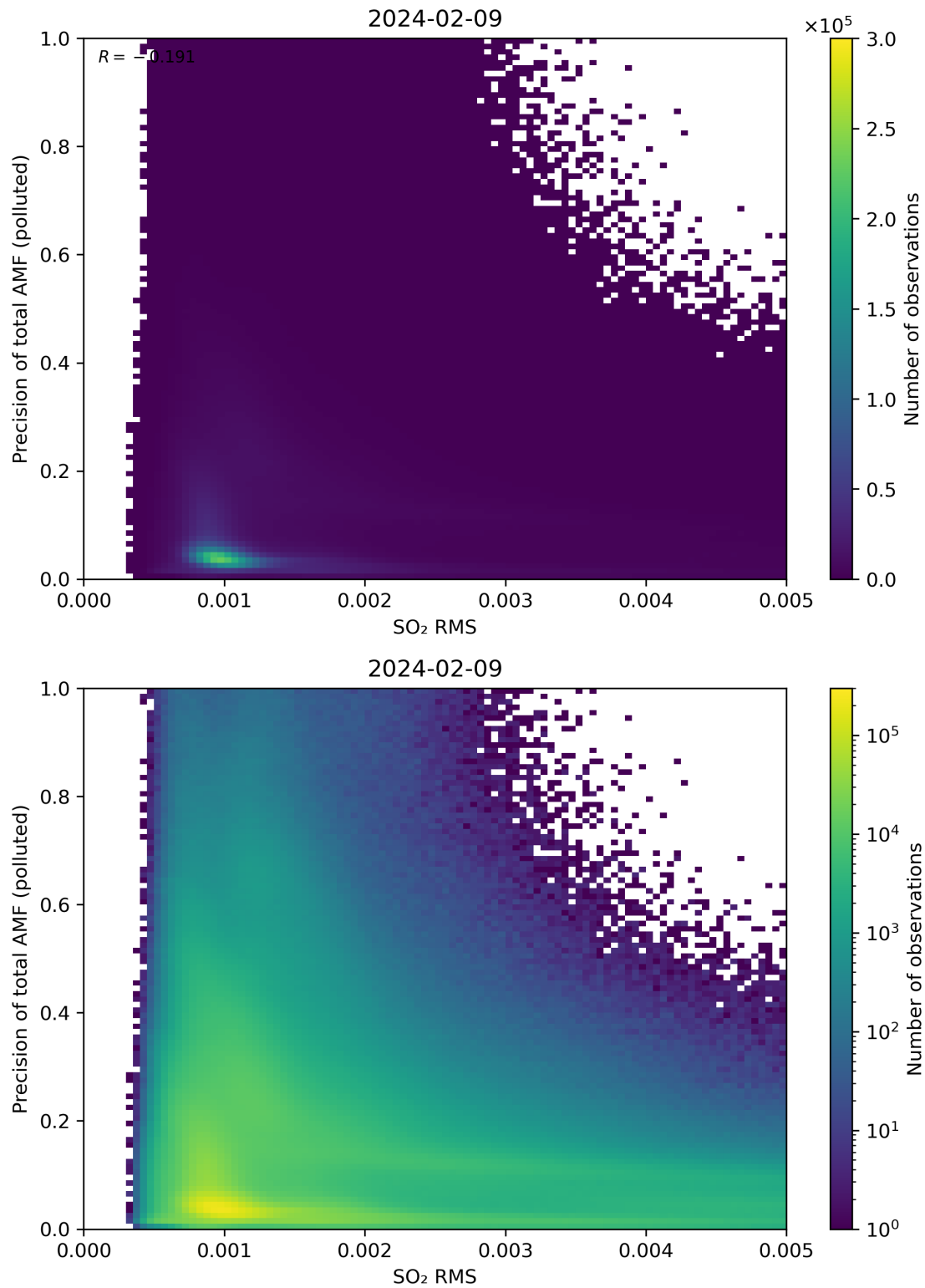
Figure 138: Scatter density plot of “SO 2 RMS” against “Precision of total AMF (polluted)” for 2024-02-08 to 2024-02-10.
