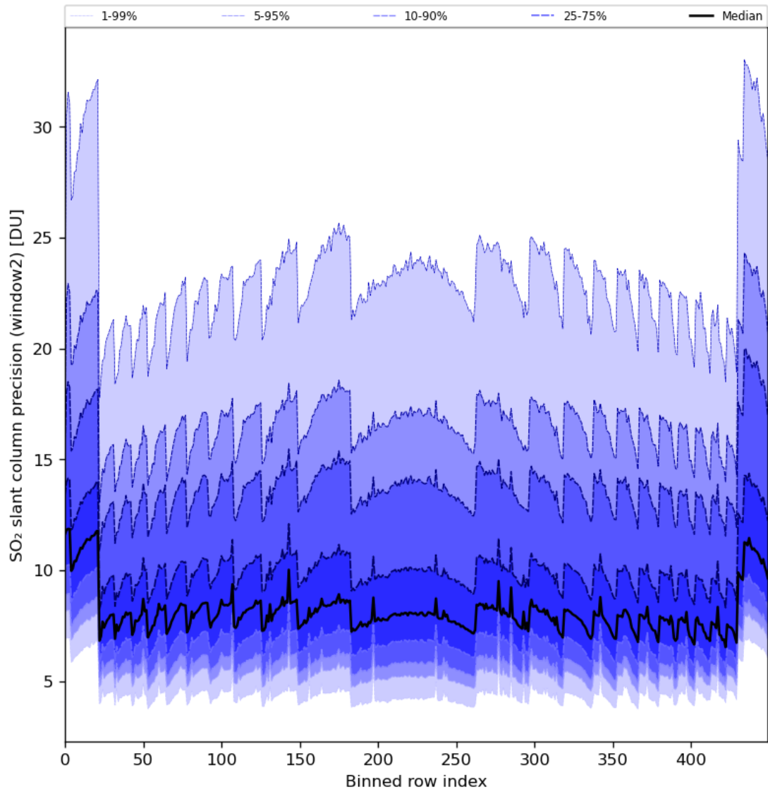
Figure 84: Along track statistics of “SO 2 slant column precision (window2)” for 2024-02-08 to 2024-02-10
