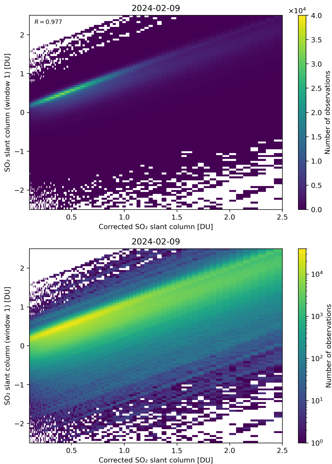
Figure 187: Scatter density plot of “Corrected SO 2 slant column” against “SO 2 slant column (window 1)” for 2024-02-08 to 2024-02-10.
