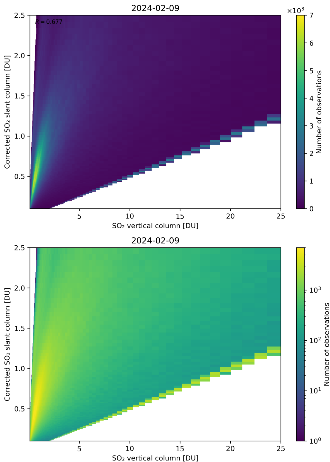
Figure 297: Scatter density plot of “SO 2 vertical column” against “Corrected SO 2 slant column” for 2024-02-08 to 2024-02-10.
