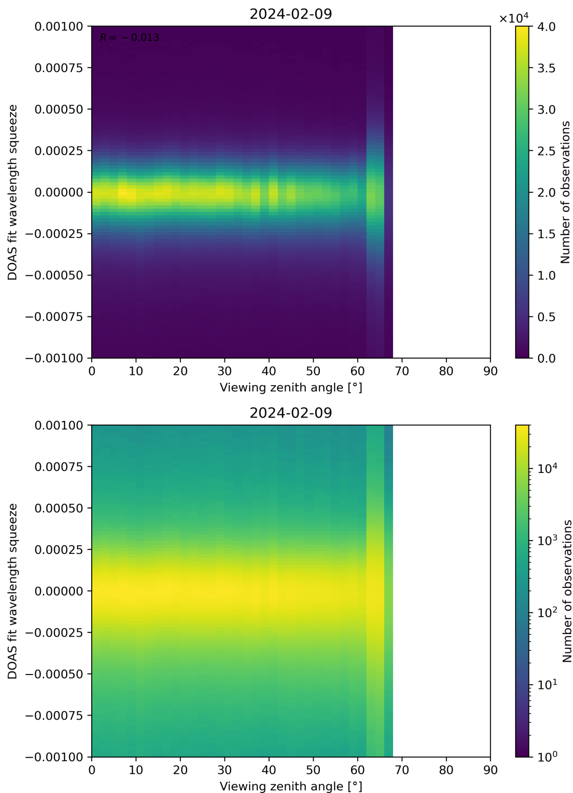
Figure 312: Scatter density plot of “Viewing zenith angle” against “DOAS fit wavelength squeeze” for 2024-02-08 to 2024-02-10.
