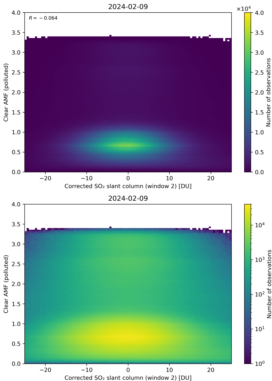
Figure 199: Scatter density plot of “Corrected SO 2 slant column (window 2)” against “Clear AMF (polluted)” for 2024-02-08 to 2024-02-10.
