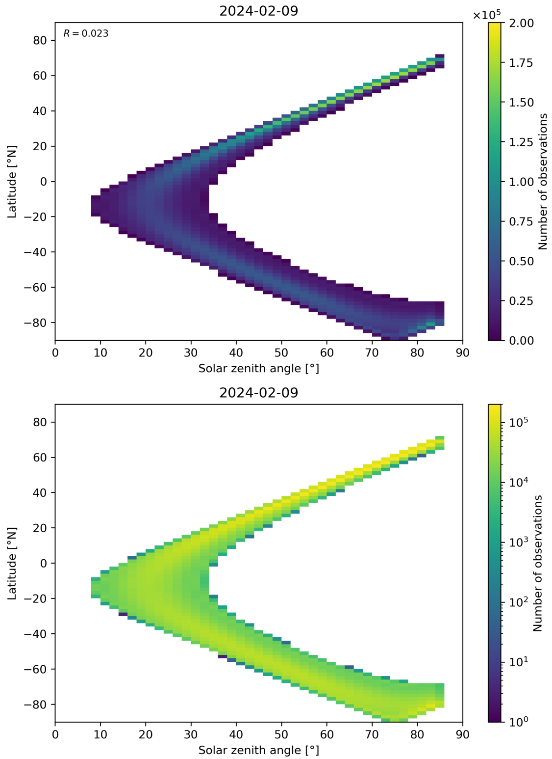
Figure 164: Scatter density plot of “Solar zenith angle” against “Latitude” for 2024-02-08 to 2024-02-10.
