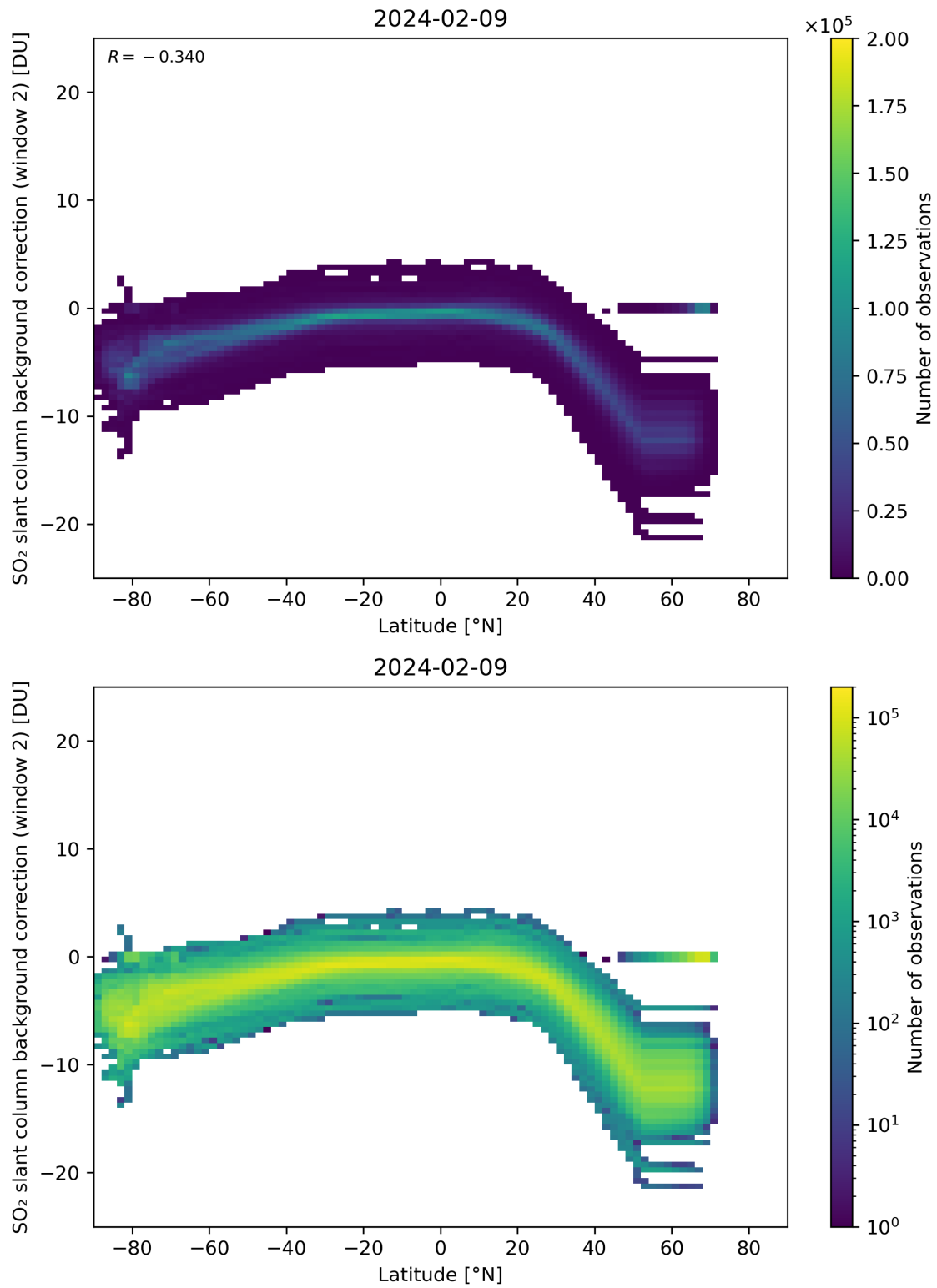
Figure 140: Scatter density plot of “Latitude” against “SO 2 slant column background correction (window 2)” for 2024-02-08 to 2024-02-10.
