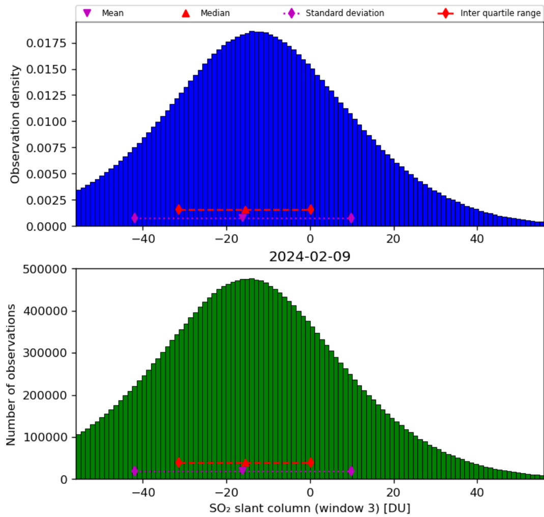
Figure 64: Histogram of “SO 2 slant column (window 3)” for 2024-02-08 to 2024-02-10
