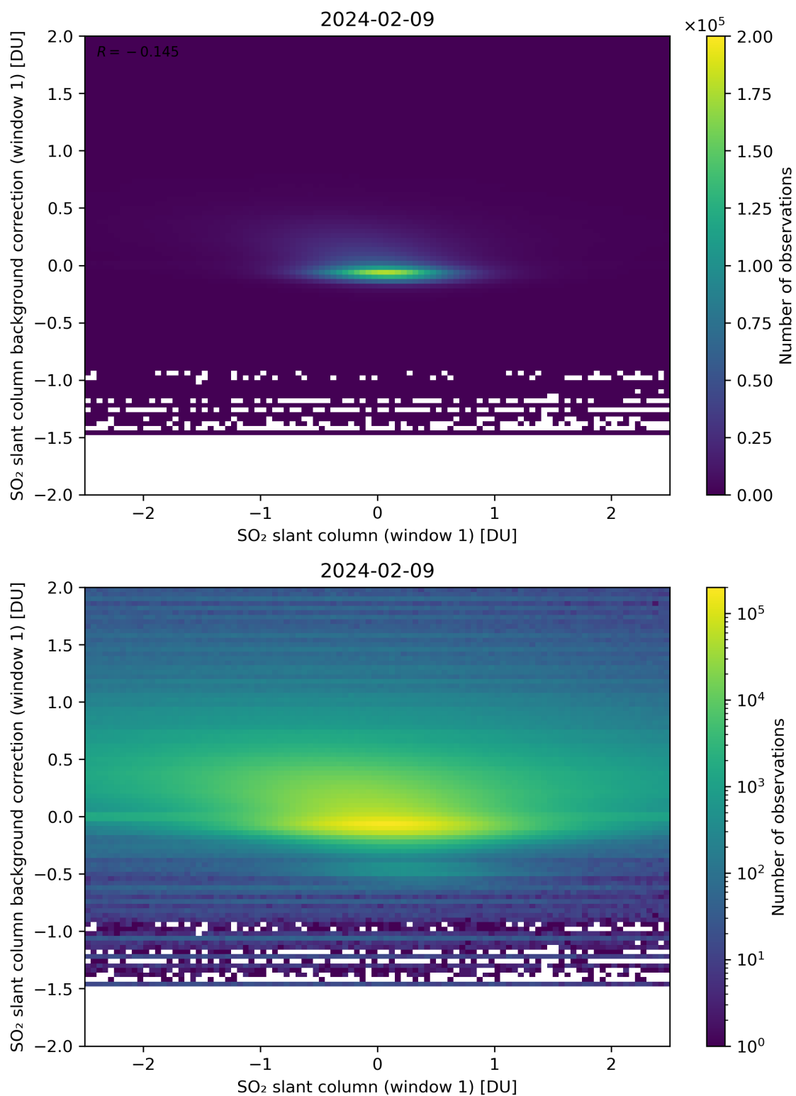
Figure 212: Scatter density plot of “SO 2 slant column (window 1)” against “SO 2 slant column background correction (window 1)” for 2024-02-08 to 2024-02-10.
