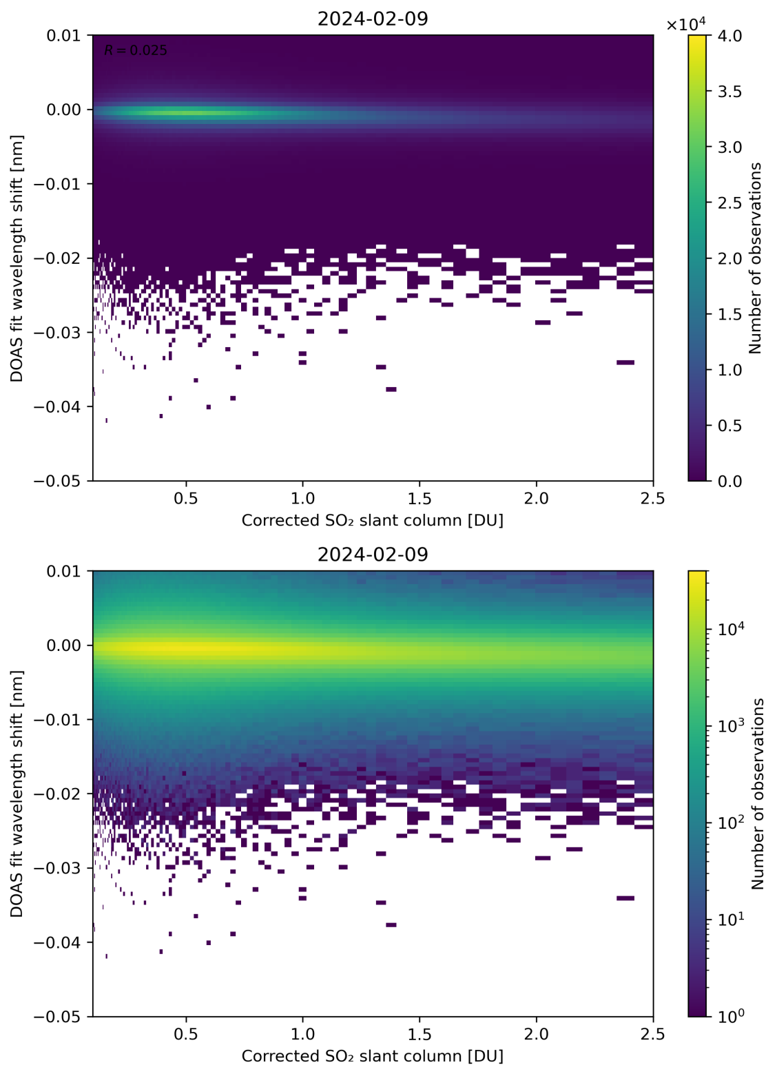
Figure 181: Scatter density plot of “Corrected SO 2 slant column” against “DOAS fit wavelength shift” for 2024-02-08 to 2024-02-10.
