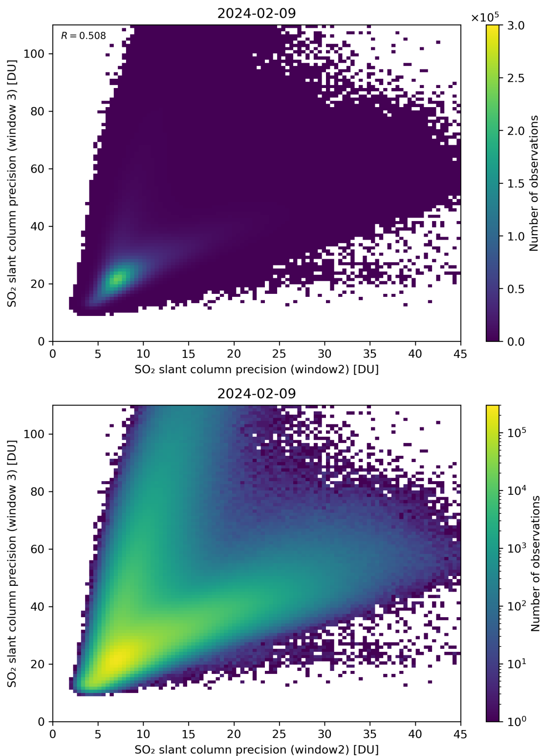
Figure 250: Scatter density plot of “SO 2 slant column precision (window2)” against “SO 2 slant column precision (window 3)” for 2024-02-08 to 2024-02-10.
