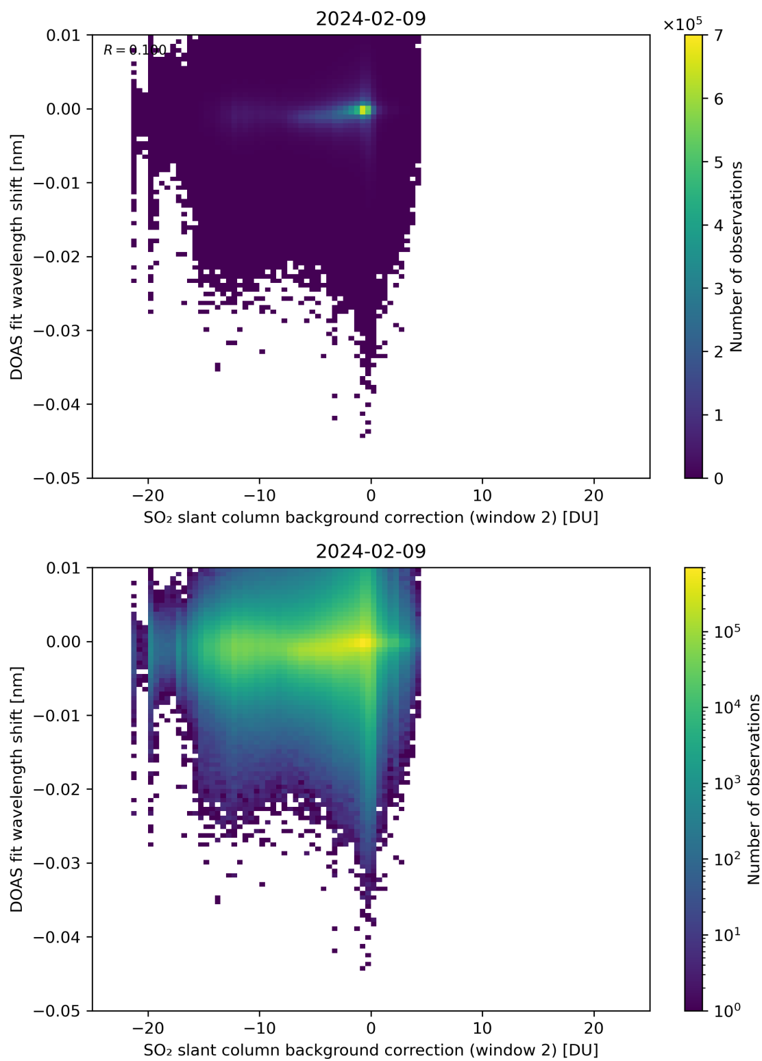
Figure 112: Scatter density plot of “SO 2 slant column background correction (window 2)” against “DOAS fit wavelength shift” for 2024-02-08 to 2024-02-10.
