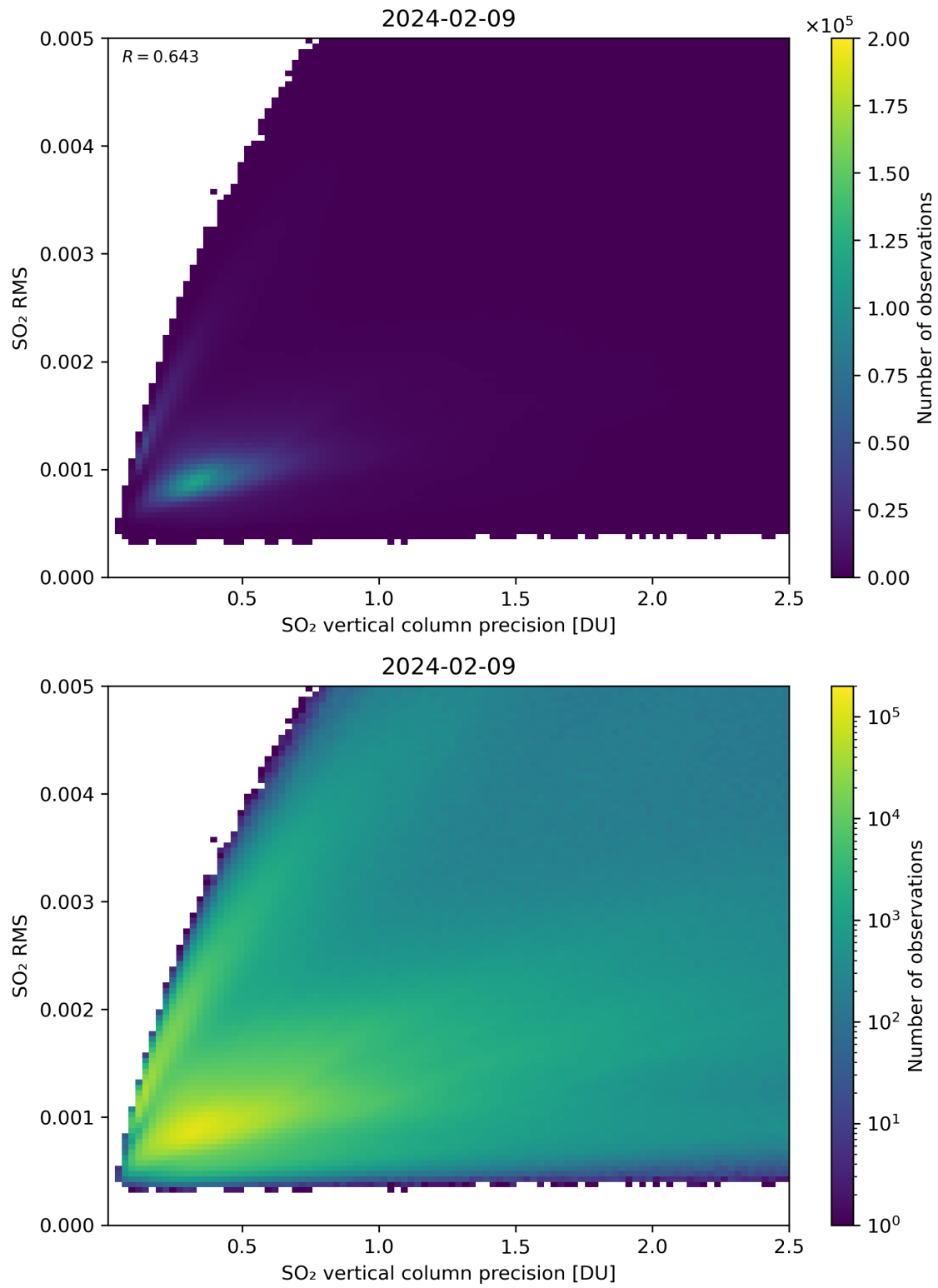
Figure 284: Scatter density plot of “SO 2 vertical column precision” against “SO 2 RMS” for 2024-02-08 to 2024-02-10.
