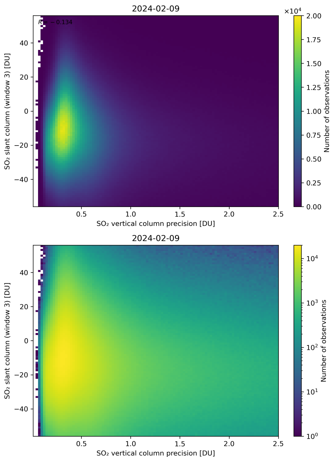
Figure 292: Scatter density plot of “SO 2 vertical column precision” against “SO 2 slant column (window 3)” for 2024-02-08 to 2024-02-10.
