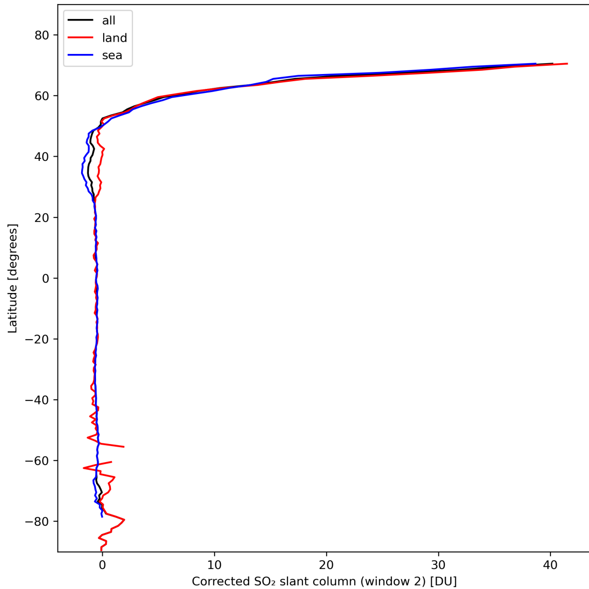
Figure 39: Zonal average of “Corrected SO 2 slant column (window 2)” for 2024-02-08 to 2024-02-10.
