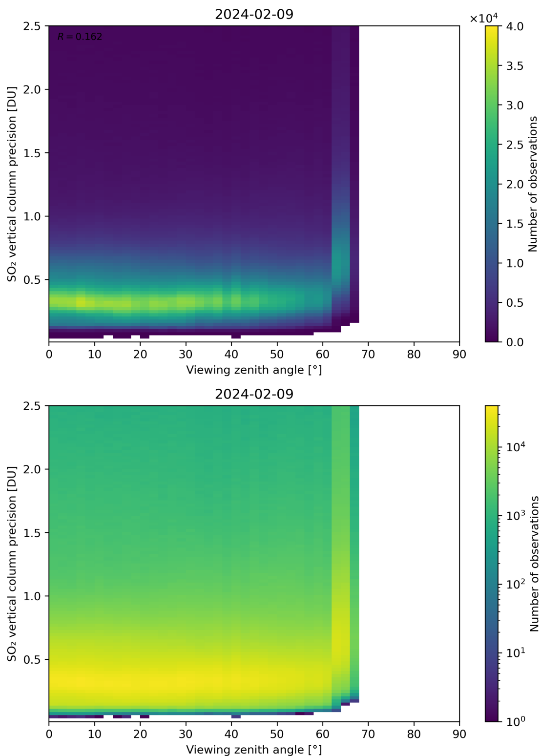
Figure 328: Scatter density plot of “Viewing zenith angle” against “SO 2 vertical column precision” for 2024-02-08 to 2024-02-10.
