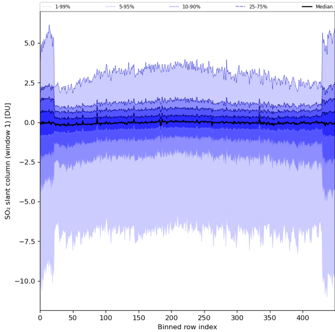
Figure 79: Along track statistics of “SO 2 slant column (window 1)” for 2024-02-08 to 2024-02-10
