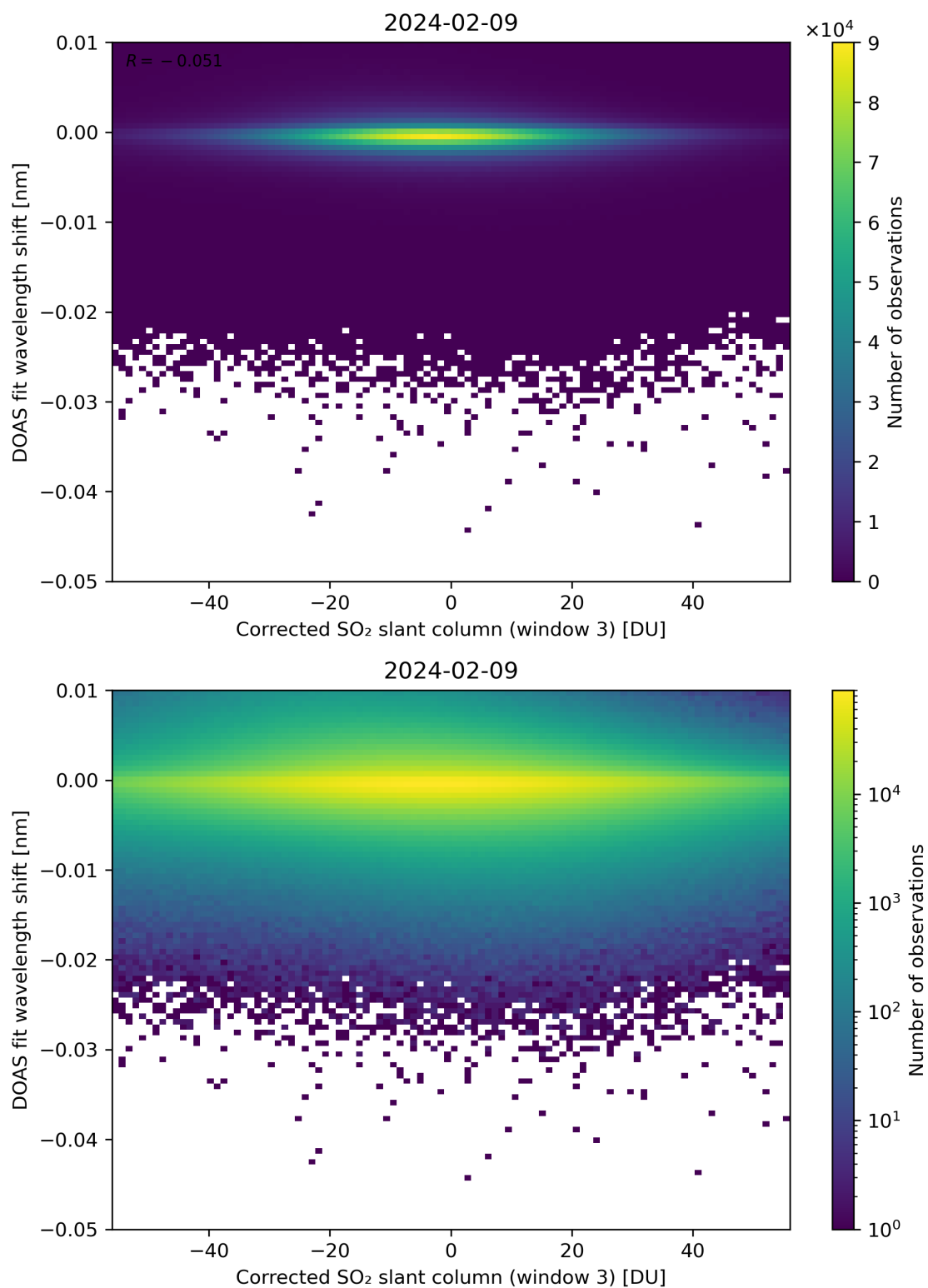
Figure 206: Scatter density plot of “Corrected SO 2 slant column (window 3)” against “DOAS fit wavelength shift” for 2024-02-08 to 2024-02-10.
