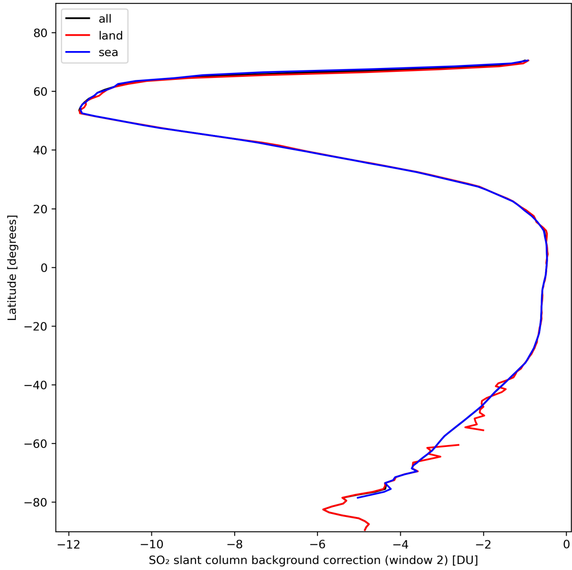
Figure 40: Zonal average of “SO 2 slant column background correction (window 2)” for 2024-02-08 to 2024-02-10.
