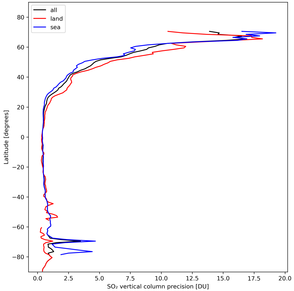
Figure 31: Zonal average of “SO 2 vertical column precision” for 2024-02-08 to 2024-02-10.
