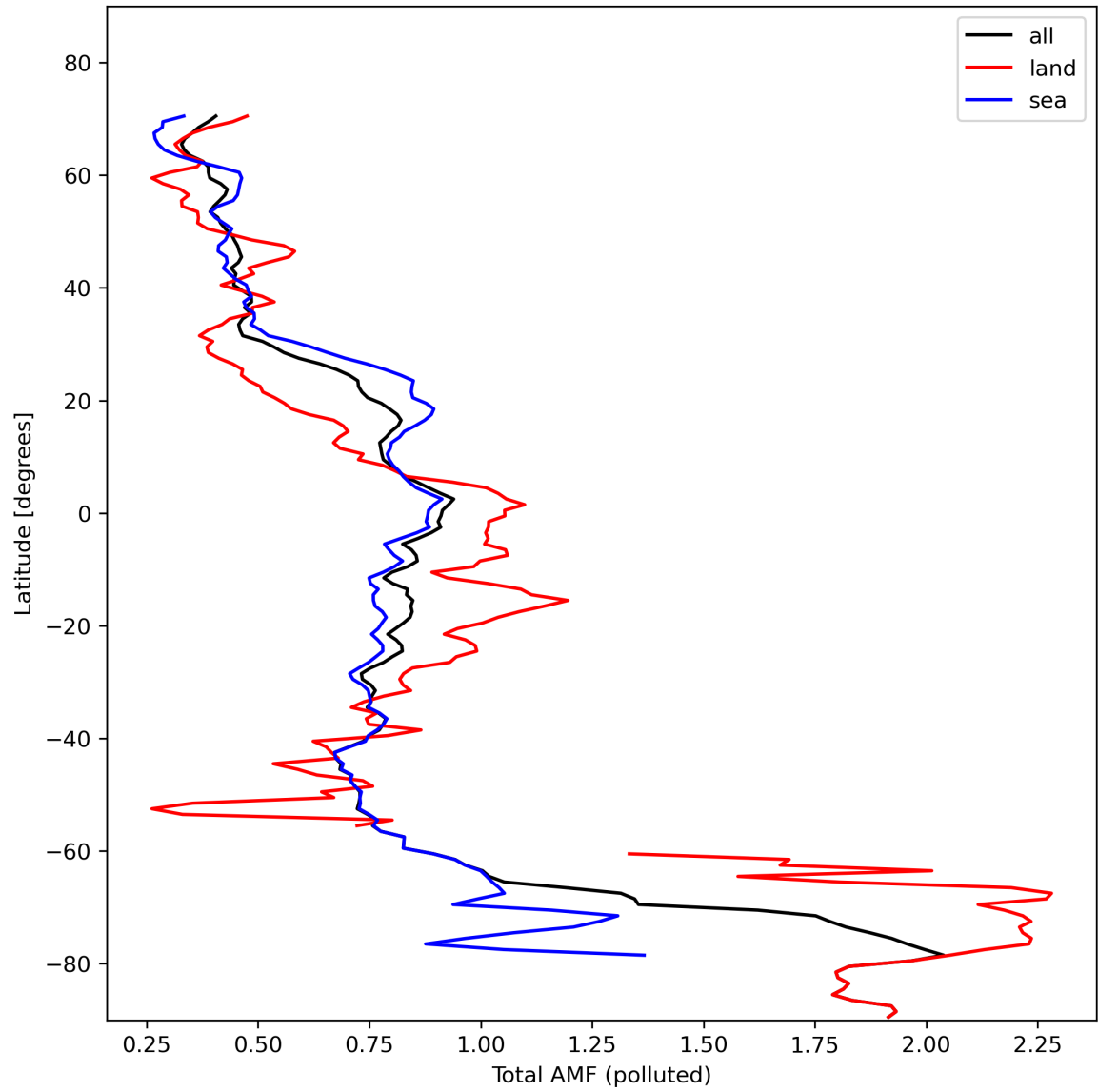
Figure 48: Zonal average of “Total AMF (polluted)” for 2024-02-08 to 2024-02-10.
