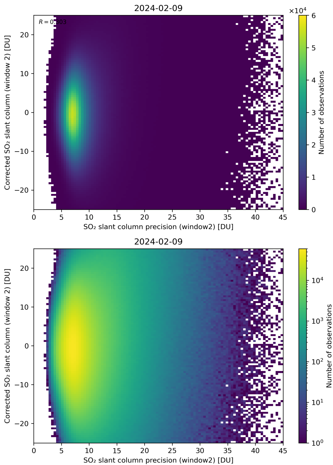
Figure 247: Scatter density plot of “SO 2 slant column precision (window2)” against “Corrected SO 2 slant column (window 2)” for 2024-02-08 to 2024-02-10.
