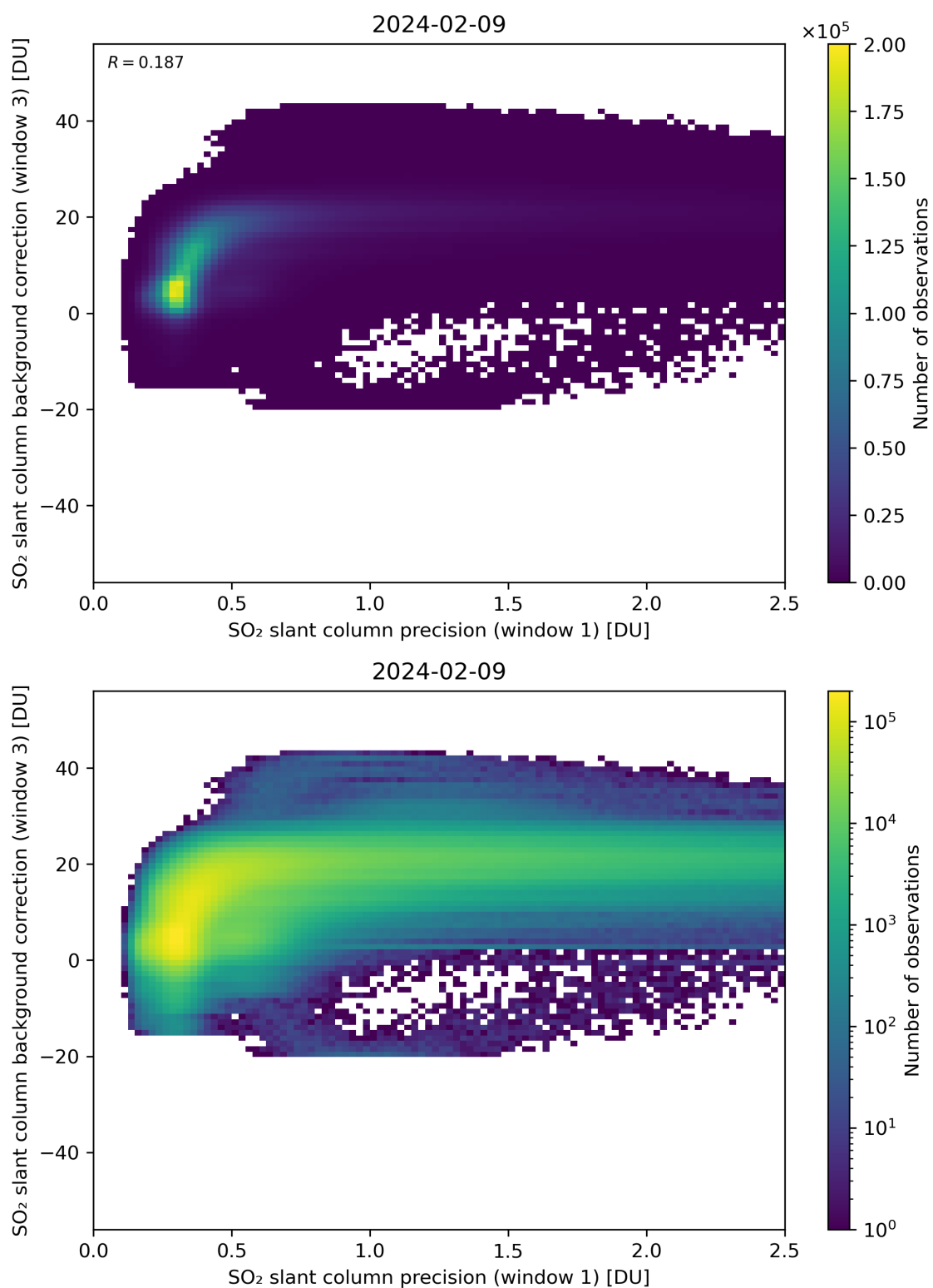
Figure 220: Scatter density plot of “SO 2 slant column precision (window 1)” against “SO 2 slant column background correction (window 3)” for 2024-02-08 to 2024-02-10.
