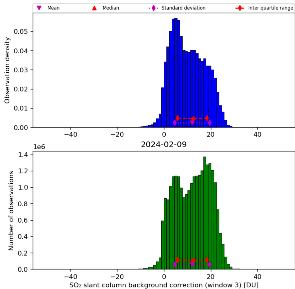
Figure 67: Histogram of “SO 2 slant column background correction (window 3)” for 2024-02-08 to 2024-02-10
