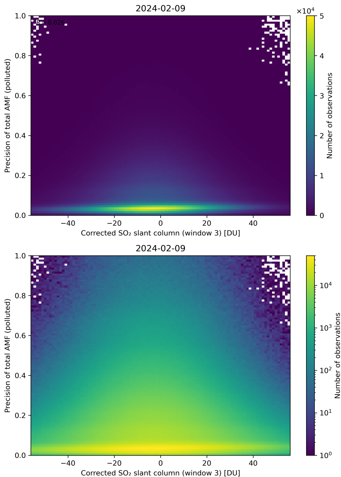
Figure 211: Scatter density plot of “Corrected SO 2 slant column (window 3)” against “Precision of total AMF (polluted)” for 2024-02-08 to 2024-02-10.
