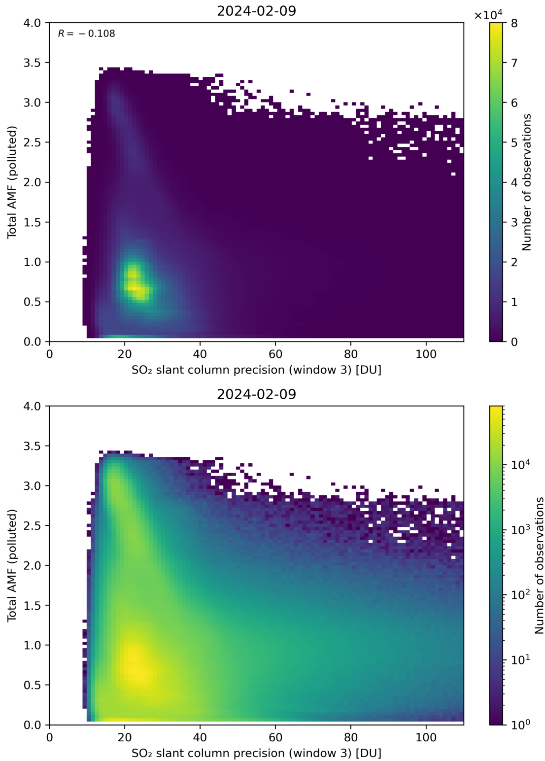
Figure 263: Scatter density plot of “SO 2 slant column precision (window 3)” against “Total AMF (polluted)” for 2024-02-08 to 2024-02-10.
