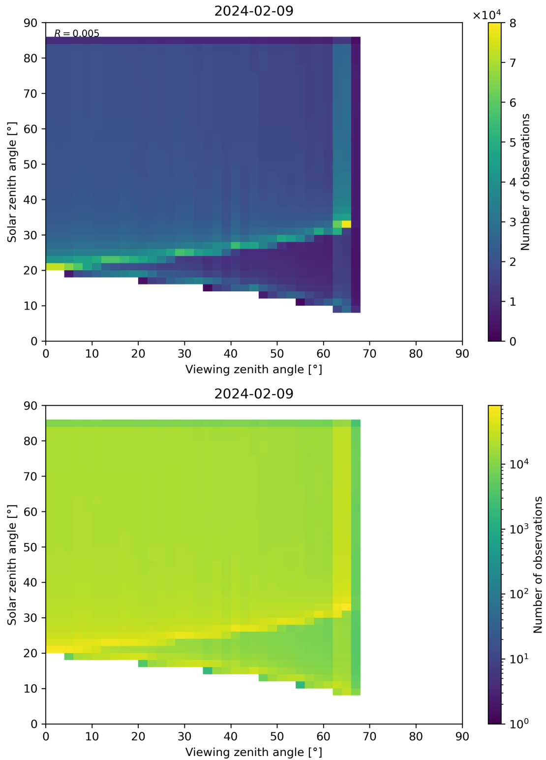
Figure 315: Scatter density plot of “Viewing zenith angle” against “Solar zenith angle” for 2024-02-08 to 2024-02-10.
