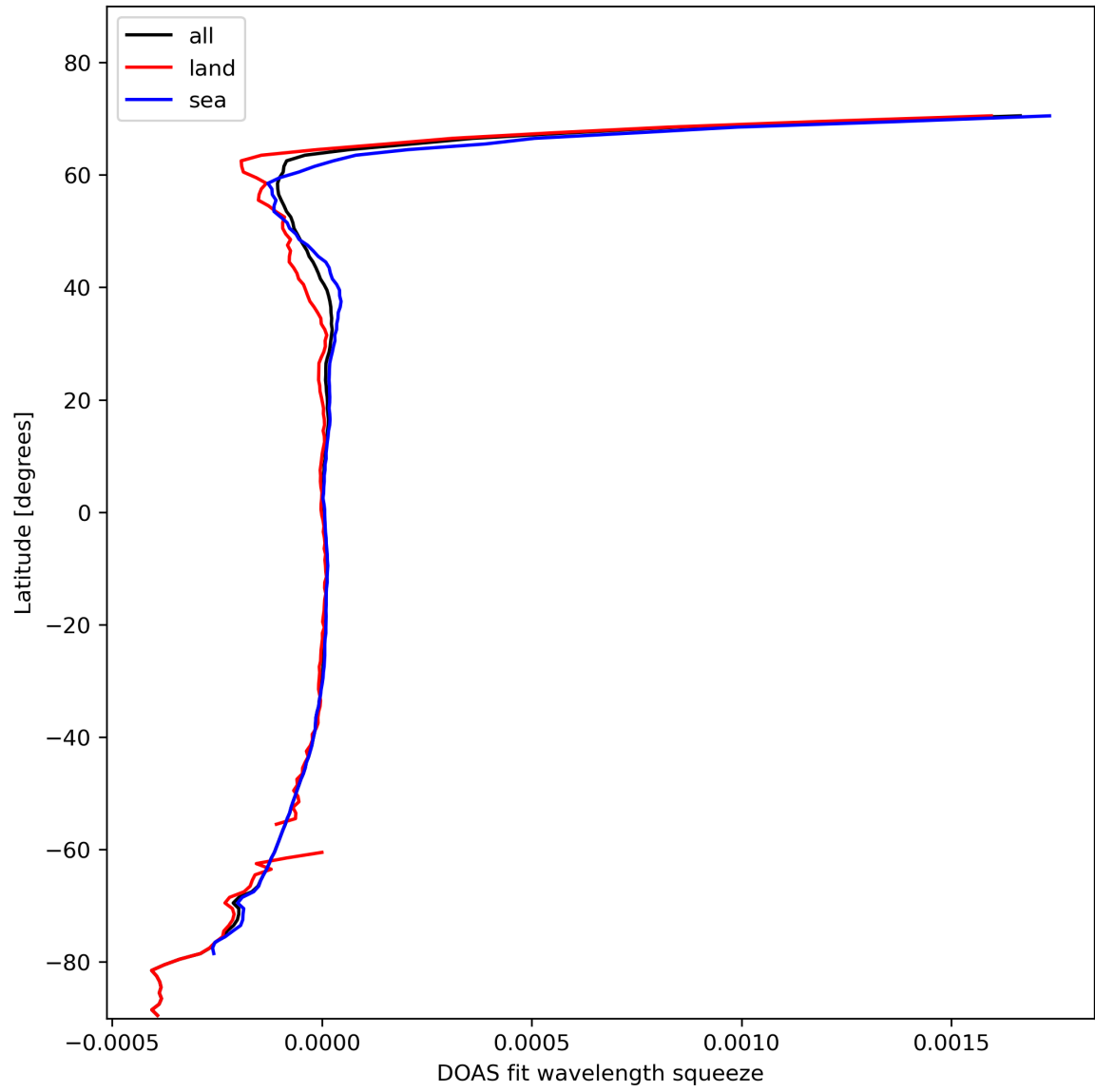
Figure 46: Zonal average of “DOAS fit wavelength squeeze” for 2024-02-08 to 2024-02-10.
