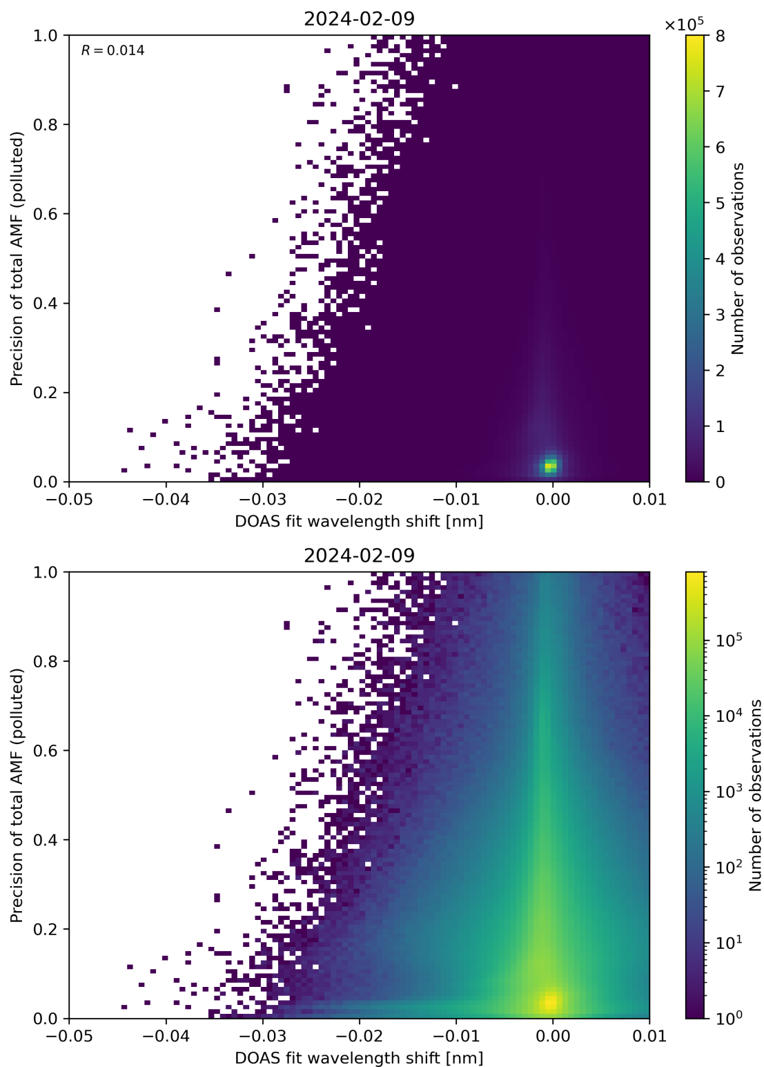
Figure 131: Scatter density plot of “DOAS fit wavelength shift” against “Precision of total AMF (polluted)” for 2024-02-08 to 2024-02-10.
