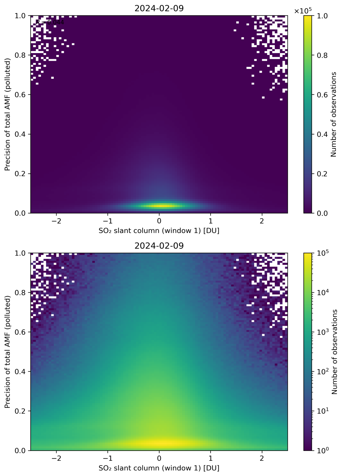
Figure 240: Scatter density plot of “SO 2 slant column (window 1)” against “Precision of total AMF (polluted)” for 2024-02-08 to 2024-02-10.
