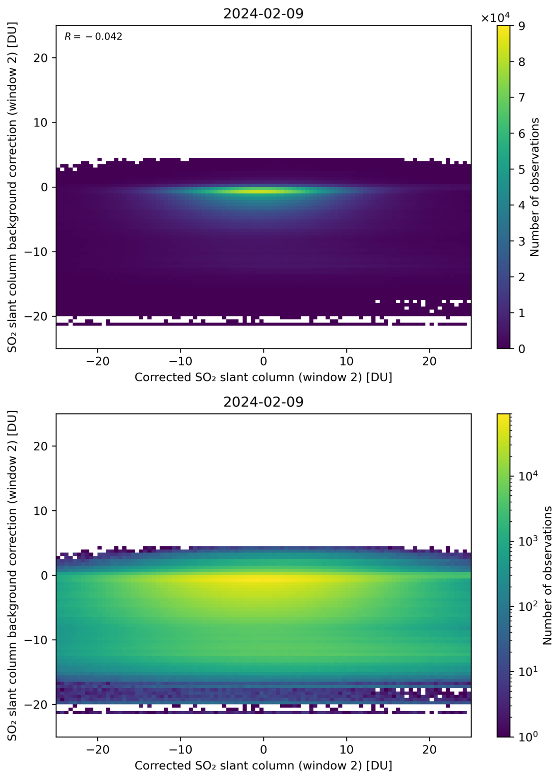
Figure 194: Scatter density plot of “Corrected SO 2 slant column (window 2)” against “SO 2 slant column background correction (window 2)” for 2024-02-08 to 2024-02-10.
