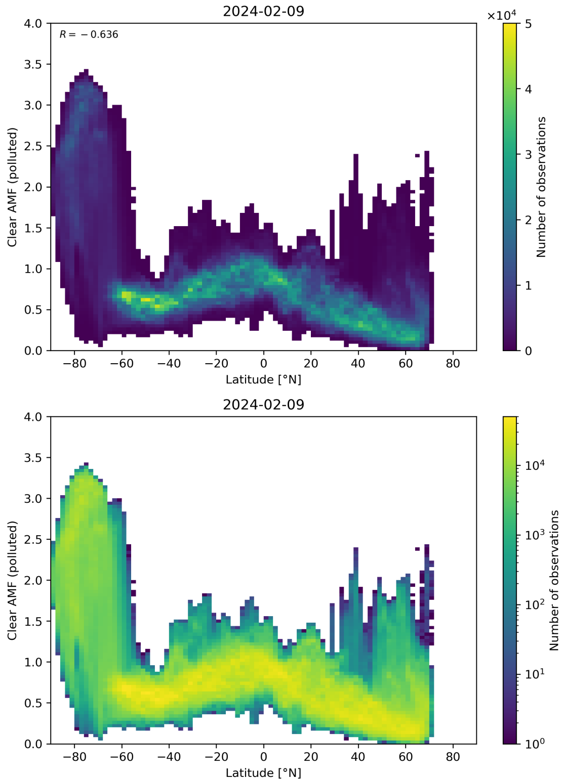
Figure 145: Scatter density plot of “Latitude” against “Clear AMF (polluted)” for 2024-02-08 to 2024-02-10.
