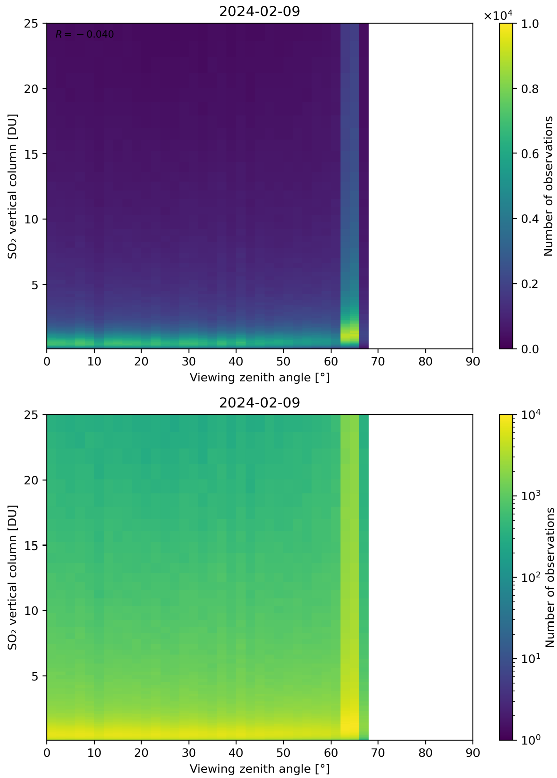
Figure 327: Scatter density plot of “Viewing zenith angle” against “SO 2 vertical column” for 2024-02-08 to 2024-02-10.
