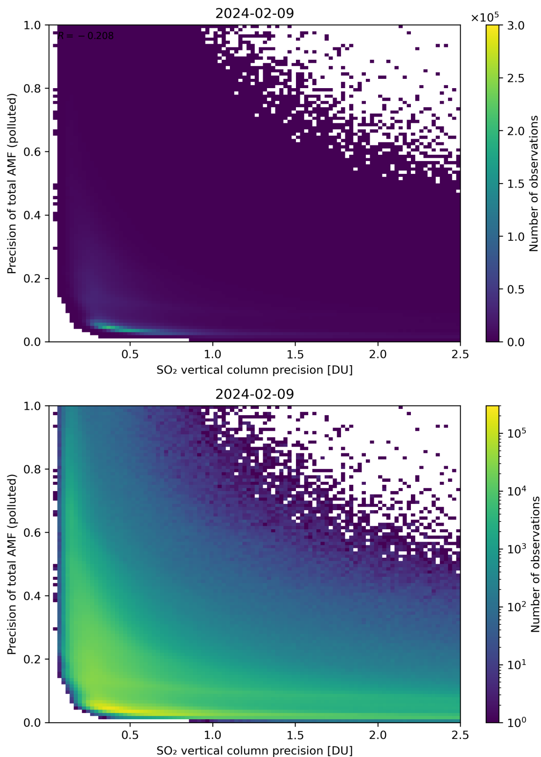
Figure 295: Scatter density plot of “SO 2 vertical column precision” against “Precision of total AMF (polluted)” for 2024-02-08 to 2024-02-10.
