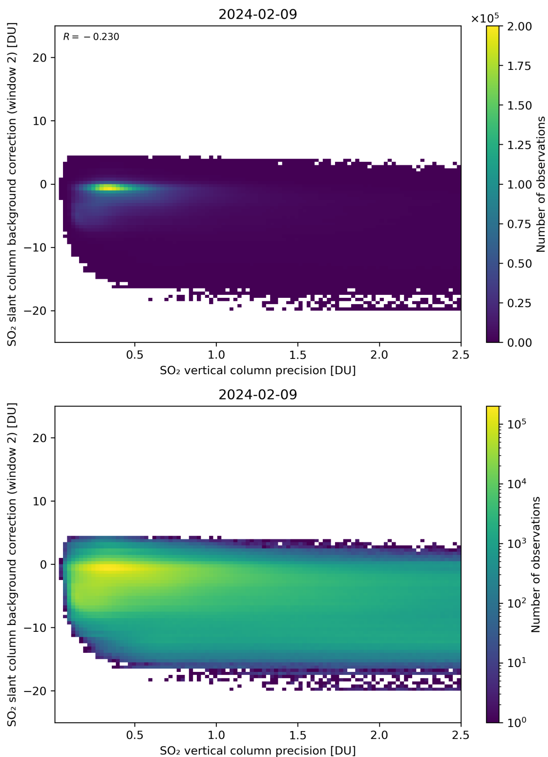
Figure 280: Scatter density plot of “SO 2 vertical column precision” against “SO 2 slant column background correction (window 2)” for 2024-02-08 to 2024-02-10.
