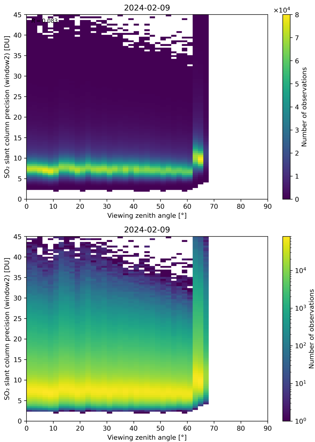
Figure 322: Scatter density plot of “Viewing zenith angle” against “SO 2 slant column precision (window2)” for 2024-02-08 to 2024-02-10.
