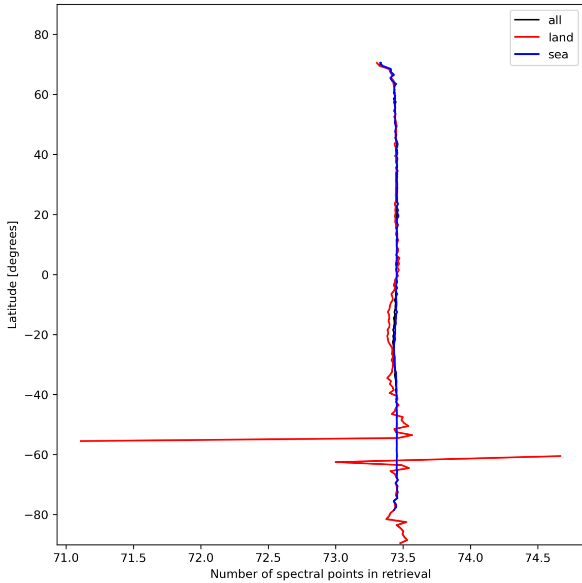
Figure 51: Zonal average of “Number of spectral points in retrieval” for 2024-02-08 to 2024-02-10.
