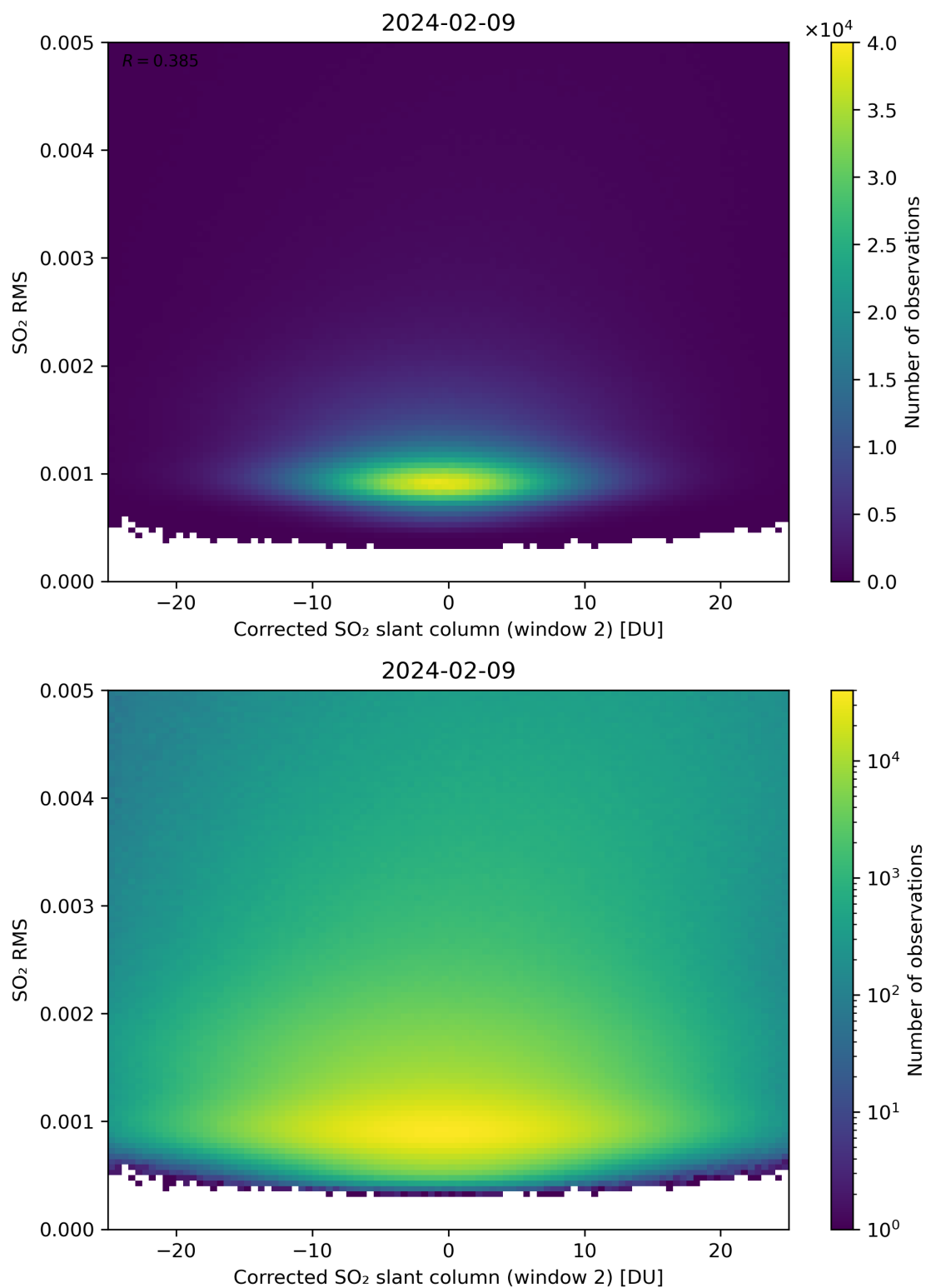
Figure 198: Scatter density plot of “Corrected SO 2 slant column (window 2)” against “SO 2 RMS” for 2024-02-08 to 2024-02-10.
