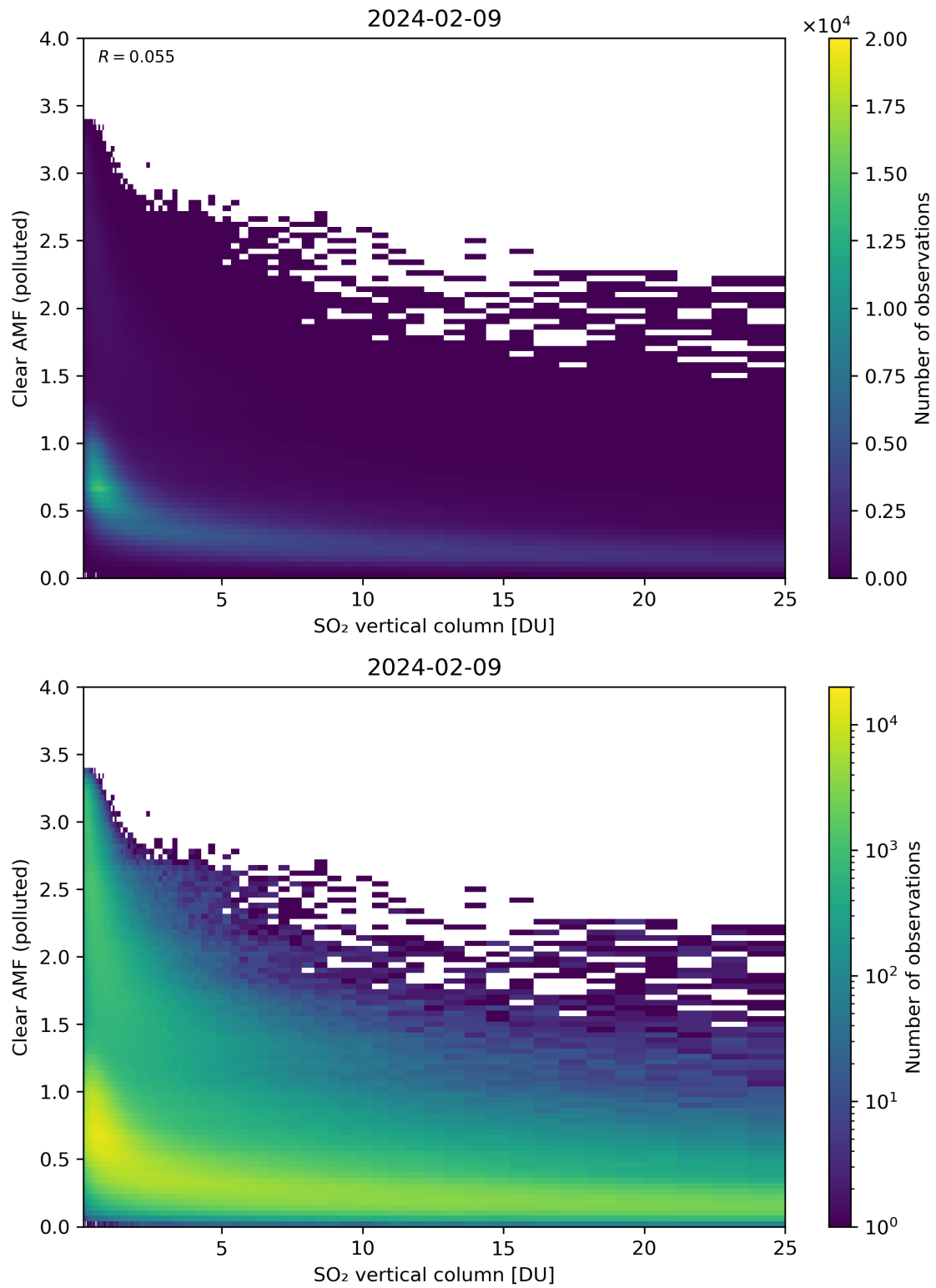
Figure 296: Scatter density plot of “SO 2 vertical column” against “Clear AMF (polluted)” for 2024-02-08 to 2024-02-10.
