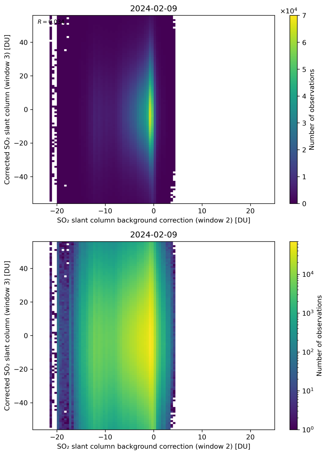
Figure 116: Scatter density plot of “SO 2 slant column background correction (window 2)” against “Corrected SO 2 slant column (window 3)” for 2024-02-08 to 2024-02-10.
