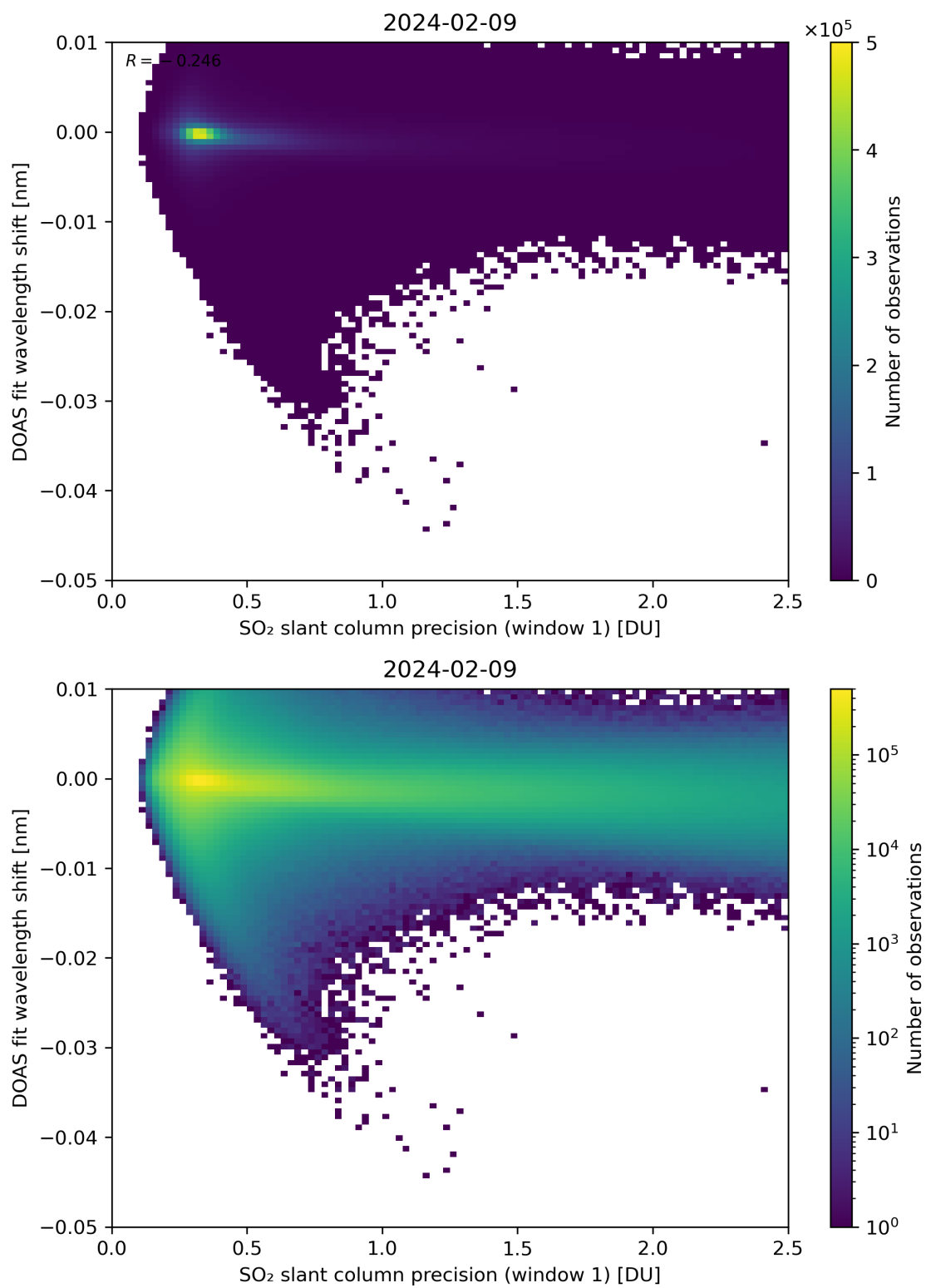
Figure 221: Scatter density plot of “SO 2 slant column precision (window 1)” against “DOAS fit wavelength shift” for 2024-02-08 to 2024-02-10.
