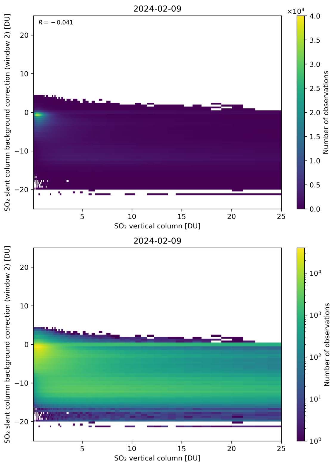
Figure 274: Scatter density plot of “SO 2 vertical column” against “SO 2 slant column background correction (window 2)” for 2024-02-08 to 2024-02-10.
