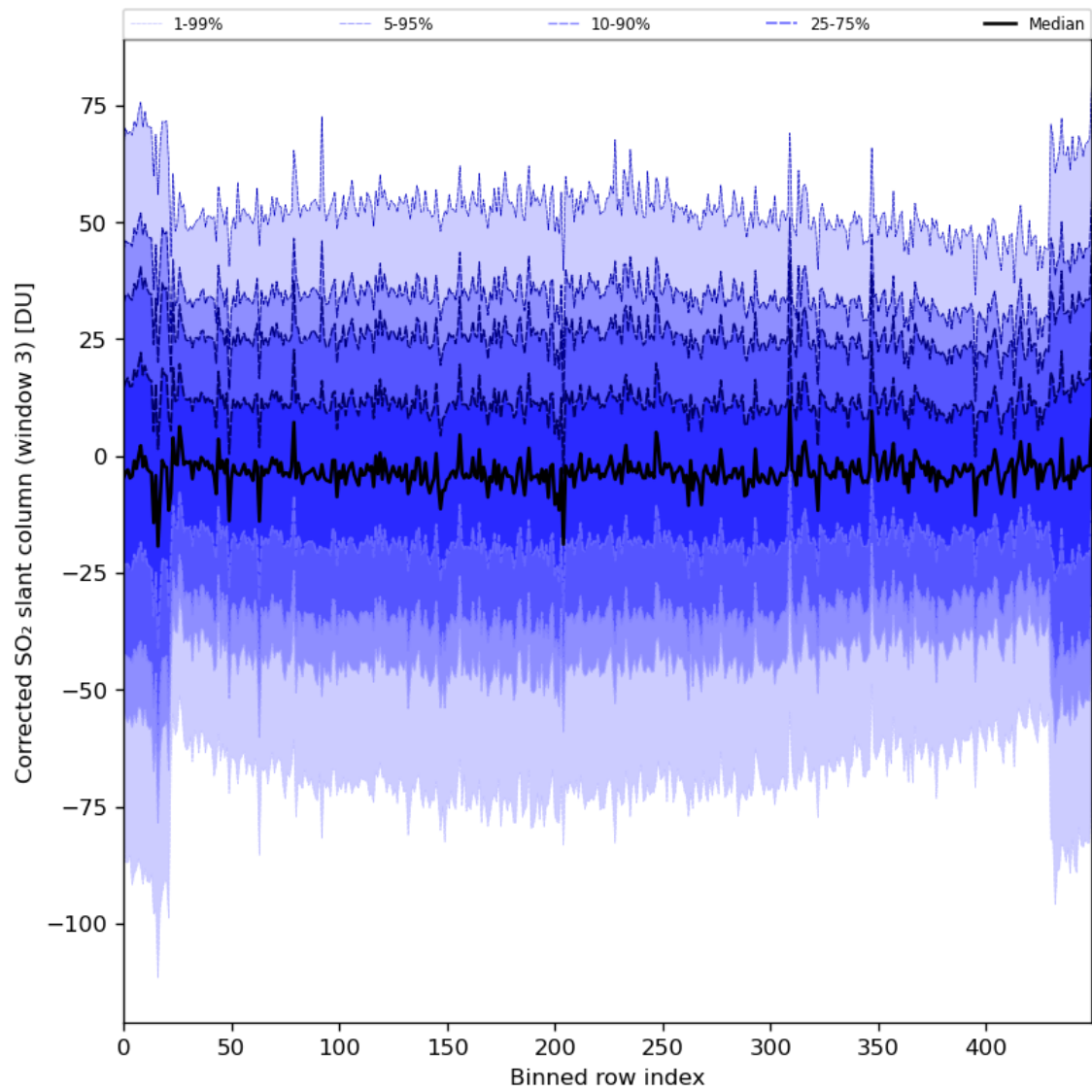
Figure 89: Along track statistics of “Corrected SO 2 slant column (window 3)” for 2024-02-08 to 2024-02-10
