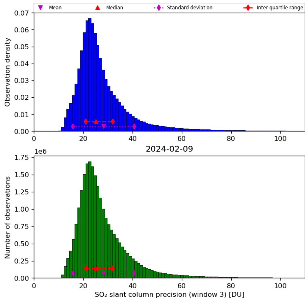
Figure 65: Histogram of “SO 2 slant column precision (window 3)” for 2024-02-08 to 2024-02-10
