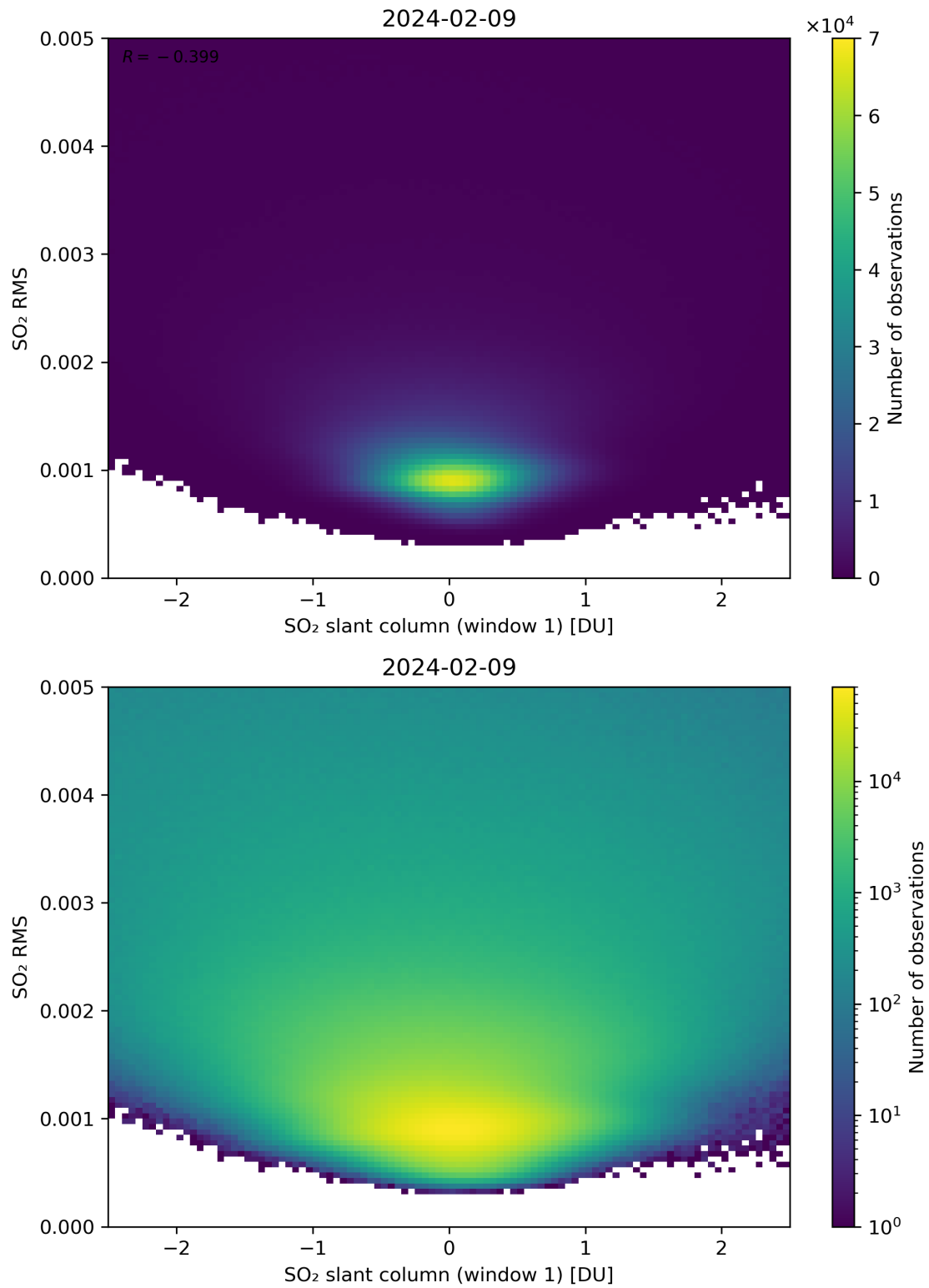
Figure 217: Scatter density plot of “SO 2 slant column (window 1)” against “SO 2 RMS” for 2024-02-08 to 2024-02-10.
