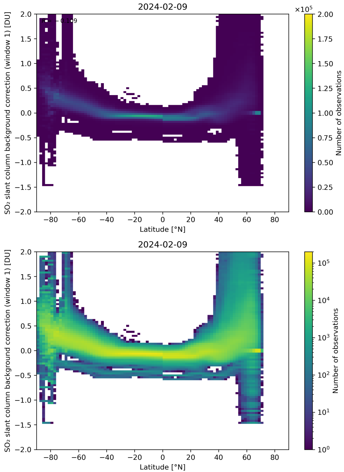
Figure 139: Scatter density plot of “Latitude” against “SO 2 slant column background correction (window 1)” for 2024-02-08 to 2024-02-10.
