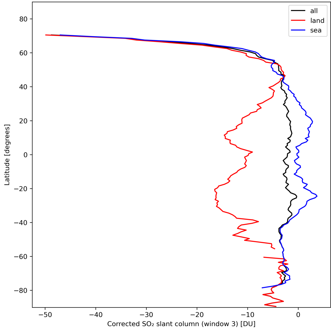
Figure 43: Zonal average of “Corrected SO 2 slant column (window 3)” for 2024-02-08 to 2024-02-10.
