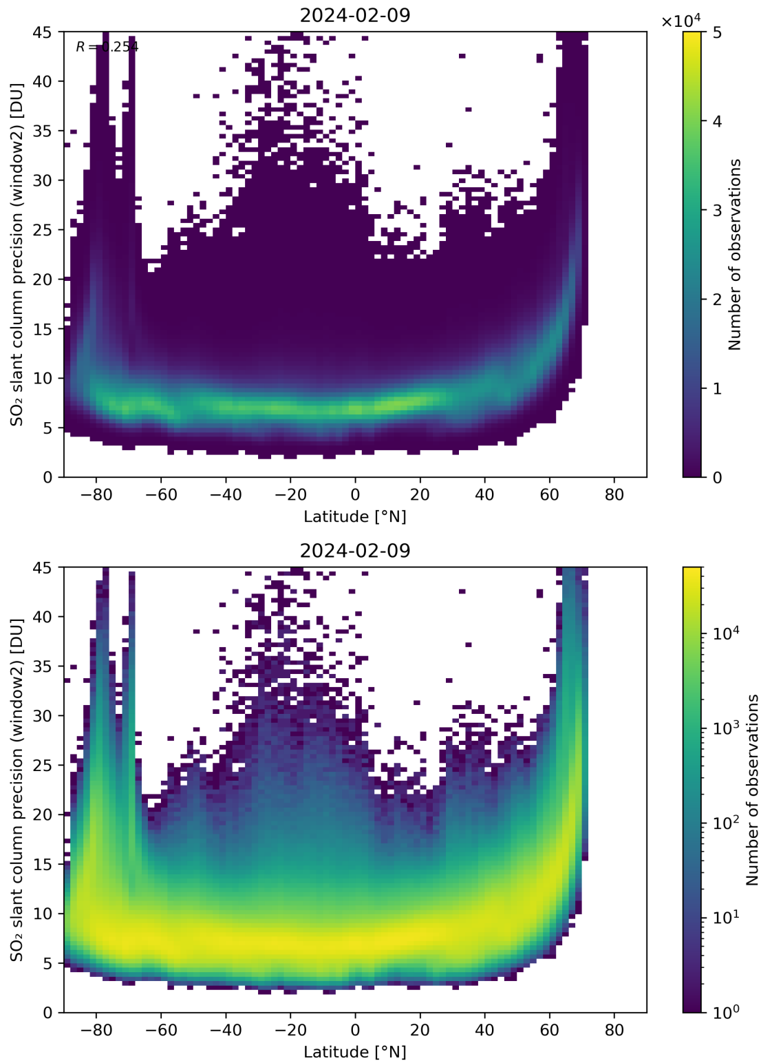
Figure 151: Scatter density plot of “Latitude” against “SO 2 slant column precision (window2)” for 2024-02-08 to 2024-02-10.
