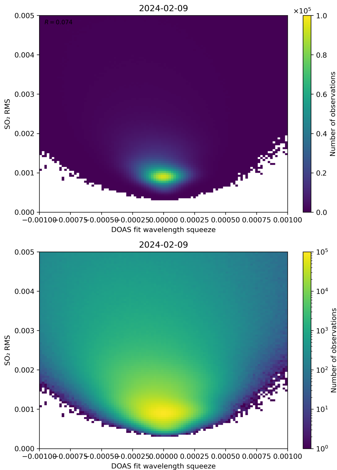
Figure 132: Scatter density plot of “DOAS fit wavelength squeeze” against “SO 2 RMS” for 2024-02-08 to 2024-02-10.
