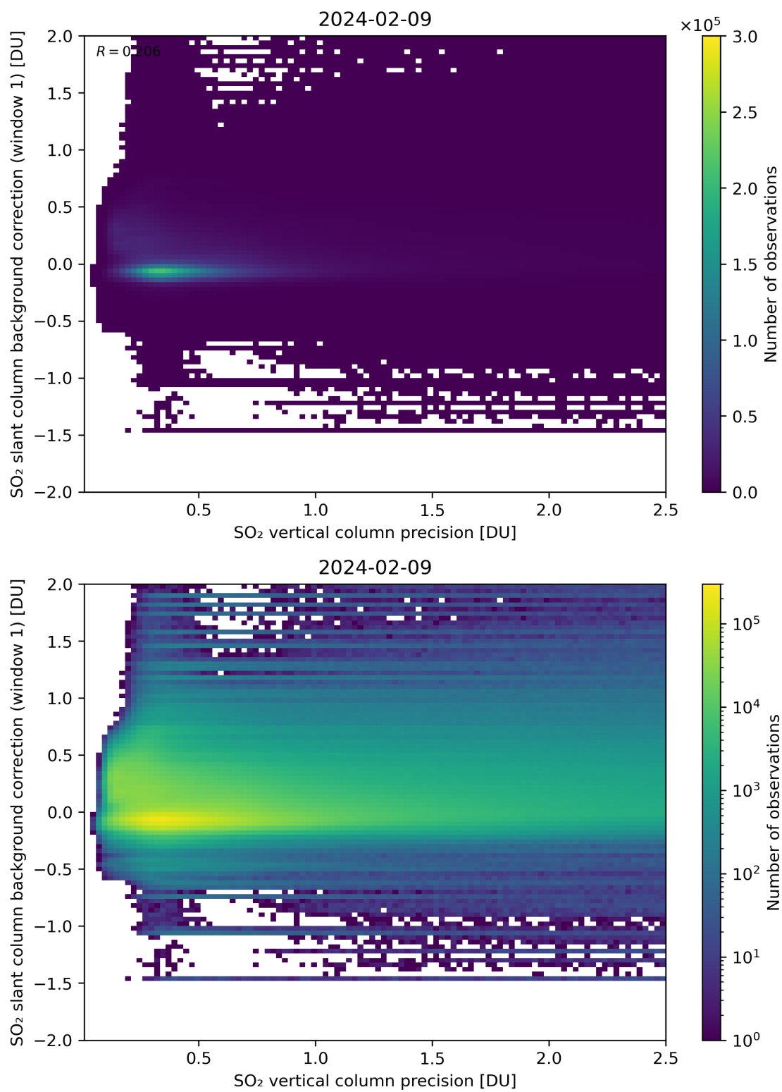
Figure 279: Scatter density plot of “SO 2 vertical column precision” against “SO 2 slant column background correction (window 1)” for 2024-02-08 to 2024-02-10.
