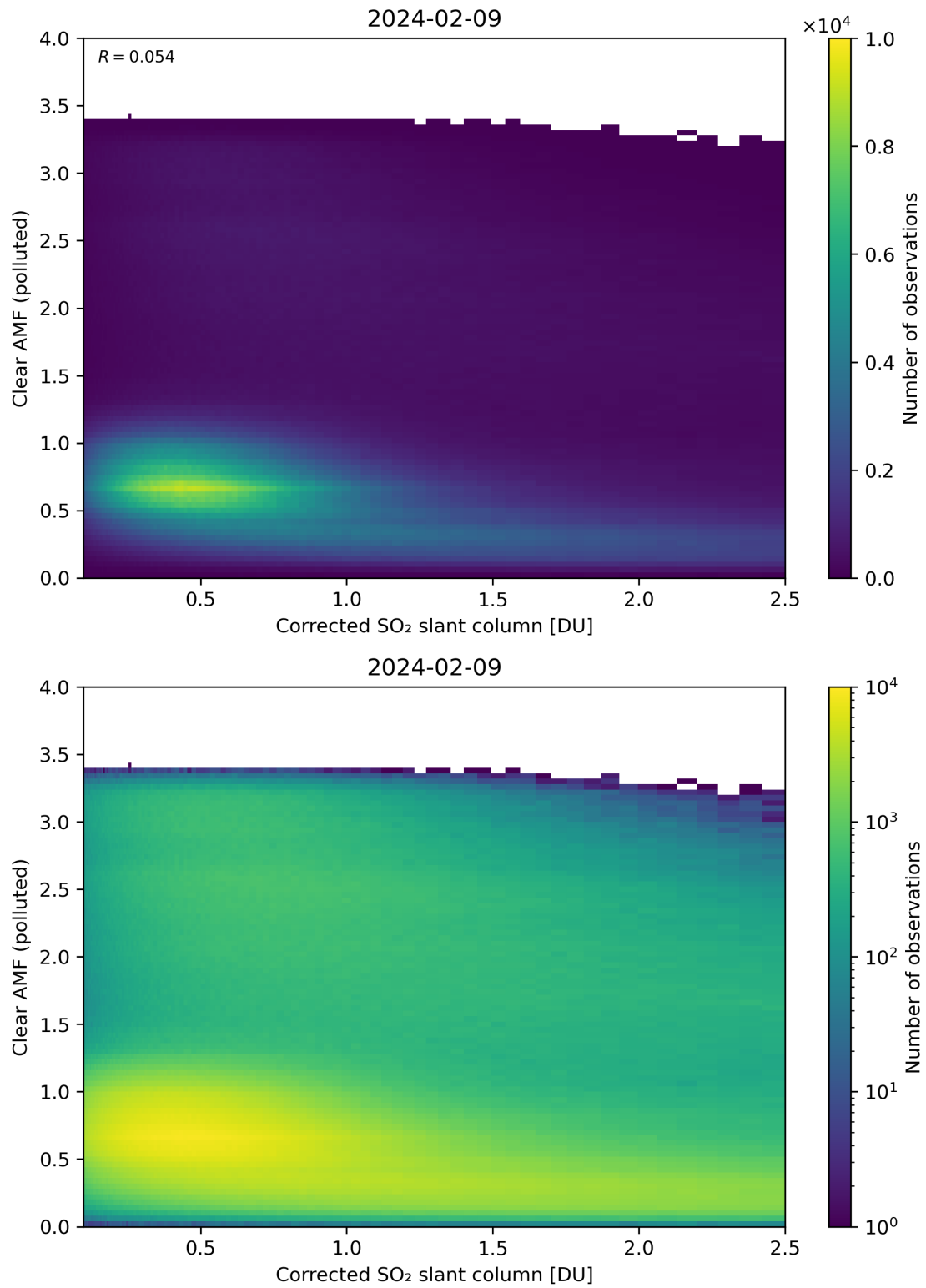
Figure 184: Scatter density plot of “Corrected SO 2 slant column” against “Clear AMF (polluted)” for 2024-02-08 to 2024-02-10.
