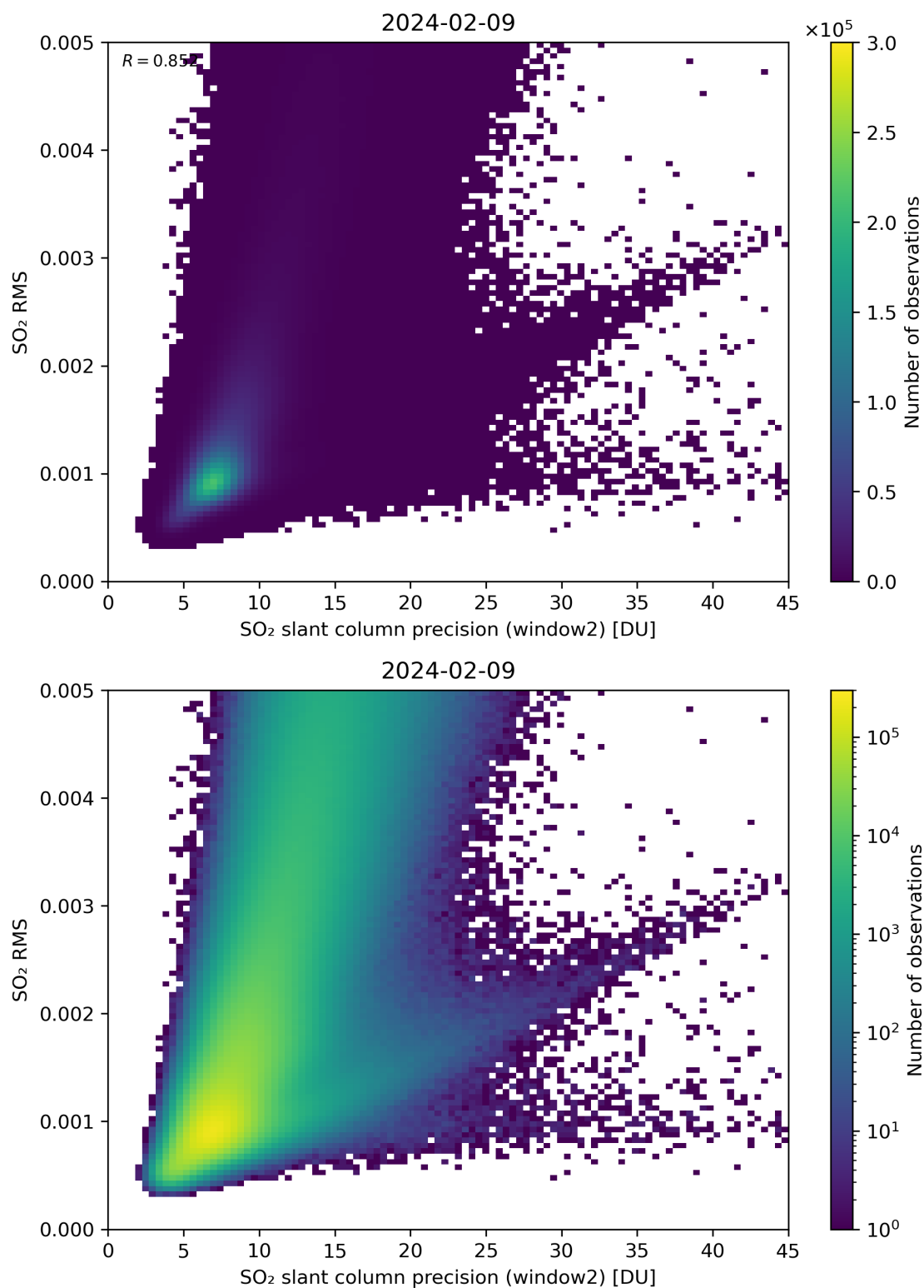
Figure 245: Scatter density plot of “SO 2 slant column precision (window2)” against “SO 2 RMS” for 2024-02-08 to 2024-02-10.
