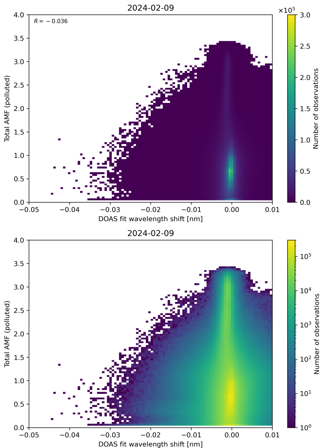
Figure 130: Scatter density plot of “DOAS fit wavelength shift” against “Total AMF (polluted)” for 2024-02-08 to 2024-02-10.
