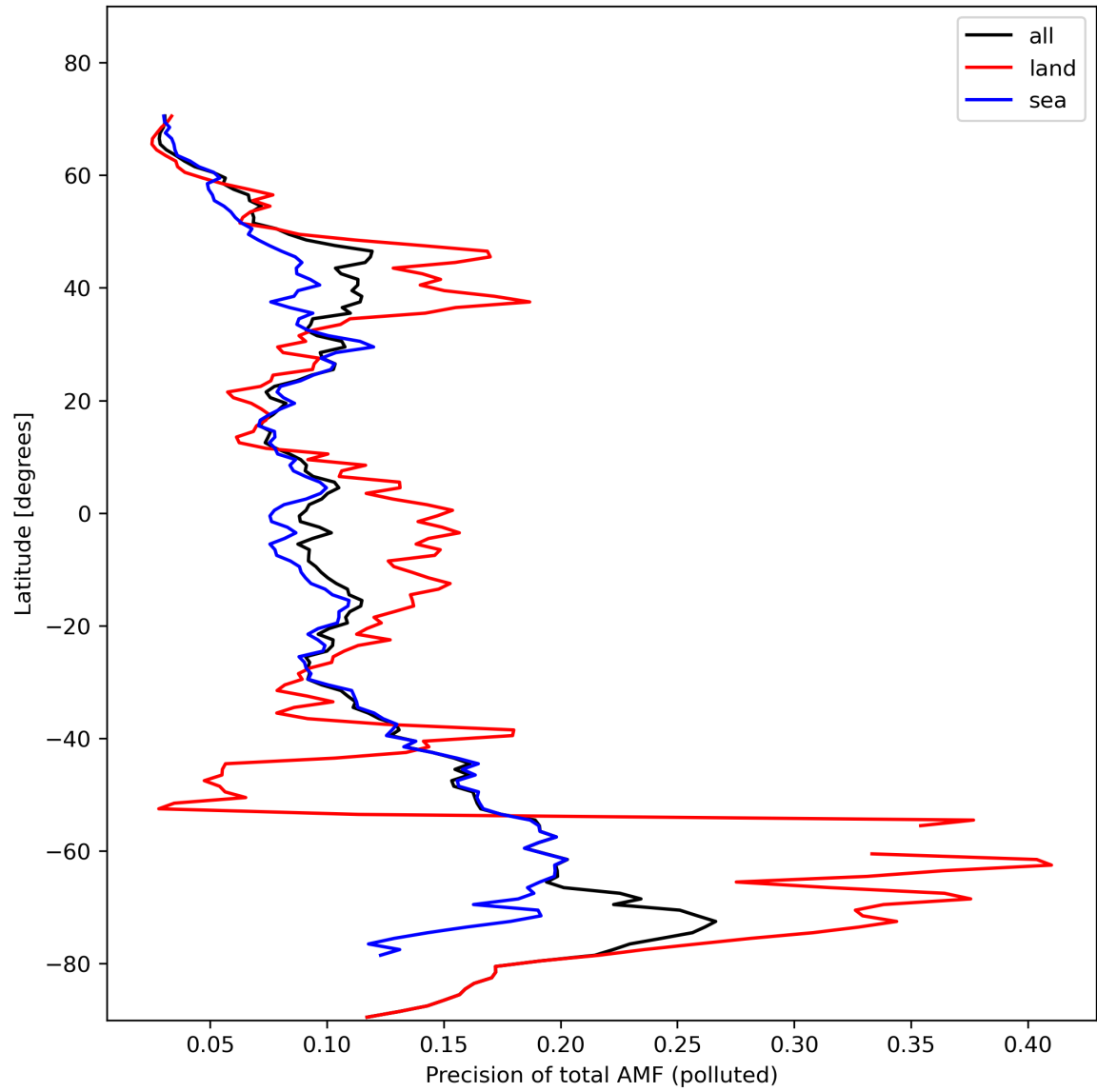
Figure 49: Zonal average of “Precision of total AMF (polluted)” for 2024-02-08 to 2024-02-10.
