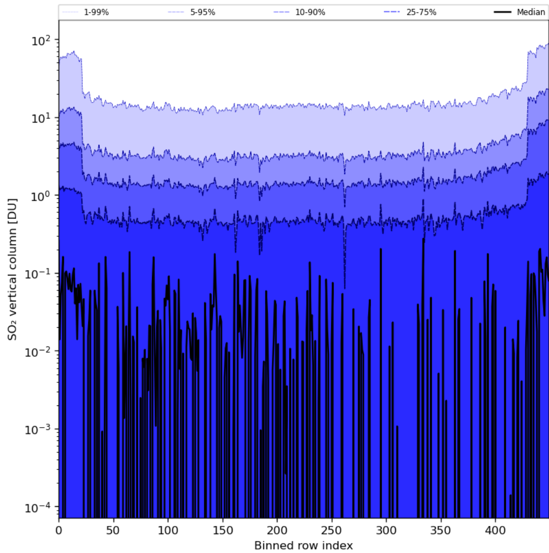
Figure 76: Along track statistics of “SO 2 vertical column” for 2024-02-08 to 2024-02-10
