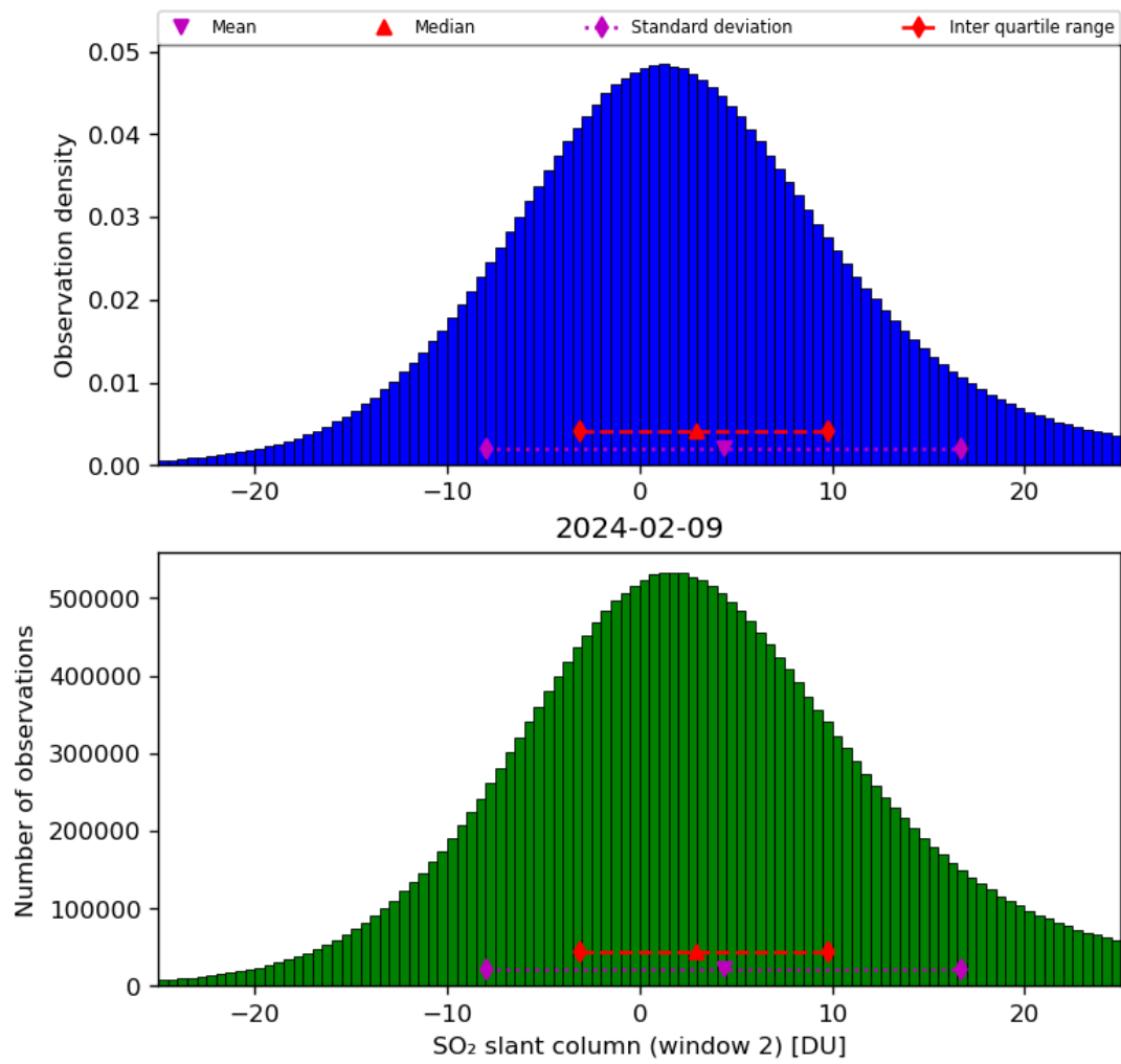
Figure 60: Histogram of “SO 2 slant column (window 2)” for 2024-02-08 to 2024-02-10
