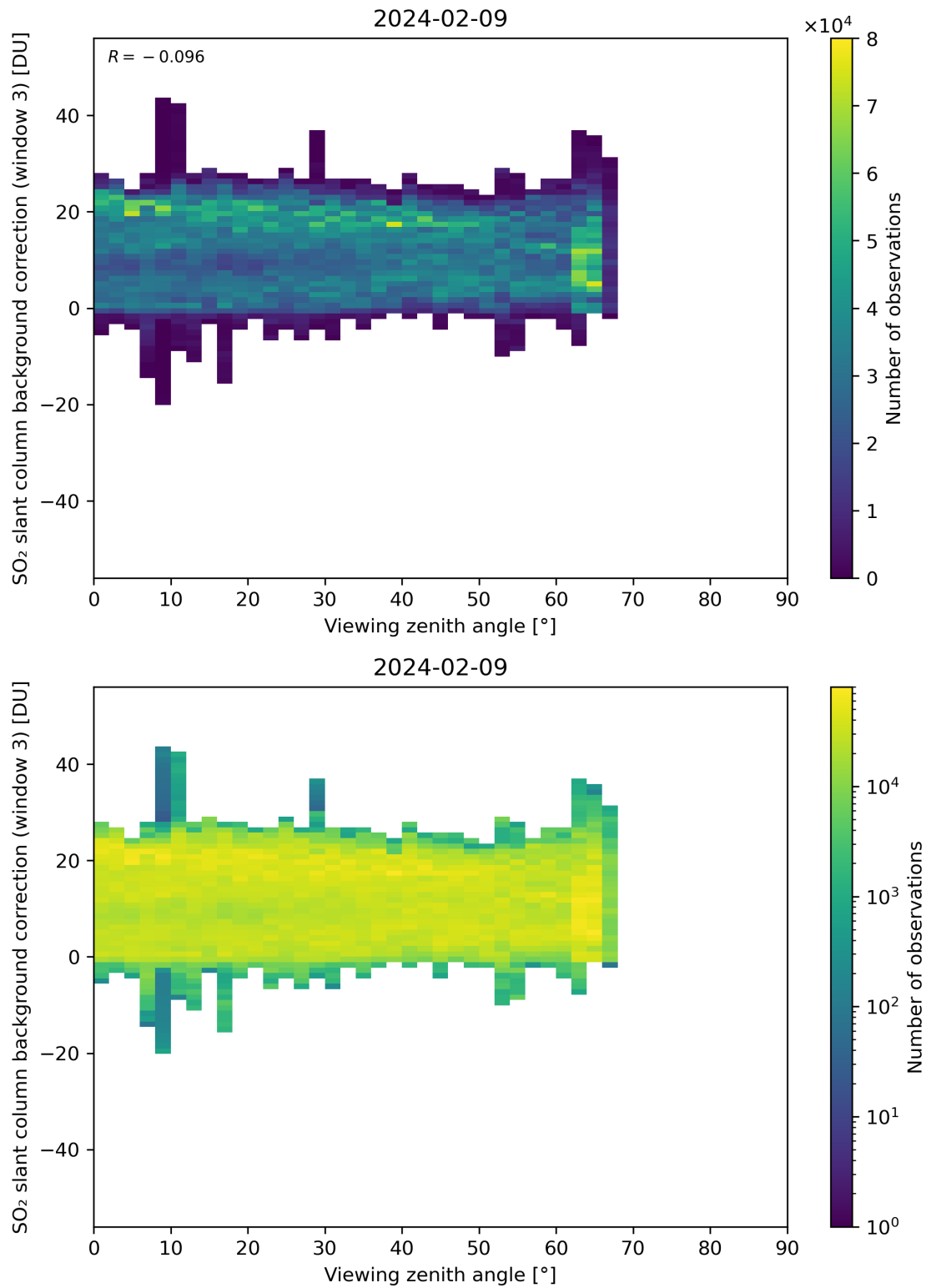
Figure 310: Scatter density plot of “Viewing zenith angle” against “SO 2 slant column background correction (window 3)” for 2024-02-08 to 2024-02-10.
