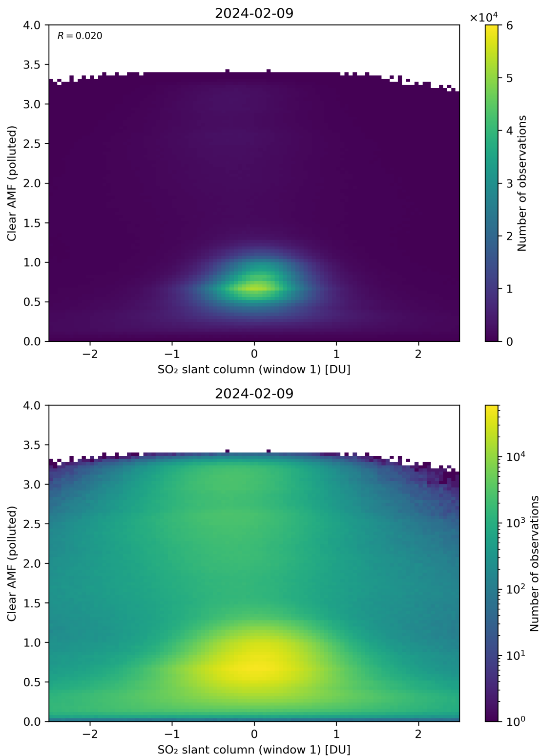
Figure 232: Scatter density plot of “SO 2 slant column (window 1)” against “Clear AMF (polluted)” for 2024-02-08 to 2024-02-10.
