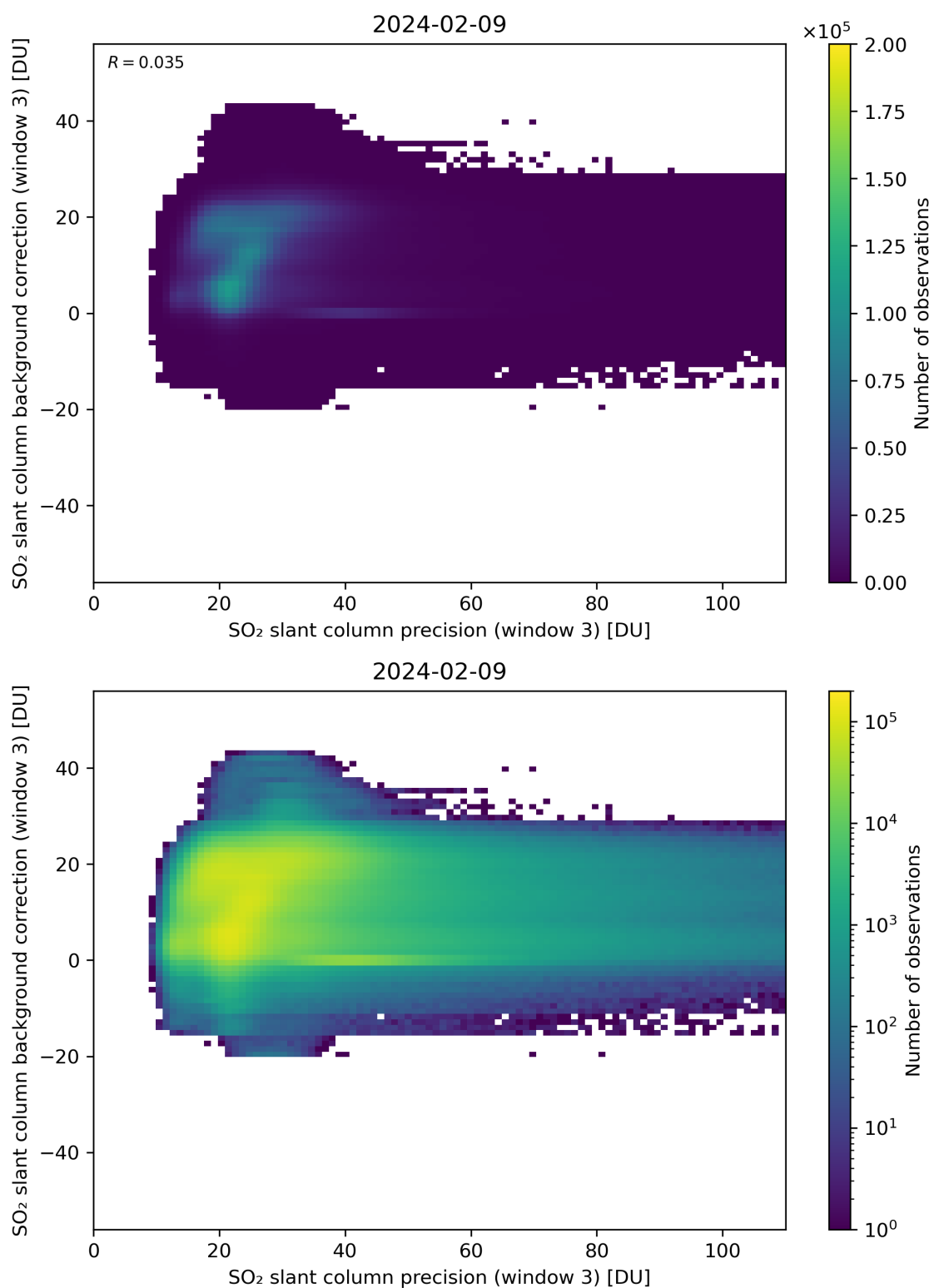
Figure 257: Scatter density plot of “SO 2 slant column precision (window 3)” against “SO 2 slant column background correction (window 3)” for 2024-02-08 to 2024-02-10.
