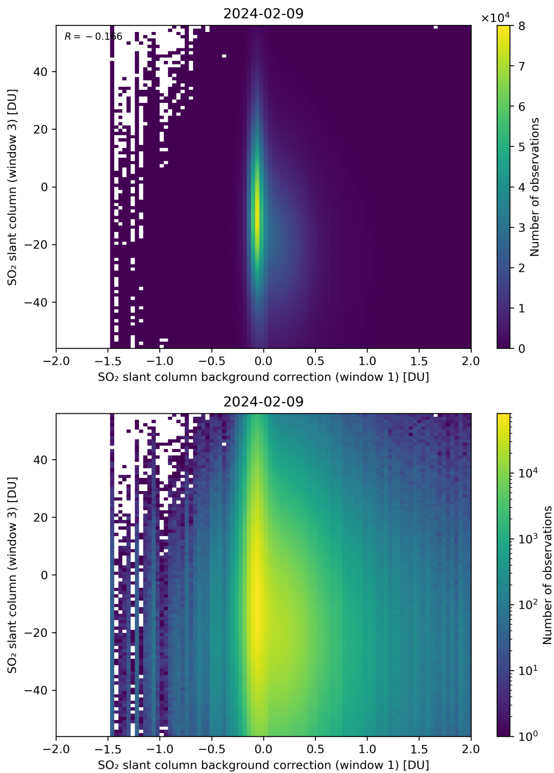
Figure 107: Scatter density plot of “SO 2 slant column background correction (window 1)” against “SO 2 slant column (window 3)” for 2024-02-08 to 2024-02-10.
