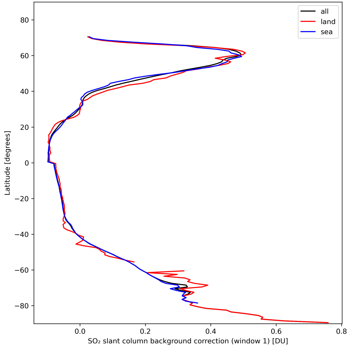
Figure 36: Zonal average of “SO 2 slant column background correction (window 1)” for 2024-02-08 to 2024-02-10.
