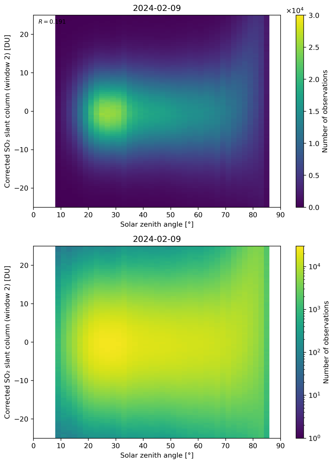
Figure 167: Scatter density plot of “Solar zenith angle” against “Corrected SO 2 slant column (window 2)” for 2024-02-08 to 2024-02-10.
