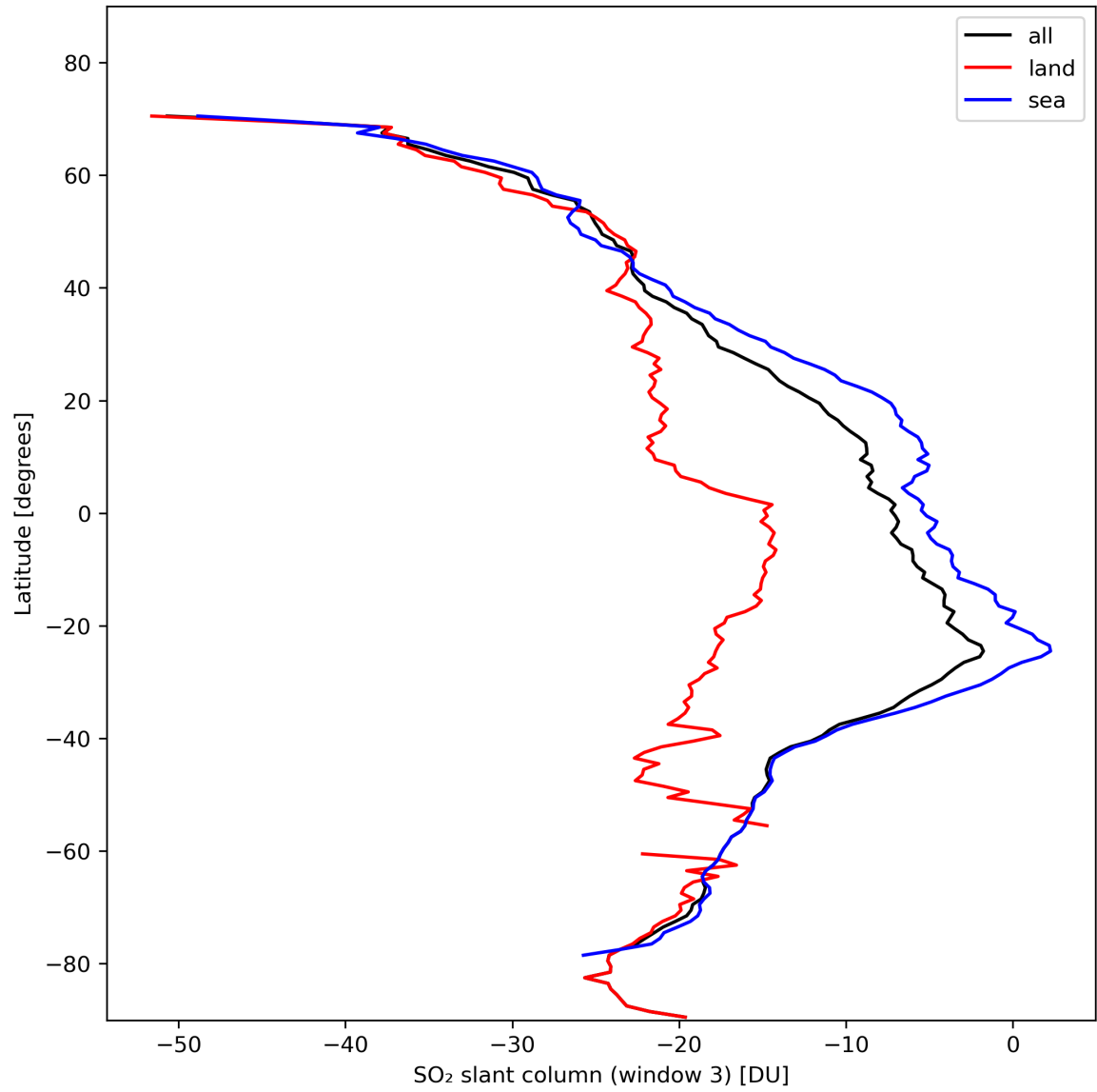
Figure 41: Zonal average of “SO 2 slant column (window 3)” for 2024-02-08 to 2024-02-10.
