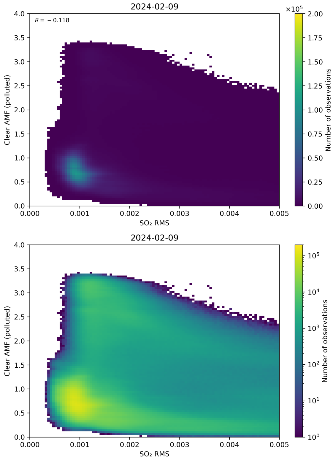
Figure 136: Scatter density plot of “SO 2 RMS” against “Clear AMF (polluted)” for 2024-02-08 to 2024-02-10.
