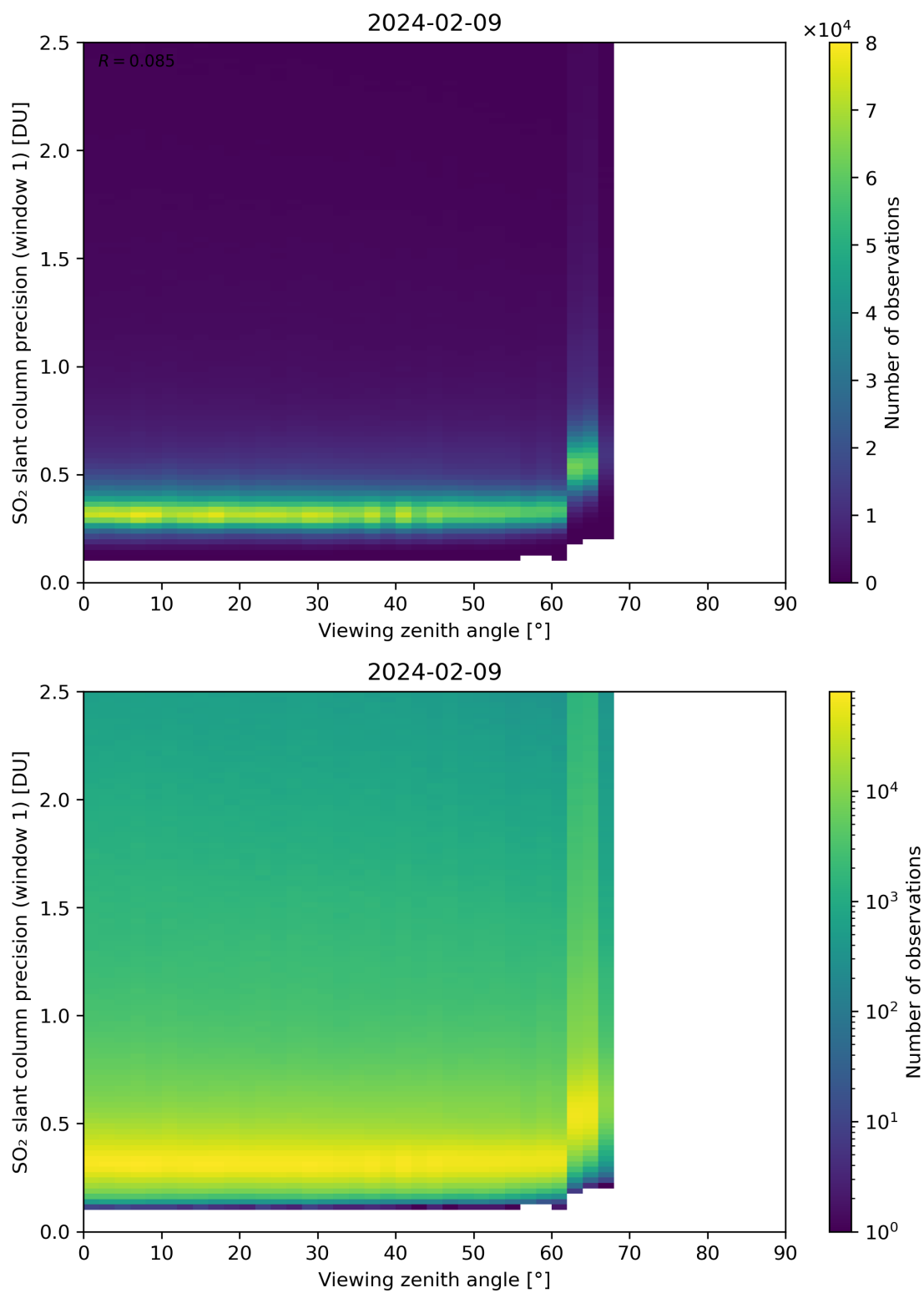
Figure 321: Scatter density plot of “Viewing zenith angle” against “SO 2 slant column precision (window 1)” for 2024-02-08 to 2024-02-10.
