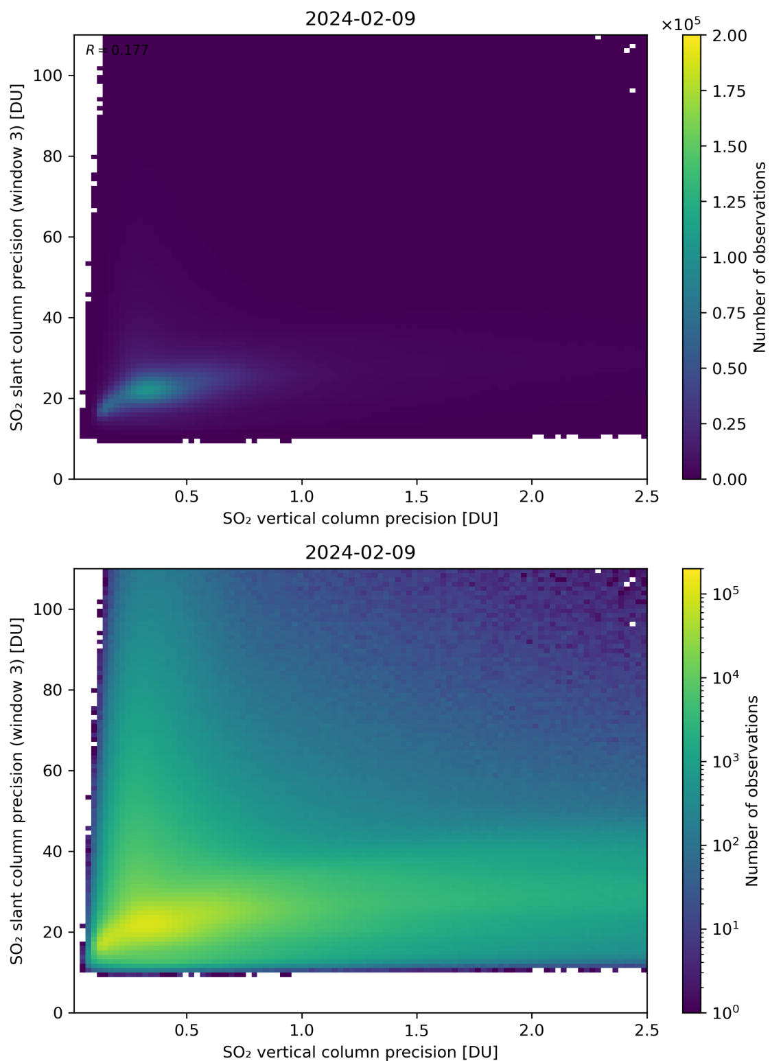
Figure 293: Scatter density plot of “SO 2 vertical column precision” against “SO 2 slant column precision (window 3)” for 2024-02-08 to 2024-02-10.
