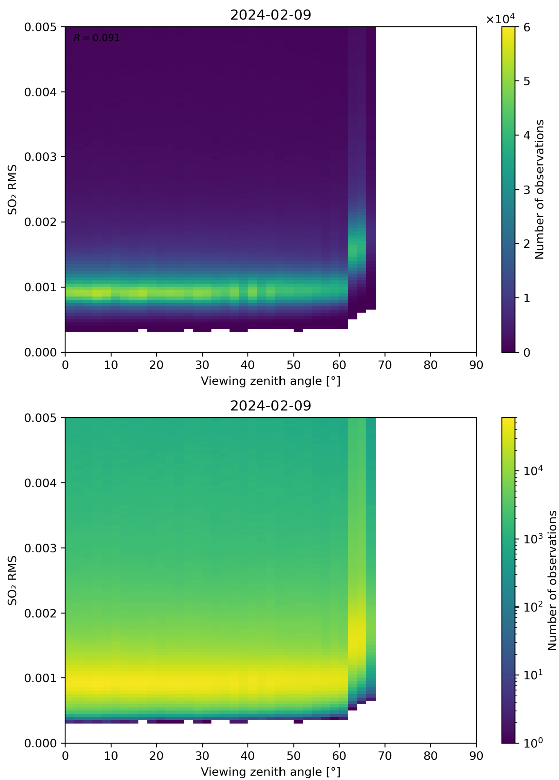
Figure 313: Scatter density plot of “Viewing zenith angle” against “SO 2 RMS” for 2024-02-08 to 2024-02-10.
