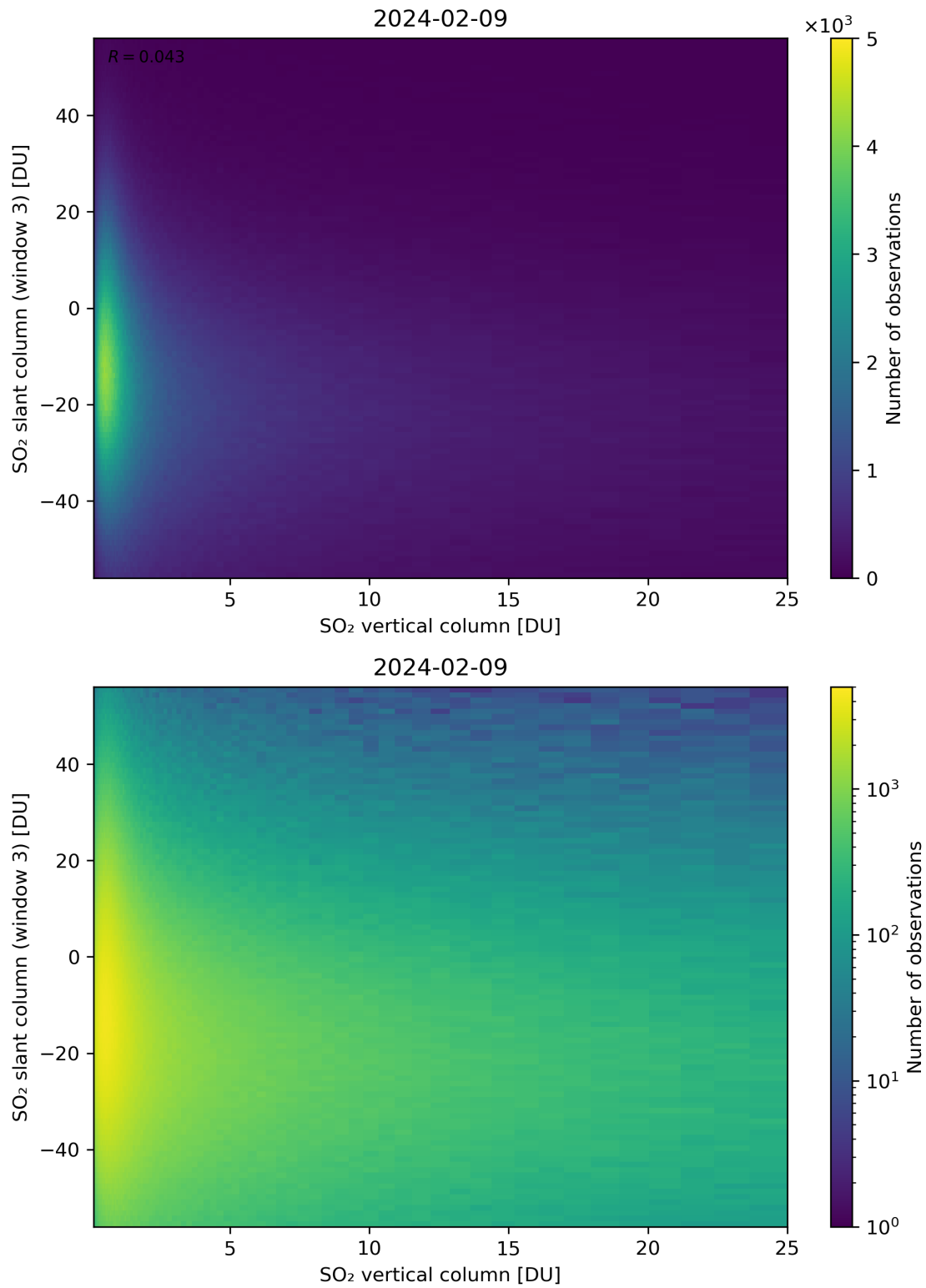
Figure 303: Scatter density plot of “SO 2 vertical column” against “SO 2 slant column (window 3)” for 2024-02-08 to 2024-02-10.
