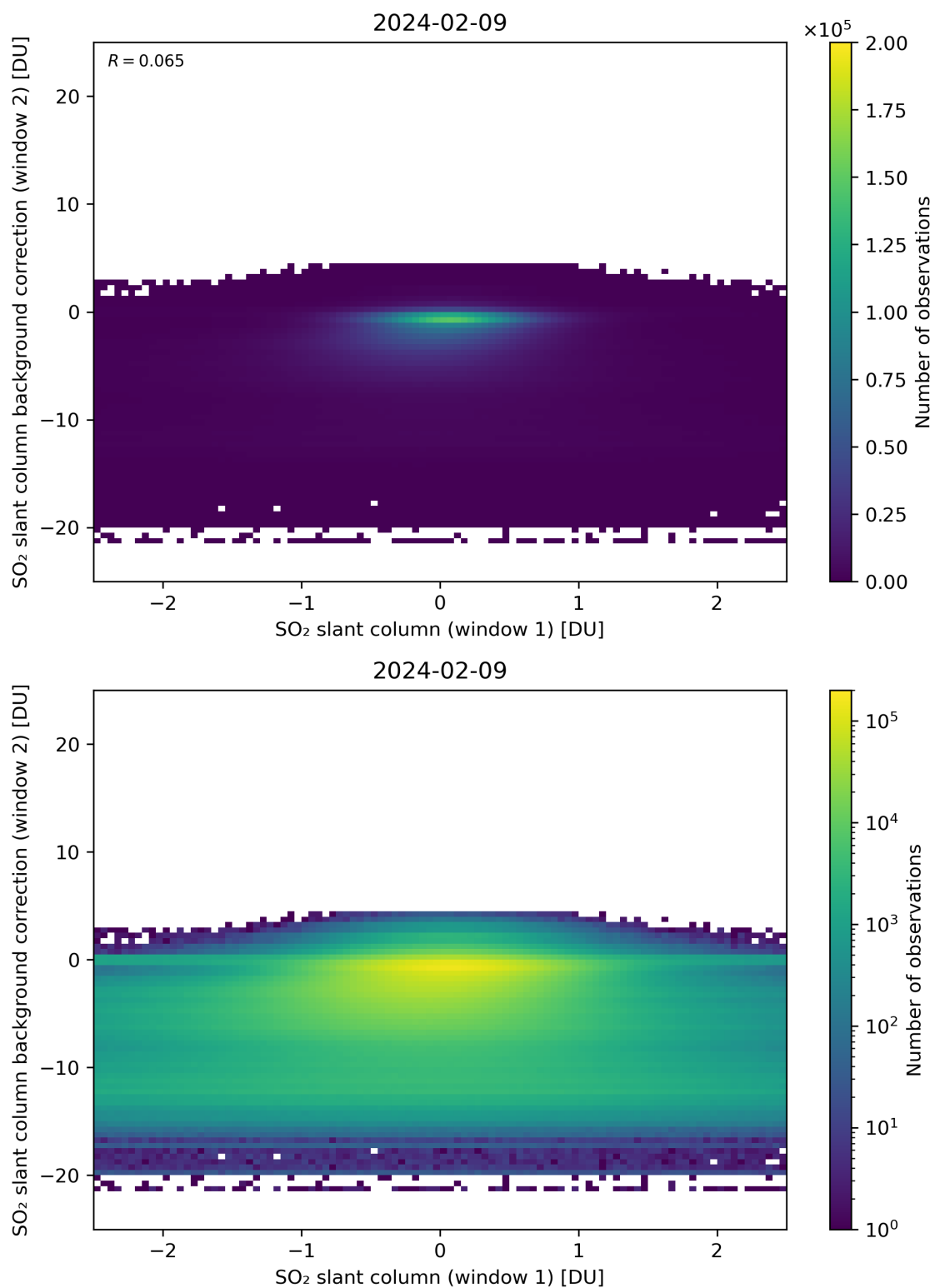
Figure 213: Scatter density plot of “SO 2 slant column (window 1)” against “SO 2 slant column background correction (window 2)” for 2024-02-08 to 2024-02-10.
