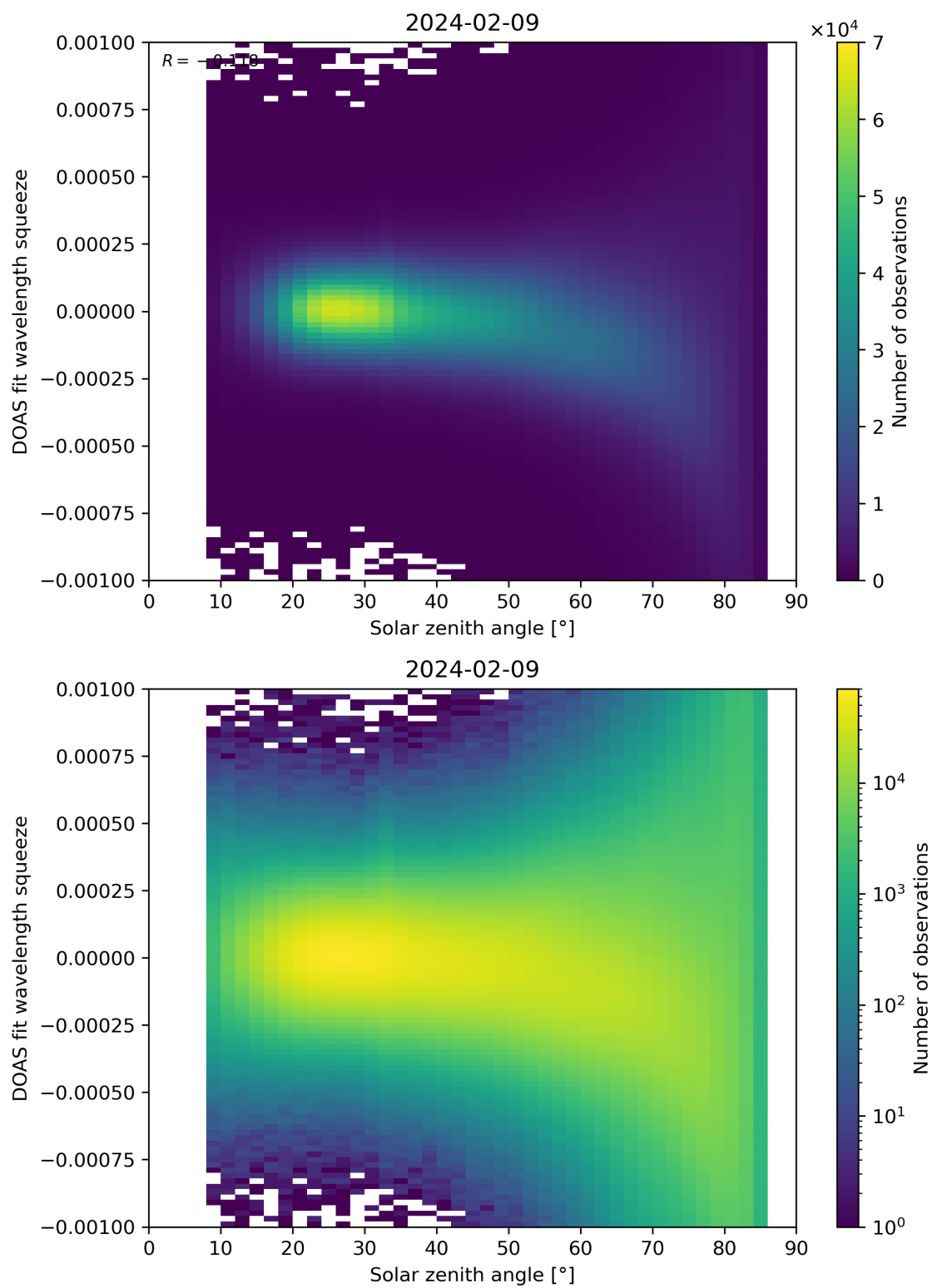
Figure 162: Scatter density plot of “Solar zenith angle” against “DOAS fit wavelength squeeze” for 2024-02-08 to 2024-02-10.
