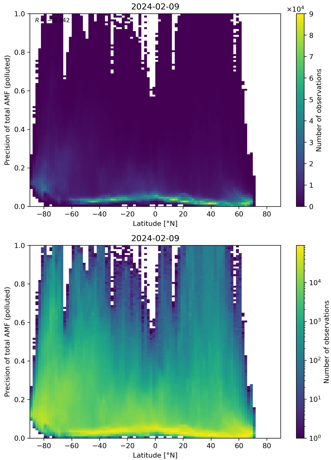
Figure 155: Scatter density plot of “Latitude” against “Precision of total AMF (polluted)” for 2024-02-08 to 2024-02-10.
