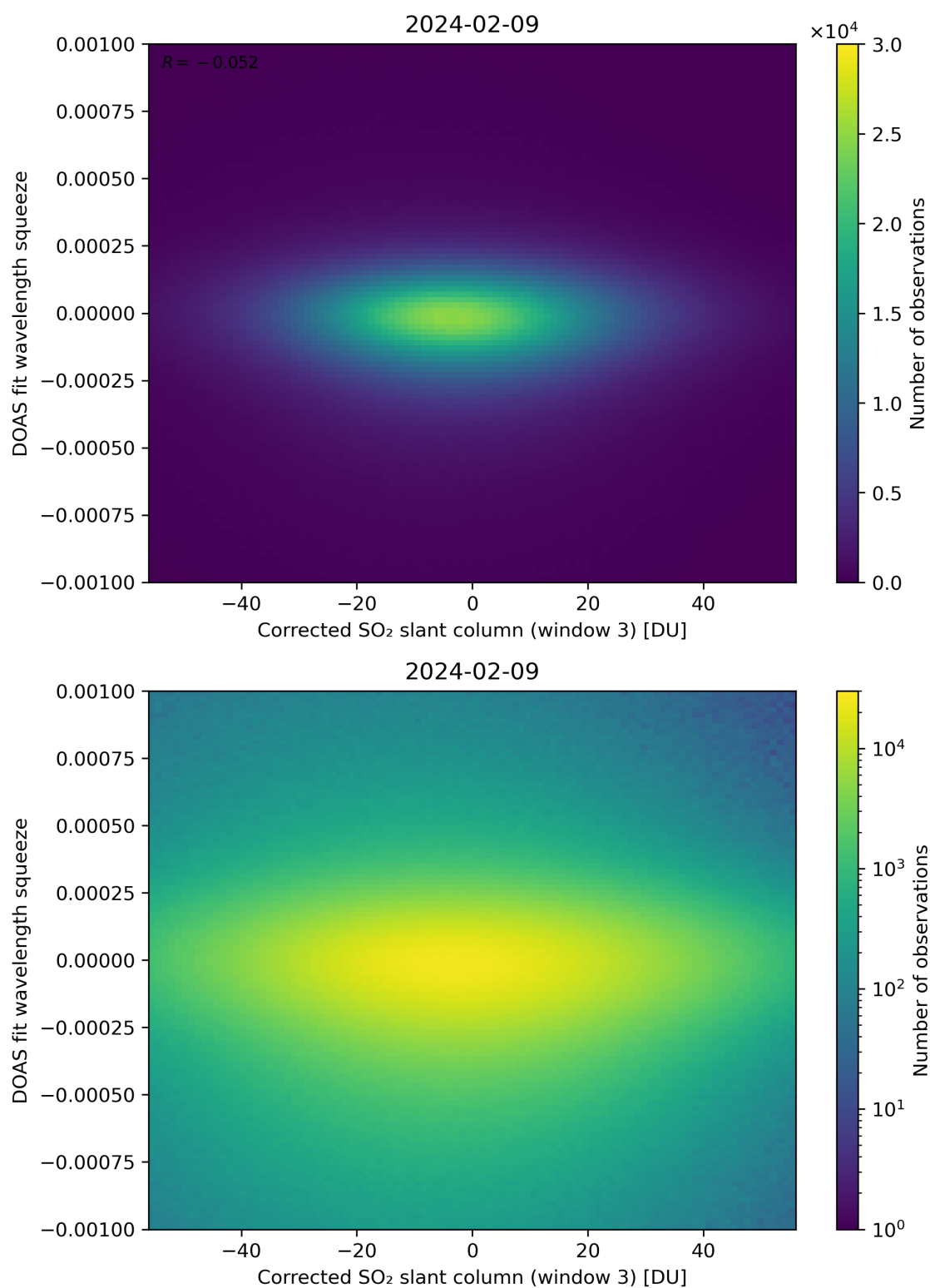
Figure 207: Scatter density plot of “Corrected SO 2 slant column (window 3)” against “DOAS fit wavelength squeeze” for 2024-02-08 to 2024-02-10.
