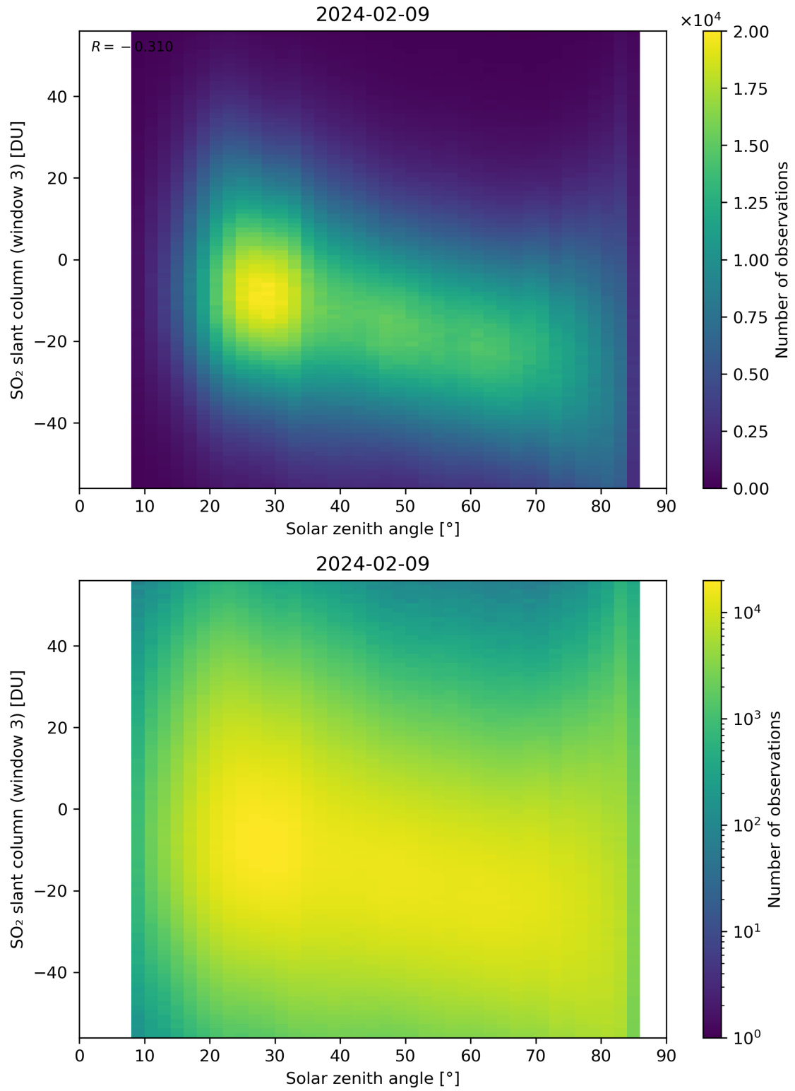
Figure 172: Scatter density plot of “Solar zenith angle” against “SO 2 slant column (window 3)” for 2024-02-08 to 2024-02-10.
