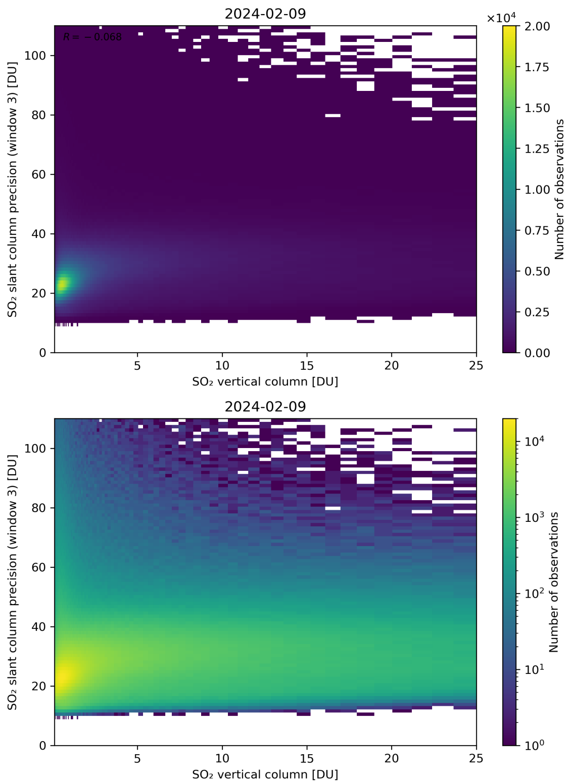
Figure 304: Scatter density plot of “SO 2 vertical column” against “SO 2 slant column precision (window 3)” for 2024-02-08 to 2024-02-10.
