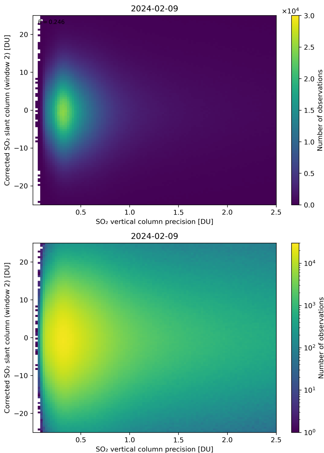
Figure 287: Scatter density plot of “SO 2 vertical column precision” against “Corrected SO 2 slant column (window 2)” for 2024-02-08 to 2024-02-10.
