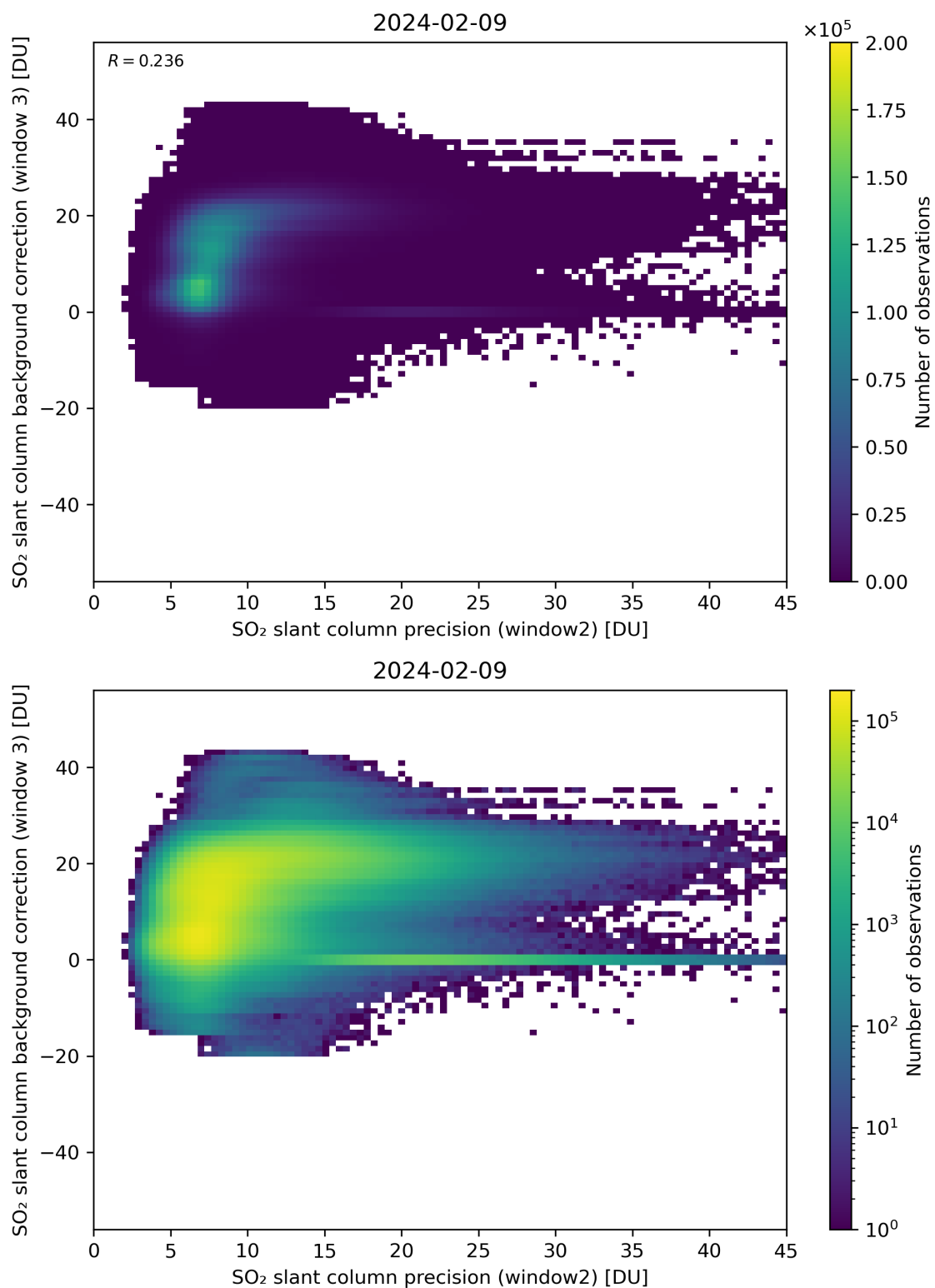
Figure 242: Scatter density plot of “SO 2 slant column precision (window2)” against “SO 2 slant column background correction (window 3)” for 2024-02-08 to 2024-02-10.
