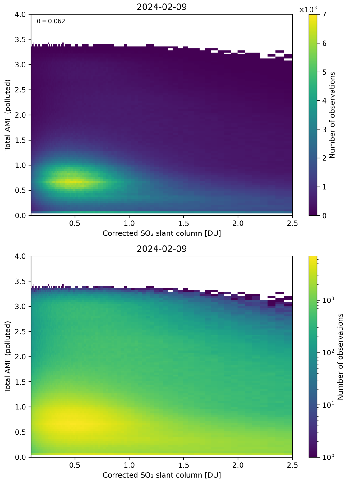
Figure 192: Scatter density plot of “Corrected SO 2 slant column” against “Total AMF (polluted)” for 2024-02-08 to 2024-02-10.
