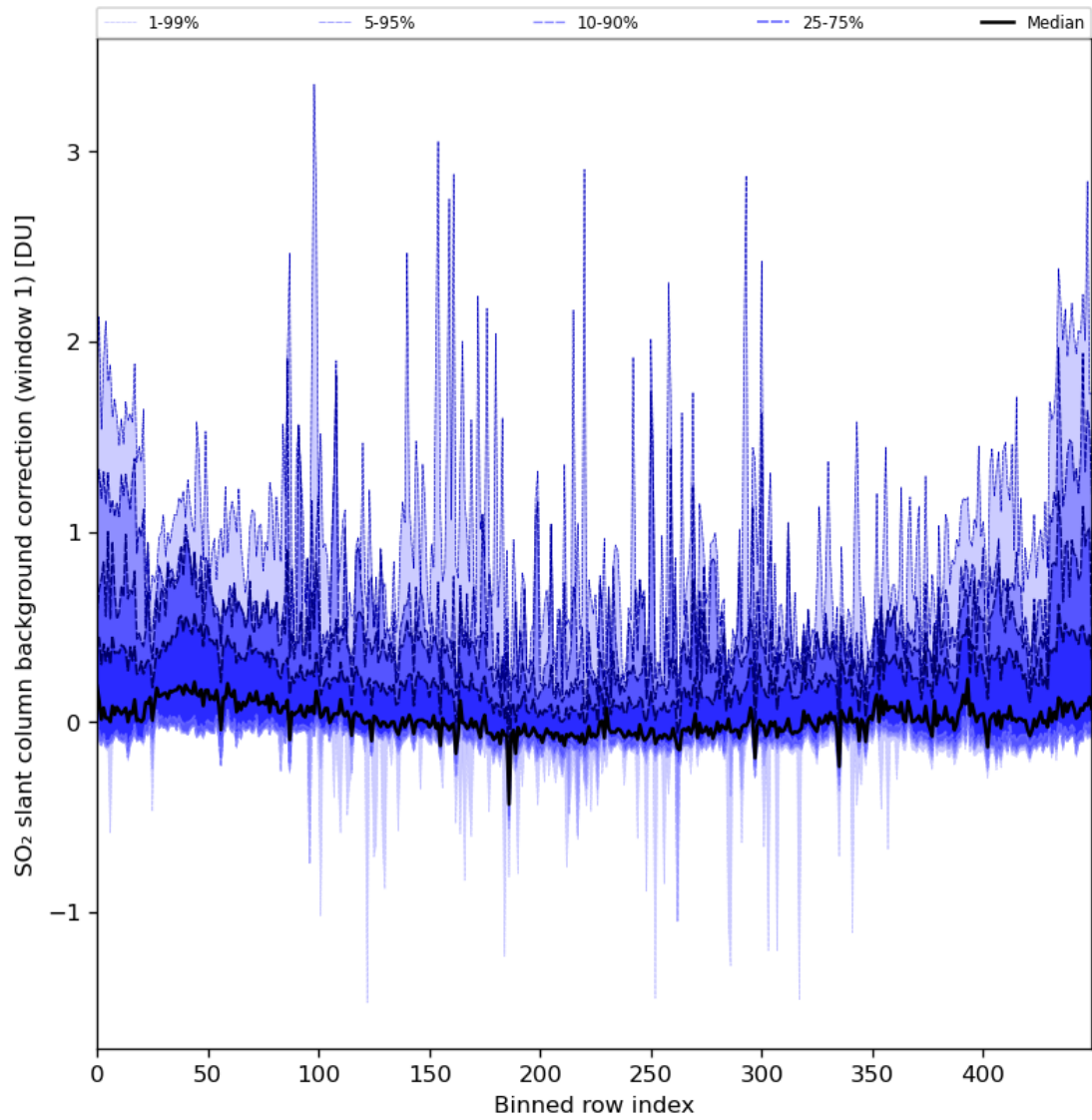
Figure 82: Along track statistics of “SO 2 slant column background correction (window 1)” for 2024-02-08 to 2024-02-10
