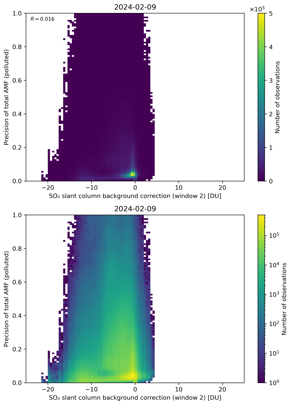
Figure 120: Scatter density plot of “SO 2 slant column background correction (window 2)” against “Precision of total AMF (polluted)” for 2024-02-08 to 2024-02-10.
