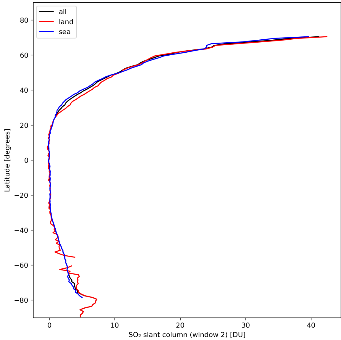
Figure 37: Zonal average of “SO 2 slant column (window 2)” for 2024-02-08 to 2024-02-10.
