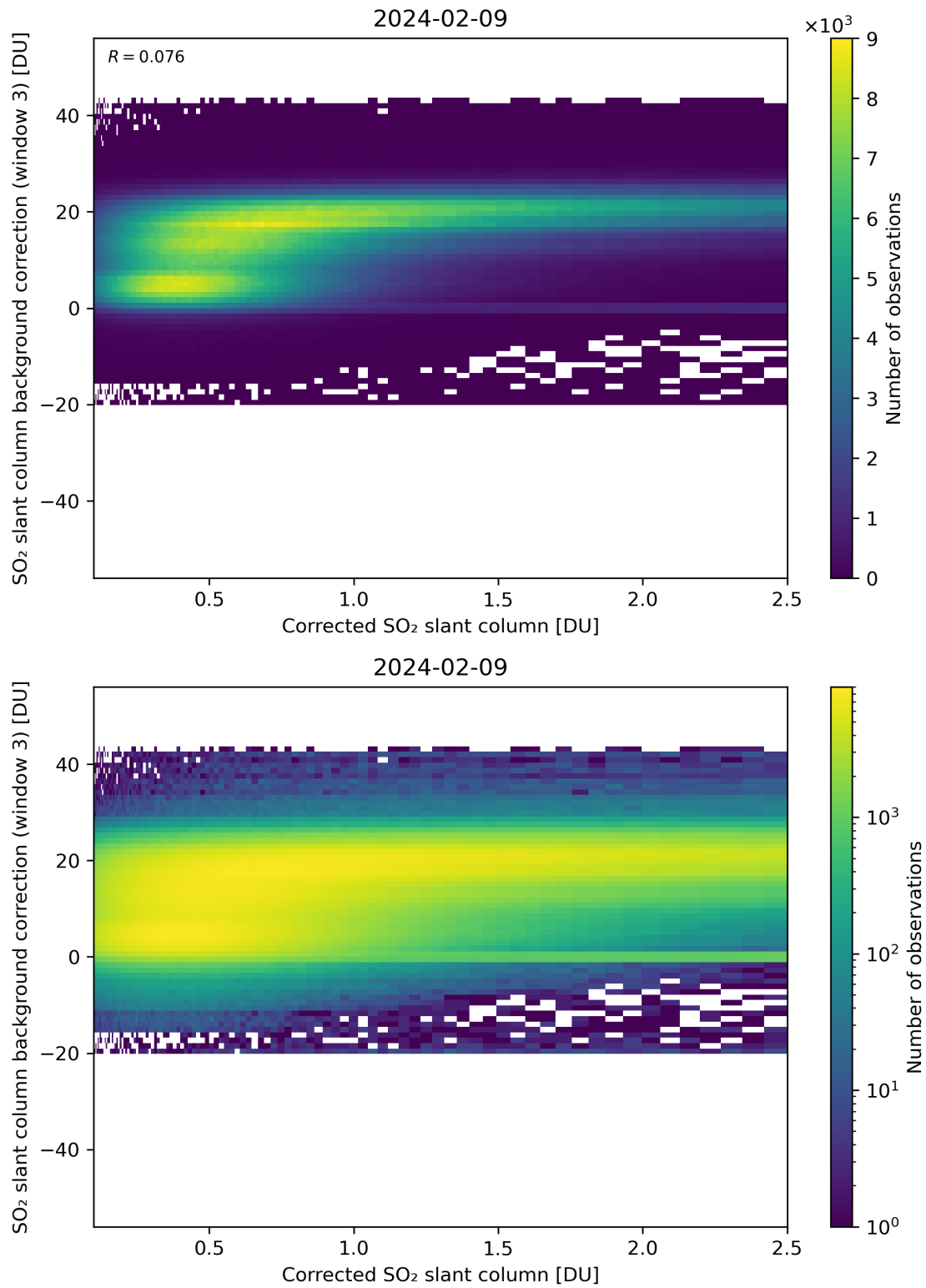
Figure 180: Scatter density plot of “Corrected SO 2 slant column” against “SO 2 slant column background correction (window 3)” for 2024-02-08 to 2024-02-10.
