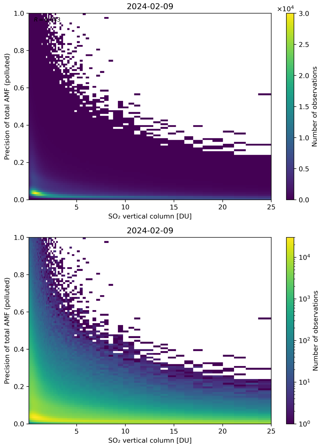
Figure 306: Scatter density plot of “SO 2 vertical column” against “Precision of total AMF (polluted)” for 2024-02-08 to 2024-02-10.
