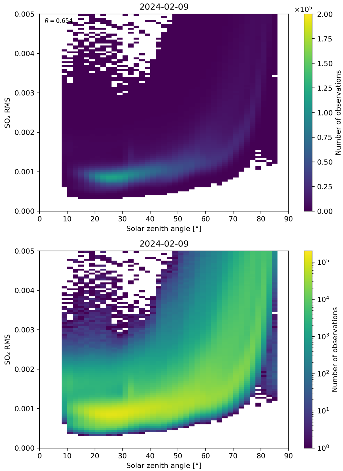
Figure 163: Scatter density plot of “Solar zenith angle” against “SO 2 RMS” for 2024-02-08 to 2024-02-10.
