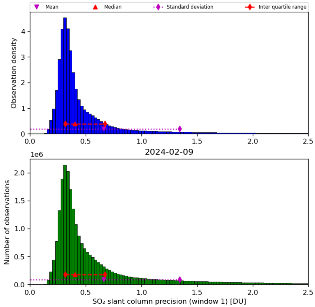
Figure 57: Histogram of “SO 2 slant column precision (window 1)” for 2024-02-08 to 2024-02-10
