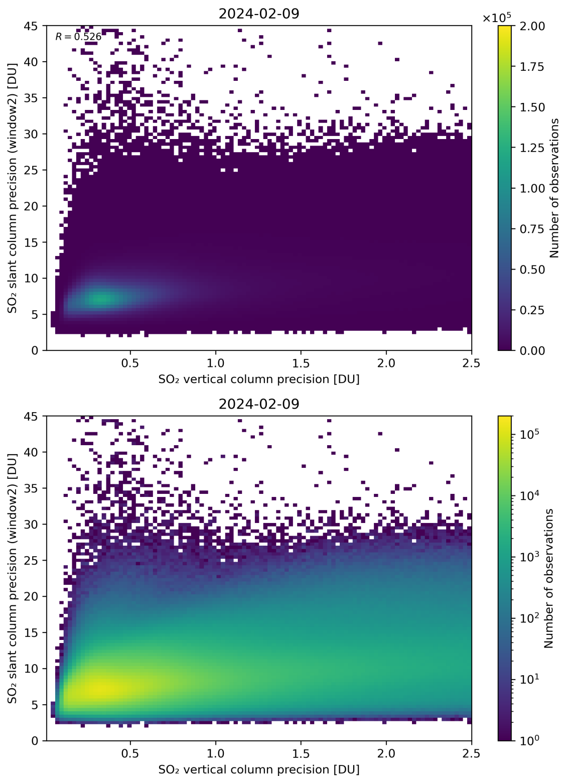
Figure 291: Scatter density plot of “SO 2 vertical column precision” against “SO 2 slant column precision (window2)” for 2024-02-08 to 2024-02-10.
