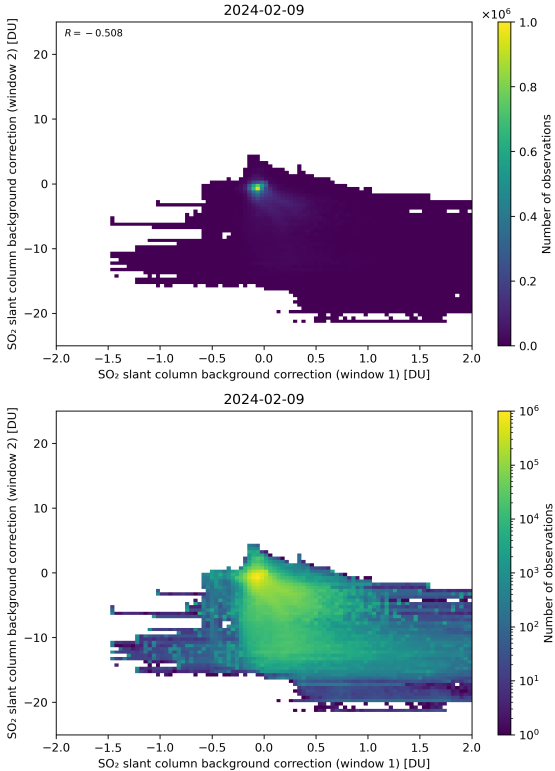
Figure 98: Scatter density plot of “SO 2 slant column background correction (window 1)” against “SO 2 slant column background correction (window 2)” for 2024-02-08 to 2024-02-10.
