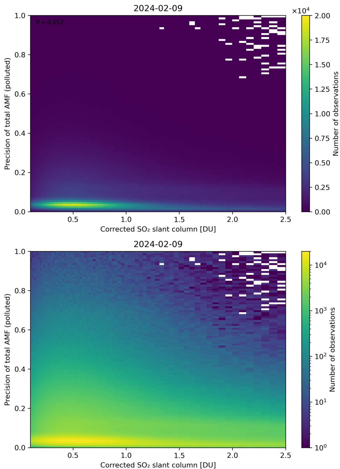
Figure 193: Scatter density plot of “Corrected SO 2 slant column” against “Precision of total AMF (polluted)” for 2024-02-08 to 2024-02-10.
