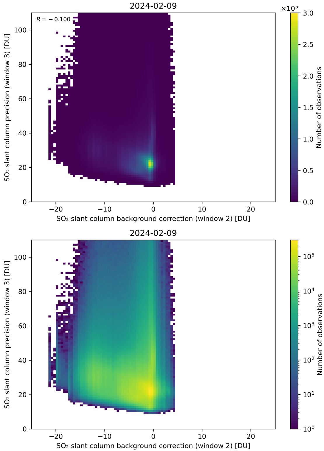
Figure 118: Scatter density plot of “SO 2 slant column background correction (window 2)” against “SO 2 slant column precision (window 3)” for 2024-02-08 to 2024-02-10.
