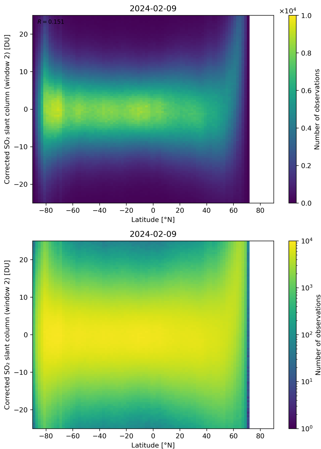
Figure 147: Scatter density plot of “Latitude” against “Corrected SO 2 slant column (window 2)” for 2024-02-08 to 2024-02-10.
