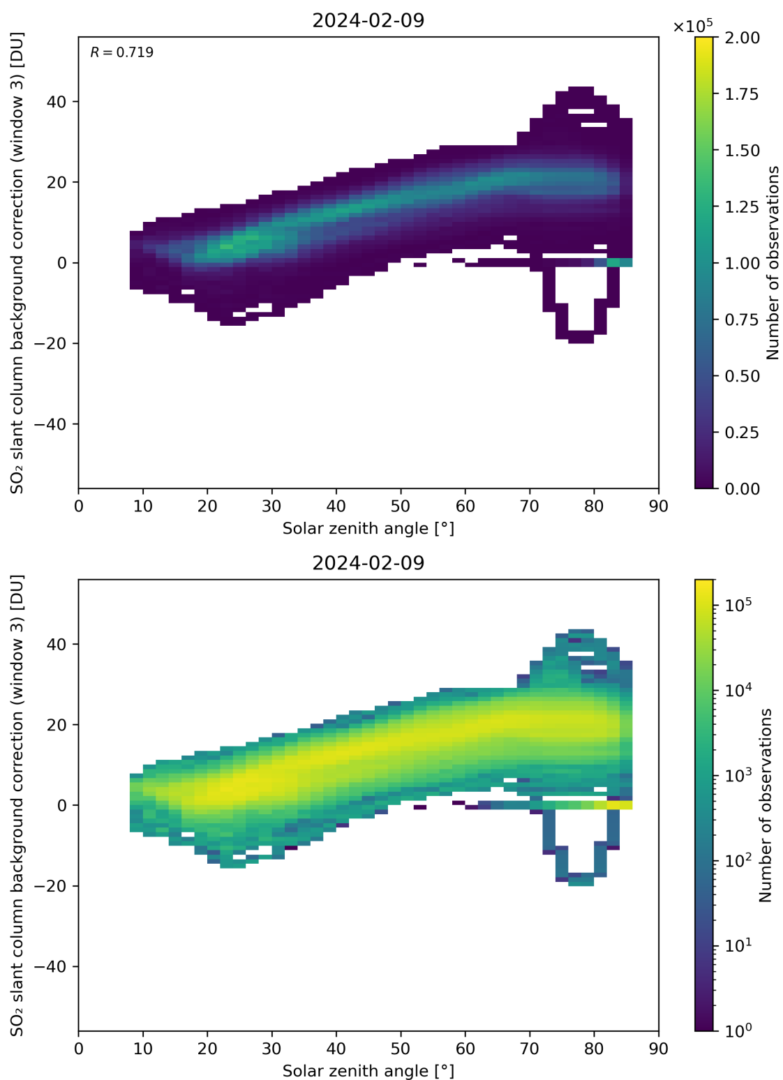
Figure 160: Scatter density plot of “Solar zenith angle” against “SO 2 slant column background correction (window 3)” for 2024-02-08 to 2024-02-10.
