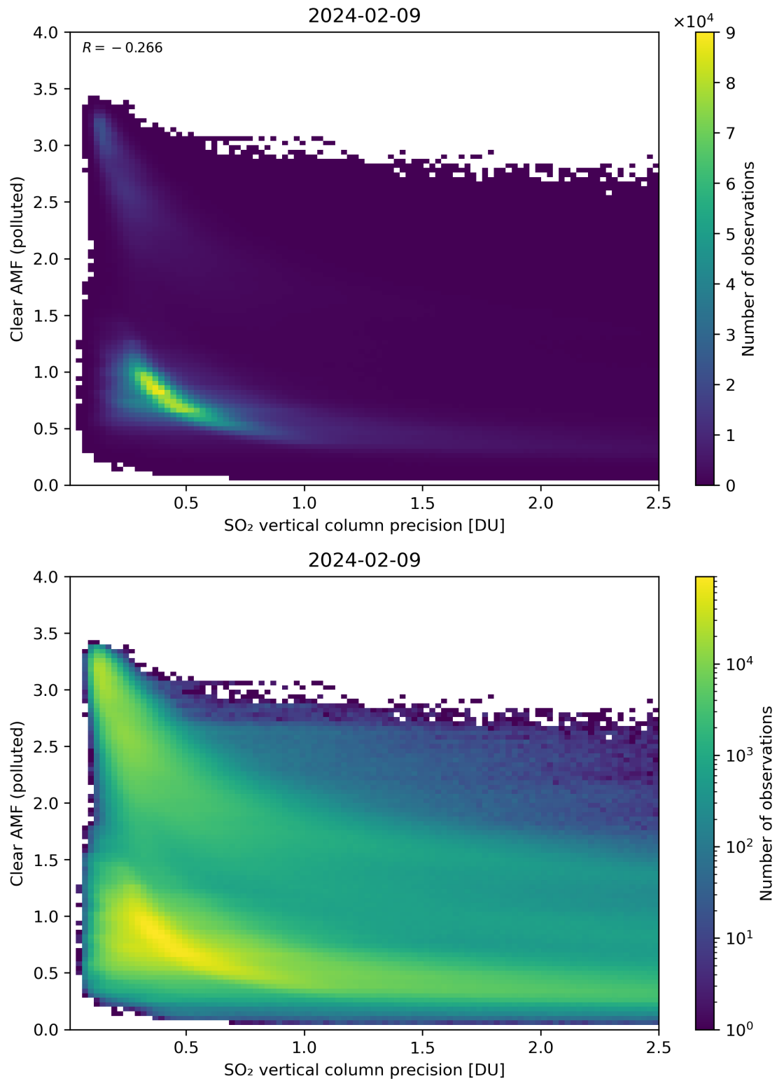
Figure 285: Scatter density plot of “SO 2 vertical column precision” against “Clear AMF (polluted)” for 2024-02-08 to 2024-02-10.
