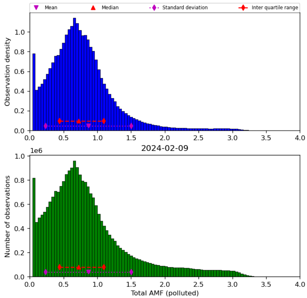
Figure 71: Histogram of “Total AMF (polluted)” for 2024-02-08 to 2024-02-10
