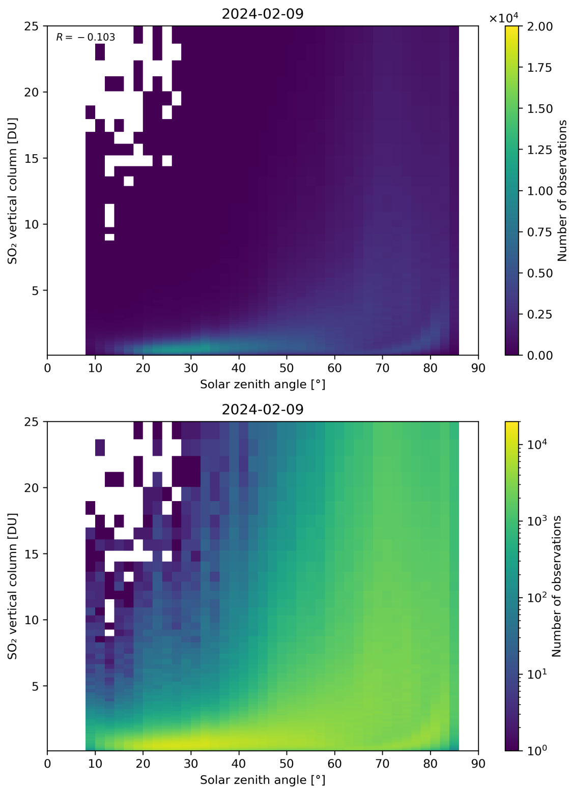
Figure 176: Scatter density plot of “Solar zenith angle” against “SO 2 vertical column” for 2024-02-08 to 2024-02-10.
