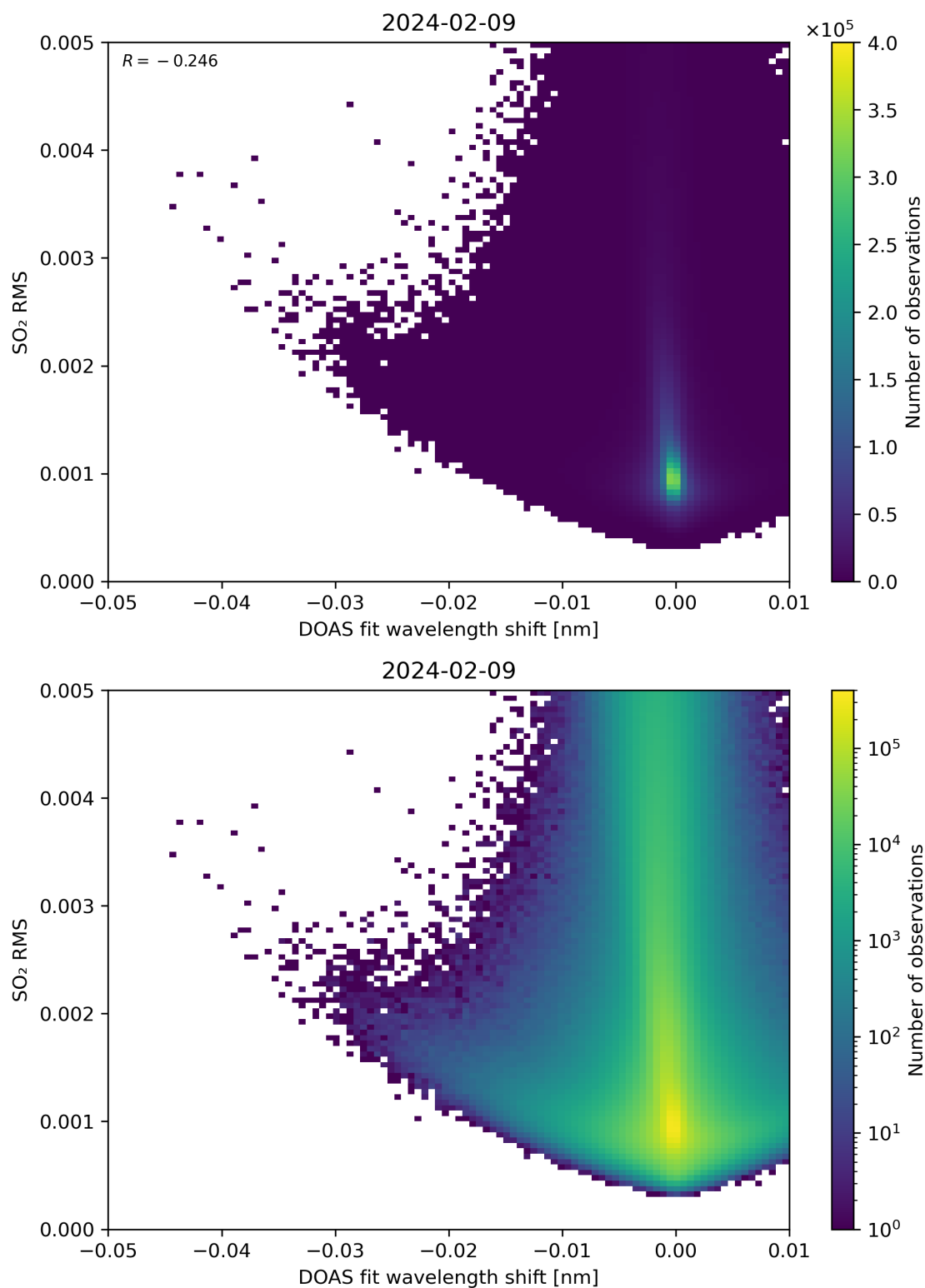
Figure 128: Scatter density plot of “DOAS fit wavelength shift” against “SO 2 RMS” for 2024-02-08 to 2024-02-10.
