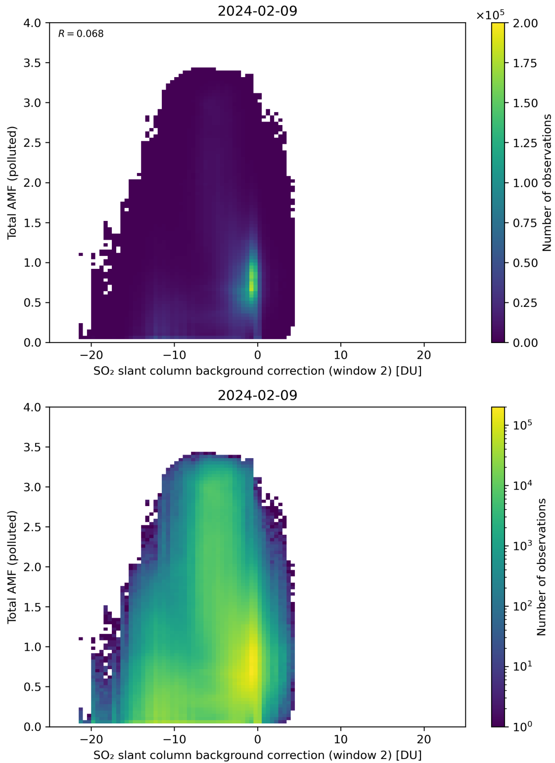
Figure 119: Scatter density plot of “SO 2 slant column background correction (window 2)” against “Total AMF (polluted)” for 2024-02-08 to 2024-02-10.
