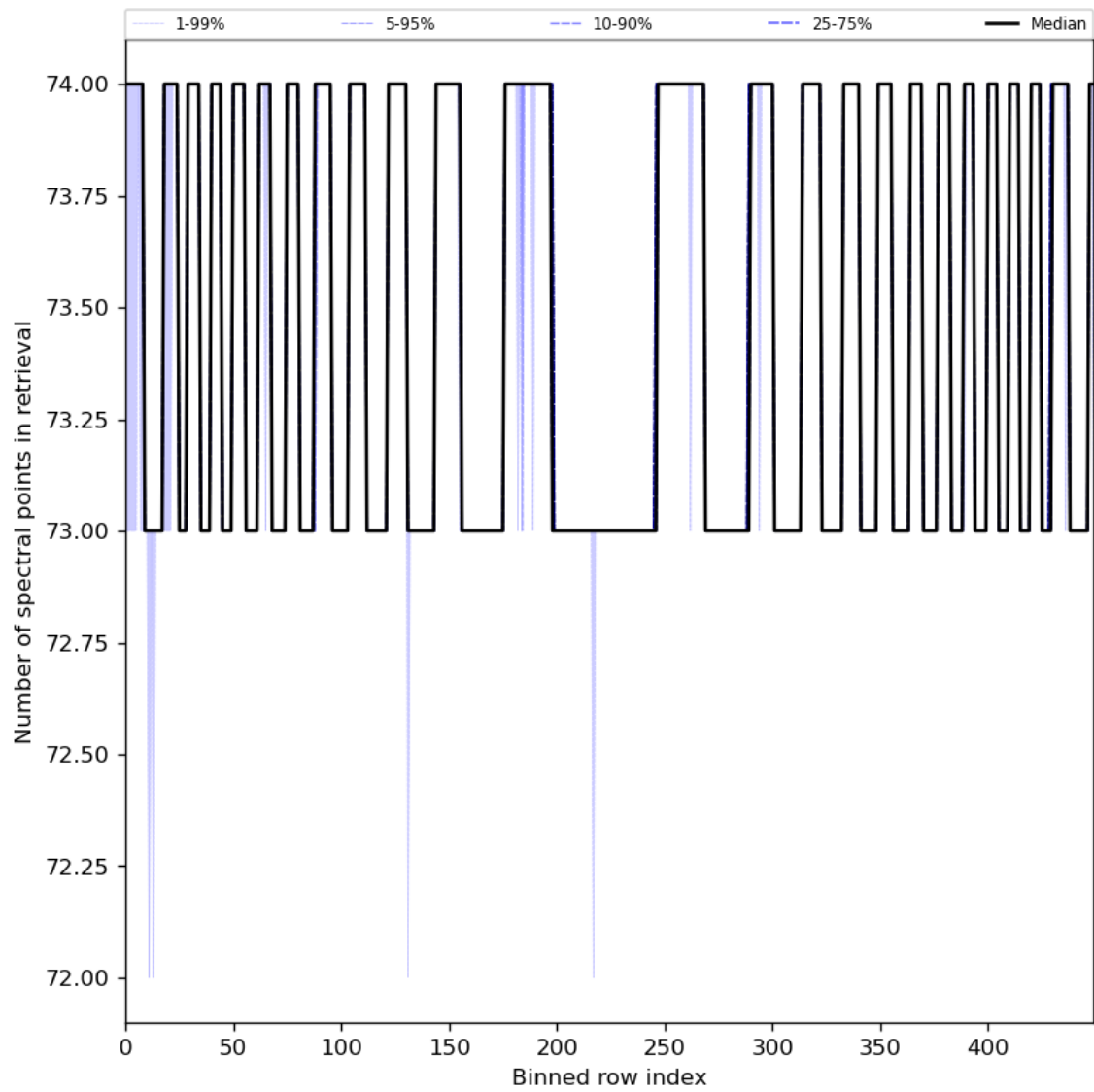
Figure 97: Along track statistics of “Number of spectral points in retrieval” for 2024-02-08 to 2024-02-10
