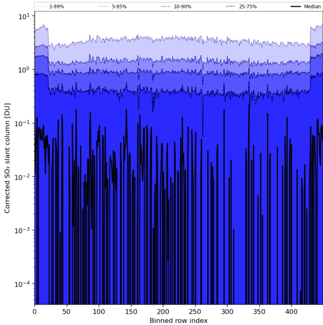
Figure 78: Along track statistics of “Corrected SO 2 slant column” for 2024-02-08 to 2024-02-10
