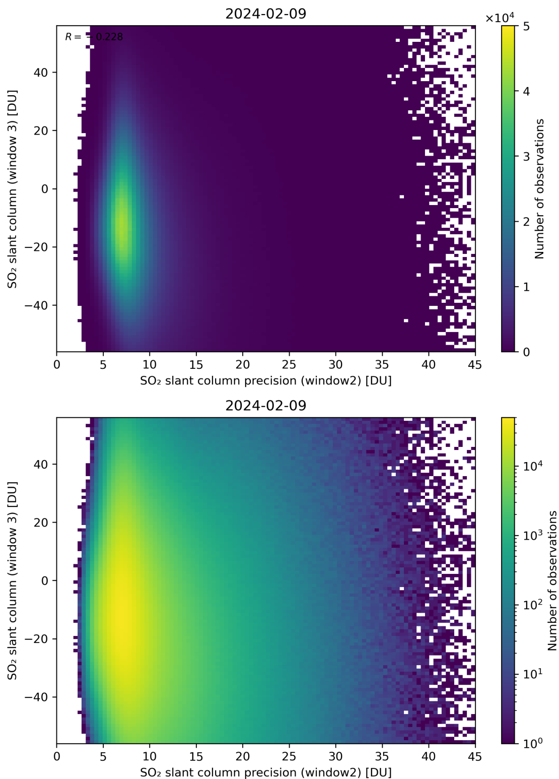
Figure 249: Scatter density plot of “SO 2 slant column precision (window2)” against “SO 2 slant column (window 3)” for 2024-02-08 to 2024-02-10.
