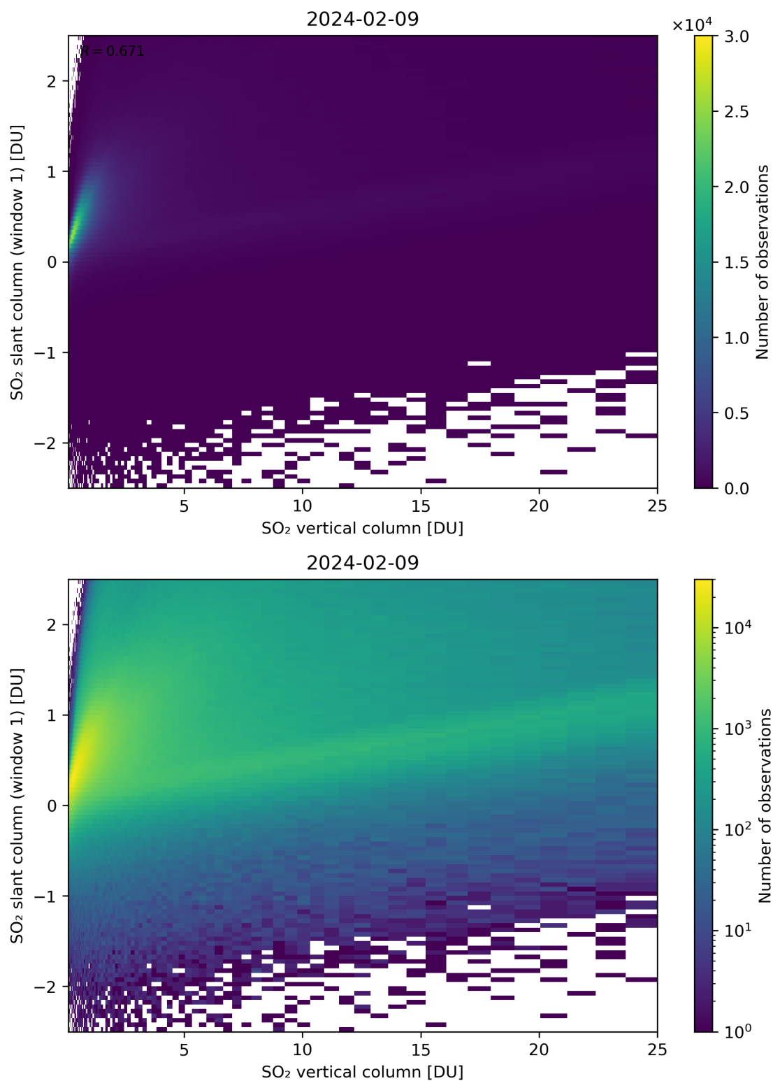
Figure 300: Scatter density plot of “SO 2 vertical column” against “SO 2 slant column (window 1)” for 2024-02-08 to 2024-02-10.
