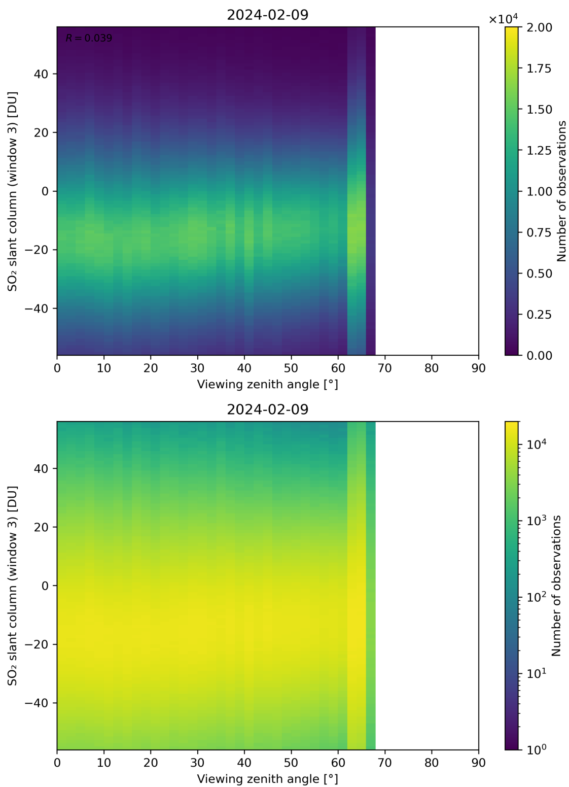
Figure 323: Scatter density plot of “Viewing zenith angle” against “SO 2 slant column (window 3)” for 2024-02-08 to 2024-02-10.
