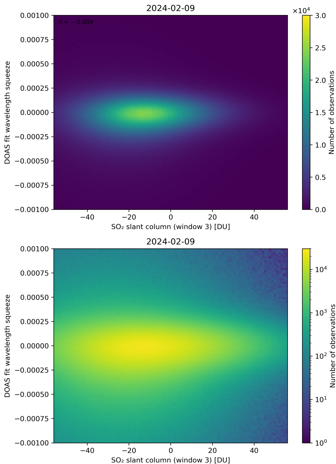
Figure 255: Scatter density plot of “SO 2 slant column (window 3)” against “DOAS fit wavelength squeeze” for 2024-02-08 to 2024-02-10.
