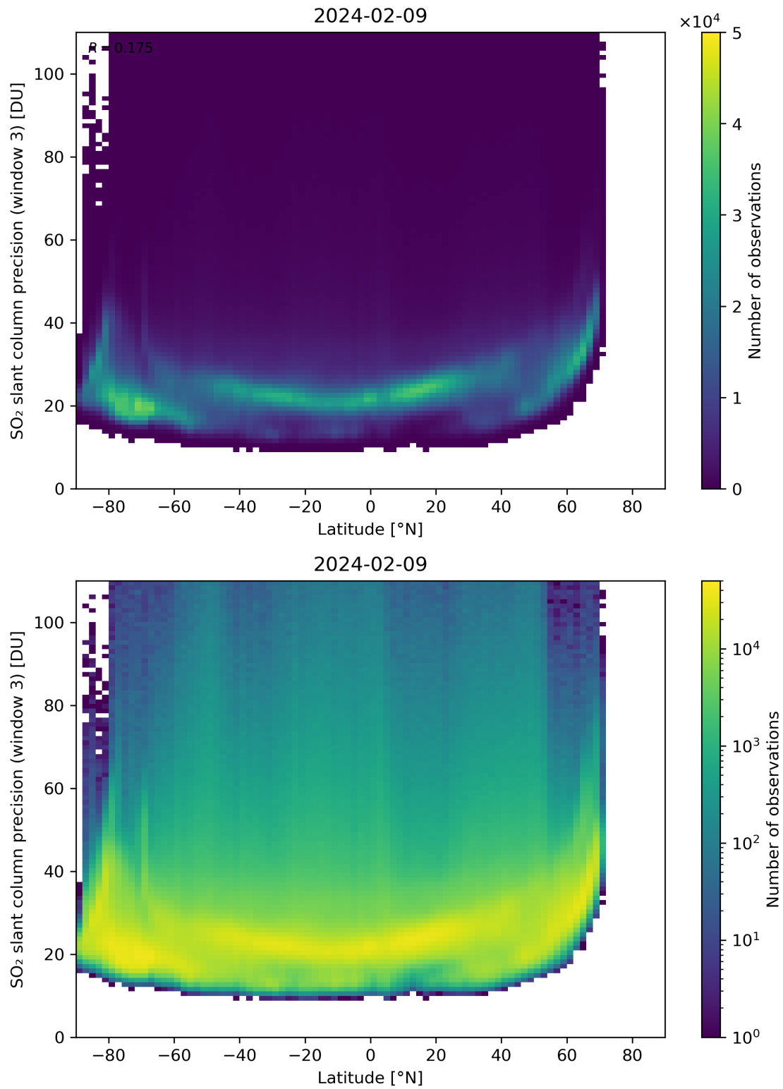
Figure 153: Scatter density plot of “Latitude” against “SO 2 slant column precision (window 3)” for 2024-02-08 to 2024-02-10.
