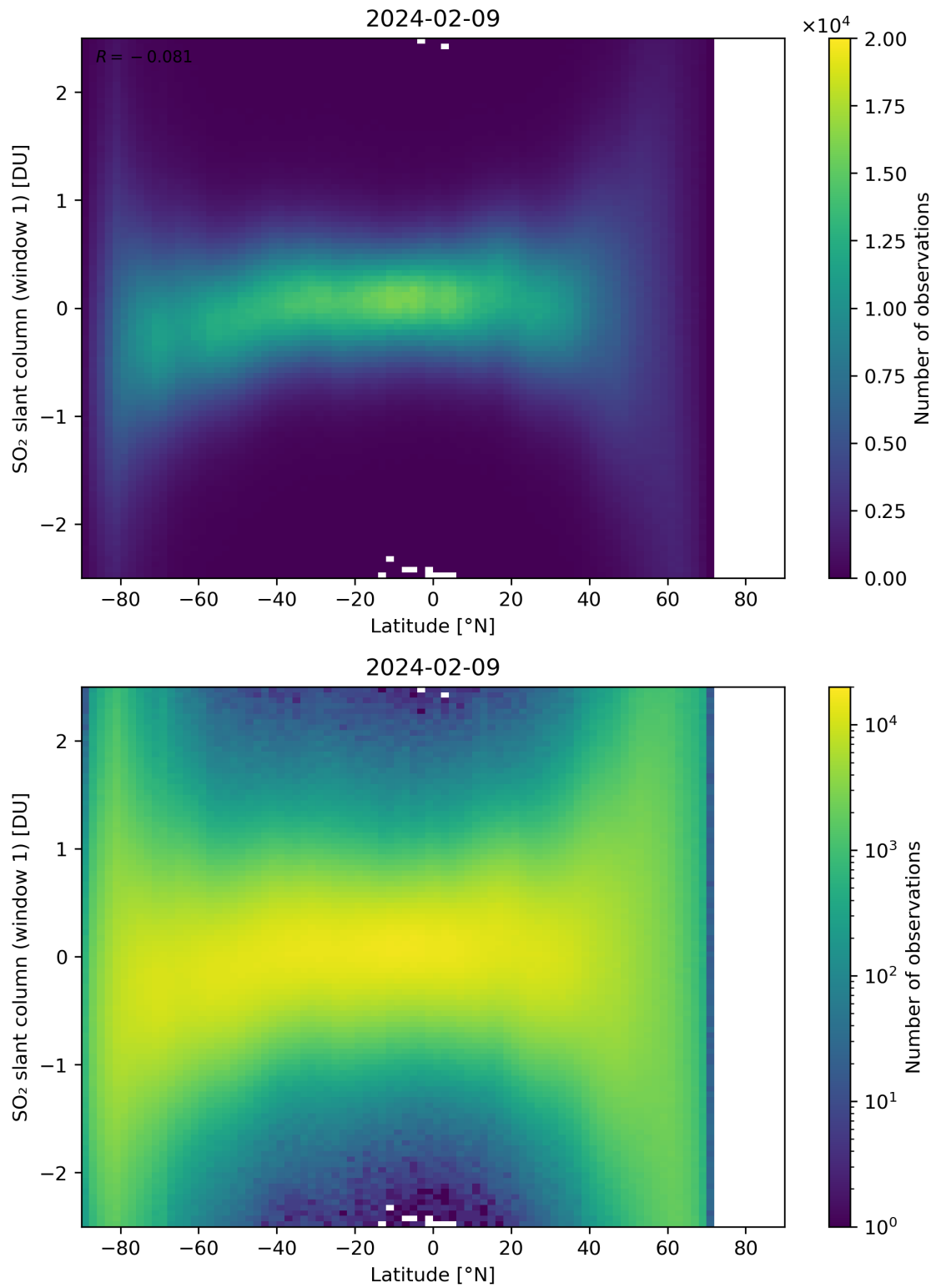
Figure 149: Scatter density plot of “Latitude” against “SO 2 slant column (window 1)” for 2024-02-08 to 2024-02-10.
