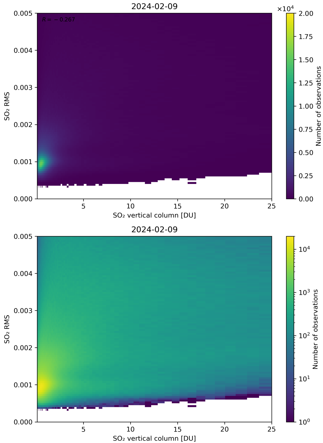
Figure 278: Scatter density plot of “SO 2 vertical column” against “SO 2 RMS” for 2024-02-08 to 2024-02-10.
