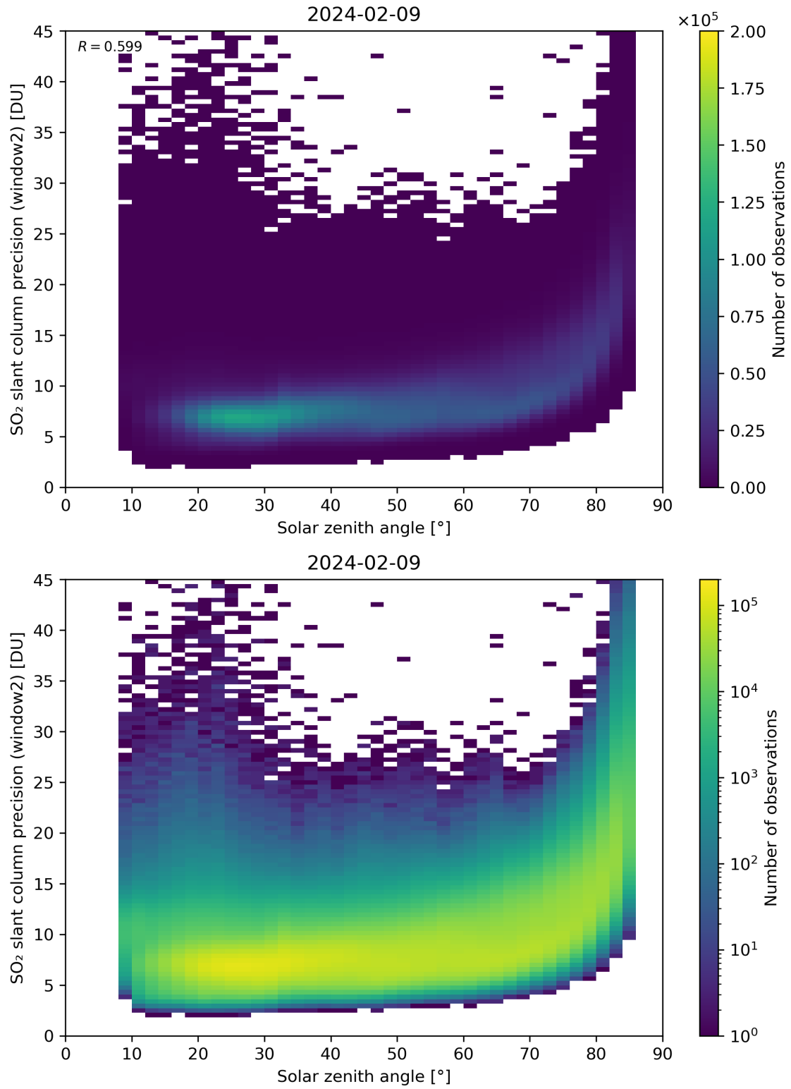
Figure 171: Scatter density plot of “Solar zenith angle” against “SO 2 slant column precision (window2)” for 2024-02-08 to 2024-02-10.
