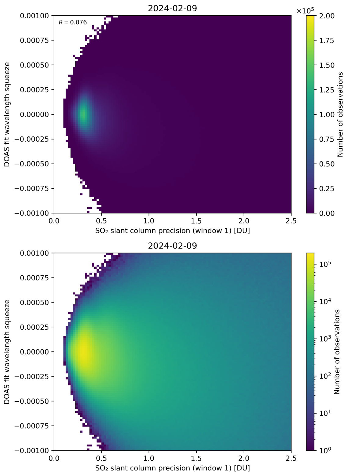
Figure 222: Scatter density plot of “SO 2 slant column precision (window 1)” against “DOAS fit wavelength squeeze” for 2024-02-08 to 2024-02-10.
