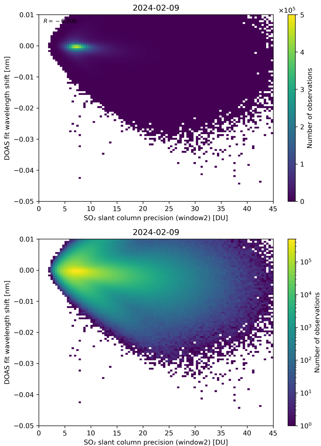
Figure 243: Scatter density plot of “SO 2 slant column precision (window2)” against “DOAS fit wavelength shift” for 2024-02-08 to 2024-02-10.
