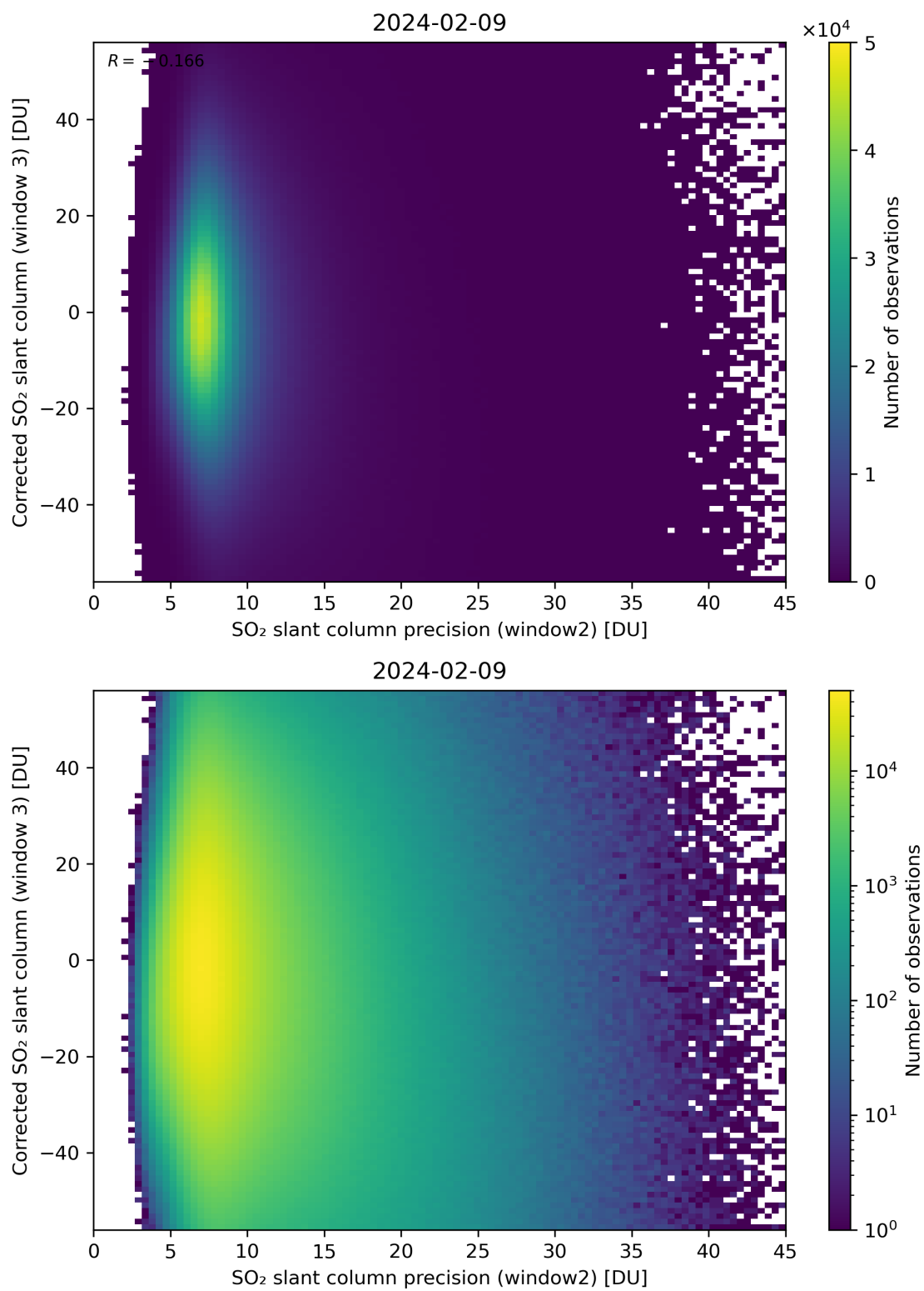
Figure 248: Scatter density plot of “SO 2 slant column precision (window2)” against “Corrected SO 2 slant column (window 3)” for 2024-02-08 to 2024-02-10.
