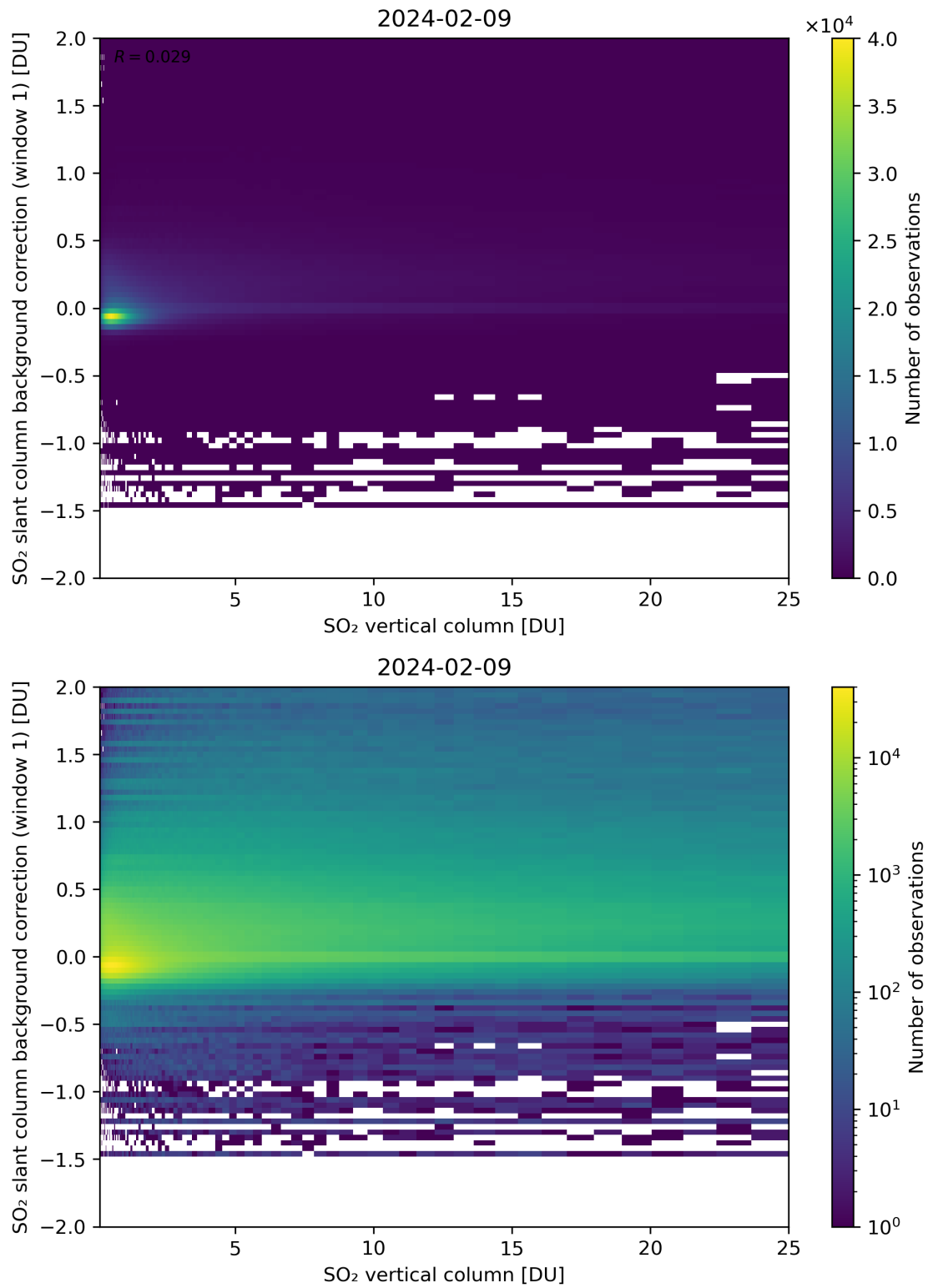
Figure 273: Scatter density plot of “SO 2 vertical column” against “SO 2 slant column background correction (window 1)” for 2024-02-08 to 2024-02-10.
