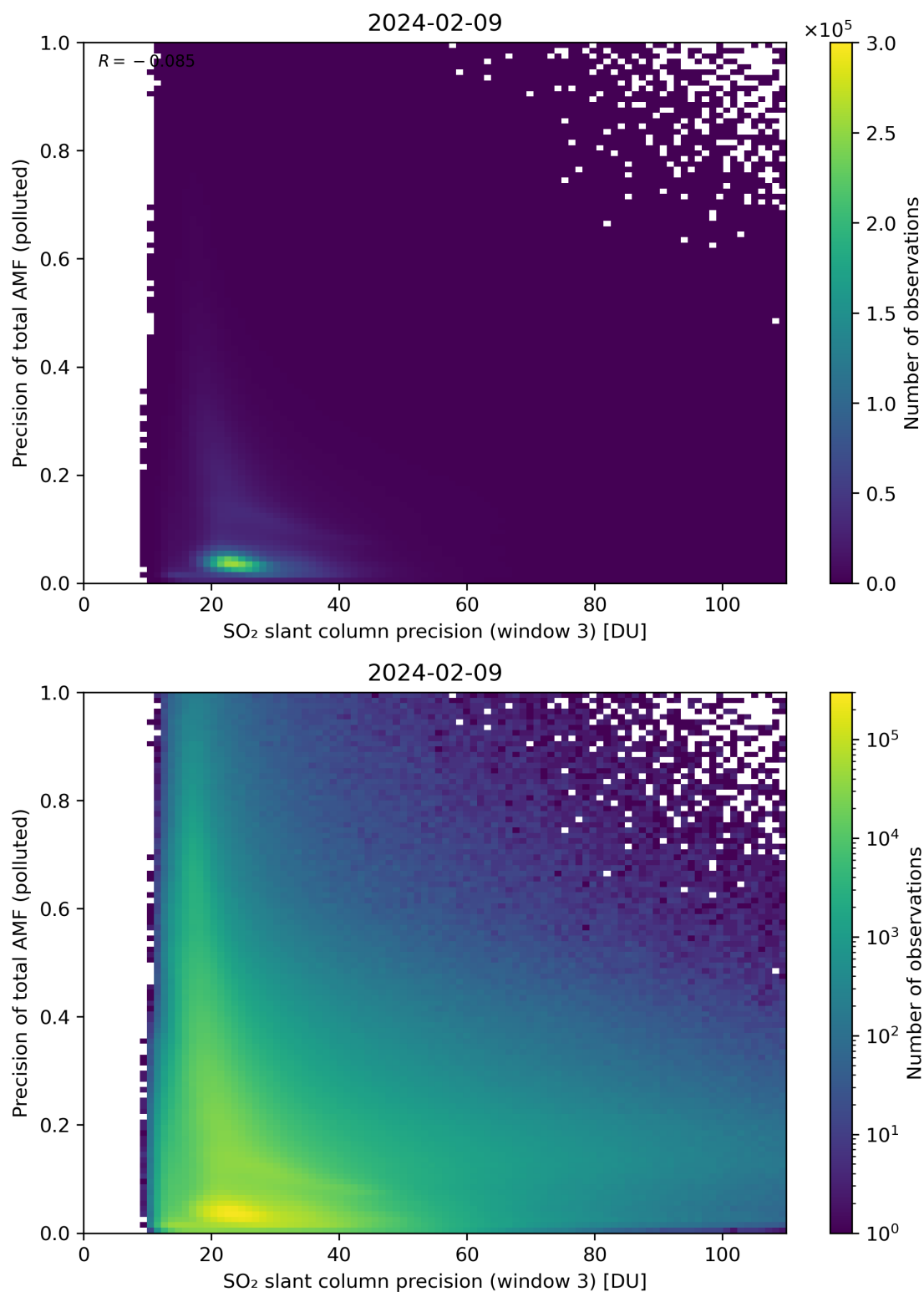
Figure 264: Scatter density plot of “SO 2 slant column precision (window 3)” against “Precision of total AMF (polluted)” for 2024-02-08 to 2024-02-10.
