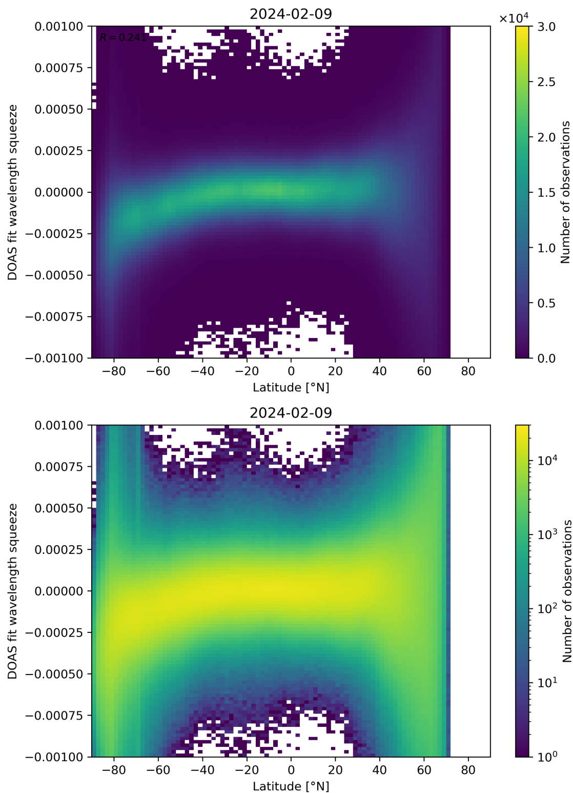
Figure 143: Scatter density plot of “Latitude” against “DOAS fit wavelength squeeze” for 2024-02-08 to 2024-02-10.
