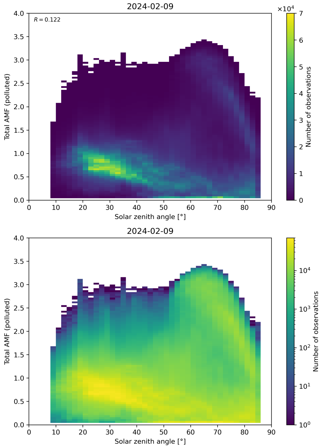
Figure 174: Scatter density plot of “Solar zenith angle” against “Total AMF (polluted)” for 2024-02-08 to 2024-02-10.
