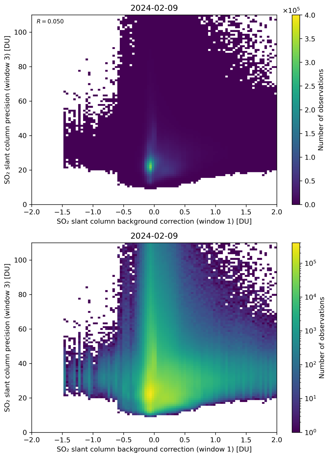
Figure 108: Scatter density plot of “SO 2 slant column background correction (window 1)” against “SO 2 slant column precision (window 3)” for 2024-02-08 to 2024-02-10.
