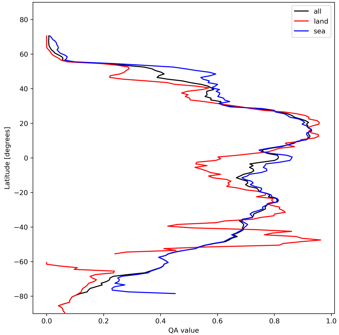
Figure 29: Zonal average of “QA value” for 2024-02-08 to 2024-02-10.
