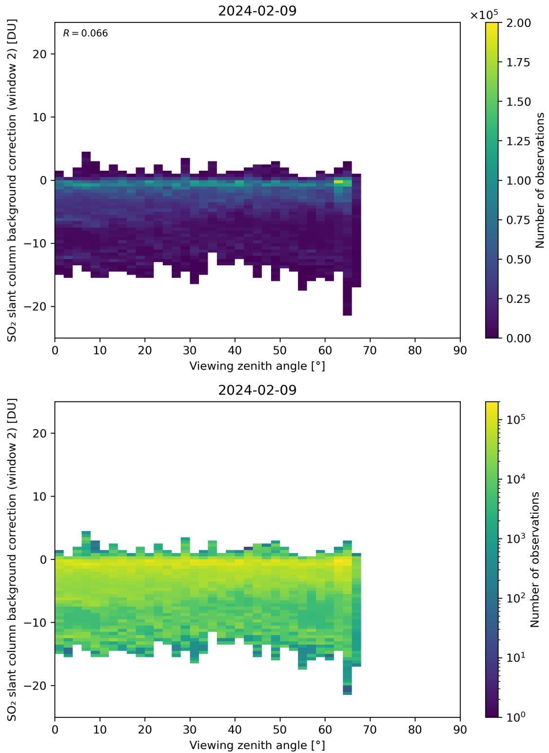
Figure 309: Scatter density plot of “Viewing zenith angle” against “SO 2 slant column background correction (window 2)” for 2024-02-08 to 2024-02-10.
