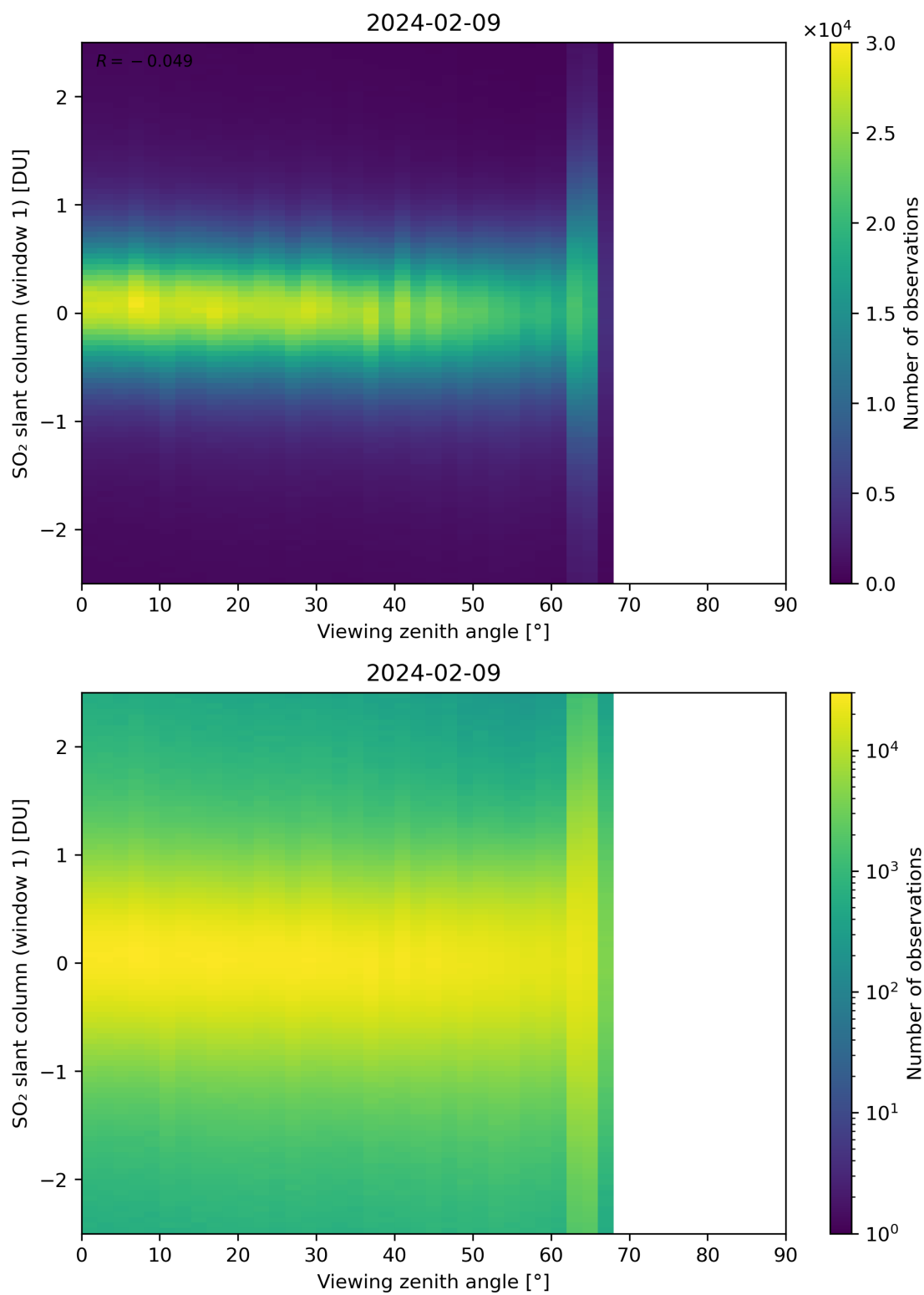
Figure 320: Scatter density plot of “Viewing zenith angle” against “SO 2 slant column (window 1)” for 2024-02-08 to 2024-02-10.
