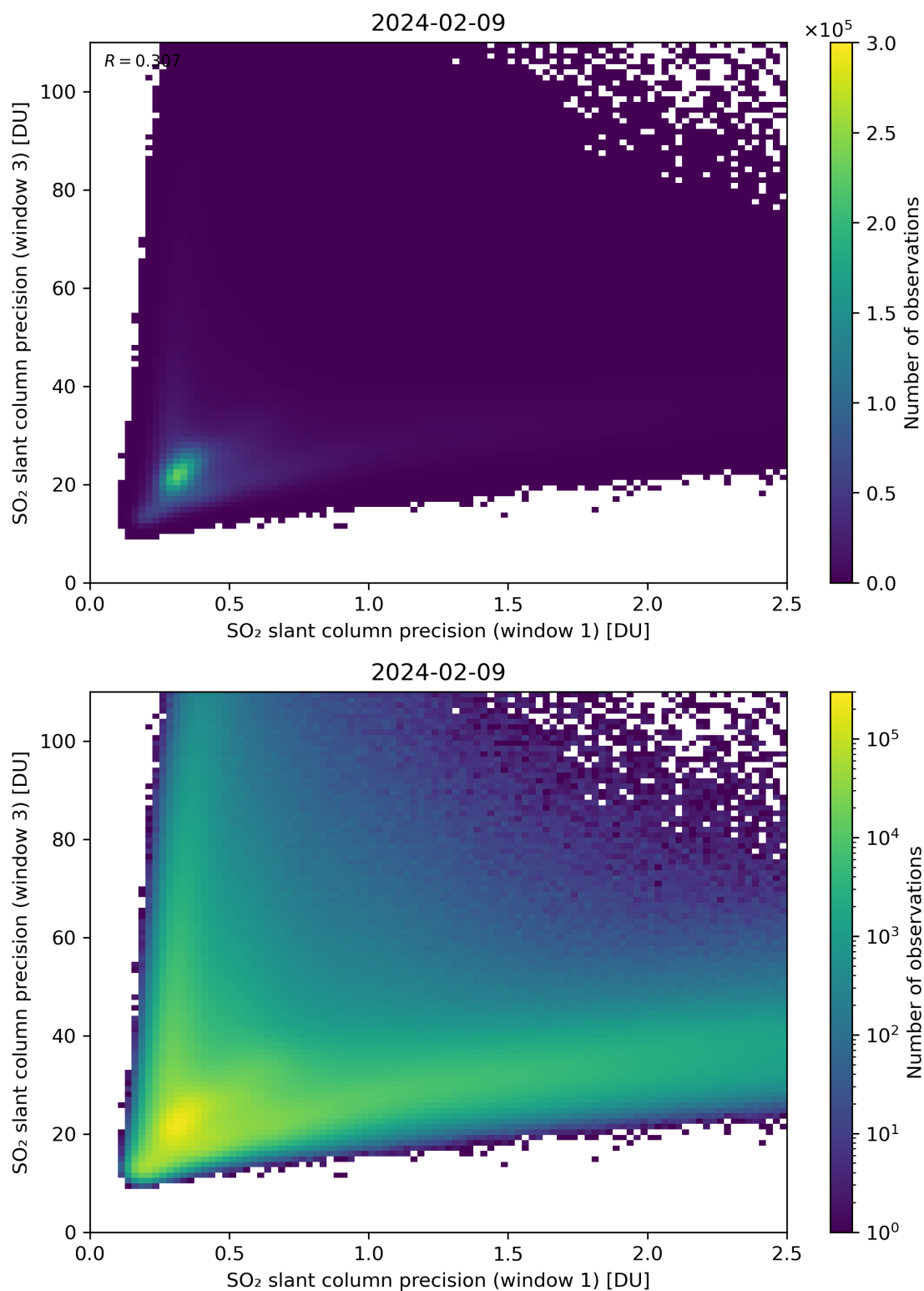
Figure 229: Scatter density plot of “SO 2 slant column precision (window 1)” against “SO 2 slant column precision (window 3)” for 2024-02-08 to 2024-02-10.
