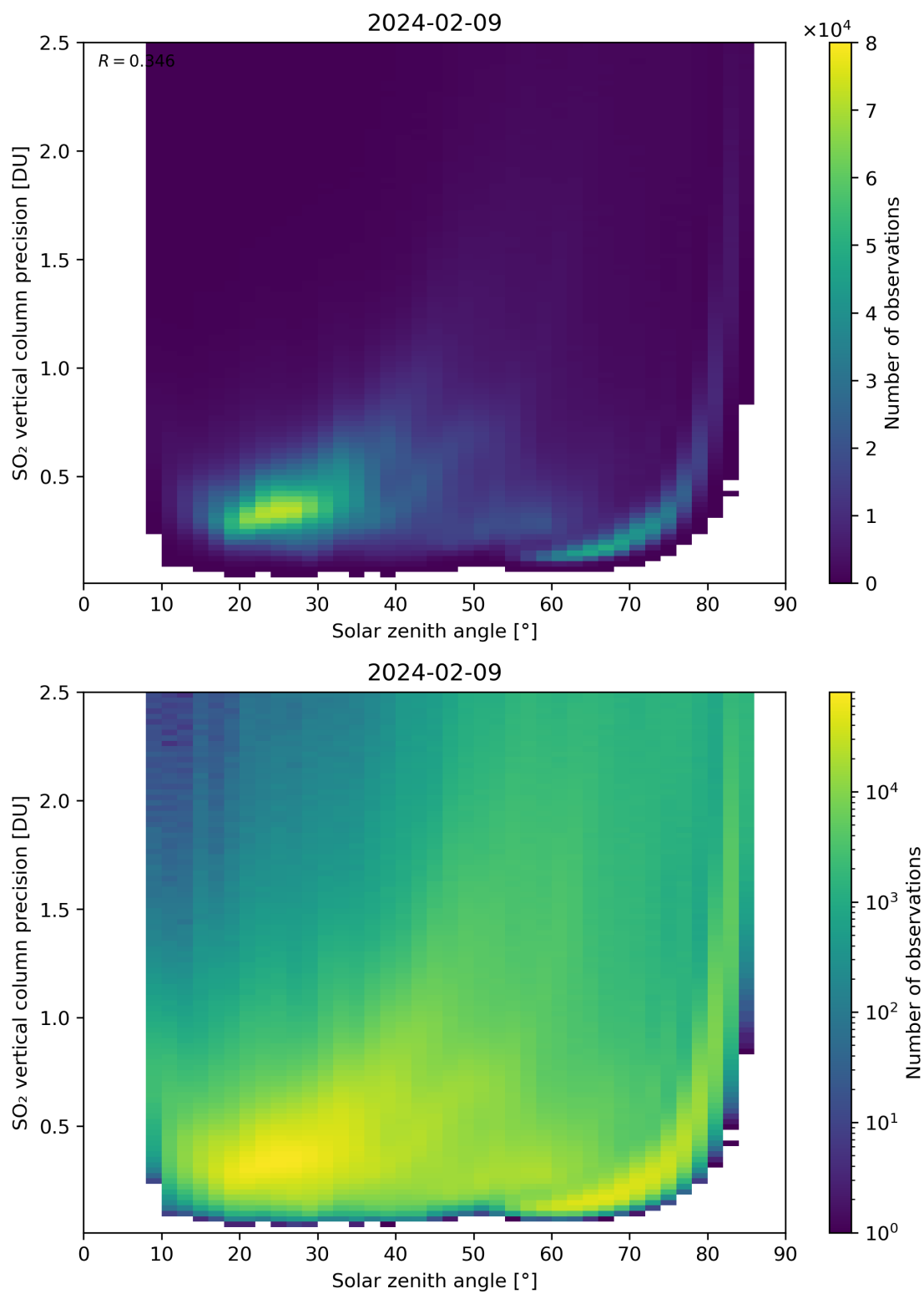
Figure 177: Scatter density plot of “Solar zenith angle” against “SO 2 vertical column precision” for 2024-02-08 to 2024-02-10.
