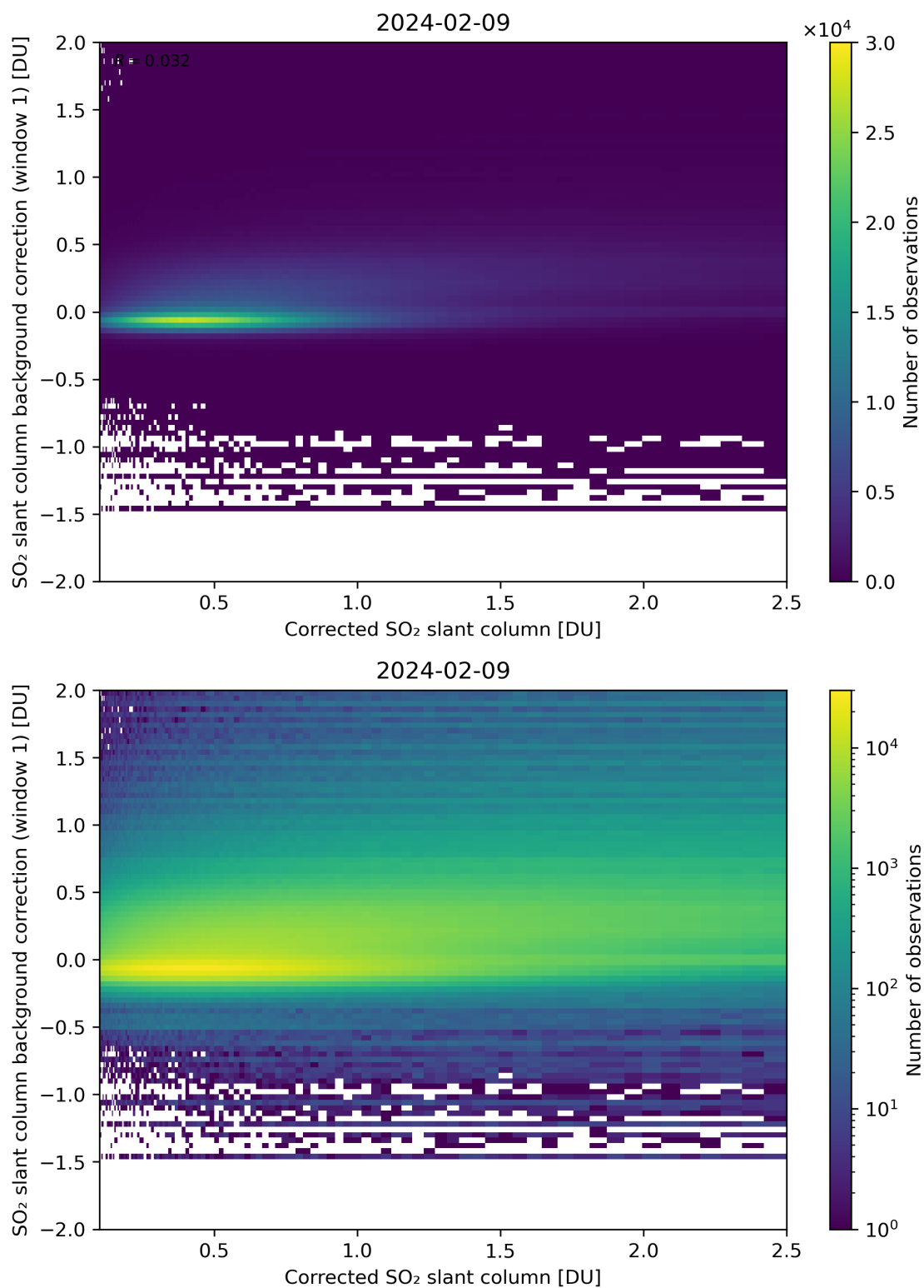
Figure 178: Scatter density plot of “Corrected SO 2 slant column” against “SO 2 slant column background correction (window 1)” for 2024-02-08 to 2024-02-10.
