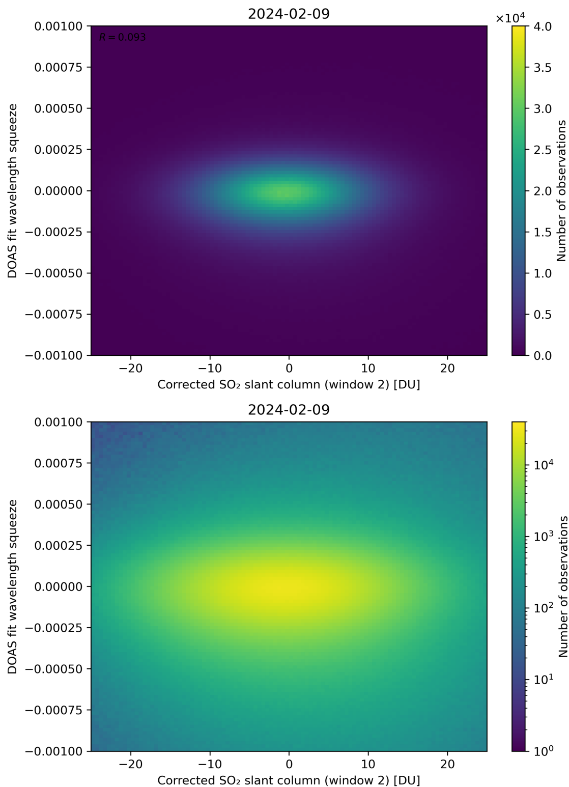
Figure 197: Scatter density plot of “Corrected SO 2 slant column (window 2)” against “DOAS fit wavelength squeeze” for 2024-02-08 to 2024-02-10.
