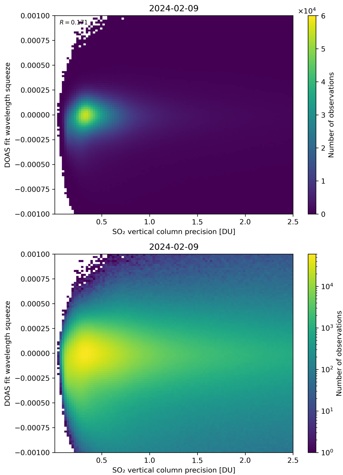
Figure 283: Scatter density plot of “SO 2 vertical column precision” against “DOAS fit wavelength squeeze” for 2024-02-08 to 2024-02-10.
