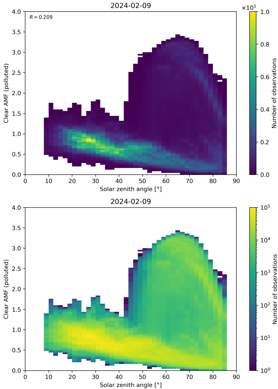
Figure 165: Scatter density plot of “Solar zenith angle” against “Clear AMF (polluted)” for 2024-02-08 to 2024-02-10.
