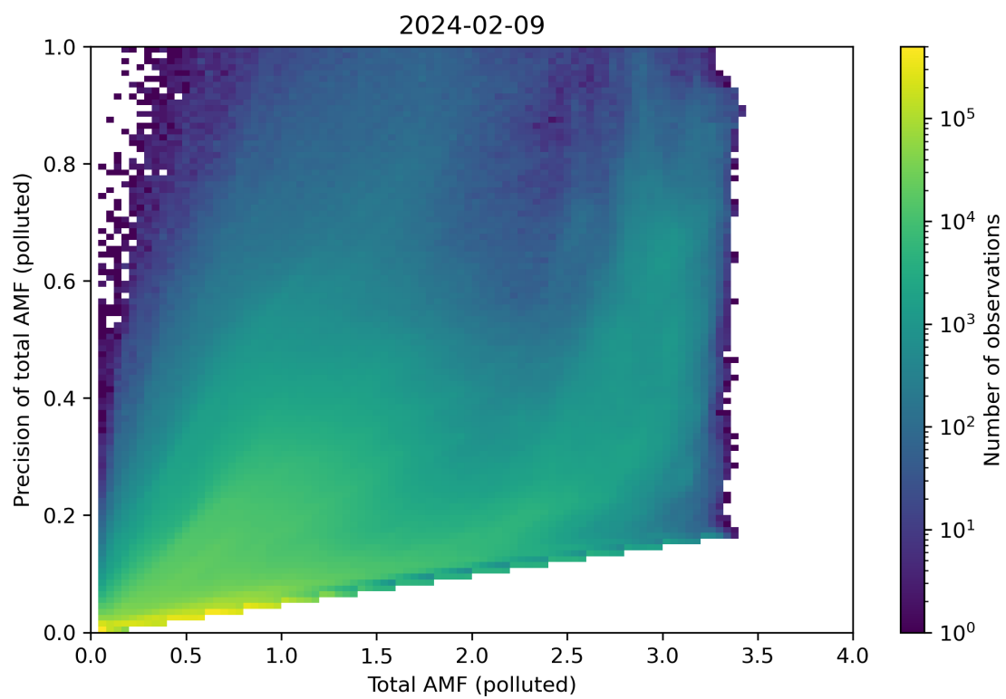
Figure 272: Scatter density plot of “Total AMF (polluted)” against “Precision of total AMF (polluted)” for 2024-02-08 to 2024-02-10.
