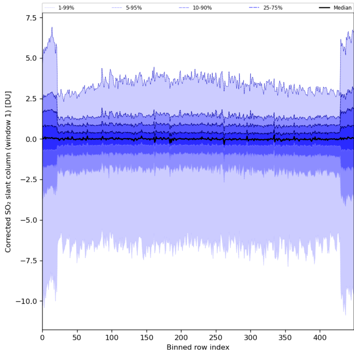
Figure 81: Along track statistics of “Corrected SO 2 slant column (window 1)” for 2024-02-08 to 2024-02-10
