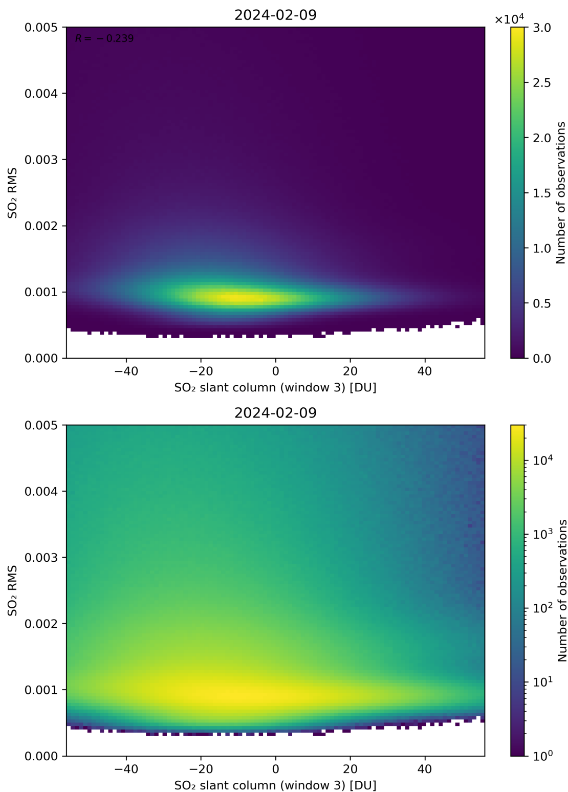
Figure 256: Scatter density plot of “SO 2 slant column (window 3)” against “SO 2 RMS” for 2024-02-08 to 2024-02-10.
