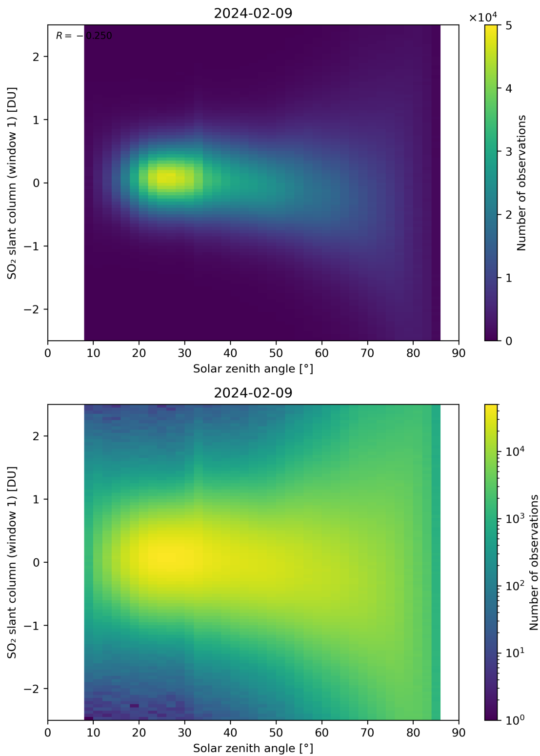
Figure 169: Scatter density plot of “Solar zenith angle” against “SO 2 slant column (window 1)” for 2024-02-08 to 2024-02-10.
