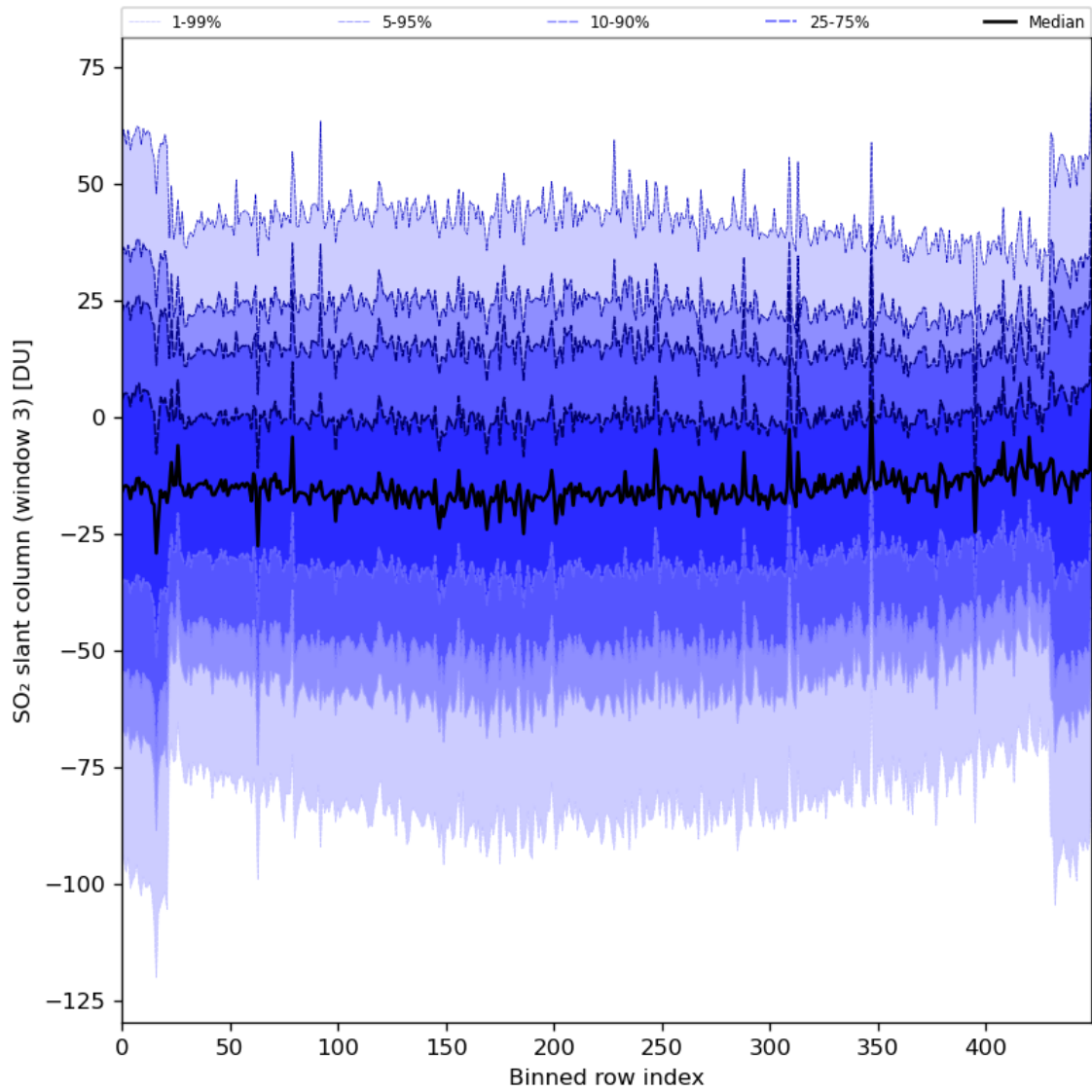
Figure 87: Along track statistics of “SO 2 slant column (window 3)” for 2024-02-08 to 2024-02-10
