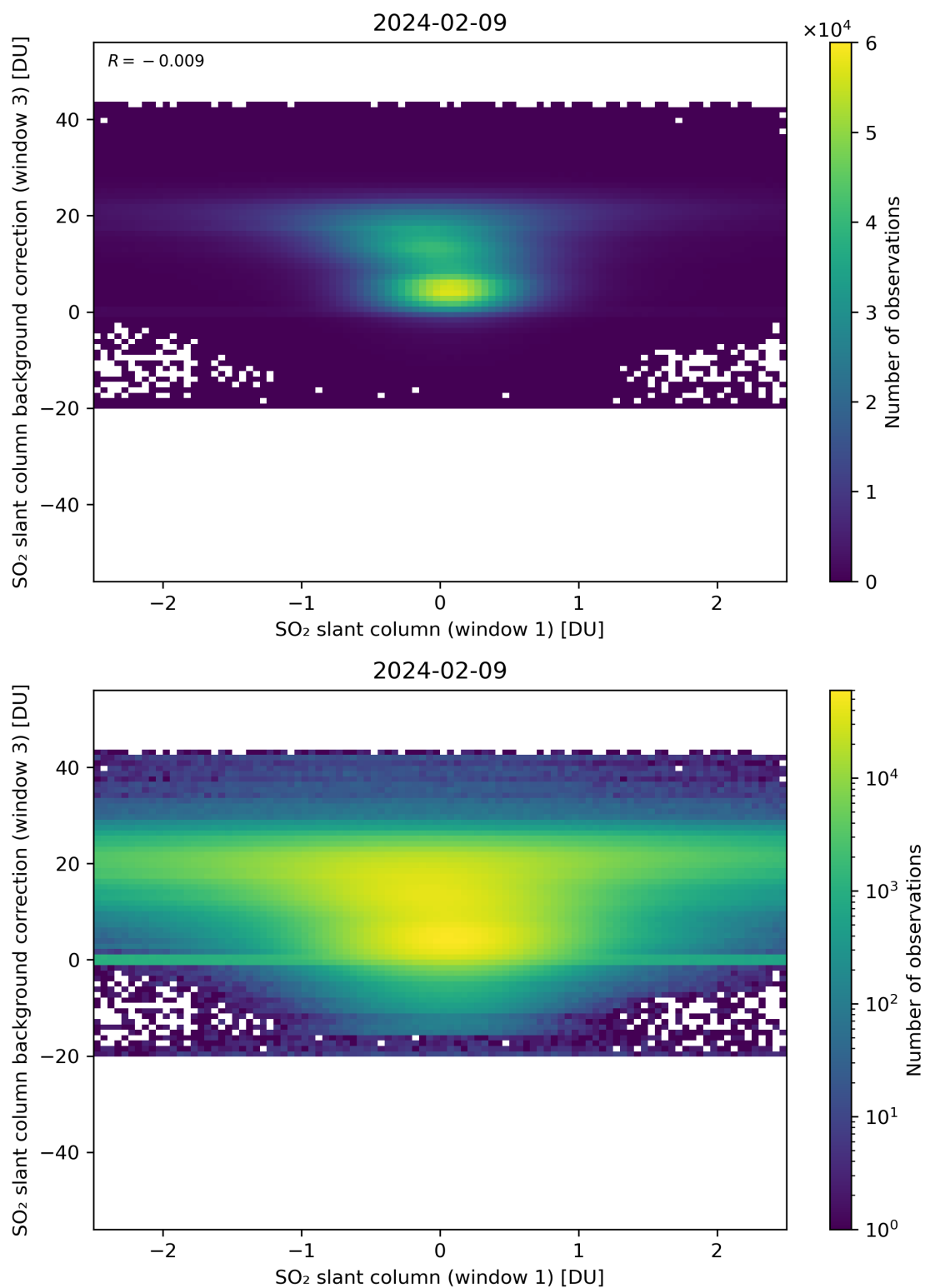
Figure 214: Scatter density plot of “SO 2 slant column (window 1)” against “SO 2 slant column background correction (window 3)” for 2024-02-08 to 2024-02-10.
