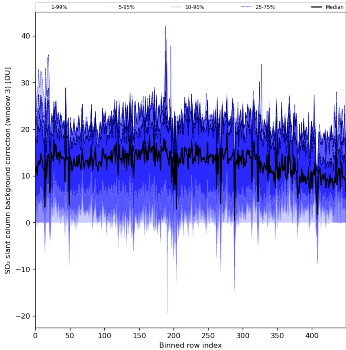
Figure 90: Along track statistics of “SO 2 slant column background correction (window 3)” for 2024-02-08 to 2024-02-10
