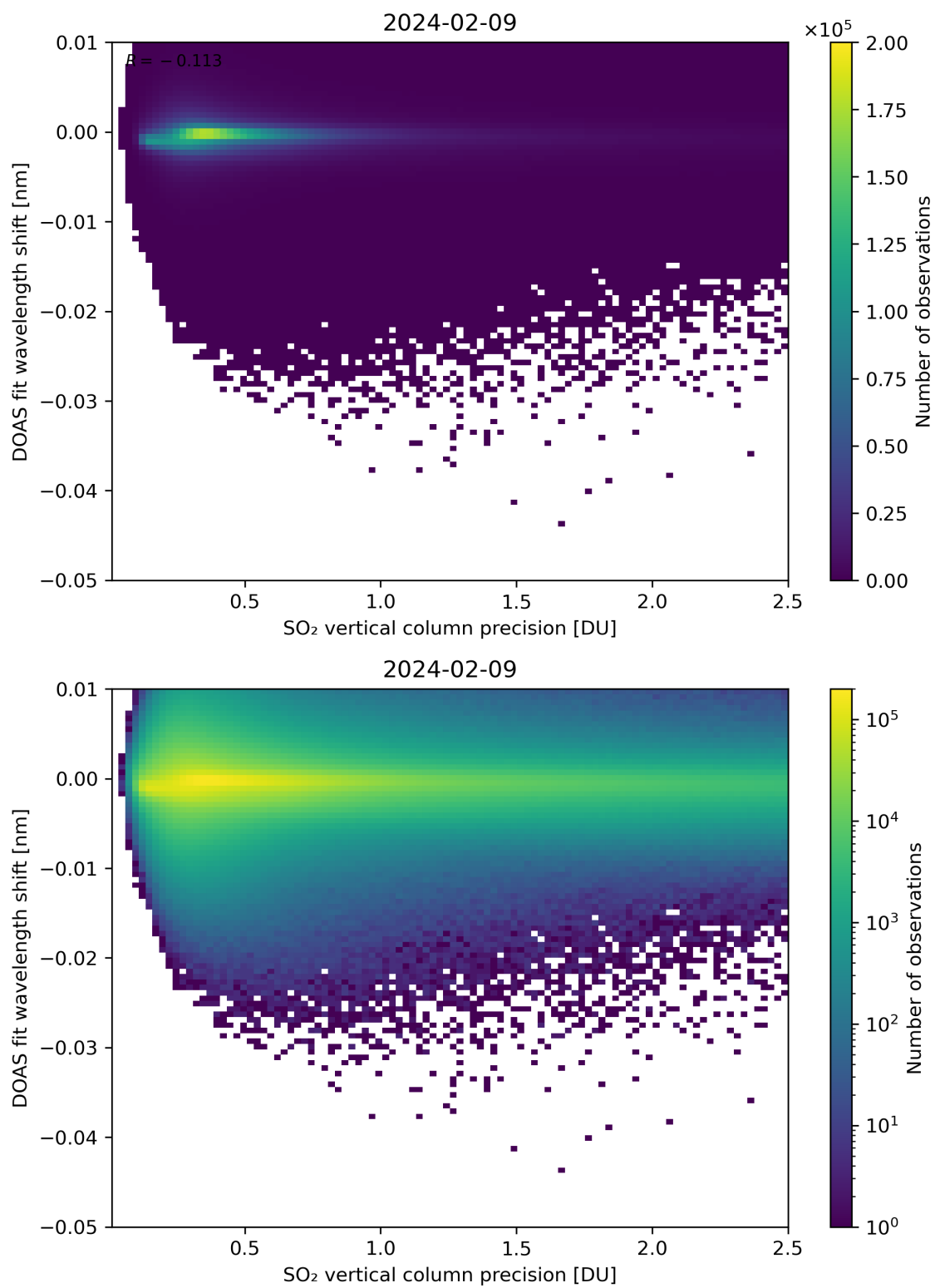
Figure 282: Scatter density plot of “SO 2 vertical column precision” against “DOAS fit wavelength shift” for 2024-02-08 to 2024-02-10.
