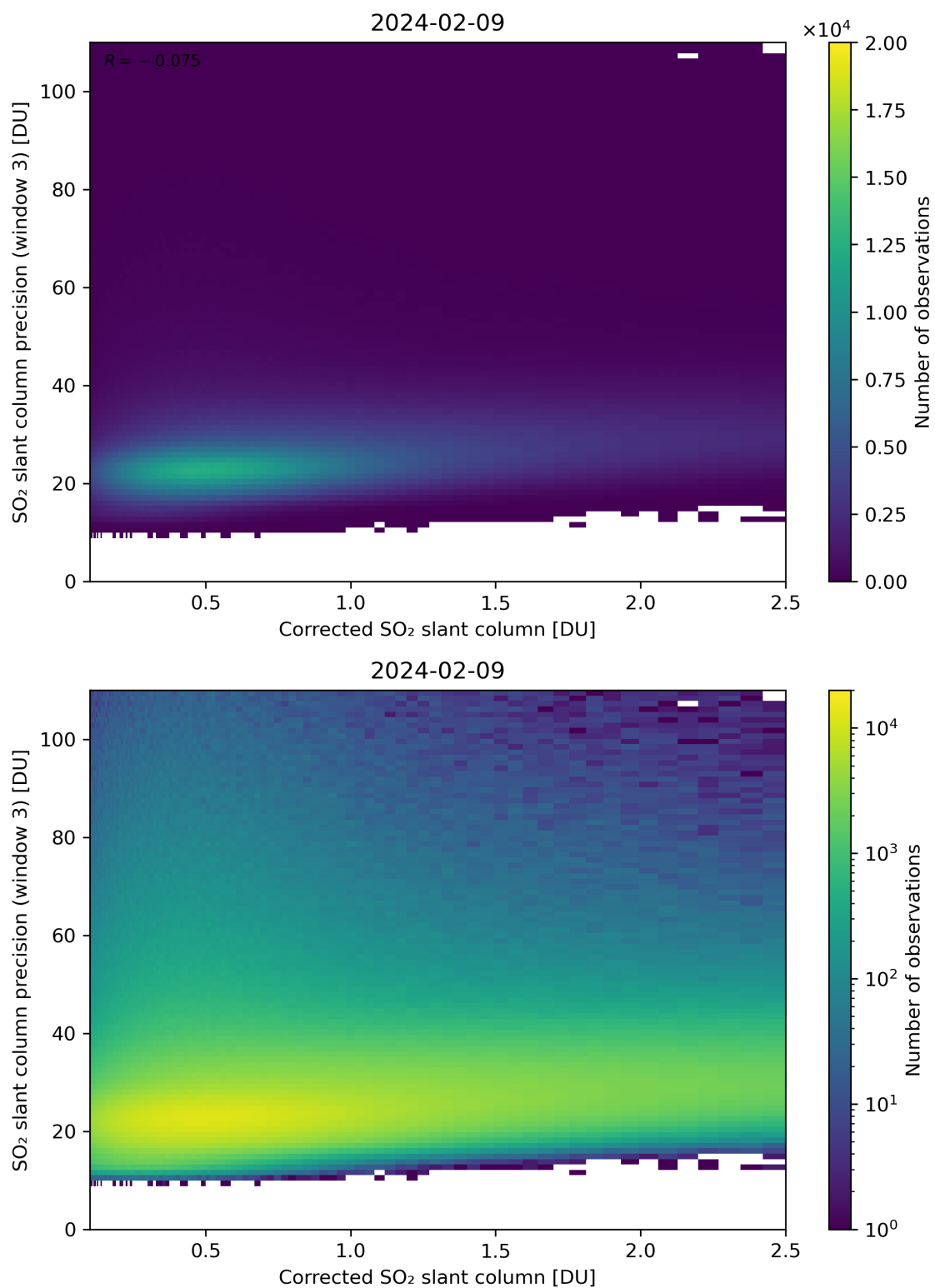
Figure 191: Scatter density plot of “Corrected SO 2 slant column” against “SO 2 slant column precision (window 3)” for 2024-02-08 to 2024-02-10.
