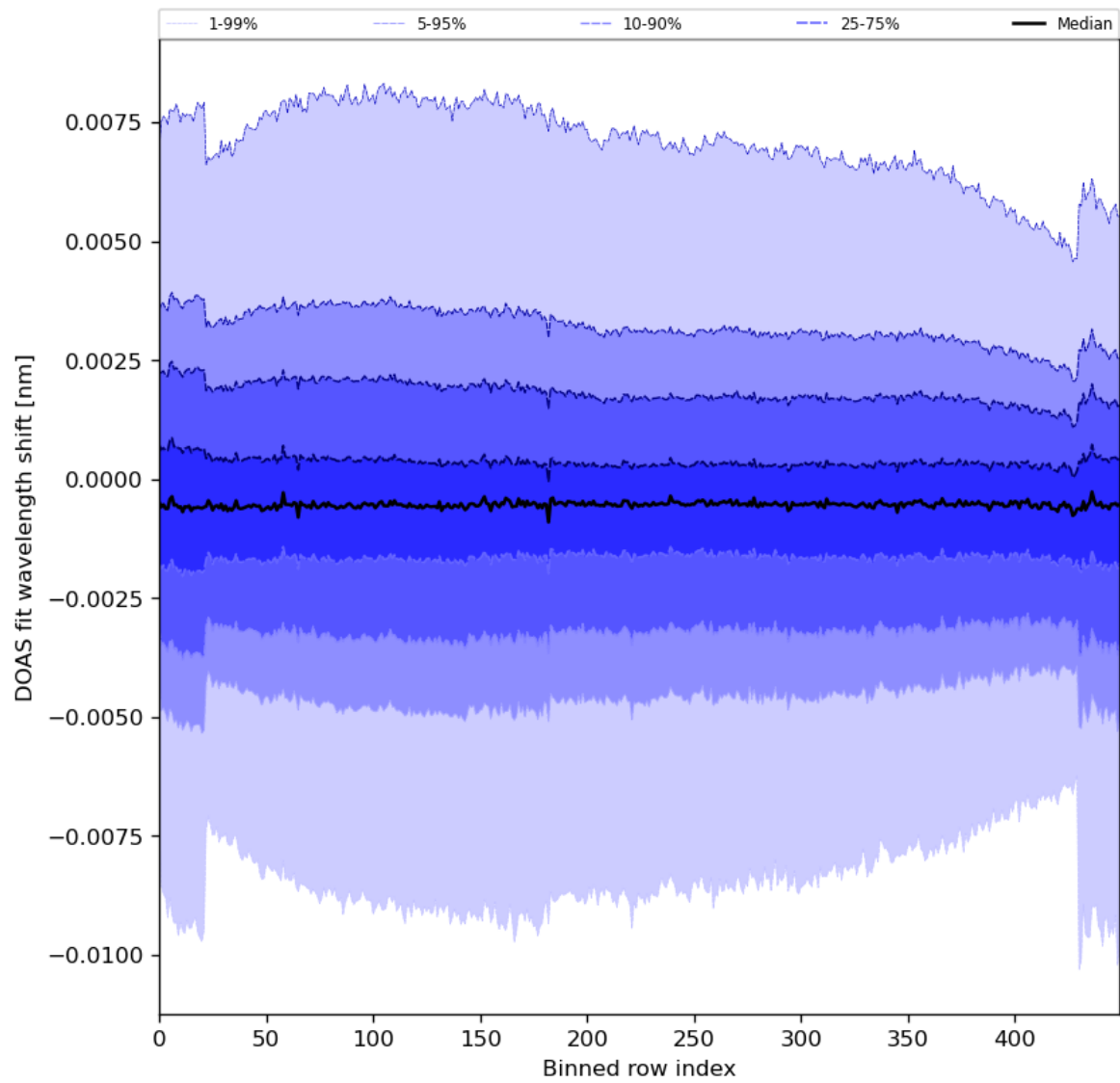
Figure 91: Along track statistics of “DOAS fit wavelength shift” for 2024-02-08 to 2024-02-10
