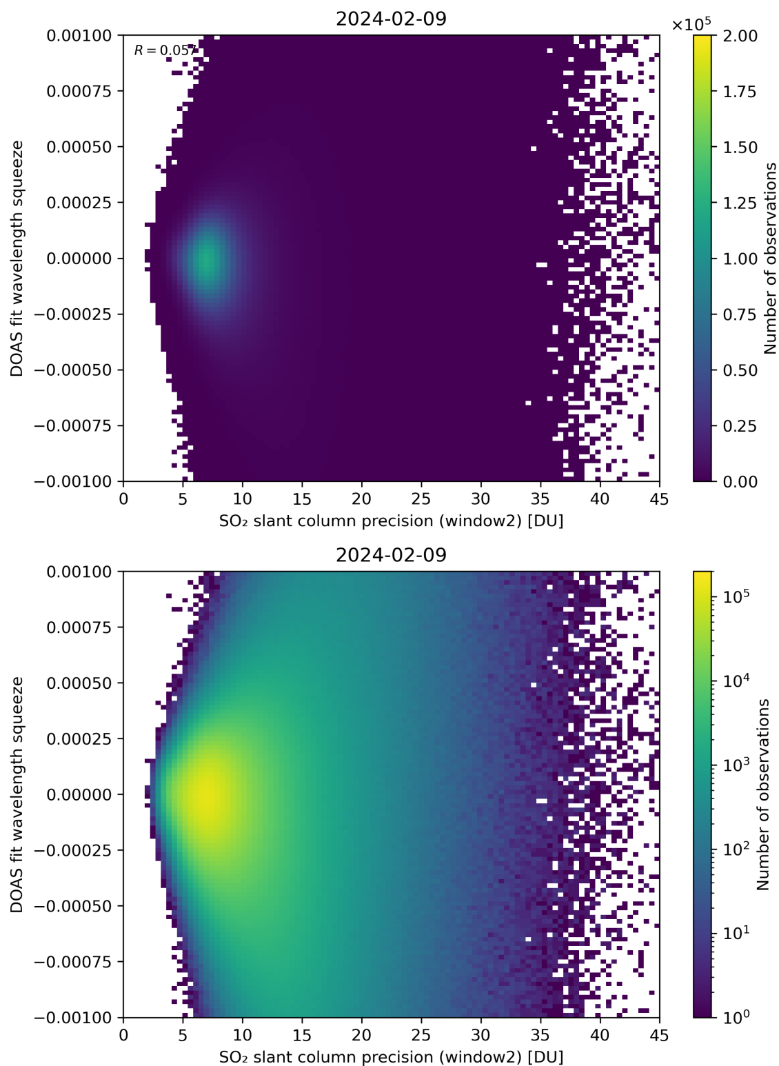
Figure 244: Scatter density plot of “SO 2 slant column precision (window2)” against “DOAS fit wavelength squeeze” for 2024-02-08 to 2024-02-10.
