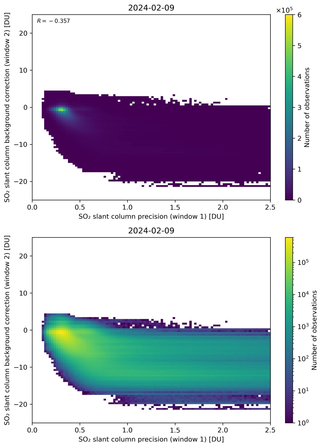
Figure 219: Scatter density plot of “SO 2 slant column precision (window 1)” against “SO 2 slant column background correction (window 2)” for 2024-02-08 to 2024-02-10.
