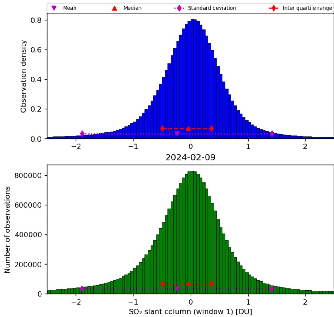
Figure 56: Histogram of “SO 2 slant column (window 1)” for 2024-02-08 to 2024-02-10
