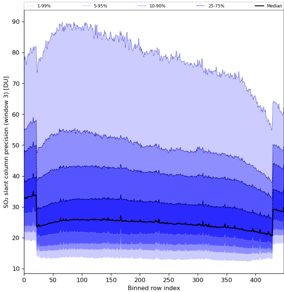
Figure 88: Along track statistics of “SO 2 slant column precision (window 3)” for 2024-02-08 to 2024-02-10
