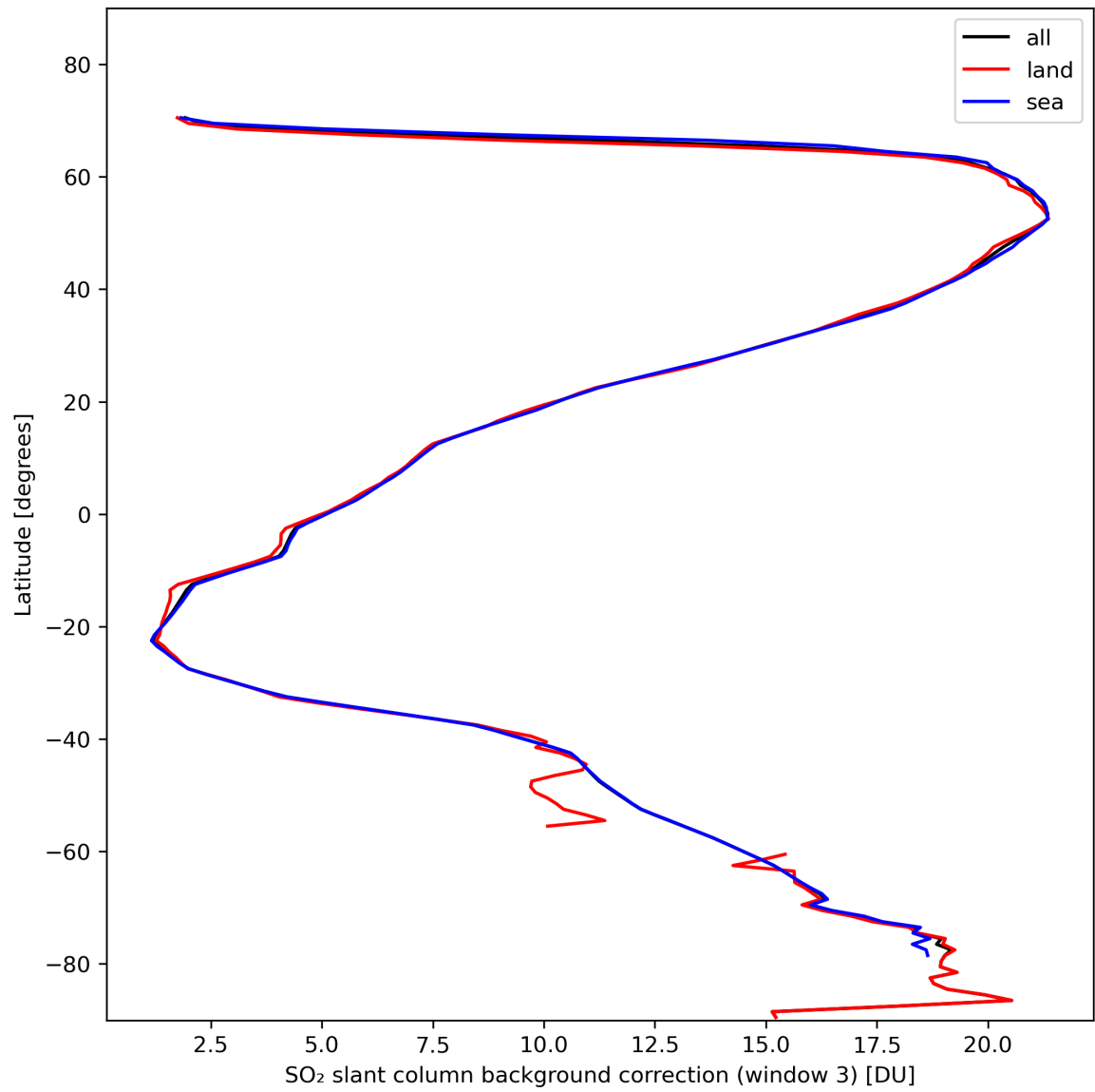
Figure 44: Zonal average of “SO 2 slant column background correction (window 3)” for 2024-02-08 to 2024-02-10.
