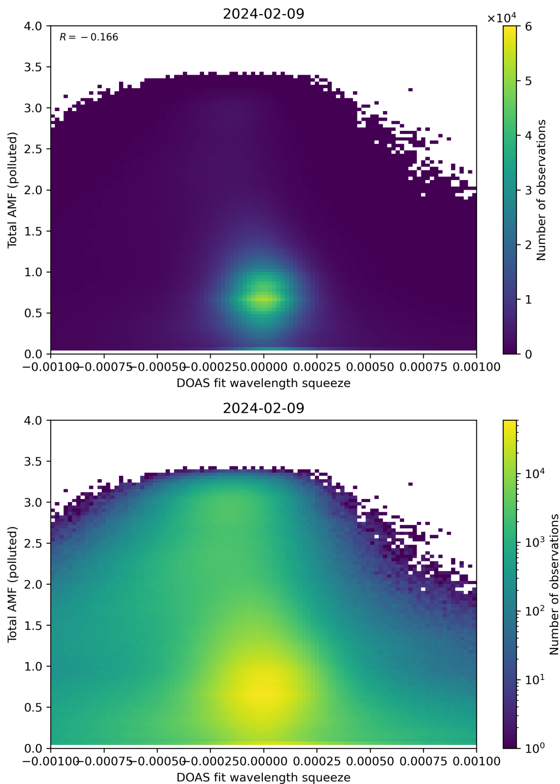
Figure 134: Scatter density plot of “DOAS fit wavelength squeeze” against “Total AMF (polluted)” for 2024-02-08 to 2024-02-10.
