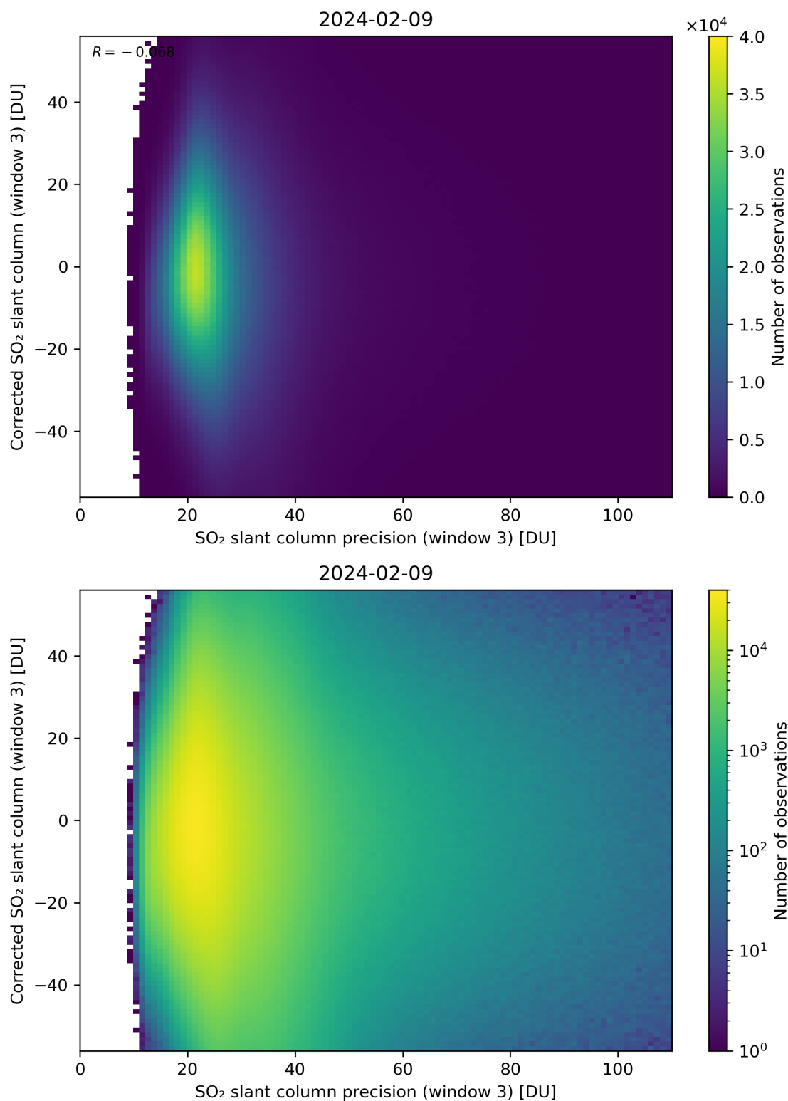
Figure 262: Scatter density plot of “SO 2 slant column precision (window 3)” against “Corrected SO 2 slant column (window 3)” for 2024-02-08 to 2024-02-10.
