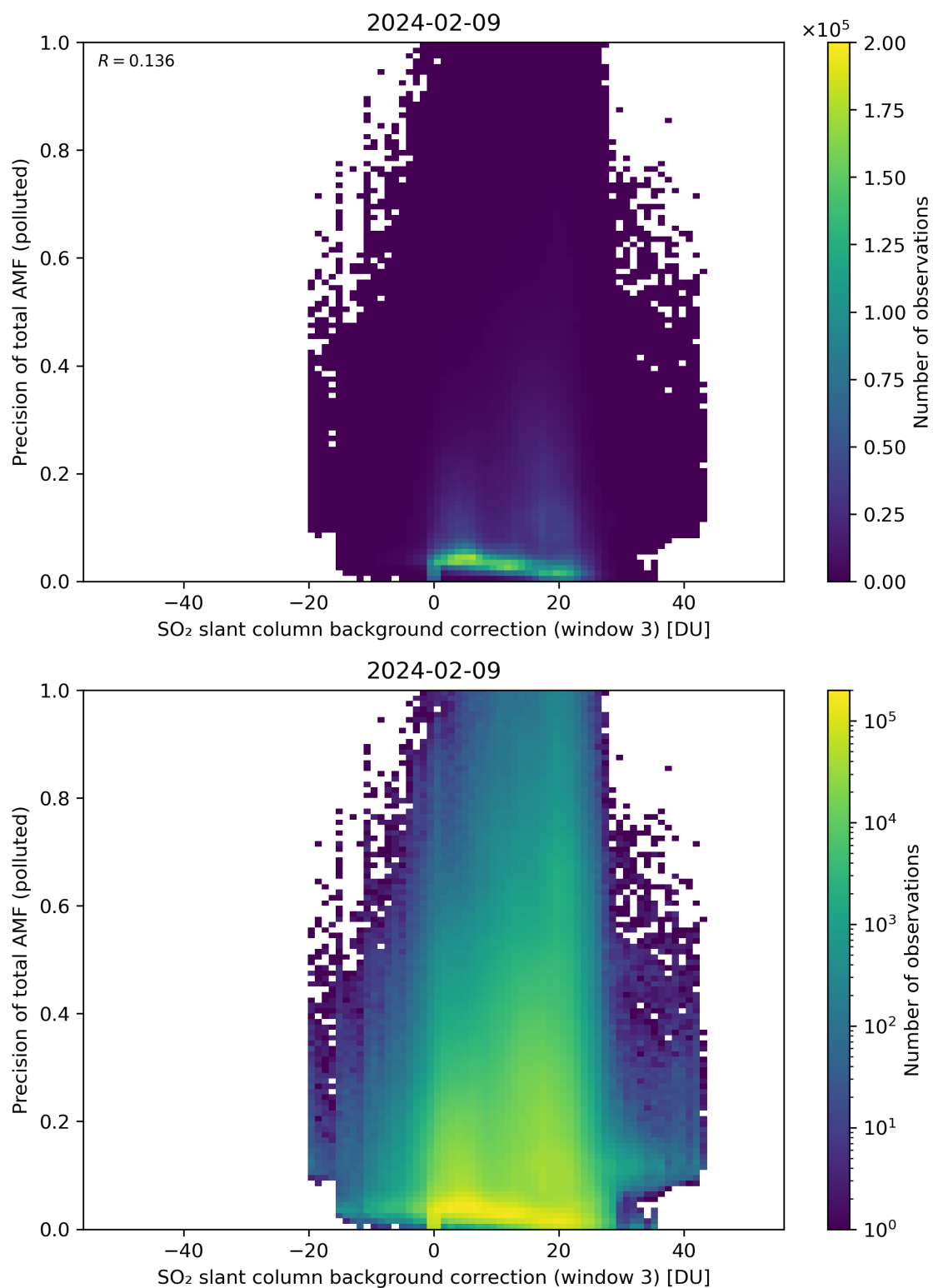
Figure 126: Scatter density plot of “SO 2 slant column background correction (window 3)” against “Precision of total AMF (polluted)” for 2024-02-08 to 2024-02-10.
