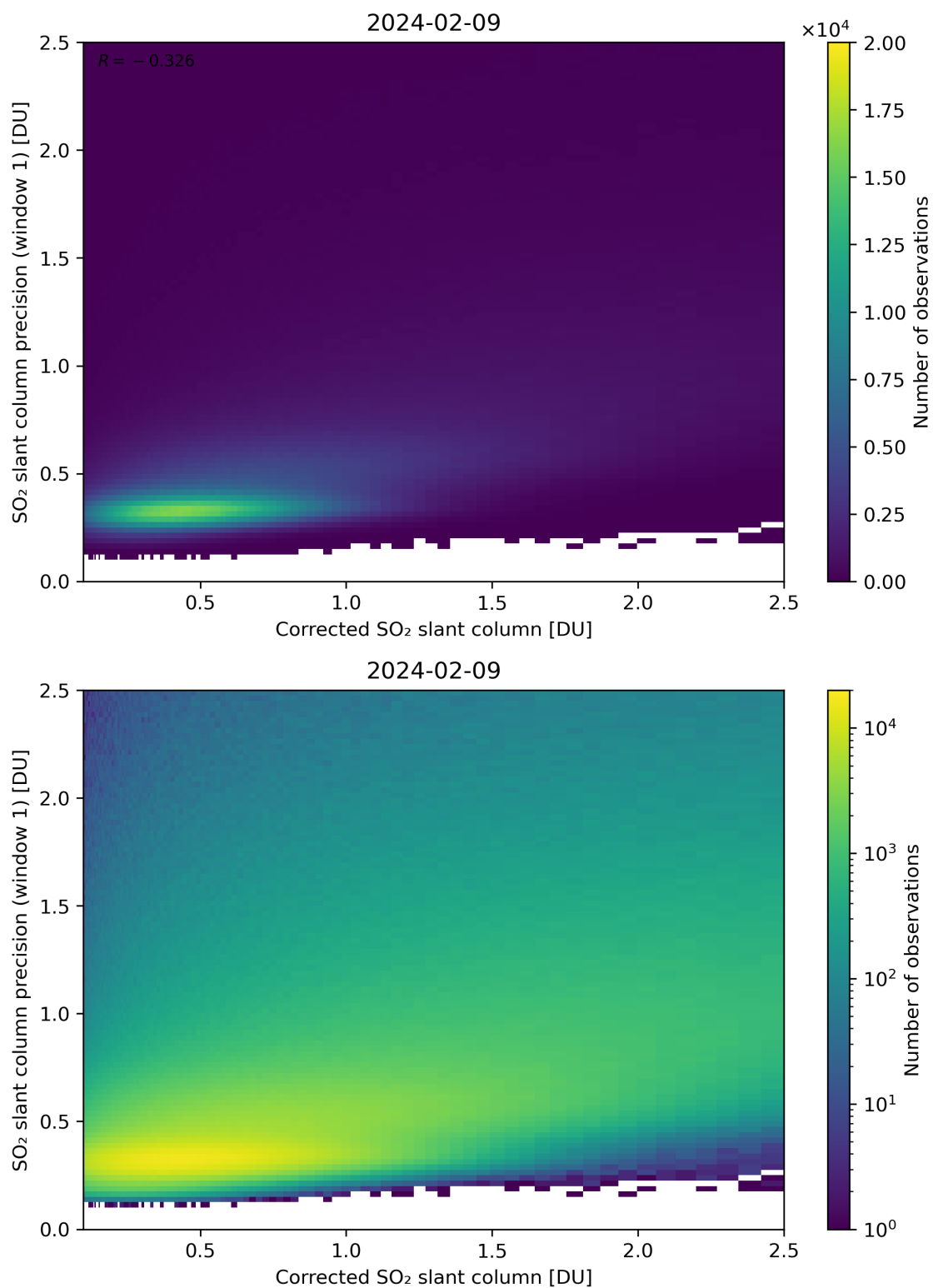
Figure 188: Scatter density plot of “Corrected SO 2 slant column” against “SO 2 slant column precision (window 1)” for 2024-02-08 to 2024-02-10.
