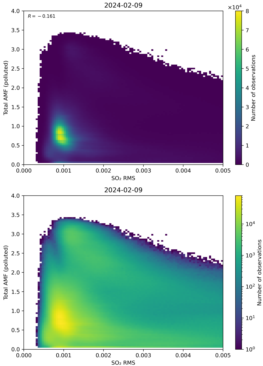
Figure 137: Scatter density plot of “SO 2 RMS” against “Total AMF (polluted)” for 2024-02-08 to 2024-02-10.
