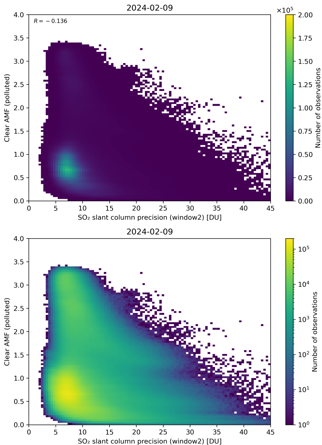
Figure 246: Scatter density plot of “SO 2 slant column precision (window2)” against “Clear AMF (polluted)” for 2024-02-08 to 2024-02-10.
