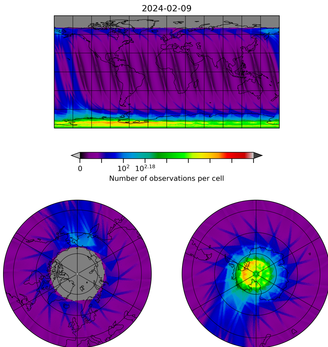
Figure 28: Map of the number of observations for 2024-02-08 to 2024-02-10
