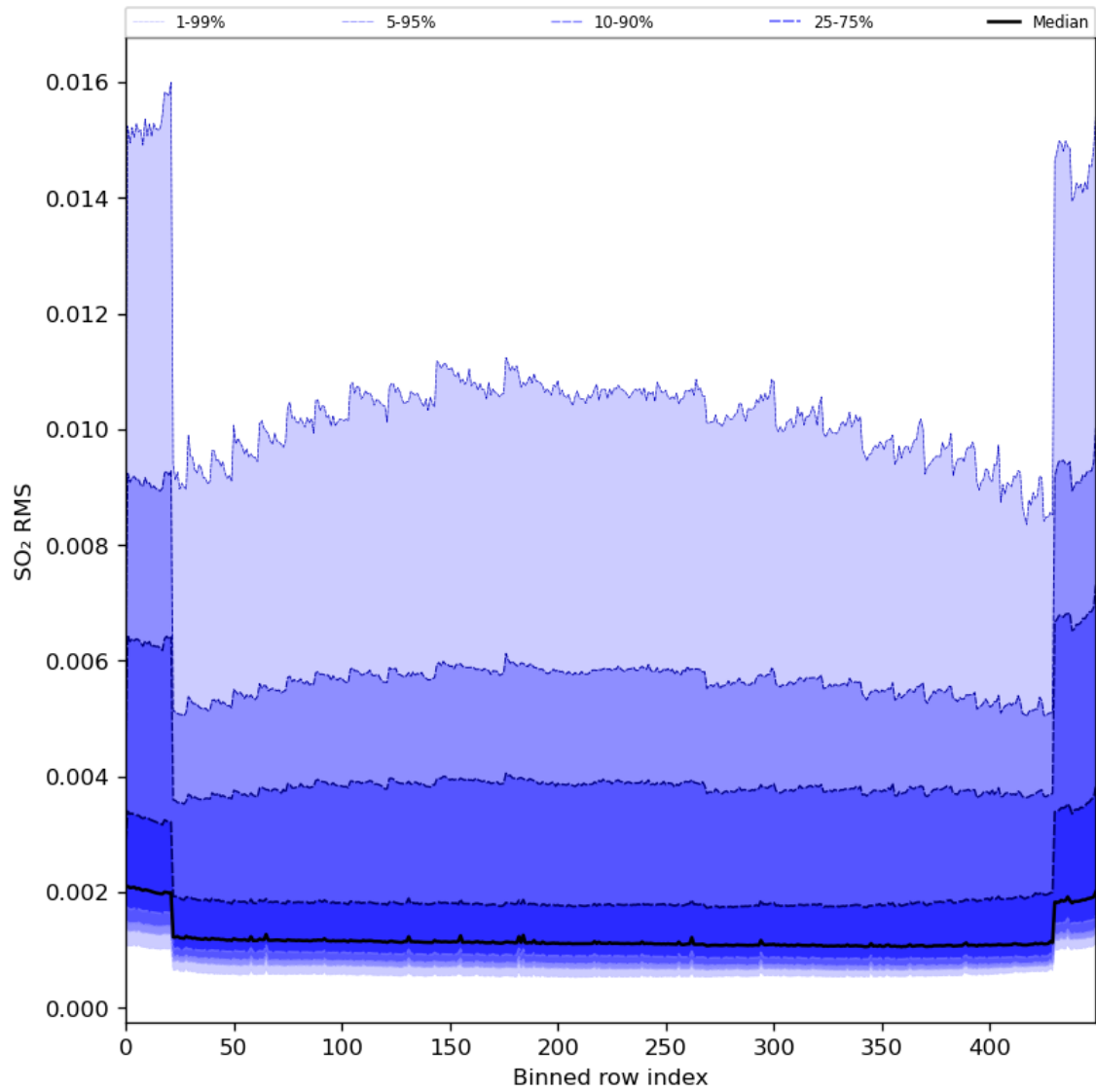
Figure 93: Along track statistics of “SO 2 RMS” for 2024-02-08 to 2024-02-10
