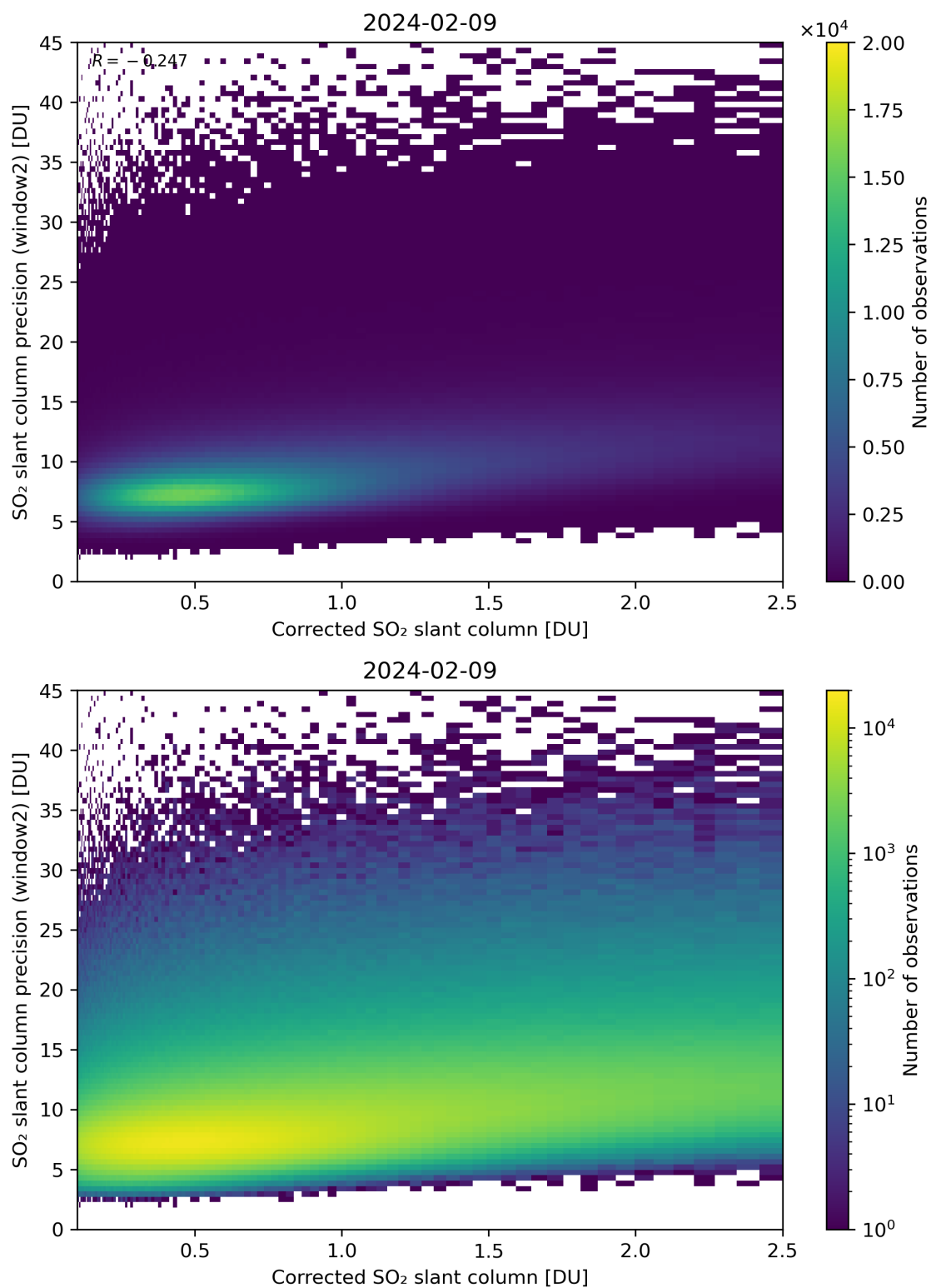
Figure 189: Scatter density plot of “Corrected SO 2 slant column” against “SO 2 slant column precision (window2)” for 2024-02-08 to 2024-02-10.
