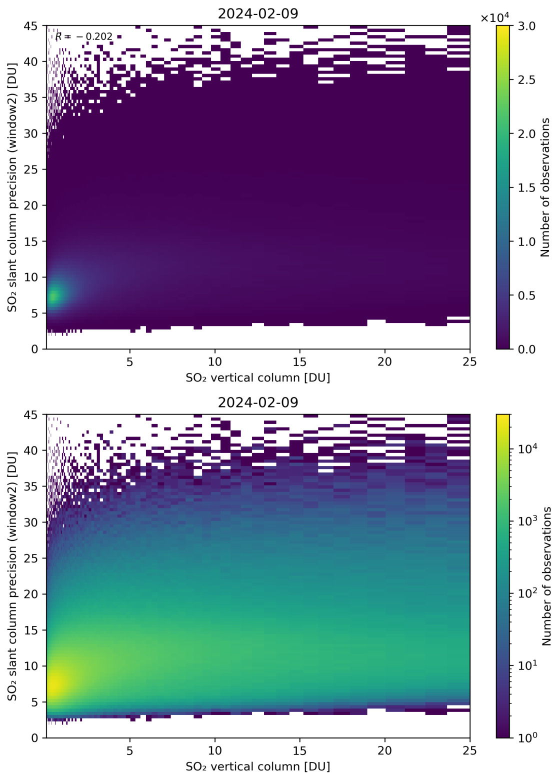
Figure 302: Scatter density plot of “SO 2 vertical column” against “SO 2 slant column precision (window2)” for 2024-02-08 to 2024-02-10.
