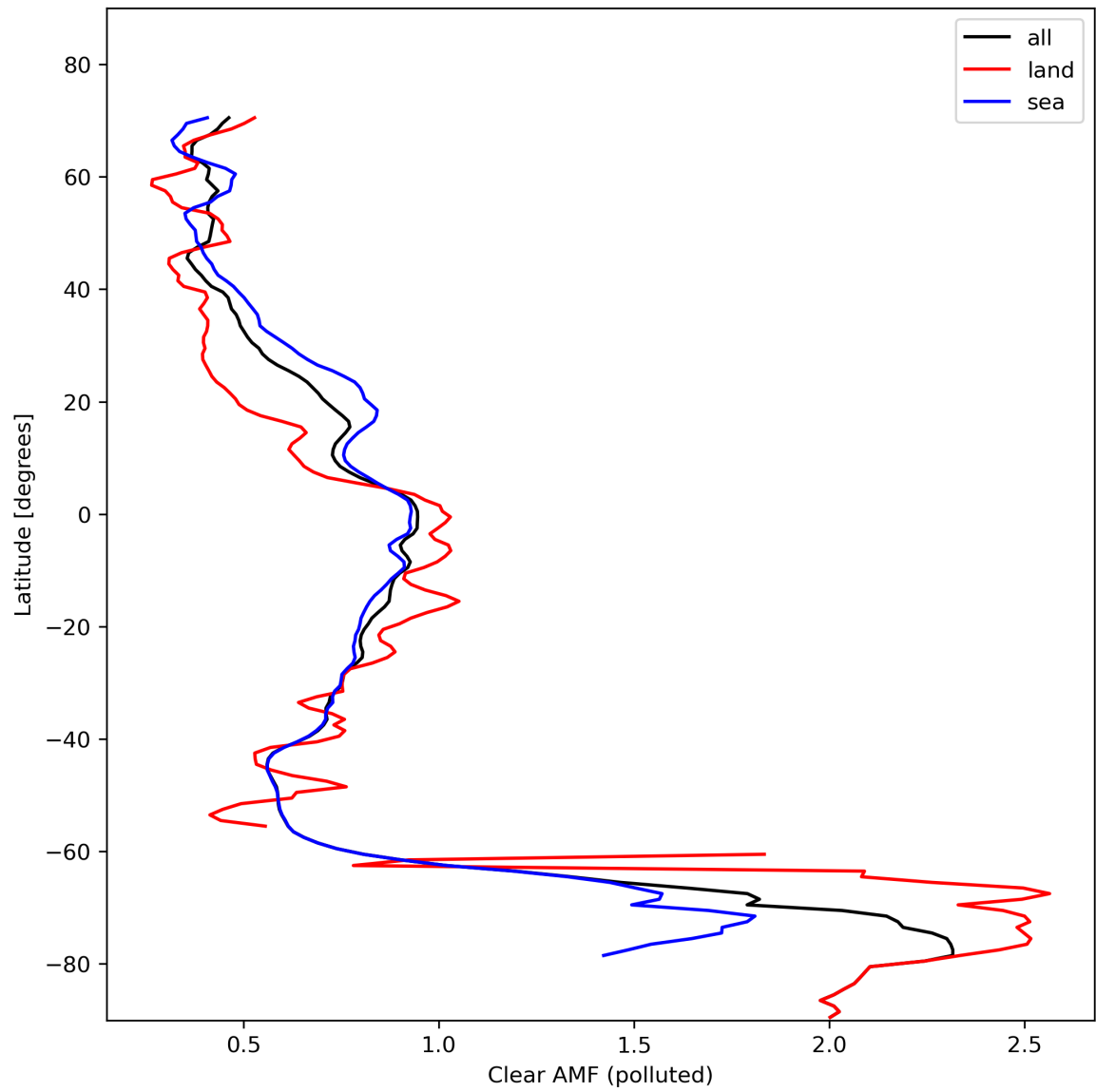
Figure 50: Zonal average of “Clear AMF (polluted)” for 2024-02-08 to 2024-02-10.
