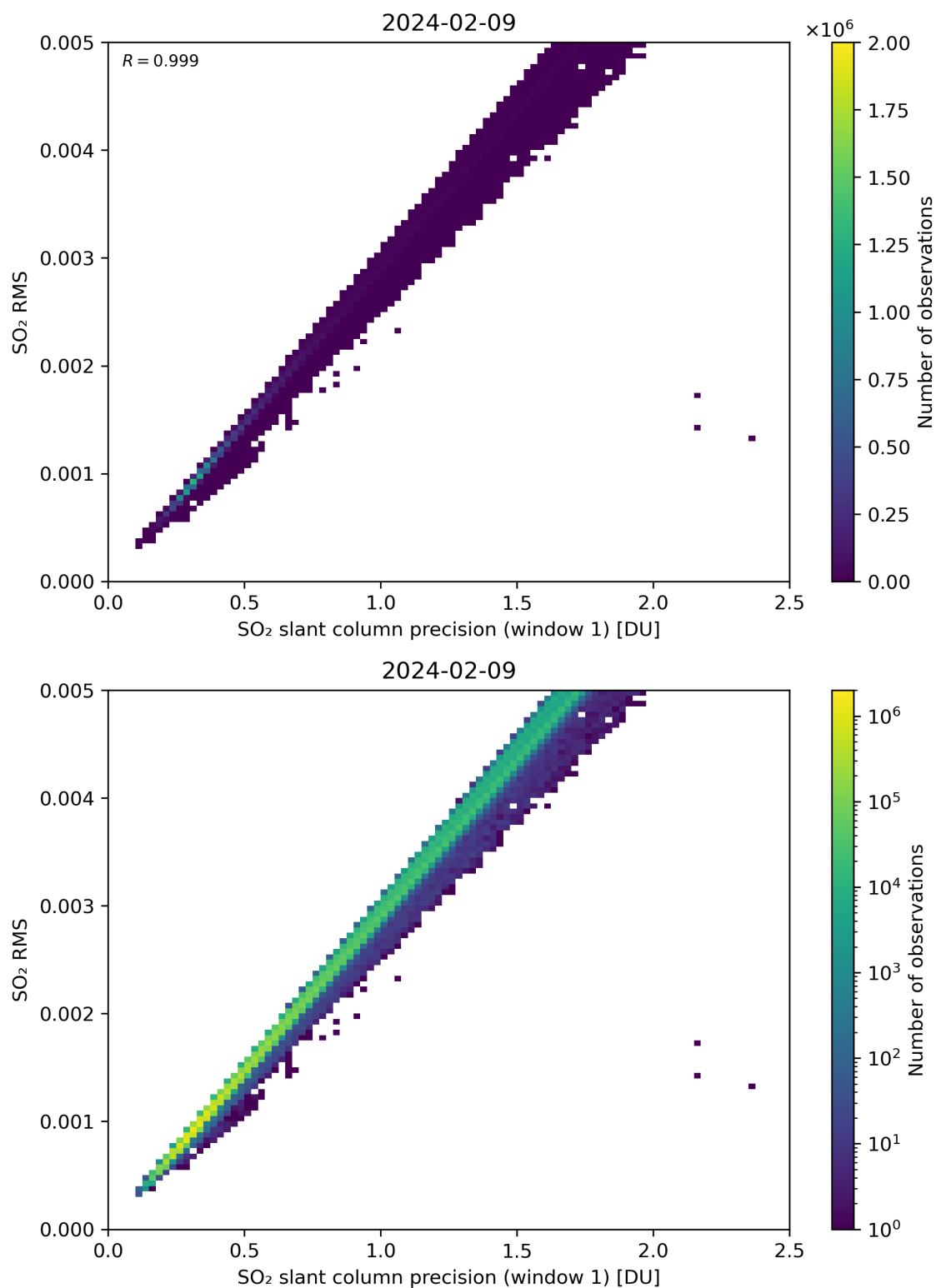
Figure 223: Scatter density plot of “SO 2 slant column precision (window 1)” against “SO 2 RMS” for 2024-02-08 to 2024-02-10.
