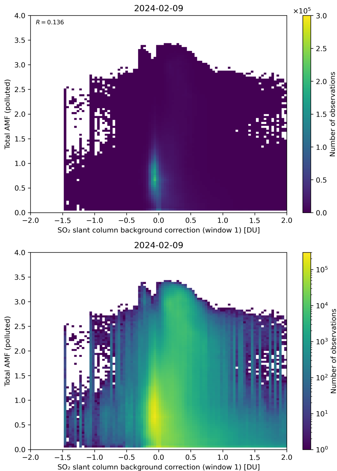
Figure 109: Scatter density plot of “SO 2 slant column background correction (window 1)” against “Total AMF (polluted)” for 2024-02-08 to 2024-02-10.
