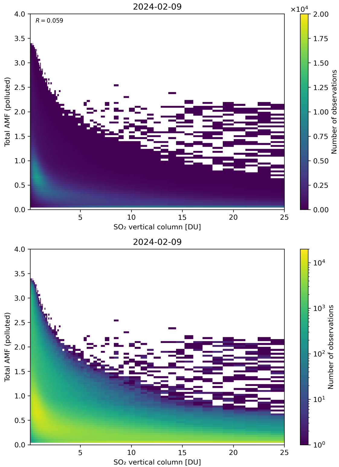
Figure 305: Scatter density plot of “SO 2 vertical column” against “Total AMF (polluted)” for 2024-02-08 to 2024-02-10.
