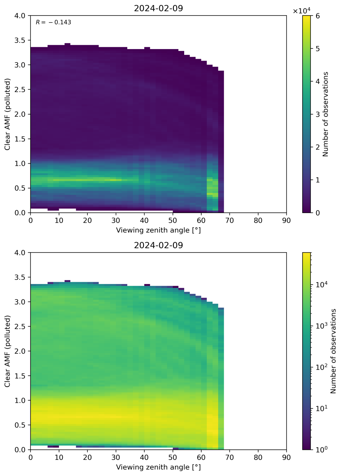
Figure 316: Scatter density plot of “Viewing zenith angle” against “Clear AMF (polluted)” for 2024-02-08 to 2024-02-10.
