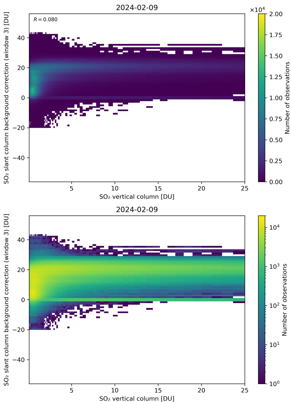
Figure 275: Scatter density plot of “SO 2 vertical column” against “SO 2 slant column background correction (window 3)” for 2024-02-08 to 2024-02-10.
