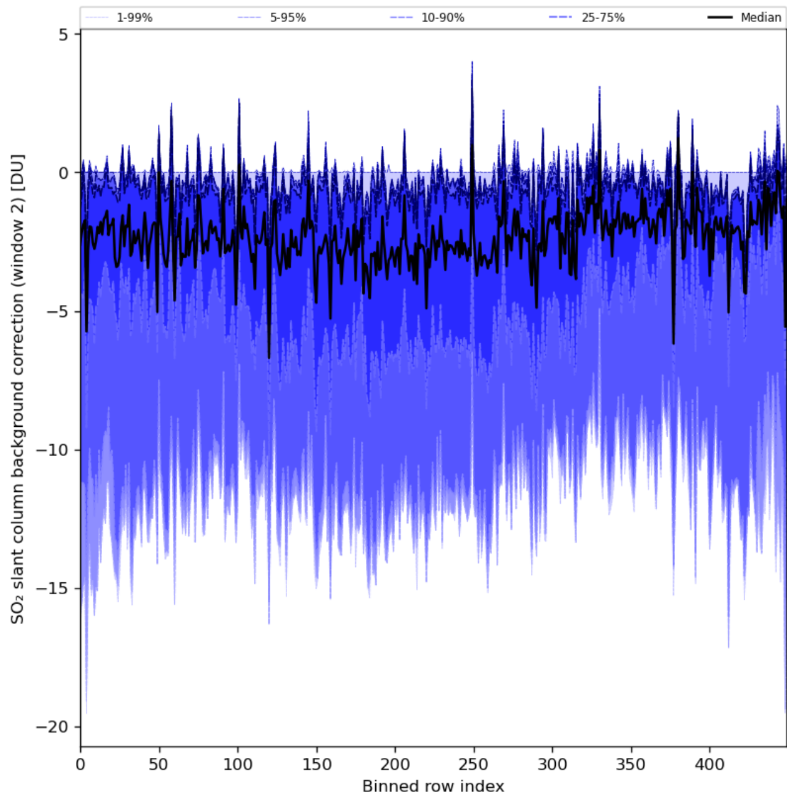
Figure 86: Along track statistics of “SO 2 slant column background correction (window 2)” for 2024-02-08 to 2024-02-10
