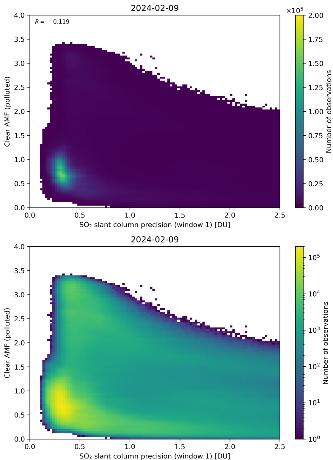
Figure 224: Scatter density plot of “SO 2 slant column precision (window 1)” against “Clear AMF (polluted)” for 2024-02-08 to 2024-02-10.
