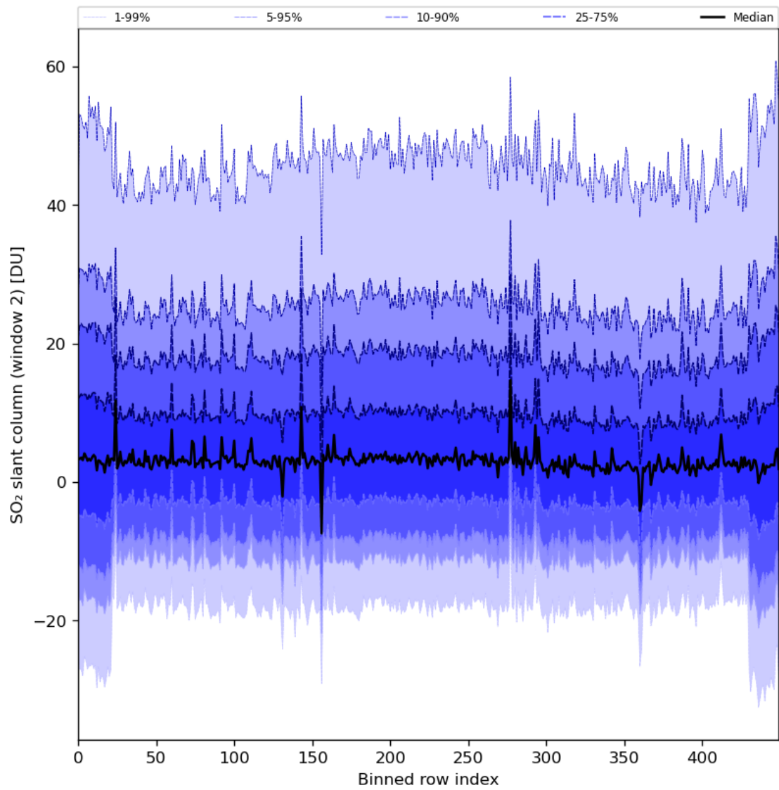
Figure 83: Along track statistics of “SO 2 slant column (window 2)” for 2024-02-08 to 2024-02-10
