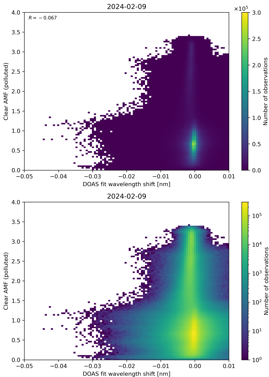
Figure 129: Scatter density plot of “DOAS fit wavelength shift” against “Clear AMF (polluted)” for 2024-02-08 to 2024-02-10.
