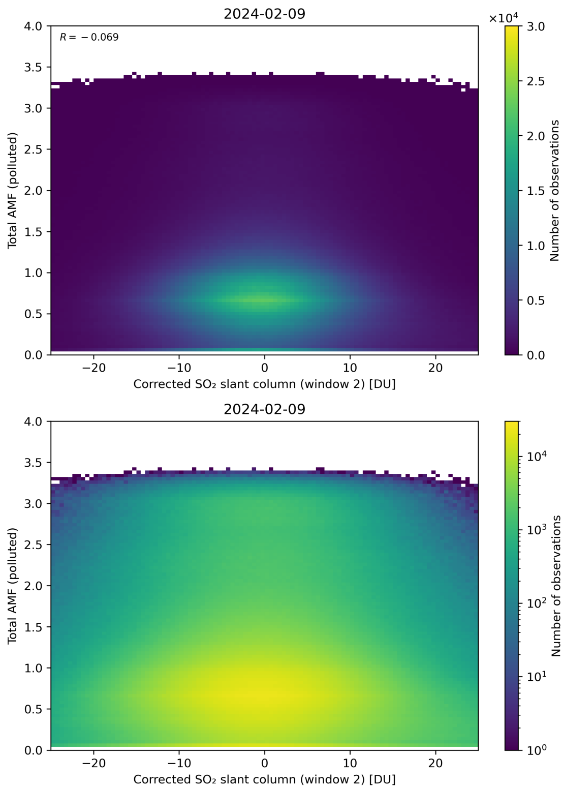
Figure 203: Scatter density plot of “Corrected SO 2 slant column (window 2)” against “Total AMF (polluted)” for 2024-02-08 to 2024-02-10.
