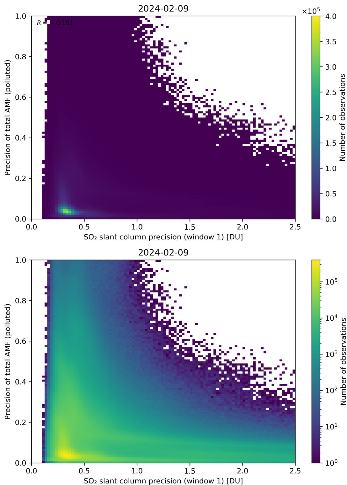
Figure 231: Scatter density plot of “SO 2 slant column precision (window 1)” against “Precision of total AMF (polluted)” for 2024-02-08 to 2024-02-10.
