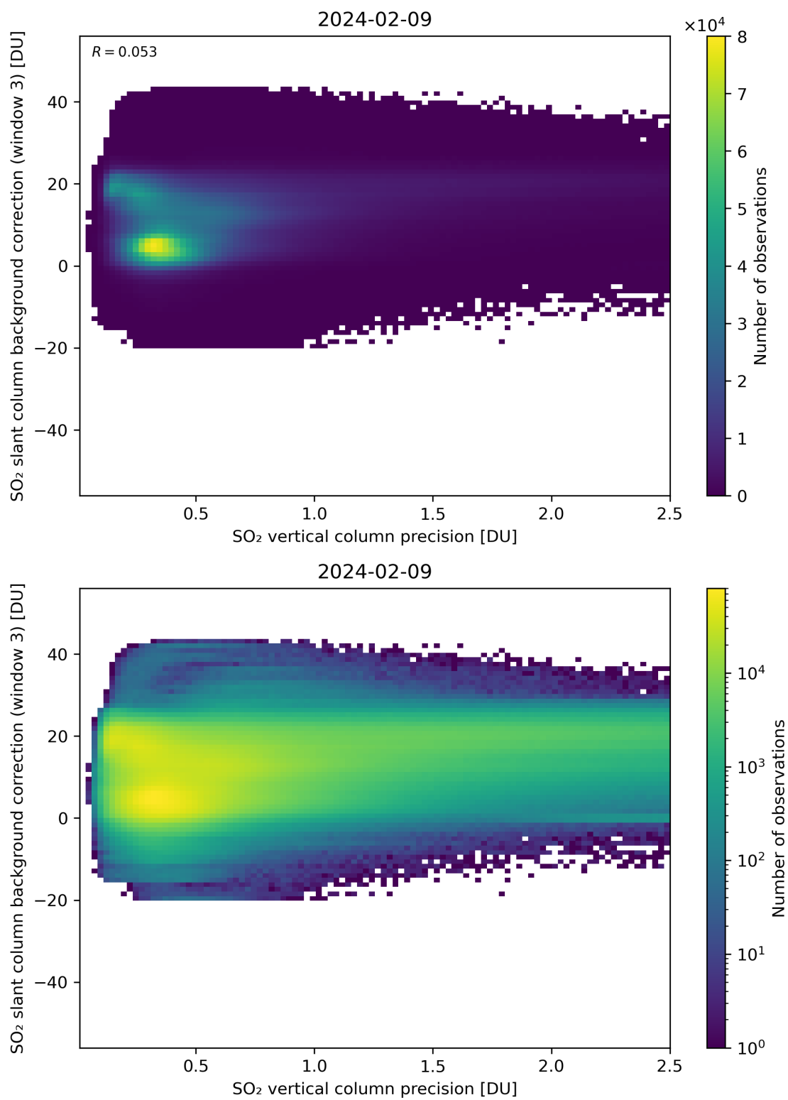
Figure 281: Scatter density plot of “SO 2 vertical column precision” against “SO 2 slant column background correction (window 3)” for 2024-02-08 to 2024-02-10.
