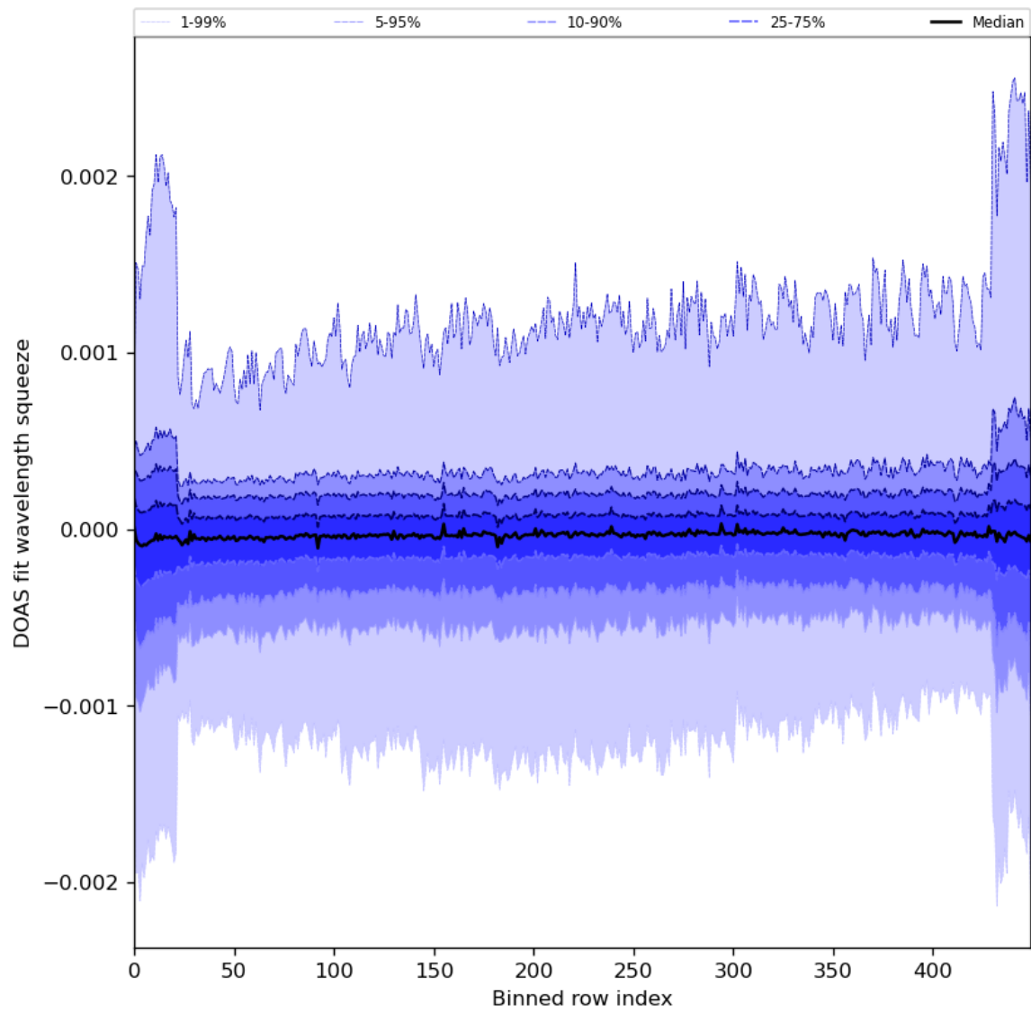
Figure 92: Along track statistics of “DOAS fit wavelength squeeze” for 2024-02-08 to 2024-02-10
