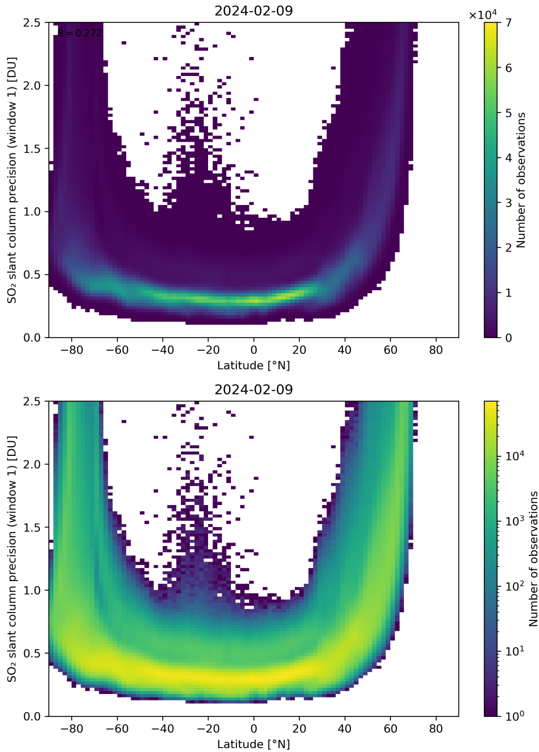
Figure 150: Scatter density plot of “Latitude” against “SO 2 slant column precision (window 1)” for 2024-02-08 to 2024-02-10.
