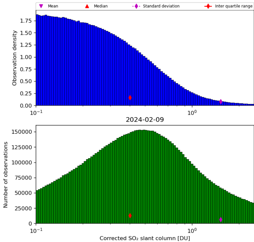
Figure 55: Histogram of “Corrected SO 2 slant column” for 2024-02-08 to 2024-02-10
