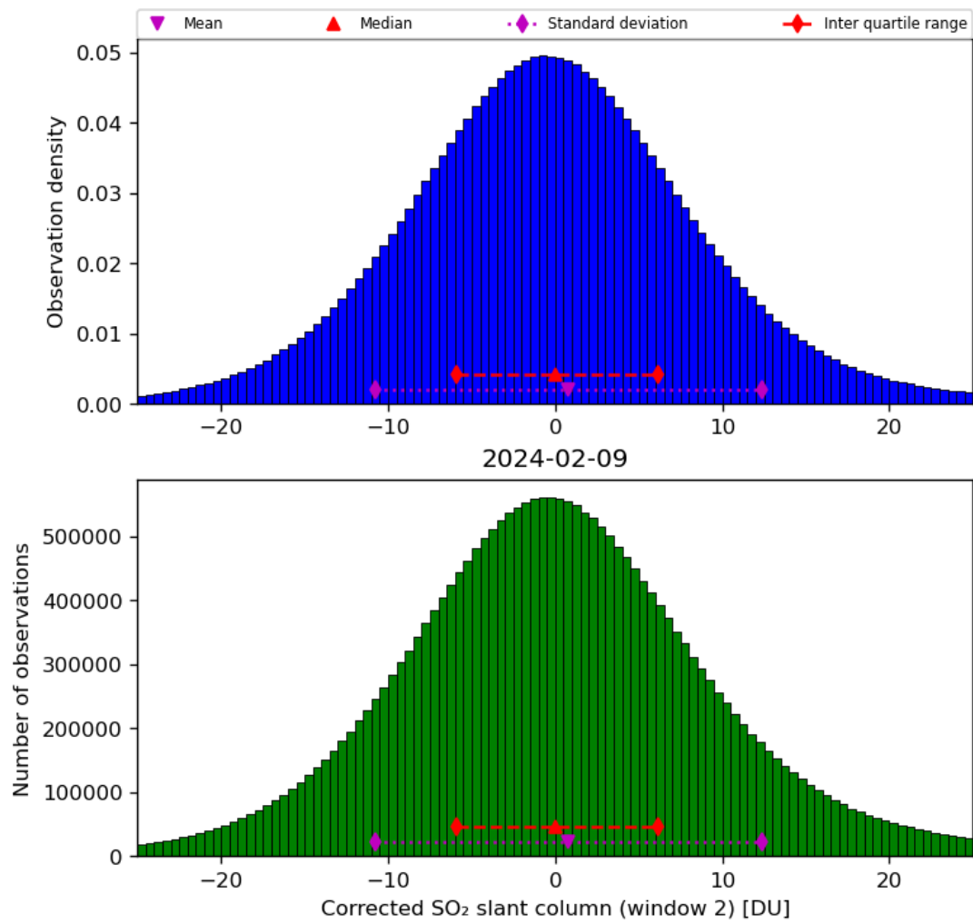
Figure 62: Histogram of “Corrected SO 2 slant column (window 2)” for 2024-02-08 to 2024-02-10
