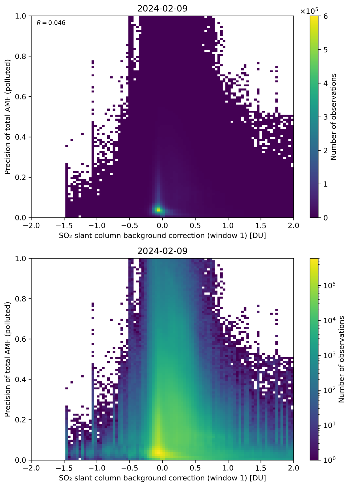
Figure 110: Scatter density plot of “SO 2 slant column background correction (window 1)” against “Precision of total AMF (polluted)” for 2024-02-08 to 2024-02-10.
