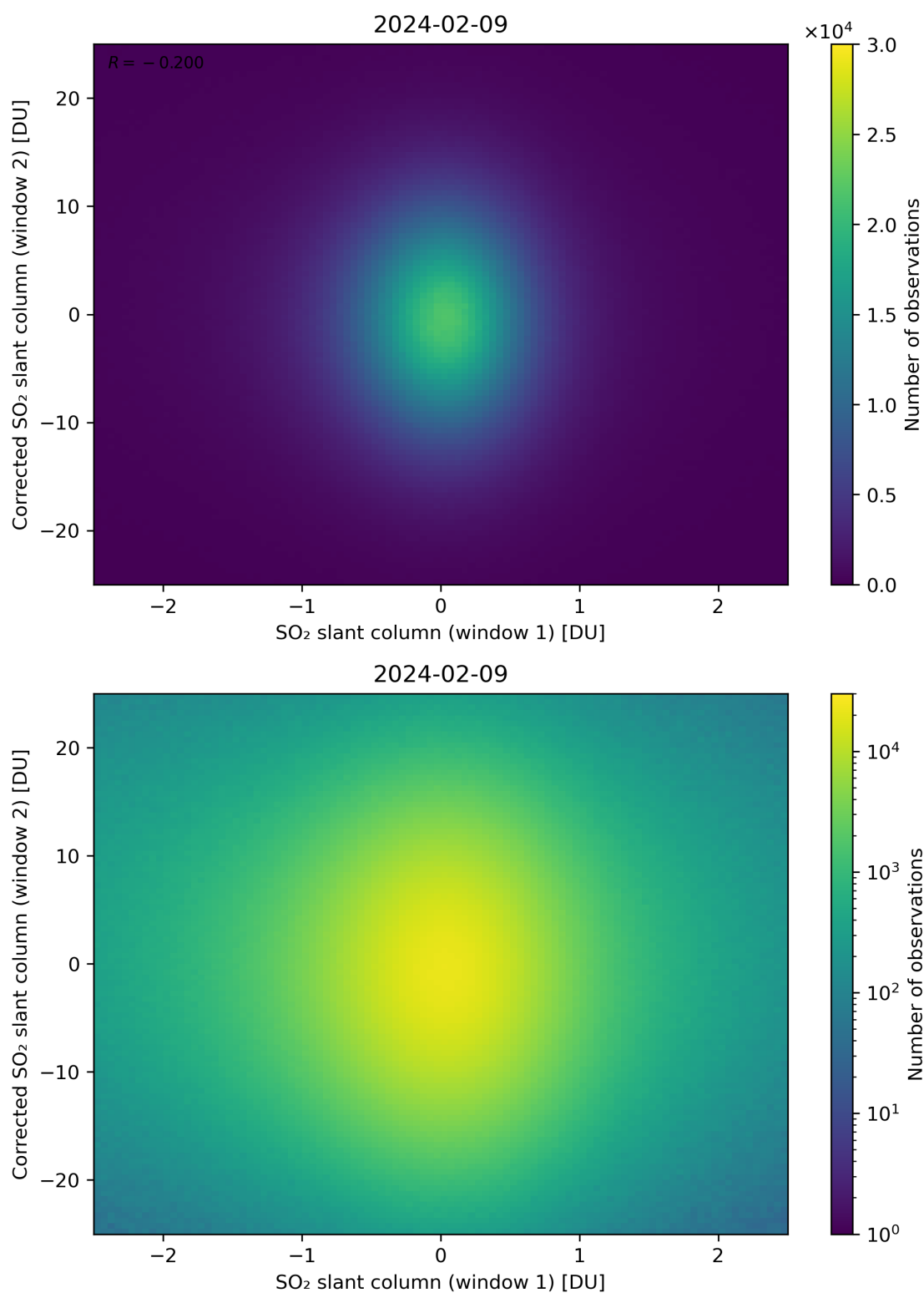
Figure 233: Scatter density plot of “SO 2 slant column (window 1)” against “Corrected SO 2 slant column (window 2)” for 2024-02-08 to 2024-02-10.
