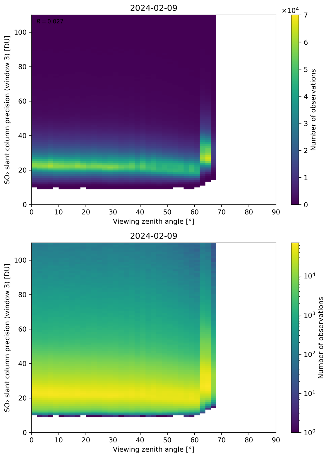
Figure 324: Scatter density plot of “Viewing zenith angle” against “SO 2 slant column precision (window 3)” for 2024-02-08 to 2024-02-10.
