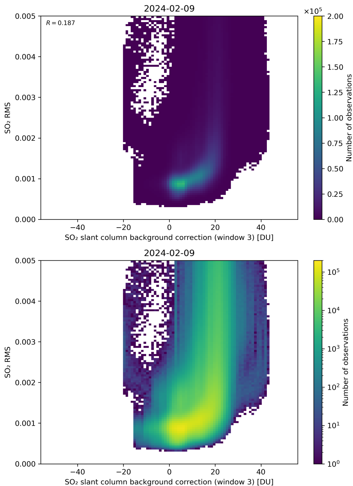
Figure 123: Scatter density plot of “SO 2 slant column background correction (window 3)” against “SO 2 RMS” for 2024-02-08 to 2024-02-10.
