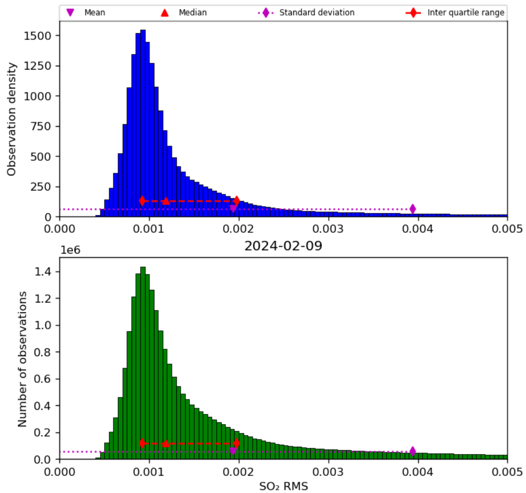
Figure 70: Histogram of “SO 2 RMS” for 2024-02-08 to 2024-02-10
