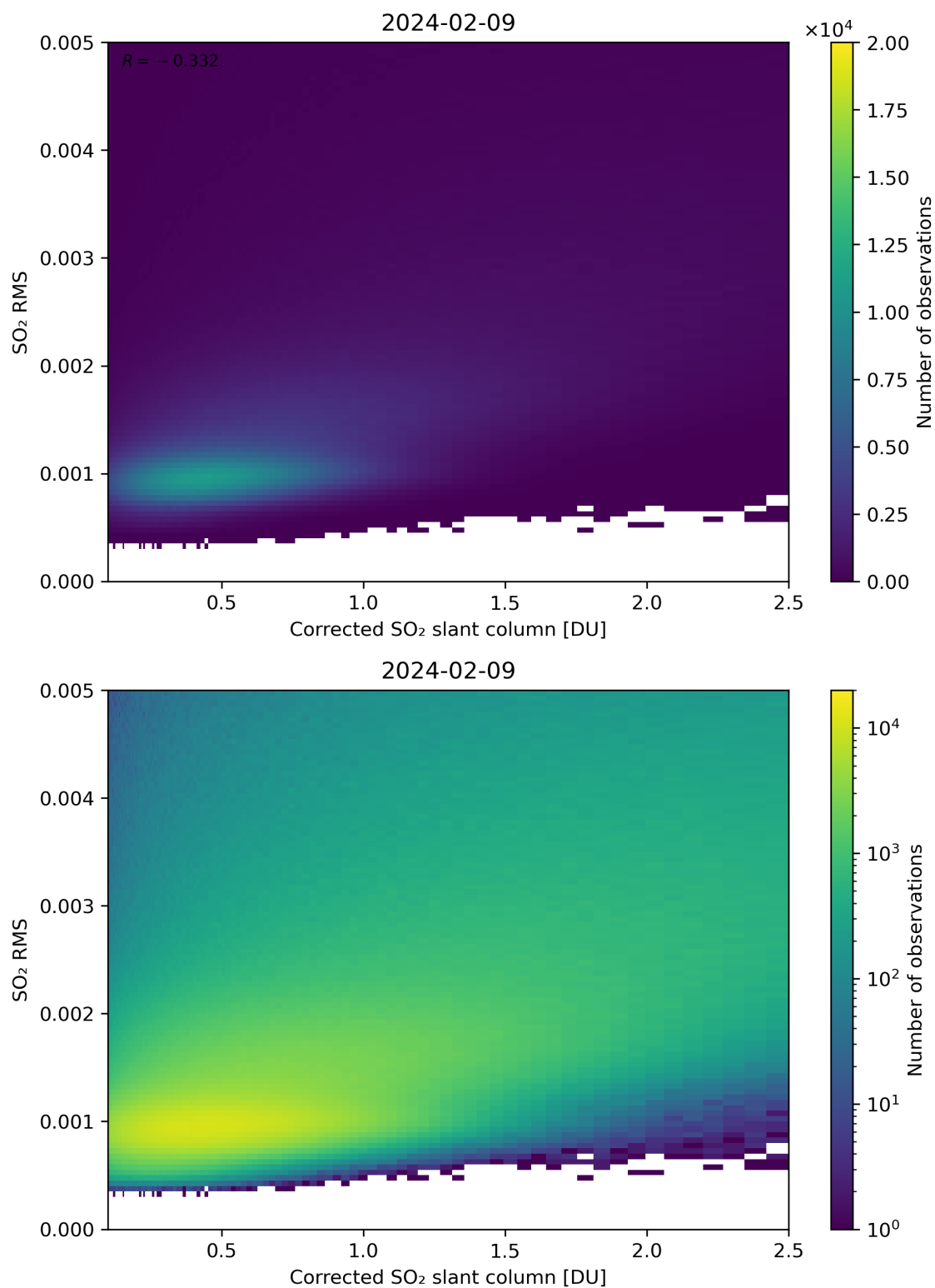
Figure 183: Scatter density plot of “Corrected SO 2 slant column” against “SO 2 RMS” for 2024-02-08 to 2024-02-10.
