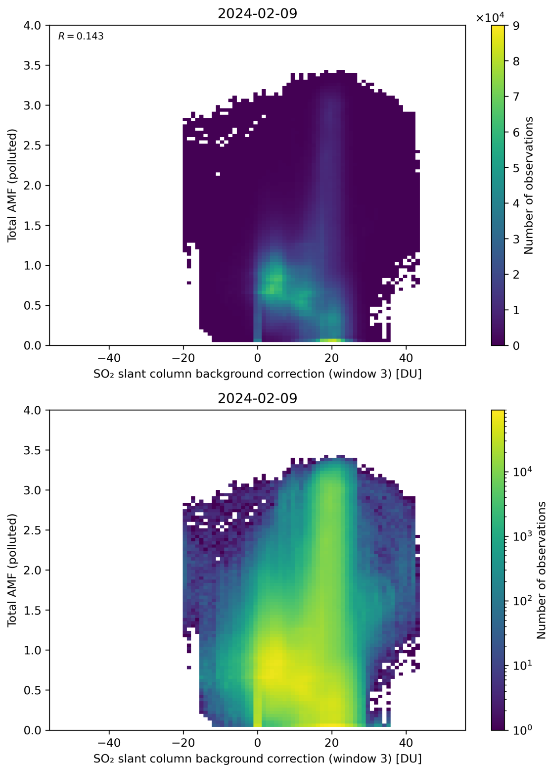
Figure 125: Scatter density plot of “SO 2 slant column background correction (window 3)” against “Total AMF (polluted)” for 2024-02-08 to 2024-02-10.
