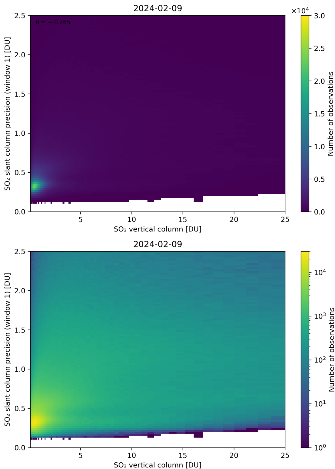
Figure 301: Scatter density plot of “SO 2 vertical column” against “SO 2 slant column precision (window 1)” for 2024-02-08 to 2024-02-10.
