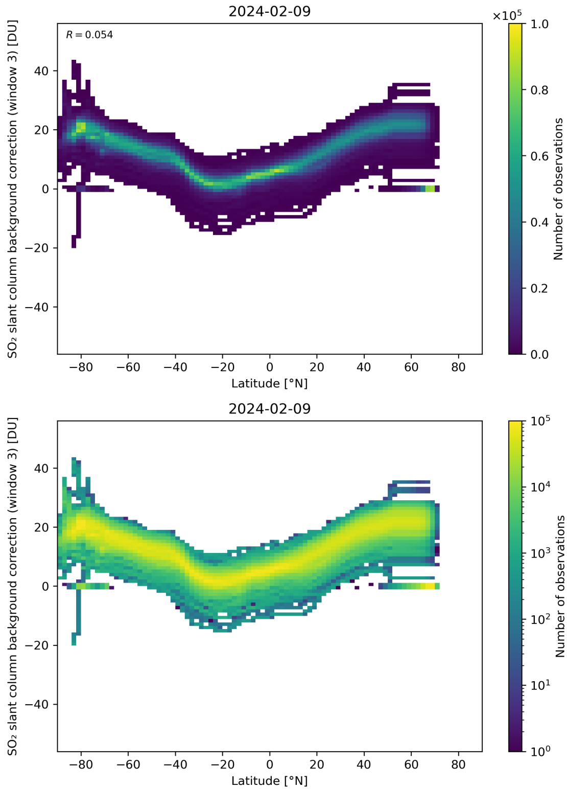
Figure 141: Scatter density plot of “Latitude” against “SO 2 slant column background correction (window 3)” for 2024-02-08 to 2024-02-10.
