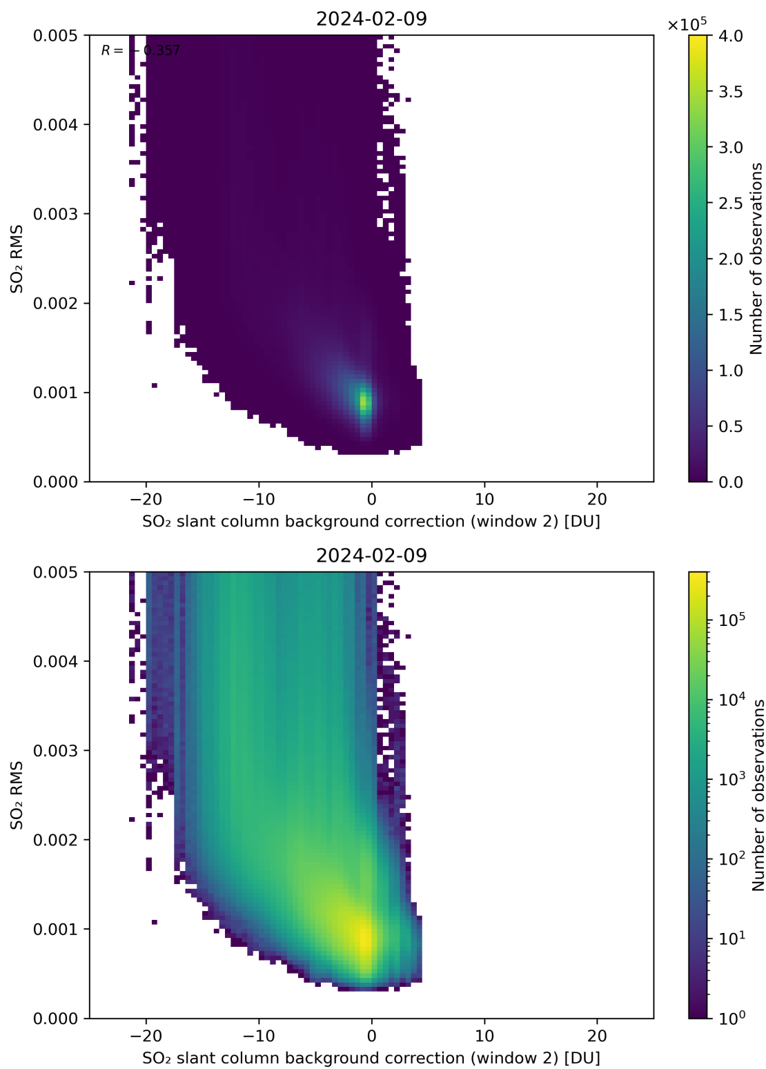
Figure 114: Scatter density plot of “SO 2 slant column background correction (window 2)” against “SO 2 RMS” for 2024-02-08 to 2024-02-10.
