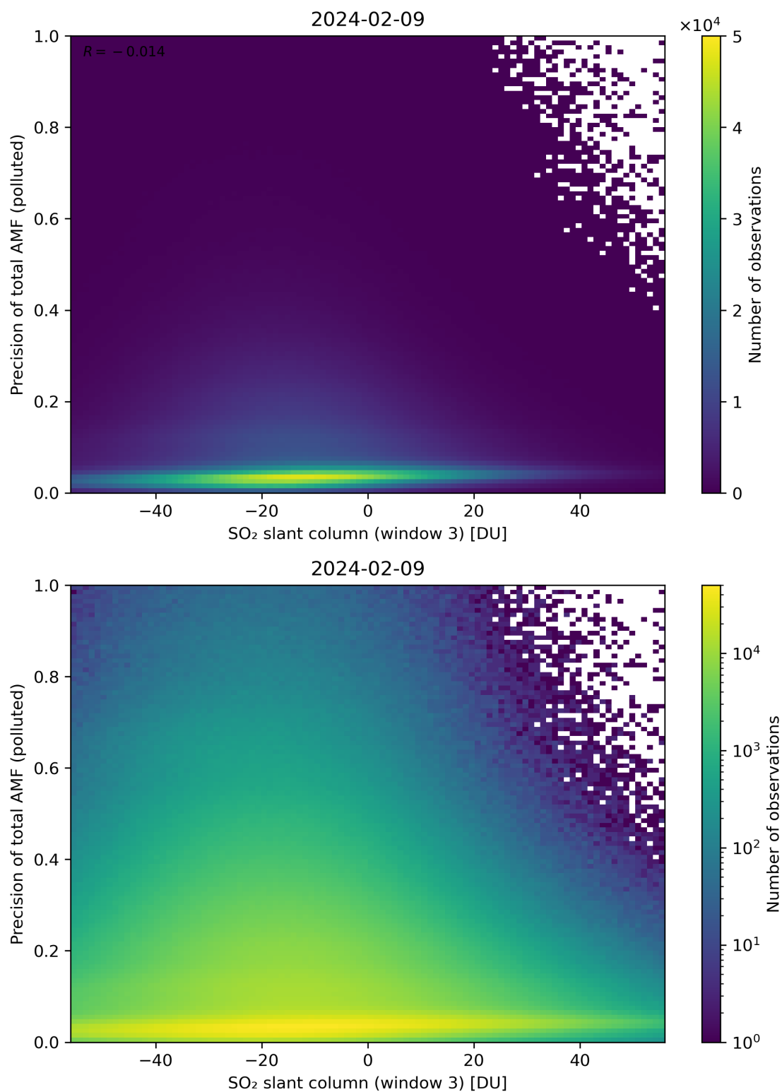
Figure 269: Scatter density plot of “SO 2 slant column (window 3)” against “Precision of total AMF (polluted)” for 2024-02-08 to 2024-02-10.
