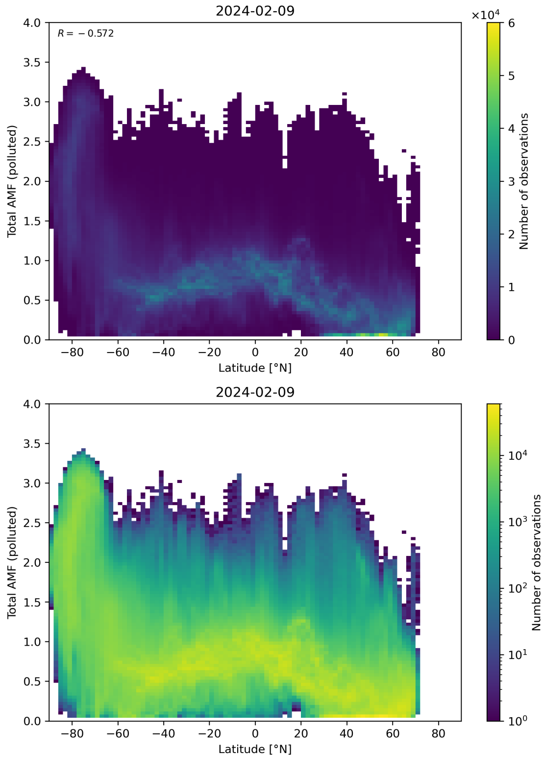
Figure 154: Scatter density plot of “Latitude” against “Total AMF (polluted)” for 2024-02-08 to 2024-02-10.
