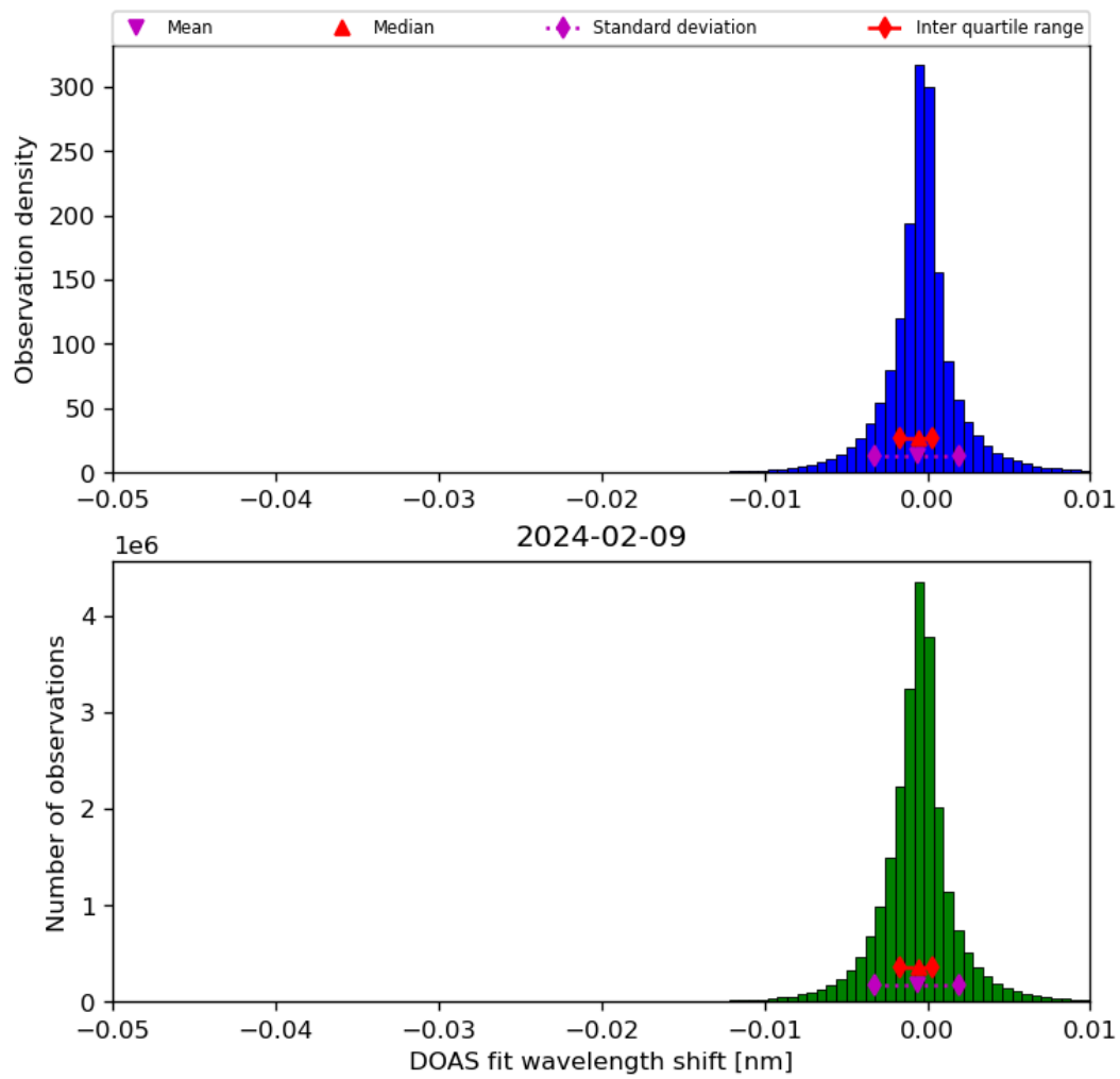
Figure 68: Histogram of “DOAS fit wavelength shift” for 2024-02-08 to 2024-02-10
