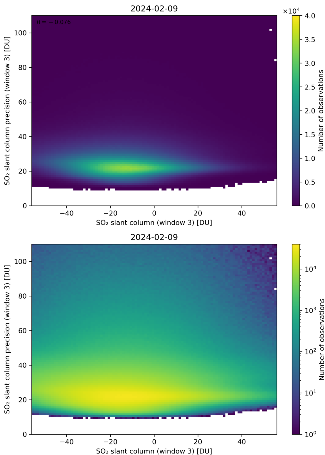
Figure 267: Scatter density plot of “SO 2 slant column (window 3)” against “SO 2 slant column precision (window 3)” for 2024-02-08 to 2024-02-10.
