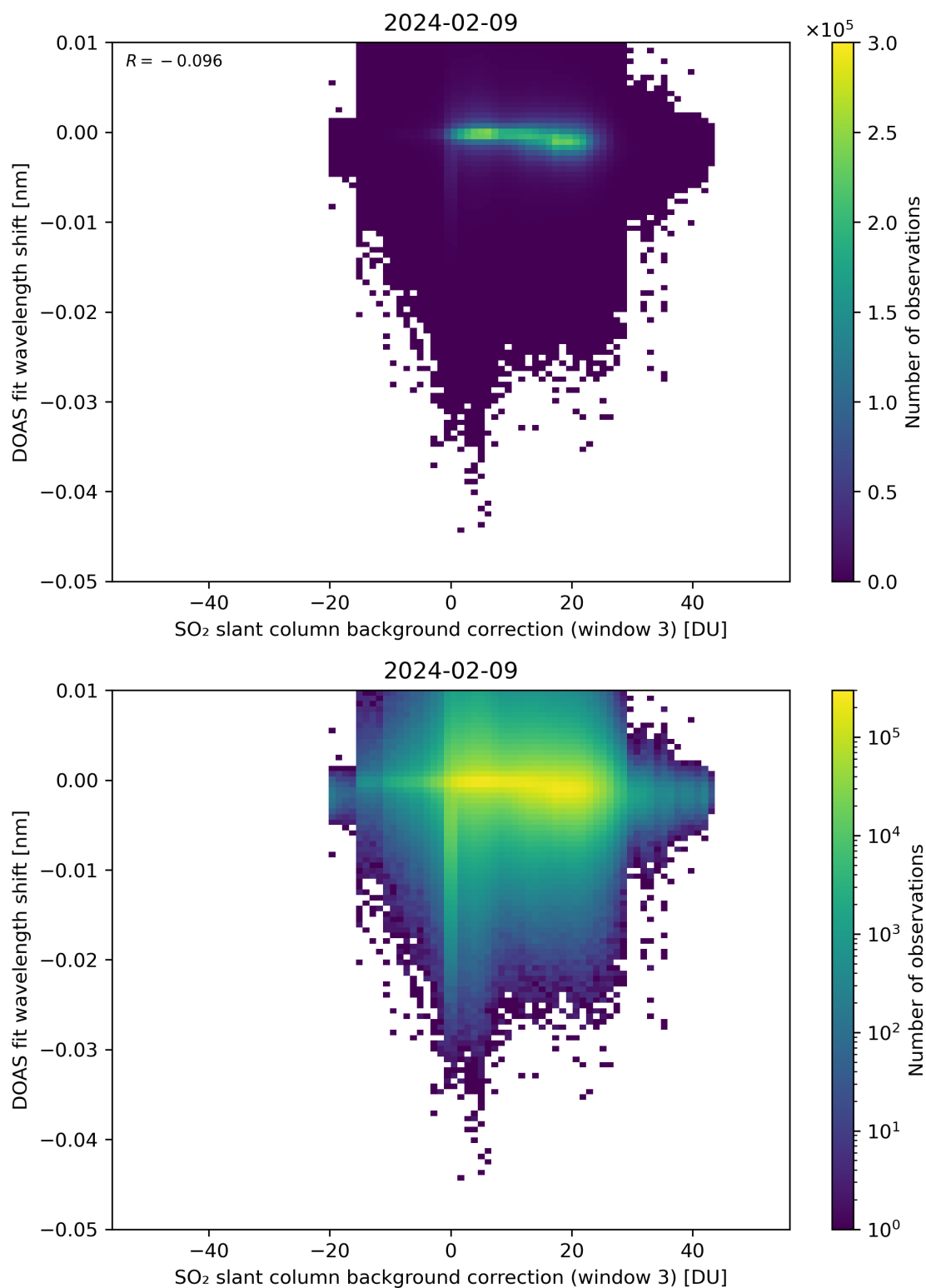
Figure 121: Scatter density plot of “SO 2 slant column background correction (window 3)” against “DOAS fit wavelength shift” for 2024-02-08 to 2024-02-10.
