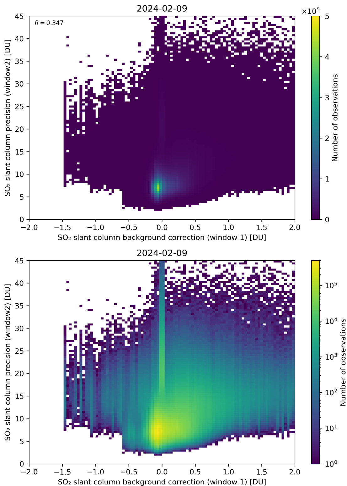
Figure 106: Scatter density plot of “SO 2 slant column background correction (window 1)” against “SO 2 slant column precision (window2)” for 2024-02-08 to 2024-02-10.
