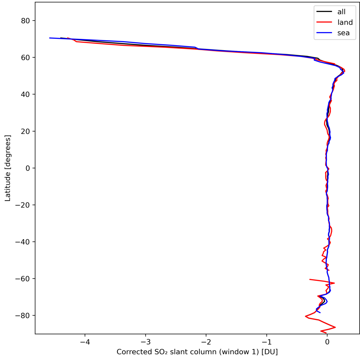
Figure 35: Zonal average of “Corrected SO 2 slant column (window 1)” for 2024-02-08 to 2024-02-10.
