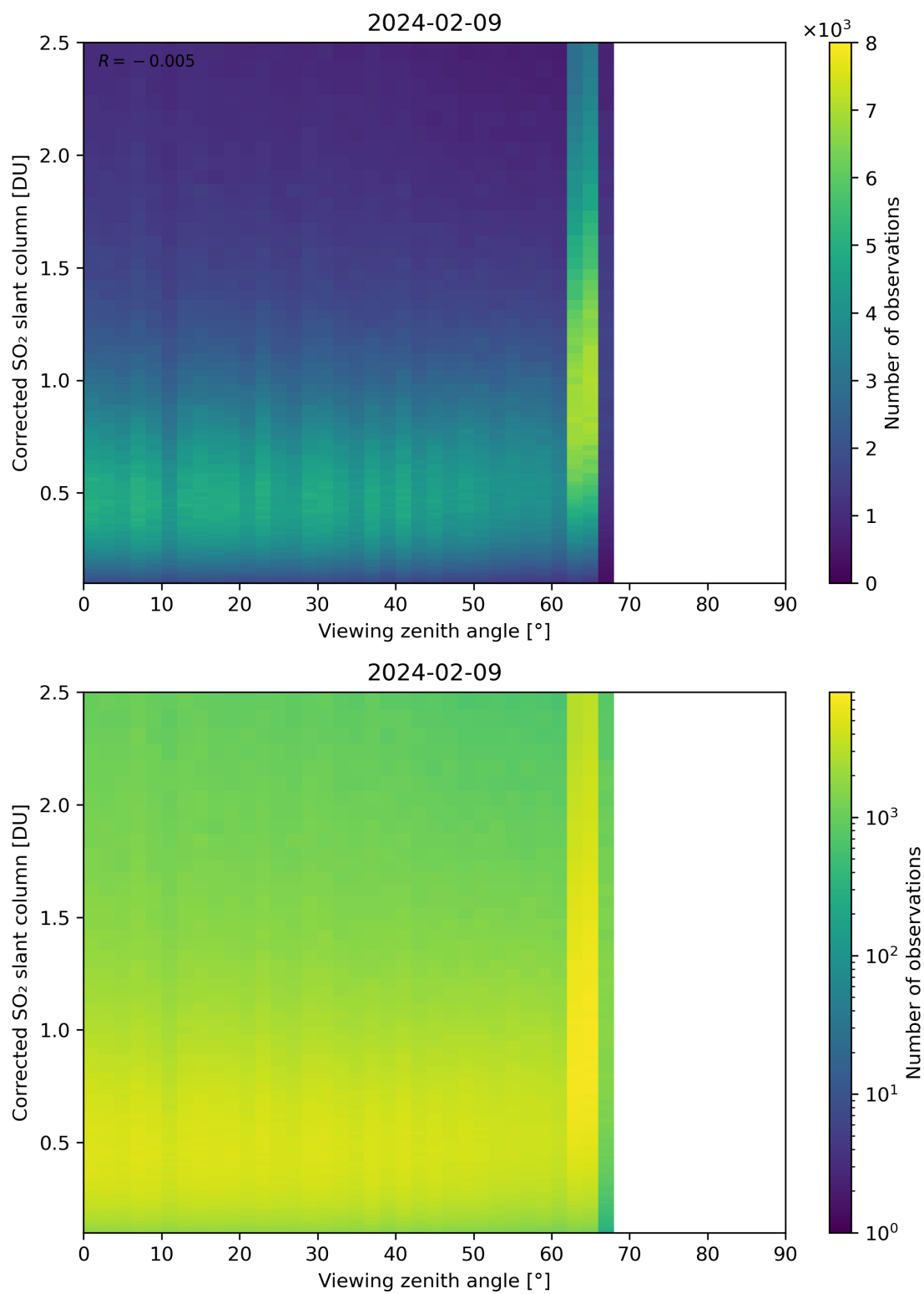
Figure 317: Scatter density plot of “Viewing zenith angle” against “Corrected SO 2 slant column” for 2024-02-08 to 2024-02-10.
