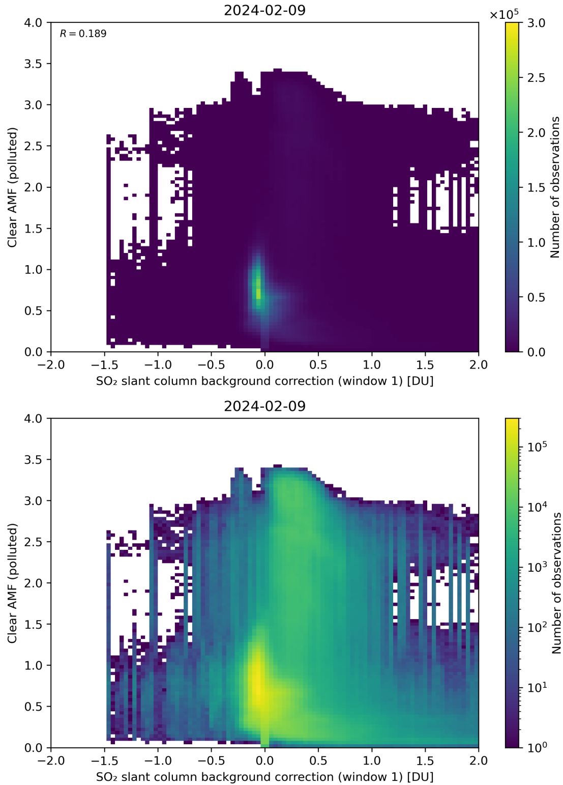
Figure 103: Scatter density plot of “SO 2 slant column background correction (window 1)” against “Clear AMF (polluted)” for 2024-02-08 to 2024-02-10.
