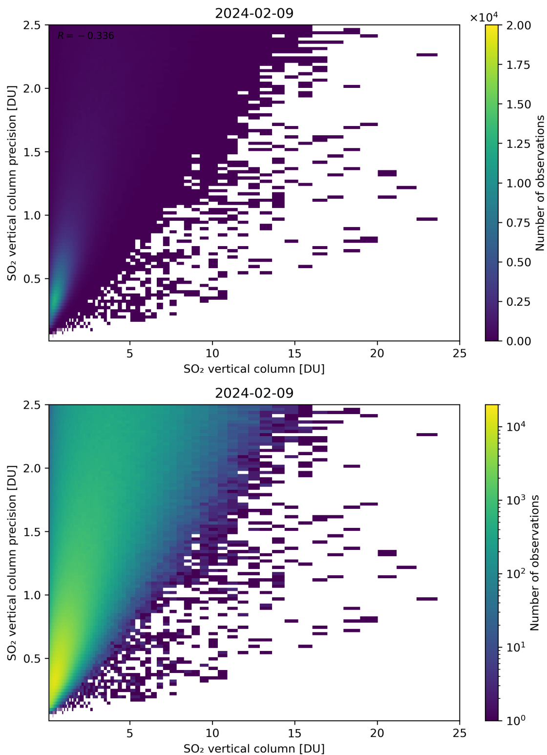
Figure 307: Scatter density plot of “SO 2 vertical column” against “SO 2 vertical column precision” for 2024-02-08 to 2024-02-10.
