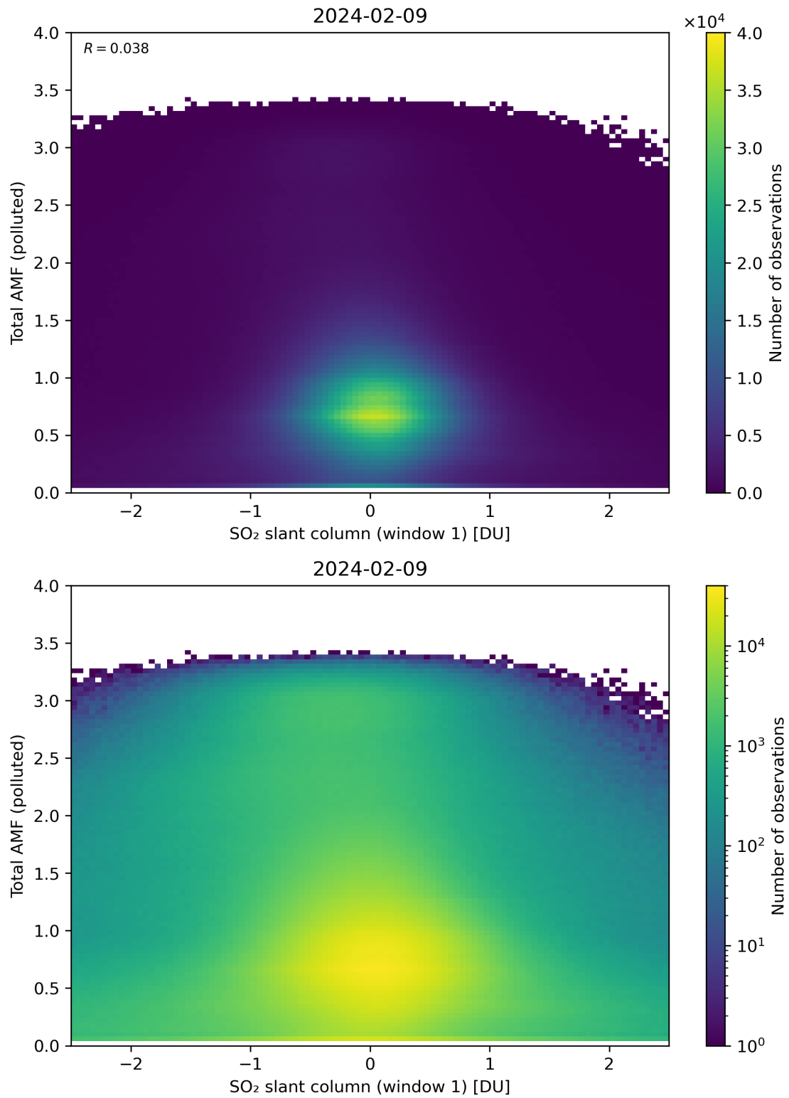
Figure 239: Scatter density plot of “SO 2 slant column (window 1)” against “Total AMF (polluted)” for 2024-02-08 to 2024-02-10.
