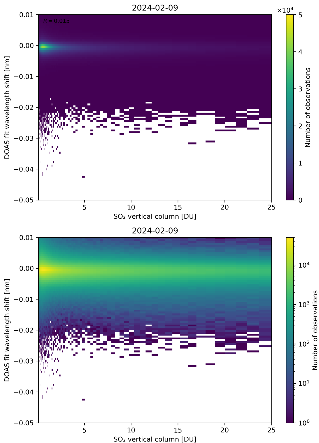
Figure 276: Scatter density plot of “SO 2 vertical column” against “DOAS fit wavelength shift” for 2024-02-08 to 2024-02-10.
