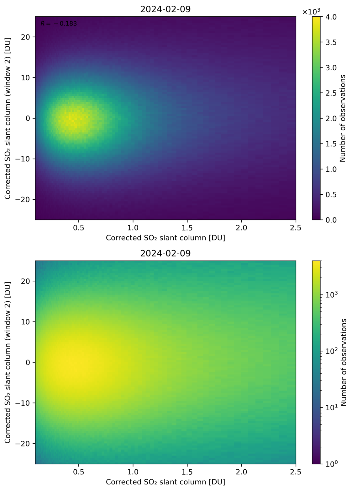
Figure 185: Scatter density plot of “Corrected SO 2 slant column” against “Corrected SO 2 slant column (window 2)” for 2024-02-08 to 2024-02-10.
