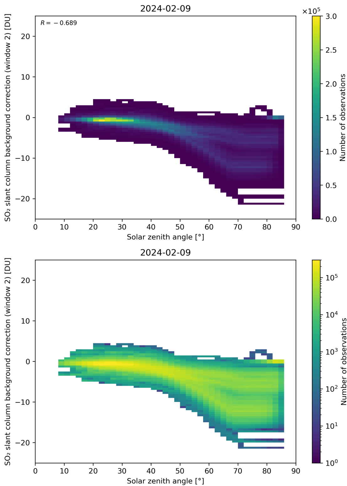
Figure 159: Scatter density plot of “Solar zenith angle” against “SO 2 slant column background correction (window 2)” for 2024-02-08 to 2024-02-10.
