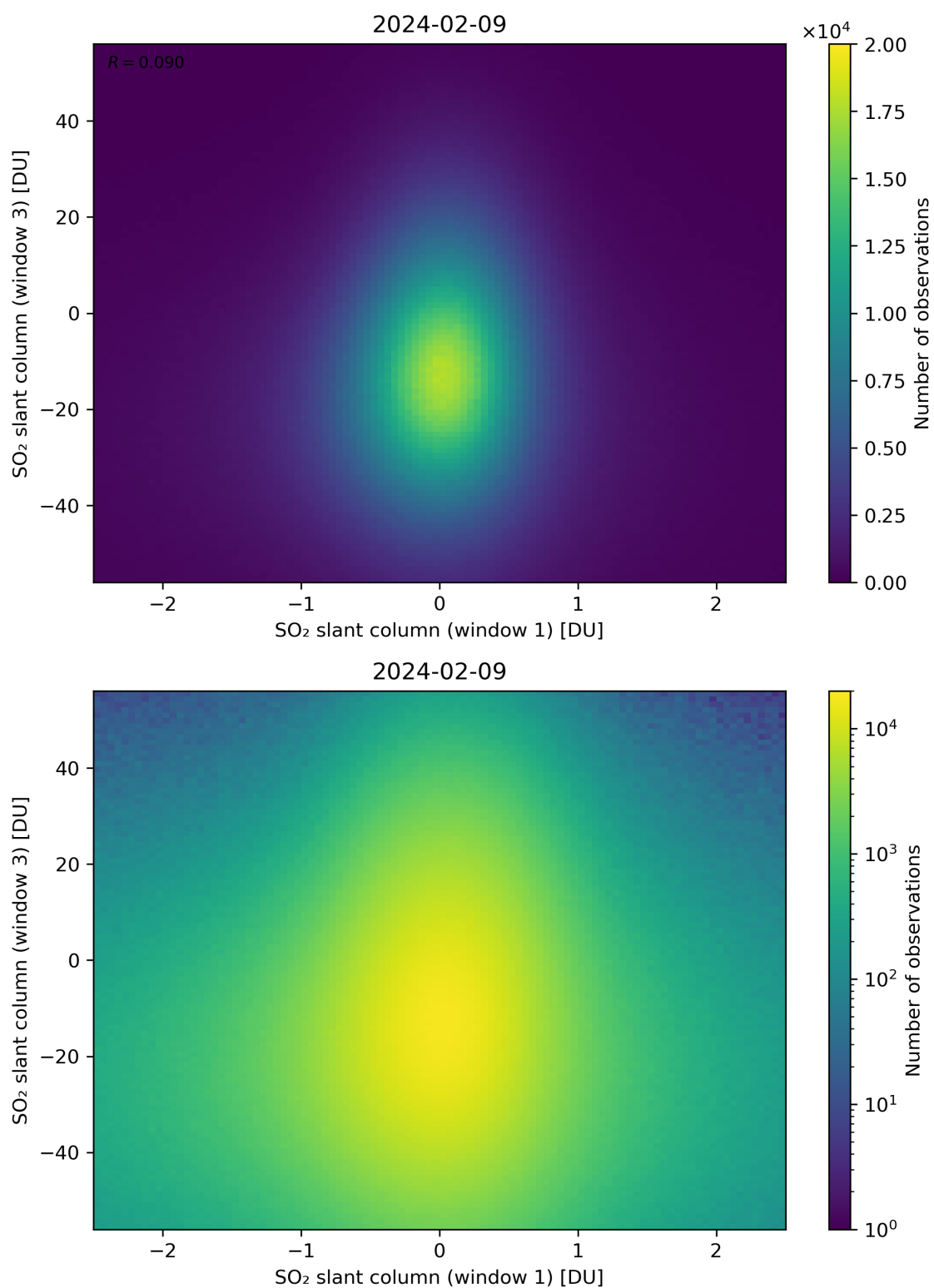
Figure 237: Scatter density plot of “SO 2 slant column (window 1)” against “SO 2 slant column (window 3)” for 2024-02-08 to 2024-02-10.
