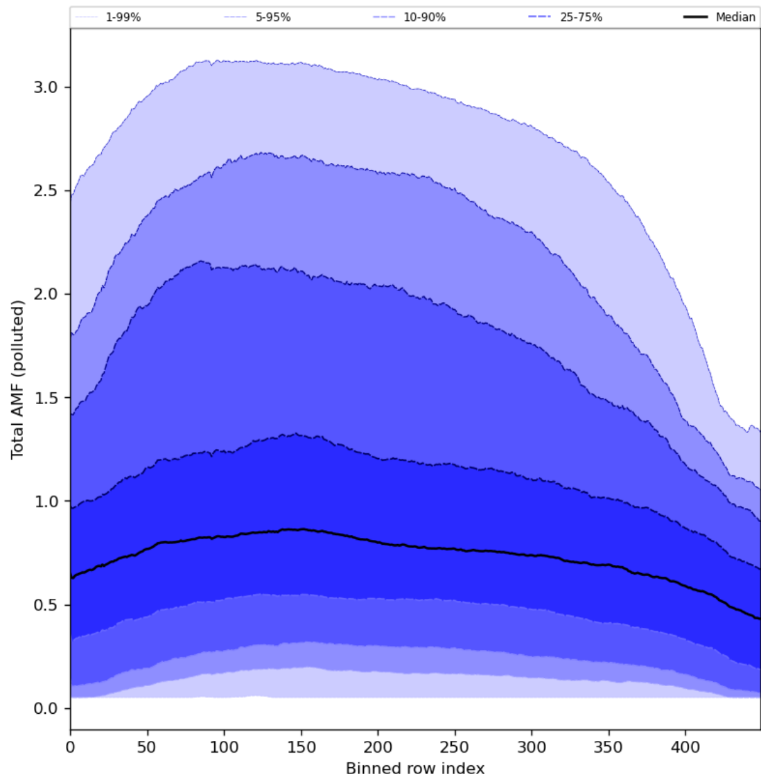
Figure 94: Along track statistics of “Total AMF (polluted)” for 2024-02-08 to 2024-02-10
