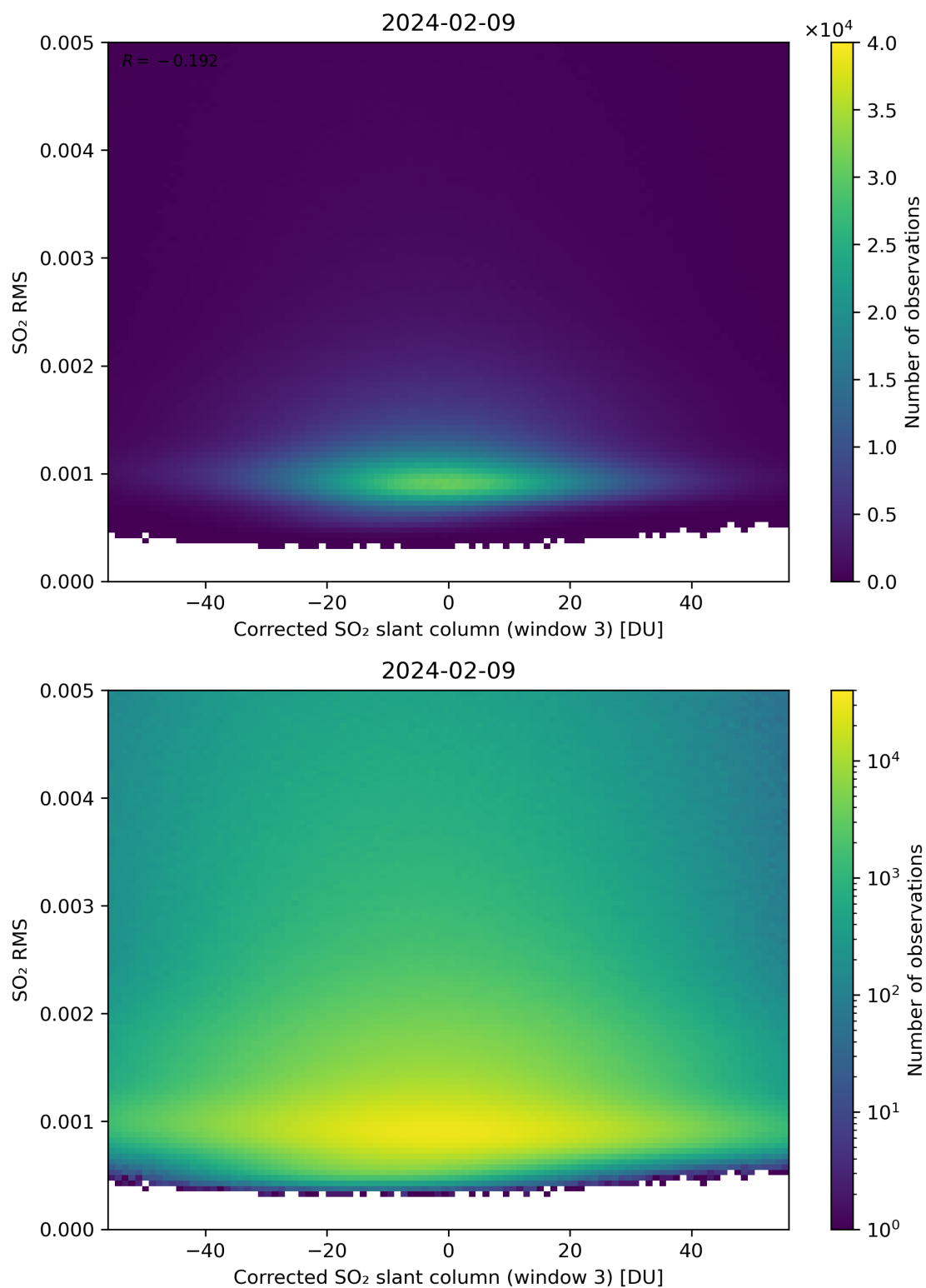
Figure 208: Scatter density plot of “Corrected SO 2 slant column (window 3)” against “SO 2 RMS” for 2024-02-08 to 2024-02-10.
