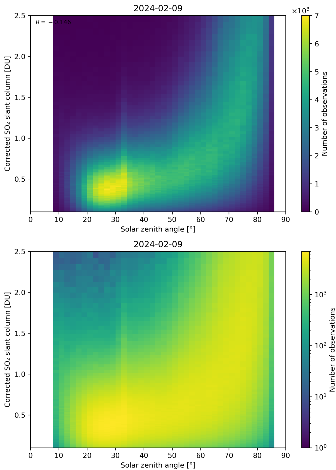
Figure 166: Scatter density plot of “Solar zenith angle” against “Corrected SO 2 slant column” for 2024-02-08 to 2024-02-10.
