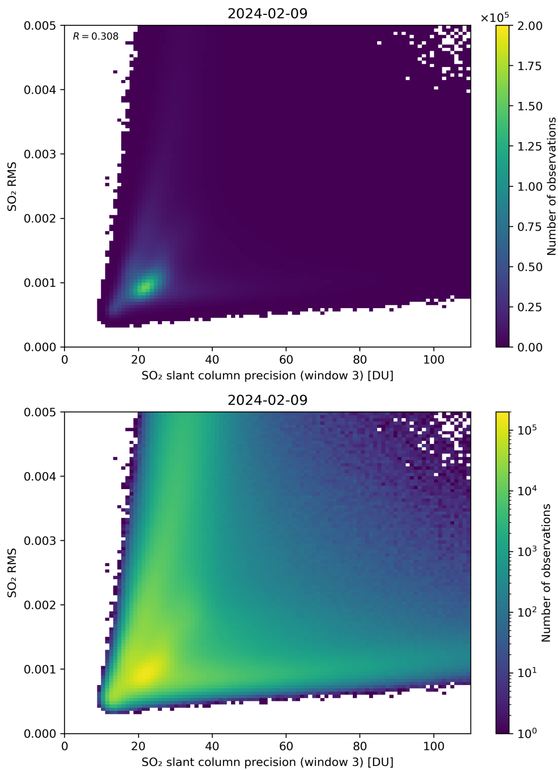
Figure 260: Scatter density plot of “SO 2 slant column precision (window 3)” against “SO 2 RMS” for 2024-02-08 to 2024-02-10.
