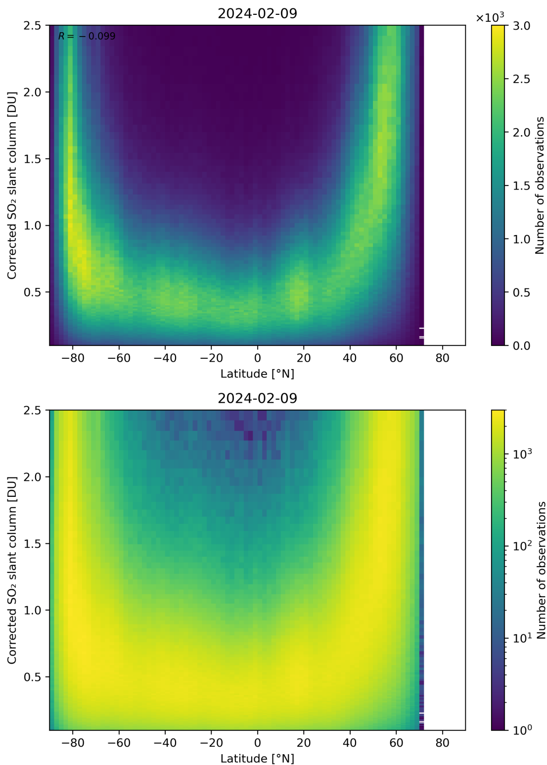
Figure 146: Scatter density plot of “Latitude” against “Corrected SO 2 slant column” for 2024-02-08 to 2024-02-10.
