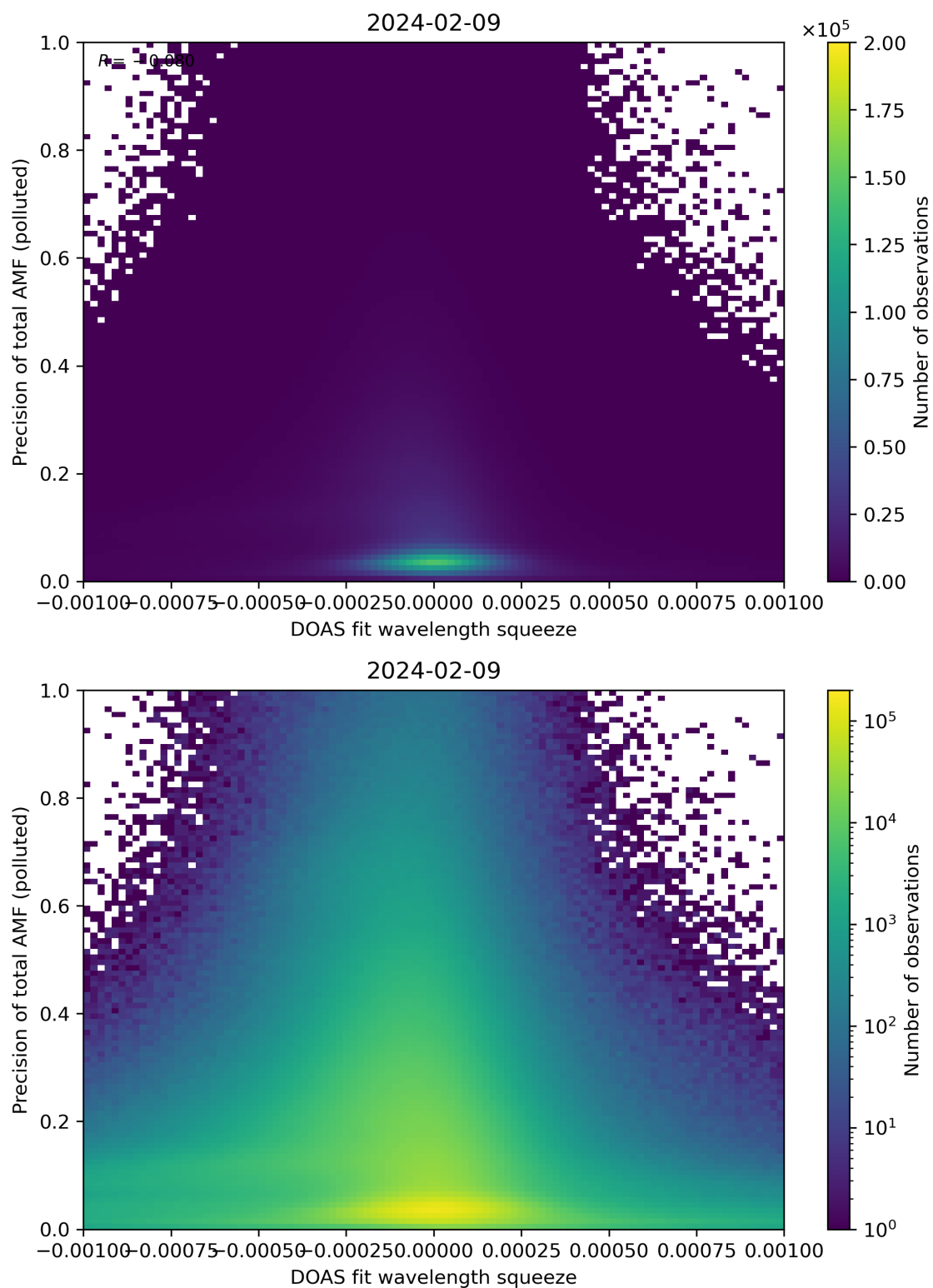
Figure 135: Scatter density plot of “DOAS fit wavelength squeeze” against “Precision of total AMF (polluted)” for 2024-02-08 to 2024-02-10.
