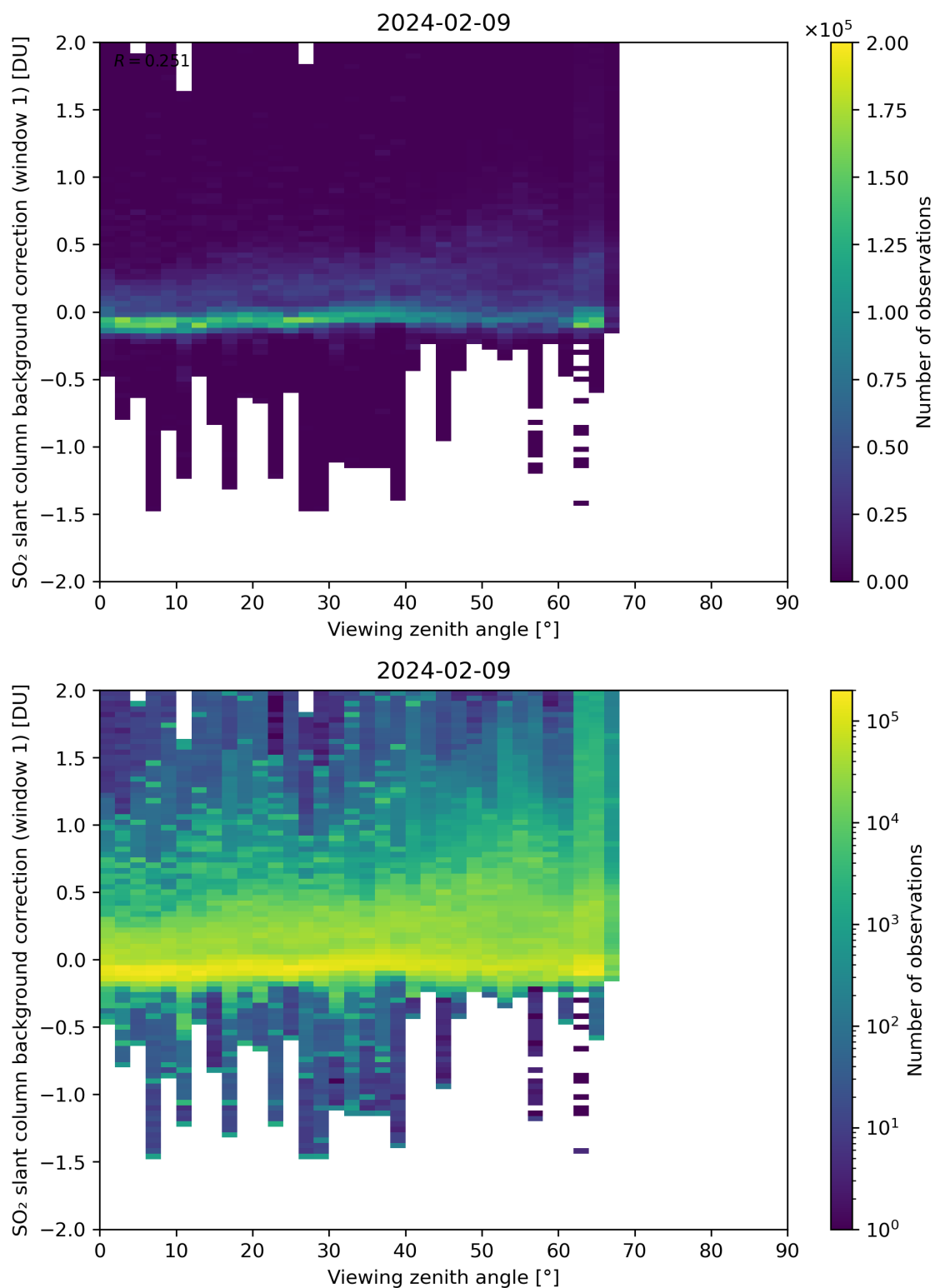
Figure 308: Scatter density plot of “Viewing zenith angle” against “SO 2 slant column background correction (window 1)” for 2024-02-08 to 2024-02-10.
