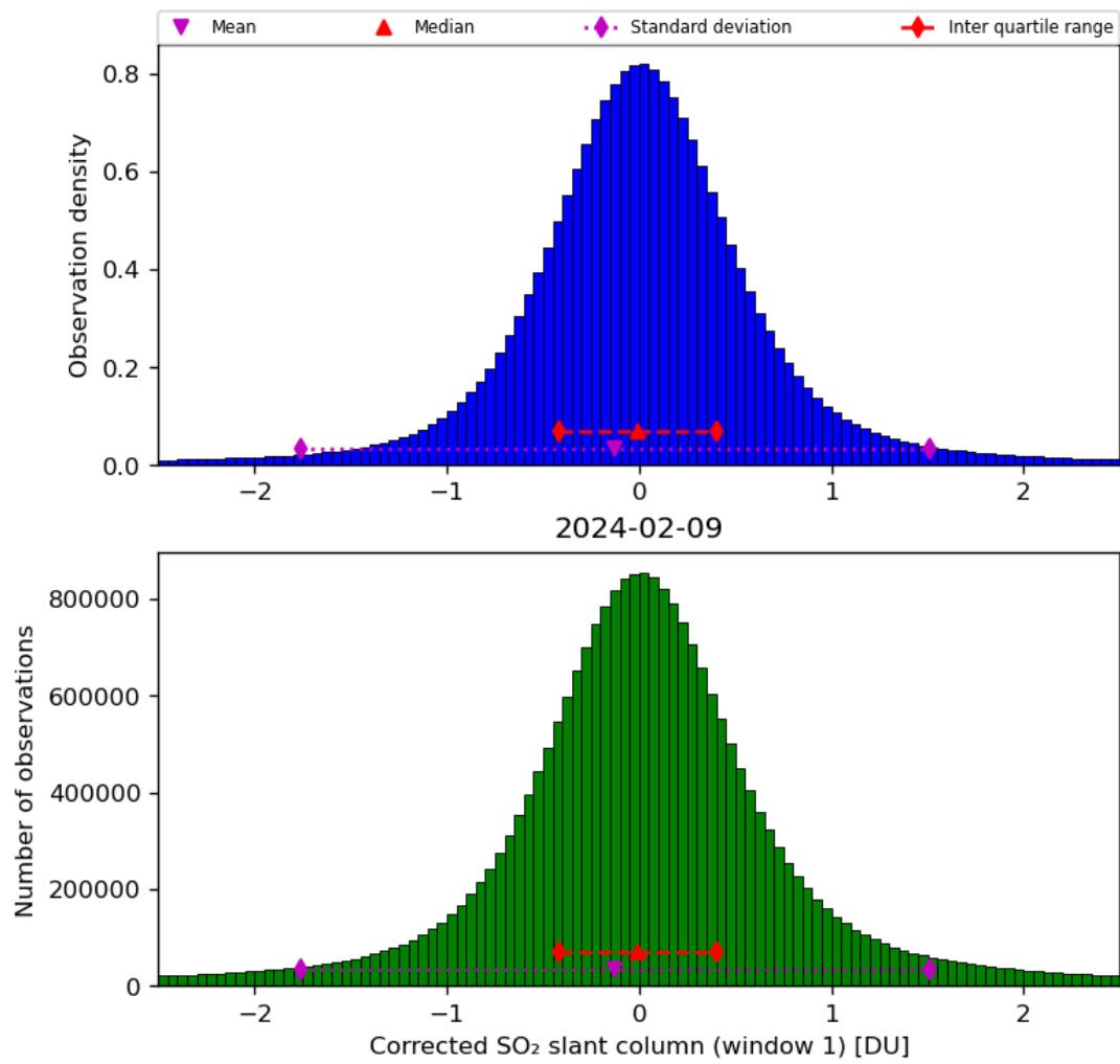
Figure 58: Histogram of “Corrected SO 2 slant column (window 1)” for 2024-02-08 to 2024-02-10
