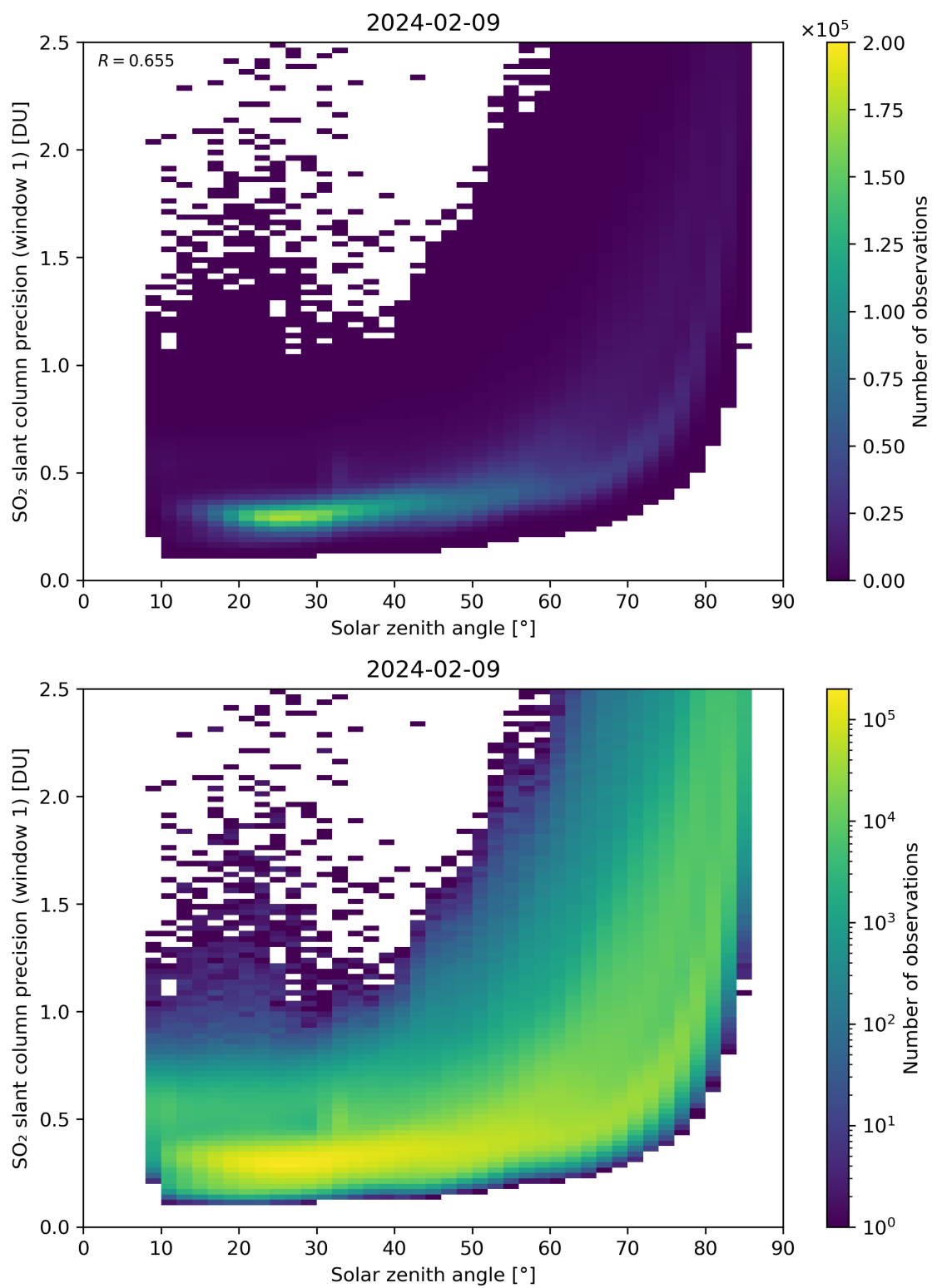
Figure 170: Scatter density plot of “Solar zenith angle” against “SO 2 slant column precision (window 1)” for 2024-02-08 to 2024-02-10.
