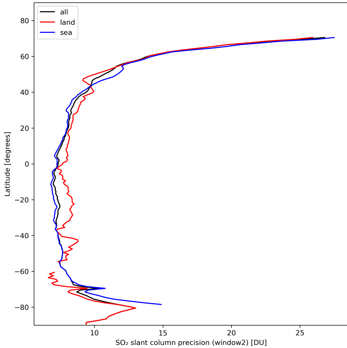
Figure 38: Zonal average of “SO 2 slant column precision (window2)” for 2024-02-08 to 2024-02-10.
