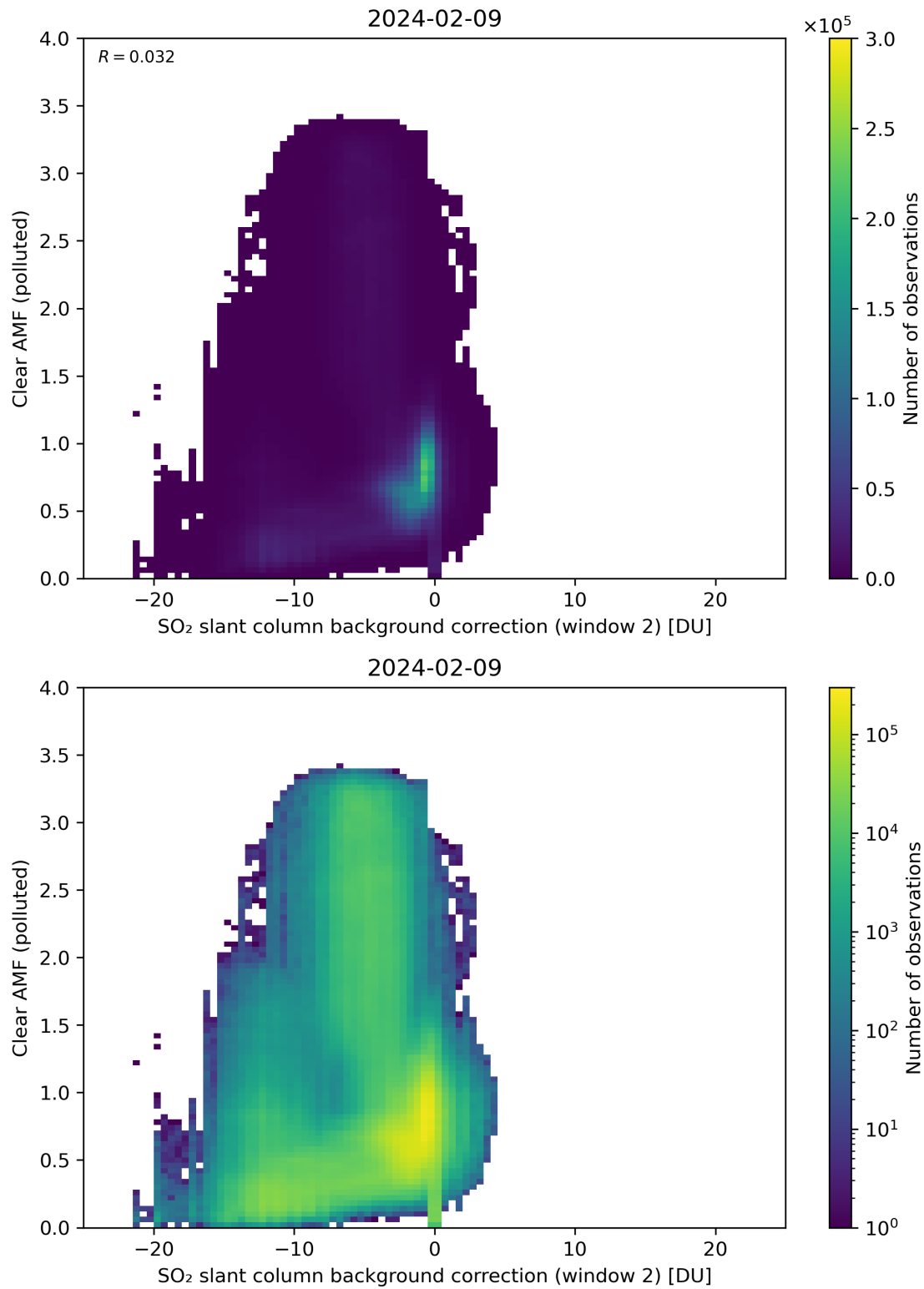
Figure 115: Scatter density plot of “SO 2 slant column background correction (window 2)” against “Clear AMF (polluted)” for 2024-02-08 to 2024-02-10.
