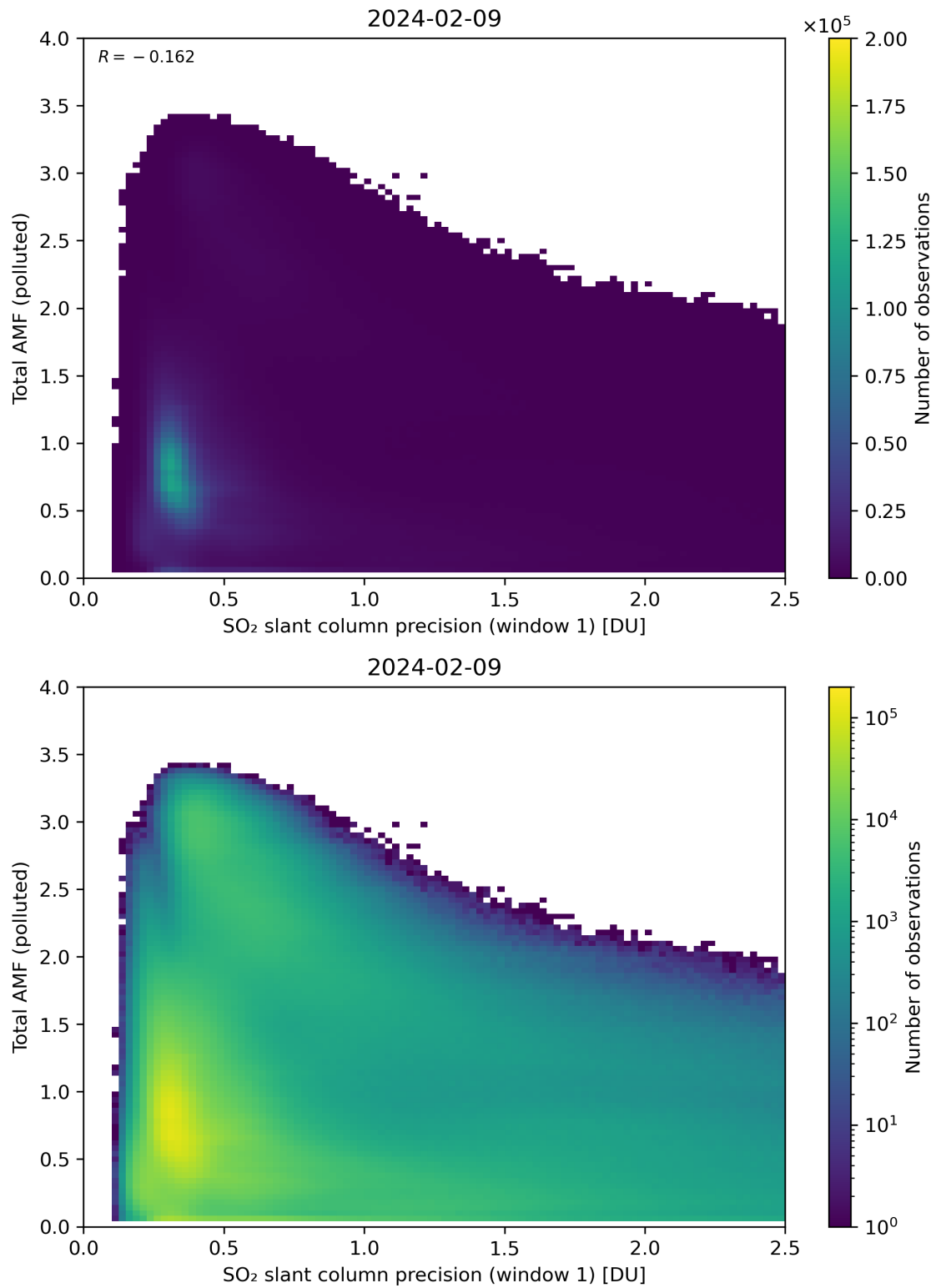
Figure 230: Scatter density plot of “SO 2 slant column precision (window 1)” against “Total AMF (polluted)” for 2024-02-08 to 2024-02-10.
