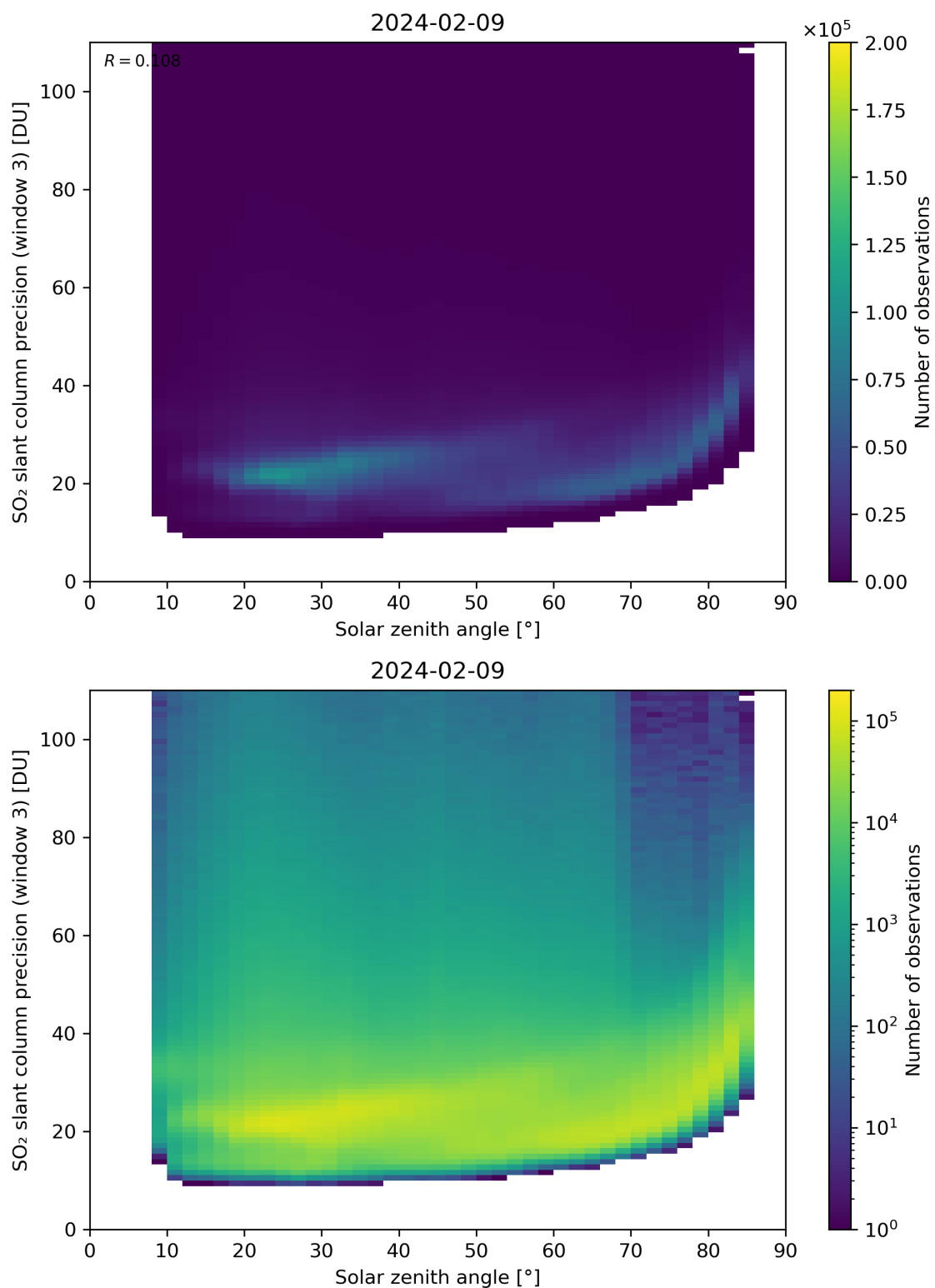
Figure 173: Scatter density plot of “Solar zenith angle” against “SO 2 slant column precision (window 3)” for 2024-02-08 to 2024-02-10.
