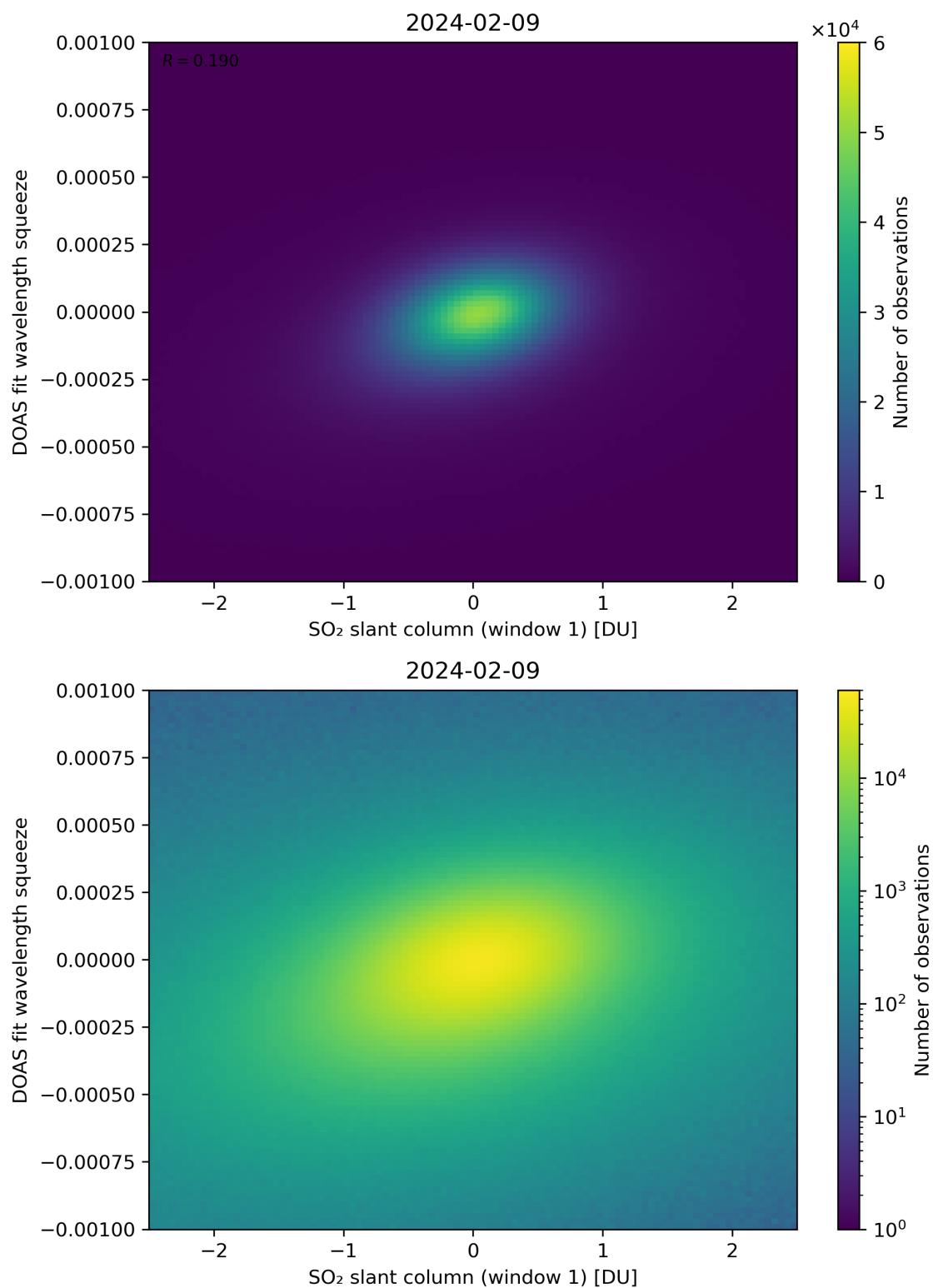
Figure 216: Scatter density plot of “SO 2 slant column (window 1)” against “DOAS fit wavelength squeeze” for 2024-02-08 to 2024-02-10.
