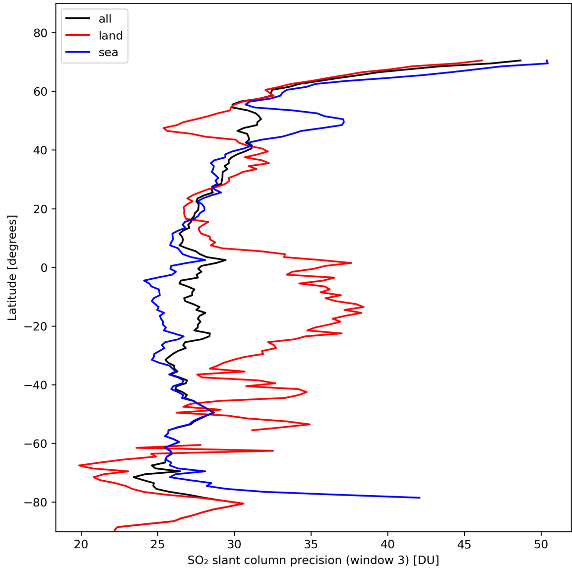
Figure 42: Zonal average of “SO 2 slant column precision (window 3)” for 2024-02-08 to 2024-02-10.
