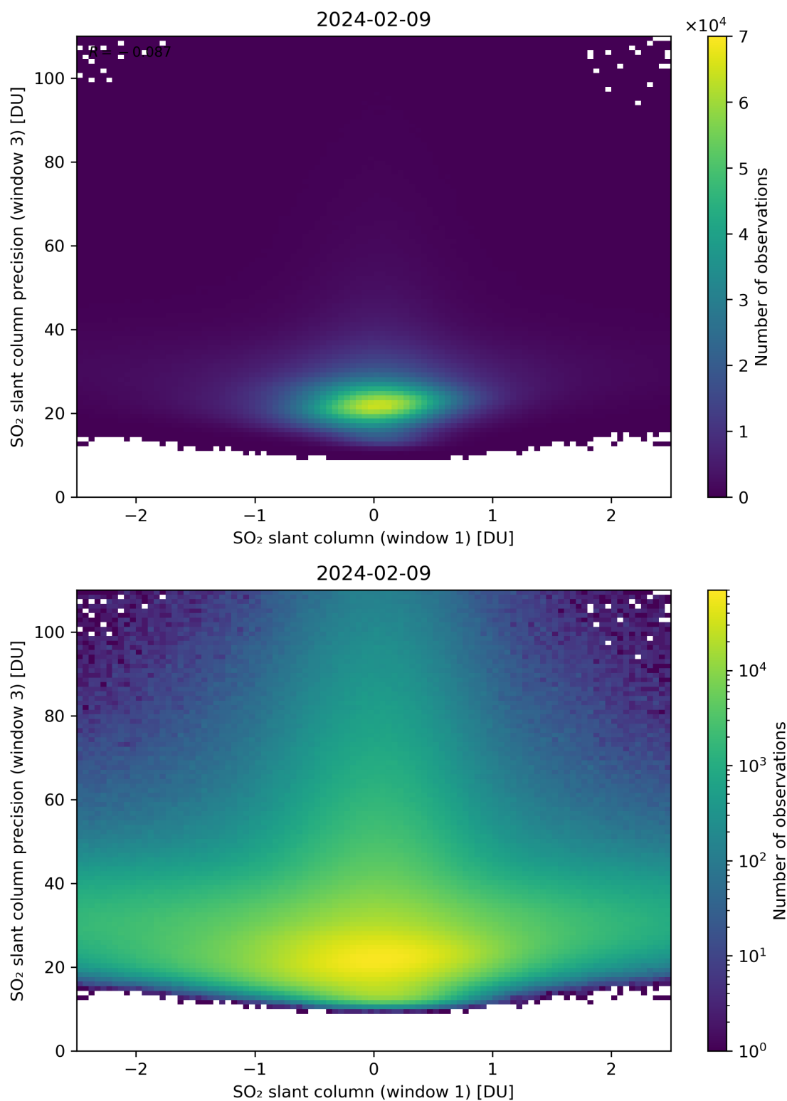
Figure 238: Scatter density plot of “SO 2 slant column (window 1)” against “SO 2 slant column precision (window 3)” for 2024-02-08 to 2024-02-10.
