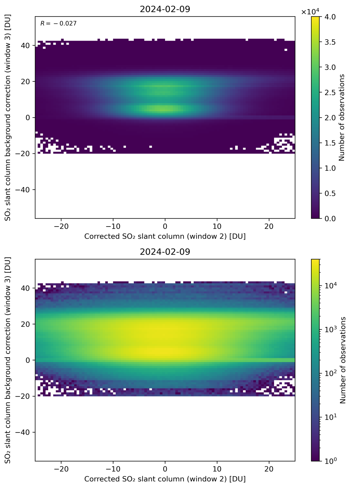
Figure 195: Scatter density plot of “Corrected SO 2 slant column (window 2)” against “SO 2 slant column background correction (window 3)” for 2024-02-08 to 2024-02-10.
