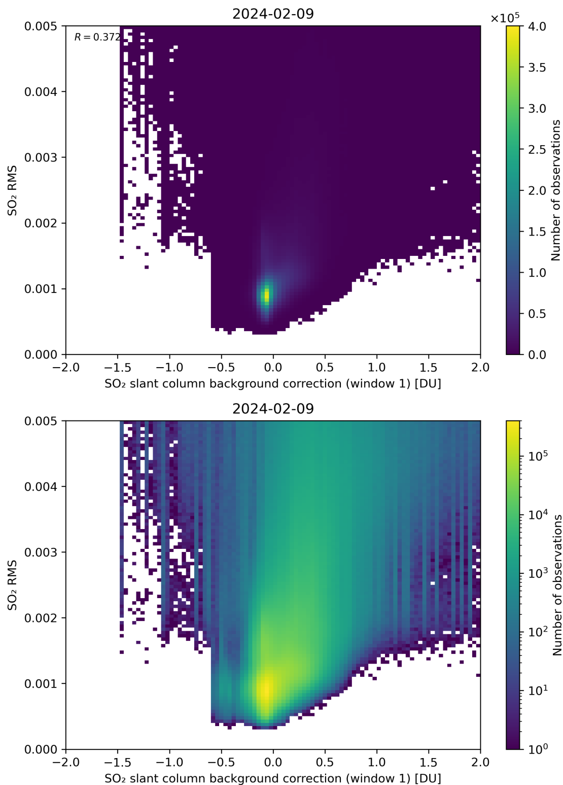
Figure 102: Scatter density plot of “SO 2 slant column background correction (window 1)” against “SO 2 RMS” for 2024-02-08 to 2024-02-10.
