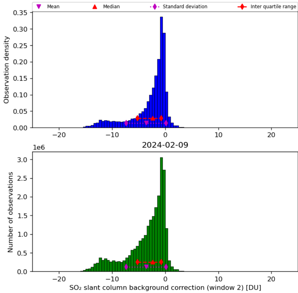
Figure 63: Histogram of “SO 2 slant column background correction (window 2)” for 2024-02-08 to 2024-02-10
