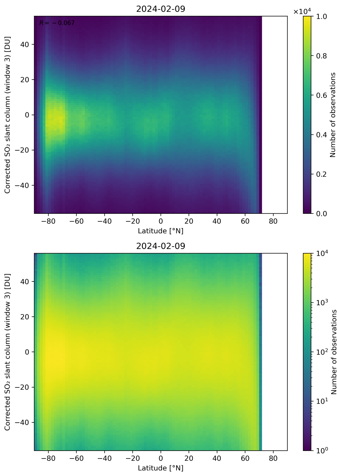
Figure 148: Scatter density plot of “Latitude” against “Corrected SO 2 slant column (window 3)” for 2024-02-08 to 2024-02-10.
