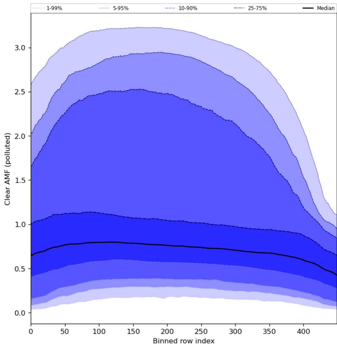
Figure 96: Along track statistics of “Clear AMF (polluted)” for 2024-02-08 to 2024-02-10
