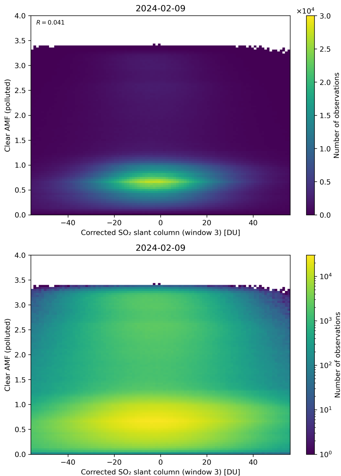
Figure 209: Scatter density plot of “Corrected SO 2 slant column (window 3)” against “Clear AMF (polluted)” for 2024-02-08 to 2024-02-10.
