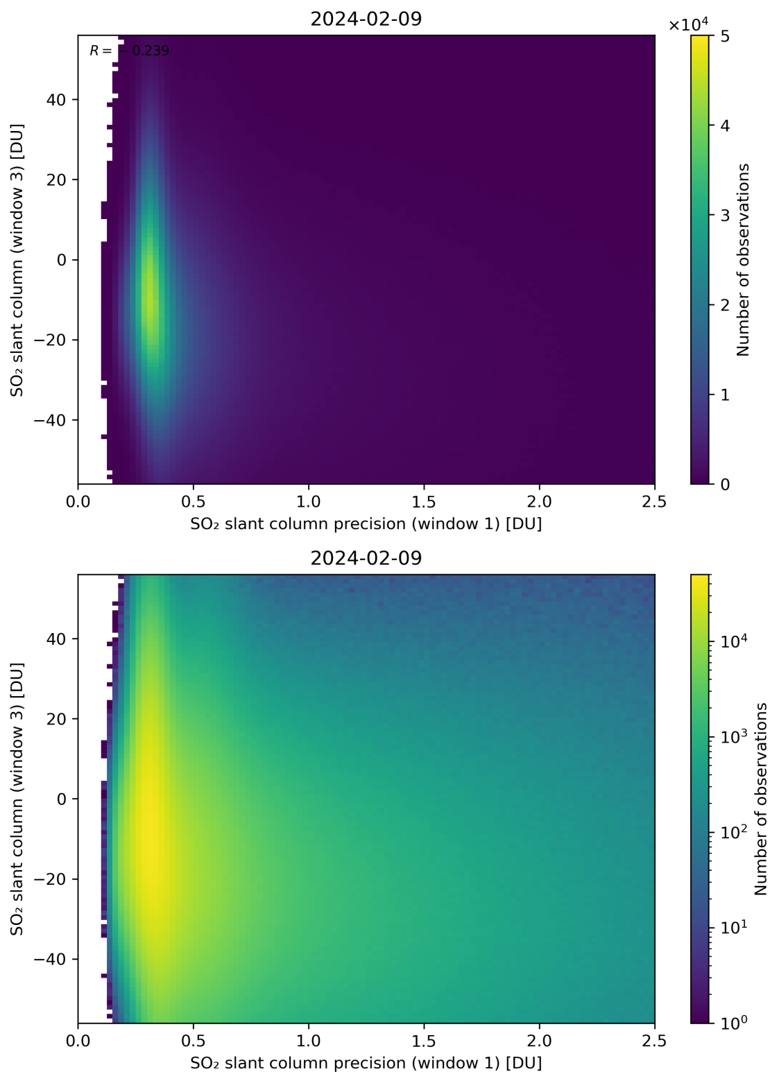
Figure 228: Scatter density plot of “SO 2 slant column precision (window 1)” against “SO 2 slant column (window 3)” for 2024-02-08 to 2024-02-10.
