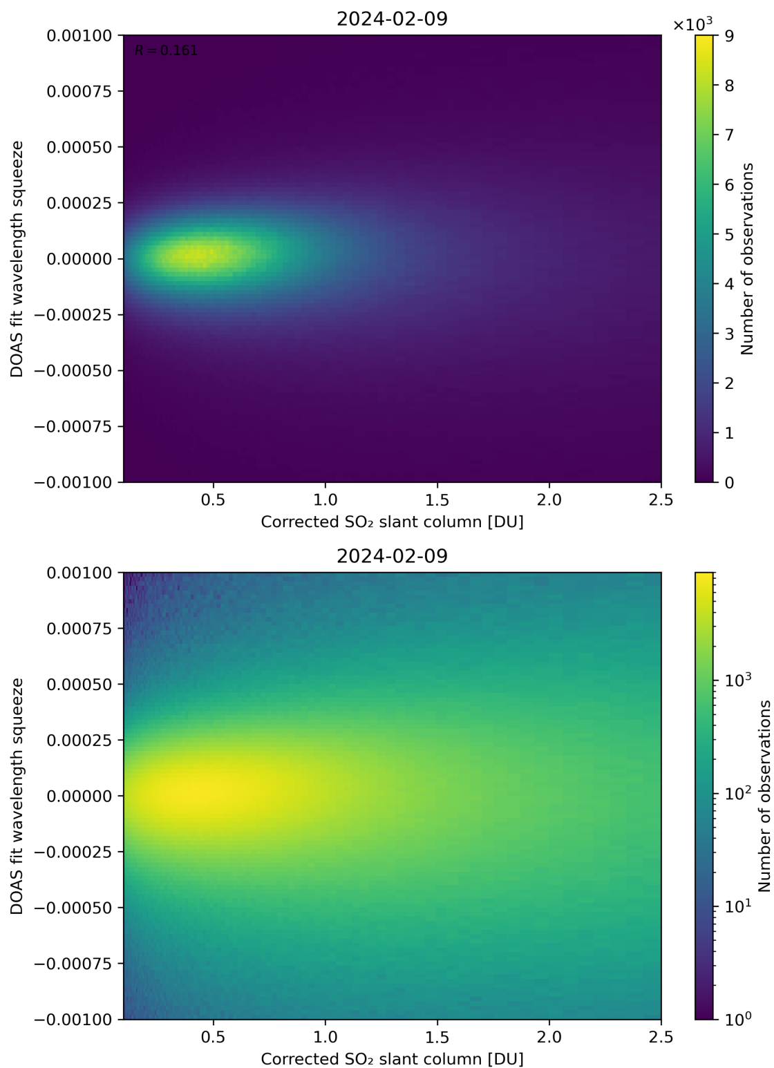
Figure 182: Scatter density plot of “Corrected SO 2 slant column” against “DOAS fit wavelength squeeze” for 2024-02-08 to 2024-02-10.
