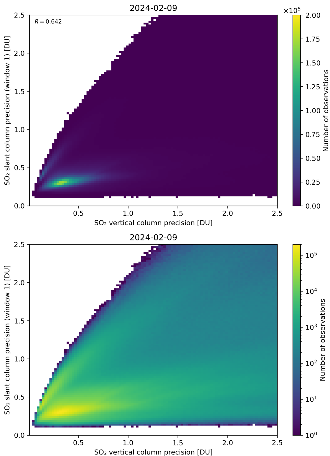
Figure 290: Scatter density plot of “SO 2 vertical column precision” against “SO 2 slant column precision (window 1)” for 2024-02-08 to 2024-02-10.
