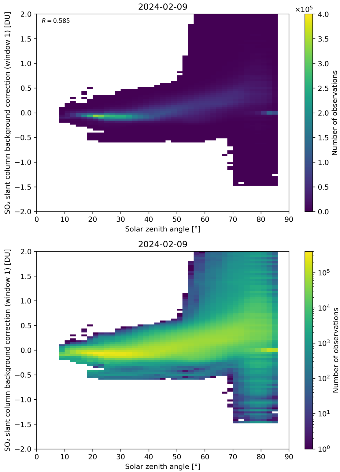
Figure 158: Scatter density plot of “Solar zenith angle” against “SO 2 slant column background correction (window 1)” for 2024-02-08 to 2024-02-10.
