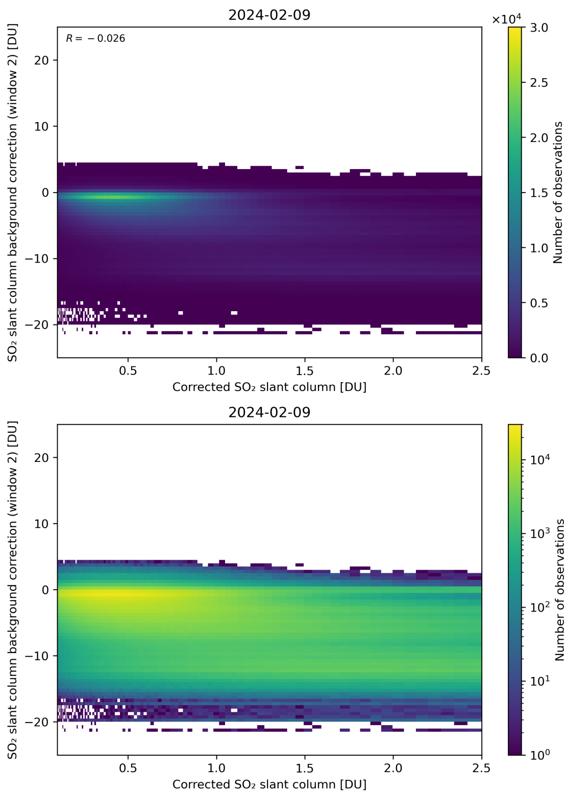
Figure 179: Scatter density plot of “Corrected SO 2 slant column” against “SO 2 slant column background correction (window 2)” for 2024-02-08 to 2024-02-10.
