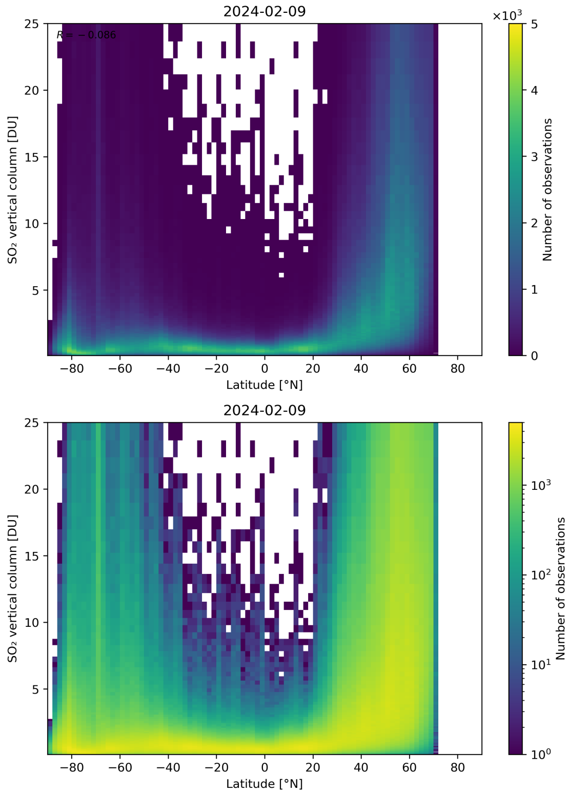
Figure 156: Scatter density plot of “Latitude” against “SO 2 vertical column” for 2024-02-08 to 2024-02-10.
