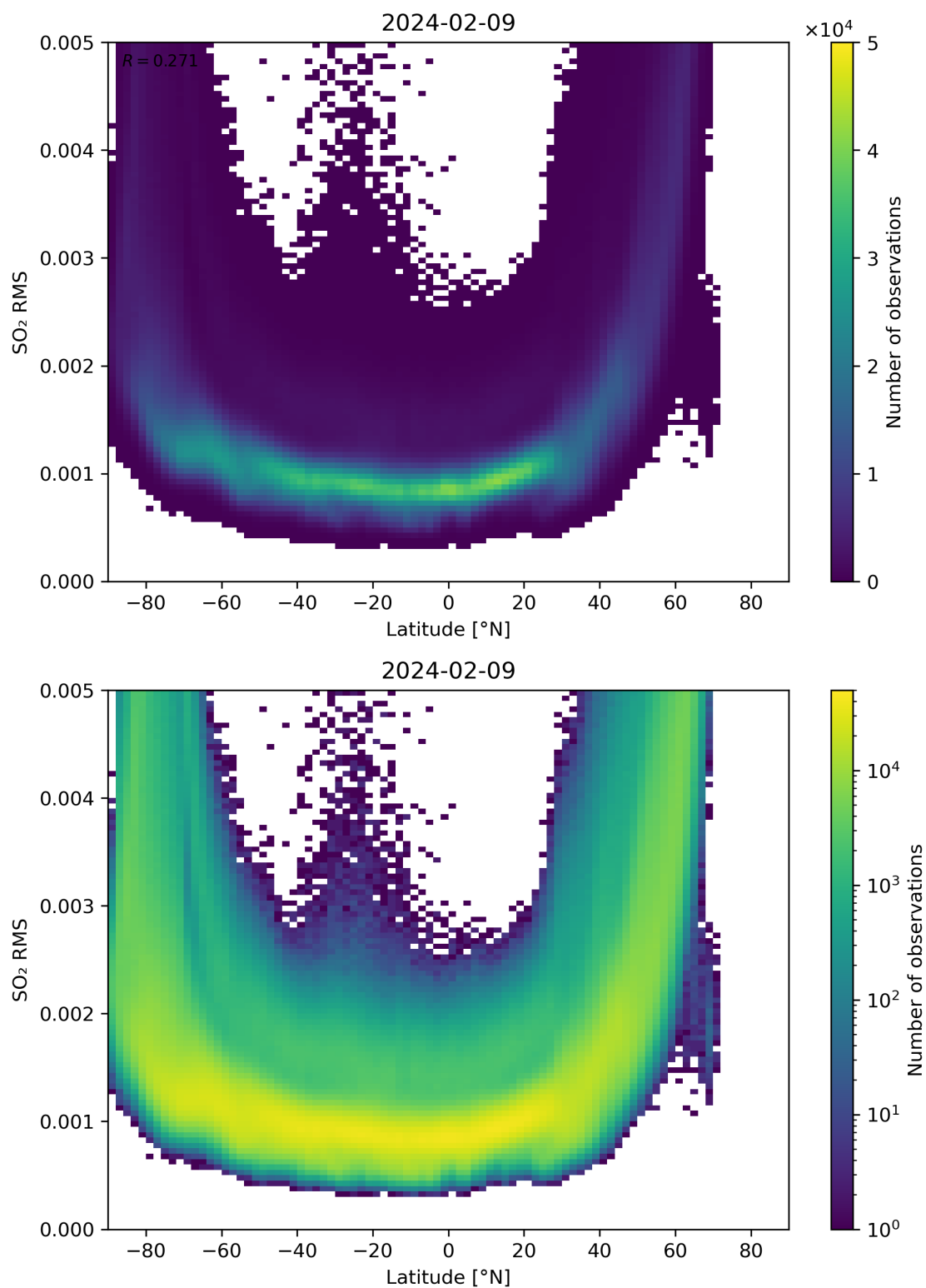
Figure 144: Scatter density plot of “Latitude” against “SO 2 RMS” for 2024-02-08 to 2024-02-10.
