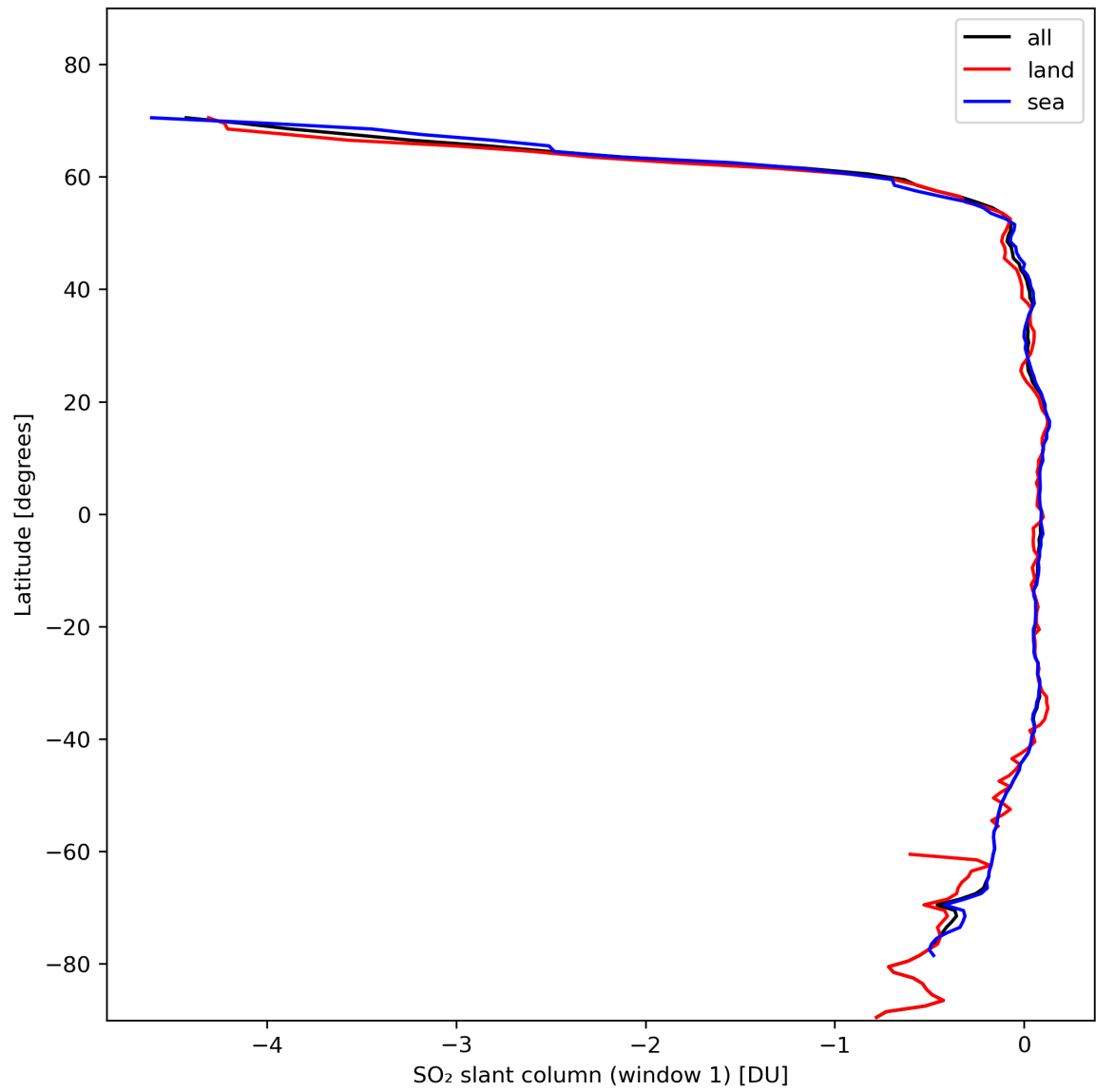
Figure 33: Zonal average of “SO 2 slant column (window 1)” for 2024-02-08 to 2024-02-10.
