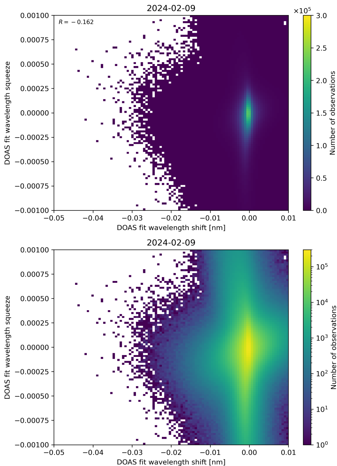
Figure 127: Scatter density plot of “DOAS fit wavelength shift” against “DOAS fit wavelength squeeze” for 2024-02-08 to 2024-02-10.
