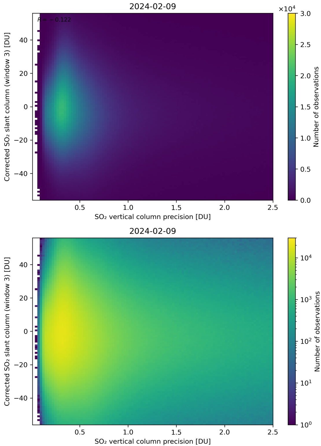
Figure 288: Scatter density plot of “SO 2 vertical column precision” against “Corrected SO 2 slant column (window 3)” for 2024-02-08 to 2024-02-10.
