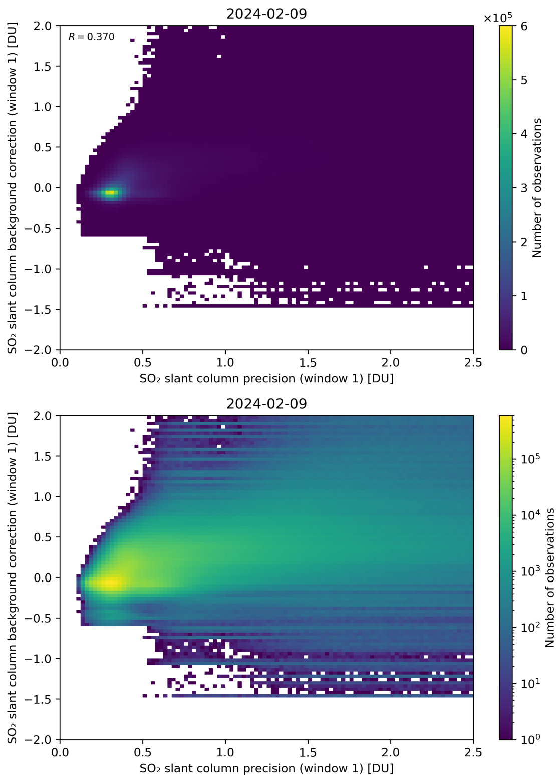
Figure 218: Scatter density plot of “SO 2 slant column precision (window 1)” against “SO 2 slant column background correction (window 1)” for 2024-02-08 to 2024-02-10.
