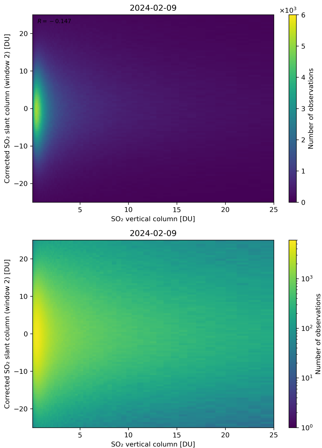
Figure 298: Scatter density plot of “SO 2 vertical column” against “Corrected SO 2 slant column (window 2)” for 2024-02-08 to 2024-02-10.
