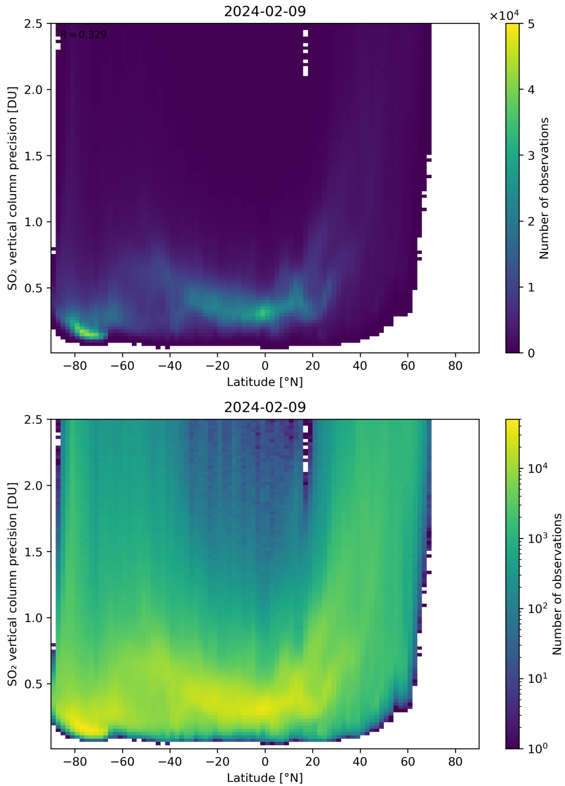
Figure 157: Scatter density plot of “Latitude” against “SO 2 vertical column precision” for 2024-02-08 to 2024-02-10.
