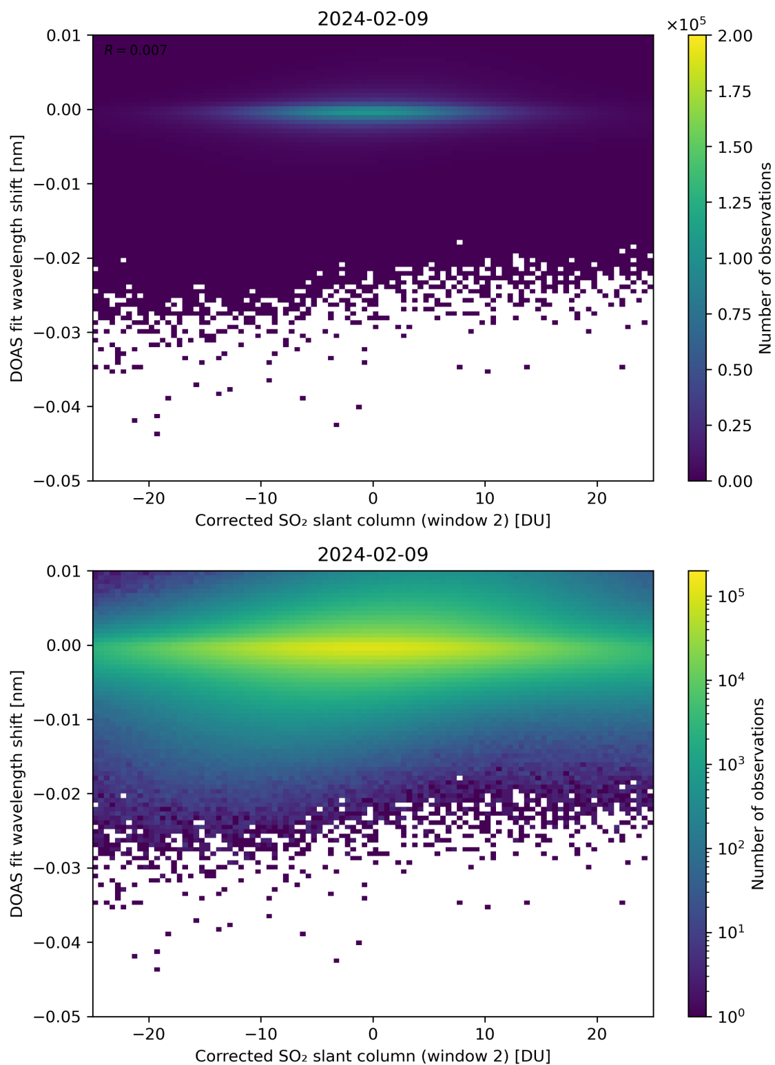
Figure 196: Scatter density plot of “Corrected SO 2 slant column (window 2)” against “DOAS fit wavelength shift” for 2024-02-08 to 2024-02-10.
