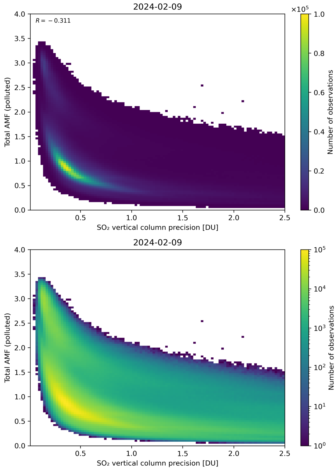
Figure 294: Scatter density plot of “SO 2 vertical column precision” against “Total AMF (polluted)” for 2024-02-08 to 2024-02-10.
