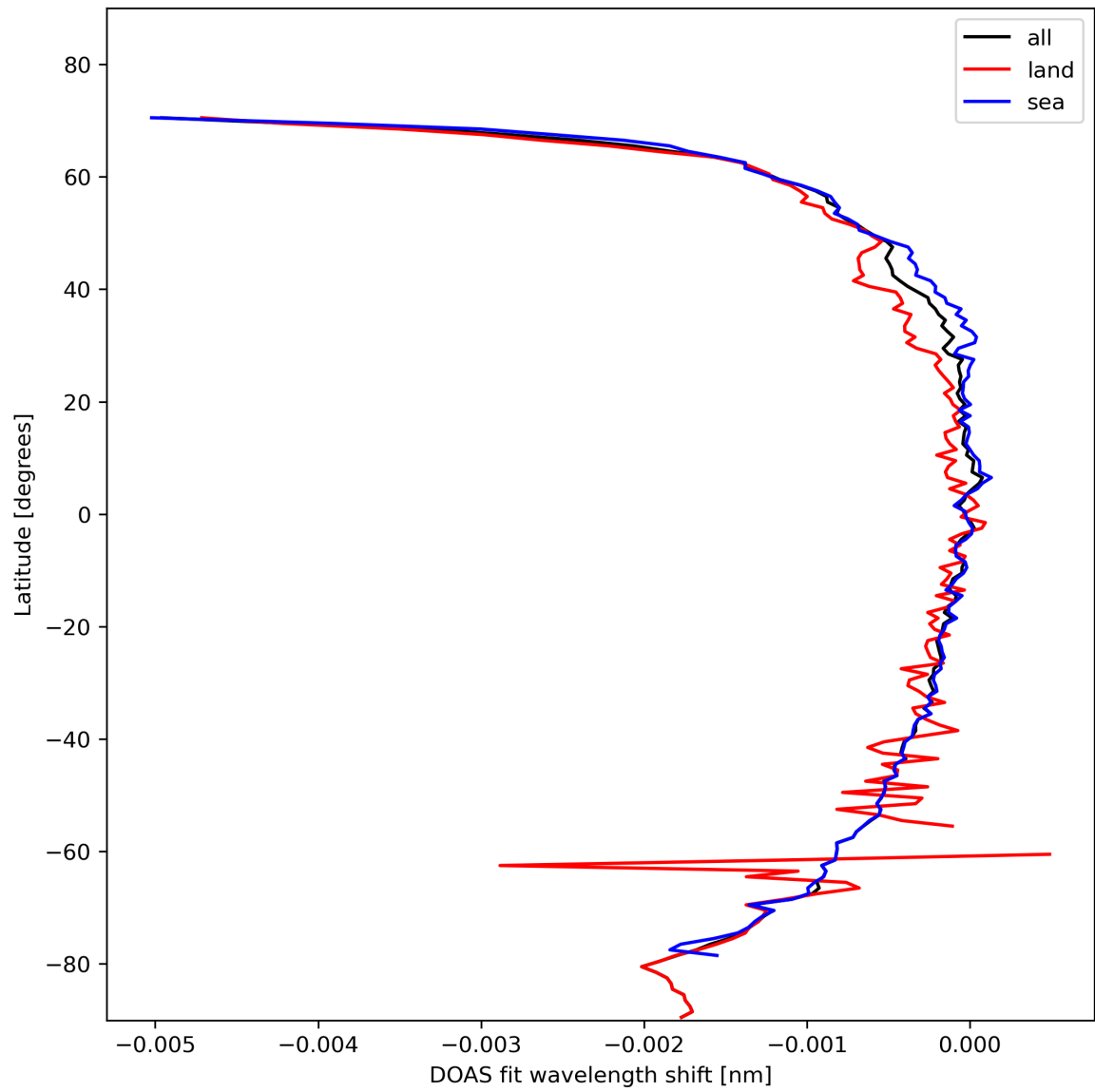
Figure 45: Zonal average of “DOAS fit wavelength shift” for 2024-02-08 to 2024-02-10.
