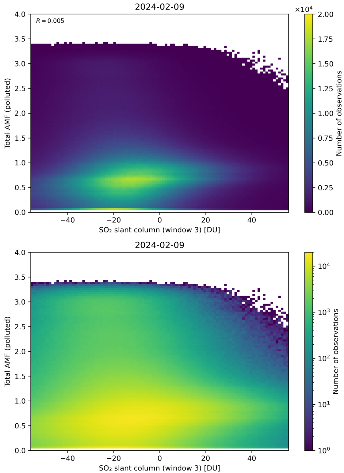
Figure 268: Scatter density plot of “SO 2 slant column (window 3)” against “Total AMF (polluted)” for 2024-02-08 to 2024-02-10.
