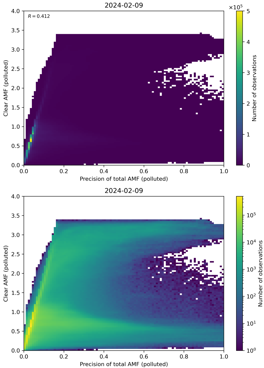
Figure 270: Scatter density plot of “Precision of total AMF (polluted)” against “Clear AMF (polluted)” for 2024-02-08 to 2024-02-10.
