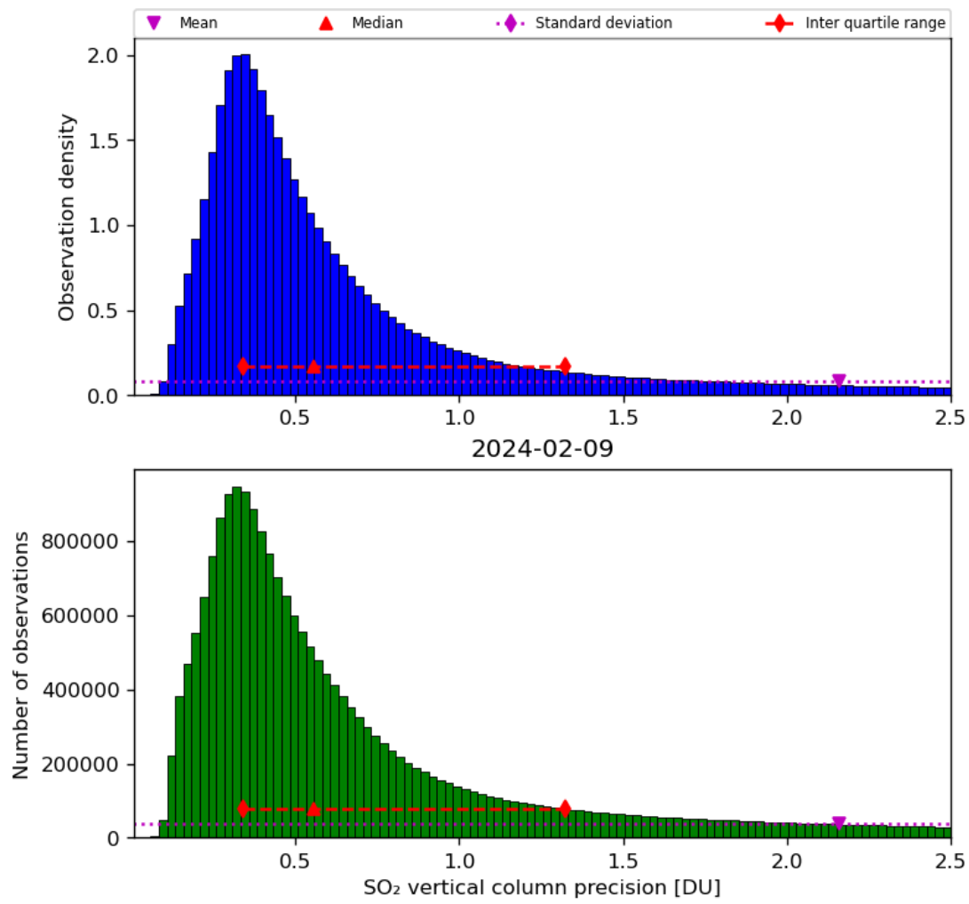
Figure 54: Histogram of “SO 2 vertical column precision” for 2024-02-08 to 2024-02-10
