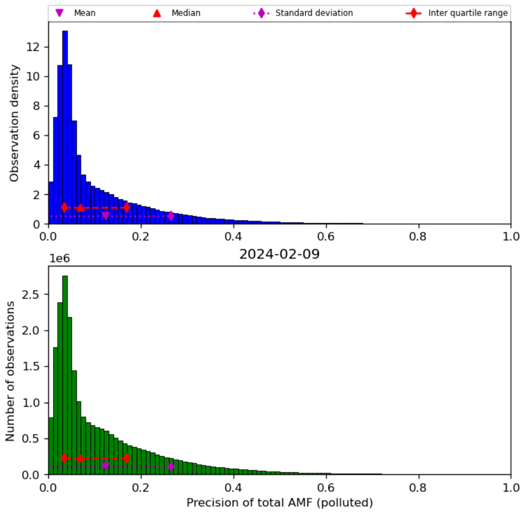
Figure 72: Histogram of “Precision of total AMF (polluted)” for 2024-02-08 to 2024-02-10
