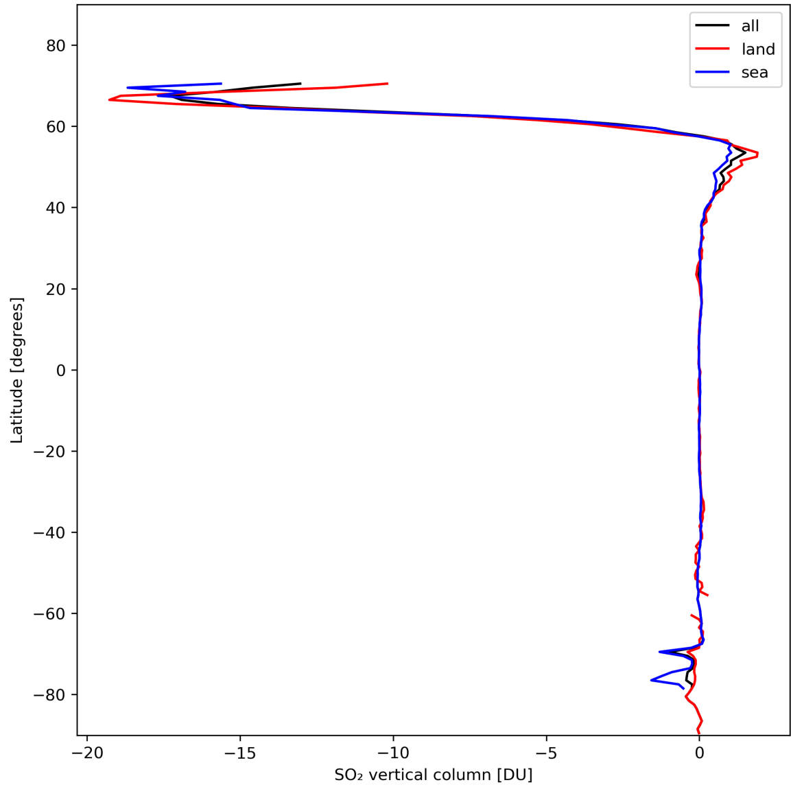
Figure 30: Zonal average of “SO 2 vertical column” for 2024-02-08 to 2024-02-10.
