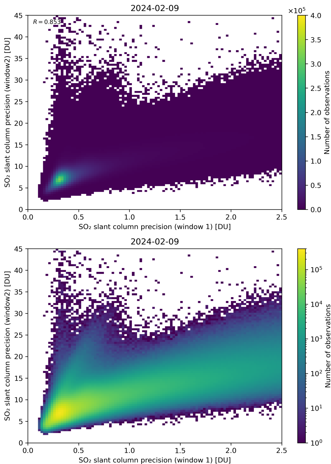
Figure 227: Scatter density plot of “SO 2 slant column precision (window 1)” against “SO 2 slant column precision (window2)” for 2024-02-08 to 2024-02-10.
