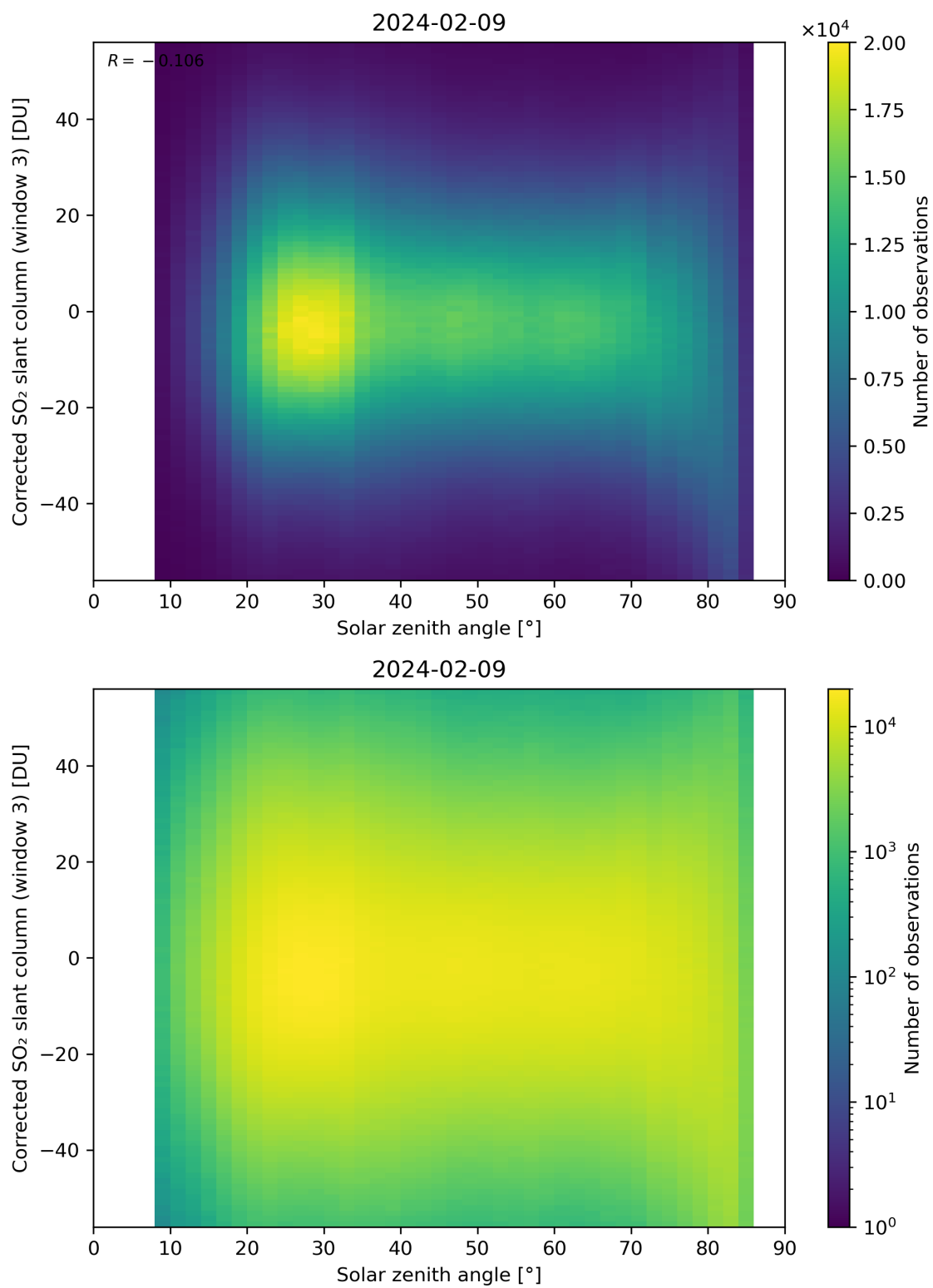
Figure 168: Scatter density plot of “Solar zenith angle” against “Corrected SO 2 slant column (window 3)” for 2024-02-08 to 2024-02-10.
