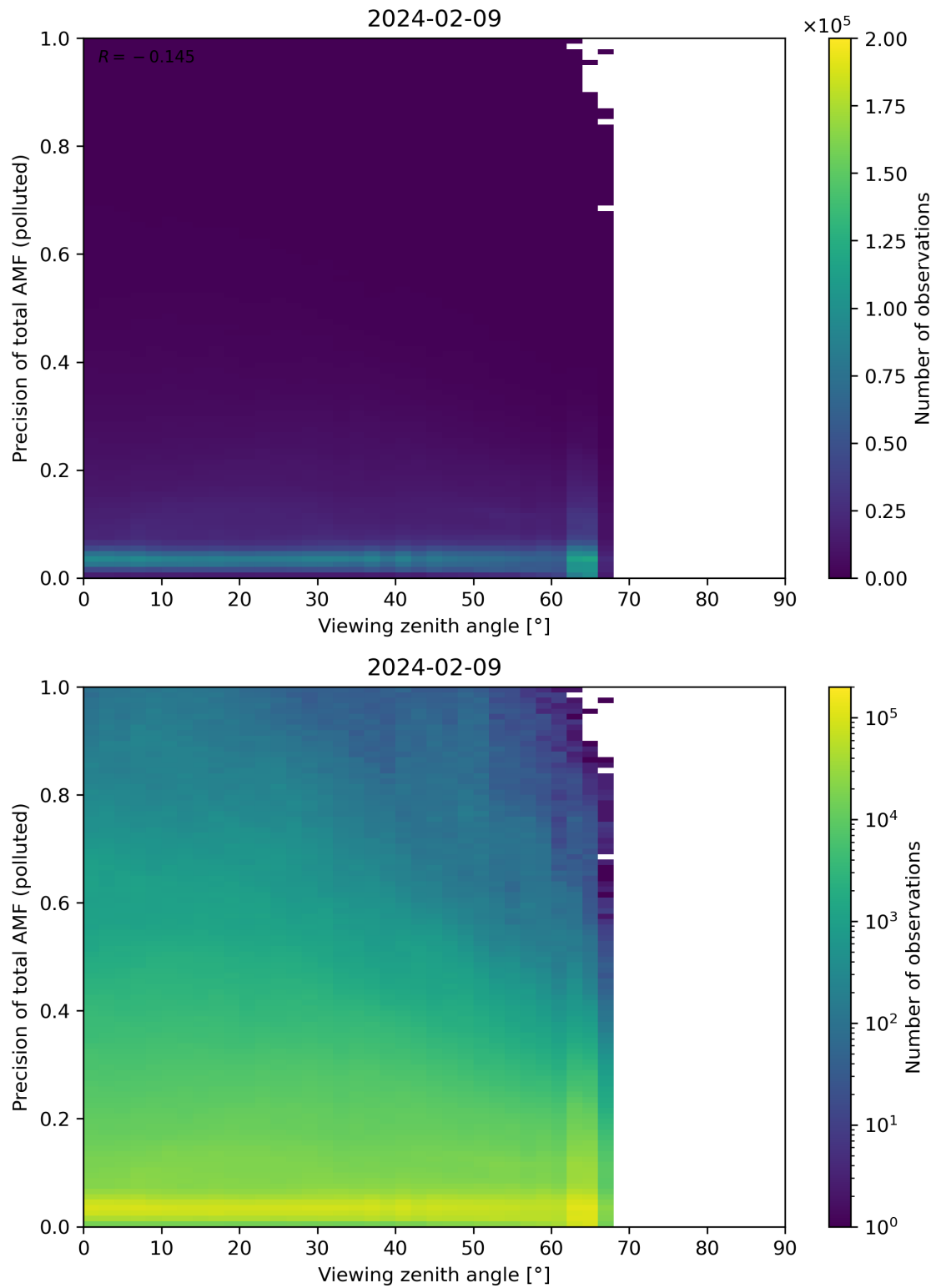
Figure 326: Scatter density plot of “Viewing zenith angle” against “Precision of total AMF (polluted)” for 2024-02-08 to 2024-02-10.
