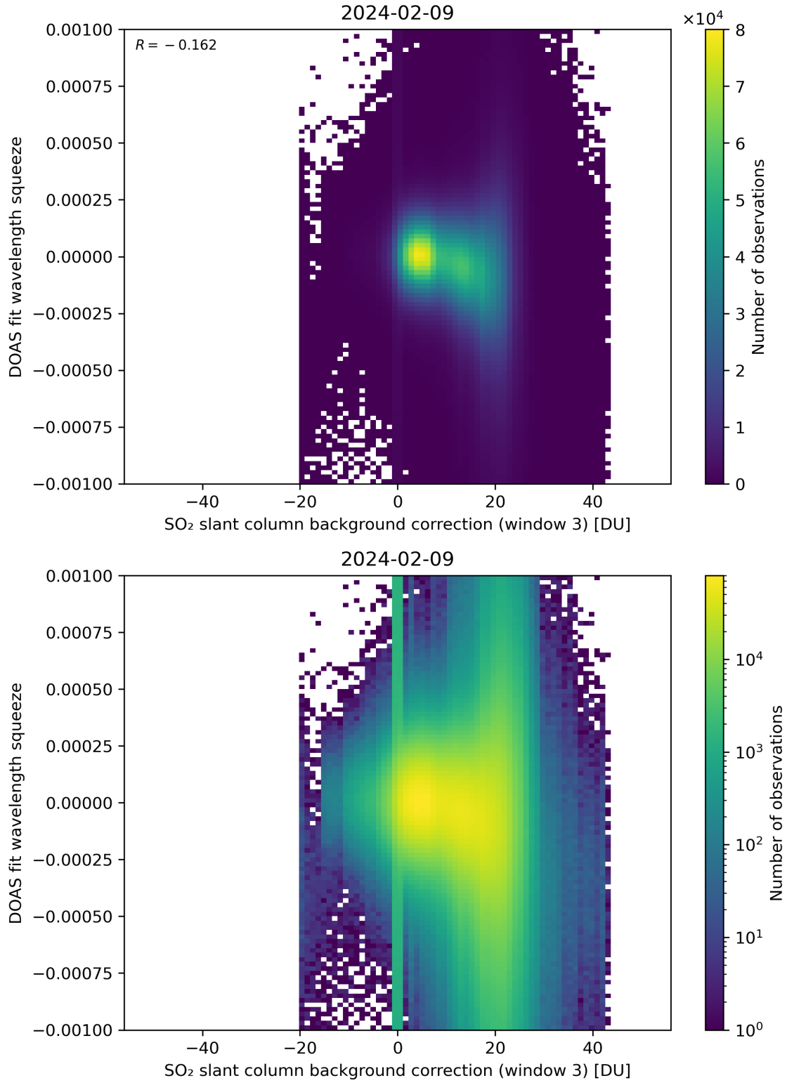
Figure 122: Scatter density plot of “SO 2 slant column background correction (window 3)” against “DOAS fit wavelength squeeze” for 2024-02-08 to 2024-02-10.
