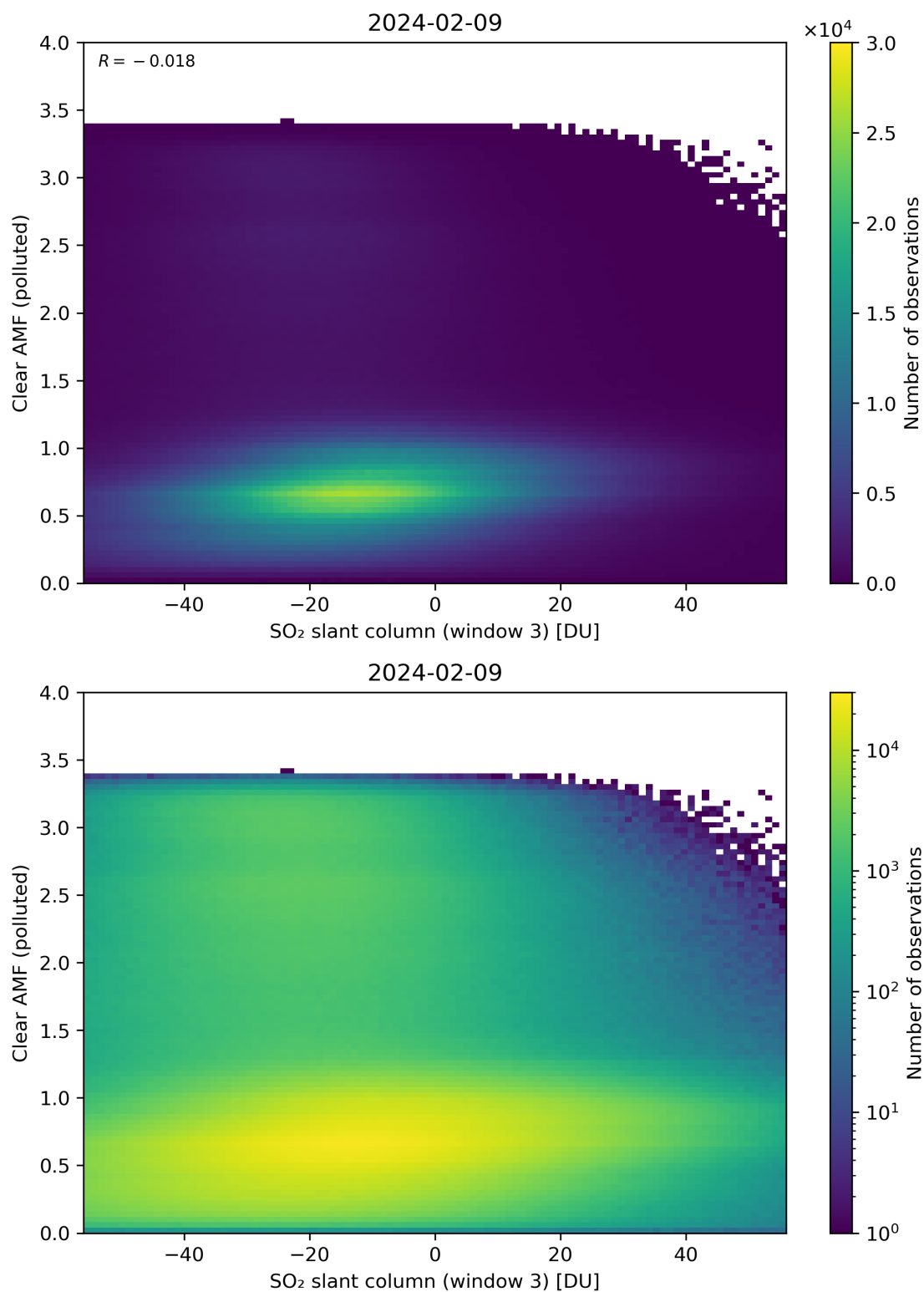
Figure 265: Scatter density plot of “SO 2 slant column (window 3)” against “Clear AMF (polluted)” for 2024-02-08 to 2024-02-10.
