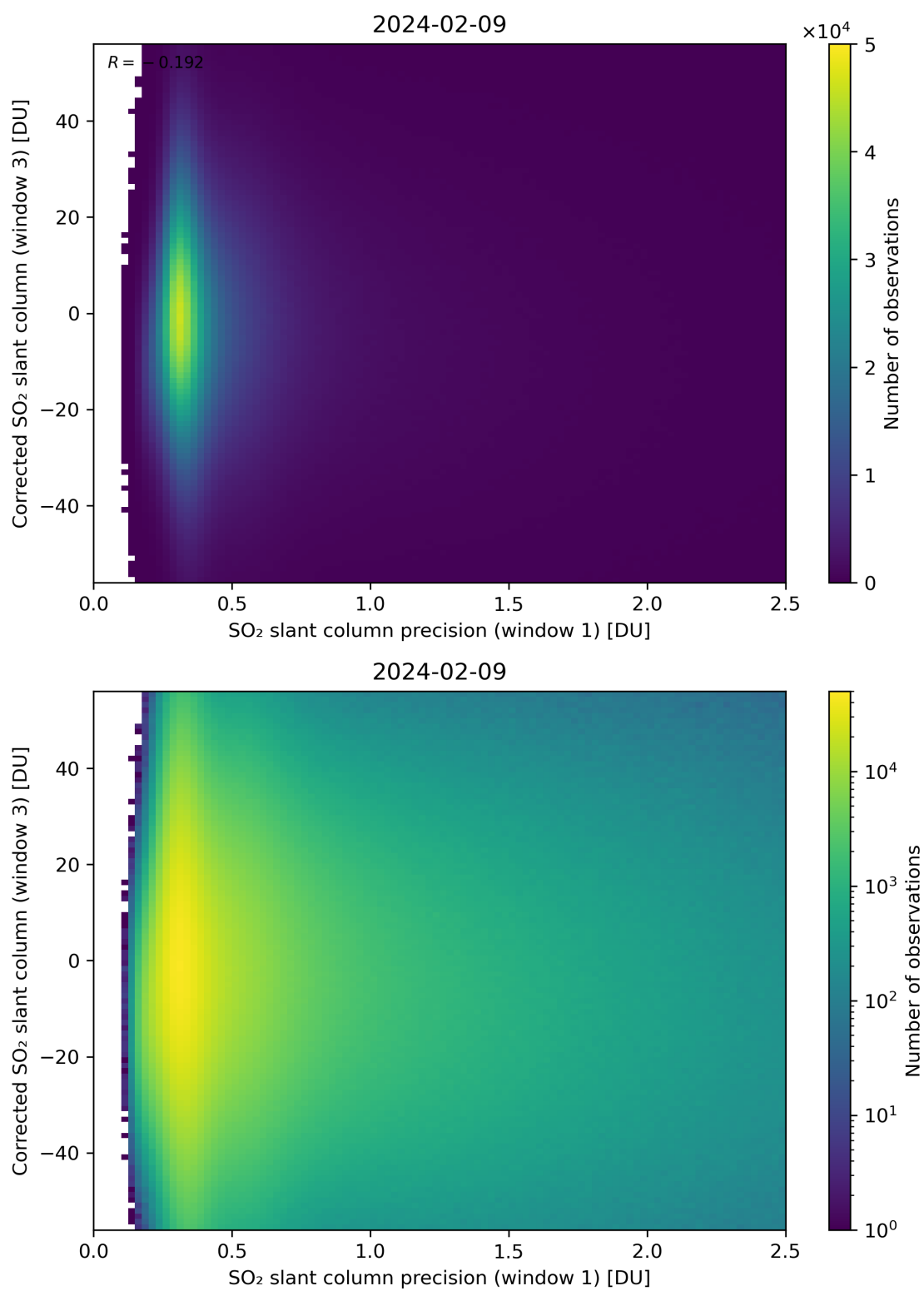
Figure 226: Scatter density plot of “SO 2 slant column precision (window 1)” against “Corrected SO 2 slant column (window 3)” for 2024-02-08 to 2024-02-10.
