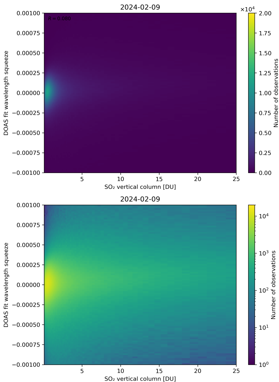
Figure 277: Scatter density plot of “SO 2 vertical column” against “DOAS fit wavelength squeeze” for 2024-02-08 to 2024-02-10.
