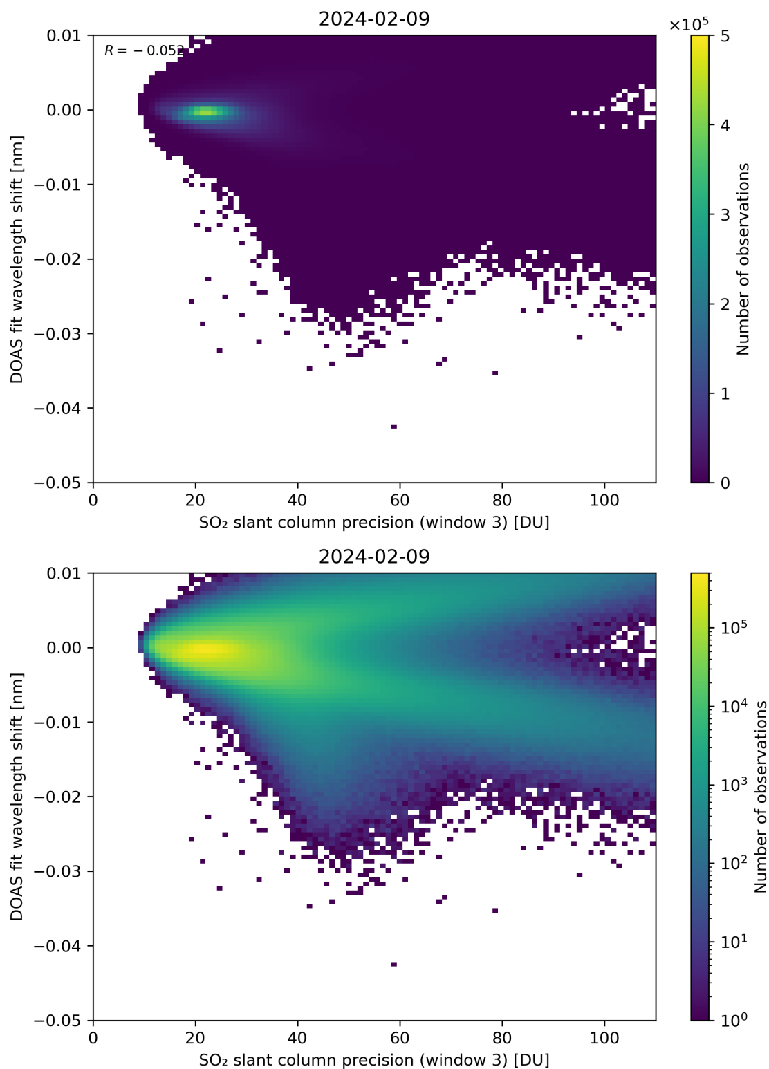
Figure 258: Scatter density plot of “SO 2 slant column precision (window 3)” against “DOAS fit wavelength shift” for 2024-02-08 to 2024-02-10.
