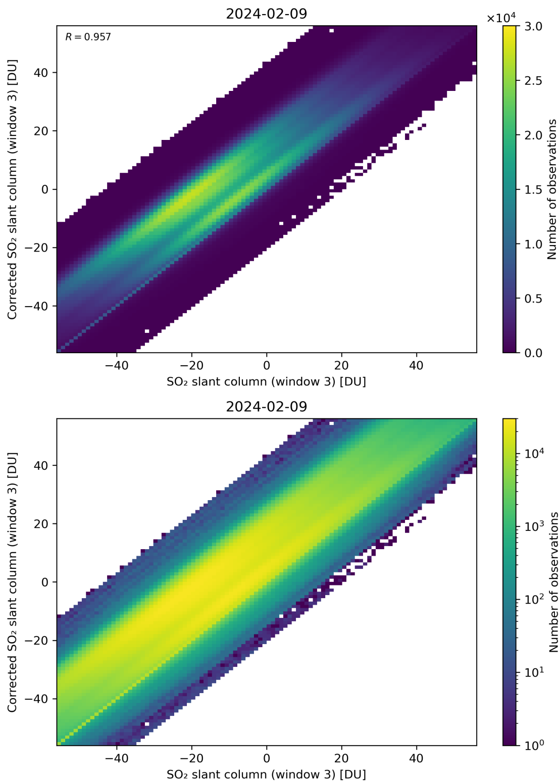
Figure 266: Scatter density plot of “SO 2 slant column (window 3)” against “Corrected SO 2 slant column (window 3)” for 2024-02-08 to 2024-02-10.
