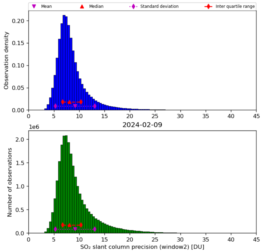
Figure 61: Histogram of “SO 2 slant column precision (window2)” for 2024-02-08 to 2024-02-10
