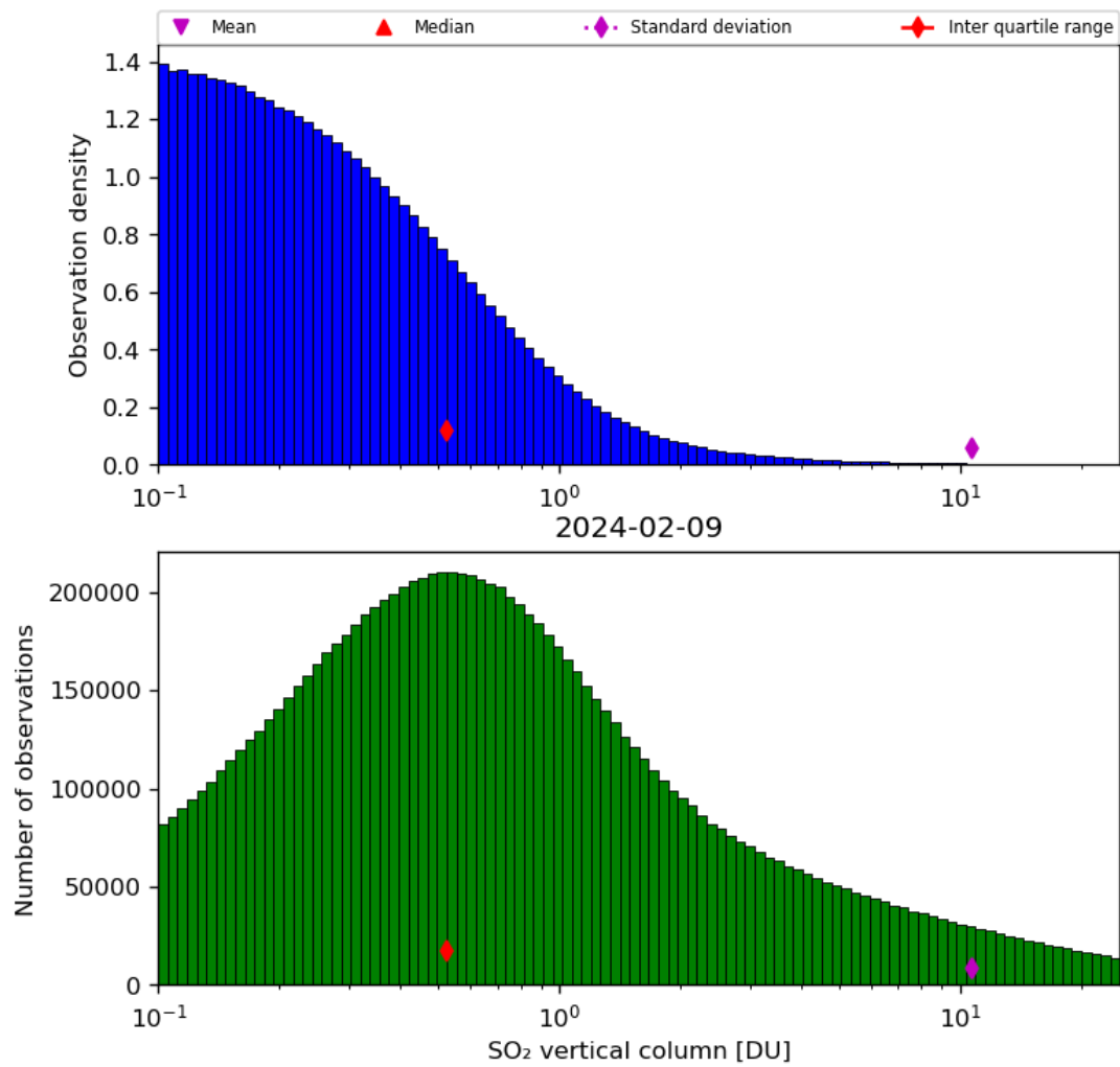
Figure 53: Histogram of “SO 2 vertical column” for 2024-02-08 to 2024-02-10
