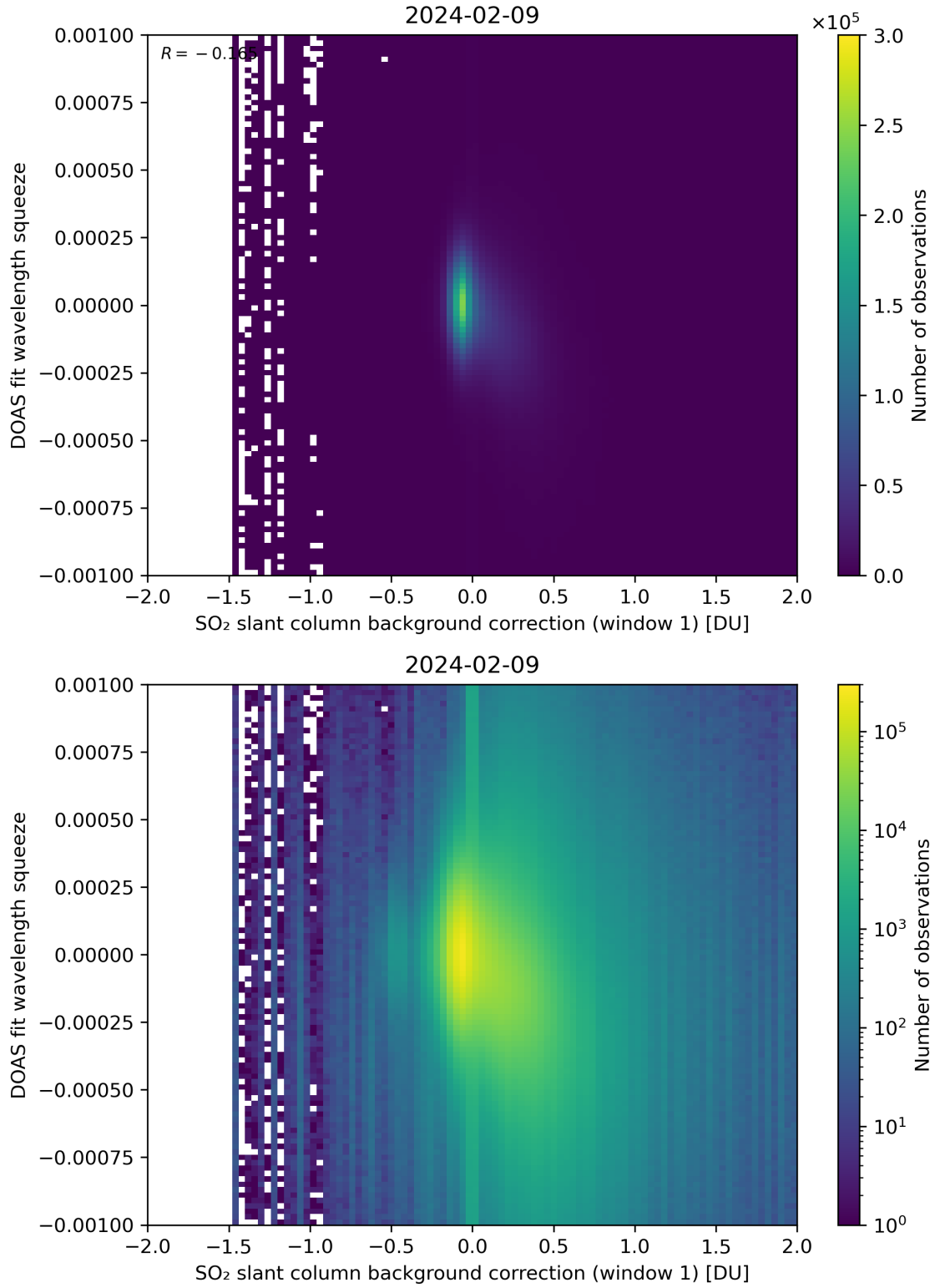
Figure 101: Scatter density plot of “SO 2 slant column background correction (window 1)” against “DOAS fit wavelength squeeze” for 2024-02-08 to 2024-02-10.
