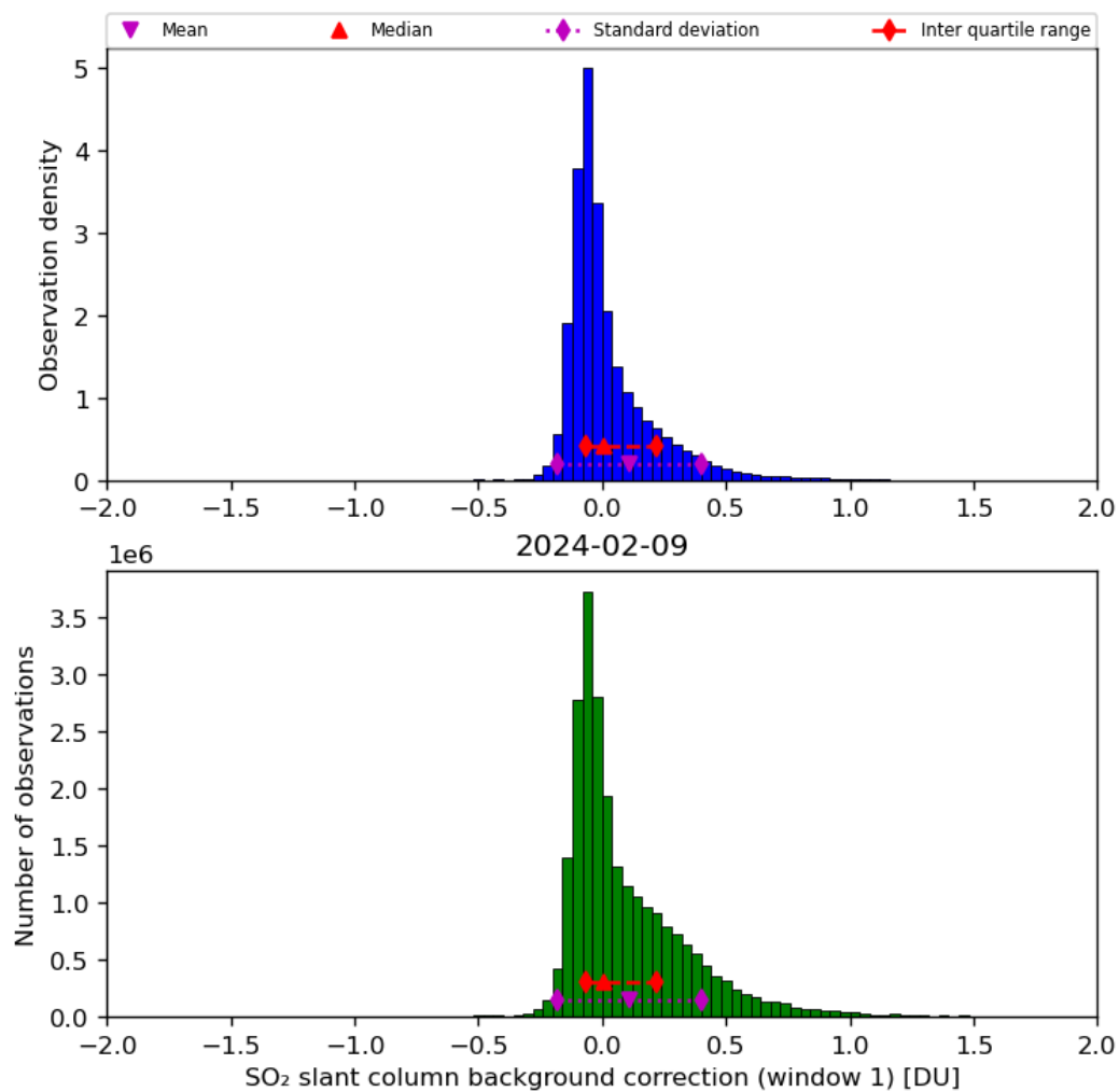
Figure 59: Histogram of “SO 2 slant column background correction (window 1)” for 2024-02-08 to 2024-02-10
