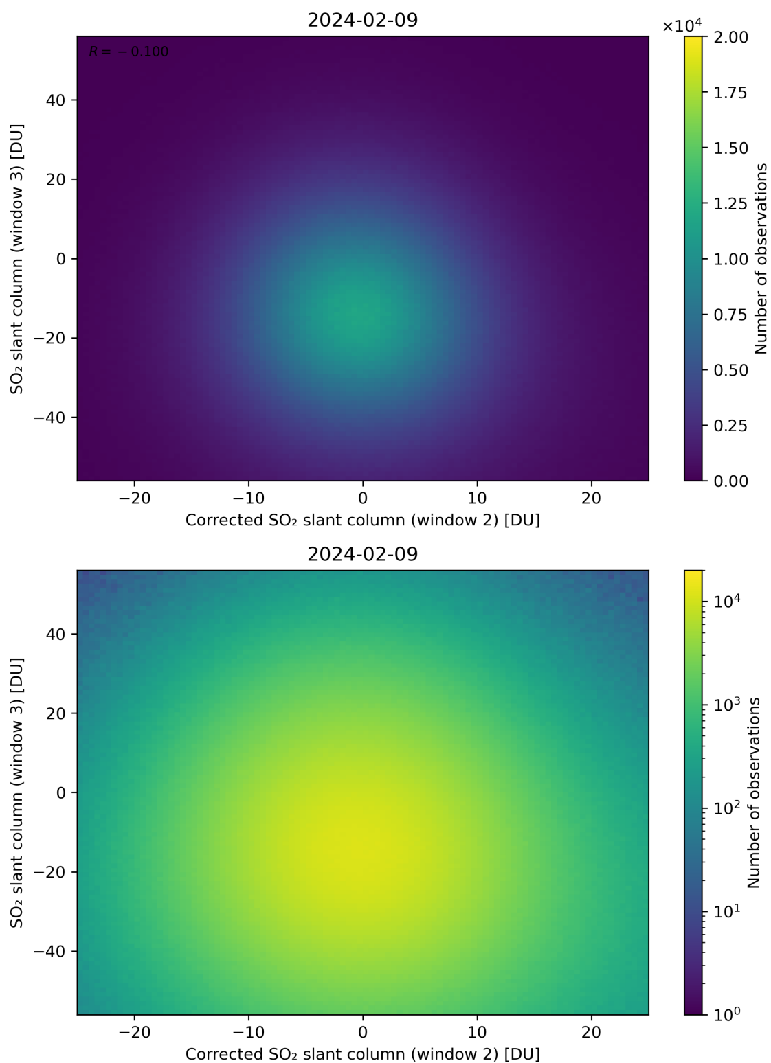
Figure 201: Scatter density plot of “Corrected SO 2 slant column (window 2)” against “SO 2 slant column (window 3)” for 2024-02-08 to 2024-02-10.
