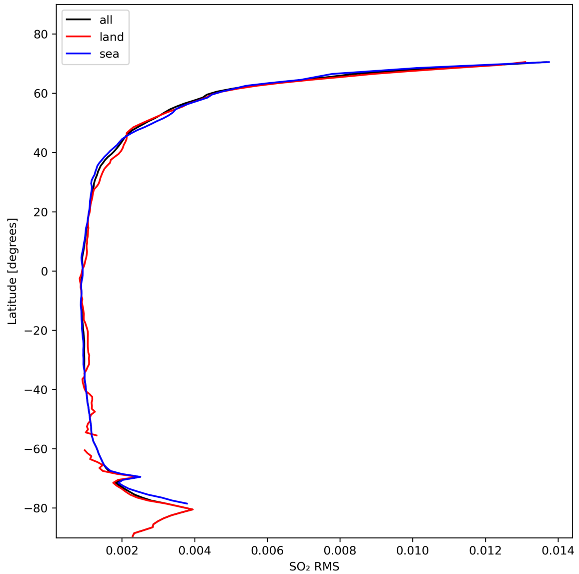
Figure 47: Zonal average of “SO 2 RMS” for 2024-02-08 to 2024-02-10.
