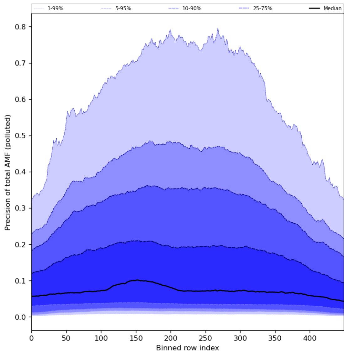
Figure 95: Along track statistics of “Precision of total AMF (polluted)” for 2024-02-08 to 2024-02-10
