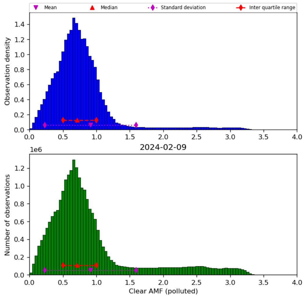
Figure 73: Histogram of “Clear AMF (polluted)” for 2024-02-08 to 2024-02-10
