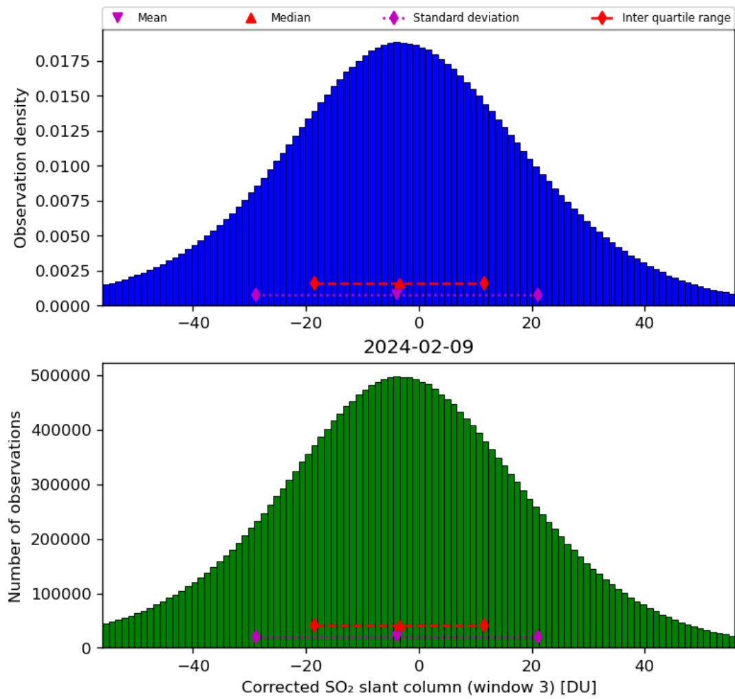
Figure 66: Histogram of “Corrected SO 2 slant column (window 3)” for 2024-02-08 to 2024-02-10
