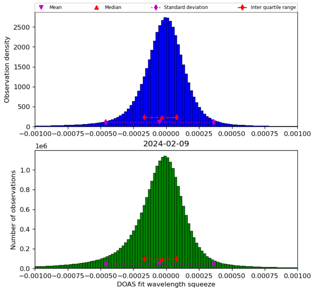
Figure 69: Histogram of “DOAS fit wavelength squeeze” for 2024-02-08 to 2024-02-10
