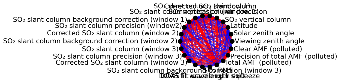
Figure 1: Map of correlation graph for 2024-02-08 to 2024-02-10.
