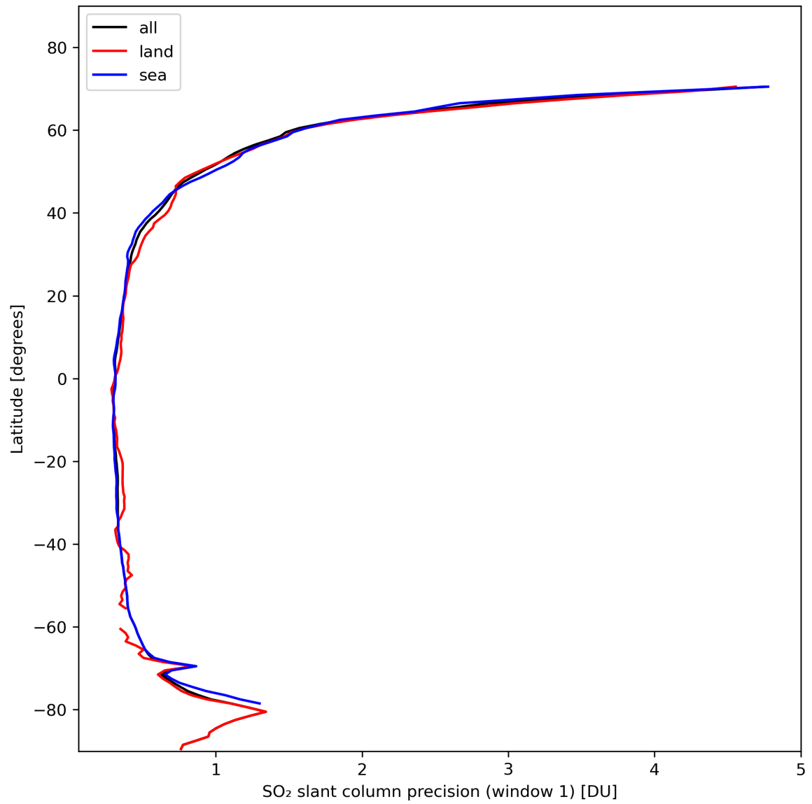
Figure 34: Zonal average of “SO 2 slant column precision (window 1)” for 2024-02-08 to 2024-02-10.
