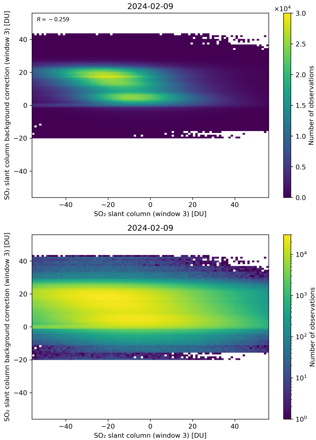
Figure 253: Scatter density plot of “SO 2 slant column (window 3)” against “SO 2 slant column background correction (window 3)” for 2024-02-08 to 2024-02-10.
