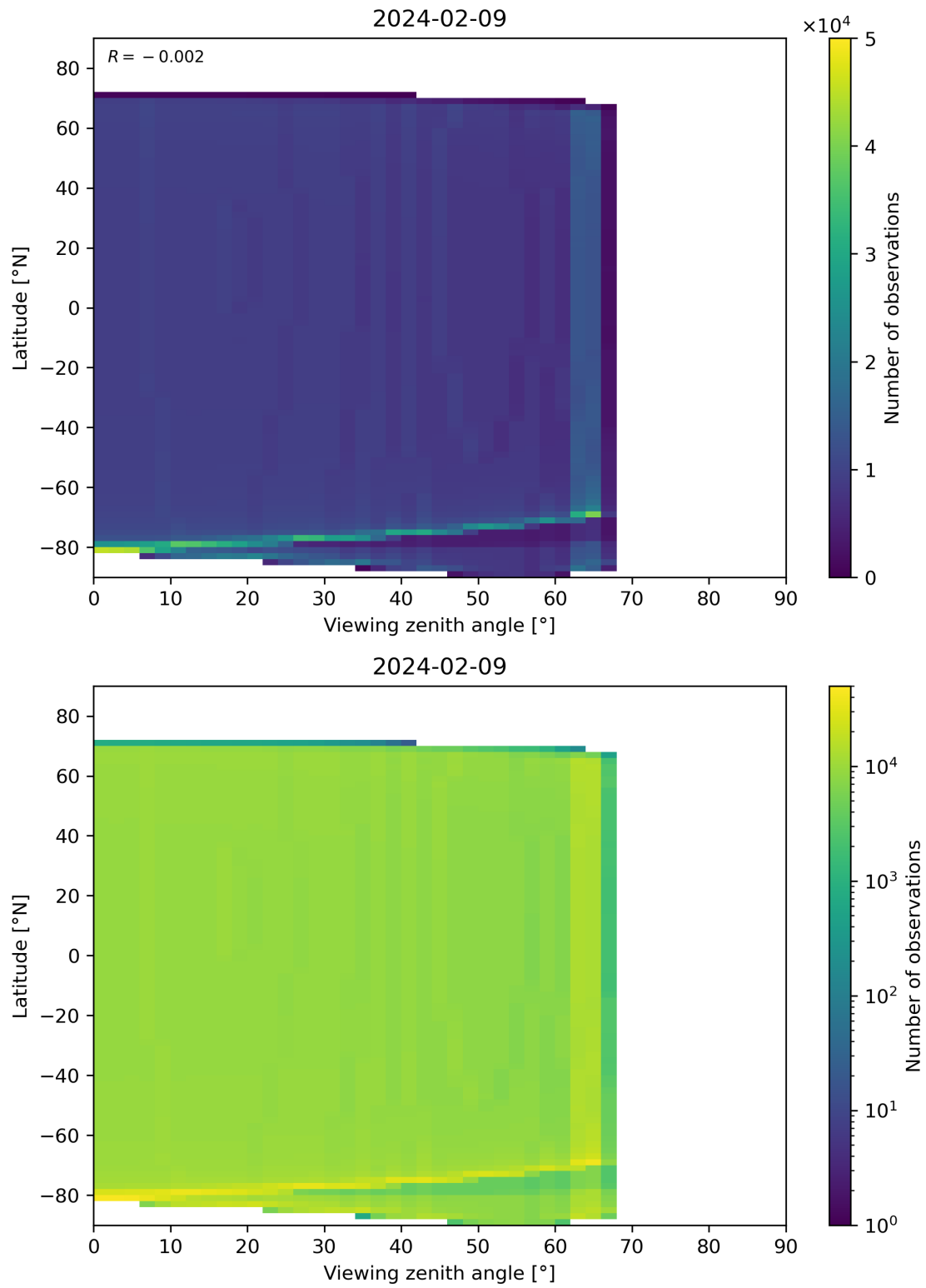
Figure 314: Scatter density plot of “Viewing zenith angle” against “Latitude” for 2024-02-08 to 2024-02-10.
