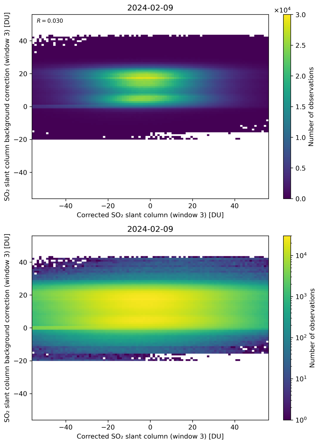
Figure 205: Scatter density plot of “Corrected SO 2 slant column (window 3)” against “SO 2 slant column background correction (window 3)” for 2024-02-08 to 2024-02-10.
