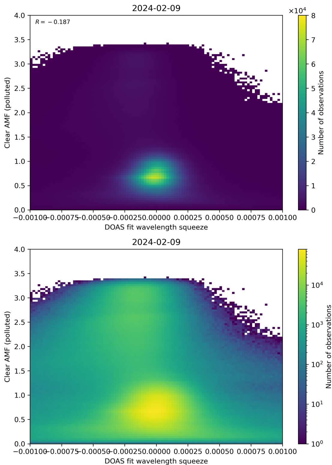
Figure 133: Scatter density plot of “DOAS fit wavelength squeeze” against “Clear AMF (polluted)” for 2024-02-08 to 2024-02-10.
