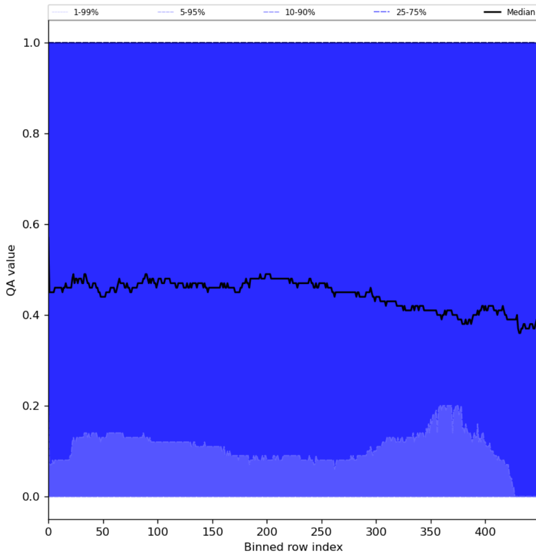
Figure 75: Along track statistics of “QA value” for 2024-02-08 to 2024-02-10
