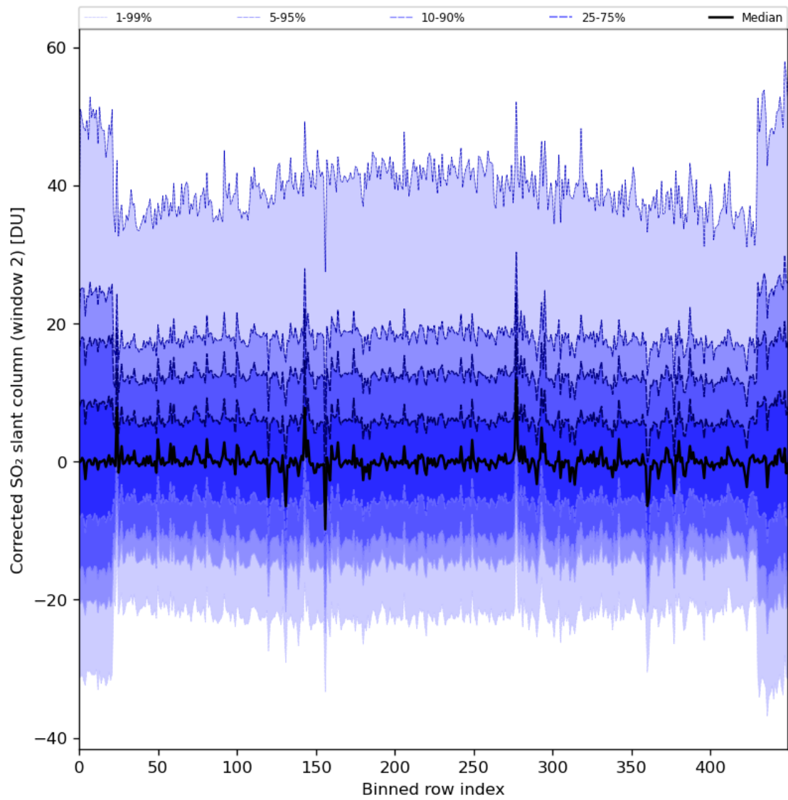
Figure 85: Along track statistics of “Corrected SO 2 slant column (window 2)” for 2024-02-08 to 2024-02-10
