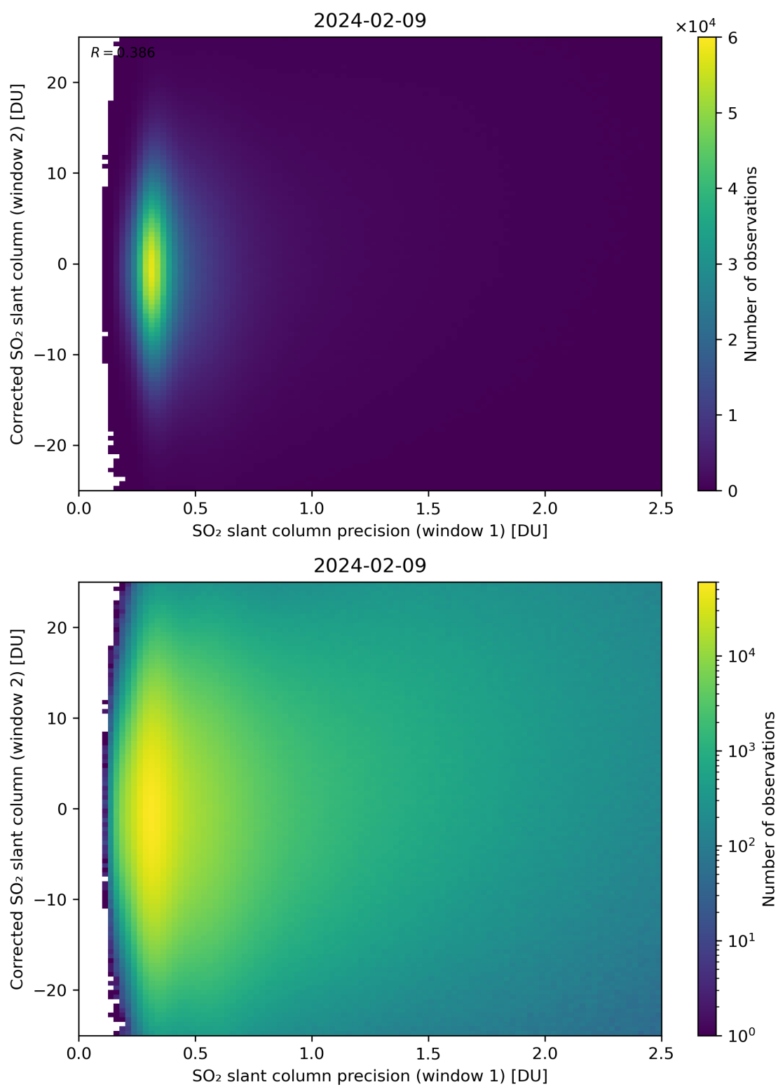
Figure 225: Scatter density plot of “SO 2 slant column precision (window 1)” against “Corrected SO 2 slant column (window 2)” for 2024-02-08 to 2024-02-10.
