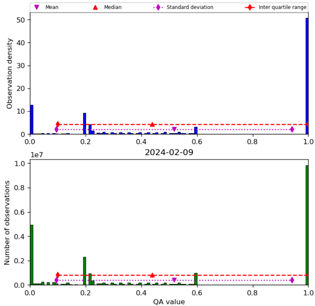
Figure 52: Histogram of “QA value” for 2024-02-08 to 2024-02-10
