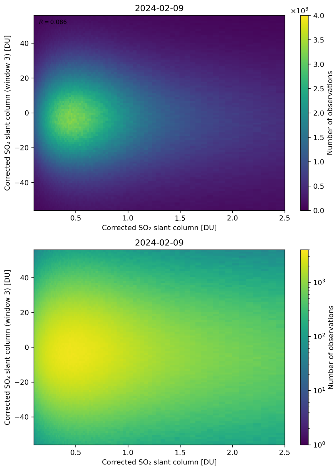
Figure 186: Scatter density plot of “Corrected SO 2 slant column” against “Corrected SO 2 slant column (window 3)” for 2024-02-08 to 2024-02-10.
