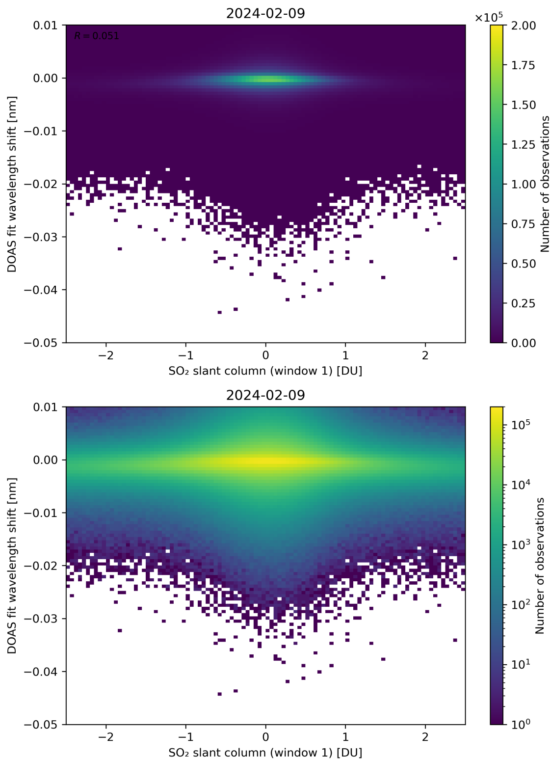
Figure 215: Scatter density plot of “SO 2 slant column (window 1)” against “DOAS fit wavelength shift” for 2024-02-08 to 2024-02-10.
