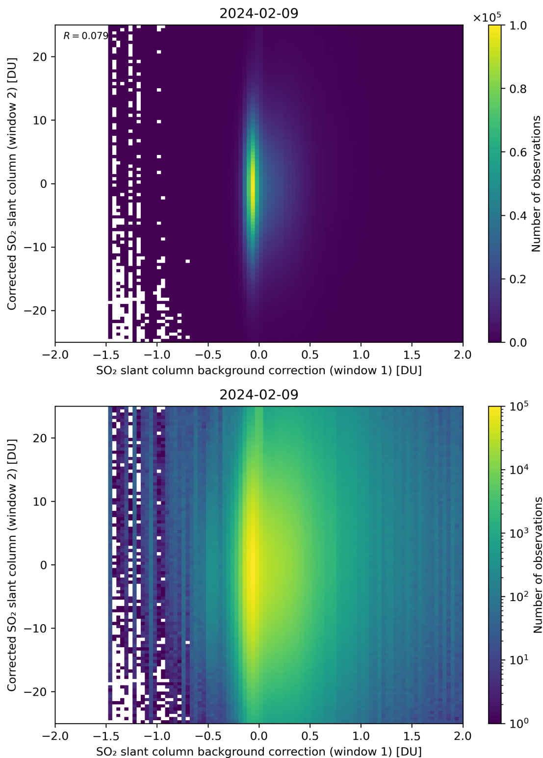
Figure 104: Scatter density plot of “SO 2 slant column background correction (window 1)” against “Corrected SO 2 slant column (window 2)” for 2024-02-08 to 2024-02-10.
