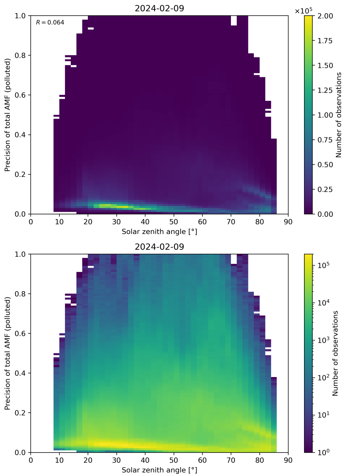
Figure 175: Scatter density plot of “Solar zenith angle” against “Precision of total AMF (polluted)” for 2024-02-08 to 2024-02-10.
