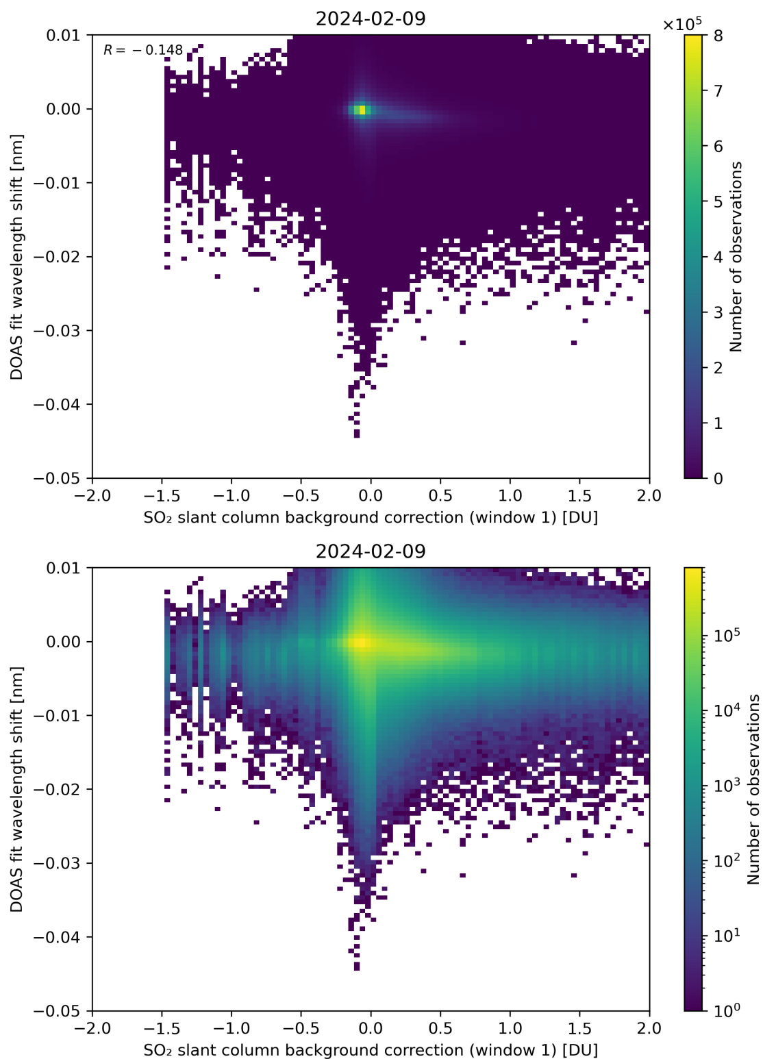
Figure 100: Scatter density plot of “SO 2 slant column background correction (window 1)” against “DOAS fit wavelength shift” for 2024-02-08 to 2024-02-10.
