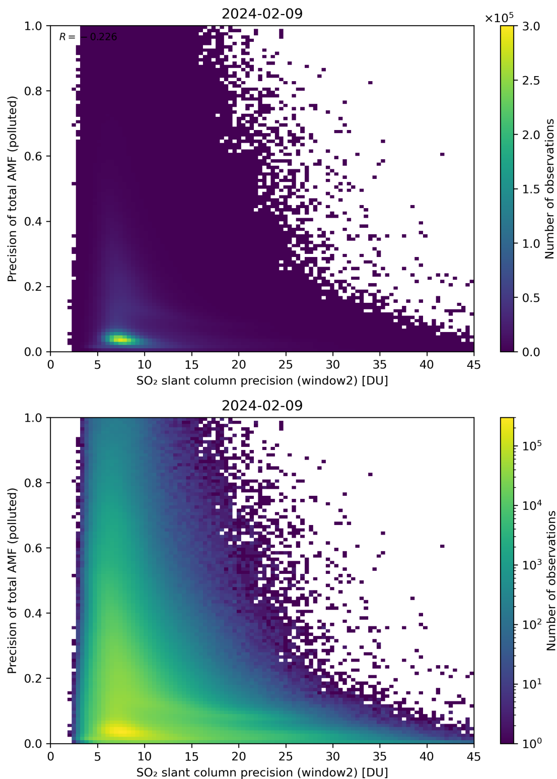
Figure 252: Scatter density plot of “SO 2 slant column precision (window2)” against “Precision of total AMF (polluted)” for 2024-02-08 to 2024-02-10.
