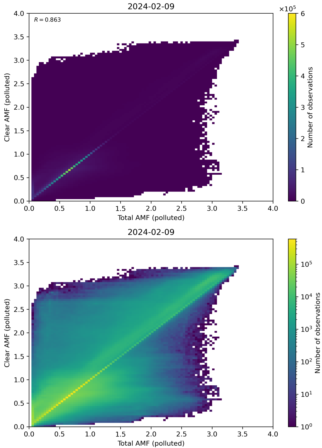
Figure 271: Scatter density plot of “Total AMF (polluted)” against “Clear AMF (polluted)” for 2024-02-08 to 2024-02-10.
