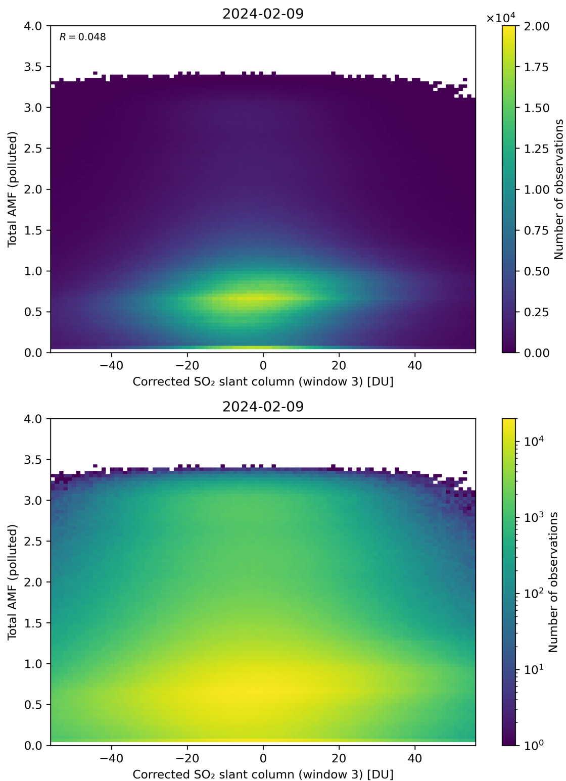
Figure 210: Scatter density plot of “Corrected SO 2 slant column (window 3)” against “Total AMF (polluted)” for 2024-02-08 to 2024-02-10.
