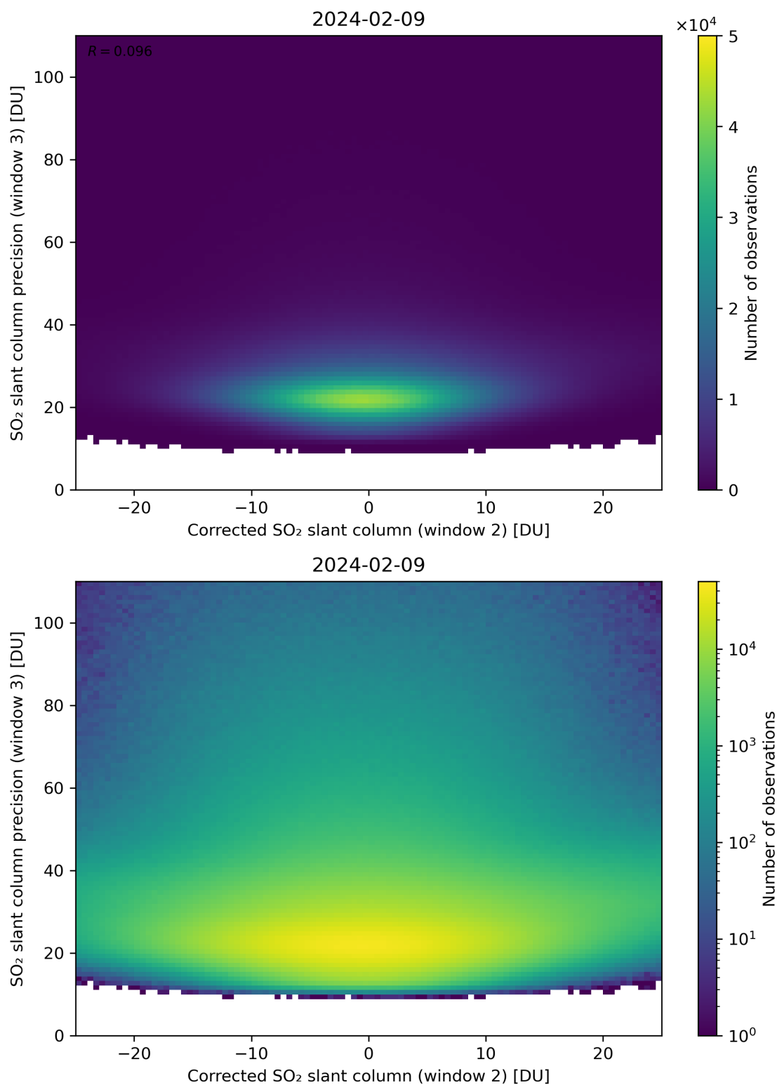
Figure 202: Scatter density plot of “Corrected SO 2 slant column (window 2)” against “SO 2 slant column precision (window 3)” for 2024-02-08 to 2024-02-10.
