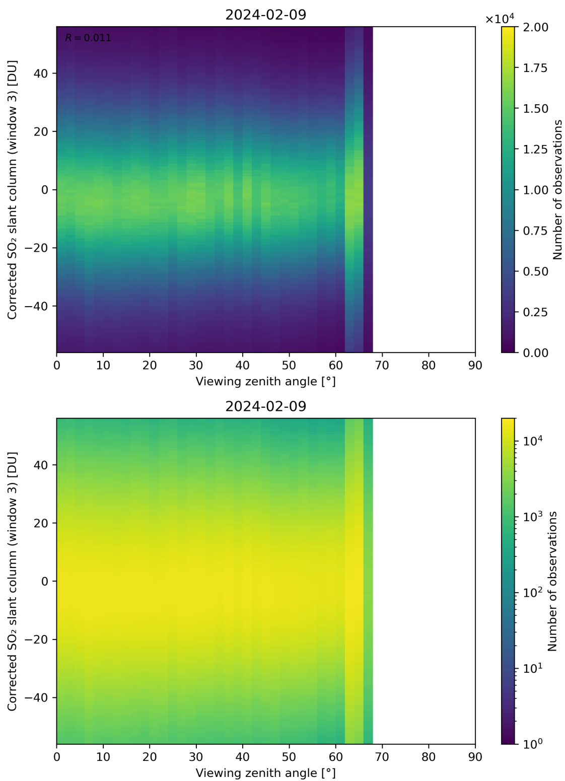
Figure 319: Scatter density plot of “Viewing zenith angle” against “Corrected SO 2 slant column (window 3)” for 2024-02-08 to 2024-02-10.
