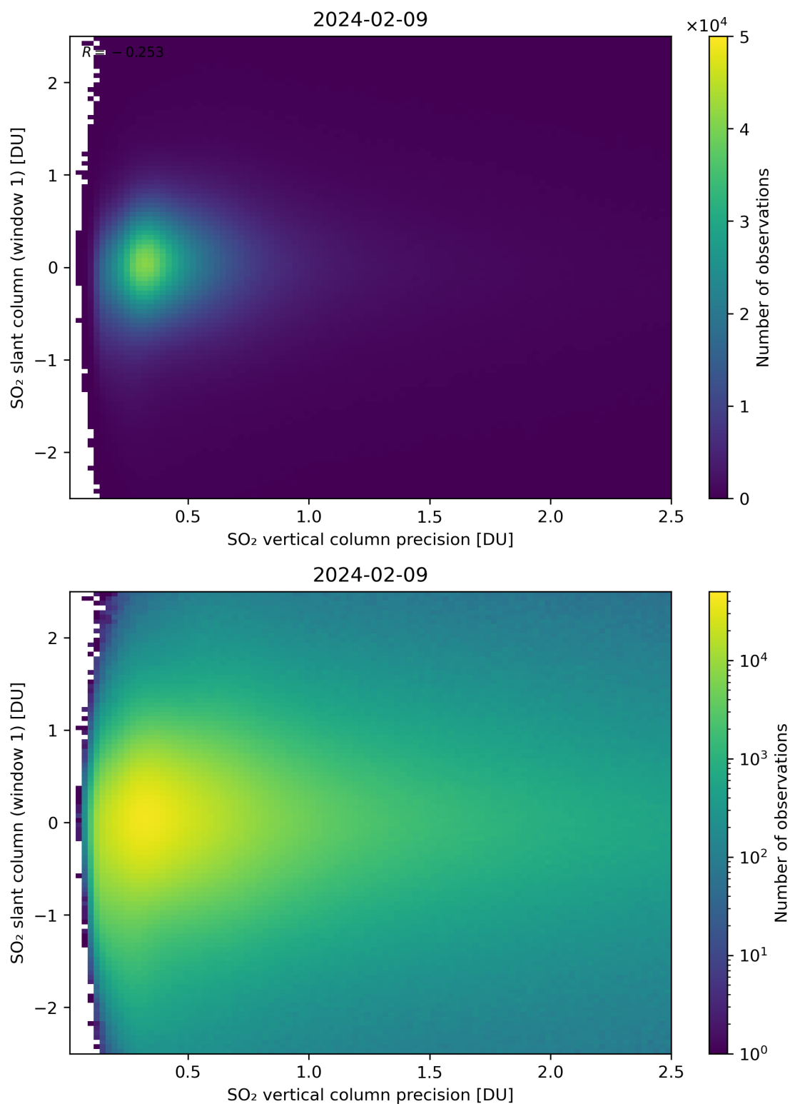
Figure 289: Scatter density plot of “SO 2 vertical column precision” against “SO 2 slant column (window 1)” for 2024-02-08 to 2024-02-10.
