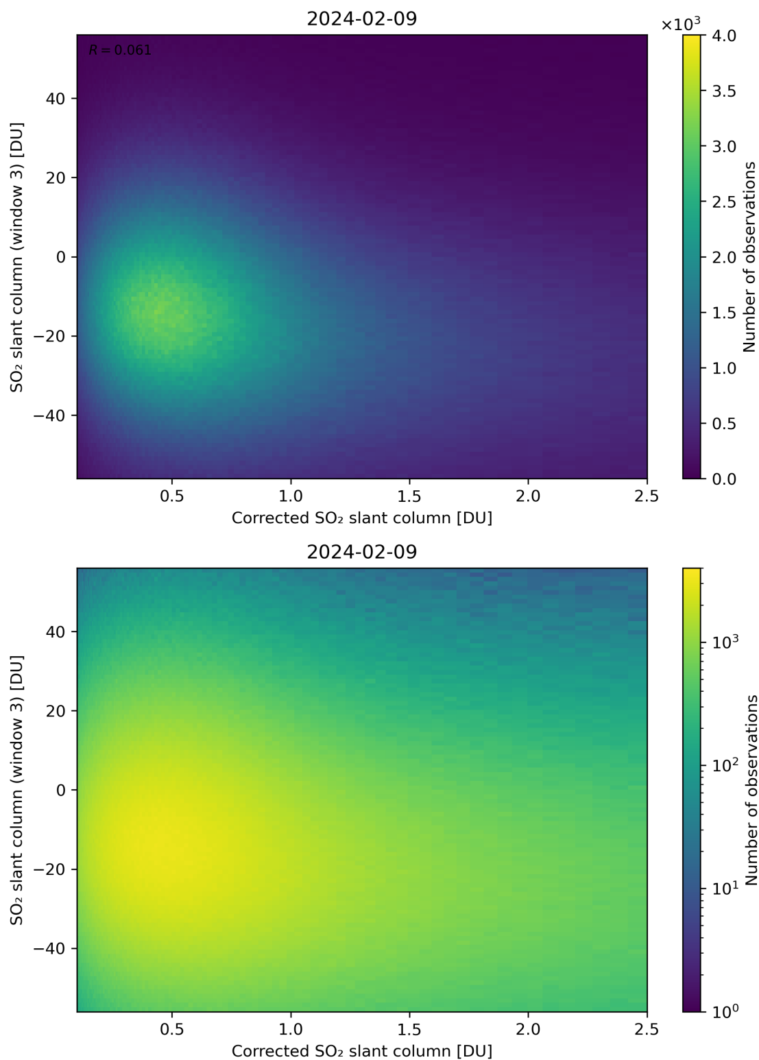
Figure 190: Scatter density plot of “Corrected SO 2 slant column” against “SO 2 slant column (window 3)” for 2024-02-08 to 2024-02-10.
