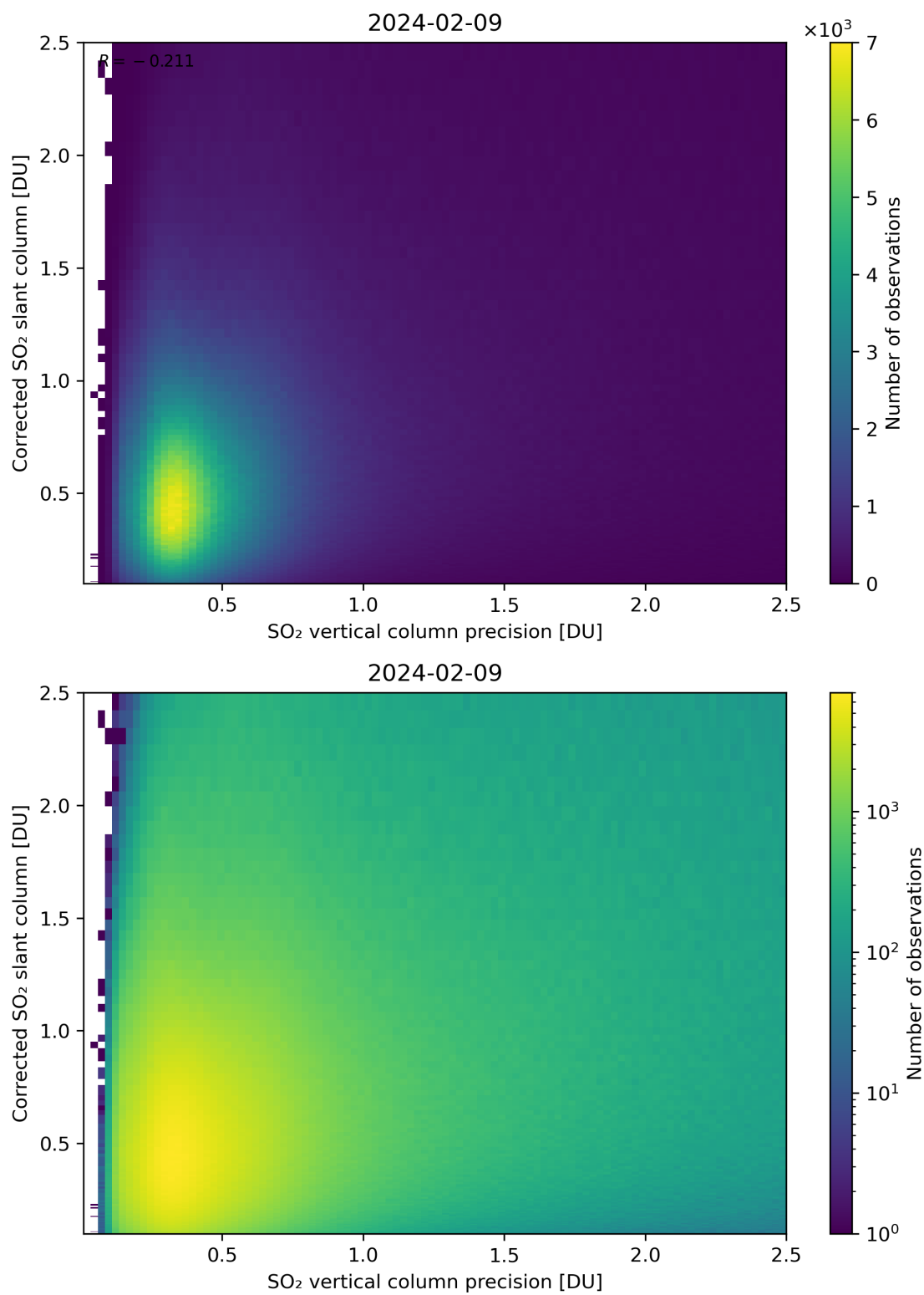
Figure 286: Scatter density plot of “SO 2 vertical column precision” against “Corrected SO 2 slant column” for 2024-02-08 to 2024-02-10.
