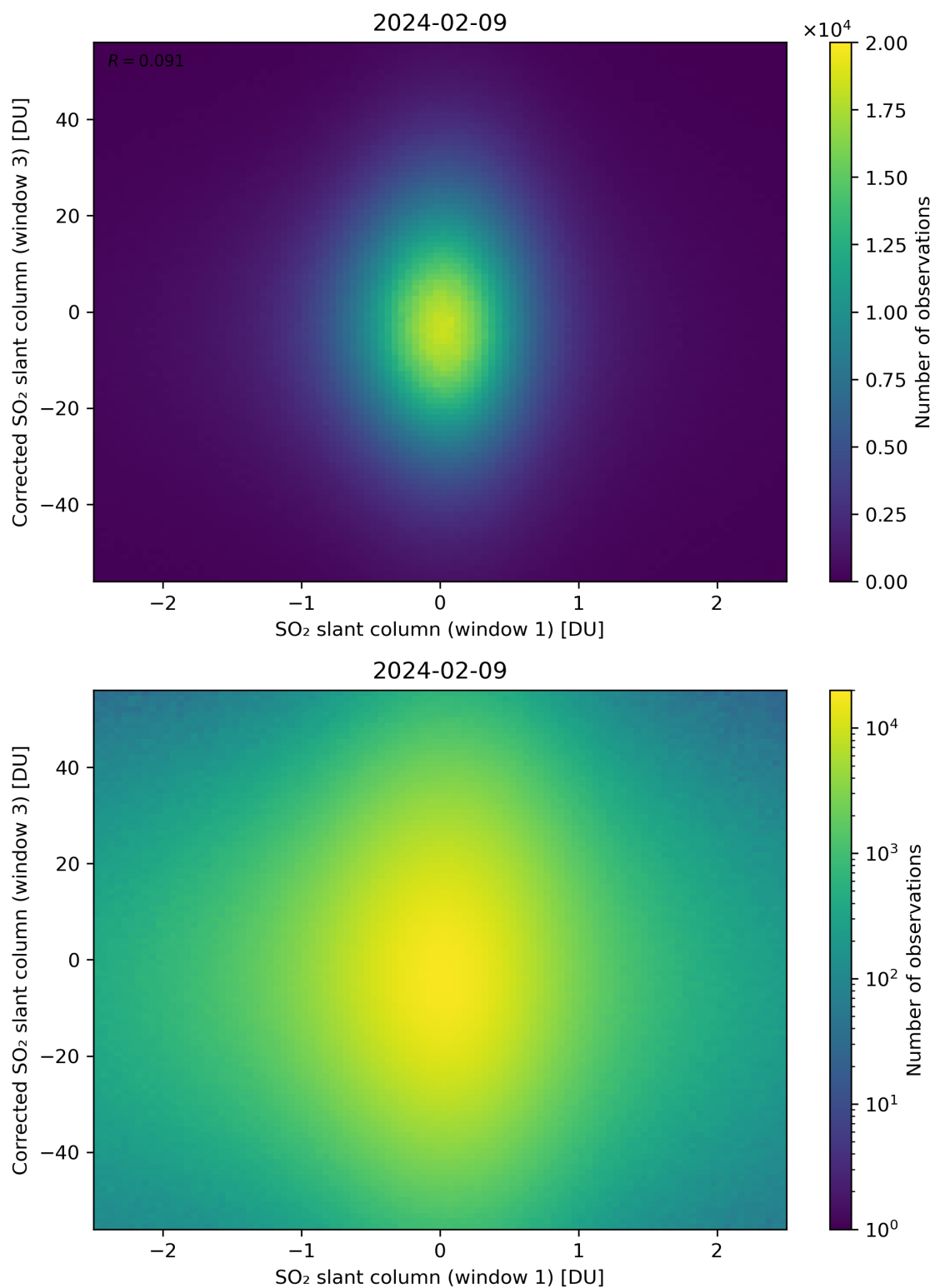
Figure 234: Scatter density plot of “SO 2 slant column (window 1)” against “Corrected SO 2 slant column (window 3)” for 2024-02-08 to 2024-02-10.
