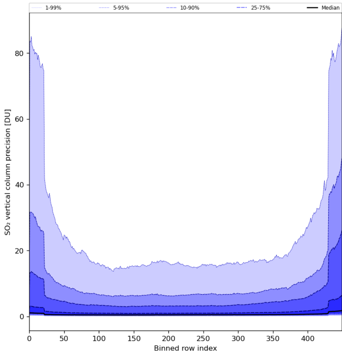
Figure 77: Along track statistics of “SO 2 vertical column precision” for 2024-02-08 to 2024-02-10
