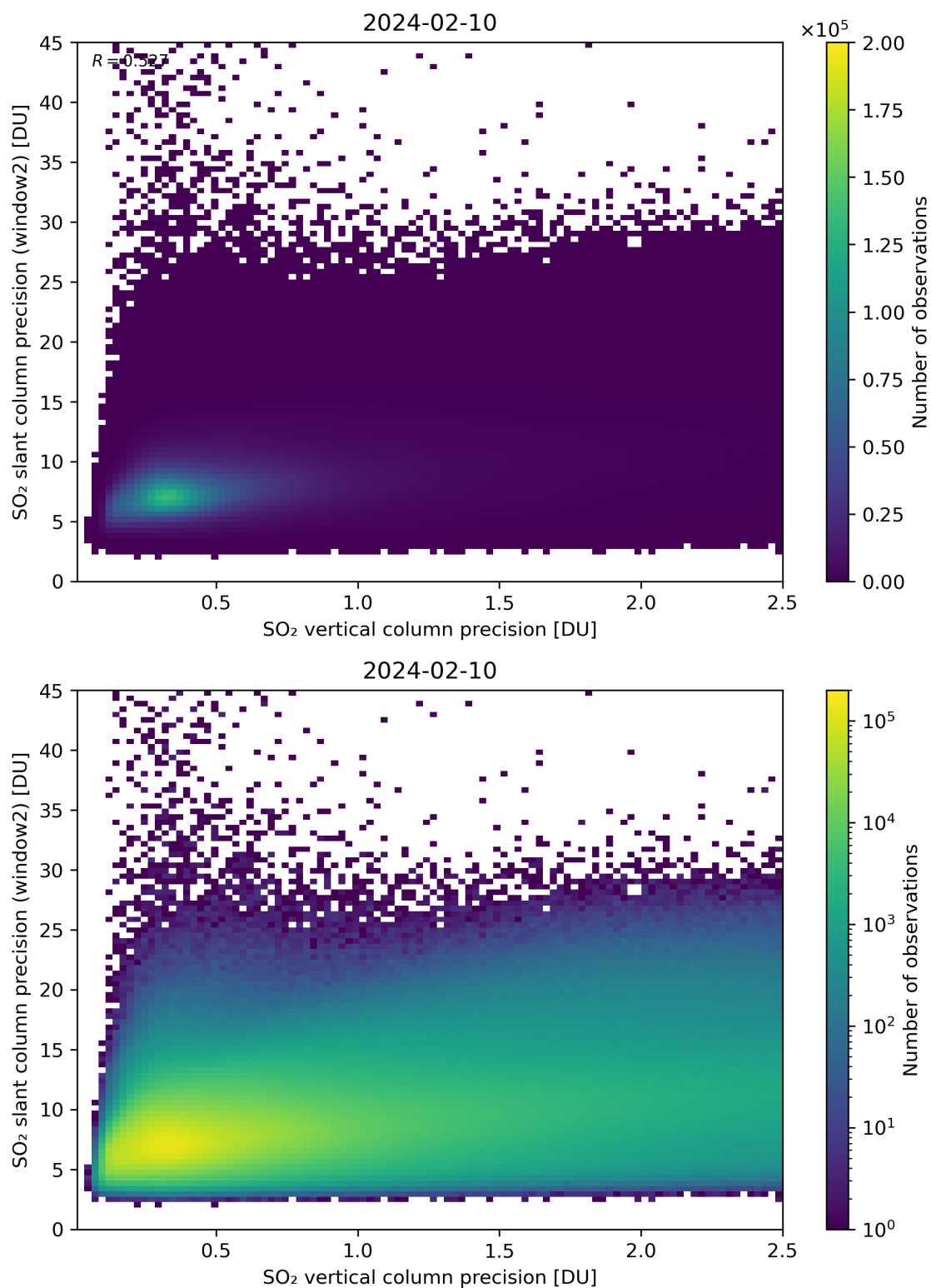
Figure 291: Scatter density plot of “SO 2 vertical column precision” against “SO 2 slant column precision (window2)” for 2024-02-09 to 2024-02-11.
