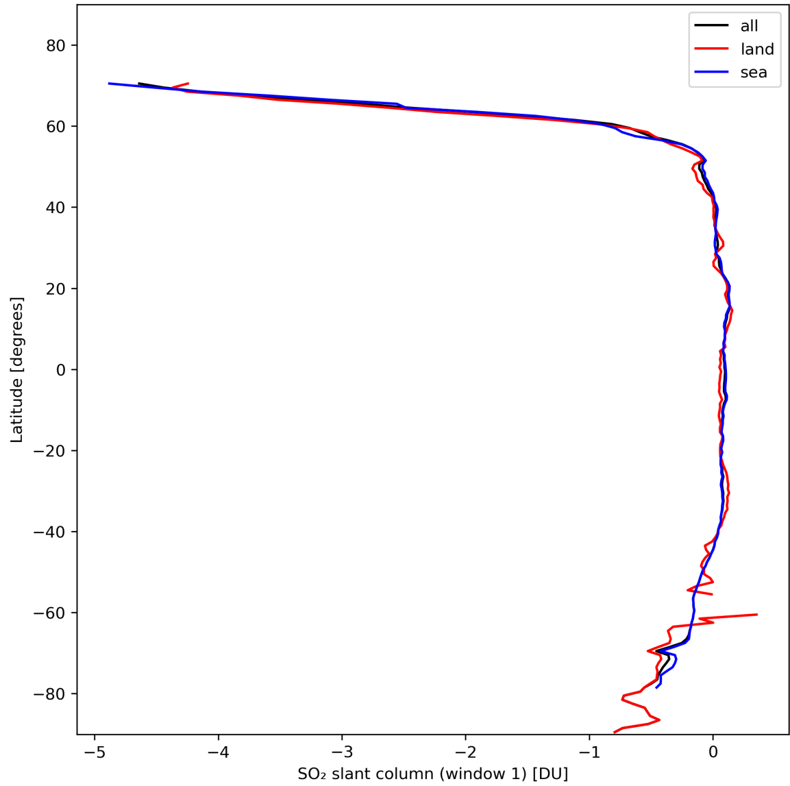
Figure 33: Zonal average of “SO 2 slant column (window 1)” for 2024-02-09 to 2024-02-11.
