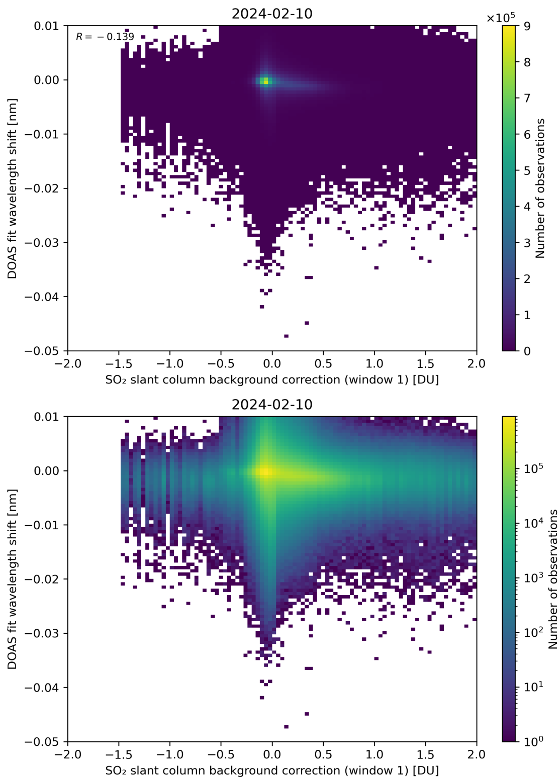
Figure 100: Scatter density plot of “SO 2 slant column background correction (window 1)” against “DOAS fit wavelength shift” for 2024-02-09 to 2024-02-11.
