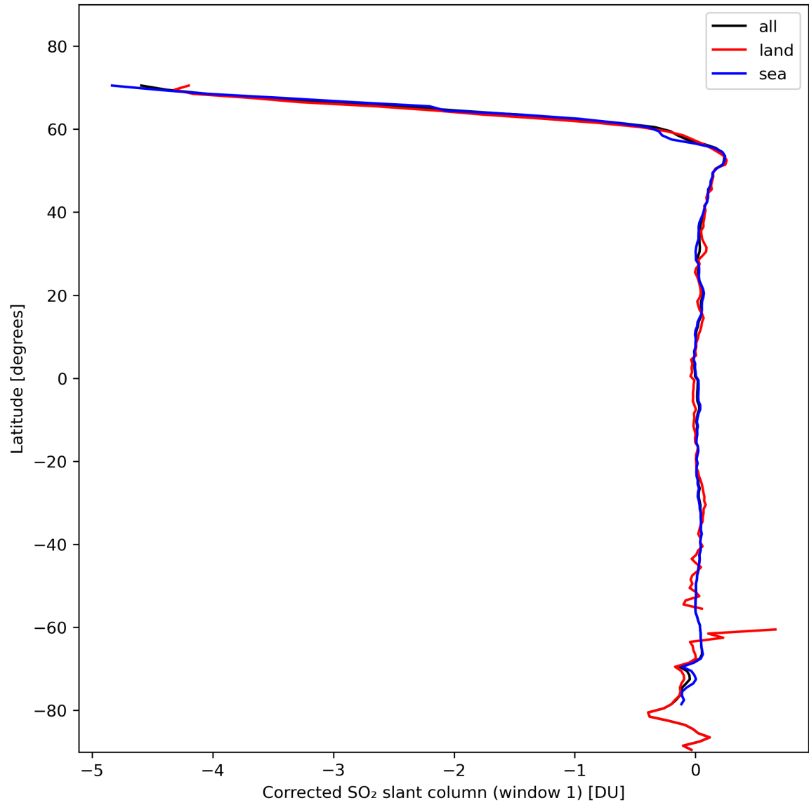
Figure 35: Zonal average of “Corrected SO 2 slant column (window 1)” for 2024-02-09 to 2024-02-11.
