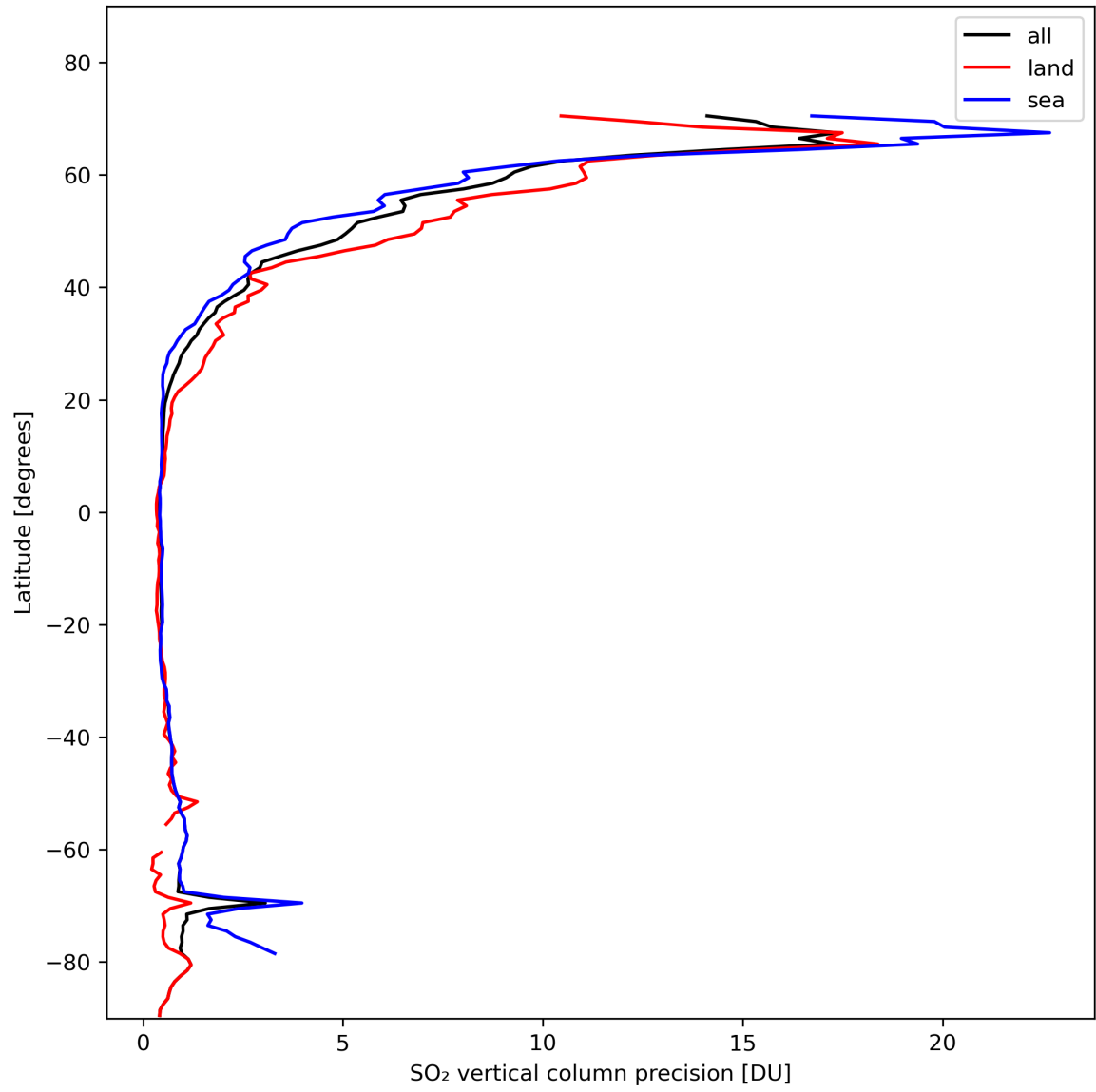
Figure 31: Zonal average of “SO 2 vertical column precision” for 2024-02-09 to 2024-02-11.
