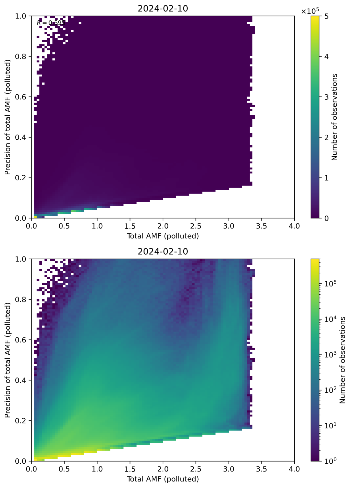
Figure 272: Scatter density plot of “Total AMF (polluted)” against “Precision of total AMF (polluted)” for 2024-02-09 to 2024-02-11.
