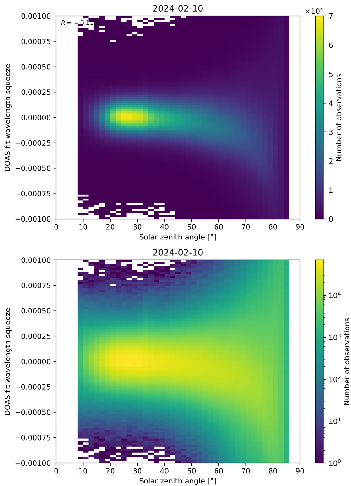
Figure 162: Scatter density plot of “Solar zenith angle” against “DOAS fit wavelength squeeze” for 2024-02-09 to 2024-02-11.
