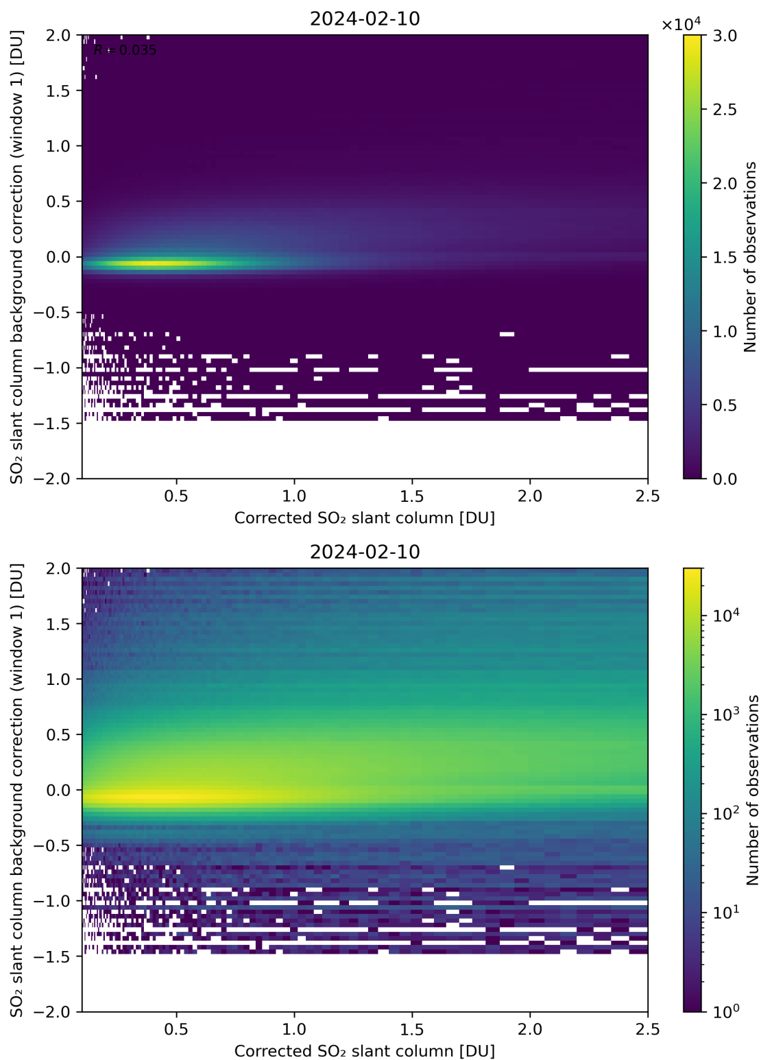
Figure 178: Scatter density plot of “Corrected SO 2 slant column” against “SO 2 slant column background correction (window 1)” for 2024-02-09 to 2024-02-11.
