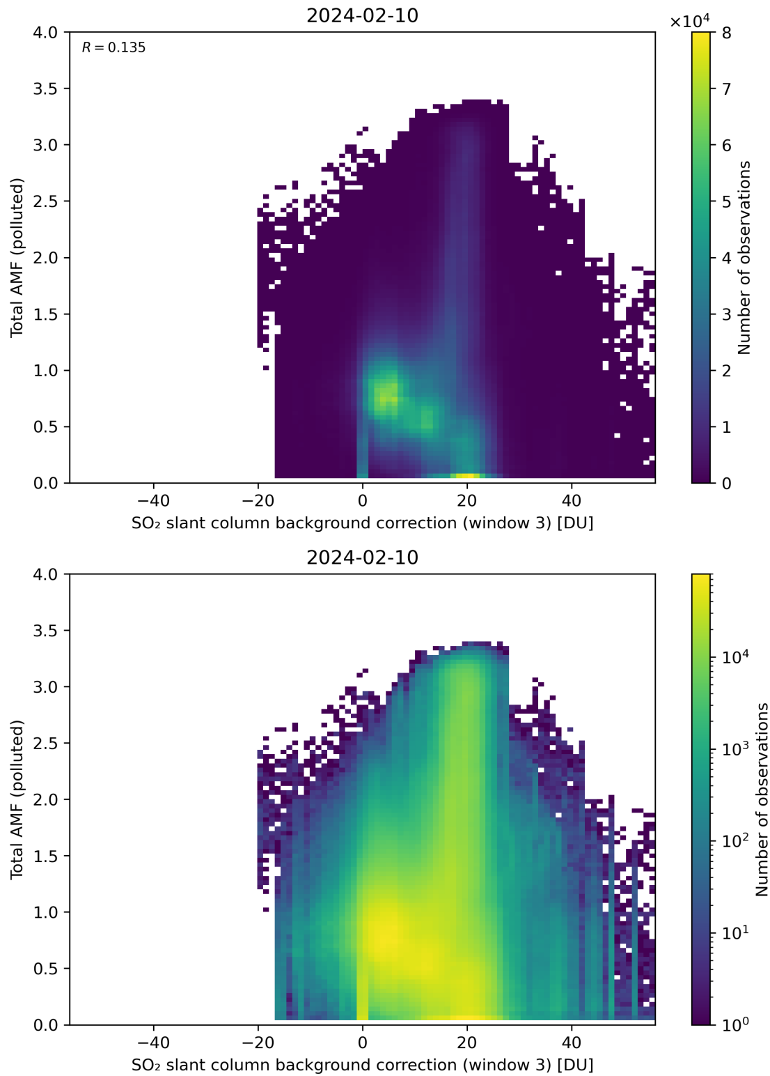
Figure 125: Scatter density plot of “SO 2 slant column background correction (window 3)” against “Total AMF (polluted)” for 2024-02-09 to 2024-02-11.
