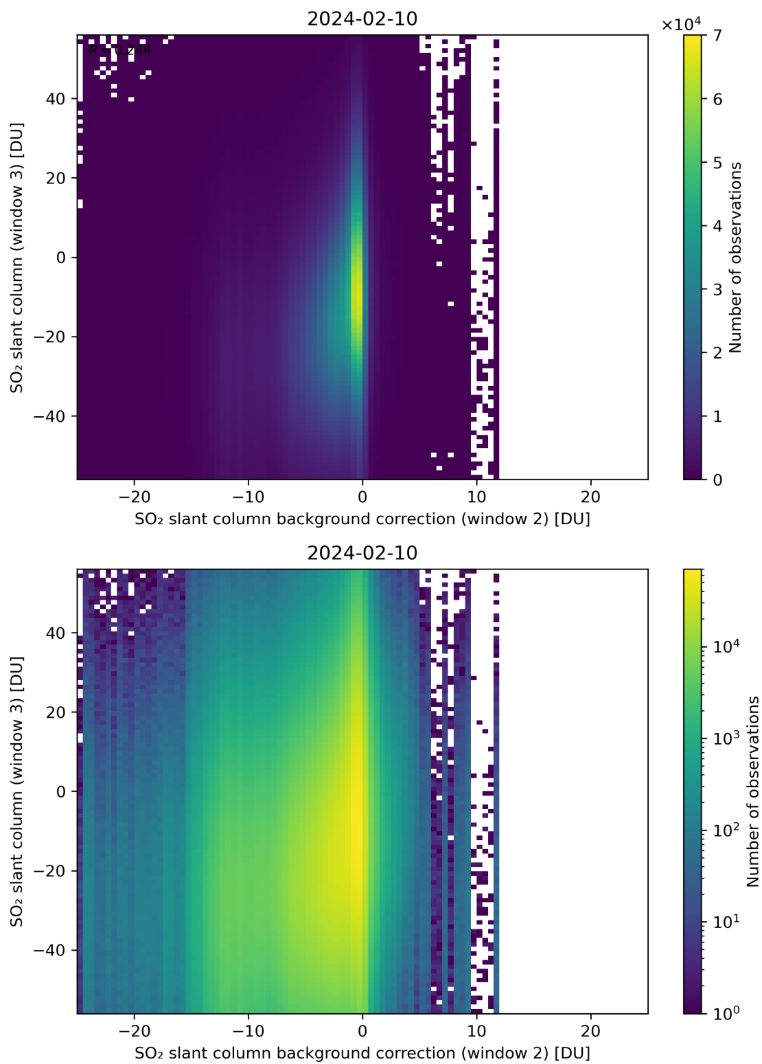
Figure 117: Scatter density plot of “SO 2 slant column background correction (window 2)” against “SO 2 slant column (window 3)” for 2024-02-09 to 2024-02-11.
