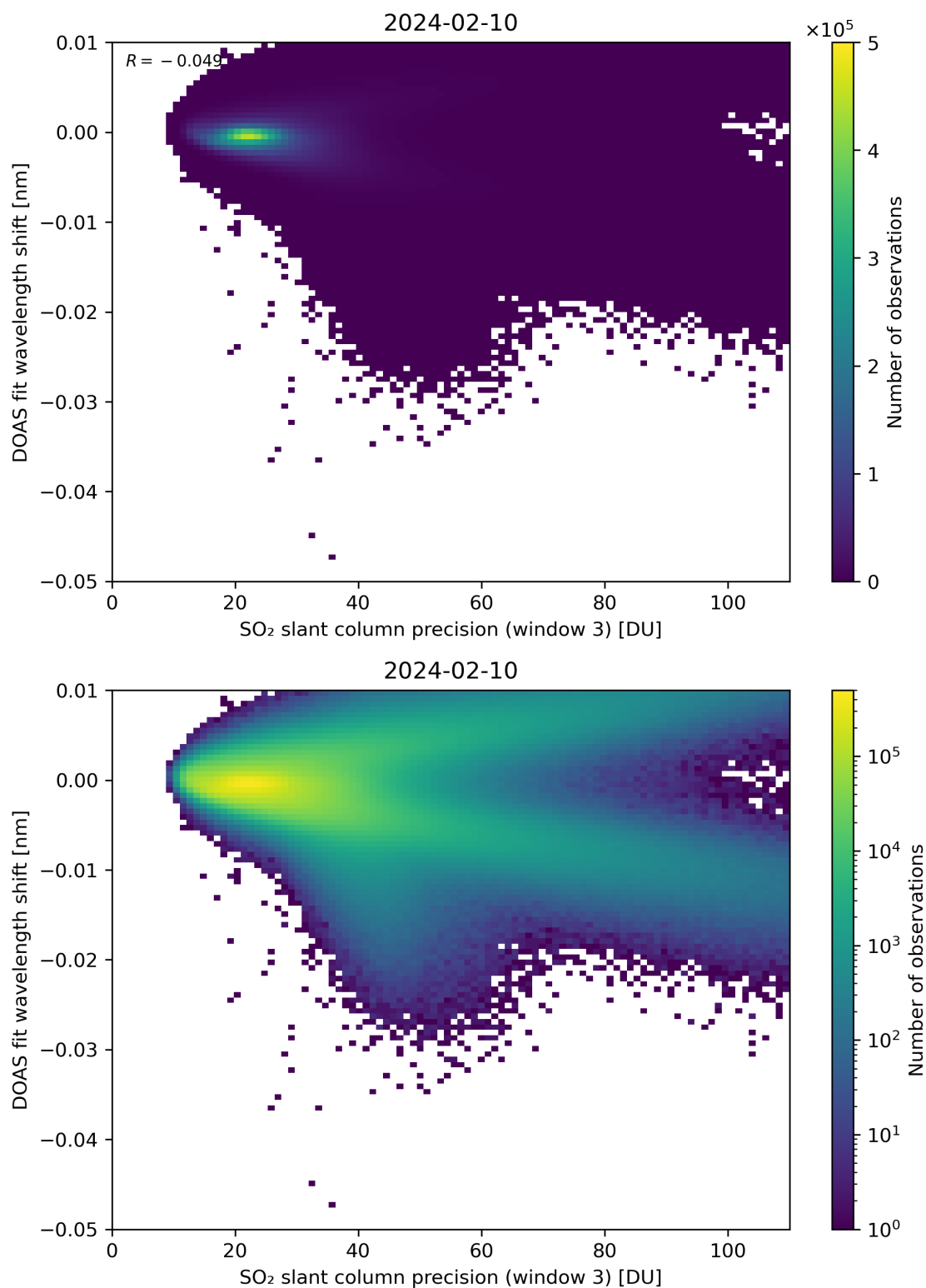
Figure 258: Scatter density plot of “SO 2 slant column precision (window 3)” against “DOAS fit wavelength shift” for 2024-02-09 to 2024-02-11.
