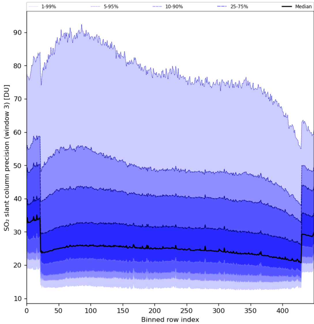
Figure 88: Along track statistics of “SO 2 slant column precision (window 3)” for 2024-02-09 to 2024-02-11
