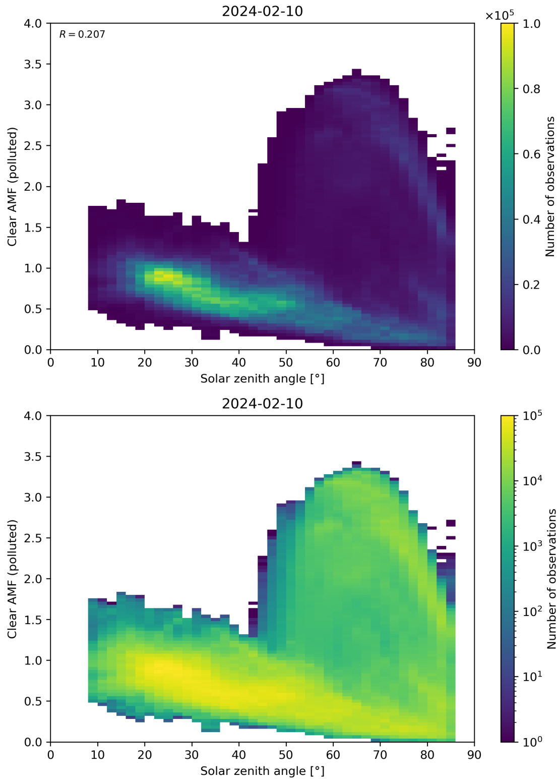
Figure 165: Scatter density plot of “Solar zenith angle” against “Clear AMF (polluted)” for 2024-02-09 to 2024-02-11.
