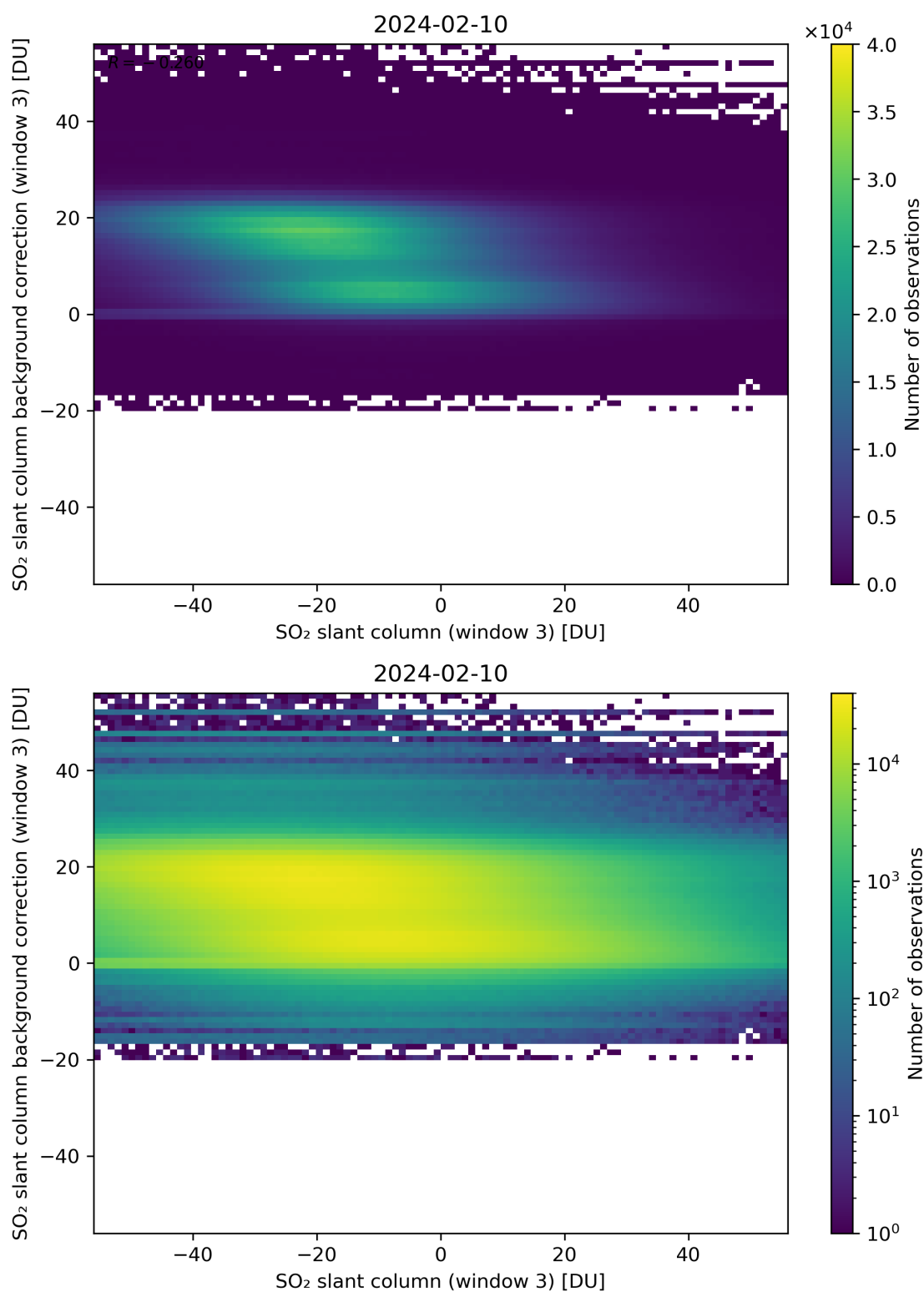
Figure 253: Scatter density plot of “SO 2 slant column (window 3)” against “SO 2 slant column background correction (window 3)” for 2024-02-09 to 2024-02-11.
