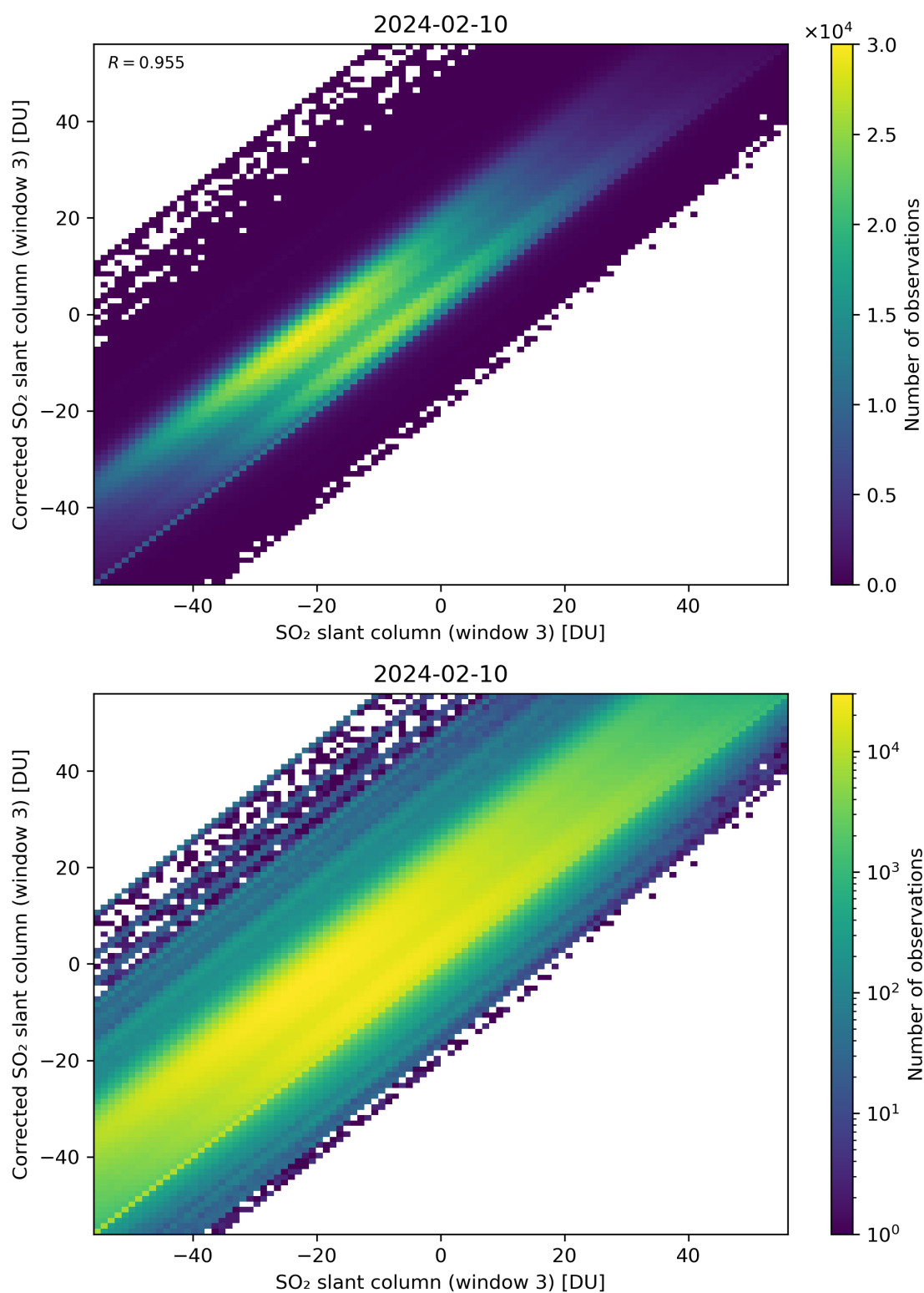
Figure 266: Scatter density plot of “SO 2 slant column (window 3)” against “Corrected SO 2 slant column (window 3)” for 2024-02-09 to 2024-02-11.
