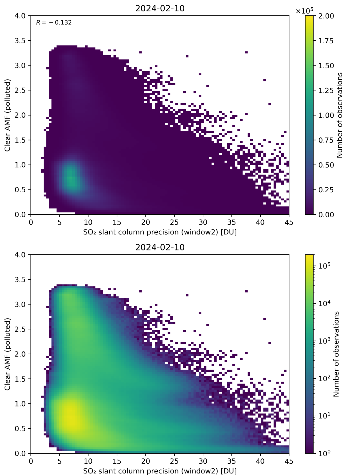
Figure 246: Scatter density plot of “SO 2 slant column precision (window2)” against “Clear AMF (polluted)” for 2024-02-09 to 2024-02-11.
