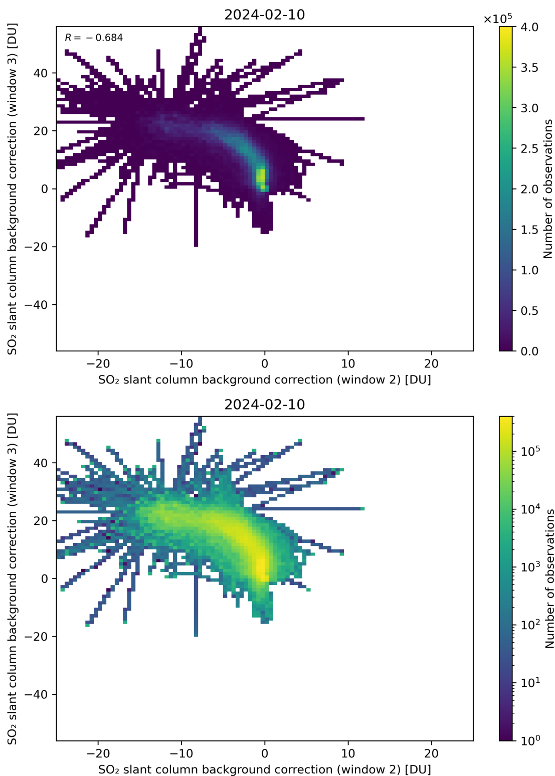
Figure 111: Scatter density plot of “SO 2 slant column background correction (window 2)” against “SO 2 slant column background correction (window 3)” for 2024-02-09 to 2024-02-11.
