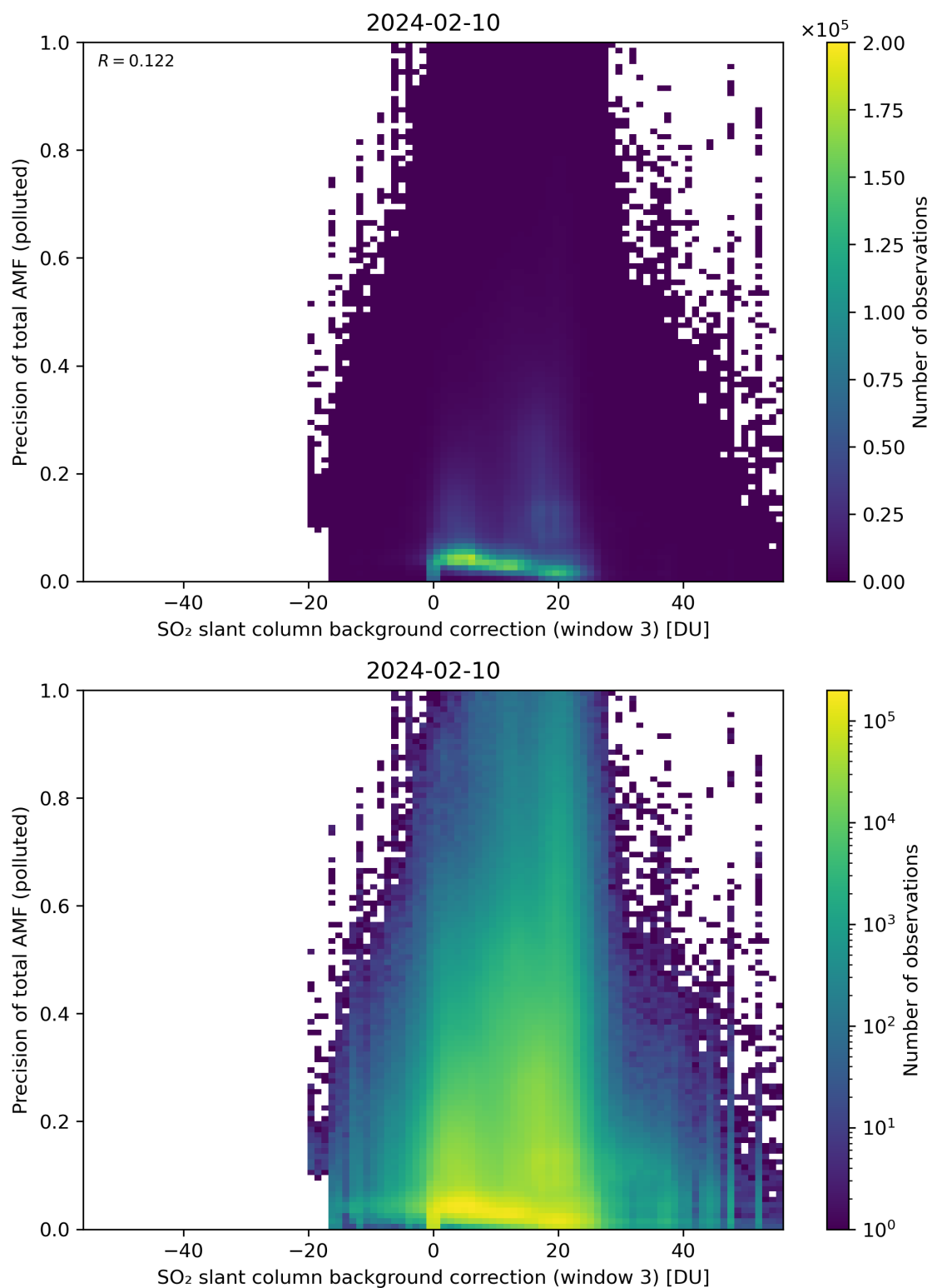
Figure 126: Scatter density plot of “SO 2 slant column background correction (window 3)” against “Precision of total AMF (polluted)” for 2024-02-09 to 2024-02-11.
