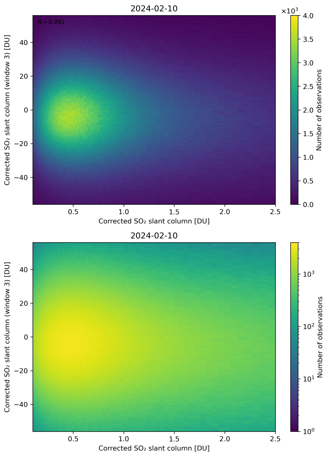
Figure 186: Scatter density plot of “Corrected SO 2 slant column” against “Corrected SO 2 slant column (window 3)” for 2024-02-09 to 2024-02-11.
