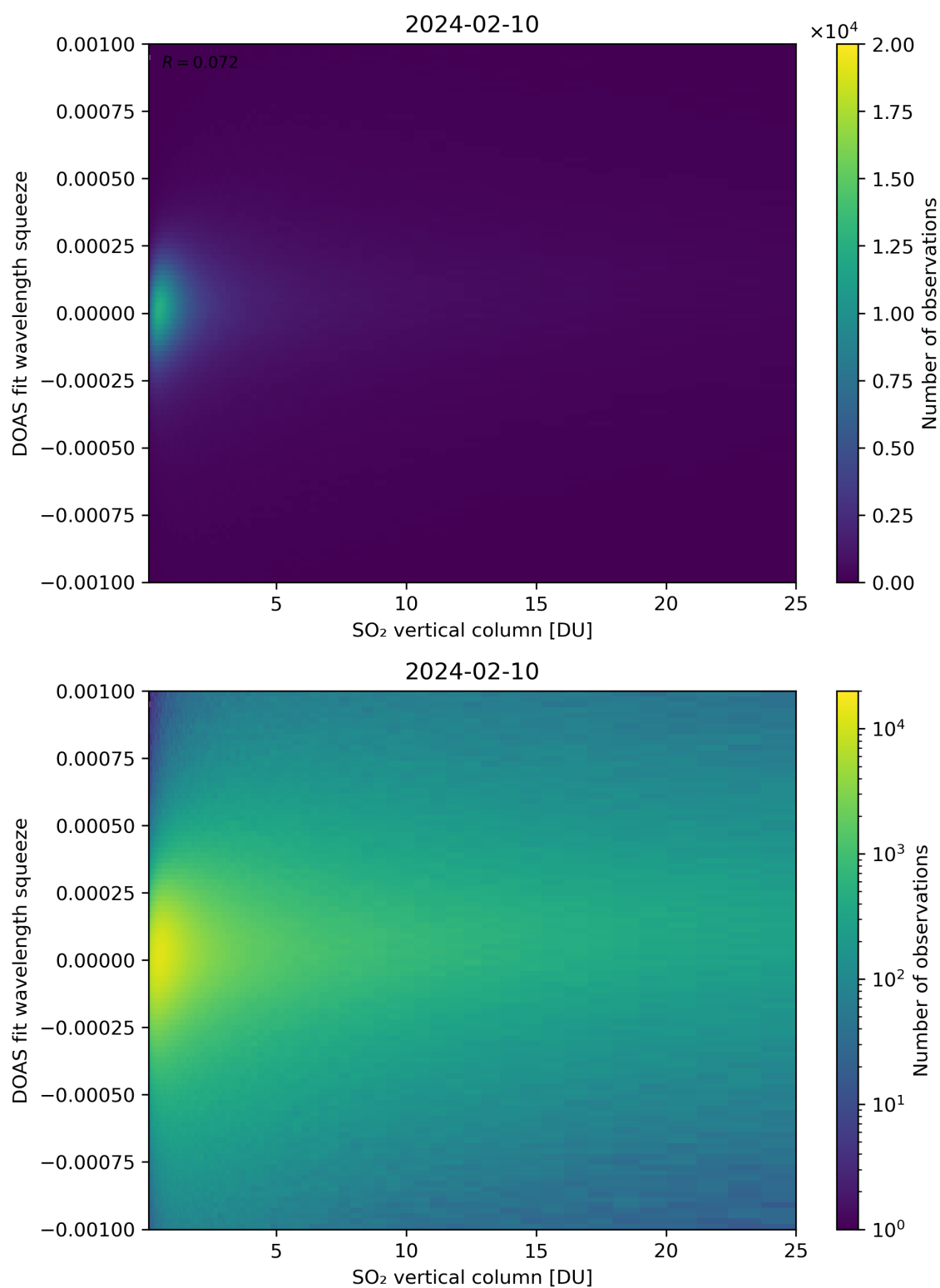
Figure 277: Scatter density plot of “SO 2 vertical column” against “DOAS fit wavelength squeeze” for 2024-02-09 to 2024-02-11.
