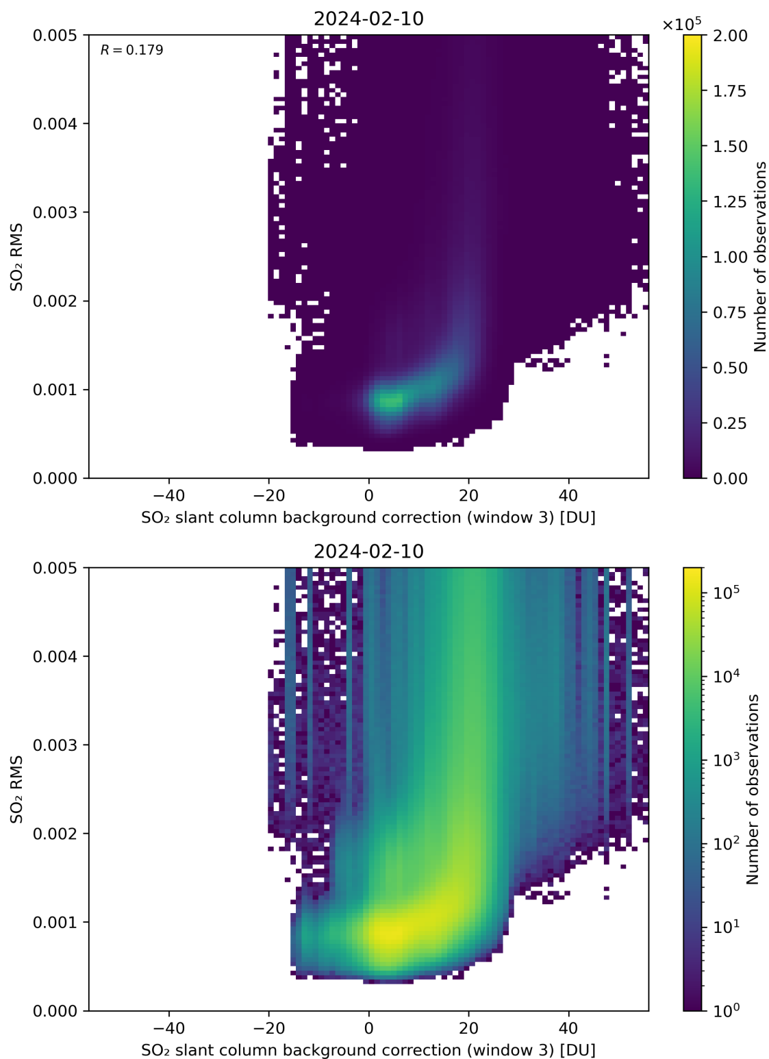
Figure 123: Scatter density plot of “SO 2 slant column background correction (window 3)” against “SO 2 RMS” for 2024-02-09 to 2024-02-11.
