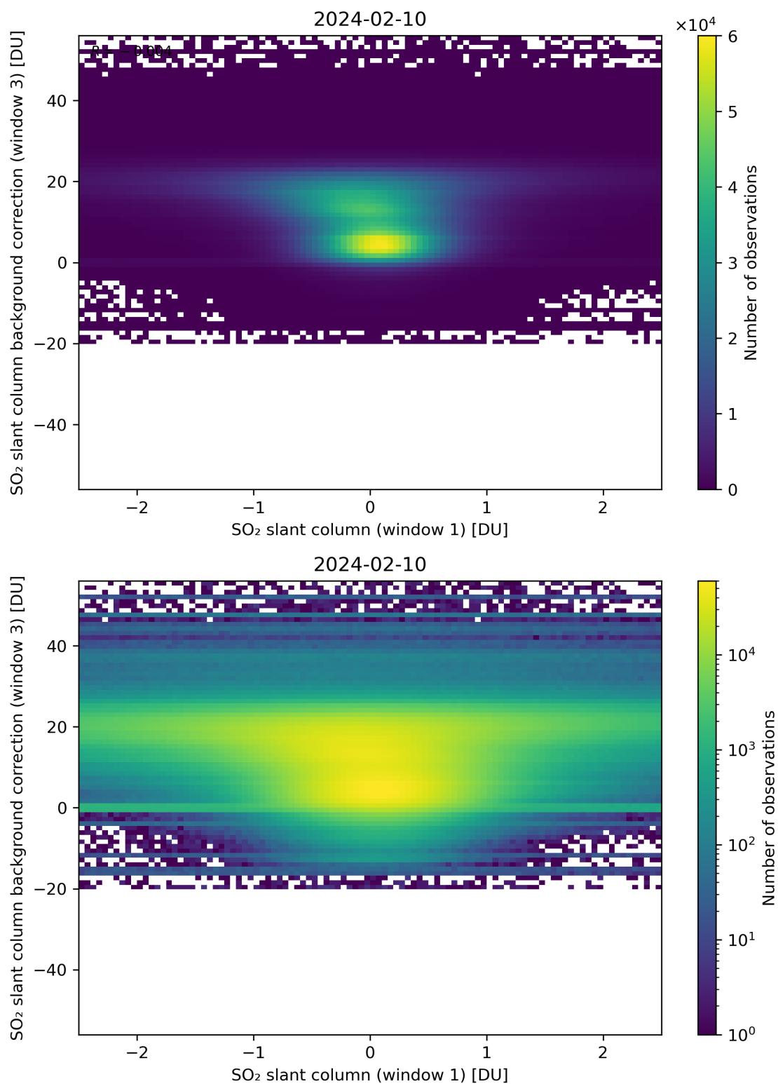
Figure 214: Scatter density plot of “SO 2 slant column (window 1)” against “SO 2 slant column background correction (window 3)” for 2024-02-09 to 2024-02-11.
