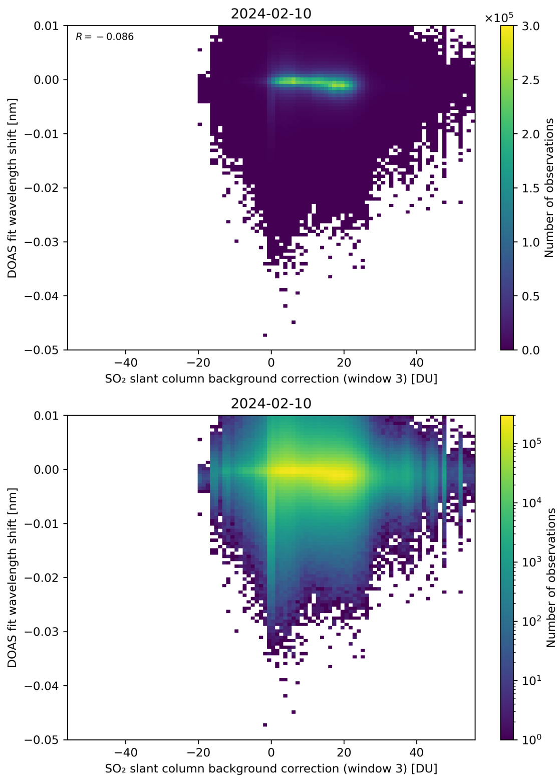
Figure 121: Scatter density plot of “SO 2 slant column background correction (window 3)” against “DOAS fit wavelength shift” for 2024-02-09 to 2024-02-11.
