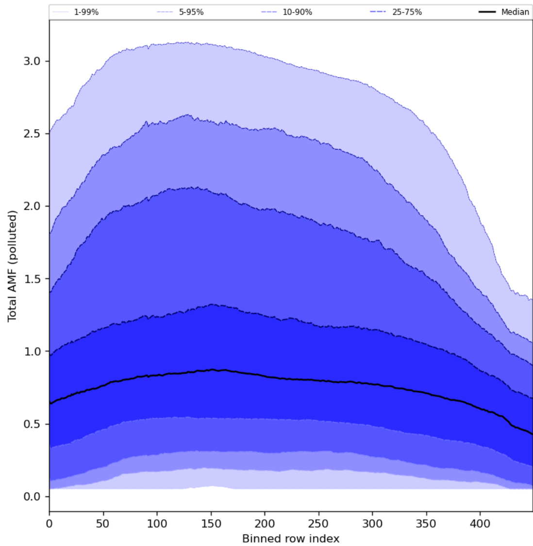
Figure 94: Along track statistics of “Total AMF (polluted)” for 2024-02-09 to 2024-02-11
