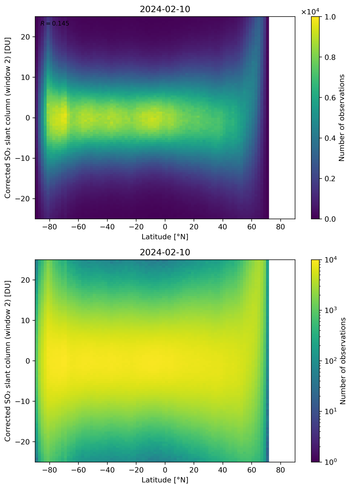
Figure 147: Scatter density plot of “Latitude” against “Corrected SO 2 slant column (window 2)” for 2024-02-09 to 2024-02-11.
