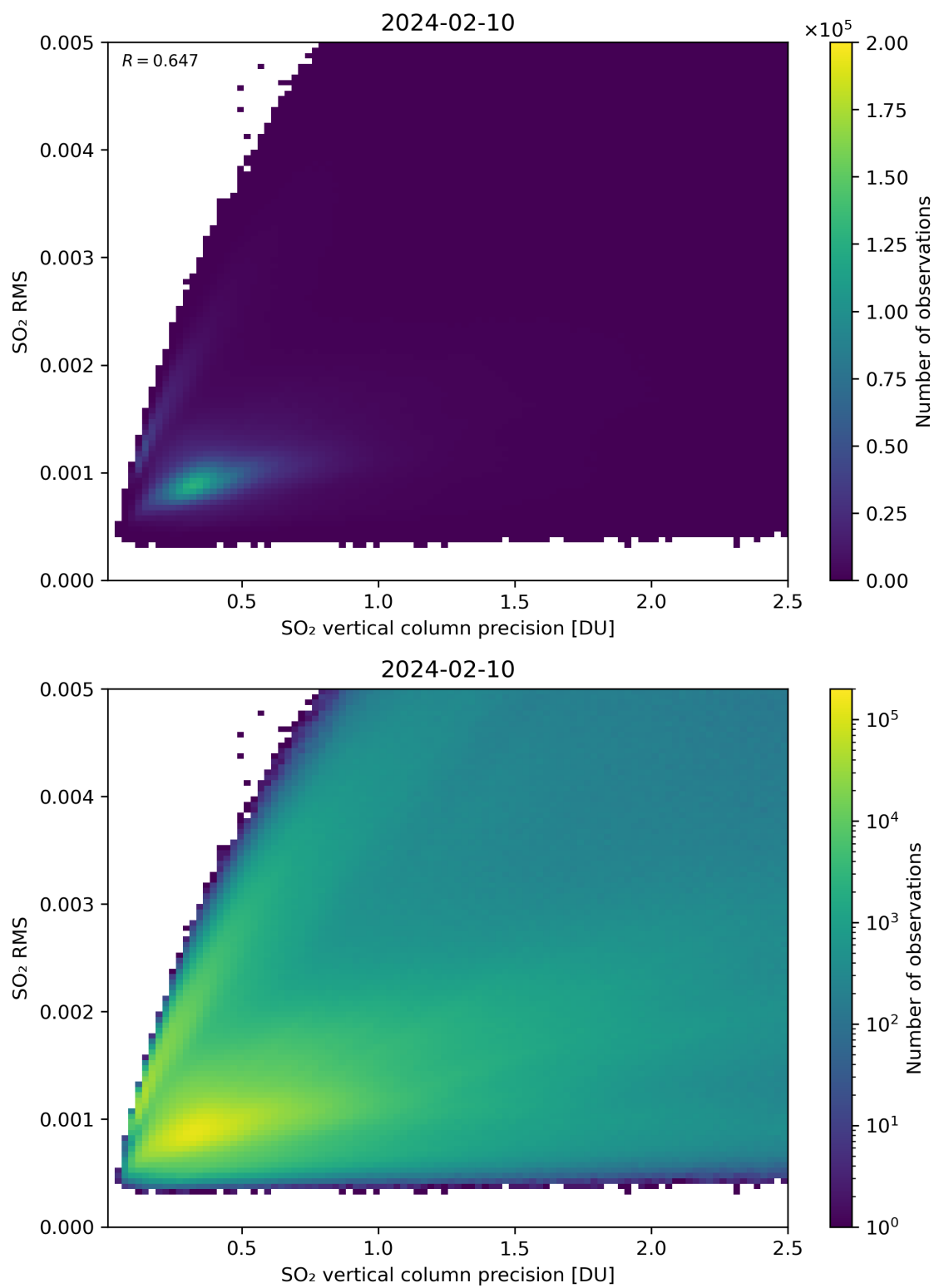
Figure 284: Scatter density plot of “SO 2 vertical column precision” against “SO 2 RMS” for 2024-02-09 to 2024-02-11.
