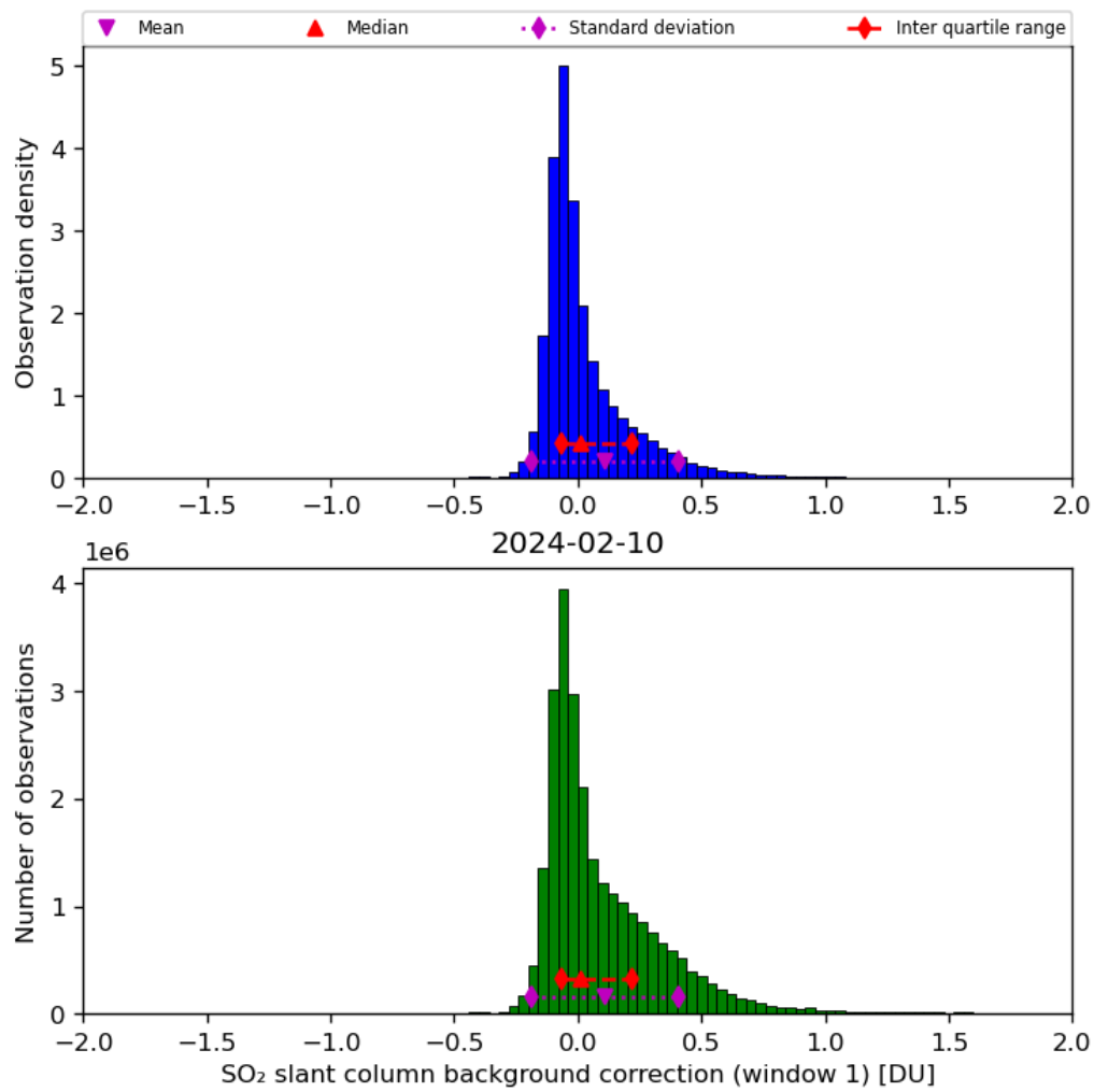
Figure 59: Histogram of “SO 2 slant column background correction (window 1)” for 2024-02-09 to 2024-02-11
