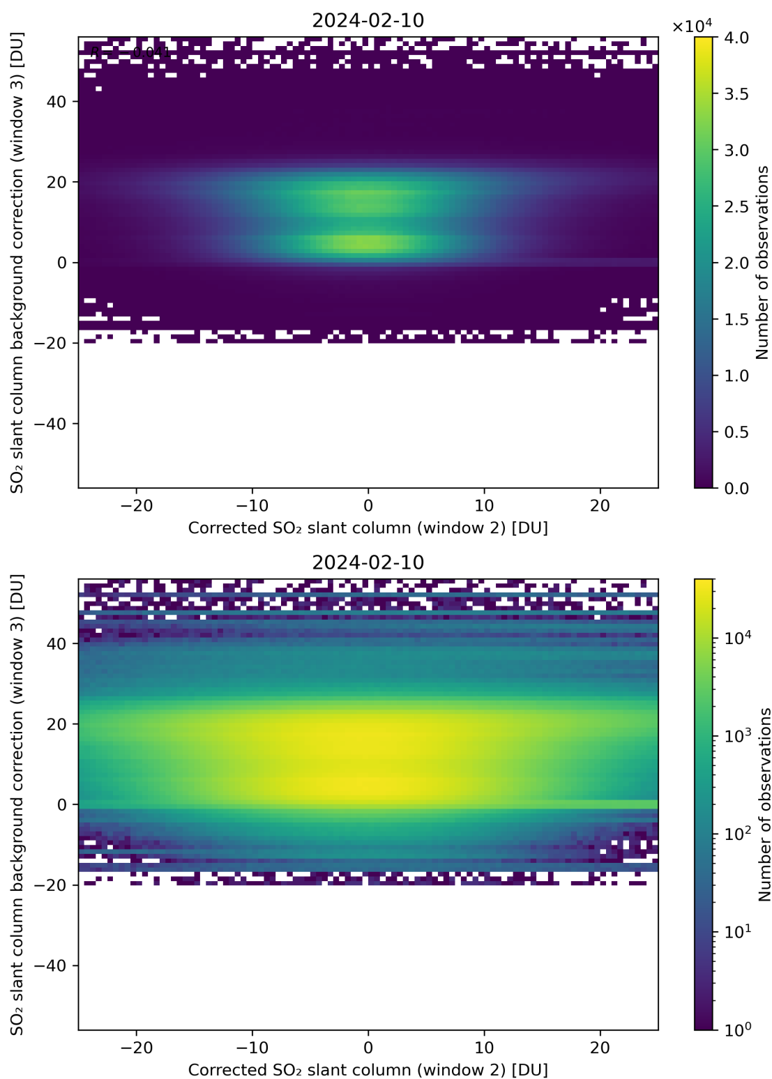
Figure 195: Scatter density plot of “Corrected SO 2 slant column (window 2)” against “SO 2 slant column background correction (window 3)” for 2024-02-09 to 2024-02-11.
