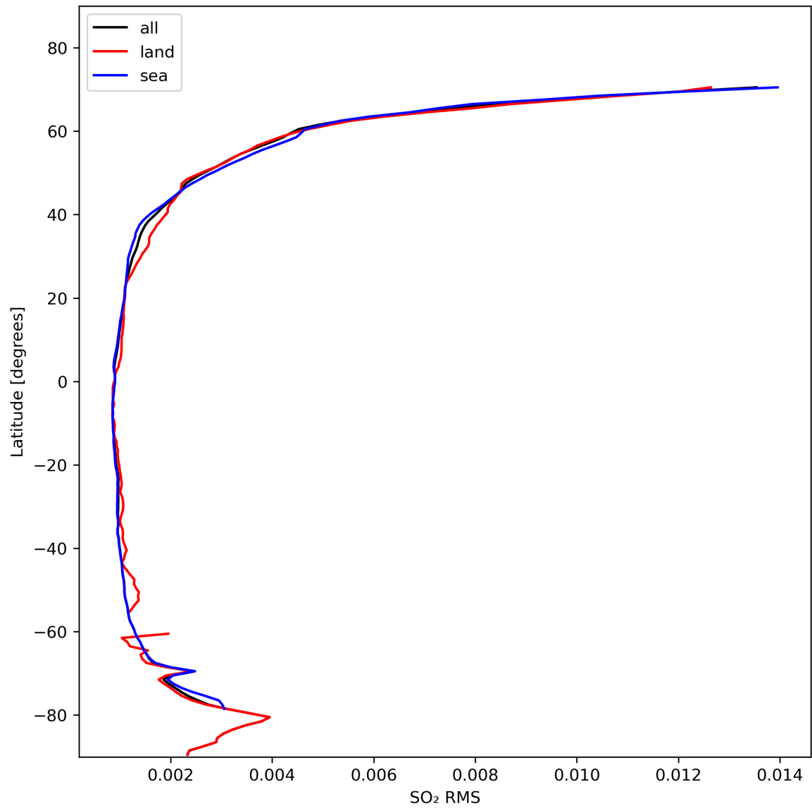
Figure 47: Zonal average of “SO 2 RMS” for 2024-02-09 to 2024-02-11.
