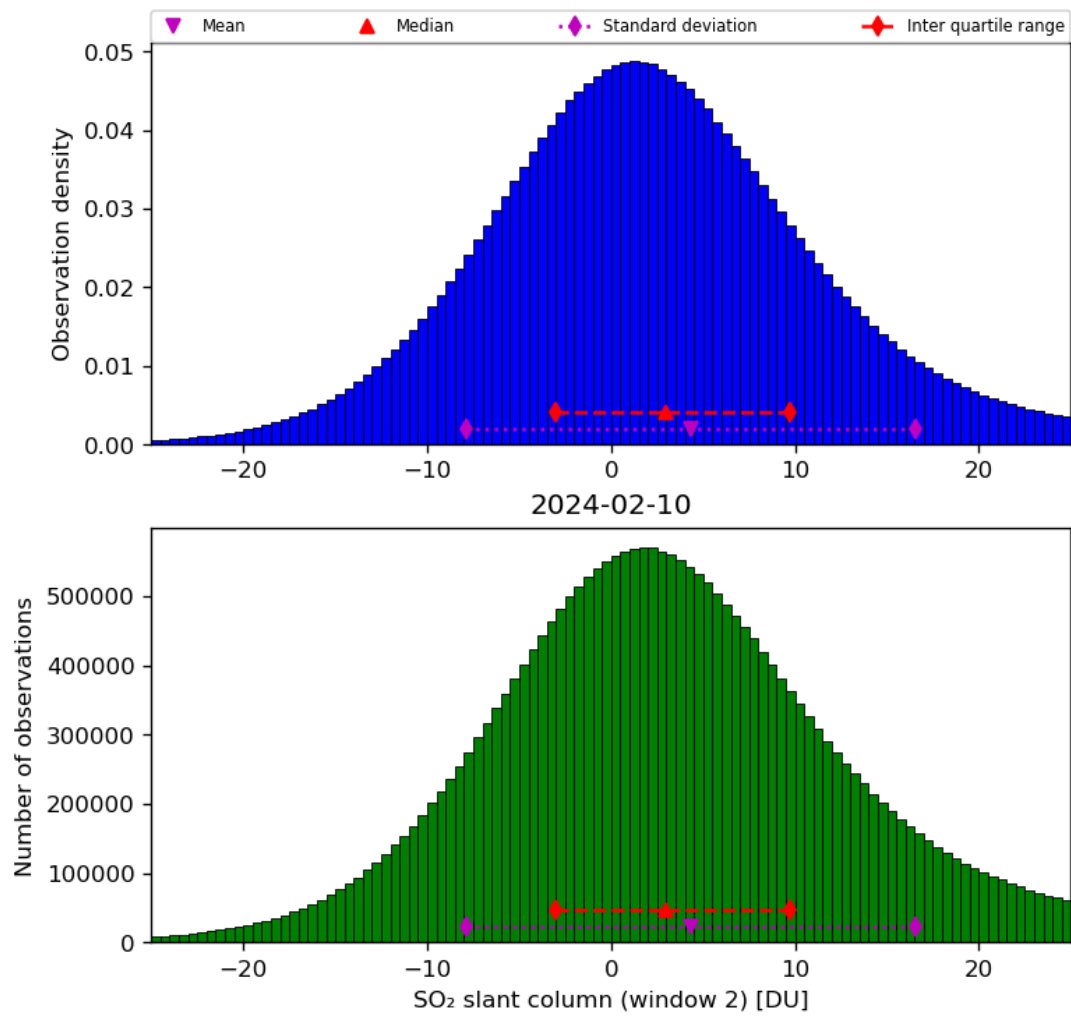
Figure 60: Histogram of “SO 2 slant column (window 2)” for 2024-02-09 to 2024-02-11
