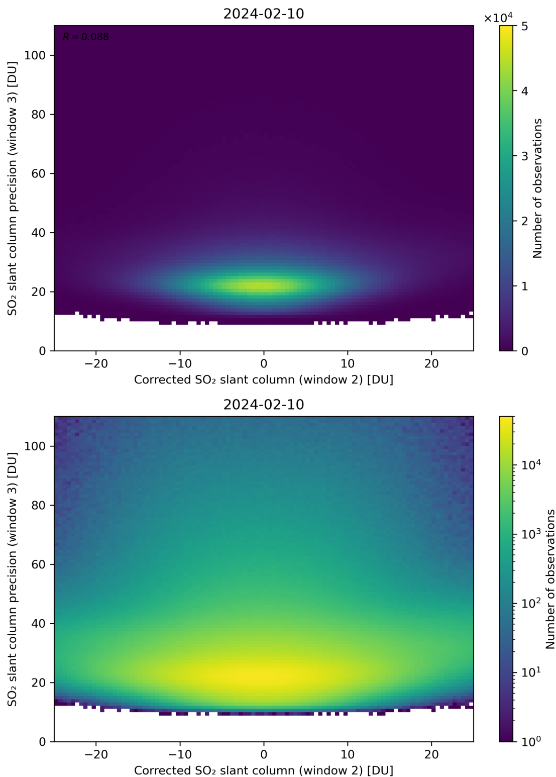
Figure 202: Scatter density plot of “Corrected SO 2 slant column (window 2)” against “SO 2 slant column precision (window 3)” for 2024-02-09 to 2024-02-11.
