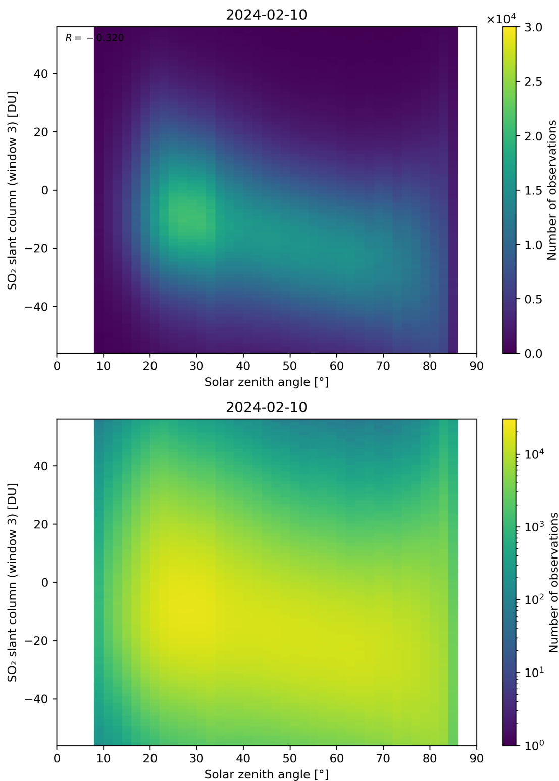
Figure 172: Scatter density plot of “Solar zenith angle” against “SO 2 slant column (window 3)” for 2024-02-09 to 2024-02-11.
