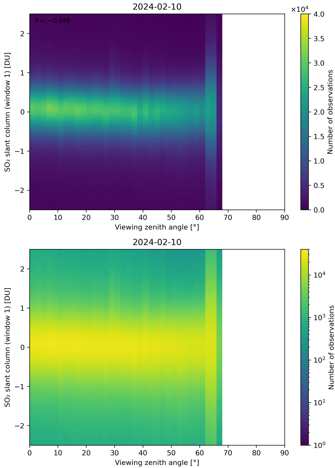
Figure 320: Scatter density plot of “Viewing zenith angle” against “SO 2 slant column (window 1)” for 2024-02-09 to 2024-02-11.
