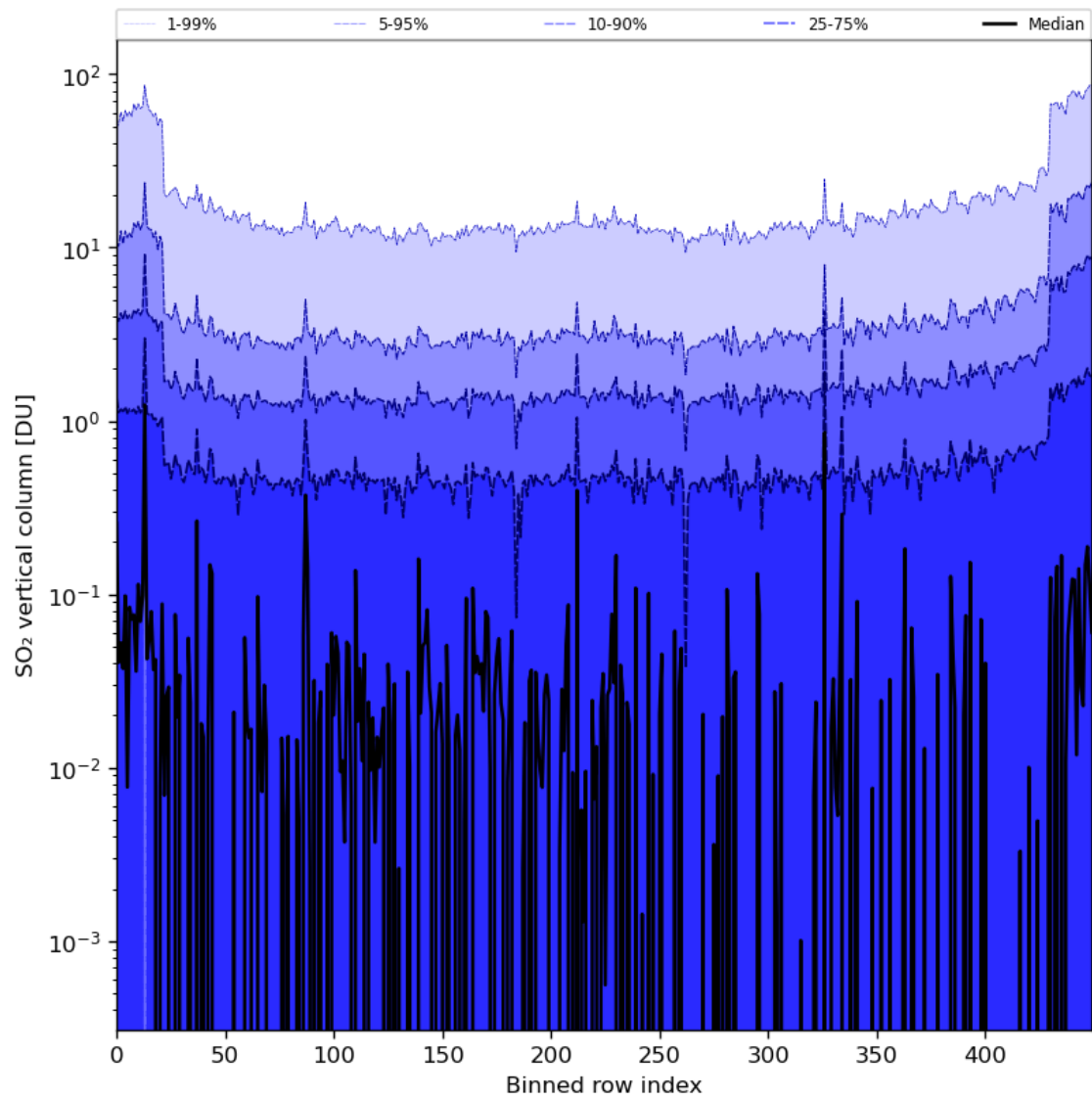
Figure 76: Along track statistics of “SO 2 vertical column” for 2024-02-09 to 2024-02-11
