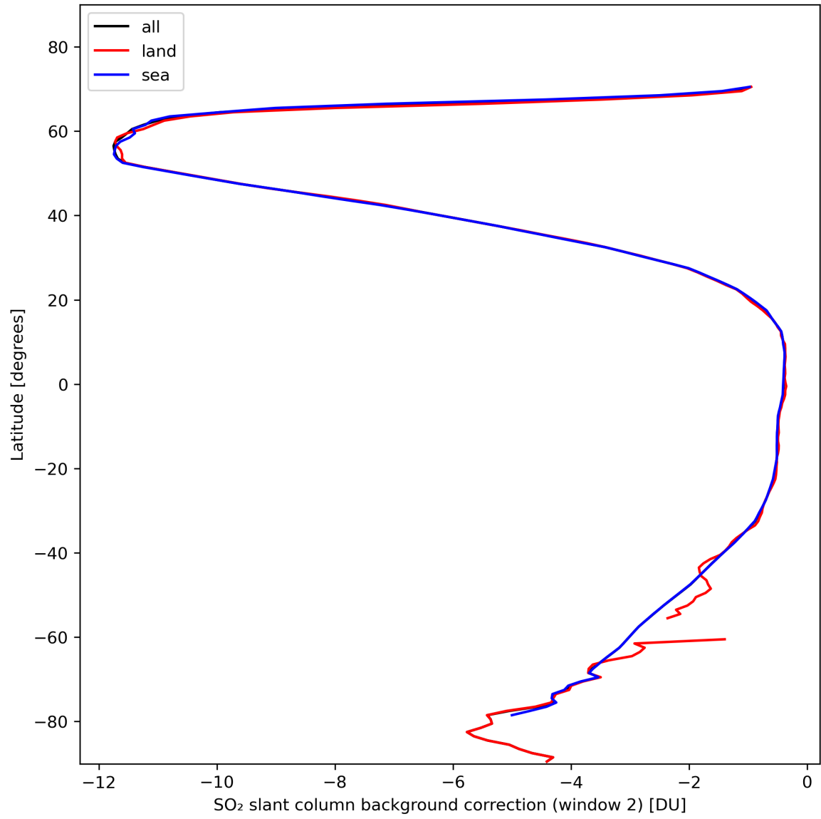
Figure 40: Zonal average of “SO 2 slant column background correction (window 2)” for 2024-02-09 to 2024-02-11.
