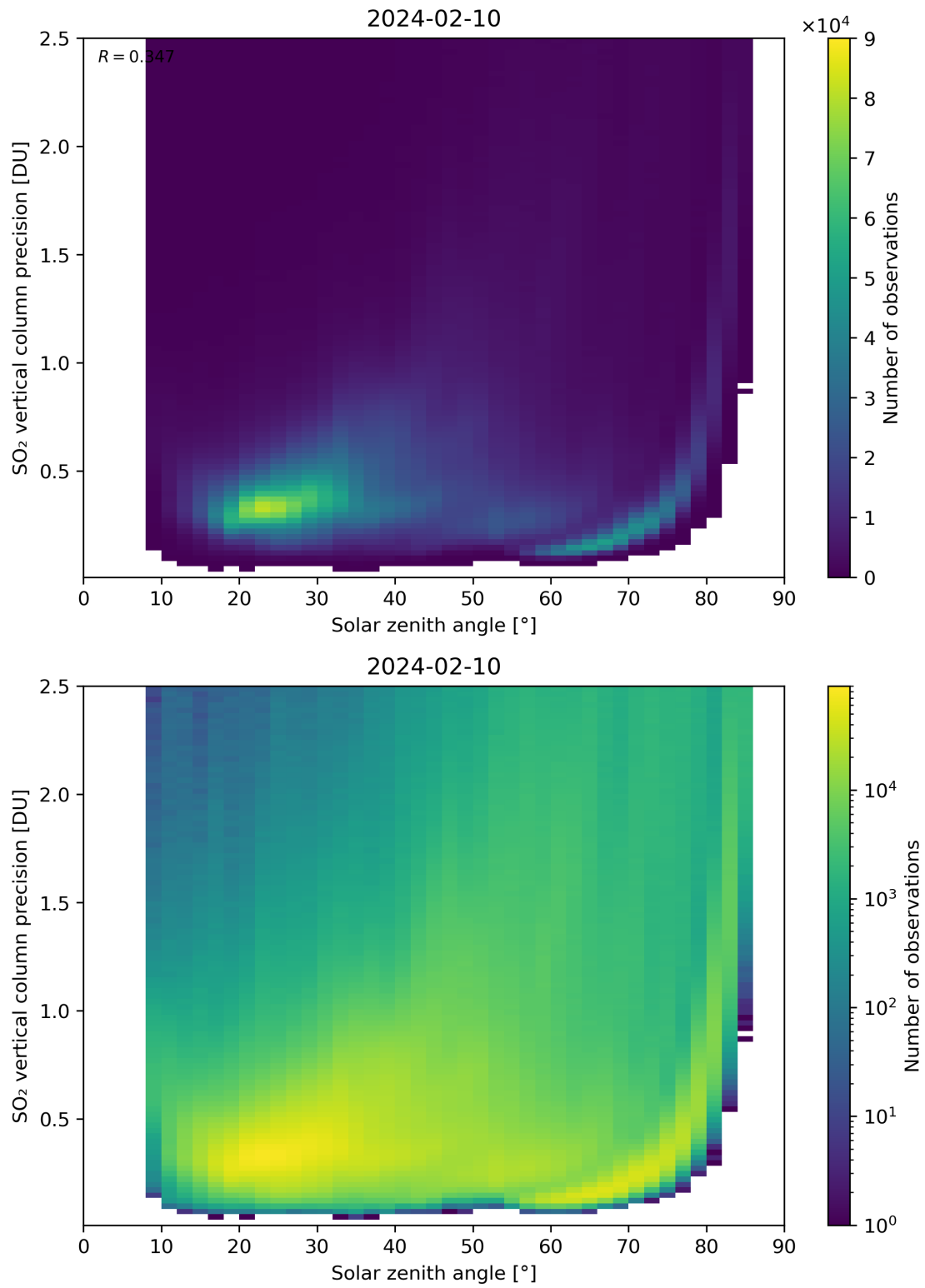
Figure 177: Scatter density plot of “Solar zenith angle” against “SO 2 vertical column precision” for 2024-02-09 to 2024-02-11.
