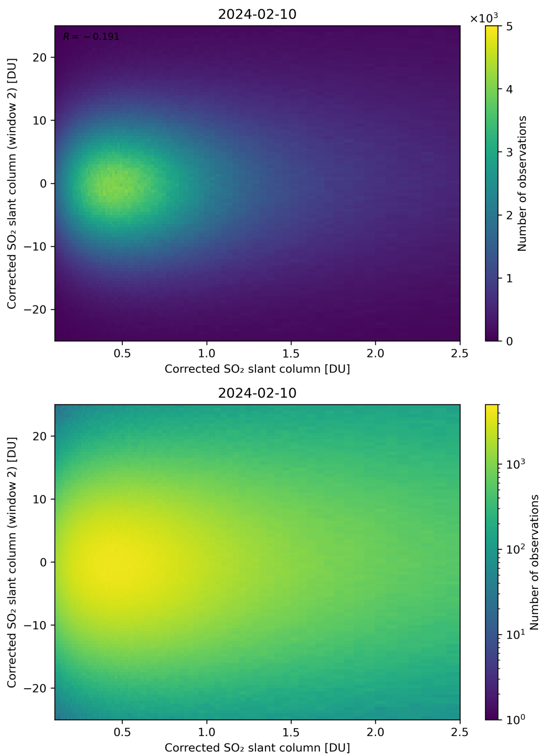
Figure 185: Scatter density plot of “Corrected SO 2 slant column” against “Corrected SO 2 slant column (window 2)” for 2024-02-09 to 2024-02-11.
