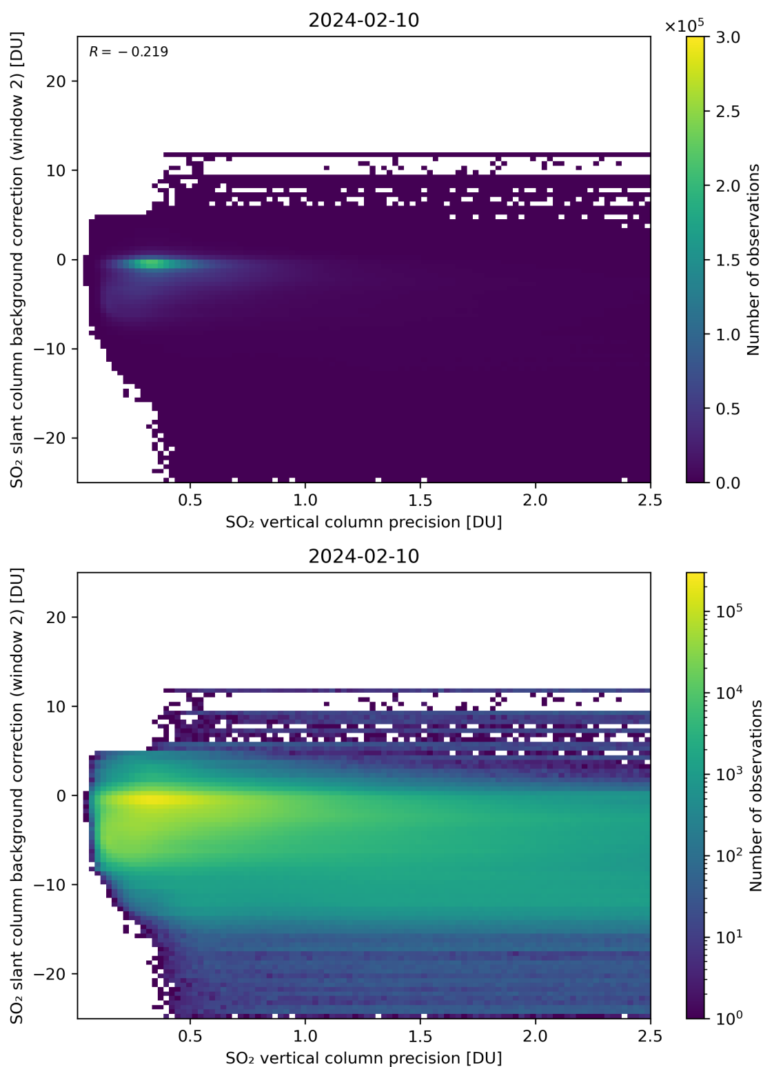
Figure 280: Scatter density plot of “SO 2 vertical column precision” against “SO 2 slant column background correction (window 2)” for 2024-02-09 to 2024-02-11.
