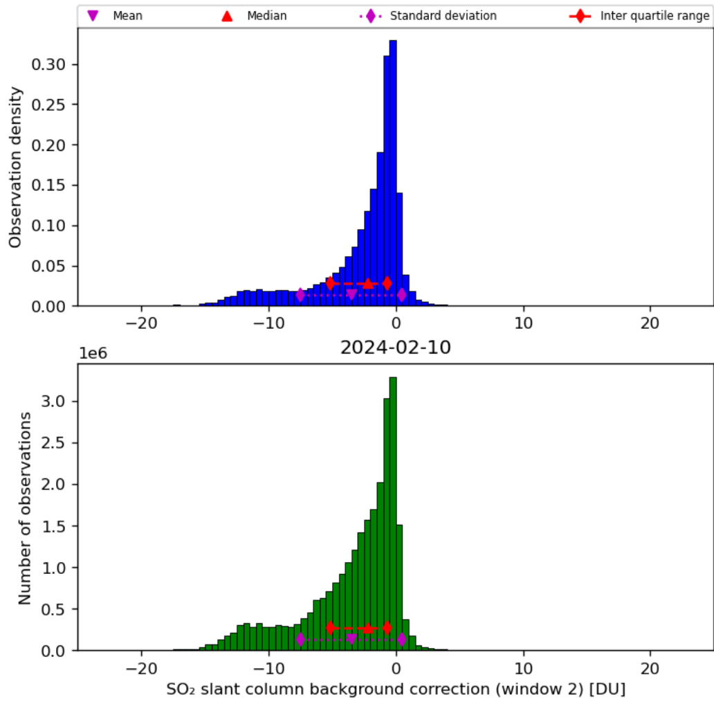
Figure 63: Histogram of “SO 2 slant column background correction (window 2)” for 2024-02-09 to 2024-02-11
