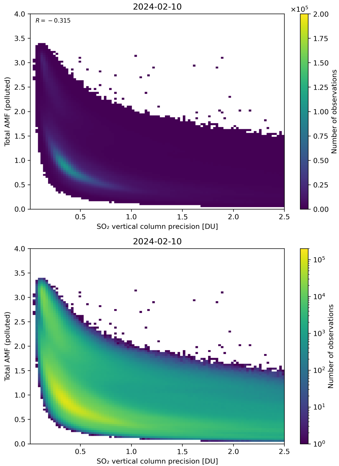
Figure 294: Scatter density plot of “SO 2 vertical column precision” against “Total AMF (polluted)” for 2024-02-09 to 2024-02-11.
