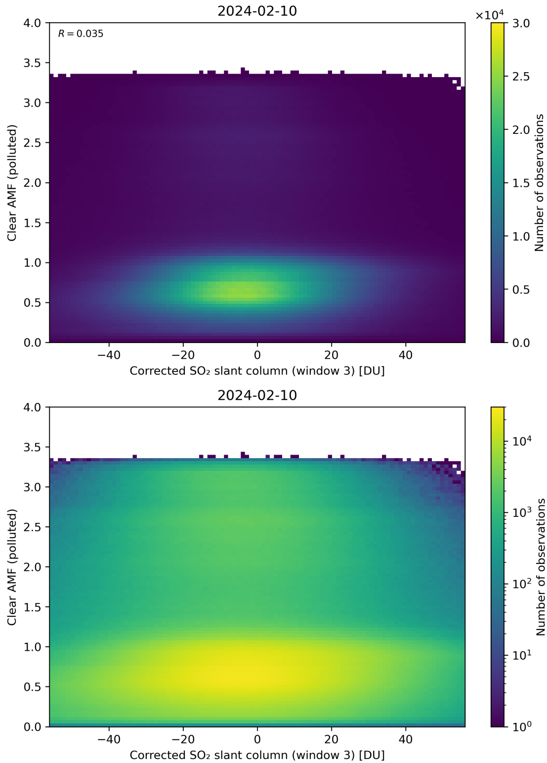
Figure 209: Scatter density plot of “Corrected SO 2 slant column (window 3)” against “Clear AMF (polluted)” for 2024-02-09 to 2024-02-11.
