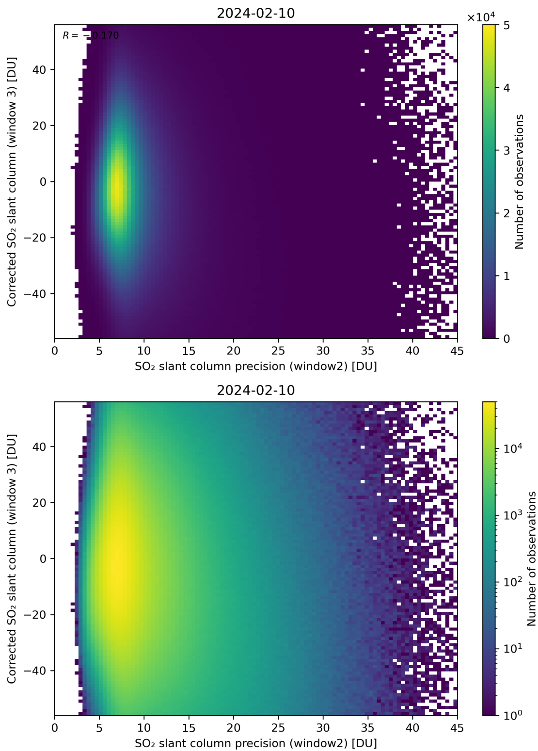
Figure 248: Scatter density plot of “SO 2 slant column precision (window2)” against “Corrected SO 2 slant column (window 3)” for 2024-02-09 to 2024-02-11.
