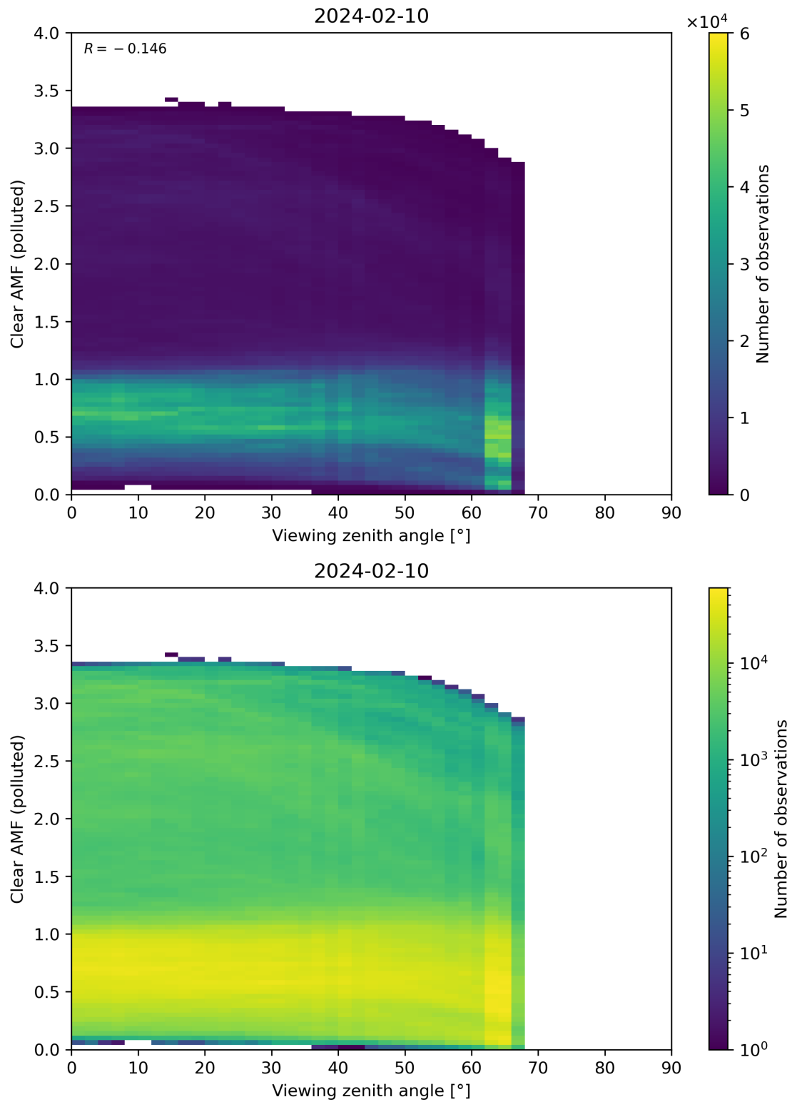
Figure 316: Scatter density plot of “Viewing zenith angle” against “Clear AMF (polluted)” for 2024-02-09 to 2024-02-11.
