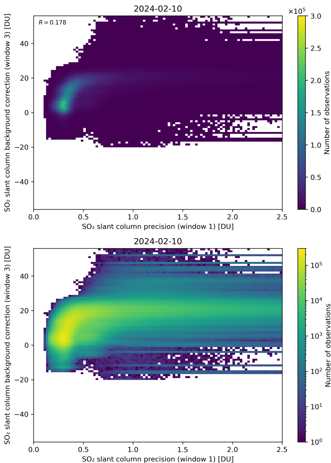
Figure 220: Scatter density plot of “SO 2 slant column precision (window 1)” against “SO 2 slant column background correction (window 3)” for 2024-02-09 to 2024-02-11.
