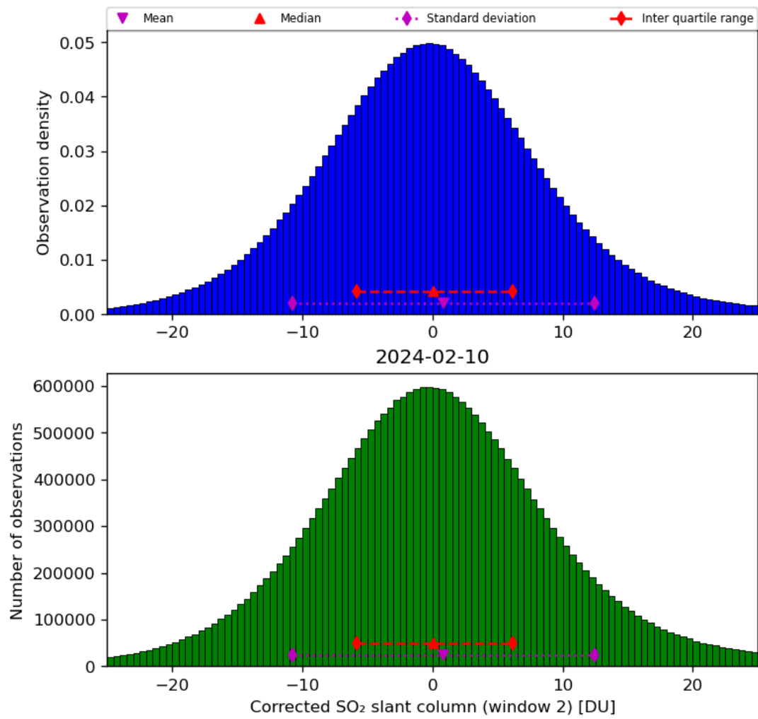
Figure 62: Histogram of “Corrected SO 2 slant column (window 2)” for 2024-02-09 to 2024-02-11
