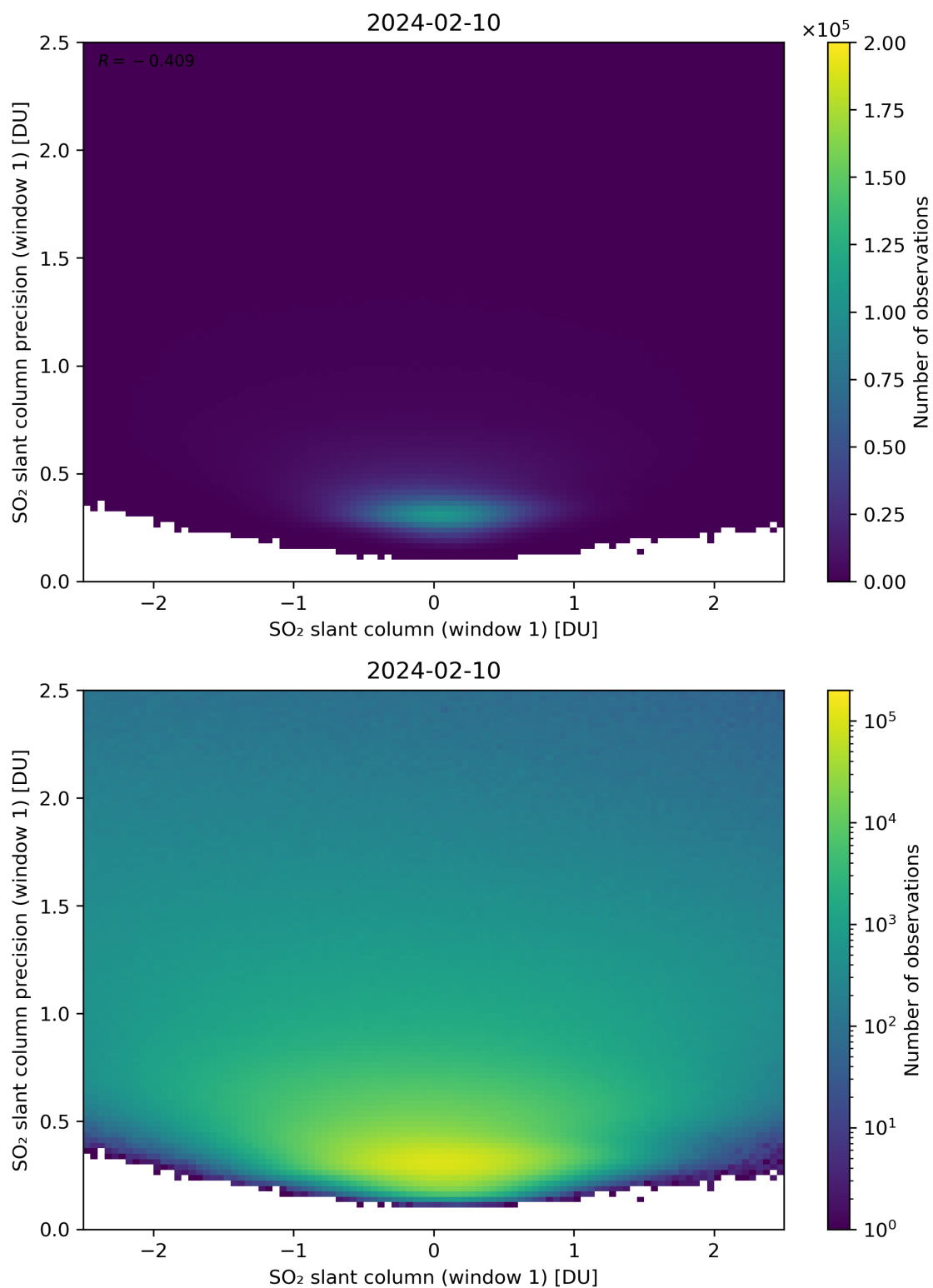
Figure 235: Scatter density plot of “SO 2 slant column (window 1)” against “SO 2 slant column precision (window 1)” for 2024-02-09 to 2024-02-11.
