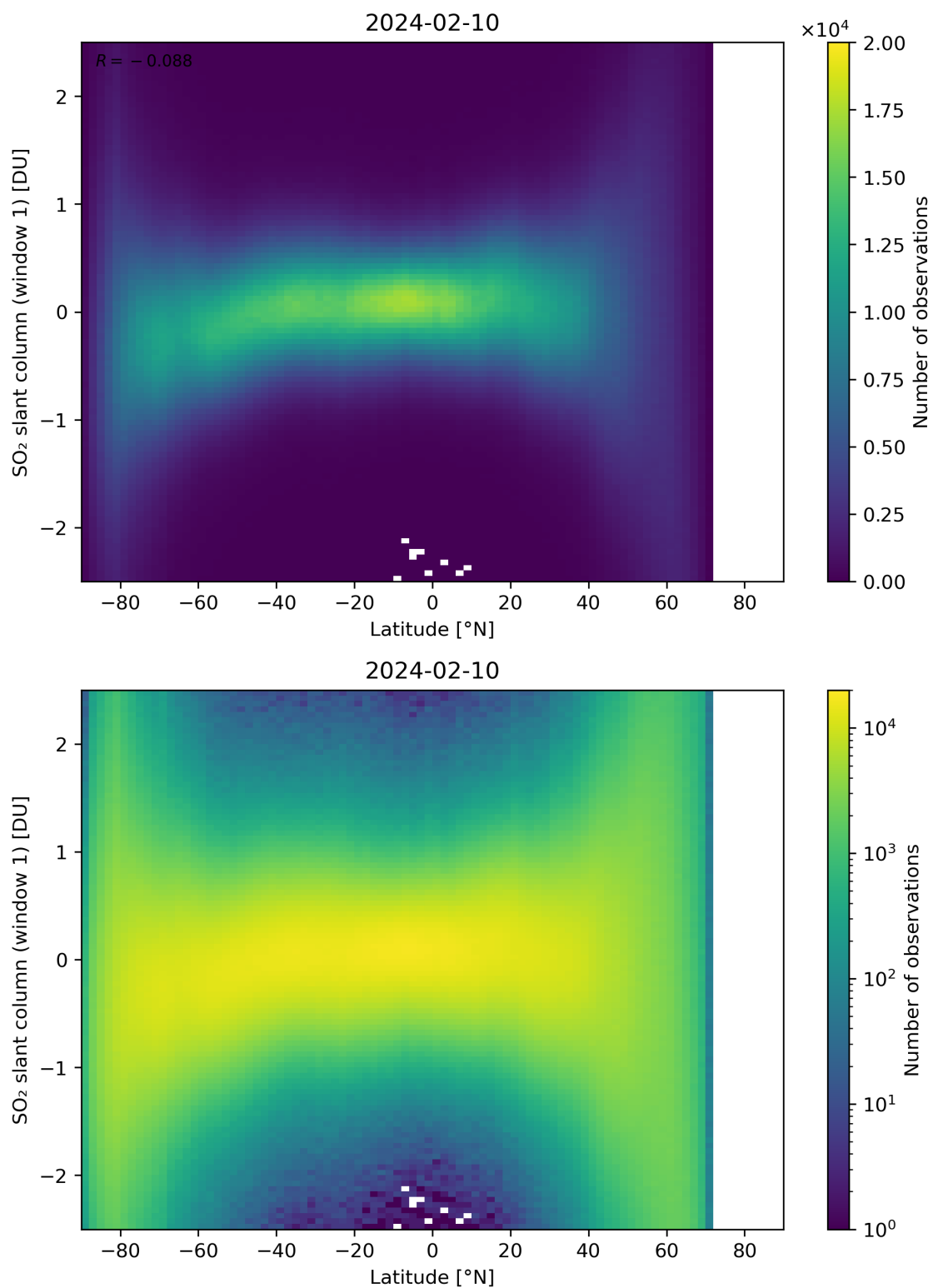
Figure 149: Scatter density plot of “Latitude” against “SO 2 slant column (window 1)” for 2024-02-09 to 2024-02-11.
