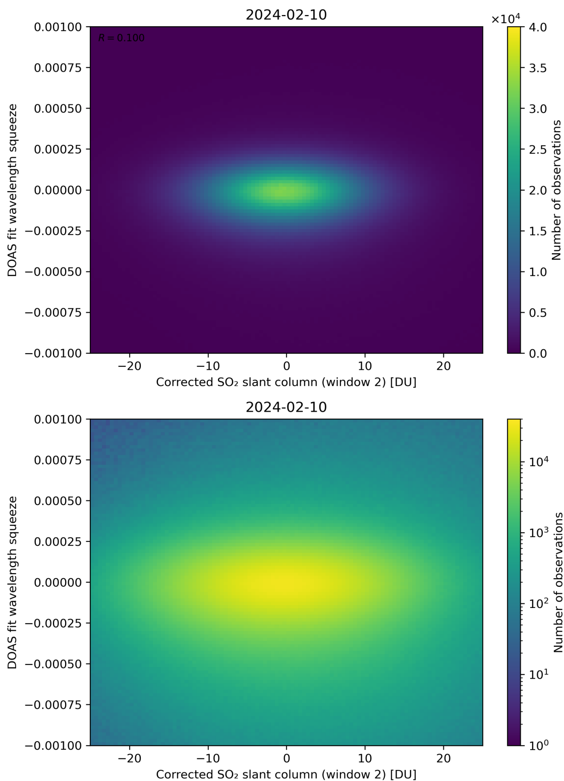
Figure 197: Scatter density plot of “Corrected SO 2 slant column (window 2)” against “DOAS fit wavelength squeeze” for 2024-02-09 to 2024-02-11.
