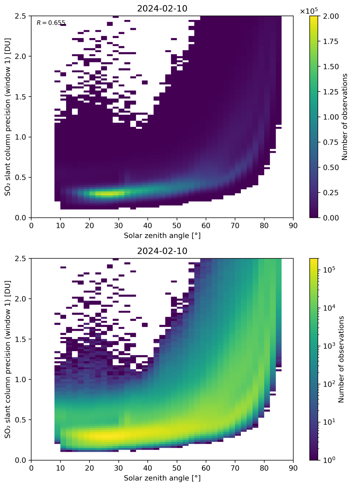
Figure 170: Scatter density plot of “Solar zenith angle” against “SO 2 slant column precision (window 1)” for 2024-02-09 to 2024-02-11.
