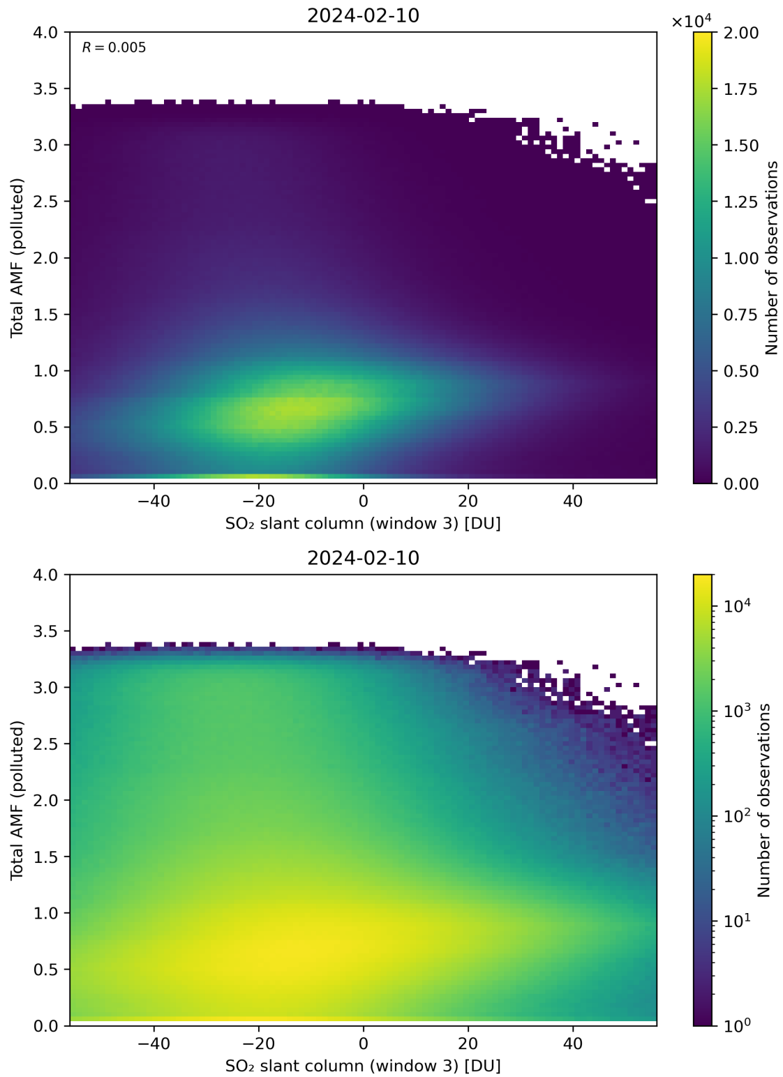
Figure 268: Scatter density plot of “SO 2 slant column (window 3)” against “Total AMF (polluted)” for 2024-02-09 to 2024-02-11.
