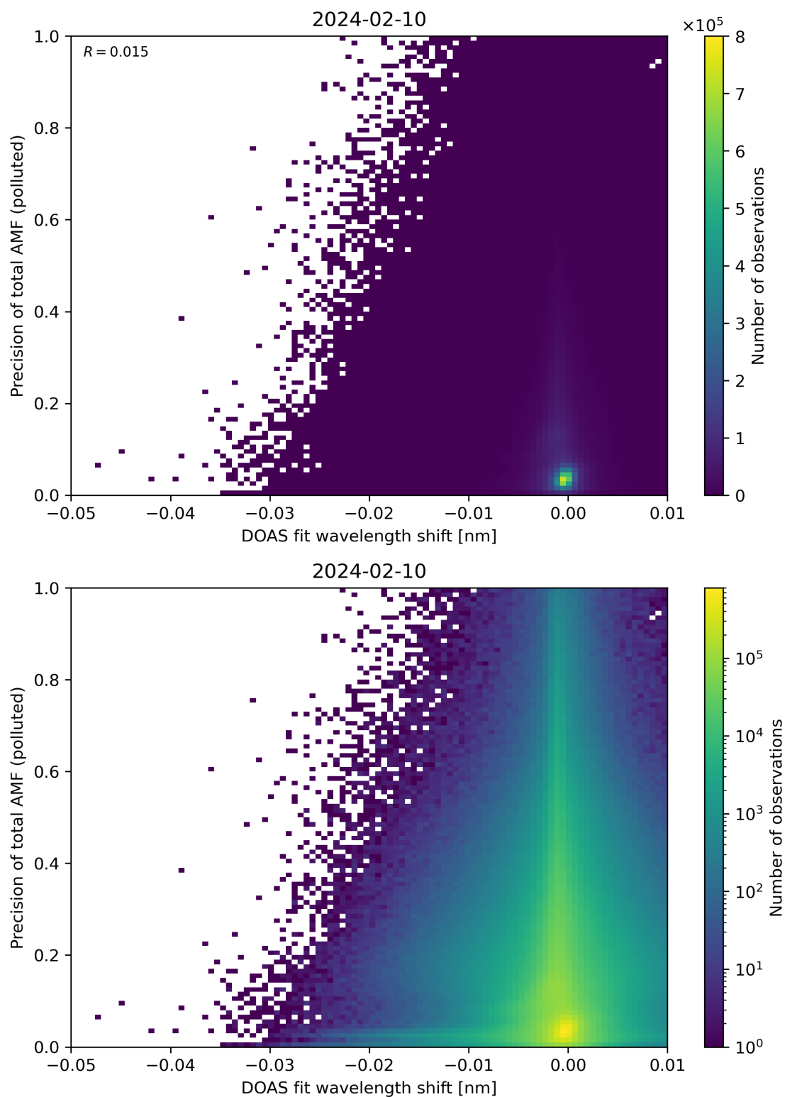
Figure 131: Scatter density plot of “DOAS fit wavelength shift” against “Precision of total AMF (polluted)” for 2024-02-09 to 2024-02-11.
