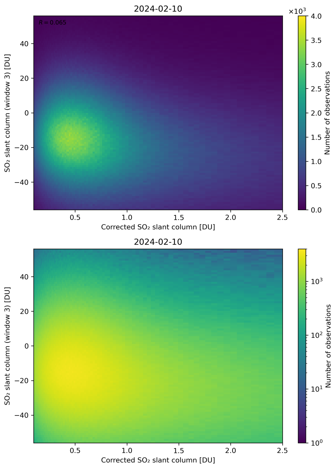
Figure 190: Scatter density plot of “Corrected SO 2 slant column” against “SO 2 slant column (window 3)” for 2024-02-09 to 2024-02-11.
