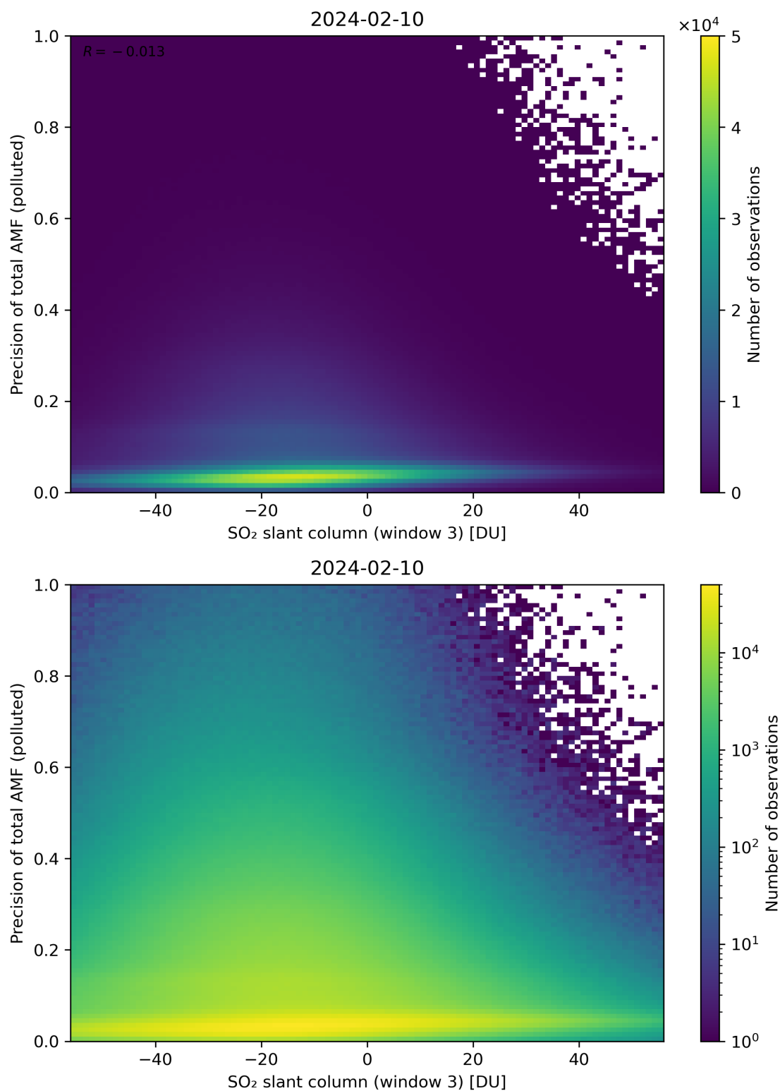
Figure 269: Scatter density plot of “SO 2 slant column (window 3)” against “Precision of total AMF (polluted)” for 2024-02-09 to 2024-02-11.
