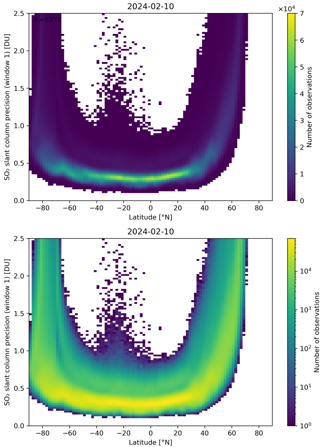
Figure 150: Scatter density plot of “Latitude” against “SO 2 slant column precision (window 1)” for 2024-02-09 to 2024-02-11.
