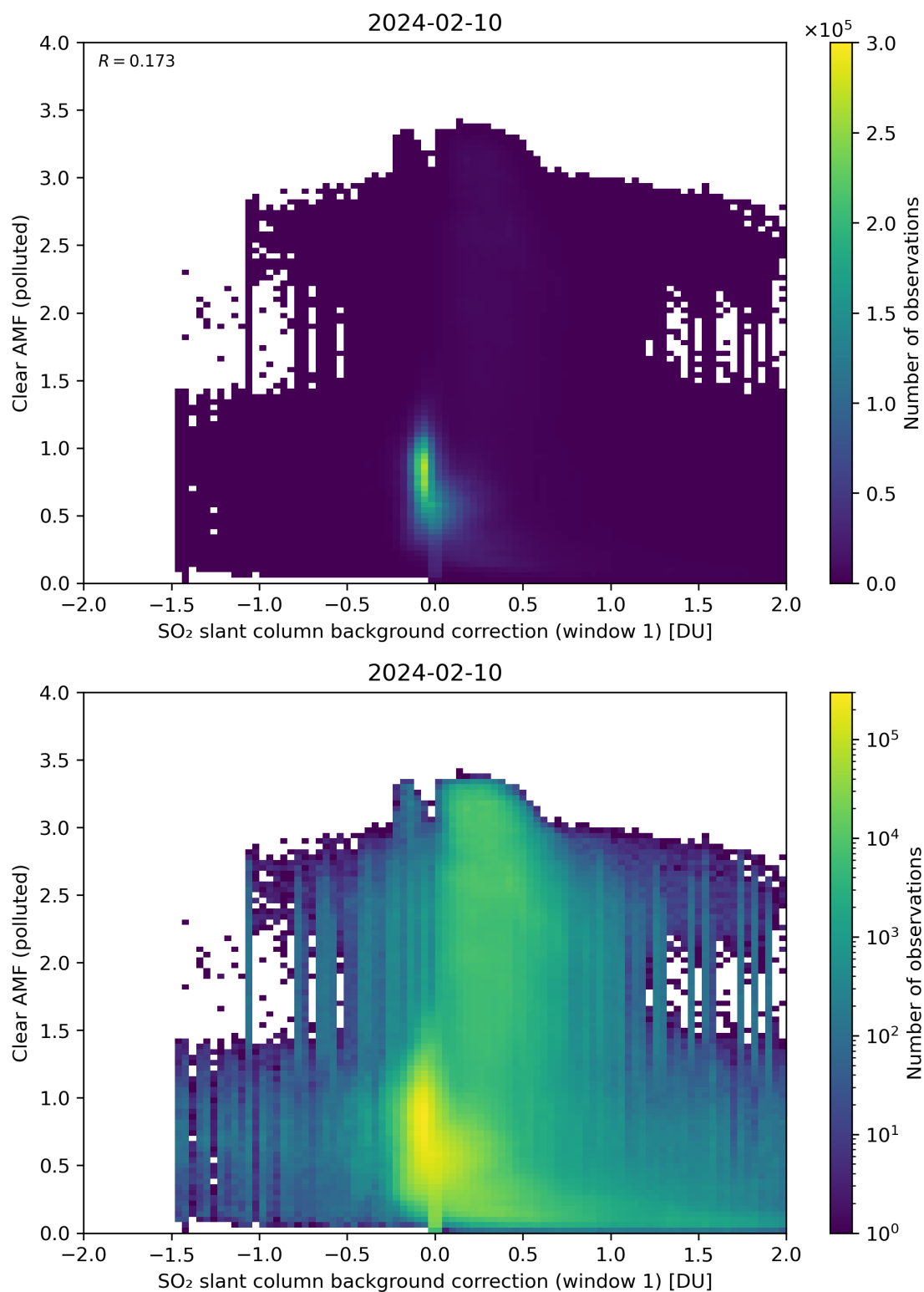
Figure 103: Scatter density plot of “SO 2 slant column background correction (window 1)” against “Clear AMF (polluted)” for 2024-02-09 to 2024-02-11.
