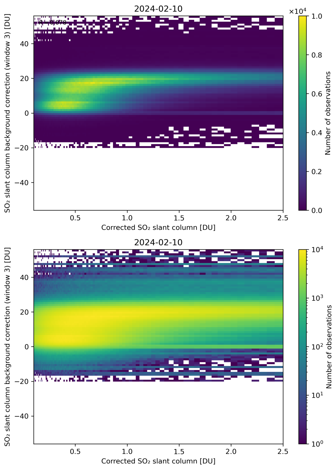
Figure 180: Scatter density plot of “Corrected SO 2 slant column” against “SO 2 slant column background correction (window 3)” for 2024-02-09 to 2024-02-11.
