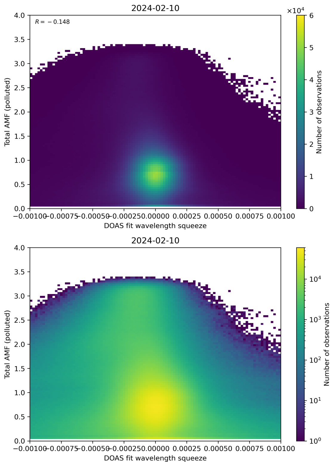
Figure 134: Scatter density plot of “DOAS fit wavelength squeeze” against “Total AMF (polluted)” for 2024-02-09 to 2024-02-11.
