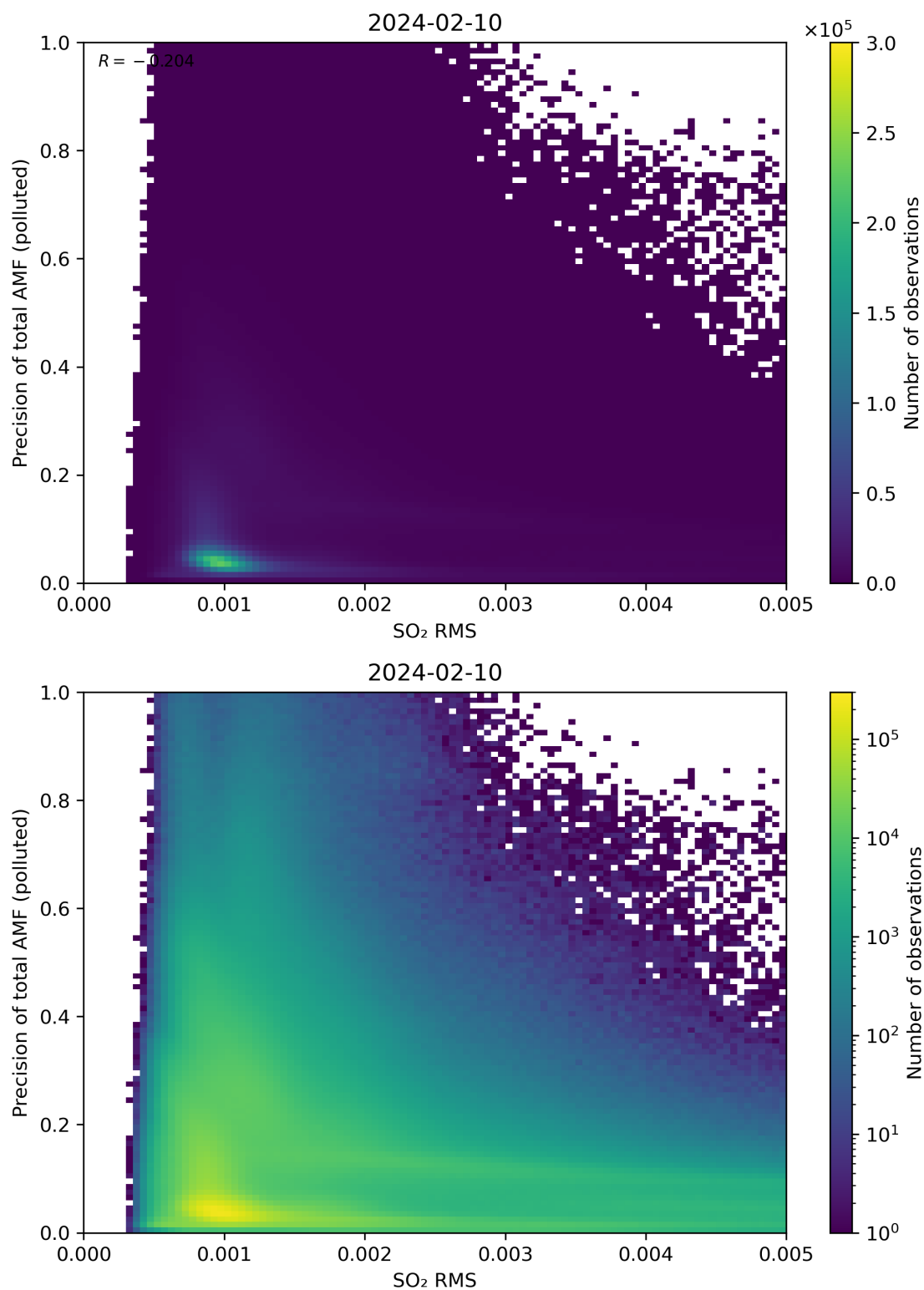
Figure 138: Scatter density plot of “SO 2 RMS” against “Precision of total AMF (polluted)” for 2024-02-09 to 2024-02-11.
