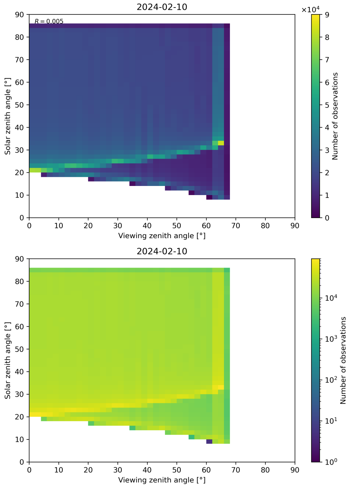
Figure 315: Scatter density plot of “Viewing zenith angle” against “Solar zenith angle” for 2024-02-09 to 2024-02-11.
