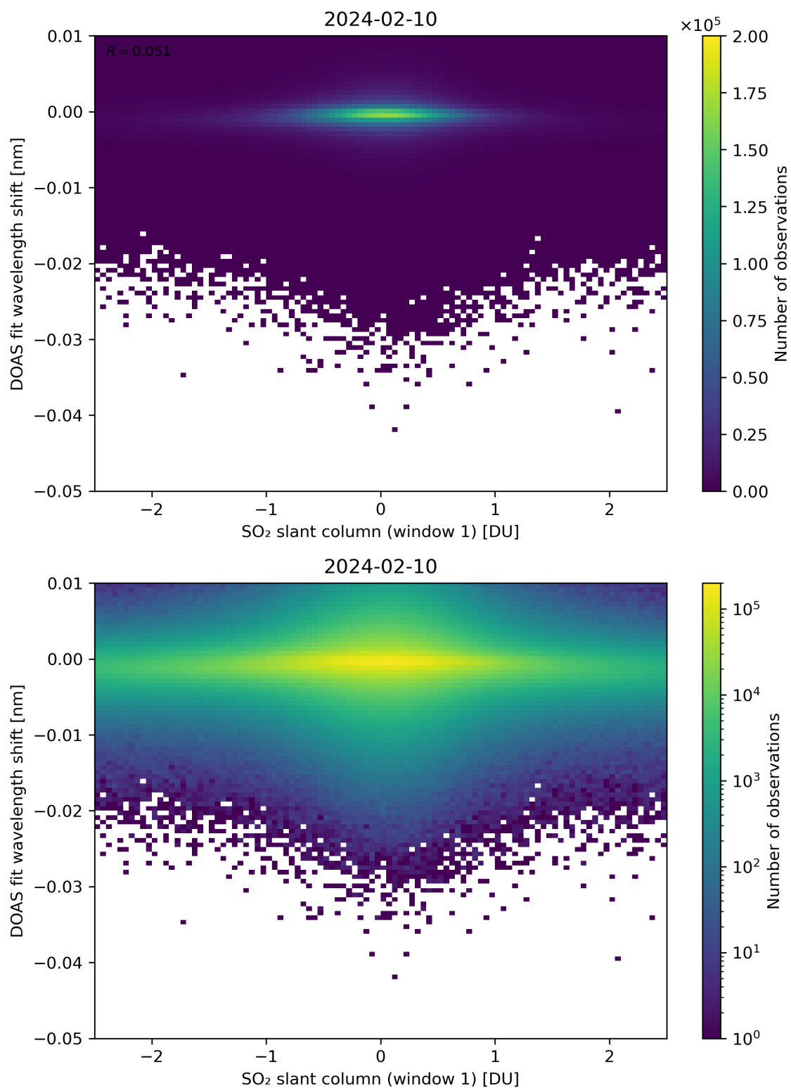
Figure 215: Scatter density plot of “SO 2 slant column (window 1)” against “DOAS fit wavelength shift” for 2024-02-09 to 2024-02-11.
