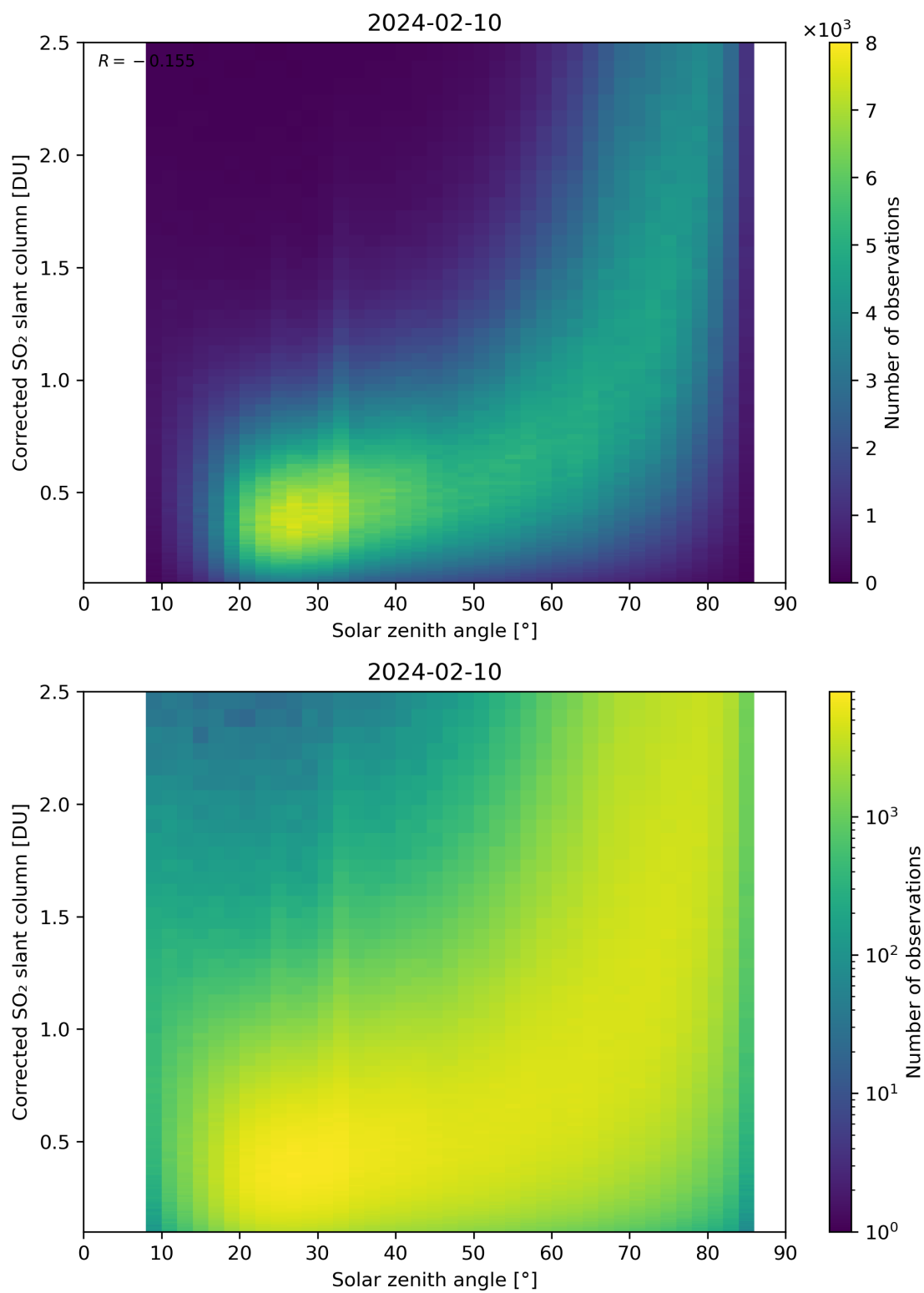
Figure 166: Scatter density plot of “Solar zenith angle” against “Corrected SO 2 slant column” for 2024-02-09 to 2024-02-11.
