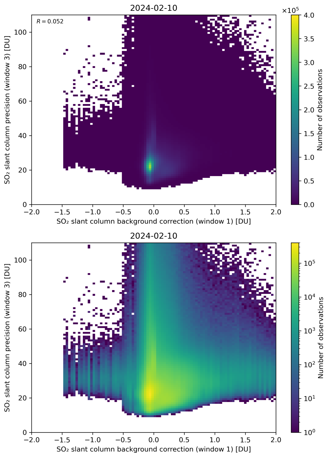
Figure 108: Scatter density plot of “SO 2 slant column background correction (window 1)” against “SO 2 slant column precision (window 3)” for 2024-02-09 to 2024-02-11.
