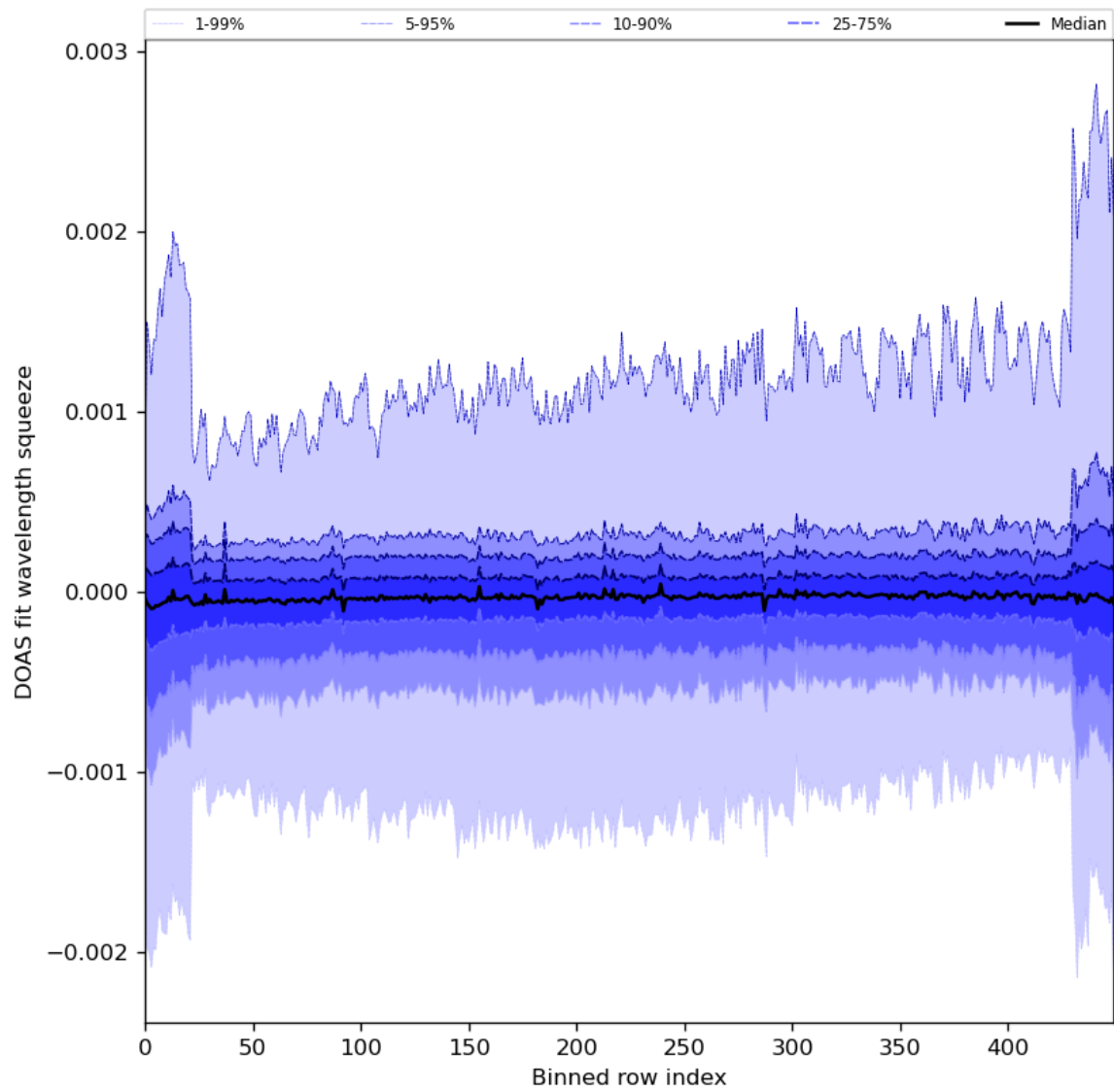
Figure 92: Along track statistics of “DOAS fit wavelength squeeze” for 2024-02-09 to 2024-02-11
