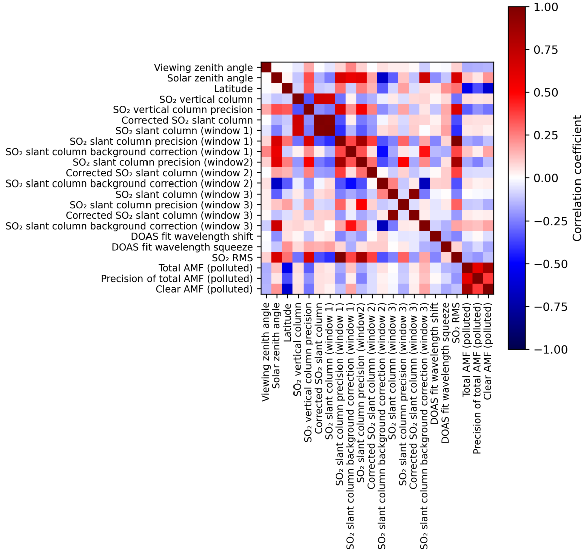
Figure 2: Map of correlation matrix for 2024-02-09 to 2024-02-11.
