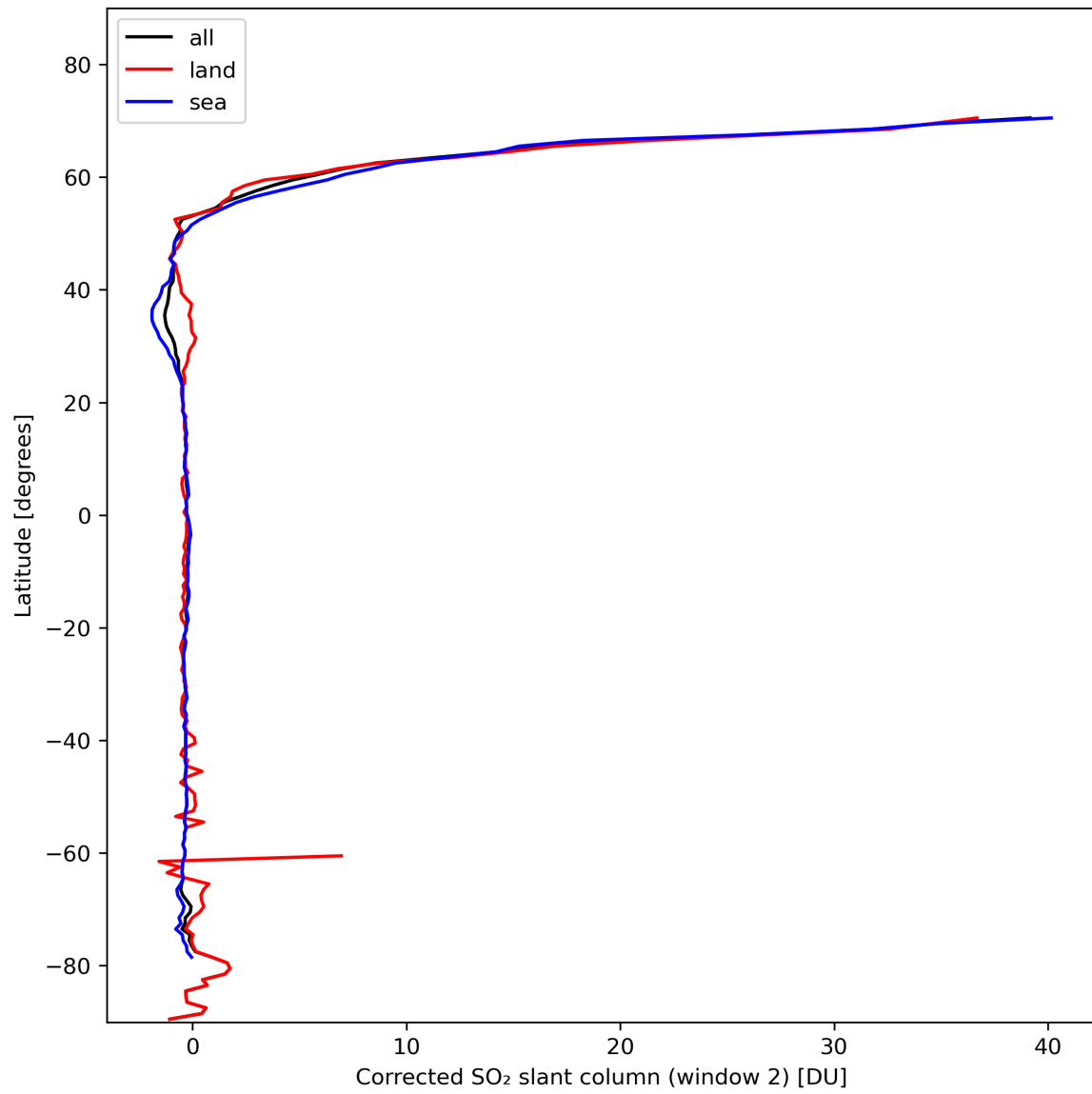
Figure 39: Zonal average of “Corrected SO 2 slant column (window 2)” for 2024-02-09 to 2024-02-11.
