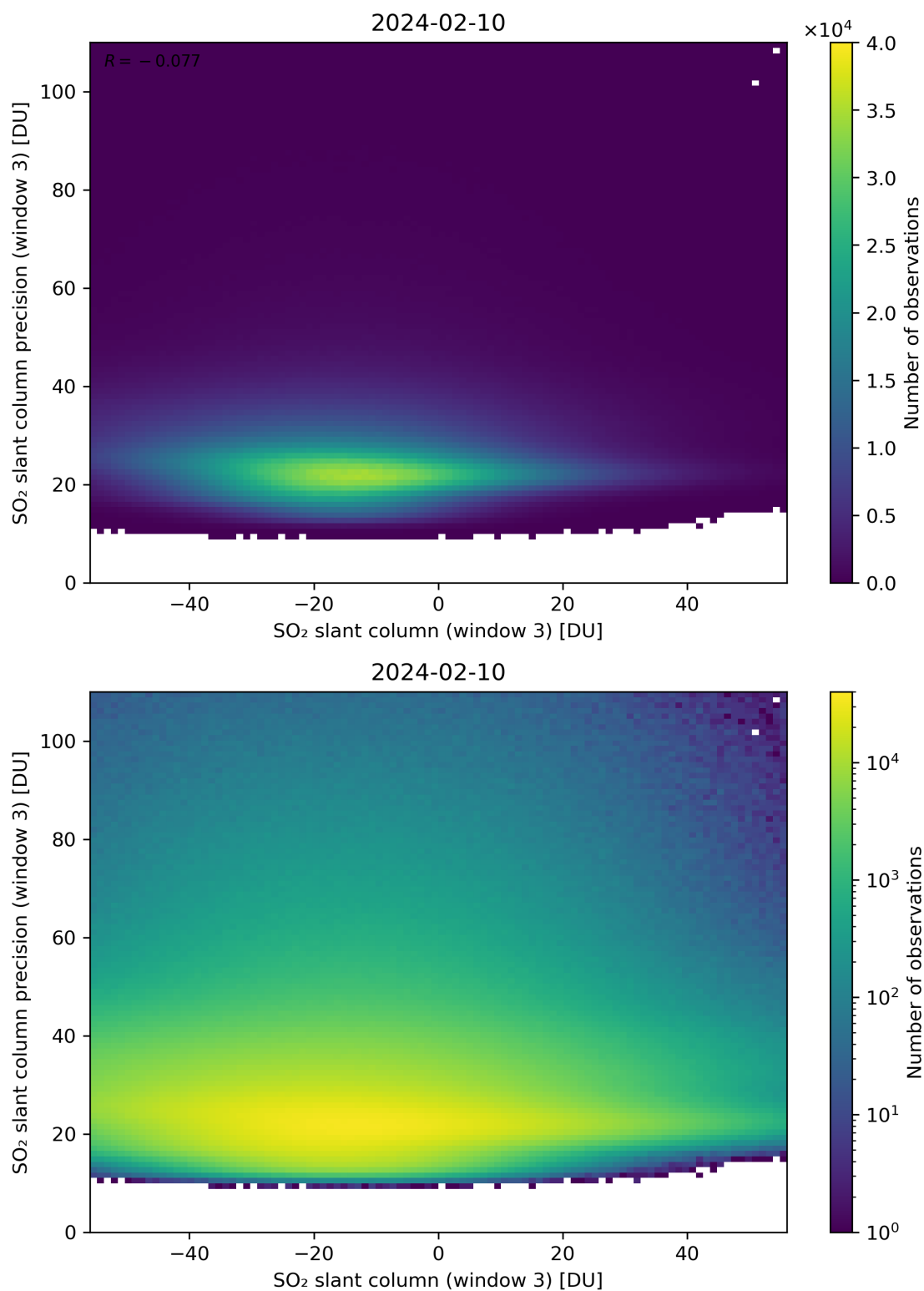
Figure 267: Scatter density plot of “SO 2 slant column (window 3)” against “SO 2 slant column precision (window 3)” for 2024-02-09 to 2024-02-11.
