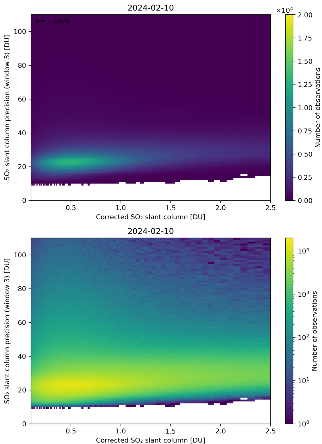
Figure 191: Scatter density plot of “Corrected SO 2 slant column” against “SO 2 slant column precision (window 3)” for 2024-02-09 to 2024-02-11.
