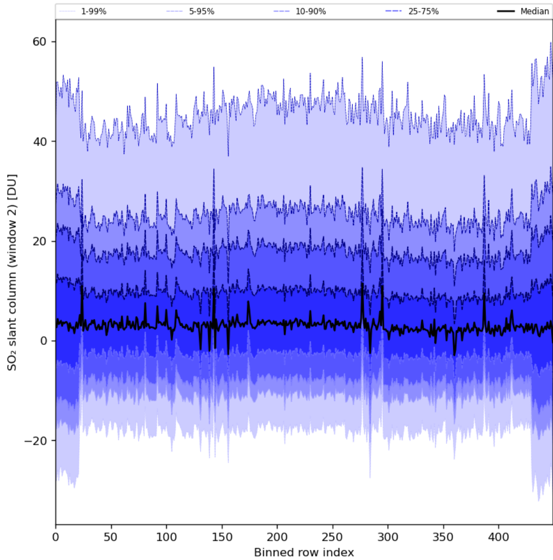
Figure 83: Along track statistics of “SO 2 slant column (window 2)” for 2024-02-09 to 2024-02-11
