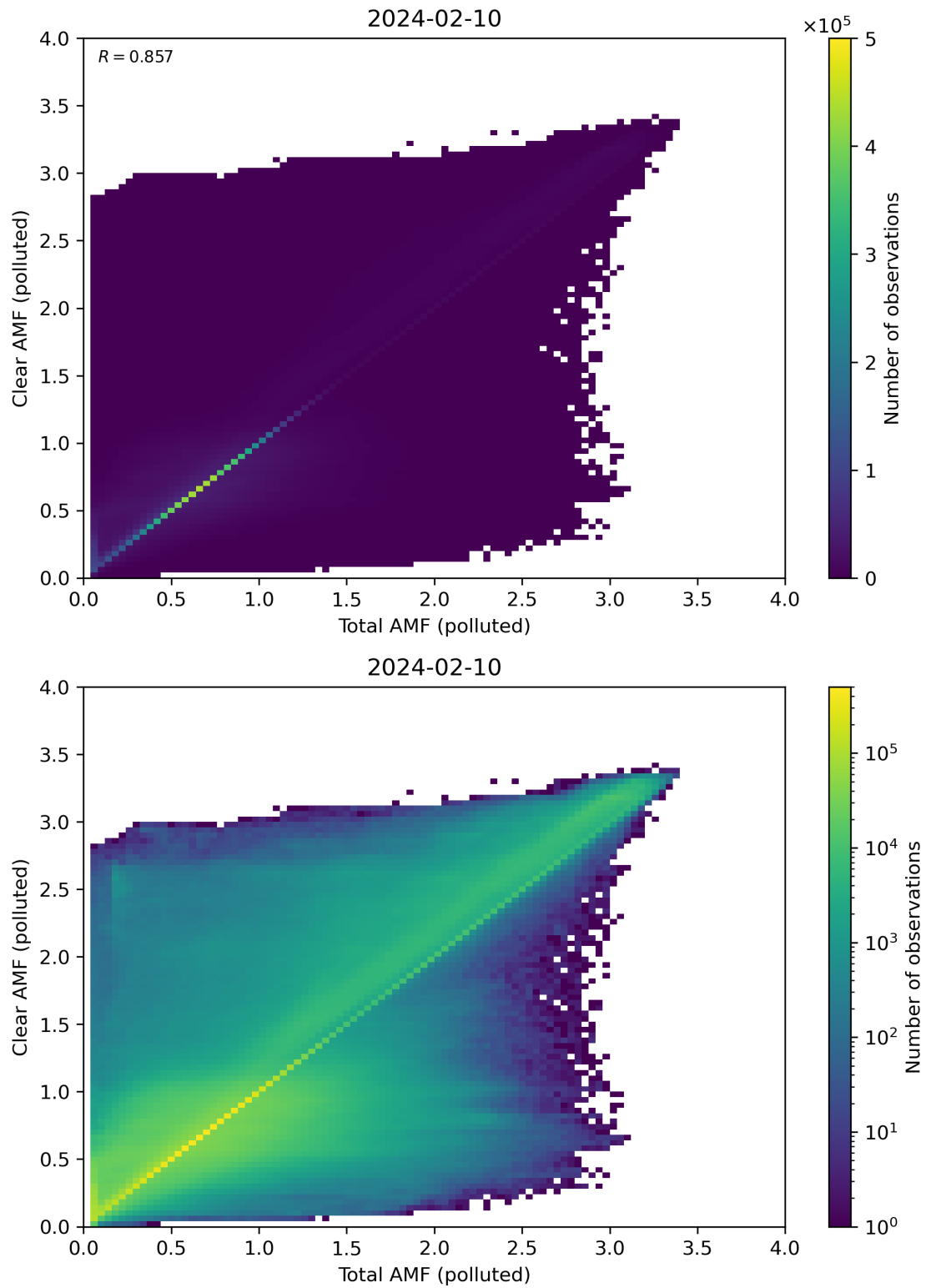
Figure 271: Scatter density plot of “Total AMF (polluted)” against “Clear AMF (polluted)” for 2024-02-09 to 2024-02-11.
