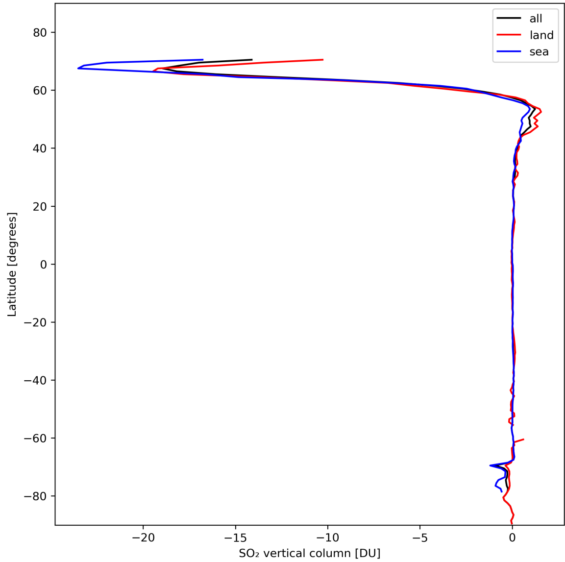
Figure 30: Zonal average of “SO 2 vertical column” for 2024-02-09 to 2024-02-11.
