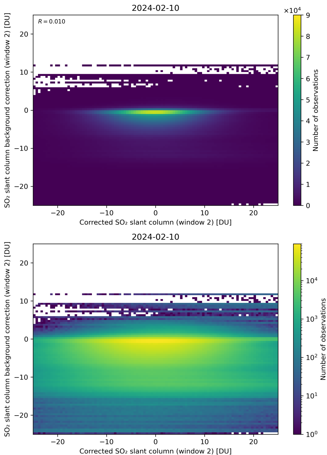
Figure 194: Scatter density plot of “Corrected SO 2 slant column (window 2)” against “SO 2 slant column background correction (window 2)” for 2024-02-09 to 2024-02-11.
