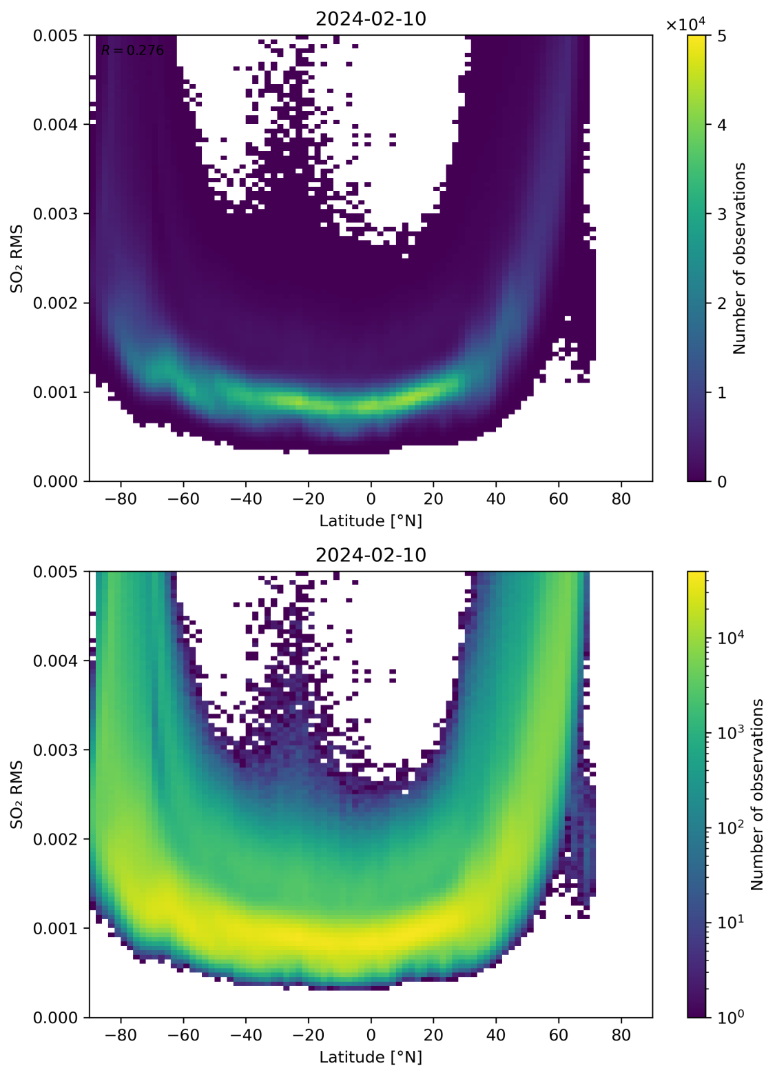
Figure 144: Scatter density plot of “Latitude” against “SO 2 RMS” for 2024-02-09 to 2024-02-11.
