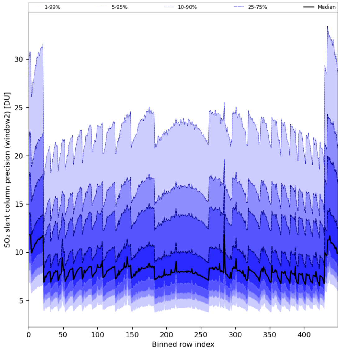
Figure 84: Along track statistics of “SO 2 slant column precision (window2)” for 2024-02-09 to 2024-02-11
