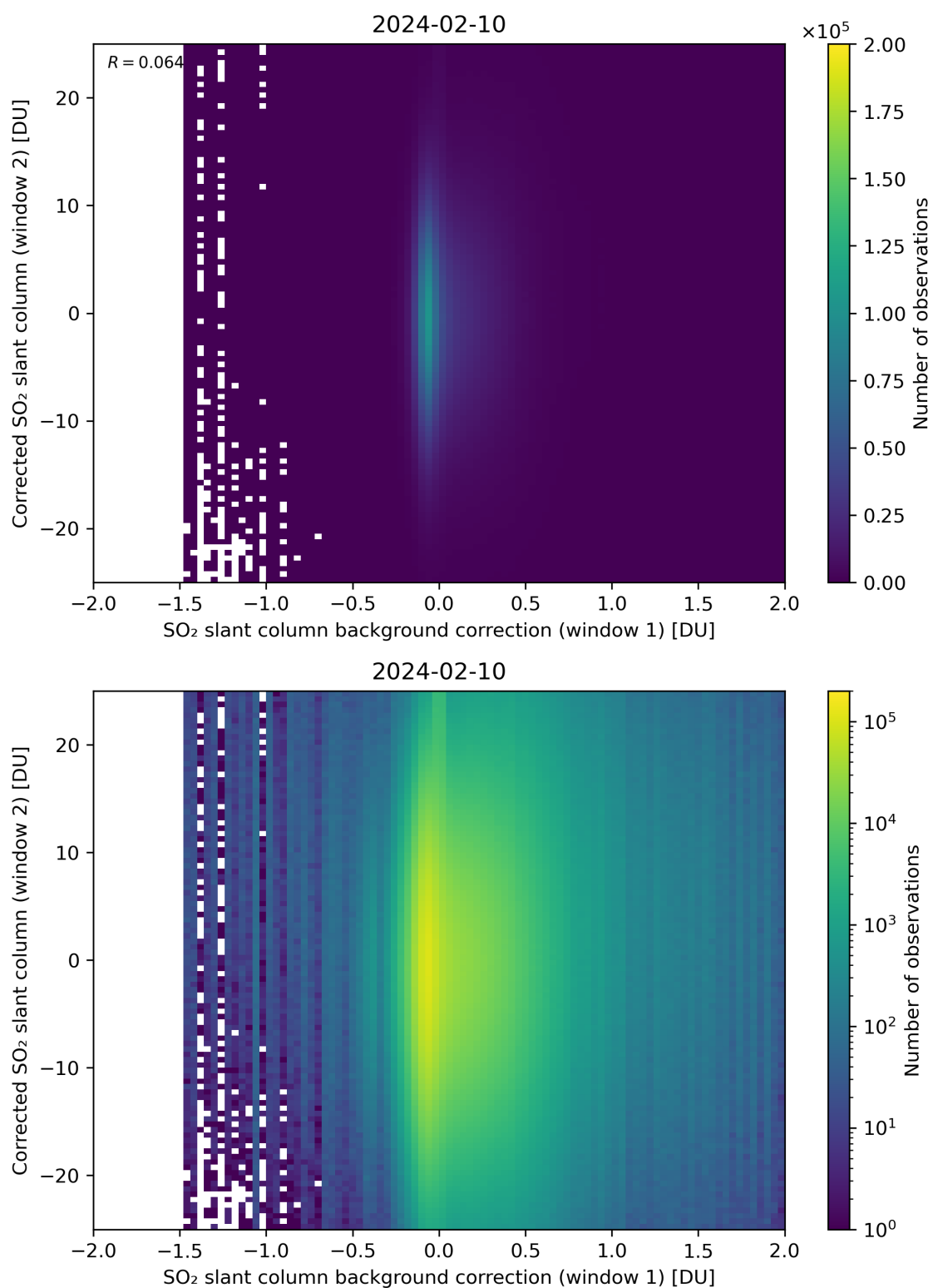
Figure 104: Scatter density plot of “SO 2 slant column background correction (window 1)” against “Corrected SO 2 slant column (window 2)” for 2024-02-09 to 2024-02-11.
