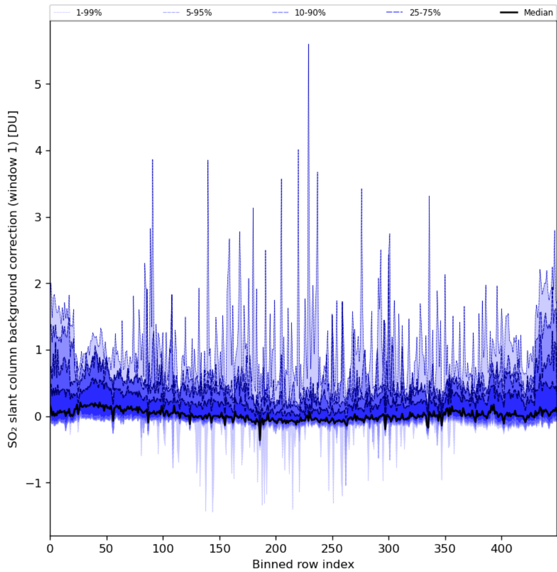
Figure 82: Along track statistics of “SO 2 slant column background correction (window 1)” for 2024-02-09 to 2024-02-11
