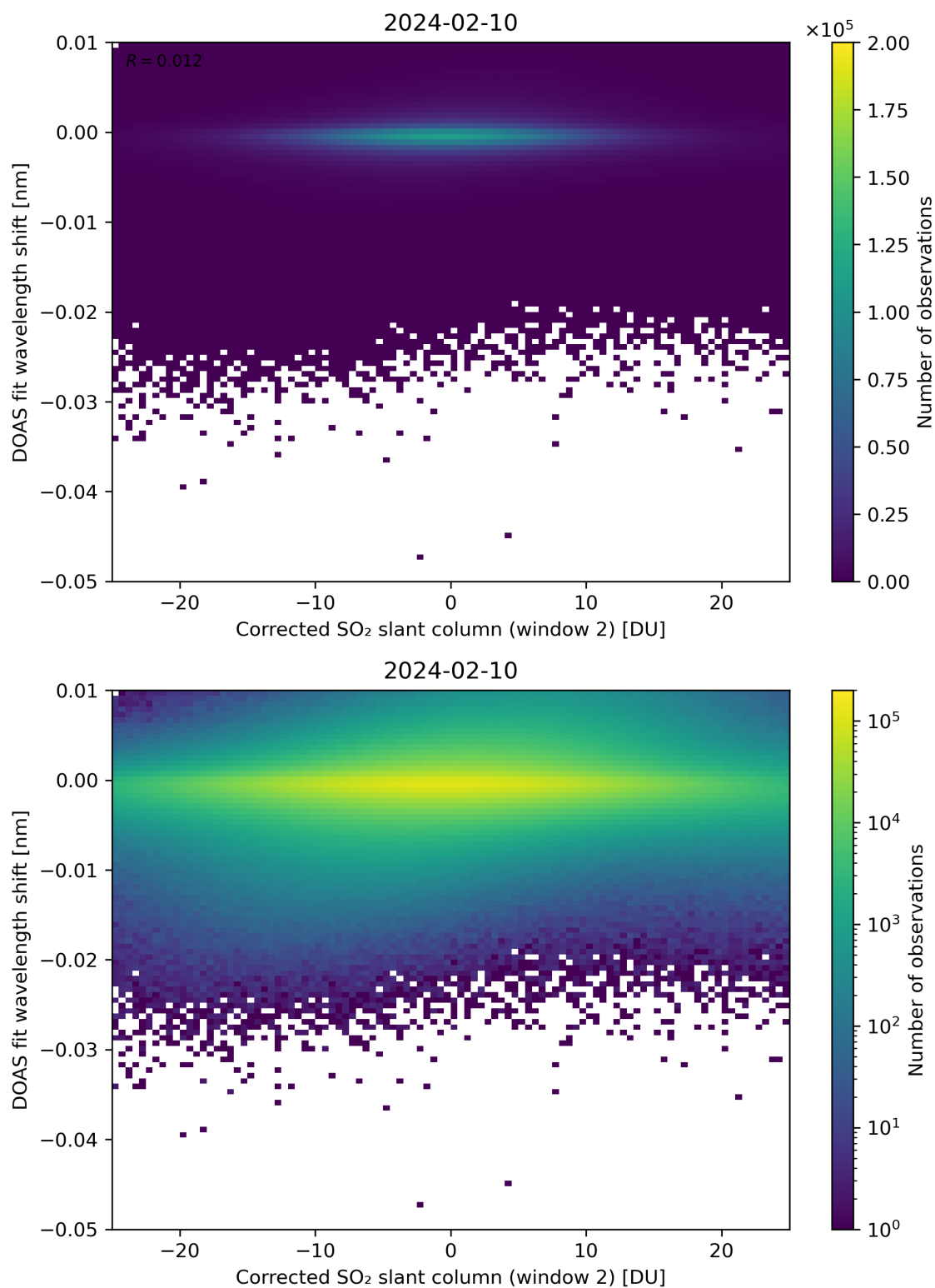
Figure 196: Scatter density plot of “Corrected SO 2 slant column (window 2)” against “DOAS fit wavelength shift” for 2024-02-09 to 2024-02-11.
