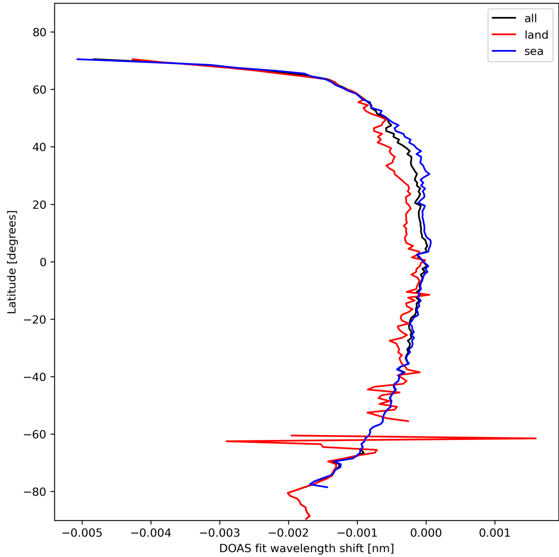
Figure 45: Zonal average of “DOAS fit wavelength shift” for 2024-02-09 to 2024-02-11.
