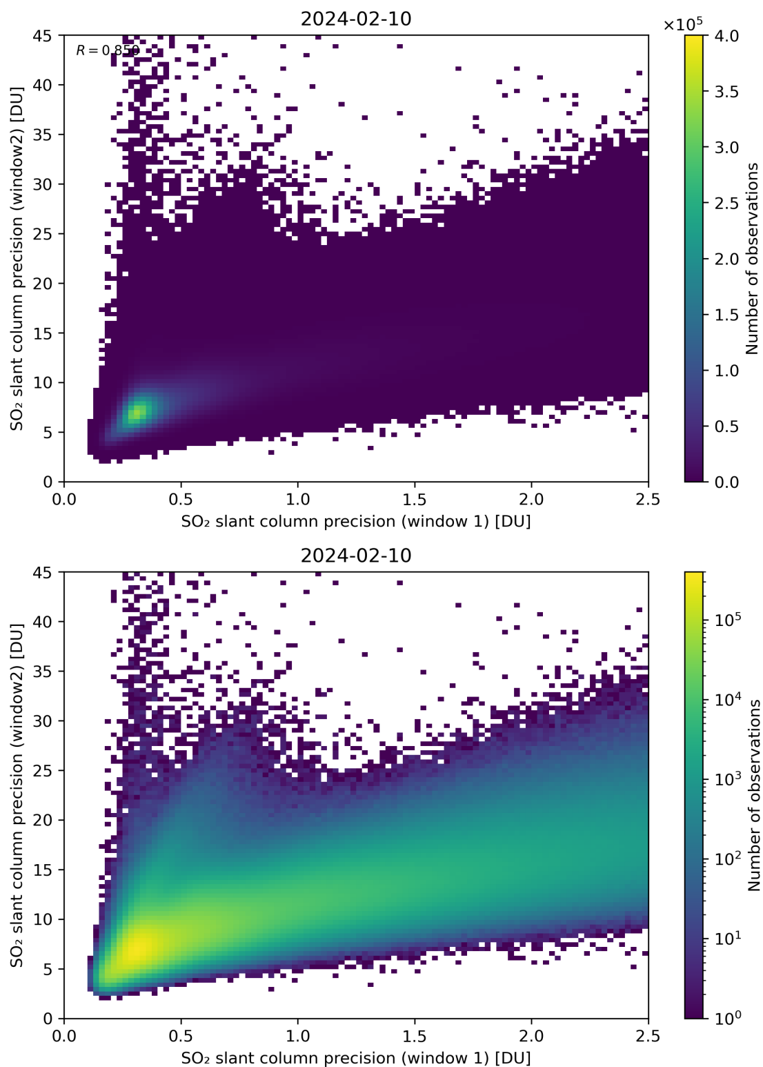
Figure 227: Scatter density plot of “SO 2 slant column precision (window 1)” against “SO 2 slant column precision (window 2)” for 2024-02-09 to 2024-02-11.
