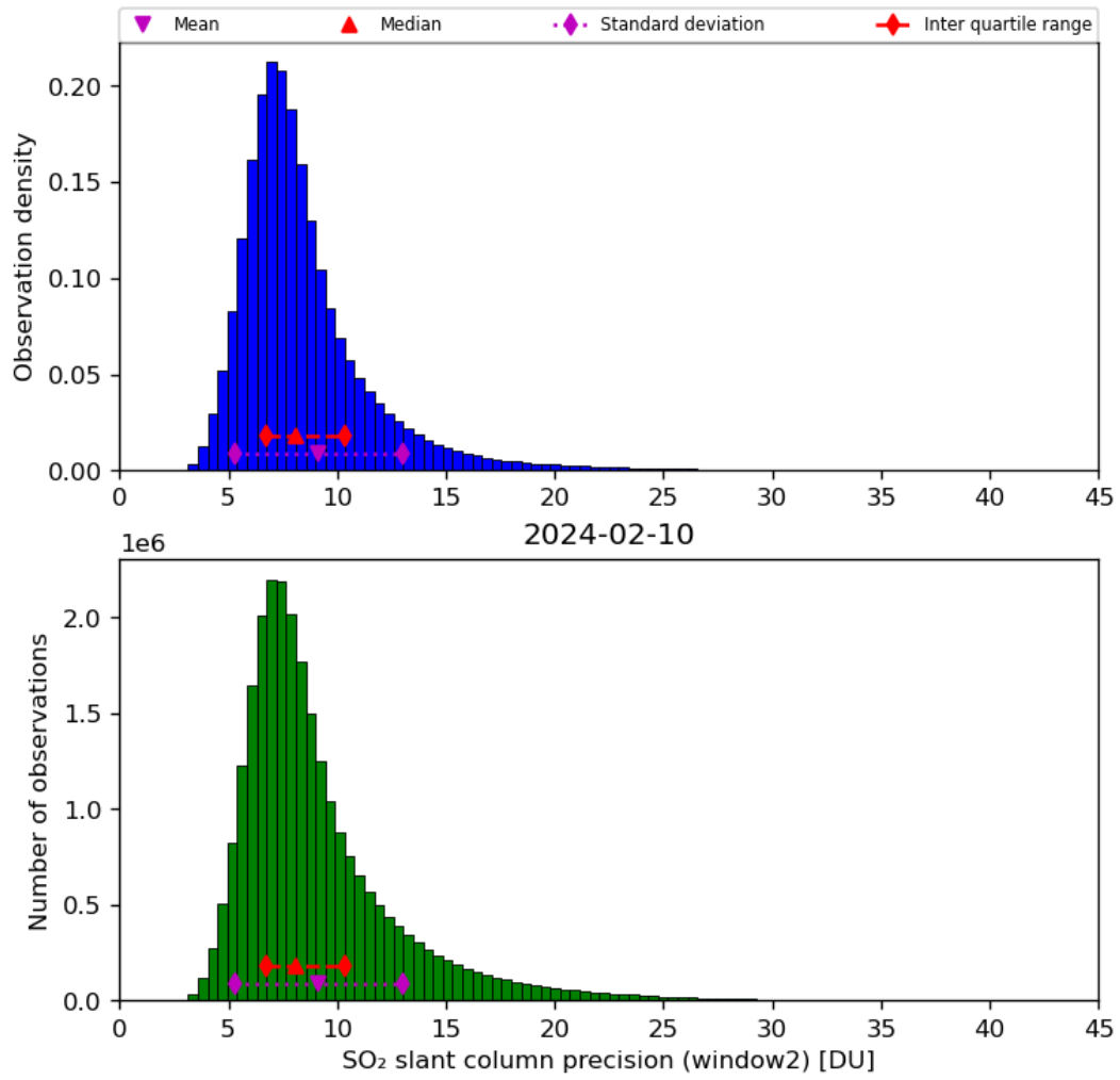
Figure 61: Histogram of “SO 2 slant column precision (window2)” for 2024-02-09 to 2024-02-11
