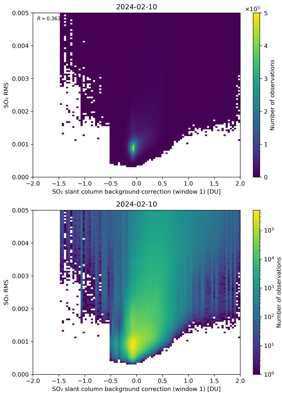
Figure 102: Scatter density plot of “SO 2 slant column background correction (window 1)” against “SO 2 RMS” for 2024-02-09 to 2024-02-11.
