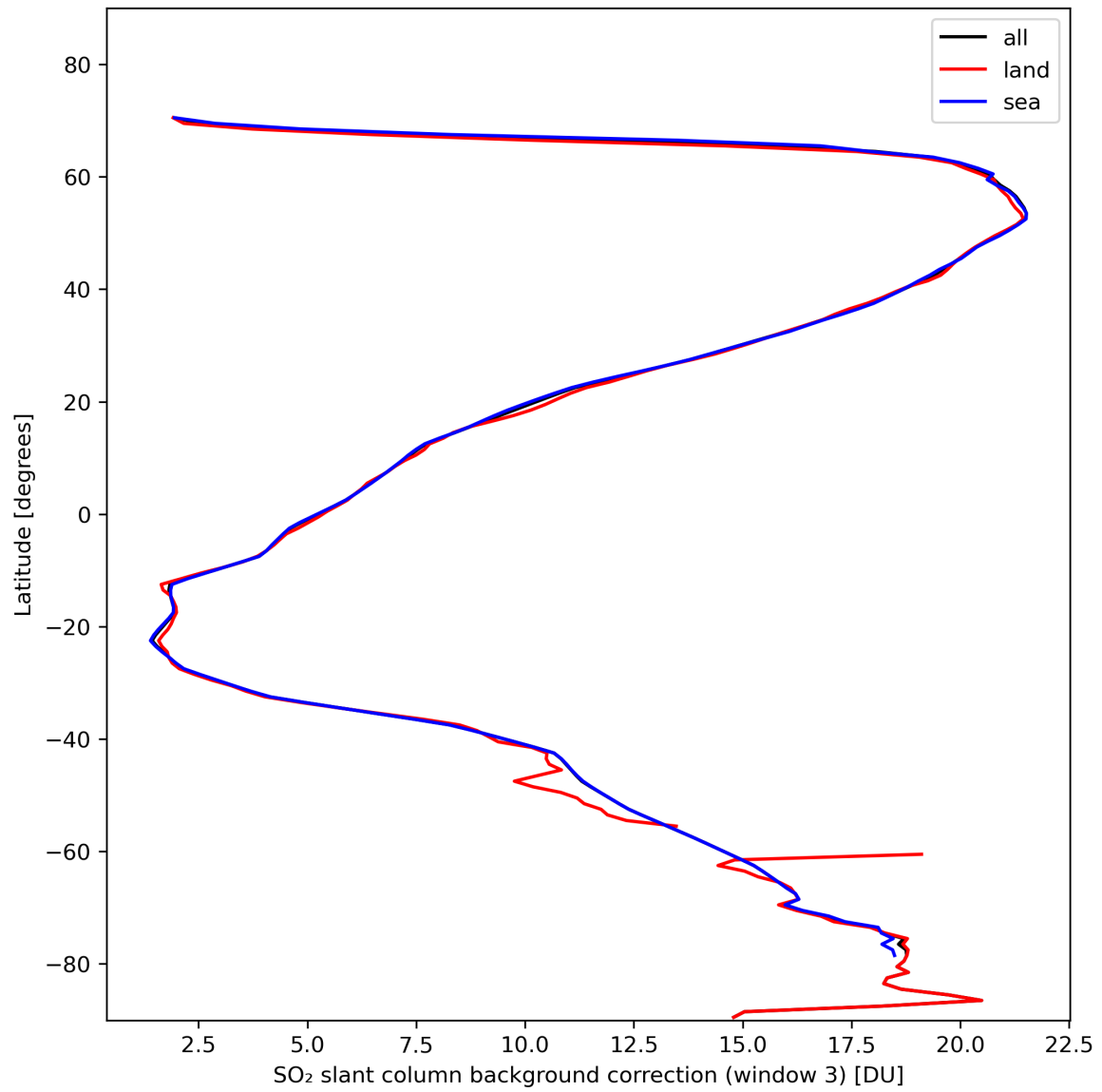
Figure 44: Zonal average of “SO 2 slant column background correction (window 3)” for 2024-02-09 to 2024-02-11.
