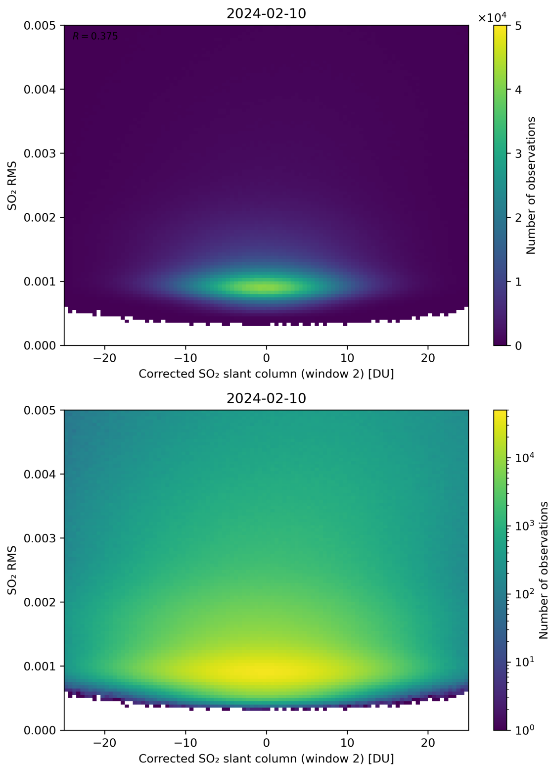
Figure 198: Scatter density plot of “Corrected SO 2 slant column (window 2)” against “SO 2 RMS” for 2024-02-09 to 2024-02-11.
