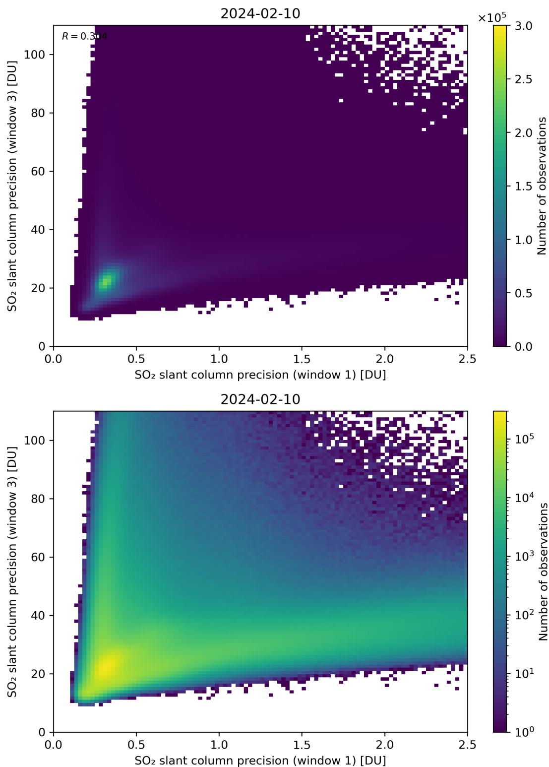
Figure 229: Scatter density plot of “SO 2 slant column precision (window 1)” against “SO 2 slant column precision (window 3)” for 2024-02-09 to 2024-02-11.
