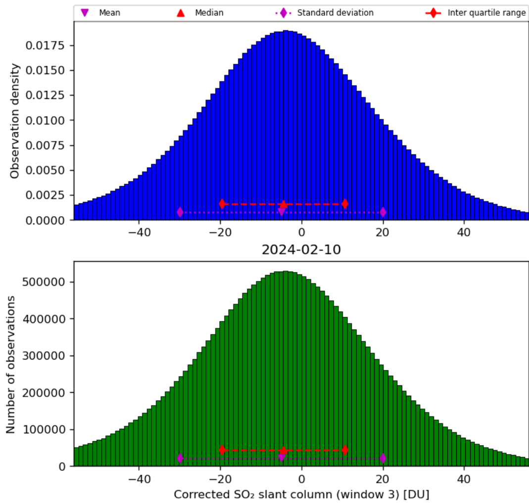
Figure 66: Histogram of “Corrected SO 2 slant column (window 3)” for 2024-02-09 to 2024-02-11
