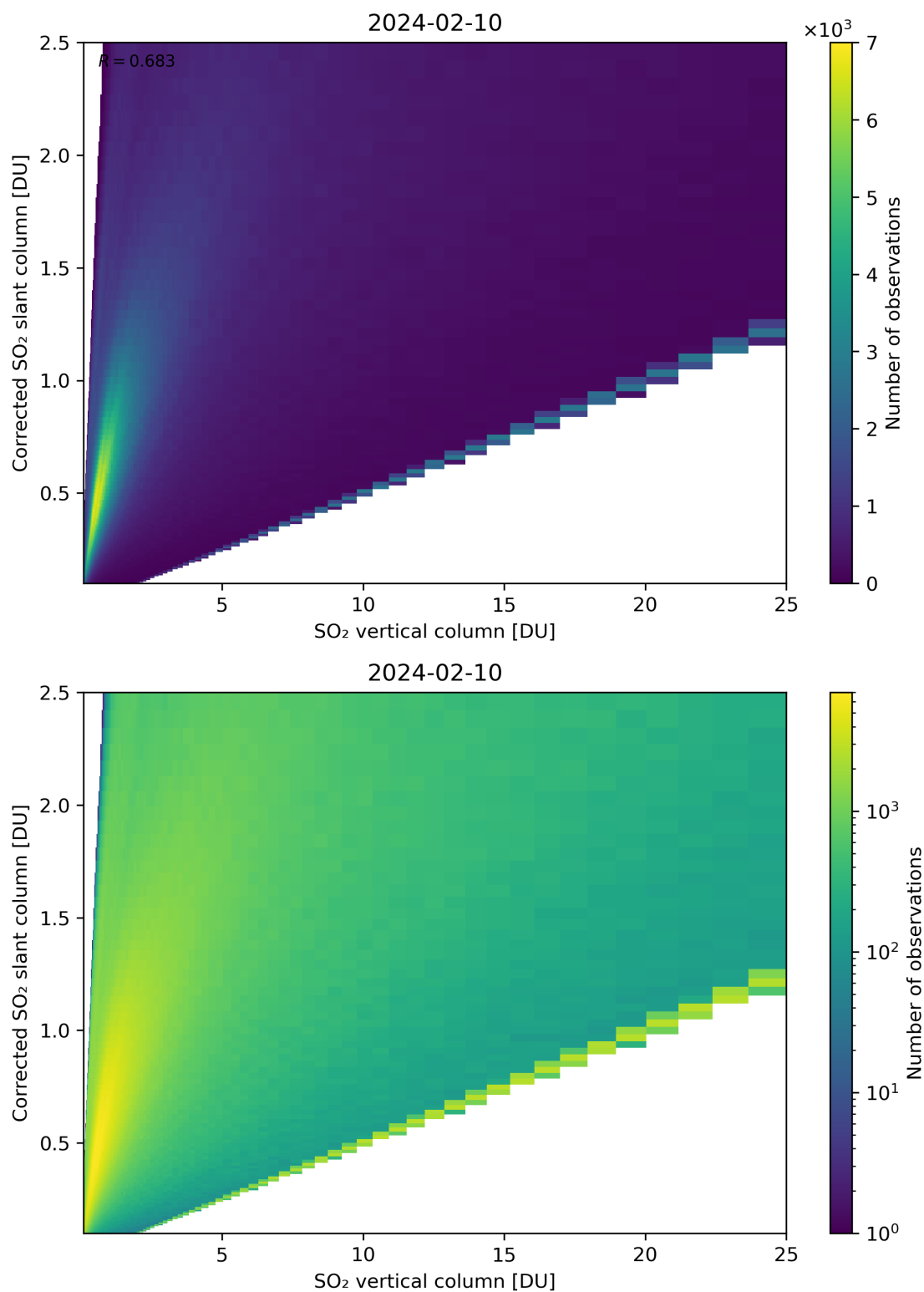
Figure 297: Scatter density plot of “SO 2 vertical column” against “Corrected SO 2 slant column” for 2024-02-09 to 2024-02-11.
