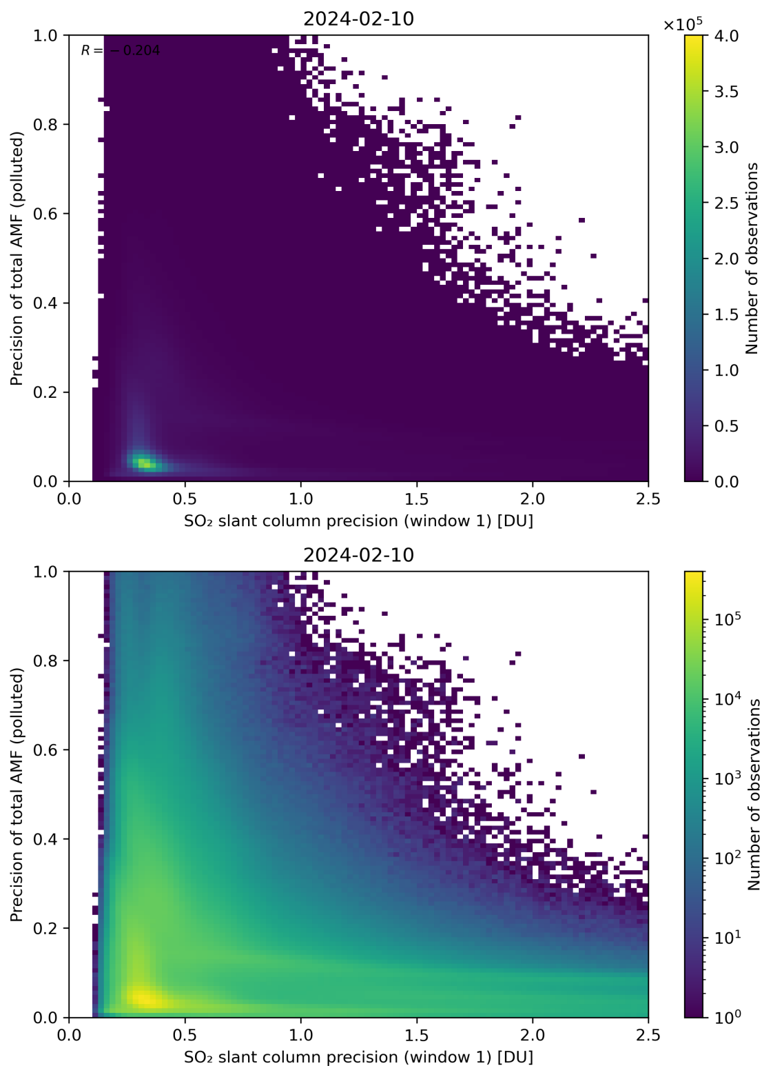
Figure 231: Scatter density plot of “SO 2 slant column precision (window 1)” against “Precision of total AMF (polluted)” for 2024-02-09 to 2024-02-11.
