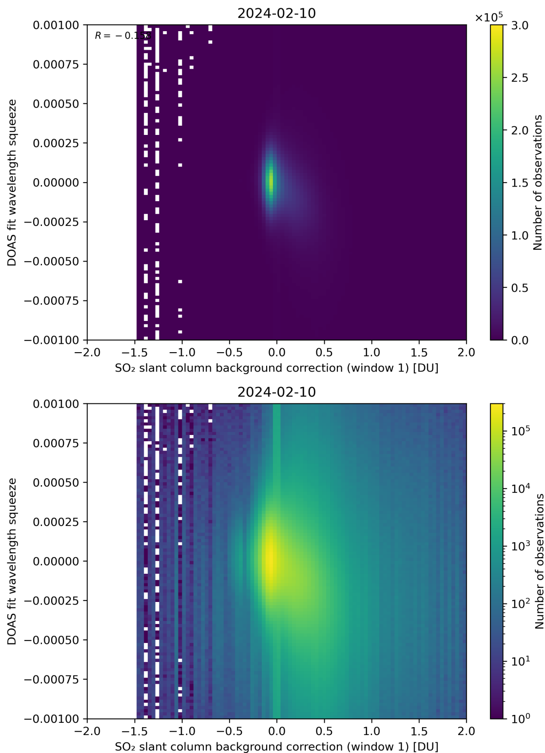
Figure 101: Scatter density plot of “SO 2 slant column background correction (window 1)” against “DOAS fit wavelength squeeze” for 2024-02-09 to 2024-02-11.
