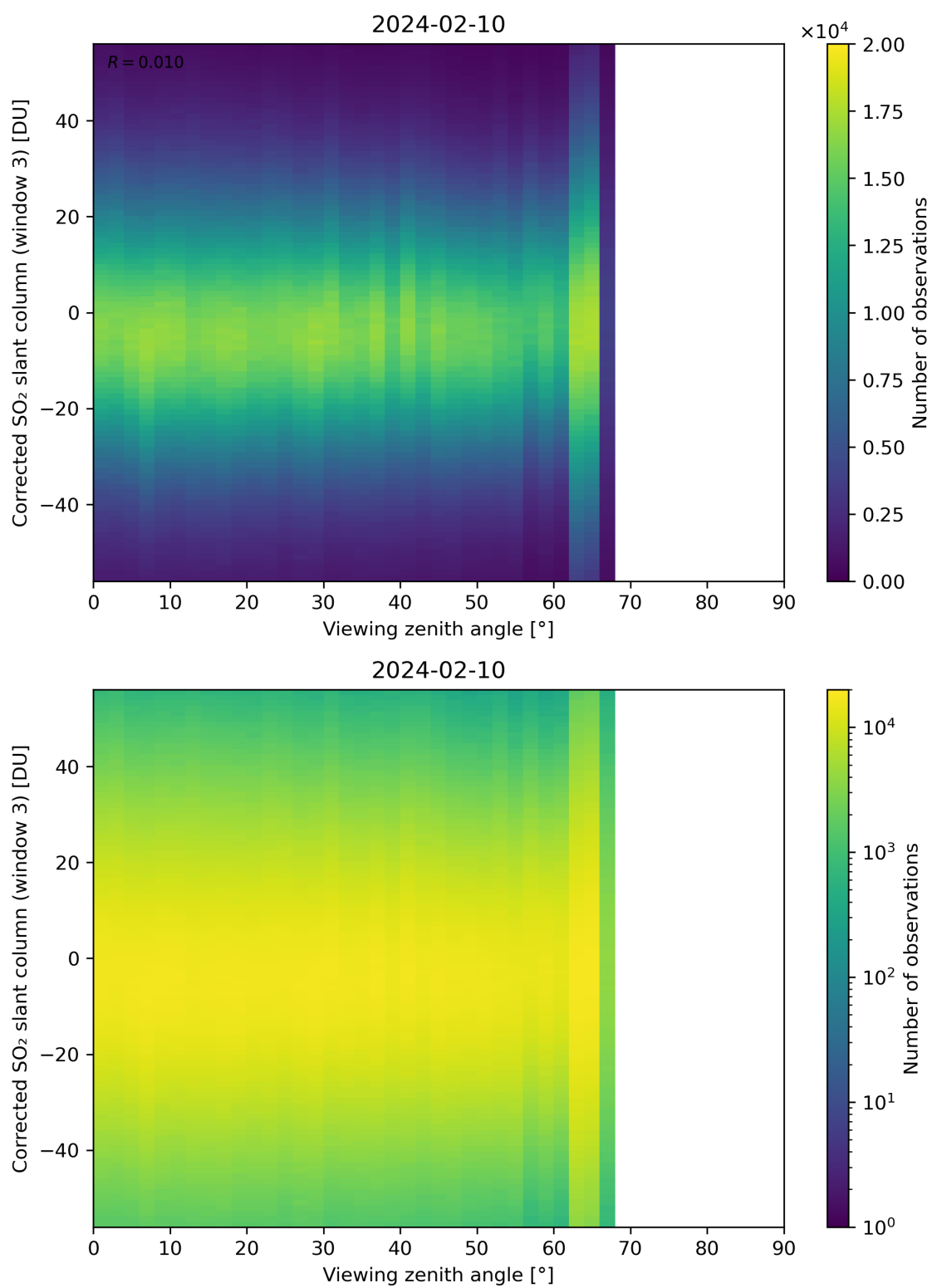
Figure 319: Scatter density plot of “Viewing zenith angle” against “Corrected SO 2 slant column (window 3)” for 2024-02-09 to 2024-02-11.
