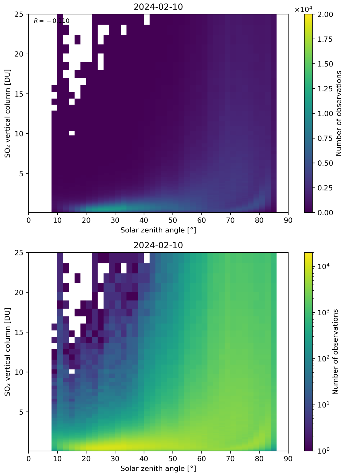
Figure 176: Scatter density plot of “Solar zenith angle” against “SO 2 vertical column” for 2024-02-09 to 2024-02-11.
