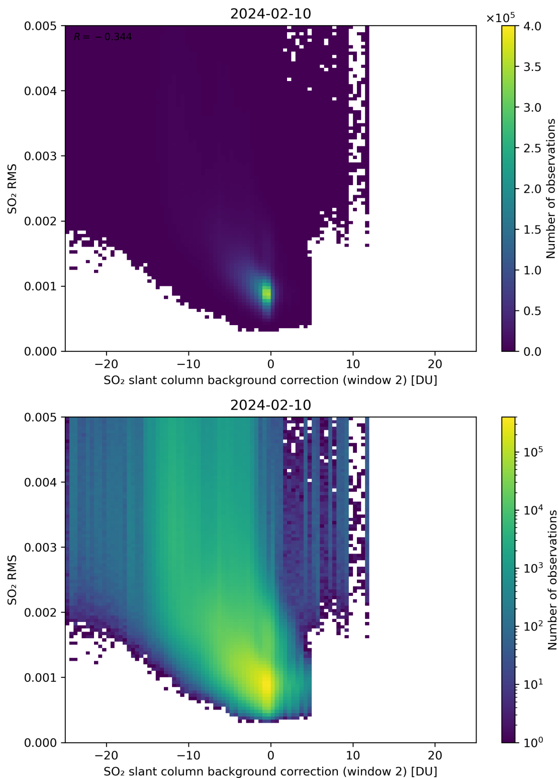
Figure 114: Scatter density plot of “SO 2 slant column background correction (window 2)” against “SO 2 RMS” for 2024-02-09 to 2024-02-11.
