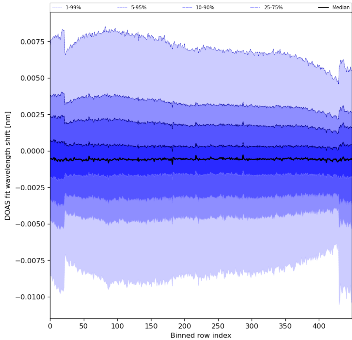
Figure 91: Along track statistics of “DOAS fit wavelength shift” for 2024-02-09 to 2024-02-11
