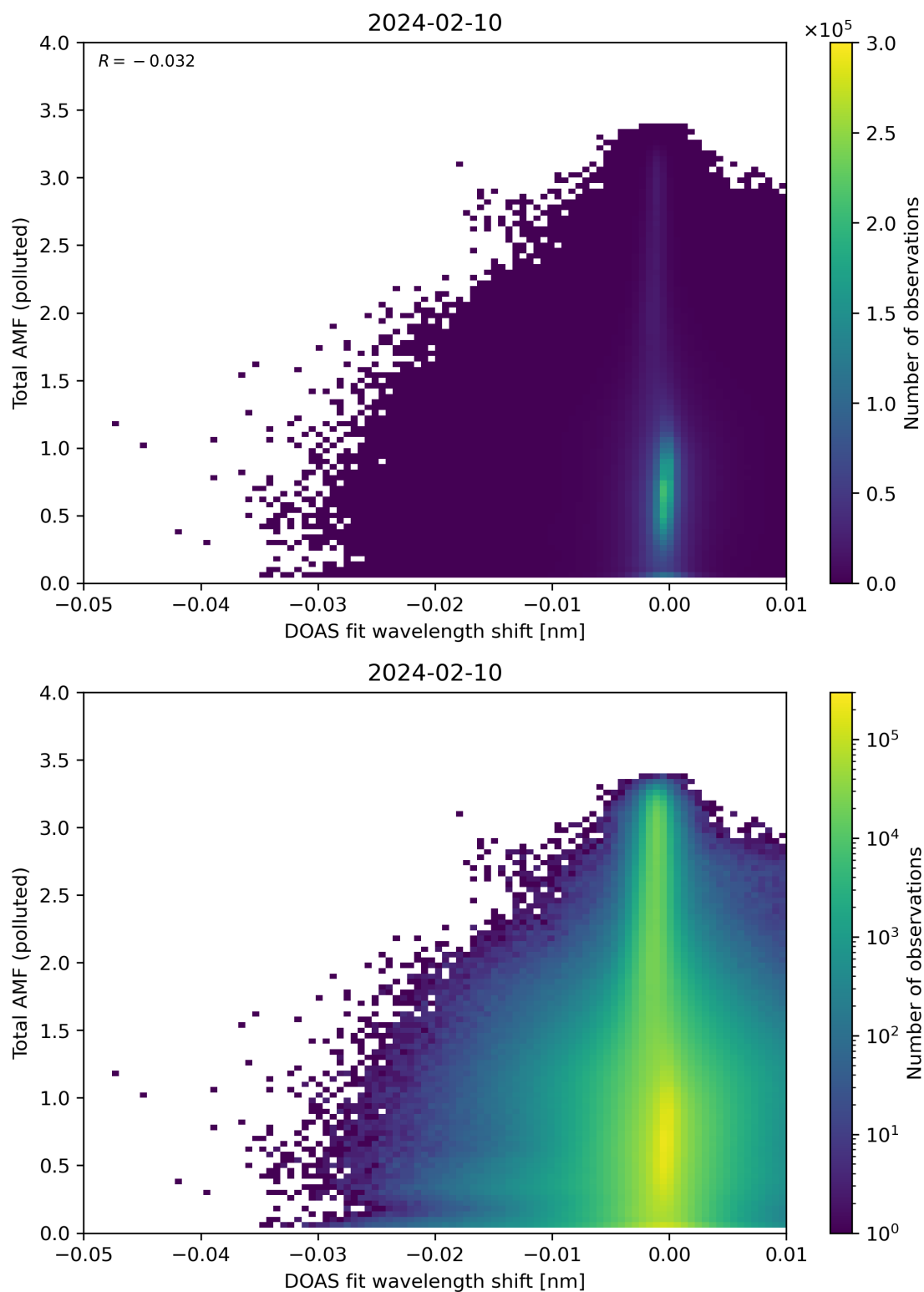
Figure 130: Scatter density plot of “DOAS fit wavelength shift” against “Total AMF (polluted)” for 2024-02-09 to 2024-02-11.
