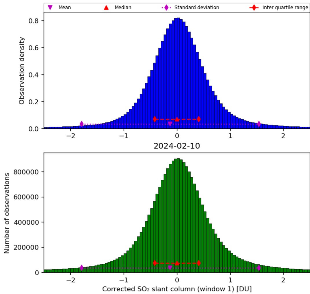
Figure 58: Histogram of “Corrected SO 2 slant column (window 1)” for 2024-02-09 to 2024-02-11
