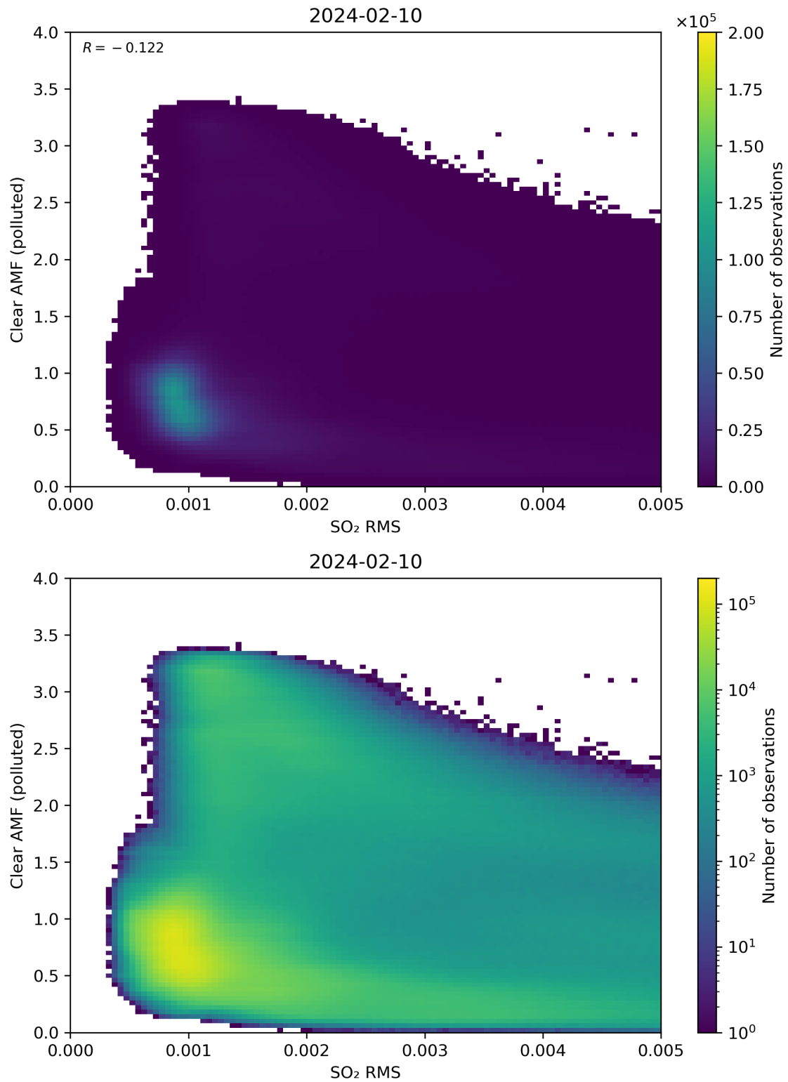
Figure 136: Scatter density plot of “SO 2 RMS” against “Clear AMF (polluted)” for 2024-02-09 to 2024-02-11.
