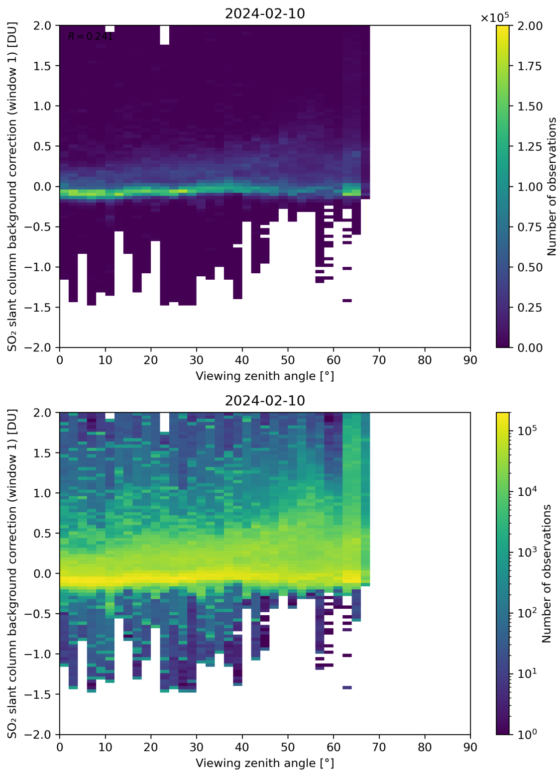
Figure 308: Scatter density plot of “Viewing zenith angle” against “SO 2 slant column background correction (window 1)” for 2024-02-09 to 2024-02-11.
