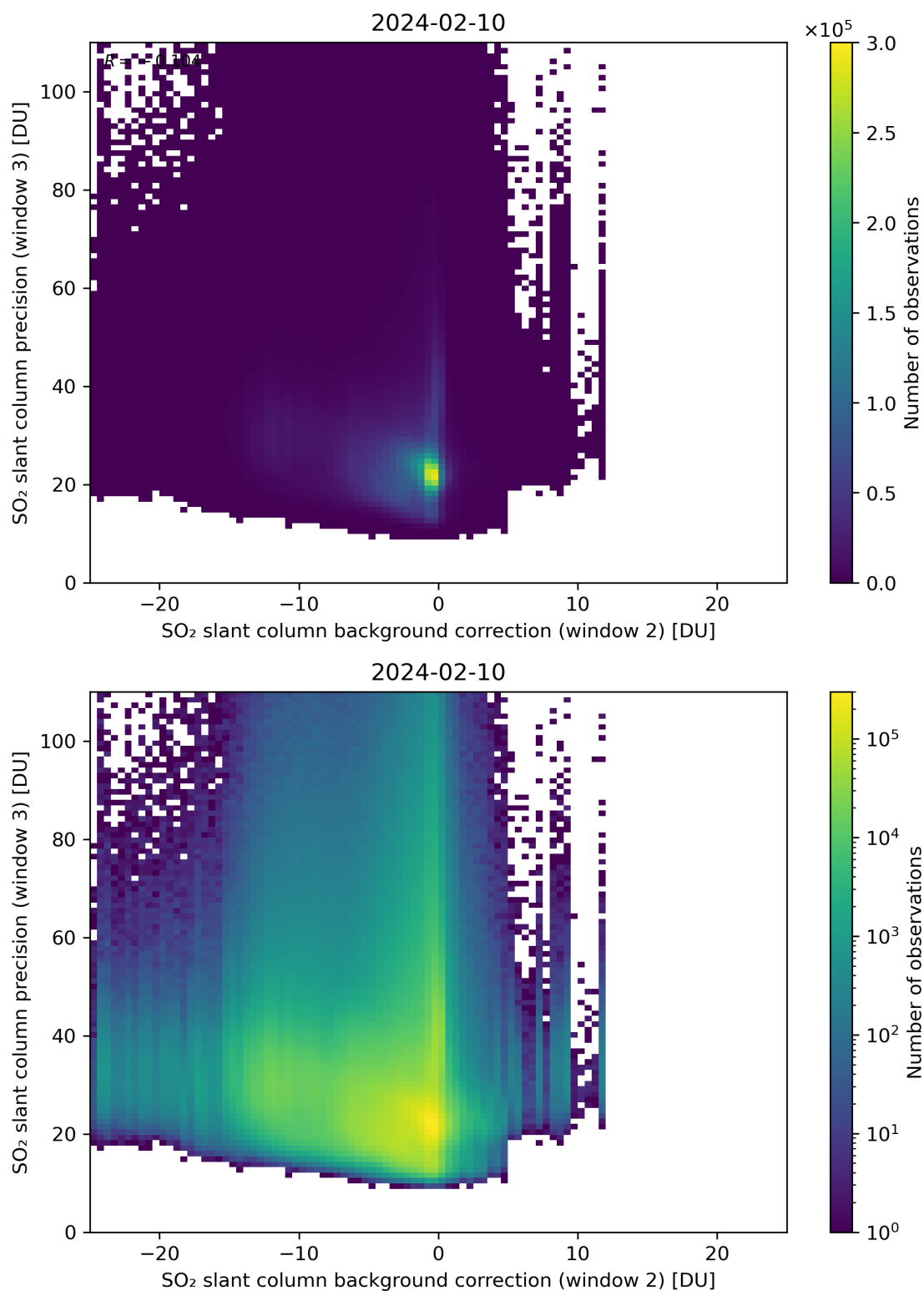
Figure 118: Scatter density plot of “SO 2 slant column background correction (window 2)” against “SO 2 slant column precision (window 3)” for 2024-02-09 to 2024-02-11.
