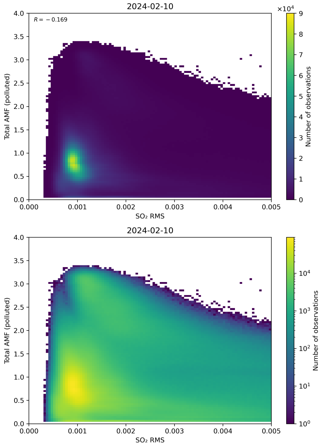
Figure 137: Scatter density plot of “SO 2 RMS” against “Total AMF (polluted)” for 2024-02-09 to 2024-02-11.
