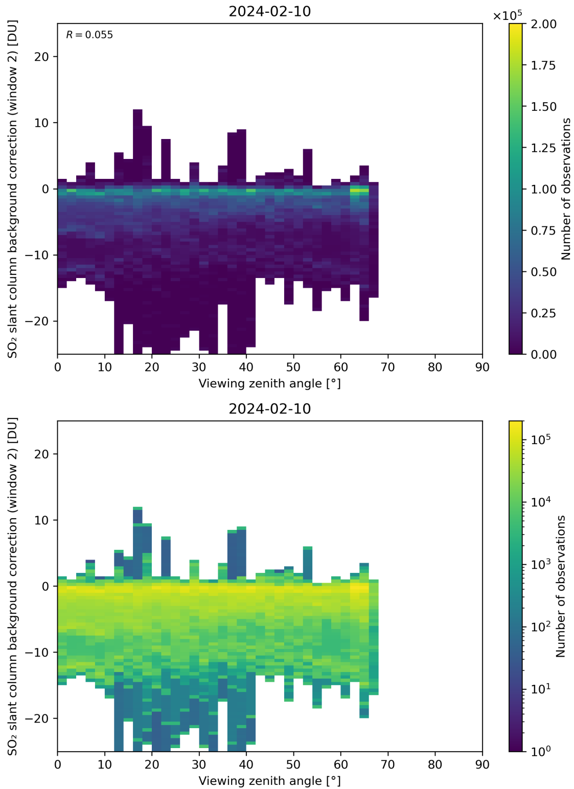
Figure 309: Scatter density plot of “Viewing zenith angle” against “SO 2 slant column background correction (window 2)” for 2024-02-09 to 2024-02-11.
