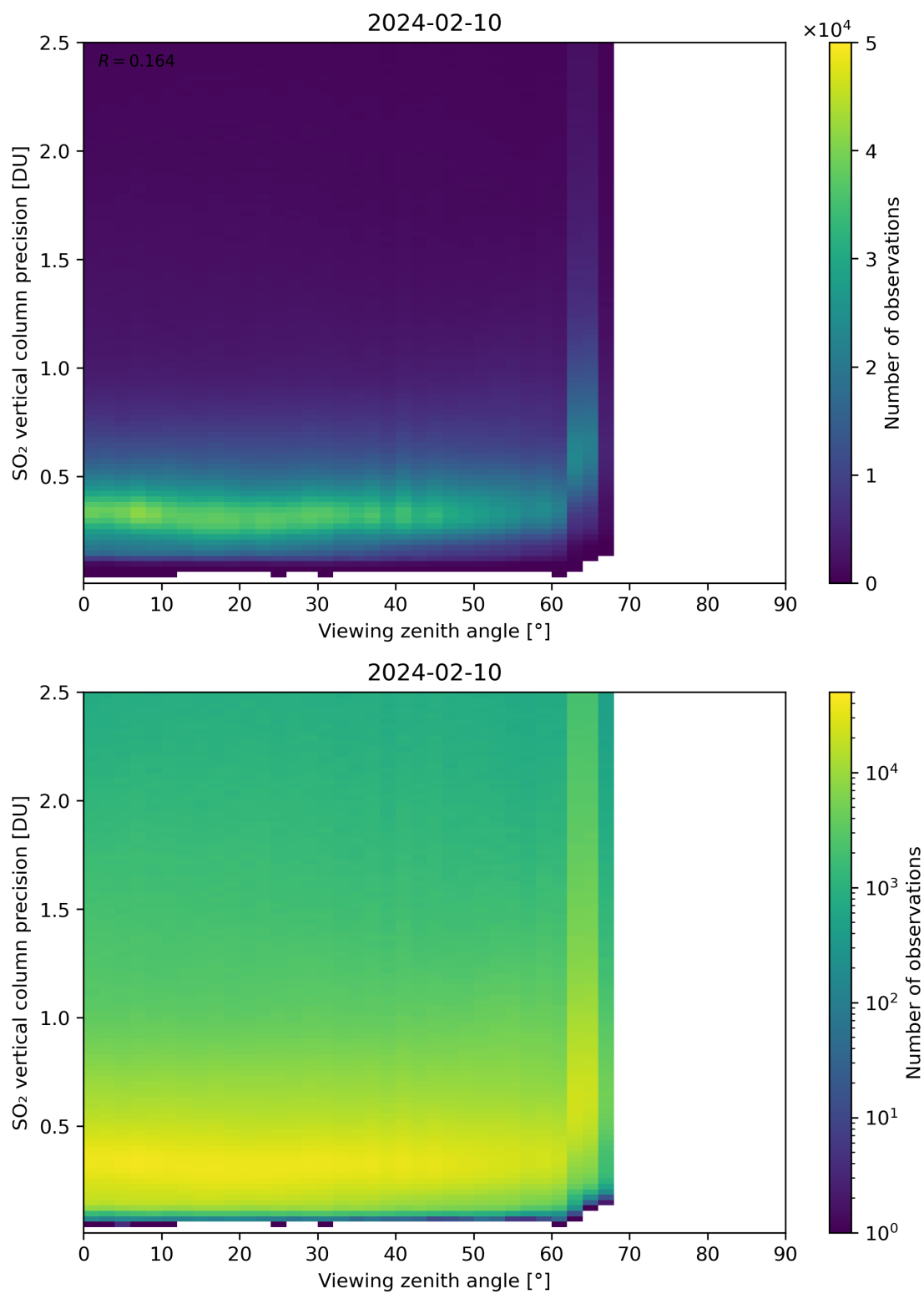
Figure 328: Scatter density plot of “Viewing zenith angle” against “SO 2 vertical column precision” for 2024-02-09 to 2024-02-11.
