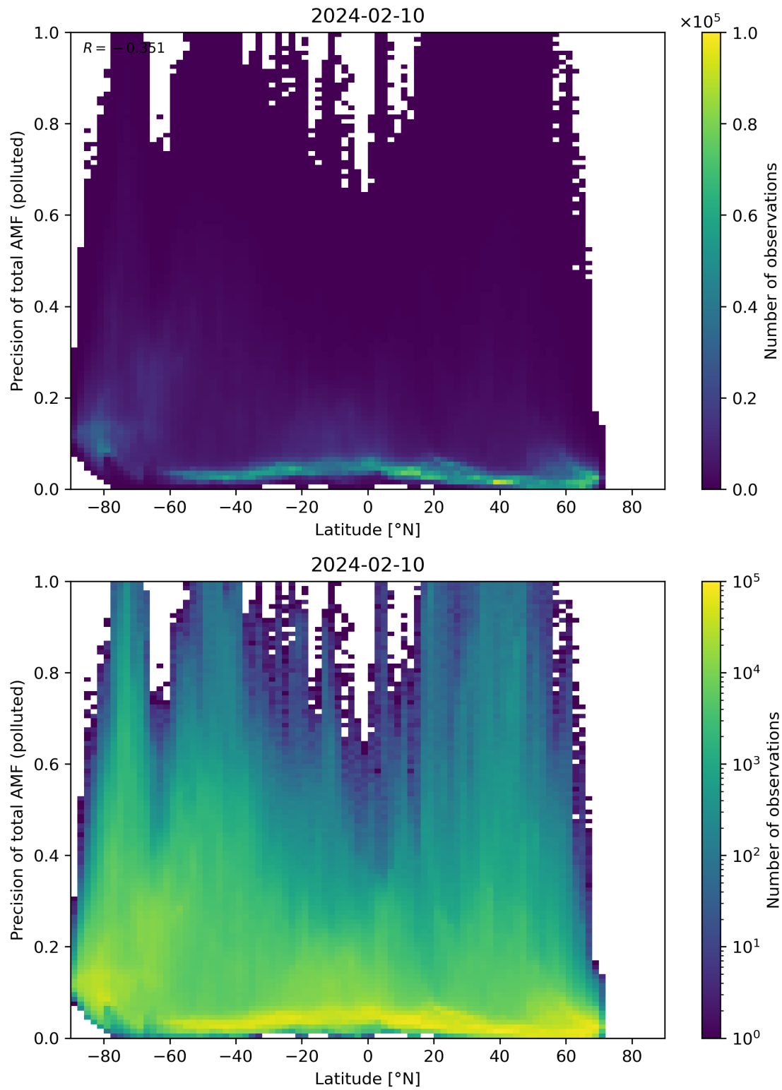
Figure 155: Scatter density plot of “Latitude” against “Precision of total AMF (polluted)” for 2024-02-09 to 2024-02-11.
