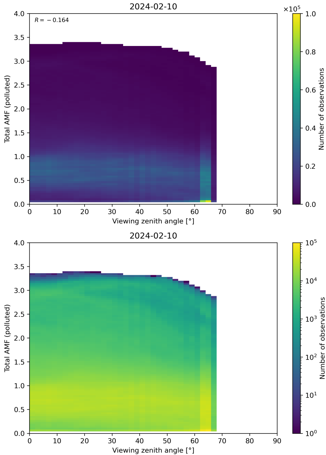
Figure 325: Scatter density plot of “Viewing zenith angle” against “Total AMF (polluted)” for 2024-02-09 to 2024-02-11.
