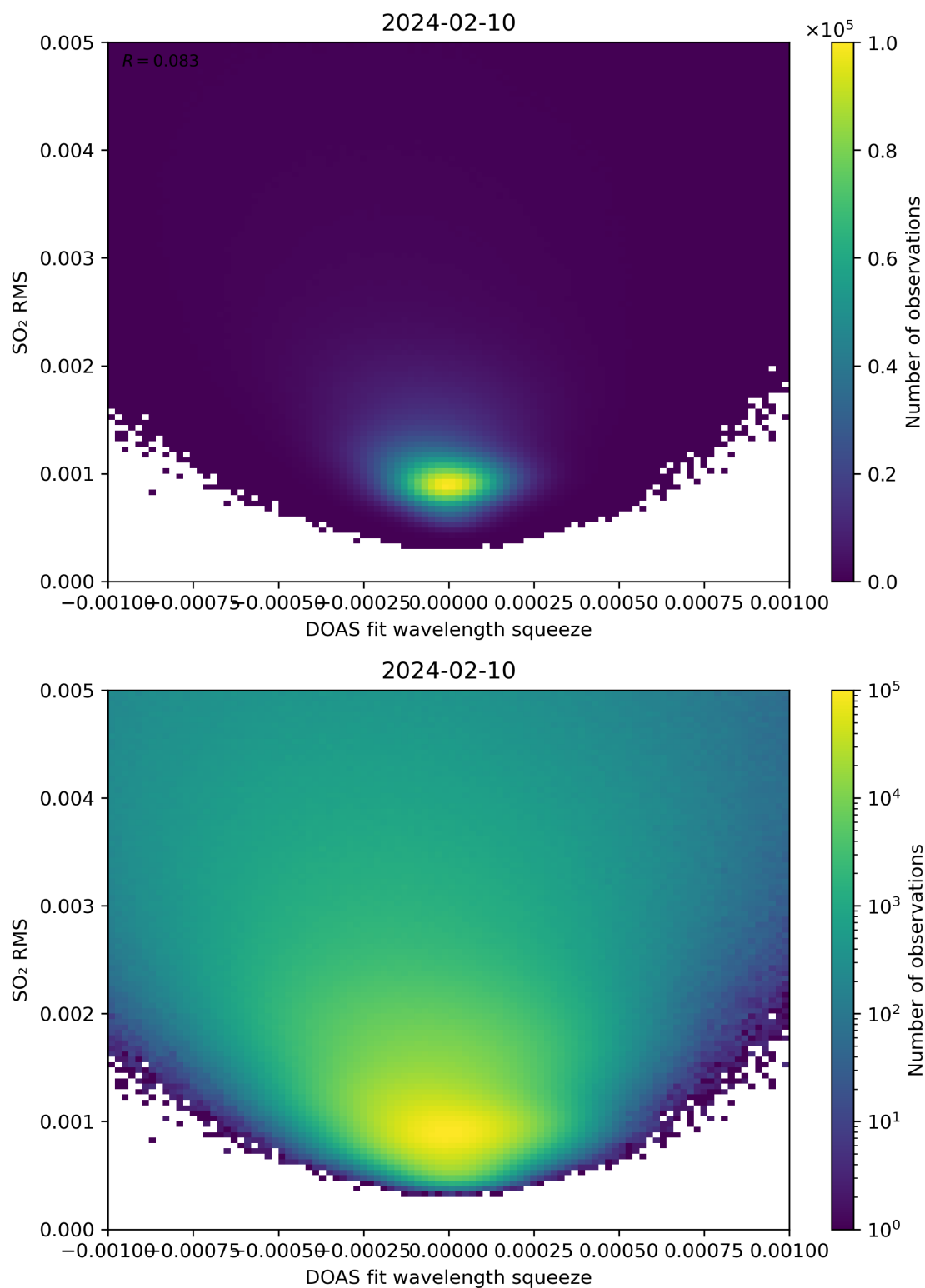
Figure 132: Scatter density plot of “DOAS fit wavelength squeeze” against “SO 2 RMS” for 2024-02-09 to 2024-02-11.
