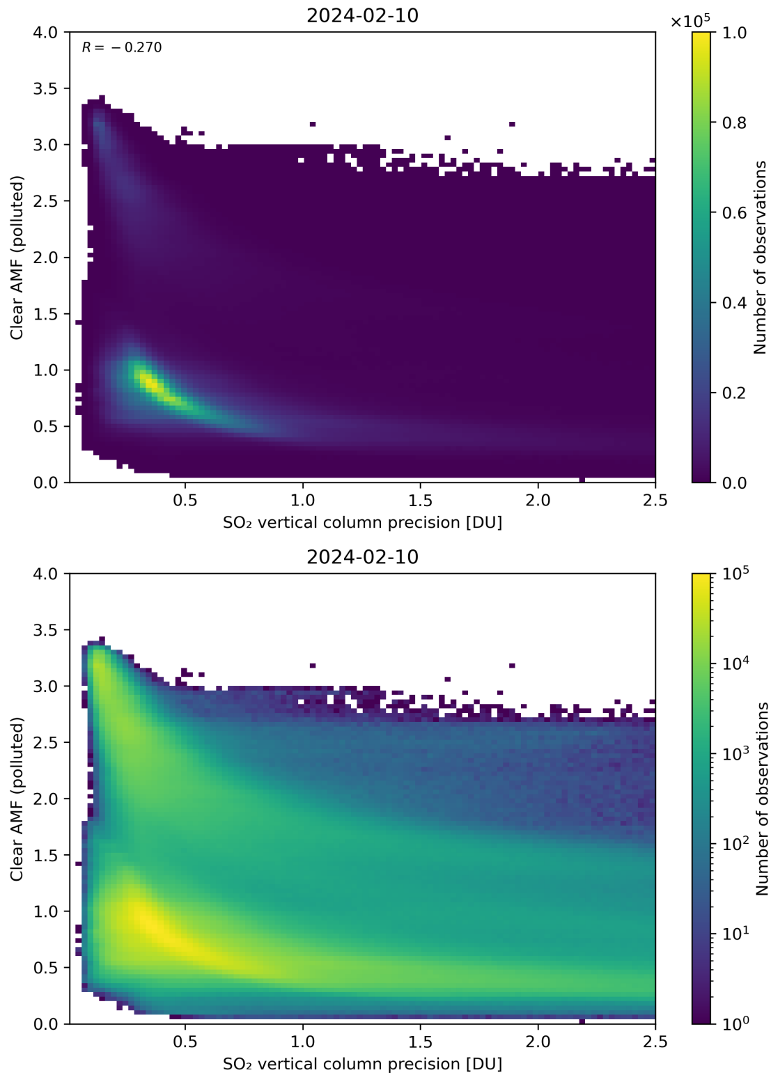
Figure 285: Scatter density plot of “SO 2 vertical column precision” against “Clear AMF (polluted)” for 2024-02-09 to 2024-02-11.
