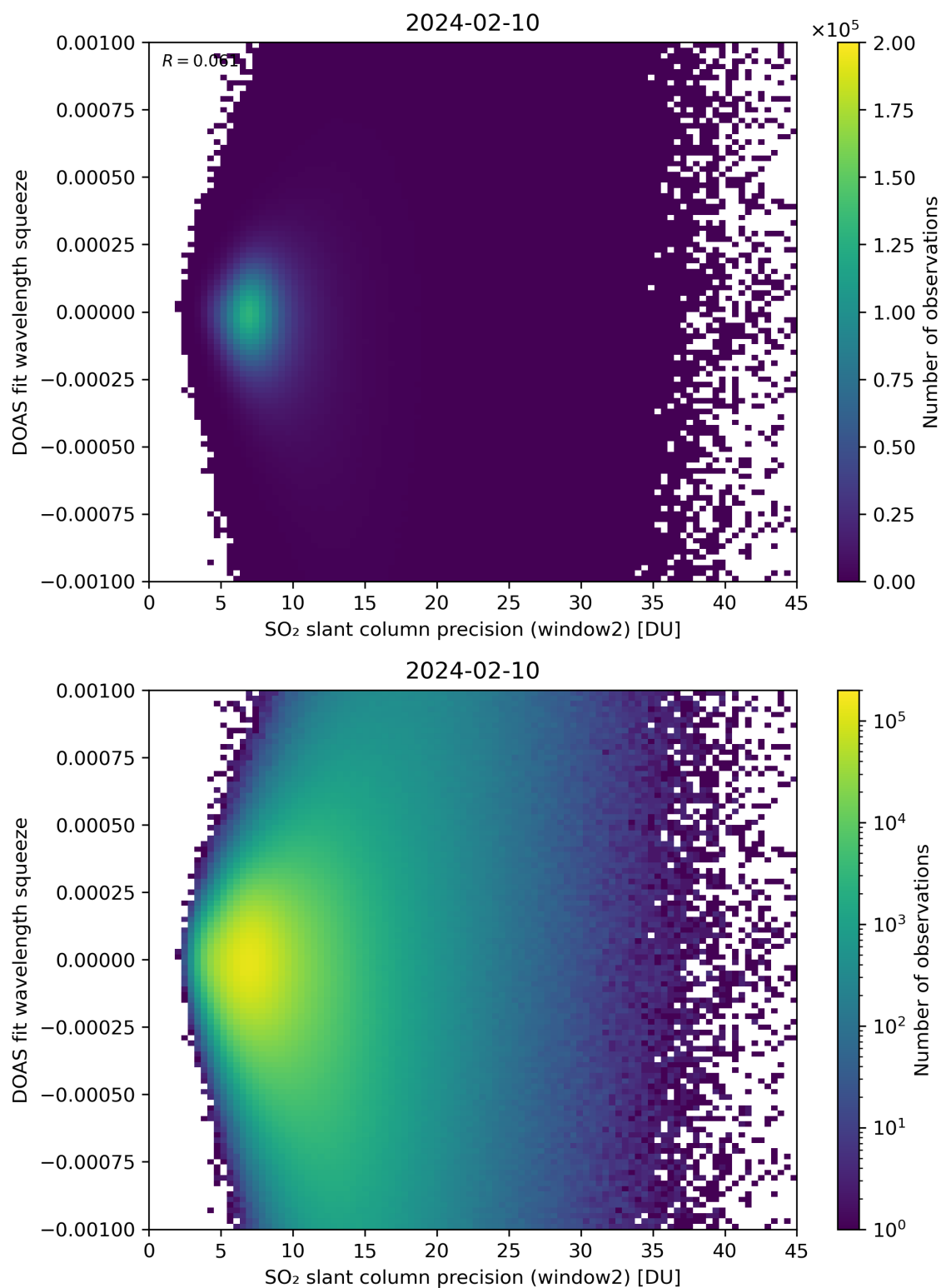
Figure 244: Scatter density plot of “SO 2 slant column precision (window2)” against “DOAS fit wavelength squeeze” for 2024-02-09 to 2024-02-11.
