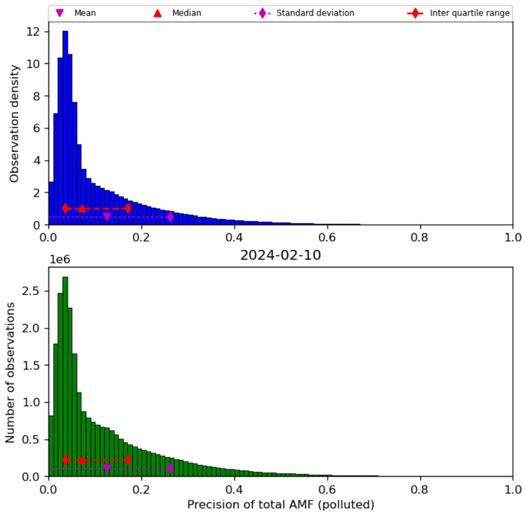
Figure 72: Histogram of “Precision of total AMF (polluted)” for 2024-02-09 to 2024-02-11
