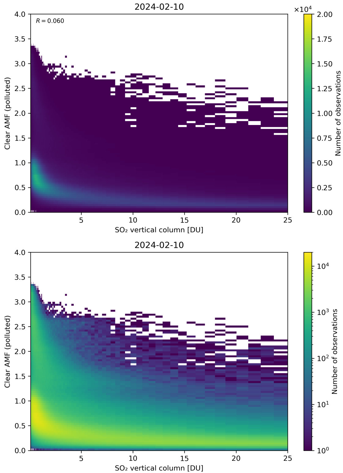
Figure 296: Scatter density plot of “SO 2 vertical column” against “Clear AMF (polluted)” for 2024-02-09 to 2024-02-11.
