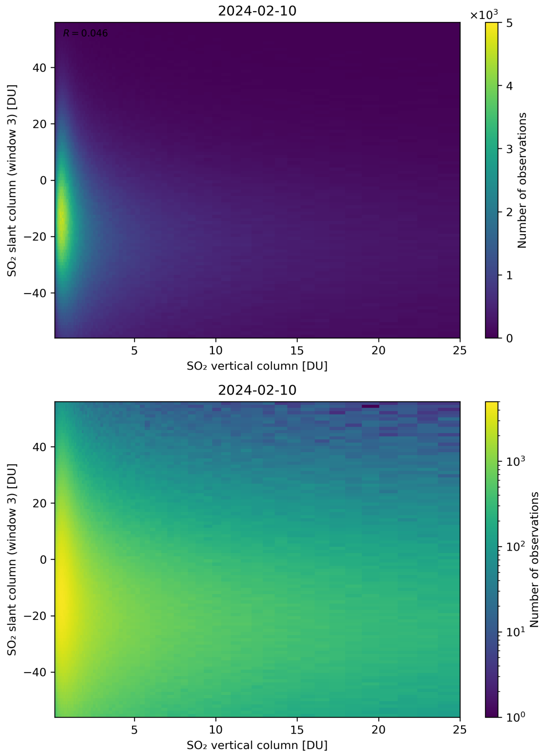
Figure 303: Scatter density plot of “SO 2 vertical column” against “SO 2 slant column (window 3)” for 2024-02-09 to 2024-02-11.
