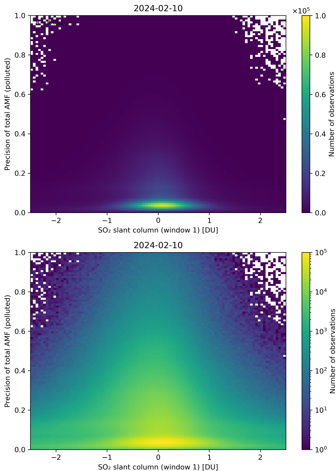
Figure 240: Scatter density plot of “SO 2 slant column (window 1)” against “Precision of total AMF (polluted)” for 2024-02-09 to 2024-02-11.
