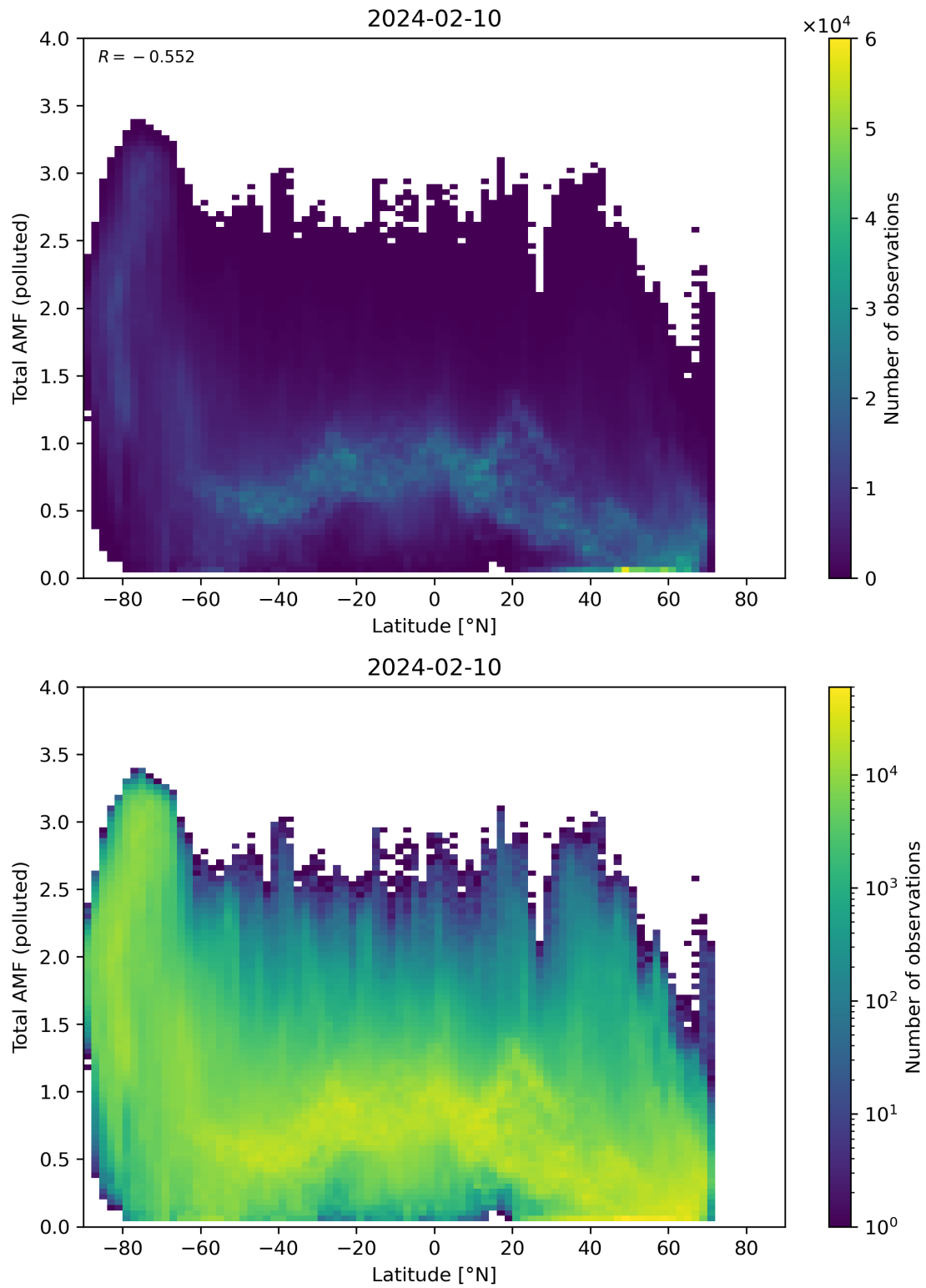
Figure 154: Scatter density plot of “Latitude” against “Total AMF (polluted)” for 2024-02-09 to 2024-02-11.
