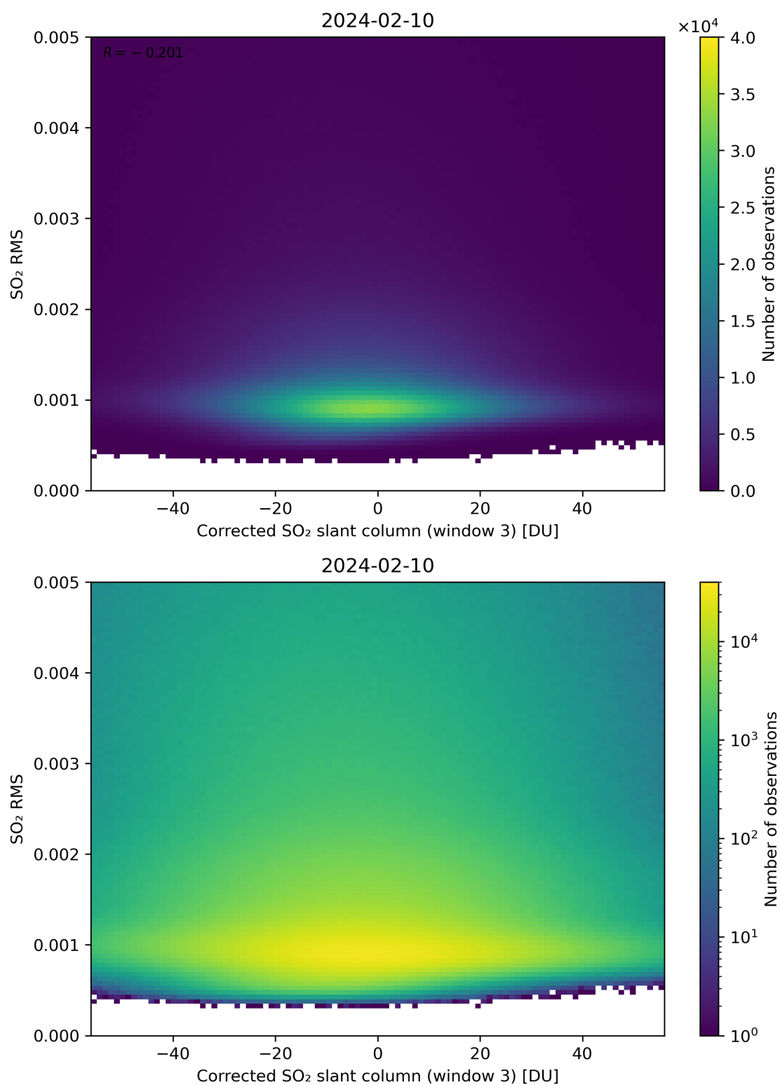
Figure 208: Scatter density plot of “Corrected SO 2 slant column (window 3)” against “SO 2 RMS” for 2024-02-09 to 2024-02-11.
