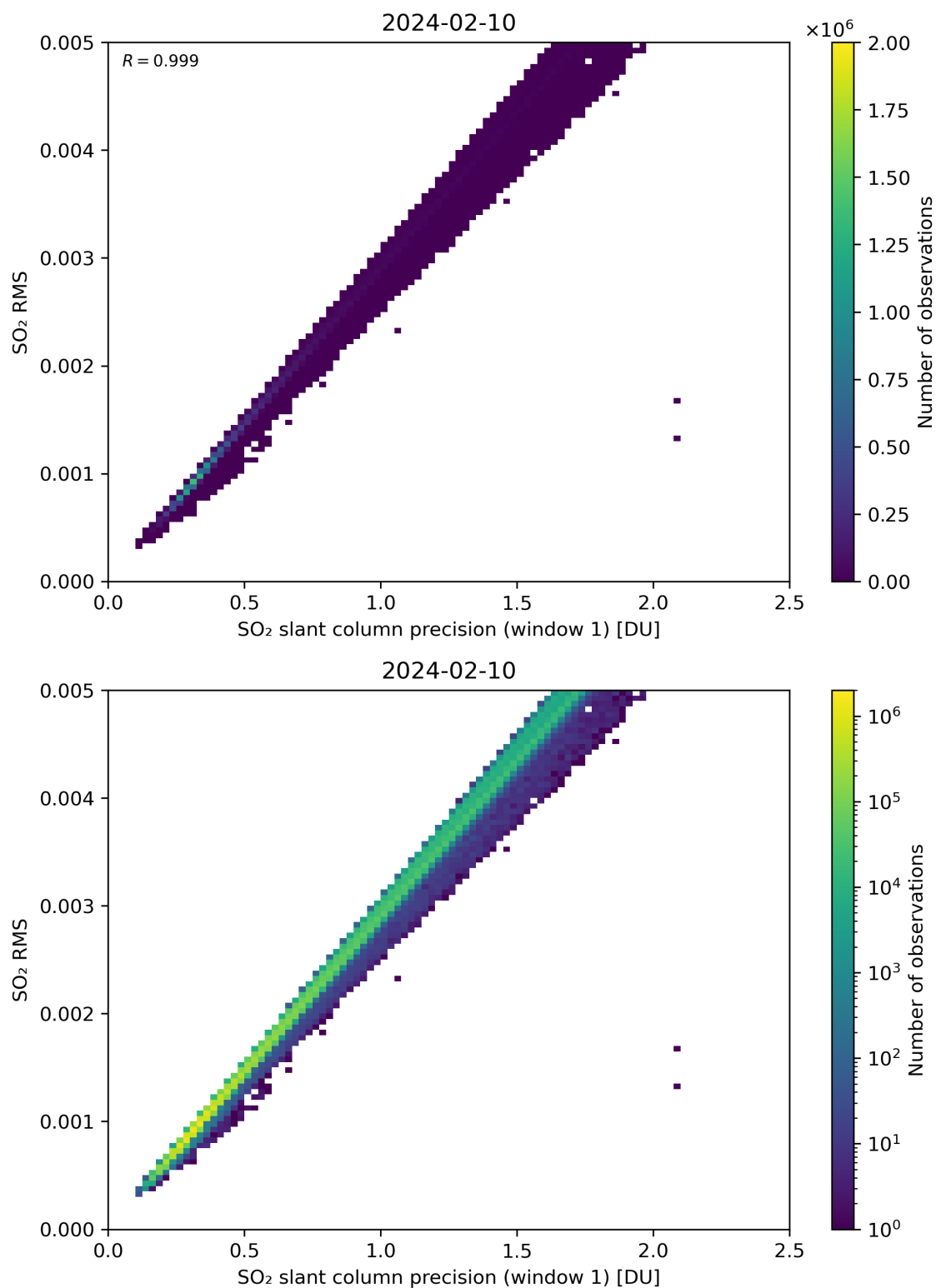
Figure 223: Scatter density plot of “SO 2 slant column precision (window 1)” against “SO 2 RMS” for 2024-02-09 to 2024-02-11.
