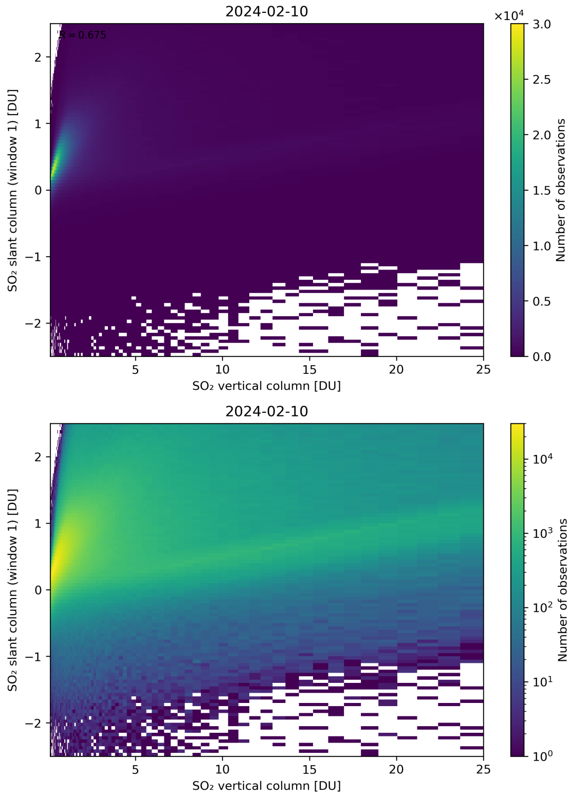
Figure 300: Scatter density plot of “SO 2 vertical column” against “SO 2 slant column (window 1)” for 2024-02-09 to 2024-02-11.
