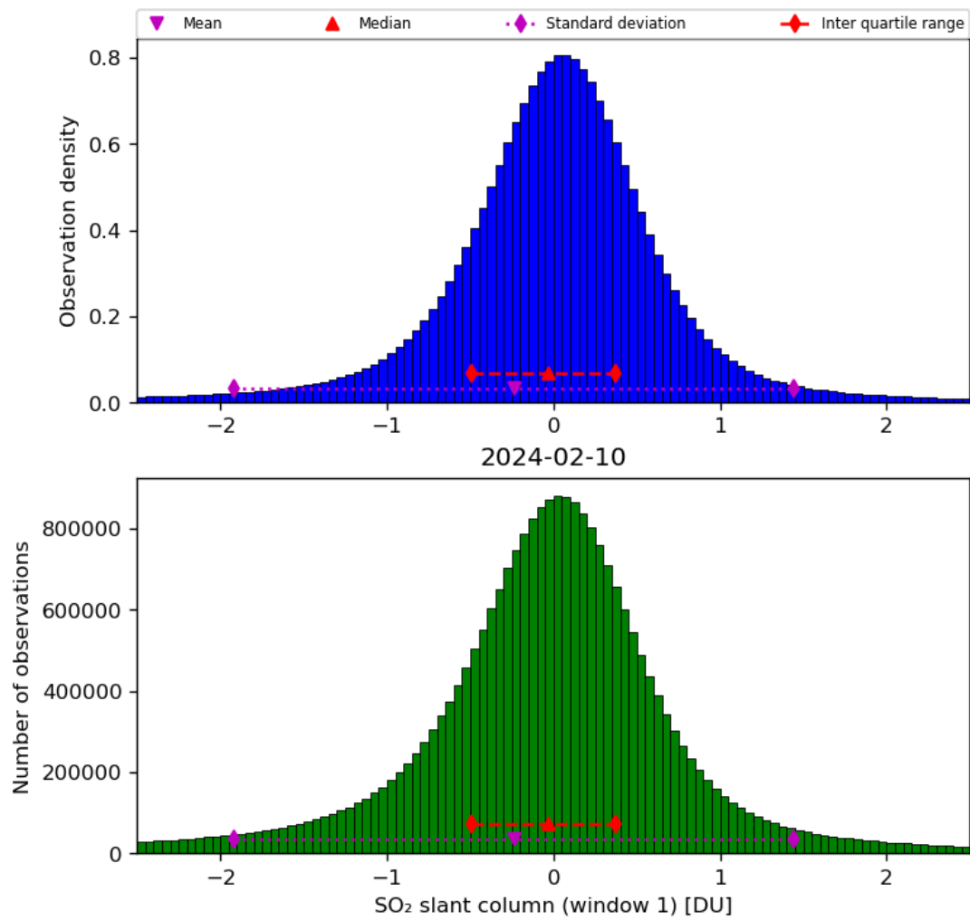
Figure 56: Histogram of “SO 2 slant column (window 1)” for 2024-02-09 to 2024-02-11
