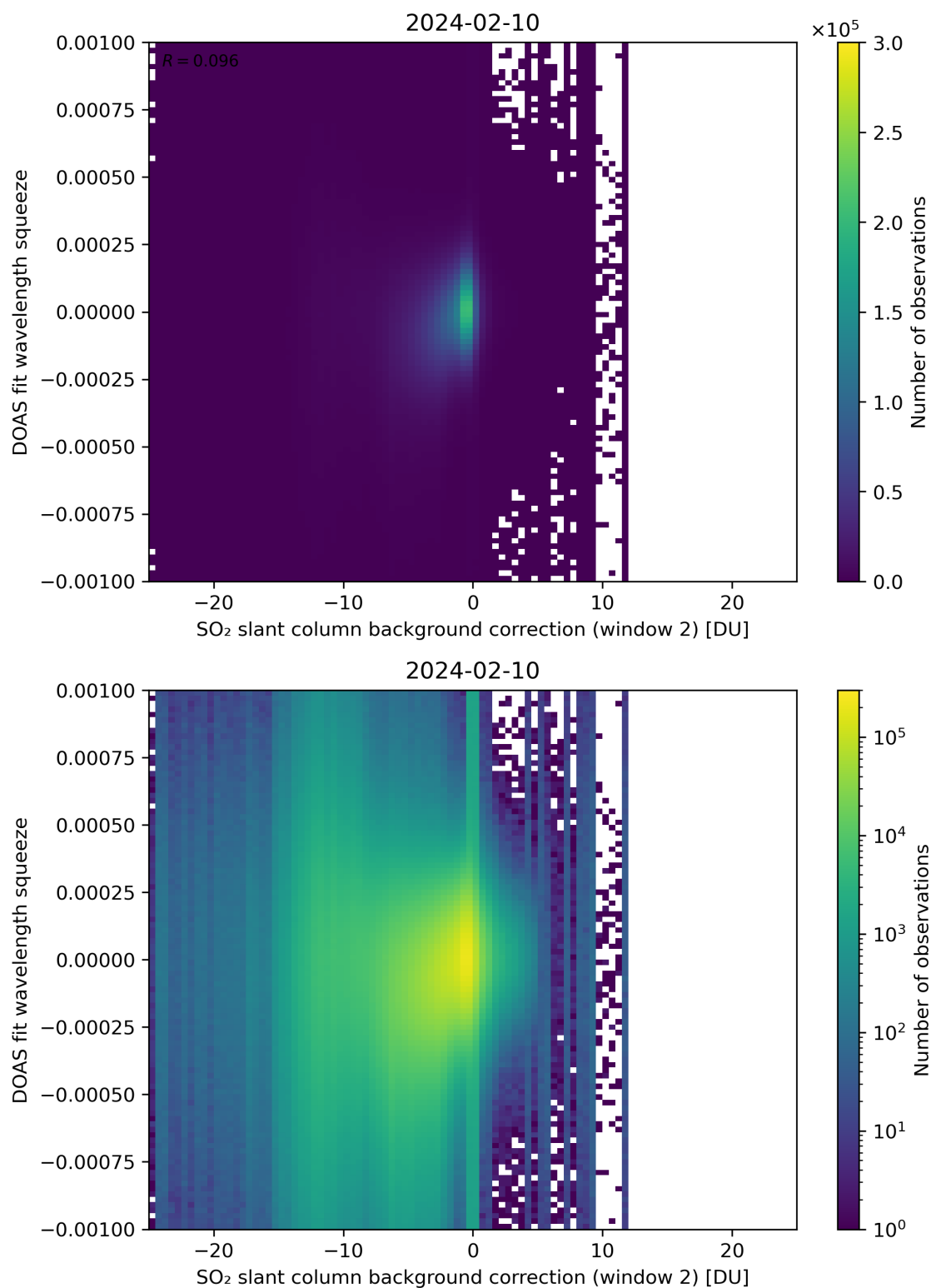
Figure 113: Scatter density plot of “SO 2 slant column background correction (window 2)” against “DOAS fit wavelength squeeze” for 2024-02-09 to 2024-02-11.
