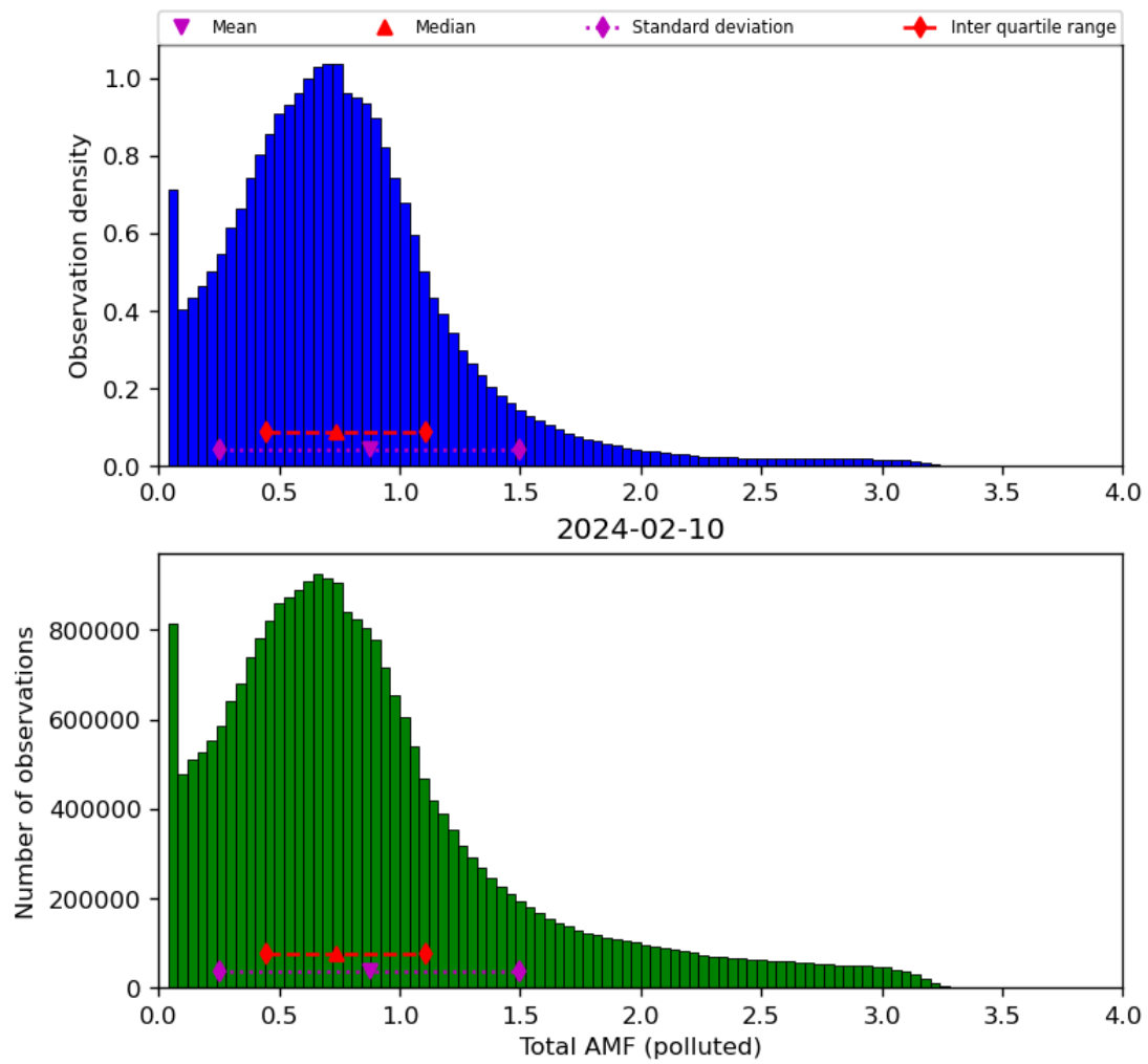
Figure 71: Histogram of “Total AMF (polluted)” for 2024-02-09 to 2024-02-11
