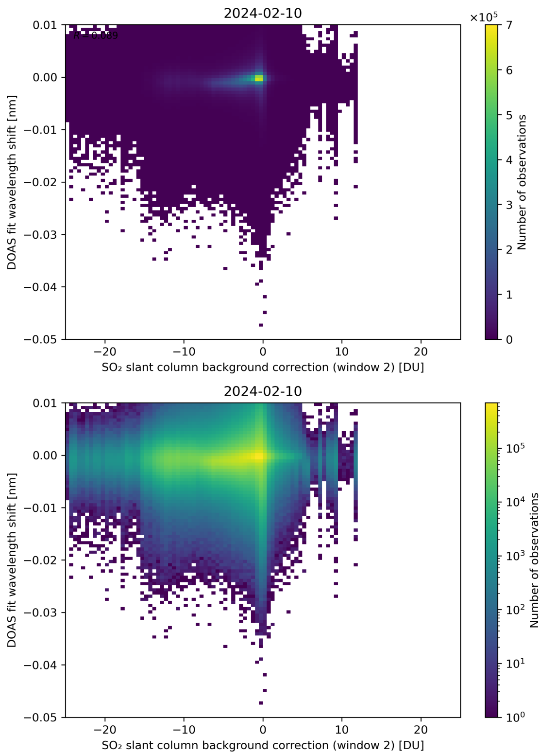
Figure 112: Scatter density plot of “SO 2 slant column background correction (window 2)” against “DOAS fit wavelength shift” for 2024-02-09 to 2024-02-11.
