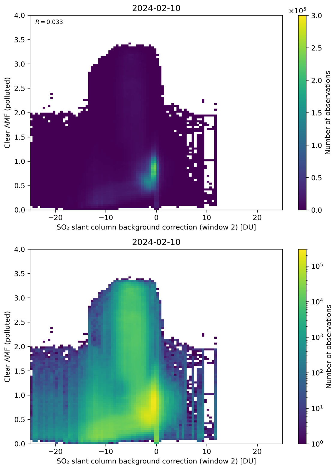
Figure 115: Scatter density plot of “SO 2 slant column background correction (window 2)” against “Clear AMF (polluted)” for 2024-02-09 to 2024-02-11.
