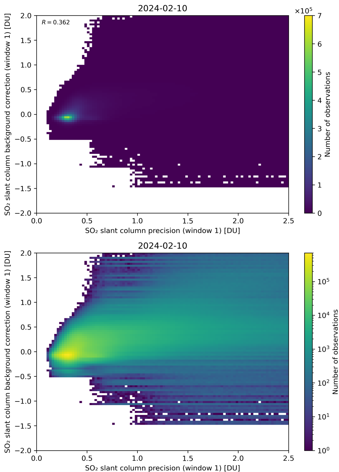
Figure 218: Scatter density plot of “SO 2 slant column precision (window 1)” against “SO 2 slant column background correction (window 1)” for 2024-02-09 to 2024-02-11.
