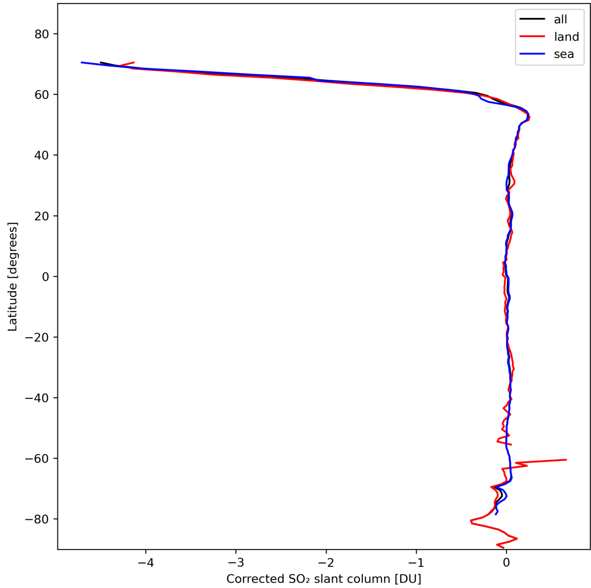
Figure 32: Zonal average of “Corrected SO 2 slant column” for 2024-02-09 to 2024-02-11.
