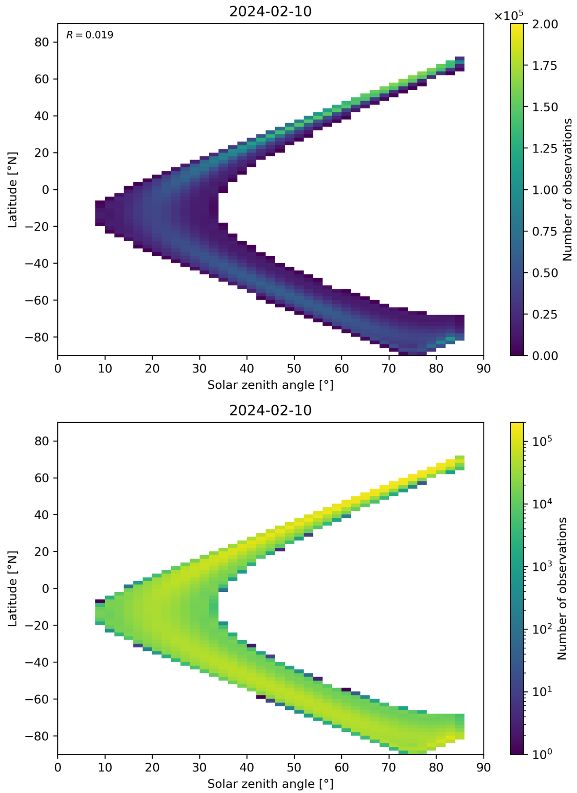
Figure 164: Scatter density plot of “Solar zenith angle” against “Latitude” for 2024-02-09 to 2024-02-11.
