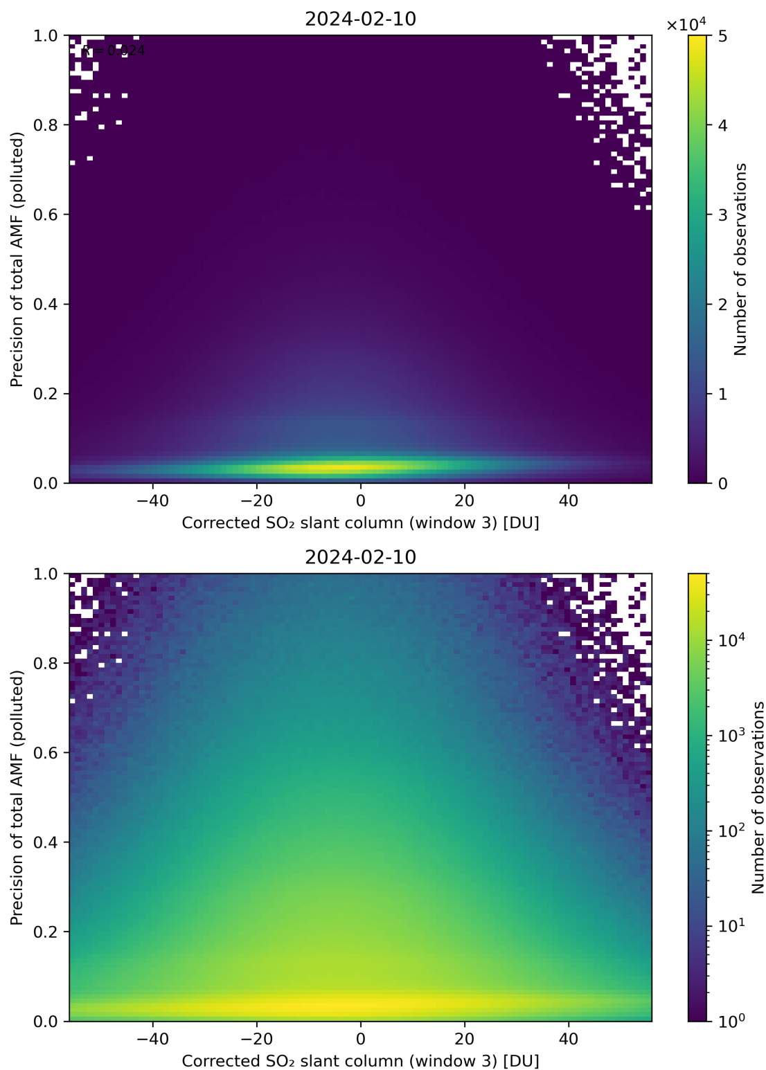
Figure 211: Scatter density plot of “Corrected SO 2 slant column (window 3)” against “Precision of total AMF (polluted)” for 2024-02-09 to 2024-02-11.
