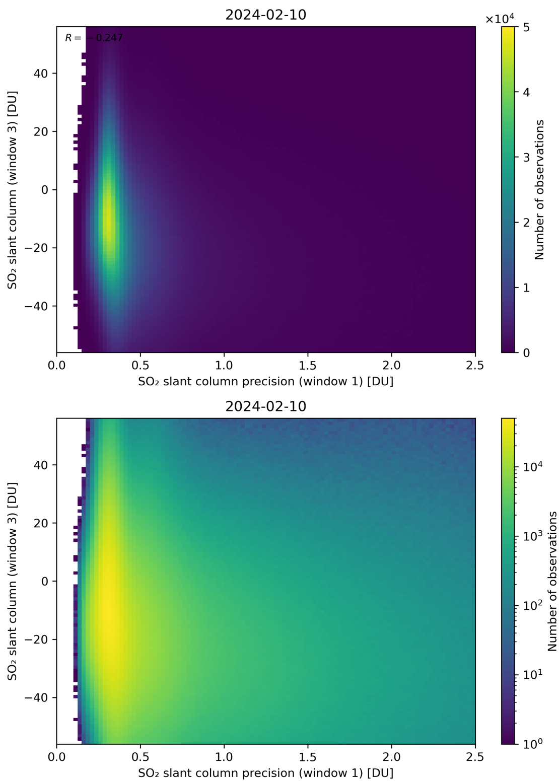
Figure 228: Scatter density plot of “SO 2 slant column precision (window 1)” against “SO 2 slant column (window 3)” for 2024-02-09 to 2024-02-11.
