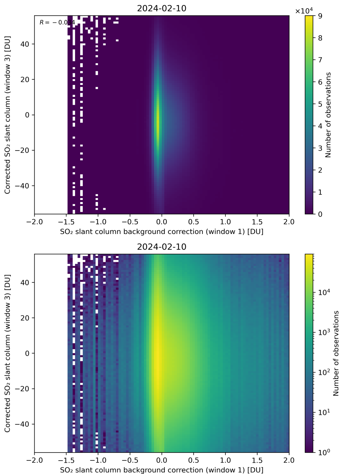
Figure 105: Scatter density plot of “SO 2 slant column background correction (window 1)” against “Corrected SO 2 slant column (window 3)” for 2024-02-09 to 2024-02-11.
