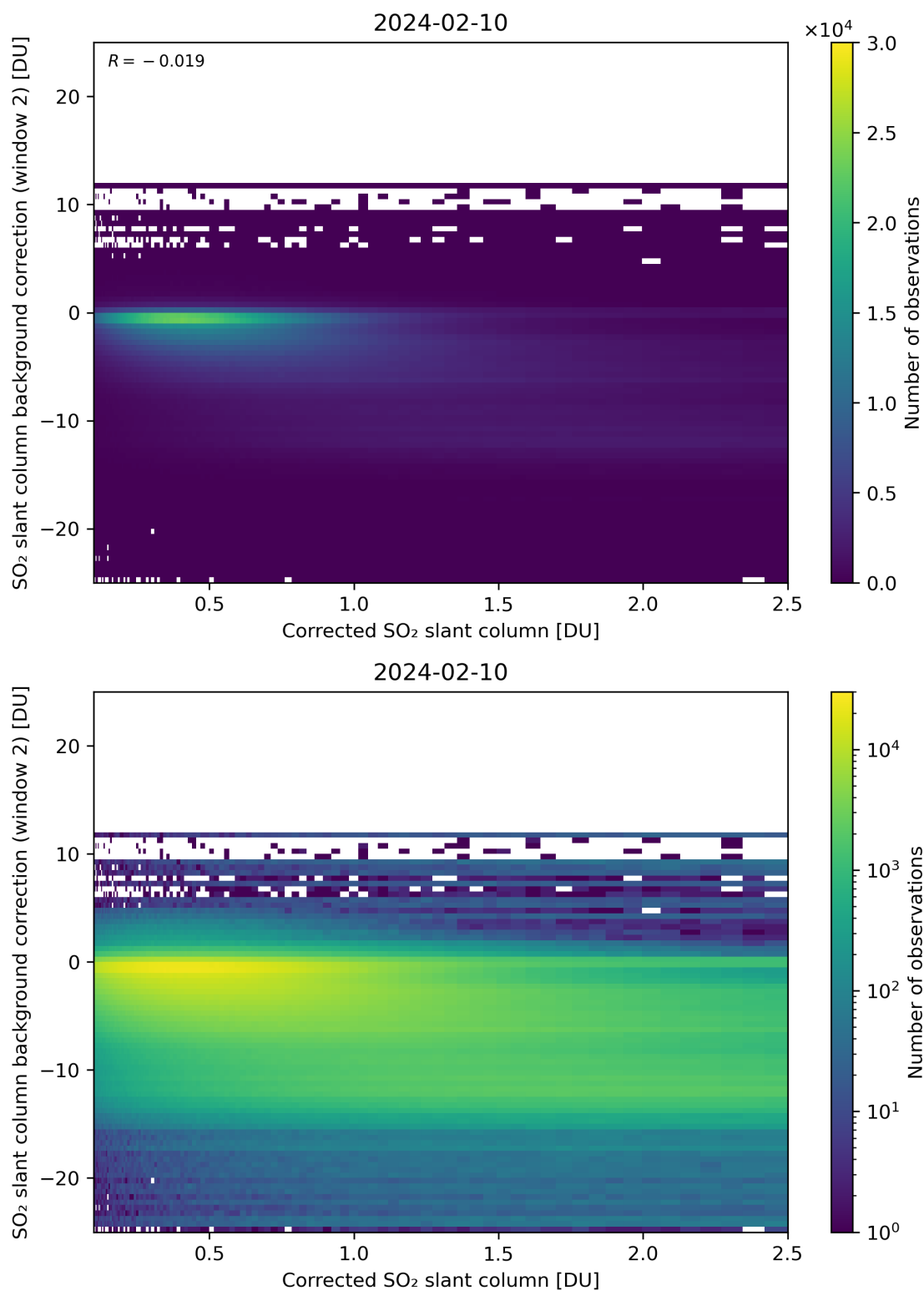
Figure 179: Scatter density plot of “Corrected SO 2 slant column” against “SO 2 slant column background correction (window 2)” for 2024-02-09 to 2024-02-11.
