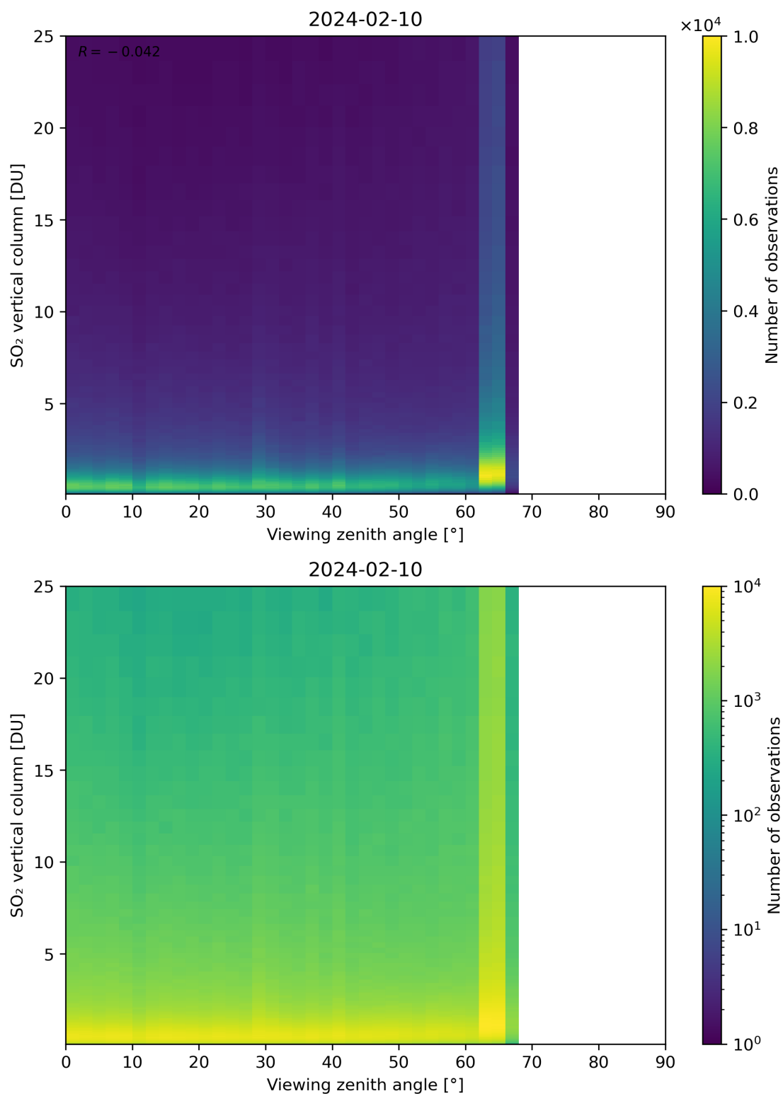
Figure 327: Scatter density plot of “Viewing zenith angle” against “SO 2 vertical column” for 2024-02-09 to 2024-02-11.
