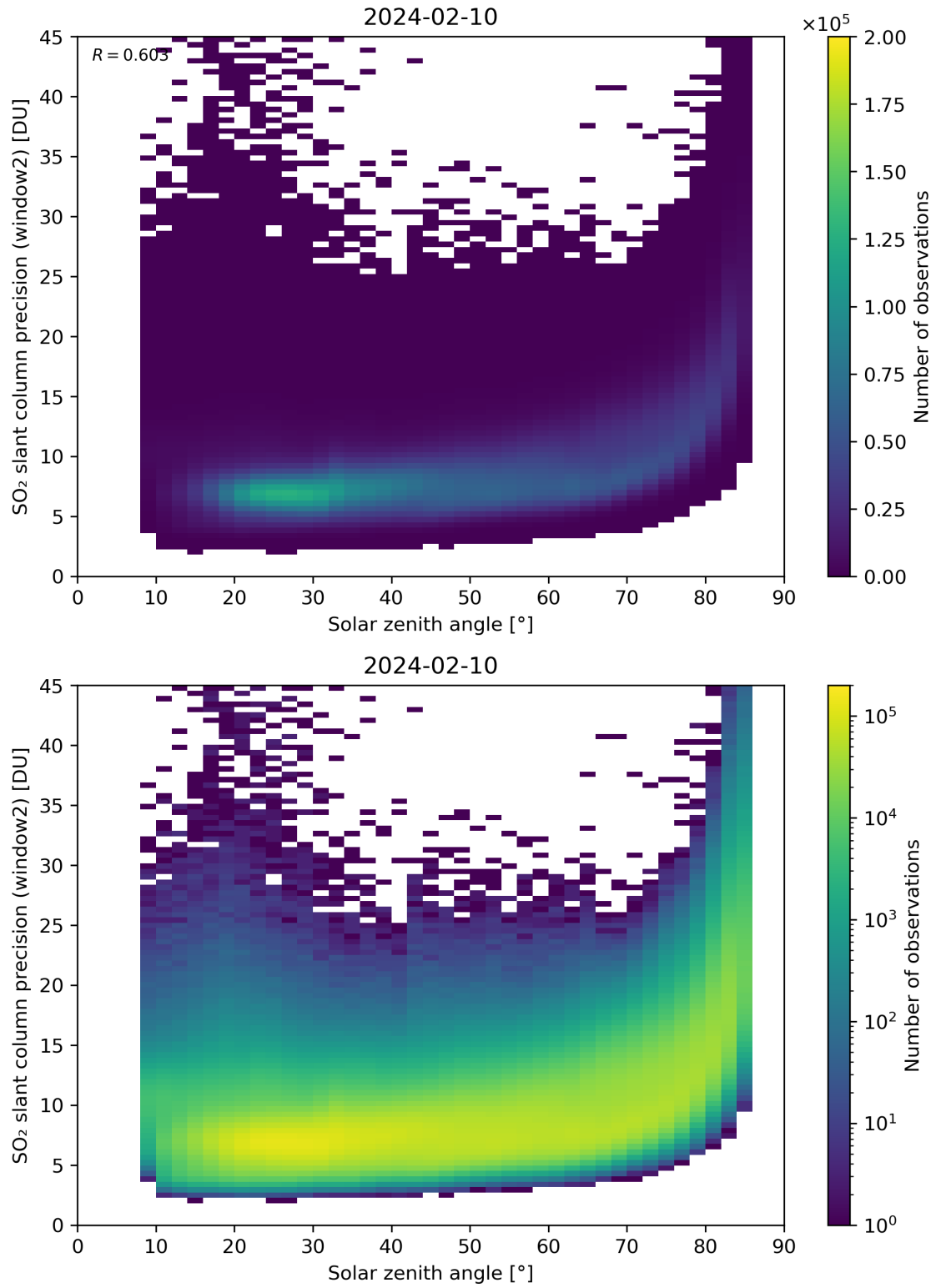
Figure 171: Scatter density plot of “Solar zenith angle” against “SO 2 slant column precision (window2)” for 2024-02-09 to 2024-02-11.
