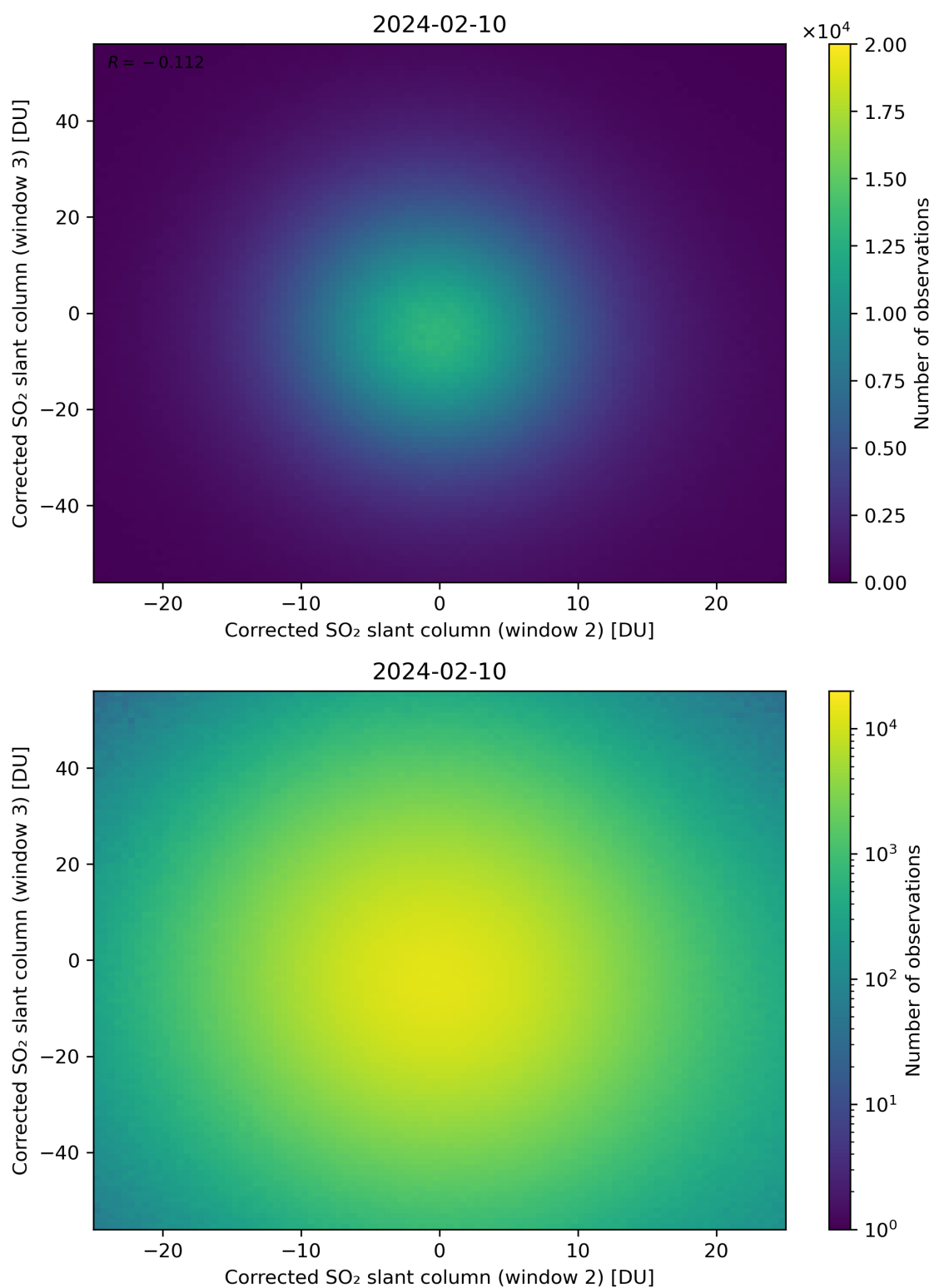
Figure 200: Scatter density plot of “Corrected SO 2 slant column (window 2)” against “Corrected SO 2 slant column (window 3)” for 2024-02-09 to 2024-02-11.
