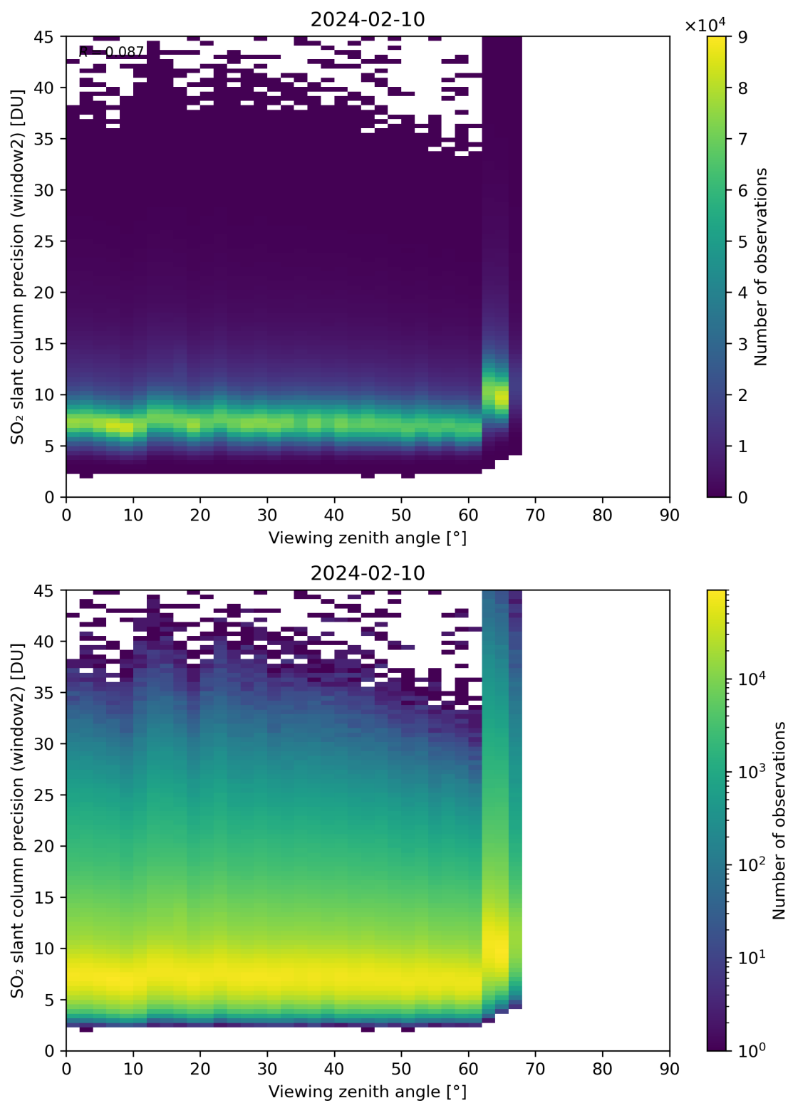
Figure 322: Scatter density plot of “Viewing zenith angle” against “SO 2 slant column precision (window2)” for 2024-02-09 to 2024-02-11.
