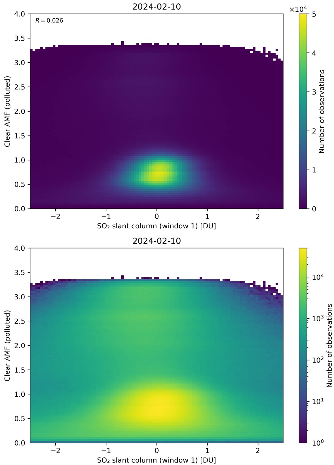
Figure 232: Scatter density plot of “SO 2 slant column (window 1)” against “Clear AMF (polluted)” for 2024-02-09 to 2024-02-11.
