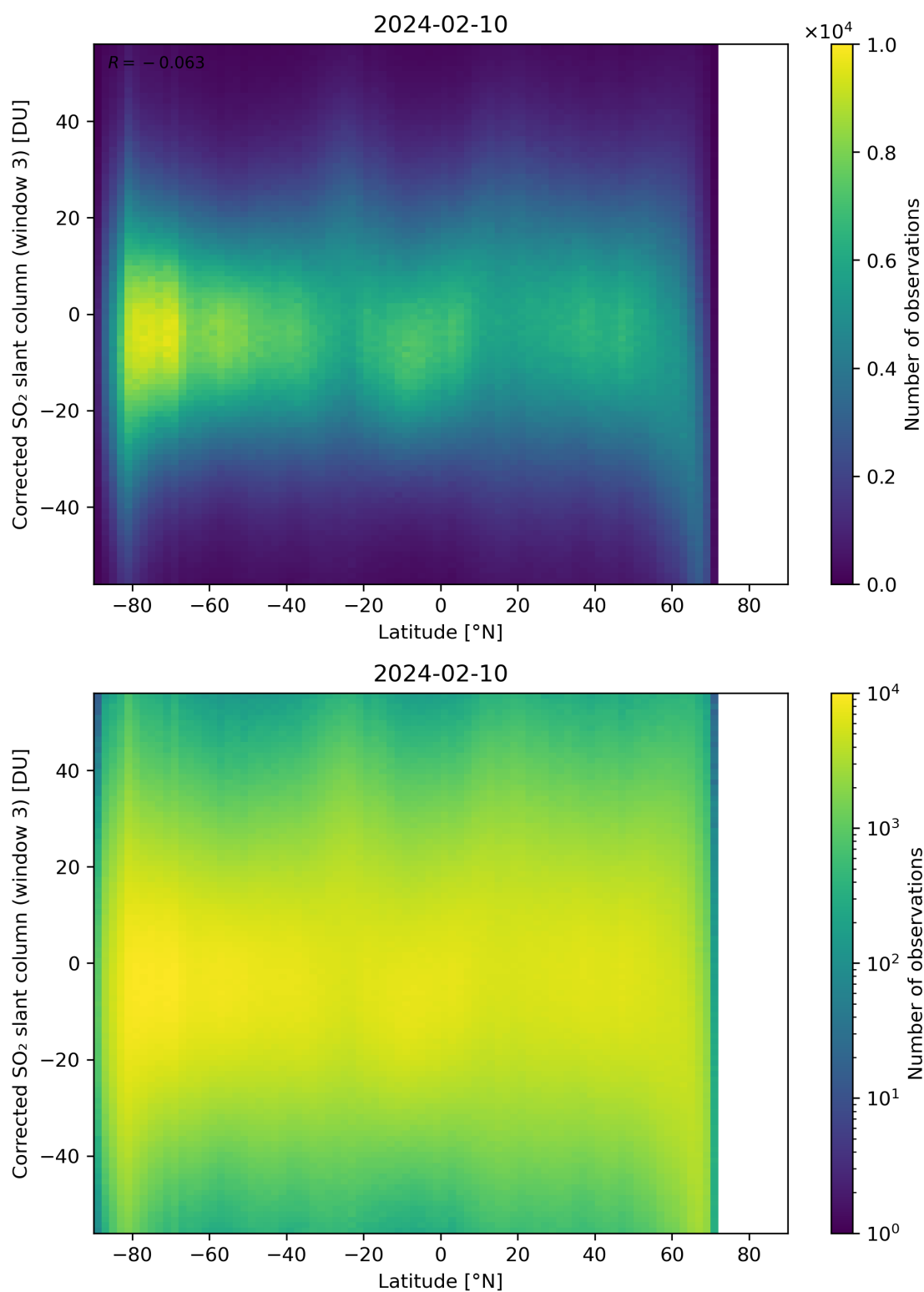
Figure 148: Scatter density plot of “Latitude” against “Corrected SO 2 slant column (window 3)” for 2024-02-09 to 2024-02-11.
