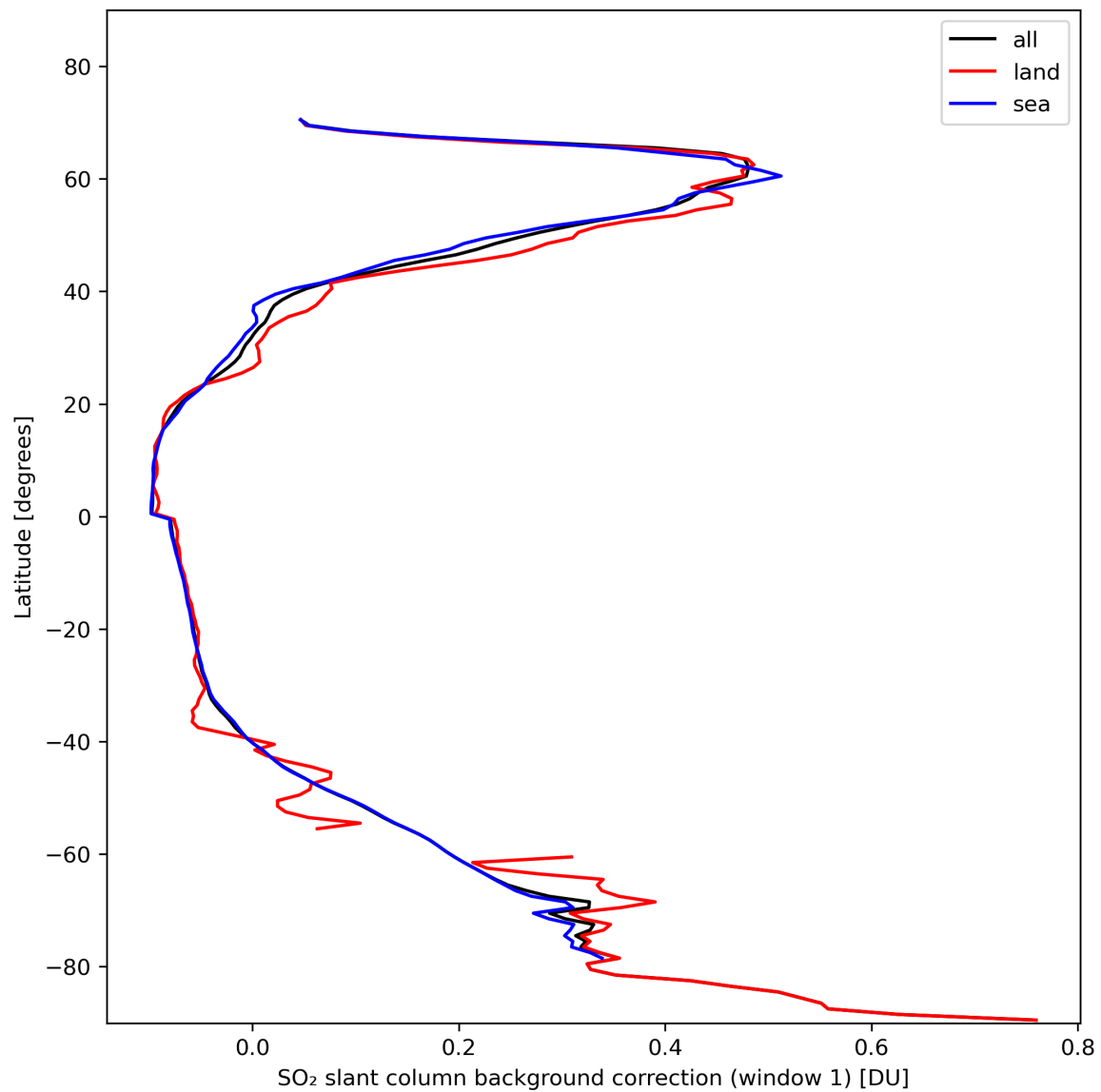
Figure 36: Zonal average of “SO 2 slant column background correction (window 1)” for 2024-02-09 to 2024-02-11.
