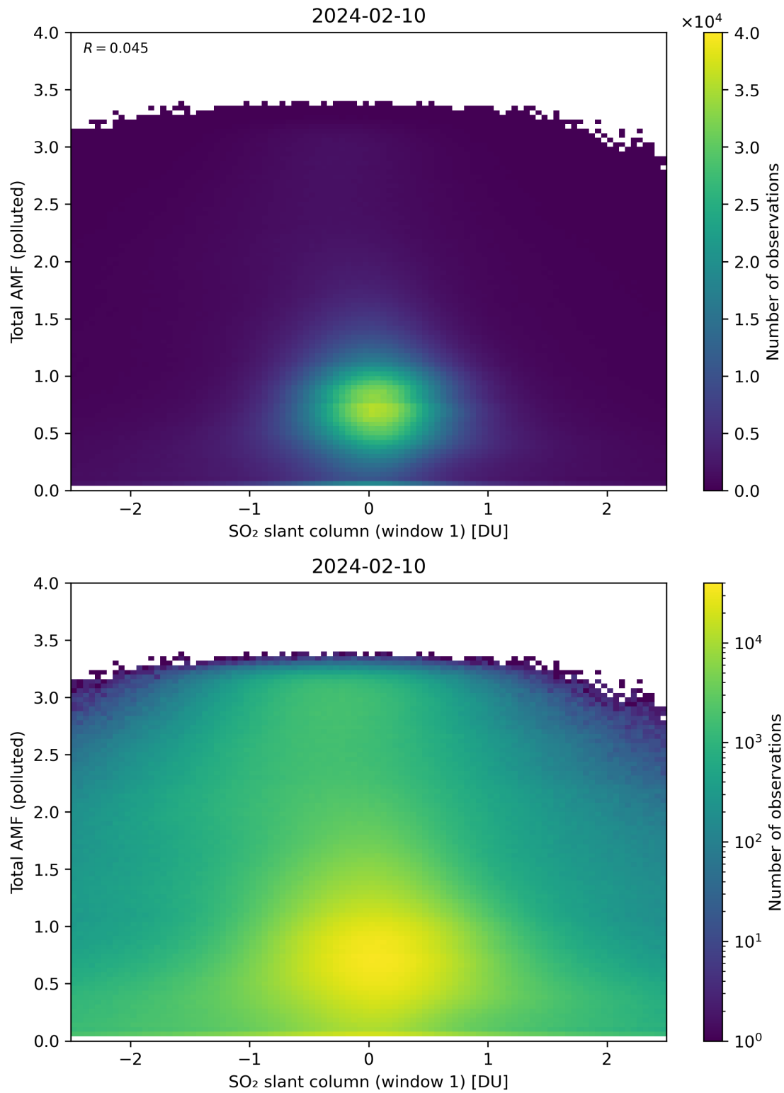
Figure 239: Scatter density plot of “SO 2 slant column (window 1)” against “Total AMF (polluted)” for 2024-02-09 to 2024-02-11.
