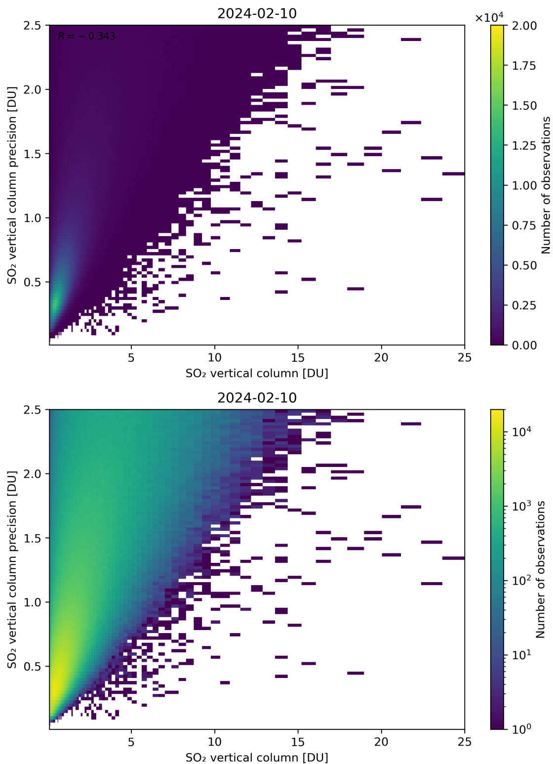
Figure 307: Scatter density plot of “SO 2 vertical column” against “SO 2 vertical column precision” for 2024-02-09 to 2024-02-11.
