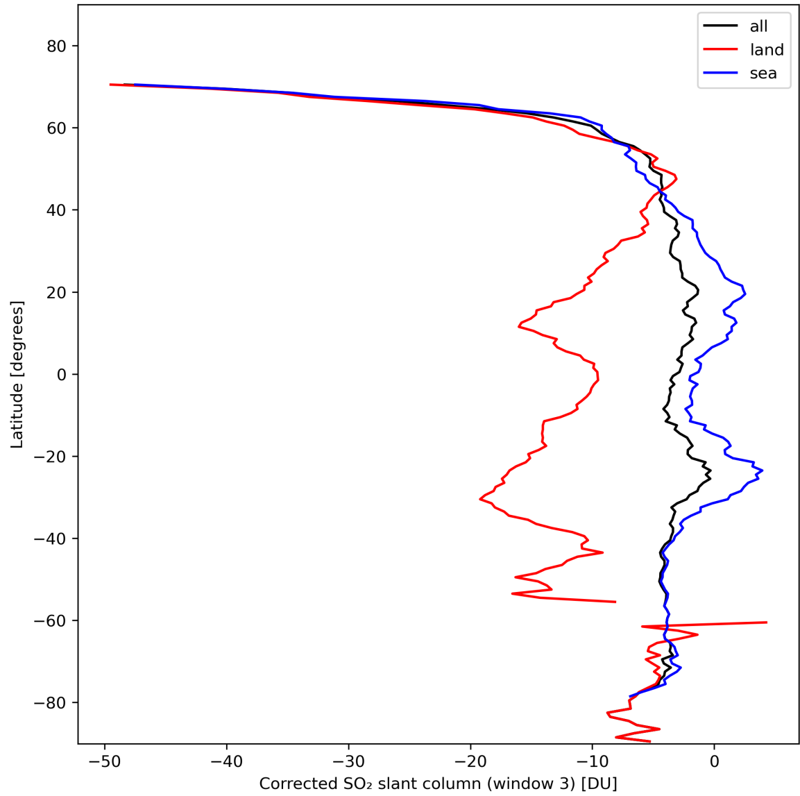
Figure 43: Zonal average of “Corrected SO 2 slant column (window 3)” for 2024-02-09 to 2024-02-11.
