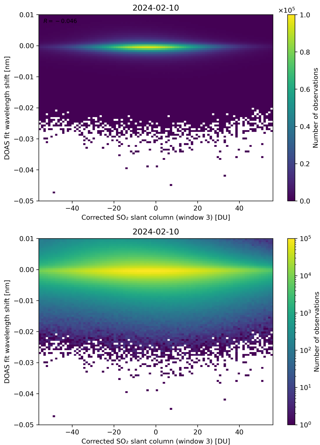
Figure 206: Scatter density plot of “Corrected SO 2 slant column (window 3)” against “DOAS fit wavelength shift” for 2024-02-09 to 2024-02-11.
