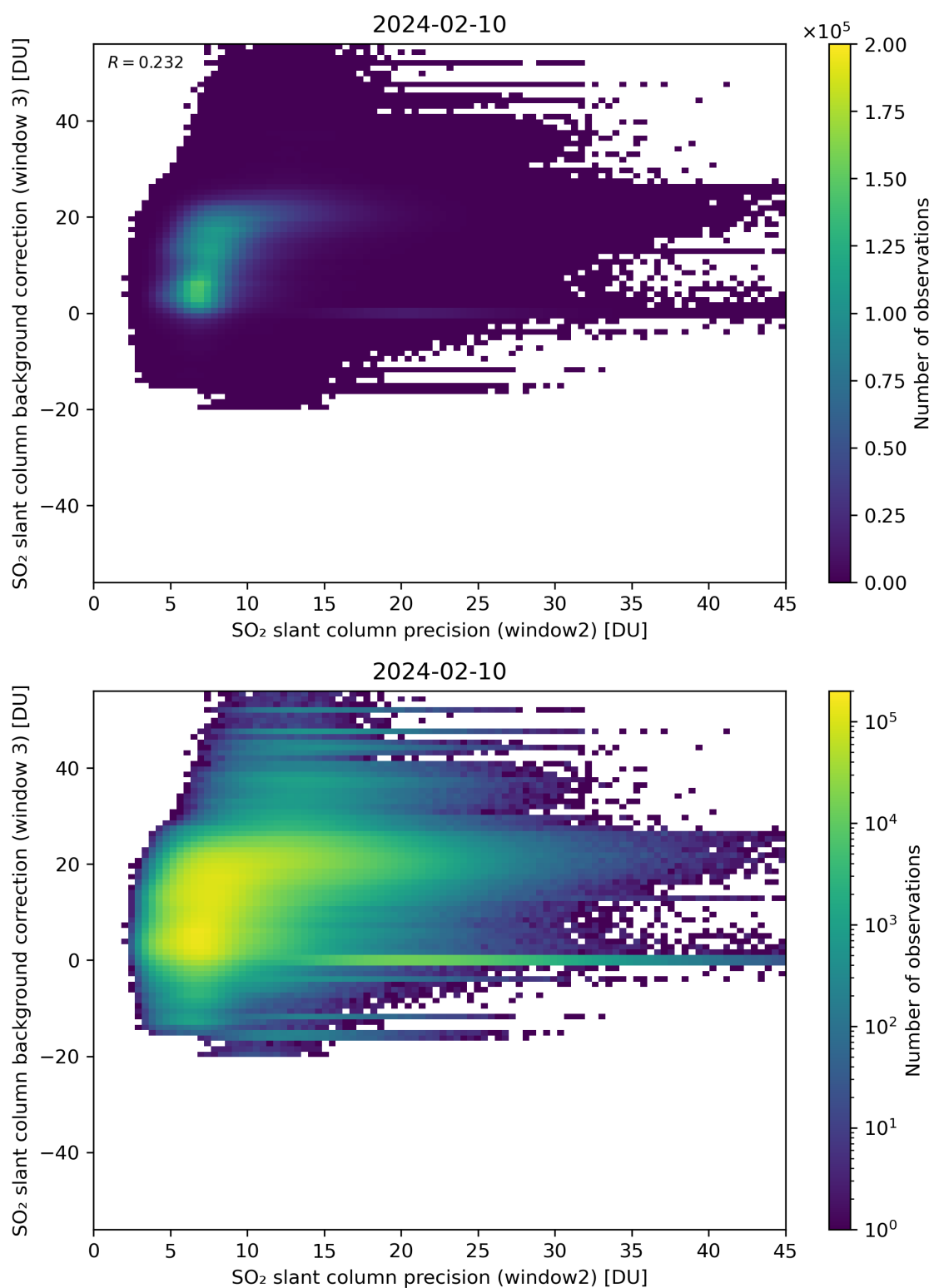
Figure 242: Scatter density plot of “SO 2 slant column precision (window2)” against “SO 2 slant column background correction (window 3)” for 2024-02-09 to 2024-02-11.
