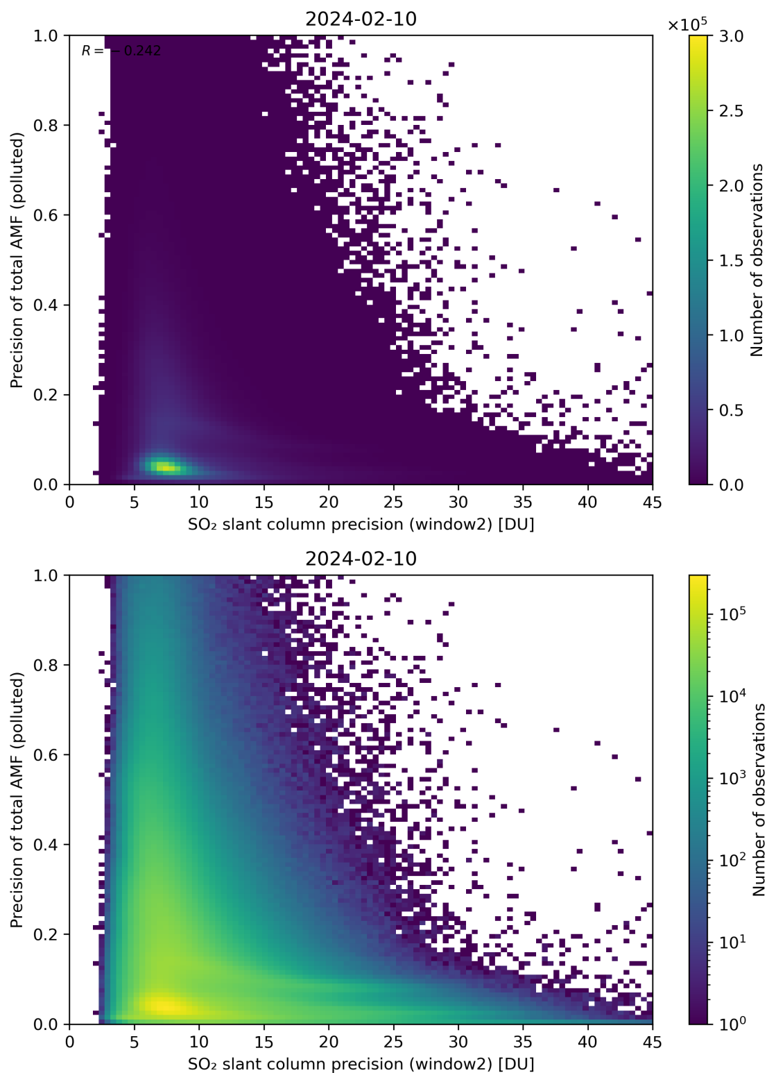
Figure 252: Scatter density plot of “SO 2 slant column precision (window2)” against “Precision of total AMF (polluted)” for 2024-02-09 to 2024-02-11.
