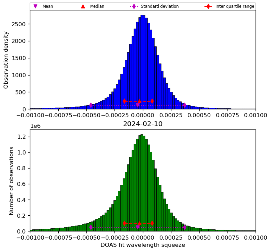
Figure 69: Histogram of “DOAS fit wavelength squeeze” for 2024-02-09 to 2024-02-11
