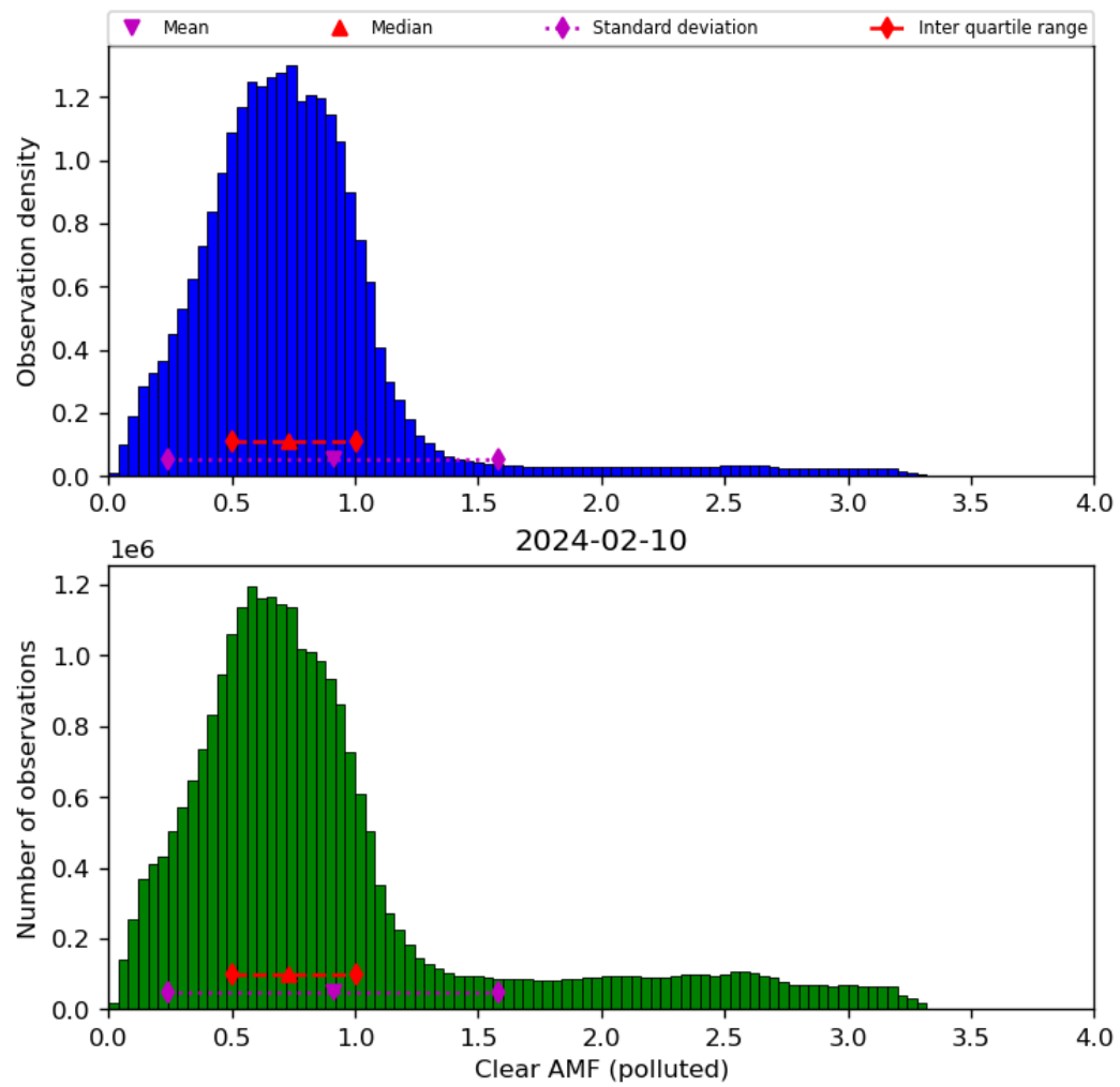
Figure 73: Histogram of “Clear AMF (polluted)” for 2024-02-09 to 2024-02-11
