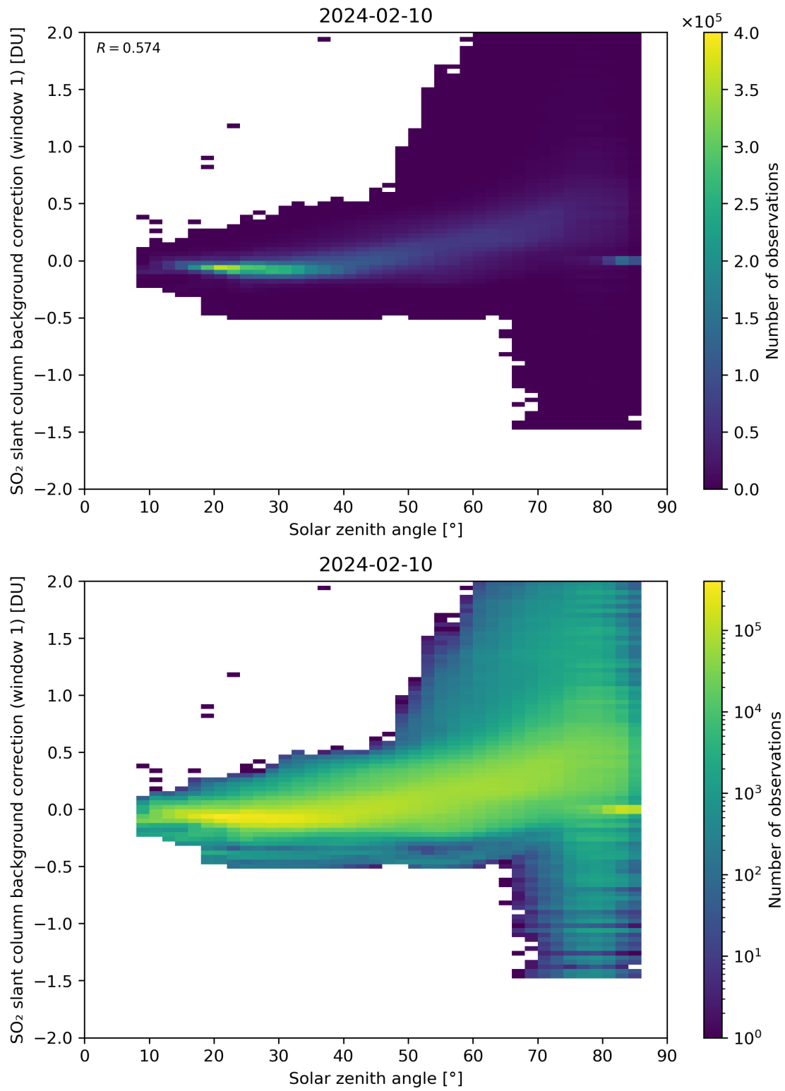
Figure 158: Scatter density plot of “Solar zenith angle” against “SO 2 slant column background correction (window 1)” for 2024-02-09 to 2024-02-11.
