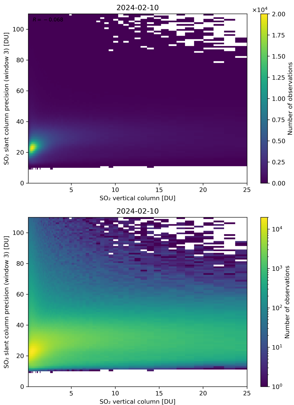
Figure 304: Scatter density plot of “SO 2 vertical column” against “SO 2 slant column precision (window 3)” for 2024-02-09 to 2024-02-11.
