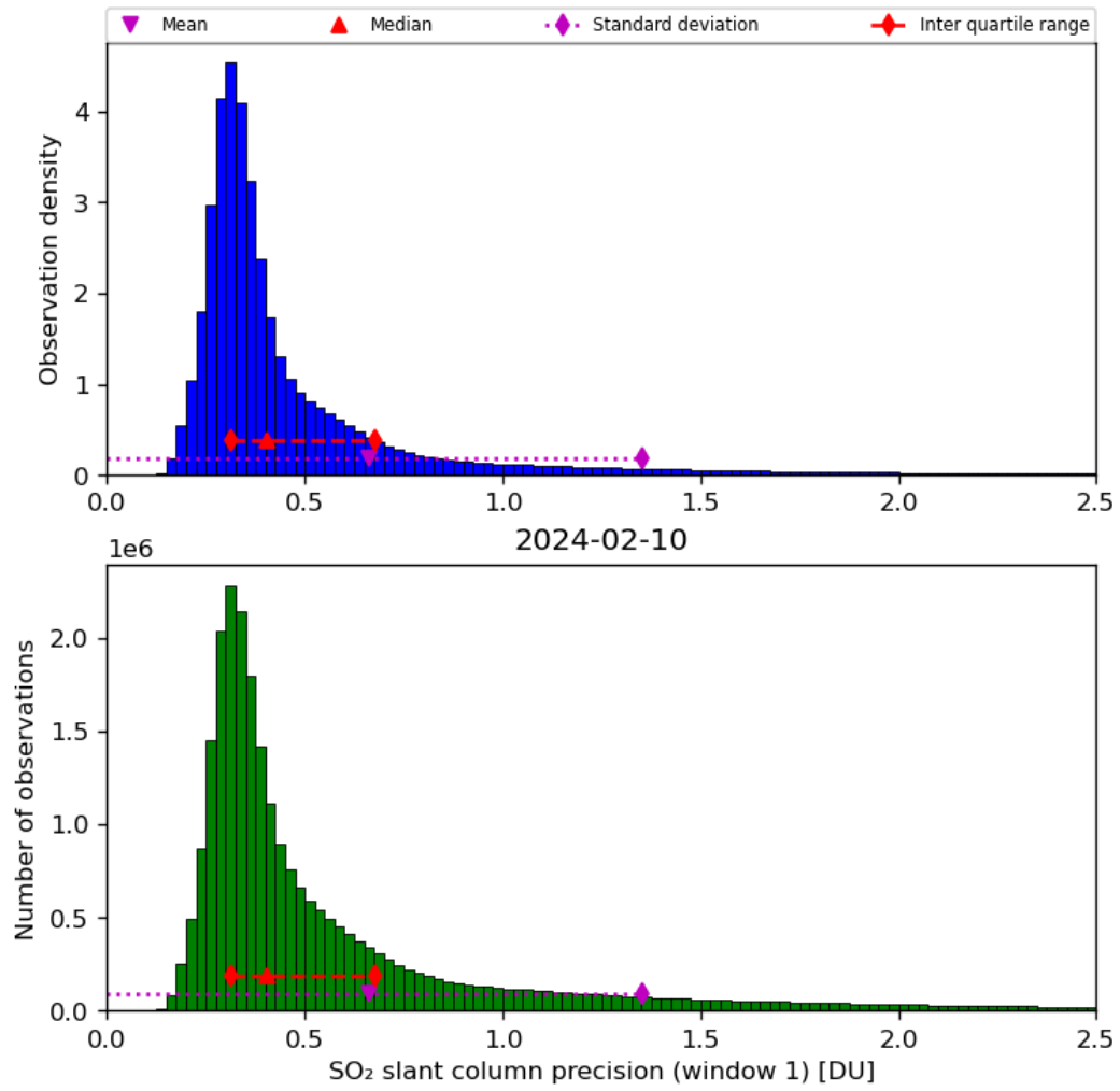
Figure 57: Histogram of “SO 2 slant column precision (window 1)” for 2024-02-09 to 2024-02-11
