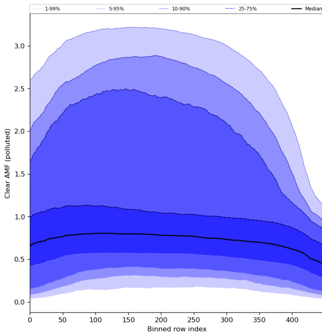
Figure 96: Along track statistics of “Clear AMF (polluted)” for 2024-02-09 to 2024-02-11
