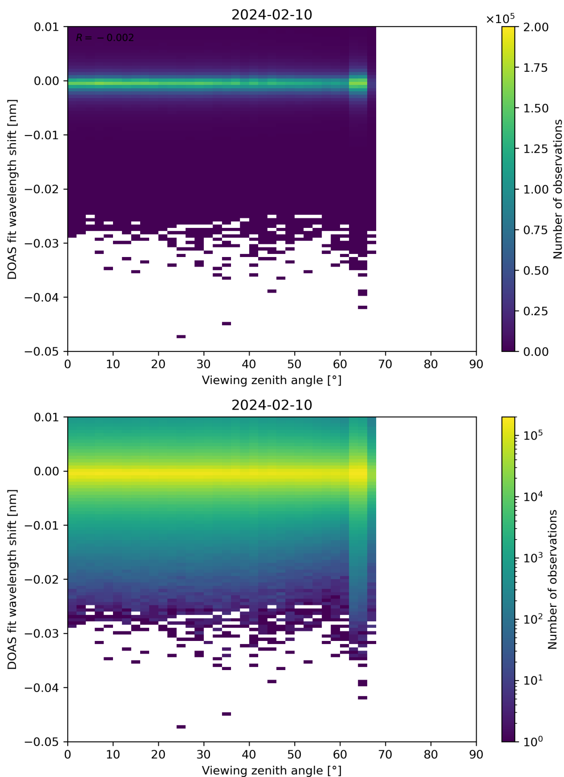
Figure 311: Scatter density plot of “Viewing zenith angle” against “DOAS fit wavelength shift” for 2024-02-09 to 2024-02-11.
