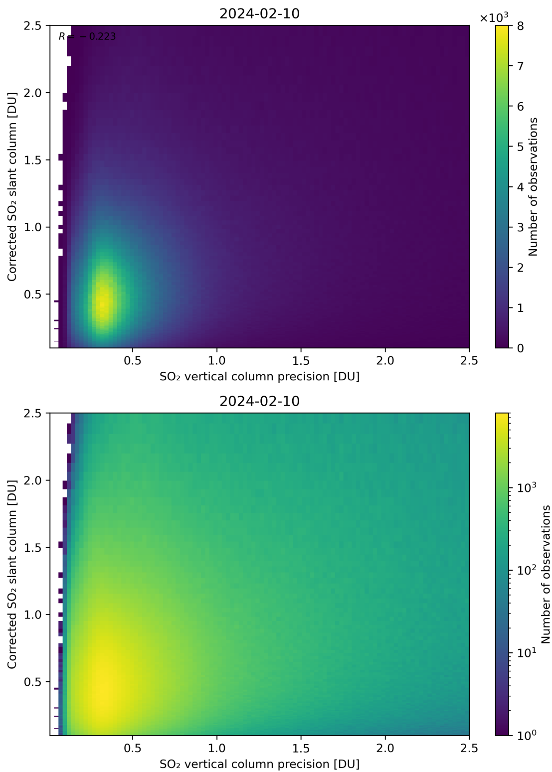
Figure 286: Scatter density plot of “SO 2 vertical column precision” against “Corrected SO 2 slant column” for 2024-02-09 to 2024-02-11.
