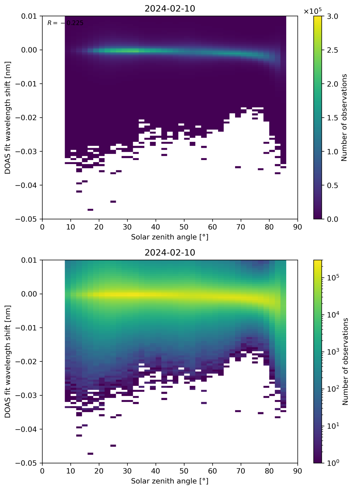
Figure 161: Scatter density plot of “Solar zenith angle” against “DOAS fit wavelength shift” for 2024-02-09 to 2024-02-11.
