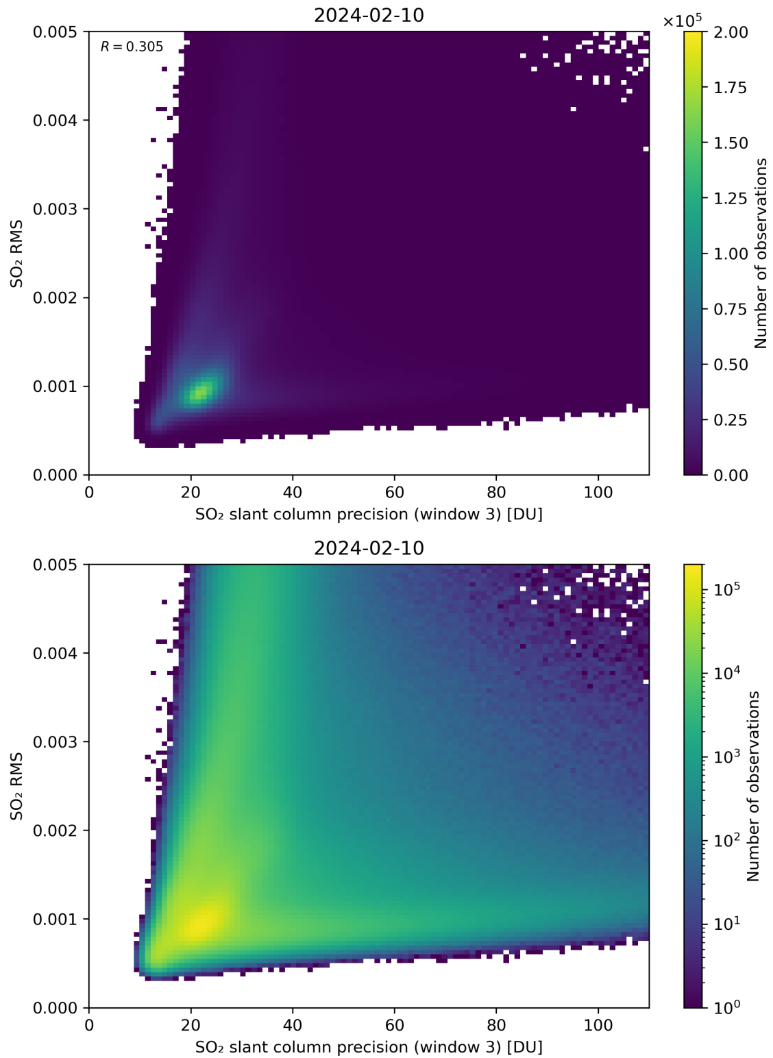
Figure 260: Scatter density plot of “SO 2 slant column precision (window 3)” against “SO 2 RMS” for 2024-02-09 to 2024-02-11.
