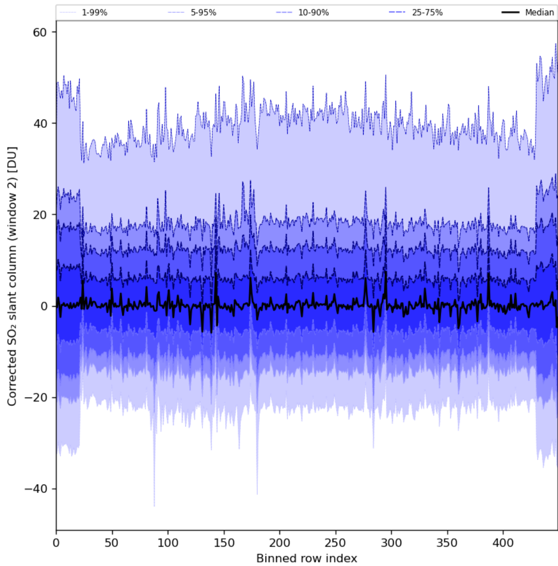
Figure 85: Along track statistics of "Corrected SO 2 slant column (window 2)" for 2024-02-09 to 2024-02-11
