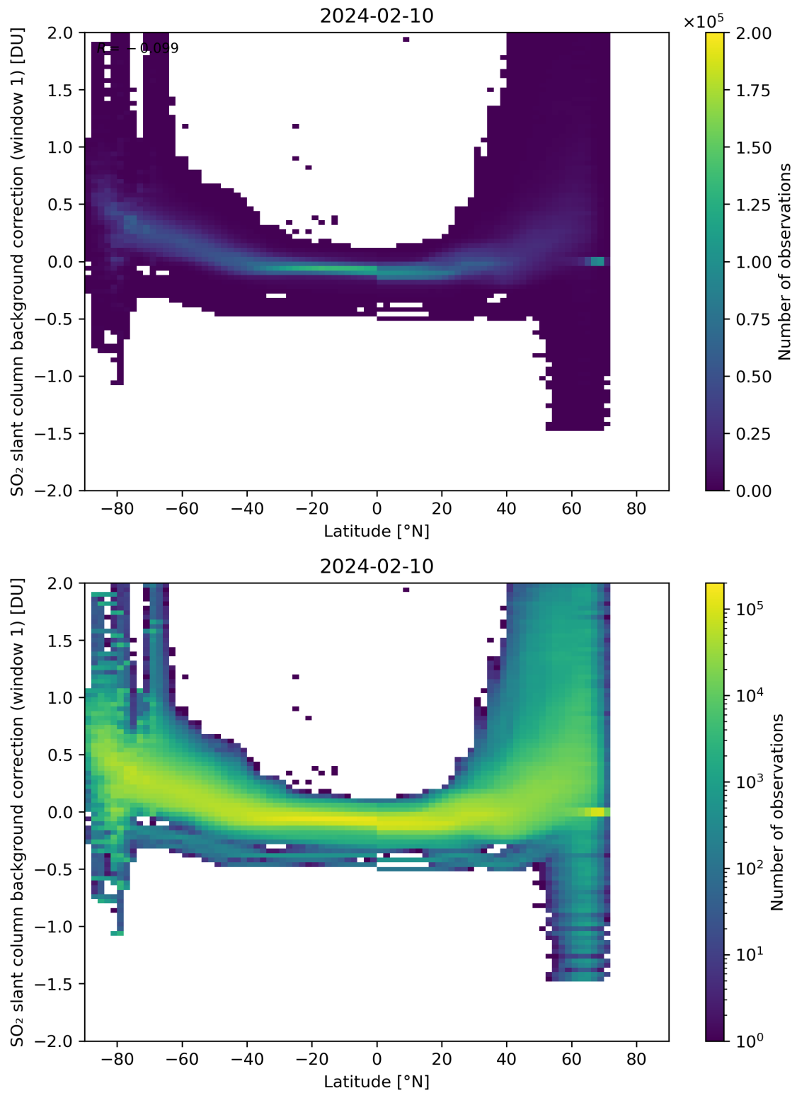
Figure 139: Scatter density plot of “Latitude” against “SO 2 slant column background correction (window 1)” for 2024-02-09 to 2024-02-11.
