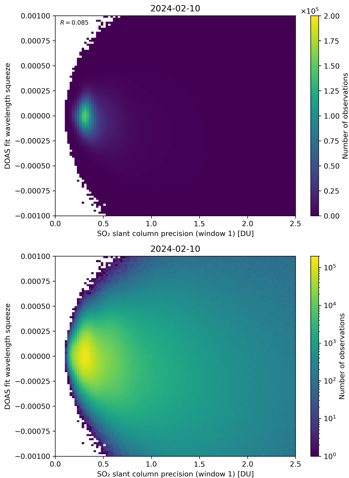
Figure 222: Scatter density plot of “SO 2 slant column precision (window 1)” against “DOAS fit wavelength squeeze” for 2024-02-09 to 2024-02-11.
