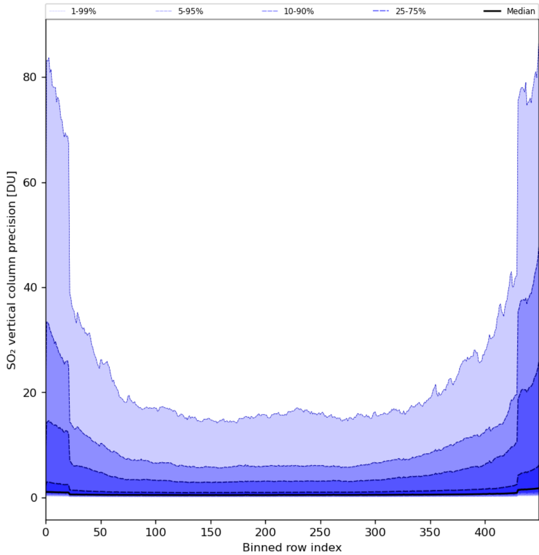
Figure 77: Along track statistics of “SO 2 vertical column precision” for 2024-02-09 to 2024-02-11
