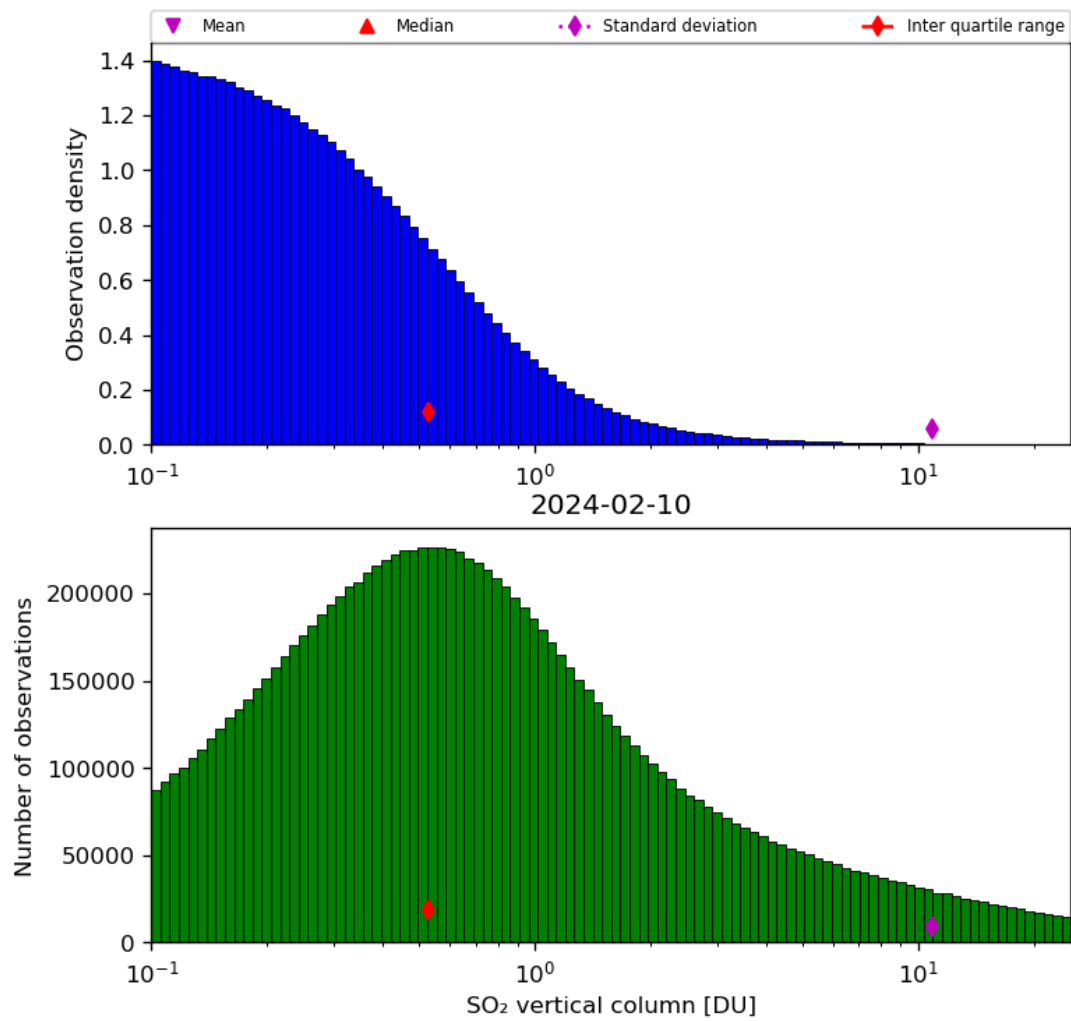
Figure 53: Histogram of “SO 2 vertical column” for 2024-02-09 to 2024-02-11
