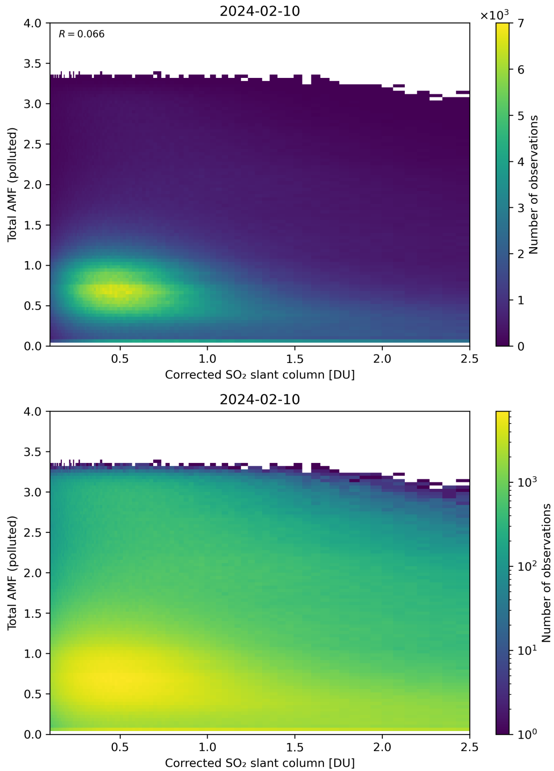
Figure 192: Scatter density plot of “Corrected SO 2 slant column” against “Total AMF (polluted)” for 2024-02-09 to 2024-02-11.
