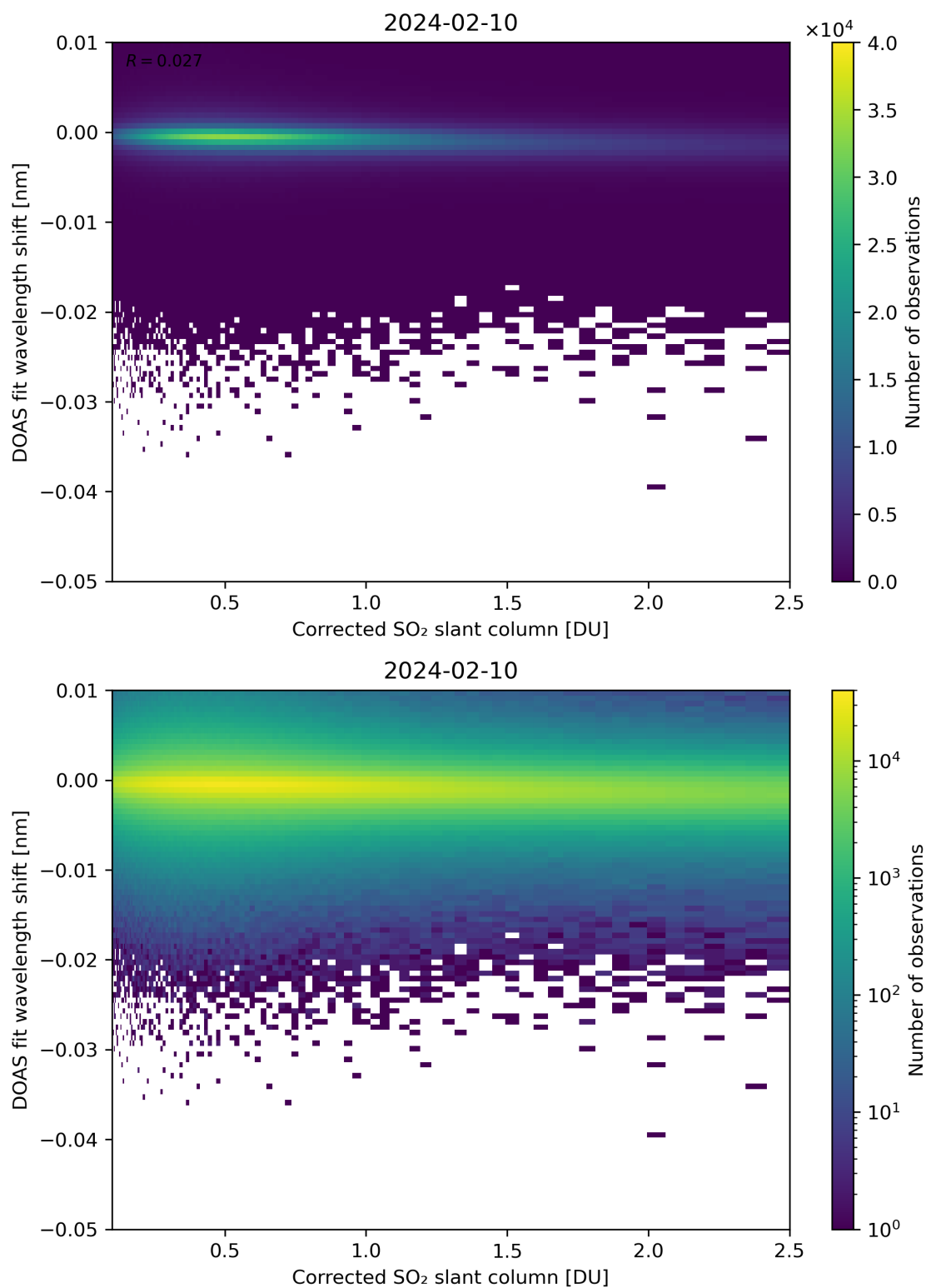
Figure 181: Scatter density plot of “Corrected SO 2 slant column” against “DOAS fit wavelength shift” for 2024-02-09 to 2024-02-11.
