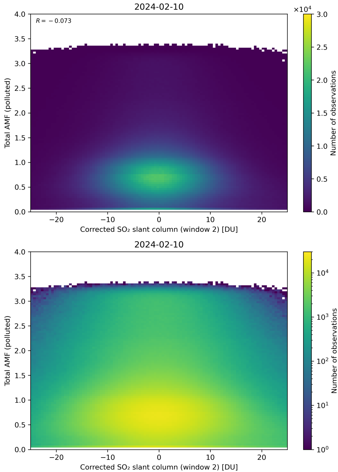
Figure 203: Scatter density plot of “Corrected SO 2 slant column (window 2)” against “Total AMF (polluted)” for 2024-02-09 to 2024-02-11.
