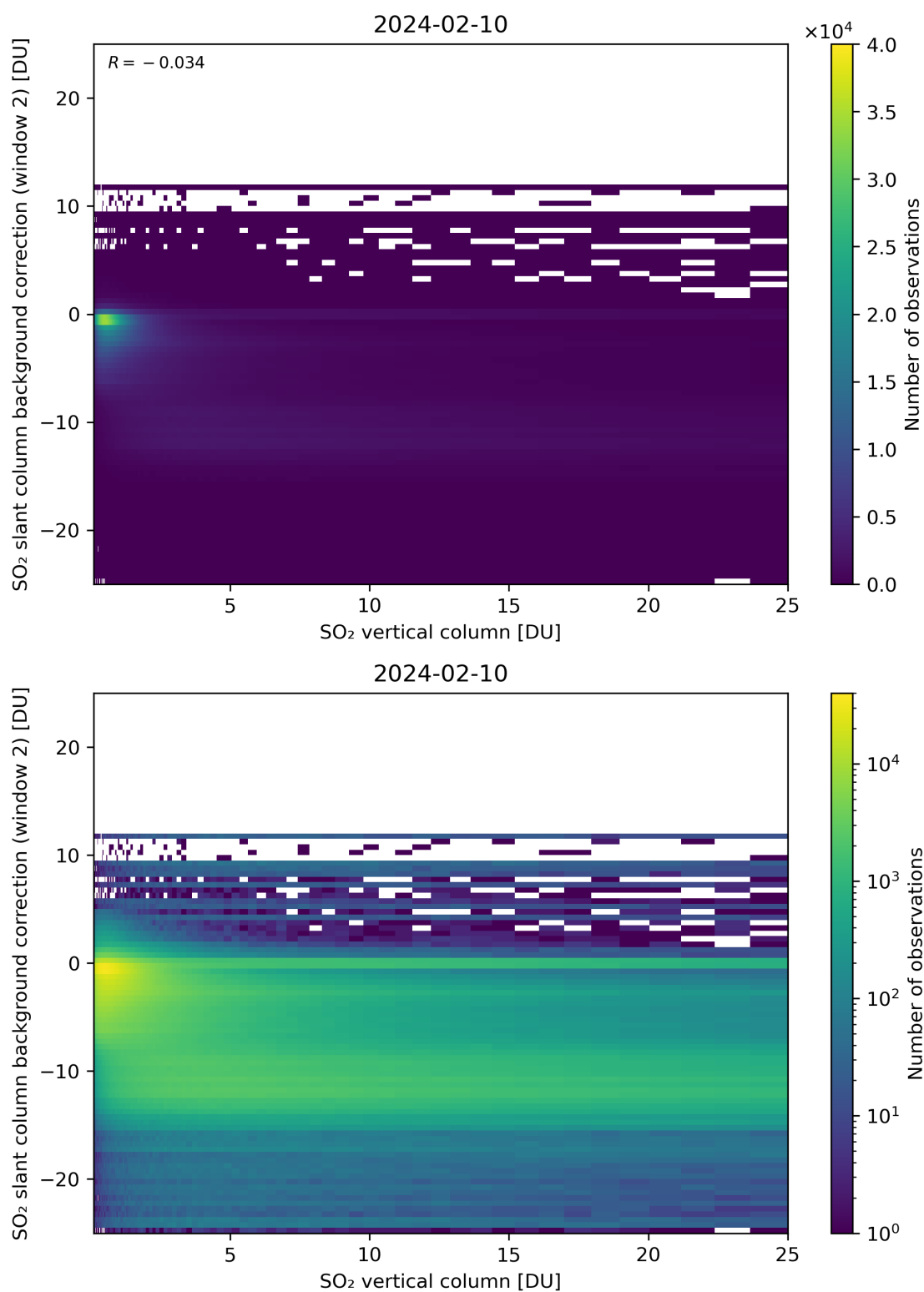
Figure 274: Scatter density plot of “SO 2 vertical column” against “SO 2 slant column background correction (window 2)” for 2024-02-09 to 2024-02-11.
