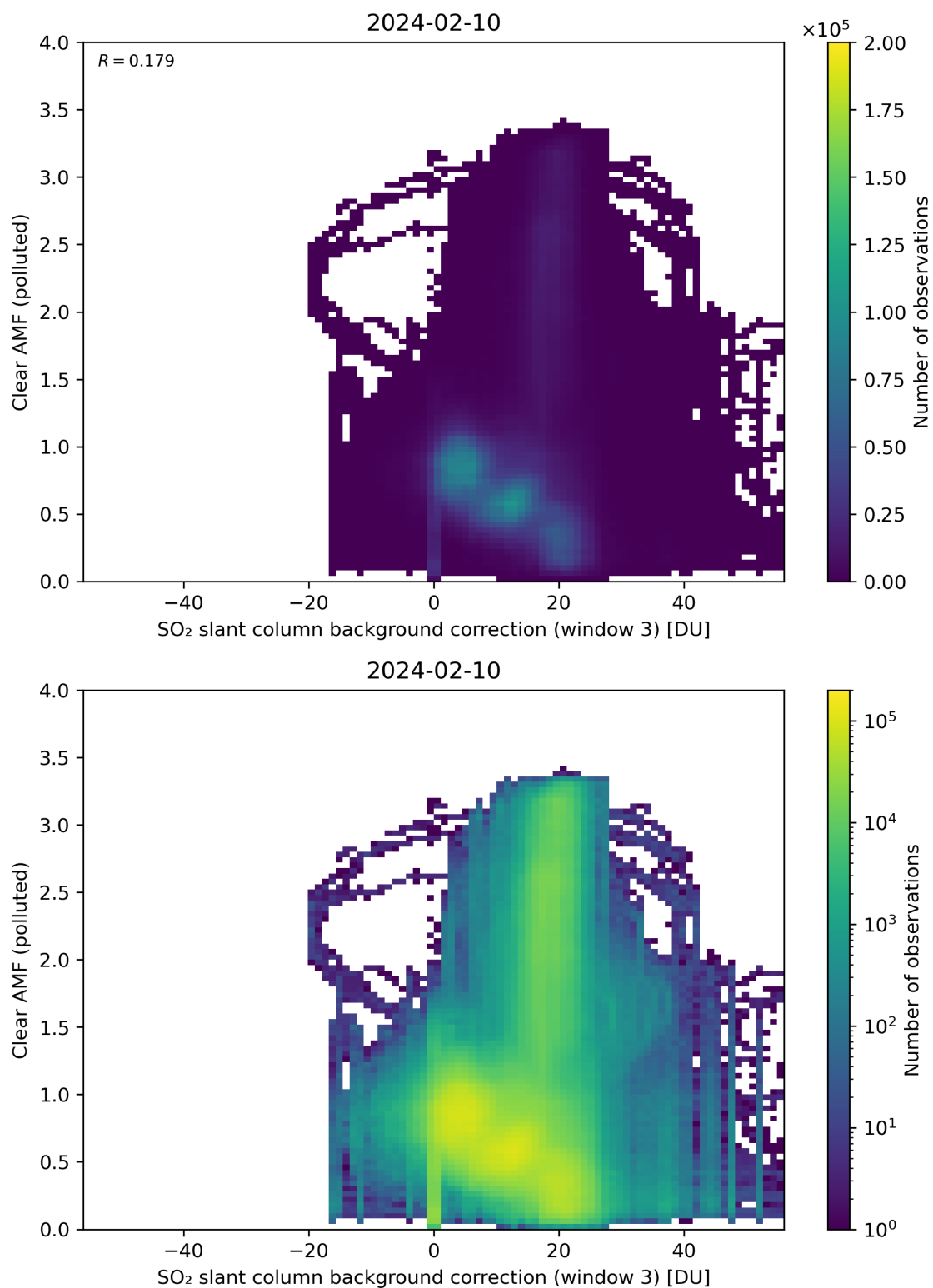
Figure 124: Scatter density plot of “SO 2 slant column background correction (window 3)” against “Clear AMF (polluted)” for 2024-02-09 to 2024-02-11.
