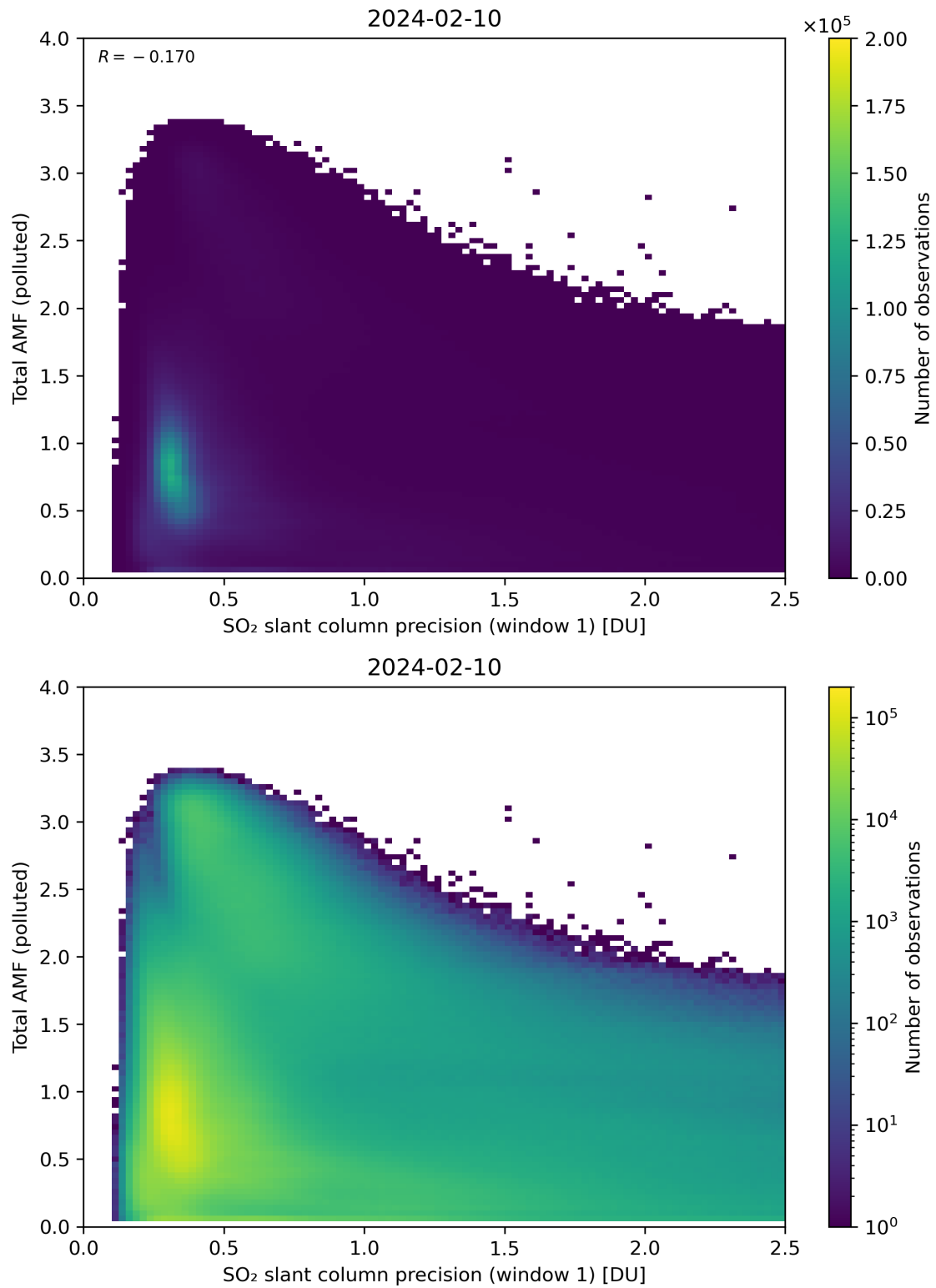
Figure 230: Scatter density plot of “SO 2 slant column precision (window 1)” against “Total AMF (polluted)” for 2024-02-09 to 2024-02-11.
