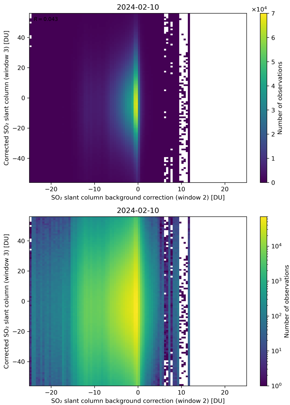
Figure 116: Scatter density plot of “SO 2 slant column background correction (window 2)” against “Corrected SO 2 slant column (window 3)” for 2024-02-09 to 2024-02-11.
