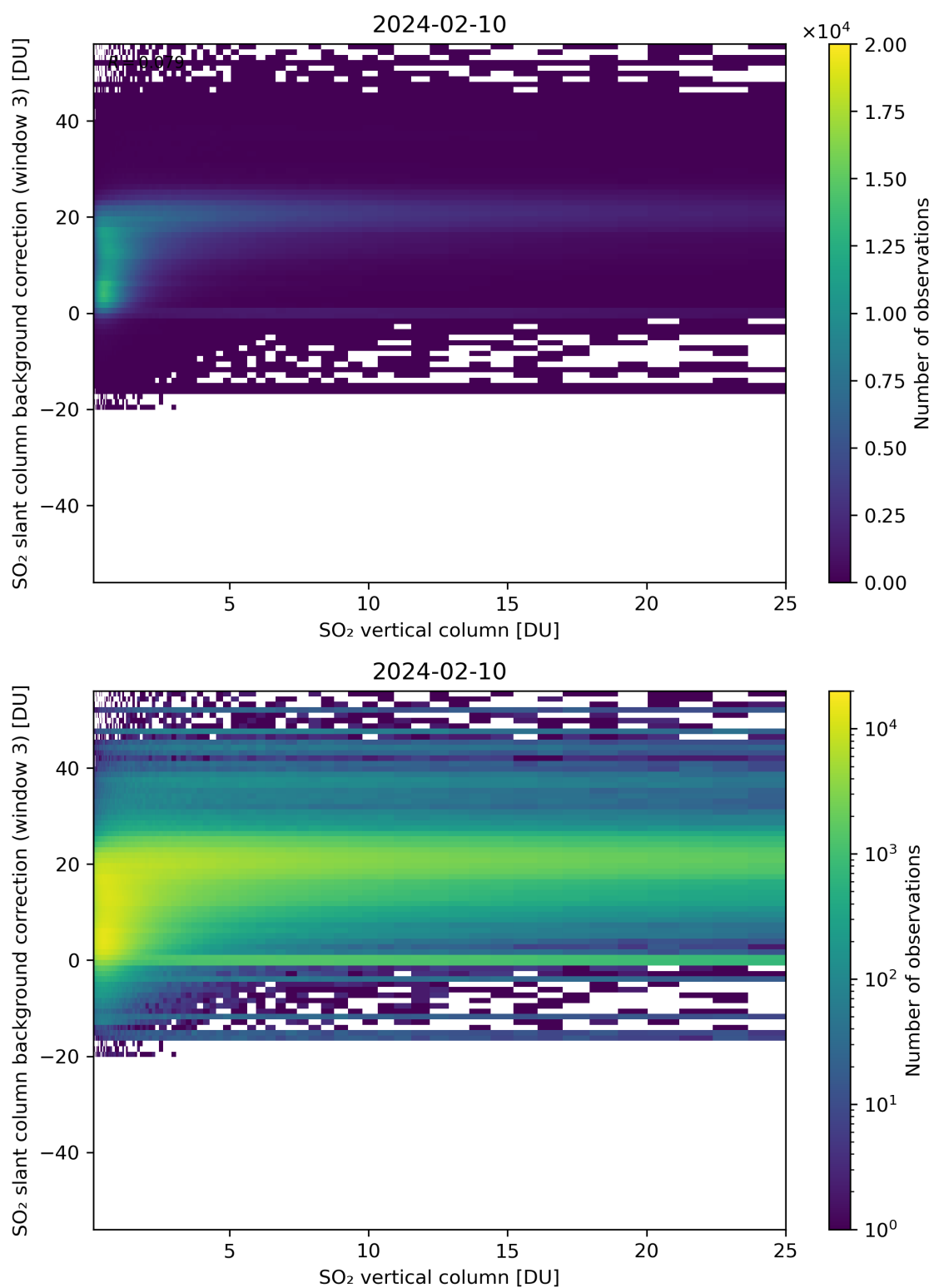
Figure 275: Scatter density plot of “SO 2 vertical column” against “SO 2 slant column background correction (window 3)” for 2024-02-09 to 2024-02-11.
