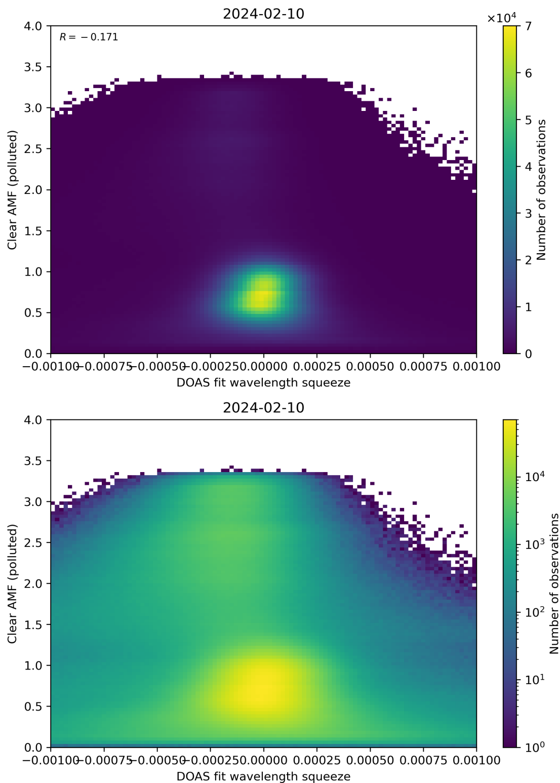
Figure 133: Scatter density plot of “DOAS fit wavelength squeeze” against “Clear AMF (polluted)” for 2024-02-09 to 2024-02-11.
