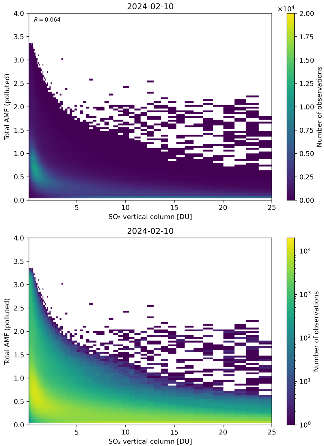
Figure 305: Scatter density plot of “SO 2 vertical column” against “Total AMF (polluted)” for 2024-02-09 to 2024-02-11.
