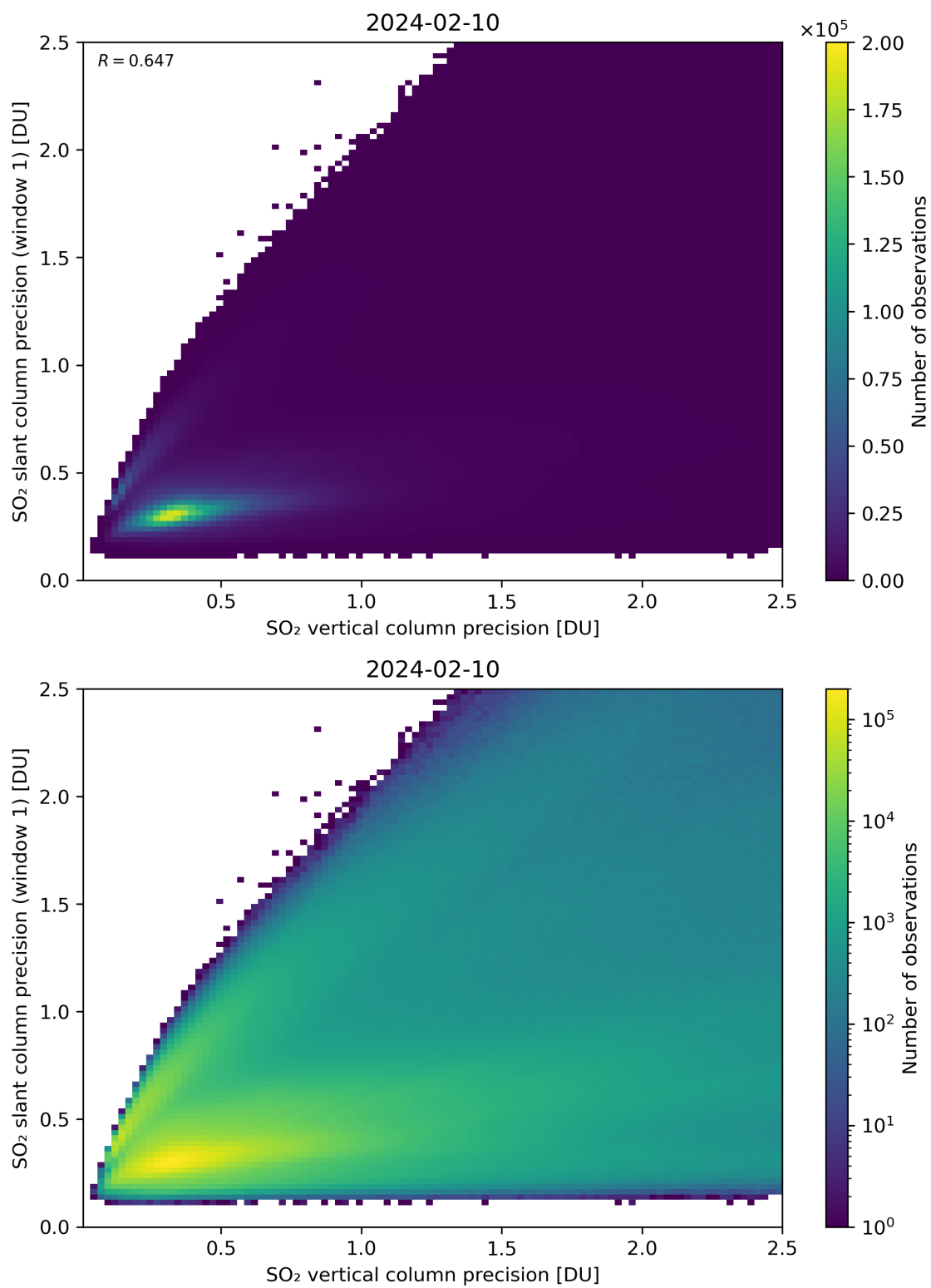
Figure 290: Scatter density plot of “SO 2 vertical column precision” against “SO 2 slant column precision (window 1)” for 2024-02-09 to 2024-02-11.
