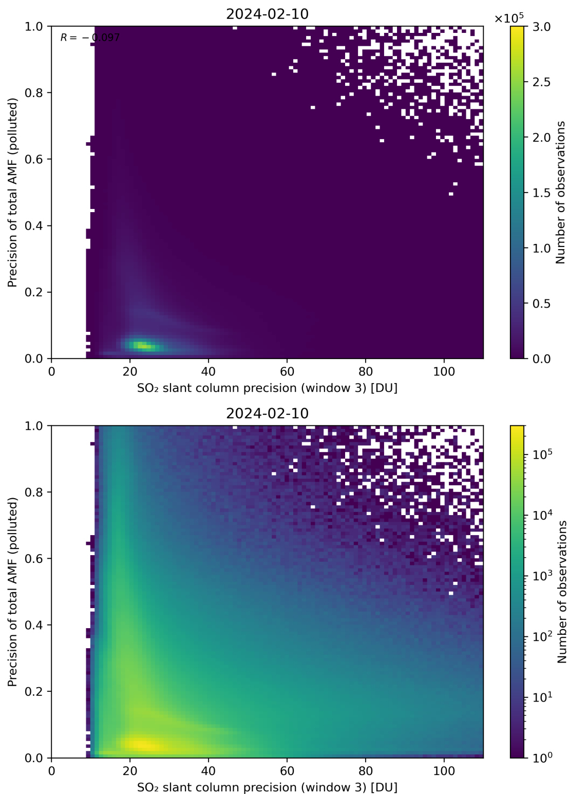
Figure 264: Scatter density plot of “SO 2 slant column precision (window 3)” against “Precision of total AMF (polluted)” for 2024-02-09 to 2024-02-11.
