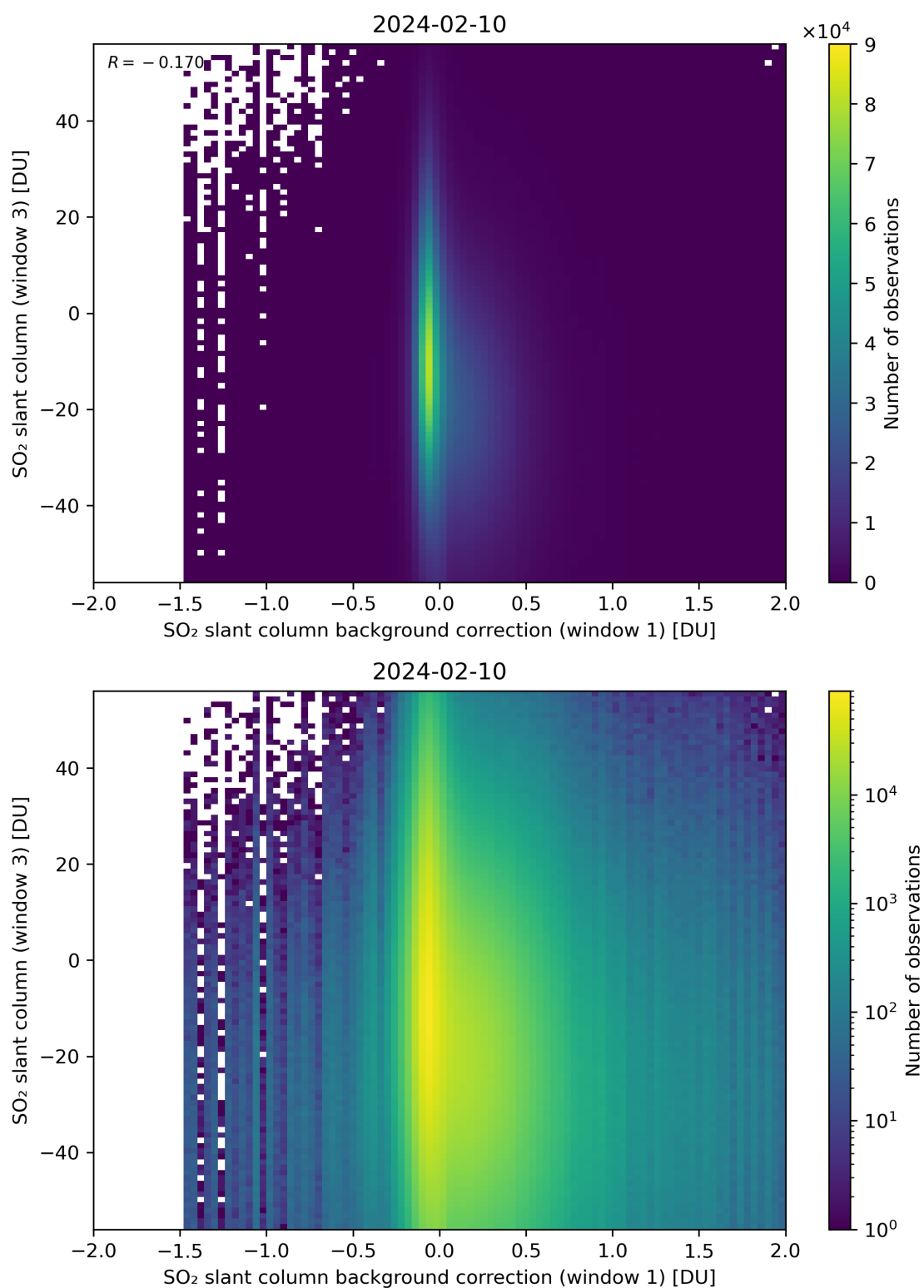
Figure 107: Scatter density plot of “SO 2 slant column background correction (window 1)” against “SO 2 slant column (window 3)” for 2024-02-09 to 2024-02-11.
