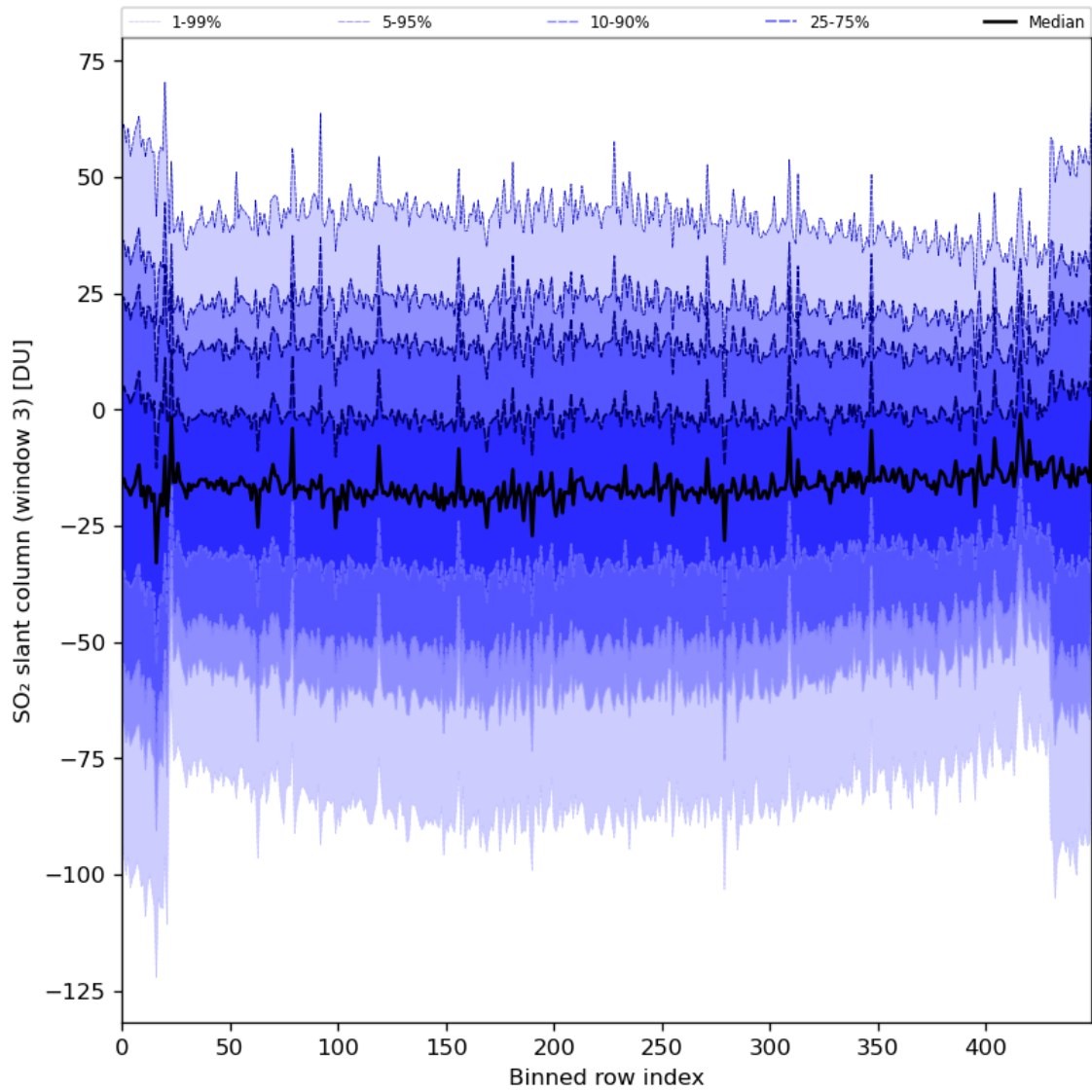
Figure 87: Along track statistics of “SO 2 slant column (window 3)” for 2024-02-09 to 2024-02-11
