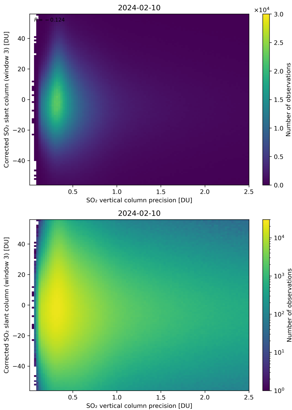
Figure 288: Scatter density plot of “SO 2 vertical column precision” against “Corrected SO 2 slant column (window 3)” for 2024-02-09 to 2024-02-11.
