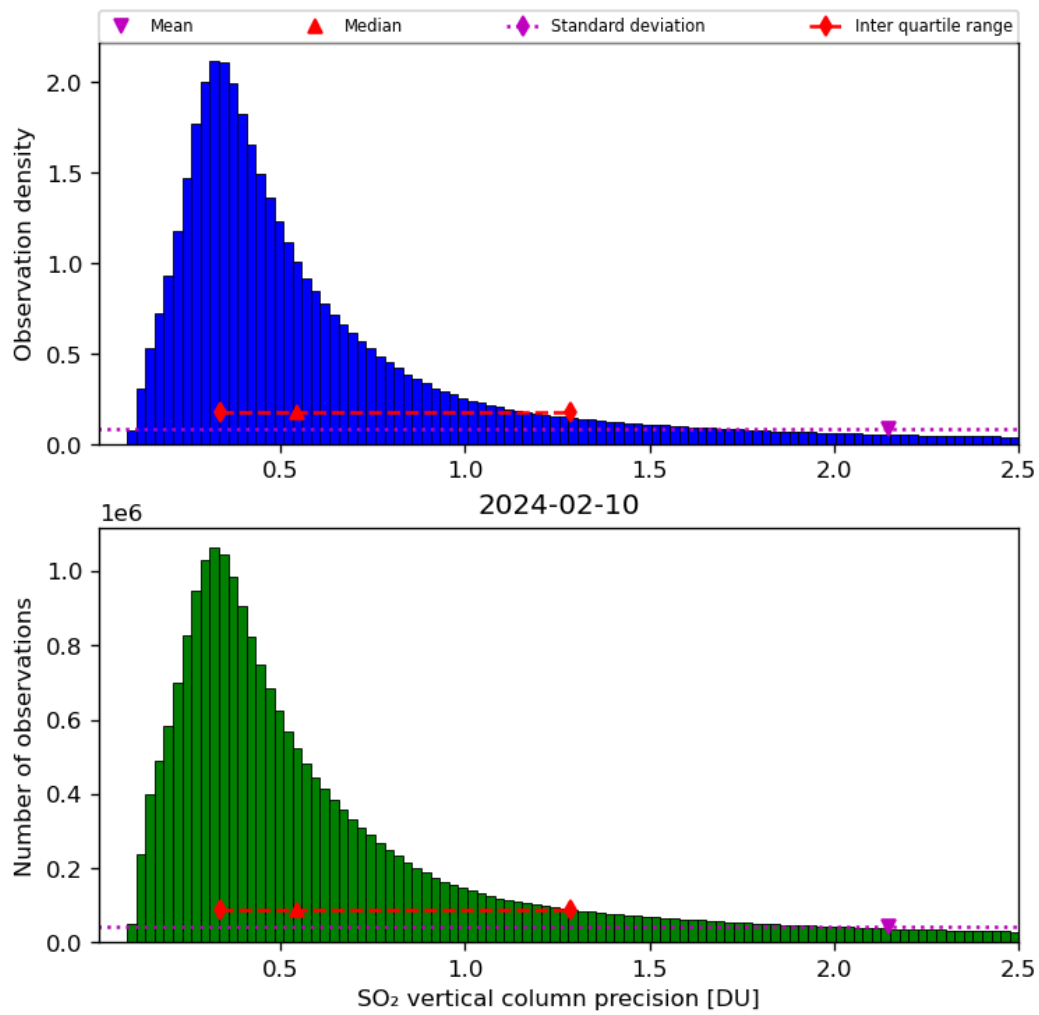
Figure 54: Histogram of “SO 2 vertical column precision” for 2024-02-09 to 2024-02-11
