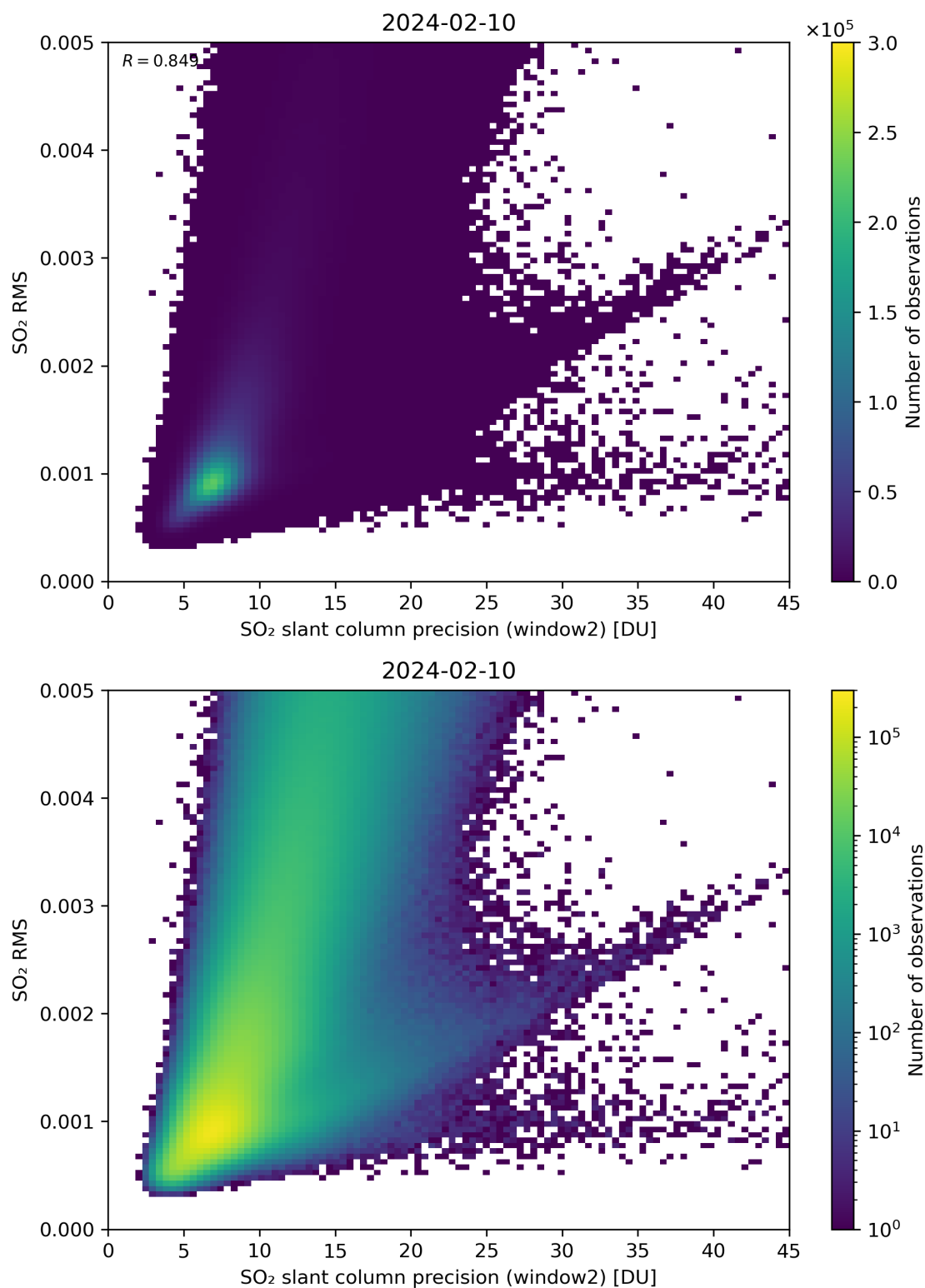
Figure 245: Scatter density plot of “SO 2 slant column precision (window2)” against “SO 2 RMS” for 2024-02-09 to 2024-02-11.
