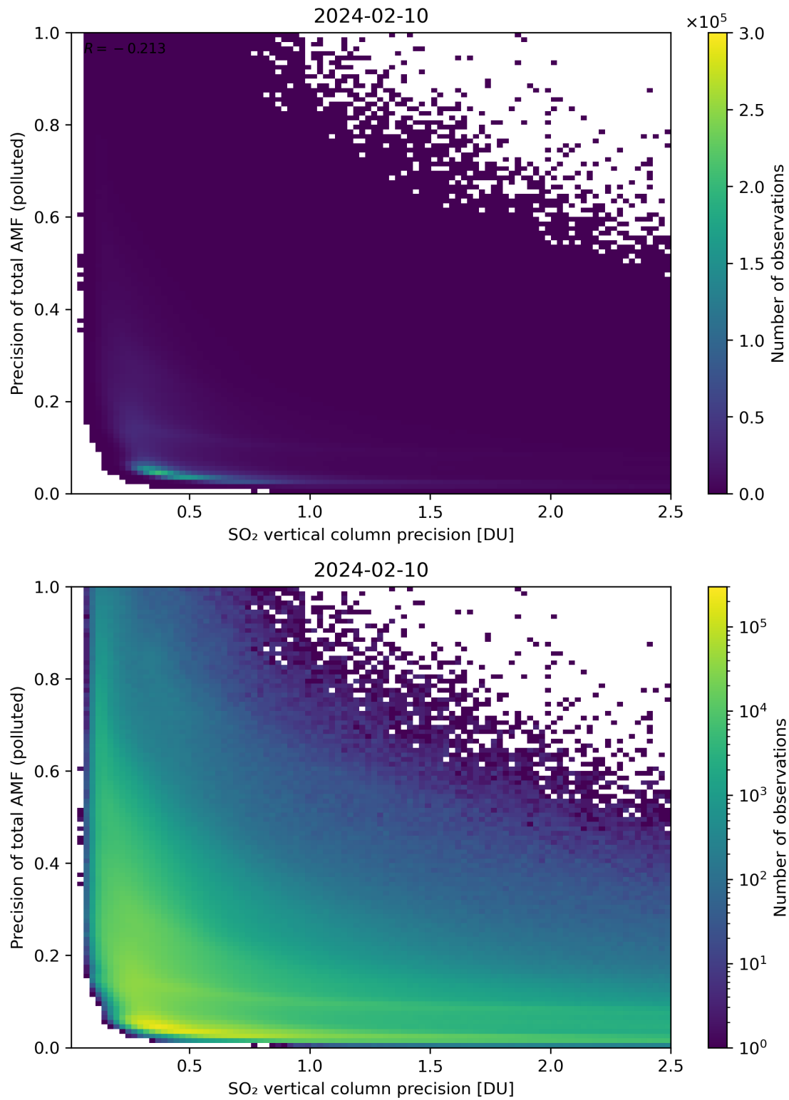
Figure 295: Scatter density plot of “SO 2 vertical column precision” against “Precision of total AMF (polluted)” for 2024-02-09 to 2024-02-11.
