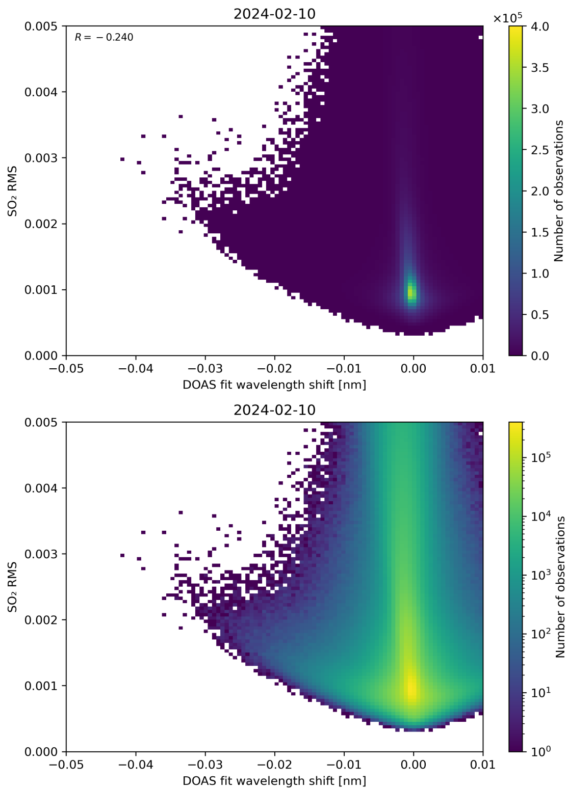
Figure 128: Scatter density plot of “DOAS fit wavelength shift” against “SO 2 RMS” for 2024-02-09 to 2024-02-11.
