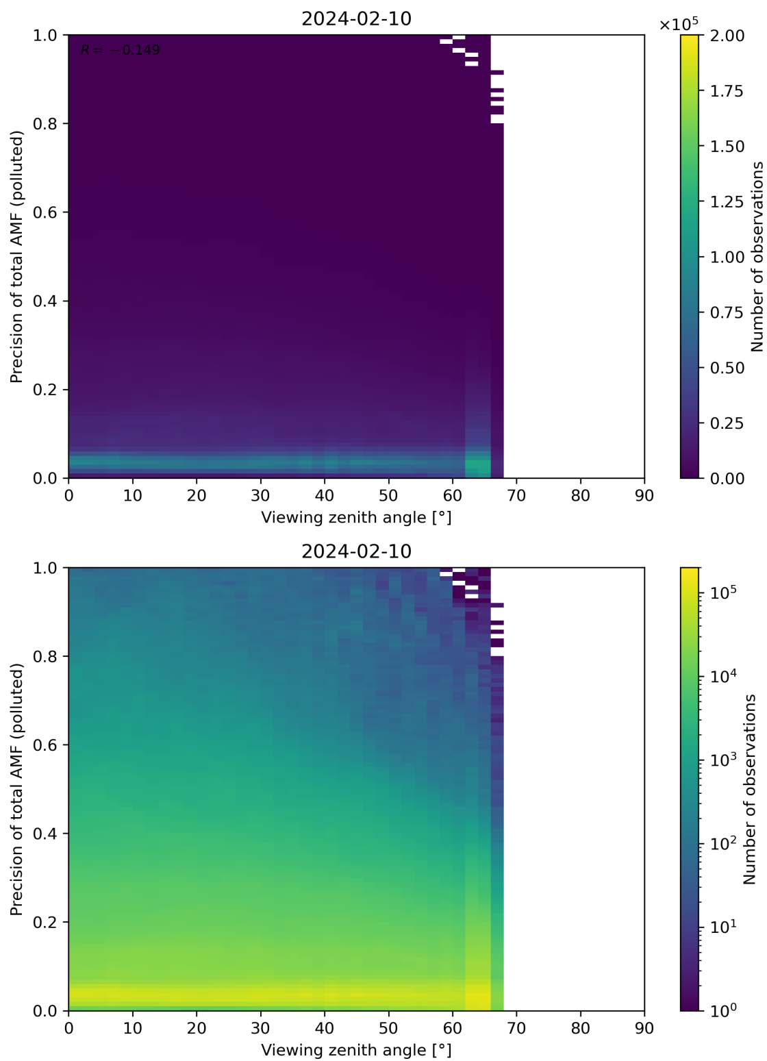
Figure 326: Scatter density plot of “Viewing zenith angle” against “Precision of total AMF (polluted)” for 2024-02-09 to 2024-02-11.
