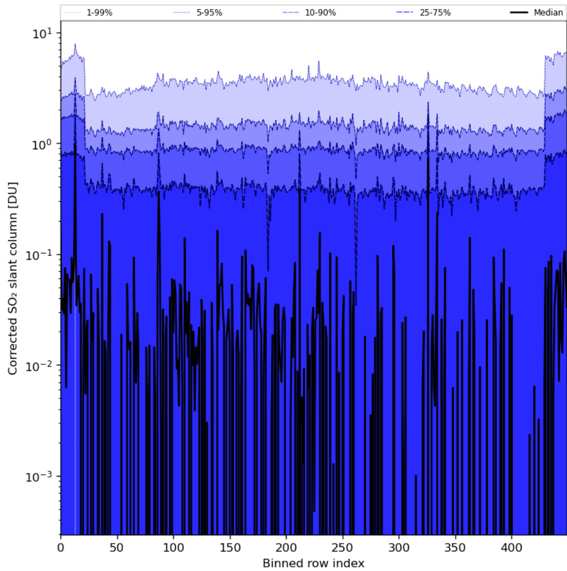
Figure 78: Along track statistics of “Corrected SO 2 slant column” for 2024-02-09 to 2024-02-11
