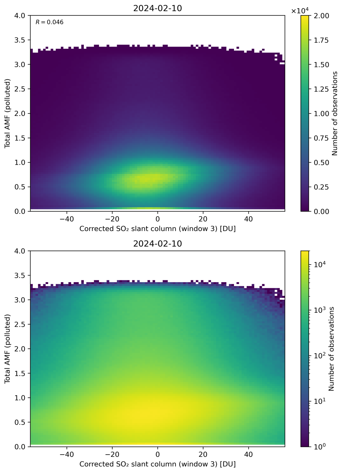
Figure 210: Scatter density plot of “Corrected SO 2 slant column (window 3)” against “Total AMF (polluted)” for 2024-02-09 to 2024-02-11.
