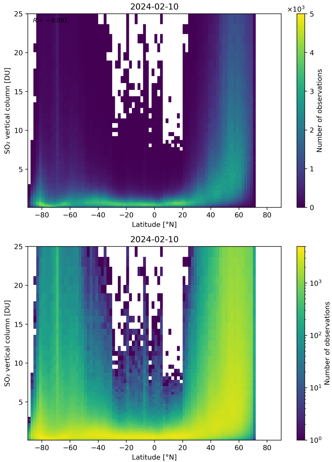
Figure 156: Scatter density plot of “Latitude” against “SO 2 vertical column” for 2024-02-09 to 2024-02-11.
