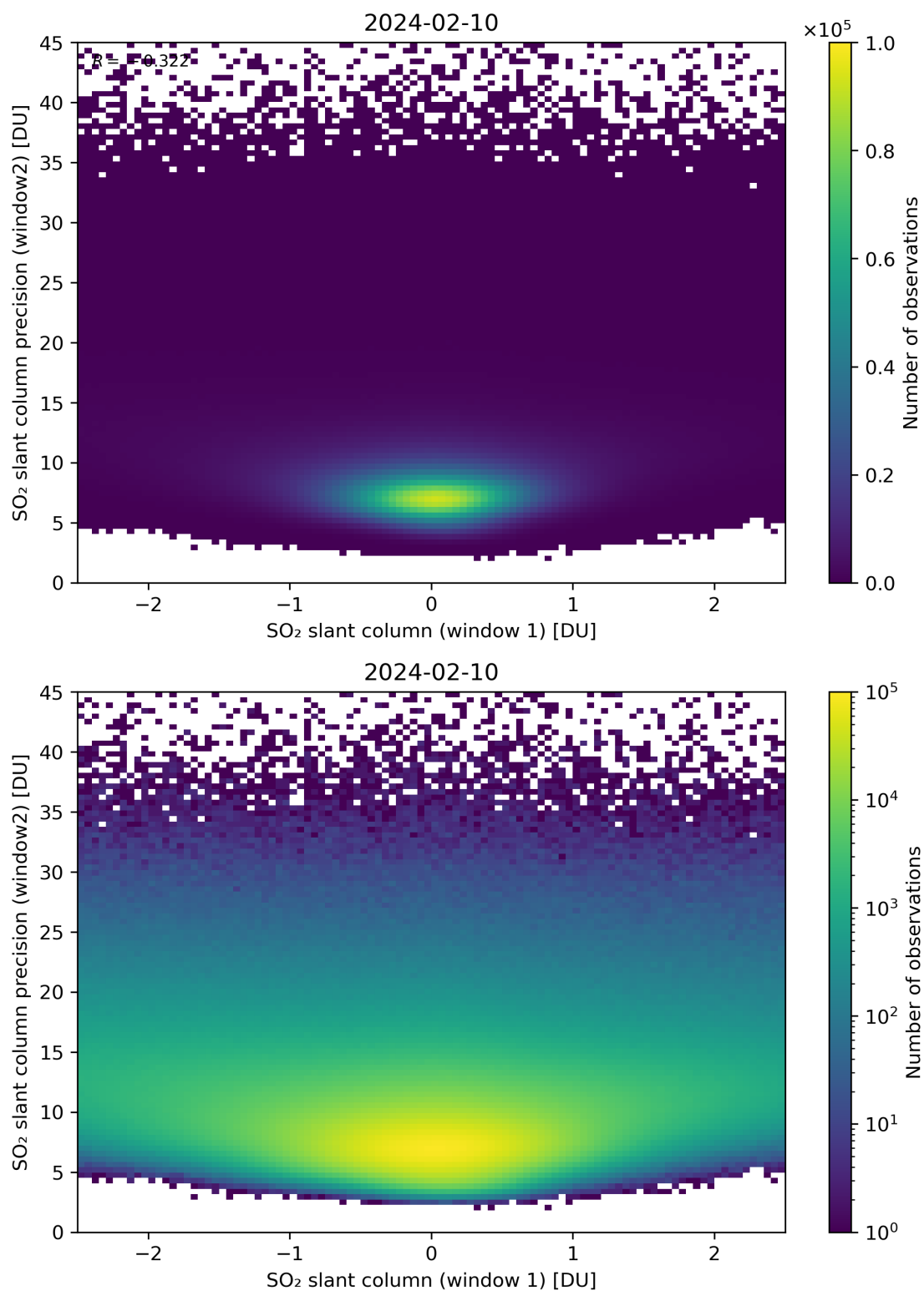
Figure 236: Scatter density plot of “SO 2 slant column (window 1)” against “SO 2 slant column precision (window2)” for 2024-02-09 to 2024-02-11.
