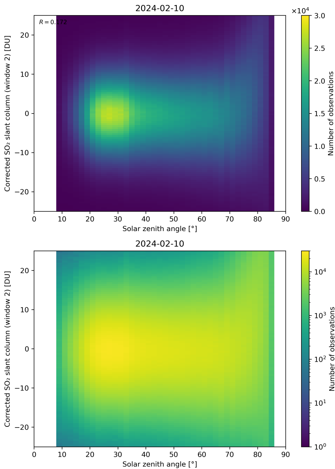
Figure 167: Scatter density plot of “Solar zenith angle” against “Corrected SO 2 slant column (window 2)” for 2024-02-09 to 2024-02-11.
