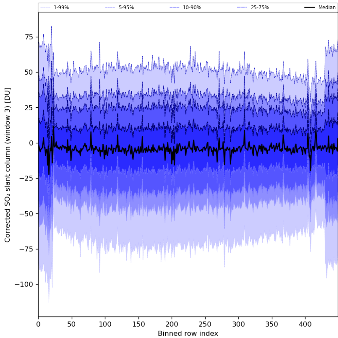
Figure 89: Along track statistics of “Corrected SO 2 slant column (window 3)” for 2024-02-09 to 2024-02-11
