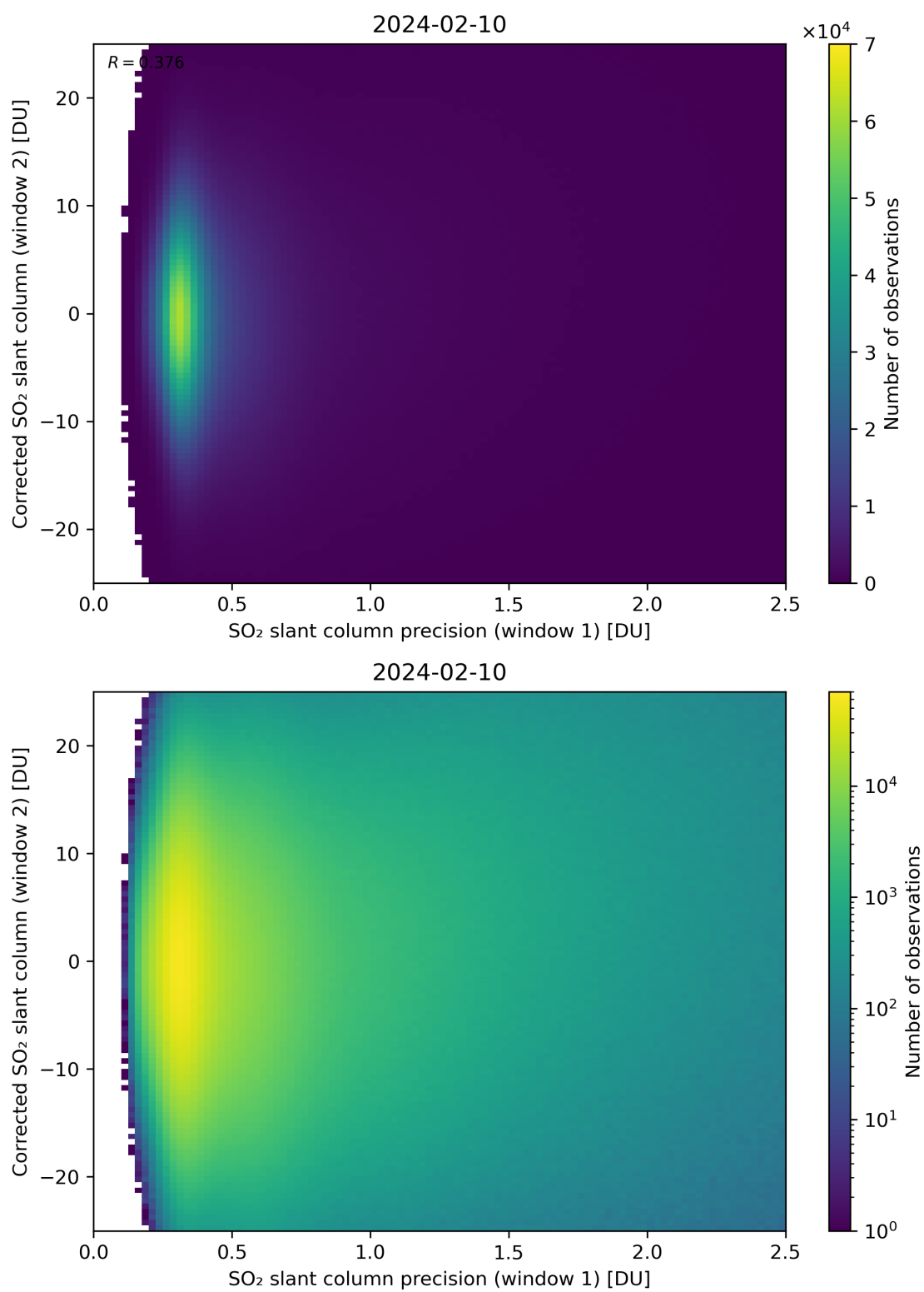
Figure 225: Scatter density plot of “SO 2 slant column precision (window 1)” against “Corrected SO 2 slant column (window 2)” for 2024-02-09 to 2024-02-11.
