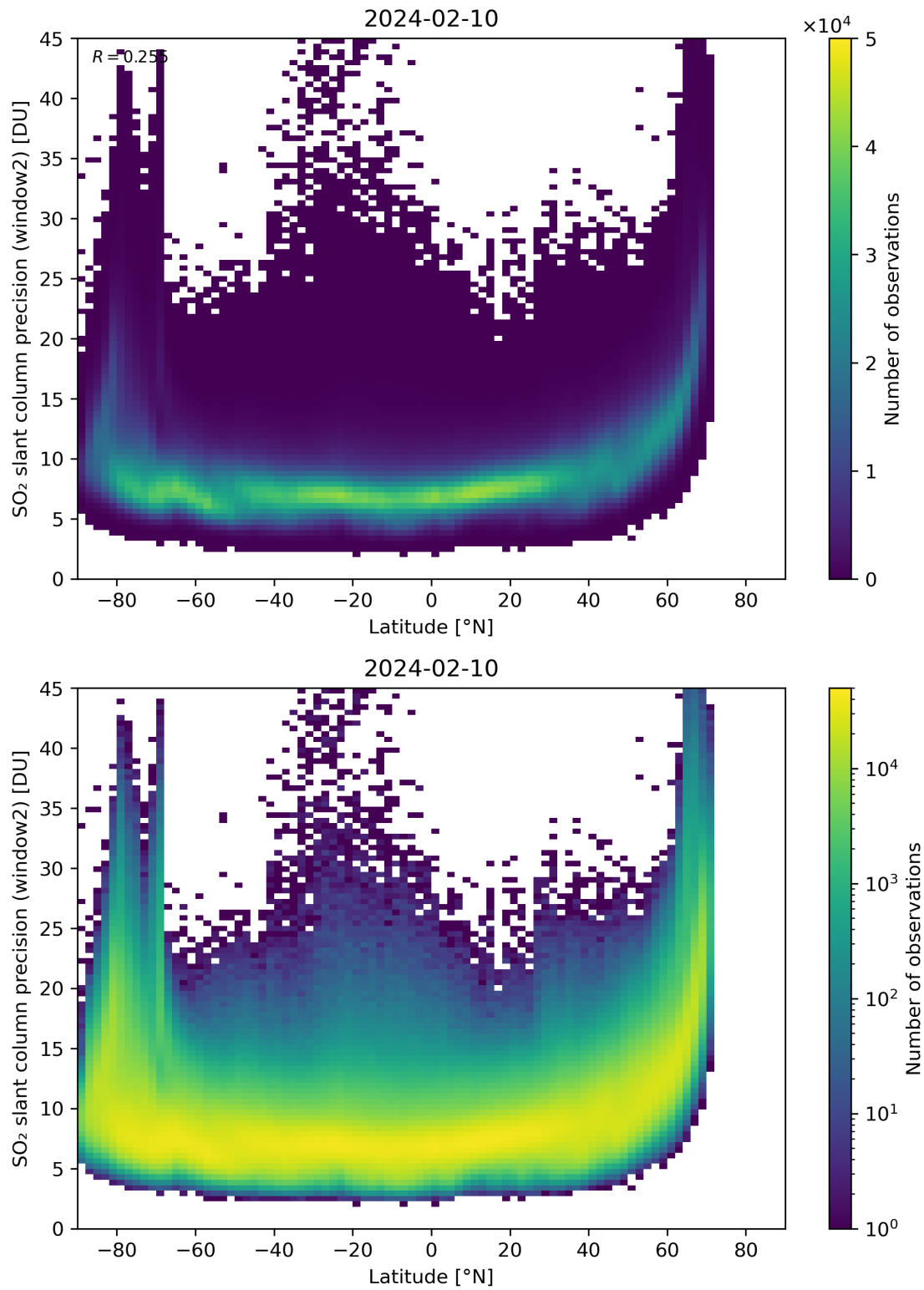
Figure 151: Scatter density plot of “Latitude” against “SO 2 slant column precision (window2)” for 2024-02-09 to 2024-02-11.
