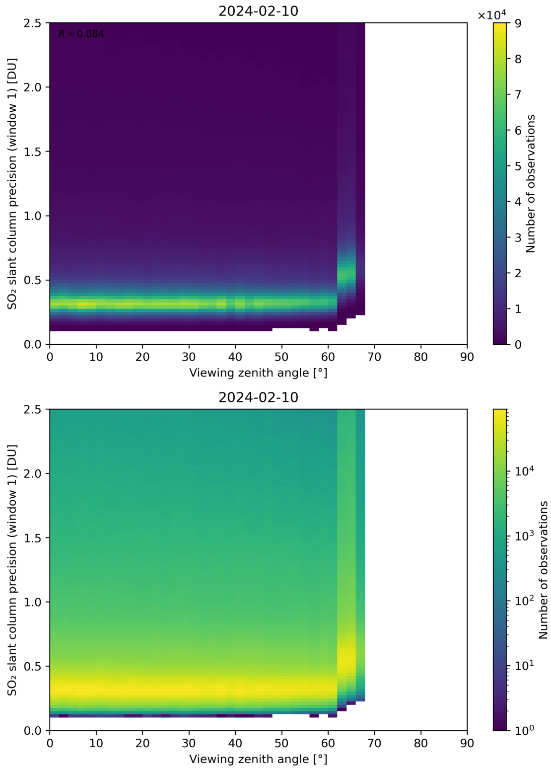
Figure 321: Scatter density plot of “Viewing zenith angle” against “SO 2 slant column precision (window 1)” for 2024-02-09 to 2024-02-11.
