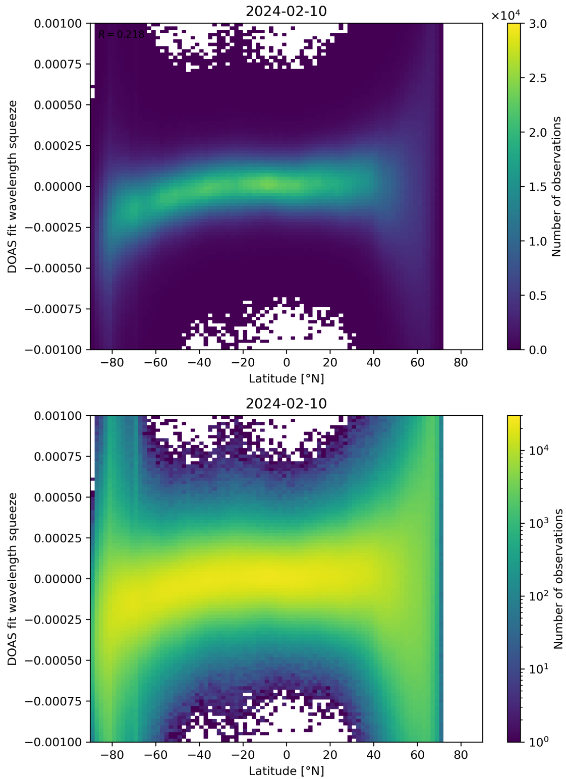
Figure 143: Scatter density plot of “Latitude” against “DOAS fit wavelength squeeze” for 2024-02-09 to 2024-02-11.
