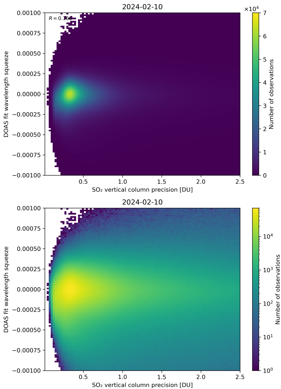
Figure 283: Scatter density plot of “SO 2 vertical column precision” against “DOAS fit wavelength squeeze” for 2024-02-09 to 2024-02-11.
