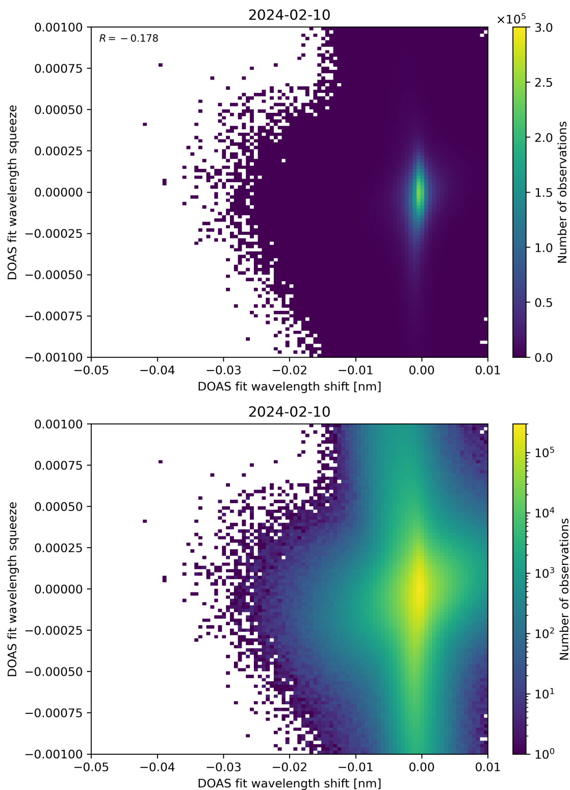
Figure 127: Scatter density plot of “DOAS fit wavelength shift” against “DOAS fit wavelength squeeze” for 2024-02-09 to 2024-02-11.
