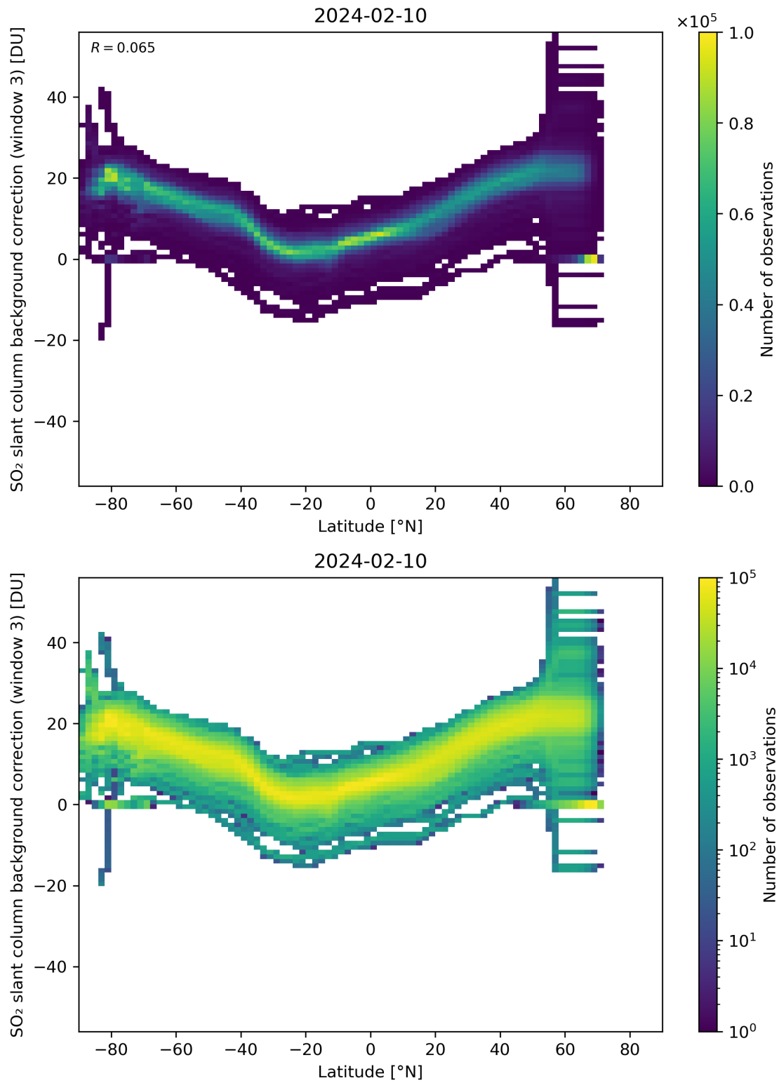
Figure 141: Scatter density plot of “Latitude” against “SO 2 slant column background correction (window 3)” for 2024-02-09 to 2024-02-11.
