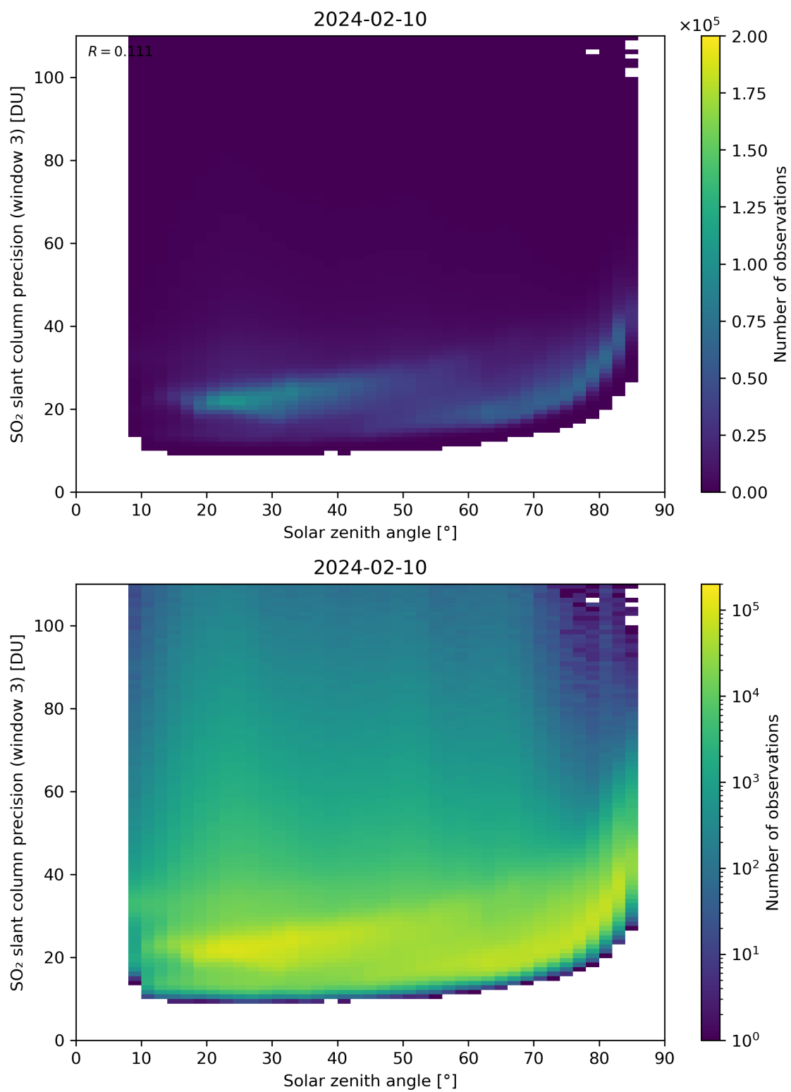
Figure 173: Scatter density plot of “Solar zenith angle” against “SO 2 slant column precision (window 3)” for 2024-02-09 to 2024-02-11.
