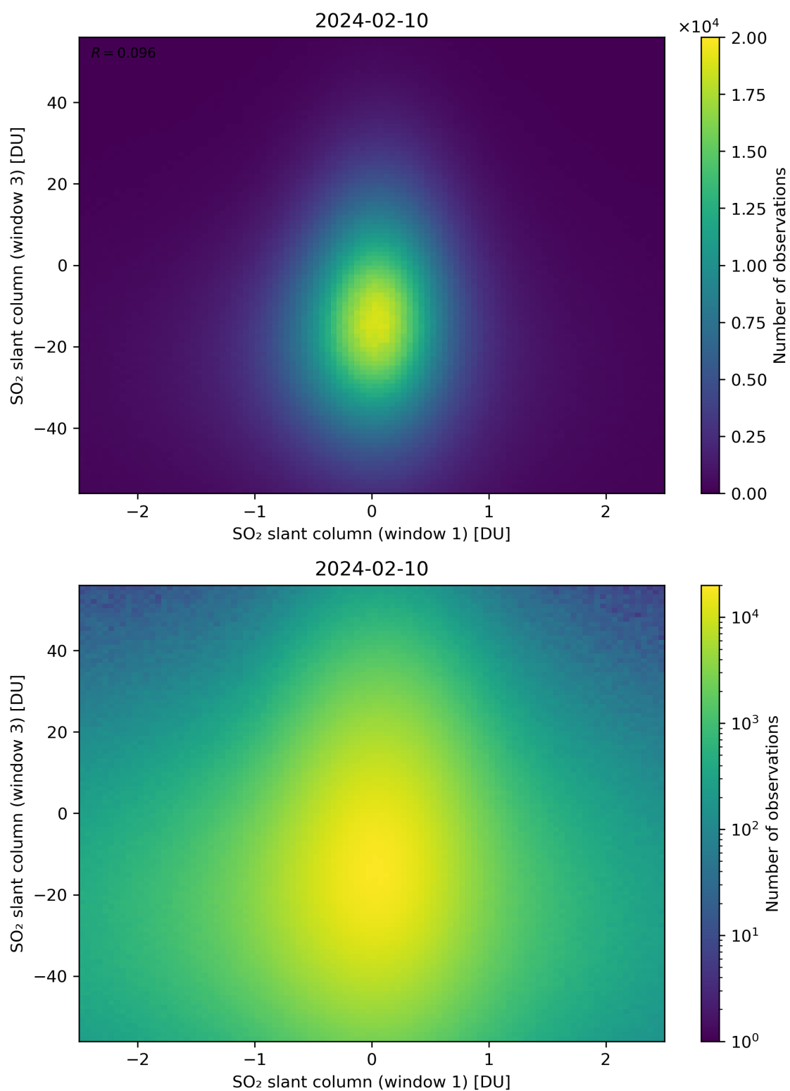
Figure 237: Scatter density plot of “SO 2 slant column (window 1)” against “SO 2 slant column (window 3)” for 2024-02-09 to 2024-02-11.
