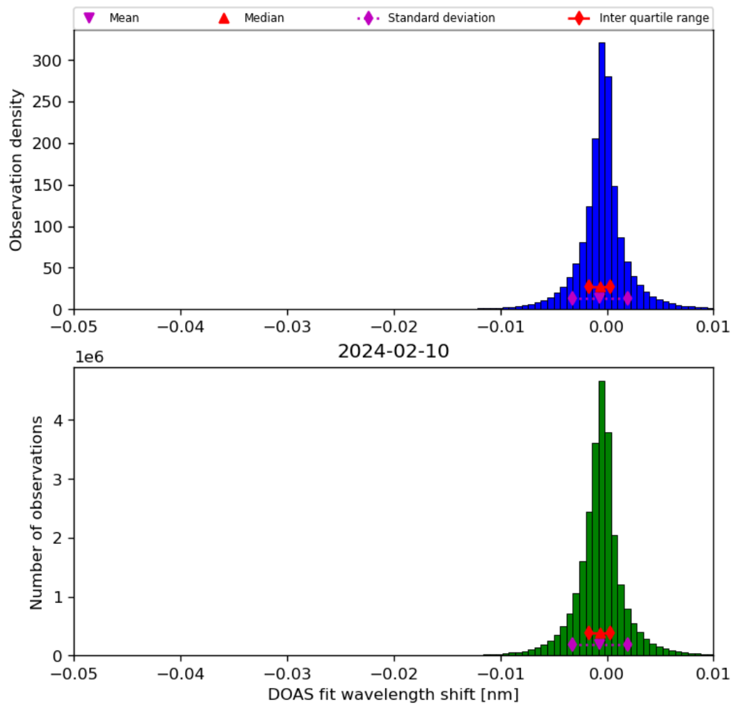
Figure 68: Histogram of “DOAS fit wavelength shift” for 2024-02-09 to 2024-02-11
