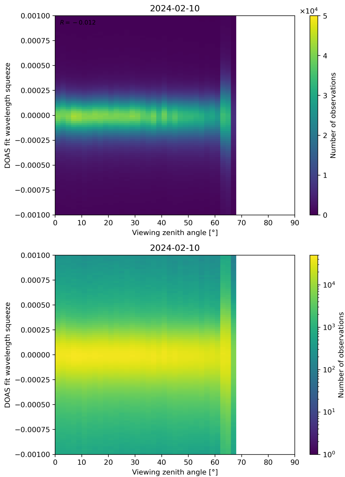
Figure 312: Scatter density plot of “Viewing zenith angle” against “DOAS fit wavelength squeeze” for 2024-02-09 to 2024-02-11.
