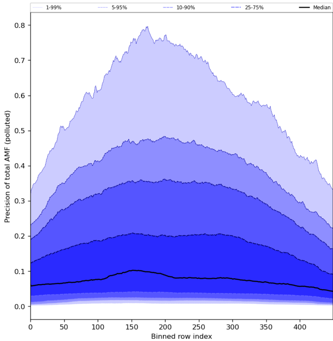
Figure 95: Along track statistics of “Precision of total AMF (polluted)” for 2024-02-09 to 2024-02-11
