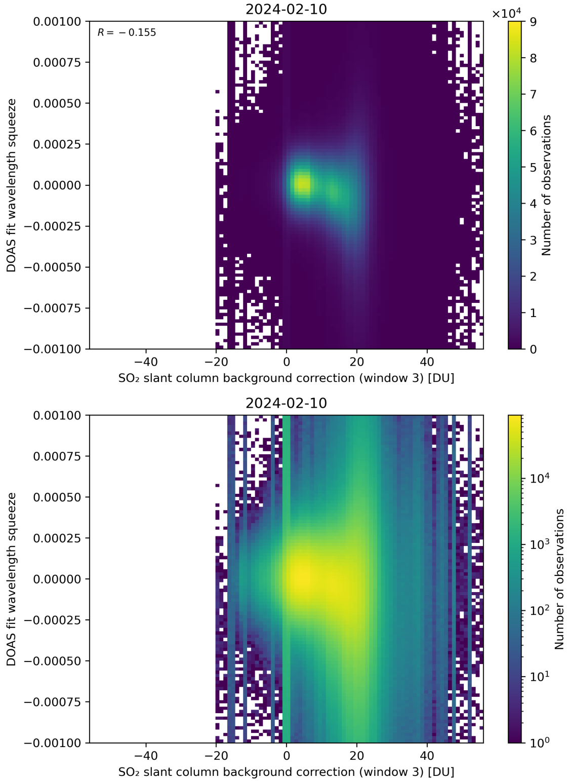
Figure 122: Scatter density plot of “SO 2 slant column background correction (window 3)” against “DOAS fit wavelength squeeze” for 2024-02-09 to 2024-02-11.
