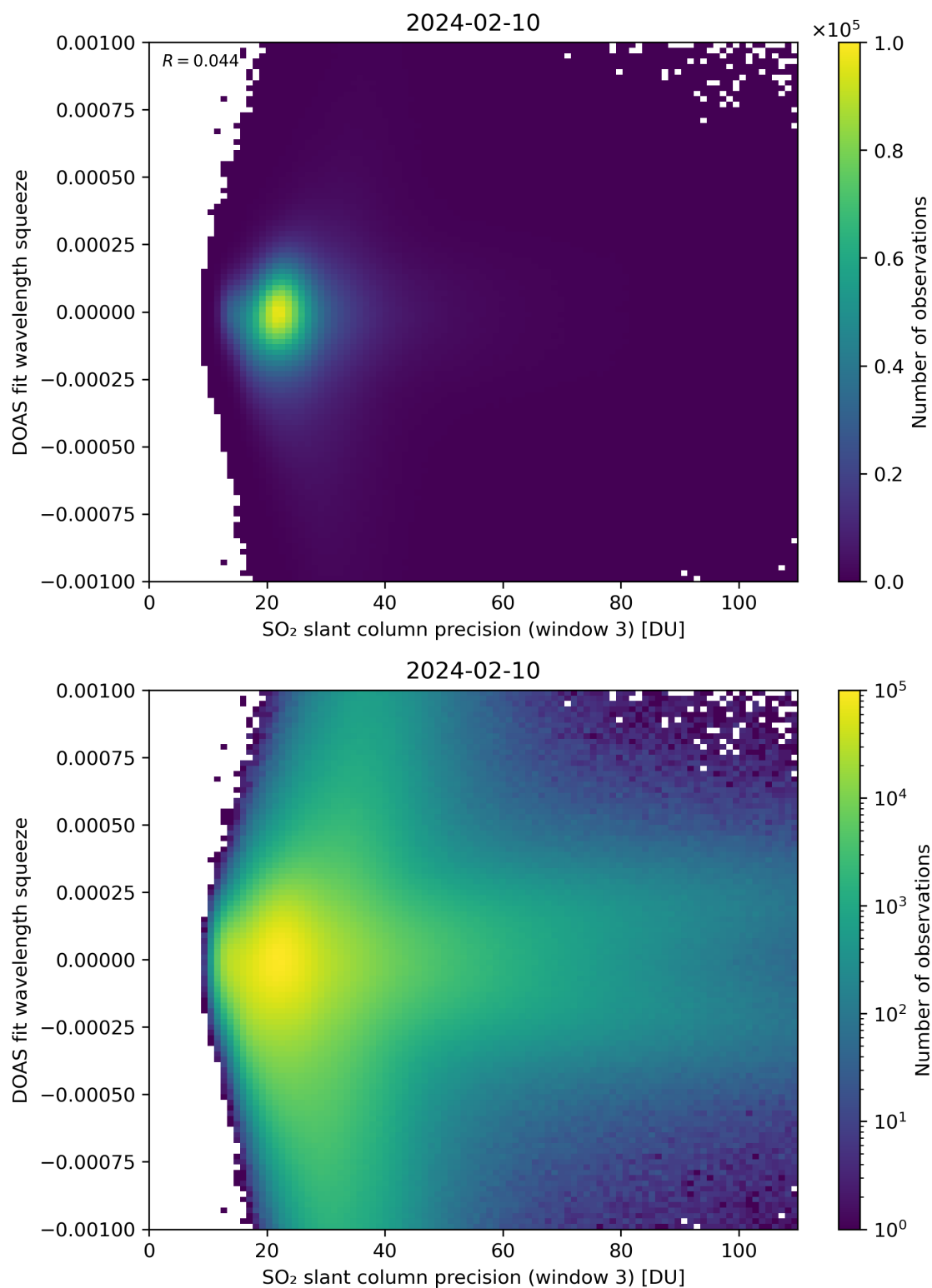
Figure 259: Scatter density plot of “SO 2 slant column precision (window 3)” against “DOAS fit wavelength squeeze” for 2024-02-09 to 2024-02-11.
