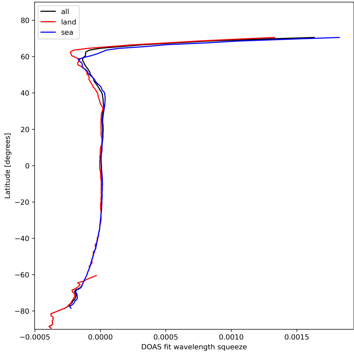
Figure 46: Zonal average of “DOAS fit wavelength squeeze” for 2024-02-09 to 2024-02-11.
