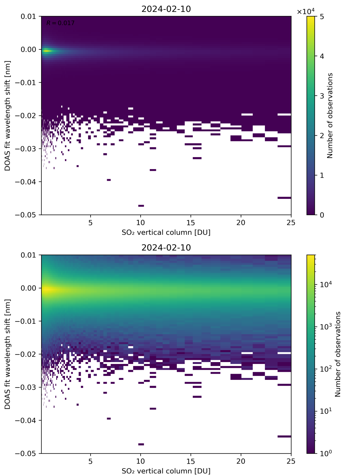
Figure 276: Scatter density plot of “SO 2 vertical column” against “DOAS fit wavelength shift” for 2024-02-09 to 2024-02-11.
