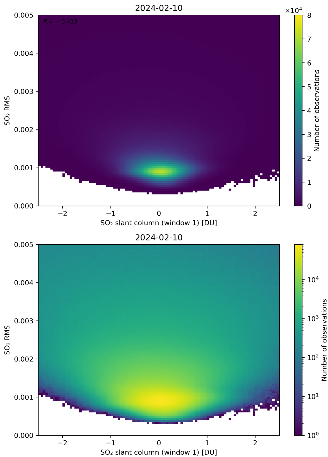
Figure 217: Scatter density plot of “SO 2 slant column (window 1)” against “SO 2 RMS” for 2024-02-09 to 2024-02-11.
