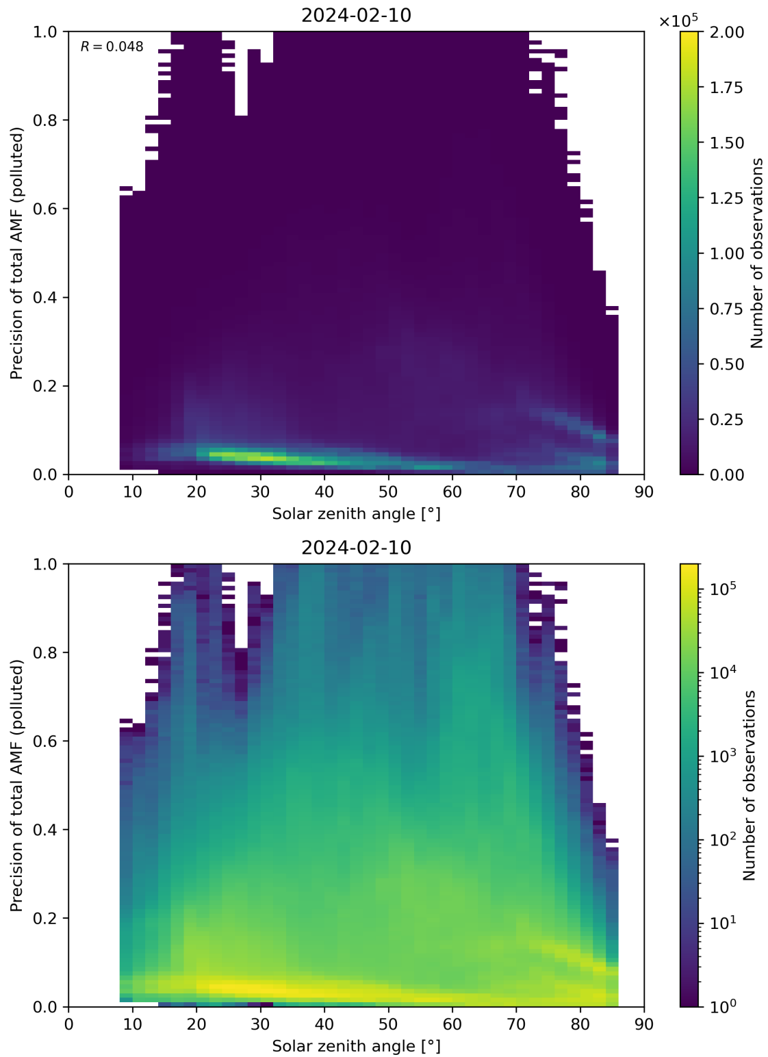
Figure 175: Scatter density plot of “Solar zenith angle” against “Precision of total AMF (polluted)” for 2024-02-09 to 2024-02-11.
