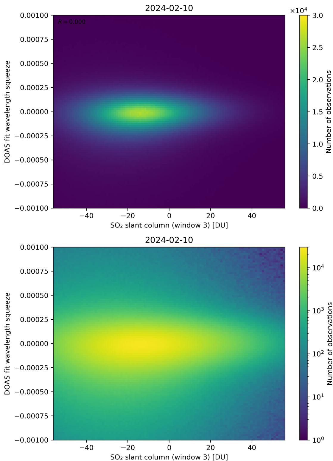
Figure 255: Scatter density plot of “SO 2 slant column (window 3)” against “DOAS fit wavelength squeeze” for 2024-02-09 to 2024-02-11.
