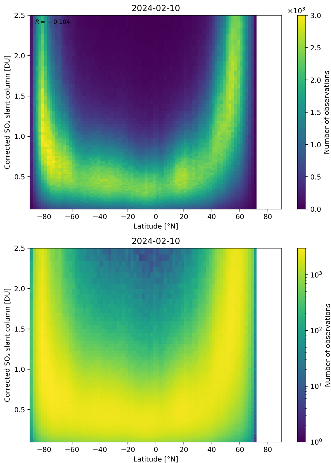
Figure 146: Scatter density plot of “Latitude” against “Corrected SO 2 slant column” for 2024-02-09 to 2024-02-11.
