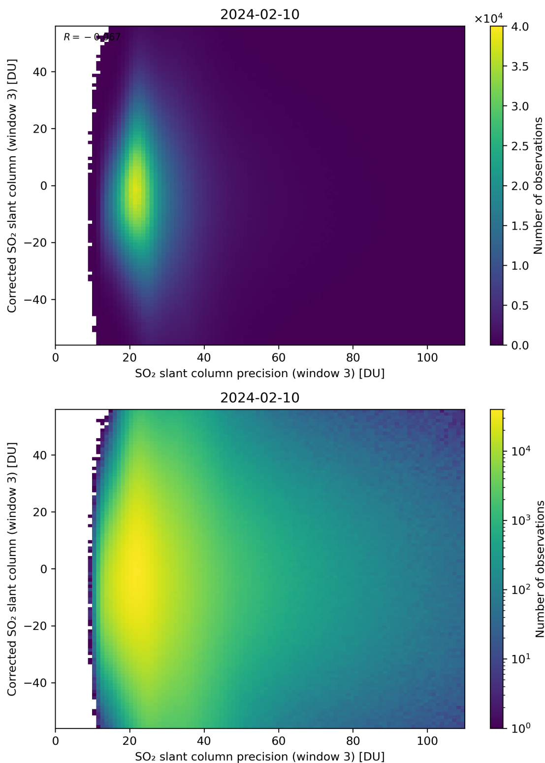
Figure 262: Scatter density plot of “SO 2 slant column precision (window 3)” against “Corrected SO 2 slant column (window 3)” for 2024-02-09 to 2024-02-11.
