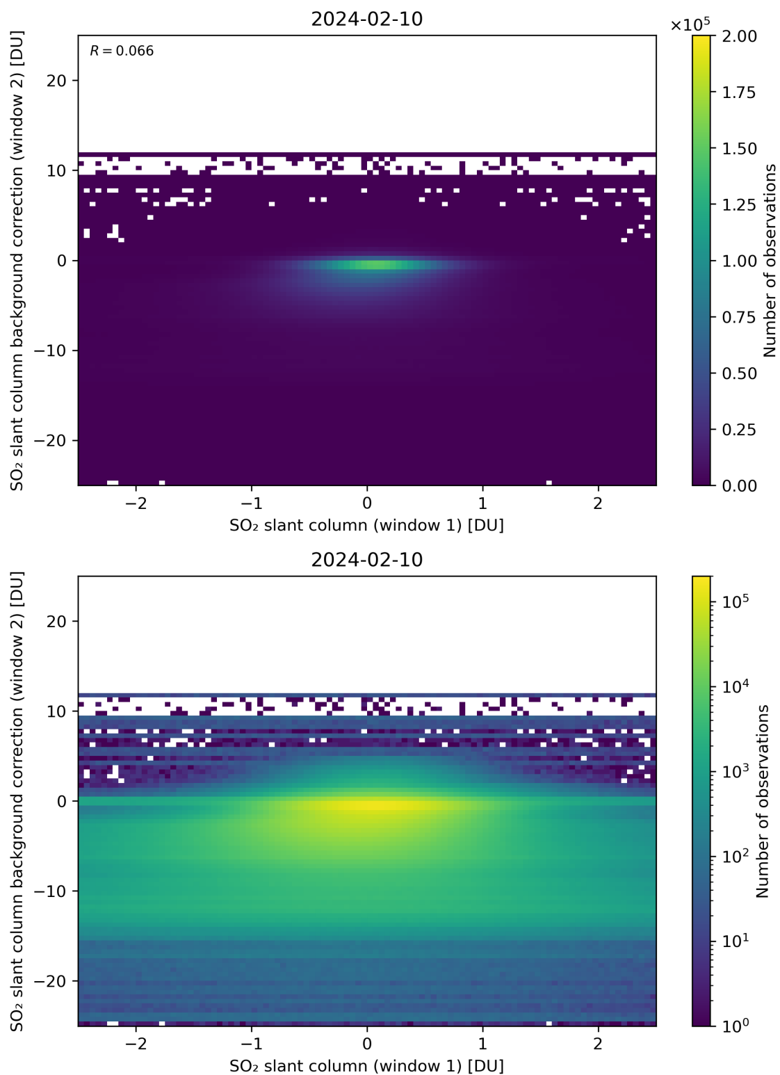
Figure 213: Scatter density plot of “SO 2 slant column (window 1)” against “SO 2 slant column background correction (window 2)” for 2024-02-09 to 2024-02-11.
