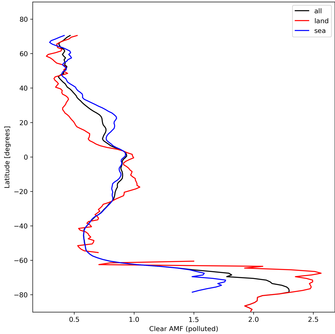
Figure 50: Zonal average of “Clear AMF (polluted)” for 2024-02-09 to 2024-02-11.
