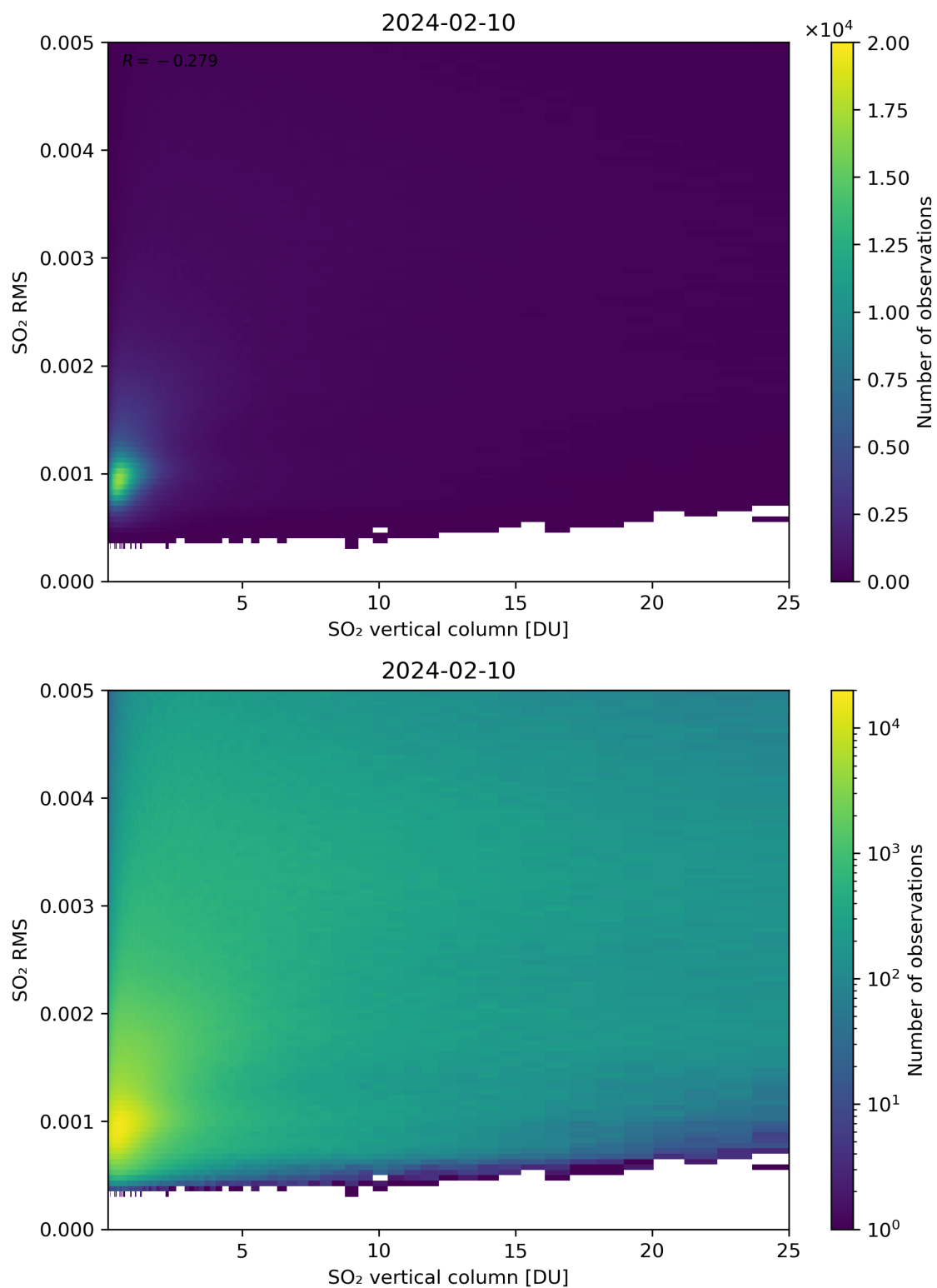
Figure 278: Scatter density plot of “SO 2 vertical column” against “SO 2 RMS” for 2024-02-09 to 2024-02-11.
