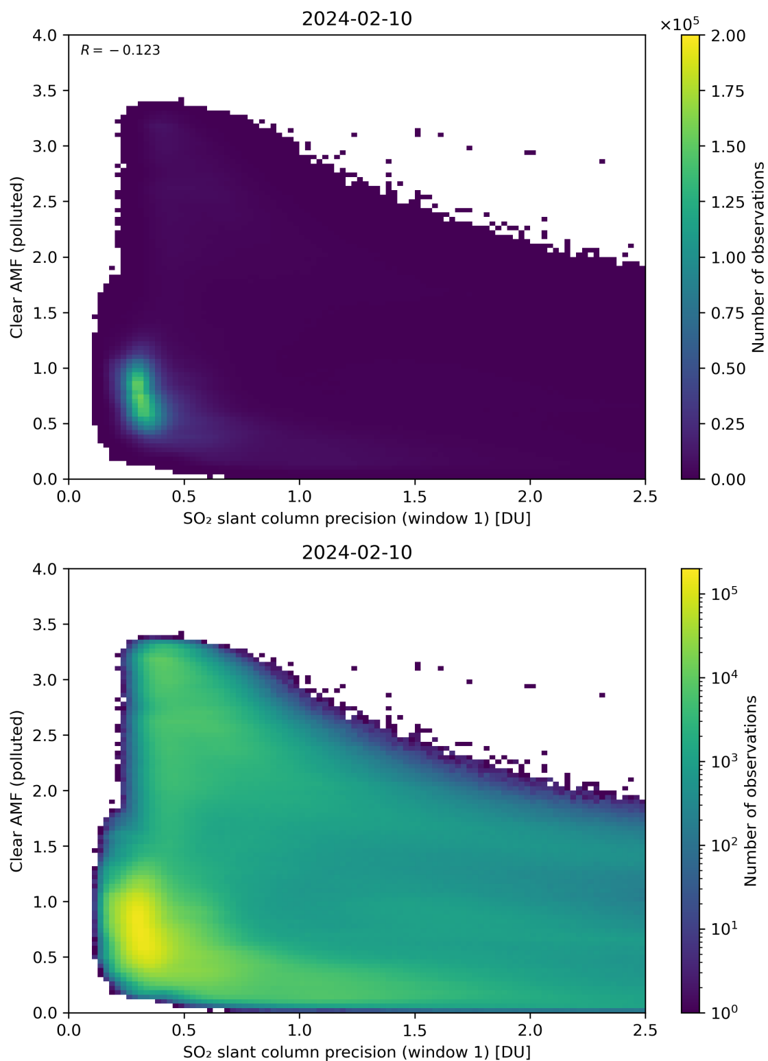
Figure 224: Scatter density plot of “SO 2 slant column precision (window 1)” against “Clear AMF (polluted)” for 2024-02-09 to 2024-02-11.
