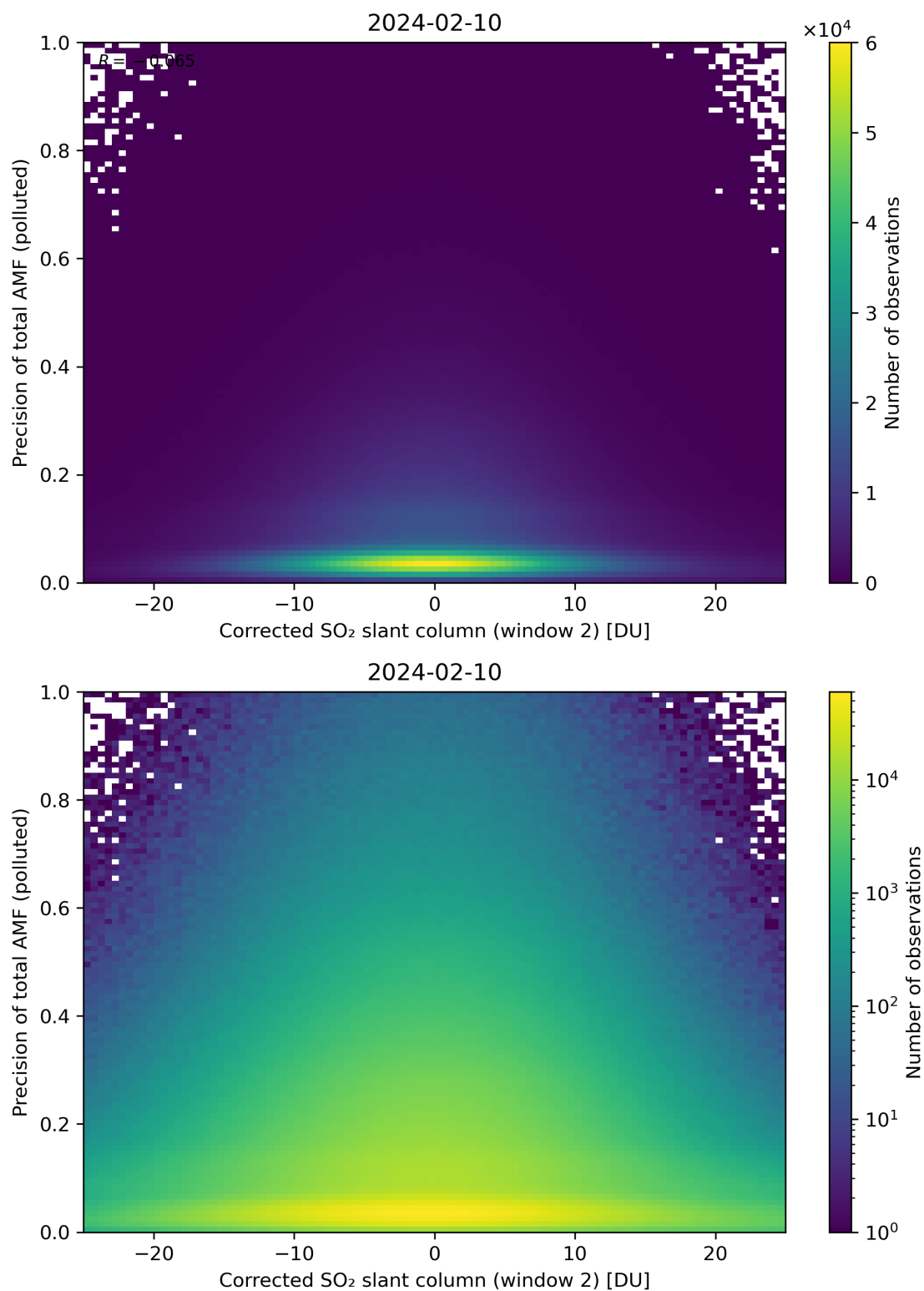
Figure 204: Scatter density plot of “Corrected SO 2 slant column (window 2)” against “Precision of total AMF (polluted)” for 2024-02-09 to 2024-02-11.
