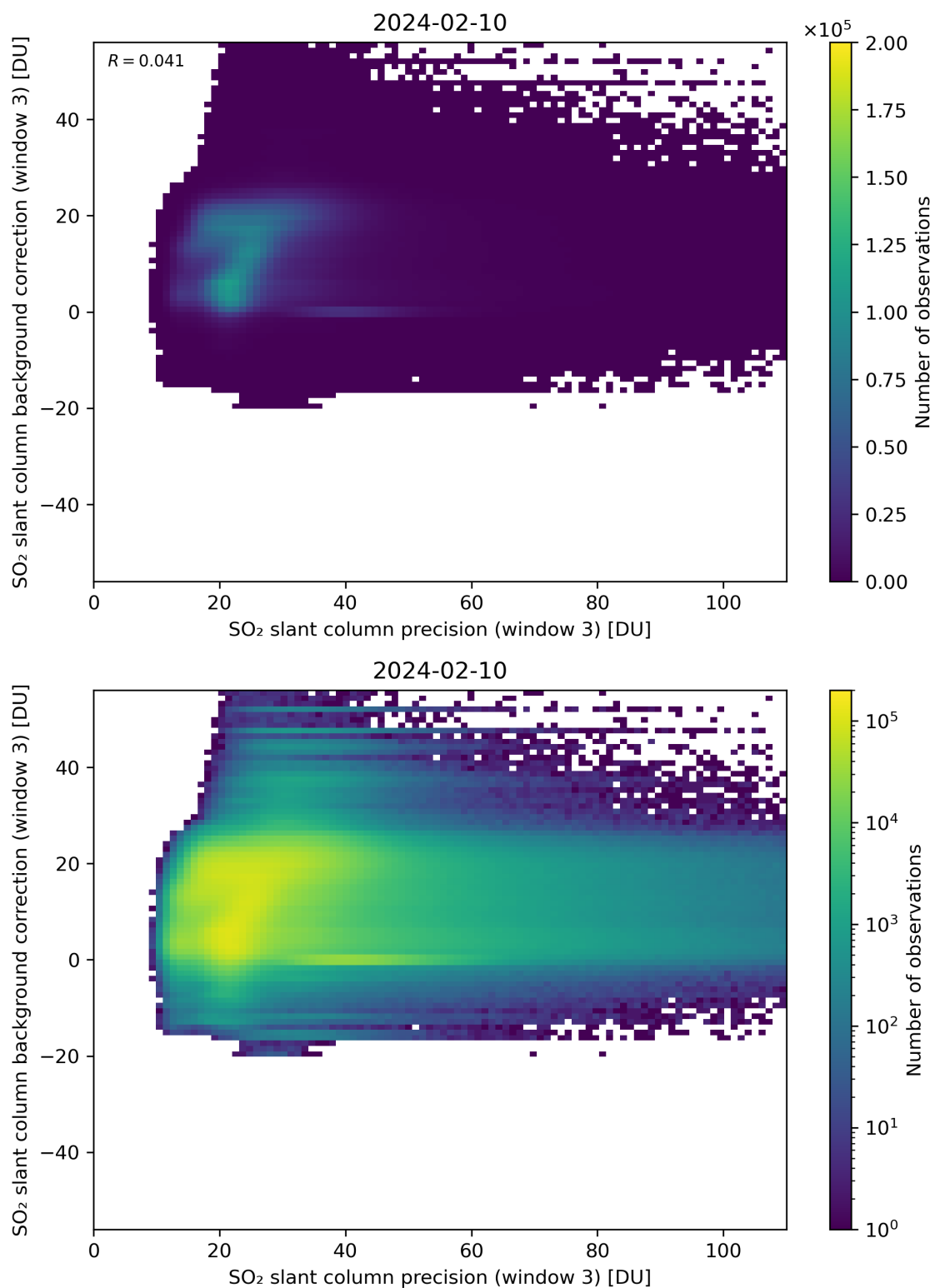
Figure 257: Scatter density plot of “SO 2 slant column precision (window 3)” against “SO 2 slant column background correction (window 3)” for 2024-02-09 to 2024-02-11.
