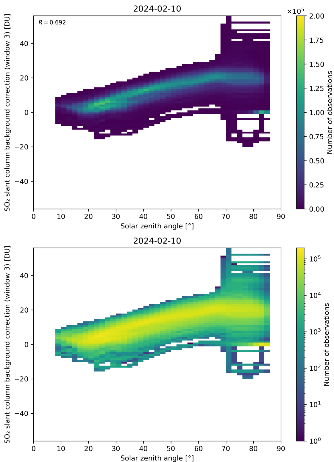
Figure 160: Scatter density plot of “Solar zenith angle” against “SO 2 slant column background correction (window 3)” for 2024-02-09 to 2024-02-11.
