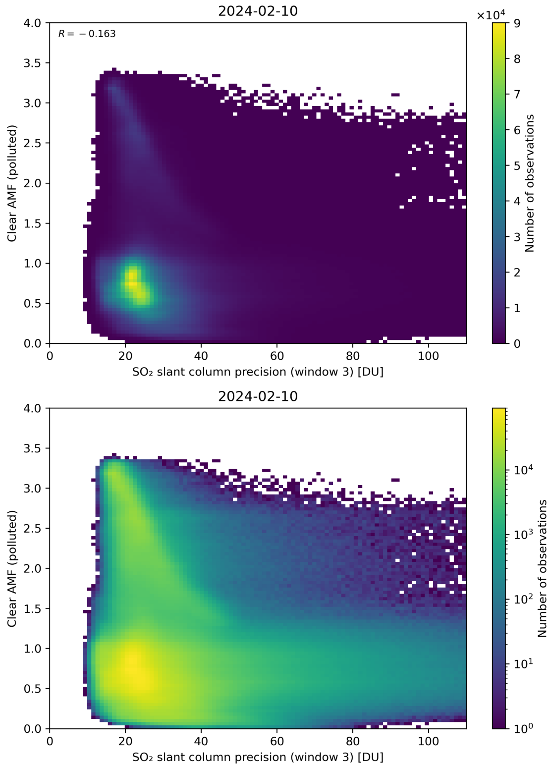
Figure 261: Scatter density plot of “SO 2 slant column precision (window 3)” against “Clear AMF (polluted)” for 2024-02-09 to 2024-02-11.
