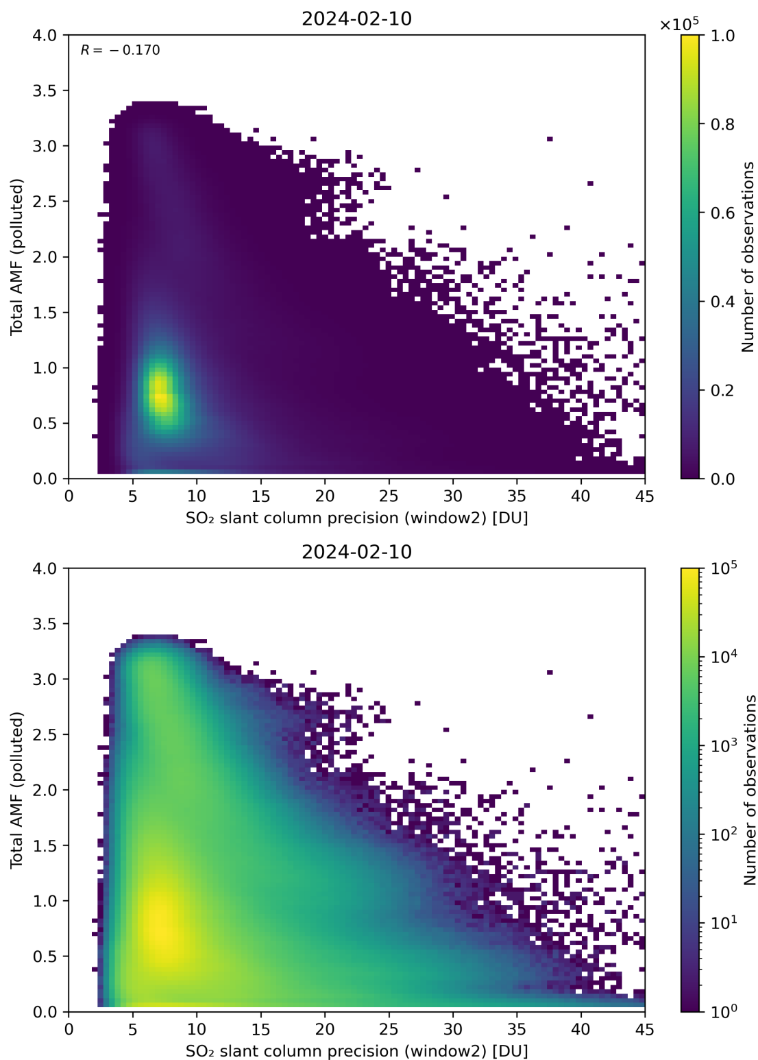
Figure 251: Scatter density plot of “SO 2 slant column precision (window2)” against “Total AMF (polluted)” for 2024-02-09 to 2024-02-11.
