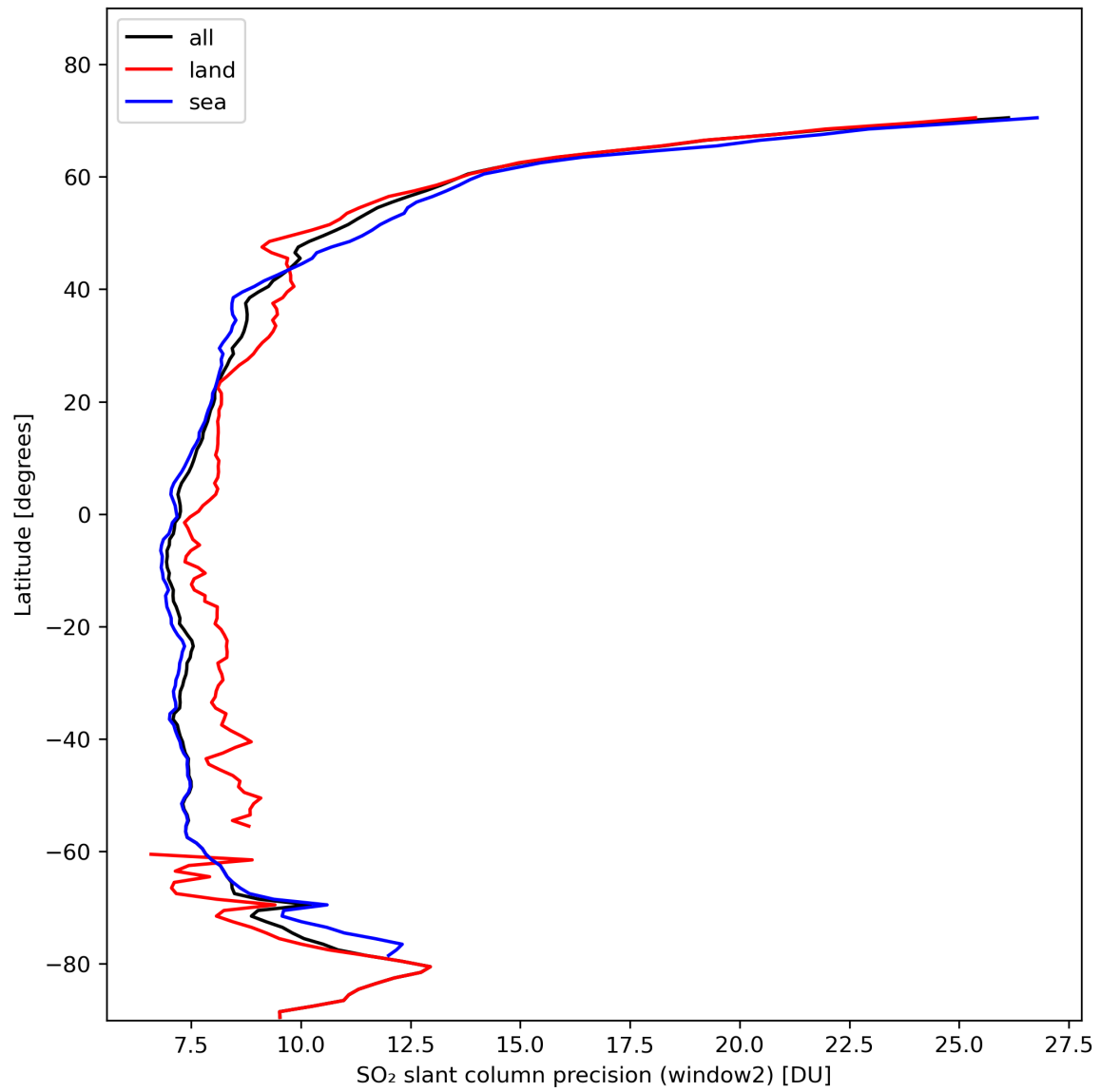
Figure 38: Zonal average of “SO 2 slant column precision (window2)” for 2024-02-09 to 2024-02-11.
