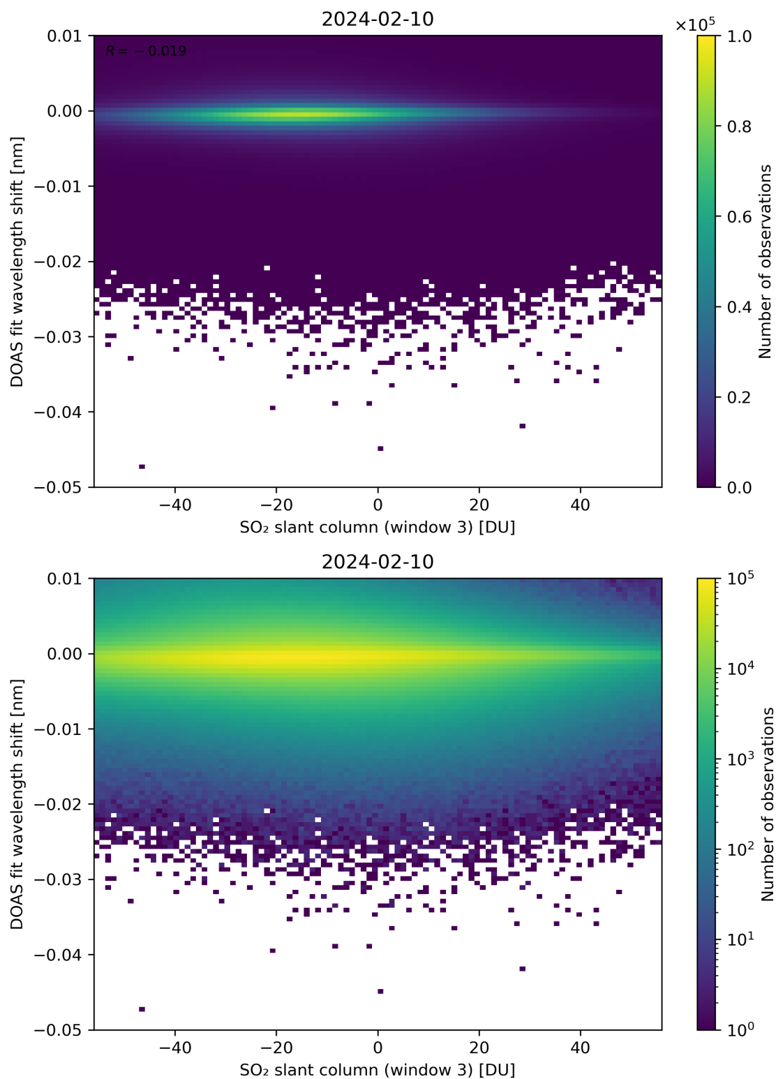
Figure 254: Scatter density plot of “SO 2 slant column (window 3)” against “DOAS fit wavelength shift” for 2024-02-09 to 2024-02-11.
