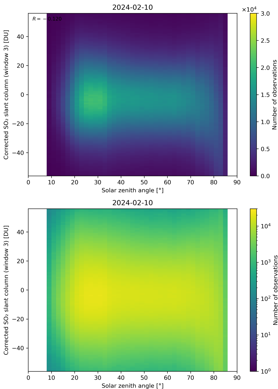
Figure 168: Scatter density plot of “Solar zenith angle” against “Corrected SO 2 slant column (window 3)” for 2024-02-09 to 2024-02-11.
