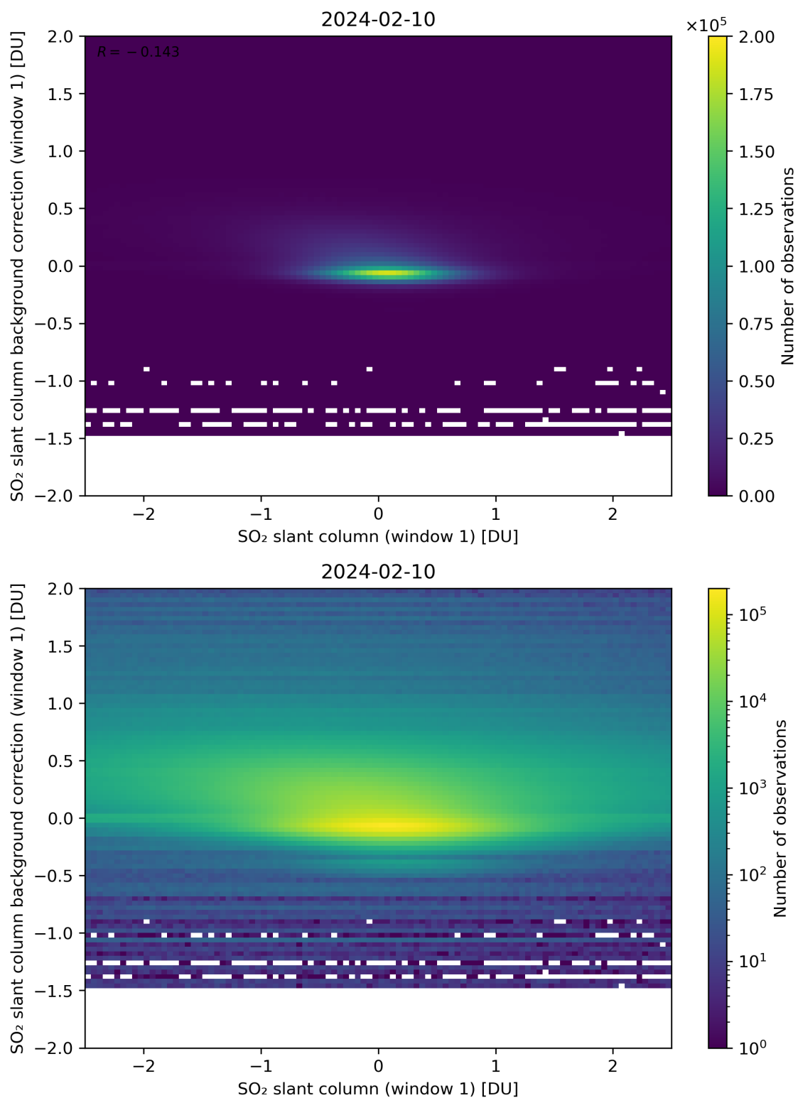
Figure 212: Scatter density plot of “SO 2 slant column (window 1)” against “SO 2 slant column background correction (window 1)” for 2024-02-09 to 2024-02-11.
