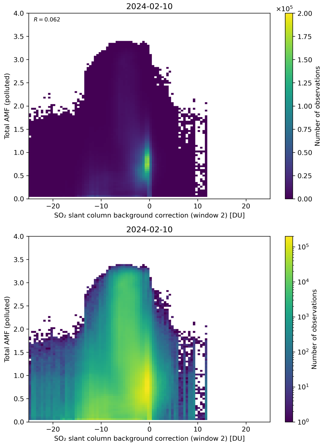
Figure 119: Scatter density plot of “SO 2 slant column background correction (window 2)” against “Total AMF (polluted)” for 2024-02-09 to 2024-02-11.
