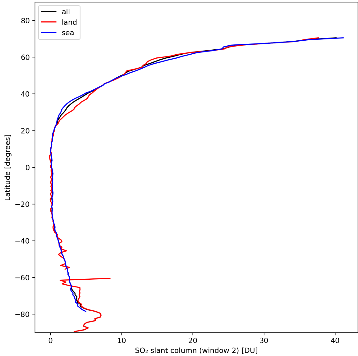
Figure 37: Zonal average of “SO 2 slant column (window 2)” for 2024-02-09 to 2024-02-11.
