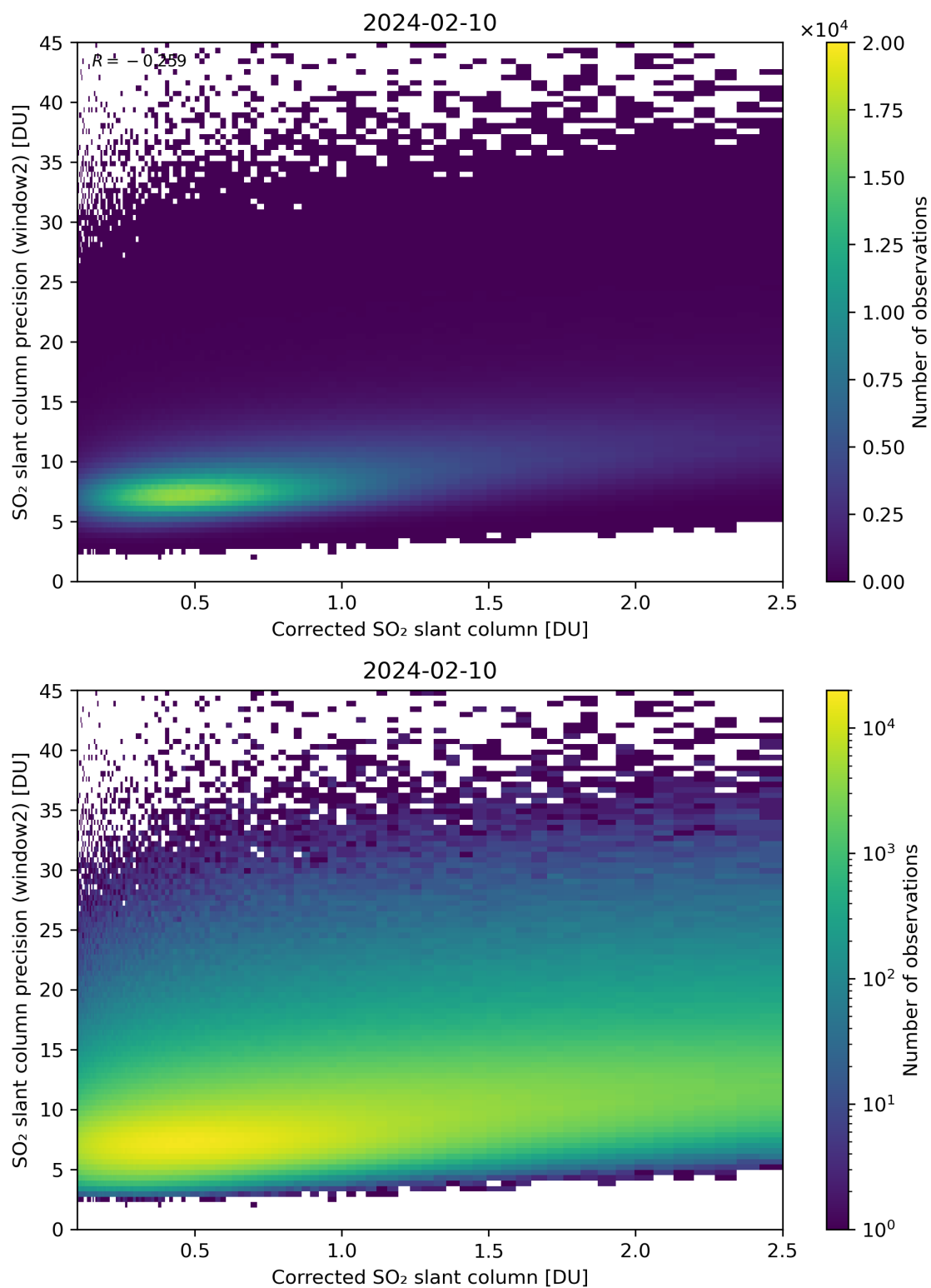
Figure 189: Scatter density plot of “Corrected SO 2 slant column” against “SO 2 slant column precision (window2)” for 2024-02-09 to 2024-02-11.
