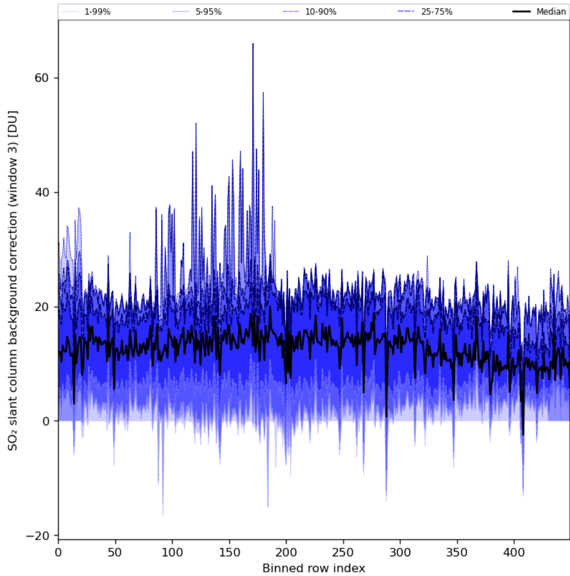
Figure 90: Along track statistics of “SO 2 slant column background correction (window 3)” for 2024-02-09 to 2024-02-11
