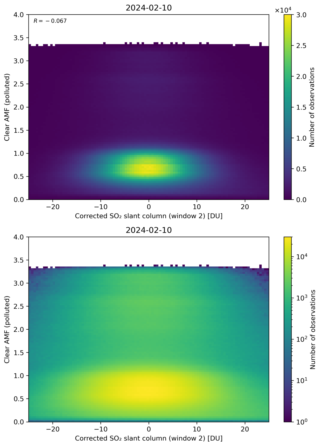
Figure 199: Scatter density plot of “Corrected SO 2 slant column (window 2)” against “Clear AMF (polluted)” for 2024-02-09 to 2024-02-11.
