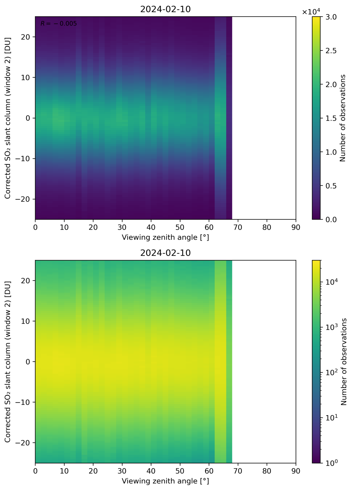
Figure 318: Scatter density plot of “Viewing zenith angle” against “Corrected SO 2 slant column (window 2)” for 2024-02-09 to 2024-02-11.
