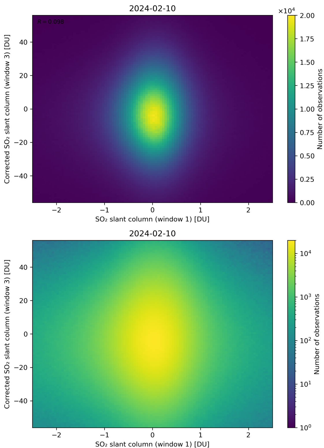
Figure 234: Scatter density plot of “SO 2 slant column (window 1)” against “Corrected SO 2 slant column (window 3)” for 2024-02-09 to 2024-02-11.
