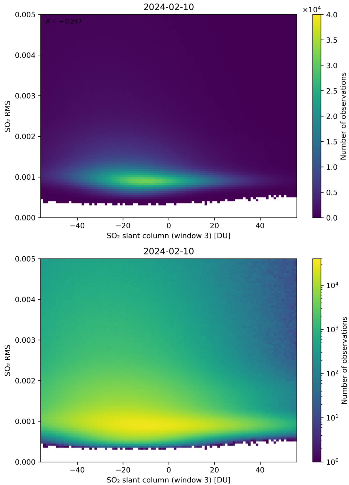
Figure 256: Scatter density plot of “SO 2 slant column (window 3)” against “SO 2 RMS” for 2024-02-09 to 2024-02-11.
