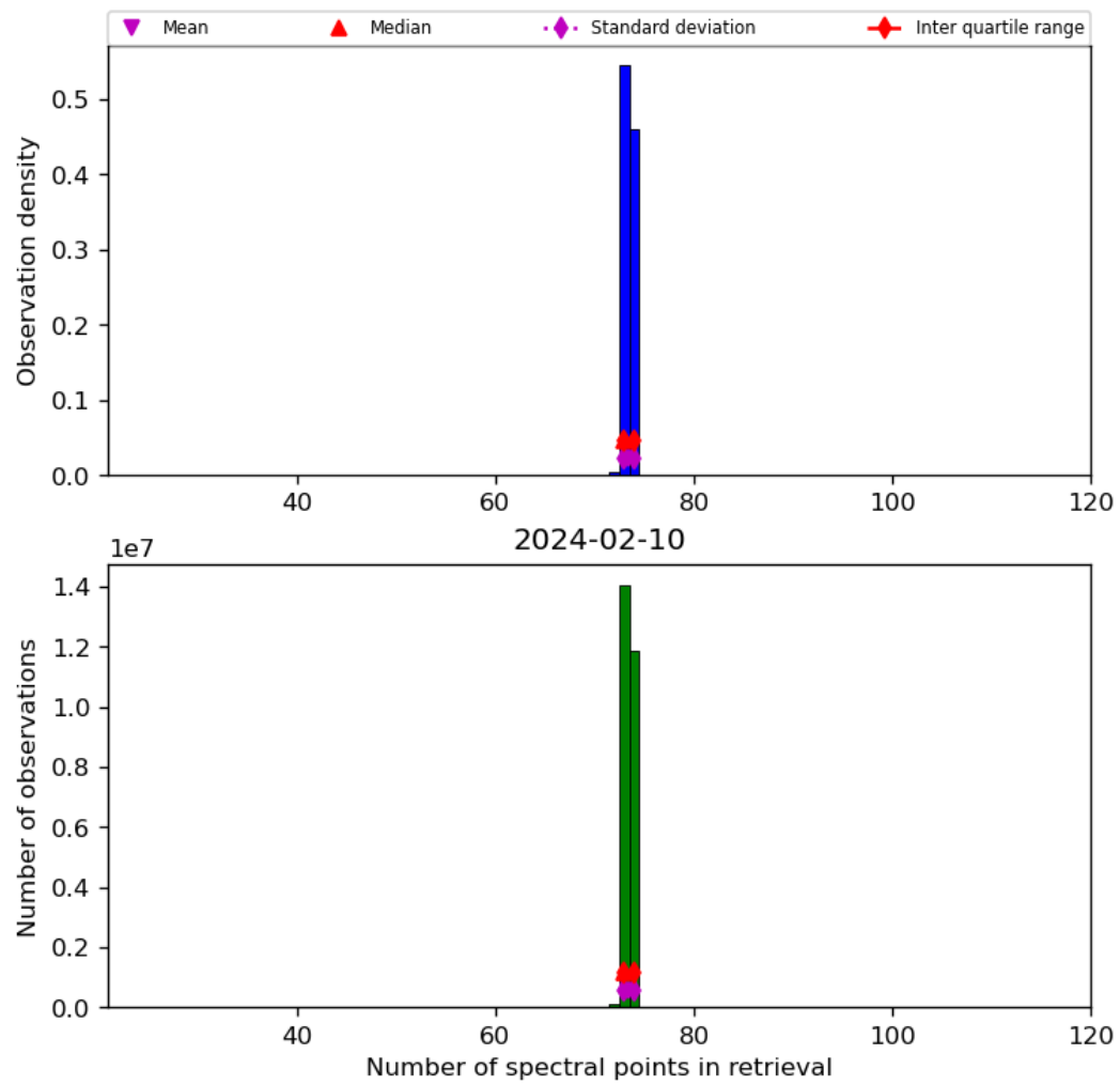
Figure 74: Histogram of “Number of spectral points in retrieval” for 2024-02-09 to 2024-02-11
