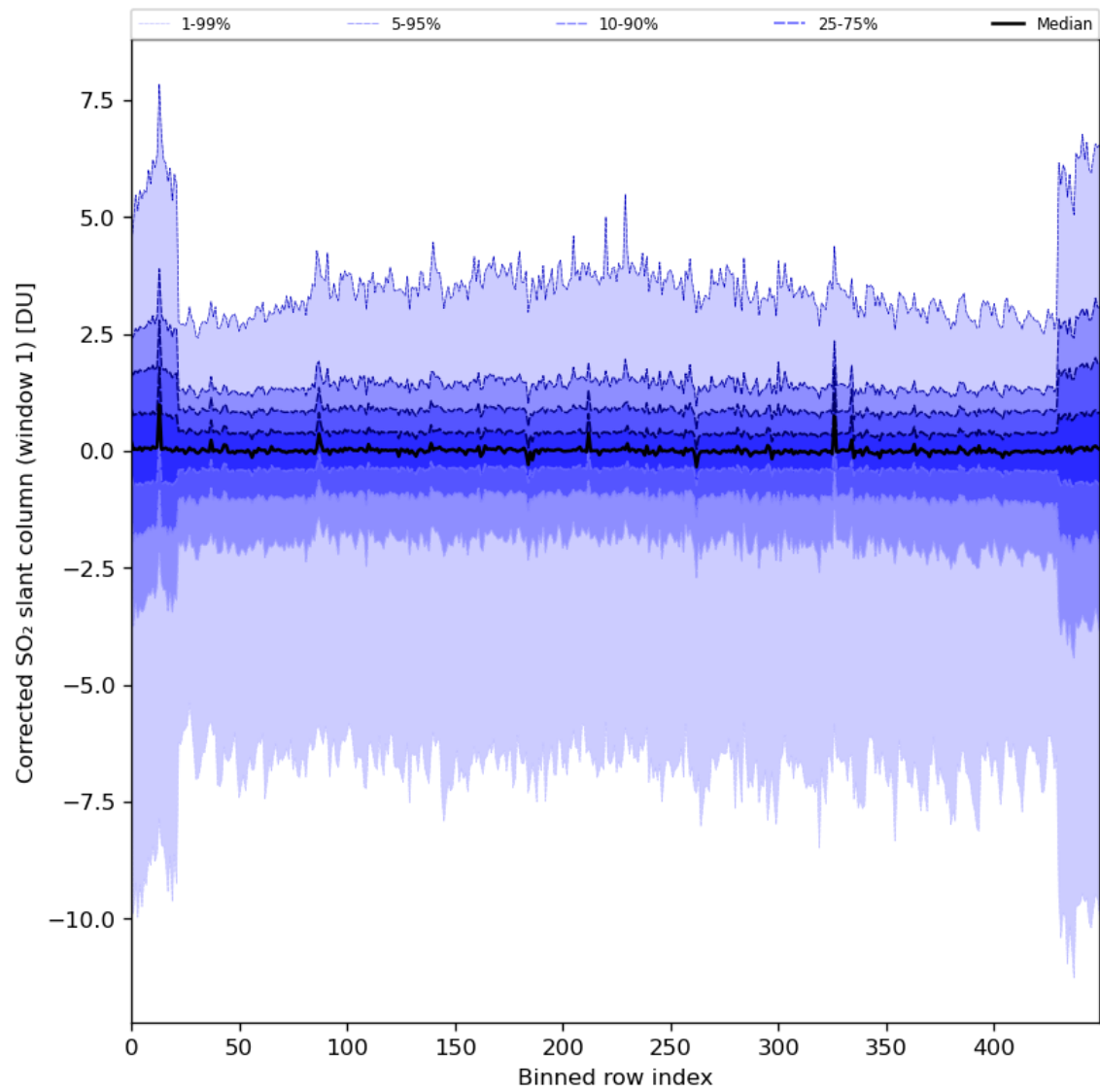
Figure 81: Along track statistics of “Corrected SO 2 slant column (window 1)” for 2024-02-09 to 2024-02-11
