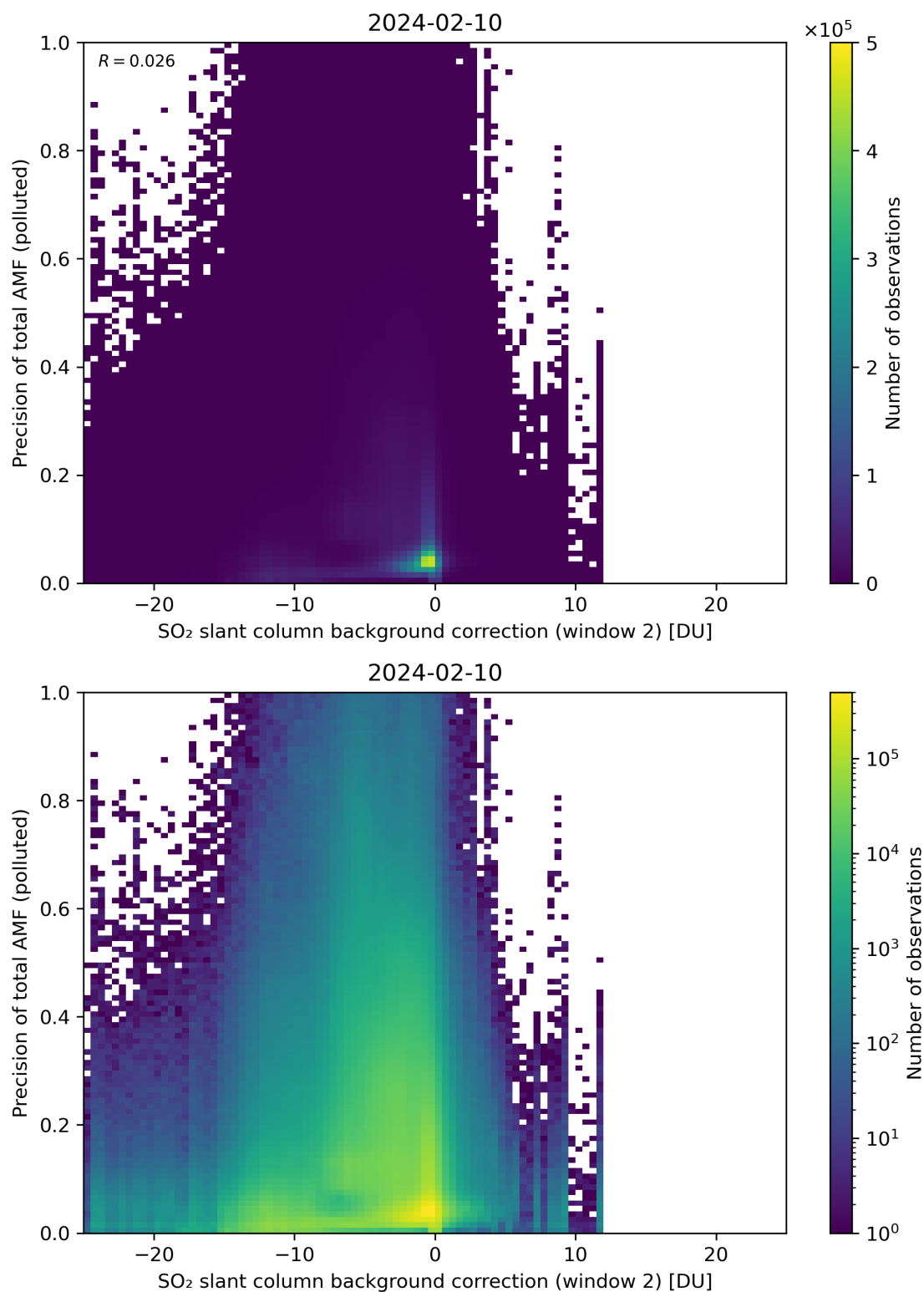
Figure 120: Scatter density plot of “SO 2 slant column background correction (window 2)” against “Precision of total AMF (polluted)” for 2024-02-09 to 2024-02-11.
