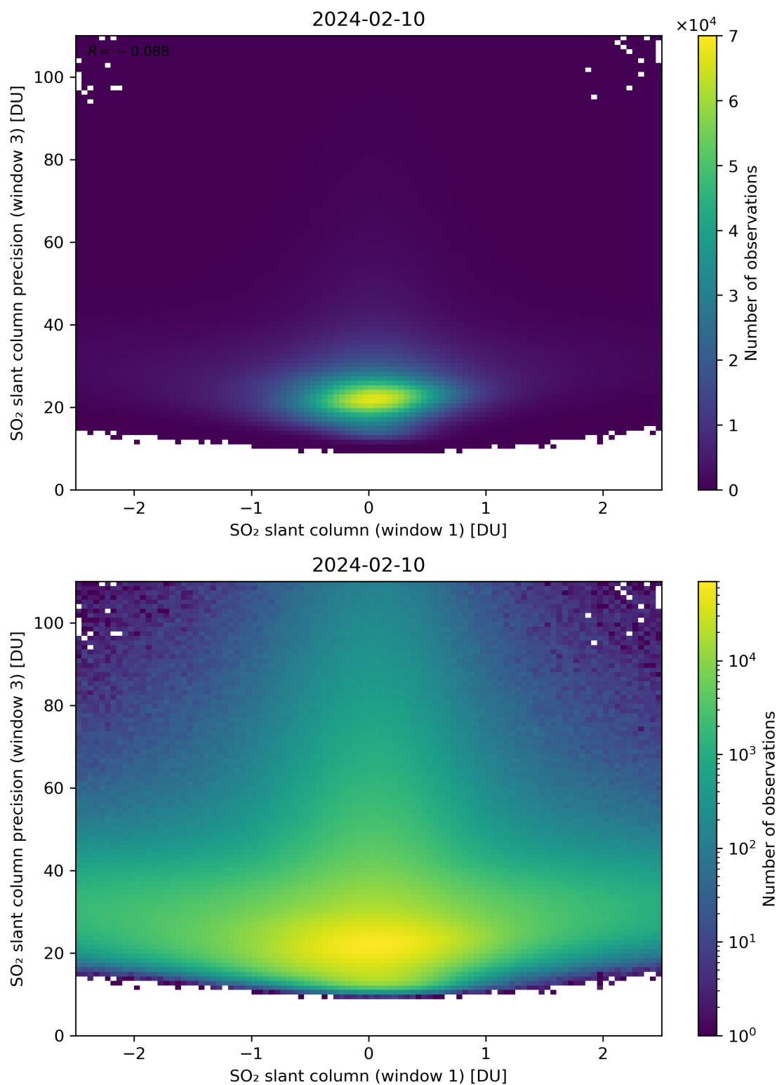
Figure 238: Scatter density plot of “SO 2 slant column (window 1)” against “SO 2 slant column precision (window 3)” for 2024-02-09 to 2024-02-11.
