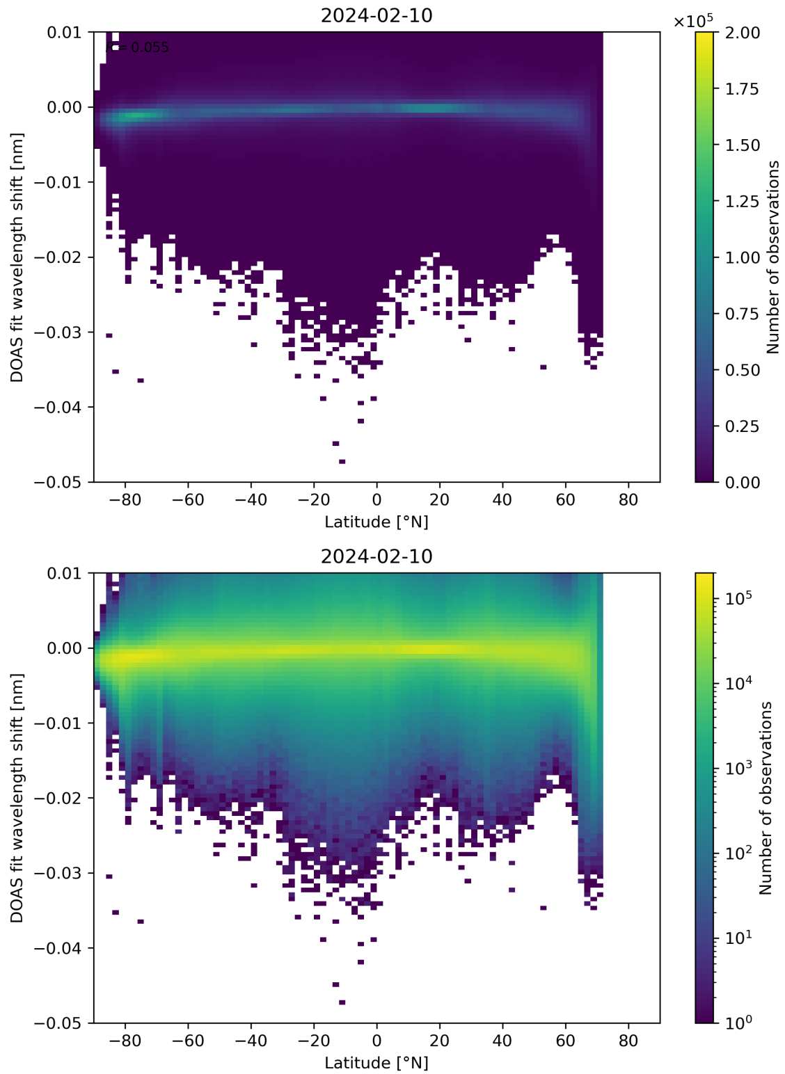
Figure 142: Scatter density plot of “Latitude” against “DOAS fit wavelength shift” for 2024-02-09 to 2024-02-11.
