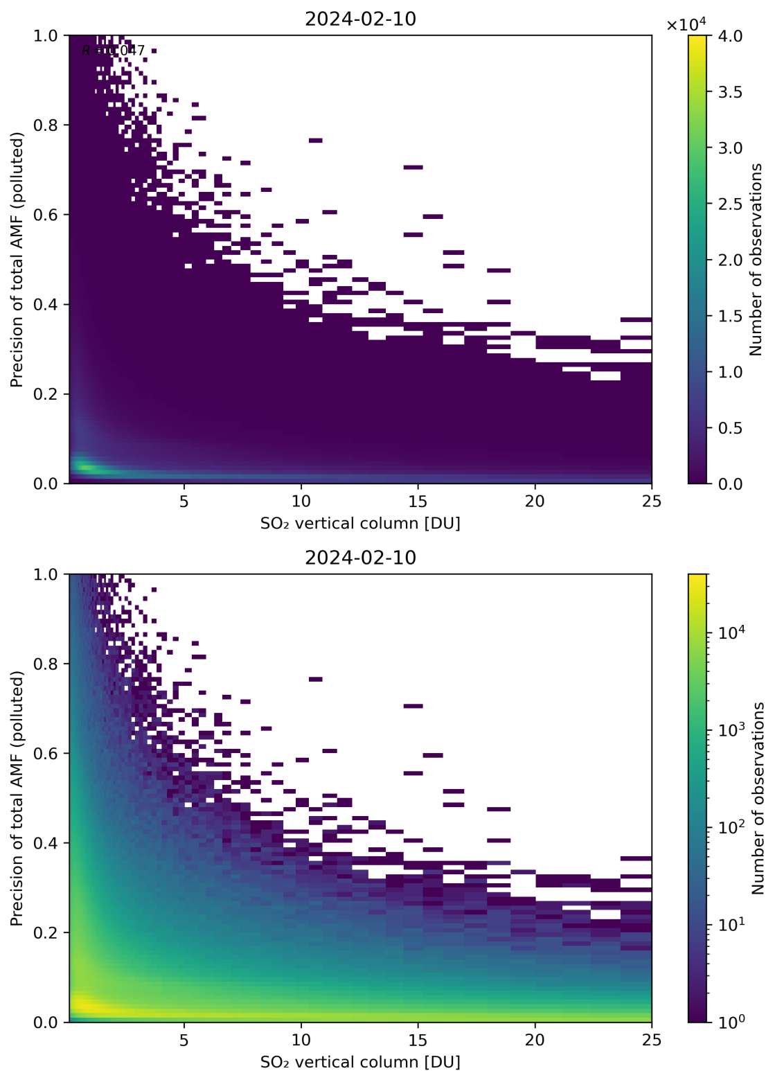
Figure 306: Scatter density plot of “SO 2 vertical column” against “Precision of total AMF (polluted)” for 2024-02-09 to 2024-02-11.
