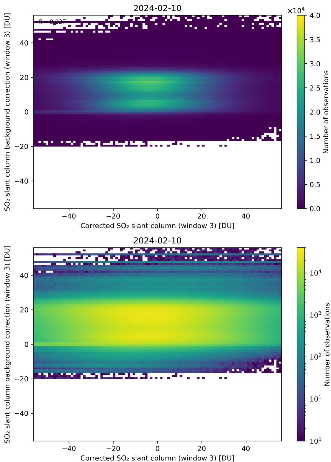
Figure 205: Scatter density plot of “Corrected SO 2 slant column (window 3)” against “SO 2 slant column background correction (window 3)” for 2024-02-09 to 2024-02-11.
