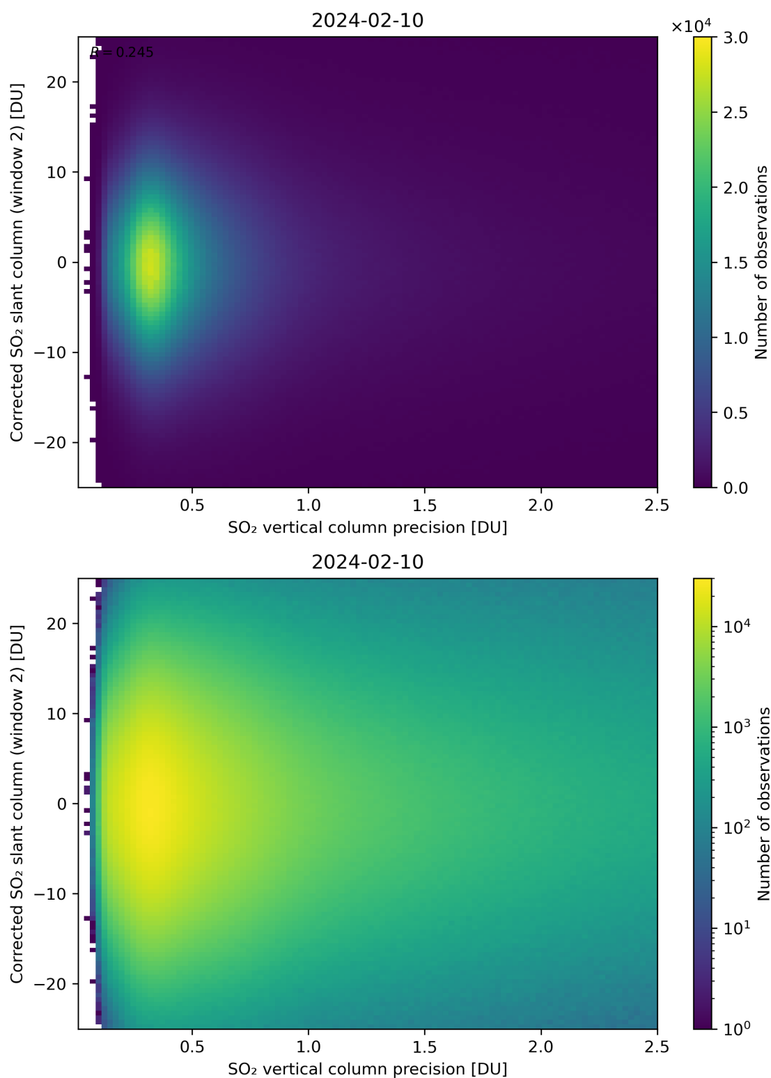
Figure 287: Scatter density plot of “SO 2 vertical column precision” against “Corrected SO 2 slant column (window 2)” for 2024-02-09 to 2024-02-11.
