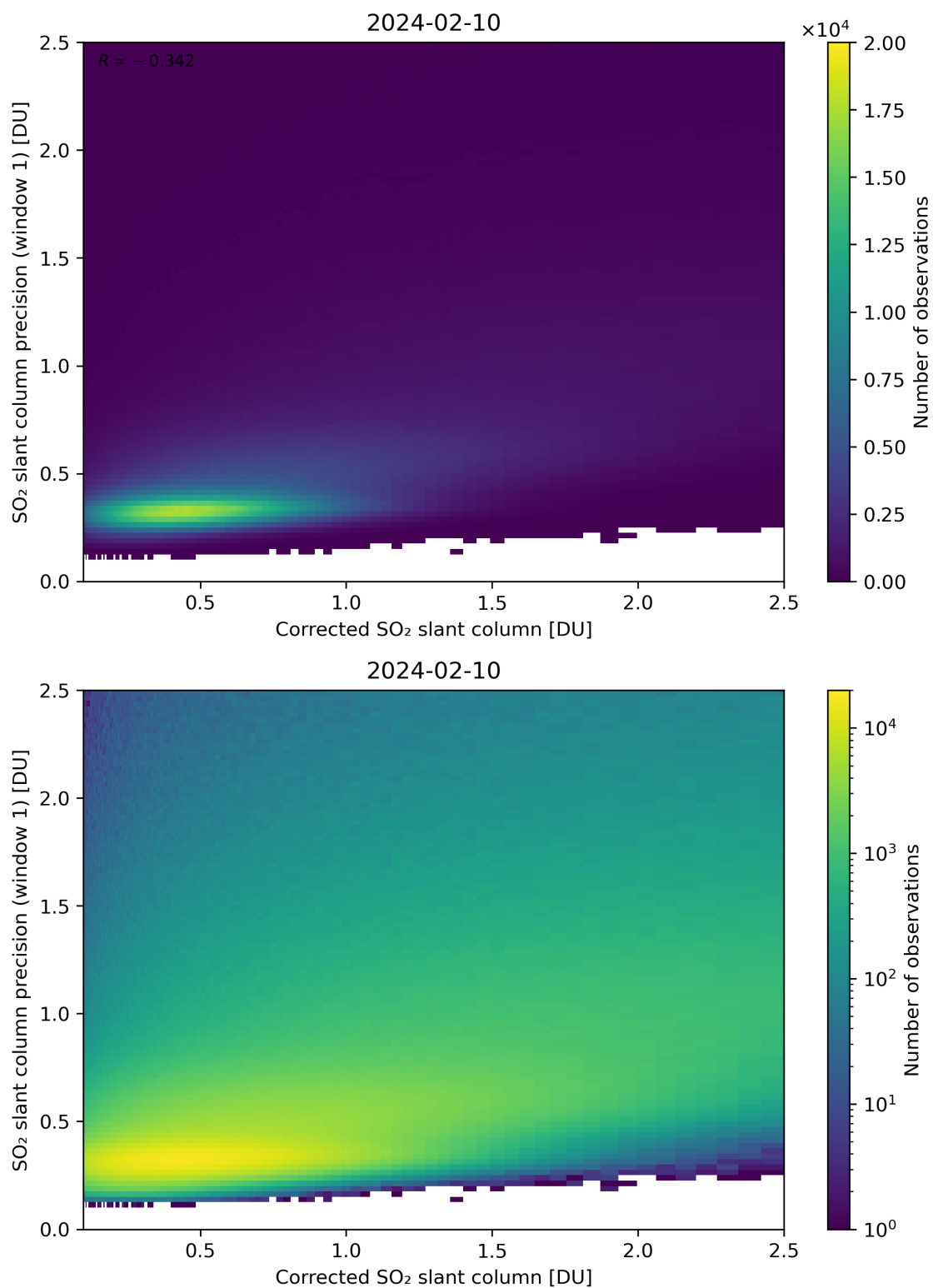
Figure 188: Scatter density plot of “Corrected SO 2 slant column” against “SO 2 slant column precision (window 1)” for 2024-02-09 to 2024-02-11.
