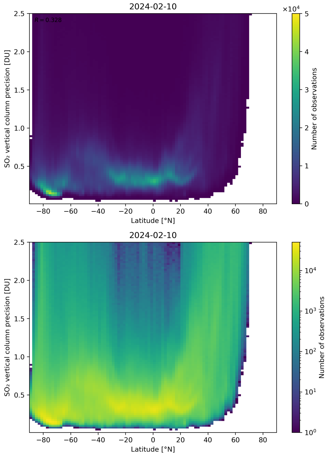
Figure 157: Scatter density plot of “Latitude” against “SO 2 vertical column precision” for 2024-02-09 to 2024-02-11.
