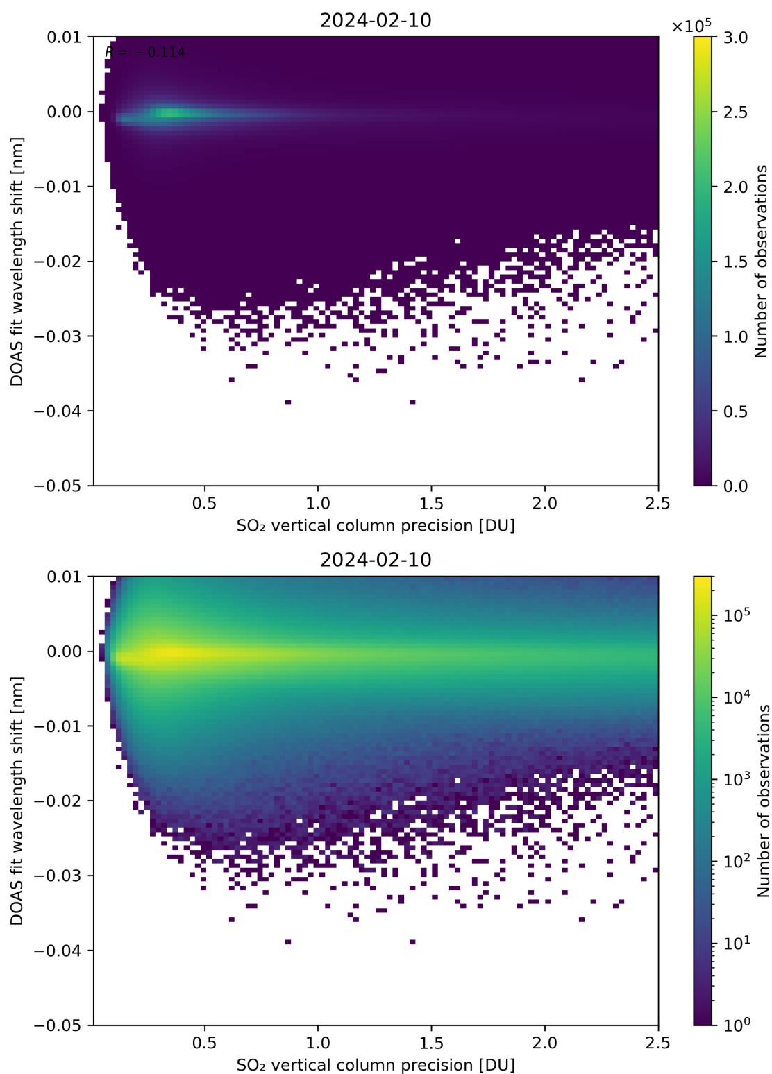
Figure 282: Scatter density plot of “SO 2 vertical column precision” against “DOAS fit wavelength shift” for 2024-02-09 to 2024-02-11.
