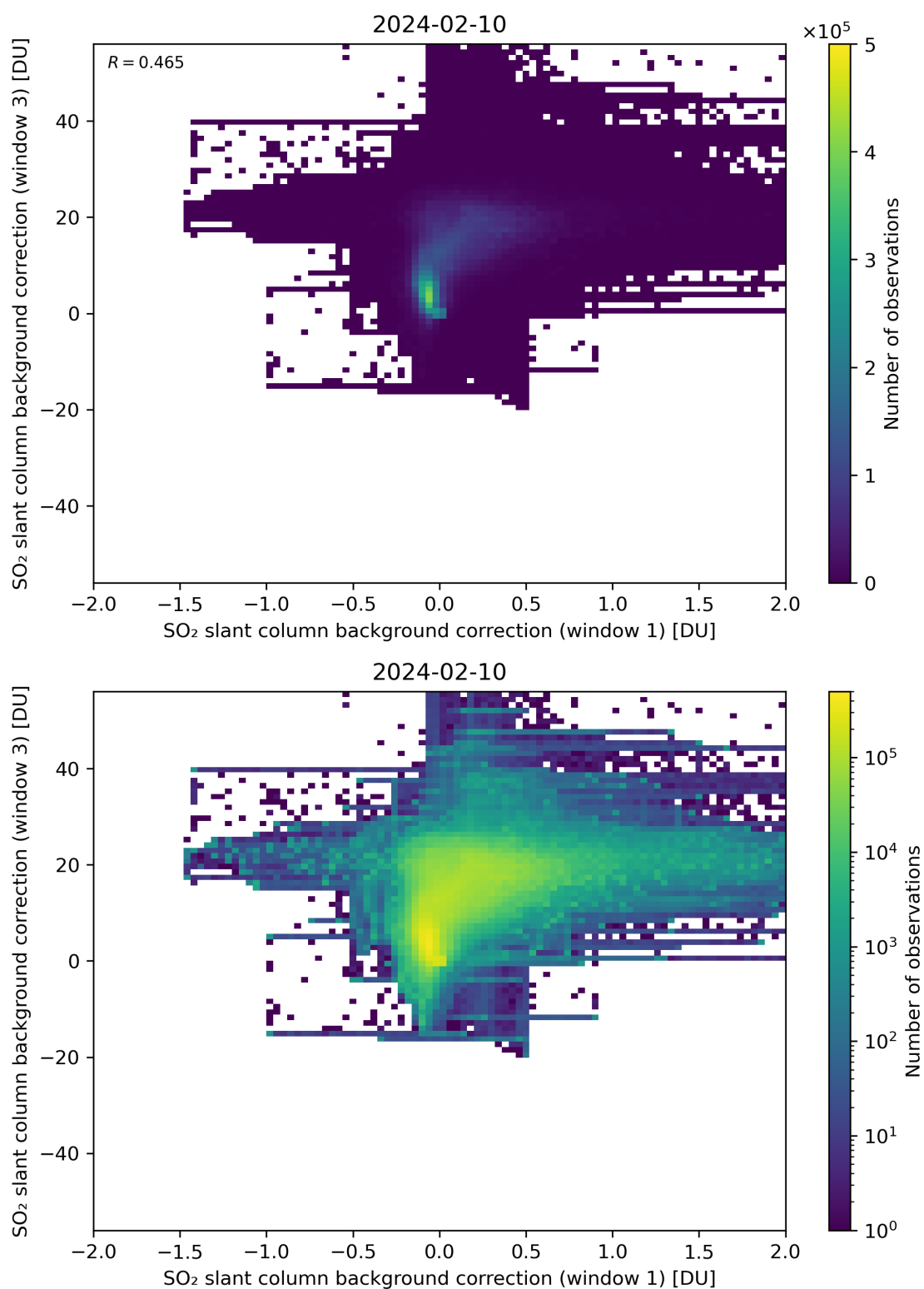
Figure 99: Scatter density plot of “SO 2 slant column background correction (window 1)” against “SO 2 slant column background correction (window 3)” for 2024-02-09 to 2024-02-11.
