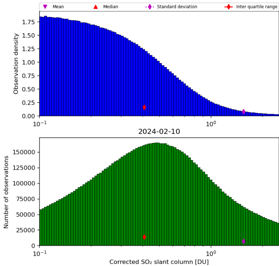
Figure 55: Histogram of “Corrected SO 2 slant column” for 2024-02-09 to 2024-02-11
