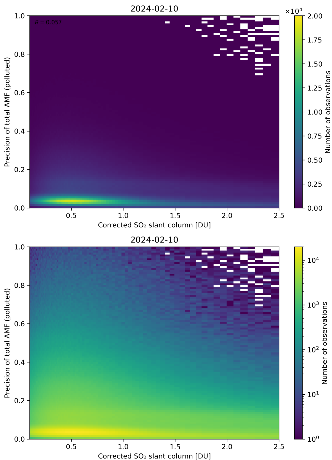
Figure 193: Scatter density plot of “Corrected SO 2 slant column” against “Precision of total AMF (polluted)” for 2024-02-09 to 2024-02-11.
