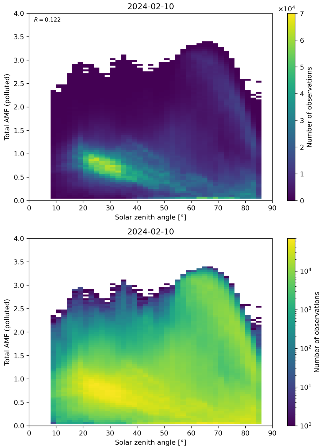
Figure 174: Scatter density plot of “Solar zenith angle” against “Total AMF (polluted)” for 2024-02-09 to 2024-02-11.
