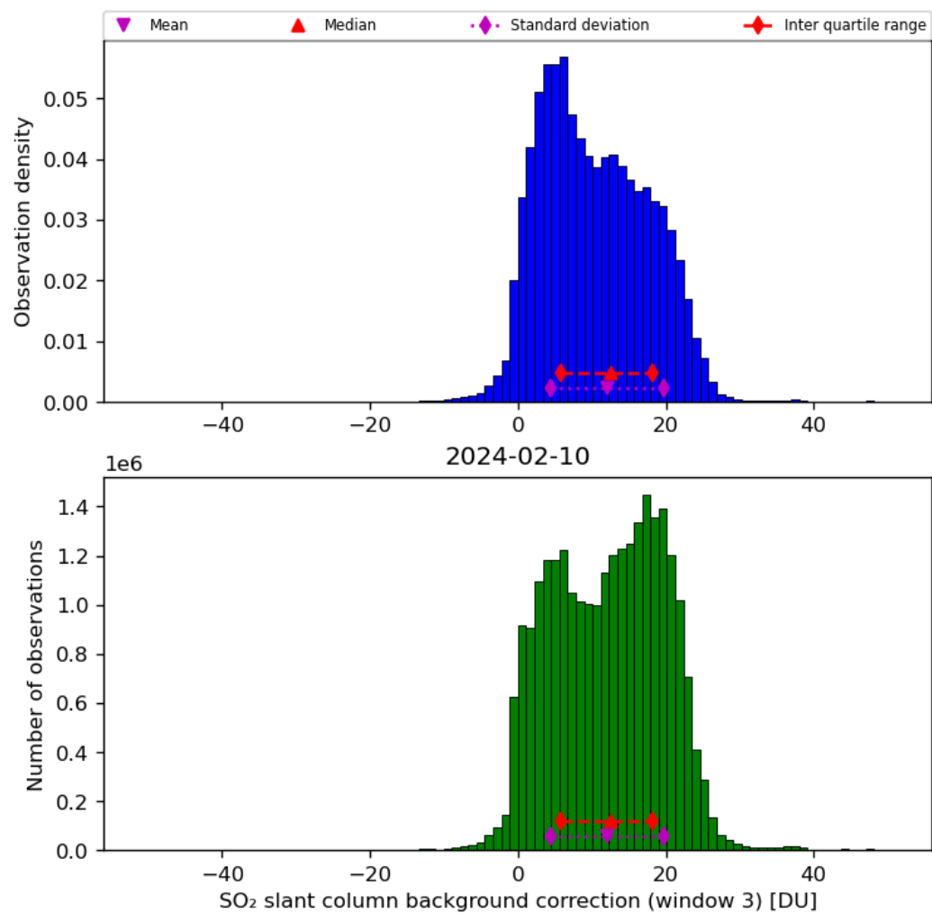
Figure 67: Histogram of “SO 2 slant column background correction (window 3)” for 2024-02-09 to 2024-02-11
