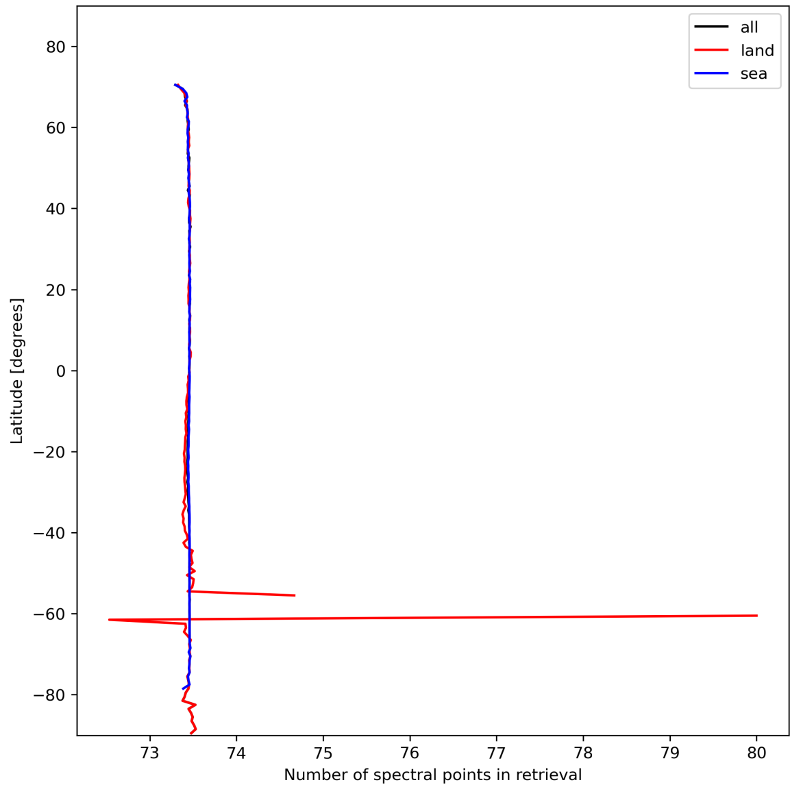
Figure 51: Zonal average of “Number of spectral points in retrieval” for 2024-02-09 to 2024-02-11.
