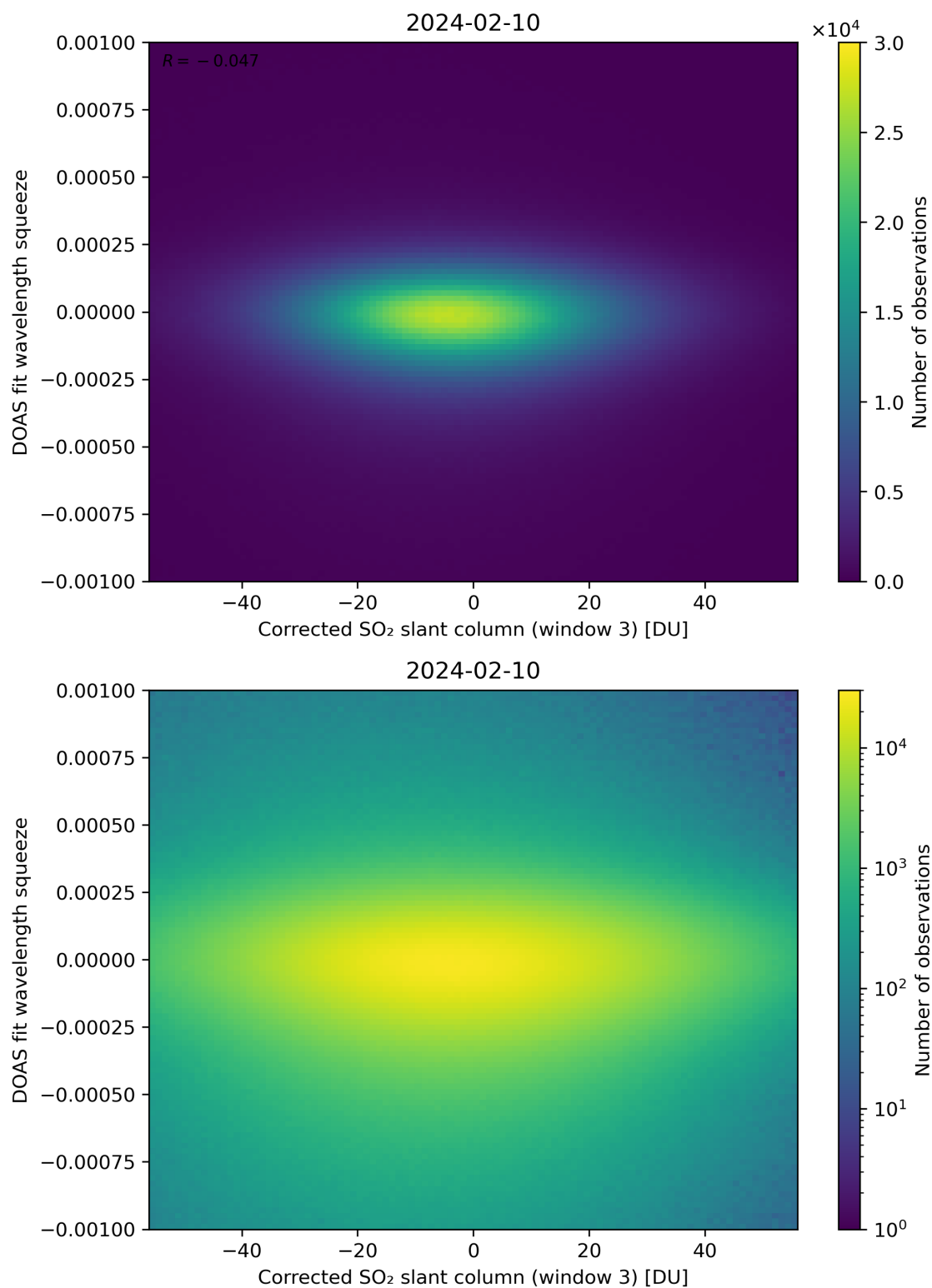
Figure 207: Scatter density plot of “Corrected SO 2 slant column (window 3)” against “DOAS fit wavelength squeeze” for 2024-02-09 to 2024-02-11.
