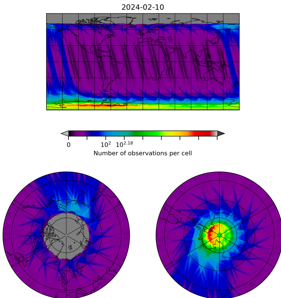
Figure 28: Map of the number of observations for 2024-02-09 to 2024-02-11
