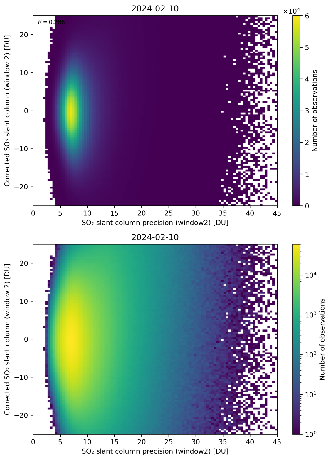
Figure 247: Scatter density plot of “SO 2 slant column precision (window2)” against “Corrected SO 2 slant column (window 2)” for 2024-02-09 to 2024-02-11.
