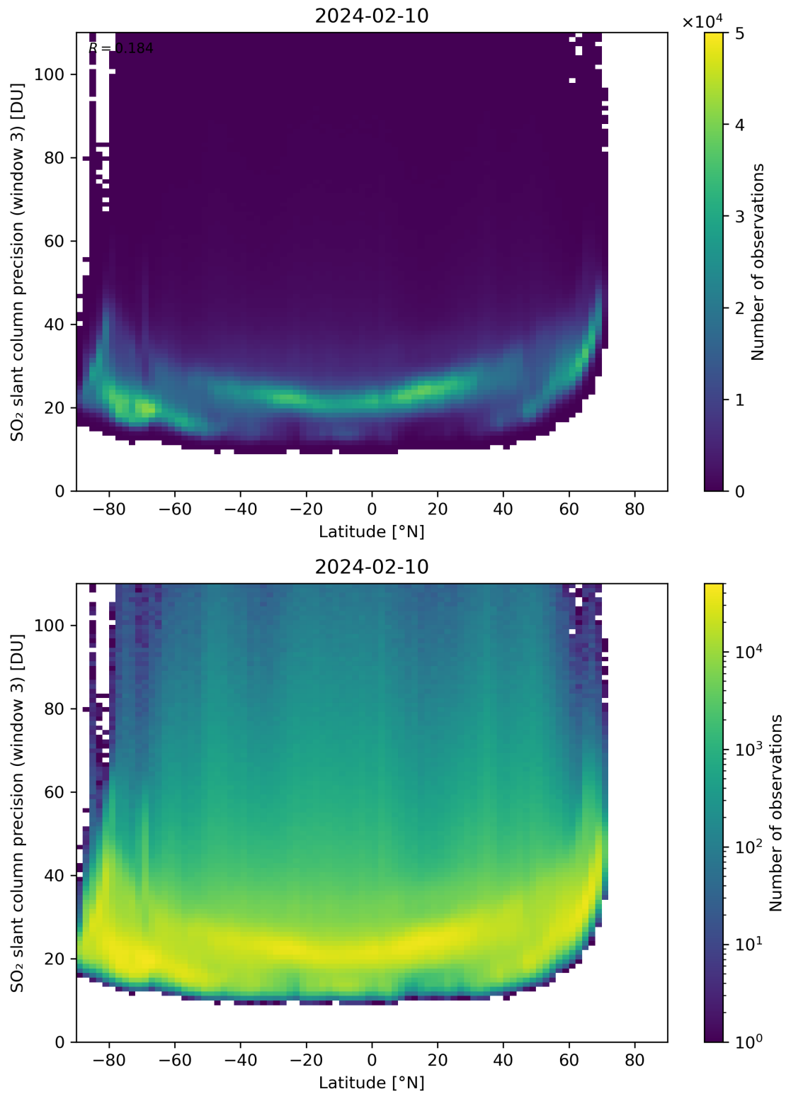
Figure 153: Scatter density plot of “Latitude” against “SO 2 slant column precision (window 3)” for 2024-02-09 to 2024-02-11.
