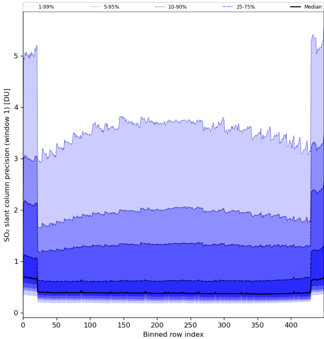
Figure 80: Along track statistics of “SO 2 slant column precision (window 1)” for 2024-02-09 to 2024-02-11
