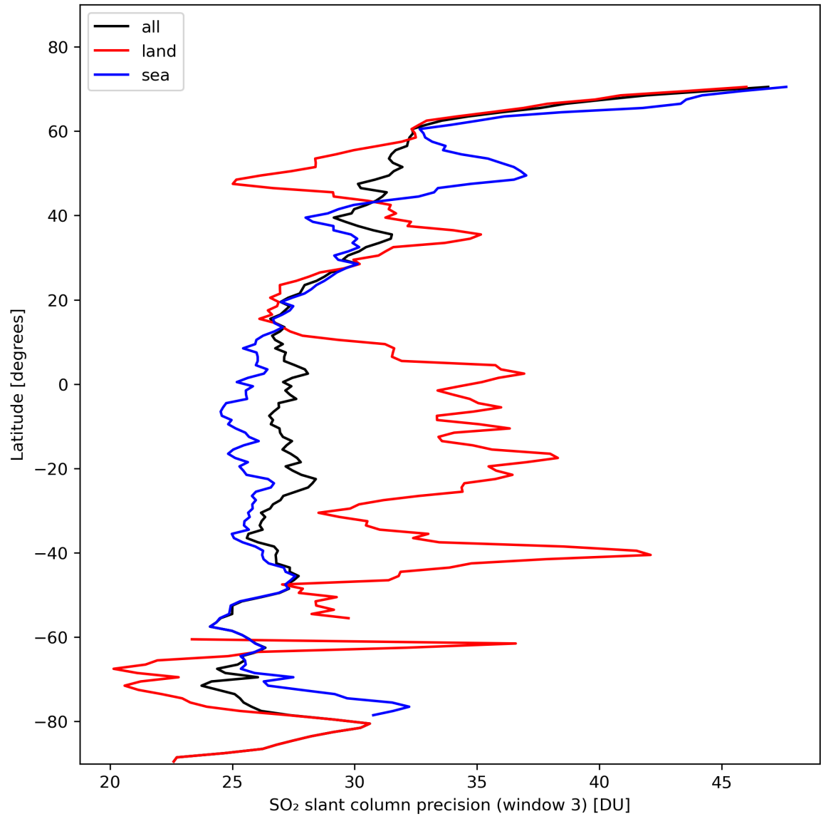
Figure 42: Zonal average of “SO 2 slant column precision (window 3)” for 2024-02-09 to 2024-02-11.
