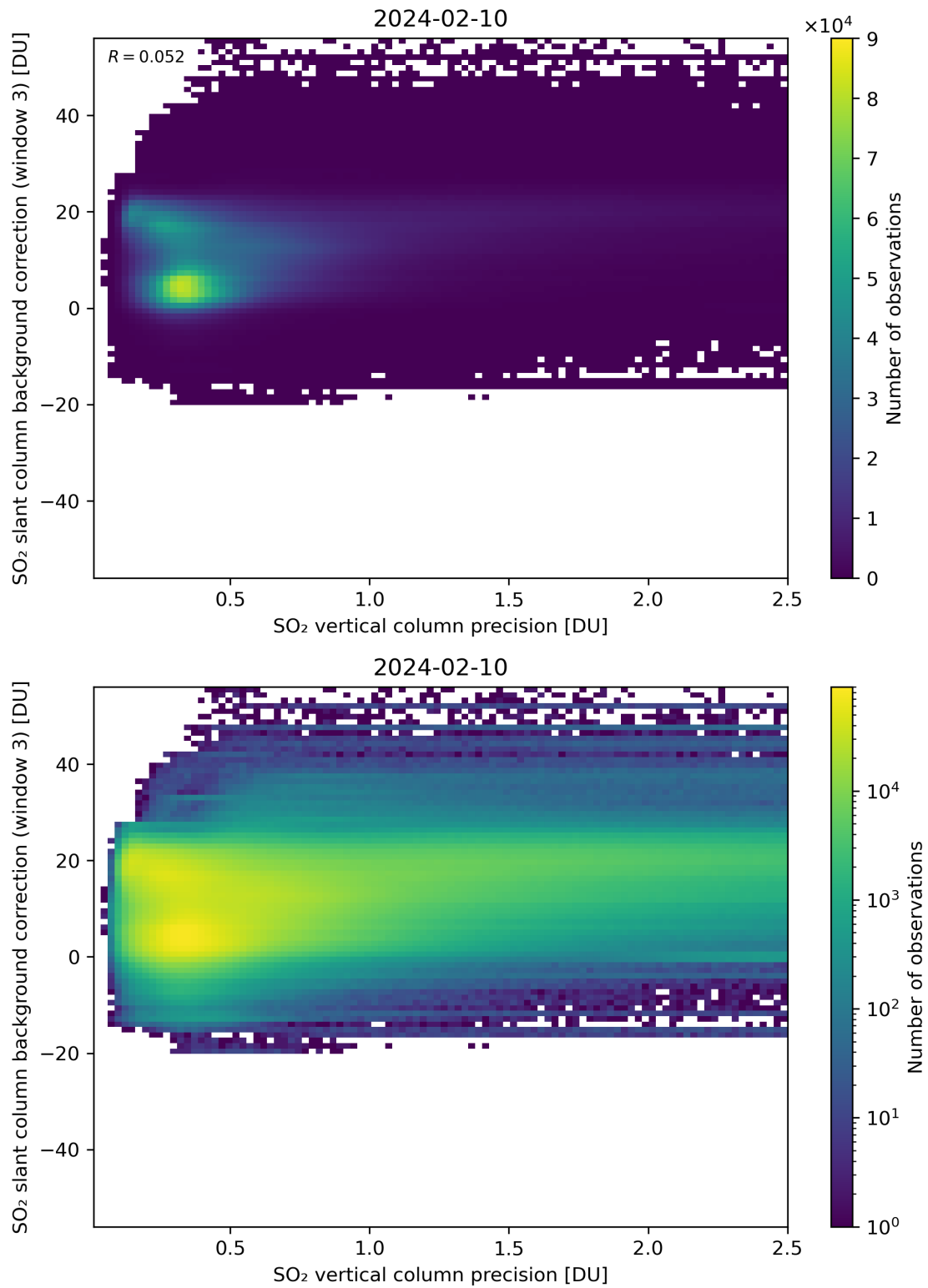
Figure 281: Scatter density plot of “SO 2 vertical column precision” against “SO 2 slant column background correction (window 3)” for 2024-02-09 to 2024-02-11.
