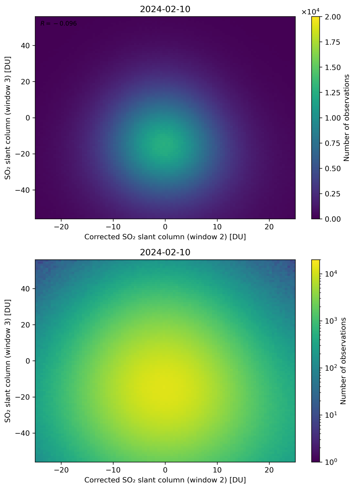
Figure 201: Scatter density plot of “Corrected SO 2 slant column (window 2)” against “SO 2 slant column (window 3)” for 2024-02-09 to 2024-02-11.
