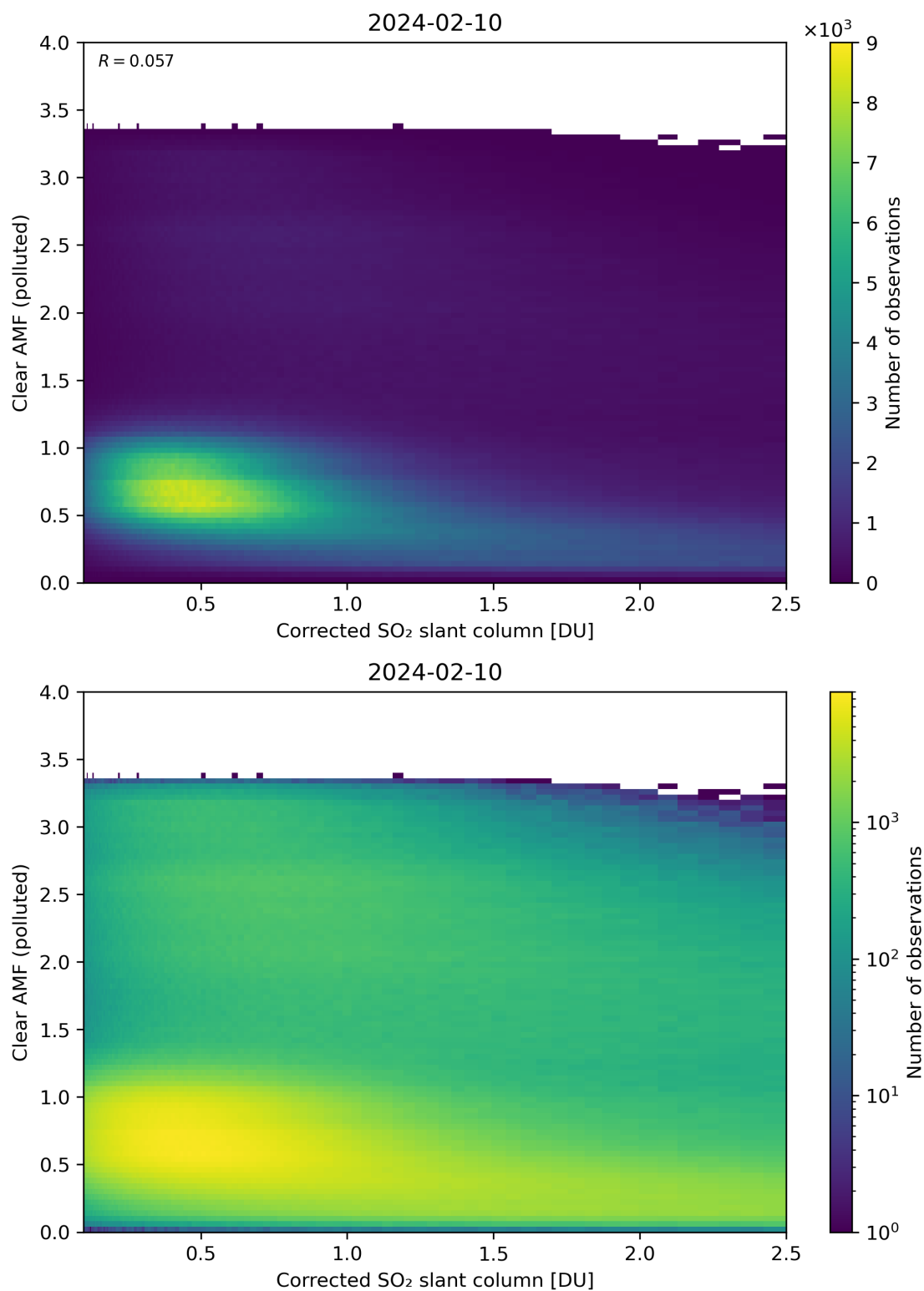
Figure 184: Scatter density plot of “Corrected SO 2 slant column” against “Clear AMF (polluted)” for 2024-02-09 to 2024-02-11.
