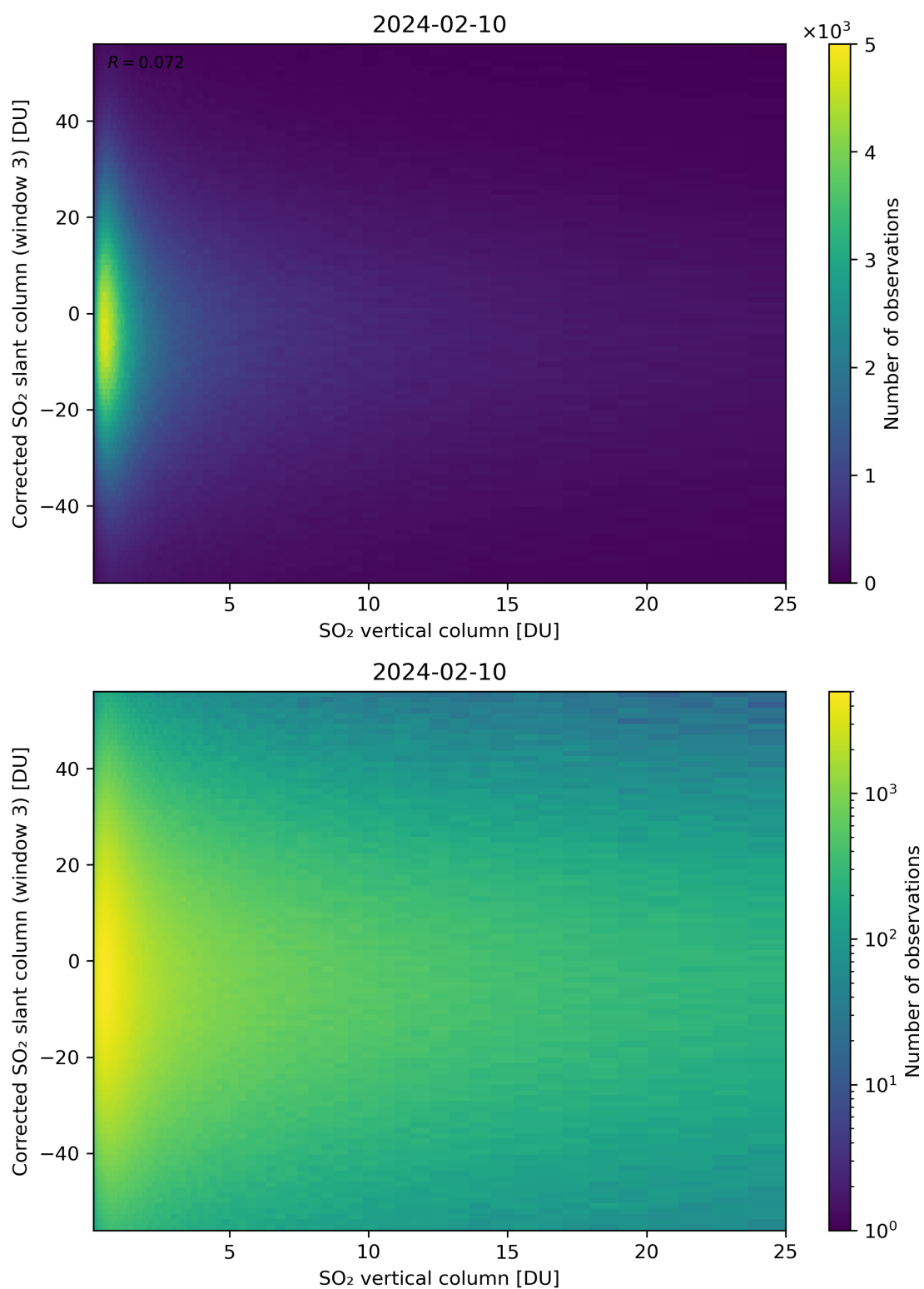
Figure 299: Scatter density plot of “SO 2 vertical column” against “Corrected SO 2 slant column (window 3)” for 2024-02-09 to 2024-02-11.
