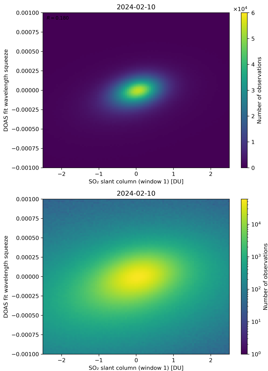
Figure 216: Scatter density plot of “SO 2 slant column (window 1)” against “DOAS fit wavelength squeeze” for 2024-02-09 to 2024-02-11.
