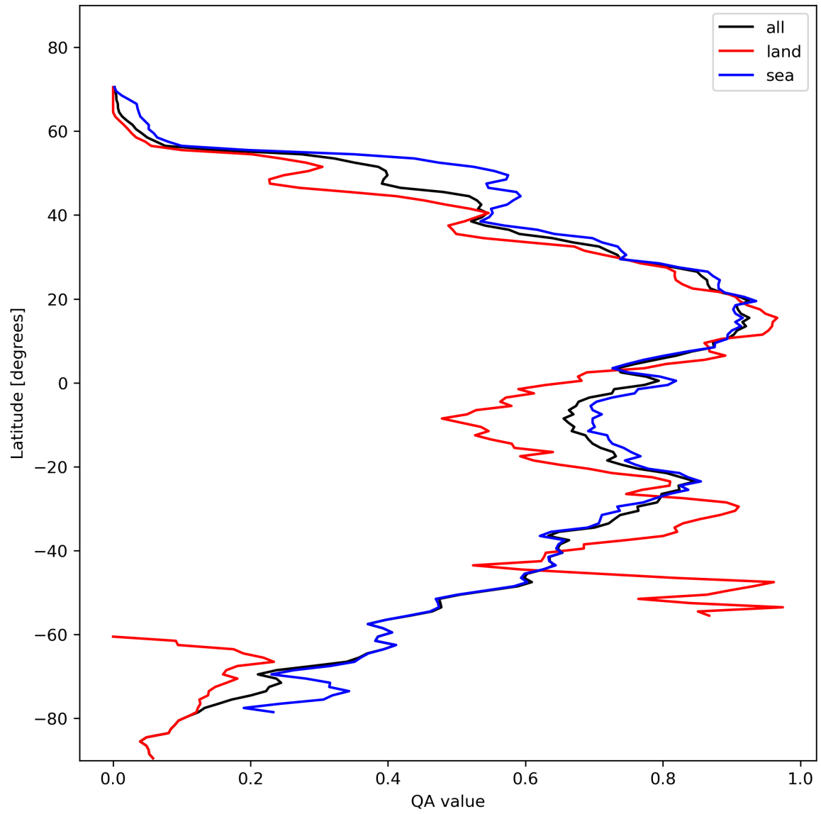
Figure 29: Zonal average of “QA value” for 2024-02-09 to 2024-02-11.
