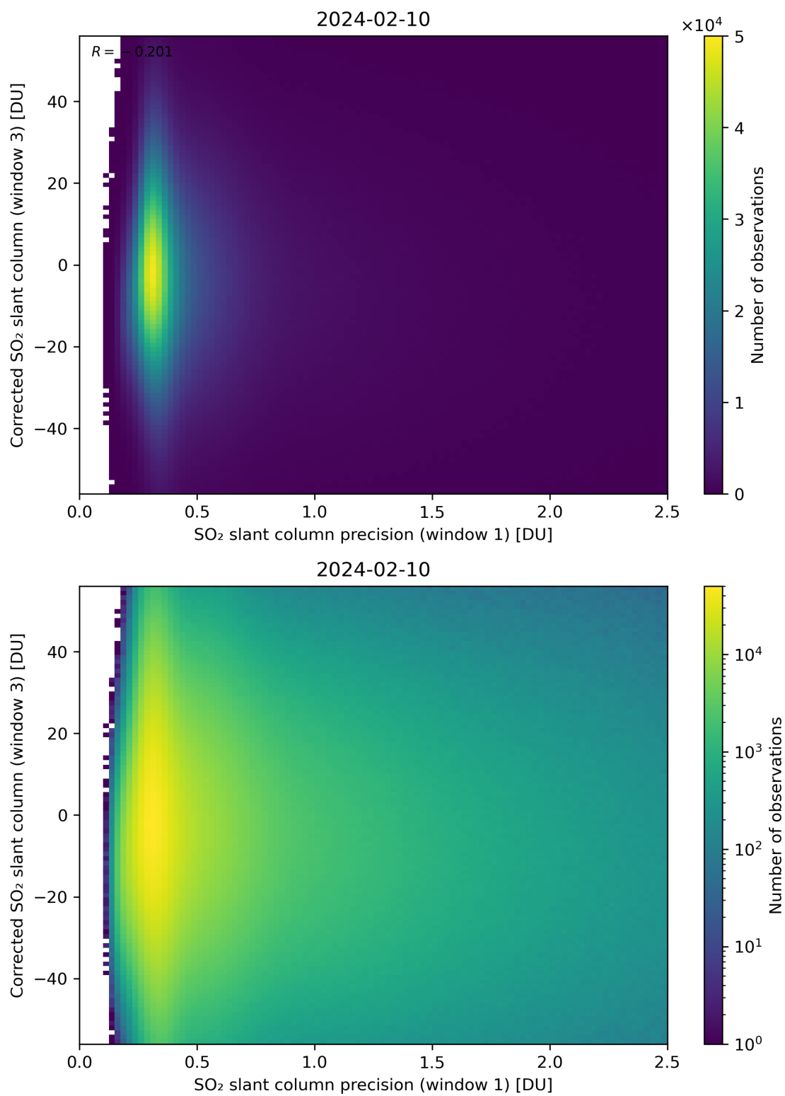
Figure 226: Scatter density plot of “SO 2 slant column precision (window 1)” against “Corrected SO 2 slant column (window 3)” for 2024-02-09 to 2024-02-11.
