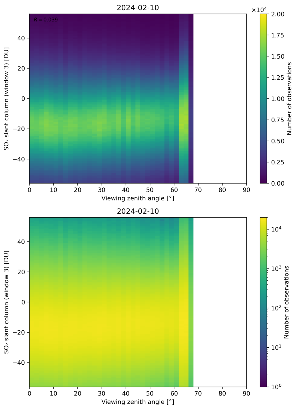
Figure 323: Scatter density plot of “Viewing zenith angle” against “SO 2 slant column (window 3)” for 2024-02-09 to 2024-02-11.
