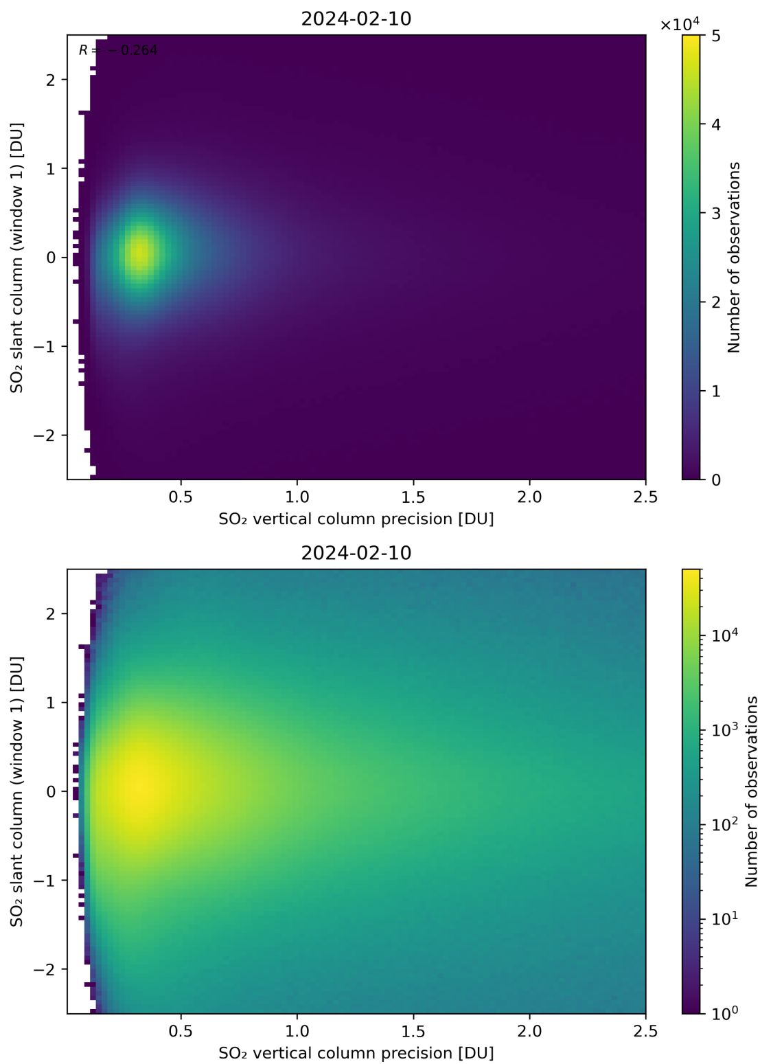
Figure 289: Scatter density plot of “SO 2 vertical column precision” against “SO 2 slant column (window 1)” for 2024-02-09 to 2024-02-11.
