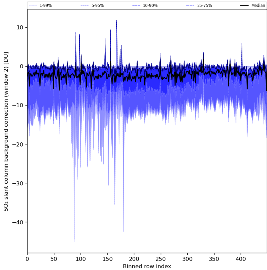
Figure 86: Along track statistics of “SO 2 slant column background correction (window 2)” for 2024-02-09 to 2024-02-11
