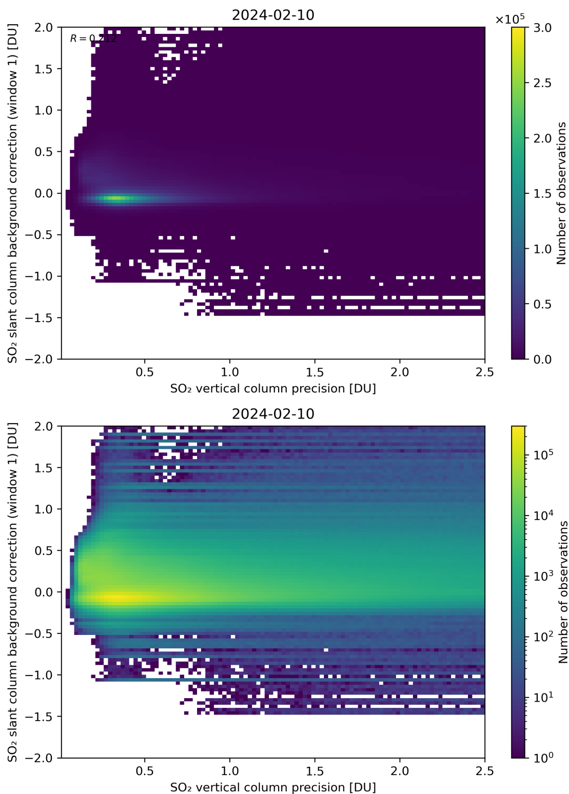
Figure 279: Scatter density plot of “SO 2 vertical column precision” against “SO 2 slant column background correction (window 1)” for 2024-02-09 to 2024-02-11.
