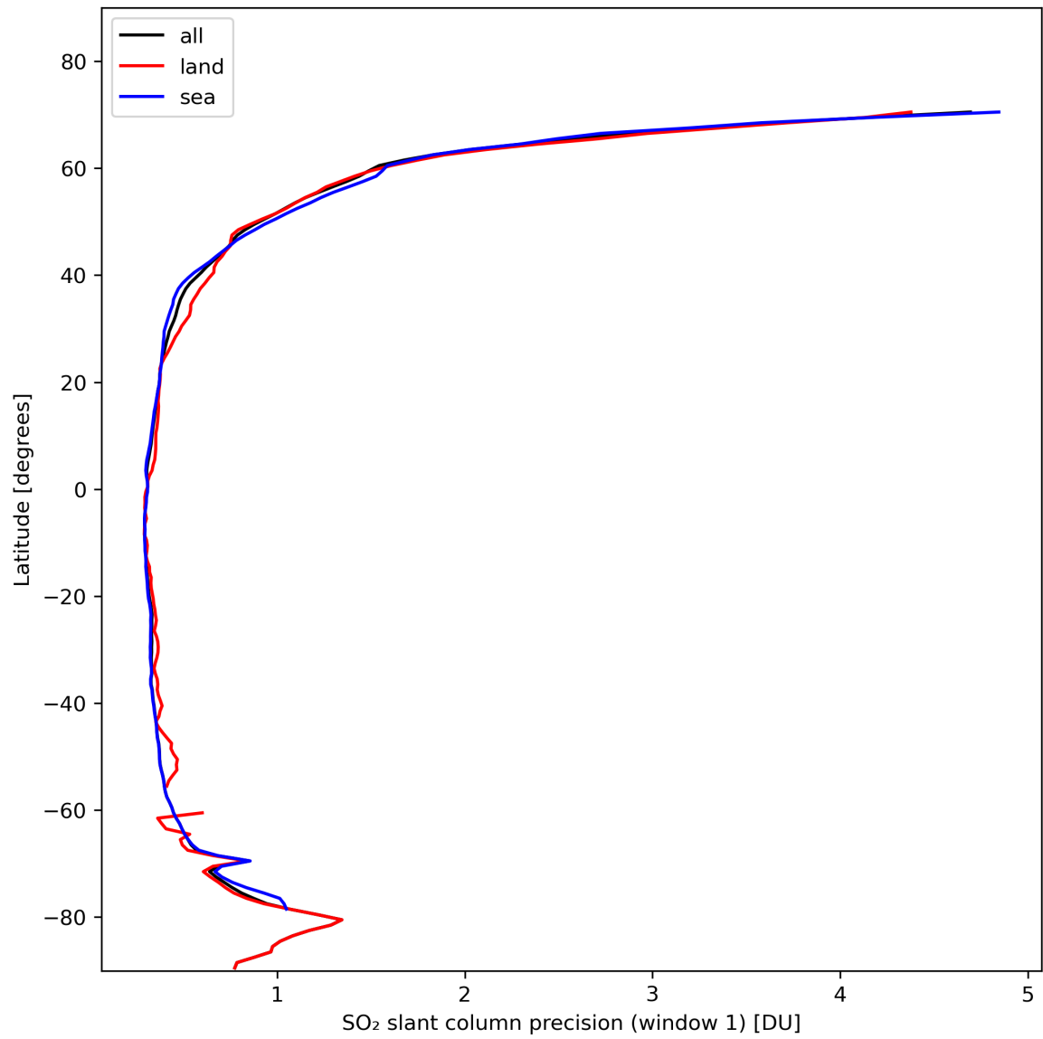
Figure 34: Zonal average of “SO 2 slant column precision (window 1)” for 2024-02-09 to 2024-02-11.
