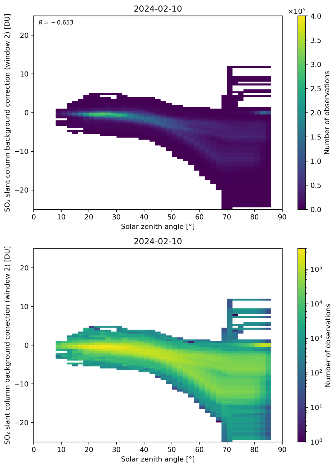
Figure 159: Scatter density plot of “Solar zenith angle” against “SO 2 slant column background correction (window 2)” for 2024-02-09 to 2024-02-11.
