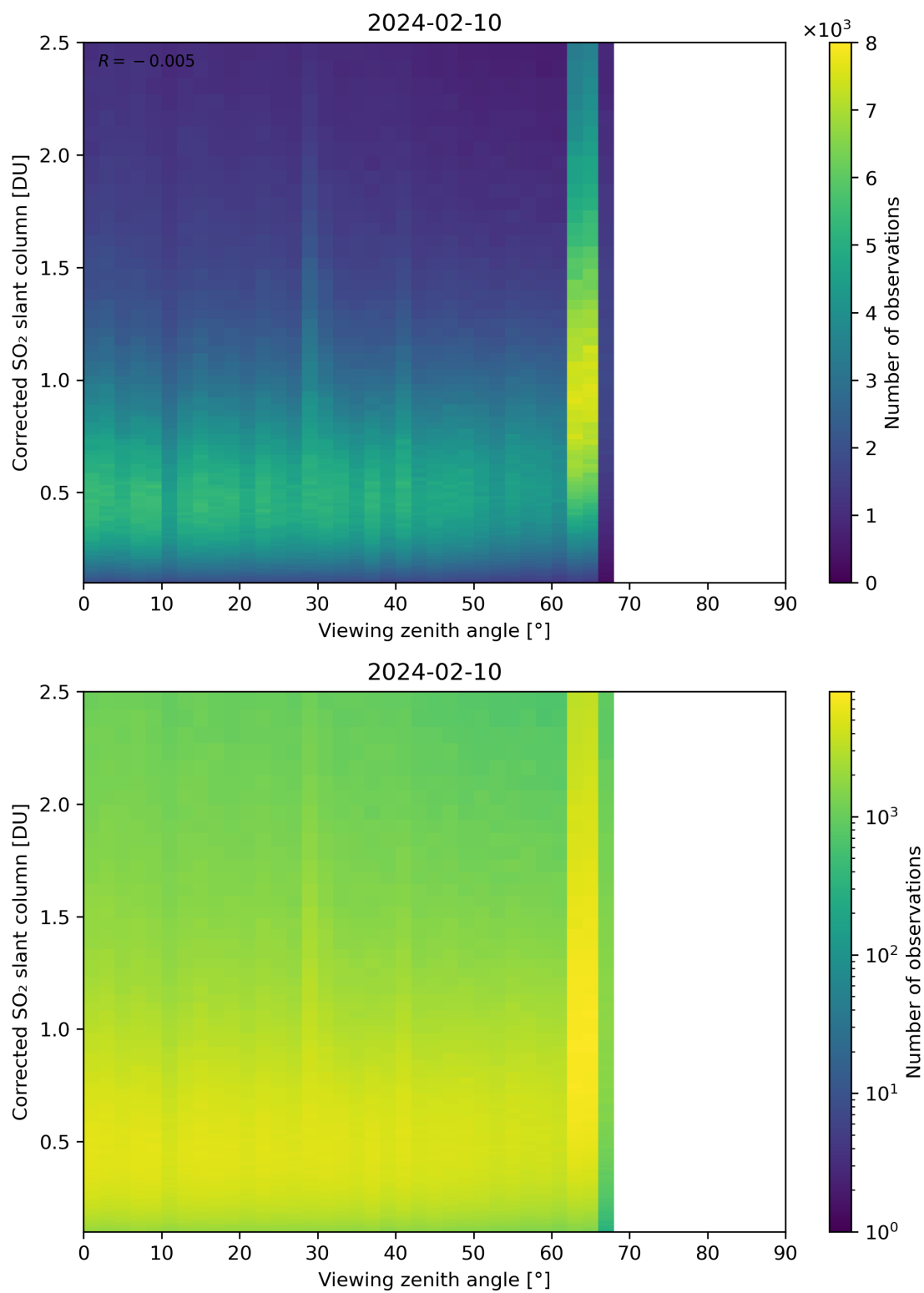
Figure 317: Scatter density plot of “Viewing zenith angle” against “Corrected SO 2 slant column” for 2024-02-09 to 2024-02-11.
