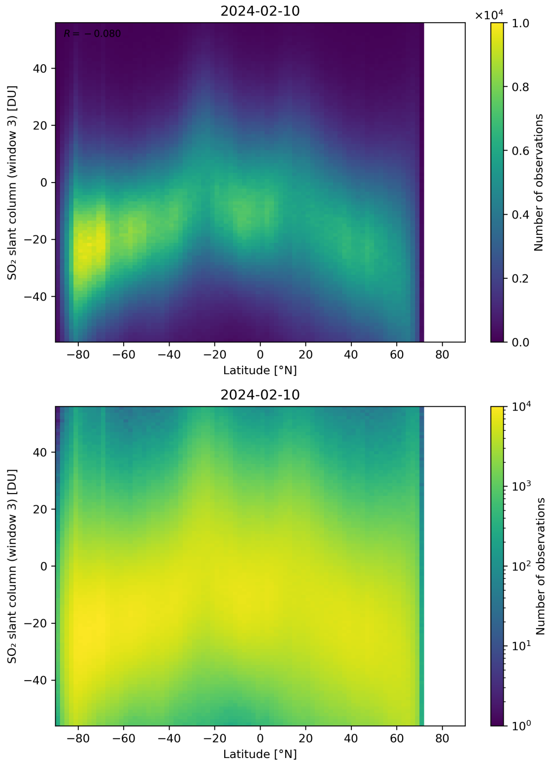
Figure 152: Scatter density plot of “Latitude” against “SO 2 slant column (window 3)” for 2024-02-09 to 2024-02-11.
