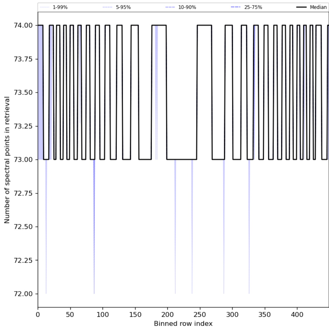
Figure 97: Along track statistics of “Number of spectral points in retrieval” for 2024-02-09 to 2024-02-11
