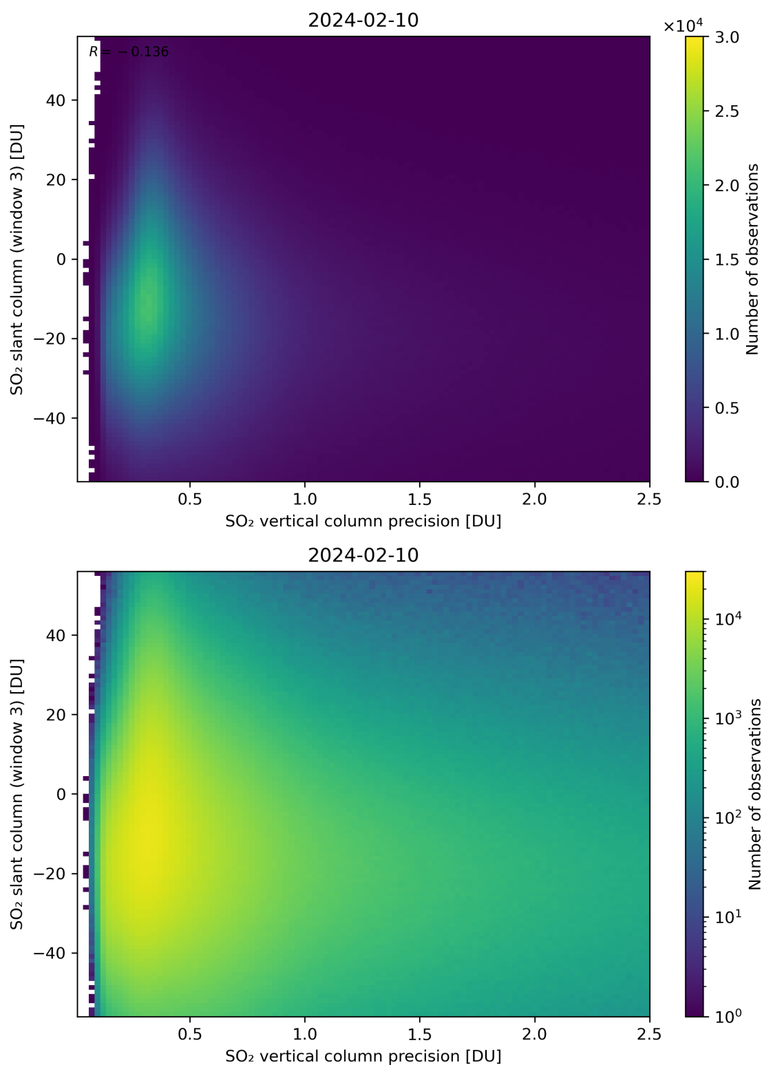
Figure 292: Scatter density plot of “SO 2 vertical column precision” against “SO 2 slant column (window 3)” for 2024-02-09 to 2024-02-11.
