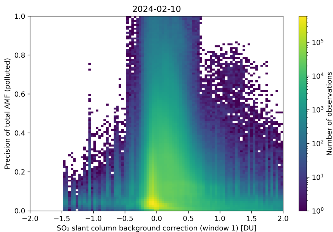
Figure 110: Scatter density plot of “SO 2 slant column background correction (window 1)” against “Precision of total AMF (polluted)” for 2024-02-09 to 2024-02-11.
