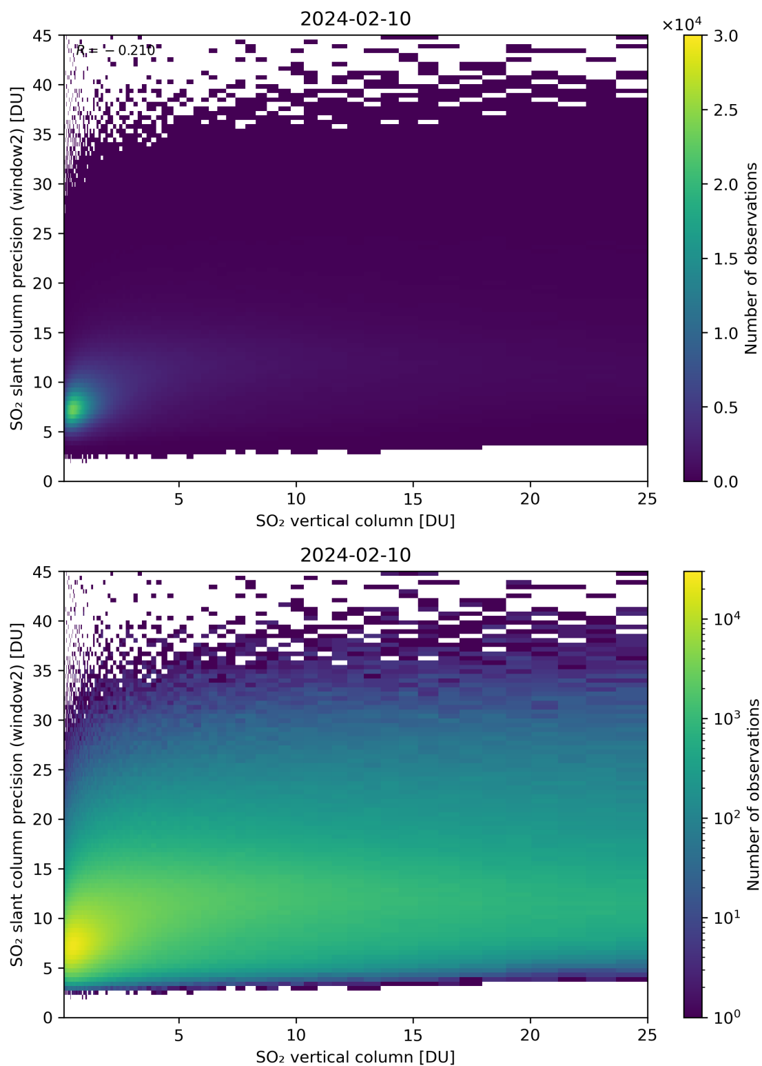
Figure 302: Scatter density plot of “SO 2 vertical column” against “SO 2 slant column precision (window2)” for 2024-02-09 to 2024-02-11.
