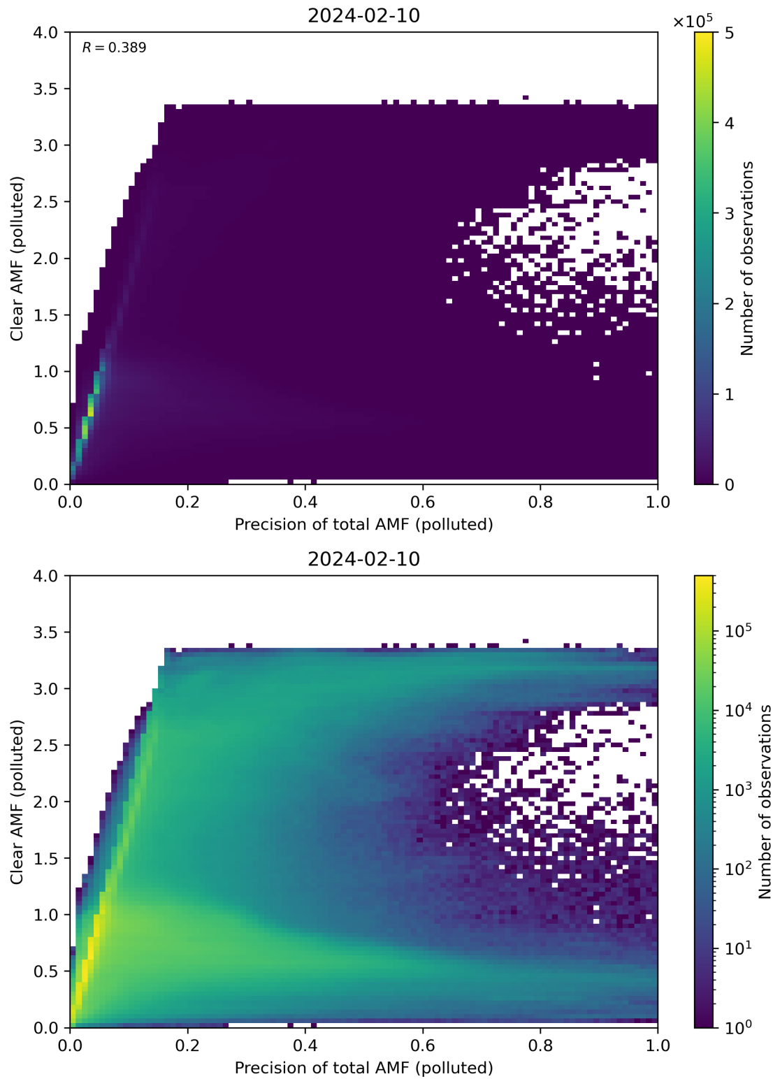
Figure 270: Scatter density plot of “Precision of total AMF (polluted)” against “Clear AMF (polluted)” for 2024-02-09 to 2024-02-11.
