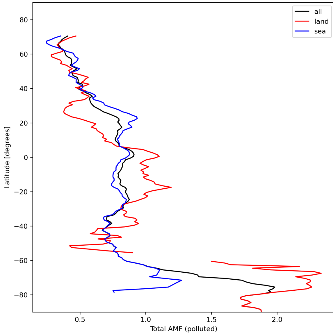
Figure 48: Zonal average of “Total AMF (polluted)” for 2024-02-09 to 2024-02-11.
