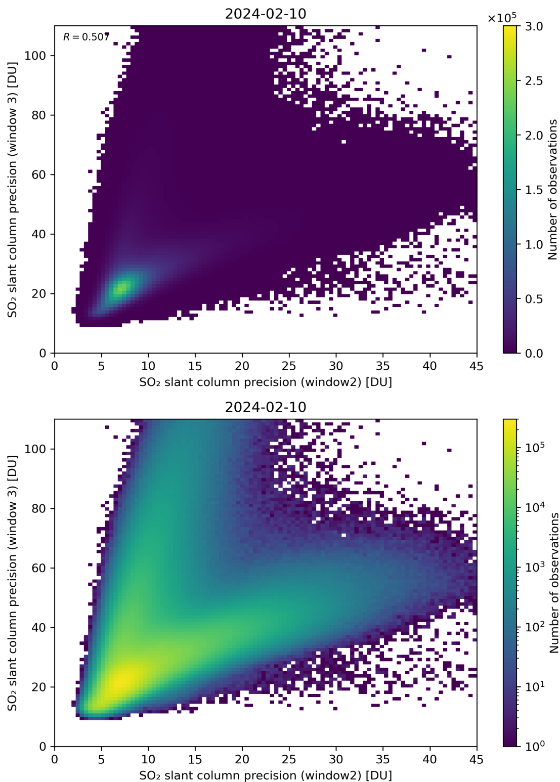
Figure 250: Scatter density plot of “SO 2 slant column precision (window2)” against “SO 2 slant column precision (window 3)” for 2024-02-09 to 2024-02-11.
