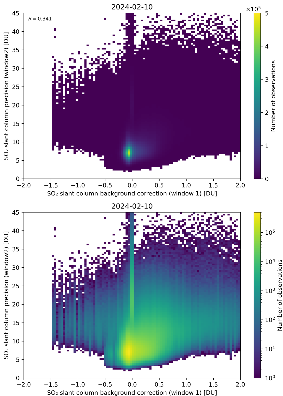
Figure 106: Scatter density plot of “SO 2 slant column background correction (window 1)” against “SO 2 slant column precision (window2)” for 2024-02-09 to 2024-02-11.
