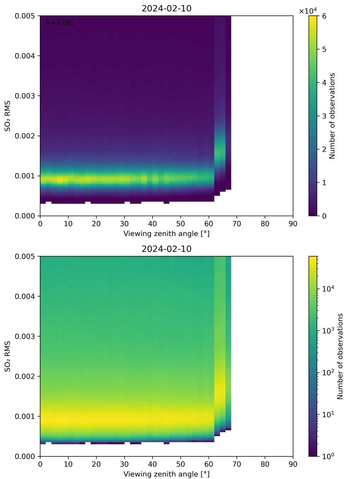
Figure 313: Scatter density plot of “Viewing zenith angle” against “SO 2 RMS” for 2024-02-09 to 2024-02-11.
