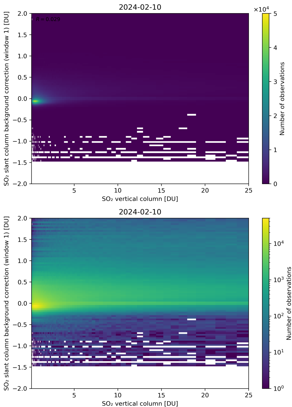
Figure 273: Scatter density plot of “SO 2 vertical column” against “SO 2 slant column background correction (window 1)” for 2024-02-09 to 2024-02-11.
