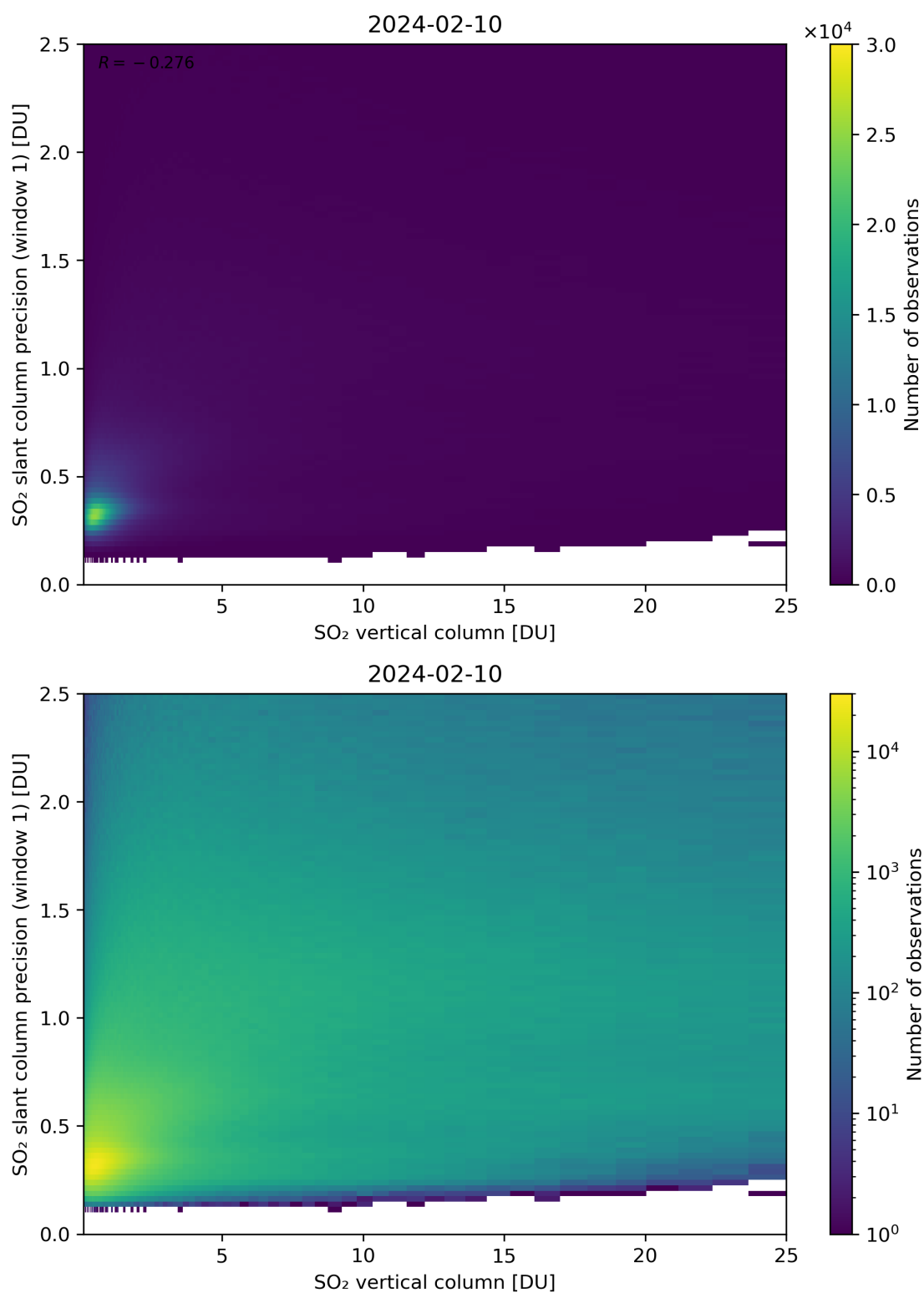
Figure 301: Scatter density plot of “SO 2 vertical column” against “SO 2 slant column precision (window 1)” for 2024-02-09 to 2024-02-11.
