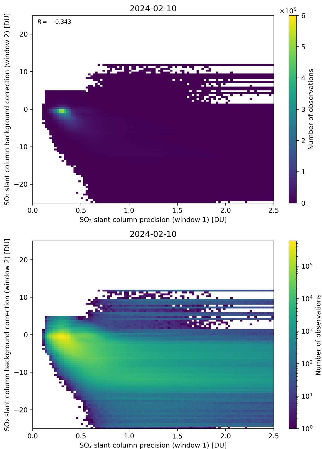
Figure 219: Scatter density plot of “SO 2 slant column precision (window 1)” against “SO 2 slant column background correction (window 2)” for 2024-02-09 to 2024-02-11.
