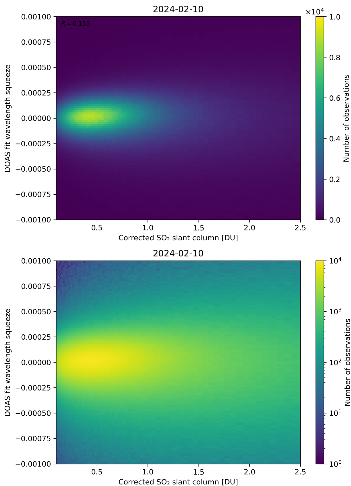
Figure 182: Scatter density plot of “Corrected SO 2 slant column” against “DOAS fit wavelength squeeze” for 2024-02-09 to 2024-02-11.
