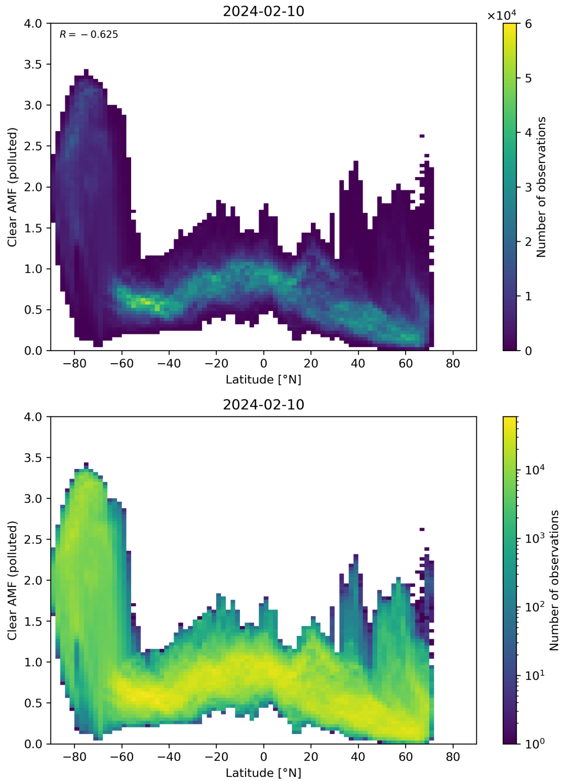
Figure 145: Scatter density plot of “Latitude” against “Clear AMF (polluted)” for 2024-02-09 to 2024-02-11.
