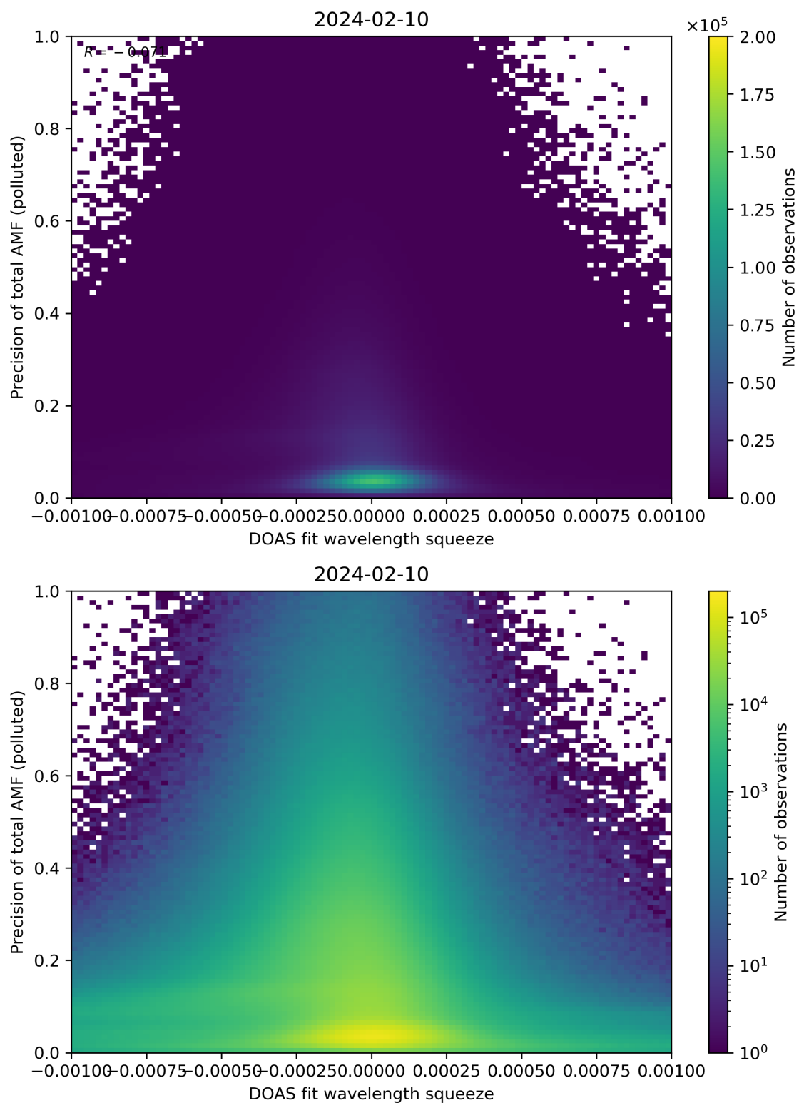
Figure 135: Scatter density plot of “DOAS fit wavelength squeeze” against “Precision of total AMF (polluted)” for 2024-02-09 to 2024-02-11.
