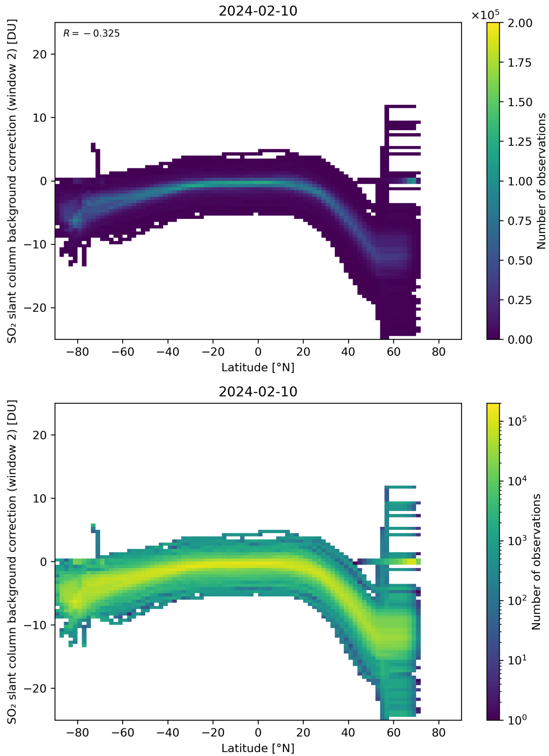
Figure 140: Scatter density plot of “Latitude” against “SO 2 slant column background correction (window 2)” for 2024-02-09 to 2024-02-11.
