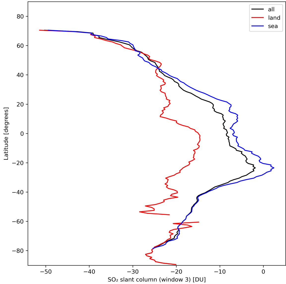
Figure 41: Zonal average of “SO 2 slant column (window 3)” for 2024-02-09 to 2024-02-11.
