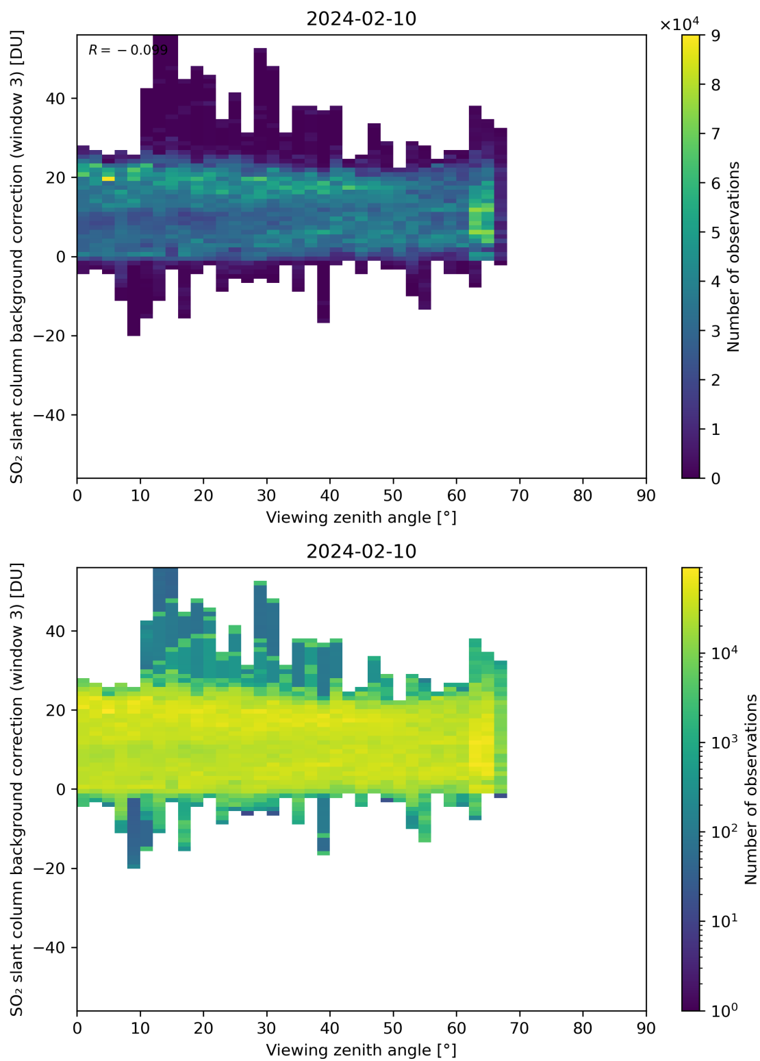
Figure 310: Scatter density plot of “Viewing zenith angle” against “SO 2 slant column background correction (window 3)” for 2024-02-09 to 2024-02-11.
