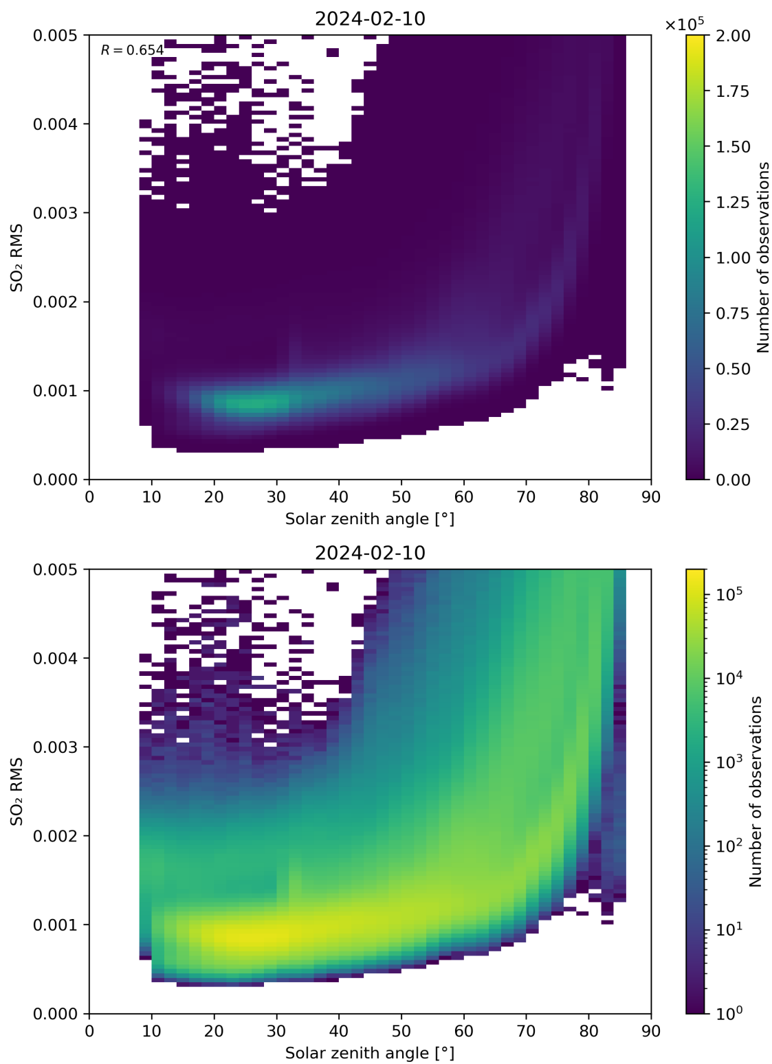
Figure 163: Scatter density plot of “Solar zenith angle” against “SO 2 RMS” for 2024-02-09 to 2024-02-11.
