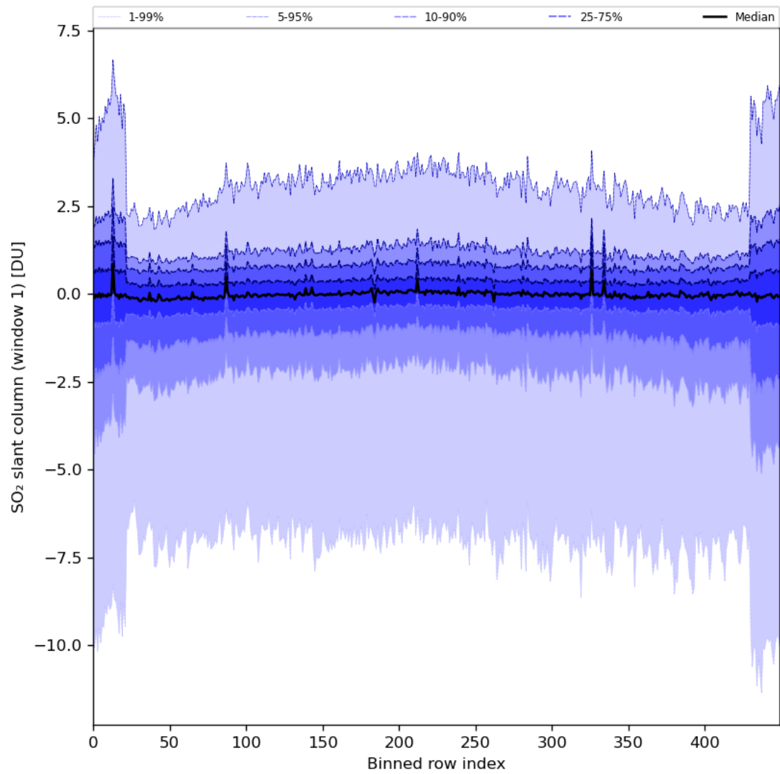
Figure 79: Along track statistics of “SO 2 slant column (window 1)” for 2024-02-09 to 2024-02-11
