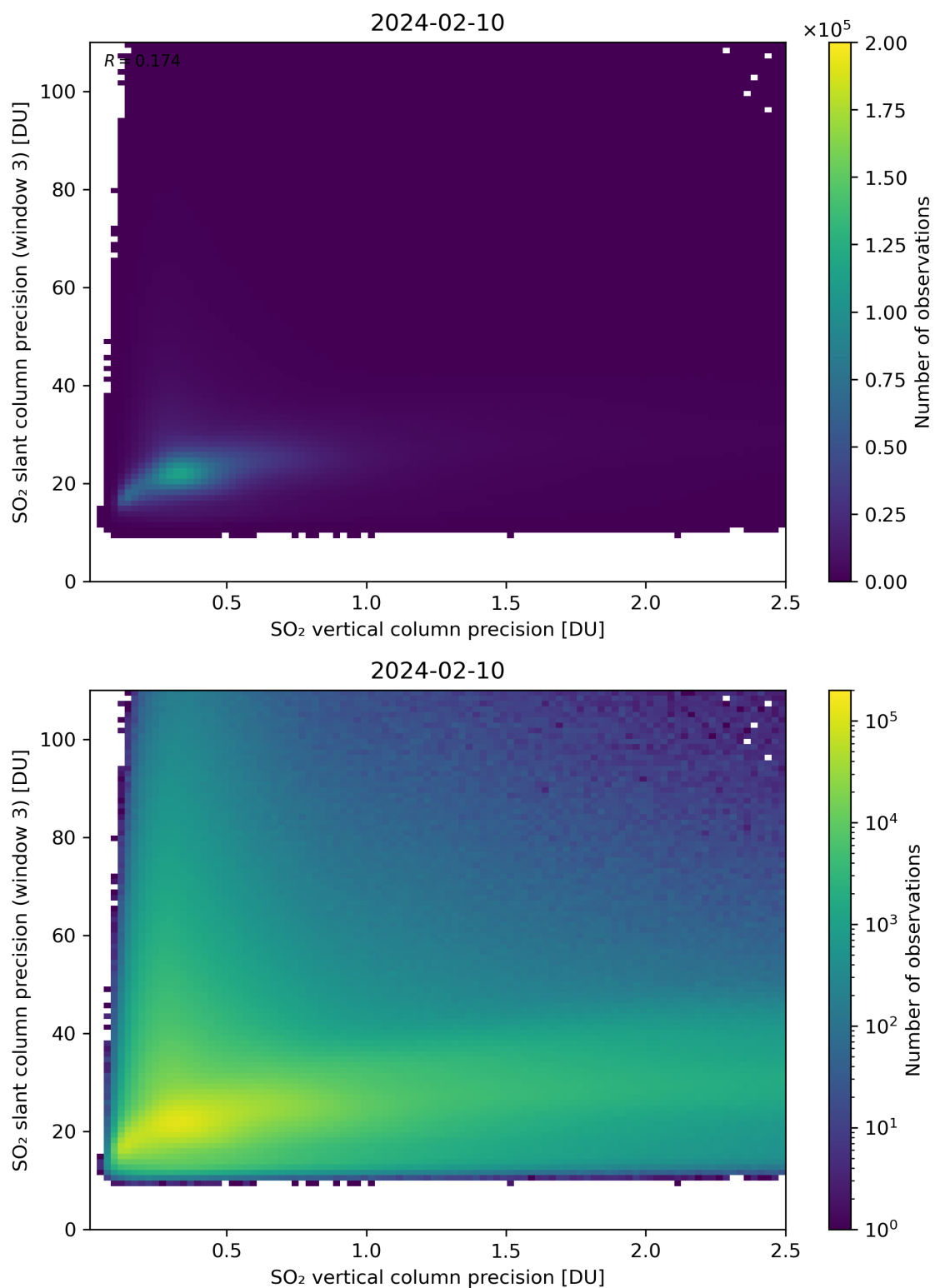
Figure 293: Scatter density plot of “SO 2 vertical column precision” against “SO 2 slant column precision (window 3)” for 2024-02-09 to 2024-02-11.
