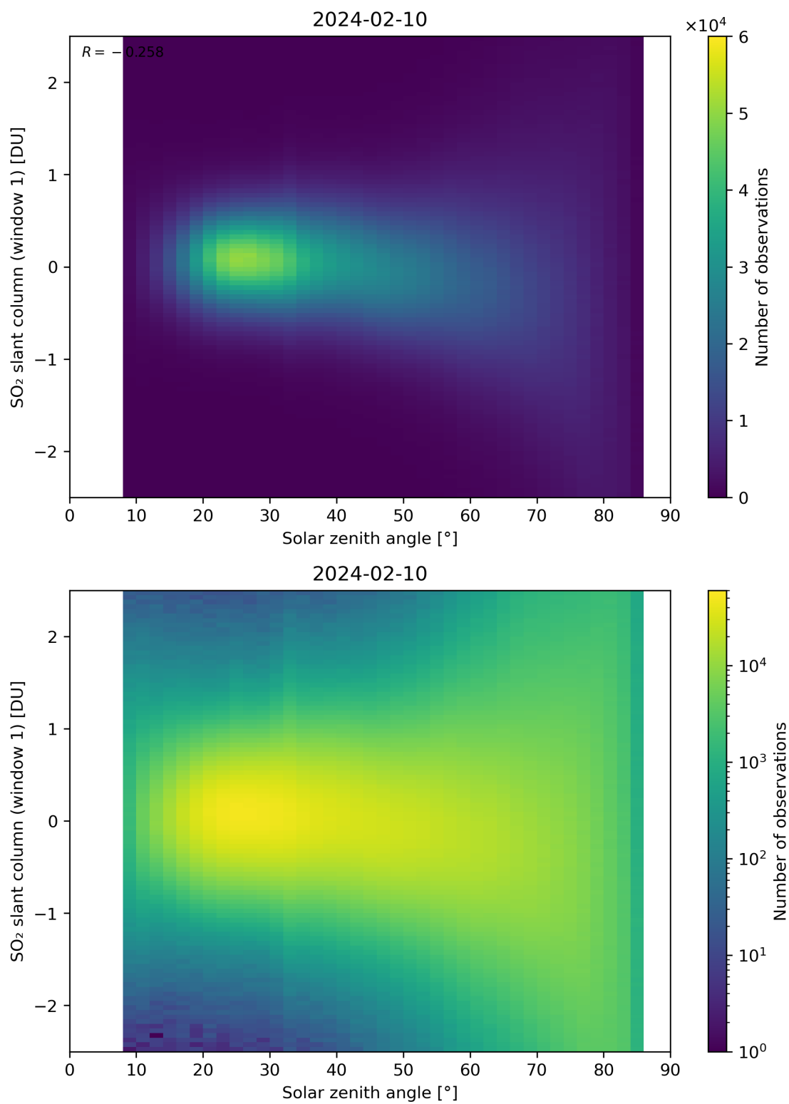
Figure 169: Scatter density plot of “Solar zenith angle” against “SO 2 slant column (window 1)” for 2024-02-09 to 2024-02-11.
