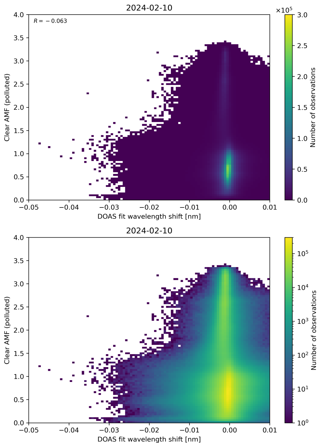
Figure 129: Scatter density plot of “DOAS fit wavelength shift” against “Clear AMF (polluted)” for 2024-02-09 to 2024-02-11.
