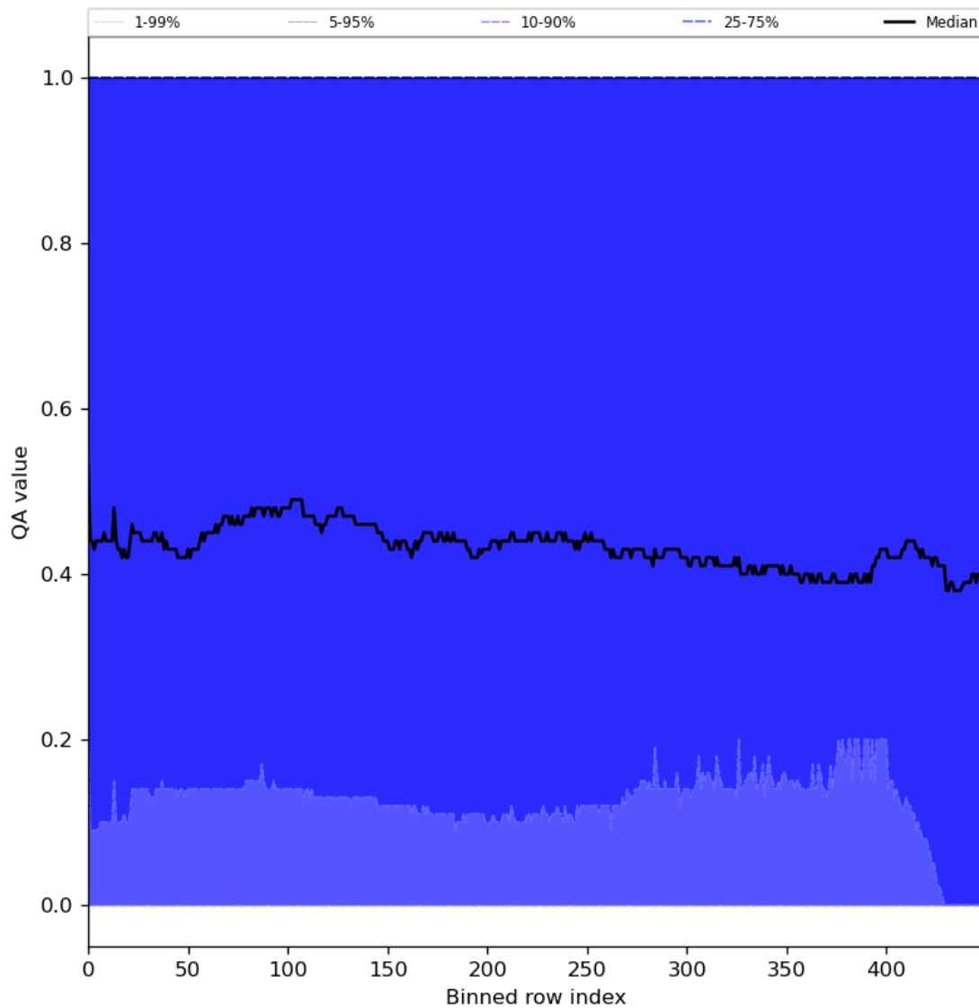
Figure 75: Along track statistics of “QA value” for 2024-02-09 to 2024-02-11
