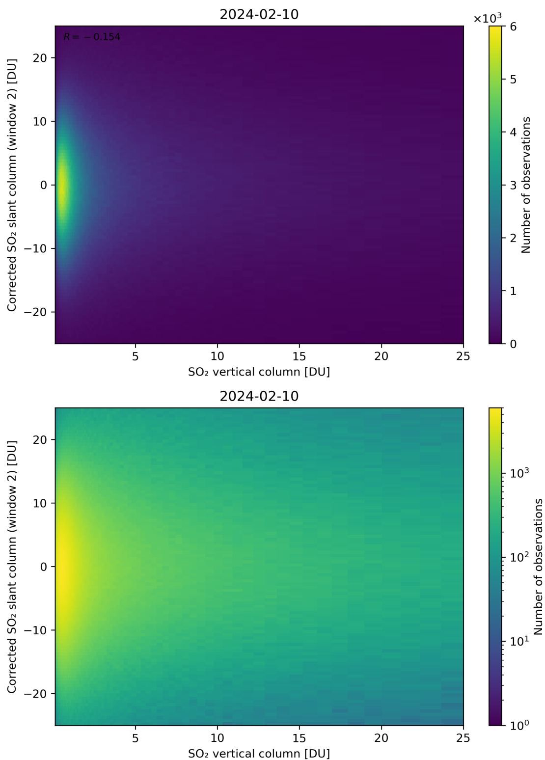
Figure 298: Scatter density plot of “SO 2 vertical column” against “Corrected SO 2 slant column (window 2)” for 2024-02-09 to 2024-02-11.
