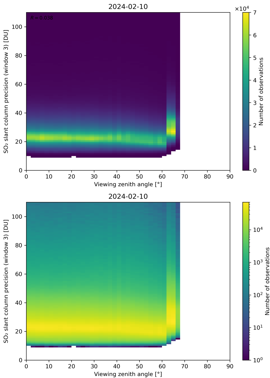
Figure 324: Scatter density plot of “Viewing zenith angle” against “SO 2 slant column precision (window 3)” for 2024-02-09 to 2024-02-11.
