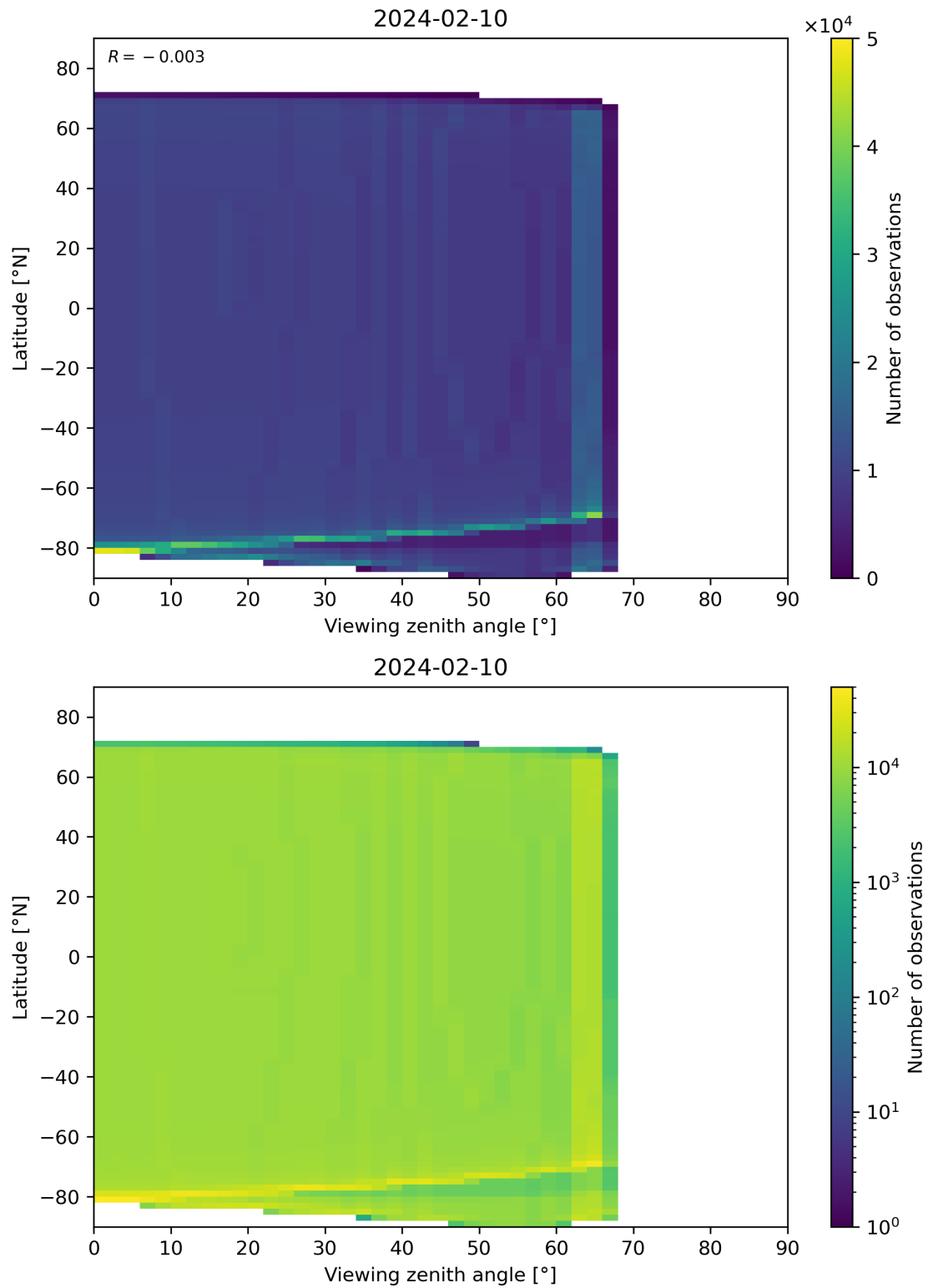
Figure 314: Scatter density plot of “Viewing zenith angle” against “Latitude” for 2024-02-09 to 2024-02-11.
