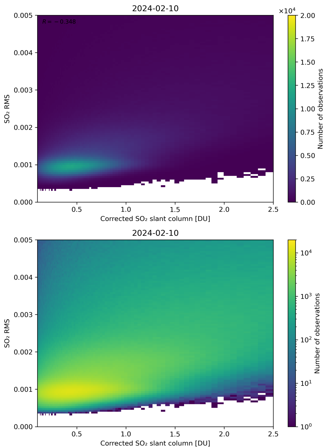
Figure 183: Scatter density plot of “Corrected SO 2 slant column” against “SO 2 RMS” for 2024-02-09 to 2024-02-11.
