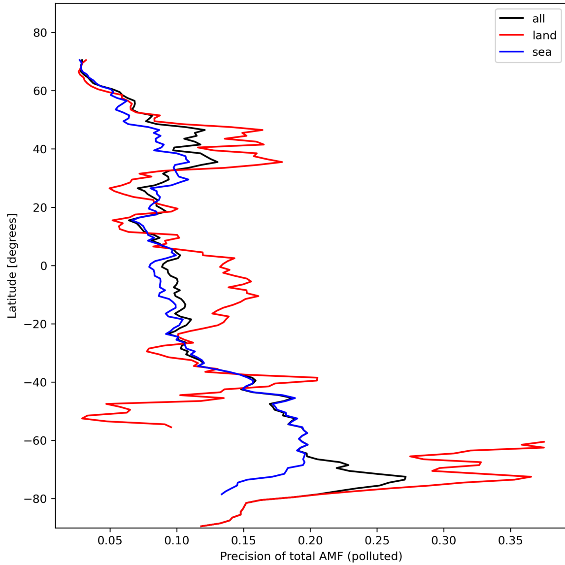
Figure 49: Zonal average of “Precision of total AMF (polluted)” for 2024-02-09 to 2024-02-11.
