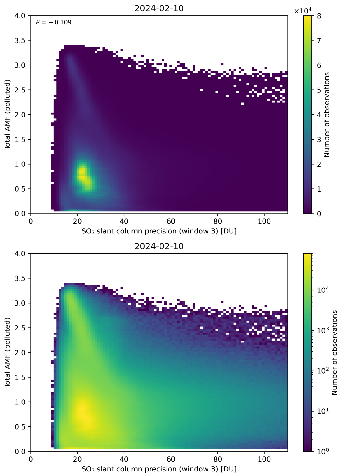
Figure 263: Scatter density plot of “SO 2 slant column precision (window 3)” against “Total AMF (polluted)” for 2024-02-09 to 2024-02-11.
