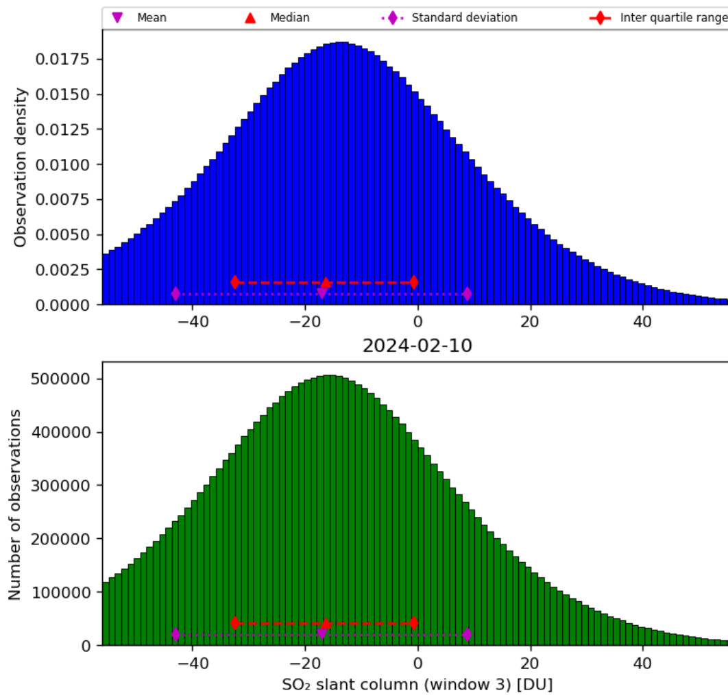
Figure 64: Histogram of “SO 2 slant column (window 3)” for 2024-02-09 to 2024-02-11
