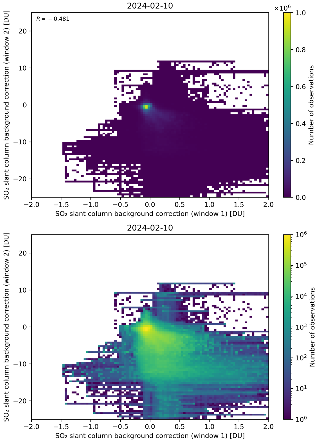
Figure 98: Scatter density plot of “SO 2 slant column background correction (window 1)” against “SO 2 slant column background correction (window 2)” for 2024-02-09 to 2024-02-11.
