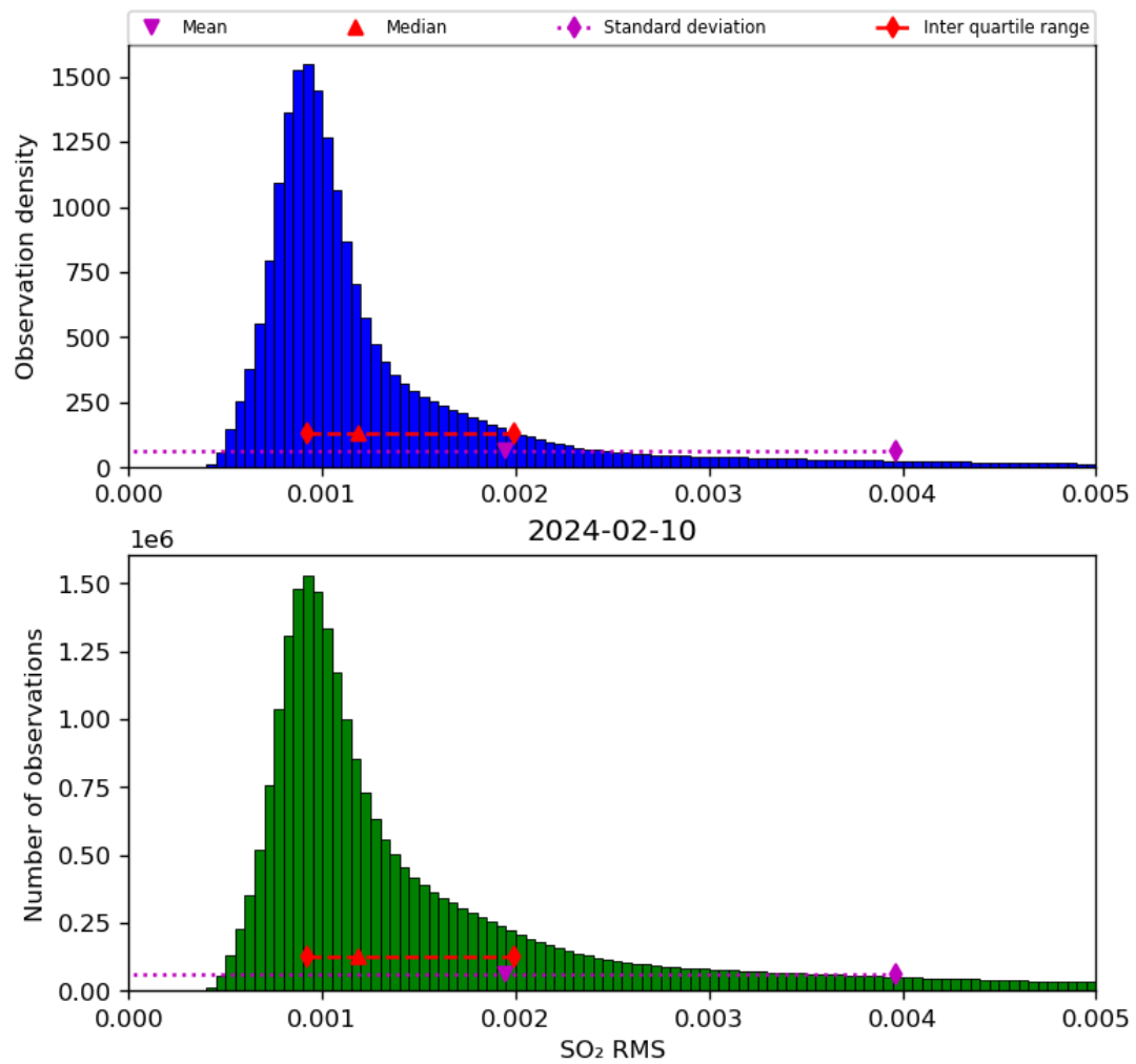
Figure 70: Histogram of “SO 2 RMS” for 2024-02-09 to 2024-02-11
