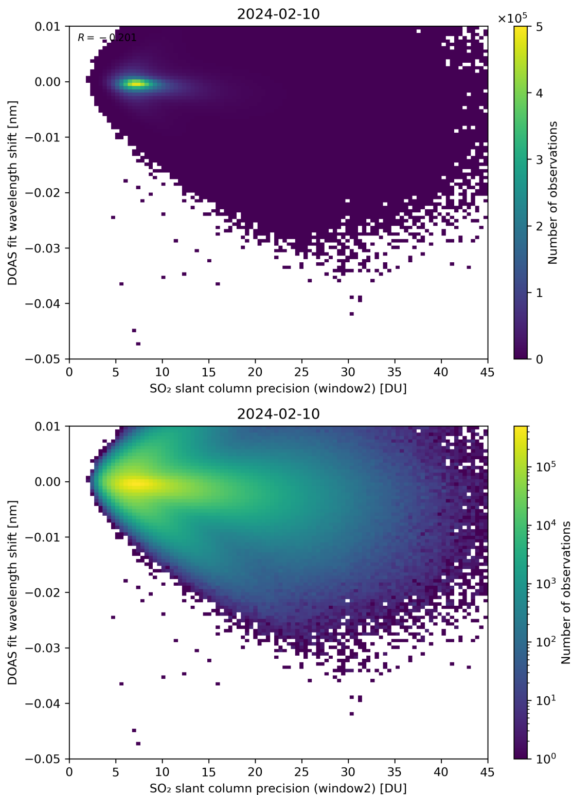
Figure 243: Scatter density plot of “SO 2 slant column precision (window2)” against “DOAS fit wavelength shift” for 2024-02-09 to 2024-02-11.
