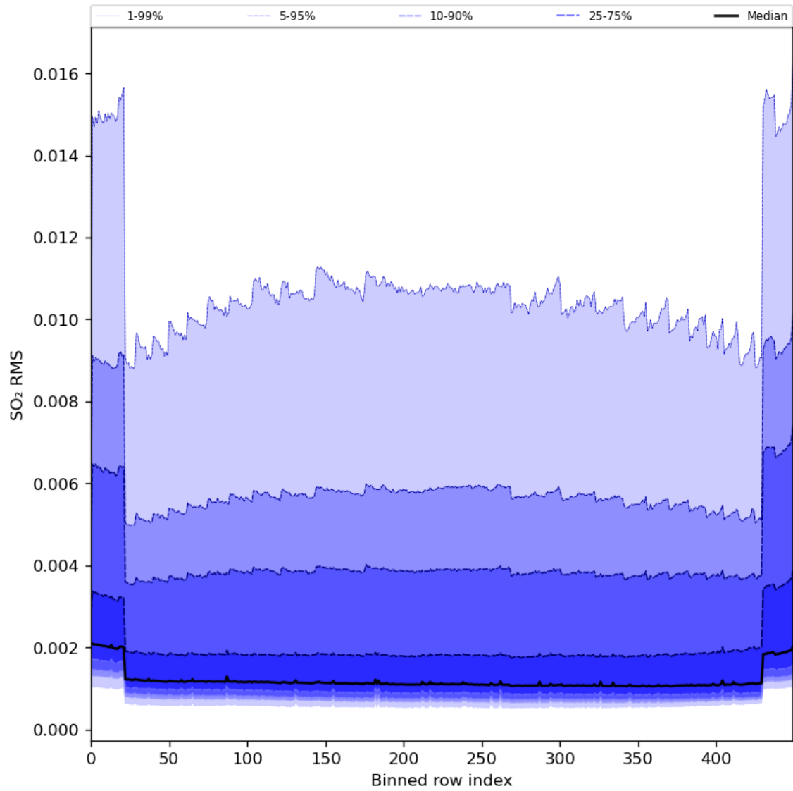
Figure 93: Along track statistics of “SO 2 RMS” for 2024-02-09 to 2024-02-11
