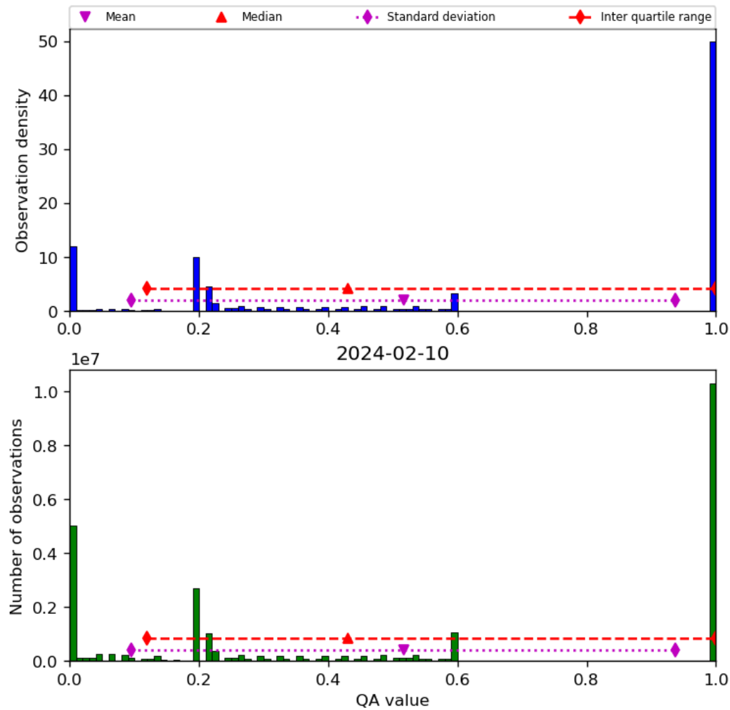
Figure 52: Histogram of “QA value” for 2024-02-09 to 2024-02-11
