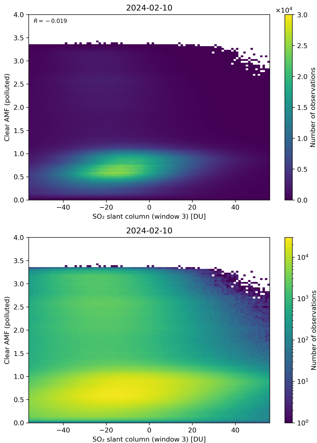
Figure 265: Scatter density plot of “SO 2 slant column (window 3)” against “Clear AMF (polluted)” for 2024-02-09 to 2024-02-11.
