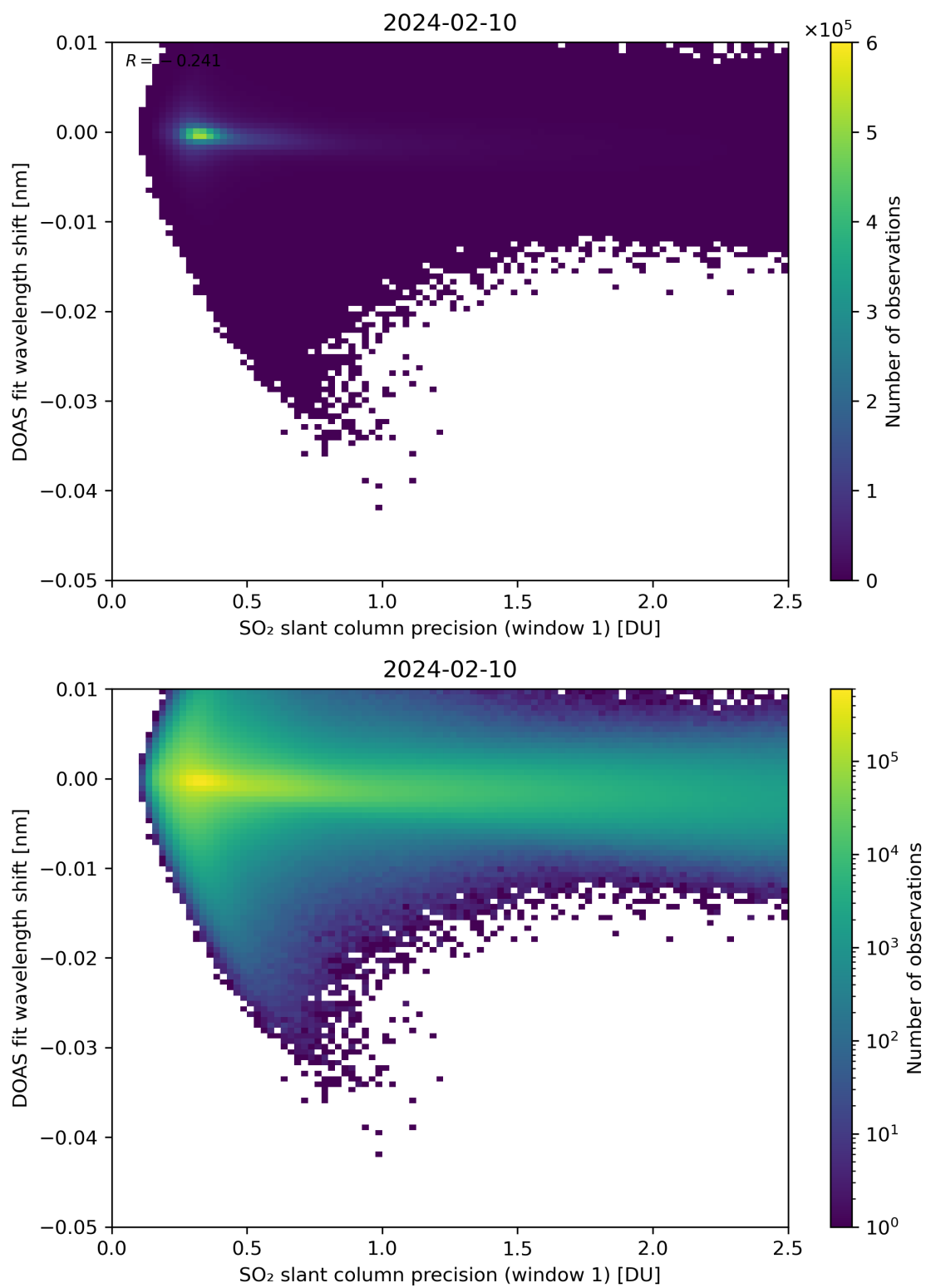
Figure 221: Scatter density plot of “SO 2 slant column precision (window 1)” against “DOAS fit wavelength shift” for 2024-02-09 to 2024-02-11.
