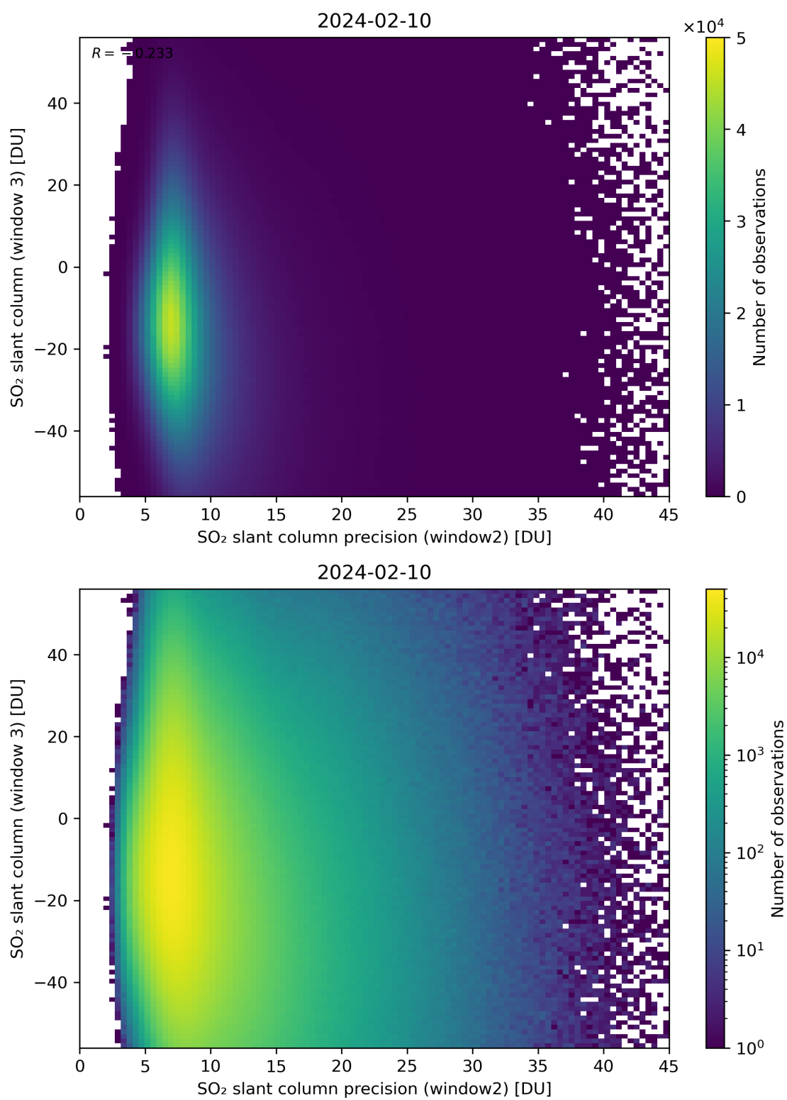
Figure 249: Scatter density plot of “SO 2 slant column precision (window2)” against “SO 2 slant column (window 3)” for 2024-02-09 to 2024-02-11.
