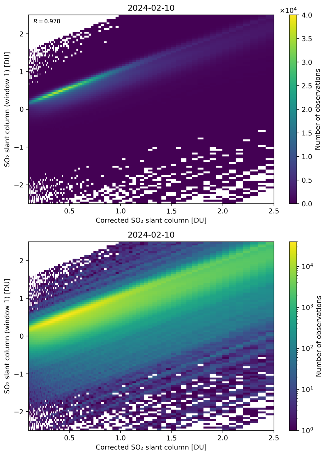
Figure 187: Scatter density plot of “Corrected SO 2 slant column” against “SO 2 slant column (window 1)” for 2024-02-09 to 2024-02-11.
