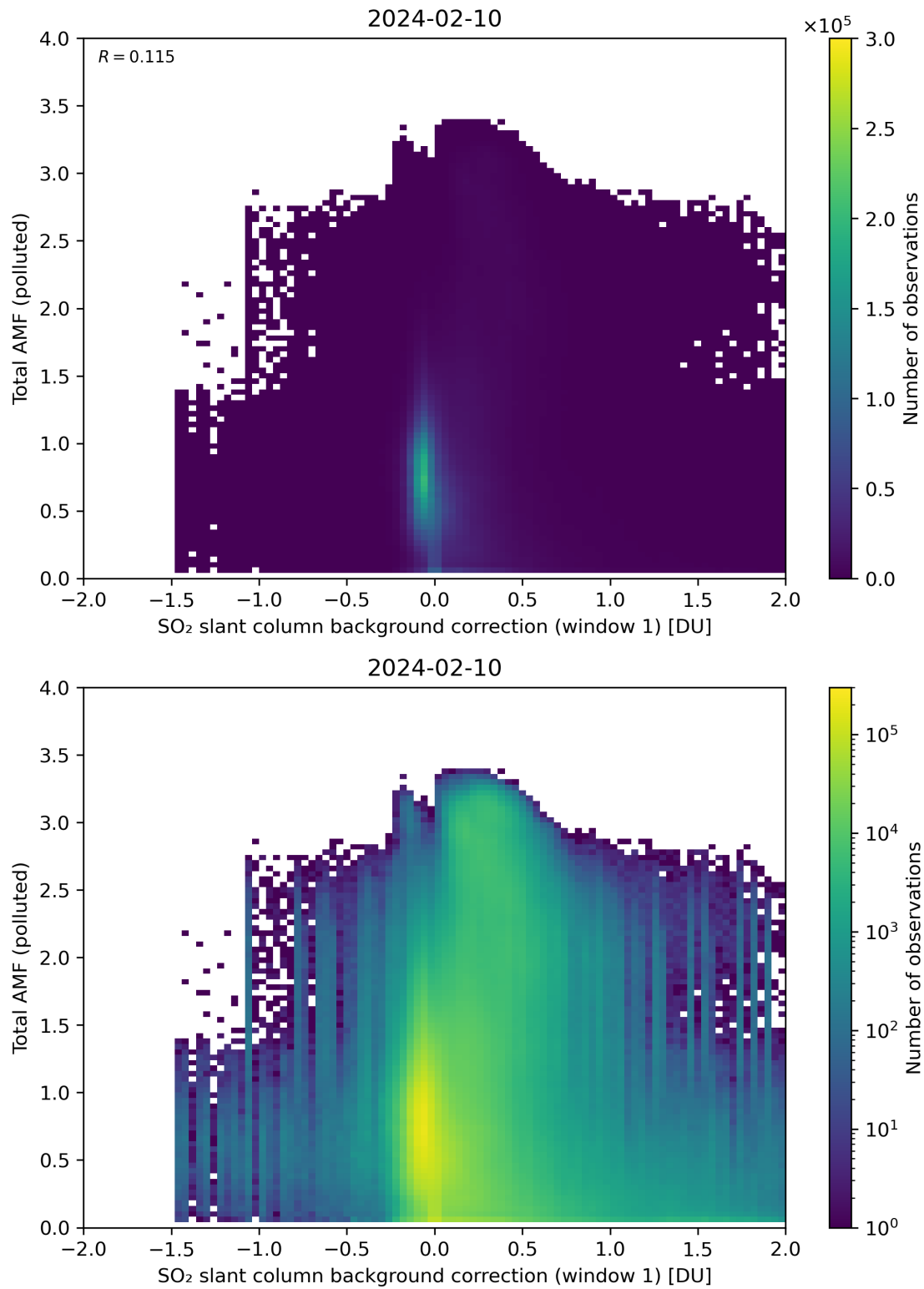
Figure 109: Scatter density plot of “SO 2 slant column background correction (window 1)” against “Total AMF (polluted)” for 2024-02-09 to 2024-02-11.
