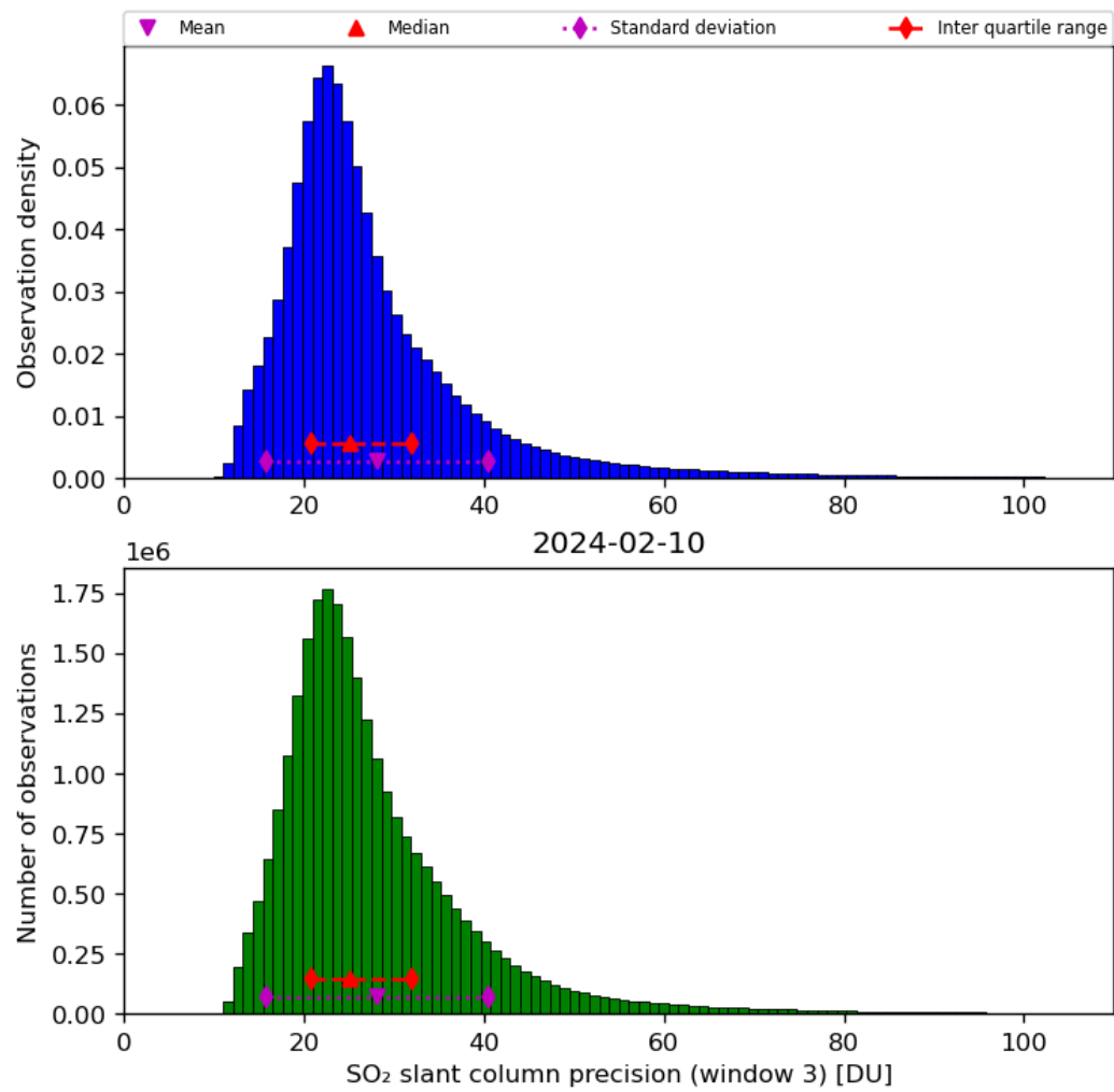
Figure 65: Histogram of “SO 2 slant column precision (window 3)” for 2024-02-09 to 2024-02-11
