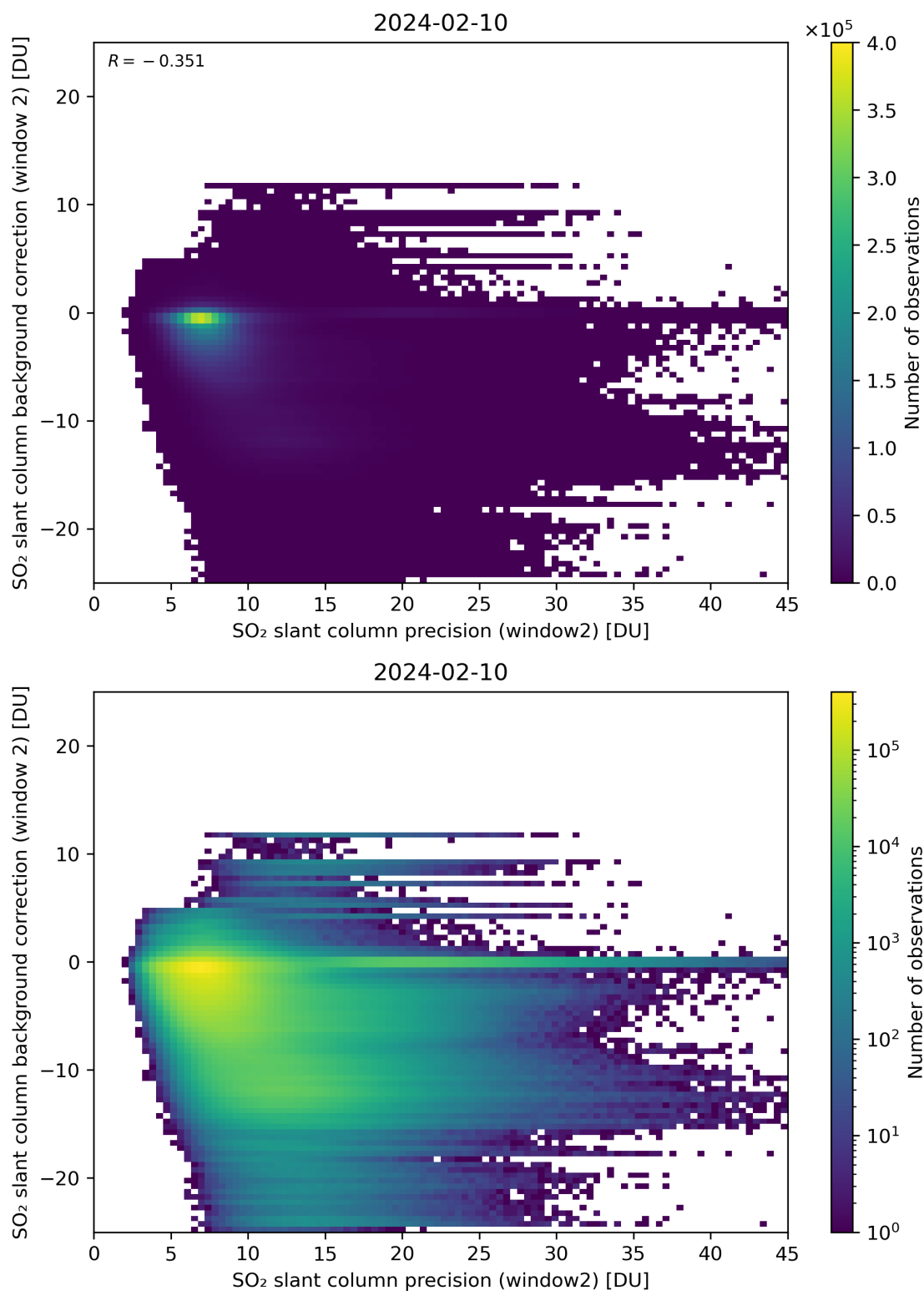
Figure 241: Scatter density plot of “SO 2 slant column precision (window2)” against “SO 2 slant column background correction (window 2)” for 2024-02-09 to 2024-02-11.
