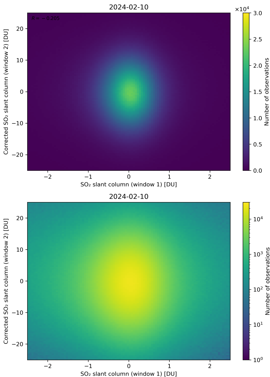
Figure 233: Scatter density plot of “SO 2 slant column (window 1)” against “Corrected SO 2 slant column (window 2)” for 2024-02-09 to 2024-02-11.
