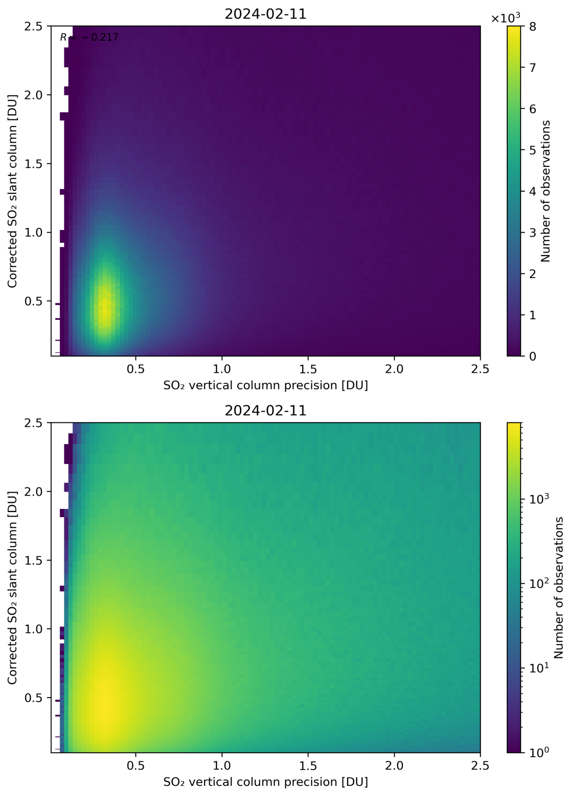
Figure 286: Scatter density plot of “SO 2 vertical column precision” against “Corrected SO 2 slant column” for 2024-02-11 to 2024-02-12.
