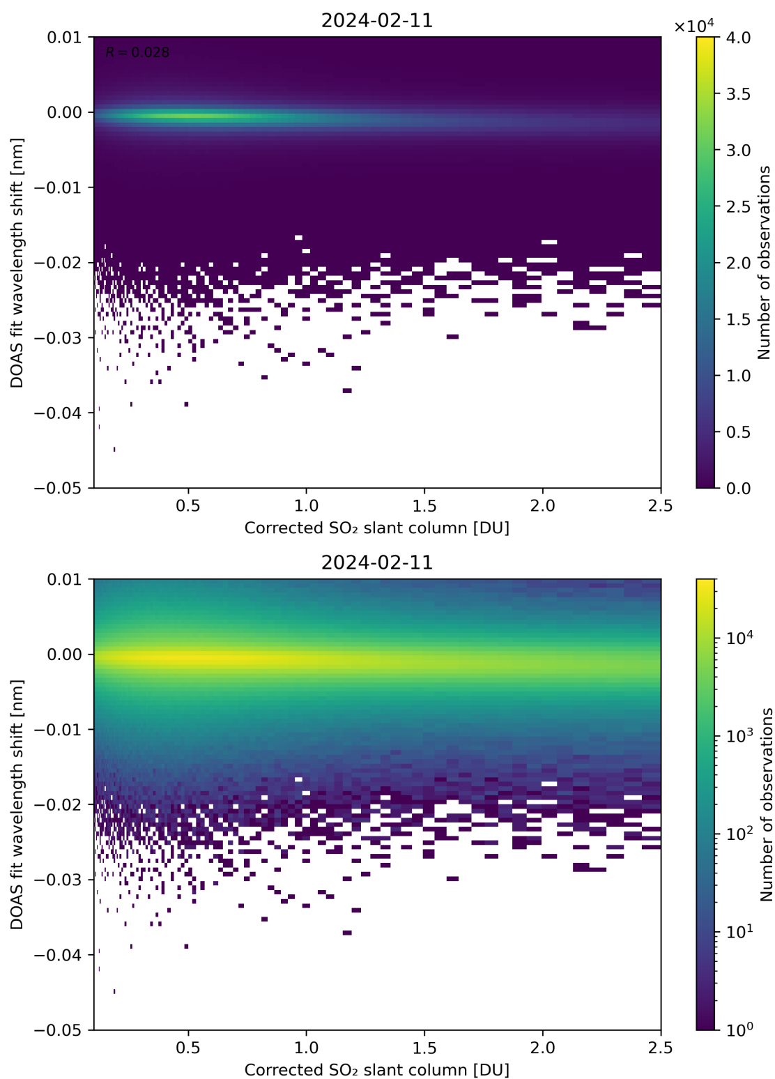
Figure 181: Scatter density plot of “Corrected SO 2 slant column” against “DOAS fit wavelength shift” for 2024-02-11 to 2024-02-12.
