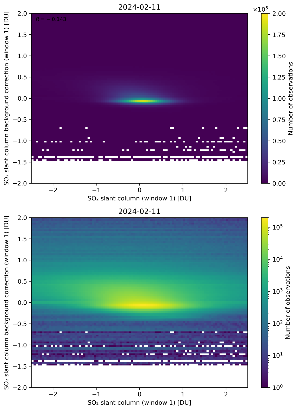
Figure 212: Scatter density plot of “SO 2 slant column (window 1)” against “SO 2 slant column background correction (window 1)” for 2024-02-11 to 2024-02-12.
