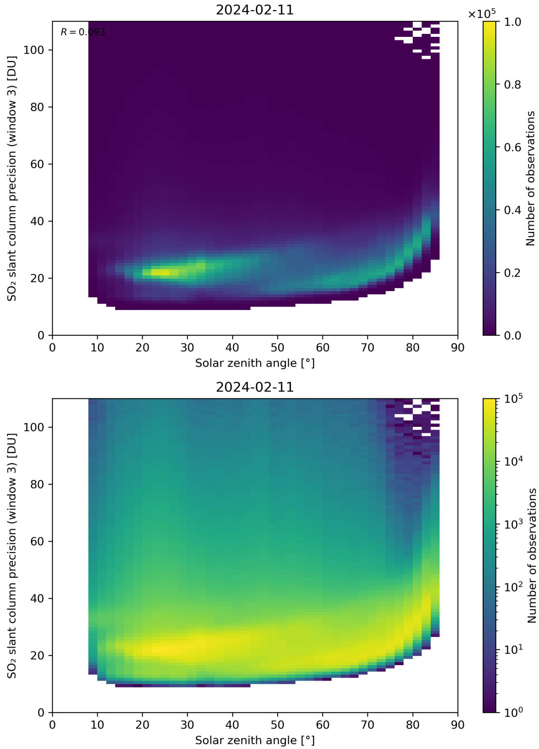
Figure 173: Scatter density plot of “Solar zenith angle” against “SO 2 slant column precision (window 3)” for 2024-02-11 to 2024-02-12.
