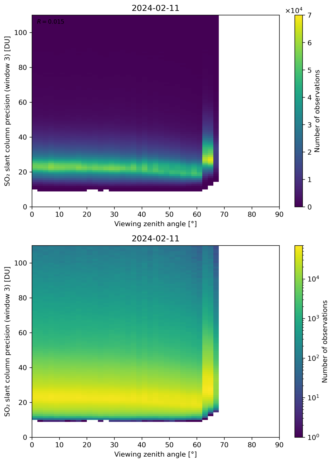
Figure 324: Scatter density plot of “Viewing zenith angle” against “SO 2 slant column precision (window 3)” for 2024-02-11 to 2024-02-12.
