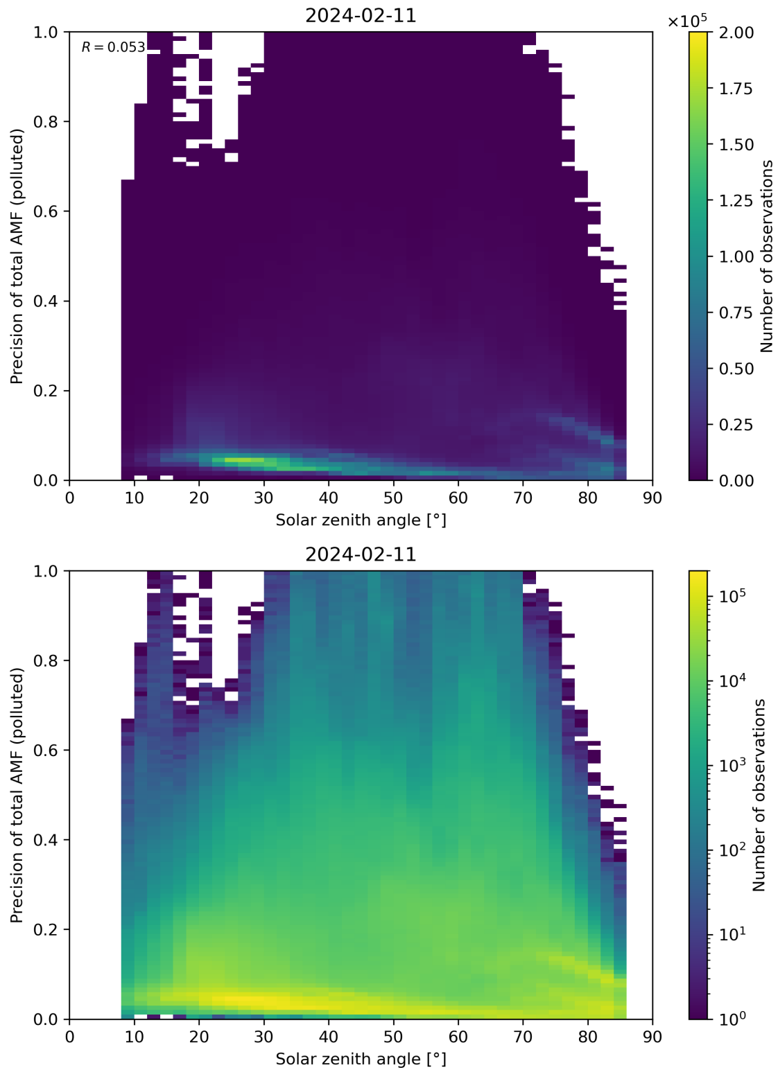
Figure 175: Scatter density plot of “Solar zenith angle” against “Precision of total AMF (polluted)” for 2024-02-11 to 2024-02-12.
