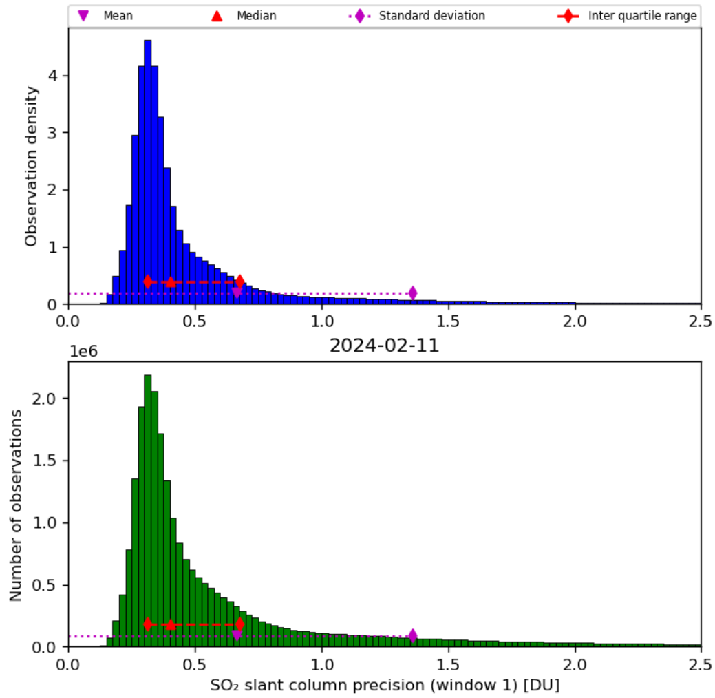
Figure 57: Histogram of “SO 2 slant column precision (window 1)” for 2024-02-11 to 2024-02-12
