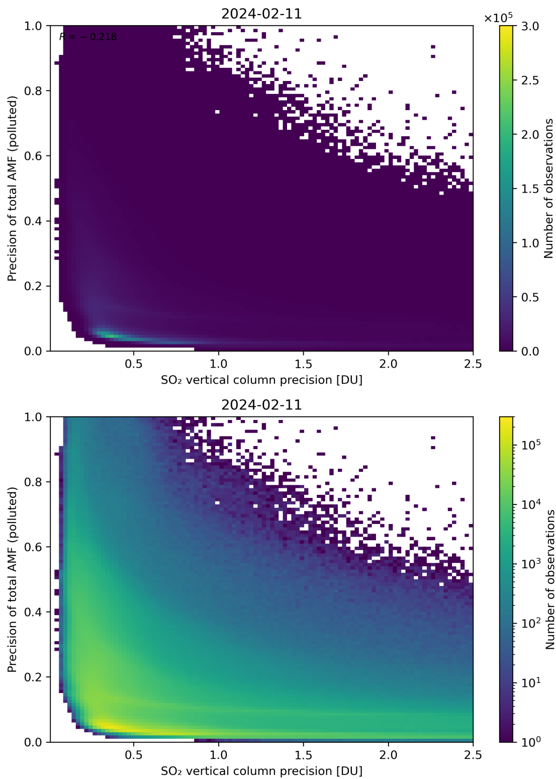
Figure 295: Scatter density plot of “SO 2 vertical column precision” against “Precision of total AMF (polluted)” for 2024-02-11 to 2024-02-12.
