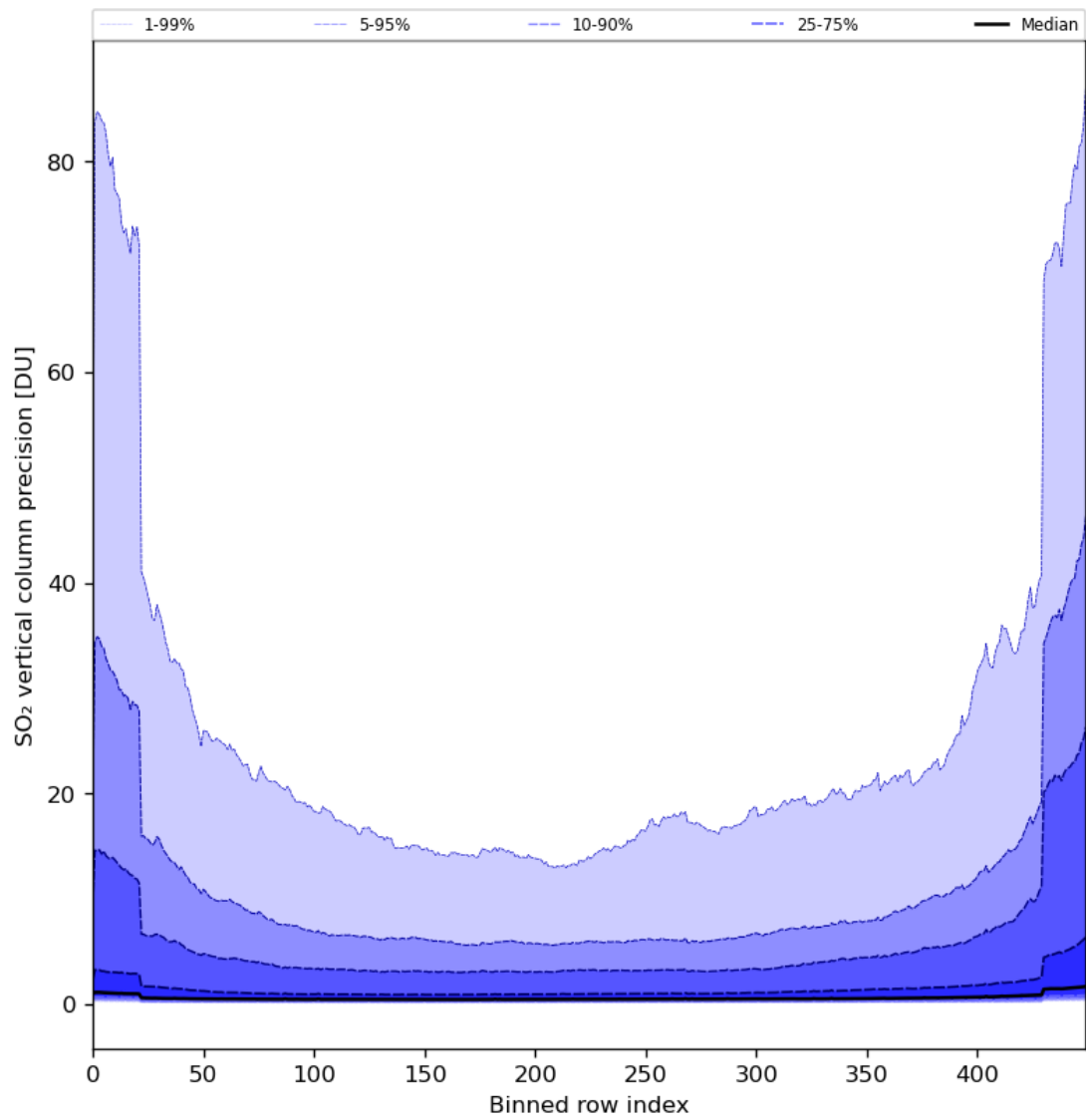
Figure 77: Along track statistics of “SO 2 vertical column precision” for 2024-02-11 to 2024-02-12
