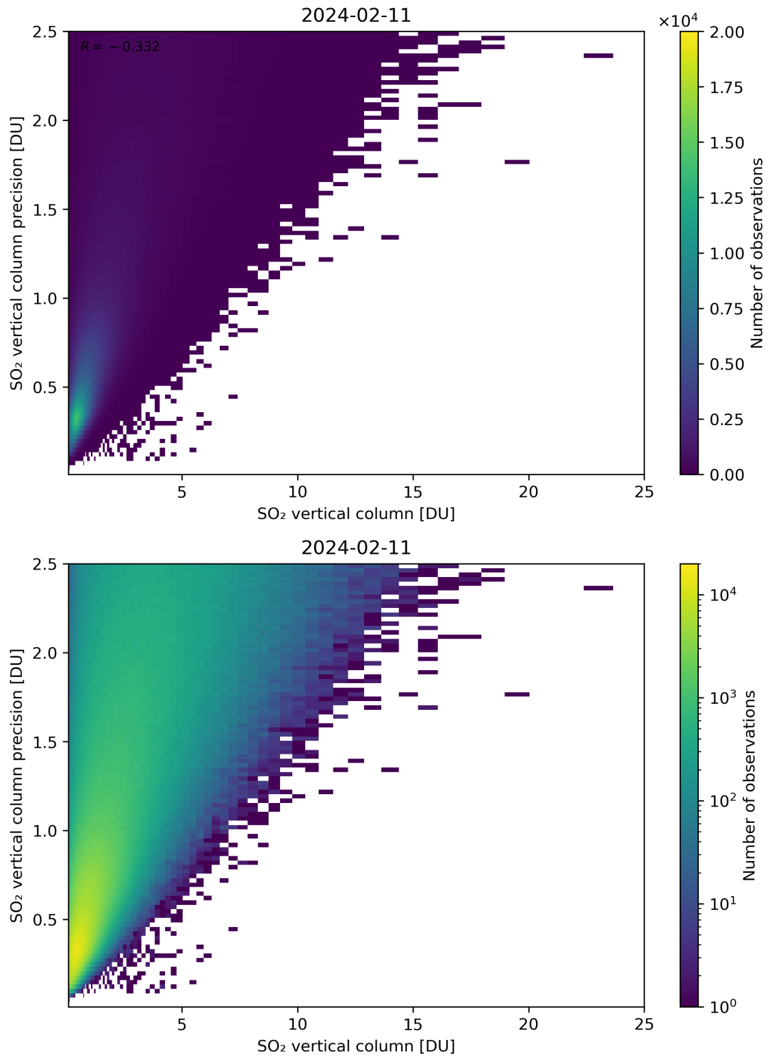
Figure 307: Scatter density plot of “SO 2 vertical column” against “SO 2 vertical column precision” for 2024-02-11 to 2024-02-12.
