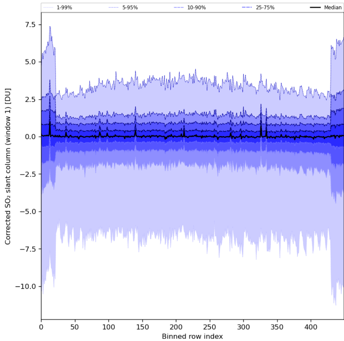
Figure 81: Along track statistics of “Corrected SO 2 slant column (window 1)” for 2024-02-11 to 2024-02-12
