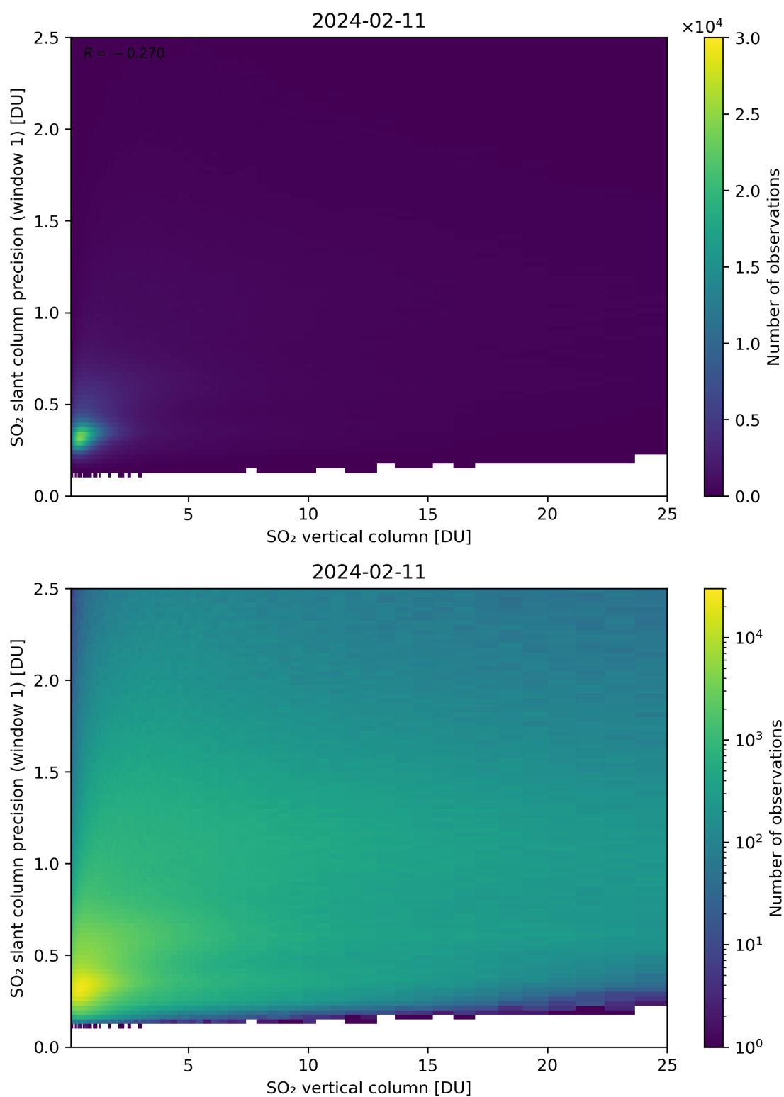
Figure 301: Scatter density plot of “SO 2 vertical column” against “SO 2 slant column precision (window 1)” for 2024-02-11 to 2024-02-12.
