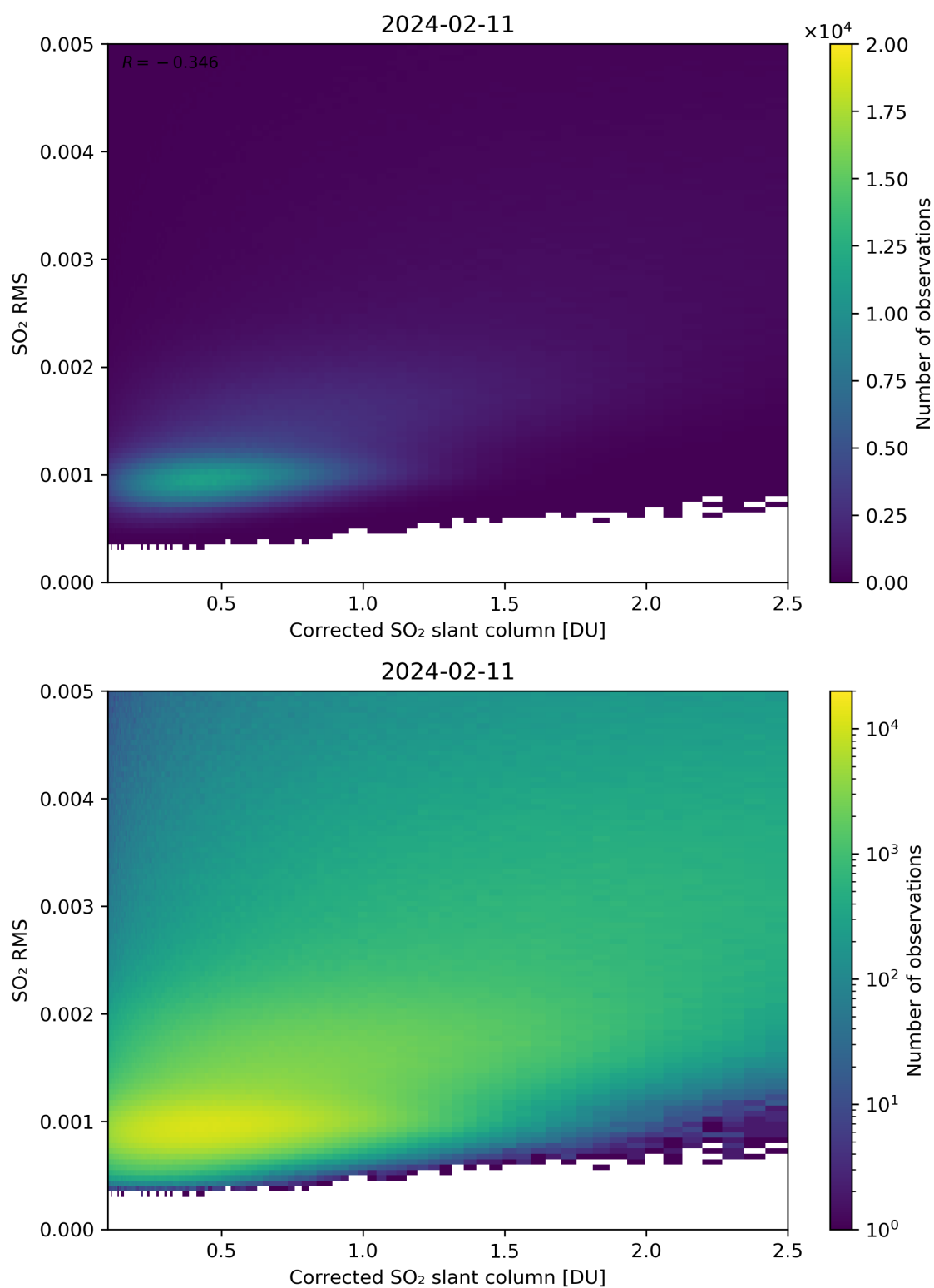
Figure 183: Scatter density plot of “Corrected SO 2 slant column” against “SO 2 RMS” for 2024-02-11 to 2024-02-12.
