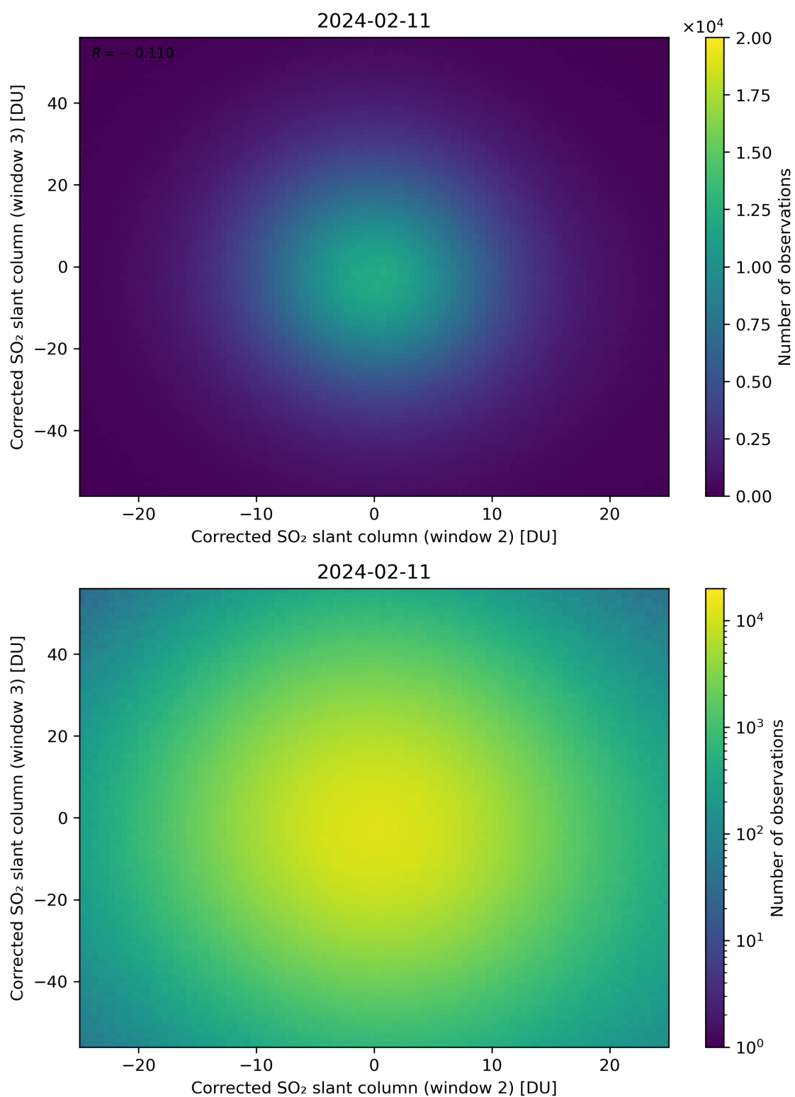
Figure 200: Scatter density plot of “Corrected SO 2 slant column (window 2)” against “Corrected SO 2 slant column (window 3)” for 2024-02-11 to 2024-02-12.
