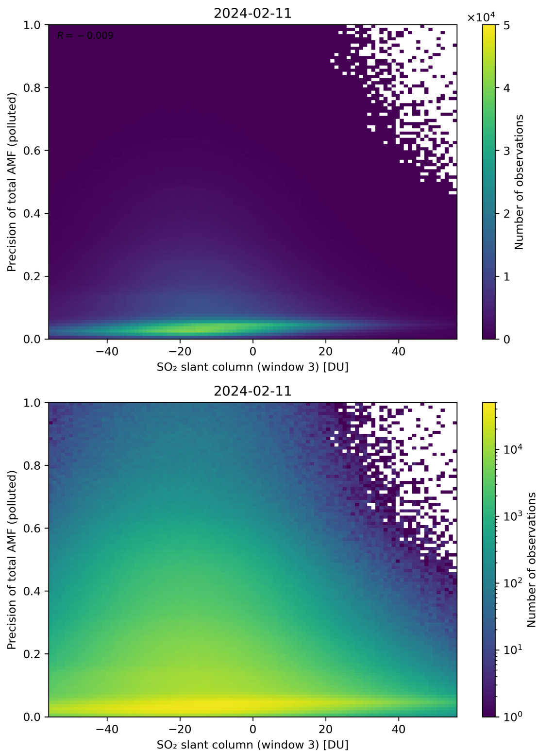
Figure 269: Scatter density plot of “SO 2 slant column (window 3)” against “Precision of total AMF (polluted)” for 2024-02-11 to 2024-02-12.
