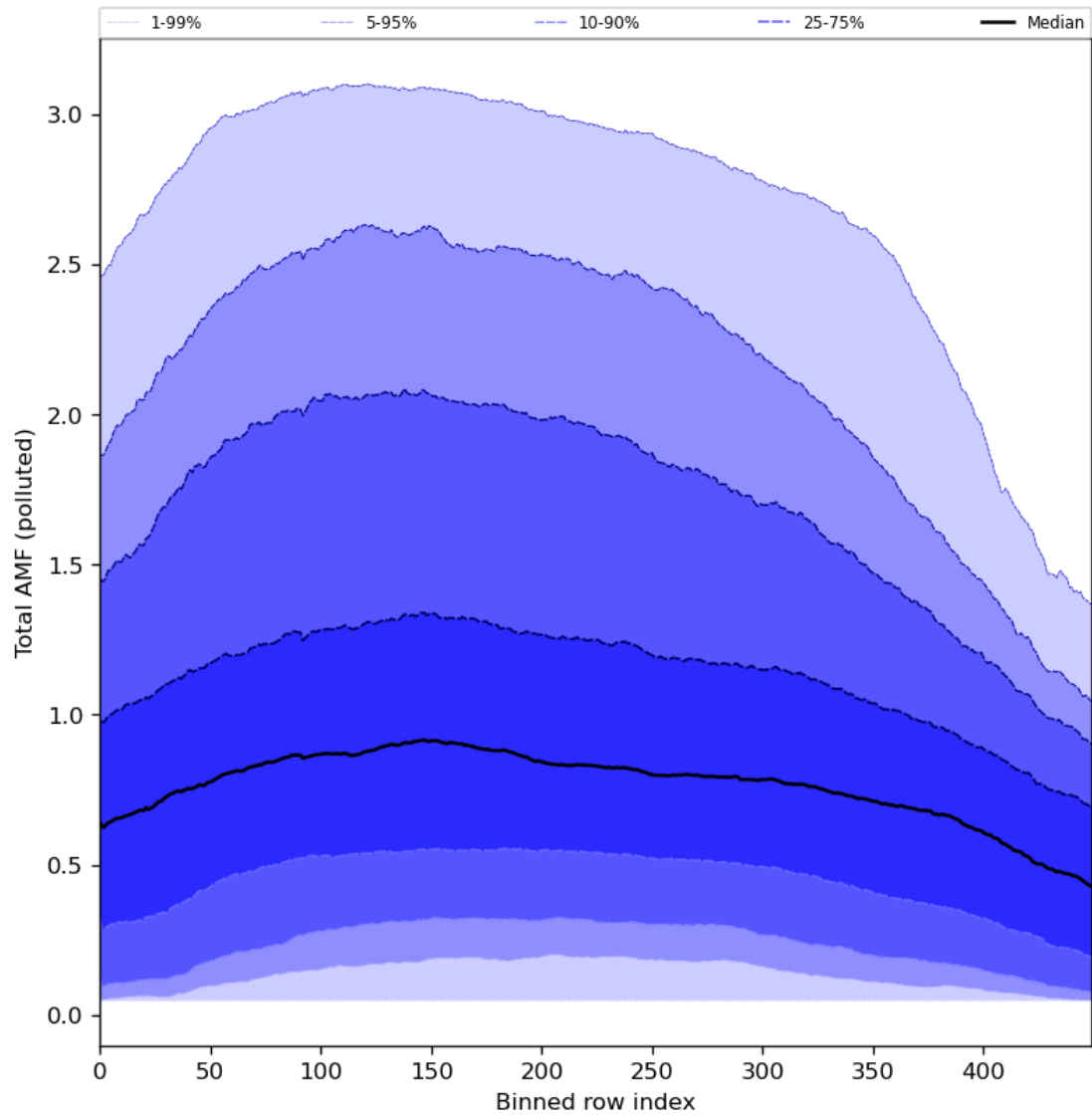
Figure 94: Along track statistics of “Total AMF (polluted)” for 2024-02-11 to 2024-02-12
