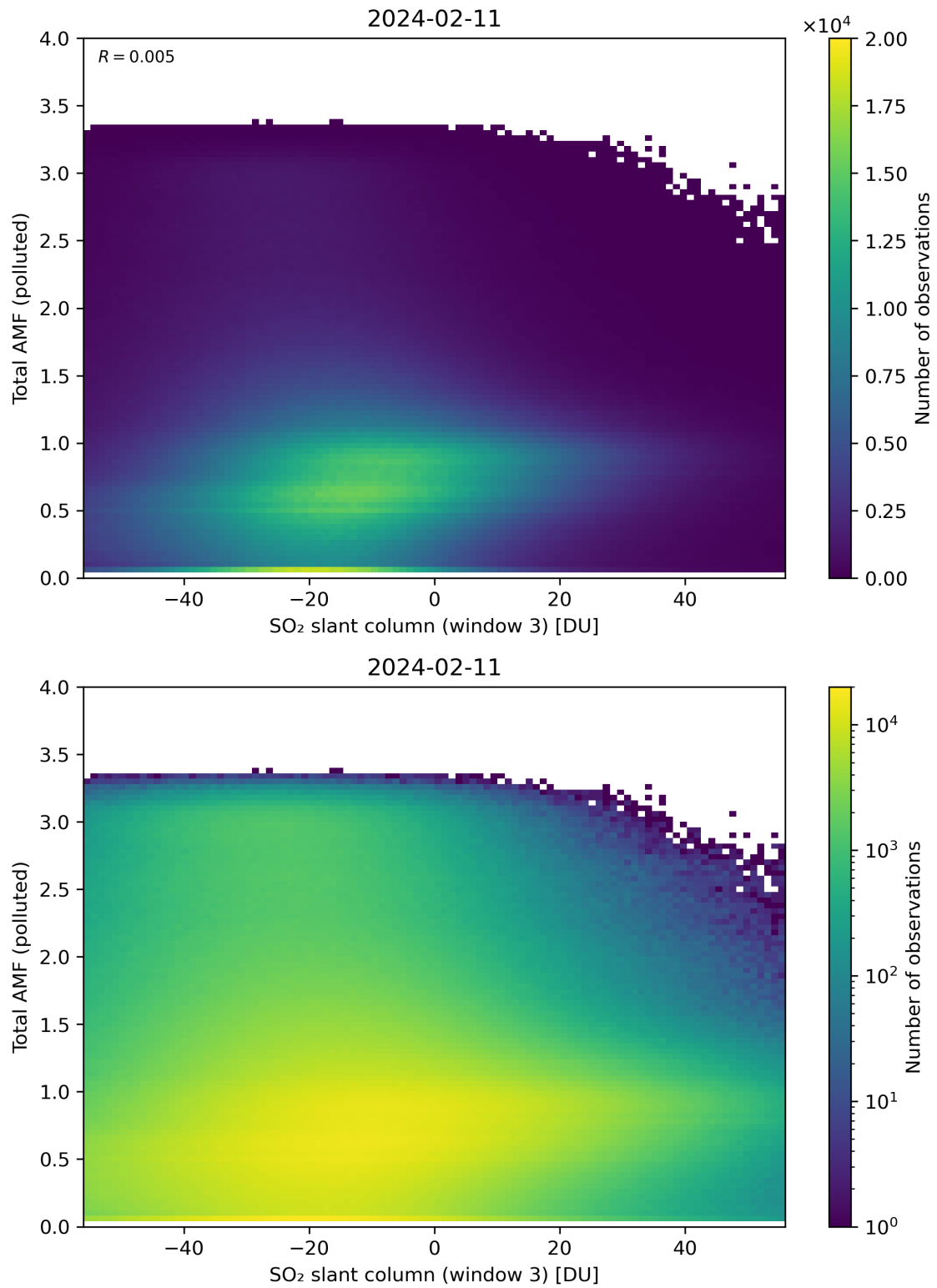
Figure 268: Scatter density plot of “SO 2 slant column (window 3)” against “Total AMF (polluted)” for 2024-02-11 to 2024-02-12.
