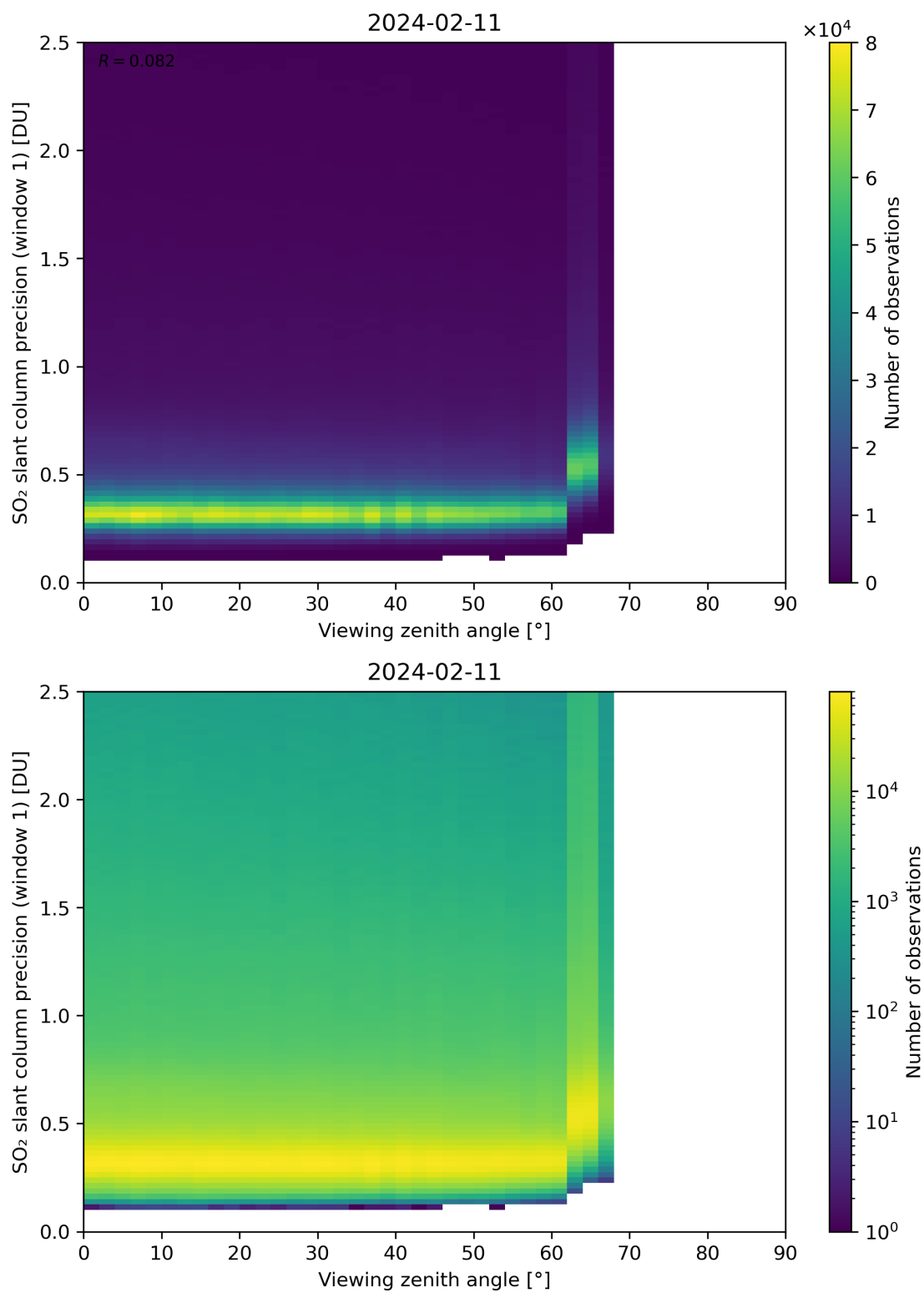
Figure 321: Scatter density plot of “Viewing zenith angle” against “SO 2 slant column precision (window 1)” for 2024-02-11 to 2024-02-12.
