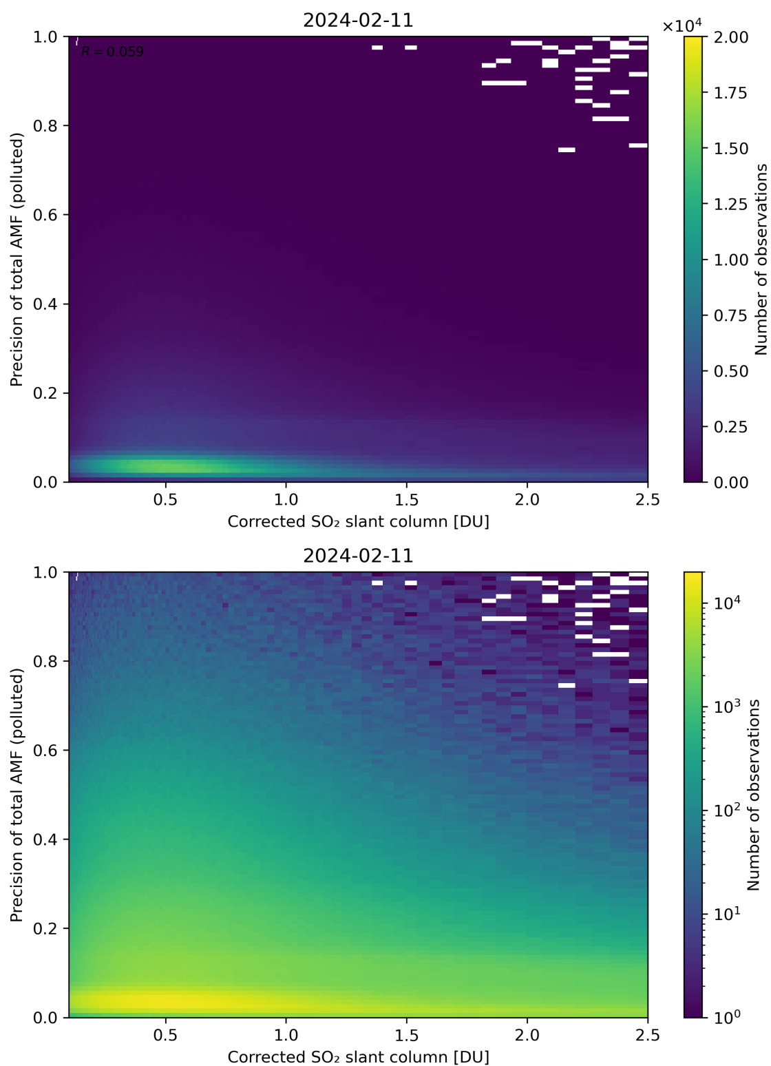
Figure 193: Scatter density plot of “Corrected SO 2 slant column” against “Precision of total AMF (polluted)” for 2024-02-11 to 2024-02-12.
