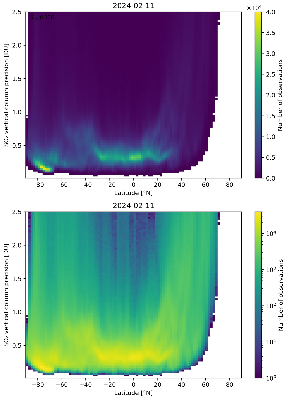
Figure 157: Scatter density plot of “Latitude” against “SO 2 vertical column precision” for 2024-02-11 to 2024-02-12.
