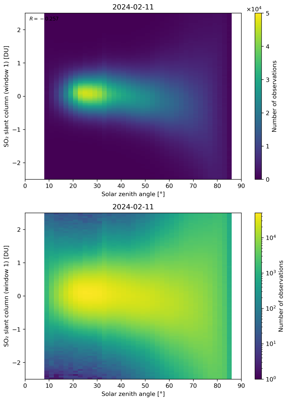
Figure 169: Scatter density plot of “Solar zenith angle” against “SO 2 slant column (window 1)” for 2024-02-11 to 2024-02-12.
