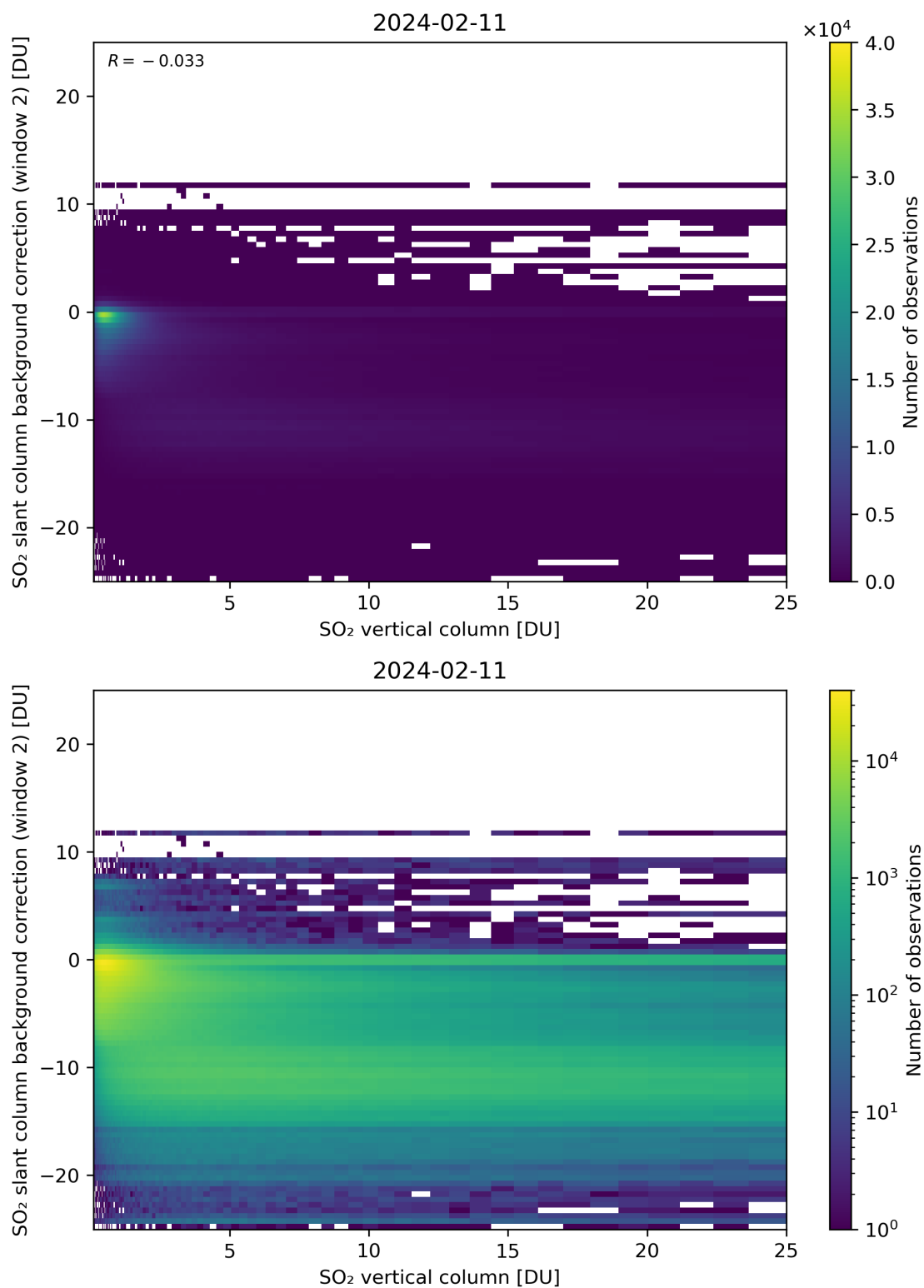
Figure 274: Scatter density plot of “SO 2 vertical column” against “SO 2 slant column background correction (window 2)” for 2024-02-11 to 2024-02-12.
