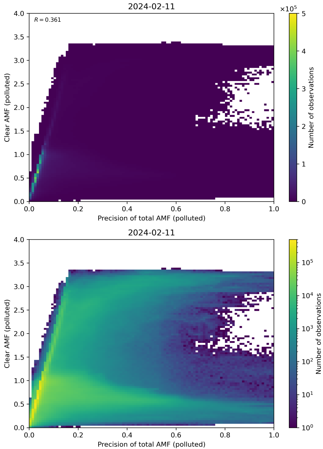
Figure 270: Scatter density plot of “Precision of total AMF (polluted)” against “Clear AMF (polluted)” for 2024-02-11 to 2024-02-12.
