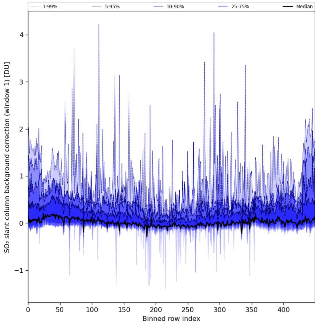
Figure 82: Along track statistics of “SO 2 slant column background correction (window 1)” for 2024-02-11 to 2024-02-12
