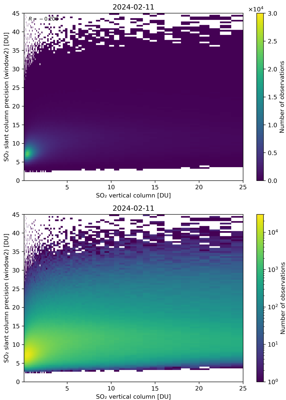
Figure 302: Scatter density plot of “SO 2 vertical column” against “SO 2 slant column precision (window2)” for 2024-02-11 to 2024-02-12.
