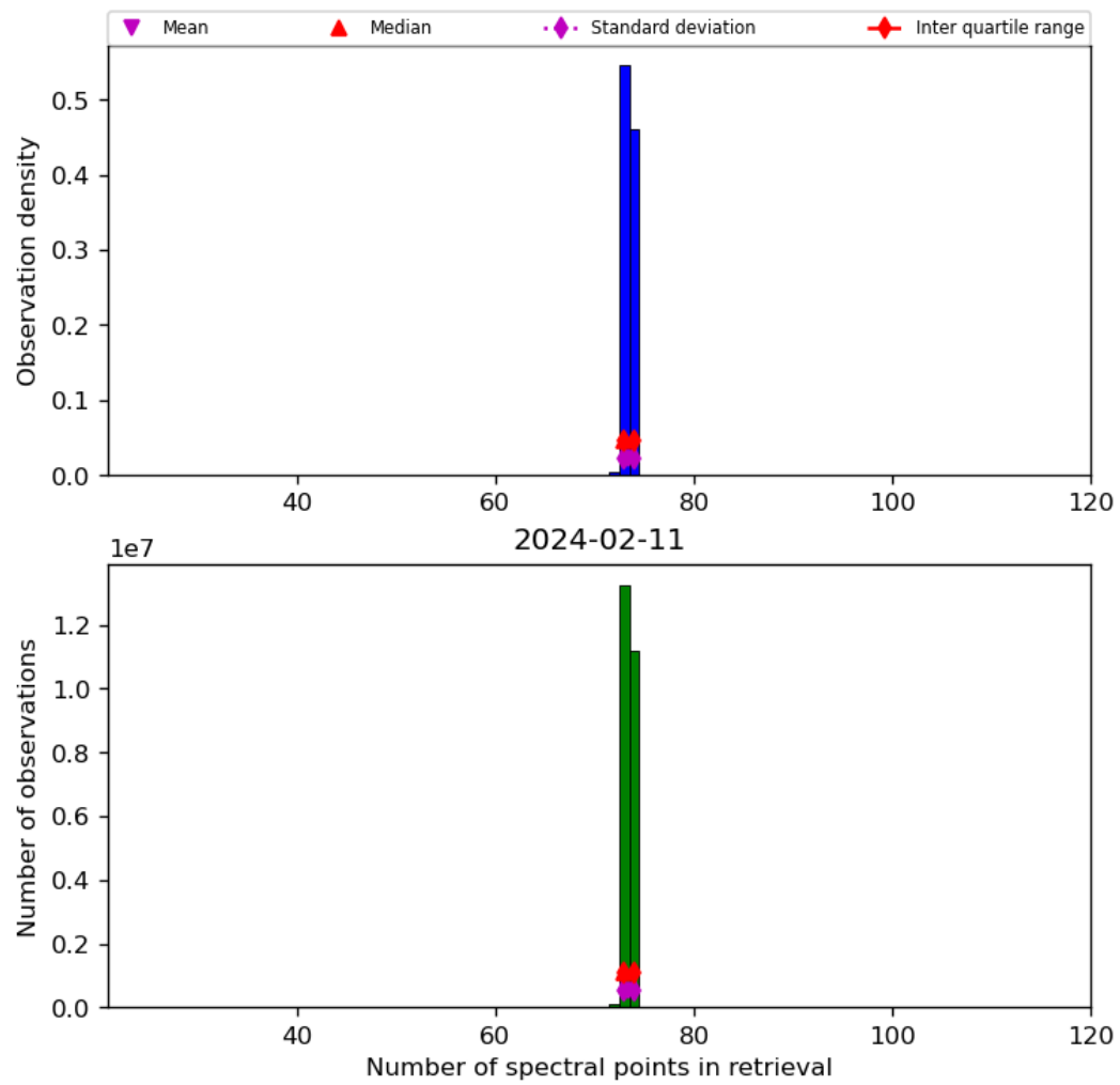
Figure 74: Histogram of “Number of spectral points in retrieval” for 2024-02-11 to 2024-02-12
