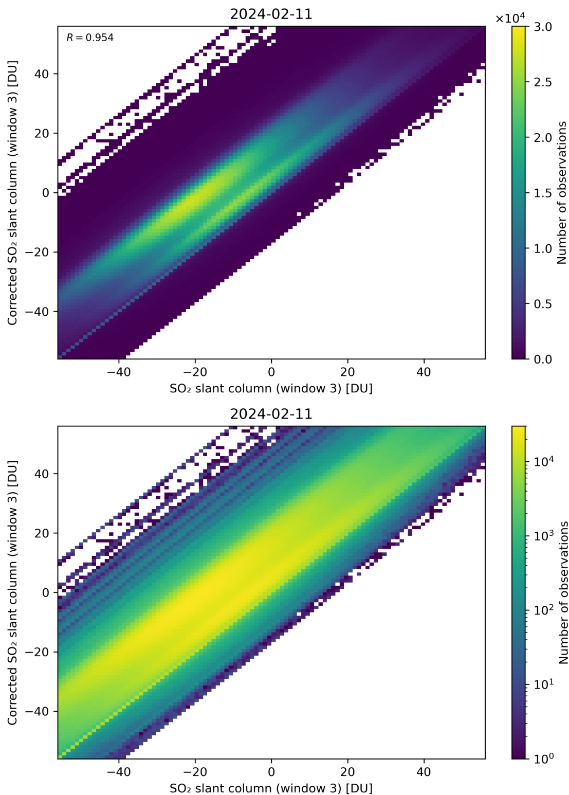
Figure 266: Scatter density plot of “SO 2 slant column (window 3)” against “Corrected SO 2 slant column (window 3)” for 2024-02-11 to 2024-02-12.
