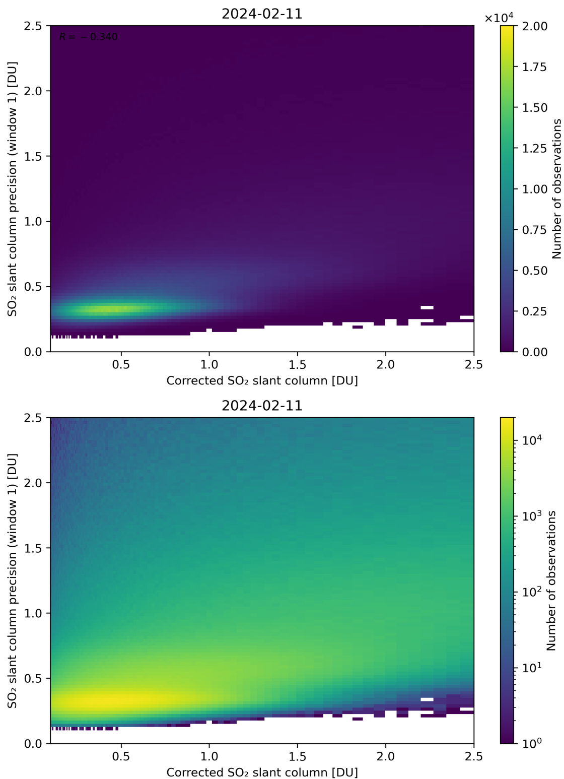
Figure 188: Scatter density plot of “Corrected SO 2 slant column” against “SO 2 slant column precision (window 1)” for 2024-02-11 to 2024-02-12.
