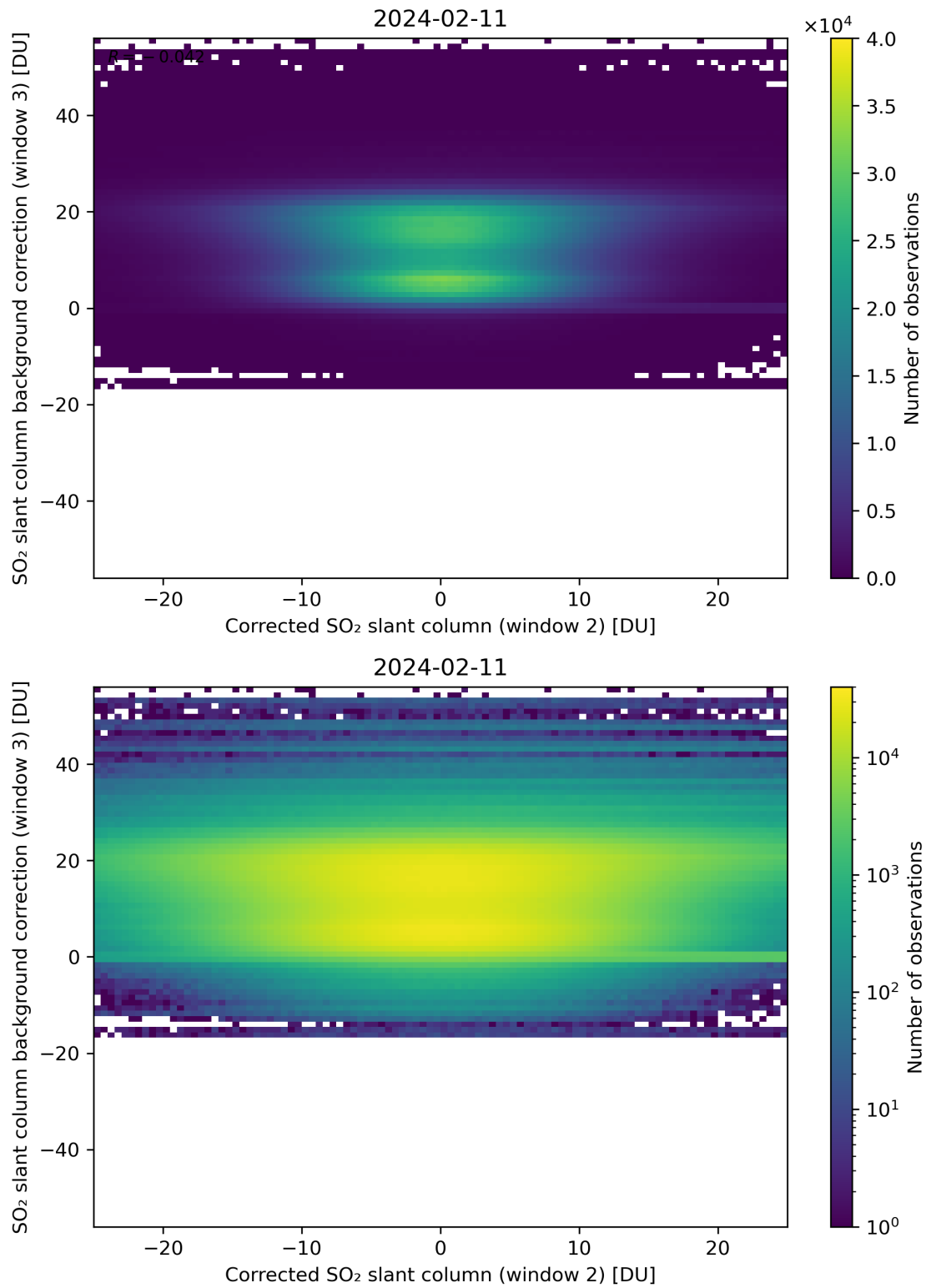
Figure 195: Scatter density plot of “Corrected SO 2 slant column (window 2)” against “SO 2 slant column background correction (window 3)” for 2024-02-11 to 2024-02-12.
