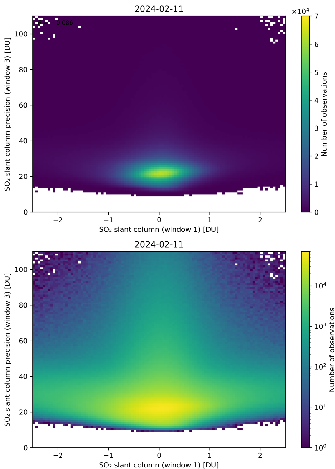
Figure 238: Scatter density plot of “SO 2 slant column (window 1)” against “SO 2 slant column precision (window 3)” for 2024-02-11 to 2024-02-12.
