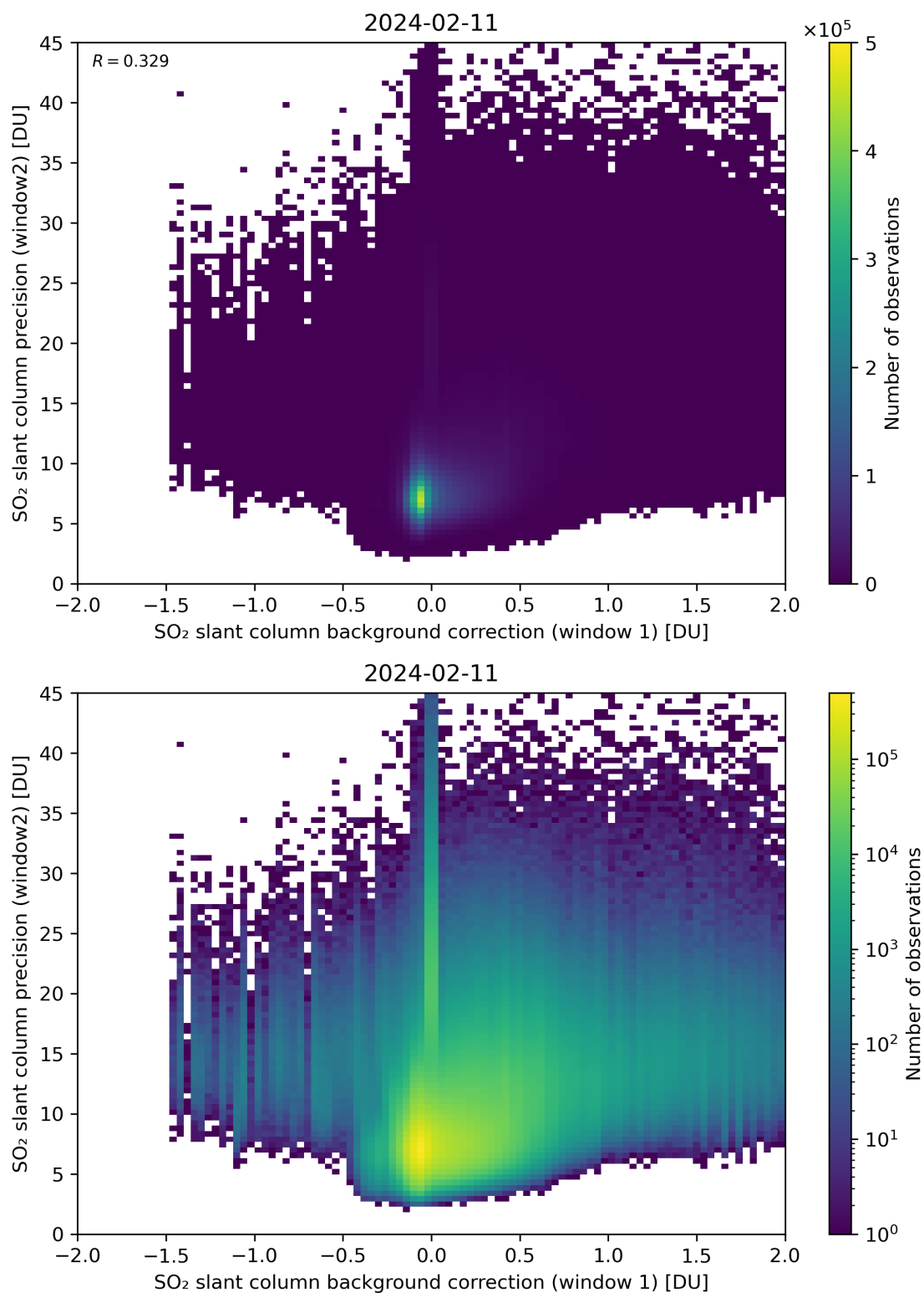
Figure 106: Scatter density plot of “SO 2 slant column background correction (window 1)” against “SO 2 slant column precision (window2)” for 2024-02-11 to 2024-02-12.
