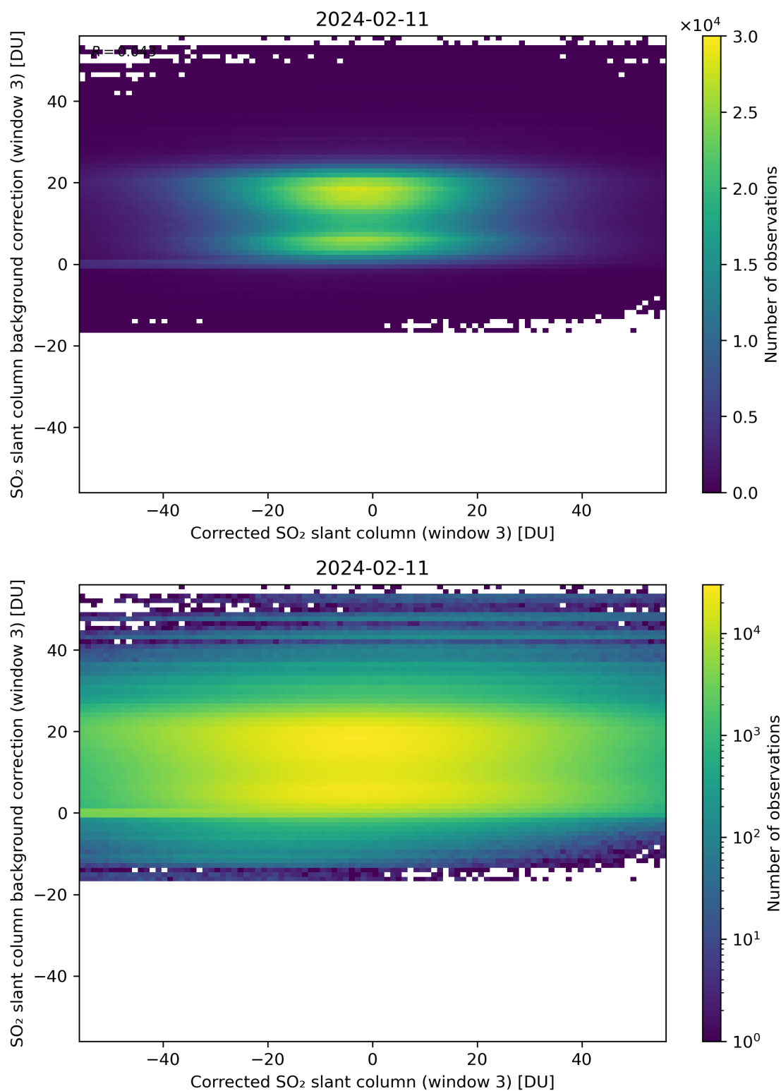
Figure 205: Scatter density plot of “Corrected SO 2 slant column (window 3)” against “SO 2 slant column background correction (window 3)” for 2024-02-11 to 2024-02-12.
