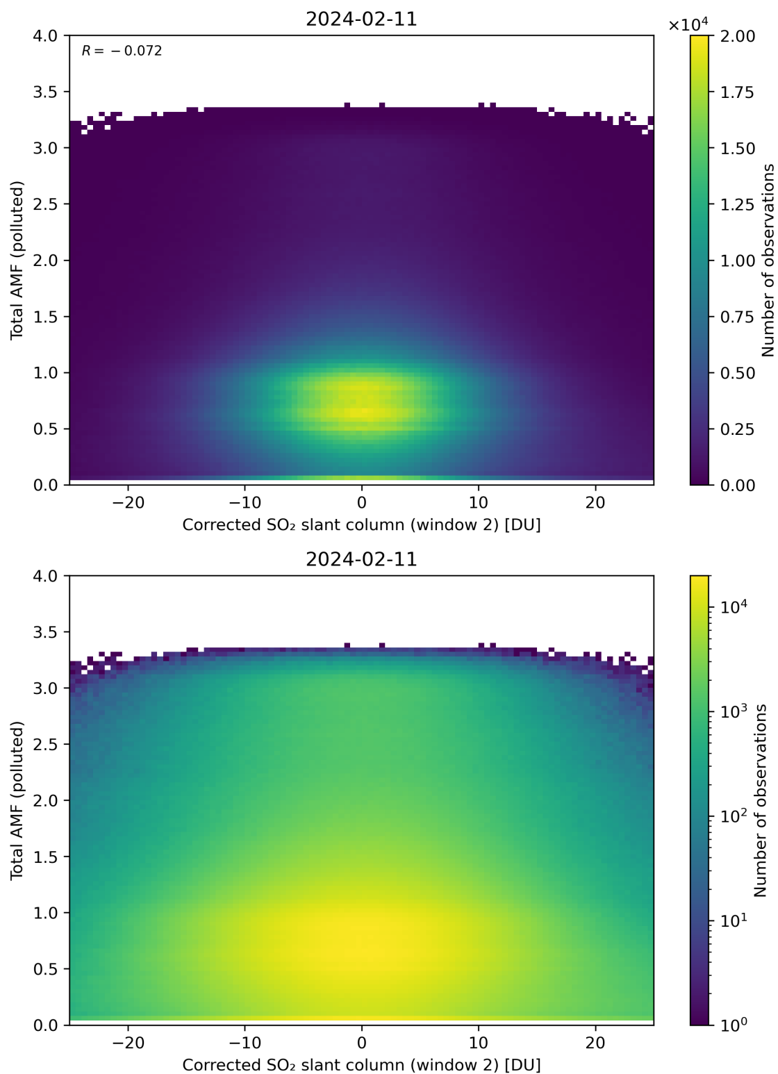
Figure 203: Scatter density plot of “Corrected SO 2 slant column (window 2)” against “Total AMF (polluted)” for 2024-02-11 to 2024-02-12.
