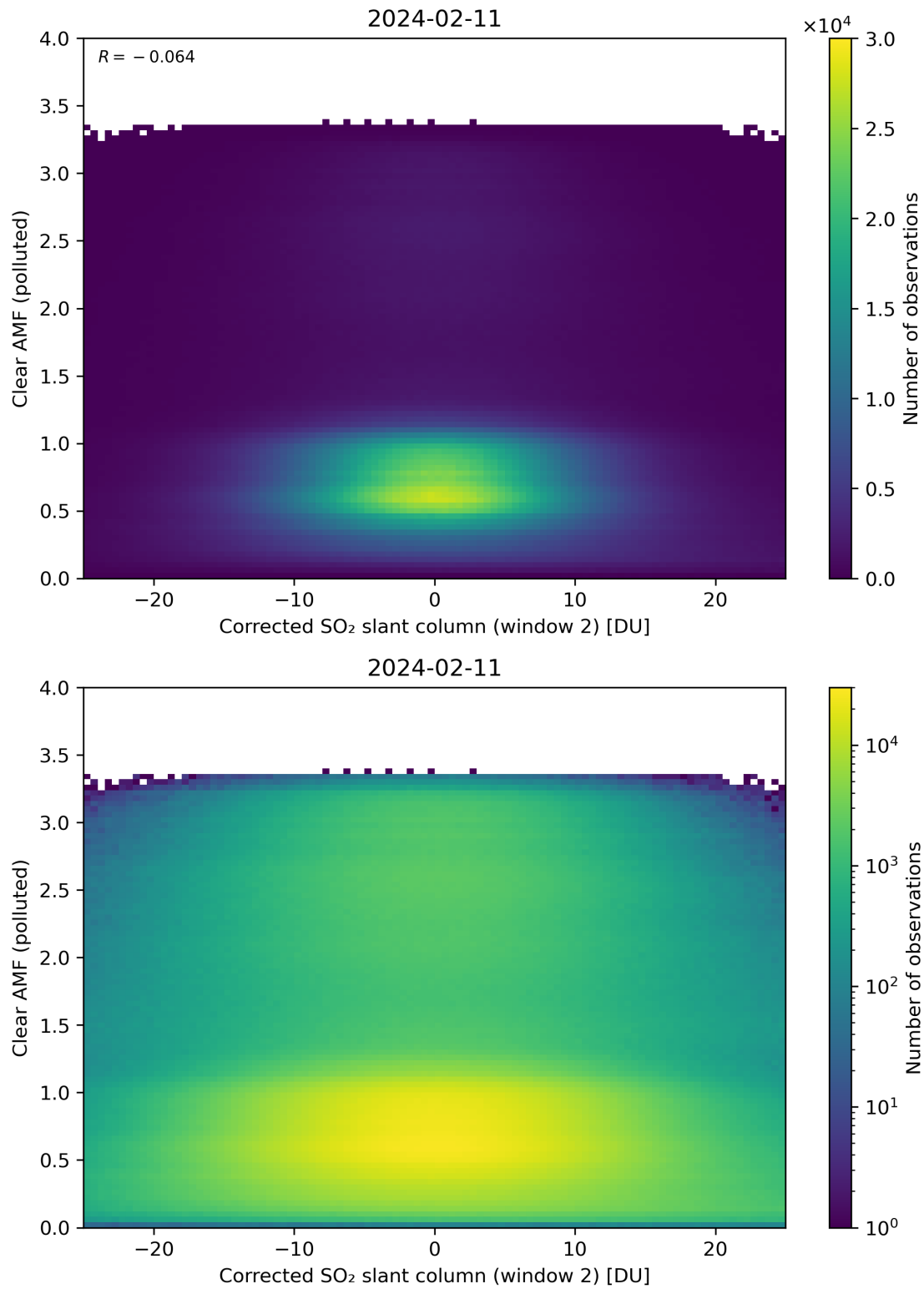
Figure 199: Scatter density plot of “Corrected SO 2 slant column (window 2)” against “Clear AMF (polluted)” for 2024-02-11 to 2024-02-12.
