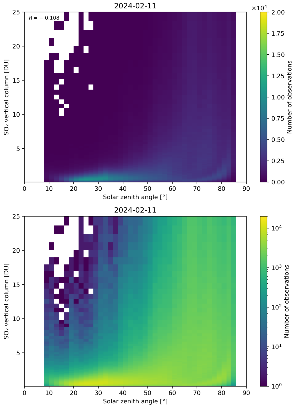
Figure 176: Scatter density plot of “Solar zenith angle” against “SO 2 vertical column” for 2024-02-11 to 2024-02-12.
