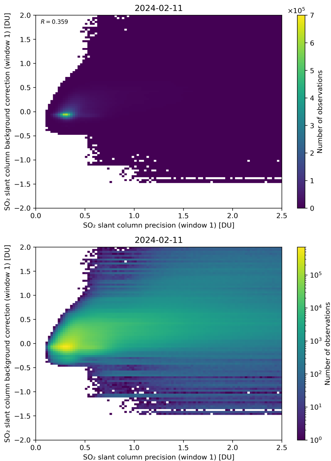
Figure 218: Scatter density plot of “SO 2 slant column precision (window 1)” against “SO 2 slant column background correction (window 1)” for 2024-02-11 to 2024-02-12.
