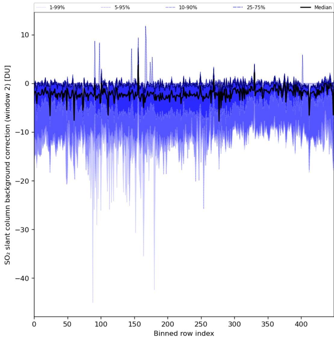
Figure 86: Along track statistics of “SO 2 slant column background correction (window 2)” for 2024-02-11 to 2024-02-12
