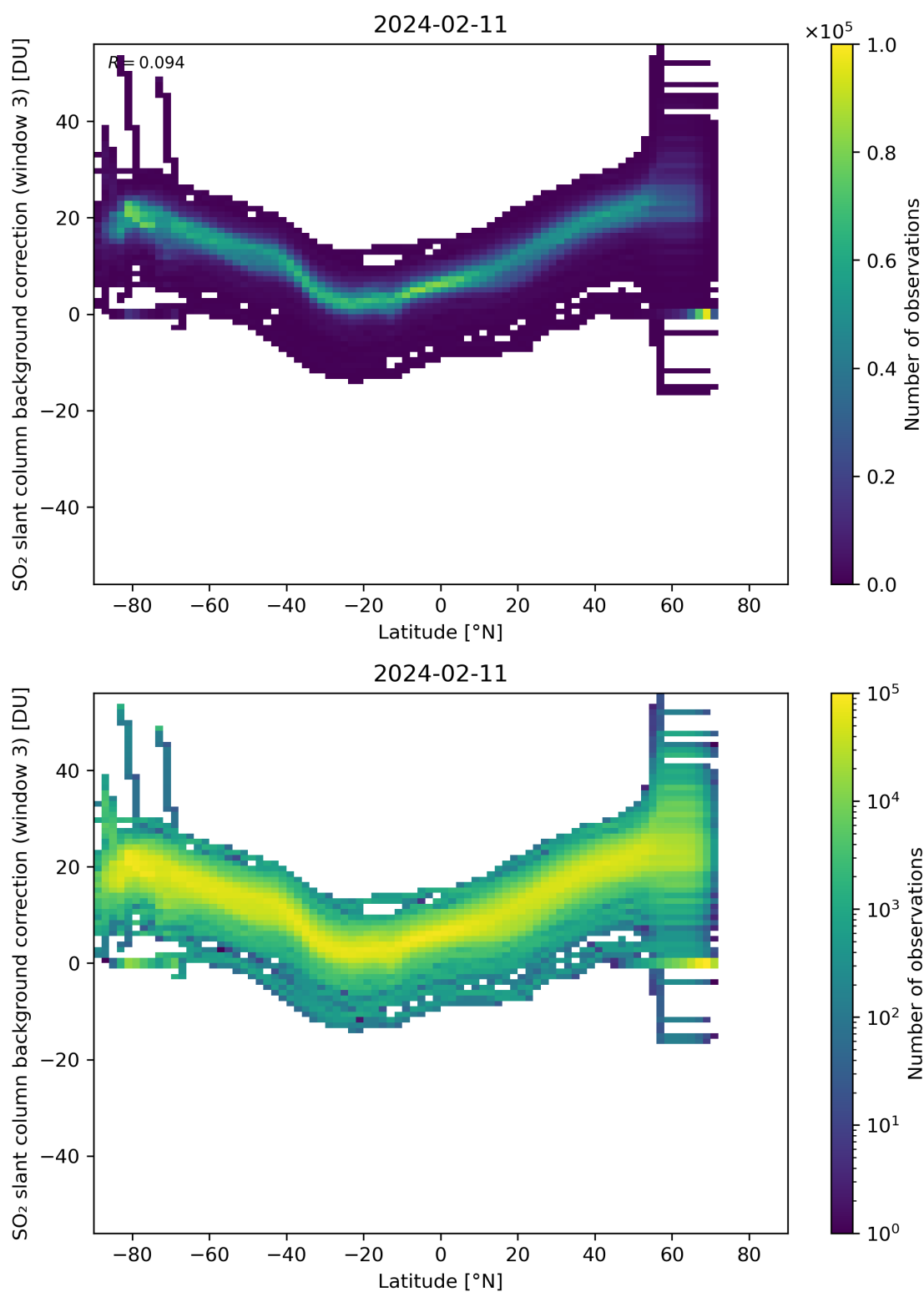
Figure 141: Scatter density plot of “Latitude” against “SO 2 slant column background correction (window 3)” for 2024-02-11 to 2024-02-12.
