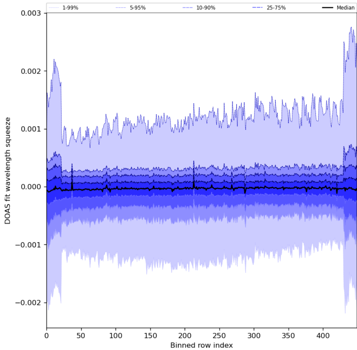
Figure 92: Along track statistics of “DOAS fit wavelength squeeze” for 2024-02-11 to 2024-02-12
