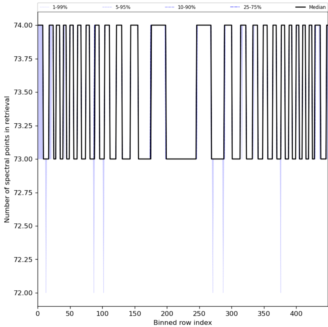
Figure 97: Along track statistics of “Number of spectral points in retrieval” for 2024-02-11 to 2024-02-12
