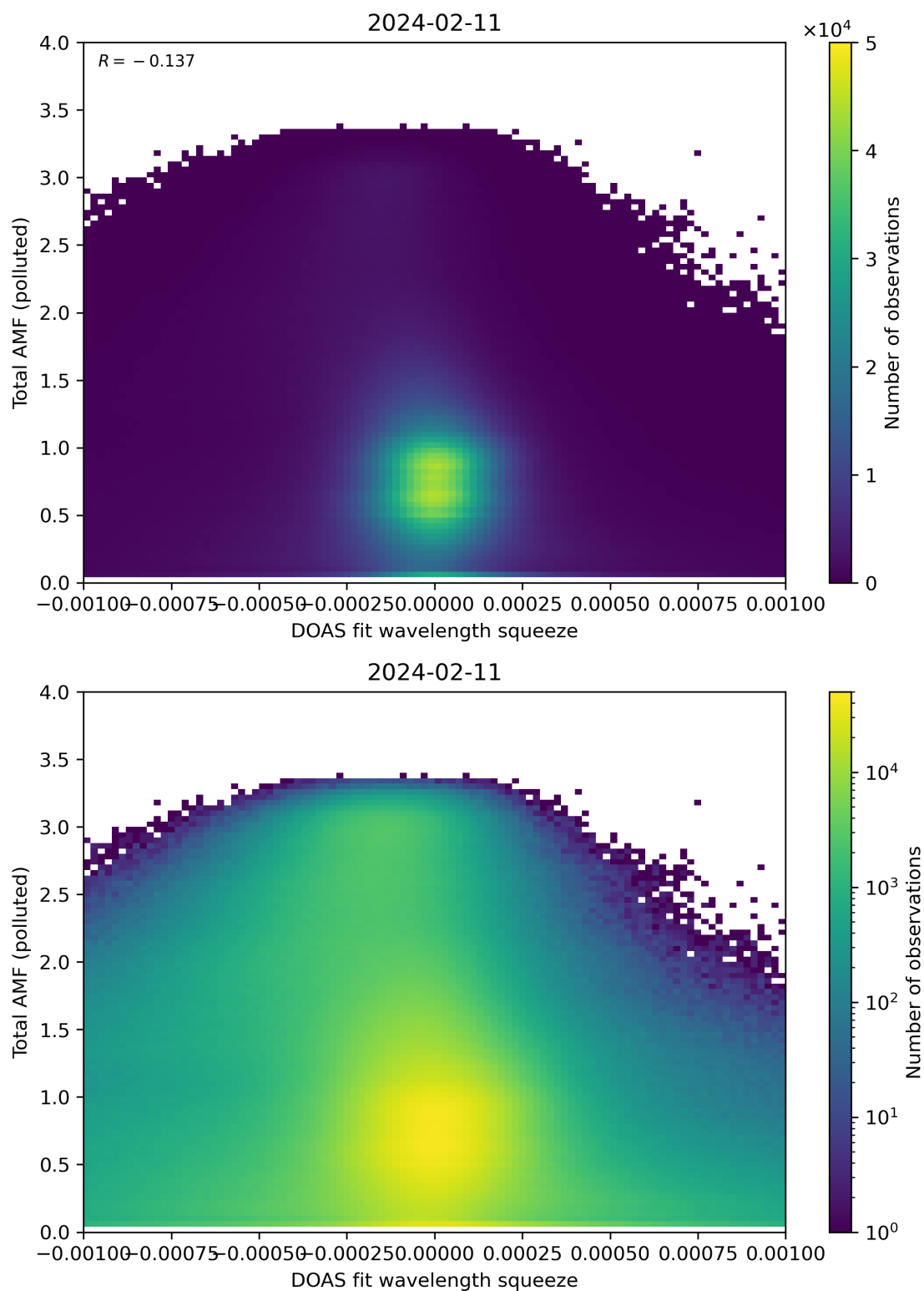
Figure 134: Scatter density plot of “DOAS fit wavelength squeeze” against “Total AMF (polluted)” for 2024-02-11 to 2024-02-12.
