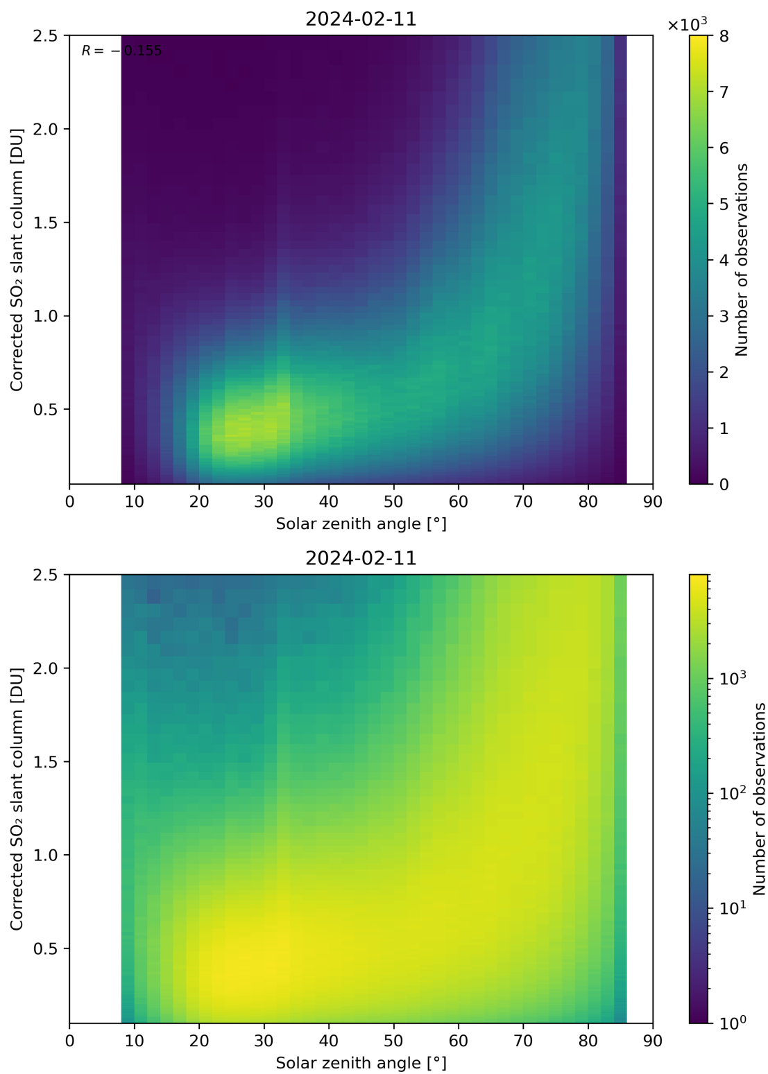
Figure 166: Scatter density plot of “Solar zenith angle” against “Corrected SO 2 slant column” for 2024-02-11 to 2024-02-12.
