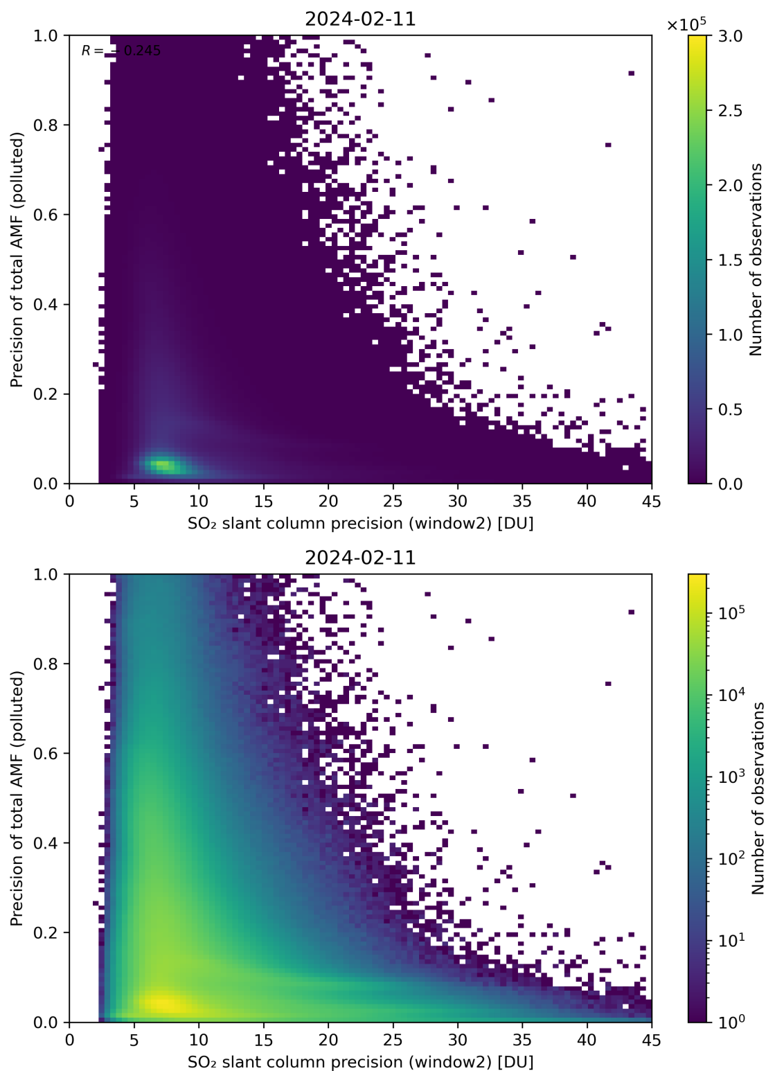
Figure 252: Scatter density plot of “SO 2 slant column precision (window2)” against “Precision of total AMF (polluted)” for 2024-02-11 to 2024-02-12.
