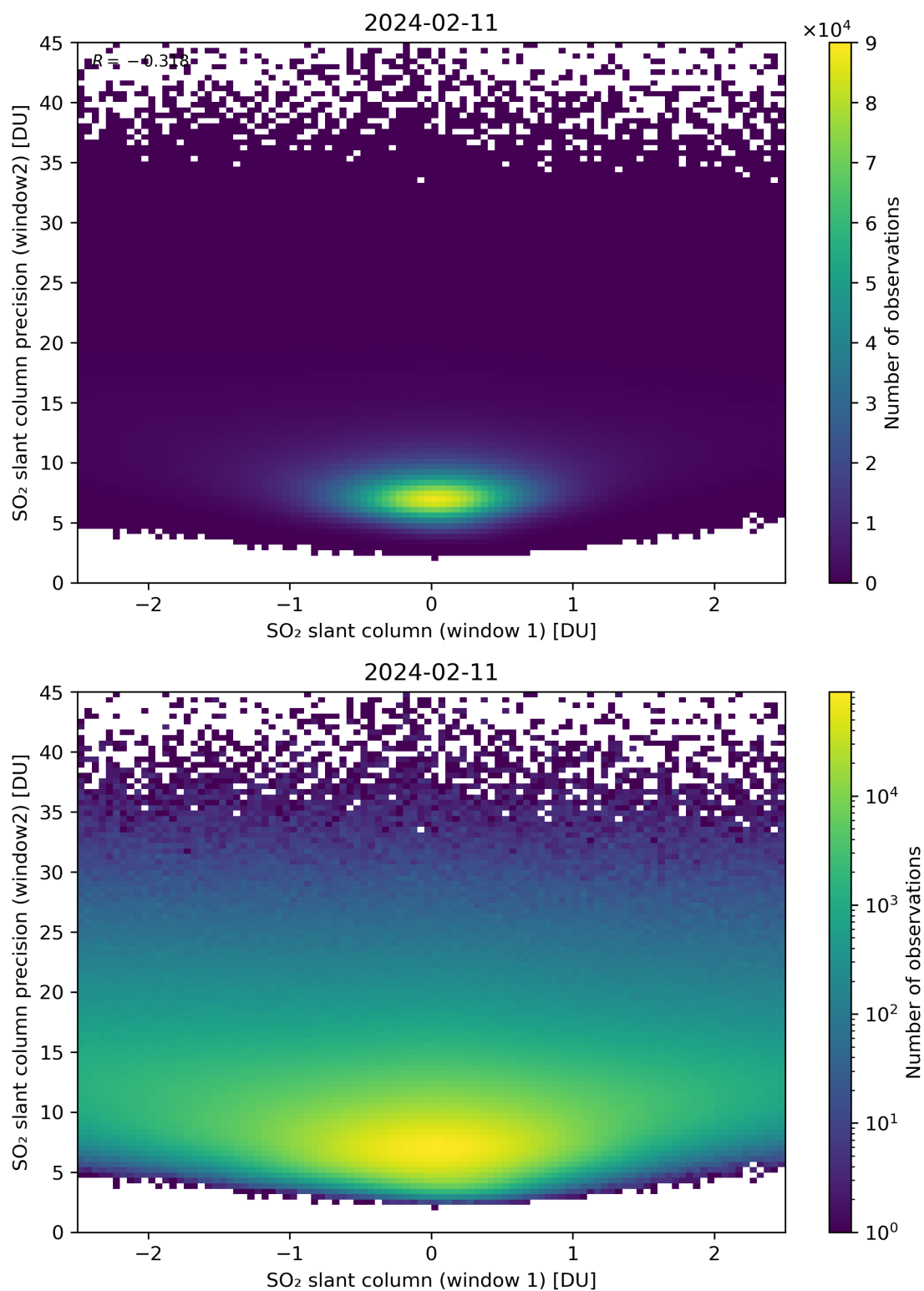
Figure 236: Scatter density plot of “SO 2 slant column (window 1)” against “SO 2 slant column precision (window2)” for 2024-02-11 to 2024-02-12.
