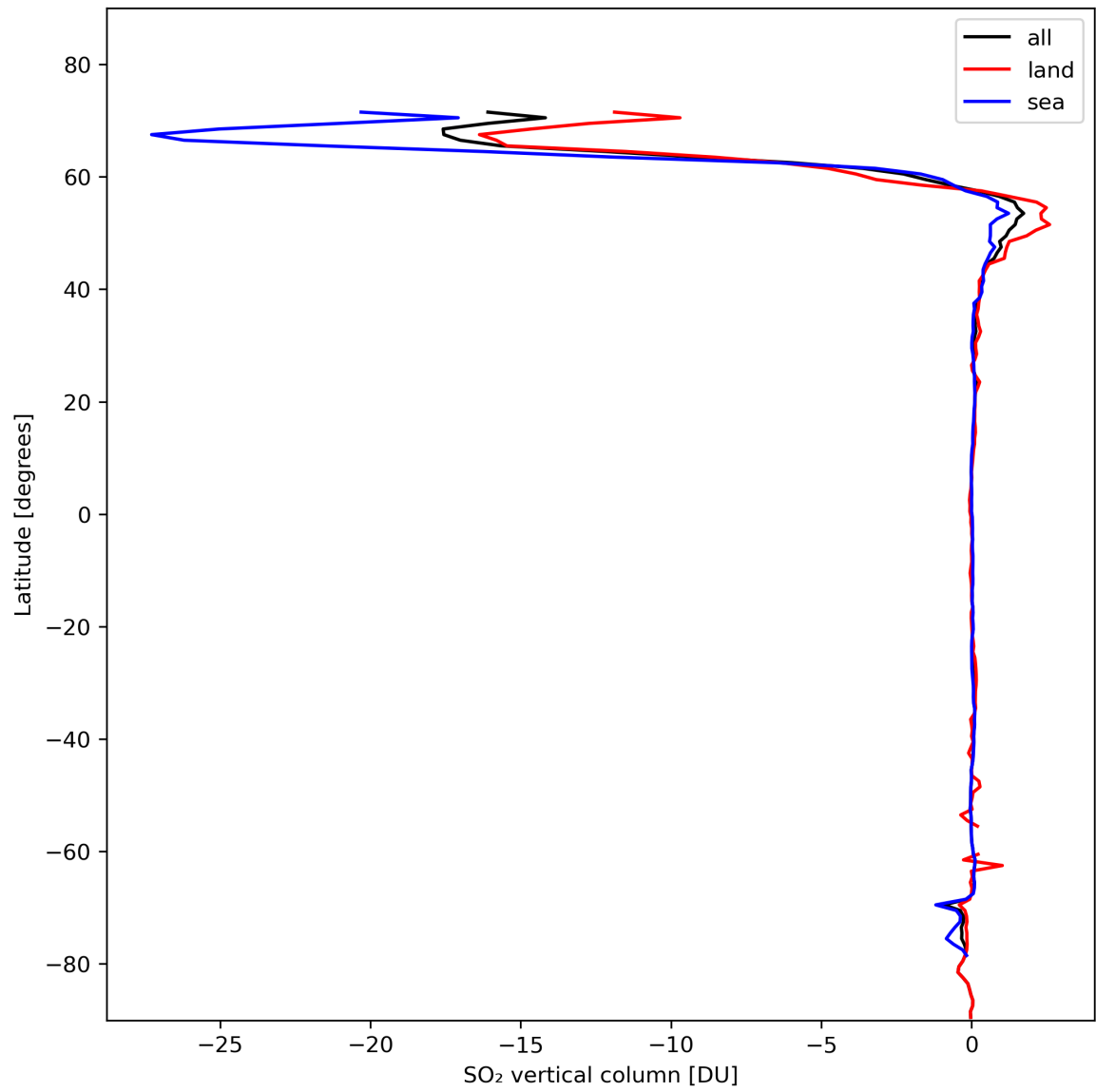
Figure 30: Zonal average of “SO 2 vertical column” for 2024-02-11 to 2024-02-12.
