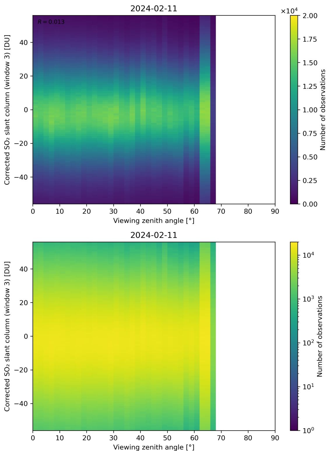
Figure 319: Scatter density plot of “Viewing zenith angle” against “Corrected SO 2 slant column (window 3)” for 2024-02-11 to 2024-02-12.
