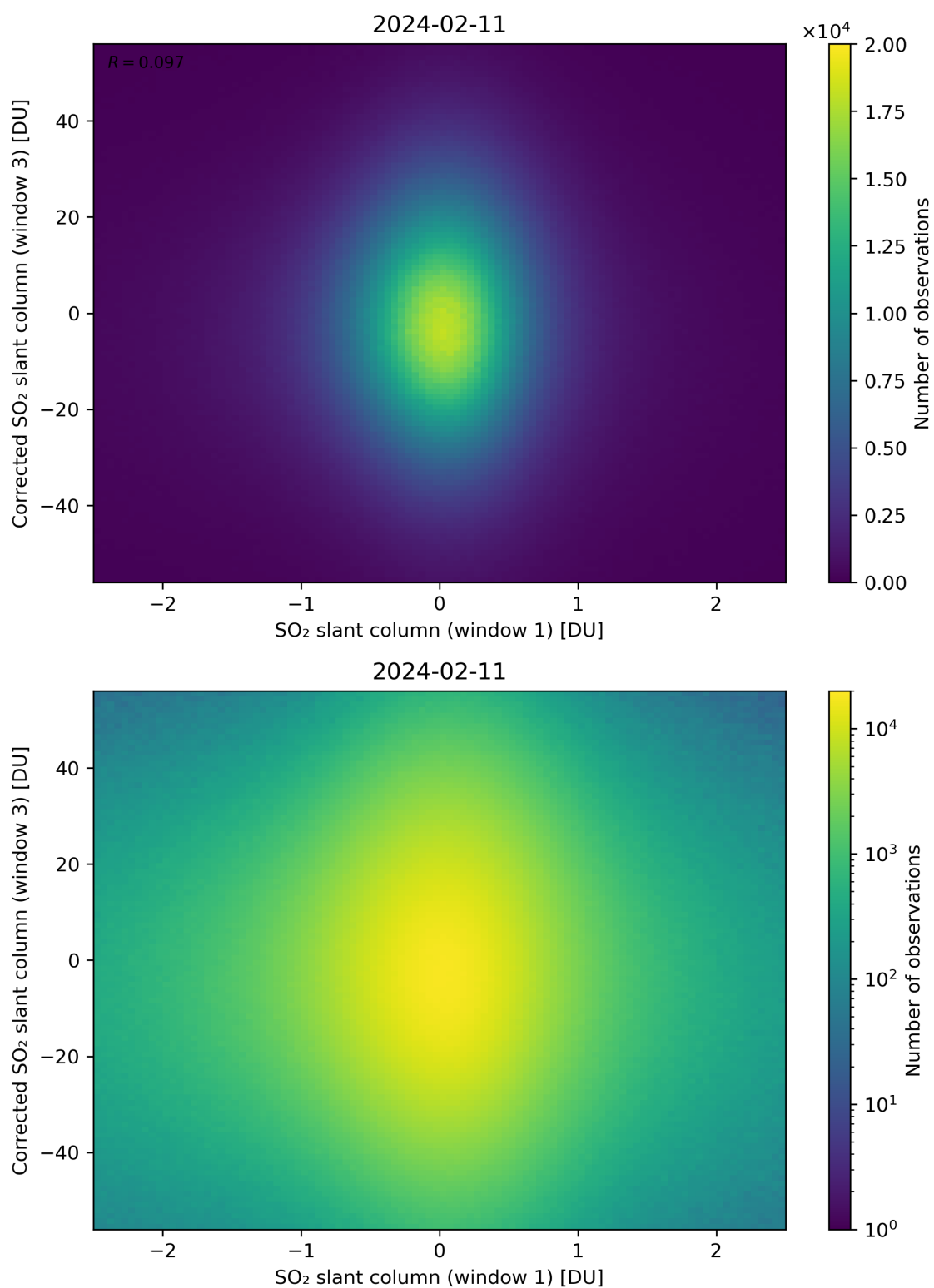
Figure 234: Scatter density plot of “SO 2 slant column (window 1)” against “Corrected SO 2 slant column (window 3)” for 2024-02-11 to 2024-02-12.
