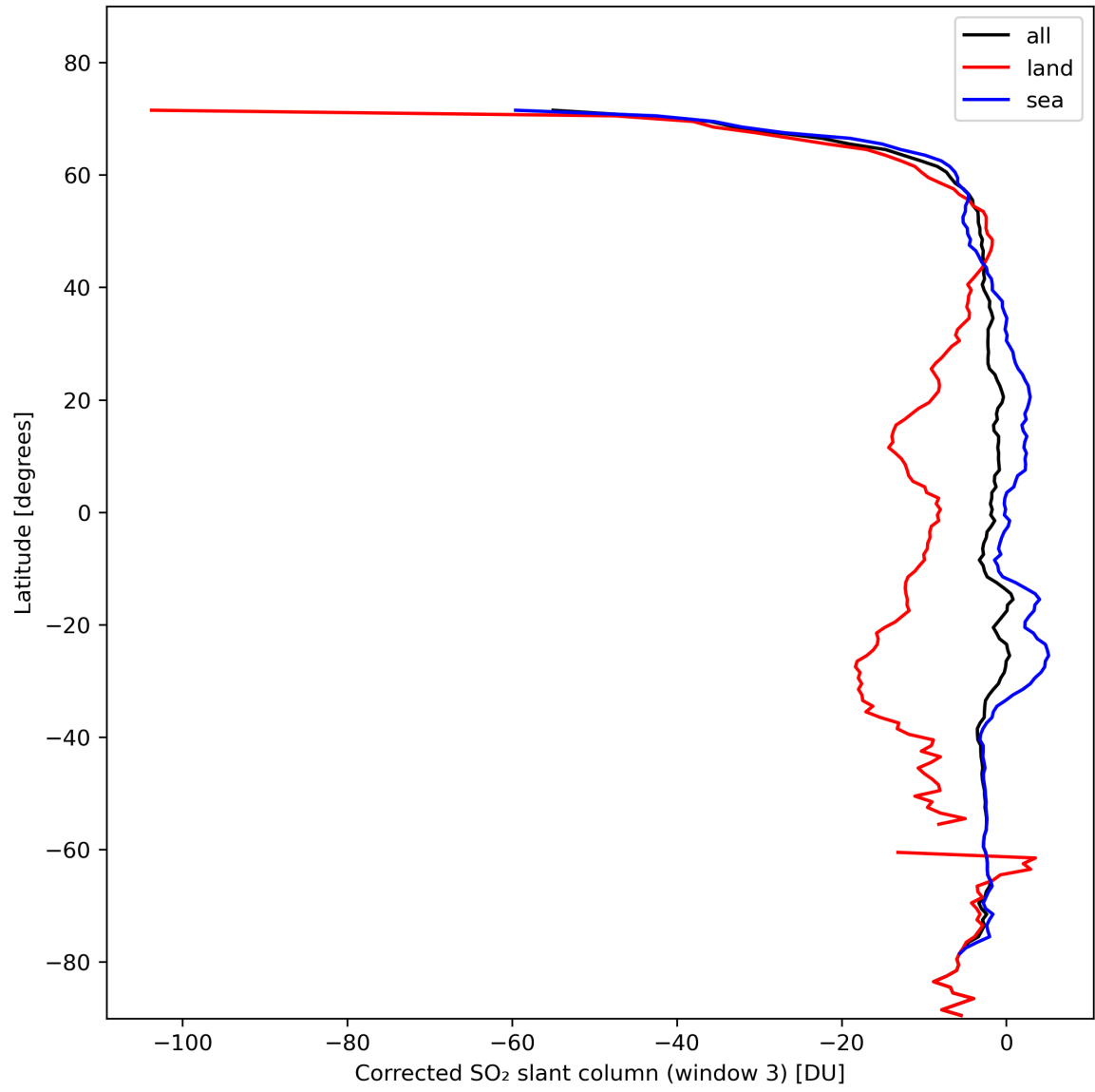
Figure 43: Zonal average of “Corrected SO 2 slant column (window 3)” for 2024-02-11 to 2024-02-12.
