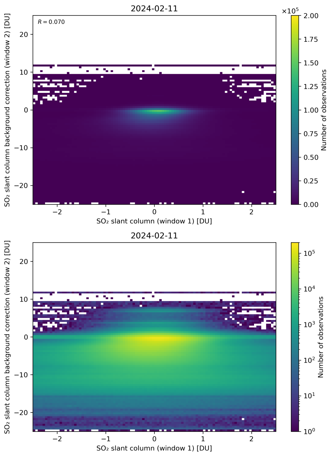
Figure 213: Scatter density plot of “SO 2 slant column (window 1)” against “SO 2 slant column background correction (window 2)” for 2024-02-11 to 2024-02-12.
