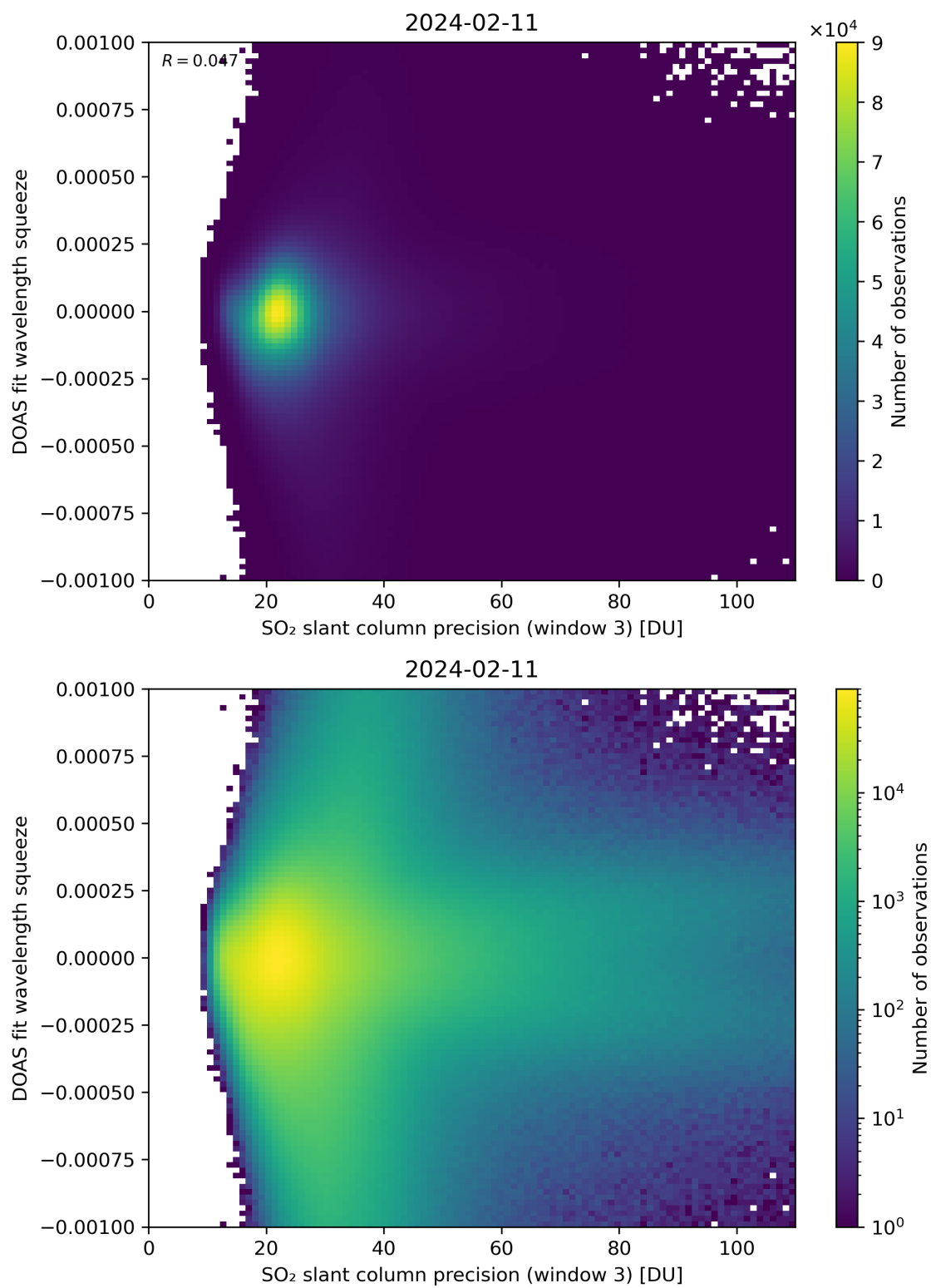
Figure 259: Scatter density plot of “SO 2 slant column precision (window 3)” against “DOAS fit wavelength squeeze” for 2024-02-11 to 2024-02-12.
