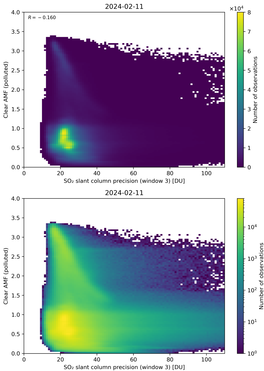
Figure 261: Scatter density plot of “SO 2 slant column precision (window 3)” against “Clear AMF (polluted)” for 2024-02-11 to 2024-02-12.
