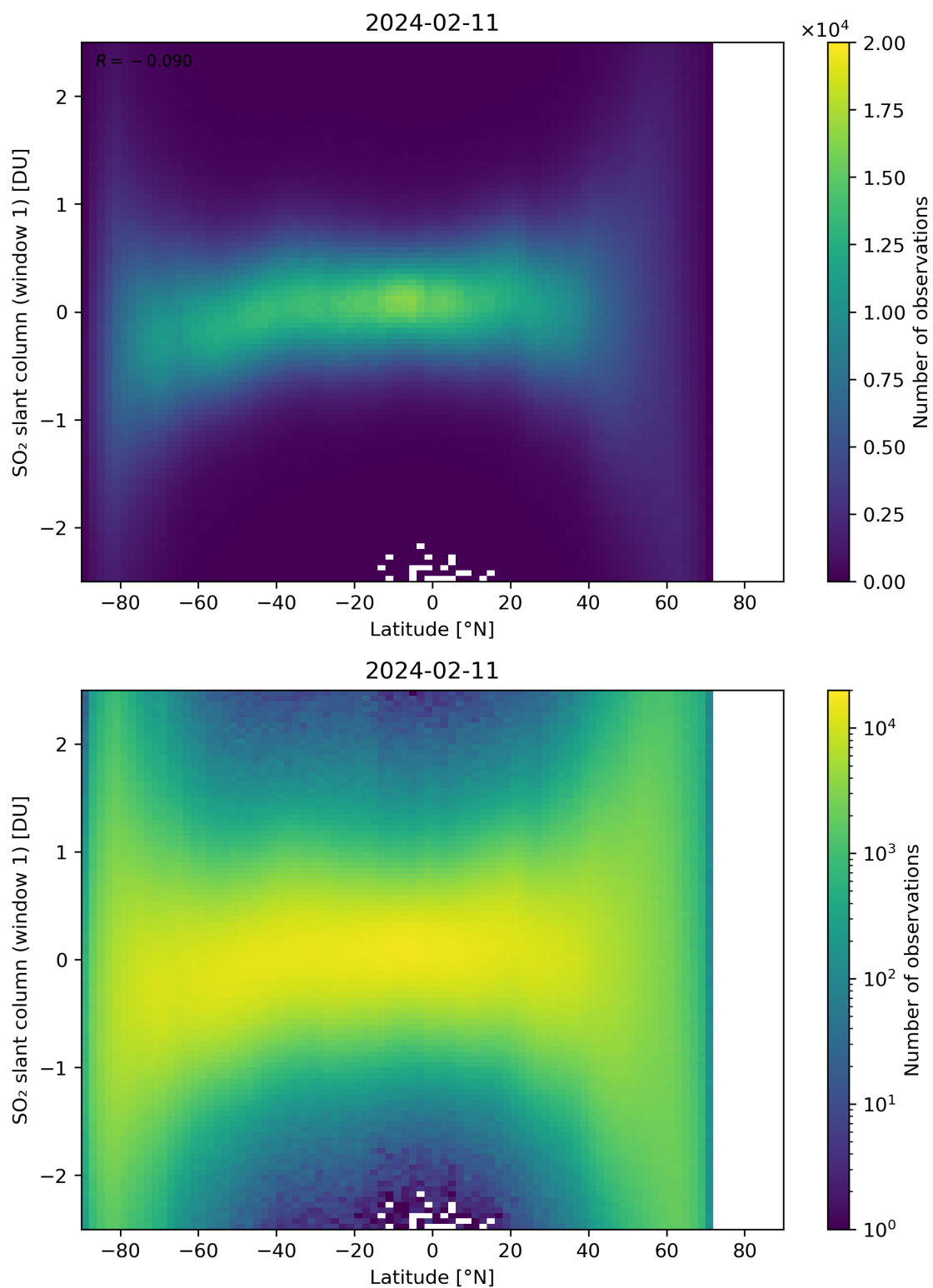
Figure 149: Scatter density plot of “Latitude” against “SO 2 slant column (window 1)” for 2024-02-11 to 2024-02-12.
