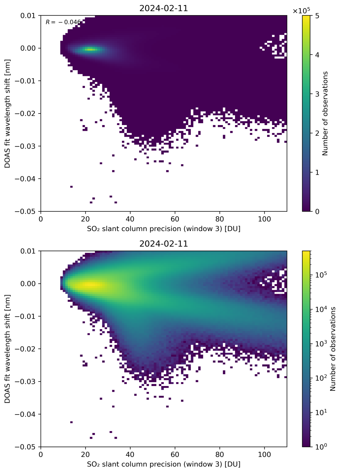
Figure 258: Scatter density plot of “SO 2 slant column precision (window 3)” against “DOAS fit wavelength shift” for 2024-02-11 to 2024-02-12.
