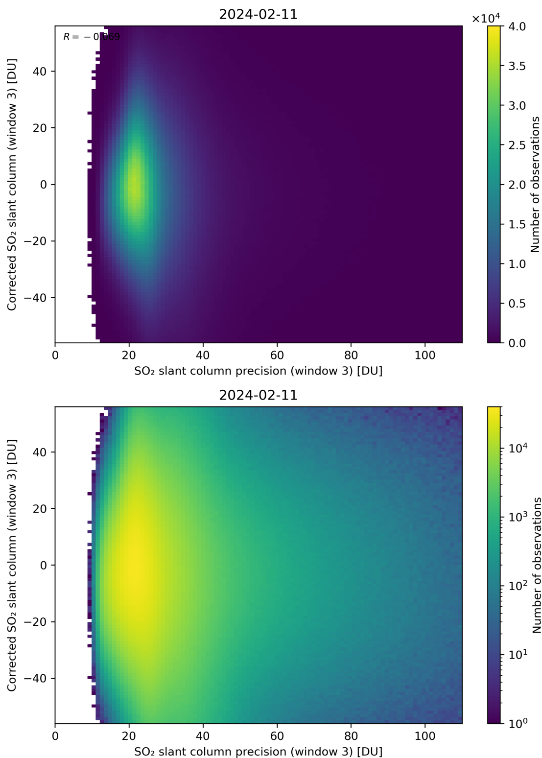
Figure 262: Scatter density plot of “SO 2 slant column precision (window 3)” against “Corrected SO 2 slant column (window 3)” for 2024-02-11 to 2024-02-12.
