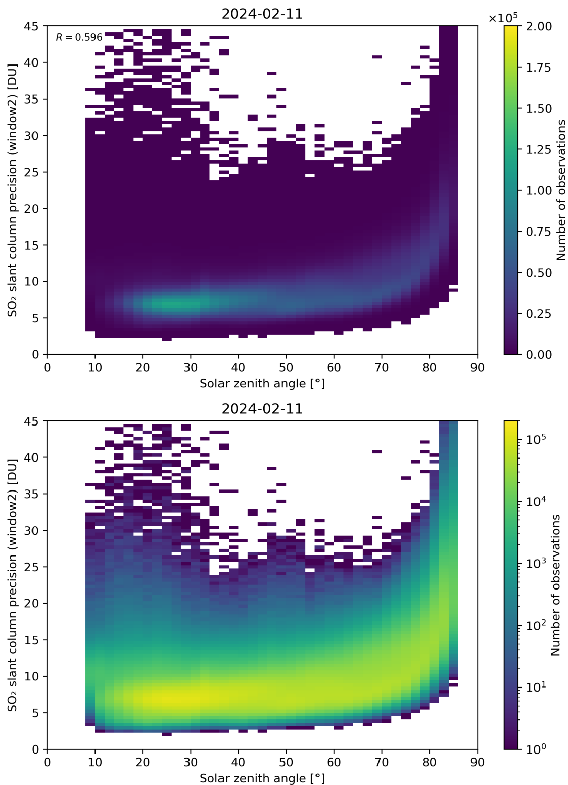
Figure 171: Scatter density plot of “Solar zenith angle” against “SO 2 slant column precision (window2)” for 2024-02-11 to 2024-02-12.
