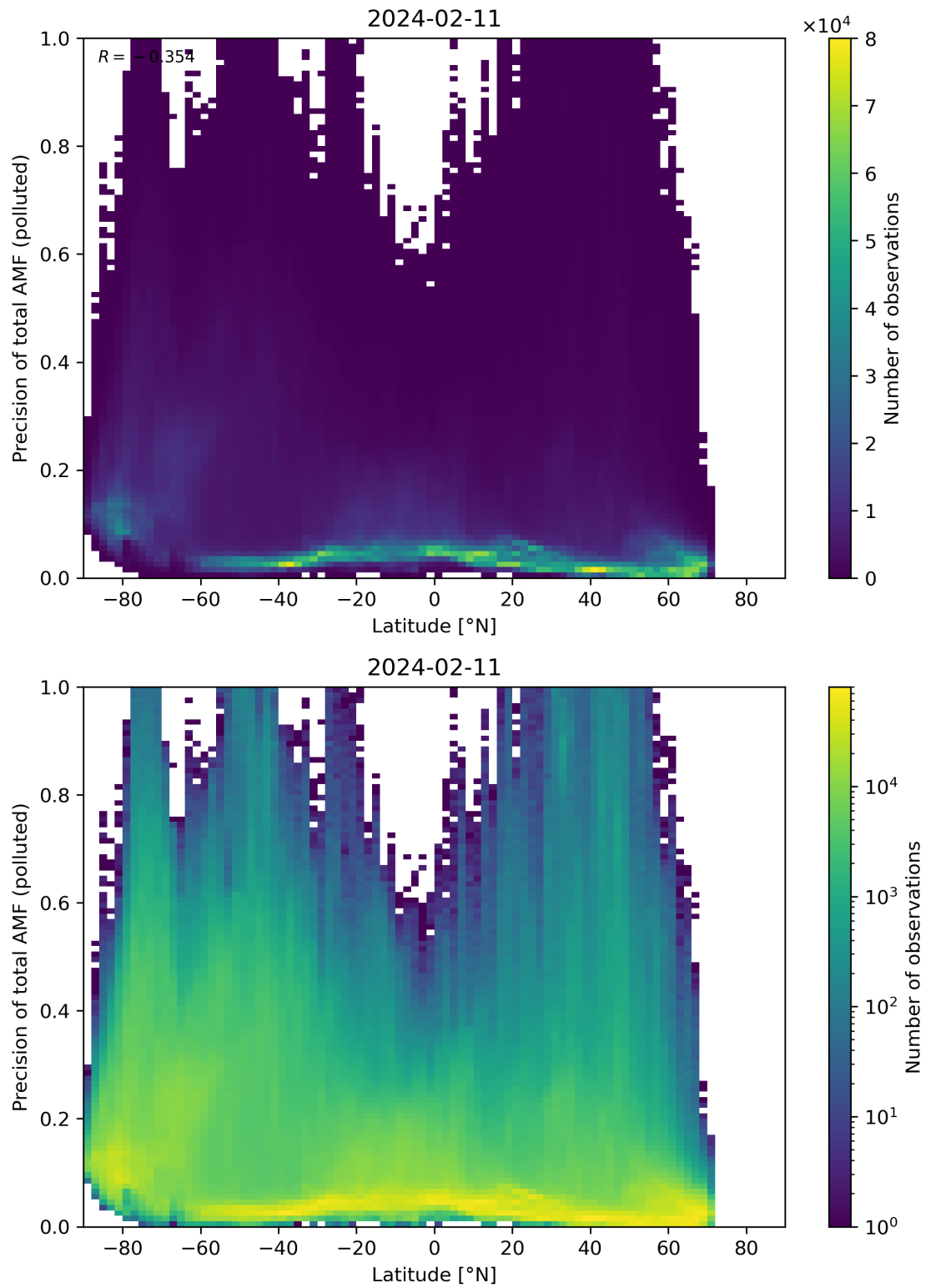
Figure 155: Scatter density plot of “Latitude” against “Precision of total AMF (polluted)” for 2024-02-11 to 2024-02-12.
