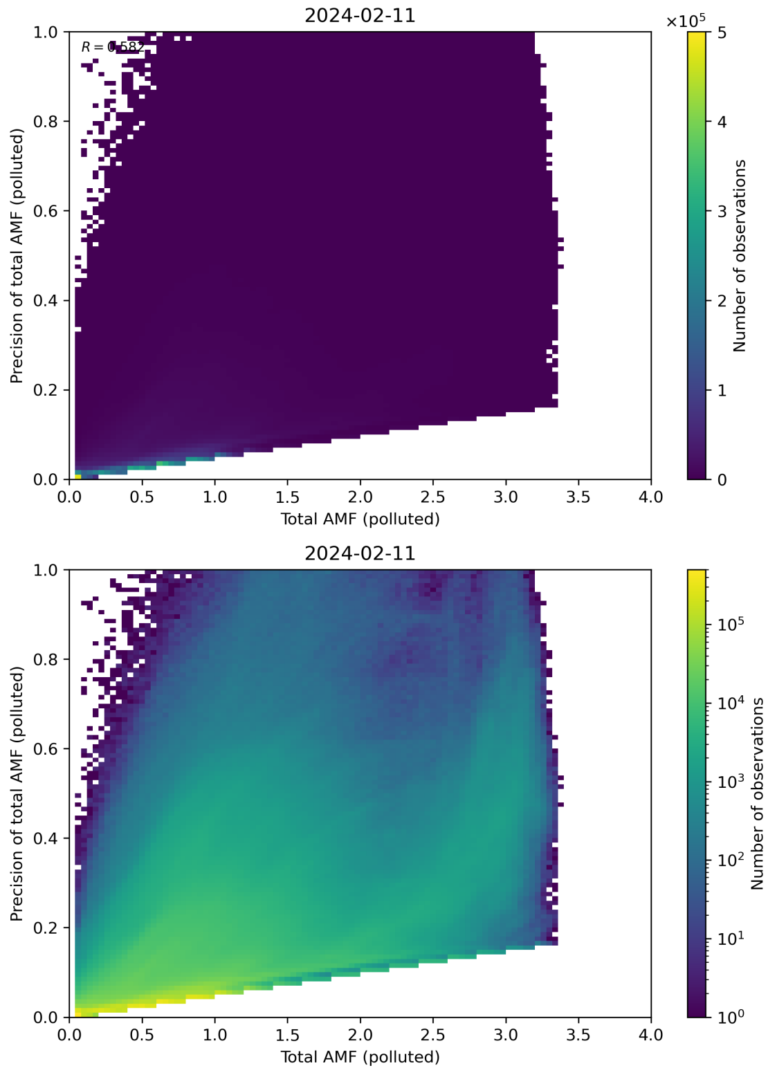
Figure 272: Scatter density plot of “Total AMF (polluted)” against “Precision of total AMF (polluted)” for 2024-02-11 to 2024-02-12.
