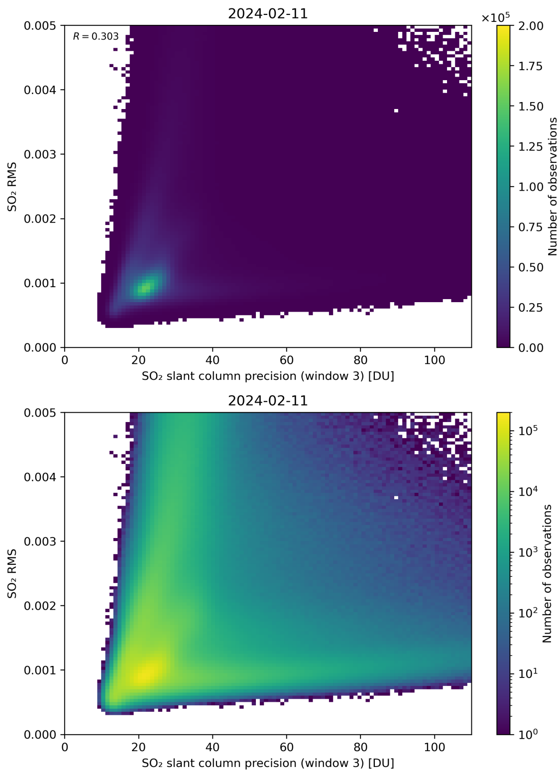
Figure 260: Scatter density plot of “SO 2 slant column precision (window 3)” against “SO 2 RMS” for 2024-02-11 to 2024-02-12.
