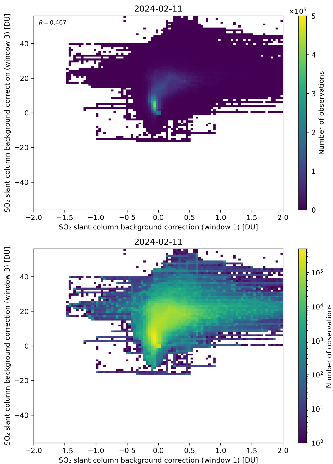
Figure 99: Scatter density plot of “SO 2 slant column background correction (window 1)” against “SO 2 slant column background correction (window 3)” for 2024-02-11 to 2024-02-12.
