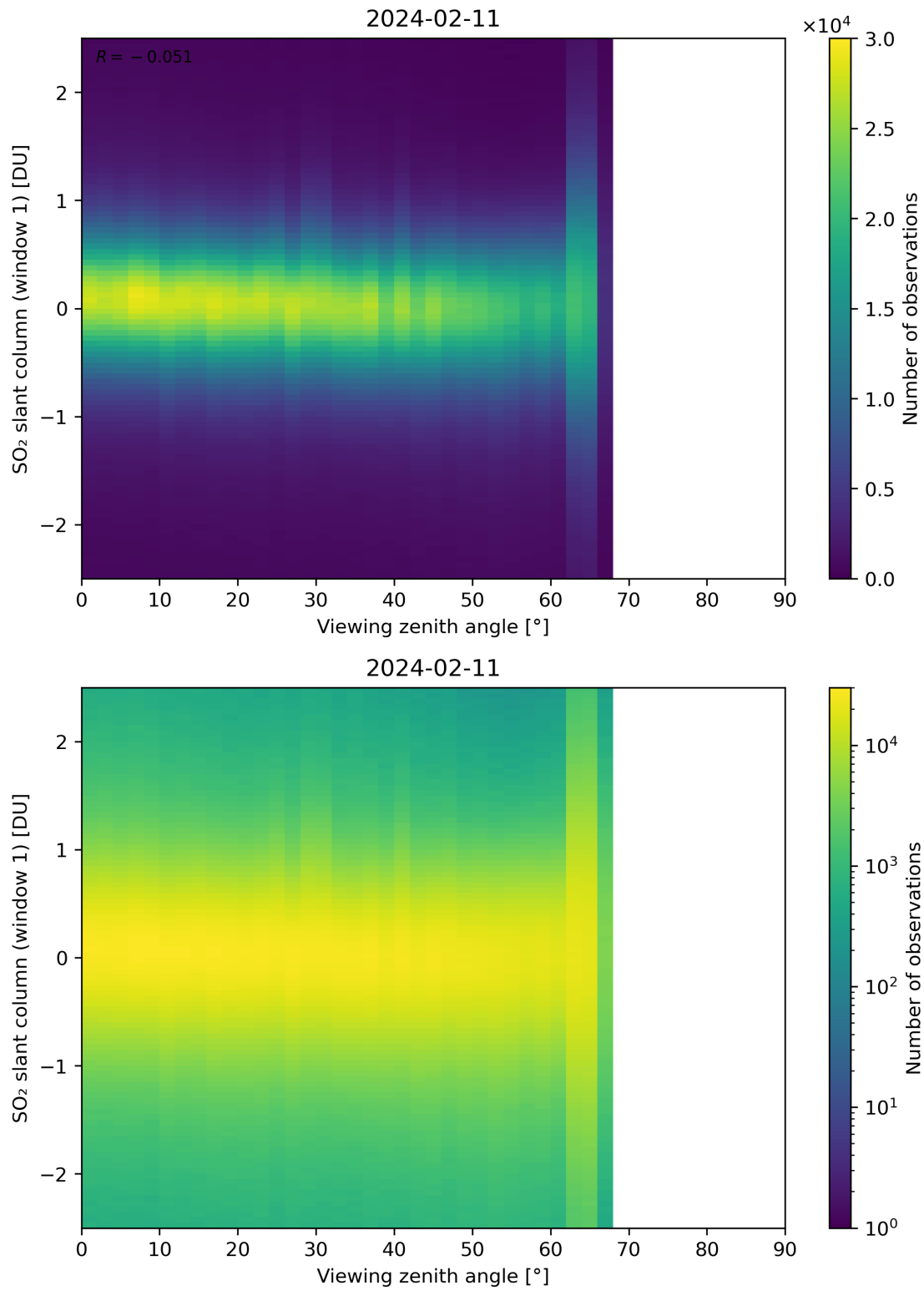
Figure 320: Scatter density plot of “Viewing zenith angle” against “SO 2 slant column (window 1)” for 2024-02-11 to 2024-02-12.
