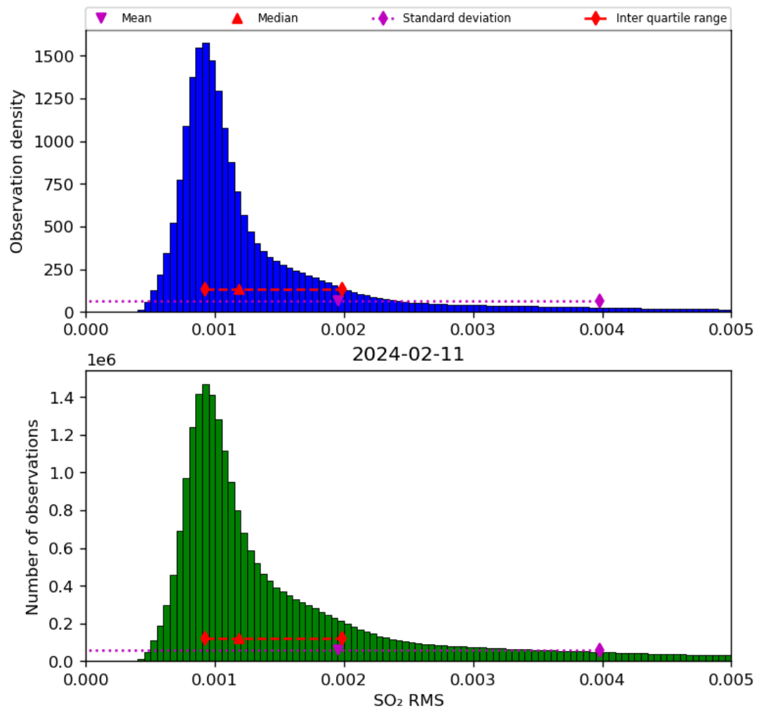
Figure 70: Histogram of “SO 2 RMS” for 2024-02-11 to 2024-02-12
