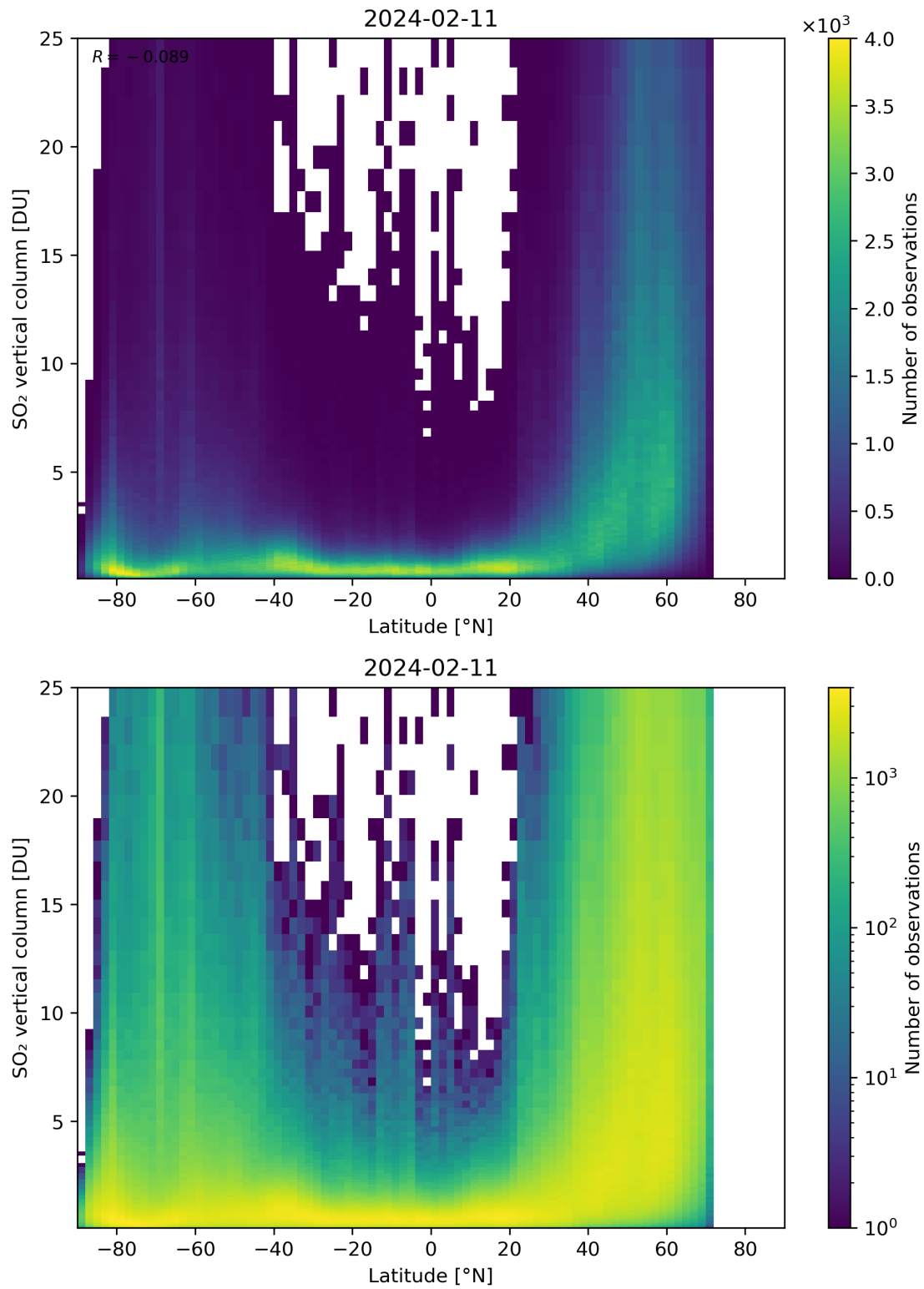
Figure 156: Scatter density plot of “Latitude” against “SO 2 vertical column” for 2024-02-11 to 2024-02-12.
