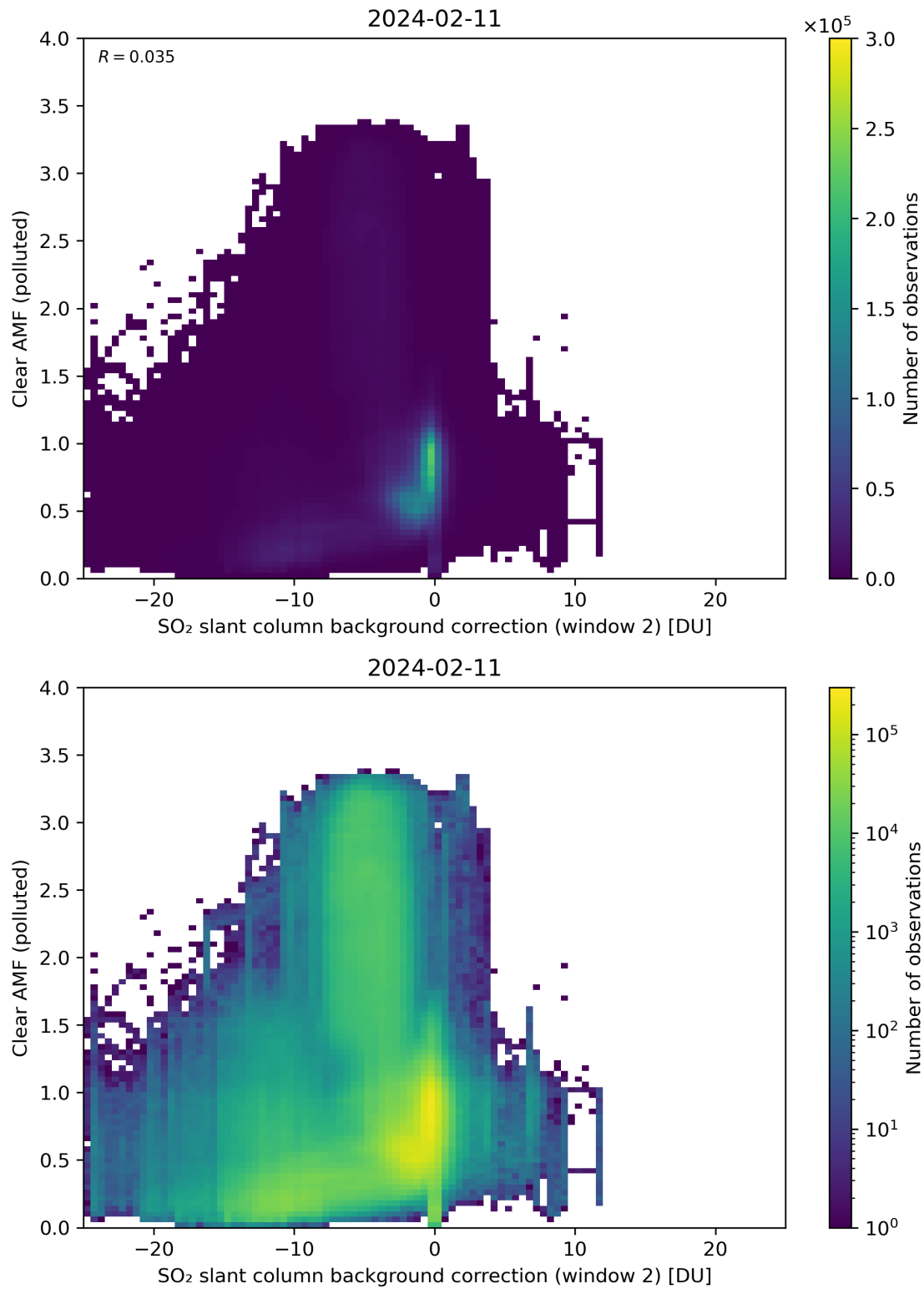
Figure 115: Scatter density plot of “SO 2 slant column background correction (window 2)” against “Clear AMF (polluted)” for 2024-02-11 to 2024-02-12.
