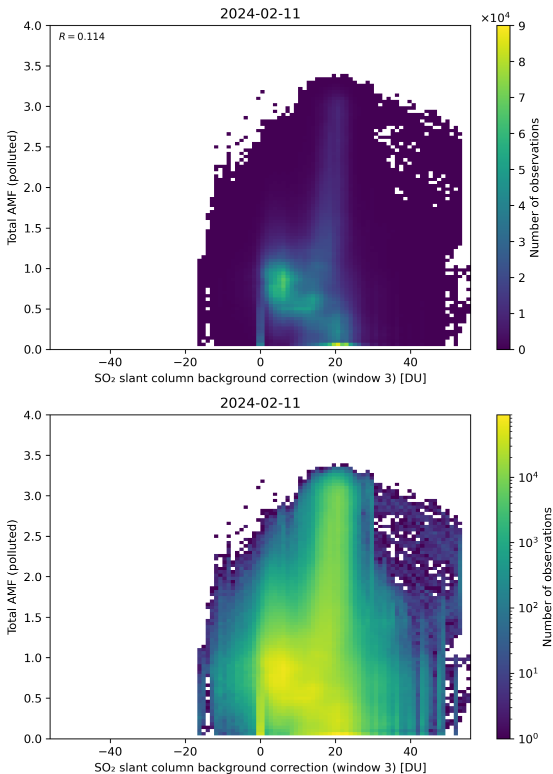
Figure 125: Scatter density plot of “SO 2 slant column background correction (window 3)” against “Total AMF (polluted)” for 2024-02-11 to 2024-02-12.
