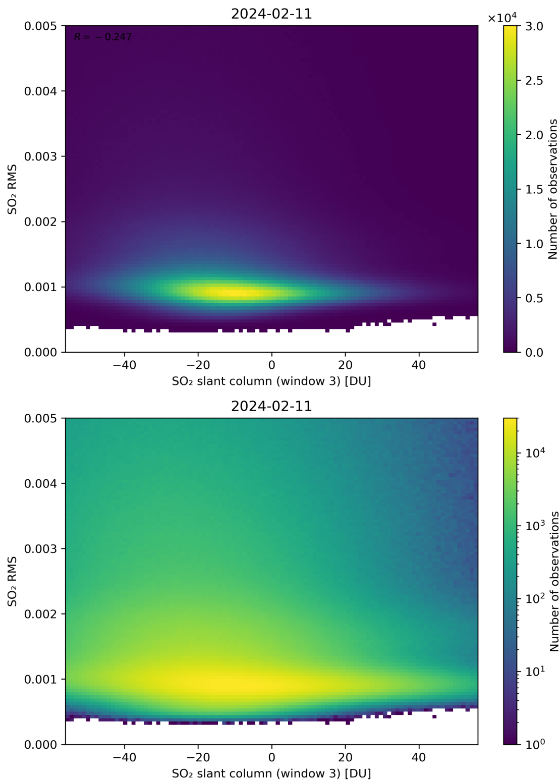
Figure 256: Scatter density plot of “SO 2 slant column (window 3)” against “SO 2 RMS” for 2024-02-11 to 2024-02-12.
