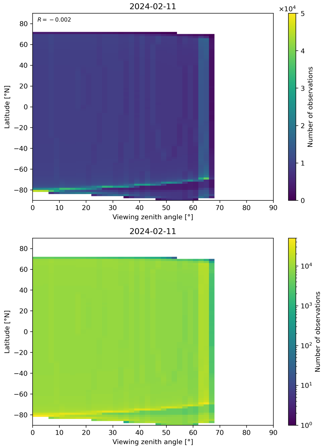
Figure 314: Scatter density plot of “Viewing zenith angle” against “Latitude” for 2024-02-11 to 2024-02-12.
