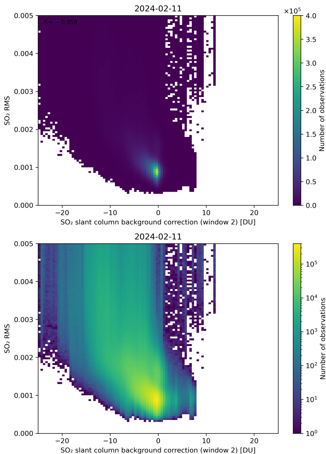
Figure 114: Scatter density plot of “SO 2 slant column background correction (window 2)” against “SO 2 RMS” for 2024-02-11 to 2024-02-12.
