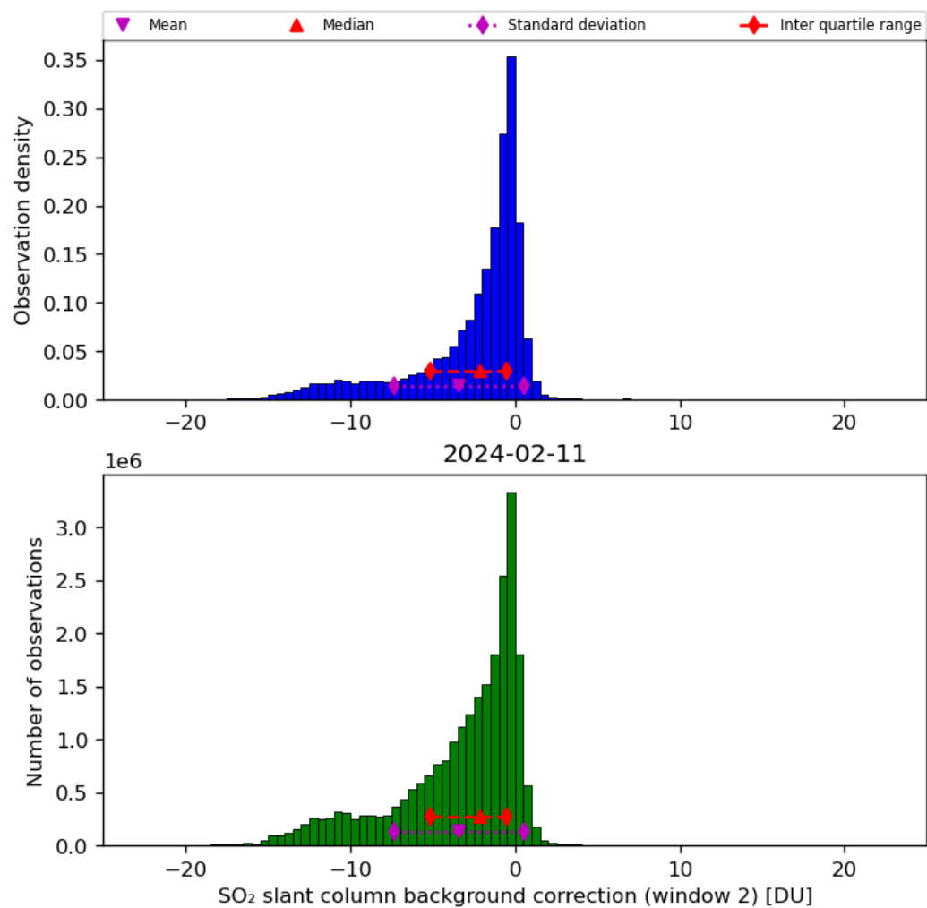
Figure 63: Histogram of “SO 2 slant column background correction (window 2)” for 2024-02-11 to 2024-02-12
