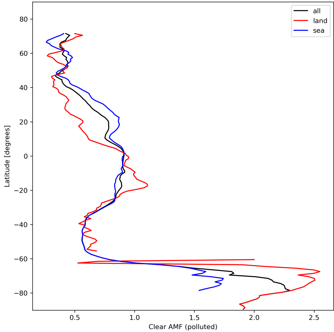
Figure 50: Zonal average of “Clear AMF (polluted)” for 2024-02-11 to 2024-02-12.
