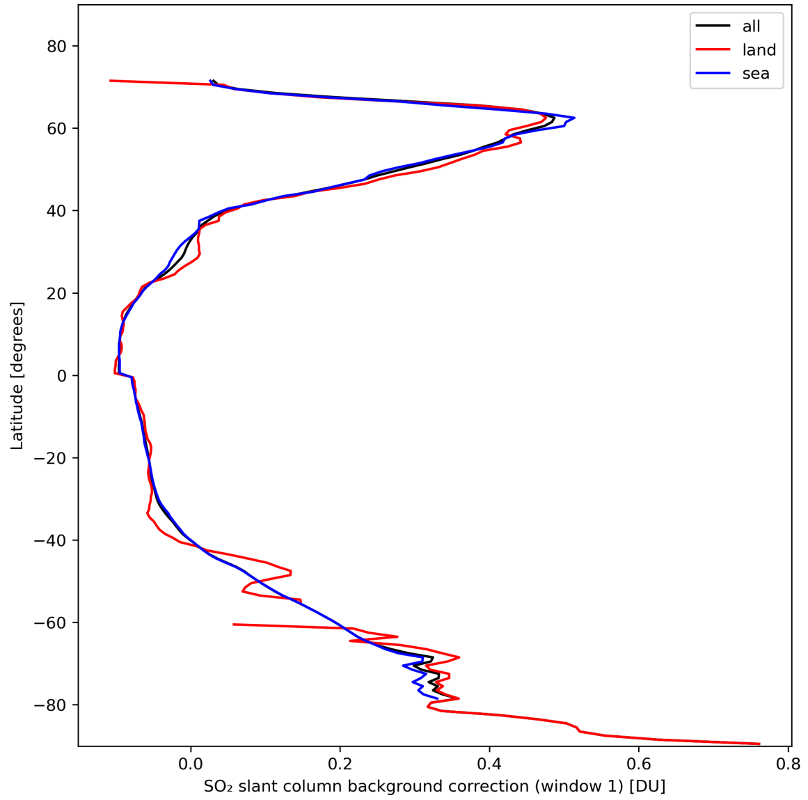
Figure 36: Zonal average of “SO 2 slant column background correction (window 1)” for 2024-02-11 to 2024-02-12.
