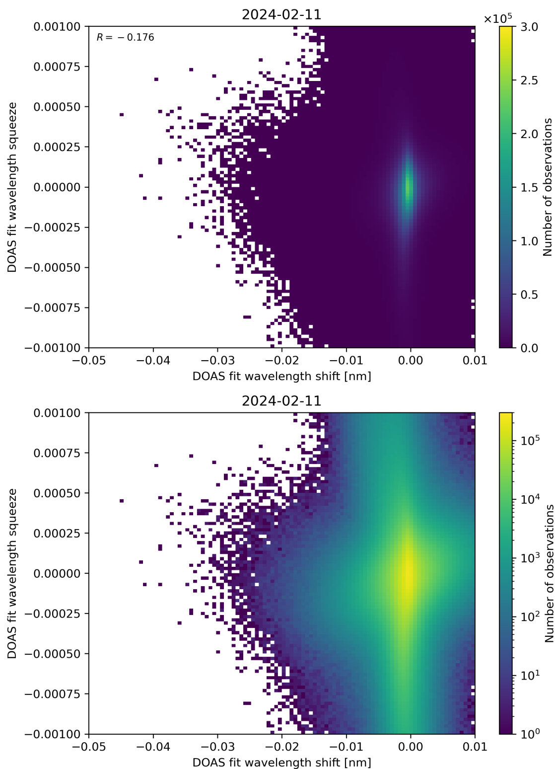
Figure 127: Scatter density plot of “DOAS fit wavelength shift” against “DOAS fit wavelength squeeze” for 2024-02-11 to 2024-02-12.
