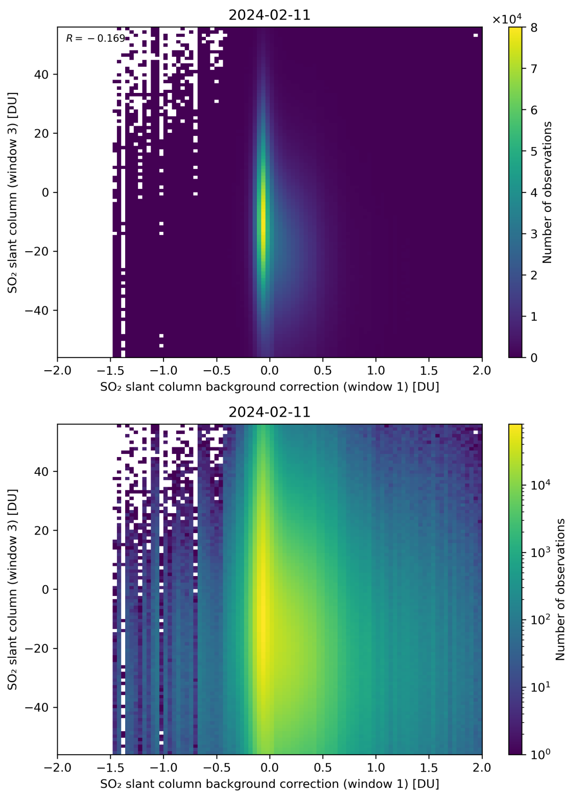
Figure 107: Scatter density plot of “SO 2 slant column background correction (window 1)” against “SO 2 slant column (window 3)” for 2024-02-11 to 2024-02-12.
