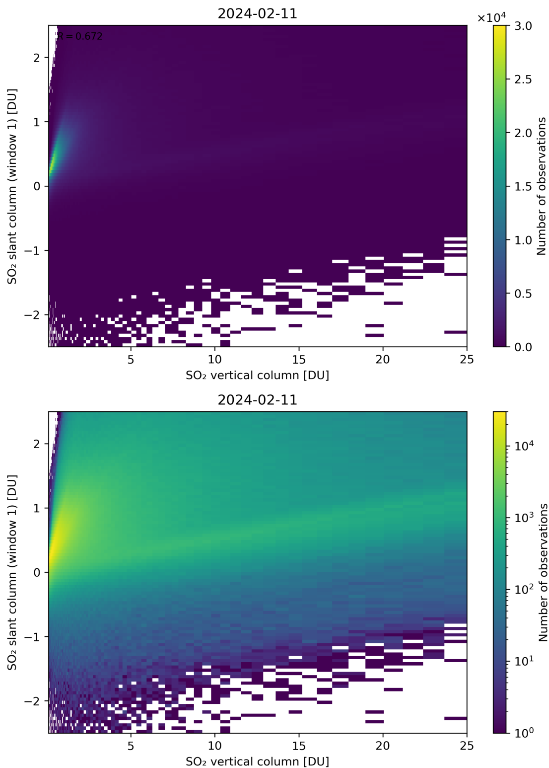
Figure 300: Scatter density plot of “SO 2 vertical column” against “SO 2 slant column (window 1)” for 2024-02-11 to 2024-02-12.
