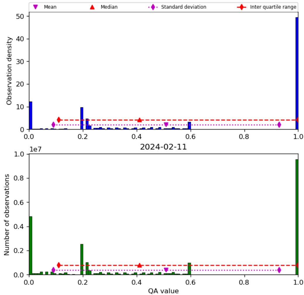
Figure 52: Histogram of “QA value” for 2024-02-11 to 2024-02-12
