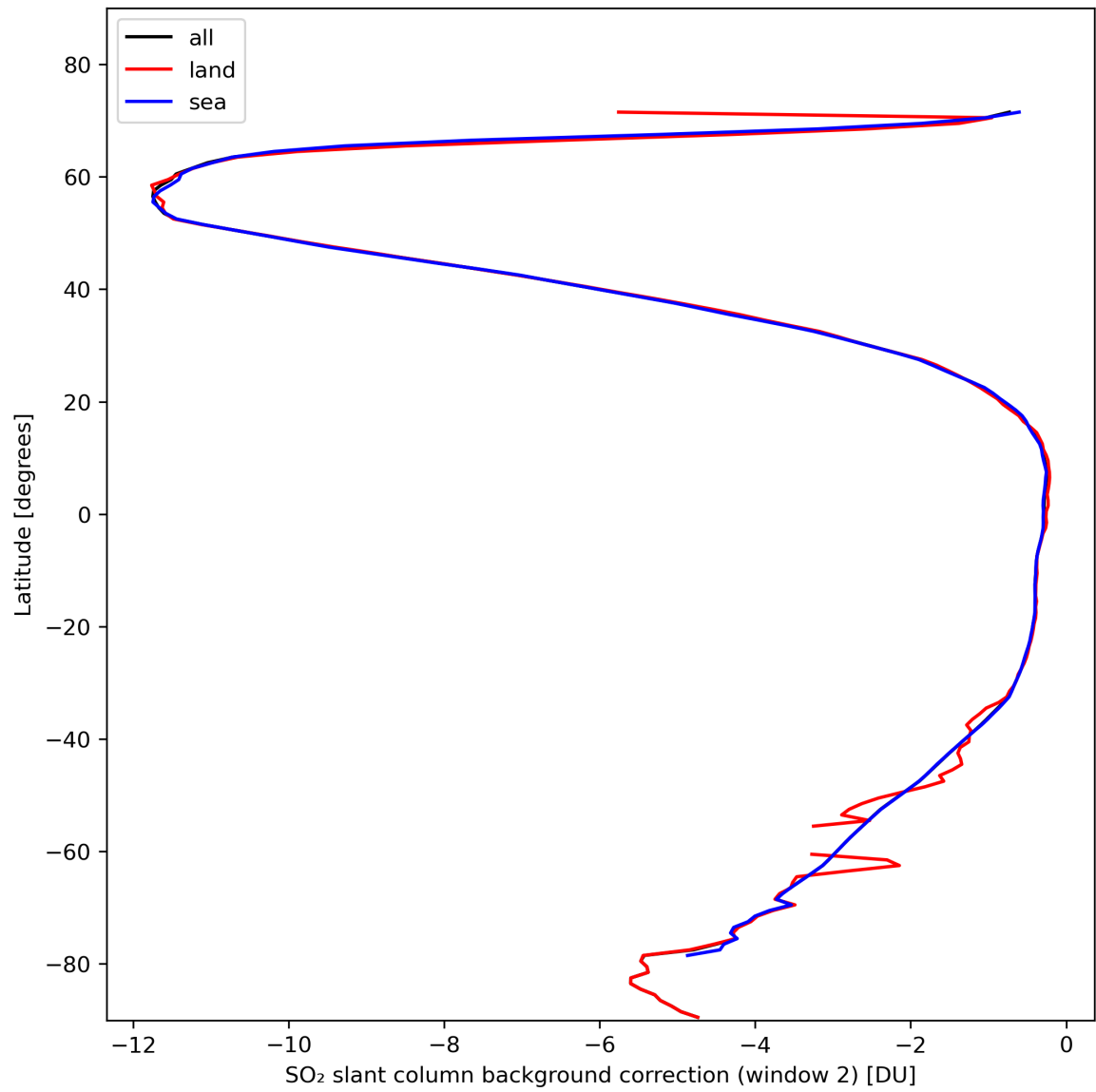
Figure 40: Zonal average of “SO 2 slant column background correction (window 2)” for 2024-02-11 to 2024-02-12.
