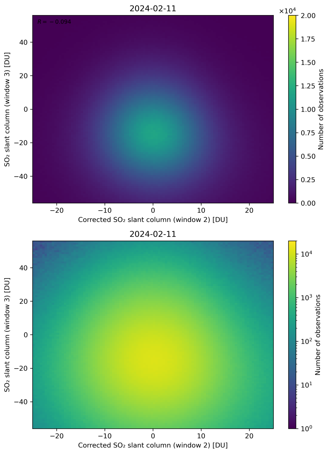
Figure 201: Scatter density plot of “Corrected SO 2 slant column (window 2)” against “SO 2 slant column (window 3)” for 2024-02-11 to 2024-02-12.
