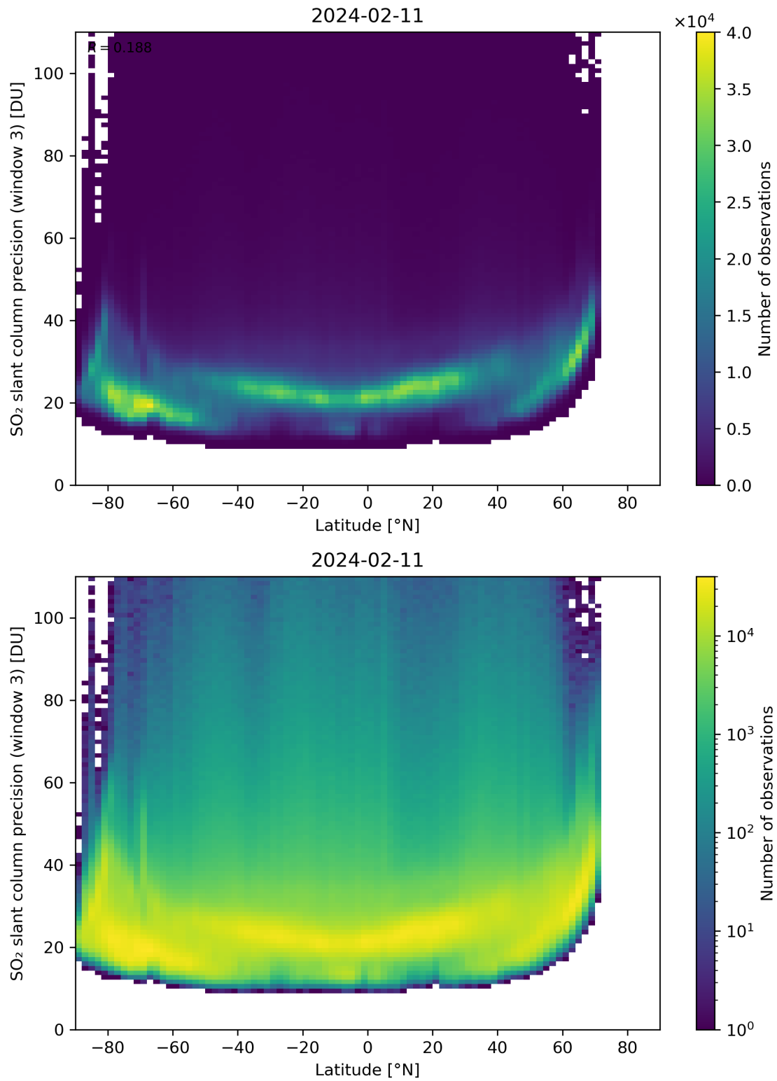
Figure 153: Scatter density plot of “Latitude” against “SO 2 slant column precision (window 3)” for 2024-02-11 to 2024-02-12.
