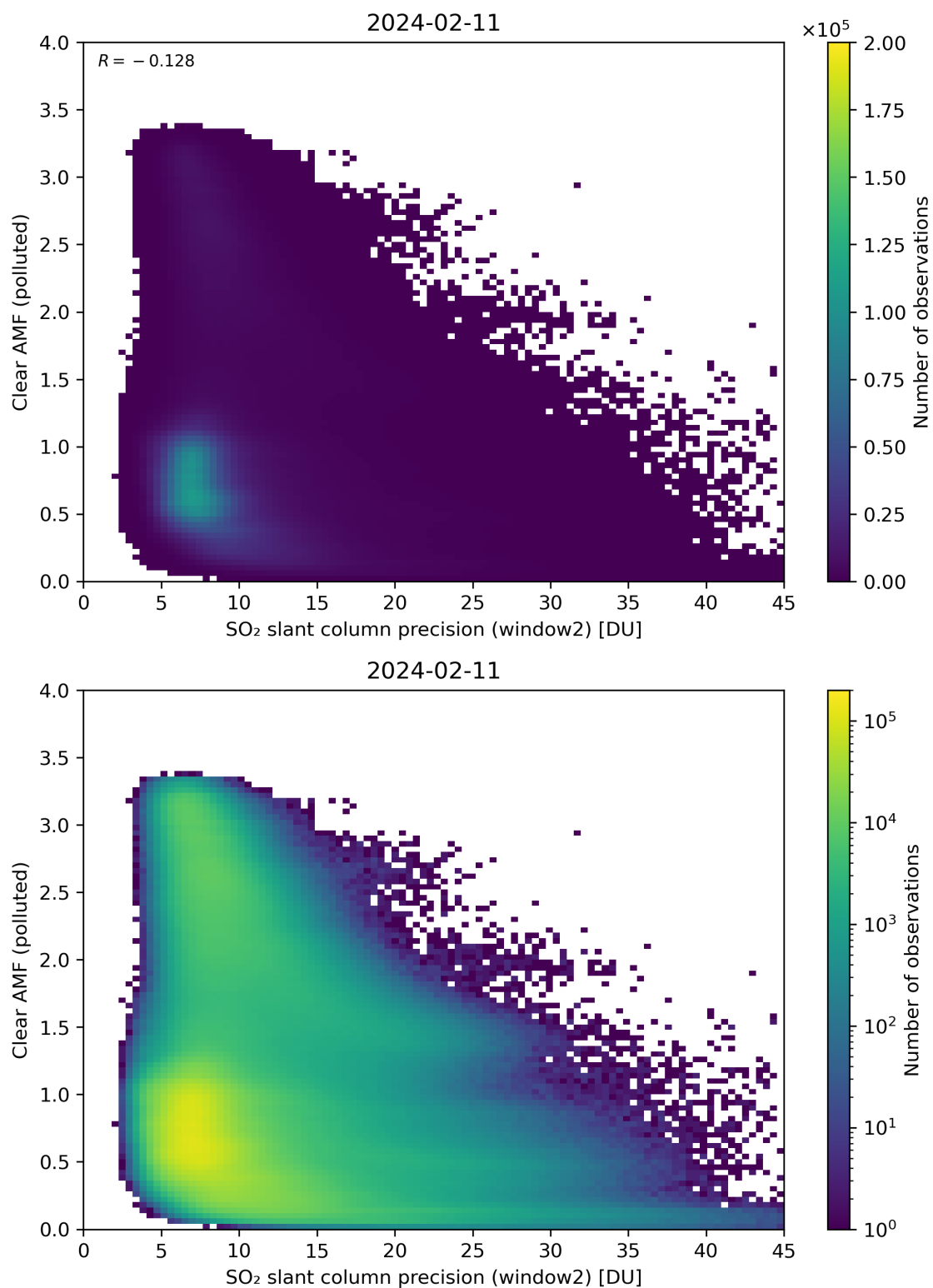
Figure 246: Scatter density plot of “SO 2 slant column precision (window2)” against “Clear AMF (polluted)” for 2024-02-11 to 2024-02-12.
