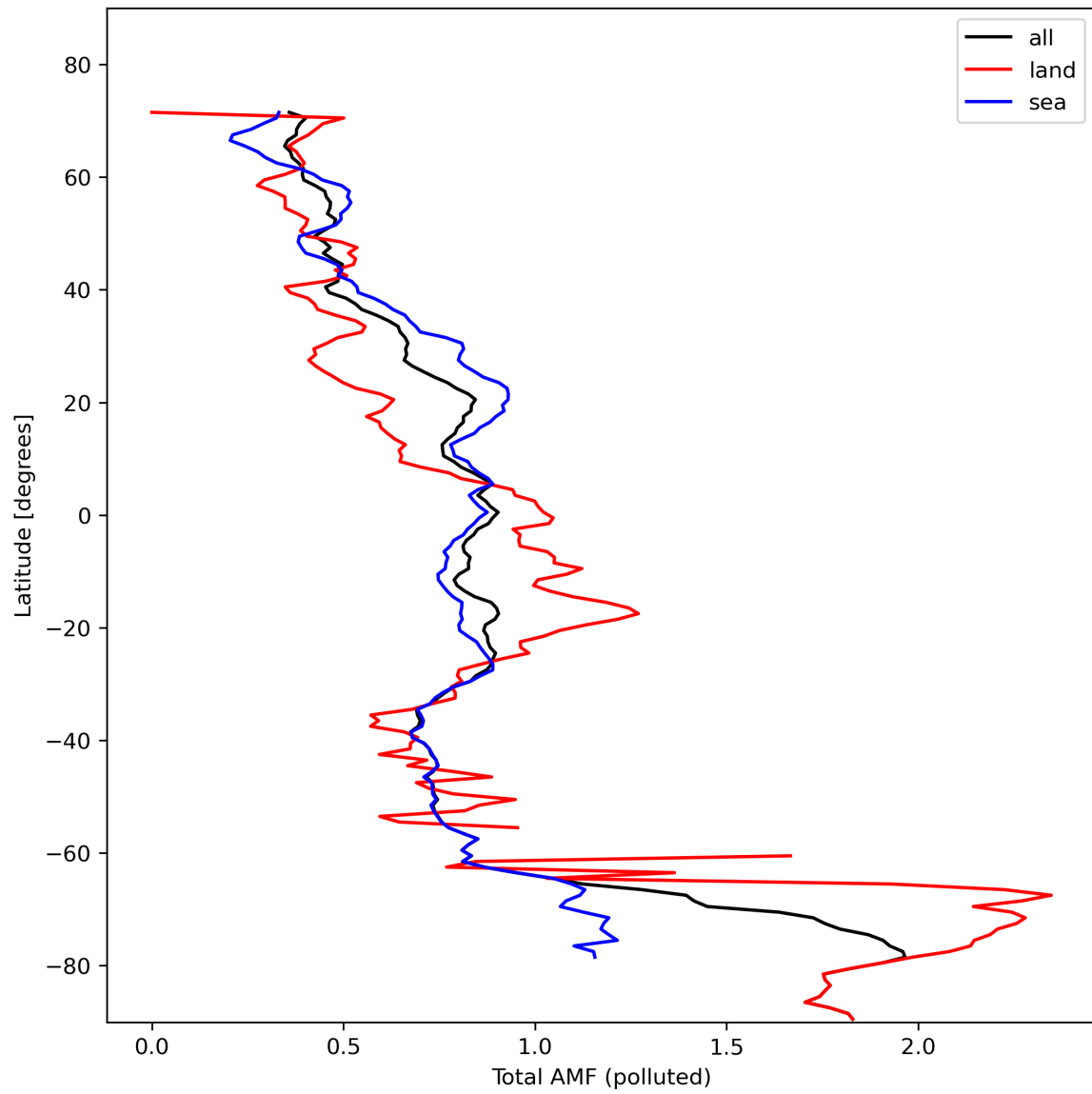
Figure 48: Zonal average of “Total AMF (polluted)” for 2024-02-11 to 2024-02-12.
