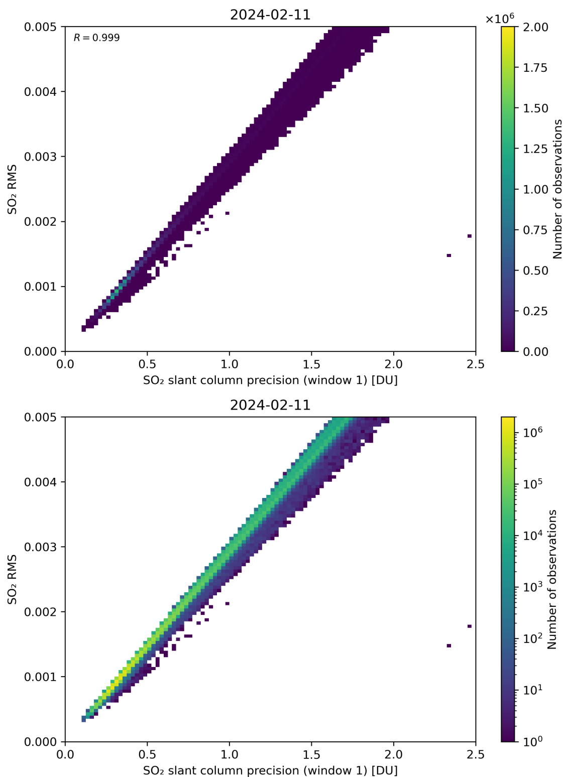
Figure 223: Scatter density plot of “SO 2 slant column precision (window 1)” against “SO 2 RMS” for 2024-02-11 to 2024-02-12.
