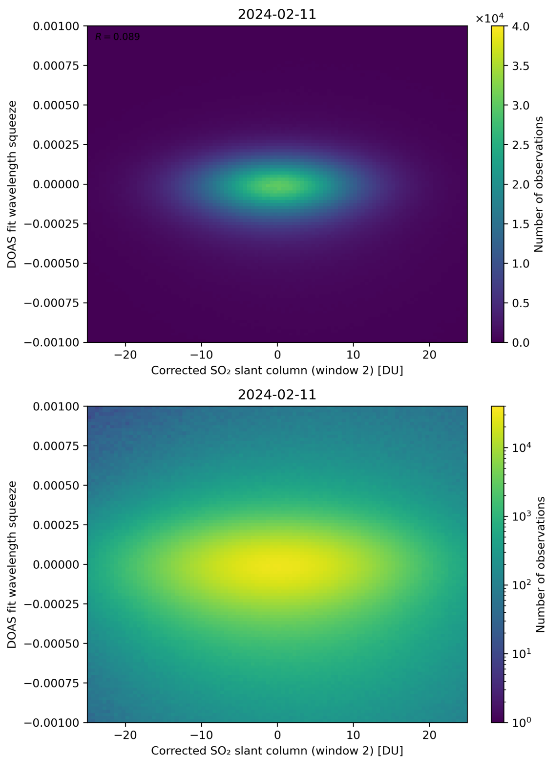
Figure 197: Scatter density plot of “Corrected SO 2 slant column (window 2)” against “DOAS fit wavelength squeeze” for 2024-02-11 to 2024-02-12.
