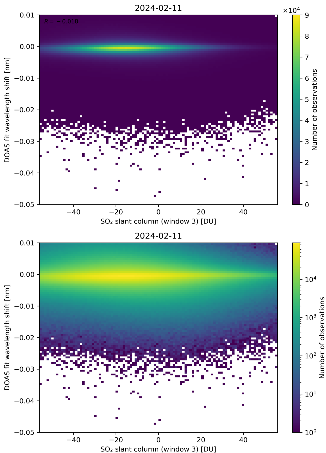
Figure 254: Scatter density plot of “SO 2 slant column (window 3)” against “DOAS fit wavelength shift” for 2024-02-11 to 2024-02-12.
