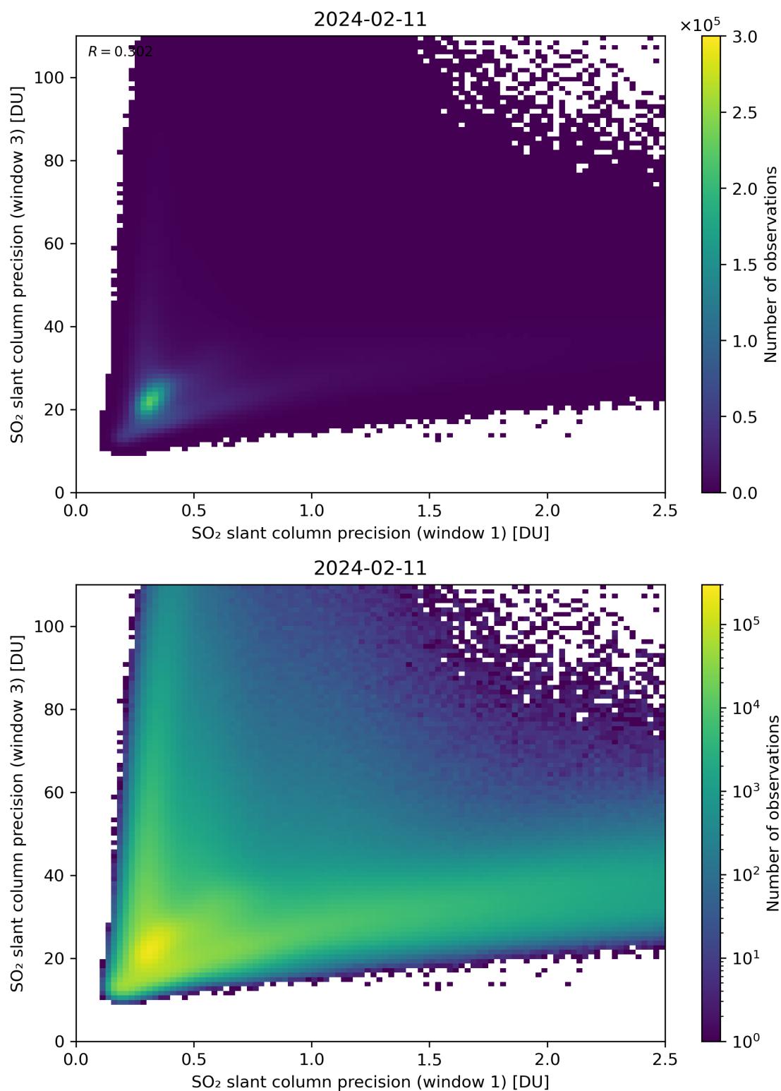
Figure 229: Scatter density plot of “SO 2 slant column precision (window 1)” against “SO 2 slant column precision (window 3)” for 2024-02-11 to 2024-02-12.
