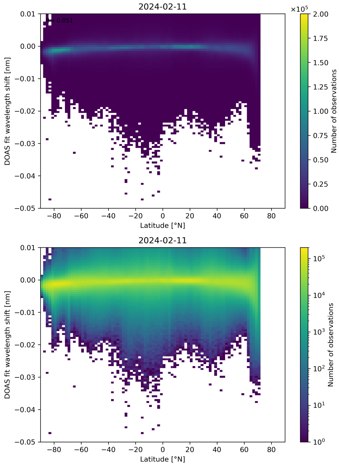
Figure 142: Scatter density plot of “Latitude” against “DOAS fit wavelength shift” for 2024-02-11 to 2024-02-12.
