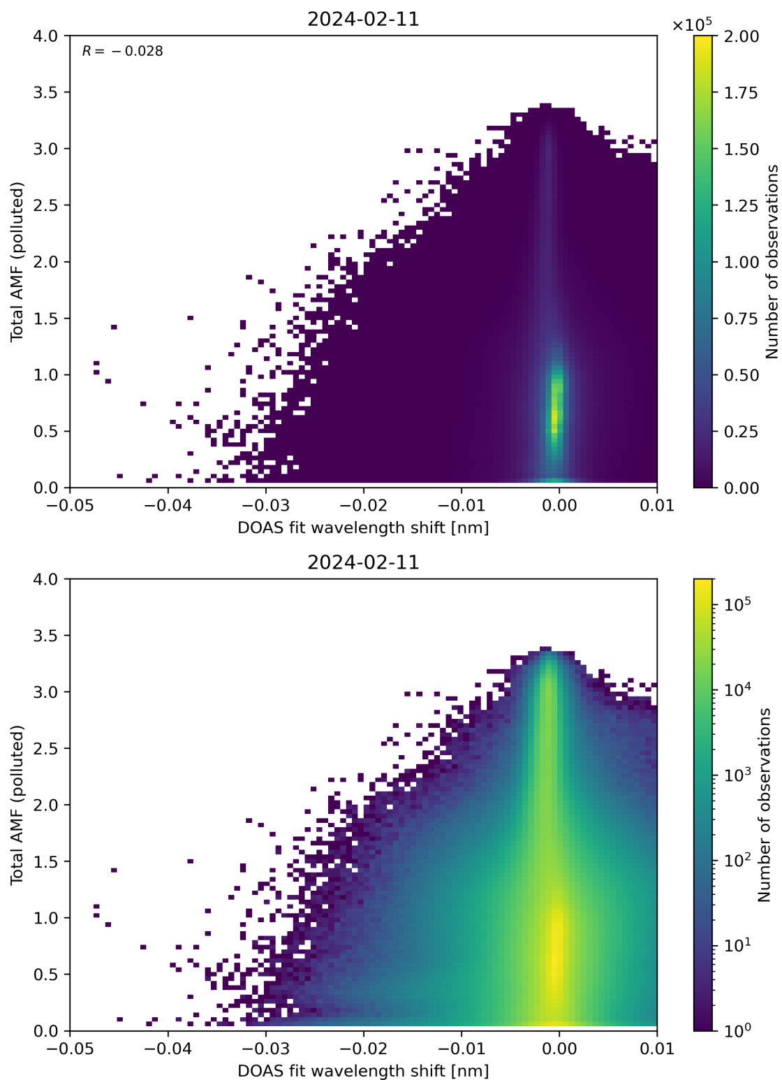
Figure 130: Scatter density plot of “DOAS fit wavelength shift” against “Total AMF (polluted)” for 2024-02-11 to 2024-02-12.
