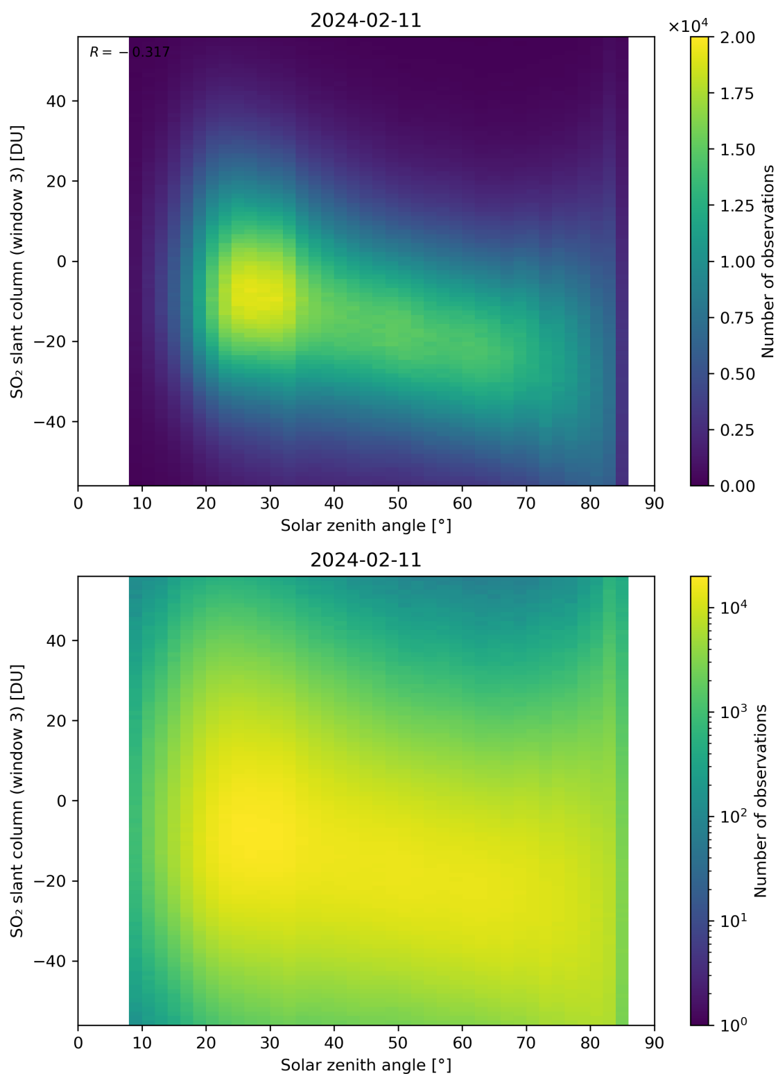
Figure 172: Scatter density plot of “Solar zenith angle” against “SO 2 slant column (window 3)” for 2024-02-11 to 2024-02-12.
