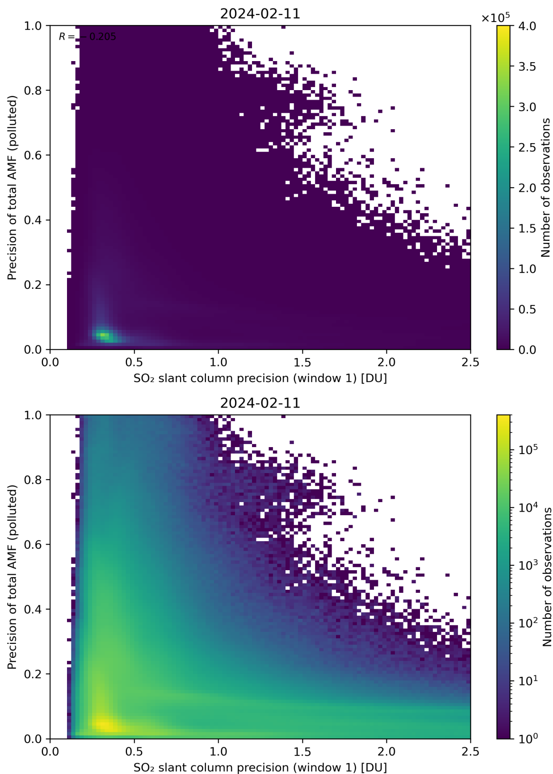
Figure 231: Scatter density plot of “SO 2 slant column precision (window 1)” against “Precision of total AMF (polluted)” for 2024-02-11 to 2024-02-12.
