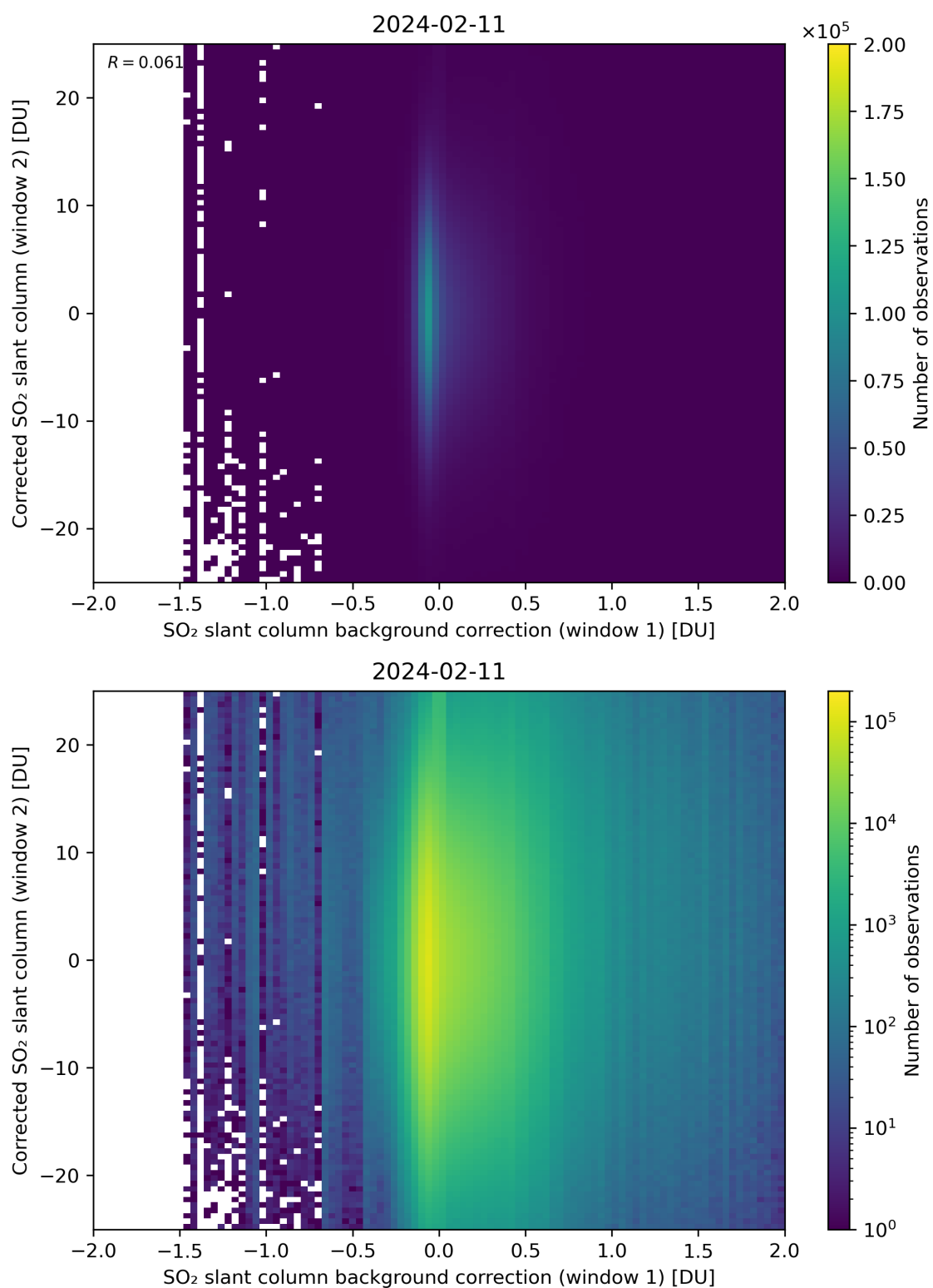
Figure 104: Scatter density plot of “SO 2 slant column background correction (window 1)” against “Corrected SO 2 slant column (window 2)” for 2024-02-11 to 2024-02-12.
