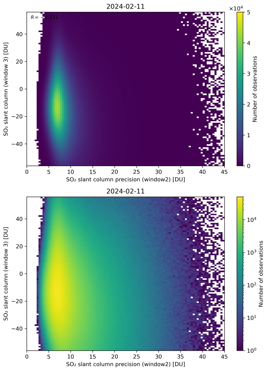
Figure 249: Scatter density plot of “SO 2 slant column precision (window2)” against “SO 2 slant column (window 3)” for 2024-02-11 to 2024-02-12.
