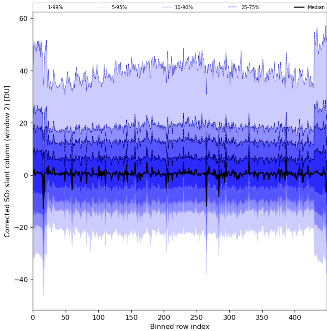
Figure 85: Along track statistics of “Corrected SO 2 slant column (window 2)” for 2024-02-11 to 2024-02-12
