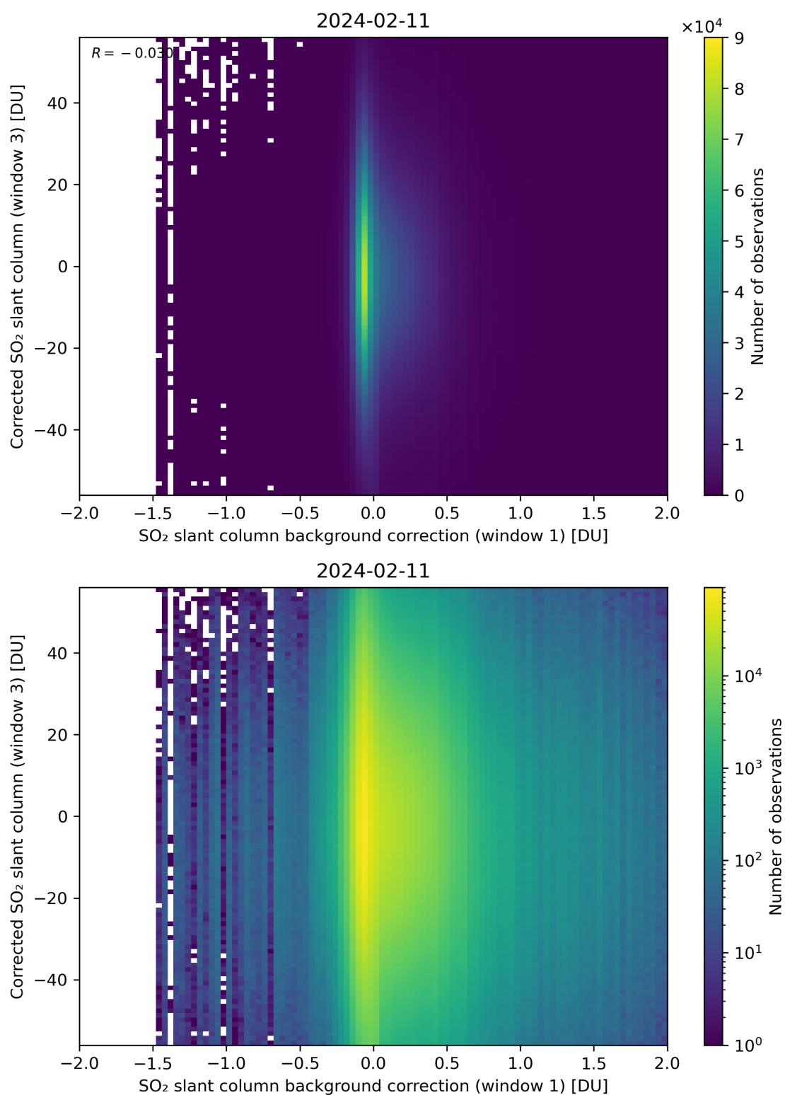
Figure 105: Scatter density plot of “SO 2 slant column background correction (window 1)” against “Corrected SO 2 slant column (window 3)” for 2024-02-11 to 2024-02-12.
