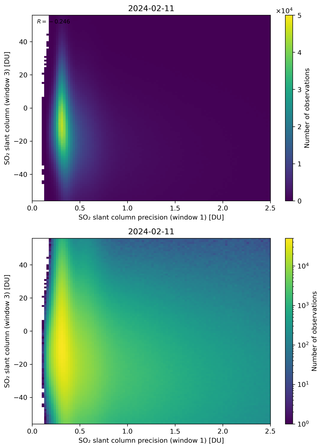
Figure 228: Scatter density plot of “SO 2 slant column precision (window 1)” against “SO 2 slant column (window 3)” for 2024-02-11 to 2024-02-12.
