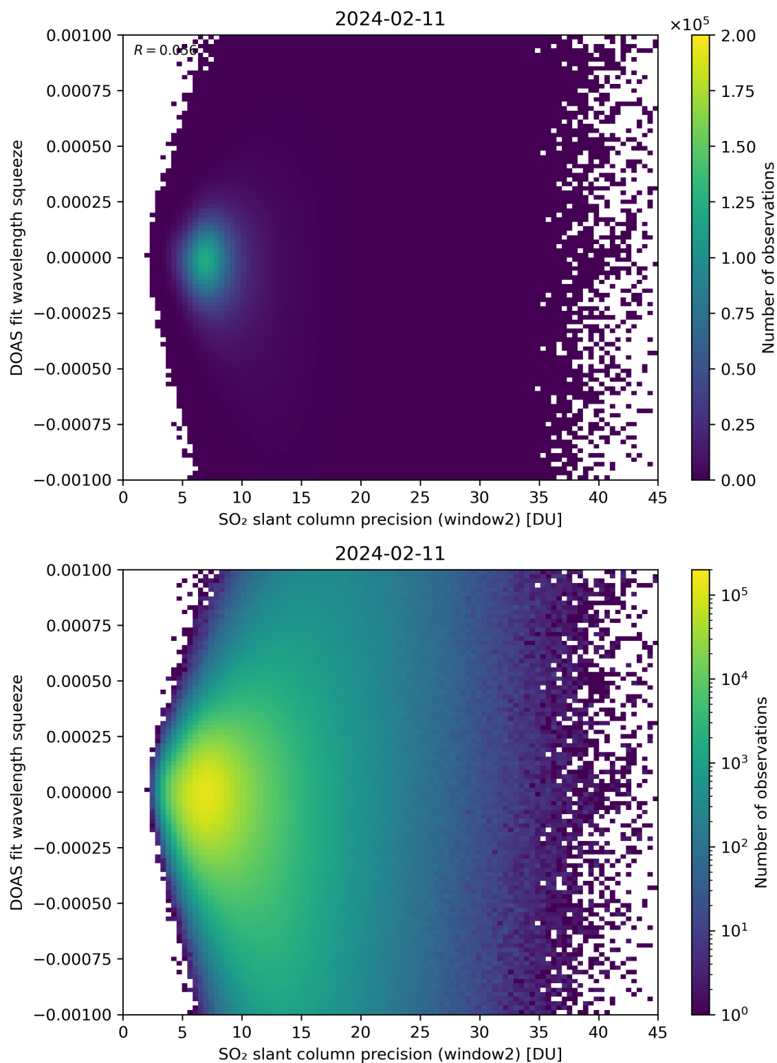
Figure 244: Scatter density plot of “SO 2 slant column precision (window2)” against “DOAS fit wavelength squeeze” for 2024-02-11 to 2024-02-12.
