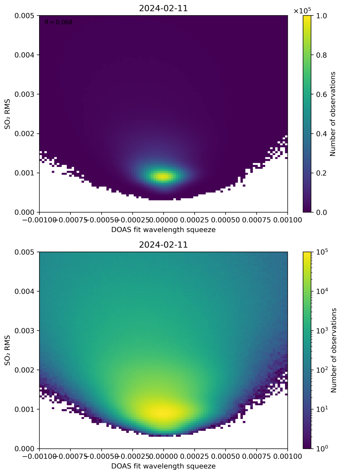
Figure 132: Scatter density plot of “DOAS fit wavelength squeeze” against “SO 2 RMS” for 2024-02-11 to 2024-02-12.
