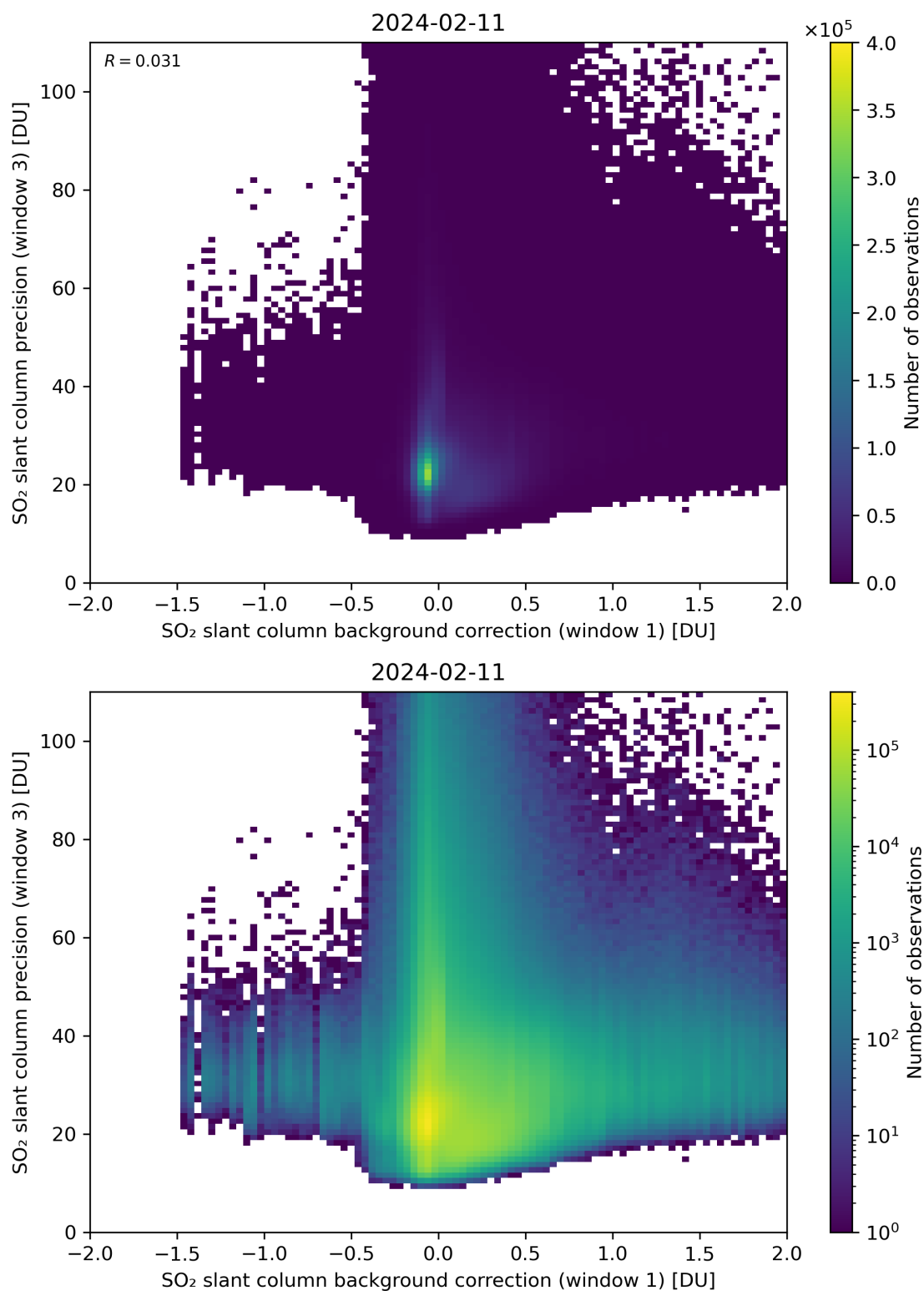
Figure 108: Scatter density plot of “SO 2 slant column background correction (window 1)” against “SO 2 slant column precision (window 3)” for 2024-02-11 to 2024-02-12.
