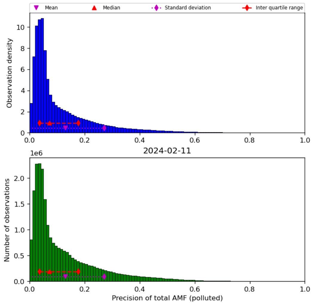
Figure 72: Histogram of “Precision of total AMF (polluted)” for 2024-02-11 to 2024-02-12
