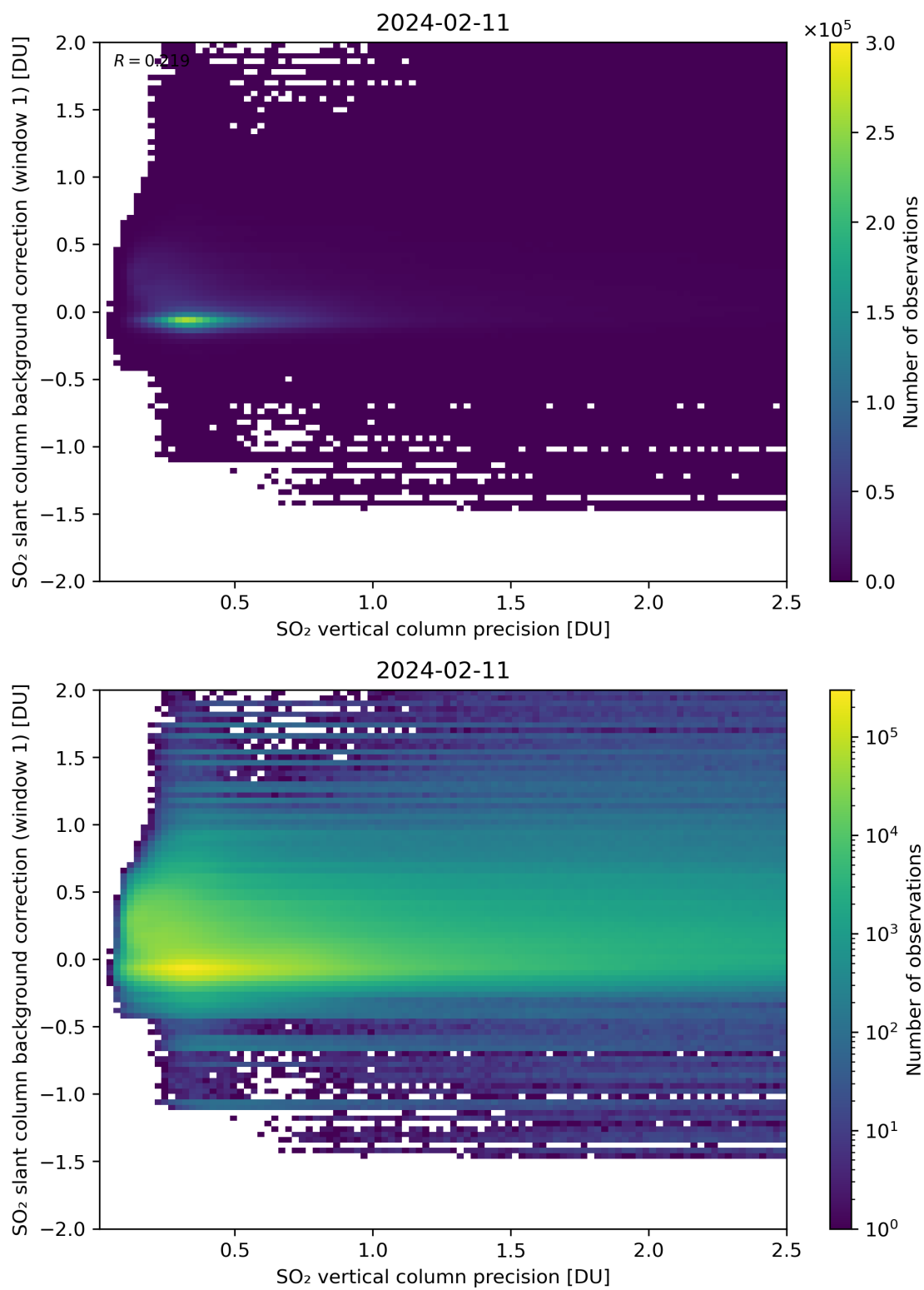
Figure 279: Scatter density plot of “SO 2 vertical column precision” against “SO 2 slant column background correction (window 1)” for 2024-02-11 to 2024-02-12.
