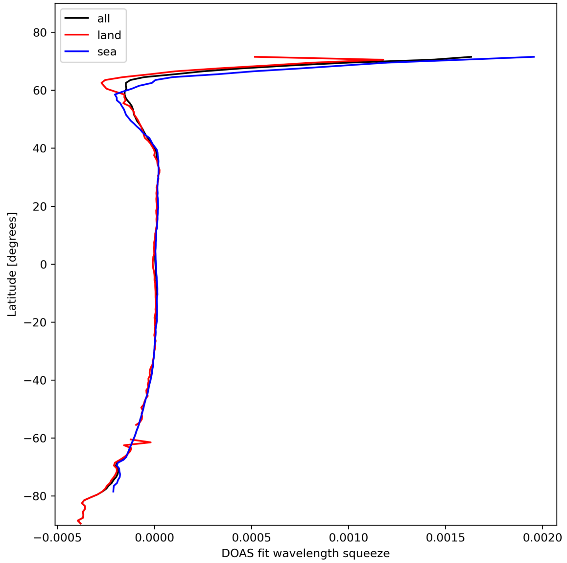
Figure 46: Zonal average of “DOAS fit wavelength squeeze” for 2024-02-11 to 2024-02-12.
