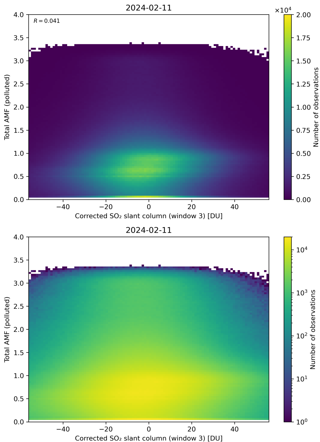
Figure 210: Scatter density plot of “Corrected SO 2 slant column (window 3)” against “Total AMF (polluted)” for 2024-02-11 to 2024-02-12.
