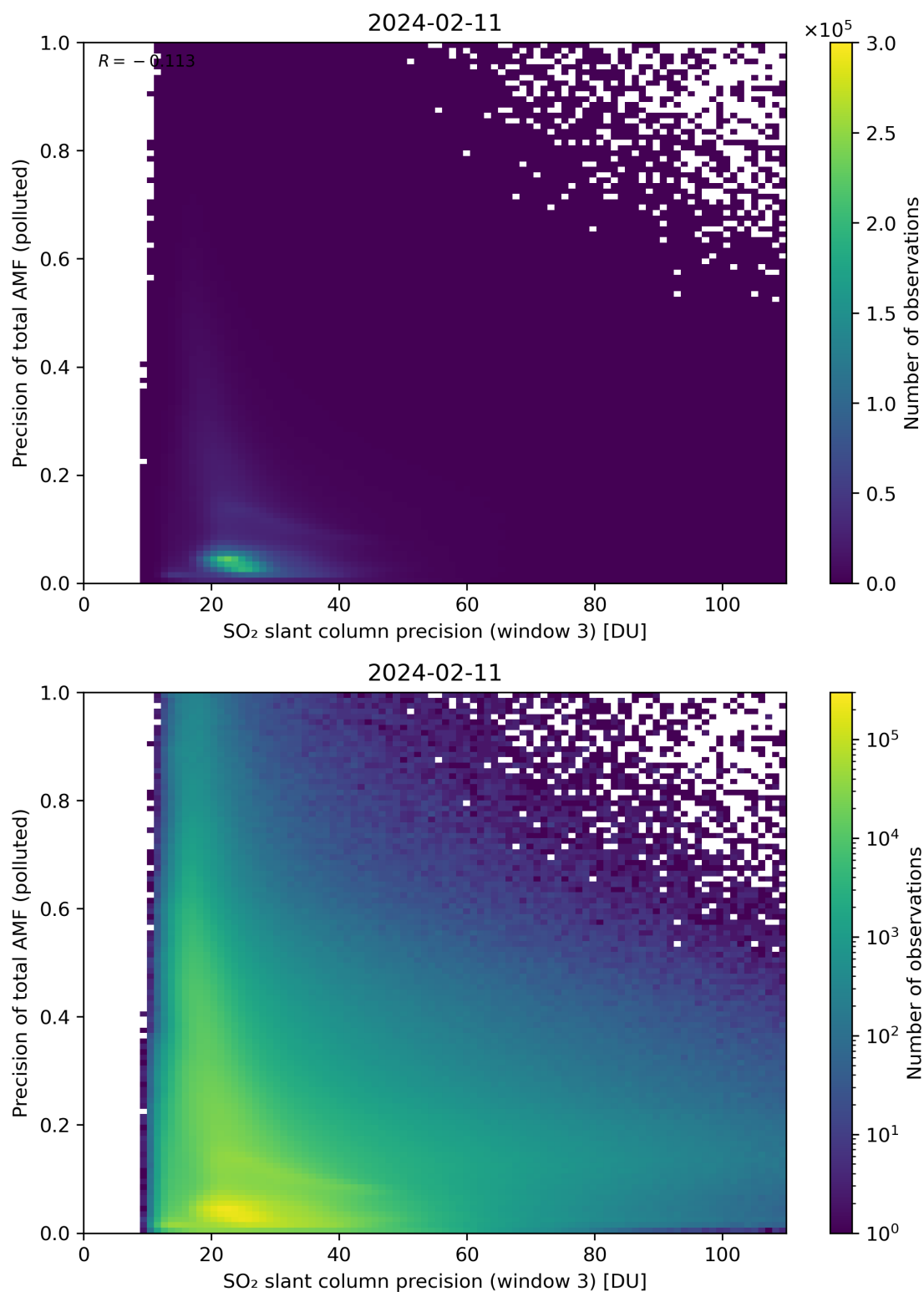
Figure 264: Scatter density plot of “SO 2 slant column precision (window 3)” against “Precision of total AMF (polluted)” for 2024-02-11 to 2024-02-12.
