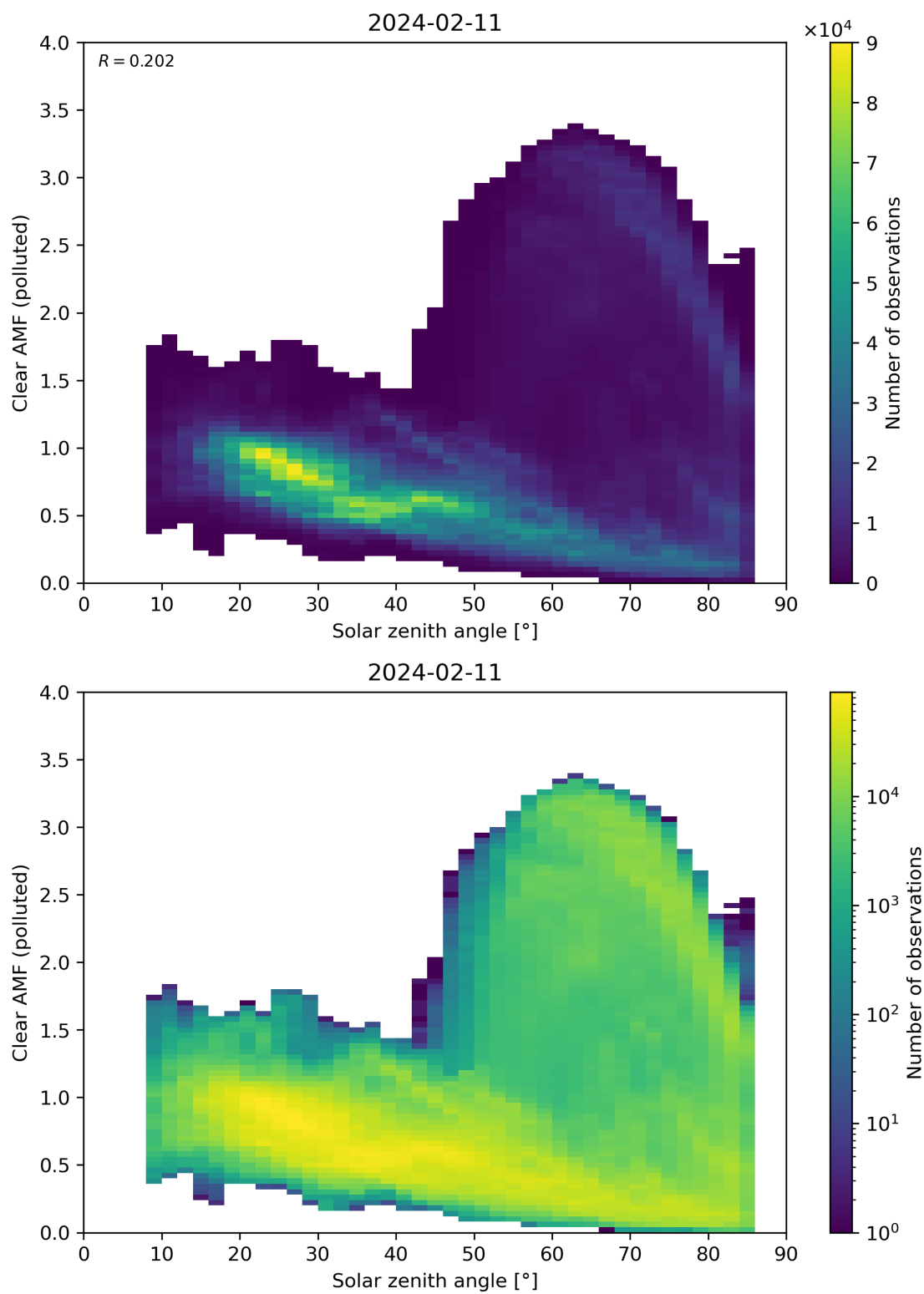
Figure 165: Scatter density plot of “Solar zenith angle” against “Clear AMF (polluted)” for 2024-02-11 to 2024-02-12.
