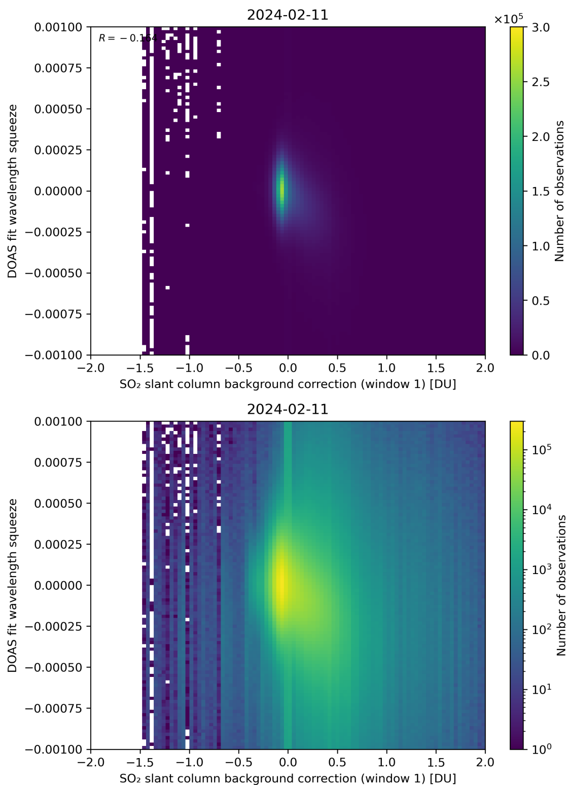
Figure 101: Scatter density plot of “SO 2 slant column background correction (window 1)” against “DOAS fit wavelength squeeze” for 2024-02-11 to 2024-02-12.
