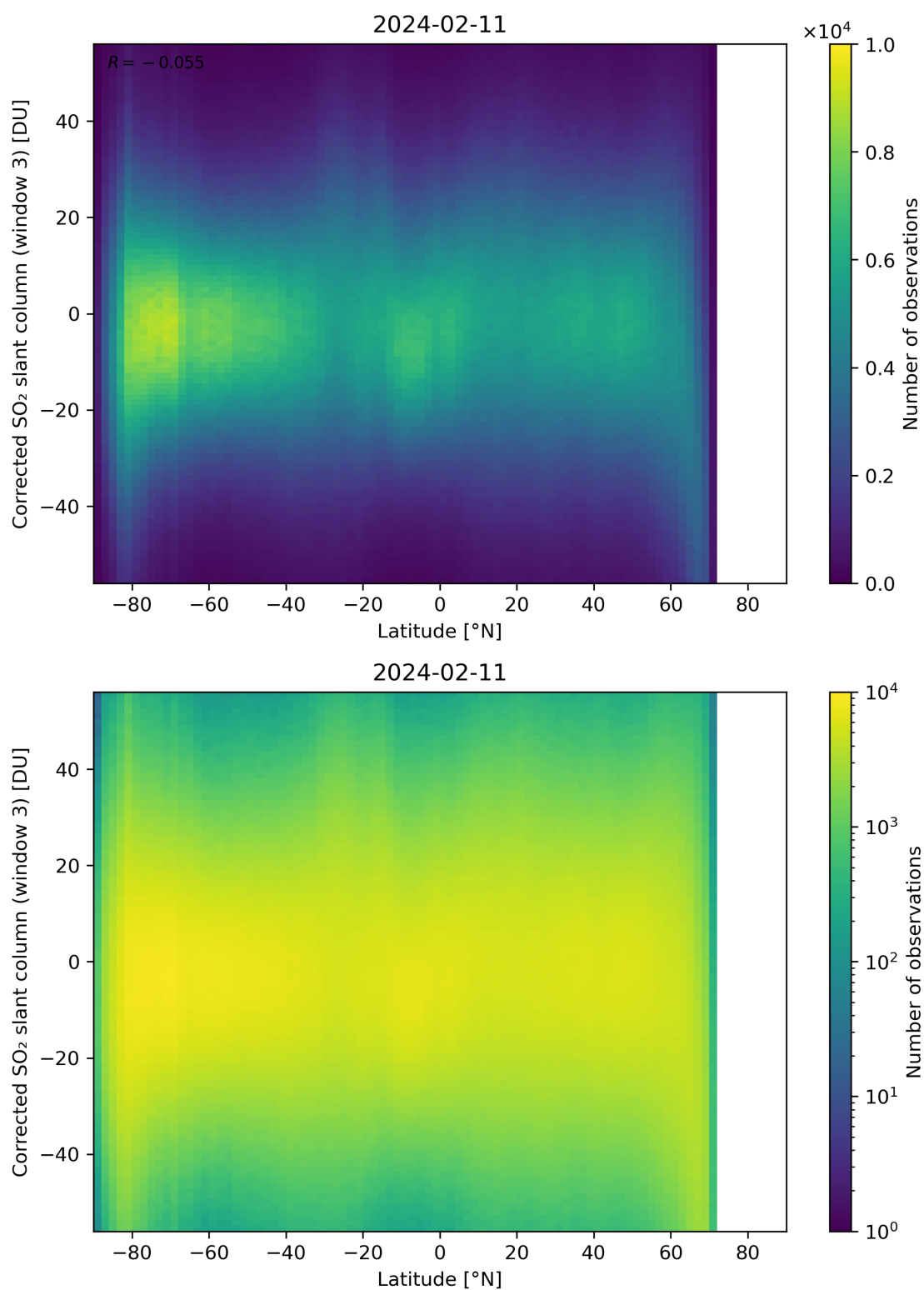
Figure 148: Scatter density plot of “Latitude” against “Corrected SO 2 slant column (window 3)” for 2024-02-11 to 2024-02-12.
