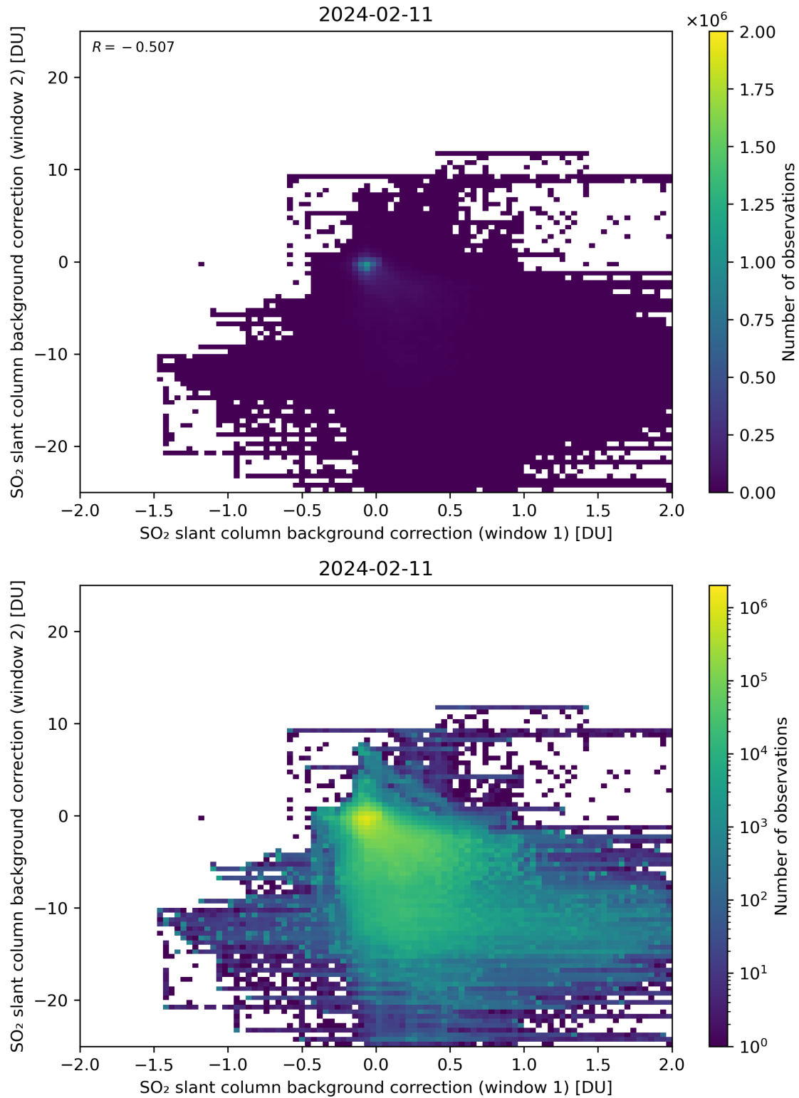
Figure 98: Scatter density plot of “SO 2 slant column background correction (window 1)” against “SO 2 slant column background correction (window 2)” for 2024-02-11 to 2024-02-12.
