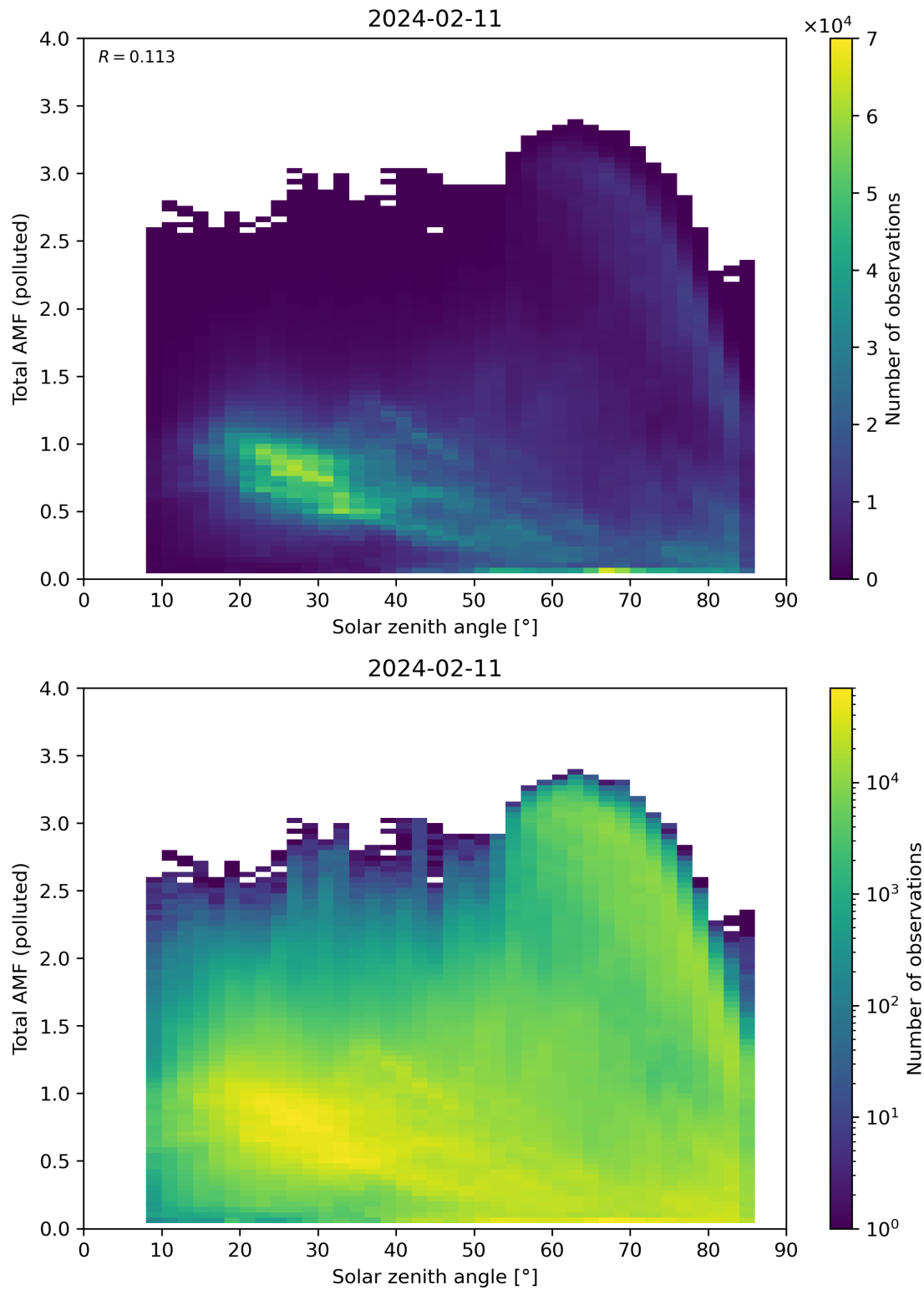
Figure 174: Scatter density plot of “Solar zenith angle” against “Total AMF (polluted)” for 2024-02-11 to 2024-02-12.
