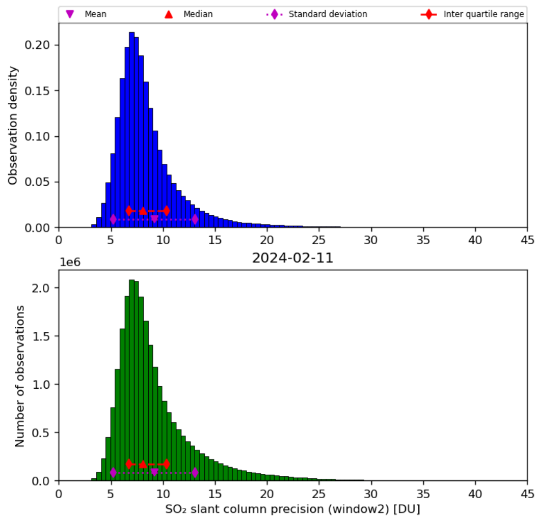
Figure 61: Histogram of “SO 2 slant column precision (window2)” for 2024-02-11 to 2024-02-12
