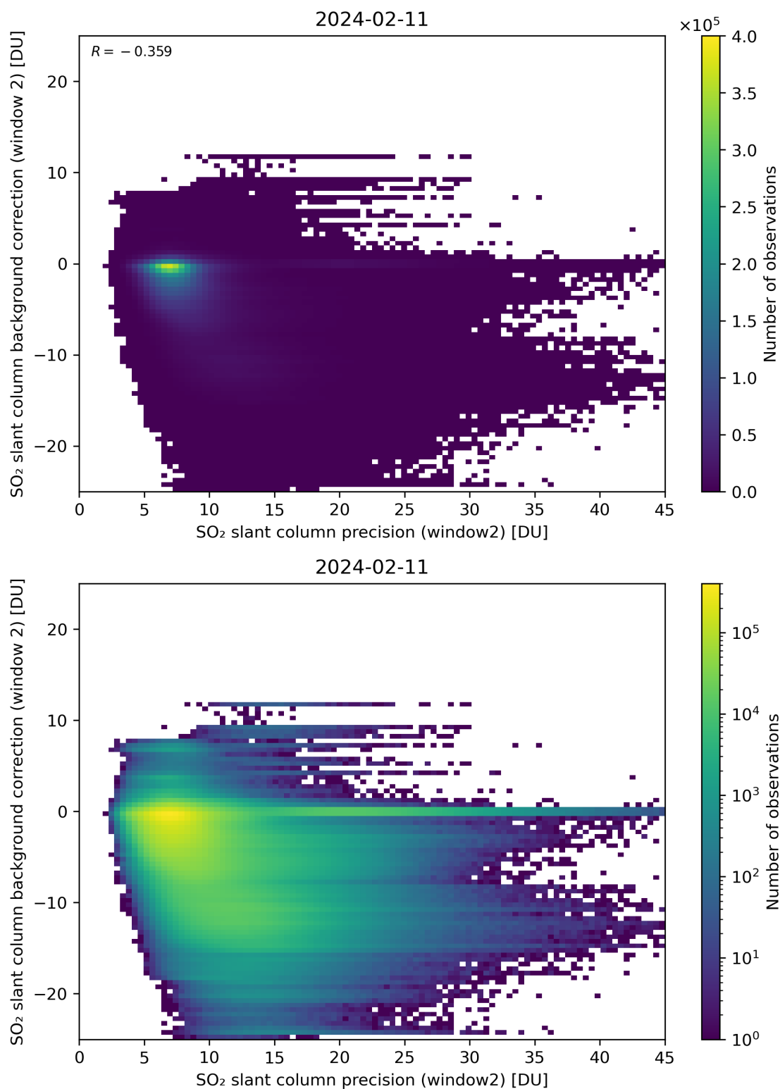
Figure 241: Scatter density plot of “SO 2 slant column precision (window2)” against “SO 2 slant column background correction (window 2)” for 2024-02-11 to 2024-02-12.
