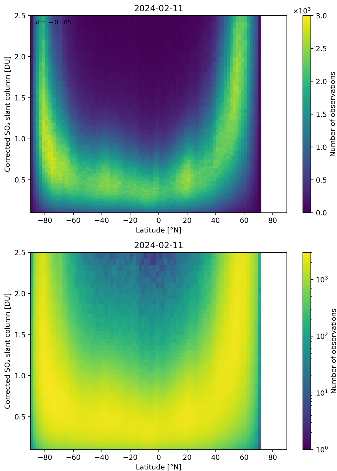
Figure 146: Scatter density plot of “Latitude” against “Corrected SO 2 slant column” for 2024-02-11 to 2024-02-12.
