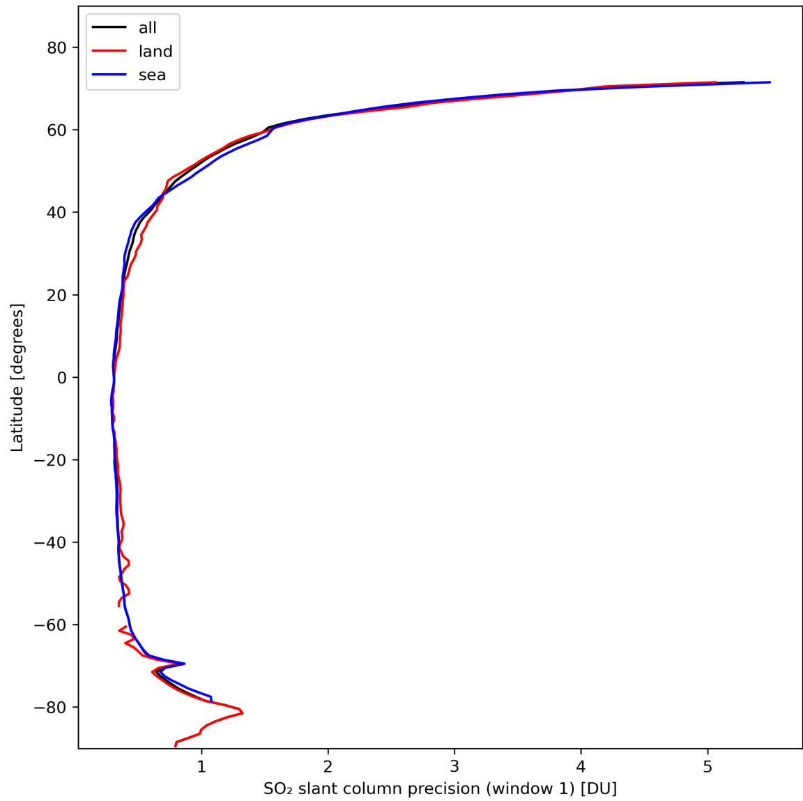
Figure 34: Zonal average of “SO 2 slant column precision (window 1)” for 2024-02-11 to 2024-02-12.
