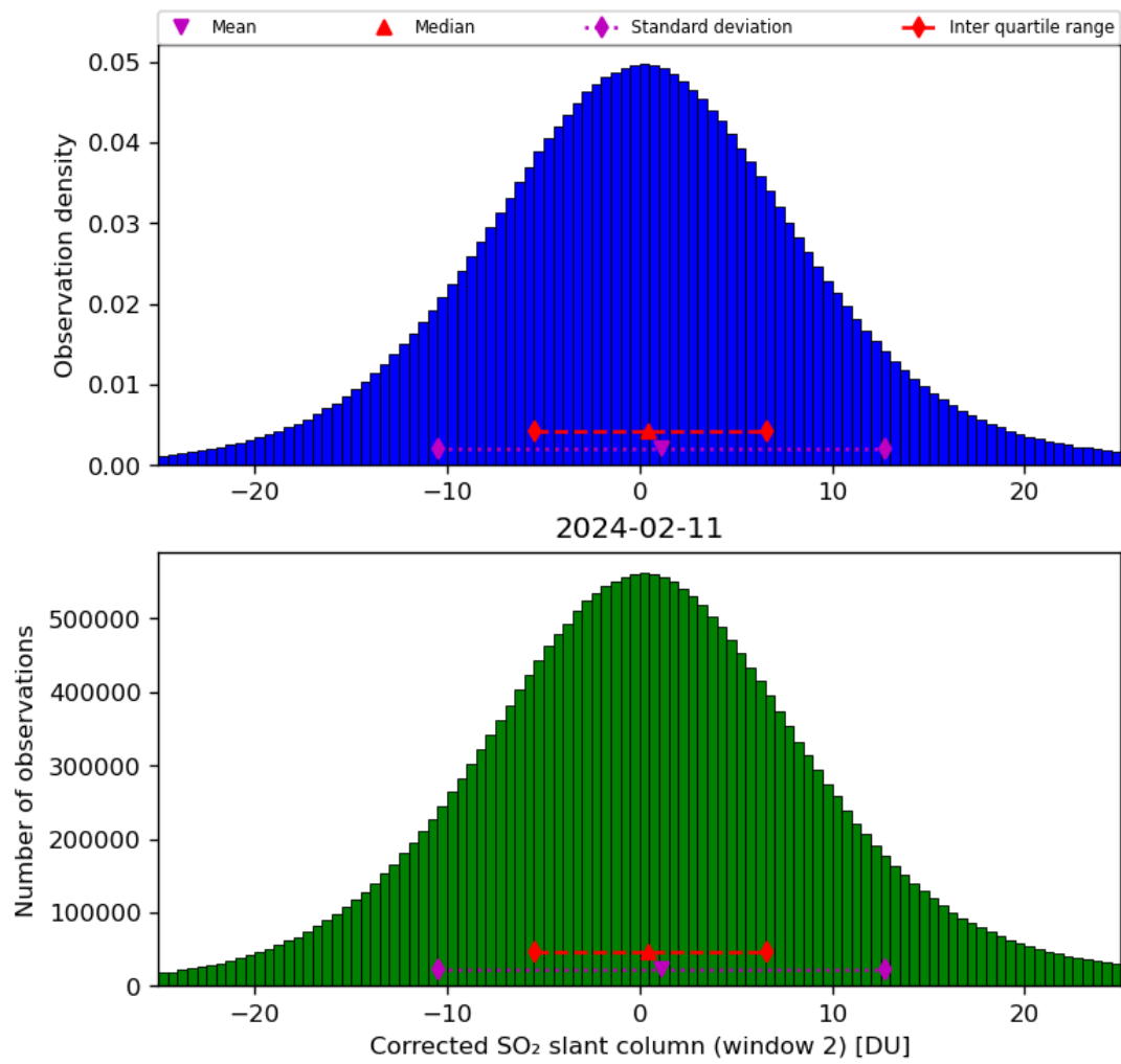
Figure 62: Histogram of “Corrected SO 2 slant column (window 2)” for 2024-02-11 to 2024-02-12
