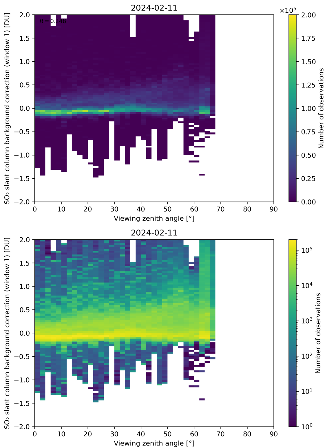
Figure 308: Scatter density plot of “Viewing zenith angle” against “SO 2 slant column background correction (window 1)” for 2024-02-11 to 2024-02-12.
