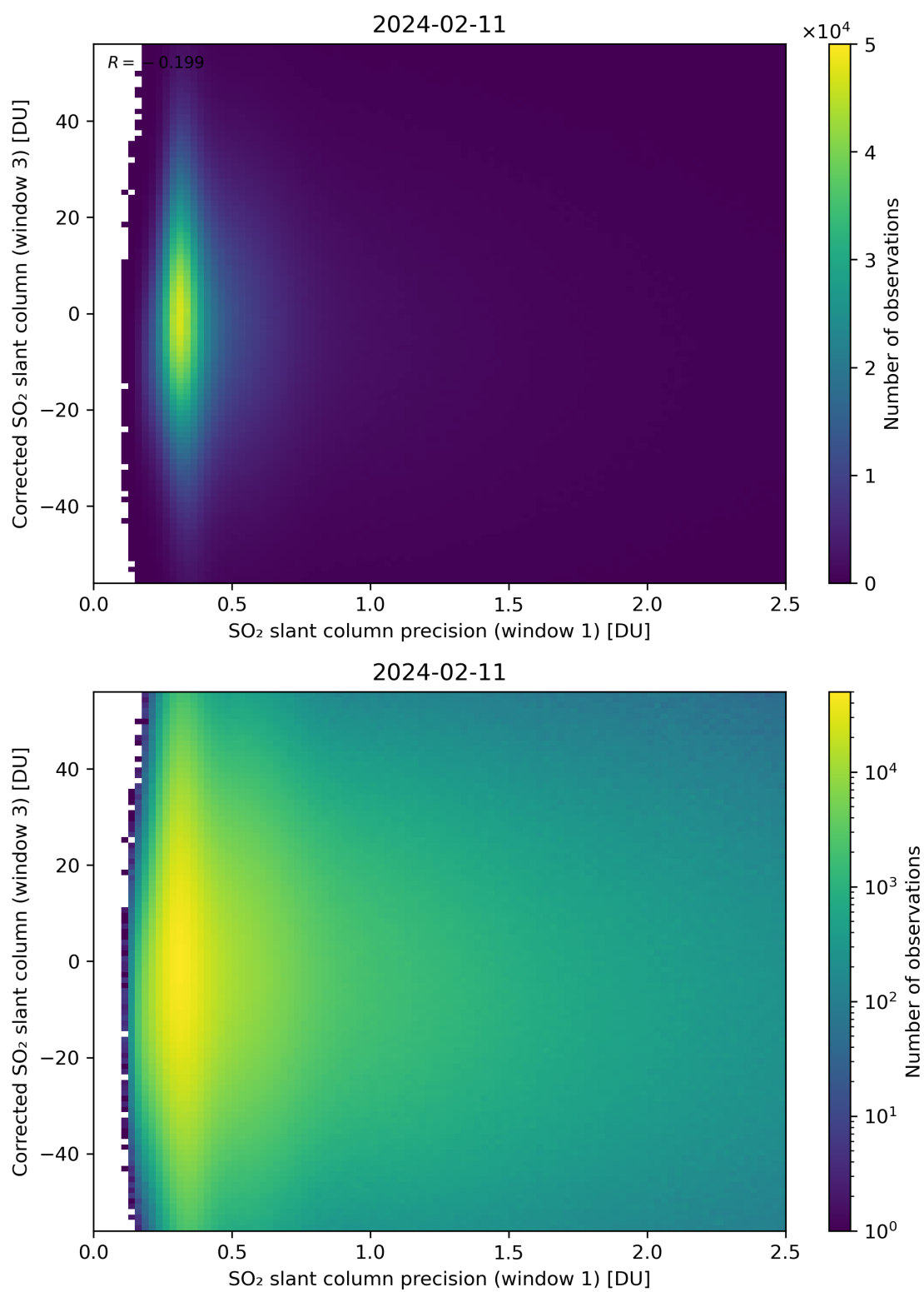
Figure 226: Scatter density plot of “SO 2 slant column precision (window 1)” against “Corrected SO 2 slant column (window 3)” for 2024-02-11 to 2024-02-12.
