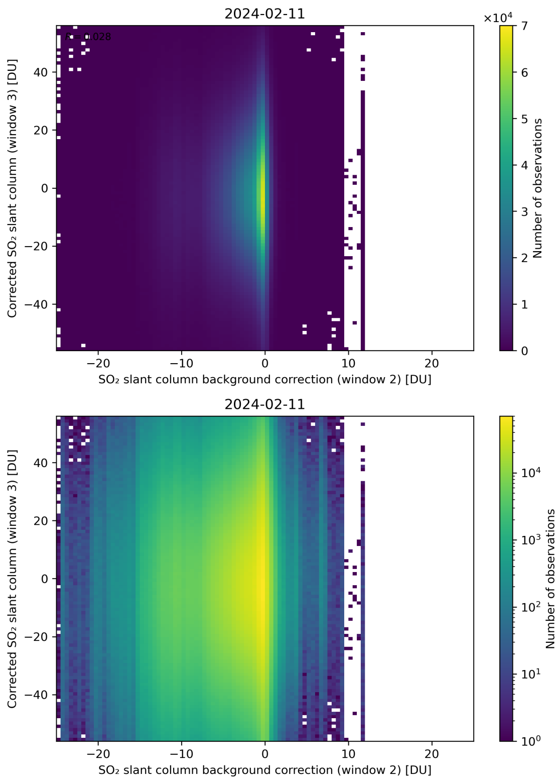
Figure 116: Scatter density plot of “SO 2 slant column background correction (window 2)” against “Corrected SO 2 slant column (window 3)” for 2024-02-11 to 2024-02-12.
