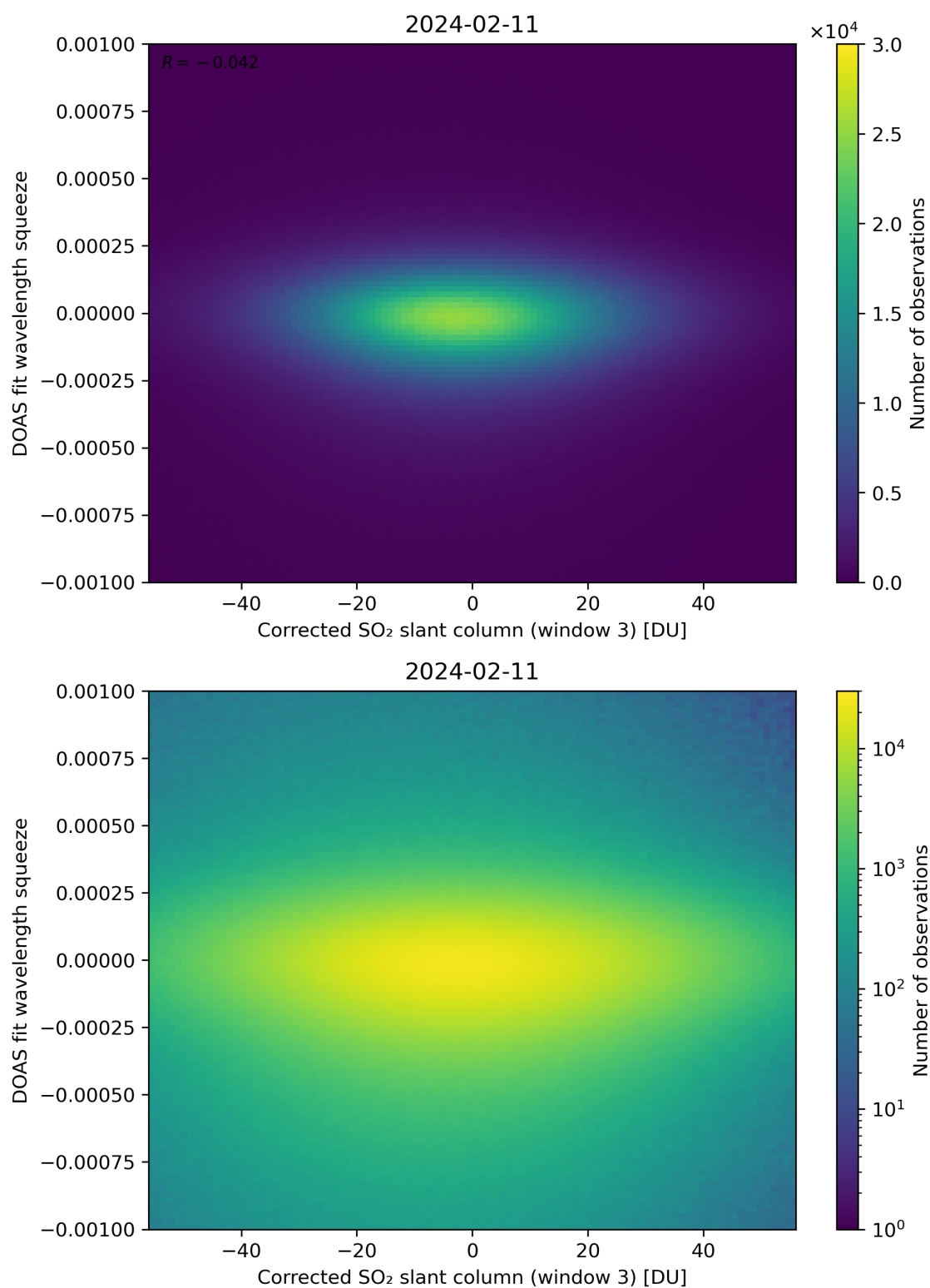
Figure 207: Scatter density plot of “Corrected SO 2 slant column (window 3)” against “DOAS fit wavelength squeeze” for 2024-02-11 to 2024-02-12.
