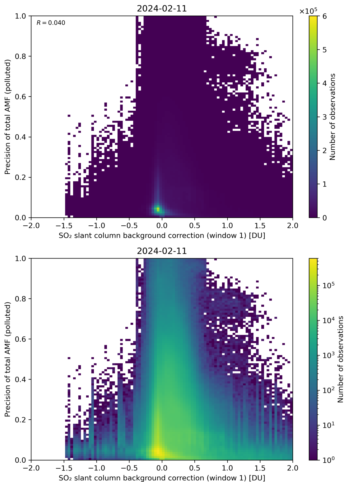
Figure 110: Scatter density plot of “SO 2 slant column background correction (window 1)” against “Precision of total AMF (polluted)” for 2024-02-11 to 2024-02-12.
