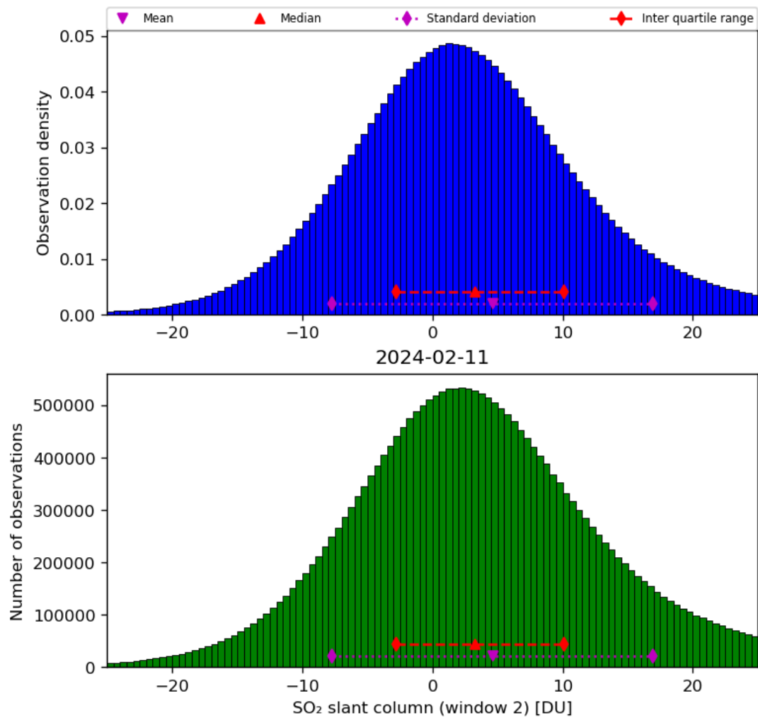
Figure 60: Histogram of “SO 2 slant column (window 2)” for 2024-02-11 to 2024-02-12
