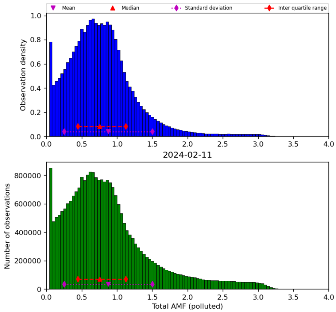
Figure 71: Histogram of “Total AMF (polluted)” for 2024-02-11 to 2024-02-12
