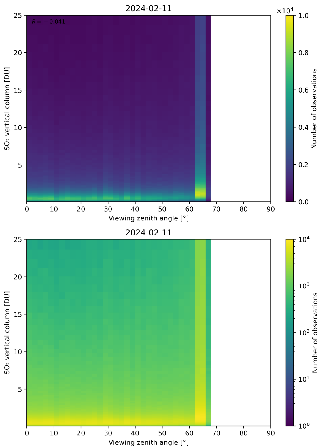
Figure 327: Scatter density plot of “Viewing zenith angle” against “SO 2 vertical column” for 2024-02-11 to 2024-02-12.
