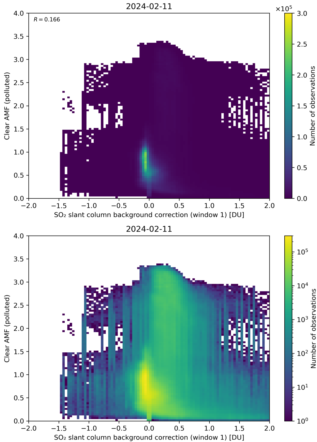
Figure 103: Scatter density plot of “SO 2 slant column background correction (window 1)” against “Clear AMF (polluted)” for 2024-02-11 to 2024-02-12.
