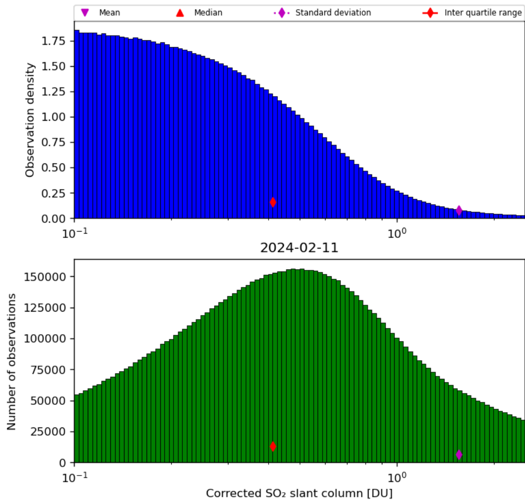
Figure 55: Histogram of “Corrected SO 2 slant column” for 2024-02-11 to 2024-02-12
