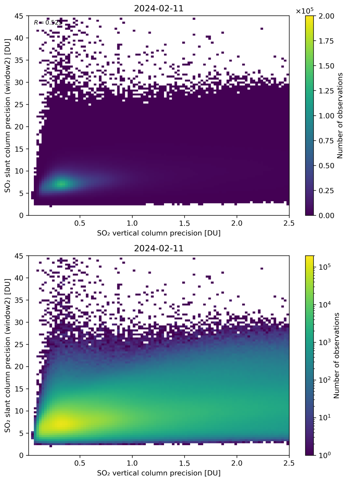
Figure 291: Scatter density plot of “SO 2 vertical column precision” against “SO 2 slant column precision (window2)” for 2024-02-11 to 2024-02-12.
