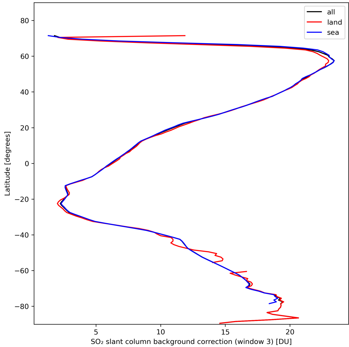
Figure 44: Zonal average of “SO 2 slant column background correction (window 3)” for 2024-02-11 to 2024-02-12.
