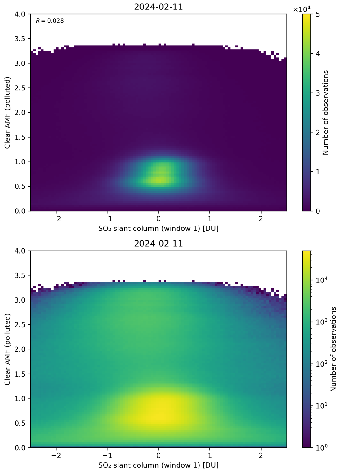
Figure 232: Scatter density plot of “SO 2 slant column (window 1)” against “Clear AMF (polluted)” for 2024-02-11 to 2024-02-12.
