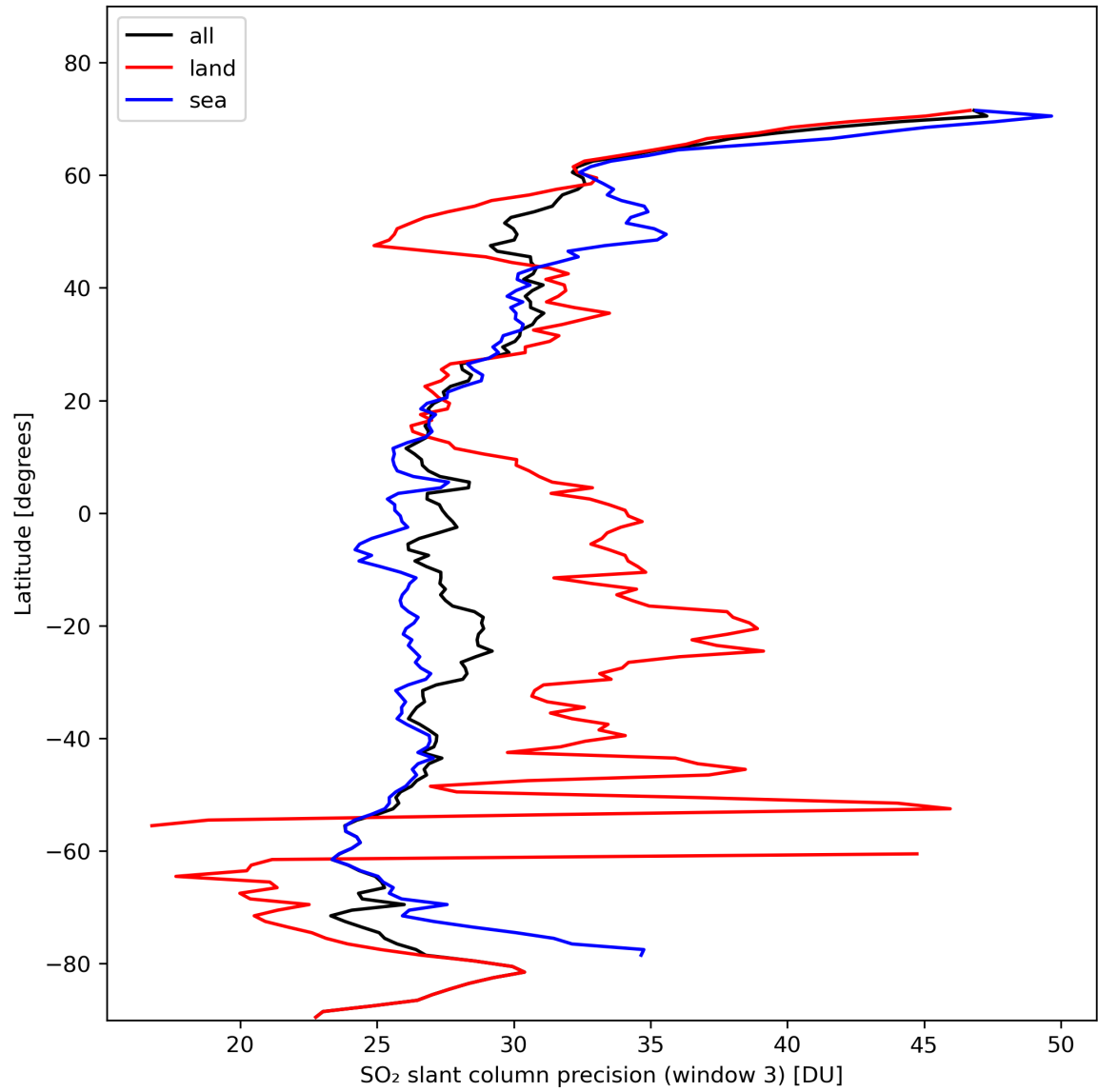
Figure 42: Zonal average of “SO 2 slant column precision (window 3)” for 2024-02-11 to 2024-02-12.
