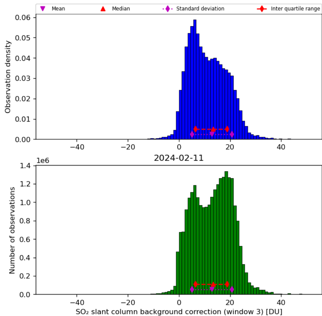
Figure 67: Histogram of “SO 2 slant column background correction (window 3)” for 2024-02-11 to 2024-02-12
