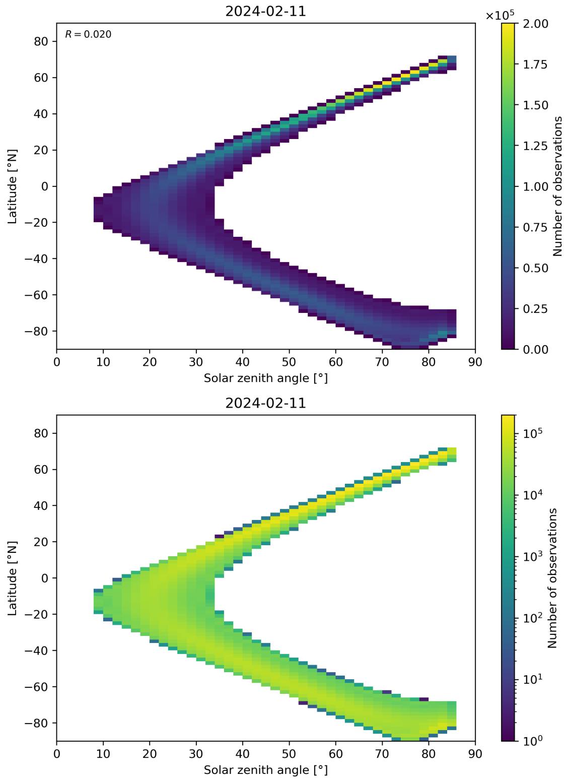
Figure 164: Scatter density plot of “Solar zenith angle” against “Latitude” for 2024-02-11 to 2024-02-12.
