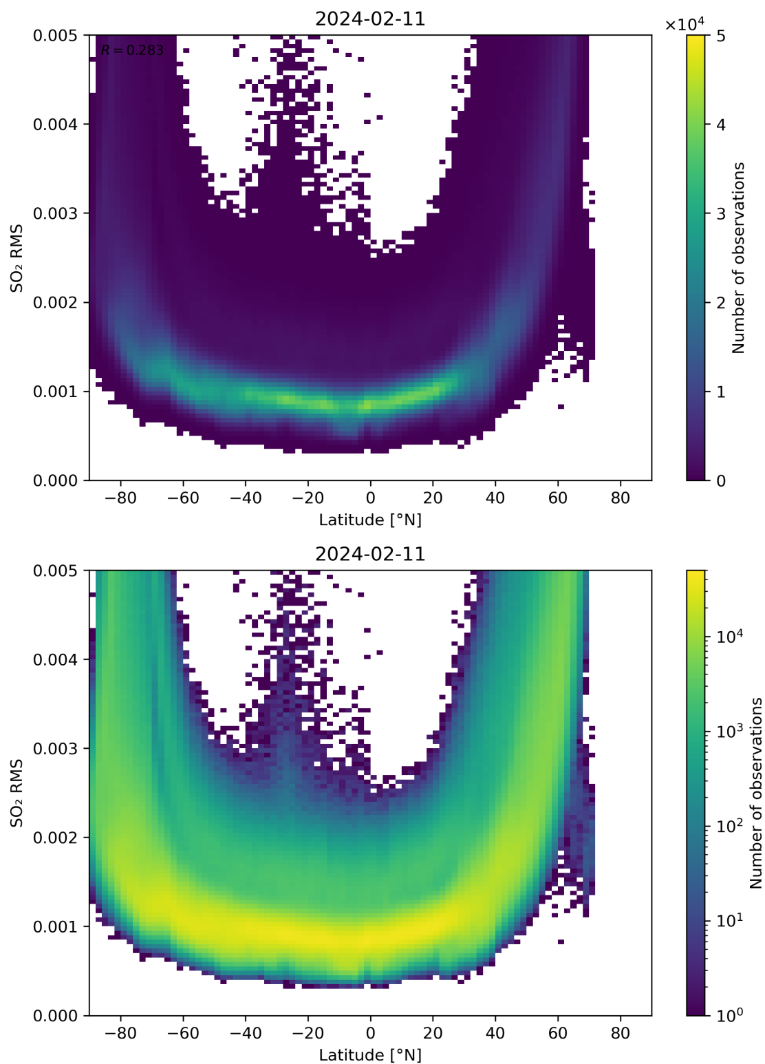
Figure 144: Scatter density plot of “Latitude” against “SO 2 RMS” for 2024-02-11 to 2024-02-12.
