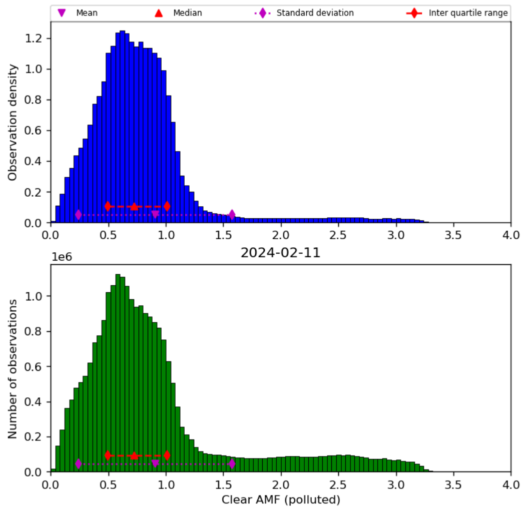
Figure 73: Histogram of “Clear AMF (polluted)” for 2024-02-11 to 2024-02-12
