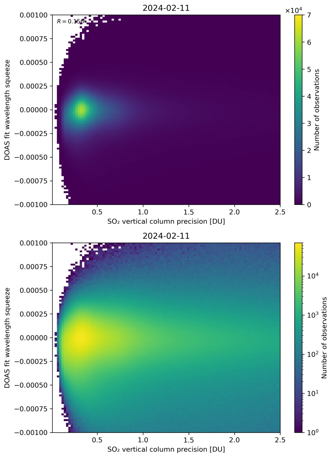
Figure 283: Scatter density plot of “SO 2 vertical column precision” against “DOAS fit wavelength squeeze” for 2024-02-11 to 2024-02-12.
