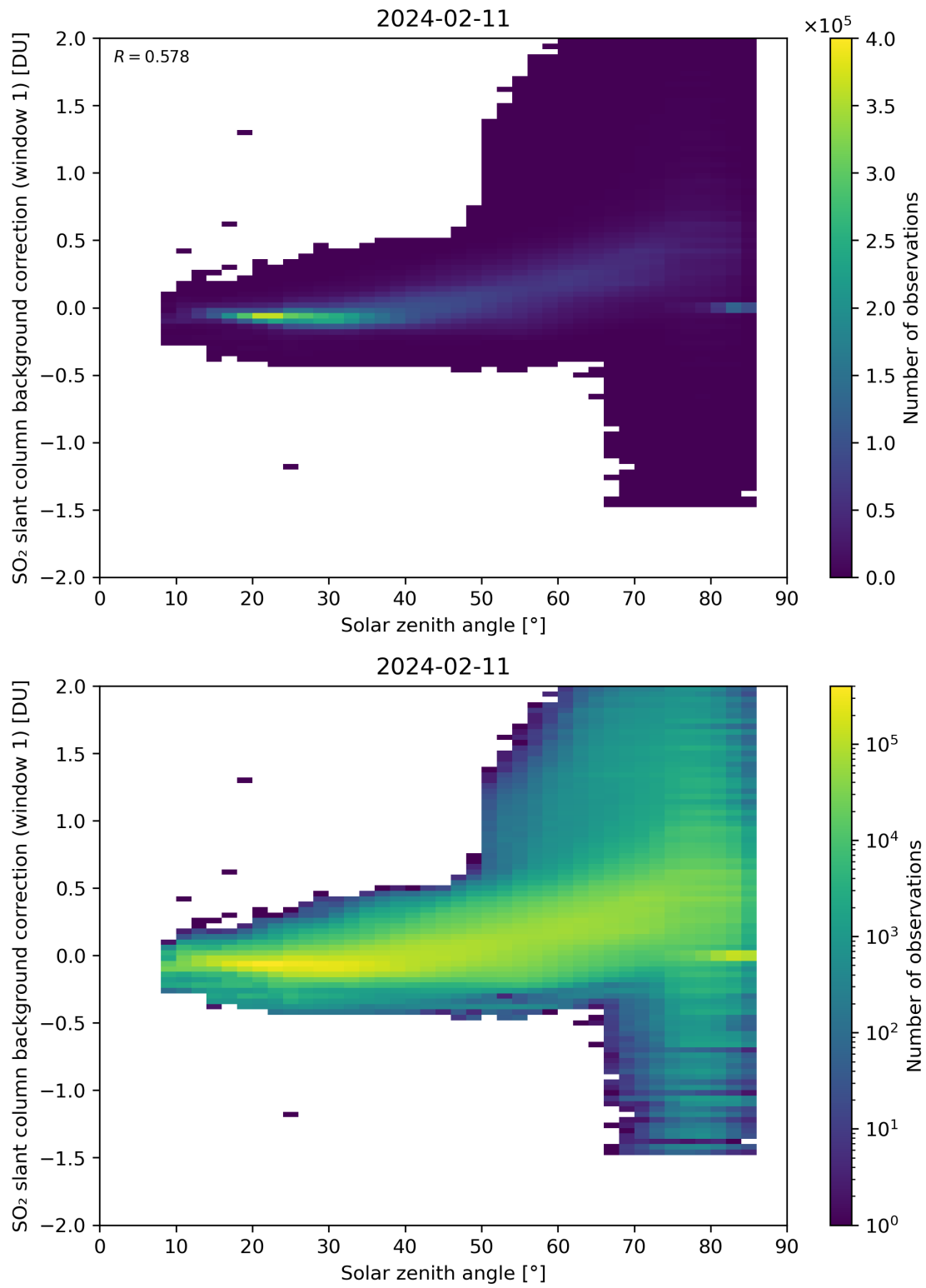
Figure 158: Scatter density plot of “Solar zenith angle” against “SO 2 slant column background correction (window 1)” for 2024-02-11 to 2024-02-12.
