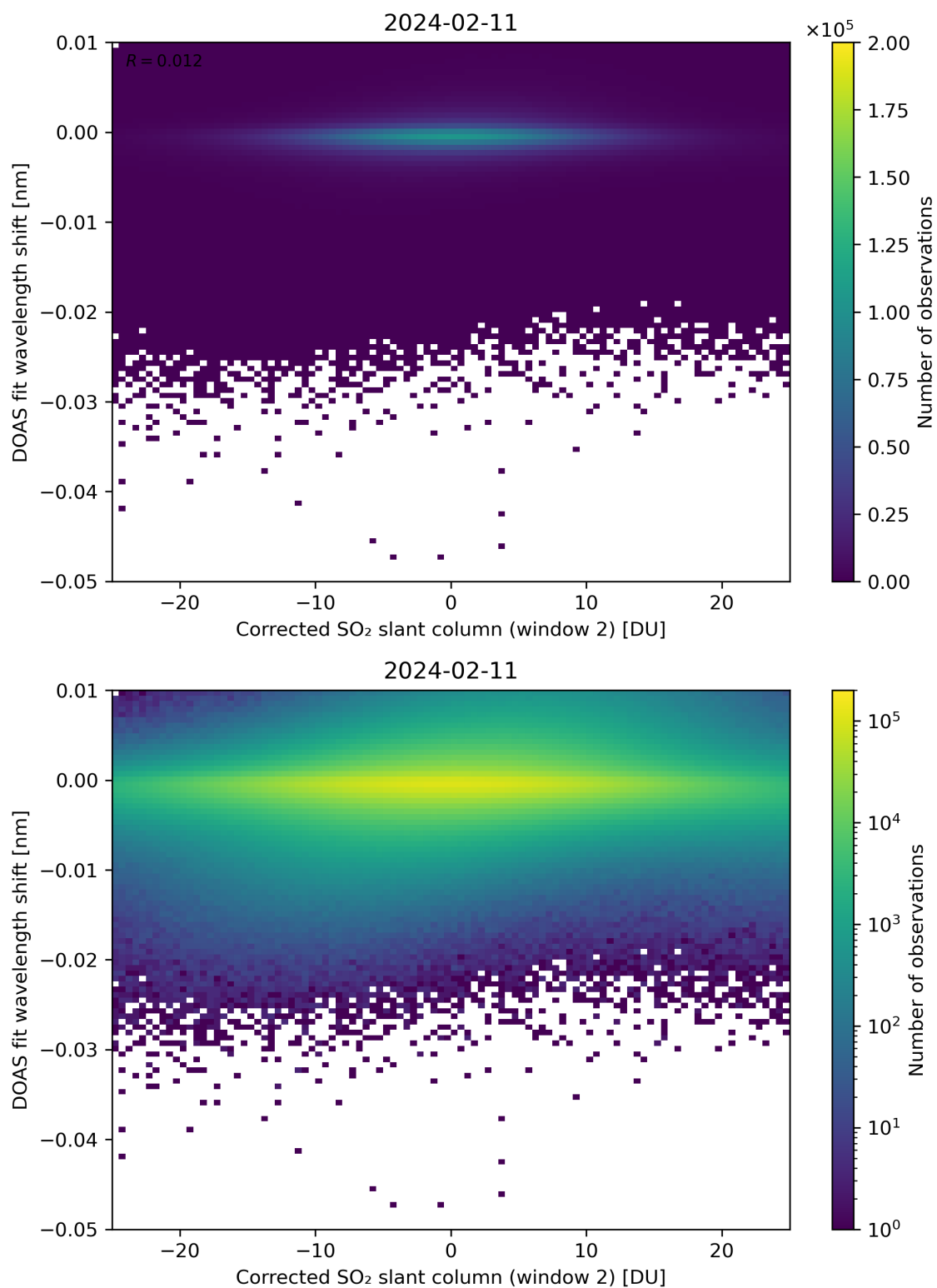
Figure 196: Scatter density plot of “Corrected SO 2 slant column (window 2)” against “DOAS fit wavelength shift” for 2024-02-11 to 2024-02-12.
