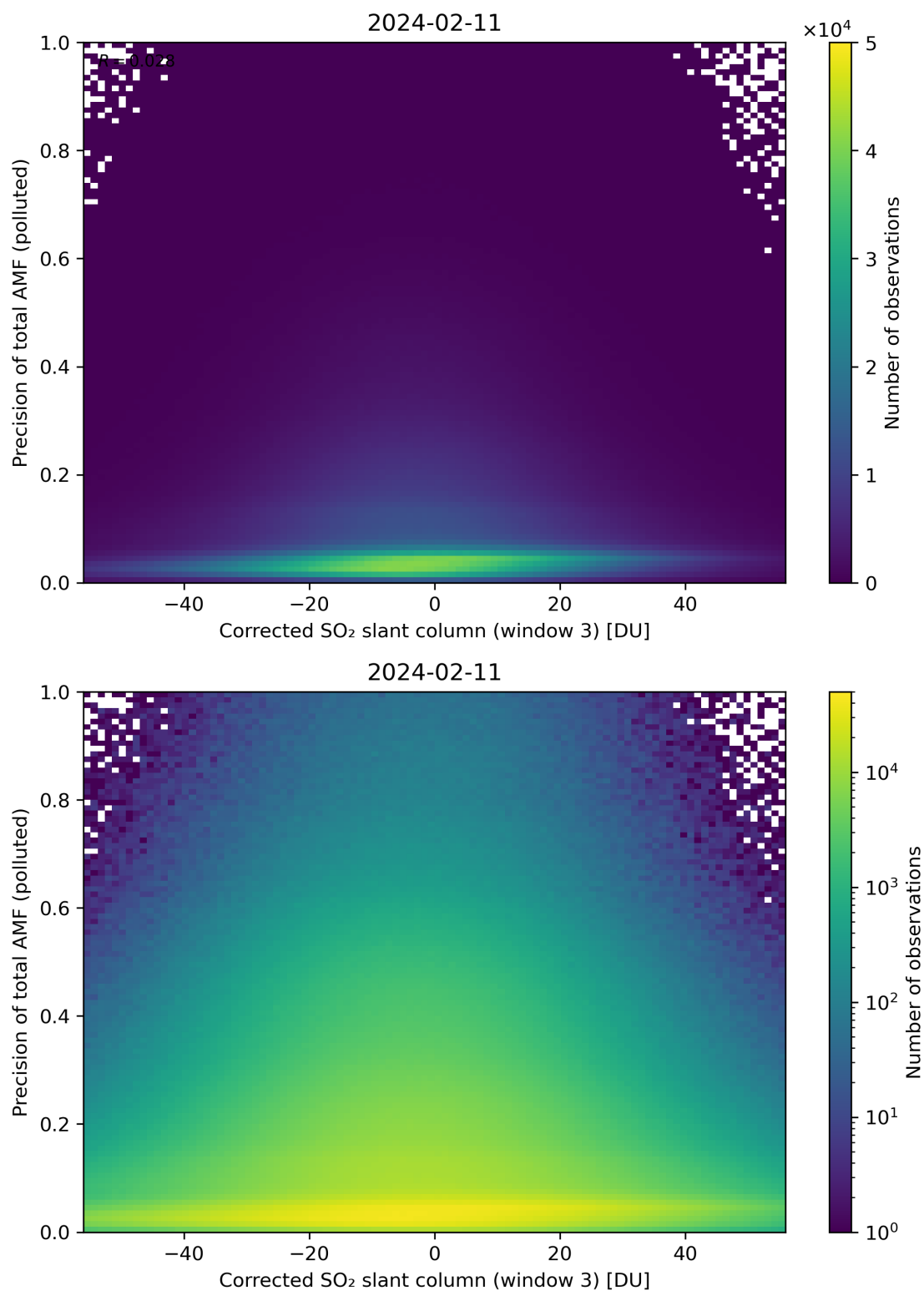
Figure 211: Scatter density plot of “Corrected SO 2 slant column (window 3)” against “Precision of total AMF (polluted)” for 2024-02-11 to 2024-02-12.
