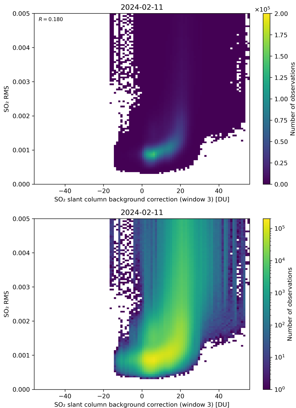
Figure 123: Scatter density plot of “SO 2 slant column background correction (window 3)” against “SO 2 RMS” for 2024-02-11 to 2024-02-12.
