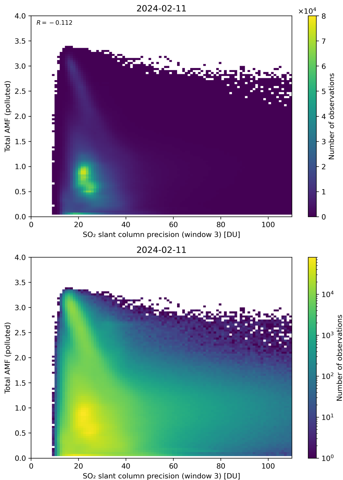
Figure 263: Scatter density plot of “SO 2 slant column precision (window 3)” against “Total AMF (polluted)” for 2024-02-11 to 2024-02-12.
