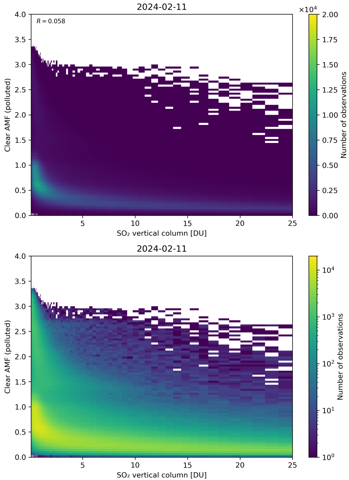
Figure 296: Scatter density plot of “SO 2 vertical column” against “Clear AMF (polluted)” for 2024-02-11 to 2024-02-12.
