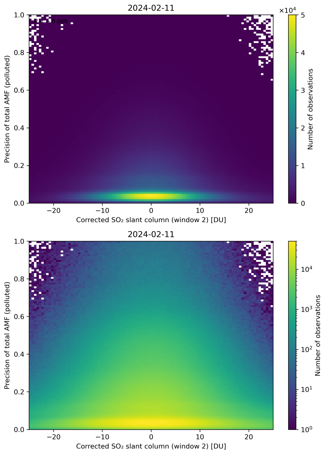
Figure 204: Scatter density plot of “Corrected SO 2 slant column (window 2)” against “Precision of total AMF (polluted)” for 2024-02-11 to 2024-02-12.
