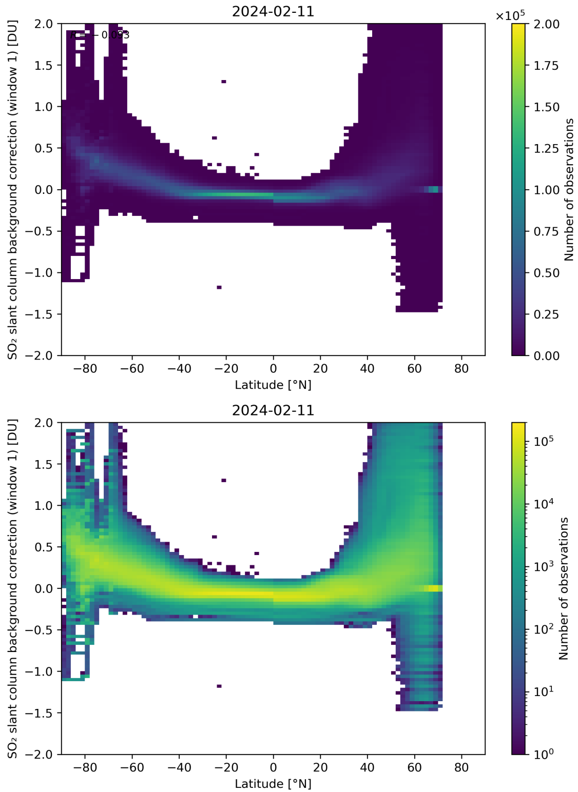
Figure 139: Scatter density plot of “Latitude” against “SO 2 slant column background correction (window 1)” for 2024-02-11 to 2024-02-12.
