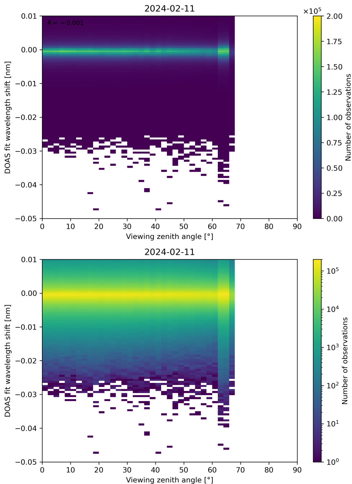
Figure 311: Scatter density plot of “Viewing zenith angle” against “DOAS fit wavelength shift” for 2024-02-11 to 2024-02-12.
