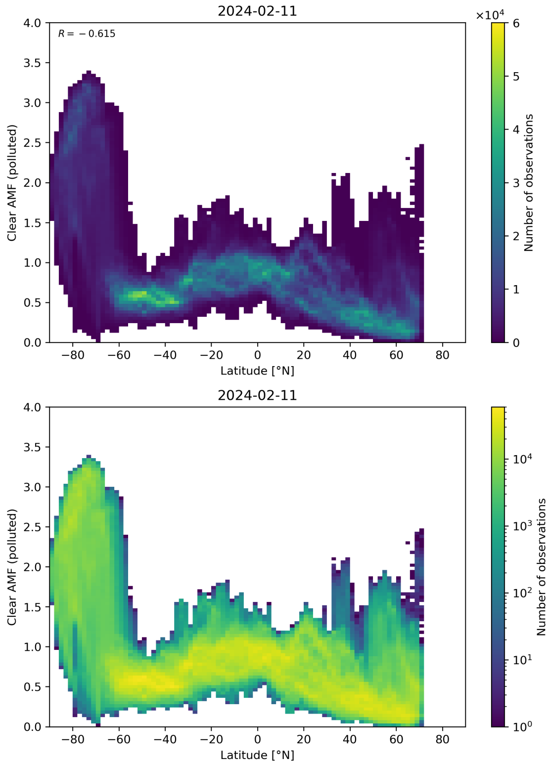
Figure 145: Scatter density plot of “Latitude” against “Clear AMF (polluted)” for 2024-02-11 to 2024-02-12.
