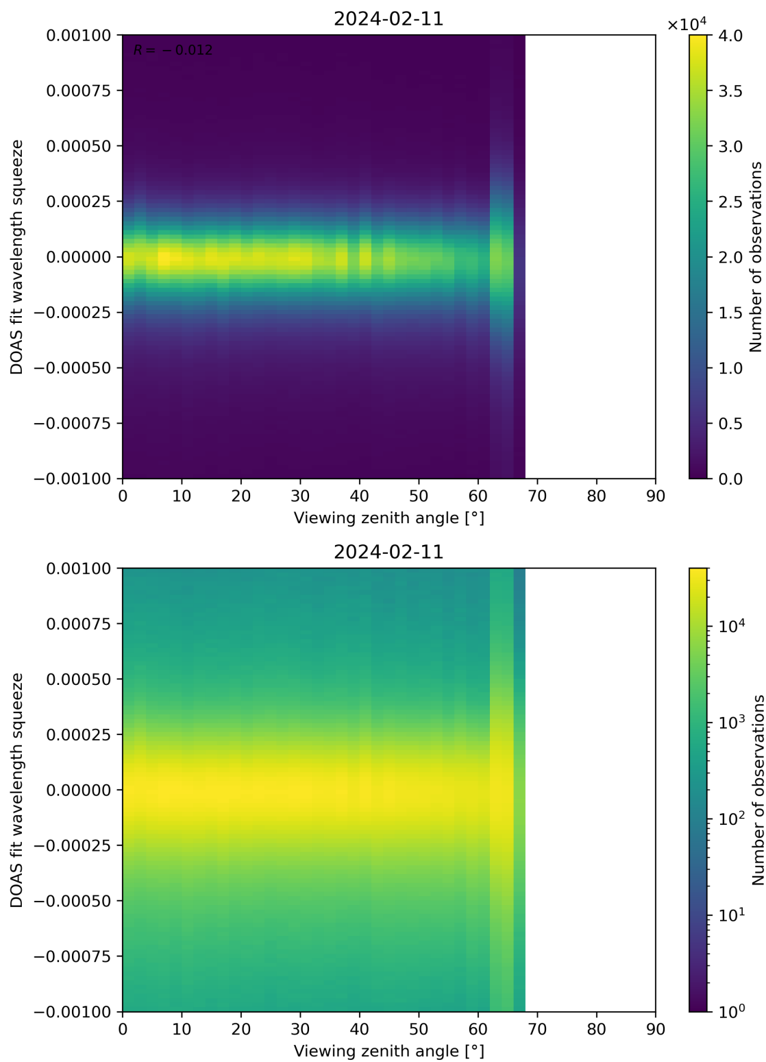
Figure 312: Scatter density plot of “Viewing zenith angle” against “DOAS fit wavelength squeeze” for 2024-02-11 to 2024-02-12.
