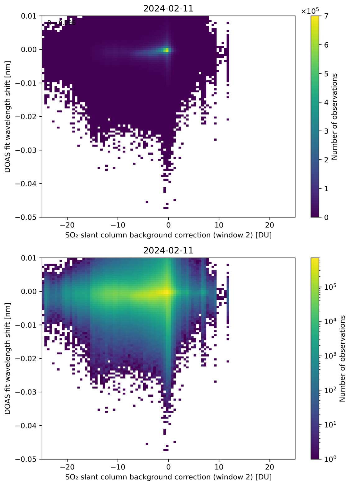
Figure 112: Scatter density plot of “SO 2 slant column background correction (window 2)” against “DOAS fit wavelength shift” for 2024-02-11 to 2024-02-12.
