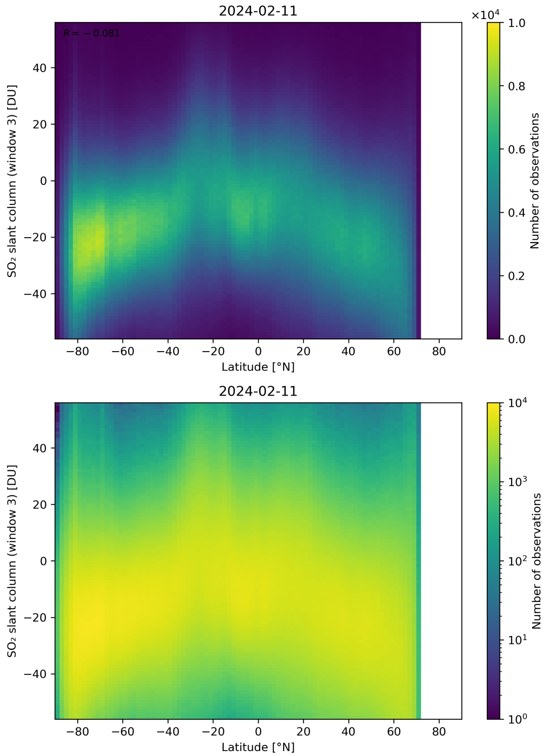
Figure 152: Scatter density plot of “Latitude” against “SO 2 slant column (window 3)” for 2024-02-11 to 2024-02-12.
