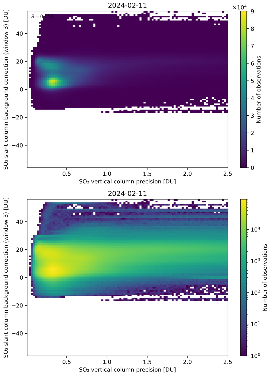
Figure 281: Scatter density plot of “SO 2 vertical column precision” against “SO 2 slant column background correction (window 3)” for 2024-02-11 to 2024-02-12.
