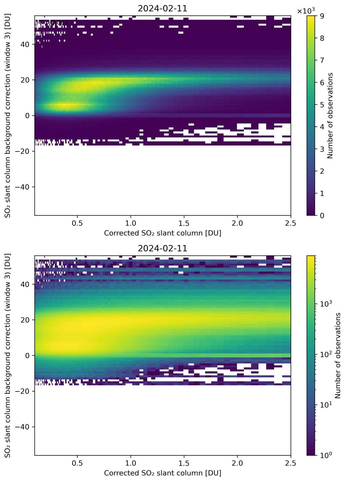
Figure 180: Scatter density plot of “Corrected SO 2 slant column” against “SO 2 slant column background correction (window 3)” for 2024-02-11 to 2024-02-12.
