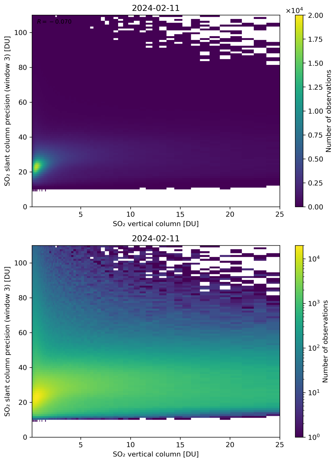
Figure 304: Scatter density plot of “SO 2 vertical column” against “SO 2 slant column precision (window 3)” for 2024-02-11 to 2024-02-12.
