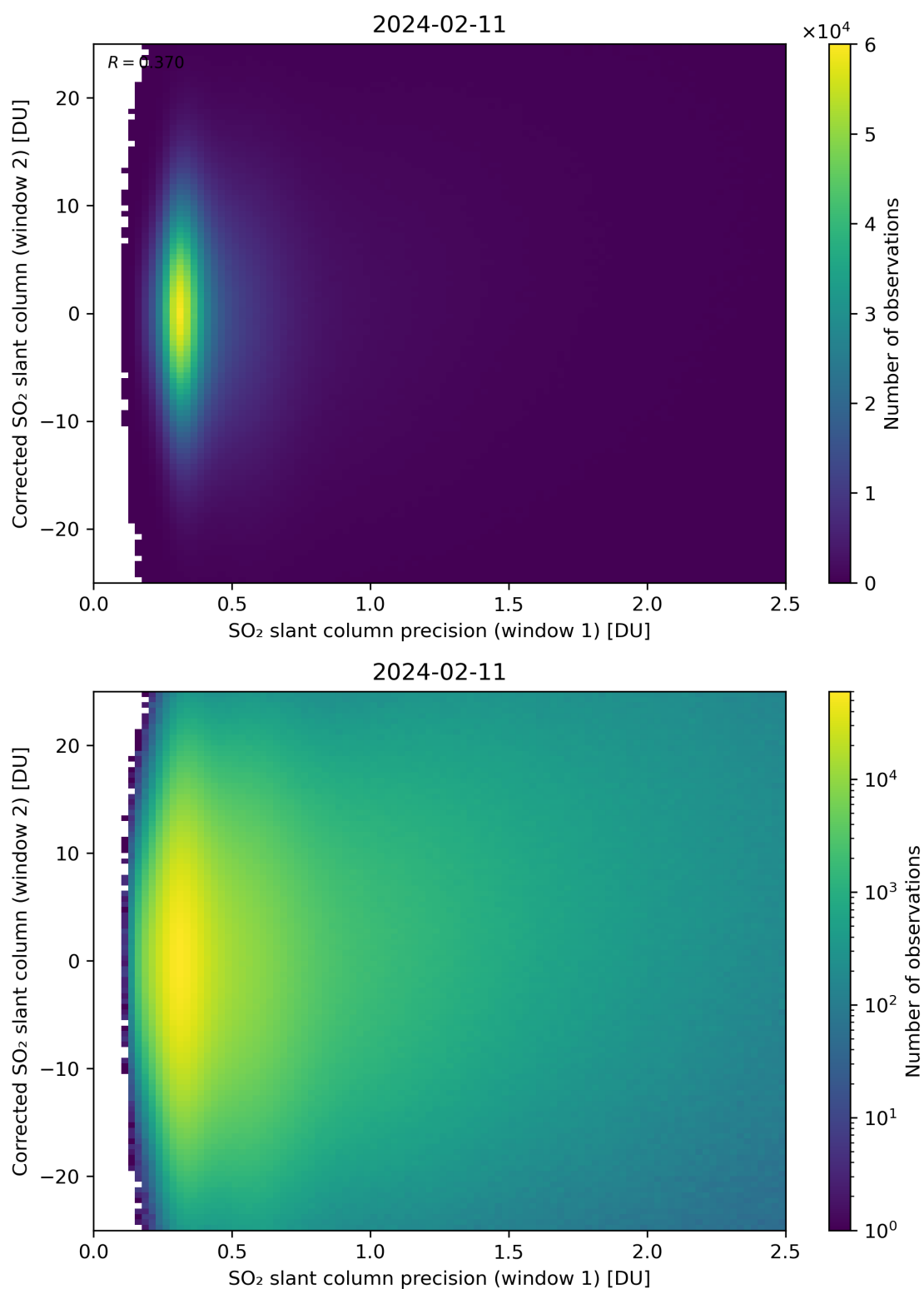
Figure 225: Scatter density plot of “SO 2 slant column precision (window 1)” against “Corrected SO 2 slant column (window 2)” for 2024-02-11 to 2024-02-12.
