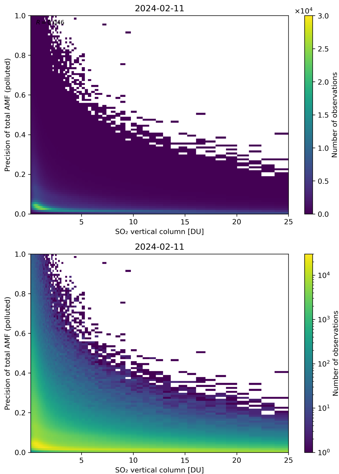
Figure 306: Scatter density plot of “SO 2 vertical column” against “Precision of total AMF (polluted)” for 2024-02-11 to 2024-02-12.
