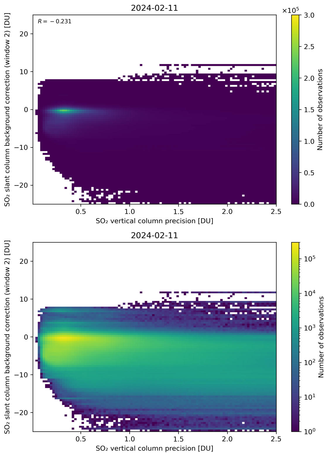
Figure 280: Scatter density plot of “SO 2 vertical column precision” against “SO 2 slant column background correction (window 2)” for 2024-02-11 to 2024-02-12.
