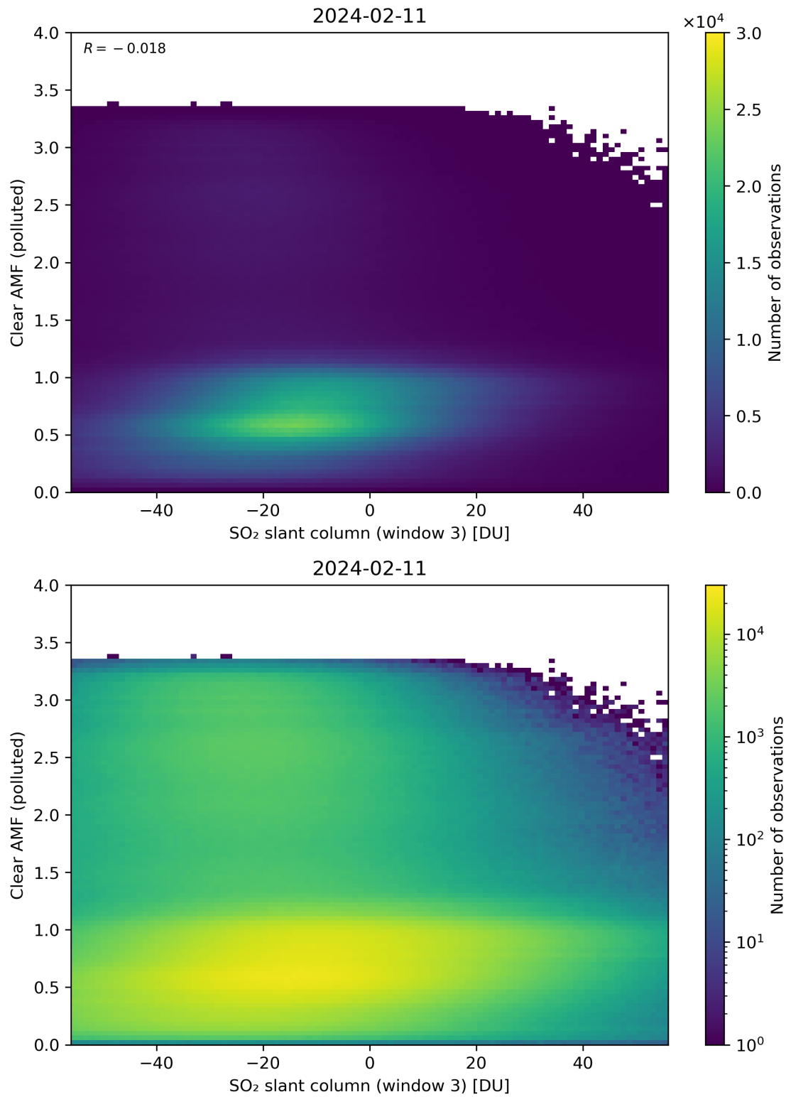
Figure 265: Scatter density plot of “SO 2 slant column (window 3)” against “Clear AMF (polluted)” for 2024-02-11 to 2024-02-12.
