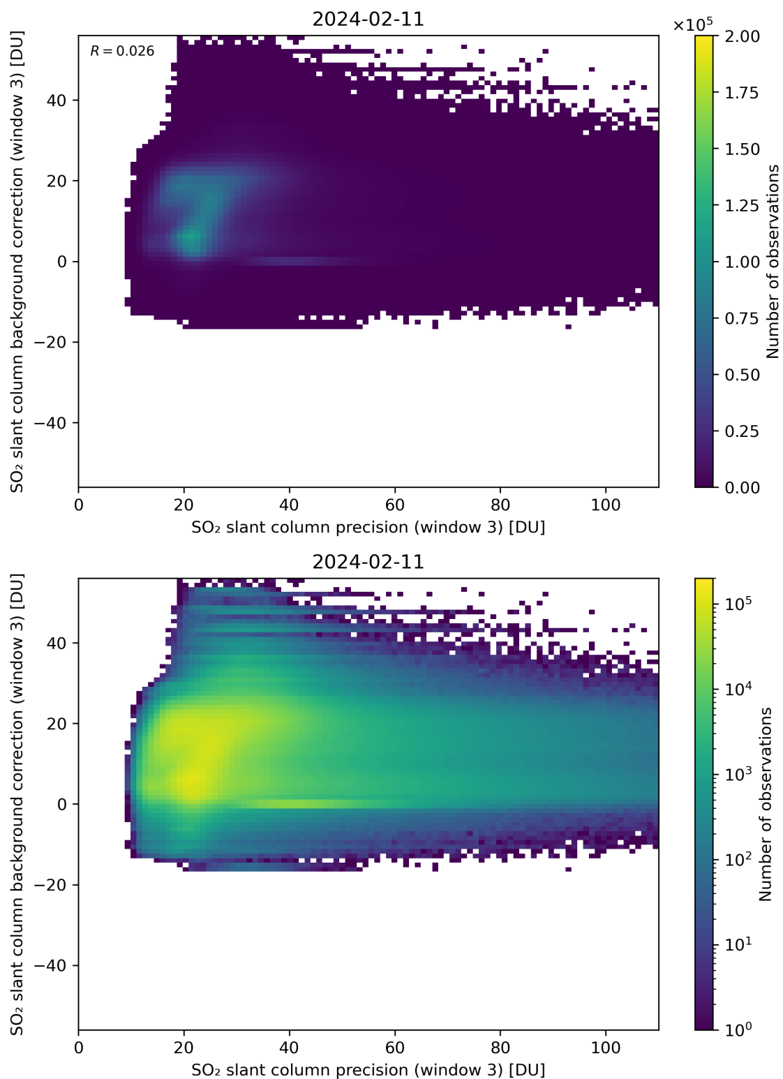
Figure 257: Scatter density plot of “SO 2 slant column precision (window 3)” against “SO 2 slant column background correction (window 3)” for 2024-02-11 to 2024-02-12.
