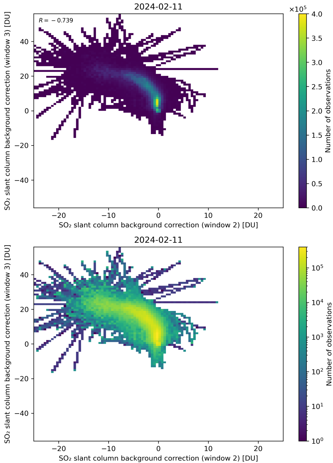
Figure 111: Scatter density plot of “SO 2 slant column background correction (window 2)” against “SO 2 slant column background correction (window 3)” for 2024-02-11 to 2024-02-12.
