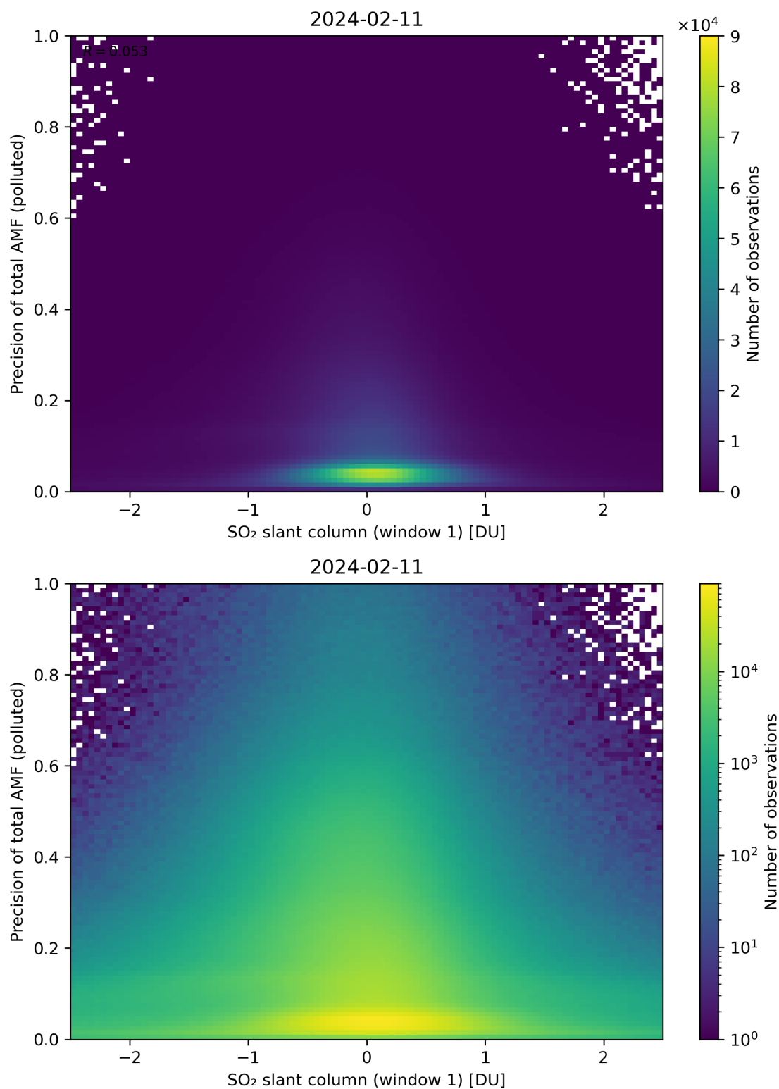
Figure 240: Scatter density plot of “SO 2 slant column (window 1)” against “Precision of total AMF (polluted)” for 2024-02-11 to 2024-02-12.
