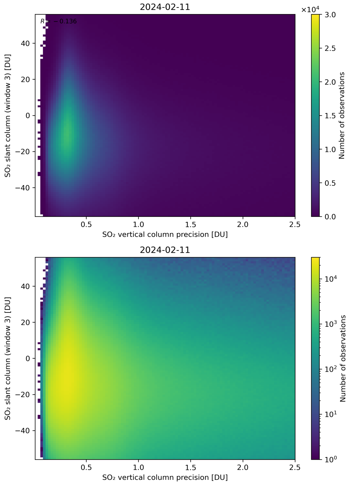
Figure 292: Scatter density plot of “SO 2 vertical column precision” against “SO 2 slant column (window 3)” for 2024-02-11 to 2024-02-12.
