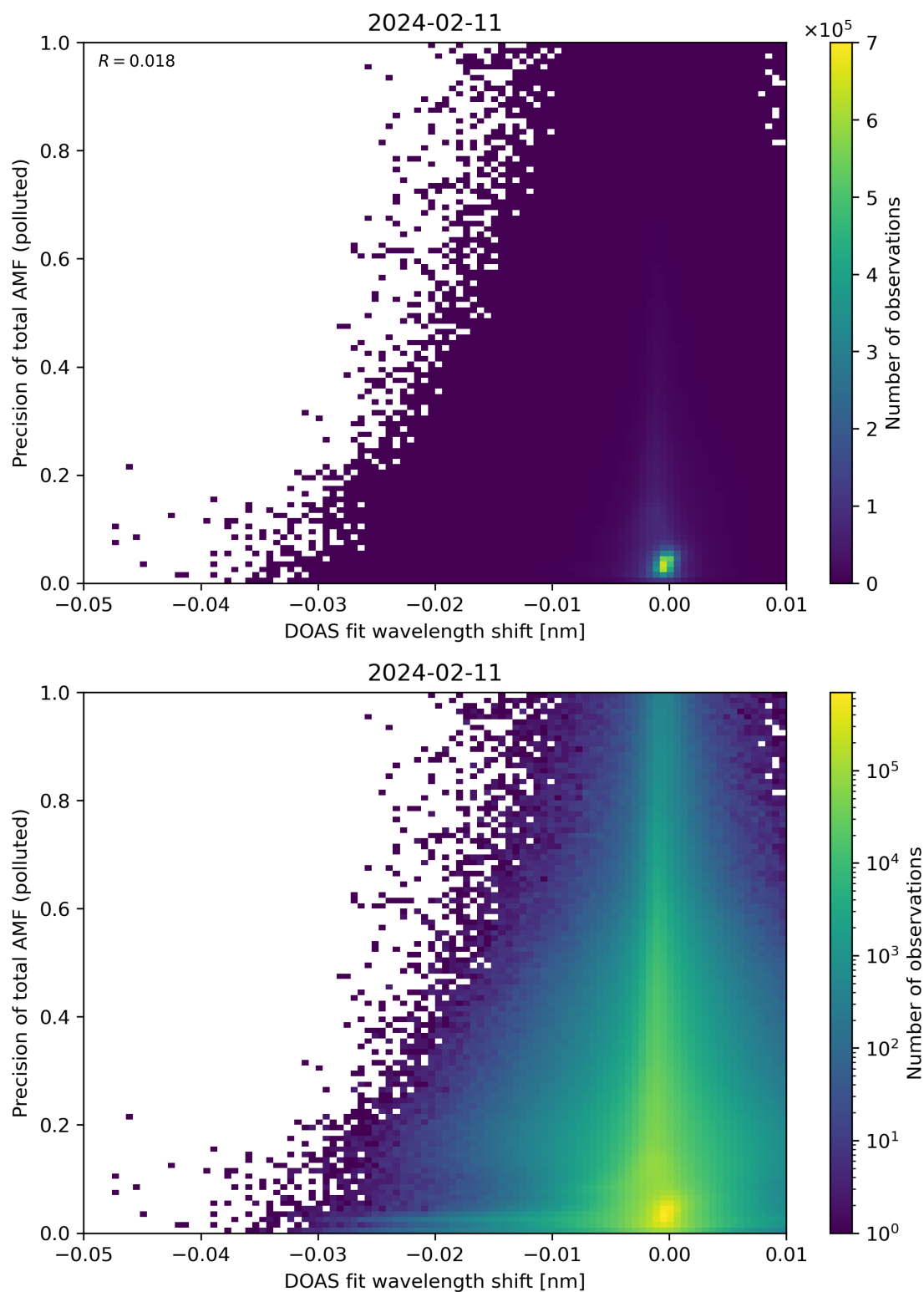
Figure 131: Scatter density plot of “DOAS fit wavelength shift” against “Precision of total AMF (polluted)” for 2024-02-11 to 2024-02-12.
