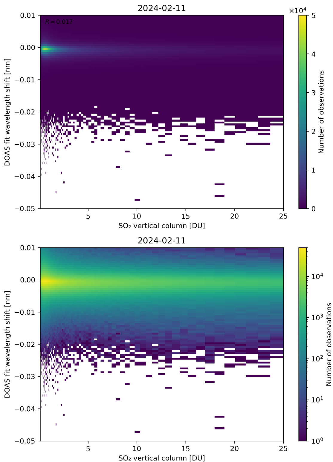
Figure 276: Scatter density plot of “SO 2 vertical column” against “DOAS fit wavelength shift” for 2024-02-11 to 2024-02-12.
