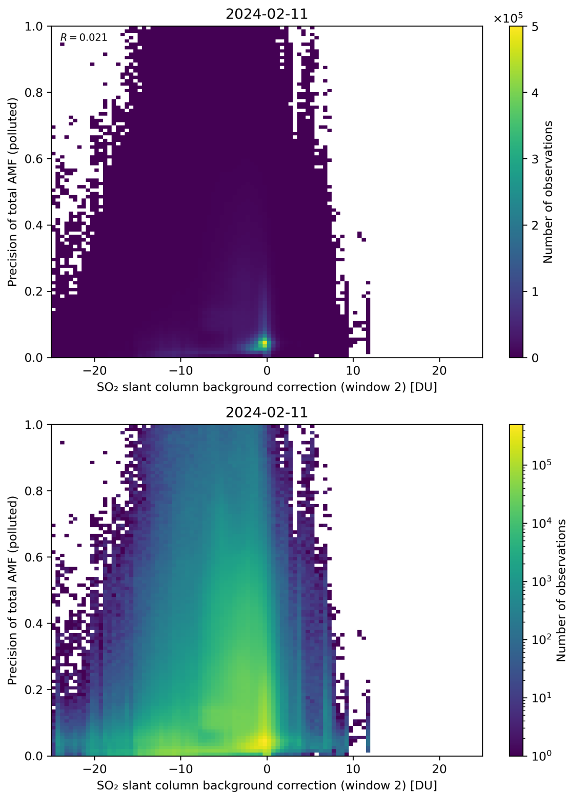
Figure 120: Scatter density plot of “SO 2 slant column background correction (window 2)” against “Precision of total AMF (polluted)” for 2024-02-11 to 2024-02-12.
