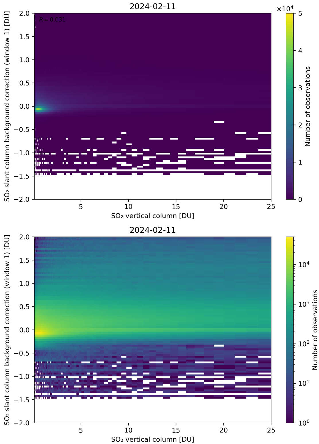
Figure 273: Scatter density plot of “SO 2 vertical column” against “SO 2 slant column background correction (window 1)” for 2024-02-11 to 2024-02-12.
