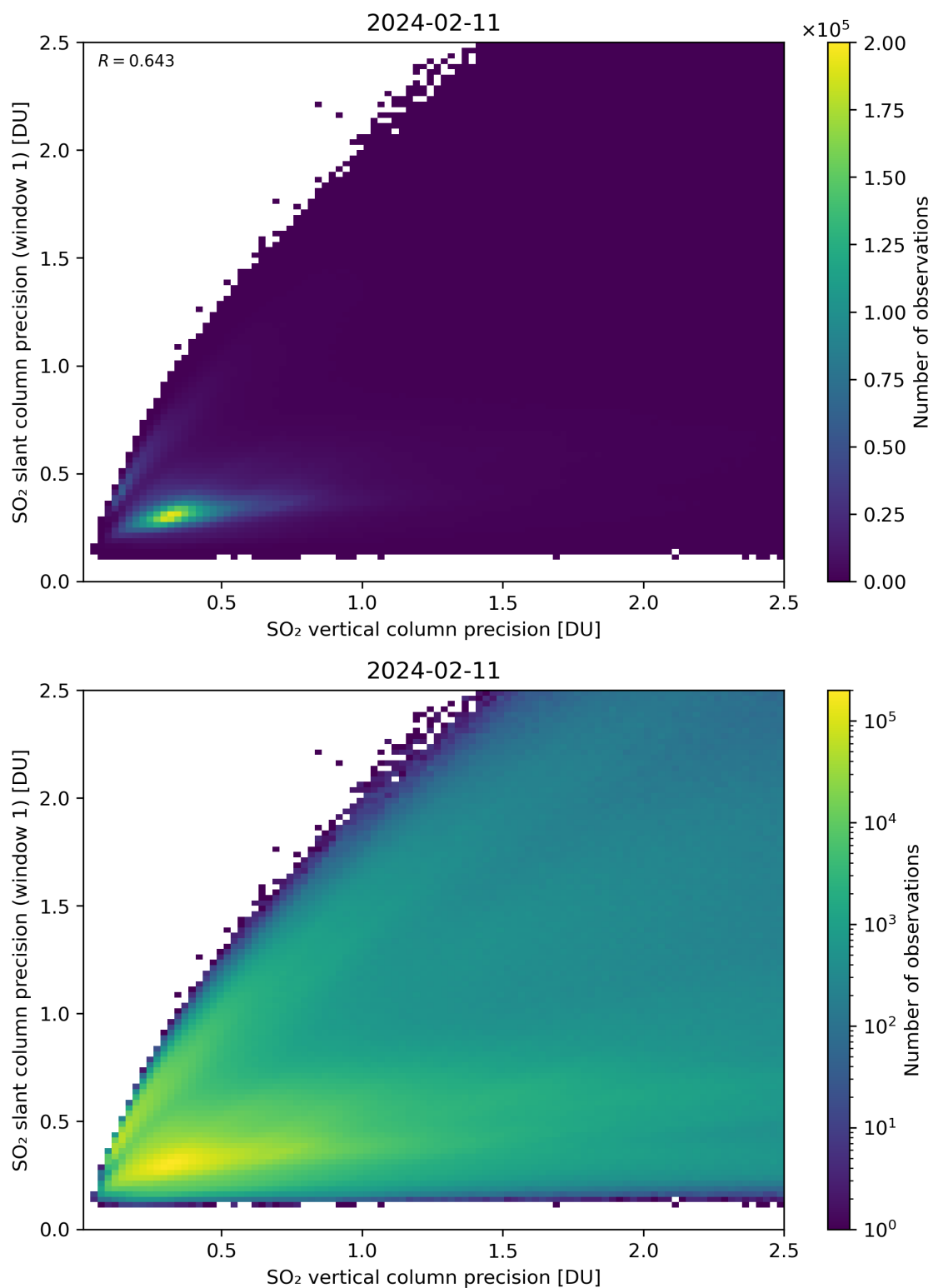
Figure 290: Scatter density plot of “SO 2 vertical column precision” against “SO 2 slant column precision (window 1)” for 2024-02-11 to 2024-02-12.
