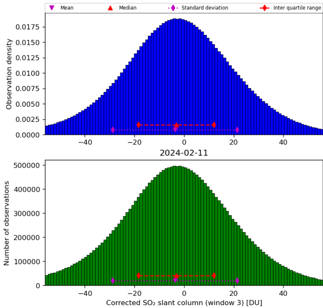
Figure 66: Histogram of “Corrected SO 2 slant column (window 3)” for 2024-02-11 to 2024-02-12
