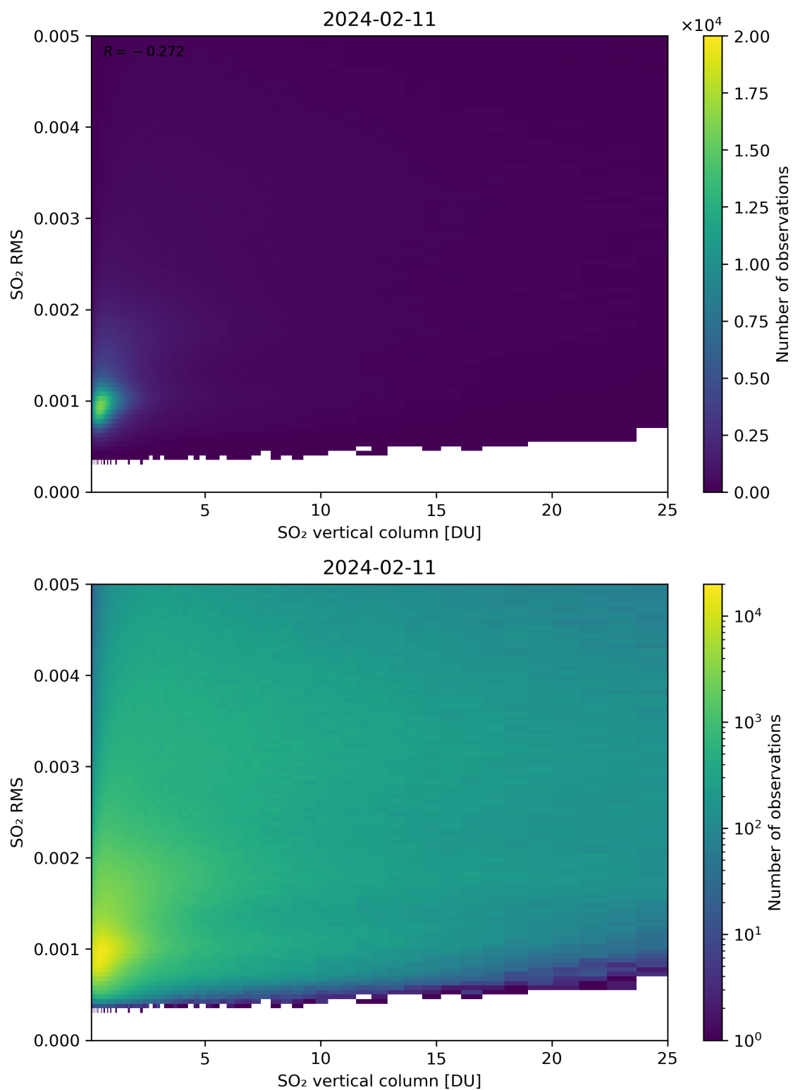
Figure 278: Scatter density plot of “SO 2 vertical column” against “SO 2 RMS” for 2024-02-11 to 2024-02-12.
