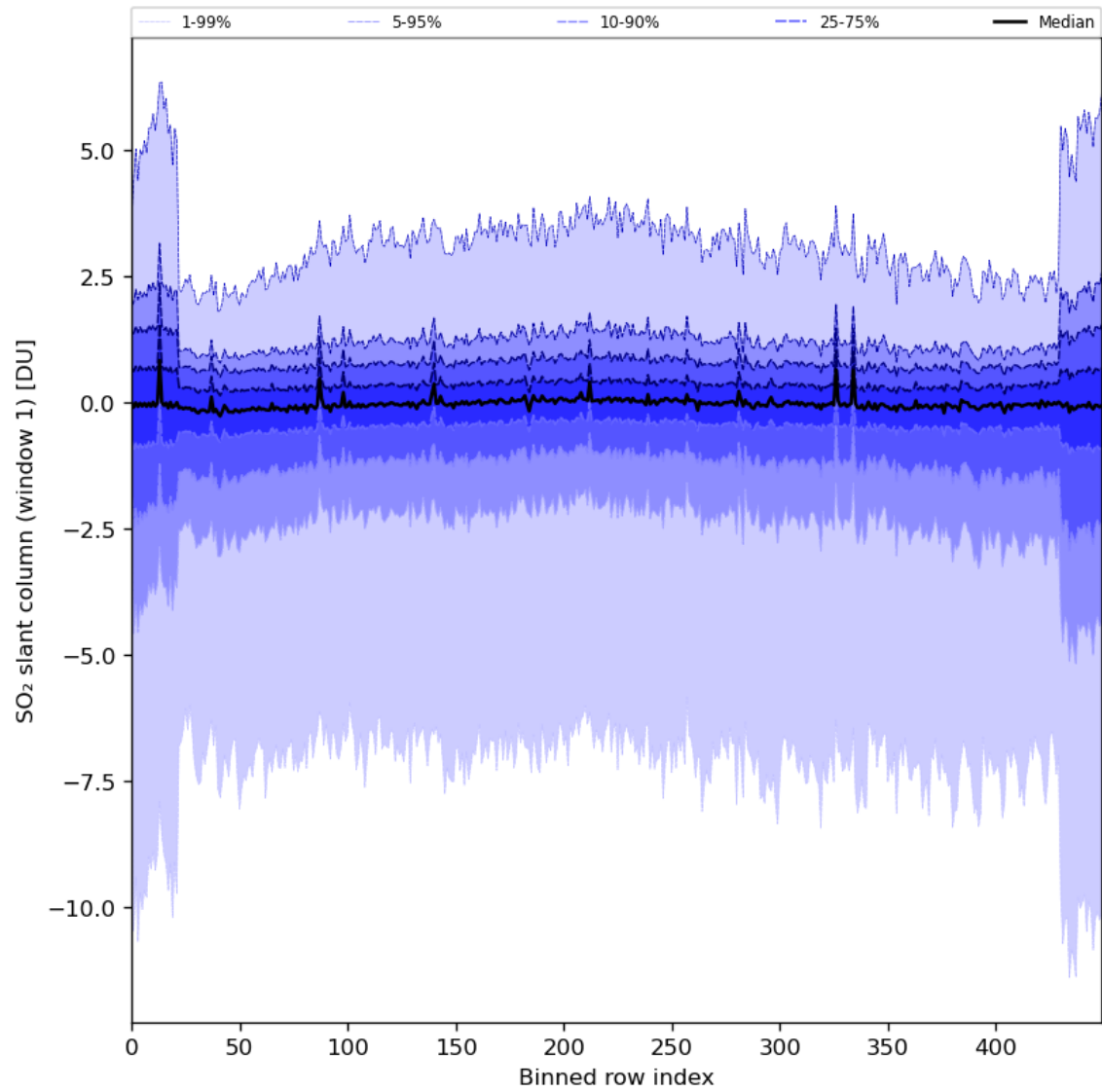
Figure 79: Along track statistics of “SO 2 slant column (window 1)” for 2024-02-11 to 2024-02-12
