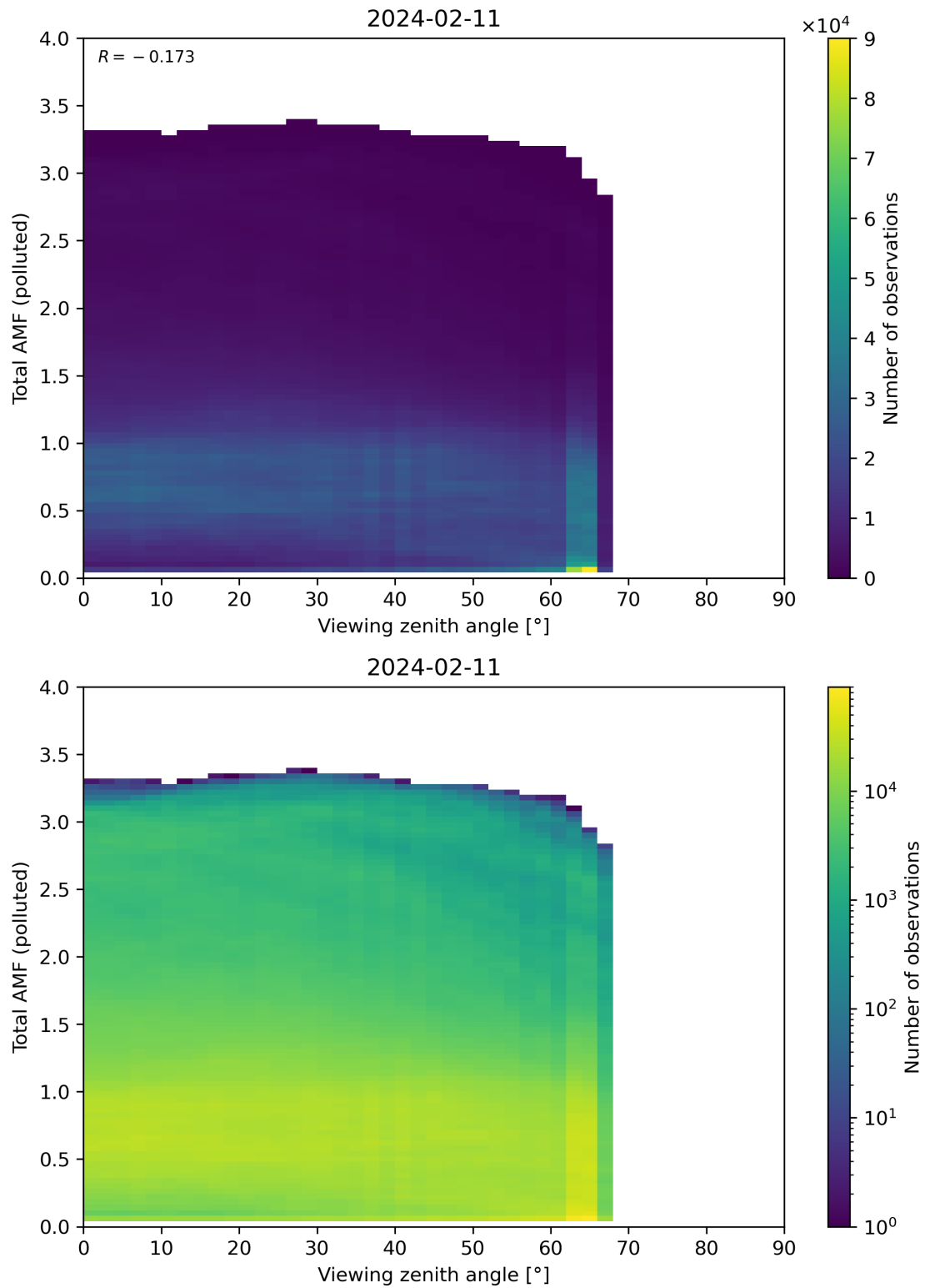
Figure 325: Scatter density plot of “Viewing zenith angle” against “Total AMF (polluted)” for 2024-02-11 to 2024-02-12.
