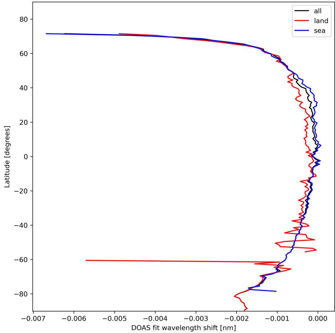
Figure 45: Zonal average of “DOAS fit wavelength shift” for 2024-02-11 to 2024-02-12.
