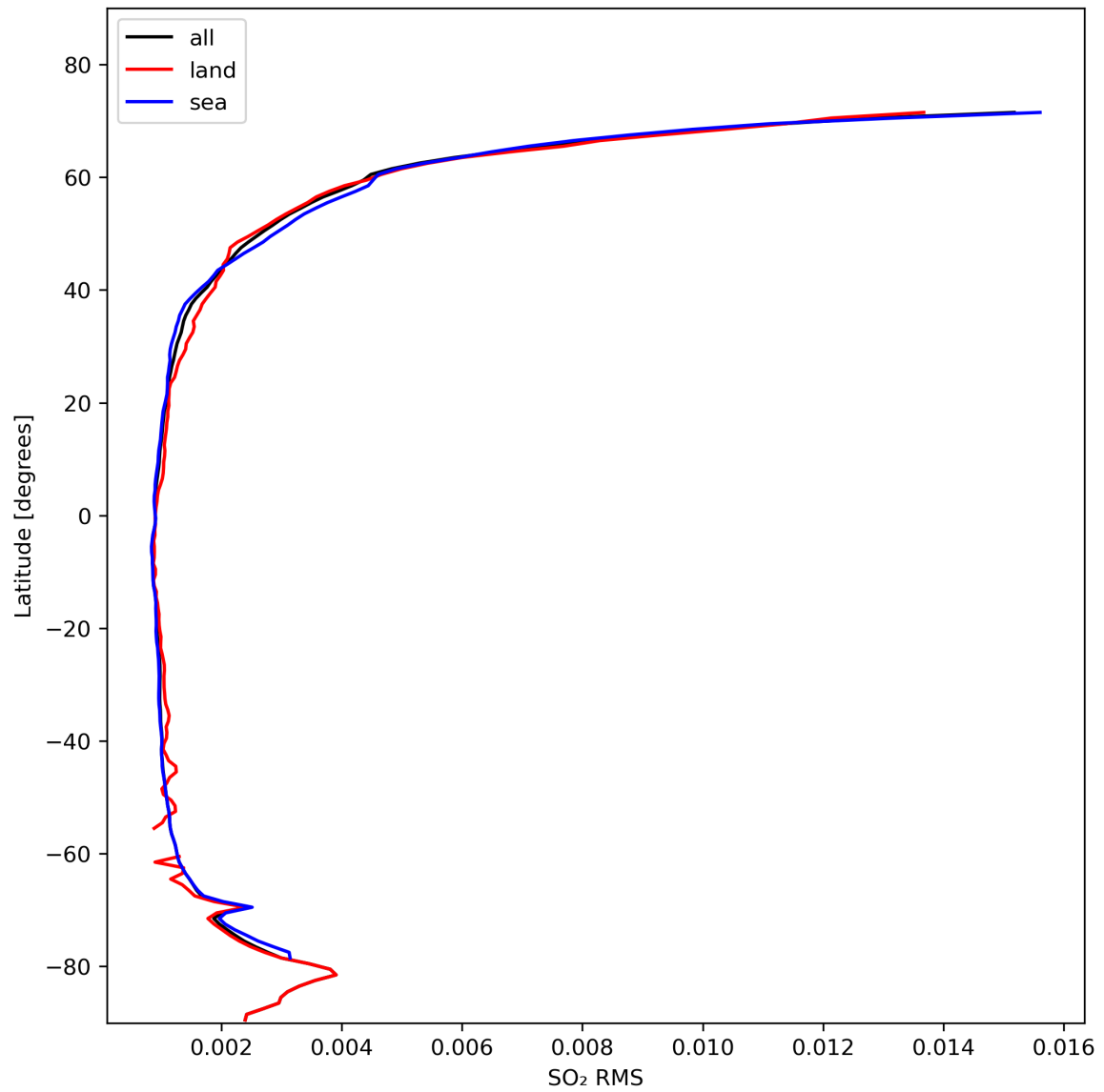
Figure 47: Zonal average of “SO 2 RMS” for 2024-02-11 to 2024-02-12.
