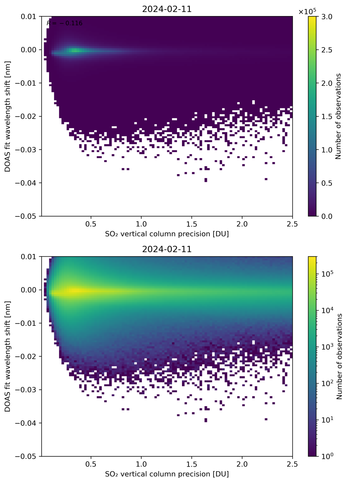
Figure 282: Scatter density plot of “SO 2 vertical column precision” against “DOAS fit wavelength shift” for 2024-02-11 to 2024-02-12.
