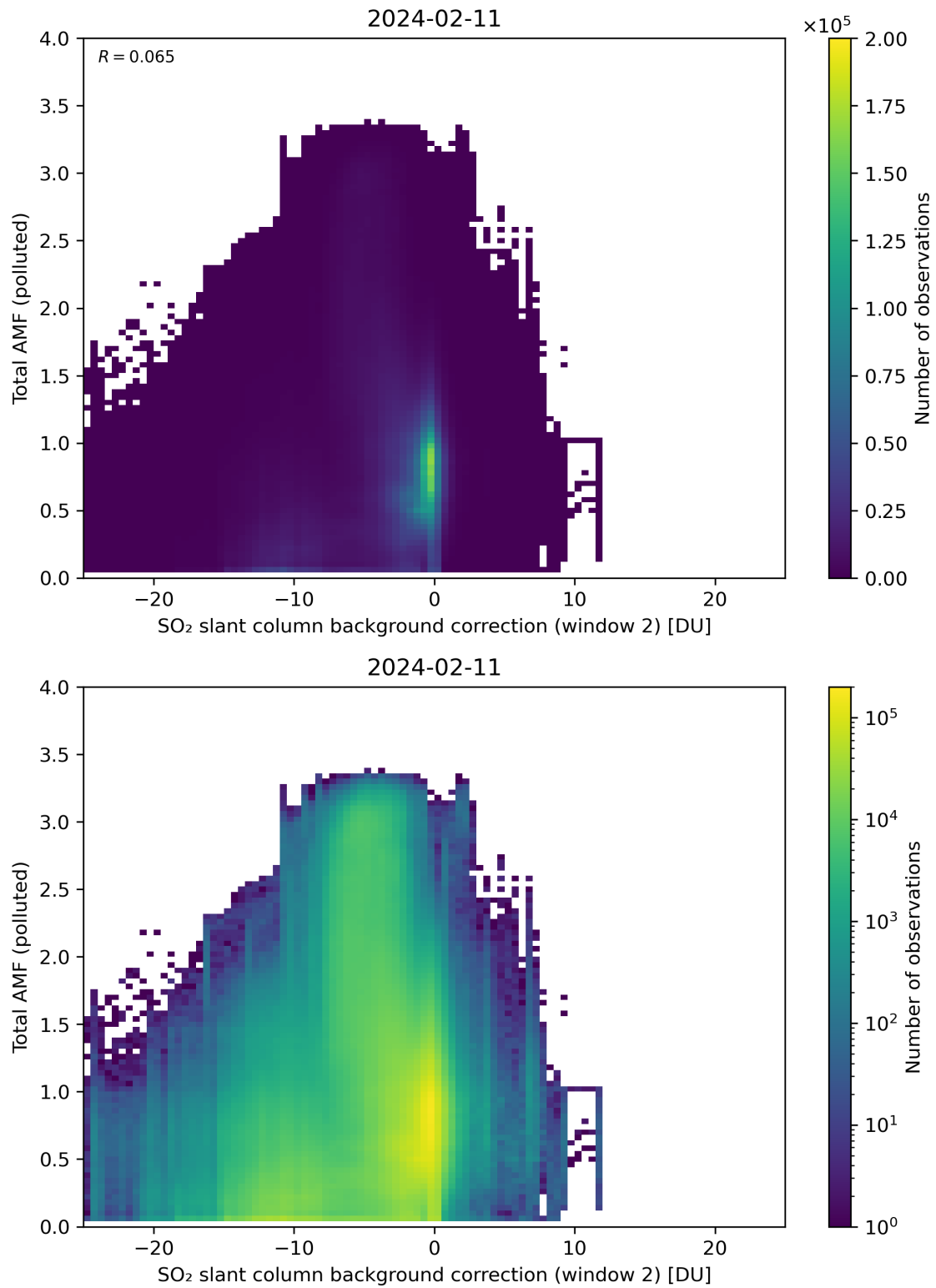
Figure 119: Scatter density plot of “SO 2 slant column background correction (window 2)” against “Total AMF (polluted)” for 2024-02-11 to 2024-02-12.
