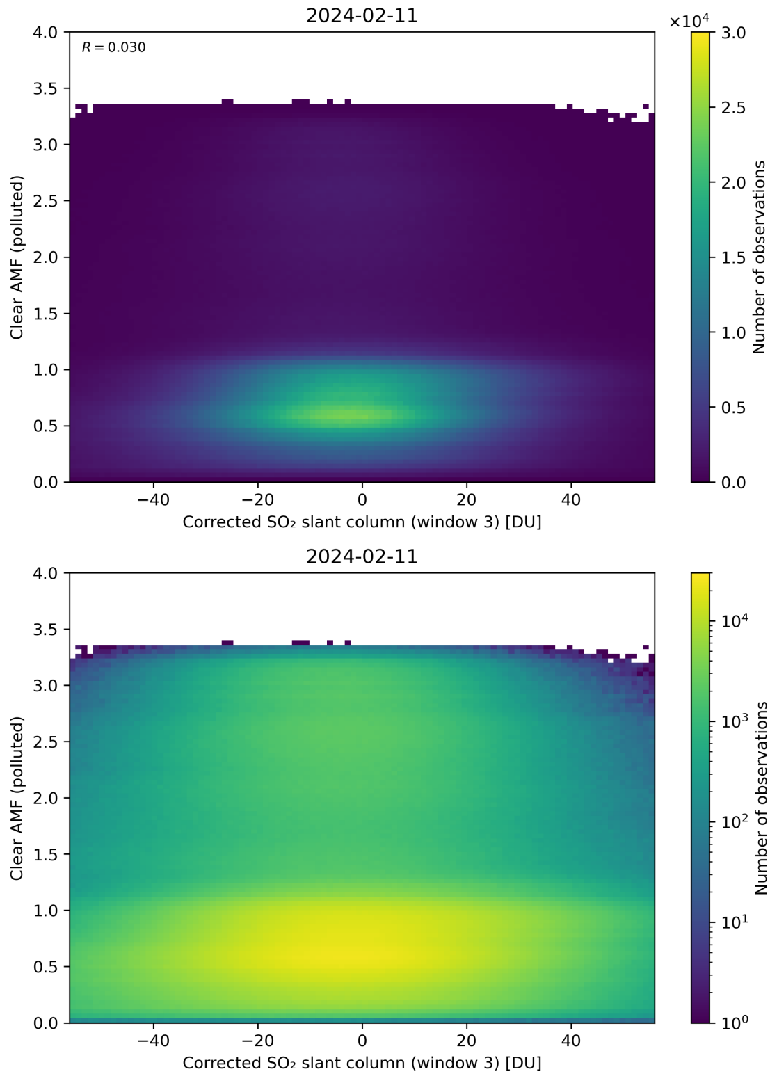
Figure 209: Scatter density plot of “Corrected SO 2 slant column (window 3)” against “Clear AMF (polluted)” for 2024-02-11 to 2024-02-12.
