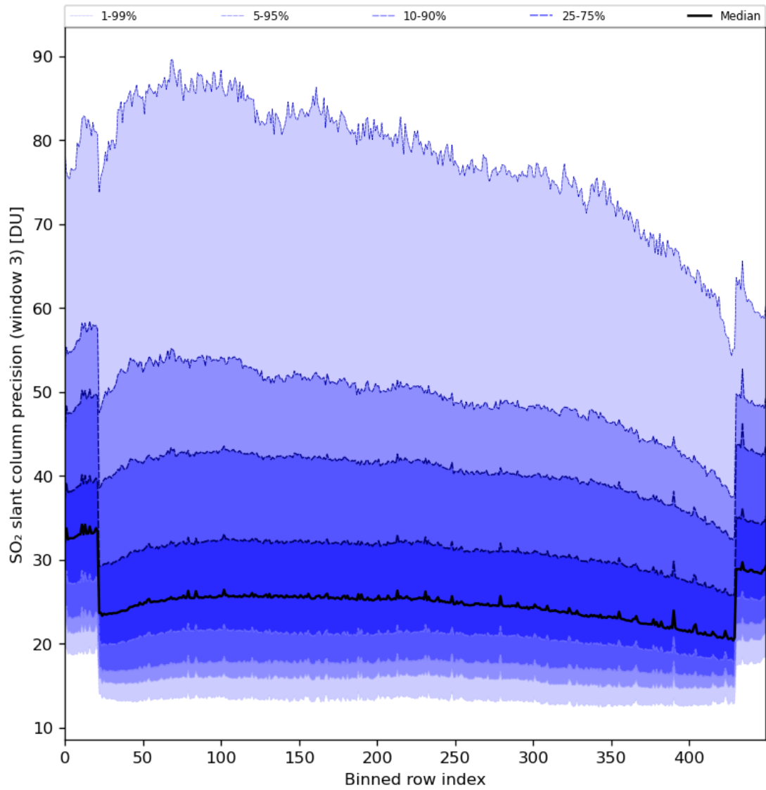
Figure 88: Along track statistics of “SO 2 slant column precision (window 3)” for 2024-02-11 to 2024-02-12
