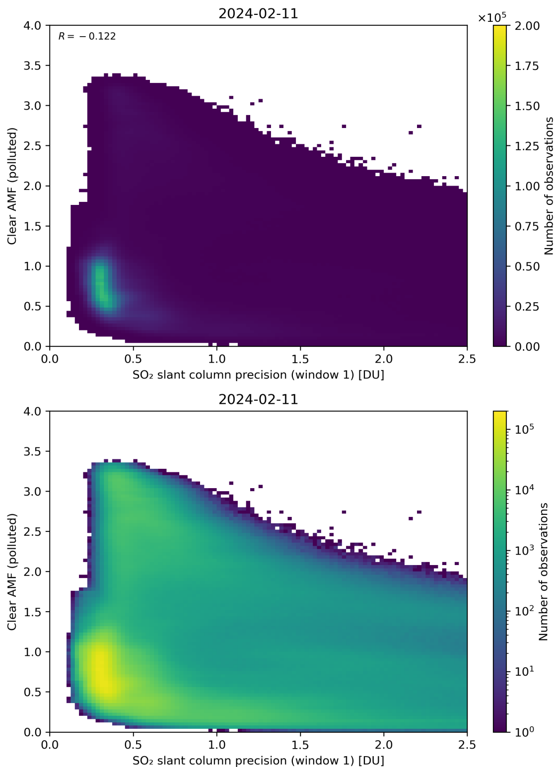
Figure 224: Scatter density plot of “SO 2 slant column precision (window 1)” against “Clear AMF (polluted)” for 2024-02-11 to 2024-02-12.
