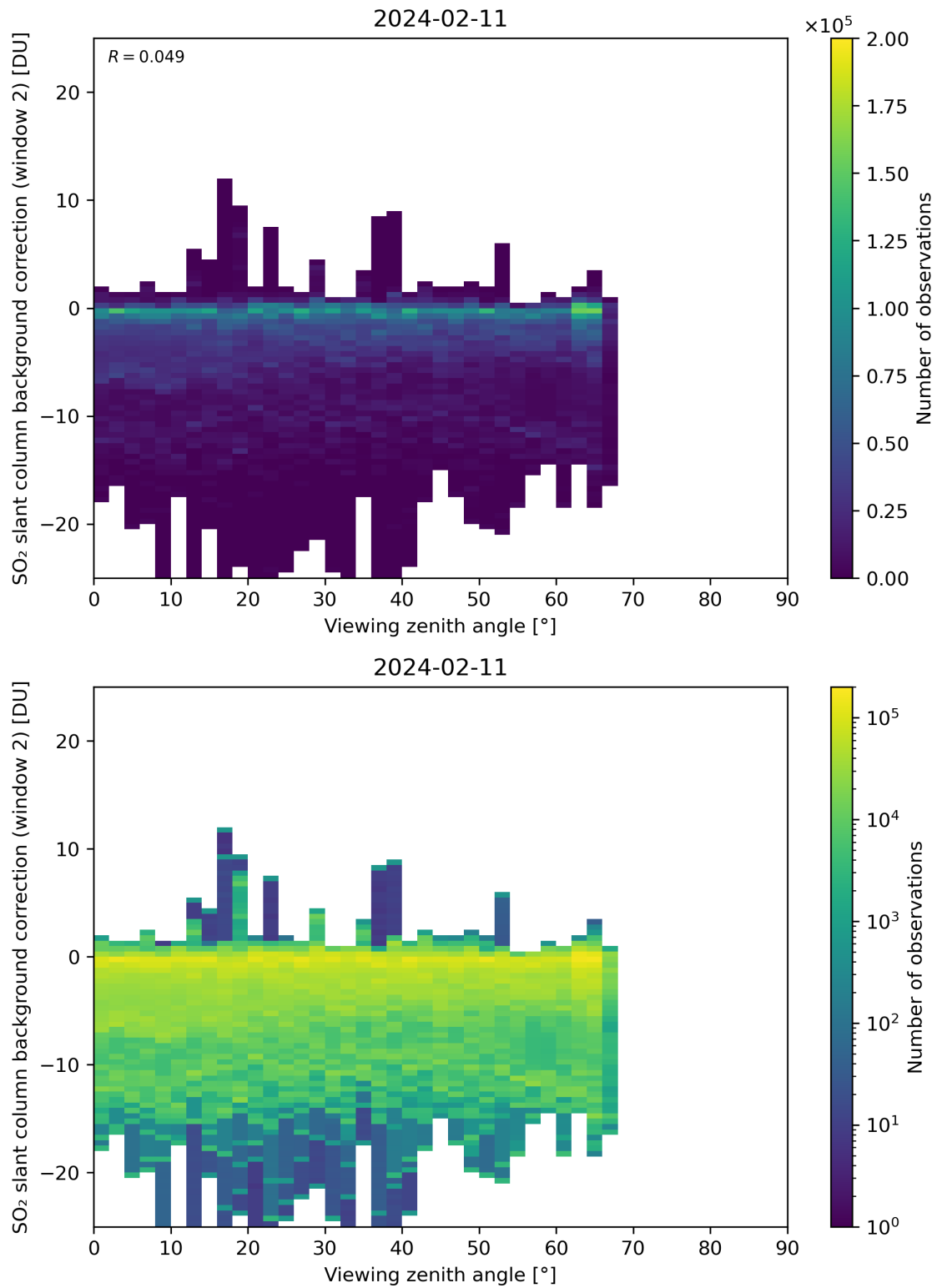
Figure 309: Scatter density plot of “Viewing zenith angle” against “SO 2 slant column background correction (window 2)” for 2024-02-11 to 2024-02-12.
