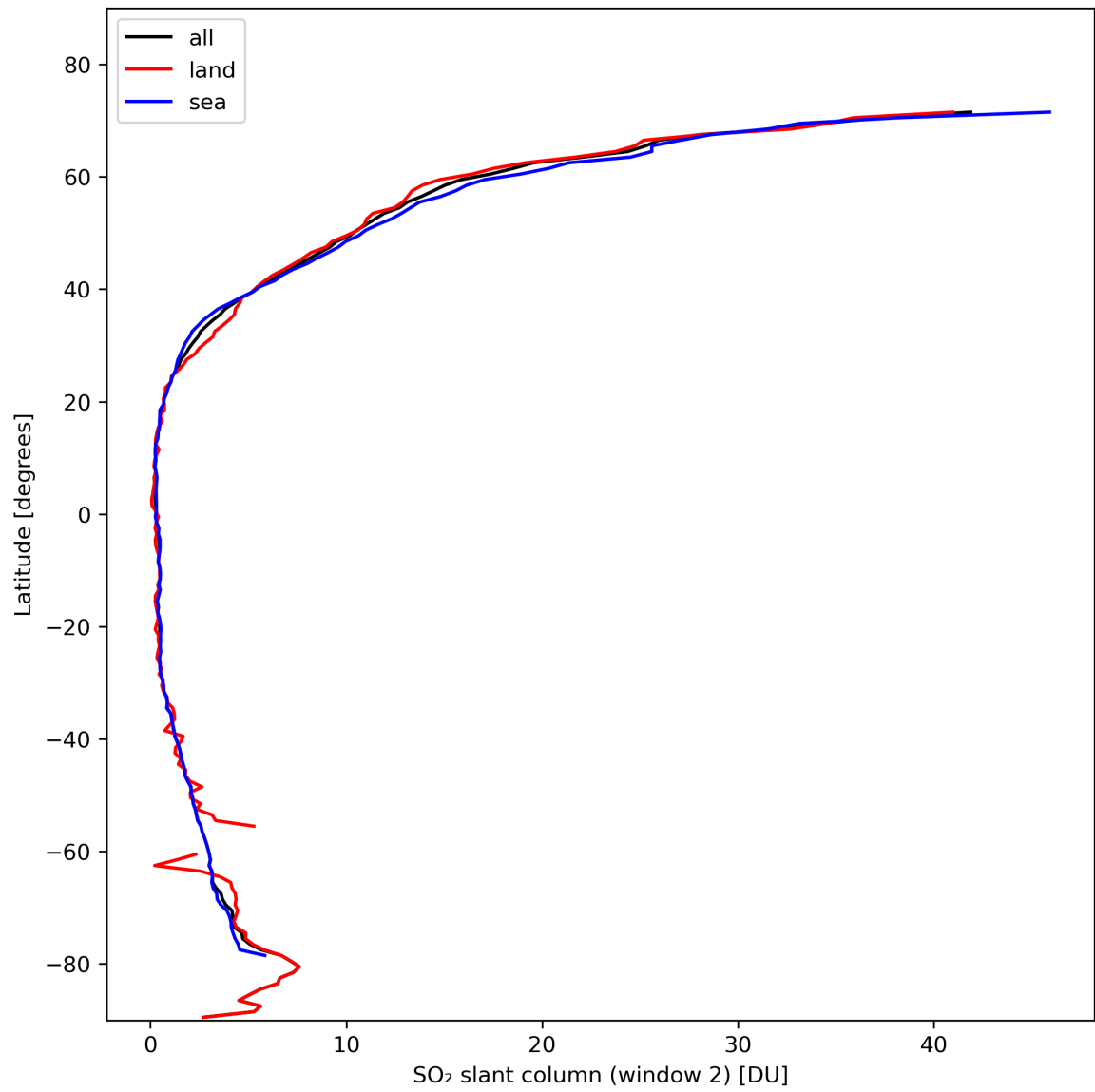
Figure 37: Zonal average of “SO 2 slant column (window 2)” for 2024-02-11 to 2024-02-12.
