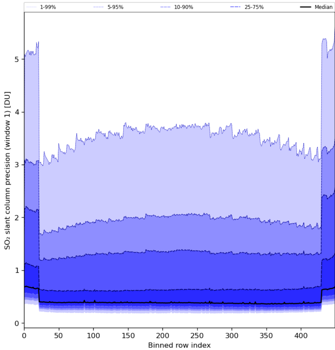
Figure 80: Along track statistics of “SO 2 slant column precision (window 1)” for 2024-02-11 to 2024-02-12
