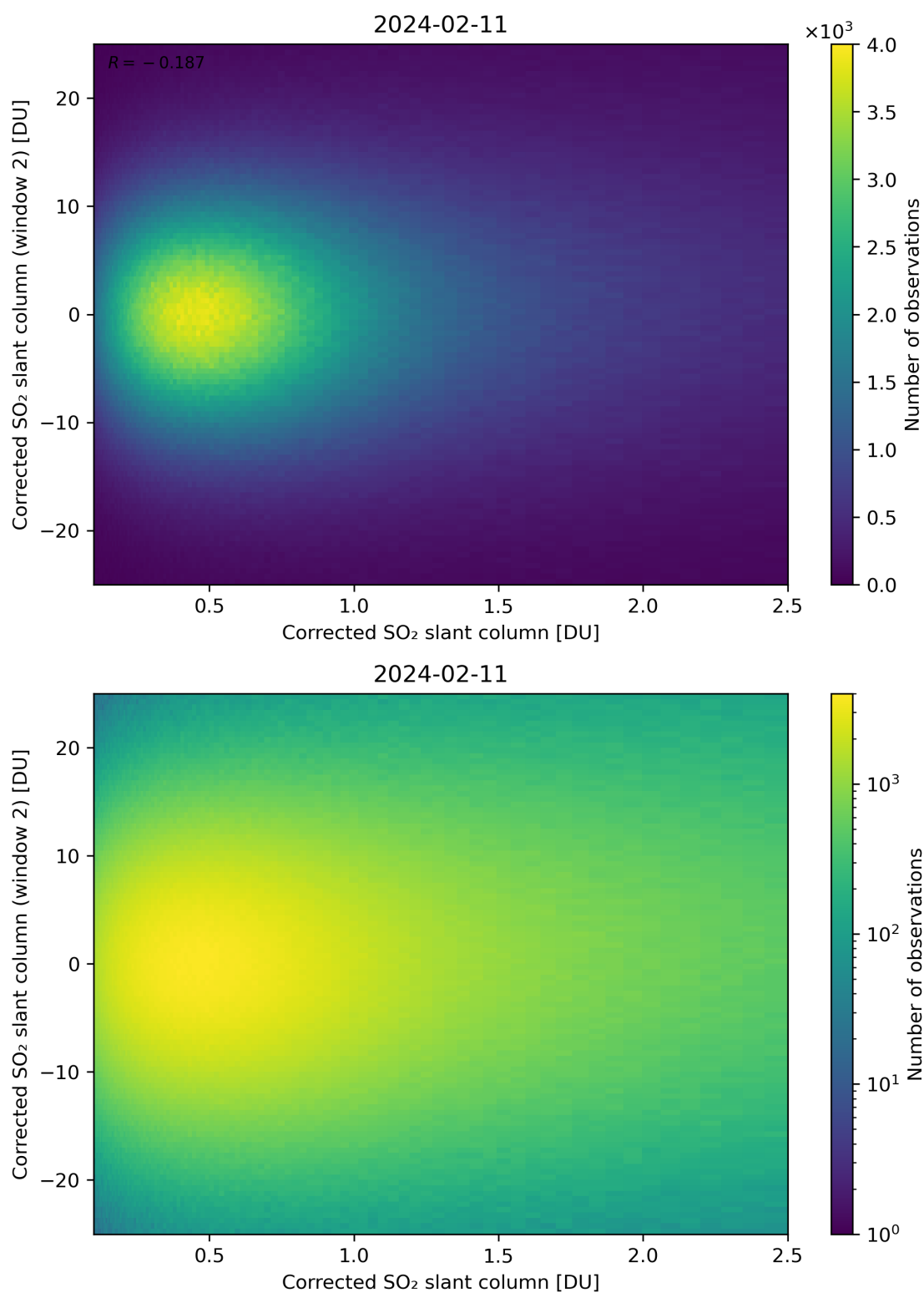
Figure 185: Scatter density plot of “Corrected SO 2 slant column” against “Corrected SO 2 slant column (window 2)” for 2024-02-11 to 2024-02-12.
