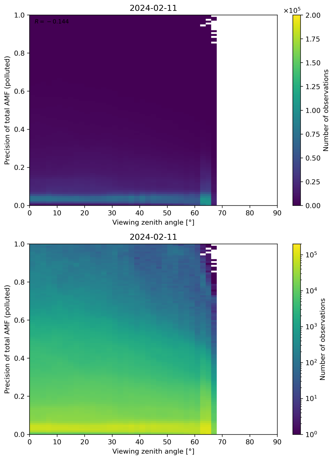
Figure 326: Scatter density plot of “Viewing zenith angle” against “Precision of total AMF (polluted)” for 2024-02-11 to 2024-02-12.
