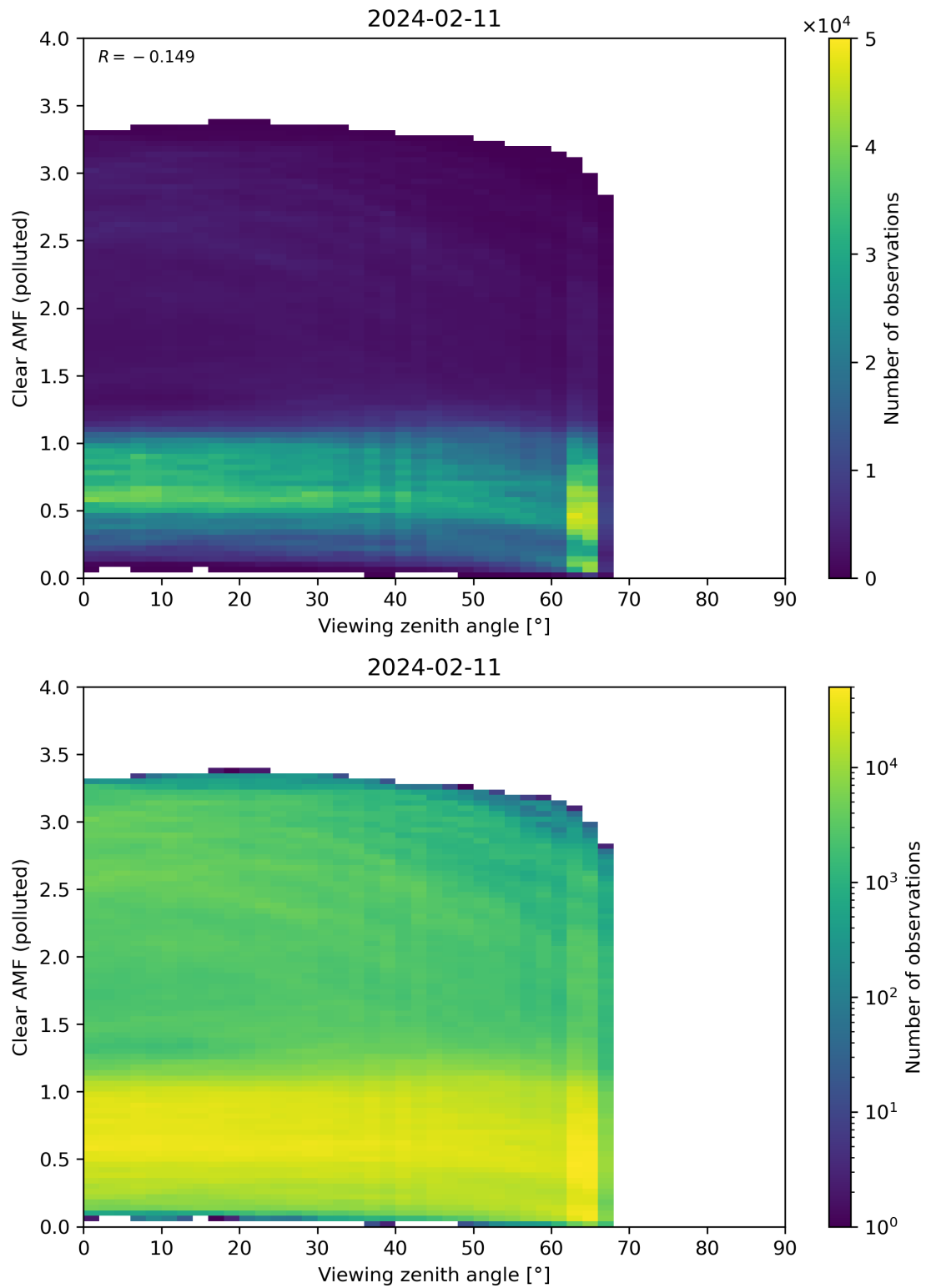
Figure 316: Scatter density plot of “Viewing zenith angle” against “Clear AMF (polluted)” for 2024-02-11 to 2024-02-12.
