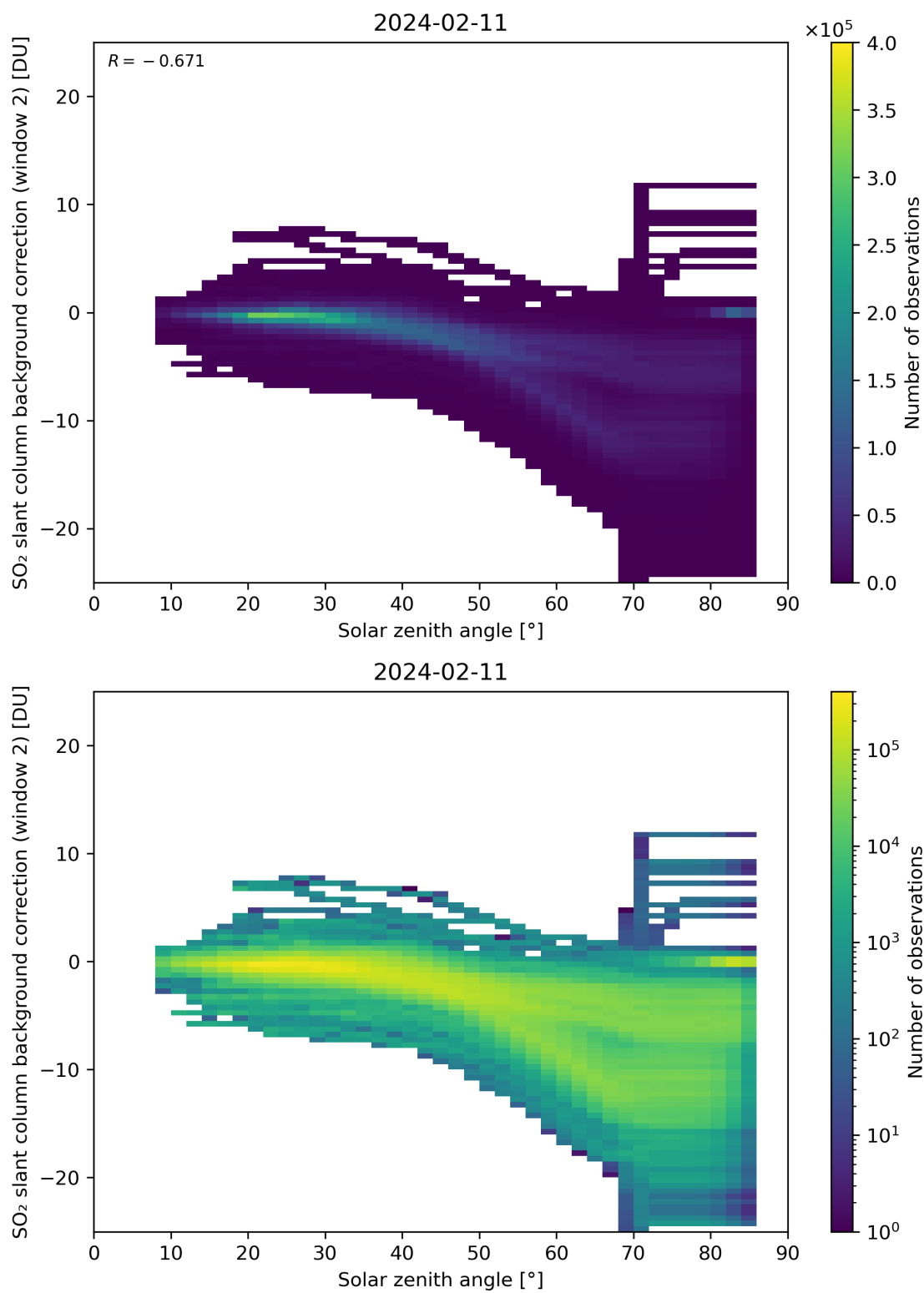
Figure 159: Scatter density plot of “Solar zenith angle” against “SO 2 slant column background correction (window 2)” for 2024-02-11 to 2024-02-12.
