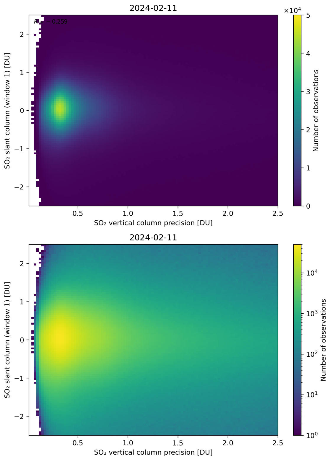
Figure 289: Scatter density plot of “SO 2 vertical column precision” against “SO 2 slant column (window 1)” for 2024-02-11 to 2024-02-12.
