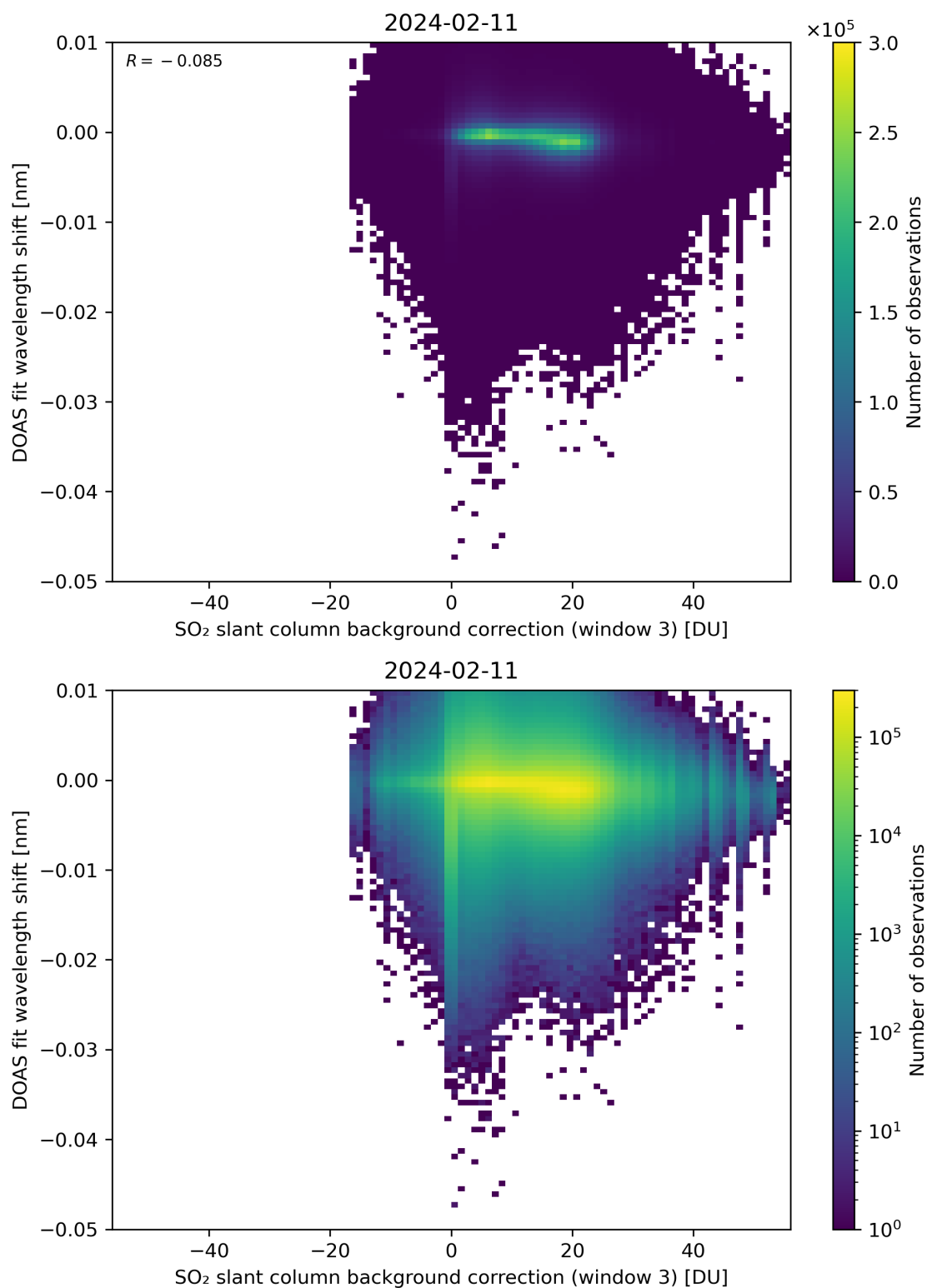
Figure 121: Scatter density plot of “SO 2 slant column background correction (window 3)” against “DOAS fit wavelength shift” for 2024-02-11 to 2024-02-12.
