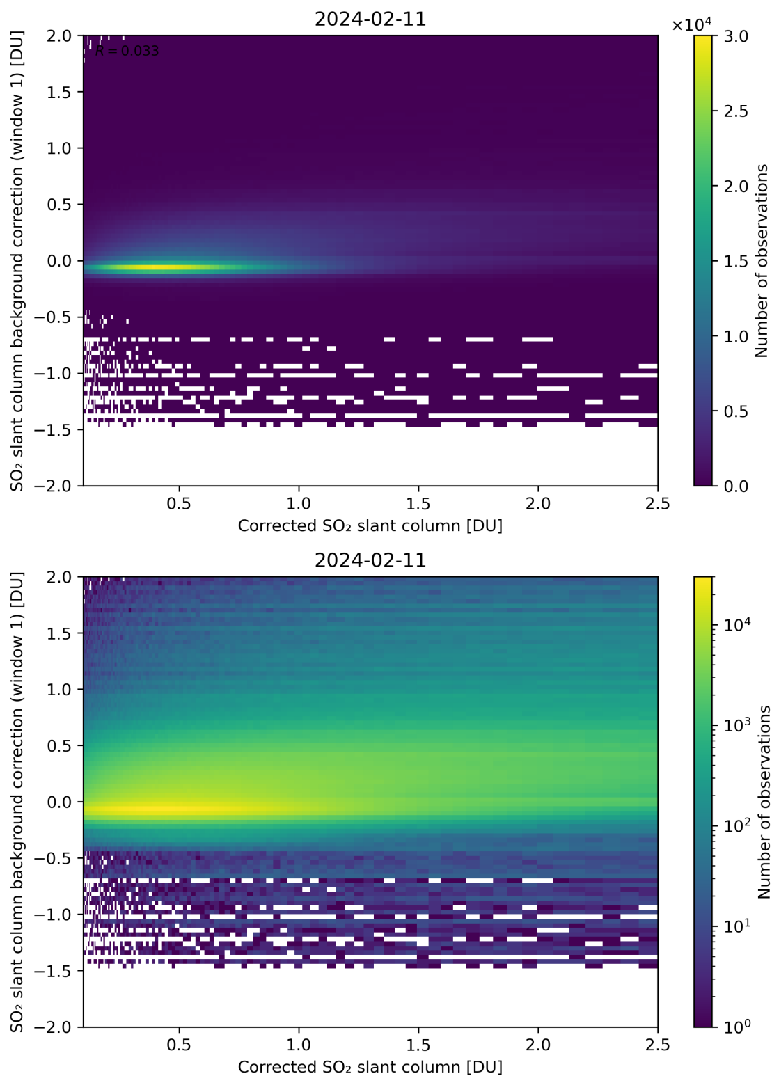
Figure 178: Scatter density plot of “Corrected SO 2 slant column” against “SO 2 slant column background correction (window 1)” for 2024-02-11 to 2024-02-12.
