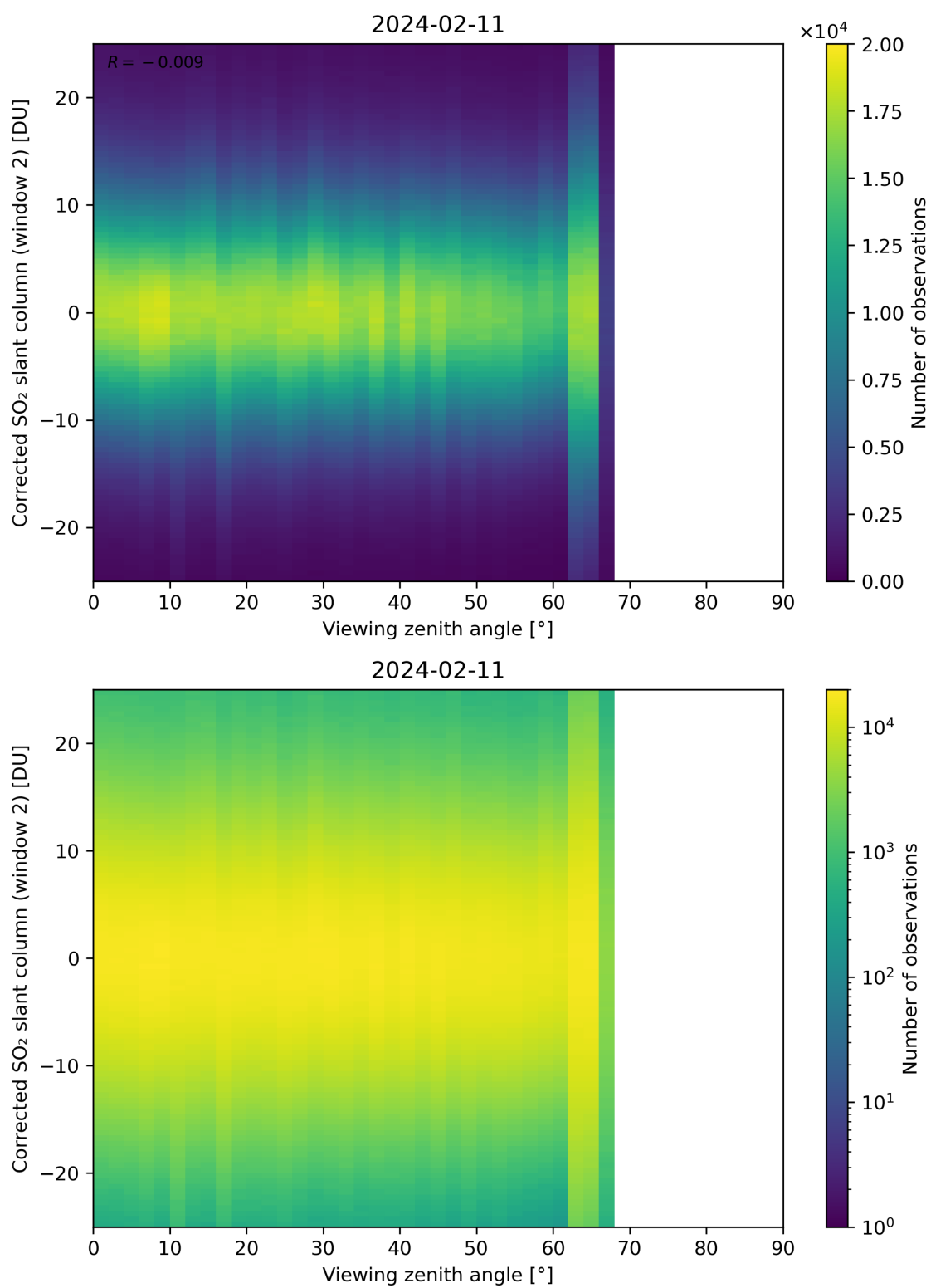
Figure 318: Scatter density plot of “Viewing zenith angle” against “Corrected SO 2 slant column (window 2)” for 2024-02-11 to 2024-02-12.
