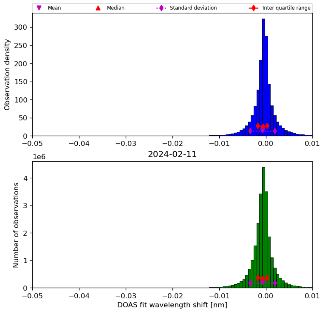
Figure 68: Histogram of “DOAS fit wavelength shift” for 2024-02-11 to 2024-02-12
