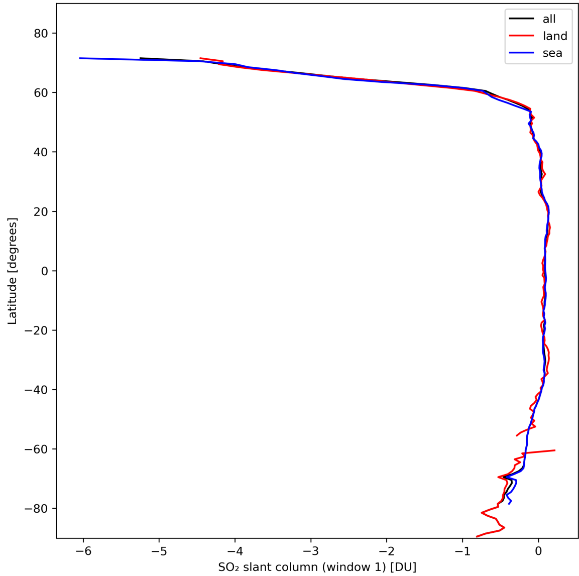
Figure 33: Zonal average of “SO 2 slant column (window 1)” for 2024-02-11 to 2024-02-12.
