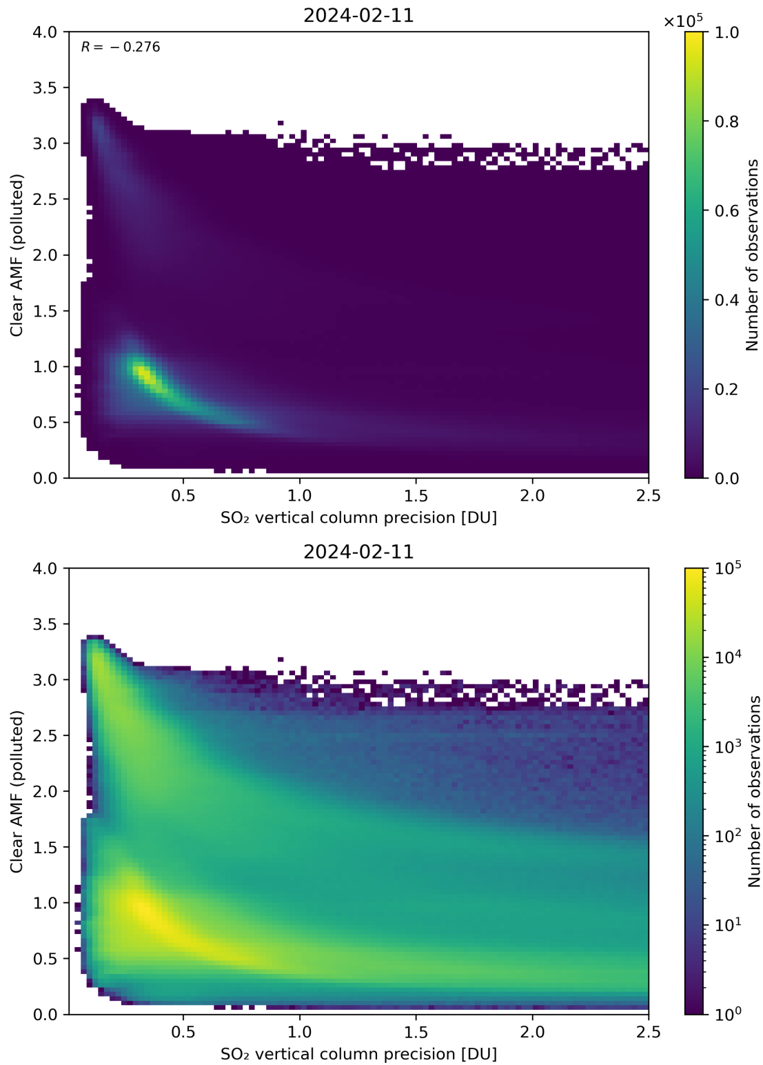
Figure 285: Scatter density plot of “SO 2 vertical column precision” against “Clear AMF (polluted)” for 2024-02-11 to 2024-02-12.
