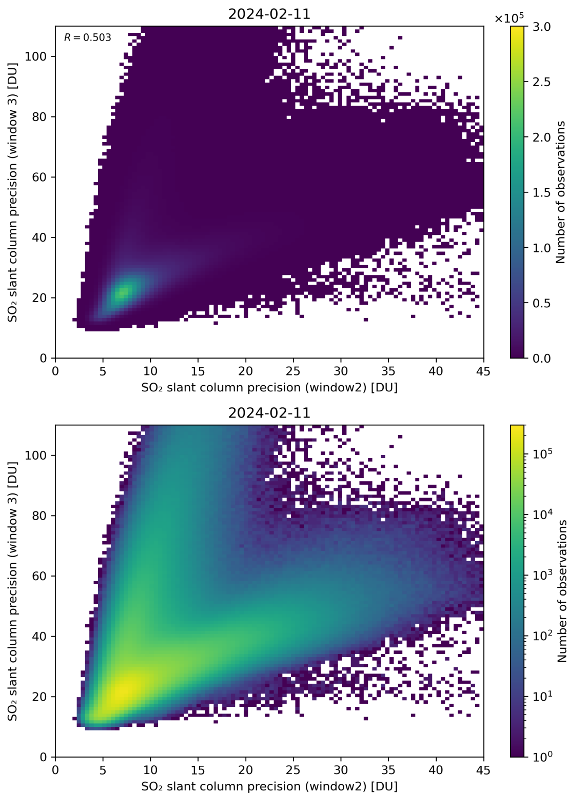
Figure 250: Scatter density plot of “SO 2 slant column precision (window2)” against “SO 2 slant column precision (window 3)” for 2024-02-11 to 2024-02-12.
