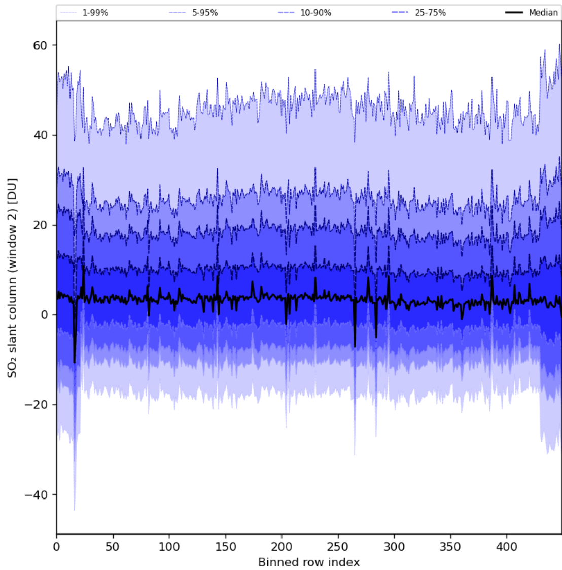
Figure 83: Along track statistics of “SO 2 slant column (window 2)” for 2024-02-11 to 2024-02-12
