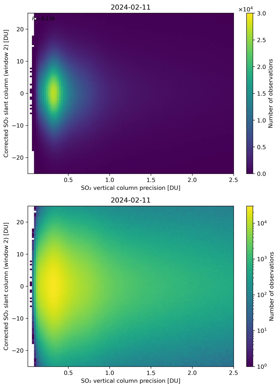
Figure 287: Scatter density plot of “SO 2 vertical column precision” against “Corrected SO 2 slant column (window 2)” for 2024-02-11 to 2024-02-12.
