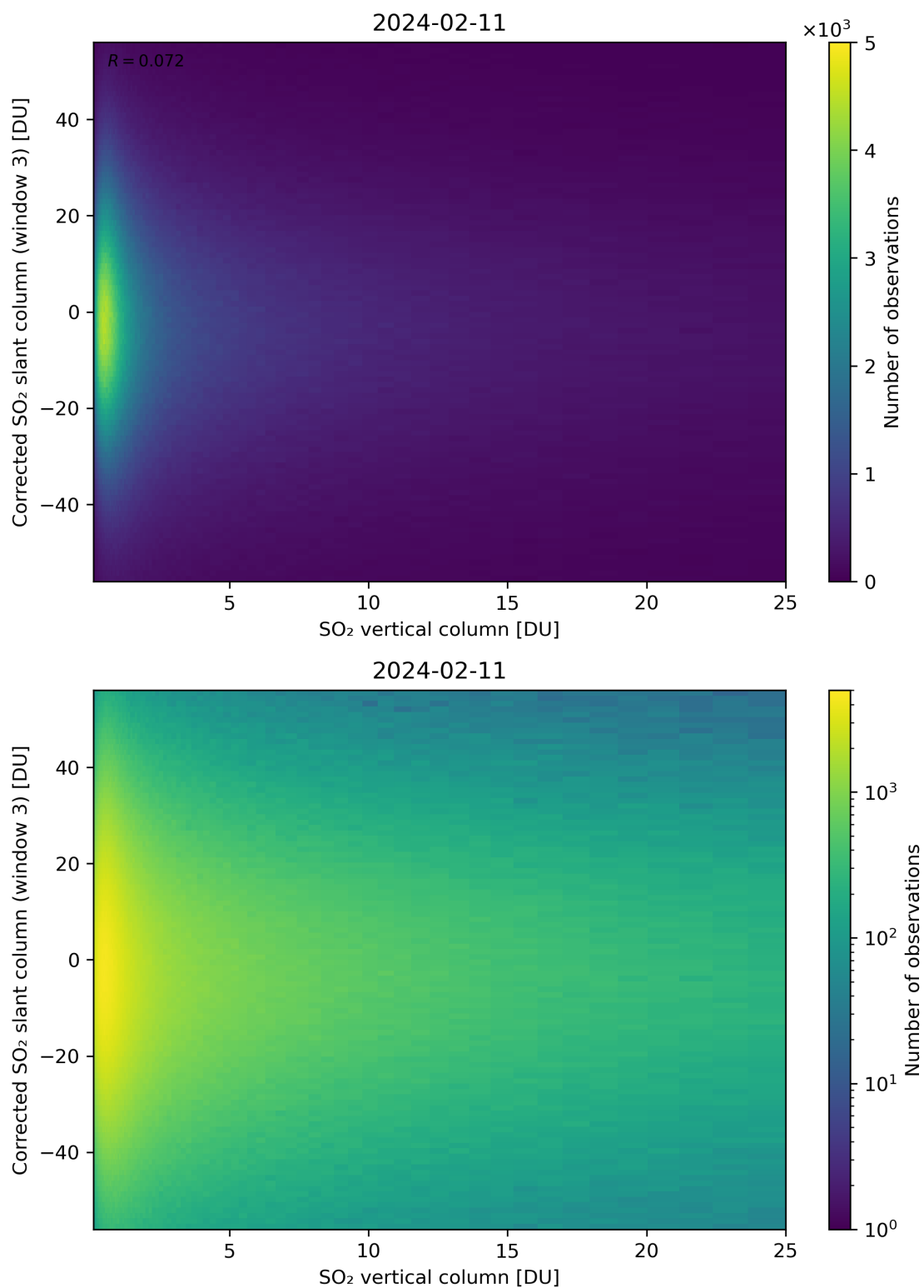
Figure 299: Scatter density plot of “SO 2 vertical column” against “Corrected SO 2 slant column (window 3)” for 2024-02-11 to 2024-02-12.
