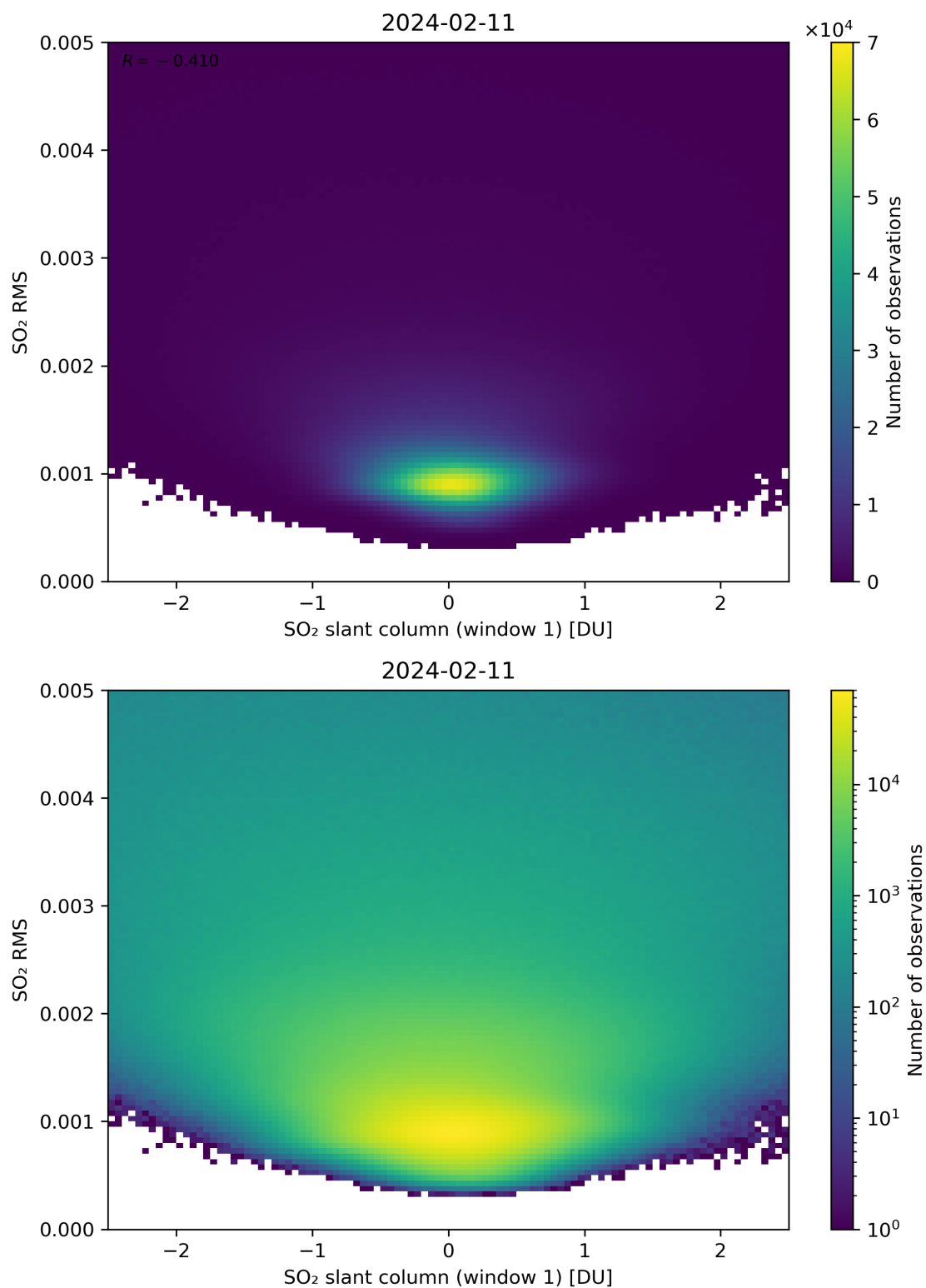
Figure 217: Scatter density plot of “SO 2 slant column (window 1)” against “SO 2 RMS” for 2024-02-11 to 2024-02-12.
