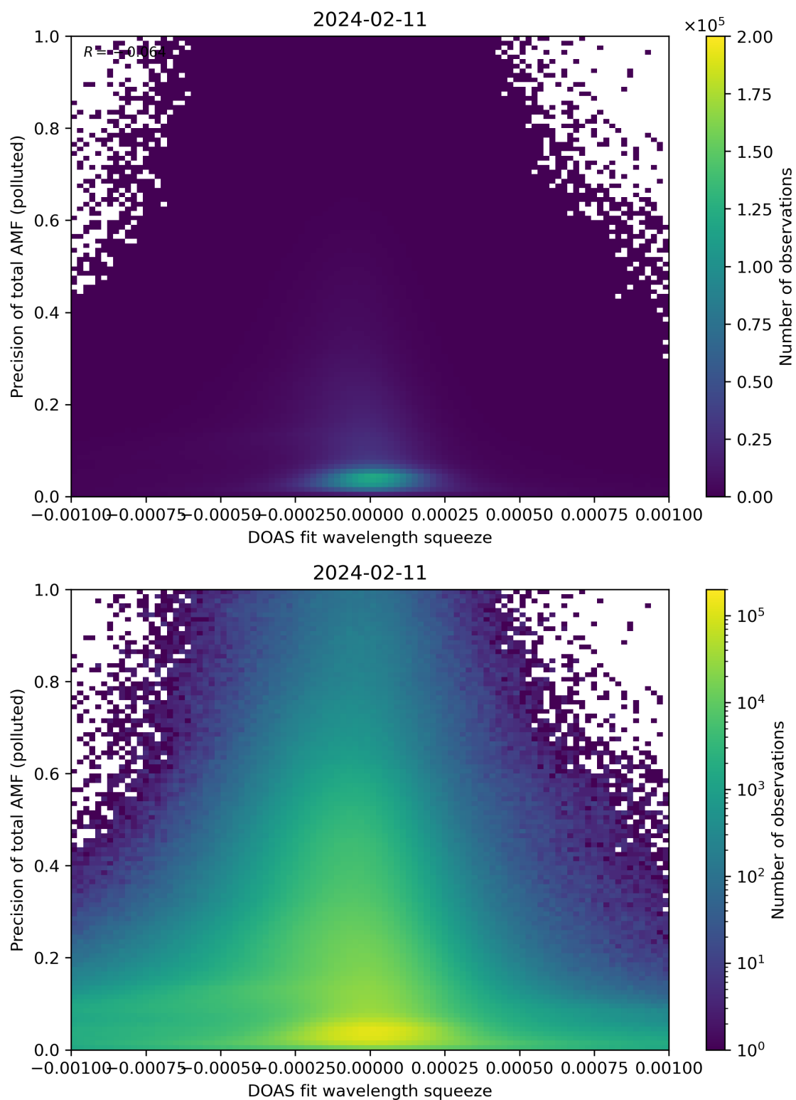
Figure 135: Scatter density plot of “DOAS fit wavelength squeeze” against “Precision of total AMF (polluted)” for 2024-02-11 to 2024-02-12.
