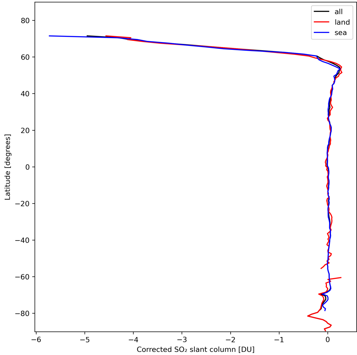
Figure 32: Zonal average of “Corrected SO 2 slant column” for 2024-02-11 to 2024-02-12.
