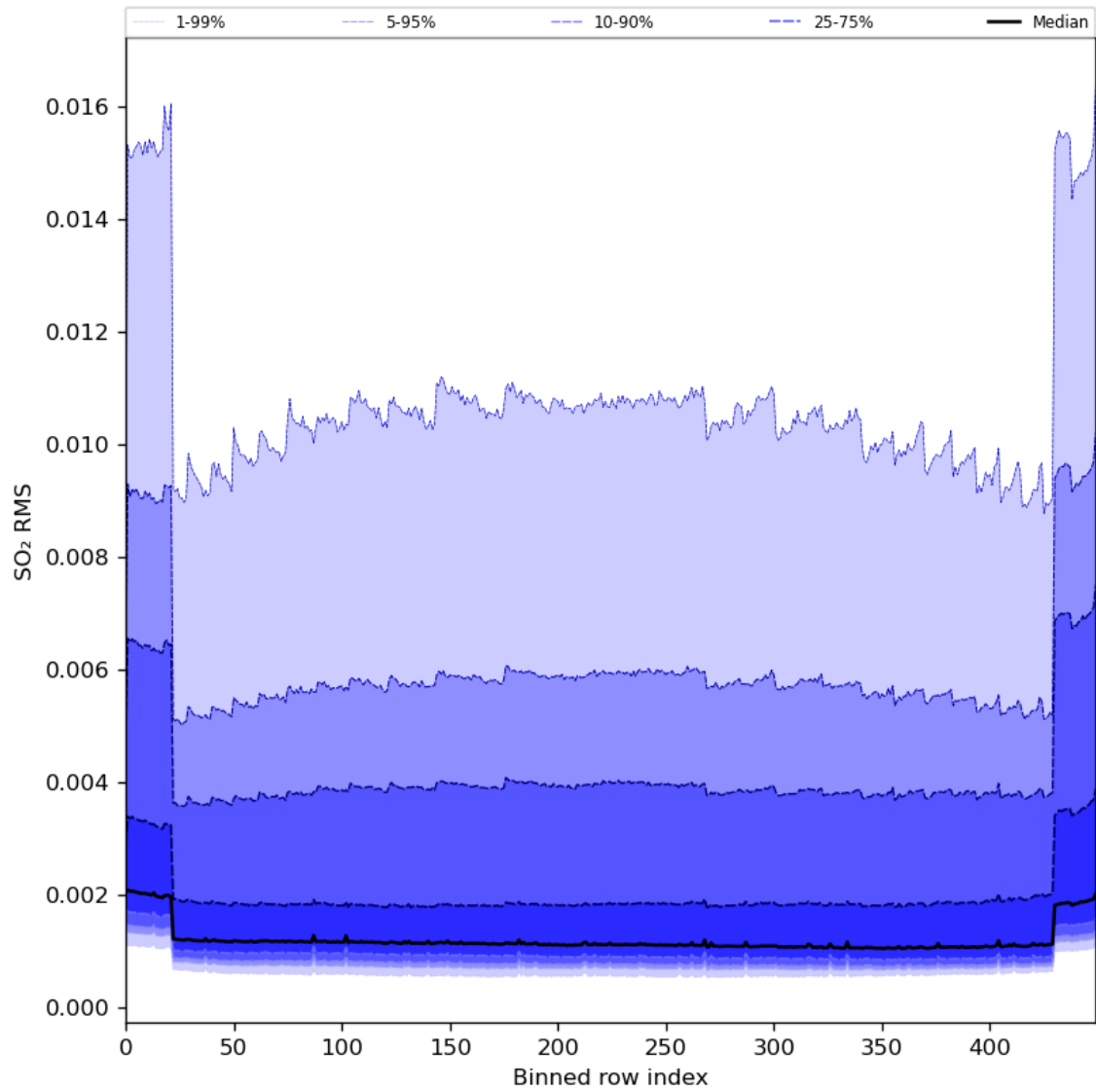
Figure 93: Along track statistics of “SO 2 RMS” for 2024-02-11 to 2024-02-12
