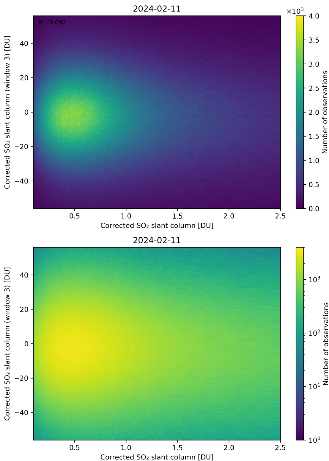
Figure 186: Scatter density plot of “Corrected SO 2 slant column” against “Corrected SO 2 slant column (window 3)” for 2024-02-11 to 2024-02-12.
