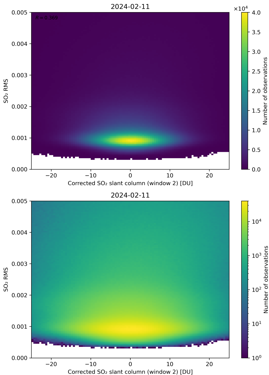
Figure 198: Scatter density plot of “Corrected SO 2 slant column (window 2)” against “SO 2 RMS” for 2024-02-11 to 2024-02-12.
