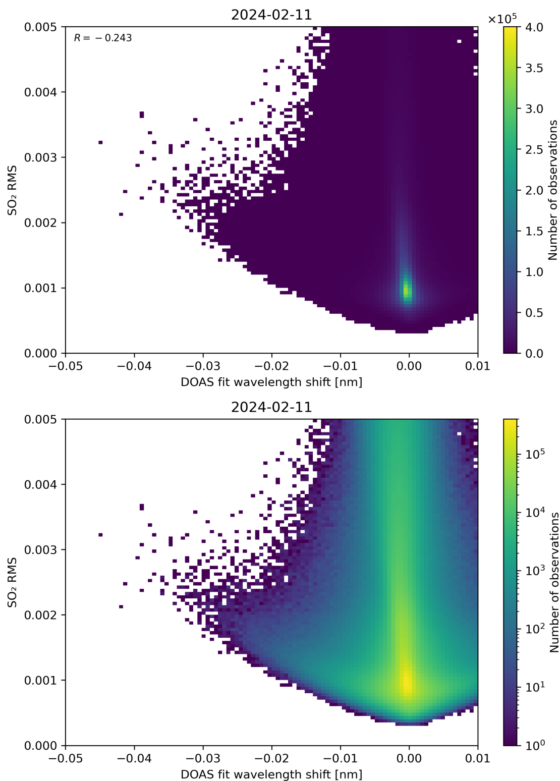
Figure 128: Scatter density plot of “DOAS fit wavelength shift” against “SO 2 RMS” for 2024-02-11 to 2024-02-12.
