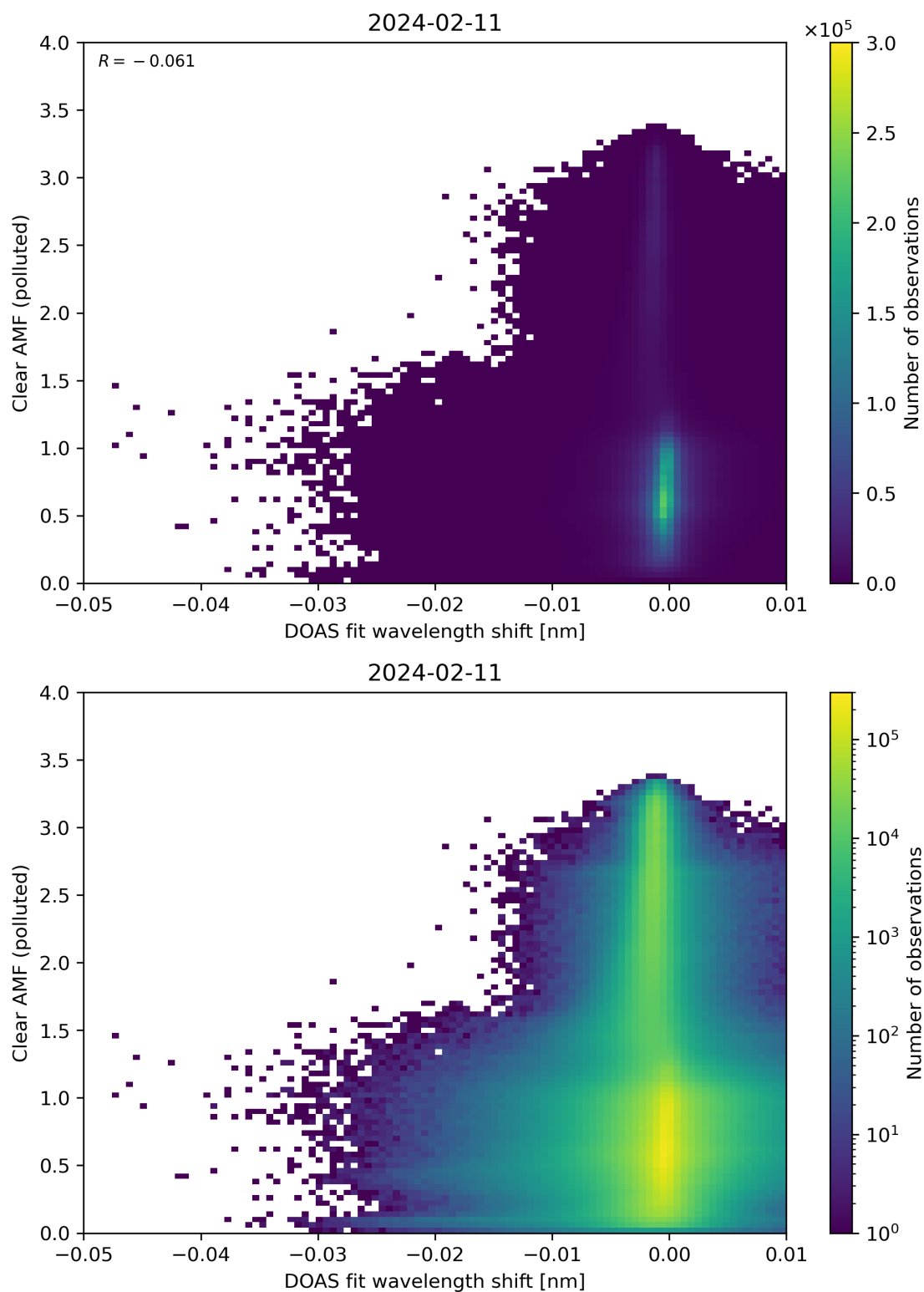
Figure 129: Scatter density plot of “DOAS fit wavelength shift” against “Clear AMF (polluted)” for 2024-02-11 to 2024-02-12.
