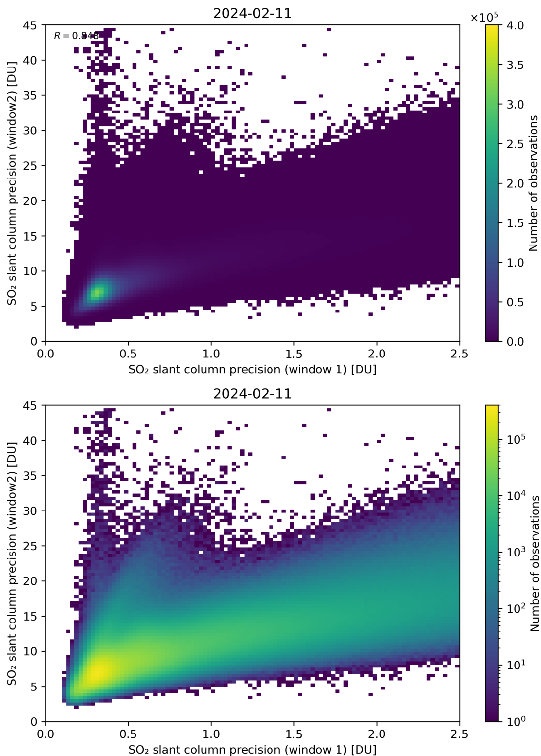
Figure 227: Scatter density plot of “SO 2 slant column precision (window 1)” against “SO 2 slant column precision (window2)” for 2024-02-11 to 2024-02-12.
