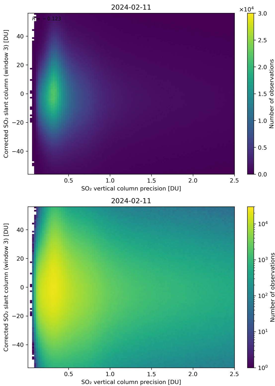
Figure 288: Scatter density plot of “SO 2 vertical column precision” against “Corrected SO 2 slant column (window 3)” for 2024-02-11 to 2024-02-12.
