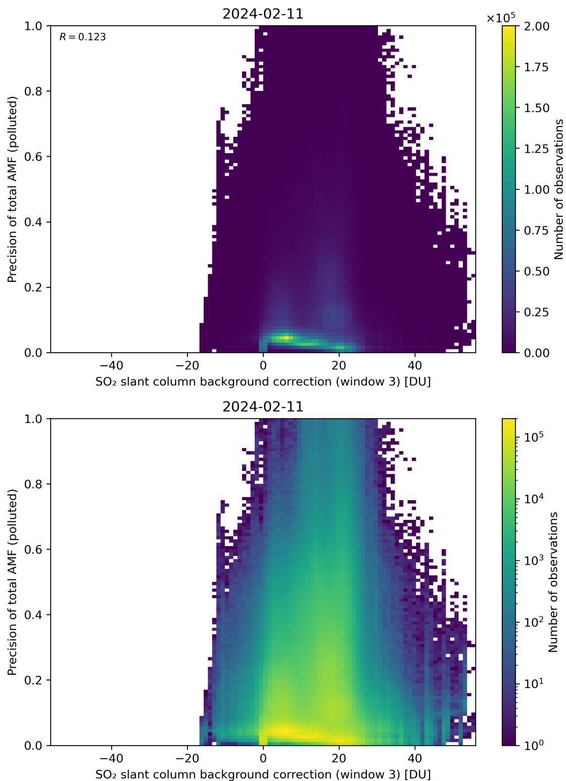
Figure 126: Scatter density plot of “SO 2 slant column background correction (window 3)” against “Precision of total AMF (polluted)” for 2024-02-11 to 2024-02-12.
