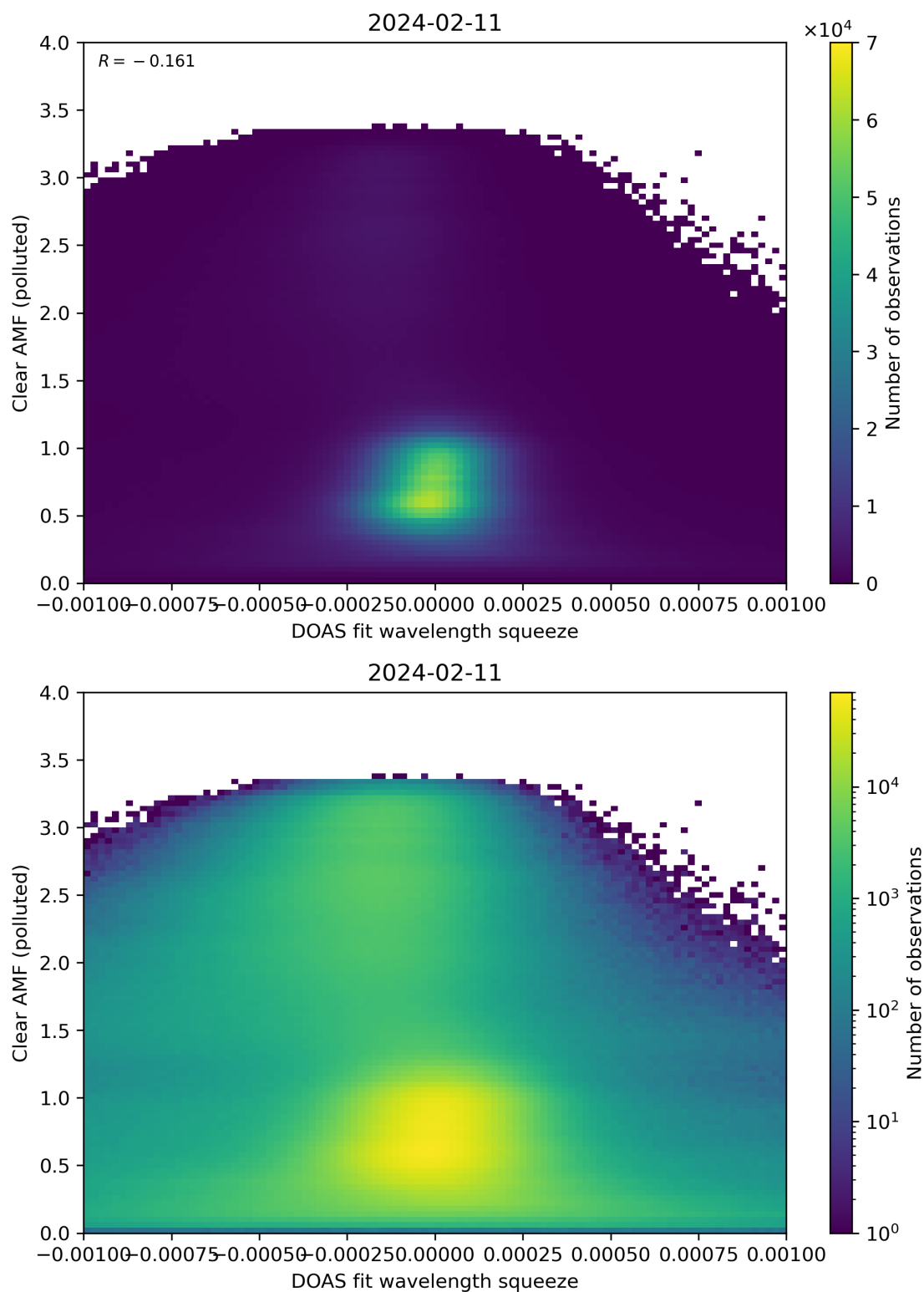
Figure 133: Scatter density plot of “DOAS fit wavelength squeeze” against “Clear AMF (polluted)” for 2024-02-11 to 2024-02-12.
