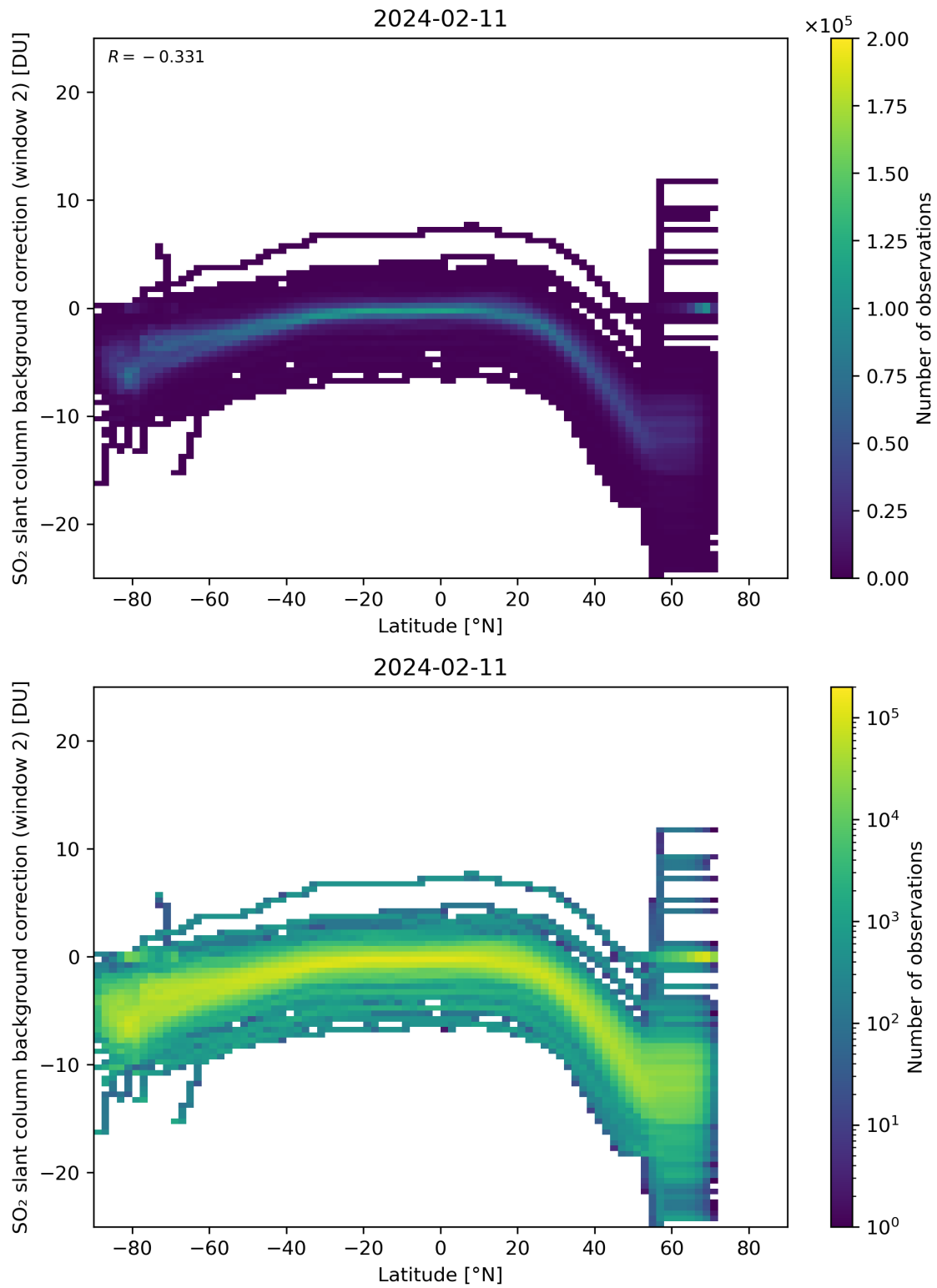
Figure 140: Scatter density plot of “Latitude” against “SO 2 slant column background correction (window 2)” for 2024-02-11 to 2024-02-12.
