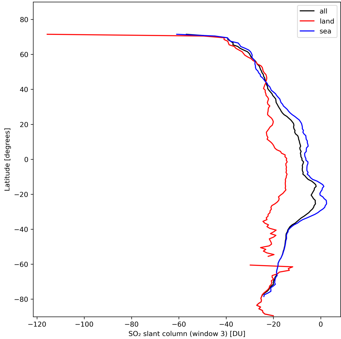
Figure 41: Zonal average of “SO 2 slant column (window 3)” for 2024-02-11 to 2024-02-12.
