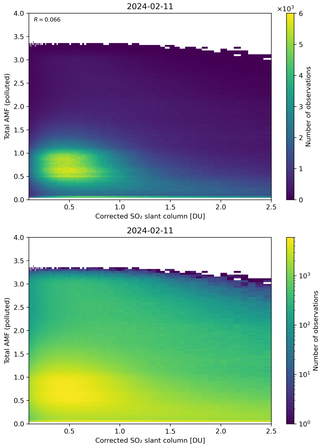
Figure 192: Scatter density plot of “Corrected SO 2 slant column” against “Total AMF (polluted)” for 2024-02-11 to 2024-02-12.
