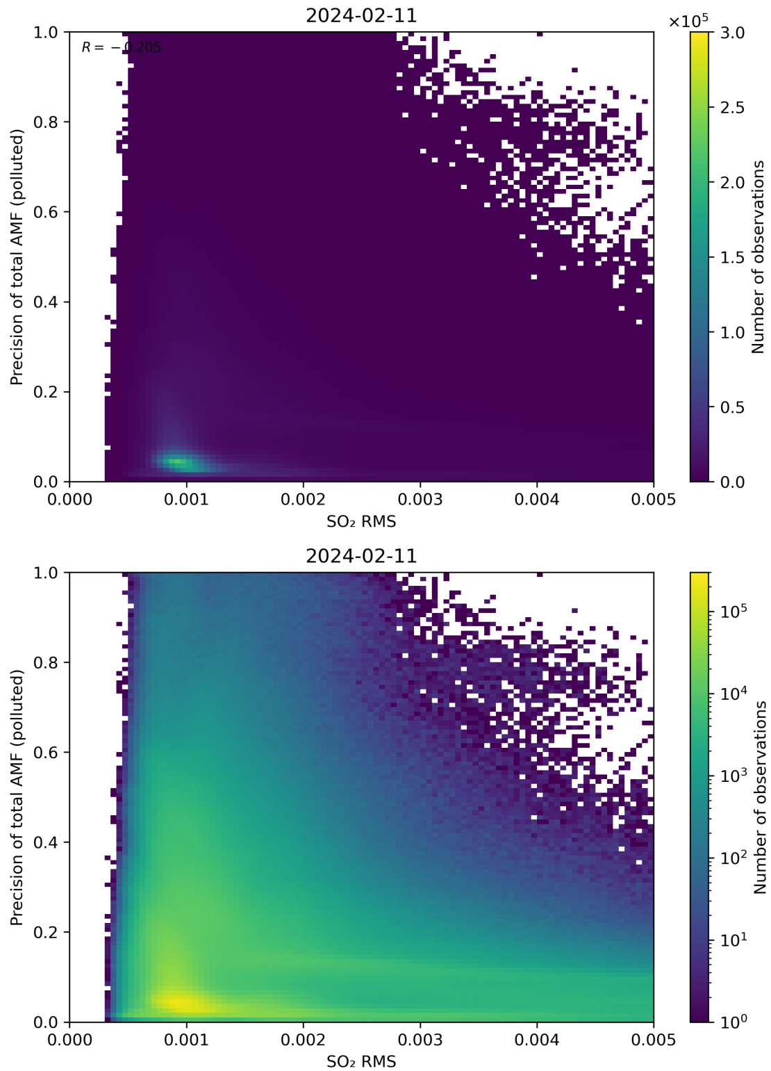
Figure 138: Scatter density plot of “SO 2 RMS” against “Precision of total AMF (polluted)” for 2024-02-11 to 2024-02-12.
