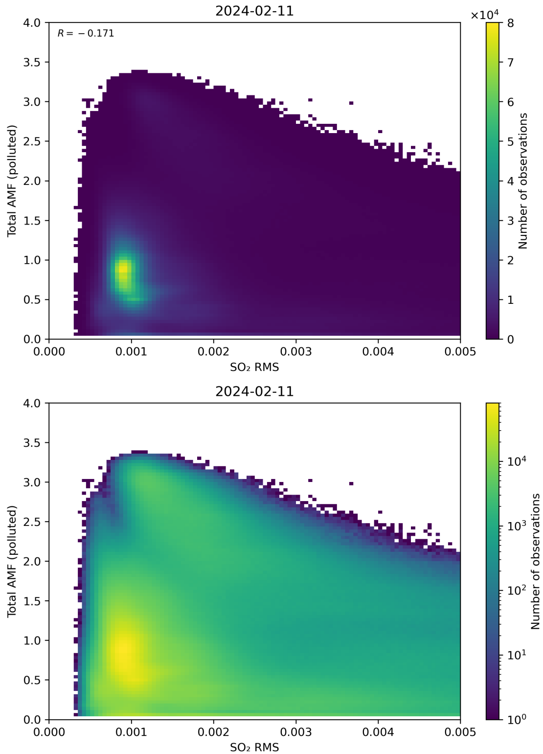
Figure 137: Scatter density plot of “SO 2 RMS” against “Total AMF (polluted)” for 2024-02-11 to 2024-02-12.
