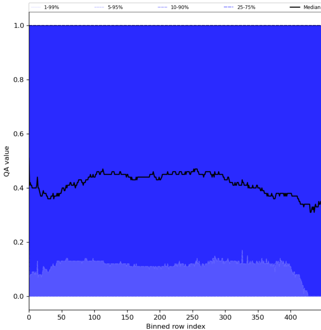
Figure 75: Along track statistics of “QA value” for 2024-02-11 to 2024-02-12
