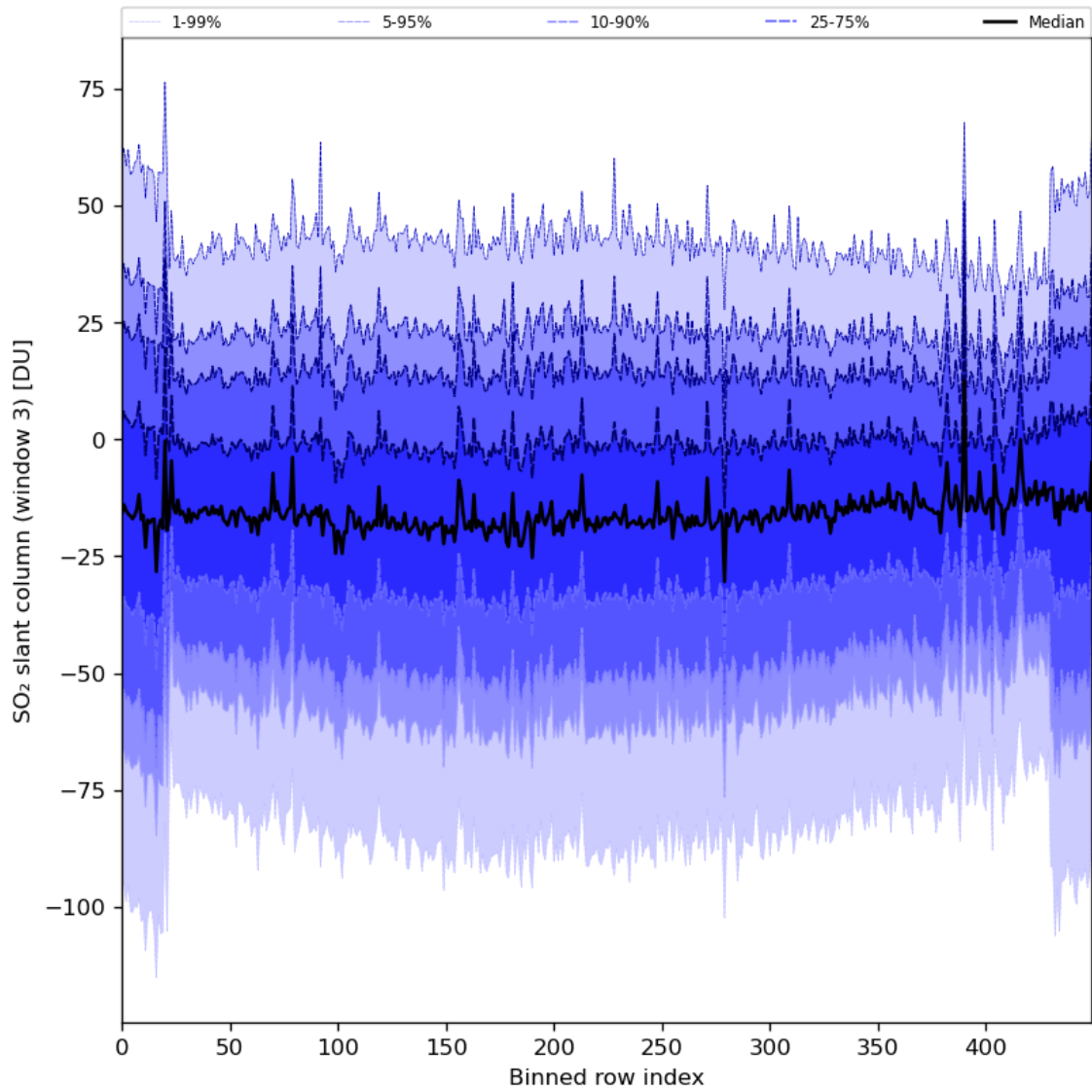
Figure 87: Along track statistics of “SO 2 slant column (window 3)” for 2024-02-11 to 2024-02-12
