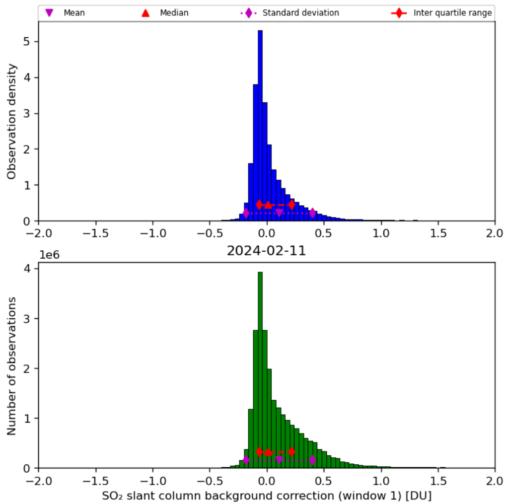
Figure 59: Histogram of “SO 2 slant column background correction (window 1)” for 2024-02-11 to 2024-02-12
