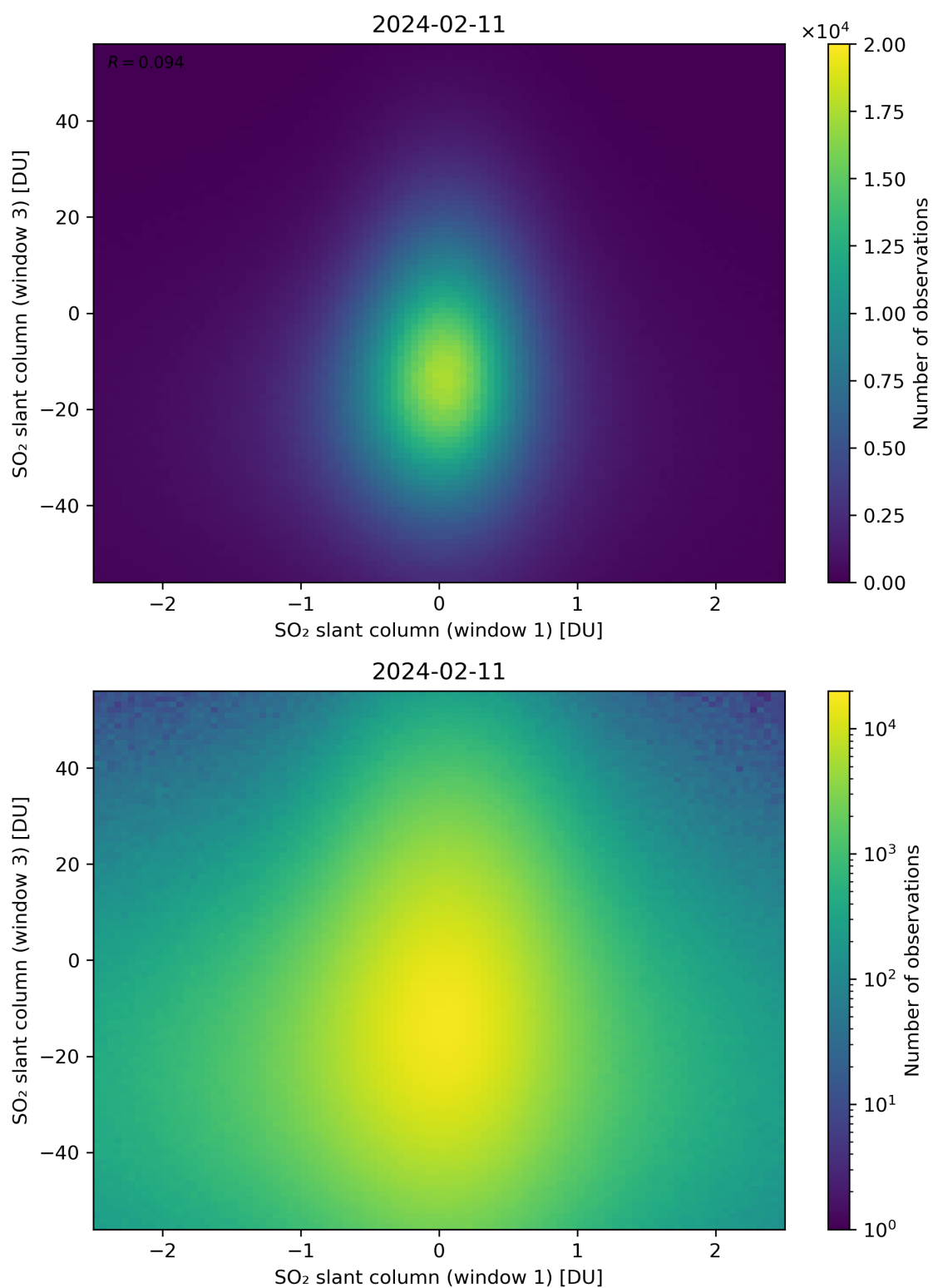
Figure 237: Scatter density plot of “SO 2 slant column (window 1)” against “SO 2 slant column (window 3)” for 2024-02-11 to 2024-02-12.
