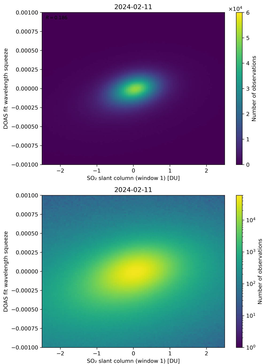
Figure 216: Scatter density plot of “SO 2 slant column (window 1)” against “DOAS fit wavelength squeeze” for 2024-02-11 to 2024-02-12.
