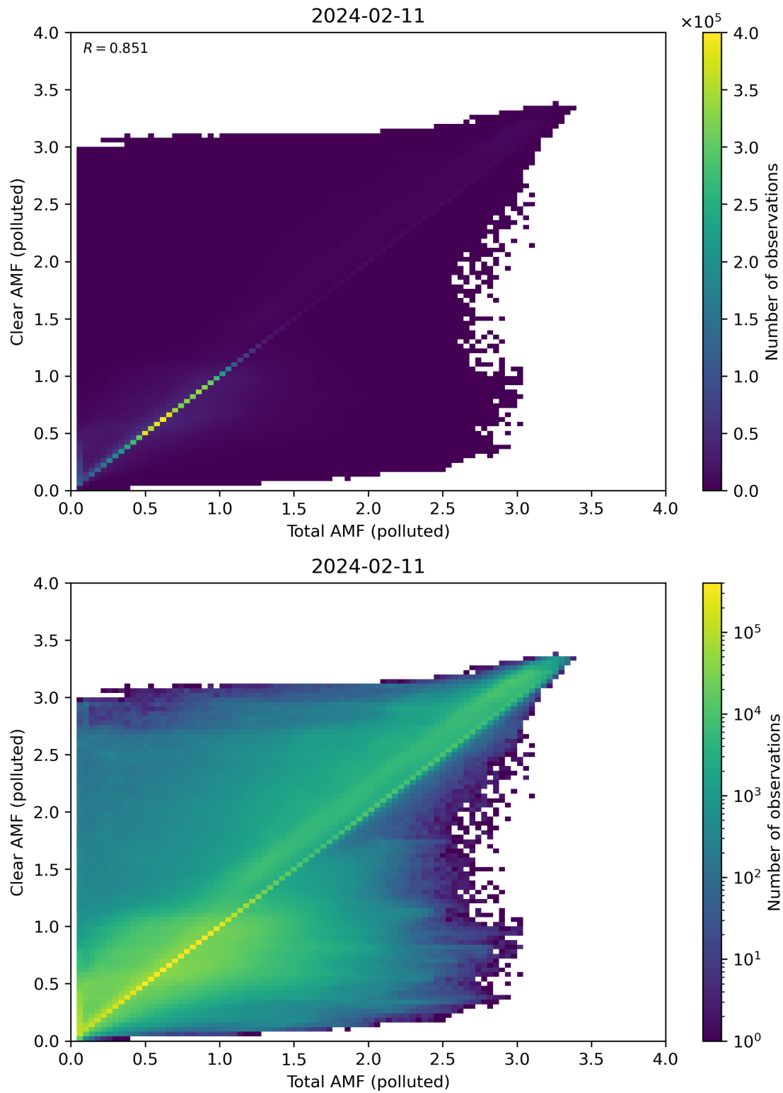
Figure 271: Scatter density plot of “Total AMF (polluted)” against “Clear AMF (polluted)” for 2024-02-11 to 2024-02-12.
