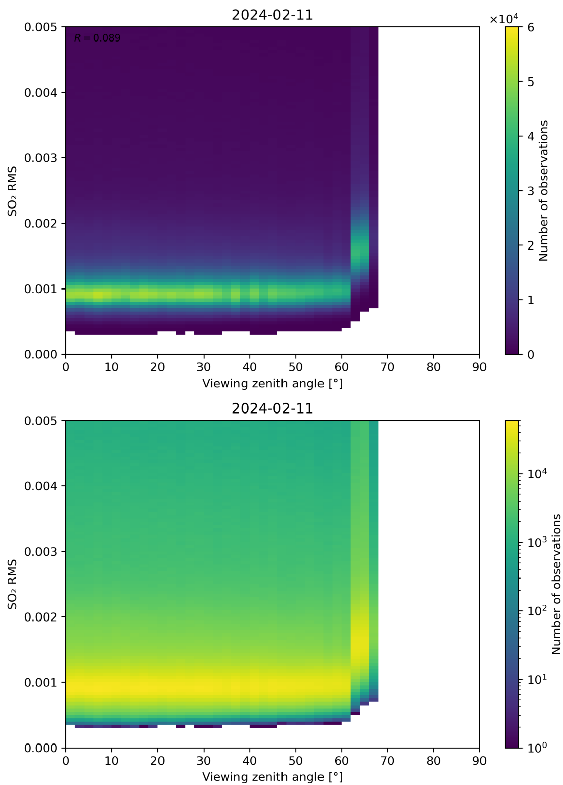
Figure 313: Scatter density plot of “Viewing zenith angle” against “SO 2 RMS” for 2024-02-11 to 2024-02-12.
