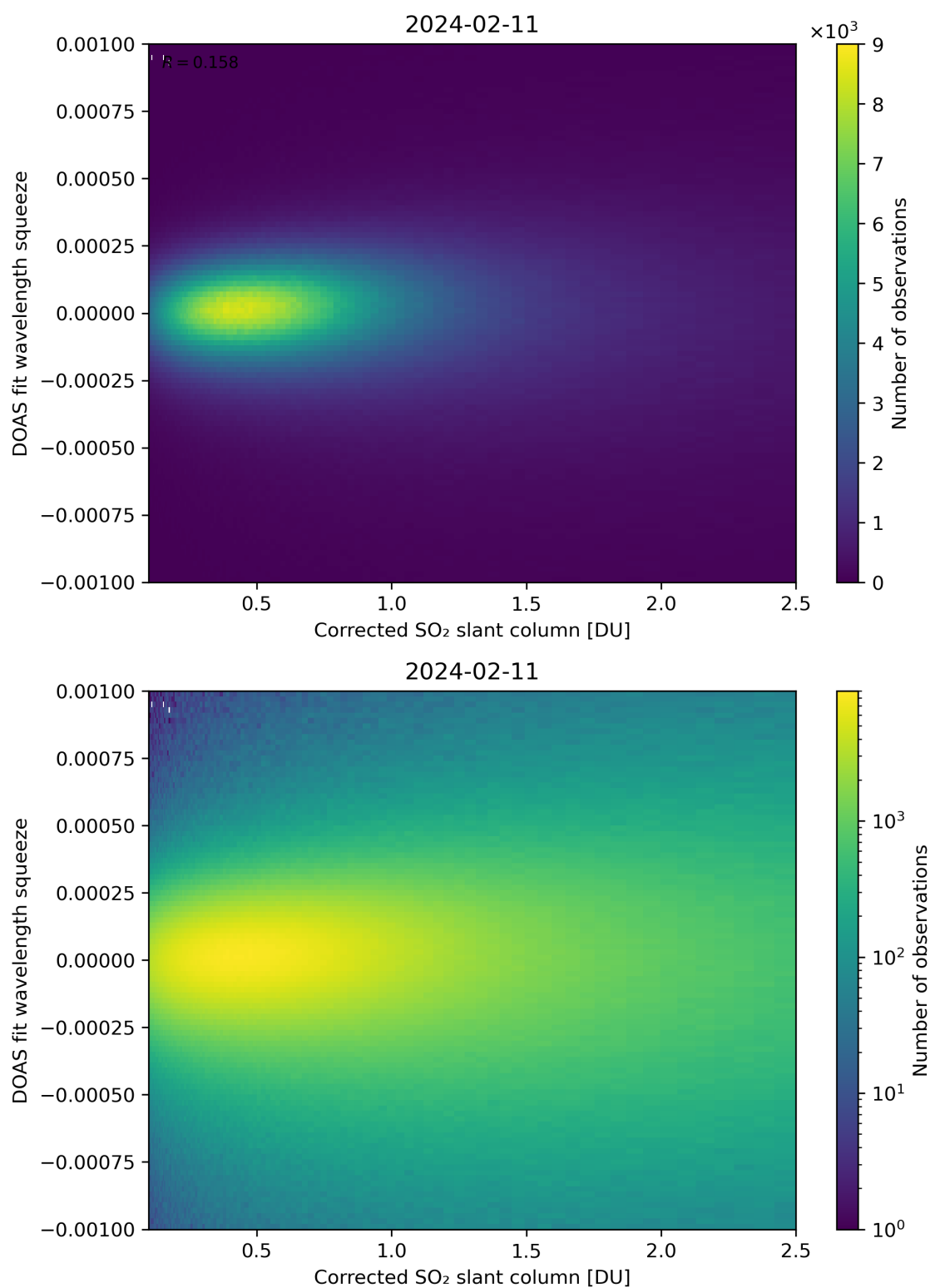
Figure 182: Scatter density plot of “Corrected SO 2 slant column” against “DOAS fit wavelength squeeze” for 2024-02-11 to 2024-02-12.
