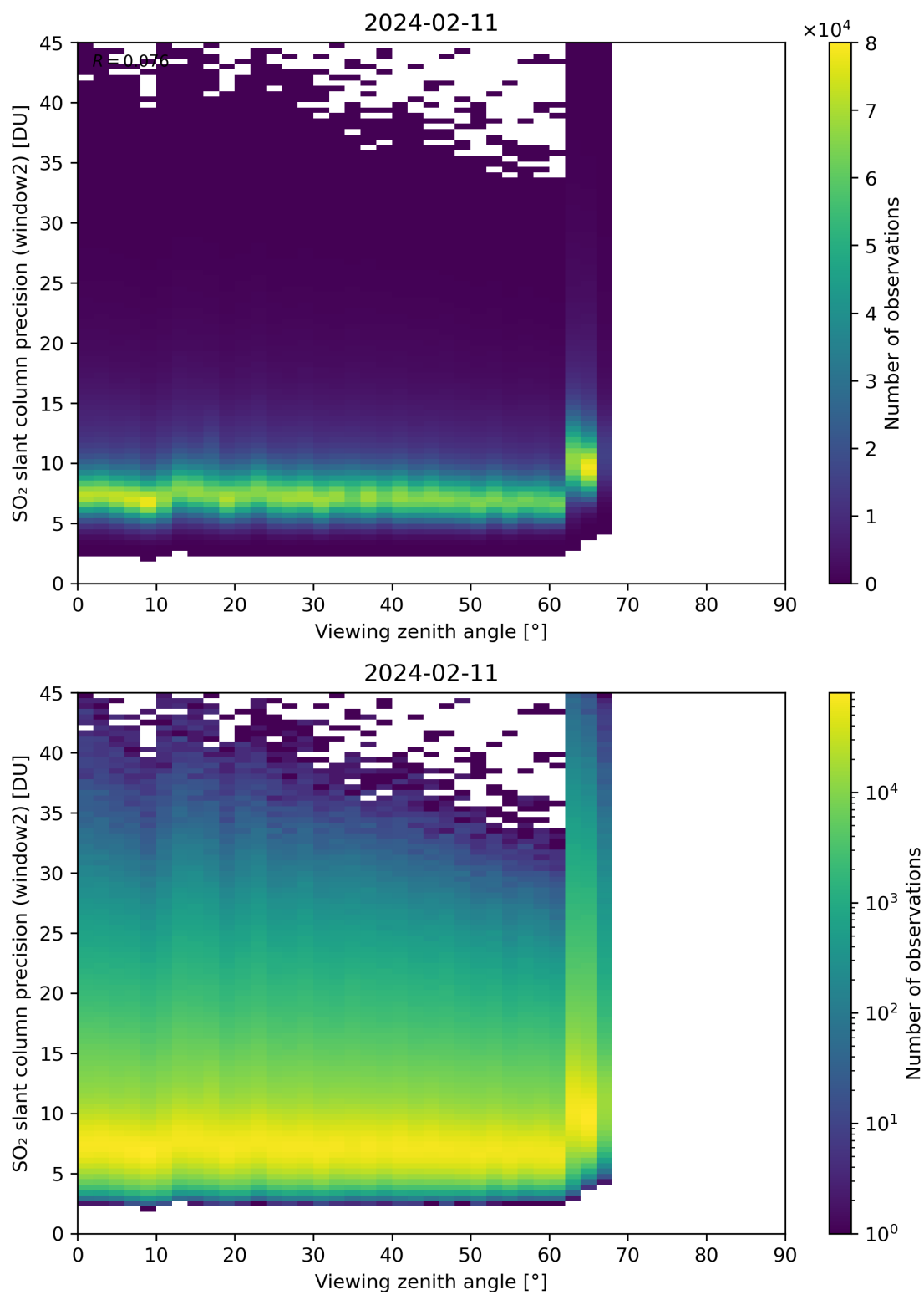
Figure 322: Scatter density plot of “Viewing zenith angle” against “SO 2 slant column precision (window2)” for 2024-02-11 to 2024-02-12.
