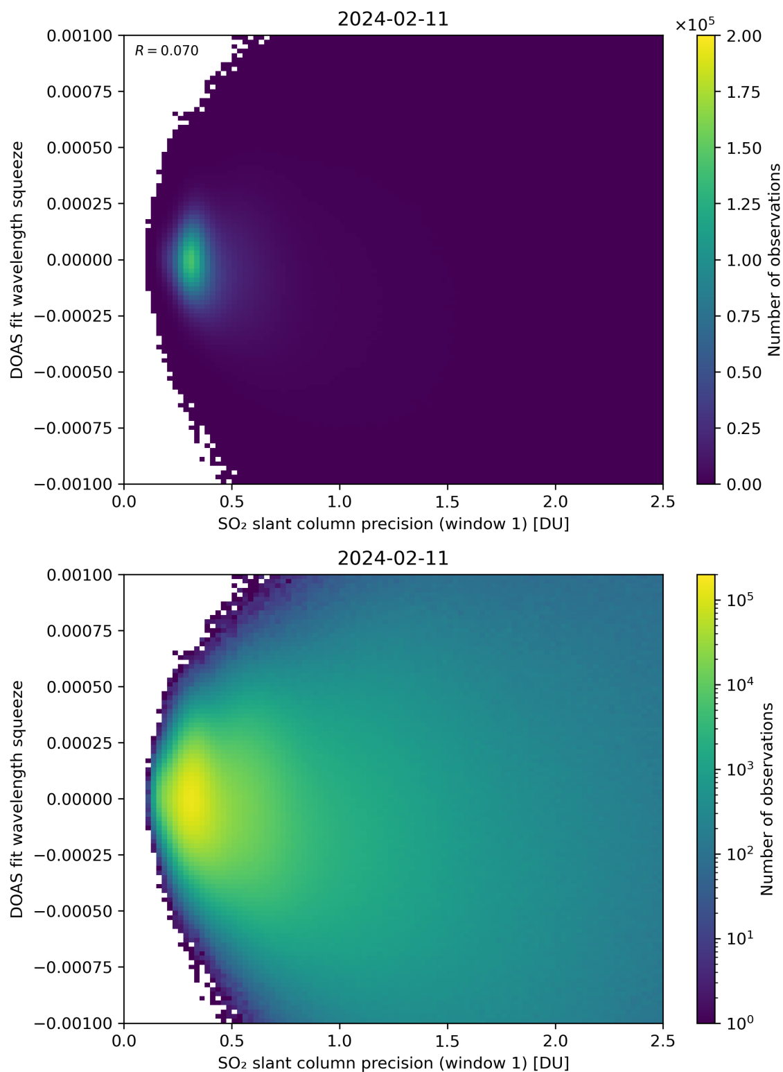
Figure 222: Scatter density plot of “SO 2 slant column precision (window 1)” against “DOAS fit wavelength squeeze” for 2024-02-11 to 2024-02-12.
