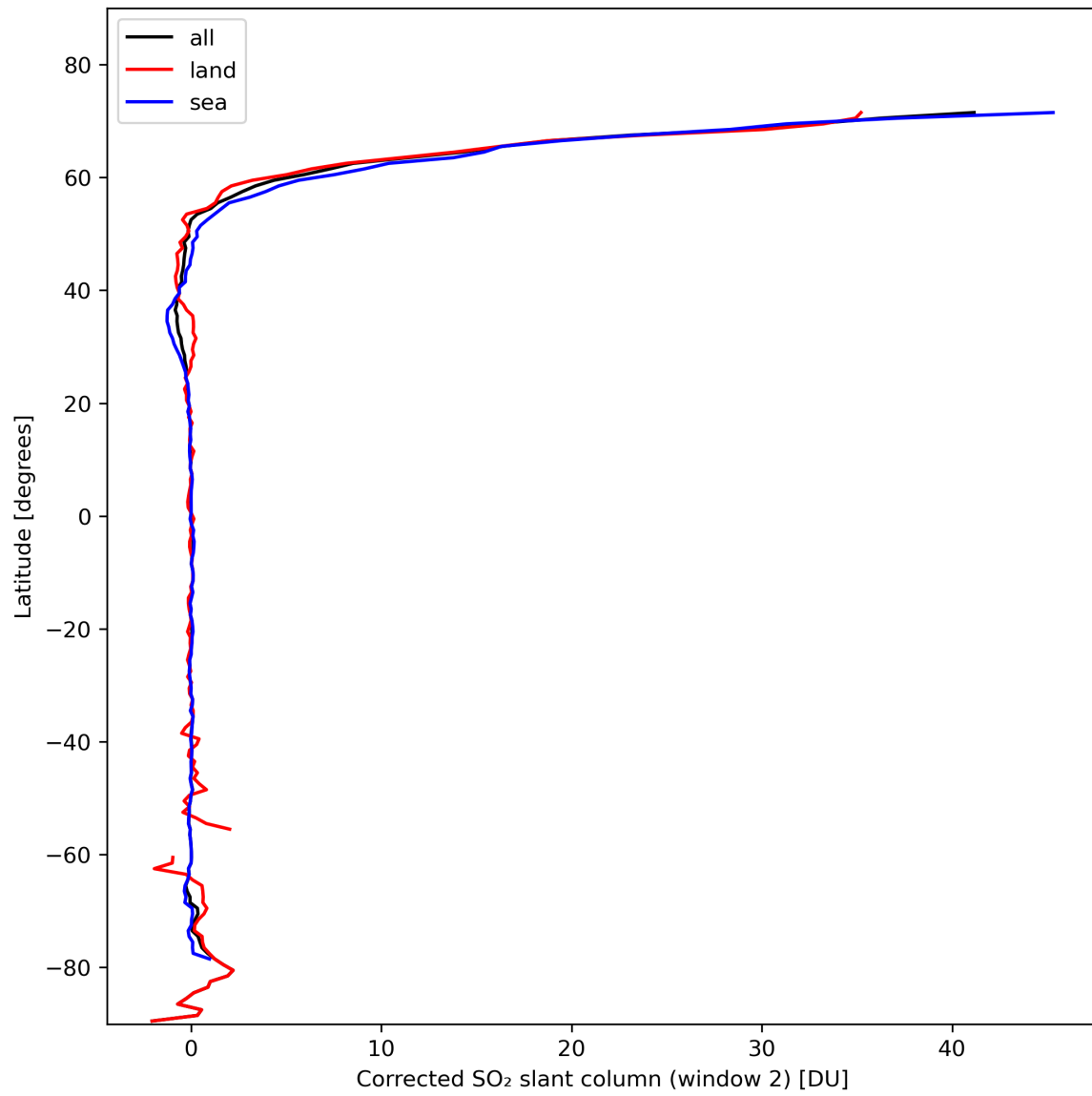
Figure 39: Zonal average of “Corrected SO 2 slant column (window 2)” for 2024-02-11 to 2024-02-12.
