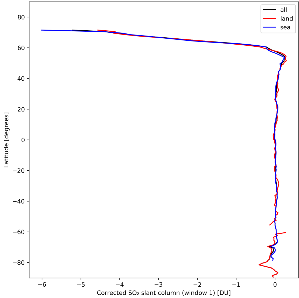
Figure 35: Zonal average of “Corrected SO 2 slant column (window 1)” for 2024-02-11 to 2024-02-12.
