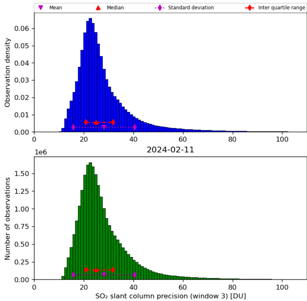
Figure 65: Histogram of “SO 2 slant column precision (window 3)” for 2024-02-11 to 2024-02-12
