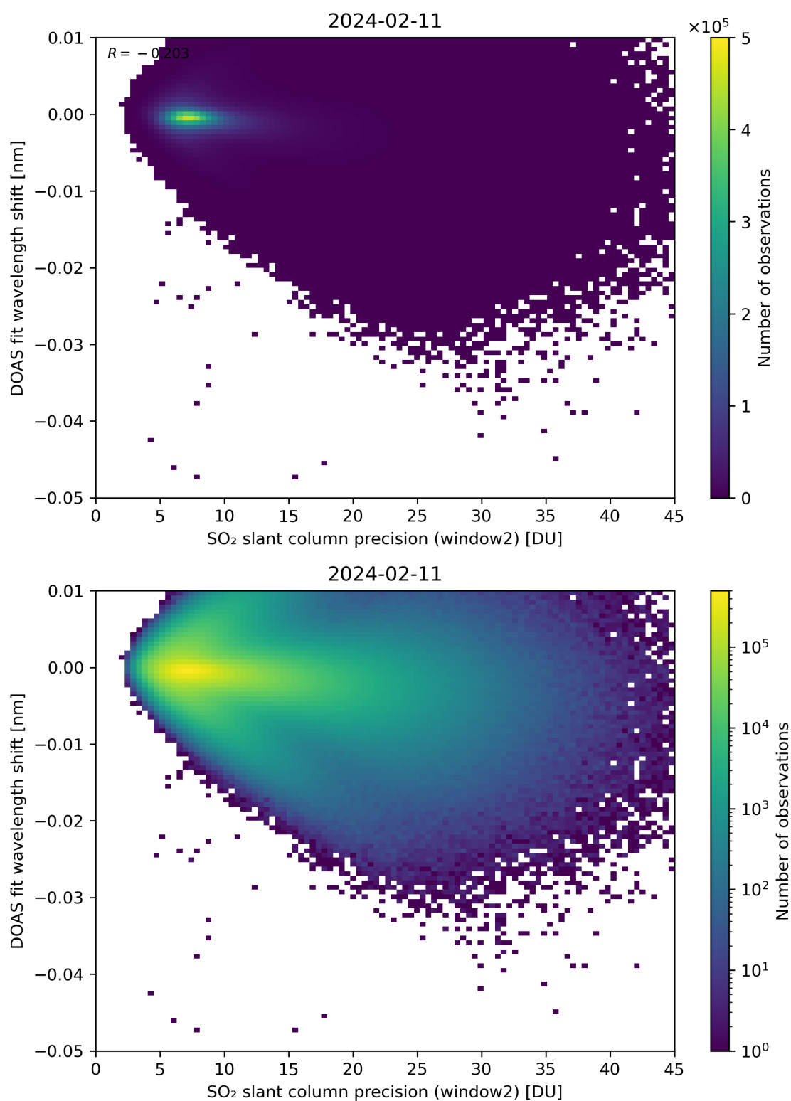
Figure 243: Scatter density plot of “SO 2 slant column precision (window2)” against “DOAS fit wavelength shift” for 2024-02-11 to 2024-02-12.
