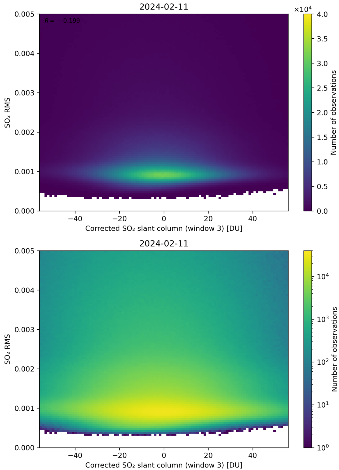
Figure 208: Scatter density plot of “Corrected SO 2 slant column (window 3)” against “SO 2 RMS” for 2024-02-11 to 2024-02-12.
