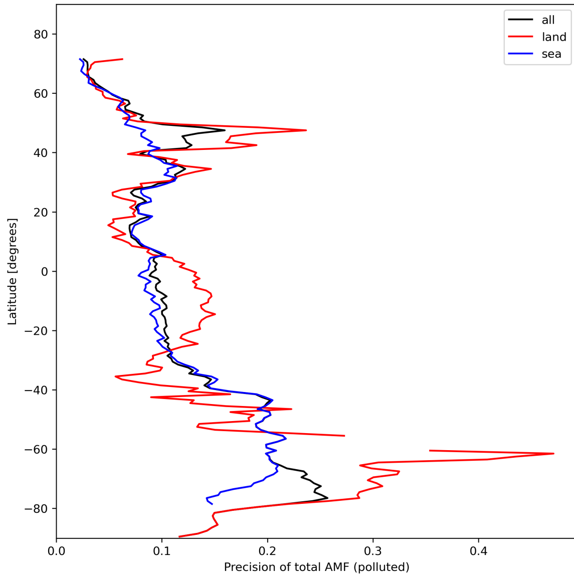
Figure 49: Zonal average of “Precision of total AMF (polluted)” for 2024-02-11 to 2024-02-12.
