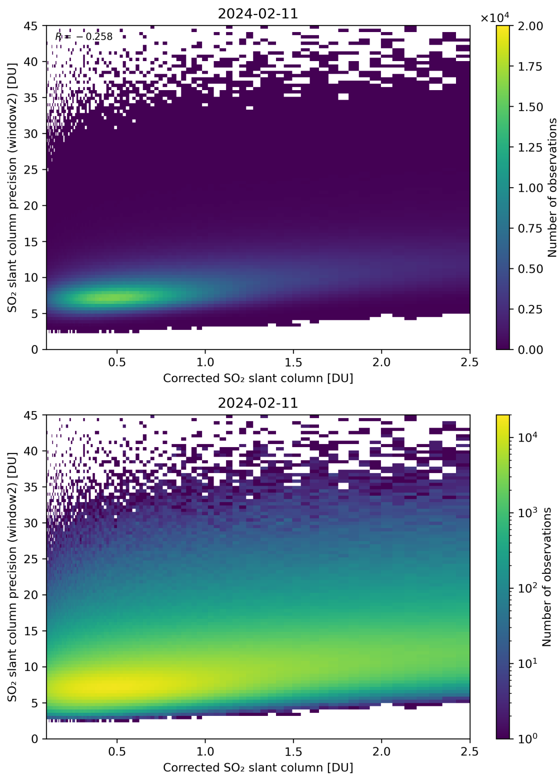
Figure 189: Scatter density plot of “Corrected SO 2 slant column” against “SO 2 slant column precision (window2)” for 2024-02-11 to 2024-02-12.
