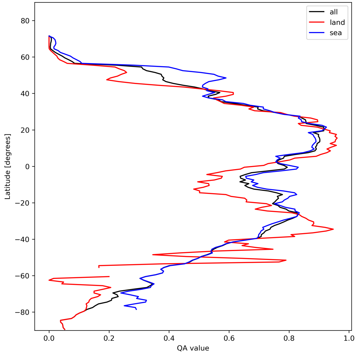
Figure 29: Zonal average of “QA value” for 2024-02-11 to 2024-02-12.
