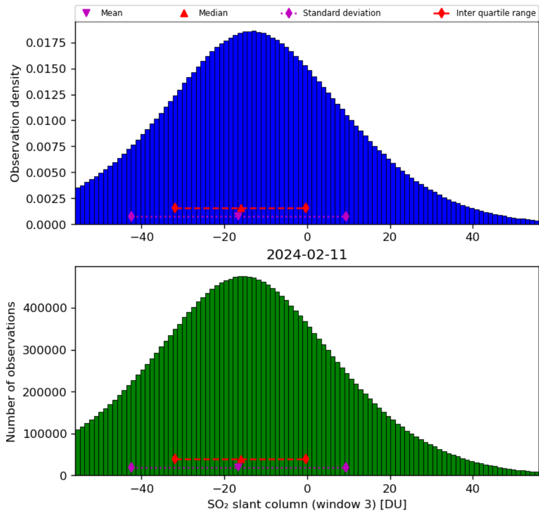
Figure 64: Histogram of “SO 2 slant column (window 3)” for 2024-02-11 to 2024-02-12
