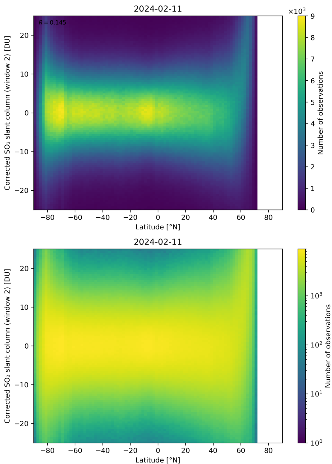
Figure 147: Scatter density plot of “Latitude” against “Corrected SO 2 slant column (window 2)” for 2024-02-11 to 2024-02-12.
