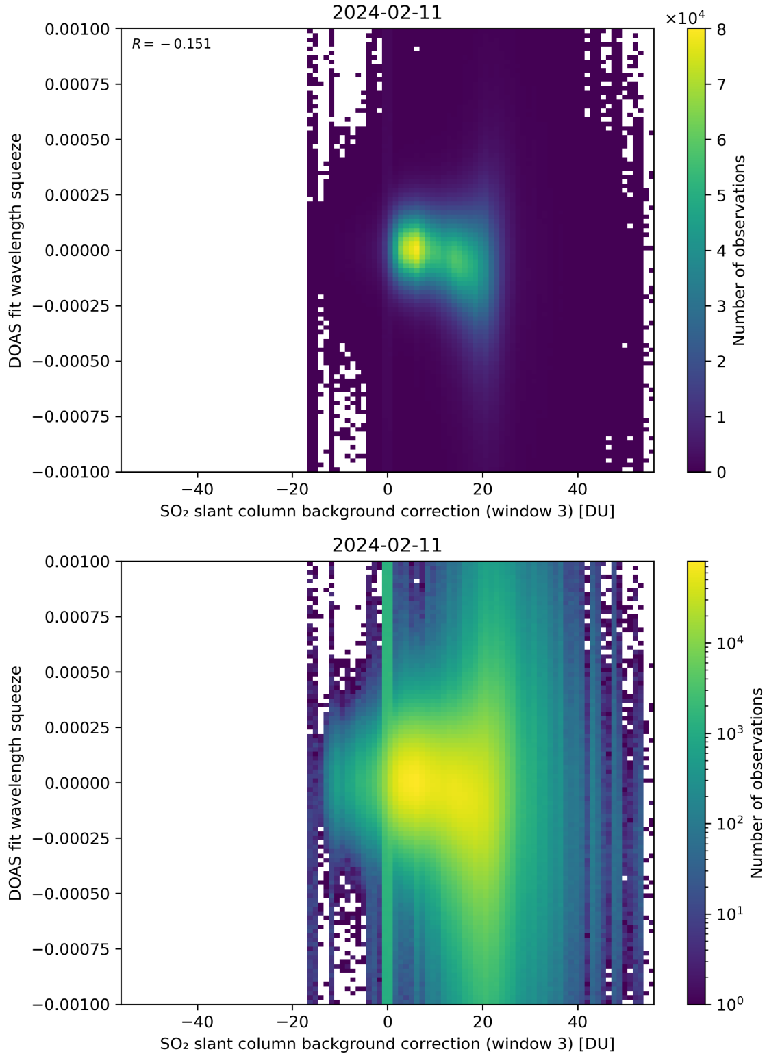
Figure 122: Scatter density plot of “SO 2 slant column background correction (window 3)” against “DOAS fit wavelength squeeze” for 2024-02-11 to 2024-02-12.
