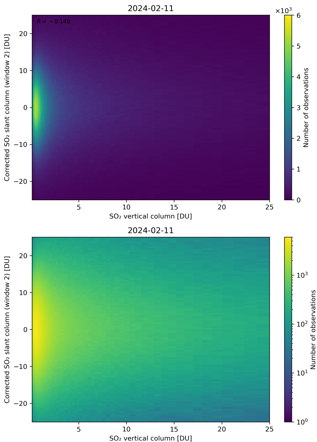
Figure 298: Scatter density plot of “SO 2 vertical column” against “Corrected SO 2 slant column (window 2)” for 2024-02-11 to 2024-02-12.
