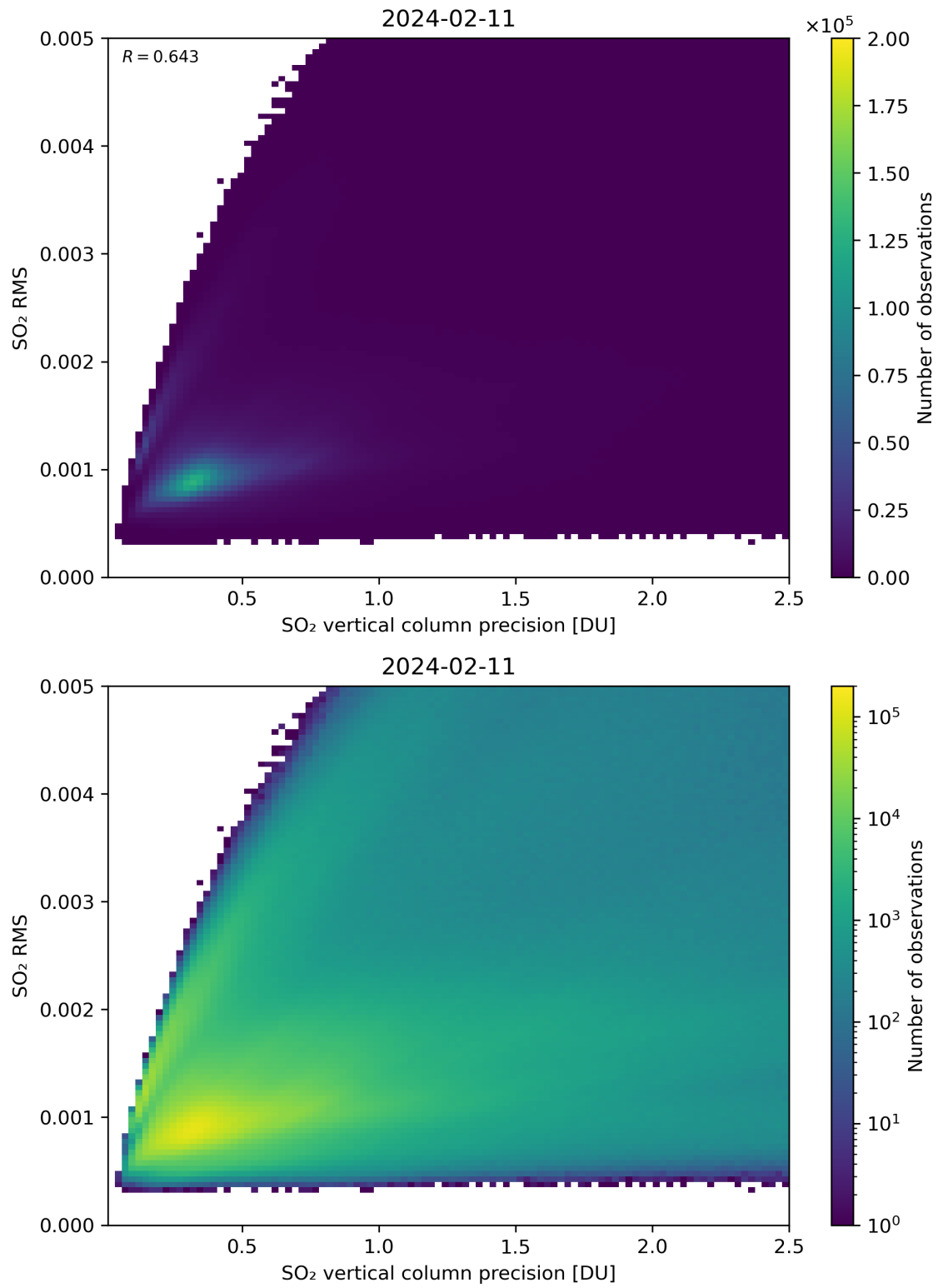
Figure 284: Scatter density plot of “SO 2 vertical column precision” against “SO 2 RMS” for 2024-02-11 to 2024-02-12.
