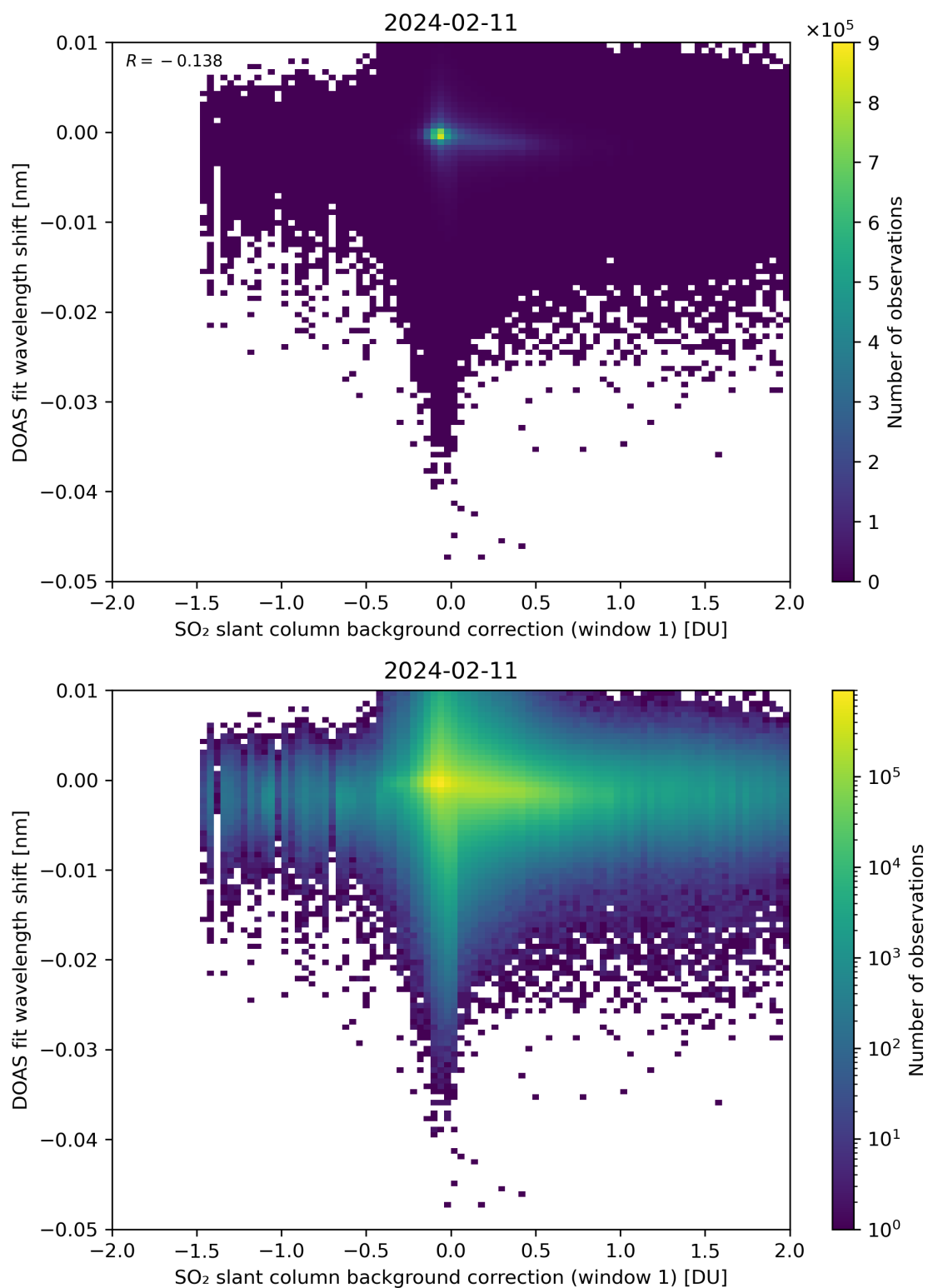
Figure 100: Scatter density plot of “SO 2 slant column background correction (window 1)” against “DOAS fit wavelength shift” for 2024-02-11 to 2024-02-12.
