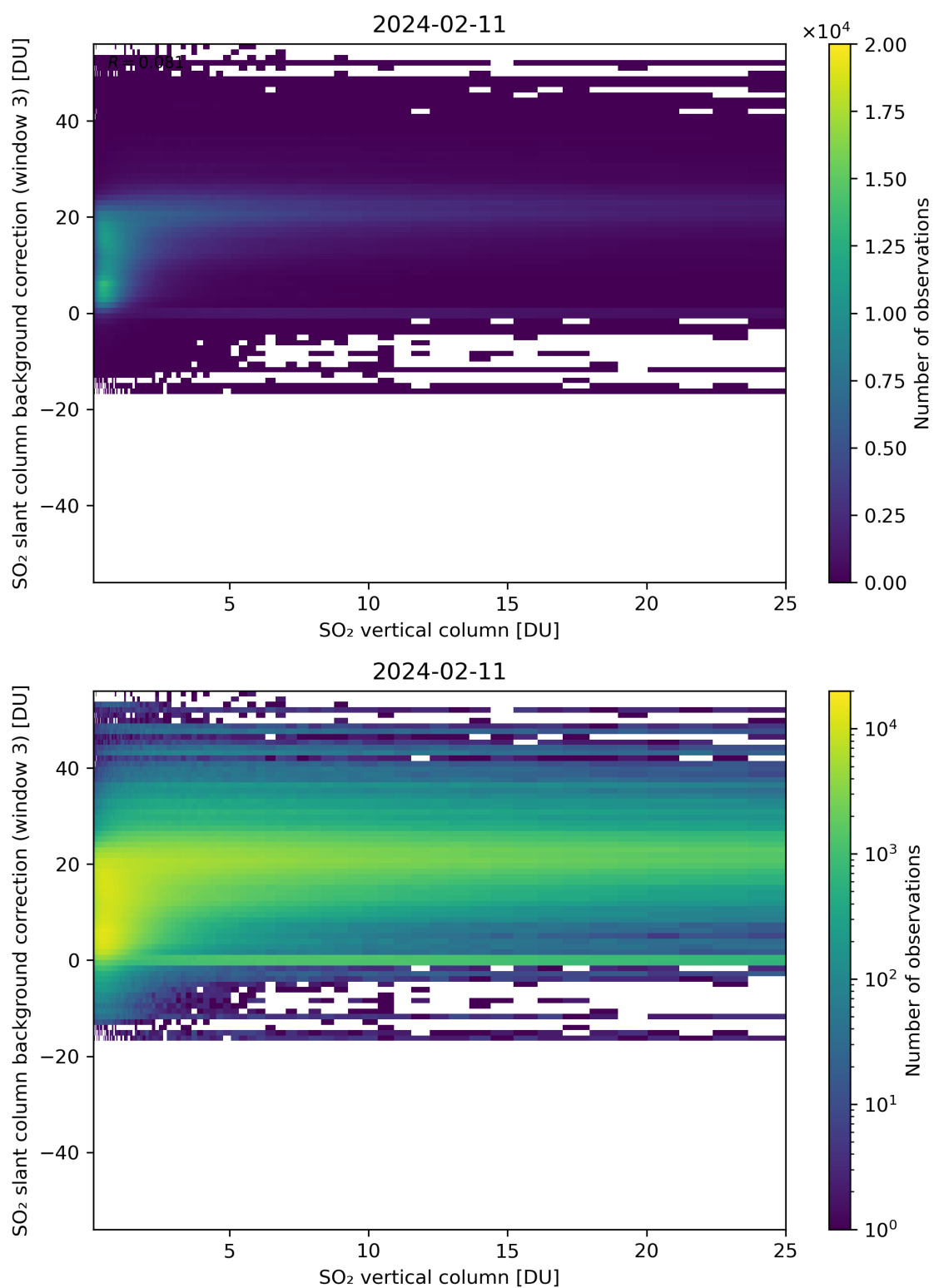
Figure 275: Scatter density plot of “SO 2 vertical column” against “SO 2 slant column background correction (window 3)” for 2024-02-11 to 2024-02-12.
