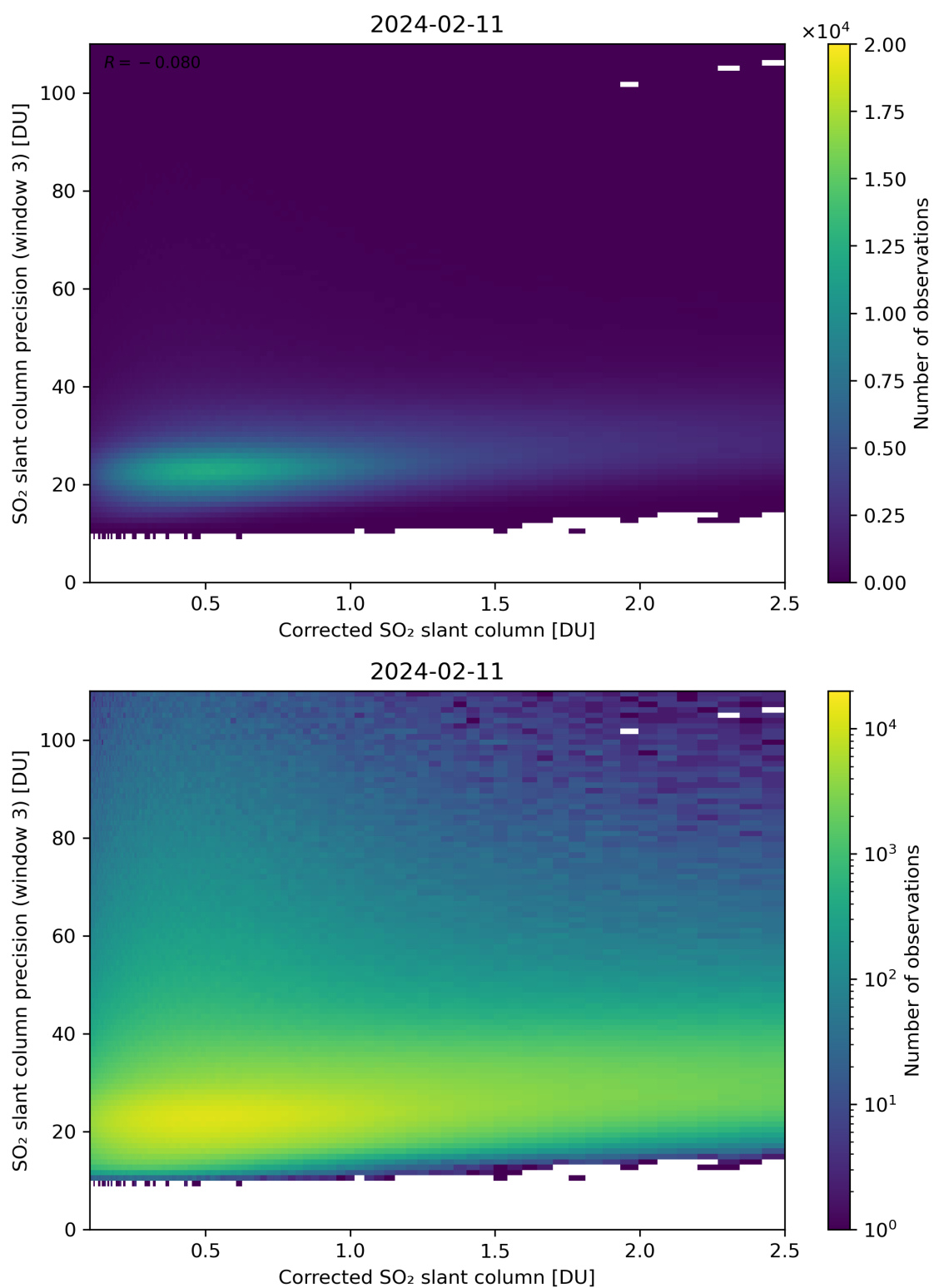
Figure 191: Scatter density plot of “Corrected SO 2 slant column” against “SO 2 slant column precision (window 3)” for 2024-02-11 to 2024-02-12.
