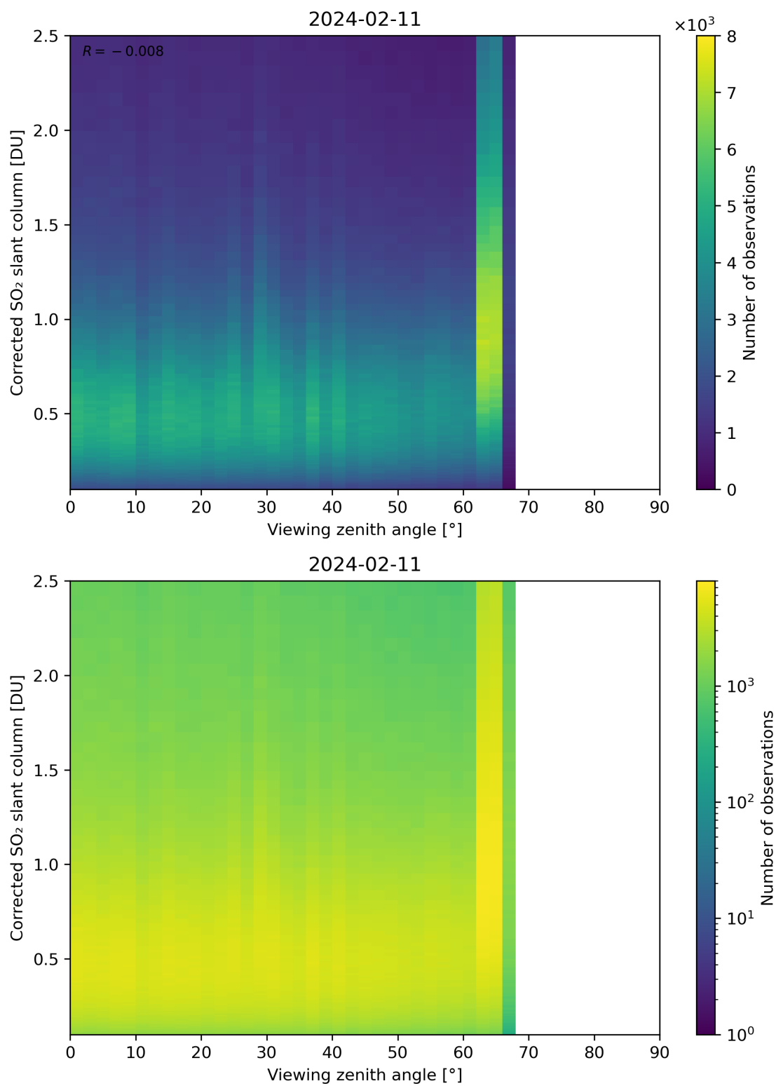
Figure 317: Scatter density plot of “Viewing zenith angle” against “Corrected SO 2 slant column” for 2024-02-11 to 2024-02-12.
