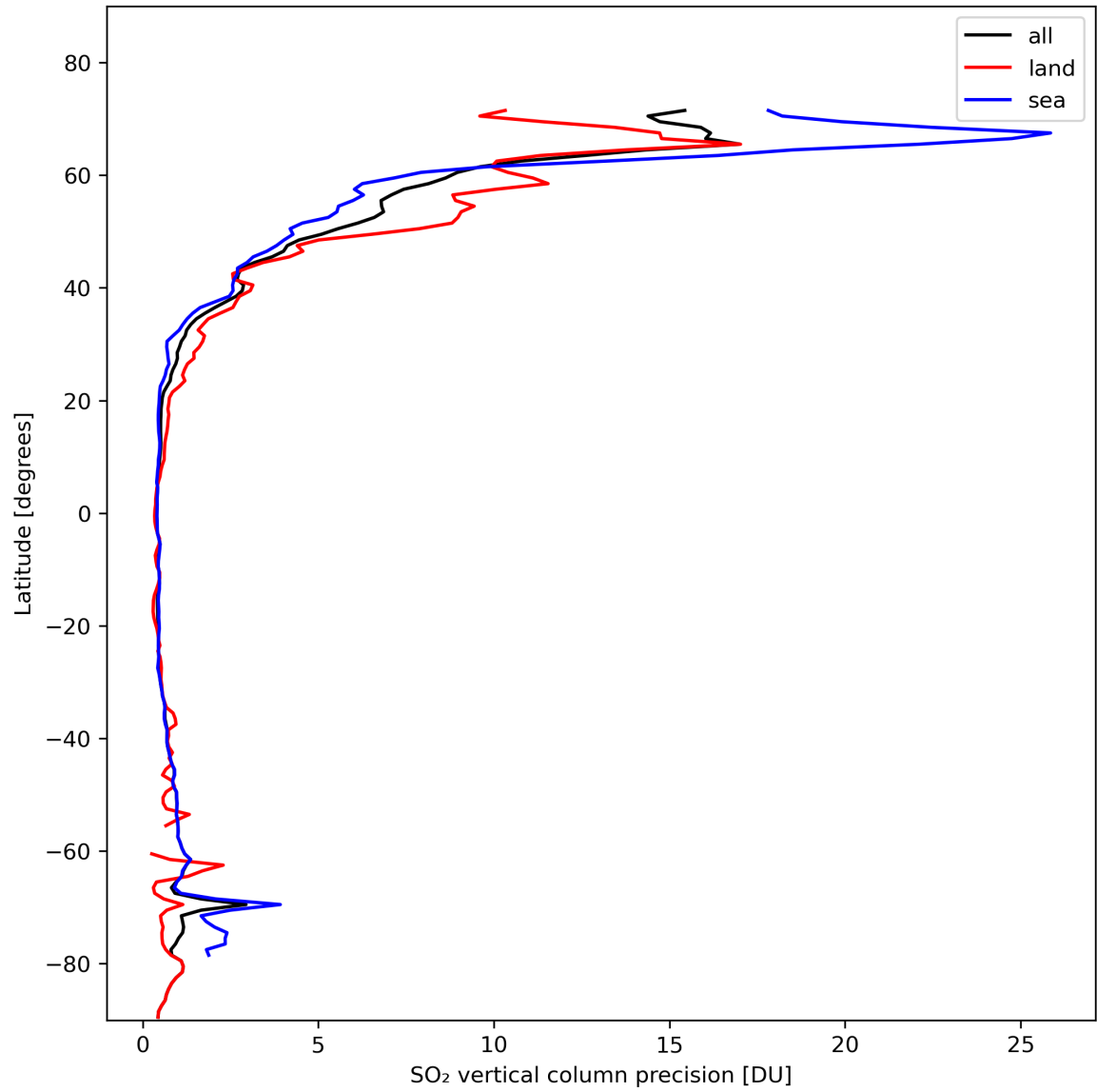
Figure 31: Zonal average of “SO 2 vertical column precision” for 2024-02-11 to 2024-02-12.
