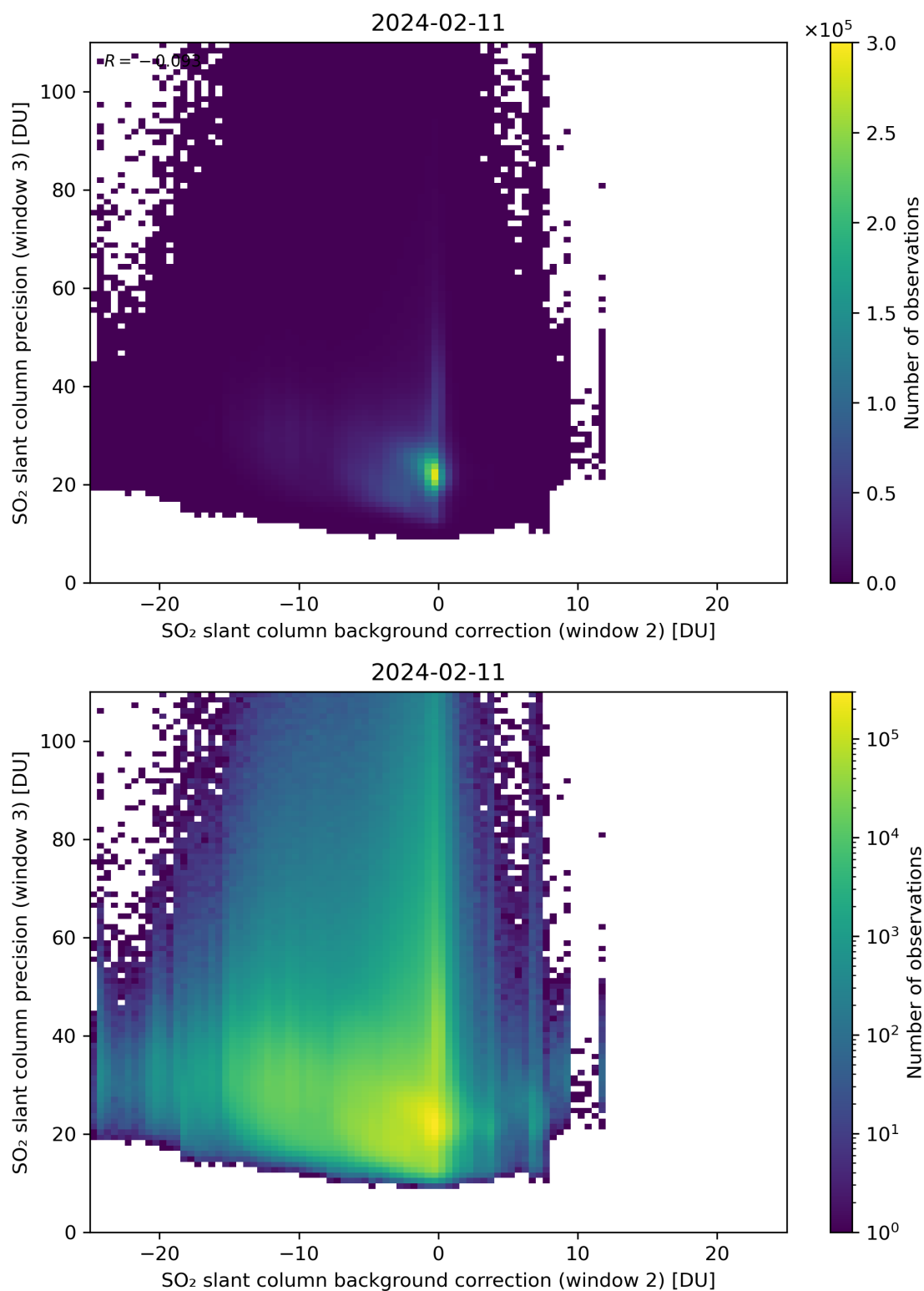
Figure 118: Scatter density plot of “SO 2 slant column background correction (window 2)” against “SO 2 slant column precision (window 3)” for 2024-02-11 to 2024-02-12.
