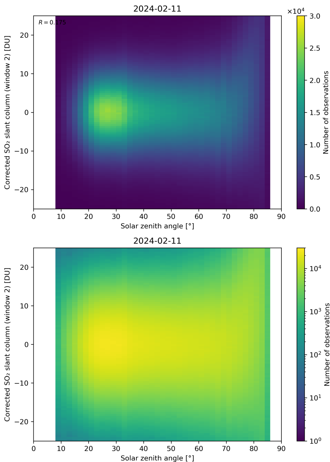
Figure 167: Scatter density plot of “Solar zenith angle” against “Corrected SO 2 slant column (window 2)” for 2024-02-11 to 2024-02-12.
