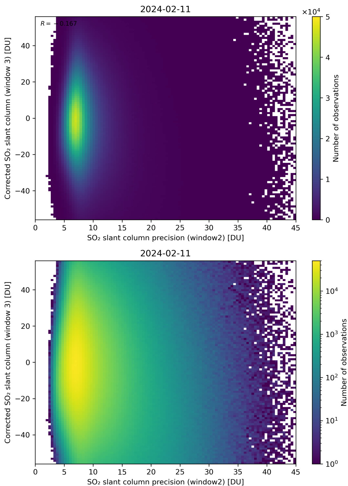
Figure 248: Scatter density plot of “SO 2 slant column precision (window2)” against “Corrected SO 2 slant column (window 3)” for 2024-02-11 to 2024-02-12.
