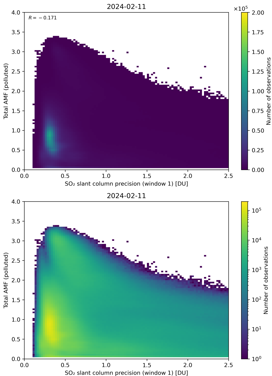
Figure 230: Scatter density plot of “SO 2 slant column precision (window 1)” against “Total AMF (polluted)” for 2024-02-11 to 2024-02-12.
