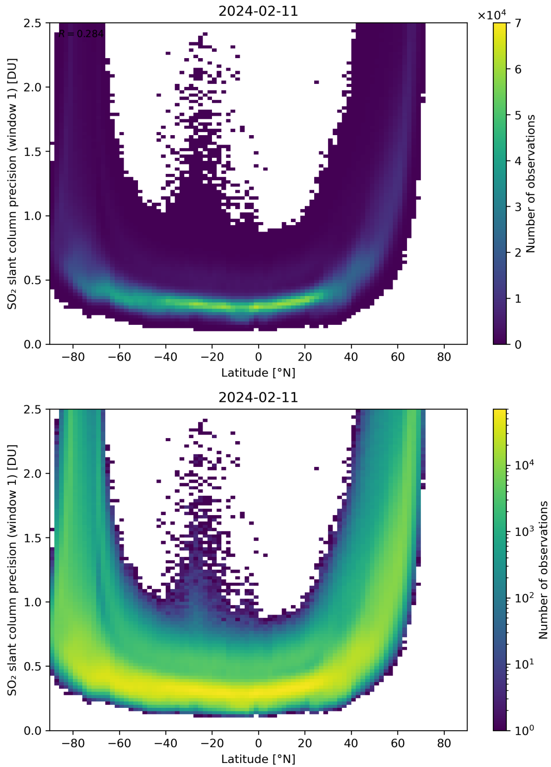
Figure 150: Scatter density plot of “Latitude” against “SO 2 slant column precision (window 1)” for 2024-02-11 to 2024-02-12.
