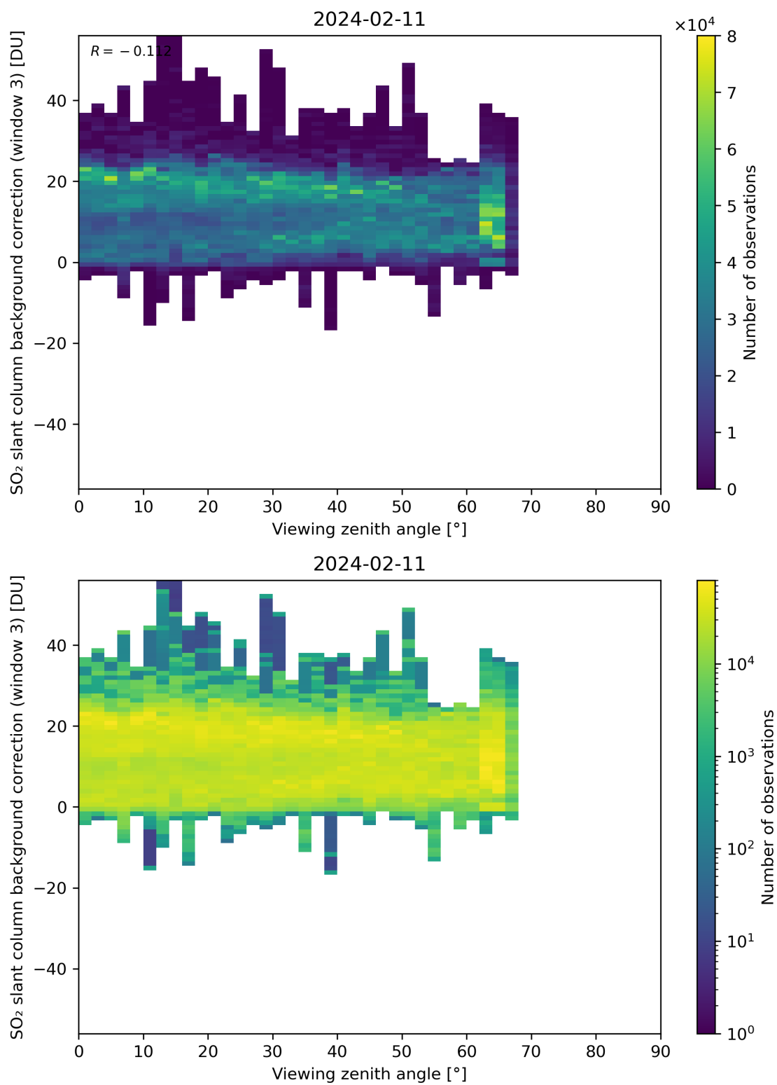
Figure 310: Scatter density plot of “Viewing zenith angle” against “SO 2 slant column background correction (window 3)” for 2024-02-11 to 2024-02-12.
