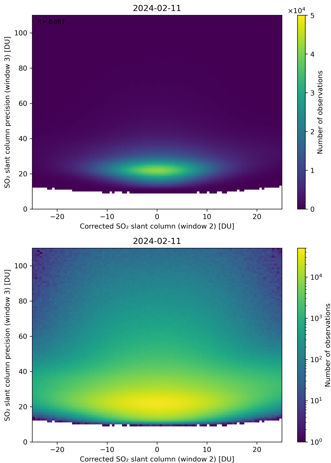
Figure 202: Scatter density plot of “Corrected SO 2 slant column (window 2)” against “SO 2 slant column precision (window 3)” for 2024-02-11 to 2024-02-12.
