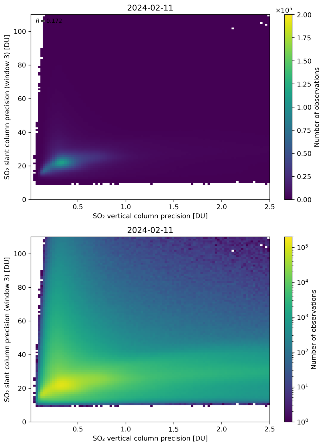
Figure 293: Scatter density plot of “SO 2 vertical column precision” against “SO 2 slant column precision (window 3)” for 2024-02-11 to 2024-02-12.
