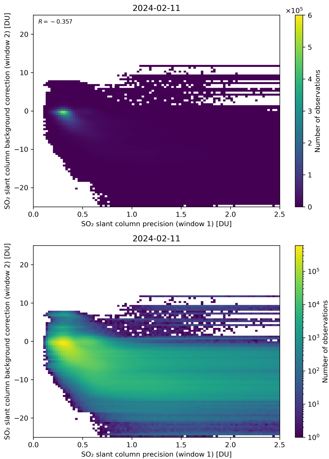
Figure 219: Scatter density plot of “SO 2 slant column precision (window 1)” against “SO 2 slant column background correction (window 2)” for 2024-02-11 to 2024-02-12.
