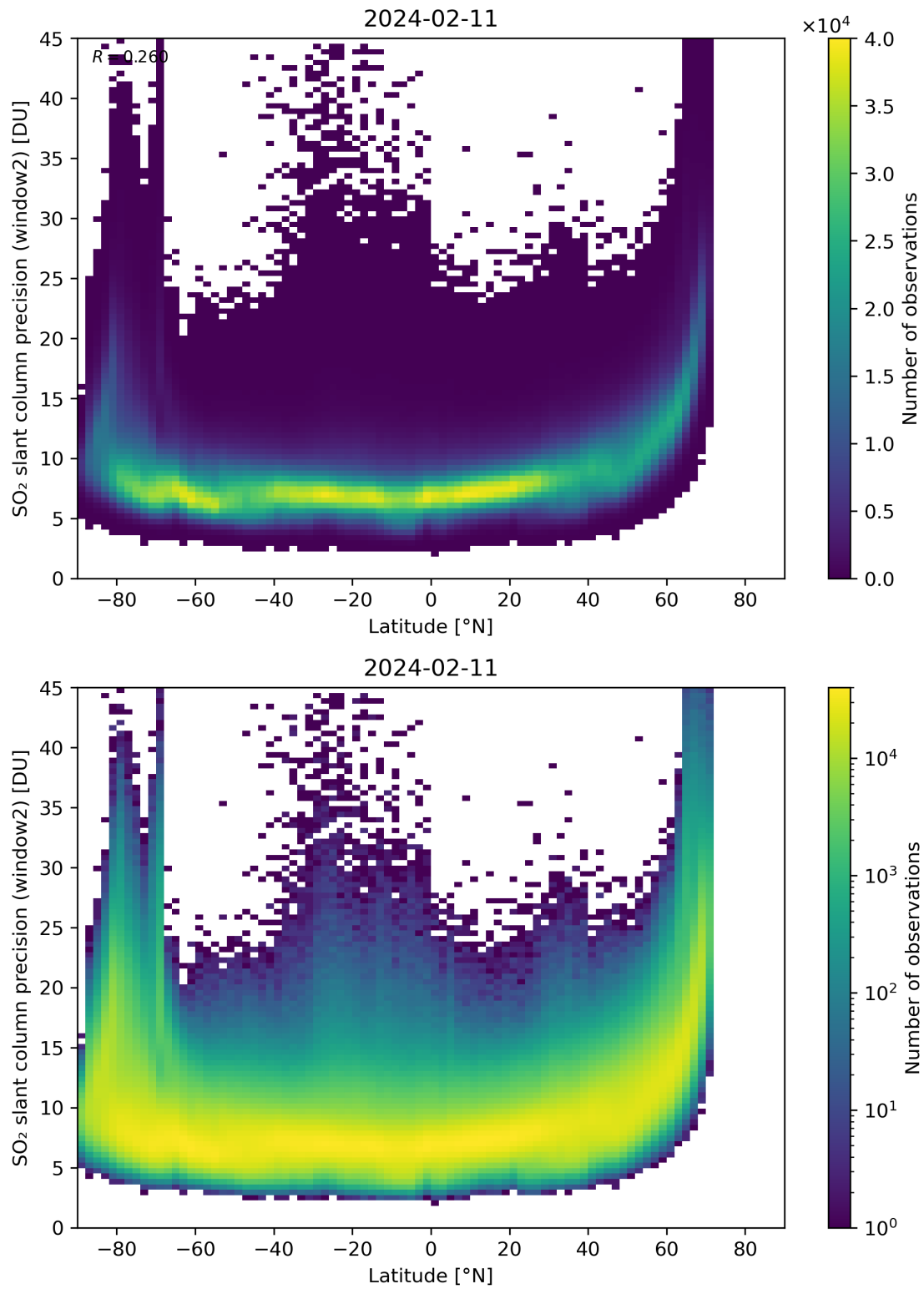
Figure 151: Scatter density plot of “Latitude” against “SO 2 slant column precision (window2)” for 2024-02-11 to 2024-02-12.
