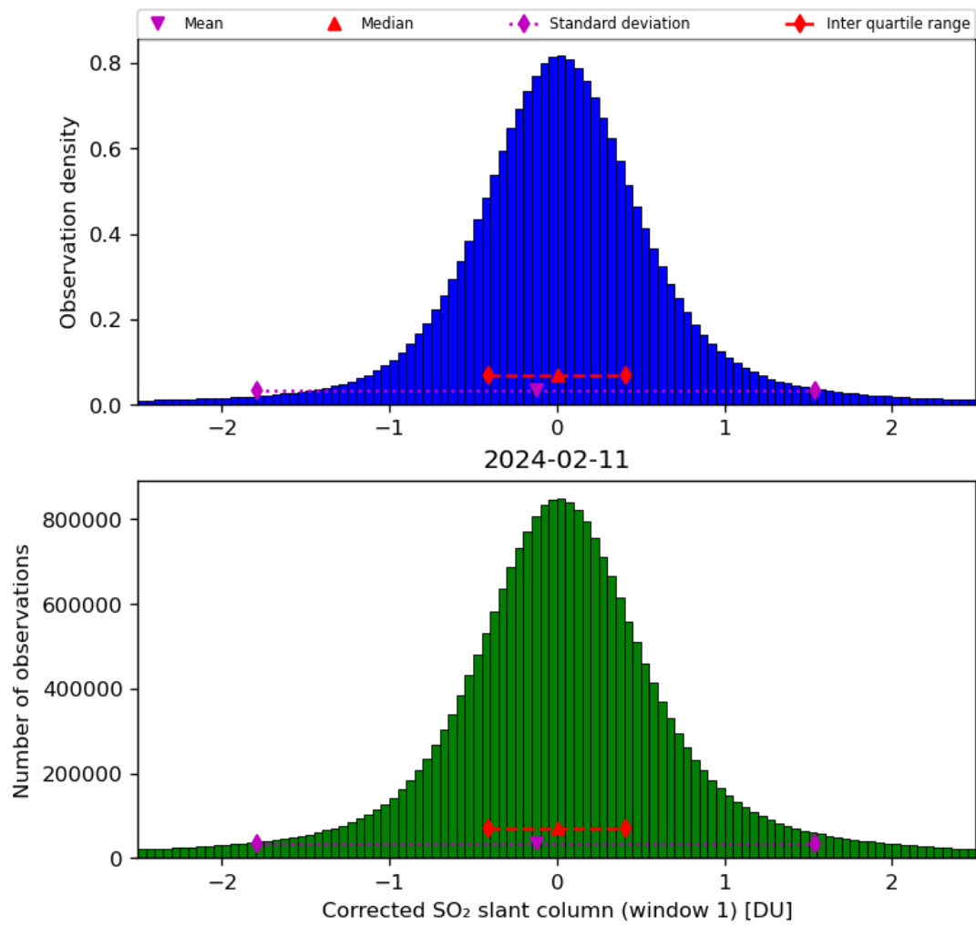
Figure 58: Histogram of “Corrected SO 2 slant column (window 1)” for 2024-02-11 to 2024-02-12
