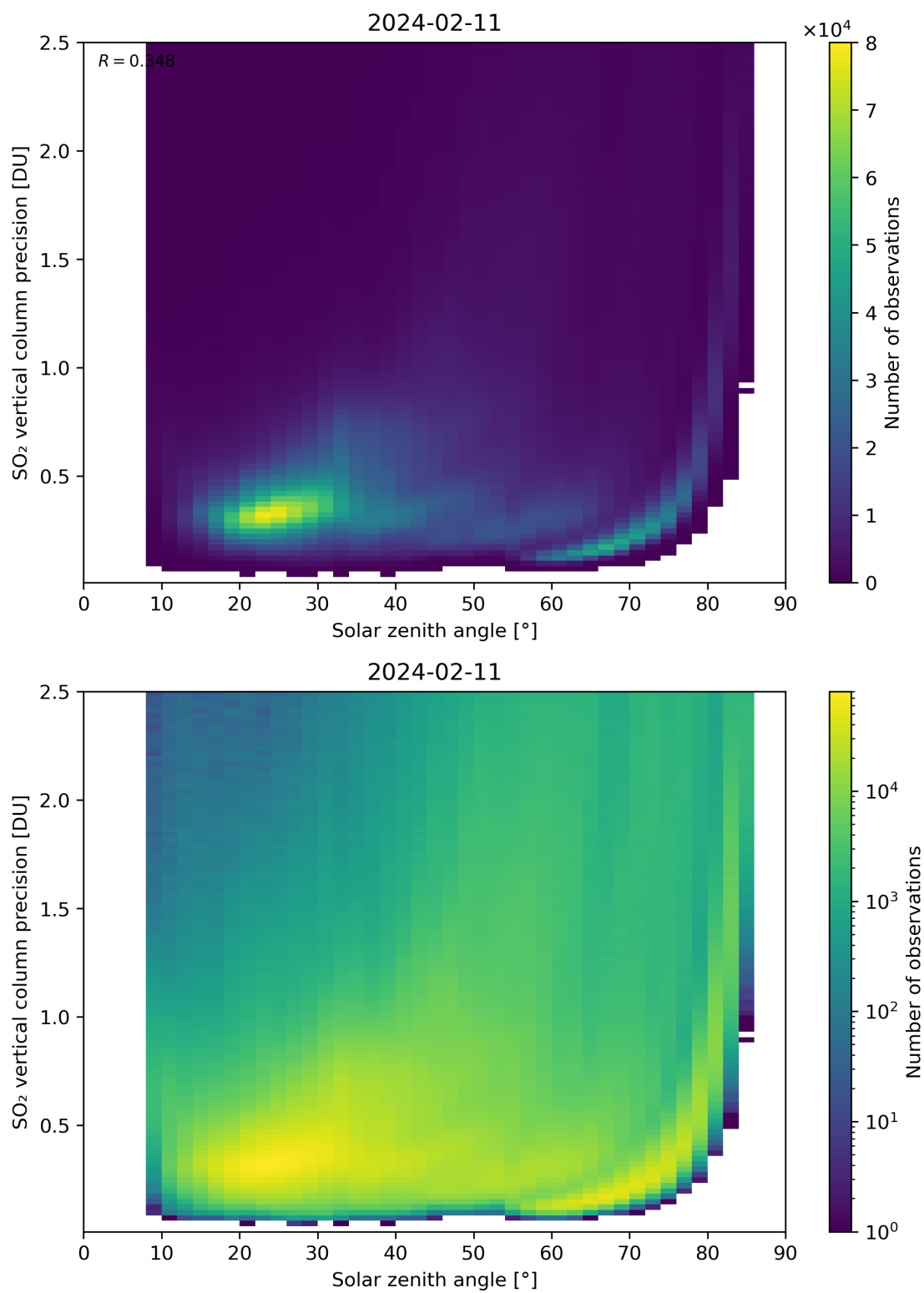
Figure 177: Scatter density plot of “Solar zenith angle” against “SO 2 vertical column precision” for 2024-02-11 to 2024-02-12.
