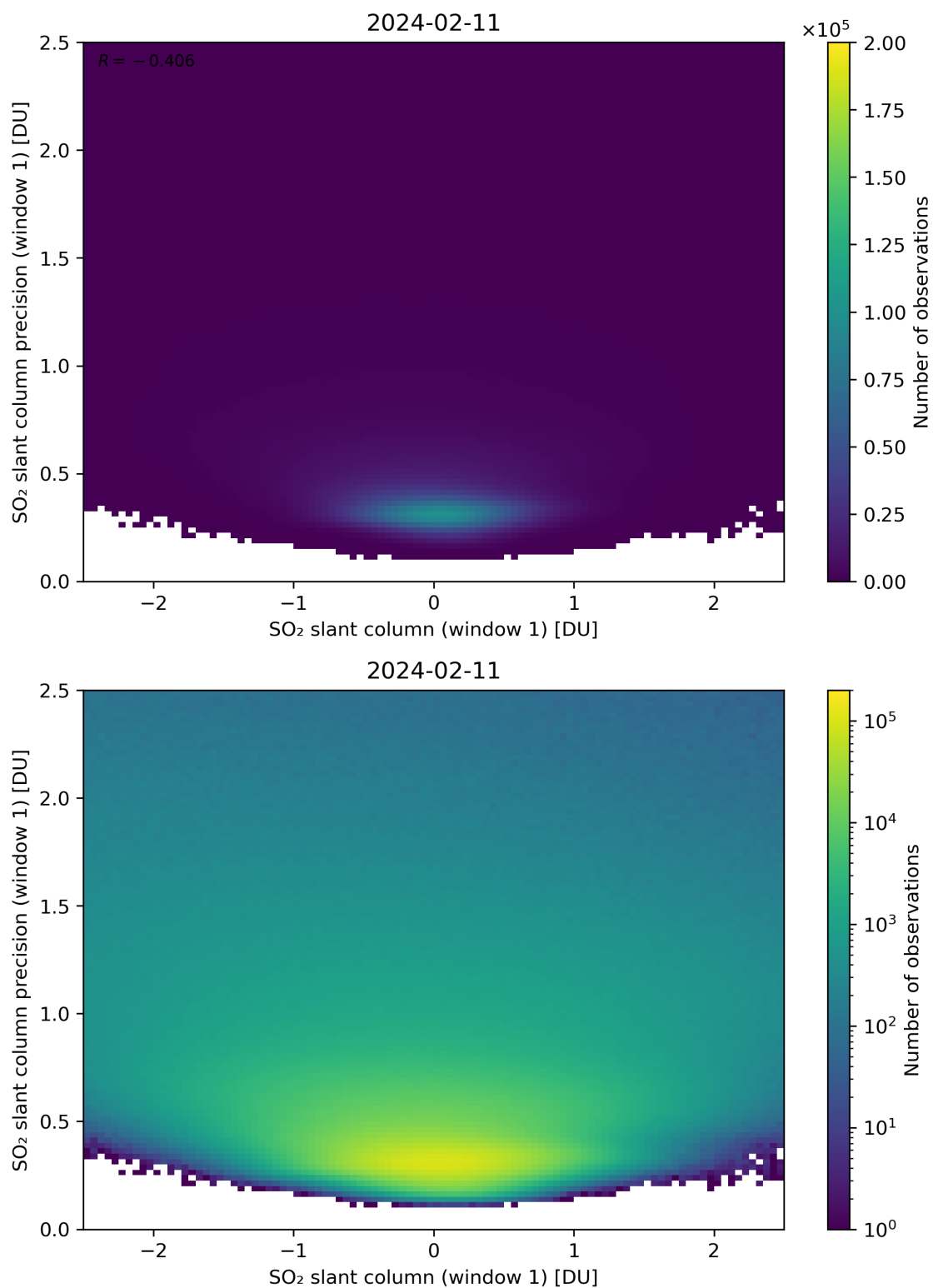
Figure 235: Scatter density plot of “SO 2 slant column (window 1)” against “SO 2 slant column precision (window 1)” for 2024-02-11 to 2024-02-12.
