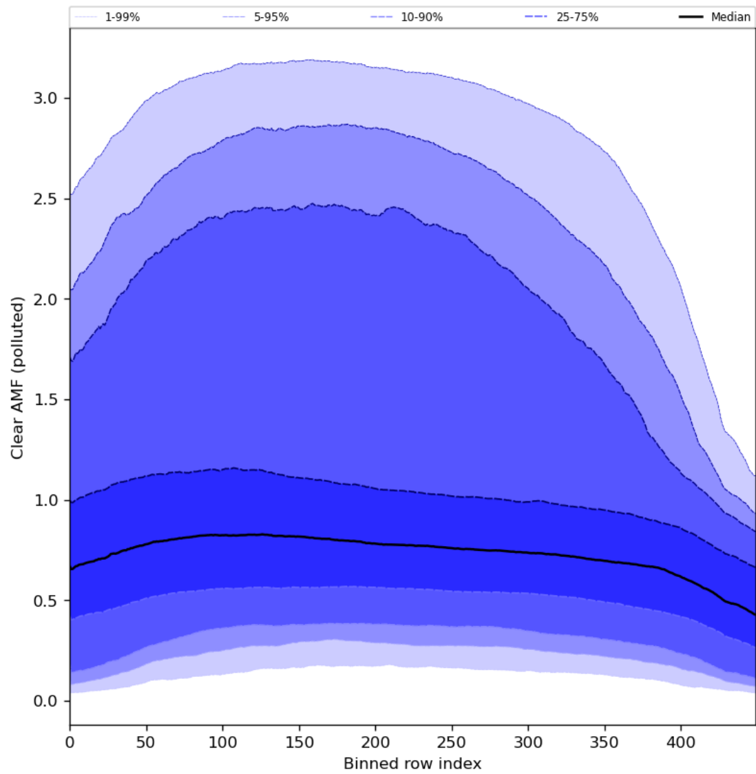
Figure 96: Along track statistics of “Clear AMF (polluted)” for 2024-02-11 to 2024-02-12
