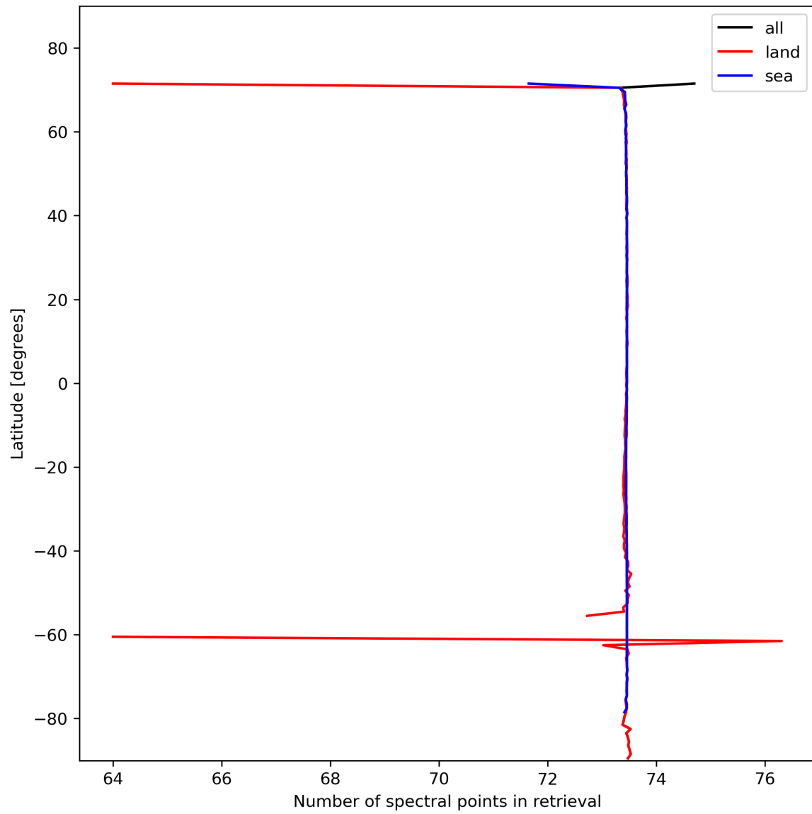
Figure 51: Zonal average of “Number of spectral points in retrieval” for 2024-02-11 to 2024-02-12.
