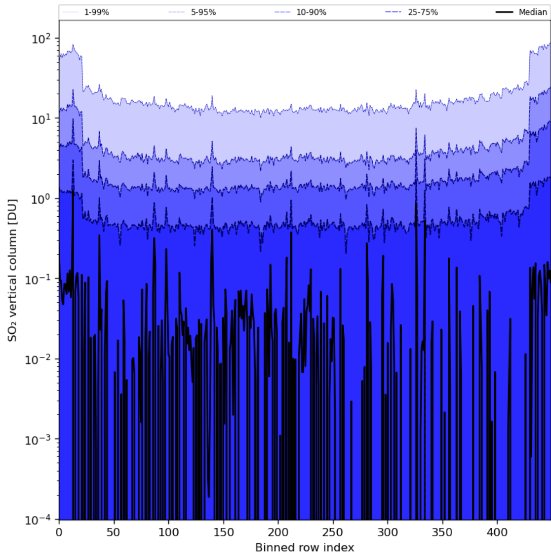
Figure 76: Along track statistics of “SO 2 vertical column” for 2024-02-11 to 2024-02-12
