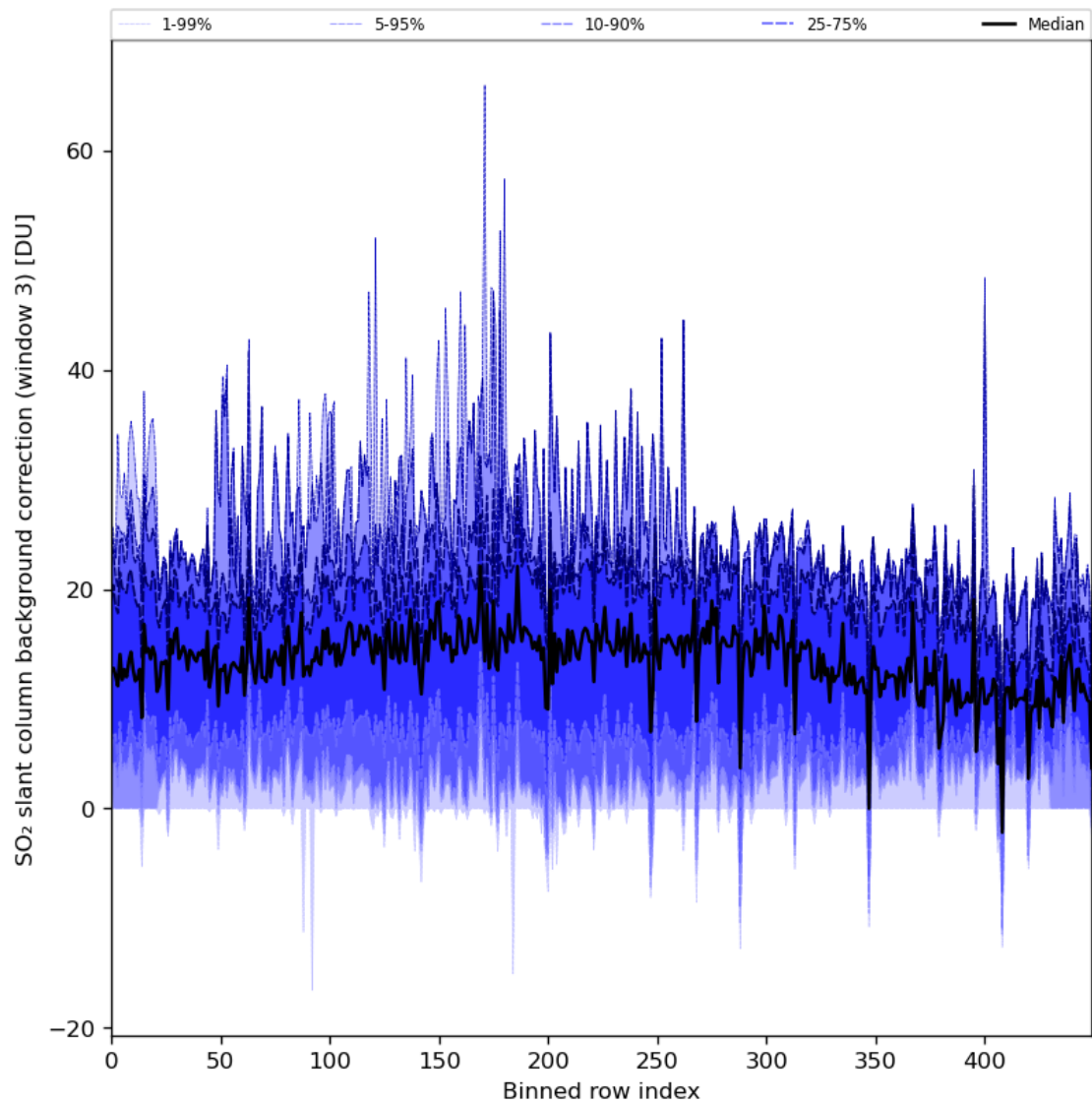
Figure 90: Along track statistics of “SO 2 slant column background correction (window 3)” for 2024-02-11 to 2024-02-12
