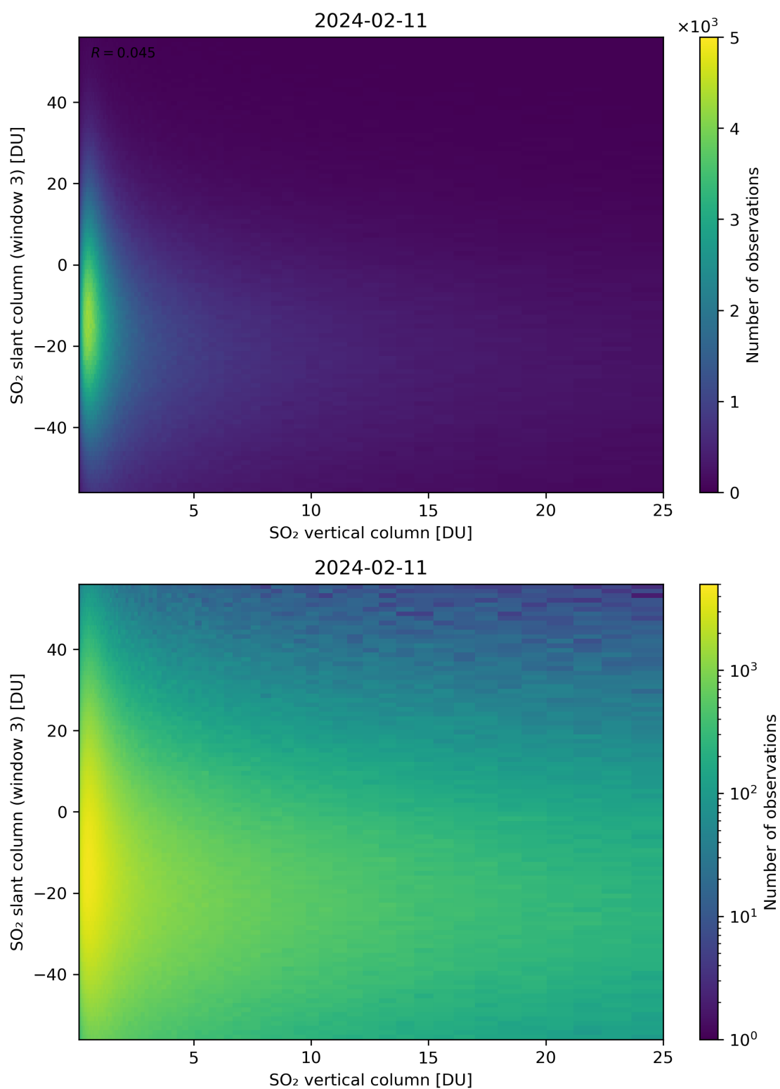
Figure 303: Scatter density plot of “SO 2 vertical column” against “SO 2 slant column (window 3)” for 2024-02-11 to 2024-02-12.
