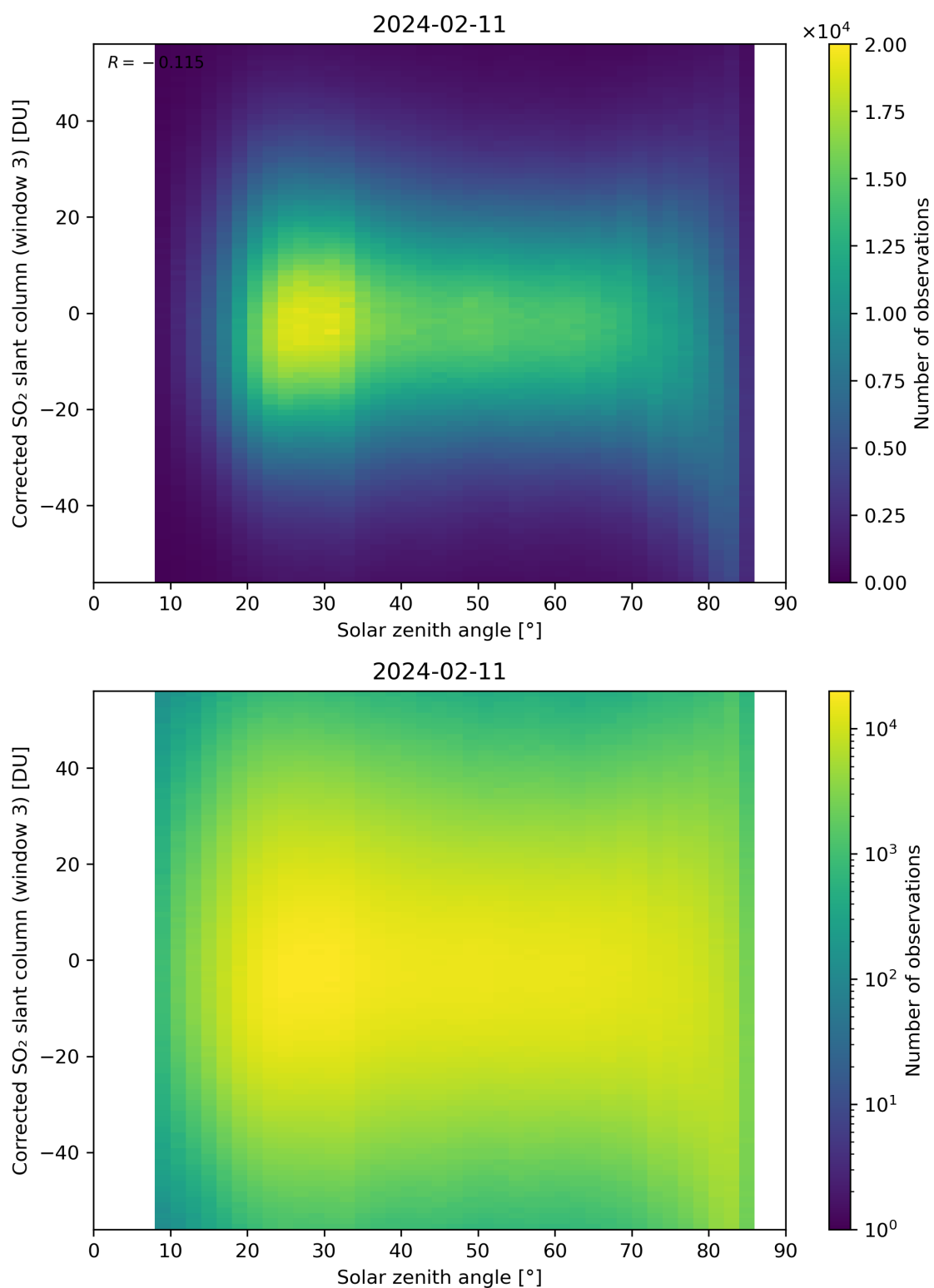
Figure 168: Scatter density plot of “Solar zenith angle” against “Corrected SO 2 slant column (window 3)” for 2024-02-11 to 2024-02-12.
