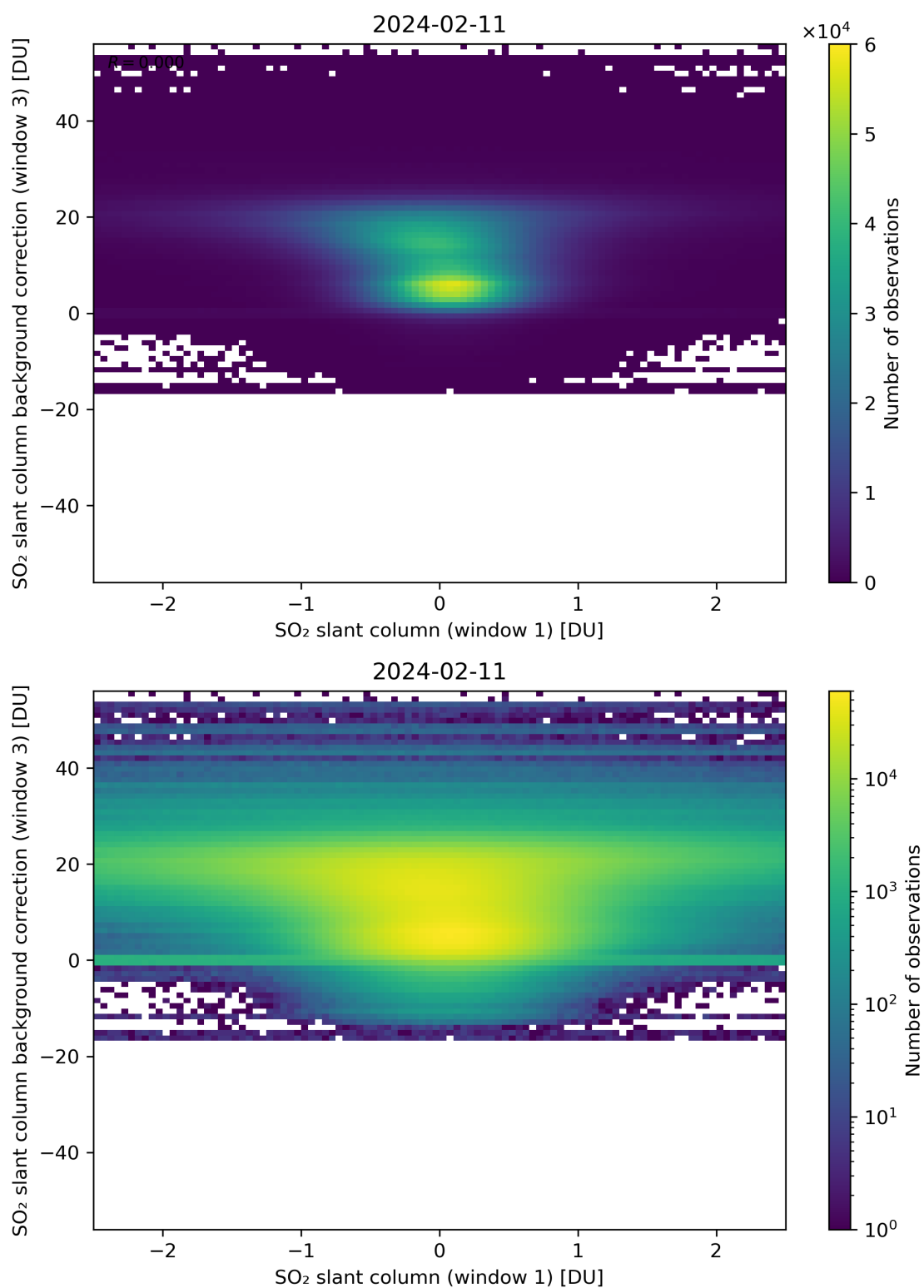
Figure 214: Scatter density plot of “SO 2 slant column (window 1)” against “SO 2 slant column background correction (window 3)” for 2024-02-11 to 2024-02-12.
