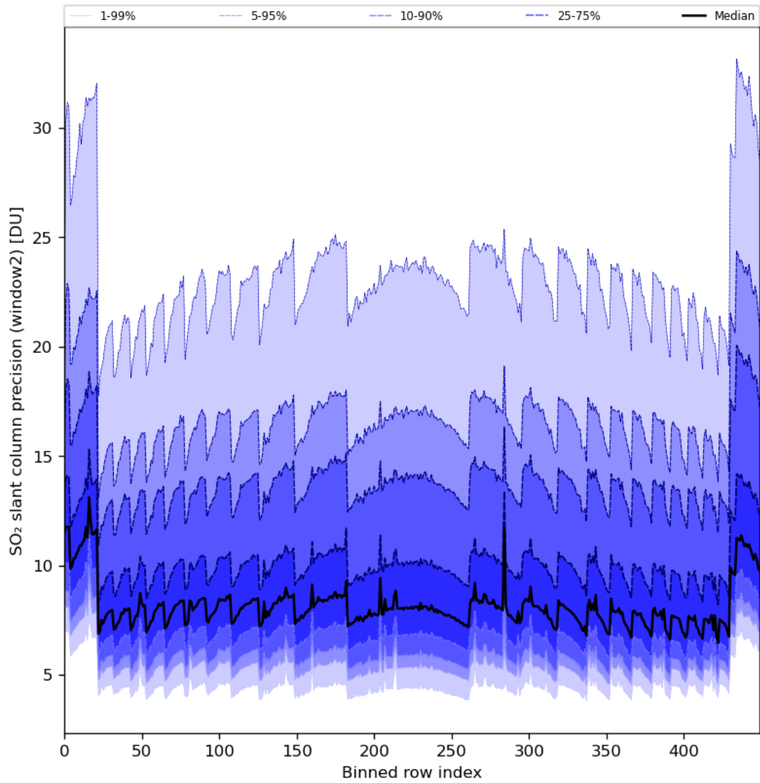
Figure 84: Along track statistics of “SO 2 slant column precision (window2)” for 2024-02-11 to 2024-02-12
