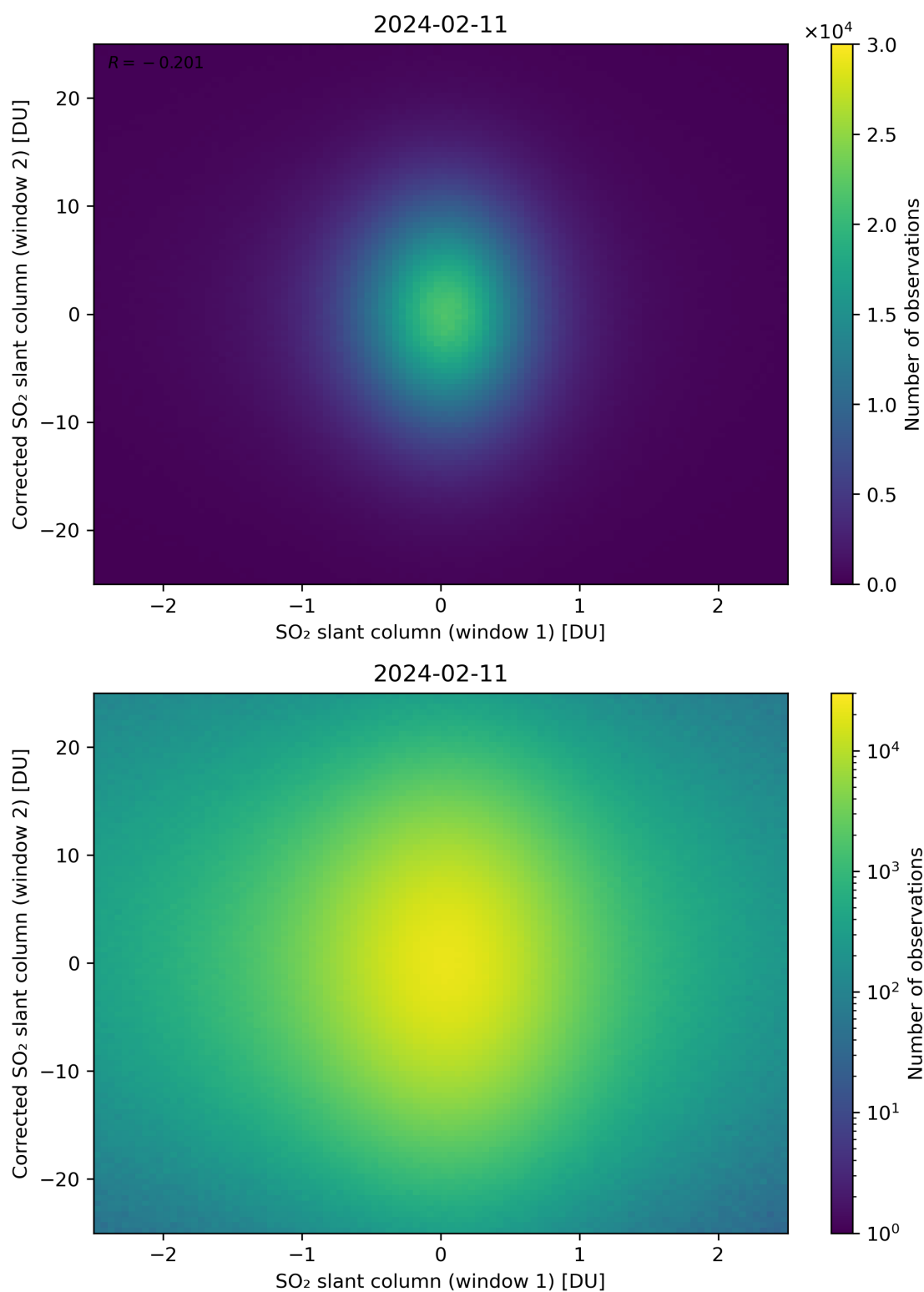
Figure 233: Scatter density plot of “SO 2 slant column (window 1)” against “Corrected SO 2 slant column (window 2)” for 2024-02-11 to 2024-02-12.
