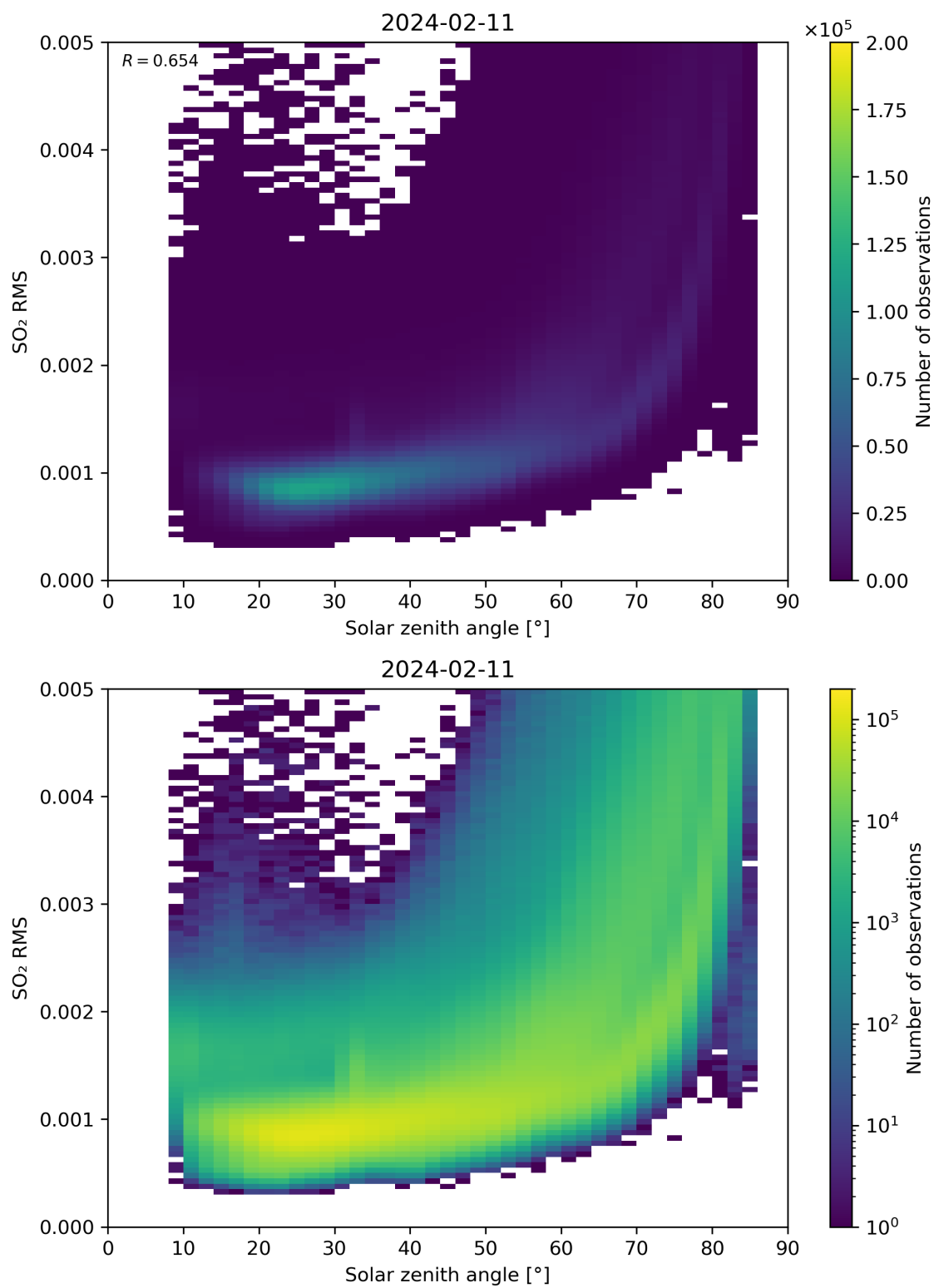
Figure 163: Scatter density plot of “Solar zenith angle” against “SO 2 RMS” for 2024-02-11 to 2024-02-12.
