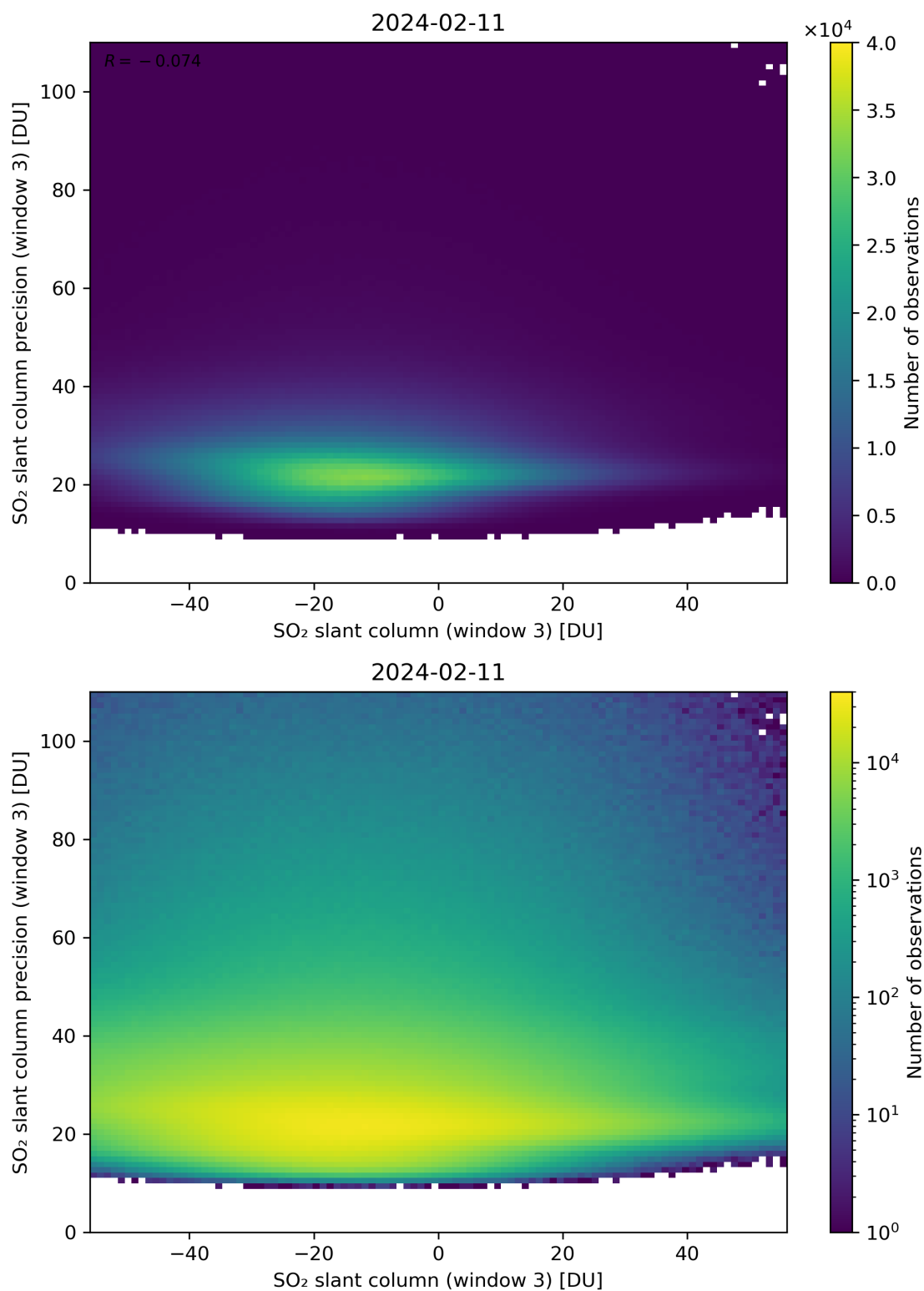
Figure 267: Scatter density plot of “SO 2 slant column (window 3)” against “SO 2 slant column precision (window 3)” for 2024-02-11 to 2024-02-12.
