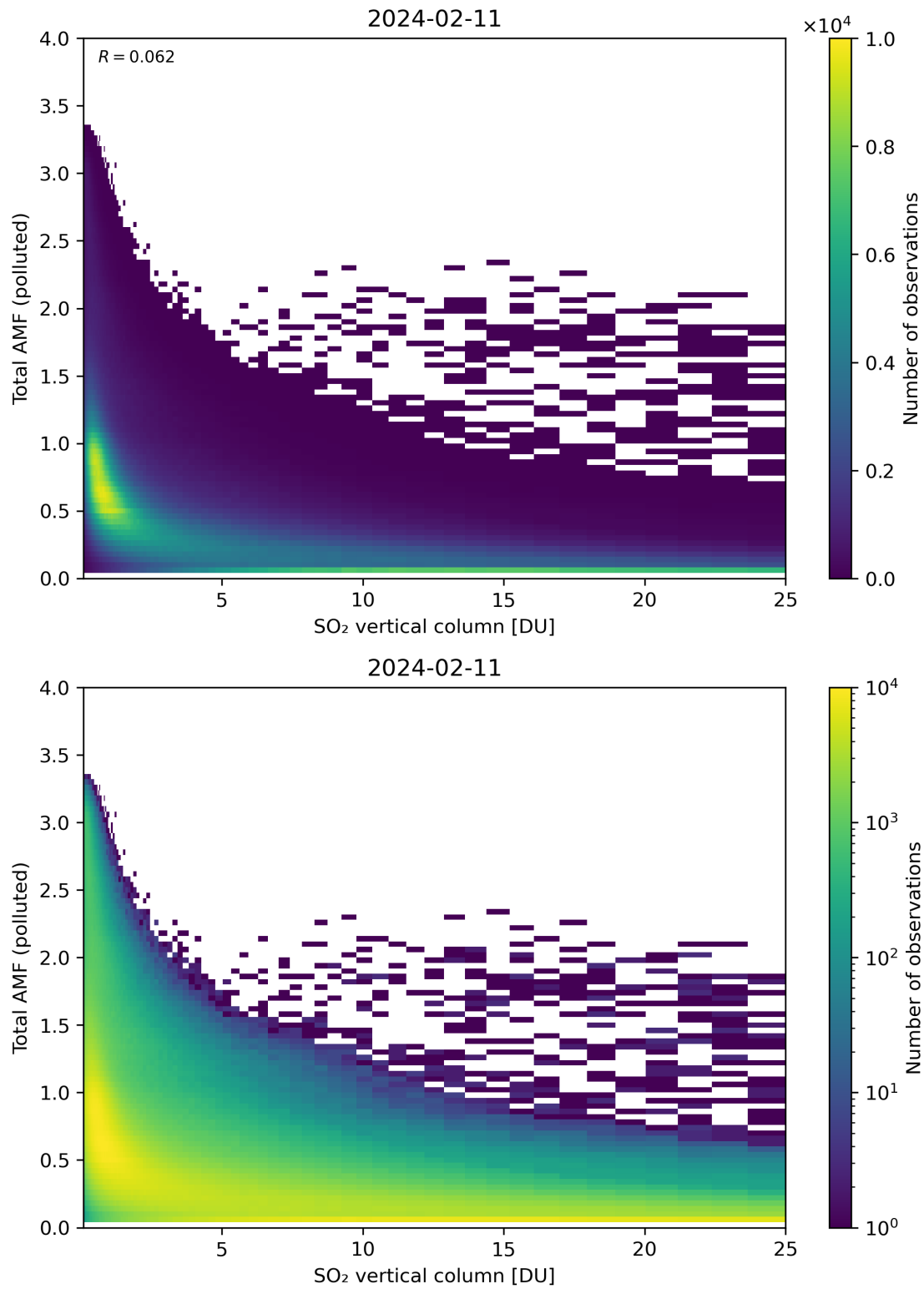
Figure 305: Scatter density plot of “SO 2 vertical column” against “Total AMF (polluted)” for 2024-02-11 to 2024-02-12.
