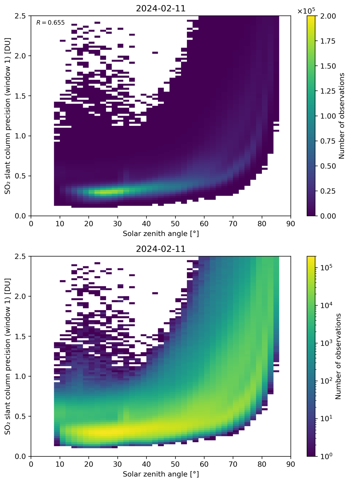
Figure 170: Scatter density plot of “Solar zenith angle” against “SO 2 slant column precision (window 1)” for 2024-02-11 to 2024-02-12.
