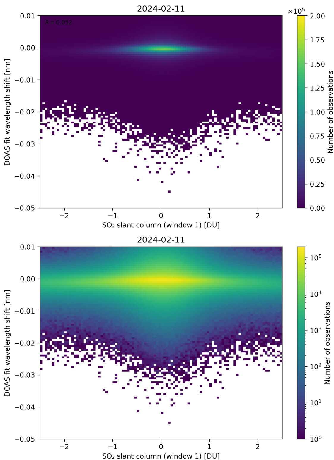
Figure 215: Scatter density plot of “SO 2 slant column (window 1)” against “DOAS fit wavelength shift” for 2024-02-11 to 2024-02-12.
