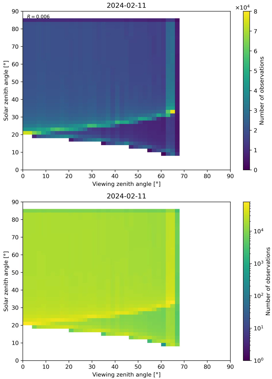
Figure 315: Scatter density plot of “Viewing zenith angle” against “Solar zenith angle” for 2024-02-11 to 2024-02-12.
