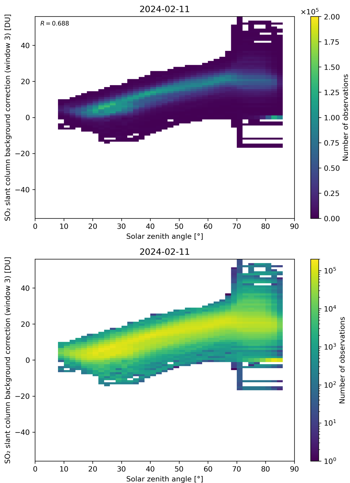
Figure 160: Scatter density plot of “Solar zenith angle” against “SO 2 slant column background correction (window 3)” for 2024-02-11 to 2024-02-12.
