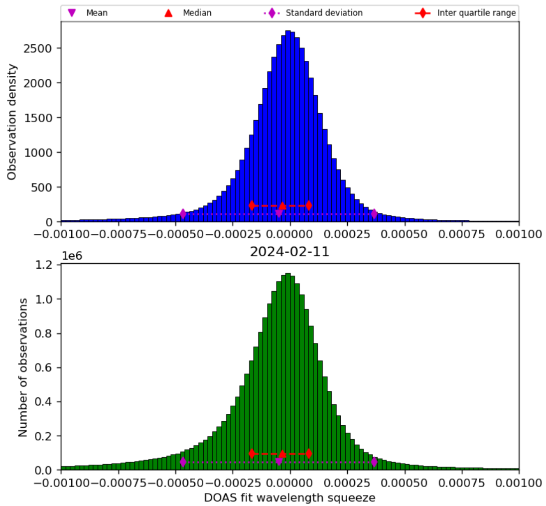
Figure 69: Histogram of “DOAS fit wavelength squeeze” for 2024-02-11 to 2024-02-12
