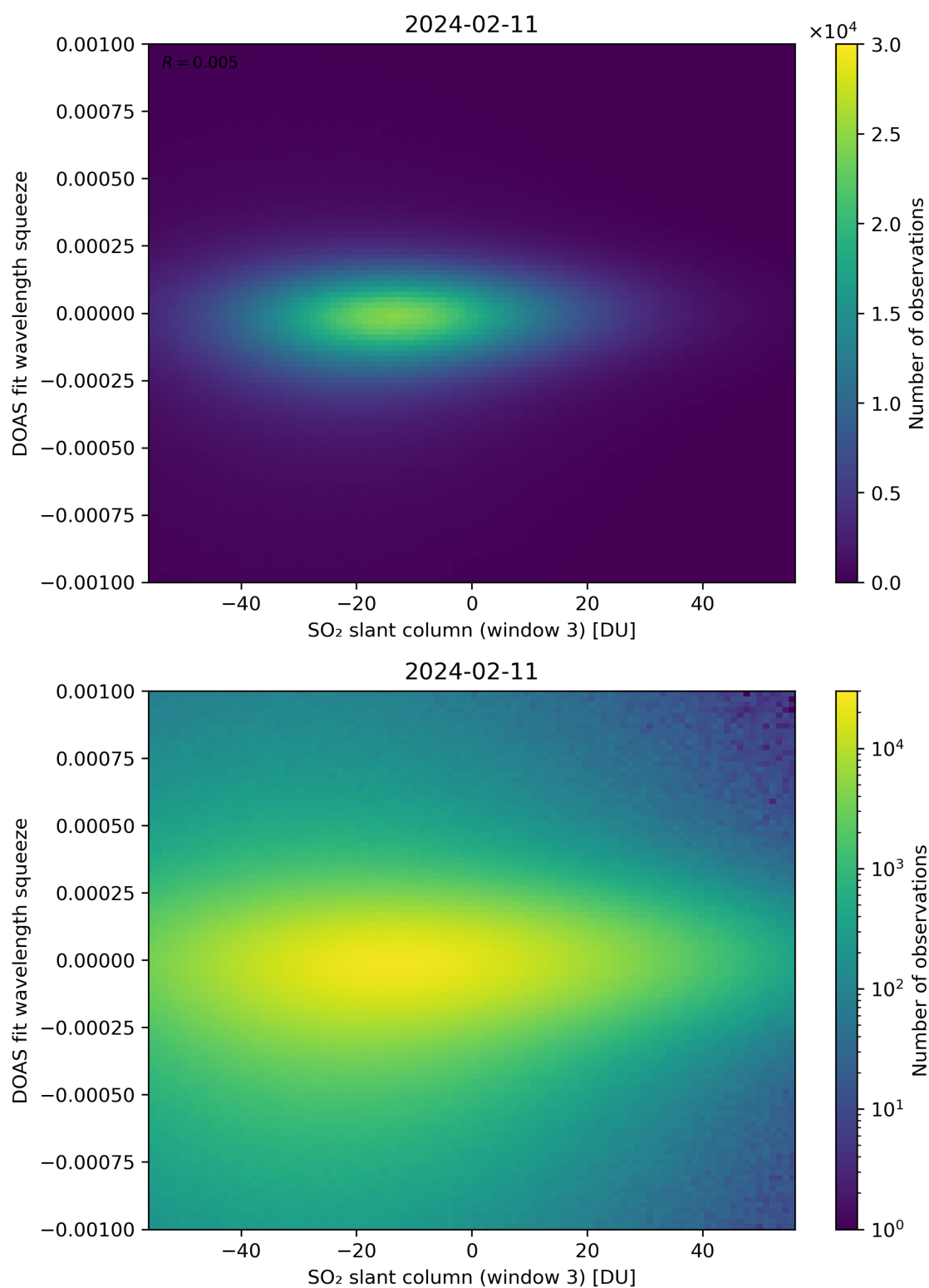
Figure 255: Scatter density plot of “SO 2 slant column (window 3)” against “DOAS fit wavelength squeeze” for 2024-02-11 to 2024-02-12.
