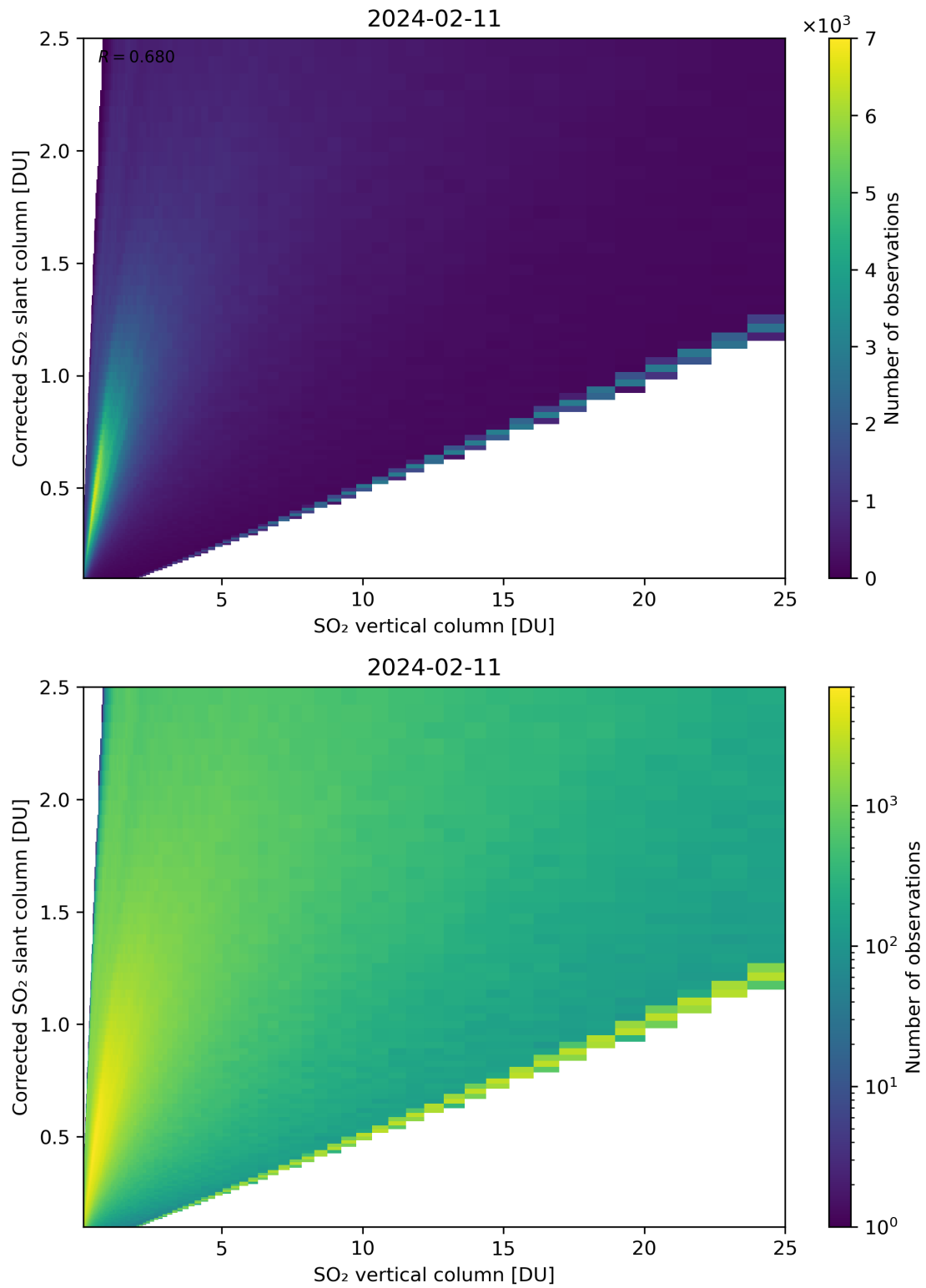
Figure 297: Scatter density plot of “SO 2 vertical column” against “Corrected SO 2 slant column” for 2024-02-11 to 2024-02-12.
