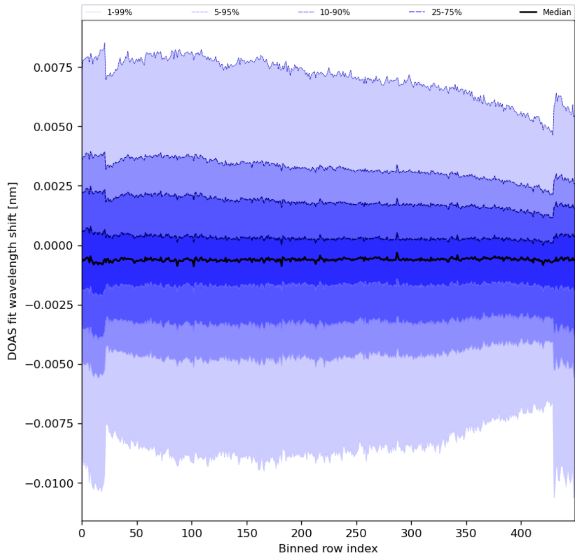
Figure 91: Along track statistics of “DOAS fit wavelength shift” for 2024-02-11 to 2024-02-12
