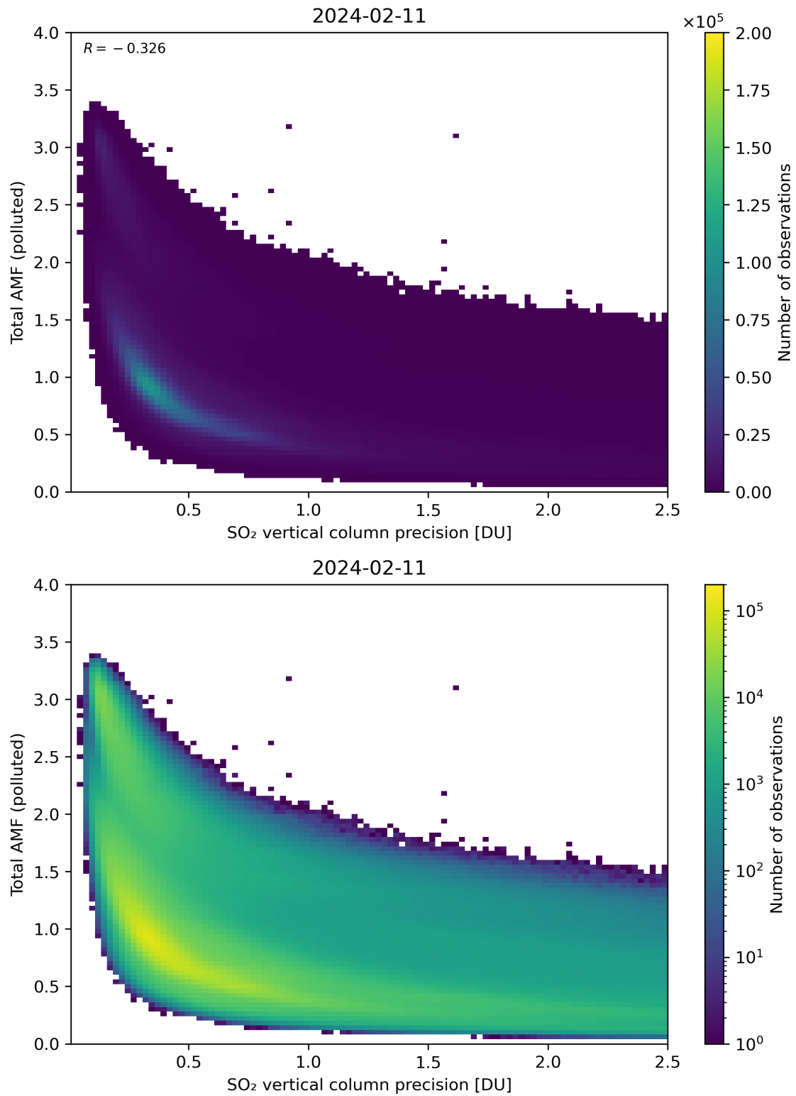
Figure 294: Scatter density plot of “SO 2 vertical column precision” against “Total AMF (polluted)” for 2024-02-11 to 2024-02-12.
