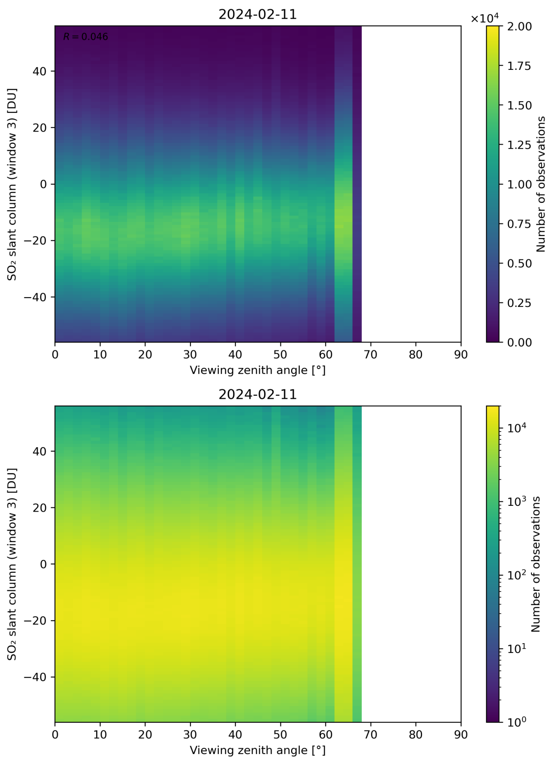
Figure 323: Scatter density plot of “Viewing zenith angle” against “SO 2 slant column (window 3)” for 2024-02-11 to 2024-02-12.
