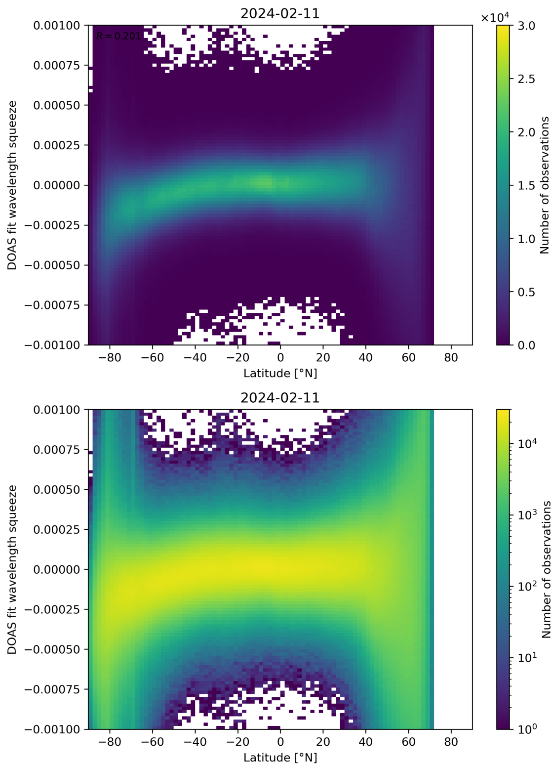
Figure 143: Scatter density plot of “Latitude” against “DOAS fit wavelength squeeze” for 2024-02-11 to 2024-02-12.
