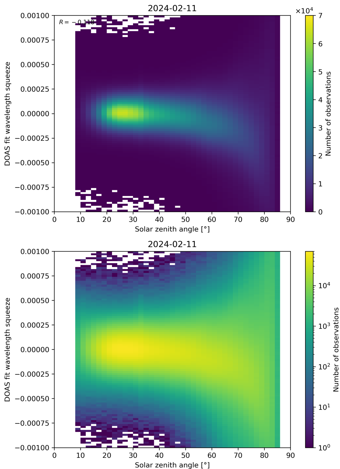
Figure 162: Scatter density plot of “Solar zenith angle” against “DOAS fit wavelength squeeze” for 2024-02-11 to 2024-02-12.
