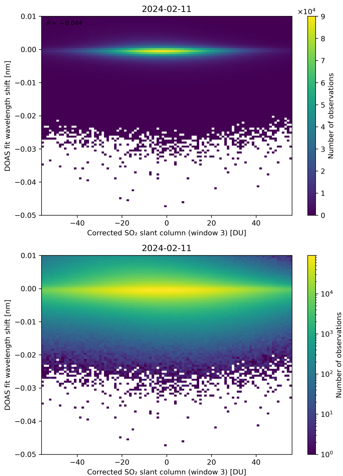
Figure 206: Scatter density plot of “Corrected SO 2 slant column (window 3)” against “DOAS fit wavelength shift” for 2024-02-11 to 2024-02-12.
