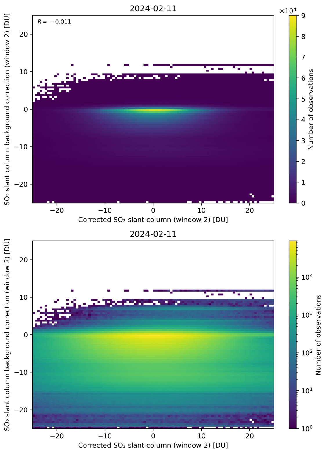
Figure 194: Scatter density plot of “Corrected SO 2 slant column (window 2)” against “SO 2 slant column background correction (window 2)” for 2024-02-11 to 2024-02-12.
