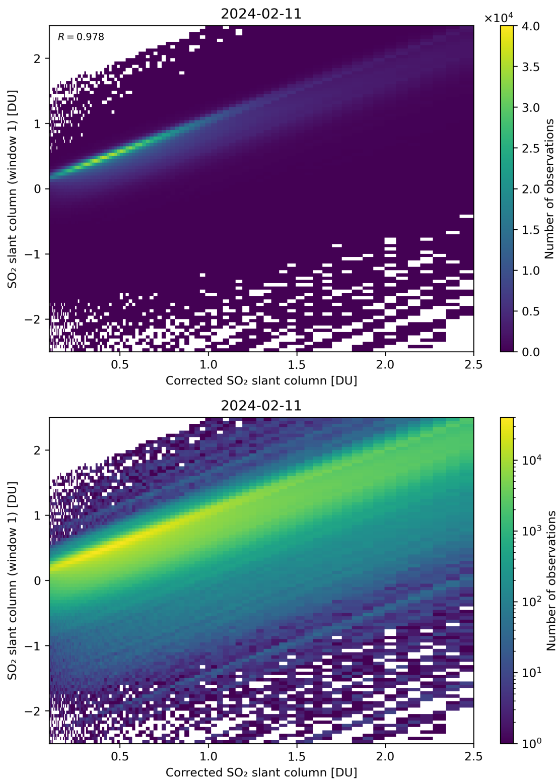
Figure 187: Scatter density plot of “Corrected SO 2 slant column” against “SO 2 slant column (window 1)” for 2024-02-11 to 2024-02-12.
