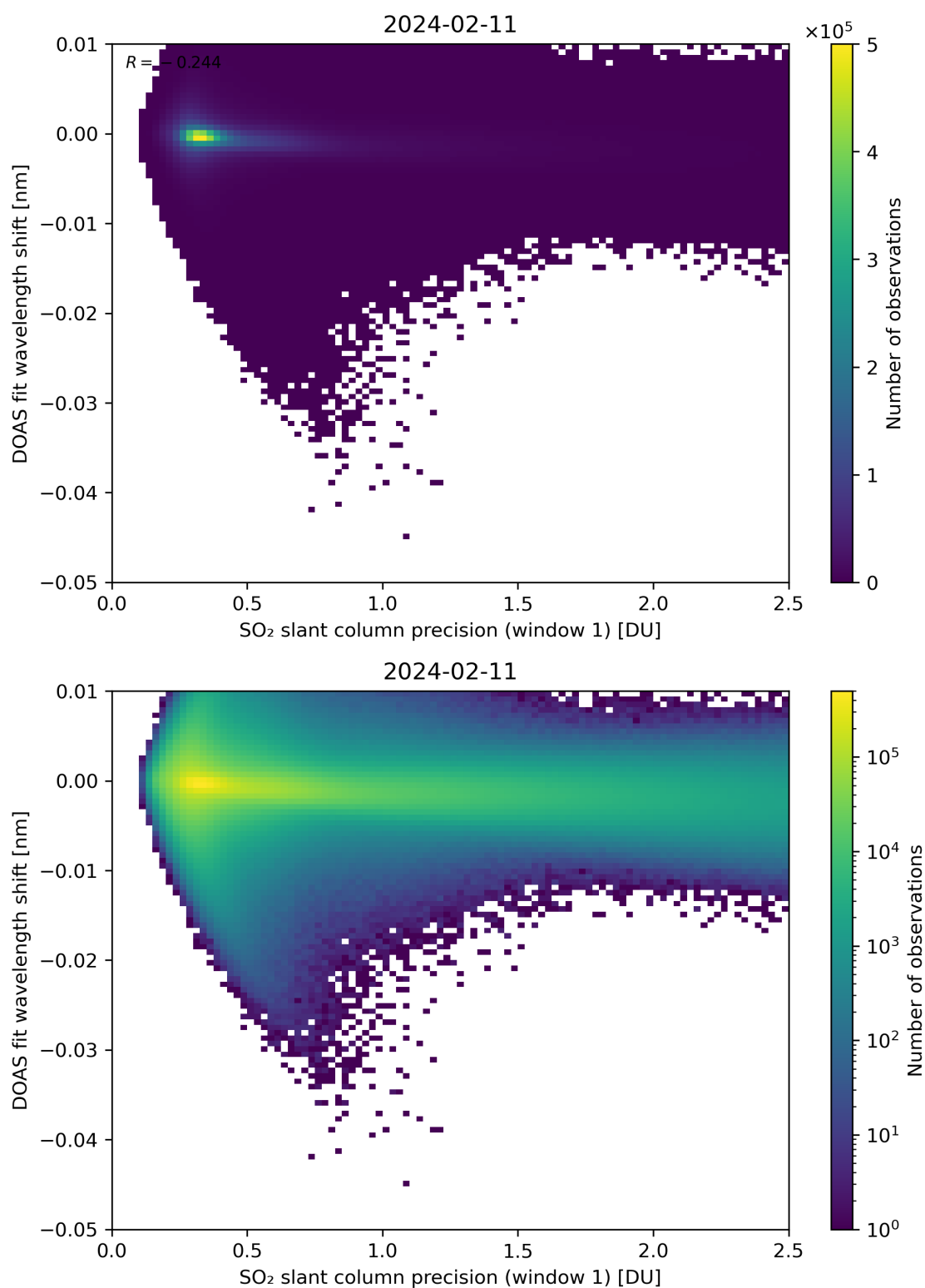
Figure 221: Scatter density plot of “SO 2 slant column precision (window 1)” against “DOAS fit wavelength shift” for 2024-02-11 to 2024-02-12.
