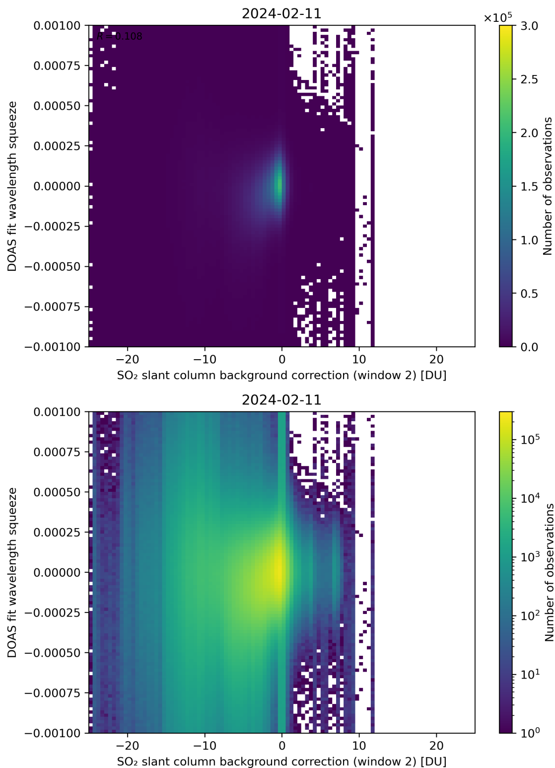
Figure 113: Scatter density plot of “SO 2 slant column background correction (window 2)” against “DOAS fit wavelength squeeze” for 2024-02-11 to 2024-02-12.
