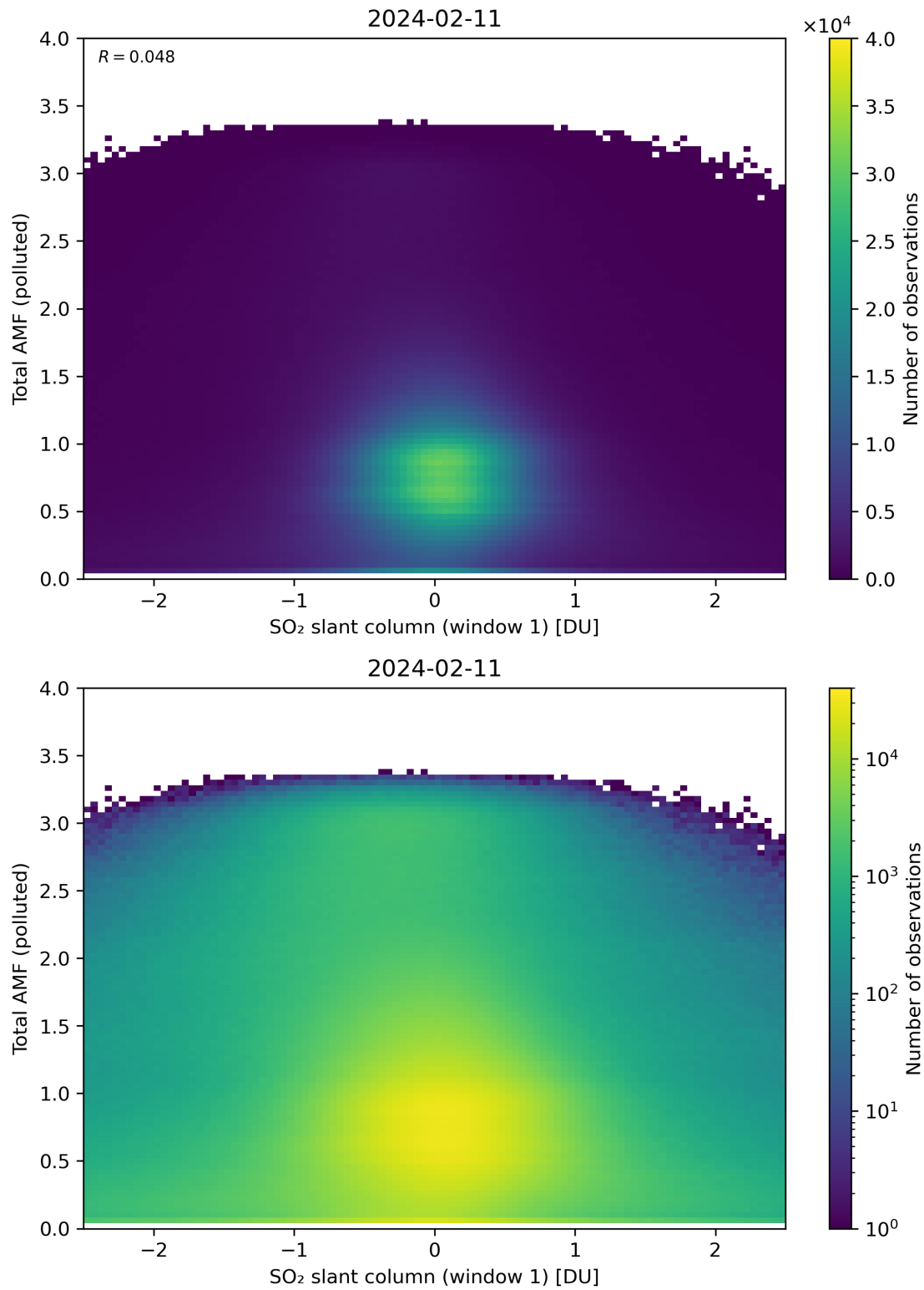
Figure 239: Scatter density plot of “SO 2 slant column (window 1)” against “Total AMF (polluted)” for 2024-02-11 to 2024-02-12.
