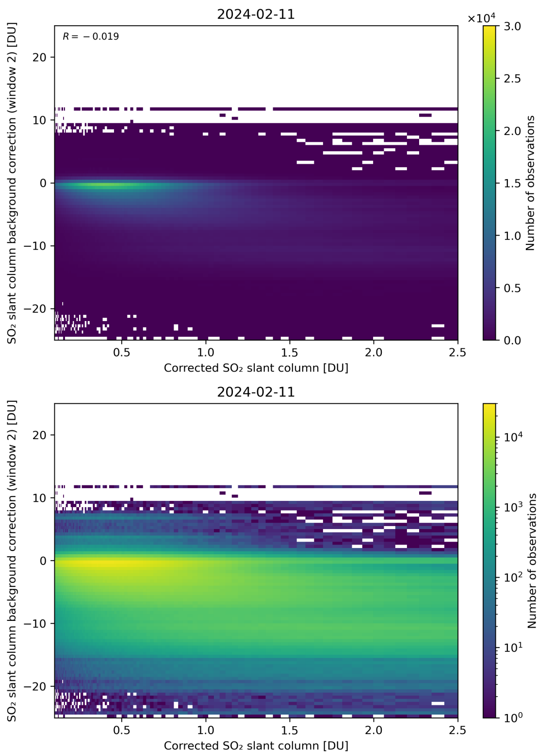
Figure 179: Scatter density plot of “Corrected SO 2 slant column” against “SO 2 slant column background correction (window 2)” for 2024-02-11 to 2024-02-12.
