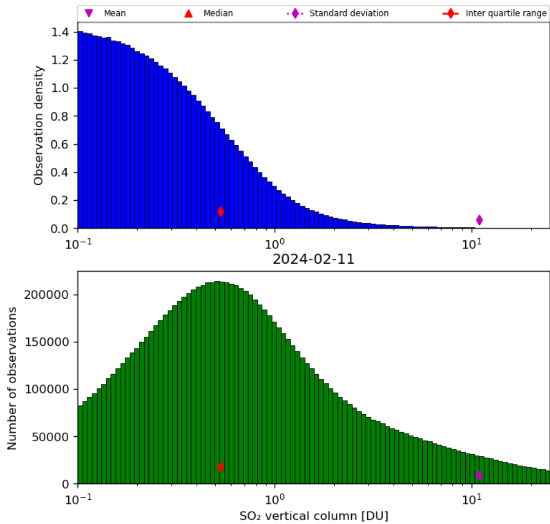
Figure 53: Histogram of “SO 2 vertical column” for 2024-02-11 to 2024-02-12
