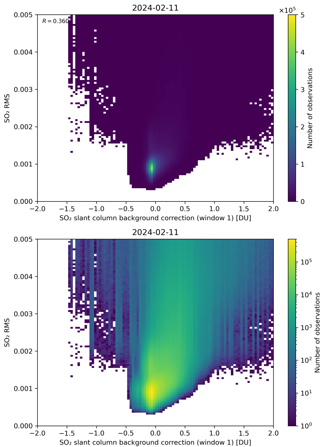
Figure 102: Scatter density plot of “SO 2 slant column background correction (window 1)” against “SO 2 RMS” for 2024-02-11 to 2024-02-12.
