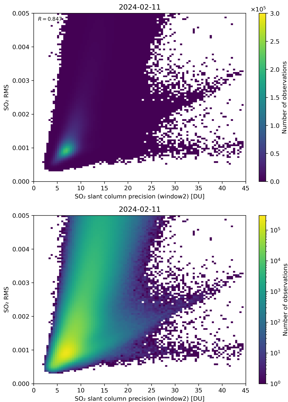
Figure 245: Scatter density plot of “SO 2 slant column precision (window2)” against “SO 2 RMS” for 2024-02-11 to 2024-02-12.
