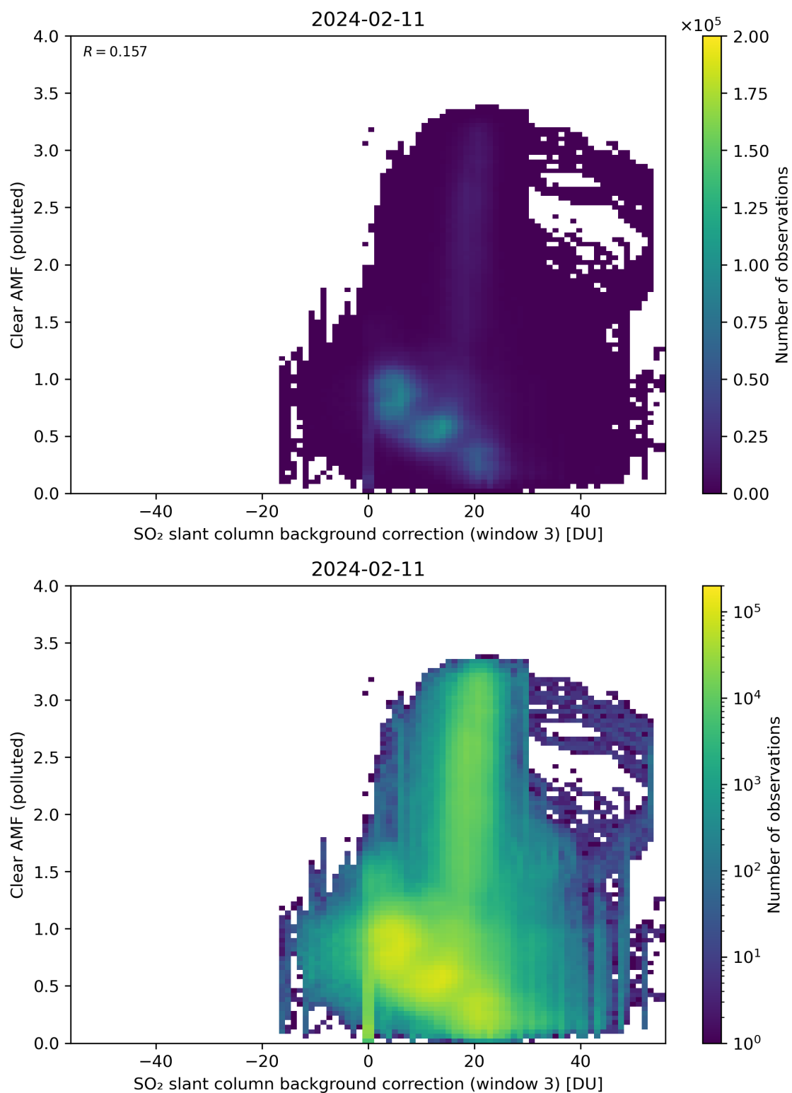
Figure 124: Scatter density plot of “SO 2 slant column background correction (window 3)” against “Clear AMF (polluted)” for 2024-02-11 to 2024-02-12.
