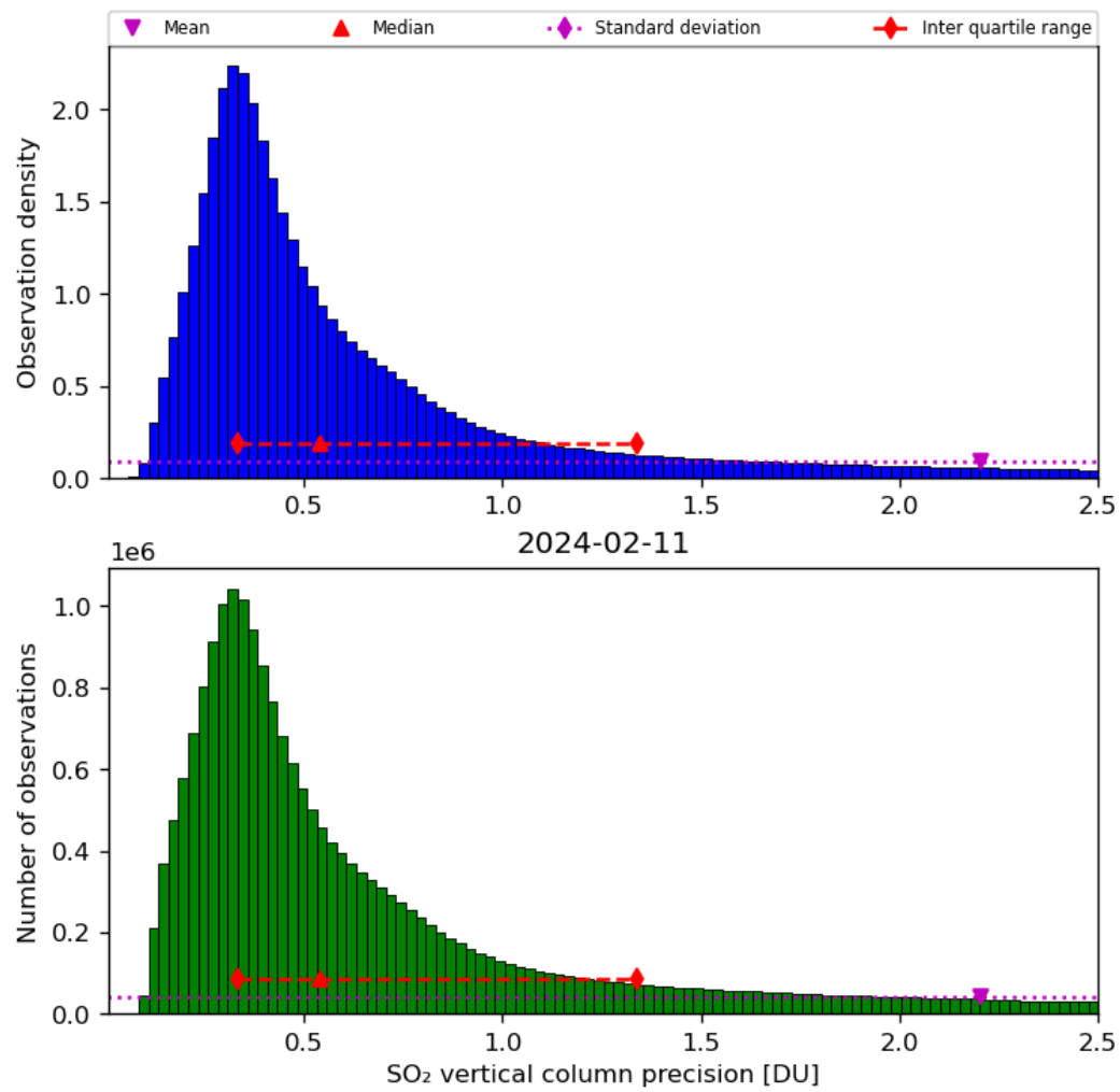
Figure 54: Histogram of “SO 2 vertical column precision” for 2024-02-11 to 2024-02-12
