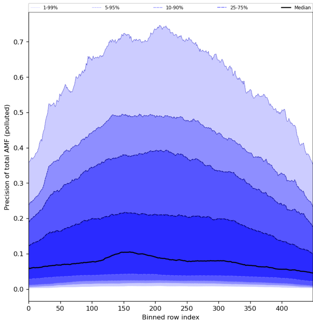
Figure 95: Along track statistics of “Precision of total AMF (polluted)” for 2024-02-11 to 2024-02-12
