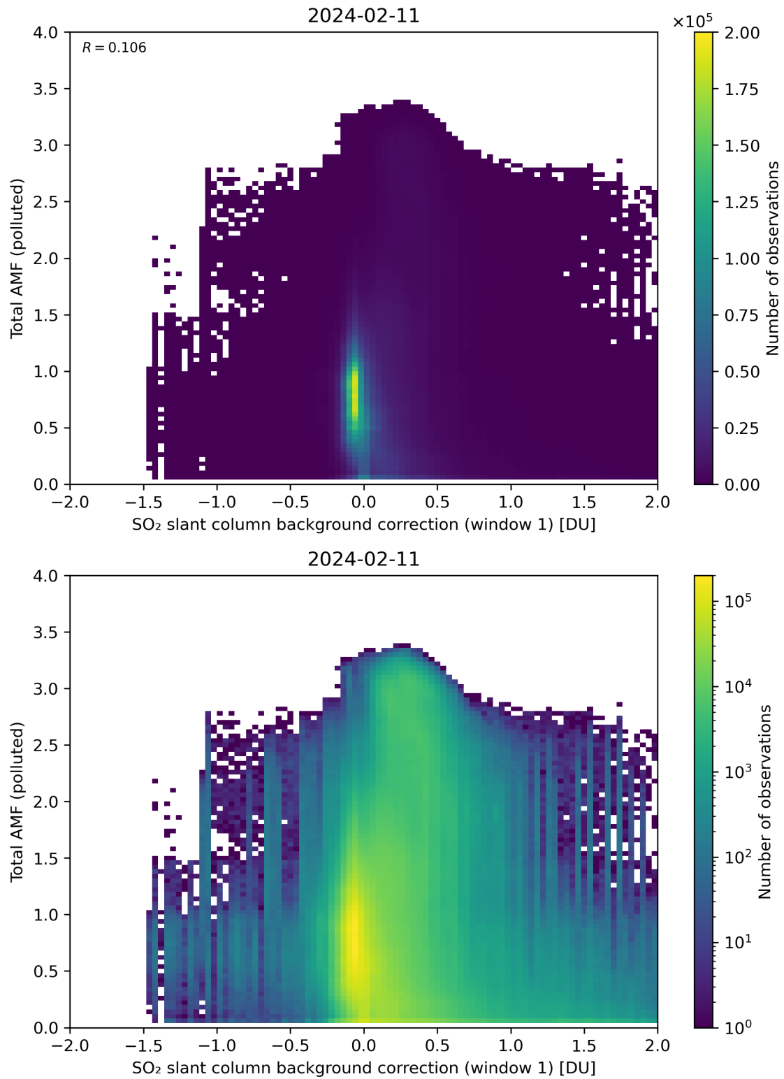
Figure 109: Scatter density plot of “SO 2 slant column background correction (window 1)” against “Total AMF (polluted)” for 2024-02-11 to 2024-02-12.
