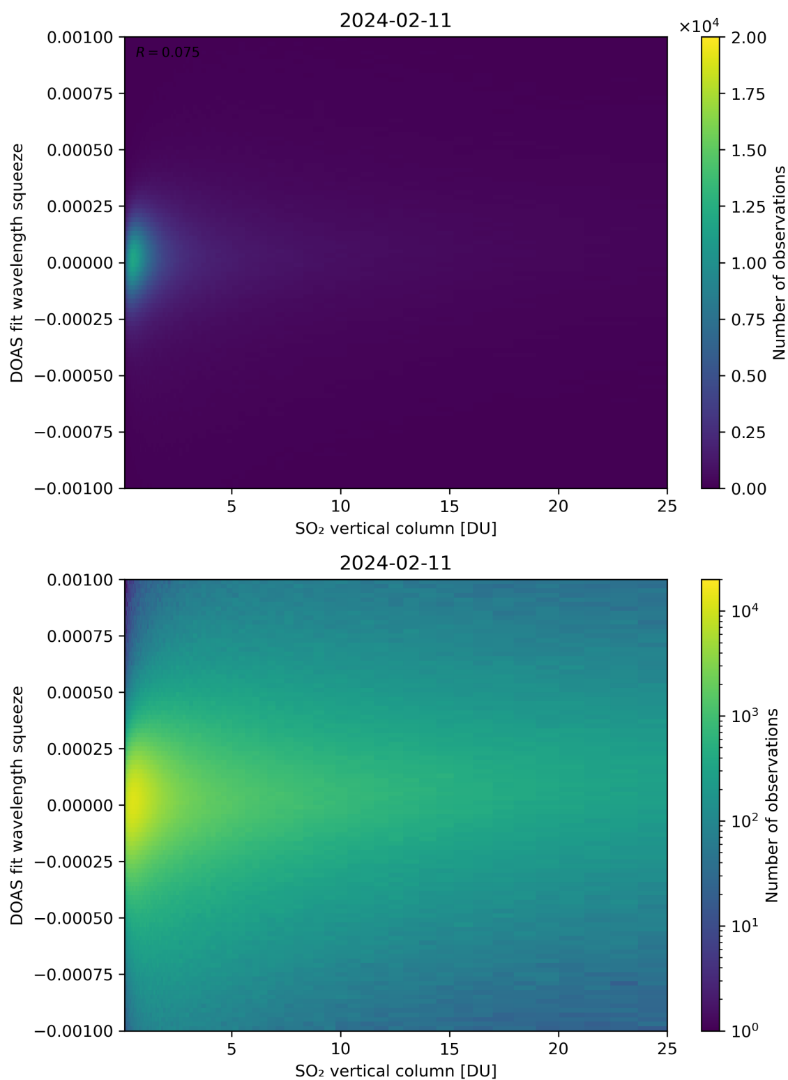
Figure 277: Scatter density plot of “SO 2 vertical column” against “DOAS fit wavelength squeeze” for 2024-02-11 to 2024-02-12.
