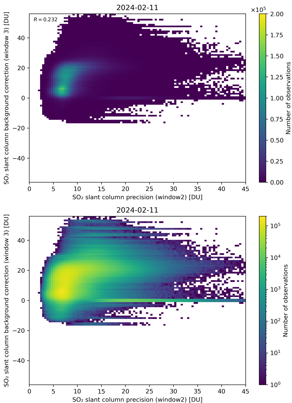
Figure 242: Scatter density plot of “SO 2 slant column precision (window2)” against “SO 2 slant column background correction (window 3)” for 2024-02-11 to 2024-02-12.
