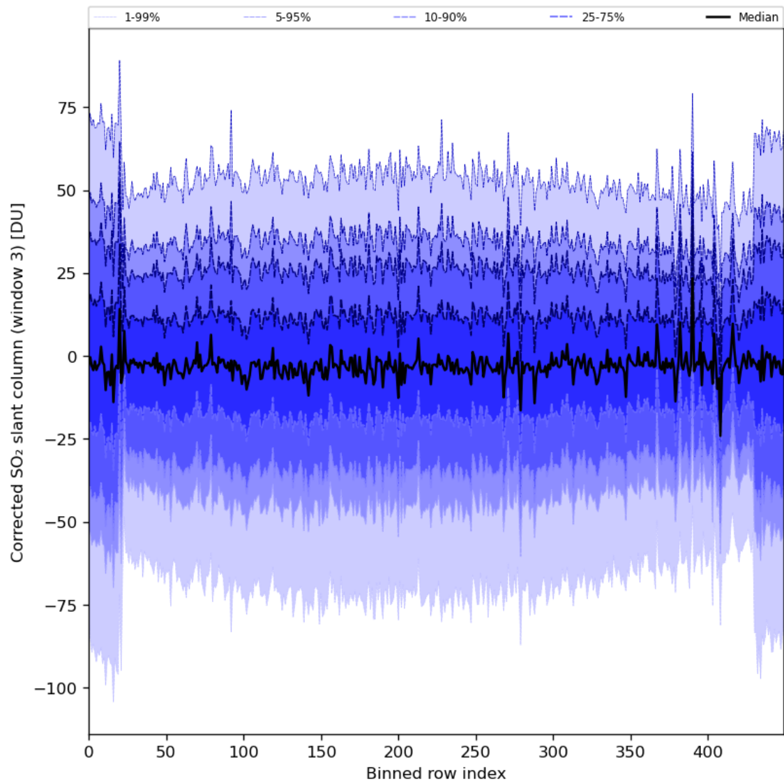
Figure 89: Along track statistics of “Corrected SO 2 slant column (window 3)” for 2024-02-11 to 2024-02-12
