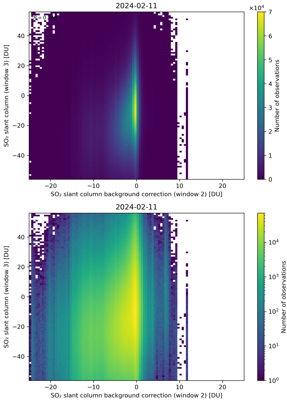
Figure 117: Scatter density plot of “SO 2 slant column background correction (window 2)” against “SO 2 slant column (window 3)” for 2024-02-11 to 2024-02-12.
