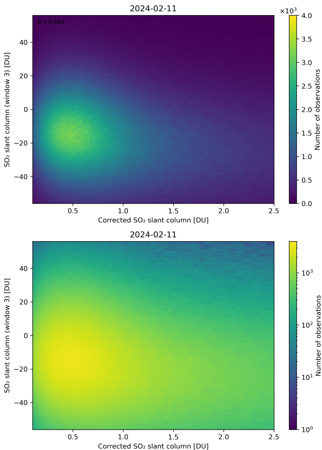
Figure 190: Scatter density plot of “Corrected SO 2 slant column” against “SO 2 slant column (window 3)” for 2024-02-11 to 2024-02-12.
