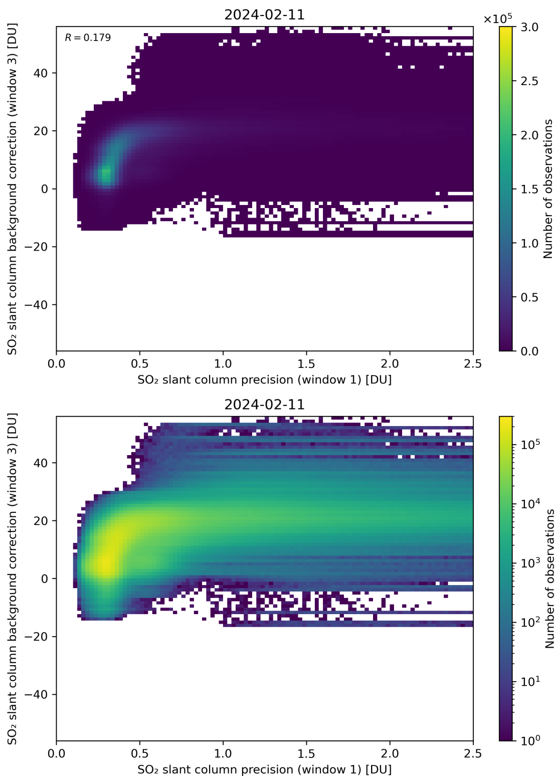
Figure 220: Scatter density plot of “SO 2 slant column precision (window 1)” against “SO 2 slant column background correction (window 3)” for 2024-02-11 to 2024-02-12.
