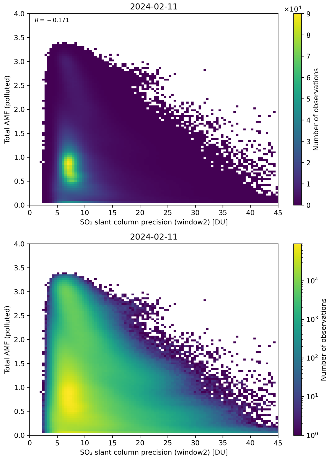
Figure 251: Scatter density plot of “SO 2 slant column precision (window2)” against “Total AMF (polluted)” for 2024-02-11 to 2024-02-12.
