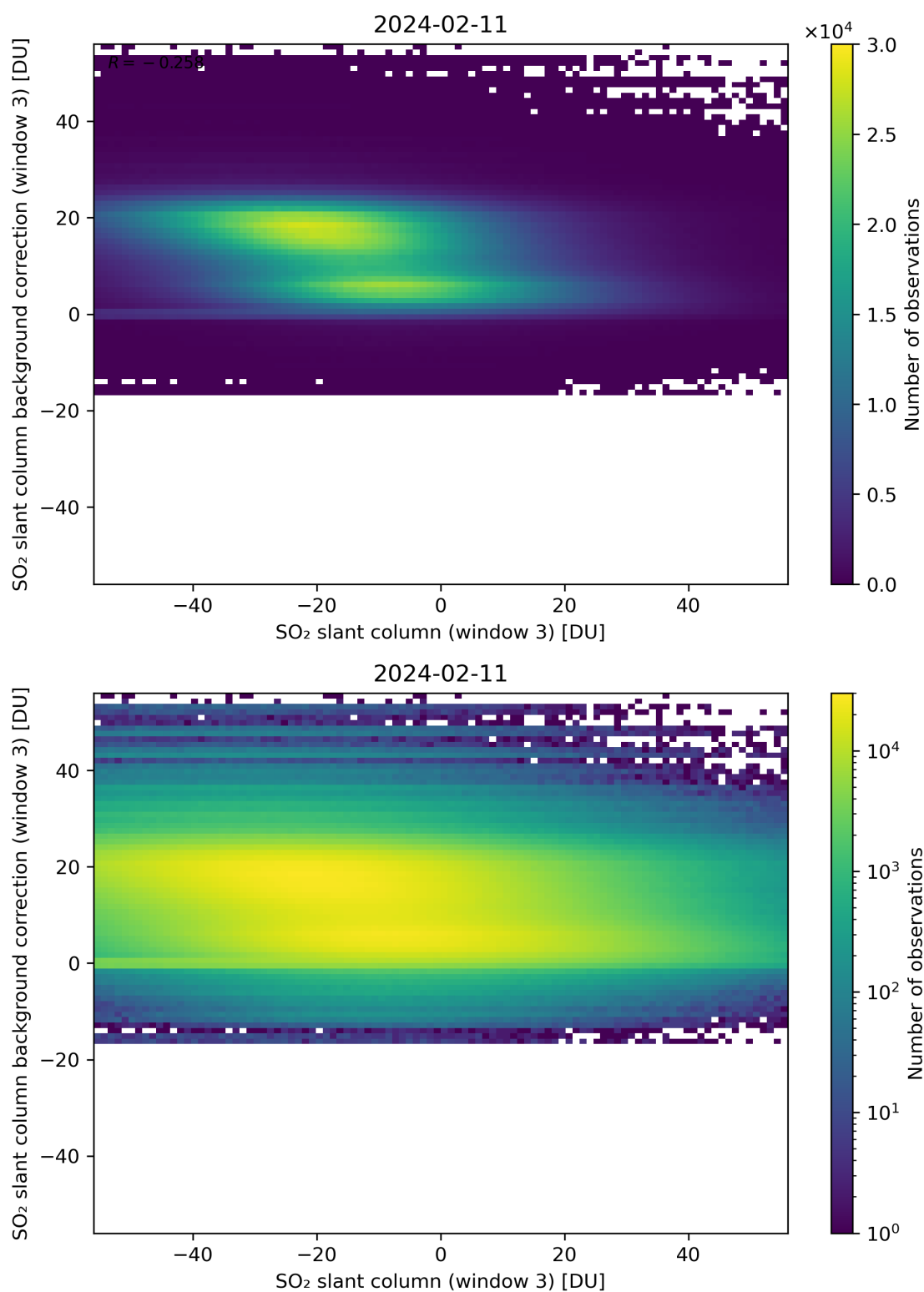
Figure 253: Scatter density plot of “SO 2 slant column (window 3)” against “SO 2 slant column background correction (window 3)” for 2024-02-11 to 2024-02-12.
