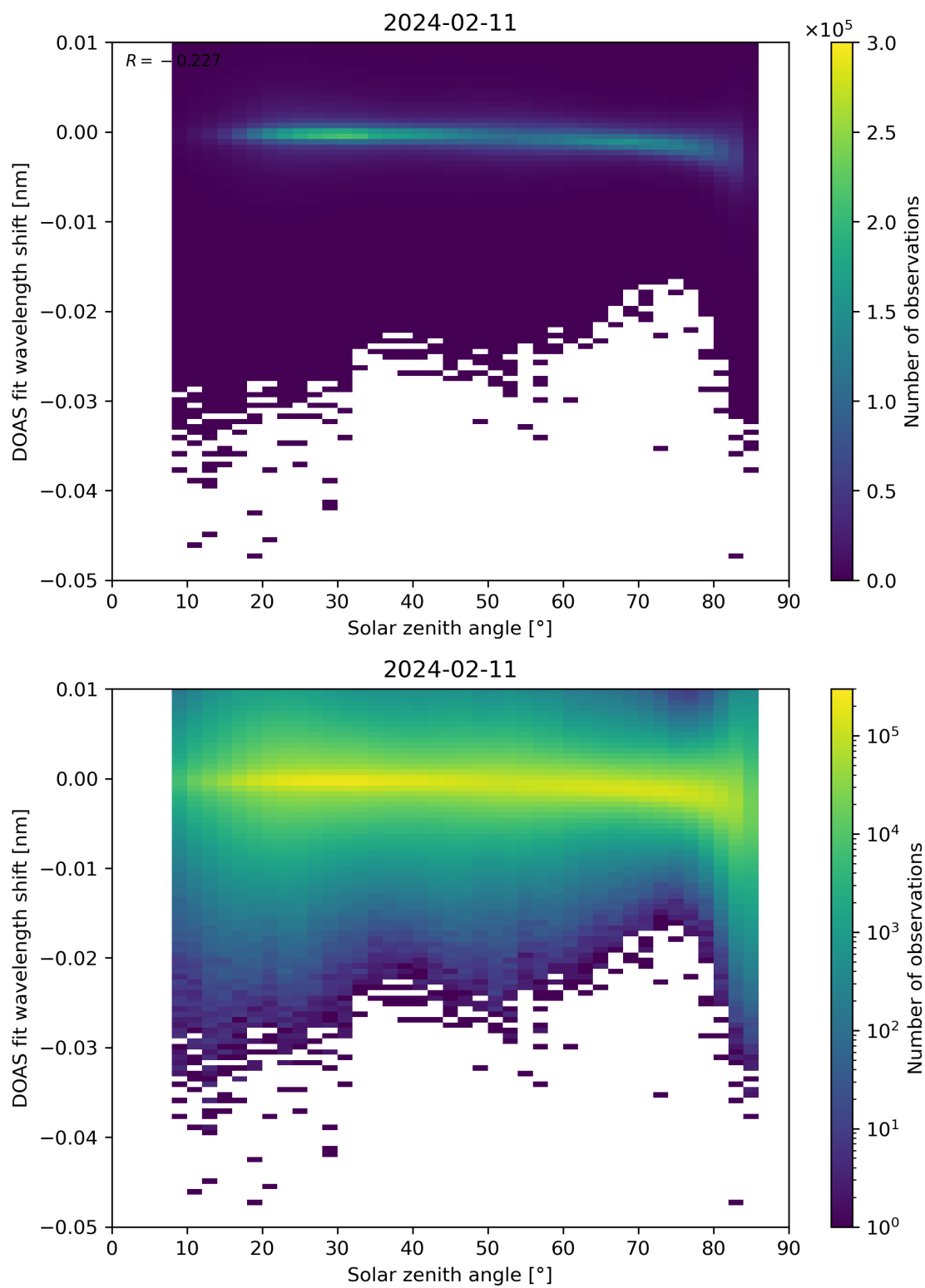
Figure 161: Scatter density plot of “Solar zenith angle” against “DOAS fit wavelength shift” for 2024-02-11 to 2024-02-12.
