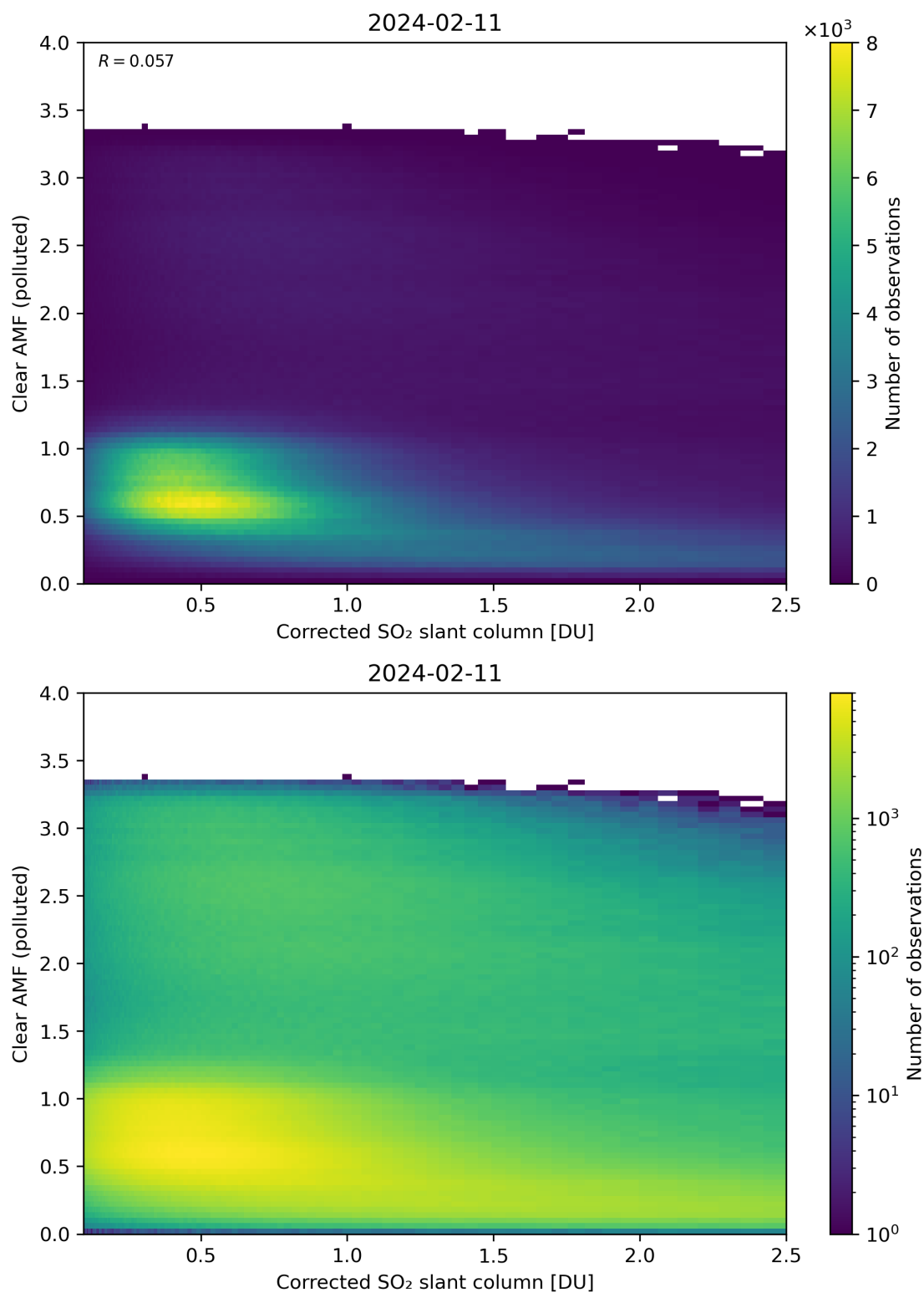
Figure 184: Scatter density plot of “Corrected SO 2 slant column” against “Clear AMF (polluted)” for 2024-02-11 to 2024-02-12.
