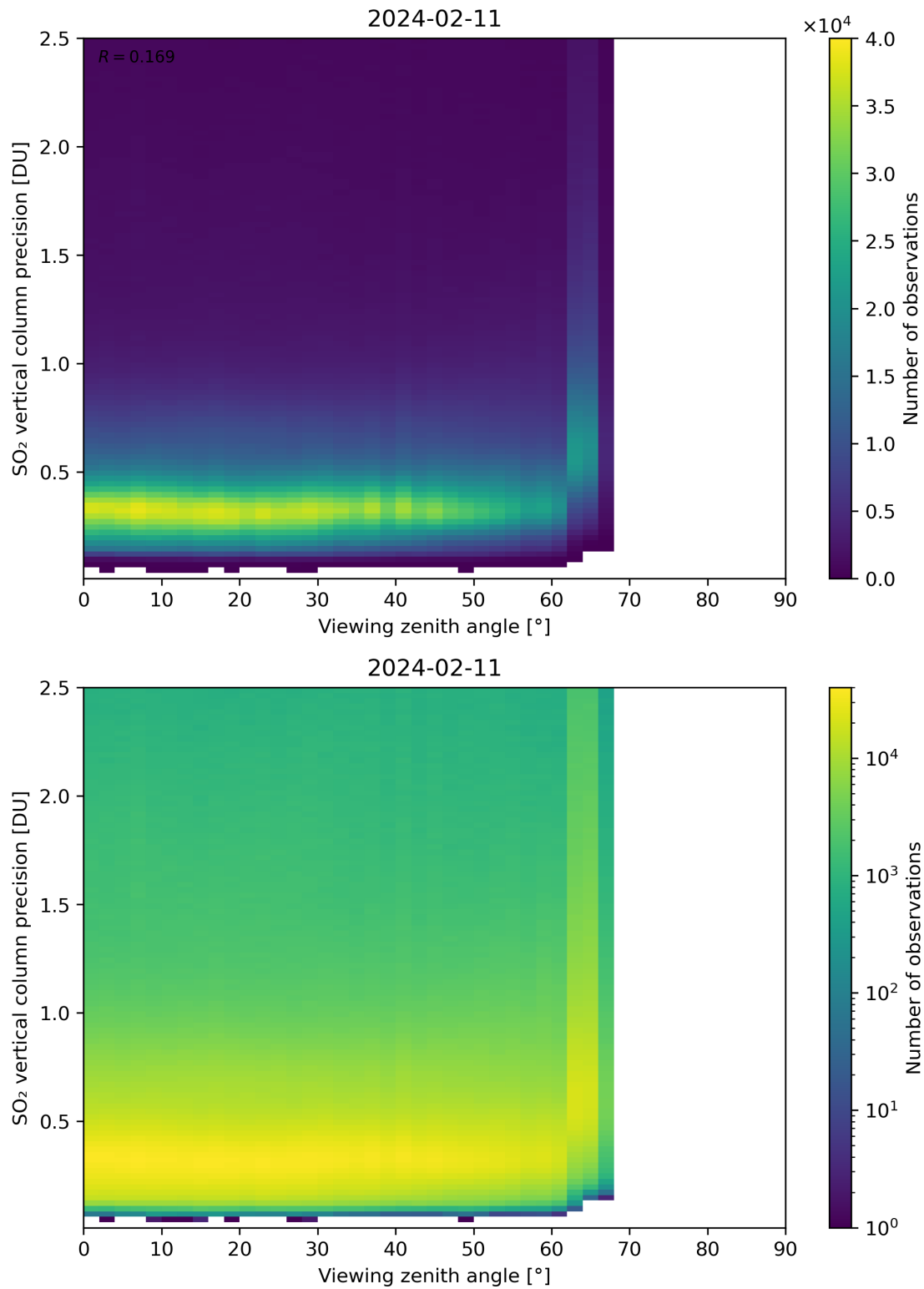
Figure 328: Scatter density plot of “Viewing zenith angle” against “SO 2 vertical column precision” for 2024-02-11 to 2024-02-12.
