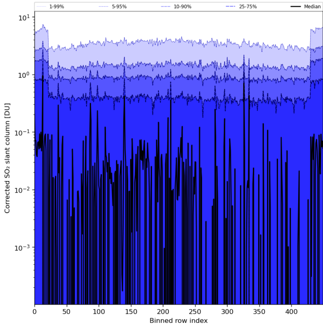
Figure 78: Along track statistics of “Corrected SO 2 slant column” for 2024-02-11 to 2024-02-12
