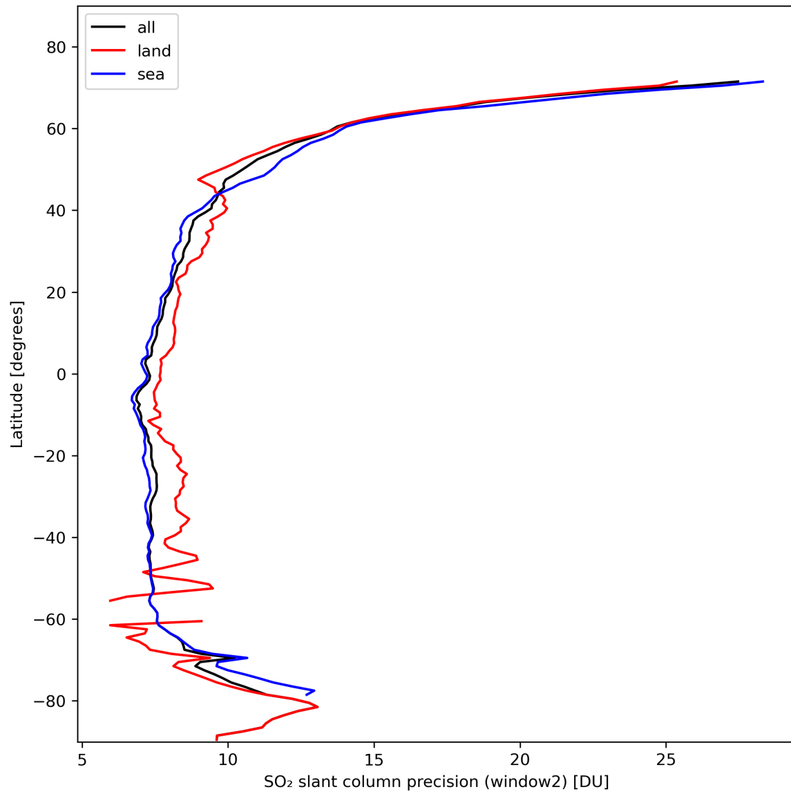
Figure 38: Zonal average of “SO 2 slant column precision (window2)” for 2024-02-11 to 2024-02-12.
