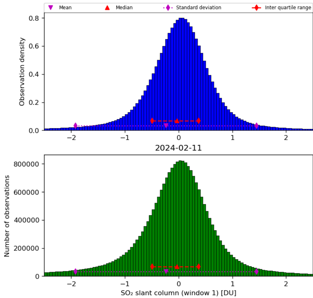
Figure 56: Histogram of “SO 2 slant column (window 1)” for 2024-02-11 to 2024-02-12
