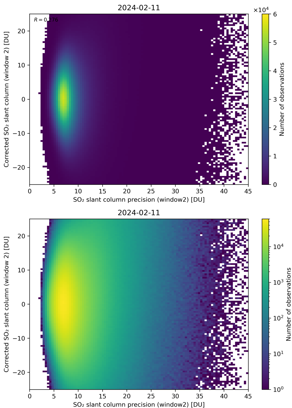
Figure 247: Scatter density plot of “SO 2 slant column precision (window2)” against “Corrected SO 2 slant column (window 2)” for 2024-02-11 to 2024-02-12.
