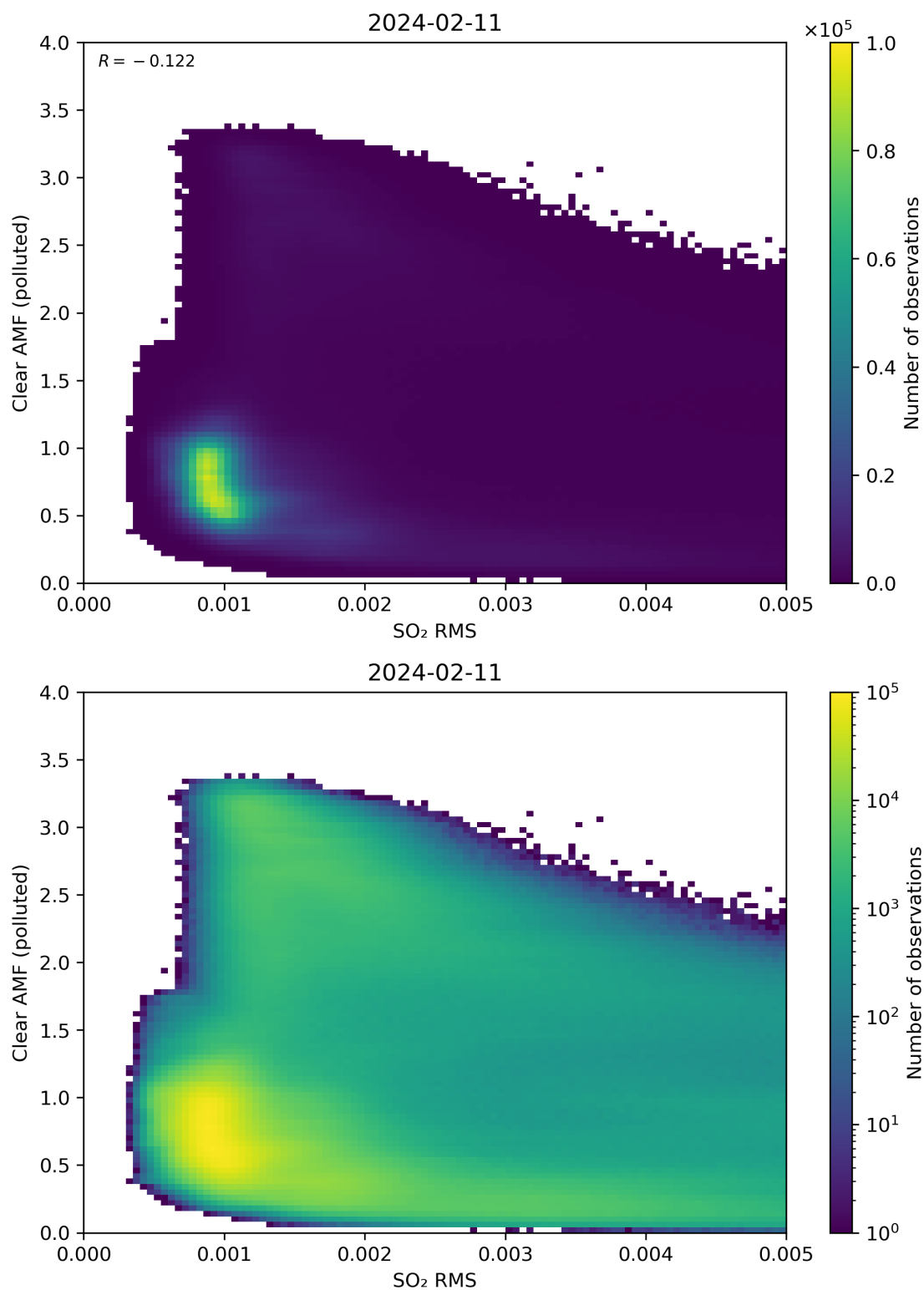
Figure 136: Scatter density plot of “SO 2 RMS” against “Clear AMF (polluted)” for 2024-02-11 to 2024-02-12.
