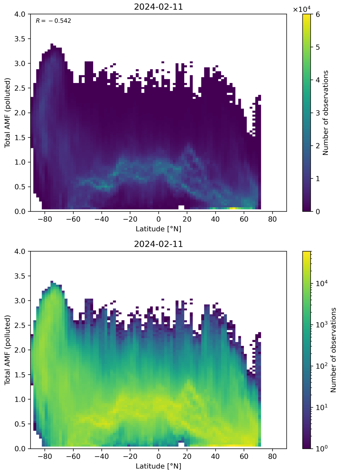
Figure 154: Scatter density plot of “Latitude” against “Total AMF (polluted)” for 2024-02-11 to 2024-02-12.
