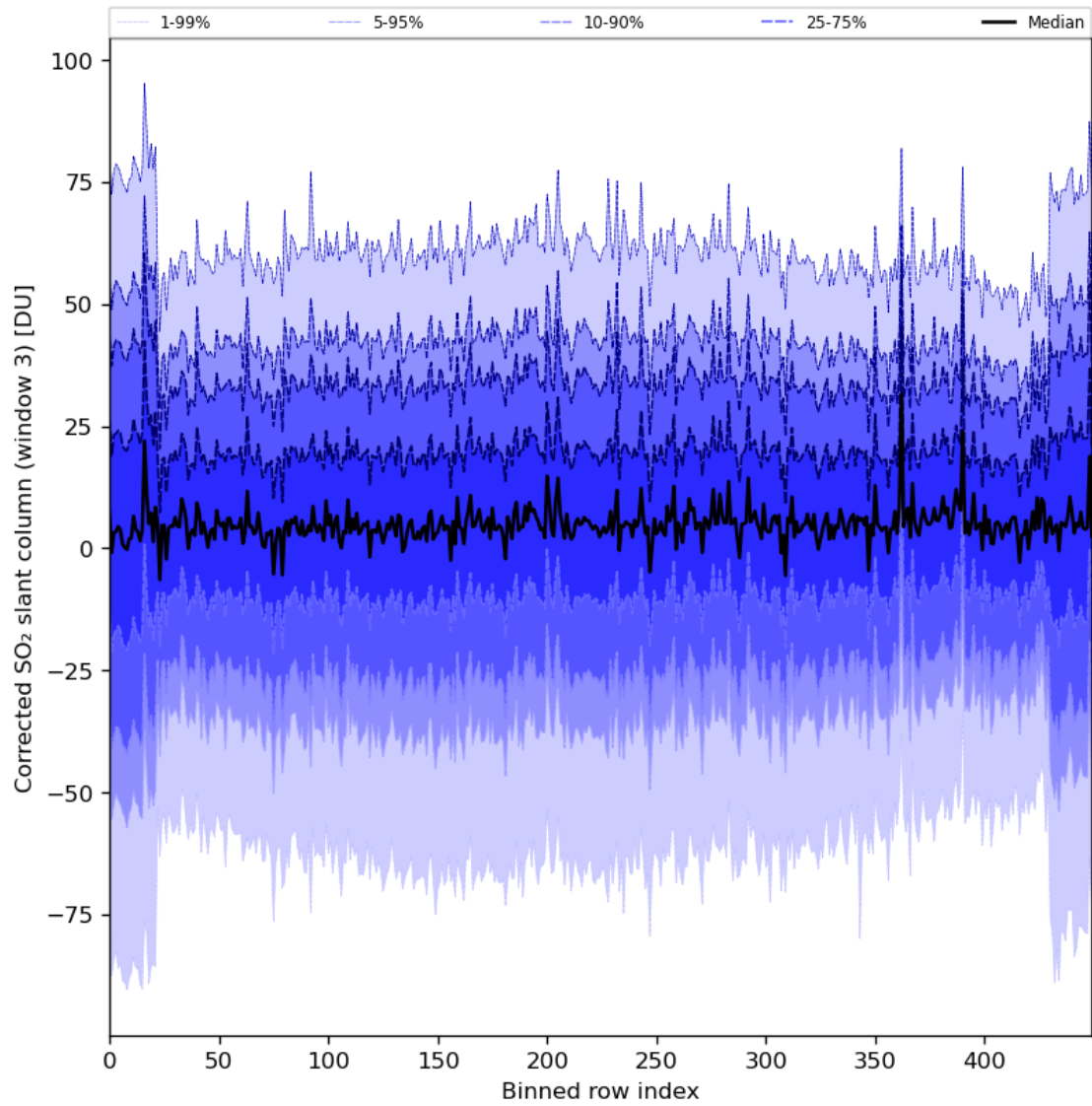
Figure 89: Along track statistics of “Corrected SO 2 slant column (window 3)” for 2024-02-13 to 2024-02-15
