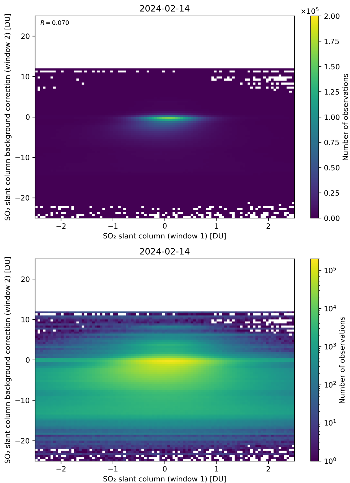
Figure 213: Scatter density plot of “SO 2 slant column (window 1)” against “SO 2 slant column background correction (window 2)” for 2024-02-13 to 2024-02-15.
