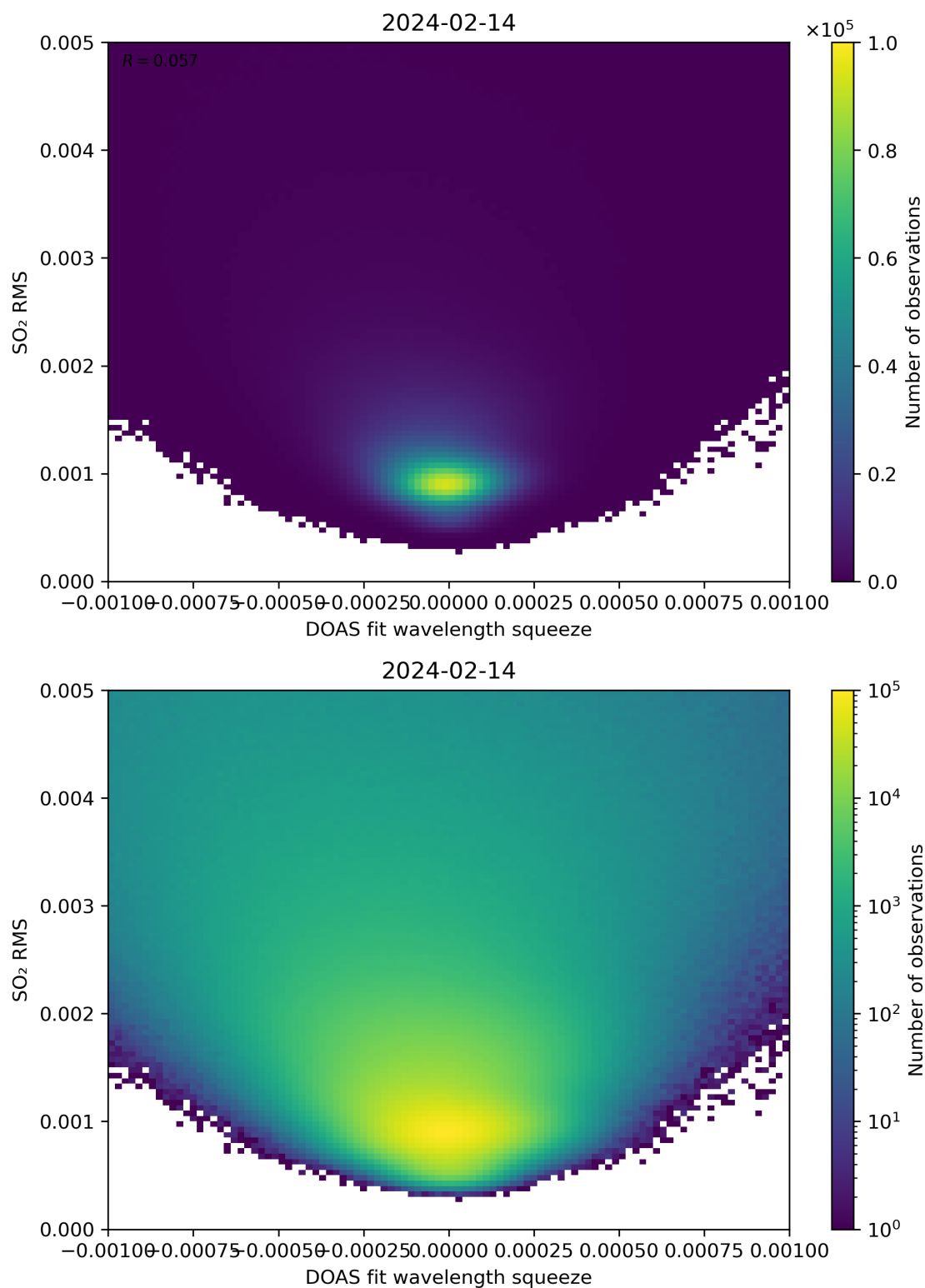
Figure 132: Scatter density plot of “DOAS fit wavelength squeeze” against “SO 2 RMS” for 2024-02-13 to 2024-02-15.
