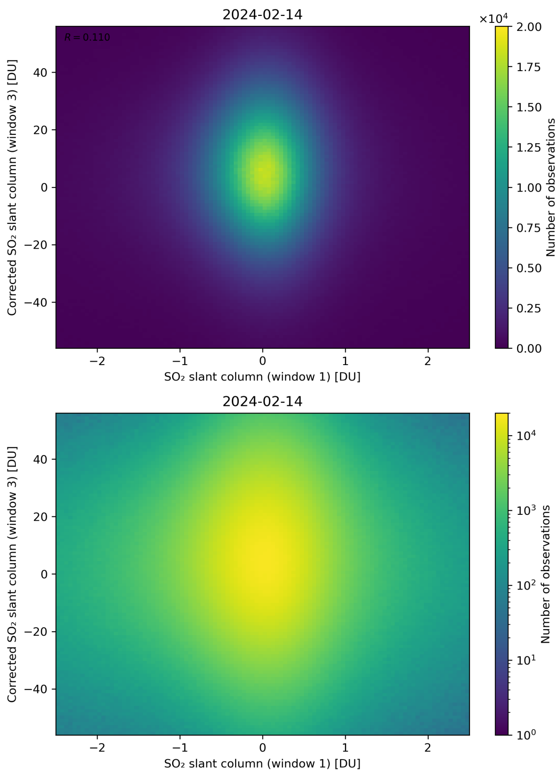
Figure 234: Scatter density plot of “SO 2 slant column (window 1)” against “Corrected SO 2 slant column (window 3)” for 2024-02-13 to 2024-02-15.
