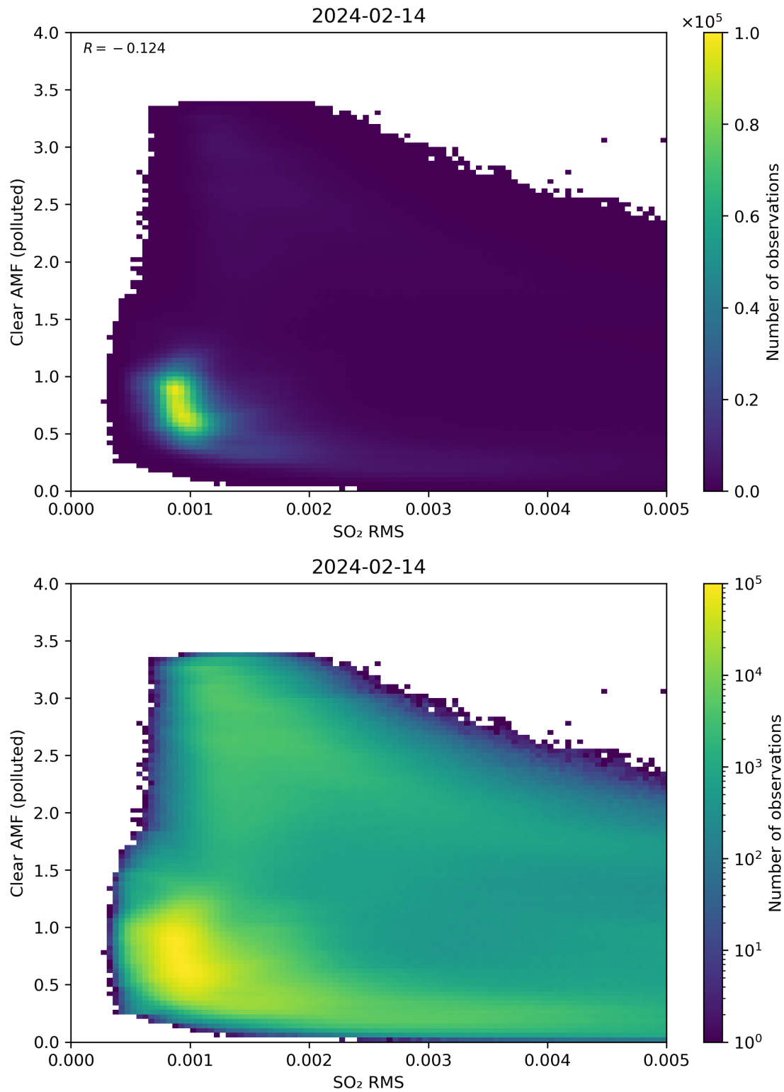
Figure 136: Scatter density plot of “SO 2 RMS” against “Clear AMF (polluted)” for 2024-02-13 to 2024-02-15.
