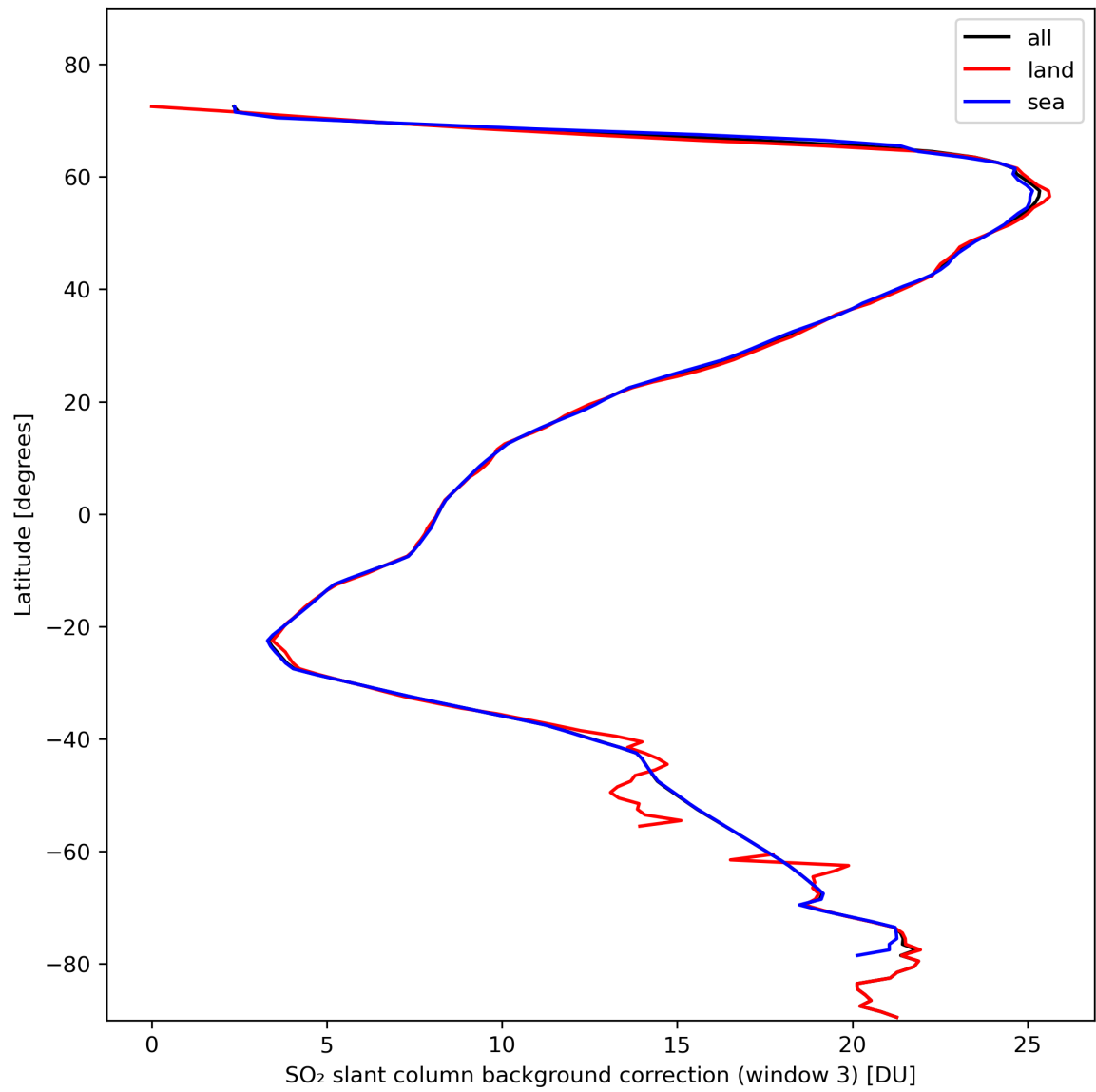
Figure 44: Zonal average of “SO 2 slant column background correction (window 3)” for 2024-02-13 to 2024-02-15.
