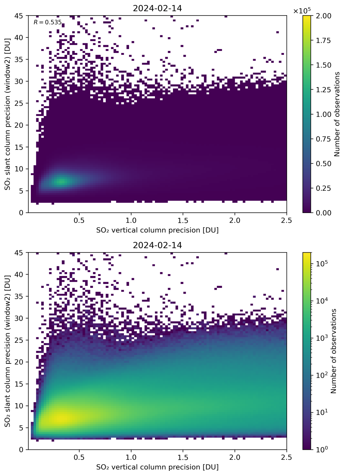
Figure 291: Scatter density plot of “SO 2 vertical column precision” against “SO 2 slant column precision (window2)” for 2024-02-13 to 2024-02-15.
