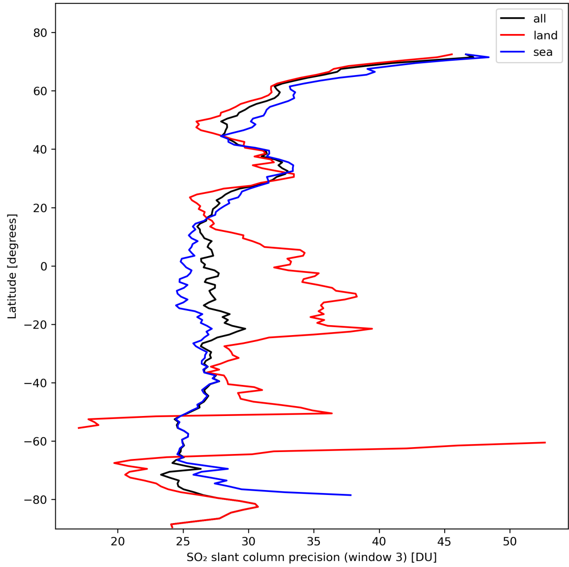
Figure 42: Zonal average of “SO 2 slant column precision (window 3)” for 2024-02-13 to 2024-02-15.
