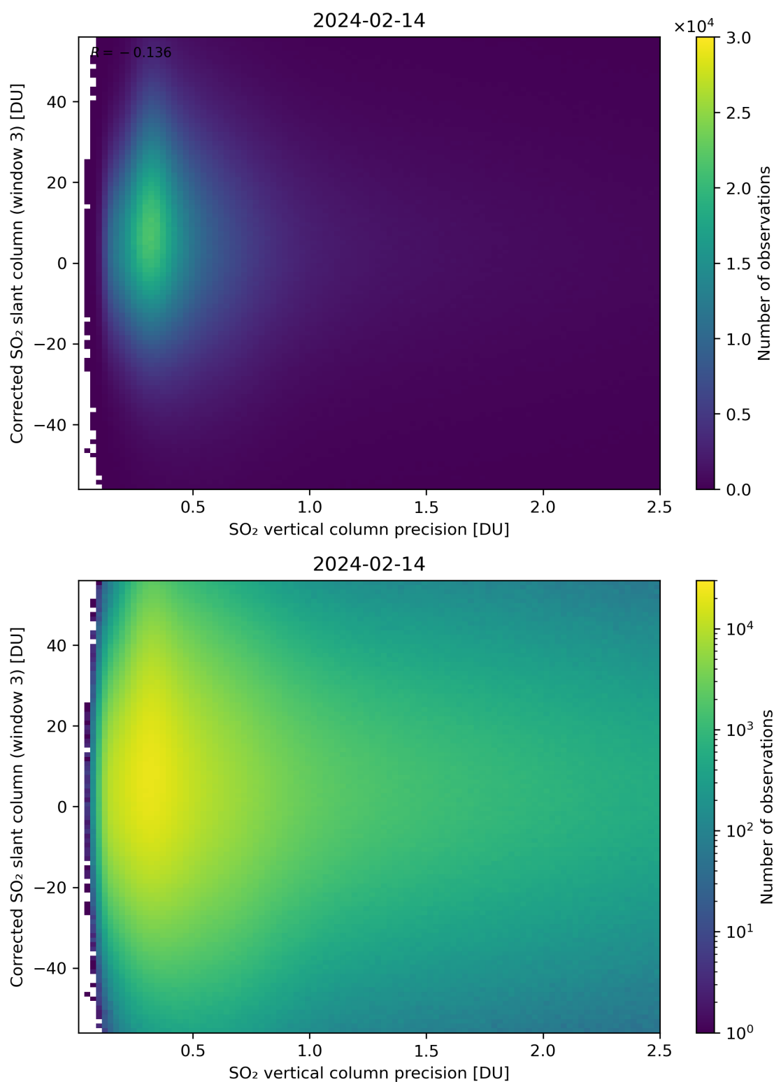
Figure 288: Scatter density plot of “SO 2 vertical column precision” against “Corrected SO 2 slant column (window 3)” for 2024-02-13 to 2024-02-15.
