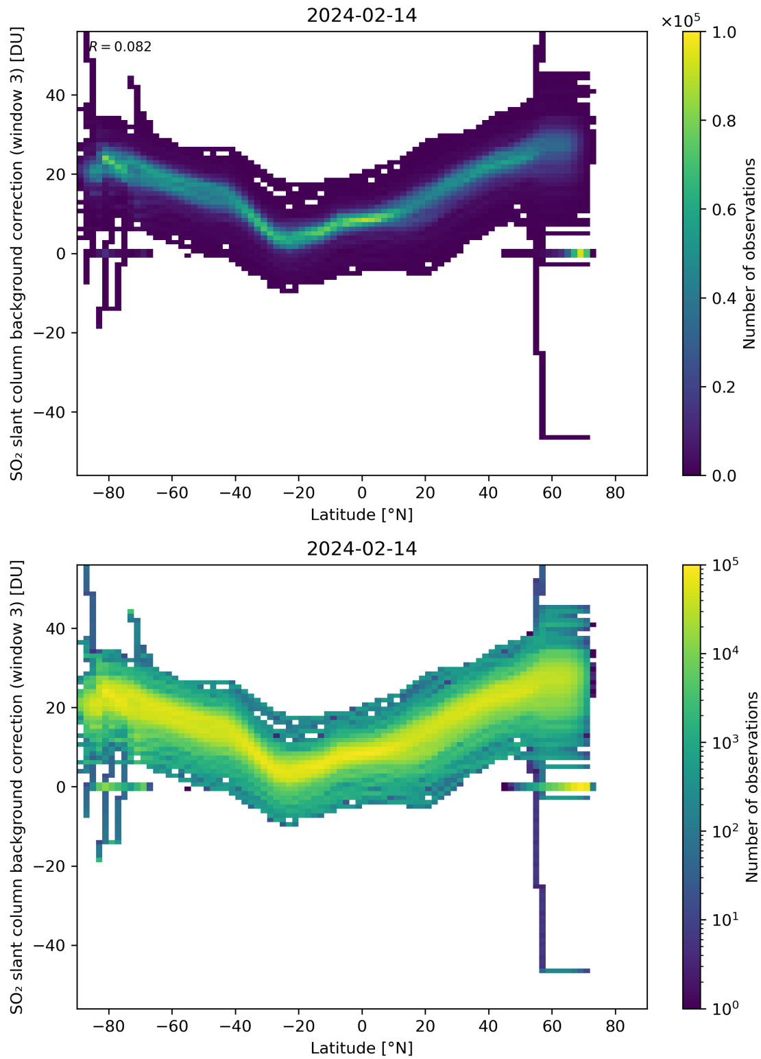
Figure 141: Scatter density plot of “Latitude” against “SO 2 slant column background correction (window 3)” for 2024-02-13 to 2024-02-15.
