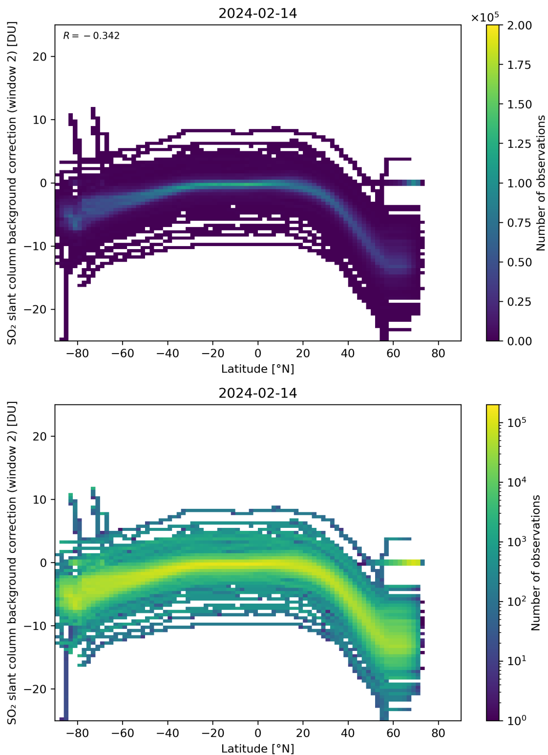
Figure 140: Scatter density plot of “Latitude” against “SO 2 slant column background correction (window 2)” for 2024-02-13 to 2024-02-15.
