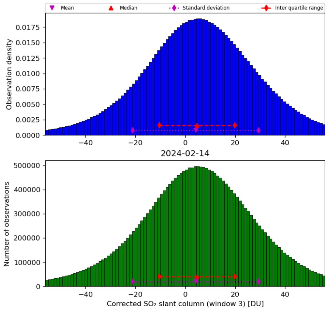
Figure 66: Histogram of "Corrected SO 2 slant column (window 3)" for 2024-02-13 to 2024-02-15
