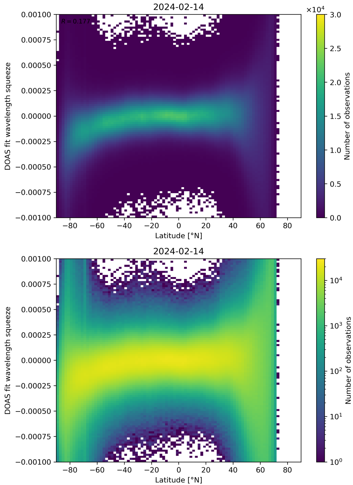
Figure 143: Scatter density plot of “Latitude” against “DOAS fit wavelength squeeze” for 2024-02-13 to 2024-02-15.
