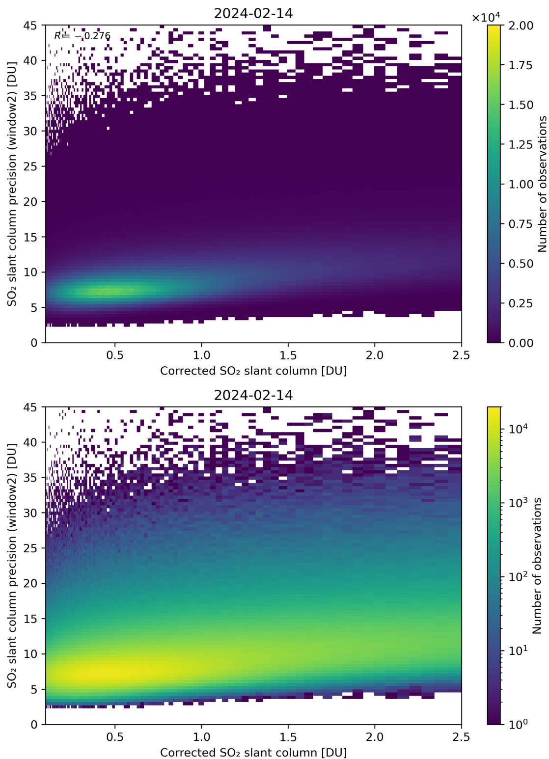
Figure 189: Scatter density plot of “Corrected SO 2 slant column” against “SO 2 slant column precision (window2)” for 2024-02-13 to 2024-02-15.
