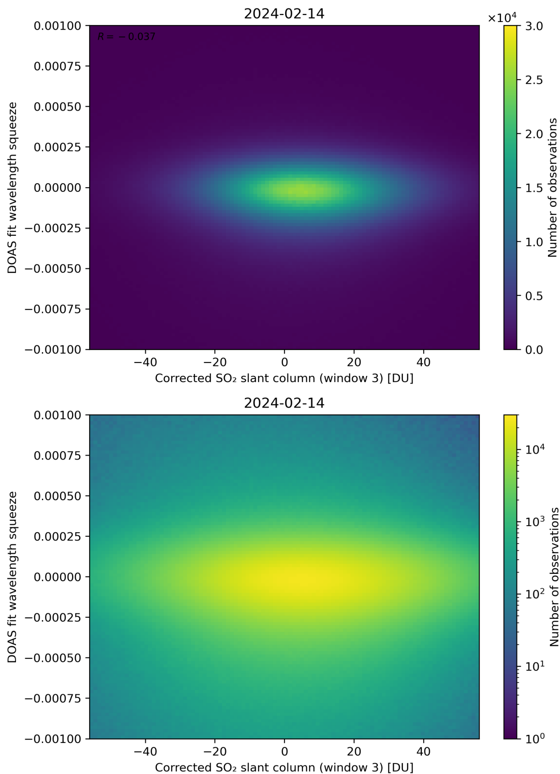
Figure 207: Scatter density plot of “Corrected SO 2 slant column (window 3)” against “DOAS fit wavelength squeeze” for 2024-02-13 to 2024-02-15.
