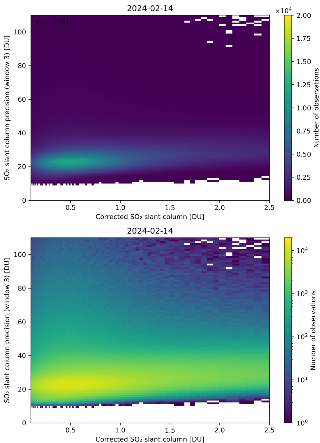
Figure 191: Scatter density plot of “Corrected SO 2 slant column” against “SO 2 slant column precision (window 3)” for 2024-02-13 to 2024-02-15.
