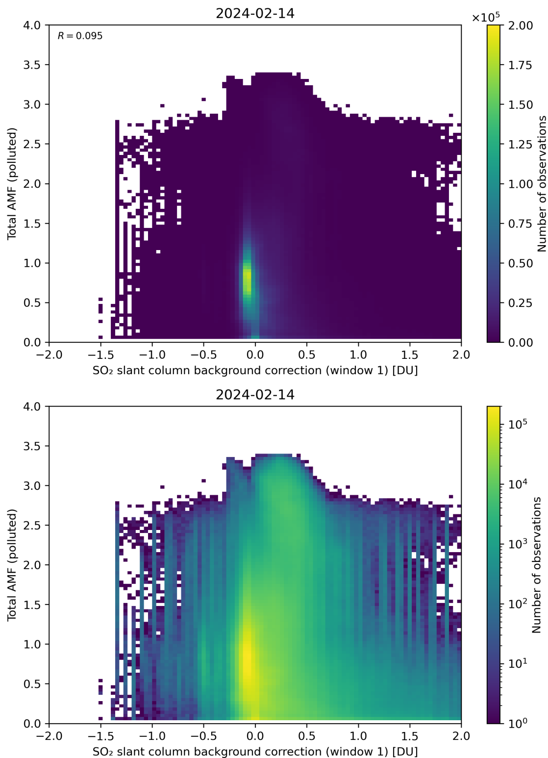
Figure 109: Scatter density plot of “SO 2 slant column background correction (window 1)” against “Total AMF (polluted)” for 2024-02-13 to 2024-02-15.
