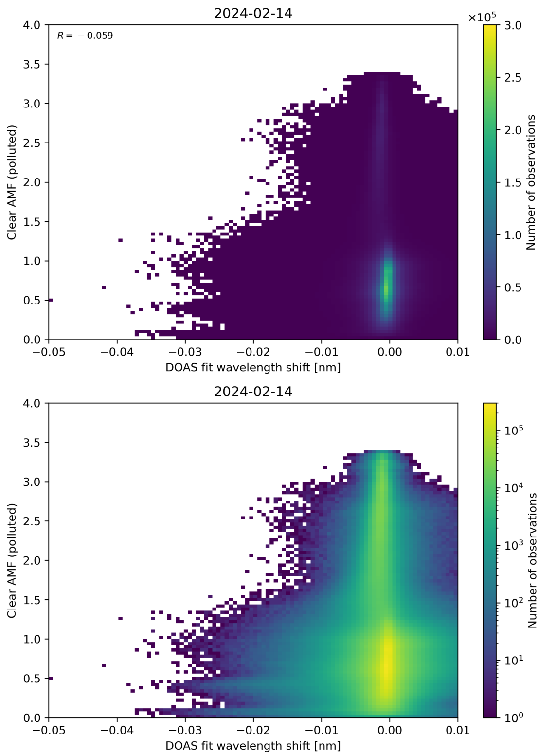
Figure 129: Scatter density plot of “DOAS fit wavelength shift” against “Clear AMF (polluted)” for 2024-02-13 to 2024-02-15.
