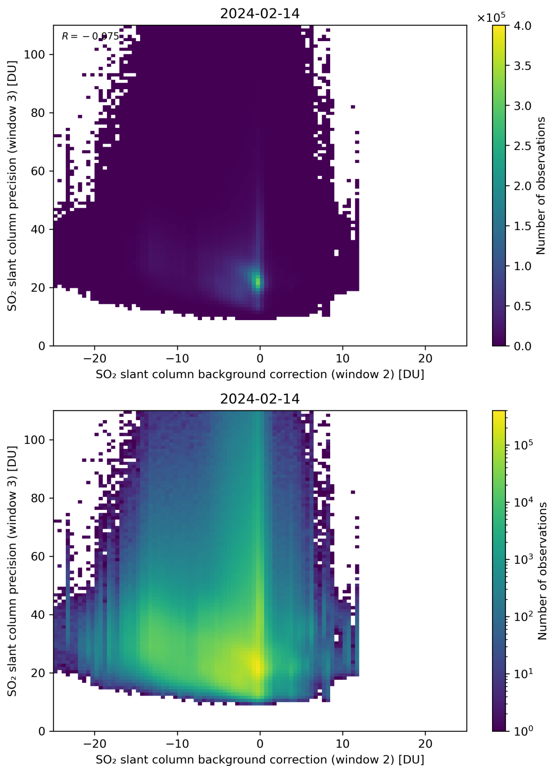
Figure 118: Scatter density plot of “SO 2 slant column background correction (window 2)” against “SO 2 slant column precision (window 3)” for 2024-02-13 to 2024-02-15.
