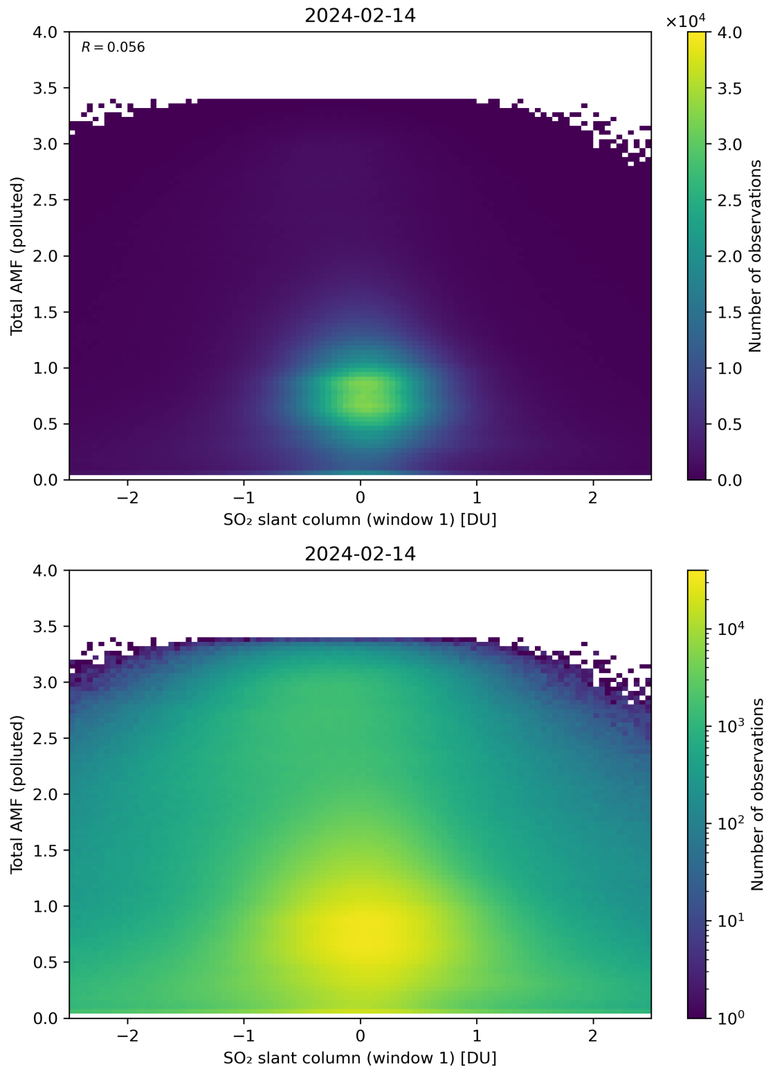
Figure 239: Scatter density plot of “SO 2 slant column (window 1)” against “Total AMF (polluted)” for 2024-02-13 to 2024-02-15.
