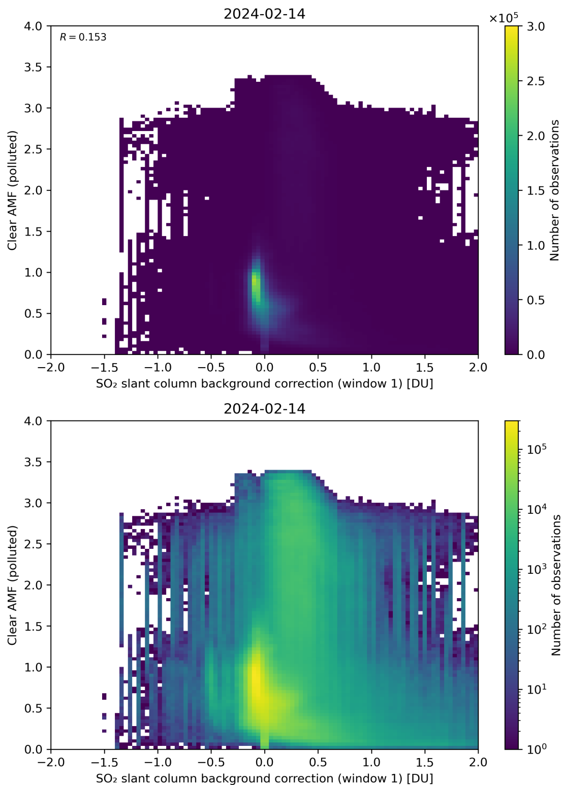
Figure 103: Scatter density plot of “SO 2 slant column background correction (window 1)” against “Clear AMF (polluted)” for 2024-02-13 to 2024-02-15.
