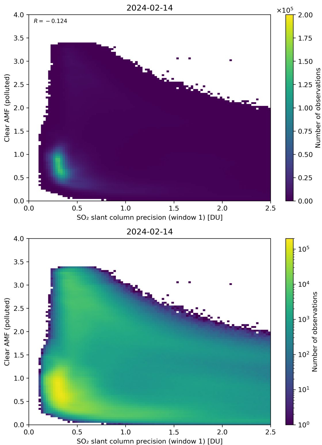
Figure 224: Scatter density plot of “SO 2 slant column precision (window 1)” against “Clear AMF (polluted)” for 2024-02-13 to 2024-02-15.
