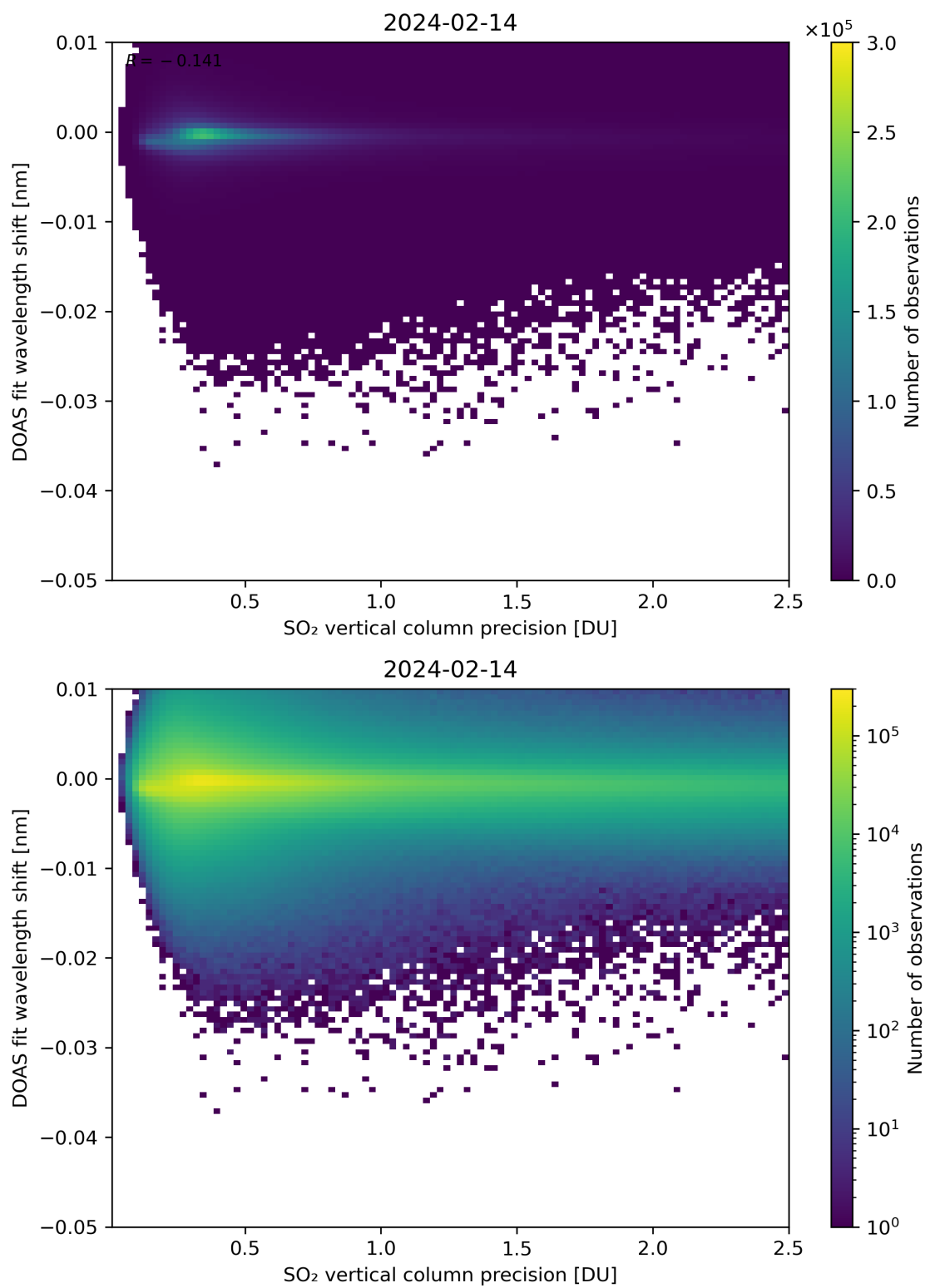
Figure 282: Scatter density plot of “SO 2 vertical column precision” against “DOAS fit wavelength shift” for 2024-02-13 to 2024-02-15.
