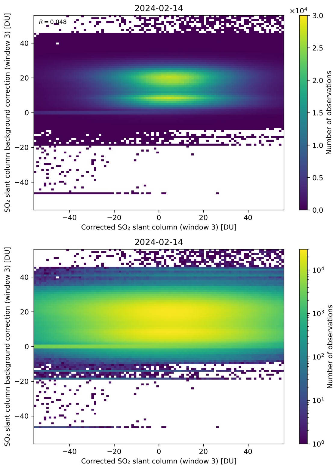
Figure 205: Scatter density plot of “Corrected SO 2 slant column (window 3)” against “SO 2 slant column background correction (window 3)” for 2024-02-13 to 2024-02-15.
