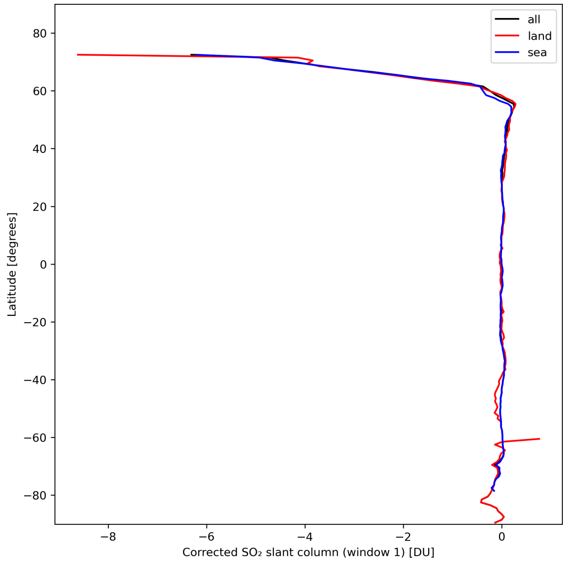
Figure 35: Zonal average of “Corrected SO 2 slant column (window 1)” for 2024-02-13 to 2024-02-15.
