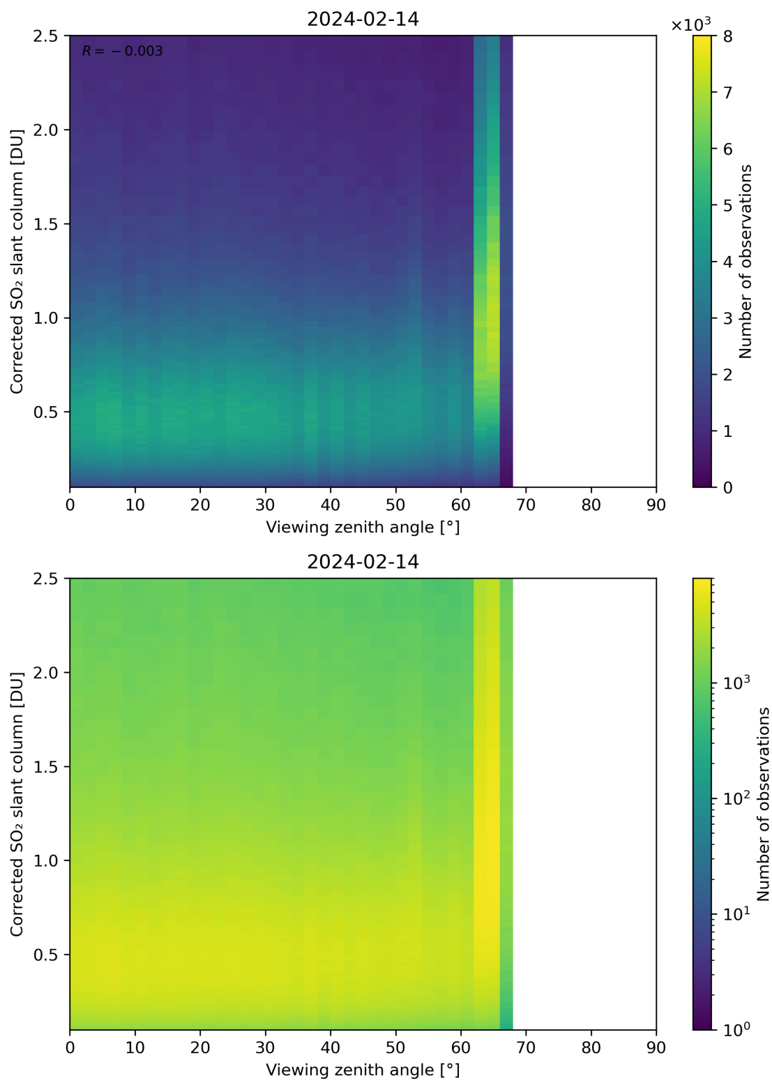
Figure 317: Scatter density plot of “Viewing zenith angle” against “Corrected SO 2 slant column” for 2024-02-13 to 2024-02-15.
