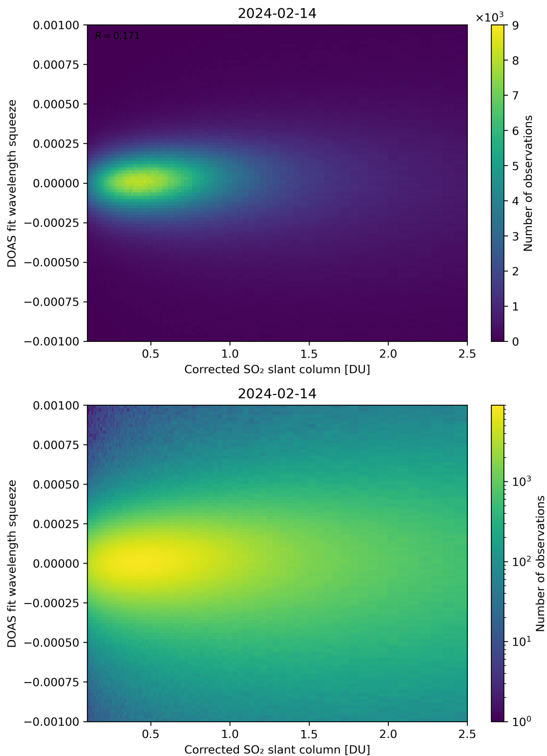
Figure 182: Scatter density plot of “Corrected SO 2 slant column” against “DOAS fit wavelength squeeze” for 2024-02-13 to 2024-02-15.
