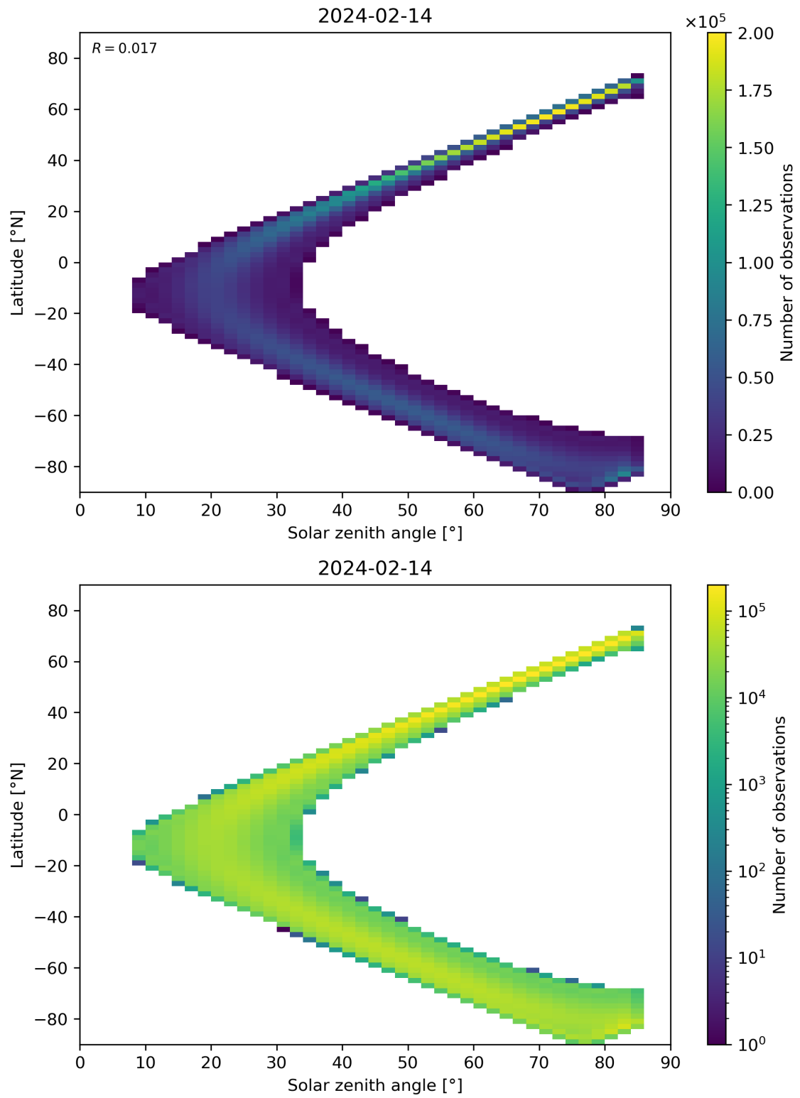
Figure 164: Scatter density plot of “Solar zenith angle” against “Latitude” for 2024-02-13 to 2024-02-15.
