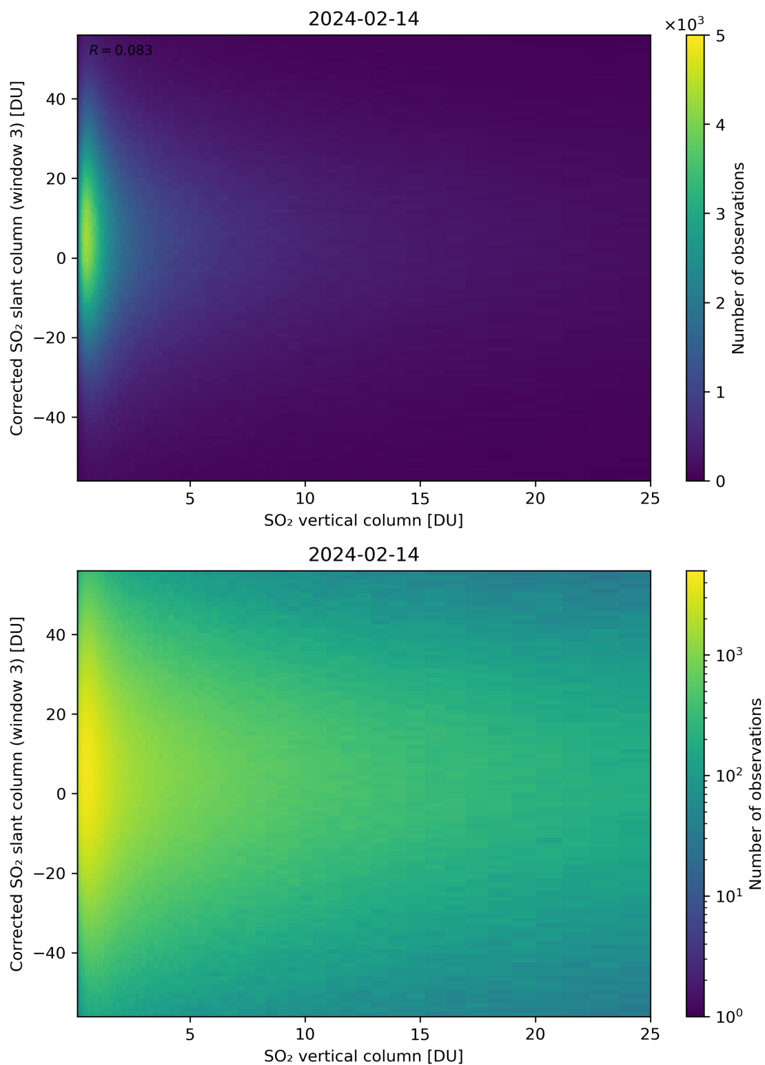
Figure 299: Scatter density plot of “SO 2 vertical column” against “Corrected SO 2 slant column (window 3)” for 2024-02-13 to 2024-02-15.
