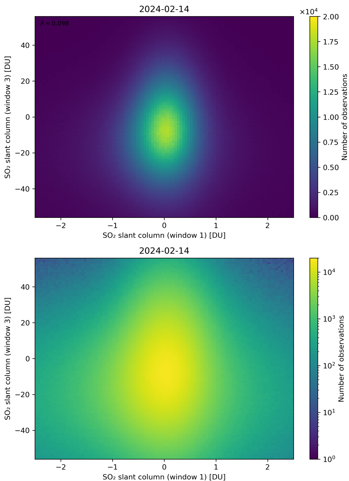
Figure 237: Scatter density plot of “SO 2 slant column (window 1)” against “SO 2 slant column (window 3)” for 2024-02-13 to 2024-02-15.
