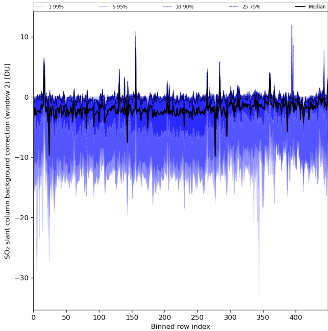
Figure 86: Along track statistics of “SO 2 slant column background correction (window 2)” for 2024-02-13 to 2024-02-15
