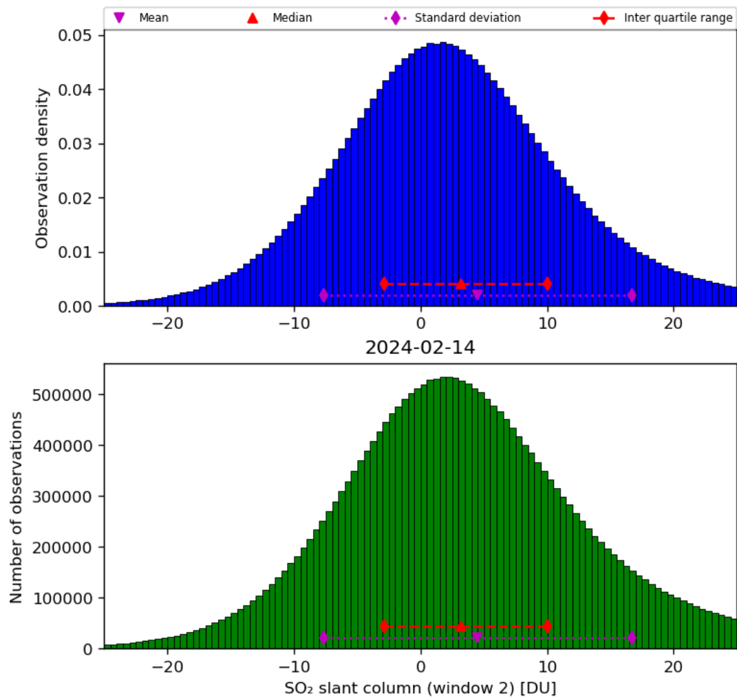
Figure 60: Histogram of “SO 2 slant column (window 2)” for 2024-02-13 to 2024-02-15
