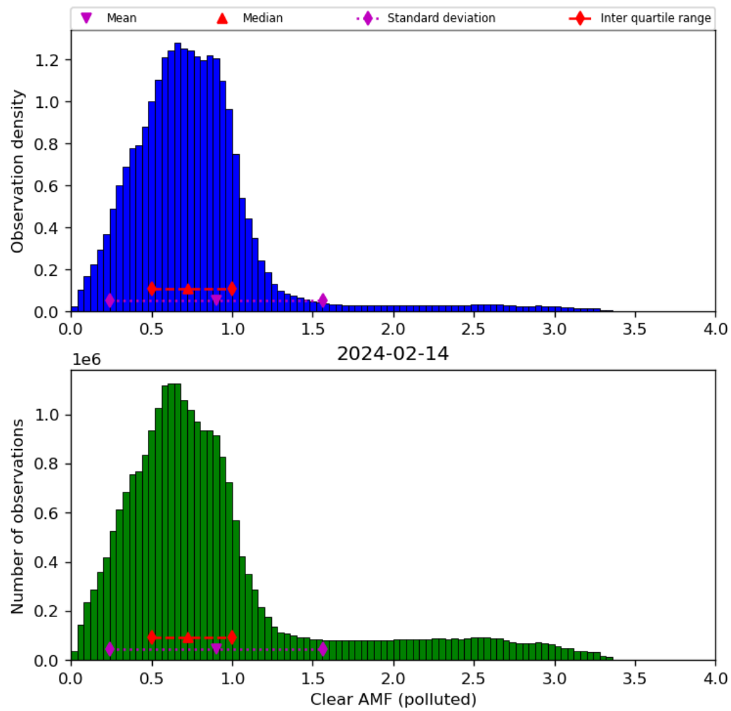
Figure 73: Histogram of “Clear AMF (polluted)” for 2024-02-13 to 2024-02-15
