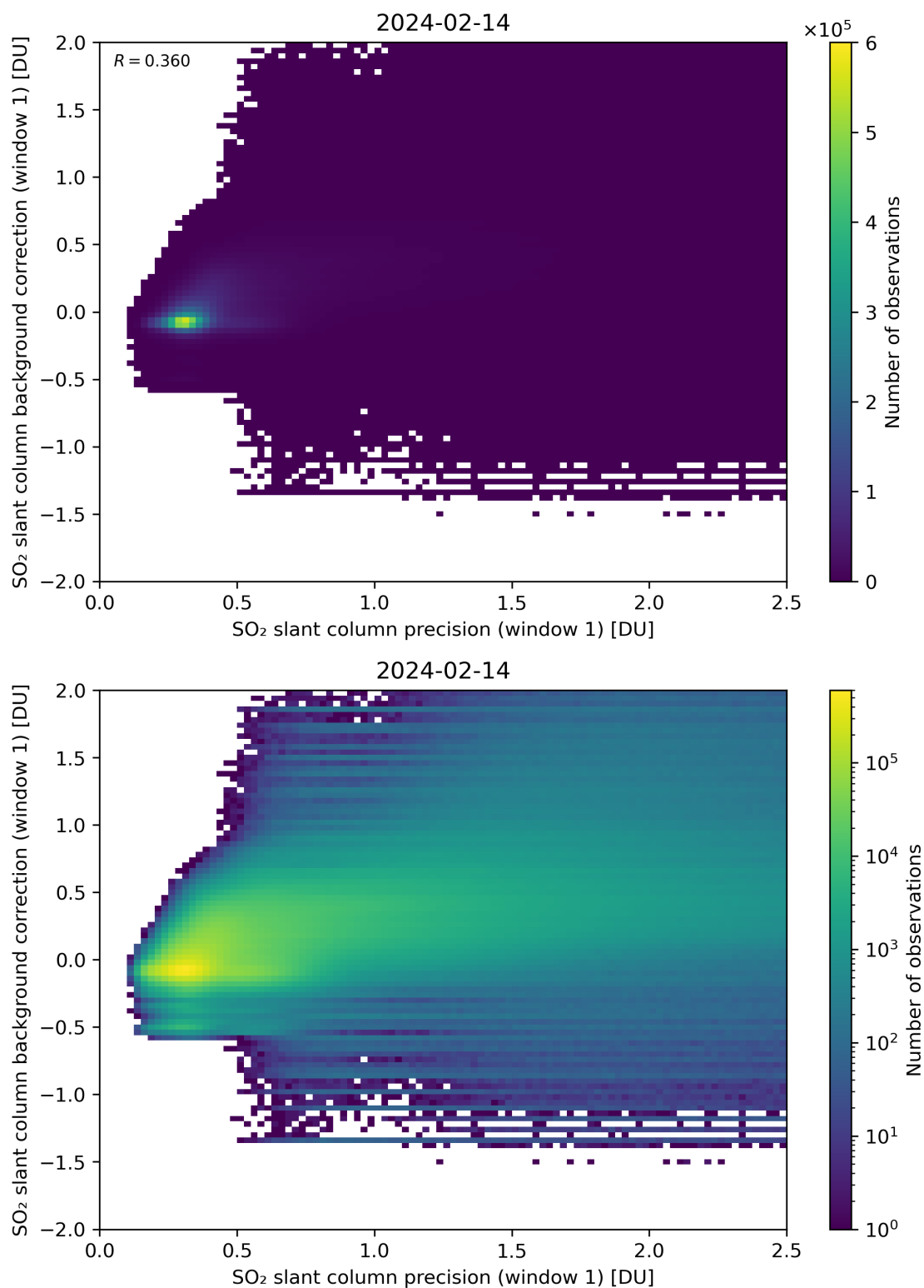
Figure 218: Scatter density plot of “SO 2 slant column precision (window 1)” against “SO 2 slant column background correction (window 1)” for 2024-02-13 to 2024-02-15.
