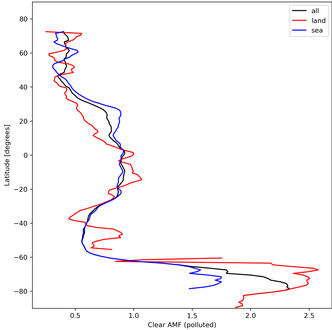
Figure 50: Zonal average of “Clear AMF (polluted)” for 2024-02-13 to 2024-02-15.
