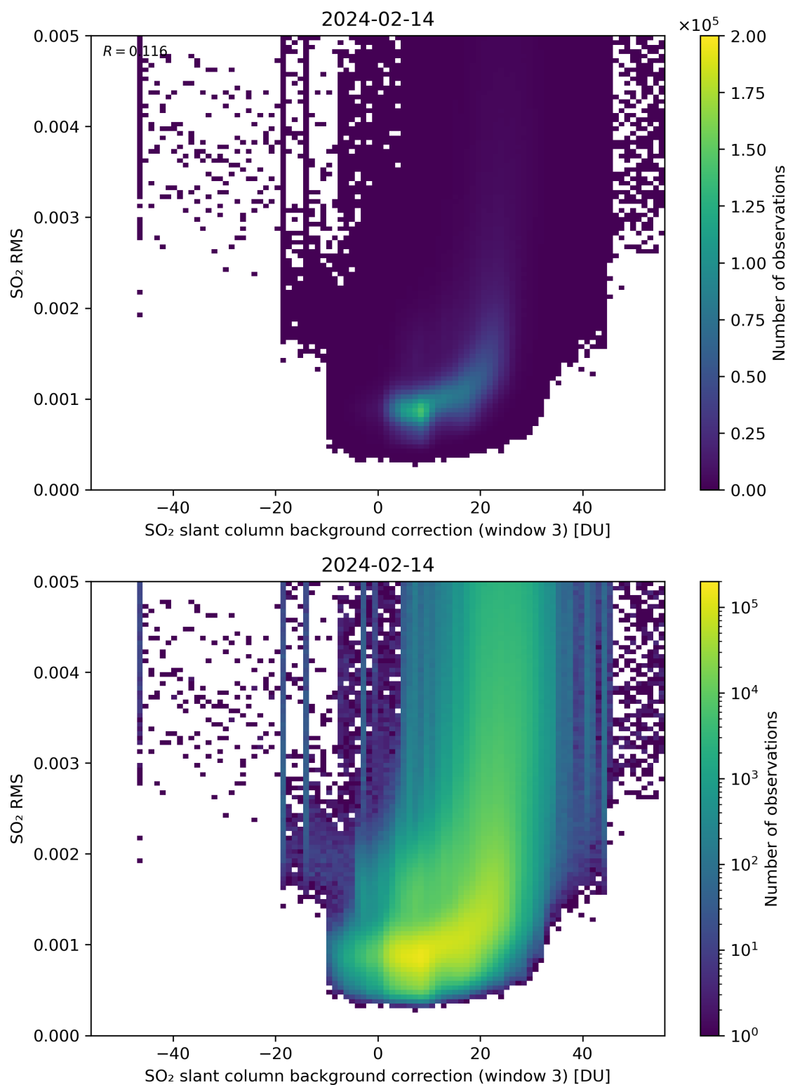
Figure 123: Scatter density plot of “SO 2 slant column background correction (window 3)” against “SO 2 RMS” for 2024-02-13 to 2024-02-15.
