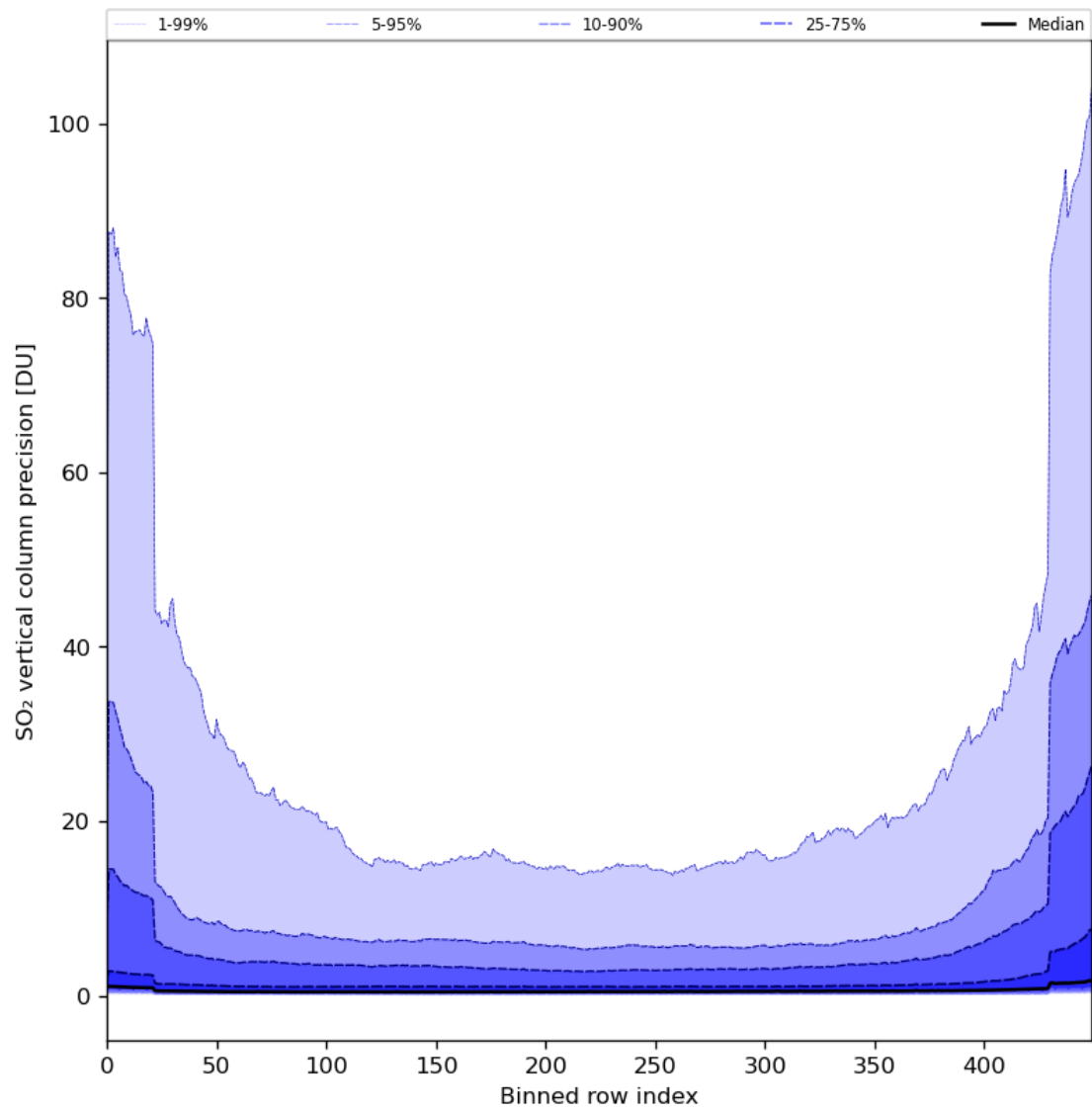
Figure 77: Along track statistics of “SO 2 vertical column precision” for 2024-02-13 to 2024-02-15
