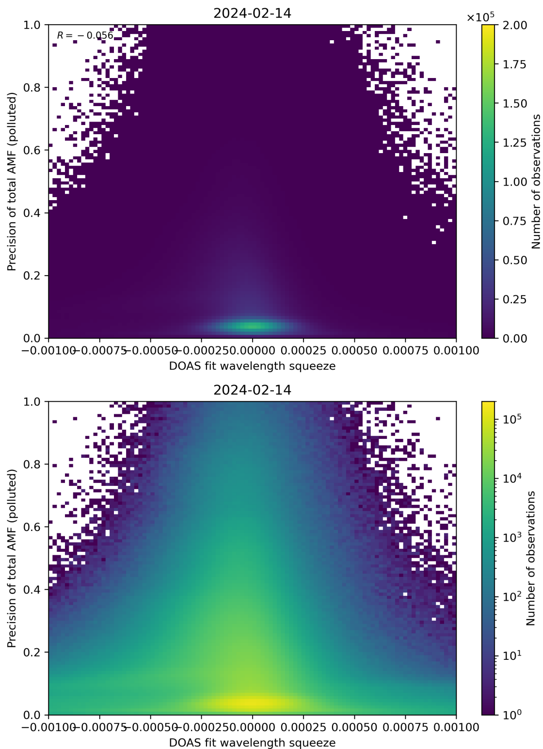
Figure 135: Scatter density plot of “DOAS fit wavelength squeeze” against “Precision of total AMF (polluted)” for 2024-02-13 to 2024-02-15.
