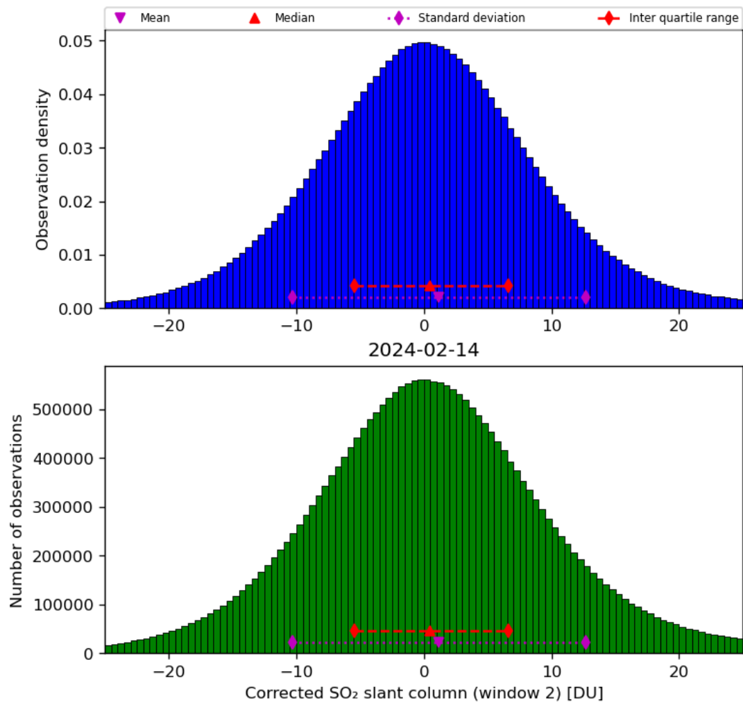
Figure 62: Histogram of “Corrected SO 2 slant column (window 2)” for 2024-02-13 to 2024-02-15
