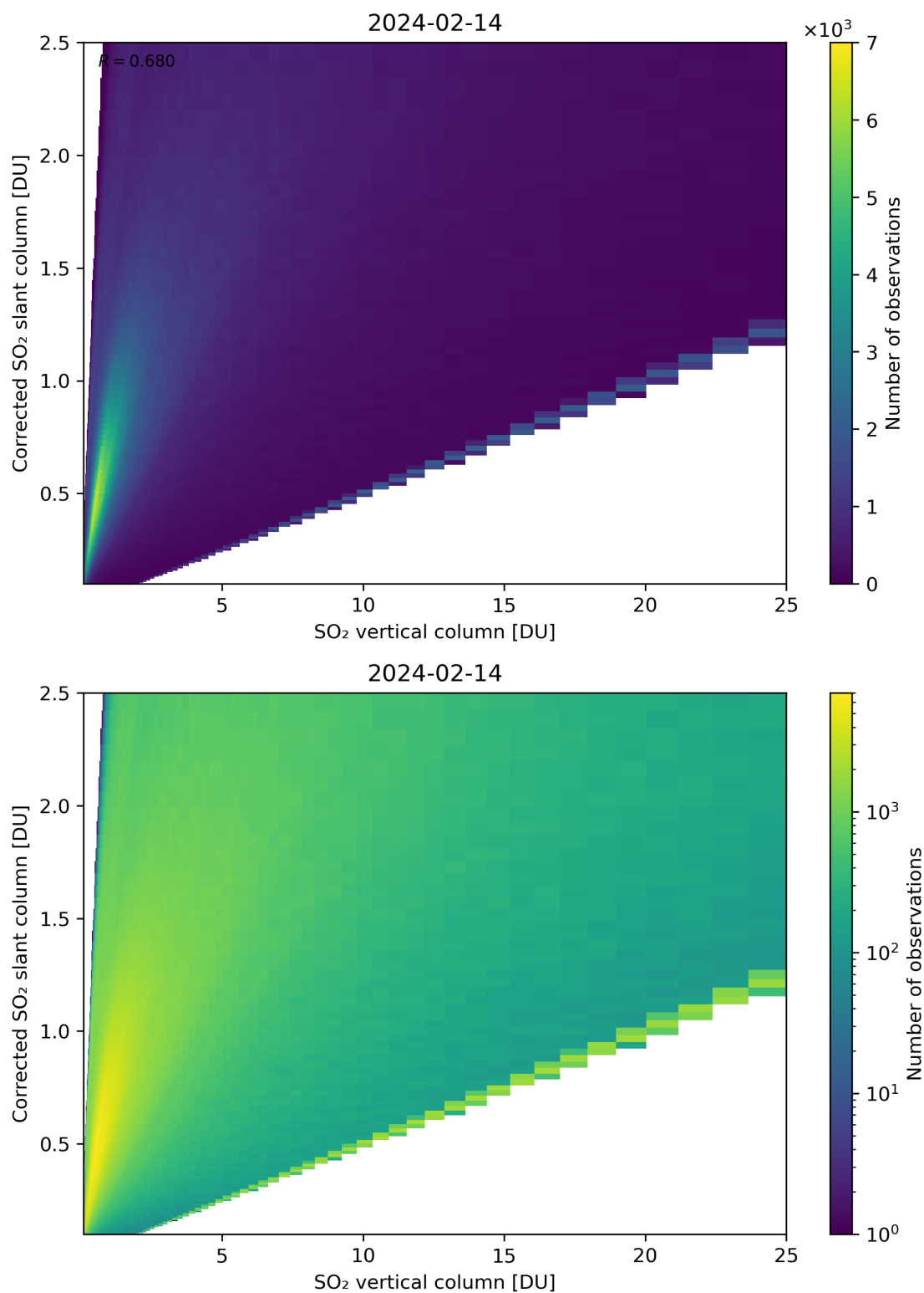
Figure 297: Scatter density plot of “SO 2 vertical column” against “Corrected SO 2 slant column” for 2024-02-13 to 2024-02-15.
