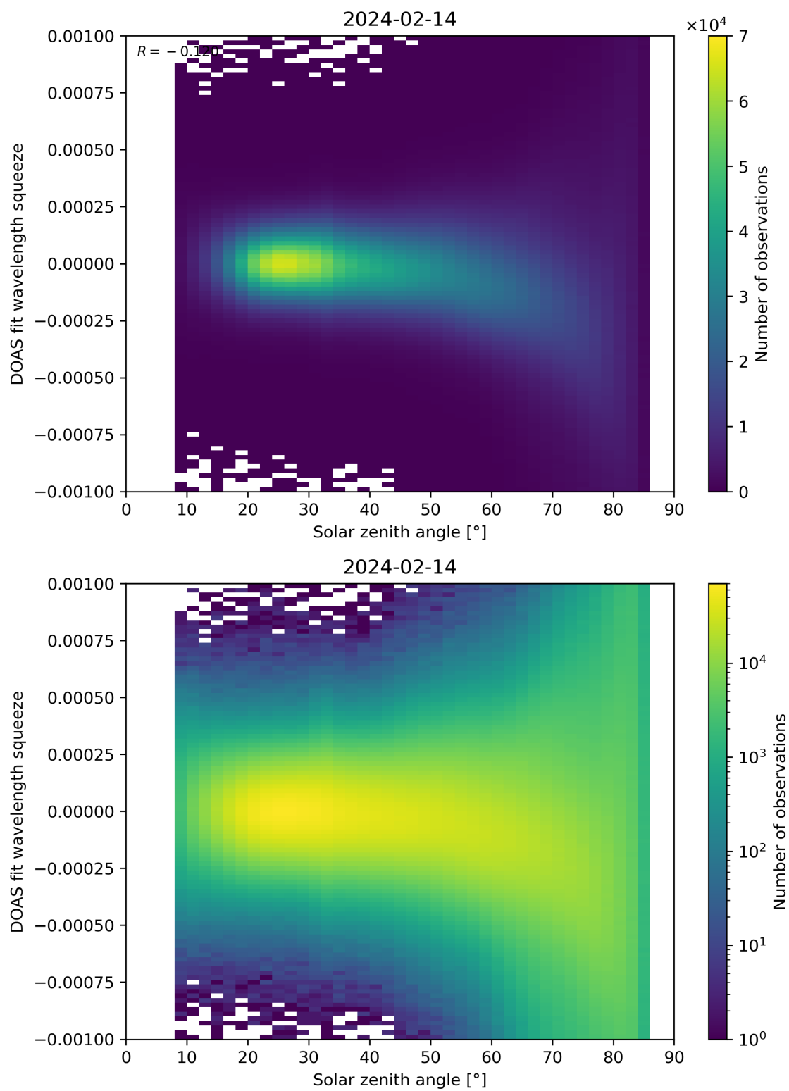
Figure 162: Scatter density plot of “Solar zenith angle” against “DOAS fit wavelength squeeze” for 2024-02-13 to 2024-02-15.
