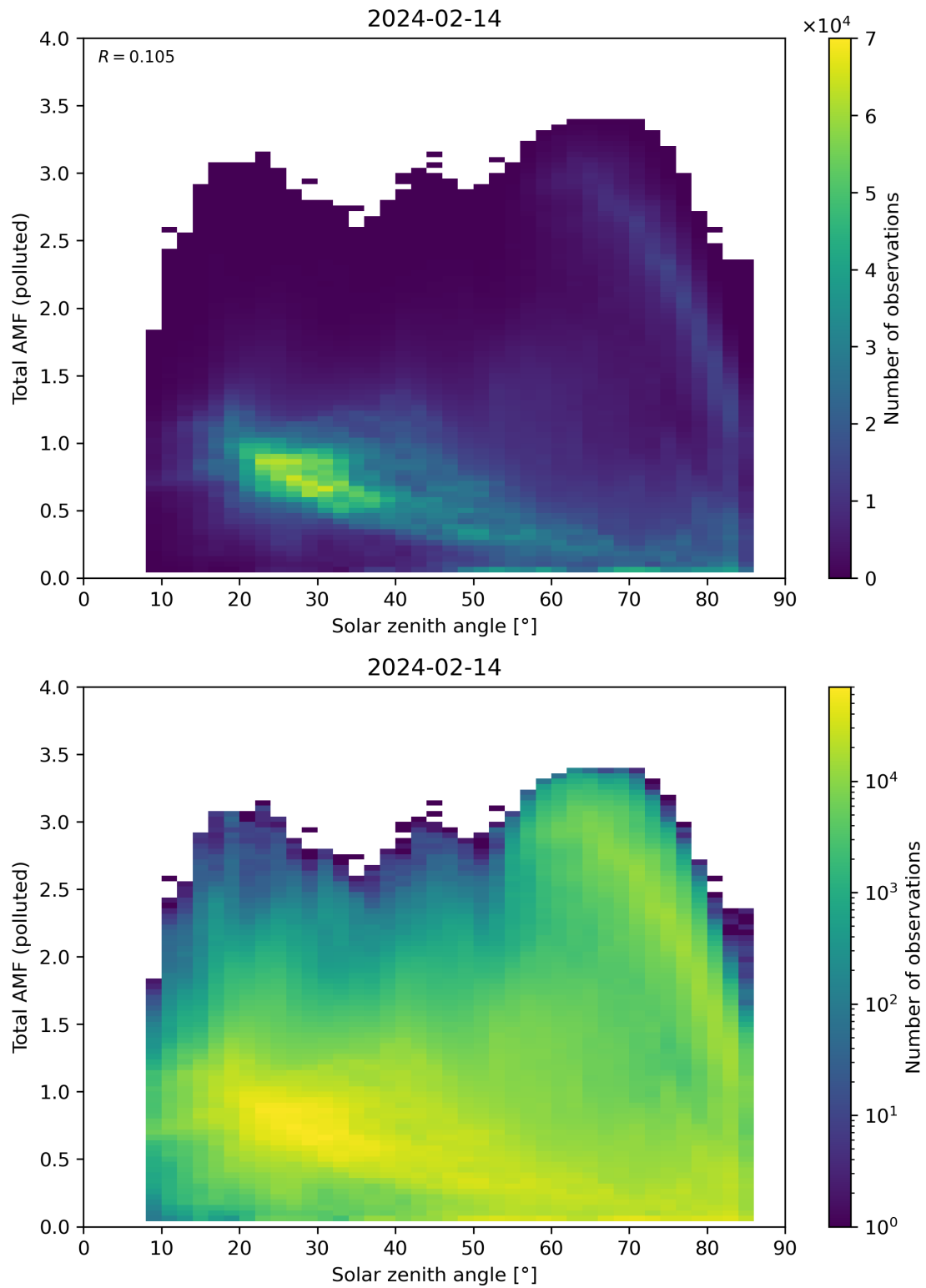
Figure 174: Scatter density plot of “Solar zenith angle” against “Total AMF (polluted)” for 2024-02-13 to 2024-02-15.
