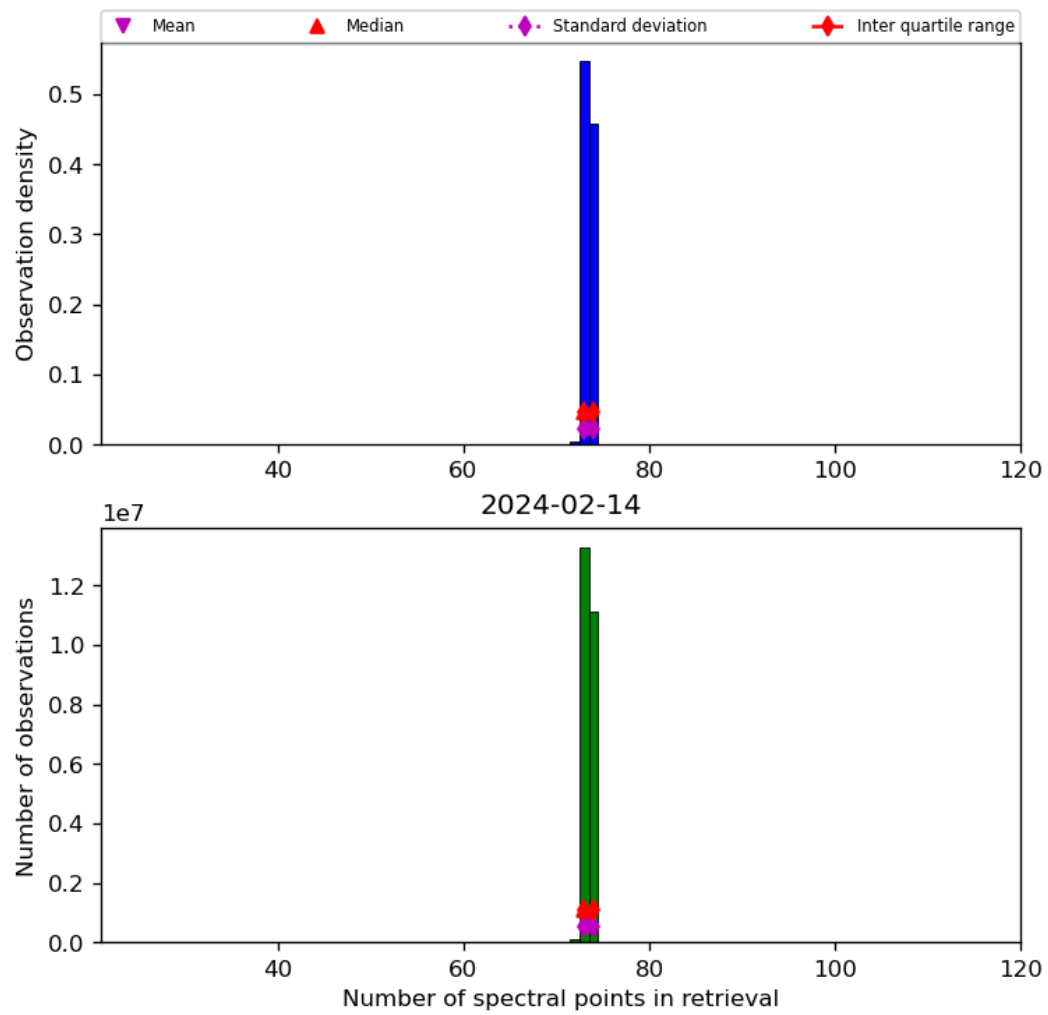
Figure 74: Histogram of “Number of spectral points in retrieval” for 2024-02-13 to 2024-02-15
