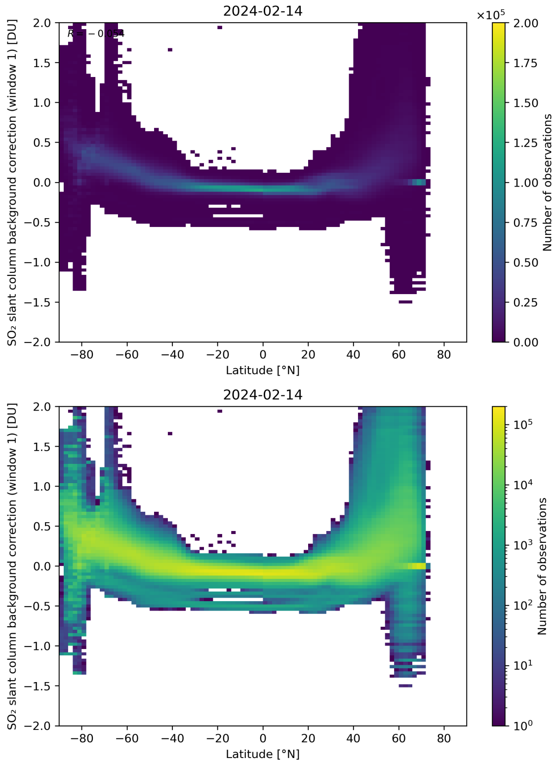
Figure 139: Scatter density plot of “Latitude” against “SO 2 slant column background correction (window 1)” for 2024-02-13 to 2024-02-15.
