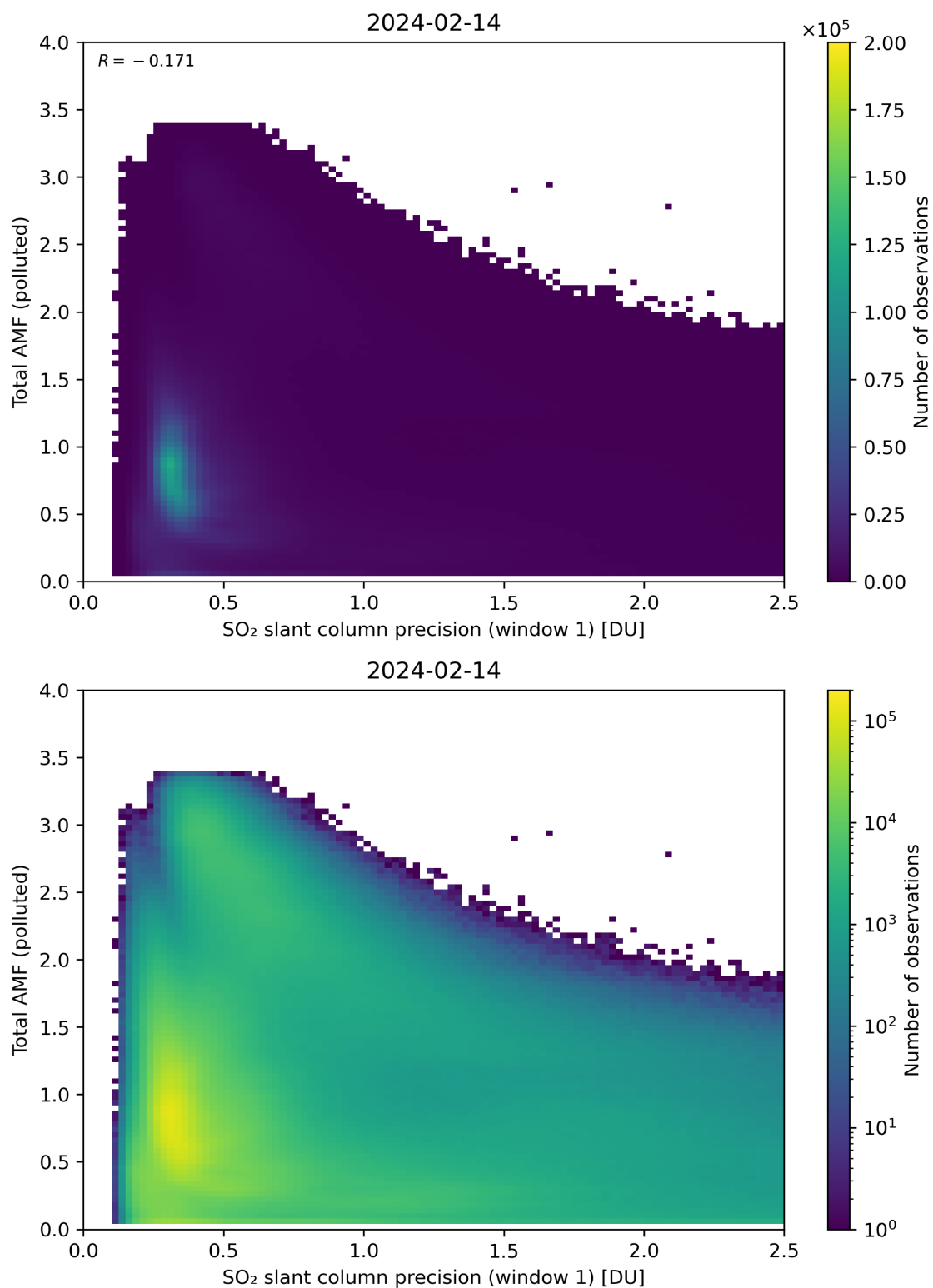
Figure 230: Scatter density plot of “SO 2 slant column precision (window 1)” against “Total AMF (polluted)” for 2024-02-13 to 2024-02-15.
