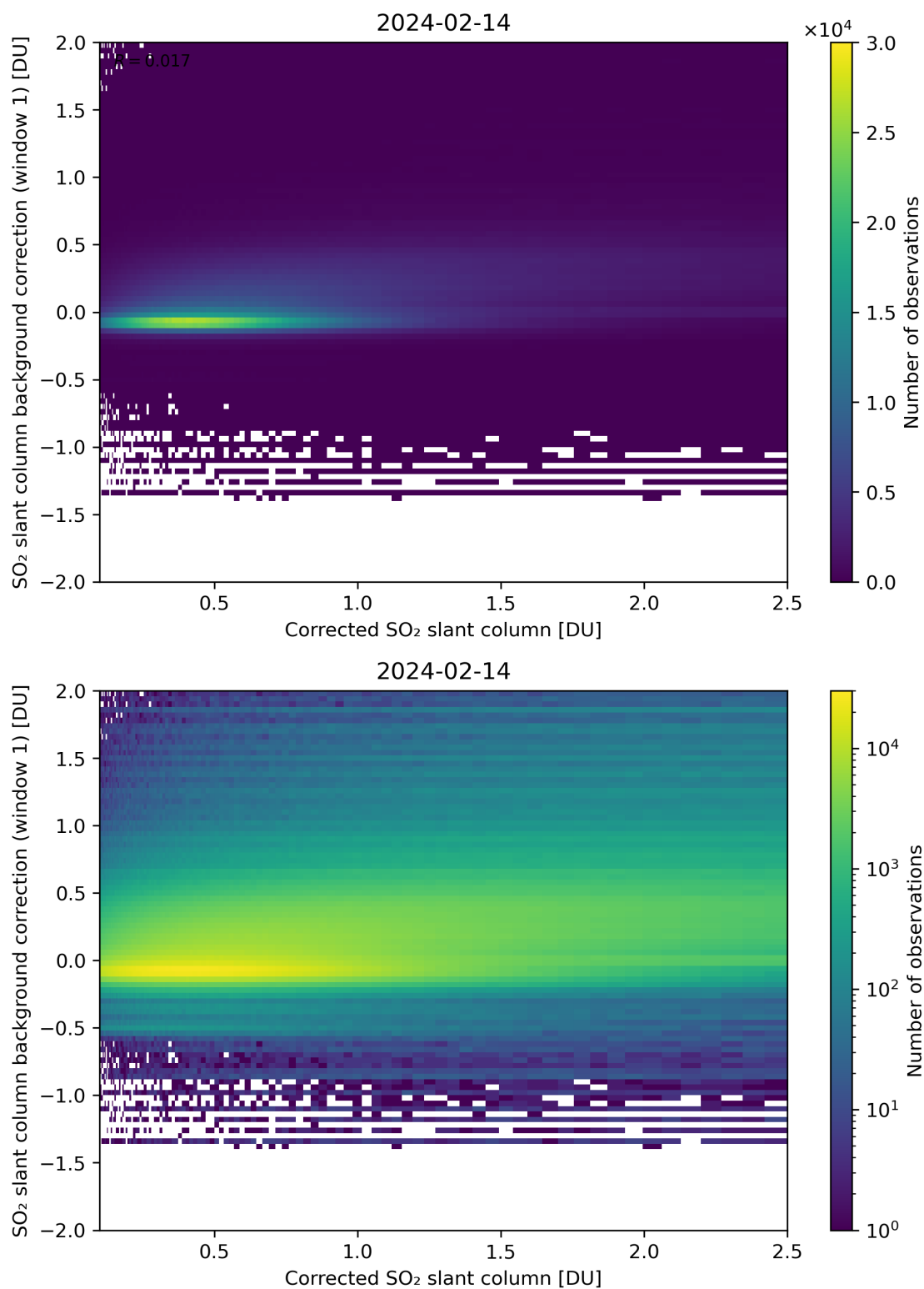
Figure 178: Scatter density plot of “Corrected SO 2 slant column” against “SO 2 slant column background correction (window 1)” for 2024-02-13 to 2024-02-15.
