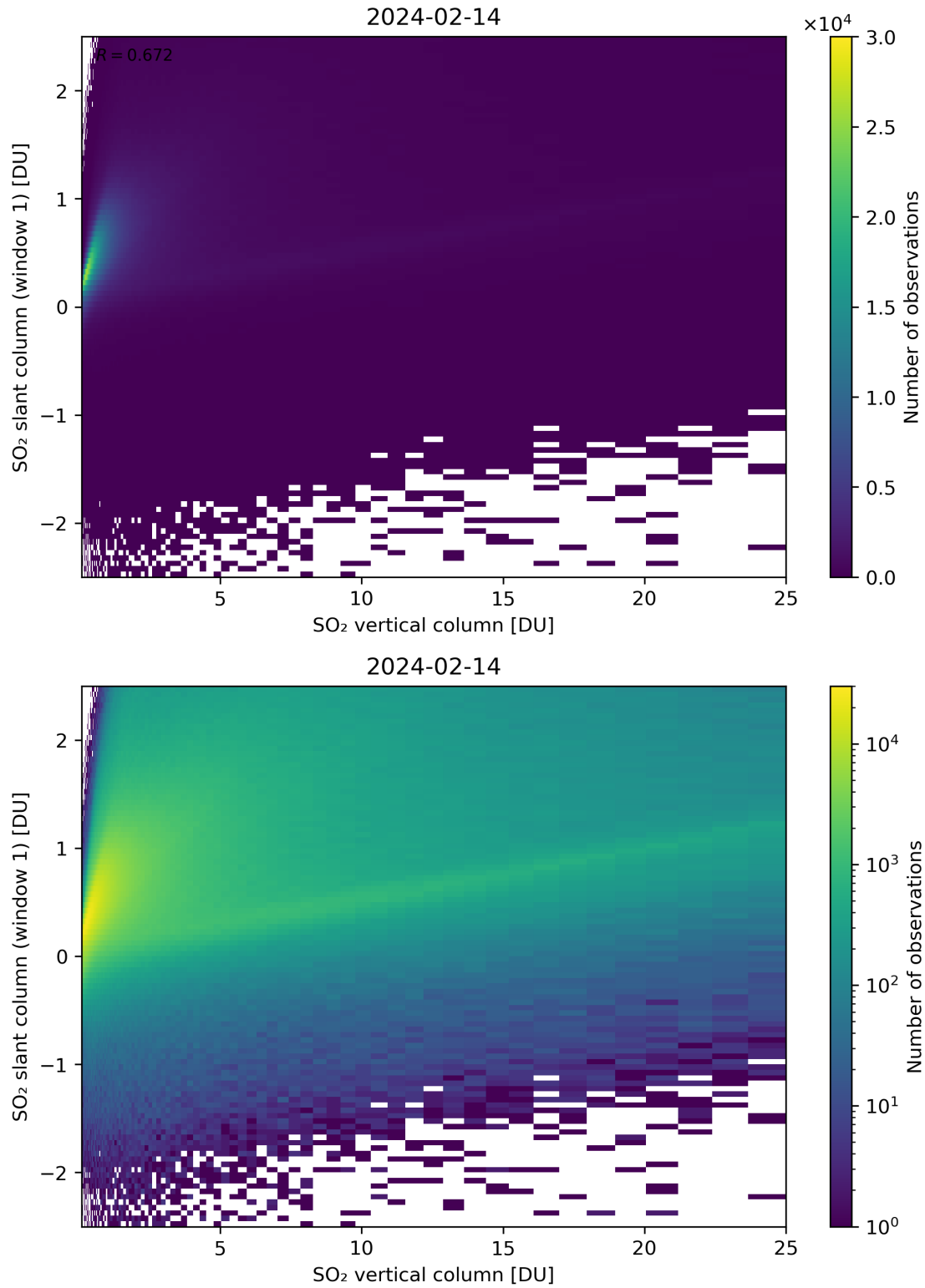
Figure 300: Scatter density plot of “SO 2 vertical column” against “SO 2 slant column (window 1)” for 2024-02-13 to 2024-02-15.
