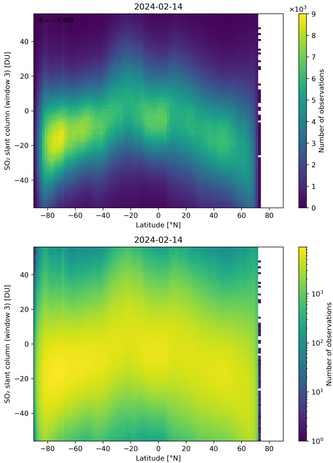
Figure 152: Scatter density plot of “Latitude” against “SO 2 slant column (window 3)” for 2024-02-13 to 2024-02-15.
