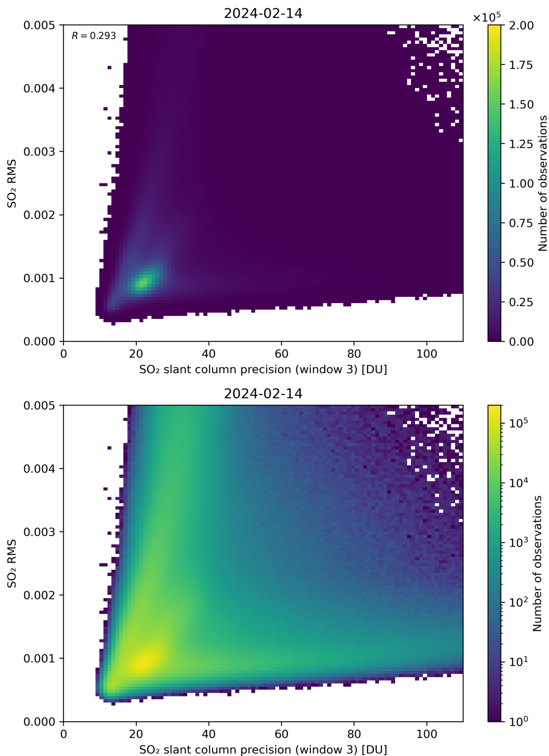
Figure 260: Scatter density plot of “SO 2 slant column precision (window 3)” against “SO 2 RMS” for 2024-02-13 to 2024-02-15.
