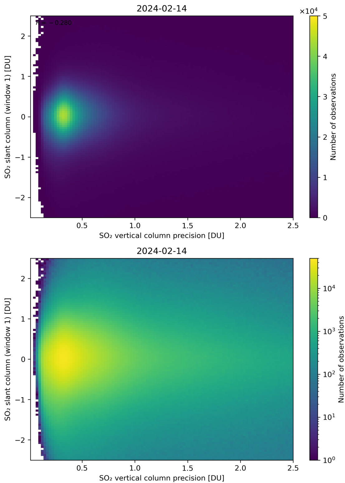
Figure 289: Scatter density plot of “SO 2 vertical column precision” against “SO 2 slant column (window 1)” for 2024-02-13 to 2024-02-15.
