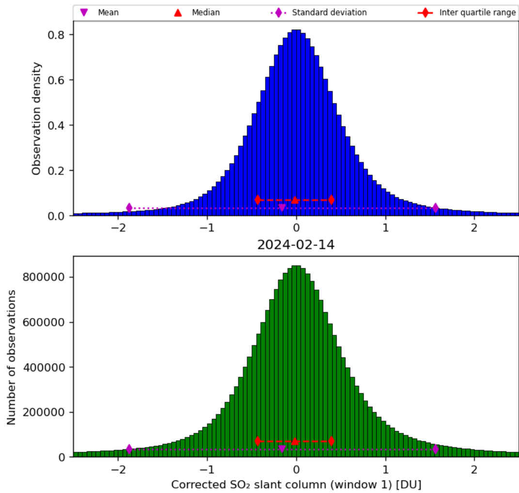
Figure 58: Histogram of “Corrected SO 2 slant column (window 1)” for 2024-02-13 to 2024-02-15
