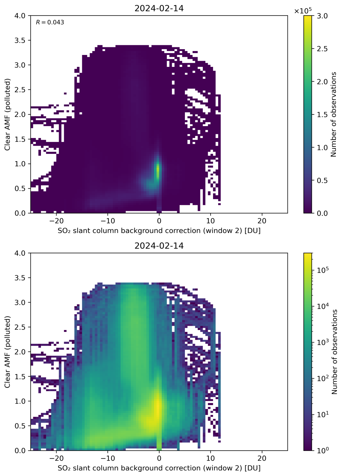
Figure 115: Scatter density plot of “SO 2 slant column background correction (window 2)” against “Clear AMF (polluted)” for 2024-02-13 to 2024-02-15.
