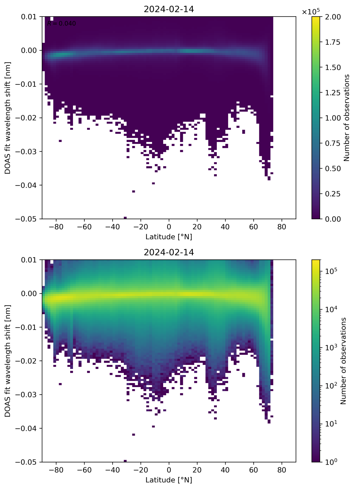
Figure 142: Scatter density plot of “Latitude” against “DOAS fit wavelength shift” for 2024-02-13 to 2024-02-15.
