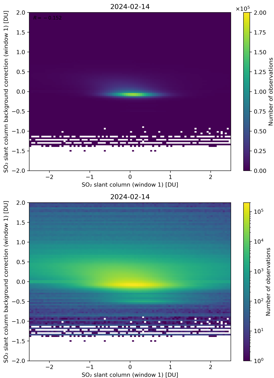
Figure 212: Scatter density plot of “SO 2 slant column (window 1)” against “SO 2 slant column background correction (window 1)” for 2024-02-13 to 2024-02-15.
