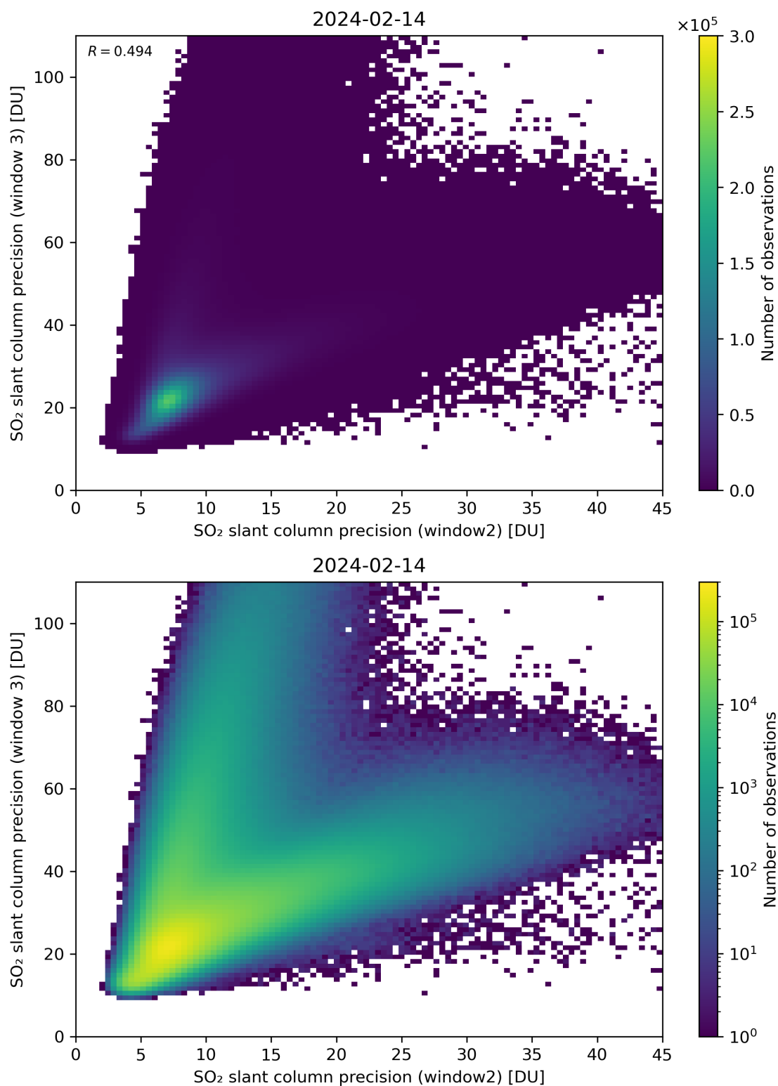
Figure 250: Scatter density plot of “SO 2 slant column precision (window2)” against “SO 2 slant column precision (window 3)” for 2024-02-13 to 2024-02-15.
