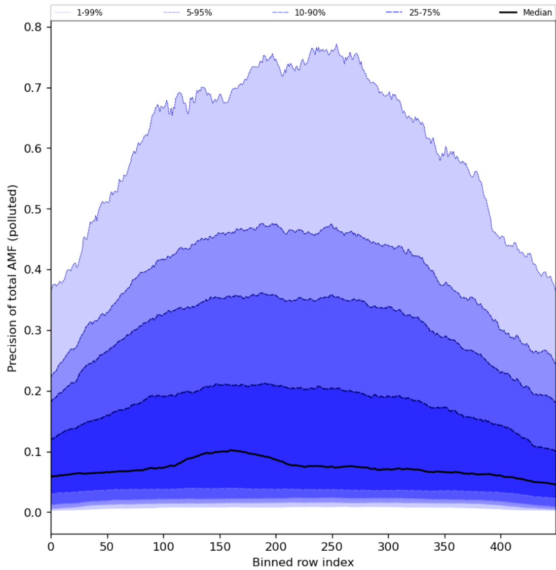
Figure 95: Along track statistics of “Precision of total AMF (polluted)” for 2024-02-13 to 2024-02-15
