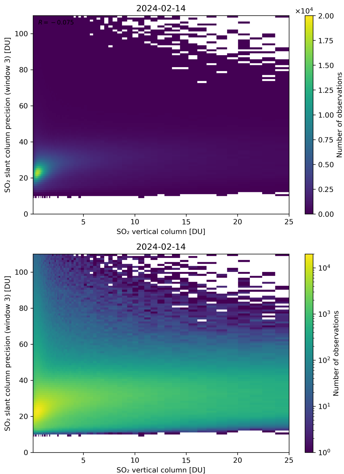
Figure 304: Scatter density plot of “SO 2 vertical column” against “SO 2 slant column precision (window 3)” for 2024-02-13 to 2024-02-15.
