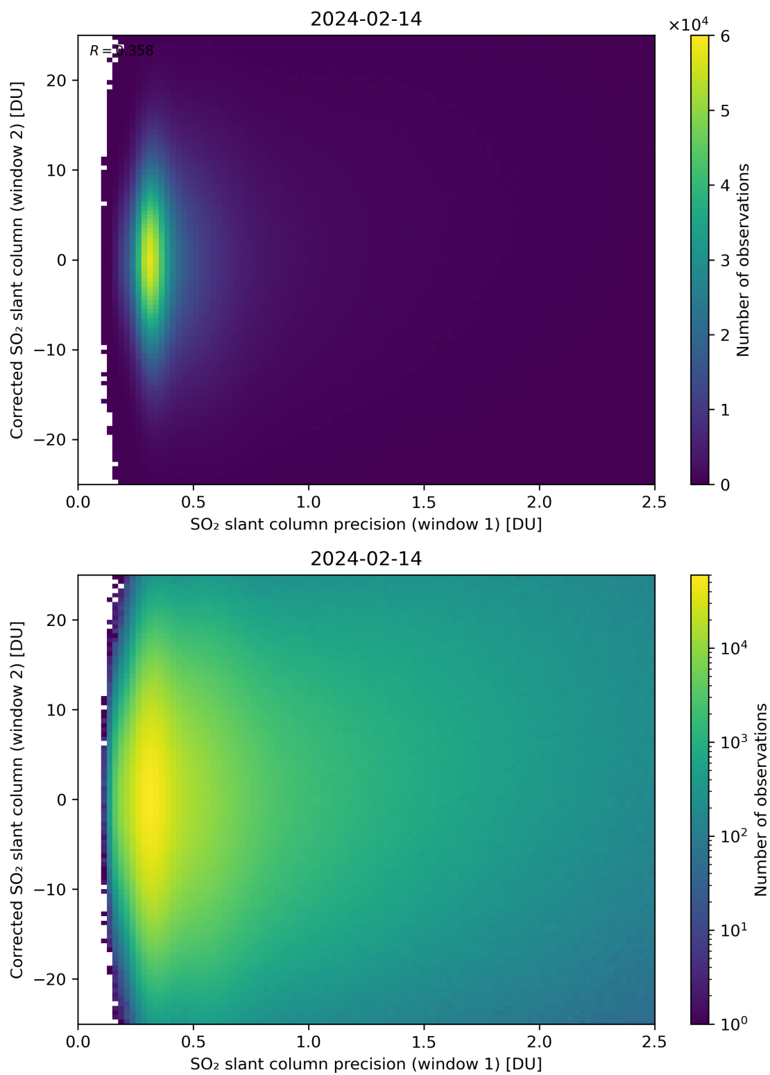
Figure 225: Scatter density plot of “SO 2 slant column precision (window 1)” against “Corrected SO 2 slant column (window 2)” for 2024-02-13 to 2024-02-15.
