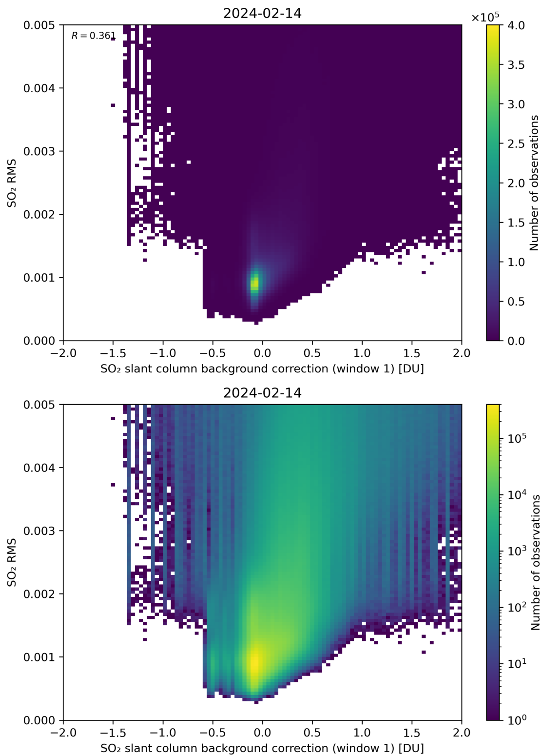
Figure 102: Scatter density plot of “SO 2 slant column background correction (window 1)” against “SO 2 RMS” for 2024-02-13 to 2024-02-15.
