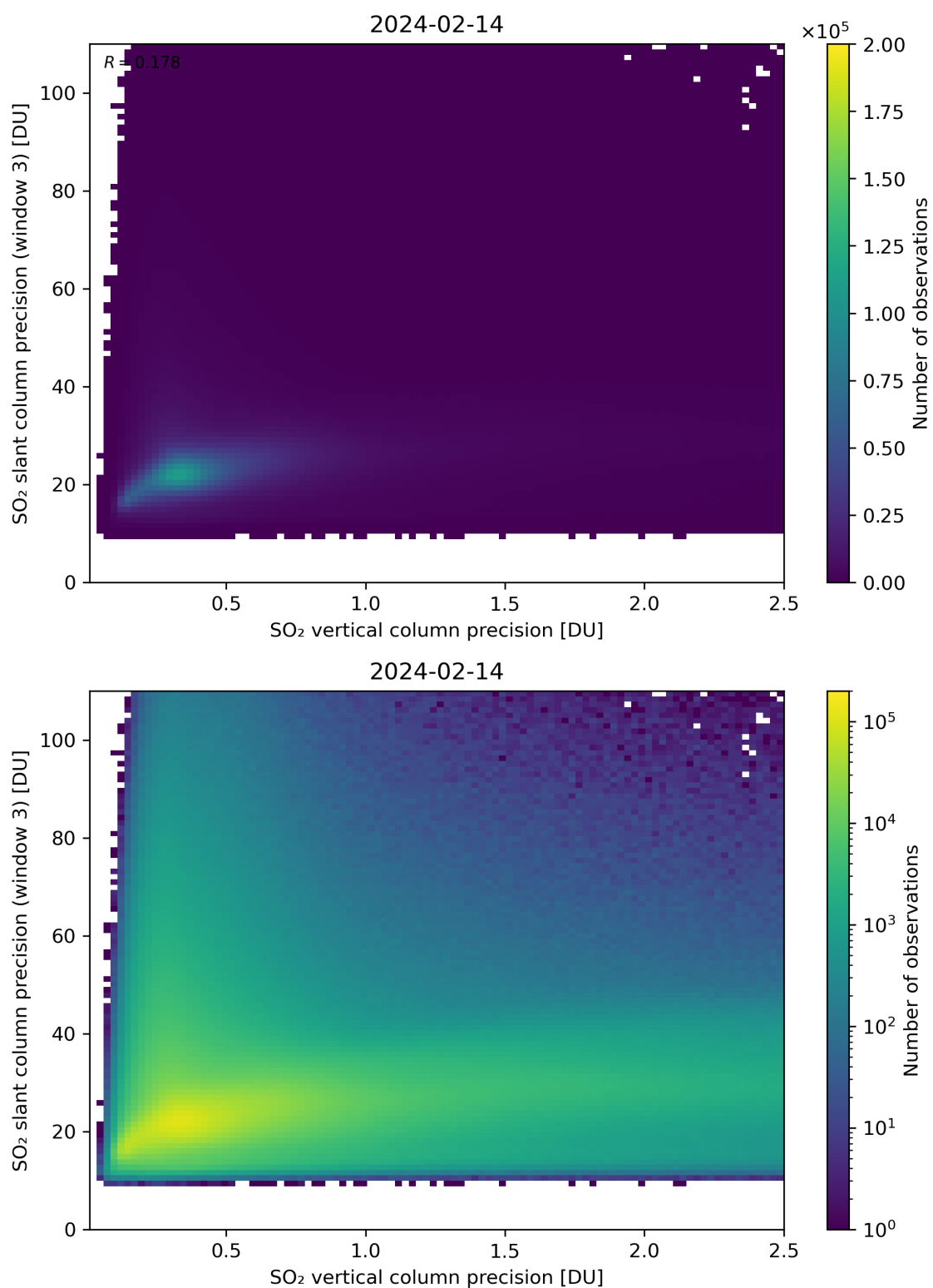
Figure 293: Scatter density plot of “SO 2 vertical column precision” against “SO 2 slant column precision (window 3)” for 2024-02-13 to 2024-02-15.
