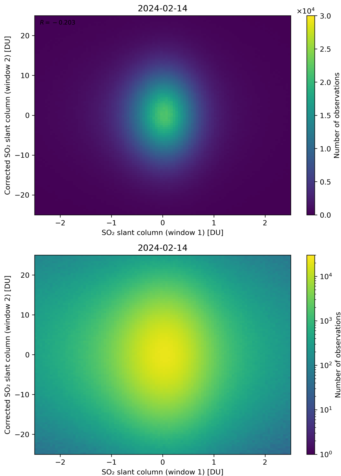
Figure 233: Scatter density plot of “SO 2 slant column (window 1)” against “Corrected SO 2 slant column (window 2)” for 2024-02-13 to 2024-02-15.
