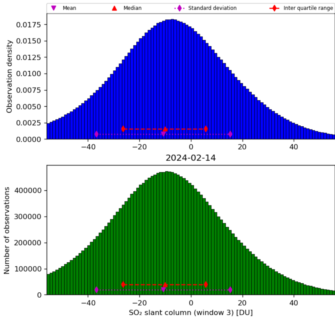
Figure 64: Histogram of “SO 2 slant column (window 3)” for 2024-02-13 to 2024-02-15
