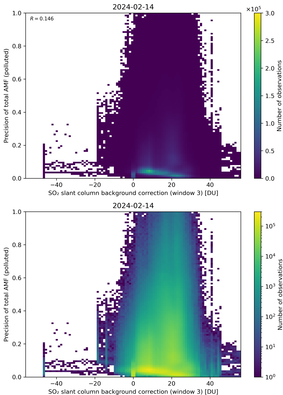
Figure 126: Scatter density plot of “SO 2 slant column background correction (window 3)” against “Precision of total AMF (polluted)” for 2024-02-13 to 2024-02-15.
