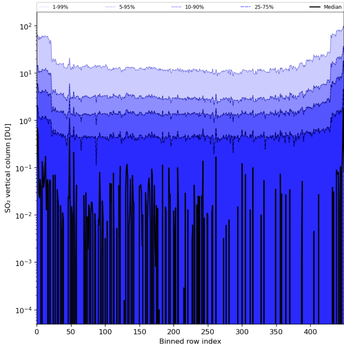
Figure 76: Along track statistics of “SO 2 vertical column” for 2024-02-13 to 2024-02-15
