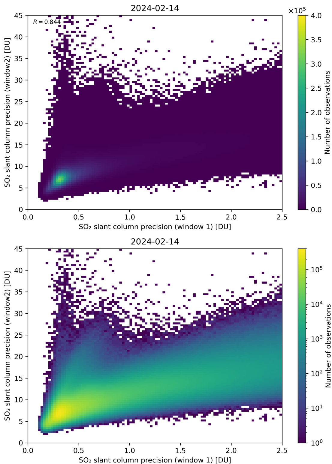
Figure 227: Scatter density plot of “SO 2 slant column precision (window 1)” against “SO 2 slant column precision (window 2)” for 2024-02-13 to 2024-02-15.
