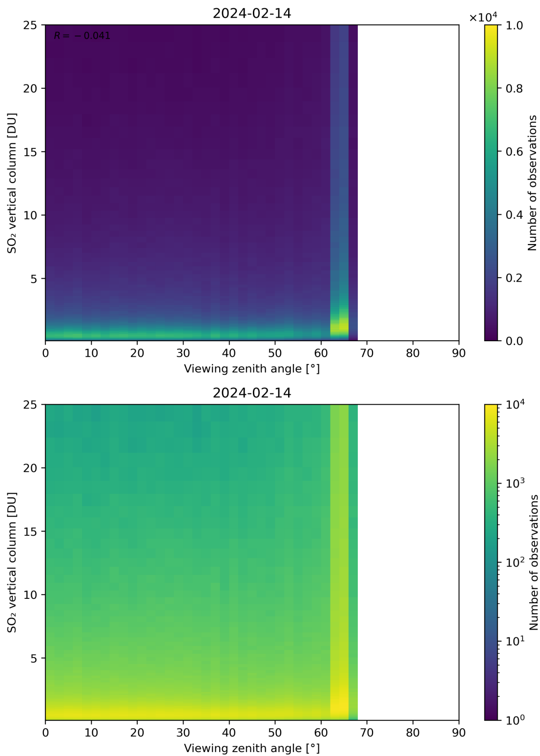
Figure 327: Scatter density plot of “Viewing zenith angle” against “SO 2 vertical column” for 2024-02-13 to 2024-02-15.
