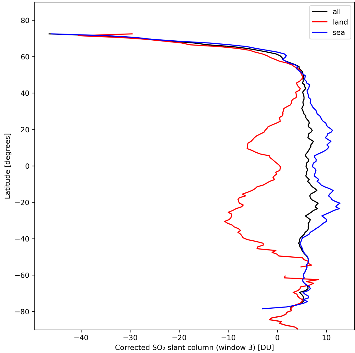
Figure 43: Zonal average of “Corrected SO 2 slant column (window 3)” for 2024-02-13 to 2024-02-15.
