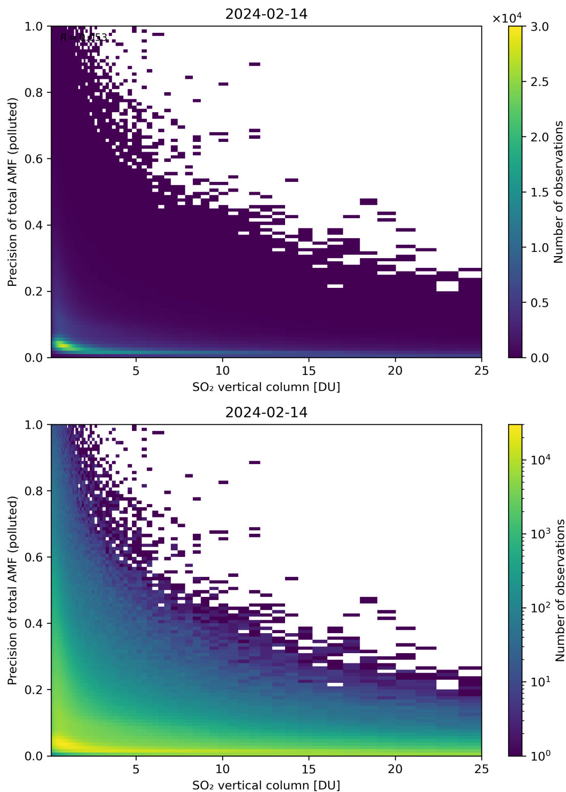
Figure 306: Scatter density plot of “SO 2 vertical column” against “Precision of total AMF (polluted)” for 2024-02-13 to 2024-02-15.
