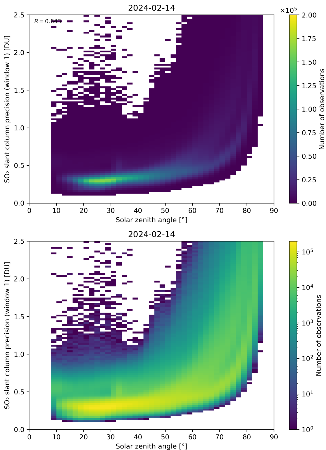
Figure 170: Scatter density plot of “Solar zenith angle” against “SO 2 slant column precision (window 1)” for 2024-02-13 to 2024-02-15.
