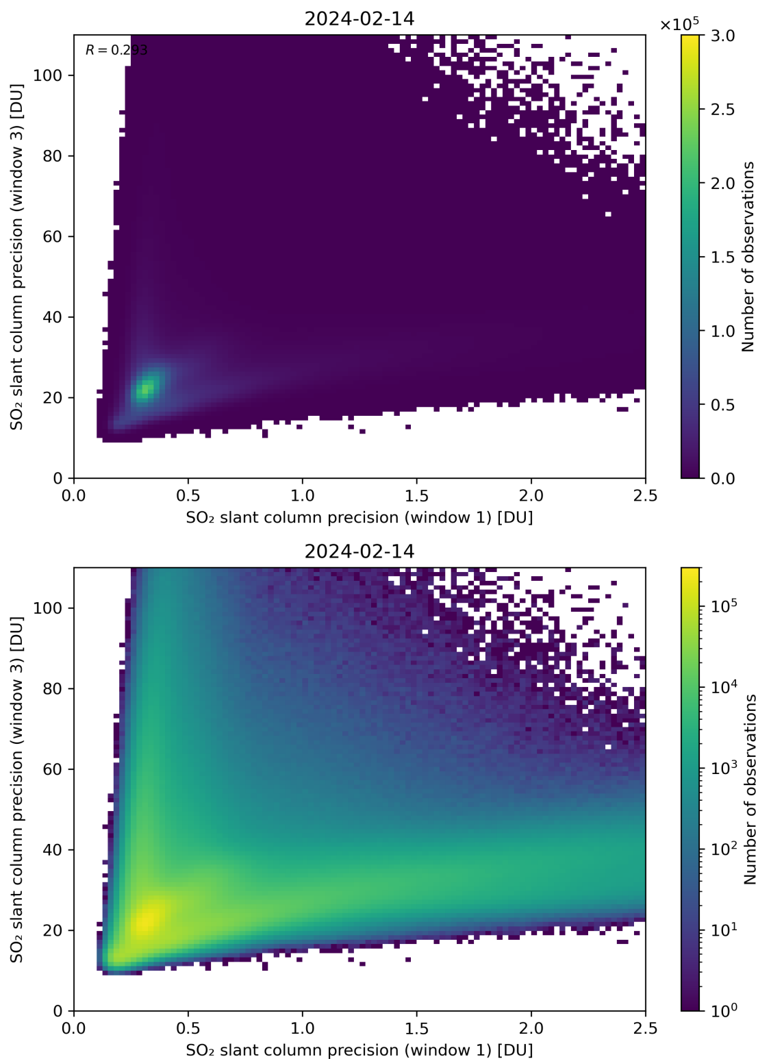
Figure 229: Scatter density plot of “SO 2 slant column precision (window 1)” against “SO 2 slant column precision (window 3)” for 2024-02-13 to 2024-02-15.
