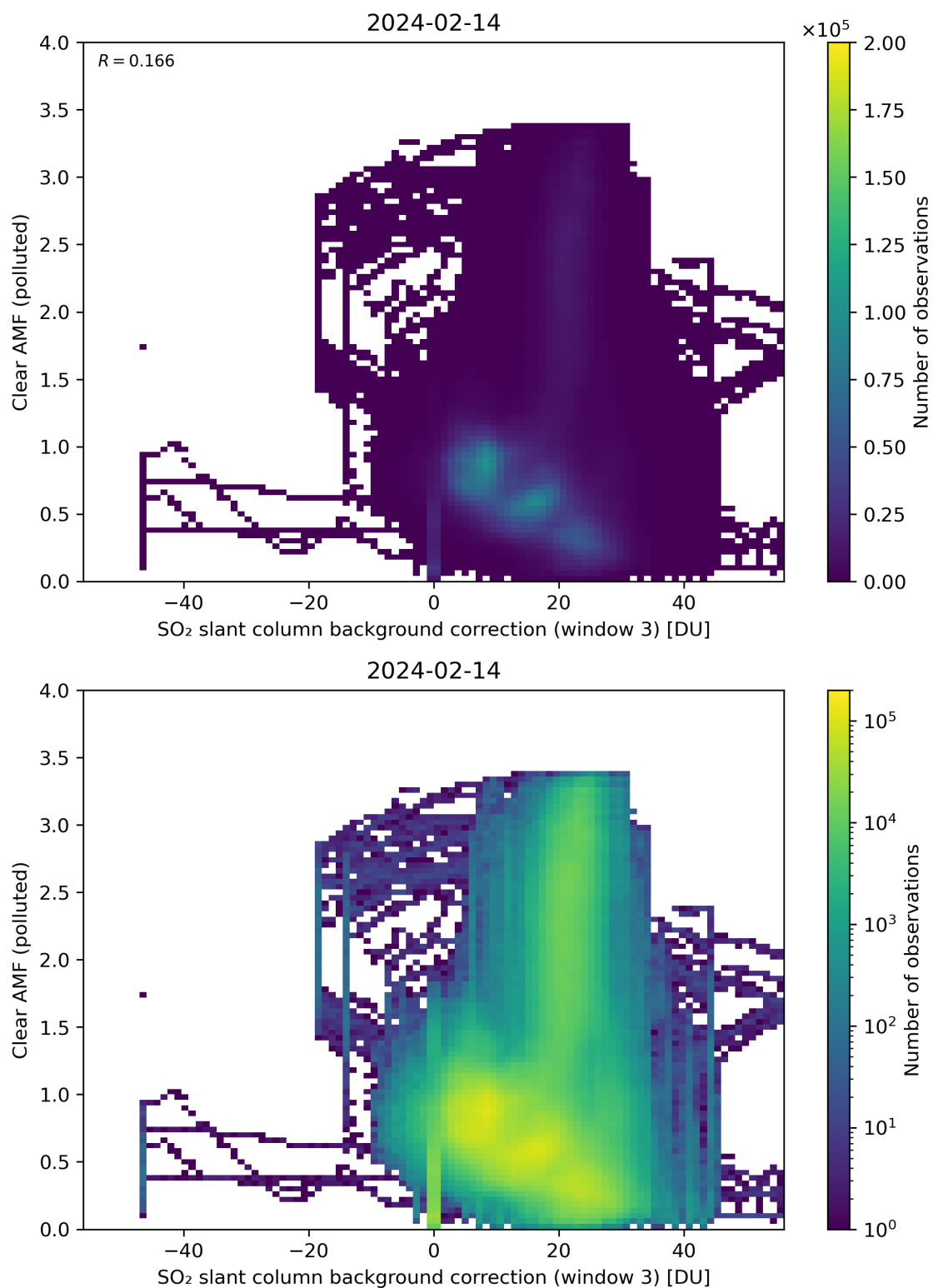
Figure 124: Scatter density plot of “SO 2 slant column background correction (window 3)” against “Clear AMF (polluted)” for 2024-02-13 to 2024-02-15.
