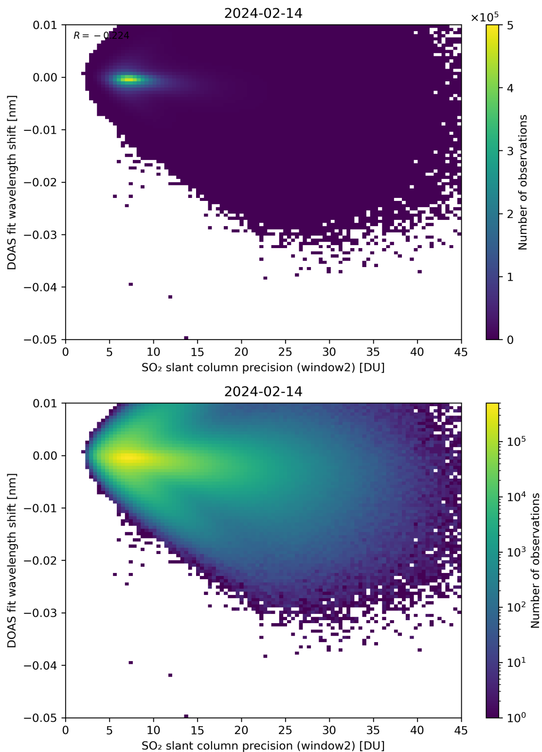
Figure 243: Scatter density plot of “SO 2 slant column precision (window2)” against “DOAS fit wavelength shift” for 2024-02-13 to 2024-02-15.
