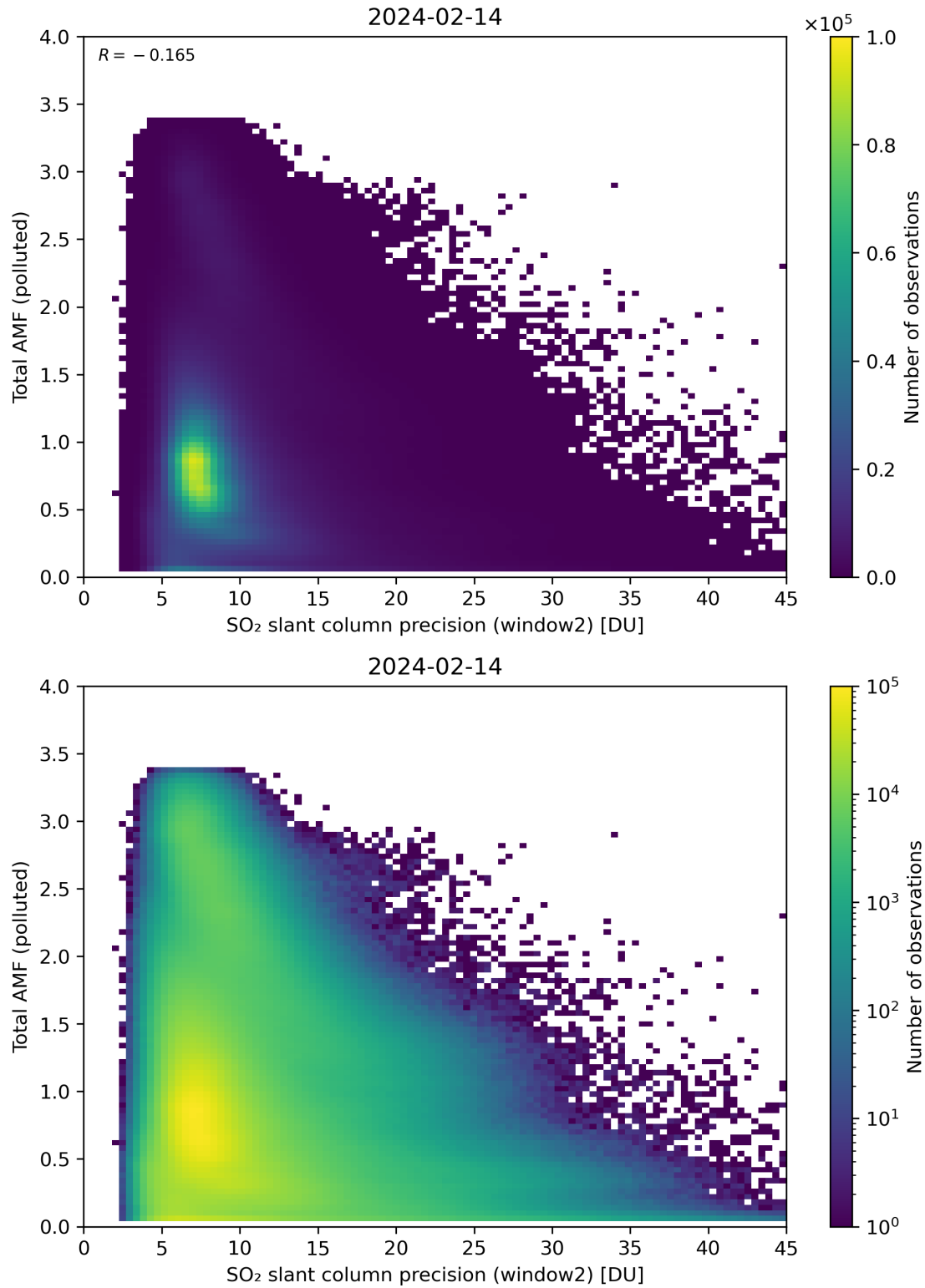
Figure 251: Scatter density plot of “SO 2 slant column precision (window2)” against “Total AMF (polluted)” for 2024-02-13 to 2024-02-15.
