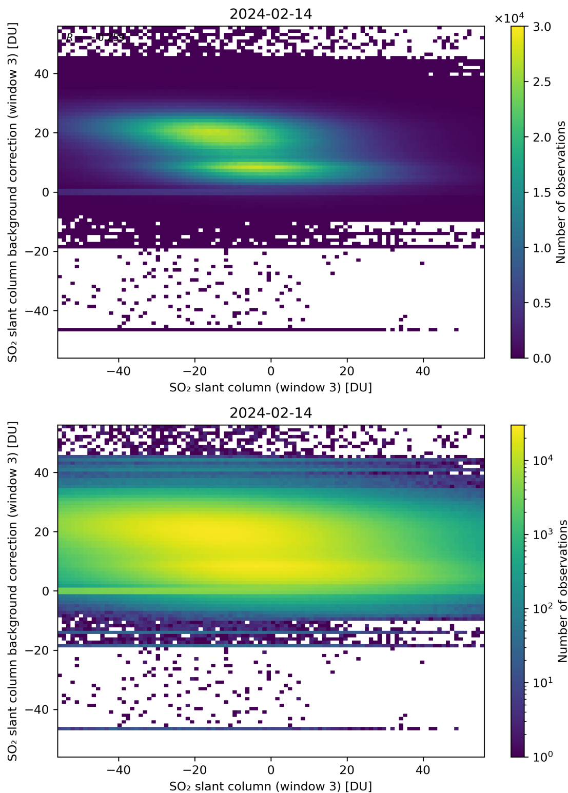
Figure 253: Scatter density plot of “SO 2 slant column (window 3)” against “SO 2 slant column background correction (window 3)” for 2024-02-13 to 2024-02-15.
