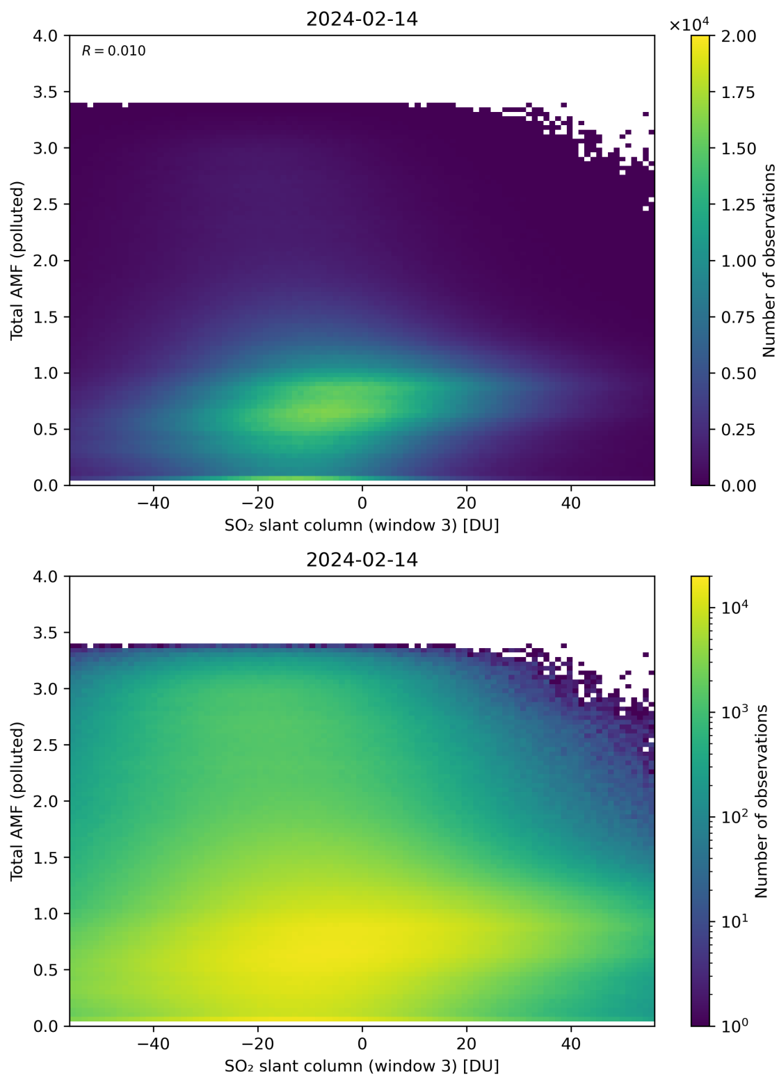
Figure 268: Scatter density plot of “SO 2 slant column (window 3)” against “Total AMF (polluted)” for 2024-02-13 to 2024-02-15.
