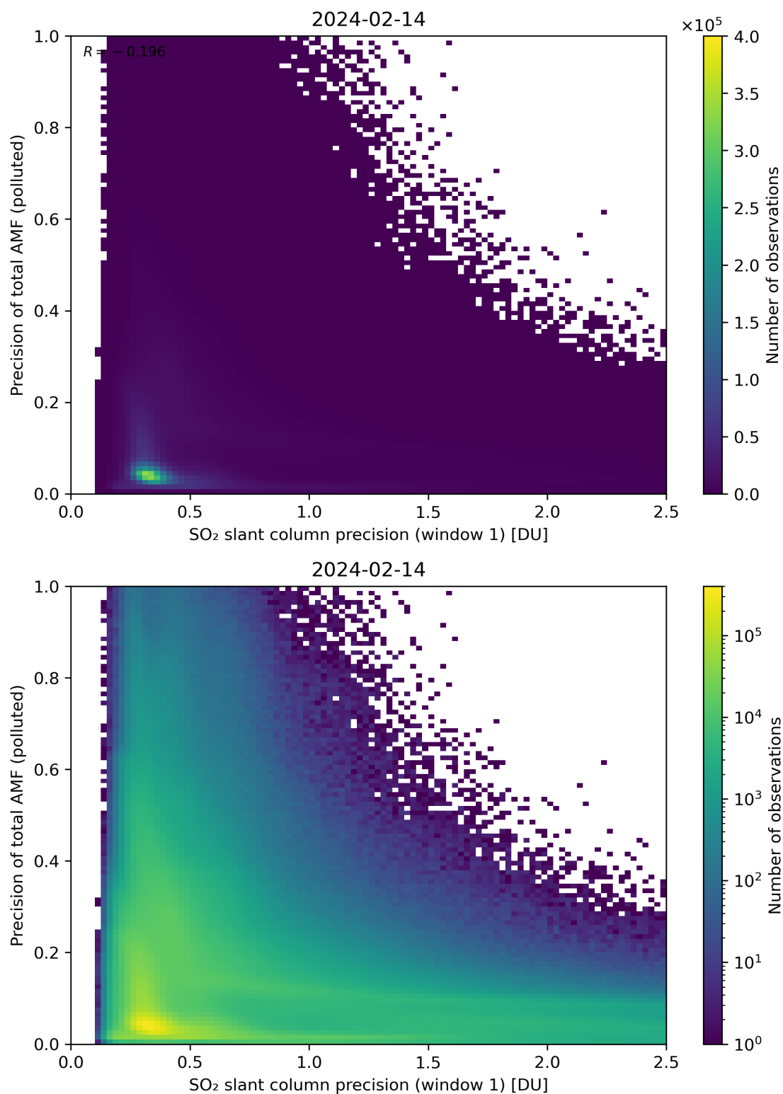
Figure 231: Scatter density plot of “SO 2 slant column precision (window 1)” against “Precision of total AMF (polluted)” for 2024-02-13 to 2024-02-15.
