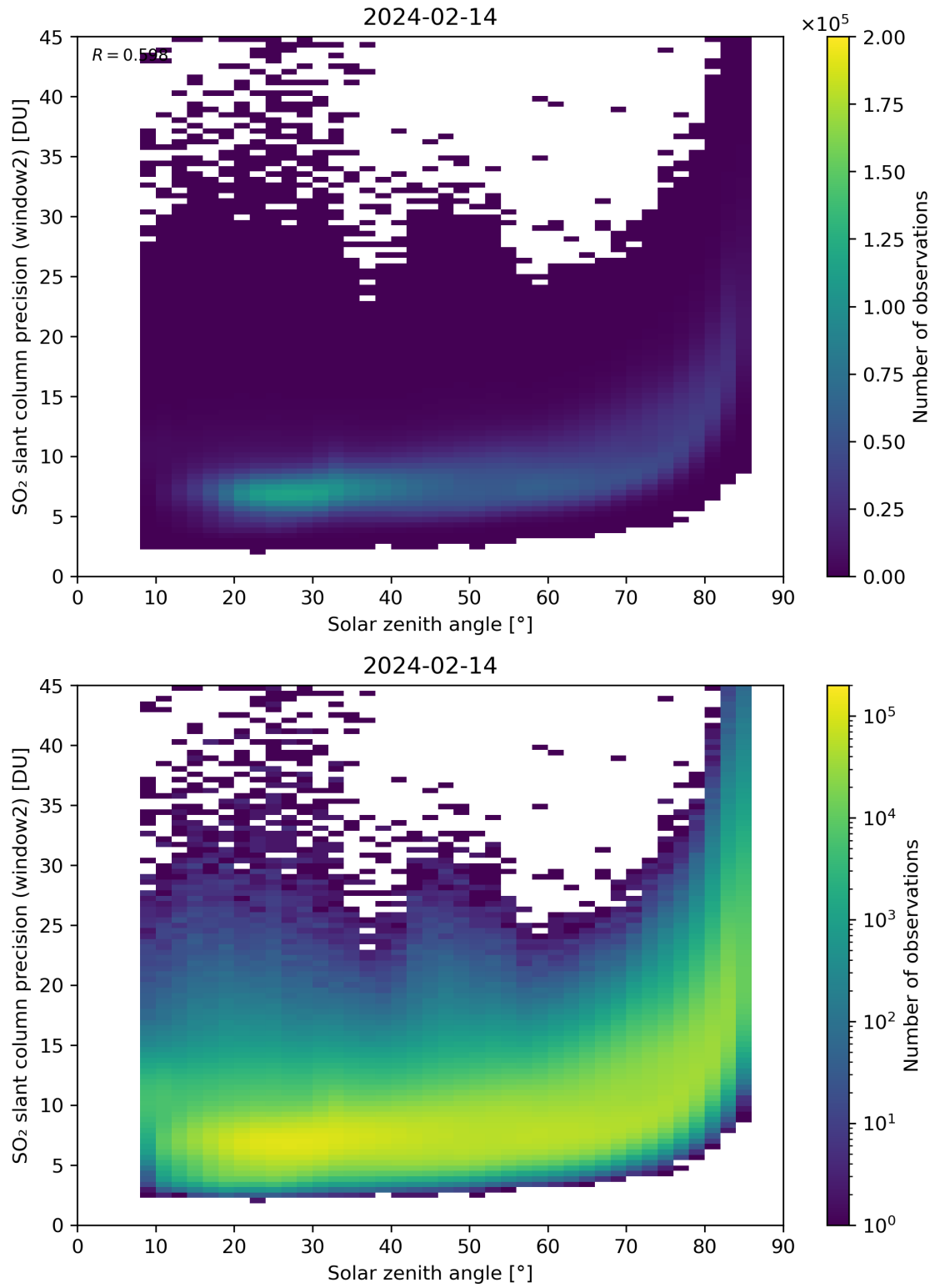
Figure 171: Scatter density plot of “Solar zenith angle” against “SO 2 slant column precision (window2)” for 2024-02-13 to 2024-02-15.
