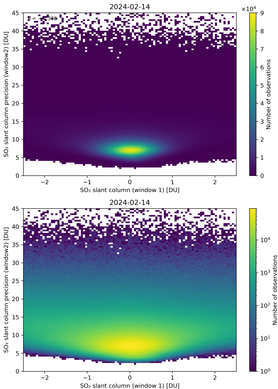
Figure 236: Scatter density plot of “SO 2 slant column (window 1)” against “SO 2 slant column precision (window2)” for 2024-02-13 to 2024-02-15.
