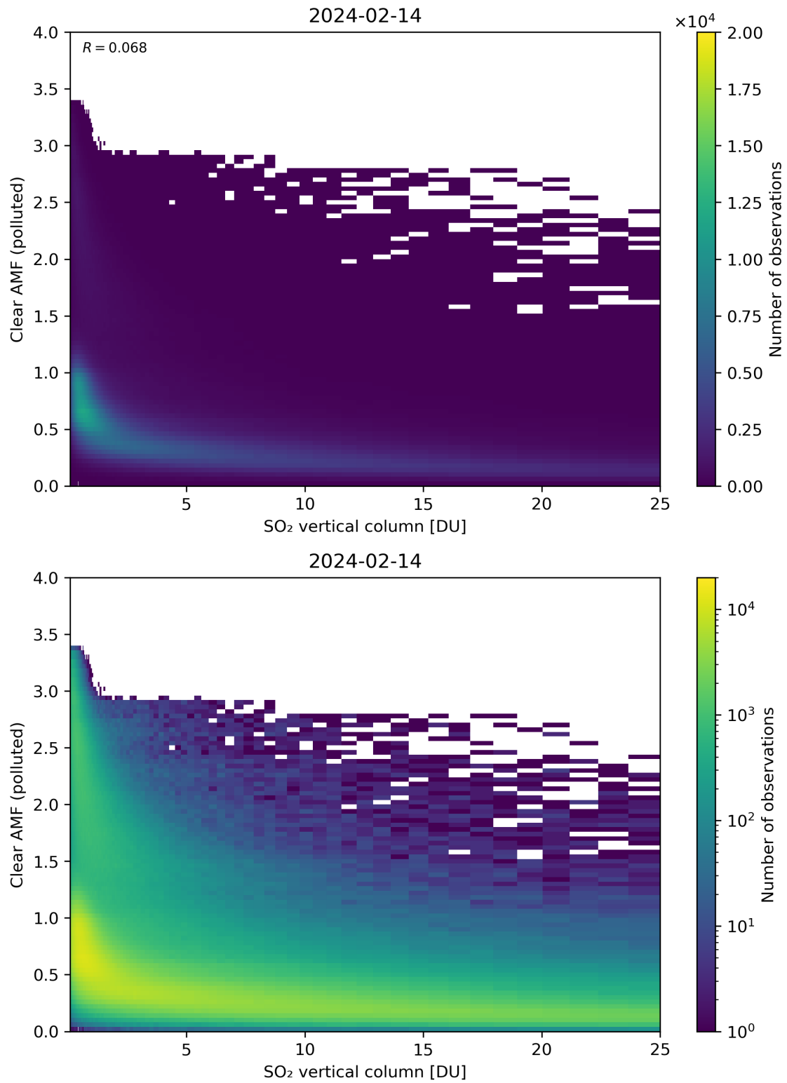
Figure 296: Scatter density plot of “SO 2 vertical column” against “Clear AMF (polluted)” for 2024-02-13 to 2024-02-15.
