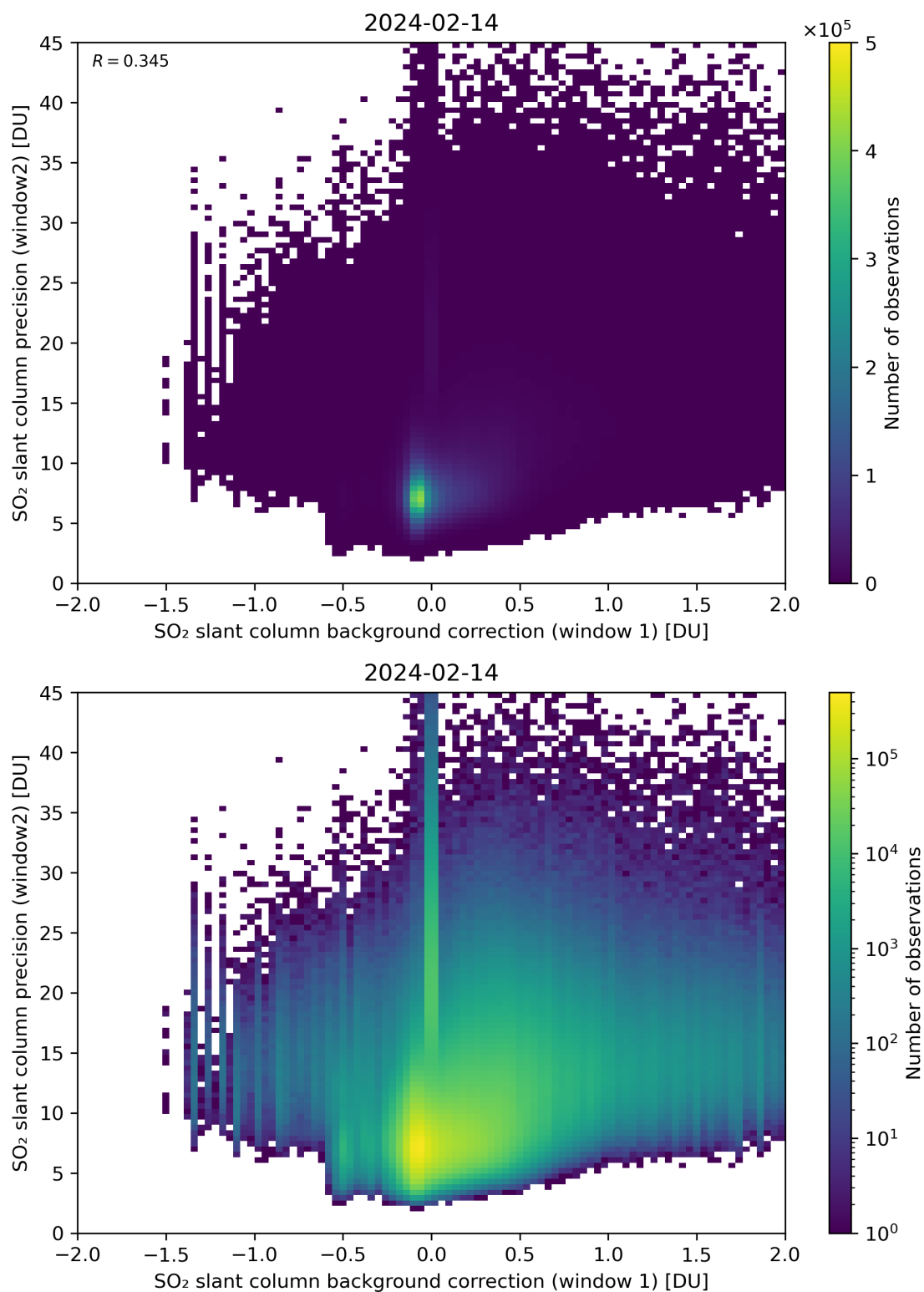
Figure 106: Scatter density plot of “SO 2 slant column background correction (window 1)” against “SO 2 slant column precision (window2)” for 2024-02-13 to 2024-02-15.
