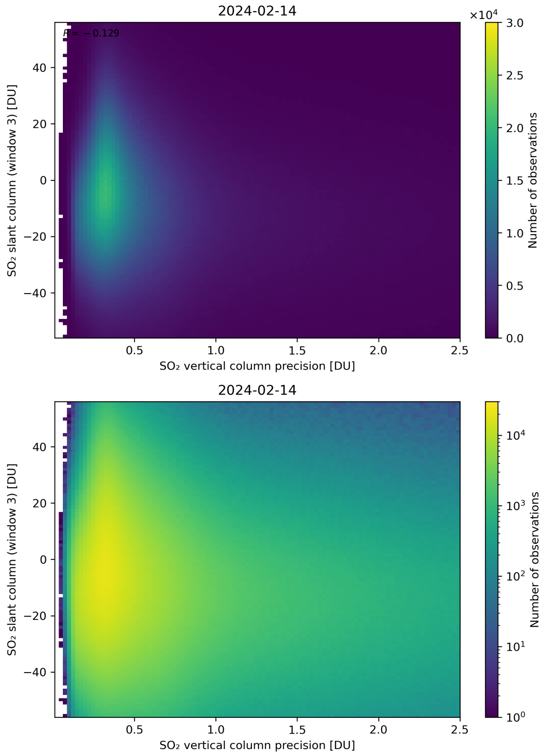
Figure 292: Scatter density plot of “SO 2 vertical column precision” against “SO 2 slant column (window 3)” for 2024-02-13 to 2024-02-15.
