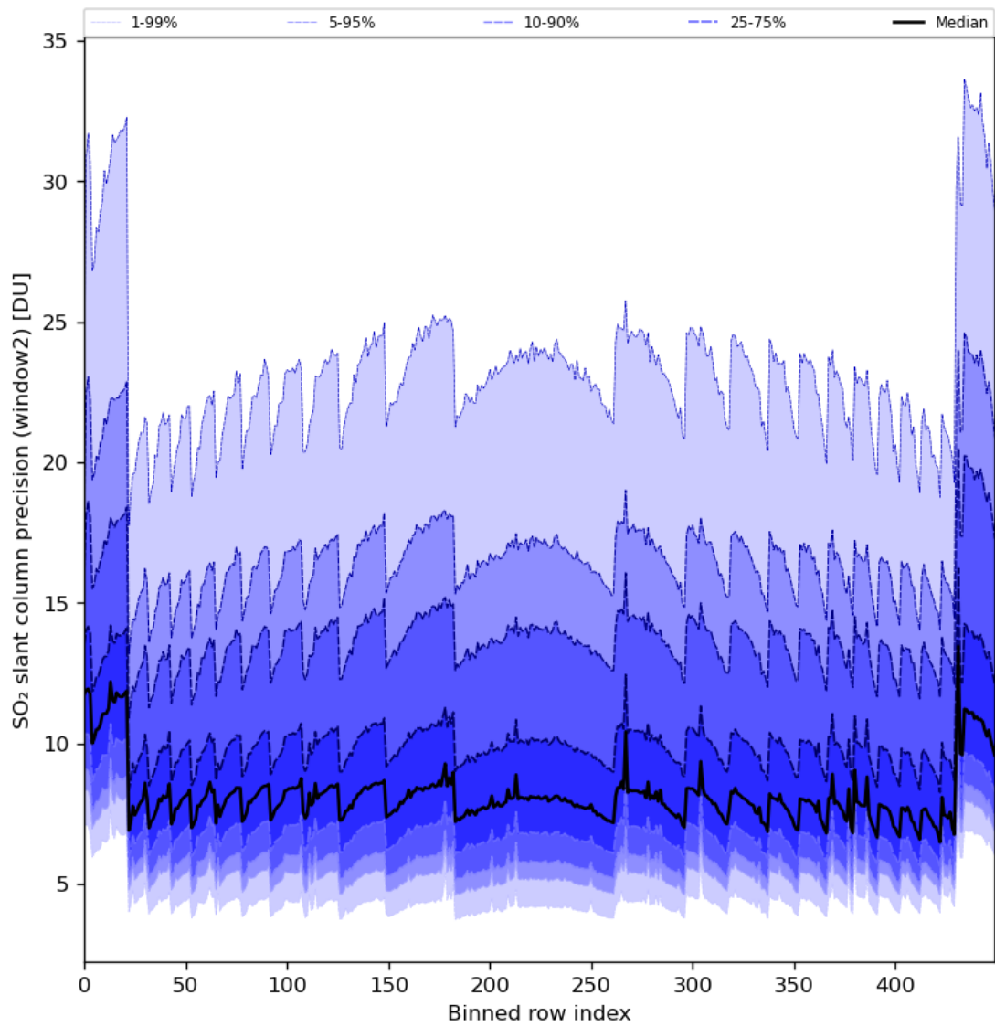
Figure 84: Along track statistics of “SO 2 slant column precision (window2)” for 2024-02-13 to 2024-02-15
