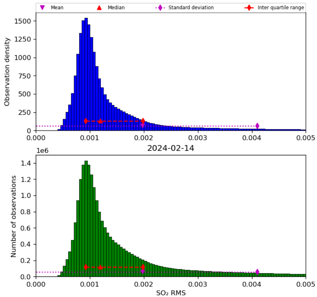
Figure 70: Histogram of “SO 2 RMS” for 2024-02-13 to 2024-02-15
