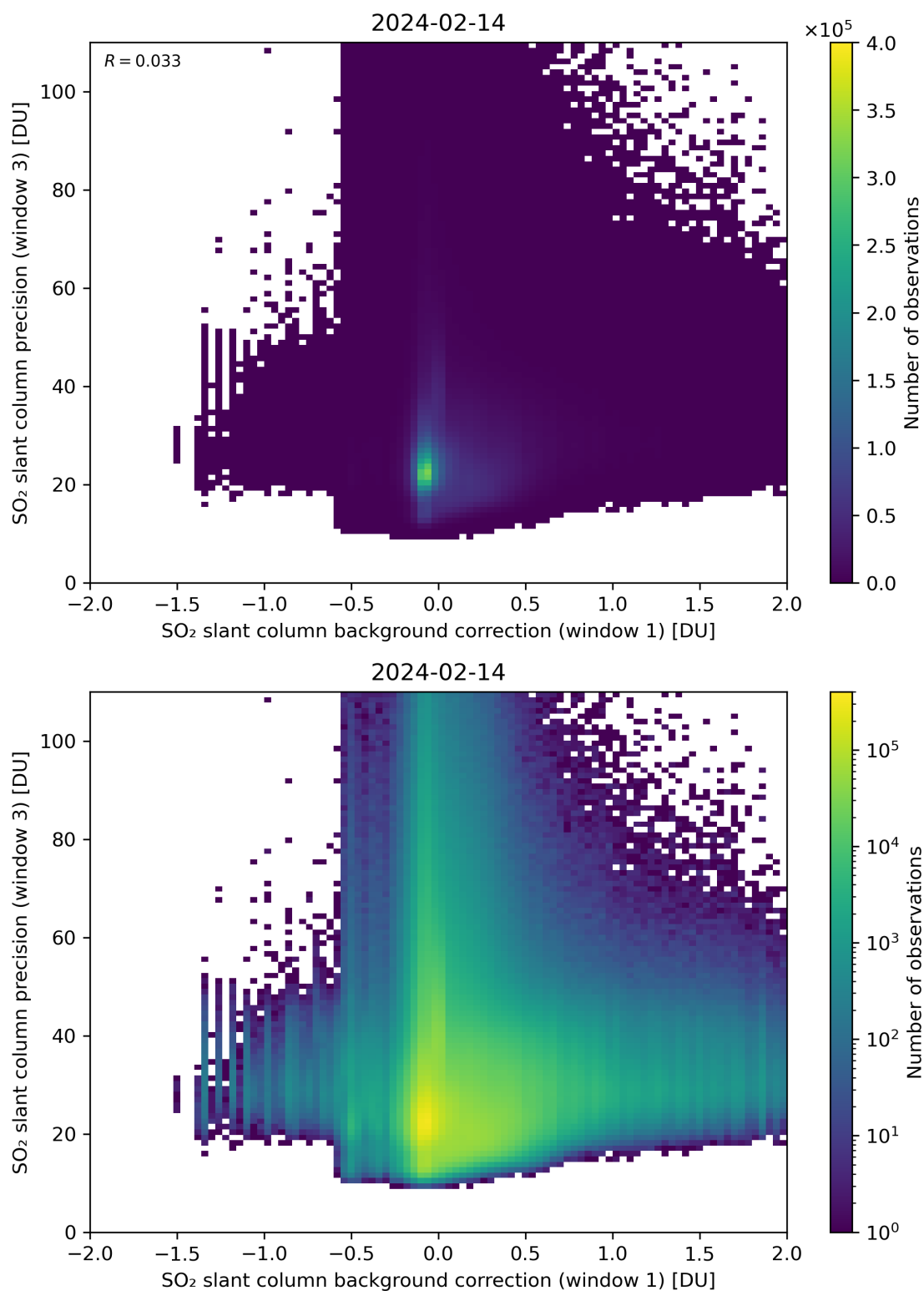
Figure 108: Scatter density plot of “SO 2 slant column background correction (window 1)” against “SO 2 slant column precision (window 3)” for 2024-02-13 to 2024-02-15.
