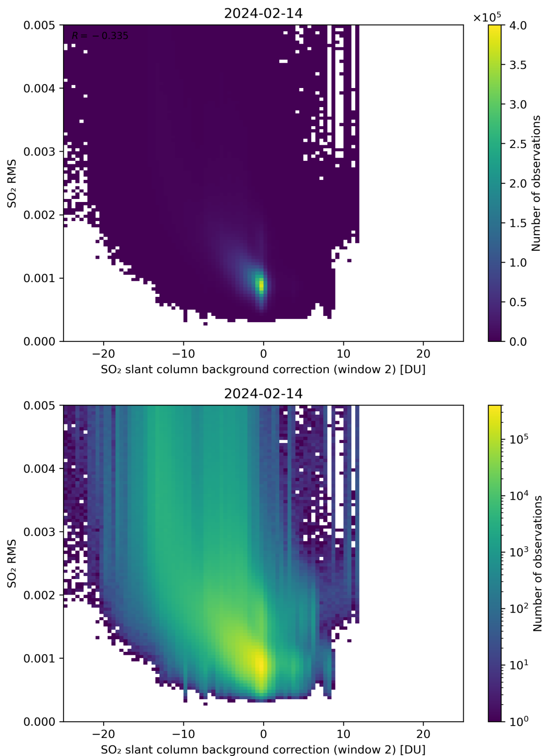
Figure 114: Scatter density plot of “SO 2 slant column background correction (window 2)” against “SO 2 RMS” for 2024-02-13 to 2024-02-15.
