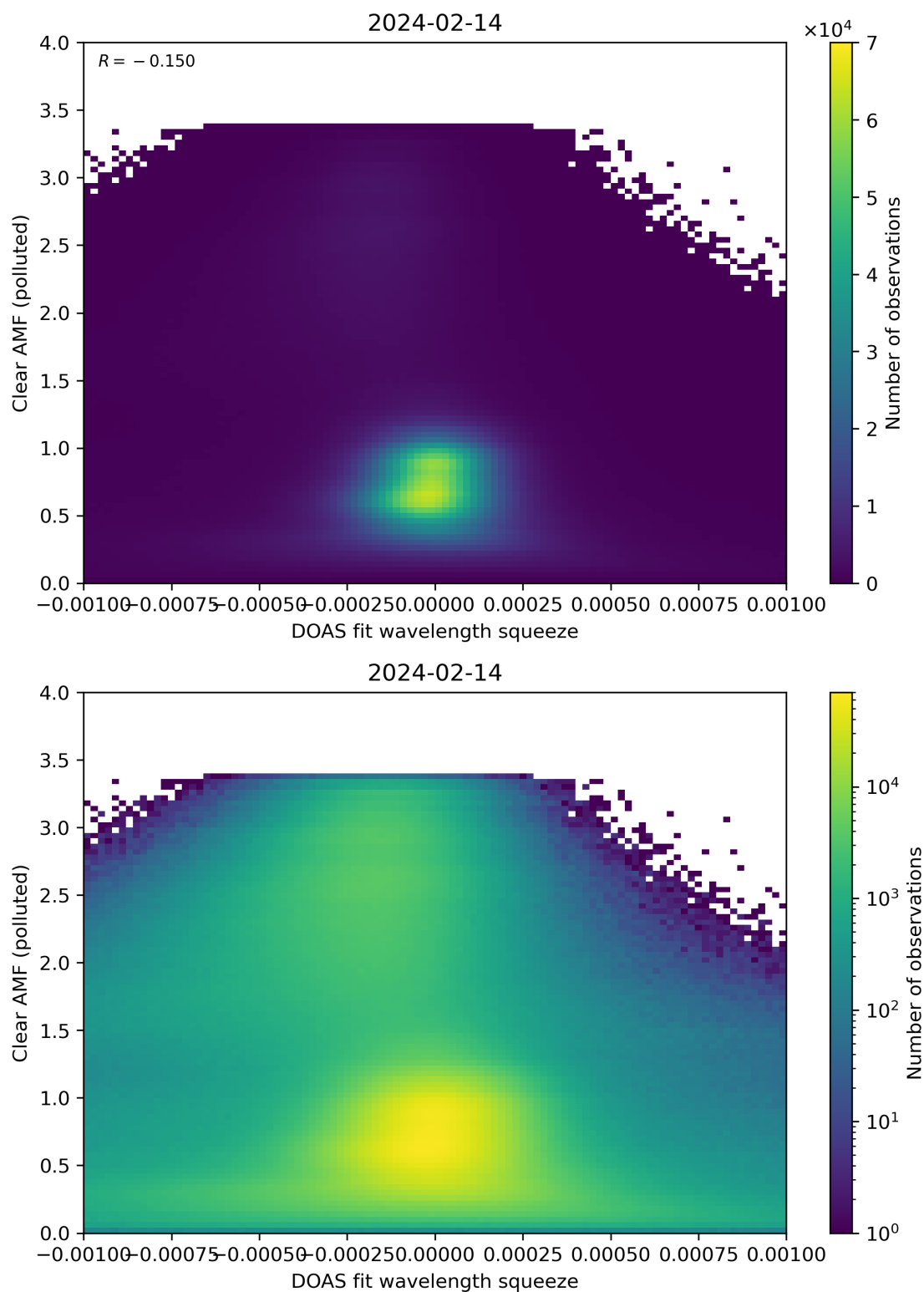
Figure 133: Scatter density plot of “DOAS fit wavelength squeeze” against “Clear AMF (polluted)” for 2024-02-13 to 2024-02-15.
