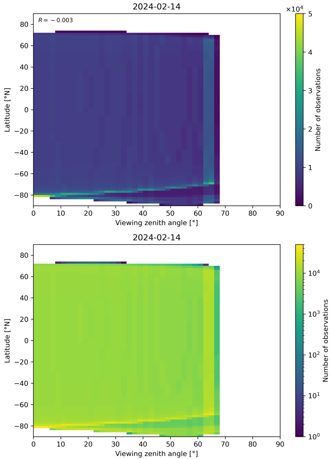
Figure 314: Scatter density plot of “Viewing zenith angle” against “Latitude” for 2024-02-13 to 2024-02-15.
