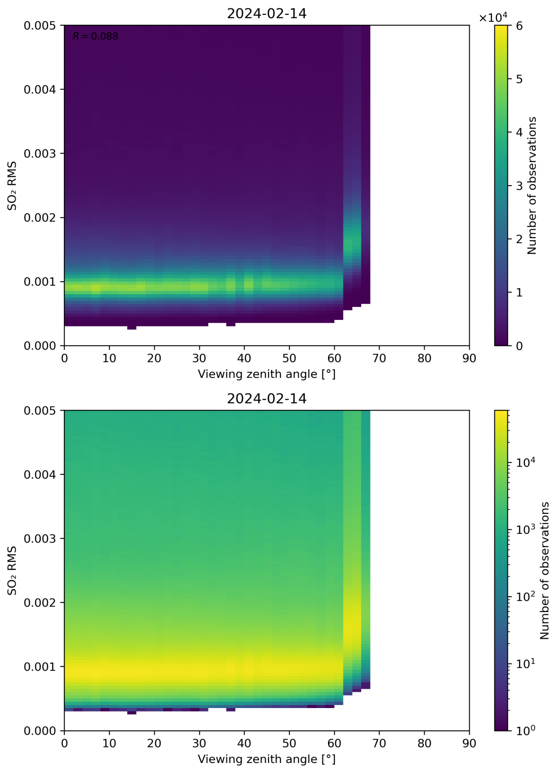
Figure 313: Scatter density plot of “Viewing zenith angle” against “SO 2 RMS” for 2024-02-13 to 2024-02-15.
