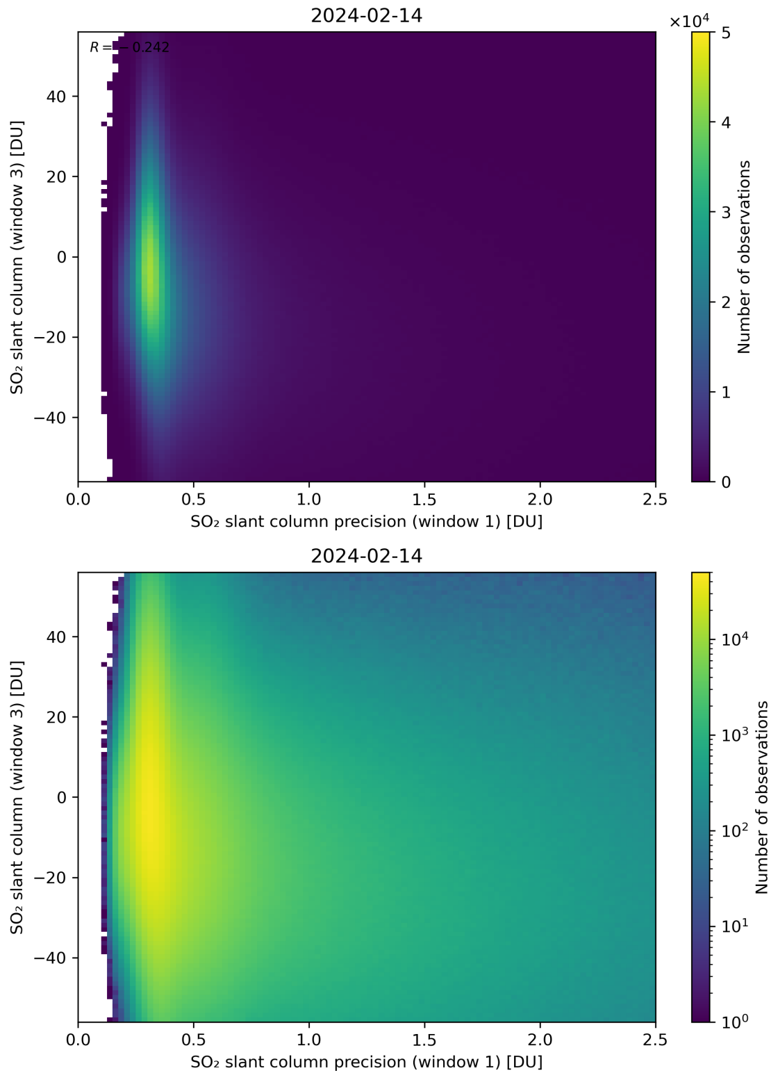
Figure 228: Scatter density plot of “SO 2 slant column precision (window 1)” against “SO 2 slant column (window 3)” for 2024-02-13 to 2024-02-15.
