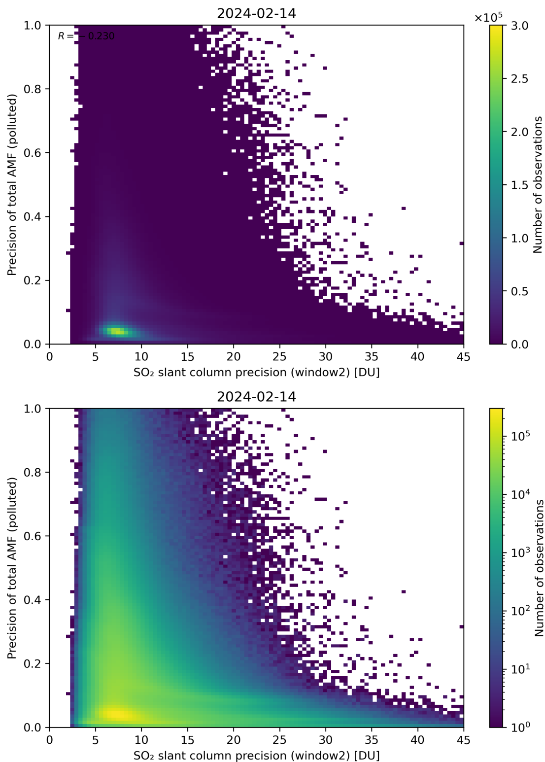
Figure 252: Scatter density plot of “SO 2 slant column precision (window2)” against “Precision of total AMF (polluted)” for 2024-02-13 to 2024-02-15.
