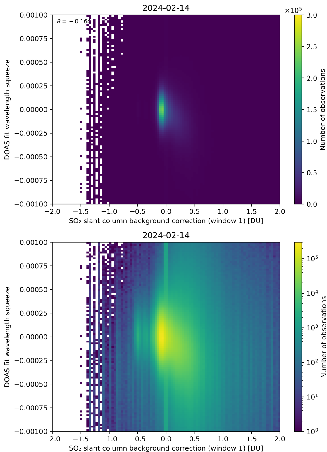
Figure 101: Scatter density plot of “SO 2 slant column background correction (window 1)” against “DOAS fit wavelength squeeze” for 2024-02-13 to 2024-02-15.
