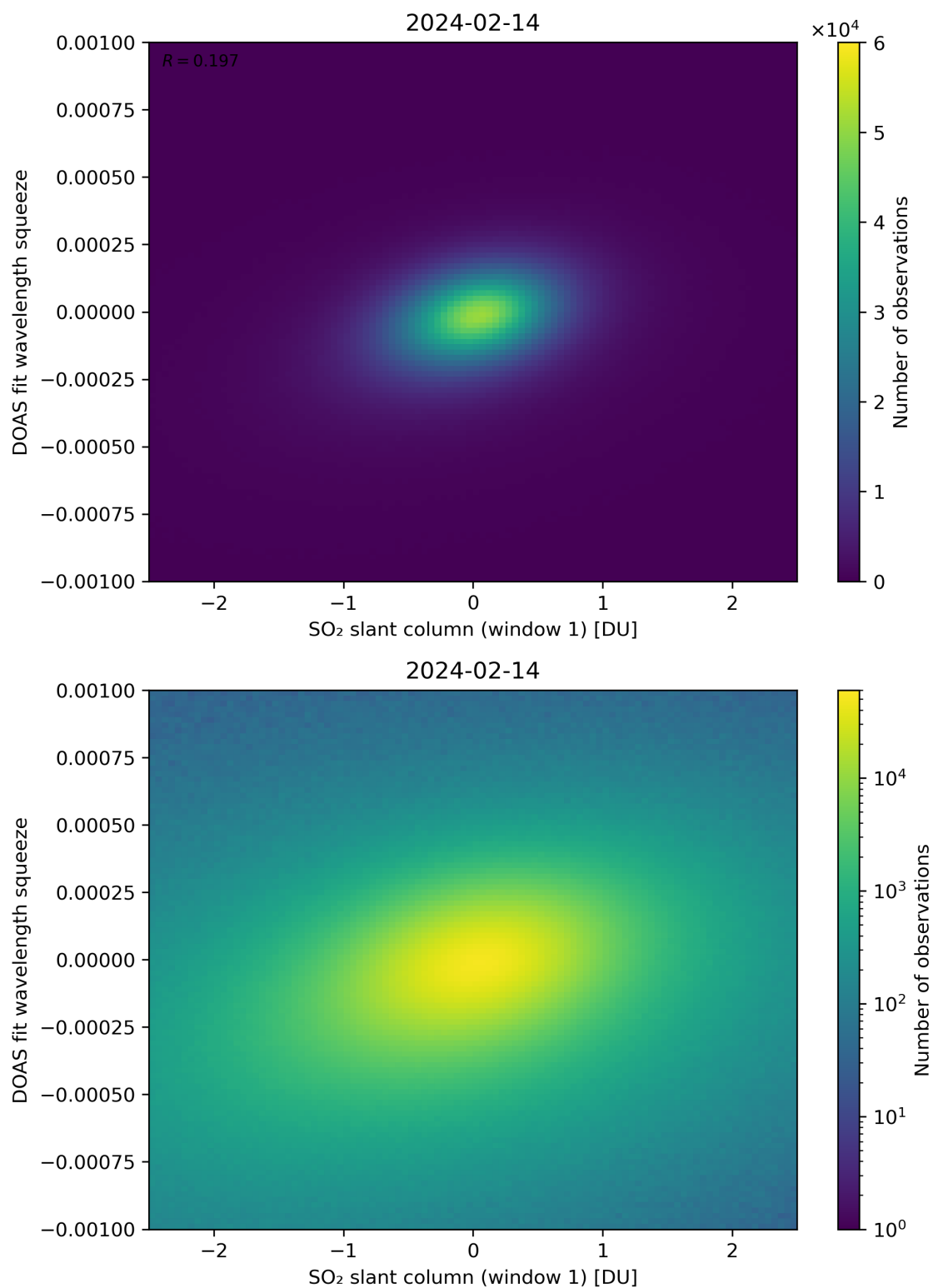
Figure 216: Scatter density plot of “SO 2 slant column (window 1)” against “DOAS fit wavelength squeeze” for 2024-02-13 to 2024-02-15.
