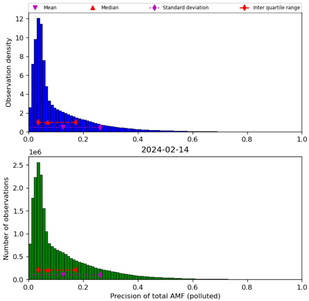
Figure 72: Histogram of “Precision of total AMF (polluted)” for 2024-02-13 to 2024-02-15
