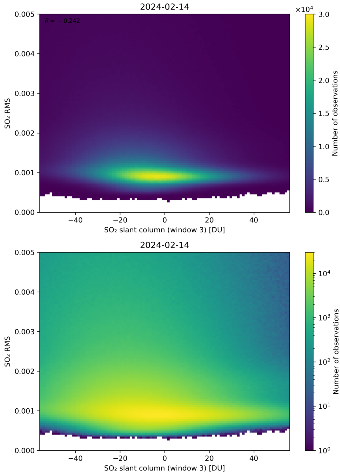
Figure 256: Scatter density plot of “SO 2 slant column (window 3)” against “SO 2 RMS” for 2024-02-13 to 2024-02-15.
