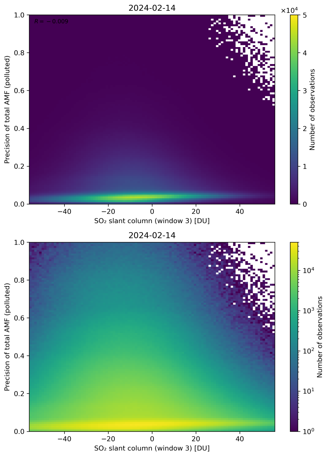
Figure 269: Scatter density plot of “SO 2 slant column (window 3)” against “Precision of total AMF (polluted)” for 2024-02-13 to 2024-02-15.
