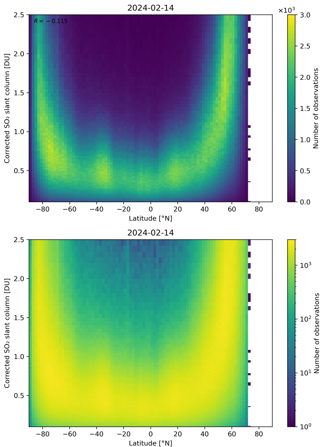
Figure 146: Scatter density plot of “Latitude” against “Corrected SO 2 slant column” for 2024-02-13 to 2024-02-15.
