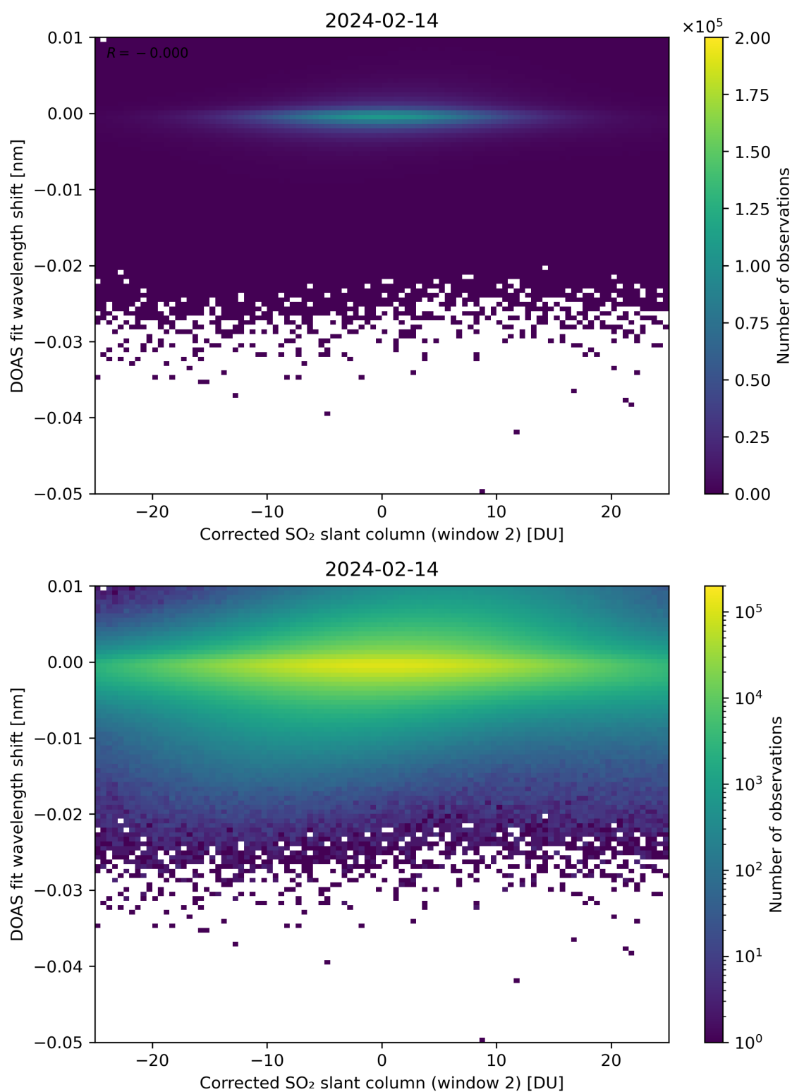
Figure 196: Scatter density plot of “Corrected SO 2 slant column (window 2)” against “DOAS fit wavelength shift” for 2024-02-13 to 2024-02-15.
