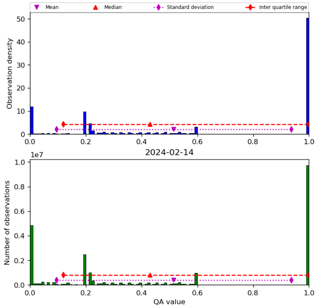
Figure 52: Histogram of “QA value” for 2024-02-13 to 2024-02-15
