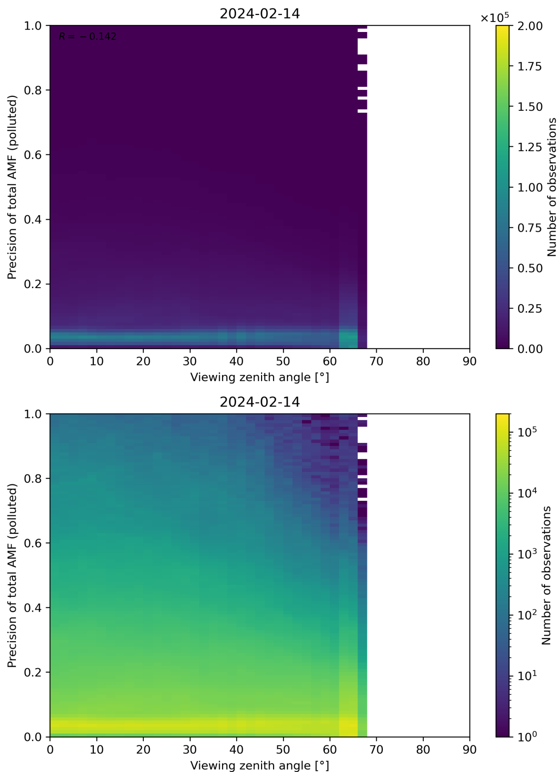
Figure 326: Scatter density plot of “Viewing zenith angle” against “Precision of total AMF (polluted)” for 2024-02-13 to 2024-02-15.
