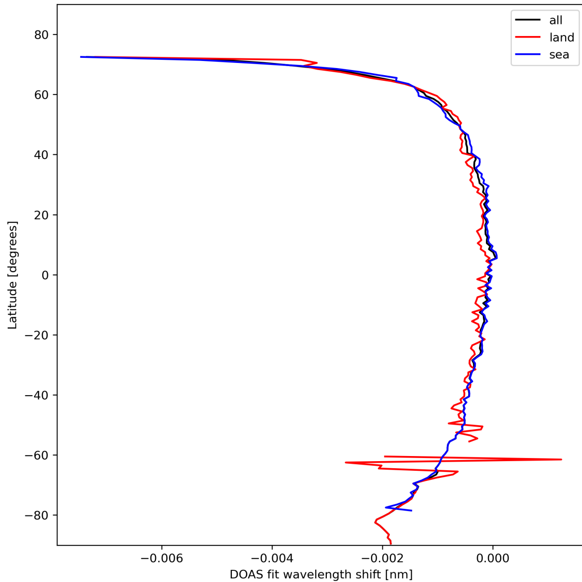
Figure 45: Zonal average of “DOAS fit wavelength shift” for 2024-02-13 to 2024-02-15.
