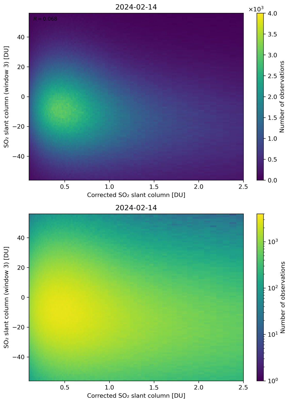
Figure 190: Scatter density plot of “Corrected SO 2 slant column” against “SO 2 slant column (window 3)” for 2024-02-13 to 2024-02-15.
