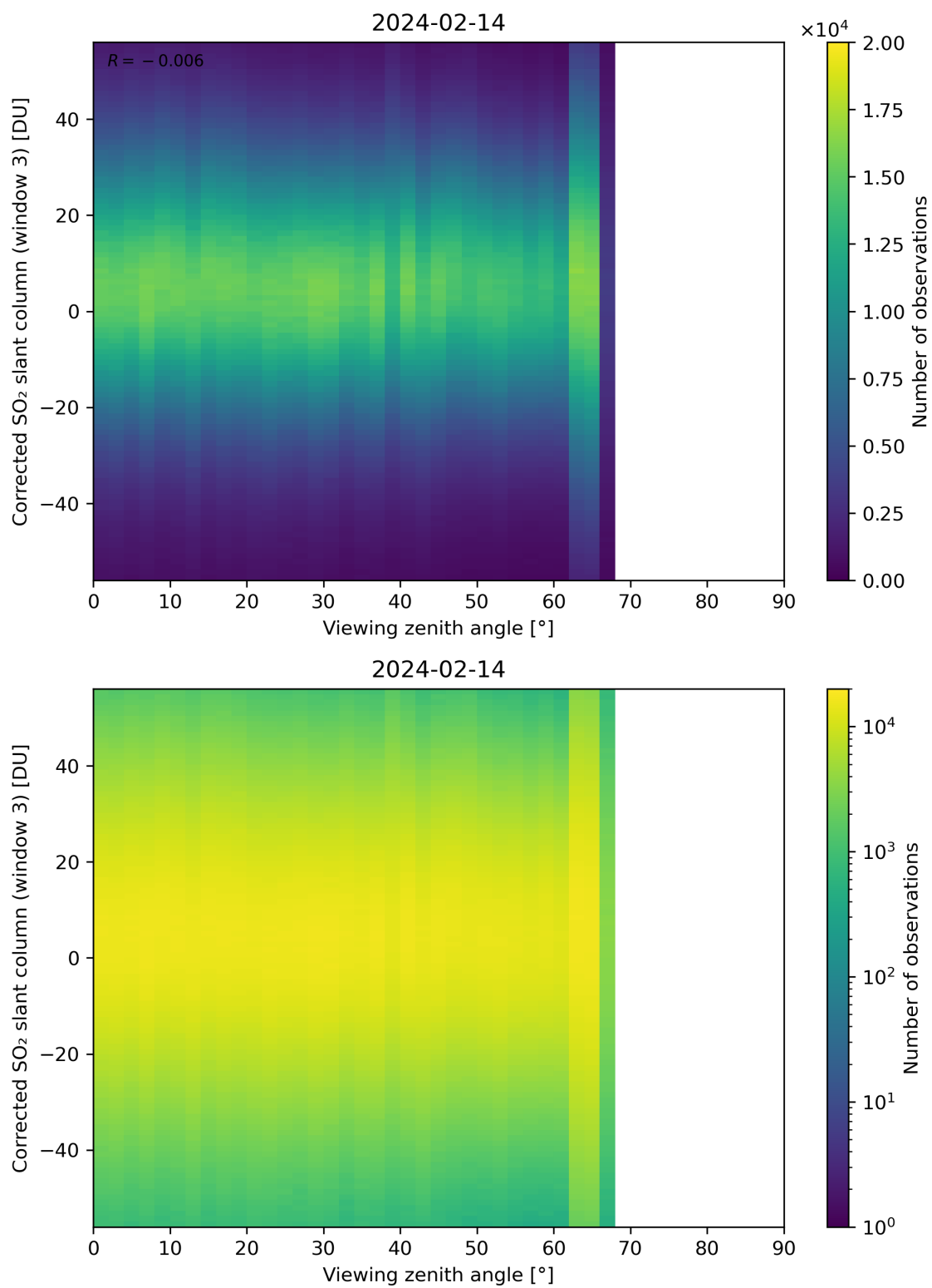
Figure 319: Scatter density plot of “Viewing zenith angle” against “Corrected SO 2 slant column (window 3)” for 2024-02-13 to 2024-02-15.
