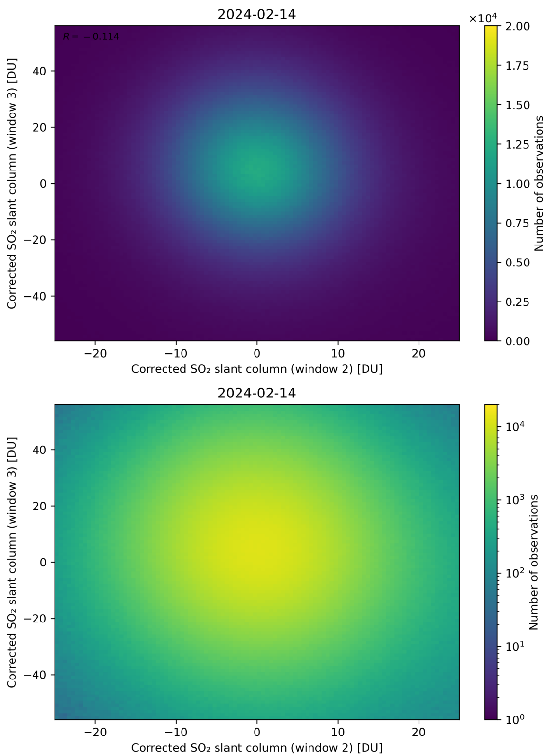
Figure 200: Scatter density plot of “Corrected SO 2 slant column (window 2)” against “Corrected SO 2 slant column (window 3)” for 2024-02-13 to 2024-02-15.
