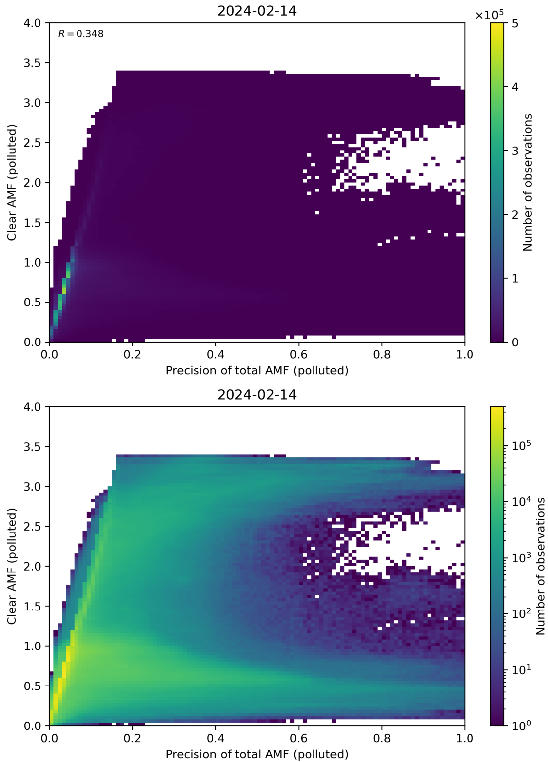
Figure 270: Scatter density plot of “Precision of total AMF (polluted)” against “Clear AMF (polluted)” for 2024-02-13 to 2024-02-15.
