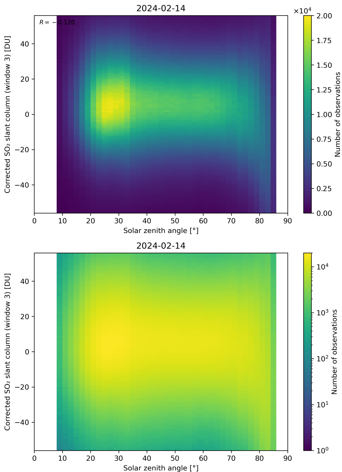
Figure 168: Scatter density plot of “Solar zenith angle” against “Corrected SO 2 slant column (window 3)” for 2024-02-13 to 2024-02-15.
