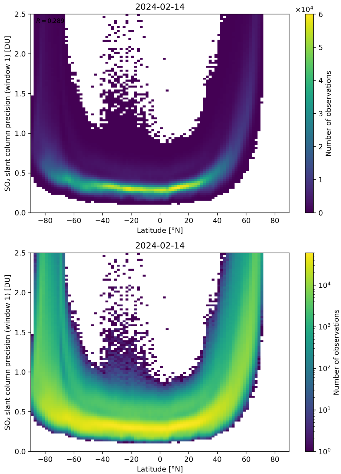
Figure 150: Scatter density plot of “Latitude” against “SO 2 slant column precision (window 1)” for 2024-02-13 to 2024-02-15.
