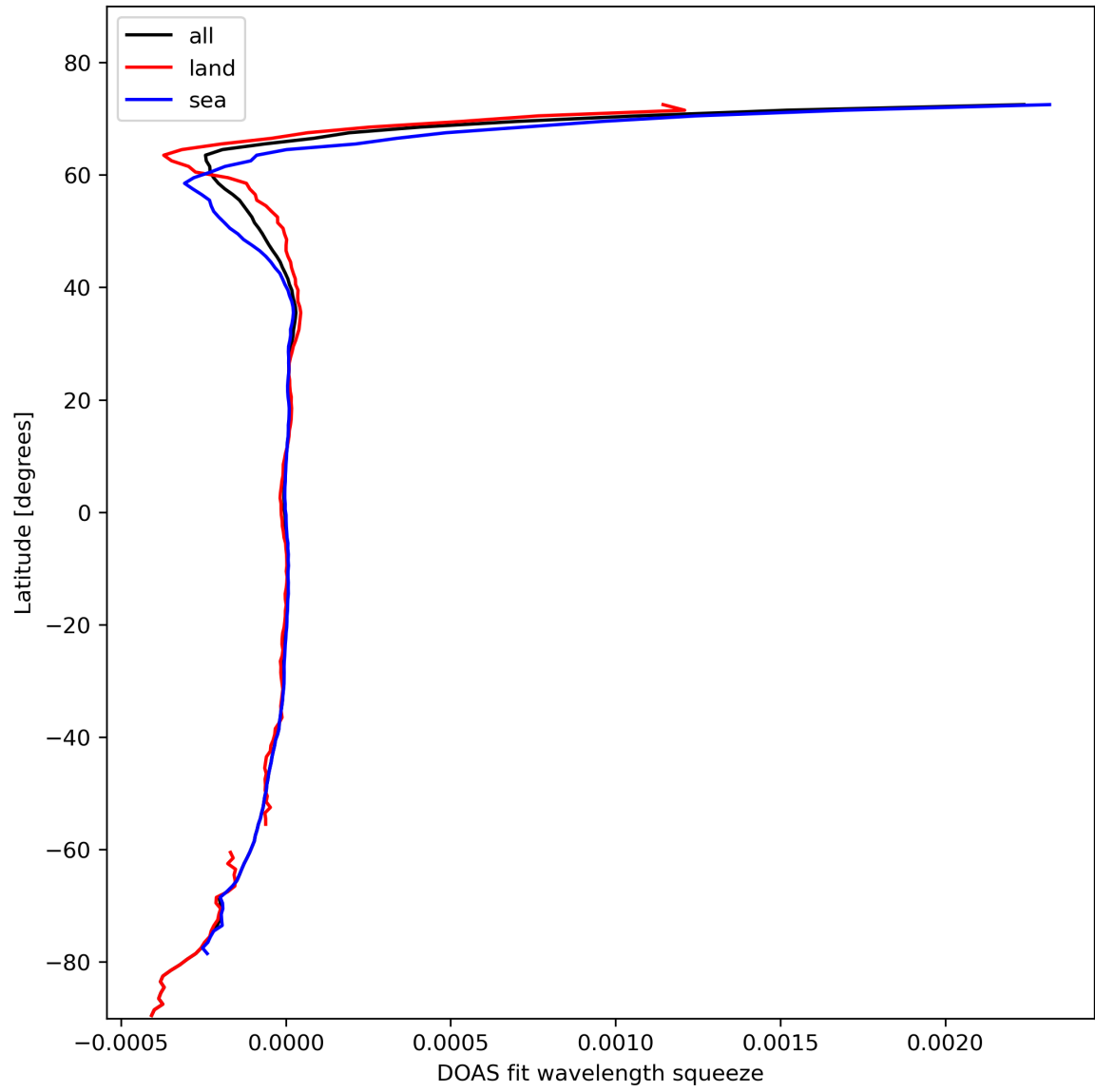
Figure 46: Zonal average of “DOAS fit wavelength squeeze” for 2024-02-13 to 2024-02-15.
