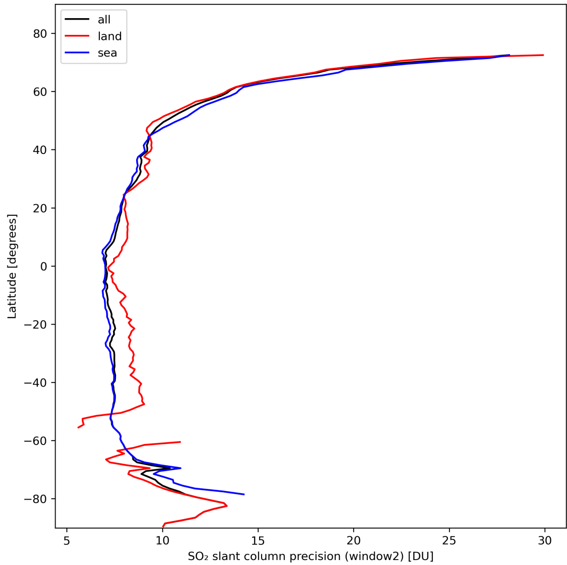
Figure 38: Zonal average of “SO 2 slant column precision (window2)” for 2024-02-13 to 2024-02-15.
