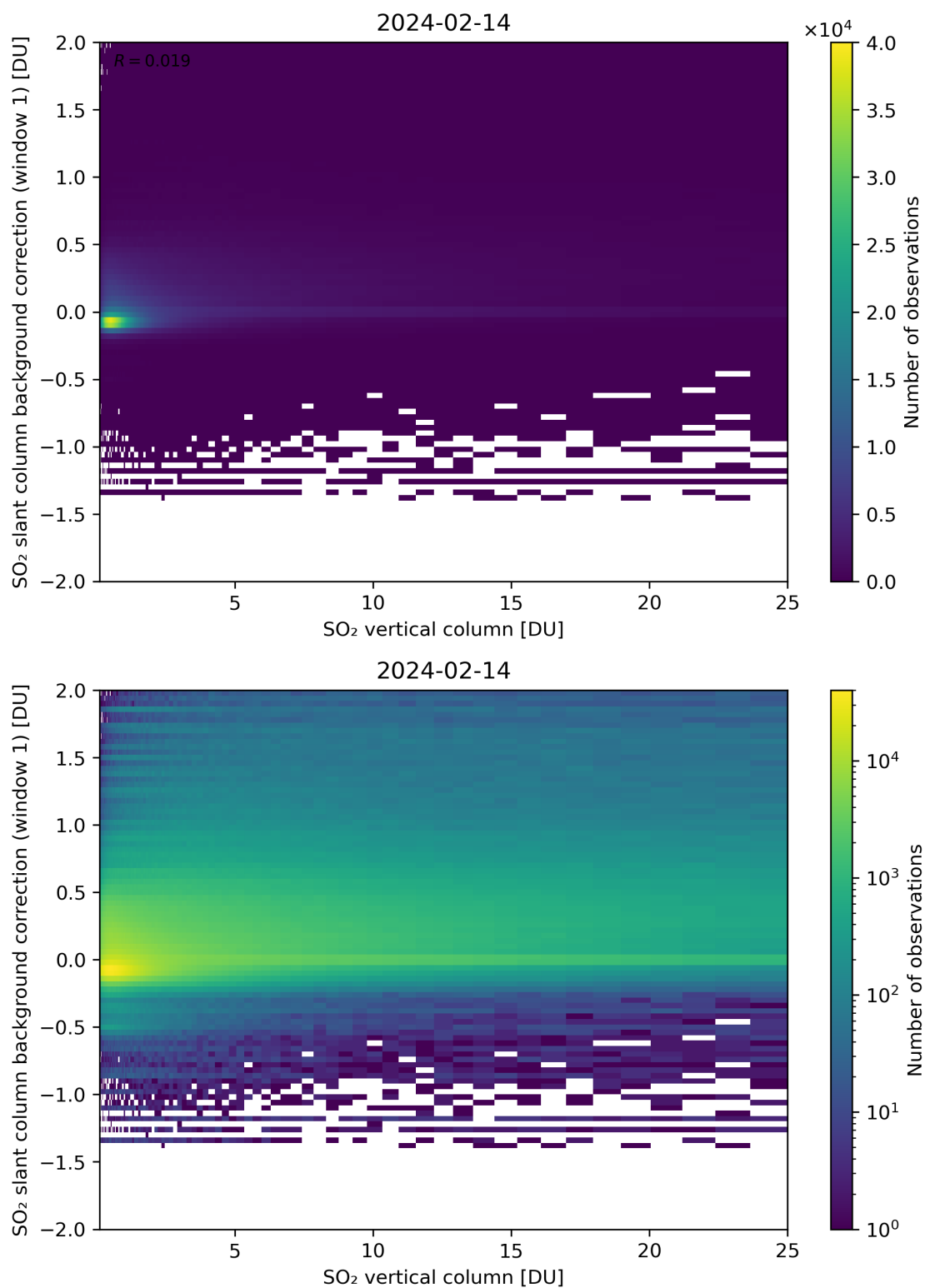
Figure 273: Scatter density plot of “SO 2 vertical column” against “SO 2 slant column background correction (window 1)” for 2024-02-13 to 2024-02-15.
