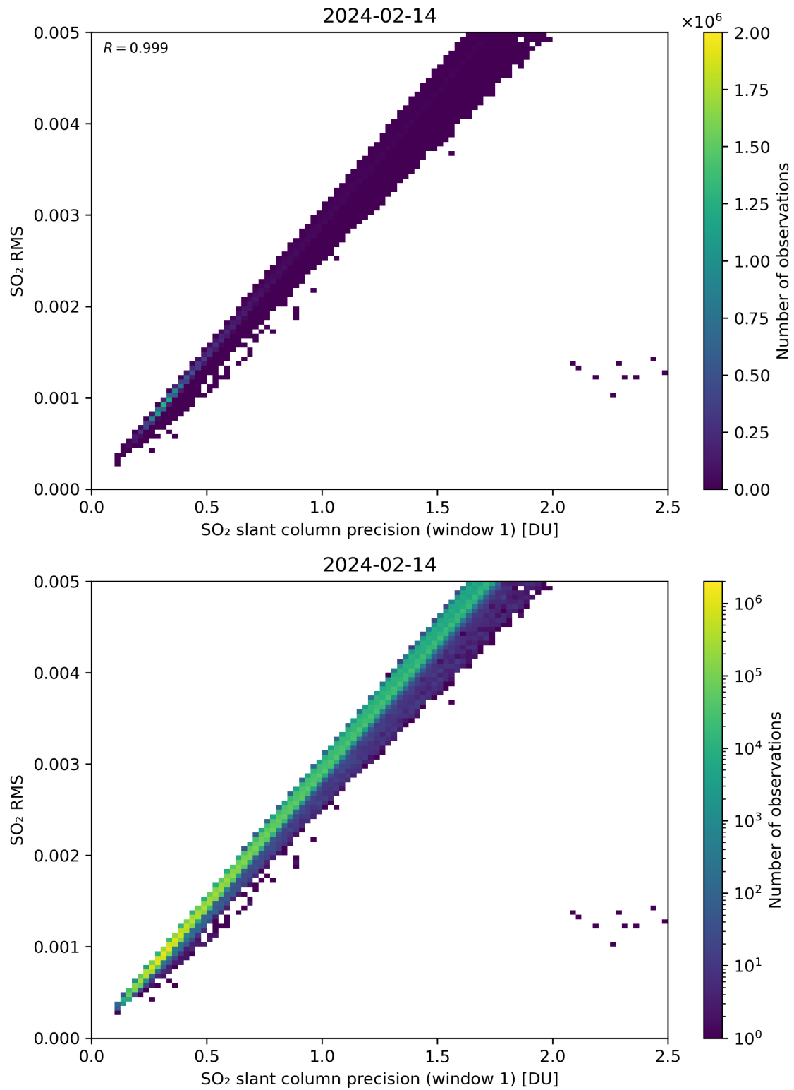
Figure 223: Scatter density plot of “SO 2 slant column precision (window 1)” against “SO 2 RMS” for 2024-02-13 to 2024-02-15.
