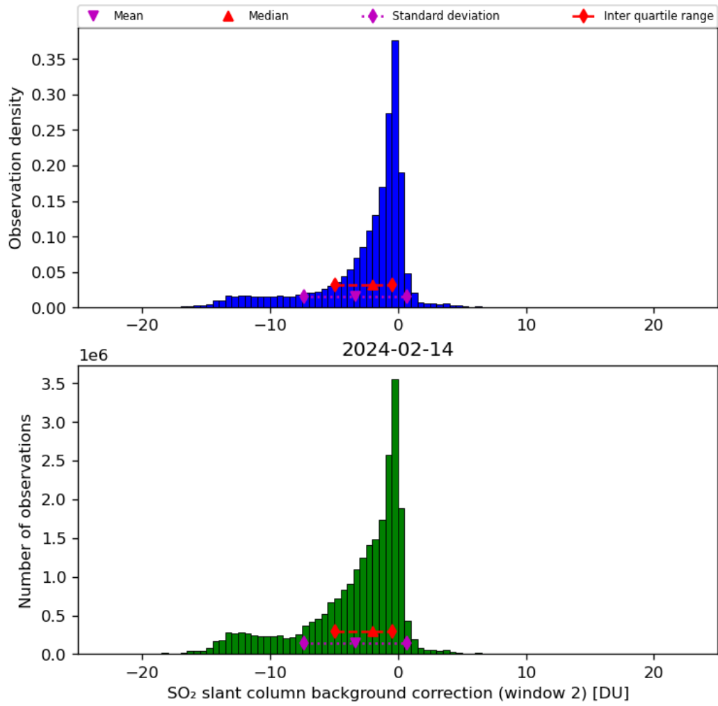
Figure 63: Histogram of “SO 2 slant column background correction (window 2)” for 2024-02-13 to 2024-02-15
