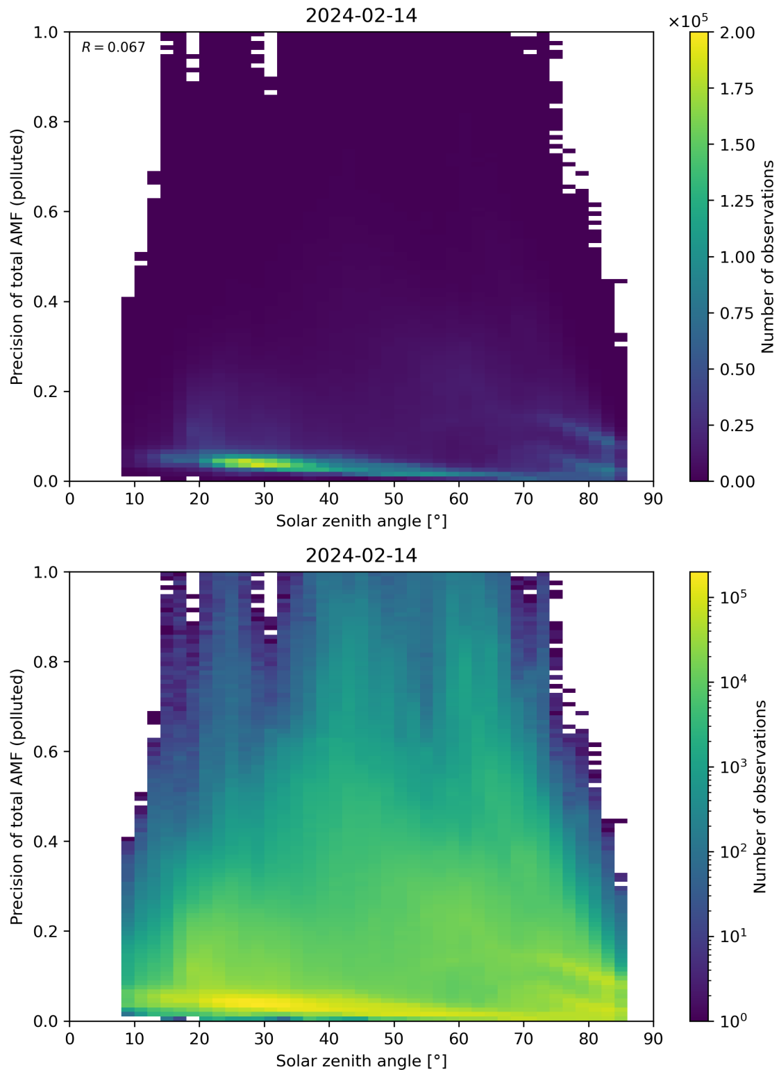
Figure 175: Scatter density plot of “Solar zenith angle” against “Precision of total AMF (polluted)” for 2024-02-13 to 2024-02-15.
