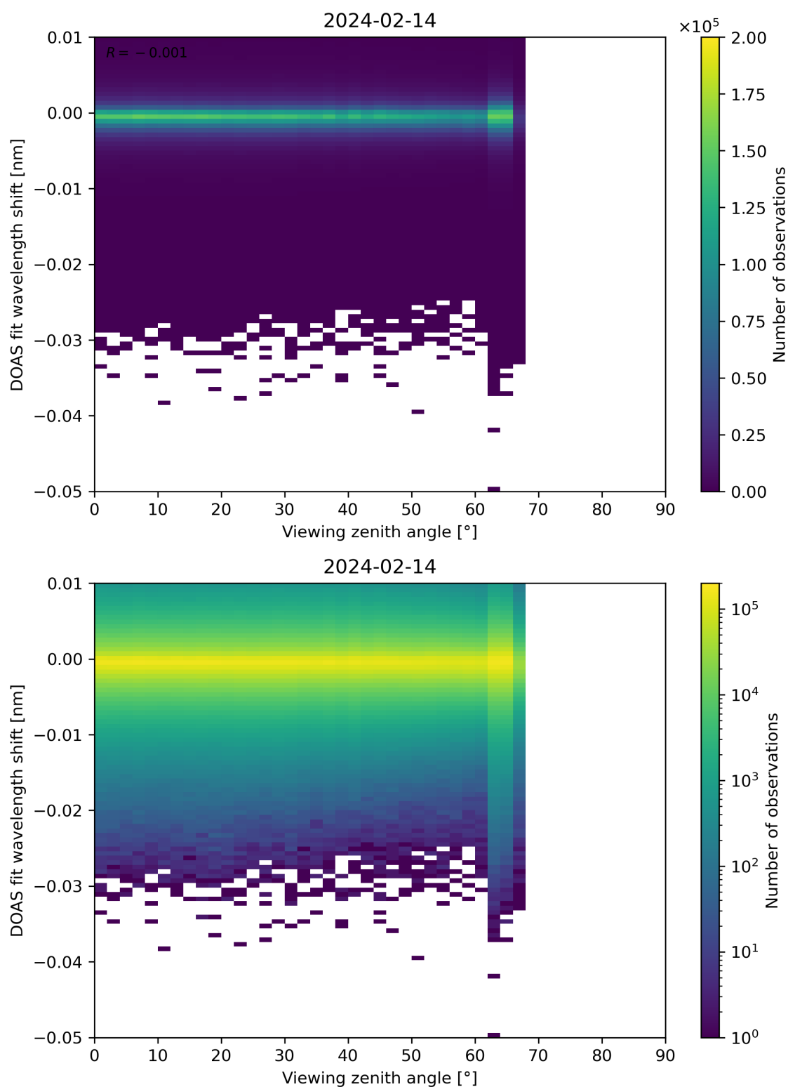
Figure 311: Scatter density plot of “Viewing zenith angle” against “DOAS fit wavelength shift” for 2024-02-13 to 2024-02-15.
