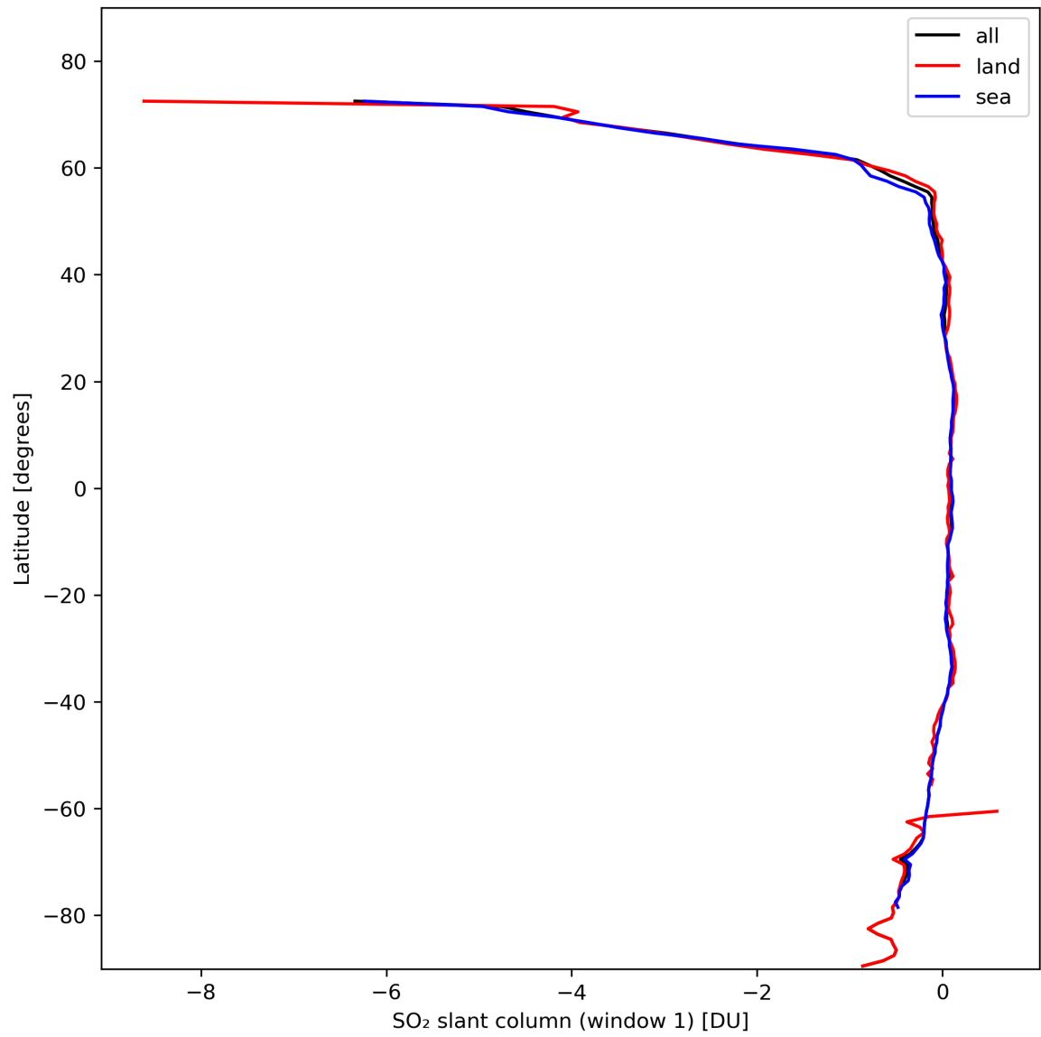
Figure 33: Zonal average of “SO 2 slant column (window 1)” for 2024-02-13 to 2024-02-15.
