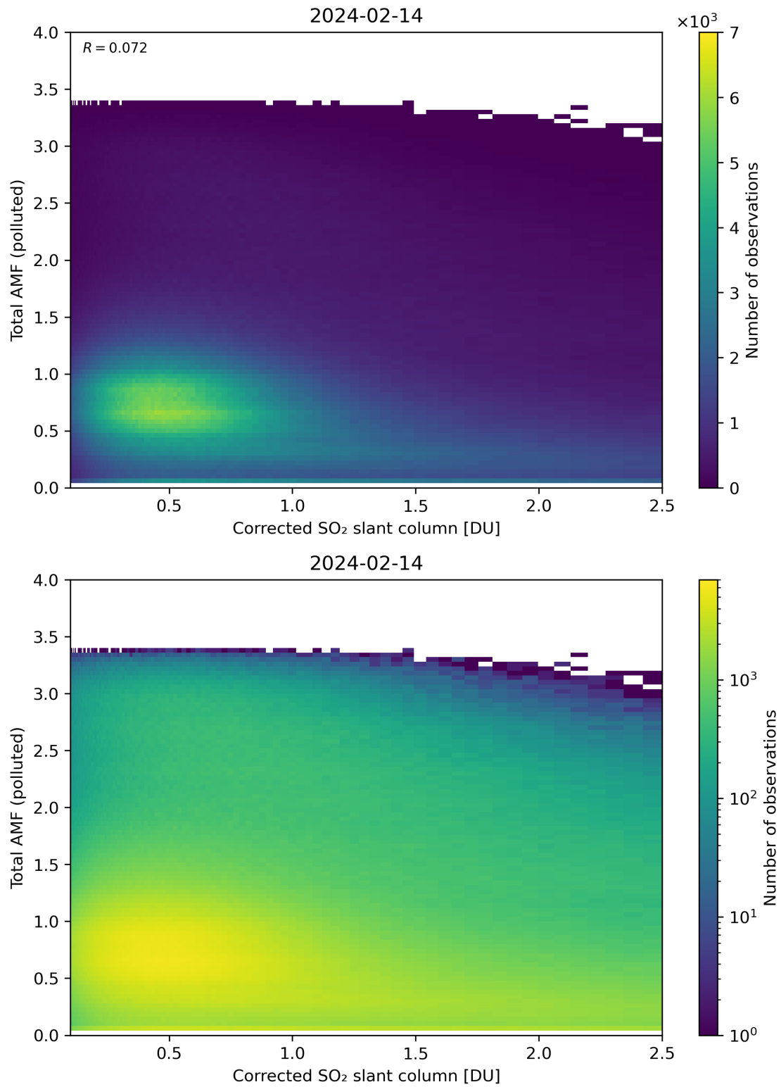
Figure 192: Scatter density plot of “Corrected SO 2 slant column” against “Total AMF (polluted)” for 2024-02-13 to 2024-02-15.
