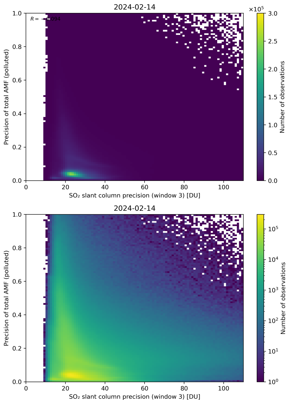
Figure 264: Scatter density plot of “SO 2 slant column precision (window 3)” against “Precision of total AMF (polluted)” for 2024-02-13 to 2024-02-15.
