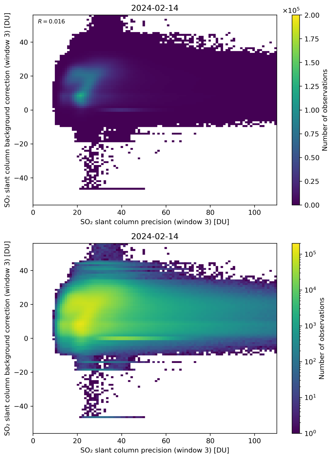
Figure 257: Scatter density plot of “SO 2 slant column precision (window 3)” against “SO 2 slant column background correction (window 3)” for 2024-02-13 to 2024-02-15.
