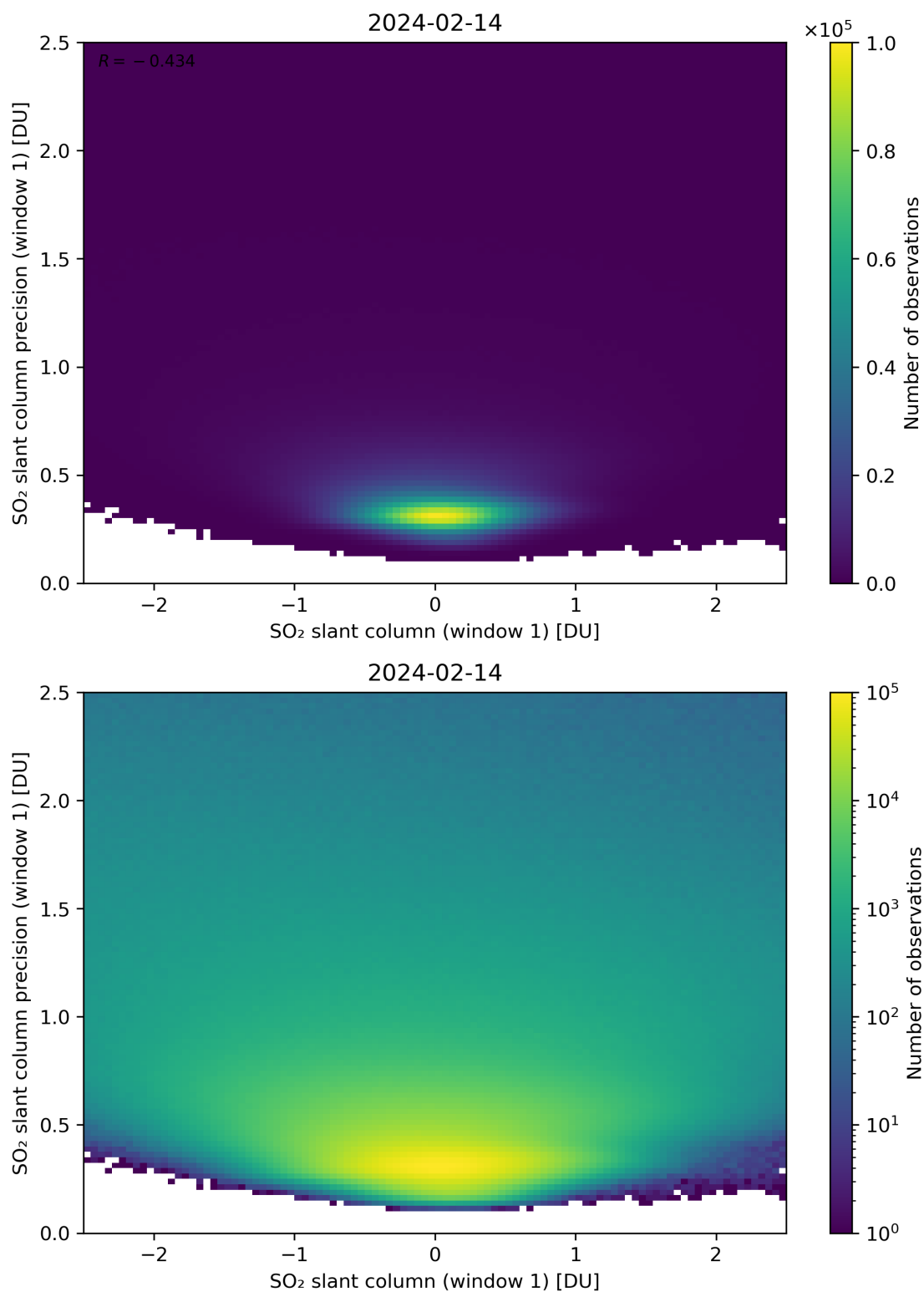
Figure 235: Scatter density plot of “SO 2 slant column (window 1)” against “SO 2 slant column precision (window 1)” for 2024-02-13 to 2024-02-15.
