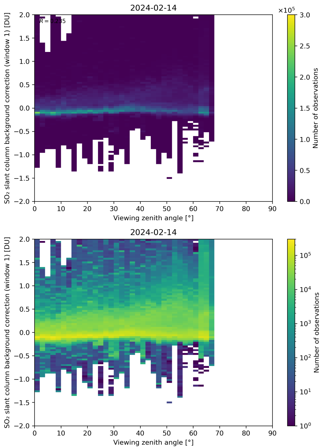
Figure 308: Scatter density plot of “Viewing zenith angle” against “SO 2 slant column background correction (window 1)” for 2024-02-13 to 2024-02-15.
