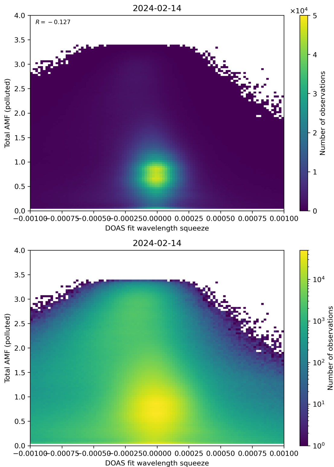
Figure 134: Scatter density plot of “DOAS fit wavelength squeeze” against “Total AMF (polluted)” for 2024-02-13 to 2024-02-15.
