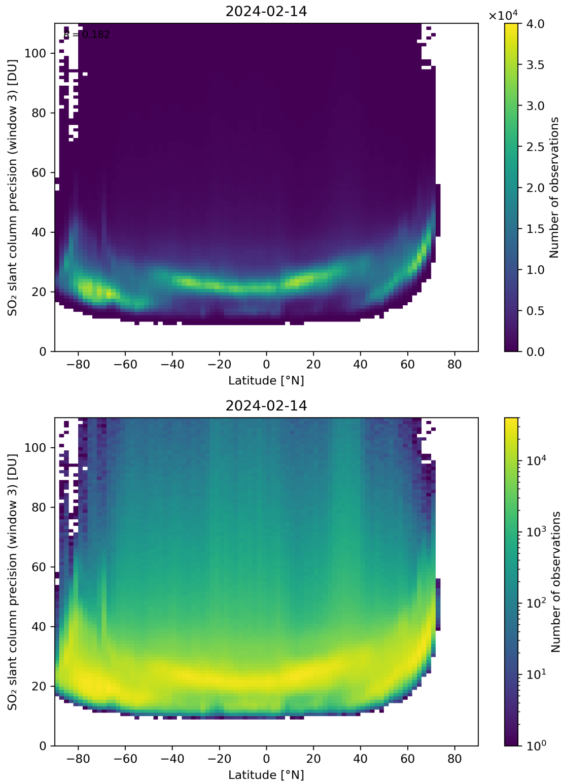
Figure 153: Scatter density plot of “Latitude” against “SO 2 slant column precision (window 3)” for 2024-02-13 to 2024-02-15.
