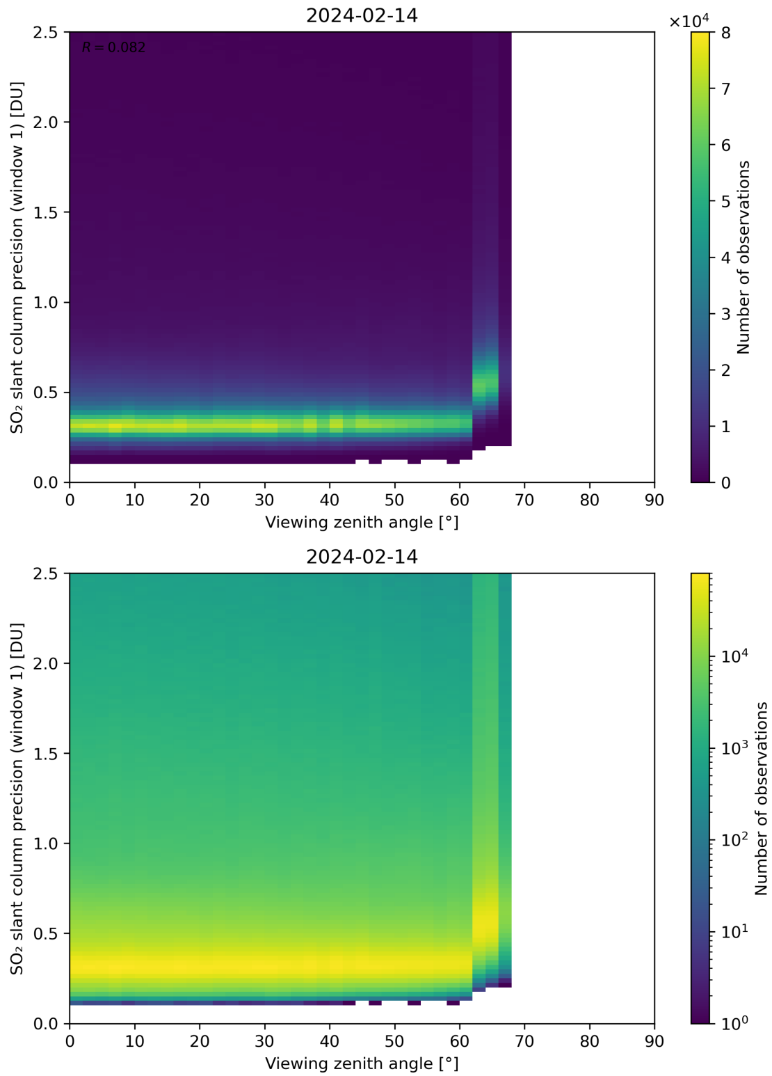
Figure 321: Scatter density plot of “Viewing zenith angle” against “SO 2 slant column precision (window 1)” for 2024-02-13 to 2024-02-15.
