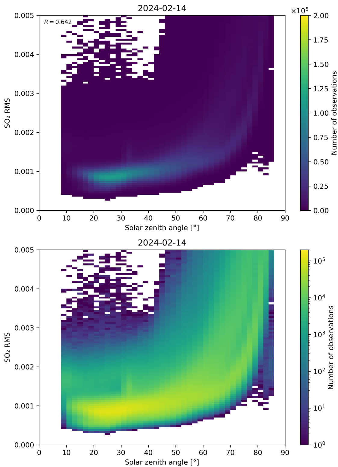
Figure 163: Scatter density plot of “Solar zenith angle” against “SO 2 RMS” for 2024-02-13 to 2024-02-15.
