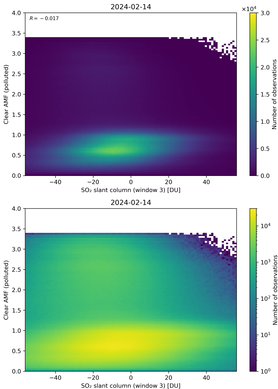
Figure 265: Scatter density plot of “SO 2 slant column (window 3)” against “Clear AMF (polluted)” for 2024-02-13 to 2024-02-15.
