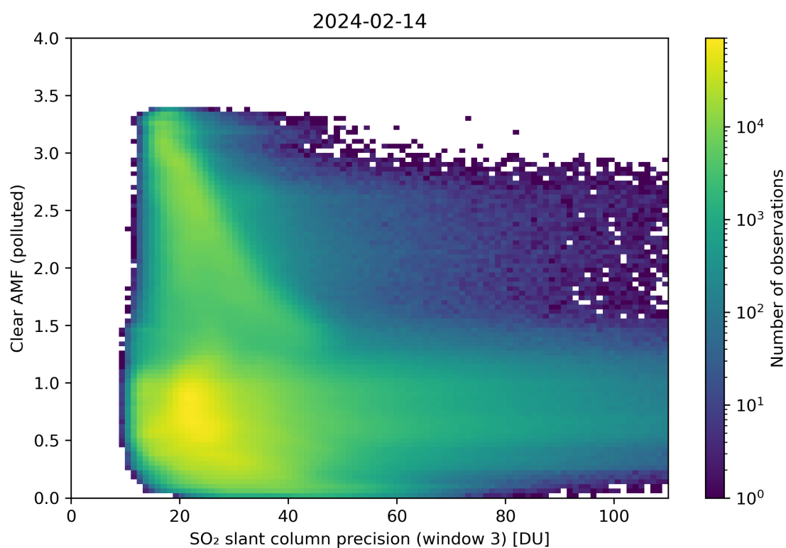
Figure 261: Scatter density plot of “SO 2 slant column precision (window 3)” against “Clear AMF (polluted)” for 2024-02-13 to 2024-02-15.
