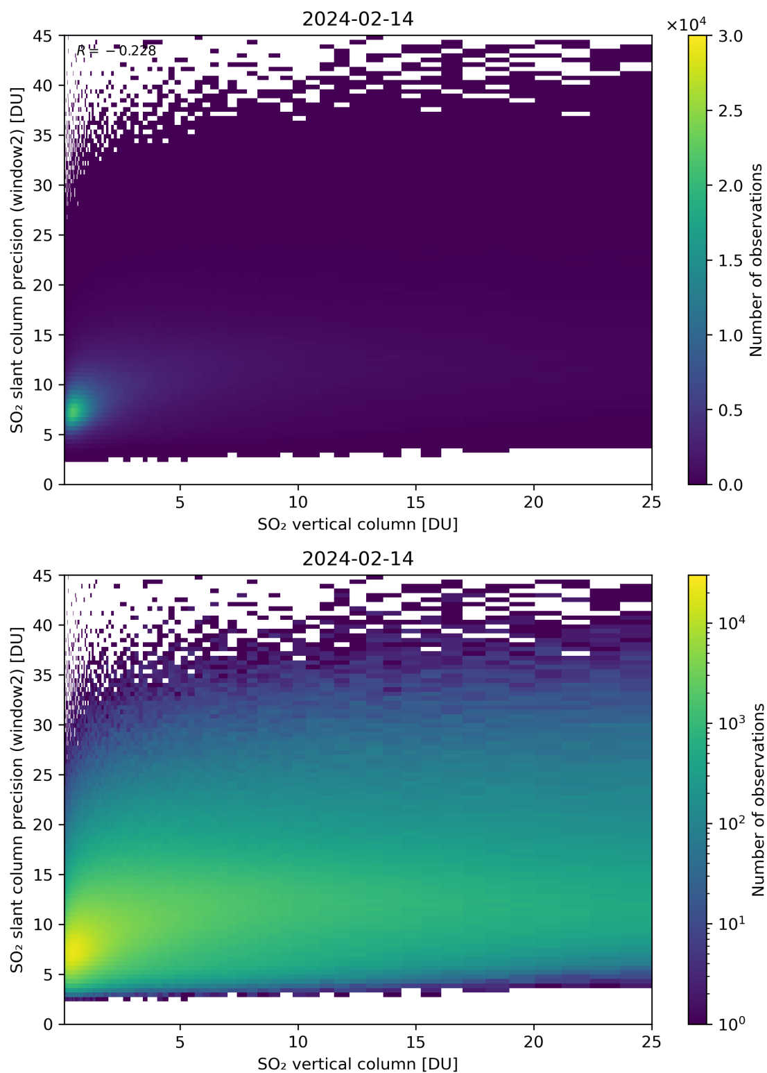
Figure 302: Scatter density plot of “SO 2 vertical column” against “SO 2 slant column precision (window2)” for 2024-02-13 to 2024-02-15.
