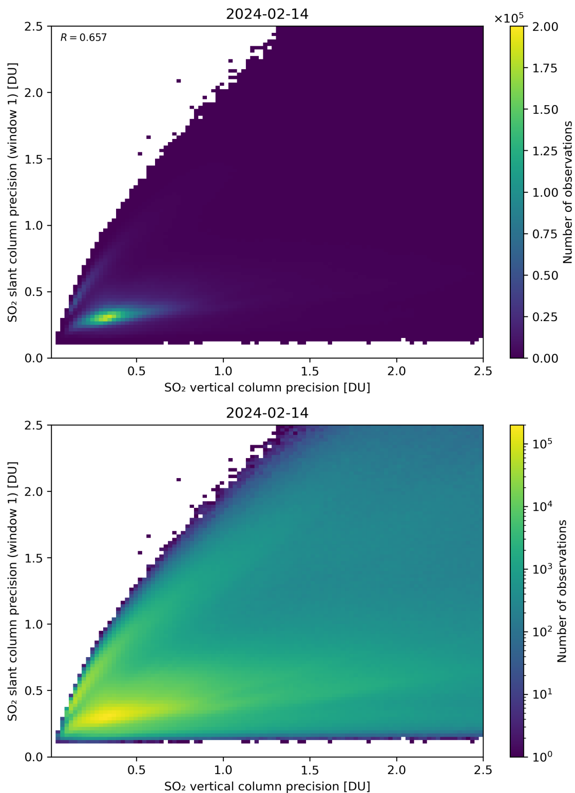
Figure 290: Scatter density plot of “SO 2 vertical column precision” against “SO 2 slant column precision (window 1)” for 2024-02-13 to 2024-02-15.
