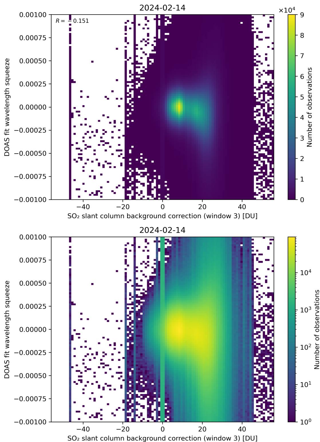
Figure 122: Scatter density plot of “SO 2 slant column background correction (window 3)” against “DOAS fit wavelength squeeze” for 2024-02-13 to 2024-02-15.
