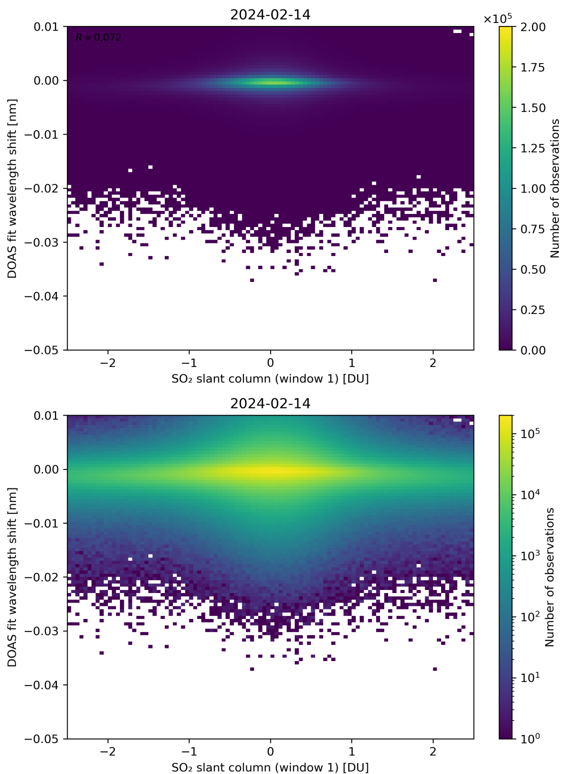
Figure 215: Scatter density plot of “SO 2 slant column (window 1)” against “DOAS fit wavelength shift” for 2024-02-13 to 2024-02-15.
