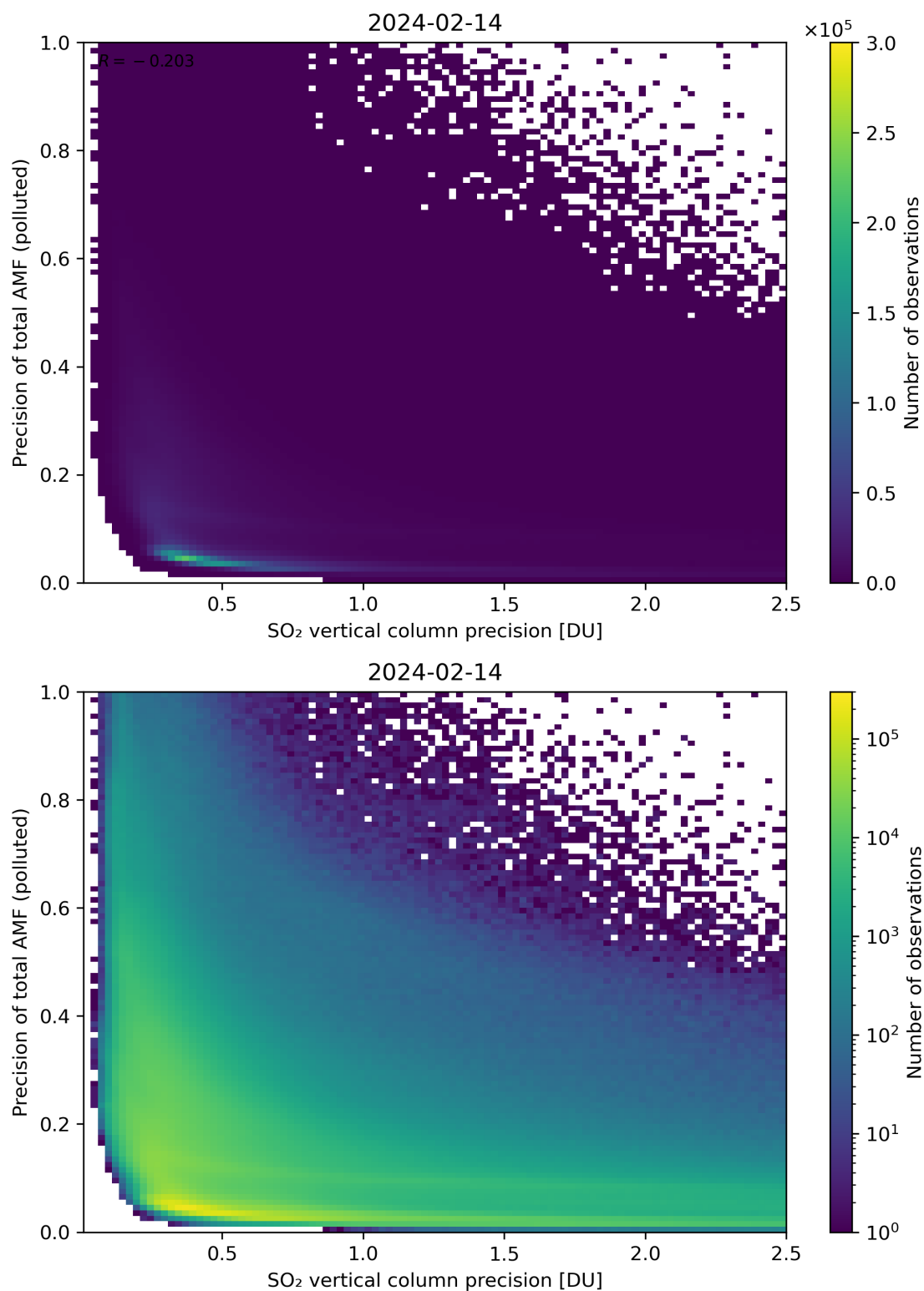
Figure 295: Scatter density plot of “SO 2 vertical column precision” against “Precision of total AMF (polluted)” for 2024-02-13 to 2024-02-15.
