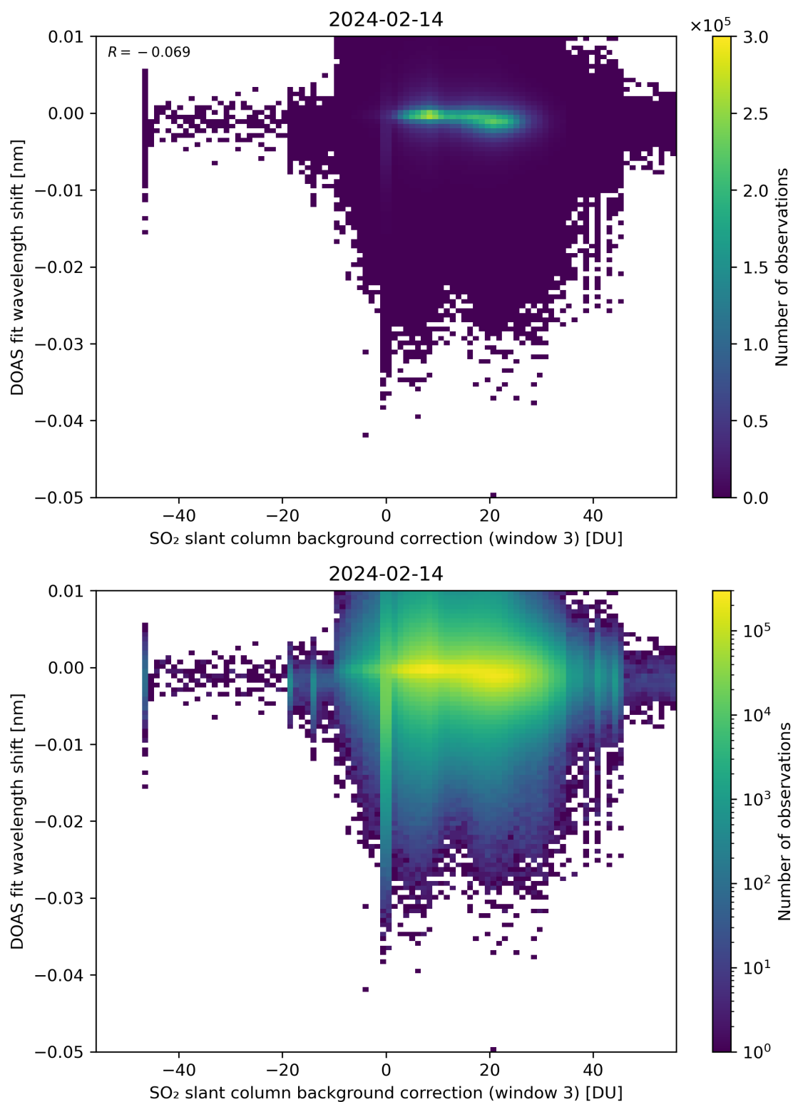
Figure 121: Scatter density plot of “SO 2 slant column background correction (window 3)” against “DOAS fit wavelength shift” for 2024-02-13 to 2024-02-15.
