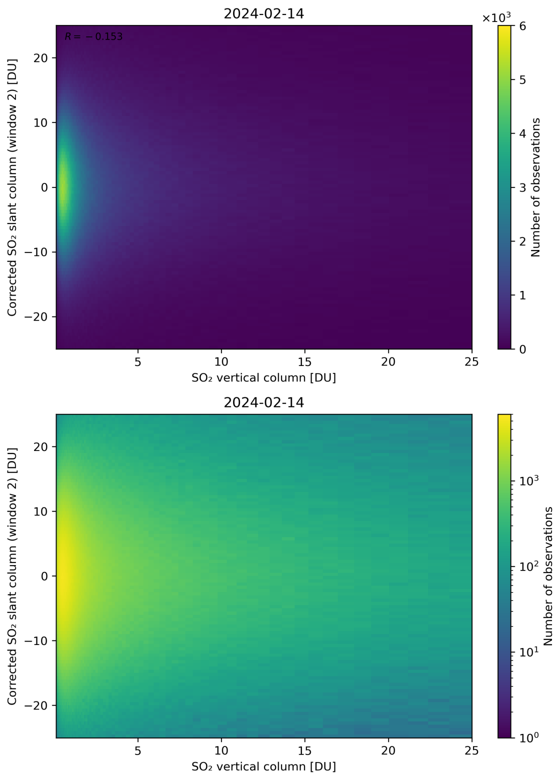
Figure 298: Scatter density plot of “SO 2 vertical column” against “Corrected SO 2 slant column (window 2)” for 2024-02-13 to 2024-02-15.
