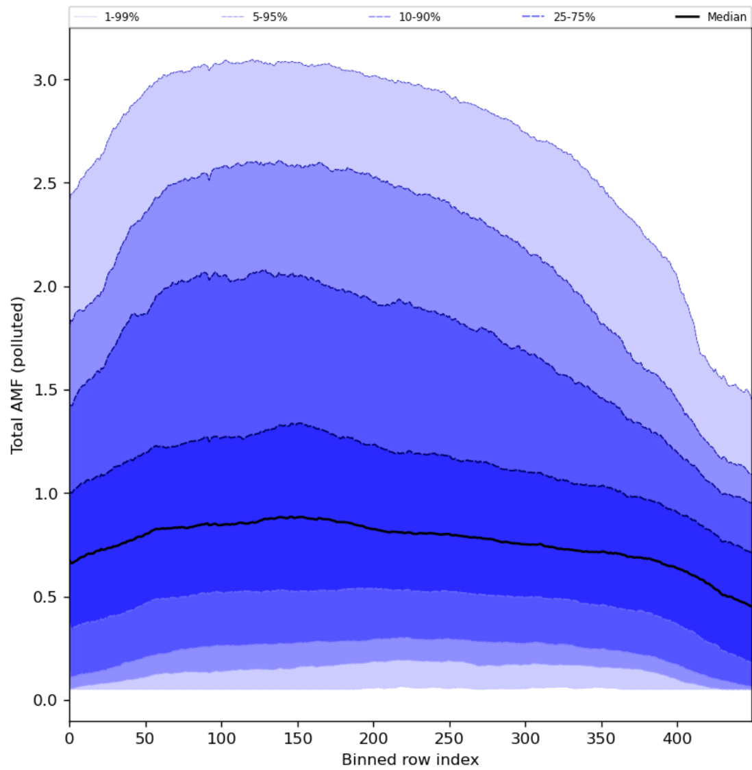
Figure 94: Along track statistics of “Total AMF (polluted)” for 2024-02-13 to 2024-02-15
