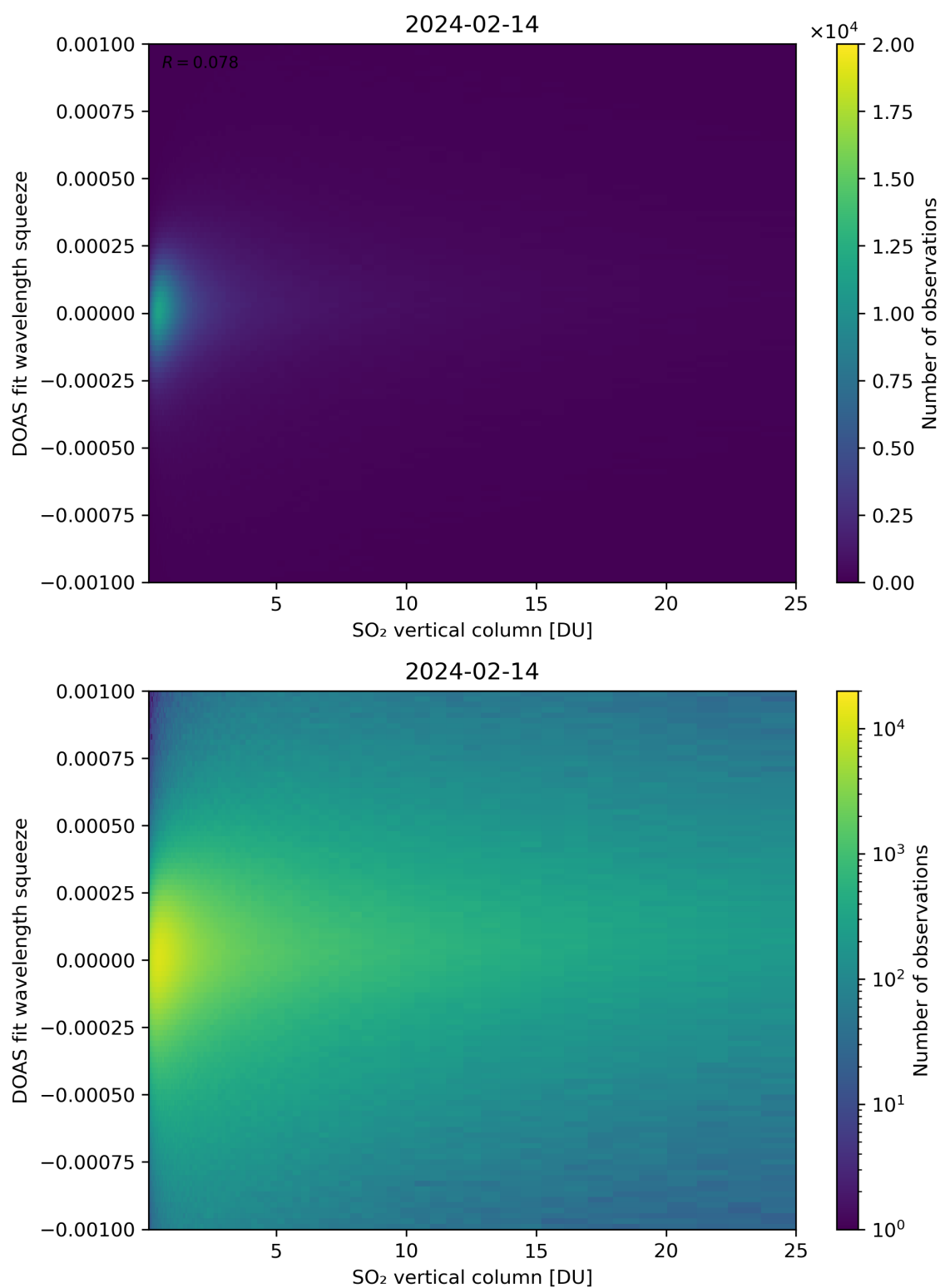
Figure 277: Scatter density plot of “SO 2 vertical column” against “DOAS fit wavelength squeeze” for 2024-02-13 to 2024-02-15.
