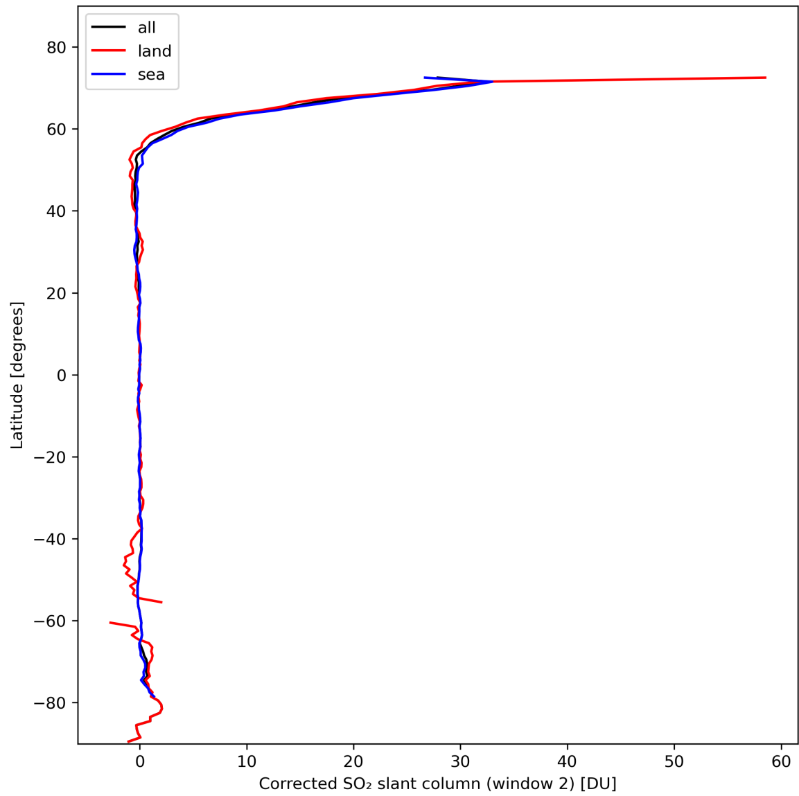
Figure 39: Zonal average of “Corrected SO 2 slant column (window 2)” for 2024-02-13 to 2024-02-15.
