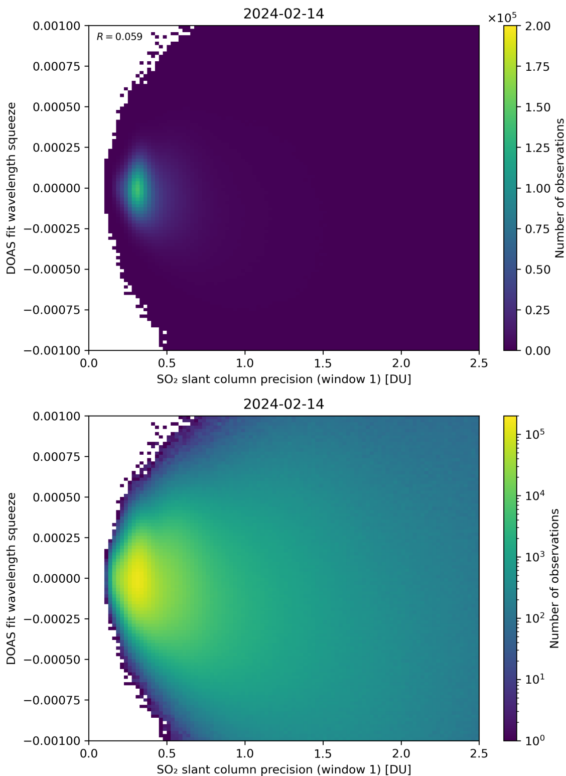
Figure 222: Scatter density plot of “SO 2 slant column precision (window 1)” against “DOAS fit wavelength squeeze” for 2024-02-13 to 2024-02-15.
