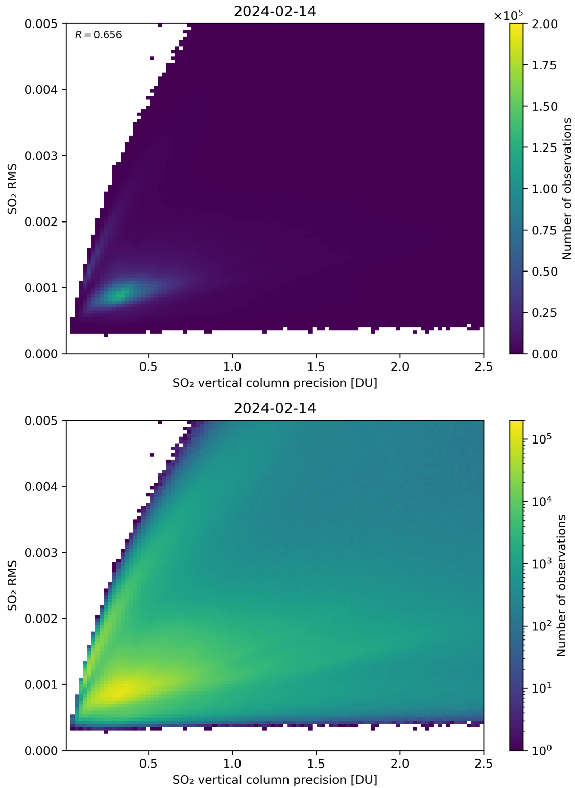
Figure 284: Scatter density plot of “SO 2 vertical column precision” against “SO 2 RMS” for 2024-02-13 to 2024-02-15.
