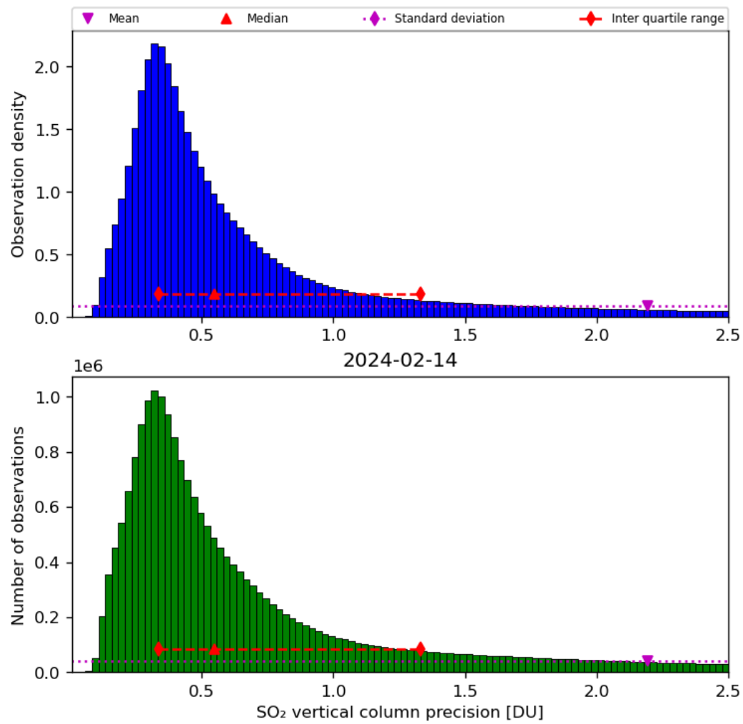
Figure 54: Histogram of “SO 2 vertical column precision” for 2024-02-13 to 2024-02-15
