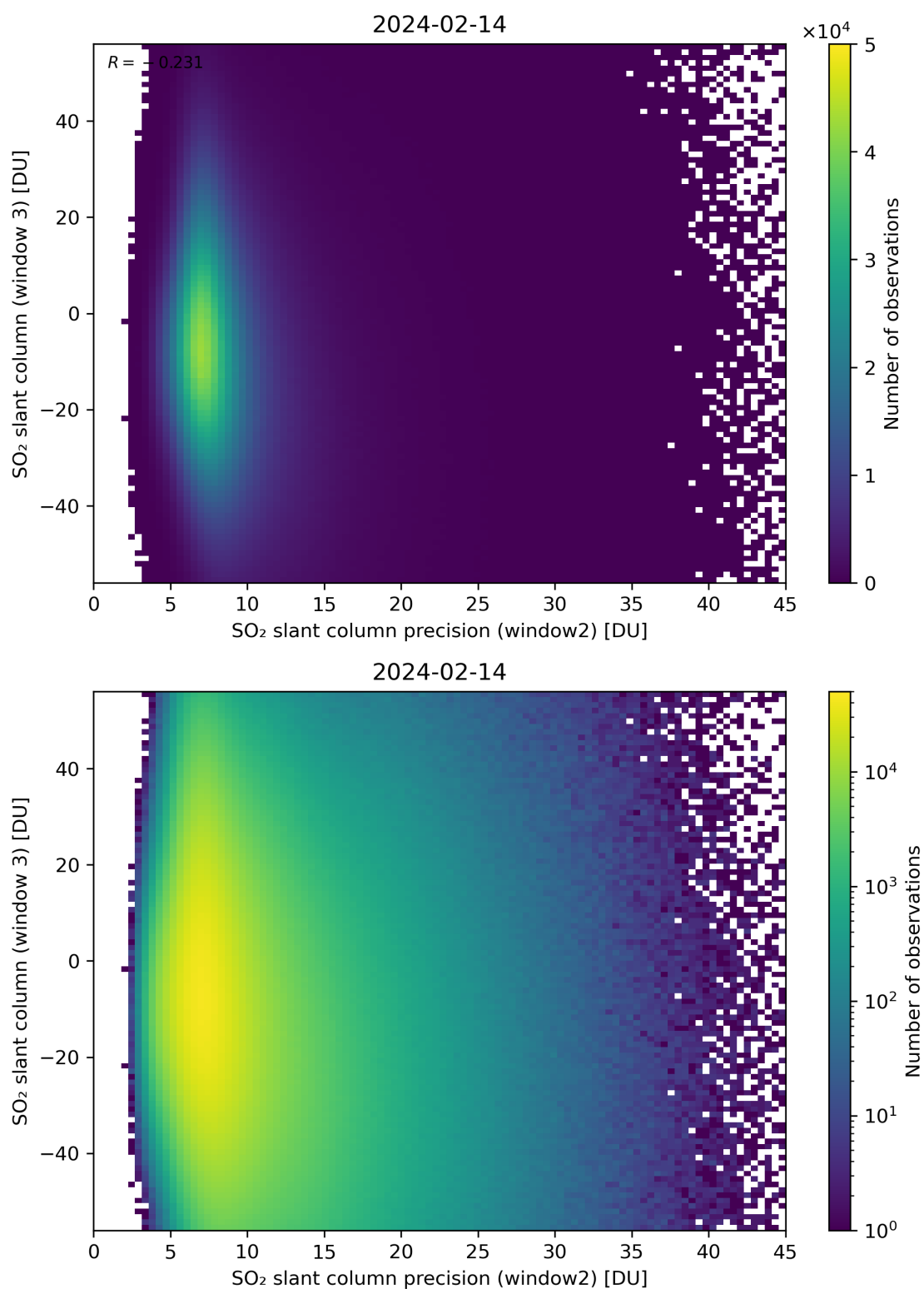
Figure 249: Scatter density plot of “SO 2 slant column precision (window2)” against “SO 2 slant column (window 3)” for 2024-02-13 to 2024-02-15.
