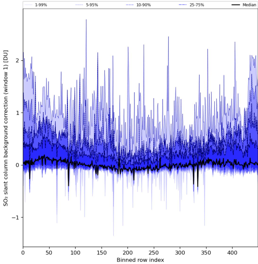
Figure 82: Along track statistics of “SO 2 slant column background correction (window 1)” for 2024-02-13 to 2024-02-15
