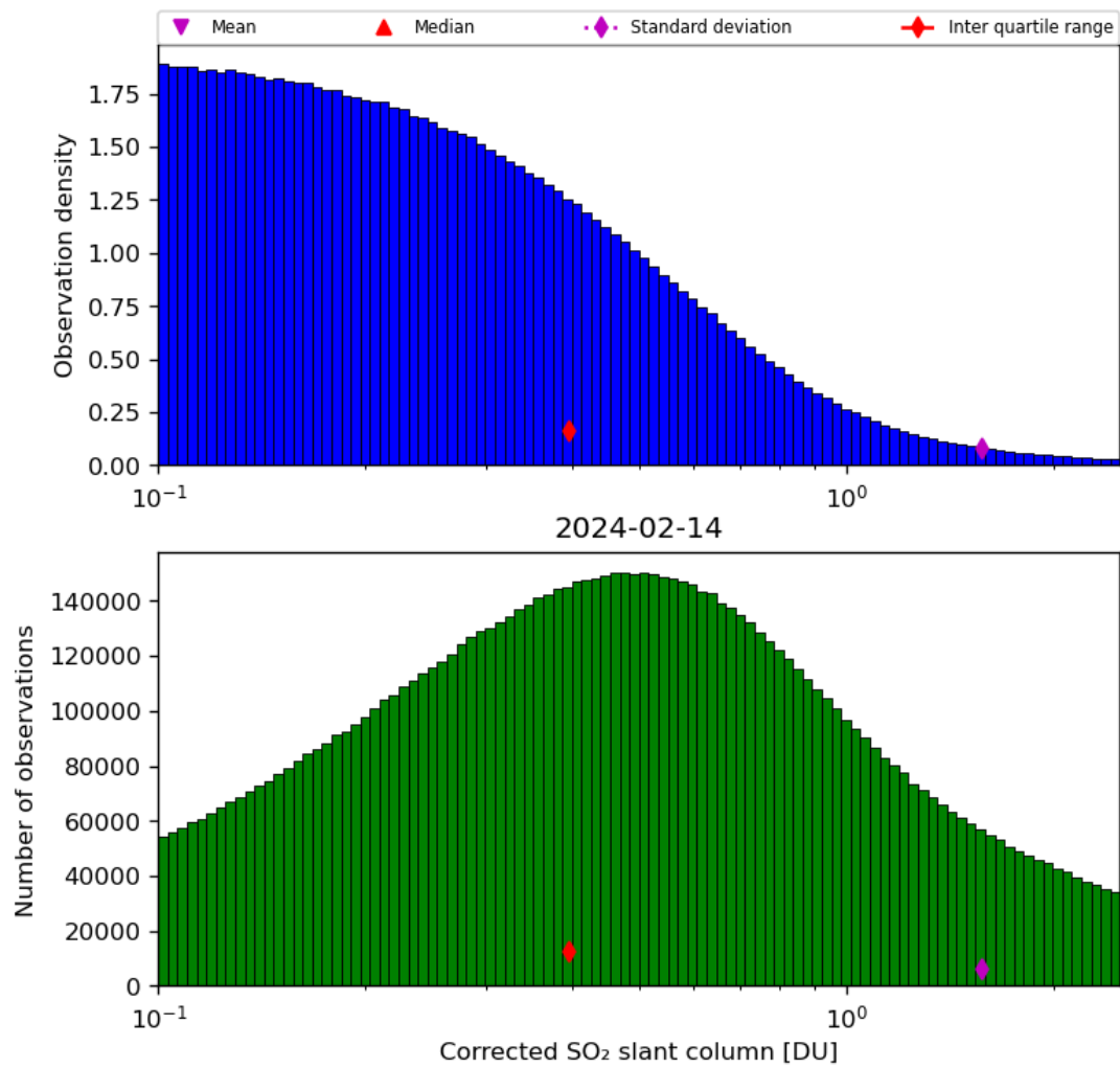
Figure 55: Histogram of “Corrected SO 2 slant column” for 2024-02-13 to 2024-02-15
