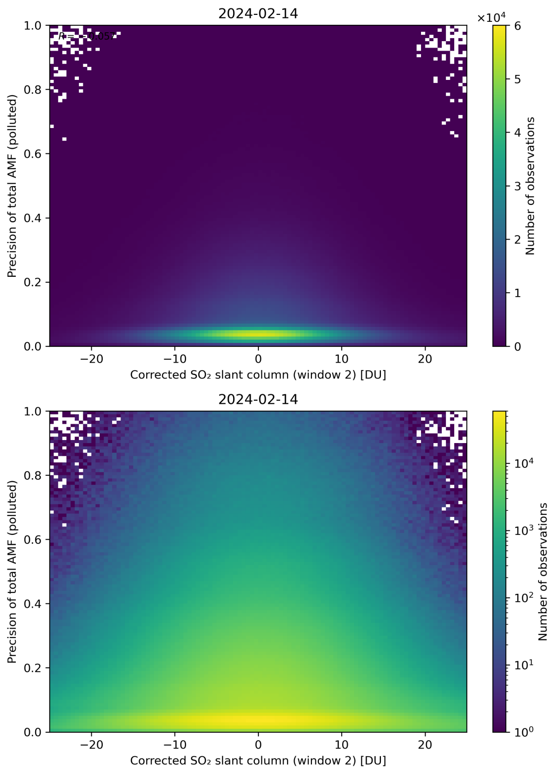
Figure 204: Scatter density plot of “Corrected SO 2 slant column (window 2)” against “Precision of total AMF (polluted)” for 2024-02-13 to 2024-02-15.
