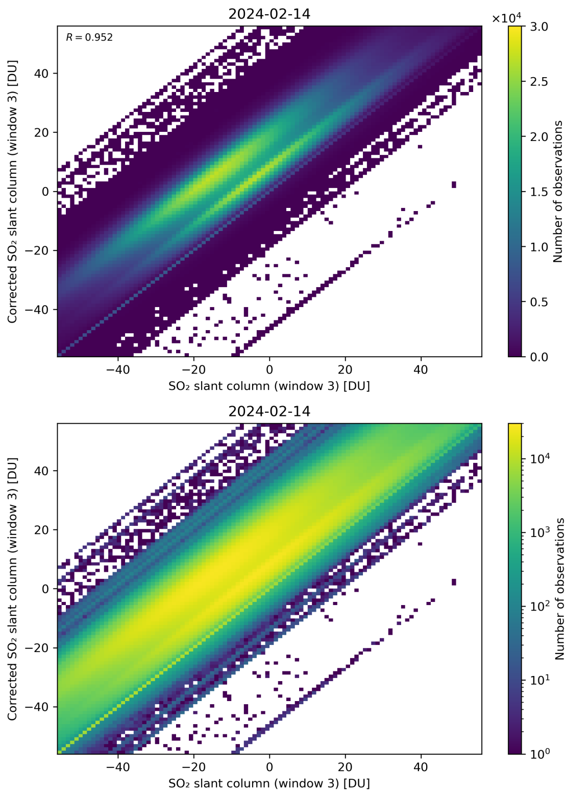
Figure 266: Scatter density plot of “SO 2 slant column (window 3)” against “Corrected SO 2 slant column (window 3)” for 2024-02-13 to 2024-02-15.
