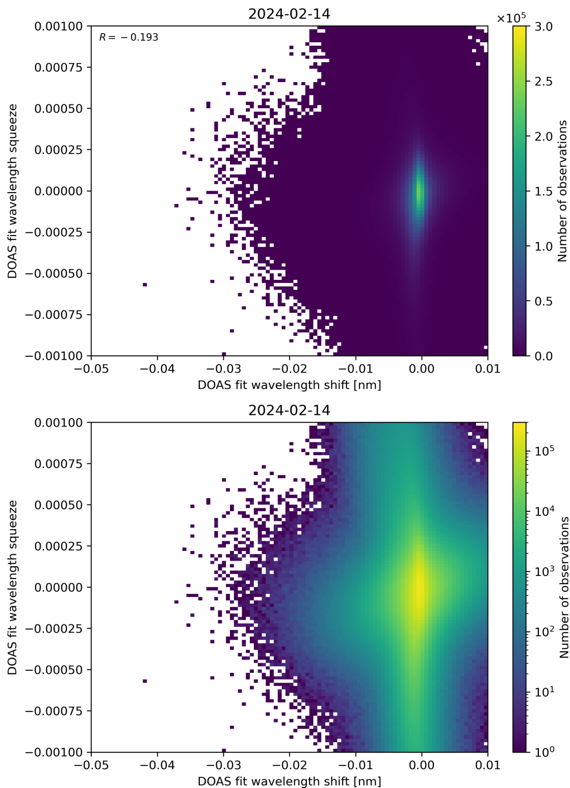
Figure 127: Scatter density plot of “DOAS fit wavelength shift” against “DOAS fit wavelength squeeze” for 2024-02-13 to 2024-02-15.
