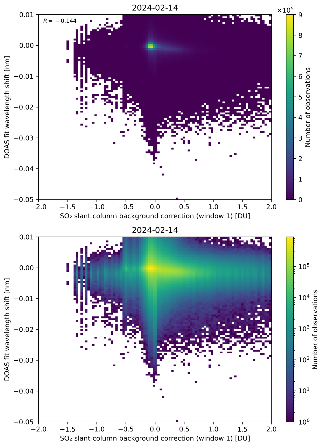
Figure 100: Scatter density plot of “SO 2 slant column background correction (window 1)” against “DOAS fit wavelength shift” for 2024-02-13 to 2024-02-15.
