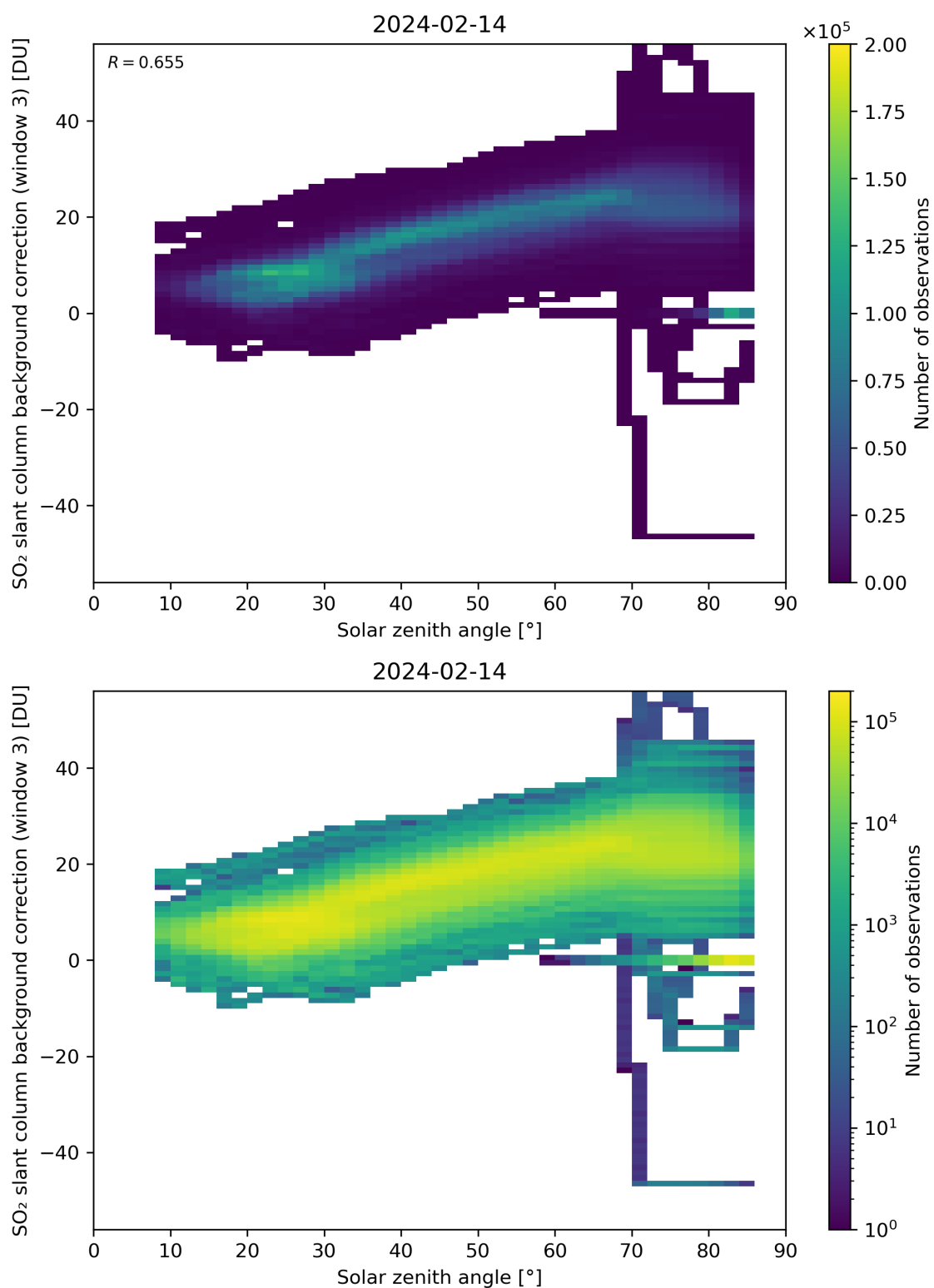
Figure 160: Scatter density plot of “Solar zenith angle” against “SO 2 slant column background correction (window 3)” for 2024-02-13 to 2024-02-15.
