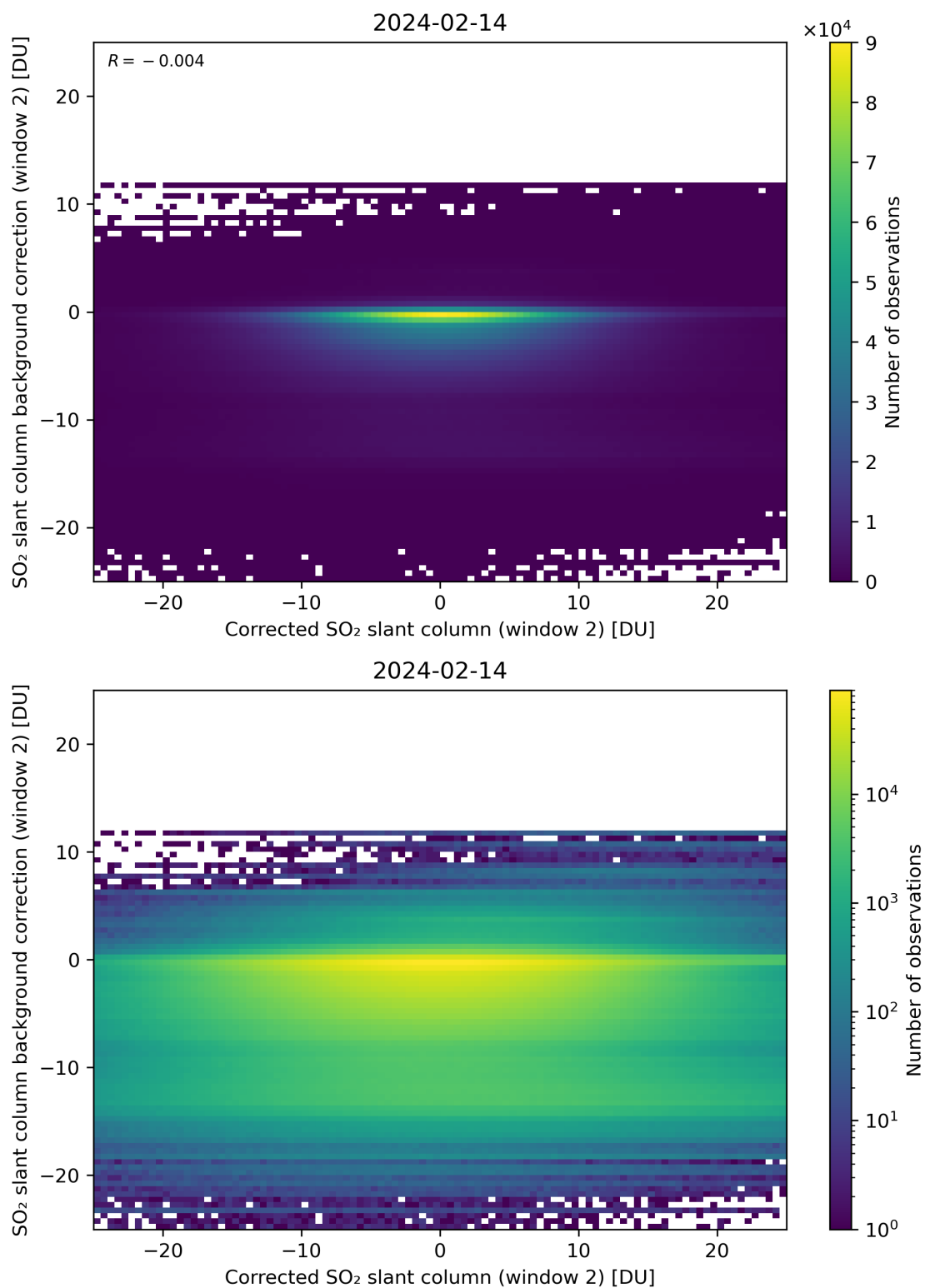
Figure 194: Scatter density plot of “Corrected SO 2 slant column (window 2)” against “SO 2 slant column background correction (window 2)” for 2024-02-13 to 2024-02-15.
