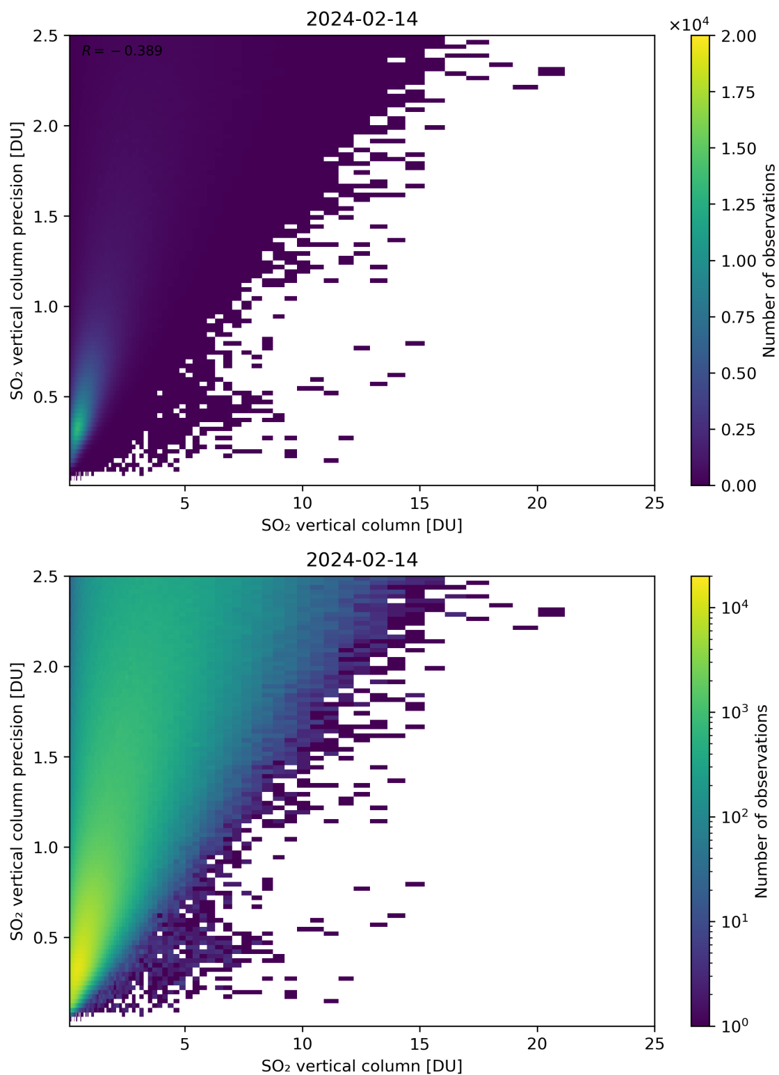
Figure 307: Scatter density plot of “SO 2 vertical column” against “SO 2 vertical column precision” for 2024-02-13 to 2024-02-15.
