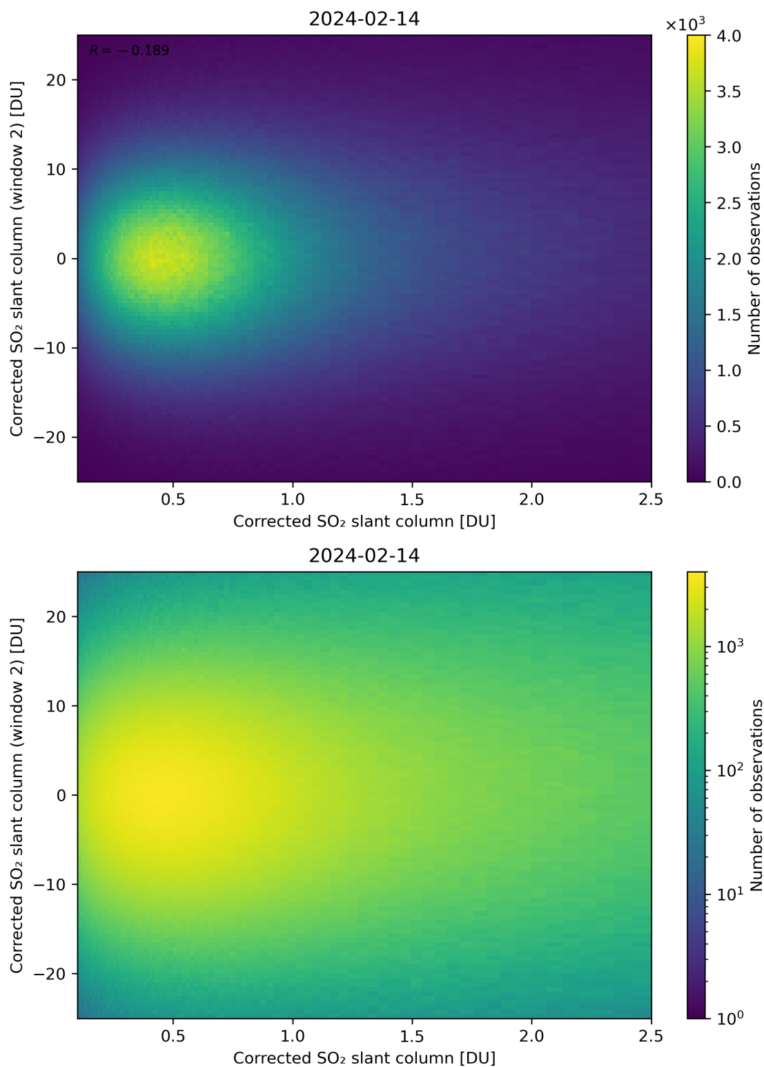
Figure 185: Scatter density plot of “Corrected SO 2 slant column” against “Corrected SO 2 slant column (window 2)” for 2024-02-13 to 2024-02-15.
