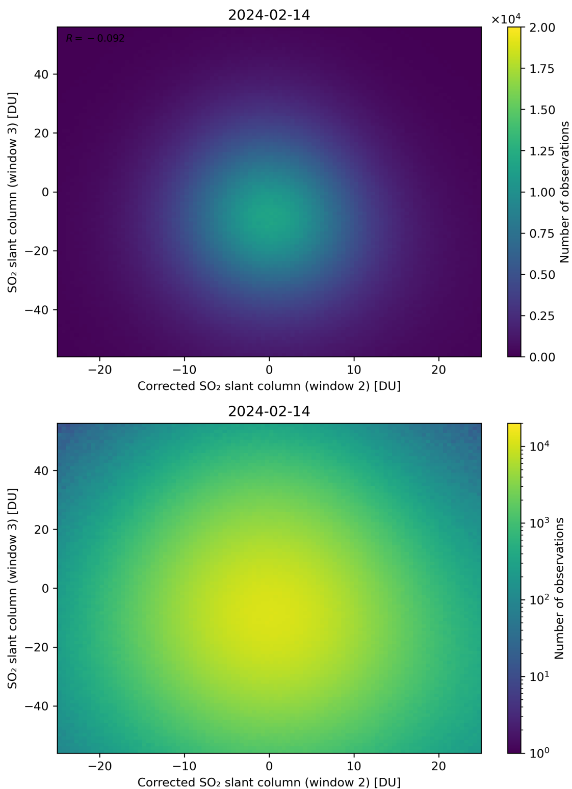
Figure 201: Scatter density plot of “Corrected SO 2 slant column (window 2)” against “SO 2 slant column (window 3)” for 2024-02-13 to 2024-02-15.
