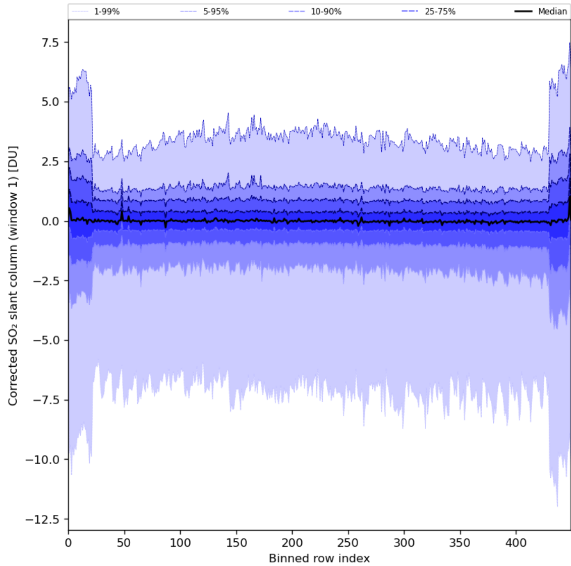
Figure 81: Along track statistics of “Corrected SO 2 slant column (window 1)” for 2024-02-13 to 2024-02-15
