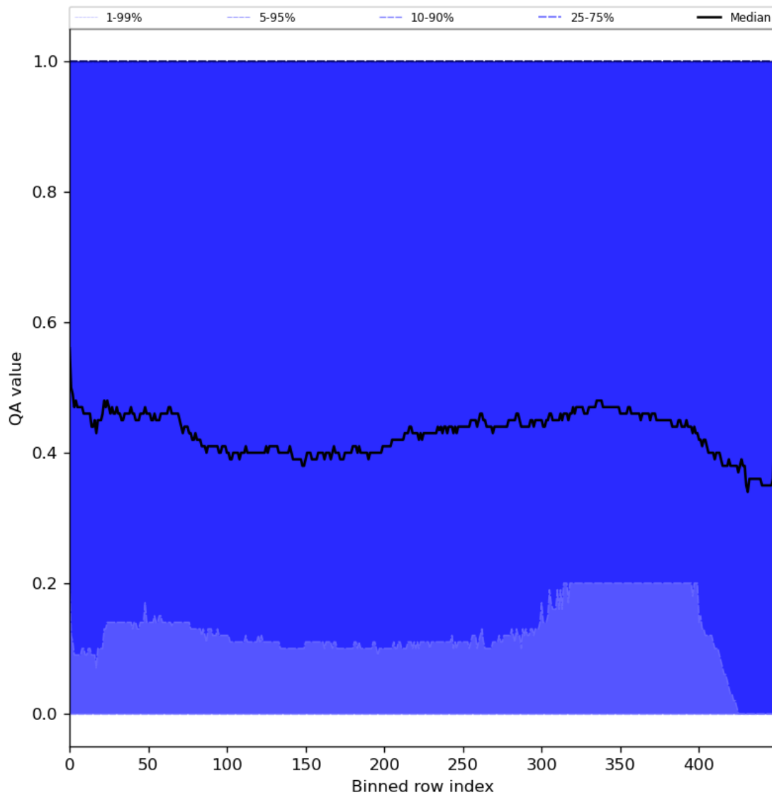
Figure 75: Along track statistics of “QA value” for 2024-02-13 to 2024-02-15
