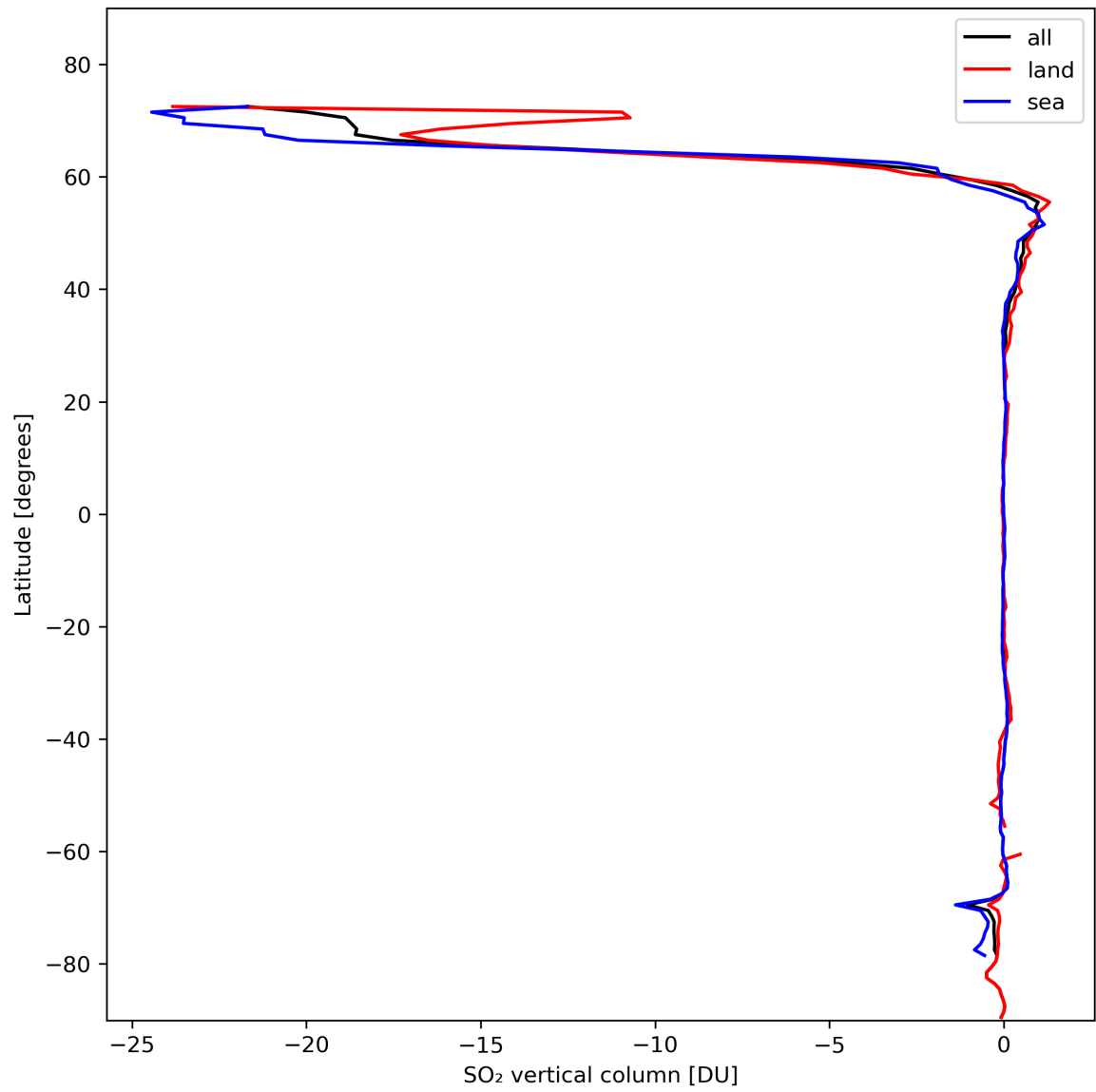
Figure 30: Zonal average of “SO 2 vertical column” for 2024-02-13 to 2024-02-15.
