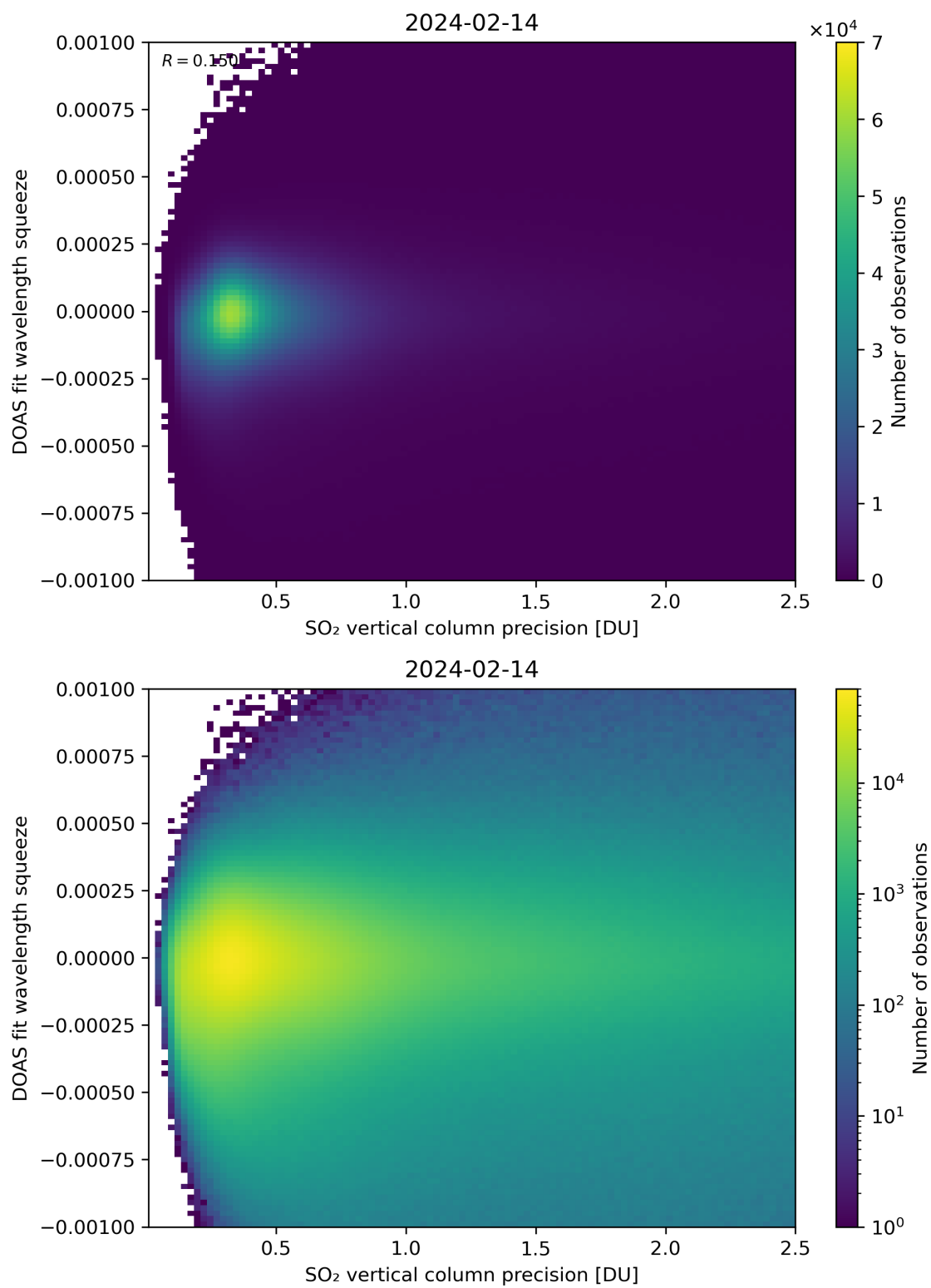
Figure 283: Scatter density plot of “SO 2 vertical column precision” against “DOAS fit wavelength squeeze” for 2024-02-13 to 2024-02-15.
