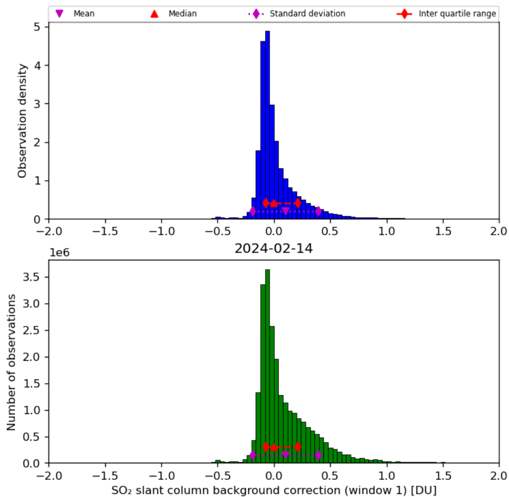
Figure 59: Histogram of “SO 2 slant column background correction (window 1)” for 2024-02-13 to 2024-02-15
