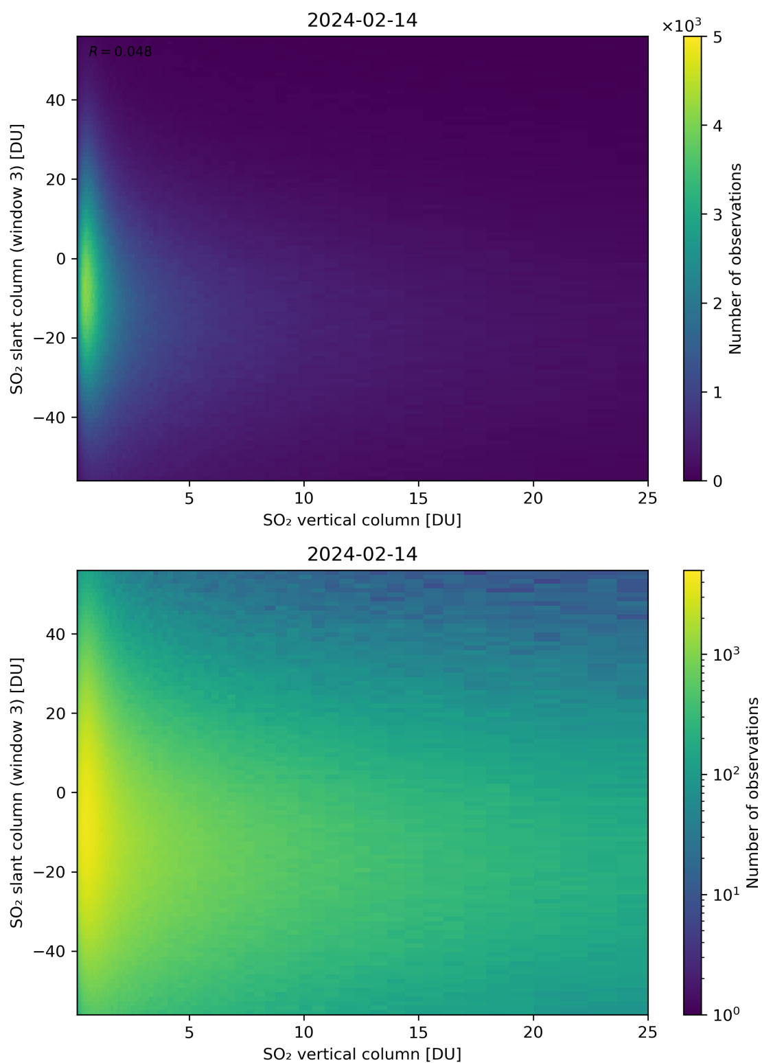
Figure 303: Scatter density plot of “SO 2 vertical column” against “SO 2 slant column (window 3)” for 2024-02-13 to 2024-02-15.
