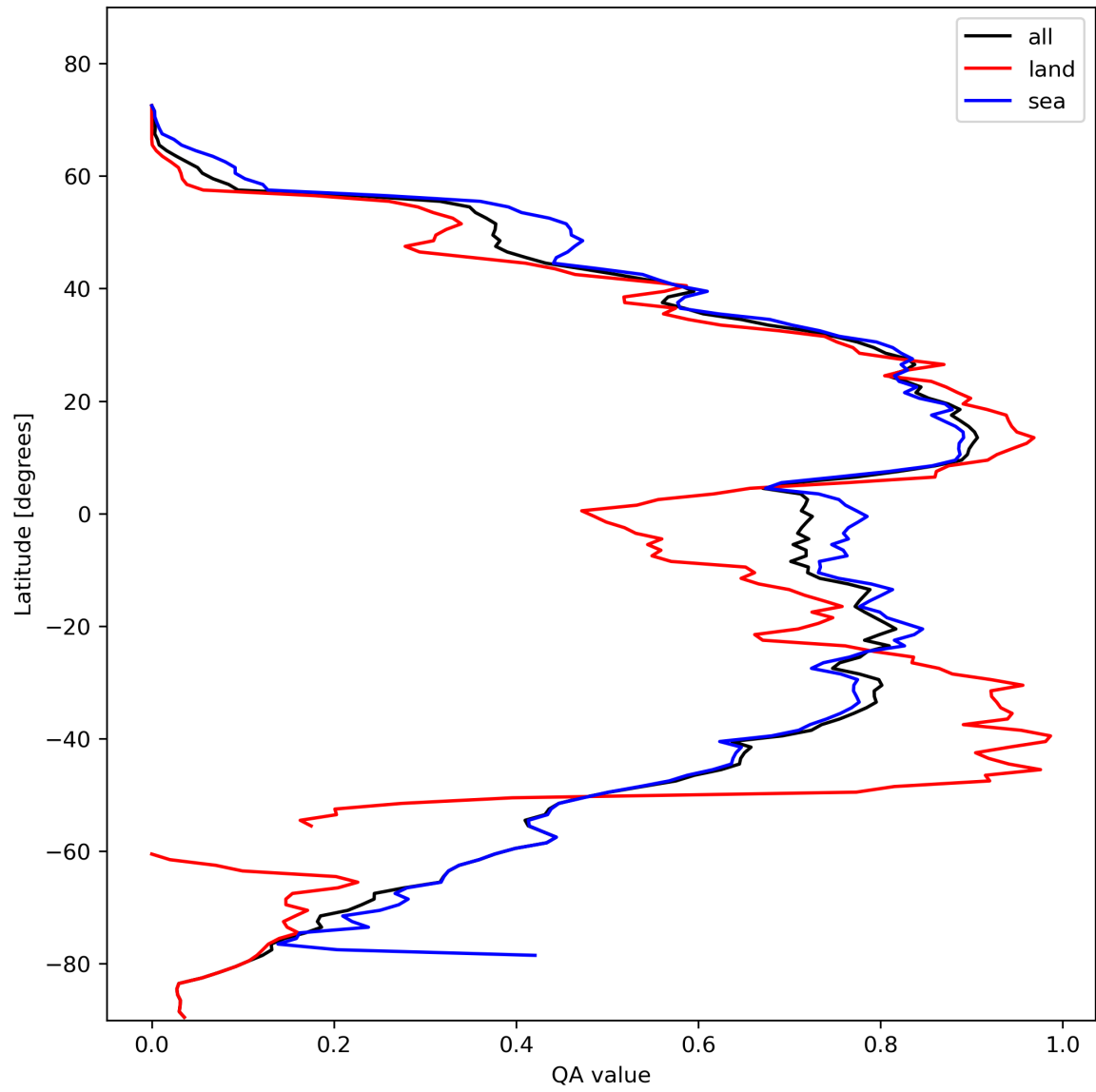
Figure 29: Zonal average of “QA value” for 2024-02-13 to 2024-02-15.
