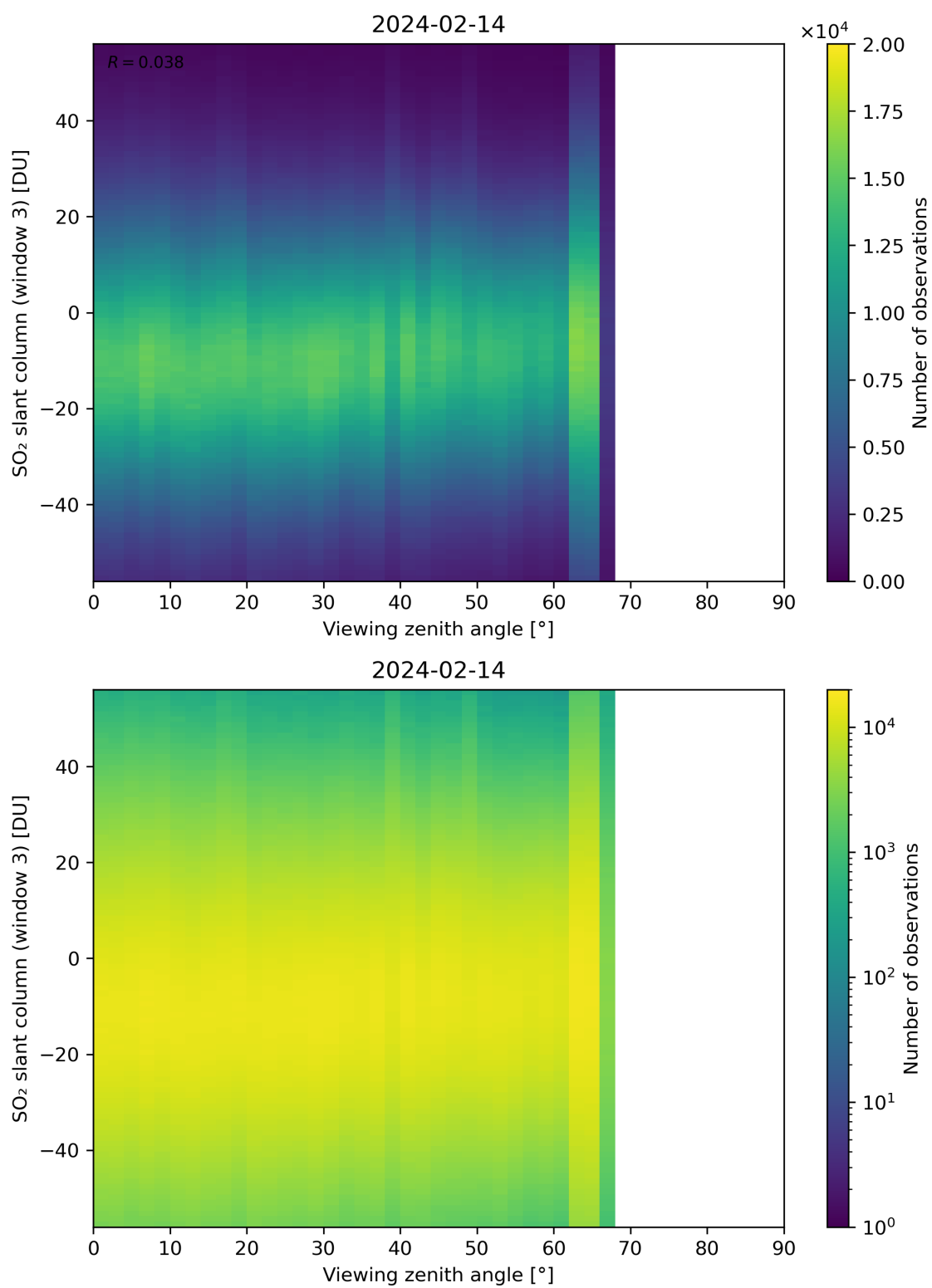
Figure 323: Scatter density plot of “Viewing zenith angle” against “SO 2 slant column (window 3)” for 2024-02-13 to 2024-02-15.
