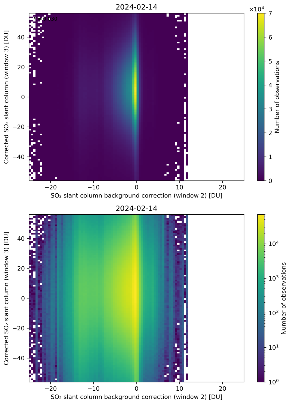
Figure 116: Scatter density plot of “SO 2 slant column background correction (window 2)” against “Corrected SO 2 slant column (window 3)” for 2024-02-13 to 2024-02-15.
