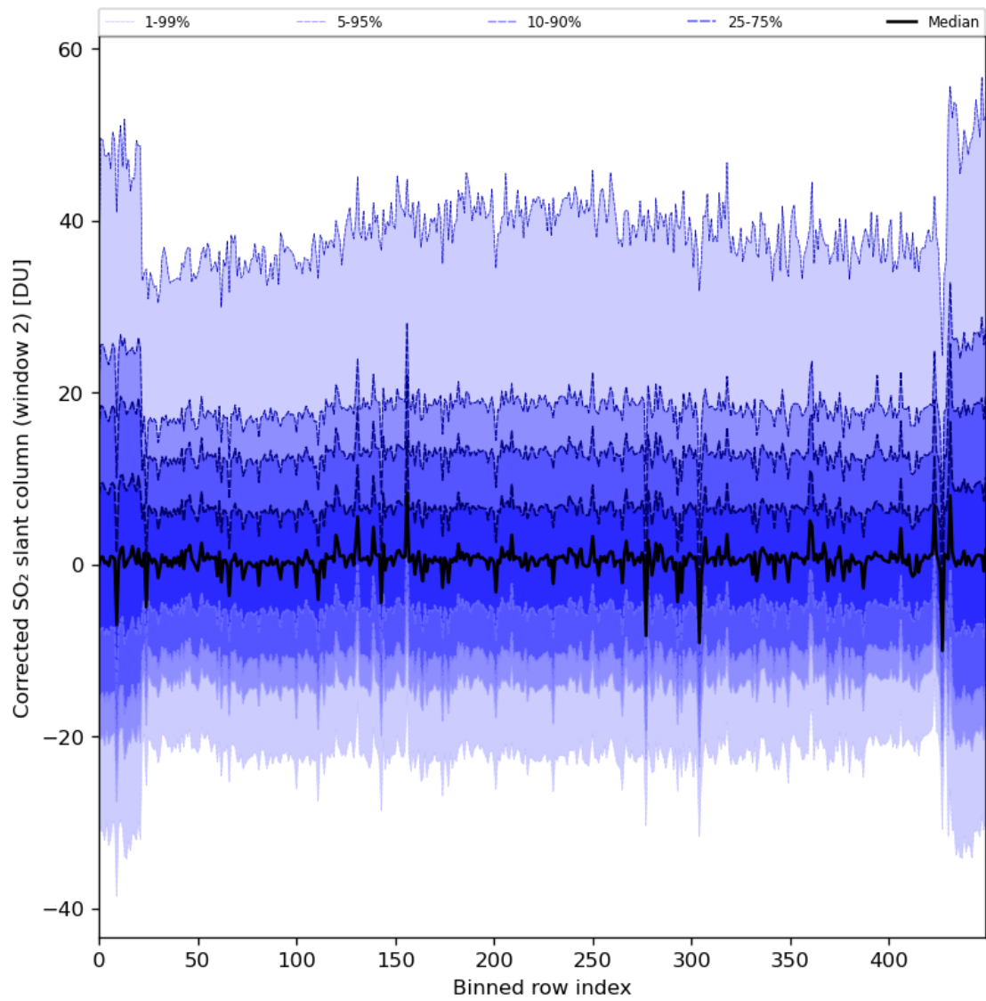
Figure 85: Along track statistics of “Corrected SO 2 slant column (window 2)” for 2024-02-13 to 2024-02-15
