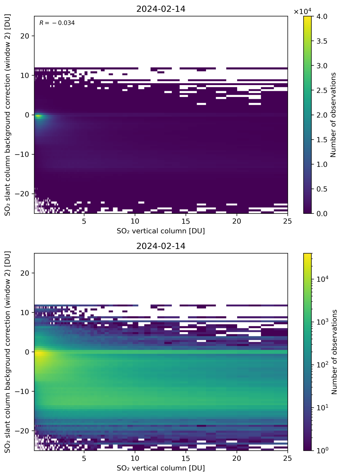
Figure 274: Scatter density plot of “SO 2 vertical column” against “SO 2 slant column background correction (window 2)” for 2024-02-13 to 2024-02-15.
