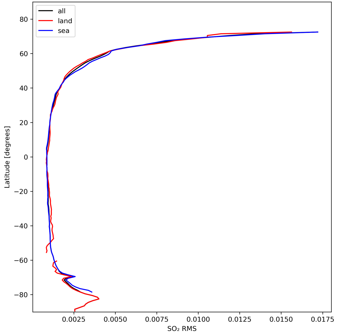
Figure 47: Zonal average of “SO 2 RMS” for 2024-02-13 to 2024-02-15.
