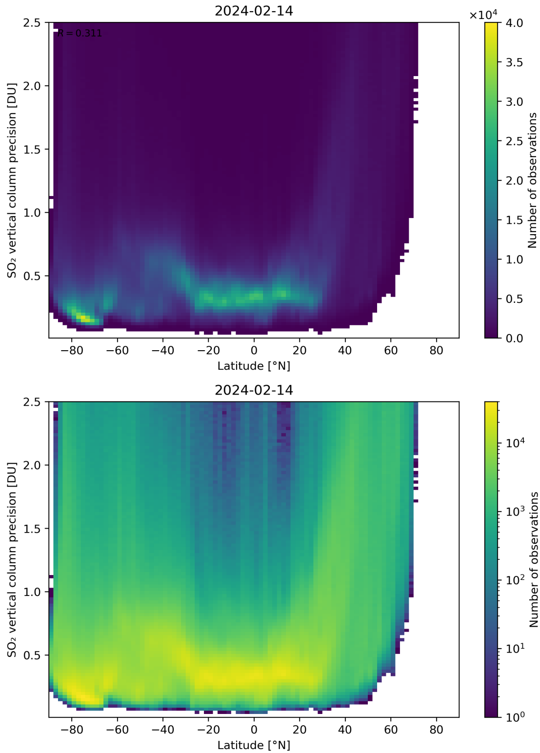
Figure 157: Scatter density plot of “Latitude” against “SO 2 vertical column precision” for 2024-02-13 to 2024-02-15.
