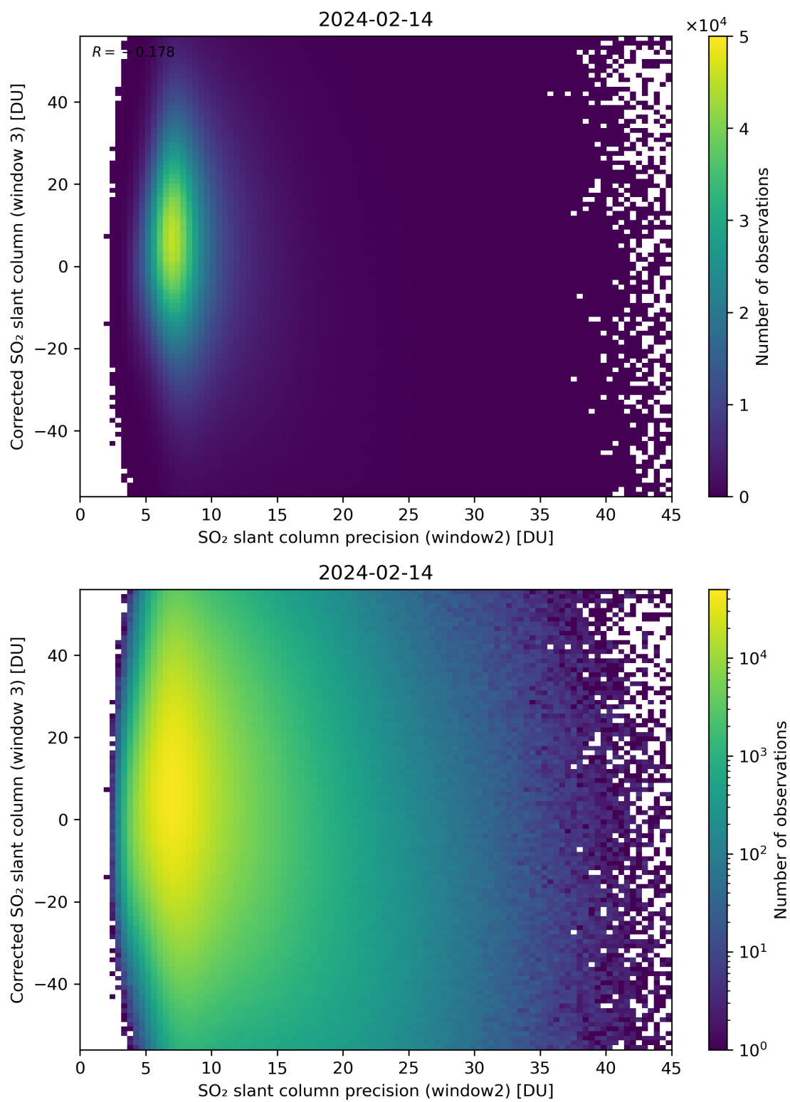
Figure 248: Scatter density plot of “SO 2 slant column precision (window2)” against “Corrected SO 2 slant column (window 3)” for 2024-02-13 to 2024-02-15.
