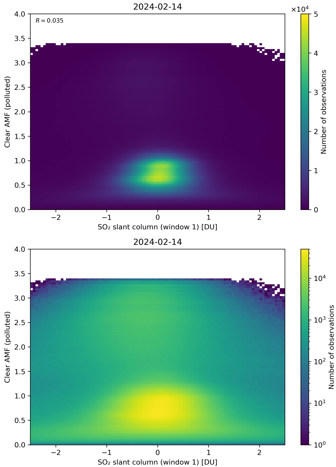
Figure 232: Scatter density plot of “SO 2 slant column (window 1)” against “Clear AMF (polluted)” for 2024-02-13 to 2024-02-15.
