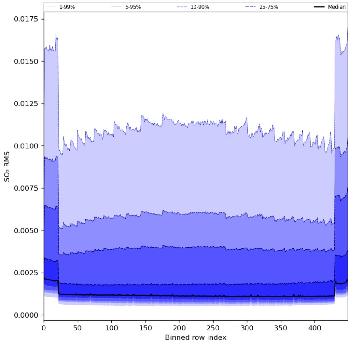
Figure 93: Along track statistics of “SO 2 RMS” for 2024-02-13 to 2024-02-15
