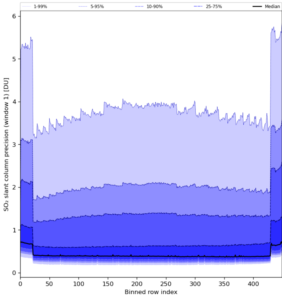
Figure 80: Along track statistics of “SO 2 slant column precision (window 1)” for 2024-02-13 to 2024-02-15
