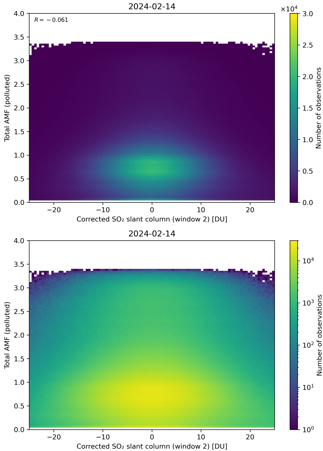
Figure 203: Scatter density plot of “Corrected SO 2 slant column (window 2)” against “Total AMF (polluted)” for 2024-02-13 to 2024-02-15.
