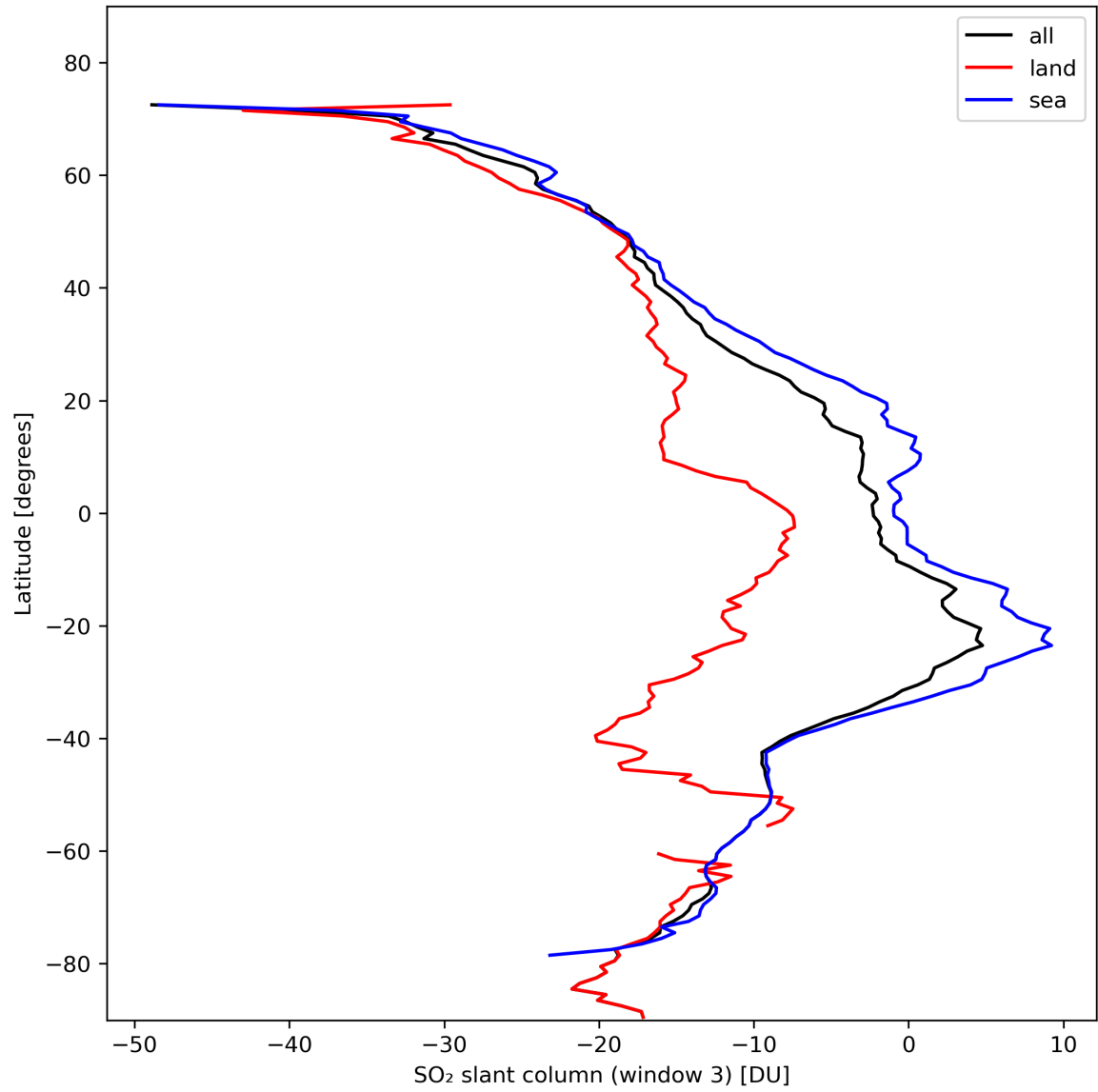
Figure 41: Zonal average of “SO 2 slant column (window 3)” for 2024-02-13 to 2024-02-15.
