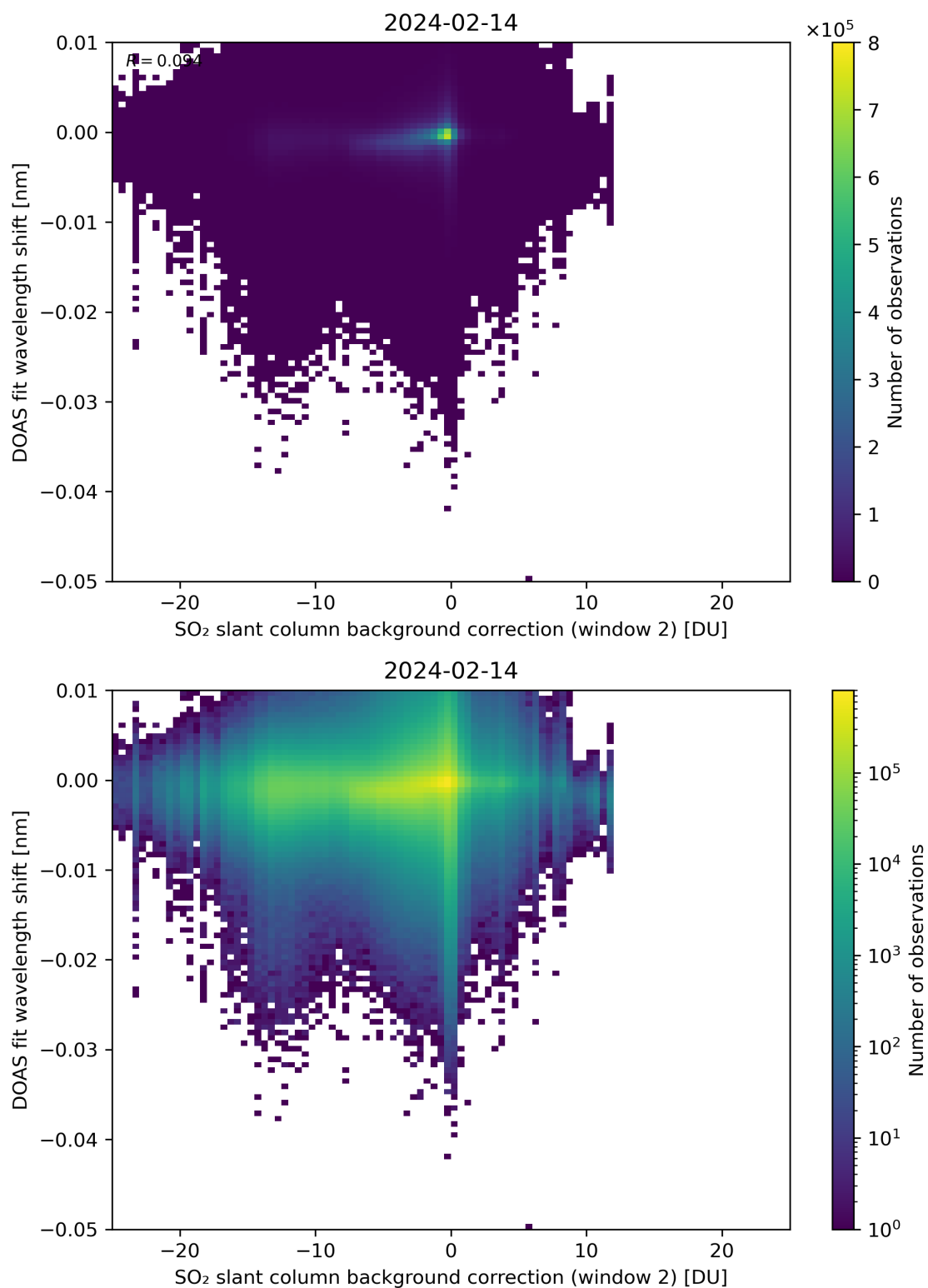
Figure 112: Scatter density plot of “SO 2 slant column background correction (window 2)” against “DOAS fit wavelength shift” for 2024-02-13 to 2024-02-15.
