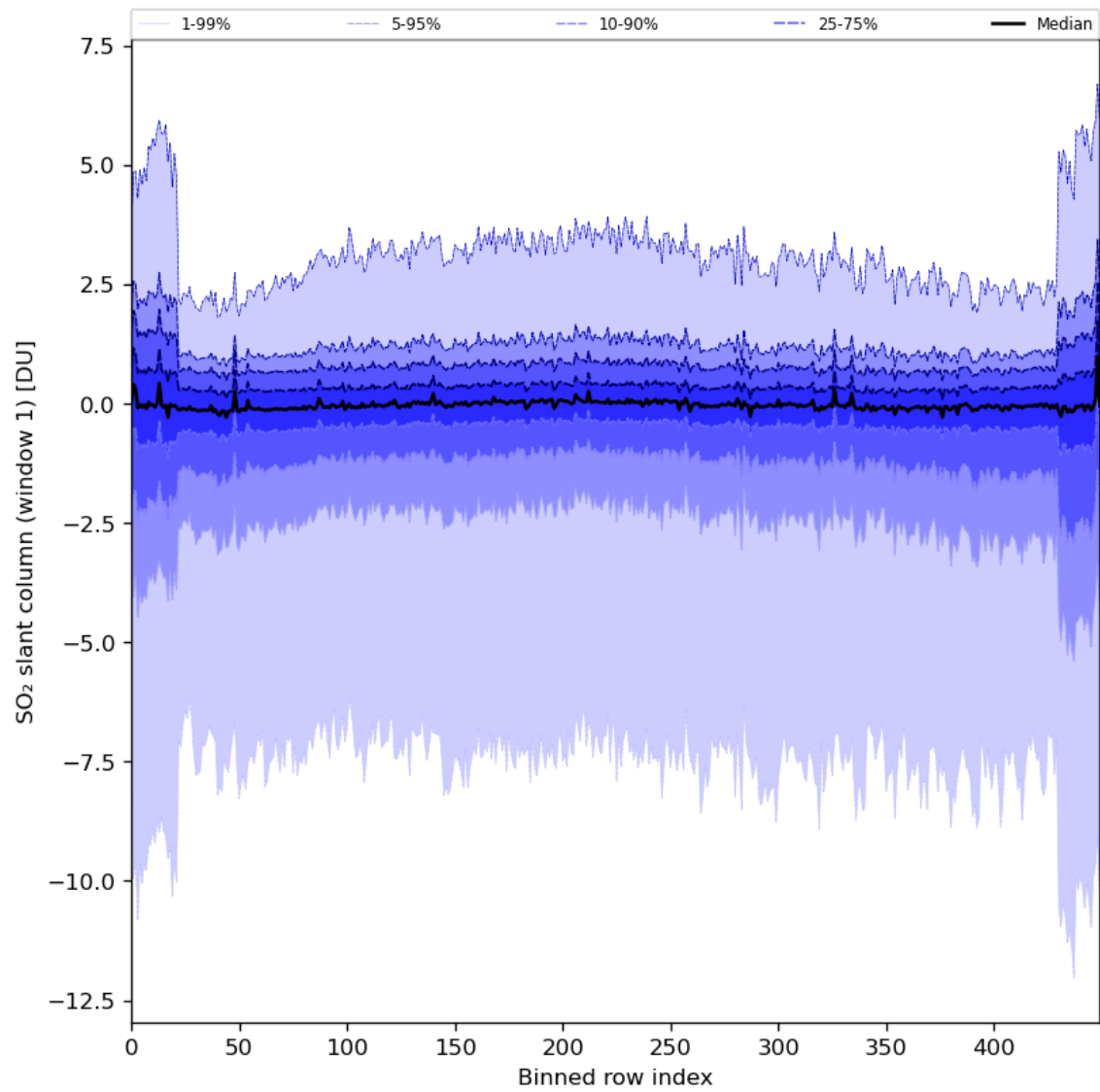
Figure 79: Along track statistics of “SO 2 slant column (window 1)” for 2024-02-13 to 2024-02-15
