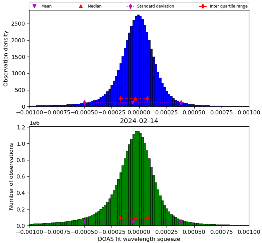
Figure 69: Histogram of “DOAS fit wavelength squeeze” for 2024-02-13 to 2024-02-15
