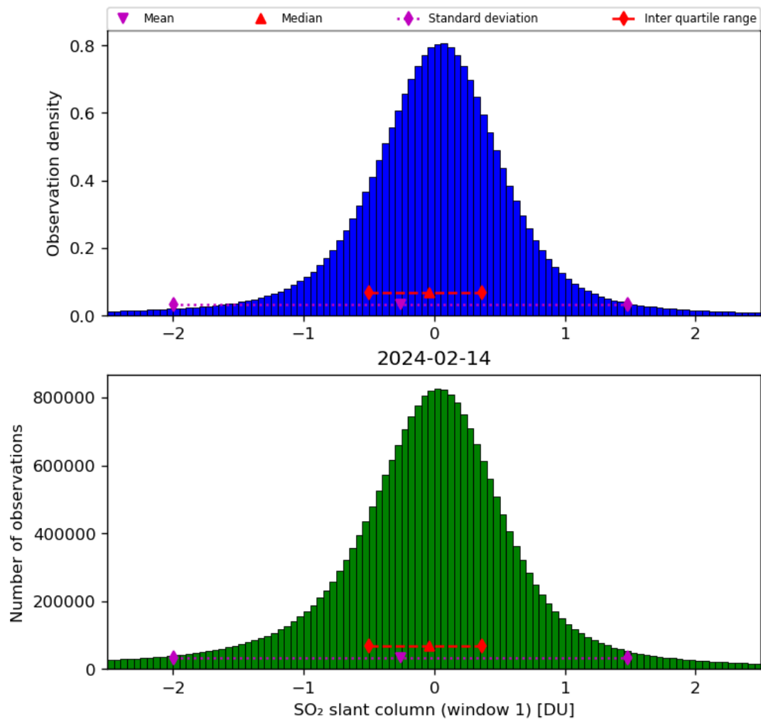
Figure 56: Histogram of “SO 2 slant column (window 1)” for 2024-02-13 to 2024-02-15
