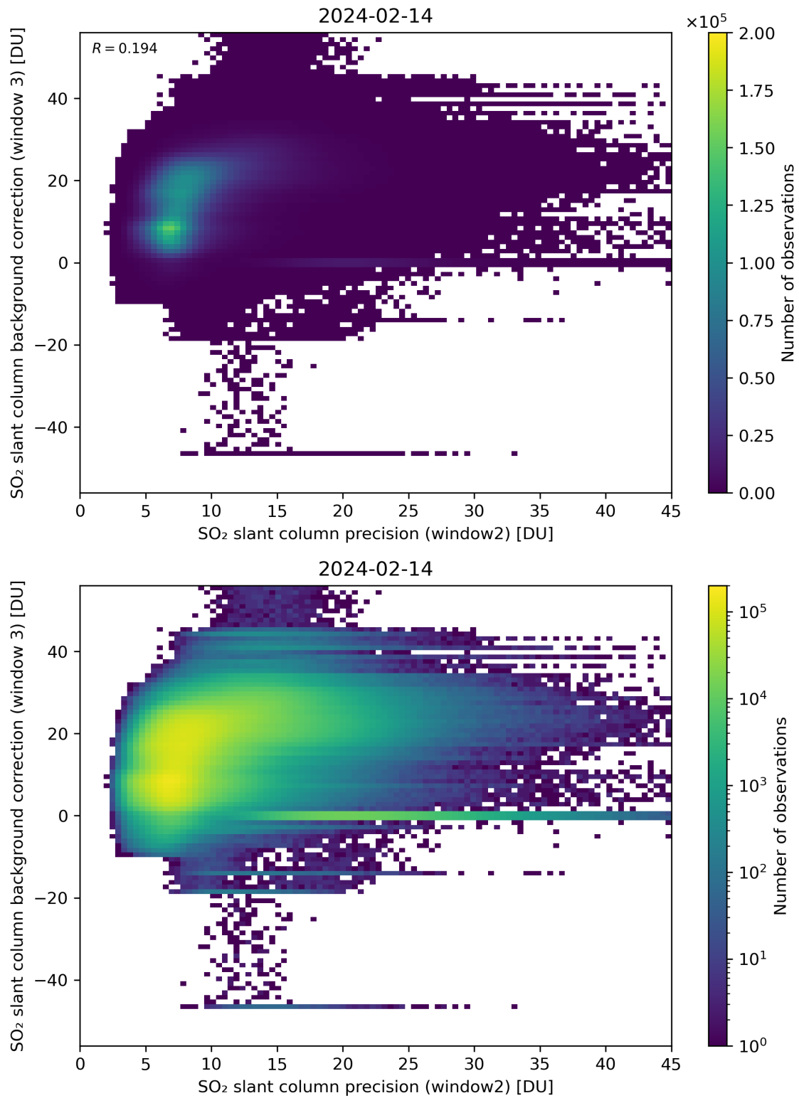
Figure 242: Scatter density plot of “SO 2 slant column precision (window2)” against “SO 2 slant column background correction (window 3)” for 2024-02-13 to 2024-02-15.
