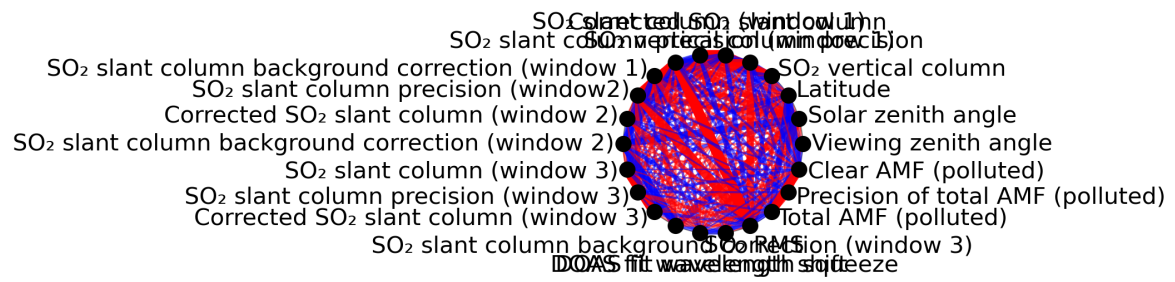
Figure 1: Map of correlation graph for 2024-02-13 to 2024-02-15.
