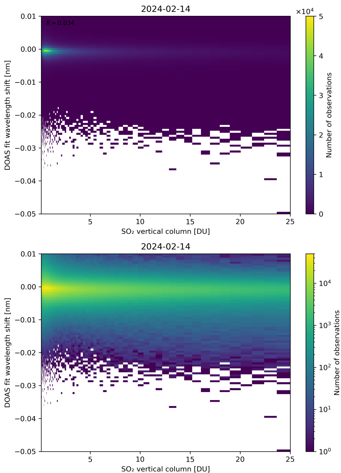
Figure 276: Scatter density plot of “SO 2 vertical column” against “DOAS fit wavelength shift” for 2024-02-13 to 2024-02-15.
