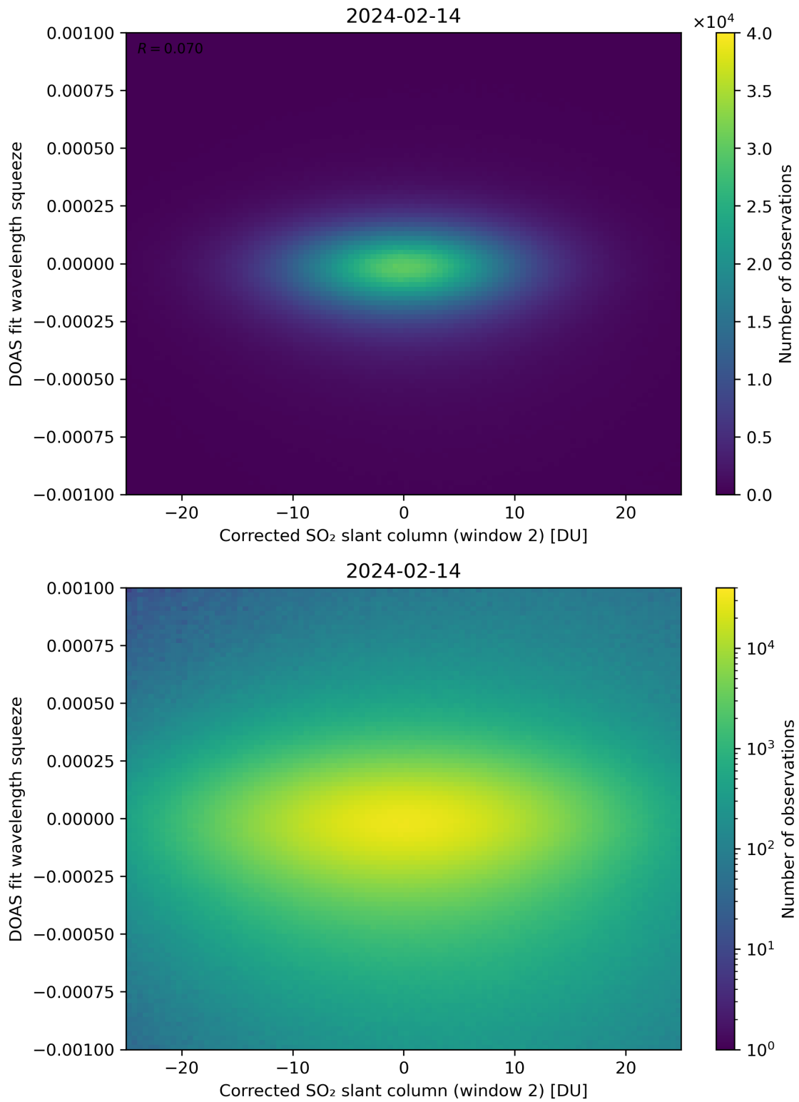
Figure 197: Scatter density plot of “Corrected SO 2 slant column (window 2)” against “DOAS fit wavelength squeeze” for 2024-02-13 to 2024-02-15.
