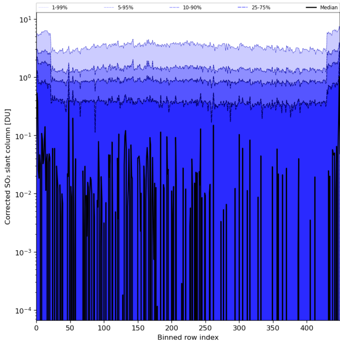
Figure 78: Along track statistics of “Corrected SO 2 slant column” for 2024-02-13 to 2024-02-15
