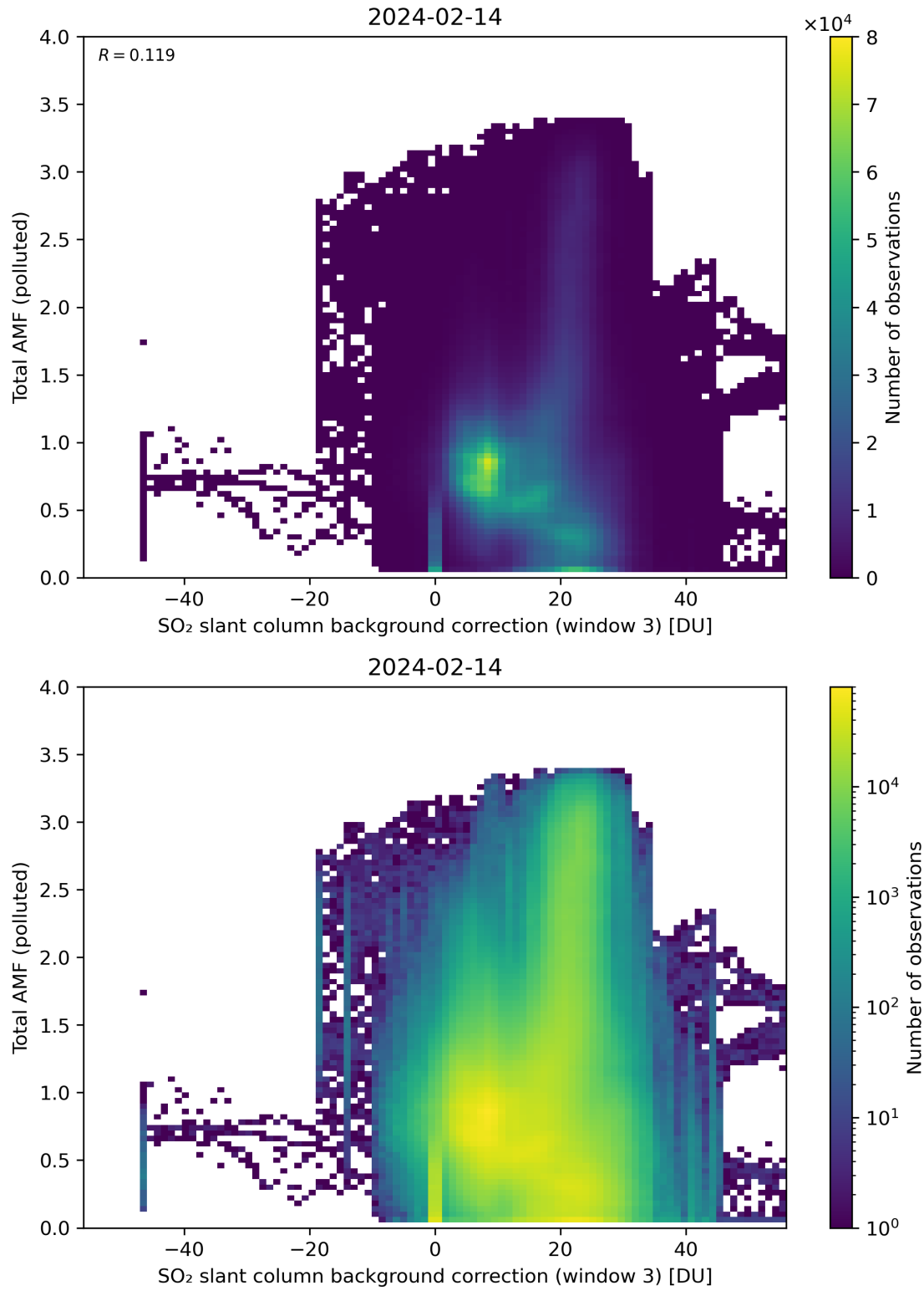
Figure 125: Scatter density plot of “SO 2 slant column background correction (window 3)” against “Total AMF (polluted)” for 2024-02-13 to 2024-02-15.
