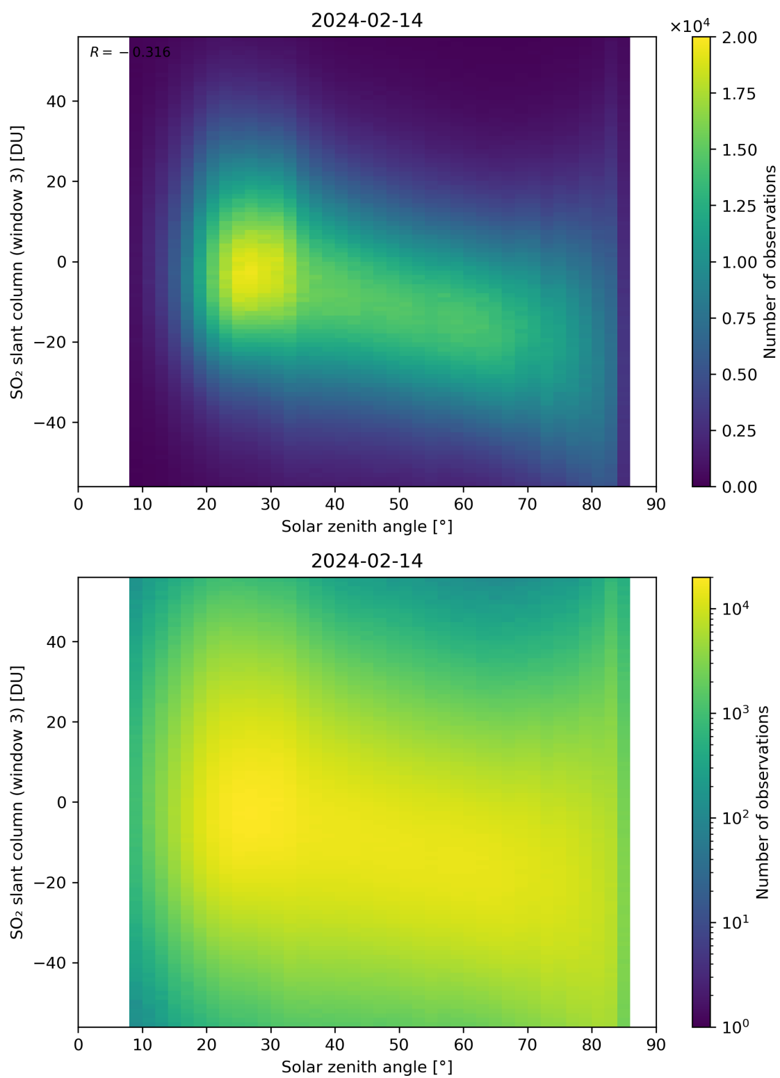
Figure 172: Scatter density plot of “Solar zenith angle” against “SO 2 slant column (window 3)” for 2024-02-13 to 2024-02-15.
