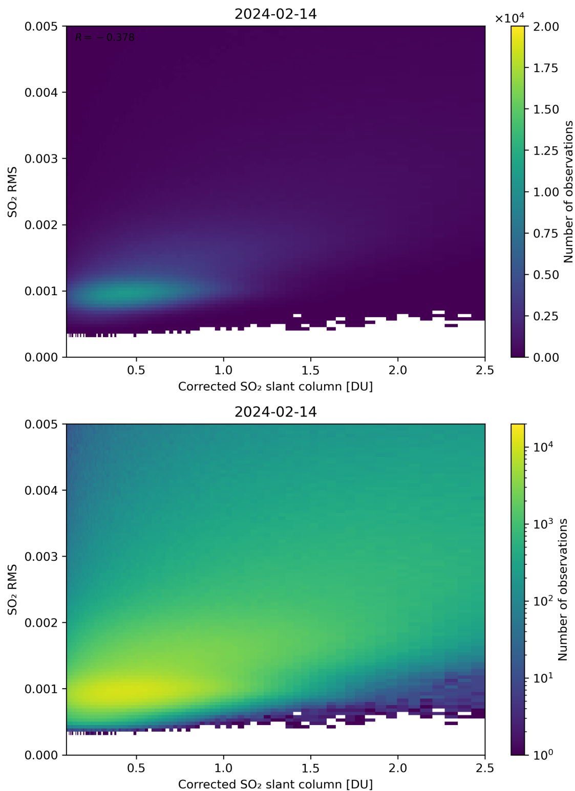
Figure 183: Scatter density plot of “Corrected SO 2 slant column” against “SO 2 RMS” for 2024-02-13 to 2024-02-15.
