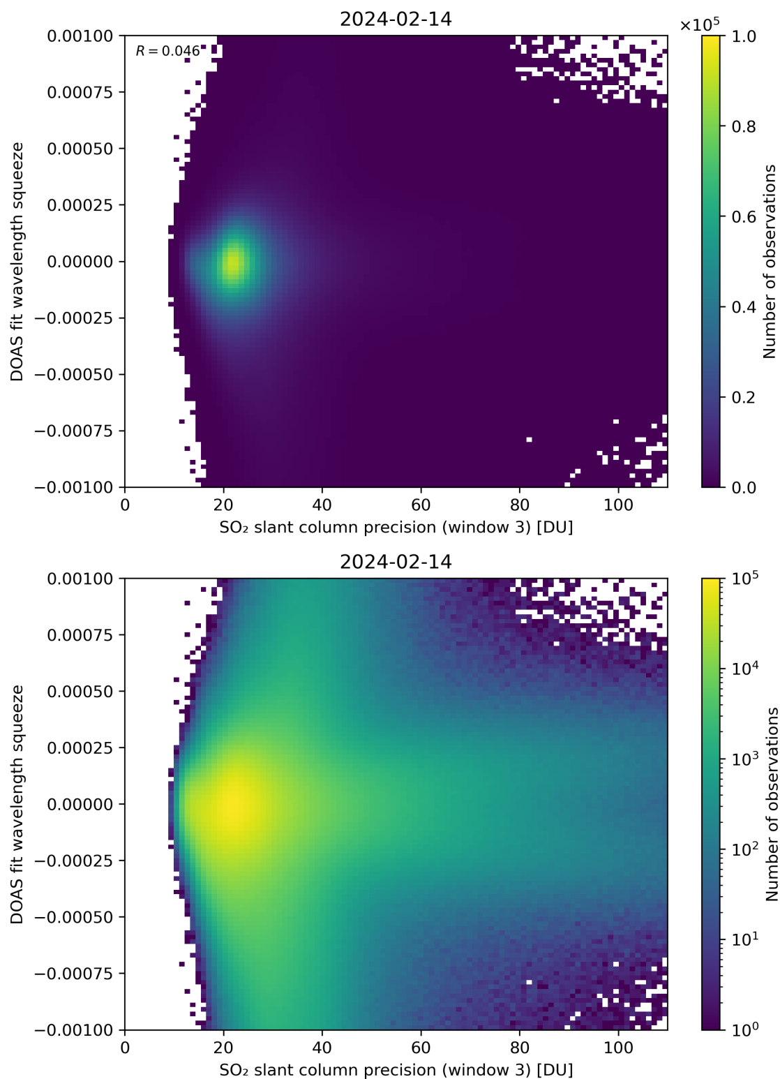
Figure 259: Scatter density plot of “SO 2 slant column precision (window 3)” against “DOAS fit wavelength squeeze” for 2024-02-13 to 2024-02-15.
