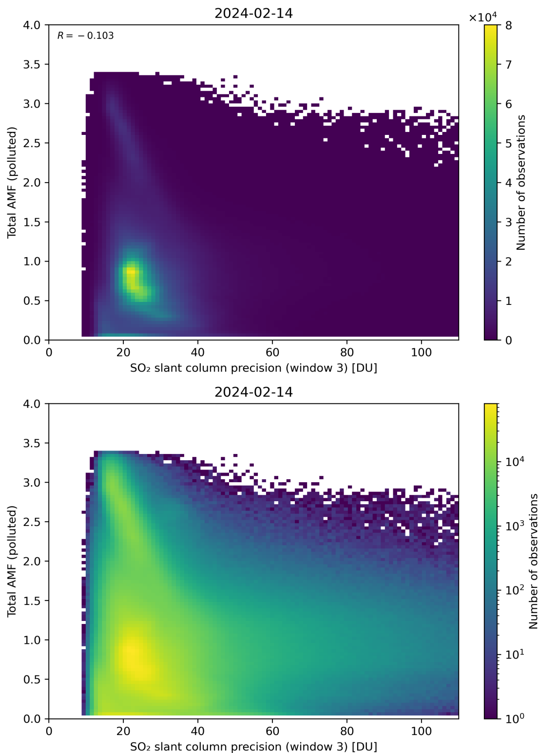
Figure 263: Scatter density plot of “SO 2 slant column precision (window 3)” against “Total AMF (polluted)” for 2024-02-13 to 2024-02-15.
