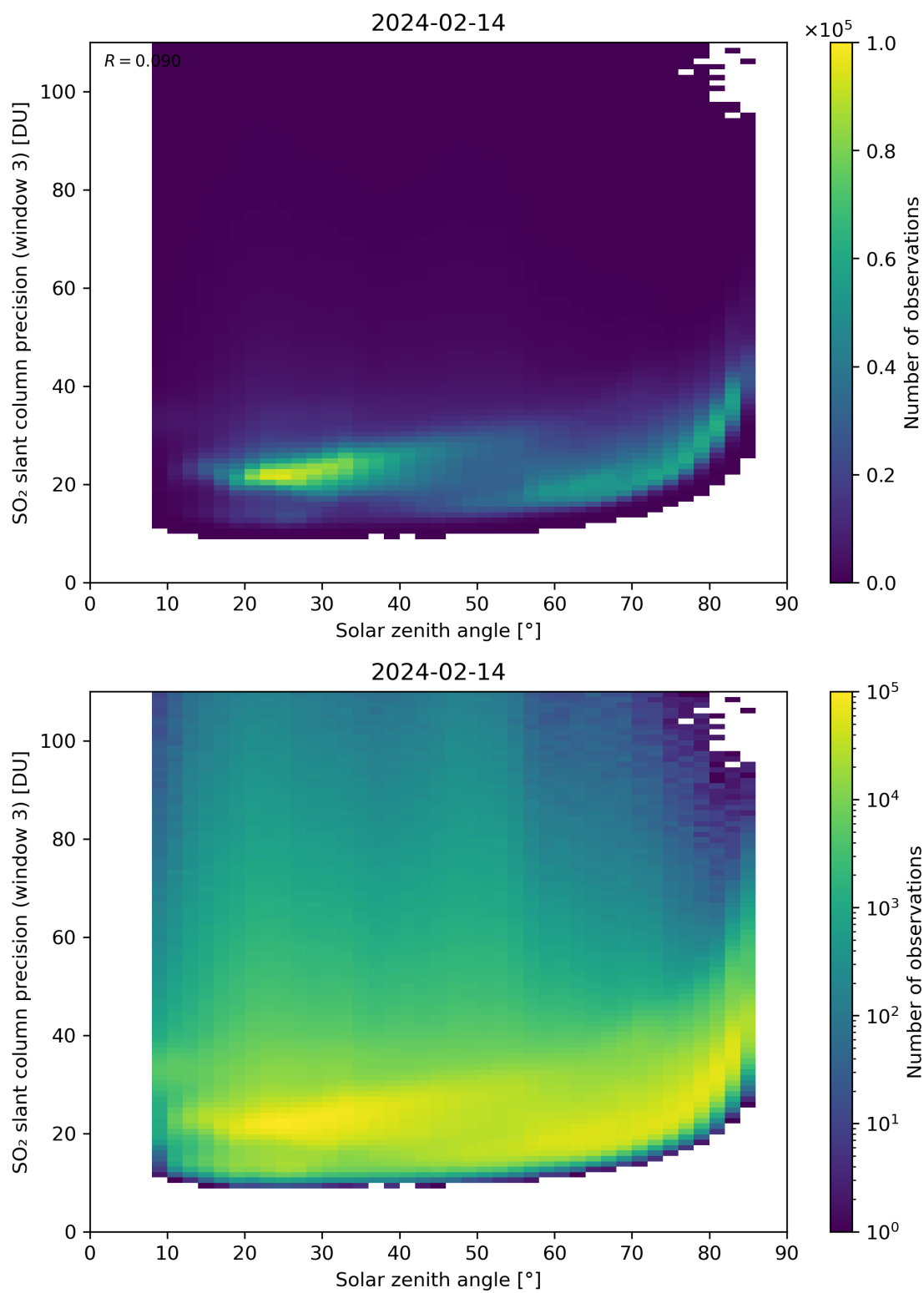
Figure 173: Scatter density plot of “Solar zenith angle” against “SO 2 slant column precision (window 3)” for 2024-02-13 to 2024-02-15.
