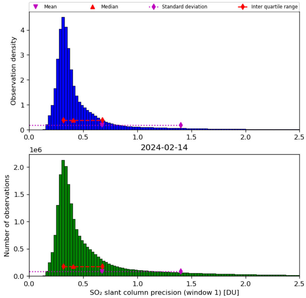
Figure 57: Histogram of “SO 2 slant column precision (window 1)” for 2024-02-13 to 2024-02-15
