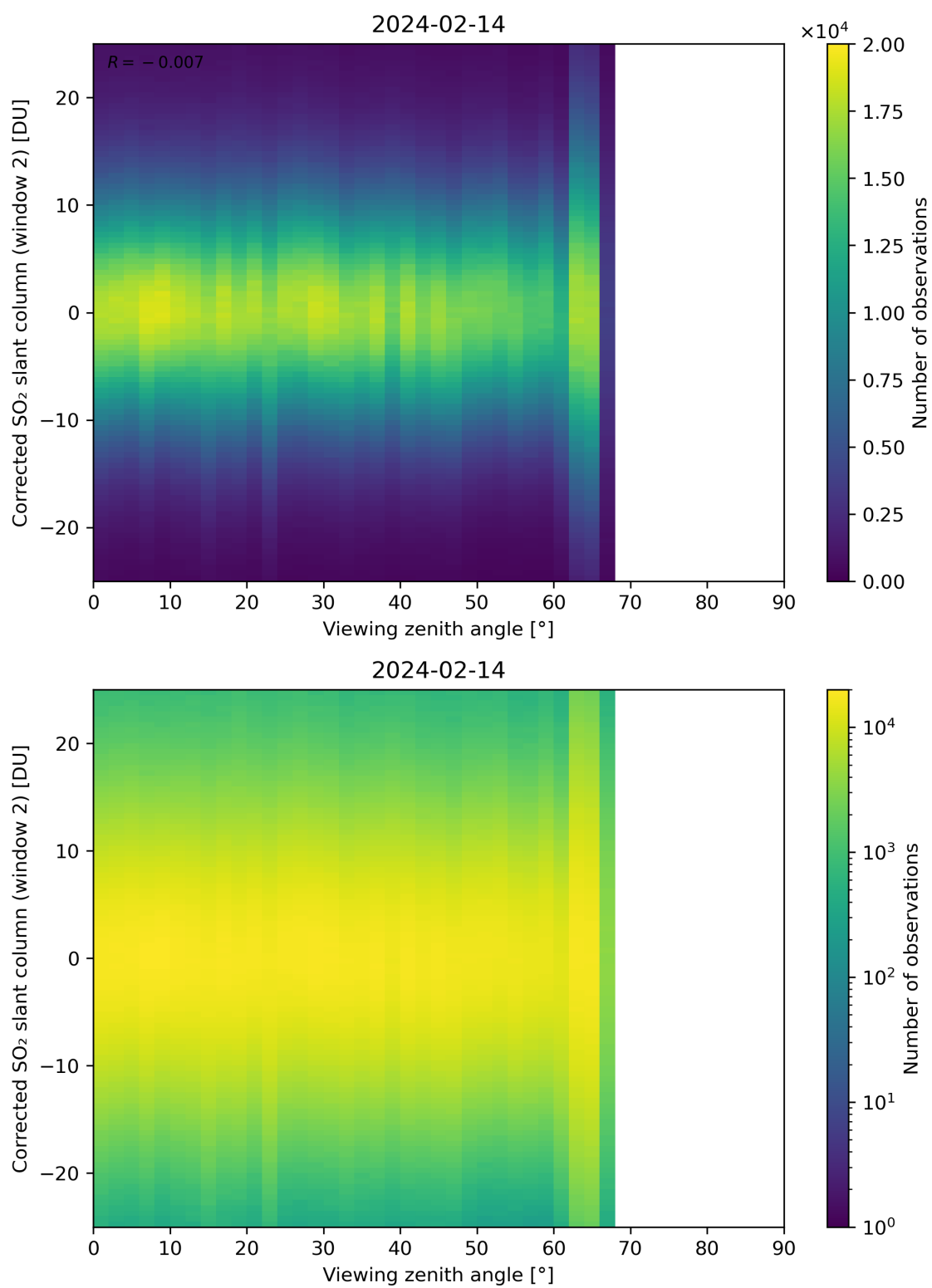
Figure 318: Scatter density plot of “Viewing zenith angle” against “Corrected SO 2 slant column (window 2)” for 2024-02-13 to 2024-02-15.
