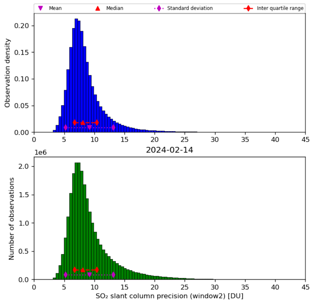
Figure 61: Histogram of “SO 2 slant column precision (window2)” for 2024-02-13 to 2024-02-15
