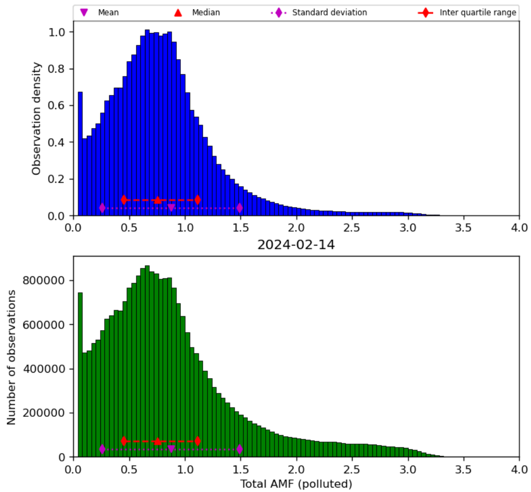
Figure 71: Histogram of “Total AMF (polluted)” for 2024-02-13 to 2024-02-15
