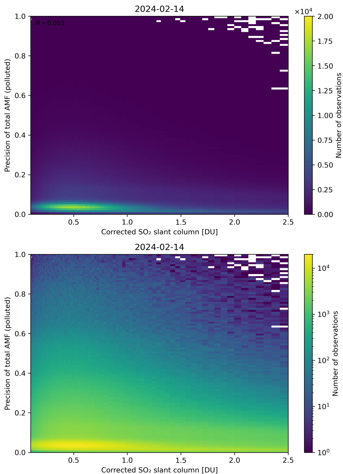
Figure 193: Scatter density plot of “Corrected SO 2 slant column” against “Precision of total AMF (polluted)” for 2024-02-13 to 2024-02-15.
