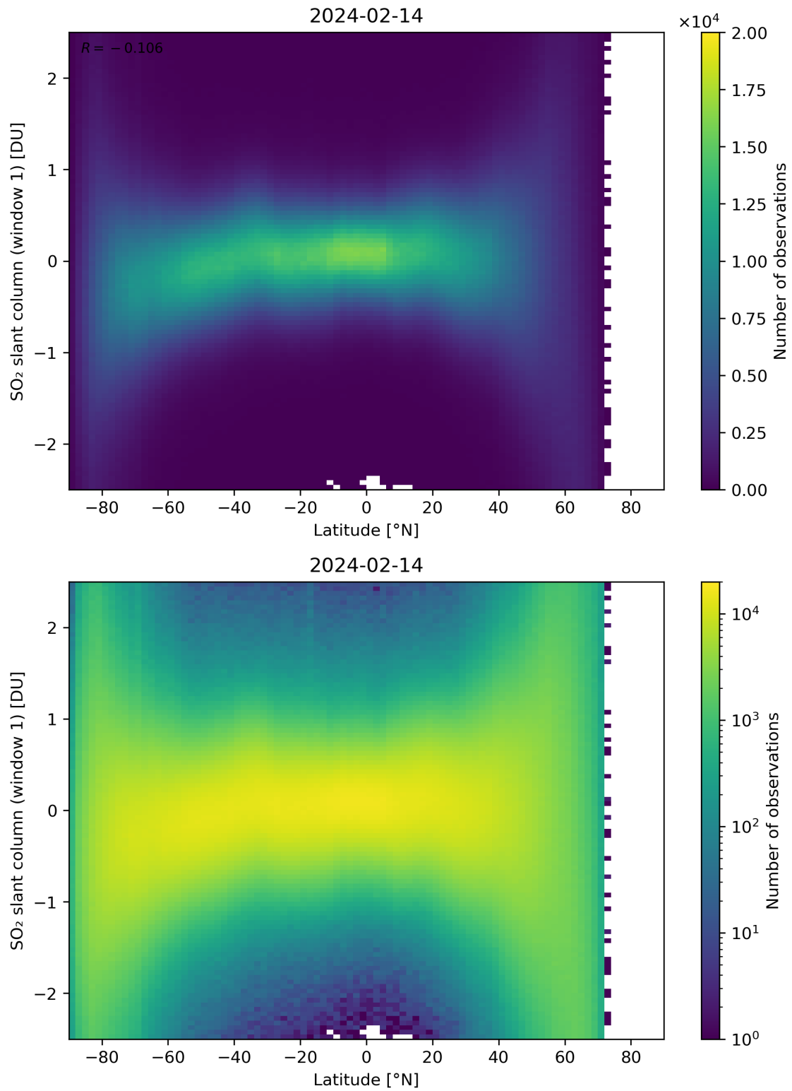
Figure 149: Scatter density plot of “Latitude” against “SO 2 slant column (window 1)” for 2024-02-13 to 2024-02-15.
