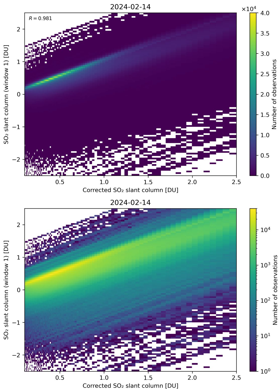
Figure 187: Scatter density plot of “Corrected SO 2 slant column” against “SO 2 slant column (window 1)” for 2024-02-13 to 2024-02-15.
