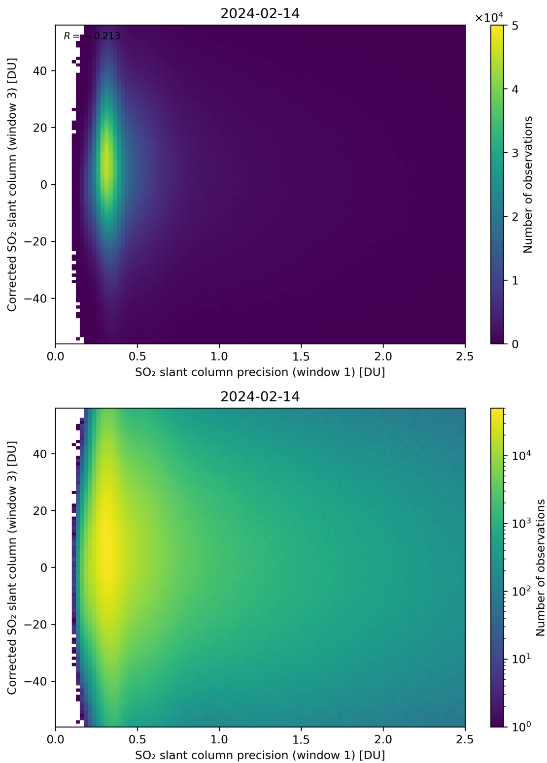
Figure 226: Scatter density plot of “SO 2 slant column precision (window 1)” against “Corrected SO 2 slant column (window 3)” for 2024-02-13 to 2024-02-15.
