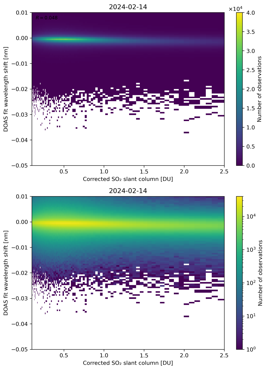
Figure 181: Scatter density plot of “Corrected SO 2 slant column” against “DOAS fit wavelength shift” for 2024-02-13 to 2024-02-15.
