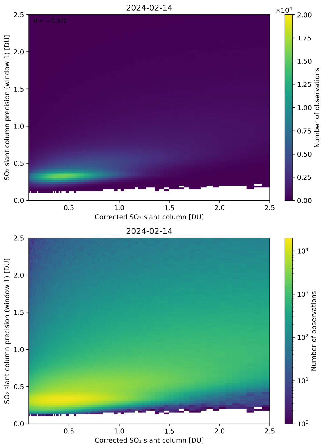
Figure 188: Scatter density plot of “Corrected SO 2 slant column” against “SO 2 slant column precision (window 1)” for 2024-02-13 to 2024-02-15.
