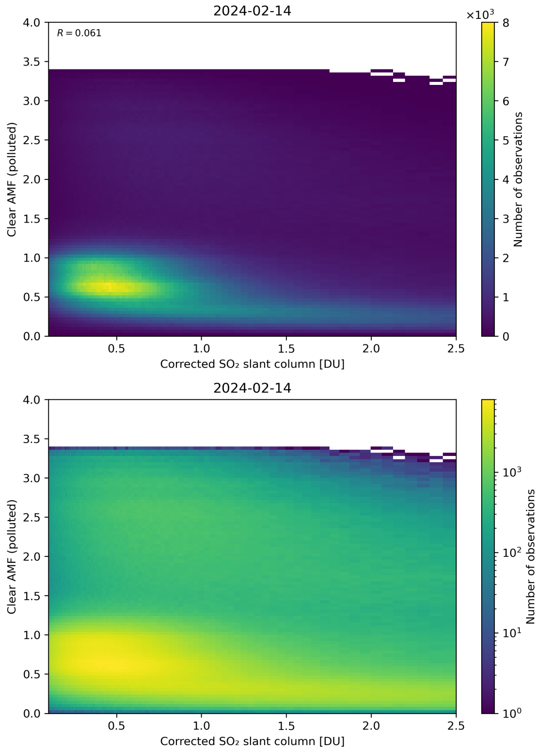
Figure 184: Scatter density plot of “Corrected SO 2 slant column” against “Clear AMF (polluted)” for 2024-02-13 to 2024-02-15.
