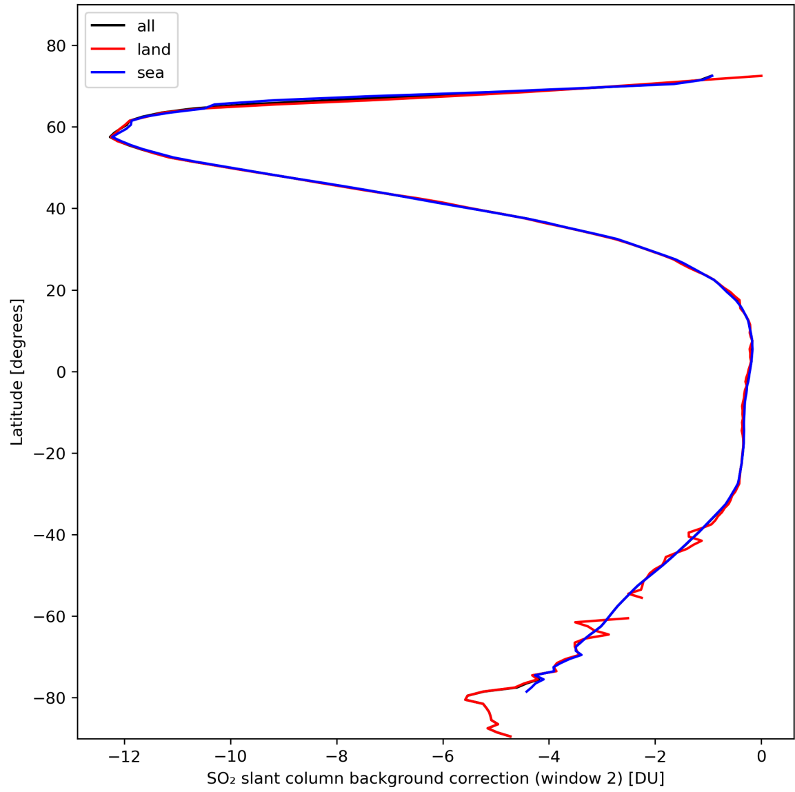
Figure 40: Zonal average of “SO 2 slant column background correction (window 2)” for 2024-02-13 to 2024-02-15.
