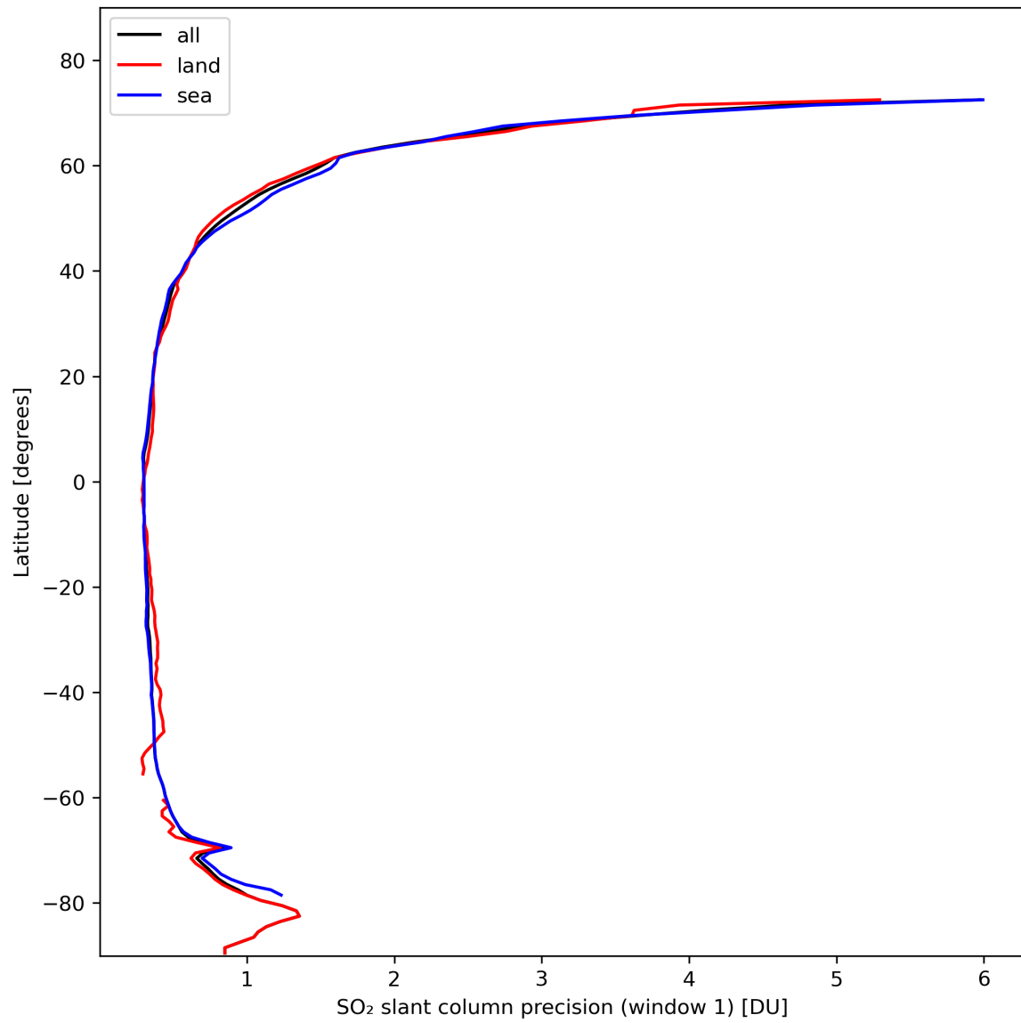
Figure 34: Zonal average of “SO 2 slant column precision (window 1)” for 2024-02-13 to 2024-02-15.
