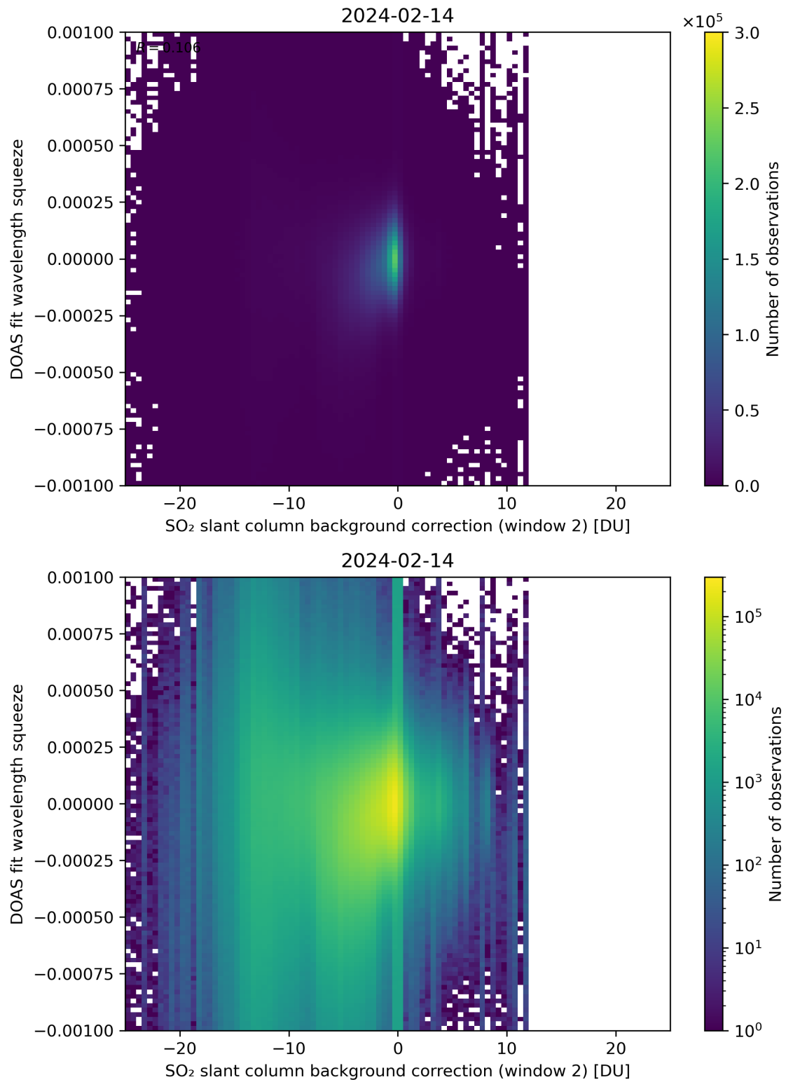
Figure 113: Scatter density plot of “SO 2 slant column background correction (window 2)” against “DOAS fit wavelength squeeze” for 2024-02-13 to 2024-02-15.
