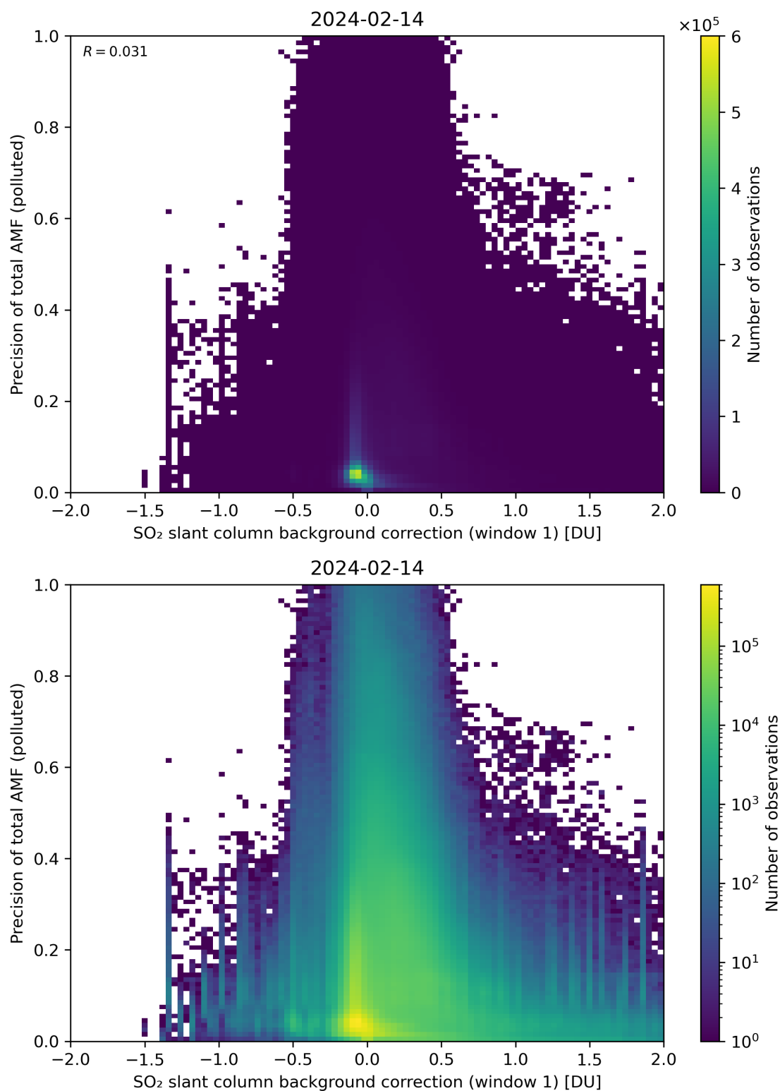
Figure 110: Scatter density plot of “SO 2 slant column background correction (window 1)” against “Precision of total AMF (polluted)” for 2024-02-13 to 2024-02-15.
