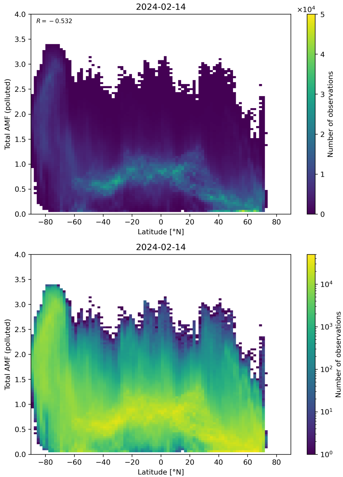
Figure 154: Scatter density plot of “Latitude” against “Total AMF (polluted)” for 2024-02-13 to 2024-02-15.
