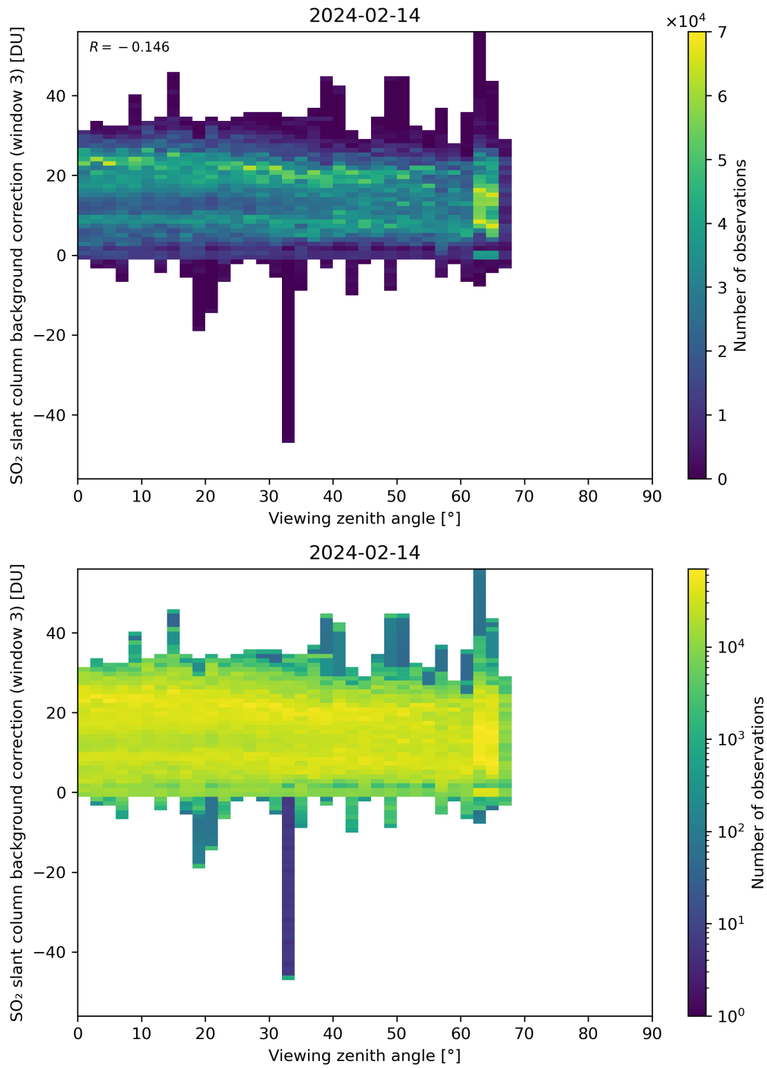
Figure 310: Scatter density plot of “Viewing zenith angle” against “SO 2 slant column background correction (window 3)” for 2024-02-13 to 2024-02-15.
