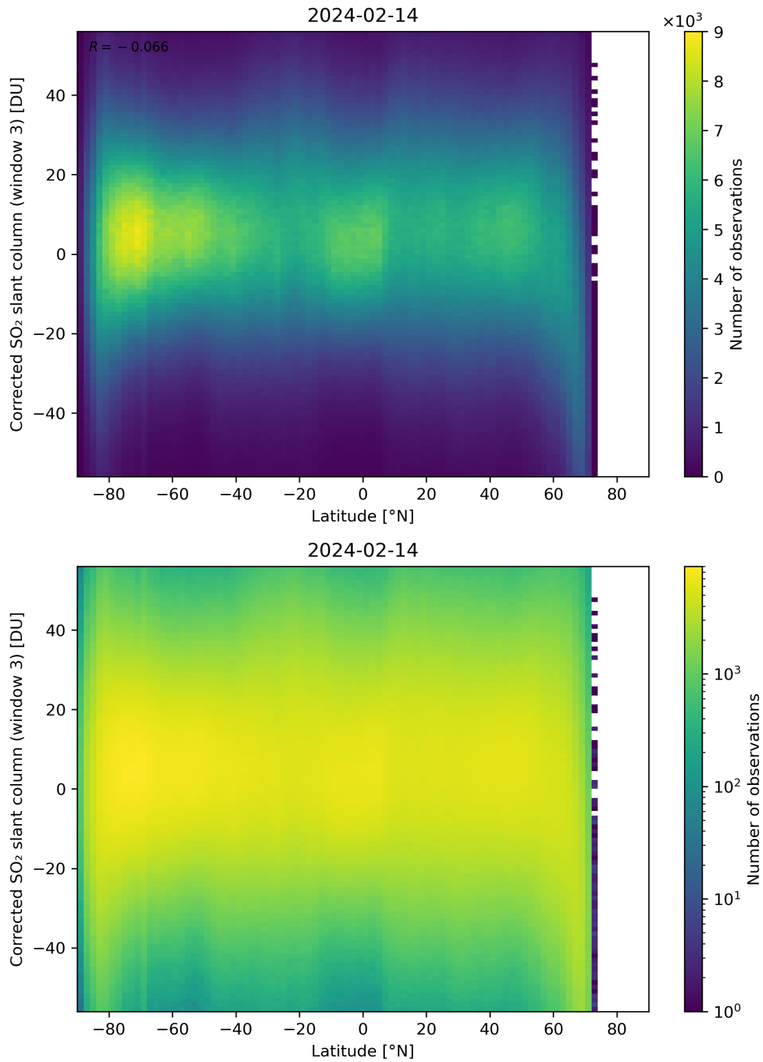
Figure 148: Scatter density plot of “Latitude” against “Corrected SO 2 slant column (window 3)” for 2024-02-13 to 2024-02-15.
