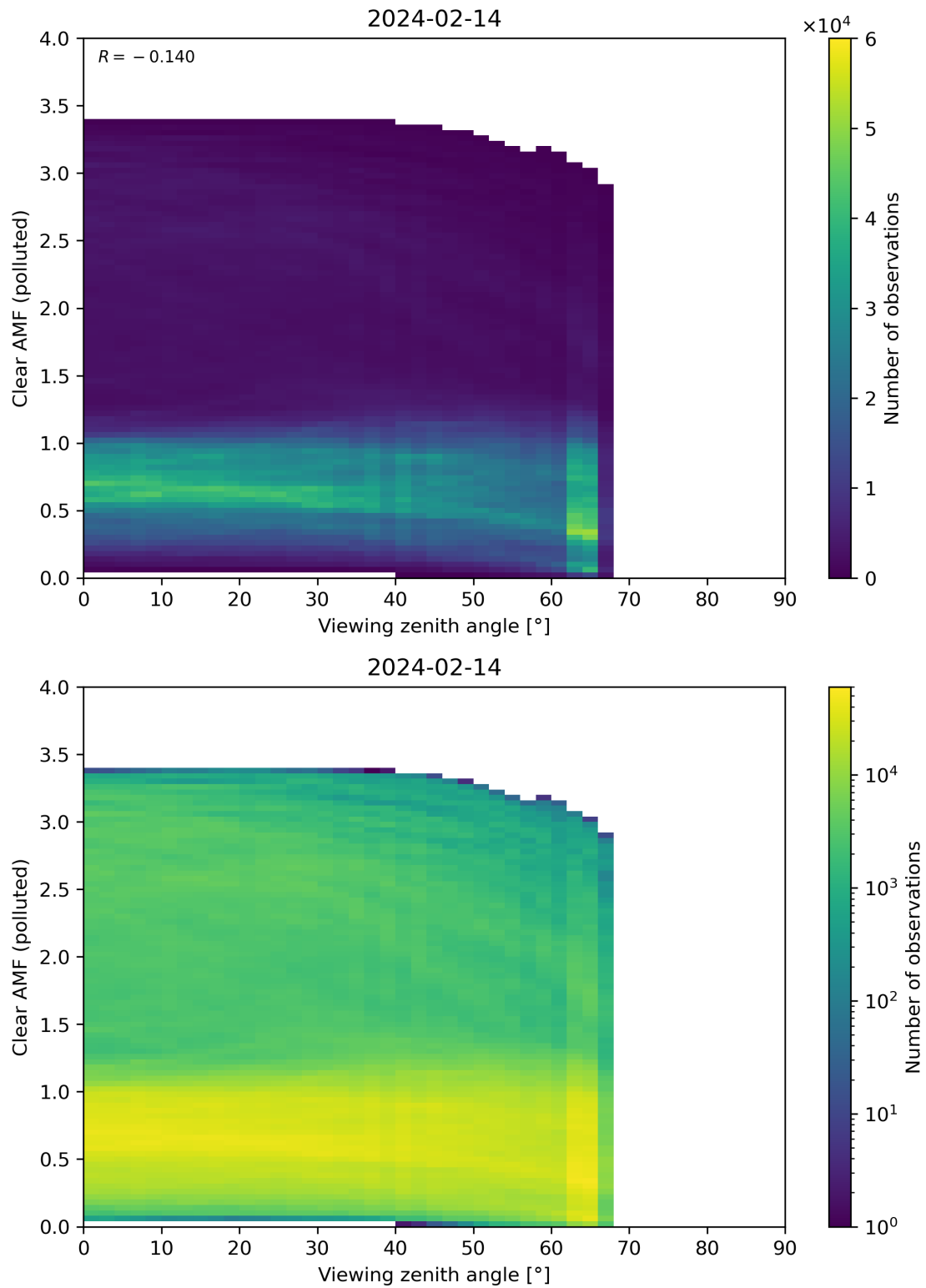
Figure 316: Scatter density plot of “Viewing zenith angle” against “Clear AMF (polluted)” for 2024-02-13 to 2024-02-15.
