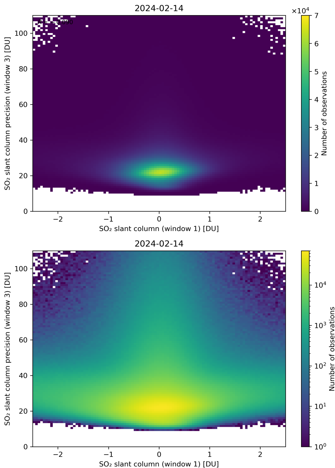
Figure 238: Scatter density plot of “SO 2 slant column (window 1)” against “SO 2 slant column precision (window 3)” for 2024-02-13 to 2024-02-15.
