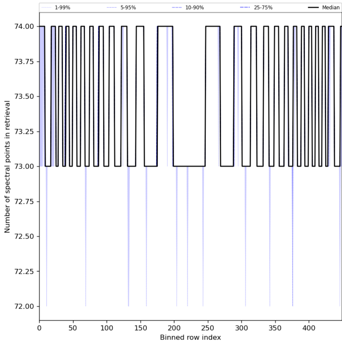
Figure 97: Along track statistics of “Number of spectral points in retrieval” for 2024-02-13 to 2024-02-15
