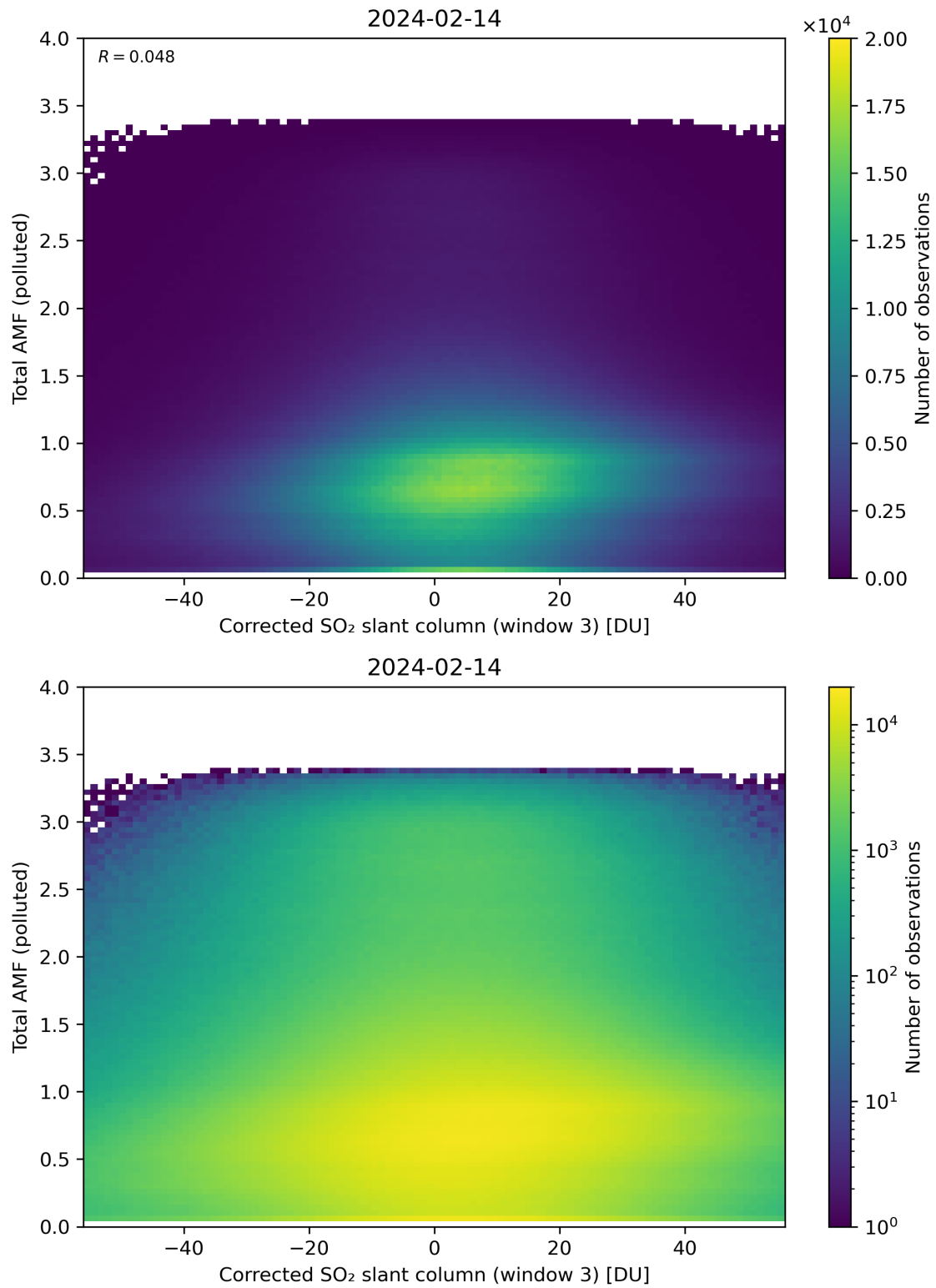
Figure 210: Scatter density plot of “Corrected SO 2 slant column (window 3)” against “Total AMF (polluted)” for 2024-02-13 to 2024-02-15.
