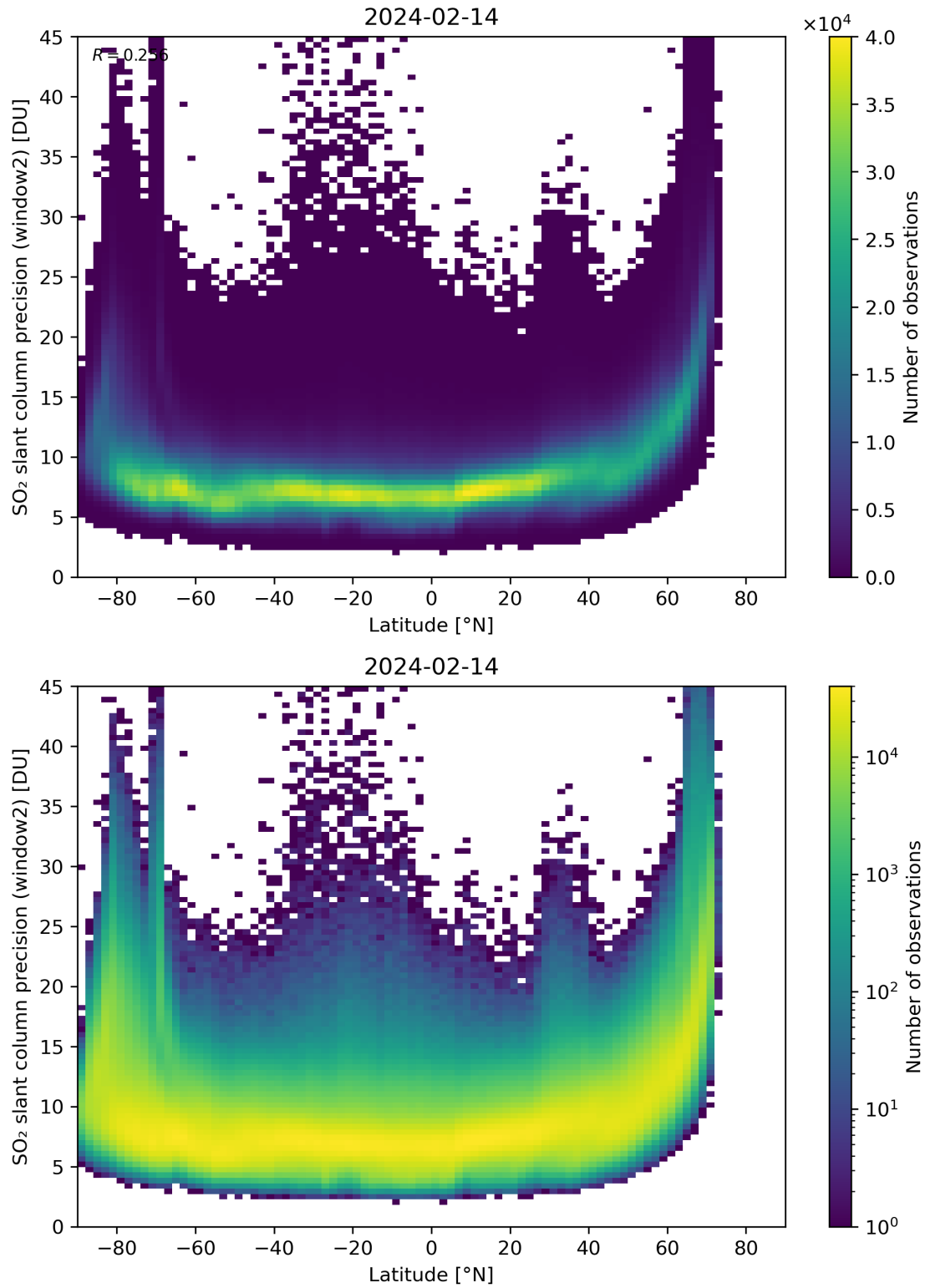
Figure 151: Scatter density plot of “Latitude” against “SO 2 slant column precision (window2)” for 2024-02-13 to 2024-02-15.
