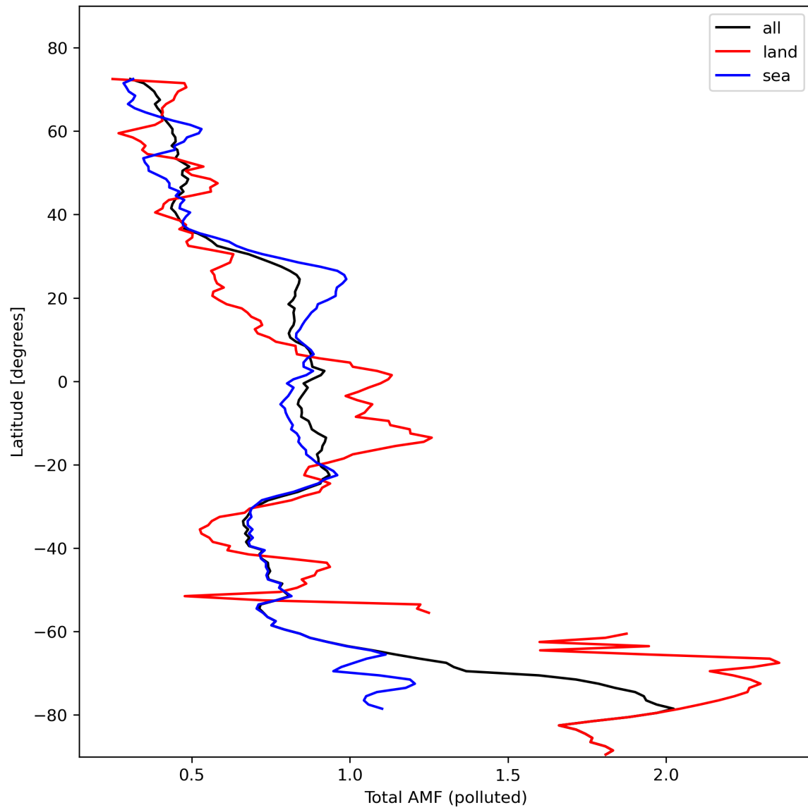
Figure 48: Zonal average of “Total AMF (polluted)” for 2024-02-13 to 2024-02-15.
