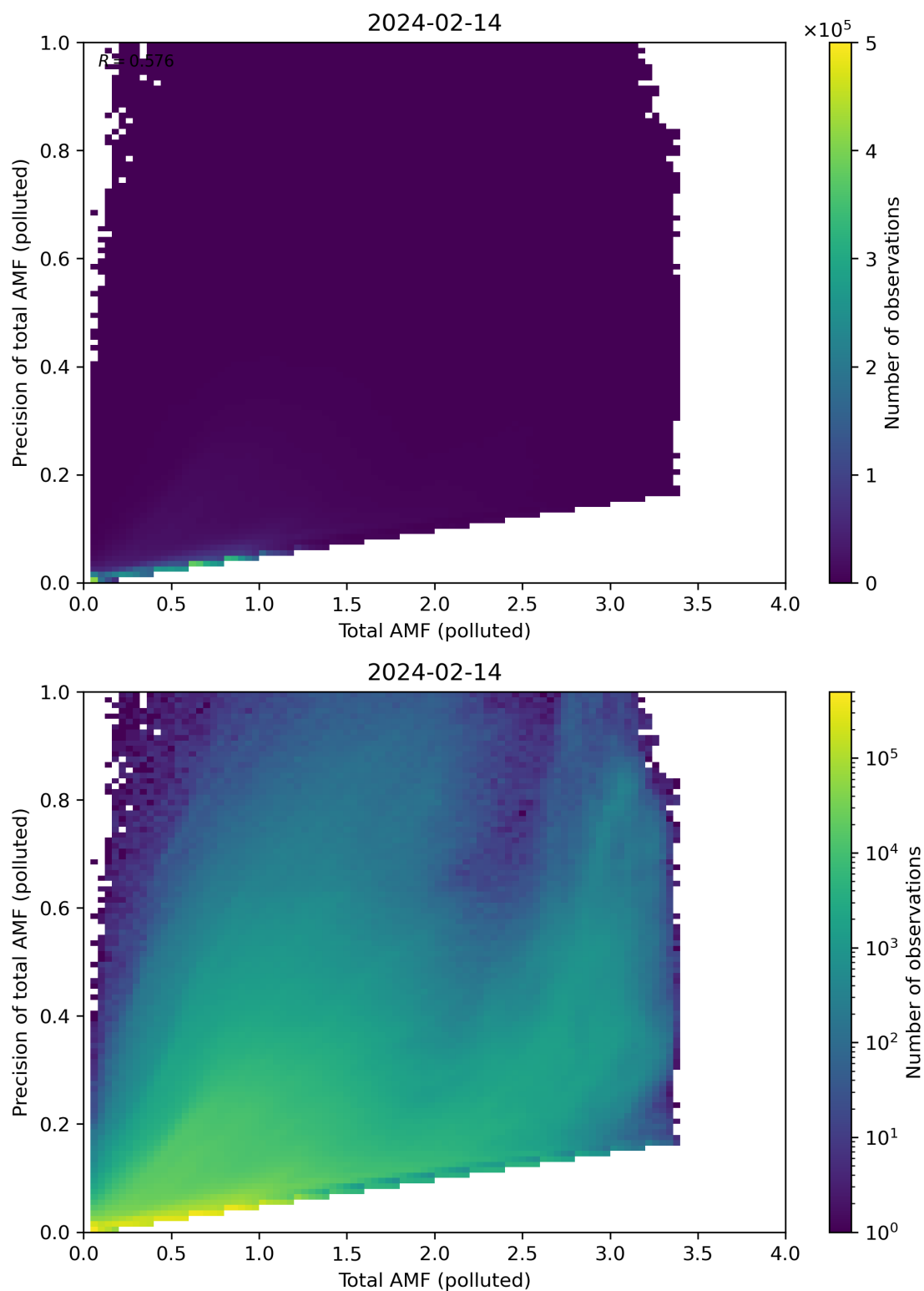
Figure 272: Scatter density plot of “Total AMF (polluted)” against “Precision of total AMF (polluted)” for 2024-02-13 to 2024-02-15.
