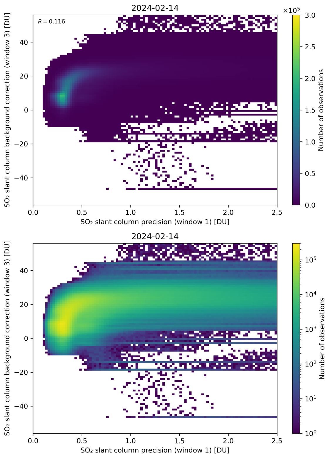
Figure 220: Scatter density plot of “SO 2 slant column precision (window 1)” against “SO 2 slant column background correction (window 3)” for 2024-02-13 to 2024-02-15.
