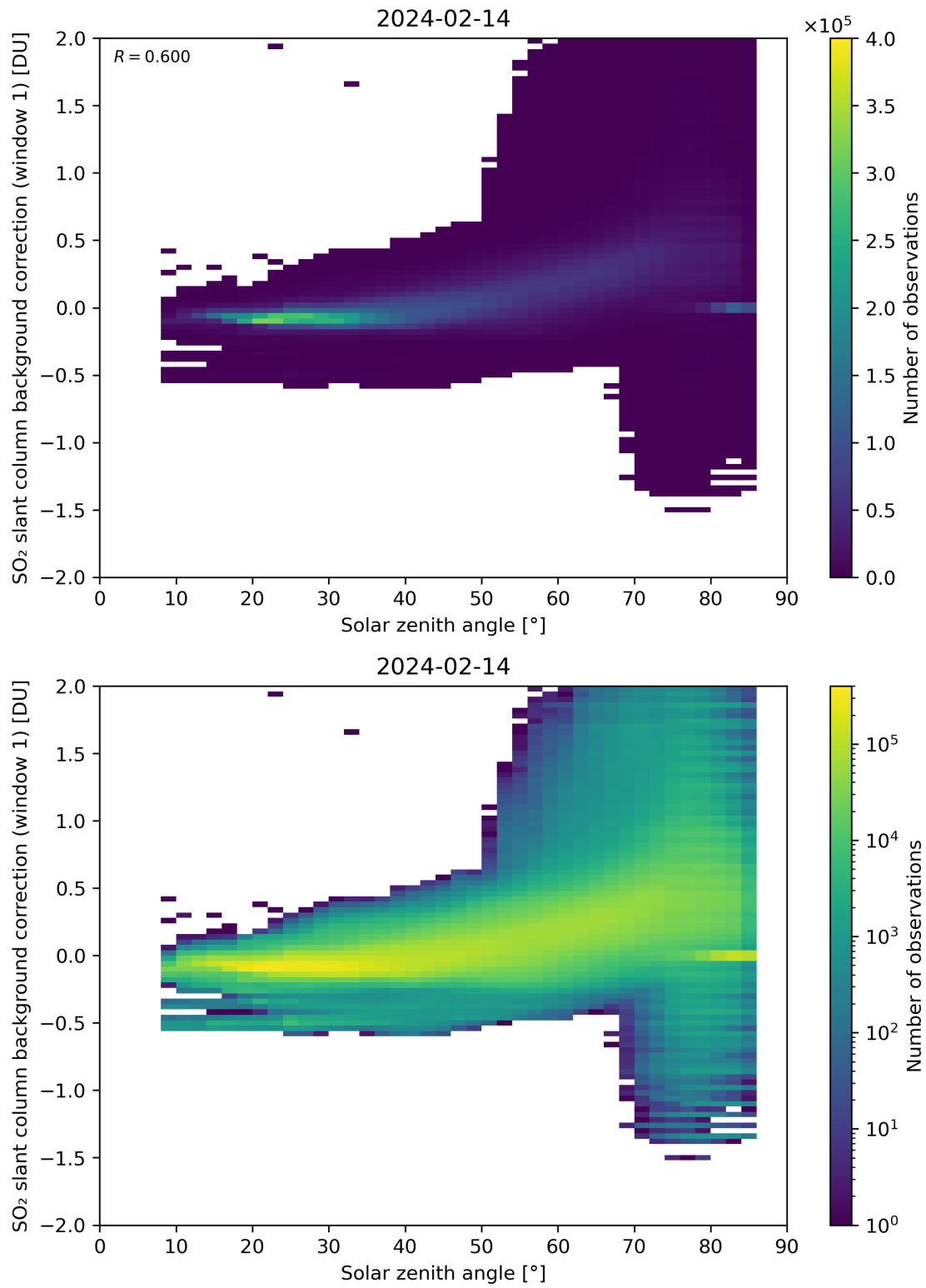
Figure 158: Scatter density plot of “Solar zenith angle” against “SO 2 slant column background correction (window 1)” for 2024-02-13 to 2024-02-15.
