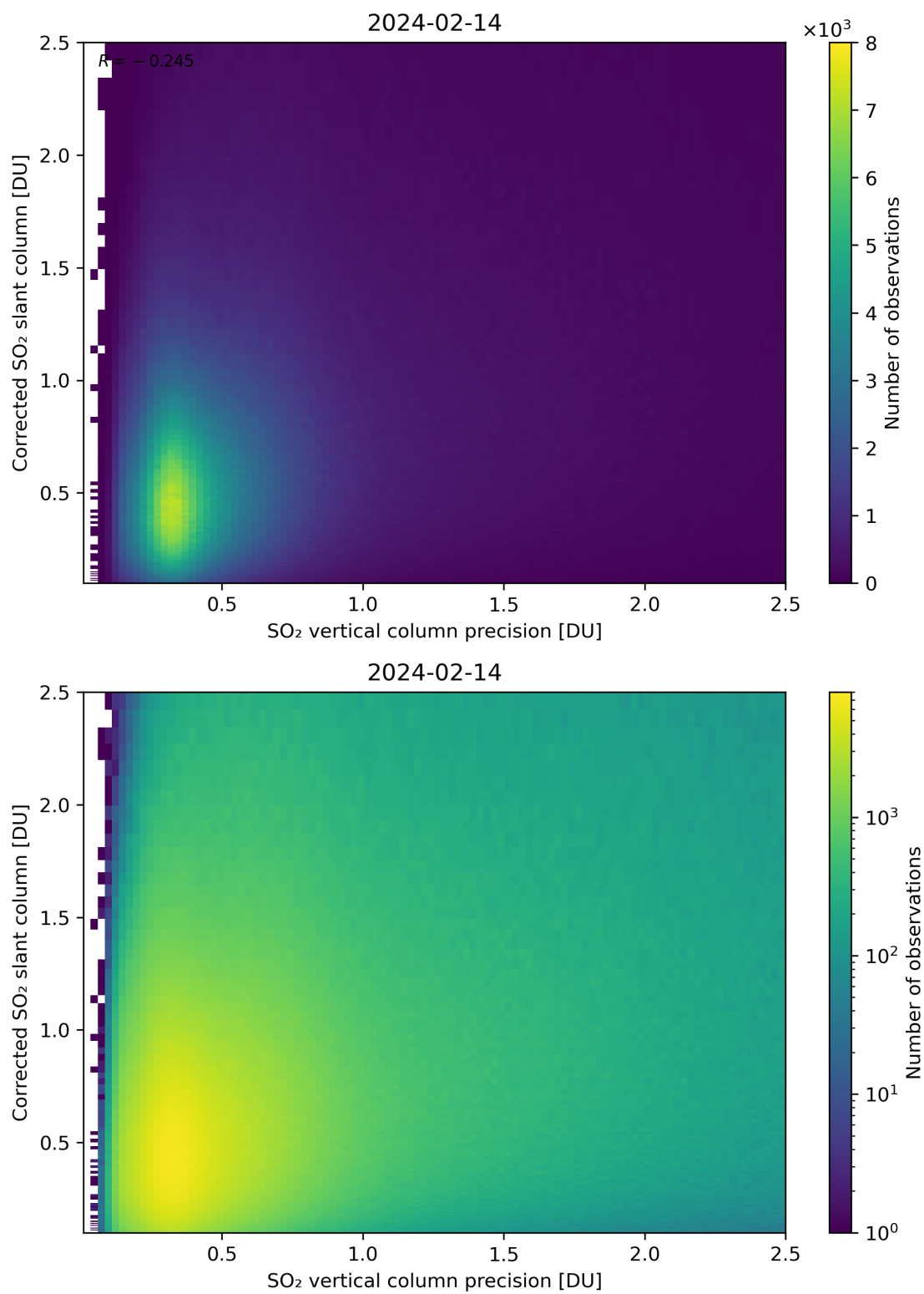
Figure 286: Scatter density plot of “SO 2 vertical column precision” against “Corrected SO 2 slant column” for 2024-02-13 to 2024-02-15.
