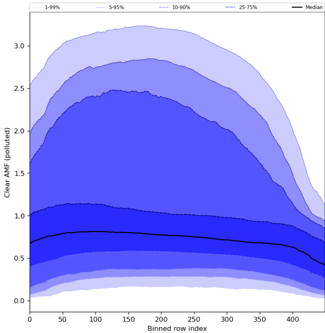
Figure 96: Along track statistics of “Clear AMF (polluted)” for 2024-02-13 to 2024-02-15
