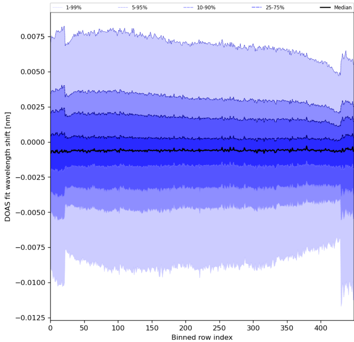
Figure 91: Along track statistics of “DOAS fit wavelength shift” for 2024-02-13 to 2024-02-15
