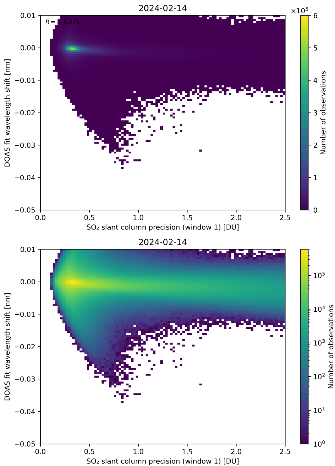
Figure 221: Scatter density plot of “SO 2 slant column precision (window 1)” against “DOAS fit wavelength shift” for 2024-02-13 to 2024-02-15.
