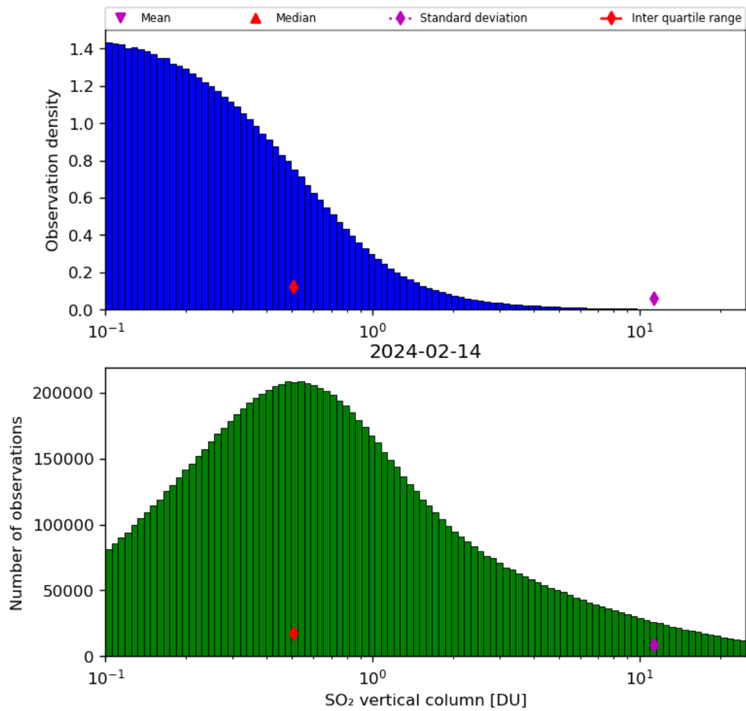
Figure 53: Histogram of “SO 2 vertical column” for 2024-02-13 to 2024-02-15
