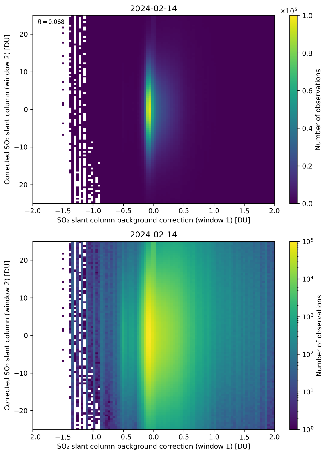
Figure 104: Scatter density plot of “SO 2 slant column background correction (window 1)” against “Corrected SO 2 slant column (window 2)” for 2024-02-13 to 2024-02-15.
