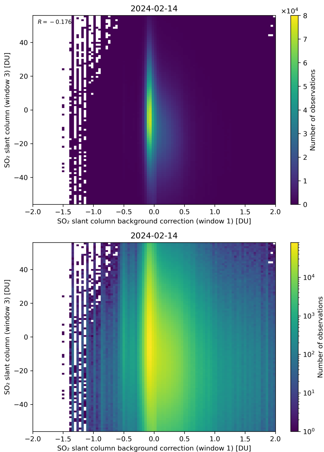
Figure 107: Scatter density plot of “SO 2 slant column background correction (window 1)” against “SO 2 slant column (window 3)” for 2024-02-13 to 2024-02-15.
