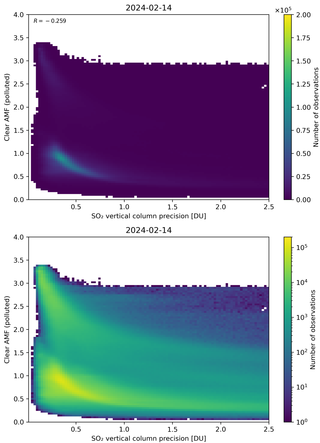
Figure 285: Scatter density plot of “SO 2 vertical column precision” against “Clear AMF (polluted)” for 2024-02-13 to 2024-02-15.
