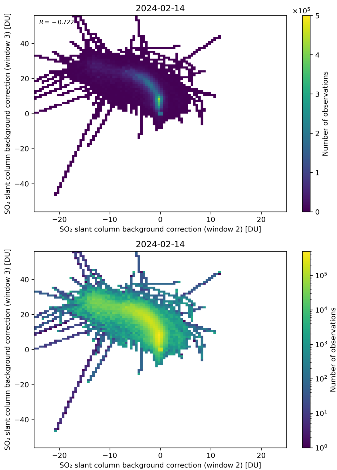
Figure 111: Scatter density plot of “SO 2 slant column background correction (window 2)” against “SO 2 slant column background correction (window 3)” for 2024-02-13 to 2024-02-15.
