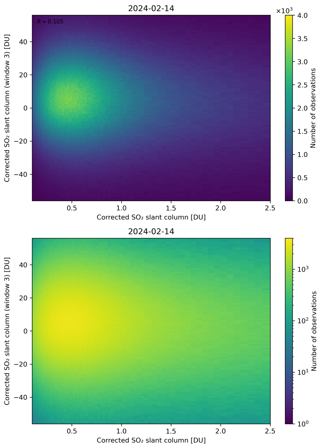
Figure 186: Scatter density plot of “Corrected SO 2 slant column” against “Corrected SO 2 slant column (window 3)” for 2024-02-13 to 2024-02-15.
