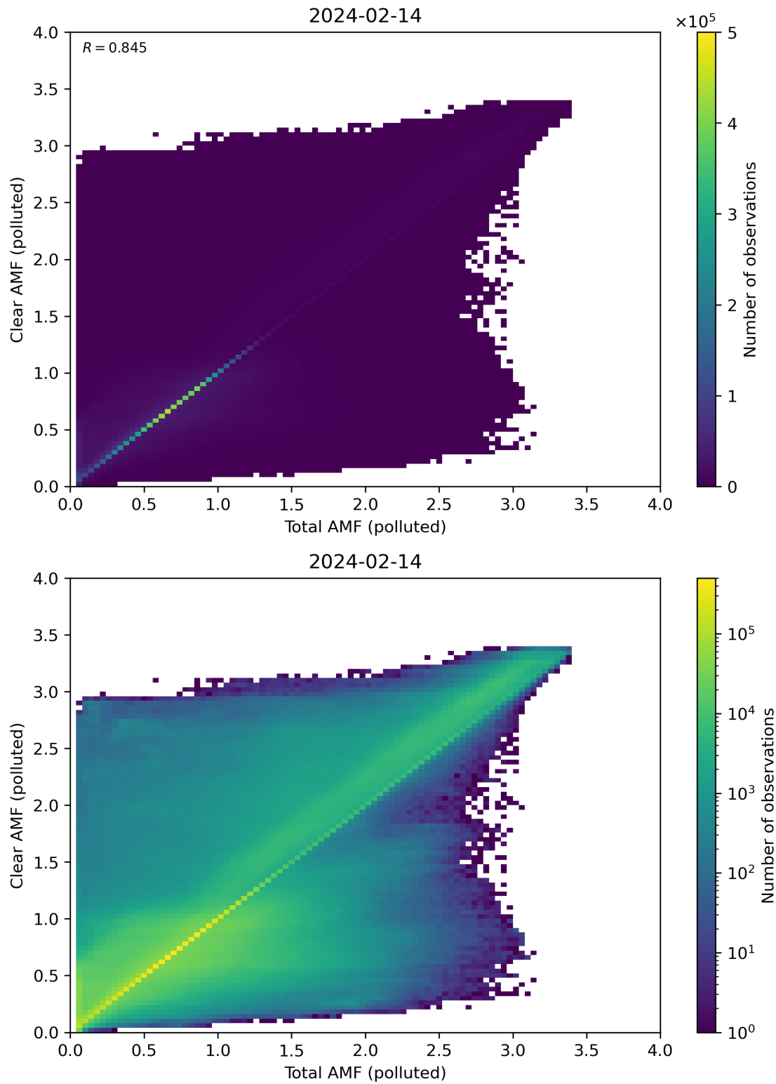
Figure 271: Scatter density plot of “Total AMF (polluted)” against “Clear AMF (polluted)” for 2024-02-13 to 2024-02-15.
