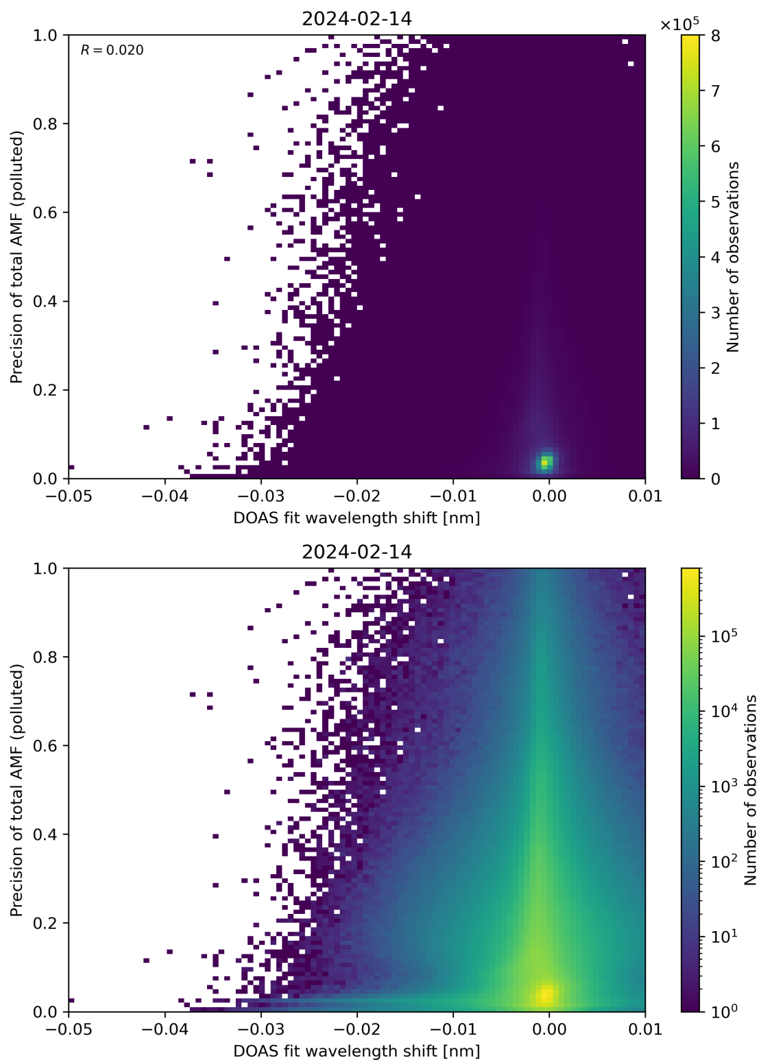
Figure 131: Scatter density plot of “DOAS fit wavelength shift” against “Precision of total AMF (polluted)” for 2024-02-13 to 2024-02-15.
