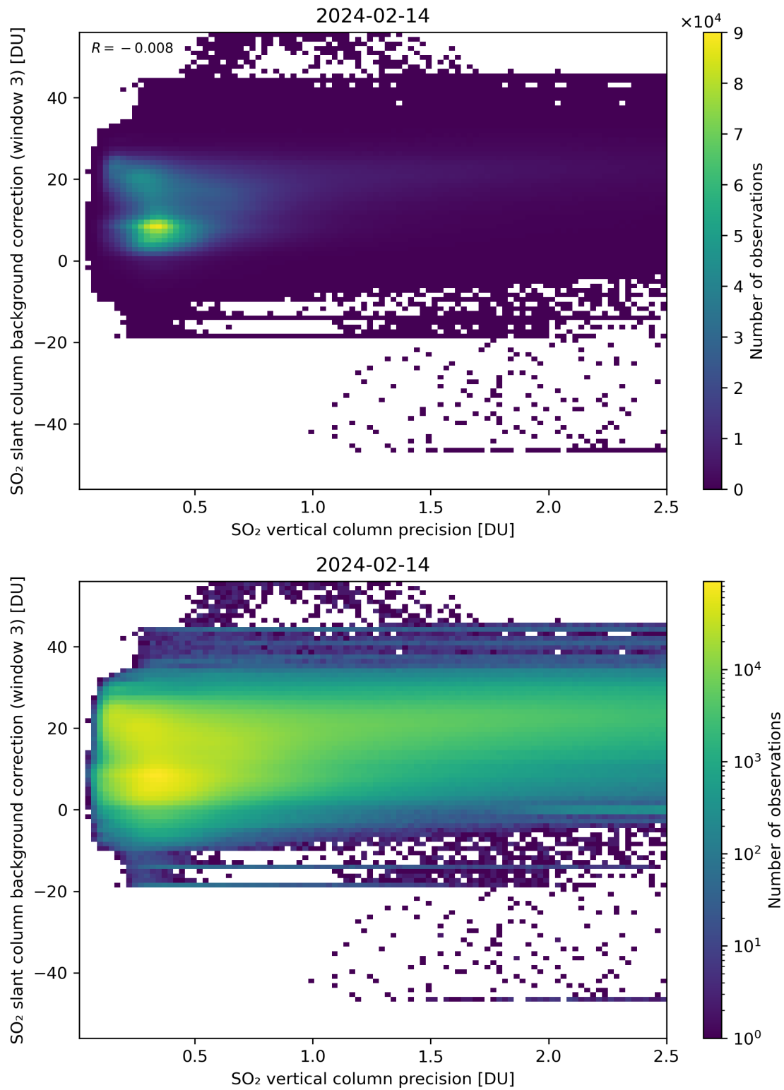
Figure 281: Scatter density plot of “SO 2 vertical column precision” against “SO 2 slant column background correction (window 3)” for 2024-02-13 to 2024-02-15.
