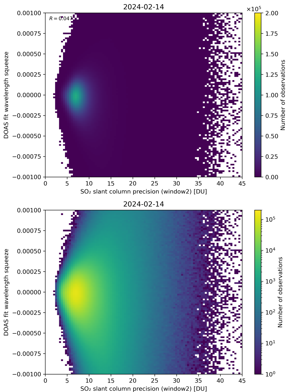
Figure 244: Scatter density plot of “SO 2 slant column precision (window2)” against “DOAS fit wavelength squeeze” for 2024-02-13 to 2024-02-15.
