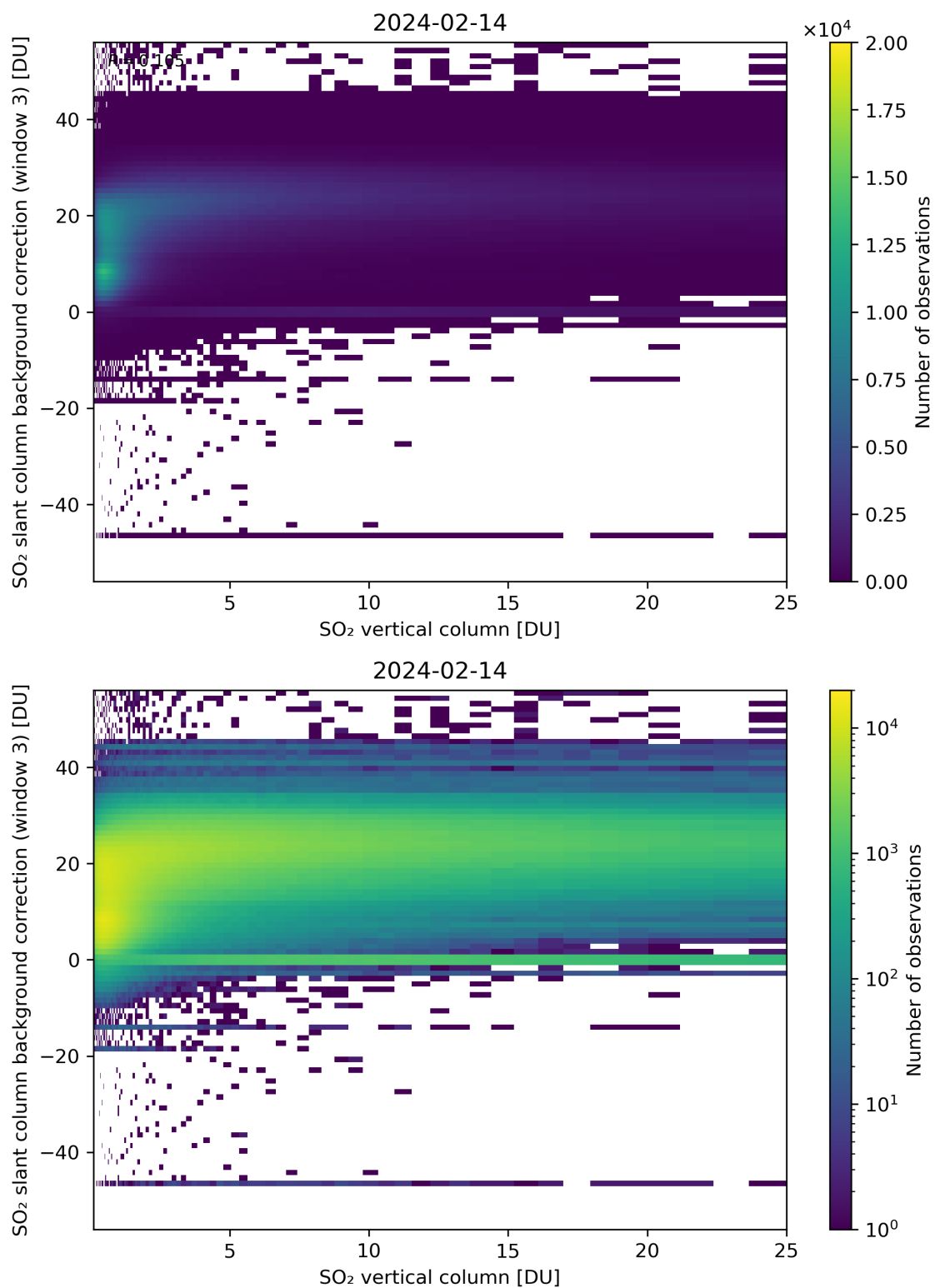
Figure 275: Scatter density plot of “SO 2 vertical column” against “SO 2 slant column background correction (window 3)” for 2024-02-13 to 2024-02-15.
