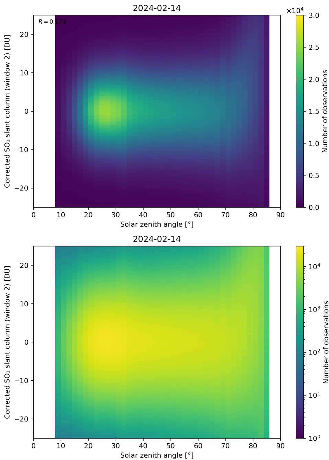
Figure 167: Scatter density plot of “Solar zenith angle” against “Corrected SO 2 slant column (window 2)” for 2024-02-13 to 2024-02-15.
