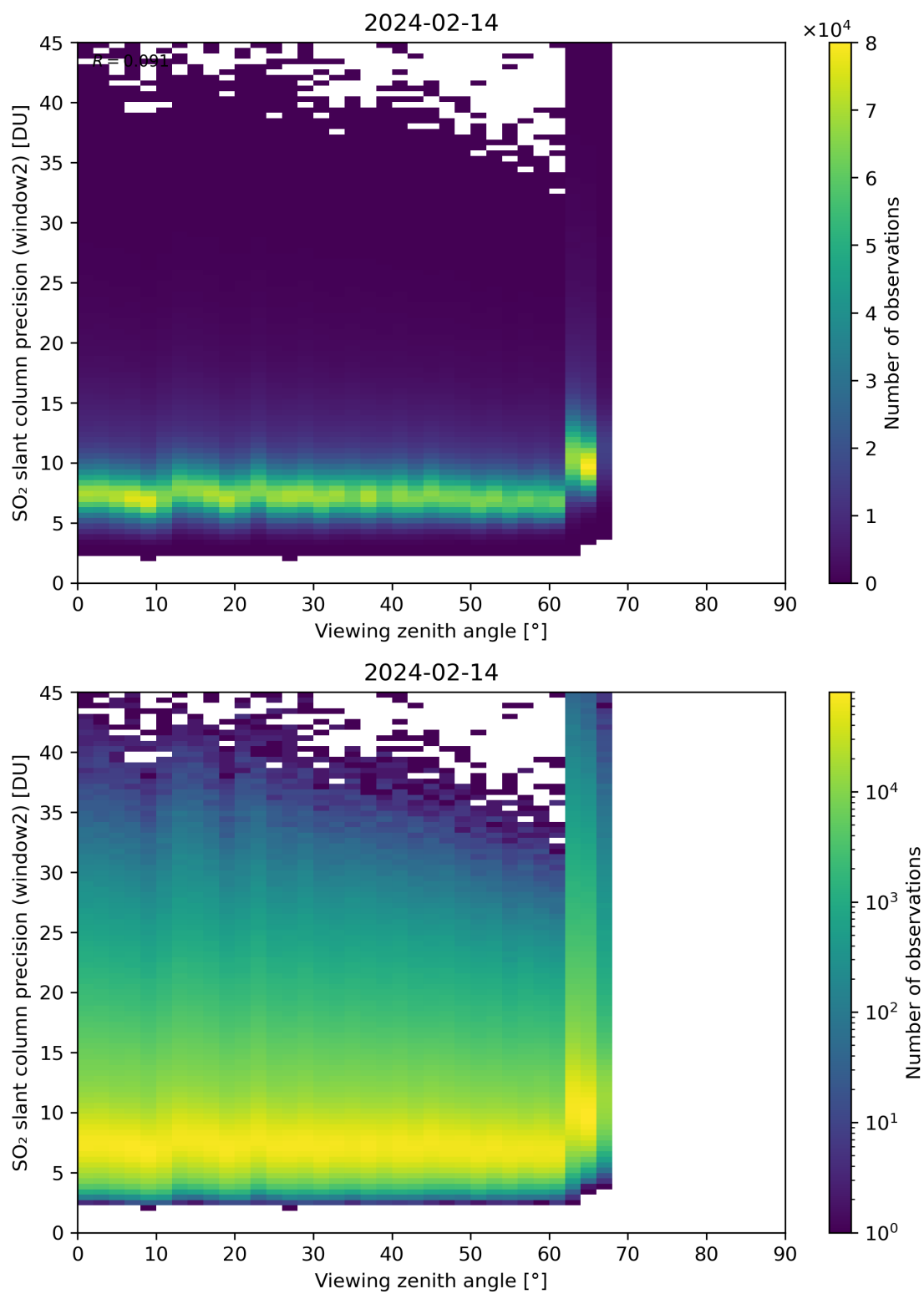
Figure 322: Scatter density plot of “Viewing zenith angle” against “SO 2 slant column precision (window2)” for 2024-02-13 to 2024-02-15.
