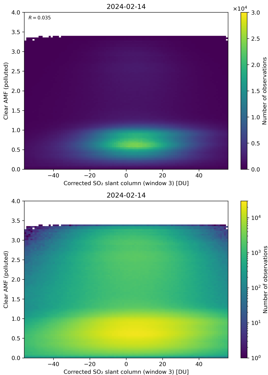
Figure 209: Scatter density plot of “Corrected SO 2 slant column (window 3)” against “Clear AMF (polluted)” for 2024-02-13 to 2024-02-15.
