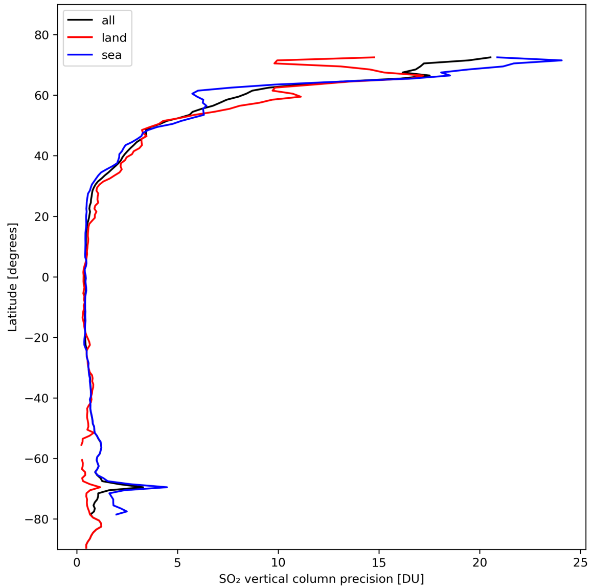
Figure 31: Zonal average of “SO 2 vertical column precision” for 2024-02-13 to 2024-02-15.
