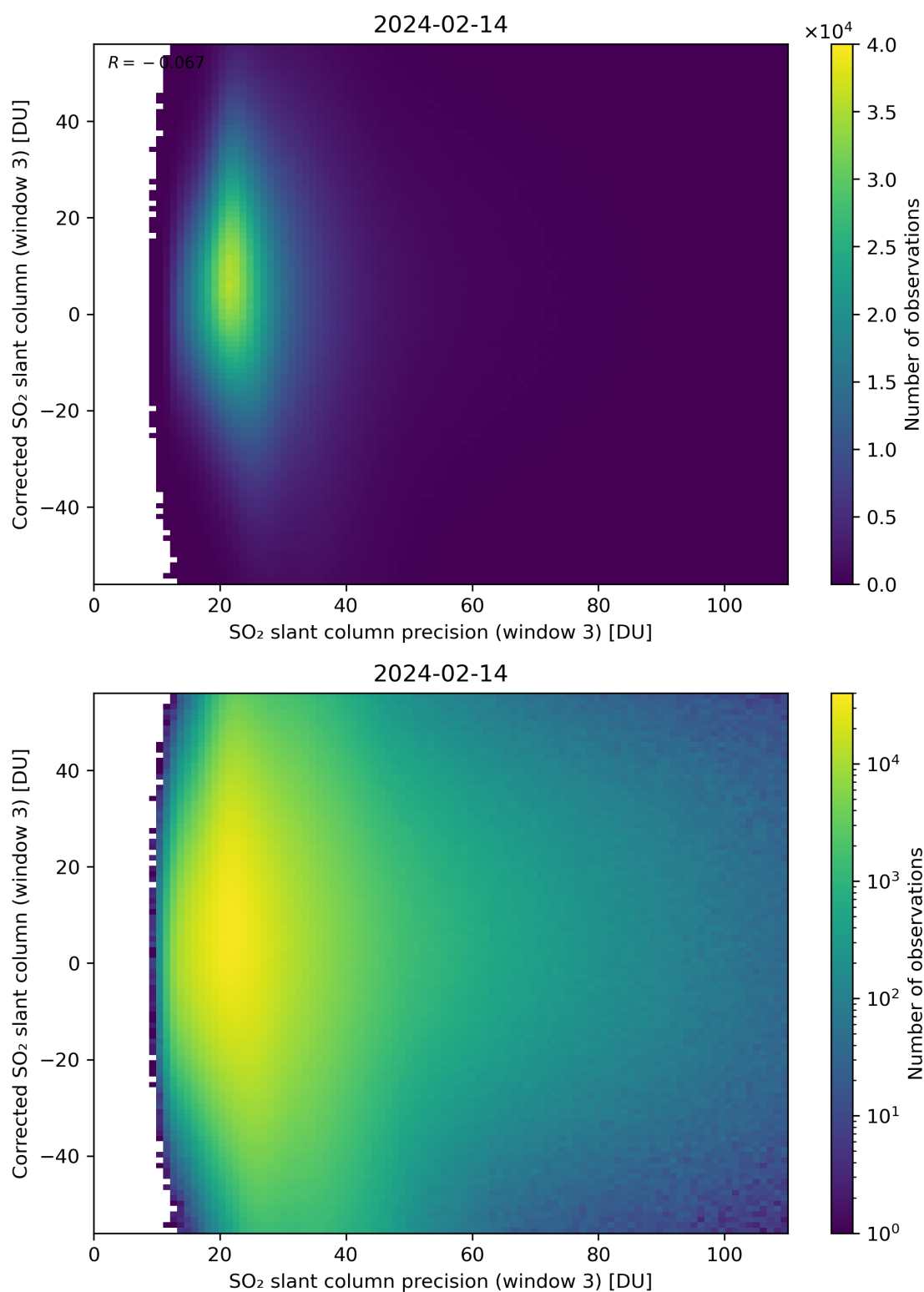
Figure 262: Scatter density plot of “SO 2 slant column precision (window 3)” against “Corrected SO 2 slant column (window 3)” for 2024-02-13 to 2024-02-15.
