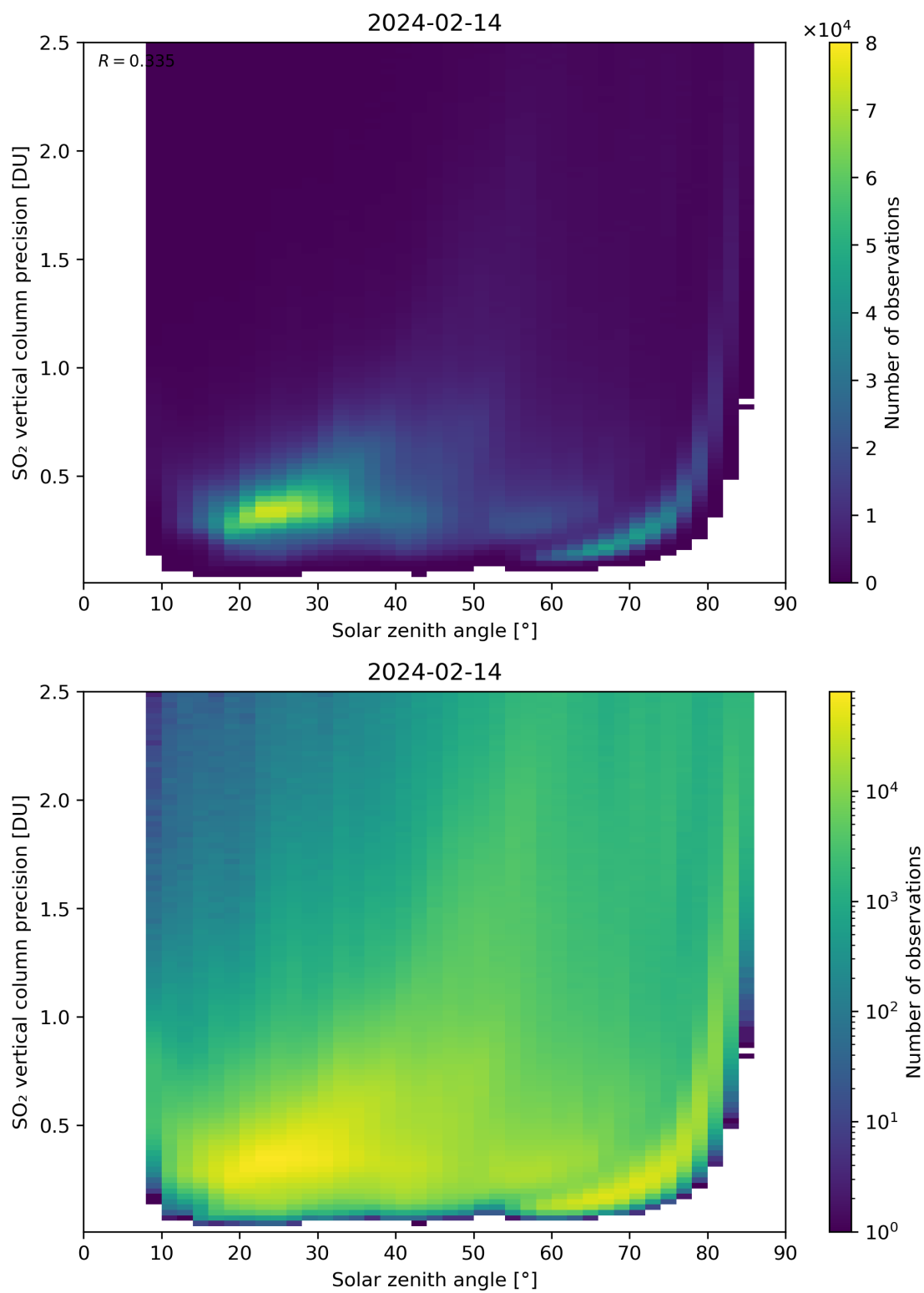
Figure 177: Scatter density plot of “Solar zenith angle” against “SO 2 vertical column precision” for 2024-02-13 to 2024-02-15.
