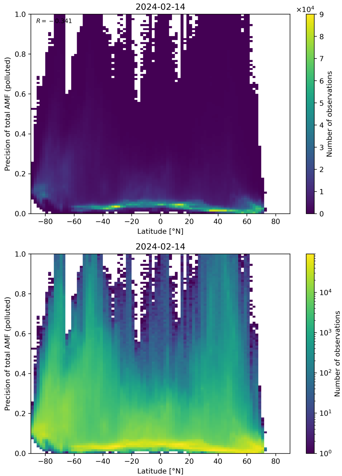
Figure 155: Scatter density plot of “Latitude” against “Precision of total AMF (polluted)” for 2024-02-13 to 2024-02-15.
