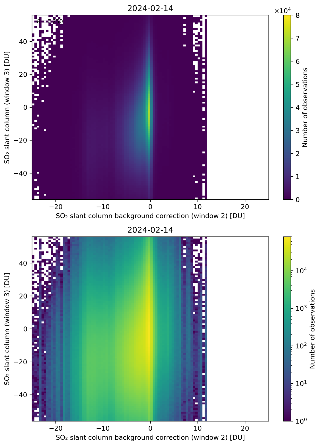
Figure 117: Scatter density plot of “SO 2 slant column background correction (window 2)” against “SO 2 slant column (window 3)” for 2024-02-13 to 2024-02-15.
