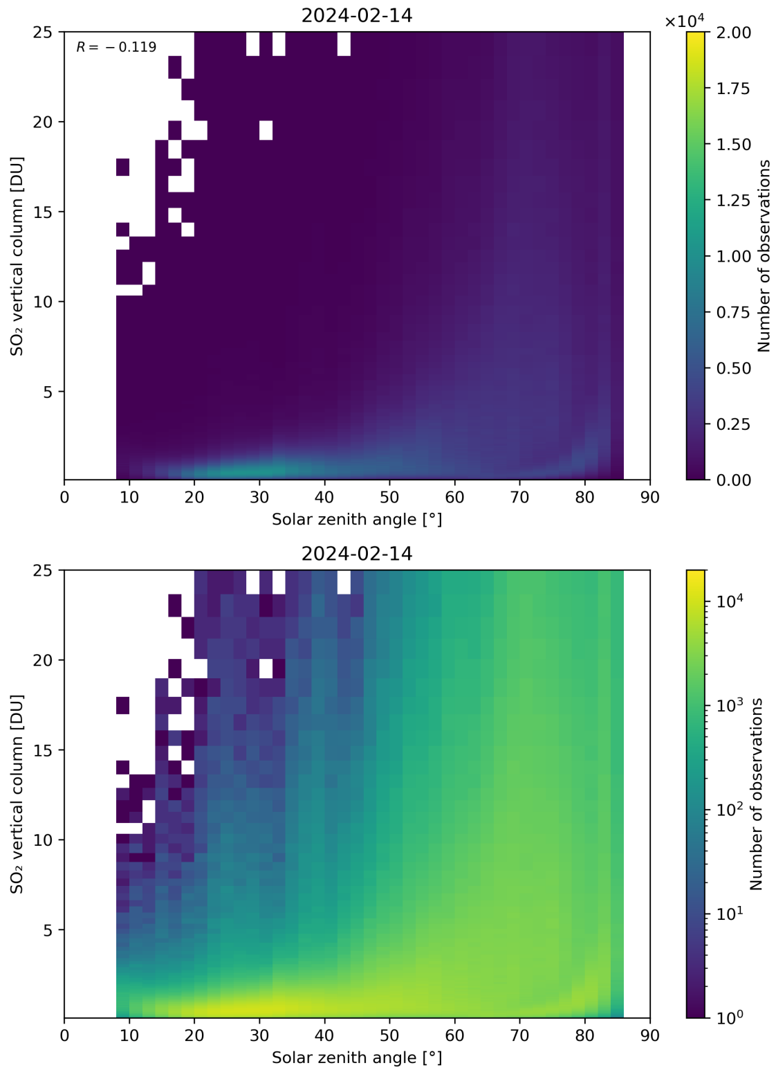
Figure 176: Scatter density plot of “Solar zenith angle” against “SO 2 vertical column” for 2024-02-13 to 2024-02-15.
