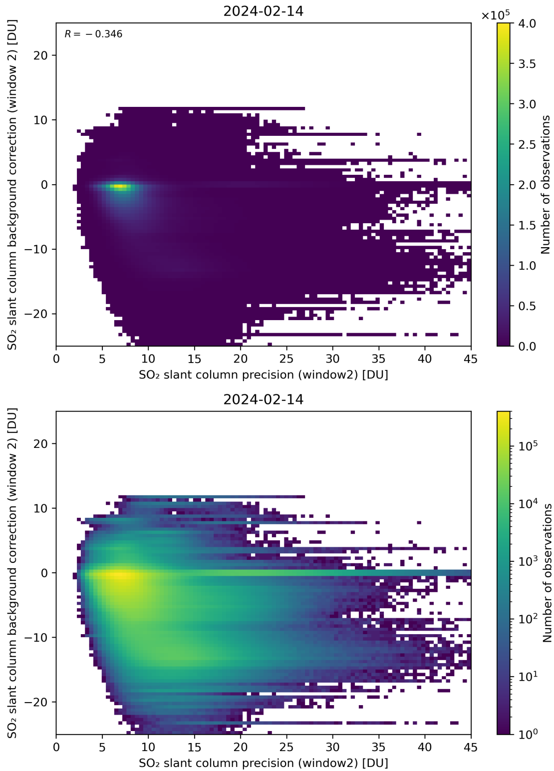
Figure 241: Scatter density plot of “SO 2 slant column precision (window2)” against “SO 2 slant column background correction (window 2)” for 2024-02-13 to 2024-02-15.
