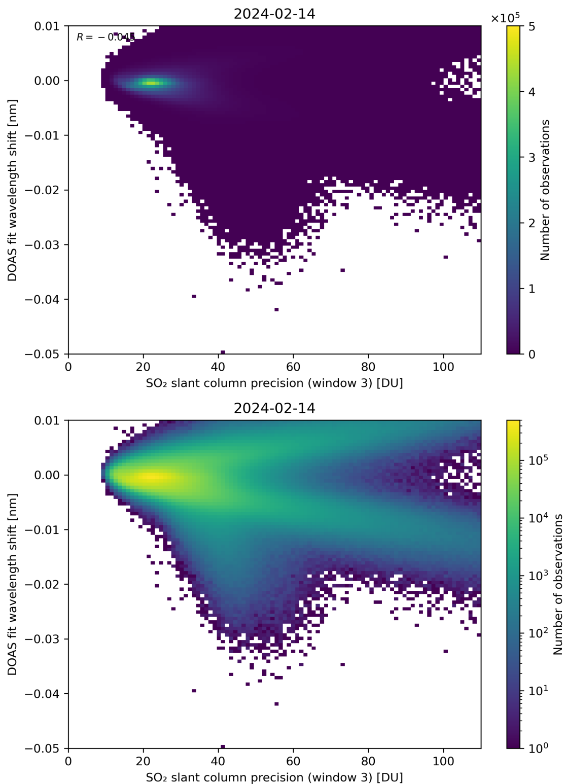
Figure 258: Scatter density plot of “SO 2 slant column precision (window 3)” against “DOAS fit wavelength shift” for 2024-02-13 to 2024-02-15.
