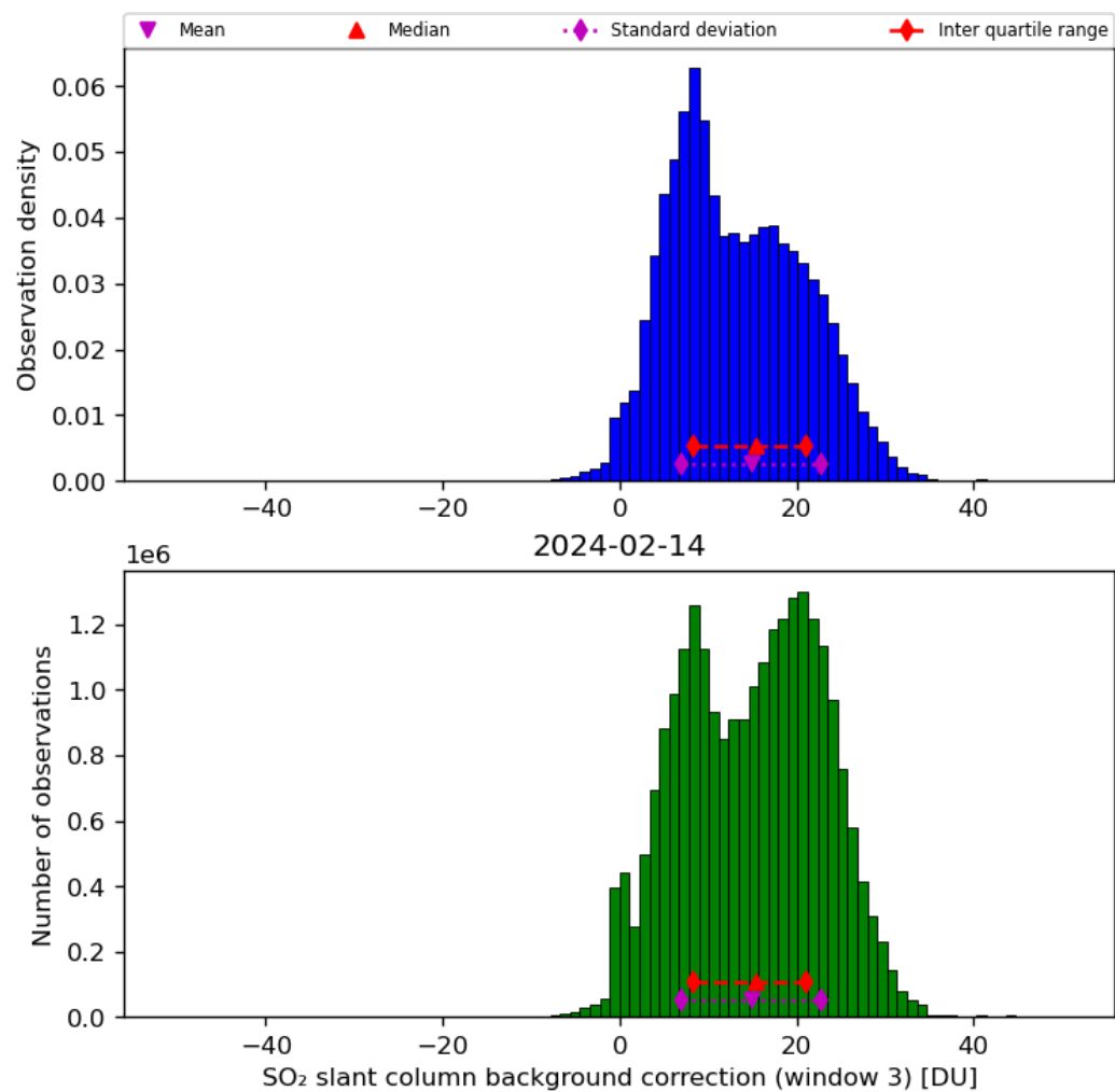
Figure 67: Histogram of “SO 2 slant column background correction (window 3)” for 2024-02-13 to 2024-02-15
