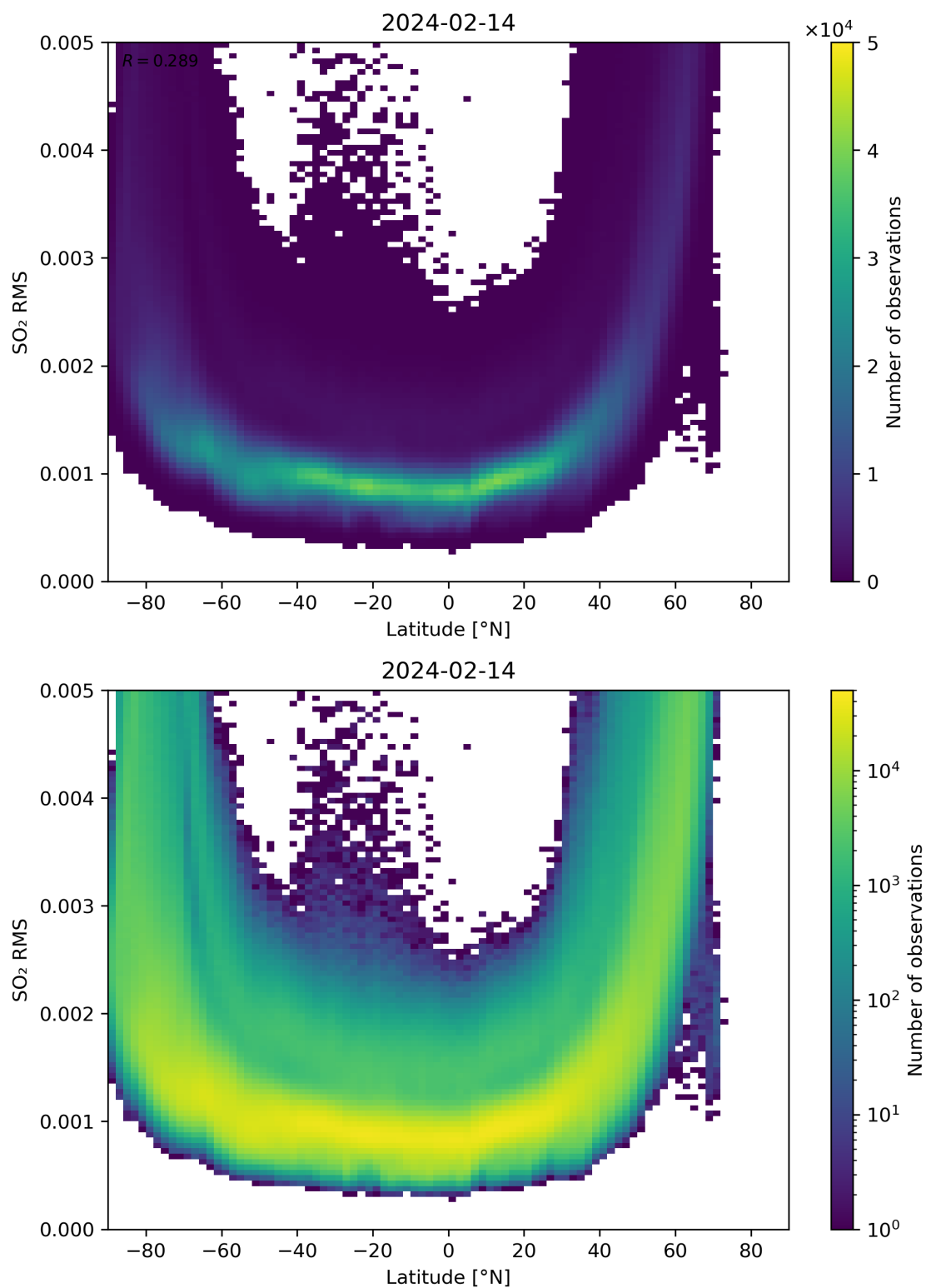
Figure 144: Scatter density plot of “Latitude” against “SO 2 RMS” for 2024-02-13 to 2024-02-15.
