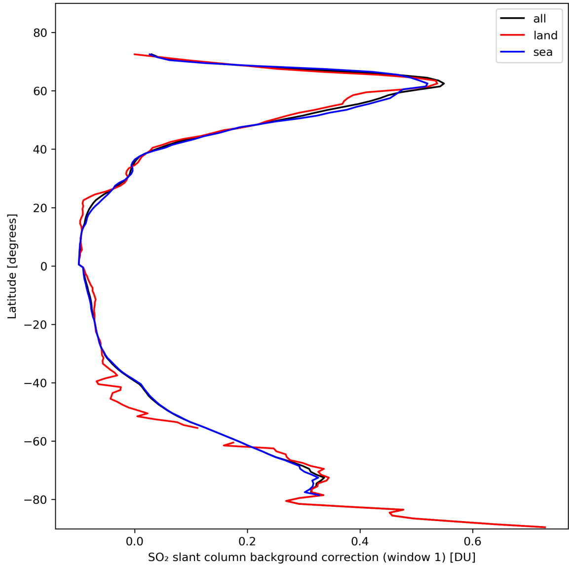
Figure 36: Zonal average of “SO 2 slant column background correction (window 1)” for 2024-02-13 to 2024-02-15.
