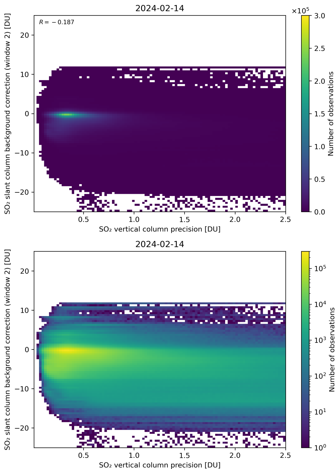
Figure 280: Scatter density plot of “SO 2 vertical column precision” against “SO 2 slant column background correction (window 2)” for 2024-02-13 to 2024-02-15.
