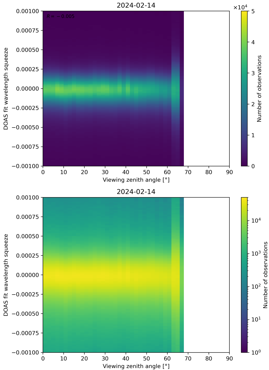
Figure 312: Scatter density plot of “Viewing zenith angle” against “DOAS fit wavelength squeeze” for 2024-02-13 to 2024-02-15.
