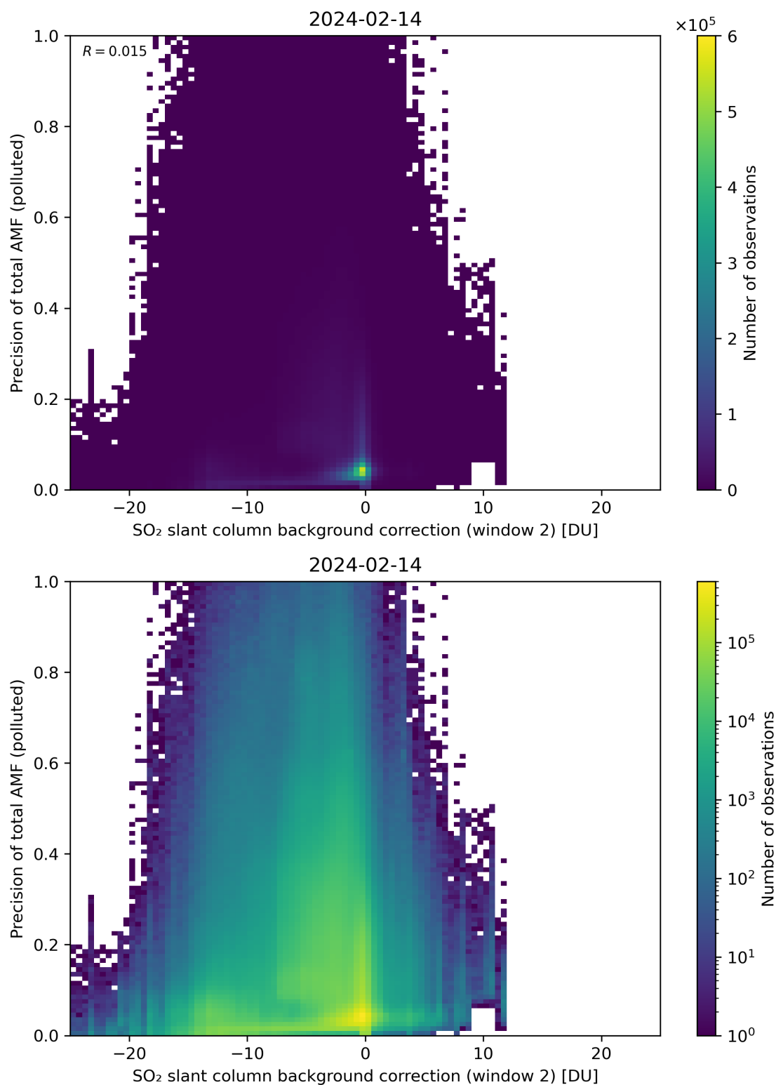
Figure 120: Scatter density plot of “SO 2 slant column background correction (window 2)” against “Precision of total AMF (polluted)” for 2024-02-13 to 2024-02-15.
