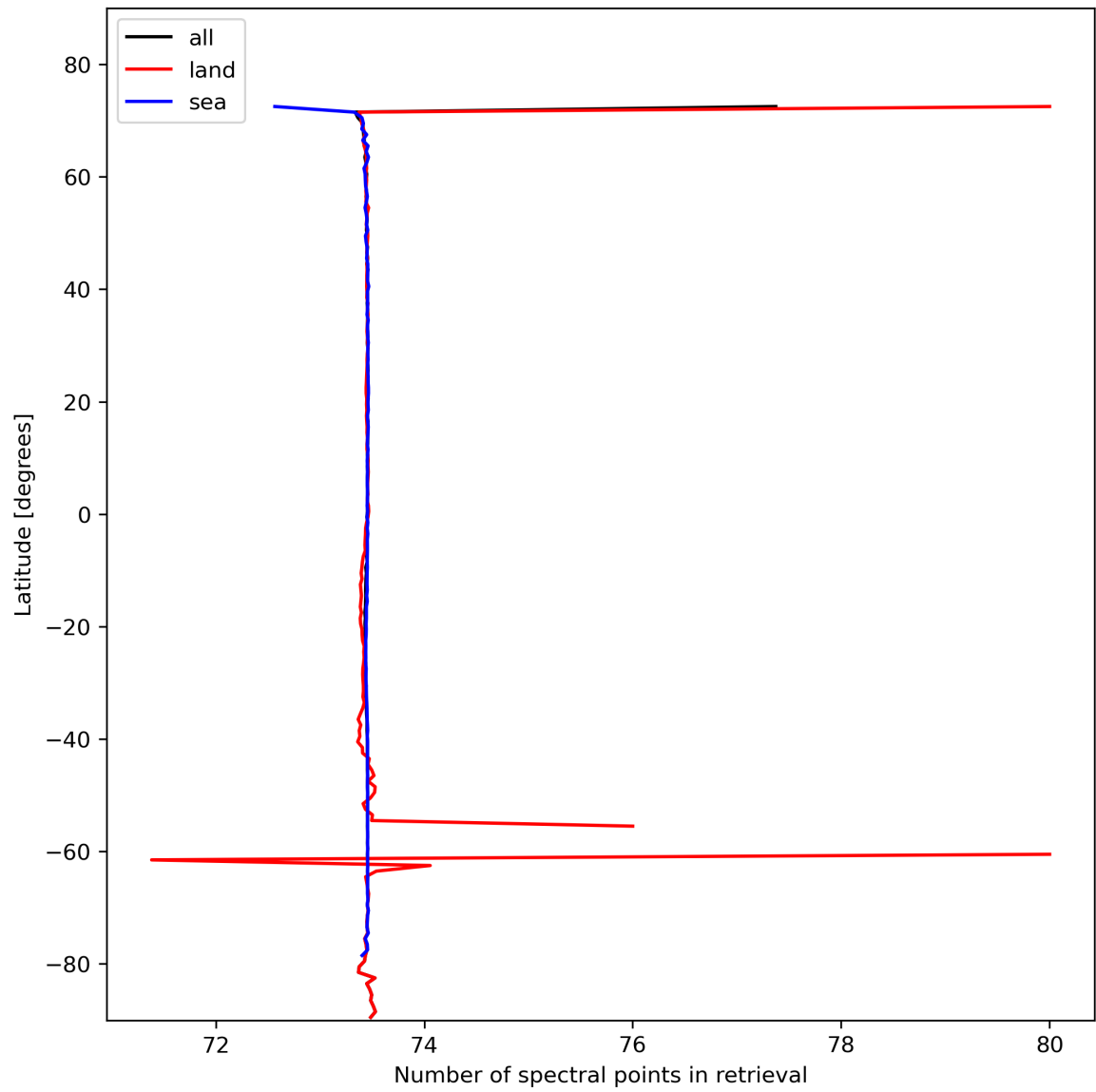
Figure 51: Zonal average of “Number of spectral points in retrieval” for 2024-02-13 to 2024-02-15.
