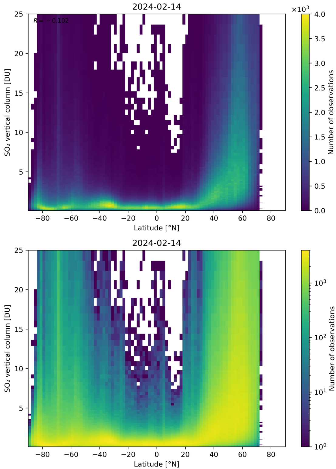
Figure 156: Scatter density plot of “Latitude” against “SO 2 vertical column” for 2024-02-13 to 2024-02-15.
