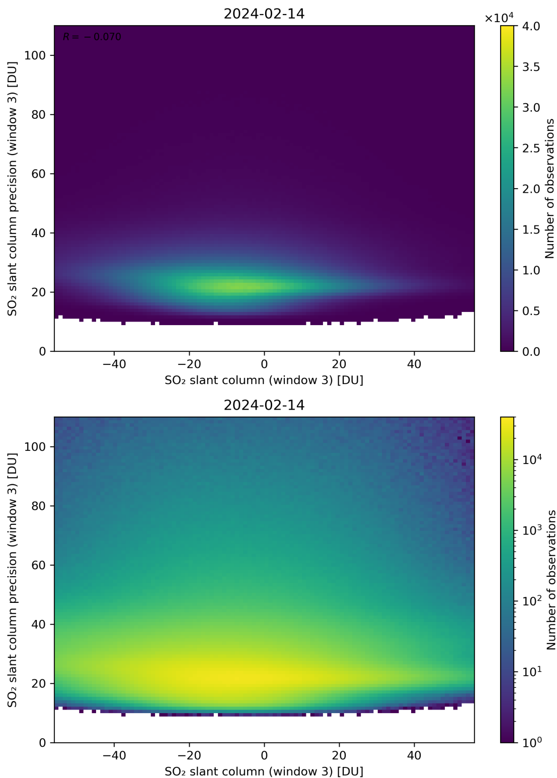
Figure 267: Scatter density plot of “SO 2 slant column (window 3)” against “SO 2 slant column precision (window 3)” for 2024-02-13 to 2024-02-15.
