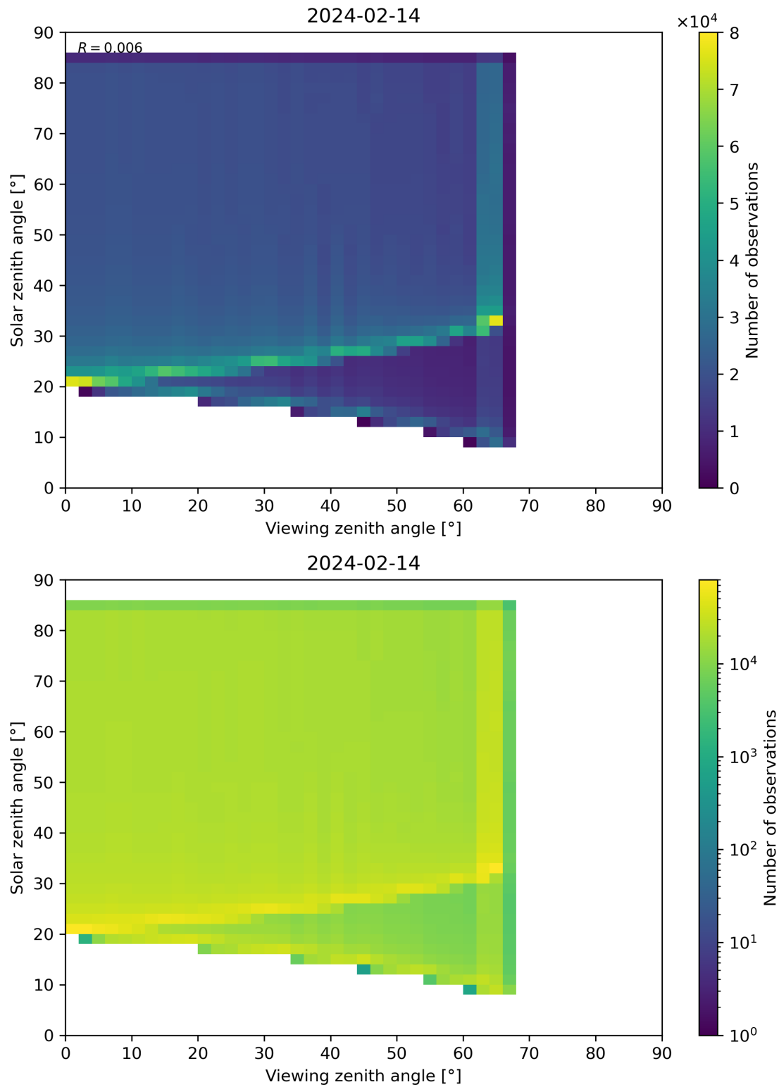
Figure 315: Scatter density plot of “Viewing zenith angle” against “Solar zenith angle” for 2024-02-13 to 2024-02-15.
