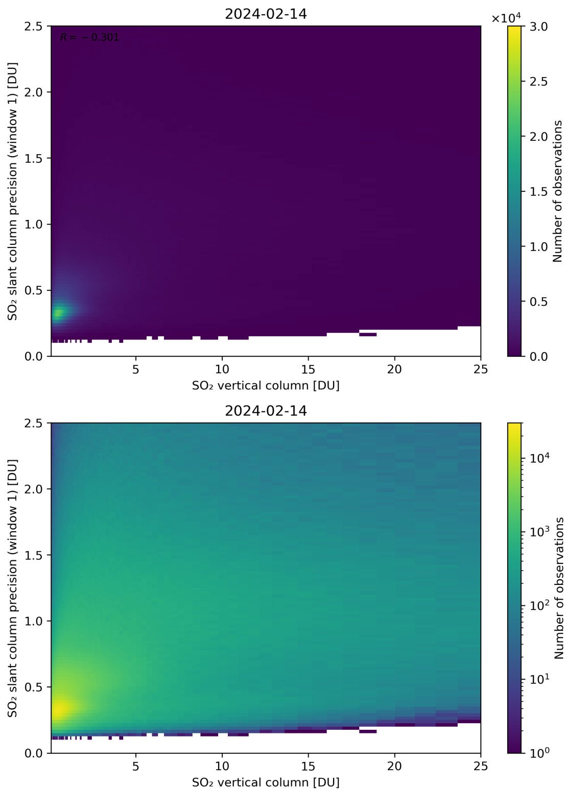
Figure 301: Scatter density plot of “SO 2 vertical column” against “SO 2 slant column precision (window 1)” for 2024-02-13 to 2024-02-15.
