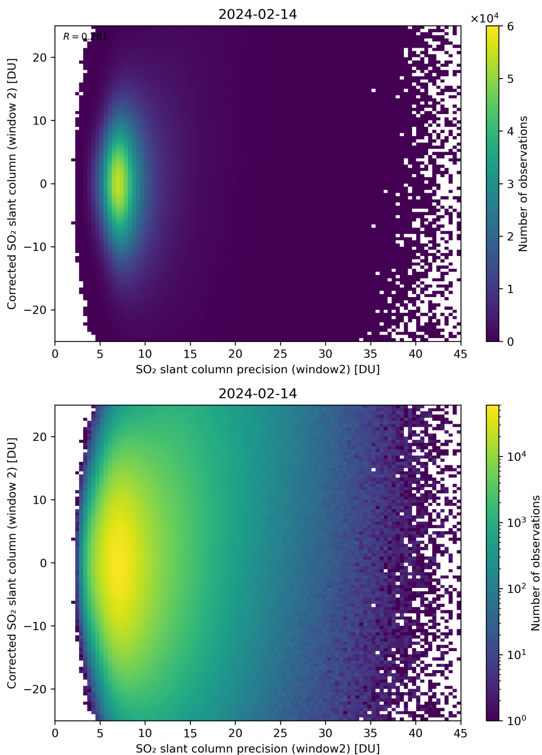
Figure 247: Scatter density plot of “SO 2 slant column precision (window2)” against “Corrected SO 2 slant column (window 2)” for 2024-02-13 to 2024-02-15.
