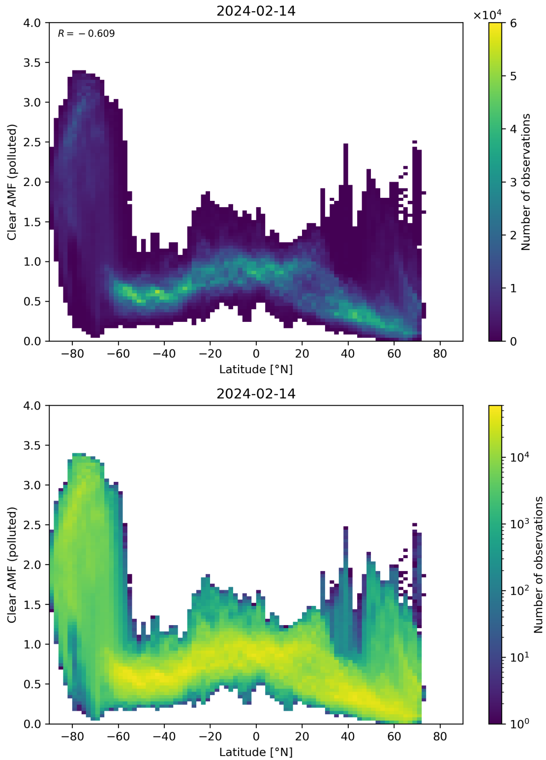
Figure 145: Scatter density plot of “Latitude” against “Clear AMF (polluted)” for 2024-02-13 to 2024-02-15.
