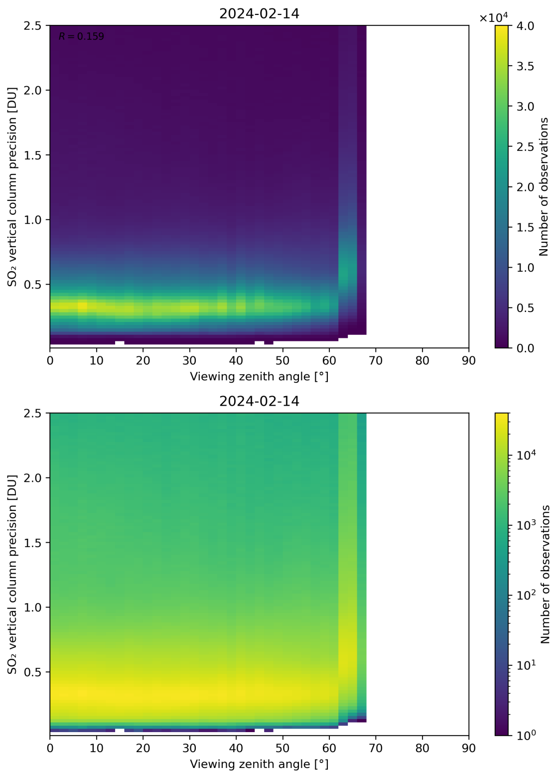
Figure 328: Scatter density plot of “Viewing zenith angle” against “SO 2 vertical column precision” for 2024-02-13 to 2024-02-15.
