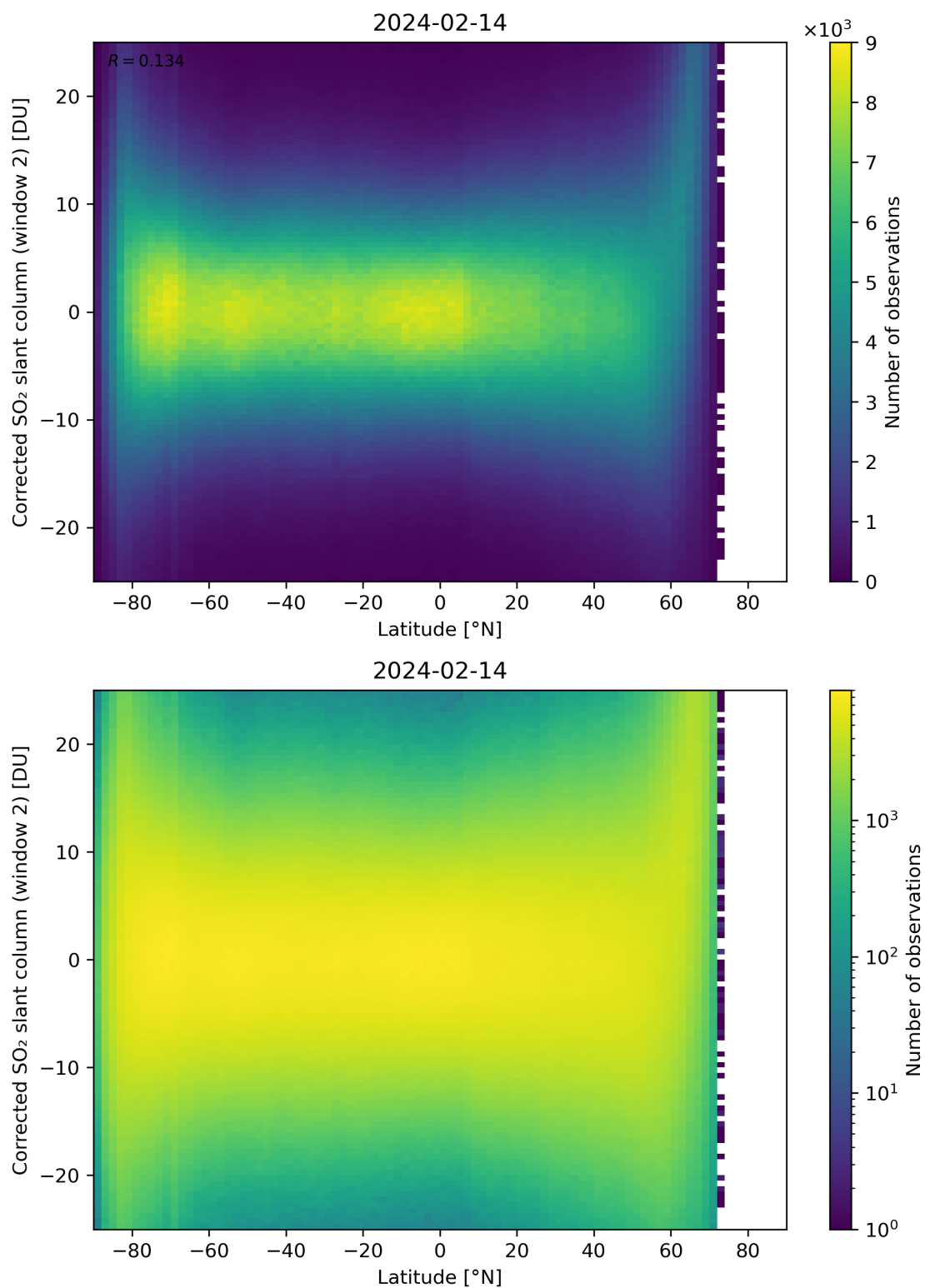
Figure 147: Scatter density plot of “Latitude” against “Corrected SO 2 slant column (window 2)” for 2024-02-13 to 2024-02-15.
