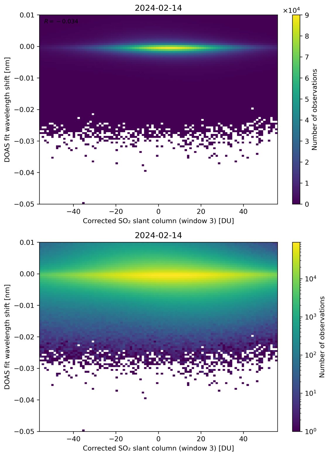
Figure 206: Scatter density plot of “Corrected SO 2 slant column (window 3)” against “DOAS fit wavelength shift” for 2024-02-13 to 2024-02-15.
