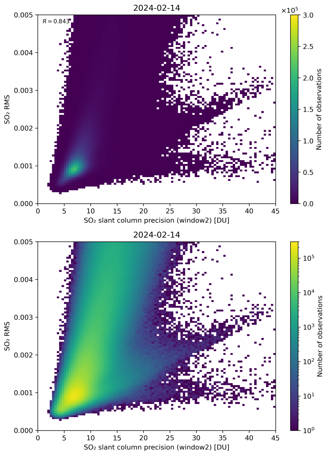
Figure 245: Scatter density plot of “SO 2 slant column precision (window2)” against “SO 2 RMS” for 2024-02-13 to 2024-02-15.
