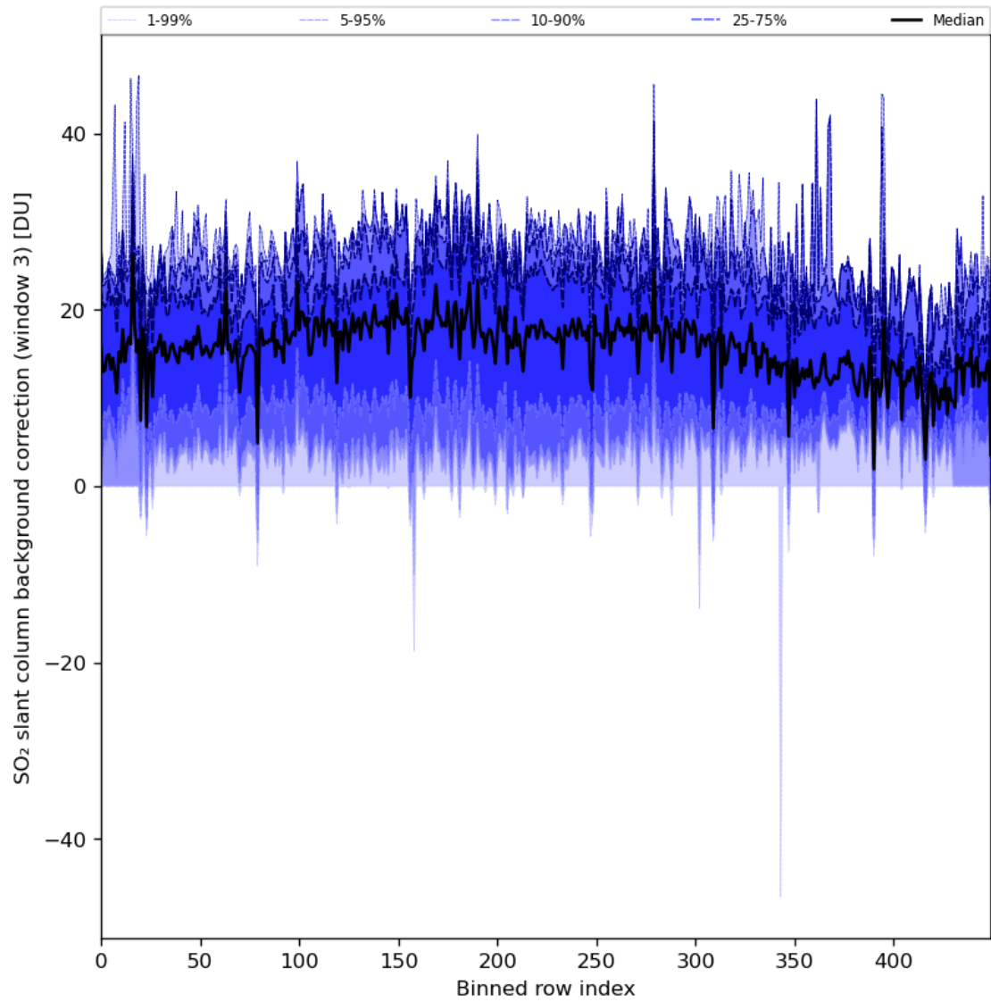
Figure 90: Along track statistics of “SO 2 slant column background correction (window 3)” for 2024-02-13 to 2024-02-15
