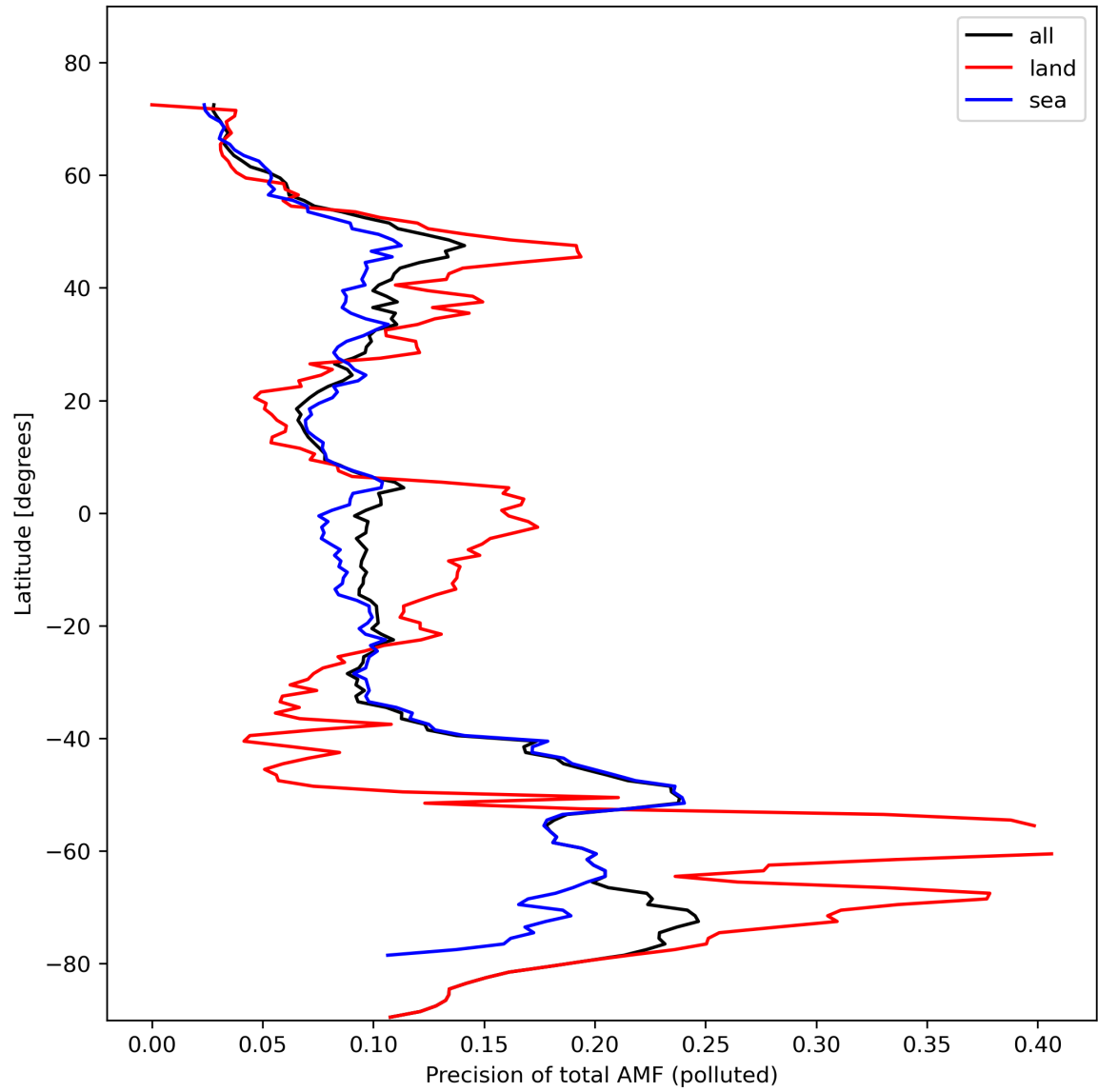
Figure 49: Zonal average of “Precision of total AMF (polluted)” for 2024-02-13 to 2024-02-15.
