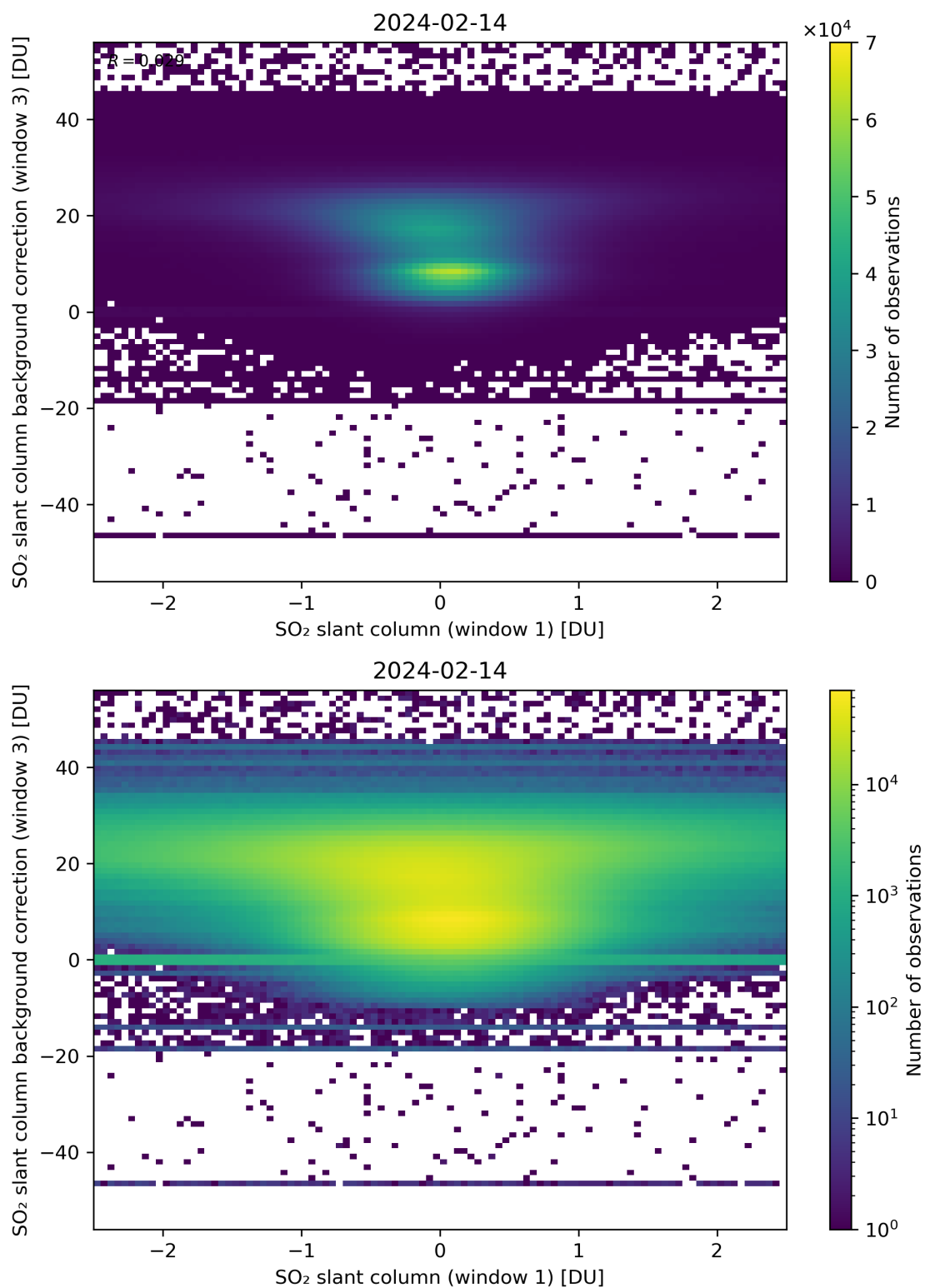
Figure 214: Scatter density plot of “SO 2 slant column (window 1)” against “SO 2 slant column background correction (window 3)” for 2024-02-13 to 2024-02-15.
