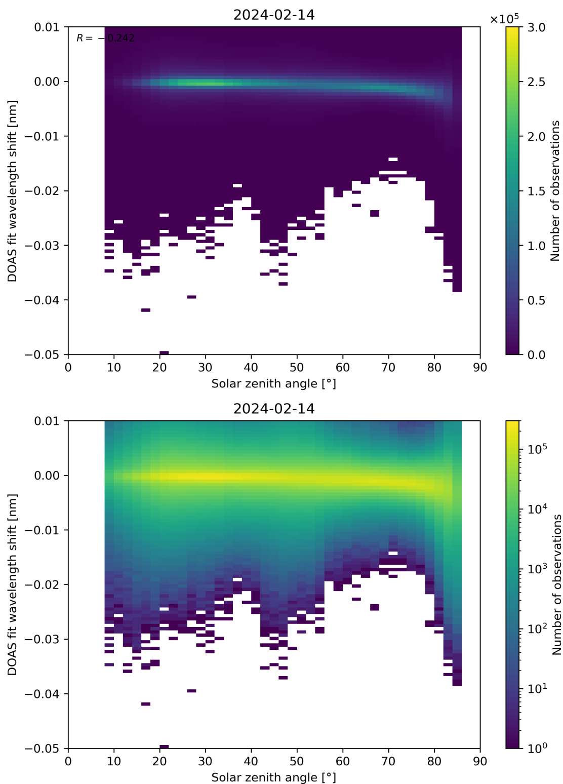
Figure 161: Scatter density plot of “Solar zenith angle” against “DOAS fit wavelength shift” for 2024-02-13 to 2024-02-15.
