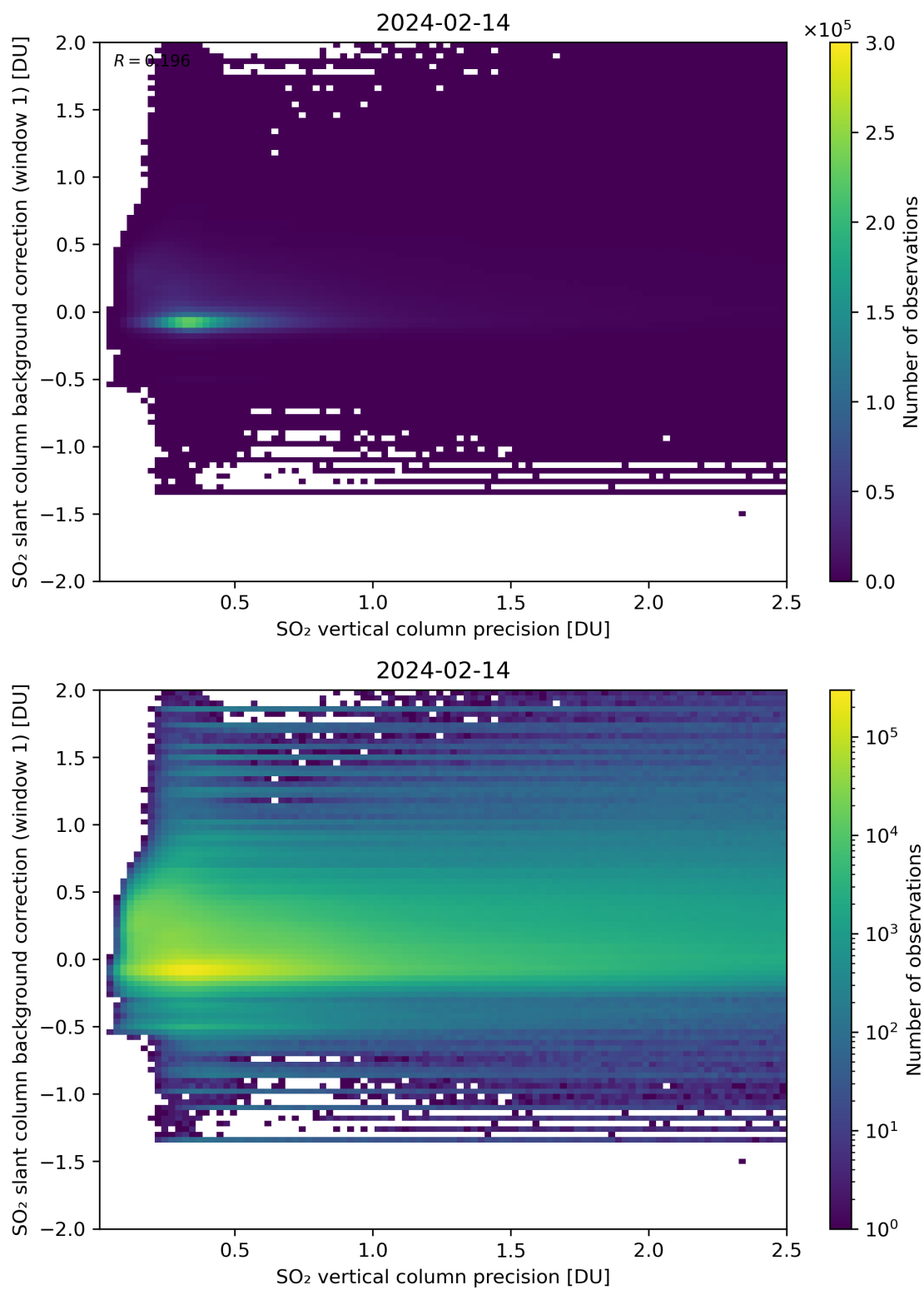
Figure 279: Scatter density plot of “SO 2 vertical column precision” against “SO 2 slant column background correction (window 1)” for 2024-02-13 to 2024-02-15.
