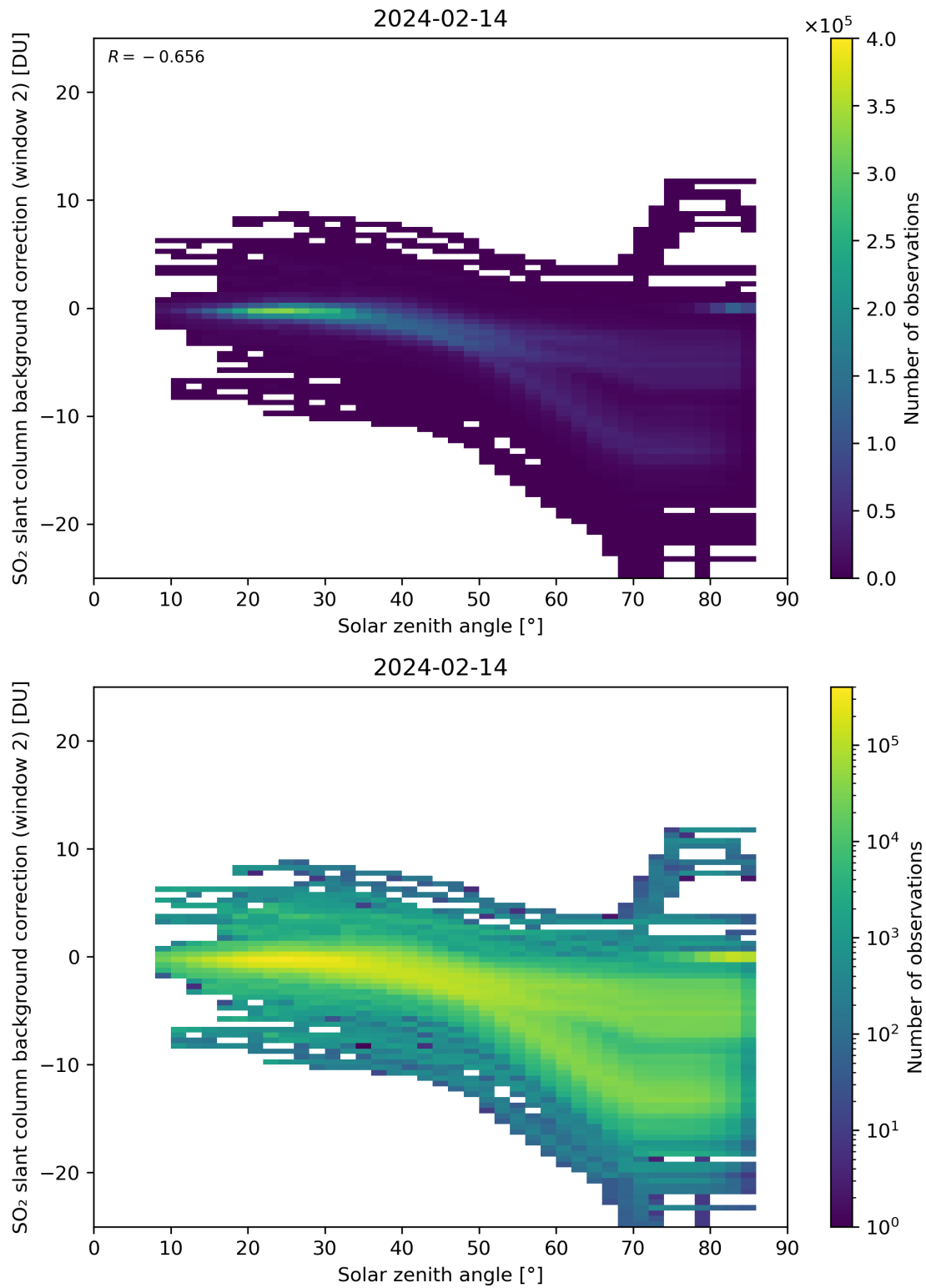
Figure 159: Scatter density plot of “Solar zenith angle” against “SO 2 slant column background correction (window 2)” for 2024-02-13 to 2024-02-15.
