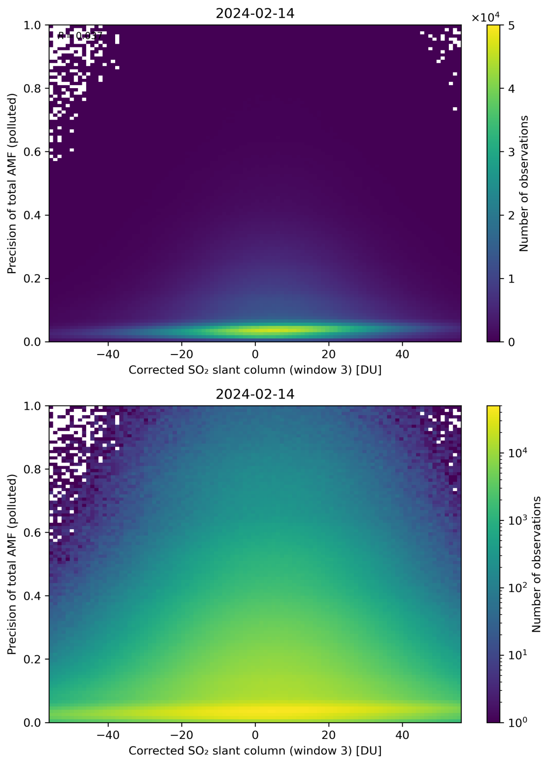
Figure 211: Scatter density plot of “Corrected SO 2 slant column (window 3)” against “Precision of total AMF (polluted)” for 2024-02-13 to 2024-02-15.
