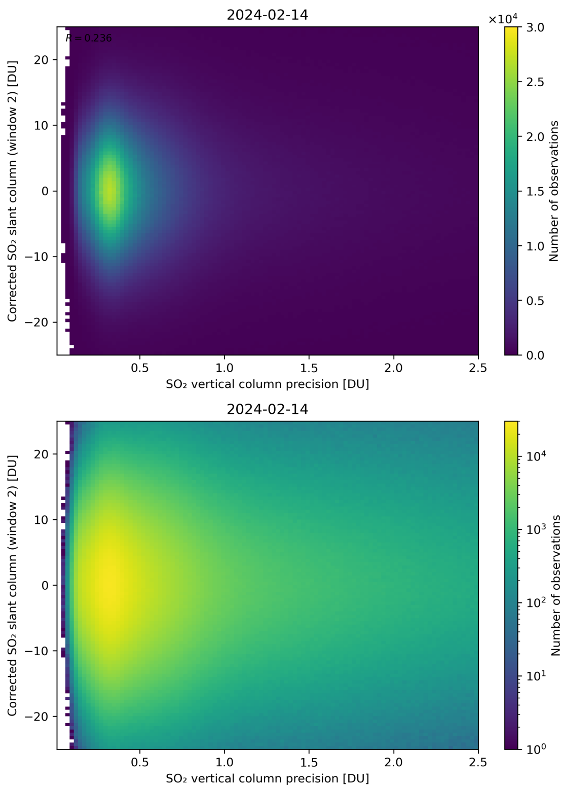
Figure 287: Scatter density plot of “SO 2 vertical column precision” against “Corrected SO 2 slant column (window 2)” for 2024-02-13 to 2024-02-15.
