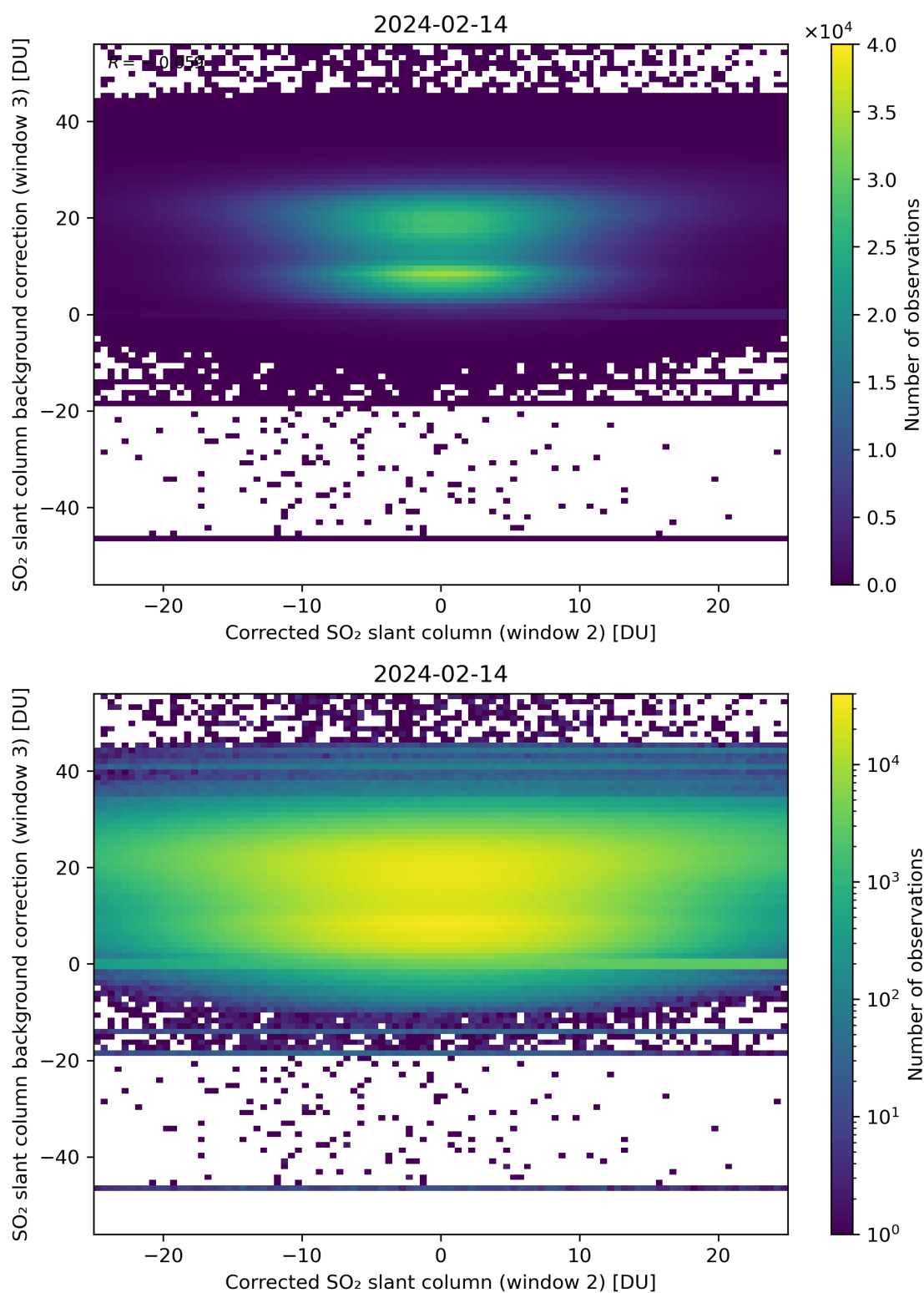
Figure 195: Scatter density plot of “Corrected SO 2 slant column (window 2)” against “SO 2 slant column background correction (window 3)” for 2024-02-13 to 2024-02-15.
