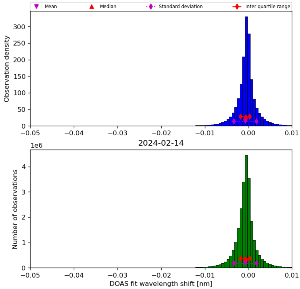
Figure 68: Histogram of “DOAS fit wavelength shift” for 2024-02-13 to 2024-02-15
