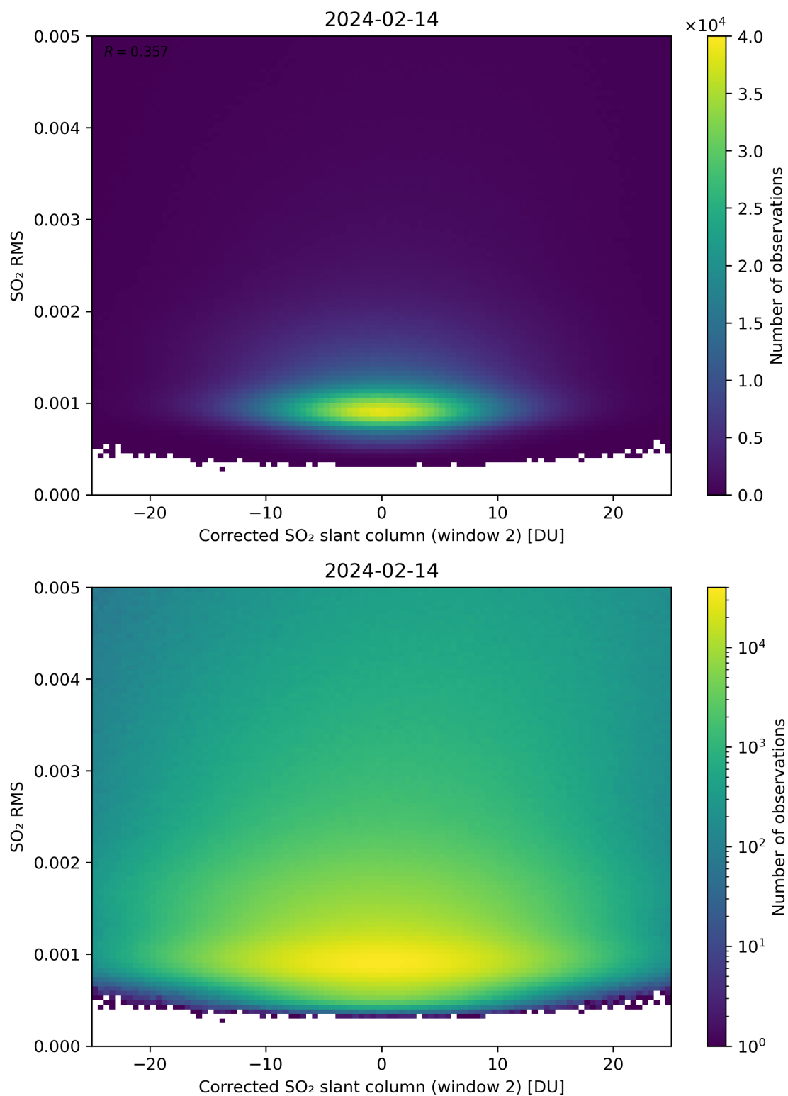
Figure 198: Scatter density plot of “Corrected SO 2 slant column (window 2)” against “SO 2 RMS” for 2024-02-13 to 2024-02-15.
