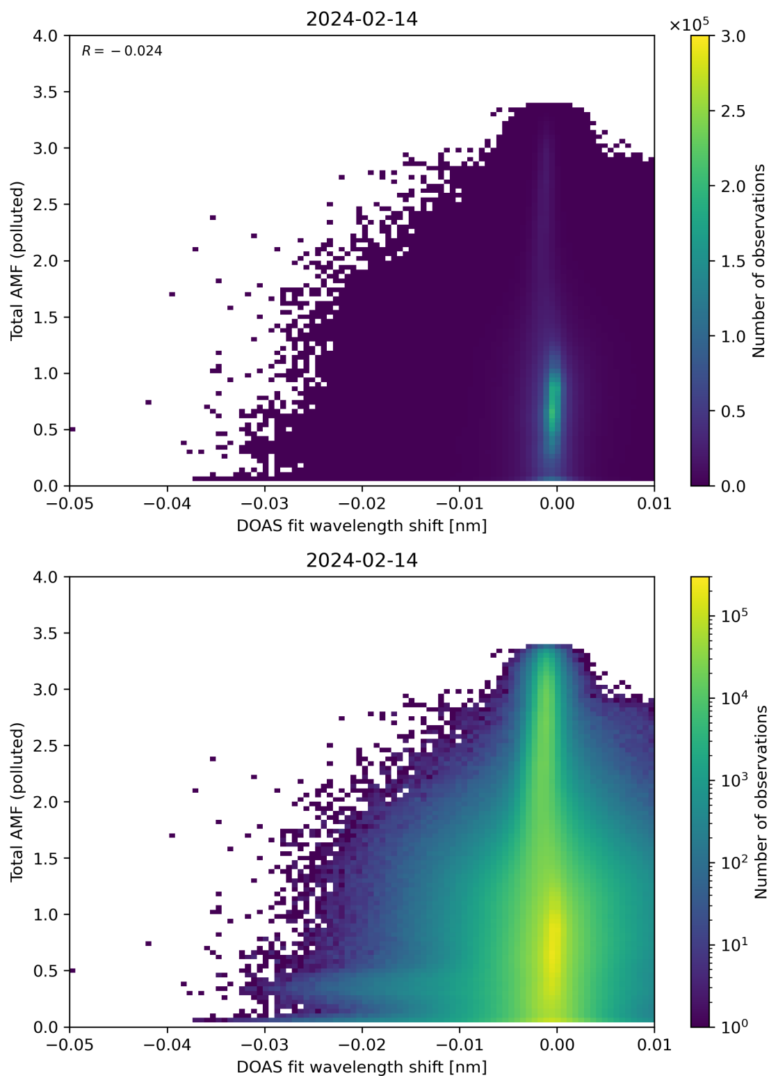
Figure 130: Scatter density plot of “DOAS fit wavelength shift” against “Total AMF (polluted)” for 2024-02-13 to 2024-02-15.
