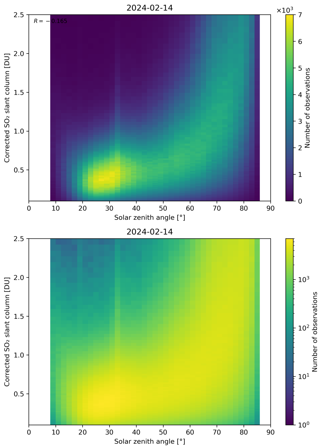
Figure 166: Scatter density plot of “Solar zenith angle” against “Corrected SO 2 slant column” for 2024-02-13 to 2024-02-15.
