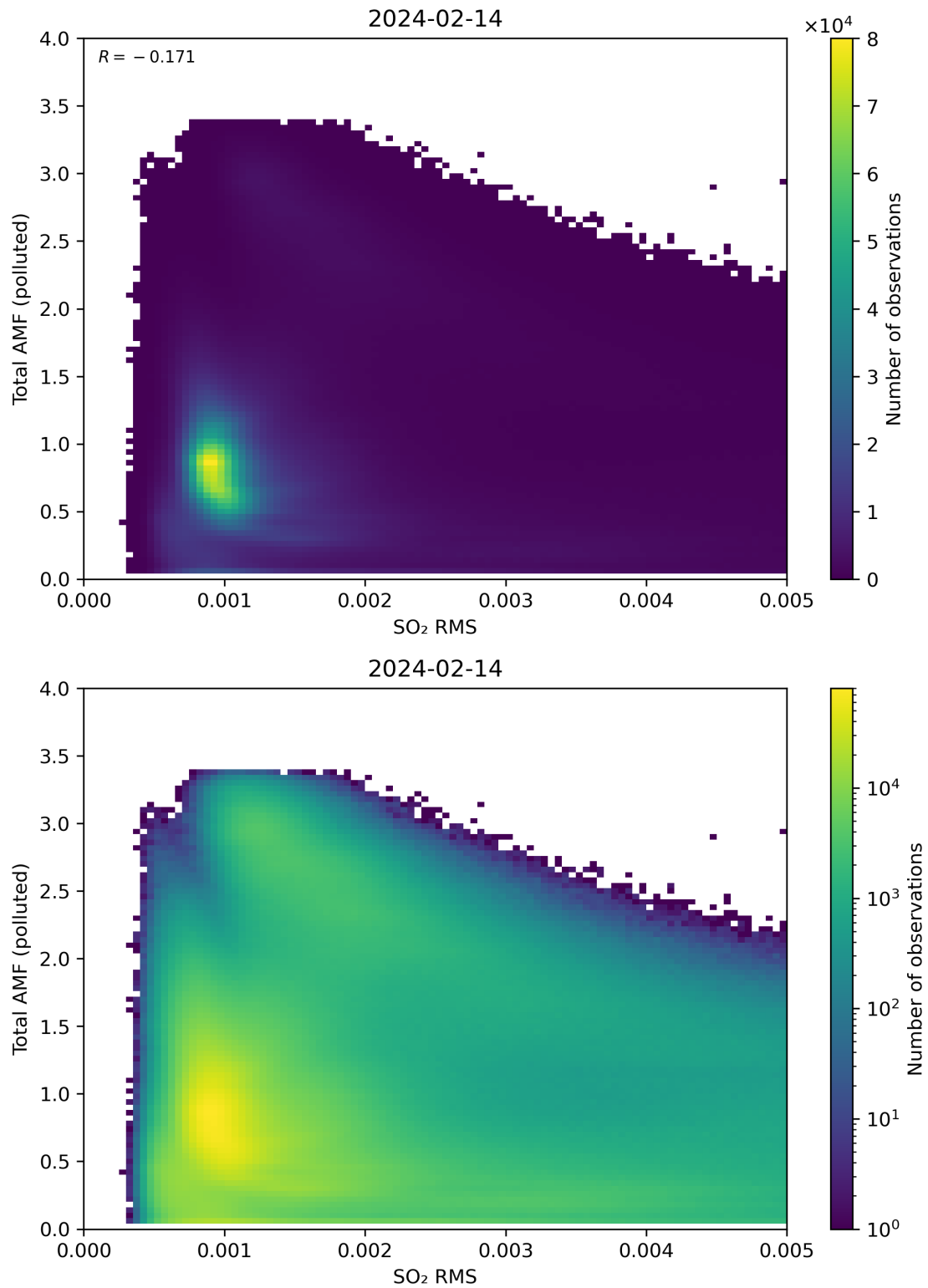
Figure 137: Scatter density plot of “SO 2 RMS” against “Total AMF (polluted)” for 2024-02-13 to 2024-02-15.
