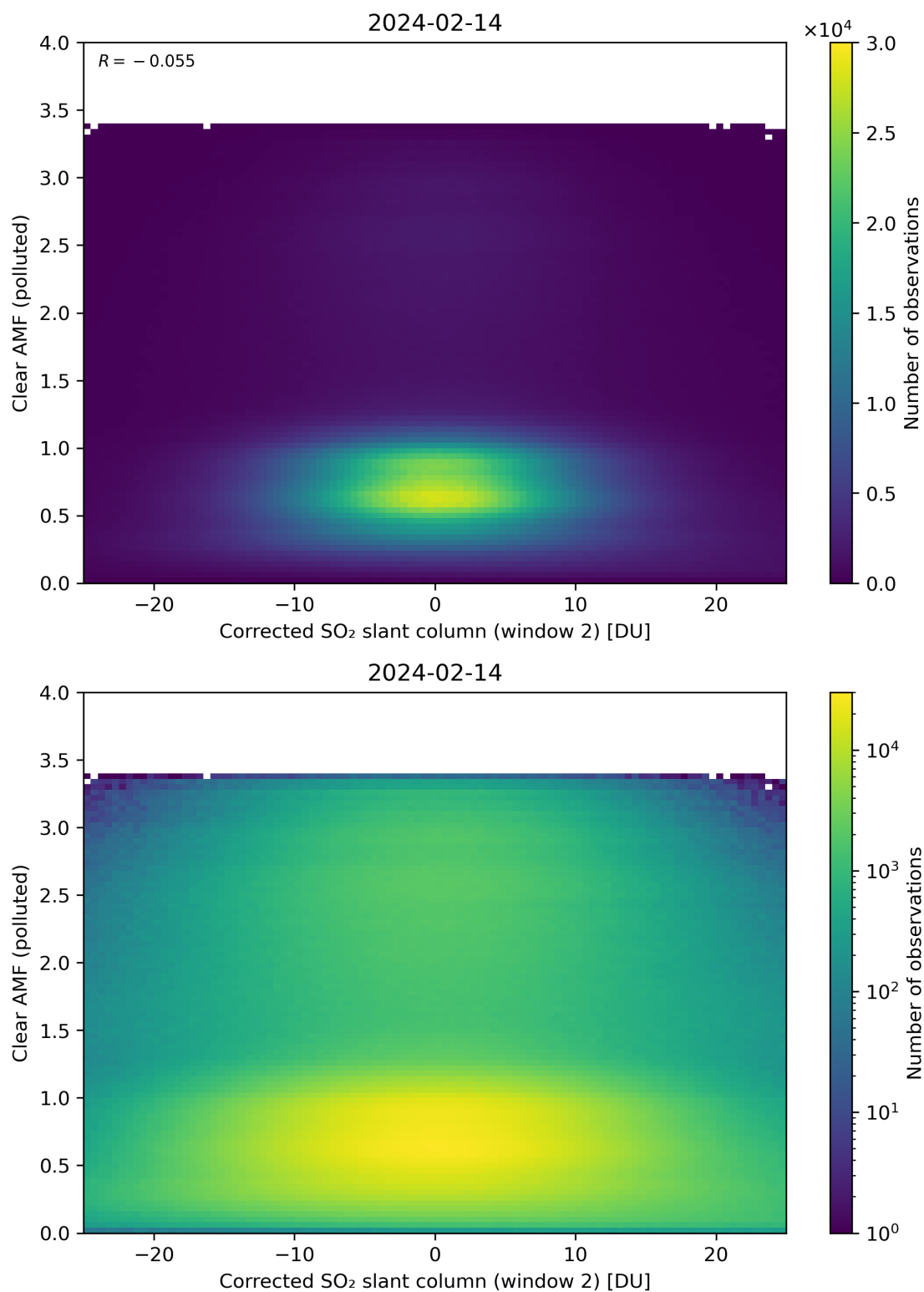
Figure 199: Scatter density plot of “Corrected SO 2 slant column (window 2)” against “Clear AMF (polluted)” for 2024-02-13 to 2024-02-15.
