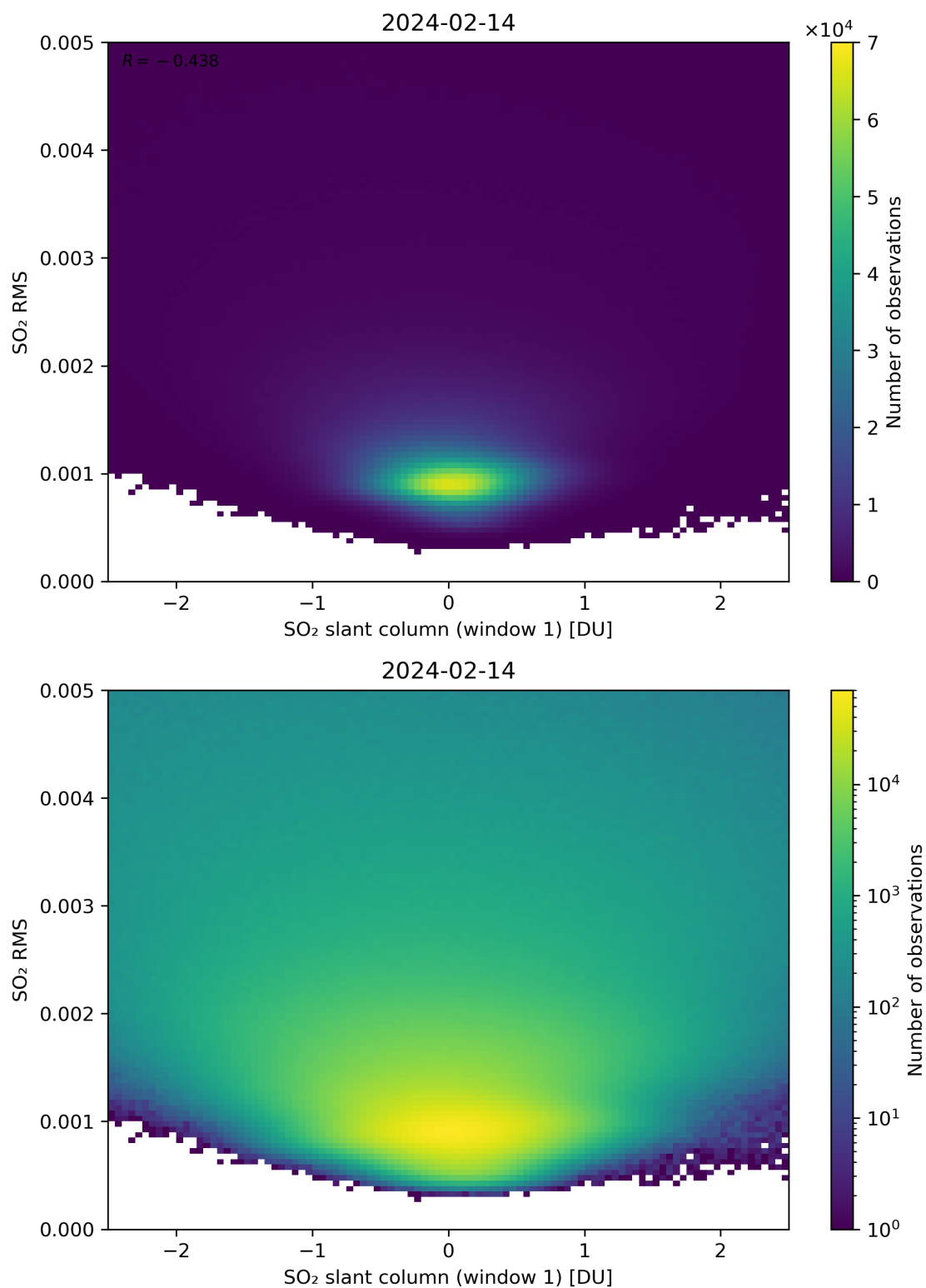
Figure 217: Scatter density plot of “SO 2 slant column (window 1)” against “SO 2 RMS” for 2024-02-13 to 2024-02-15.
