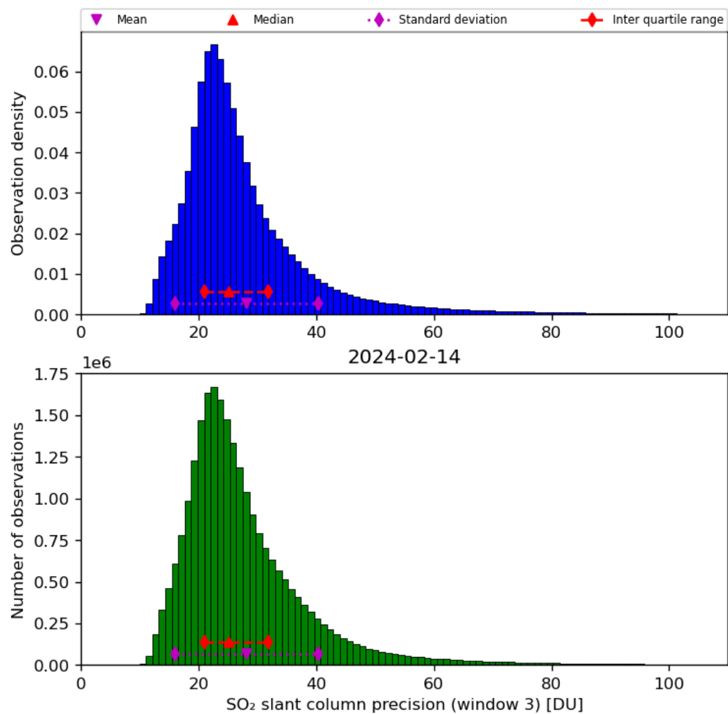
Figure 65: Histogram of “SO 2 slant column precision (window 3)” for 2024-02-13 to 2024-02-15
