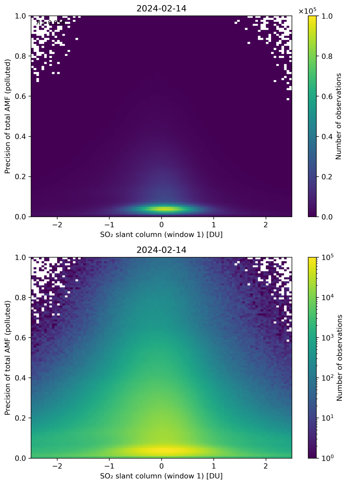
Figure 240: Scatter density plot of “SO 2 slant column (window 1)” against “Precision of total AMF (polluted)” for 2024-02-13 to 2024-02-15.
