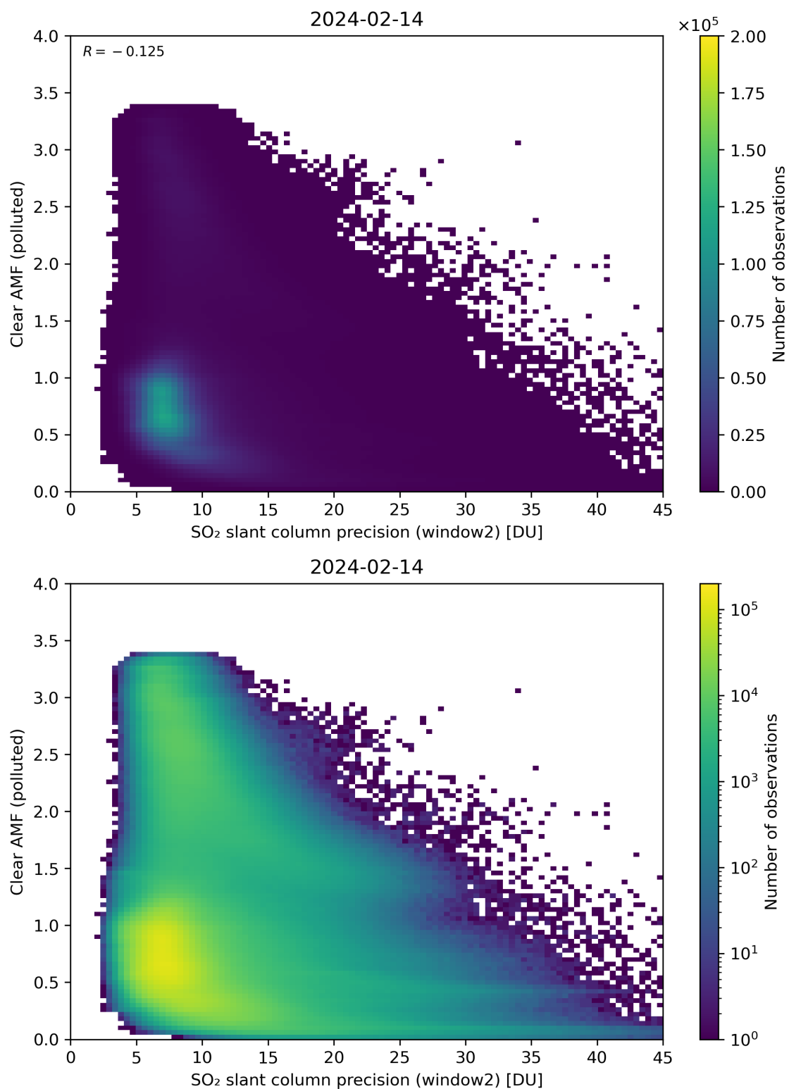
Figure 246: Scatter density plot of “SO 2 slant column precision (window2)” against “Clear AMF (polluted)” for 2024-02-13 to 2024-02-15.
