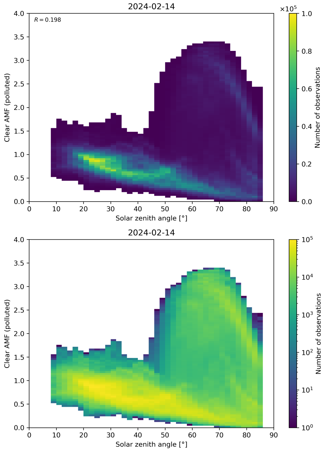
Figure 165: Scatter density plot of “Solar zenith angle” against “Clear AMF (polluted)” for 2024-02-13 to 2024-02-15.
