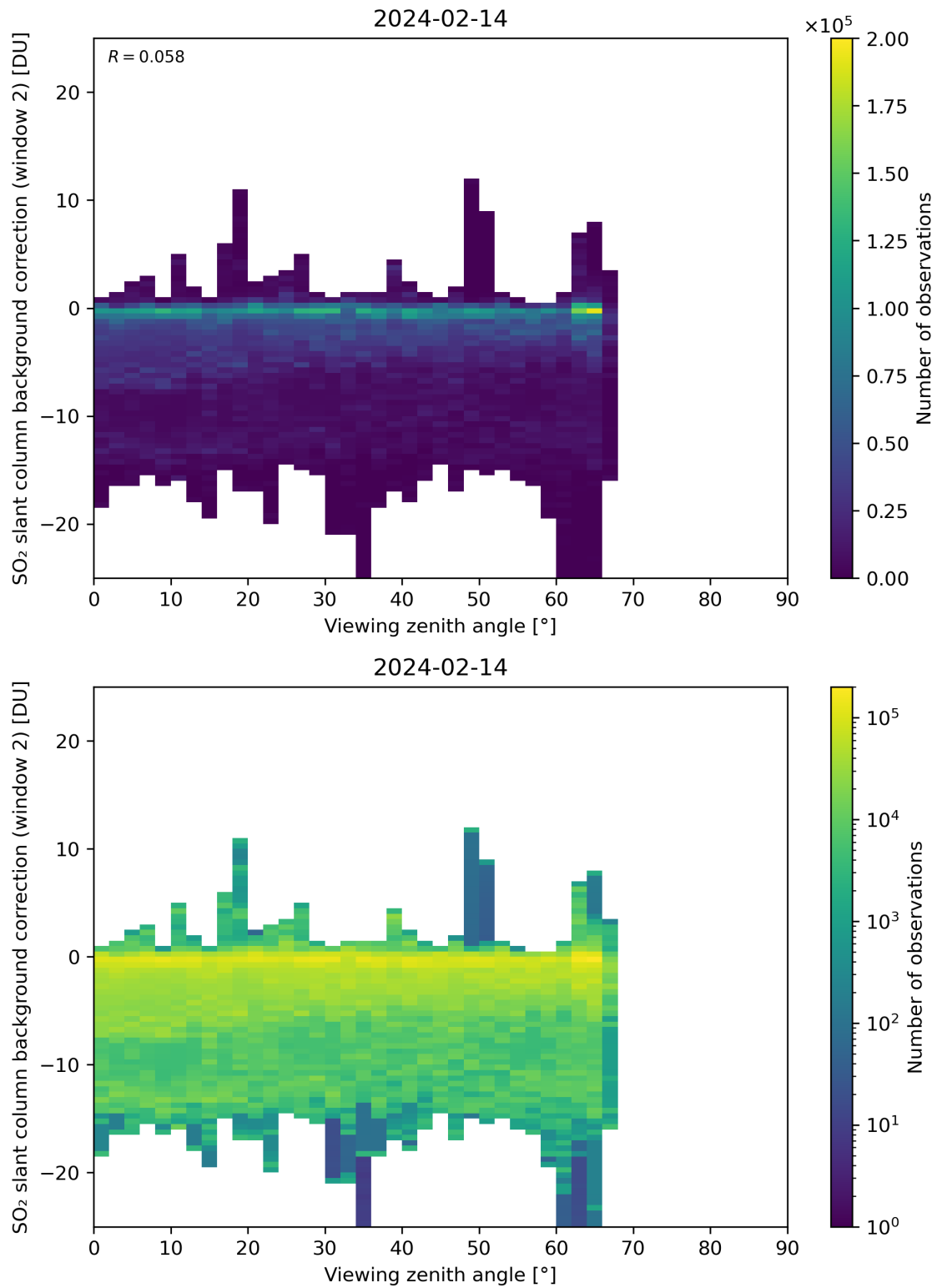
Figure 309: Scatter density plot of “Viewing zenith angle” against “SO 2 slant column background correction (window 2)” for 2024-02-13 to 2024-02-15.
