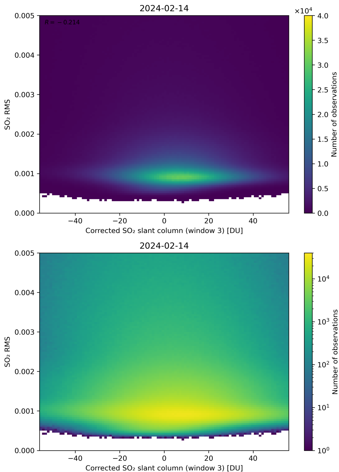
Figure 208: Scatter density plot of “Corrected SO 2 slant column (window 3)” against “SO 2 RMS” for 2024-02-13 to 2024-02-15.
