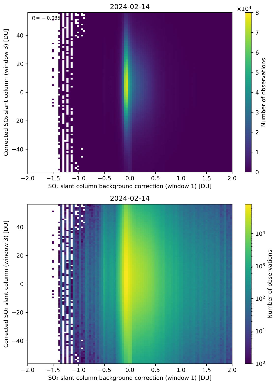
Figure 105: Scatter density plot of “SO 2 slant column background correction (window 1)” against “Corrected SO 2 slant column (window 3)” for 2024-02-13 to 2024-02-15.
