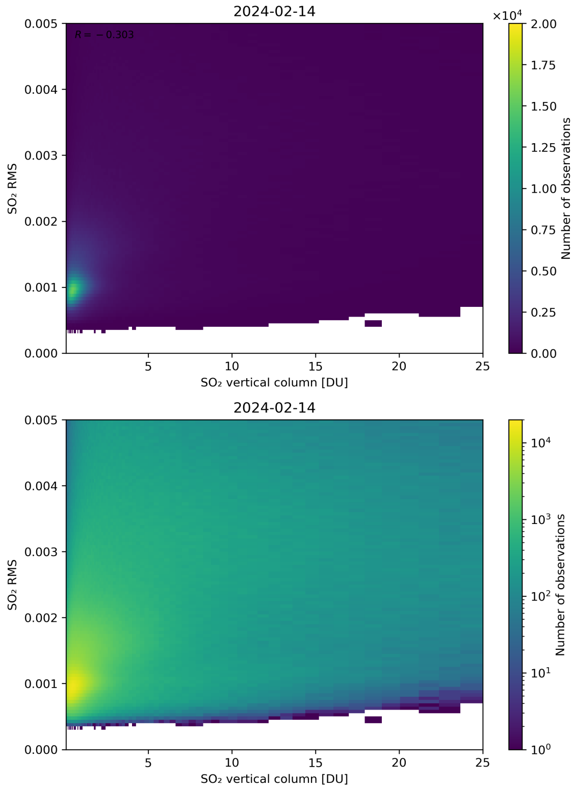
Figure 278: Scatter density plot of “SO 2 vertical column” against “SO 2 RMS” for 2024-02-13 to 2024-02-15.
