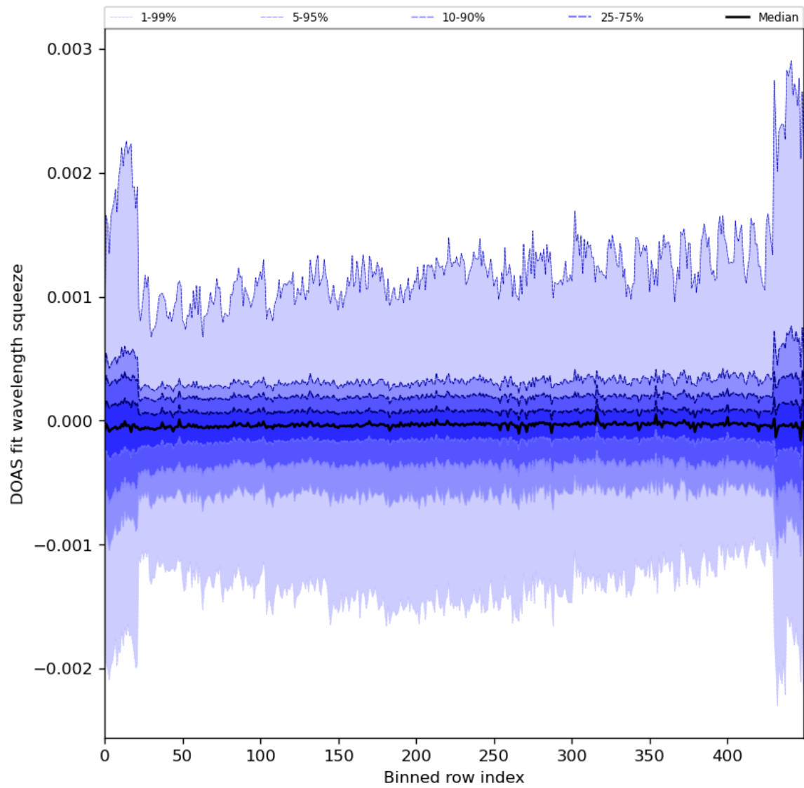
Figure 92: Along track statistics of “DOAS fit wavelength squeeze” for 2024-02-13 to 2024-02-15
