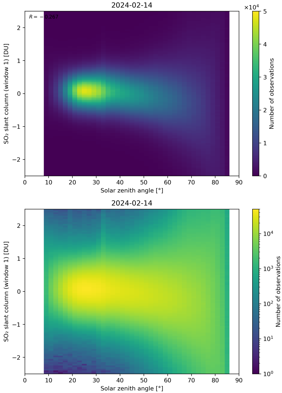
Figure 169: Scatter density plot of “Solar zenith angle” against “SO 2 slant column (window 1)” for 2024-02-13 to 2024-02-15.
