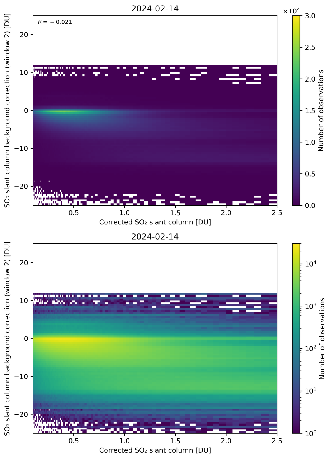
Figure 179: Scatter density plot of “Corrected SO 2 slant column” against “SO 2 slant column background correction (window 2)” for 2024-02-13 to 2024-02-15.
