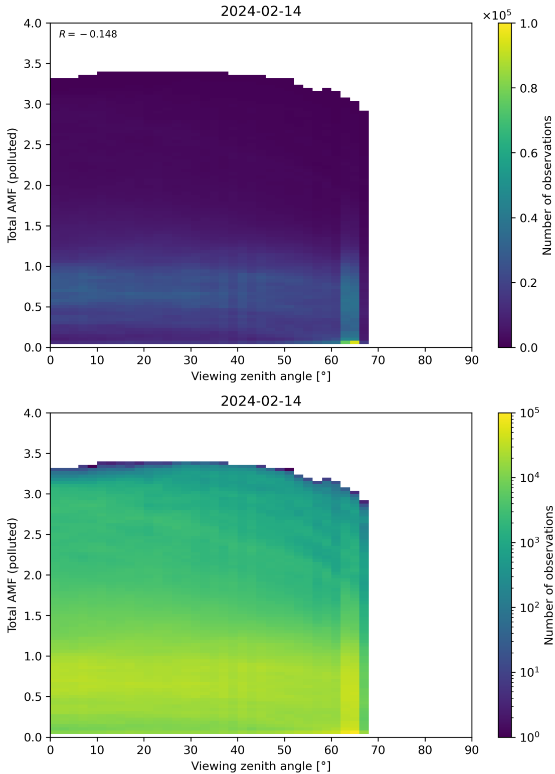
Figure 325: Scatter density plot of “Viewing zenith angle” against “Total AMF (polluted)” for 2024-02-13 to 2024-02-15.
