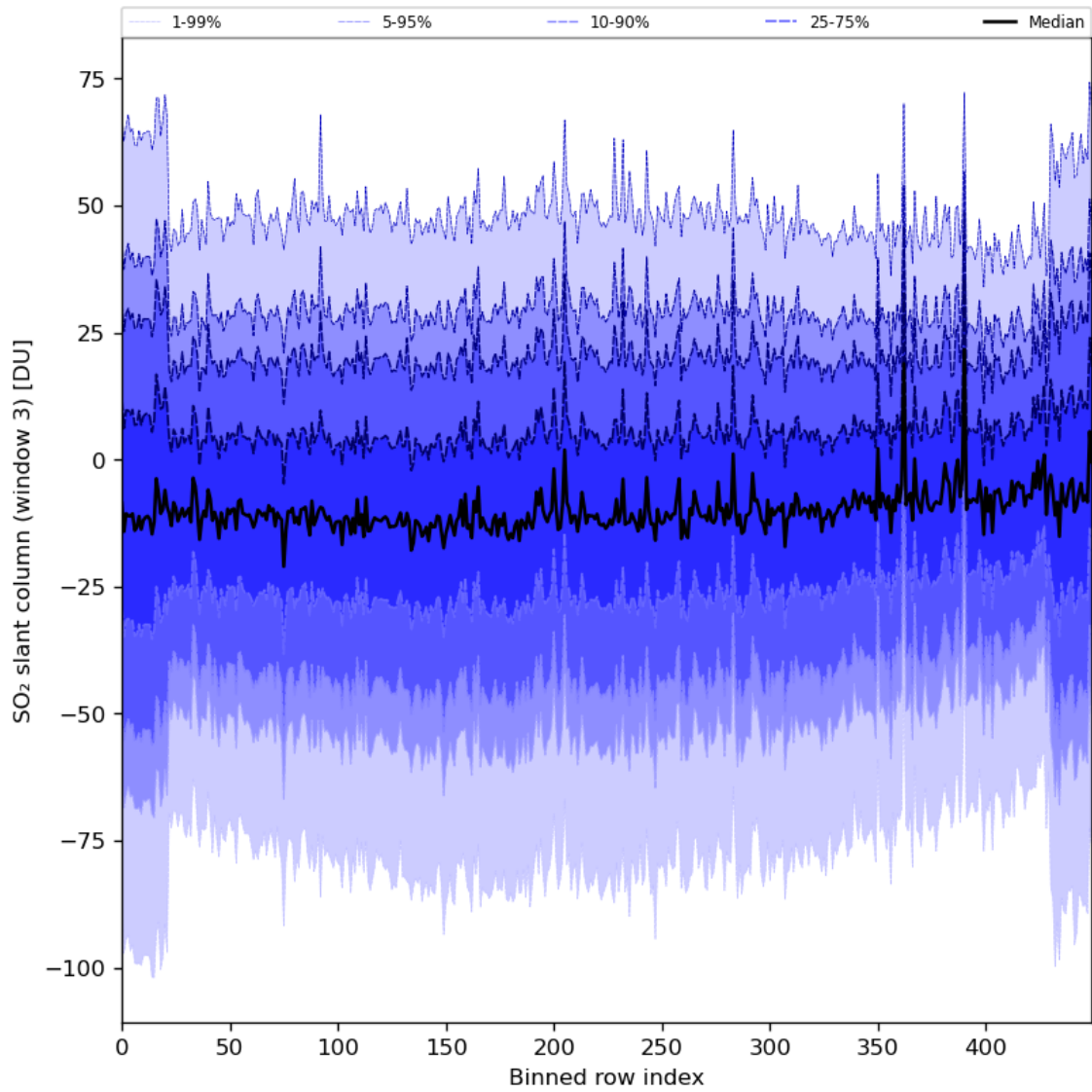
Figure 87: Along track statistics of “SO 2 slant column (window 3)” for 2024-02-13 to 2024-02-15
