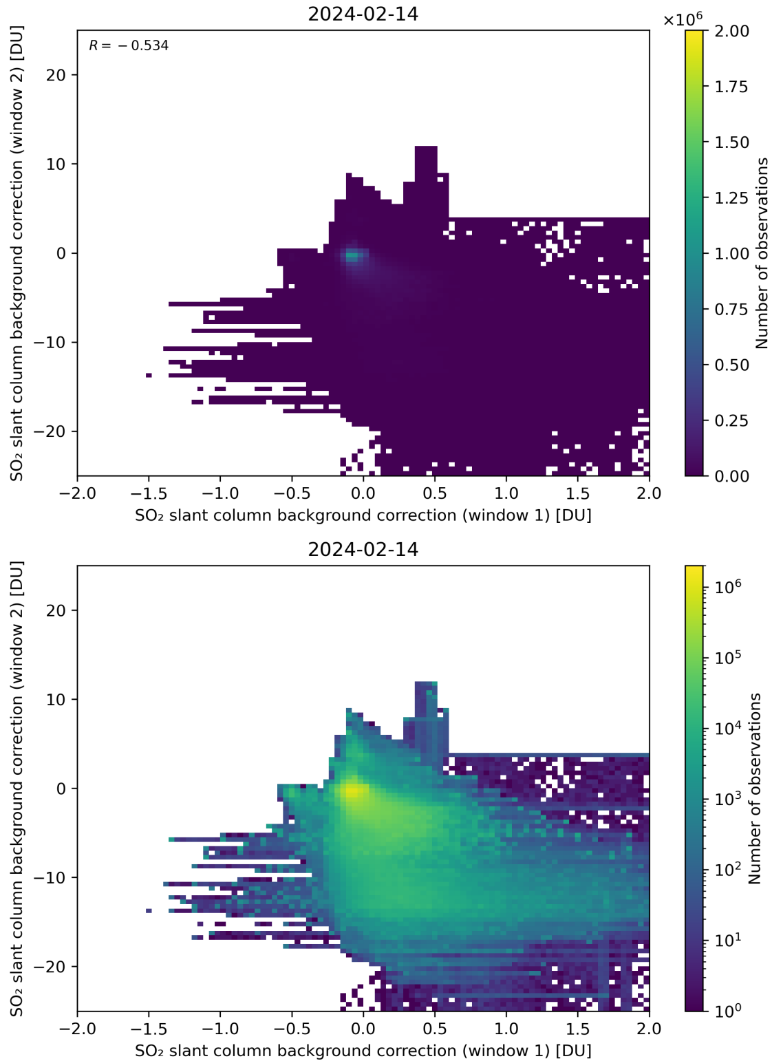
Figure 98: Scatter density plot of “SO 2 slant column background correction (window 1)” against “SO 2 slant column background correction (window 2)” for 2024-02-13 to 2024-02-15.
