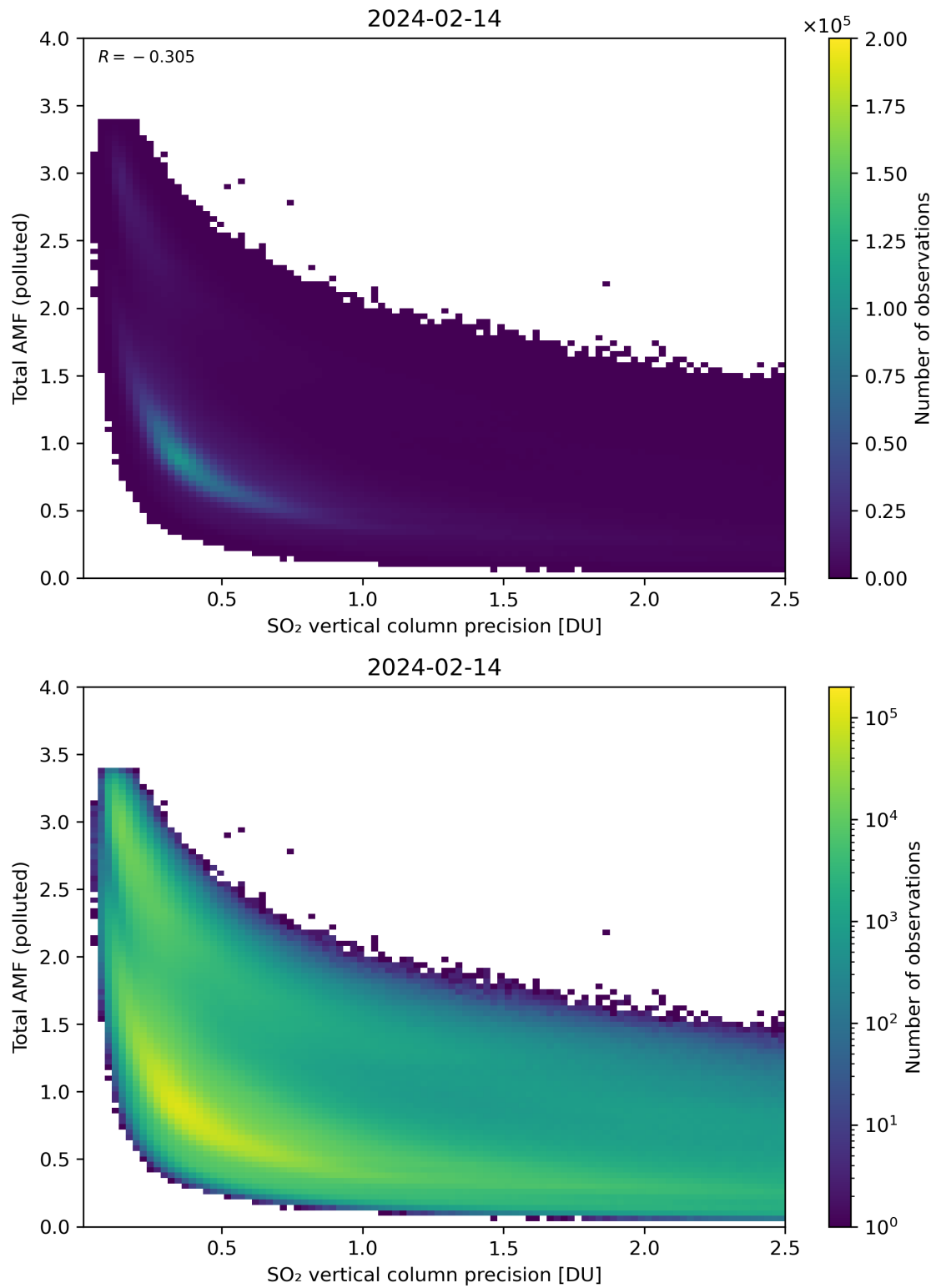
Figure 294: Scatter density plot of “SO 2 vertical column precision” against “Total AMF (polluted)” for 2024-02-13 to 2024-02-15.
