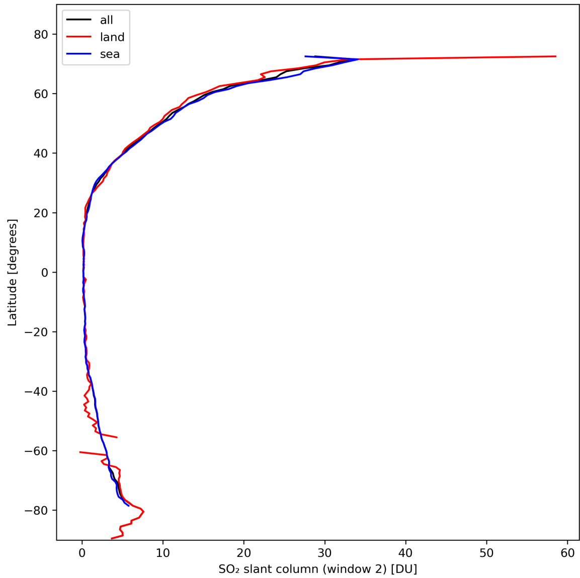
Figure 37: Zonal average of “SO 2 slant column (window 2)” for 2024-02-13 to 2024-02-15.
