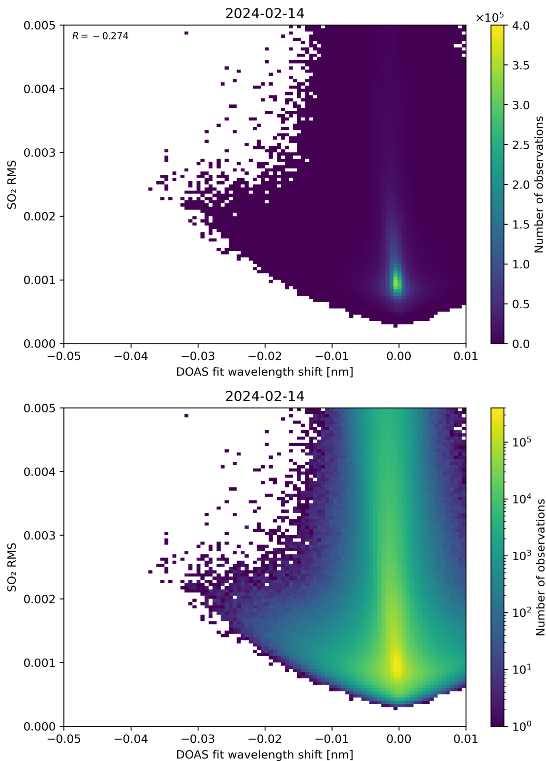
Figure 128: Scatter density plot of “DOAS fit wavelength shift” against “SO 2 RMS” for 2024-02-13 to 2024-02-15.
