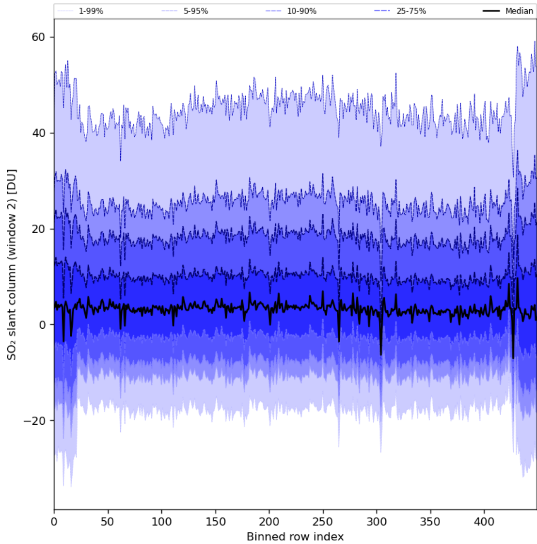
Figure 83: Along track statistics of “SO 2 slant column (window 2)” for 2024-02-13 to 2024-02-15
