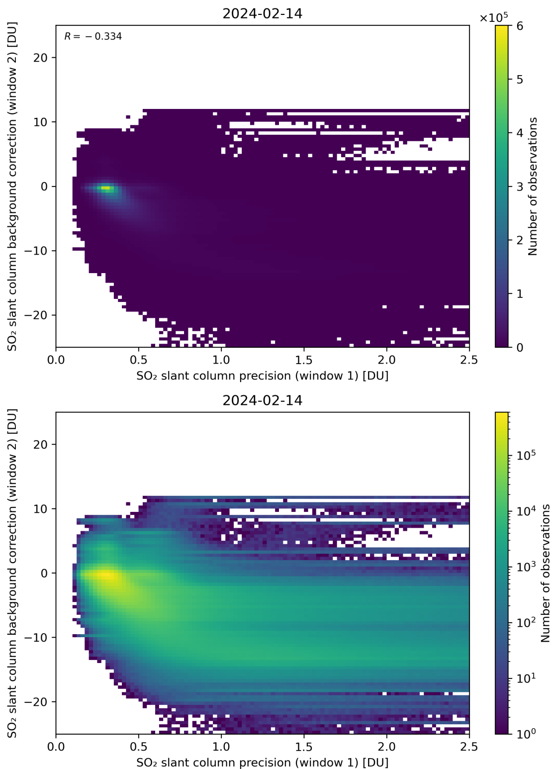
Figure 219: Scatter density plot of “SO 2 slant column precision (window 1)” against “SO 2 slant column background correction (window 2)” for 2024-02-13 to 2024-02-15.
