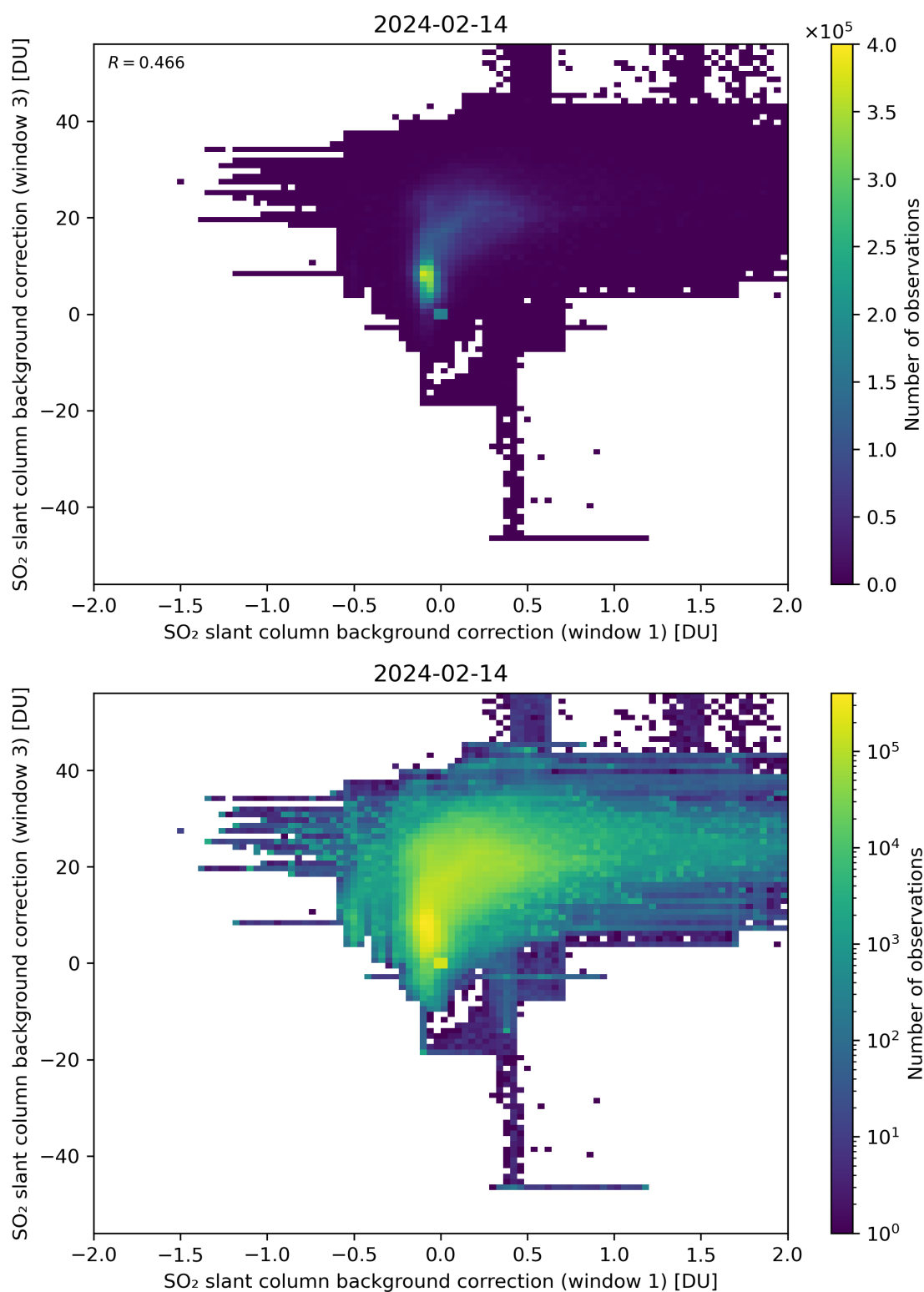
Figure 99: Scatter density plot of “SO 2 slant column background correction (window 1)” against “SO 2 slant column background correction (window 3)” for 2024-02-13 to 2024-02-15.
