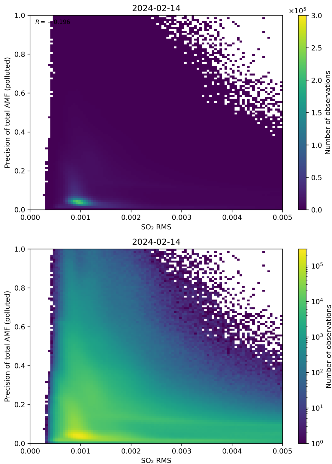
Figure 138: Scatter density plot of “SO 2 RMS” against “Precision of total AMF (polluted)” for 2024-02-13 to 2024-02-15.
