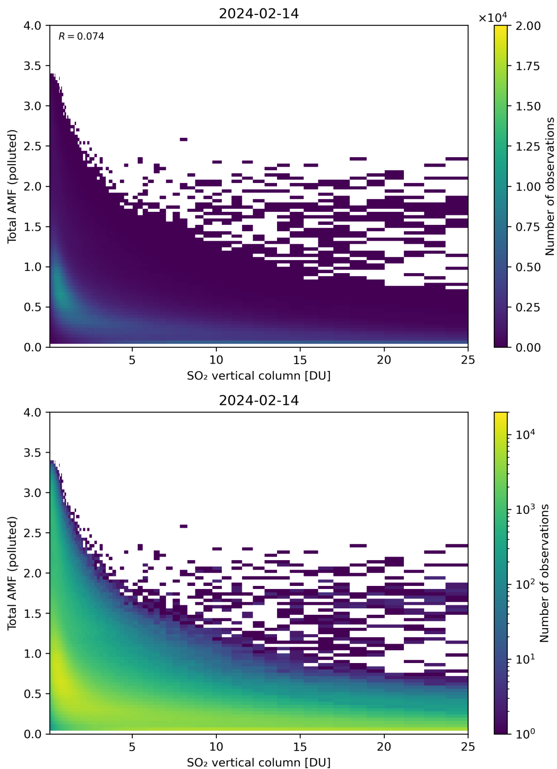
Figure 305: Scatter density plot of “SO 2 vertical column” against “Total AMF (polluted)” for 2024-02-13 to 2024-02-15.
