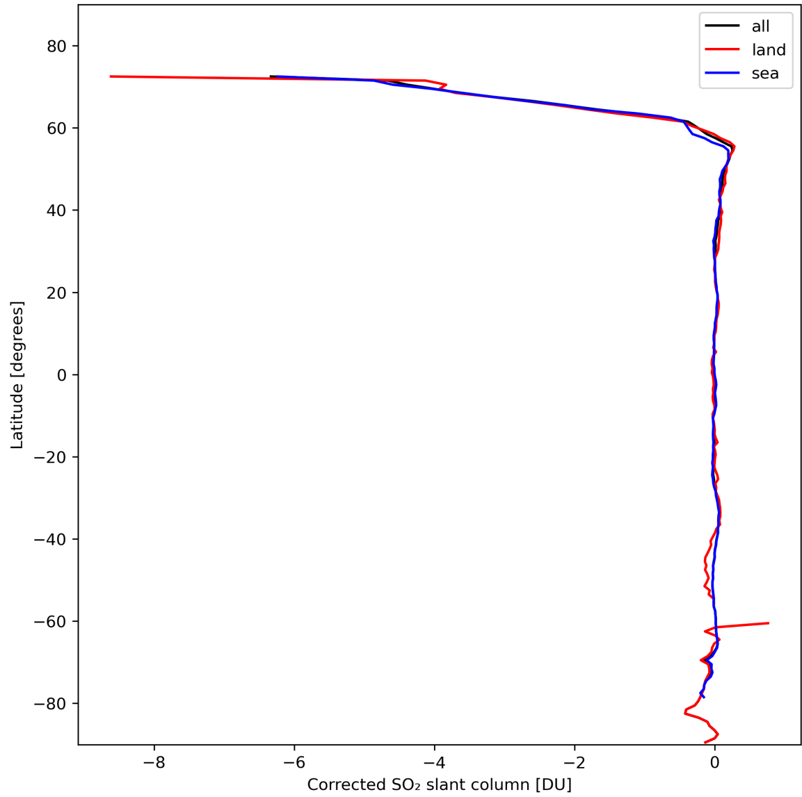
Figure 32: Zonal average of “Corrected SO 2 slant column” for 2024-02-13 to 2024-02-15.
