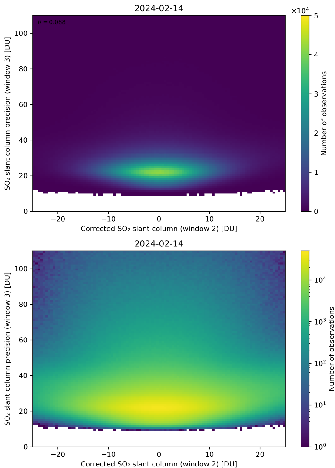
Figure 202: Scatter density plot of “Corrected SO 2 slant column (window 2)” against “SO 2 slant column precision (window 3)” for 2024-02-13 to 2024-02-15.
