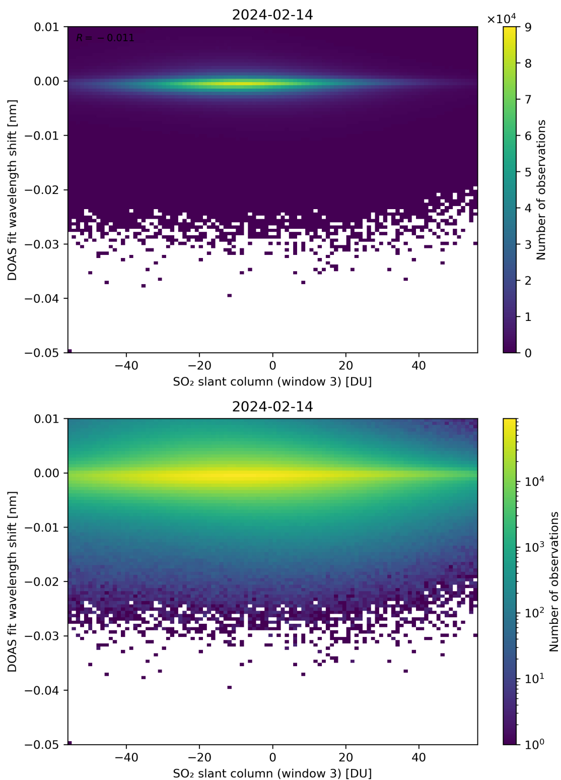
Figure 254: Scatter density plot of “SO 2 slant column (window 3)” against “DOAS fit wavelength shift” for 2024-02-13 to 2024-02-15.
