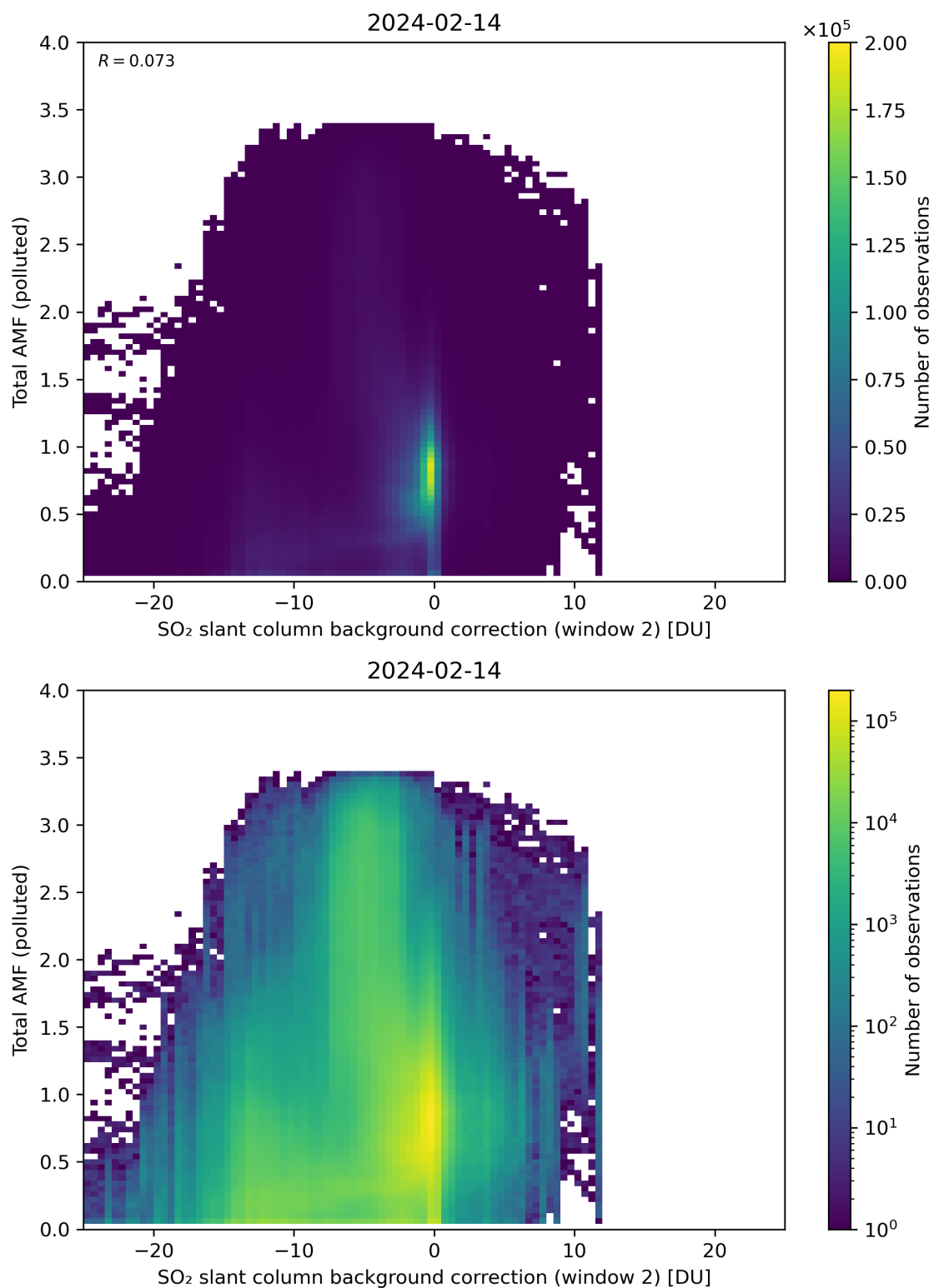
Figure 119: Scatter density plot of “SO 2 slant column background correction (window 2)” against “Total AMF (polluted)” for 2024-02-13 to 2024-02-15.
