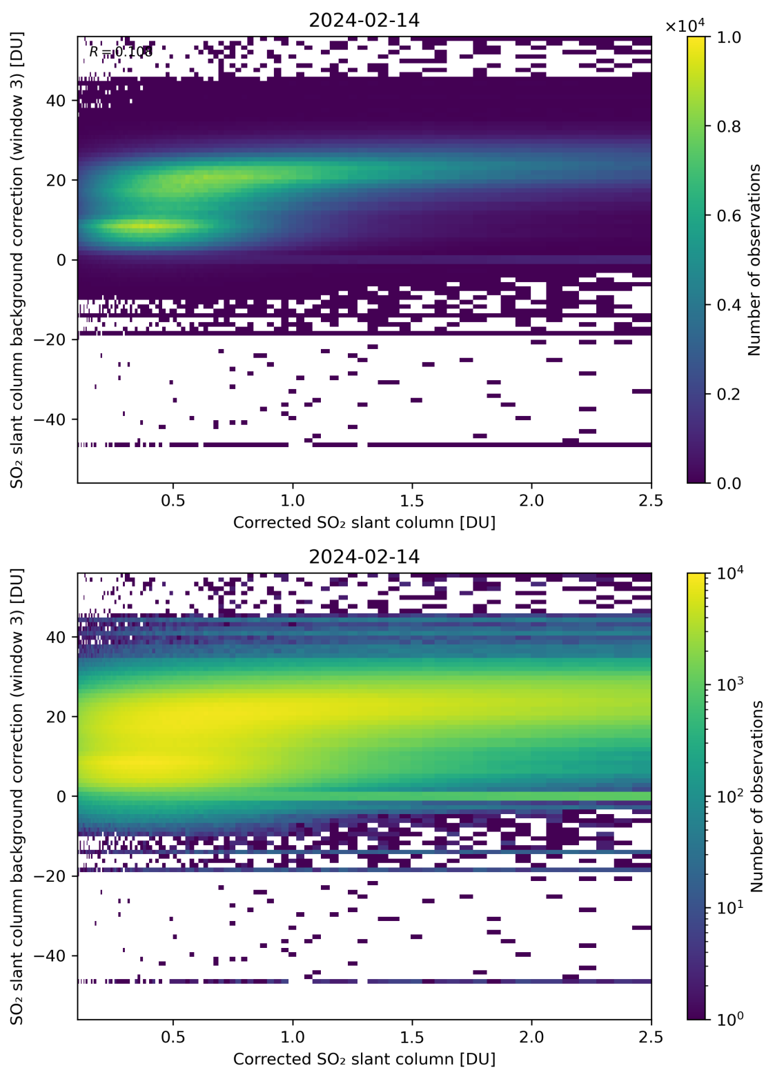
Figure 180: Scatter density plot of “Corrected SO 2 slant column” against “SO 2 slant column background correction (window 3)” for 2024-02-13 to 2024-02-15.
