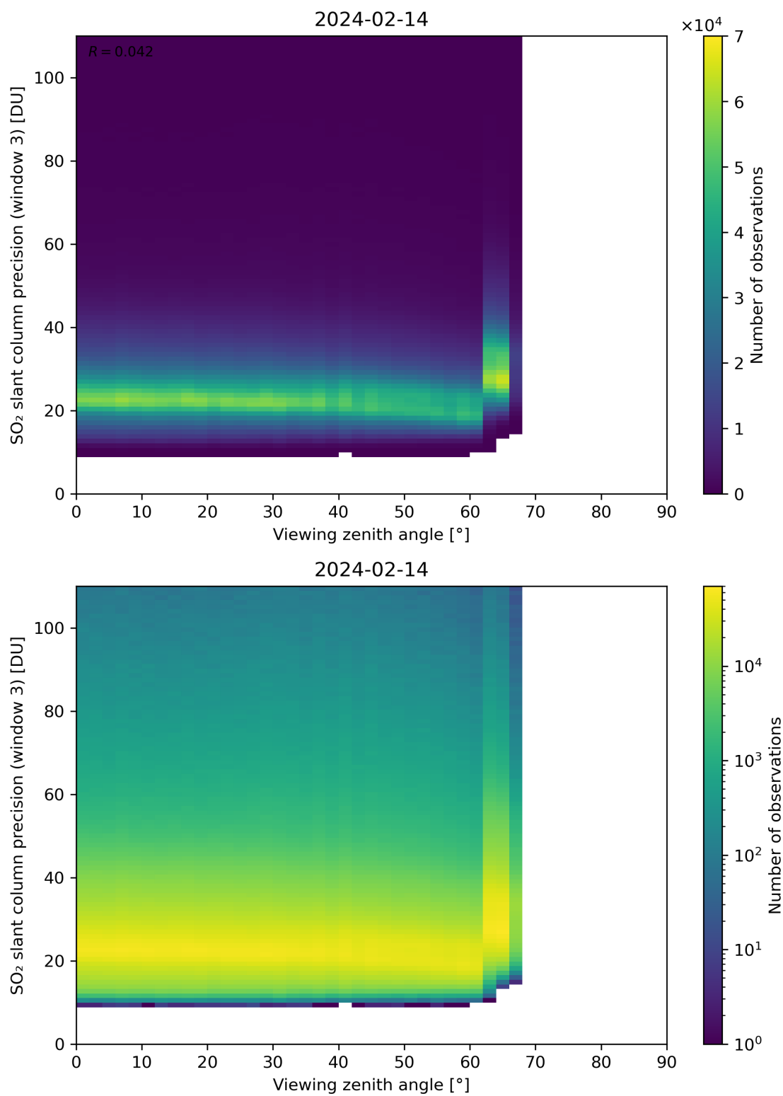
Figure 324: Scatter density plot of “Viewing zenith angle” against “SO 2 slant column precision (window 3)” for 2024-02-13 to 2024-02-15.
