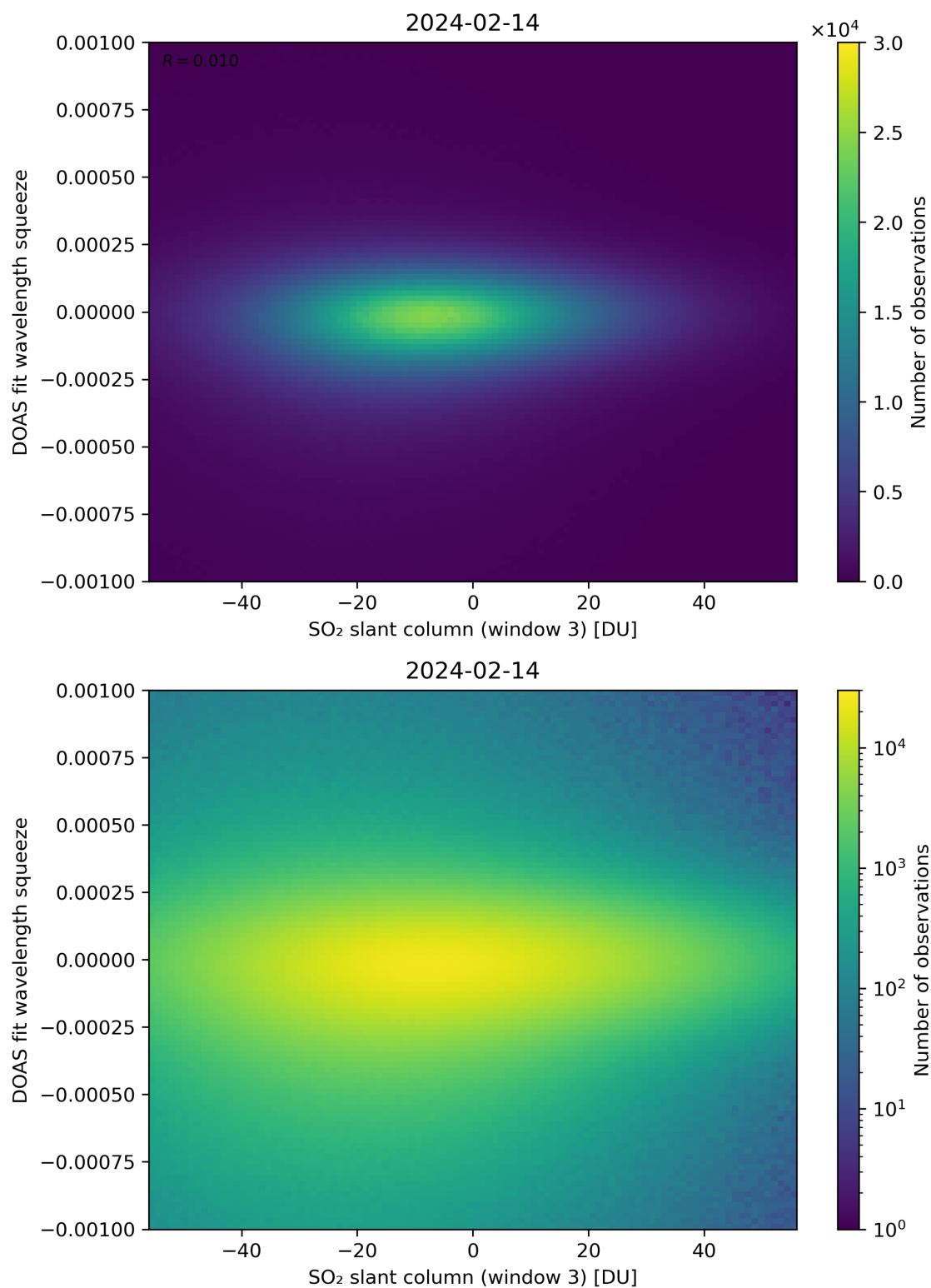
Figure 255: Scatter density plot of “SO 2 slant column (window 3)” against “DOAS fit wavelength squeeze” for 2024-02-13 to 2024-02-15.
