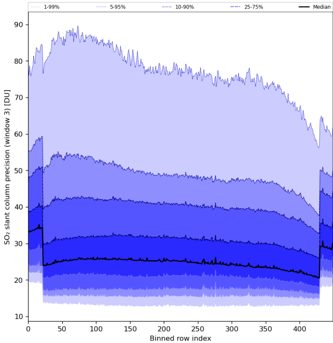
Figure 88: Along track statistics of “SO 2 slant column precision (window 3)” for 2024-02-13 to 2024-02-15
