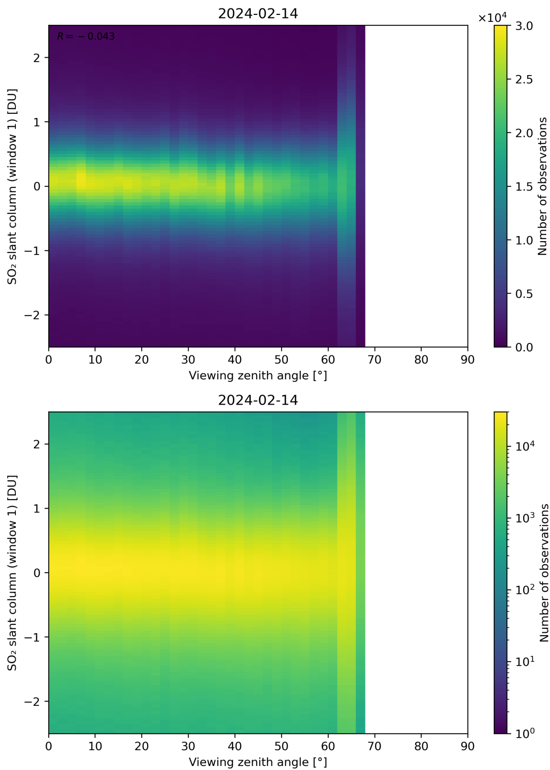
Figure 320: Scatter density plot of “Viewing zenith angle” against “SO 2 slant column (window 1)” for 2024-02-13 to 2024-02-15.
