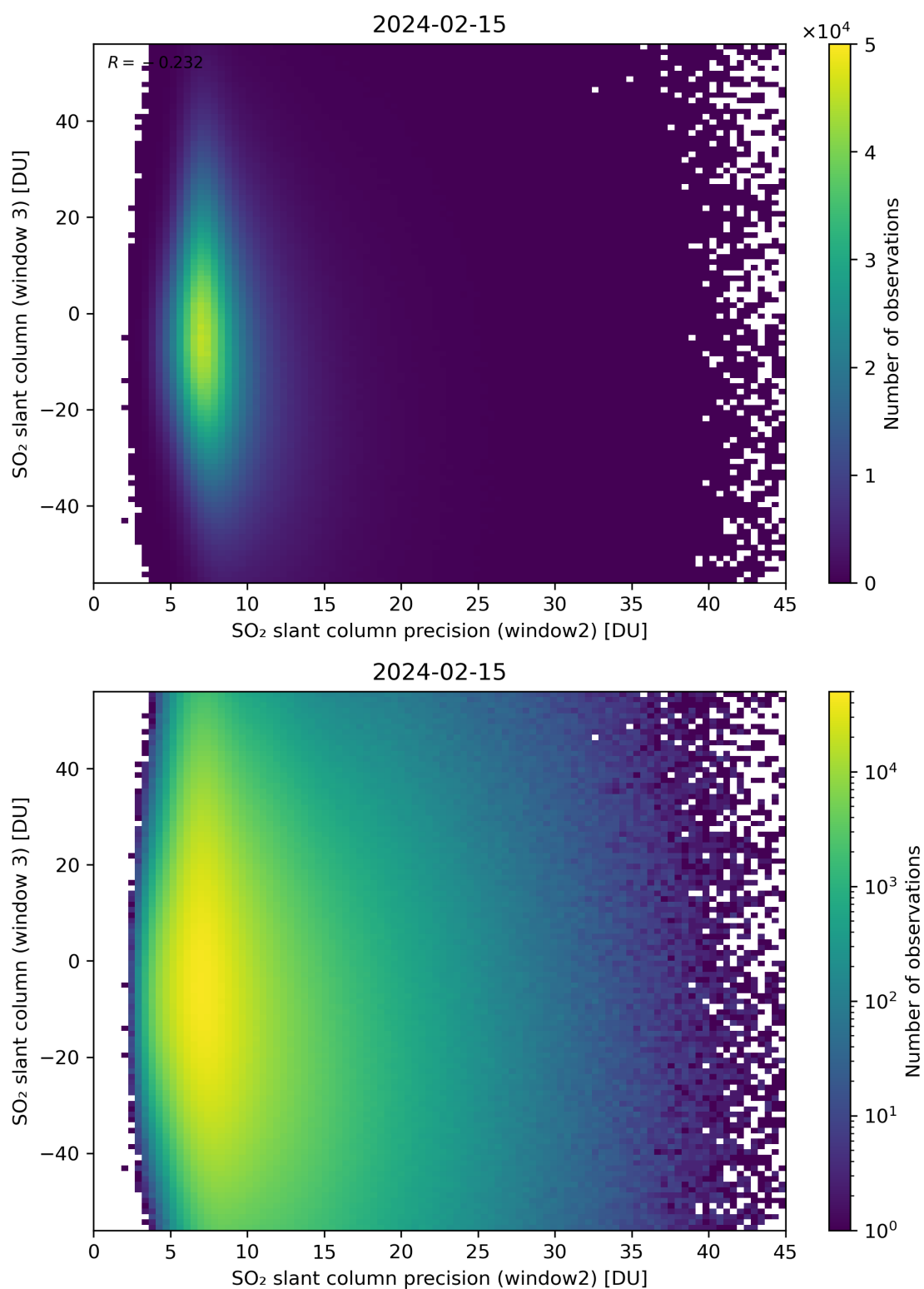
Figure 249: Scatter density plot of “SO 2 slant column precision (window2)” against “SO 2 slant column (window 3)” for 2024-02-14 to 2024-02-16.
