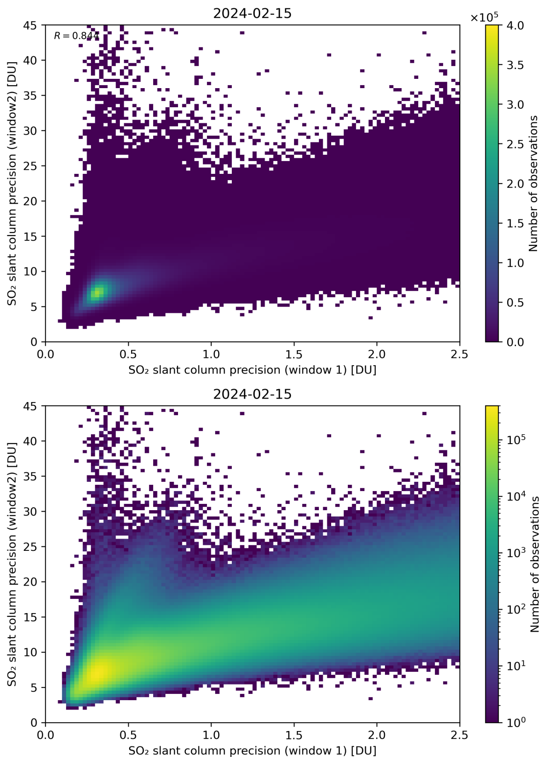
Figure 227: Scatter density plot of “SO 2 slant column precision (window 1)” against “SO 2 slant column precision (window2)” for 2024-02-14 to 2024-02-16.
