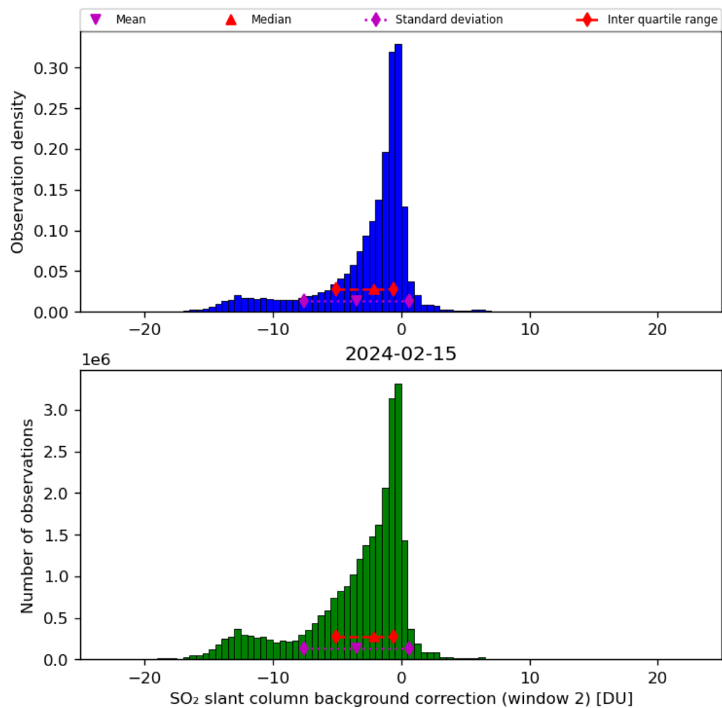
Figure 63: Histogram of “SO 2 slant column background correction (window 2)” for 2024-02-14 to 2024-02-16
