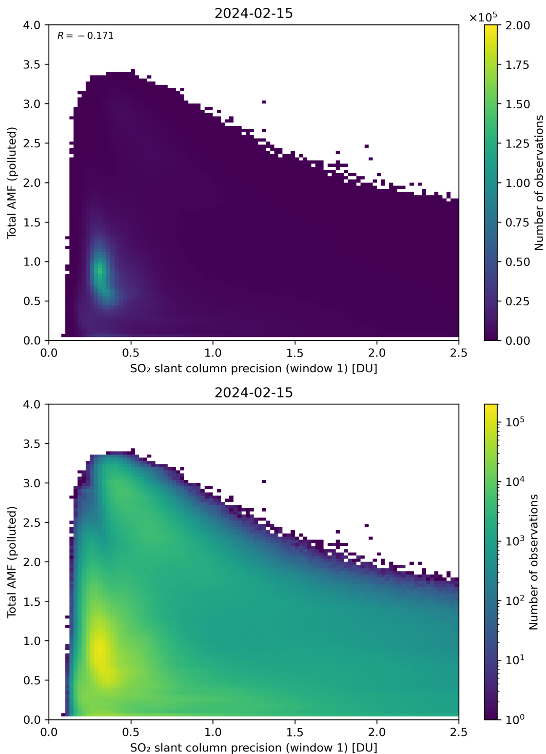
Figure 230: Scatter density plot of “SO 2 slant column precision (window 1)” against “Total AMF (polluted)” for 2024-02-14 to 2024-02-16.
