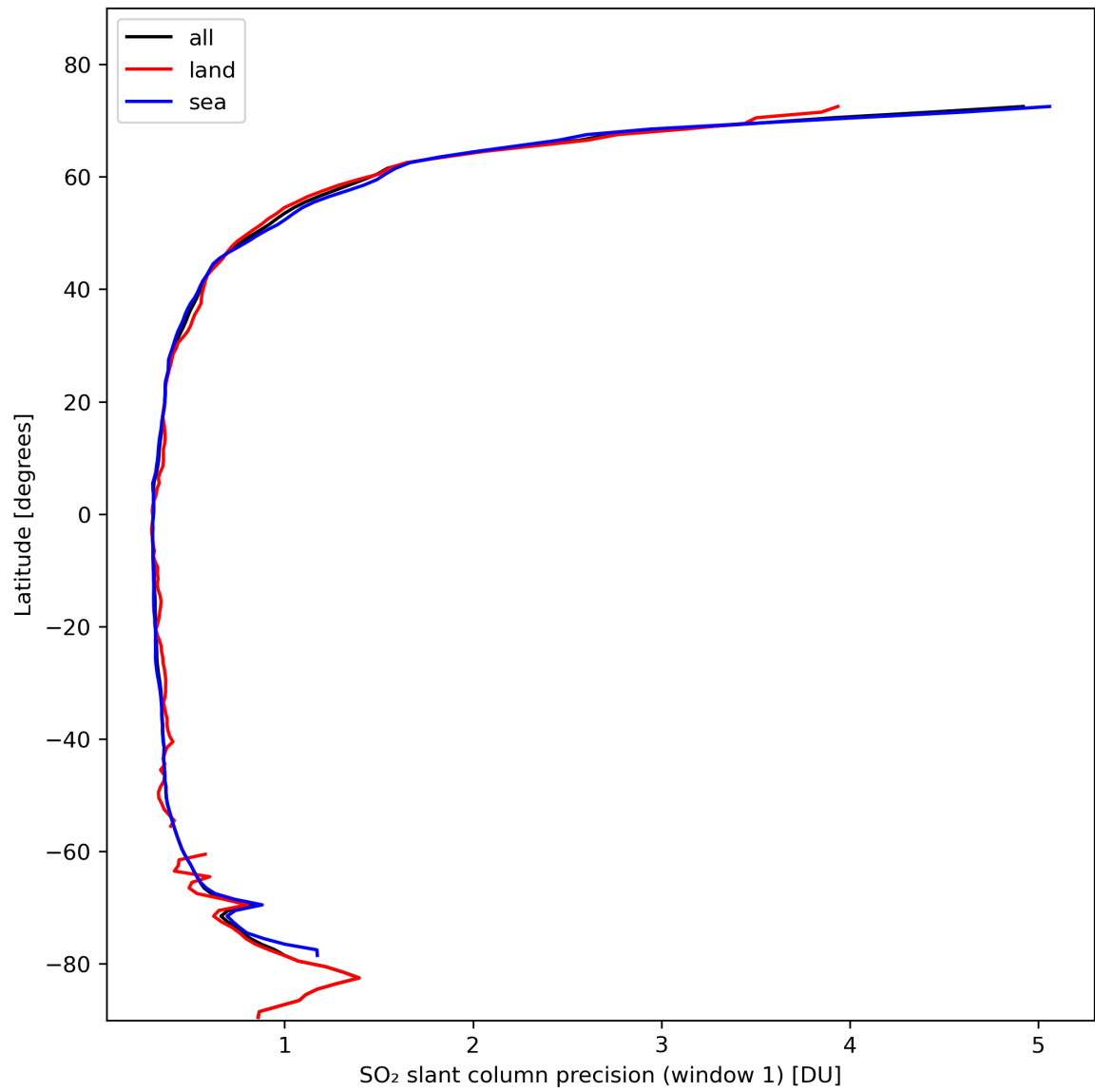
Figure 34: Zonal average of “SO 2 slant column precision (window 1)” for 2024-02-14 to 2024-02-16.
