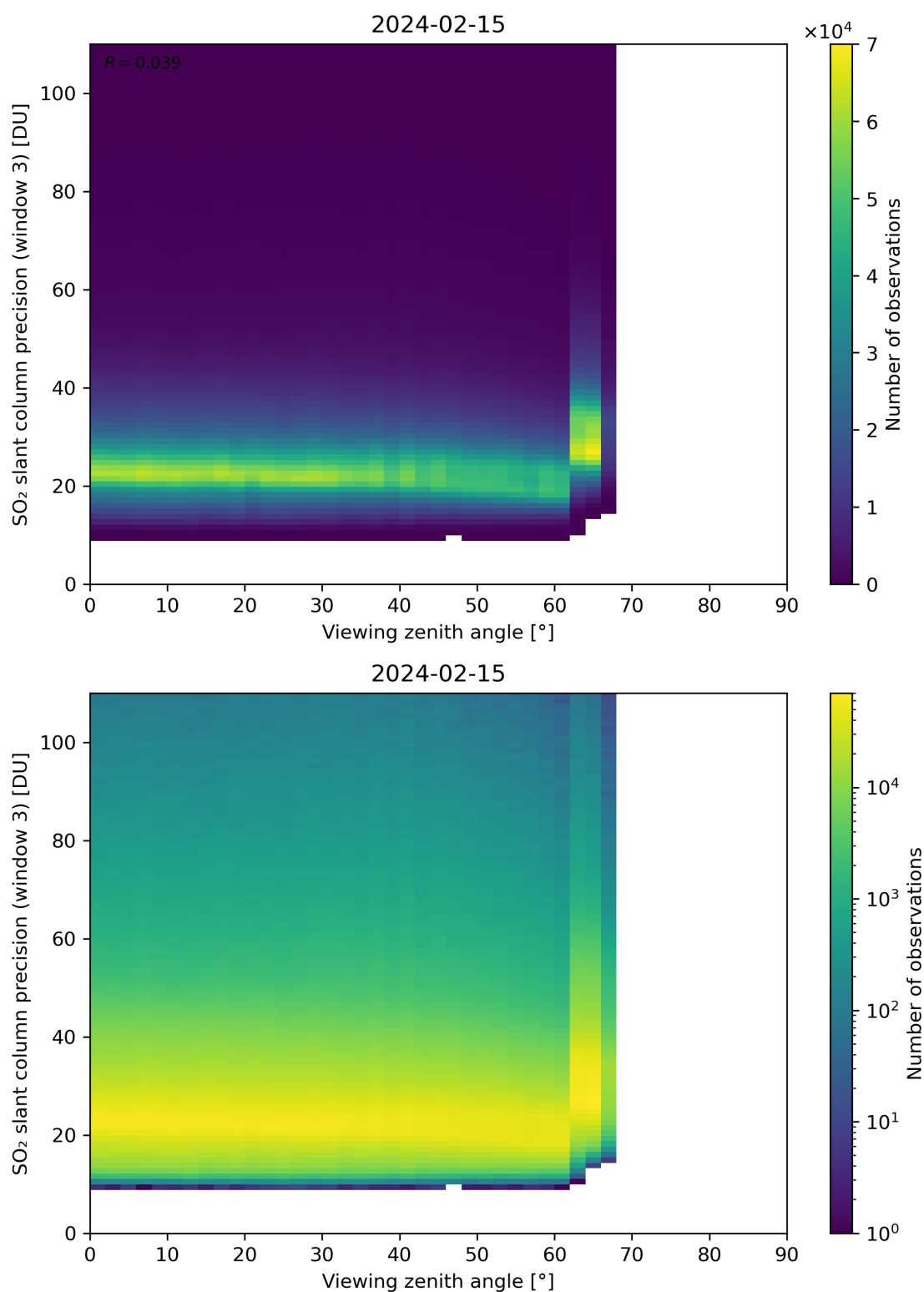
Figure 324: Scatter density plot of “Viewing zenith angle” against “SO 2 slant column precision (window 3)” for 2024-02-14 to 2024-02-16.
