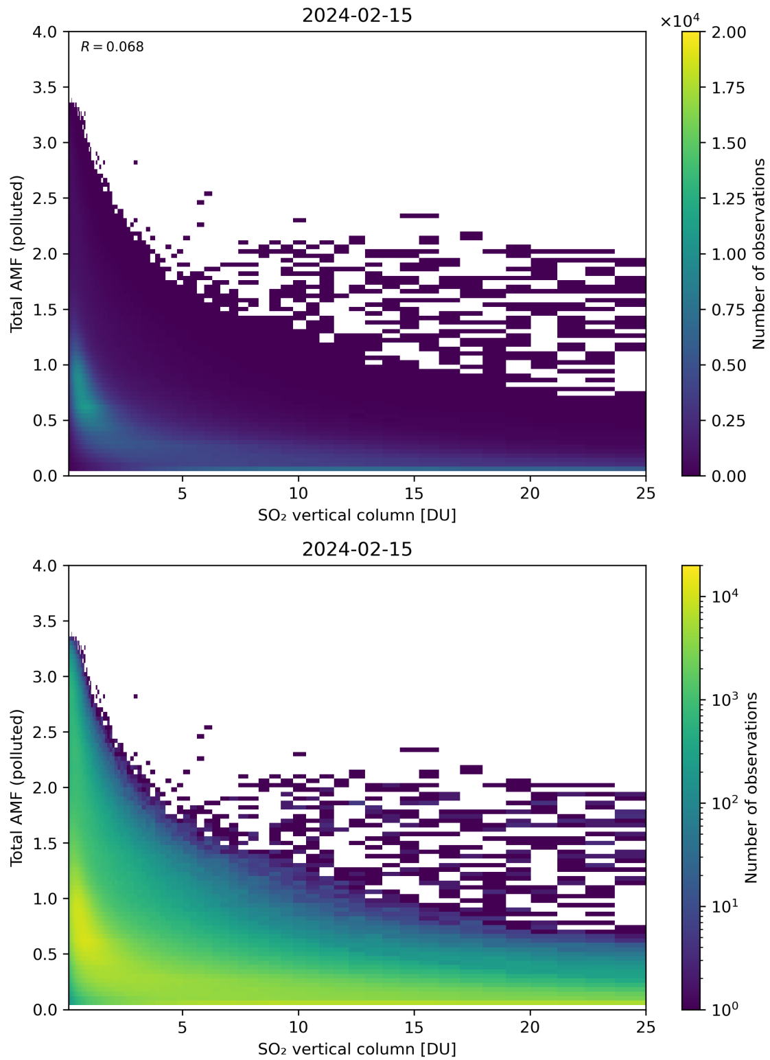
Figure 305: Scatter density plot of “SO 2 vertical column” against “Total AMF (polluted)” for 2024-02-14 to 2024-02-16.
