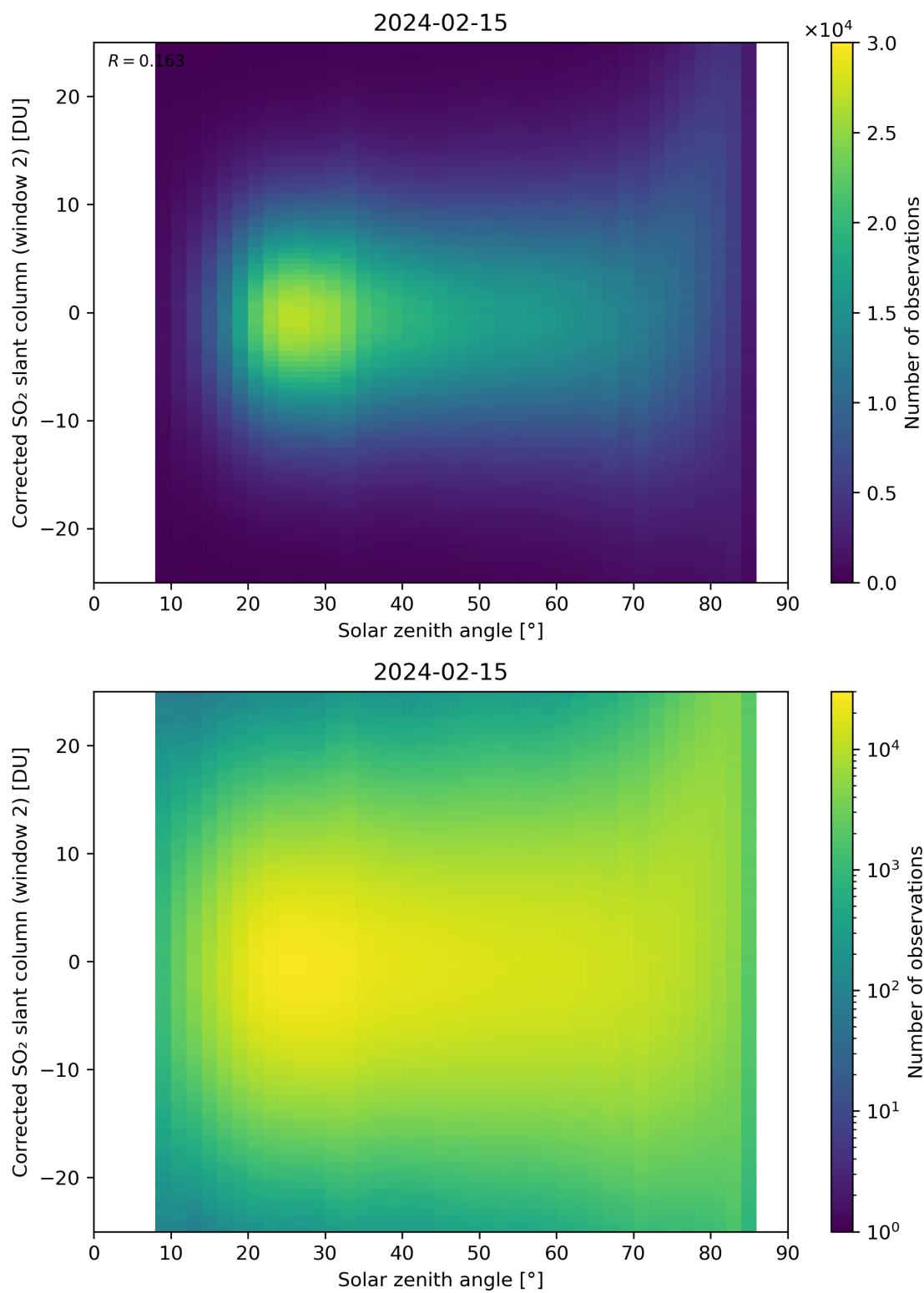
Figure 167: Scatter density plot of “Solar zenith angle” against “Corrected SO 2 slant column (window 2)” for 2024-02-14 to 2024-02-16.
