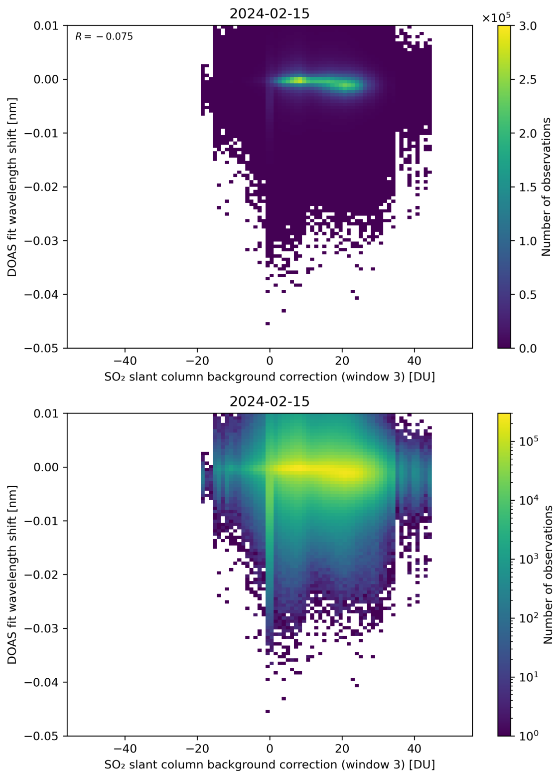
Figure 121: Scatter density plot of “SO 2 slant column background correction (window 3)” against “DOAS fit wavelength shift” for 2024-02-14 to 2024-02-16.
