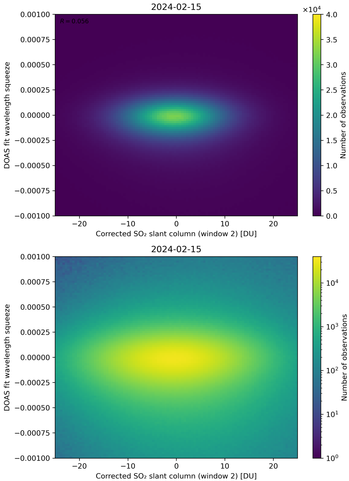
Figure 197: Scatter density plot of “Corrected SO 2 slant column (window 2)” against “DOAS fit wavelength squeeze” for 2024-02-14 to 2024-02-16.
