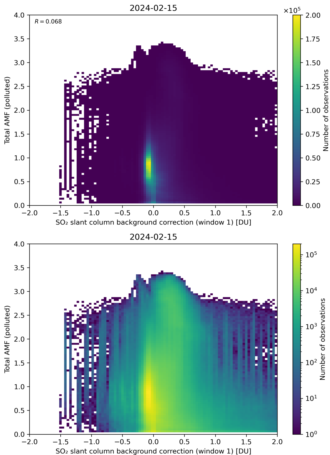
Figure 109: Scatter density plot of “SO 2 slant column background correction (window 1)” against “Total AMF (polluted)” for 2024-02-14 to 2024-02-16.
