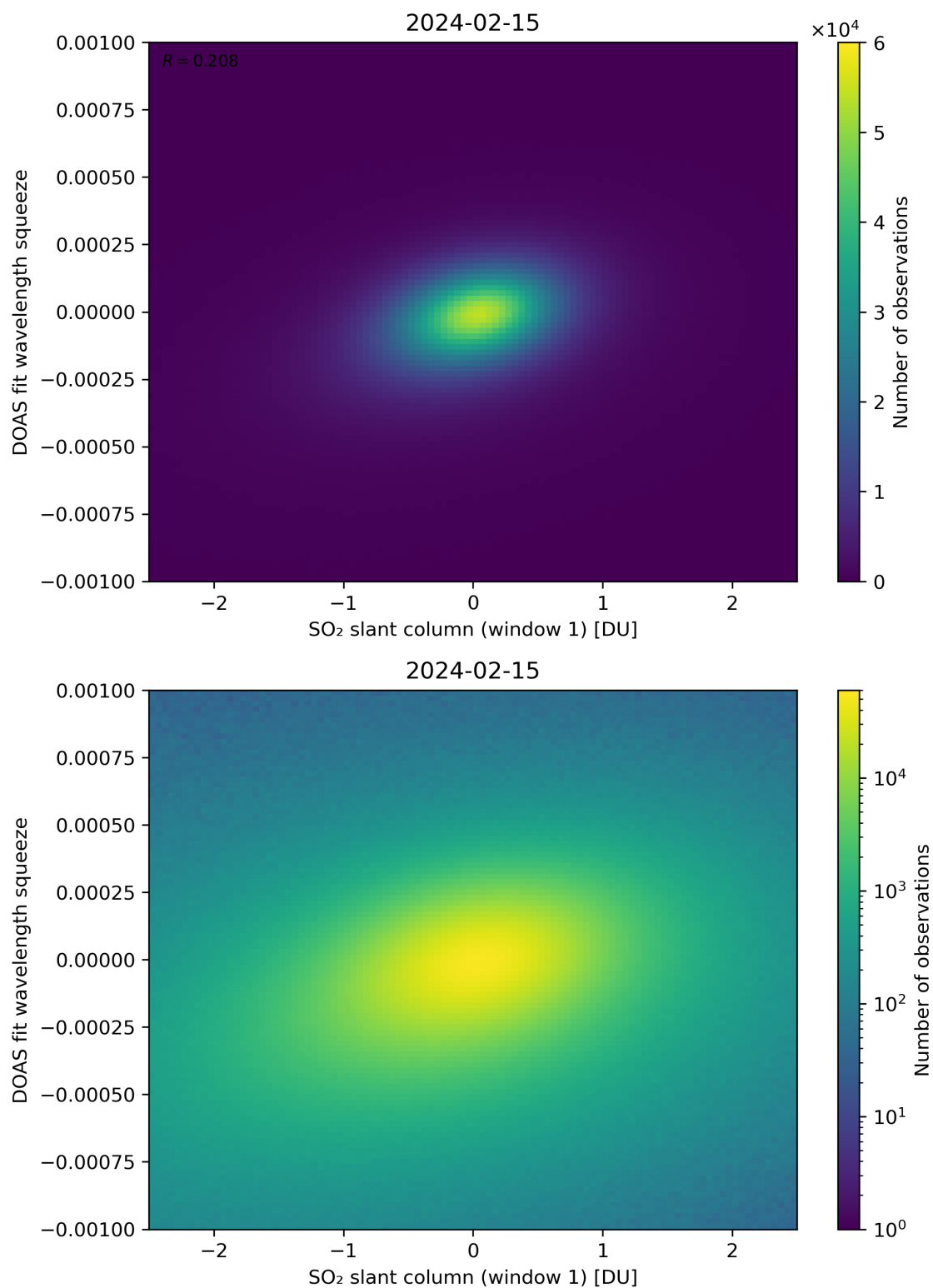
Figure 216: Scatter density plot of “SO 2 slant column (window 1)” against “DOAS fit wavelength squeeze” for 2024-02-14 to 2024-02-16.
