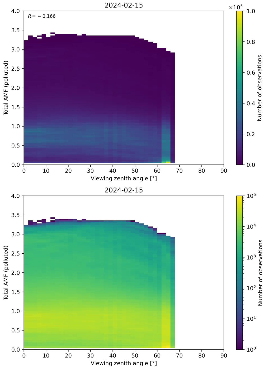
Figure 325: Scatter density plot of “Viewing zenith angle” against “Total AMF (polluted)” for 2024-02-14 to 2024-02-16.
