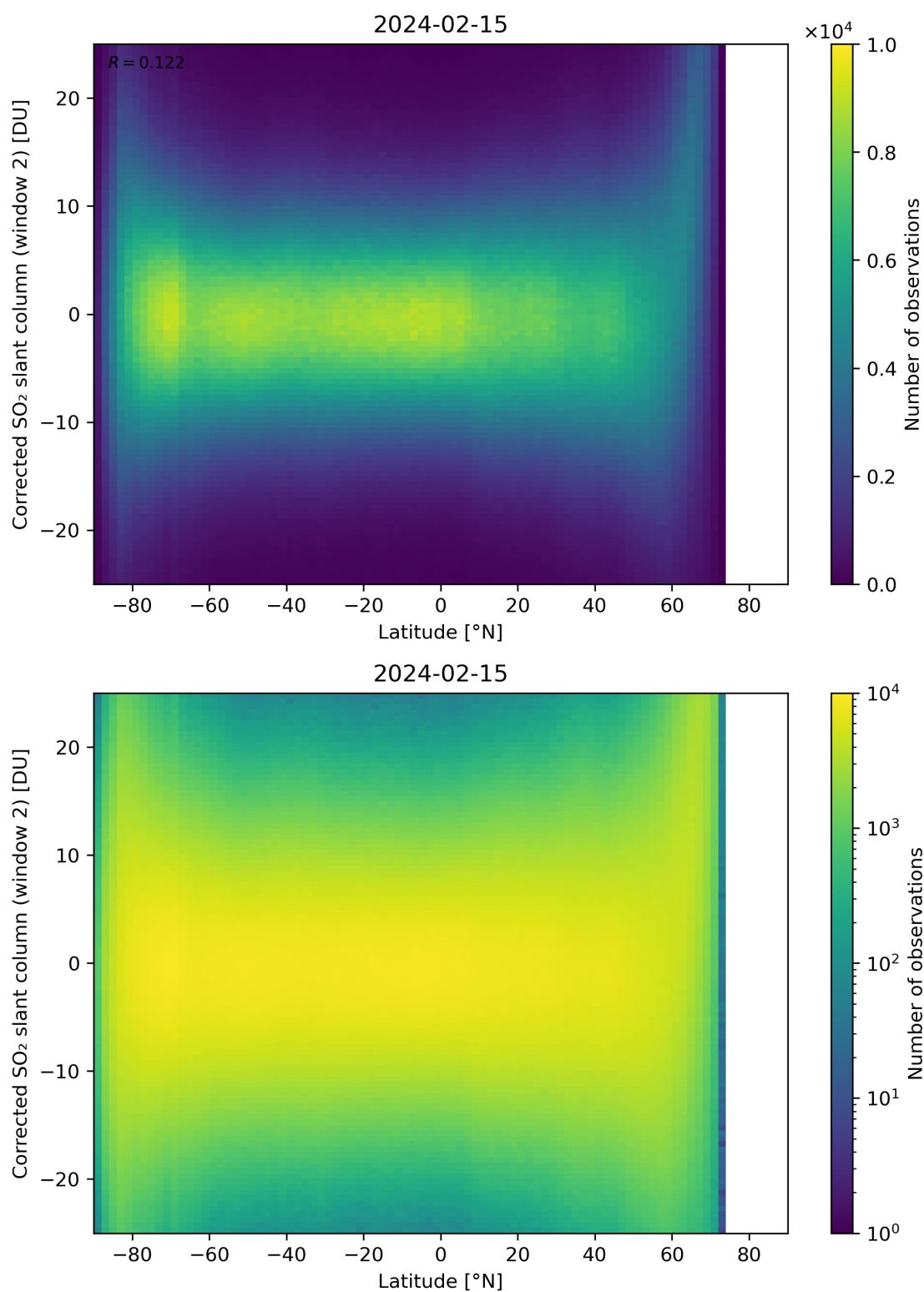
Figure 147: Scatter density plot of “Latitude” against “Corrected SO 2 slant column (window 2)” for 2024-02-14 to 2024-02-16.
