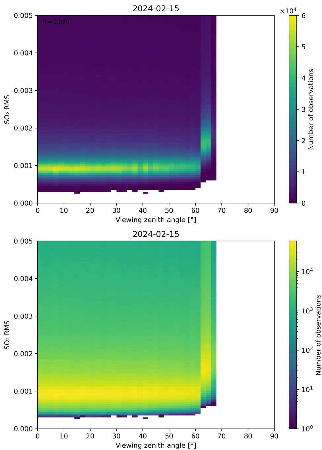
Figure 313: Scatter density plot of “Viewing zenith angle” against “SO 2 RMS” for 2024-02-14 to 2024-02-16.
