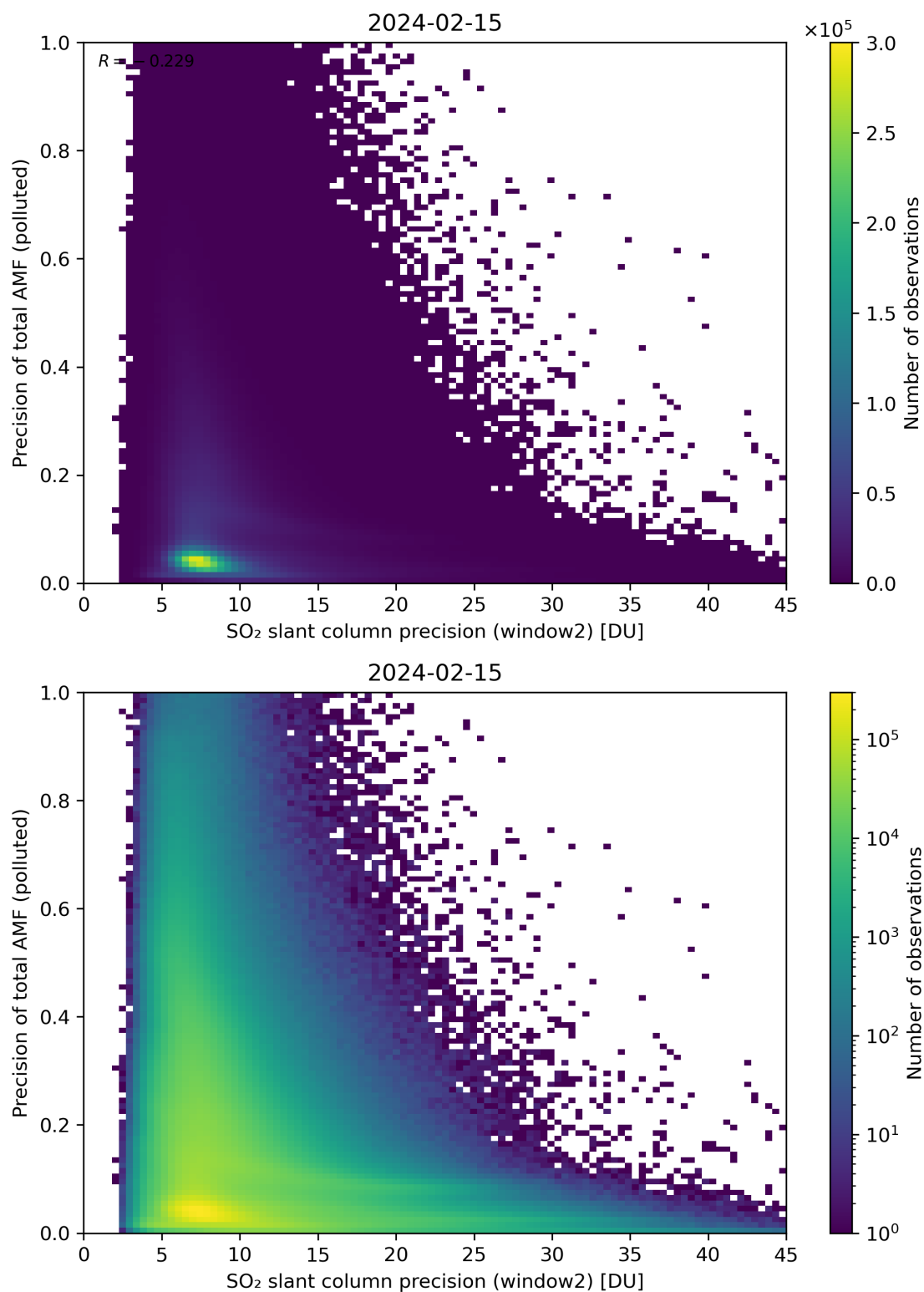
Figure 252: Scatter density plot of “SO 2 slant column precision (window2)” against “Precision of total AMF (polluted)” for 2024-02-14 to 2024-02-16.
