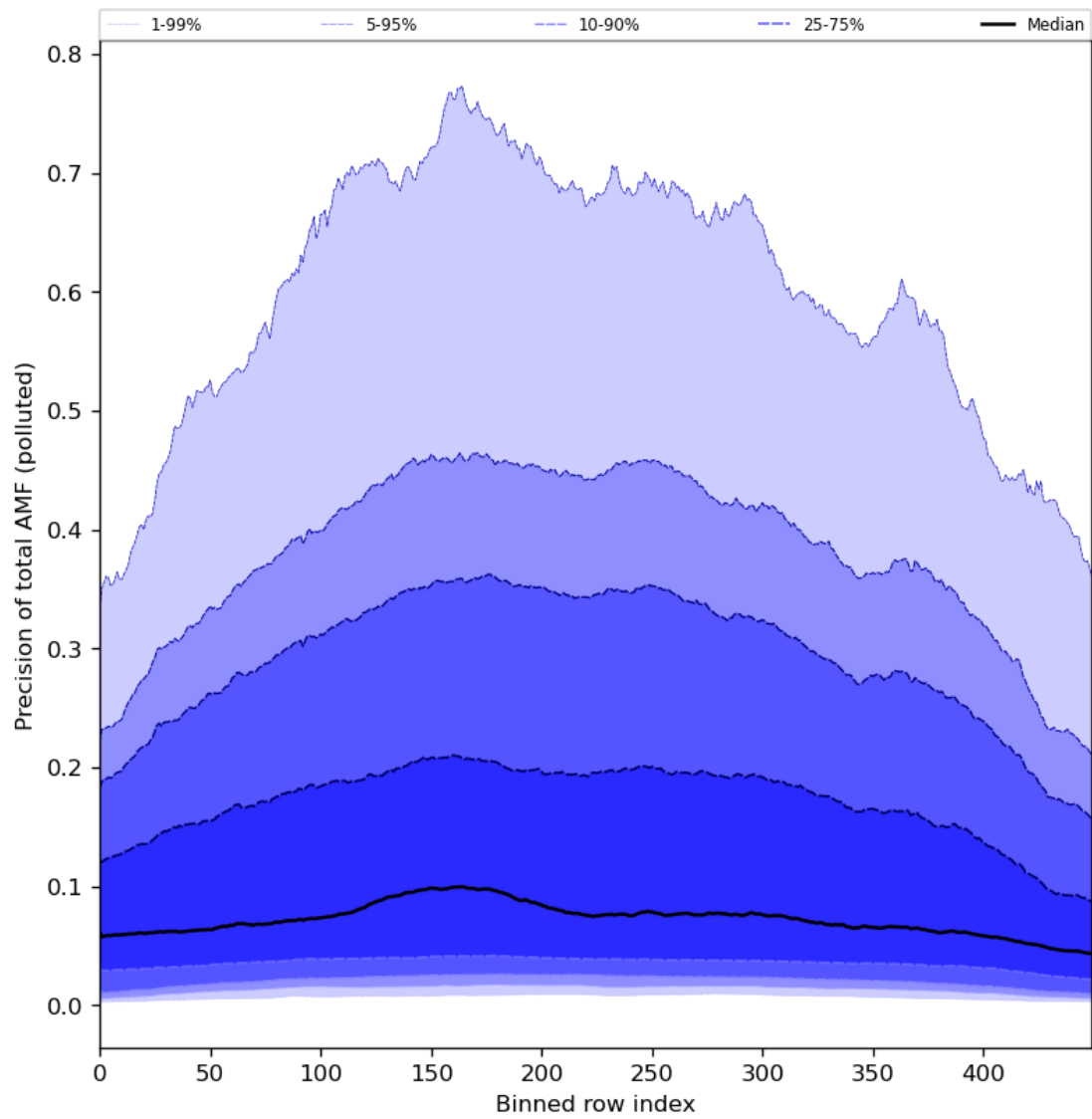
Figure 95: Along track statistics of “Precision of total AMF (polluted)” for 2024-02-14 to 2024-02-16
