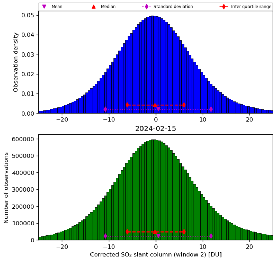
Figure 62: Histogram of “Corrected SO 2 slant column (window 2)” for 2024-02-14 to 2024-02-16
