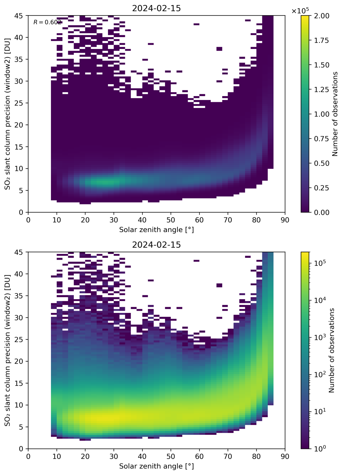
Figure 171: Scatter density plot of “Solar zenith angle” against “SO 2 slant column precision (window2)” for 2024-02-14 to 2024-02-16.
