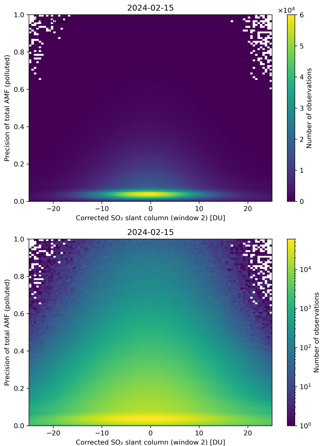
Figure 204: Scatter density plot of “Corrected SO 2 slant column (window 2)” against “Precision of total AMF (polluted)” for 2024-02-14 to 2024-02-16.
