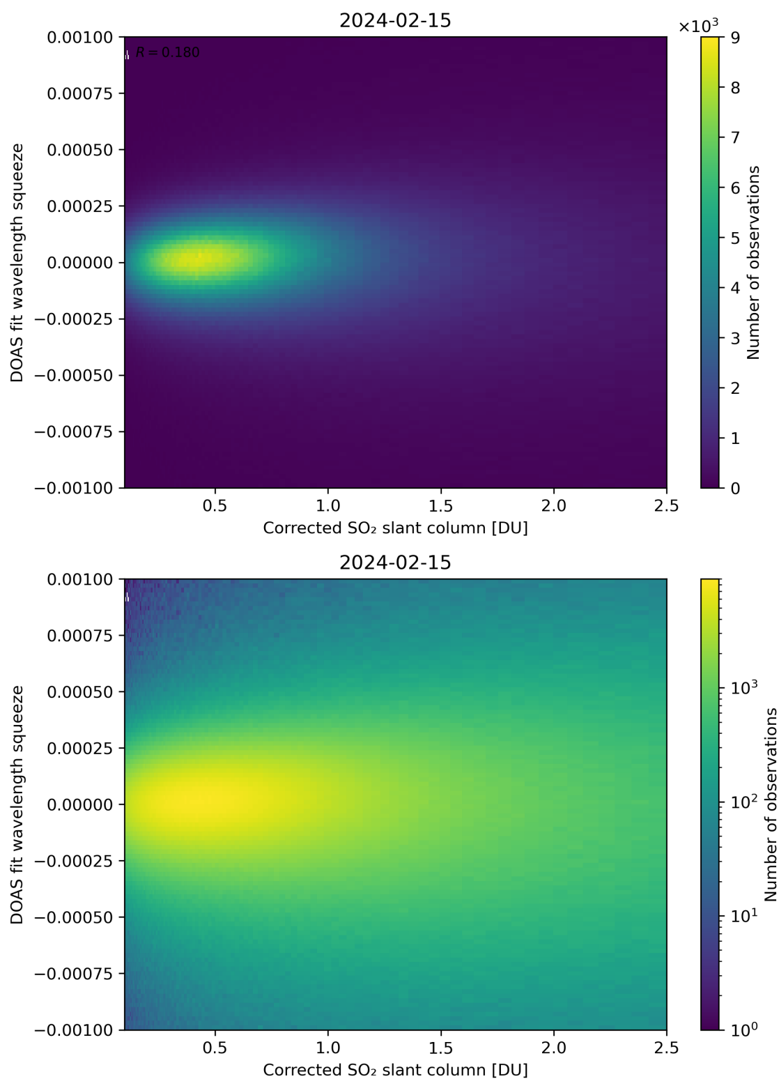
Figure 182: Scatter density plot of “Corrected SO 2 slant column” against “DOAS fit wavelength squeeze” for 2024-02-14 to 2024-02-16.
