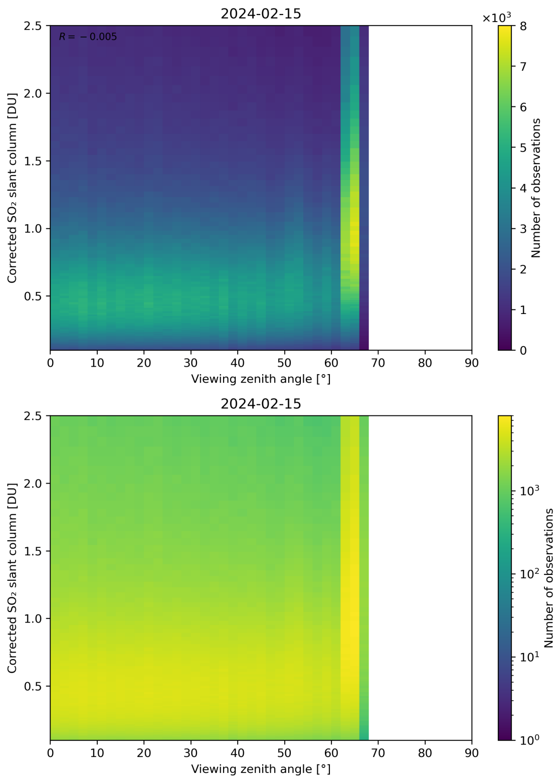
Figure 317: Scatter density plot of “Viewing zenith angle” against “Corrected SO 2 slant column” for 2024-02-14 to 2024-02-16.
