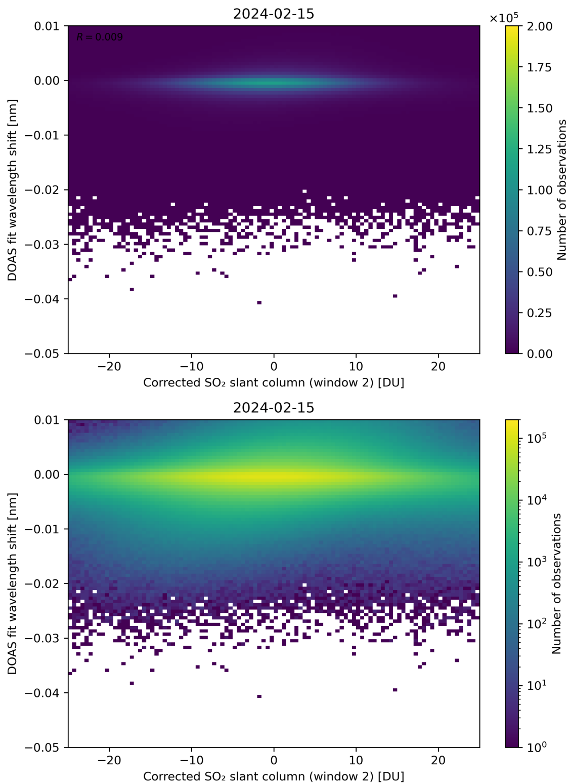
Figure 196: Scatter density plot of “Corrected SO 2 slant column (window 2)” against “DOAS fit wavelength shift” for 2024-02-14 to 2024-02-16.
