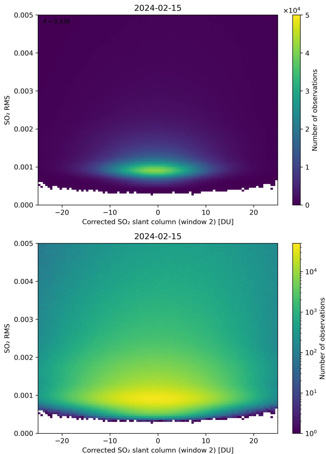
Figure 198: Scatter density plot of “Corrected SO 2 slant column (window 2)” against “SO 2 RMS” for 2024-02-14 to 2024-02-16.
