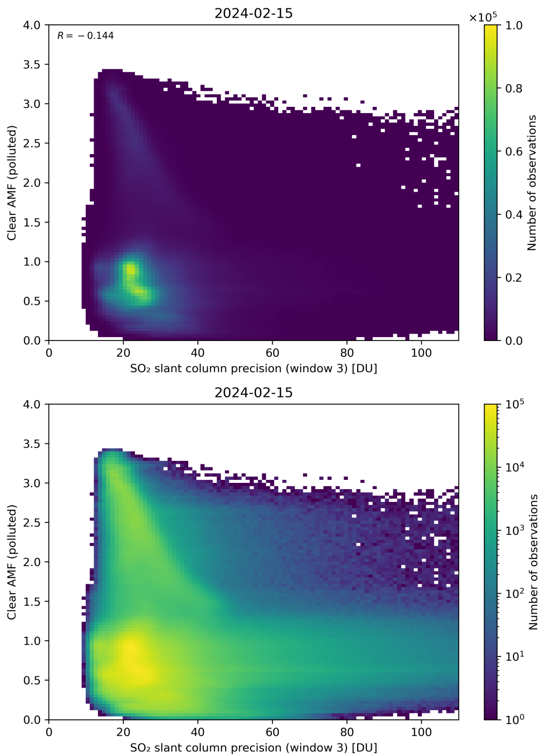
Figure 261: Scatter density plot of “SO 2 slant column precision (window 3)” against “Clear AMF (polluted)” for 2024-02-14 to 2024-02-16.
