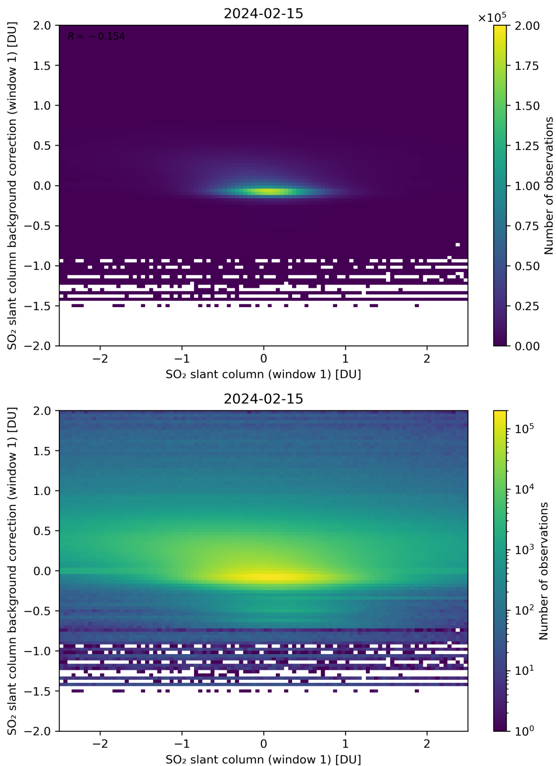
Figure 212: Scatter density plot of “SO 2 slant column (window 1)” against “SO 2 slant column background correction (window 1)” for 2024-02-14 to 2024-02-16.
