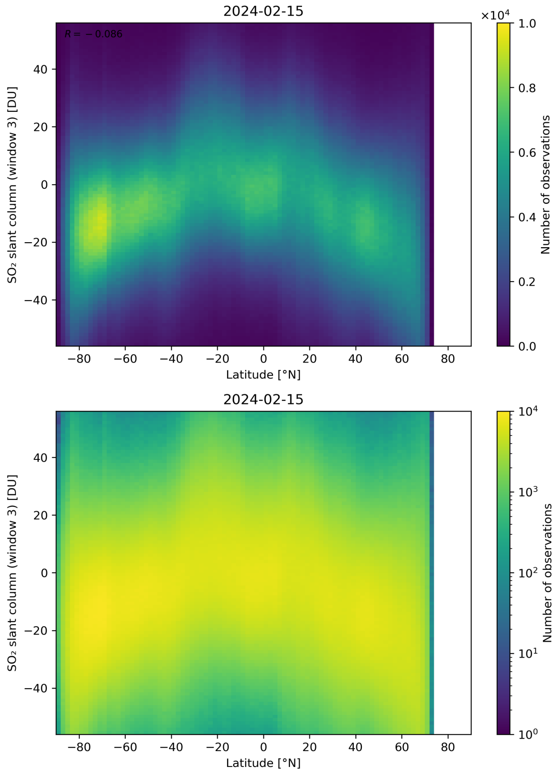
Figure 152: Scatter density plot of “Latitude” against “SO 2 slant column (window 3)” for 2024-02-14 to 2024-02-16.
