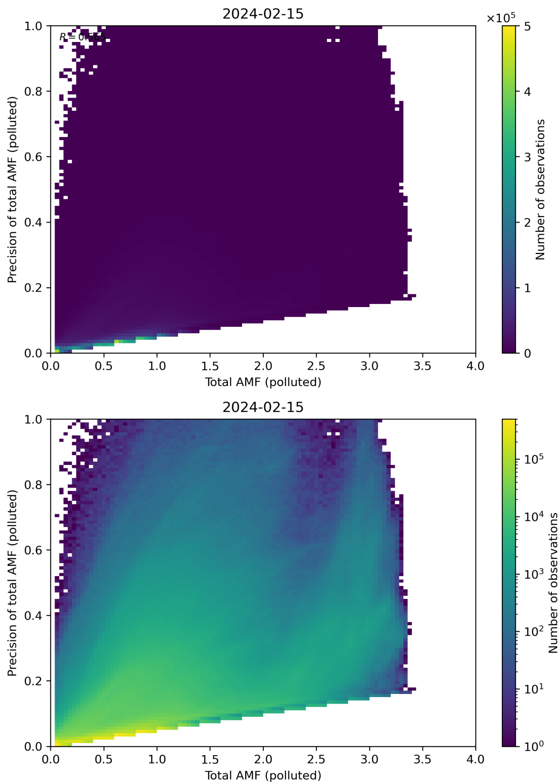
Figure 272: Scatter density plot of “Total AMF (polluted)” against “Precision of total AMF (polluted)” for 2024-02-14 to 2024-02-16.
