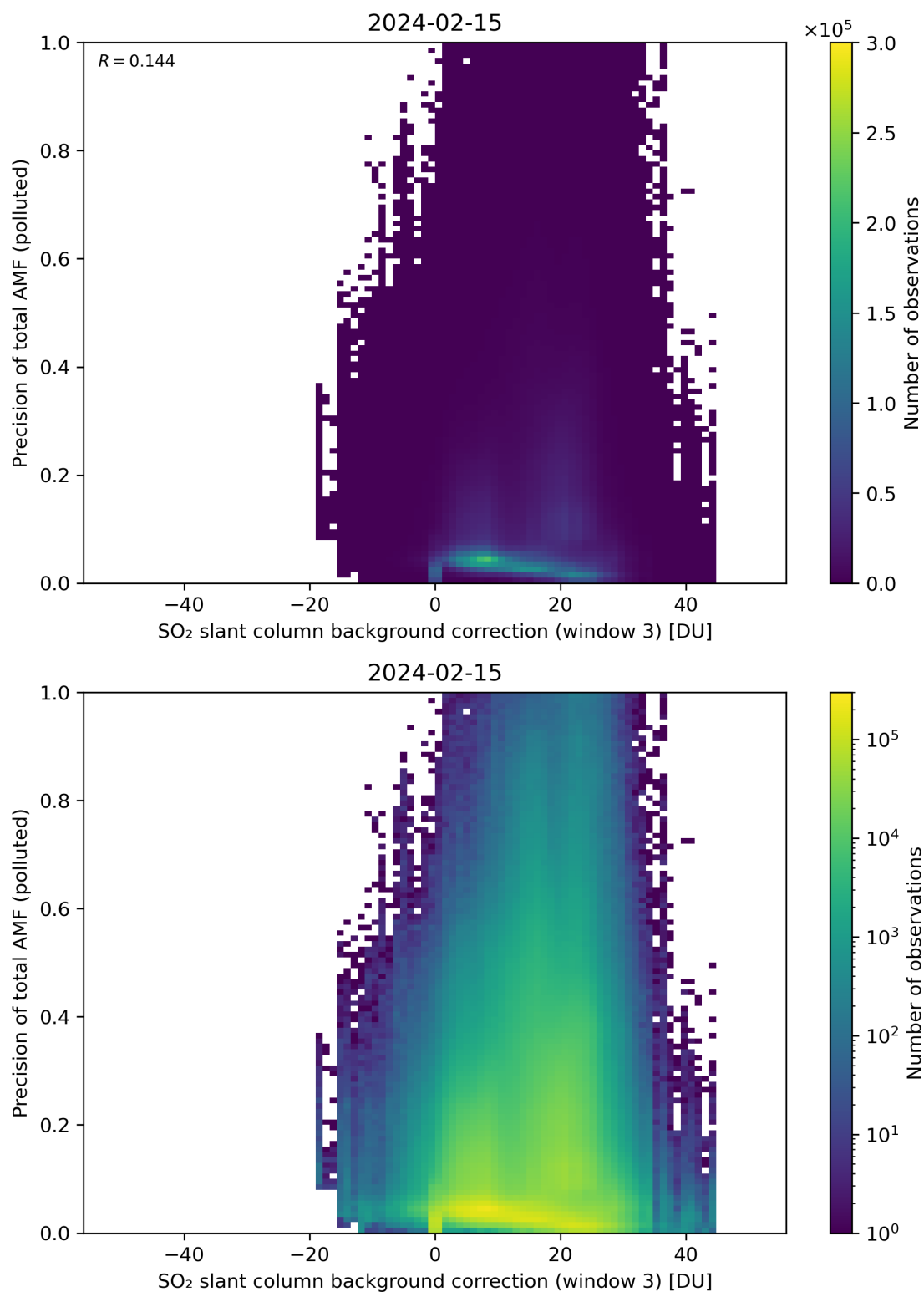
Figure 126: Scatter density plot of “SO 2 slant column background correction (window 3)” against “Precision of total AMF (polluted)” for 2024-02-14 to 2024-02-16.
