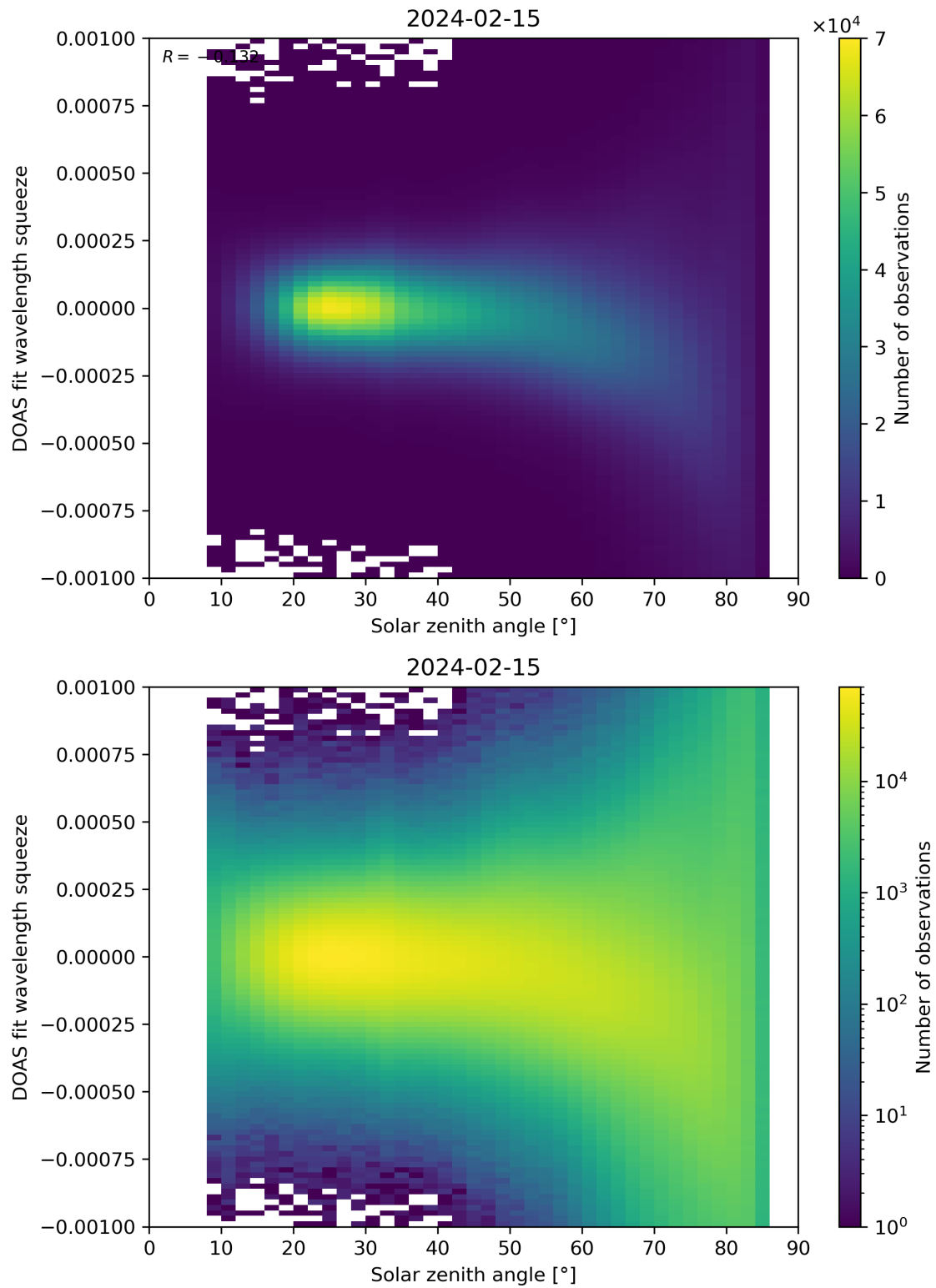
Figure 162: Scatter density plot of “Solar zenith angle” against “DOAS fit wavelength squeeze” for 2024-02-14 to 2024-02-16.
