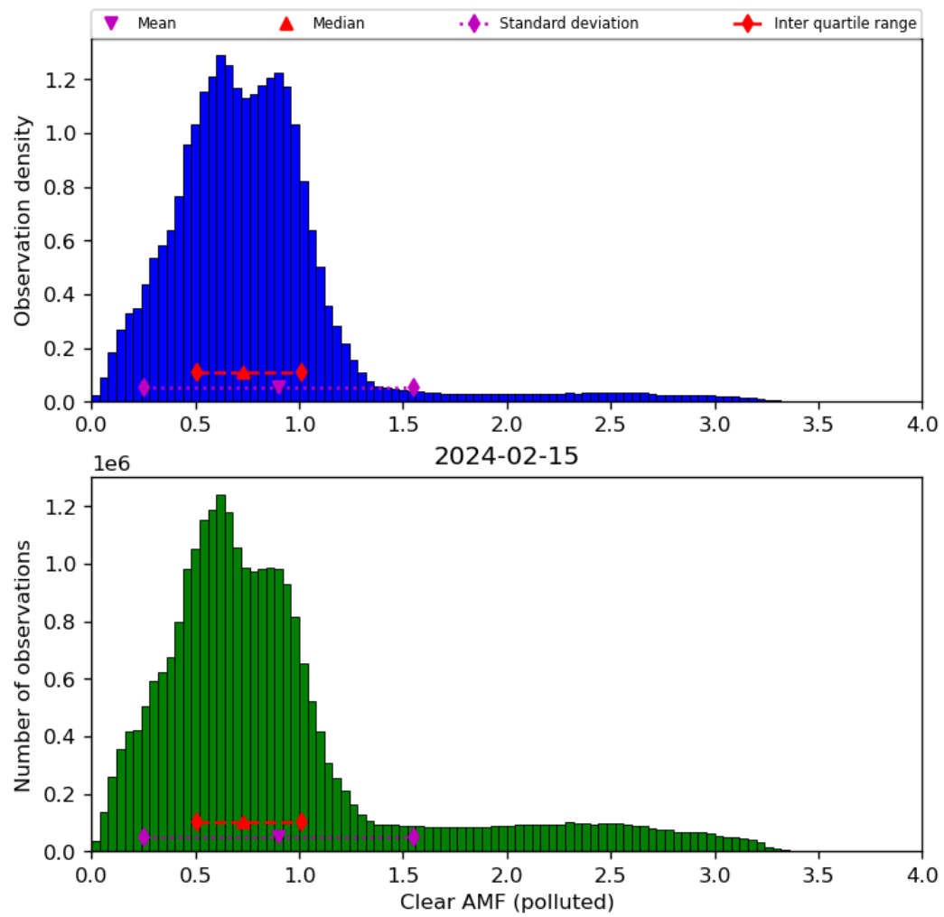
Figure 73: Histogram of “Clear AMF (polluted)” for 2024-02-14 to 2024-02-16
