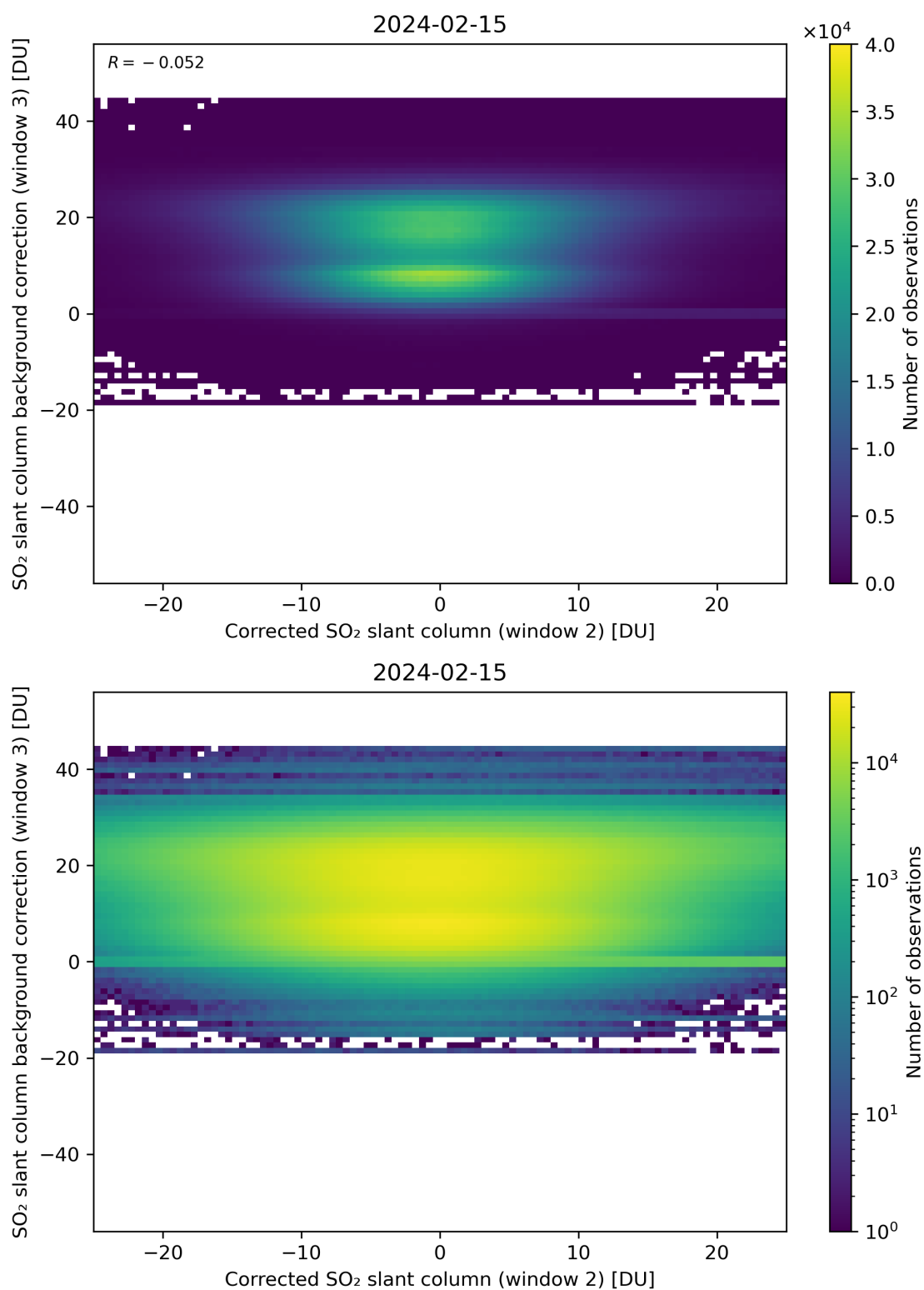
Figure 195: Scatter density plot of “Corrected SO 2 slant column (window 2)” against “SO 2 slant column background correction (window 3)” for 2024-02-14 to 2024-02-16.
