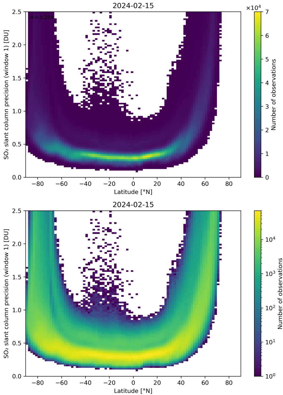
Figure 150: Scatter density plot of “Latitude” against “SO 2 slant column precision (window 1)” for 2024-02-14 to 2024-02-16.
