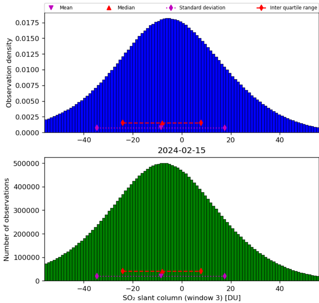
Figure 64: Histogram of “SO 2 slant column (window 3)” for 2024-02-14 to 2024-02-16
