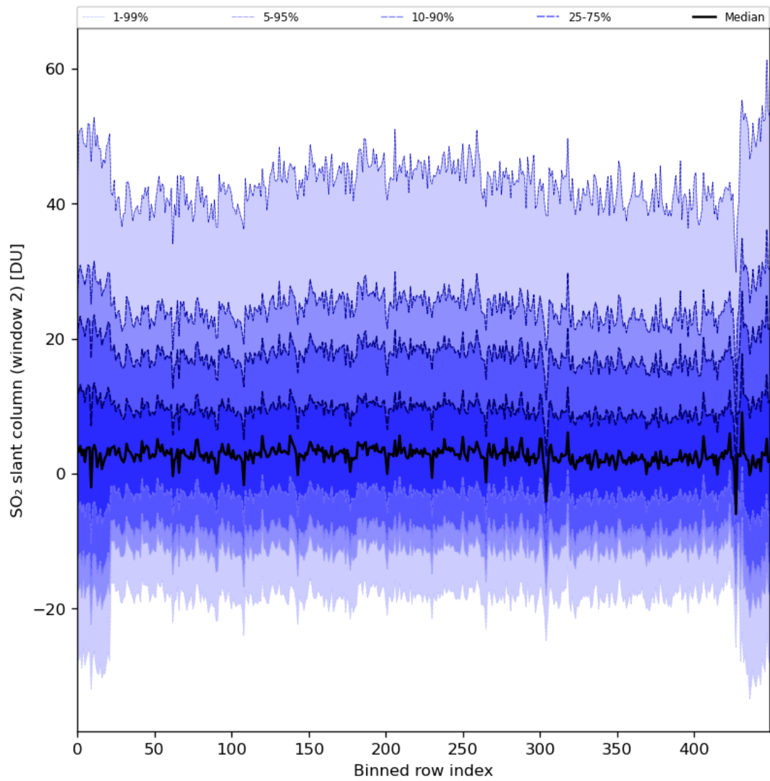
Figure 83: Along track statistics of “SO 2 slant column (window 2)” for 2024-02-14 to 2024-02-16
