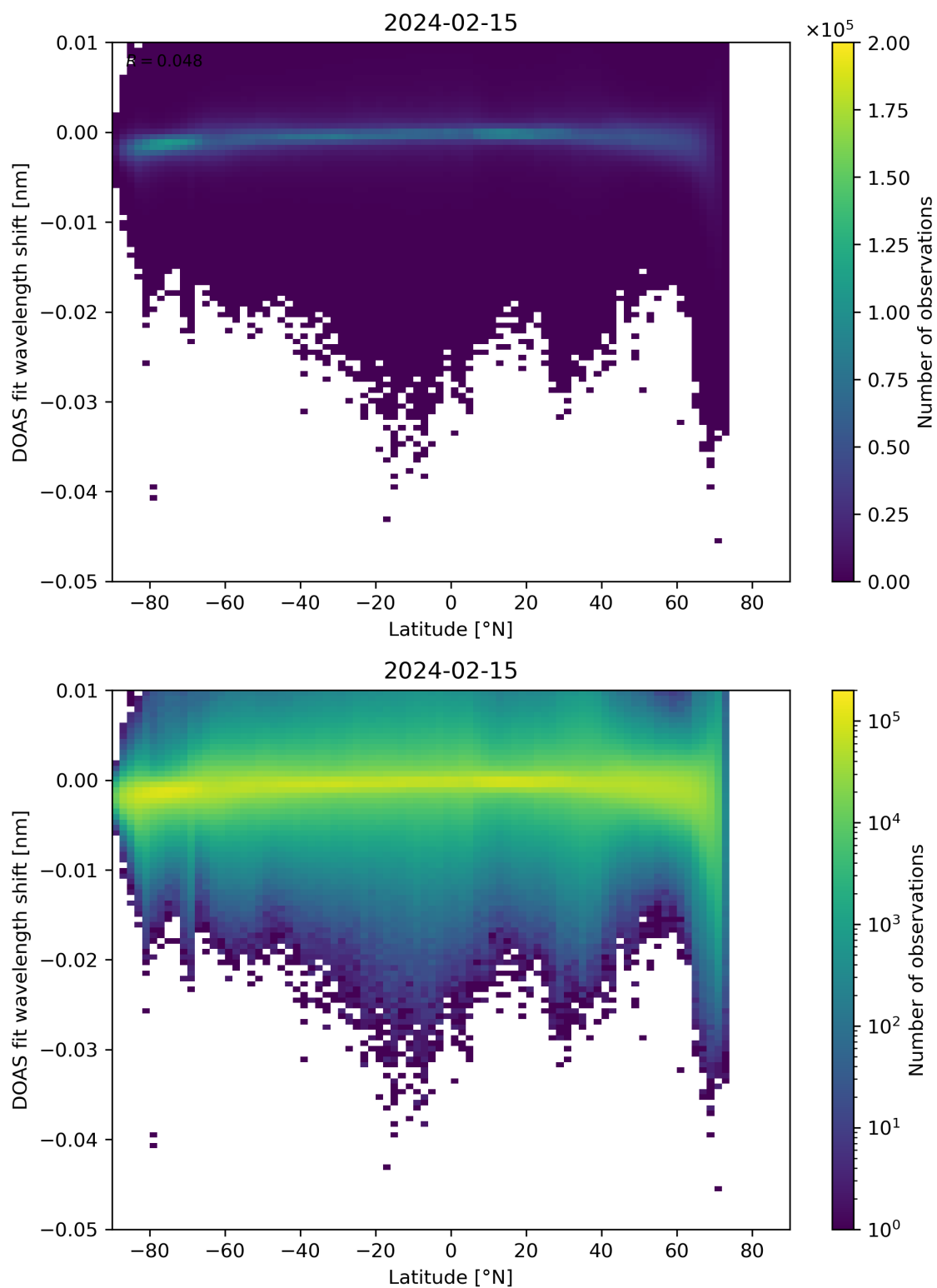
Figure 142: Scatter density plot of “Latitude” against “DOAS fit wavelength shift” for 2024-02-14 to 2024-02-16.
