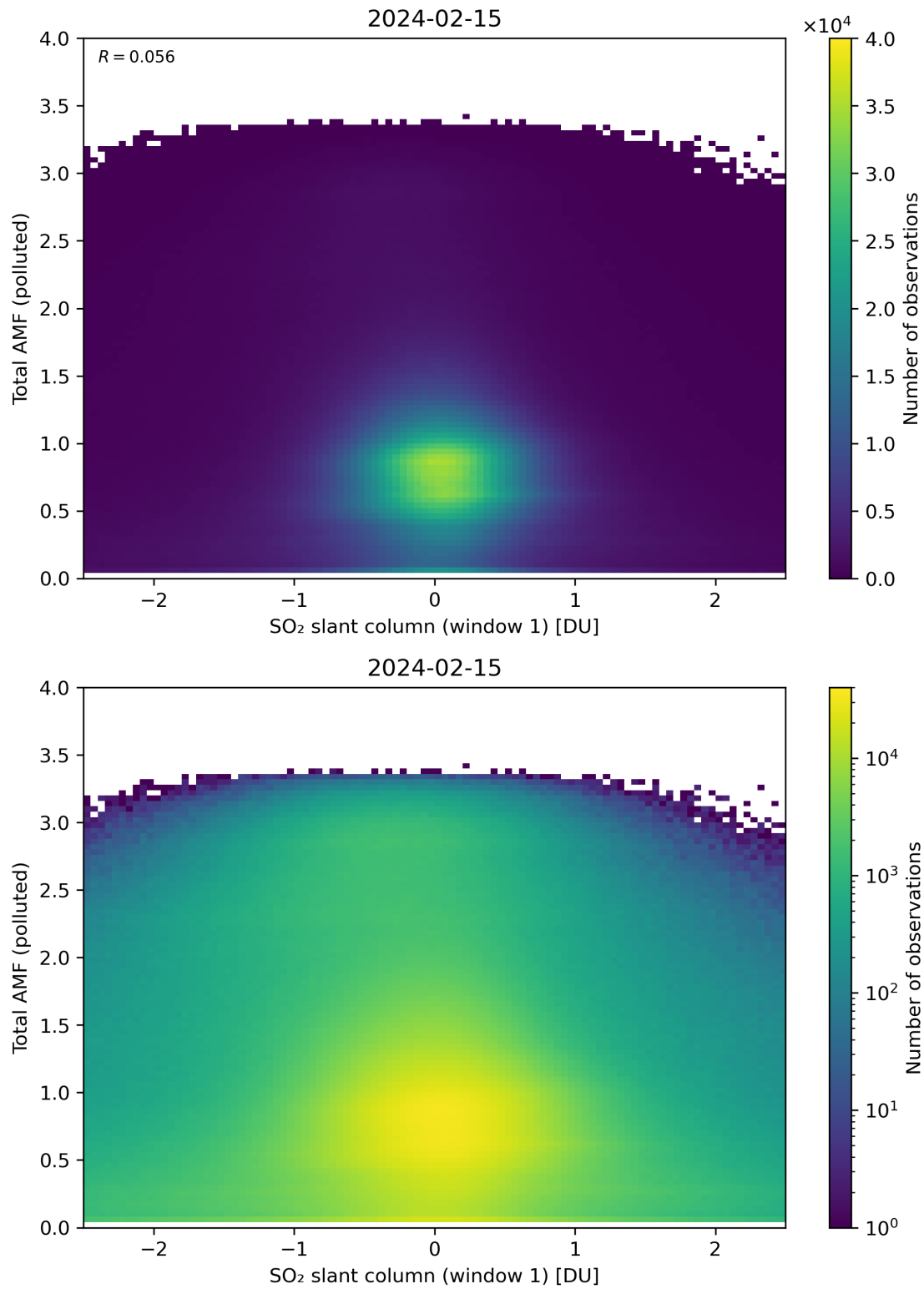
Figure 239: Scatter density plot of “SO 2 slant column (window 1)” against “Total AMF (polluted)” for 2024-02-14 to 2024-02-16.
