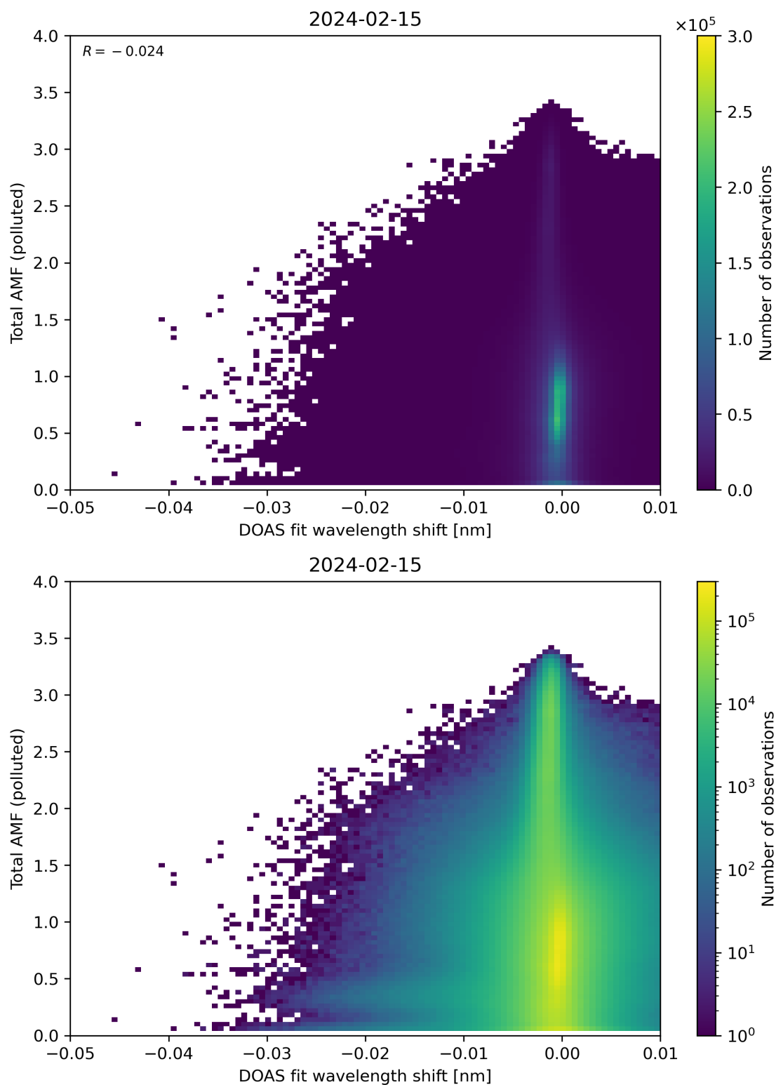
Figure 130: Scatter density plot of “DOAS fit wavelength shift” against “Total AMF (polluted)” for 2024-02-14 to 2024-02-16.
