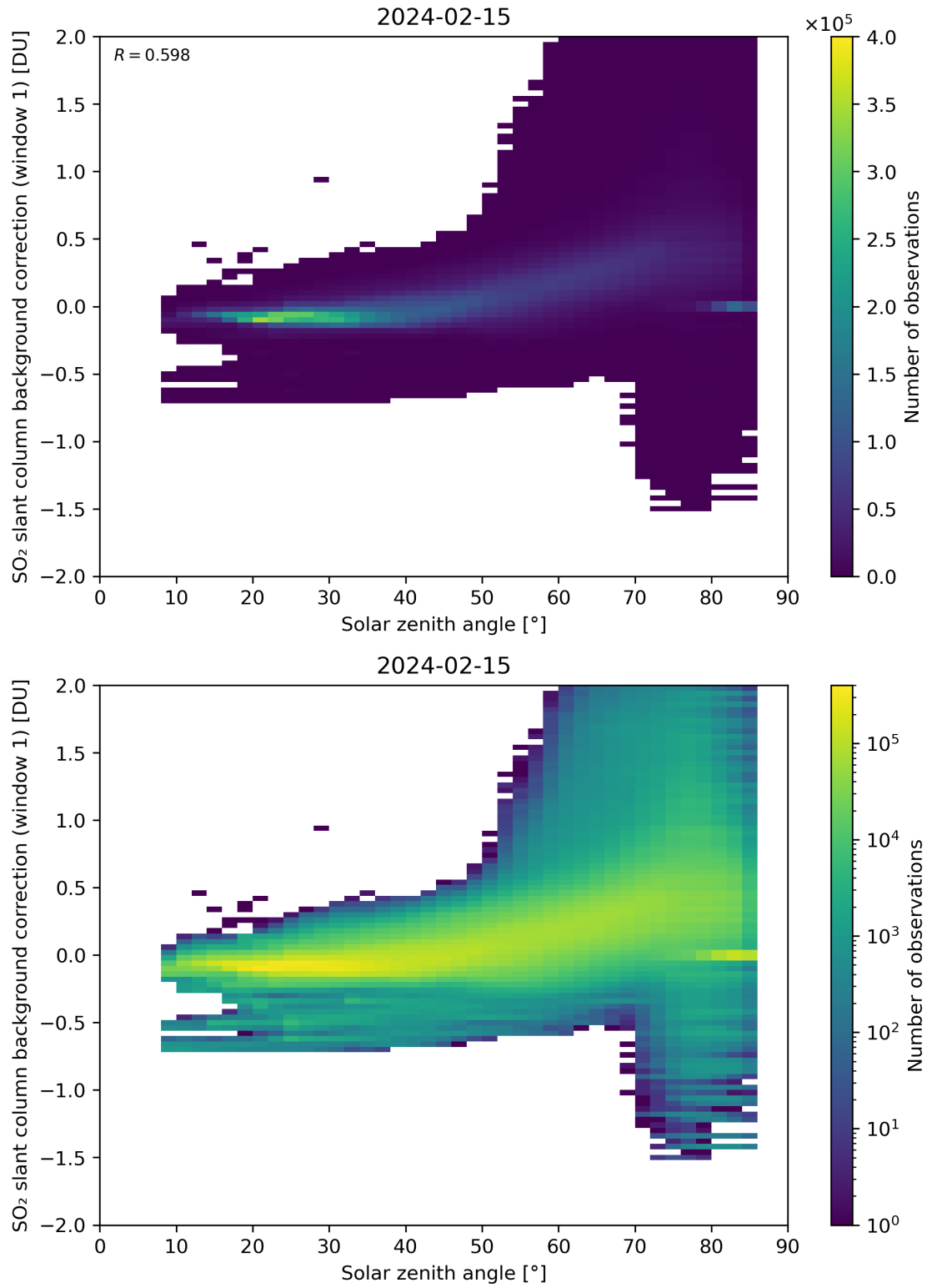
Figure 158: Scatter density plot of “Solar zenith angle” against “SO 2 slant column background correction (window 1)” for 2024-02-14 to 2024-02-16.
