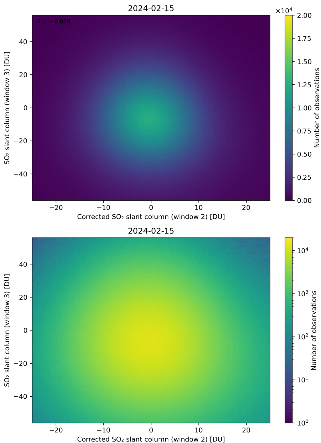
Figure 201: Scatter density plot of “Corrected SO 2 slant column (window 2)” against “SO 2 slant column (window 3)” for 2024-02-14 to 2024-02-16.
