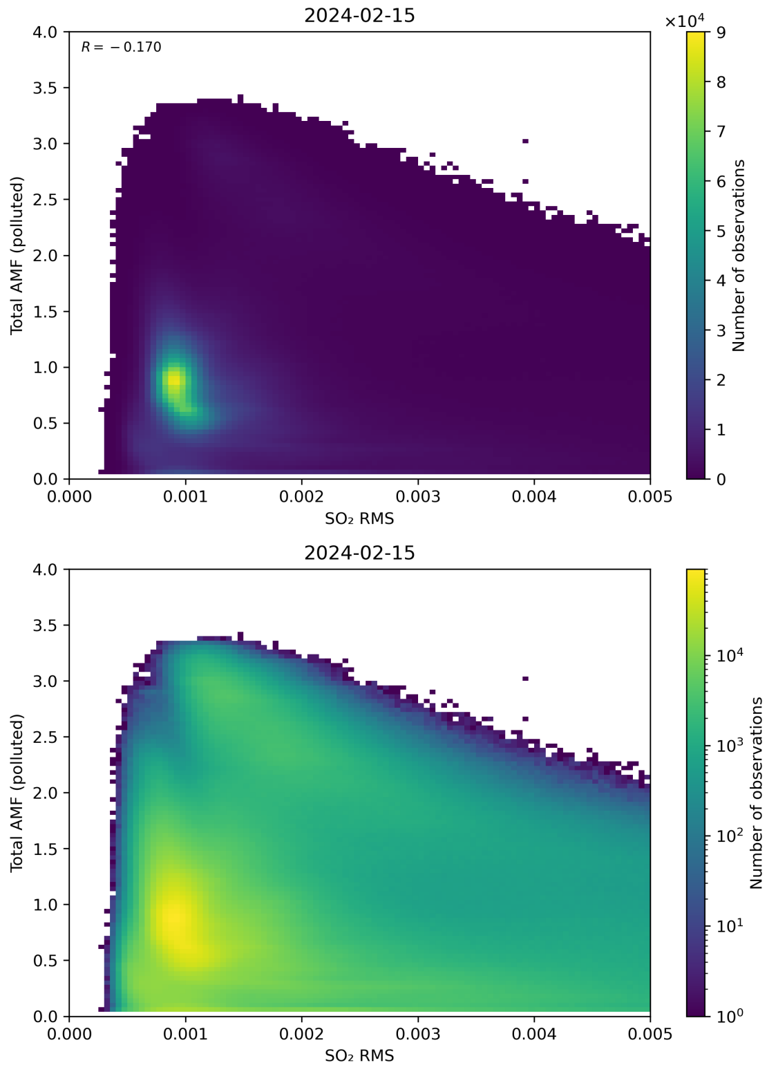
Figure 137: Scatter density plot of “SO 2 RMS” against “Total AMF (polluted)” for 2024-02-14 to 2024-02-16.
