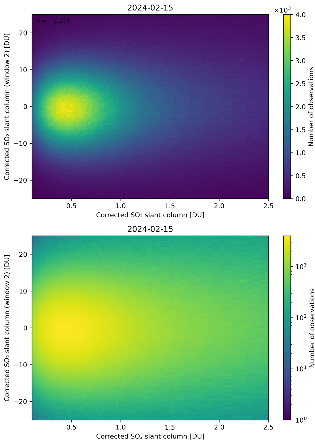
Figure 185: Scatter density plot of “Corrected SO 2 slant column” against “Corrected SO 2 slant column (window 2)” for 2024-02-14 to 2024-02-16.
