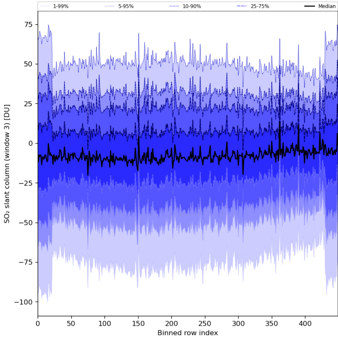
Figure 87: Along track statistics of “SO 2 slant column (window 3)” for 2024-02-14 to 2024-02-16
