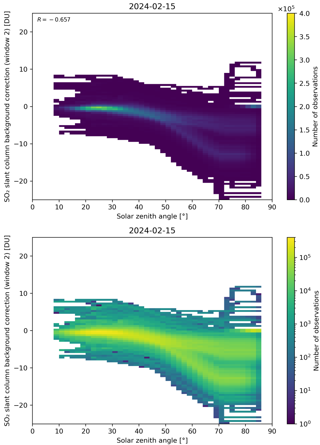
Figure 159: Scatter density plot of “Solar zenith angle” against “SO 2 slant column background correction (window 2)” for 2024-02-14 to 2024-02-16.
