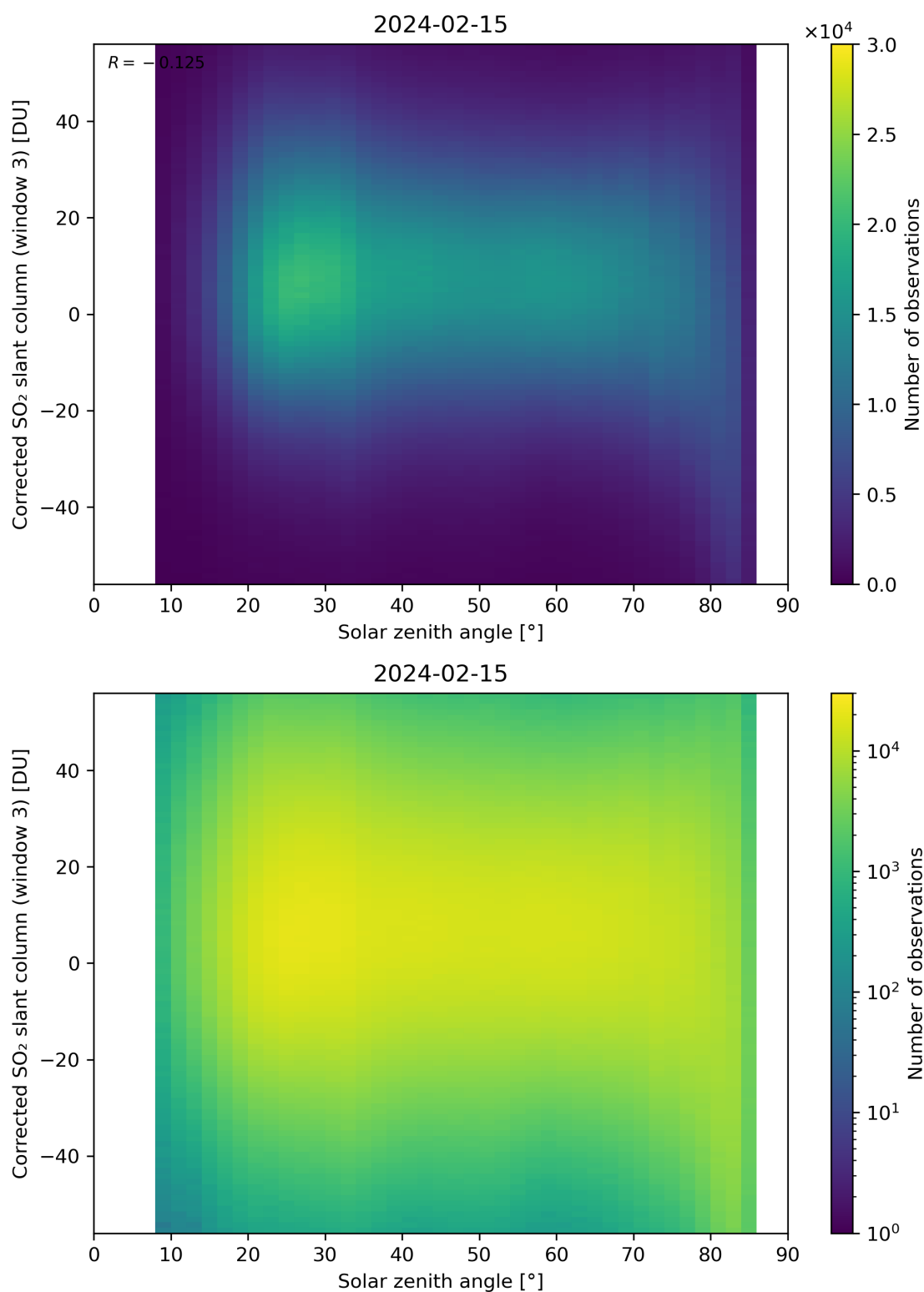
Figure 168: Scatter density plot of “Solar zenith angle” against “Corrected SO 2 slant column (window 3)” for 2024-02-14 to 2024-02-16.
