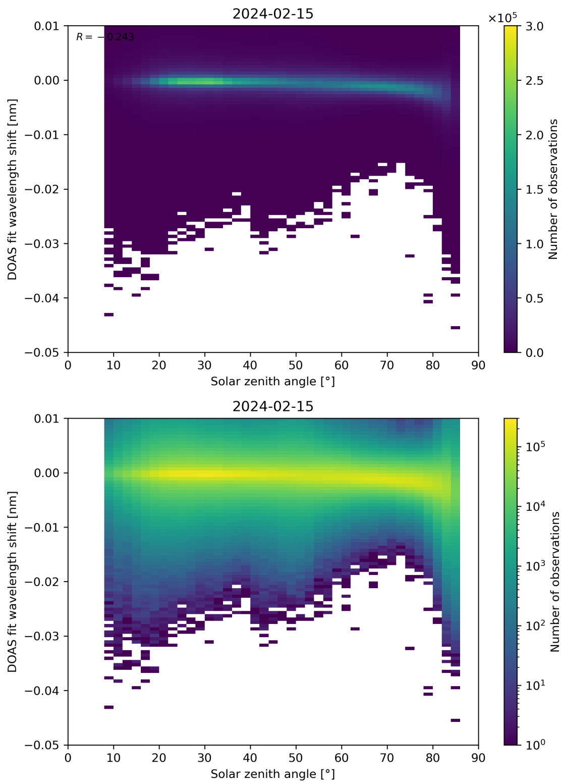
Figure 161: Scatter density plot of “Solar zenith angle” against “DOAS fit wavelength shift” for 2024-02-14 to 2024-02-16.
