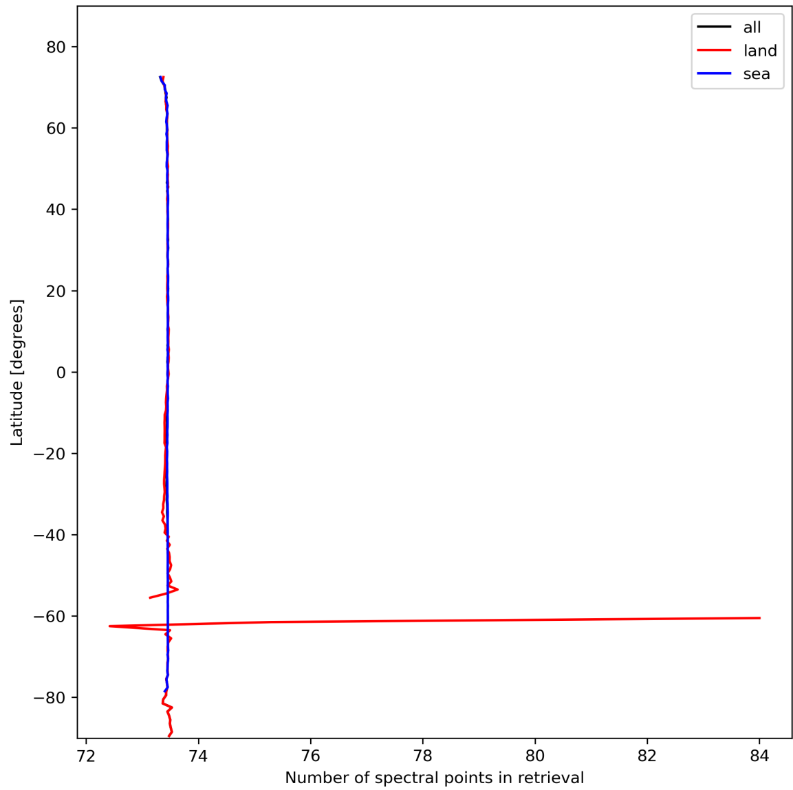
Figure 51: Zonal average of “Number of spectral points in retrieval” for 2024-02-14 to 2024-02-16.
