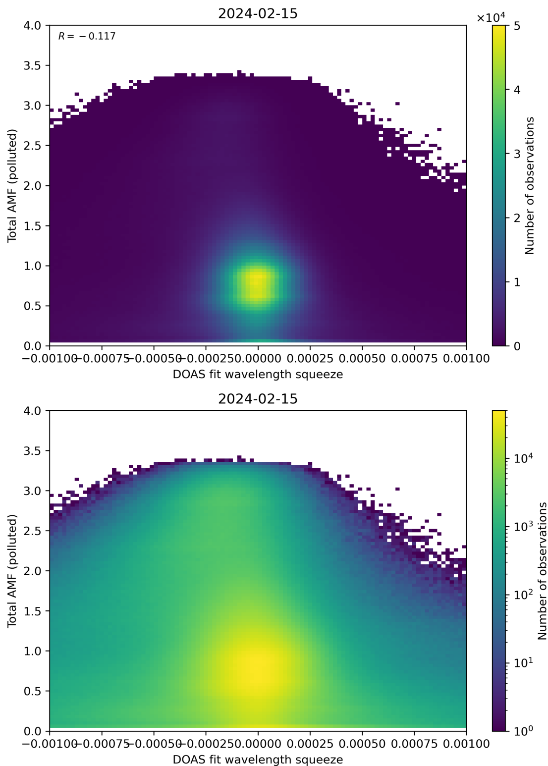
Figure 134: Scatter density plot of “DOAS fit wavelength squeeze” against “Total AMF (polluted)” for 2024-02-14 to 2024-02-16.
