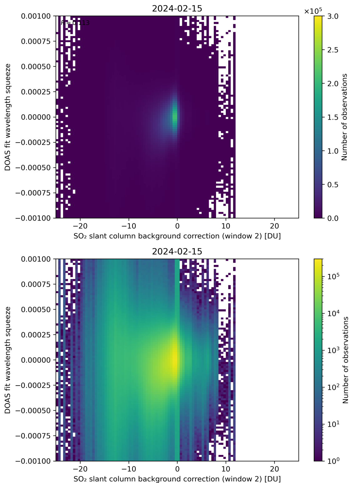
Figure 113: Scatter density plot of “SO 2 slant column background correction (window 2)” against “DOAS fit wavelength squeeze” for 2024-02-14 to 2024-02-16.
