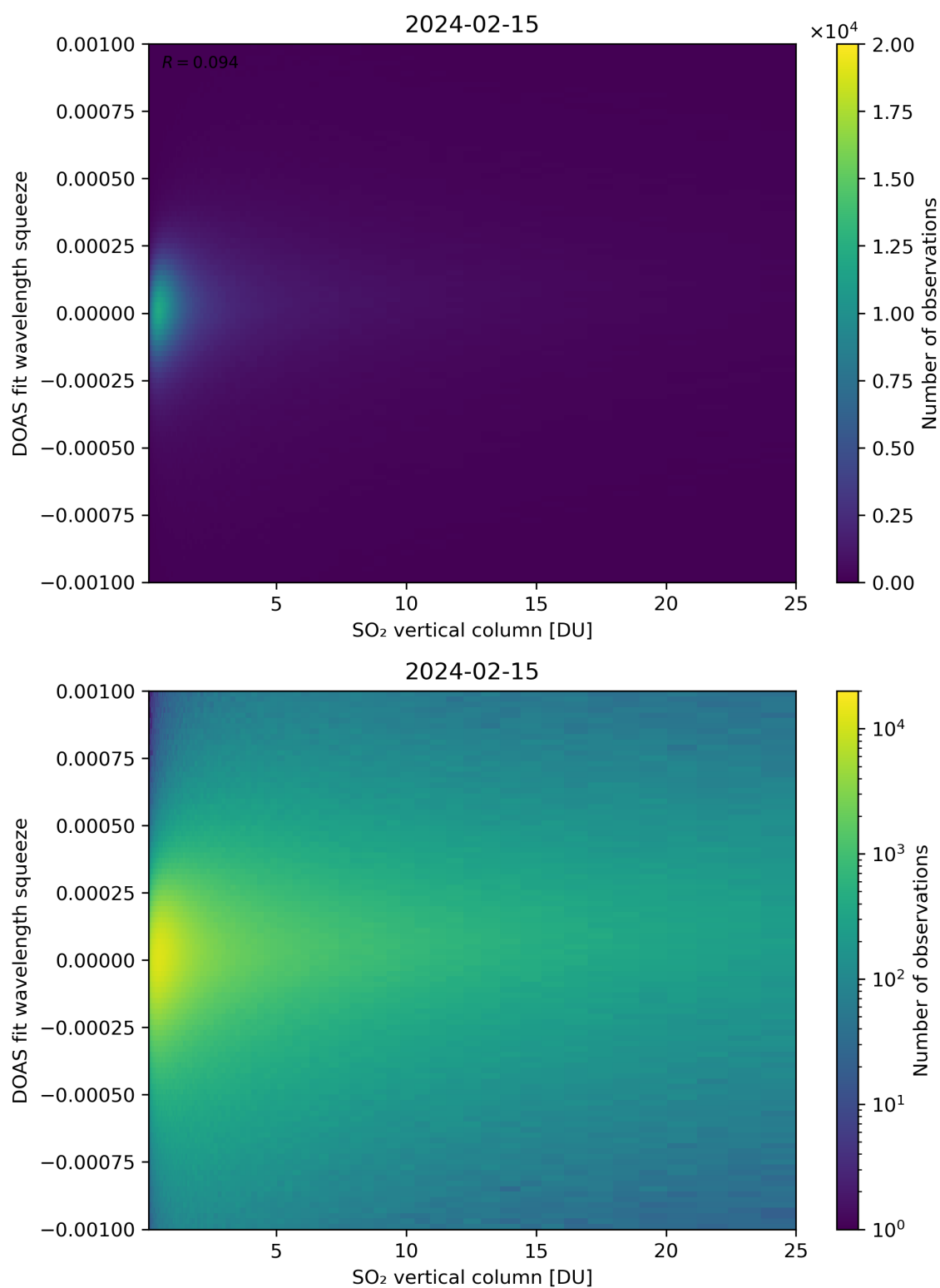
Figure 277: Scatter density plot of “SO 2 vertical column” against “DOAS fit wavelength squeeze” for 2024-02-14 to 2024-02-16.
