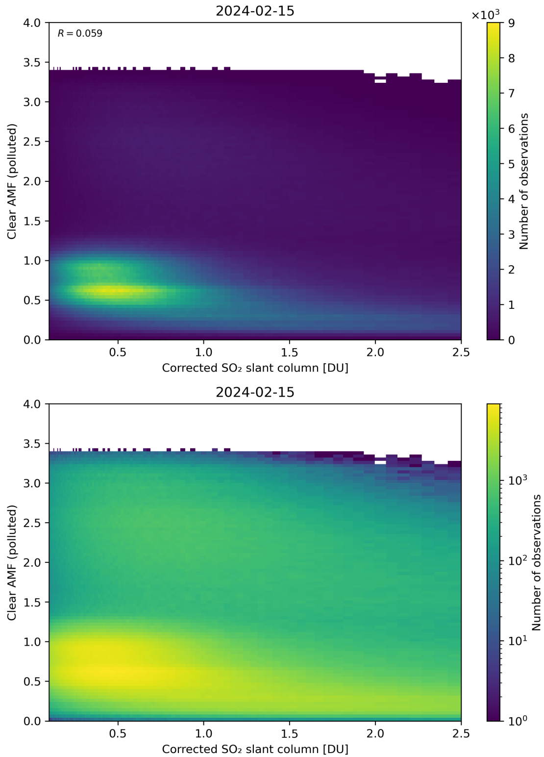
Figure 184: Scatter density plot of “Corrected SO 2 slant column” against “Clear AMF (polluted)” for 2024-02-14 to 2024-02-16.
