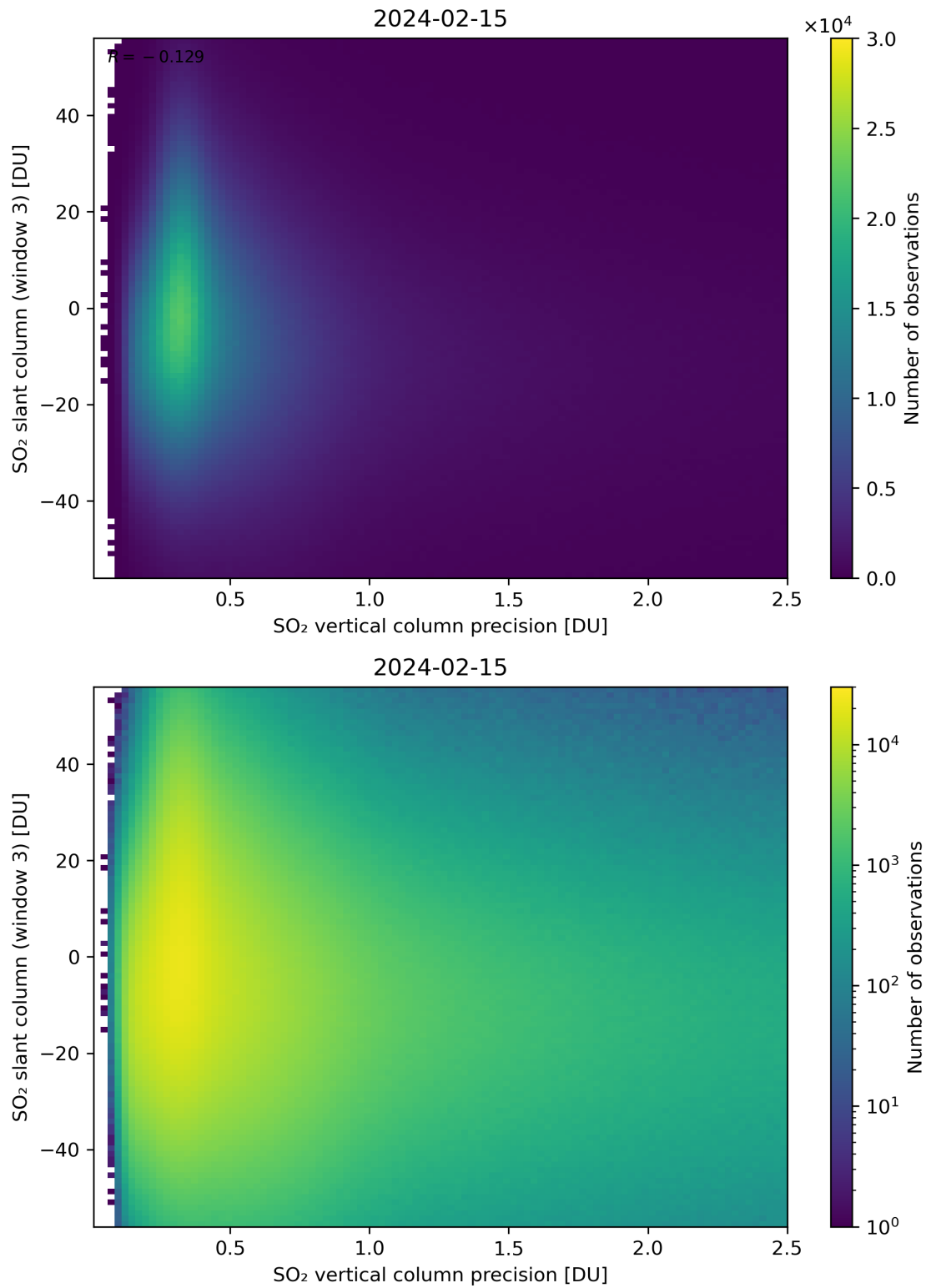
Figure 292: Scatter density plot of “SO 2 vertical column precision” against “SO 2 slant column (window 3)” for 2024-02-14 to 2024-02-16.
