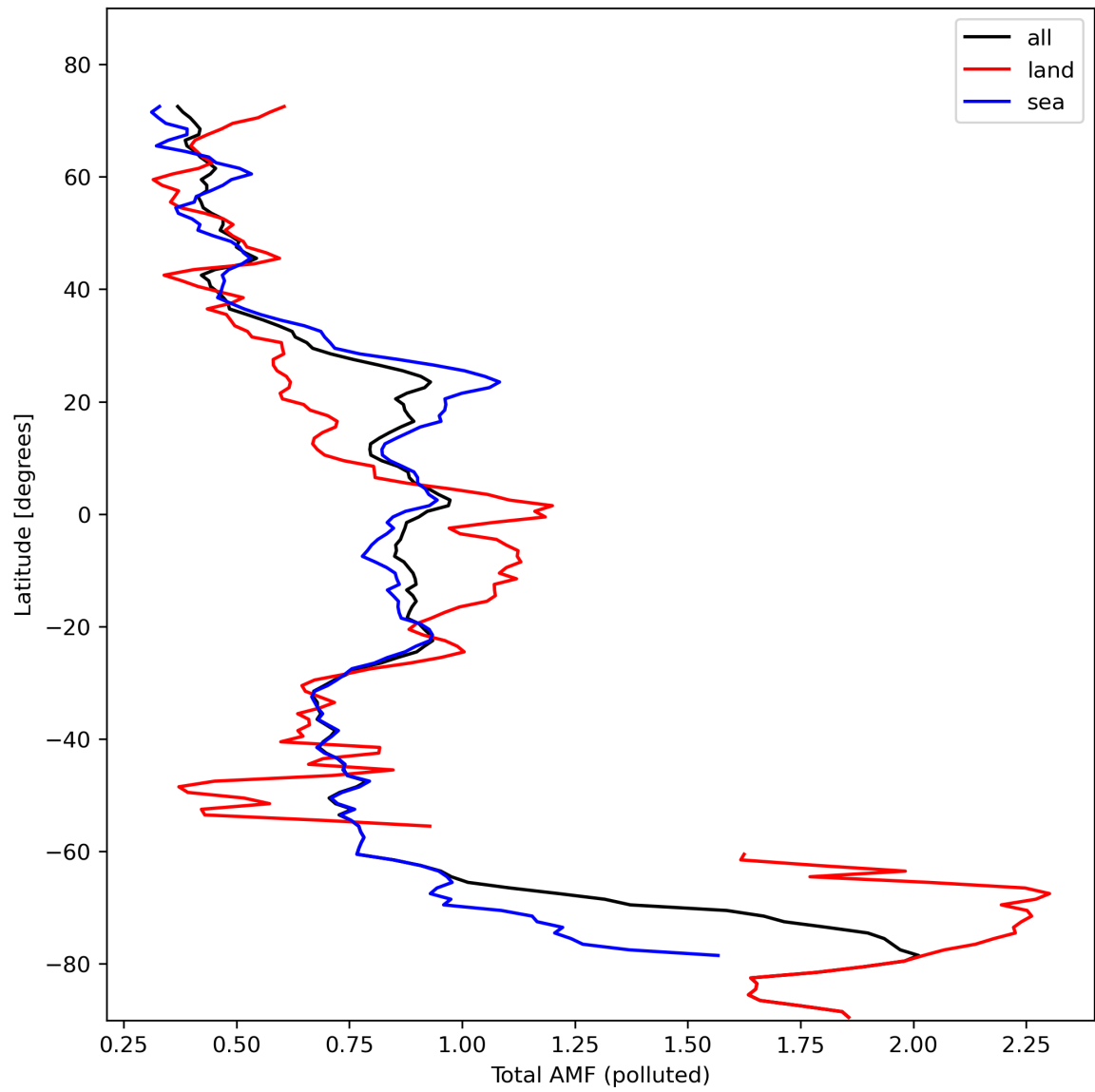
Figure 48: Zonal average of “Total AMF (polluted)” for 2024-02-14 to 2024-02-16.
