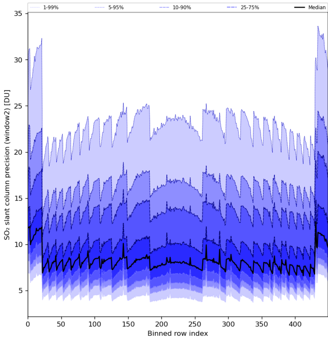
Figure 84: Along track statistics of “SO 2 slant column precision (window2)” for 2024-02-14 to 2024-02-16
