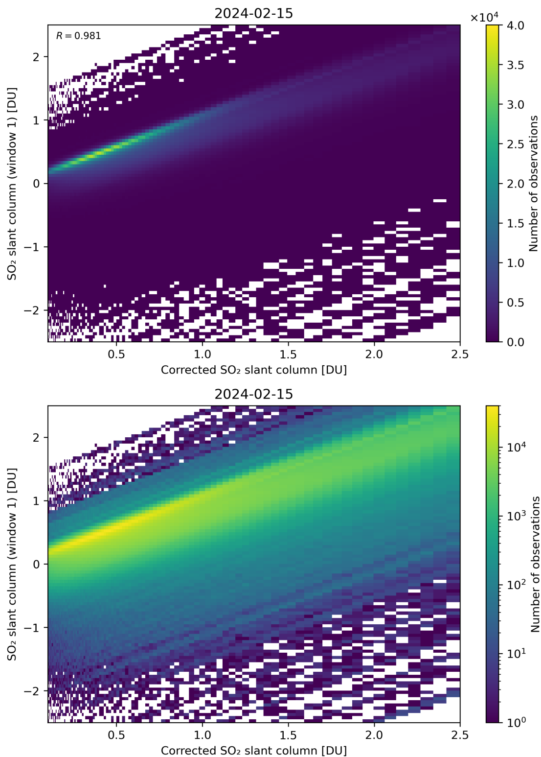
Figure 187: Scatter density plot of “Corrected SO 2 slant column” against “SO 2 slant column (window 1)” for 2024-02-14 to 2024-02-16.
