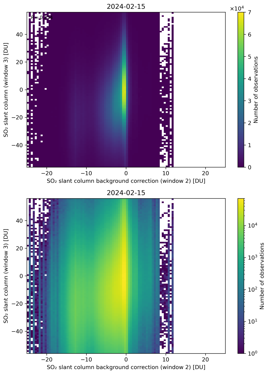
Figure 117: Scatter density plot of “SO 2 slant column background correction (window 2)” against “SO 2 slant column (window 3)” for 2024-02-14 to 2024-02-16.
