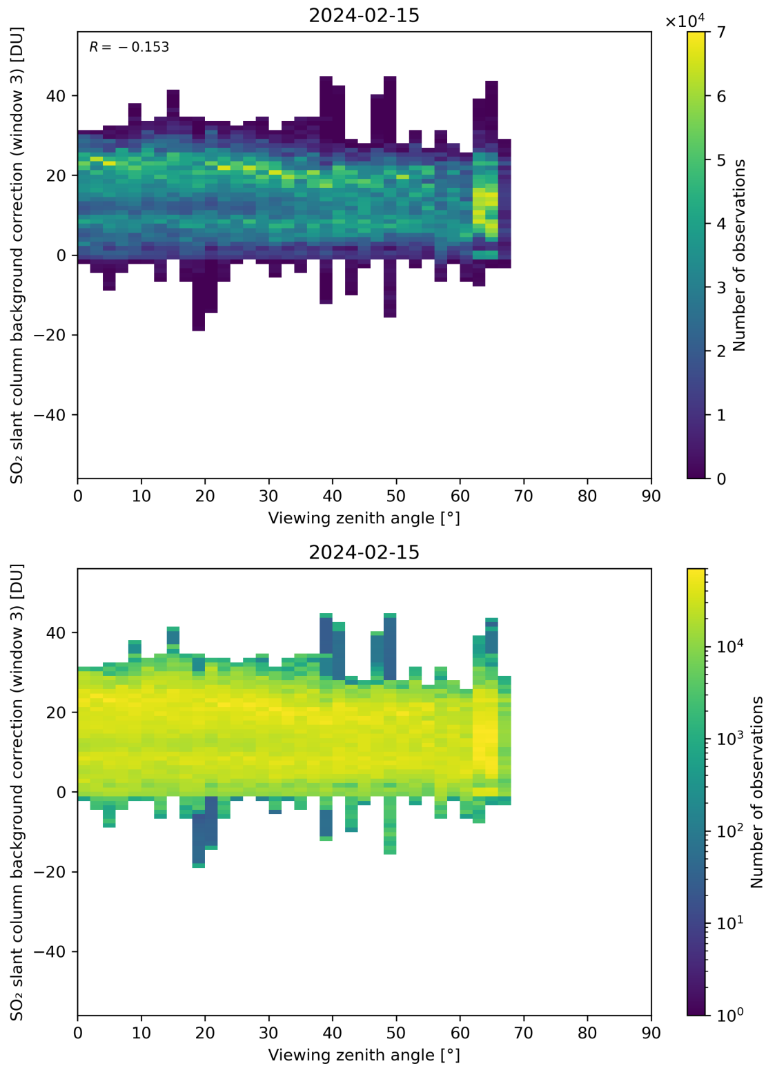
Figure 310: Scatter density plot of “Viewing zenith angle” against “SO 2 slant column background correction (window 3)” for 2024-02-14 to 2024-02-16.
