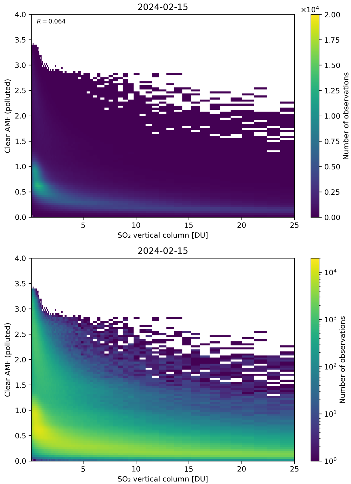
Figure 296: Scatter density plot of “SO 2 vertical column” against “Clear AMF (polluted)” for 2024-02-14 to 2024-02-16.
