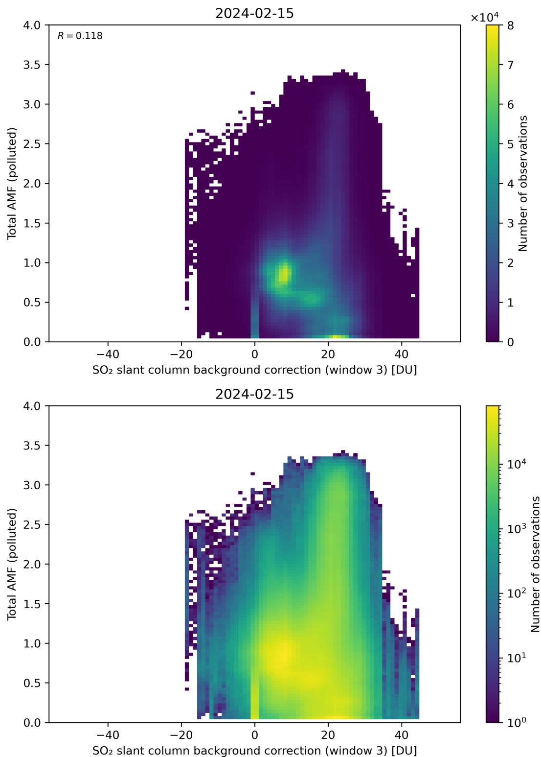
Figure 125: Scatter density plot of “SO 2 slant column background correction (window 3)” against “Total AMF (polluted)” for 2024-02-14 to 2024-02-16.
