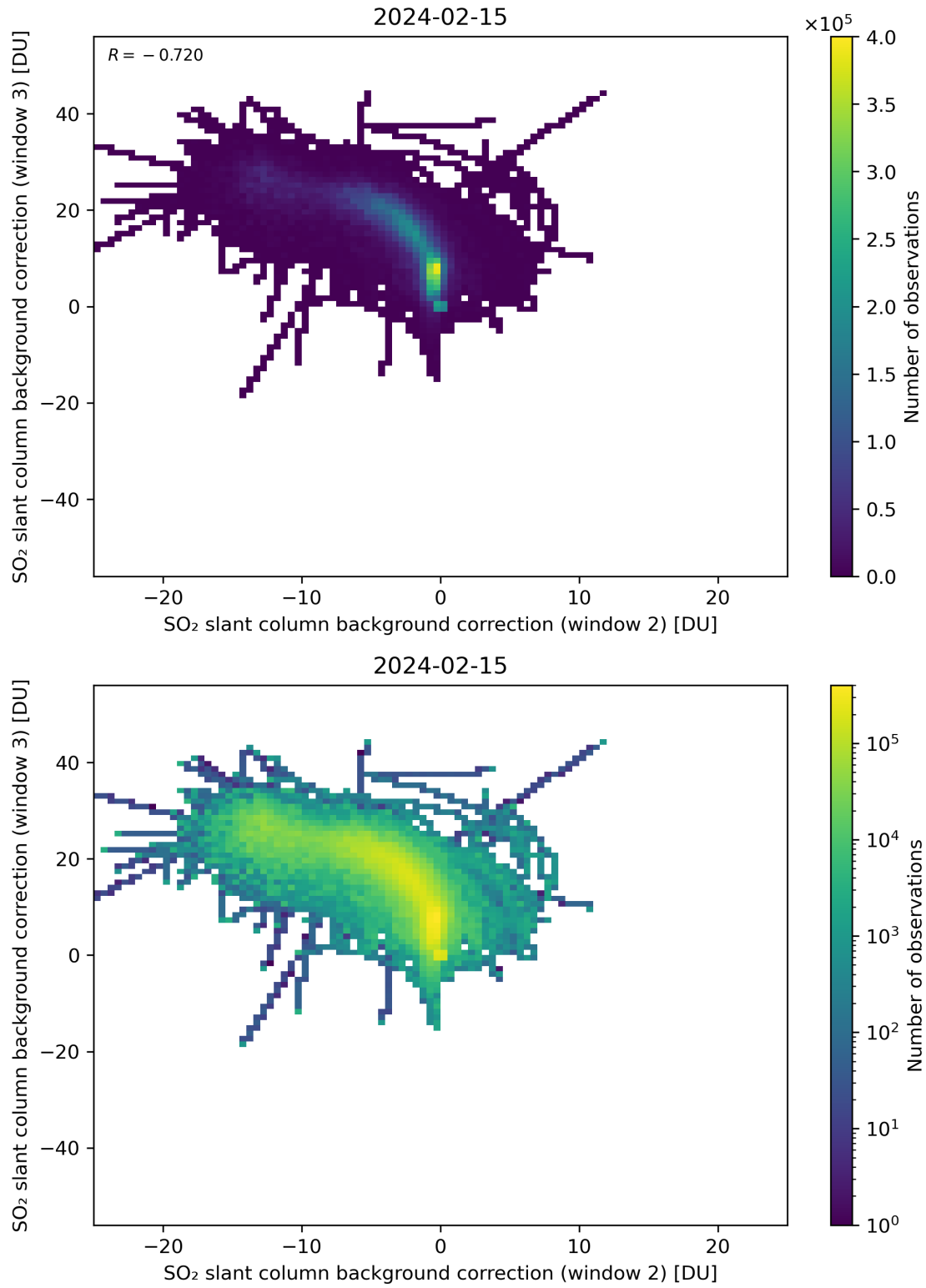
Figure 111: Scatter density plot of “SO 2 slant column background correction (window 2)” against “SO 2 slant column background correction (window 3)” for 2024-02-14 to 2024-02-16.
