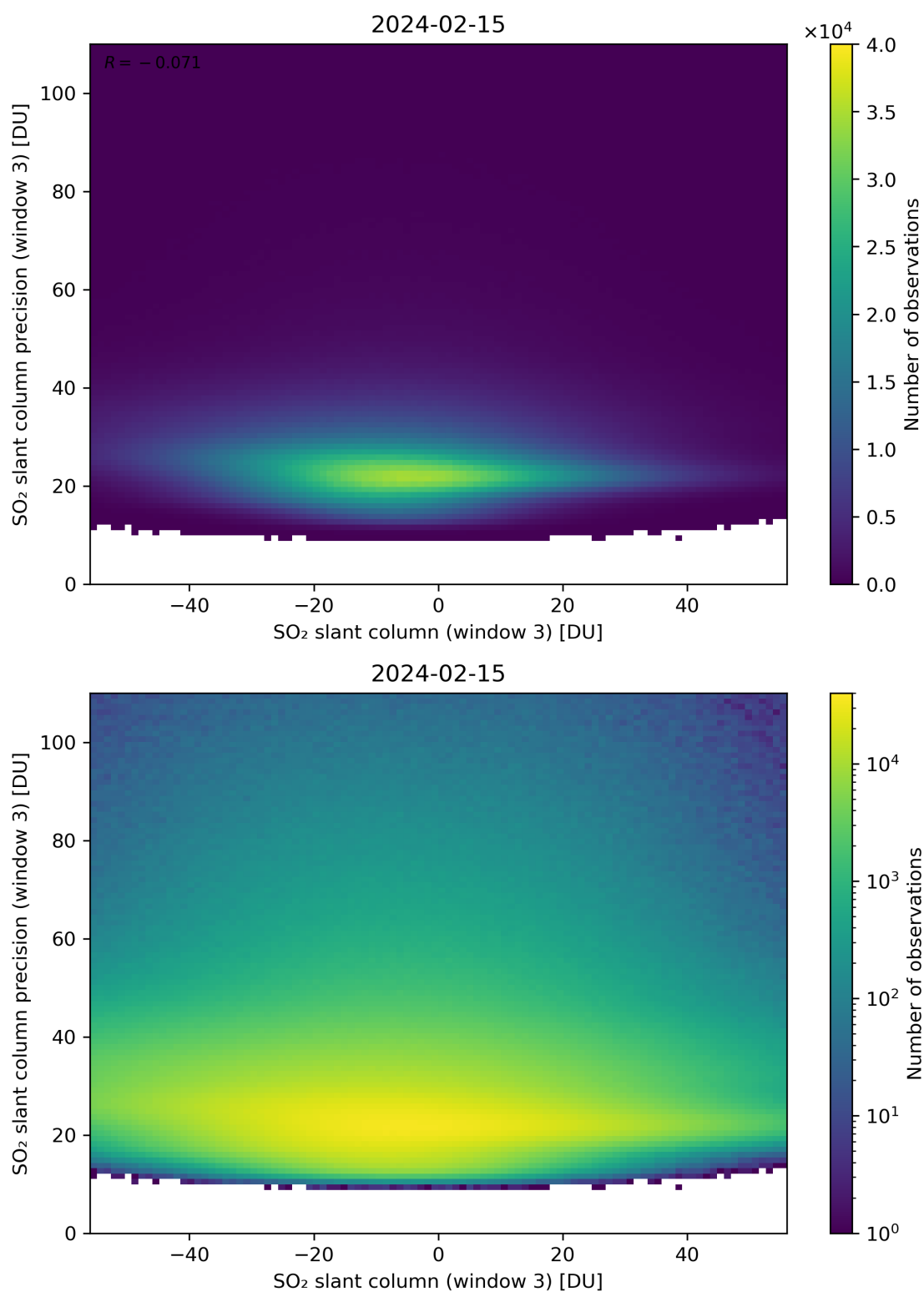
Figure 267: Scatter density plot of “SO 2 slant column (window 3)” against “SO 2 slant column precision (window 3)” for 2024-02-14 to 2024-02-16.
