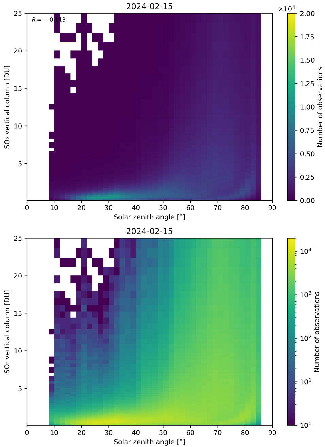
Figure 176: Scatter density plot of “Solar zenith angle” against “SO 2 vertical column” for 2024-02-14 to 2024-02-16.
