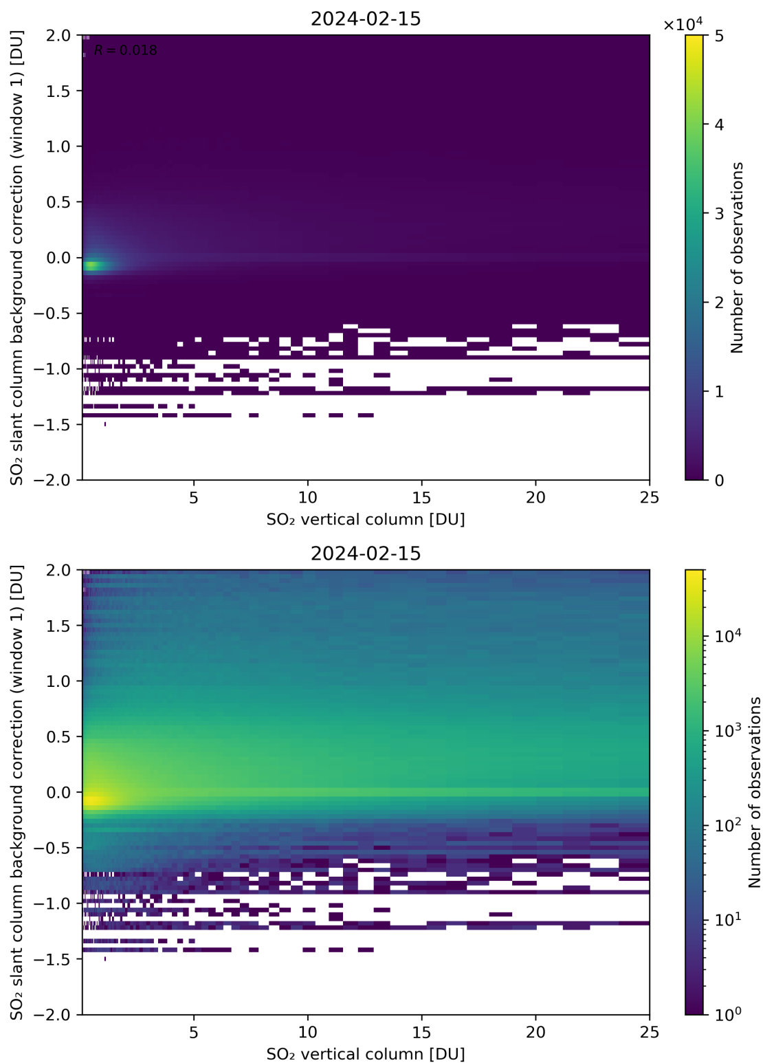
Figure 273: Scatter density plot of “SO 2 vertical column” against “SO 2 slant column background correction (window 1)” for 2024-02-14 to 2024-02-16.
