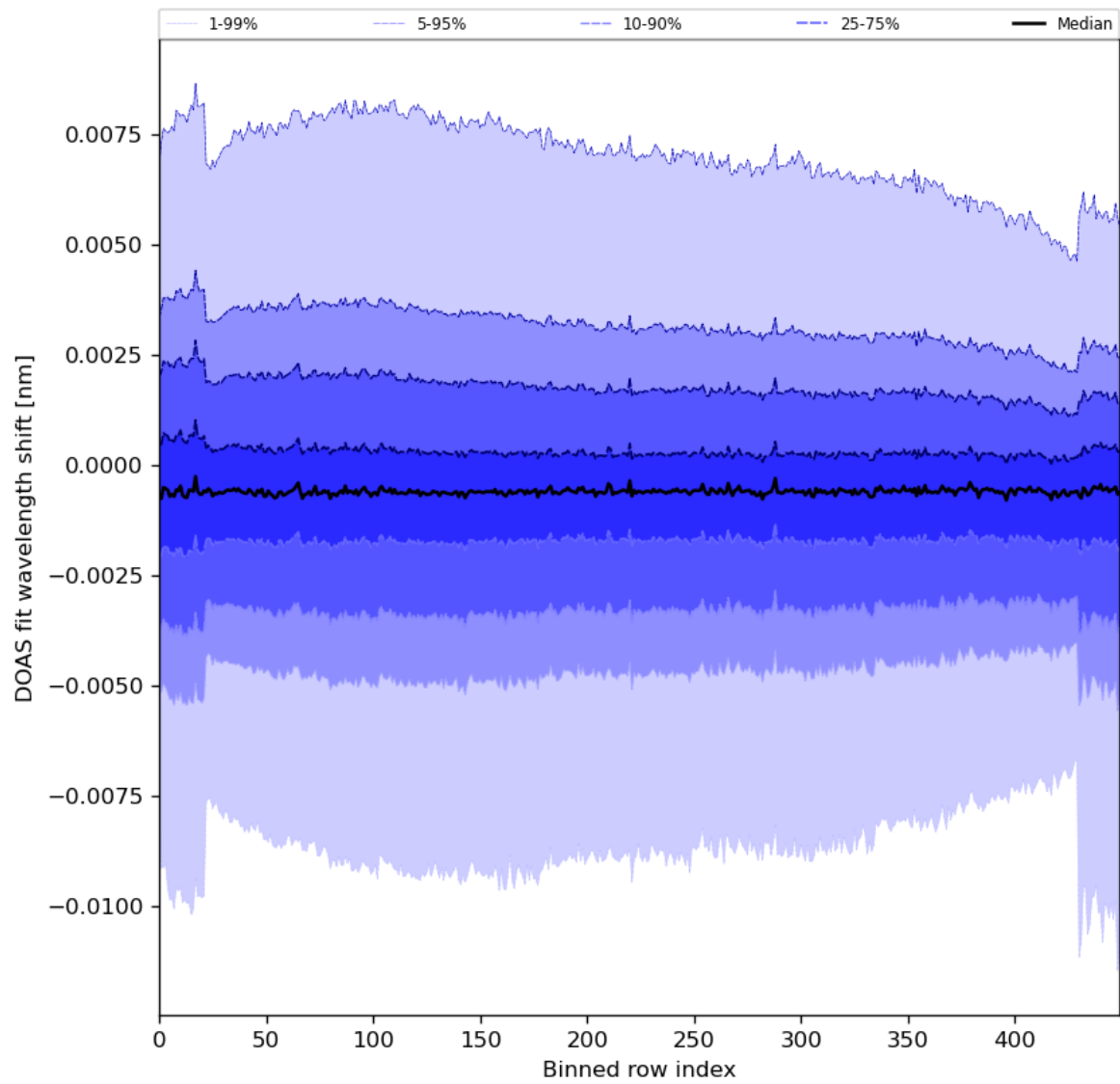
Figure 91: Along track statistics of “DOAS fit wavelength shift” for 2024-02-14 to 2024-02-16
