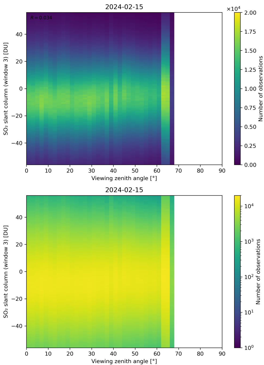
Figure 323: Scatter density plot of “Viewing zenith angle” against “SO 2 slant column (window 3)” for 2024-02-14 to 2024-02-16.
