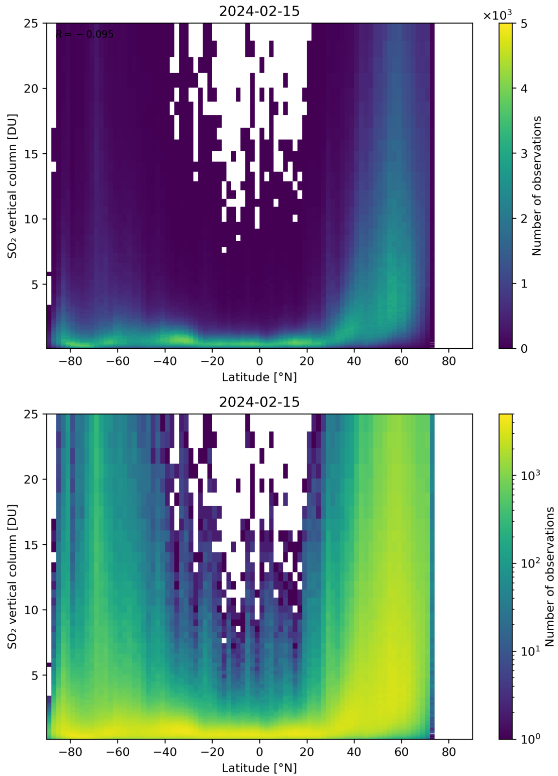
Figure 156: Scatter density plot of “Latitude” against “SO 2 vertical column” for 2024-02-14 to 2024-02-16.
