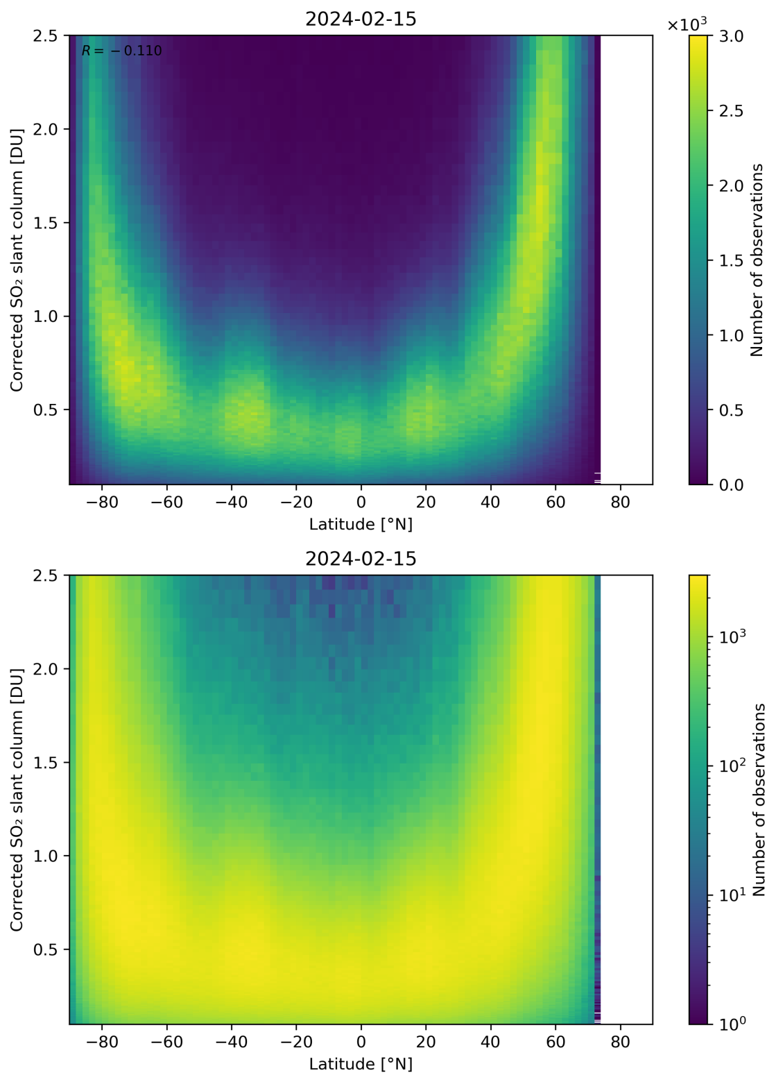
Figure 146: Scatter density plot of “Latitude” against “Corrected SO 2 slant column” for 2024-02-14 to 2024-02-16.
