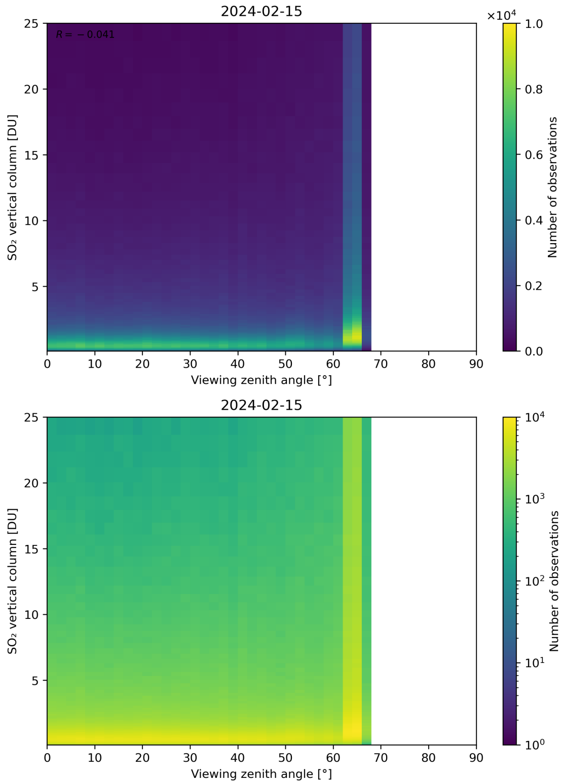
Figure 327: Scatter density plot of “Viewing zenith angle” against “SO 2 vertical column” for 2024-02-14 to 2024-02-16.
