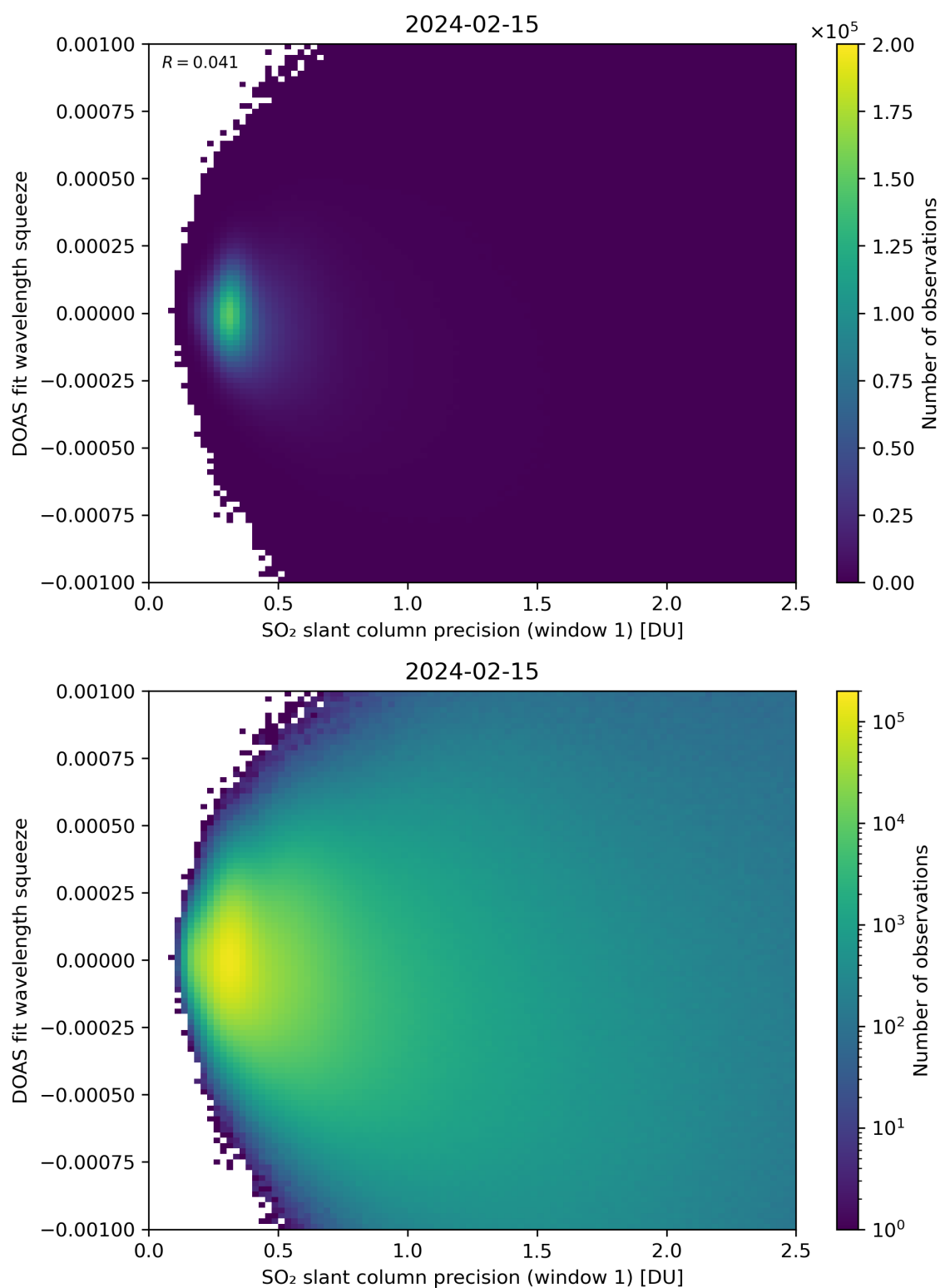
Figure 222: Scatter density plot of “SO 2 slant column precision (window 1)” against “DOAS fit wavelength squeeze” for 2024-02-14 to 2024-02-16.
