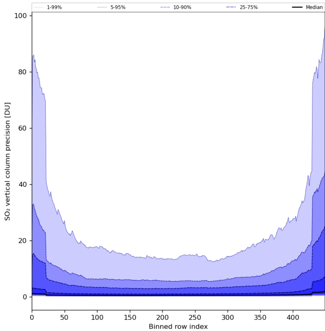
Figure 77: Along track statistics of “SO 2 vertical column precision” for 2024-02-14 to 2024-02-16
