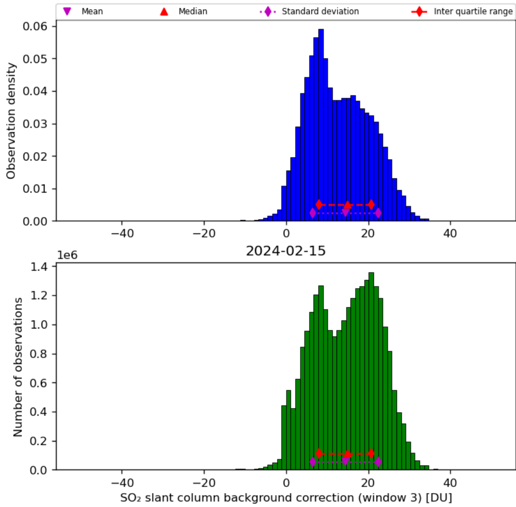
Figure 67: Histogram of “SO 2 slant column background correction (window 3)” for 2024-02-14 to 2024-02-16
