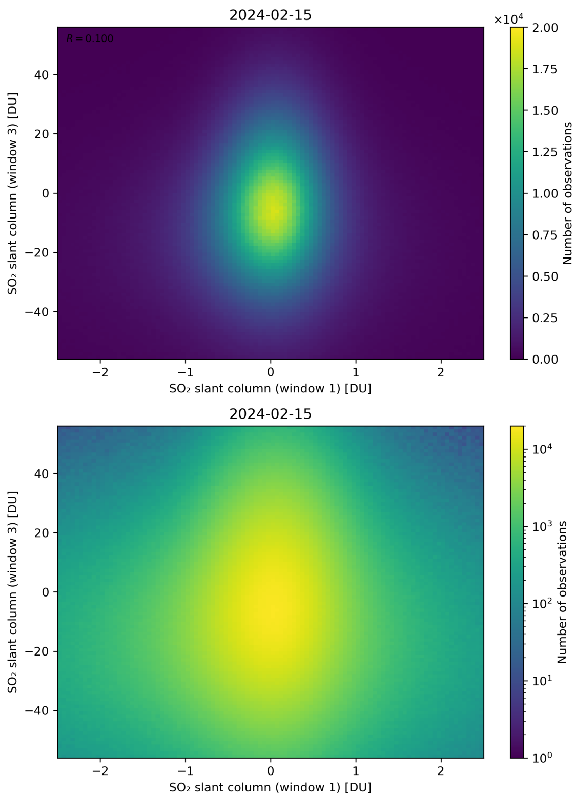
Figure 237: Scatter density plot of “SO 2 slant column (window 1)” against “SO 2 slant column (window 3)” for 2024-02-14 to 2024-02-16.
