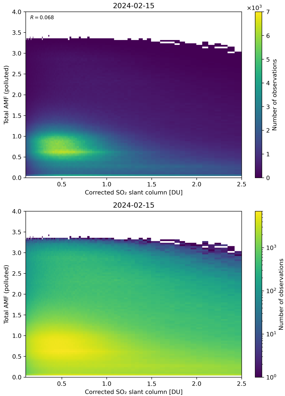
Figure 192: Scatter density plot of “Corrected SO 2 slant column” against “Total AMF (polluted)” for 2024-02-14 to 2024-02-16.
