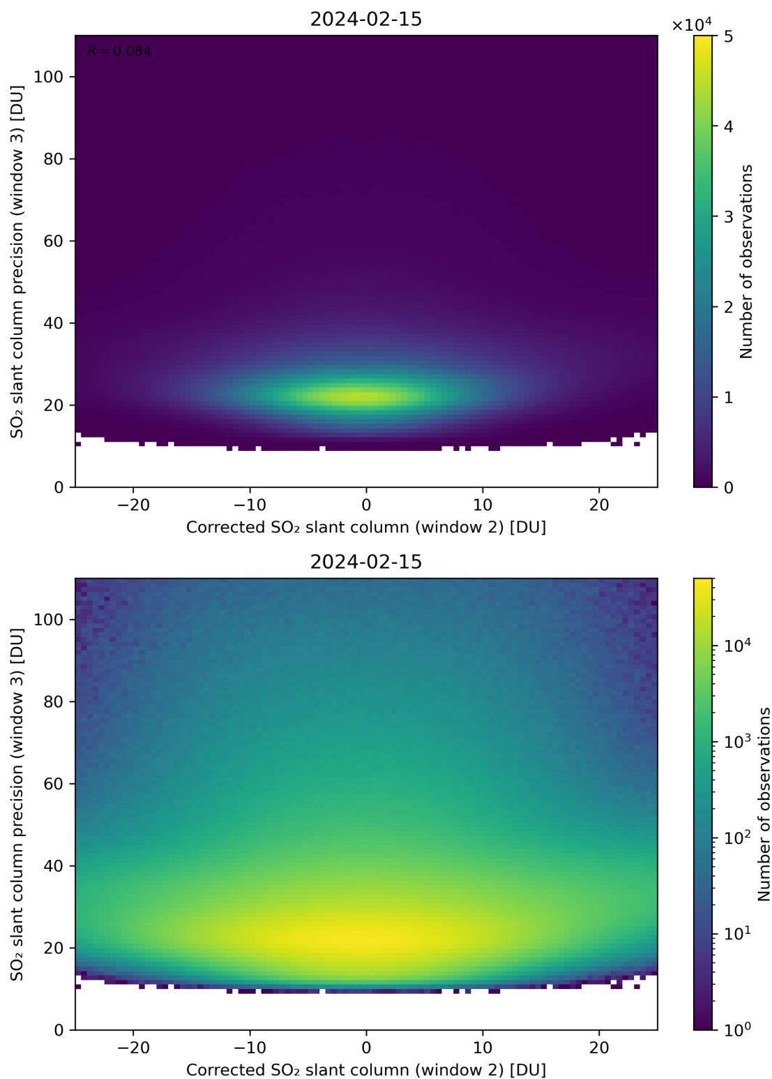
Figure 202: Scatter density plot of “Corrected SO 2 slant column (window 2)” against “SO 2 slant column precision (window 3)” for 2024-02-14 to 2024-02-16.
