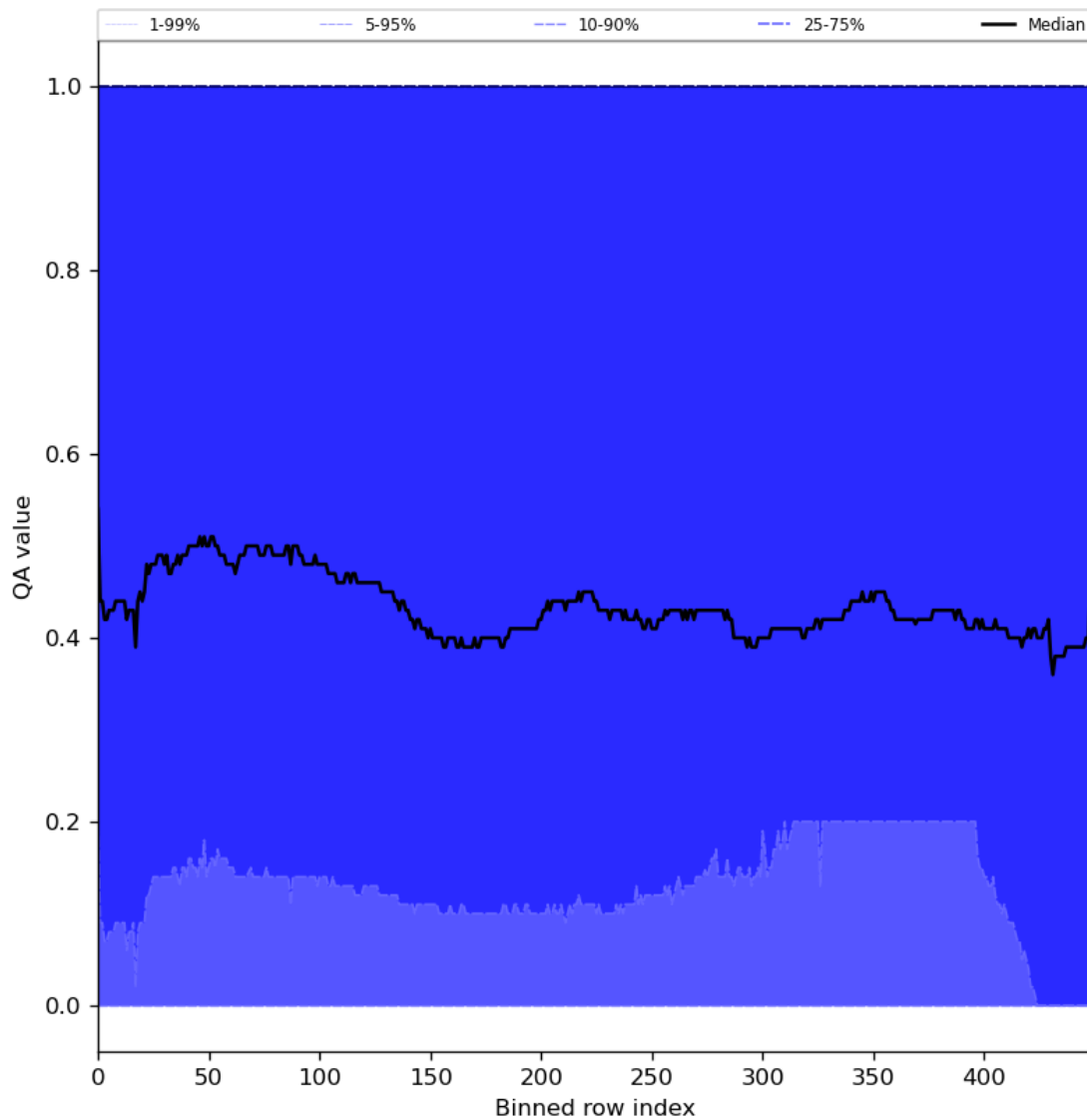
Figure 75: Along track statistics of “QA value” for 2024-02-14 to 2024-02-16
