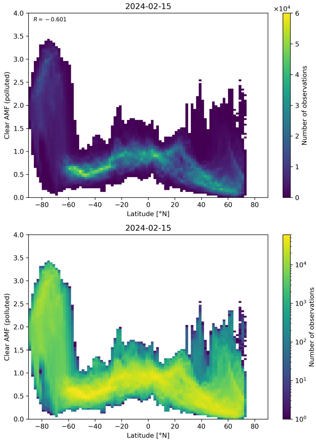
Figure 145: Scatter density plot of “Latitude” against “Clear AMF (polluted)” for 2024-02-14 to 2024-02-16.
