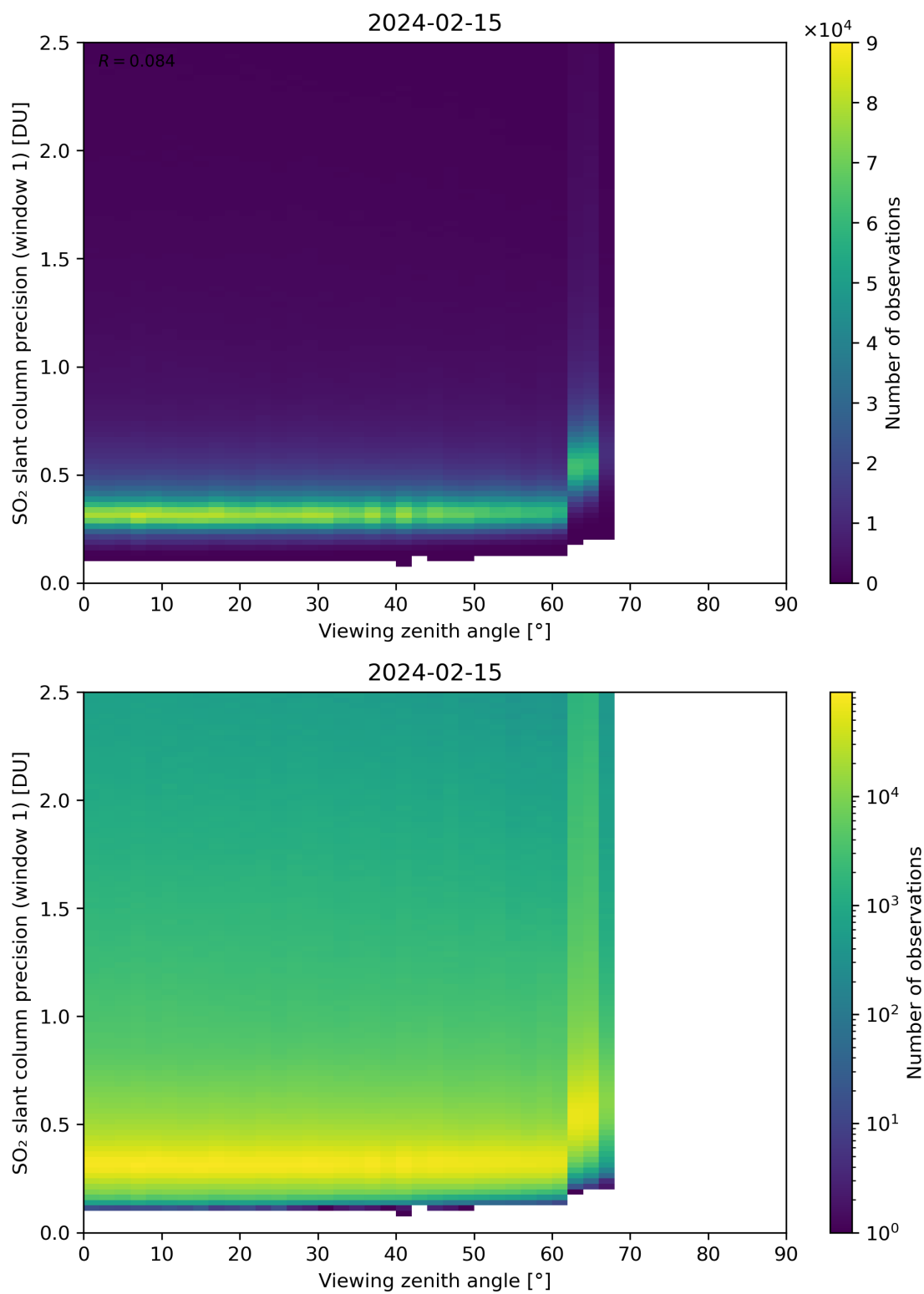
Figure 321: Scatter density plot of “Viewing zenith angle” against “SO 2 slant column precision (window 1)” for 2024-02-14 to 2024-02-16.
