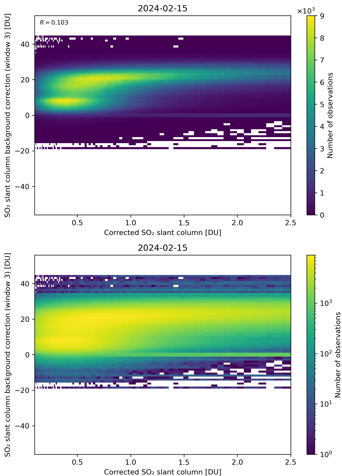
Figure 180: Scatter density plot of “Corrected SO 2 slant column” against “SO 2 slant column background correction (window 3)” for 2024-02-14 to 2024-02-16.
