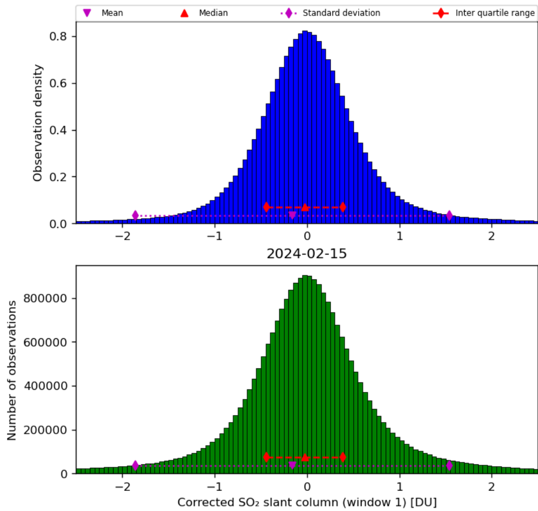
Figure 58: Histogram of “Corrected SO 2 slant column (window 1)” for 2024-02-14 to 2024-02-16
