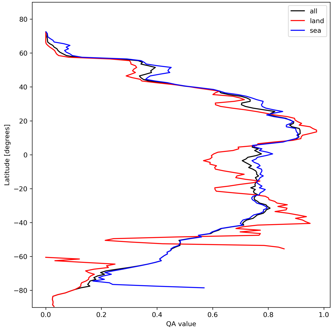
Figure 29: Zonal average of “QA value” for 2024-02-14 to 2024-02-16.
