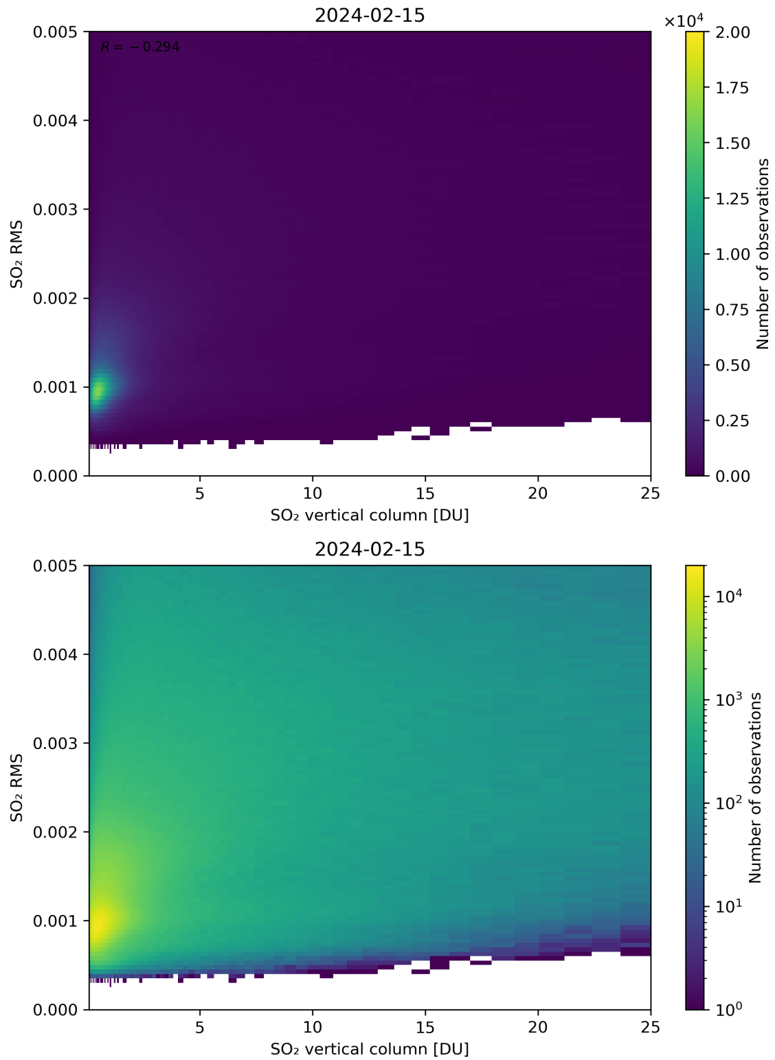
Figure 278: Scatter density plot of “SO 2 vertical column” against “SO 2 RMS” for 2024-02-14 to 2024-02-16.
