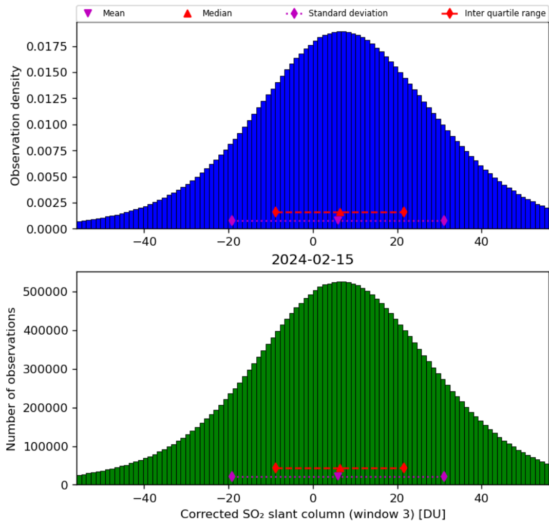
Figure 66: Histogram of “Corrected SO 2 slant column (window 3)” for 2024-02-14 to 2024-02-16
