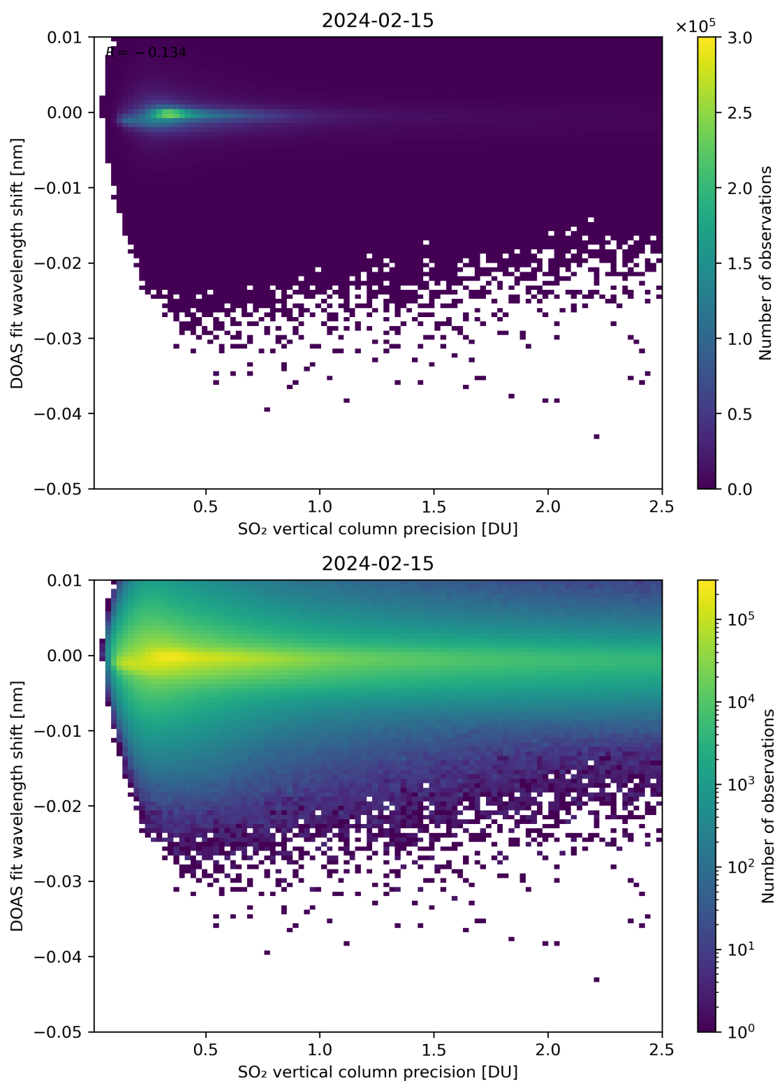
Figure 282: Scatter density plot of “SO 2 vertical column precision” against “DOAS fit wavelength shift” for 2024-02-14 to 2024-02-16.
