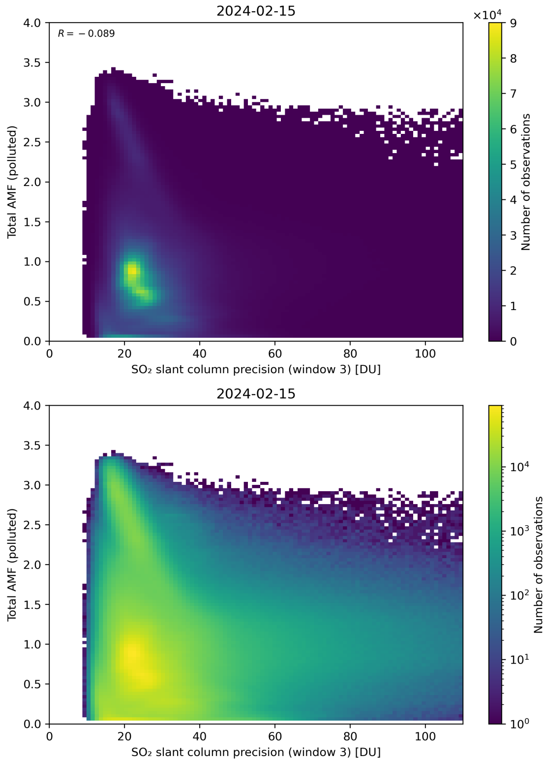
Figure 263: Scatter density plot of “SO 2 slant column precision (window 3)” against “Total AMF (polluted)” for 2024-02-14 to 2024-02-16.
