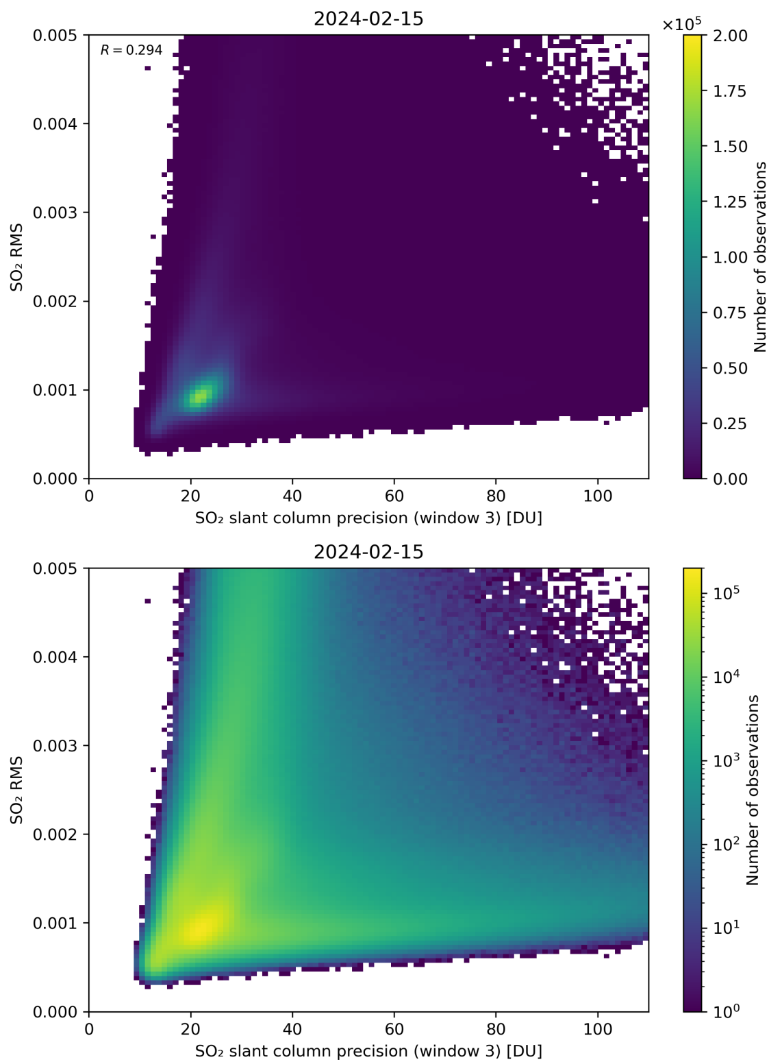
Figure 260: Scatter density plot of “SO 2 slant column precision (window 3)” against “SO 2 RMS” for 2024-02-14 to 2024-02-16.
