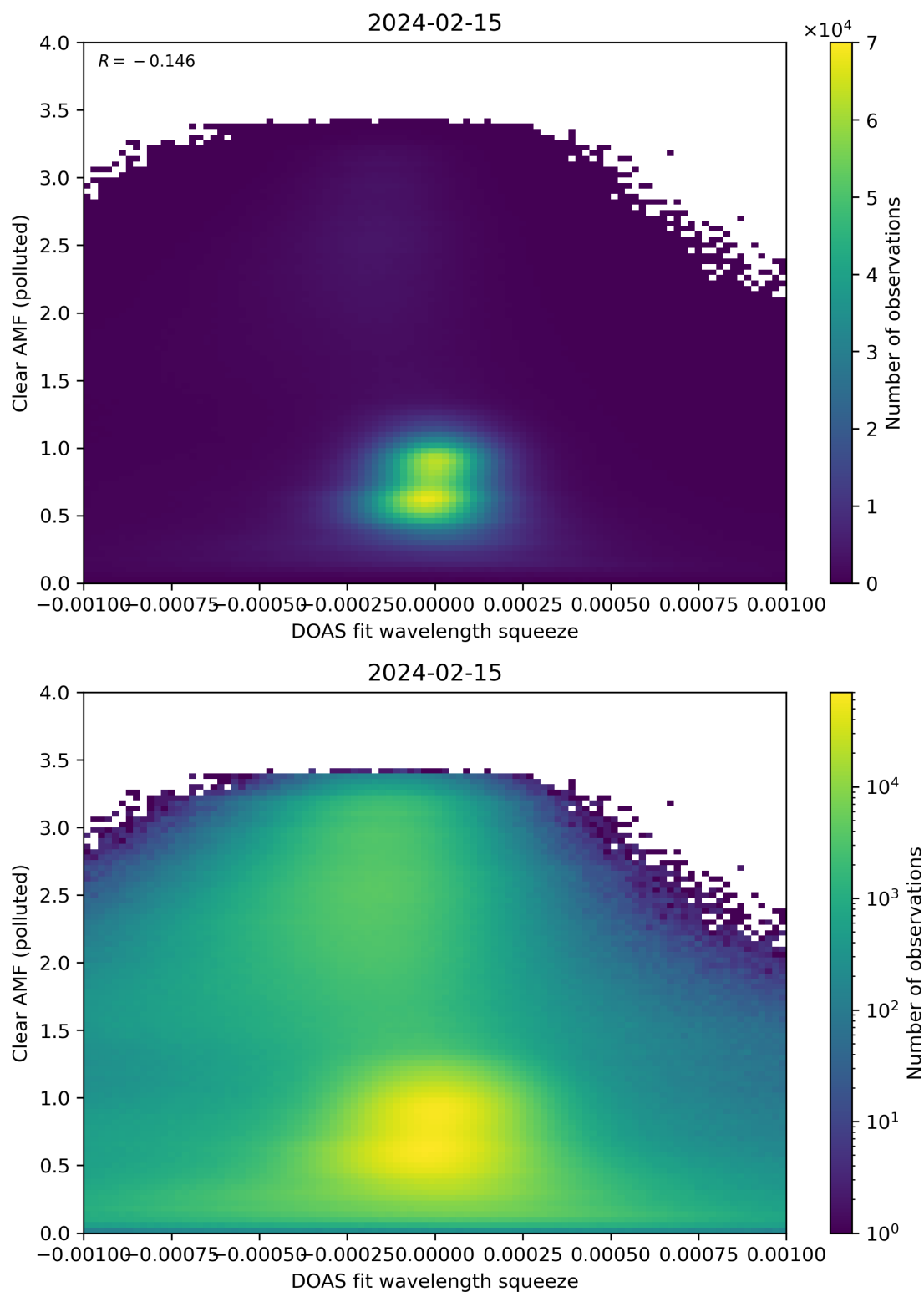
Figure 133: Scatter density plot of “DOAS fit wavelength squeeze” against “Clear AMF (polluted)” for 2024-02-14 to 2024-02-16.
