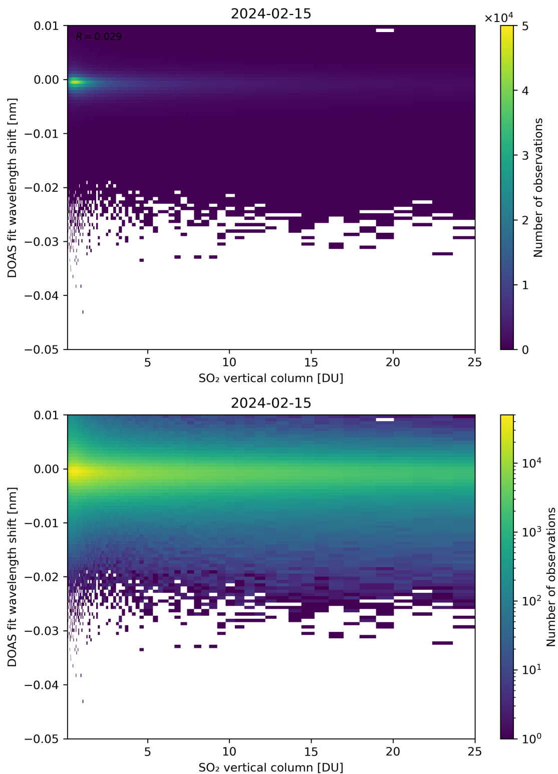
Figure 276: Scatter density plot of “SO 2 vertical column” against “DOAS fit wavelength shift” for 2024-02-14 to 2024-02-16.
