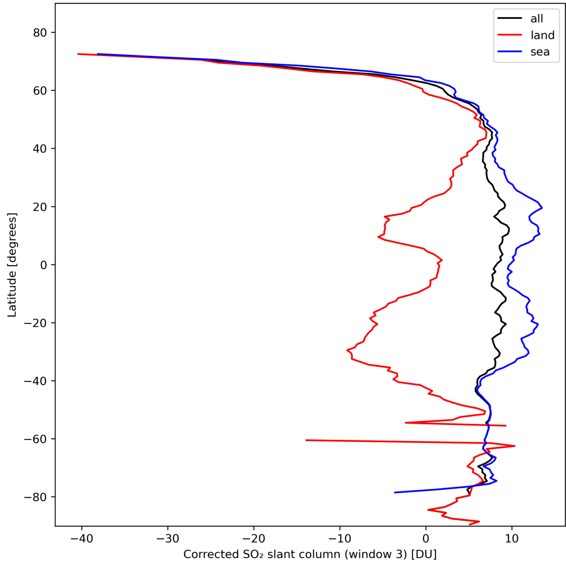
Figure 43: Zonal average of “Corrected SO 2 slant column (window 3)” for 2024-02-14 to 2024-02-16.
