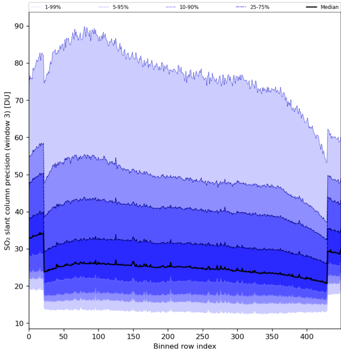
Figure 88: Along track statistics of “SO 2 slant column precision (window 3)” for 2024-02-14 to 2024-02-16
