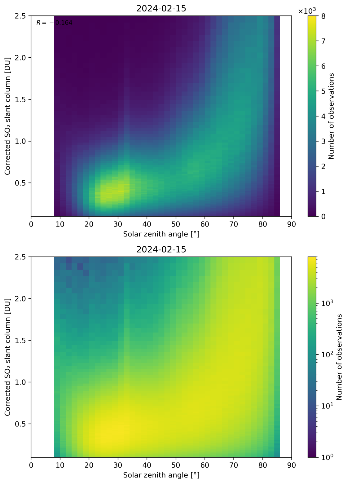
Figure 166: Scatter density plot of “Solar zenith angle” against “Corrected SO 2 slant column” for 2024-02-14 to 2024-02-16.
