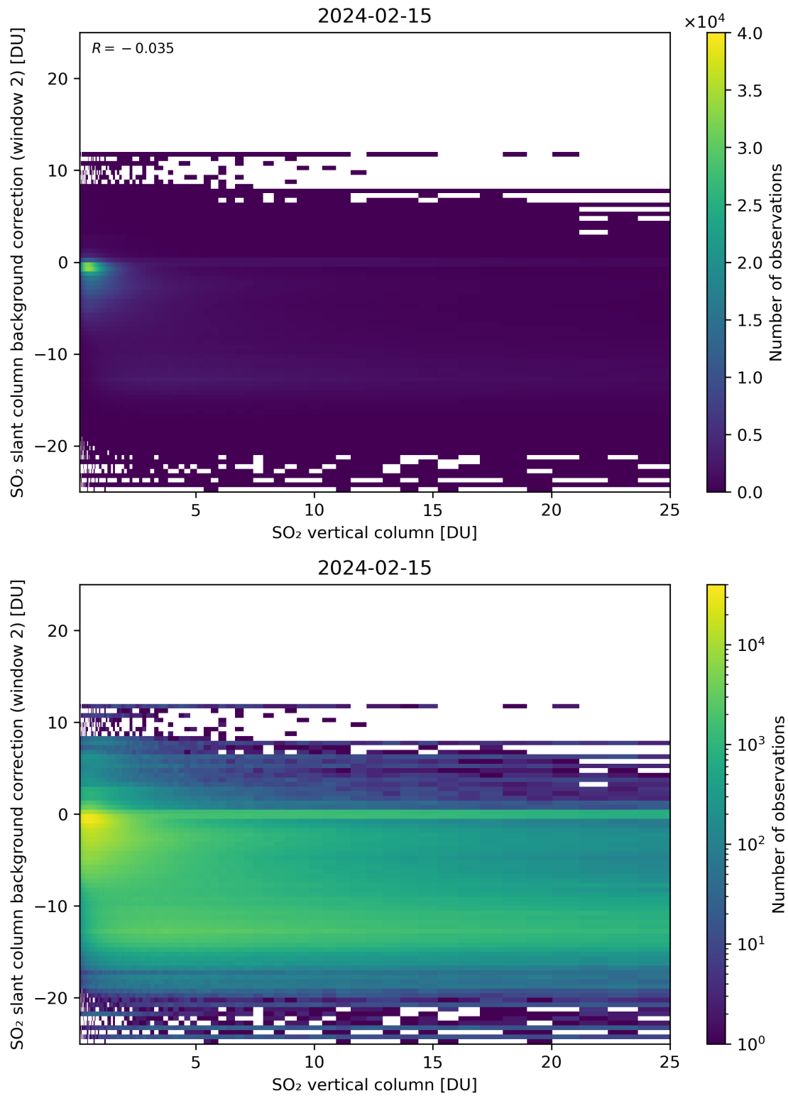
Figure 274: Scatter density plot of “SO 2 vertical column” against “SO 2 slant column background correction (window 2)” for 2024-02-14 to 2024-02-16.
