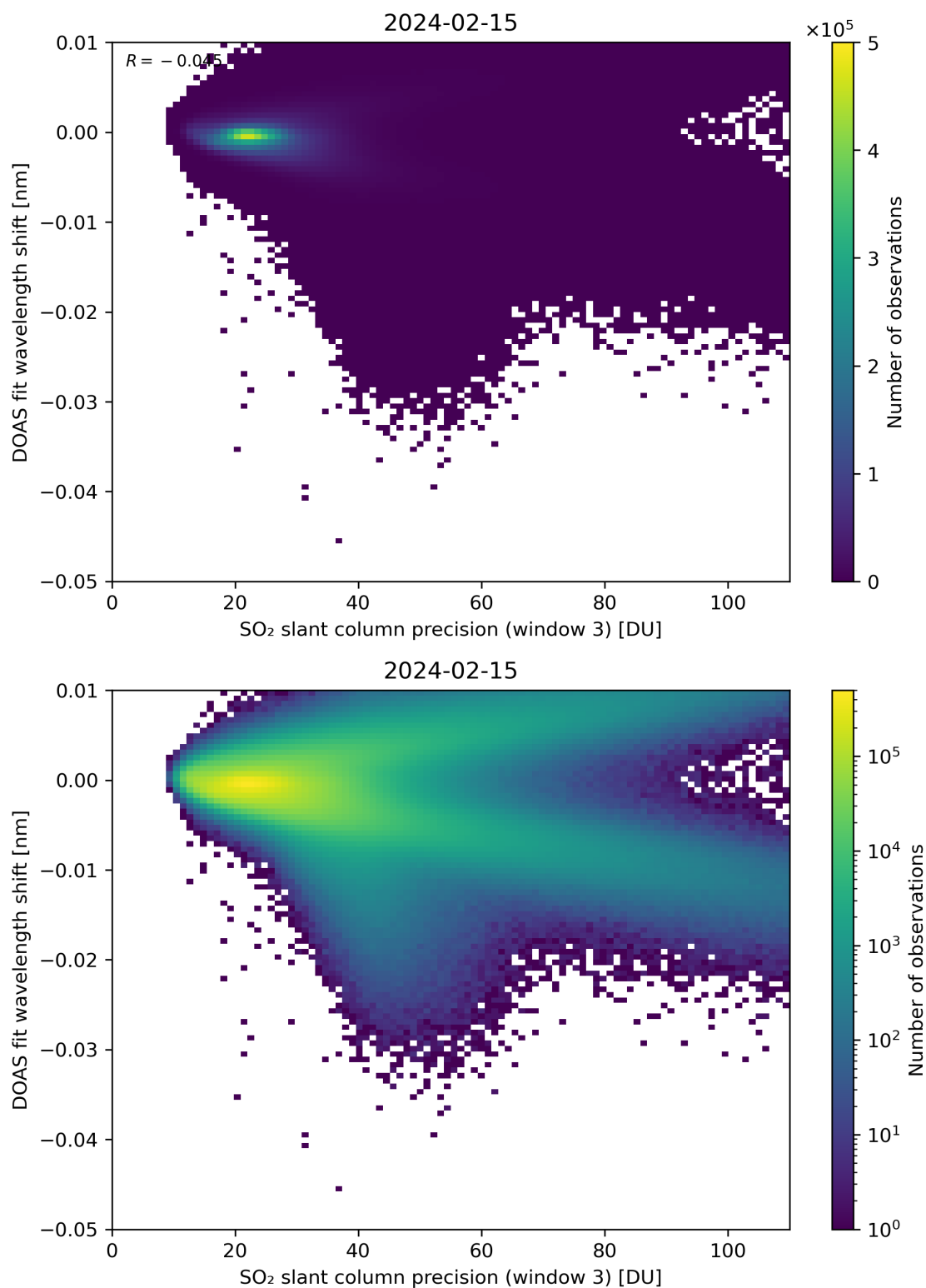
Figure 258: Scatter density plot of “SO 2 slant column precision (window 3)” against “DOAS fit wavelength shift” for 2024-02-14 to 2024-02-16.
