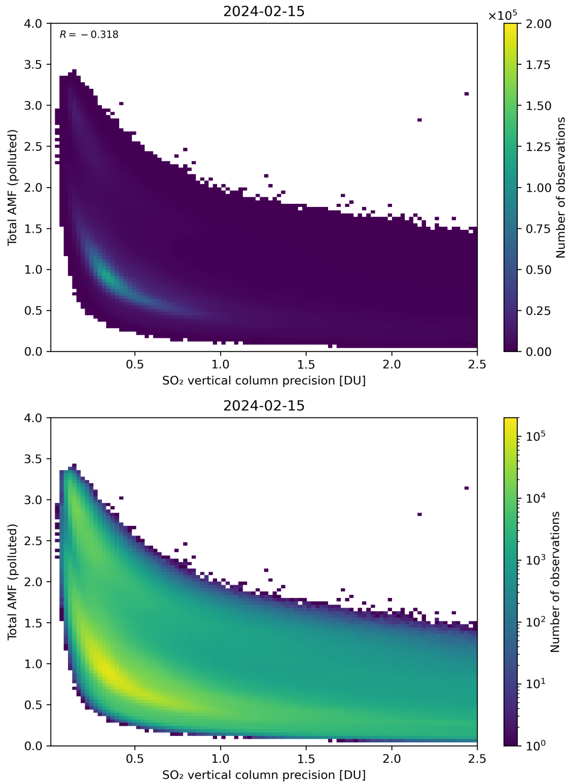
Figure 294: Scatter density plot of “SO 2 vertical column precision” against “Total AMF (polluted)” for 2024-02-14 to 2024-02-16.
