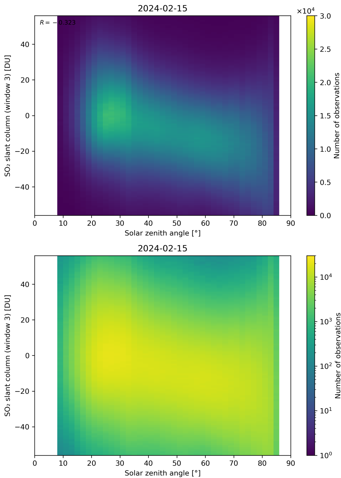
Figure 172: Scatter density plot of “Solar zenith angle” against “SO 2 slant column (window 3)” for 2024-02-14 to 2024-02-16.
