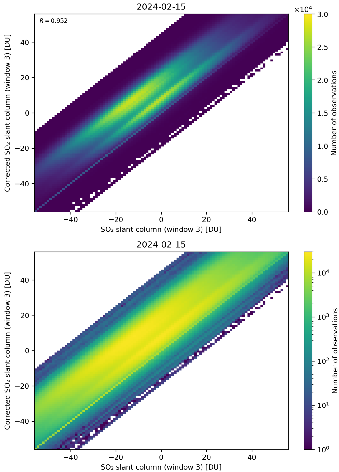
Figure 266: Scatter density plot of “SO 2 slant column (window 3)” against “Corrected SO 2 slant column (window 3)” for 2024-02-14 to 2024-02-16.
