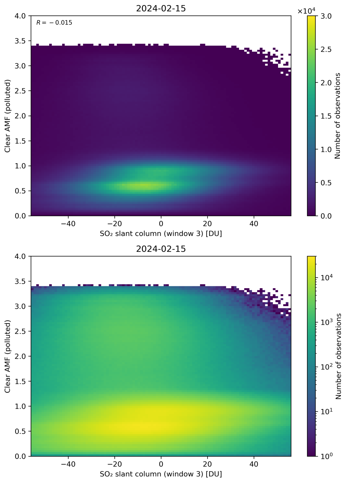
Figure 265: Scatter density plot of “SO 2 slant column (window 3)” against “Clear AMF (polluted)” for 2024-02-14 to 2024-02-16.
