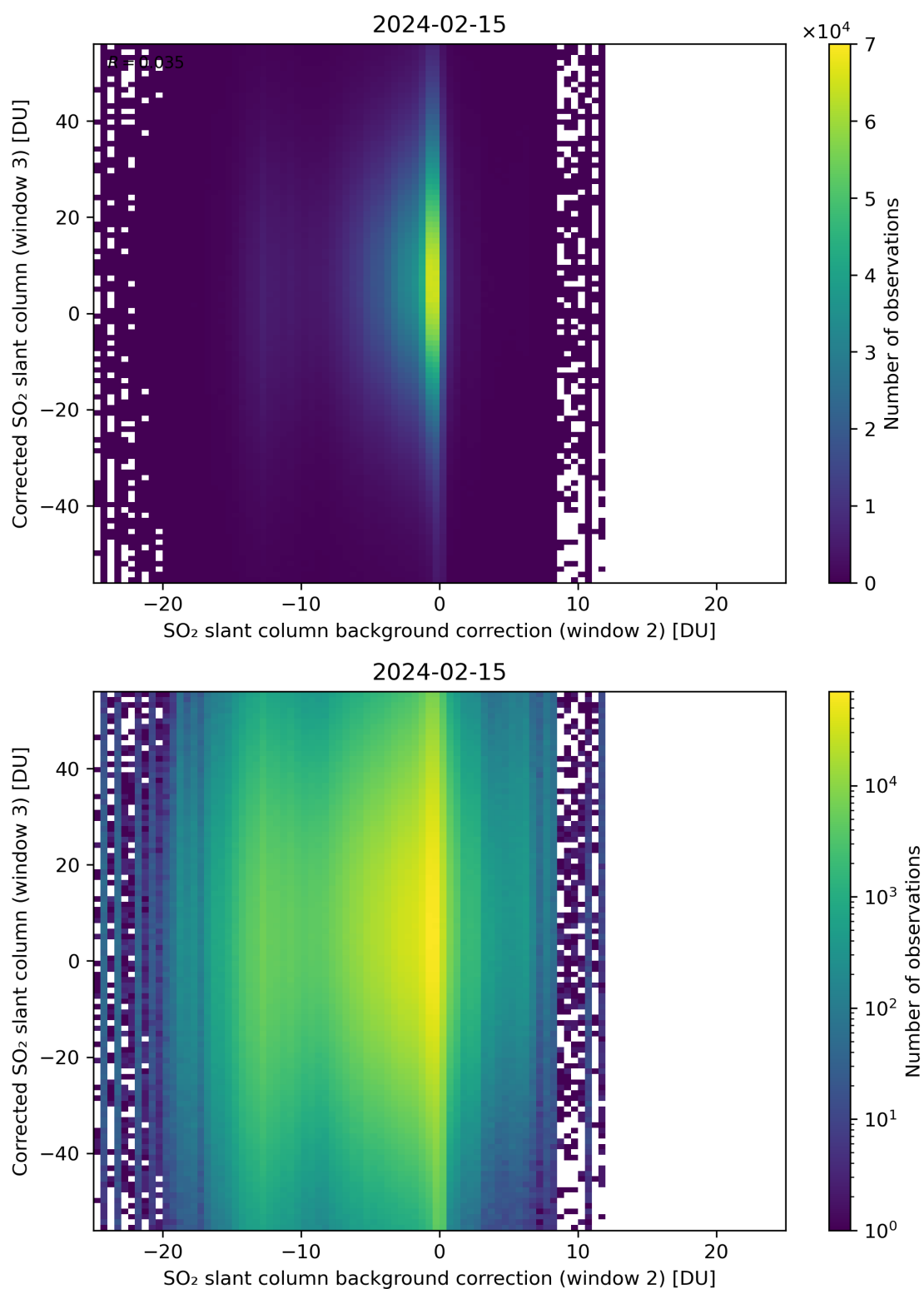
Figure 116: Scatter density plot of “SO 2 slant column background correction (window 2)” against “Corrected SO 2 slant column (window 3)” for 2024-02-14 to 2024-02-16.
