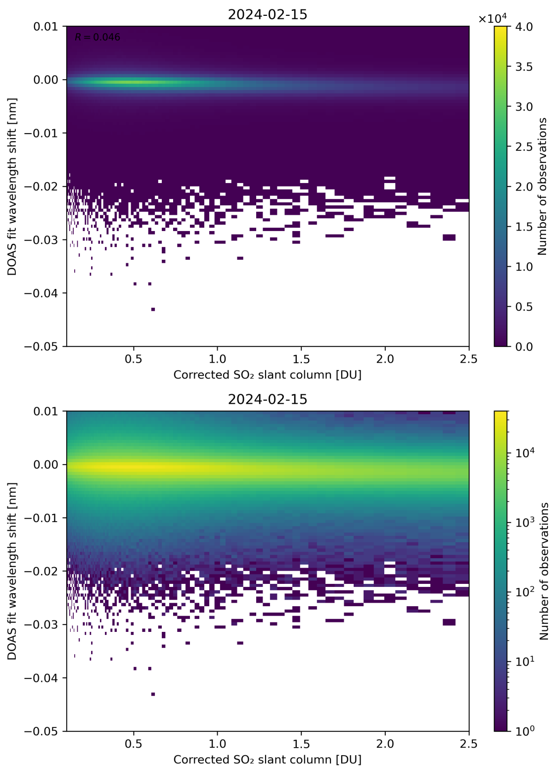
Figure 181: Scatter density plot of “Corrected SO 2 slant column” against “DOAS fit wavelength shift” for 2024-02-14 to 2024-02-16.
