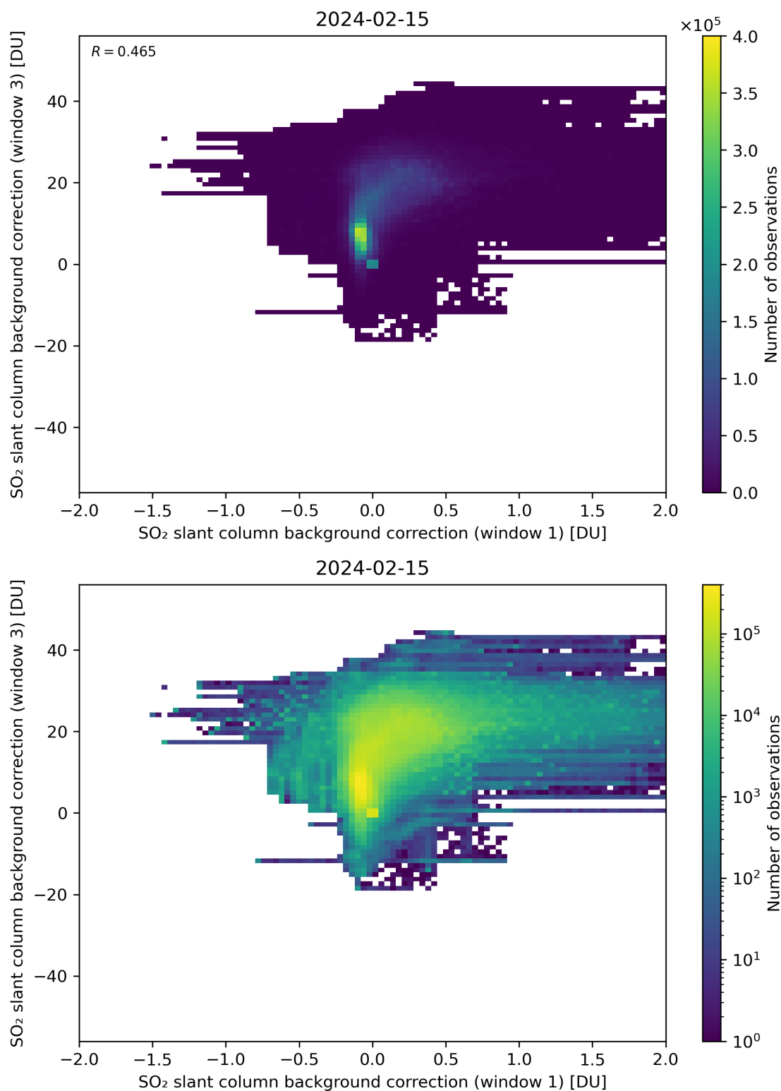
Figure 99: Scatter density plot of “SO 2 slant column background correction (window 1)” against “SO 2 slant column background correction (window 3)” for 2024-02-14 to 2024-02-16.
