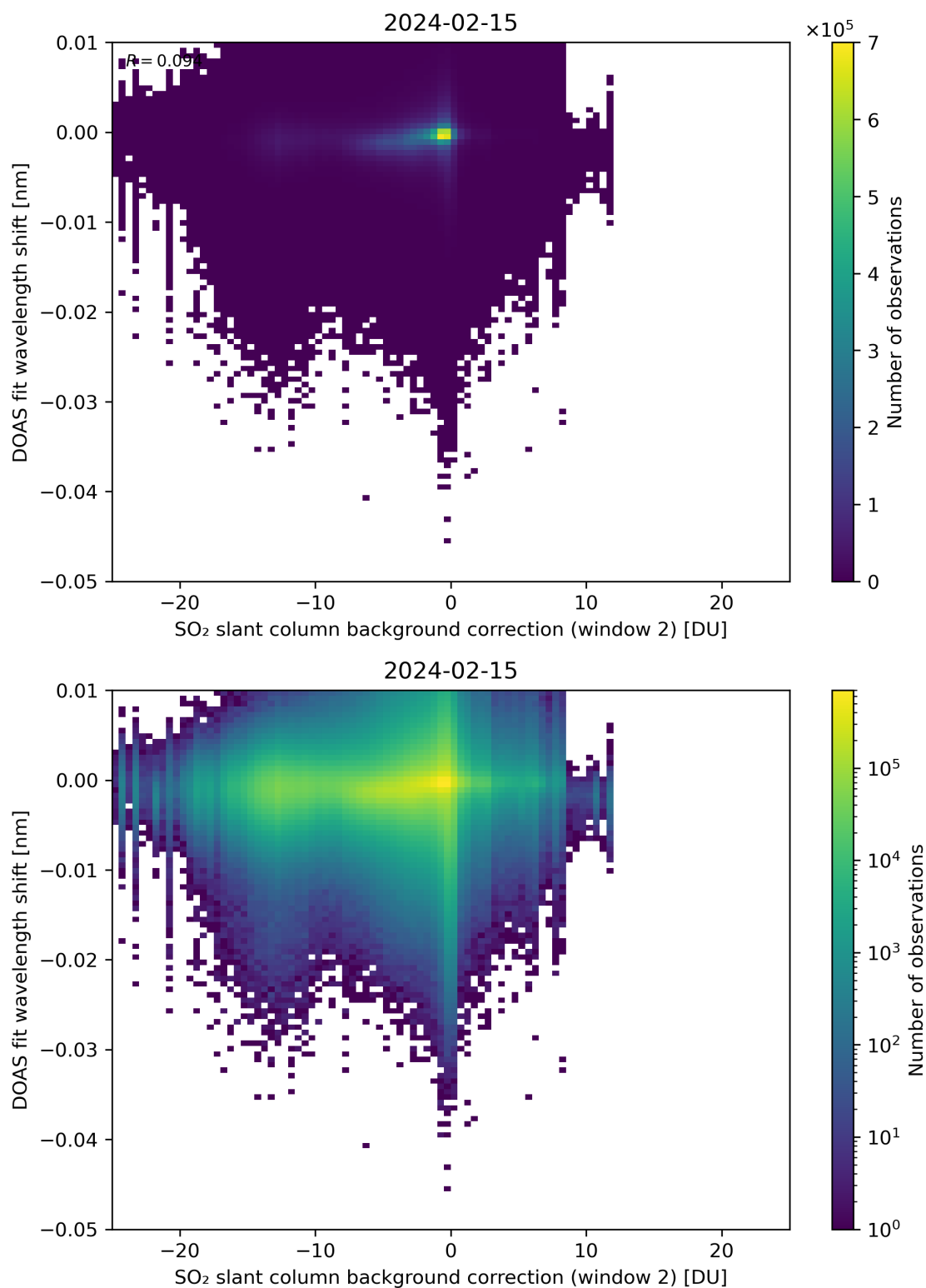
Figure 112: Scatter density plot of “SO 2 slant column background correction (window 2)” against “DOAS fit wavelength shift” for 2024-02-14 to 2024-02-16.
