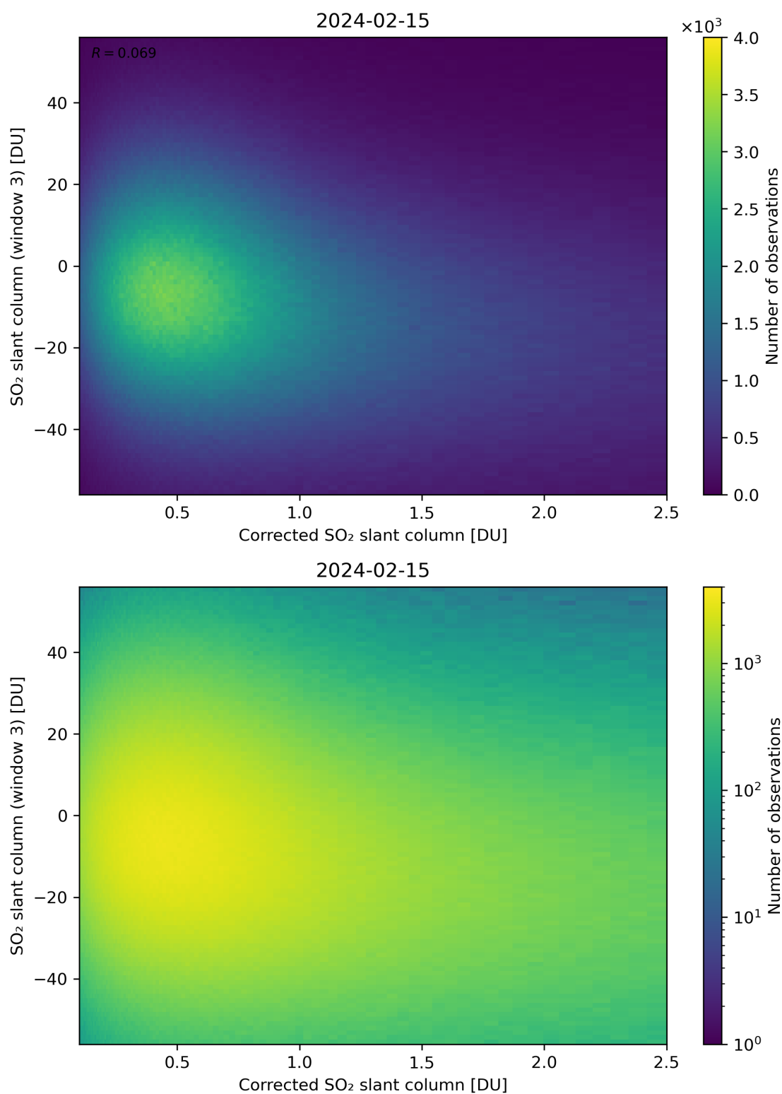
Figure 190: Scatter density plot of “Corrected SO 2 slant column” against “SO 2 slant column (window 3)” for 2024-02-14 to 2024-02-16.
