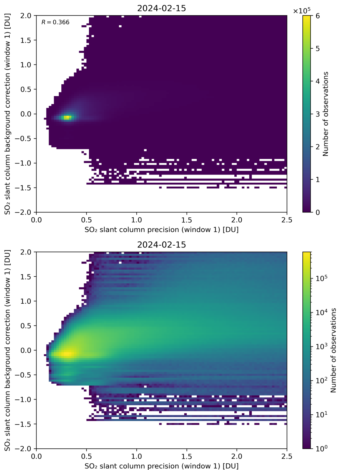
Figure 218: Scatter density plot of “SO 2 slant column precision (window 1)” against “SO 2 slant column background correction (window 1)” for 2024-02-14 to 2024-02-16.
