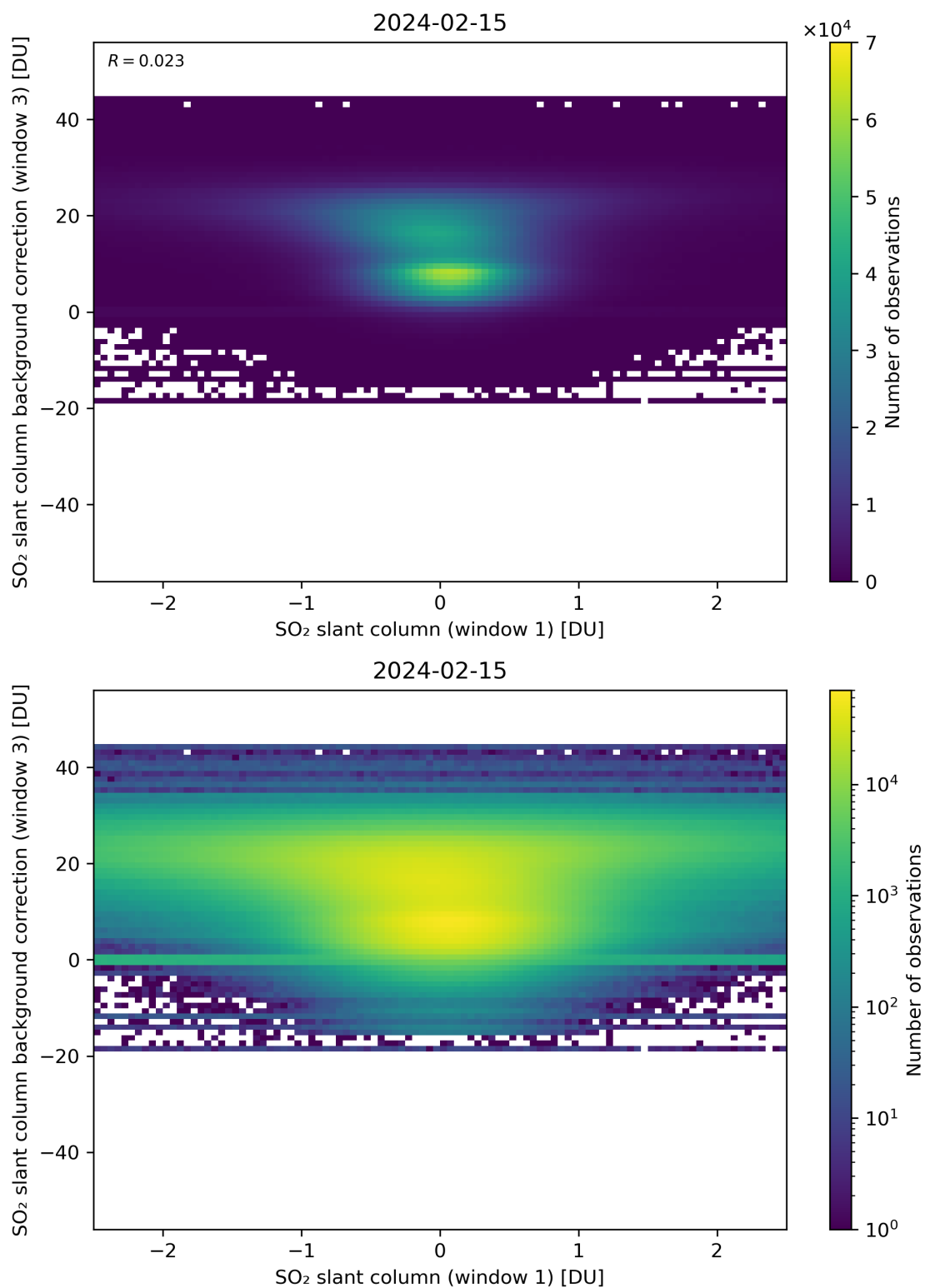
Figure 214: Scatter density plot of “SO 2 slant column (window 1)” against “SO 2 slant column background correction (window 3)” for 2024-02-14 to 2024-02-16.
