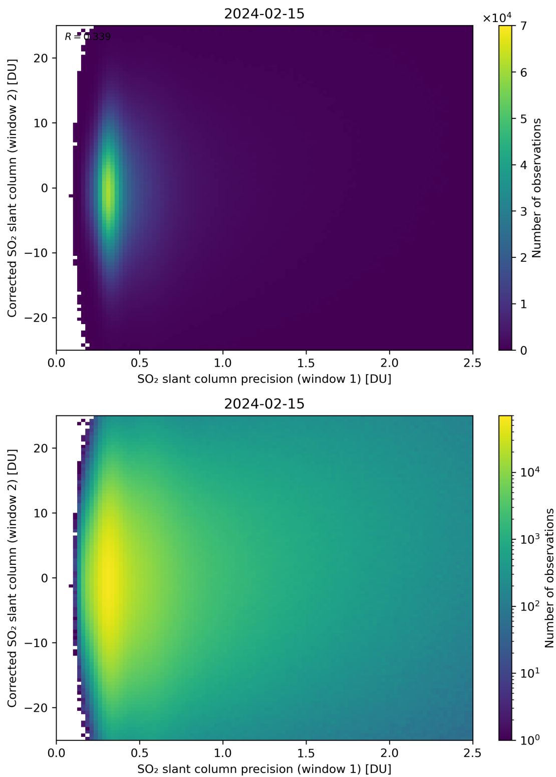
Figure 225: Scatter density plot of “SO 2 slant column precision (window 1)” against “Corrected SO 2 slant column (window 2)” for 2024-02-14 to 2024-02-16.
