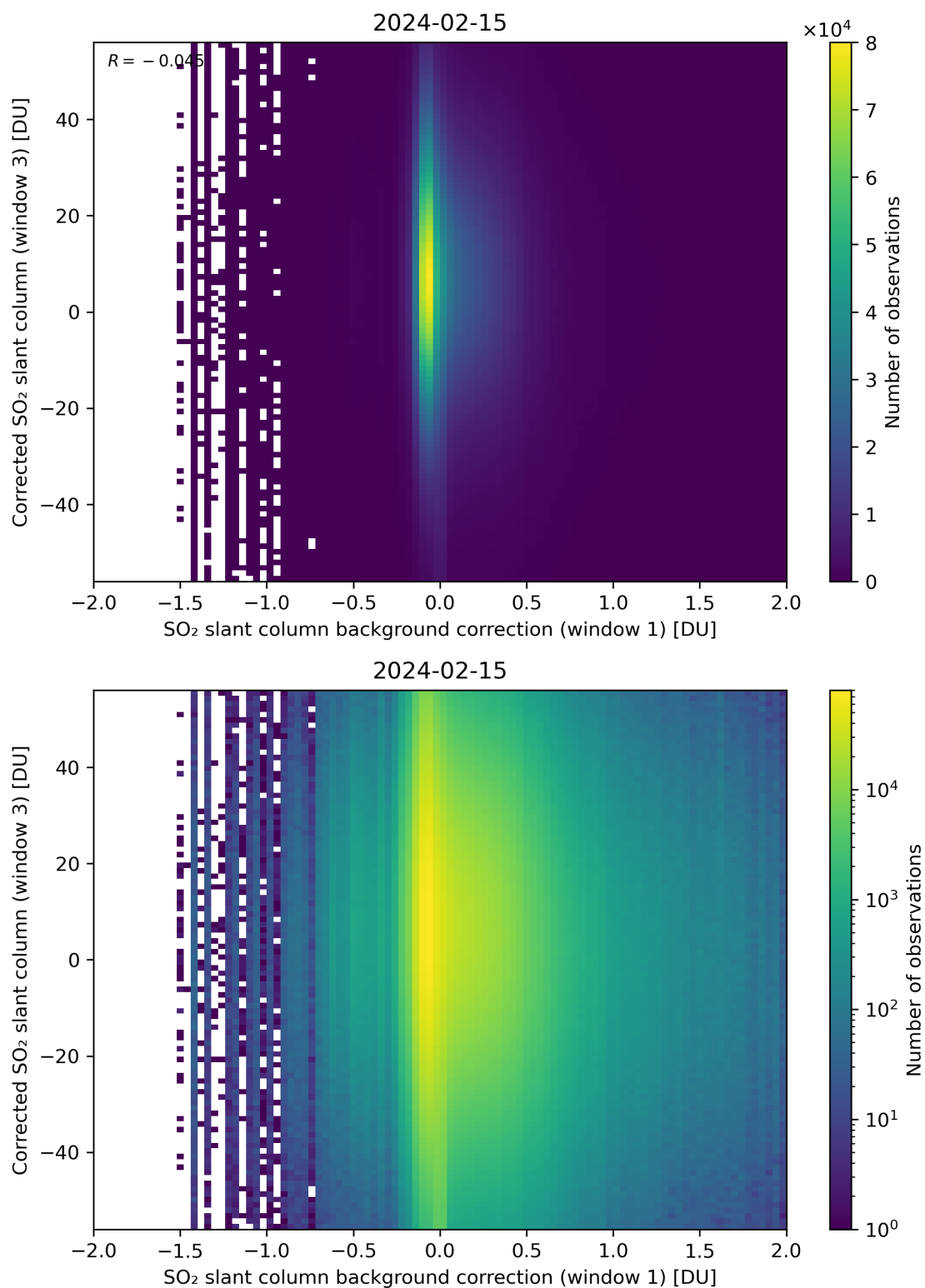
Figure 105: Scatter density plot of “SO 2 slant column background correction (window 1)” against “Corrected SO 2 slant column (window 3)” for 2024-02-14 to 2024-02-16.
