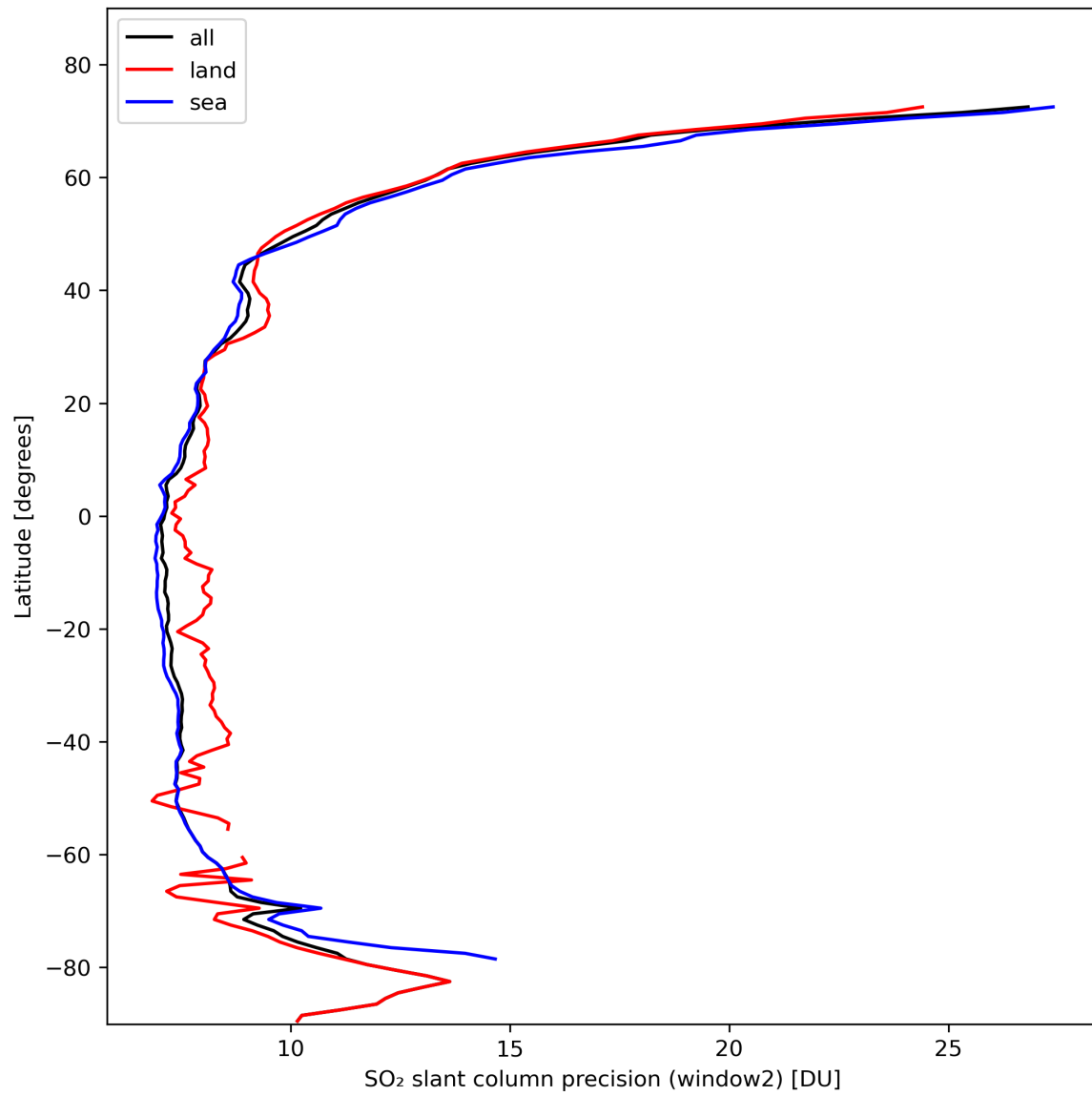
Figure 38: Zonal average of “SO 2 slant column precision (window2)” for 2024-02-14 to 2024-02-16.
