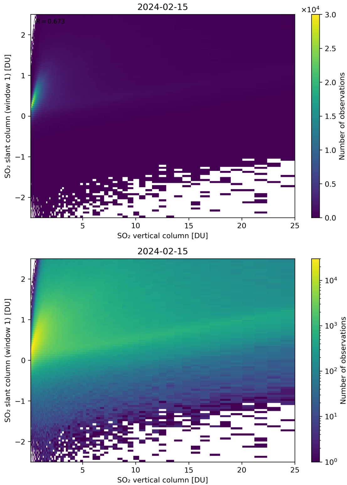
Figure 300: Scatter density plot of “SO 2 vertical column” against “SO 2 slant column (window 1)” for 2024-02-14 to 2024-02-16.
