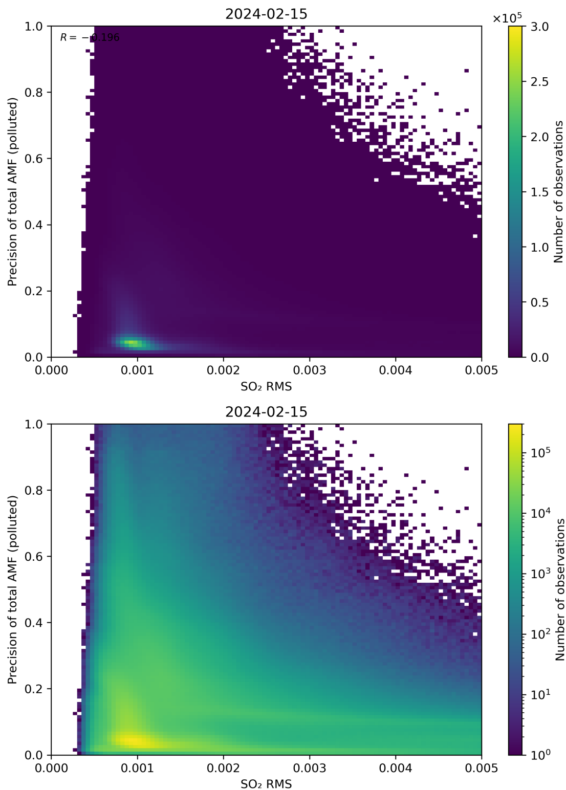
Figure 138: Scatter density plot of “SO 2 RMS” against “Precision of total AMF (polluted)” for 2024-02-14 to 2024-02-16.
