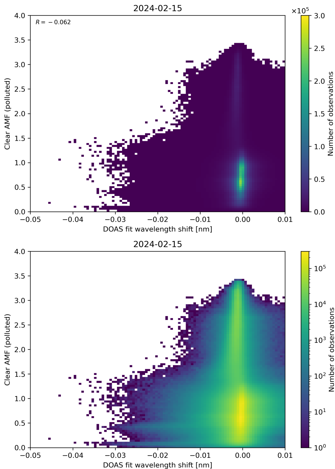
Figure 129: Scatter density plot of “DOAS fit wavelength shift” against “Clear AMF (polluted)” for 2024-02-14 to 2024-02-16.
