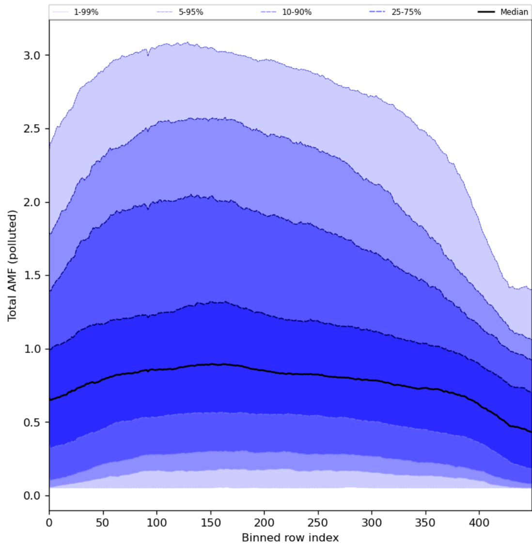
Figure 94: Along track statistics of “Total AMF (polluted)” for 2024-02-14 to 2024-02-16
