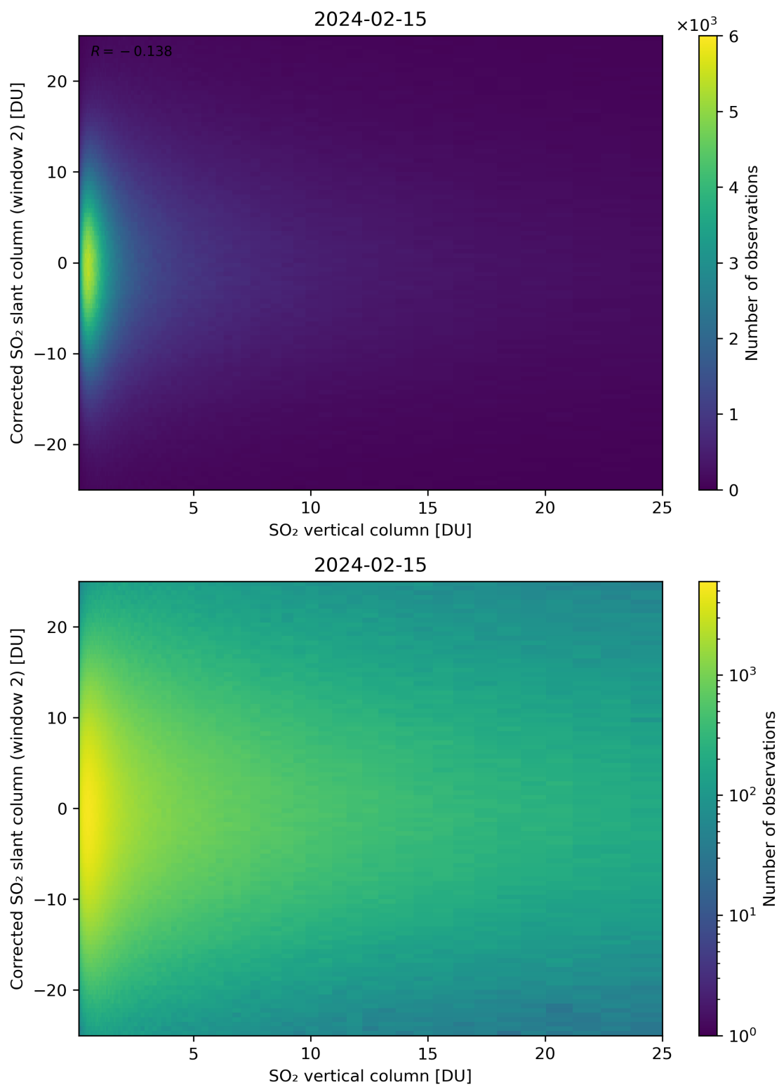
Figure 298: Scatter density plot of “SO 2 vertical column” against “Corrected SO 2 slant column (window 2)” for 2024-02-14 to 2024-02-16.
