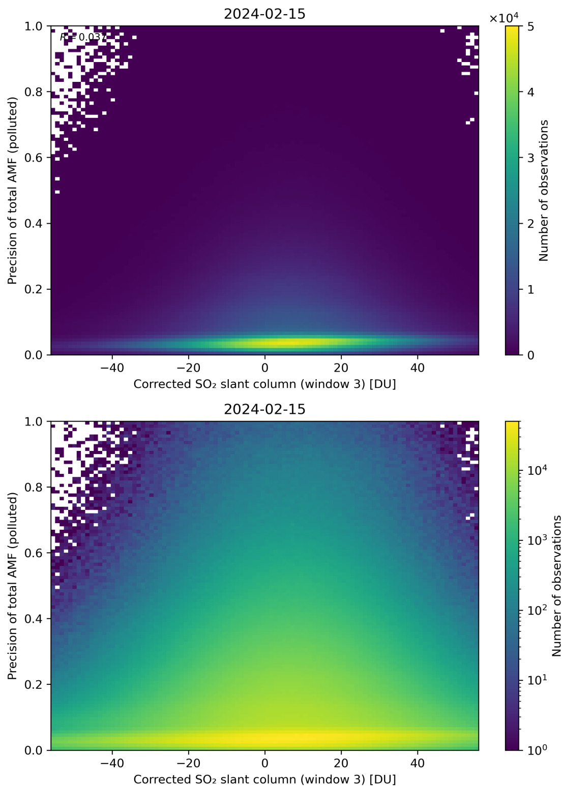
Figure 211: Scatter density plot of “Corrected SO 2 slant column (window 3)” against “Precision of total AMF (polluted)” for 2024-02-14 to 2024-02-16.
