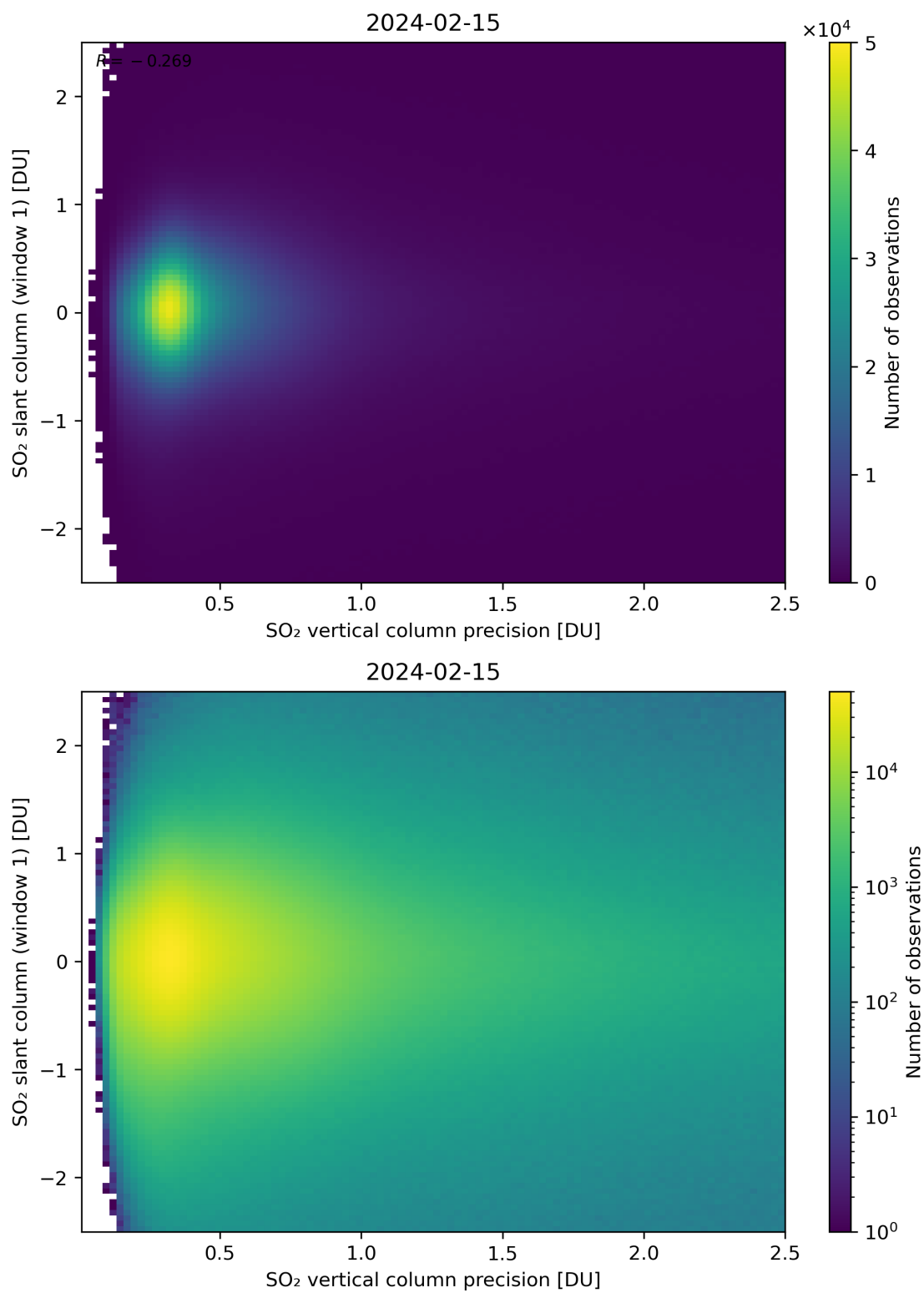
Figure 289: Scatter density plot of “SO 2 vertical column precision” against “SO 2 slant column (window 1)” for 2024-02-14 to 2024-02-16.
