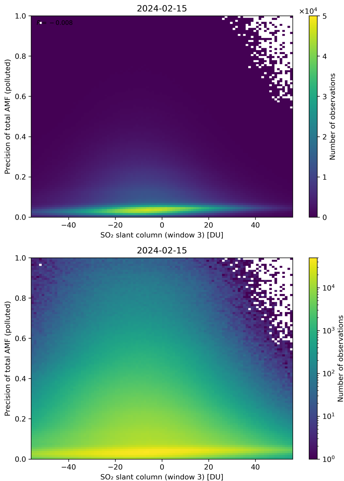
Figure 269: Scatter density plot of “SO 2 slant column (window 3)” against “Precision of total AMF (polluted)” for 2024-02-14 to 2024-02-16.
