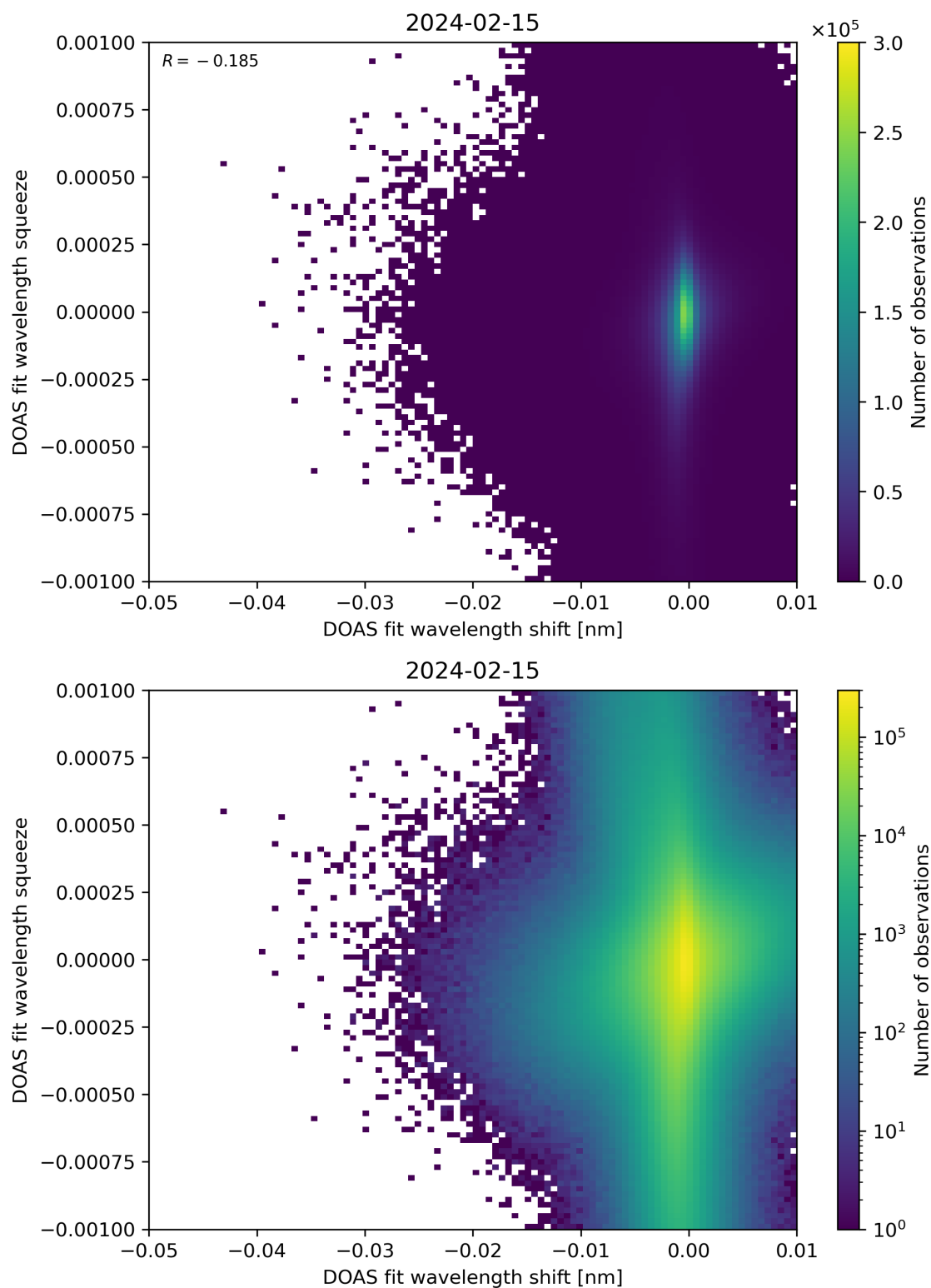
Figure 127: Scatter density plot of “DOAS fit wavelength shift” against “DOAS fit wavelength squeeze” for 2024-02-14 to 2024-02-16.
