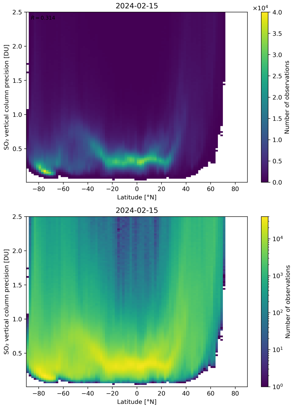
Figure 157: Scatter density plot of “Latitude” against “SO 2 vertical column precision” for 2024-02-14 to 2024-02-16.
