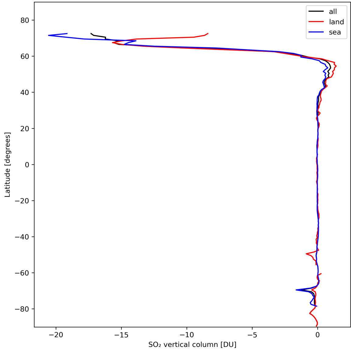
Figure 30: Zonal average of “SO 2 vertical column” for 2024-02-14 to 2024-02-16.
