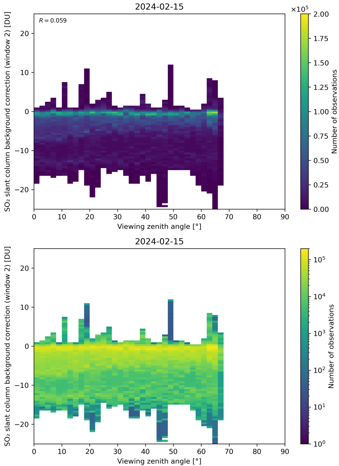
Figure 309: Scatter density plot of “Viewing zenith angle” against “SO 2 slant column background correction (window 2)” for 2024-02-14 to 2024-02-16.
