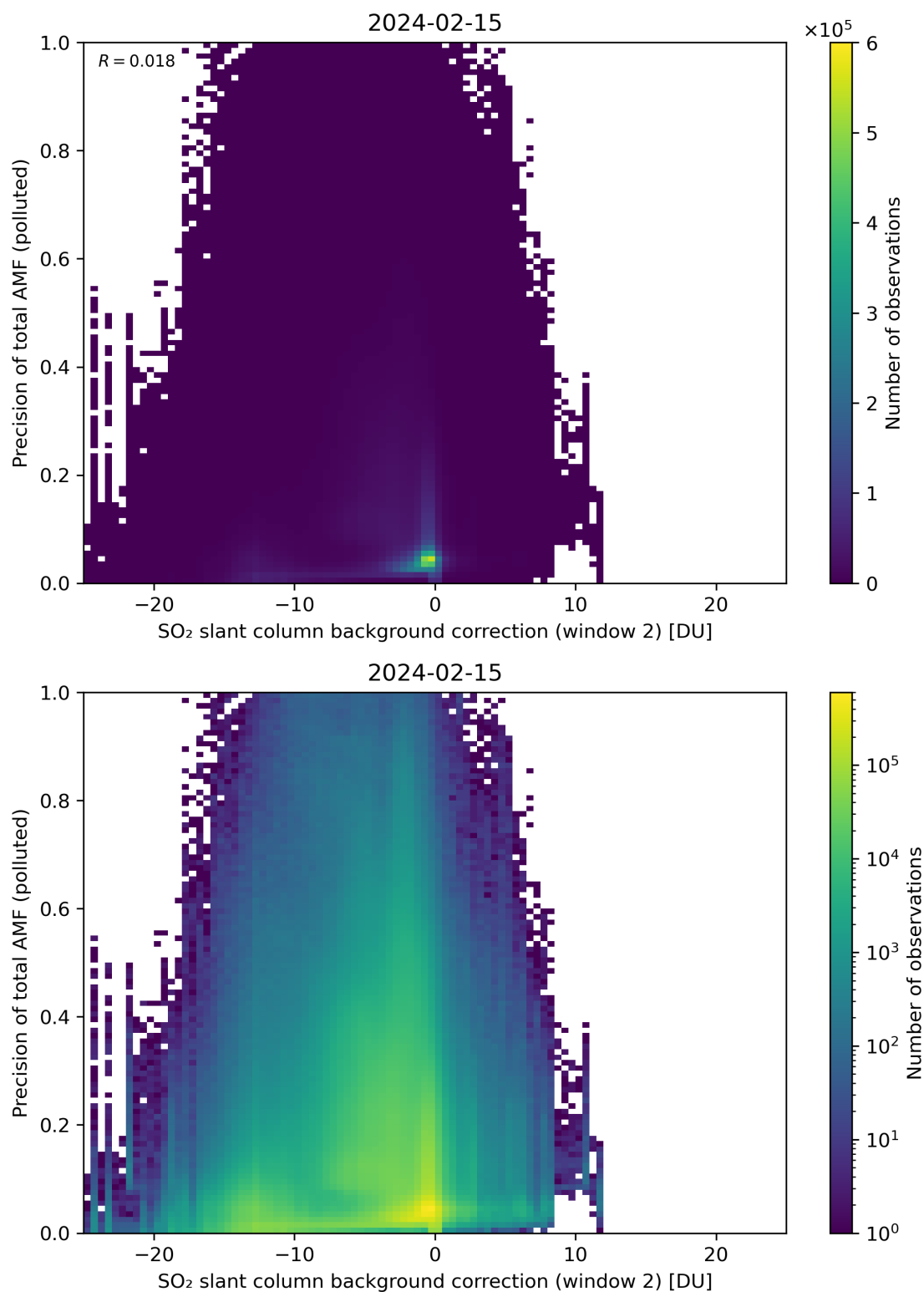
Figure 120: Scatter density plot of “SO 2 slant column background correction (window 2)” against “Precision of total AMF (polluted)” for 2024-02-14 to 2024-02-16.
