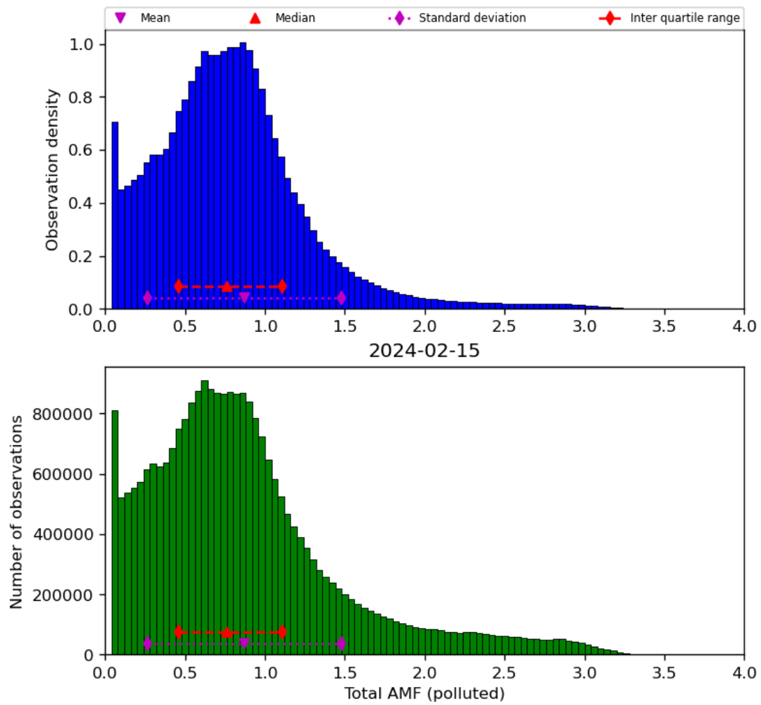
Figure 71: Histogram of “Total AMF (polluted)” for 2024-02-14 to 2024-02-16
