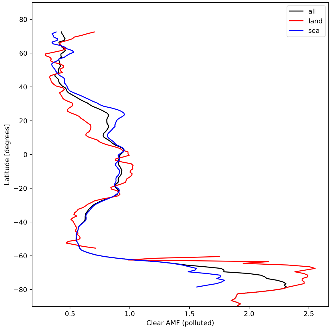
Figure 50: Zonal average of “Clear AMF (polluted)” for 2024-02-14 to 2024-02-16.
