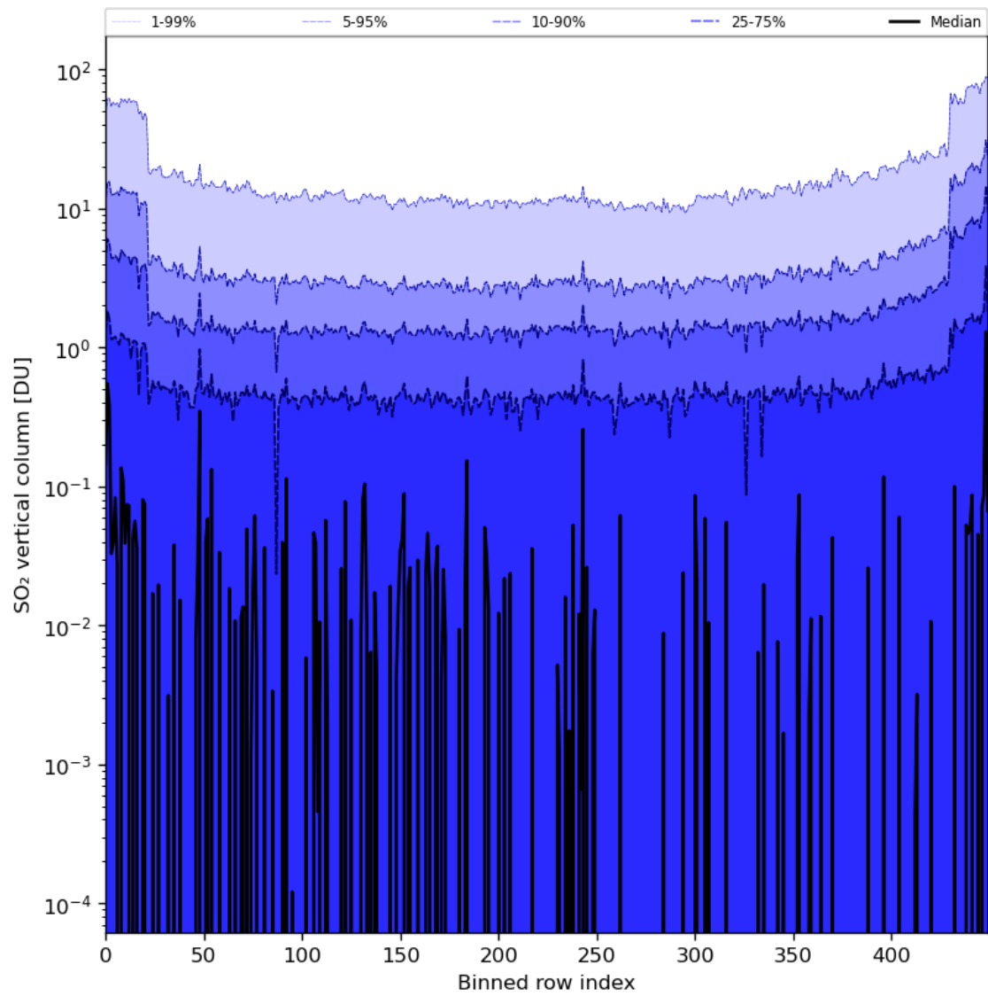
Figure 76: Along track statistics of “SO 2 vertical column” for 2024-02-14 to 2024-02-16
