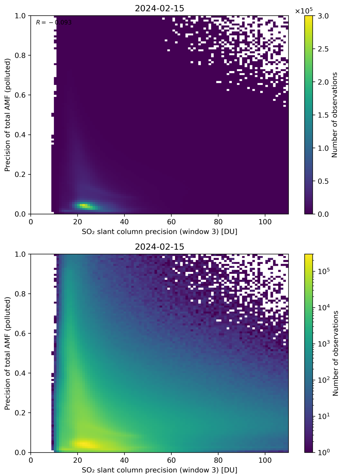
Figure 264: Scatter density plot of “SO 2 slant column precision (window 3)” against “Precision of total AMF (polluted)” for 2024-02-14 to 2024-02-16.
