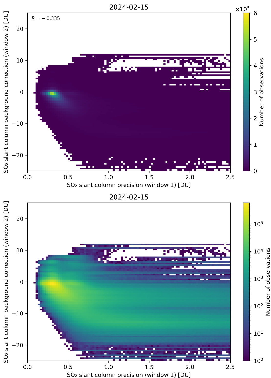
Figure 219: Scatter density plot of “SO 2 slant column precision (window 1)” against “SO 2 slant column background correction (window 2)” for 2024-02-14 to 2024-02-16.
