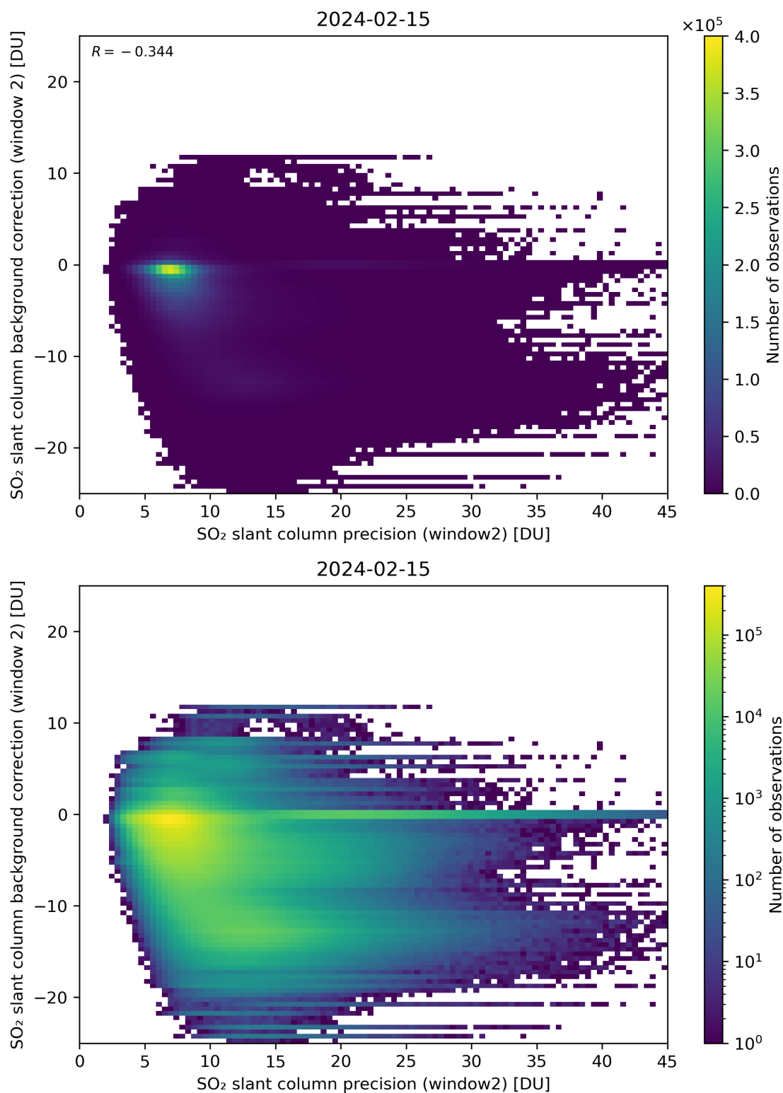
Figure 241: Scatter density plot of “SO 2 slant column precision (window2)” against “SO 2 slant column background correction (window 2)” for 2024-02-14 to 2024-02-16.
