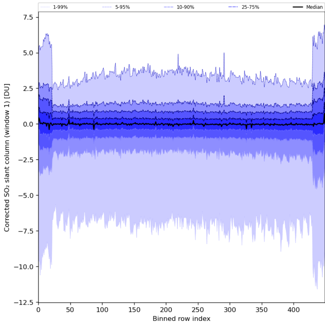
Figure 81: Along track statistics of “Corrected SO 2 slant column (window 1)” for 2024-02-14 to 2024-02-16
