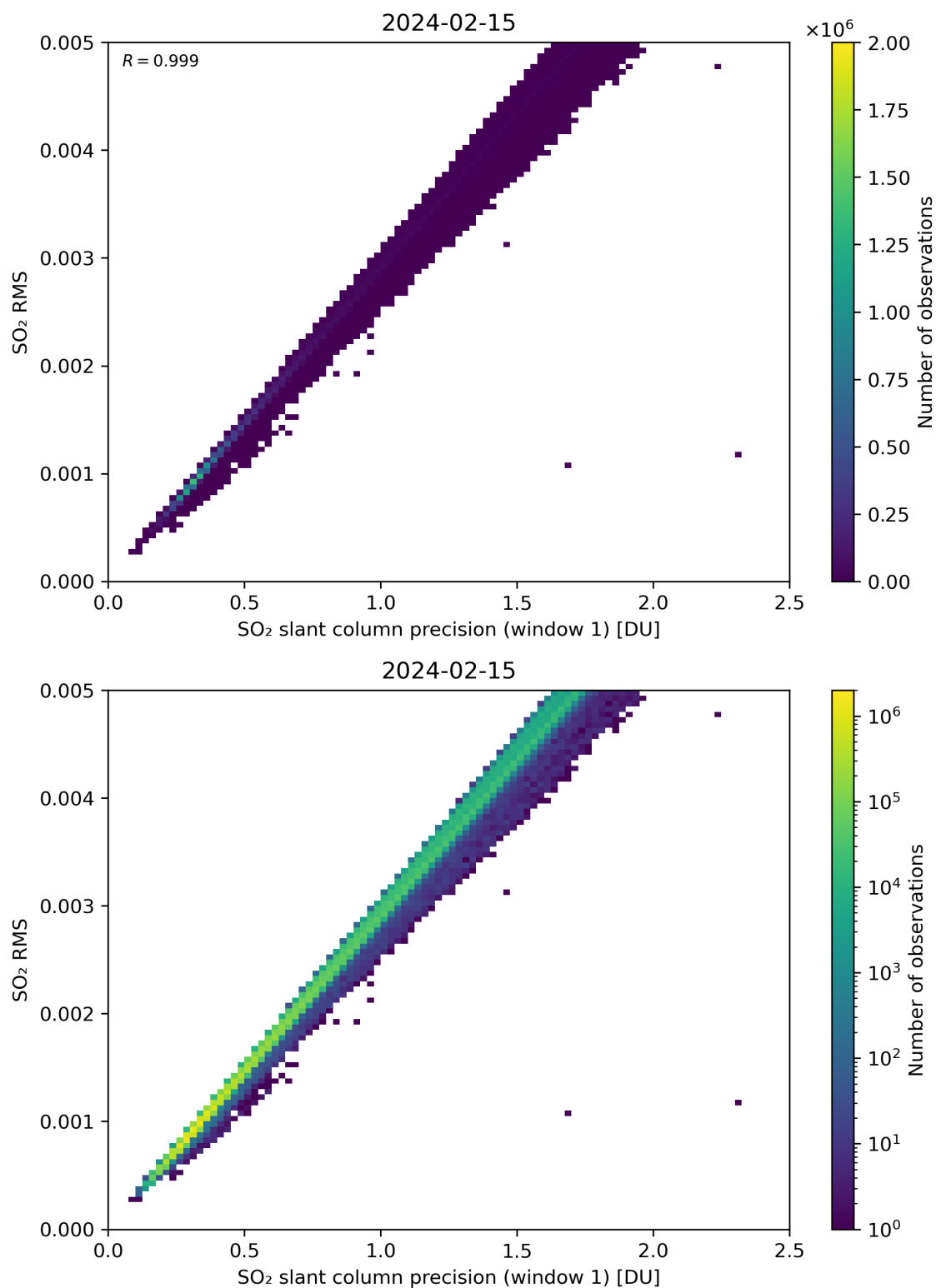
Figure 223: Scatter density plot of “SO 2 slant column precision (window 1)” against “SO 2 RMS” for 2024-02-14 to 2024-02-16.
