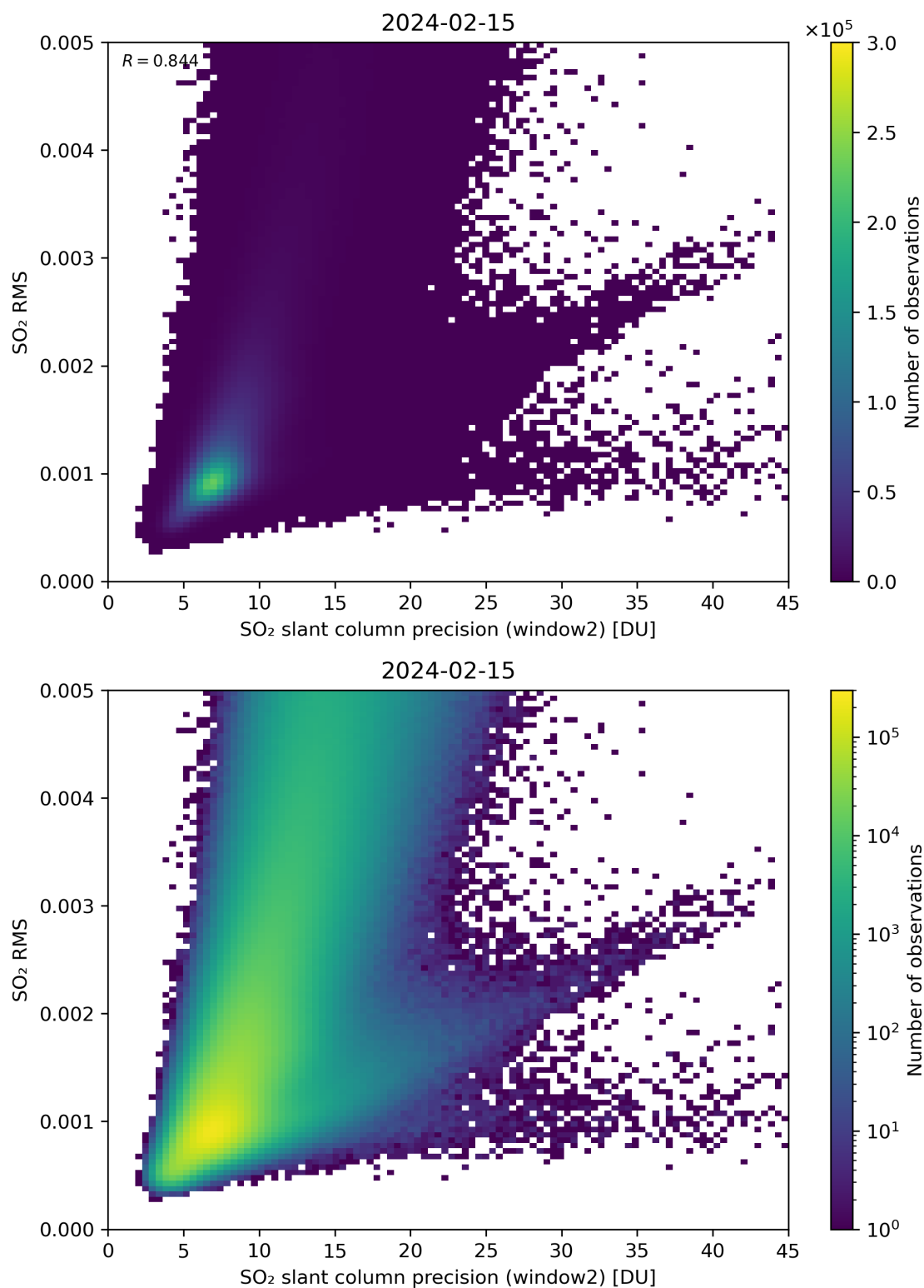
Figure 245: Scatter density plot of “SO 2 slant column precision (window2)” against “SO 2 RMS” for 2024-02-14 to 2024-02-16.
