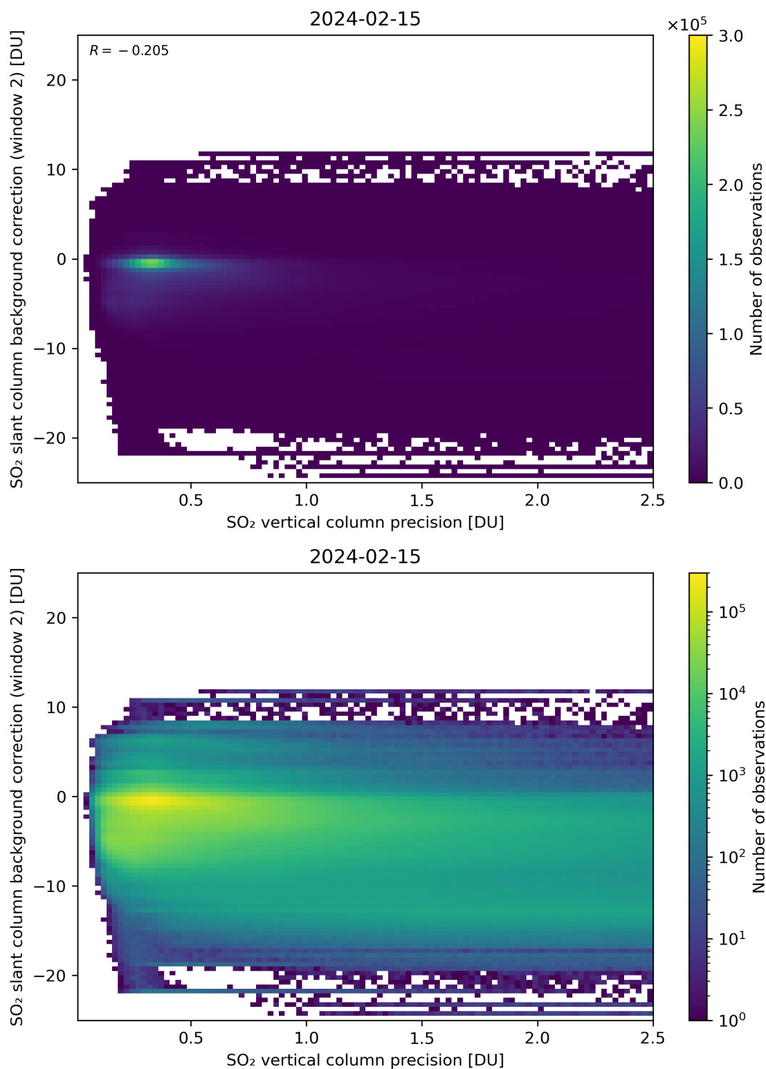
Figure 280: Scatter density plot of “SO 2 vertical column precision” against “SO 2 slant column background correction (window 2)” for 2024-02-14 to 2024-02-16.
