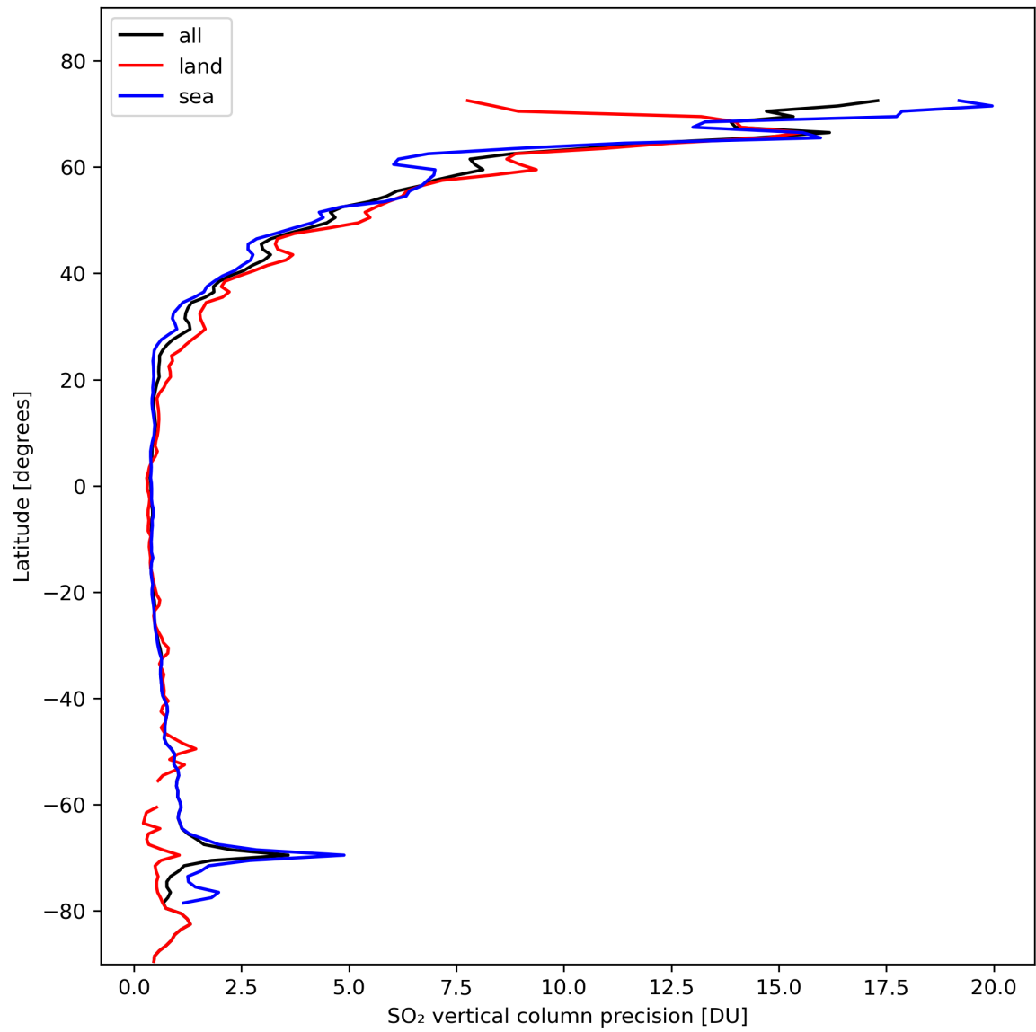
Figure 31: Zonal average of “SO 2 vertical column precision” for 2024-02-14 to 2024-02-16.
