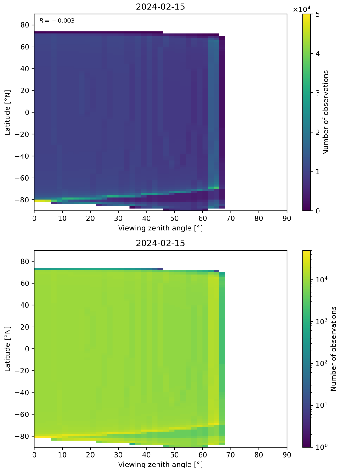
Figure 314: Scatter density plot of “Viewing zenith angle” against “Latitude” for 2024-02-14 to 2024-02-16.
