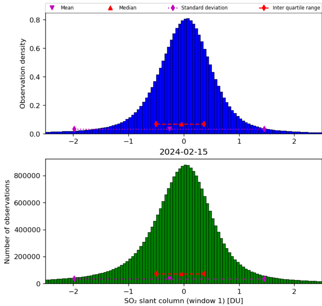
Figure 56: Histogram of “SO 2 slant column (window 1)” for 2024-02-14 to 2024-02-16
