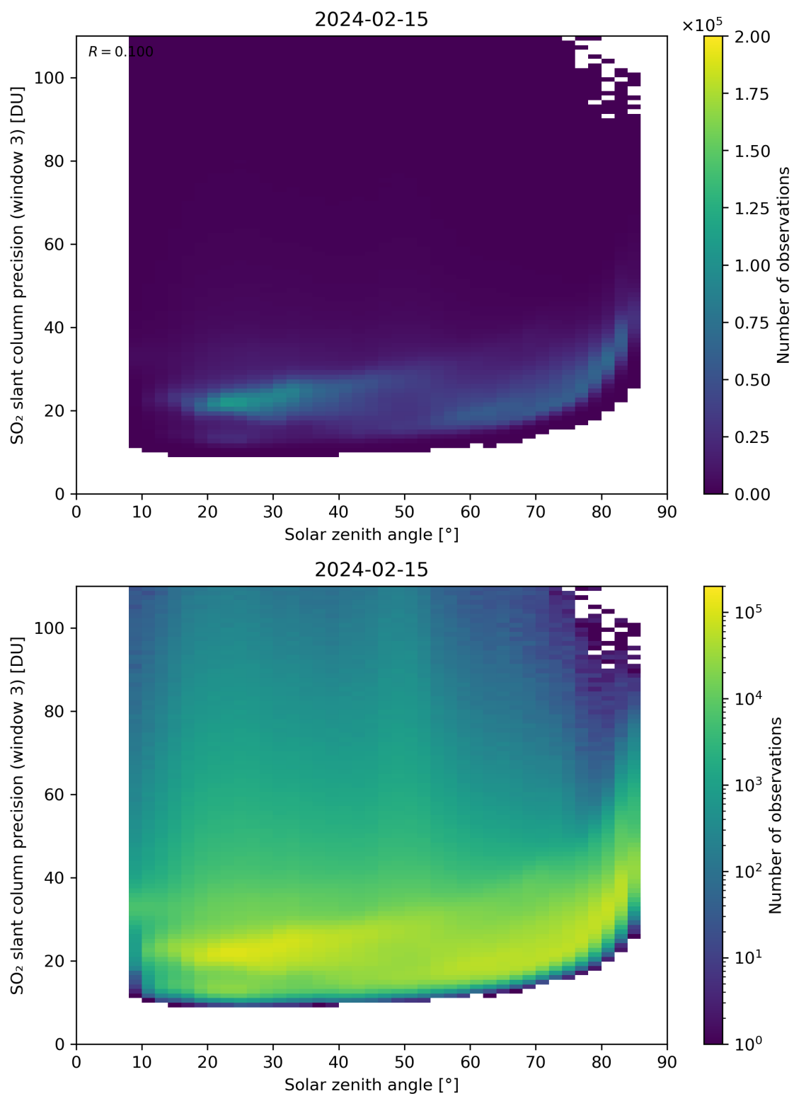
Figure 173: Scatter density plot of “Solar zenith angle” against “SO 2 slant column precision (window 3)” for 2024-02-14 to 2024-02-16.
