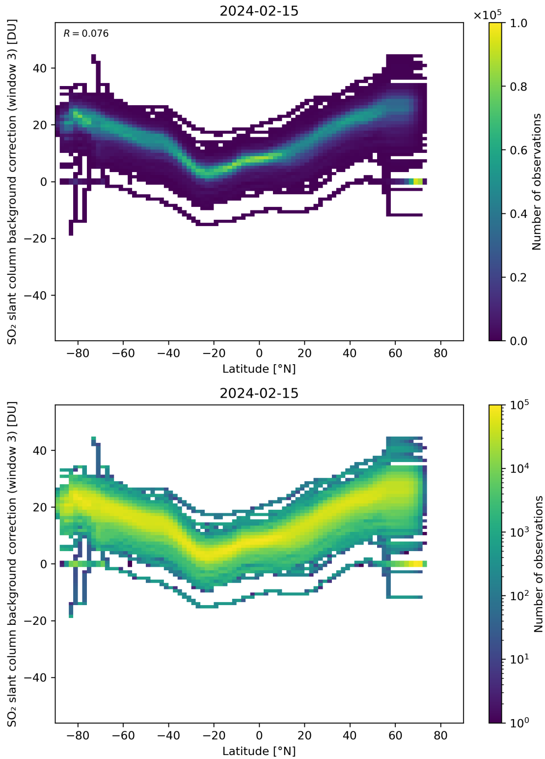
Figure 141: Scatter density plot of “Latitude” against “SO 2 slant column background correction (window 3)” for 2024-02-14 to 2024-02-16.
