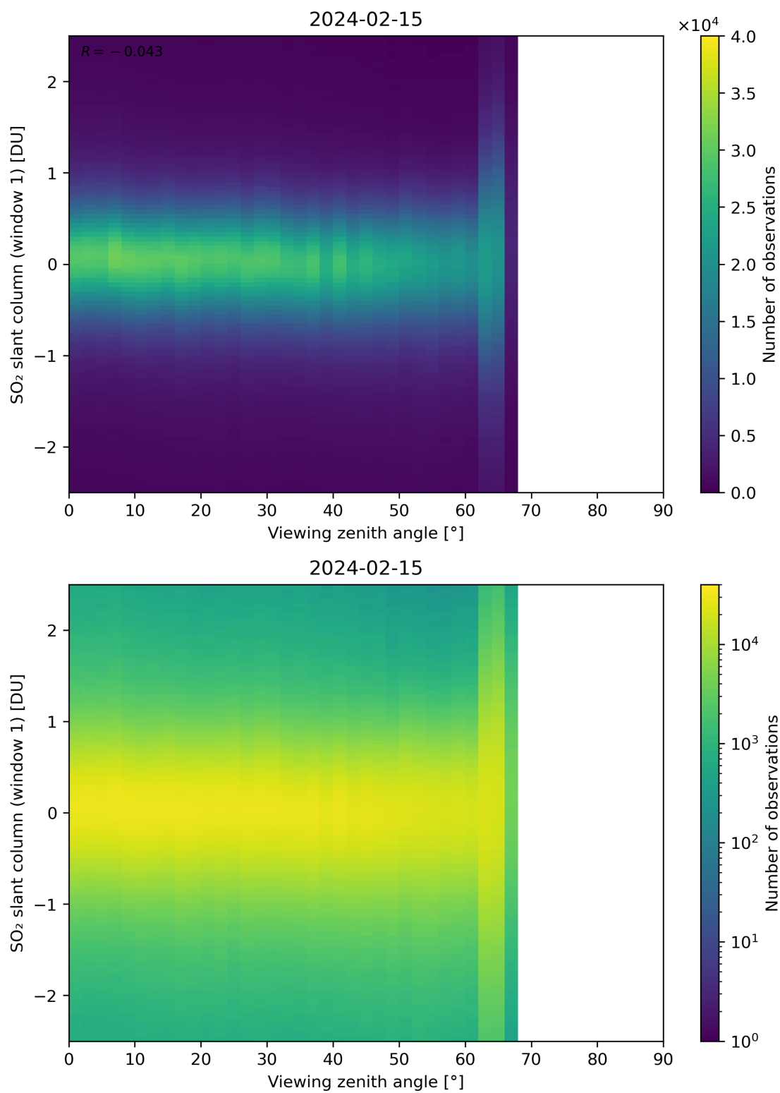
Figure 320: Scatter density plot of “Viewing zenith angle” against “SO 2 slant column (window 1)” for 2024-02-14 to 2024-02-16.
