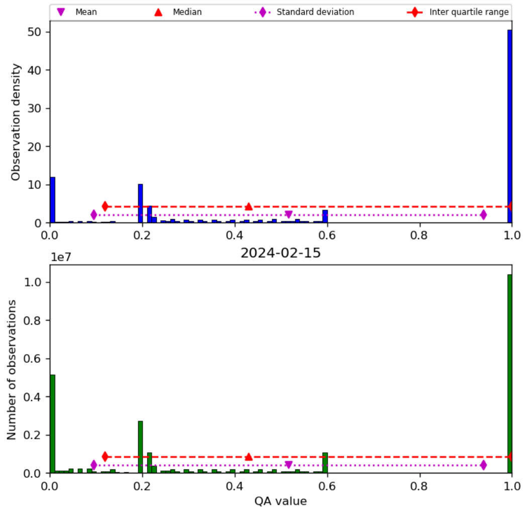
Figure 52: Histogram of “QA value” for 2024-02-14 to 2024-02-16
