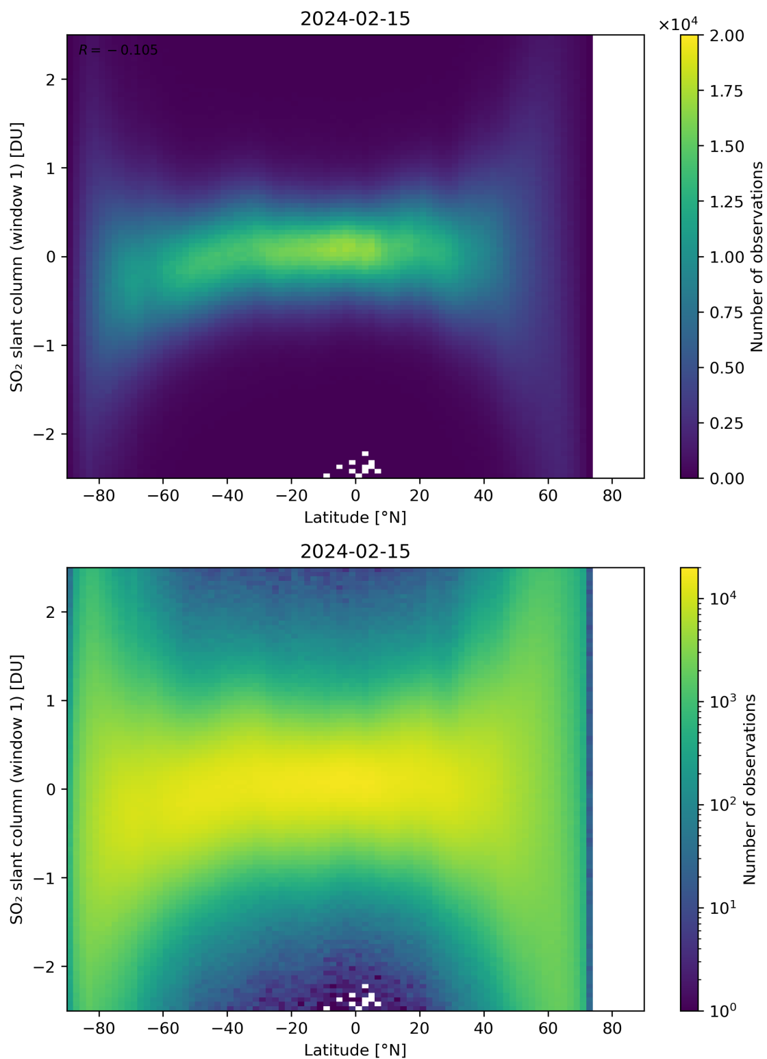
Figure 149: Scatter density plot of “Latitude” against “SO 2 slant column (window 1)” for 2024-02-14 to 2024-02-16.
