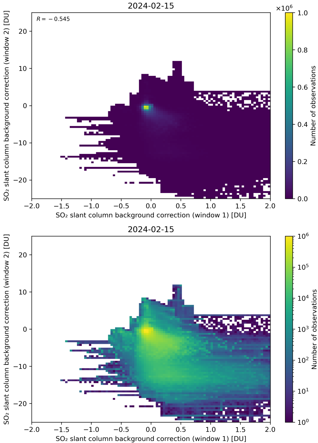
Figure 98: Scatter density plot of “SO 2 slant column background correction (window 1)” against “SO 2 slant column background correction (window 2)” for 2024-02-14 to 2024-02-16.
