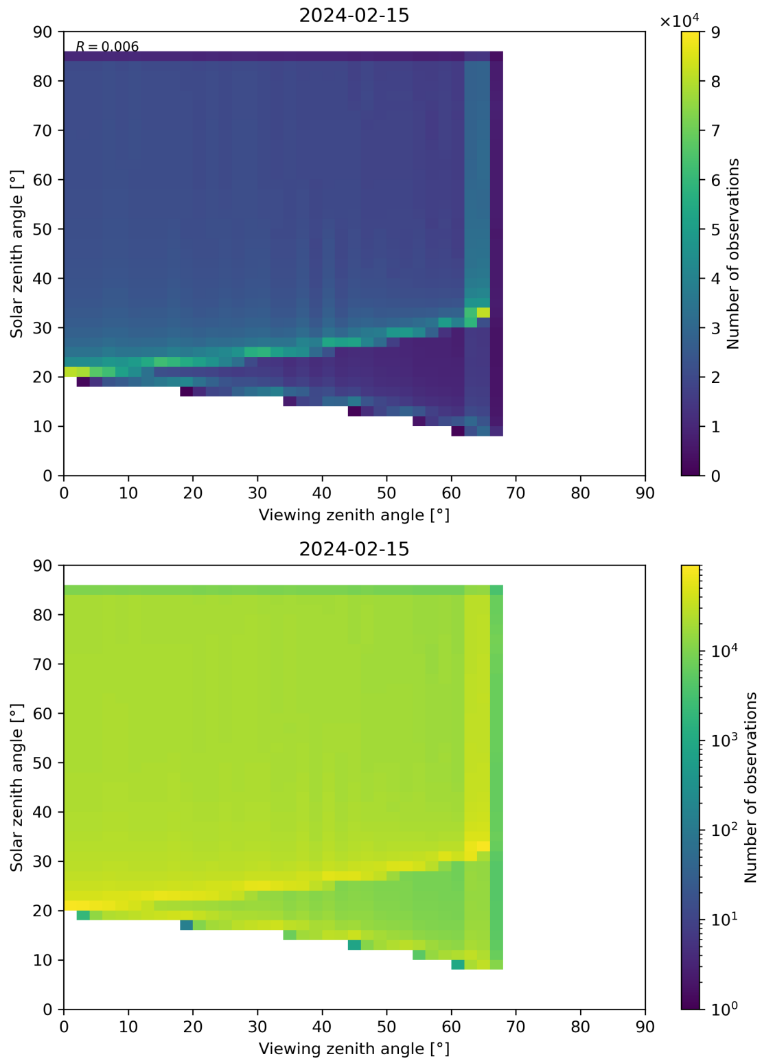
Figure 315: Scatter density plot of “Viewing zenith angle” against “Solar zenith angle” for 2024-02-14 to 2024-02-16.
