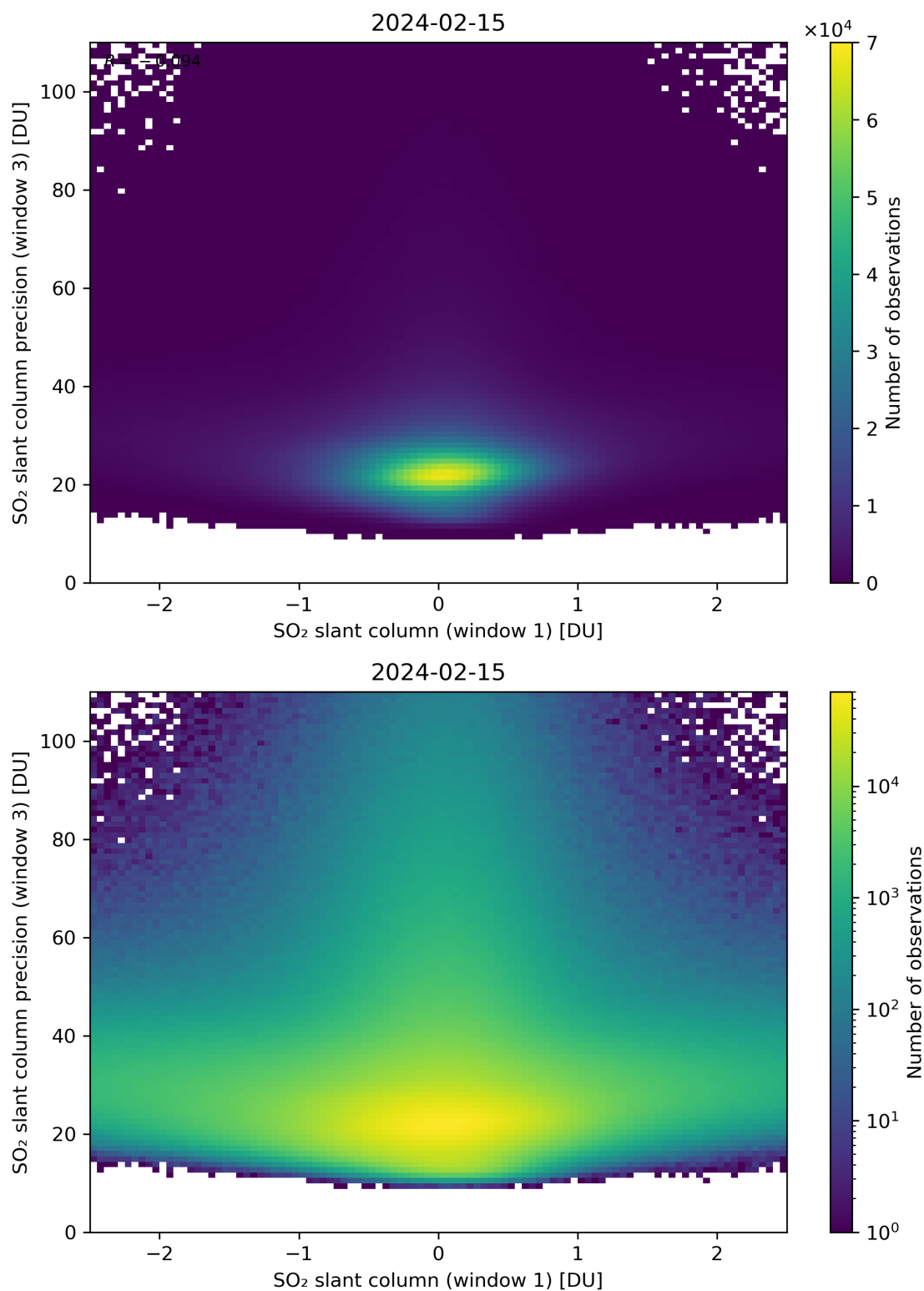
Figure 238: Scatter density plot of “SO 2 slant column (window 1)” against “SO 2 slant column precision (window 3)” for 2024-02-14 to 2024-02-16.
