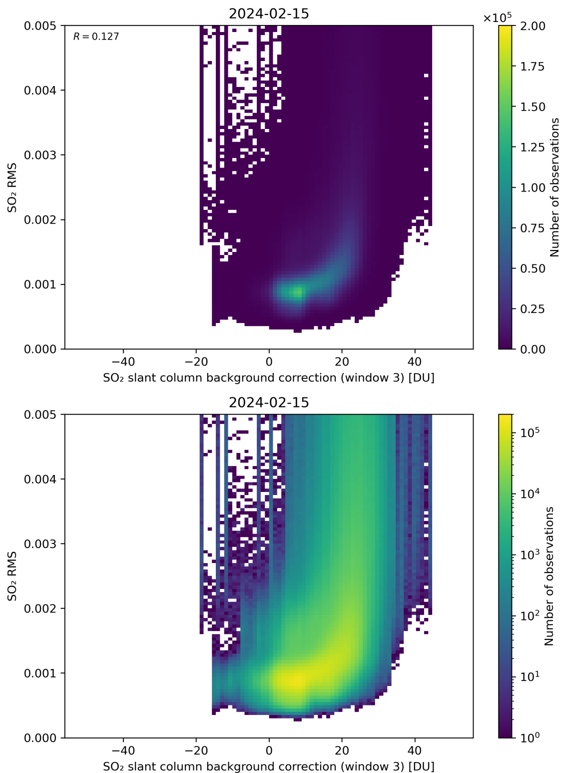
Figure 123: Scatter density plot of “SO 2 slant column background correction (window 3)” against “SO 2 RMS” for 2024-02-14 to 2024-02-16.
