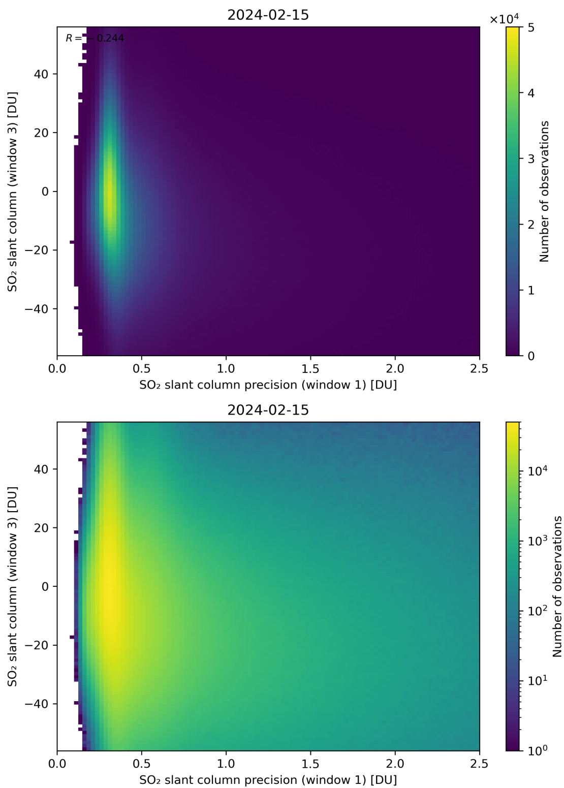
Figure 228: Scatter density plot of “SO 2 slant column precision (window 1)” against “SO 2 slant column (window 3)” for 2024-02-14 to 2024-02-16.
