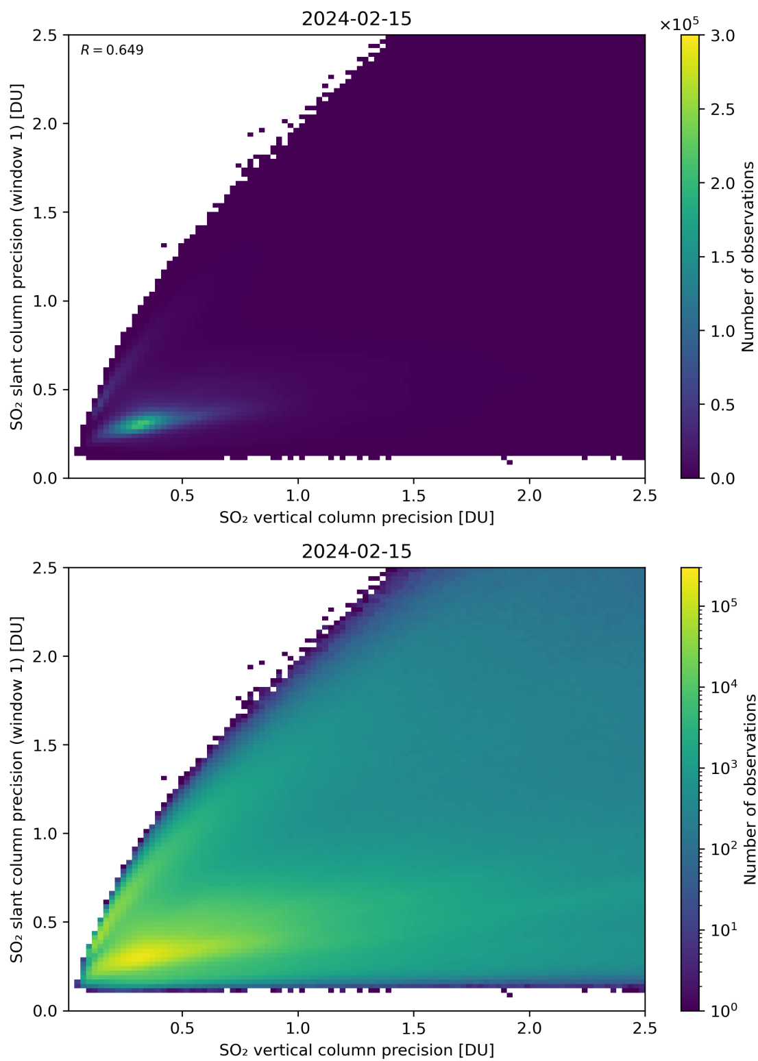
Figure 290: Scatter density plot of “SO 2 vertical column precision” against “SO 2 slant column precision (window 1)” for 2024-02-14 to 2024-02-16.
