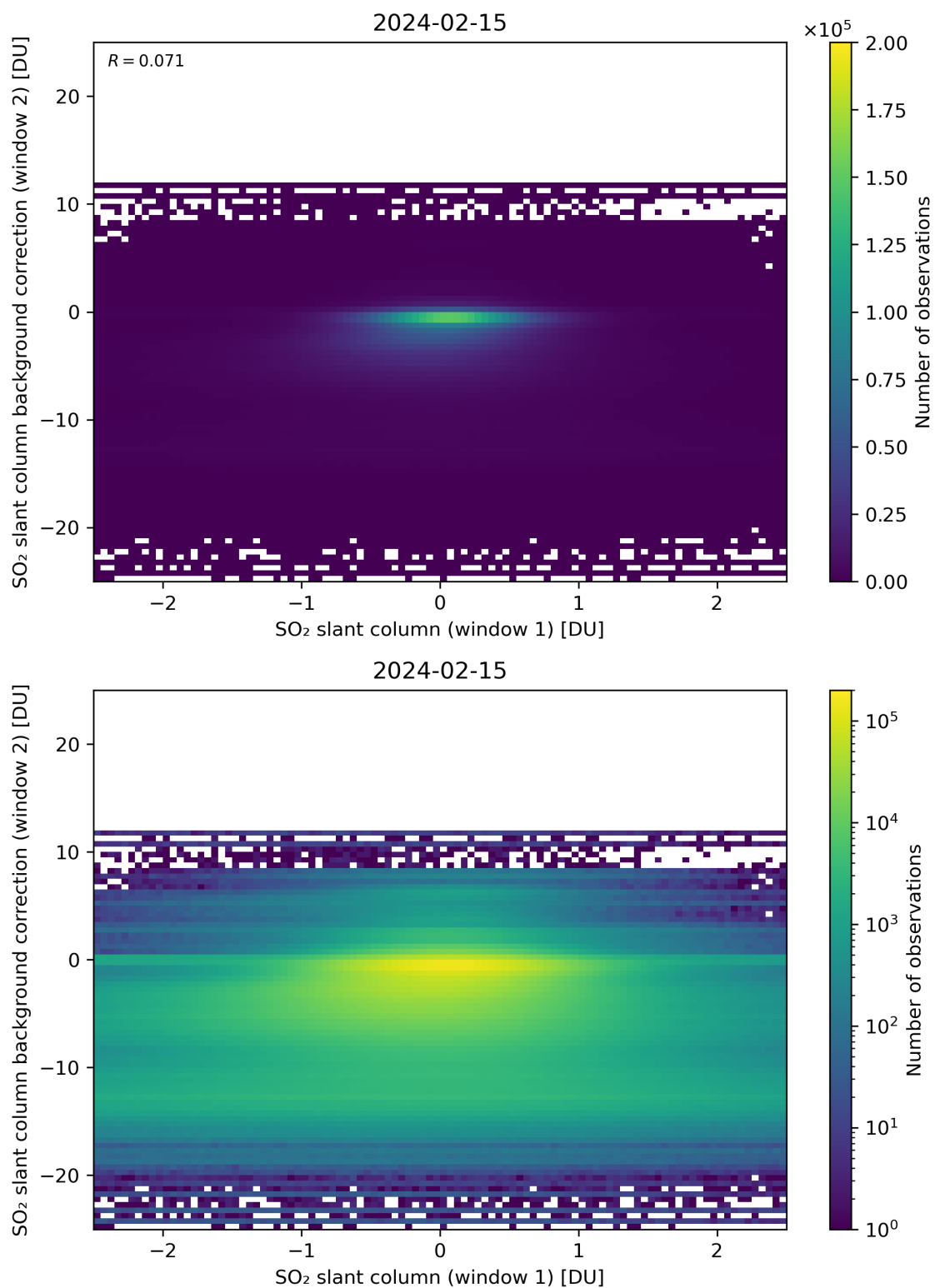
Figure 213: Scatter density plot of “SO 2 slant column (window 1)” against “SO 2 slant column background correction (window 2)” for 2024-02-14 to 2024-02-16.
