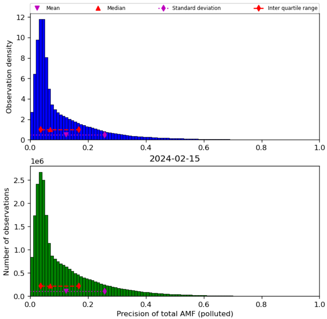
Figure 72: Histogram of “Precision of total AMF (polluted)” for 2024-02-14 to 2024-02-16
