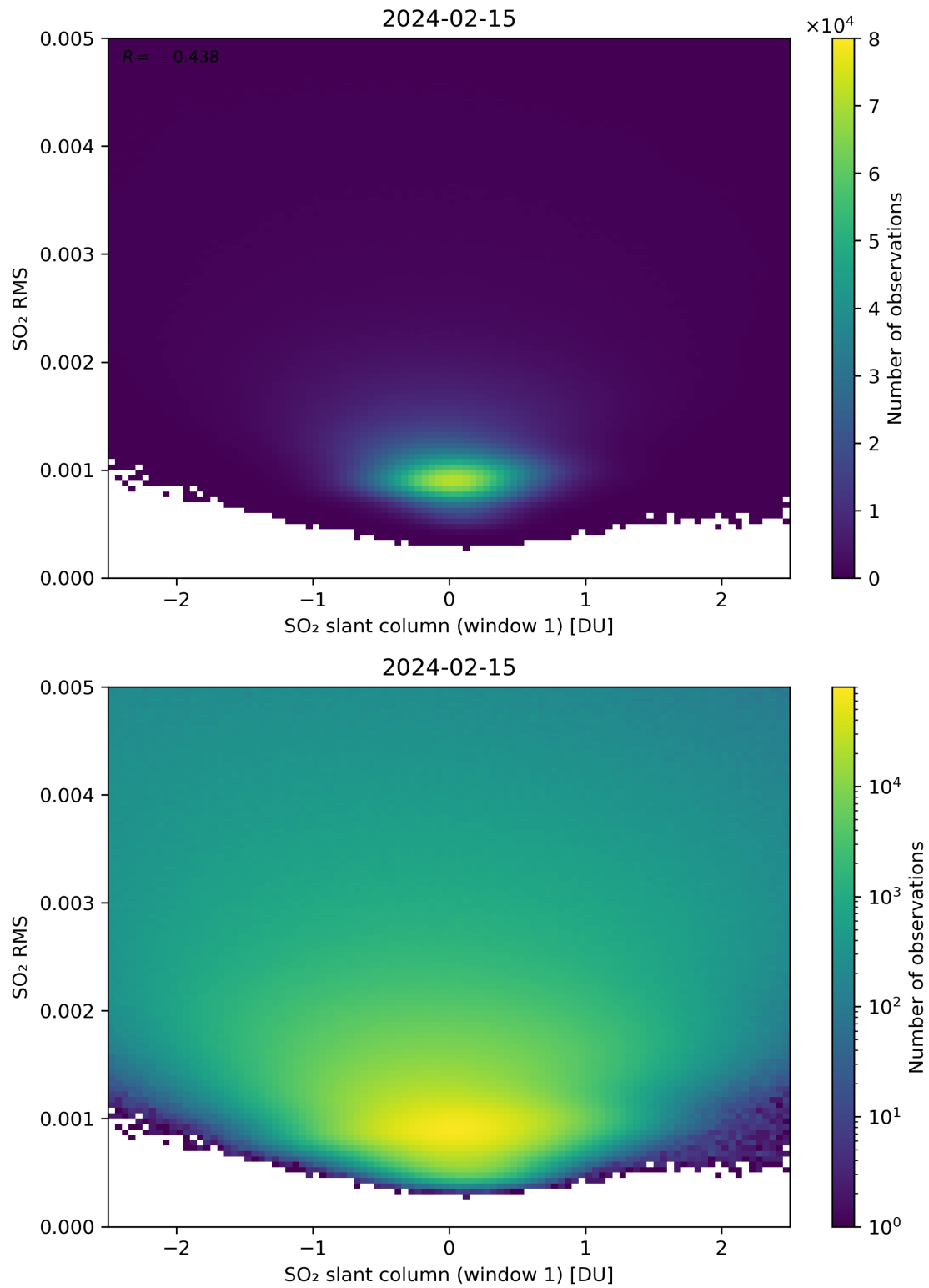
Figure 217: Scatter density plot of “SO 2 slant column (window 1)” against “SO 2 RMS” for 2024-02-14 to 2024-02-16.
