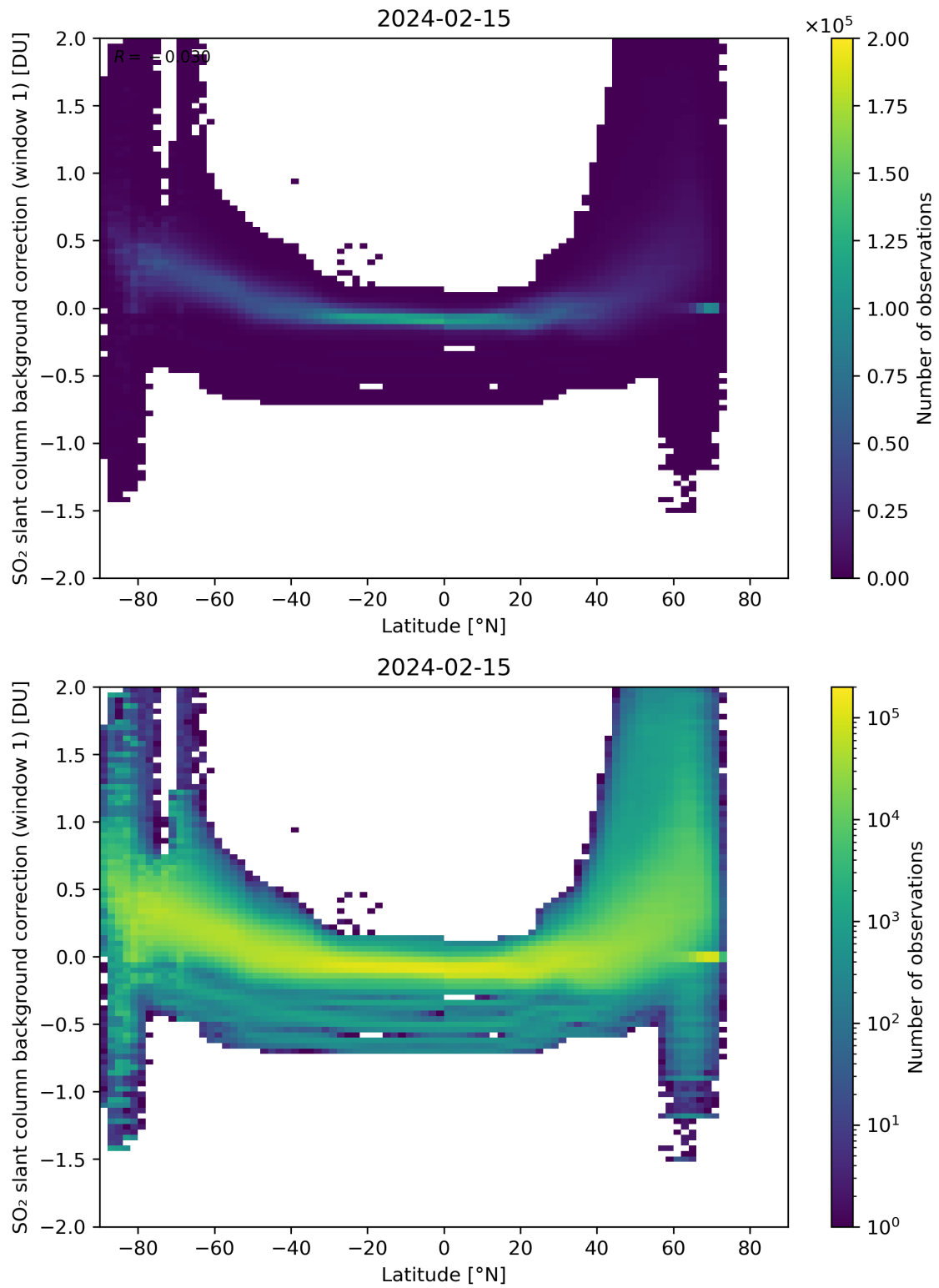
Figure 139: Scatter density plot of “Latitude” against “SO 2 slant column background correction (window 1)” for 2024-02-14 to 2024-02-16.
