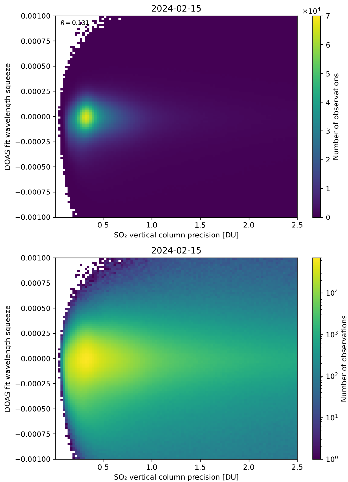
Figure 283: Scatter density plot of “SO 2 vertical column precision” against “DOAS fit wavelength squeeze” for 2024-02-14 to 2024-02-16.
