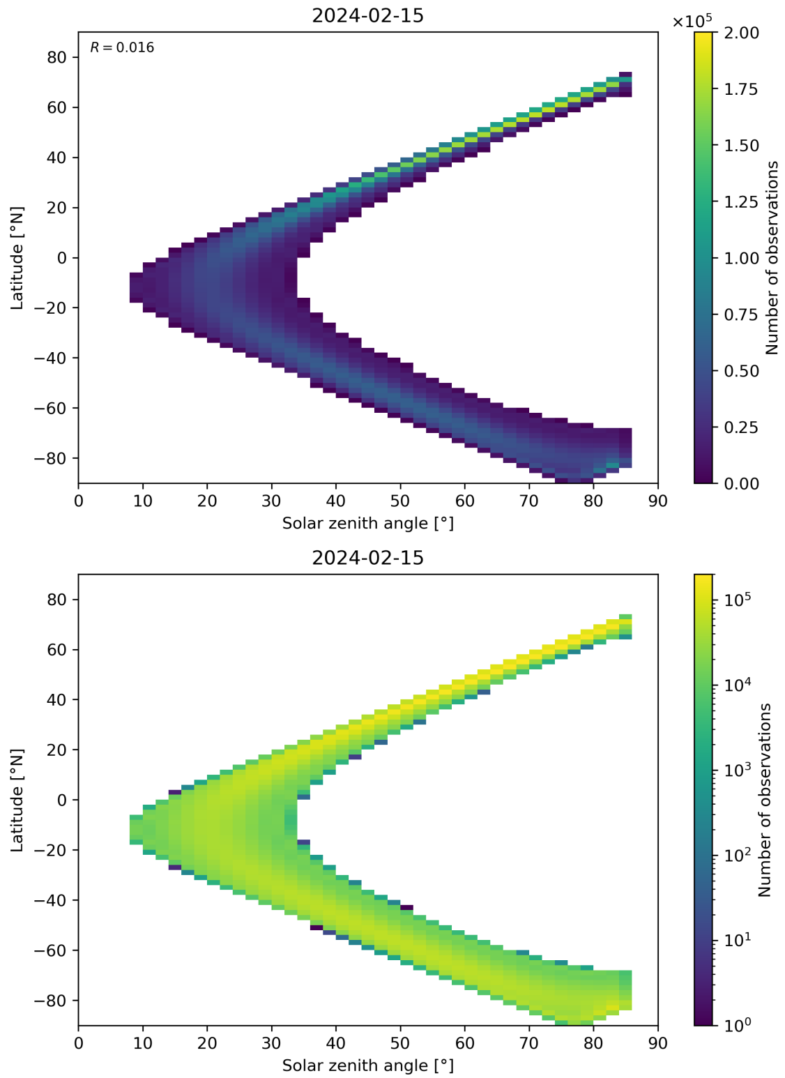
Figure 164: Scatter density plot of “Solar zenith angle” against “Latitude” for 2024-02-14 to 2024-02-16.
