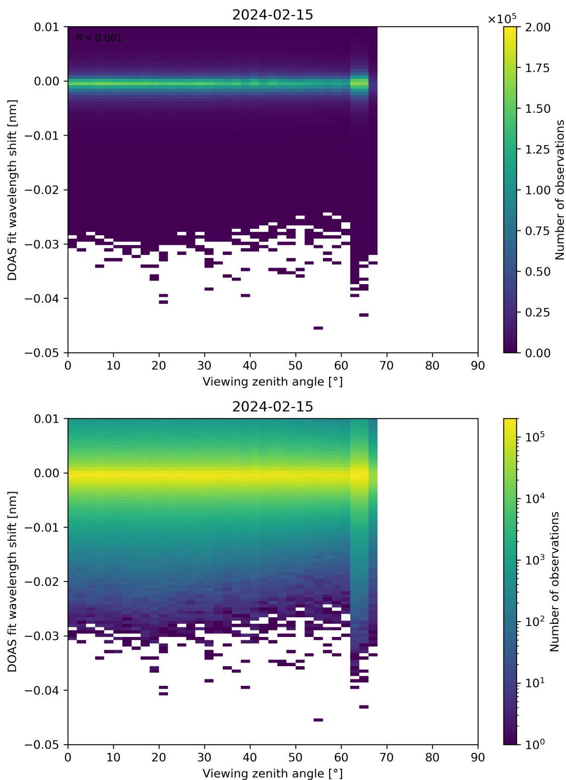
Figure 311: Scatter density plot of “Viewing zenith angle” against “DOAS fit wavelength shift” for 2024-02-14 to 2024-02-16.
