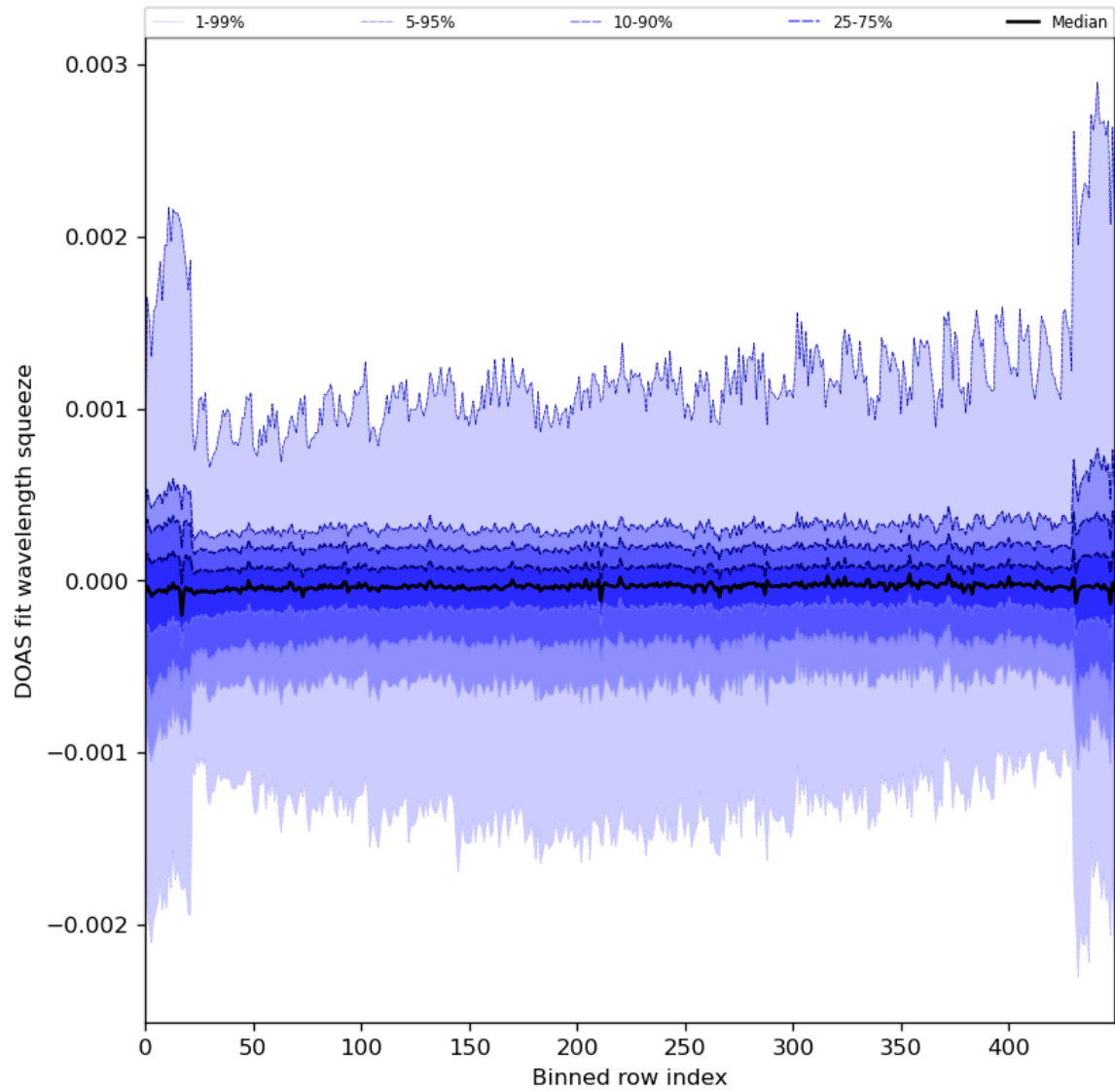
Figure 92: Along track statistics of “DOAS fit wavelength squeeze” for 2024-02-14 to 2024-02-16
