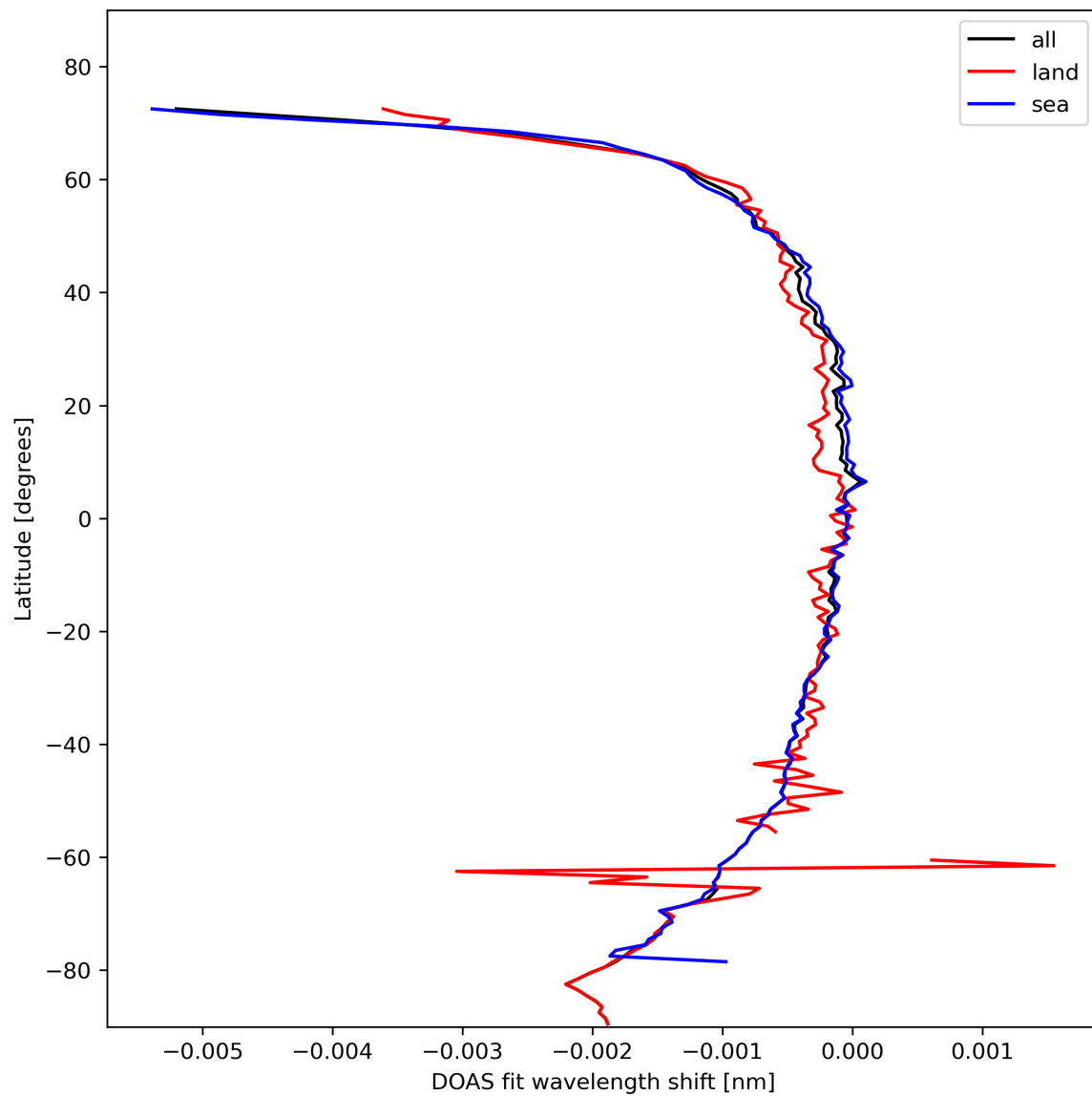
Figure 45: Zonal average of “DOAS fit wavelength shift” for 2024-02-14 to 2024-02-16.
