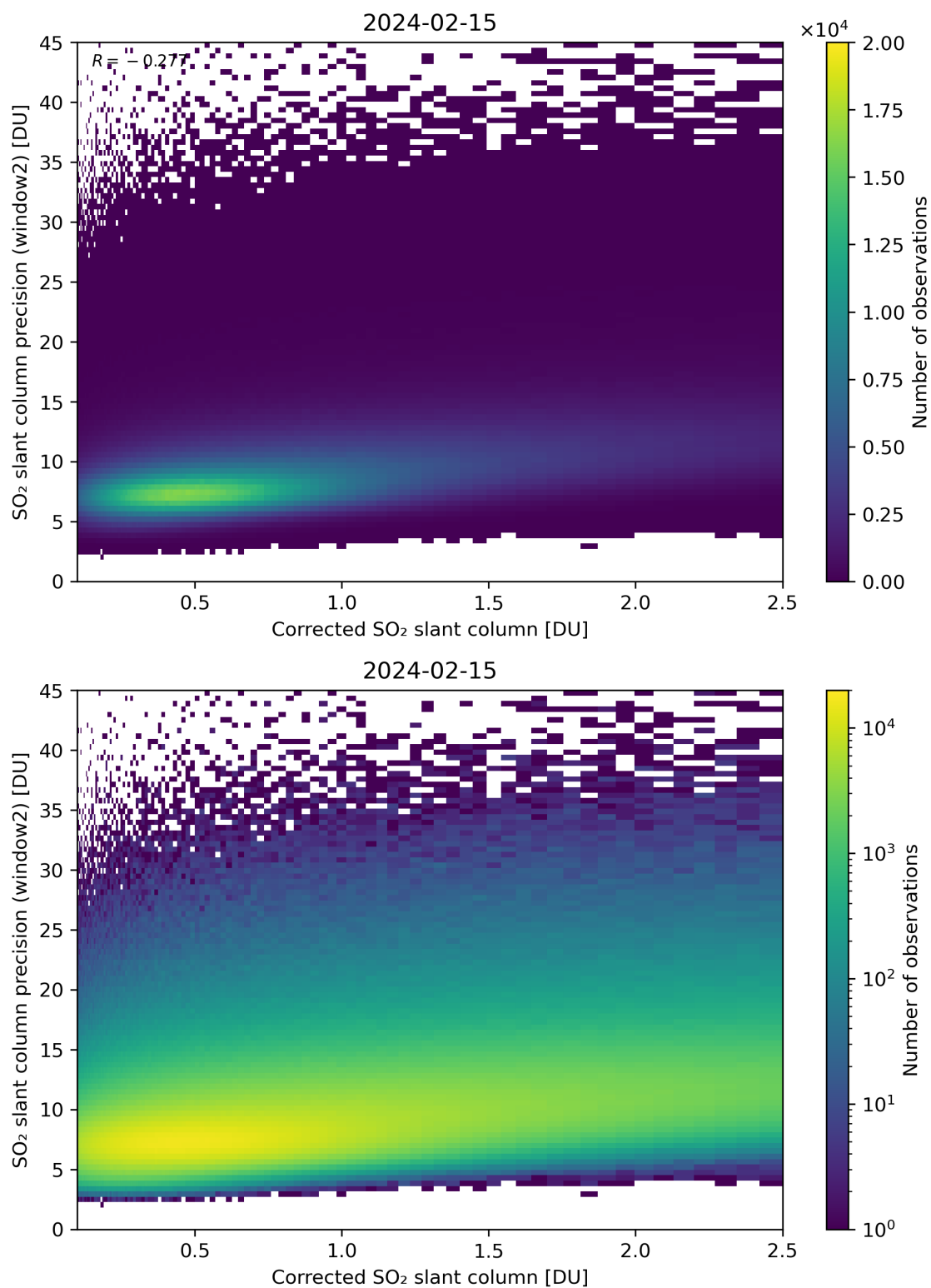
Figure 189: Scatter density plot of “Corrected SO 2 slant column” against “SO 2 slant column precision (window2)” for 2024-02-14 to 2024-02-16.
