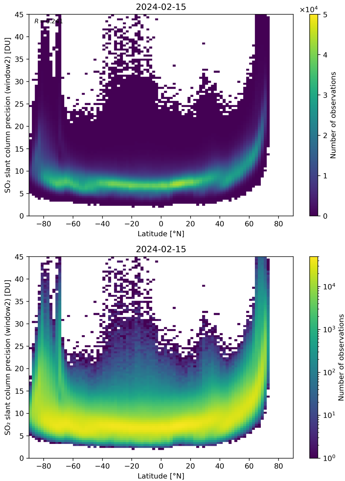
Figure 151: Scatter density plot of “Latitude” against “SO 2 slant column precision (window2)” for 2024-02-14 to 2024-02-16.
