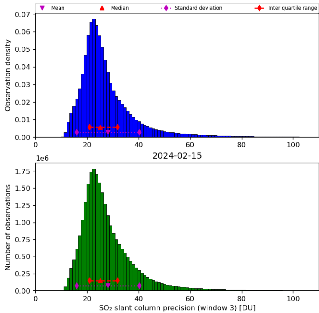
Figure 65: Histogram of “SO 2 slant column precision (window 3)” for 2024-02-14 to 2024-02-16
