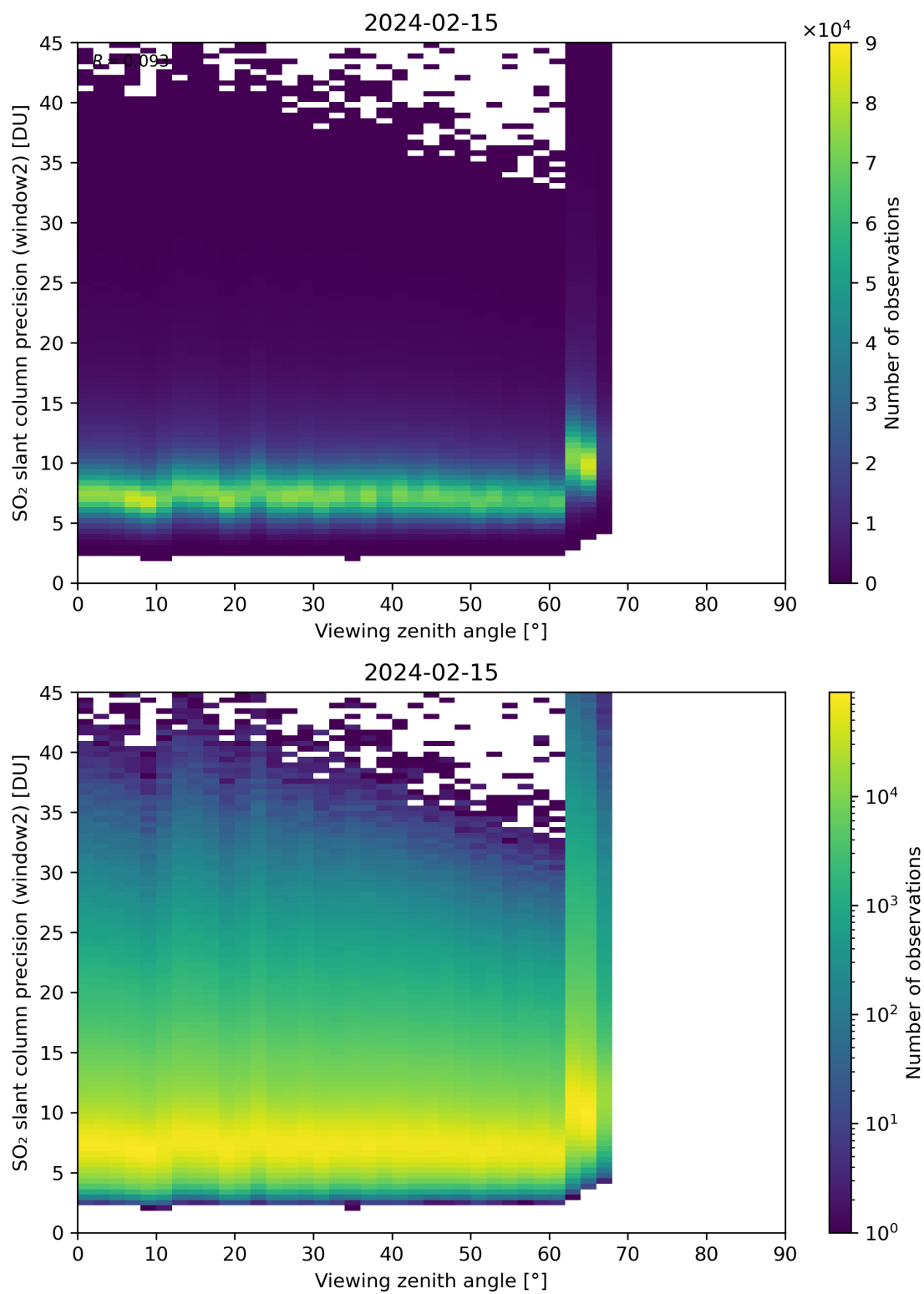
Figure 322: Scatter density plot of “Viewing zenith angle” against “SO 2 slant column precision (window2)” for 2024-02-14 to 2024-02-16.
