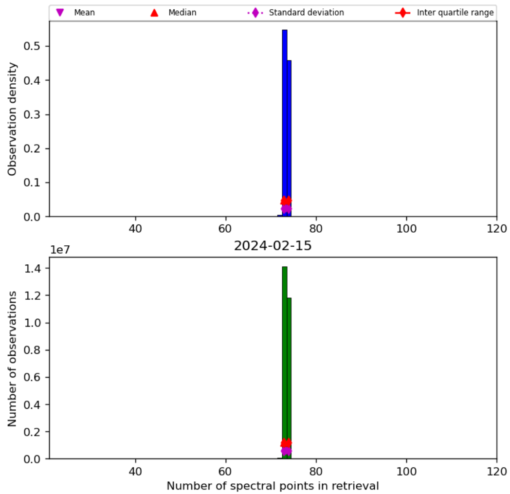
Figure 74: Histogram of “Number of spectral points in retrieval” for 2024-02-14 to 2024-02-16
