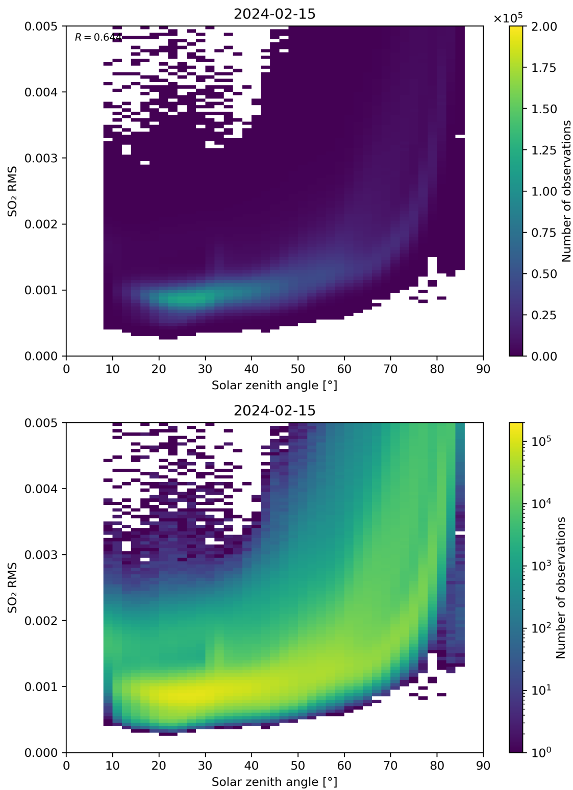
Figure 163: Scatter density plot of “Solar zenith angle” against “SO 2 RMS” for 2024-02-14 to 2024-02-16.
