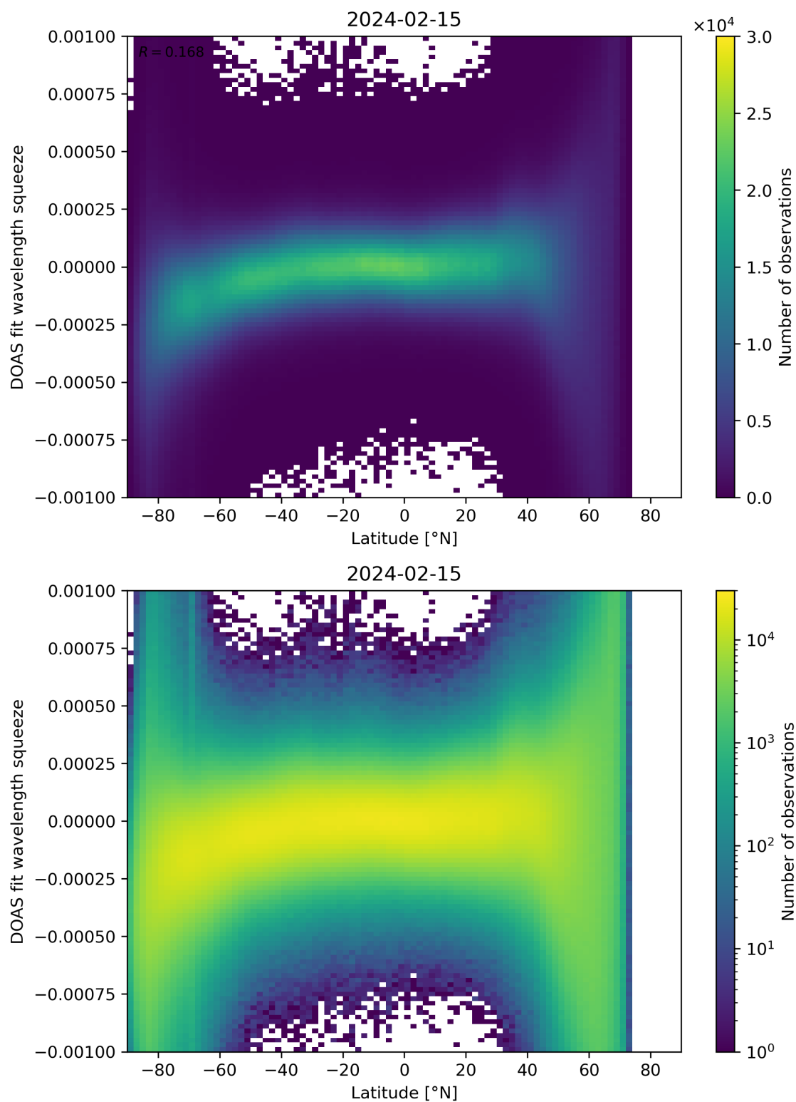
Figure 143: Scatter density plot of “Latitude” against “DOAS fit wavelength squeeze” for 2024-02-14 to 2024-02-16.
