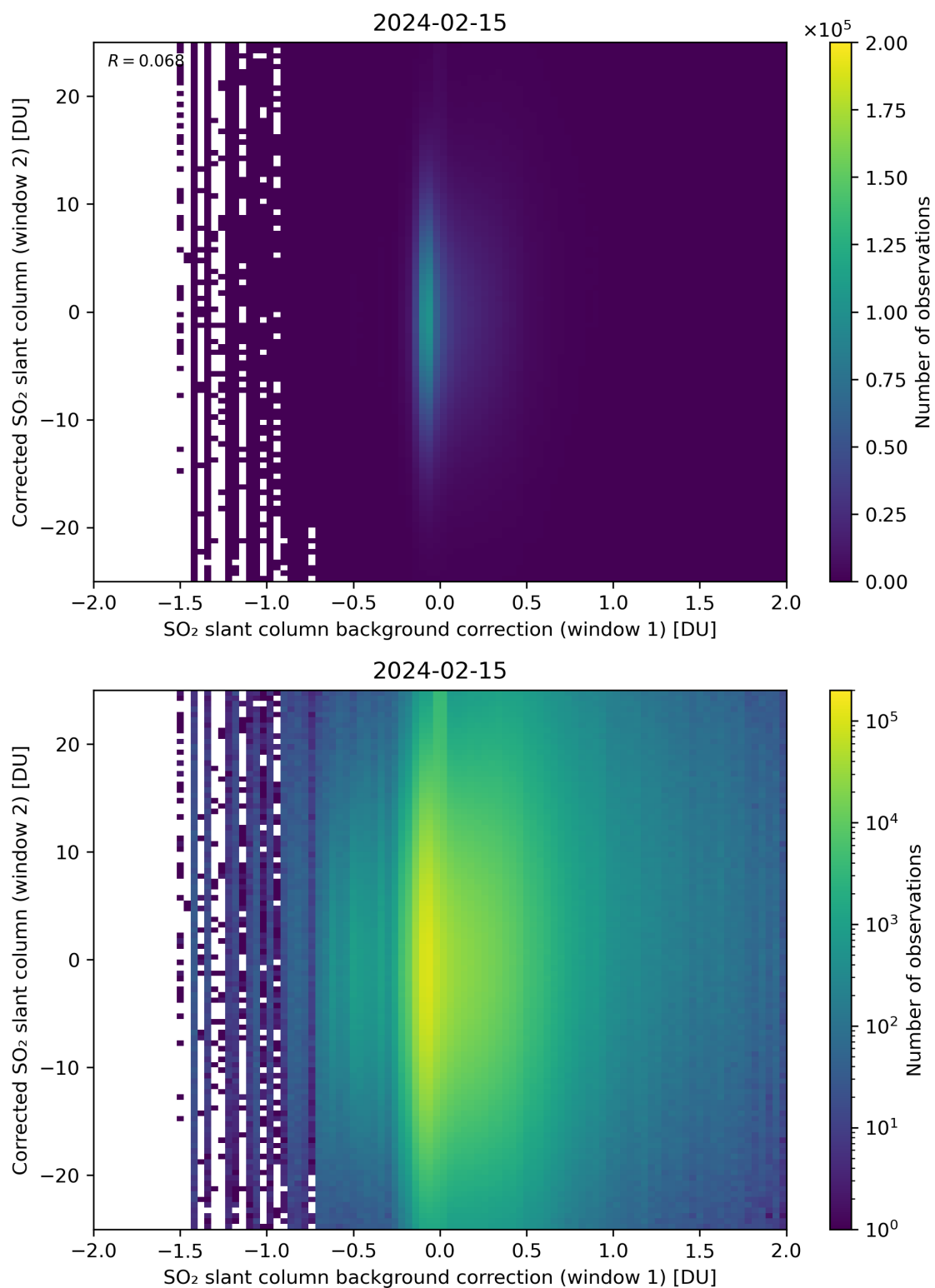
Figure 104: Scatter density plot of “SO 2 slant column background correction (window 1)” against “Corrected SO 2 slant column (window 2)” for 2024-02-14 to 2024-02-16.
