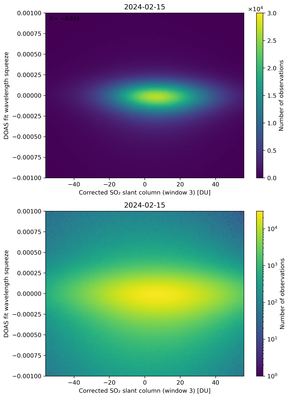
Figure 207: Scatter density plot of “Corrected SO 2 slant column (window 3)” against “DOAS fit wavelength squeeze” for 2024-02-14 to 2024-02-16.
