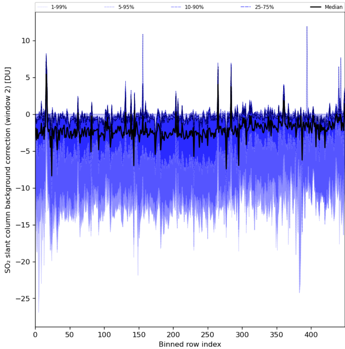
Figure 86: Along track statistics of “SO 2 slant column background correction (window 2)” for 2024-02-14 to 2024-02-16
