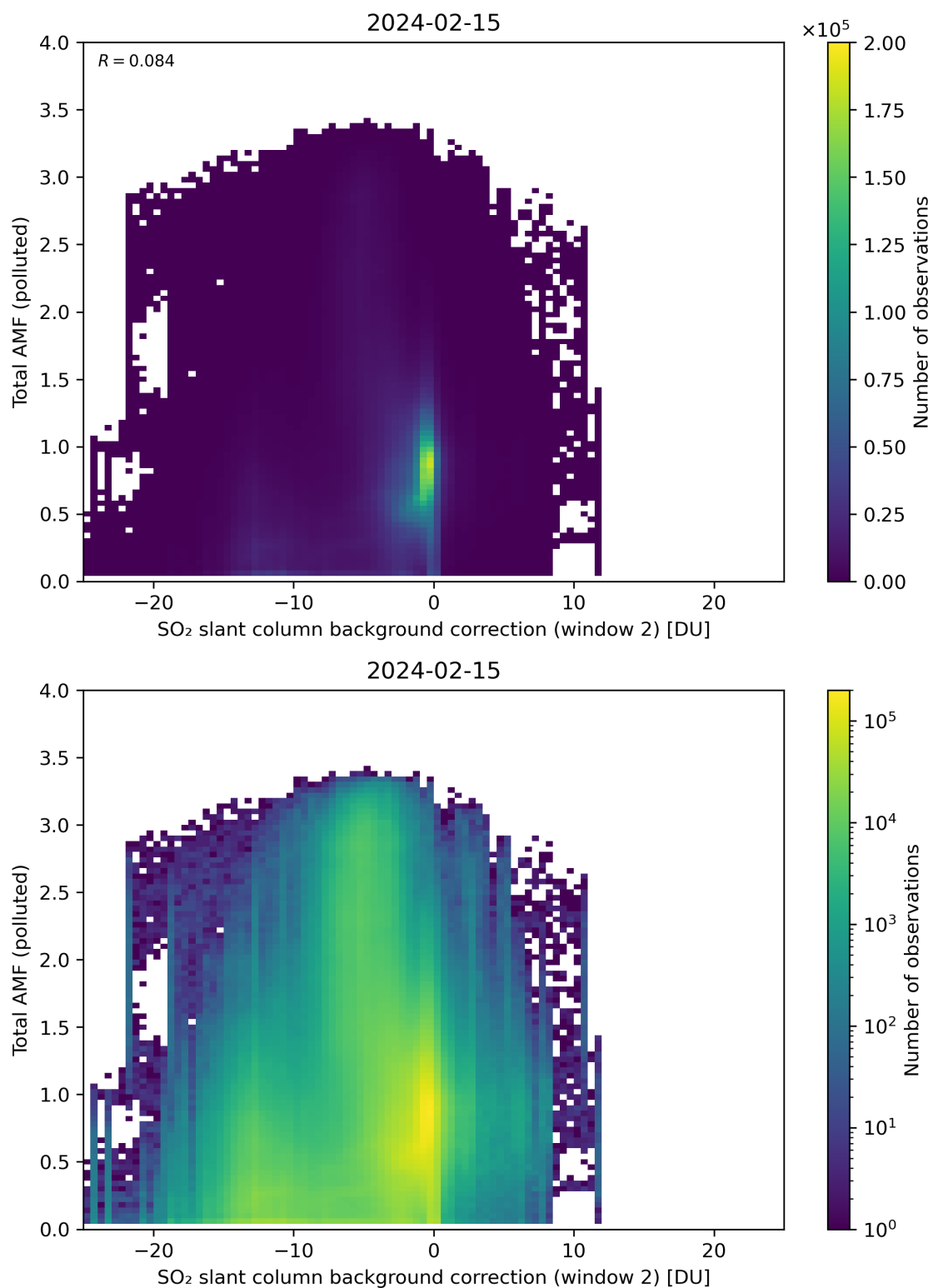
Figure 119: Scatter density plot of “SO 2 slant column background correction (window 2)” against “Total AMF (polluted)” for 2024-02-14 to 2024-02-16.
