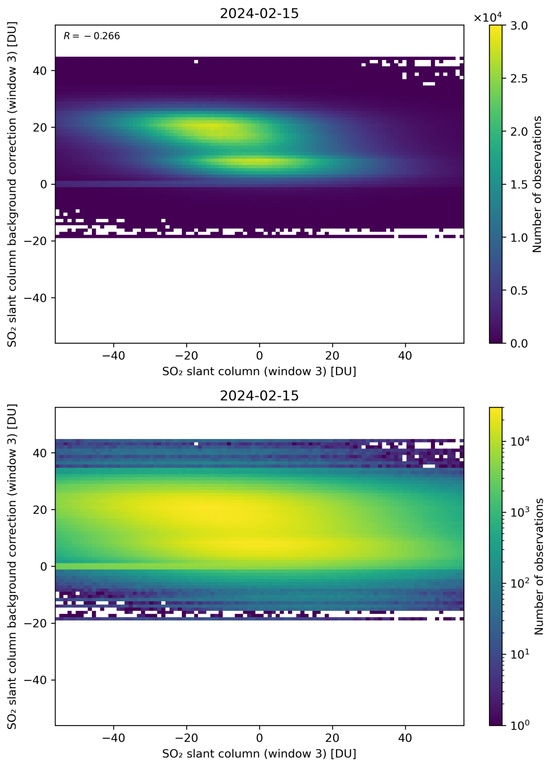
Figure 253: Scatter density plot of “SO 2 slant column (window 3)” against “SO 2 slant column background correction (window 3)” for 2024-02-14 to 2024-02-16.
