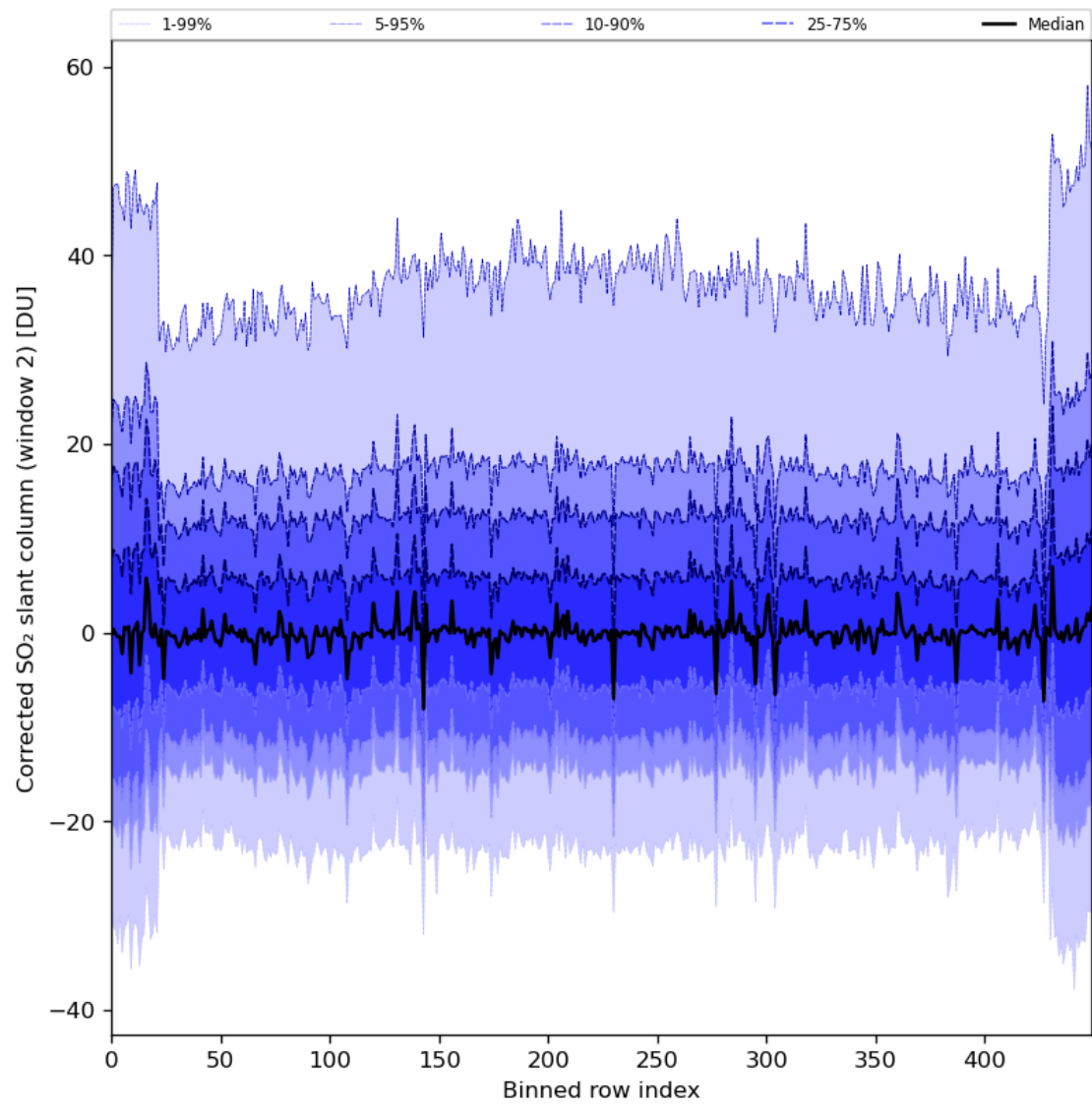
Figure 85: Along track statistics of “Corrected SO 2 slant column (window 2)” for 2024-02-14 to 2024-02-16
