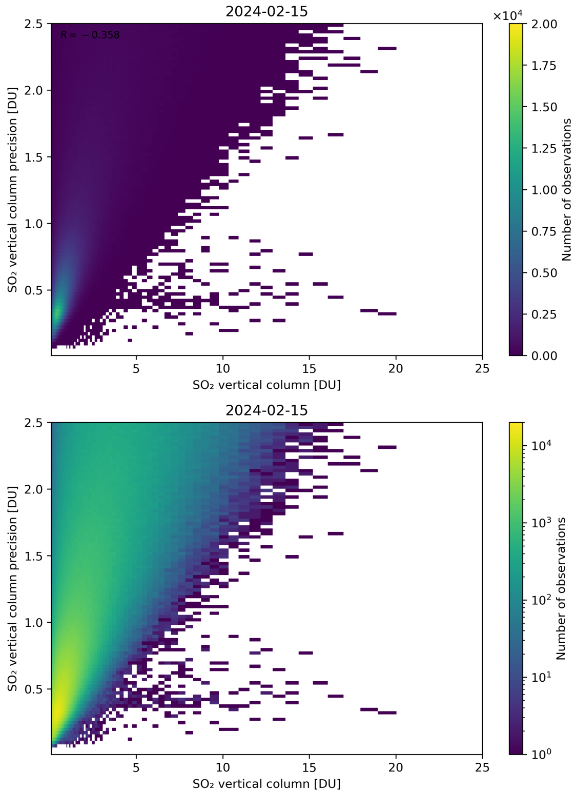
Figure 307: Scatter density plot of “SO 2 vertical column” against “SO 2 vertical column precision” for 2024-02-14 to 2024-02-16.
