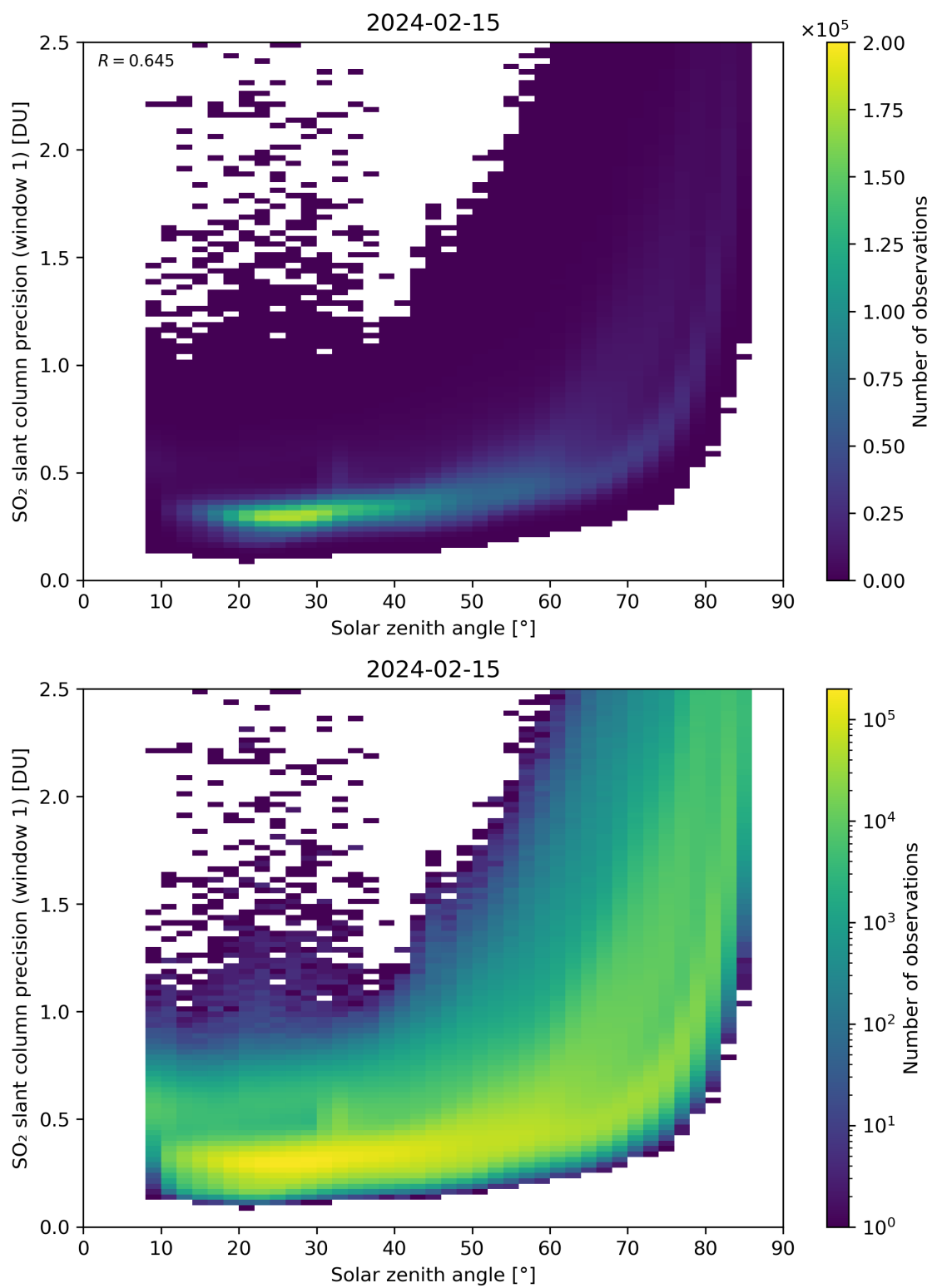
Figure 170: Scatter density plot of “Solar zenith angle” against “SO 2 slant column precision (window 1)” for 2024-02-14 to 2024-02-16.
