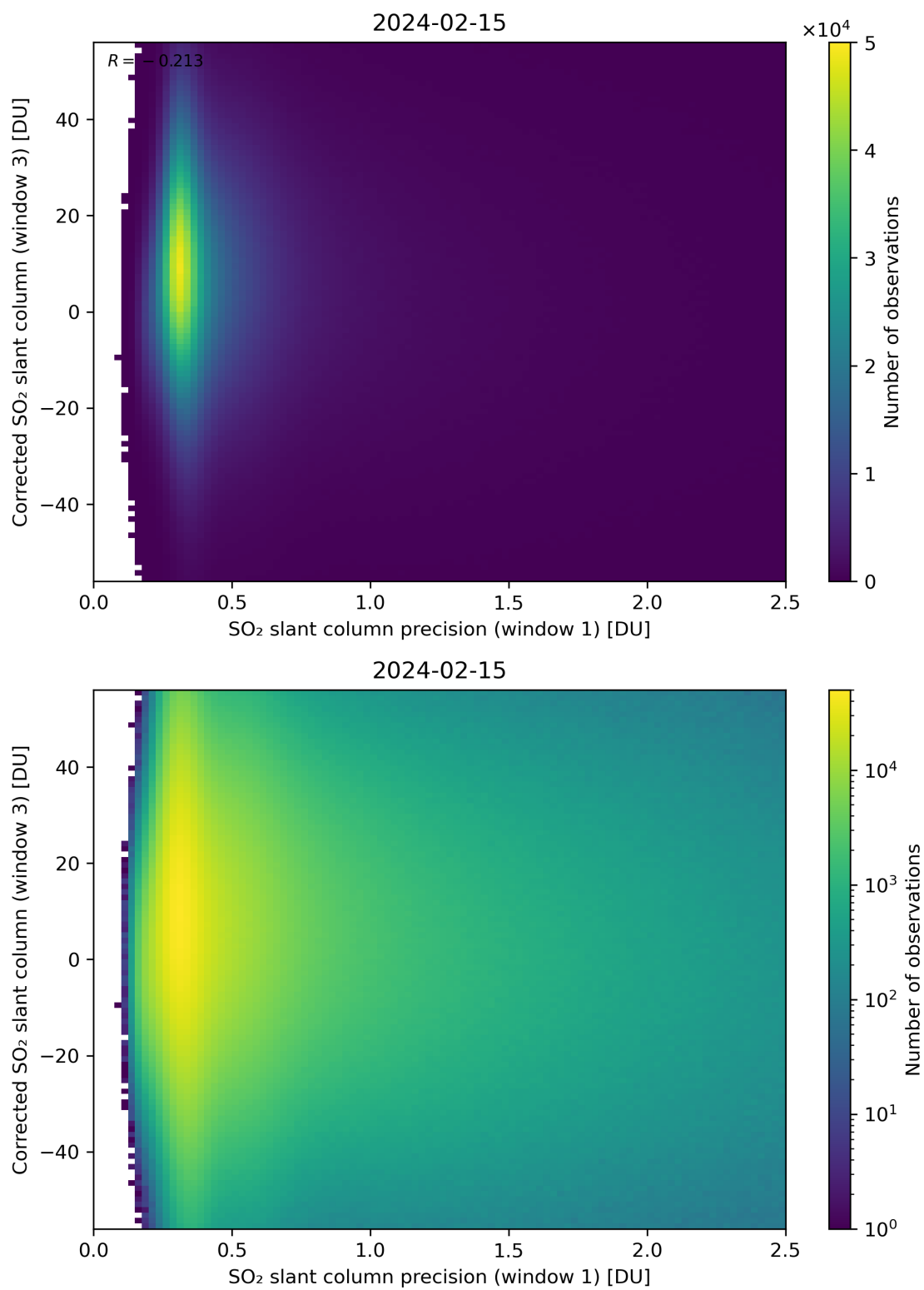
Figure 226: Scatter density plot of “SO 2 slant column precision (window 1)” against “Corrected SO 2 slant column (window 3)” for 2024-02-14 to 2024-02-16.
