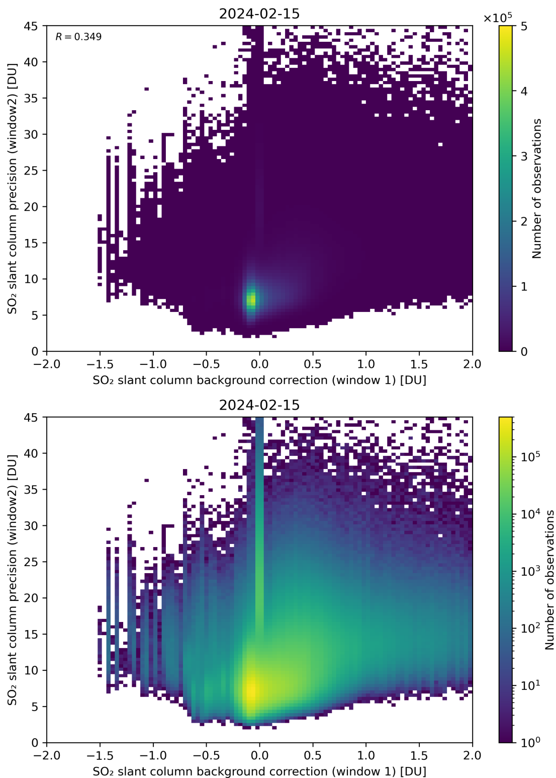
Figure 106: Scatter density plot of “SO 2 slant column background correction (window 1)” against “SO 2 slant column precision (window2)” for 2024-02-14 to 2024-02-16.
