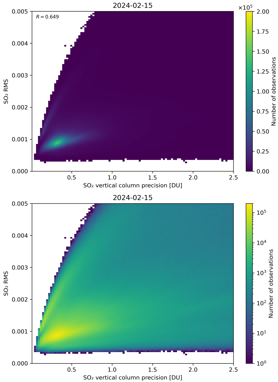
Figure 284: Scatter density plot of “SO 2 vertical column precision” against “SO 2 RMS” for 2024-02-14 to 2024-02-16.
