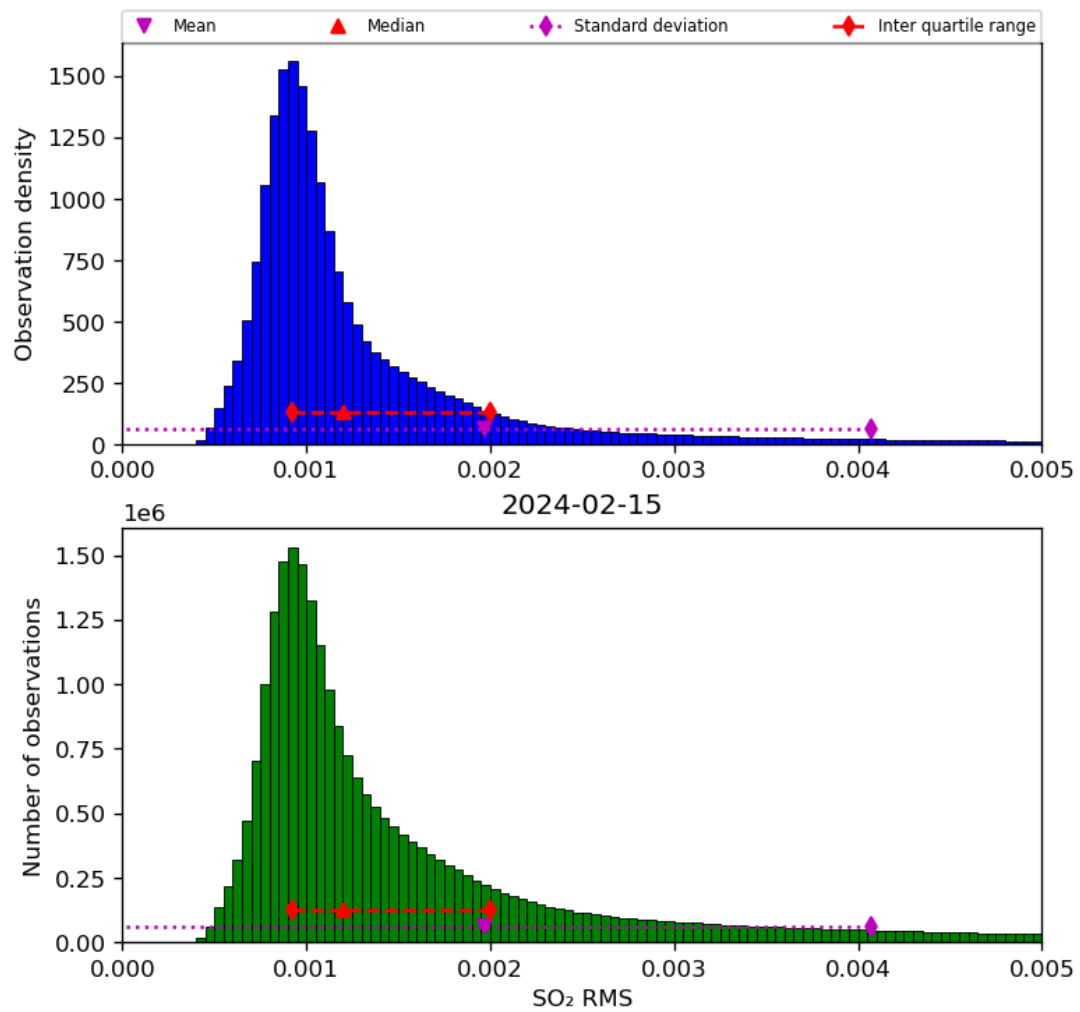
Figure 70: Histogram of “SO 2 RMS” for 2024-02-14 to 2024-02-16
