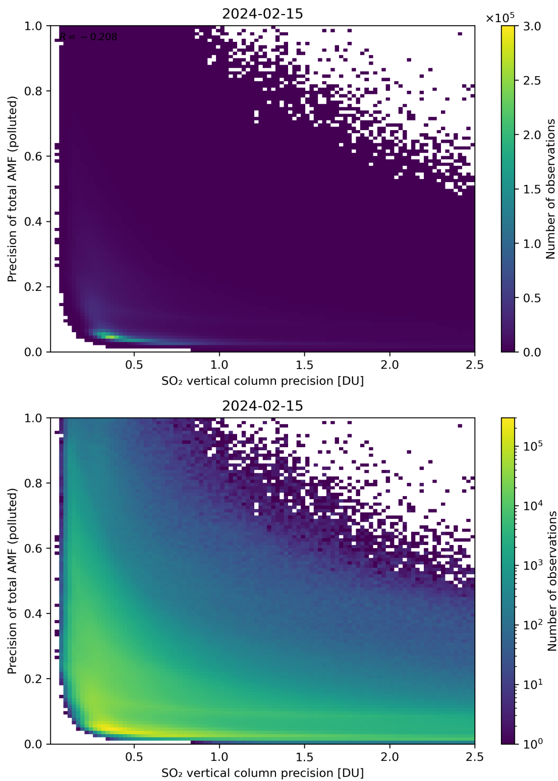
Figure 295: Scatter density plot of “SO 2 vertical column precision” against “Precision of total AMF (polluted)” for 2024-02-14 to 2024-02-16.
