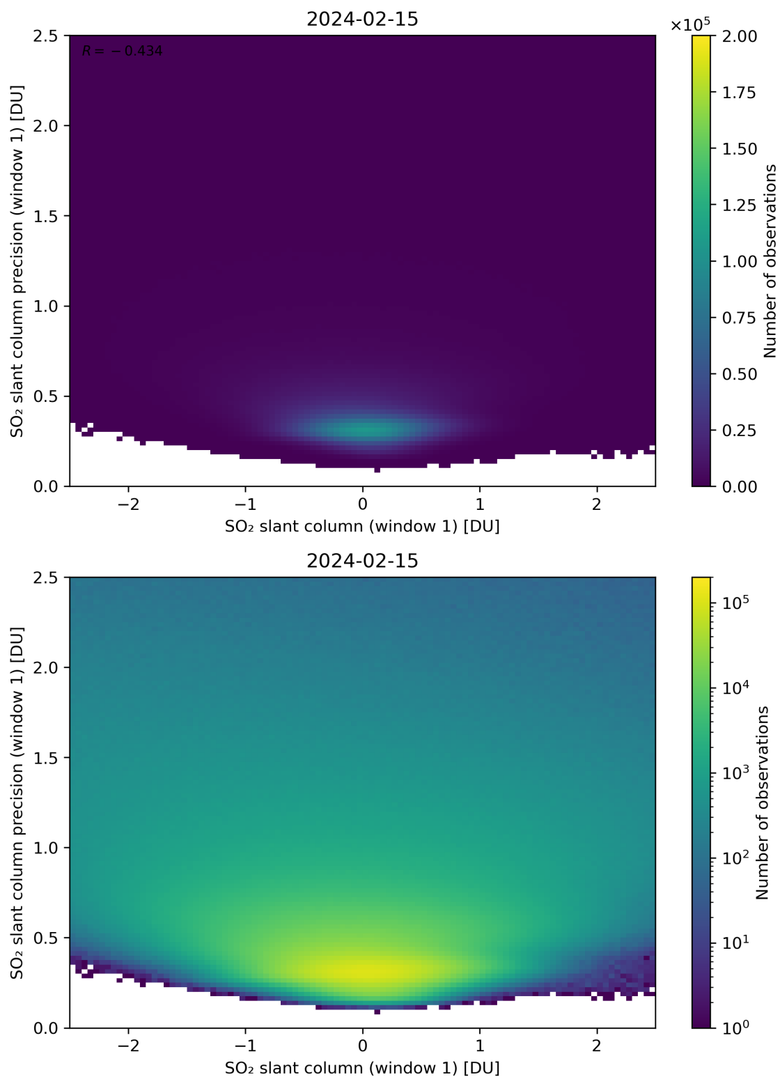
Figure 235: Scatter density plot of “SO 2 slant column (window 1)” against “SO 2 slant column precision (window 1)” for 2024-02-14 to 2024-02-16.
