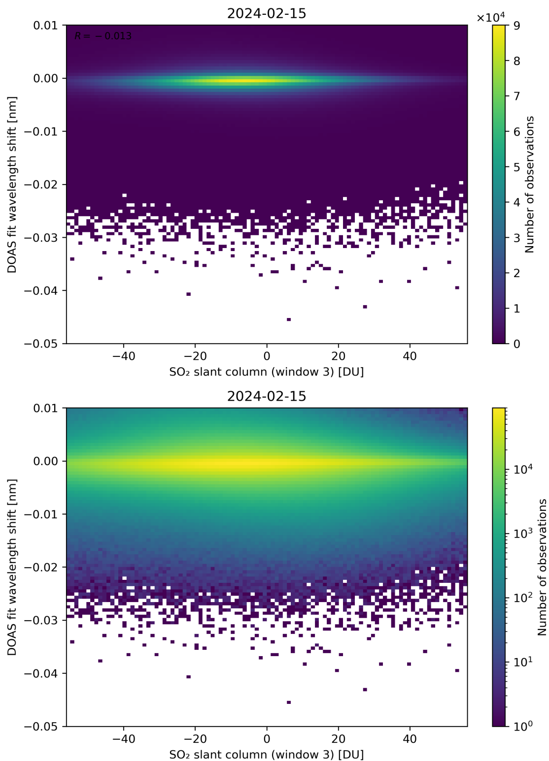
Figure 254: Scatter density plot of “SO 2 slant column (window 3)” against “DOAS fit wavelength shift” for 2024-02-14 to 2024-02-16.
