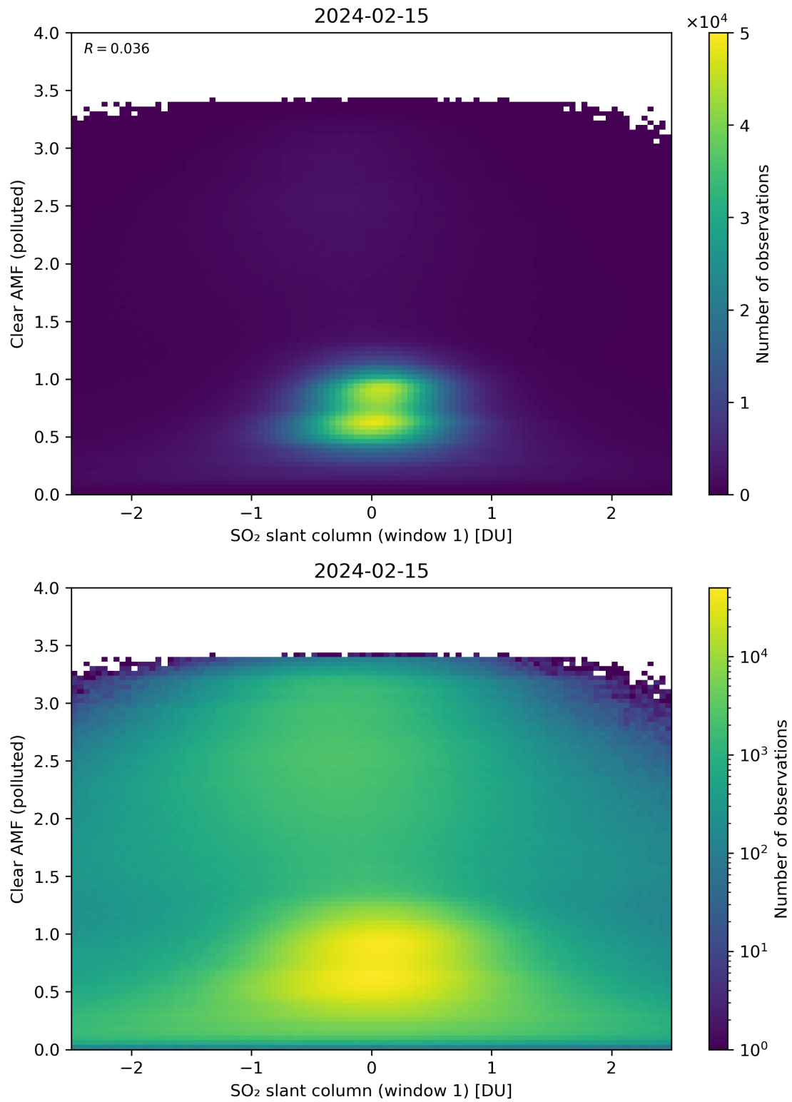
Figure 232: Scatter density plot of “SO 2 slant column (window 1)” against “Clear AMF (polluted)” for 2024-02-14 to 2024-02-16.
