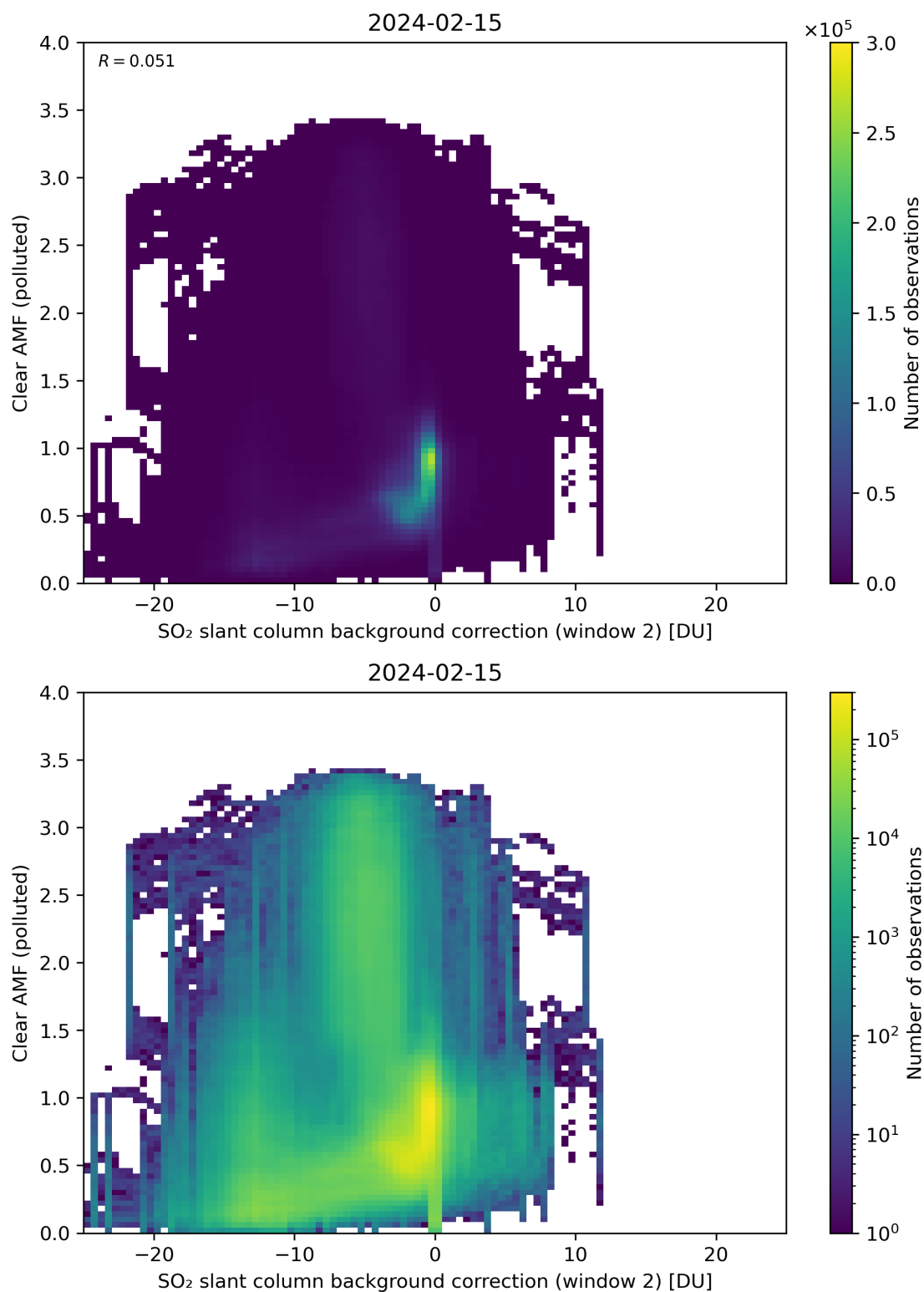
Figure 115: Scatter density plot of “SO 2 slant column background correction (window 2)” against “Clear AMF (polluted)” for 2024-02-14 to 2024-02-16.
