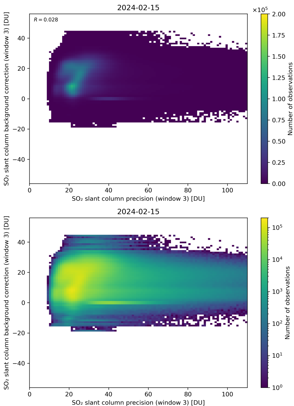
Figure 257: Scatter density plot of “SO 2 slant column precision (window 3)” against “SO 2 slant column background correction (window 3)” for 2024-02-14 to 2024-02-16.
