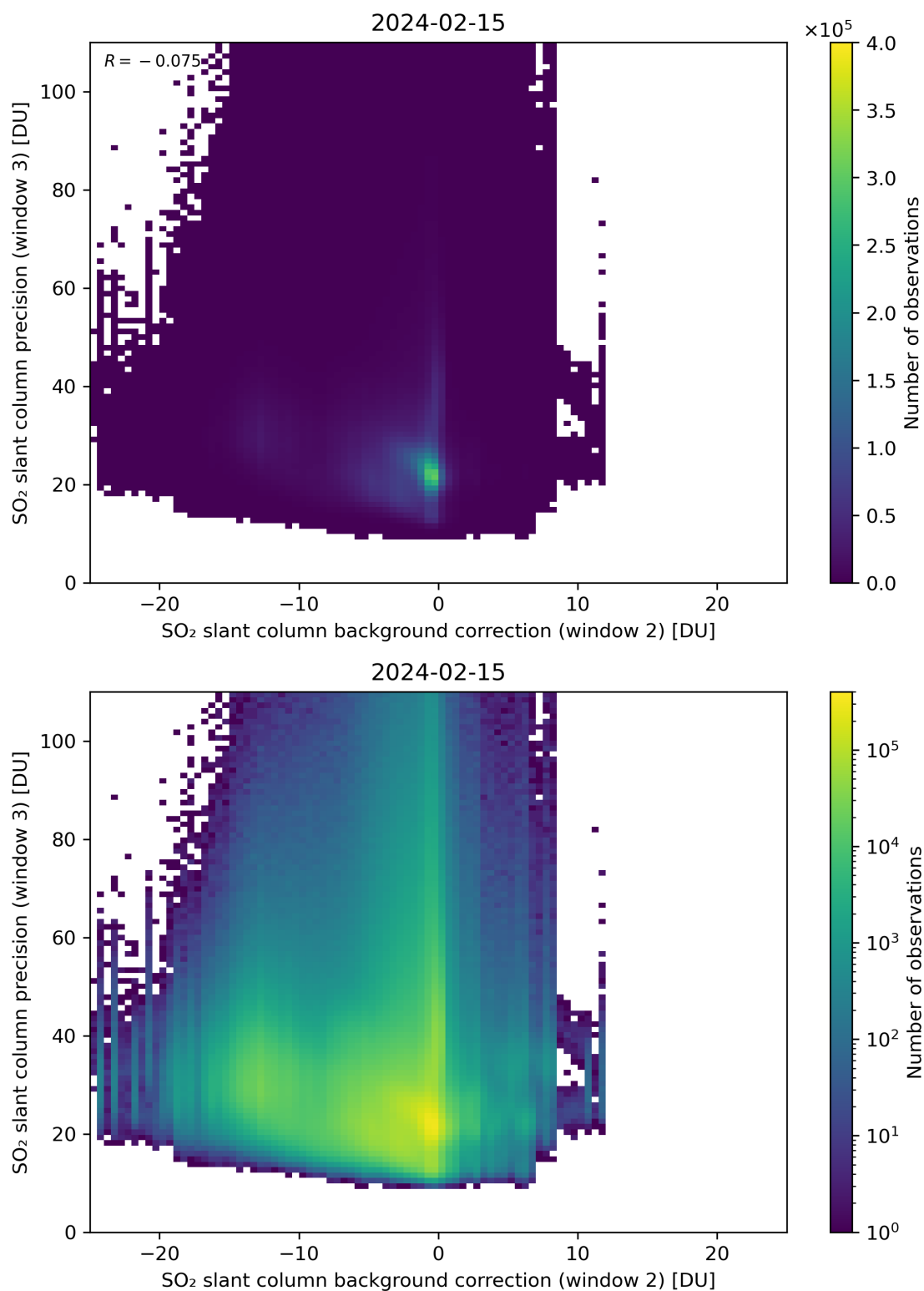
Figure 118: Scatter density plot of “SO 2 slant column background correction (window 2)” against “SO 2 slant column precision (window 3)” for 2024-02-14 to 2024-02-16.
