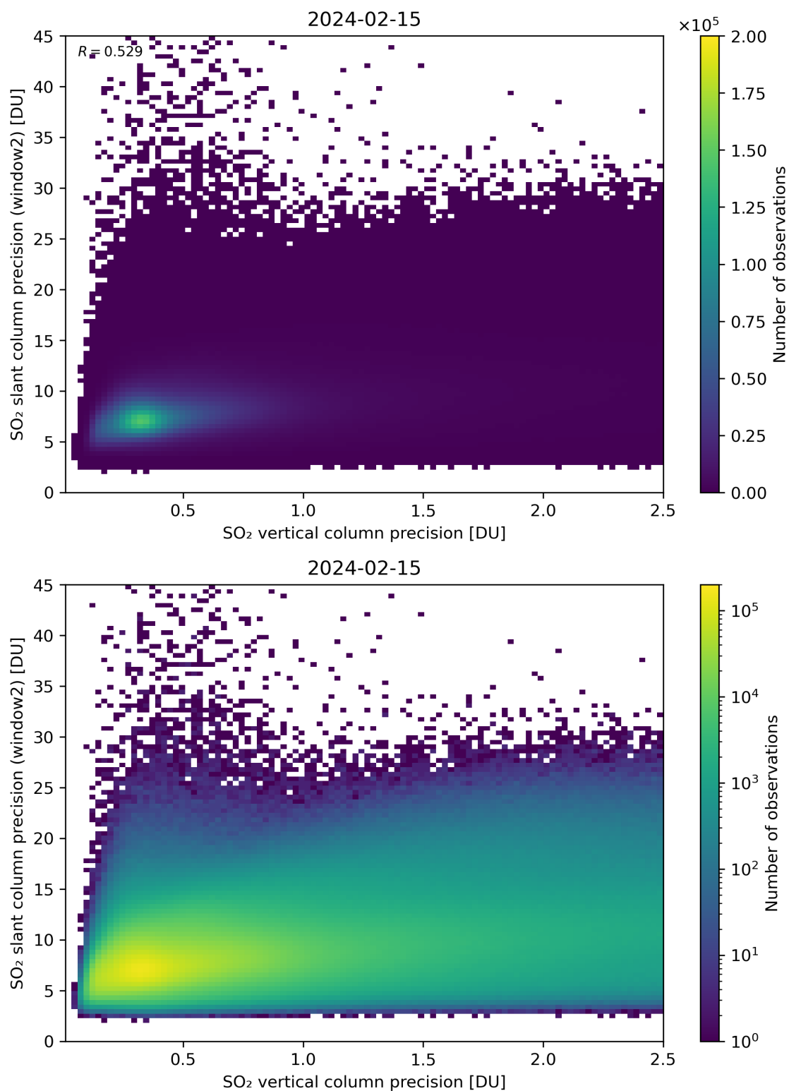
Figure 291: Scatter density plot of “SO 2 vertical column precision” against “SO 2 slant column precision (window2)” for 2024-02-14 to 2024-02-16.
