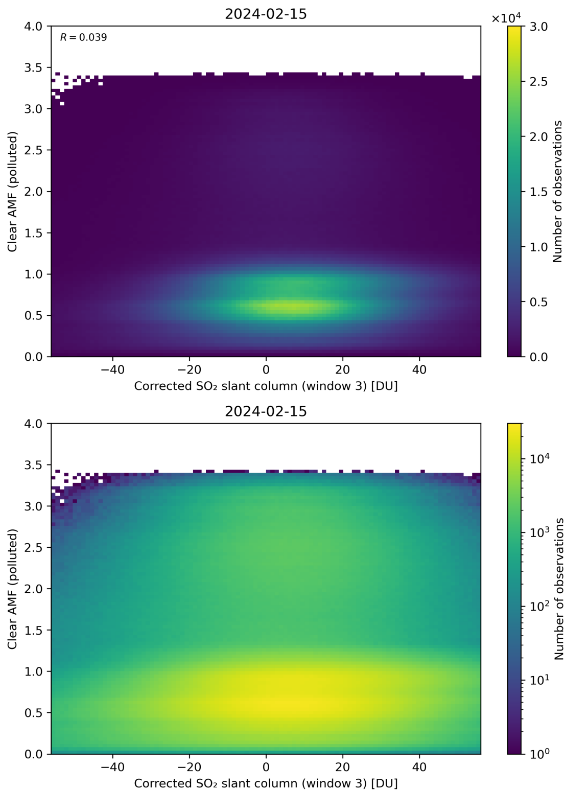
Figure 209: Scatter density plot of “Corrected SO 2 slant column (window 3)” against “Clear AMF (polluted)” for 2024-02-14 to 2024-02-16.
