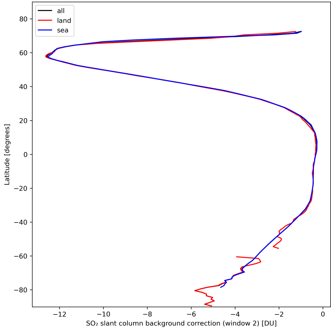
Figure 40: Zonal average of “SO 2 slant column background correction (window 2)” for 2024-02-14 to 2024-02-16.
