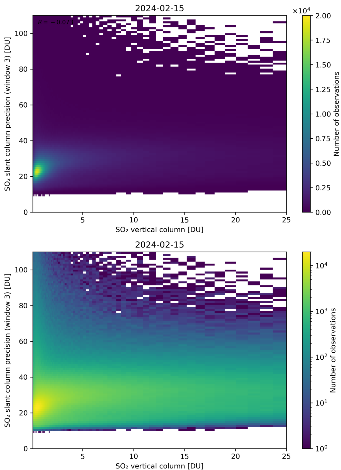
Figure 304: Scatter density plot of “SO 2 vertical column” against “SO 2 slant column precision (window 3)” for 2024-02-14 to 2024-02-16.
