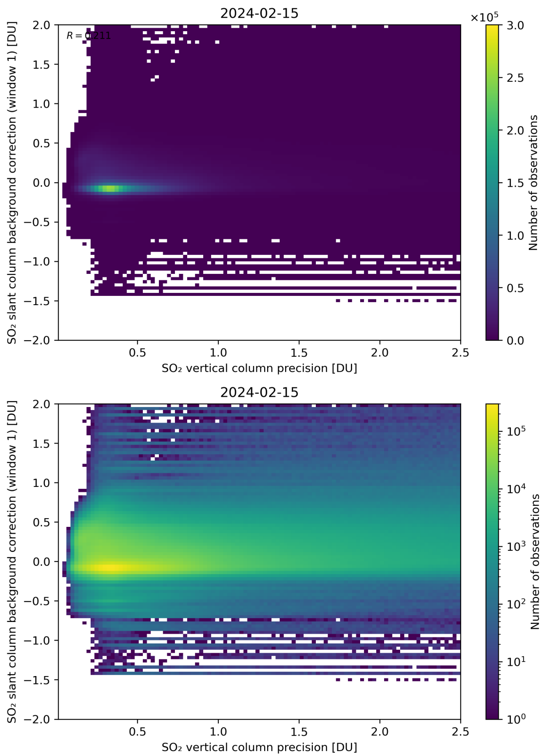
Figure 279: Scatter density plot of “SO 2 vertical column precision” against “SO 2 slant column background correction (window 1)” for 2024-02-14 to 2024-02-16.
