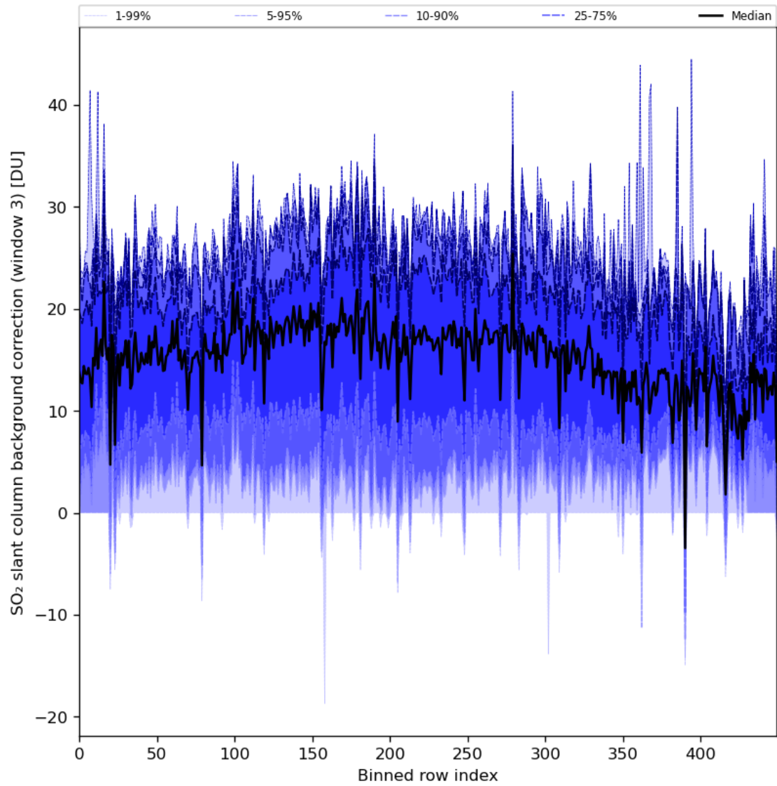
Figure 90: Along track statistics of “SO 2 slant column background correction (window 3)” for 2024-02-14 to 2024-02-16
