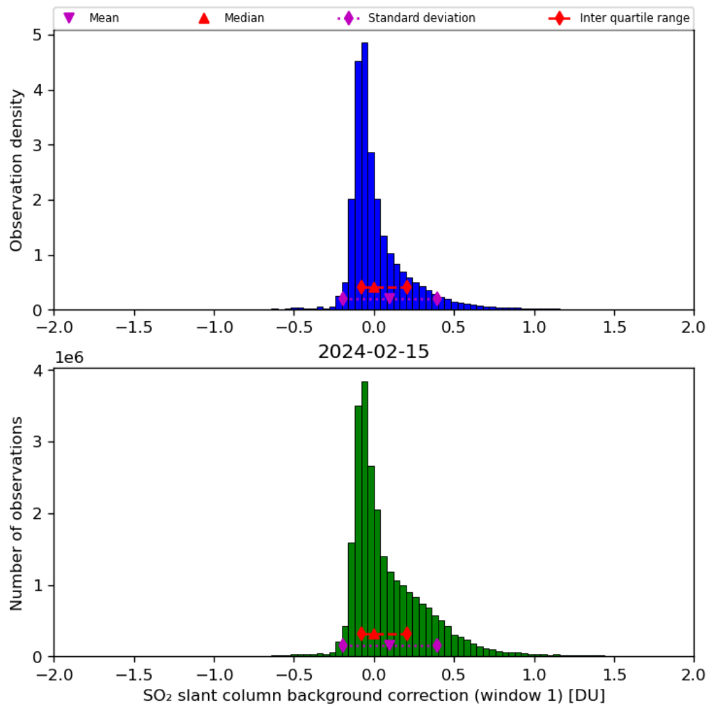
Figure 59: Histogram of “SO 2 slant column background correction (window 1)” for 2024-02-14 to 2024-02-16
