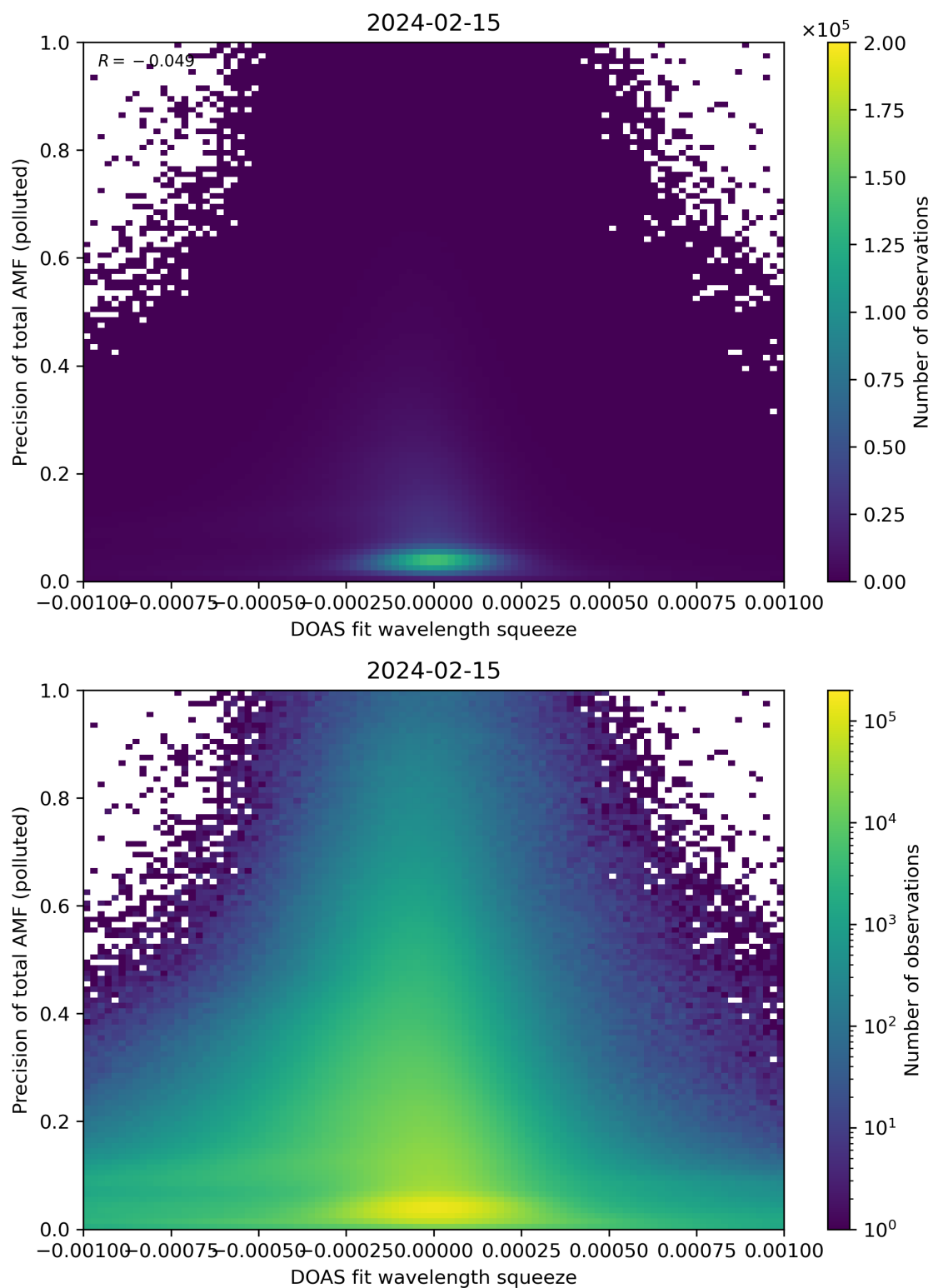
Figure 135: Scatter density plot of “DOAS fit wavelength squeeze” against “Precision of total AMF (polluted)” for 2024-02-14 to 2024-02-16.
