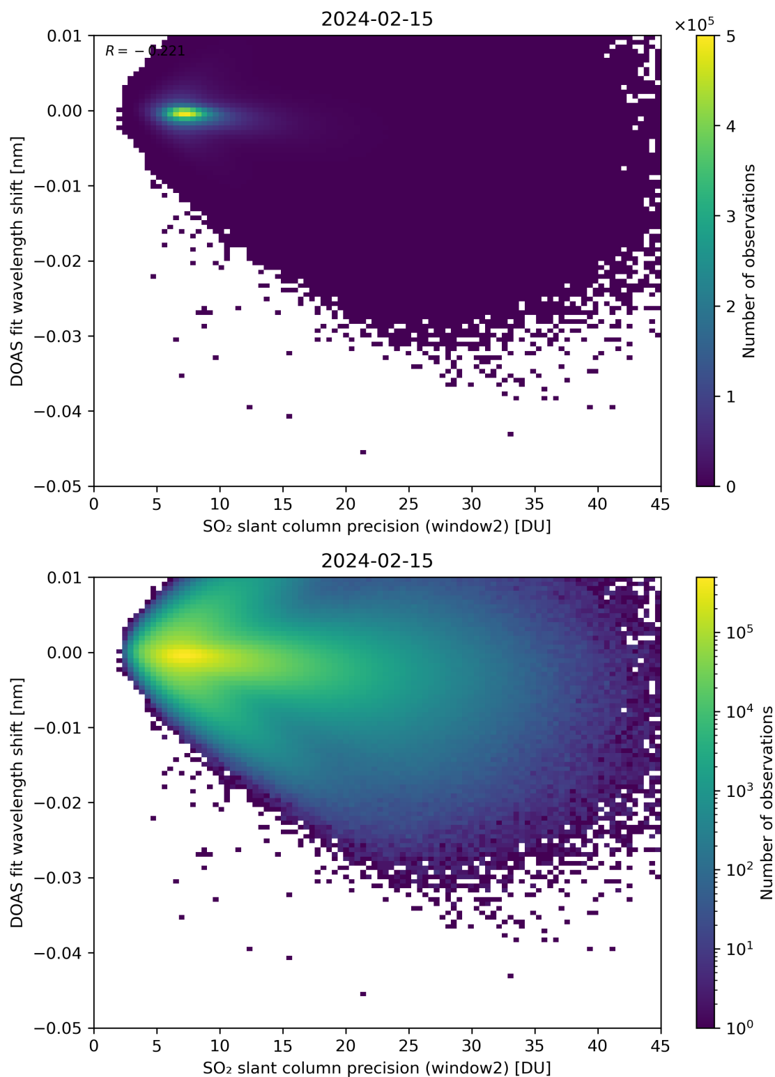
Figure 243: Scatter density plot of “SO 2 slant column precision (window2)” against “DOAS fit wavelength shift” for 2024-02-14 to 2024-02-16.
