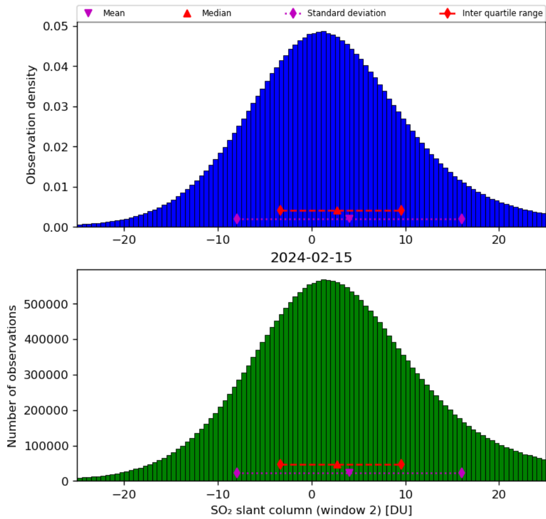
Figure 60: Histogram of “SO 2 slant column (window 2)” for 2024-02-14 to 2024-02-16
