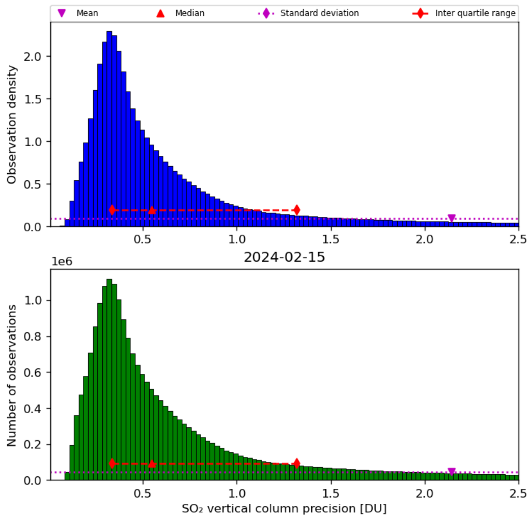
Figure 54: Histogram of “SO 2 vertical column precision” for 2024-02-14 to 2024-02-16
