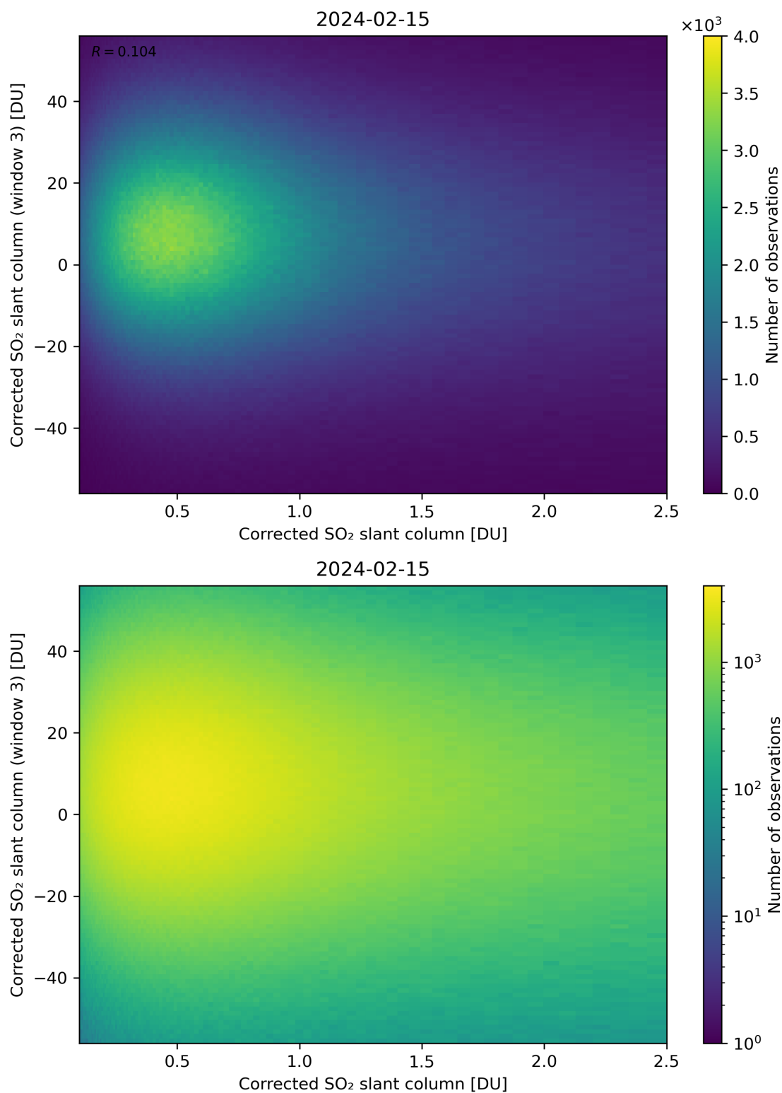
Figure 186: Scatter density plot of “Corrected SO 2 slant column” against “Corrected SO 2 slant column (window 3)” for 2024-02-14 to 2024-02-16.
