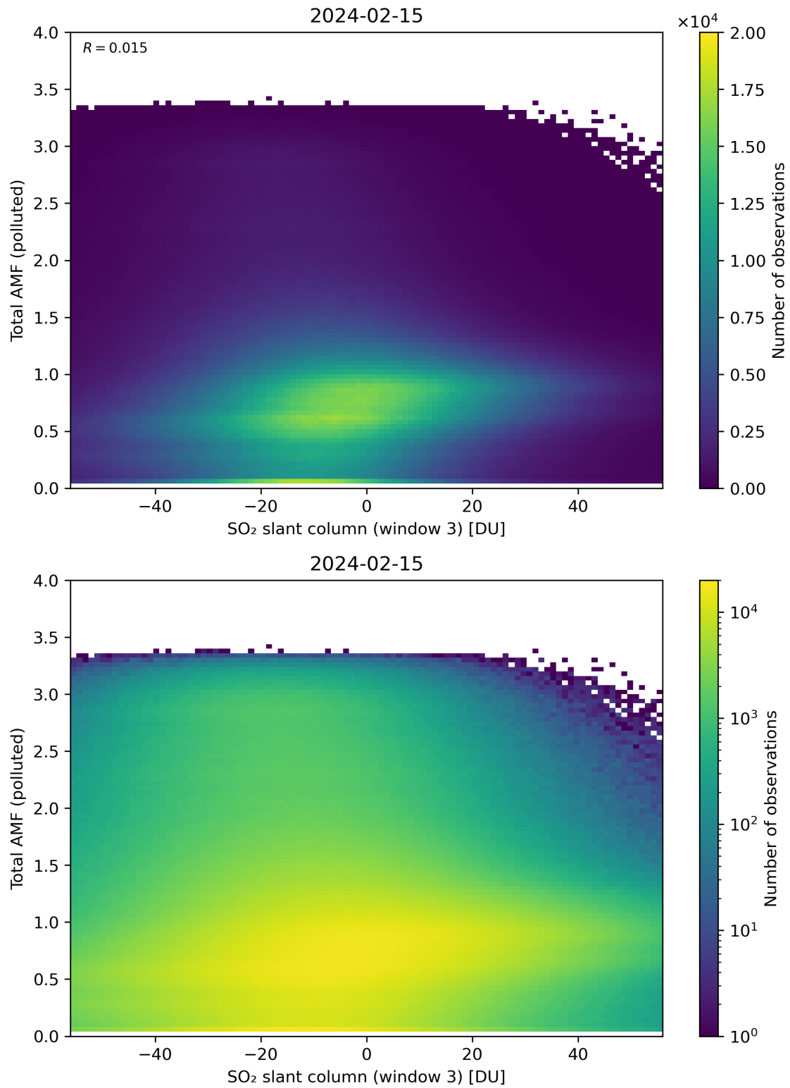
Figure 268: Scatter density plot of “SO 2 slant column (window 3)” against “Total AMF (polluted)” for 2024-02-14 to 2024-02-16.
