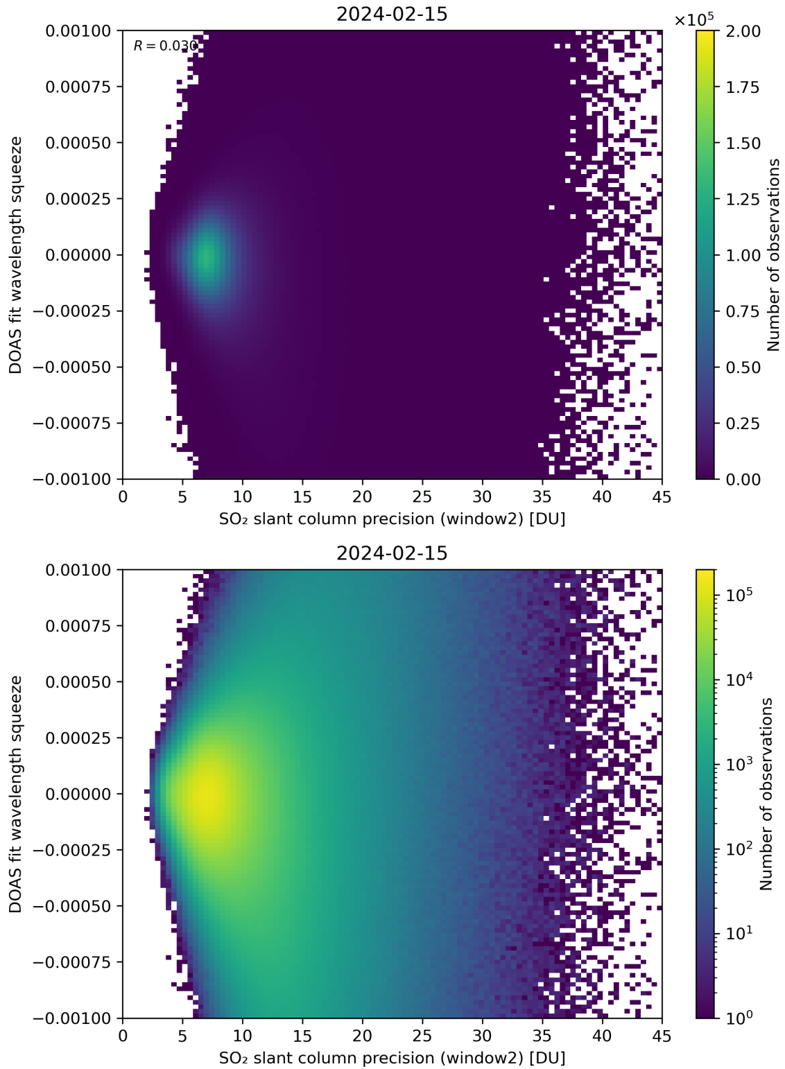
Figure 244: Scatter density plot of “SO 2 slant column precision (window2)” against “DOAS fit wavelength squeeze” for 2024-02-14 to 2024-02-16.
