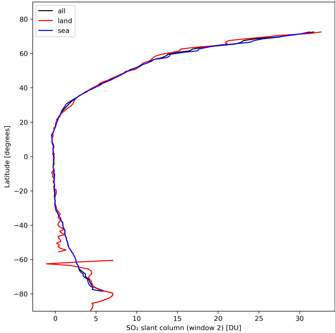
Figure 37: Zonal average of “SO 2 slant column (window 2)” for 2024-02-14 to 2024-02-16.
