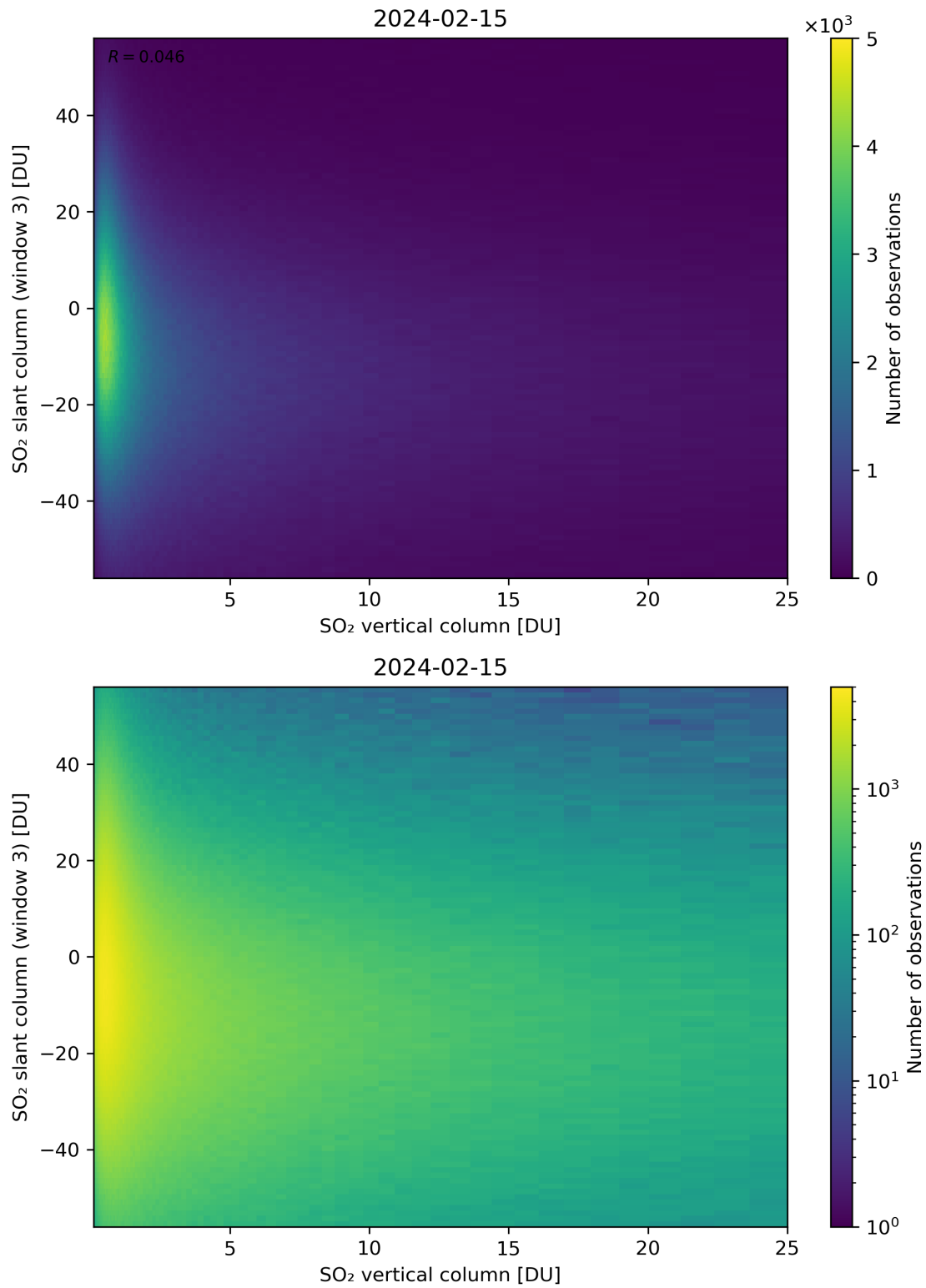
Figure 303: Scatter density plot of “SO 2 vertical column” against “SO 2 slant column (window 3)” for 2024-02-14 to 2024-02-16.
