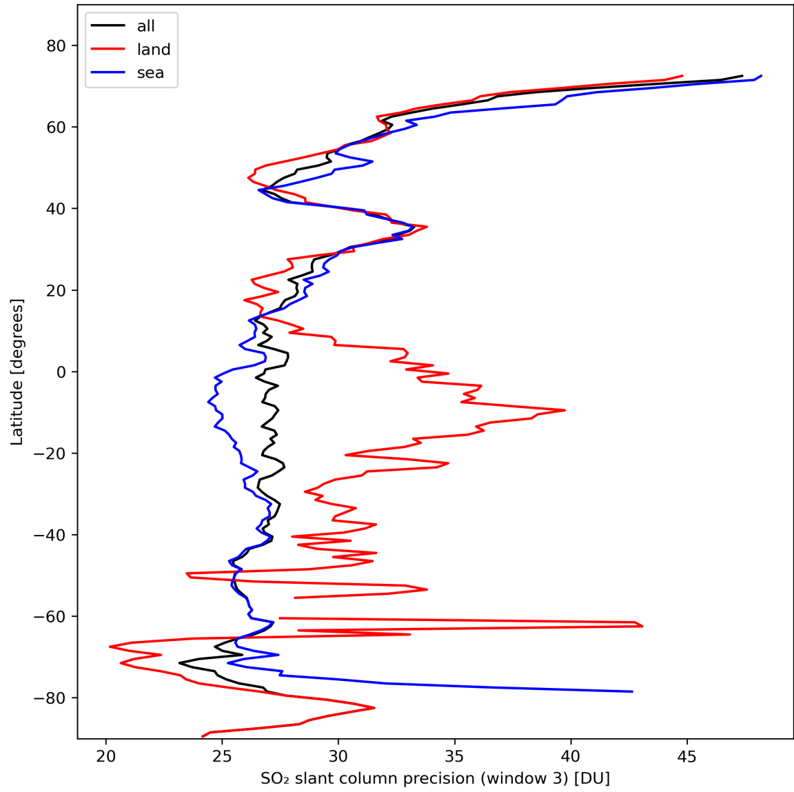
Figure 42: Zonal average of “SO 2 slant column precision (window 3)” for 2024-02-14 to 2024-02-16.
