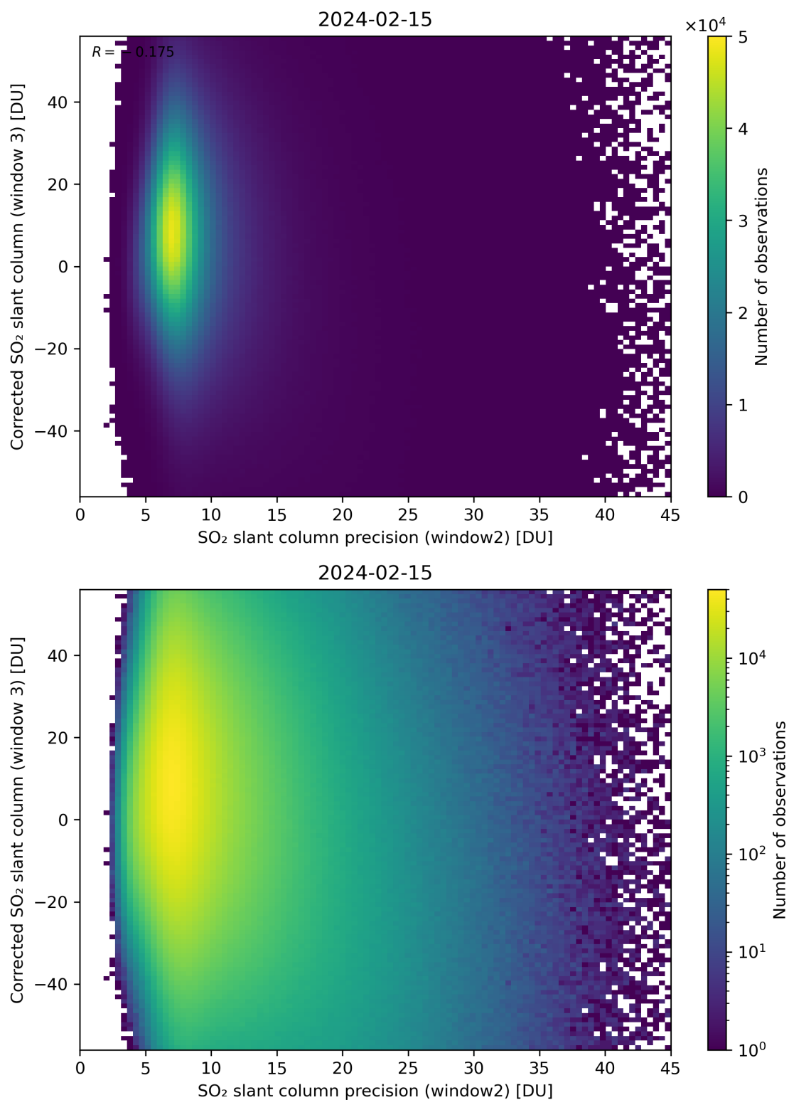
Figure 248: Scatter density plot of “SO 2 slant column precision (window2)” against “Corrected SO 2 slant column (window 3)” for 2024-02-14 to 2024-02-16.
