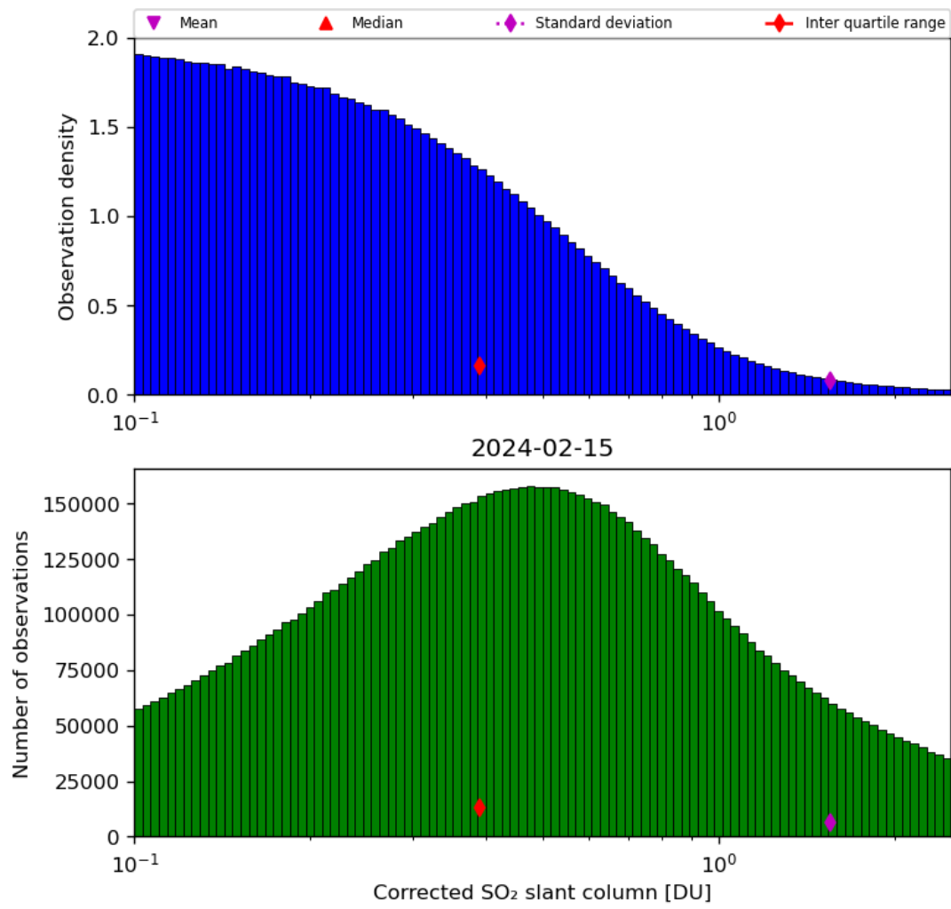
Figure 55: Histogram of “Corrected SO 2 slant column” for 2024-02-14 to 2024-02-16
