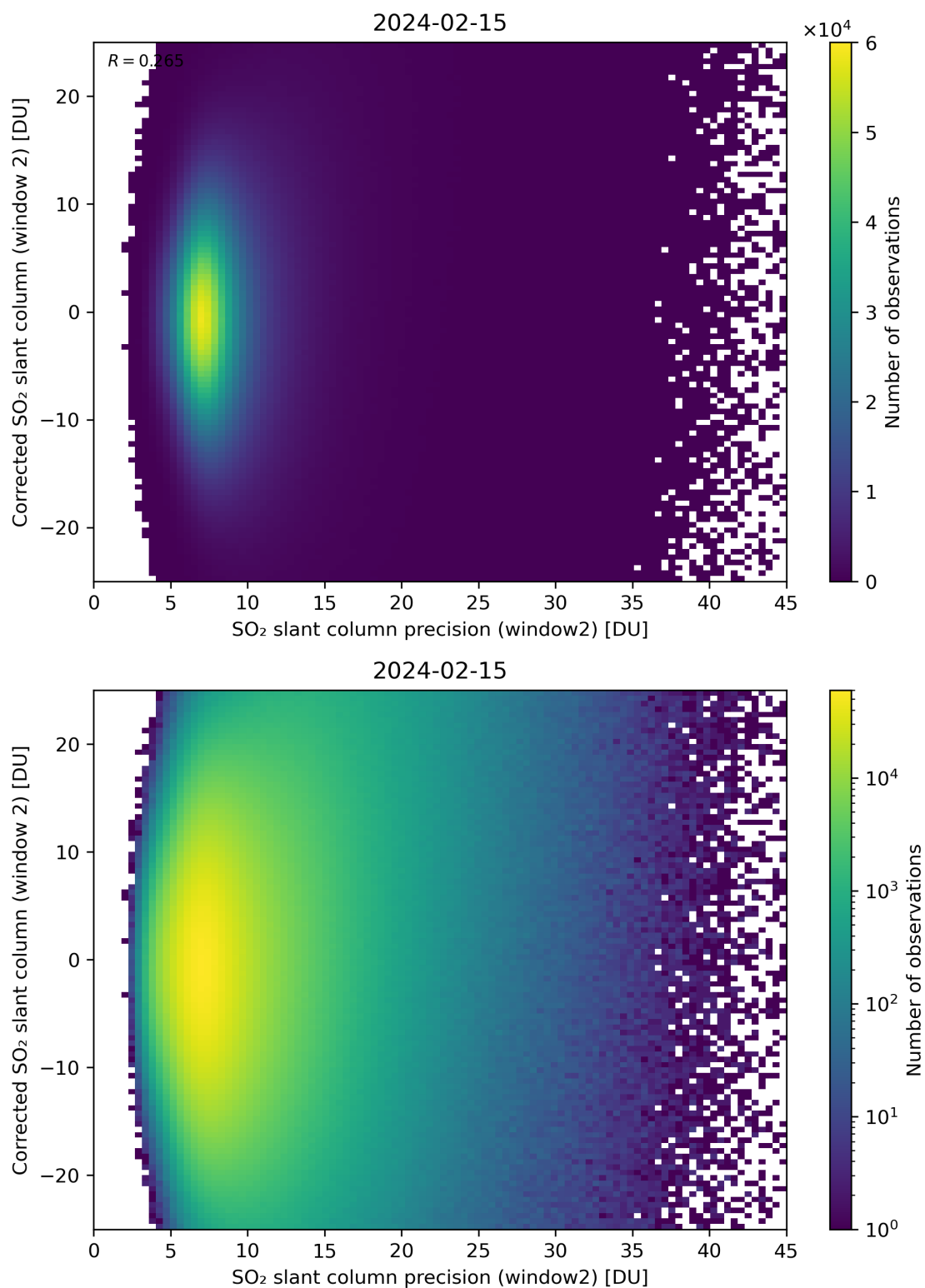
Figure 247: Scatter density plot of “SO 2 slant column precision (window2)” against “Corrected SO 2 slant column (window 2)” for 2024-02-14 to 2024-02-16.
