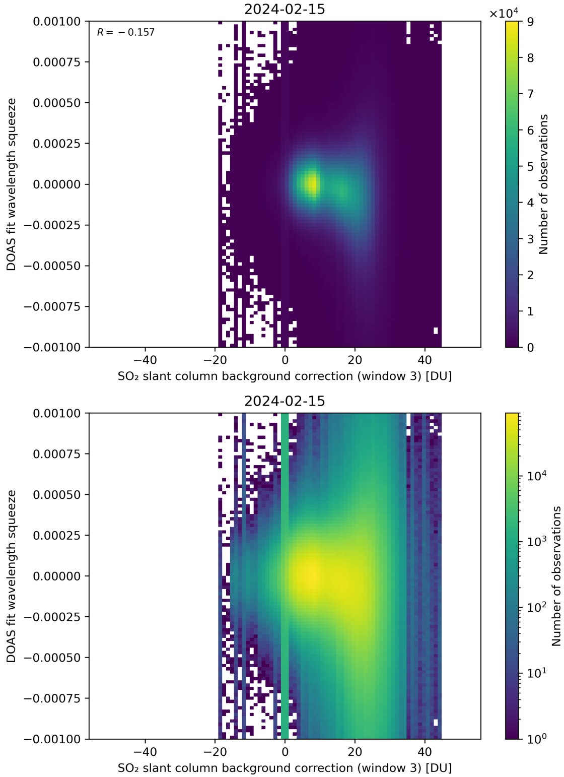
Figure 122: Scatter density plot of “SO 2 slant column background correction (window 3)” against “DOAS fit wavelength squeeze” for 2024-02-14 to 2024-02-16.
