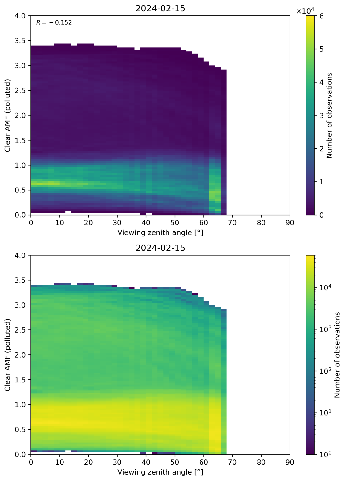
Figure 316: Scatter density plot of “Viewing zenith angle” against “Clear AMF (polluted)” for 2024-02-14 to 2024-02-16.
