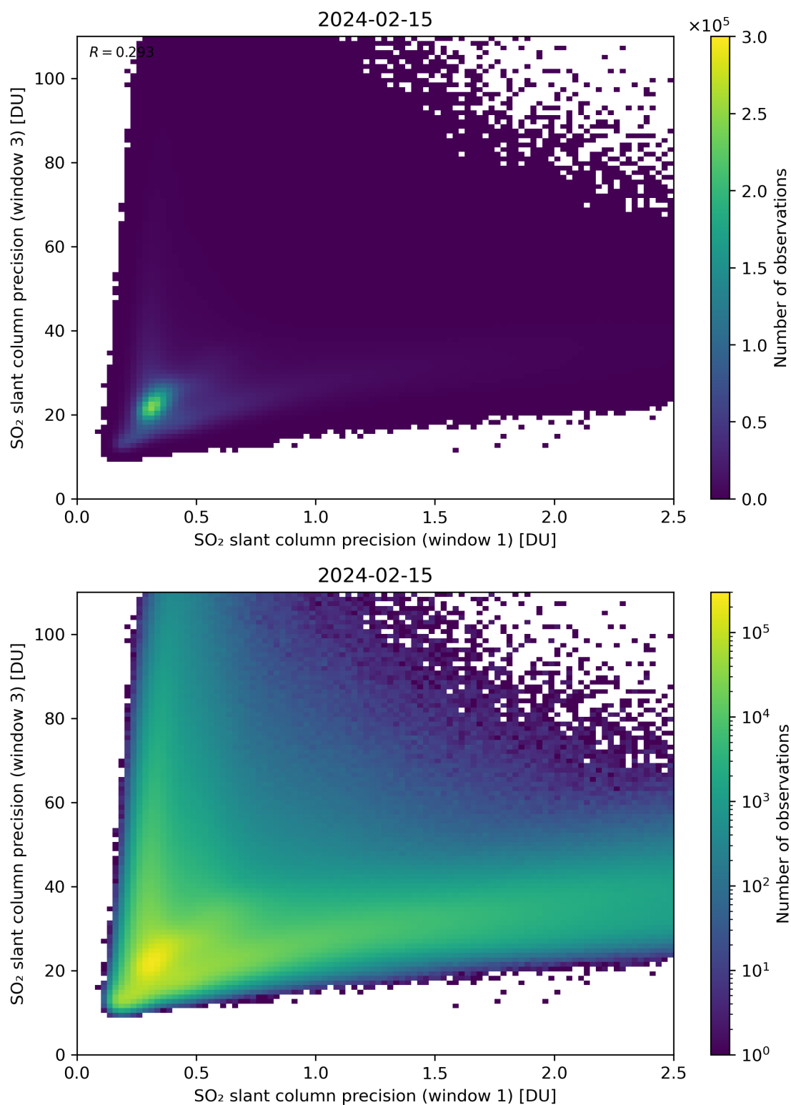
Figure 229: Scatter density plot of “SO 2 slant column precision (window 1)” against “SO 2 slant column precision (window 3)” for 2024-02-14 to 2024-02-16.
