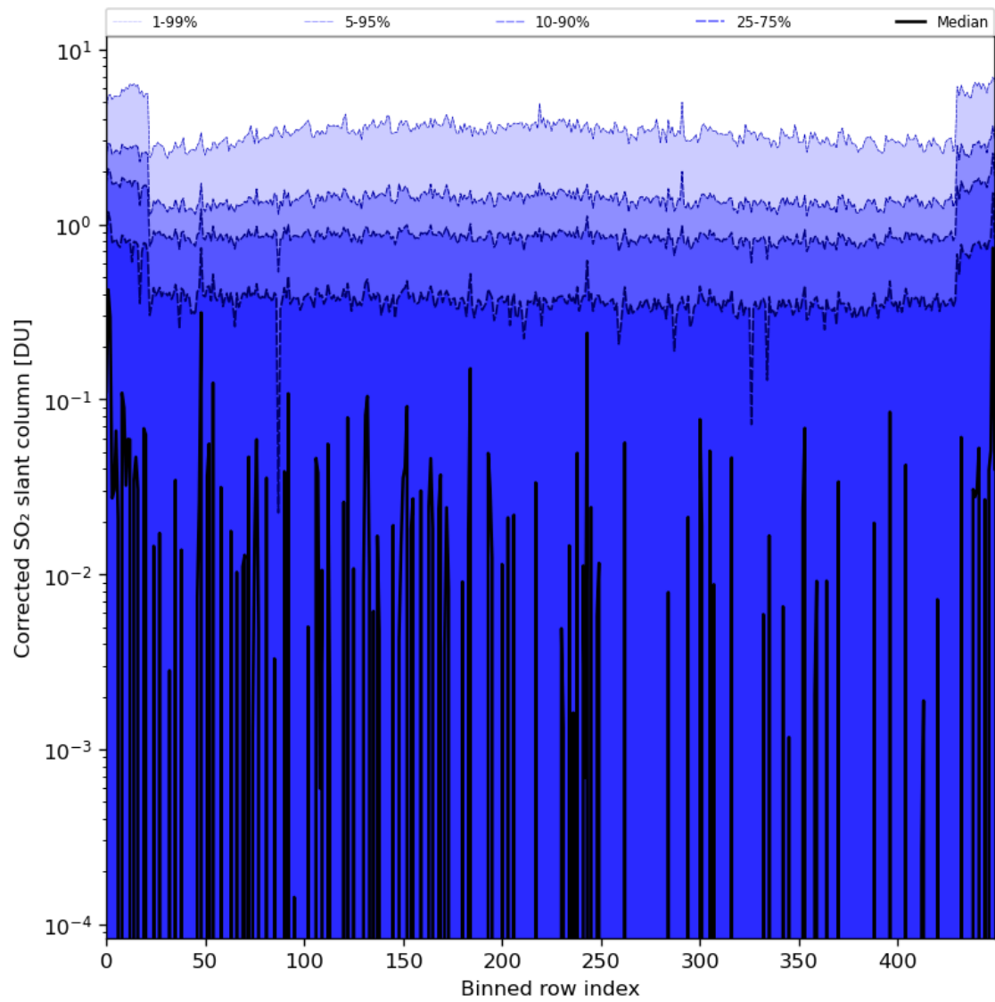
Figure 78: Along track statistics of “Corrected SO 2 slant column” for 2024-02-14 to 2024-02-16
