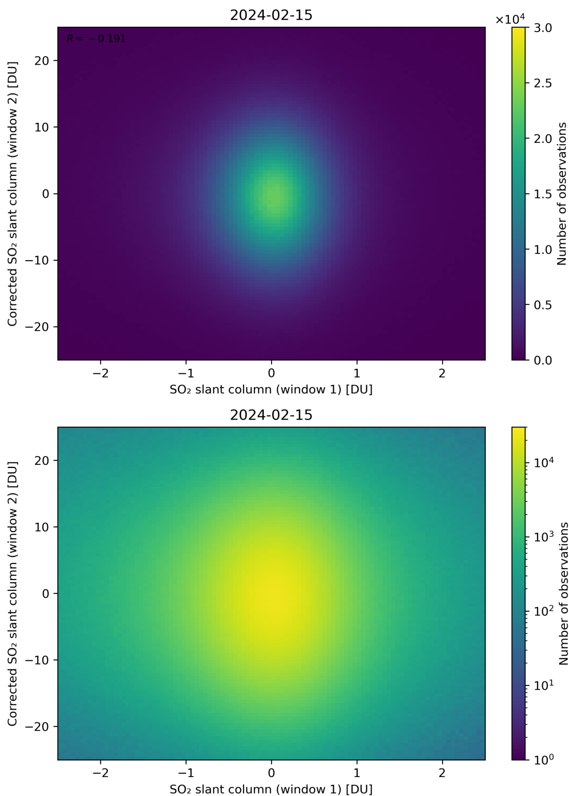
Figure 233: Scatter density plot of “SO 2 slant column (window 1)” against “Corrected SO 2 slant column (window 2)” for 2024-02-14 to 2024-02-16.
