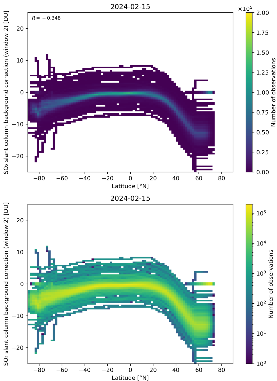
Figure 140: Scatter density plot of “Latitude” against “SO 2 slant column background correction (window 2)” for 2024-02-14 to 2024-02-16.
