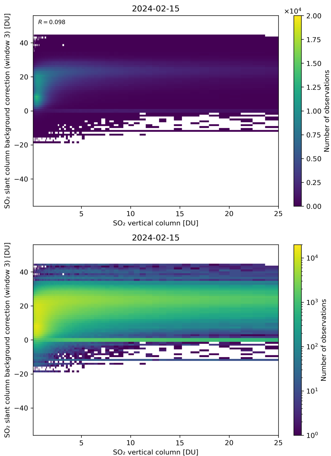
Figure 275: Scatter density plot of “SO 2 vertical column” against “SO 2 slant column background correction (window 3)” for 2024-02-14 to 2024-02-16.
