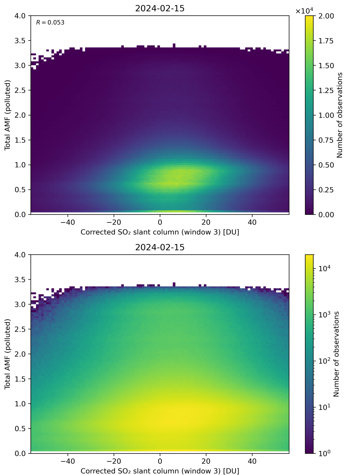
Figure 210: Scatter density plot of “Corrected SO 2 slant column (window 3)” against “Total AMF (polluted)” for 2024-02-14 to 2024-02-16.
