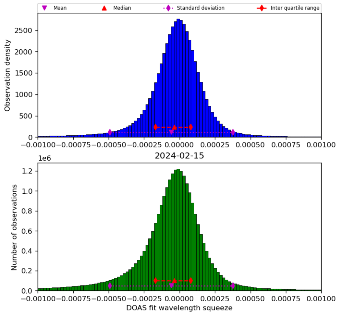
Figure 69: Histogram of “DOAS fit wavelength squeeze” for 2024-02-14 to 2024-02-16
