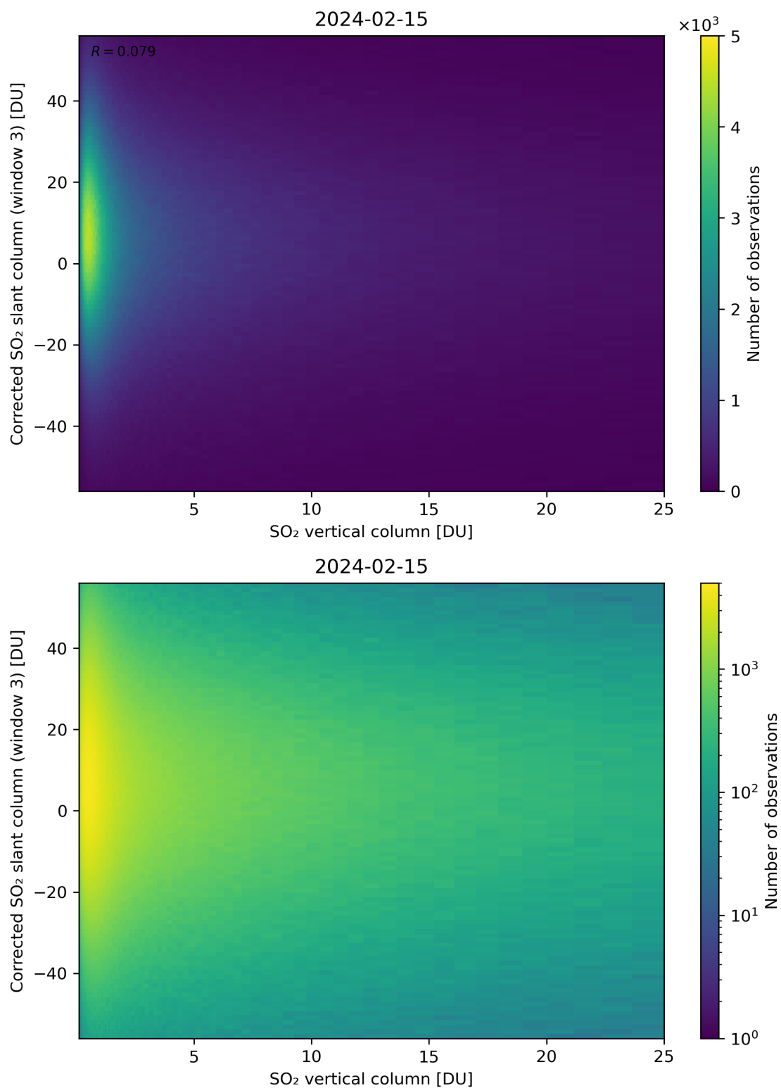
Figure 299: Scatter density plot of “SO 2 vertical column” against “Corrected SO 2 slant column (window 3)” for 2024-02-14 to 2024-02-16.
