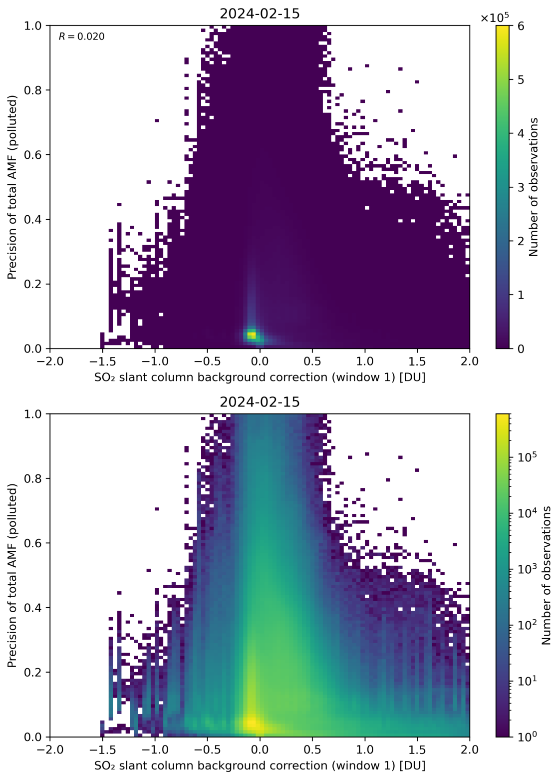
Figure 110: Scatter density plot of “SO 2 slant column background correction (window 1)” against “Precision of total AMF (polluted)” for 2024-02-14 to 2024-02-16.
