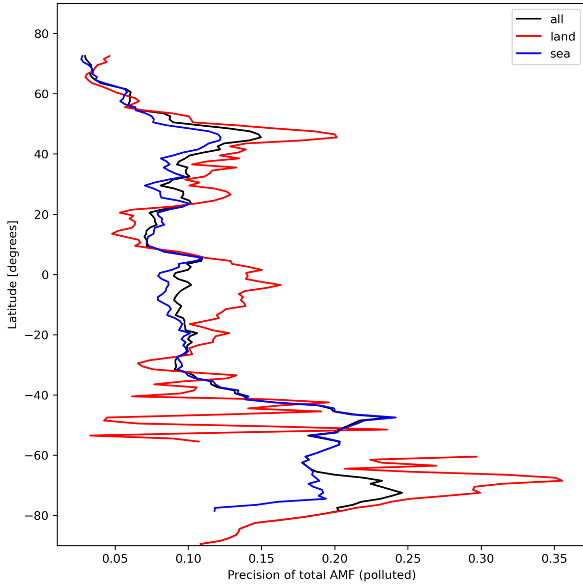
Figure 49: Zonal average of “Precision of total AMF (polluted)” for 2024-02-14 to 2024-02-16.
