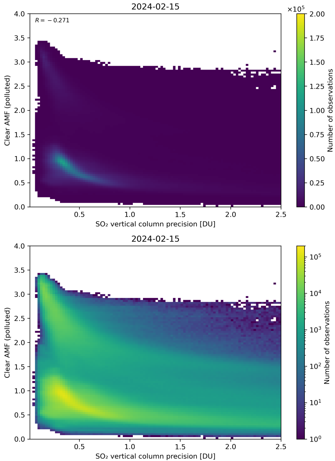
Figure 285: Scatter density plot of “SO 2 vertical column precision” against “Clear AMF (polluted)” for 2024-02-14 to 2024-02-16.
