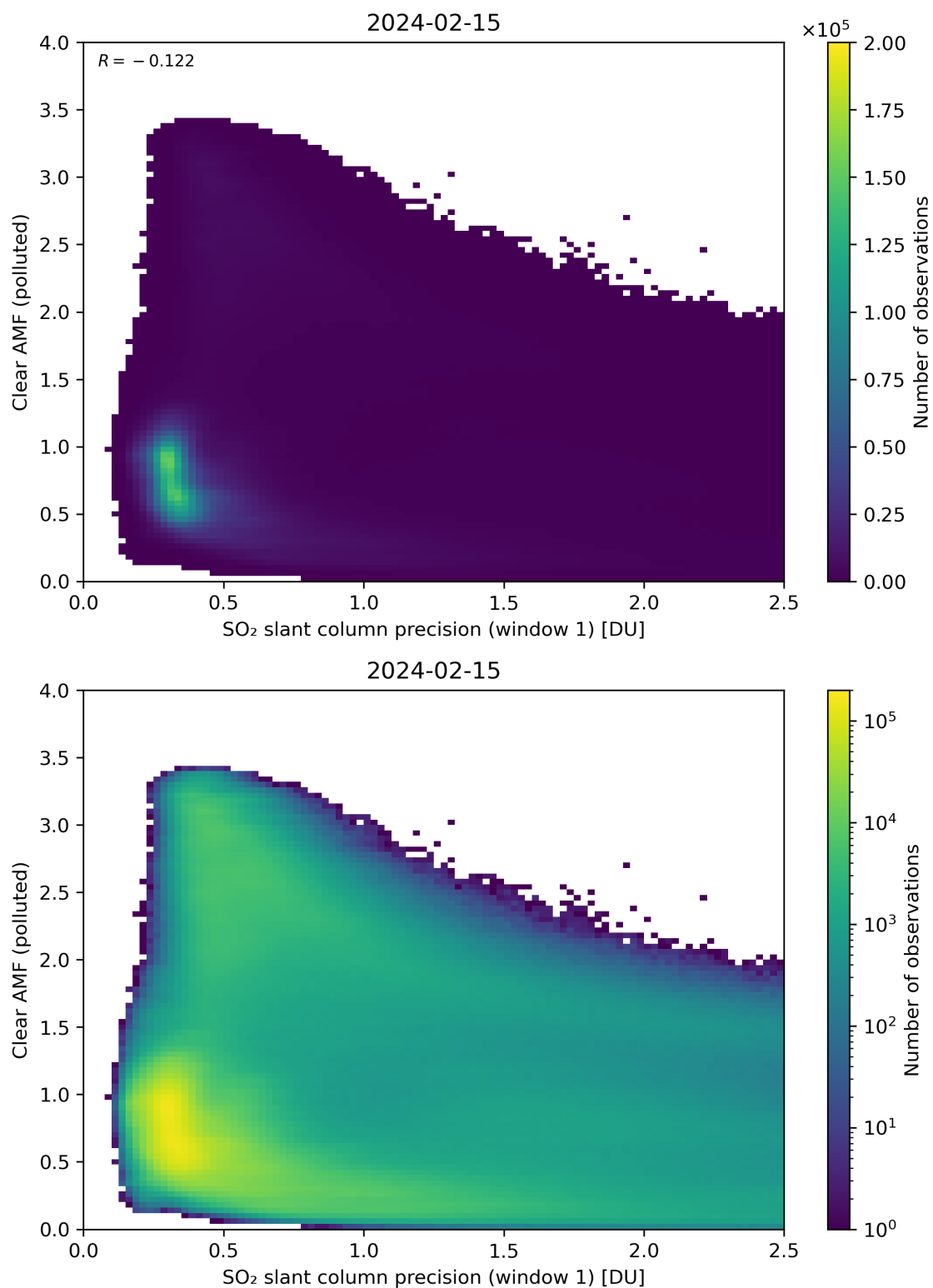
Figure 224: Scatter density plot of “SO 2 slant column precision (window 1)” against “Clear AMF (polluted)” for 2024-02-14 to 2024-02-16.
