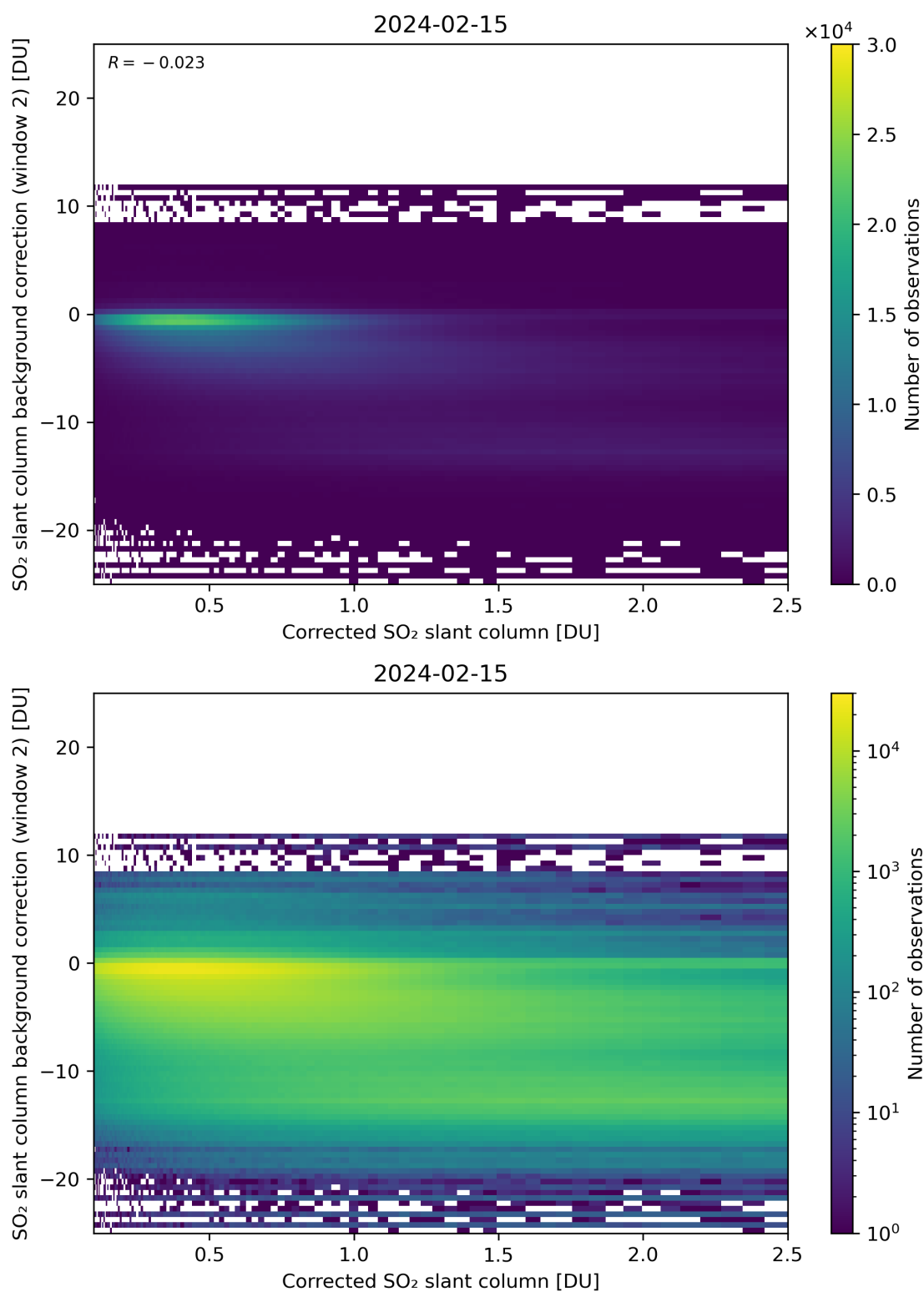
Figure 179: Scatter density plot of “Corrected SO 2 slant column” against “SO 2 slant column background correction (window 2)” for 2024-02-14 to 2024-02-16.
