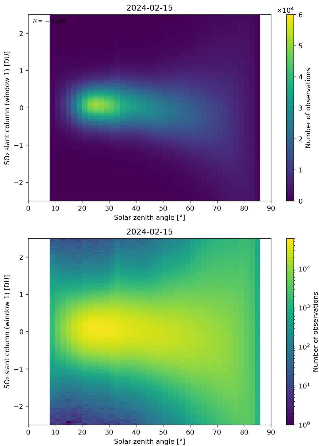
Figure 169: Scatter density plot of “Solar zenith angle” against “SO 2 slant column (window 1)” for 2024-02-14 to 2024-02-16.
