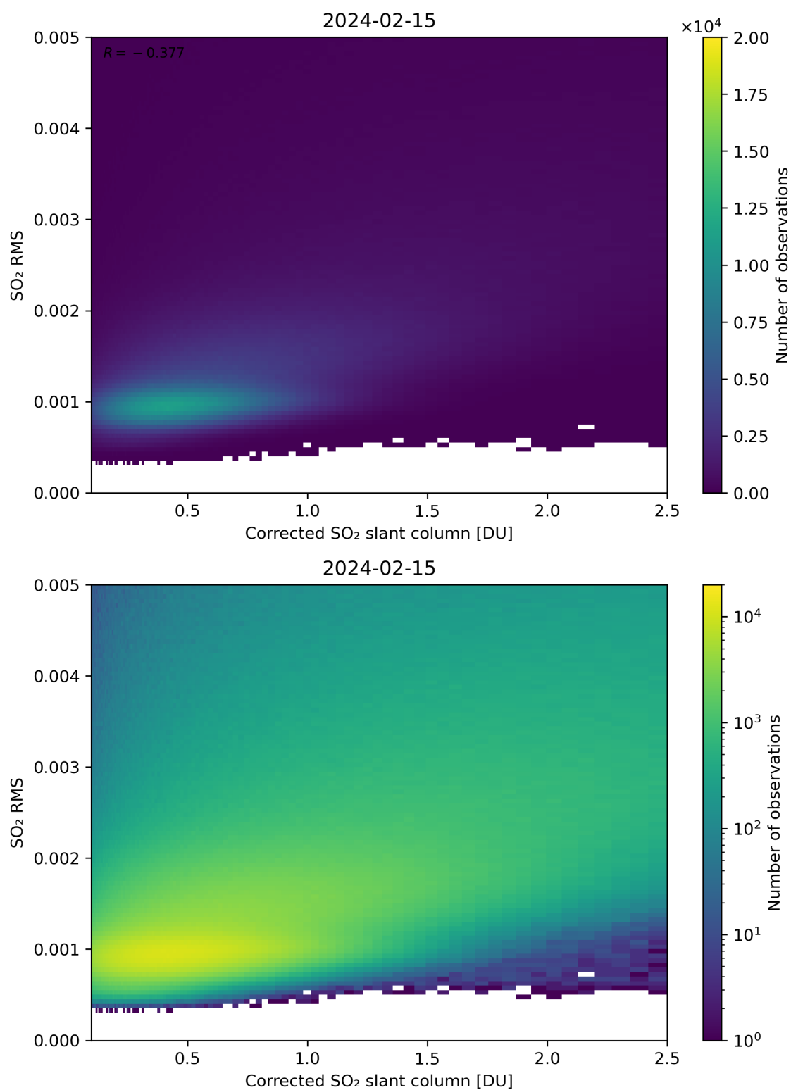
Figure 183: Scatter density plot of “Corrected SO 2 slant column” against “SO 2 RMS” for 2024-02-14 to 2024-02-16.
