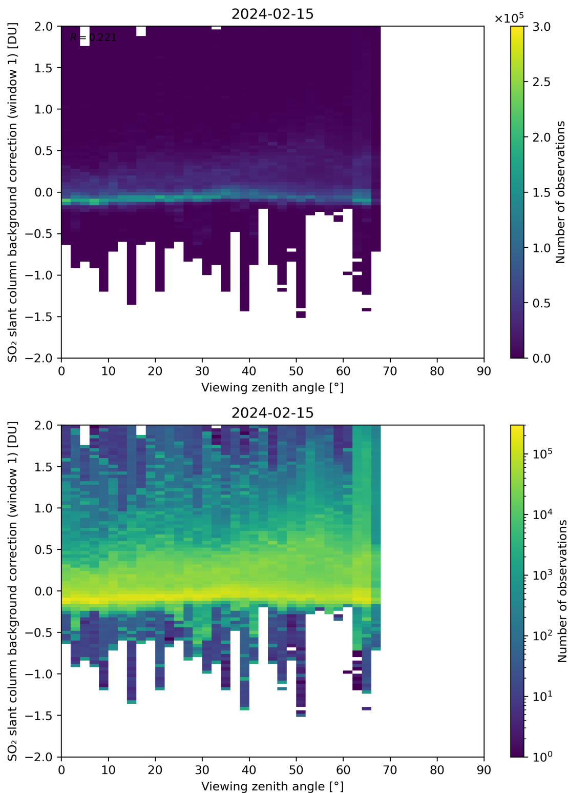
Figure 308: Scatter density plot of “Viewing zenith angle” against “SO 2 slant column background correction (window 1)” for 2024-02-14 to 2024-02-16.
