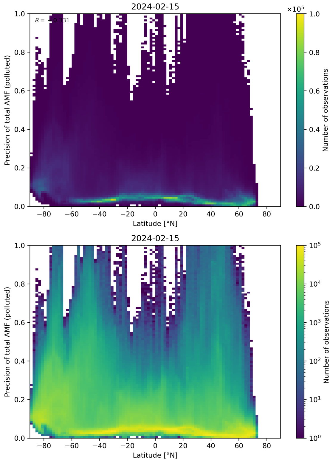
Figure 155: Scatter density plot of “Latitude” against “Precision of total AMF (polluted)” for 2024-02-14 to 2024-02-16.
