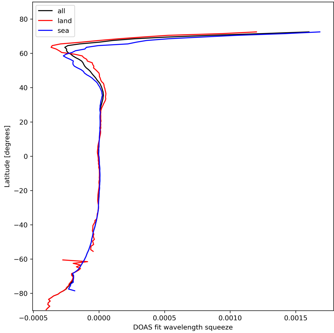
Figure 46: Zonal average of “DOAS fit wavelength squeeze” for 2024-02-14 to 2024-02-16.
