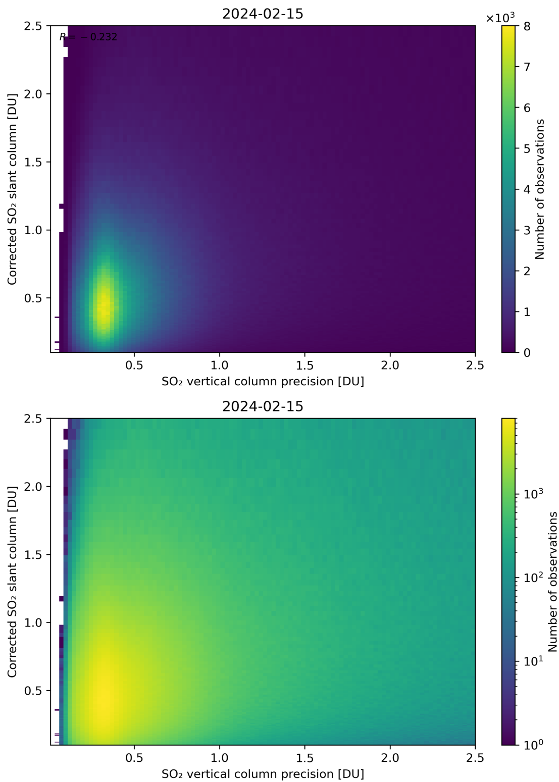
Figure 286: Scatter density plot of “SO 2 vertical column precision” against “Corrected SO 2 slant column” for 2024-02-14 to 2024-02-16.
