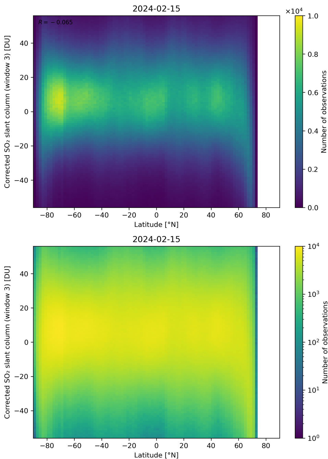
Figure 148: Scatter density plot of “Latitude” against “Corrected SO 2 slant column (window 3)” for 2024-02-14 to 2024-02-16.
