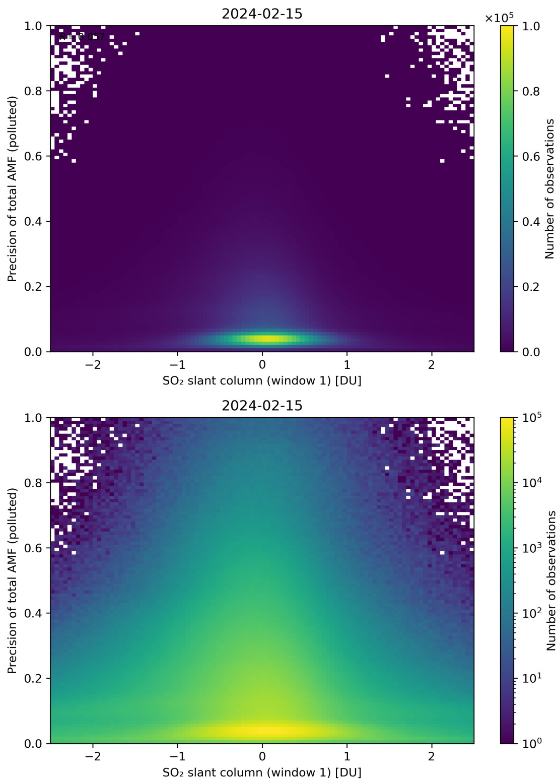
Figure 240: Scatter density plot of “SO 2 slant column (window 1)” against “Precision of total AMF (polluted)” for 2024-02-14 to 2024-02-16.
