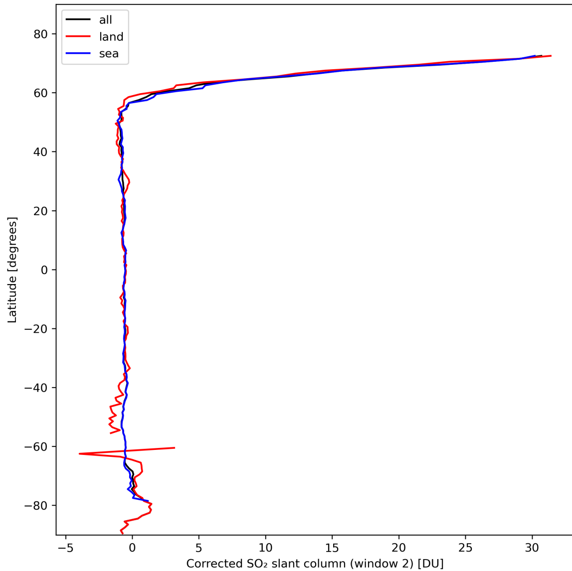
Figure 39: Zonal average of “Corrected SO 2 slant column (window 2)” for 2024-02-14 to 2024-02-16.
