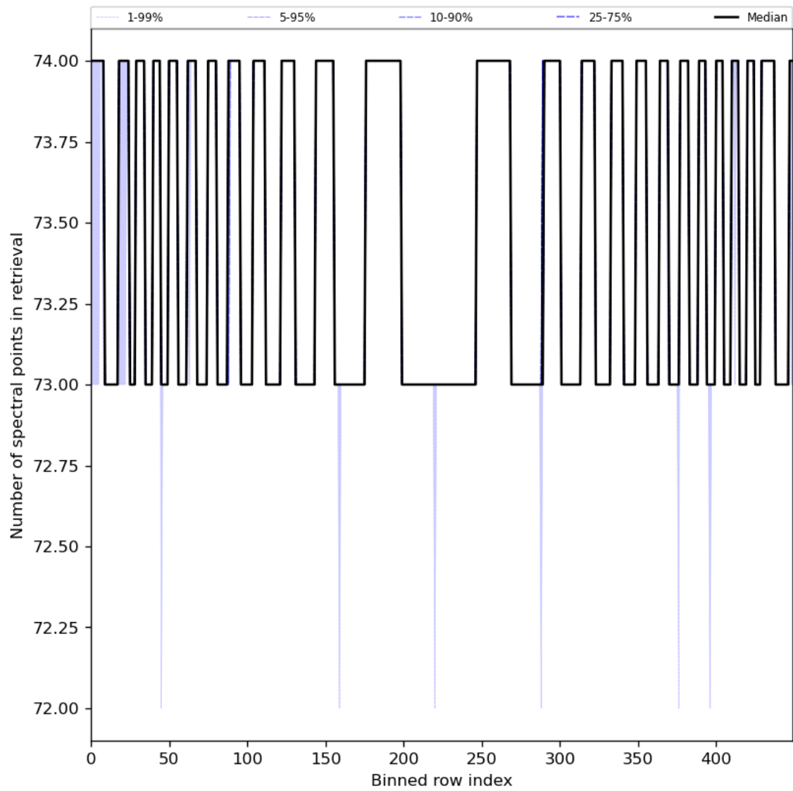
Figure 97: Along track statistics of “Number of spectral points in retrieval” for 2024-02-14 to 2024-02-16
