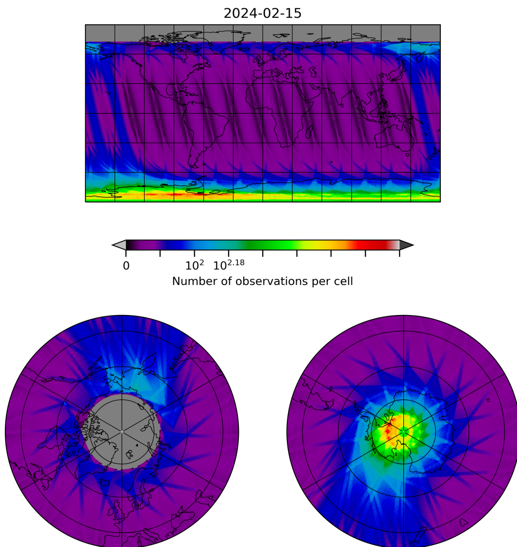
Figure 28: Map of the number of observations for 2024-02-14 to 2024-02-16
