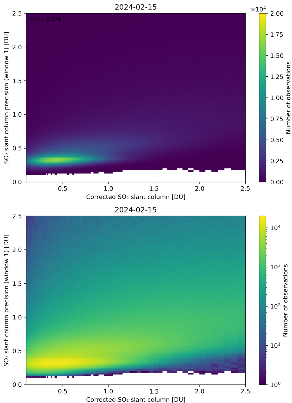
Figure 188: Scatter density plot of “Corrected SO 2 slant column” against “SO 2 slant column precision (window 1)” for 2024-02-14 to 2024-02-16.
