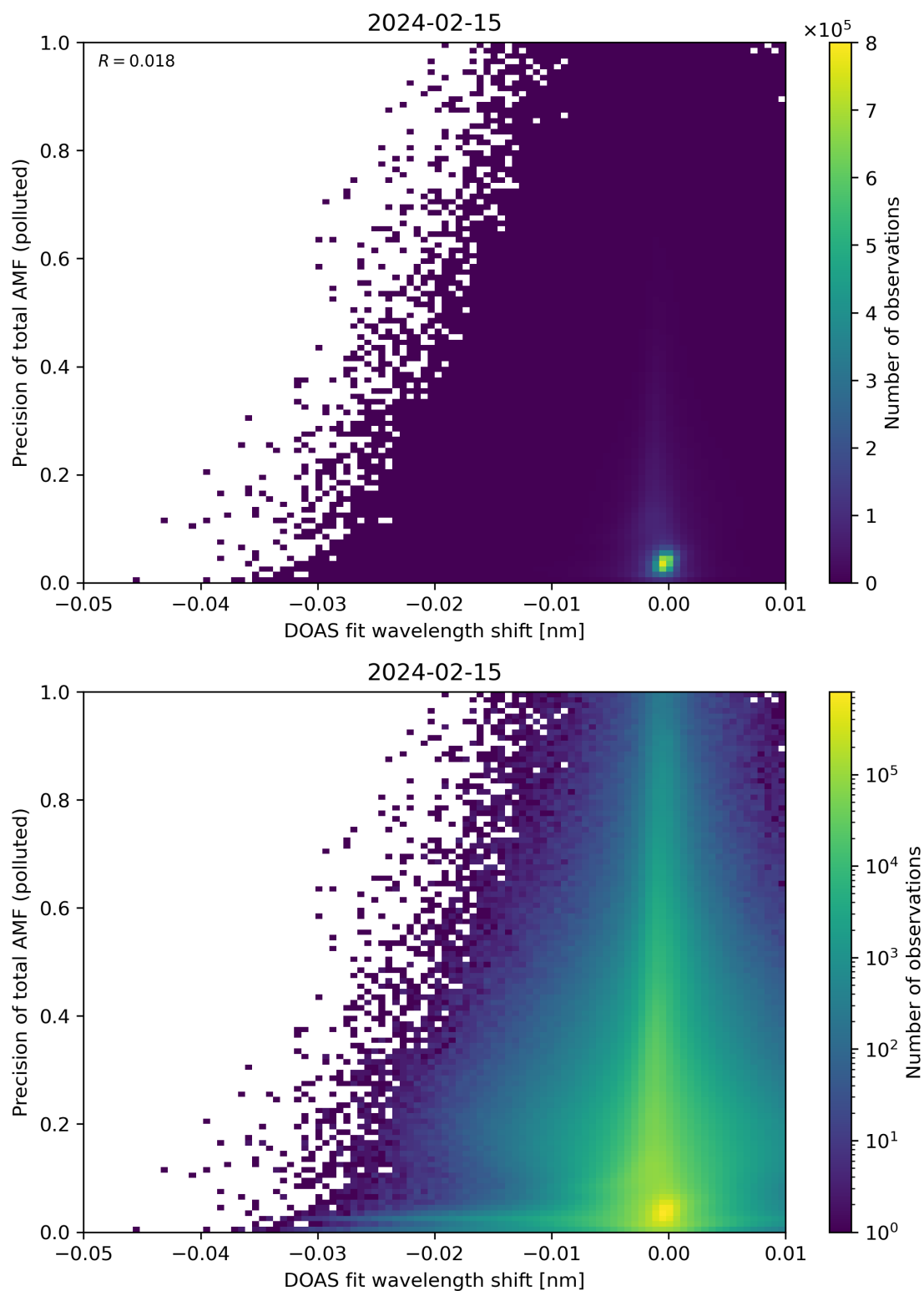
Figure 131: Scatter density plot of “DOAS fit wavelength shift” against “Precision of total AMF (polluted)” for 2024-02-14 to 2024-02-16.
