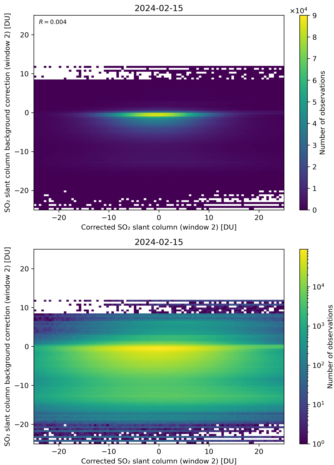
Figure 194: Scatter density plot of “Corrected SO 2 slant column (window 2)” against “SO 2 slant column background correction (window 2)” for 2024-02-14 to 2024-02-16.
