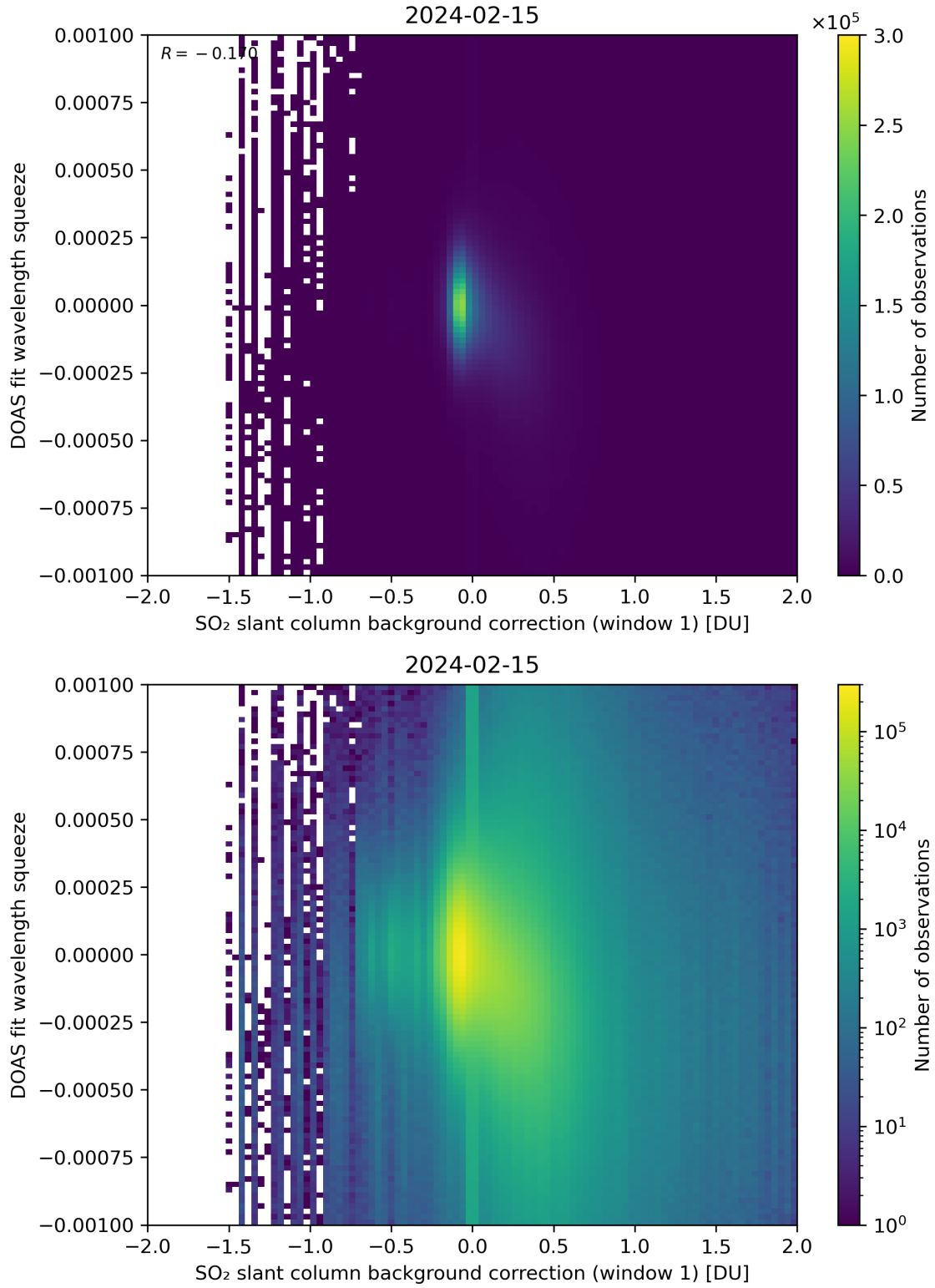
Figure 101: Scatter density plot of “SO 2 slant column background correction (window 1)” against “DOAS fit wavelength squeeze” for 2024-02-14 to 2024-02-16.
