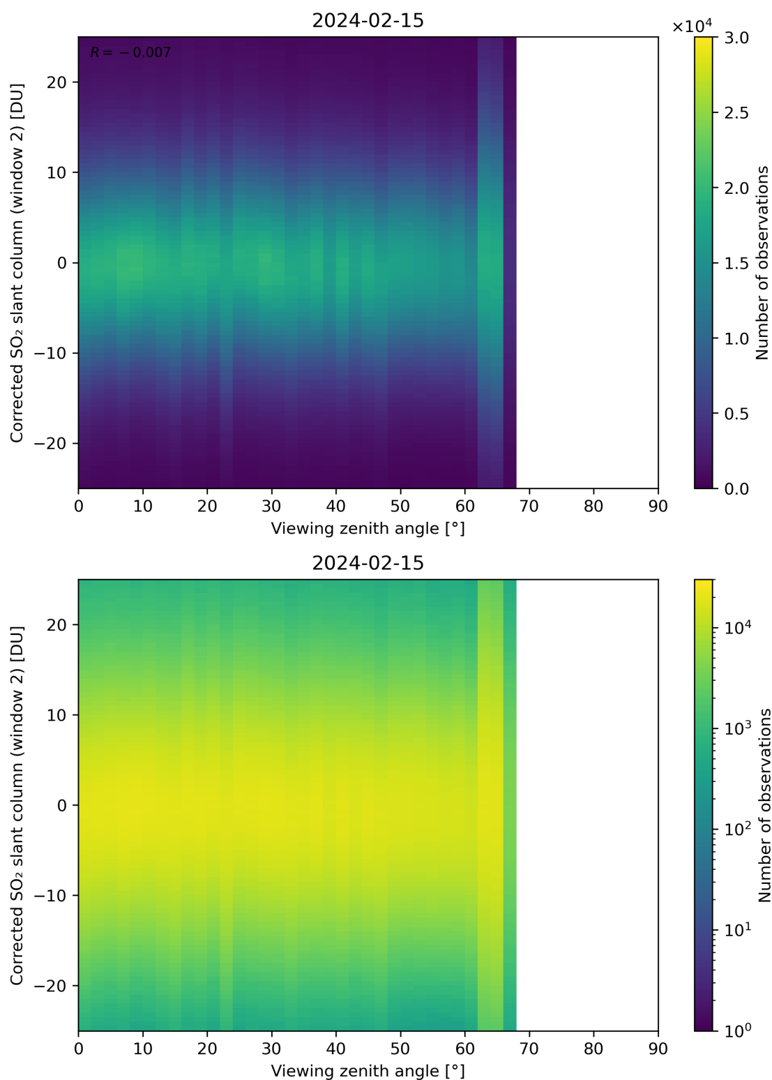
Figure 318: Scatter density plot of “Viewing zenith angle” against “Corrected SO 2 slant column (window 2)” for 2024-02-14 to 2024-02-16.
