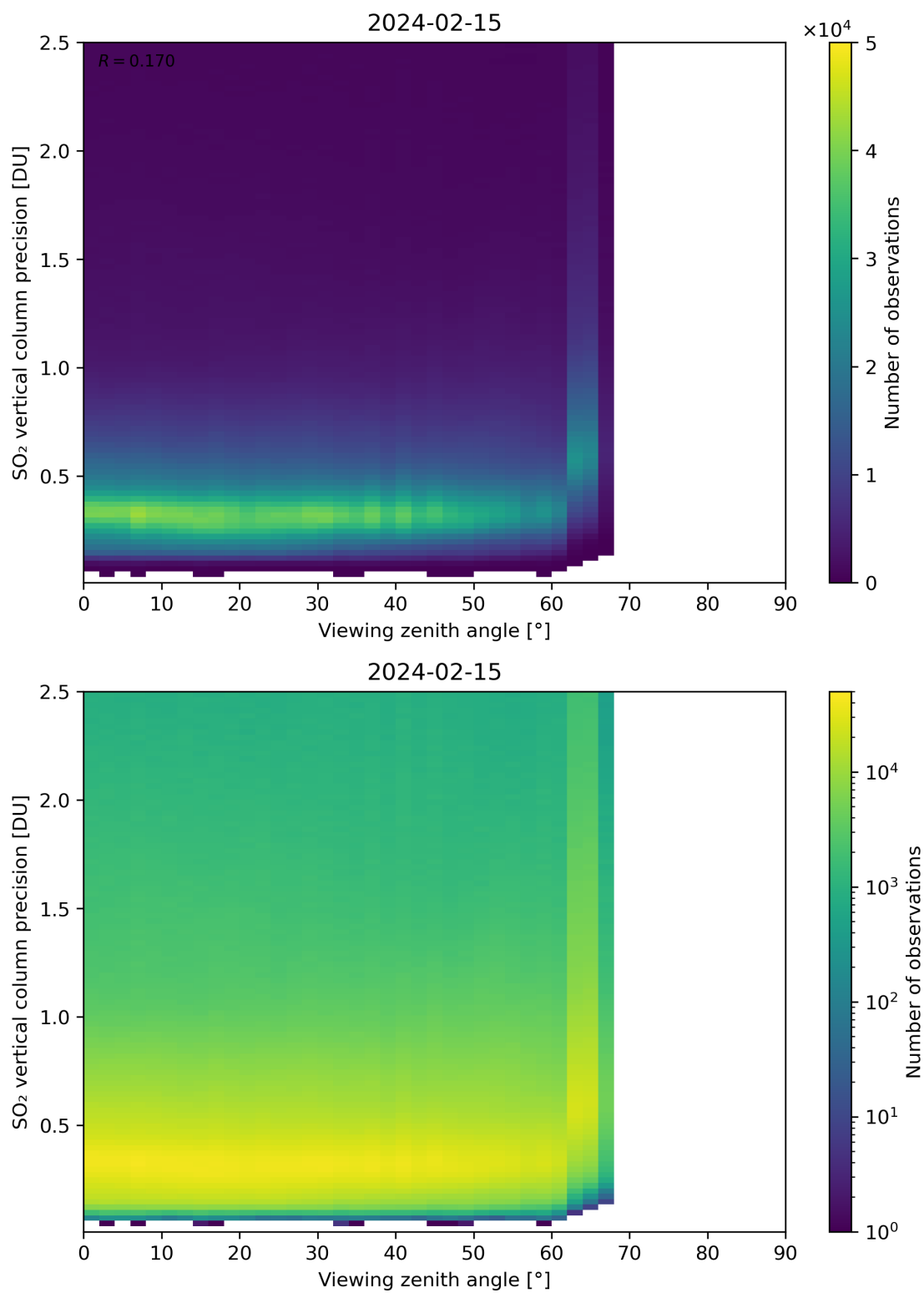
Figure 328: Scatter density plot of “Viewing zenith angle” against “SO 2 vertical column precision” for 2024-02-14 to 2024-02-16.
