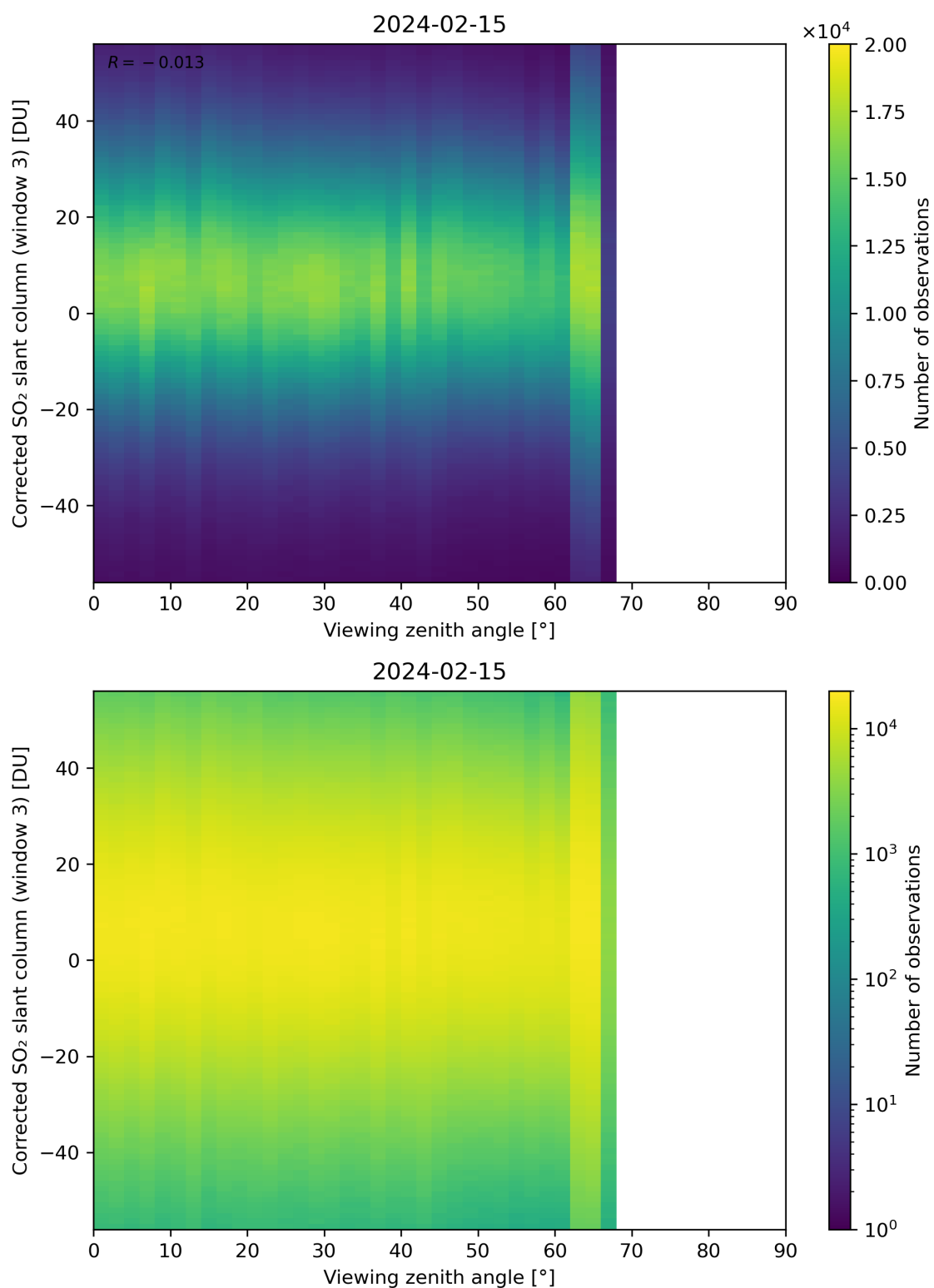
Figure 319: Scatter density plot of “Viewing zenith angle” against “Corrected SO 2 slant column (window 3)” for 2024-02-14 to 2024-02-16.
