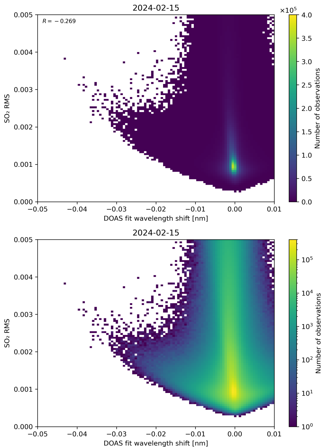
Figure 128: Scatter density plot of “DOAS fit wavelength shift” against “SO 2 RMS” for 2024-02-14 to 2024-02-16.
