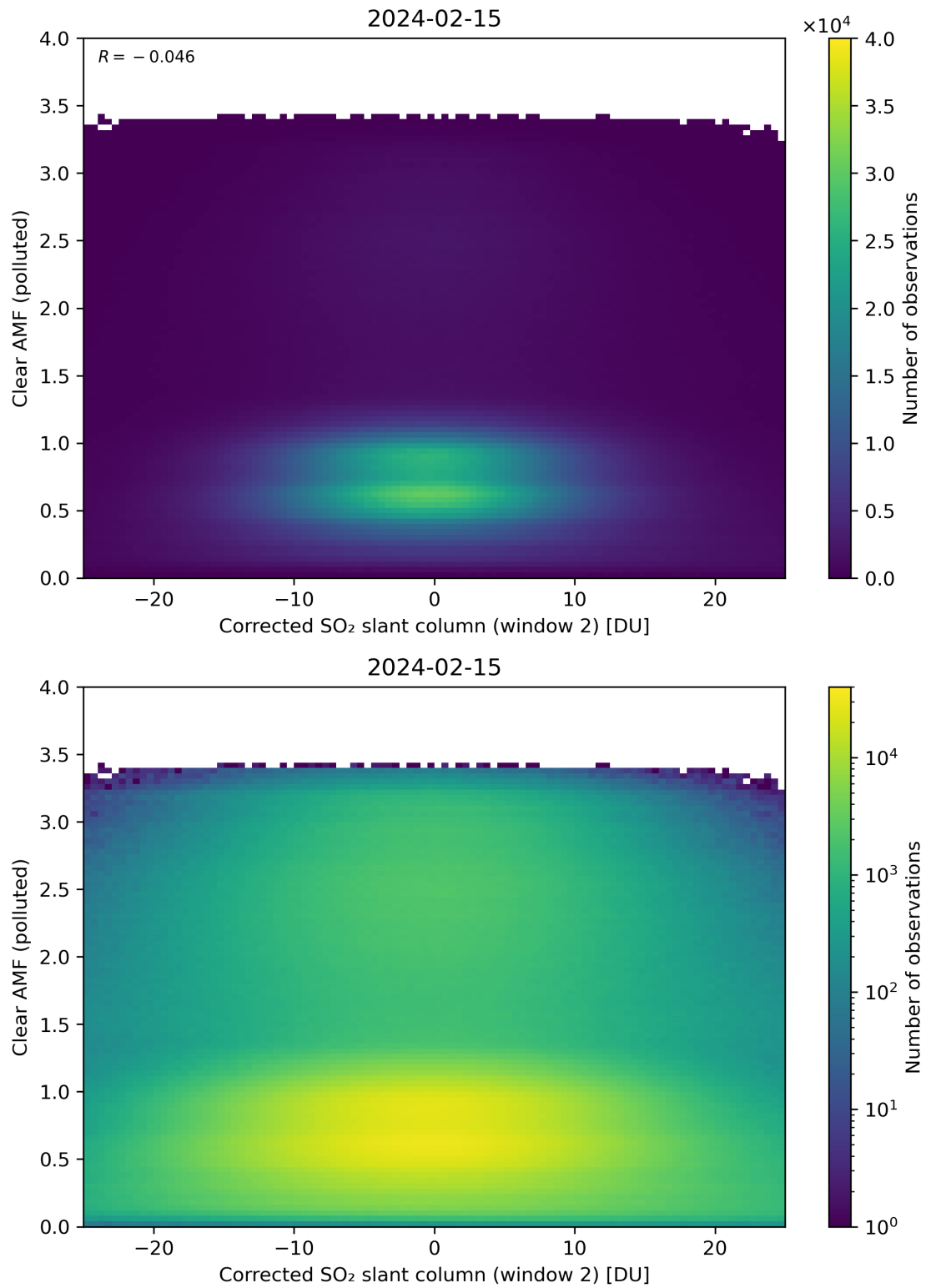
Figure 199: Scatter density plot of “Corrected SO 2 slant column (window 2)” against “Clear AMF (polluted)” for 2024-02-14 to 2024-02-16.
