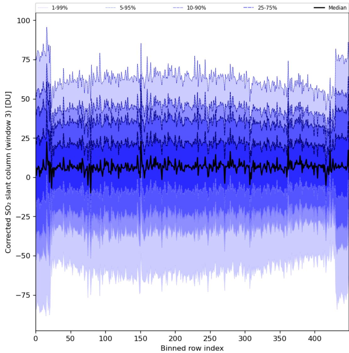
Figure 89: Along track statistics of “Corrected SO 2 slant column (window 3)” for 2024-02-14 to 2024-02-16
