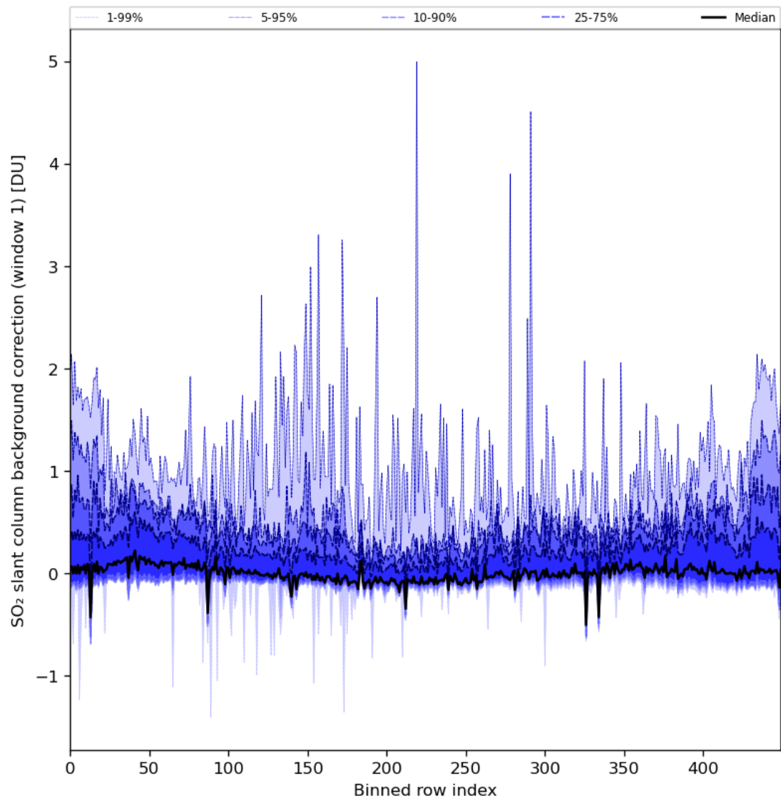
Figure 82: Along track statistics of “SO 2 slant column background correction (window 1)” for 2024-02-14 to 2024-02-16
