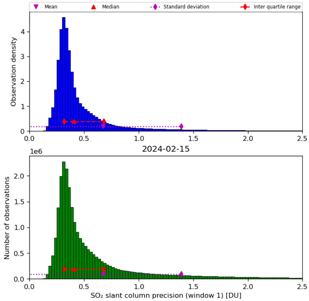
Figure 57: Histogram of “SO 2 slant column precision (window 1)” for 2024-02-14 to 2024-02-16
