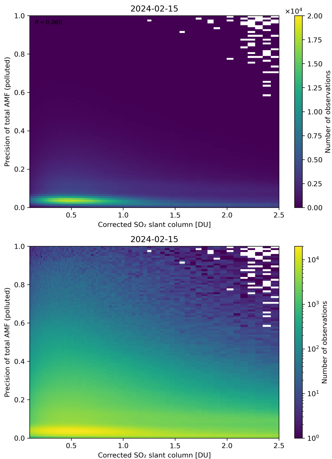
Figure 193: Scatter density plot of “Corrected SO 2 slant column” against “Precision of total AMF (polluted)” for 2024-02-14 to 2024-02-16.
