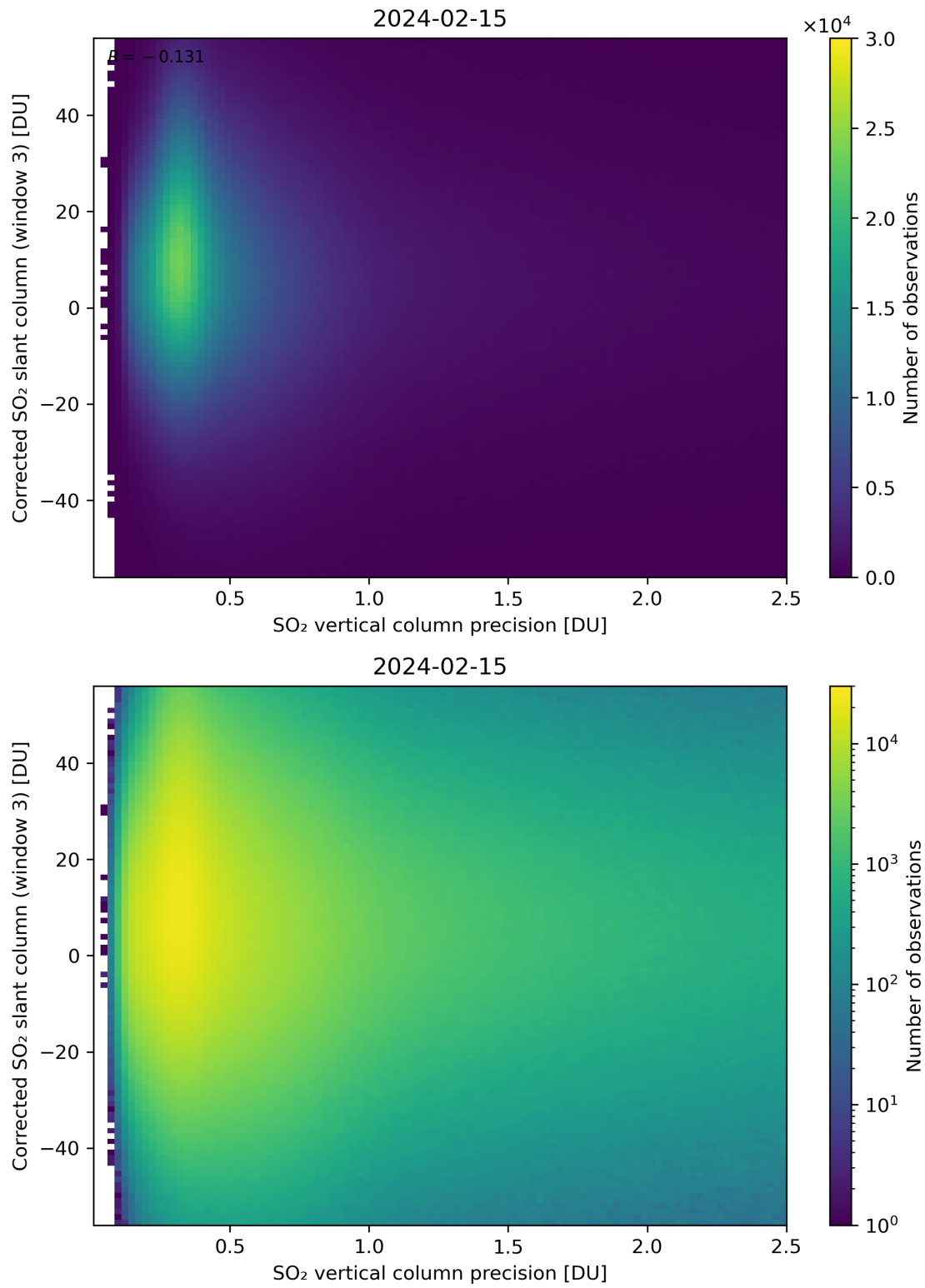
Figure 288: Scatter density plot of “SO 2 vertical column precision” against “Corrected SO 2 slant column (window 3)” for 2024-02-14 to 2024-02-16.
