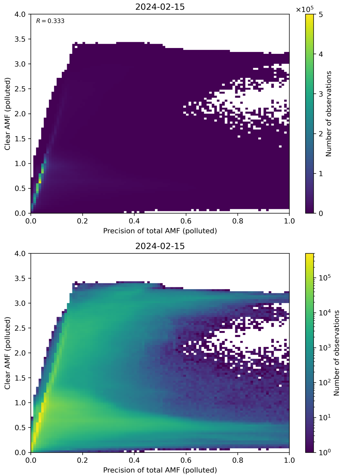
Figure 270: Scatter density plot of “Precision of total AMF (polluted)” against “Clear AMF (polluted)” for 2024-02-14 to 2024-02-16.
