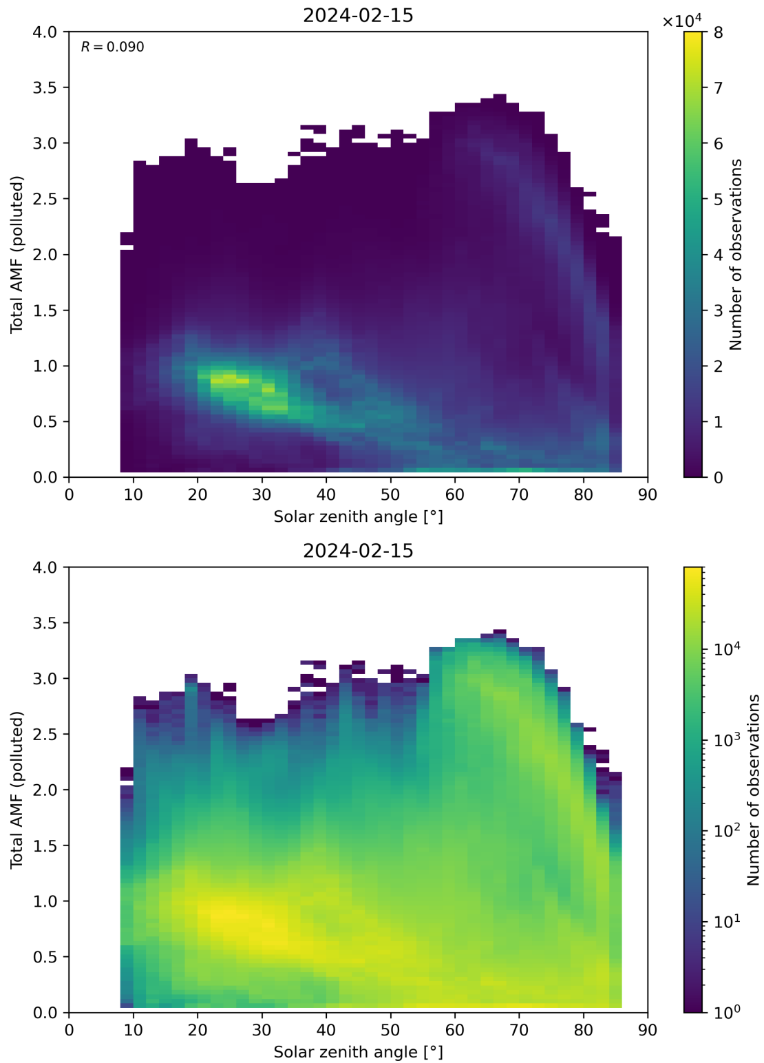
Figure 174: Scatter density plot of “Solar zenith angle” against “Total AMF (polluted)” for 2024-02-14 to 2024-02-16.
