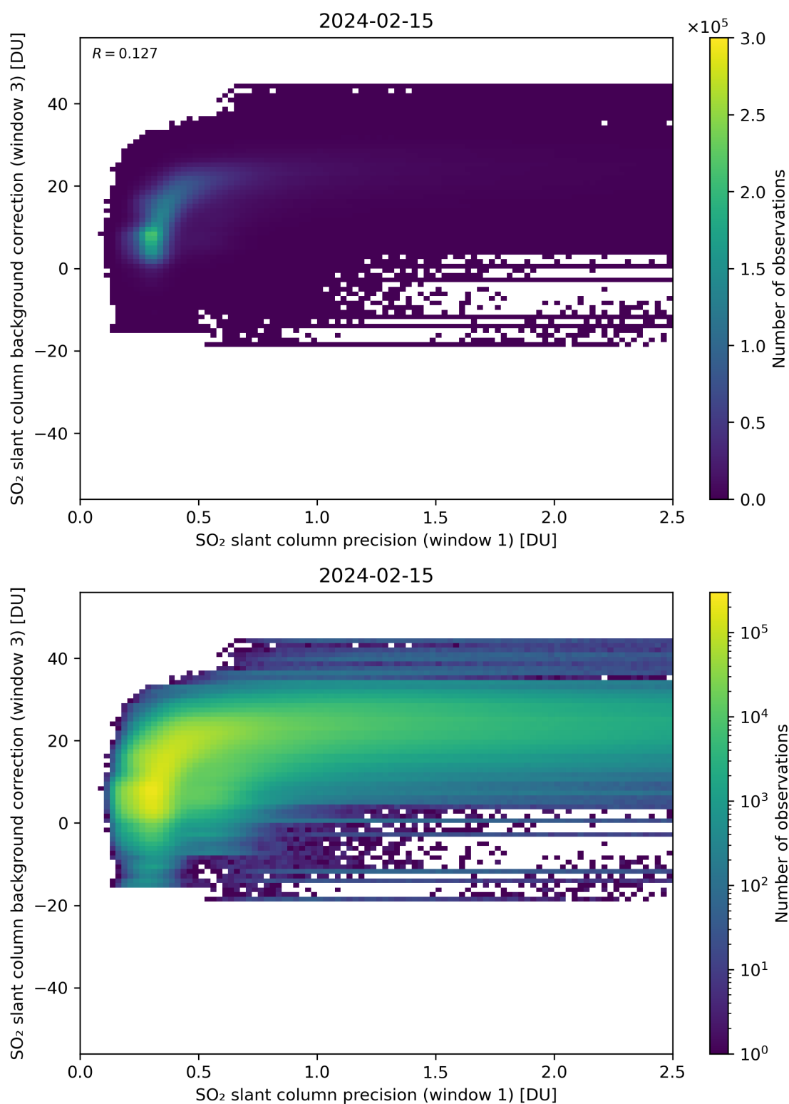
Figure 220: Scatter density plot of “SO 2 slant column precision (window 1)” against “SO 2 slant column background correction (window 3)” for 2024-02-14 to 2024-02-16.
