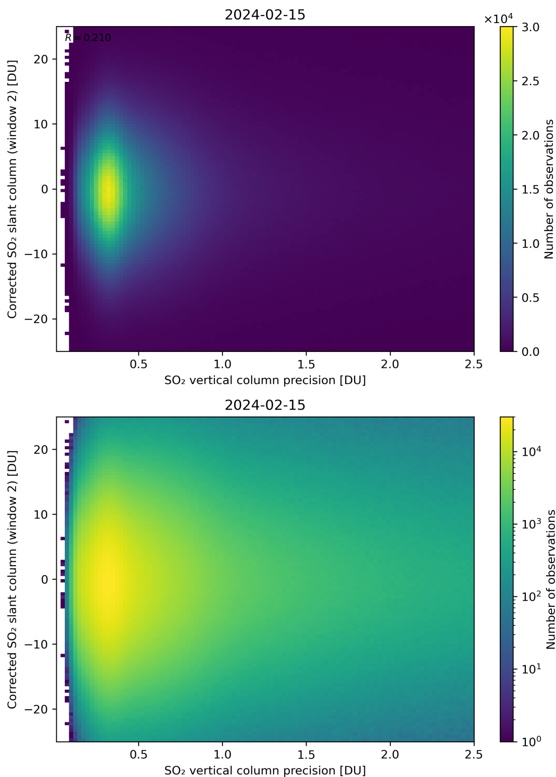
Figure 287: Scatter density plot of “SO 2 vertical column precision” against “Corrected SO 2 slant column (window 2)” for 2024-02-14 to 2024-02-16.
