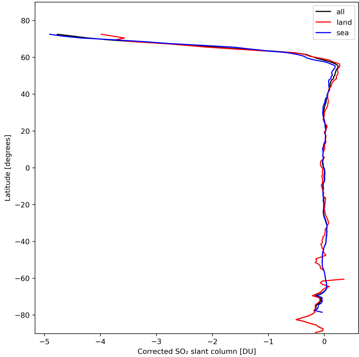
Figure 32: Zonal average of “Corrected SO 2 slant column” for 2024-02-14 to 2024-02-16.
