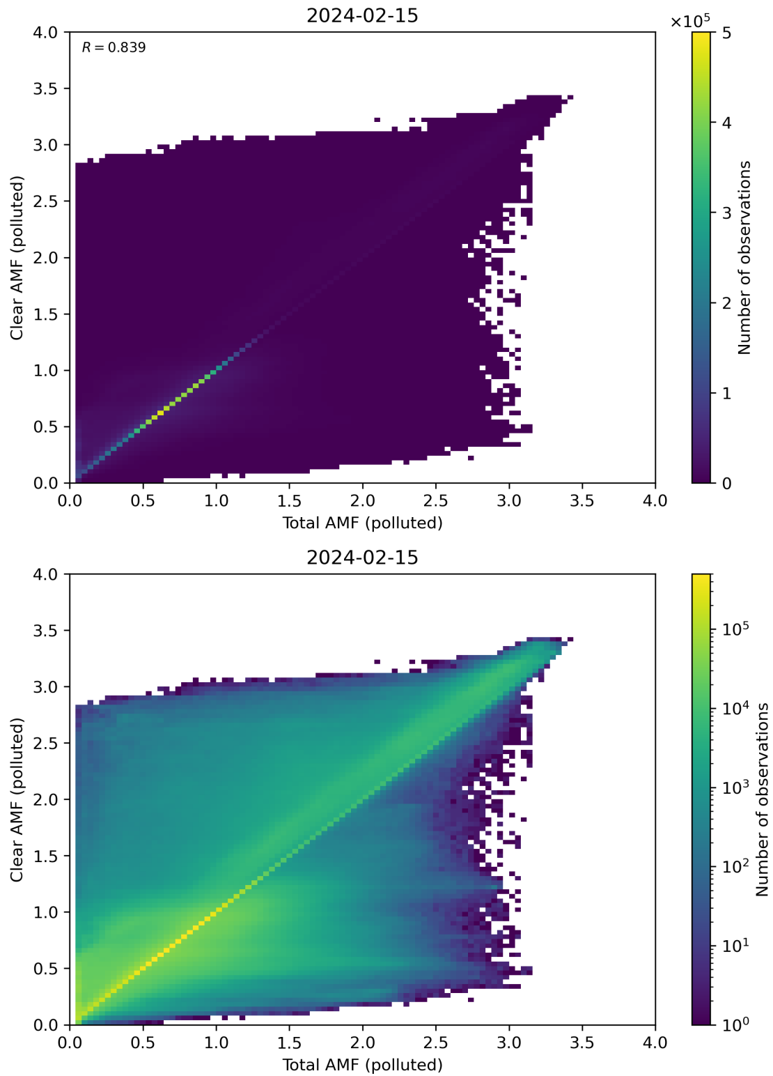
Figure 271: Scatter density plot of “Total AMF (polluted)” against “Clear AMF (polluted)” for 2024-02-14 to 2024-02-16.
