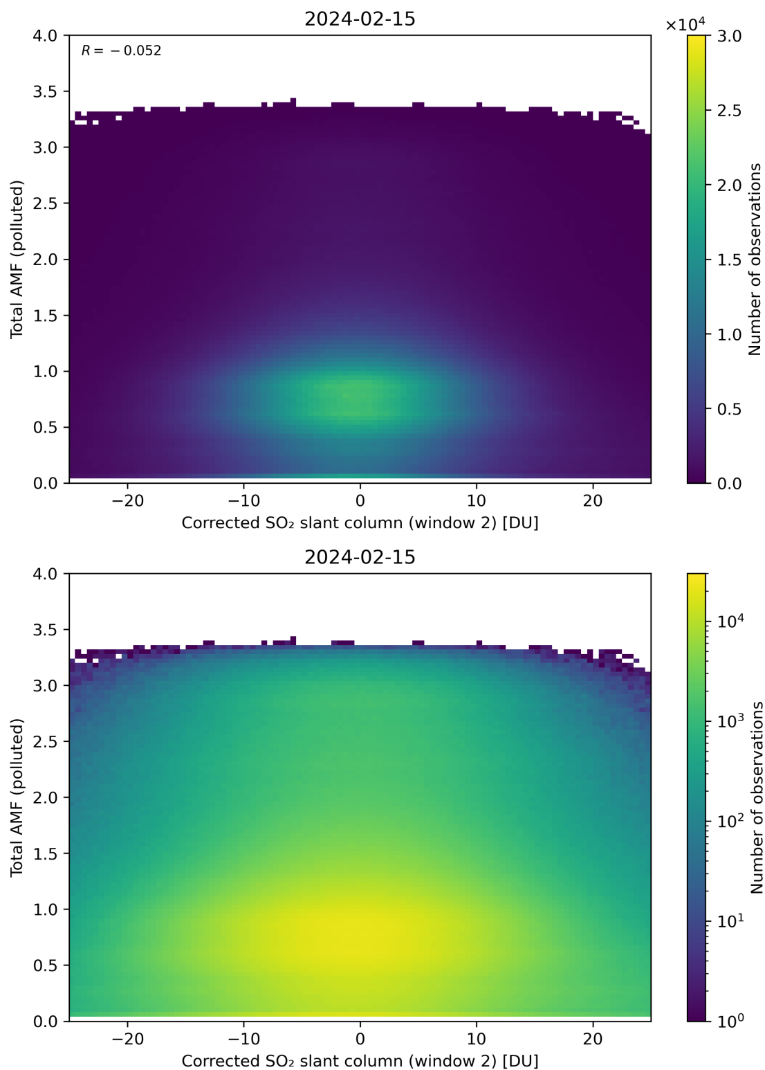
Figure 203: Scatter density plot of “Corrected SO 2 slant column (window 2)” against “Total AMF (polluted)” for 2024-02-14 to 2024-02-16.
