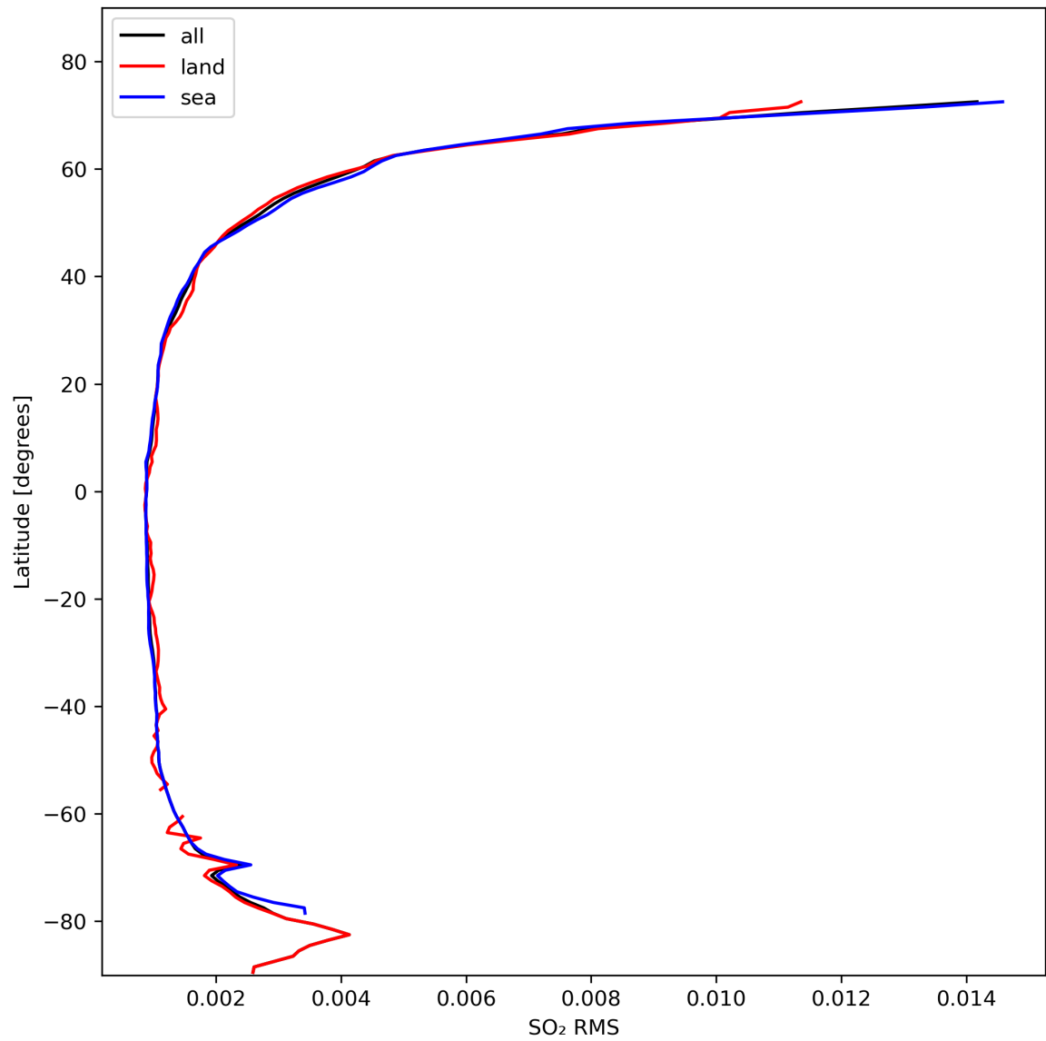
Figure 47: Zonal average of “SO 2 RMS” for 2024-02-14 to 2024-02-16.
