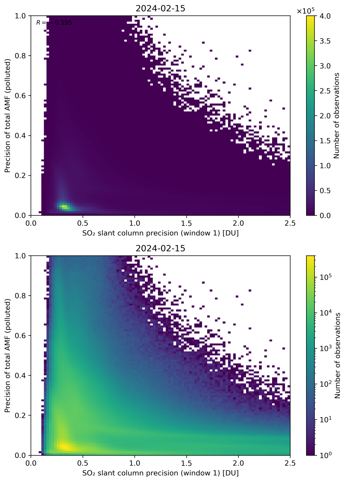
Figure 231: Scatter density plot of “SO 2 slant column precision (window 1)” against “Precision of total AMF (polluted)” for 2024-02-14 to 2024-02-16.
