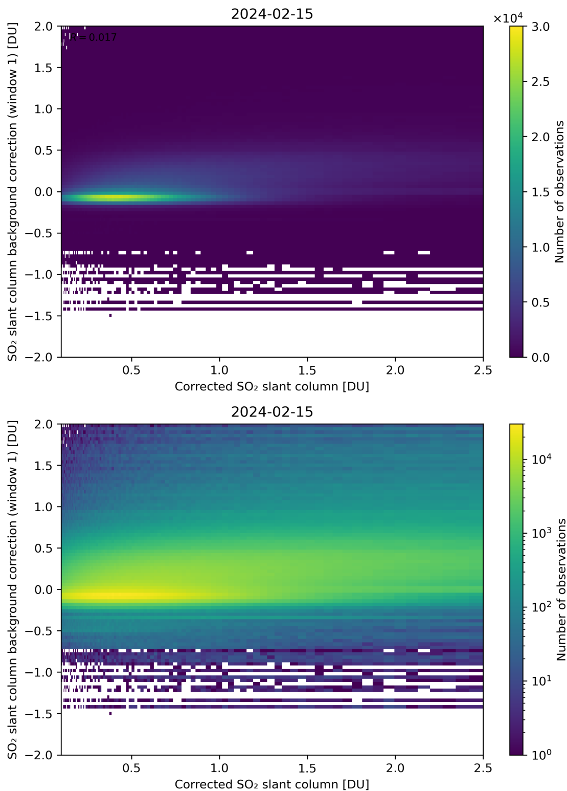
Figure 178: Scatter density plot of “Corrected SO 2 slant column” against “SO 2 slant column background correction (window 1)” for 2024-02-14 to 2024-02-16.
