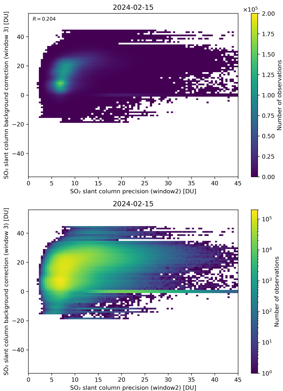
Figure 242: Scatter density plot of “SO 2 slant column precision (window2)” against “SO 2 slant column background correction (window 3)” for 2024-02-14 to 2024-02-16.
