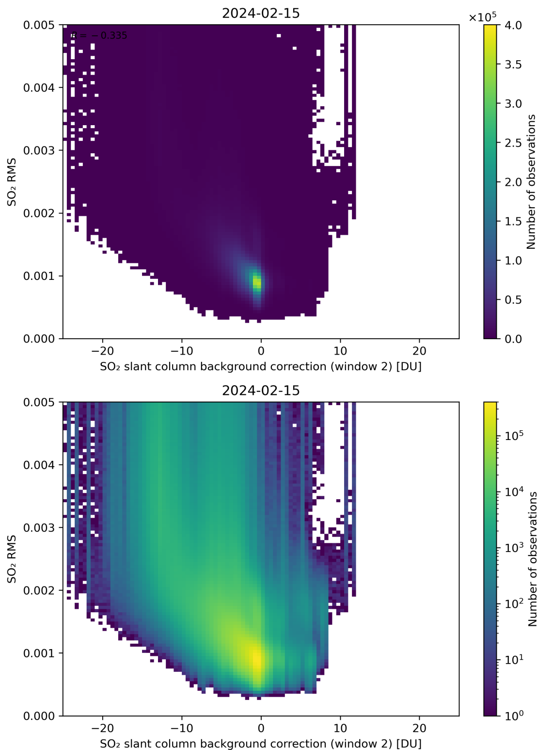
Figure 114: Scatter density plot of “SO 2 slant column background correction (window 2)” against “SO 2 RMS” for 2024-02-14 to 2024-02-16.
