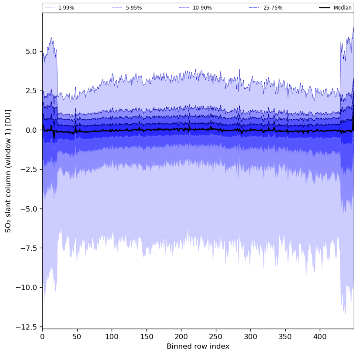
Figure 79: Along track statistics of “SO 2 slant column (window 1)” for 2024-02-14 to 2024-02-16
