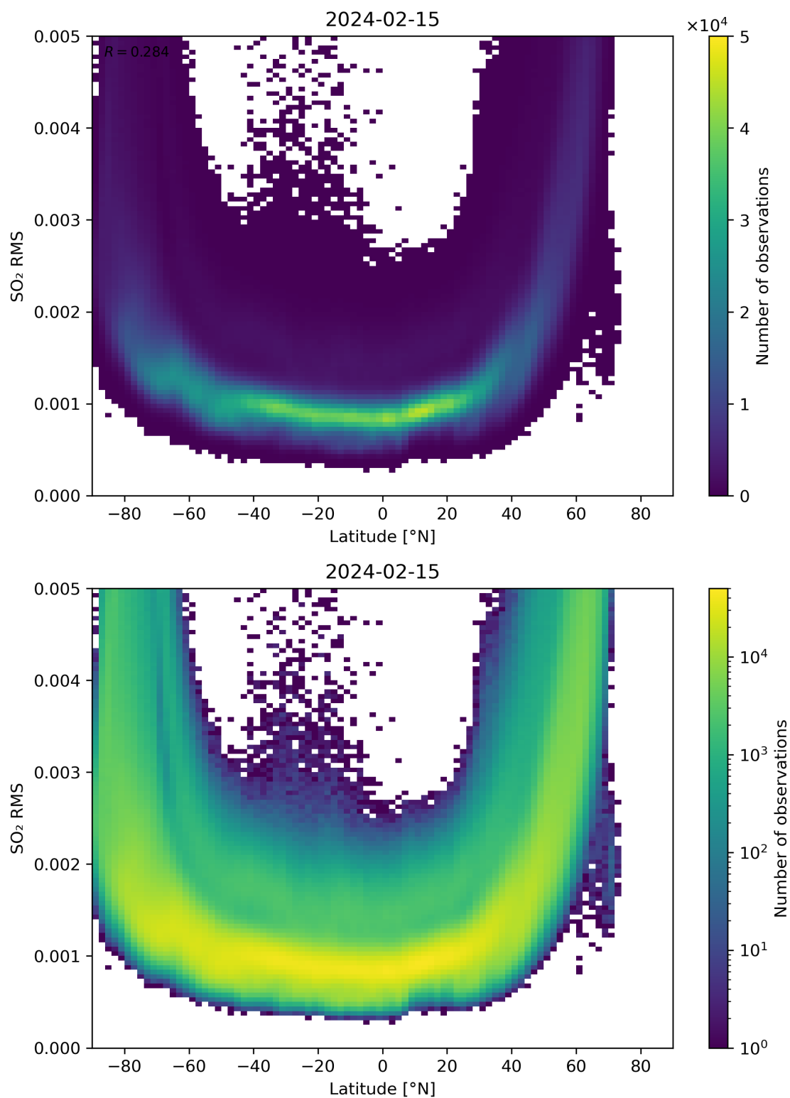
Figure 144: Scatter density plot of “Latitude” against “SO 2 RMS” for 2024-02-14 to 2024-02-16.
