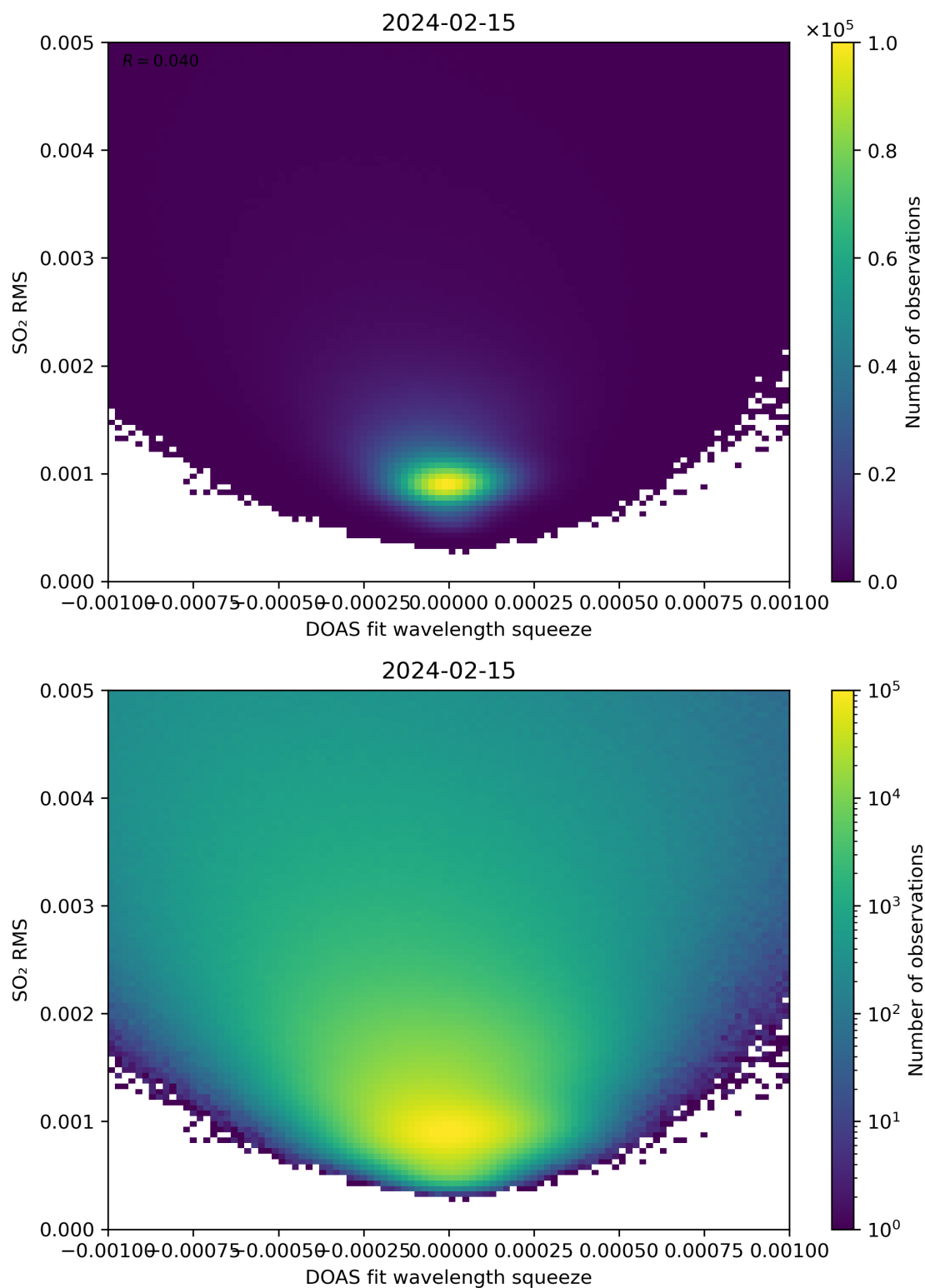
Figure 132: Scatter density plot of “DOAS fit wavelength squeeze” against “SO 2 RMS” for 2024-02-14 to 2024-02-16.
