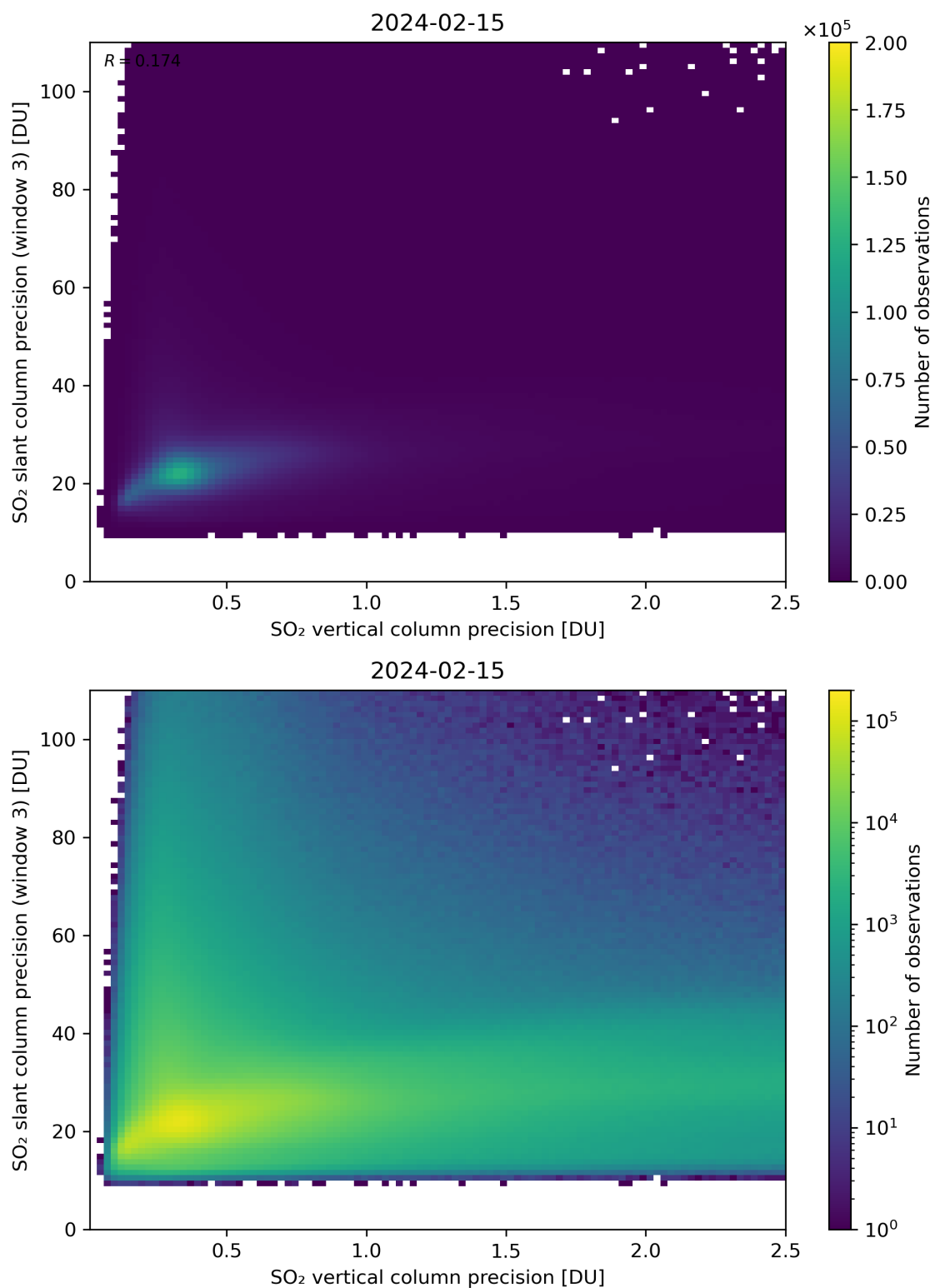
Figure 293: Scatter density plot of “SO 2 vertical column precision” against “SO 2 slant column precision (window 3)” for 2024-02-14 to 2024-02-16.
