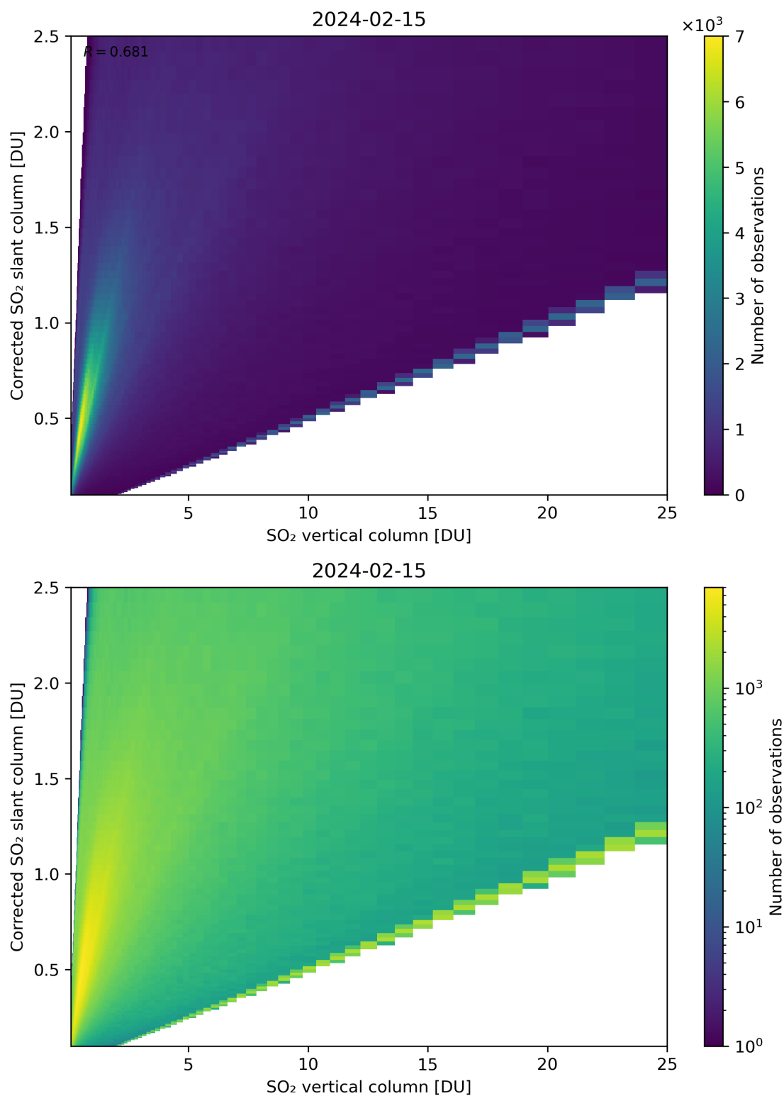
Figure 297: Scatter density plot of “SO 2 vertical column” against “Corrected SO 2 slant column” for 2024-02-14 to 2024-02-16.
