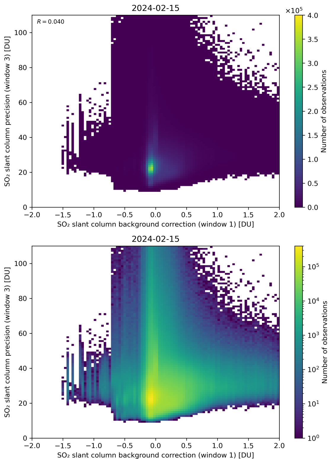
Figure 108: Scatter density plot of “SO 2 slant column background correction (window 1)” against “SO 2 slant column precision (window 3)” for 2024-02-14 to 2024-02-16.
