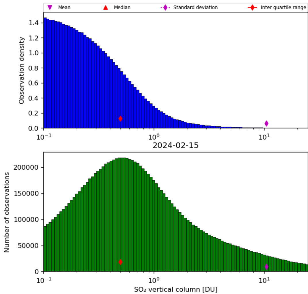
Figure 53: Histogram of “SO 2 vertical column” for 2024-02-14 to 2024-02-16
