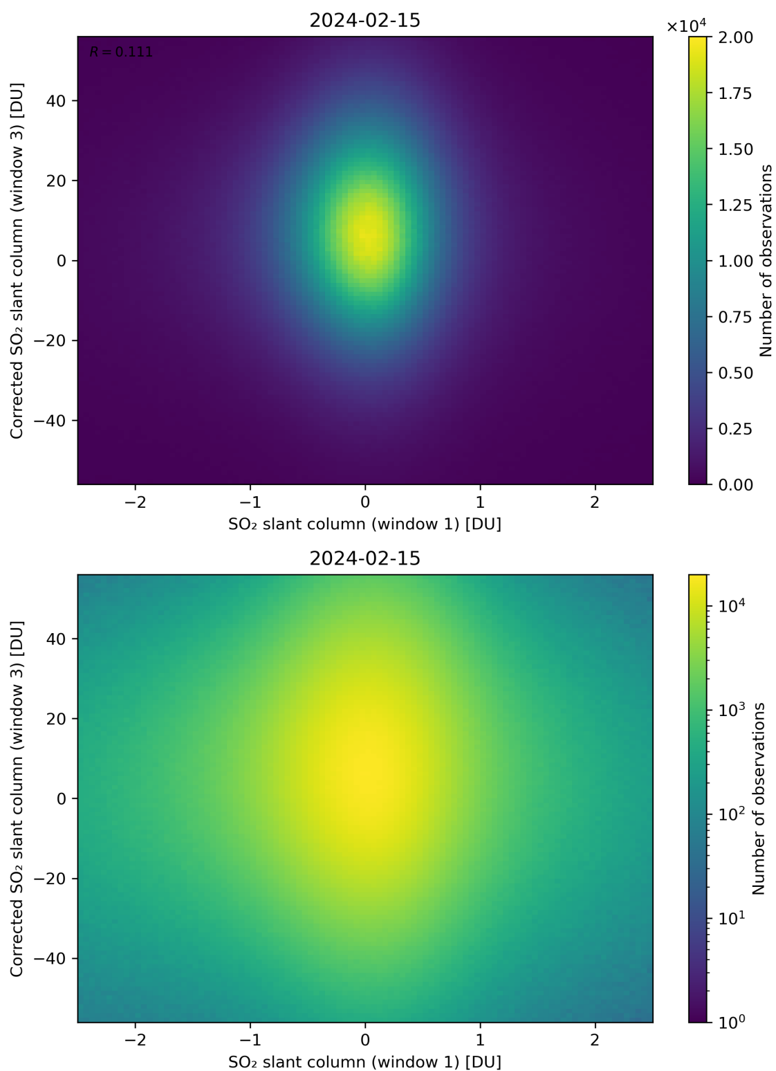
Figure 234: Scatter density plot of “SO 2 slant column (window 1)” against “Corrected SO 2 slant column (window 3)” for 2024-02-14 to 2024-02-16.
