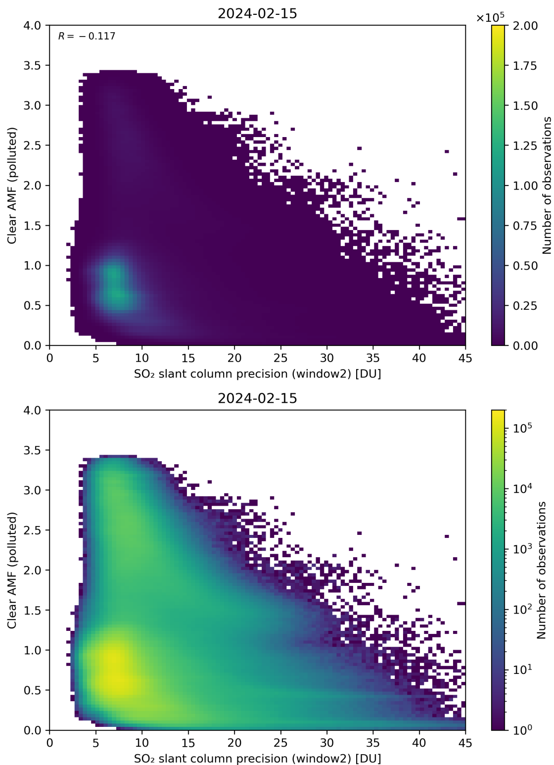
Figure 246: Scatter density plot of “SO 2 slant column precision (window2)” against “Clear AMF (polluted)” for 2024-02-14 to 2024-02-16.
