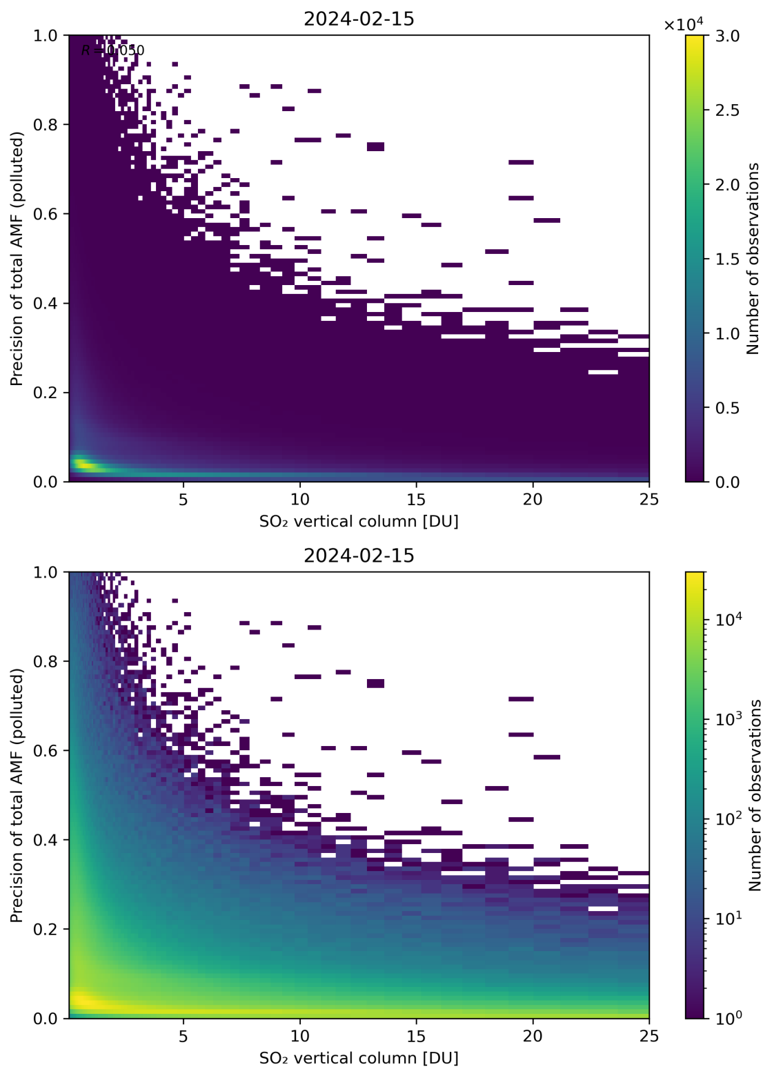
Figure 306: Scatter density plot of “SO 2 vertical column” against “Precision of total AMF (polluted)” for 2024-02-14 to 2024-02-16.
