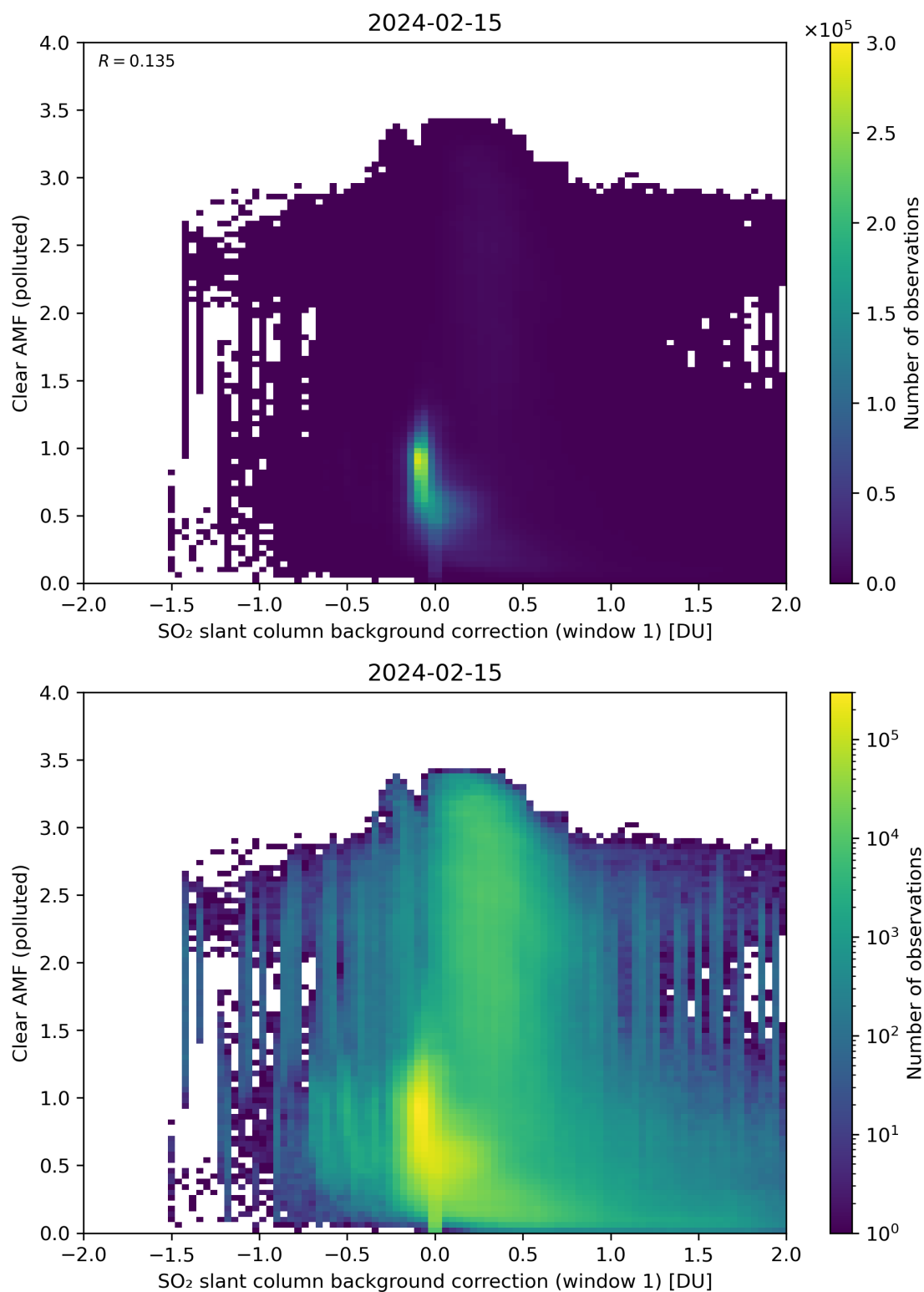
Figure 103: Scatter density plot of “SO 2 slant column background correction (window 1)” against “Clear AMF (polluted)” for 2024-02-14 to 2024-02-16.
