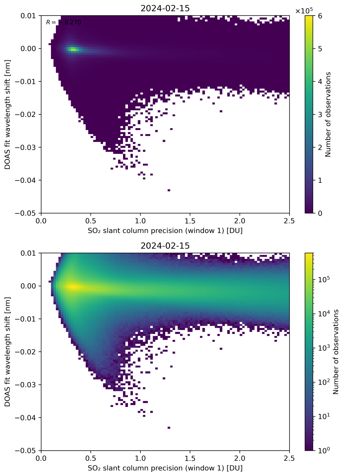
Figure 221: Scatter density plot of “SO 2 slant column precision (window 1)” against “DOAS fit wavelength shift” for 2024-02-14 to 2024-02-16.
