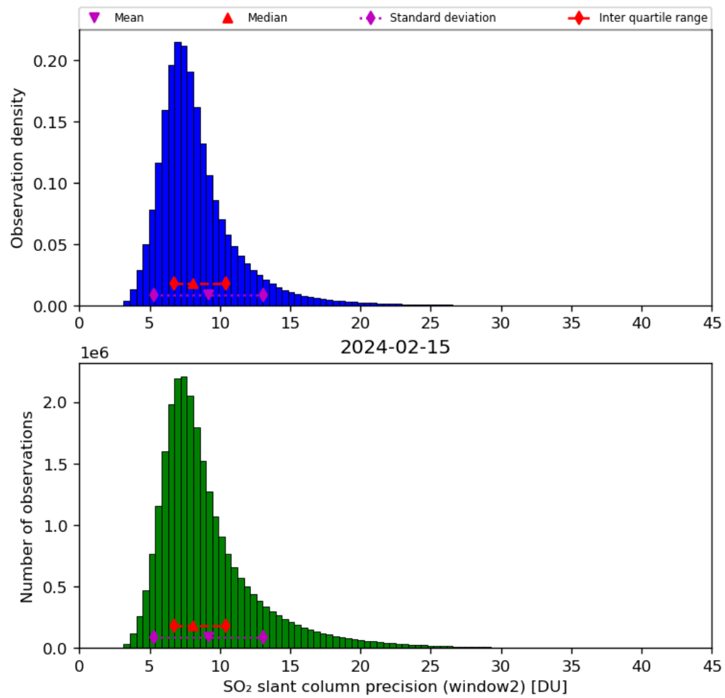
Figure 61: Histogram of “SO 2 slant column precision (window2)” for 2024-02-14 to 2024-02-16
