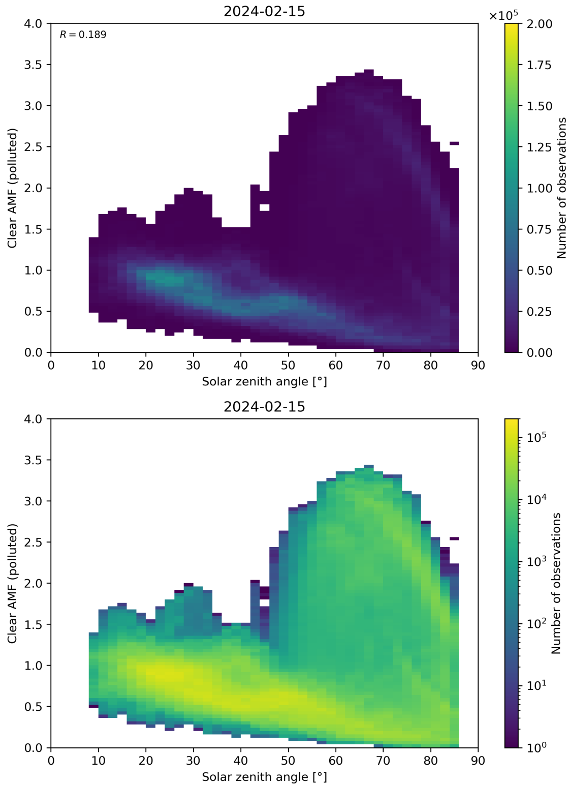
Figure 165: Scatter density plot of “Solar zenith angle” against “Clear AMF (polluted)” for 2024-02-14 to 2024-02-16.
