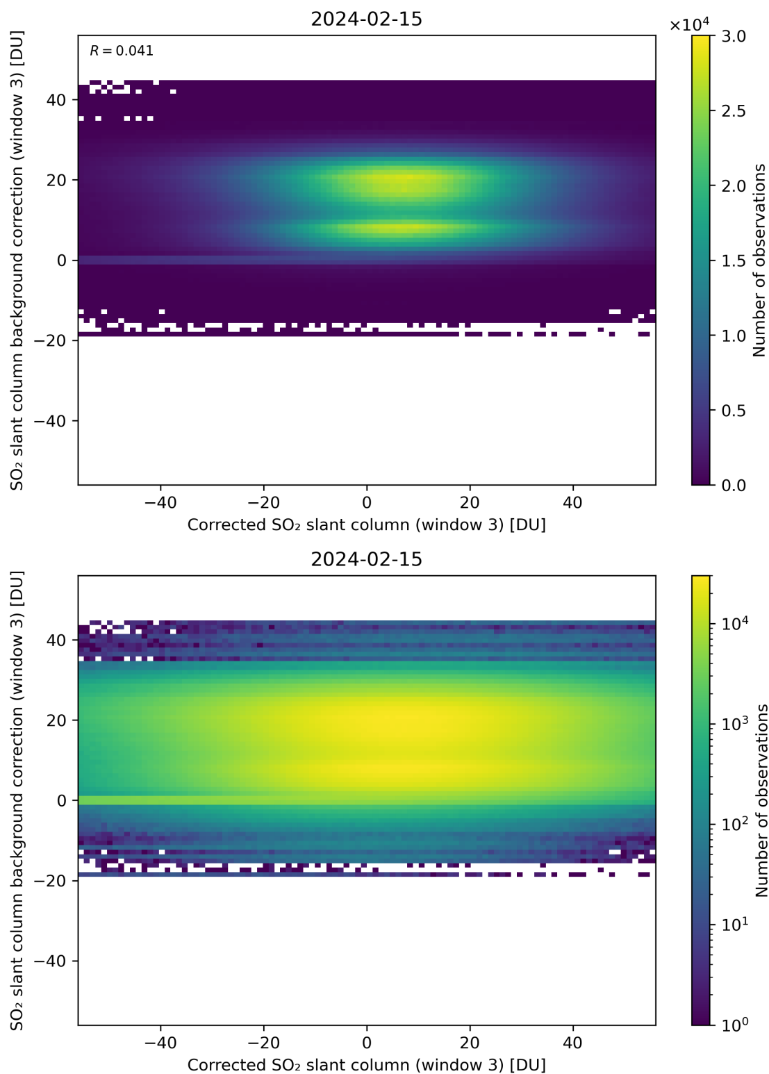
Figure 205: Scatter density plot of “Corrected SO 2 slant column (window 3)” against “SO 2 slant column background correction (window 3)” for 2024-02-14 to 2024-02-16.
