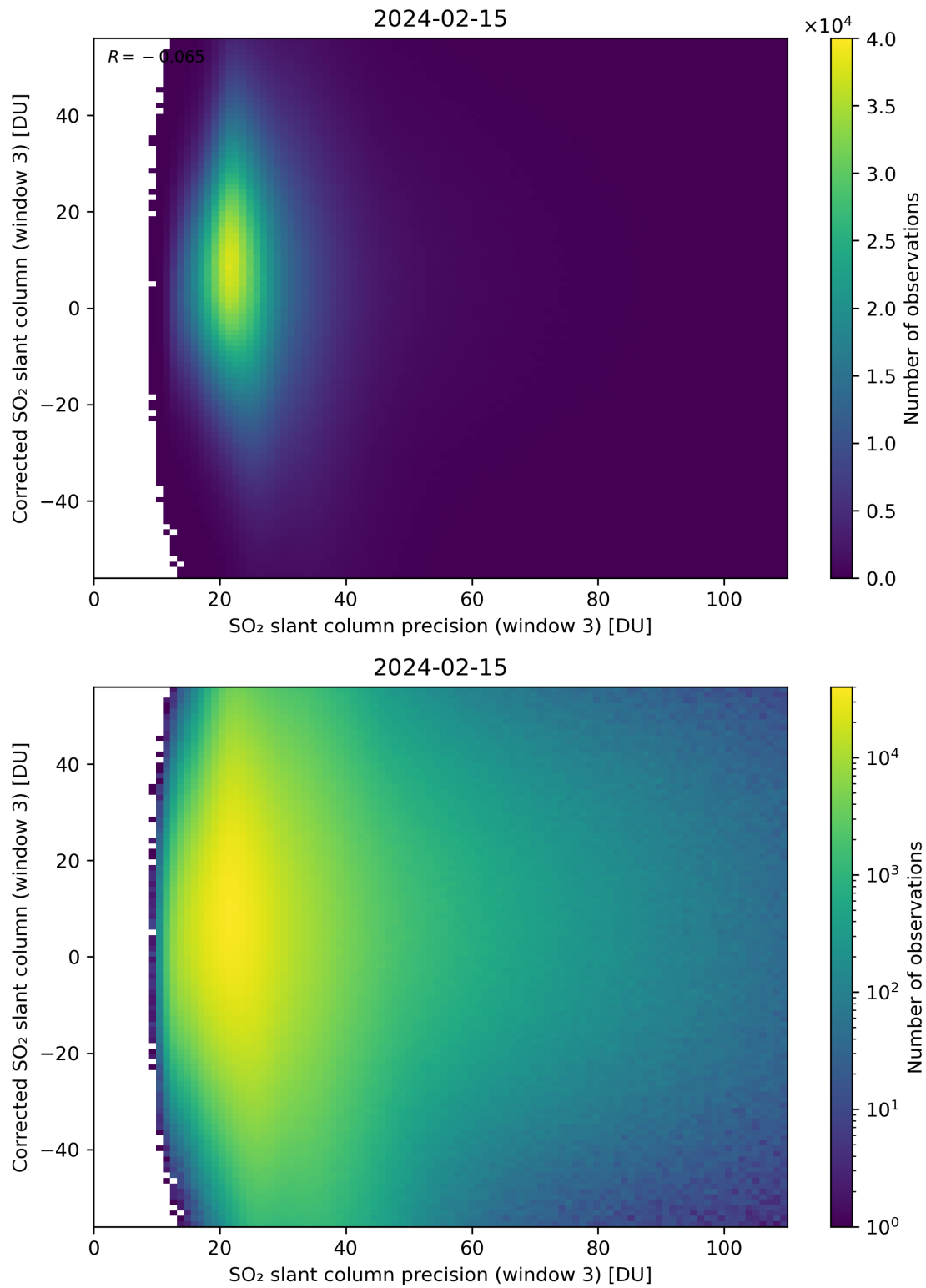
Figure 262: Scatter density plot of “SO 2 slant column precision (window 3)” against “Corrected SO 2 slant column (window 3)” for 2024-02-14 to 2024-02-16.
