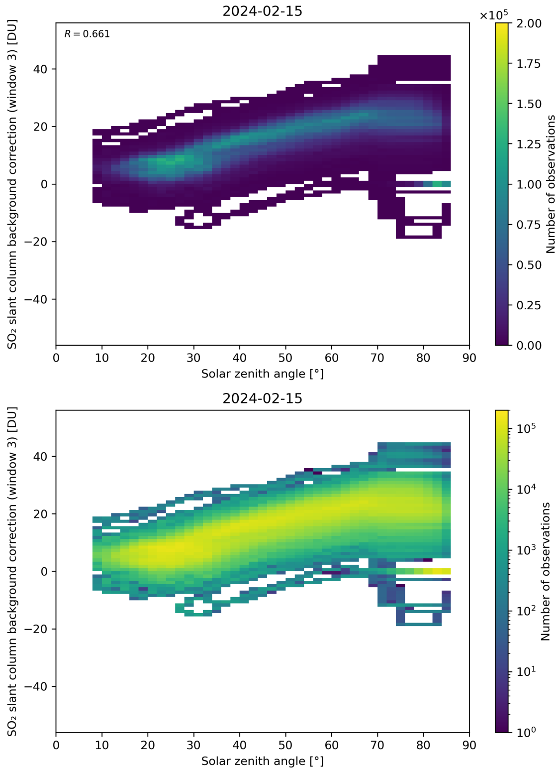
Figure 160: Scatter density plot of “Solar zenith angle” against “SO 2 slant column background correction (window 3)” for 2024-02-14 to 2024-02-16.
