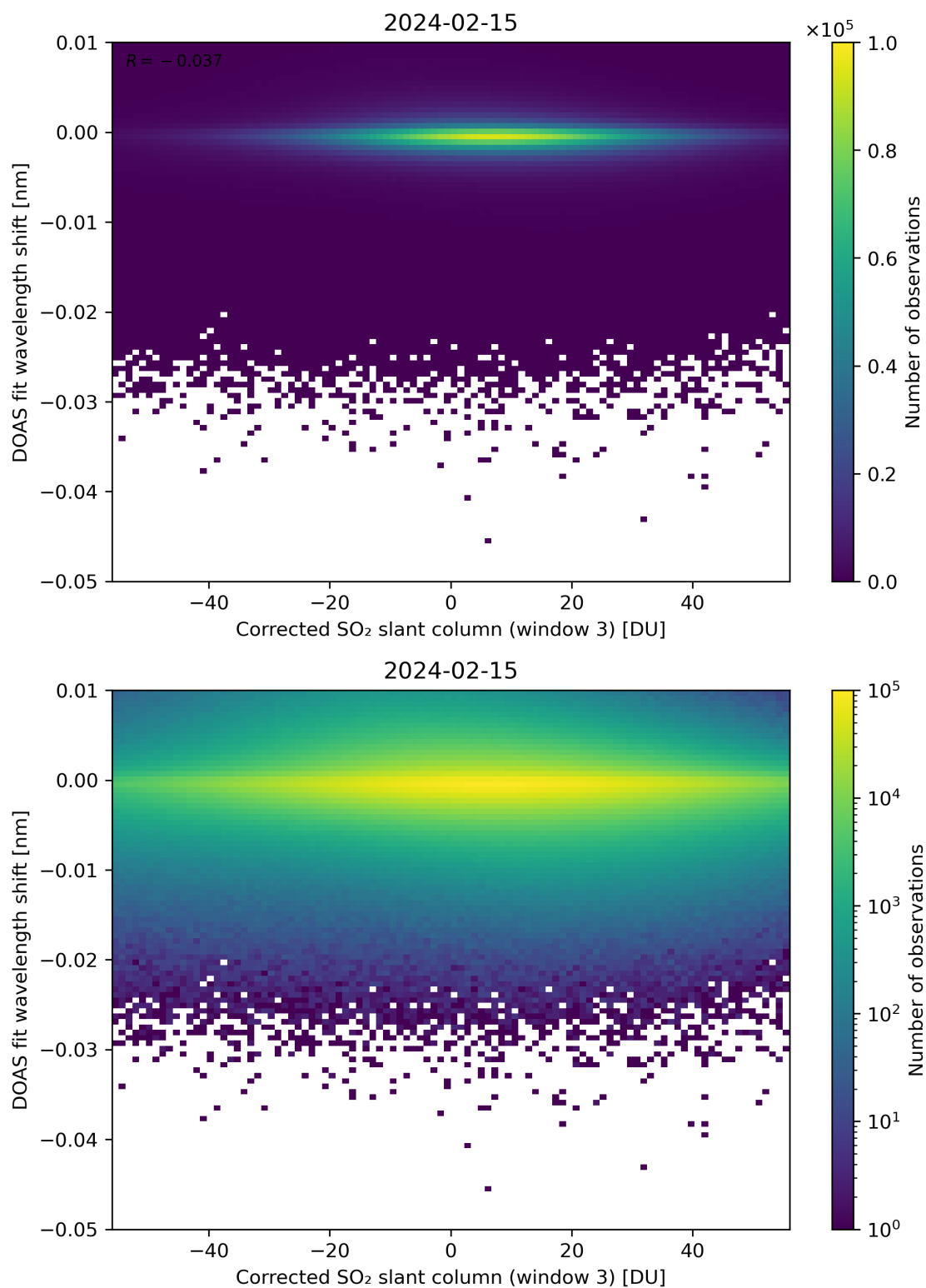
Figure 206: Scatter density plot of “Corrected SO 2 slant column (window 3)” against “DOAS fit wavelength shift” for 2024-02-14 to 2024-02-16.
