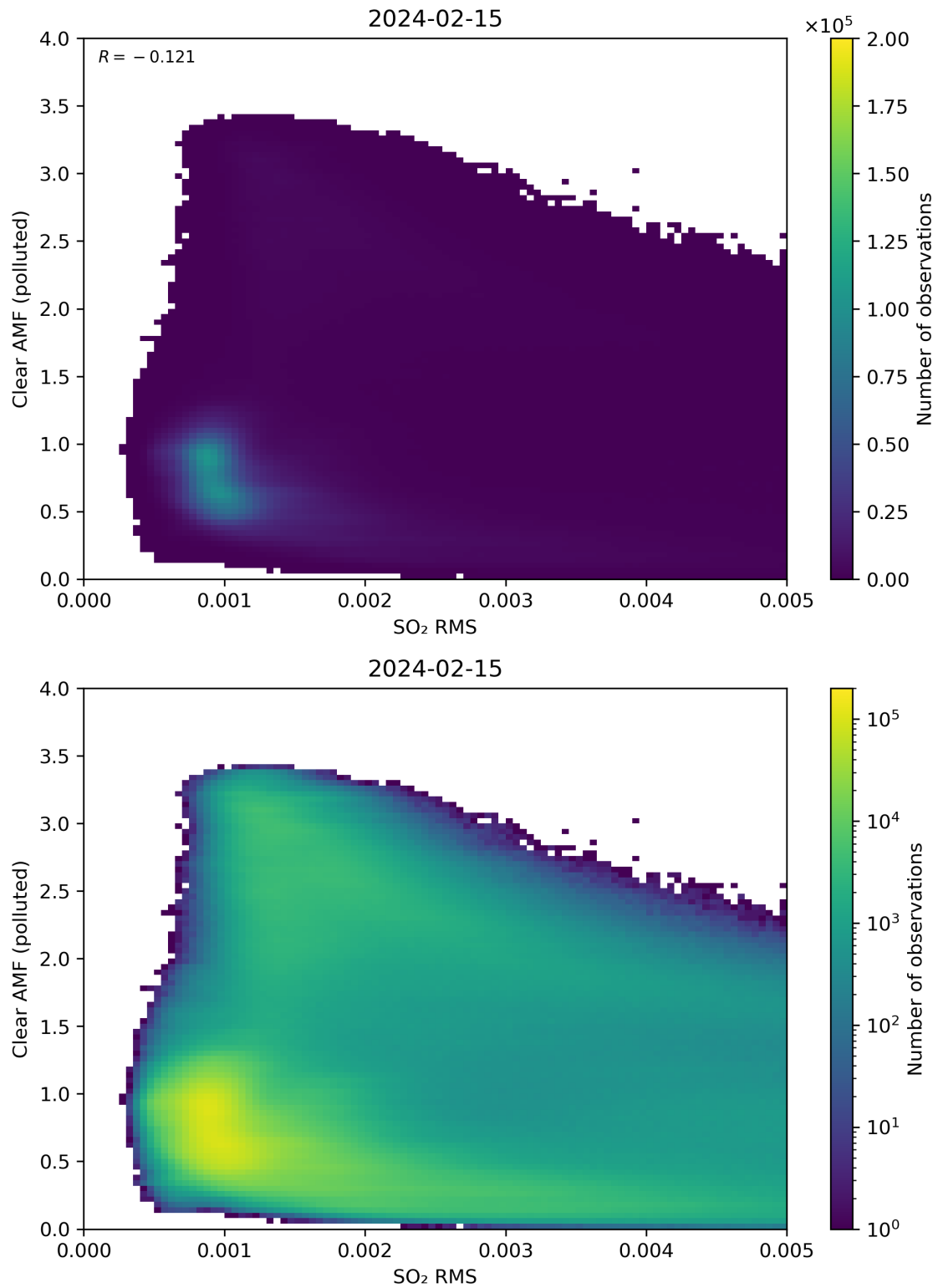
Figure 136: Scatter density plot of “SO 2 RMS” against “Clear AMF (polluted)” for 2024-02-14 to 2024-02-16.
