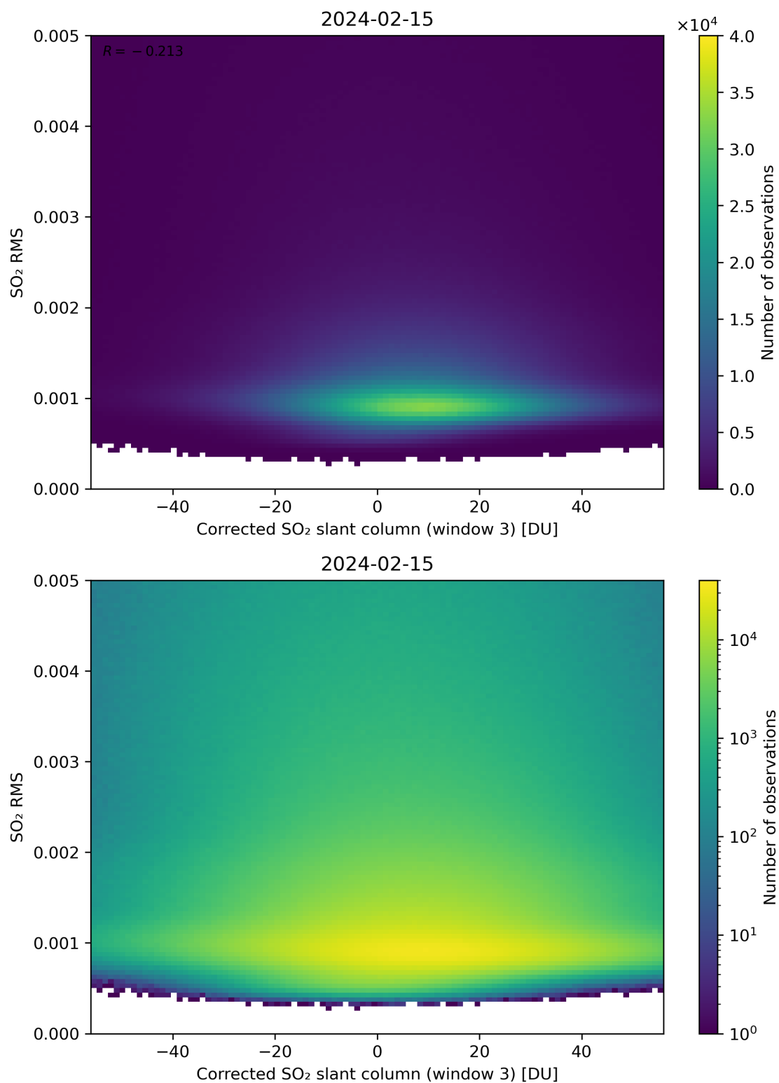
Figure 208: Scatter density plot of “Corrected SO 2 slant column (window 3)” against “SO 2 RMS” for 2024-02-14 to 2024-02-16.
