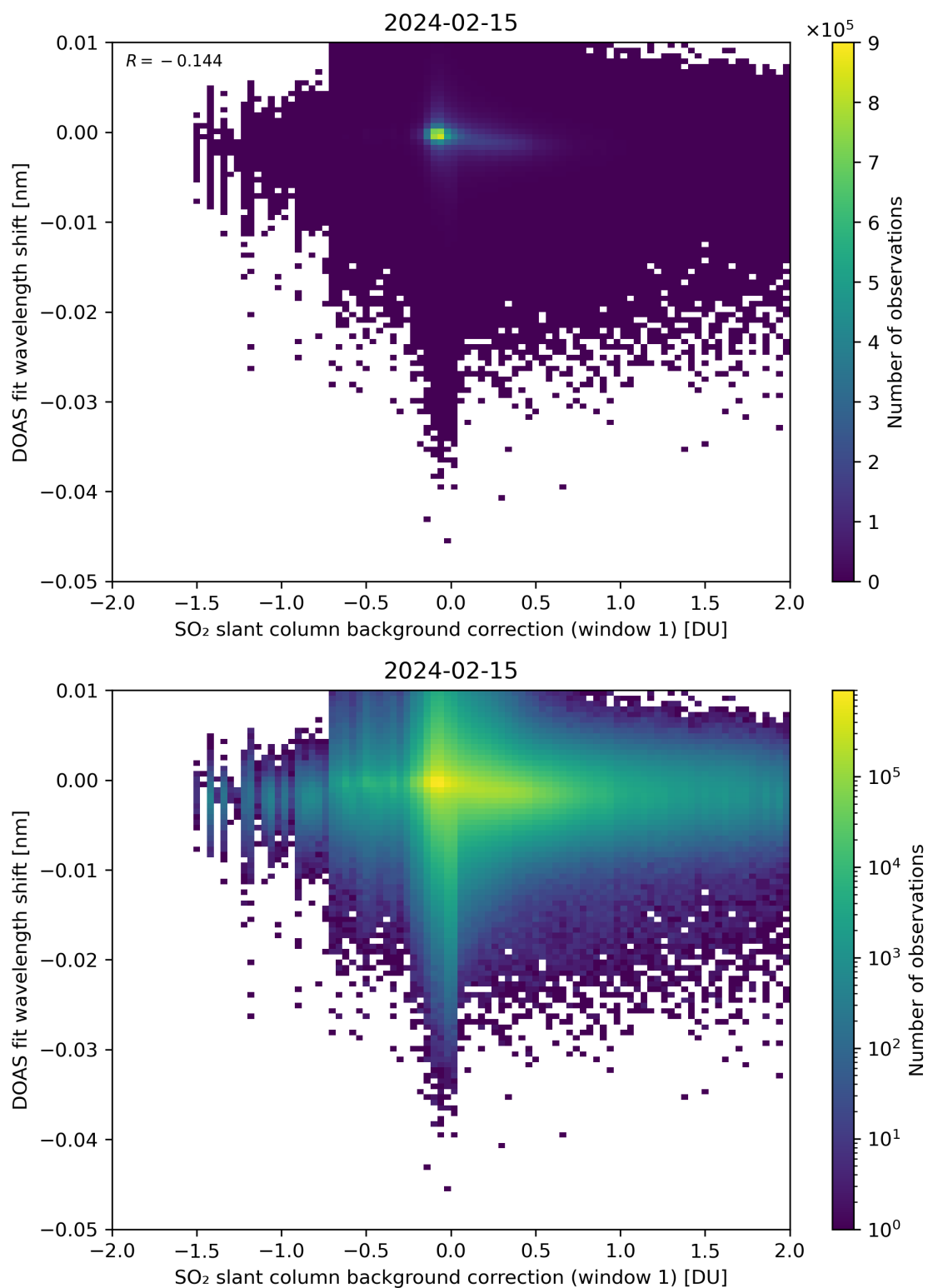
Figure 100: Scatter density plot of “SO 2 slant column background correction (window 1)” against “DOAS fit wavelength shift” for 2024-02-14 to 2024-02-16.
