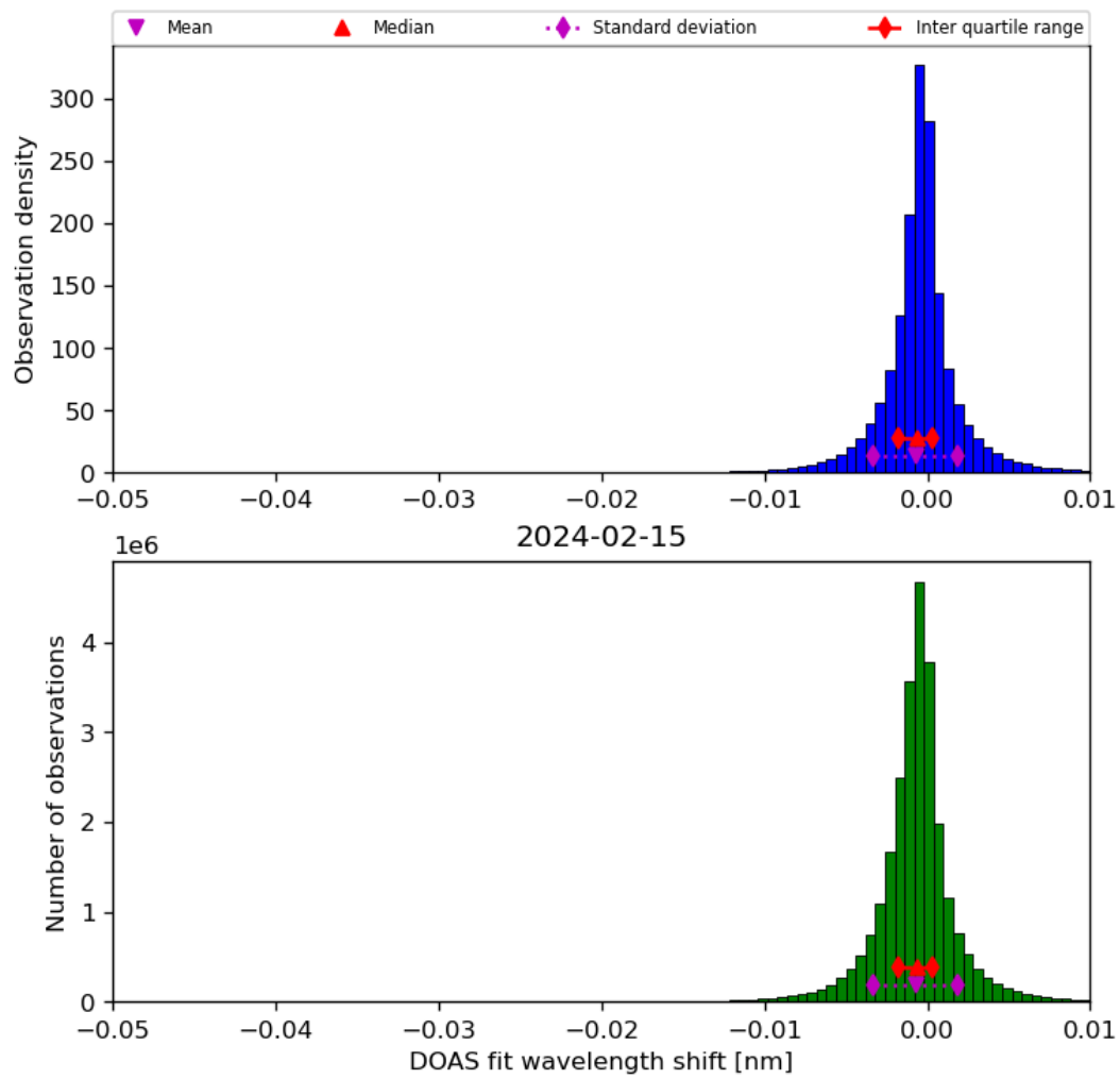
Figure 68: Histogram of “DOAS fit wavelength shift” for 2024-02-14 to 2024-02-16
