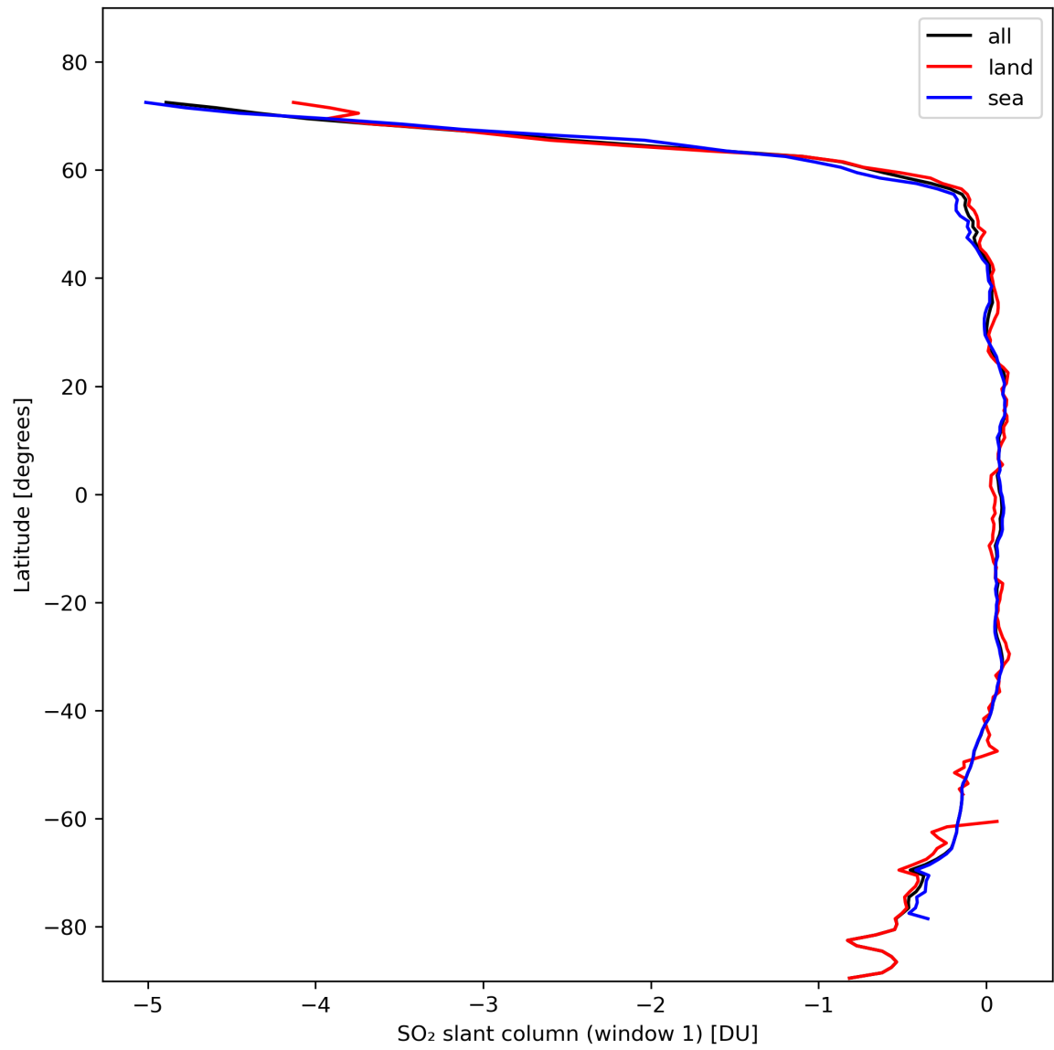
Figure 33: Zonal average of “SO 2 slant column (window 1)” for 2024-02-14 to 2024-02-16.
