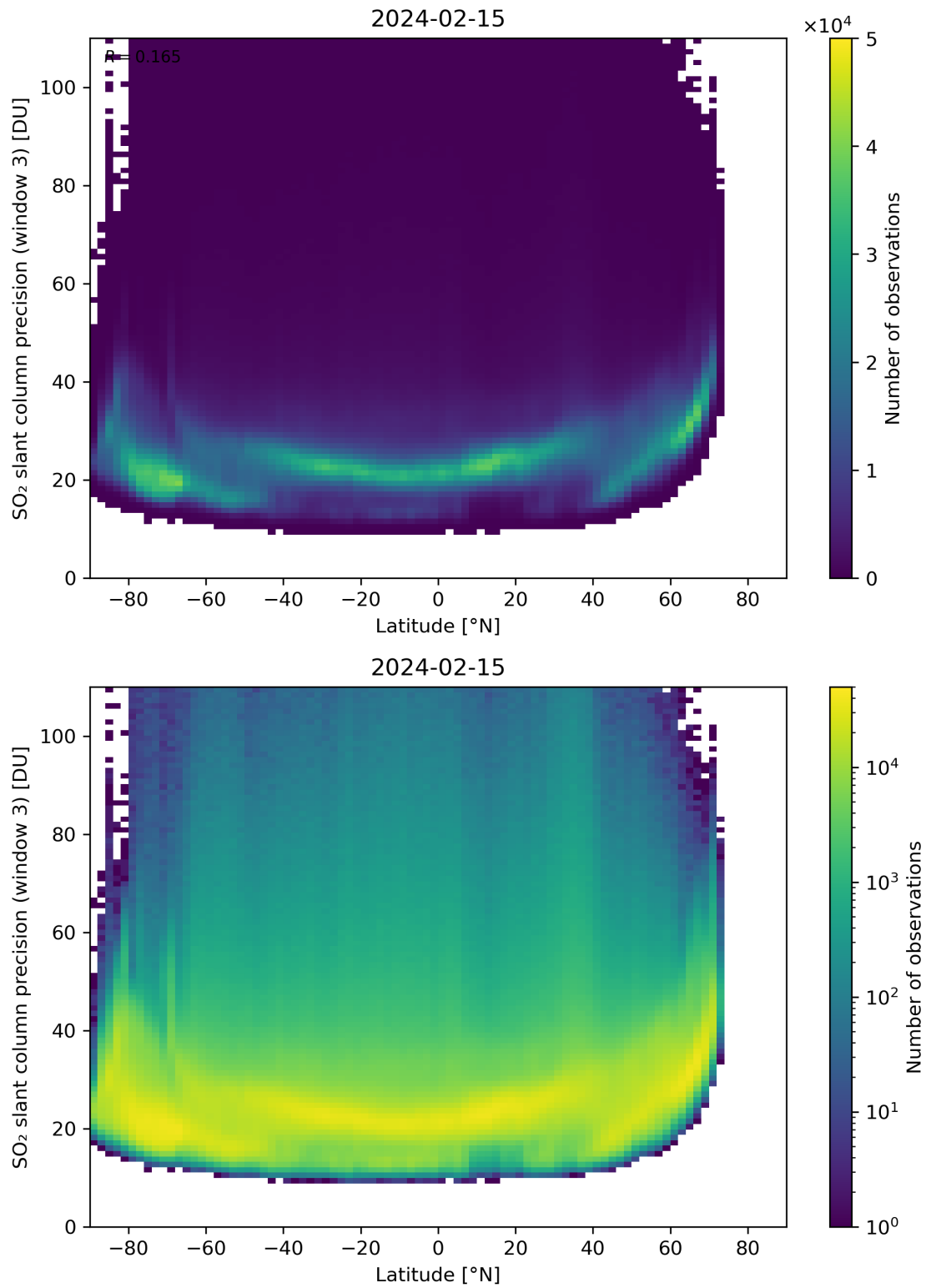
Figure 153: Scatter density plot of “Latitude” against “SO 2 slant column precision (window 3)” for 2024-02-14 to 2024-02-16.
