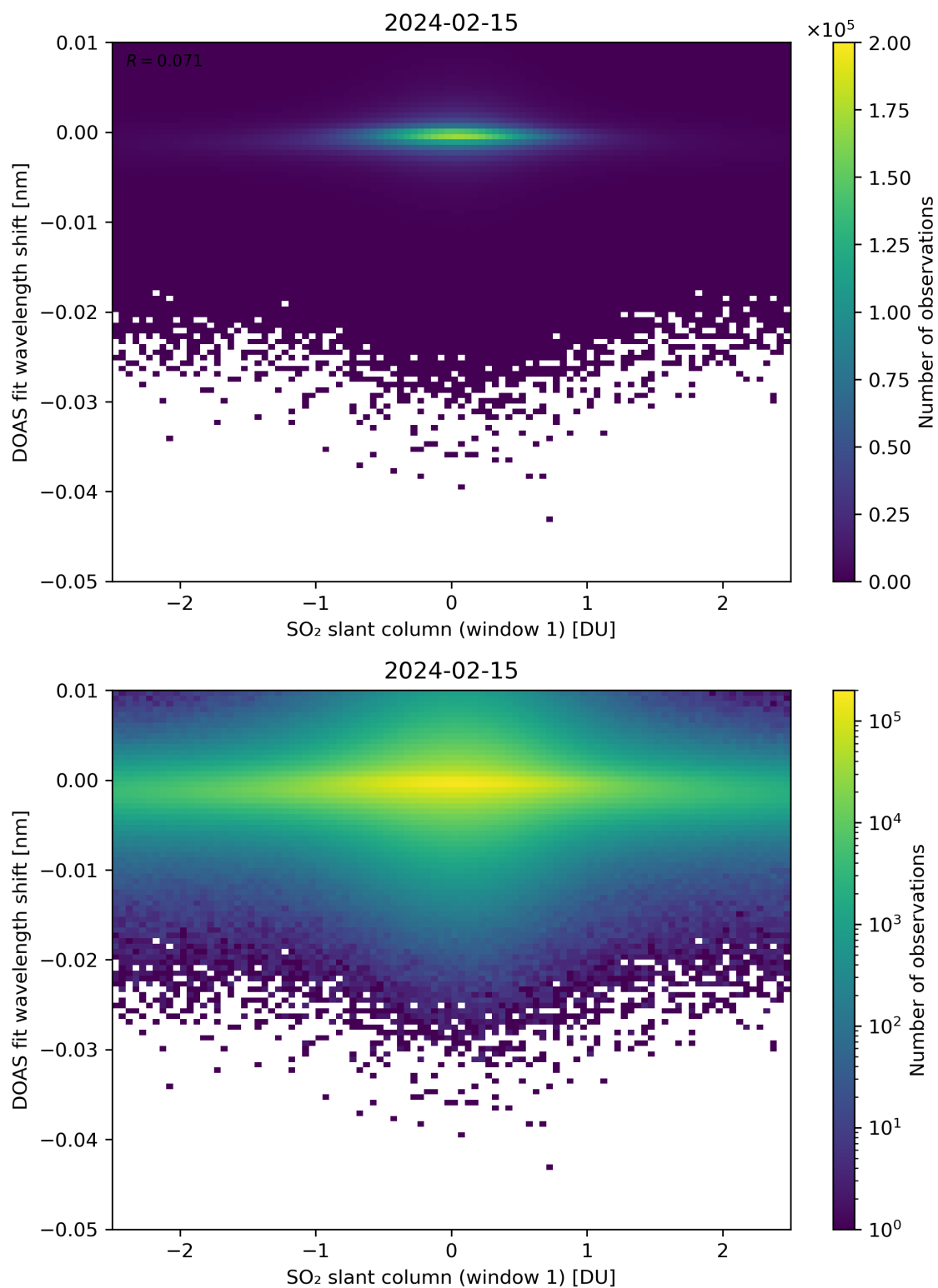
Figure 215: Scatter density plot of “SO 2 slant column (window 1)” against “DOAS fit wavelength shift” for 2024-02-14 to 2024-02-16.
