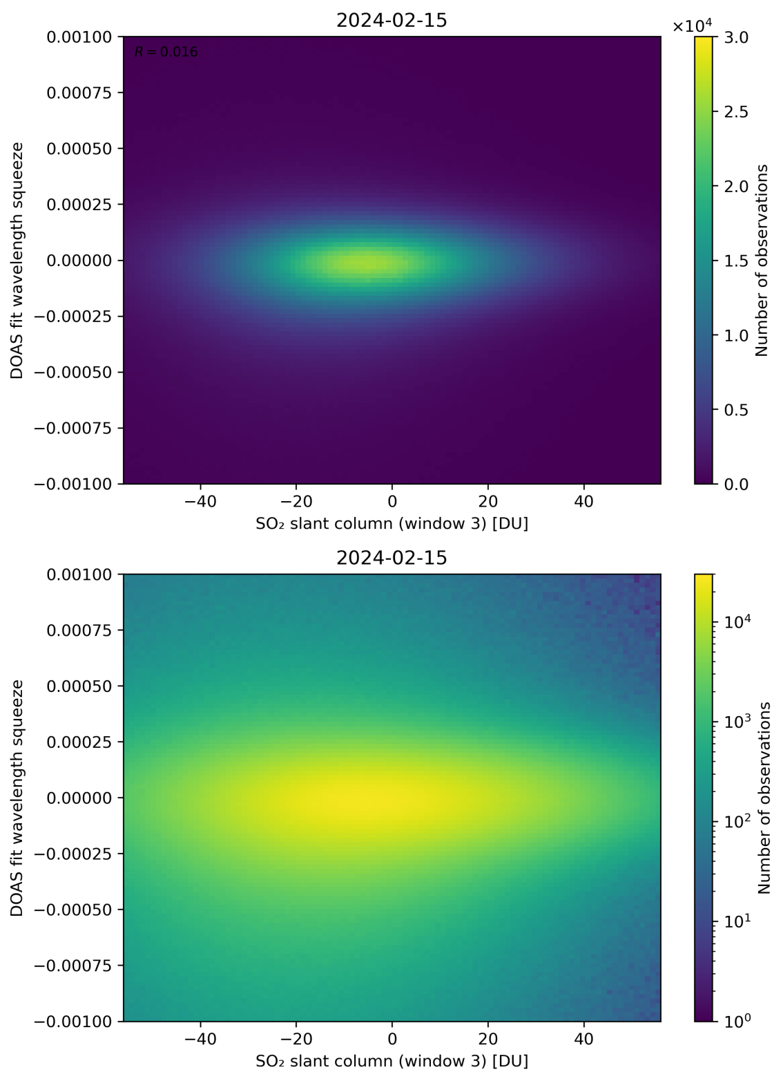
Figure 255: Scatter density plot of “SO 2 slant column (window 3)” against “DOAS fit wavelength squeeze” for 2024-02-14 to 2024-02-16.
