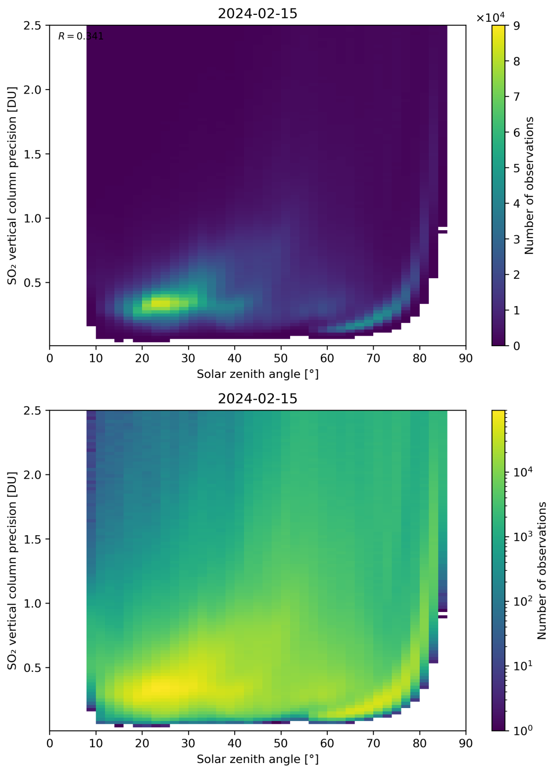
Figure 177: Scatter density plot of “Solar zenith angle” against “SO 2 vertical column precision” for 2024-02-14 to 2024-02-16.
