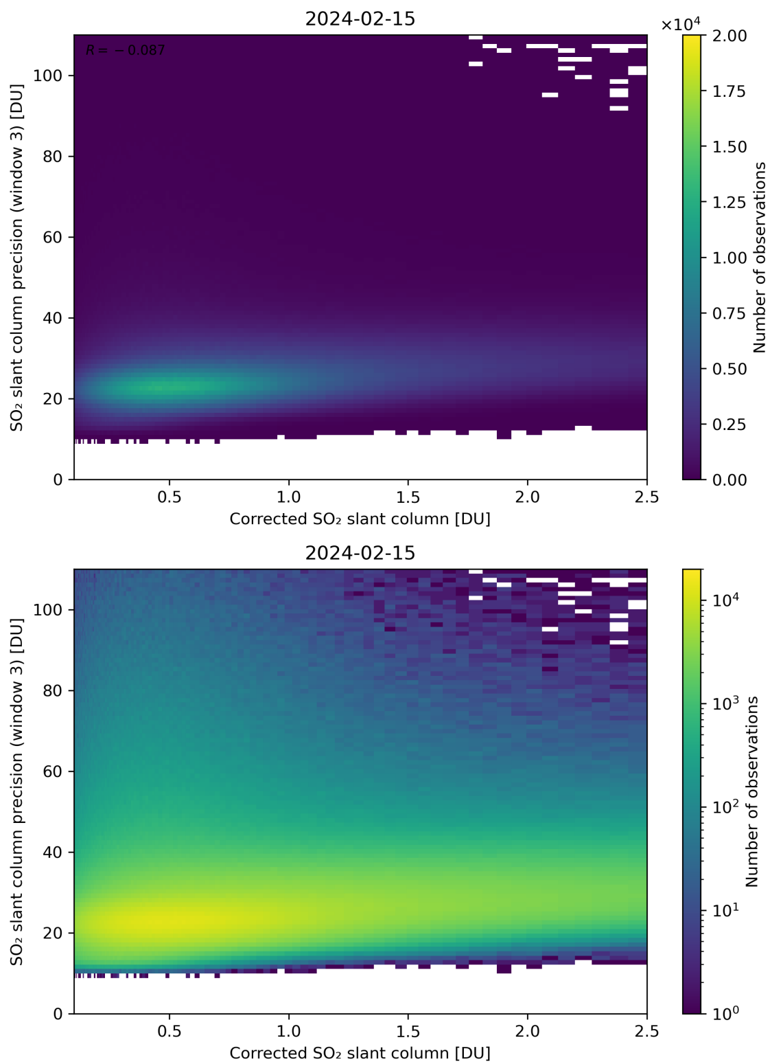
Figure 191: Scatter density plot of “Corrected SO 2 slant column” against “SO 2 slant column precision (window 3)” for 2024-02-14 to 2024-02-16.
