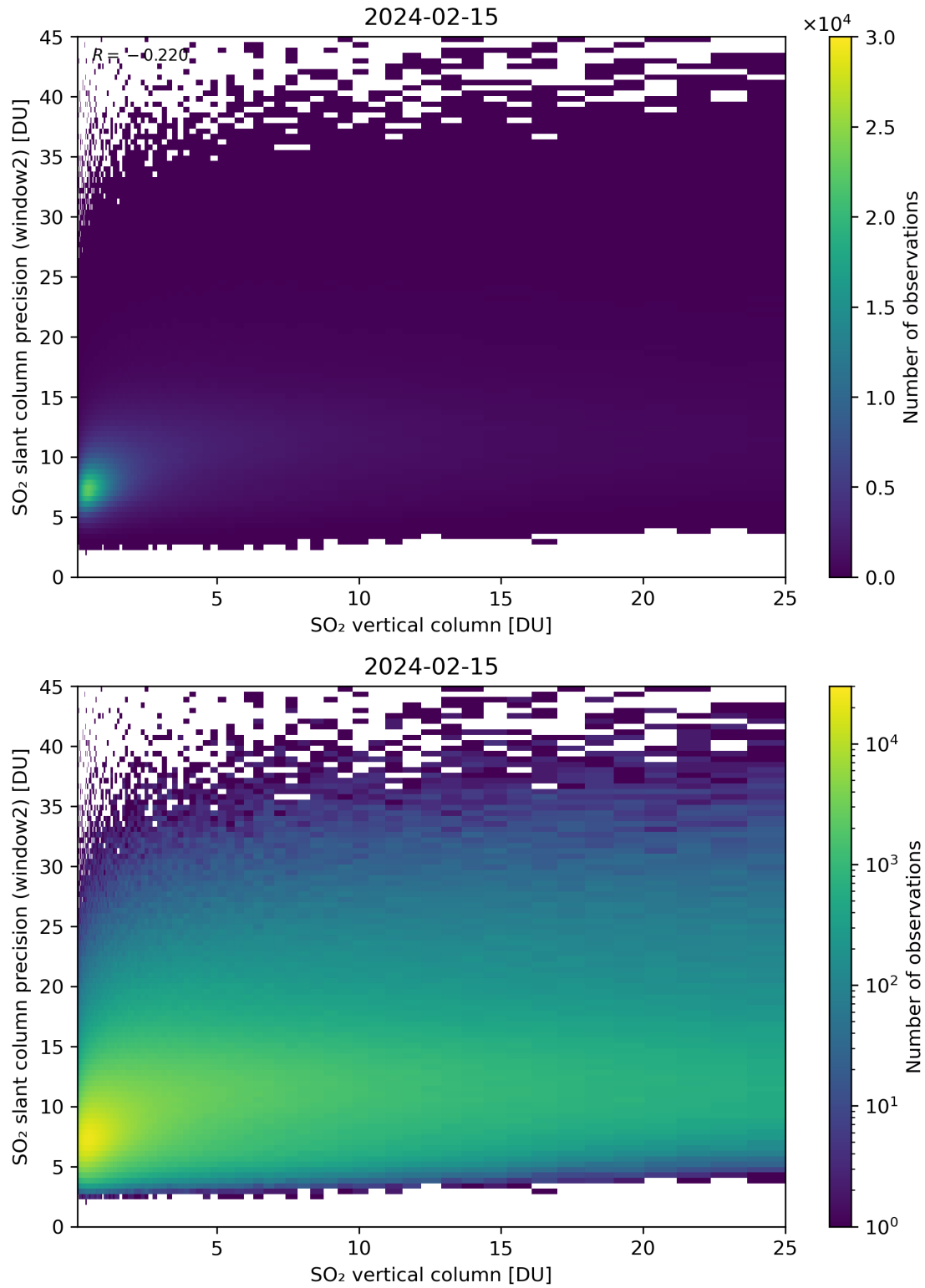
Figure 302: Scatter density plot of “SO 2 vertical column” against “SO 2 slant column precision (window2)” for 2024-02-14 to 2024-02-16.
