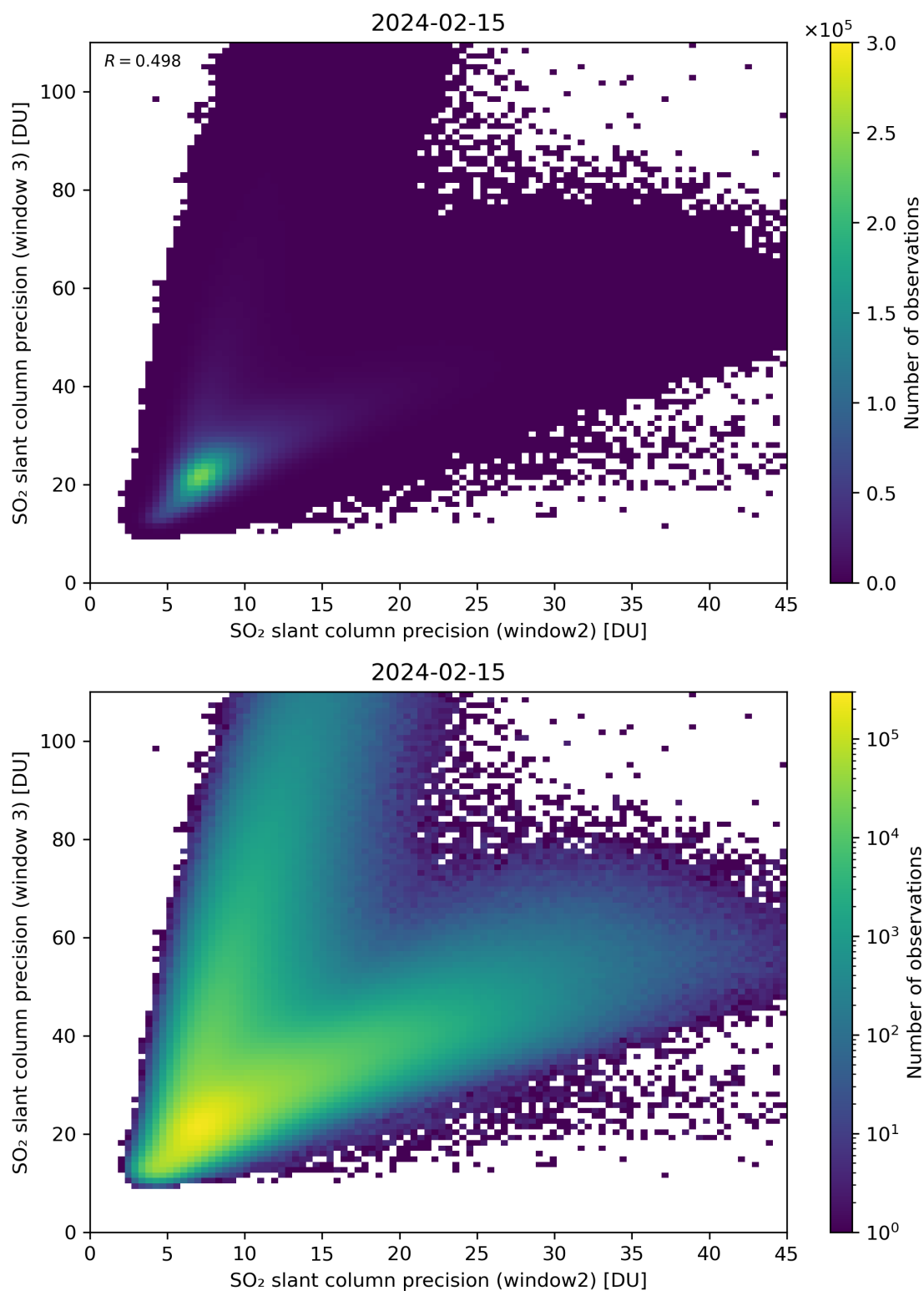
Figure 250: Scatter density plot of “SO 2 slant column precision (window2)” against “SO 2 slant column precision (window 3)” for 2024-02-14 to 2024-02-16.
