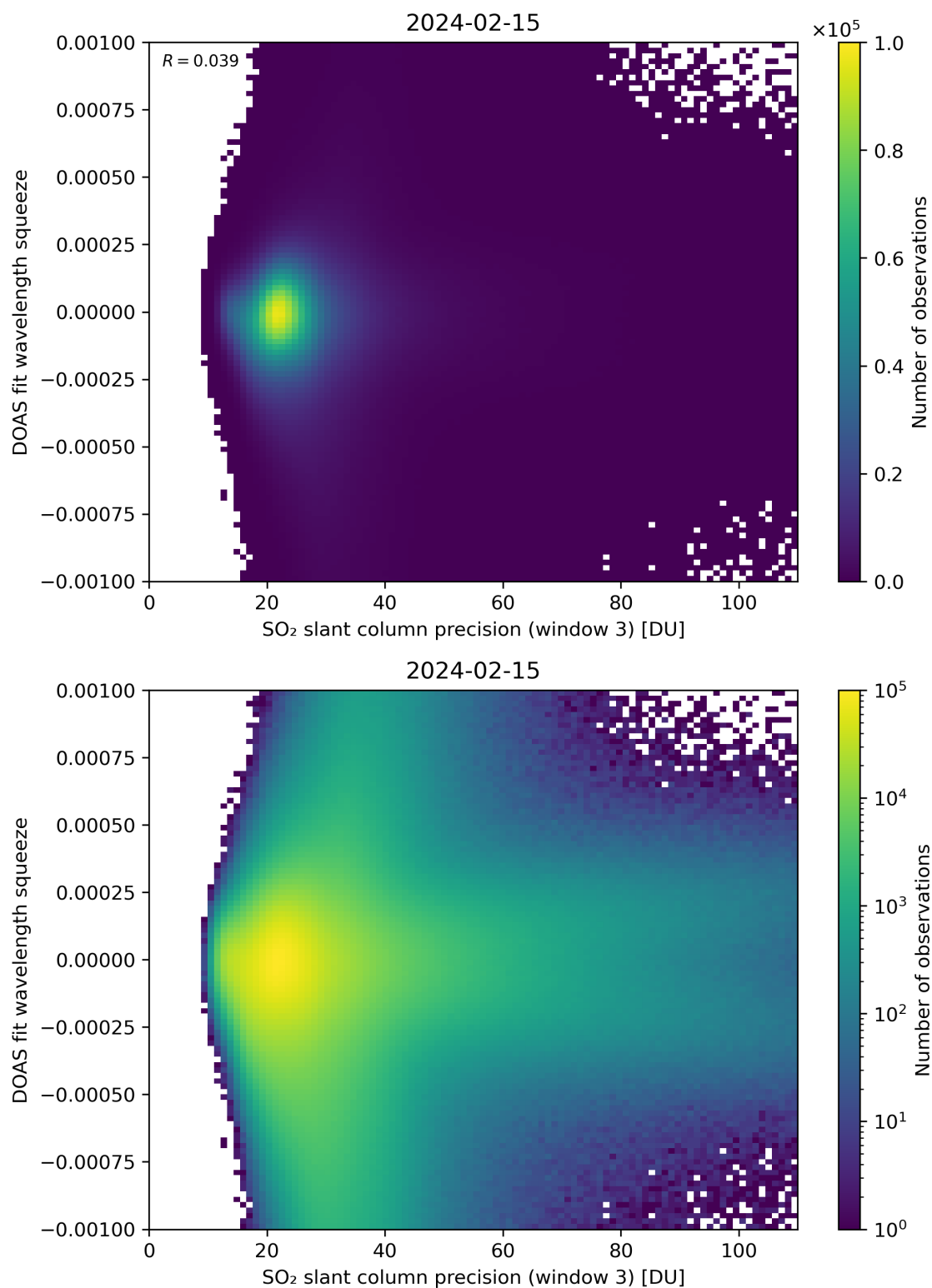
Figure 259: Scatter density plot of “SO 2 slant column precision (window 3)” against “DOAS fit wavelength squeeze” for 2024-02-14 to 2024-02-16.
