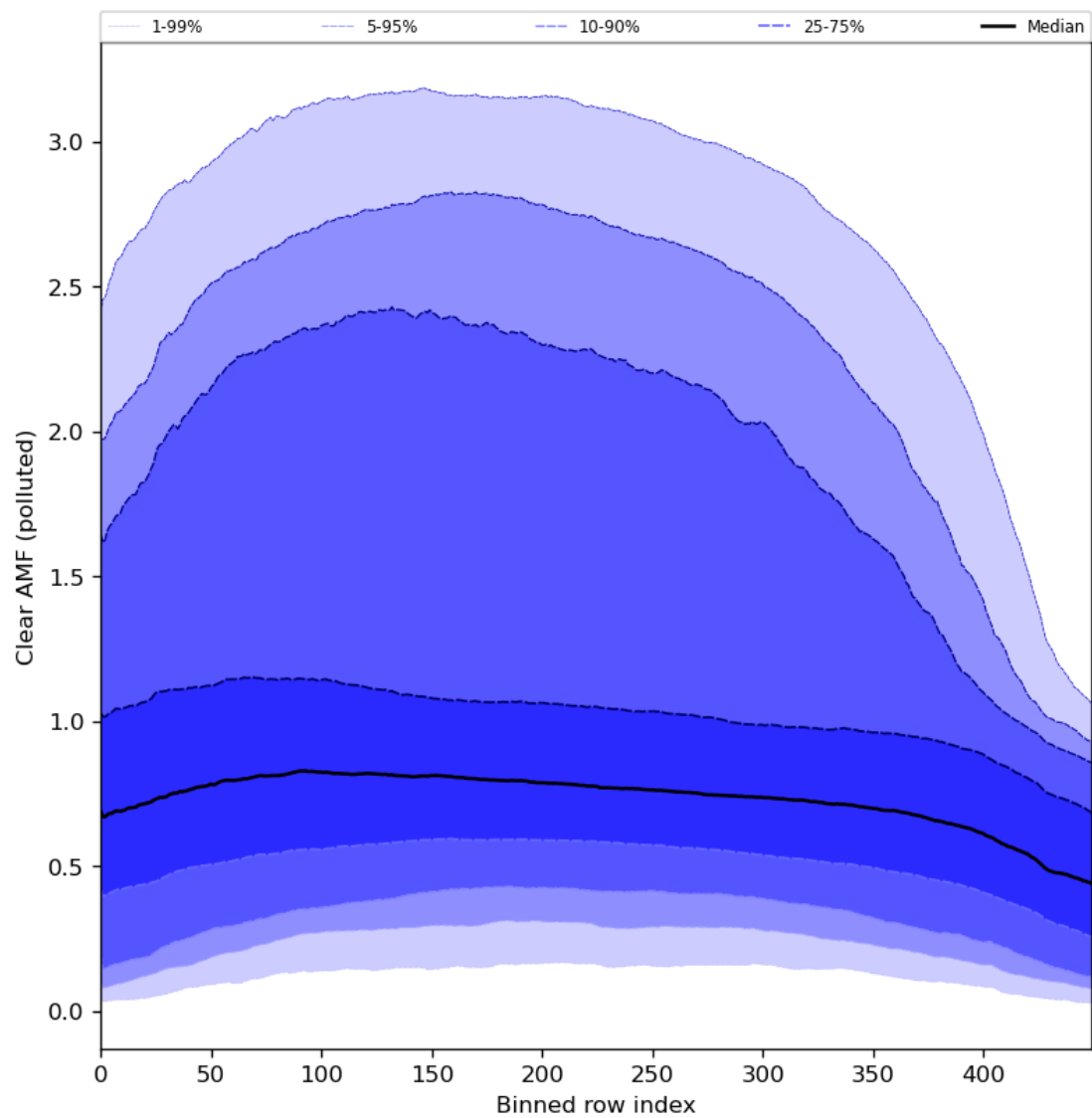
Figure 96: Along track statistics of “Clear AMF (polluted)” for 2024-02-14 to 2024-02-16
