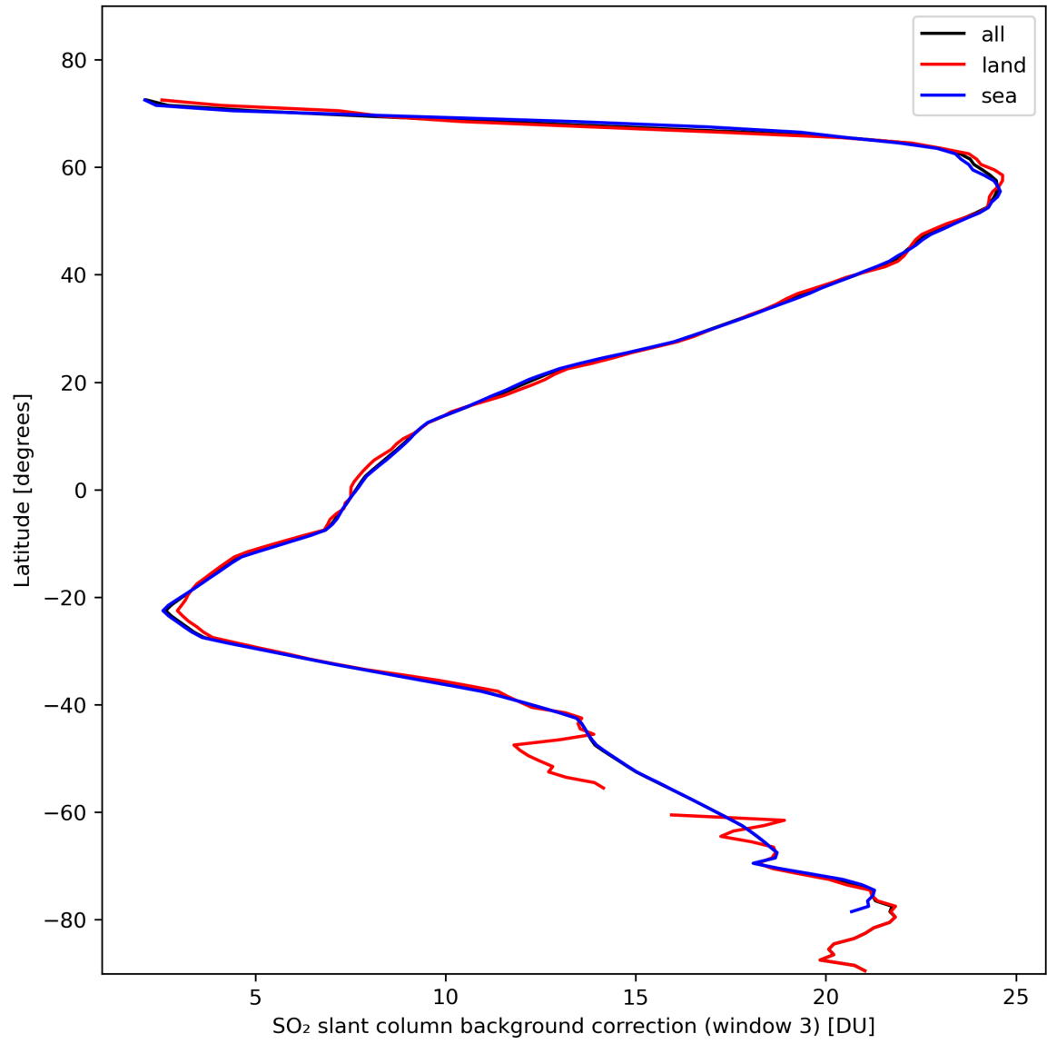
Figure 44: Zonal average of “SO 2 slant column background correction (window 3)” for 2024-02-14 to 2024-02-16.
