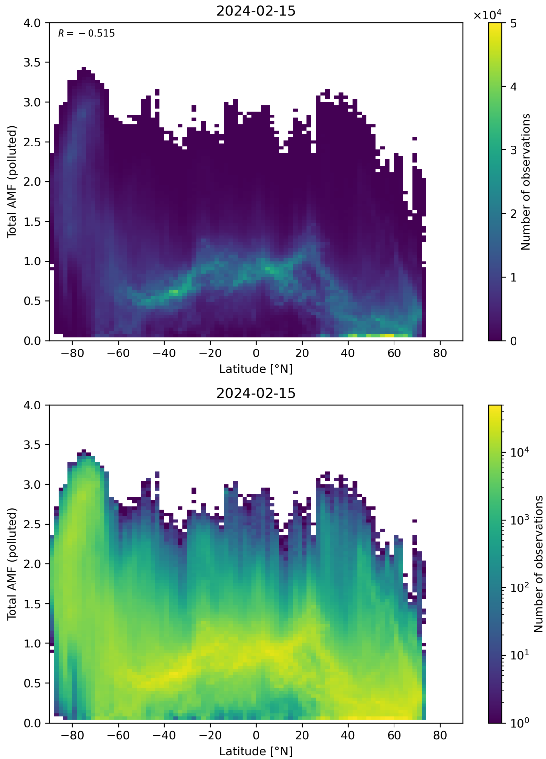
Figure 154: Scatter density plot of “Latitude” against “Total AMF (polluted)” for 2024-02-14 to 2024-02-16.
