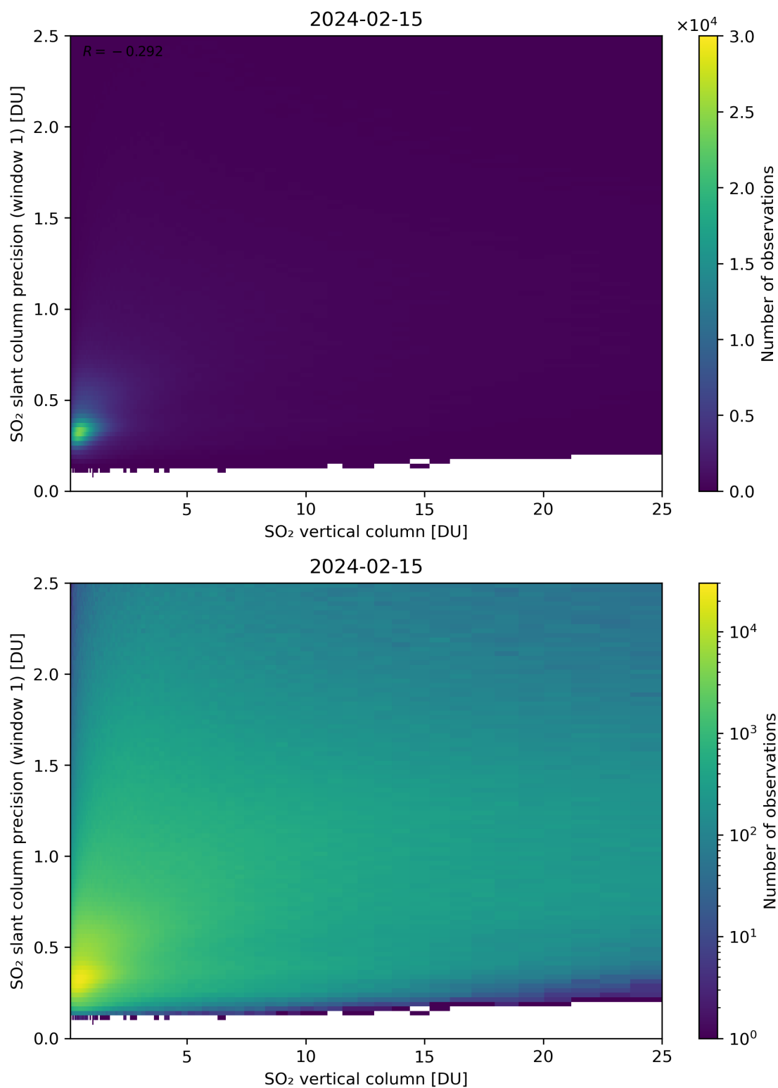
Figure 301: Scatter density plot of “SO 2 vertical column” against “SO 2 slant column precision (window 1)” for 2024-02-14 to 2024-02-16.
