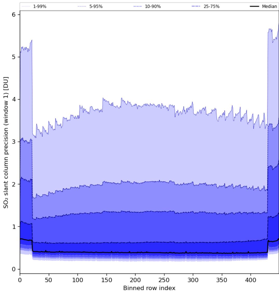
Figure 80: Along track statistics of “SO 2 slant column precision (window 1)” for 2024-02-14 to 2024-02-16
