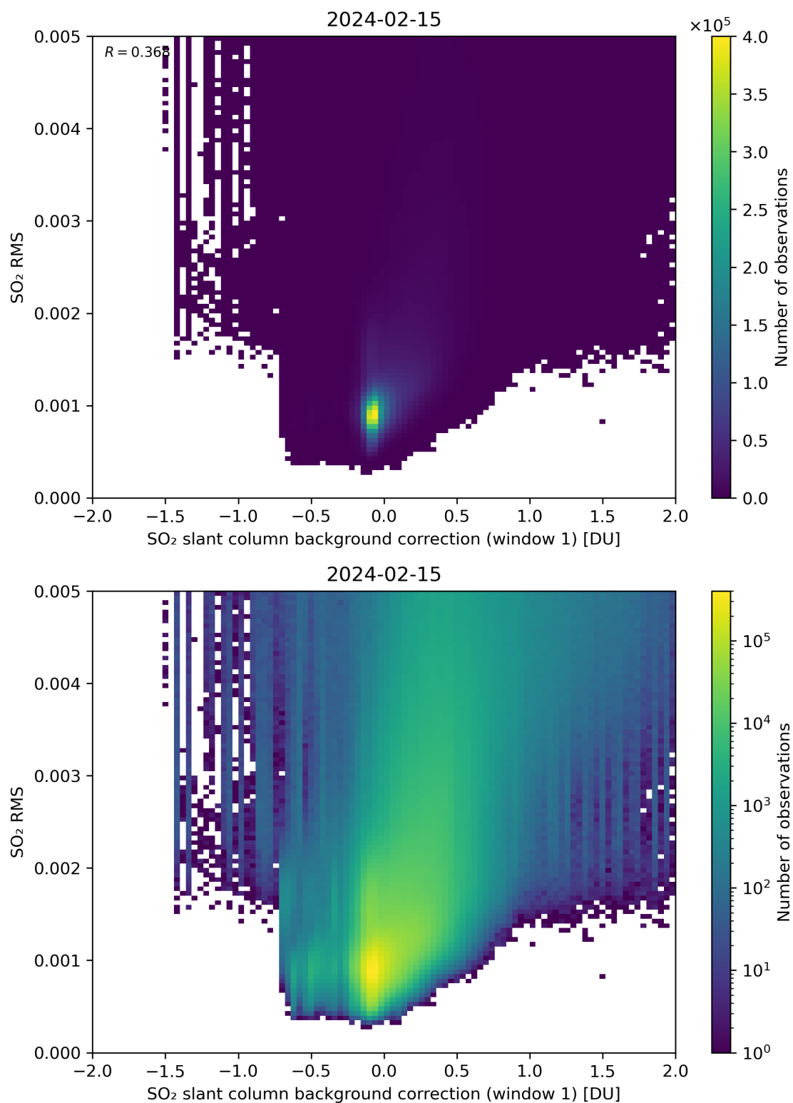
Figure 102: Scatter density plot of “SO 2 slant column background correction (window 1)” against “SO 2 RMS” for 2024-02-14 to 2024-02-16.
