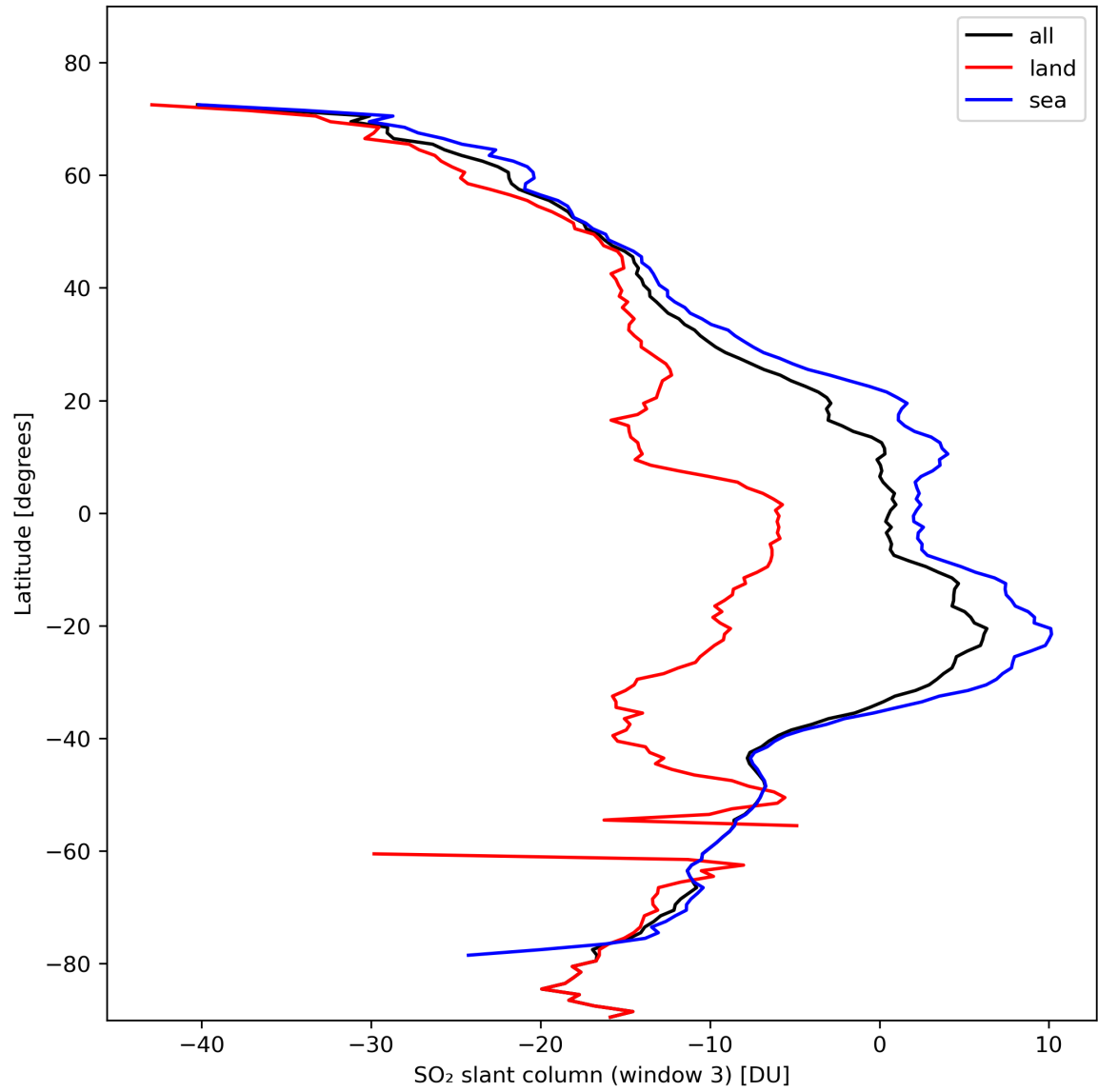
Figure 41: Zonal average of “SO 2 slant column (window 3)” for 2024-02-14 to 2024-02-16.
