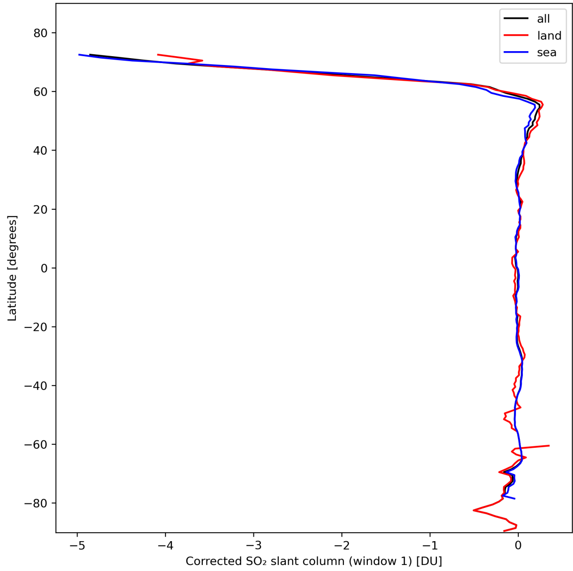
Figure 35: Zonal average of “Corrected SO 2 slant column (window 1)” for 2024-02-14 to 2024-02-16.
