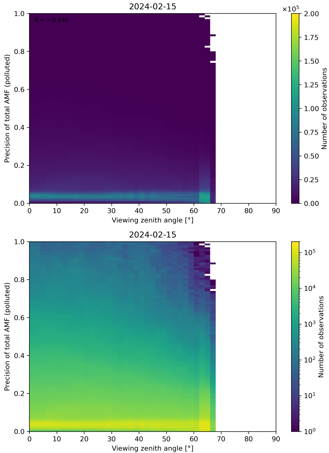
Figure 326: Scatter density plot of “Viewing zenith angle” against “Precision of total AMF (polluted)” for 2024-02-14 to 2024-02-16.
