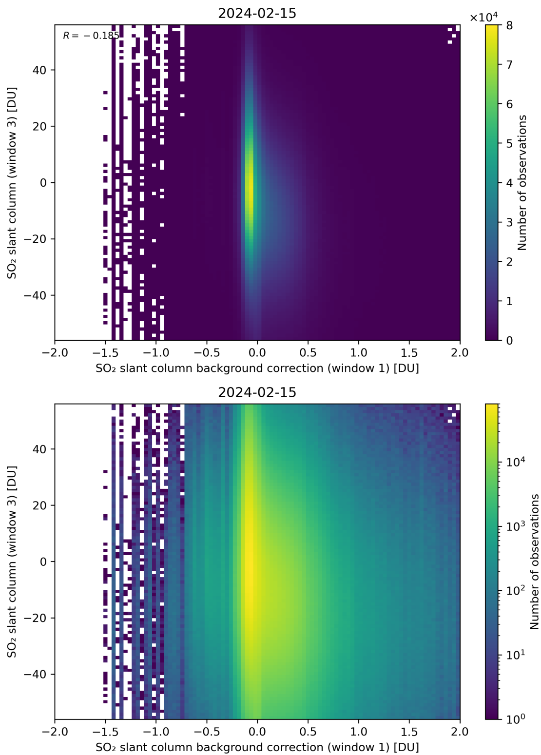
Figure 107: Scatter density plot of “SO 2 slant column background correction (window 1)” against “SO 2 slant column (window 3)” for 2024-02-14 to 2024-02-16.
