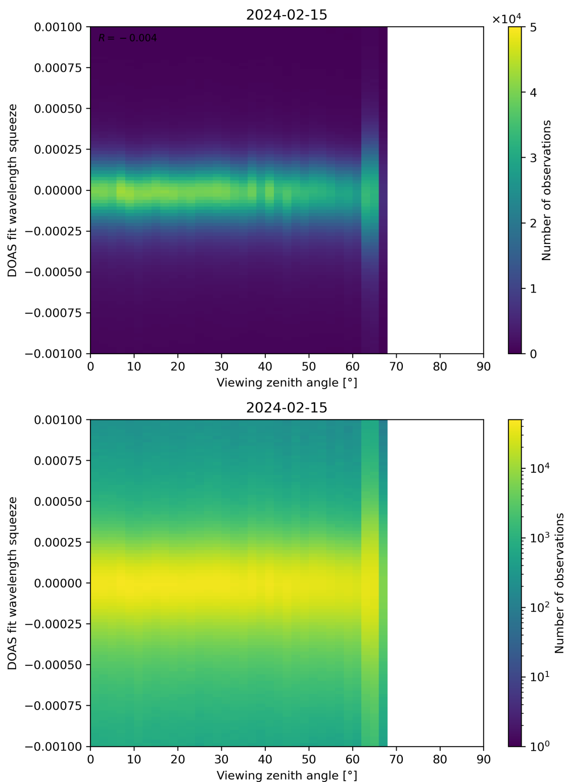
Figure 312: Scatter density plot of “Viewing zenith angle” against “DOAS fit wavelength squeeze” for 2024-02-14 to 2024-02-16.
