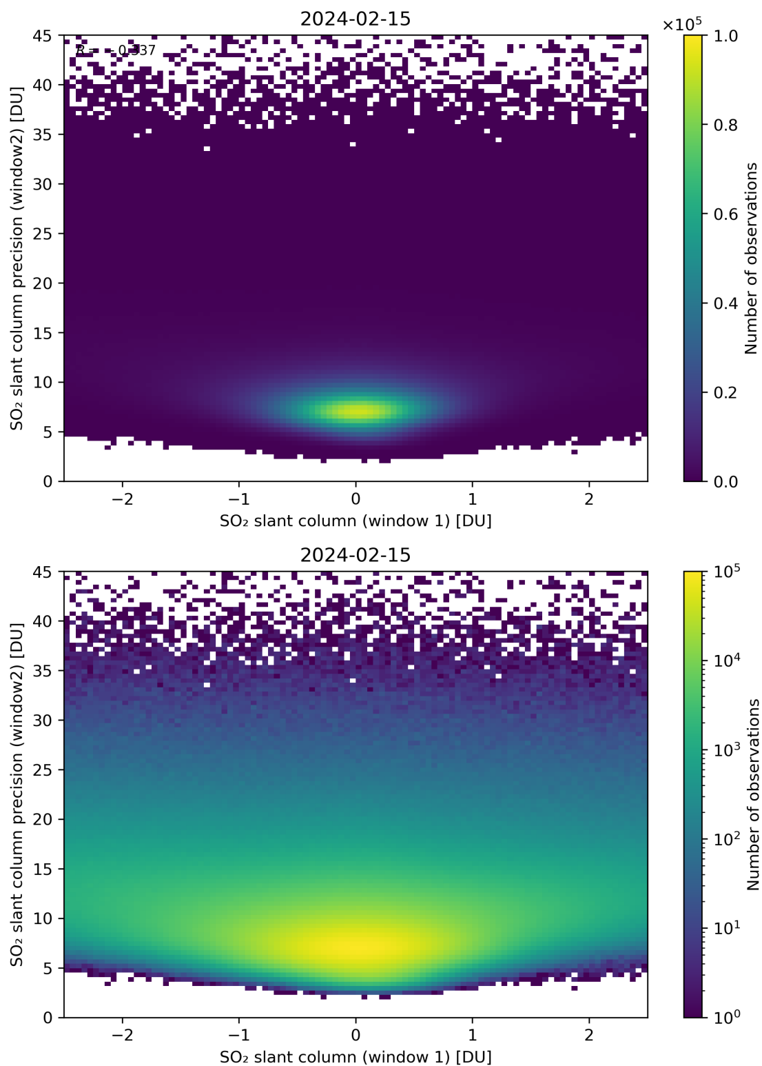
Figure 236: Scatter density plot of “SO 2 slant column (window 1)” against “SO 2 slant column precision (window2)” for 2024-02-14 to 2024-02-16.
