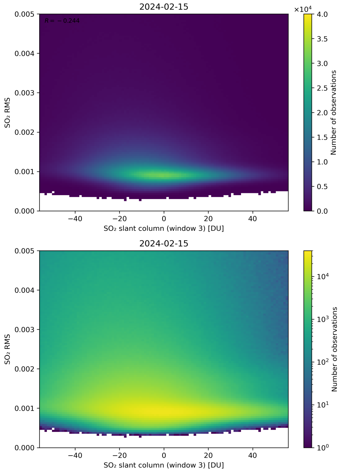
Figure 256: Scatter density plot of “SO 2 slant column (window 3)” against “SO 2 RMS” for 2024-02-14 to 2024-02-16.
