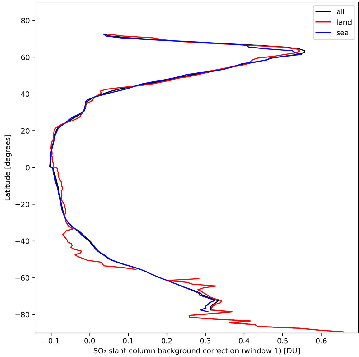
Figure 36: Zonal average of “SO 2 slant column background correction (window 1)” for 2024-02-14 to 2024-02-16.
