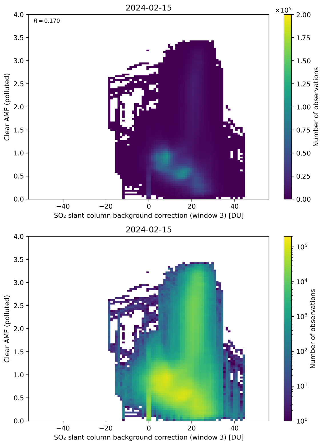
Figure 124: Scatter density plot of “SO 2 slant column background correction (window 3)” against “Clear AMF (polluted)” for 2024-02-14 to 2024-02-16.
