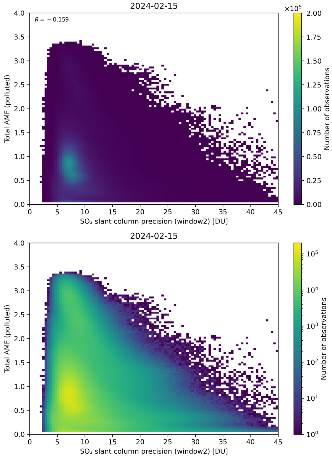
Figure 251: Scatter density plot of “SO 2 slant column precision (window2)” against “Total AMF (polluted)” for 2024-02-14 to 2024-02-16.
