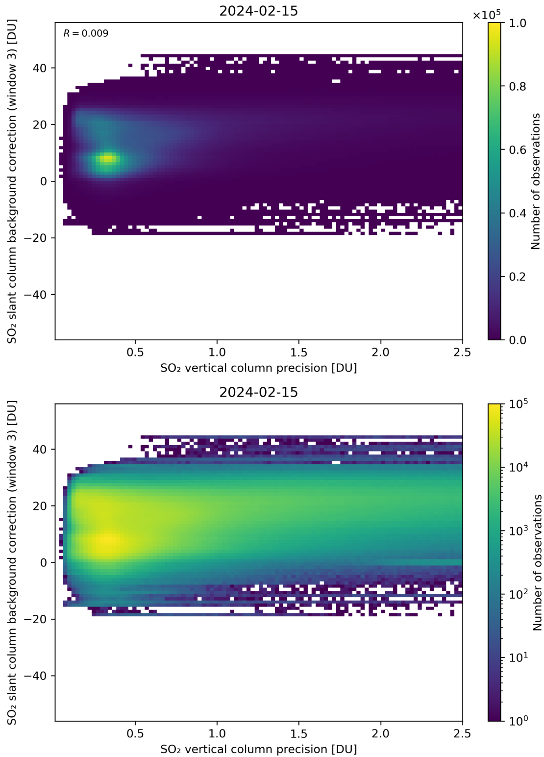
Figure 281: Scatter density plot of “SO 2 vertical column precision” against “SO 2 slant column background correction (window 3)” for 2024-02-14 to 2024-02-16.
