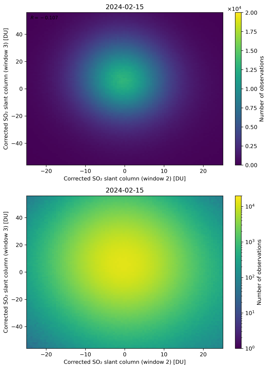
Figure 200: Scatter density plot of “Corrected SO 2 slant column (window 2)” against “Corrected SO 2 slant column (window 3)” for 2024-02-14 to 2024-02-16.
