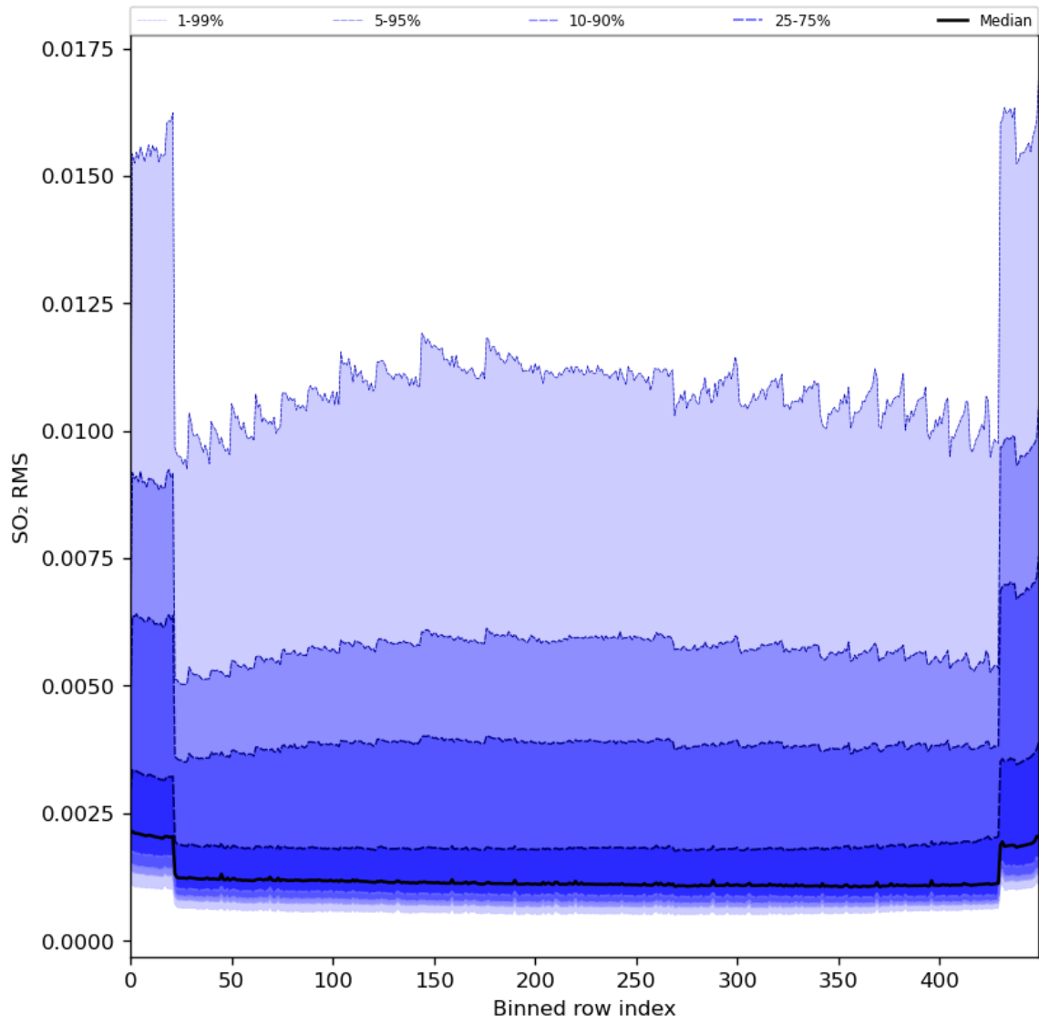
Figure 93: Along track statistics of “SO 2 RMS” for 2024-02-14 to 2024-02-16
