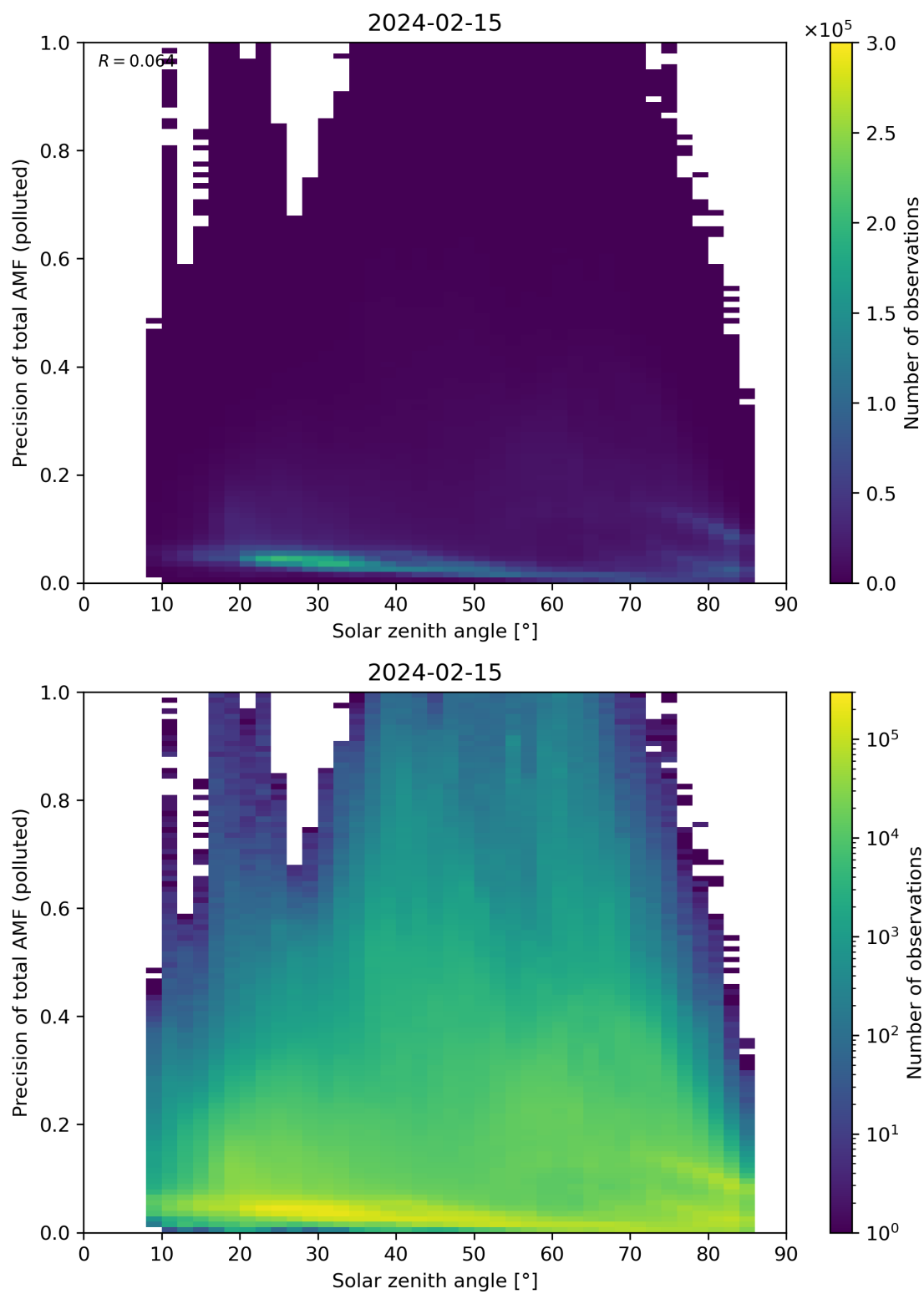
Figure 175: Scatter density plot of “Solar zenith angle” against “Precision of total AMF (polluted)” for 2024-02-14 to 2024-02-16.
