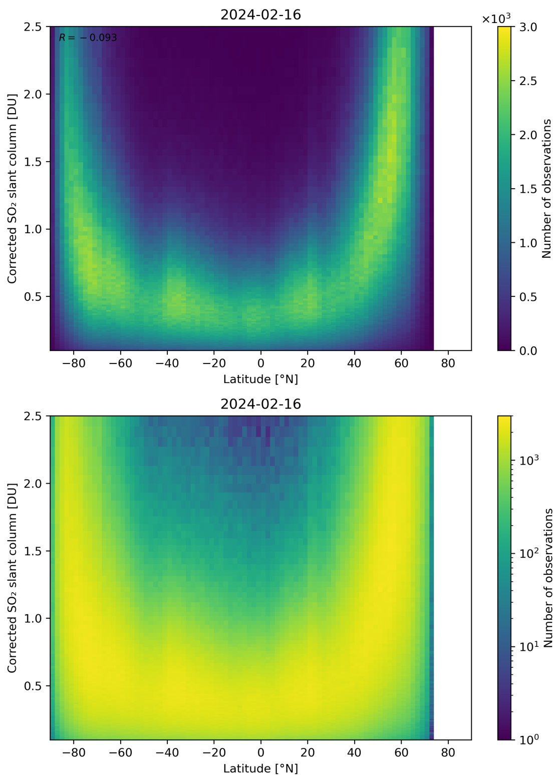
Figure 146: Scatter density plot of “Latitude” against “Corrected SO 2 slant column” for 2024-02-16 to 2024-02-17.
