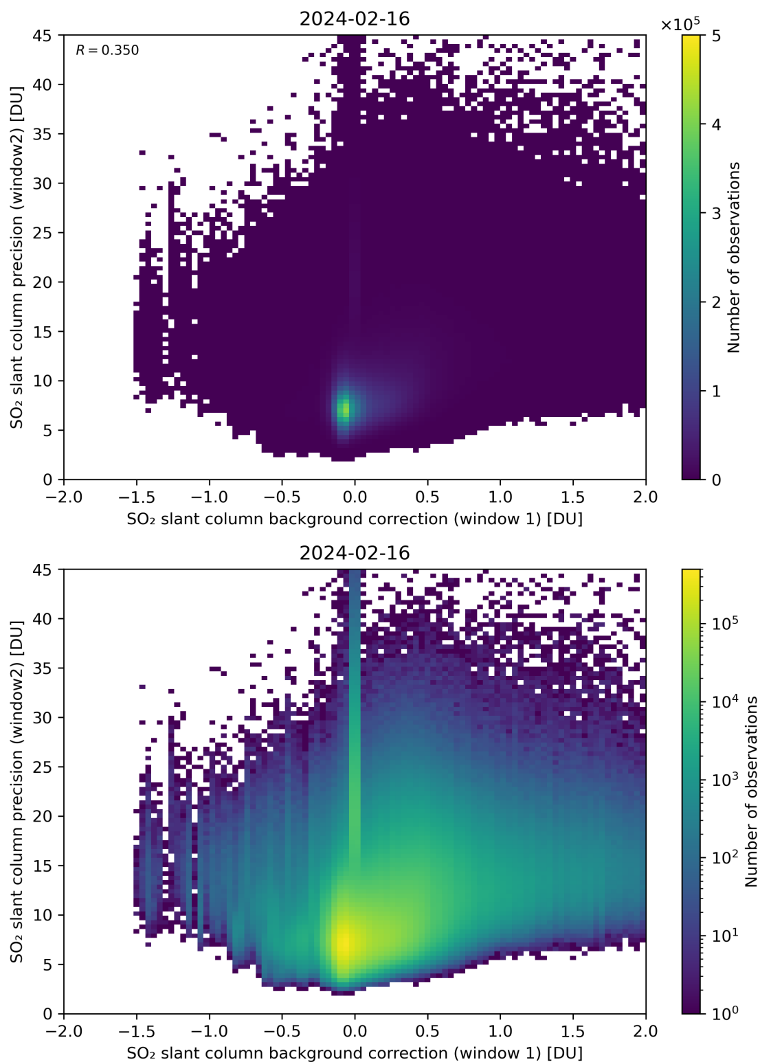
Figure 106: Scatter density plot of “SO 2 slant column background correction (window 1)” against “SO 2 slant column precision (window2)” for 2024-02-16 to 2024-02-17.
