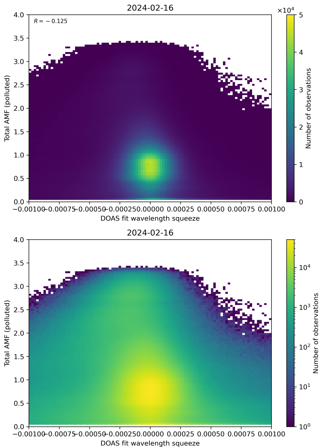
Figure 134: Scatter density plot of “DOAS fit wavelength squeeze” against “Total AMF (polluted)” for 2024-02-16 to 2024-02-17.
