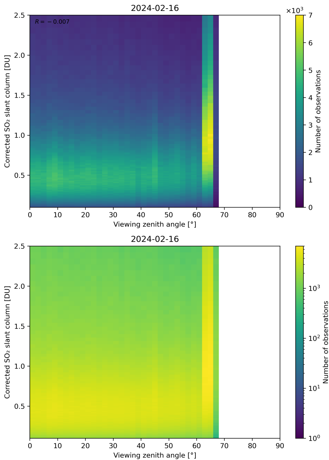
Figure 317: Scatter density plot of “Viewing zenith angle” against “Corrected SO 2 slant column” for 2024-02-16 to 2024-02-17.
