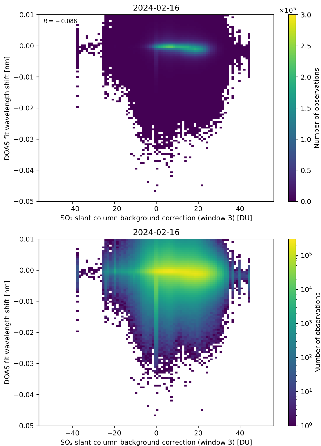
Figure 121: Scatter density plot of “SO 2 slant column background correction (window 3)” against “DOAS fit wavelength shift” for 2024-02-16 to 2024-02-17.
