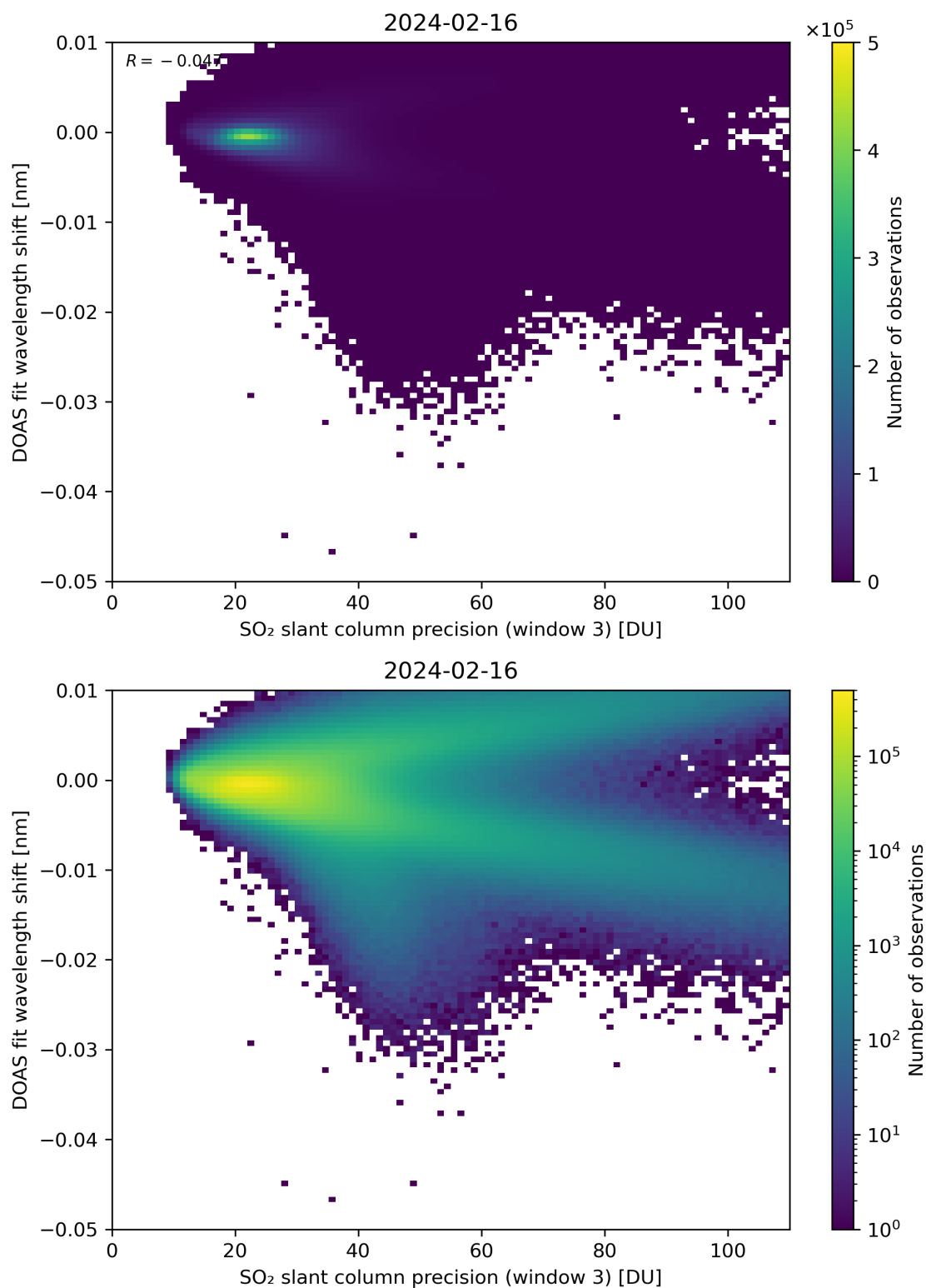
Figure 258: Scatter density plot of “SO 2 slant column precision (window 3)” against “DOAS fit wavelength shift” for 2024-02-16 to 2024-02-17.
