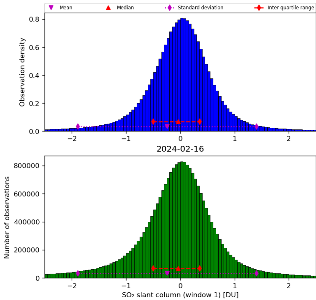
Figure 56: Histogram of “SO 2 slant column (window 1)” for 2024-02-16 to 2024-02-17
