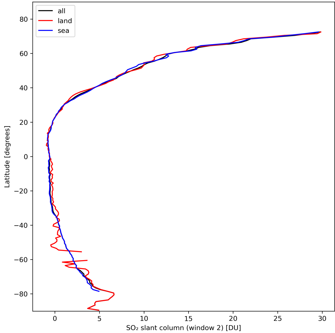
Figure 37: Zonal average of “SO 2 slant column (window 2)” for 2024-02-16 to 2024-02-17.
