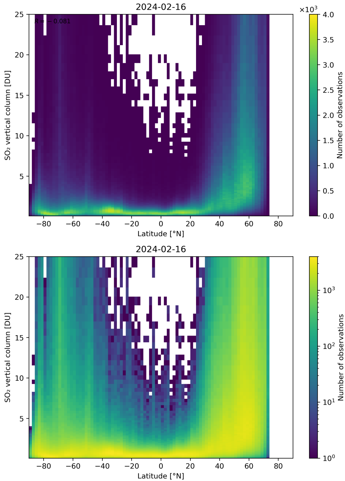
Figure 156: Scatter density plot of “Latitude” against “SO 2 vertical column” for 2024-02-16 to 2024-02-17.
