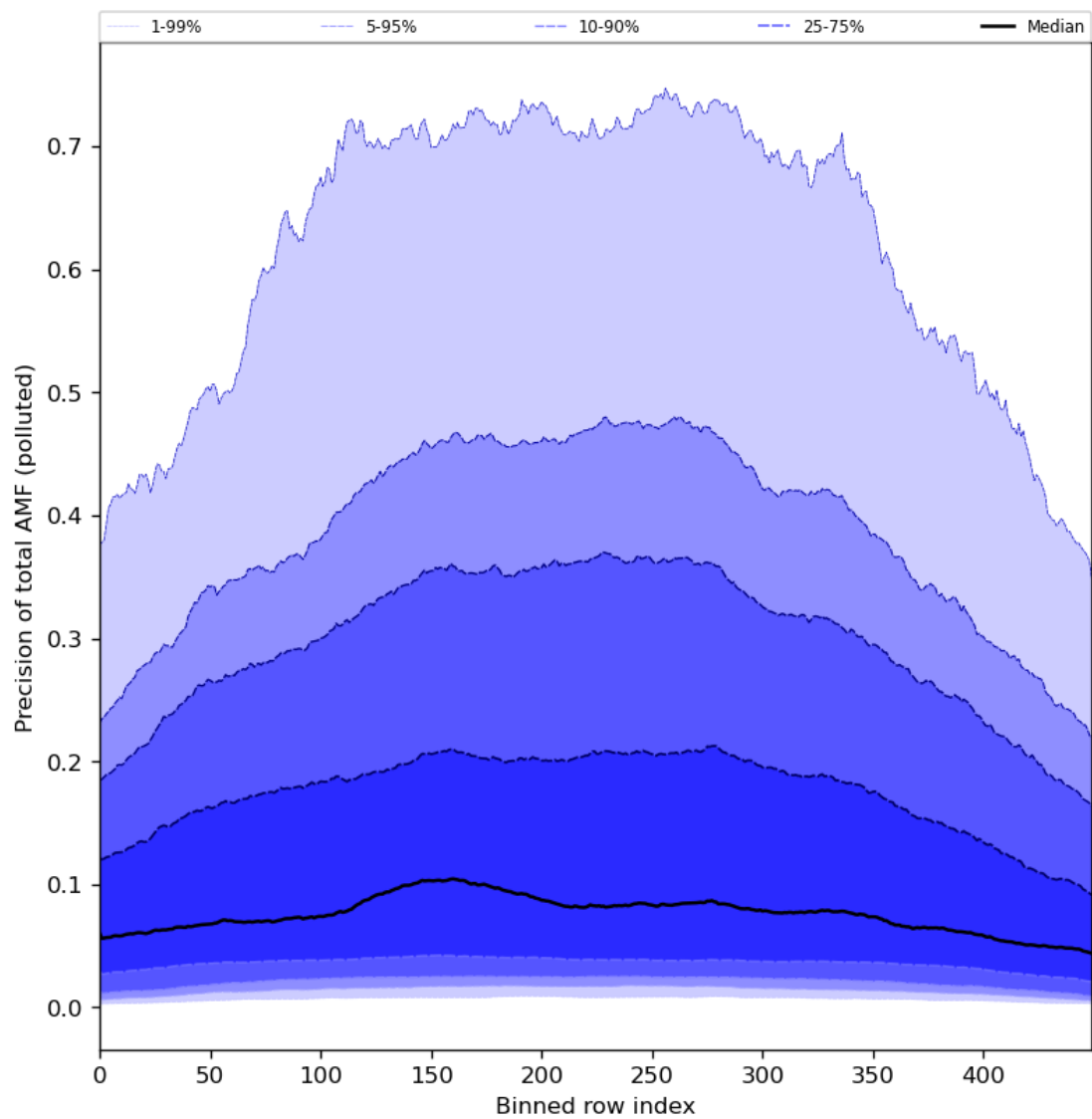
Figure 95: Along track statistics of “Precision of total AMF (polluted)” for 2024-02-16 to 2024-02-17
