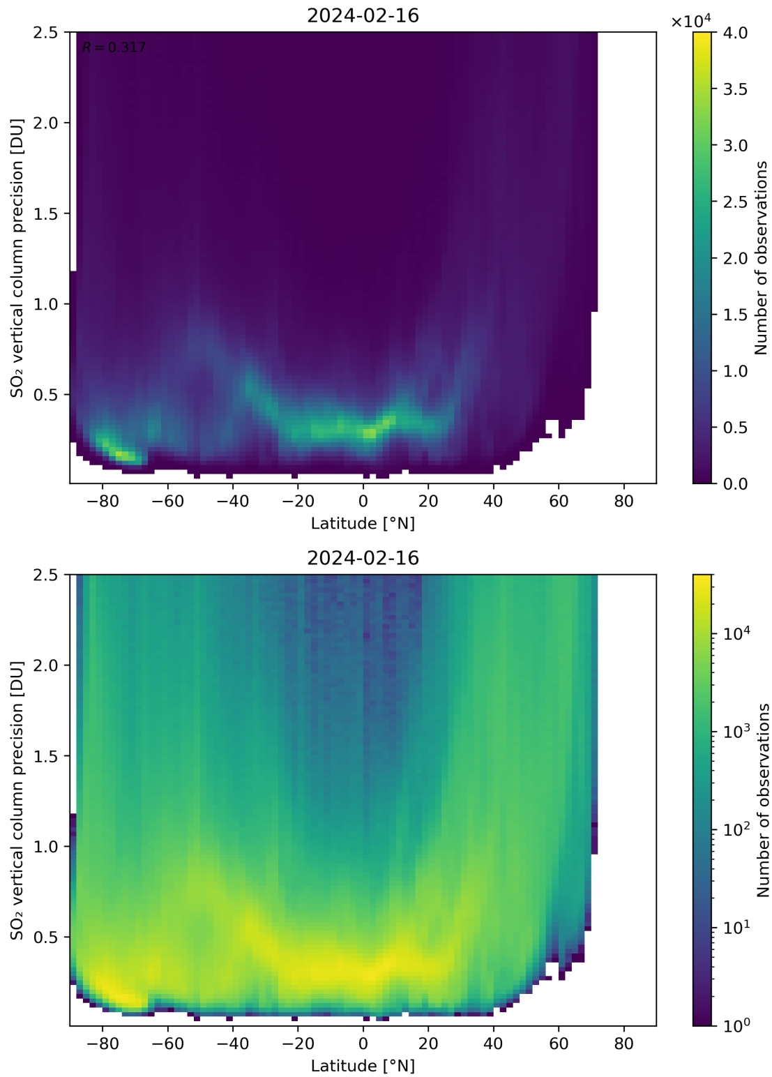
Figure 157: Scatter density plot of “Latitude” against “SO 2 vertical column precision” for 2024-02-16 to 2024-02-17.
