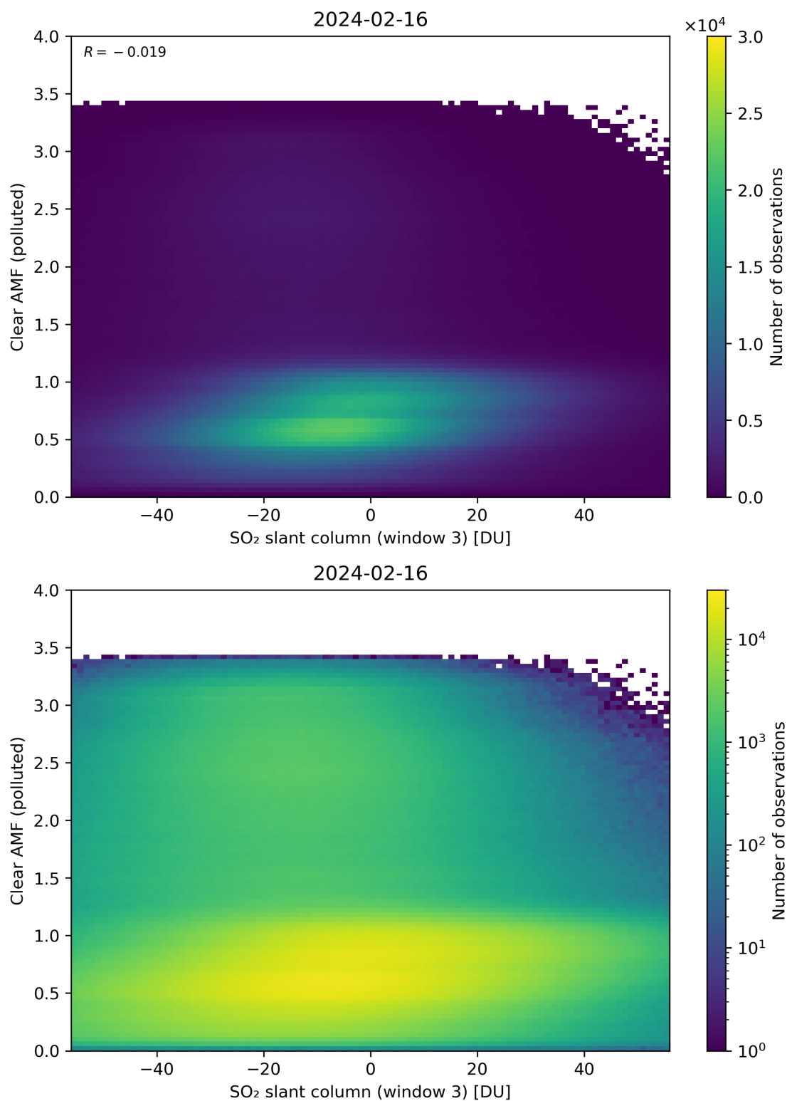
Figure 265: Scatter density plot of “SO 2 slant column (window 3)” against “Clear AMF (polluted)” for 2024-02-16 to 2024-02-17.
