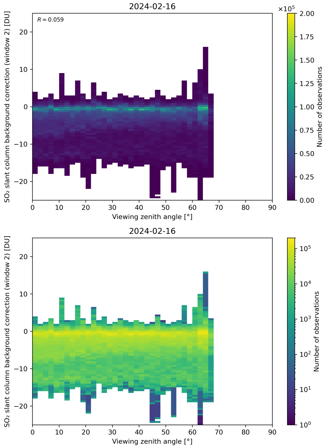
Figure 309: Scatter density plot of “Viewing zenith angle” against “SO 2 slant column background correction (window 2)” for 2024-02-16 to 2024-02-17.
