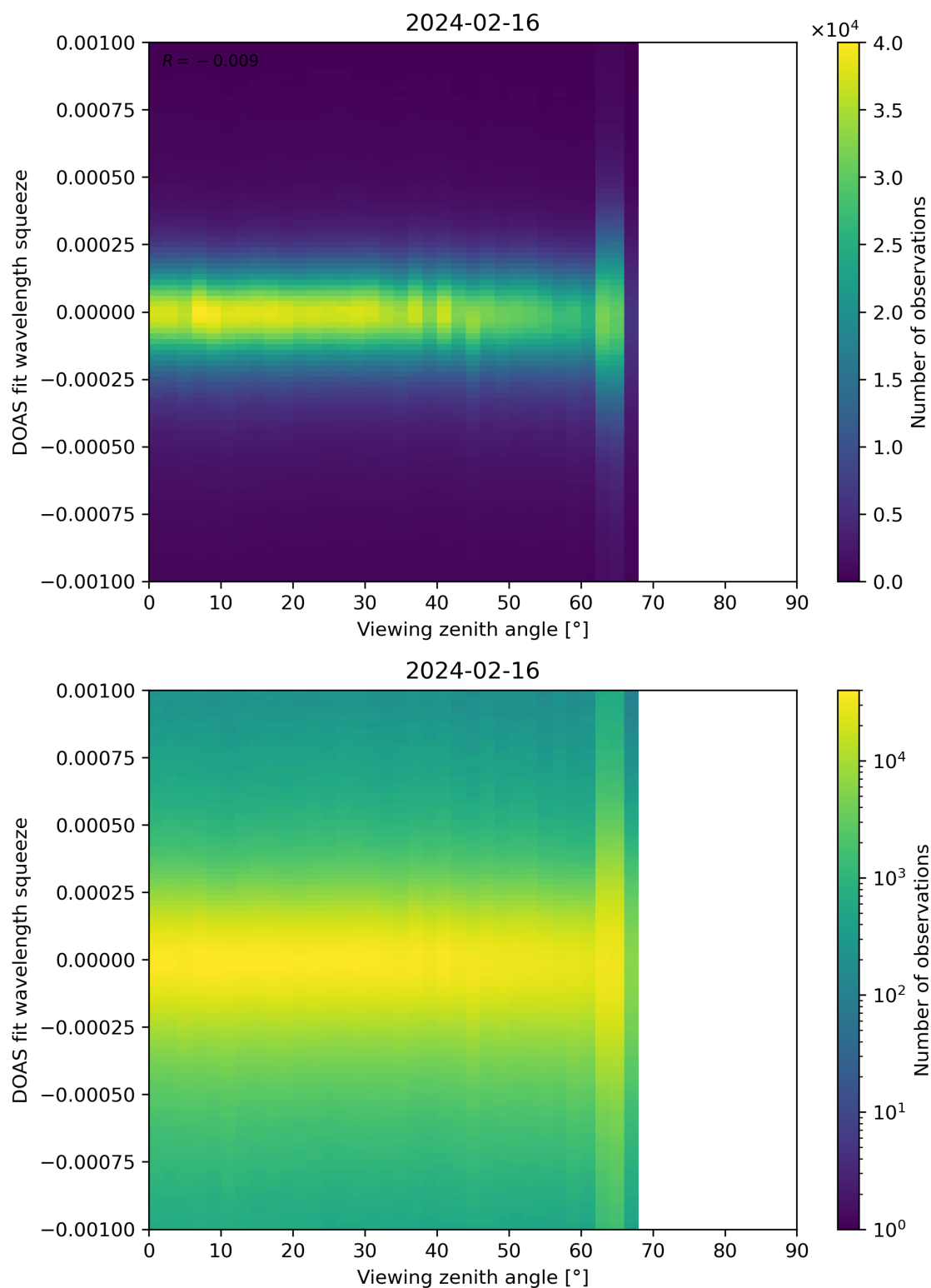
Figure 312: Scatter density plot of “Viewing zenith angle” against “DOAS fit wavelength squeeze” for 2024-02-16 to 2024-02-17.
