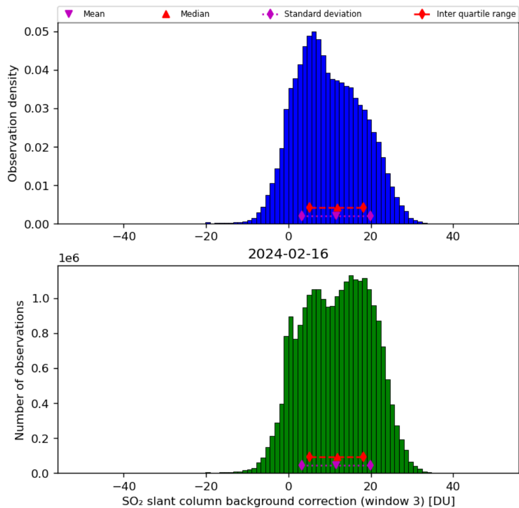
Figure 67: Histogram of “SO 2 slant column background correction (window 3)” for 2024-02-16 to 2024-02-17
