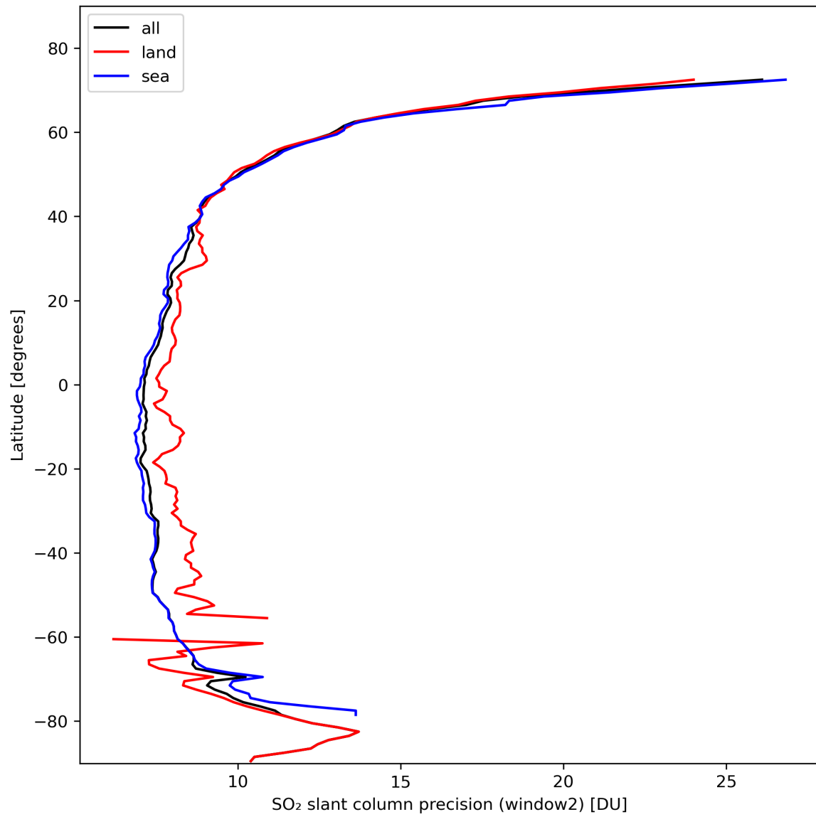
Figure 38: Zonal average of “SO 2 slant column precision (window2)” for 2024-02-16 to 2024-02-17.
