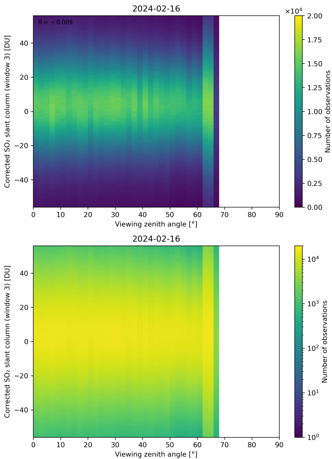
Figure 319: Scatter density plot of “Viewing zenith angle” against “Corrected SO 2 slant column (window 3)” for 2024-02-16 to 2024-02-17.
