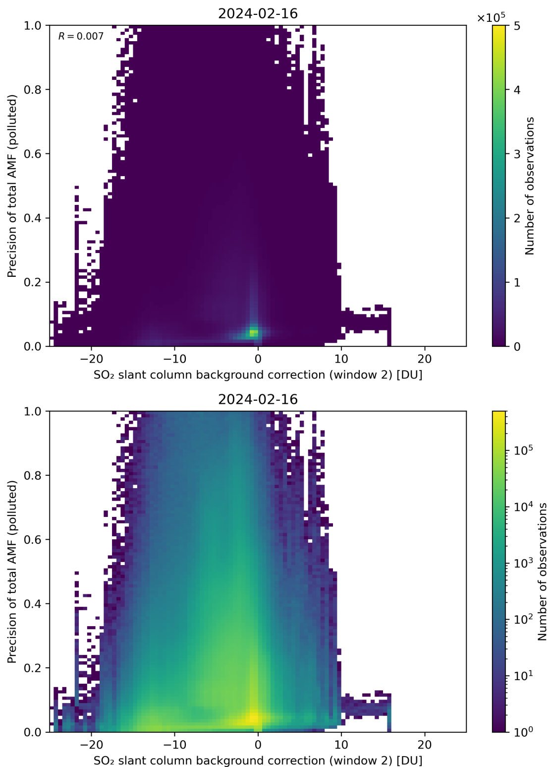
Figure 120: Scatter density plot of “SO 2 slant column background correction (window 2)” against “Precision of total AMF (polluted)” for 2024-02-16 to 2024-02-17.
