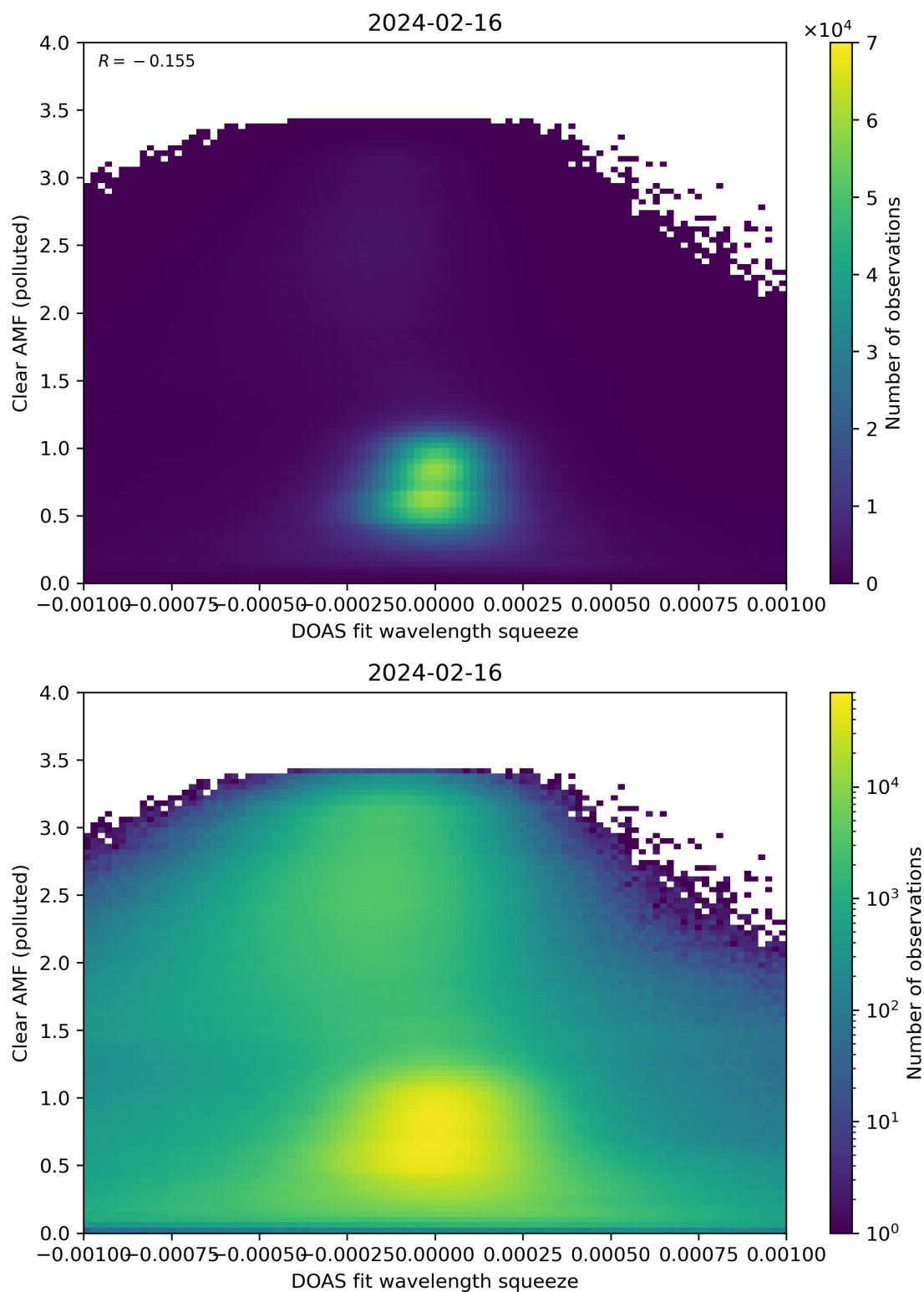
Figure 133: Scatter density plot of “DOAS fit wavelength squeeze” against “Clear AMF (polluted)” for 2024-02-16 to 2024-02-17.
