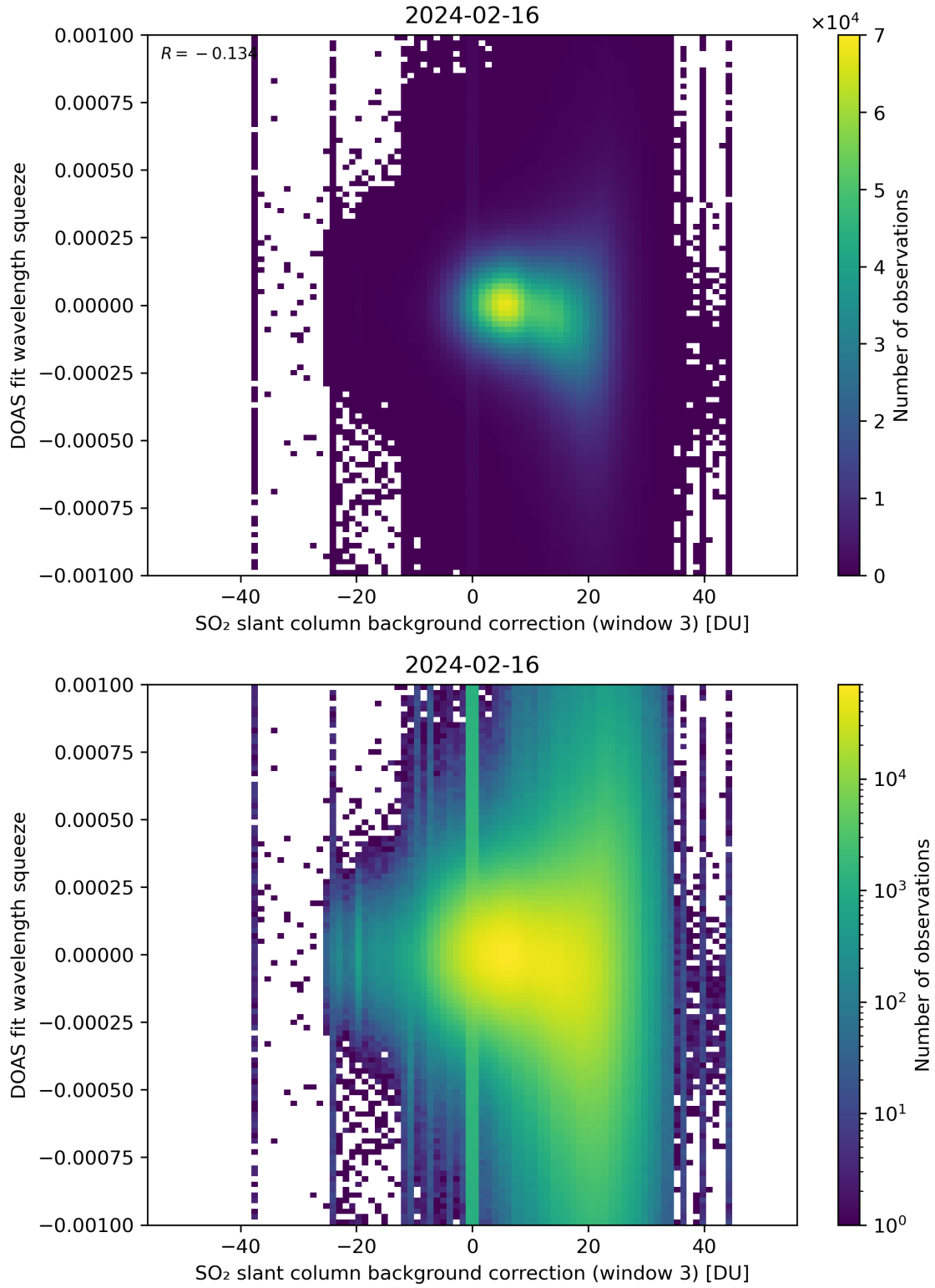
Figure 122: Scatter density plot of “SO 2 slant column background correction (window 3)” against “DOAS fit wavelength squeeze” for 2024-02-16 to 2024-02-17.
