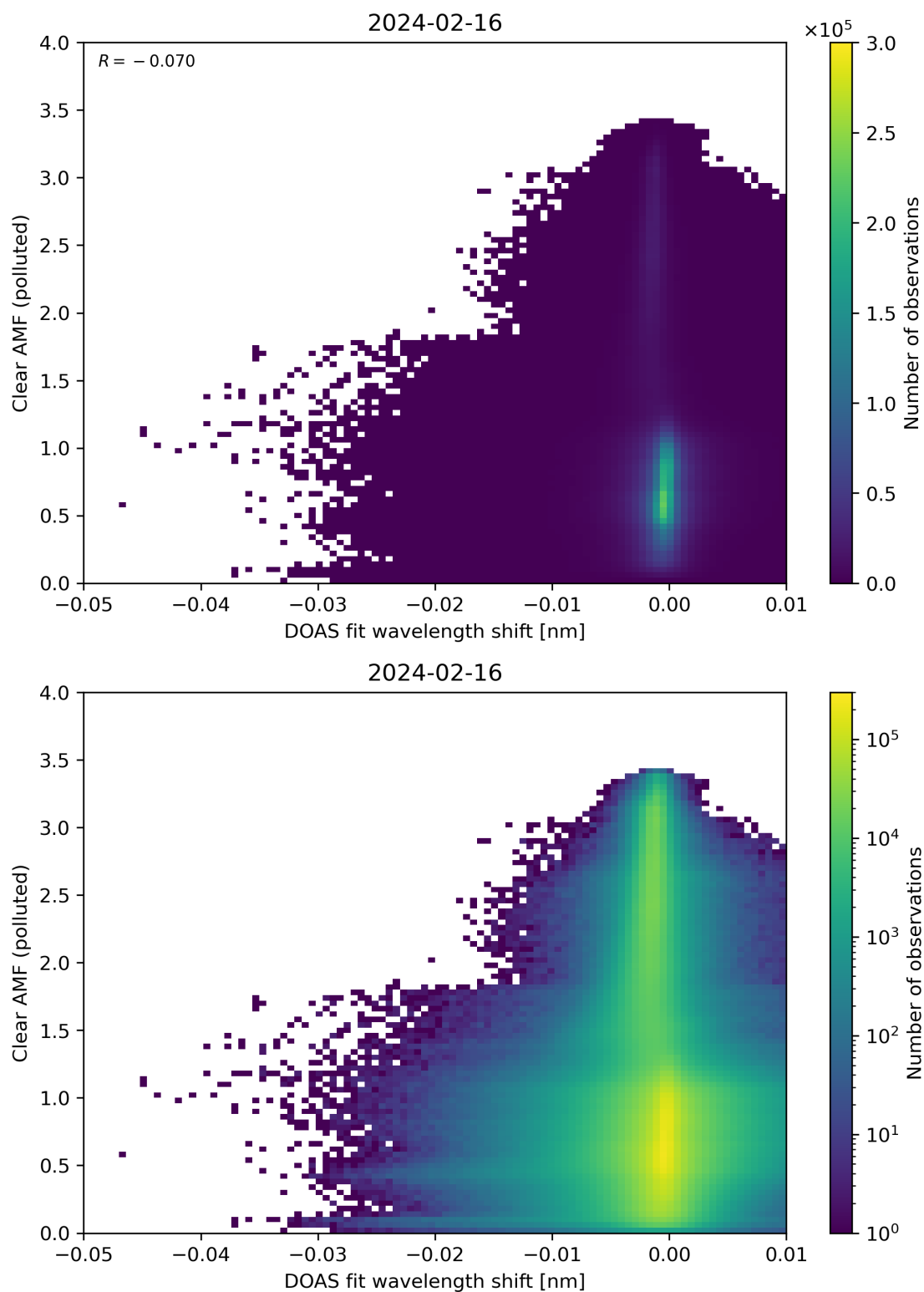
Figure 129: Scatter density plot of “DOAS fit wavelength shift” against “Clear AMF (polluted)” for 2024-02-16 to 2024-02-17.
