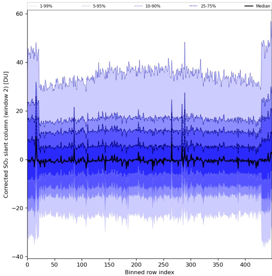
Figure 85: Along track statistics of “Corrected SO 2 slant column (window 2)” for 2024-02-16 to 2024-02-17
