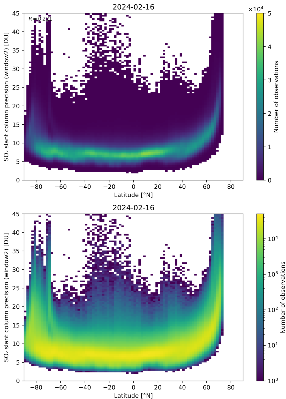
Figure 151: Scatter density plot of “Latitude” against “SO 2 slant column precision (window2)” for 2024-02-16 to 2024-02-17.
