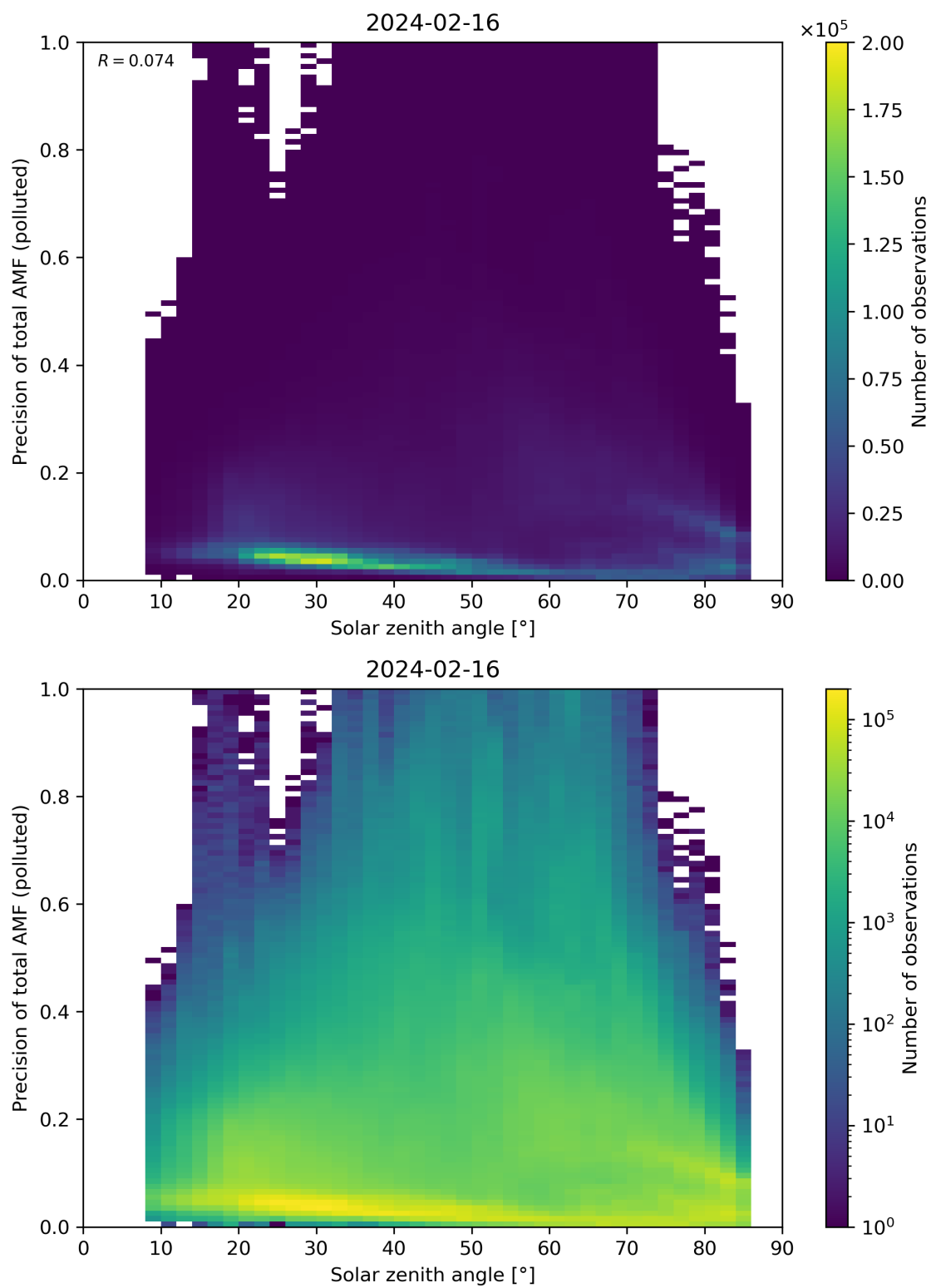
Figure 175: Scatter density plot of “Solar zenith angle” against “Precision of total AMF (polluted)” for 2024-02-16 to 2024-02-17.
