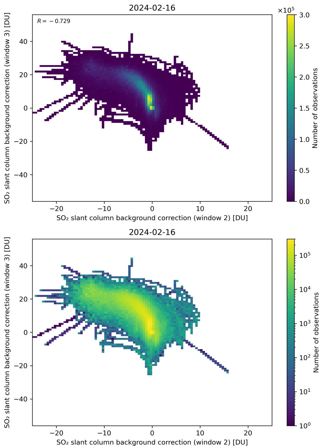
Figure 111: Scatter density plot of “SO 2 slant column background correction (window 2)” against “SO 2 slant column background correction (window 3)” for 2024-02-16 to 2024-02-17.
