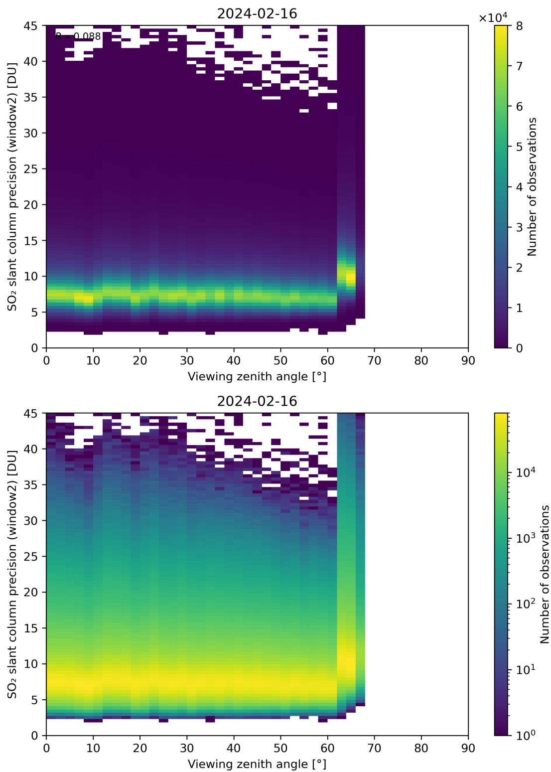
Figure 322: Scatter density plot of “Viewing zenith angle” against “SO 2 slant column precision (window2)” for 2024-02-16 to 2024-02-17.
