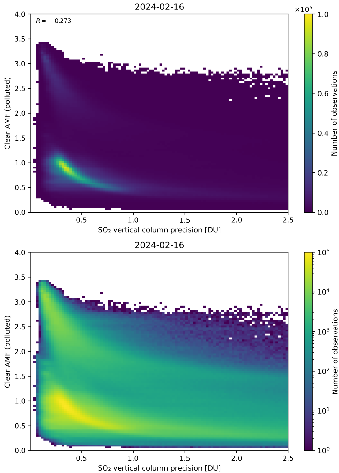
Figure 285: Scatter density plot of “SO 2 vertical column precision” against “Clear AMF (polluted)” for 2024-02-16 to 2024-02-17.
