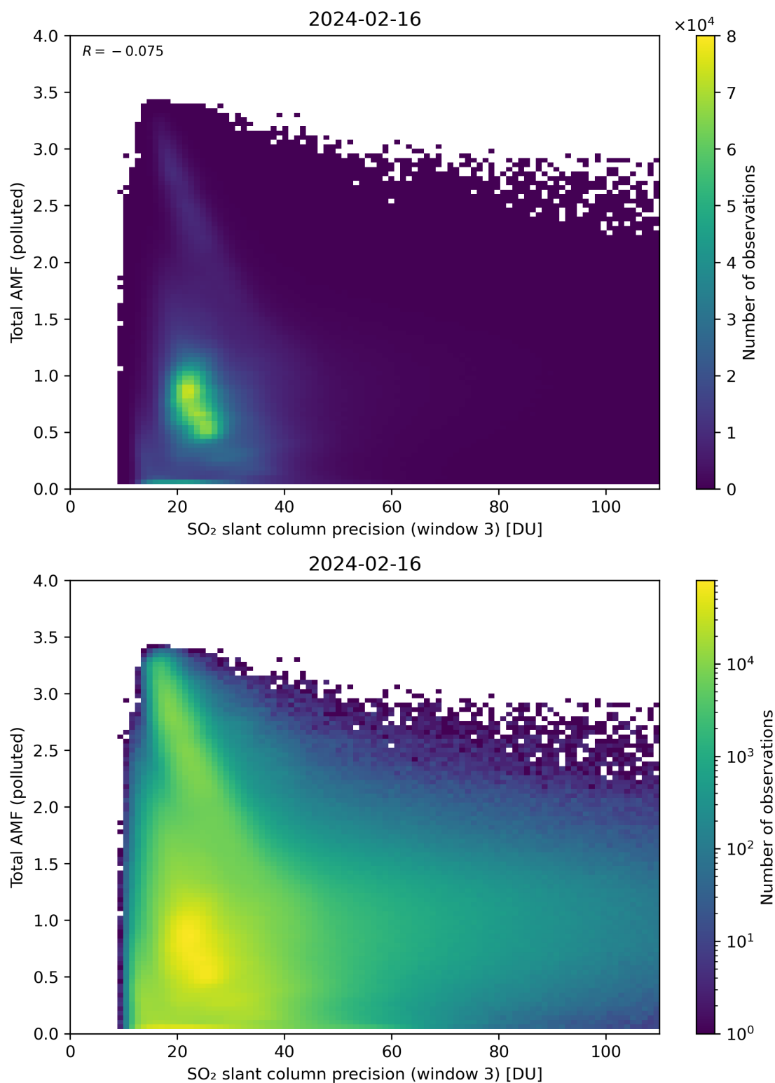
Figure 263: Scatter density plot of “SO 2 slant column precision (window 3)” against “Total AMF (polluted)” for 2024-02-16 to 2024-02-17.
