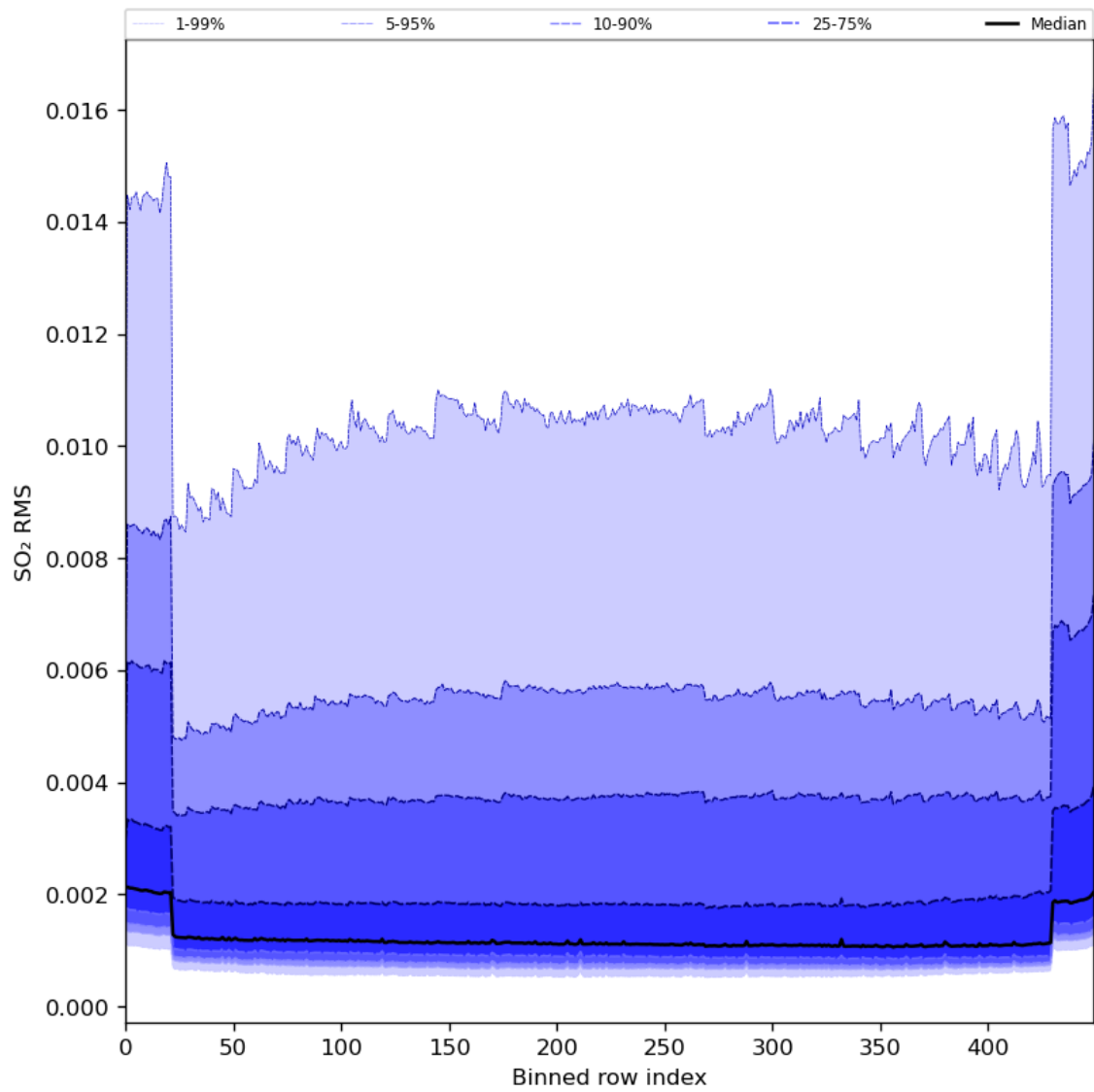
Figure 93: Along track statistics of “SO 2 RMS” for 2024-02-16 to 2024-02-17
