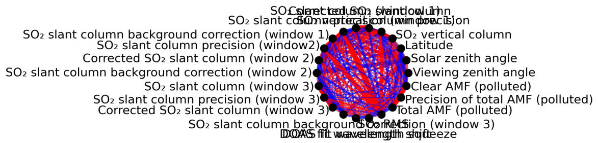
Figure 1: Map of correlation graph for 2024-02-16 to 2024-02-17.
