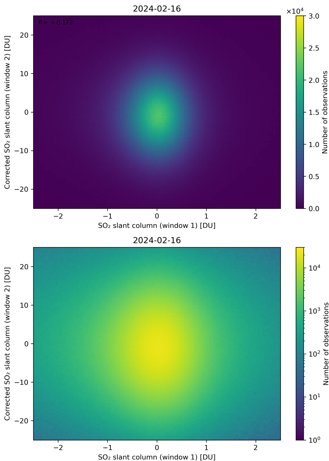
Figure 233: Scatter density plot of “SO 2 slant column (window 1)” against “Corrected SO 2 slant column (window 2)” for 2024-02-16 to 2024-02-17.
