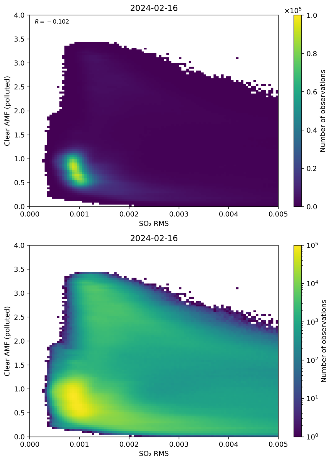
Figure 136: Scatter density plot of “SO 2 RMS” against “Clear AMF (polluted)” for 2024-02-16 to 2024-02-17.
