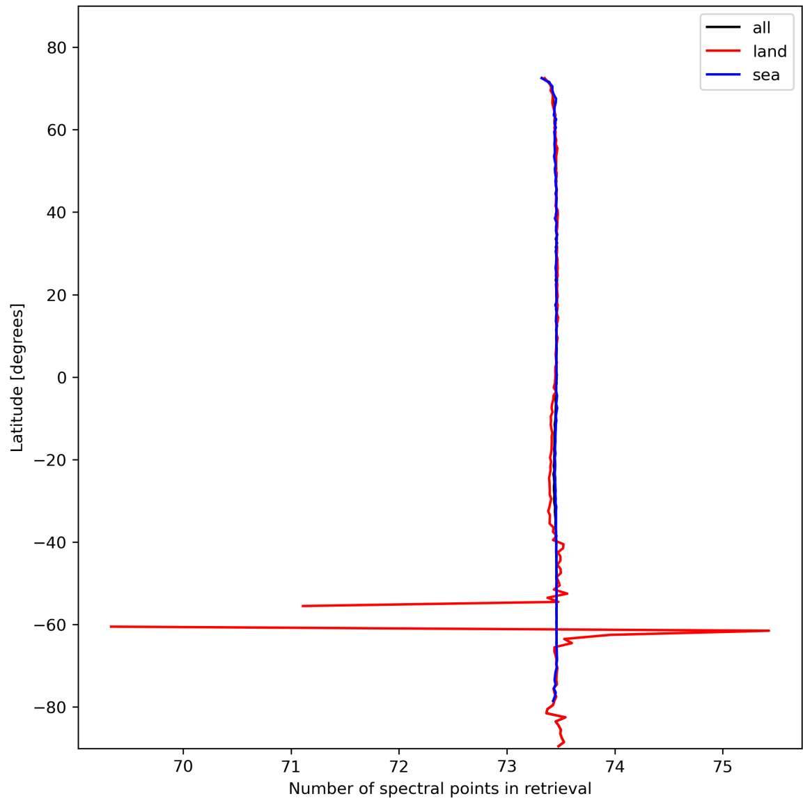
Figure 51: Zonal average of “Number of spectral points in retrieval” for 2024-02-16 to 2024-02-17.
