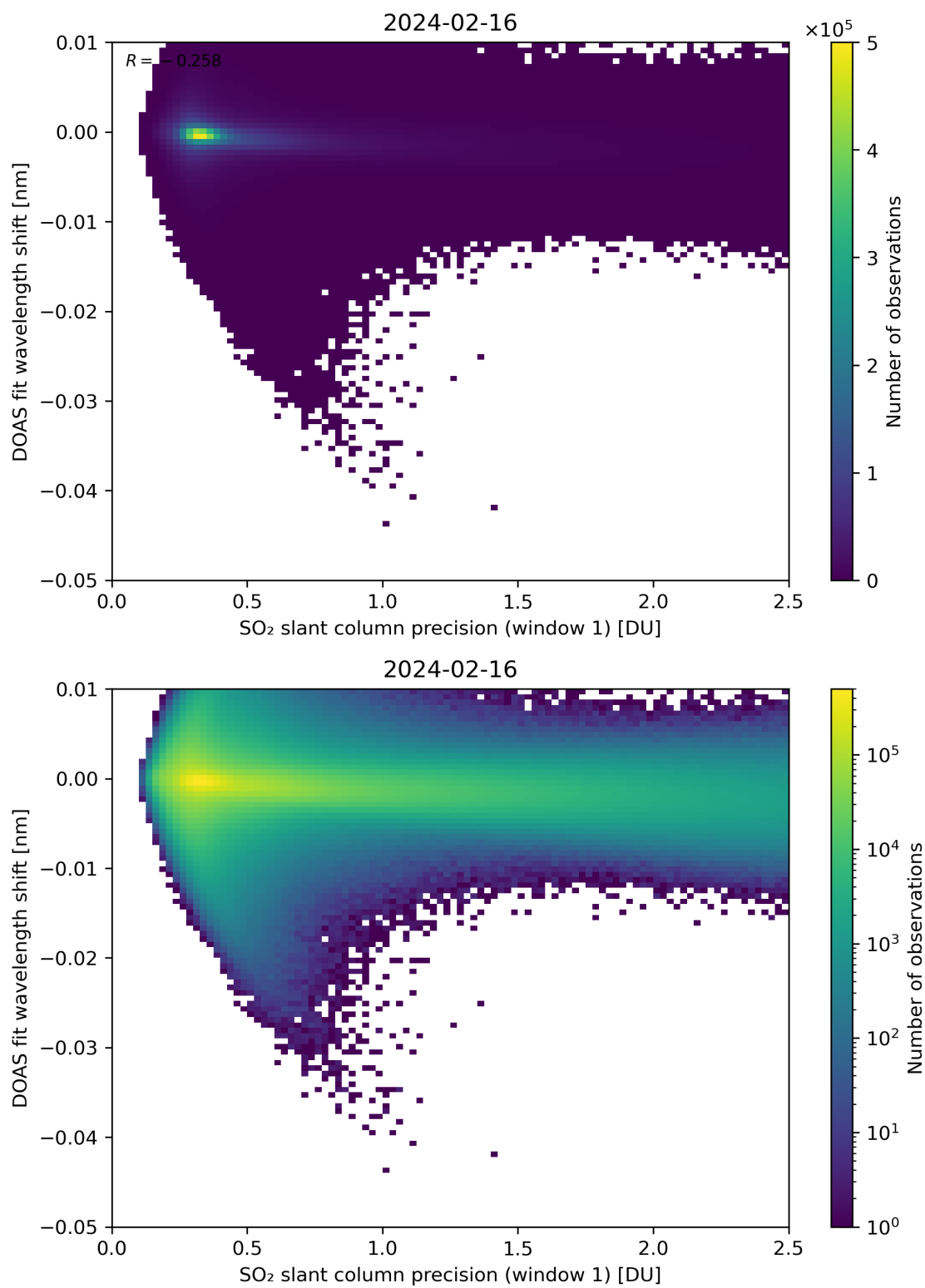
Figure 221: Scatter density plot of “SO 2 slant column precision (window 1)” against “DOAS fit wavelength shift” for 2024-02-16 to 2024-02-17.
