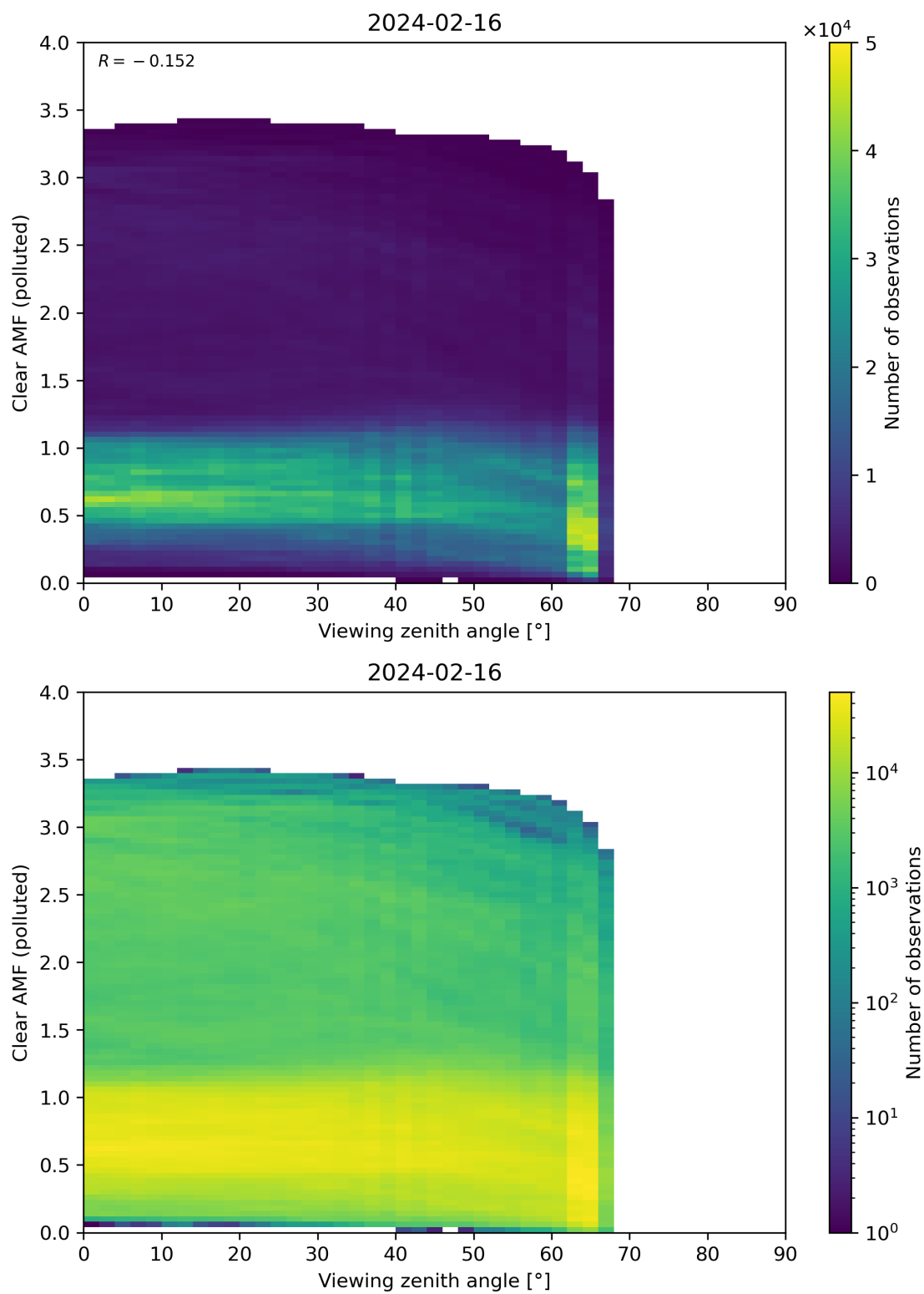
Figure 316: Scatter density plot of “Viewing zenith angle” against “Clear AMF (polluted)” for 2024-02-16 to 2024-02-17.
