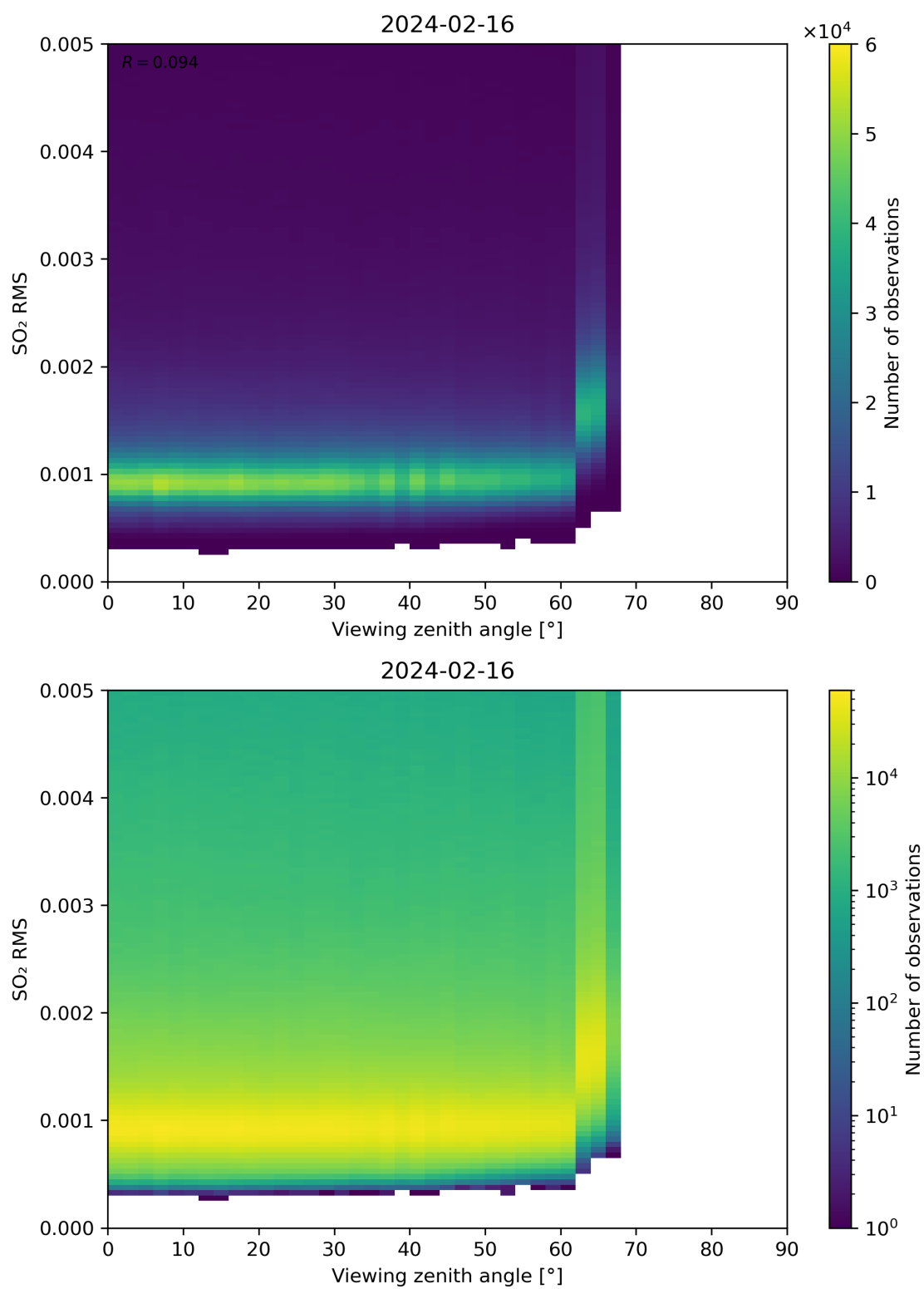
Figure 313: Scatter density plot of “Viewing zenith angle” against “SO 2 RMS” for 2024-02-16 to 2024-02-17.
