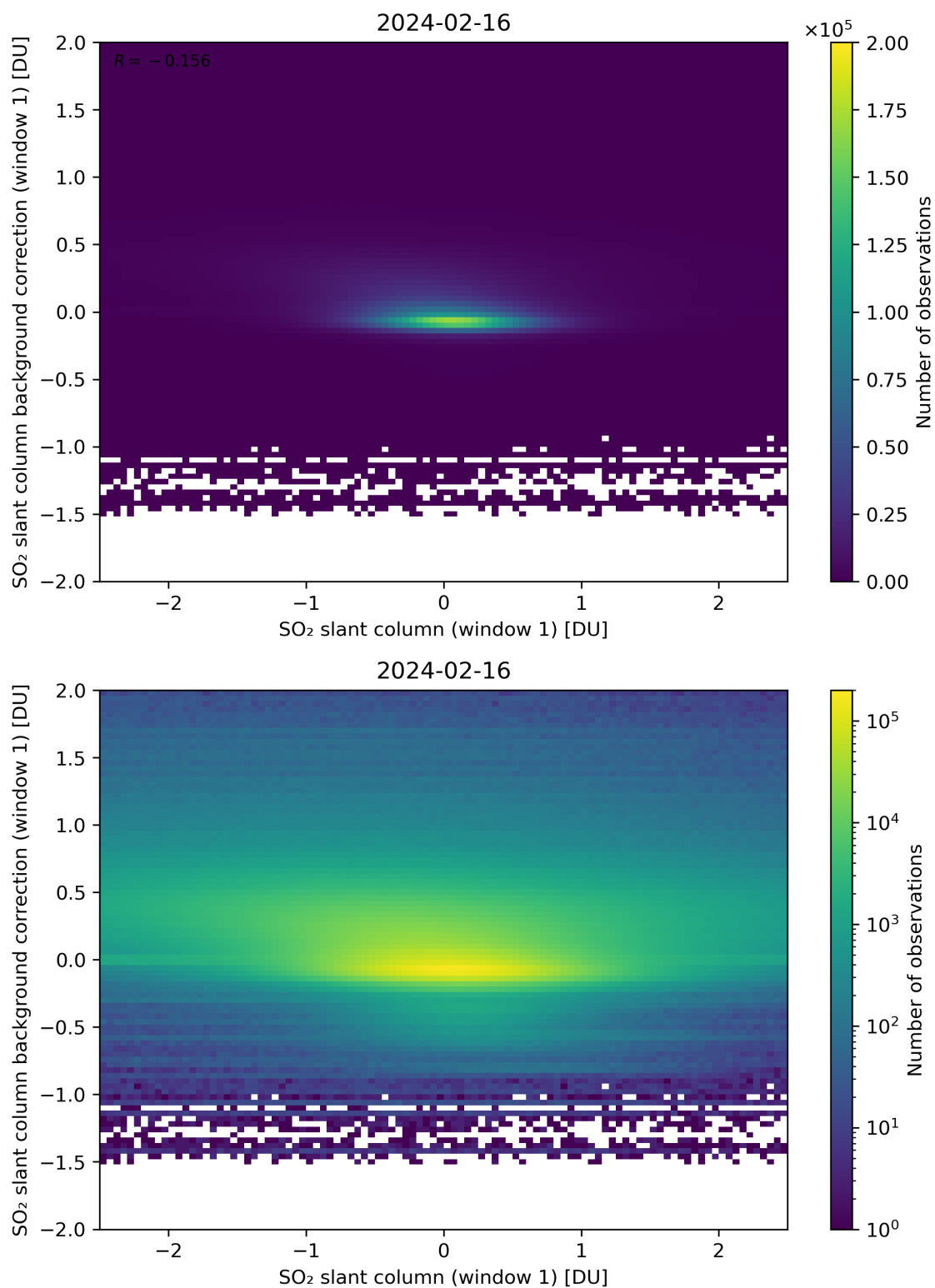
Figure 212: Scatter density plot of “SO 2 slant column (window 1)” against “SO 2 slant column background correction (window 1)” for 2024-02-16 to 2024-02-17.
