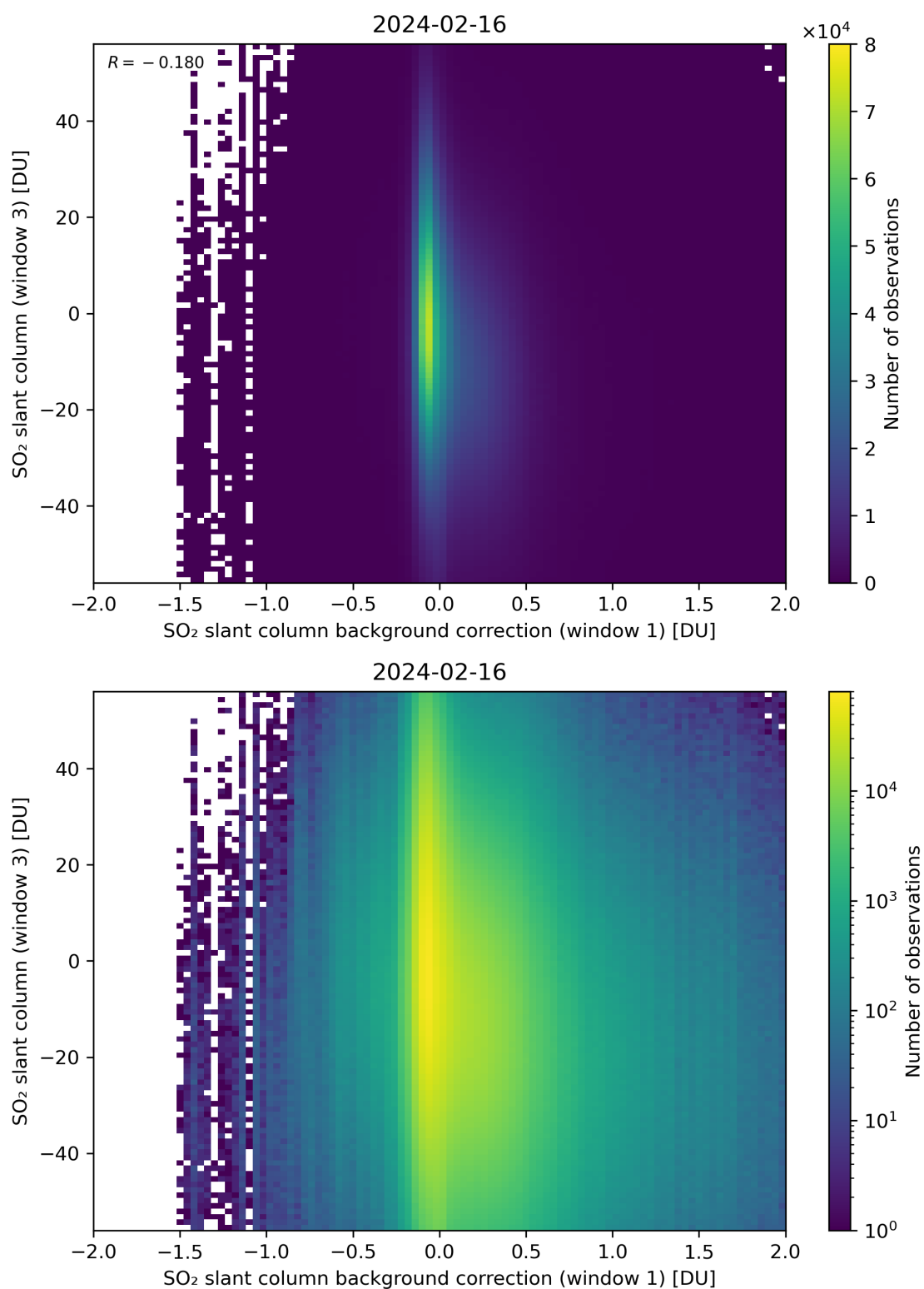
Figure 107: Scatter density plot of “SO 2 slant column background correction (window 1)” against “SO 2 slant column (window 3)” for 2024-02-16 to 2024-02-17.
