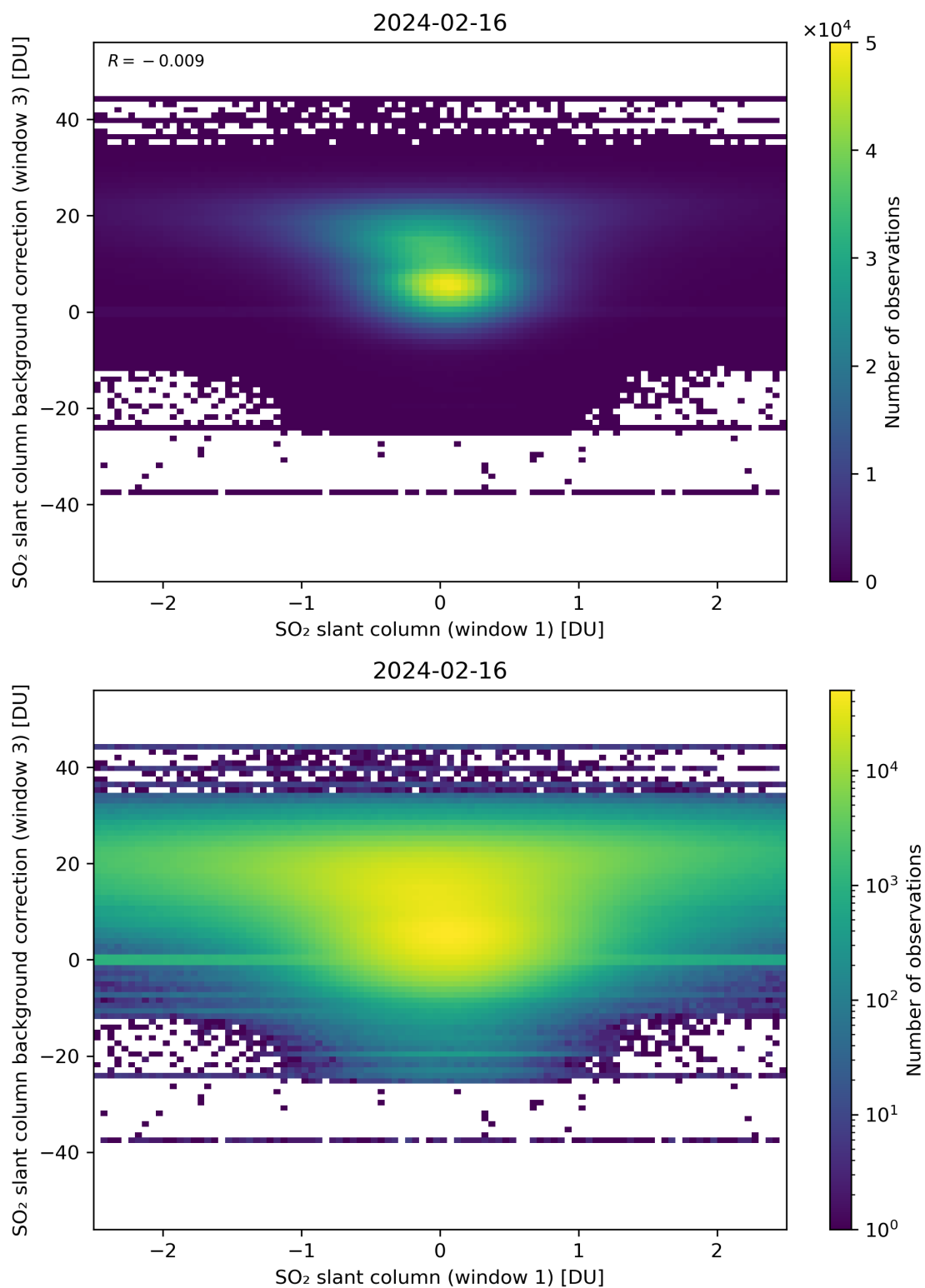
Figure 214: Scatter density plot of “SO 2 slant column (window 1)” against “SO 2 slant column background correction (window 3)” for 2024-02-16 to 2024-02-17.
