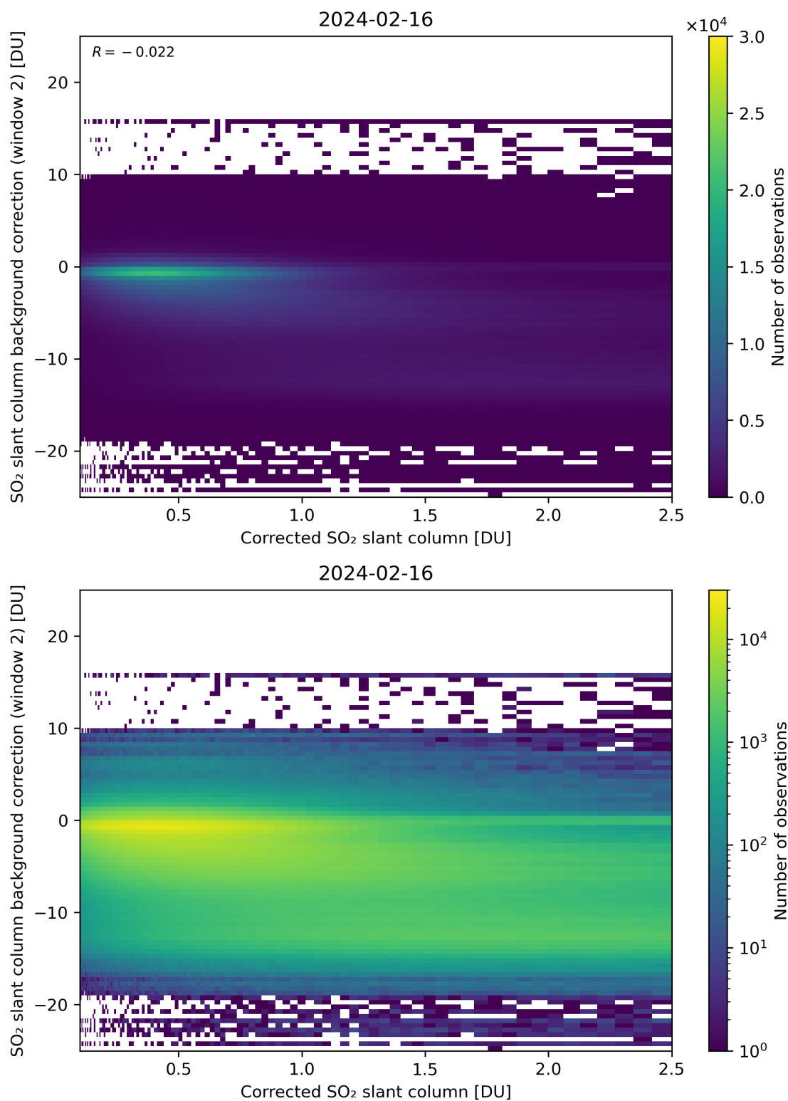
Figure 179: Scatter density plot of “Corrected SO 2 slant column” against “SO 2 slant column background correction (window 2)” for 2024-02-16 to 2024-02-17.
