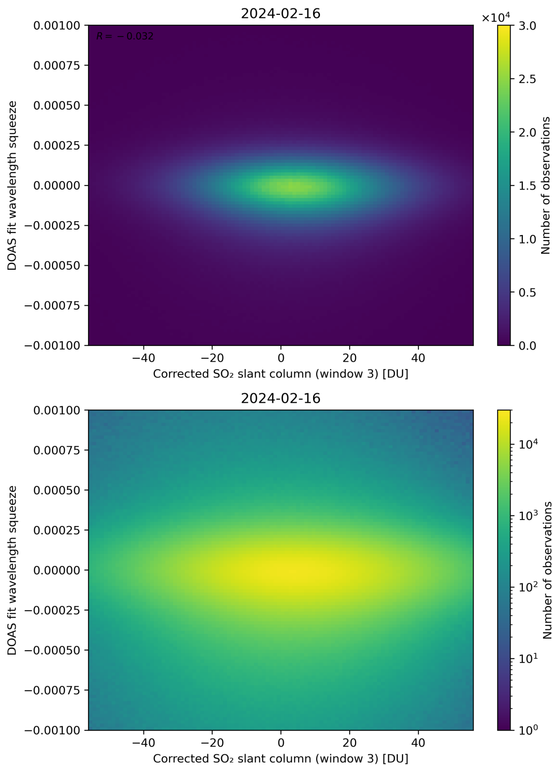
Figure 207: Scatter density plot of “Corrected SO 2 slant column (window 3)” against “DOAS fit wavelength squeeze” for 2024-02-16 to 2024-02-17.
