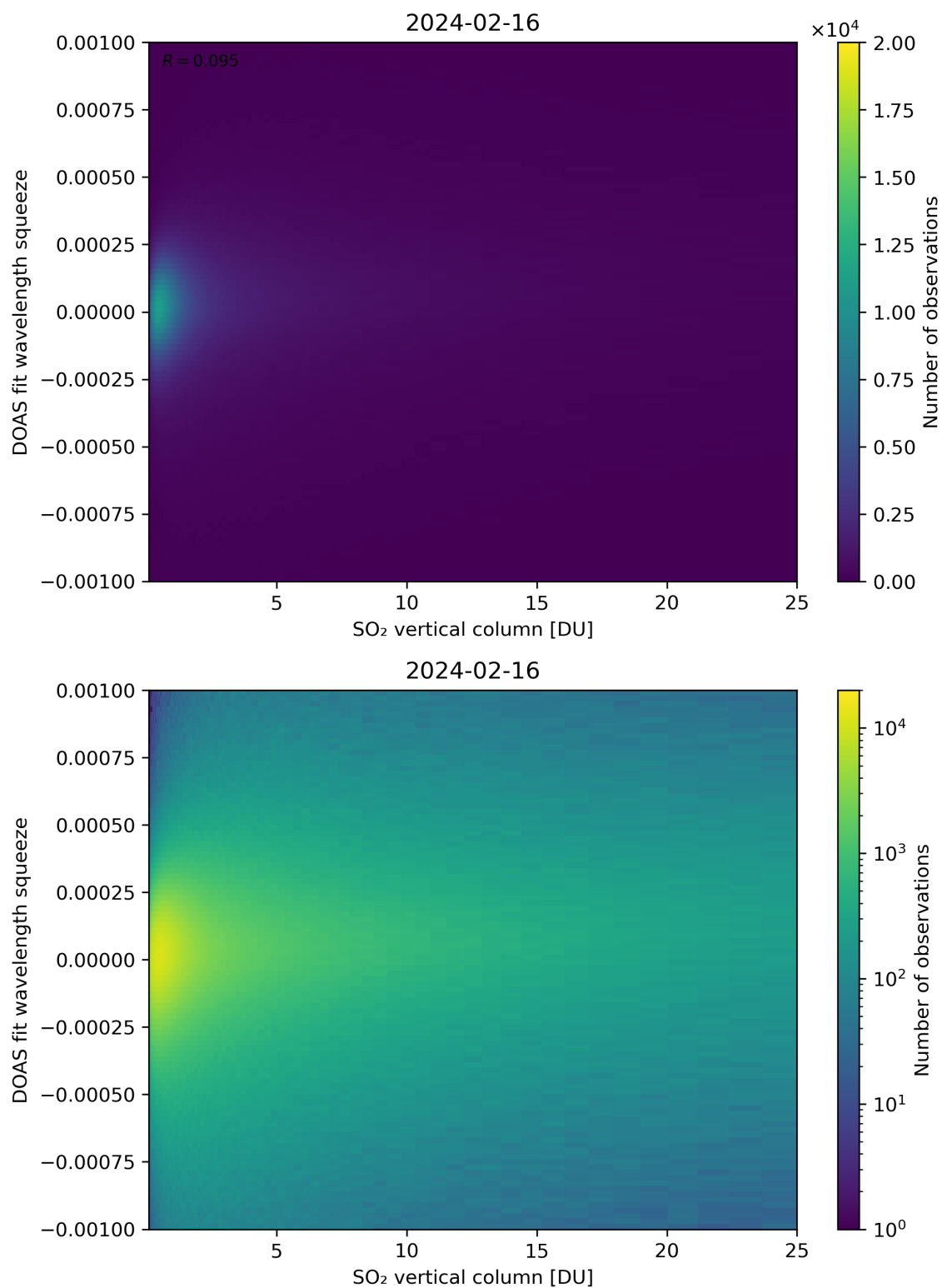
Figure 277: Scatter density plot of “SO 2 vertical column” against “DOAS fit wavelength squeeze” for 2024-02-16 to 2024-02-17.
