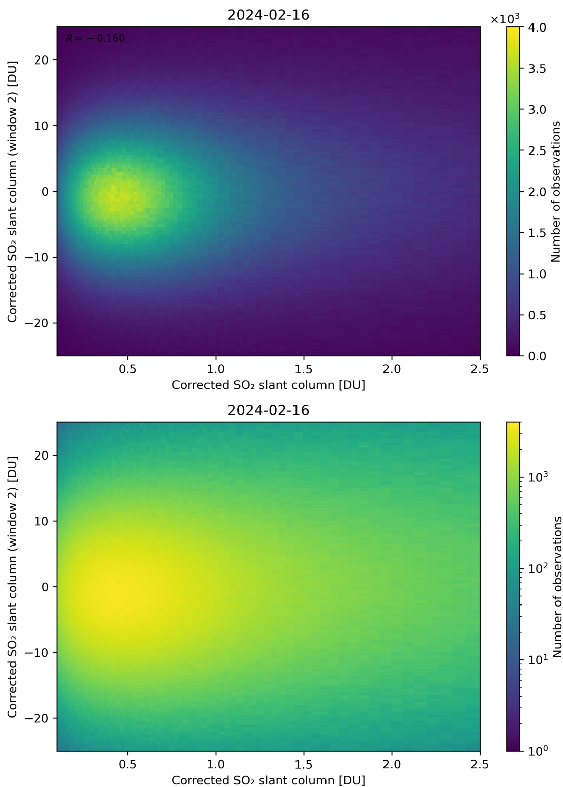
Figure 185: Scatter density plot of “Corrected SO 2 slant column” against “Corrected SO 2 slant column (window 2)” for 2024-02-16 to 2024-02-17.
