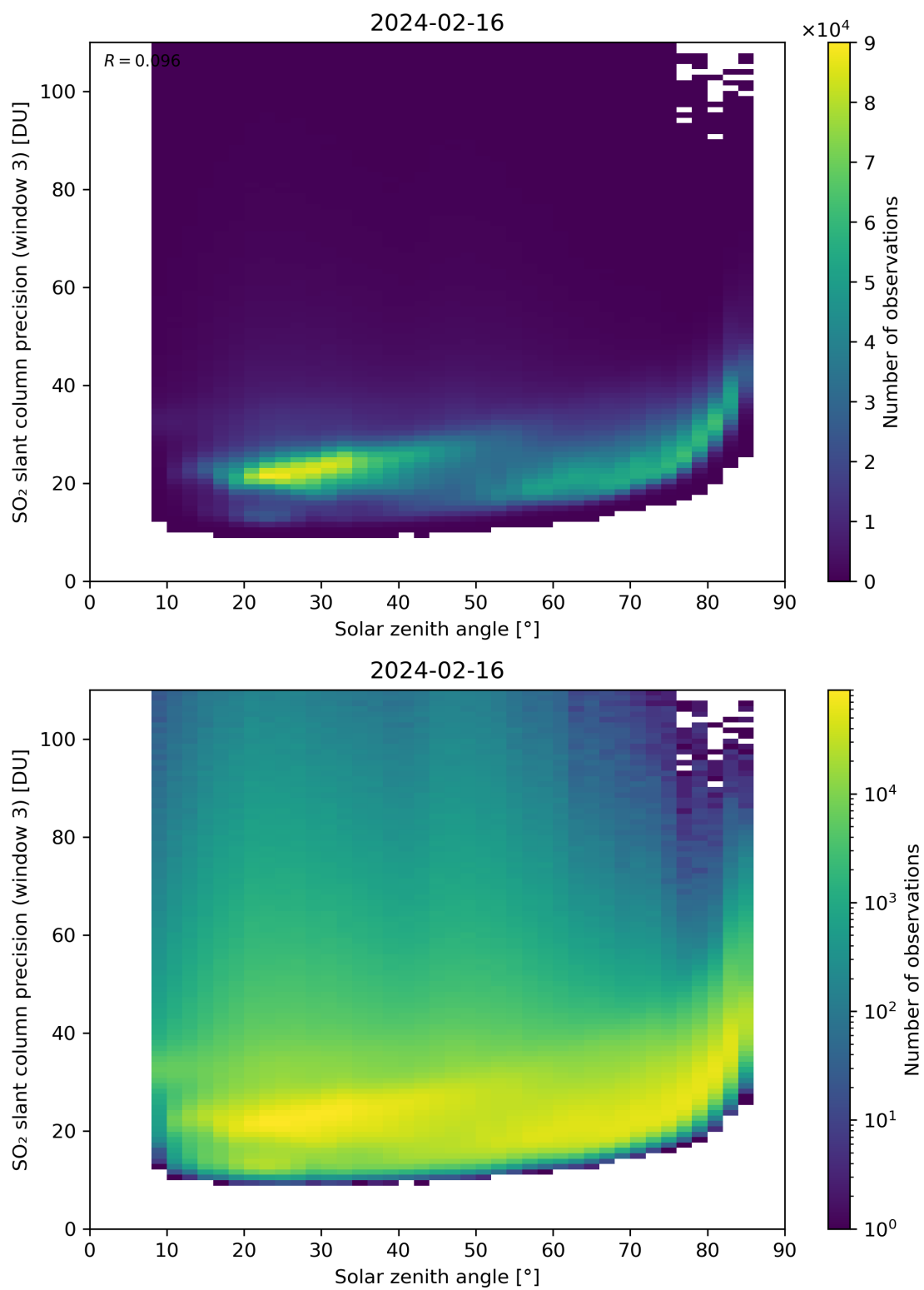
Figure 173: Scatter density plot of “Solar zenith angle” against “SO 2 slant column precision (window 3)” for 2024-02-16 to 2024-02-17.
