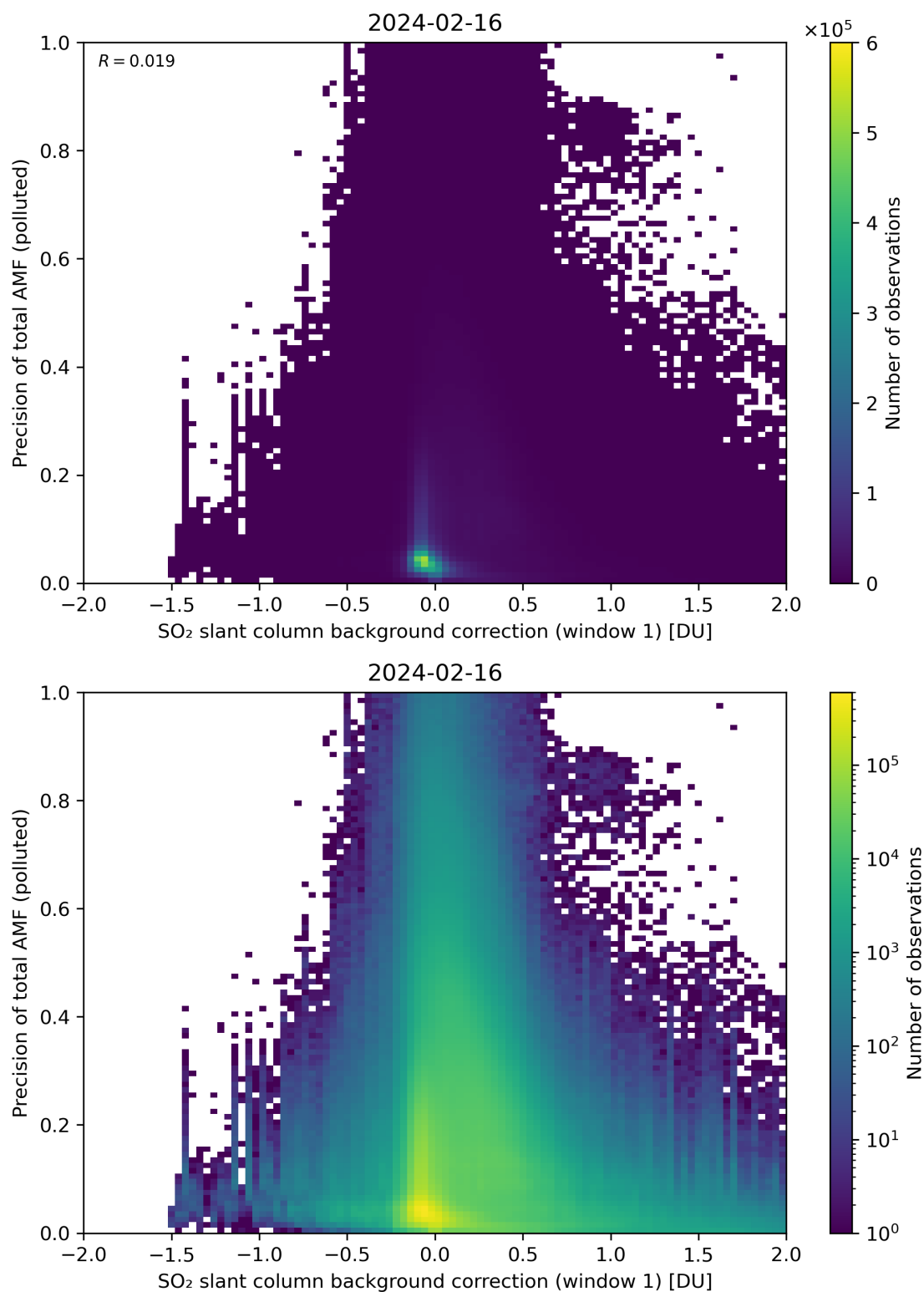
Figure 110: Scatter density plot of “SO 2 slant column background correction (window 1)” against “Precision of total AMF (polluted)” for 2024-02-16 to 2024-02-17.
