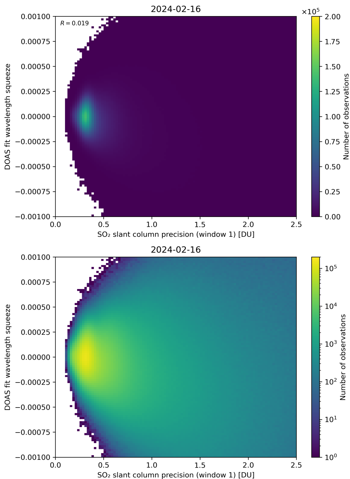
Figure 222: Scatter density plot of “SO 2 slant column precision (window 1)” against “DOAS fit wavelength squeeze” for 2024-02-16 to 2024-02-17.
