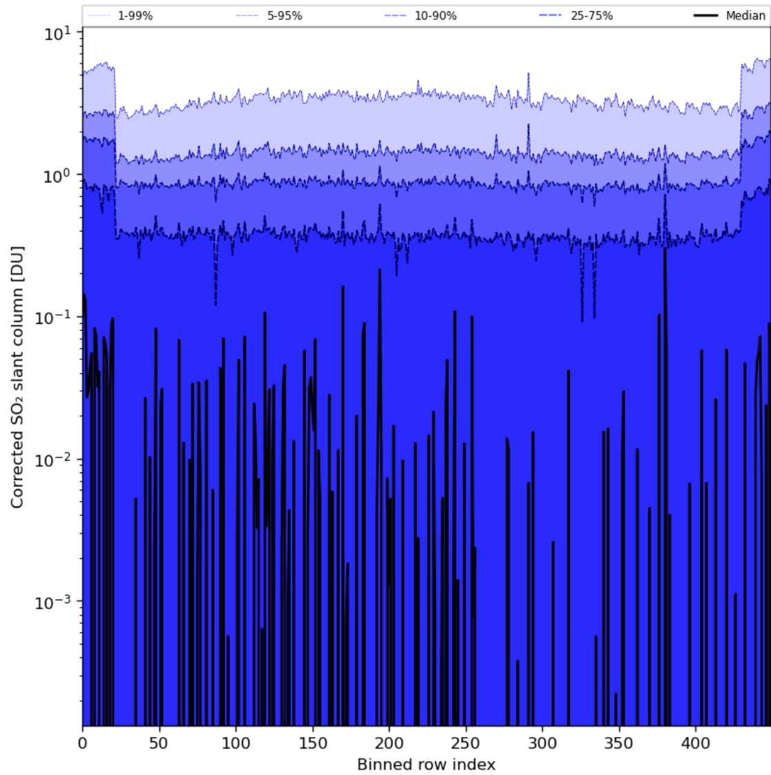
Figure 78: Along track statistics of “Corrected SO 2 slant column” for 2024-02-16 to 2024-02-17
