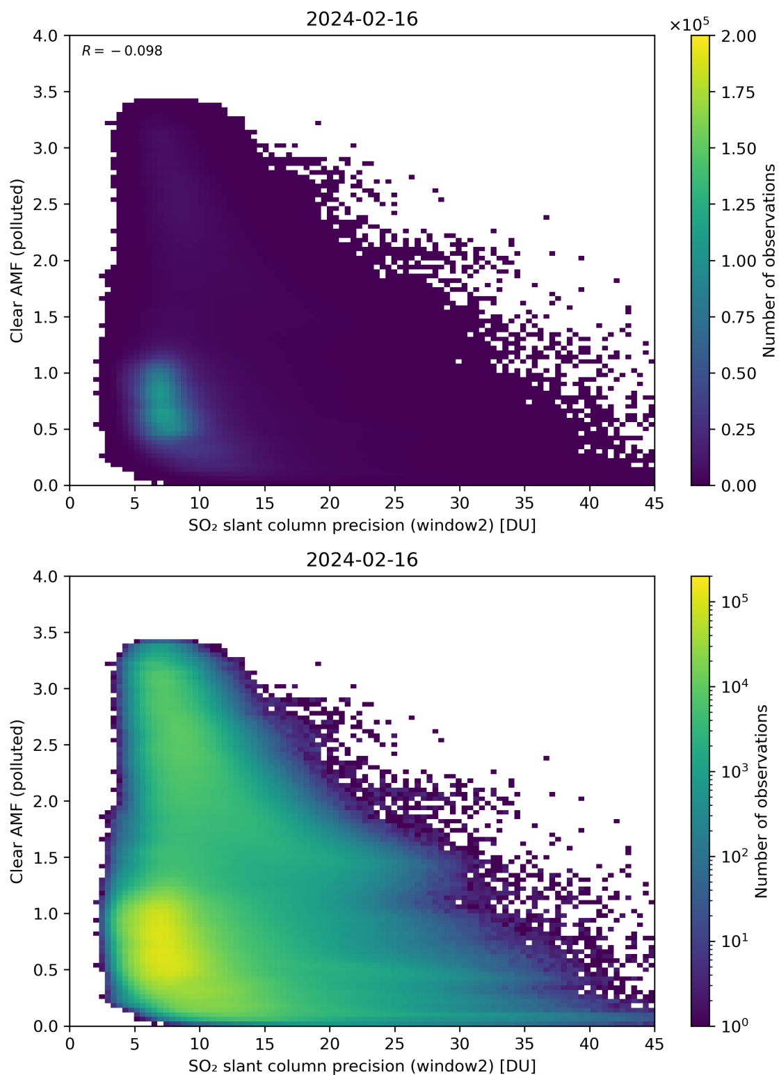
Figure 246: Scatter density plot of “SO 2 slant column precision (window2)” against “Clear AMF (polluted)” for 2024-02-16 to 2024-02-17.
