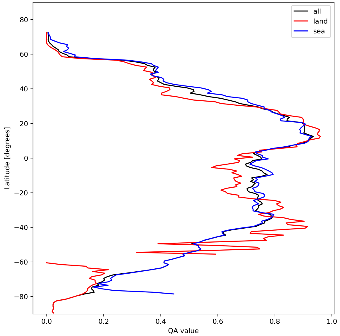
Figure 29: Zonal average of “QA value” for 2024-02-16 to 2024-02-17.
