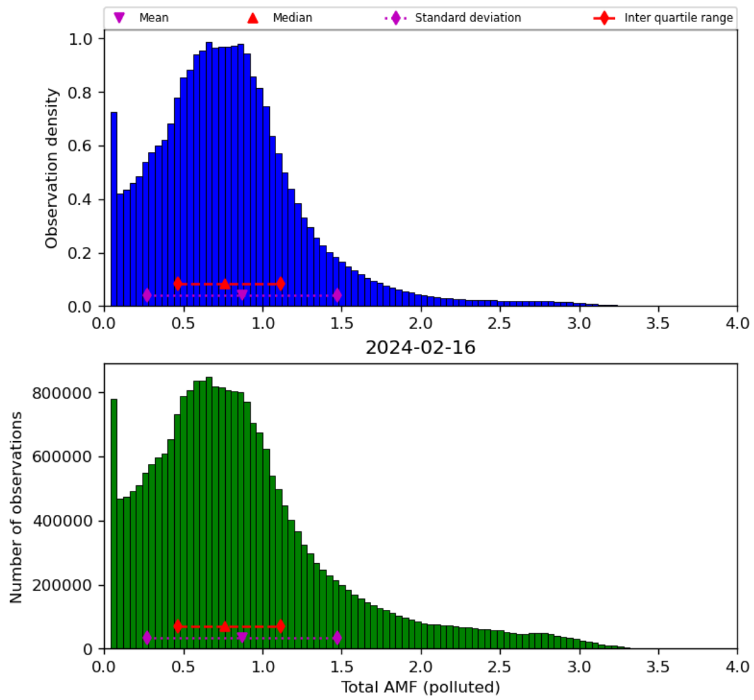
Figure 71: Histogram of “Total AMF (polluted)” for 2024-02-16 to 2024-02-17
