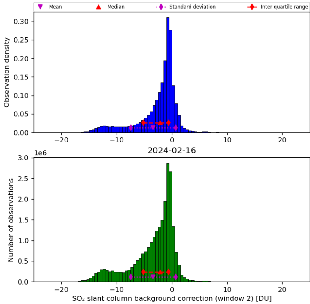
Figure 63: Histogram of “SO 2 slant column background correction (window 2)” for 2024-02-16 to 2024-02-17
