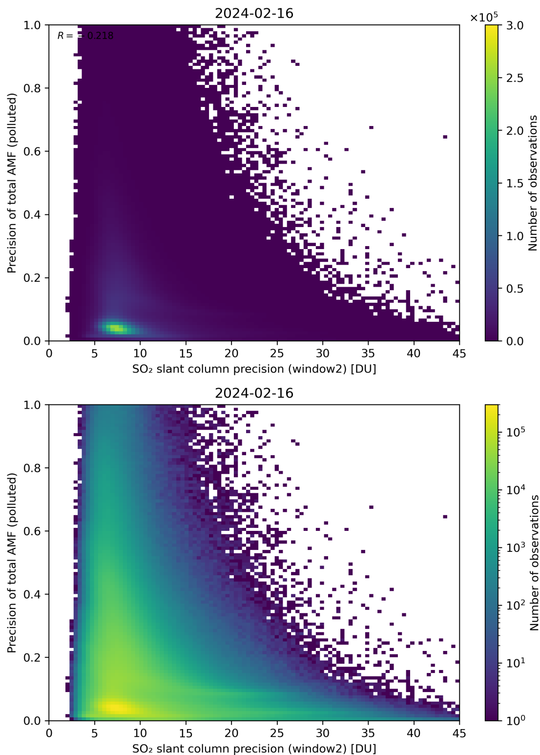
Figure 252: Scatter density plot of “SO 2 slant column precision (window2)” against “Precision of total AMF (polluted)” for 2024-02-16 to 2024-02-17.
