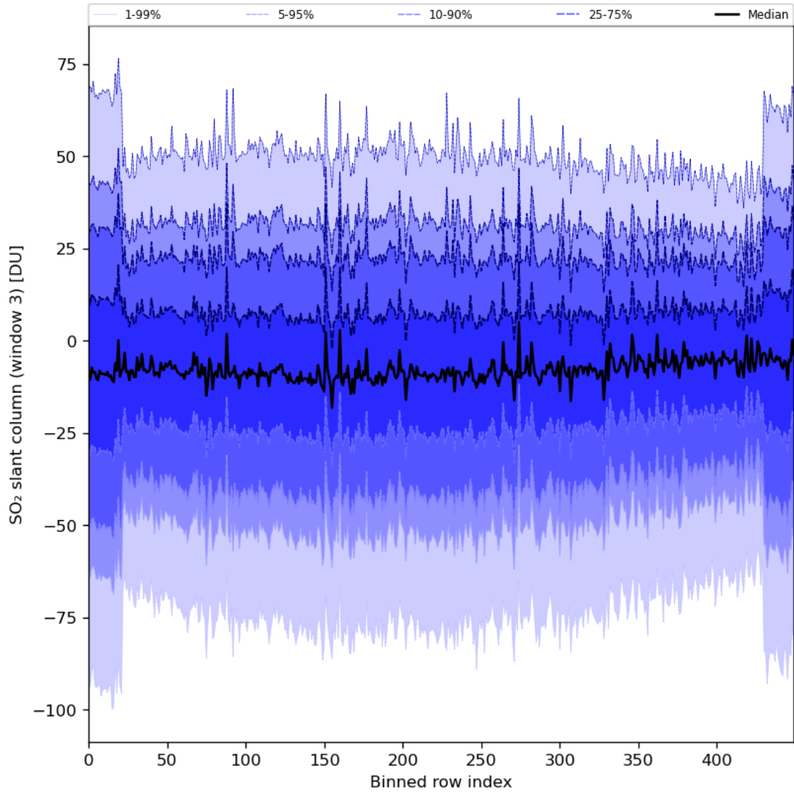
Figure 87: Along track statistics of “SO 2 slant column (window 3)” for 2024-02-16 to 2024-02-17
