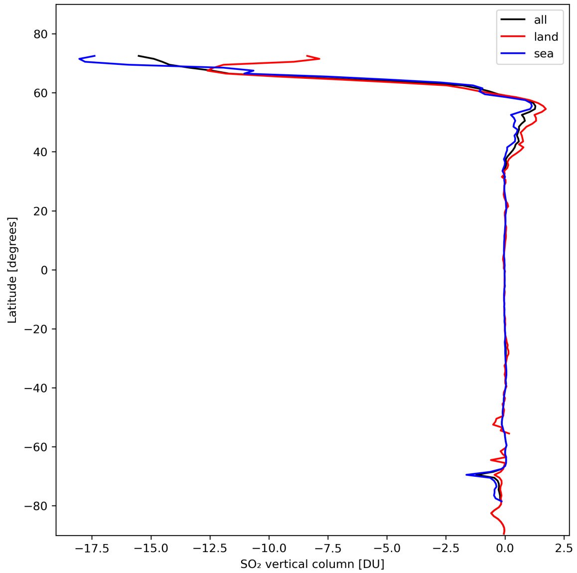
Figure 30: Zonal average of “SO 2 vertical column” for 2024-02-16 to 2024-02-17.
