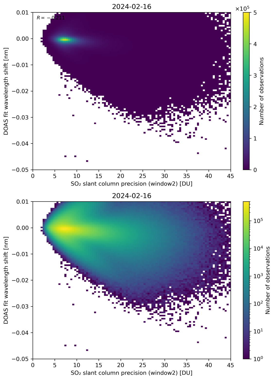
Figure 243: Scatter density plot of “SO 2 slant column precision (window2)” against “DOAS fit wavelength shift” for 2024-02-16 to 2024-02-17.
