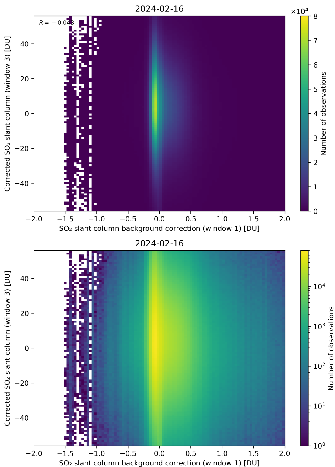
Figure 105: Scatter density plot of “SO 2 slant column background correction (window 1)” against “Corrected SO 2 slant column (window 3)” for 2024-02-16 to 2024-02-17.
