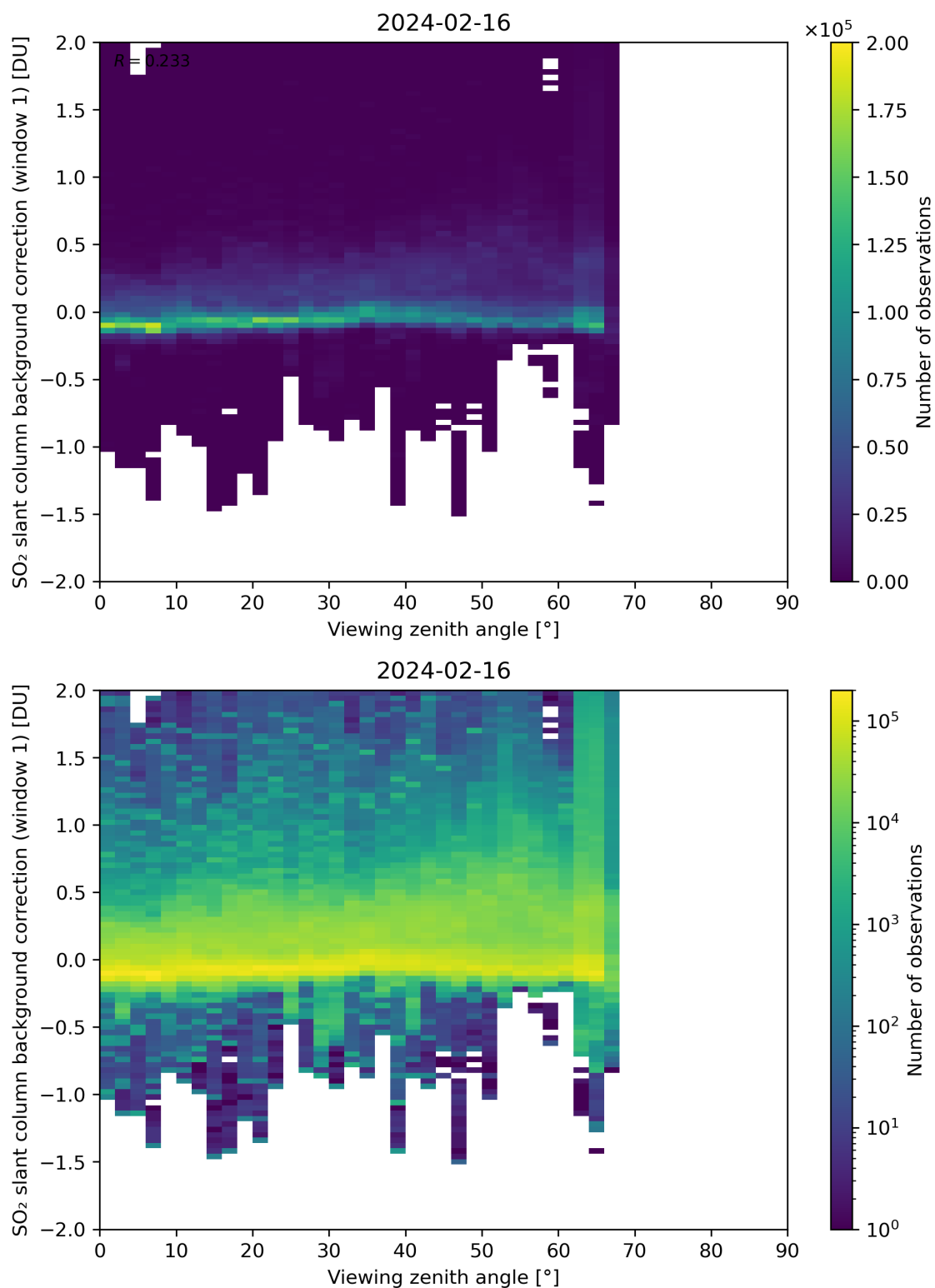
Figure 308: Scatter density plot of “Viewing zenith angle” against “SO 2 slant column background correction (window 1)” for 2024-02-16 to 2024-02-17.
