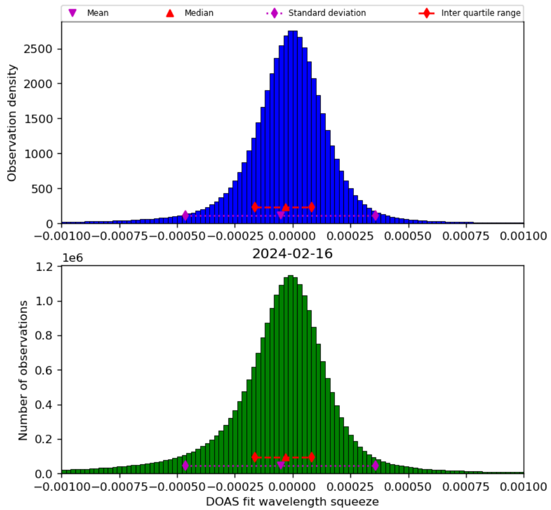
Figure 69: Histogram of “DOAS fit wavelength squeeze” for 2024-02-16 to 2024-02-17
