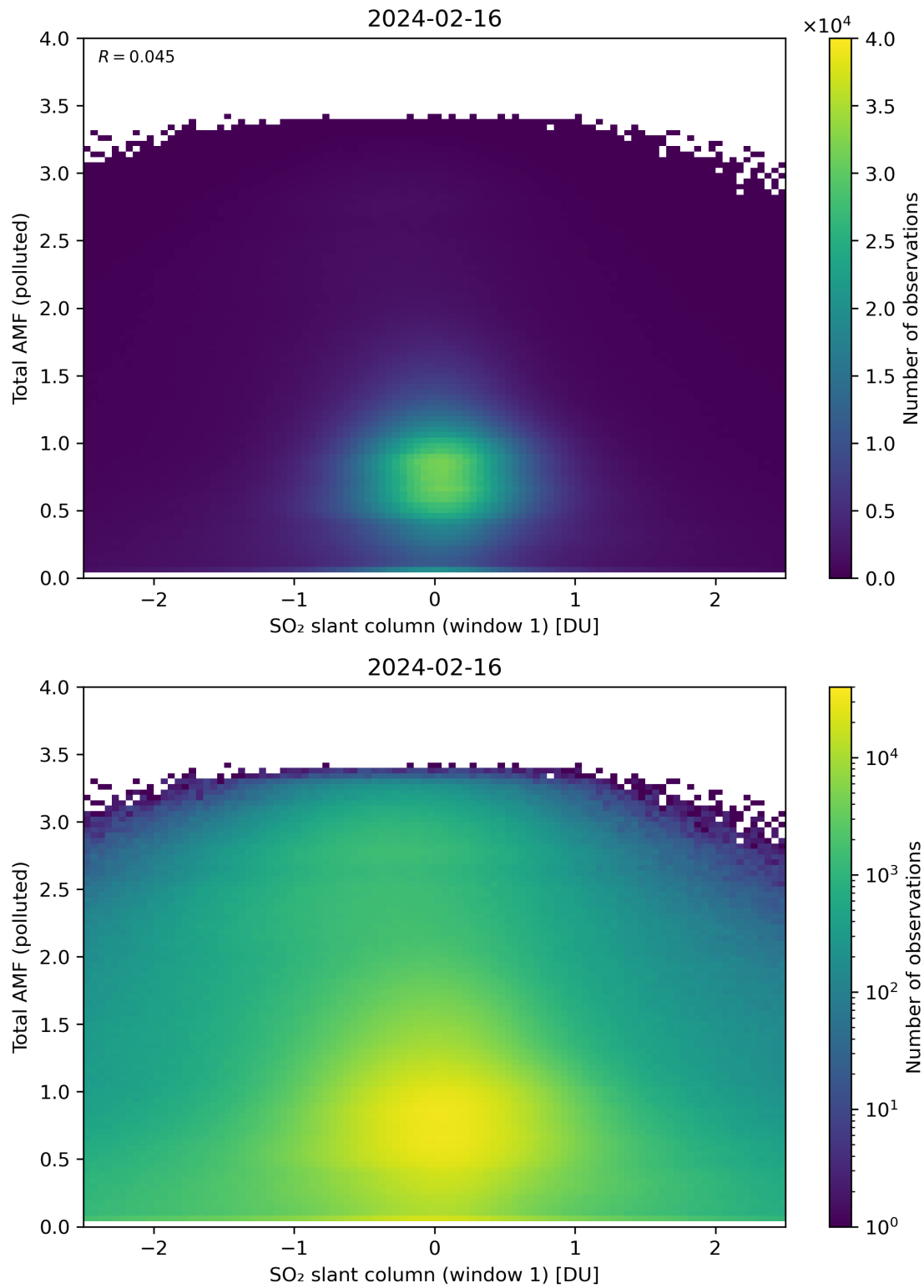
Figure 239: Scatter density plot of “SO 2 slant column (window 1)” against “Total AMF (polluted)” for 2024-02-16 to 2024-02-17.
