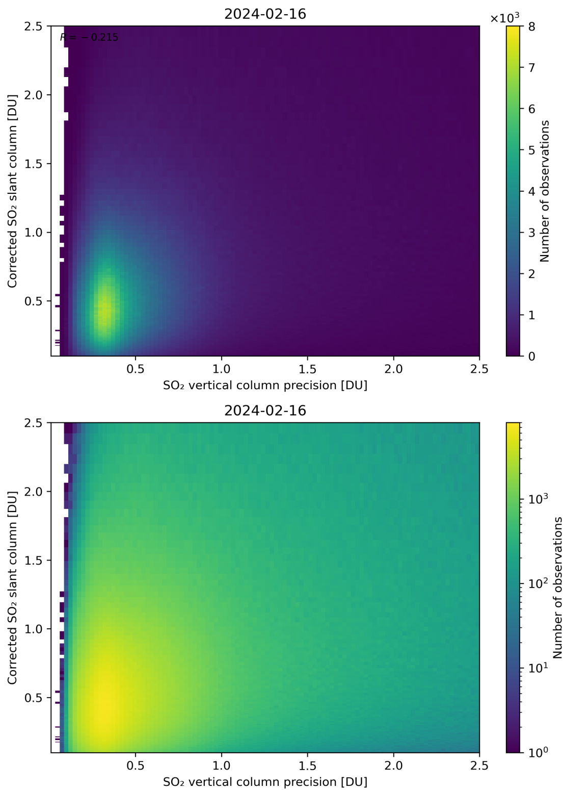
Figure 286: Scatter density plot of “SO 2 vertical column precision” against “Corrected SO 2 slant column” for 2024-02-16 to 2024-02-17.
