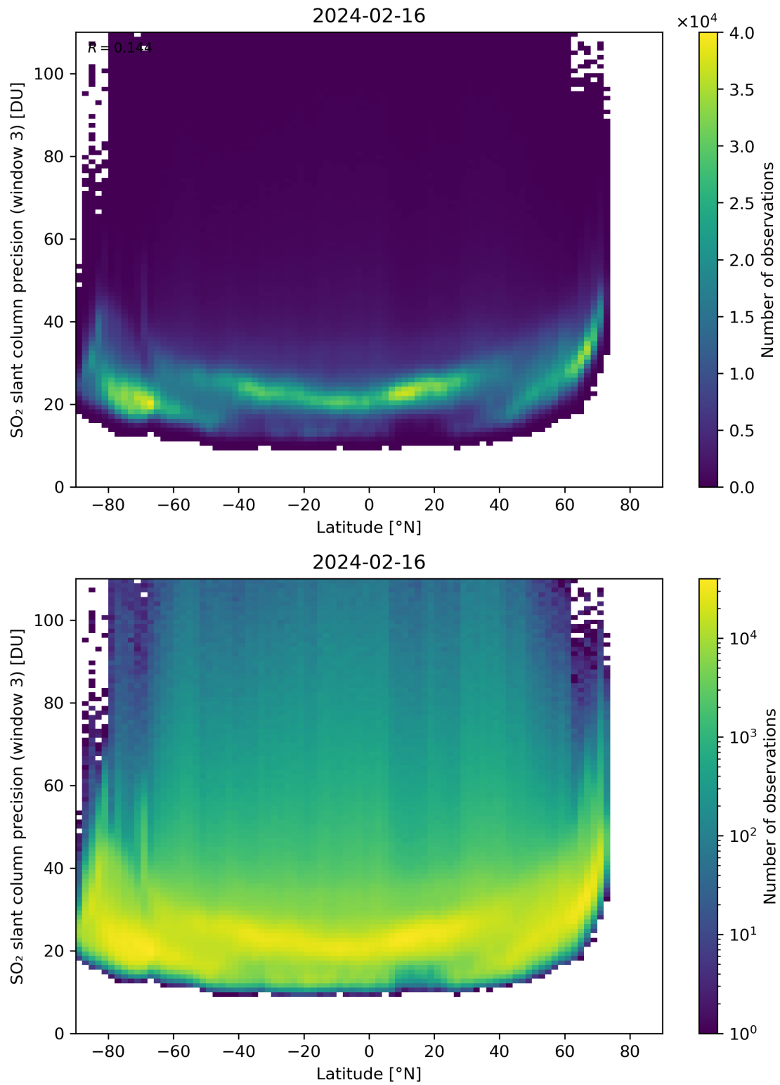
Figure 153: Scatter density plot of “Latitude” against “SO 2 slant column precision (window 3)” for 2024-02-16 to 2024-02-17.
