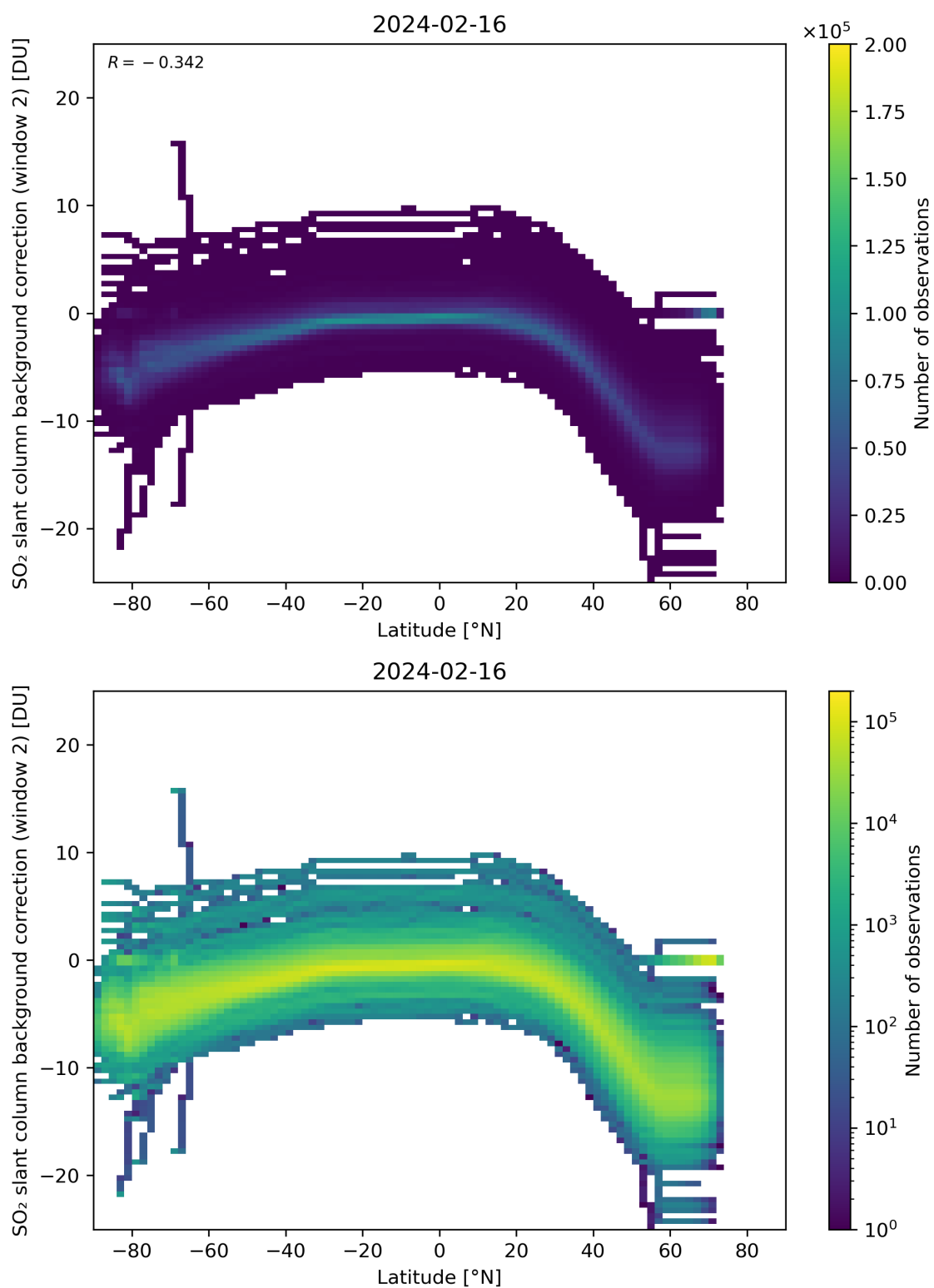
Figure 140: Scatter density plot of “Latitude” against “SO 2 slant column background correction (window 2)” for 2024-02-16 to 2024-02-17.
