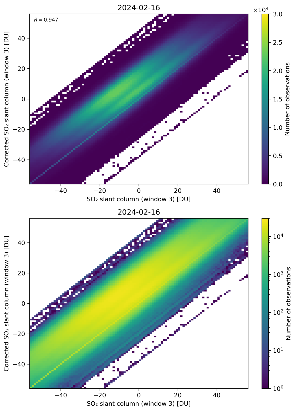
Figure 266: Scatter density plot of “SO 2 slant column (window 3)” against “Corrected SO 2 slant column (window 3)” for 2024-02-16 to 2024-02-17.
