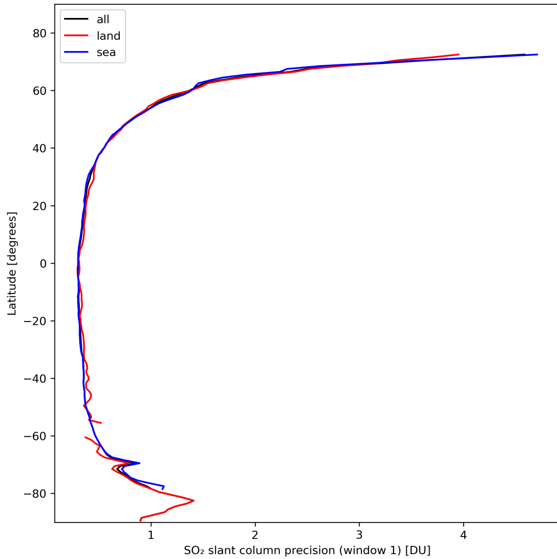
Figure 34: Zonal average of “SO 2 slant column precision (window 1)” for 2024-02-16 to 2024-02-17.
