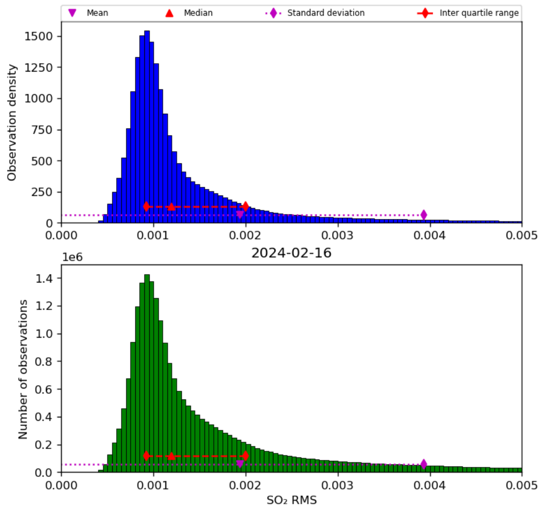
Figure 70: Histogram of “SO 2 RMS” for 2024-02-16 to 2024-02-17
