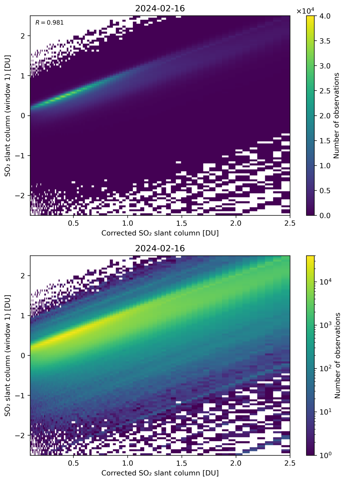
Figure 187: Scatter density plot of “Corrected SO 2 slant column” against “SO 2 slant column (window 1)” for 2024-02-16 to 2024-02-17.
