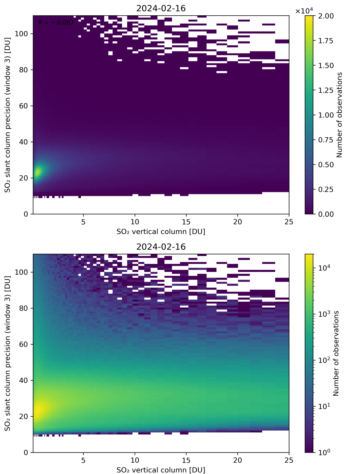
Figure 304: Scatter density plot of “SO 2 vertical column” against “SO 2 slant column precision (window 3)” for 2024-02-16 to 2024-02-17.
