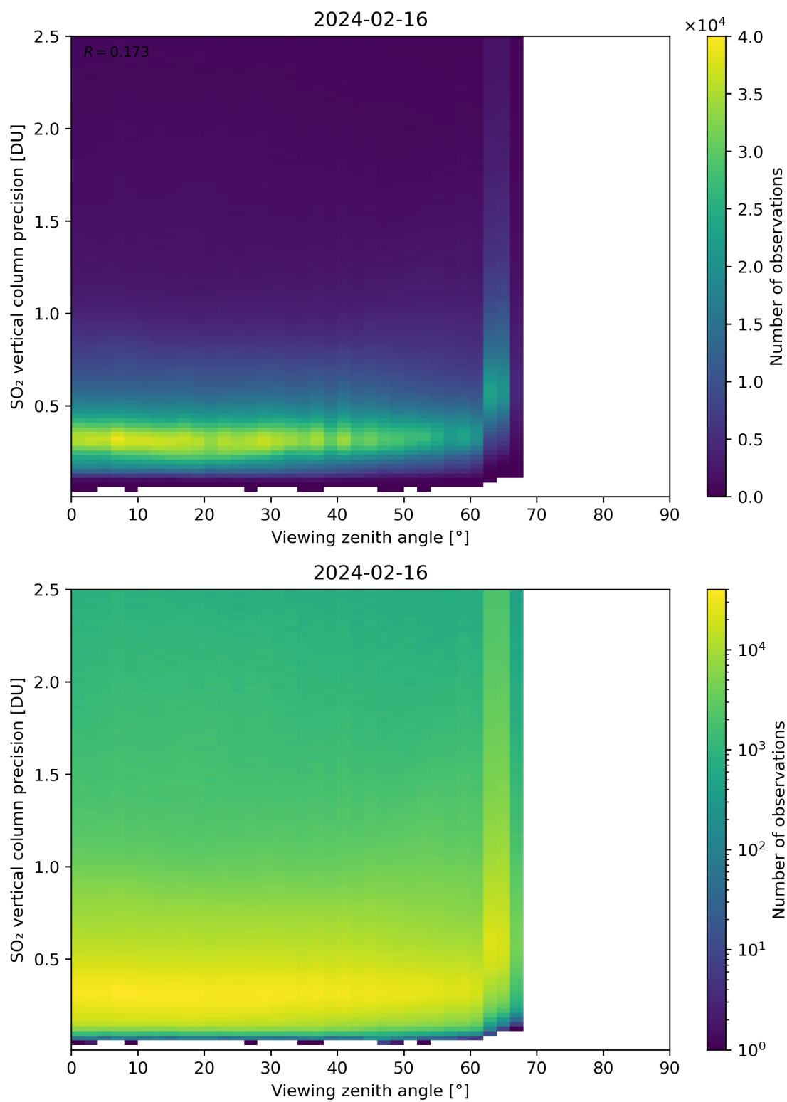
Figure 328: Scatter density plot of “Viewing zenith angle” against “SO 2 vertical column precision” for 2024-02-16 to 2024-02-17.
