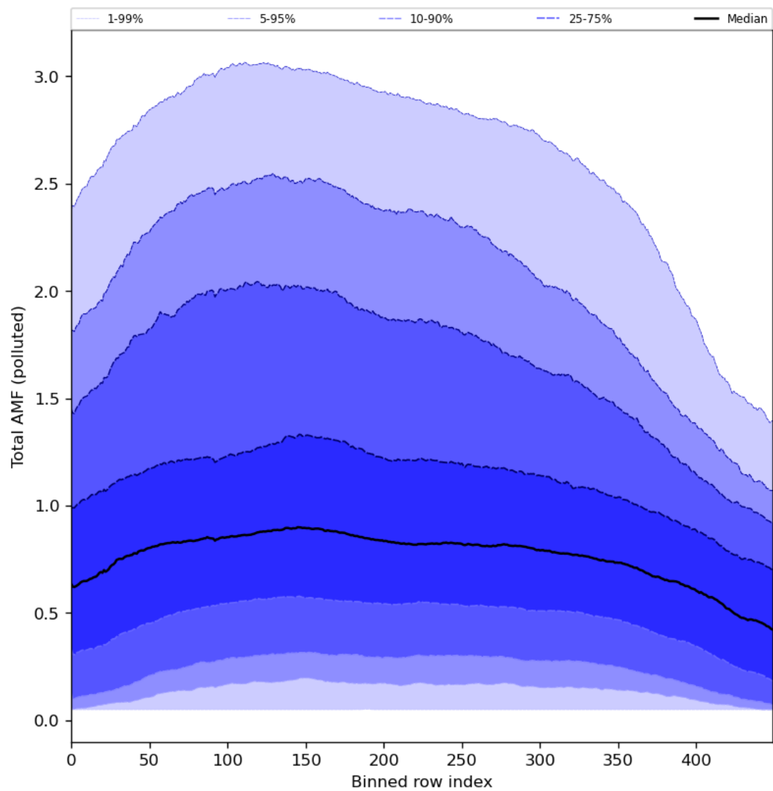
Figure 94: Along track statistics of “Total AMF (polluted)” for 2024-02-16 to 2024-02-17
