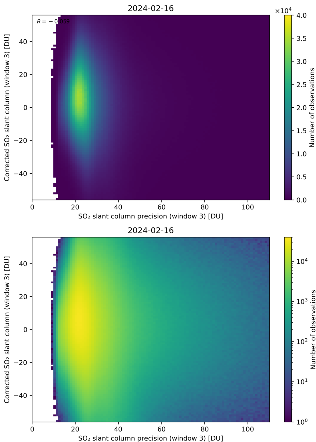
Figure 262: Scatter density plot of “SO 2 slant column precision (window 3)” against “Corrected SO 2 slant column (window 3)” for 2024-02-16 to 2024-02-17.
