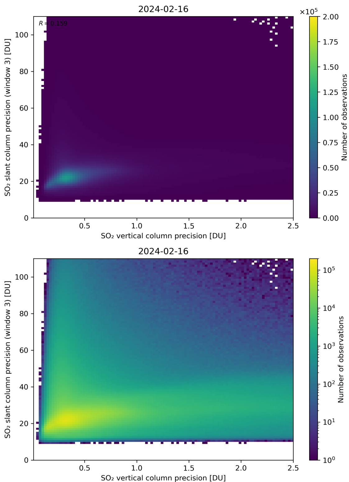
Figure 293: Scatter density plot of “SO 2 vertical column precision” against “SO 2 slant column precision (window 3)” for 2024-02-16 to 2024-02-17.
