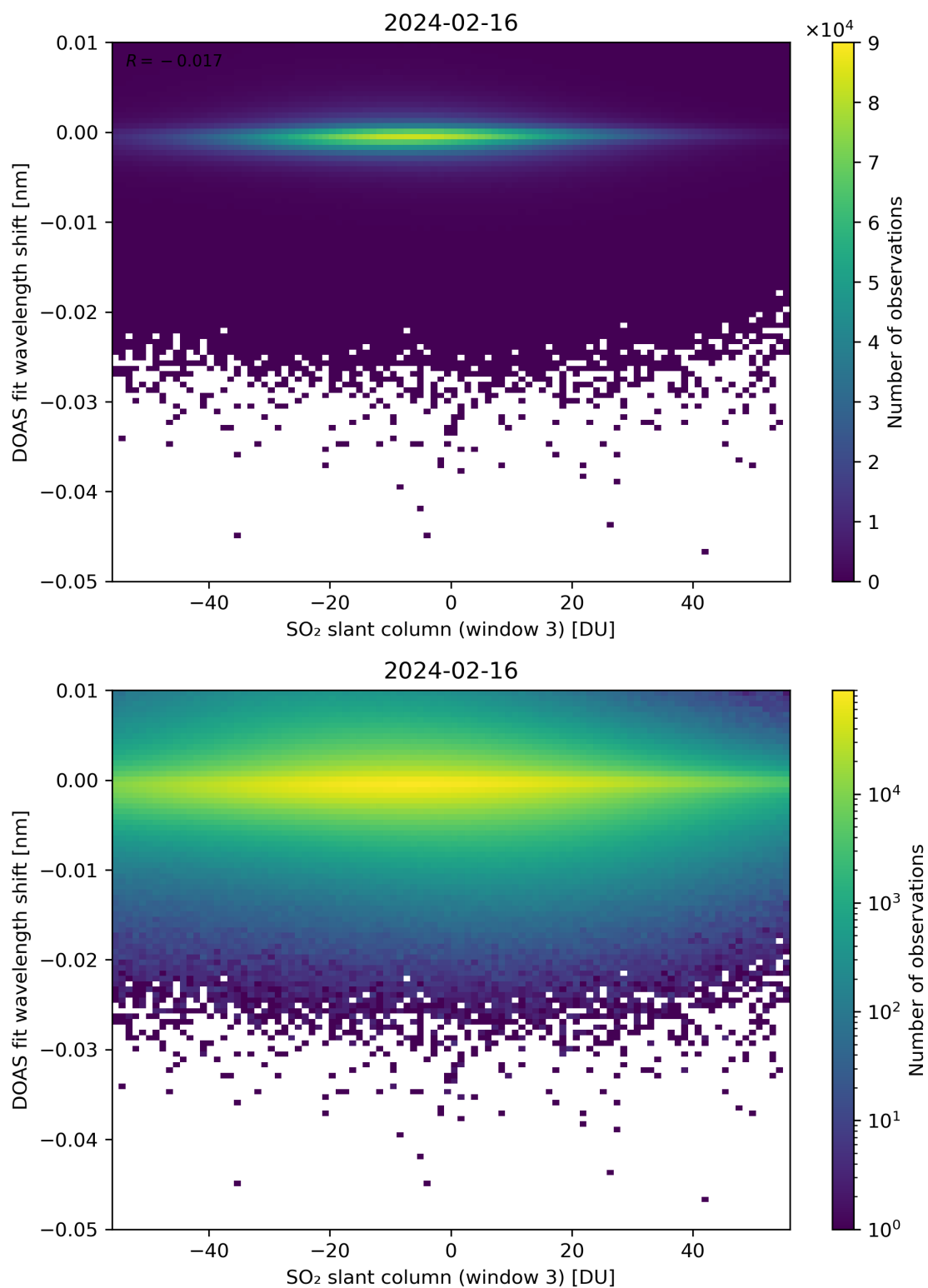
Figure 254: Scatter density plot of “SO 2 slant column (window 3)” against “DOAS fit wavelength shift” for 2024-02-16 to 2024-02-17.
