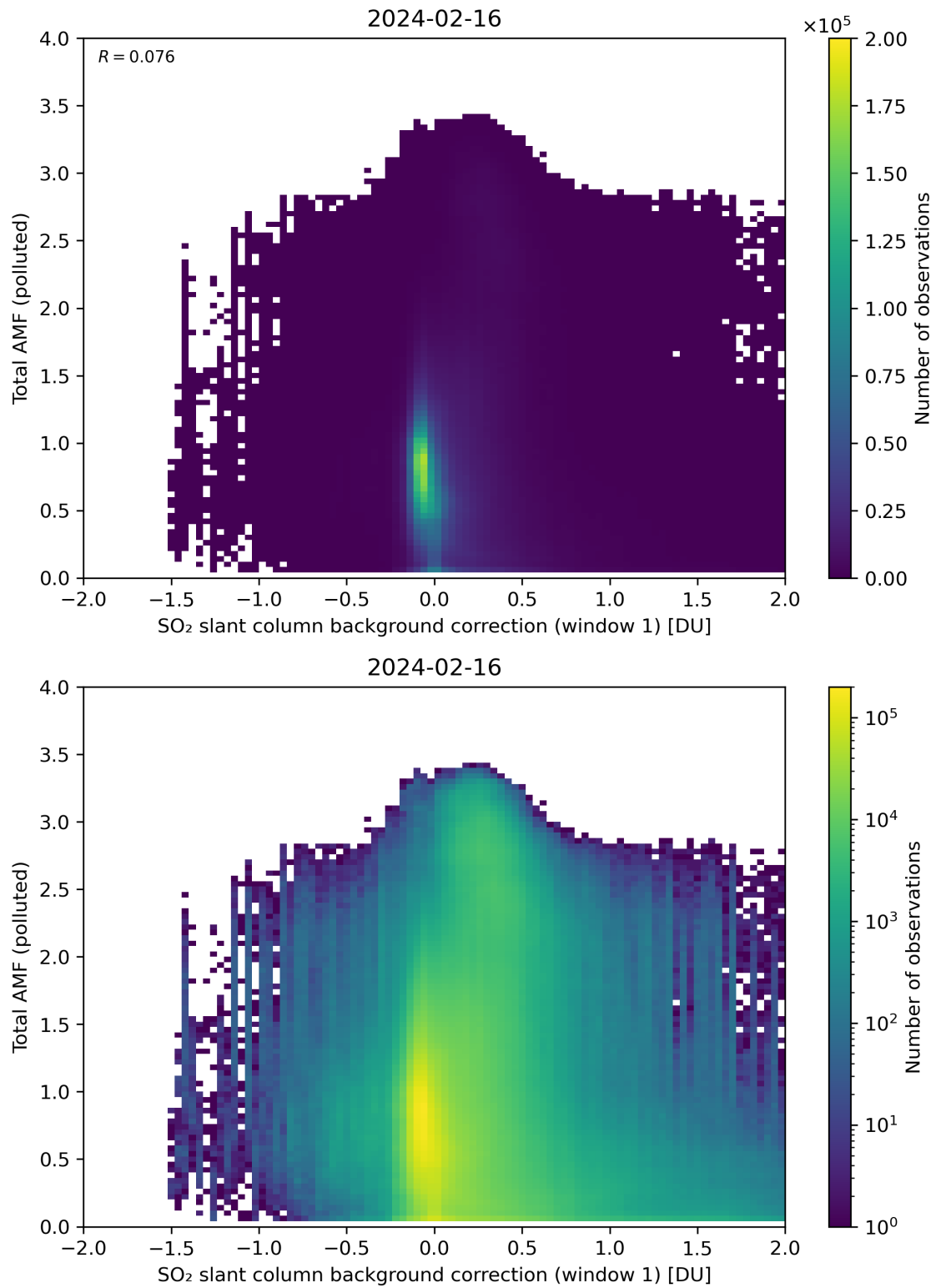
Figure 109: Scatter density plot of “SO 2 slant column background correction (window 1)” against “Total AMF (polluted)” for 2024-02-16 to 2024-02-17.
