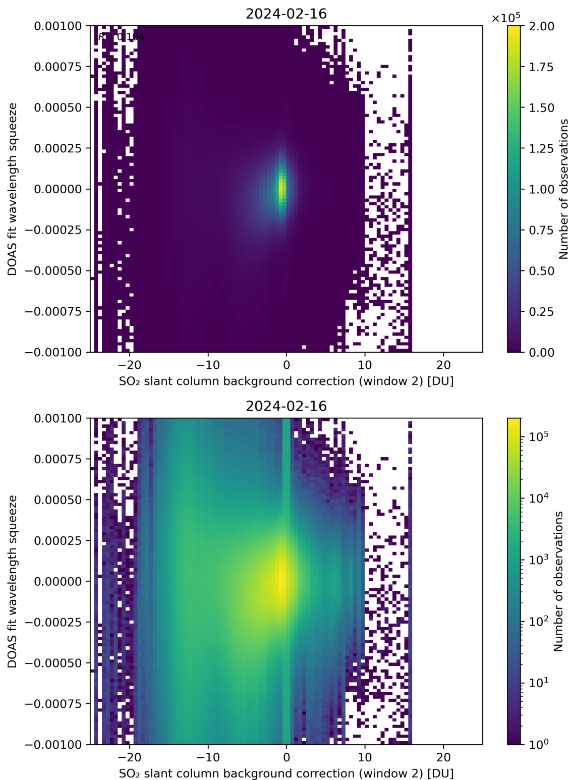
Figure 113: Scatter density plot of “SO 2 slant column background correction (window 2)” against “DOAS fit wavelength squeeze” for 2024-02-16 to 2024-02-17.
