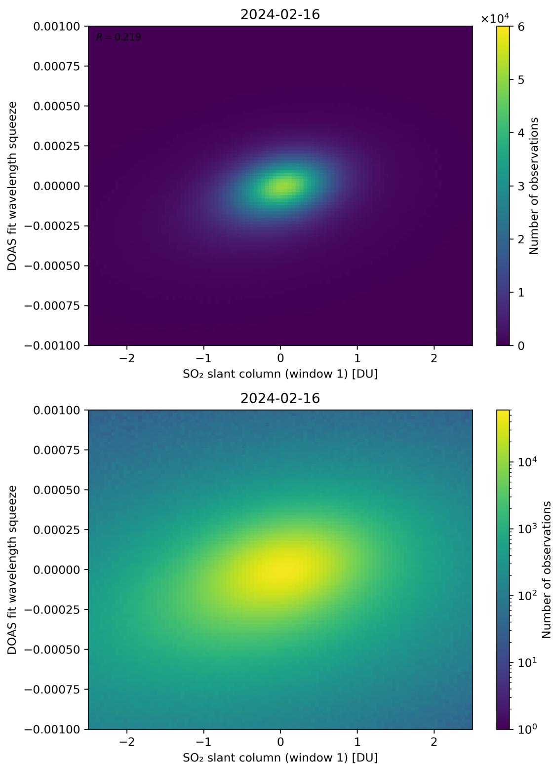
Figure 216: Scatter density plot of “SO 2 slant column (window 1)” against “DOAS fit wavelength squeeze” for 2024-02-16 to 2024-02-17.
