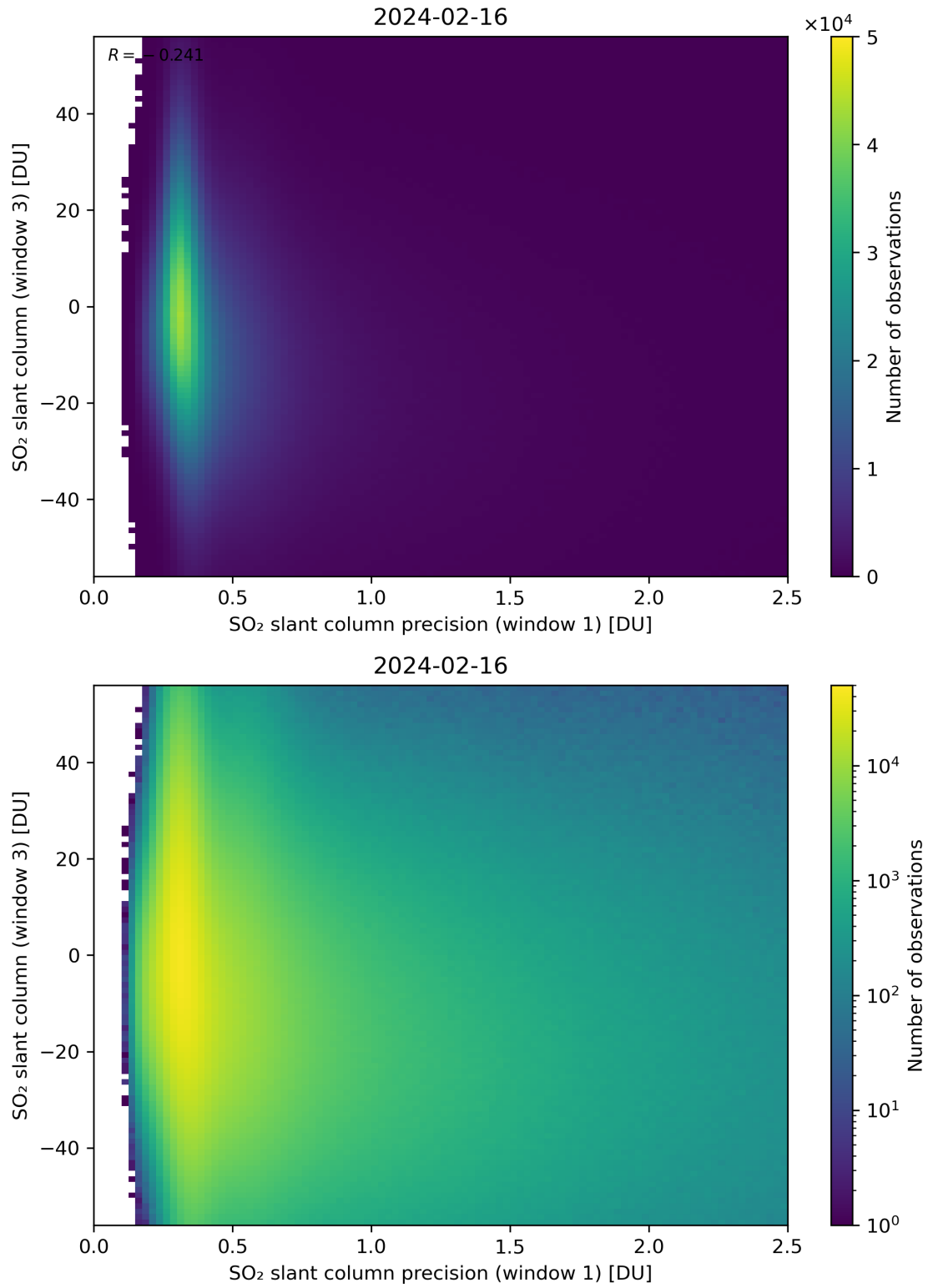
Figure 228: Scatter density plot of “SO 2 slant column precision (window 1)” against “SO 2 slant column (window 3)” for 2024-02-16 to 2024-02-17.
