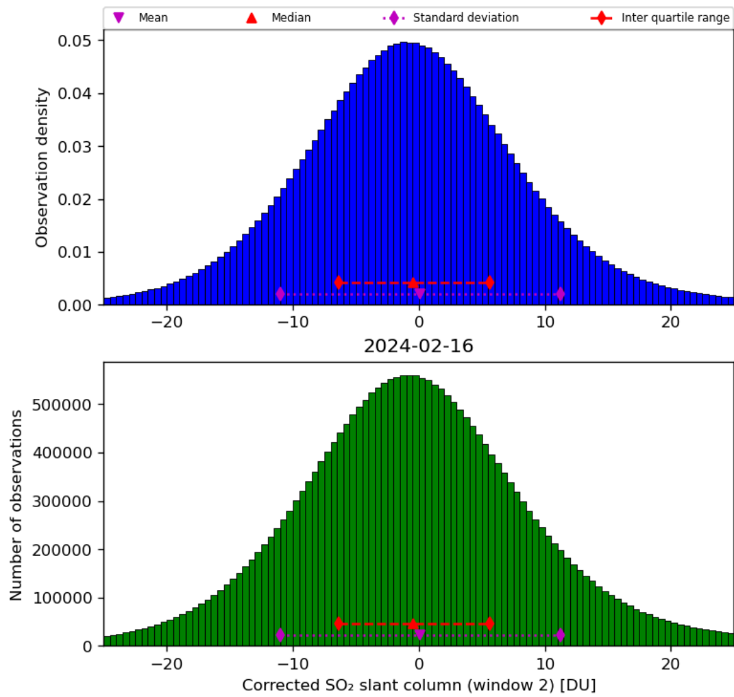
Figure 62: Histogram of “Corrected SO 2 slant column (window 2)” for 2024-02-16 to 2024-02-17
