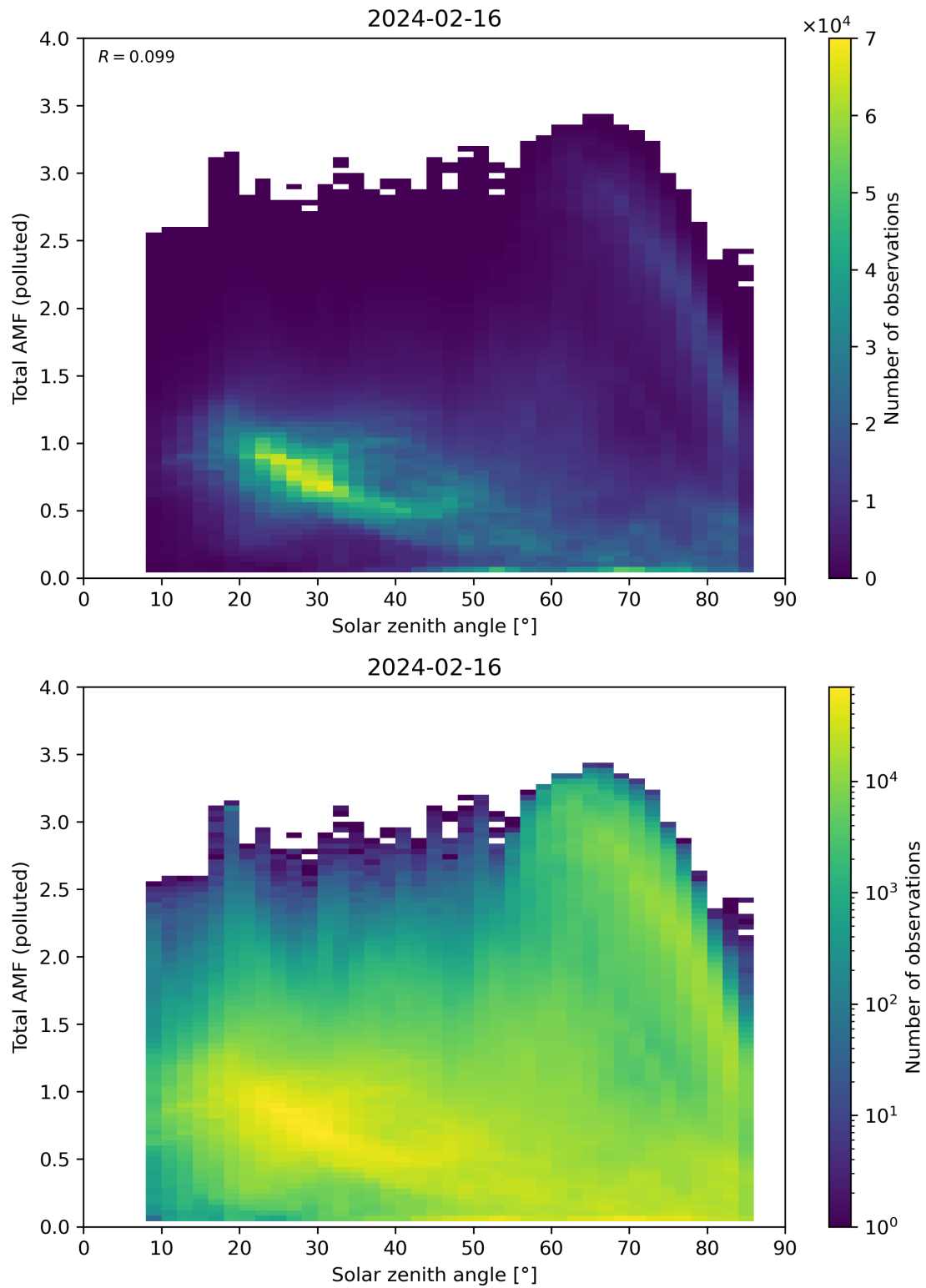
Figure 174: Scatter density plot of “Solar zenith angle” against “Total AMF (polluted)” for 2024-02-16 to 2024-02-17.
