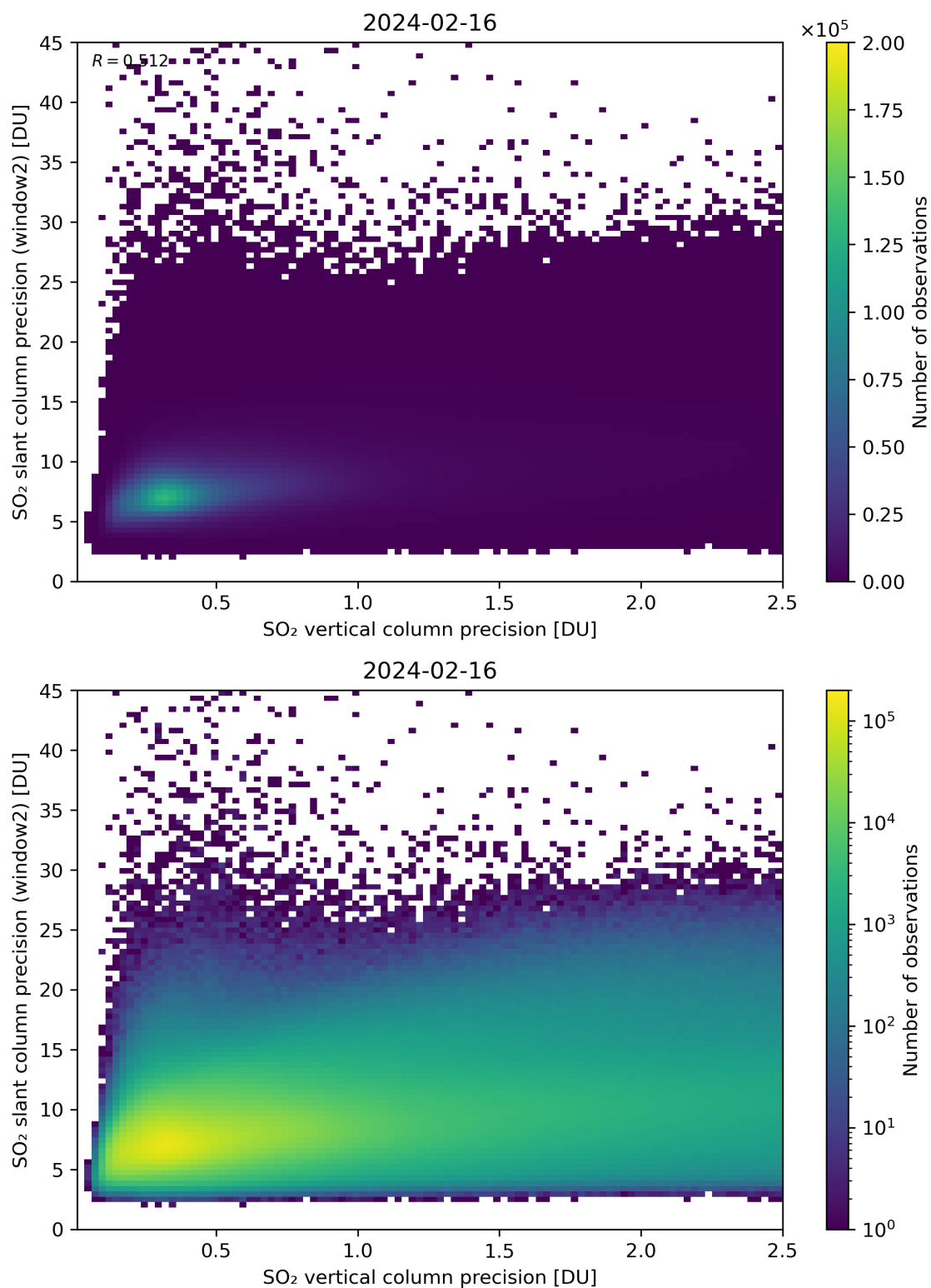
Figure 291: Scatter density plot of “SO 2 vertical column precision” against “SO 2 slant column precision (window2)” for 2024-02-16 to 2024-02-17.
