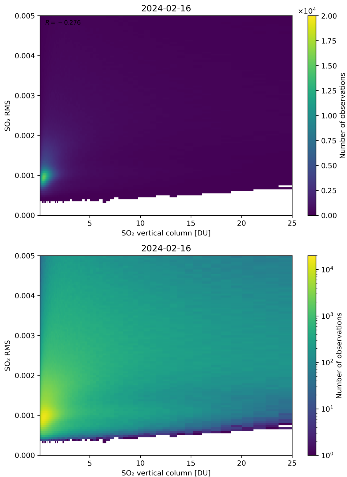
Figure 278: Scatter density plot of “SO 2 vertical column” against “SO 2 RMS” for 2024-02-16 to 2024-02-17.
