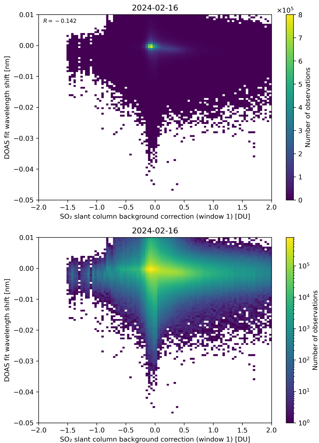
Figure 100: Scatter density plot of “SO 2 slant column background correction (window 1)” against “DOAS fit wavelength shift” for 2024-02-16 to 2024-02-17.
