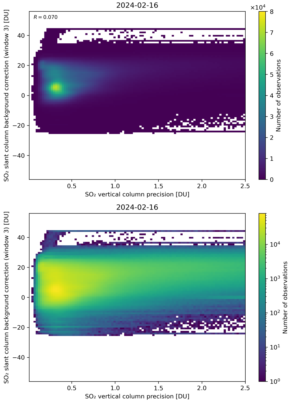
Figure 281: Scatter density plot of “SO 2 vertical column precision” against “SO 2 slant column background correction (window 3)” for 2024-02-16 to 2024-02-17.
