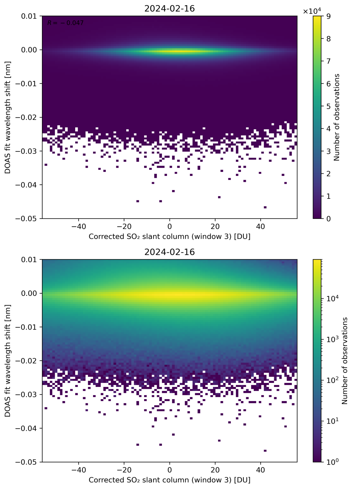
Figure 206: Scatter density plot of “Corrected SO 2 slant column (window 3)” against “DOAS fit wavelength shift” for 2024-02-16 to 2024-02-17.
