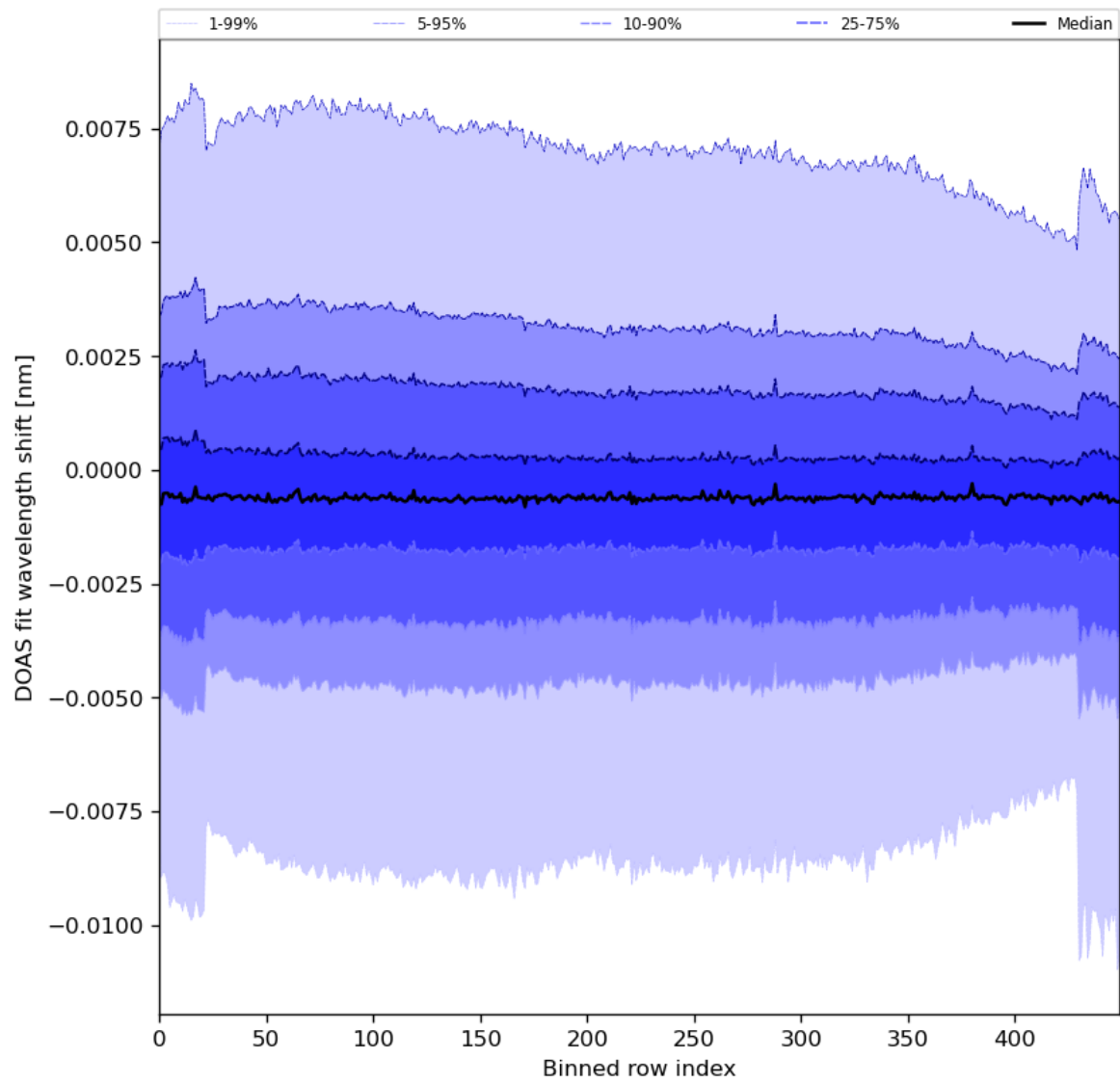
Figure 91: Along track statistics of “DOAS fit wavelength shift” for 2024-02-16 to 2024-02-17
