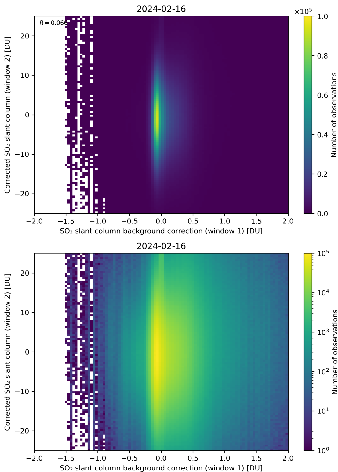
Figure 104: Scatter density plot of “SO 2 slant column background correction (window 1)” against “Corrected SO 2 slant column (window 2)” for 2024-02-16 to 2024-02-17.
