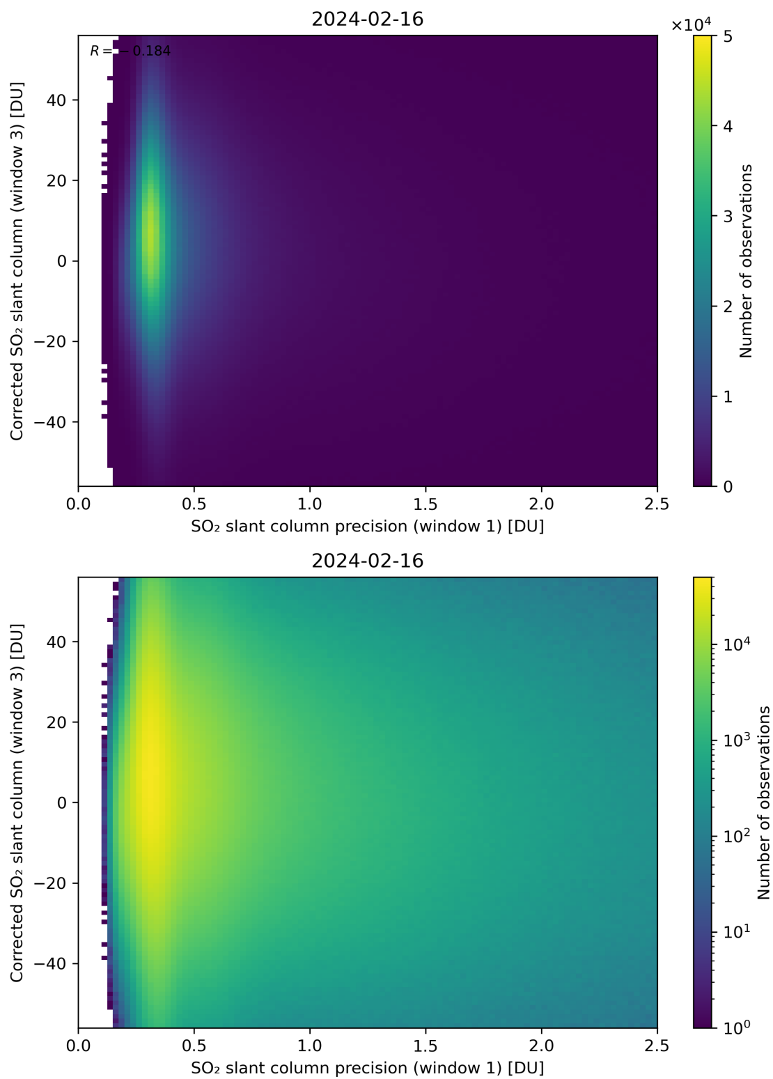
Figure 226: Scatter density plot of “SO 2 slant column precision (window 1)” against “Corrected SO 2 slant column (window 3)” for 2024-02-16 to 2024-02-17.
