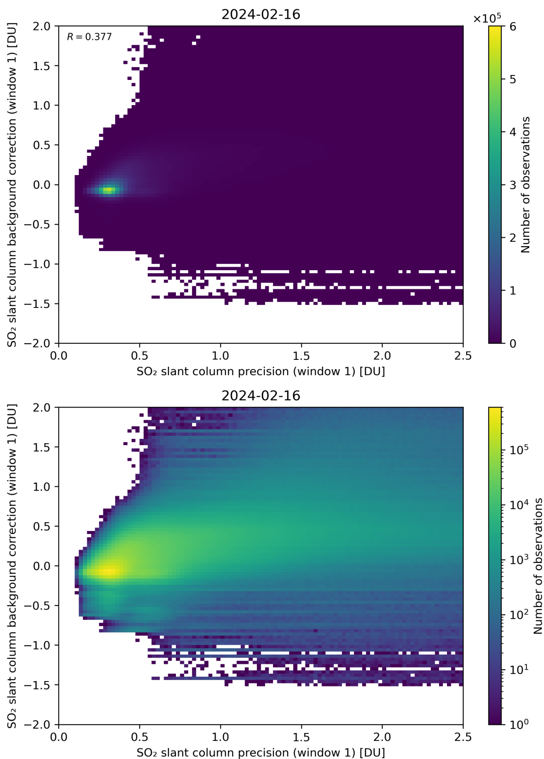
Figure 218: Scatter density plot of “SO 2 slant column precision (window 1)” against “SO 2 slant column background correction (window 1)” for 2024-02-16 to 2024-02-17.
