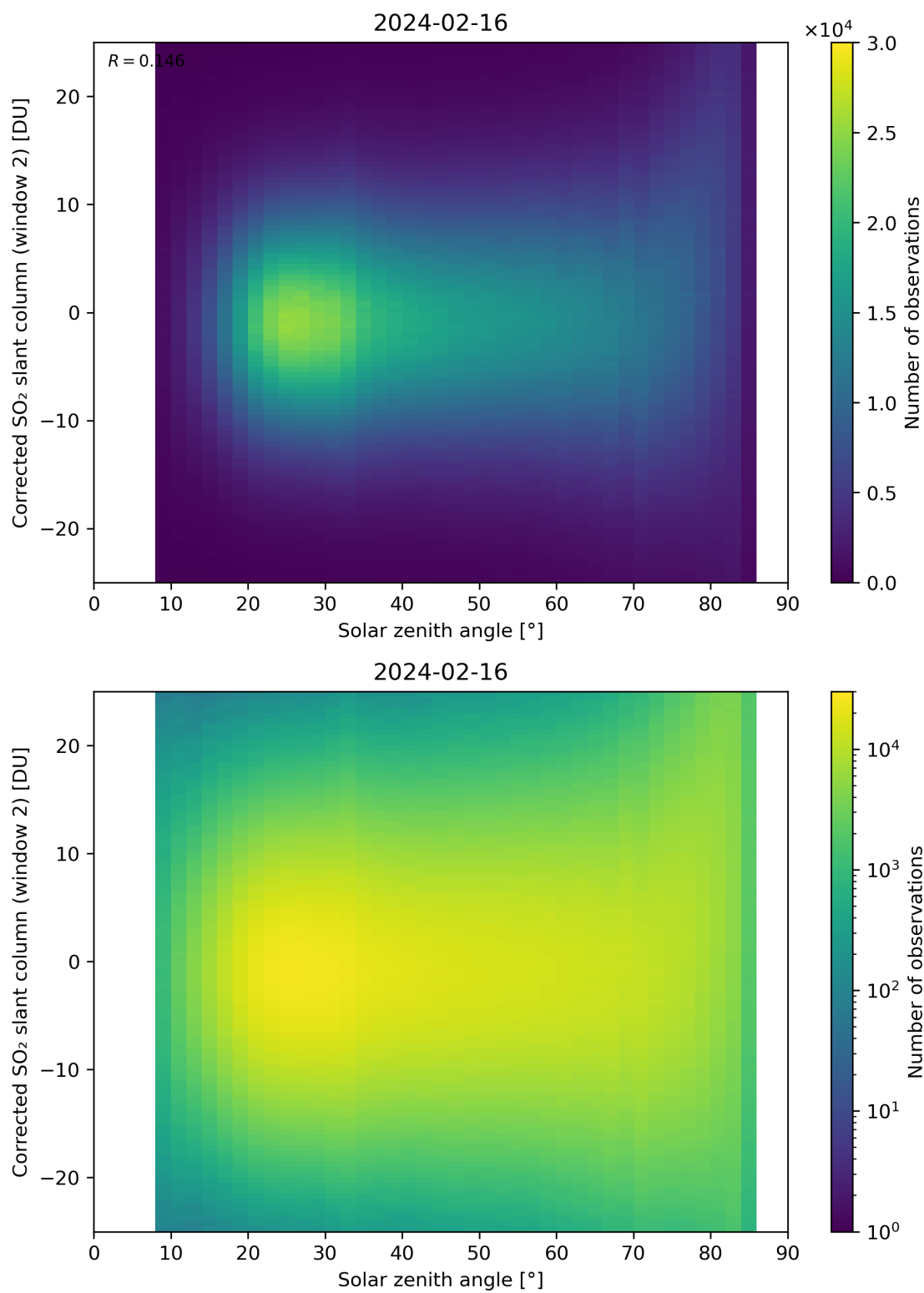
Figure 167: Scatter density plot of “Solar zenith angle” against “Corrected SO 2 slant column (window 2)” for 2024-02-16 to 2024-02-17.
