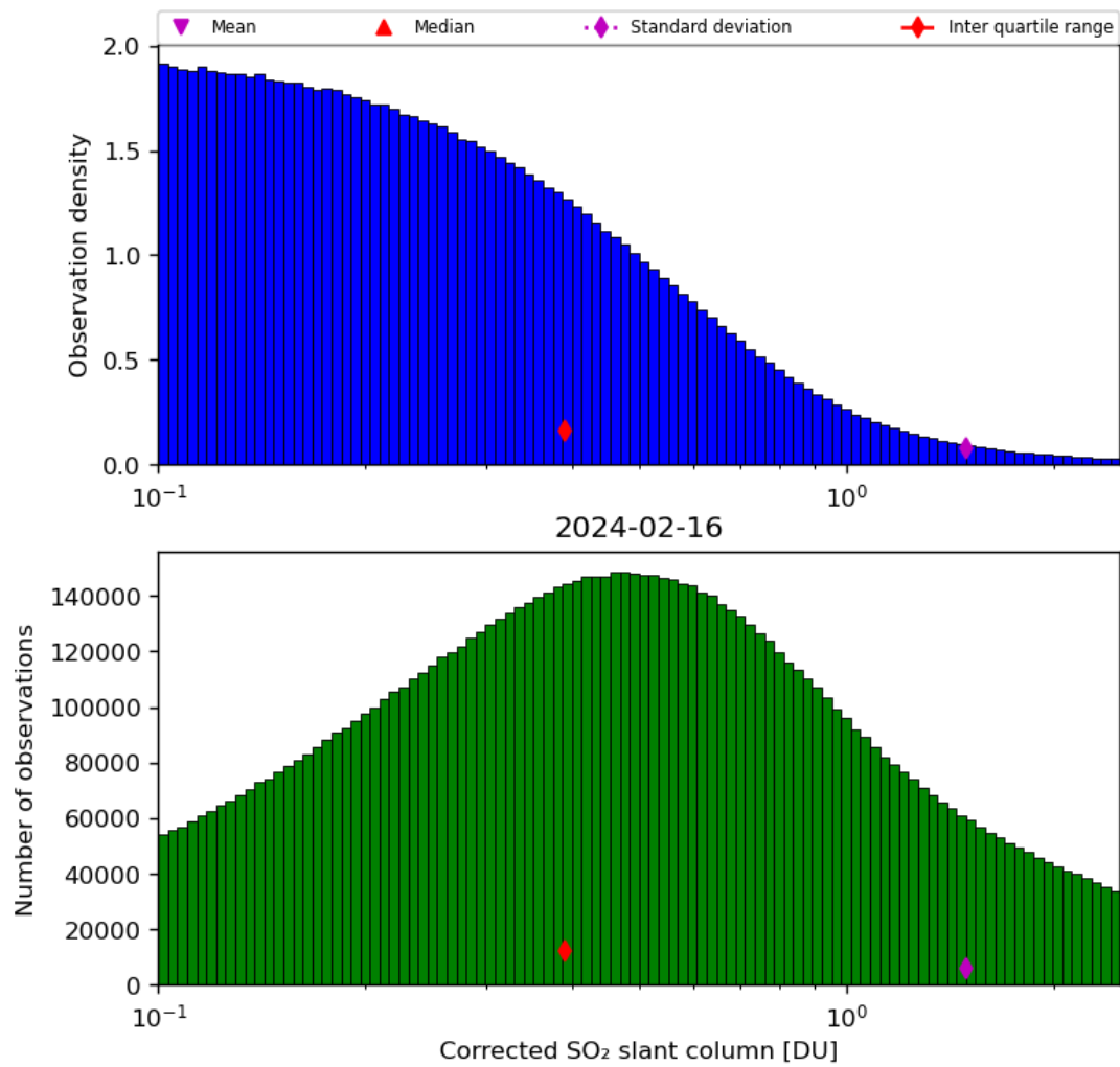
Figure 55: Histogram of “Corrected SO 2 slant column” for 2024-02-16 to 2024-02-17
