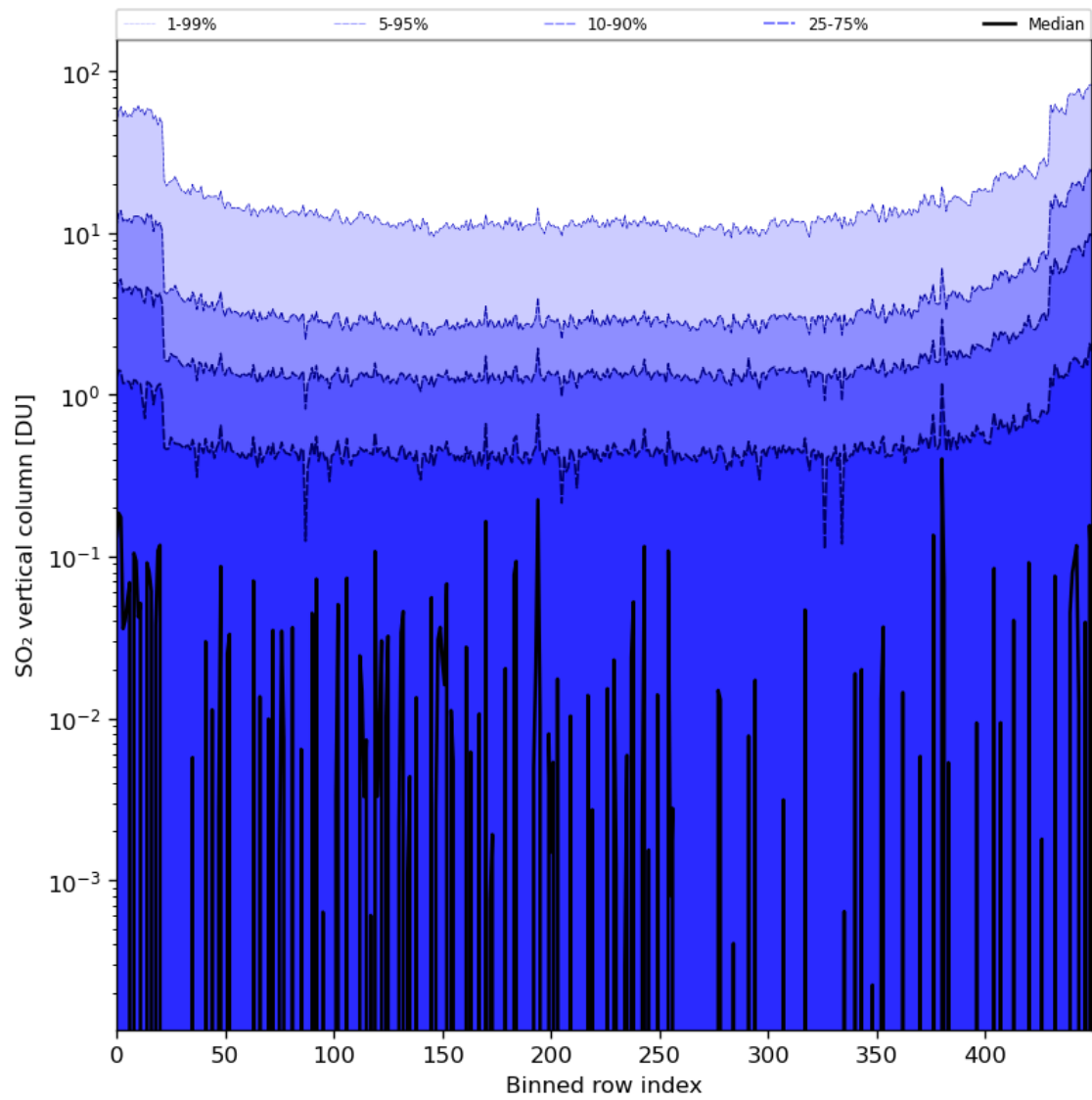
Figure 76: Along track statistics of “SO 2 vertical column” for 2024-02-16 to 2024-02-17
