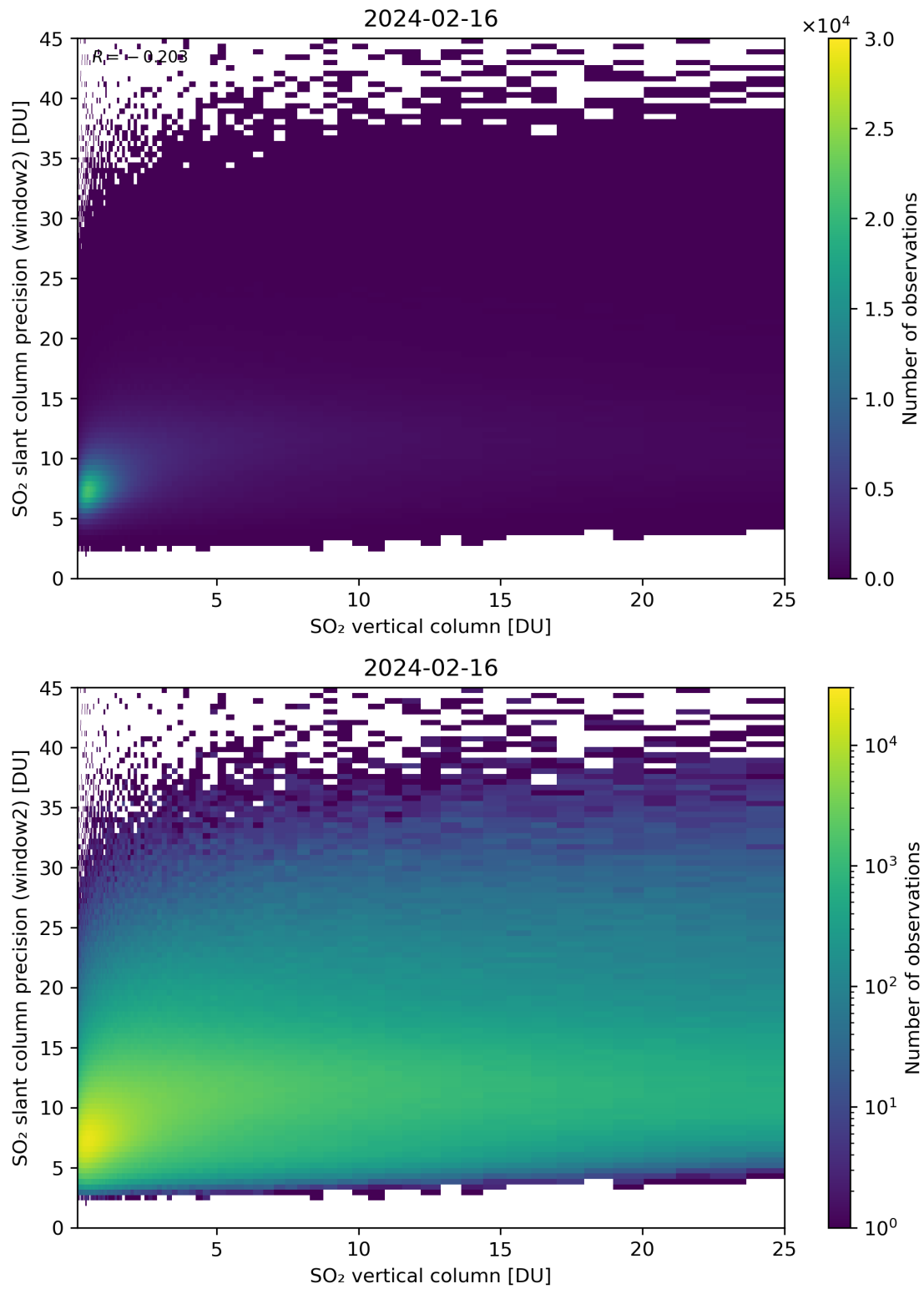
Figure 302: Scatter density plot of “SO 2 vertical column” against “SO 2 slant column precision (window2)” for 2024-02-16 to 2024-02-17.
