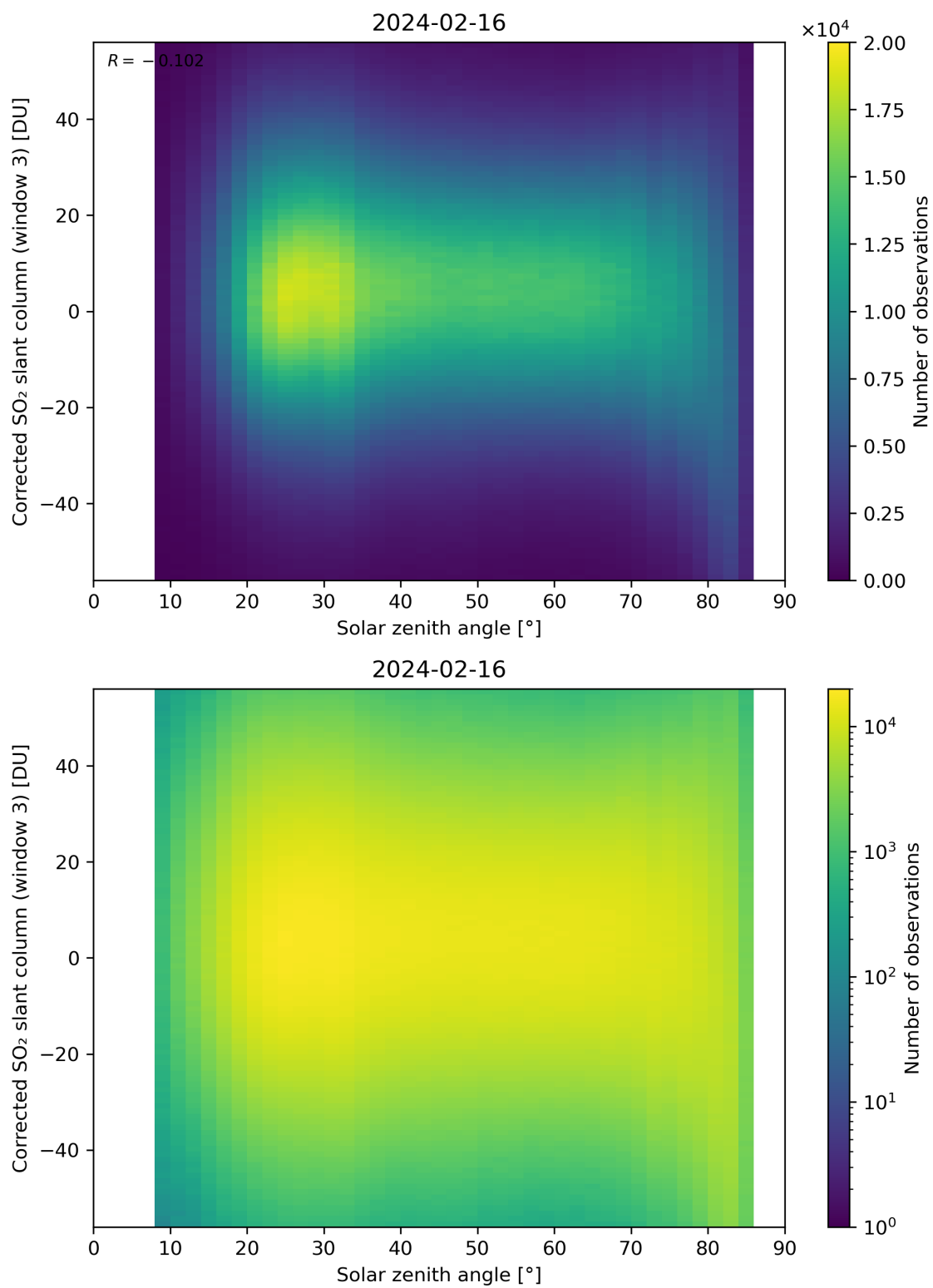
Figure 168: Scatter density plot of “Solar zenith angle” against “Corrected SO 2 slant column (window 3)” for 2024-02-16 to 2024-02-17.
