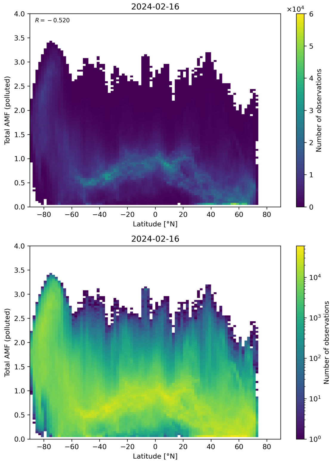
Figure 154: Scatter density plot of “Latitude” against “Total AMF (polluted)” for 2024-02-16 to 2024-02-17.
