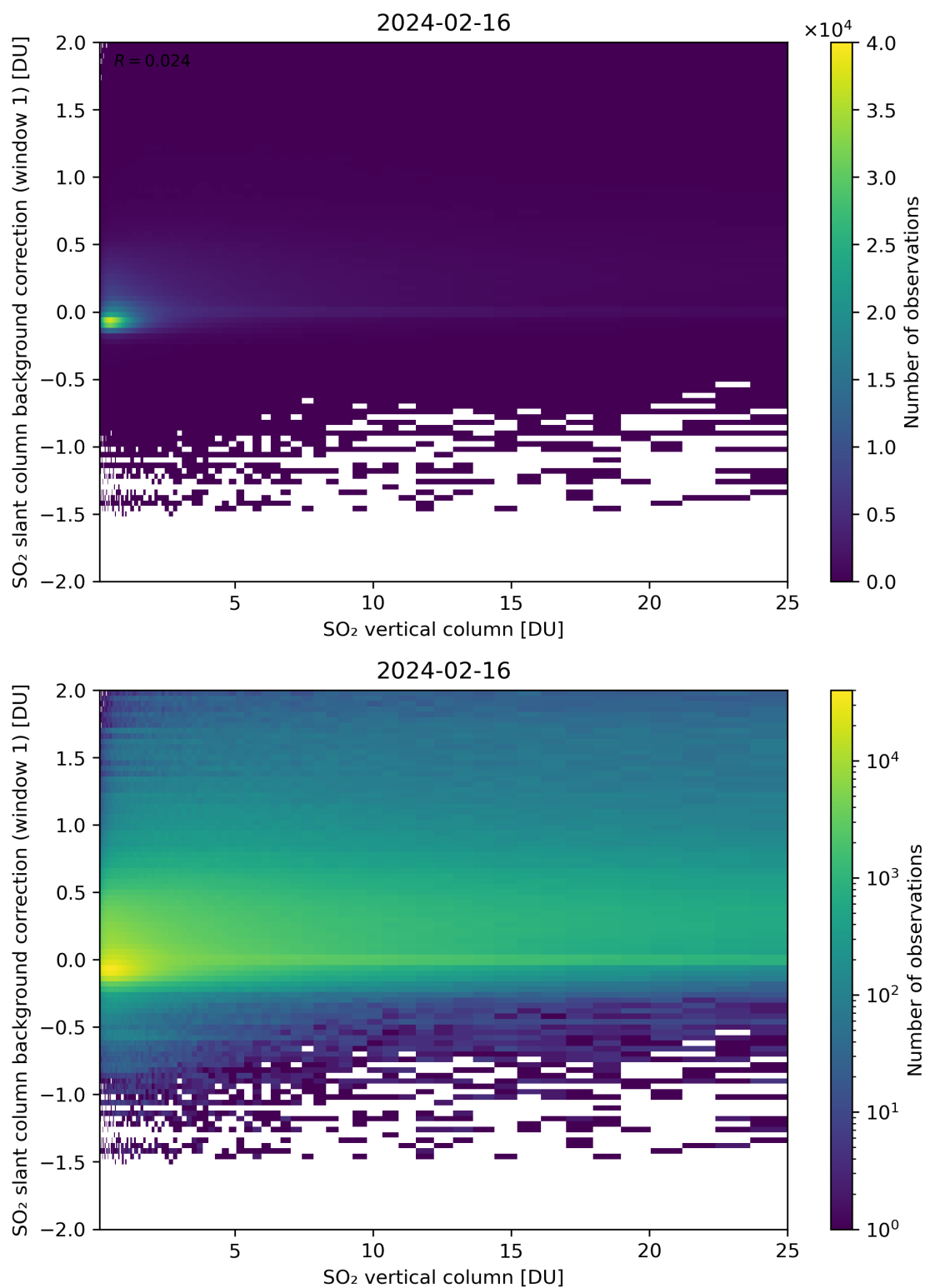
Figure 273: Scatter density plot of “SO 2 vertical column” against “SO 2 slant column background correction (window 1)” for 2024-02-16 to 2024-02-17.
