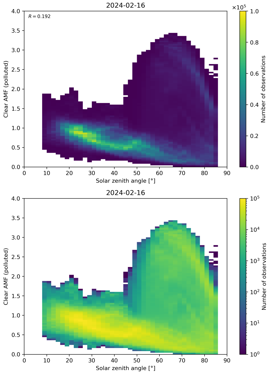
Figure 165: Scatter density plot of “Solar zenith angle” against “Clear AMF (polluted)” for 2024-02-16 to 2024-02-17.
