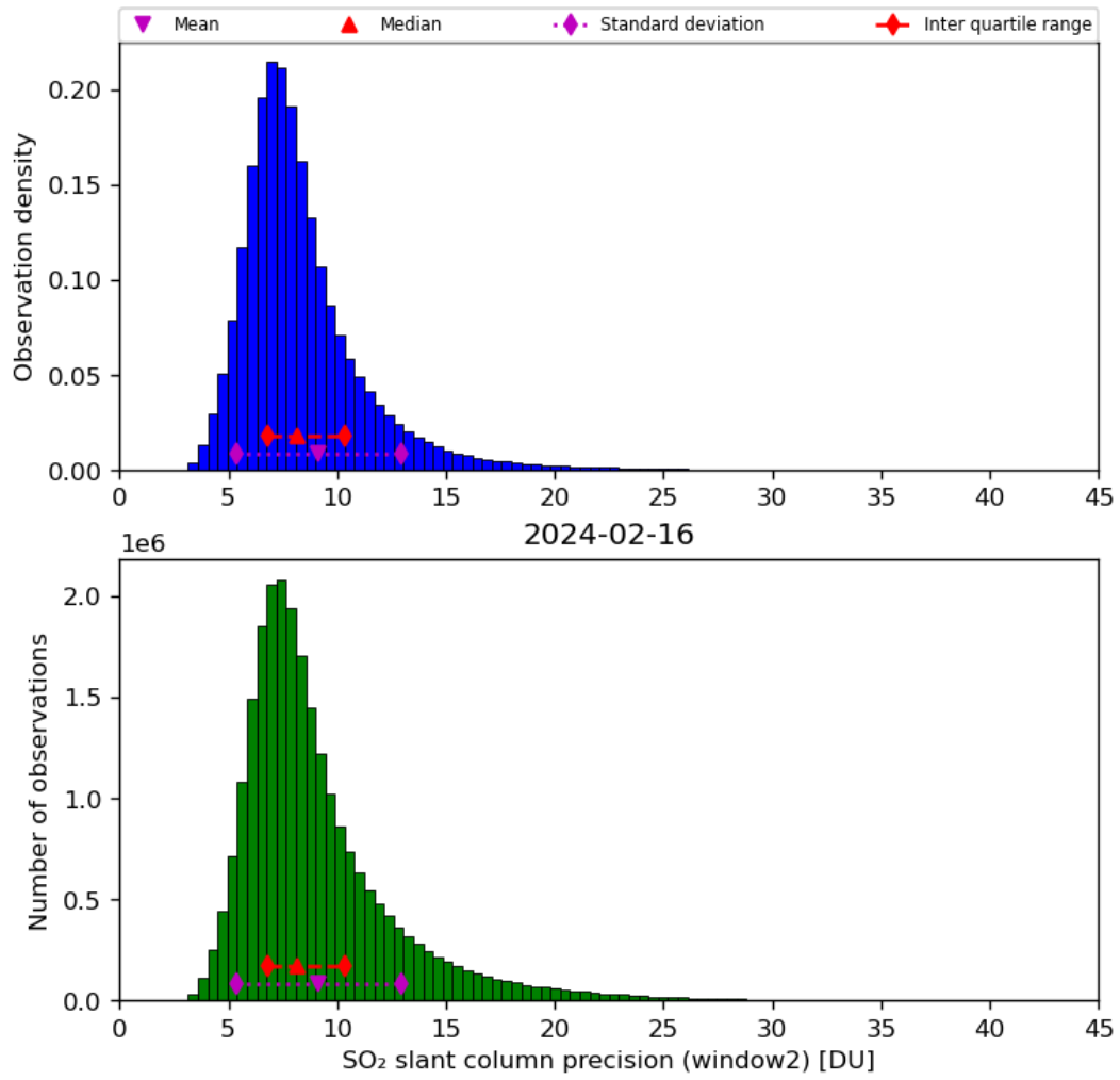
Figure 61: Histogram of “SO 2 slant column precision (window2)” for 2024-02-16 to 2024-02-17
