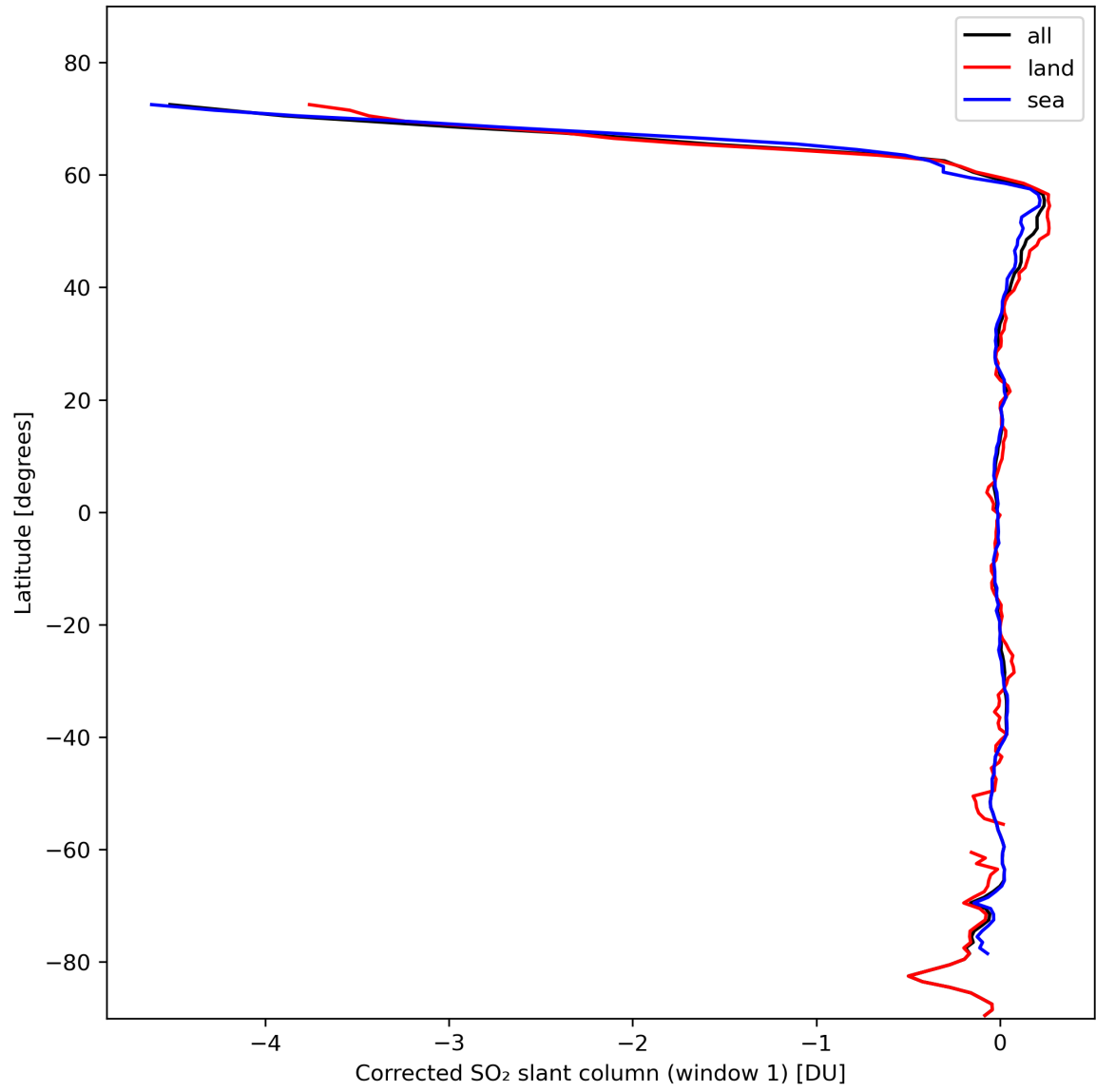
Figure 35: Zonal average of “Corrected SO 2 slant column (window 1)” for 2024-02-16 to 2024-02-17.
