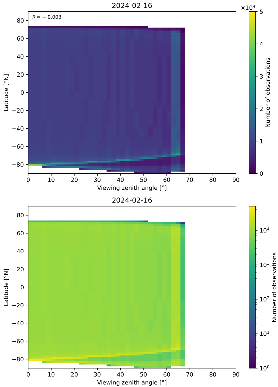
Figure 314: Scatter density plot of “Viewing zenith angle” against “Latitude” for 2024-02-16 to 2024-02-17.
