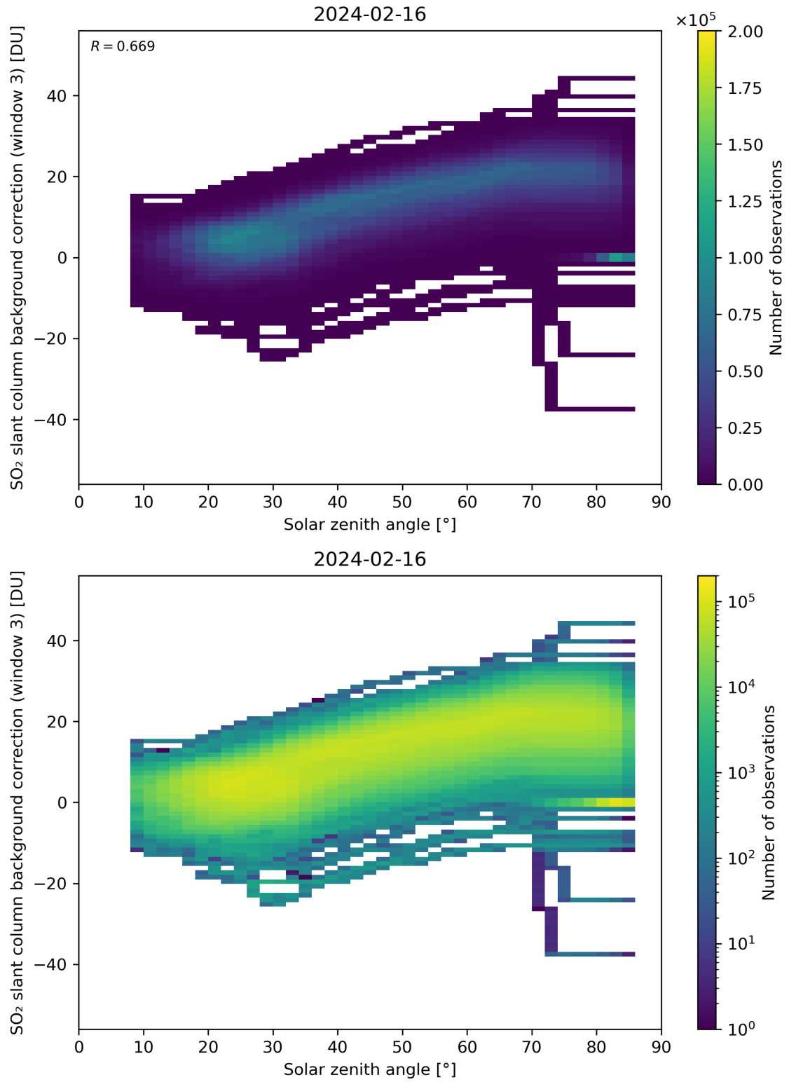
Figure 160: Scatter density plot of “Solar zenith angle” against “SO 2 slant column background correction (window 3)” for 2024-02-16 to 2024-02-17.
