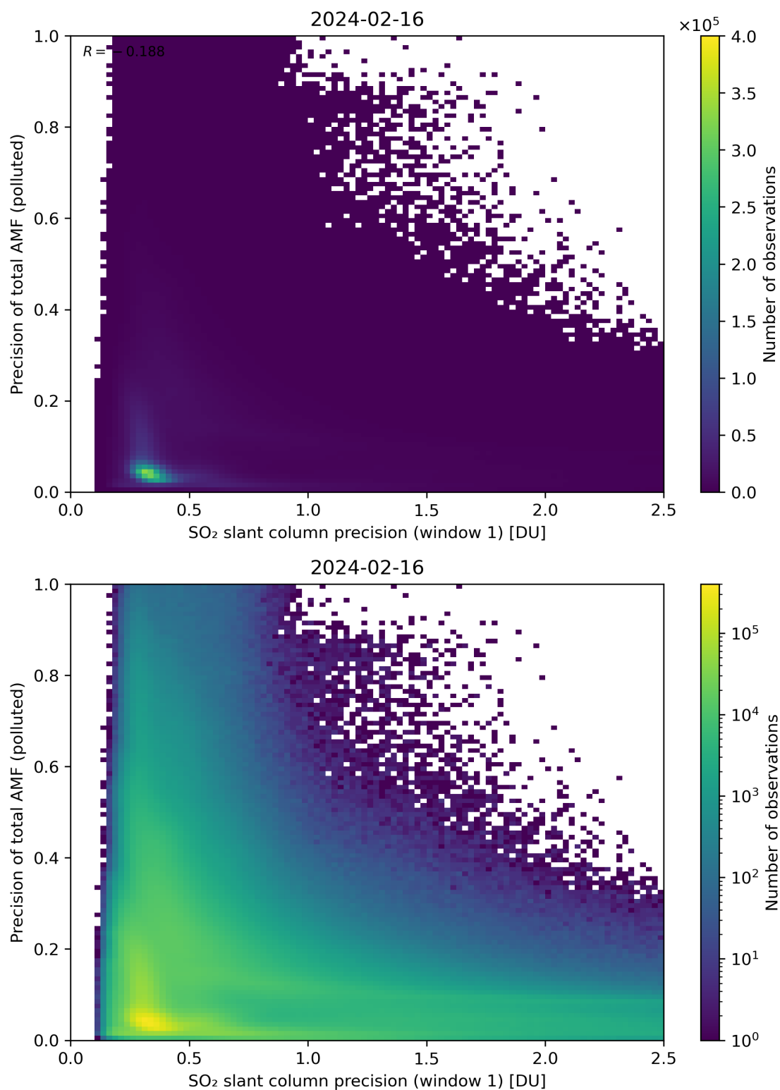
Figure 231: Scatter density plot of “SO 2 slant column precision (window 1)” against “Precision of total AMF (polluted)” for 2024-02-16 to 2024-02-17.
