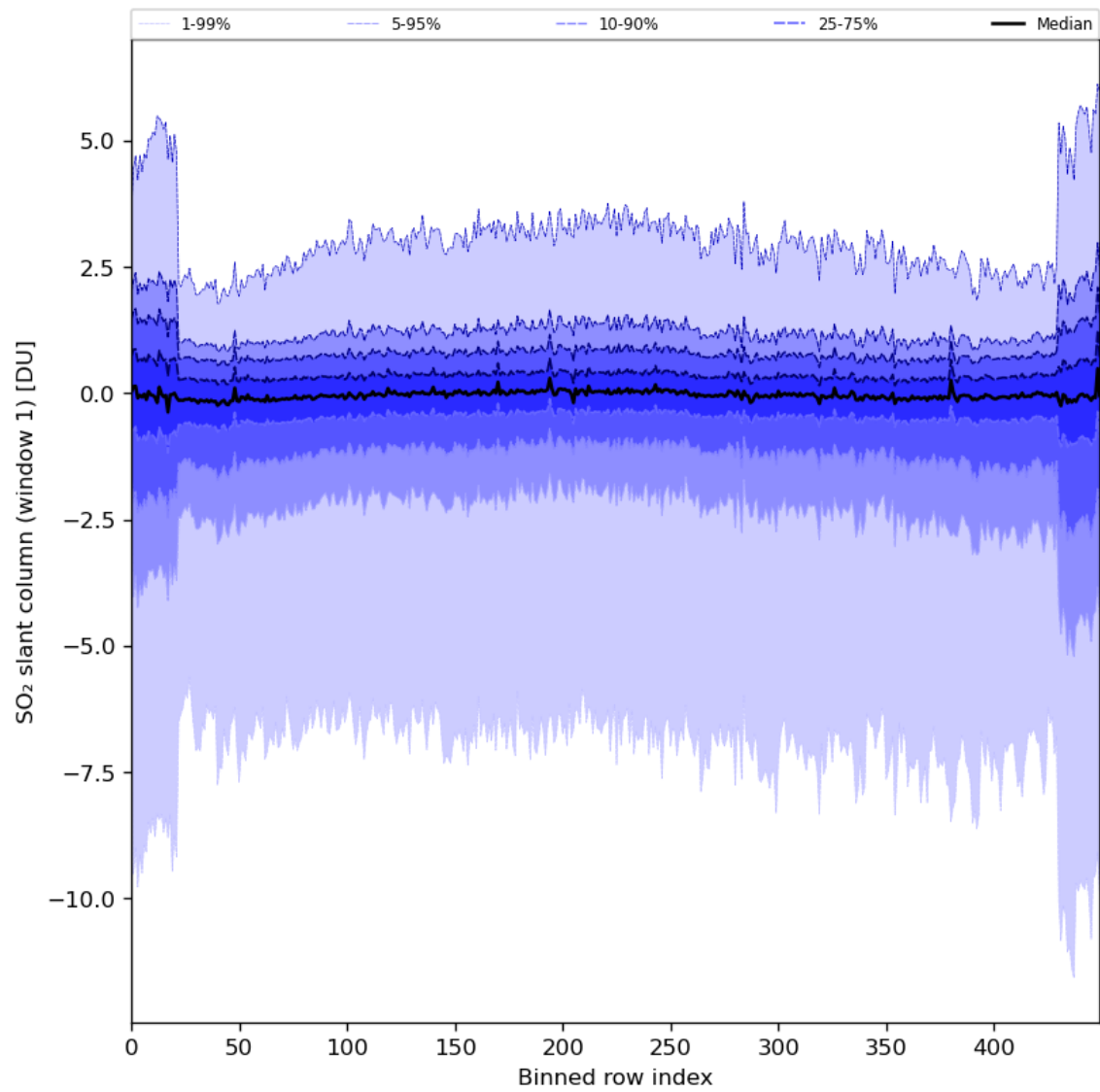
Figure 79: Along track statistics of “SO 2 slant column (window 1)” for 2024-02-16 to 2024-02-17
