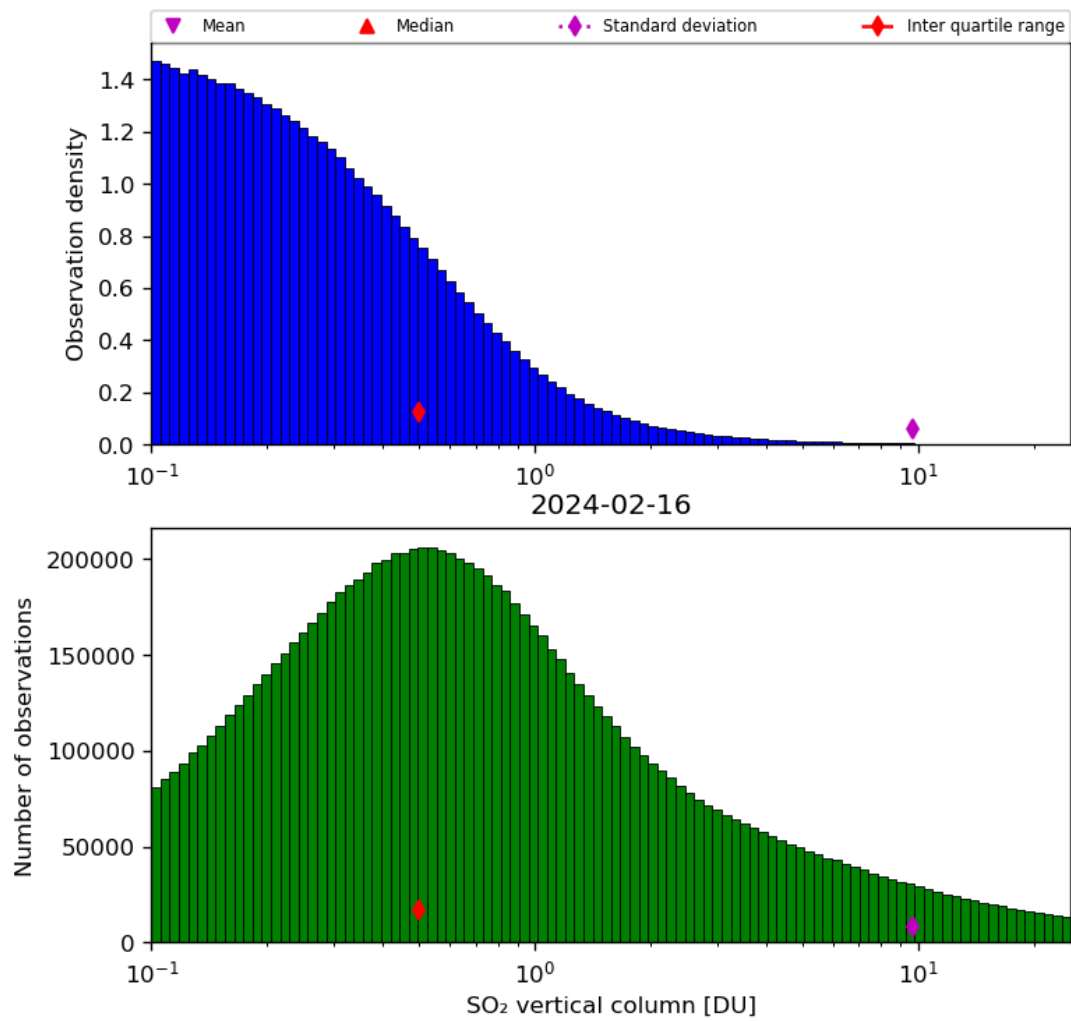
Figure 53: Histogram of “SO 2 vertical column” for 2024-02-16 to 2024-02-17
