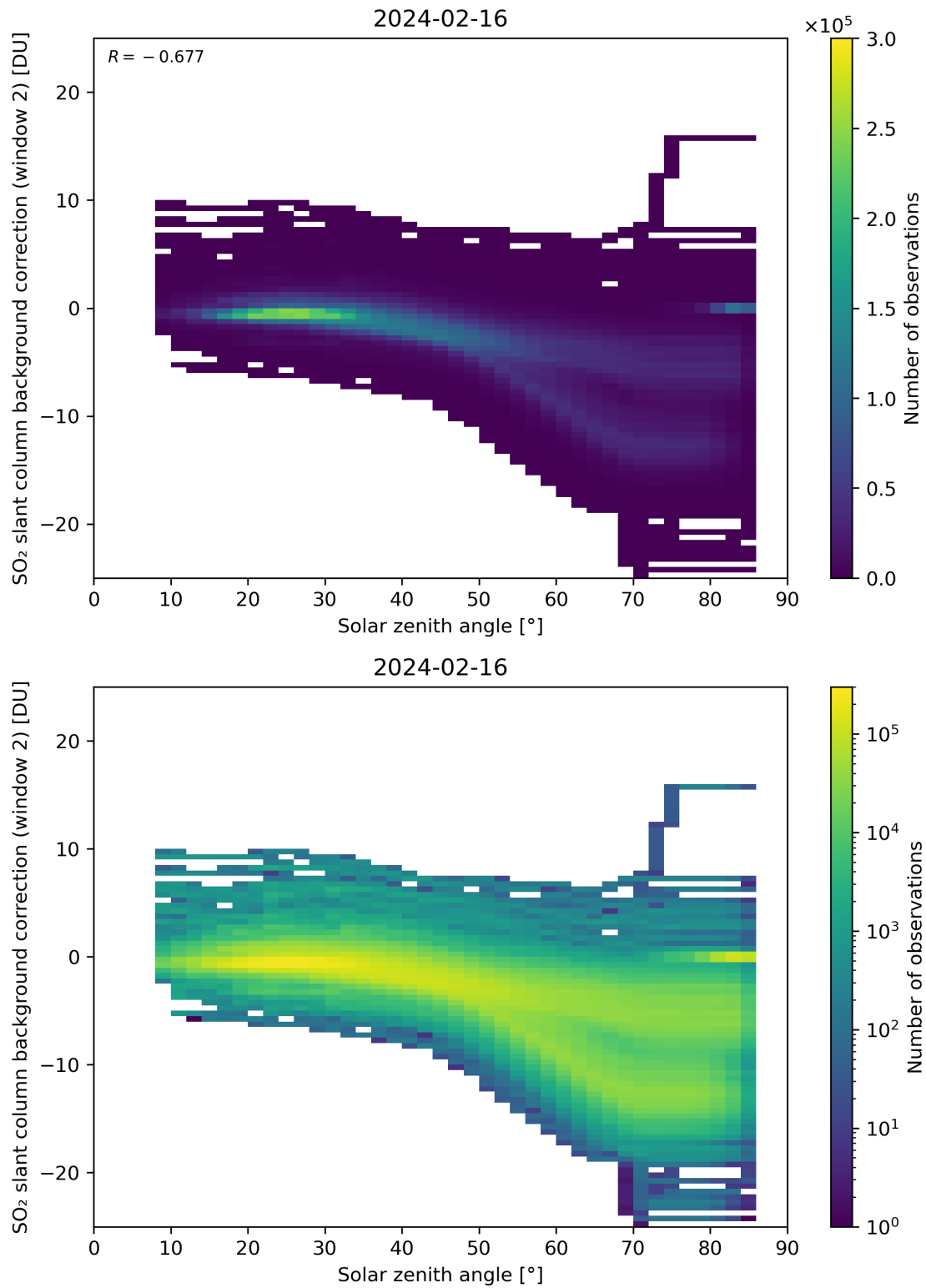
Figure 159: Scatter density plot of “Solar zenith angle” against “SO 2 slant column background correction (window 2)” for 2024-02-16 to 2024-02-17.
