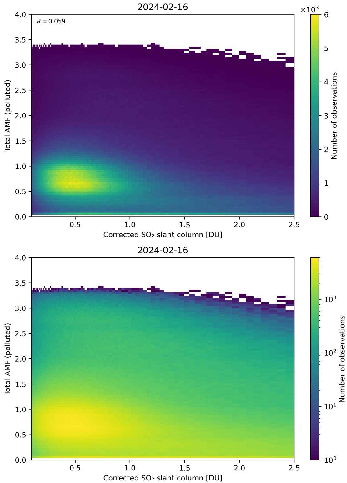
Figure 192: Scatter density plot of “Corrected SO 2 slant column” against “Total AMF (polluted)” for 2024-02-16 to 2024-02-17.
