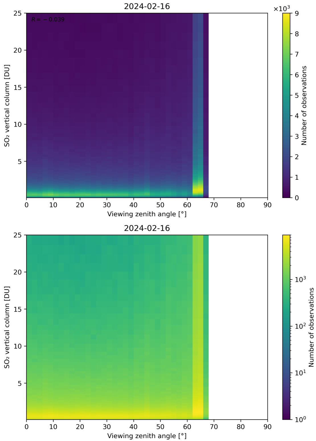
Figure 327: Scatter density plot of “Viewing zenith angle” against “SO 2 vertical column” for 2024-02-16 to 2024-02-17.
