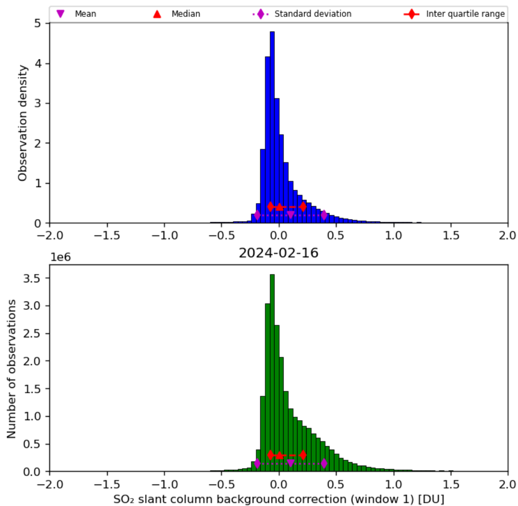
Figure 59: Histogram of “SO 2 slant column background correction (window 1)” for 2024-02-16 to 2024-02-17
