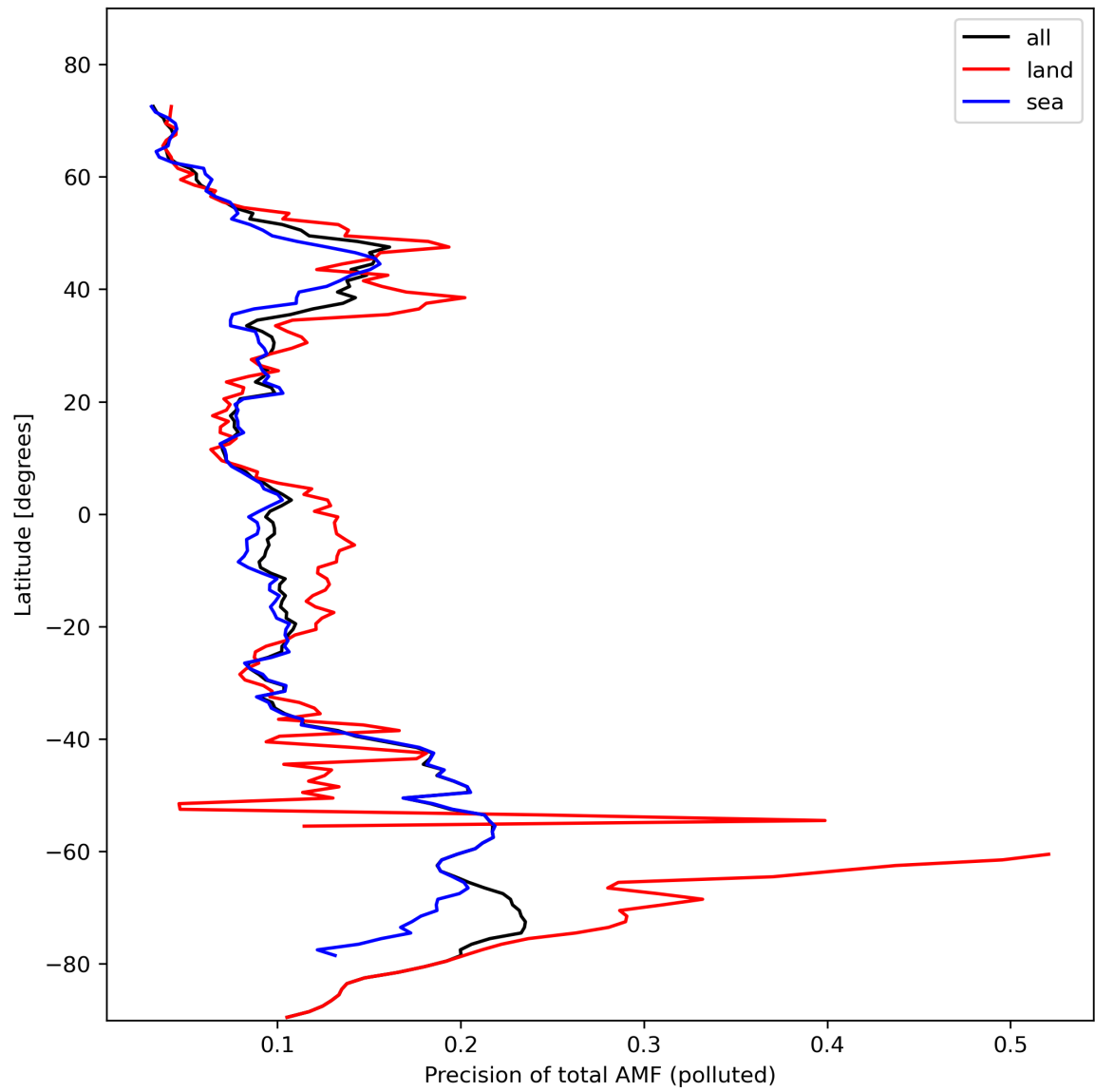
Figure 49: Zonal average of “Precision of total AMF (polluted)” for 2024-02-16 to 2024-02-17.
