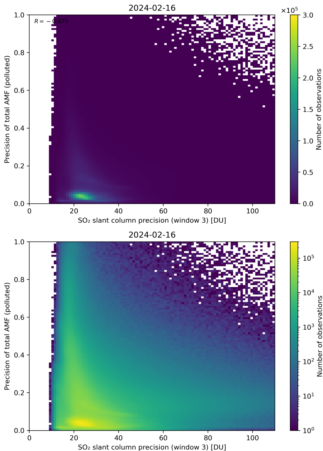
Figure 264: Scatter density plot of “SO 2 slant column precision (window 3)” against “Precision of total AMF (polluted)” for 2024-02-16 to 2024-02-17.
