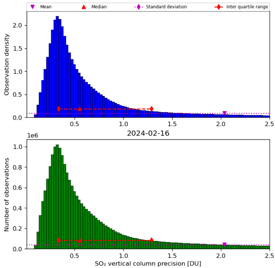
Figure 54: Histogram of “SO 2 vertical column precision” for 2024-02-16 to 2024-02-17
