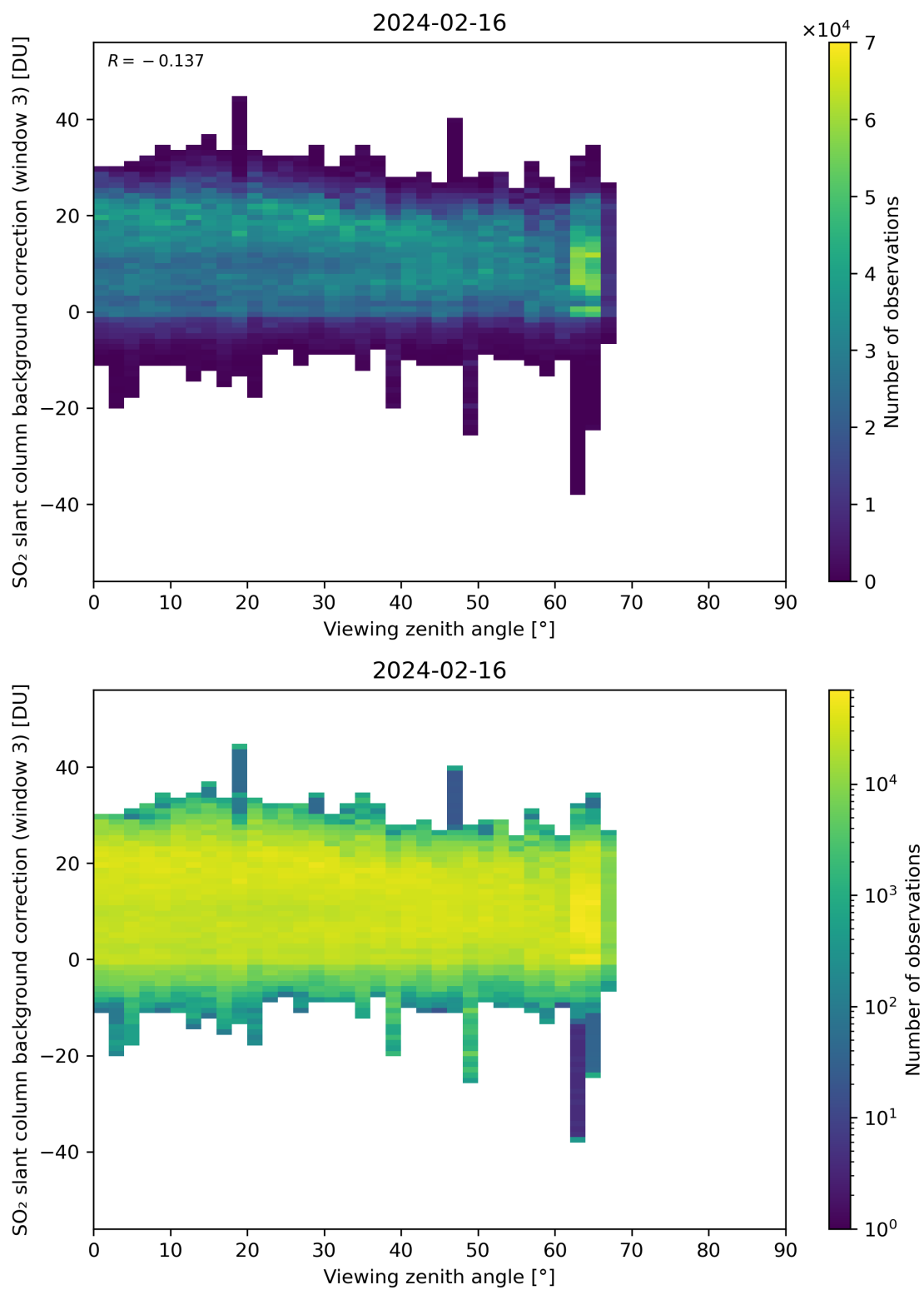
Figure 310: Scatter density plot of “Viewing zenith angle” against “SO 2 slant column background correction (window 3)” for 2024-02-16 to 2024-02-17.
