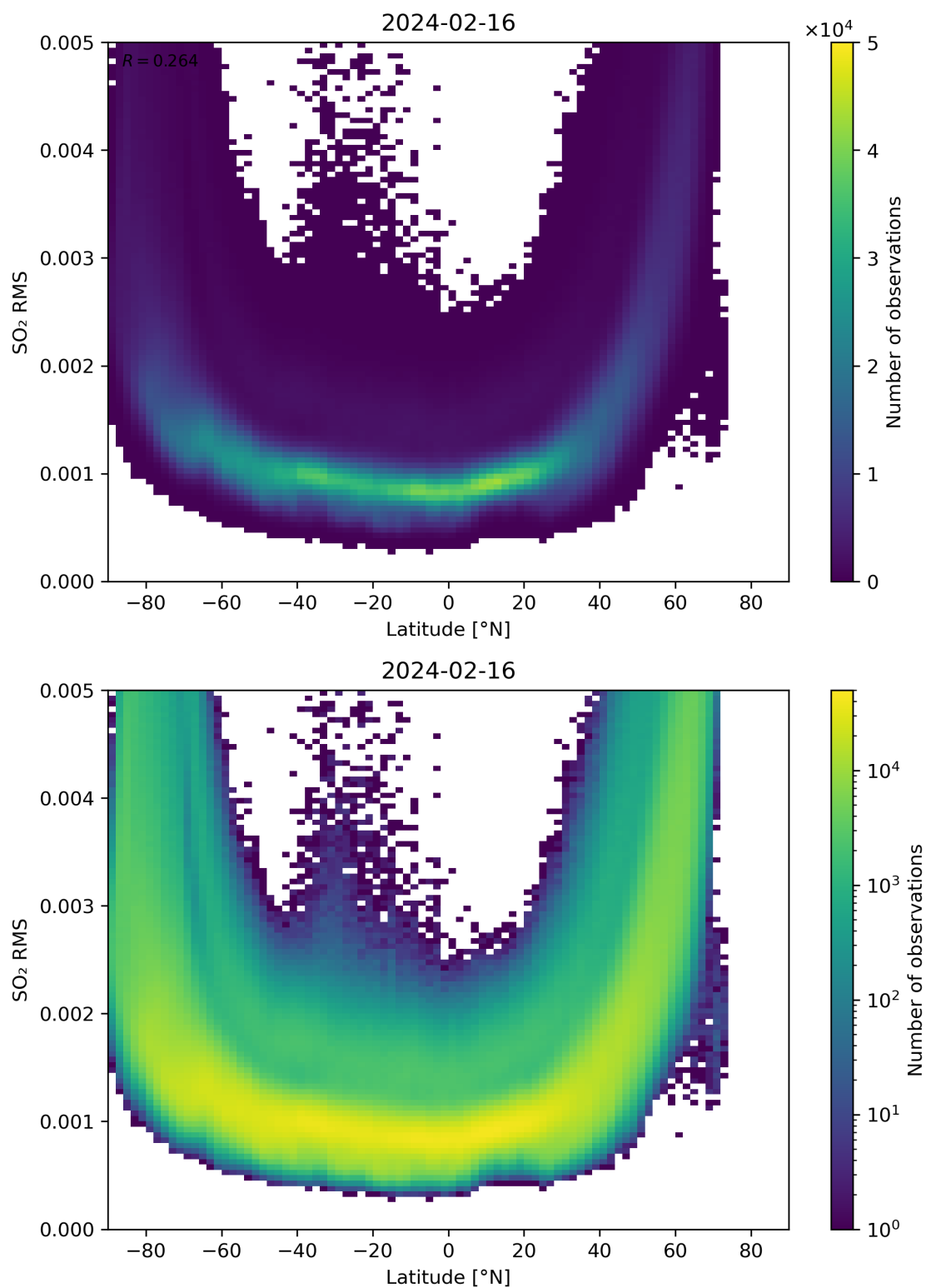
Figure 144: Scatter density plot of “Latitude” against “SO 2 RMS” for 2024-02-16 to 2024-02-17.
