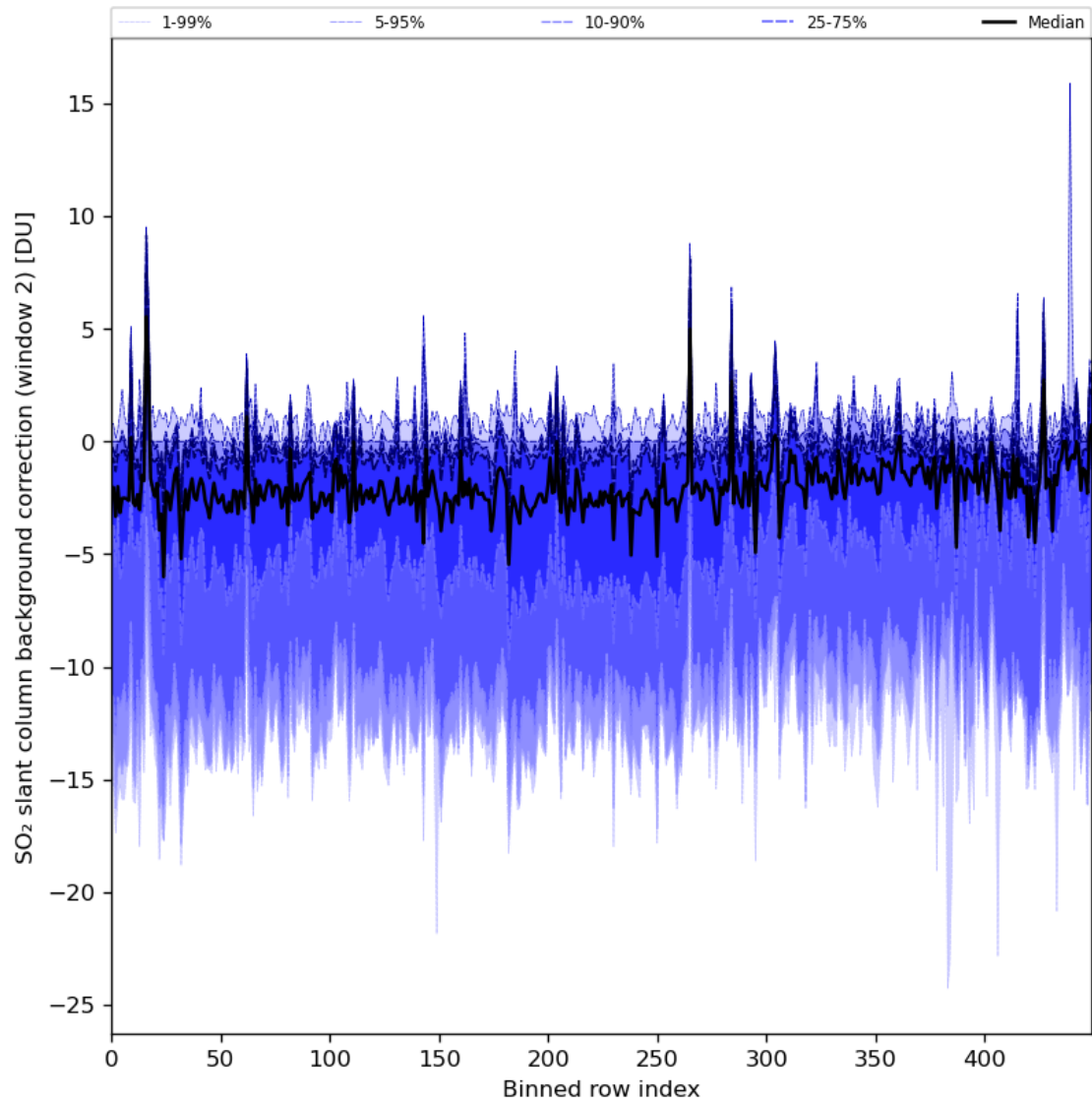
Figure 86: Along track statistics of “SO 2 slant column background correction (window 2)” for 2024-02-16 to 2024-02-17
