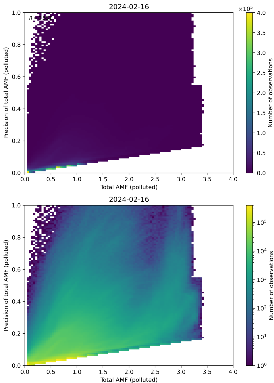
Figure 272: Scatter density plot of “Total AMF (polluted)” against “Precision of total AMF (polluted)” for 2024-02-16 to 2024-02-17.
