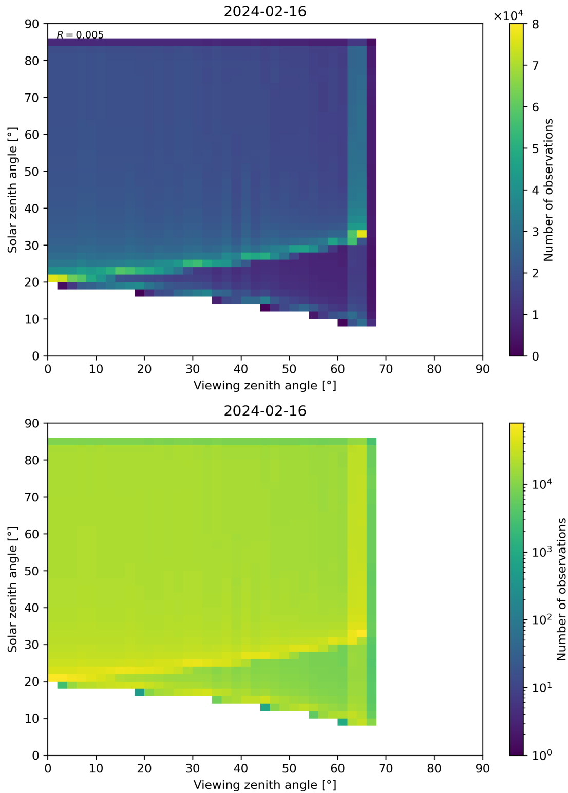
Figure 315: Scatter density plot of “Viewing zenith angle” against “Solar zenith angle” for 2024-02-16 to 2024-02-17.
