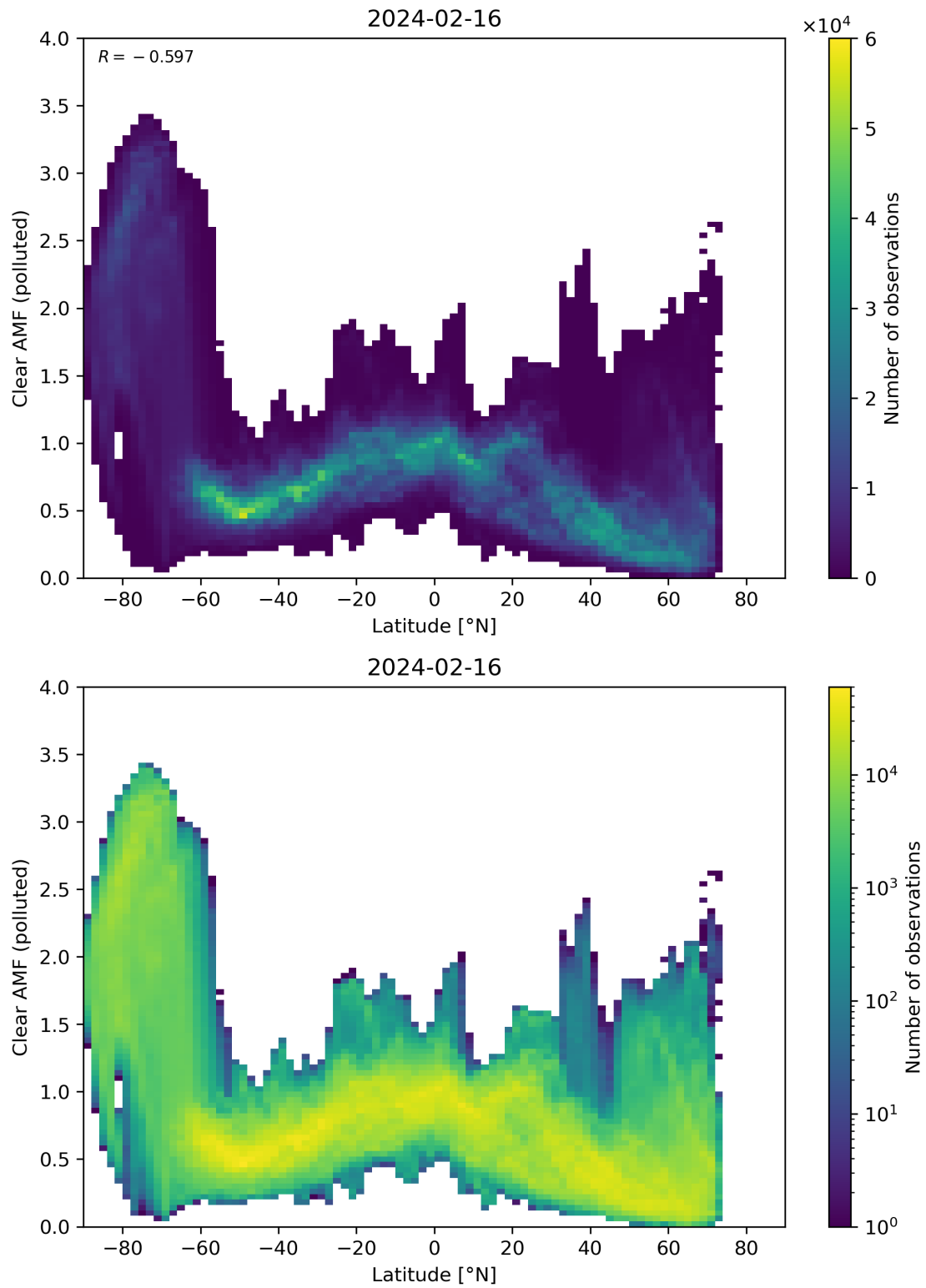
Figure 145: Scatter density plot of “Latitude” against “Clear AMF (polluted)” for 2024-02-16 to 2024-02-17.
