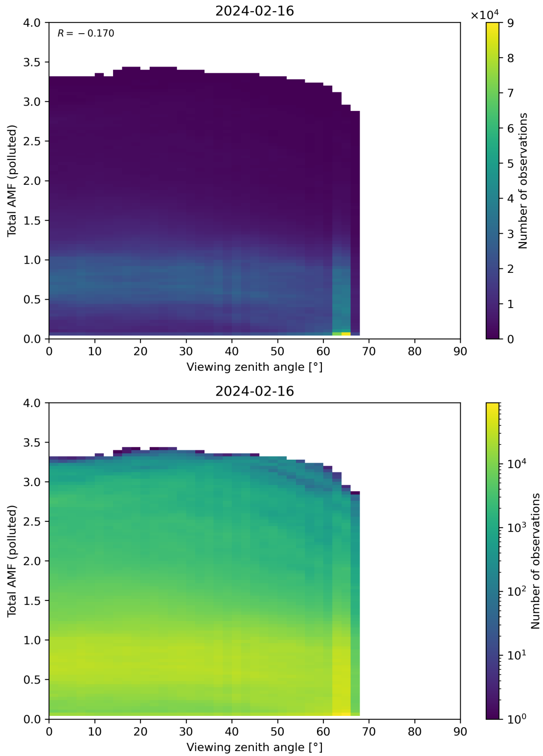
Figure 325: Scatter density plot of “Viewing zenith angle” against “Total AMF (polluted)” for 2024-02-16 to 2024-02-17.
