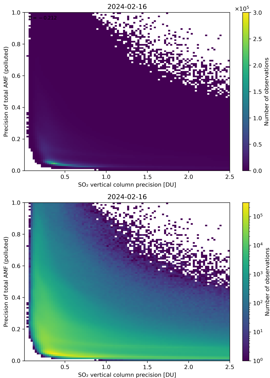
Figure 295: Scatter density plot of “SO 2 vertical column precision” against “Precision of total AMF (polluted)” for 2024-02-16 to 2024-02-17.
