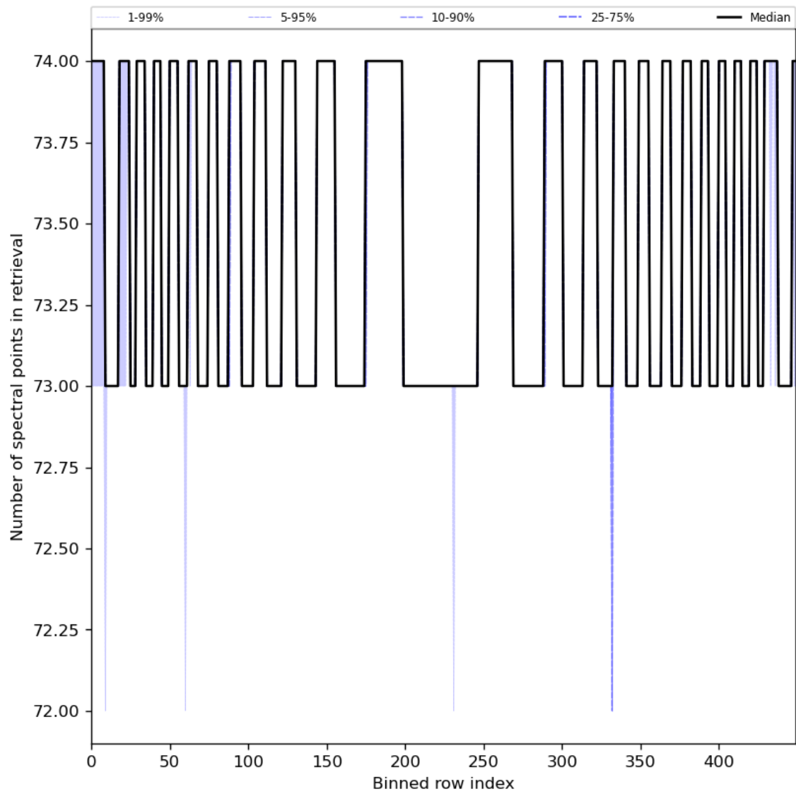
Figure 97: Along track statistics of “Number of spectral points in retrieval” for 2024-02-16 to 2024-02-17
