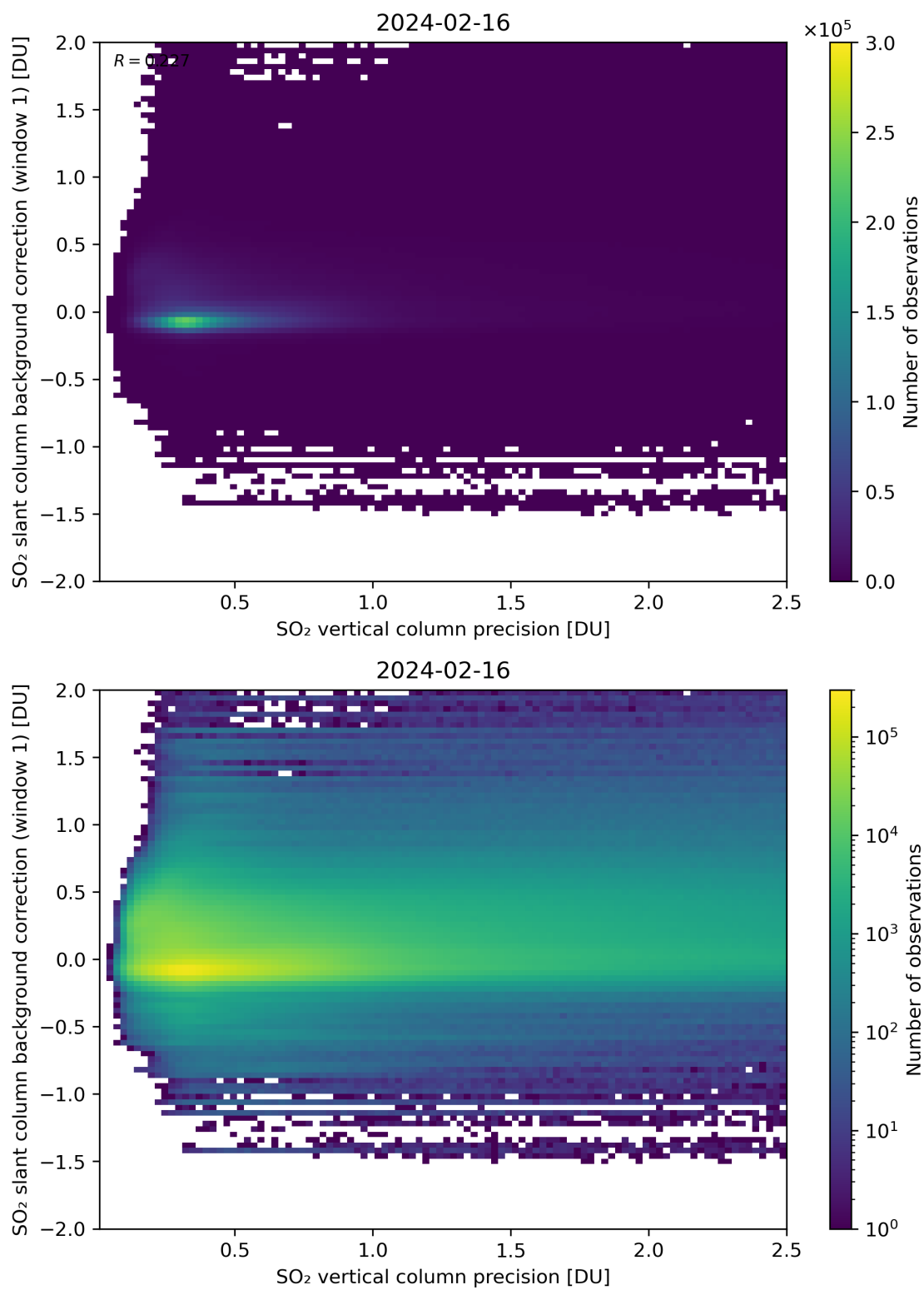
Figure 279: Scatter density plot of “SO 2 vertical column precision” against “SO 2 slant column background correction (window 1)” for 2024-02-16 to 2024-02-17.
