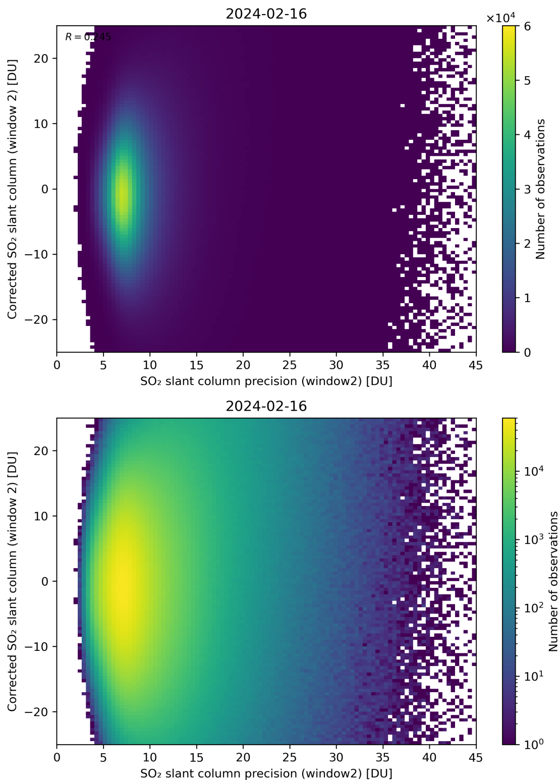
Figure 247: Scatter density plot of “SO 2 slant column precision (window2)” against “Corrected SO 2 slant column (window 2)” for 2024-02-16 to 2024-02-17.
