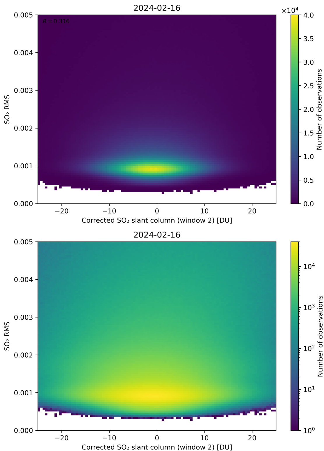
Figure 198: Scatter density plot of “Corrected SO 2 slant column (window 2)” against “SO 2 RMS” for 2024-02-16 to 2024-02-17.
