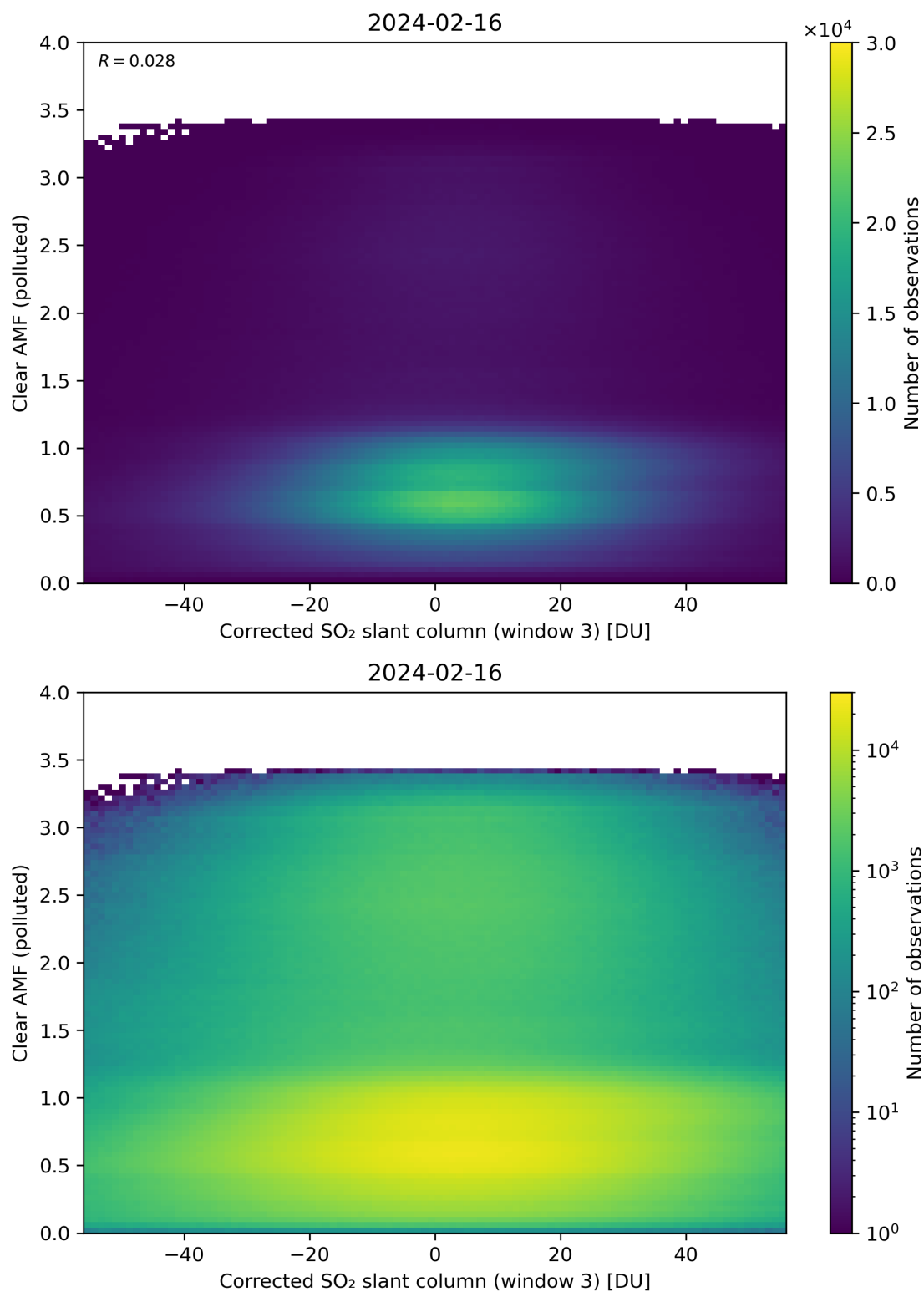
Figure 209: Scatter density plot of “Corrected SO 2 slant column (window 3)” against “Clear AMF (polluted)” for 2024-02-16 to 2024-02-17.
