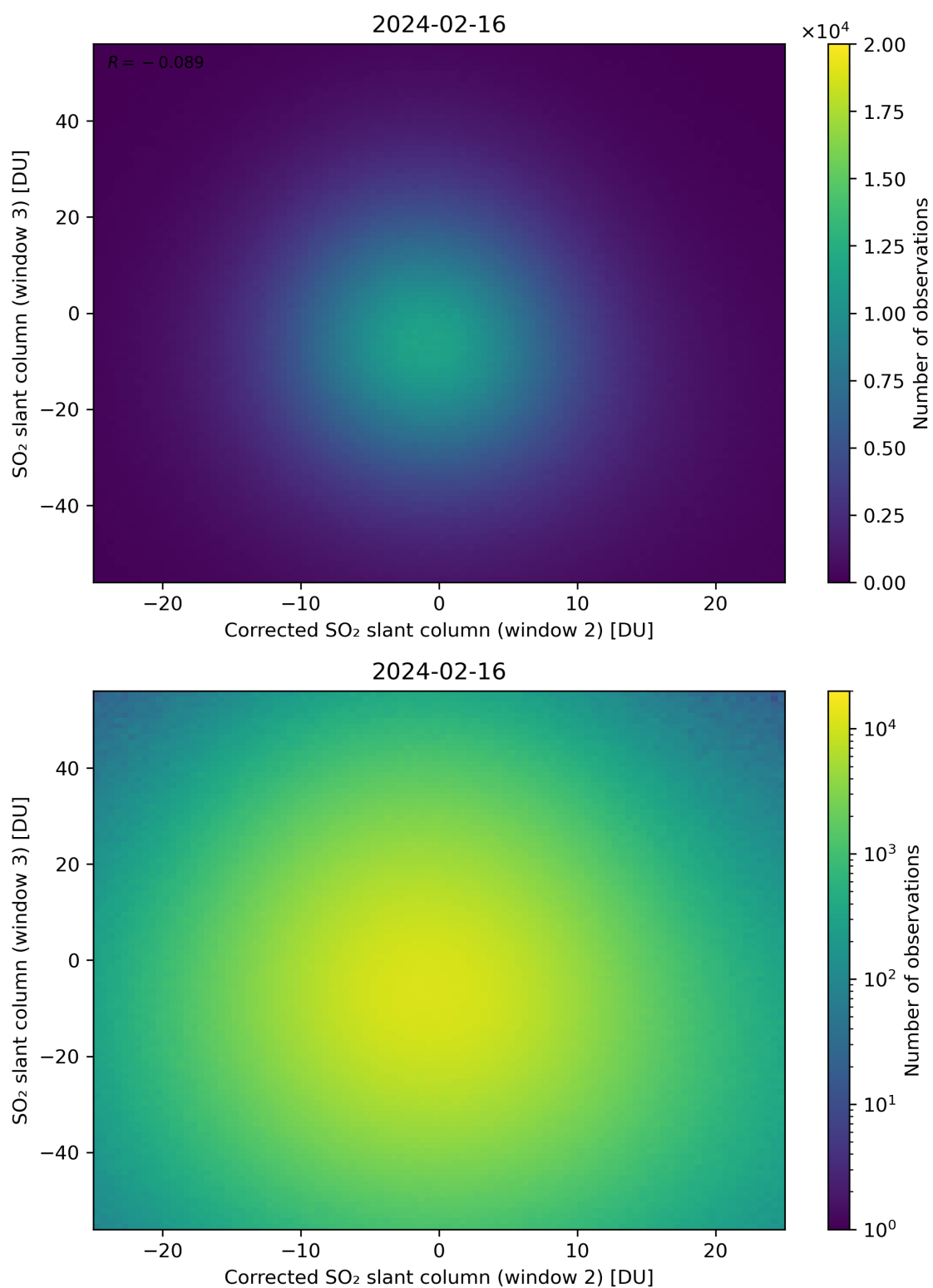
Figure 201: Scatter density plot of “Corrected SO 2 slant column (window 2)” against “SO 2 slant column (window 3)” for 2024-02-16 to 2024-02-17.
