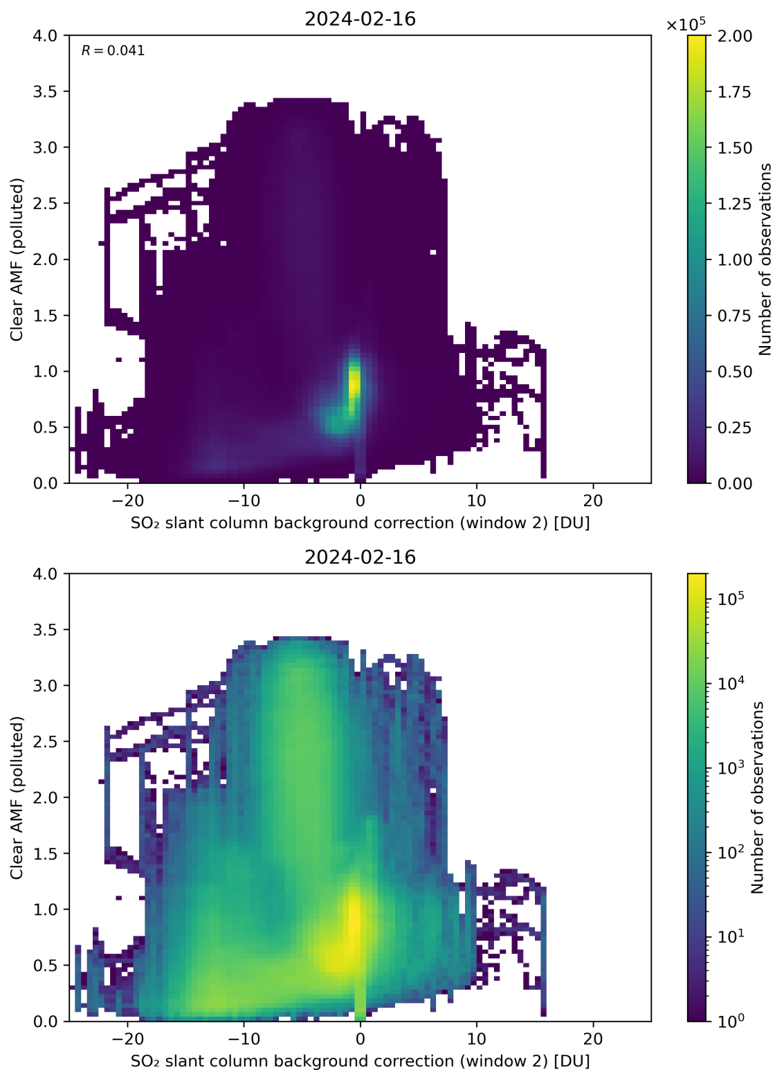
Figure 115: Scatter density plot of “SO 2 slant column background correction (window 2)” against “Clear AMF (polluted)” for 2024-02-16 to 2024-02-17.
