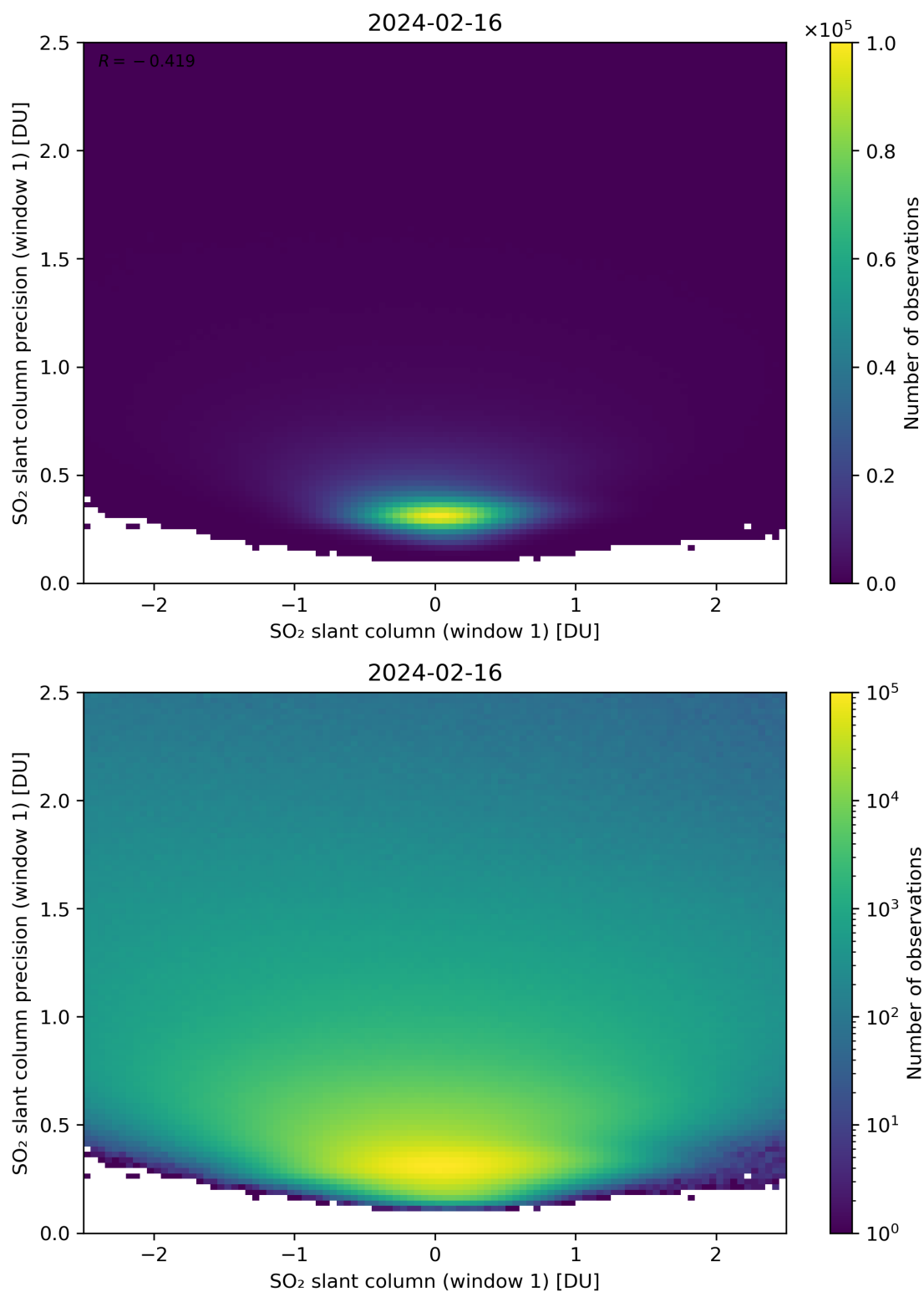
Figure 235: Scatter density plot of “SO 2 slant column (window 1)” against “SO 2 slant column precision (window 1)” for 2024-02-16 to 2024-02-17.
