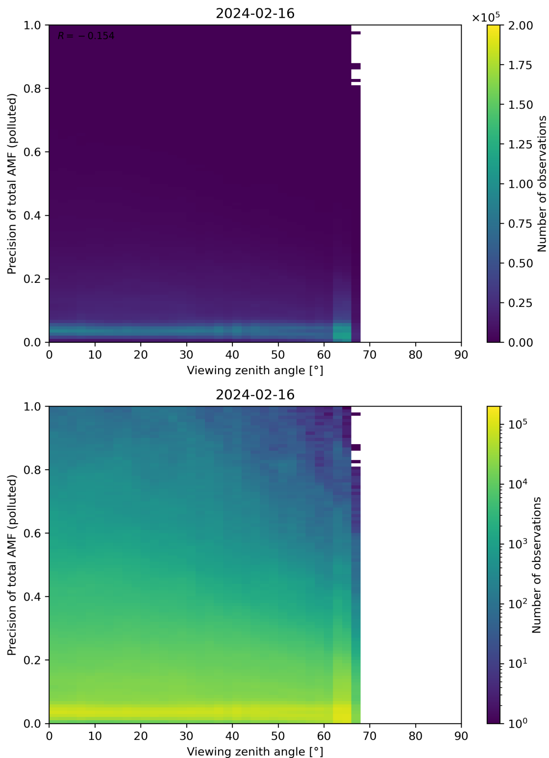
Figure 326: Scatter density plot of “Viewing zenith angle” against “Precision of total AMF (polluted)” for 2024-02-16 to 2024-02-17.
