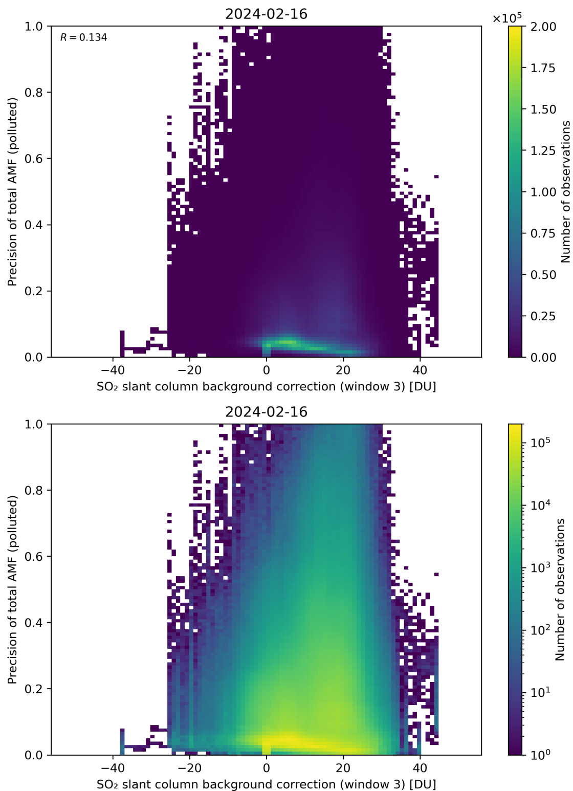
Figure 126: Scatter density plot of “SO 2 slant column background correction (window 3)” against “Precision of total AMF (polluted)” for 2024-02-16 to 2024-02-17.
