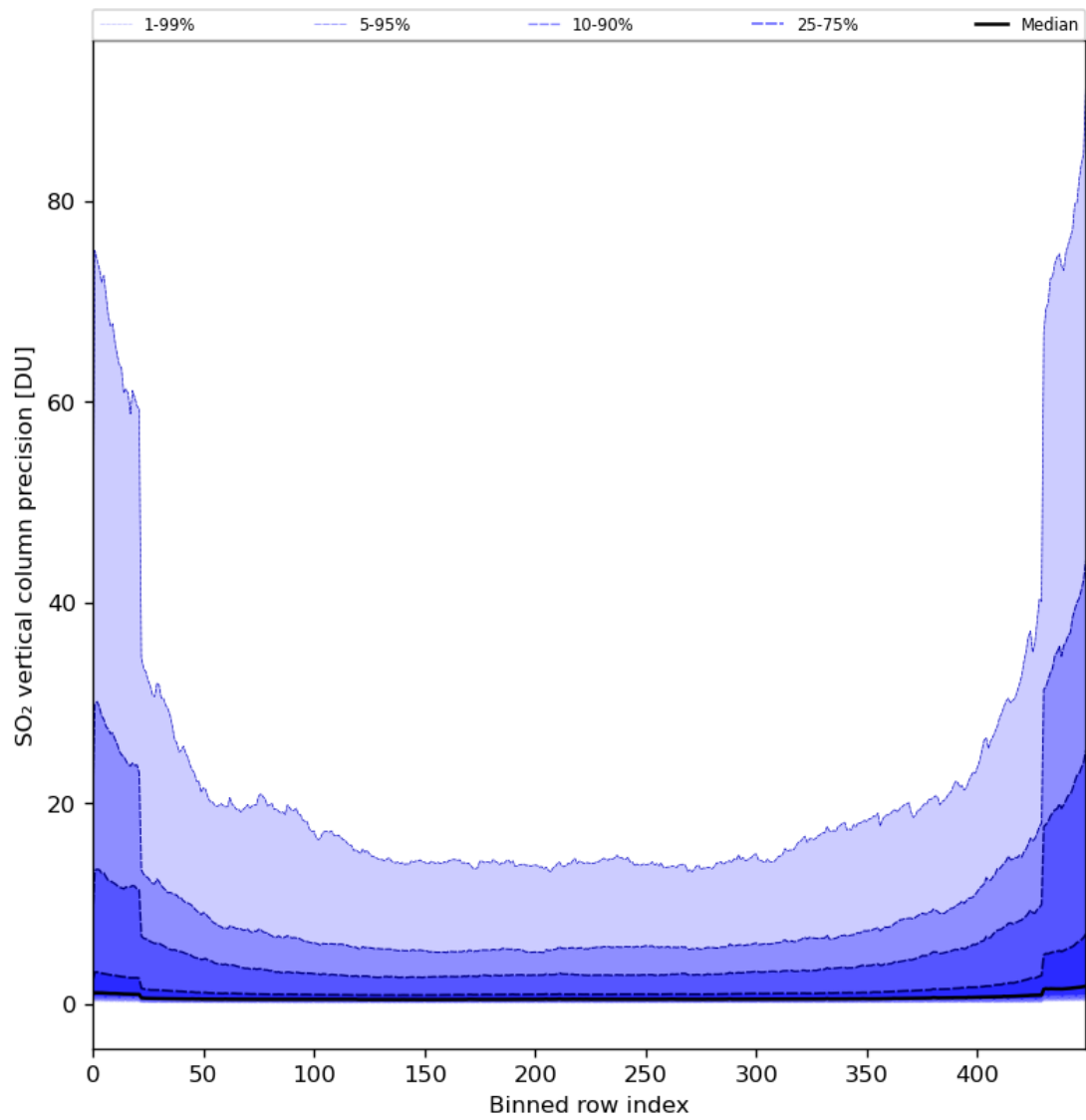
Figure 77: Along track statistics of “SO 2 vertical column precision” for 2024-02-16 to 2024-02-17
