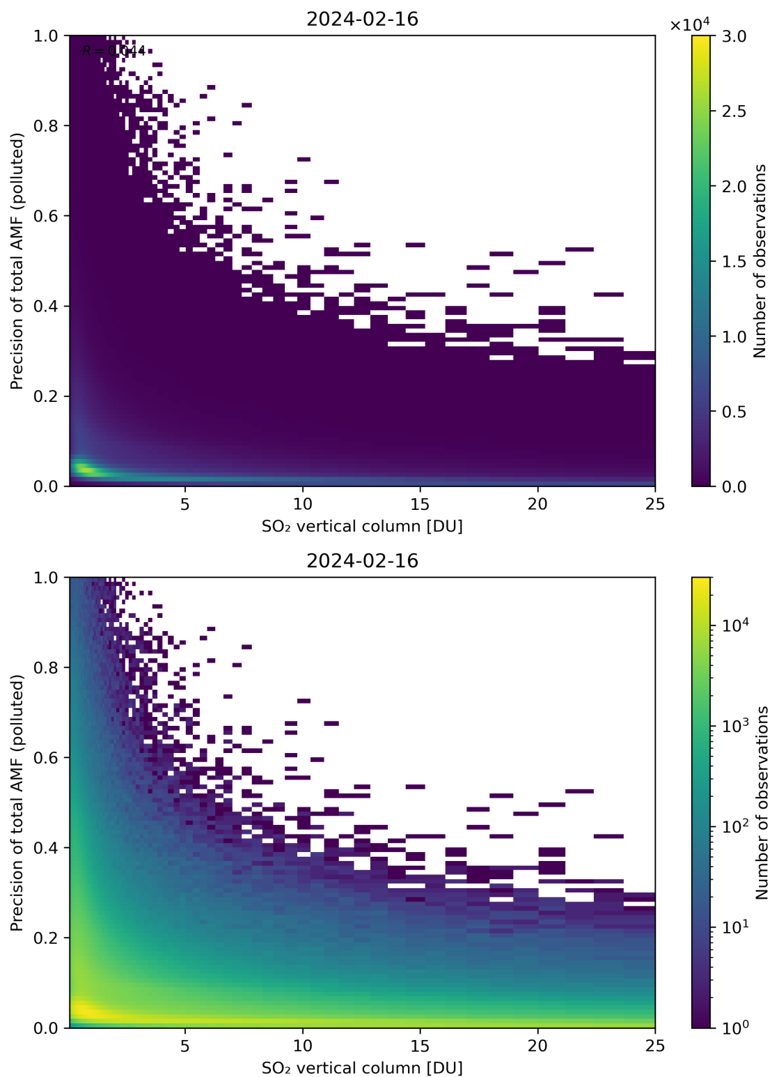
Figure 306: Scatter density plot of “SO 2 vertical column” against “Precision of total AMF (polluted)” for 2024-02-16 to 2024-02-17.
