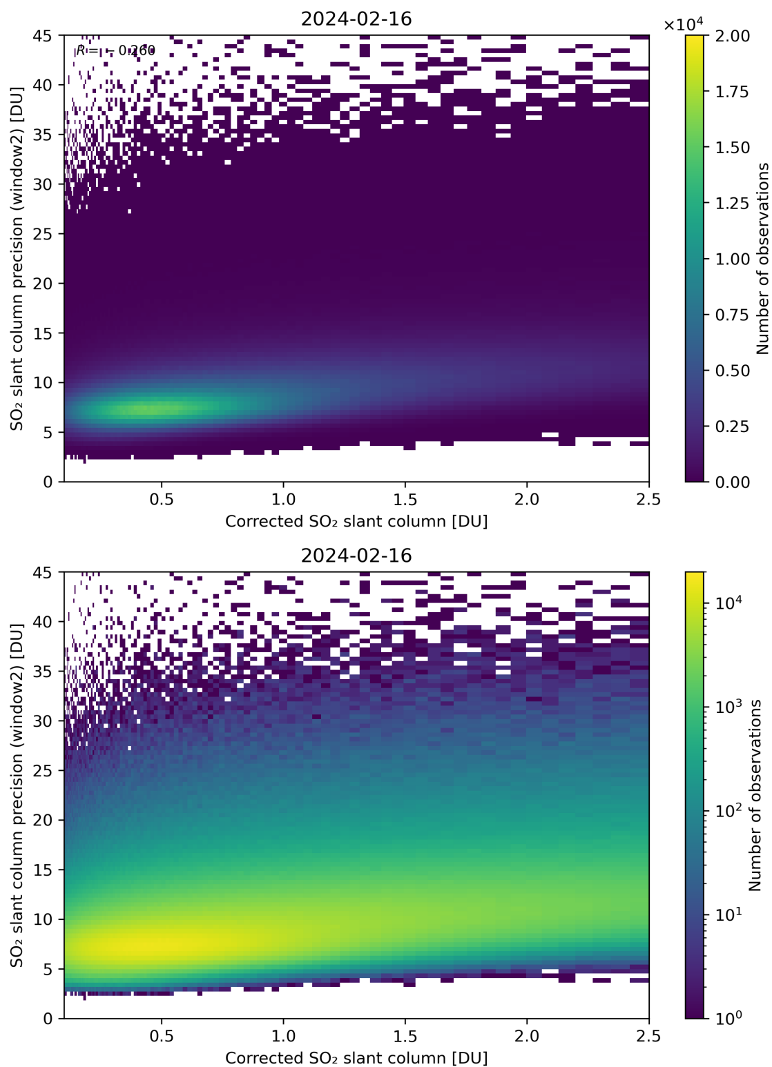
Figure 189: Scatter density plot of “Corrected SO 2 slant column” against “SO 2 slant column precision (window2)” for 2024-02-16 to 2024-02-17.
