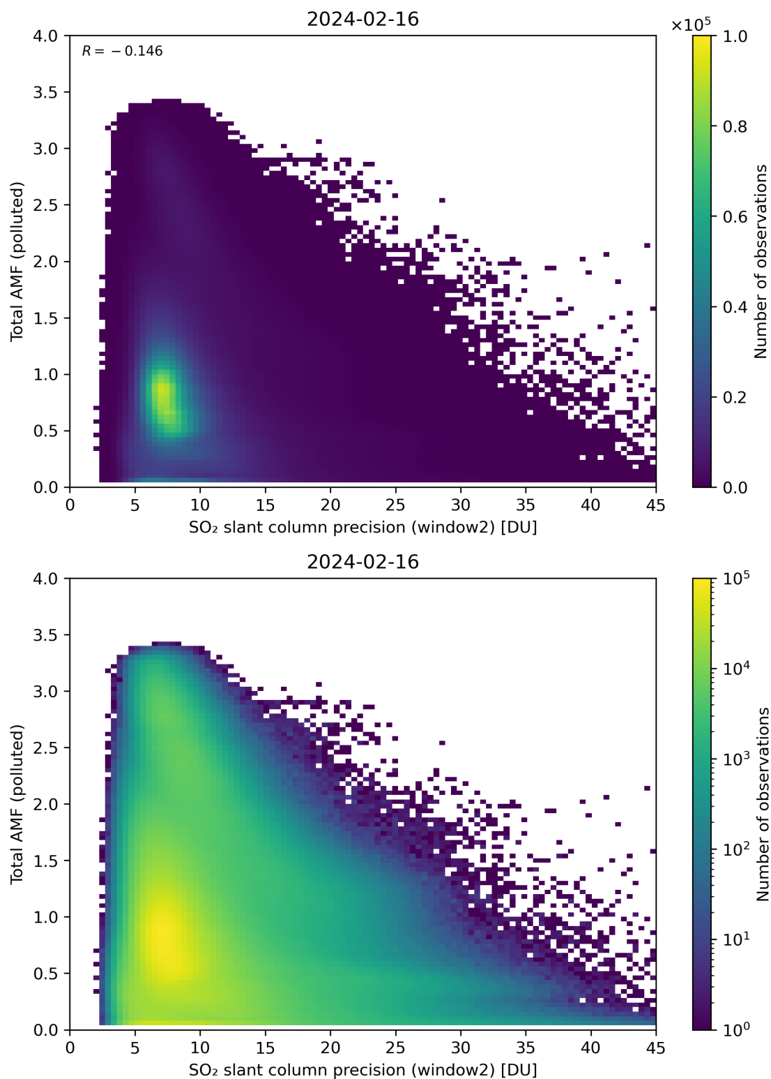
Figure 251: Scatter density plot of “SO 2 slant column precision (window2)” against “Total AMF (polluted)” for 2024-02-16 to 2024-02-17.
