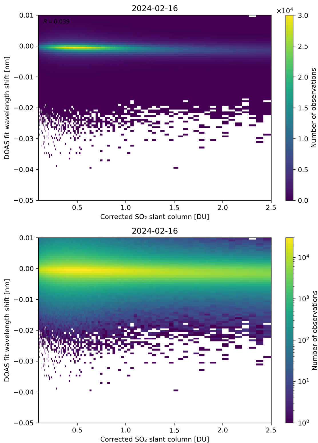
Figure 181: Scatter density plot of “Corrected SO 2 slant column” against “DOAS fit wavelength shift” for 2024-02-16 to 2024-02-17.
