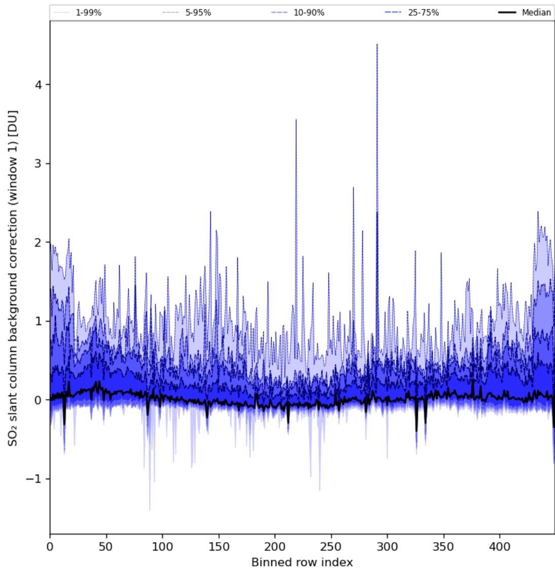
Figure 82: Along track statistics of “SO 2 slant column background correction (window 1)” for 2024-02-16 to 2024-02-17
