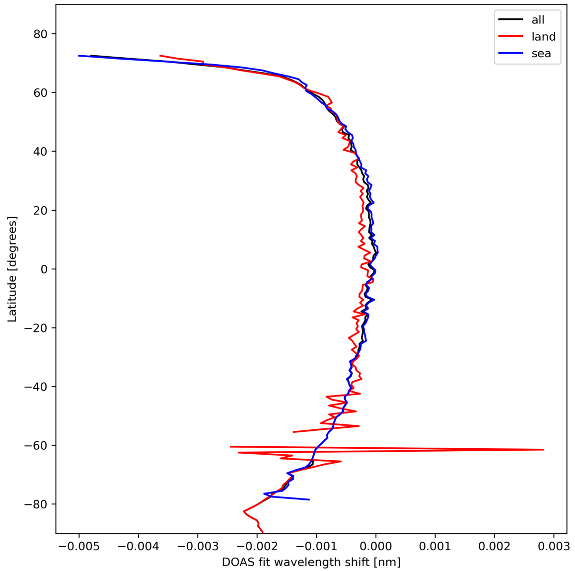
Figure 45: Zonal average of “DOAS fit wavelength shift” for 2024-02-16 to 2024-02-17.
