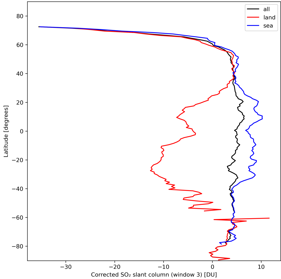
Figure 43: Zonal average of “Corrected SO 2 slant column (window 3)” for 2024-02-16 to 2024-02-17.
