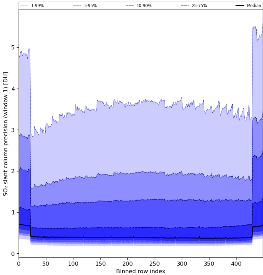
Figure 80: Along track statistics of “SO 2 slant column precision (window 1)” for 2024-02-16 to 2024-02-17
