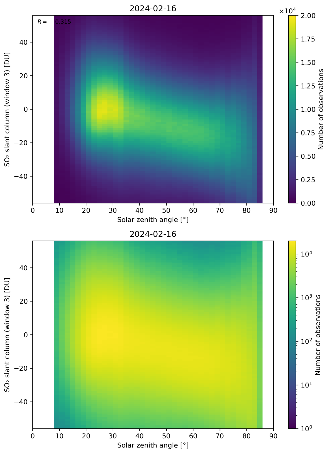
Figure 172: Scatter density plot of “Solar zenith angle” against “SO 2 slant column (window 3)” for 2024-02-16 to 2024-02-17.
