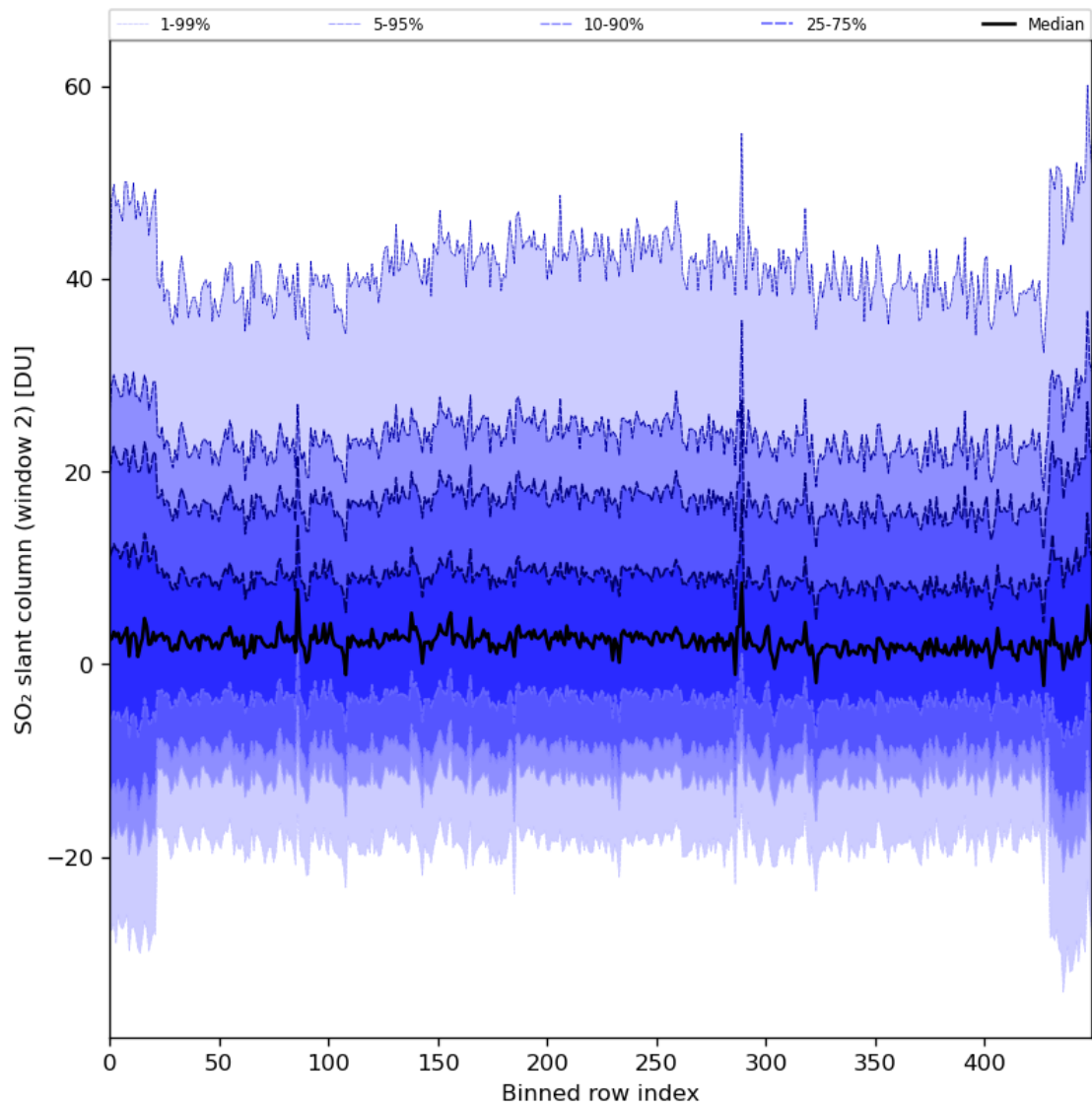
Figure 83: Along track statistics of “SO 2 slant column (window 2)” for 2024-02-16 to 2024-02-17
