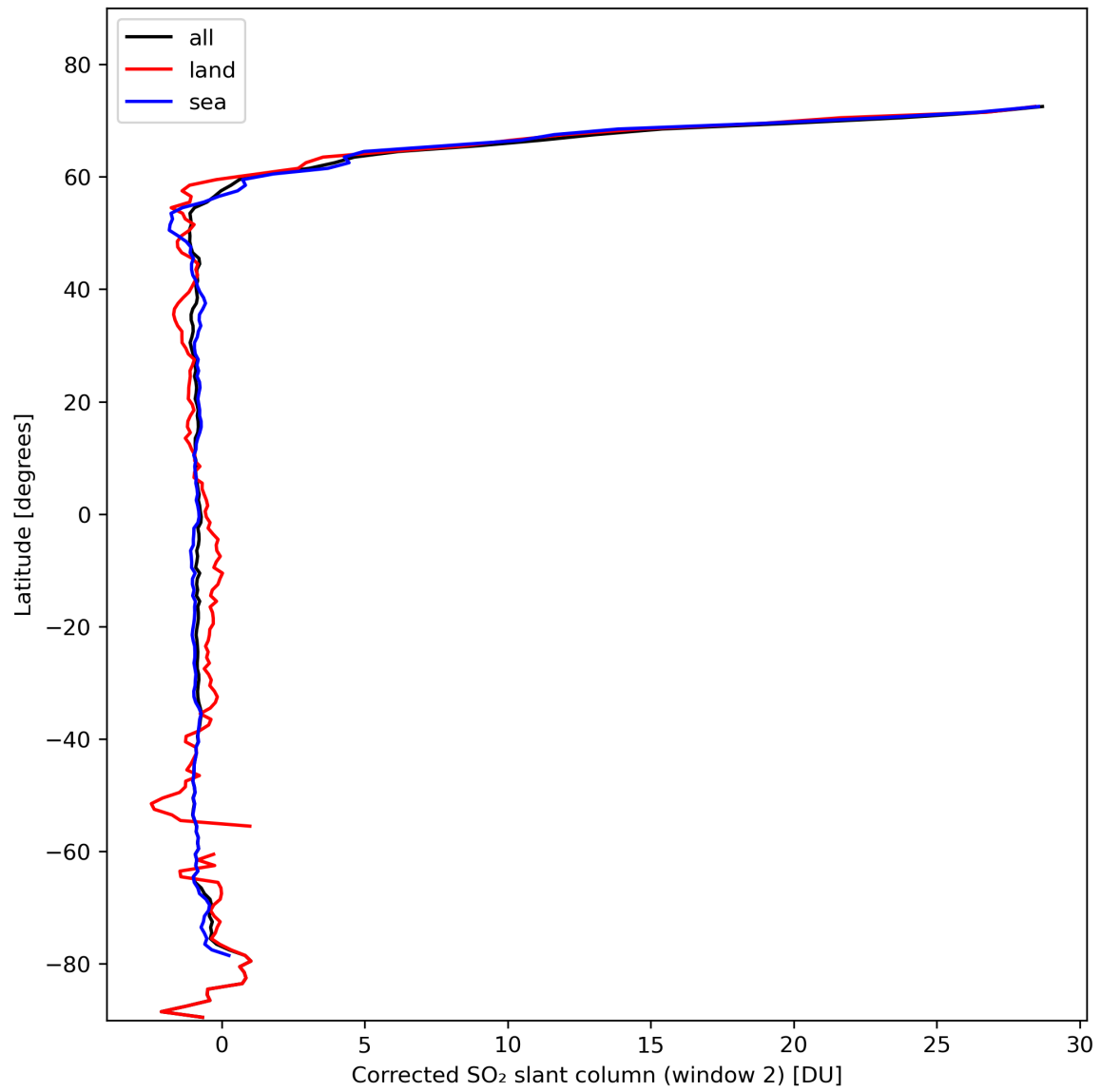
Figure 39: Zonal average of “Corrected SO 2 slant column (window 2)” for 2024-02-16 to 2024-02-17.
