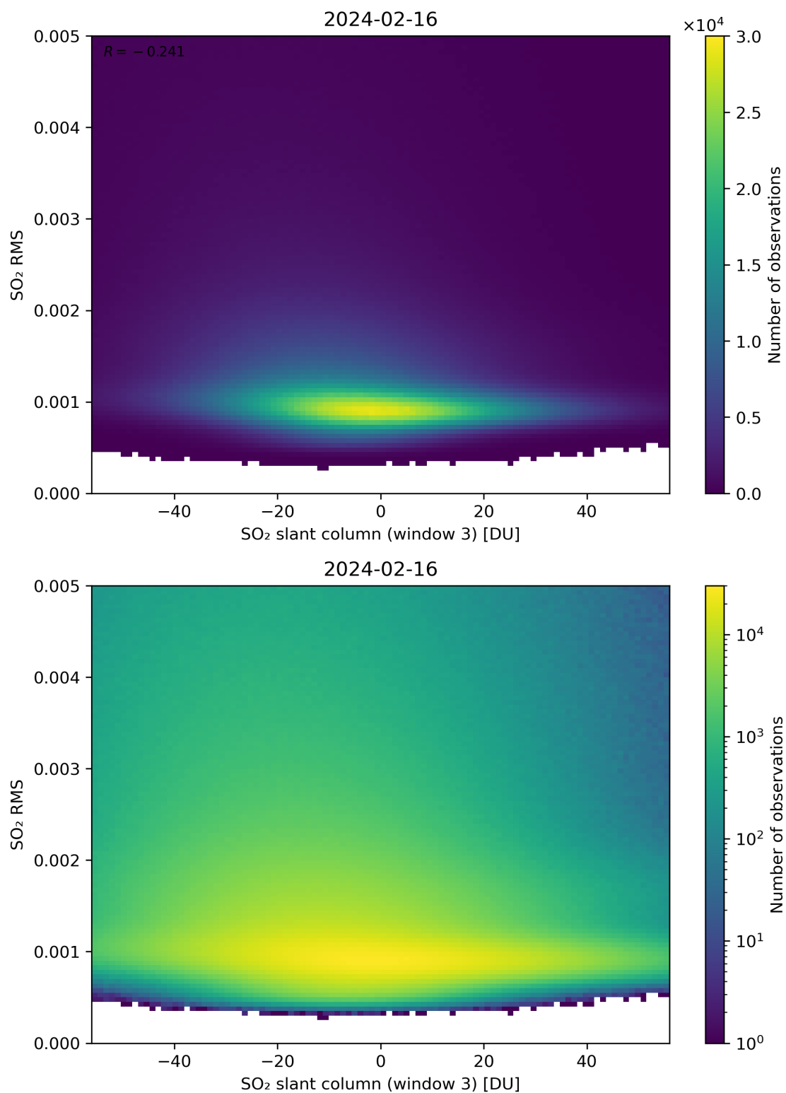
Figure 256: Scatter density plot of “SO 2 slant column (window 3)” against “SO 2 RMS” for 2024-02-16 to 2024-02-17.
