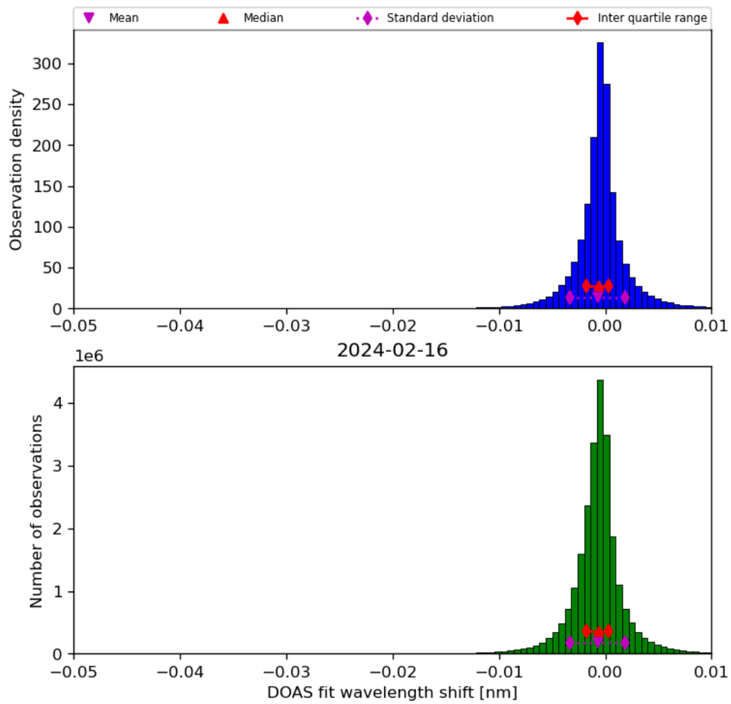
Figure 68: Histogram of “DOAS fit wavelength shift” for 2024-02-16 to 2024-02-17
