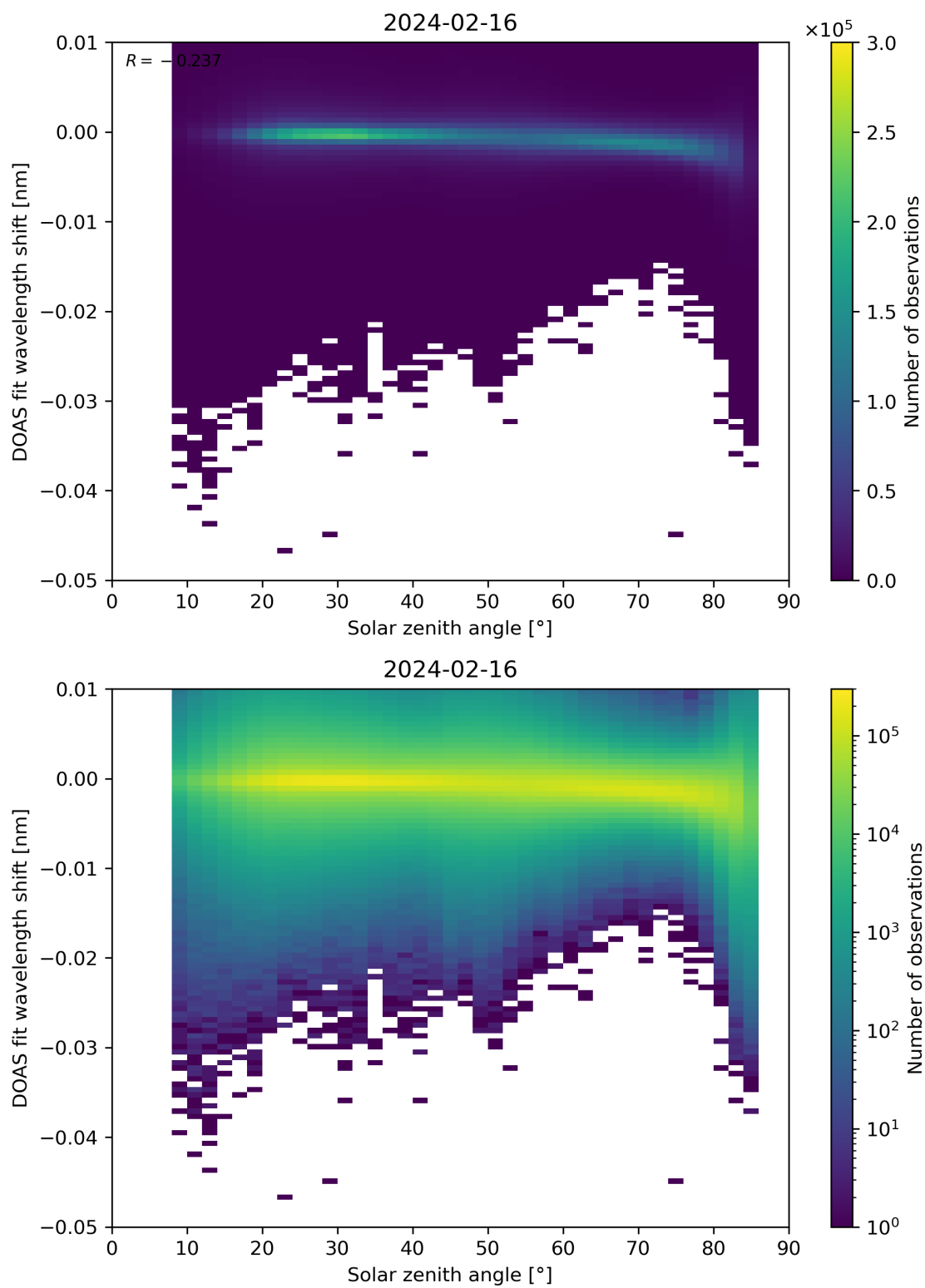
Figure 161: Scatter density plot of “Solar zenith angle” against “DOAS fit wavelength shift” for 2024-02-16 to 2024-02-17.
