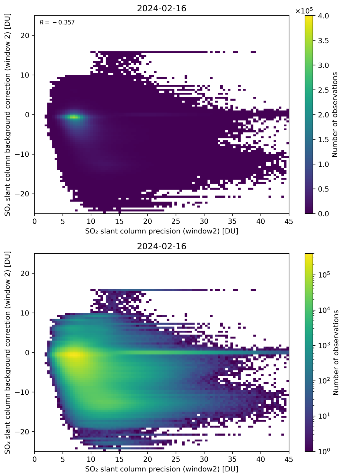
Figure 241: Scatter density plot of “SO 2 slant column precision (window2)” against “SO 2 slant column background correction (window 2)” for 2024-02-16 to 2024-02-17.
