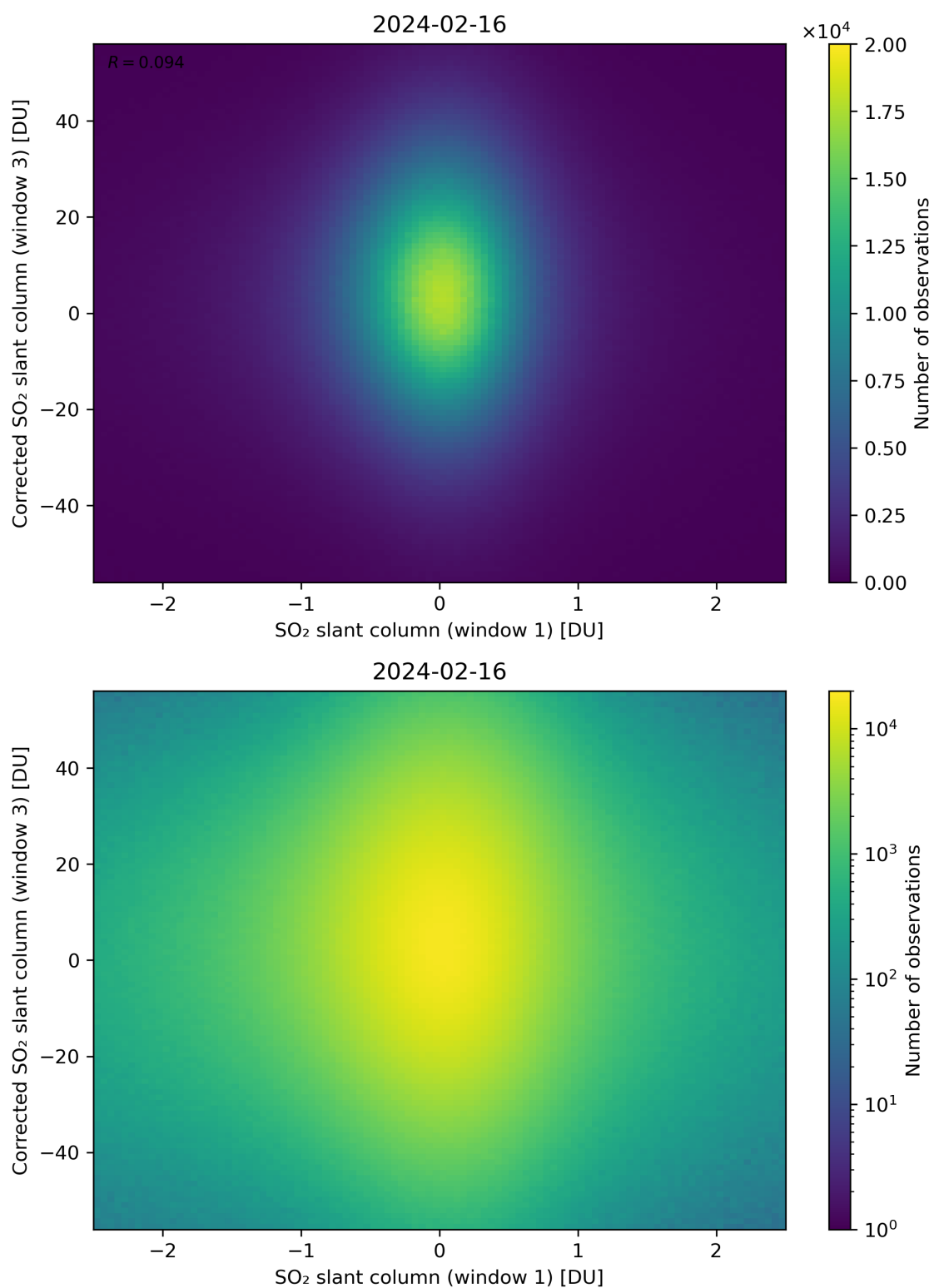
Figure 234: Scatter density plot of “SO 2 slant column (window 1)” against “Corrected SO 2 slant column (window 3)” for 2024-02-16 to 2024-02-17.
