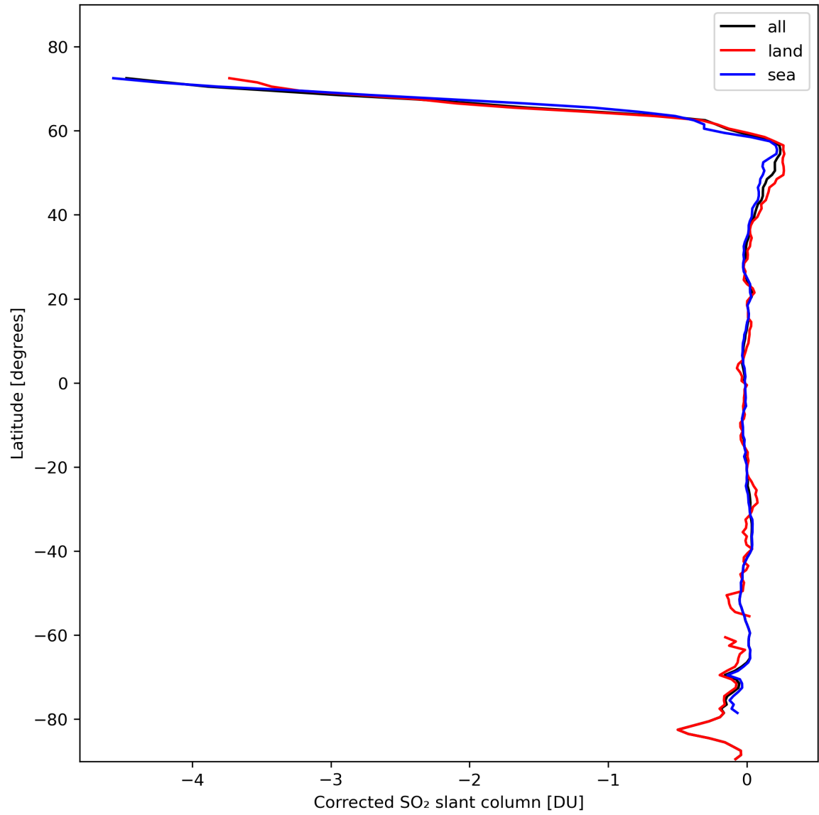
Figure 32: Zonal average of “Corrected SO 2 slant column” for 2024-02-16 to 2024-02-17.
