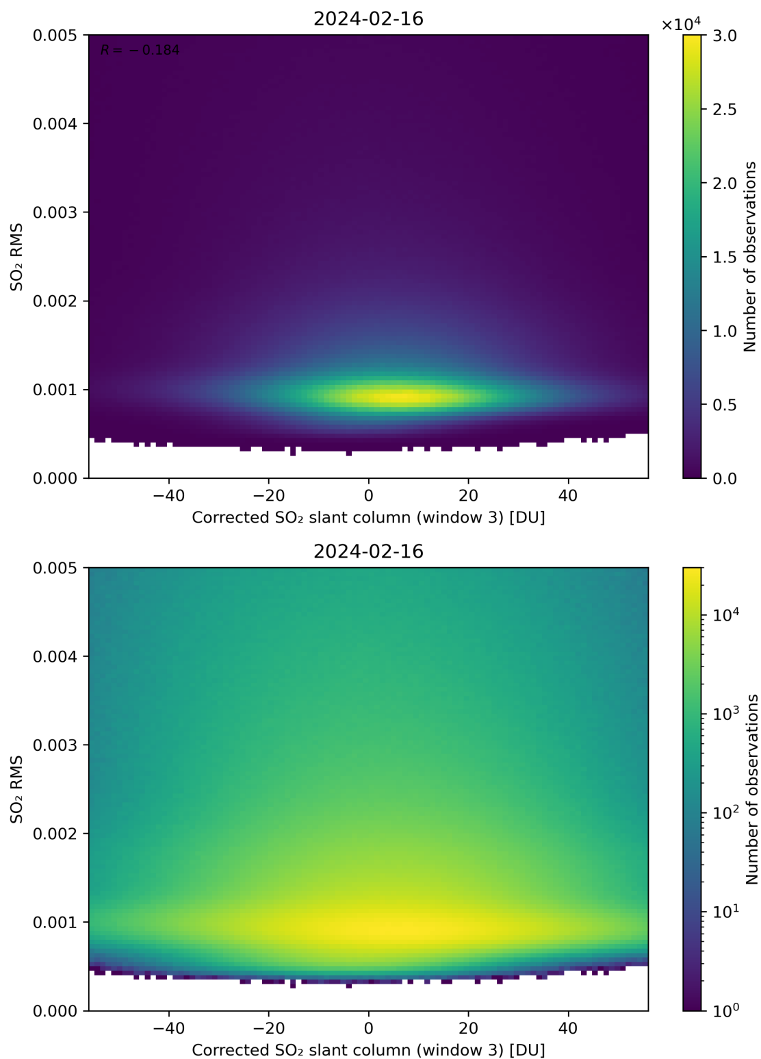
Figure 208: Scatter density plot of “Corrected SO 2 slant column (window 3)” against “SO 2 RMS” for 2024-02-16 to 2024-02-17.
