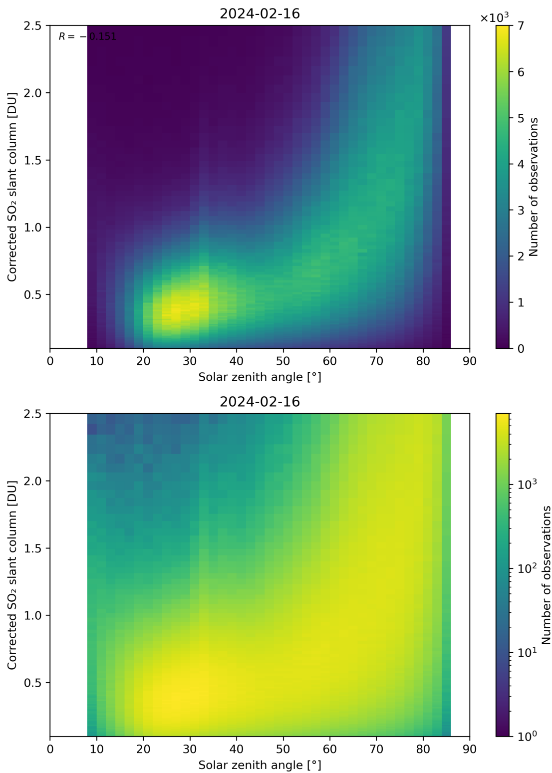
Figure 166: Scatter density plot of “Solar zenith angle” against “Corrected SO 2 slant column” for 2024-02-16 to 2024-02-17.
