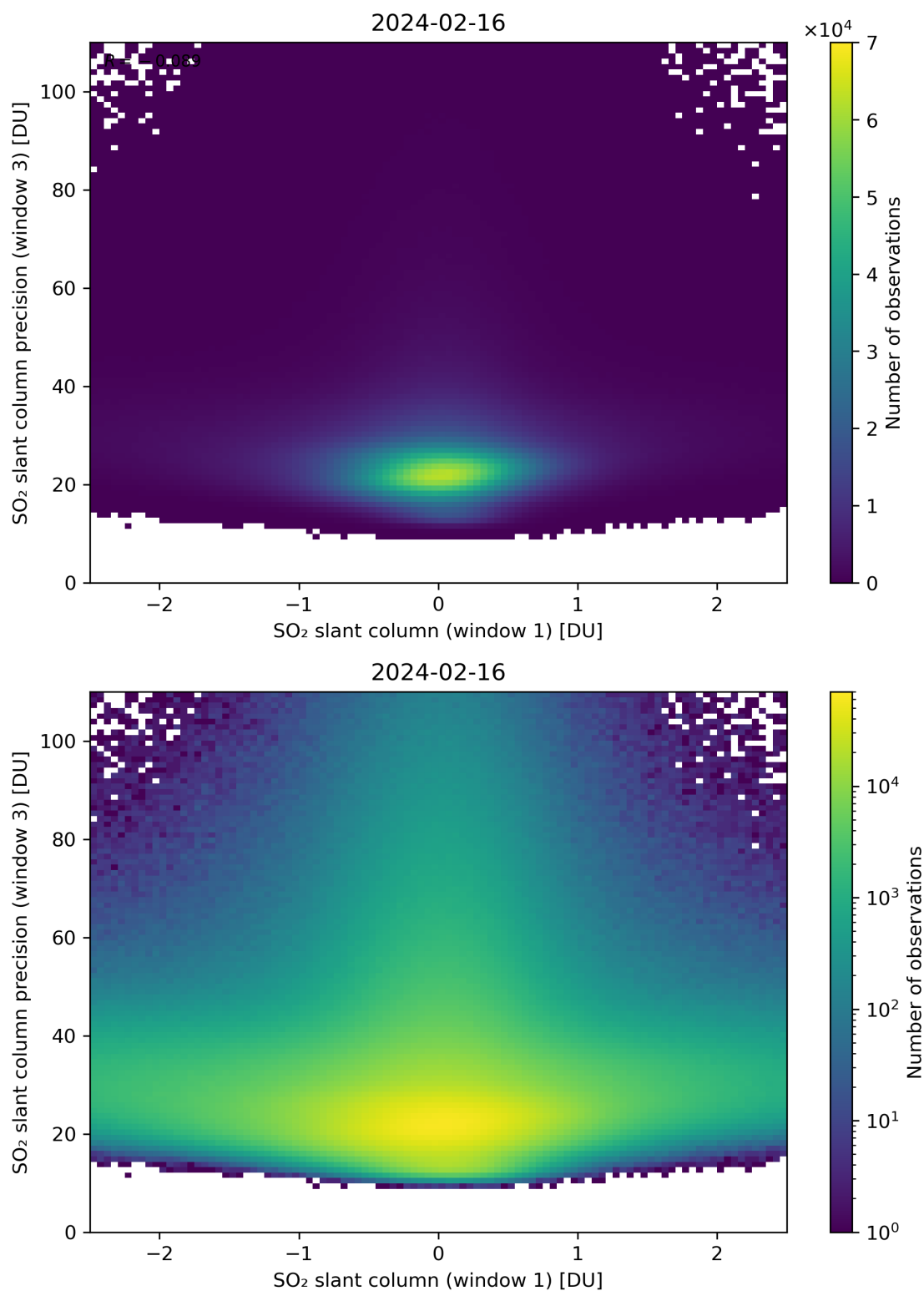
Figure 238: Scatter density plot of “SO 2 slant column (window 1)” against “SO 2 slant column precision (window 3)” for 2024-02-16 to 2024-02-17.
