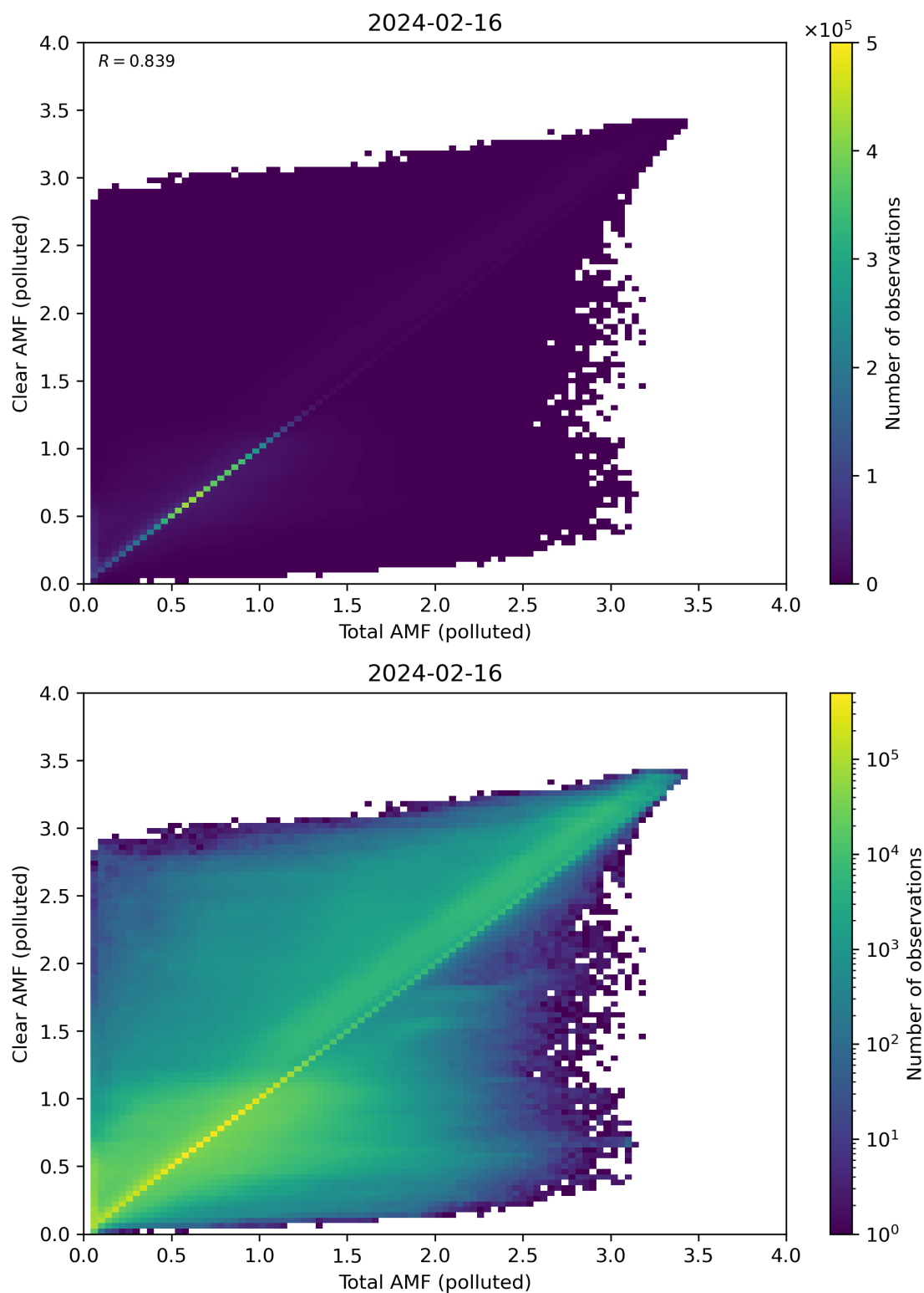
Figure 271: Scatter density plot of “Total AMF (polluted)” against “Clear AMF (polluted)” for 2024-02-16 to 2024-02-17.
