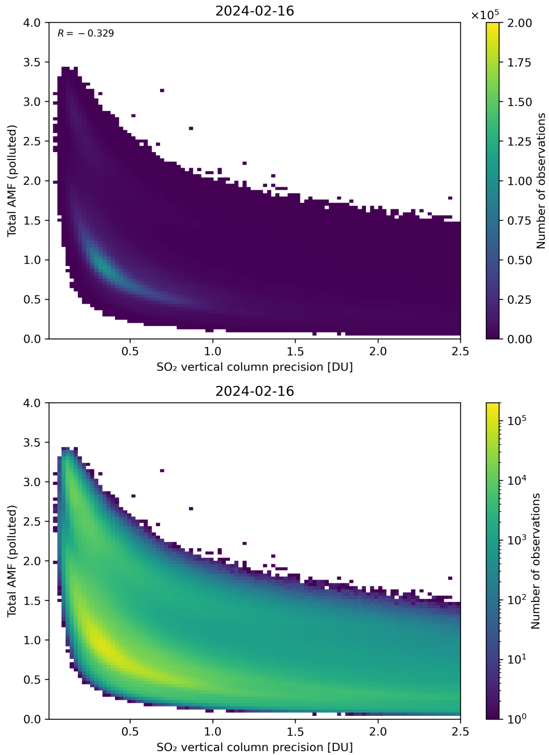
Figure 294: Scatter density plot of “SO 2 vertical column precision” against “Total AMF (polluted)” for 2024-02-16 to 2024-02-17.
