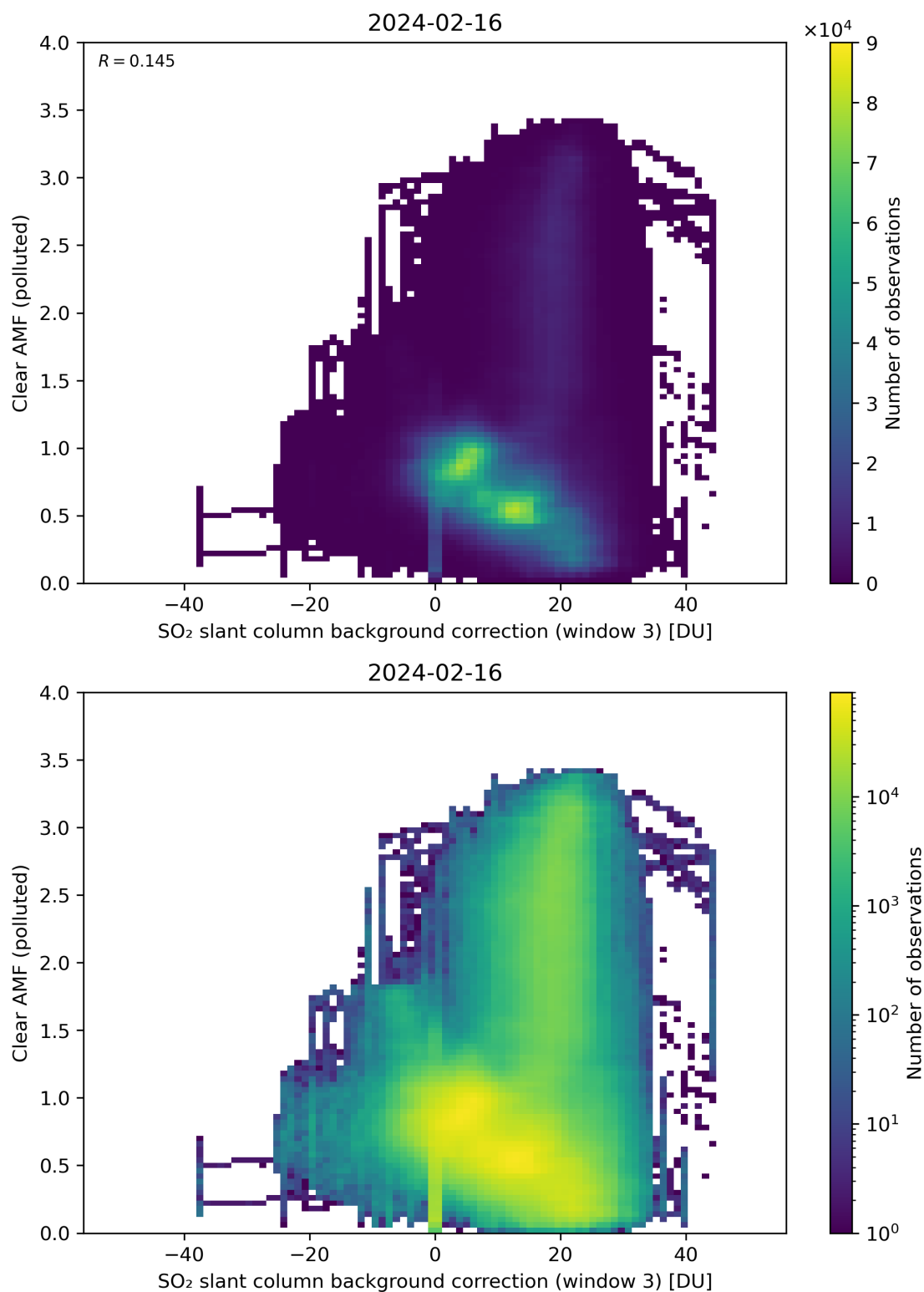
Figure 124: Scatter density plot of “SO 2 slant column background correction (window 3)” against “Clear AMF (polluted)” for 2024-02-16 to 2024-02-17.
