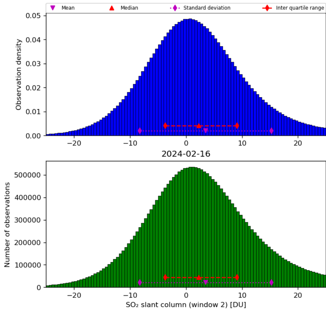
Figure 60: Histogram of “SO 2 slant column (window 2)” for 2024-02-16 to 2024-02-17
