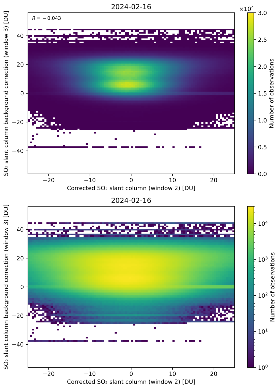
Figure 195: Scatter density plot of “Corrected SO 2 slant column (window 2)” against “SO 2 slant column background correction (window 3)” for 2024-02-16 to 2024-02-17.
