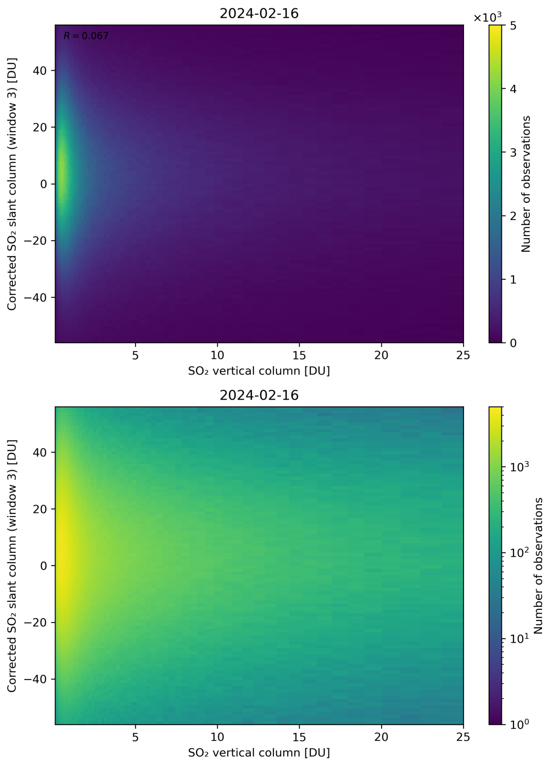
Figure 299: Scatter density plot of “SO 2 vertical column” against “Corrected SO 2 slant column (window 3)” for 2024-02-16 to 2024-02-17.
