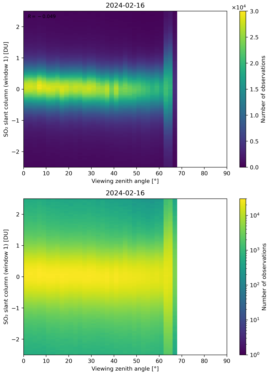
Figure 320: Scatter density plot of “Viewing zenith angle” against “SO 2 slant column (window 1)” for 2024-02-16 to 2024-02-17.
