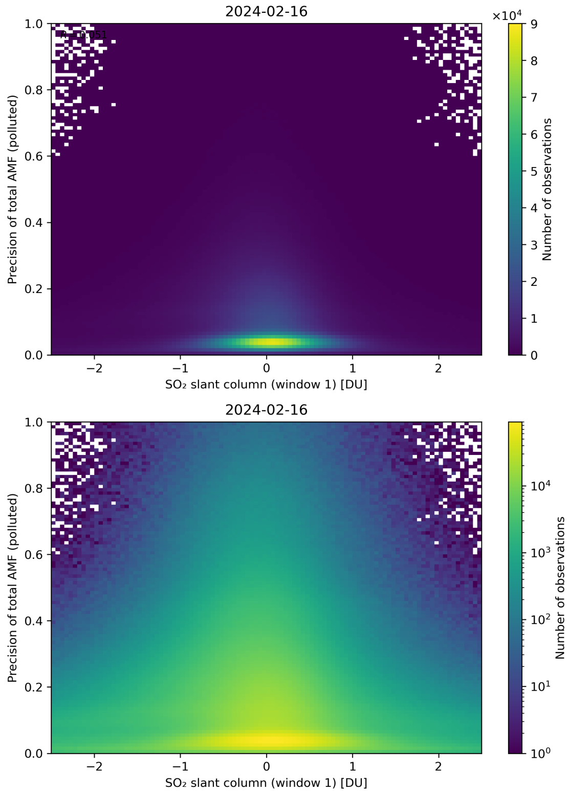
Figure 240: Scatter density plot of “SO 2 slant column (window 1)” against “Precision of total AMF (polluted)” for 2024-02-16 to 2024-02-17.
