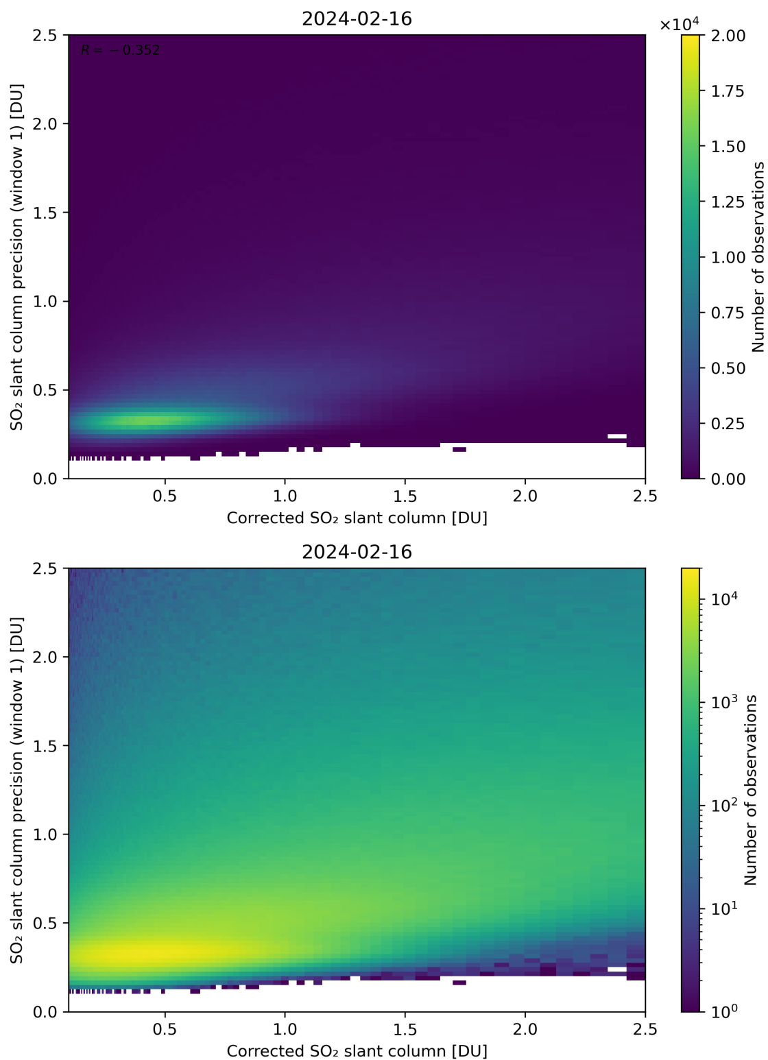
Figure 188: Scatter density plot of “Corrected SO 2 slant column” against “SO 2 slant column precision (window 1)” for 2024-02-16 to 2024-02-17.
