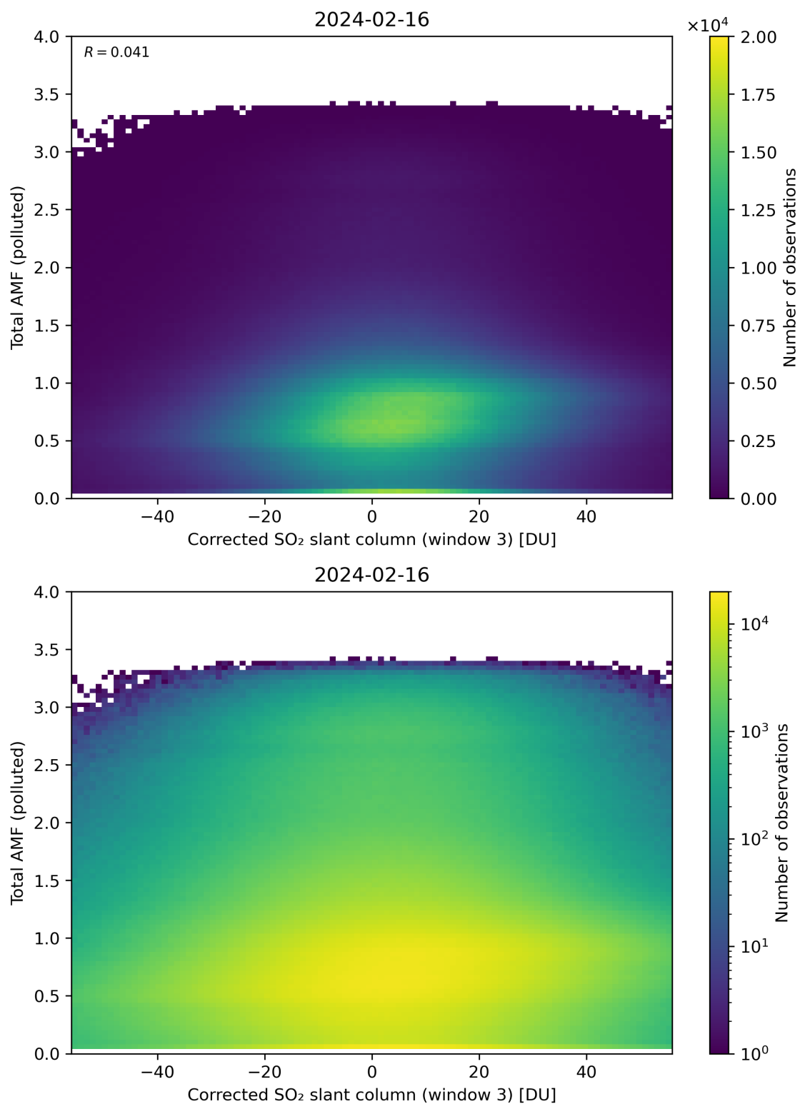
Figure 210: Scatter density plot of “Corrected SO 2 slant column (window 3)” against “Total AMF (polluted)” for 2024-02-16 to 2024-02-17.
