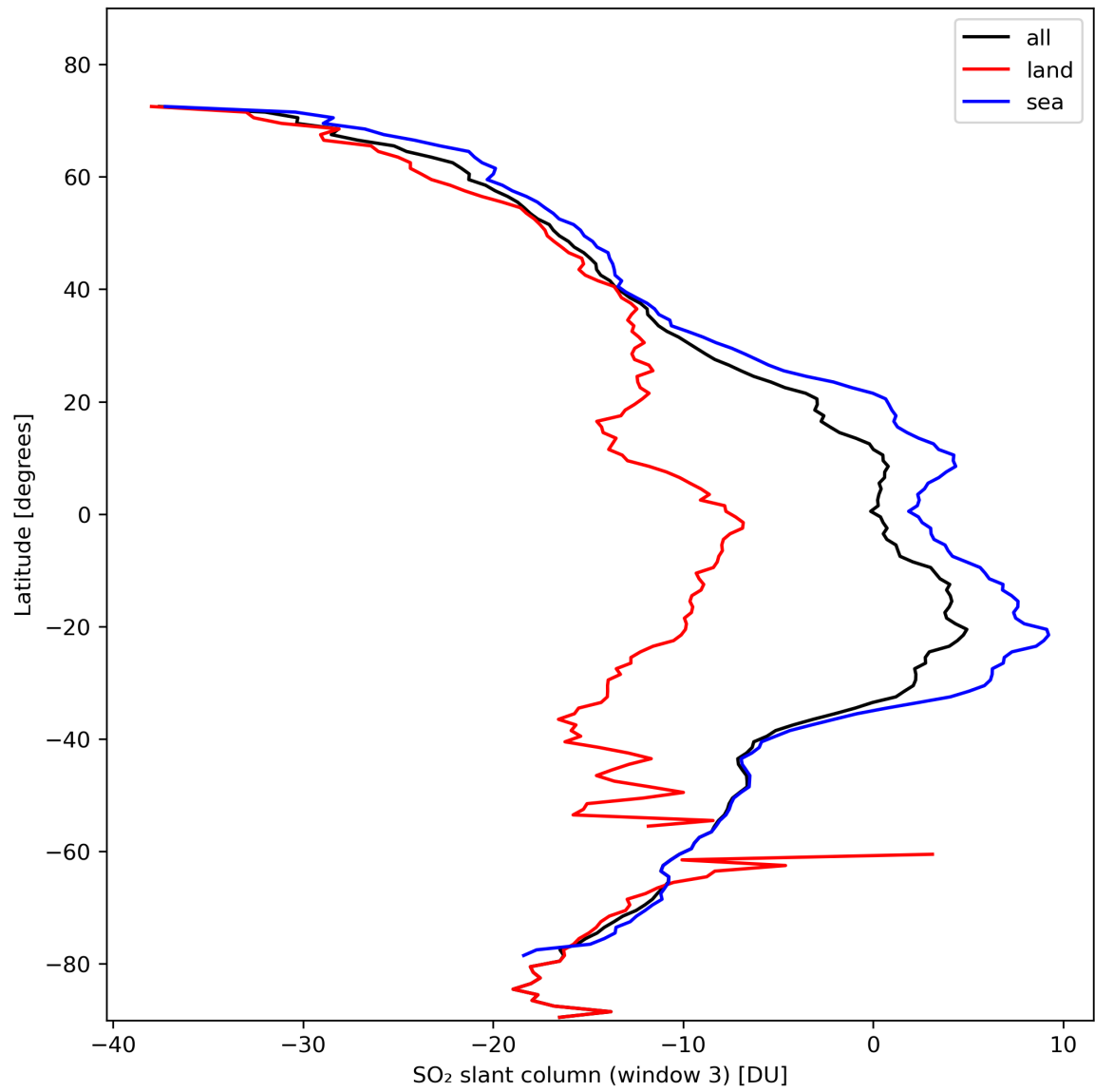
Figure 41: Zonal average of “SO 2 slant column (window 3)” for 2024-02-16 to 2024-02-17.
