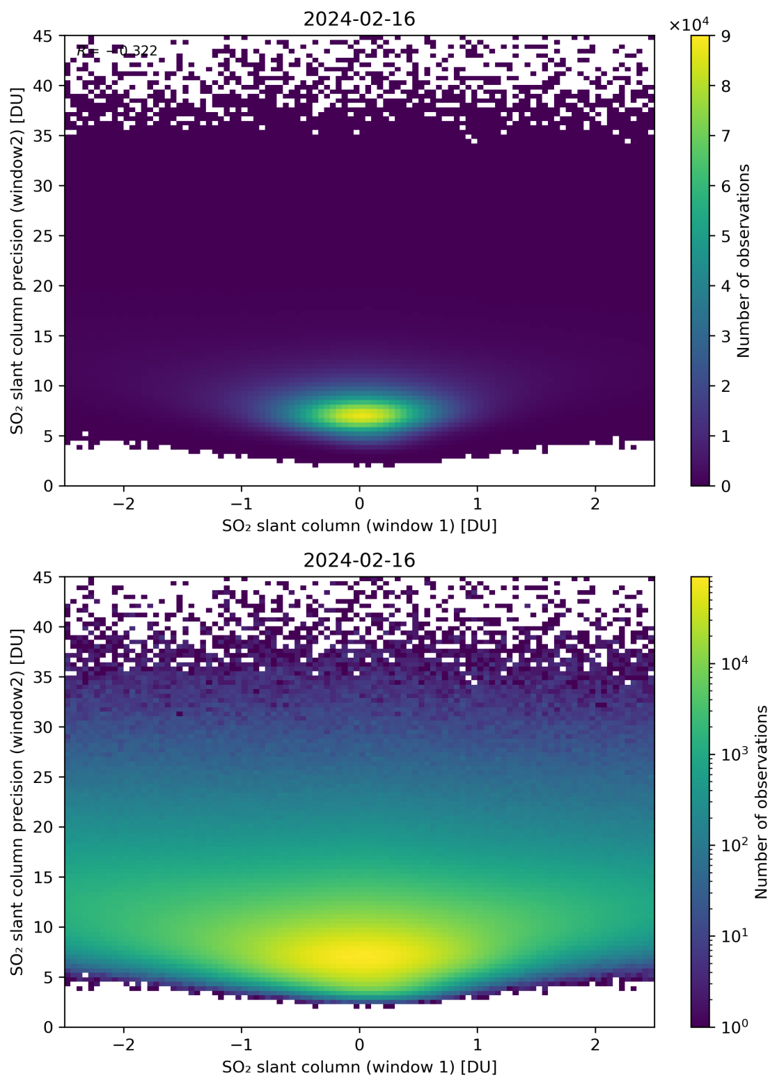
Figure 236: Scatter density plot of “SO 2 slant column (window 1)” against “SO 2 slant column precision (window2)” for 2024-02-16 to 2024-02-17.
