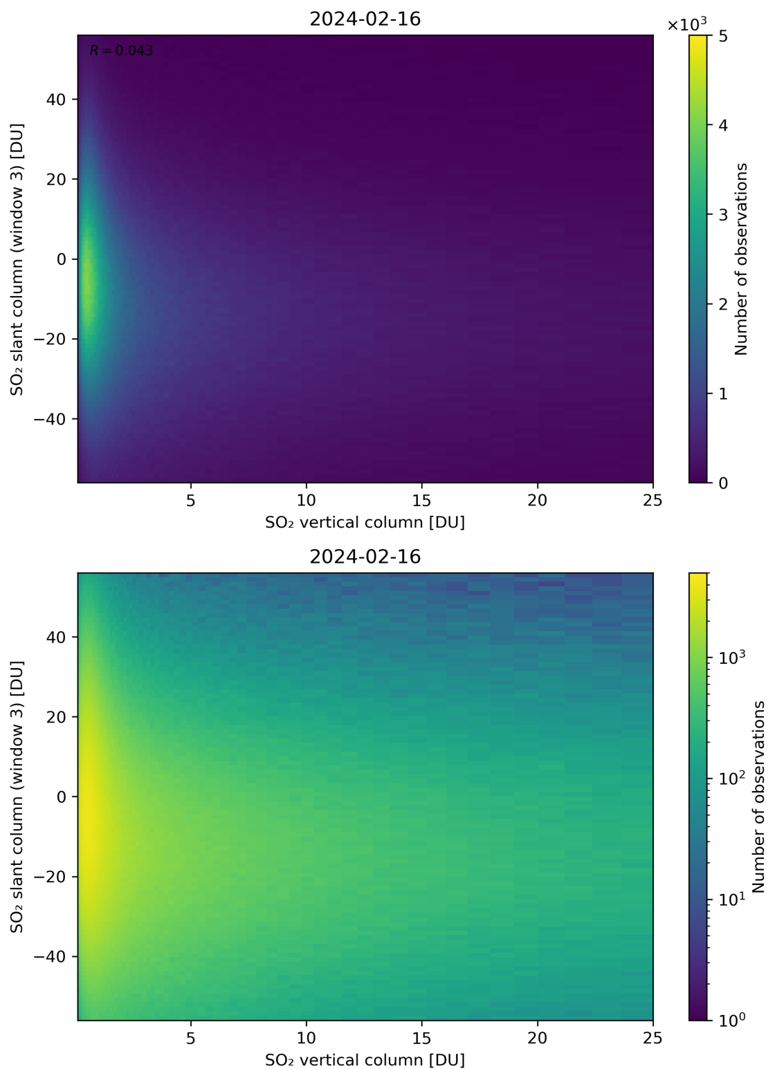
Figure 303: Scatter density plot of “SO 2 vertical column” against “SO 2 slant column (window 3)” for 2024-02-16 to 2024-02-17.
