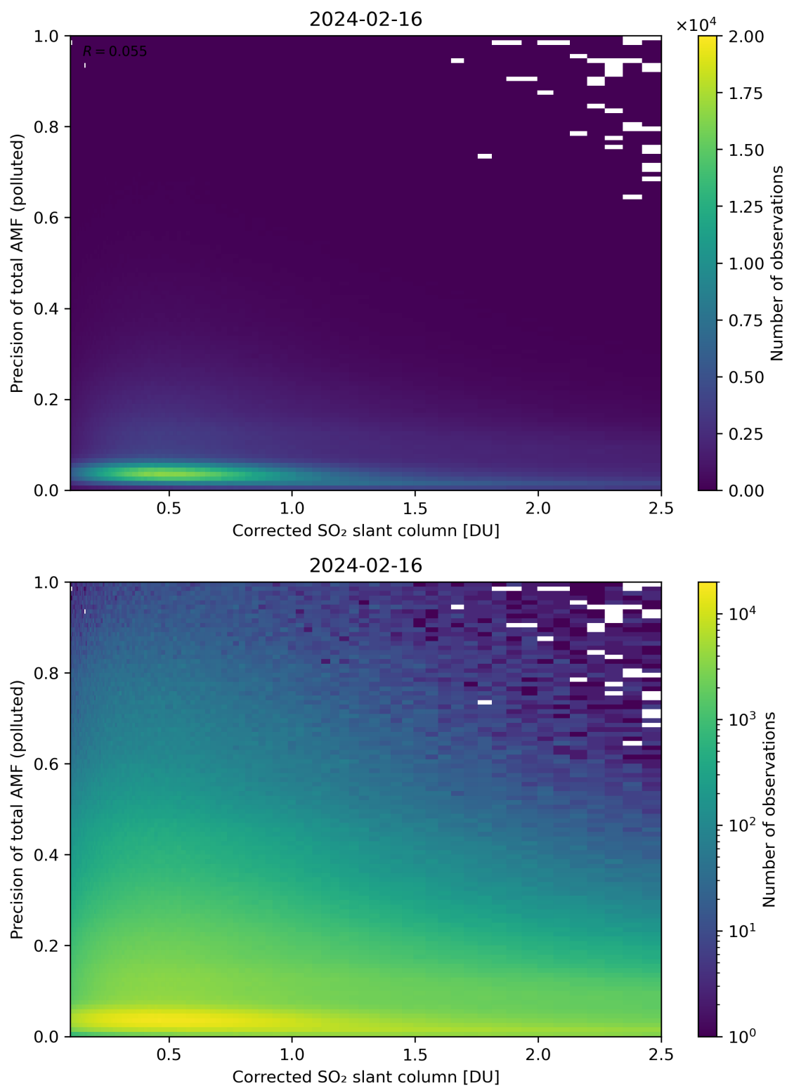
Figure 193: Scatter density plot of “Corrected SO 2 slant column” against “Precision of total AMF (polluted)” for 2024-02-16 to 2024-02-17.
