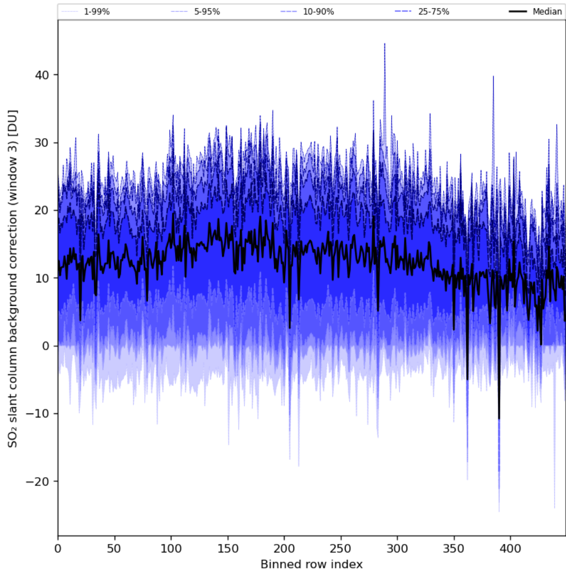
Figure 90: Along track statistics of “SO 2 slant column background correction (window 3)” for 2024-02-16 to 2024-02-17
