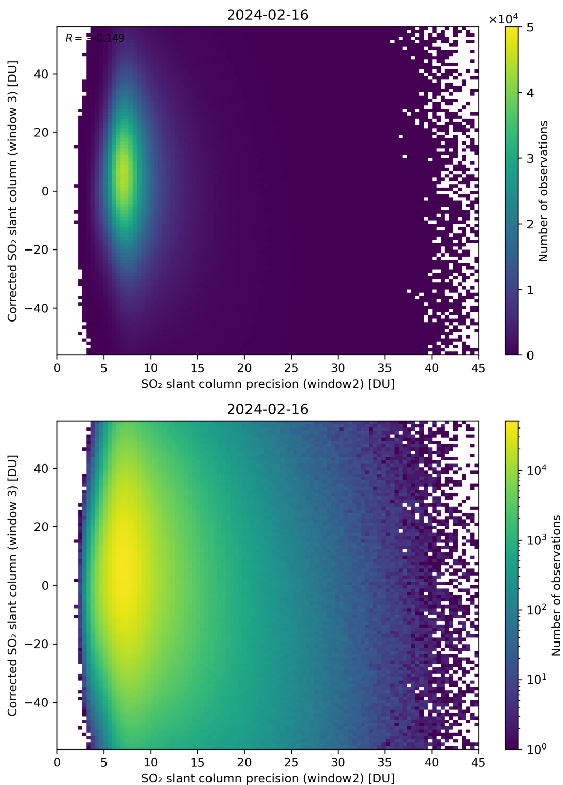
Figure 248: Scatter density plot of “SO 2 slant column precision (window2)” against “Corrected SO 2 slant column (window 3)” for 2024-02-16 to 2024-02-17.
