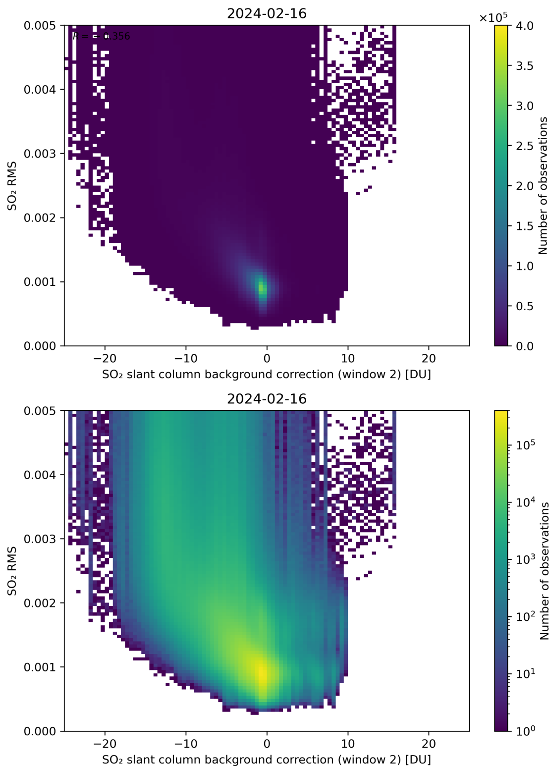
Figure 114: Scatter density plot of “SO 2 slant column background correction (window 2)” against “SO 2 RMS” for 2024-02-16 to 2024-02-17.
