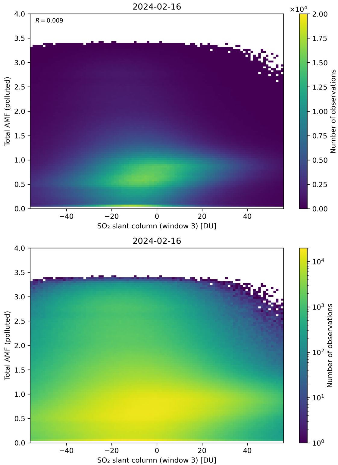
Figure 268: Scatter density plot of “SO 2 slant column (window 3)” against “Total AMF (polluted)” for 2024-02-16 to 2024-02-17.
