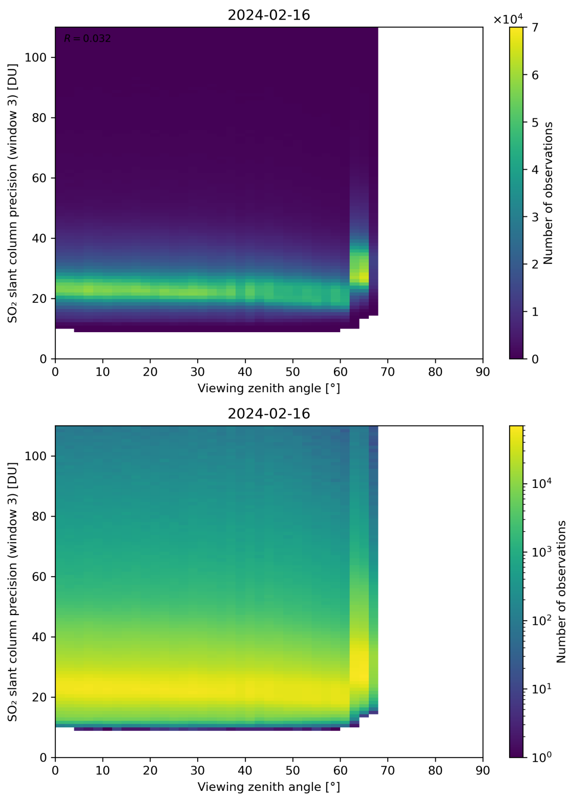
Figure 324: Scatter density plot of “Viewing zenith angle” against “SO 2 slant column precision (window 3)” for 2024-02-16 to 2024-02-17.
