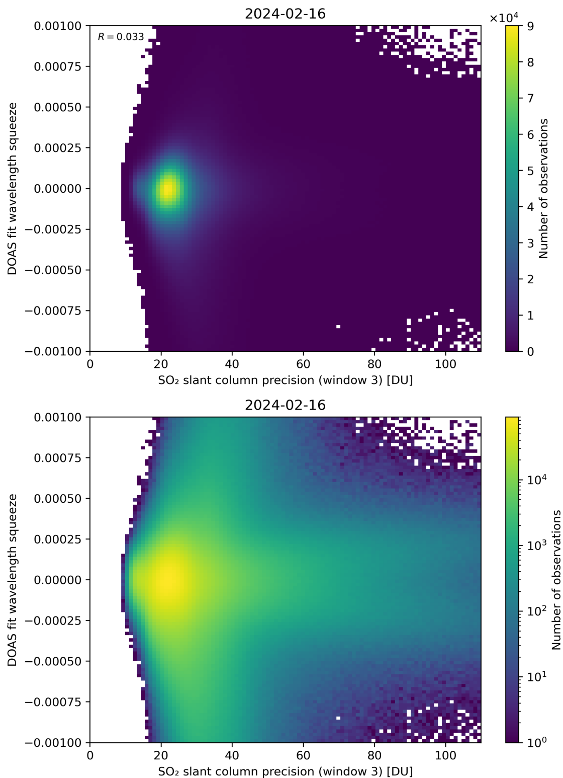
Figure 259: Scatter density plot of “SO 2 slant column precision (window 3)” against “DOAS fit wavelength squeeze” for 2024-02-16 to 2024-02-17.
