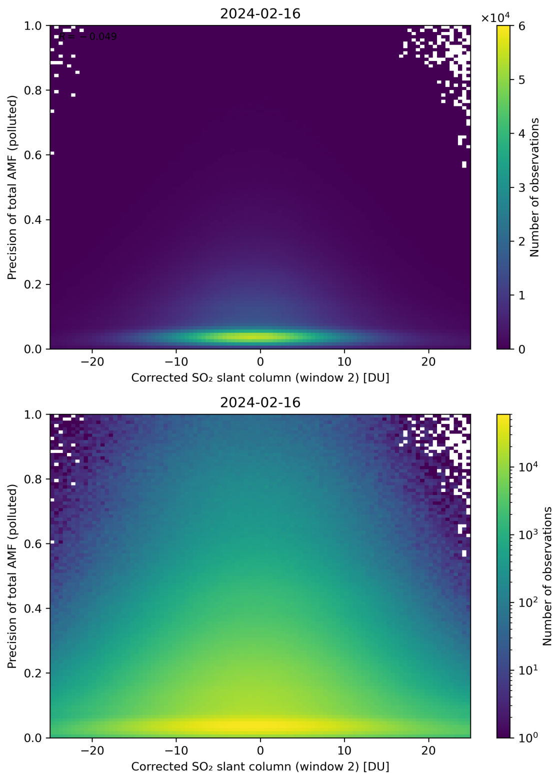
Figure 204: Scatter density plot of “Corrected SO 2 slant column (window 2)” against “Precision of total AMF (polluted)” for 2024-02-16 to 2024-02-17.
