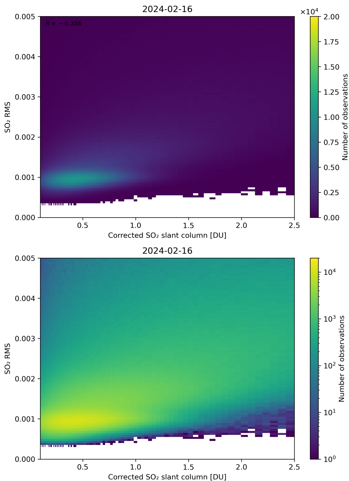
Figure 183: Scatter density plot of “Corrected SO 2 slant column” against “SO 2 RMS” for 2024-02-16 to 2024-02-17.
