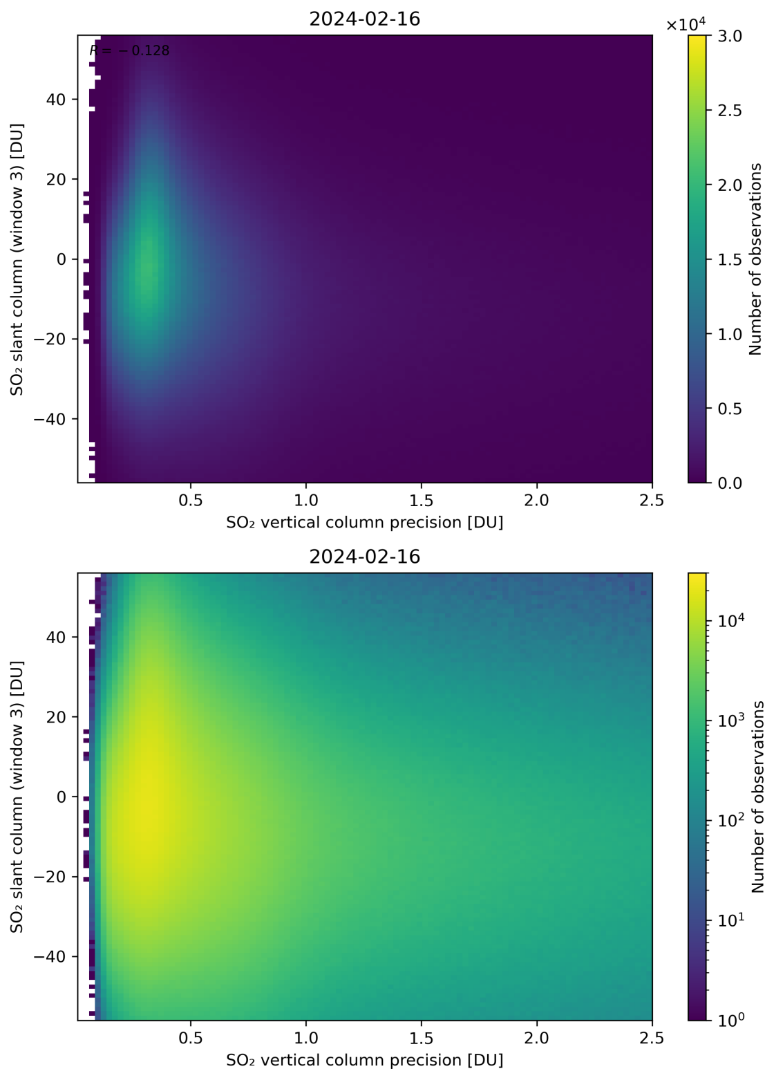
Figure 292: Scatter density plot of “SO 2 vertical column precision” against “SO 2 slant column (window 3)” for 2024-02-16 to 2024-02-17.
