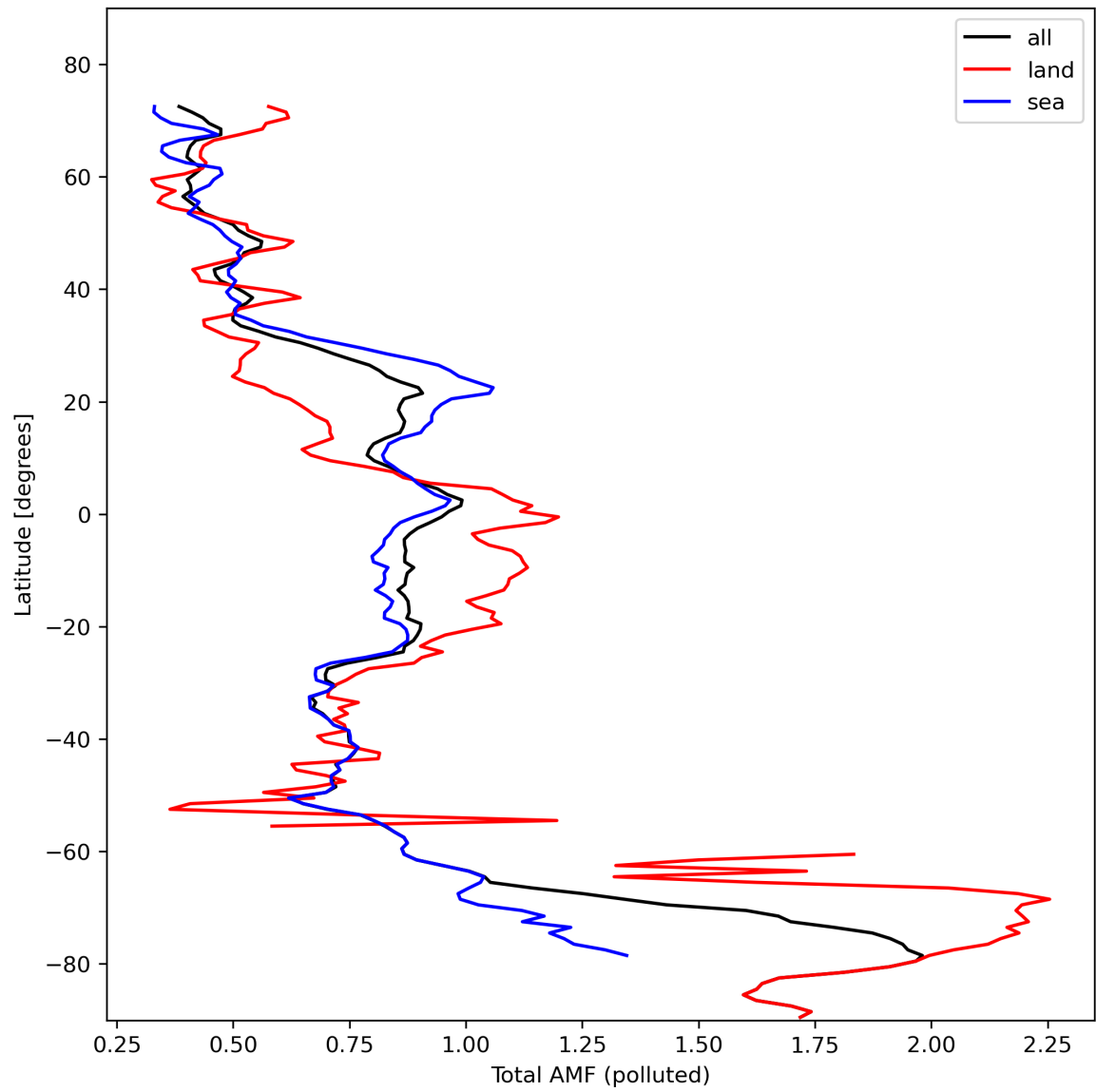
Figure 48: Zonal average of “Total AMF (polluted)” for 2024-02-16 to 2024-02-17.
