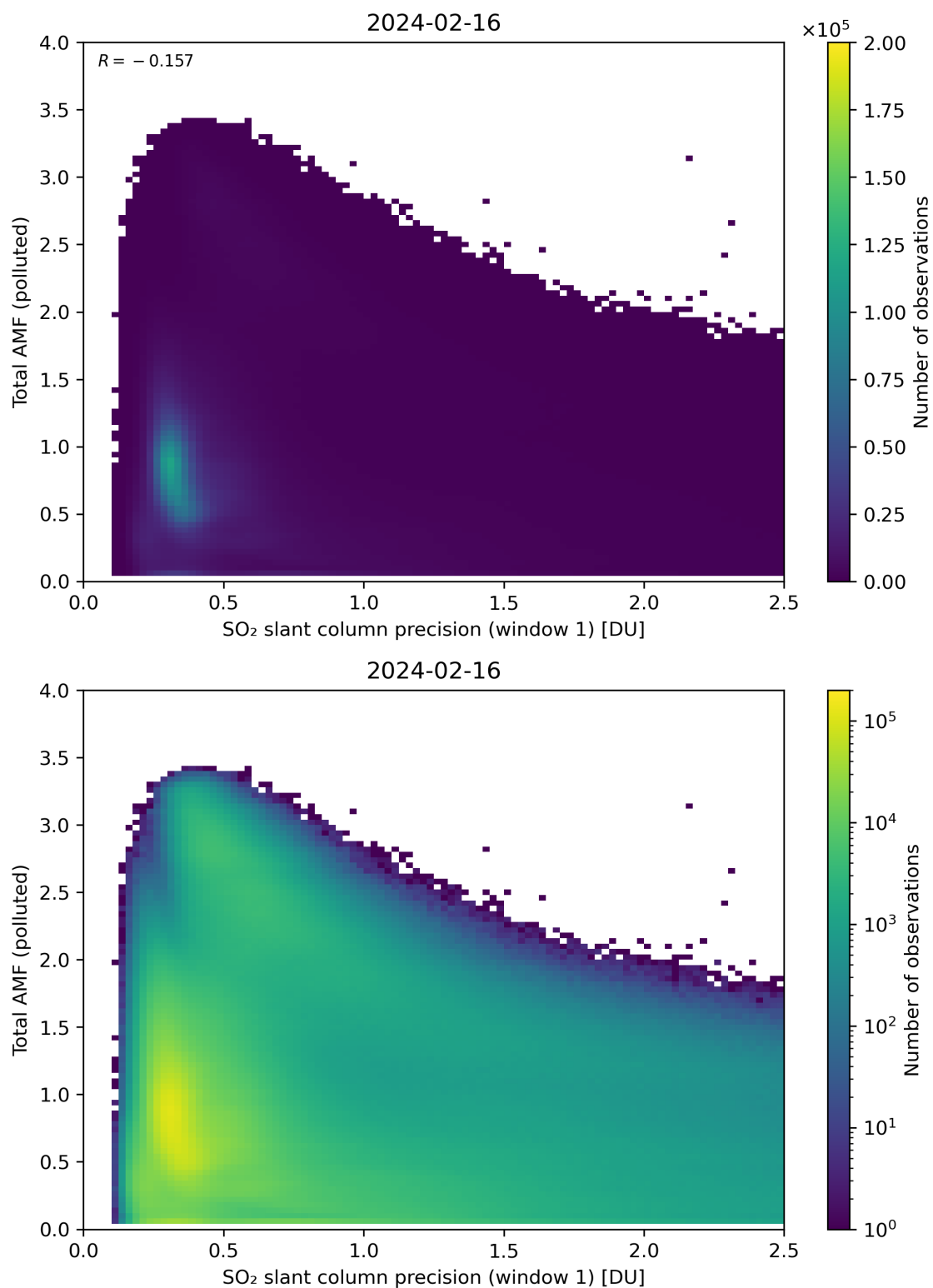
Figure 230: Scatter density plot of “SO 2 slant column precision (window 1)” against “Total AMF (polluted)” for 2024-02-16 to 2024-02-17.
