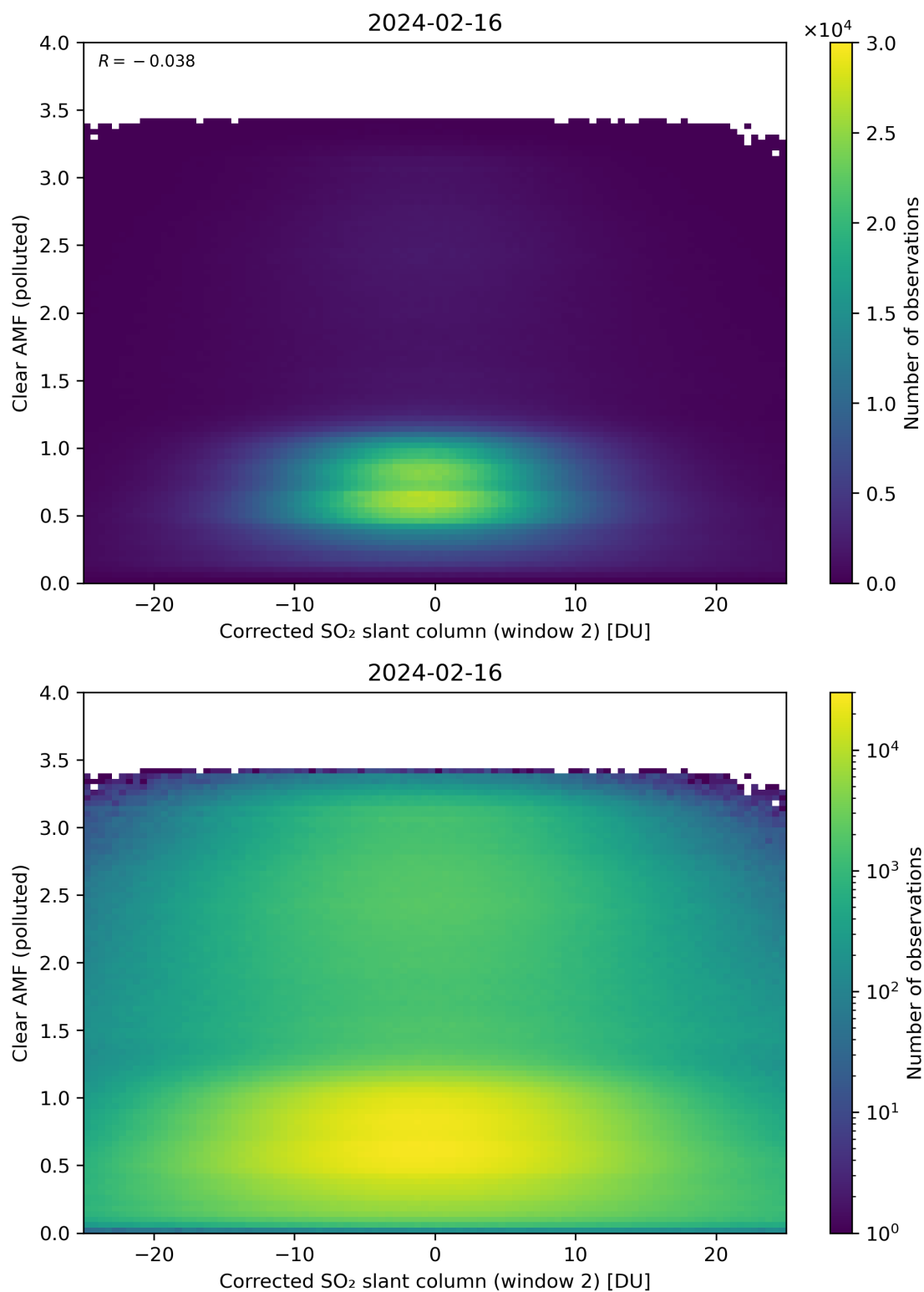
Figure 199: Scatter density plot of “Corrected SO 2 slant column (window 2)” against “Clear AMF (polluted)” for 2024-02-16 to 2024-02-17.
