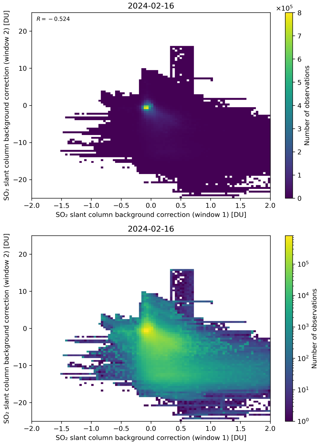
Figure 98: Scatter density plot of “SO 2 slant column background correction (window 1)” against “SO 2 slant column background correction (window 2)” for 2024-02-16 to 2024-02-17.
