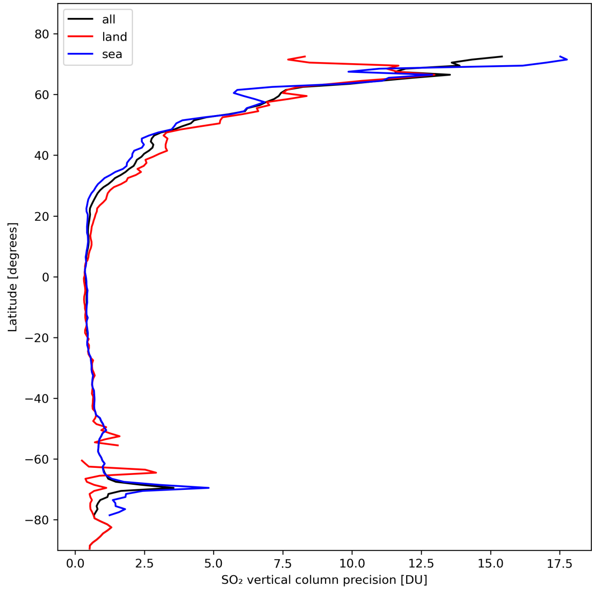
Figure 31: Zonal average of “SO 2 vertical column precision” for 2024-02-16 to 2024-02-17.
