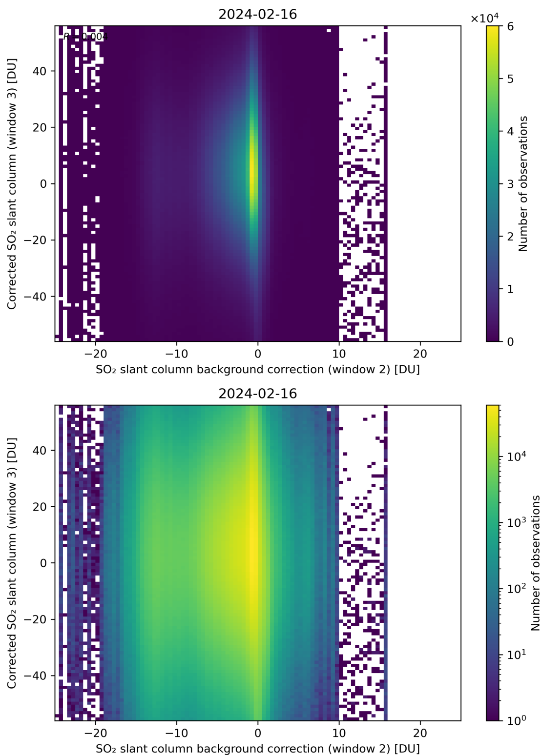
Figure 116: Scatter density plot of “SO 2 slant column background correction (window 2)” against “Corrected SO 2 slant column (window 3)” for 2024-02-16 to 2024-02-17.
