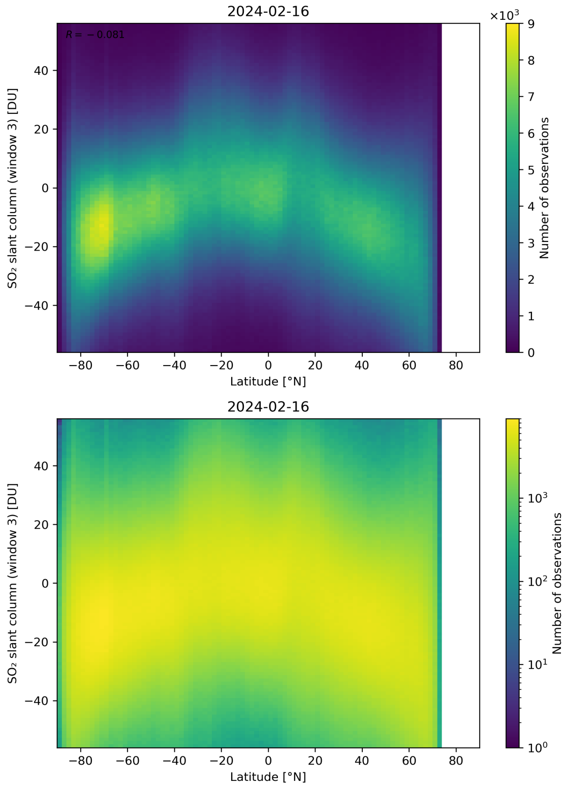
Figure 152: Scatter density plot of “Latitude” against “SO 2 slant column (window 3)” for 2024-02-16 to 2024-02-17.
