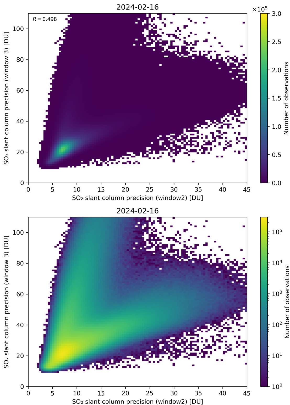
Figure 250: Scatter density plot of “SO 2 slant column precision (window2)” against “SO 2 slant column precision (window 3)” for 2024-02-16 to 2024-02-17.
