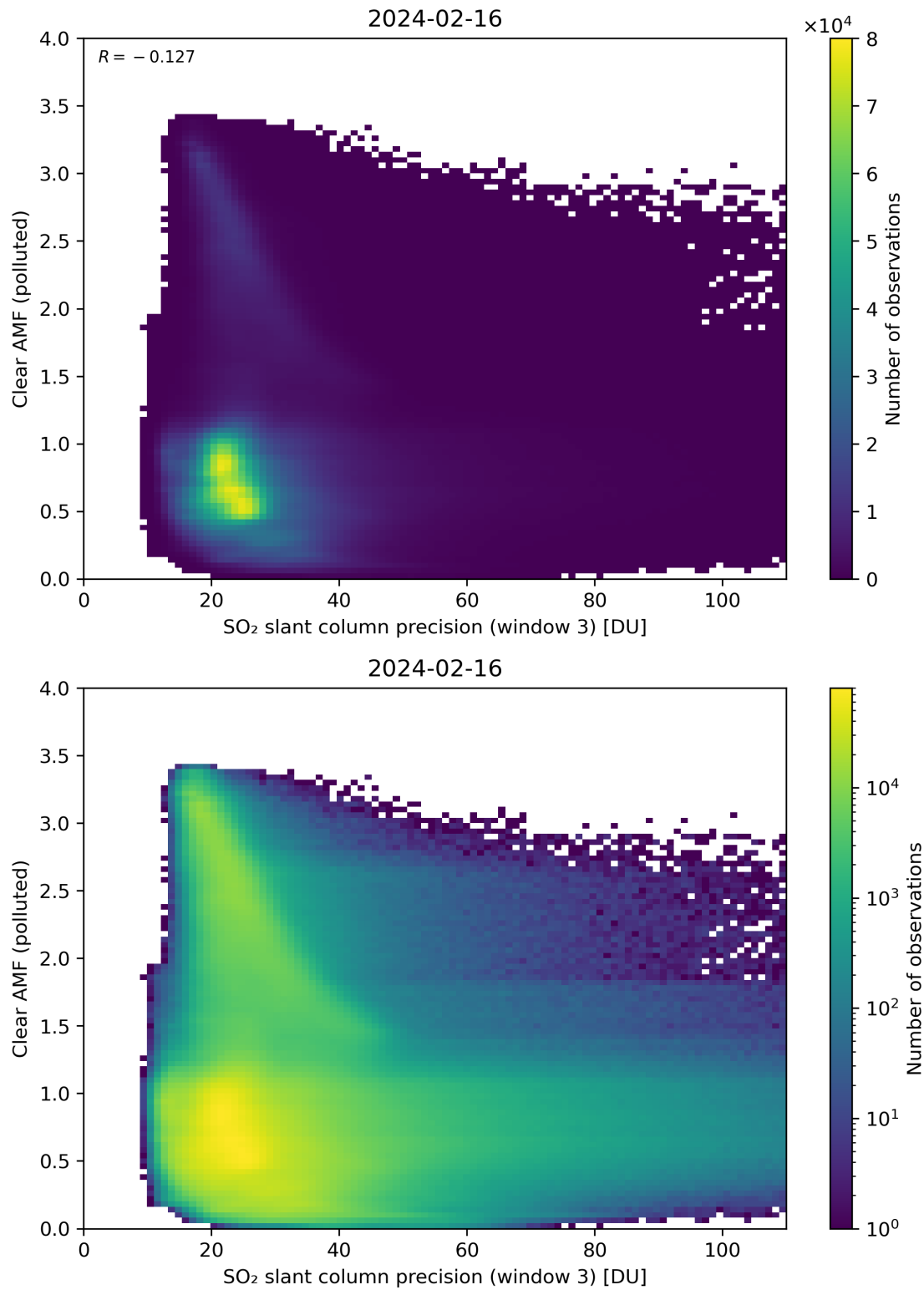
Figure 261: Scatter density plot of “SO 2 slant column precision (window 3)” against “Clear AMF (polluted)” for 2024-02-16 to 2024-02-17.
