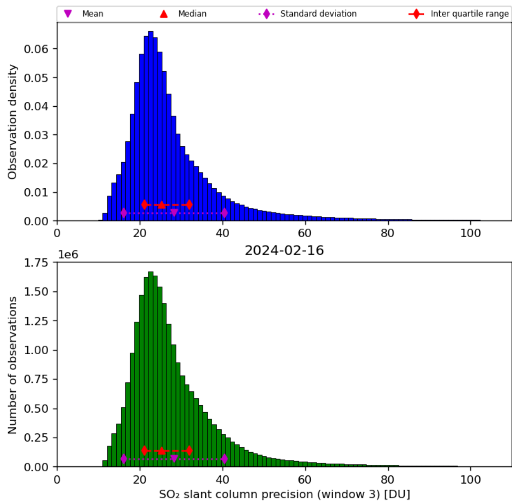
Figure 65: Histogram of “SO 2 slant column precision (window 3)” for 2024-02-16 to 2024-02-17
