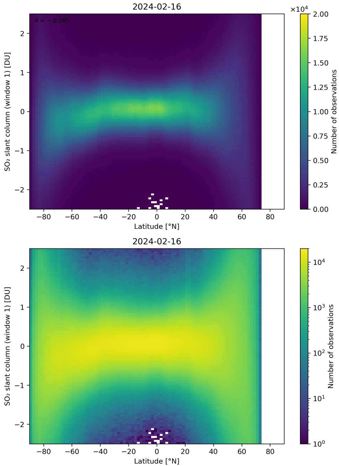
Figure 149: Scatter density plot of “Latitude” against “SO 2 slant column (window 1)” for 2024-02-16 to 2024-02-17.
