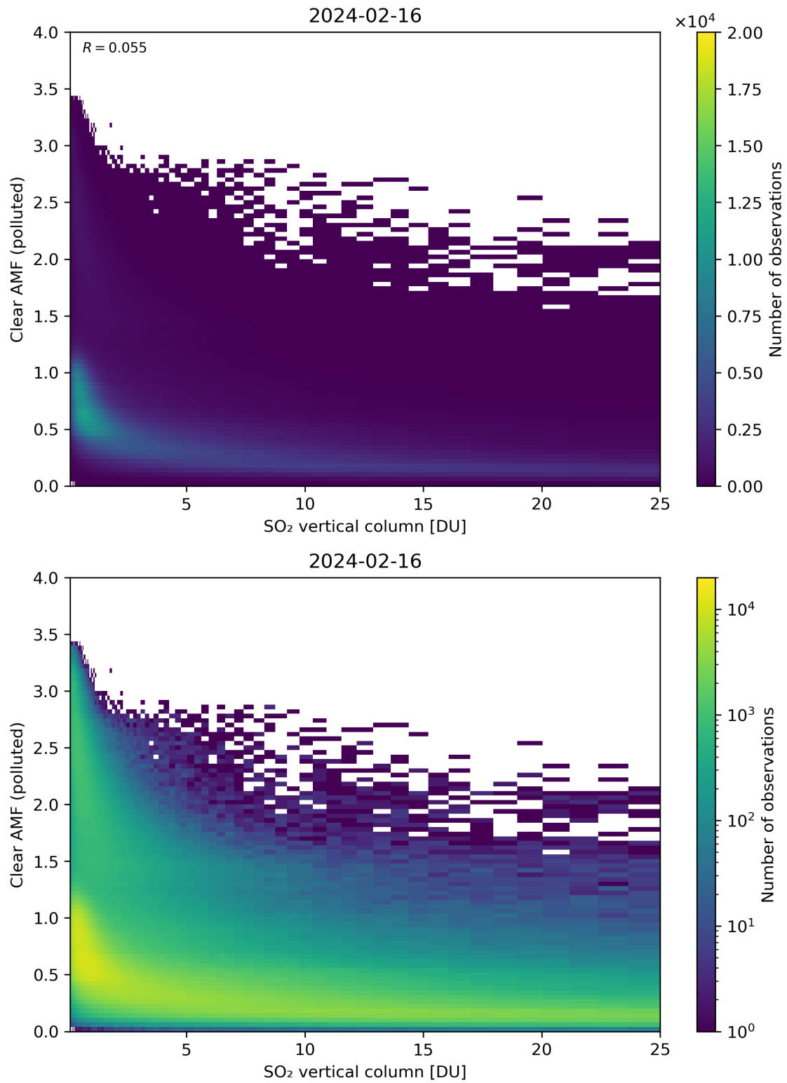
Figure 296: Scatter density plot of “SO 2 vertical column” against “Clear AMF (polluted)” for 2024-02-16 to 2024-02-17.
