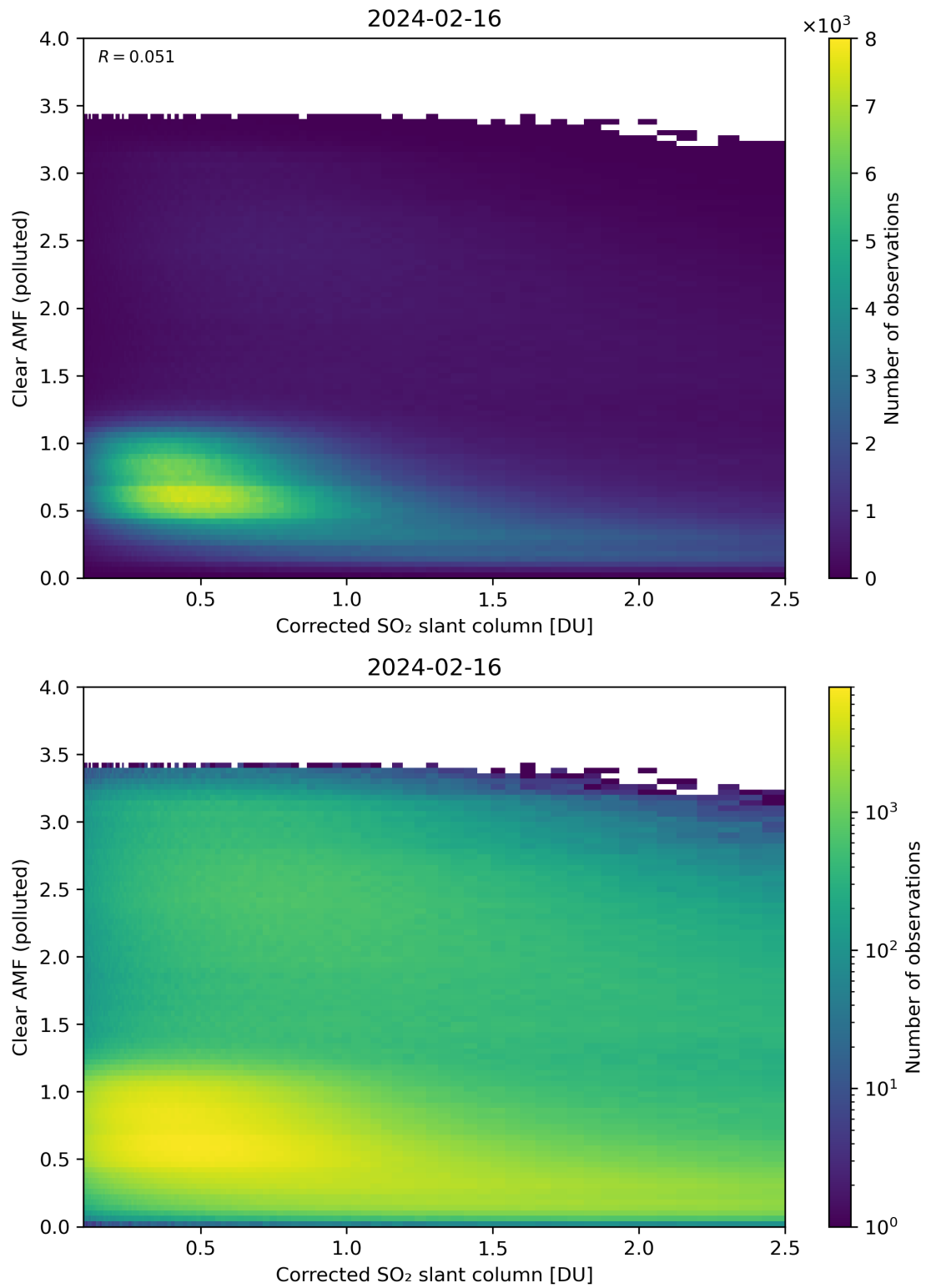
Figure 184: Scatter density plot of “Corrected SO 2 slant column” against “Clear AMF (polluted)” for 2024-02-16 to 2024-02-17.
