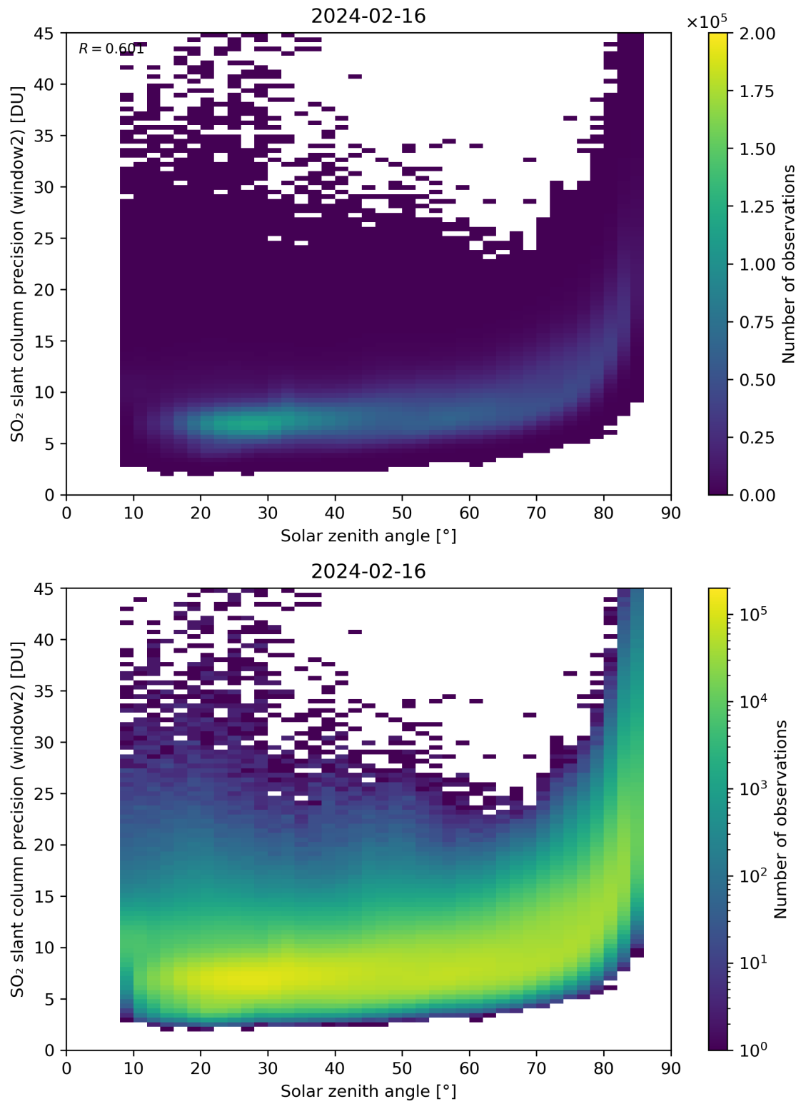
Figure 171: Scatter density plot of “Solar zenith angle” against “SO 2 slant column precision (window2)” for 2024-02-16 to 2024-02-17.
