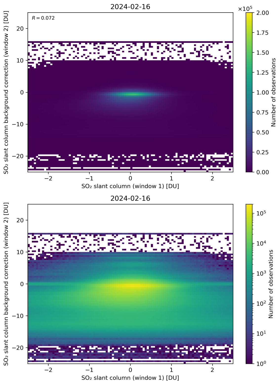
Figure 213: Scatter density plot of “SO 2 slant column (window 1)” against “SO 2 slant column background correction (window 2)” for 2024-02-16 to 2024-02-17.
