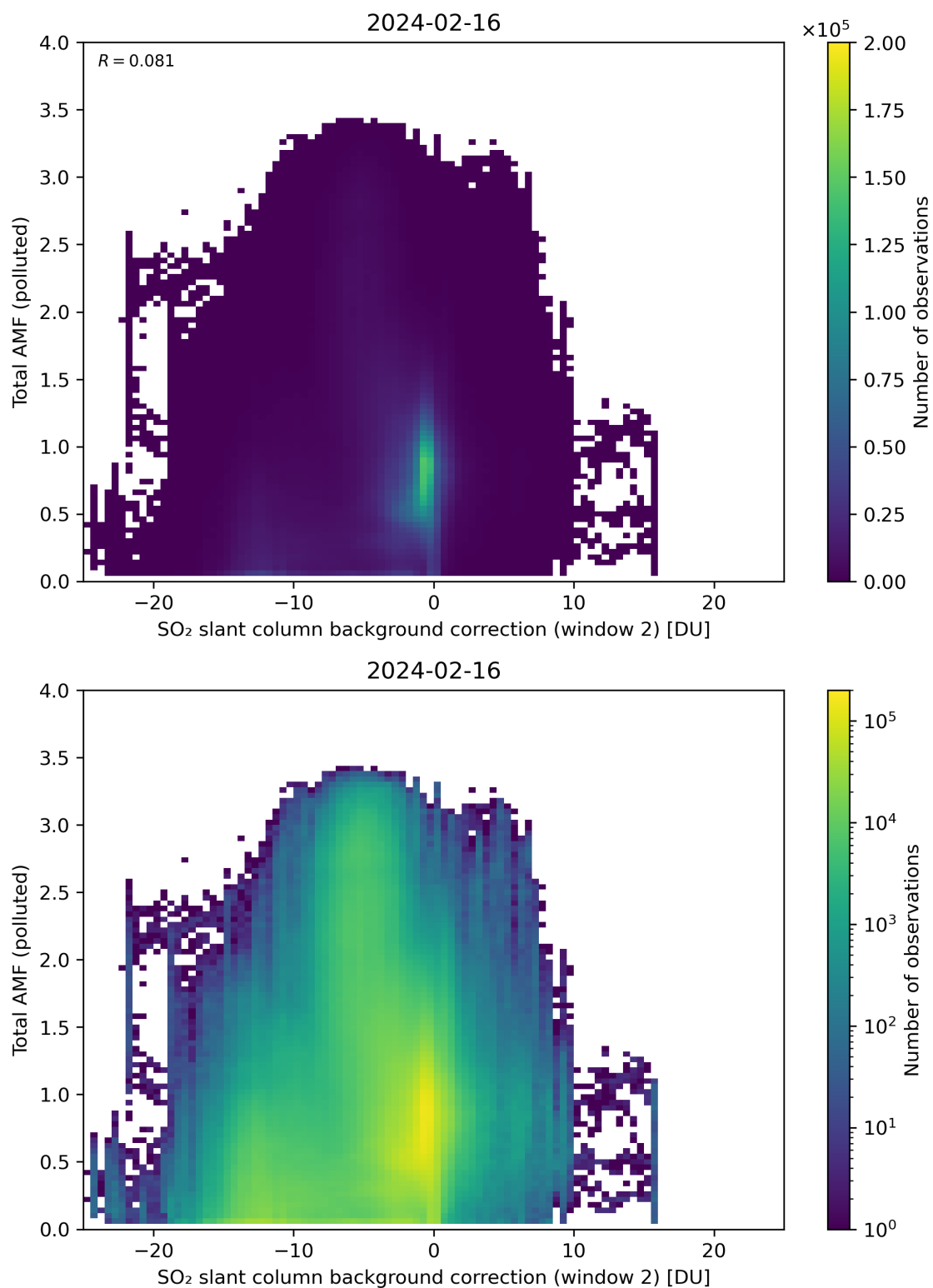
Figure 119: Scatter density plot of “SO 2 slant column background correction (window 2)” against “Total AMF (polluted)” for 2024-02-16 to 2024-02-17.
