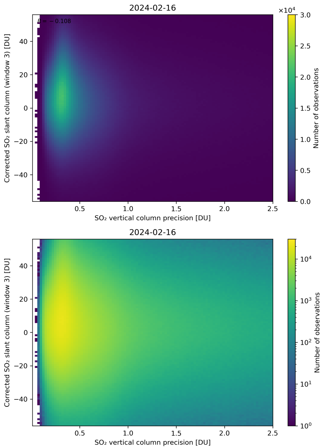
Figure 288: Scatter density plot of “SO 2 vertical column precision” against “Corrected SO 2 slant column (window 3)” for 2024-02-16 to 2024-02-17.
