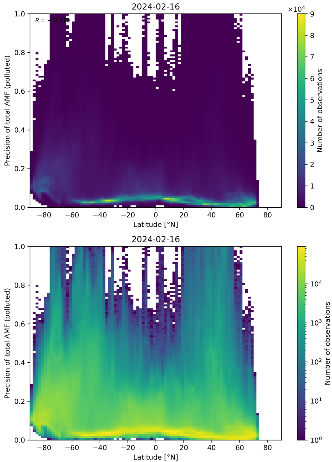
Figure 155: Scatter density plot of “Latitude” against “Precision of total AMF (polluted)” for 2024-02-16 to 2024-02-17.
