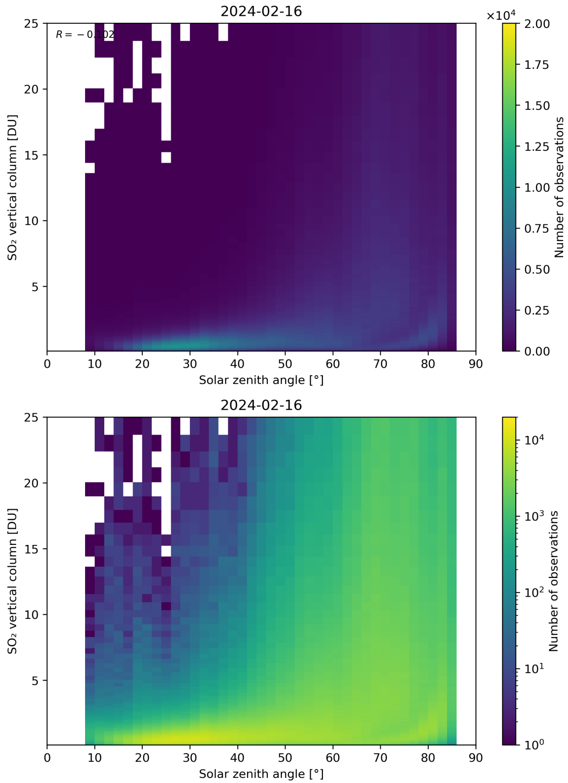
Figure 176: Scatter density plot of “Solar zenith angle” against “SO 2 vertical column” for 2024-02-16 to 2024-02-17.
