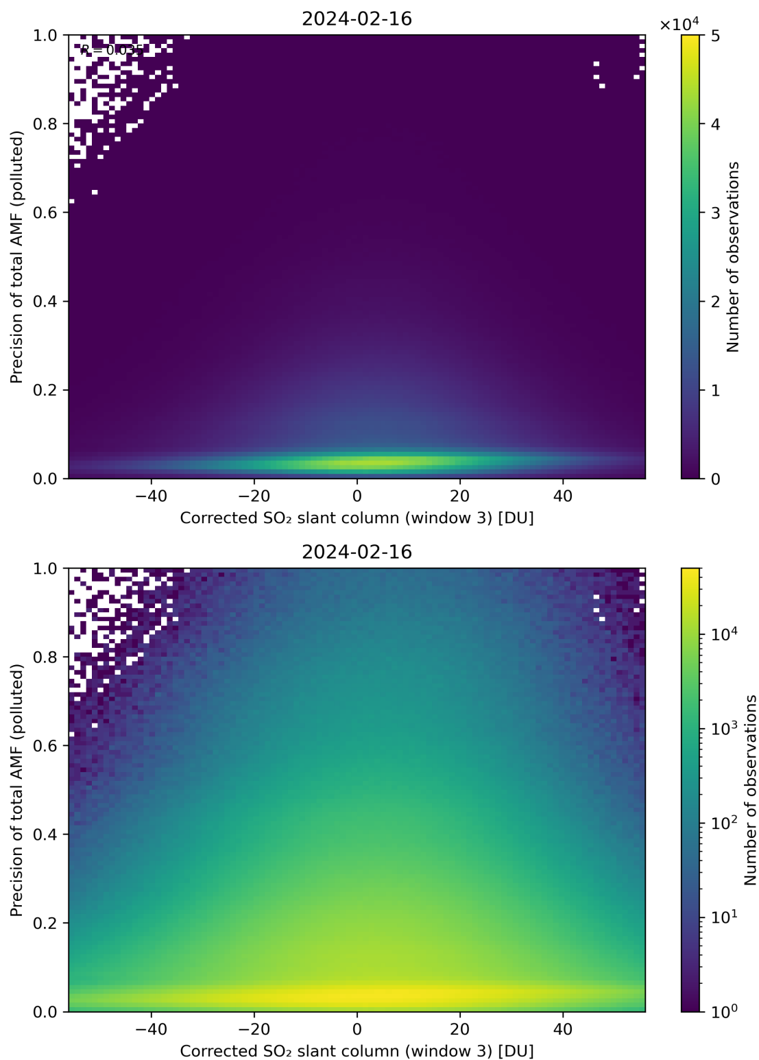
Figure 211: Scatter density plot of “Corrected SO 2 slant column (window 3)” against “Precision of total AMF (polluted)” for 2024-02-16 to 2024-02-17.
