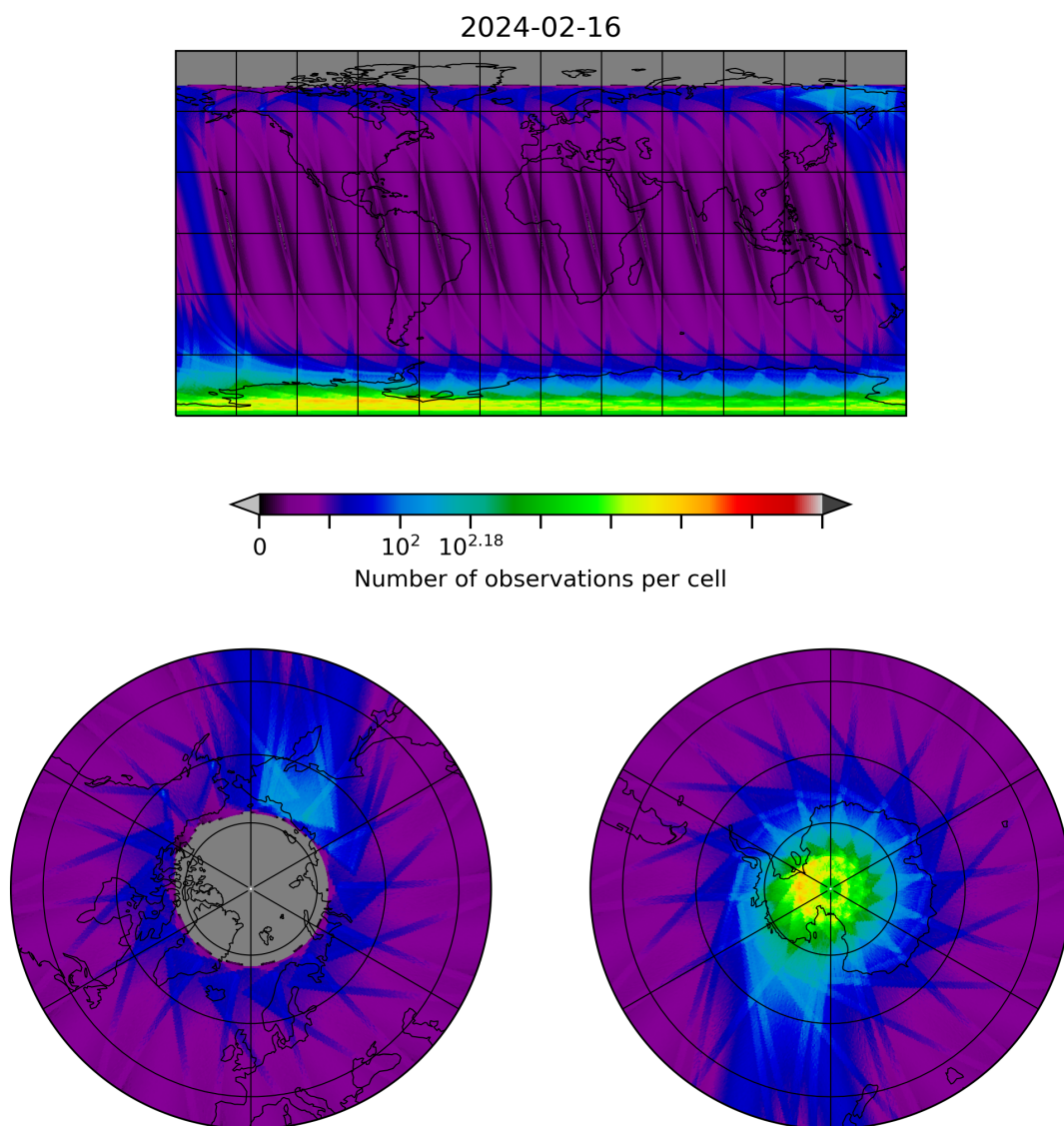
Figure 28: Map of the number of observations for 2024-02-16 to 2024-02-17
