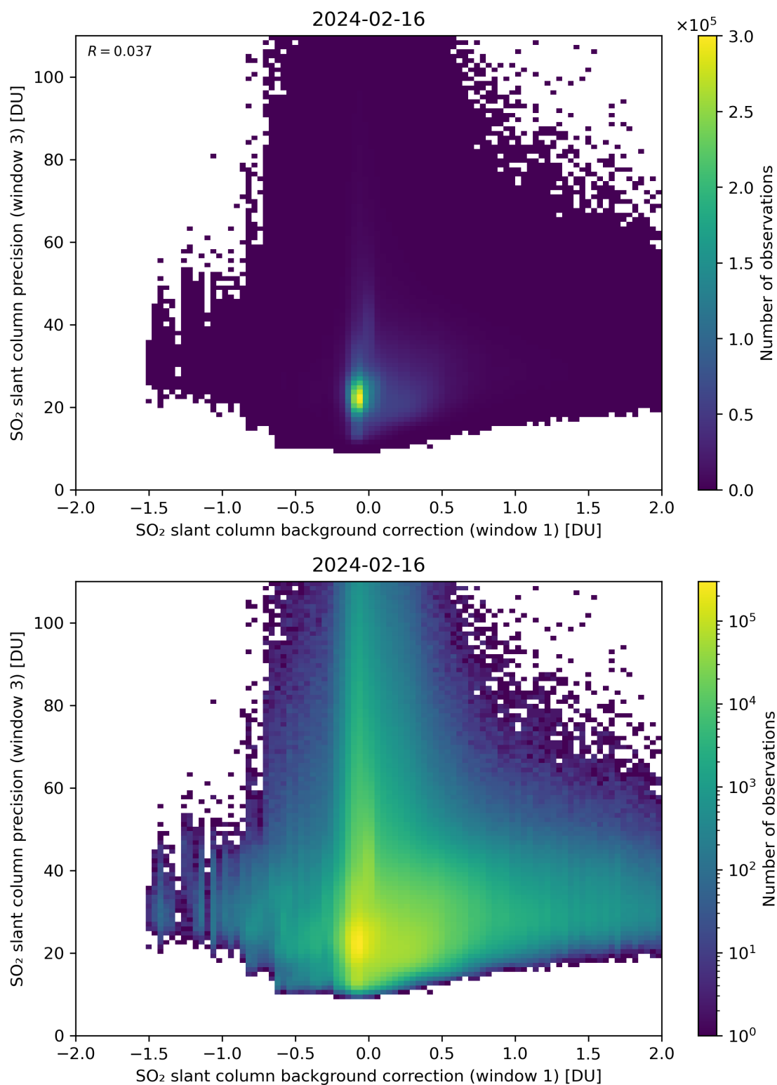
Figure 108: Scatter density plot of “SO 2 slant column background correction (window 1)” against “SO 2 slant column precision (window 3)” for 2024-02-16 to 2024-02-17.
