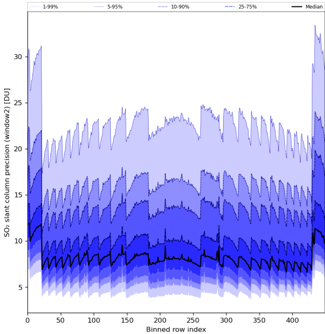
Figure 84: Along track statistics of “SO 2 slant column precision (window2)” for 2024-02-16 to 2024-02-17
