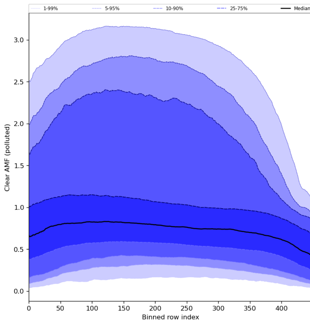
Figure 96: Along track statistics of “Clear AMF (polluted)” for 2024-02-16 to 2024-02-17
