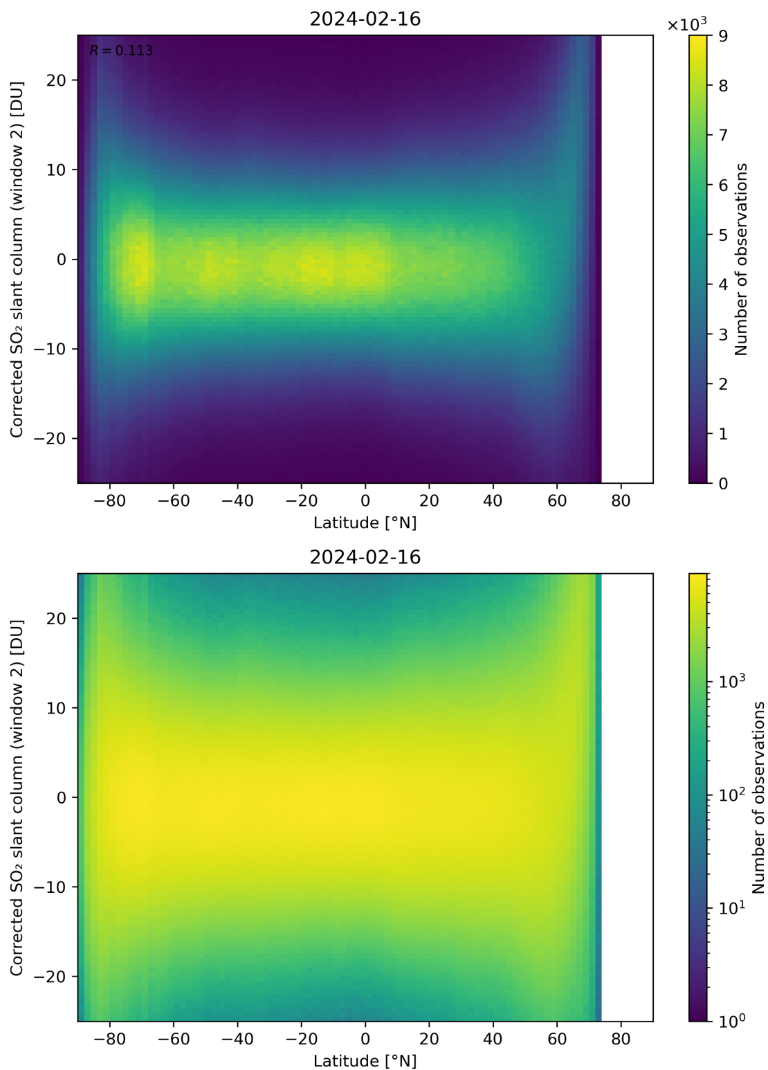
Figure 147: Scatter density plot of “Latitude” against “Corrected SO 2 slant column (window 2)” for 2024-02-16 to 2024-02-17.
