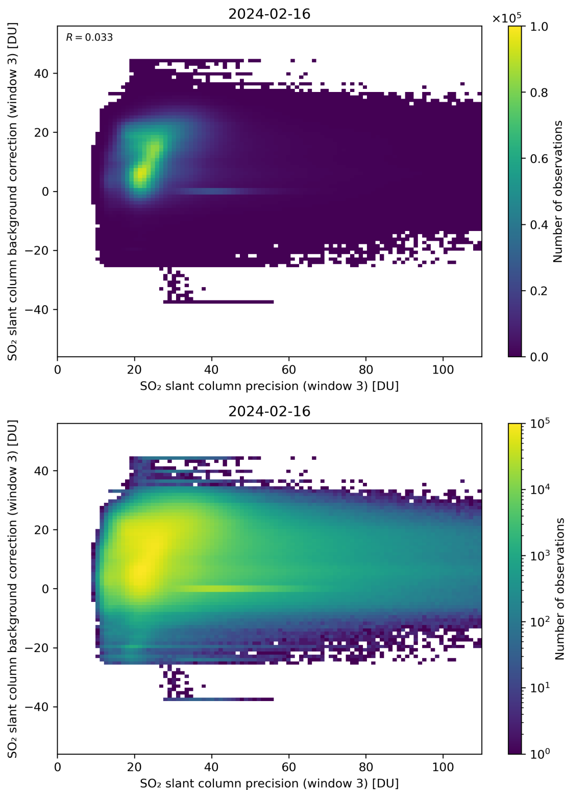
Figure 257: Scatter density plot of “SO 2 slant column precision (window 3)” against “SO 2 slant column background correction (window 3)” for 2024-02-16 to 2024-02-17.
