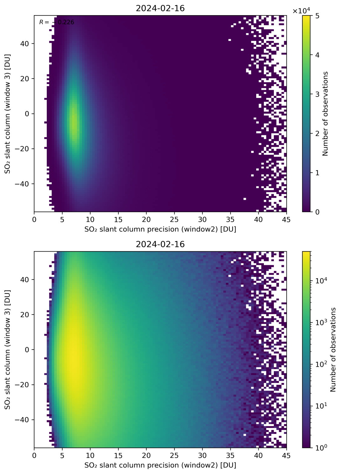
Figure 249: Scatter density plot of “SO 2 slant column precision (window2)” against “SO 2 slant column (window 3)” for 2024-02-16 to 2024-02-17.
