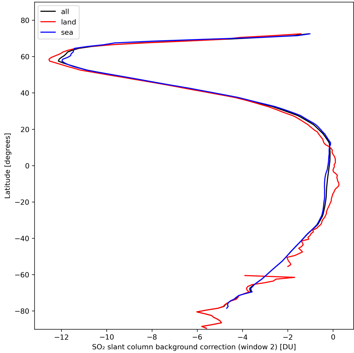
Figure 40: Zonal average of “SO 2 slant column background correction (window 2)” for 2024-02-16 to 2024-02-17.
