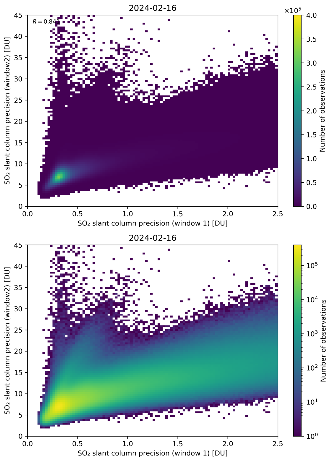
Figure 227: Scatter density plot of “SO 2 slant column precision (window 1)” against “SO 2 slant column precision (window2)” for 2024-02-16 to 2024-02-17.
