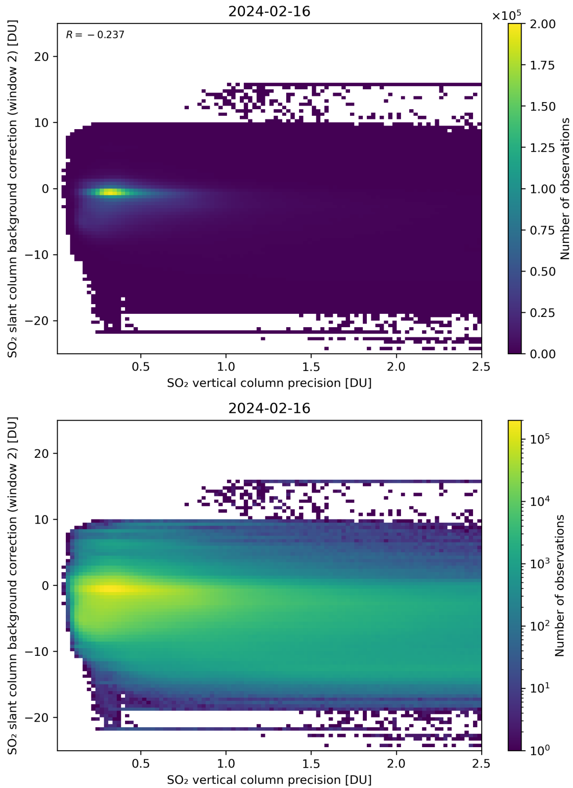
Figure 280: Scatter density plot of “SO 2 vertical column precision” against “SO 2 slant column background correction (window 2)” for 2024-02-16 to 2024-02-17.
