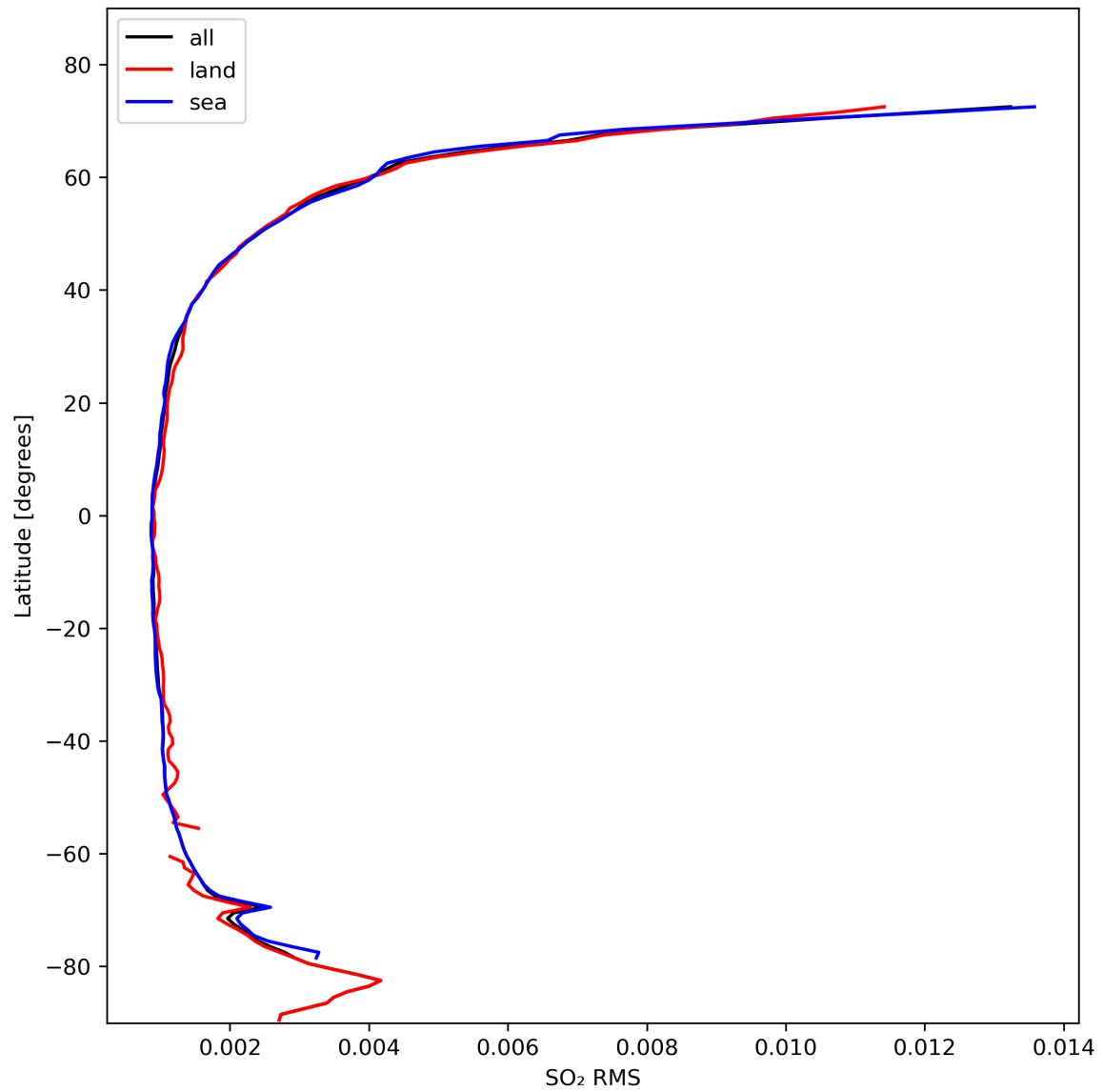
Figure 47: Zonal average of “SO 2 RMS” for 2024-02-16 to 2024-02-17.
