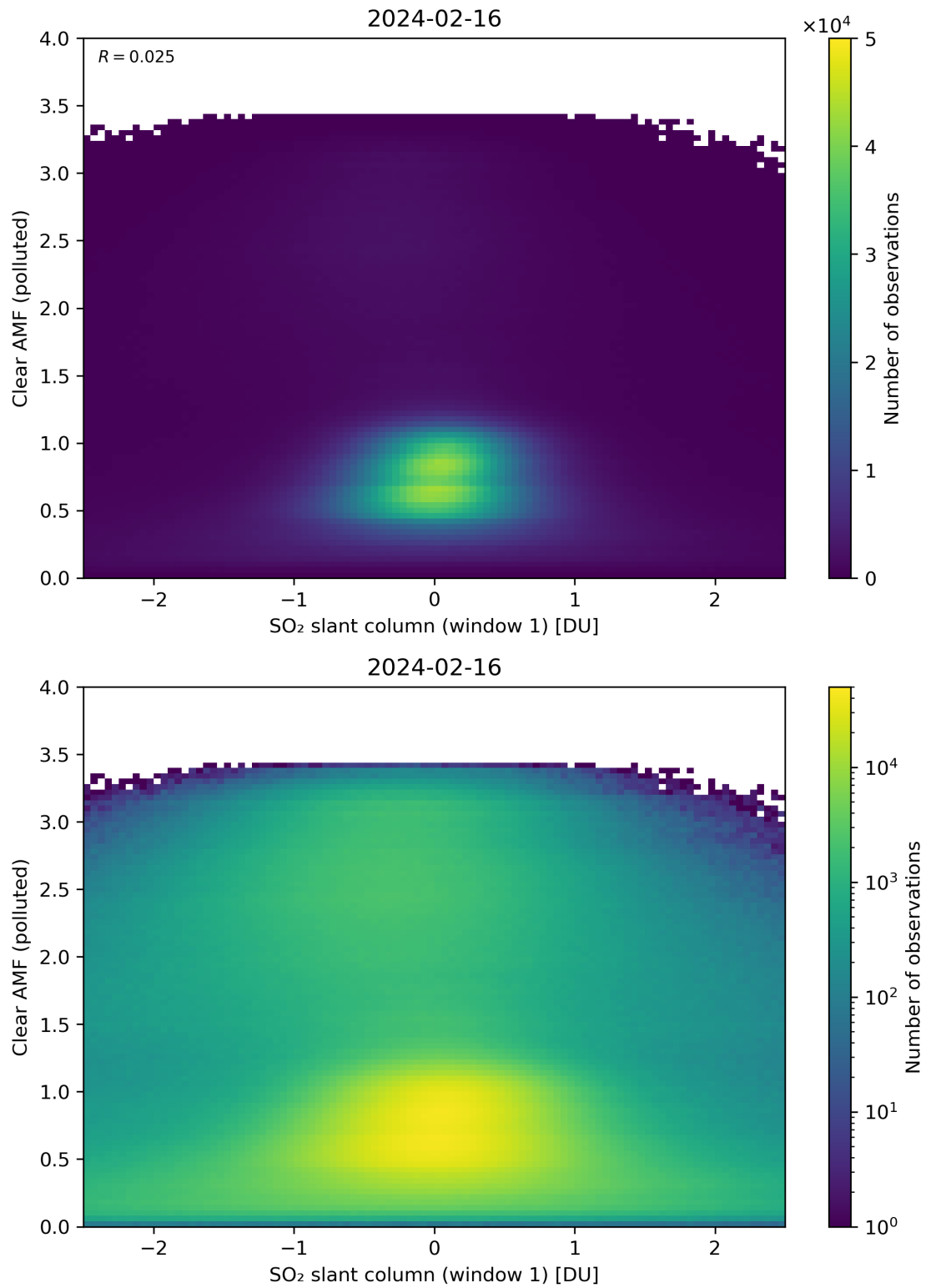
Figure 232: Scatter density plot of “SO 2 slant column (window 1)” against “Clear AMF (polluted)” for 2024-02-16 to 2024-02-17.
