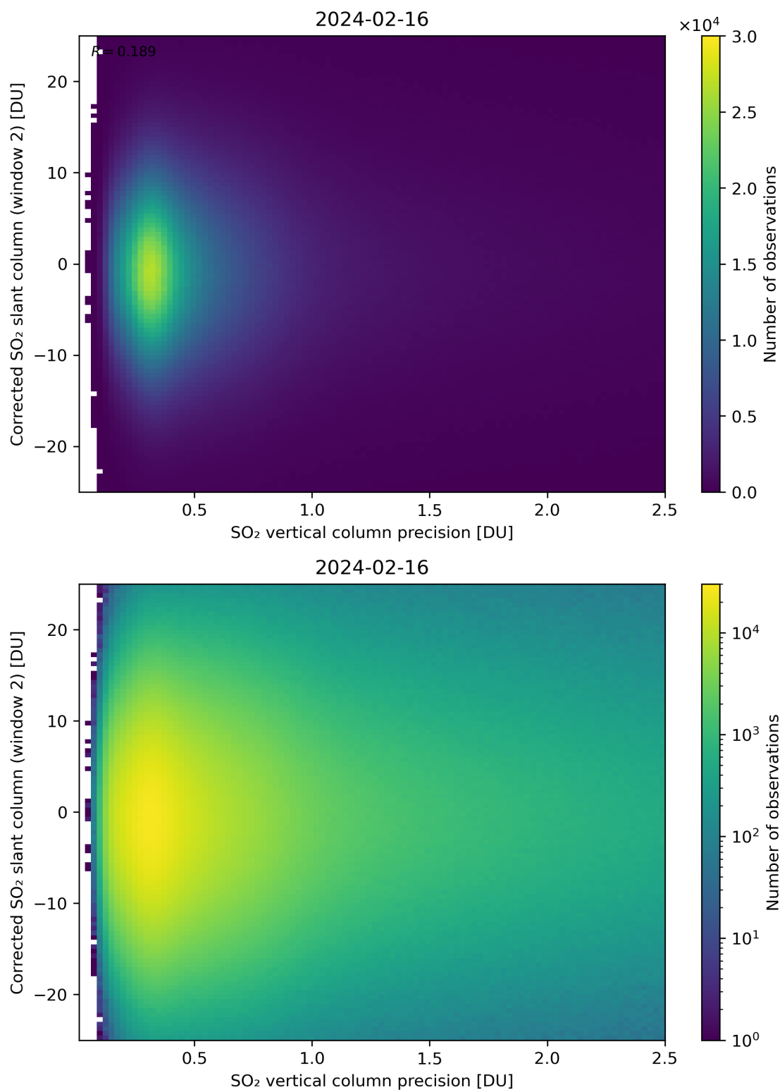
Figure 287: Scatter density plot of “SO 2 vertical column precision” against “Corrected SO 2 slant column (window 2)” for 2024-02-16 to 2024-02-17.
