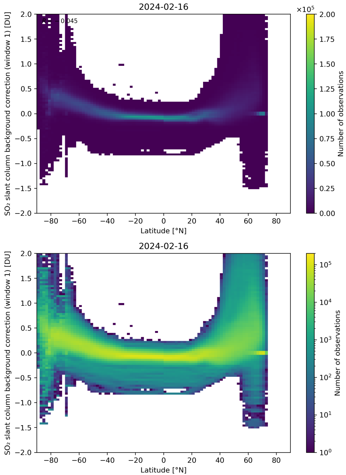
Figure 139: Scatter density plot of “Latitude” against “SO 2 slant column background correction (window 1)” for 2024-02-16 to 2024-02-17.
