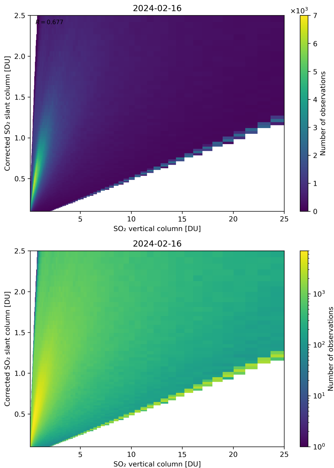
Figure 297: Scatter density plot of “SO 2 vertical column” against “Corrected SO 2 slant column” for 2024-02-16 to 2024-02-17.
