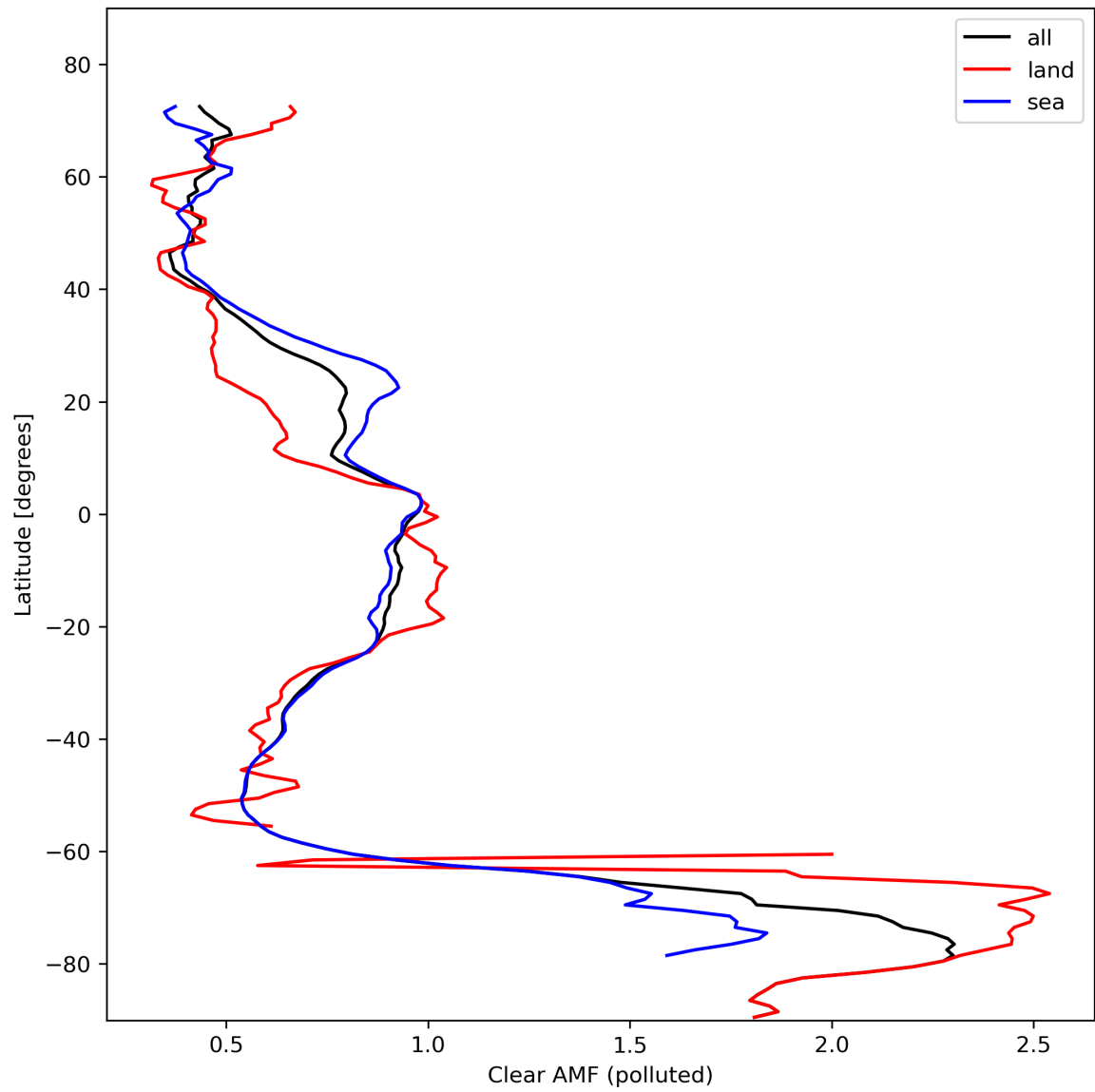
Figure 50: Zonal average of “Clear AMF (polluted)” for 2024-02-16 to 2024-02-17.
