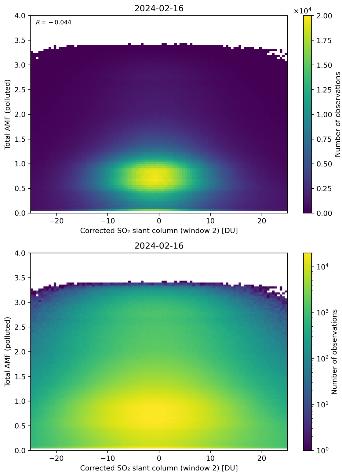
Figure 203: Scatter density plot of “Corrected SO 2 slant column (window 2)” against “Total AMF (polluted)” for 2024-02-16 to 2024-02-17.
