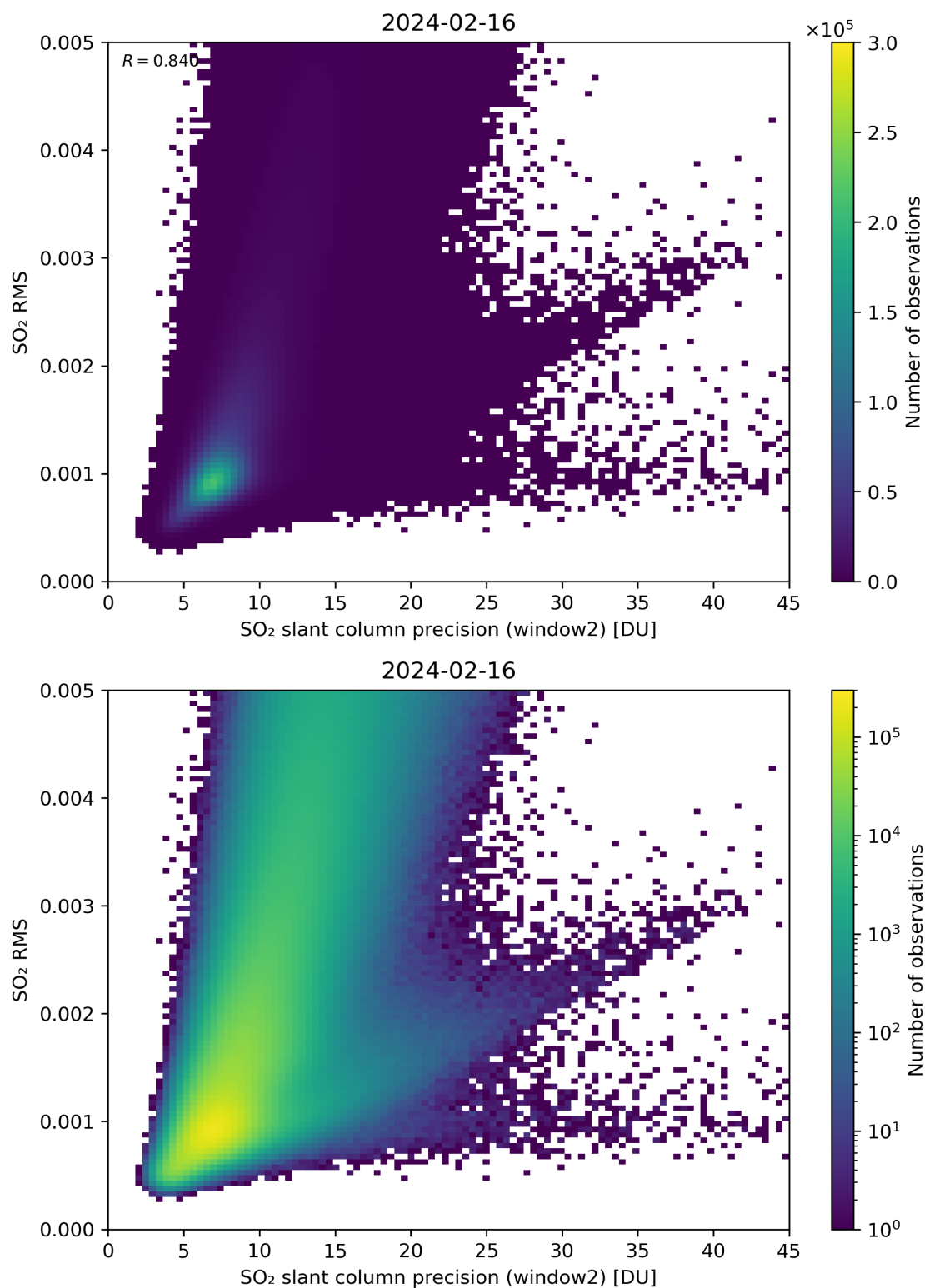
Figure 245: Scatter density plot of “SO 2 slant column precision (window2)” against “SO 2 RMS” for 2024-02-16 to 2024-02-17.
