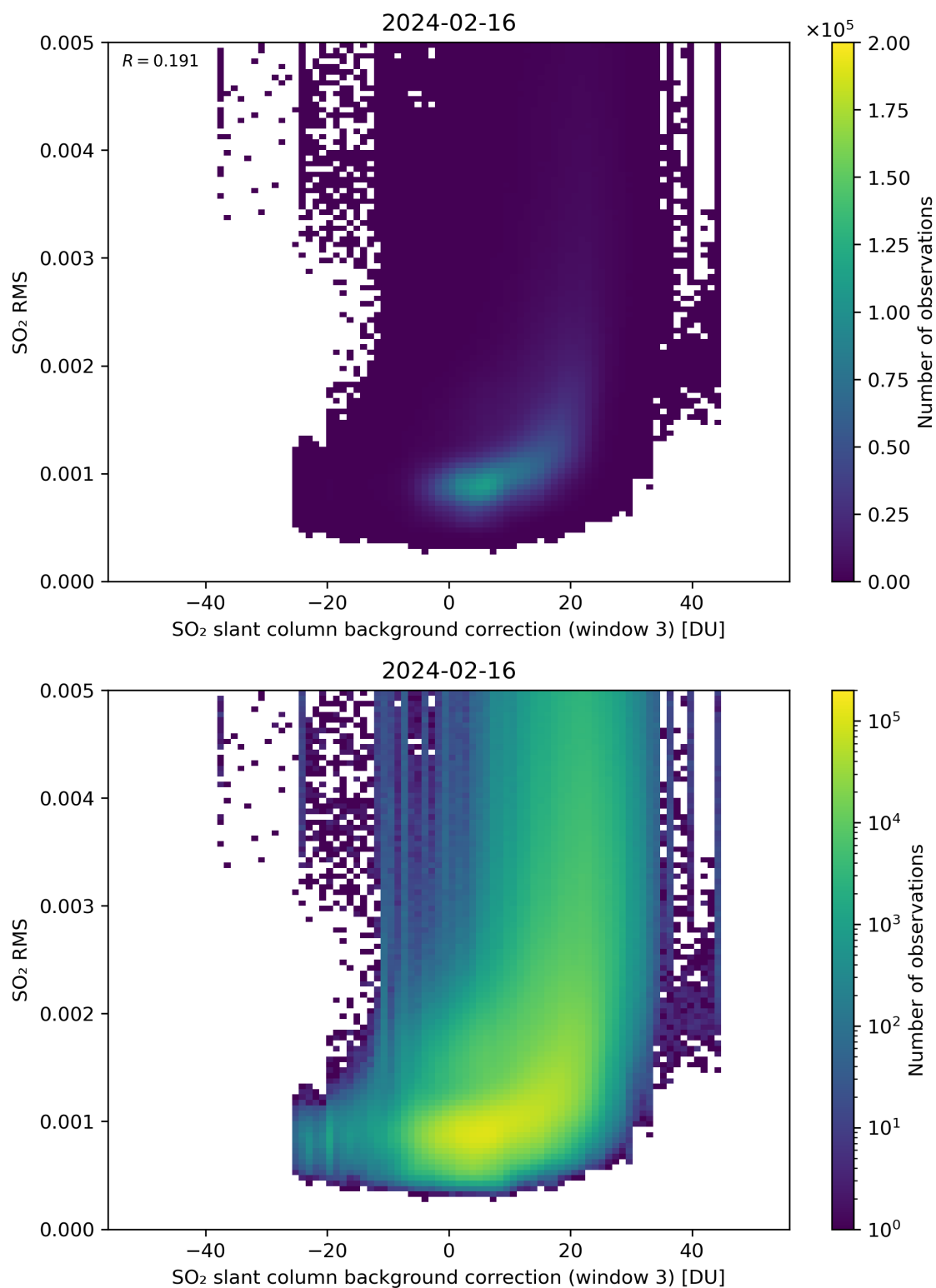
Figure 123: Scatter density plot of “SO 2 slant column background correction (window 3)” against “SO 2 RMS” for 2024-02-16 to 2024-02-17.
