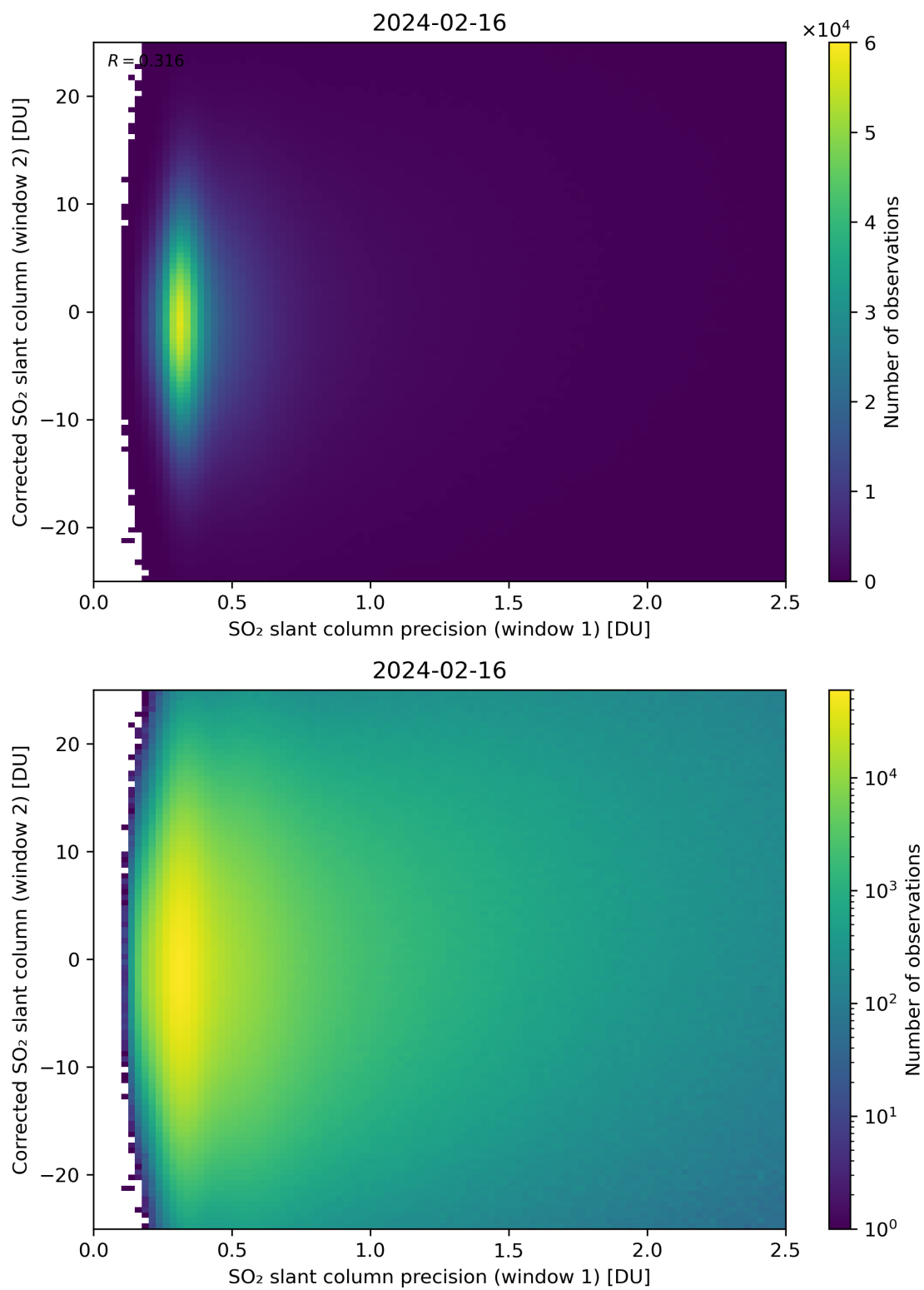
Figure 225: Scatter density plot of “SO 2 slant column precision (window 1)” against “Corrected SO 2 slant column (window 2)” for 2024-02-16 to 2024-02-17.
