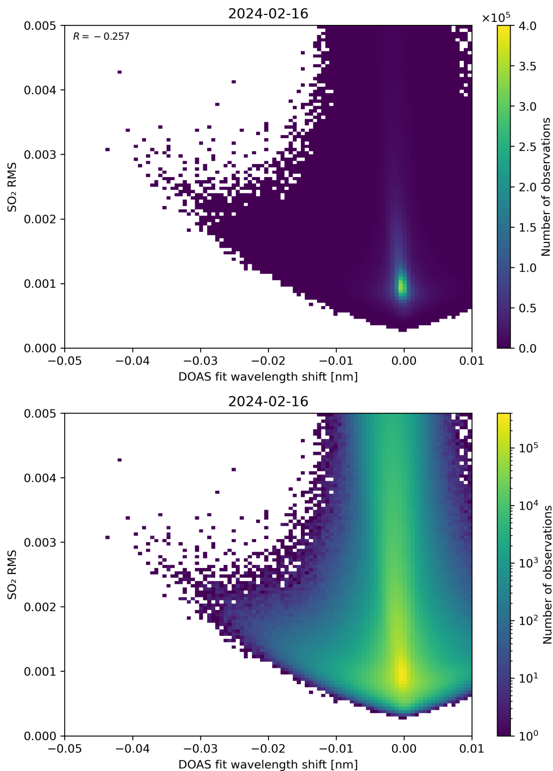
Figure 128: Scatter density plot of “DOAS fit wavelength shift” against “SO 2 RMS” for 2024-02-16 to 2024-02-17.
