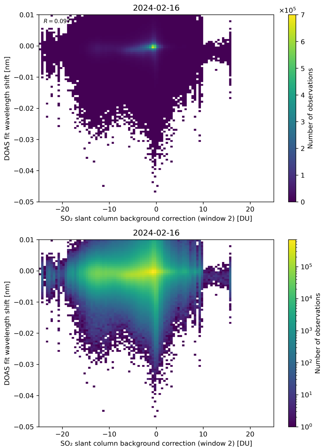
Figure 112: Scatter density plot of “SO 2 slant column background correction (window 2)” against “DOAS fit wavelength shift” for 2024-02-16 to 2024-02-17.
