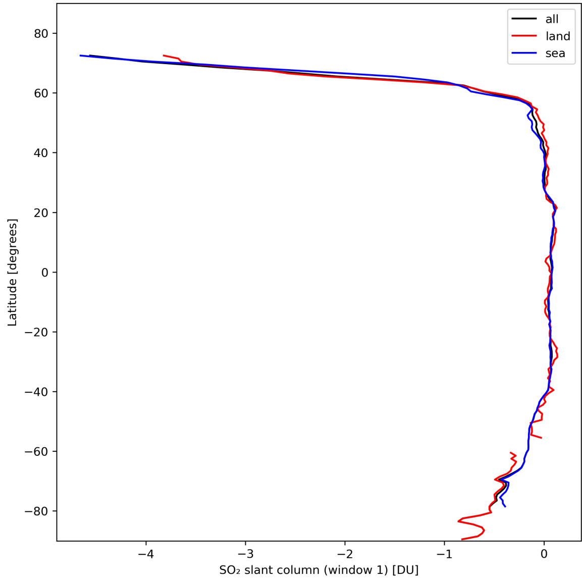
Figure 33: Zonal average of “SO 2 slant column (window 1)” for 2024-02-16 to 2024-02-17.
