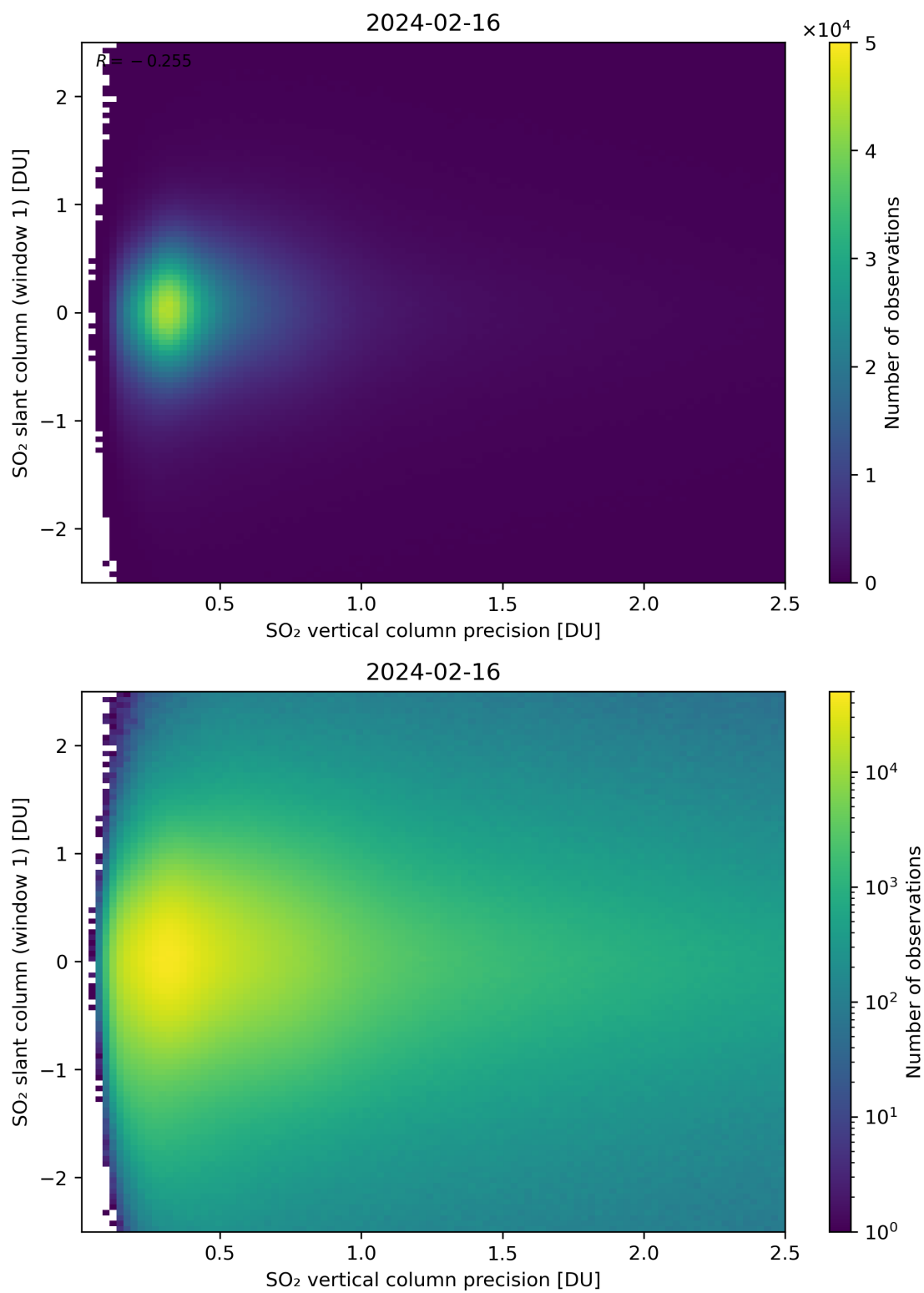
Figure 289: Scatter density plot of “SO 2 vertical column precision” against “SO 2 slant column (window 1)” for 2024-02-16 to 2024-02-17.
