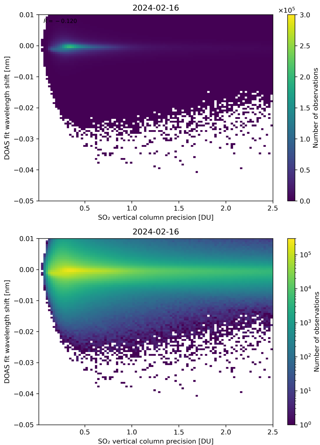
Figure 282: Scatter density plot of “SO 2 vertical column precision” against “DOAS fit wavelength shift” for 2024-02-16 to 2024-02-17.
