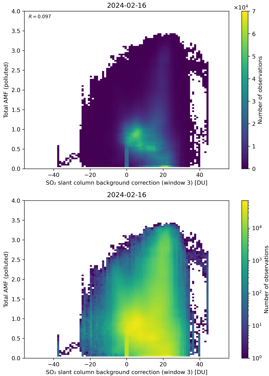
Figure 125: Scatter density plot of “SO 2 slant column background correction (window 3)” against “Total AMF (polluted)” for 2024-02-16 to 2024-02-17.
