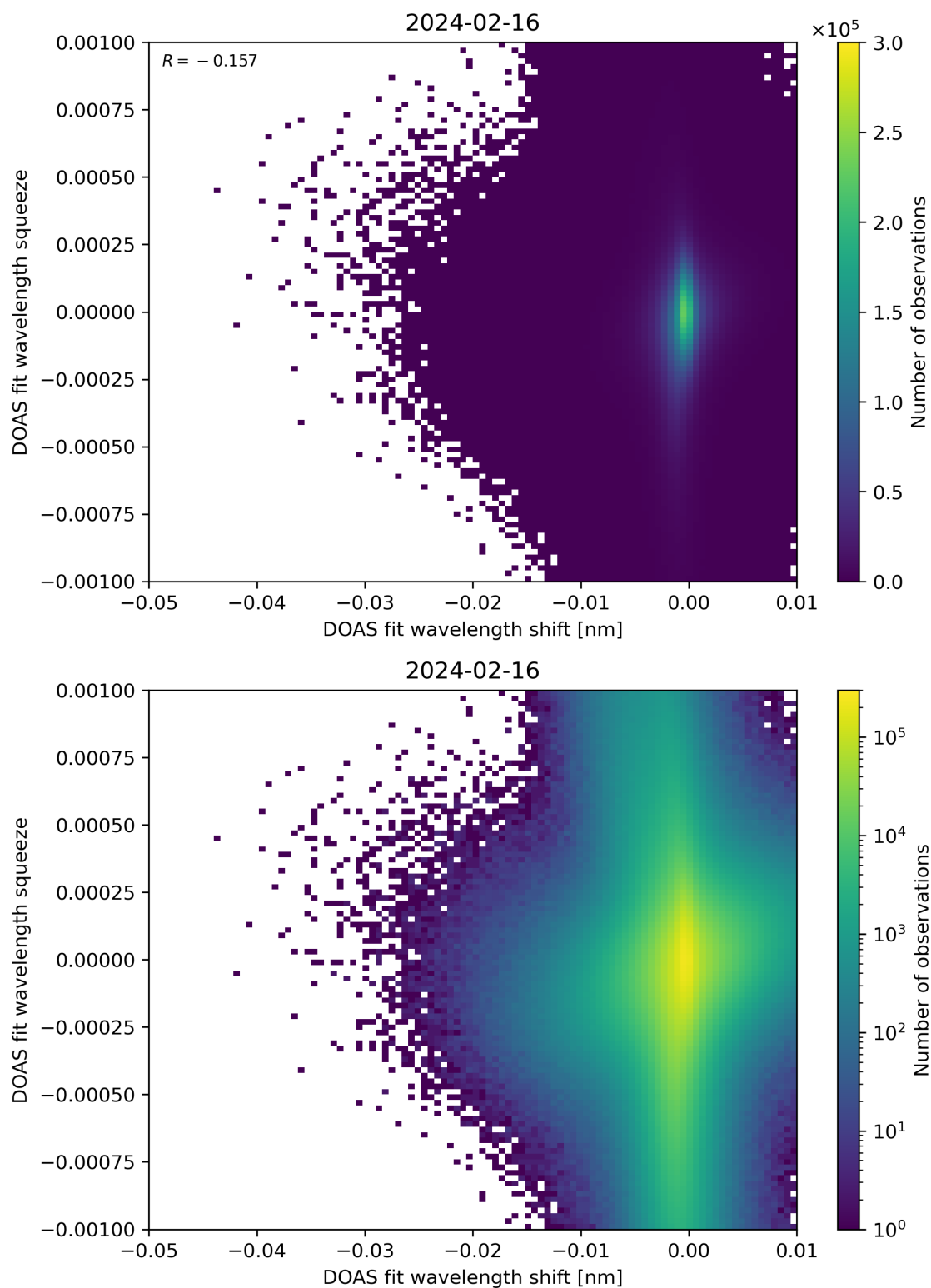
Figure 127: Scatter density plot of “DOAS fit wavelength shift” against “DOAS fit wavelength squeeze” for 2024-02-16 to 2024-02-17.
