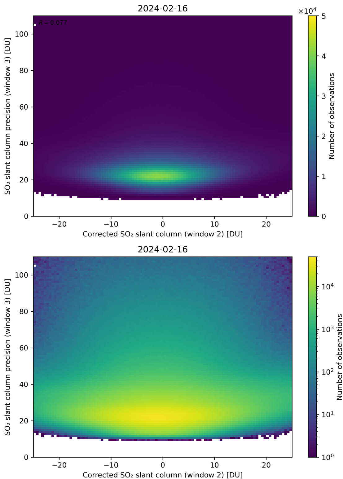
Figure 202: Scatter density plot of “Corrected SO 2 slant column (window 2)” against “SO 2 slant column precision (window 3)” for 2024-02-16 to 2024-02-17.
