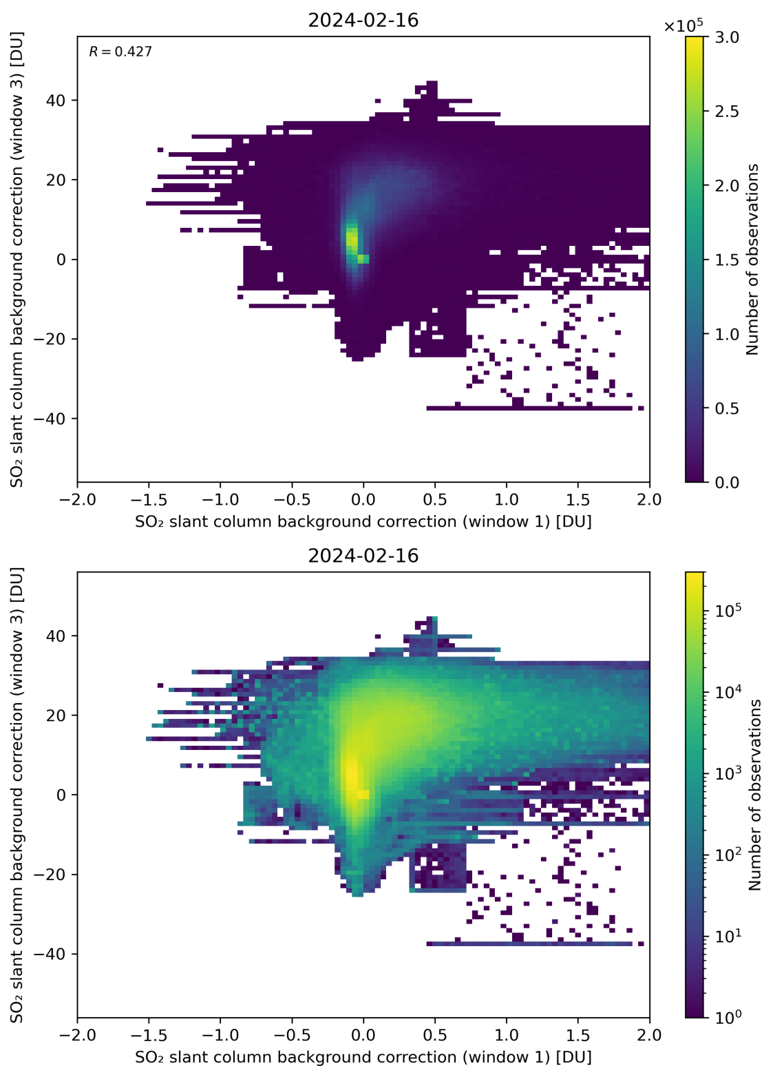
Figure 99: Scatter density plot of “SO 2 slant column background correction (window 1)” against “SO 2 slant column background correction (window 3)” for 2024-02-16 to 2024-02-17.
