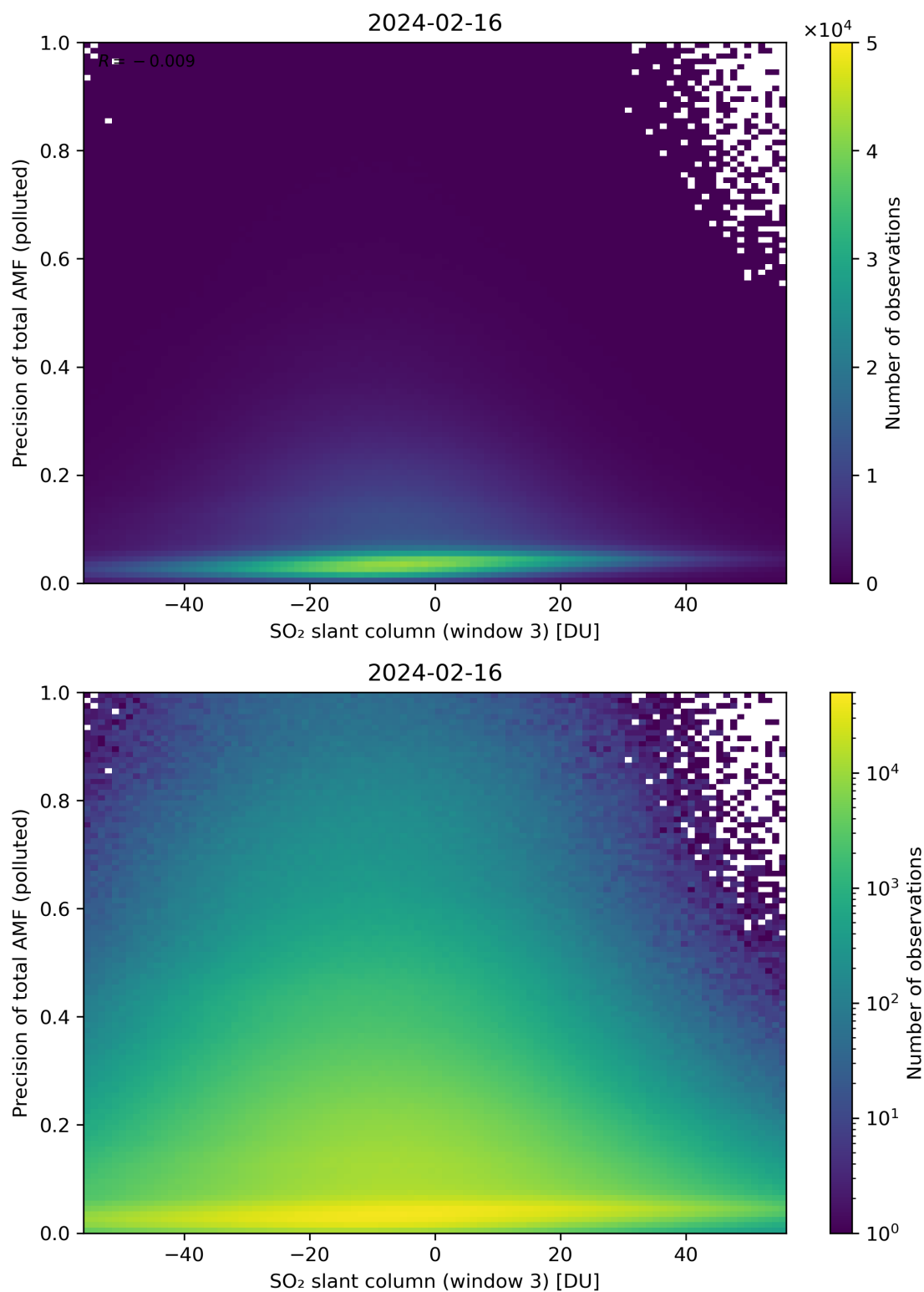
Figure 269: Scatter density plot of “SO 2 slant column (window 3)” against “Precision of total AMF (polluted)” for 2024-02-16 to 2024-02-17.
