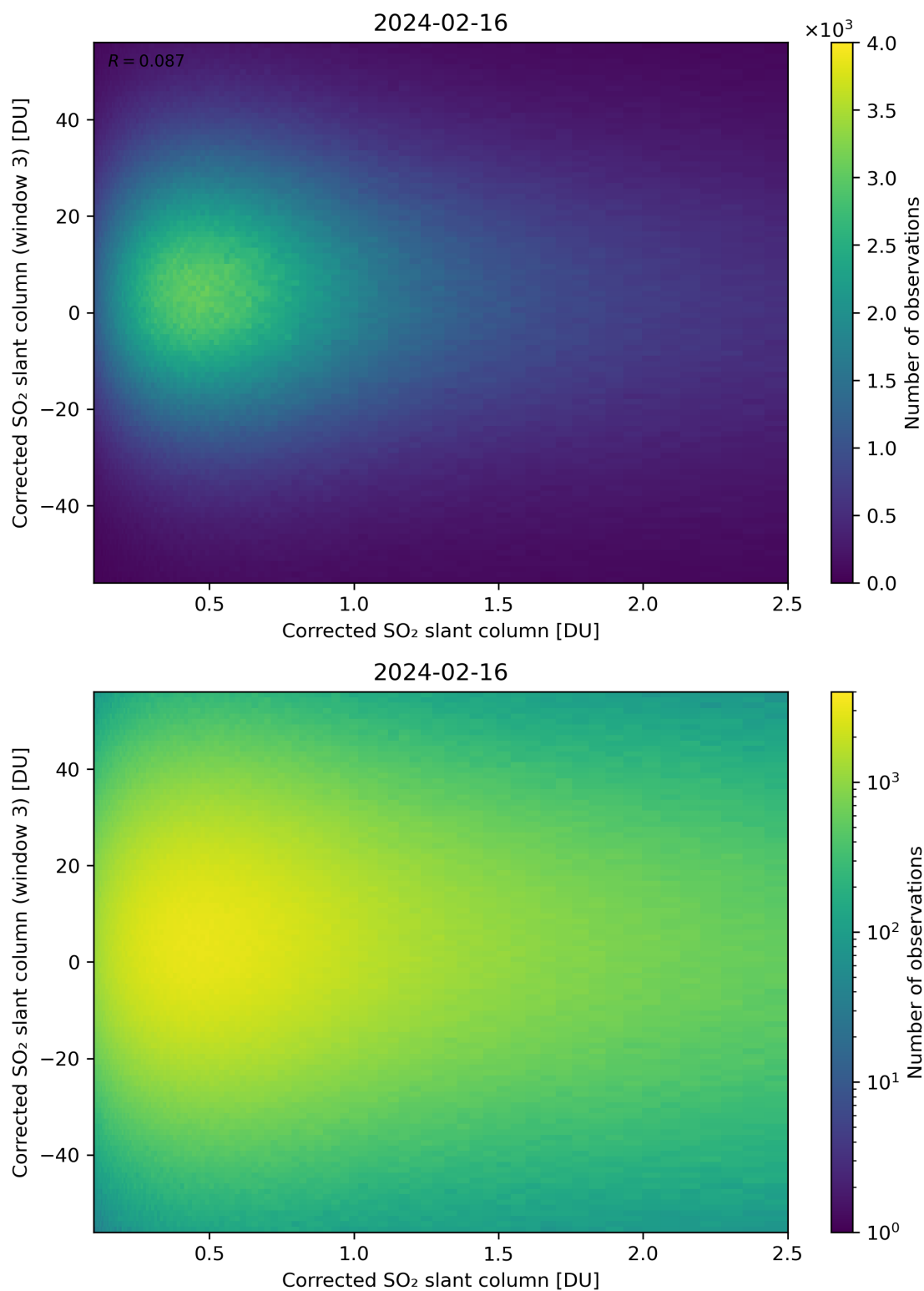
Figure 186: Scatter density plot of “Corrected SO 2 slant column” against “Corrected SO 2 slant column (window 3)” for 2024-02-16 to 2024-02-17.
