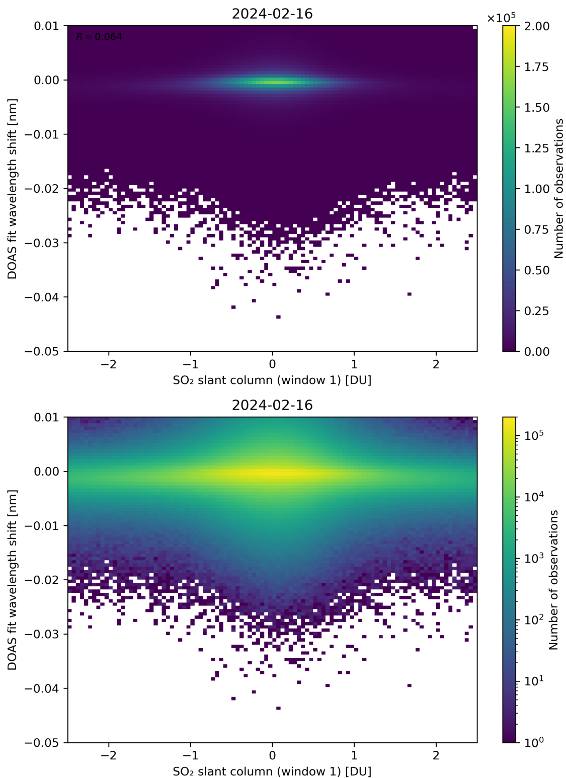
Figure 215: Scatter density plot of “SO 2 slant column (window 1)” against “DOAS fit wavelength shift” for 2024-02-16 to 2024-02-17.
