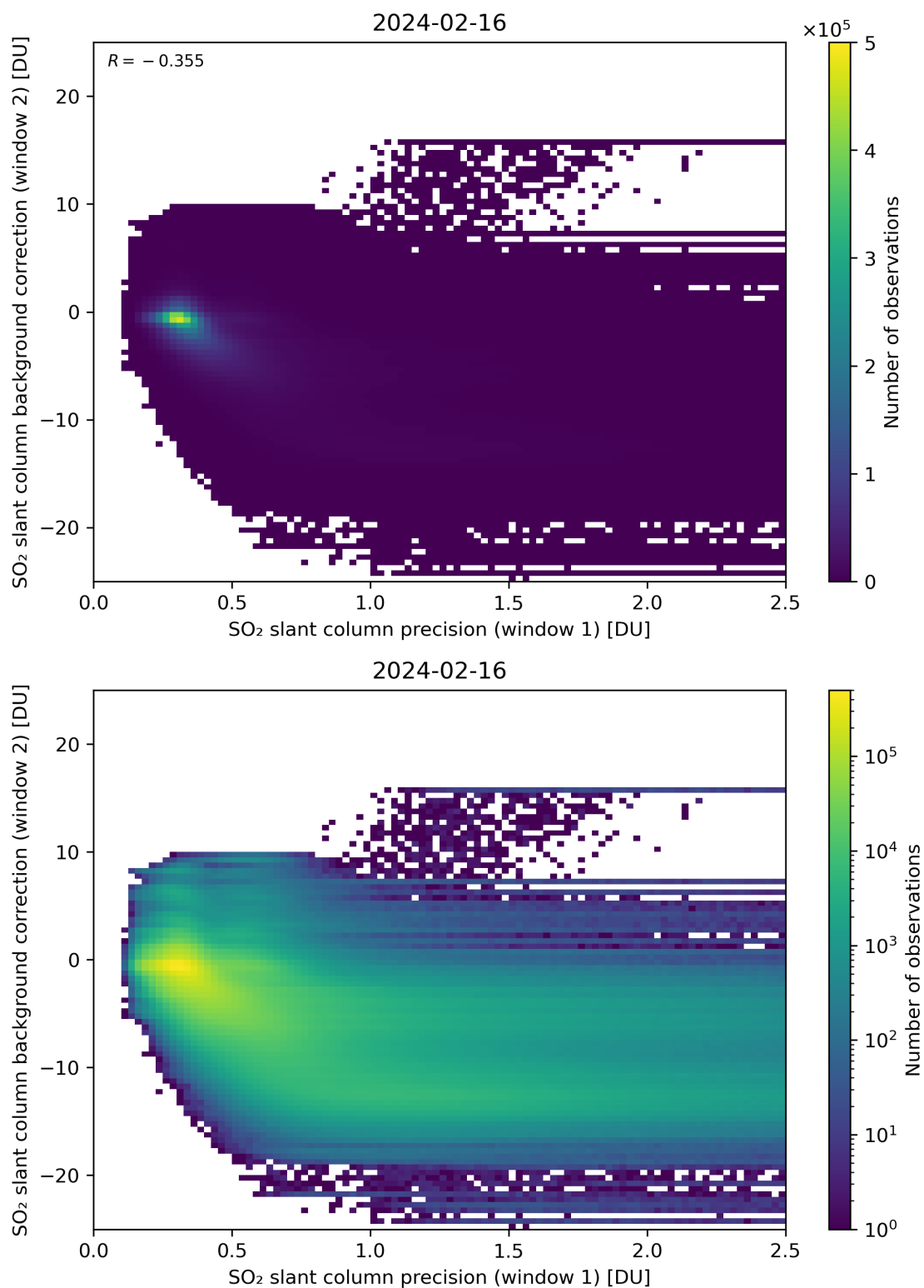
Figure 219: Scatter density plot of “SO 2 slant column precision (window 1)” against “SO 2 slant column background correction (window 2)” for 2024-02-16 to 2024-02-17.
