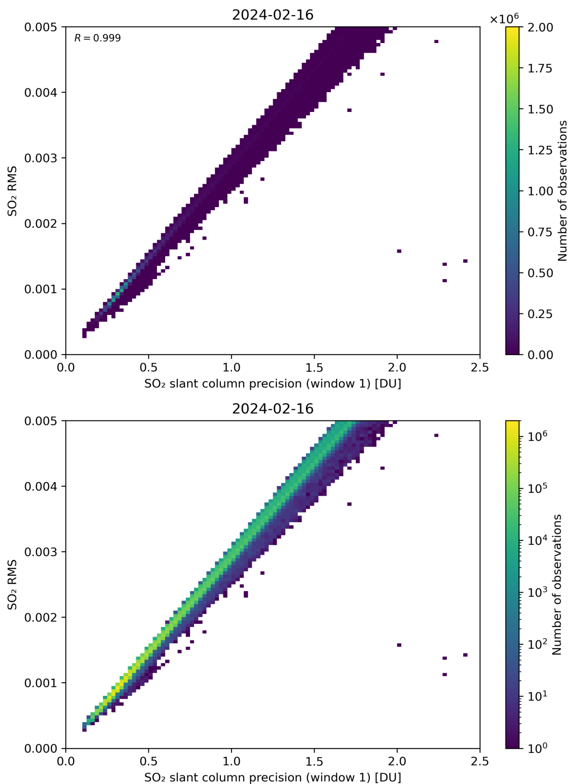
Figure 223: Scatter density plot of “SO 2 slant column precision (window 1)” against “SO 2 RMS” for 2024-02-16 to 2024-02-17.
