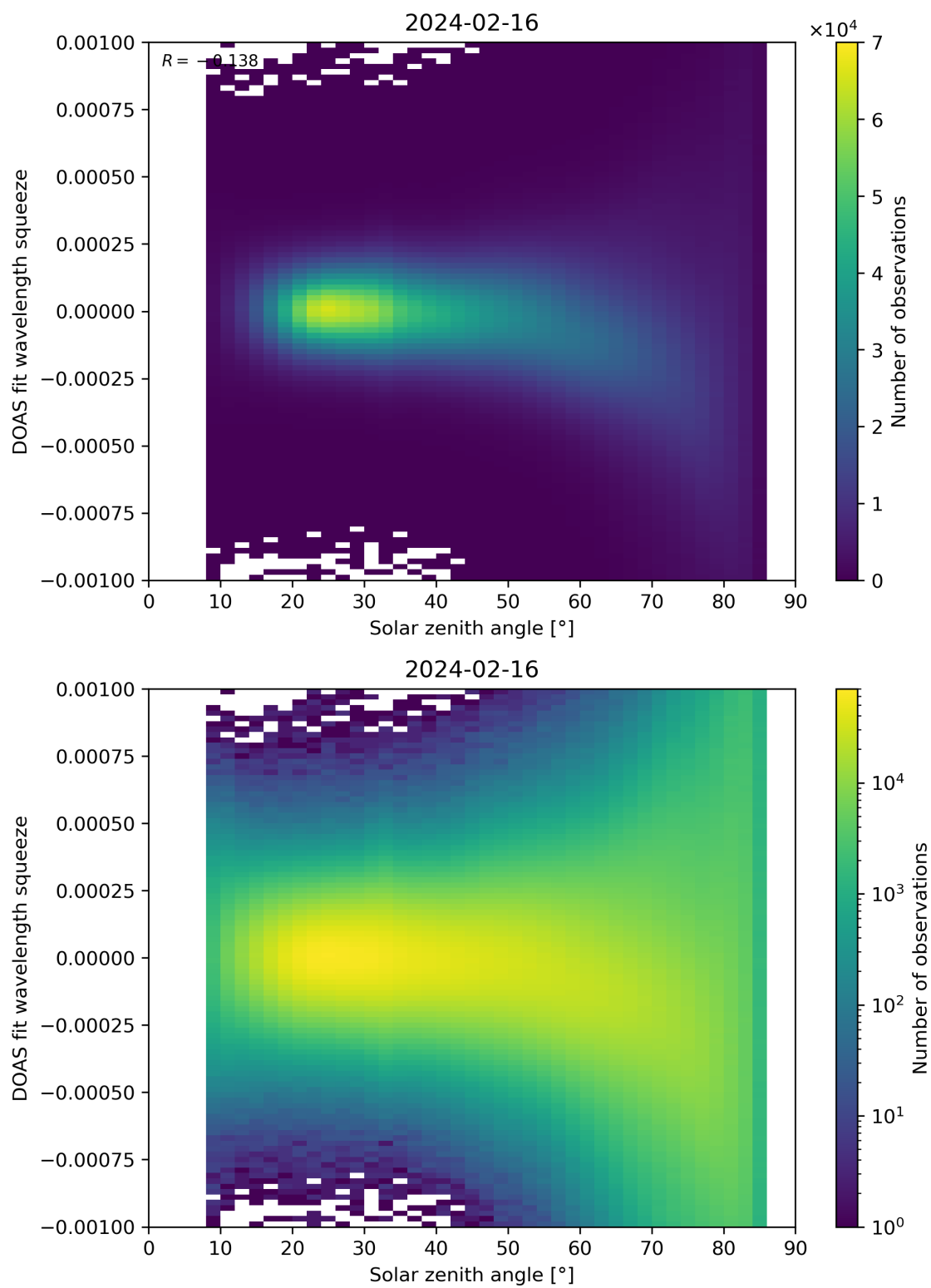
Figure 162: Scatter density plot of “Solar zenith angle” against “DOAS fit wavelength squeeze” for 2024-02-16 to 2024-02-17.
