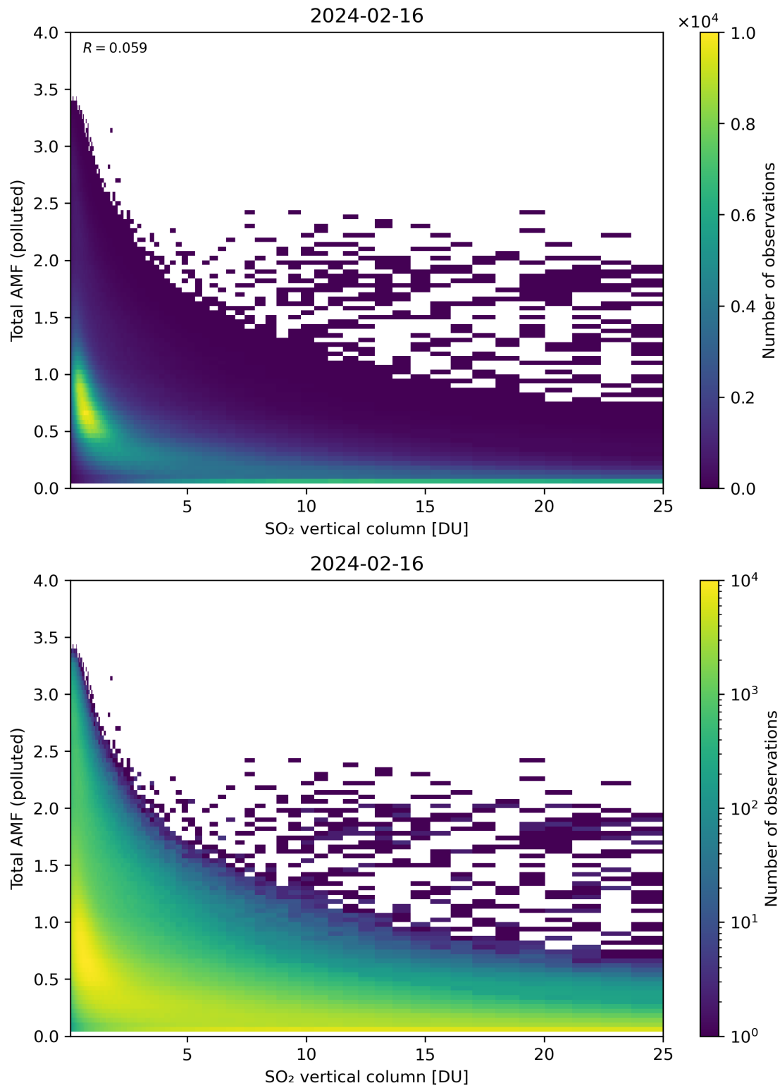
Figure 305: Scatter density plot of “SO 2 vertical column” against “Total AMF (polluted)” for 2024-02-16 to 2024-02-17.
