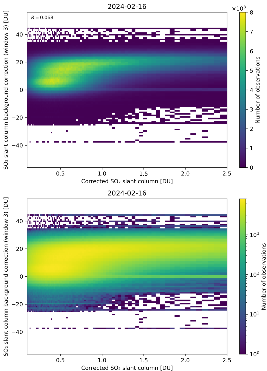
Figure 180: Scatter density plot of “Corrected SO 2 slant column” against “SO 2 slant column background correction (window 3)” for 2024-02-16 to 2024-02-17.
