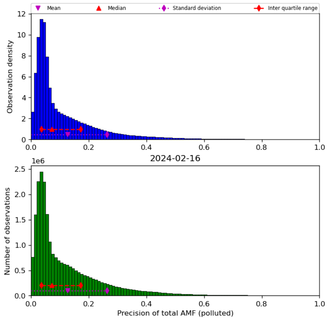
Figure 72: Histogram of “Precision of total AMF (polluted)” for 2024-02-16 to 2024-02-17
