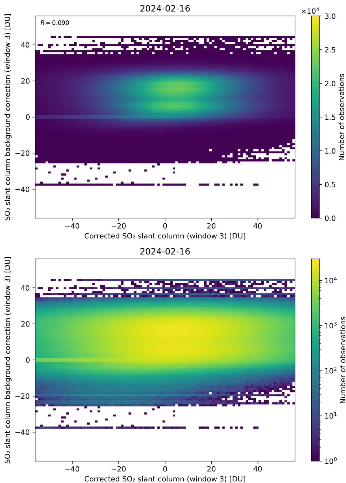
Figure 205: Scatter density plot of “Corrected SO 2 slant column (window 3)” against “SO 2 slant column background correction (window 3)” for 2024-02-16 to 2024-02-17.
