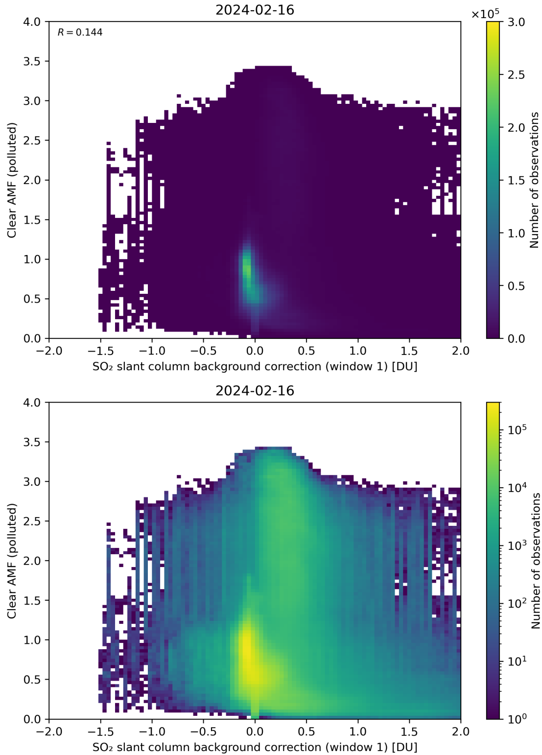
Figure 103: Scatter density plot of “SO 2 slant column background correction (window 1)” against “Clear AMF (polluted)” for 2024-02-16 to 2024-02-17.
