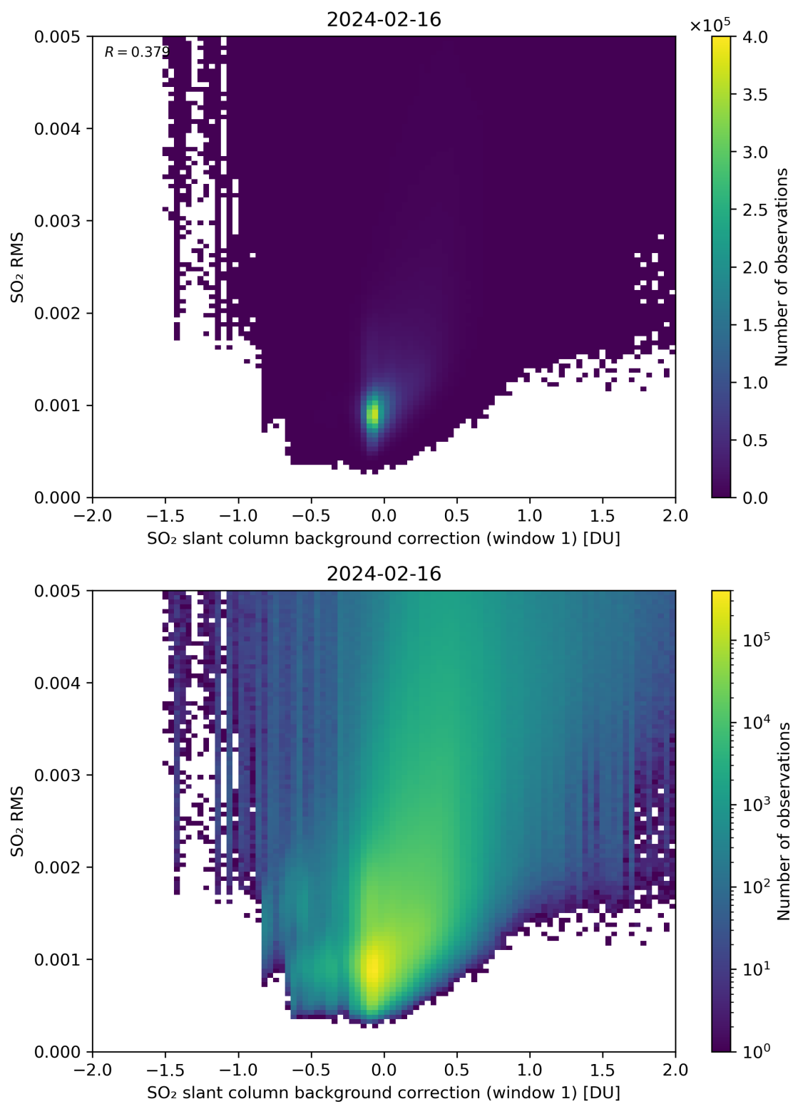
Figure 102: Scatter density plot of “SO 2 slant column background correction (window 1)” against “SO 2 RMS” for 2024-02-16 to 2024-02-17.
