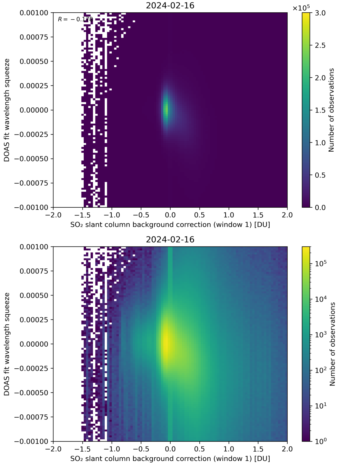
Figure 101: Scatter density plot of “SO 2 slant column background correction (window 1)” against “DOAS fit wavelength squeeze” for 2024-02-16 to 2024-02-17.
