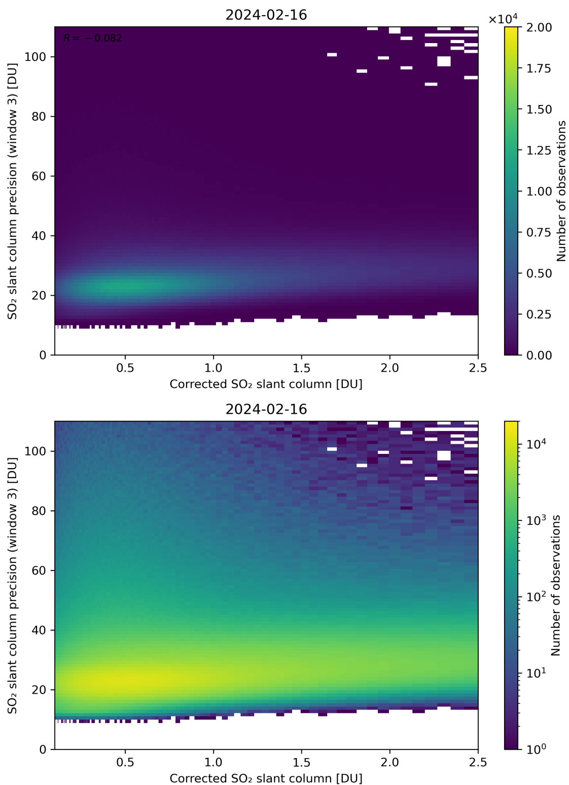
Figure 191: Scatter density plot of “Corrected SO 2 slant column” against “SO 2 slant column precision (window 3)” for 2024-02-16 to 2024-02-17.
