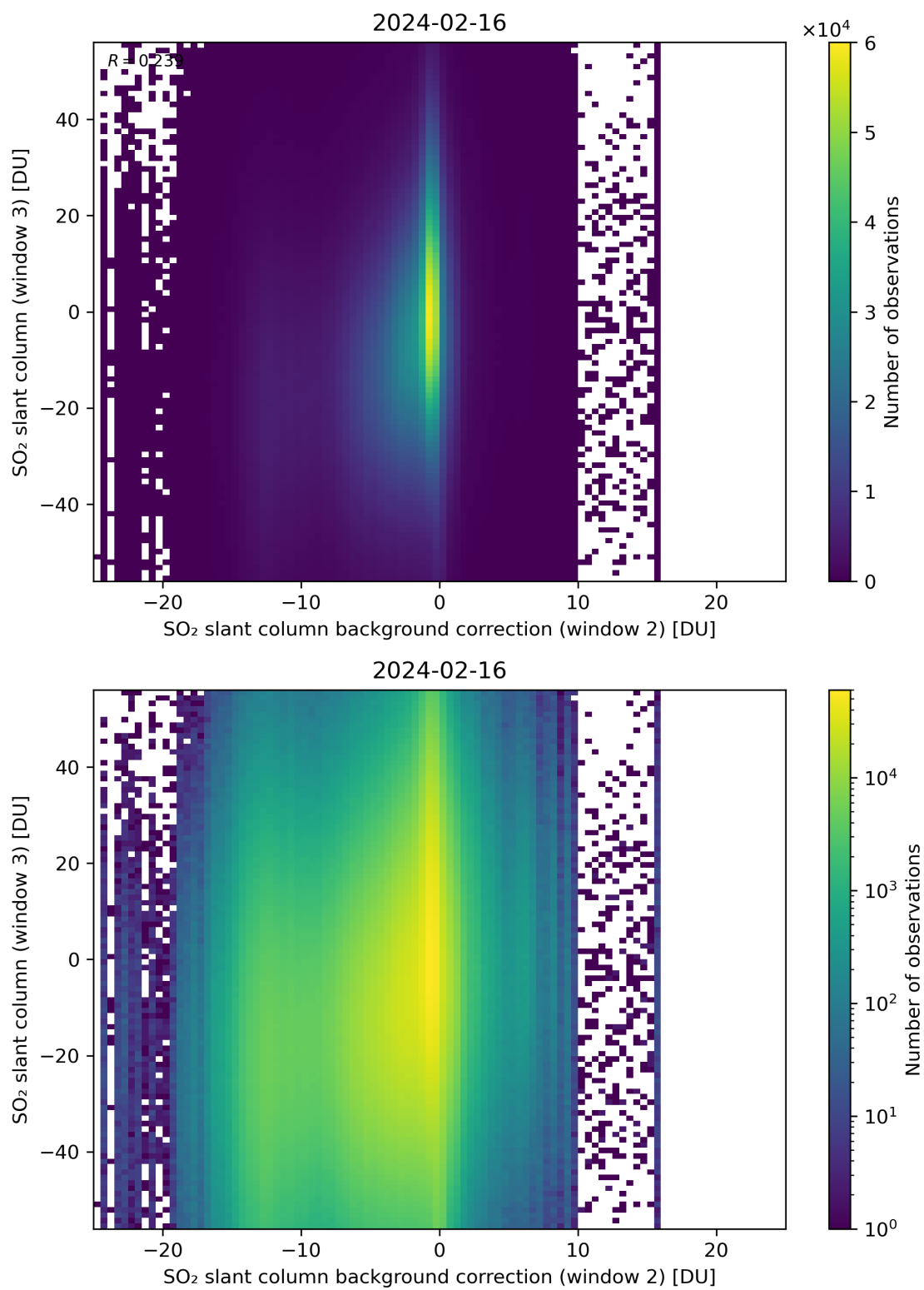
Figure 117: Scatter density plot of “SO 2 slant column background correction (window 2)” against “SO 2 slant column (window 3)” for 2024-02-16 to 2024-02-17.
