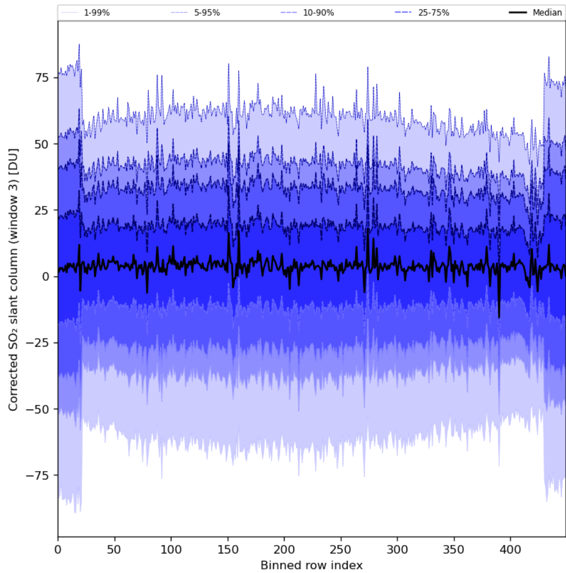
Figure 89: Along track statistics of “Corrected SO 2 slant column (window 3)” for 2024-02-16 to 2024-02-17
