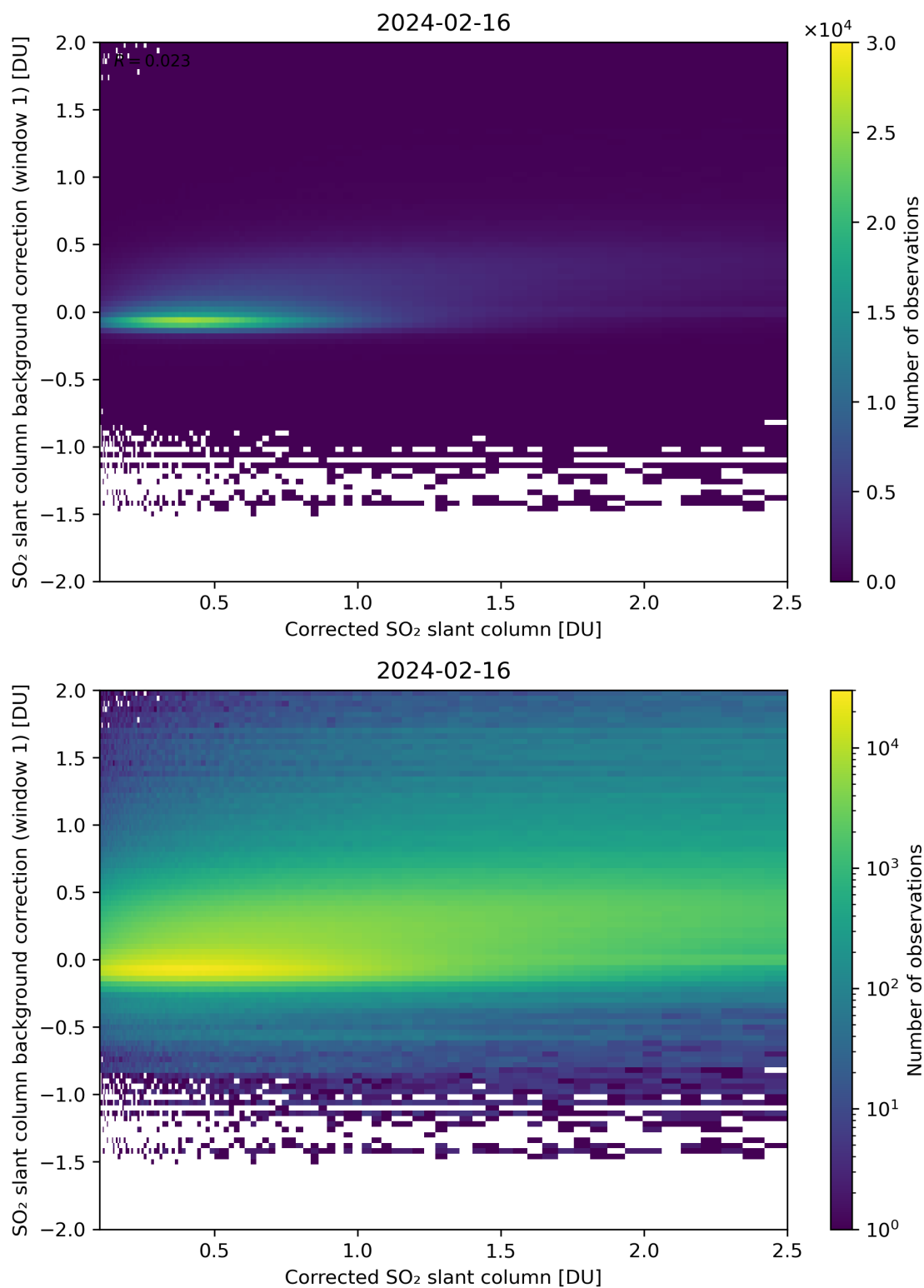
Figure 178: Scatter density plot of “Corrected SO 2 slant column” against “SO 2 slant column background correction (window 1)” for 2024-02-16 to 2024-02-17.
