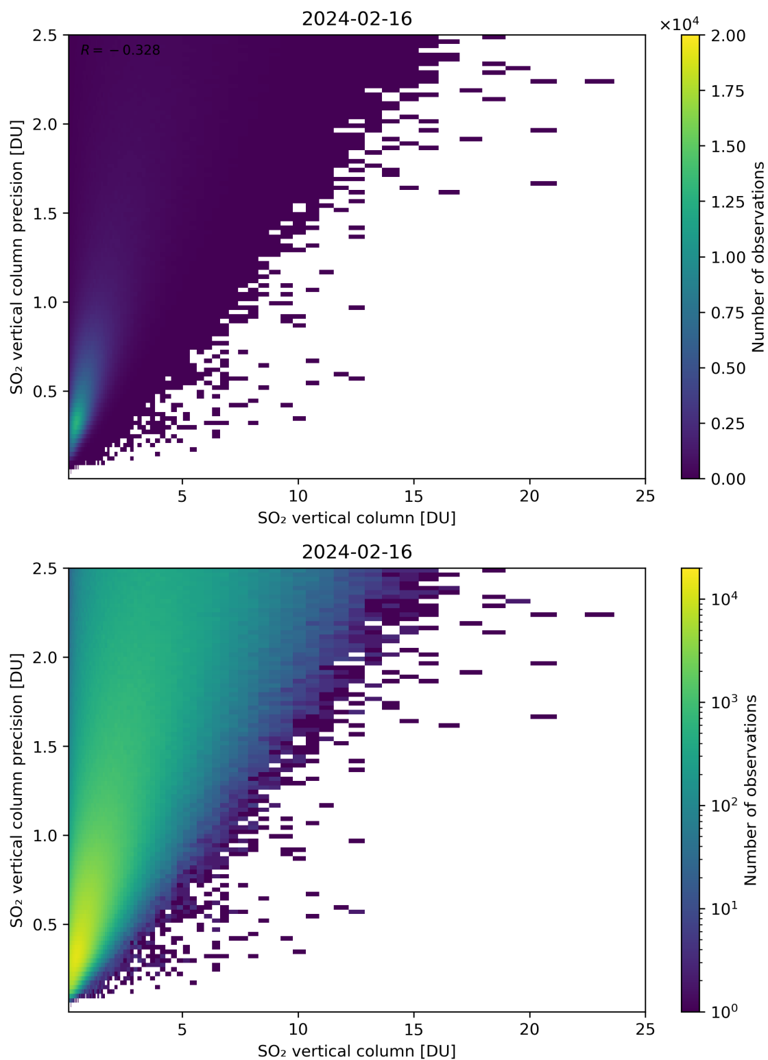
Figure 307: Scatter density plot of “SO 2 vertical column” against “SO 2 vertical column precision” for 2024-02-16 to 2024-02-17.
