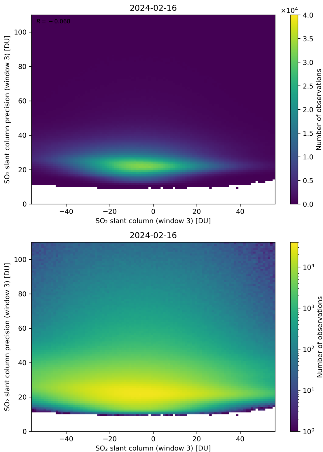
Figure 267: Scatter density plot of “SO 2 slant column (window 3)” against “SO 2 slant column precision (window 3)” for 2024-02-16 to 2024-02-17.
