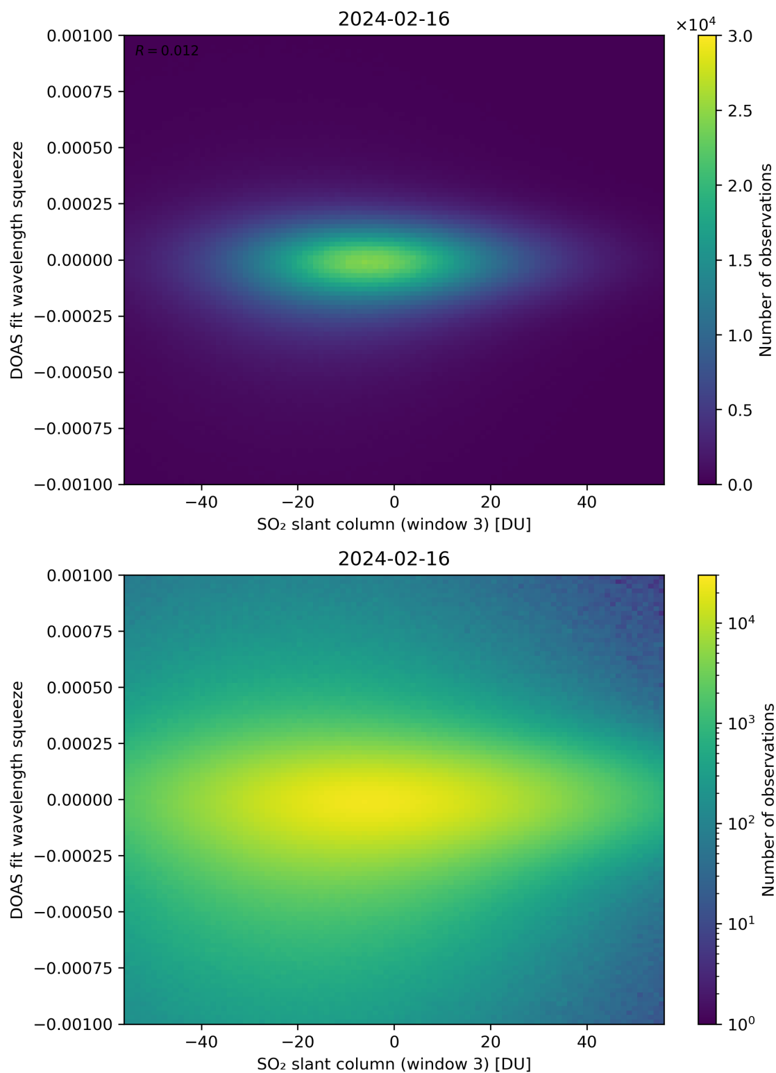
Figure 255: Scatter density plot of “SO 2 slant column (window 3)” against “DOAS fit wavelength squeeze” for 2024-02-16 to 2024-02-17.
