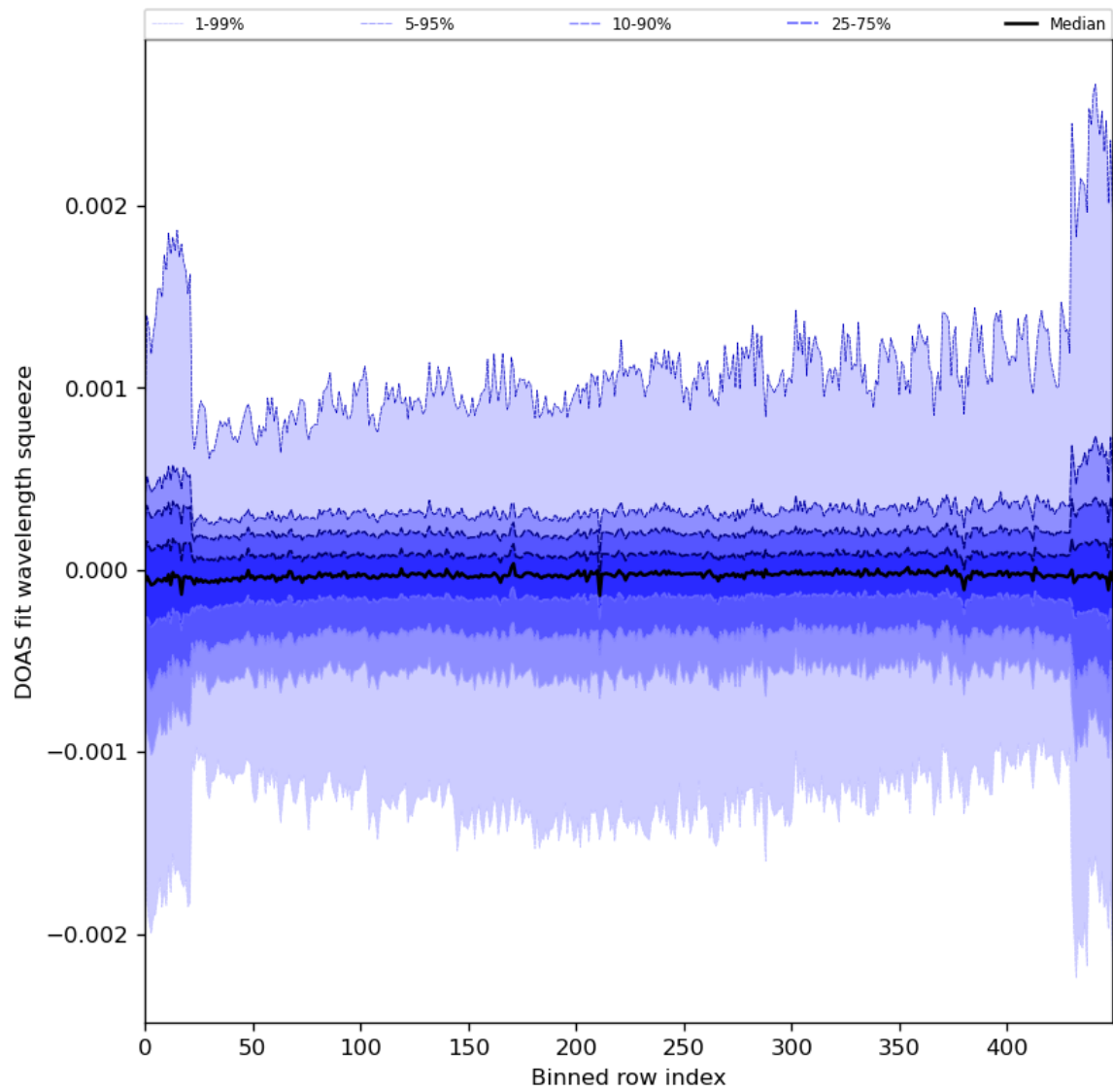
Figure 92: Along track statistics of “DOAS fit wavelength squeeze” for 2024-02-16 to 2024-02-17
