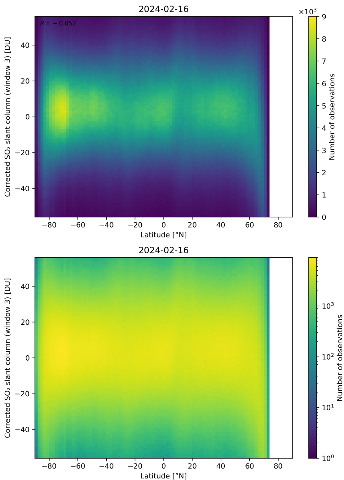
Figure 148: Scatter density plot of “Latitude” against “Corrected SO 2 slant column (window 3)” for 2024-02-16 to 2024-02-17.
