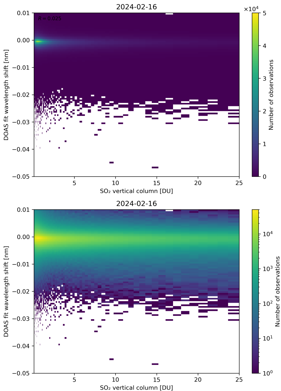
Figure 276: Scatter density plot of “SO 2 vertical column” against “DOAS fit wavelength shift” for 2024-02-16 to 2024-02-17.
