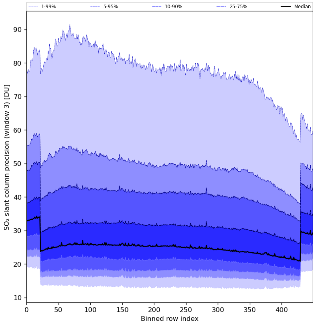
Figure 88: Along track statistics of “SO 2 slant column precision (window 3)” for 2024-02-16 to 2024-02-17
