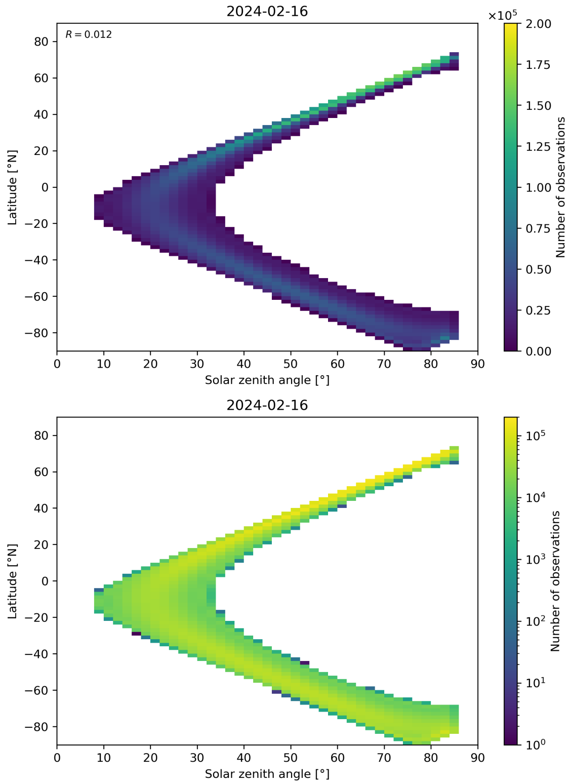
Figure 164: Scatter density plot of “Solar zenith angle” against “Latitude” for 2024-02-16 to 2024-02-17.
