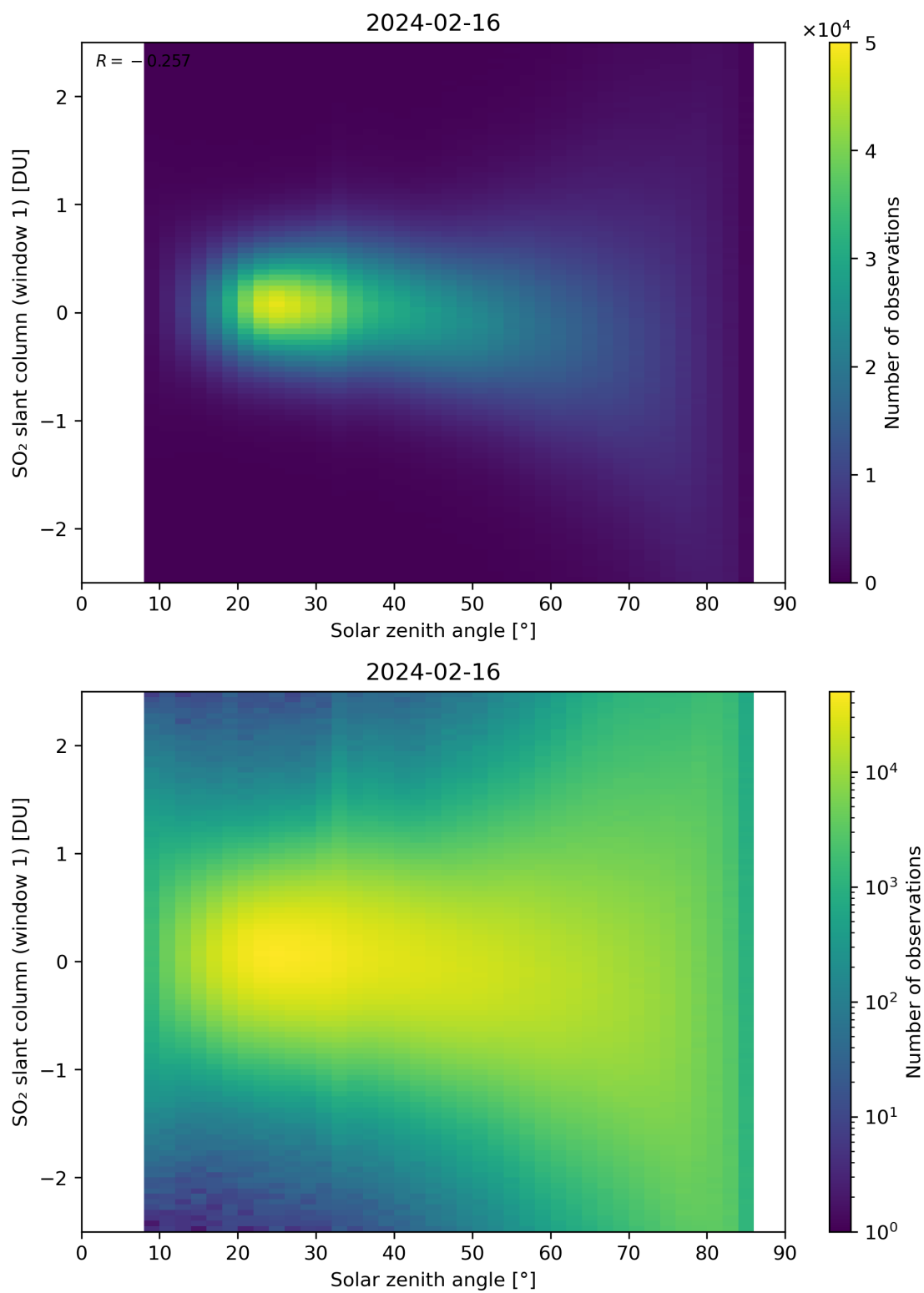
Figure 169: Scatter density plot of “Solar zenith angle” against “SO 2 slant column (window 1)” for 2024-02-16 to 2024-02-17.
