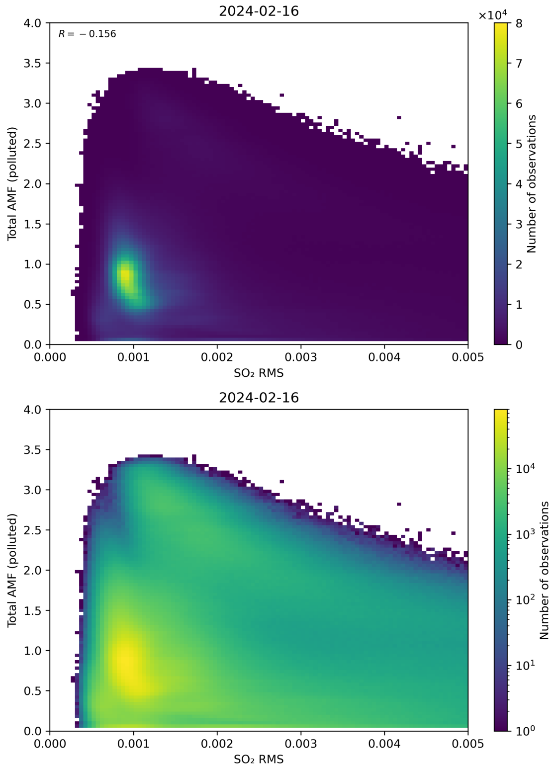
Figure 137: Scatter density plot of “SO 2 RMS” against “Total AMF (polluted)” for 2024-02-16 to 2024-02-17.
