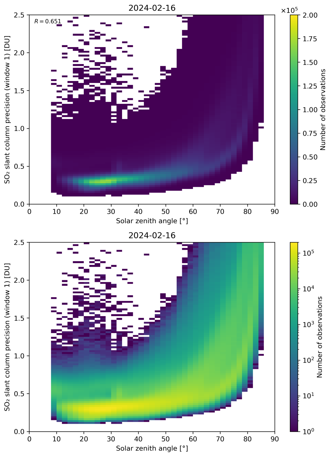
Figure 170: Scatter density plot of “Solar zenith angle” against “SO 2 slant column precision (window 1)” for 2024-02-16 to 2024-02-17.
