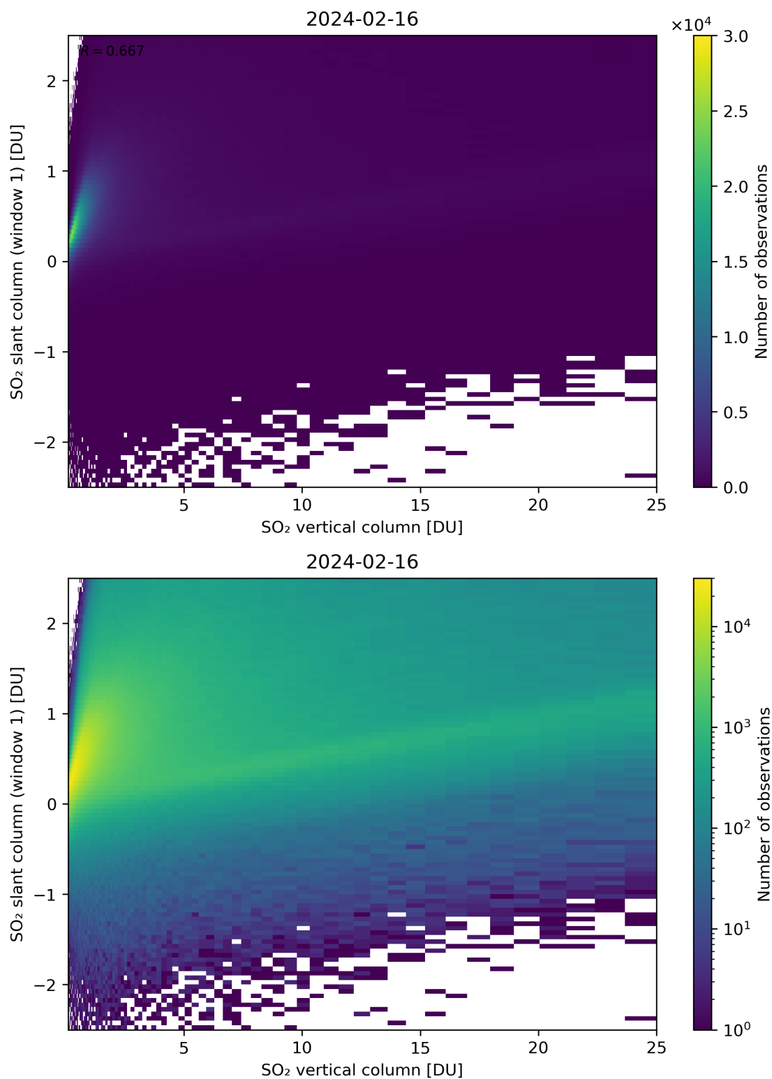
Figure 300: Scatter density plot of “SO 2 vertical column” against “SO 2 slant column (window 1)” for 2024-02-16 to 2024-02-17.
