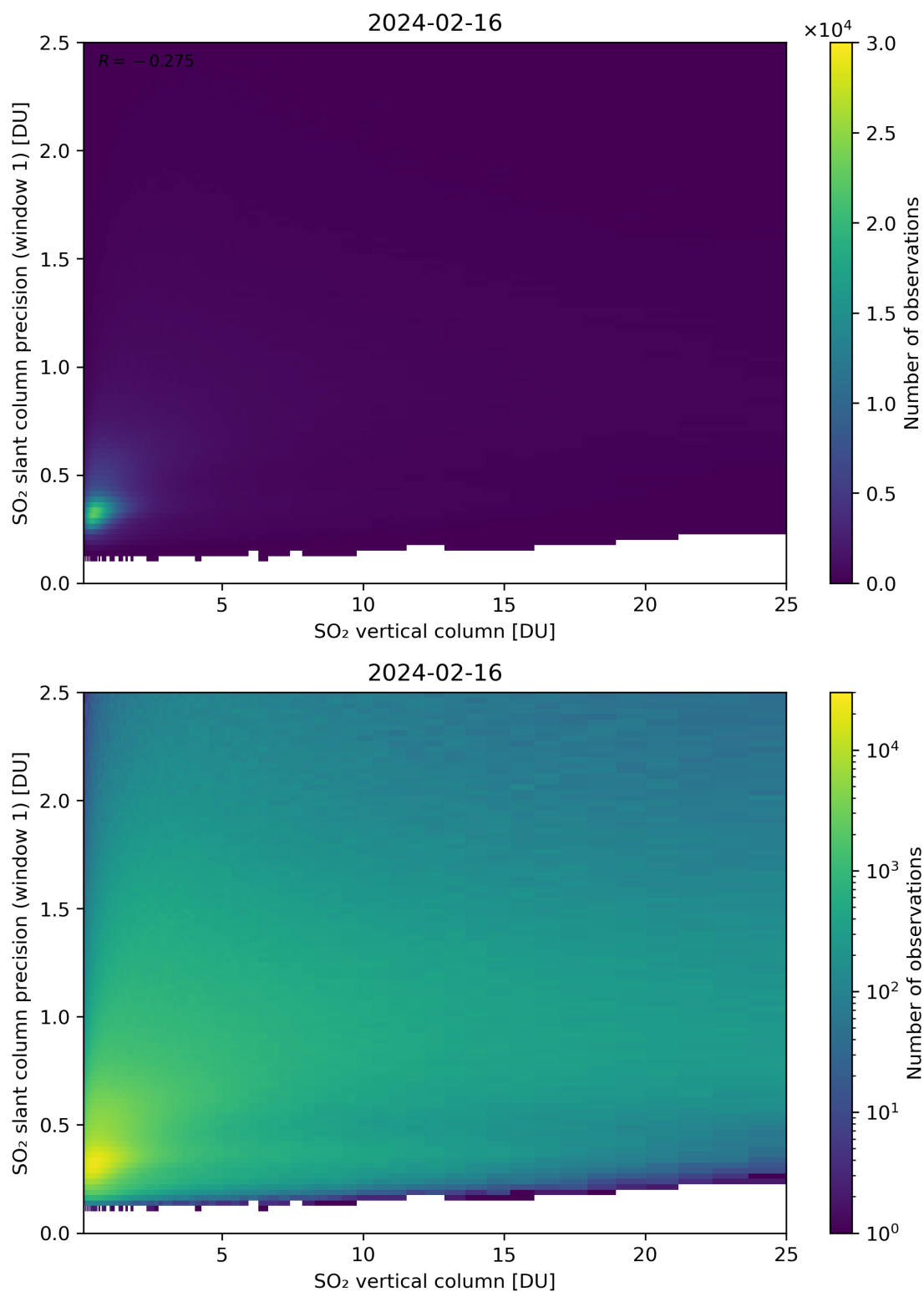
Figure 301: Scatter density plot of “SO 2 vertical column” against “SO 2 slant column precision (window 1)” for 2024-02-16 to 2024-02-17.
