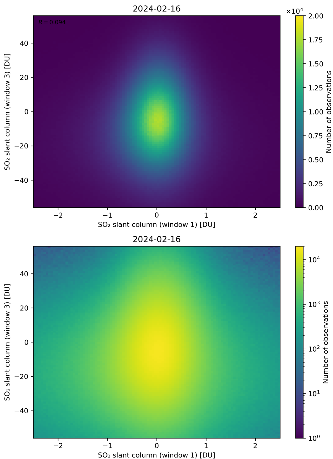
Figure 237: Scatter density plot of “SO 2 slant column (window 1)” against “SO 2 slant column (window 3)” for 2024-02-16 to 2024-02-17.
