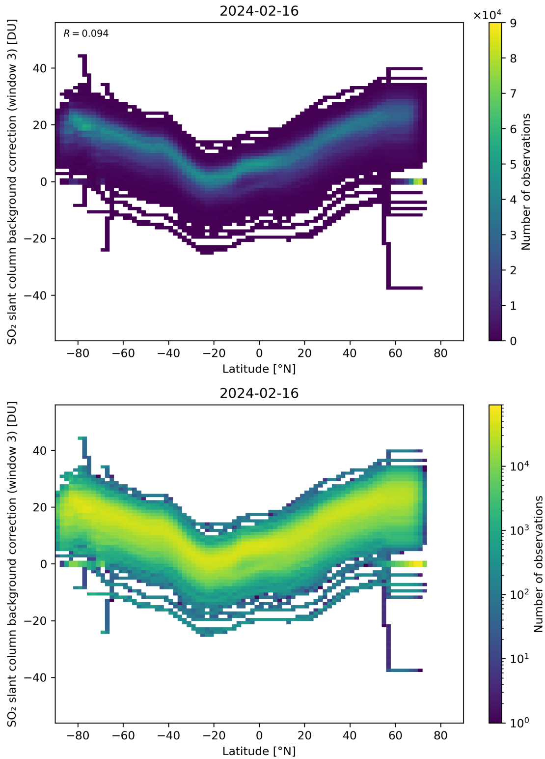
Figure 141: Scatter density plot of “Latitude” against “SO 2 slant column background correction (window 3)” for 2024-02-16 to 2024-02-17.
