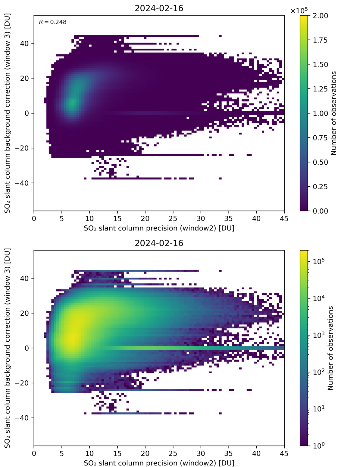
Figure 242: Scatter density plot of “SO 2 slant column precision (window2)” against “SO 2 slant column background correction (window 3)” for 2024-02-16 to 2024-02-17.
