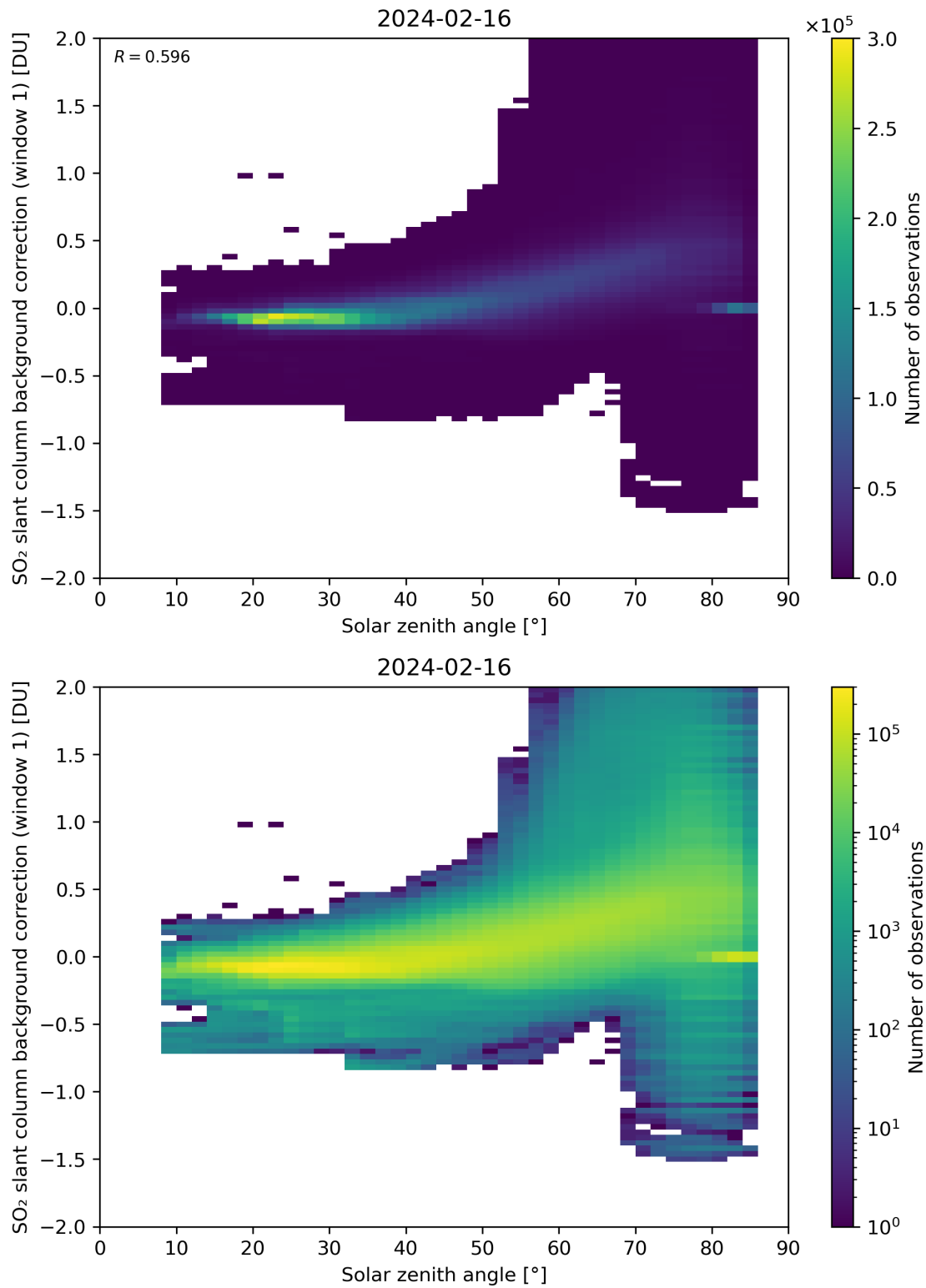
Figure 158: Scatter density plot of “Solar zenith angle” against “SO 2 slant column background correction (window 1)” for 2024-02-16 to 2024-02-17.
