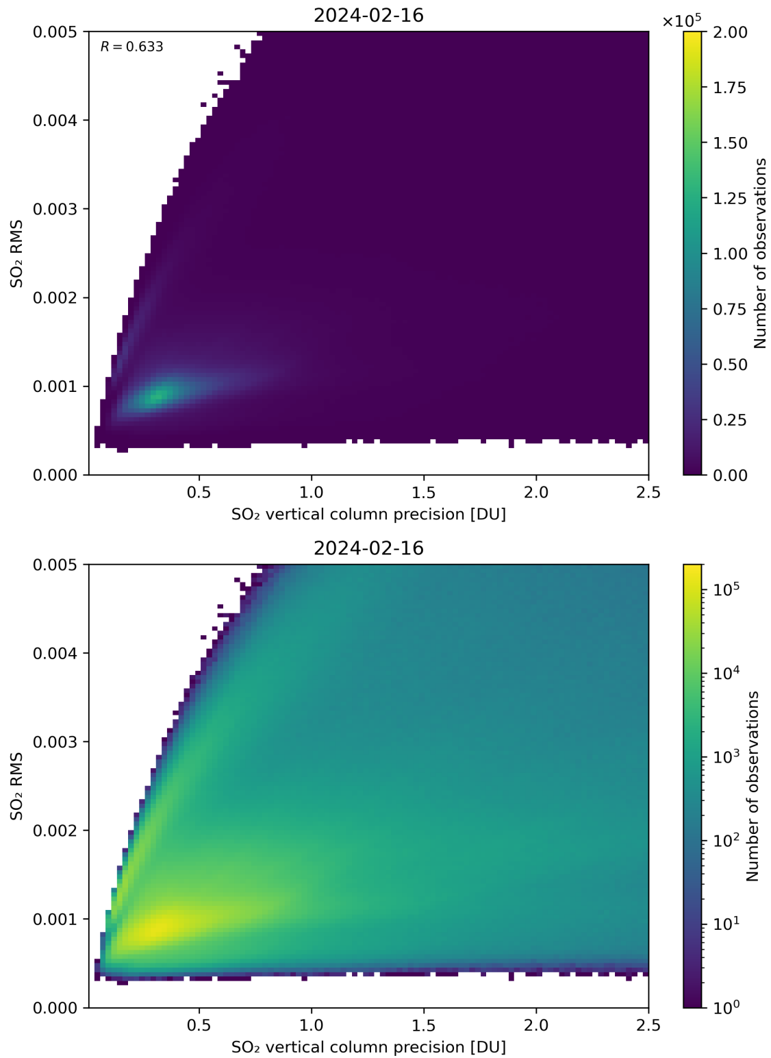
Figure 284: Scatter density plot of “SO 2 vertical column precision” against “SO 2 RMS” for 2024-02-16 to 2024-02-17.
