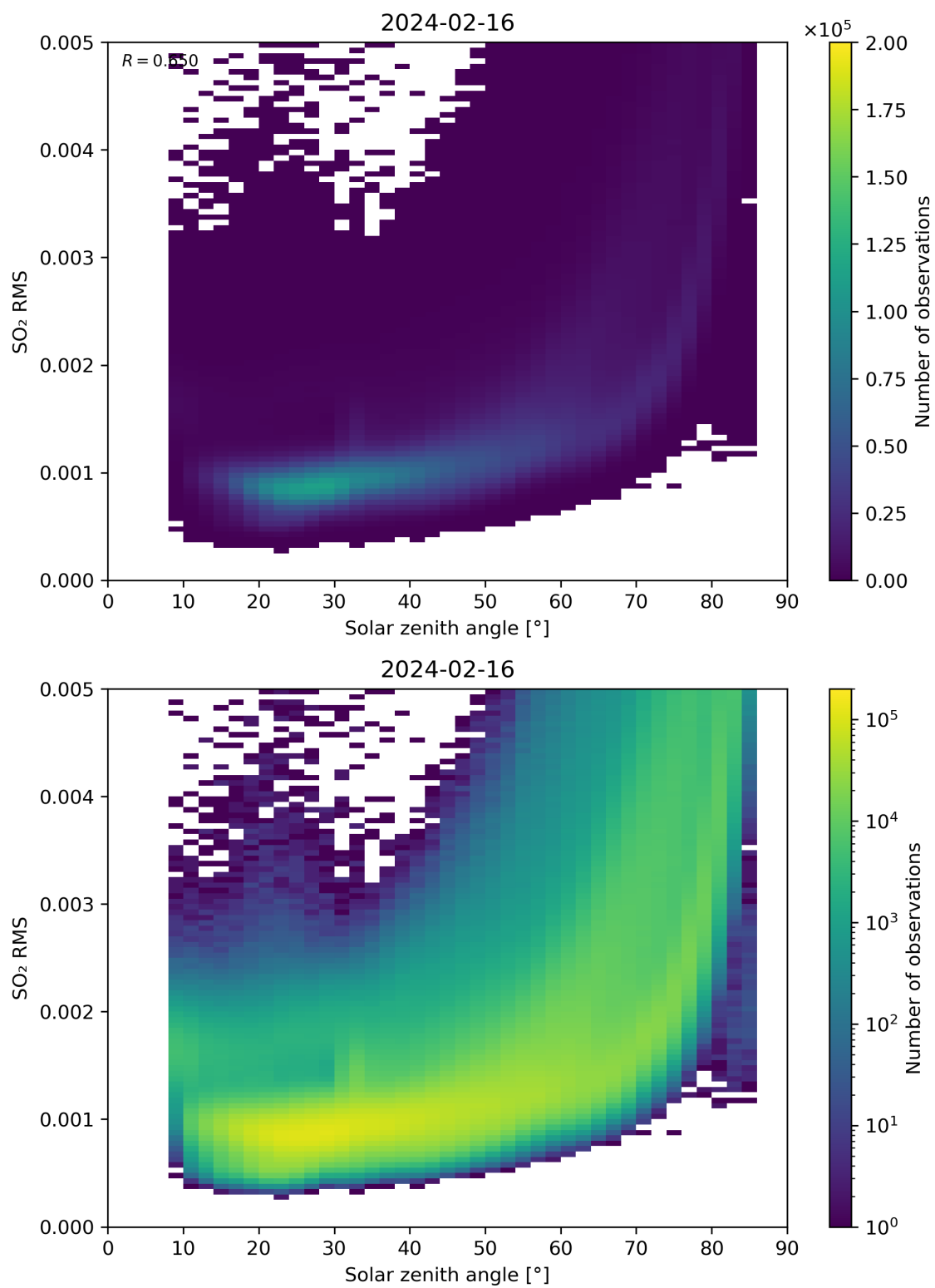
Figure 163: Scatter density plot of “Solar zenith angle” against “SO 2 RMS” for 2024-02-16 to 2024-02-17.
