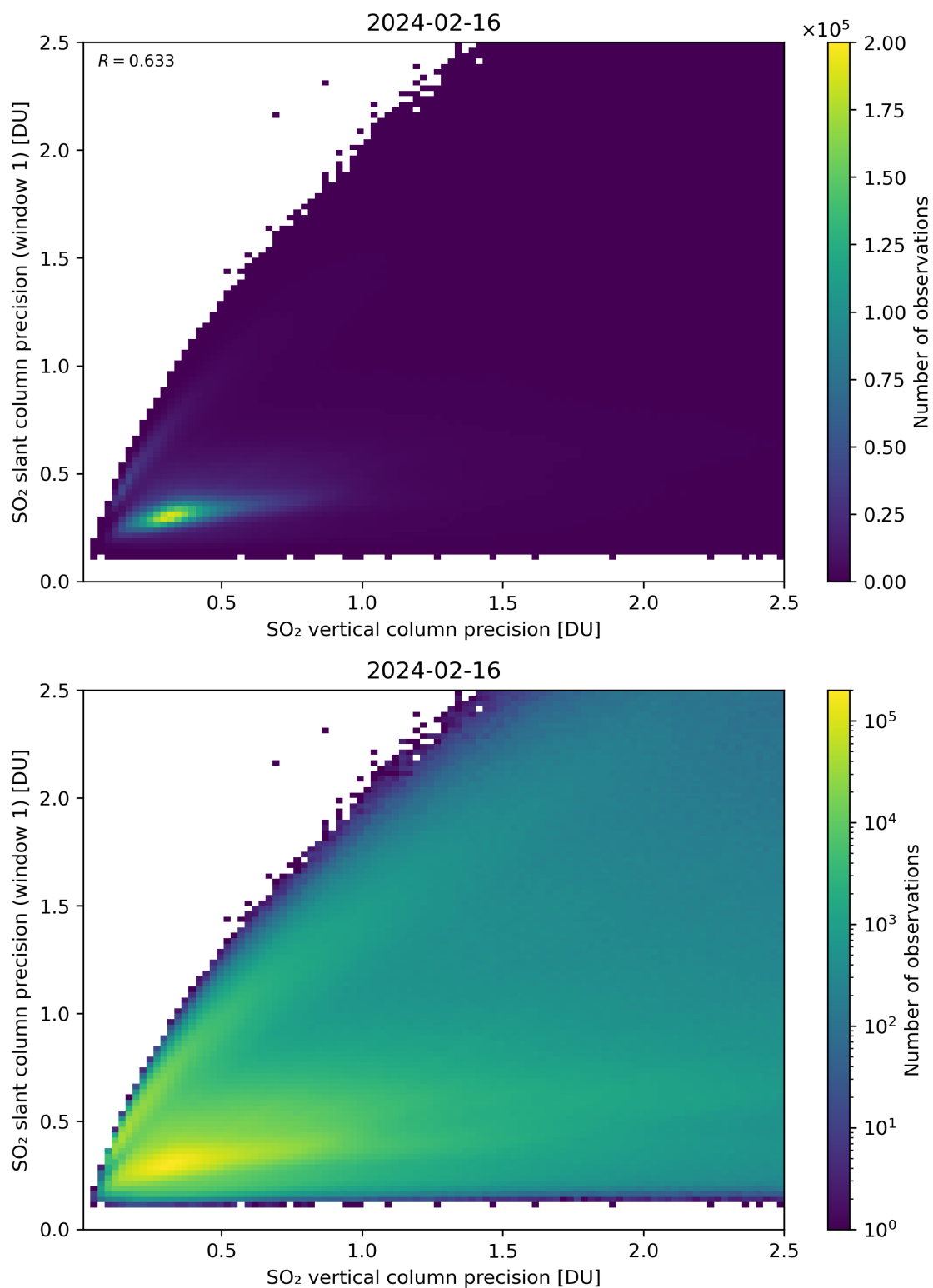
Figure 290: Scatter density plot of “SO 2 vertical column precision” against “SO 2 slant column precision (window 1)” for 2024-02-16 to 2024-02-17.
