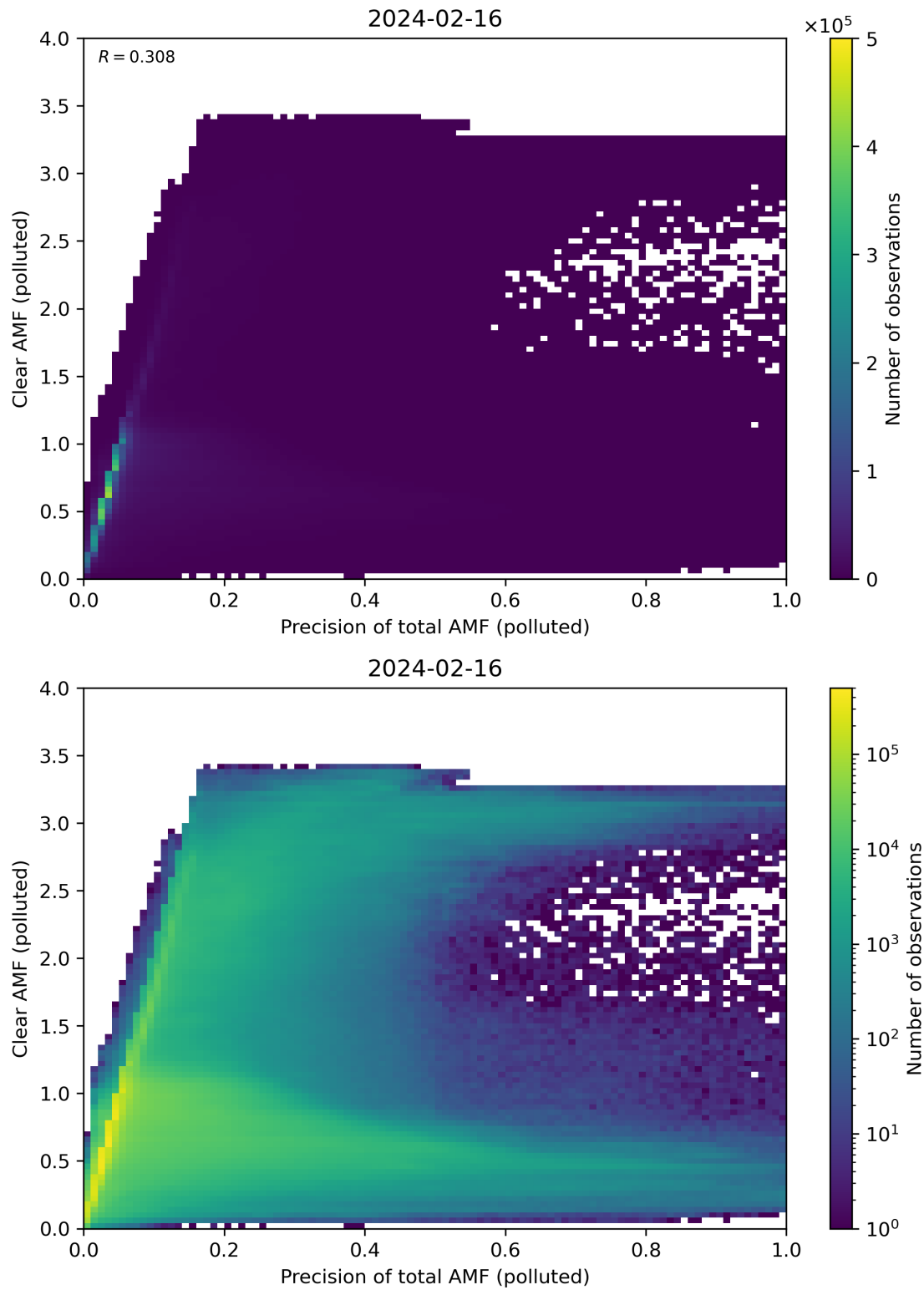
Figure 270: Scatter density plot of “Precision of total AMF (polluted)” against “Clear AMF (polluted)” for 2024-02-16 to 2024-02-17.
