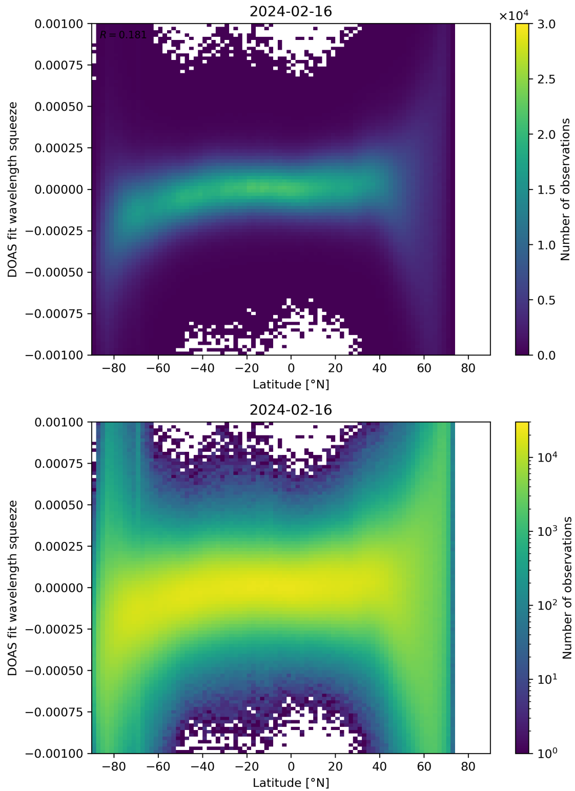
Figure 143: Scatter density plot of “Latitude” against “DOAS fit wavelength squeeze” for 2024-02-16 to 2024-02-17.
