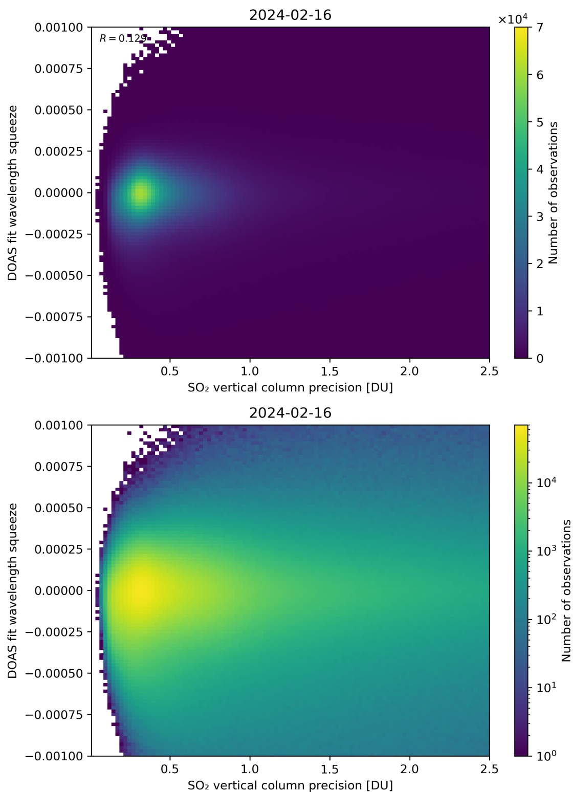
Figure 283: Scatter density plot of “SO 2 vertical column precision” against “DOAS fit wavelength squeeze” for 2024-02-16 to 2024-02-17.
