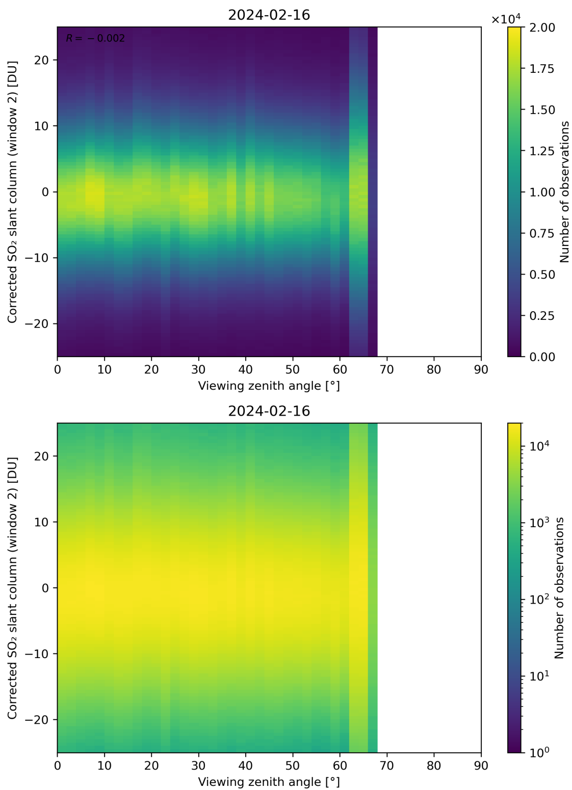
Figure 318: Scatter density plot of “Viewing zenith angle” against “Corrected SO 2 slant column (window 2)” for 2024-02-16 to 2024-02-17.
