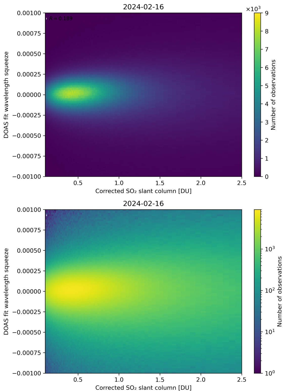
Figure 182: Scatter density plot of “Corrected SO 2 slant column” against “DOAS fit wavelength squeeze” for 2024-02-16 to 2024-02-17.
