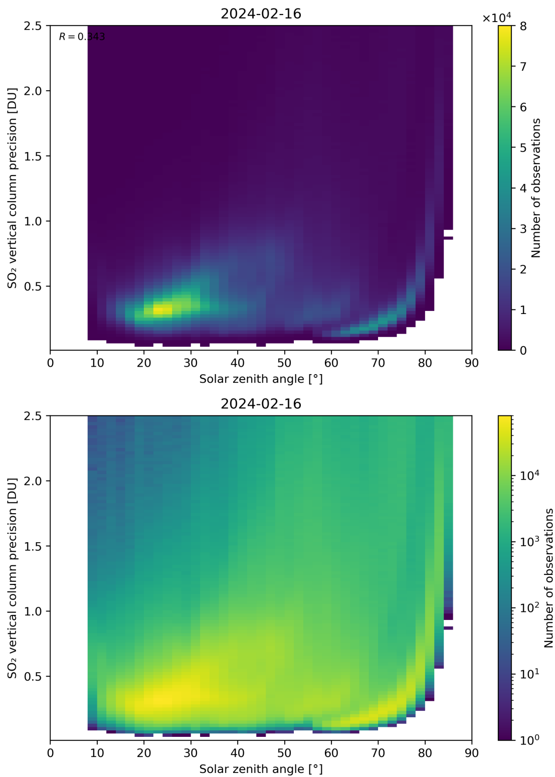
Figure 177: Scatter density plot of “Solar zenith angle” against “SO 2 vertical column precision” for 2024-02-16 to 2024-02-17.
