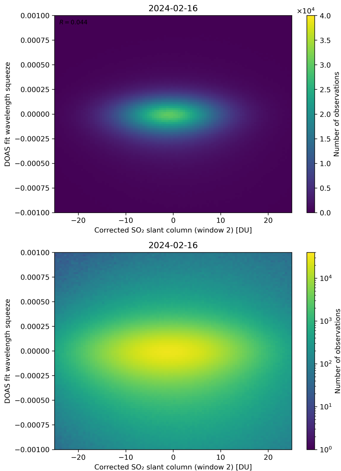
Figure 197: Scatter density plot of “Corrected SO 2 slant column (window 2)” against “DOAS fit wavelength squeeze” for 2024-02-16 to 2024-02-17.
