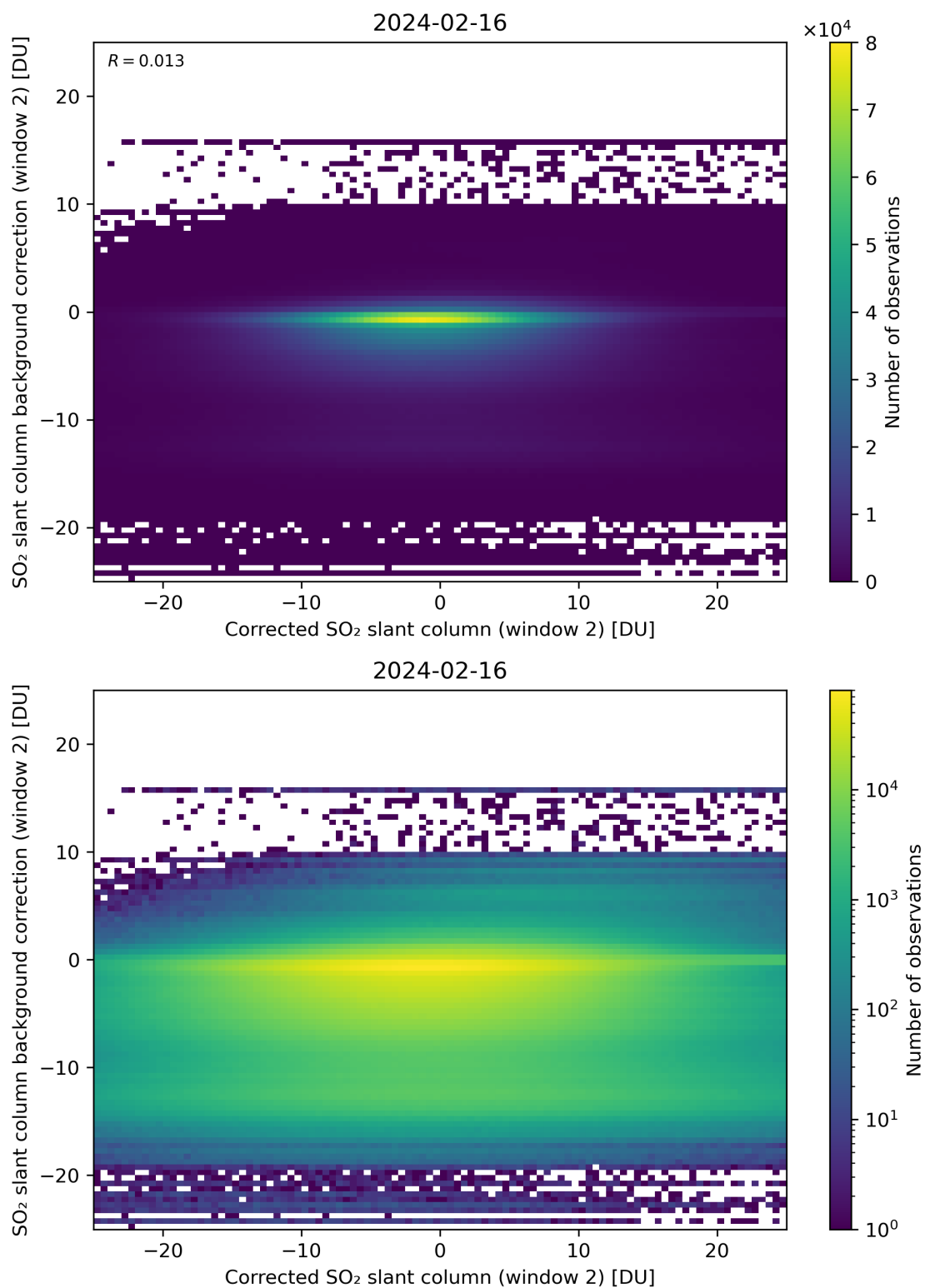
Figure 194: Scatter density plot of “Corrected SO 2 slant column (window 2)” against “SO 2 slant column background correction (window 2)” for 2024-02-16 to 2024-02-17.
