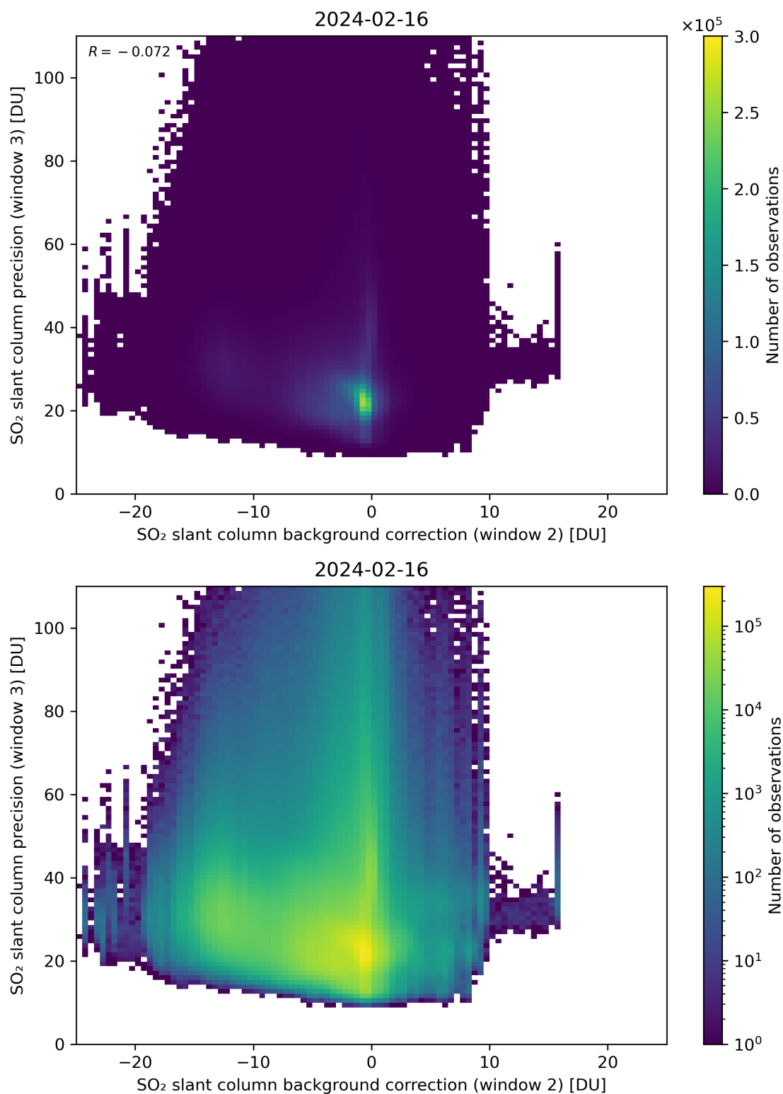
Figure 118: Scatter density plot of “SO 2 slant column background correction (window 2)” against “SO 2 slant column precision (window 3)” for 2024-02-16 to 2024-02-17.
