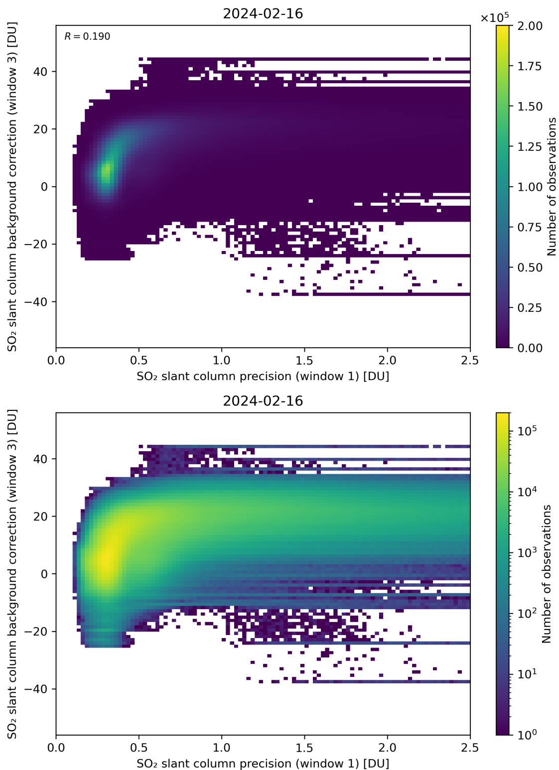
Figure 220: Scatter density plot of “SO 2 slant column precision (window 1)” against “SO 2 slant column background correction (window 3)” for 2024-02-16 to 2024-02-17.
