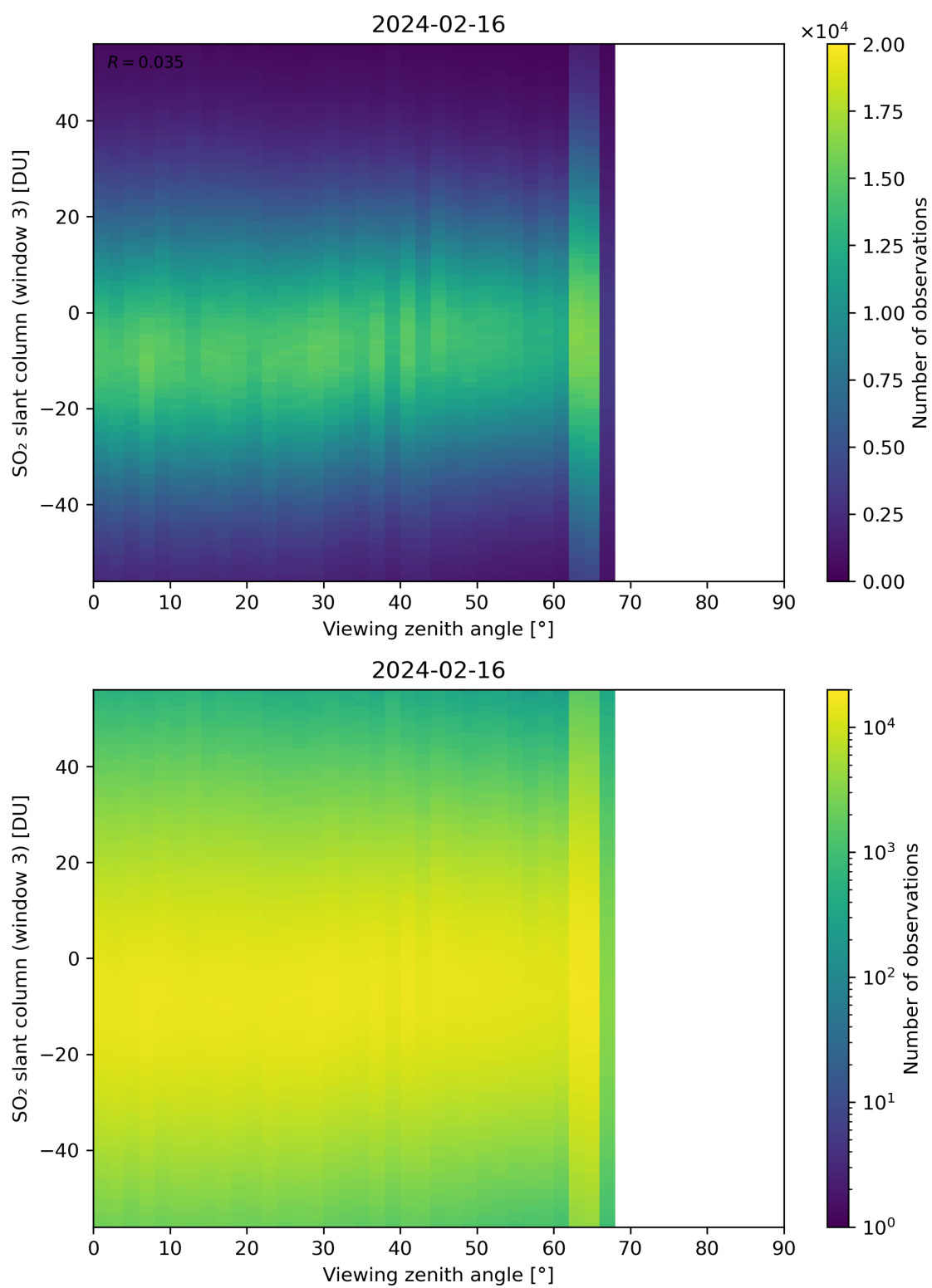
Figure 323: Scatter density plot of “Viewing zenith angle” against “SO 2 slant column (window 3)” for 2024-02-16 to 2024-02-17.
