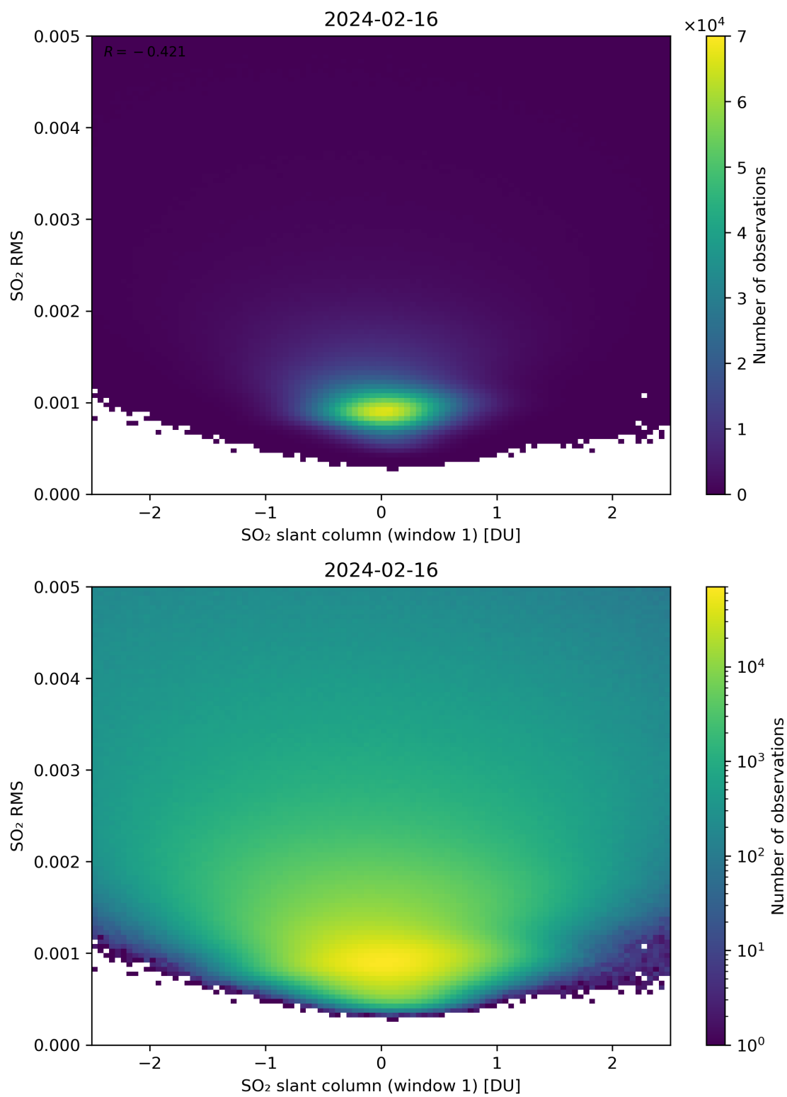
Figure 217: Scatter density plot of “SO 2 slant column (window 1)” against “SO 2 RMS” for 2024-02-16 to 2024-02-17.
