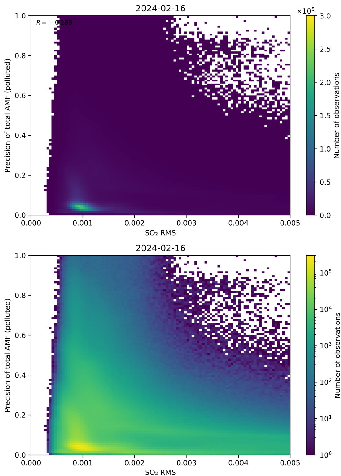
Figure 138: Scatter density plot of “SO 2 RMS” against “Precision of total AMF (polluted)” for 2024-02-16 to 2024-02-17.
