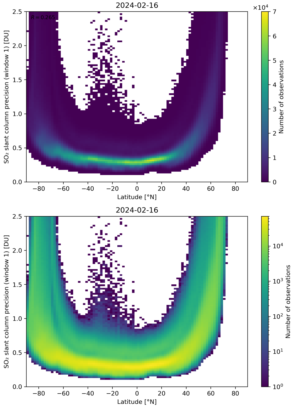
Figure 150: Scatter density plot of “Latitude” against “SO 2 slant column precision (window 1)” for 2024-02-16 to 2024-02-17.
