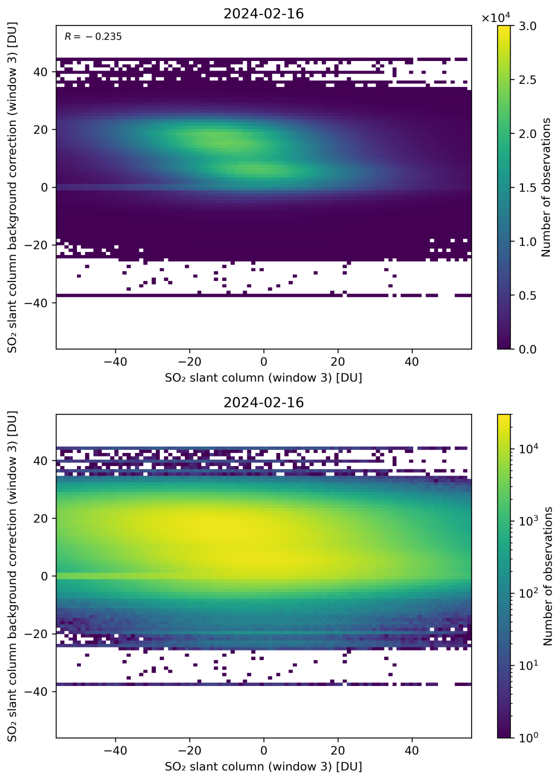
Figure 253: Scatter density plot of “SO 2 slant column (window 3)” against “SO 2 slant column background correction (window 3)” for 2024-02-16 to 2024-02-17.
