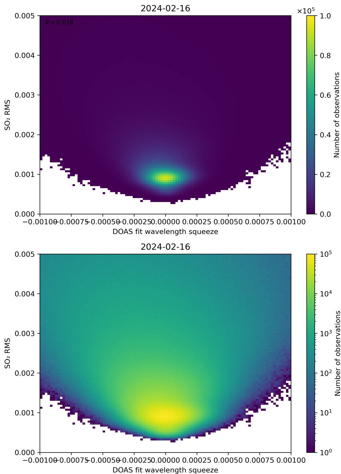
Figure 132: Scatter density plot of “DOAS fit wavelength squeeze” against “SO 2 RMS” for 2024-02-16 to 2024-02-17.
