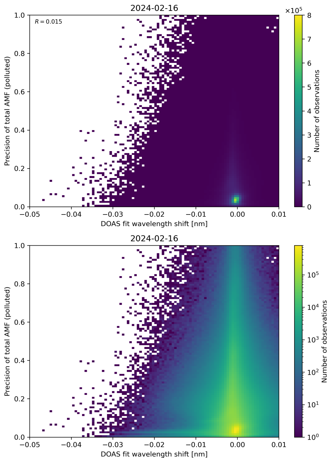
Figure 131: Scatter density plot of “DOAS fit wavelength shift” against “Precision of total AMF (polluted)” for 2024-02-16 to 2024-02-17.
