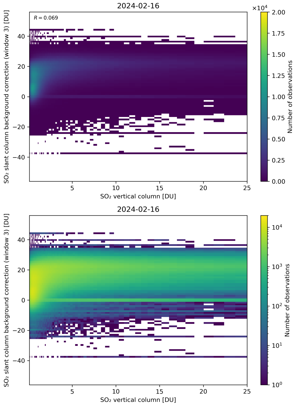
Figure 275: Scatter density plot of “SO 2 vertical column” against “SO 2 slant column background correction (window 3)” for 2024-02-16 to 2024-02-17.
