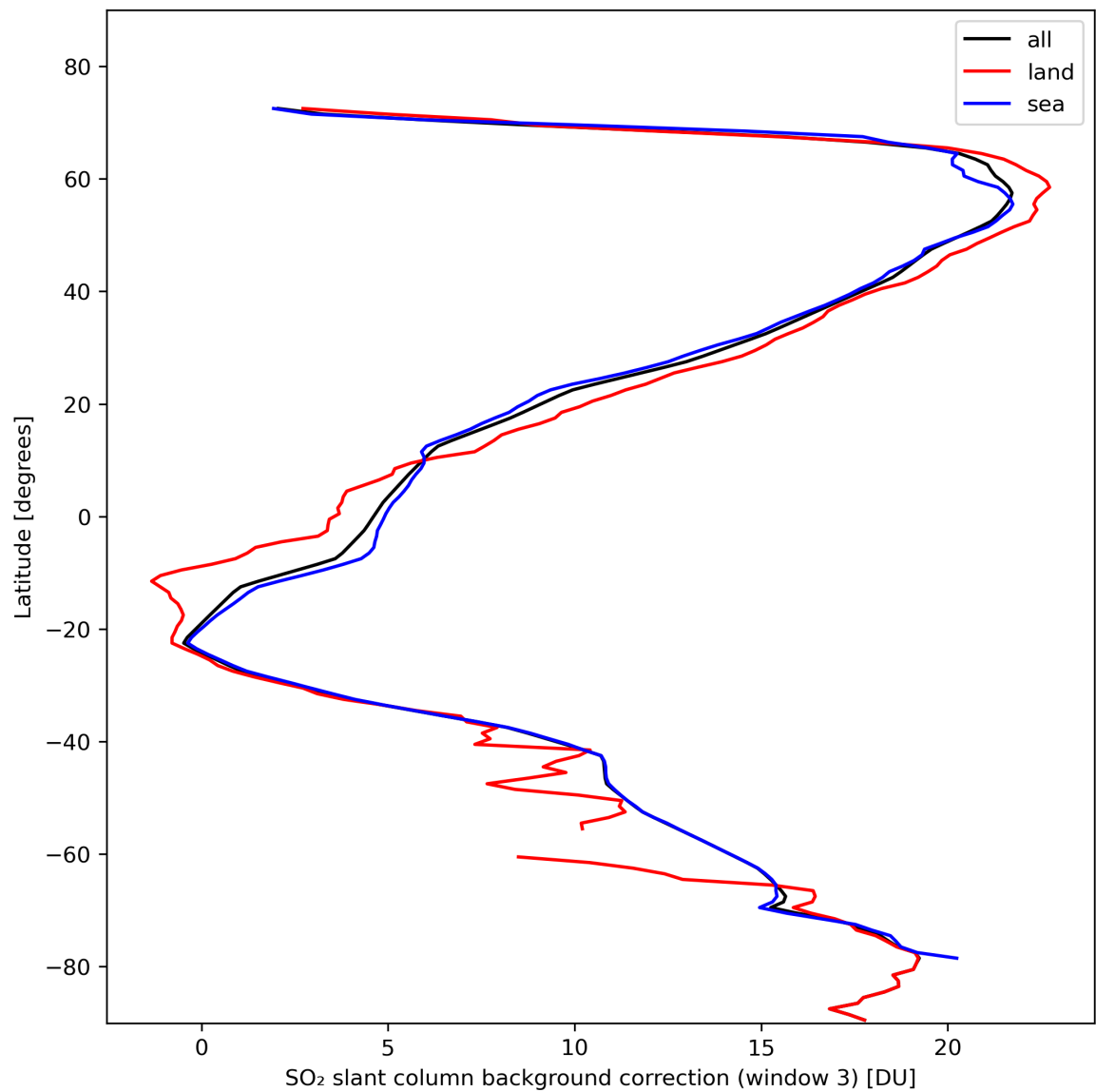
Figure 44: Zonal average of “SO 2 slant column background correction (window 3)” for 2024-02-16 to 2024-02-17.
