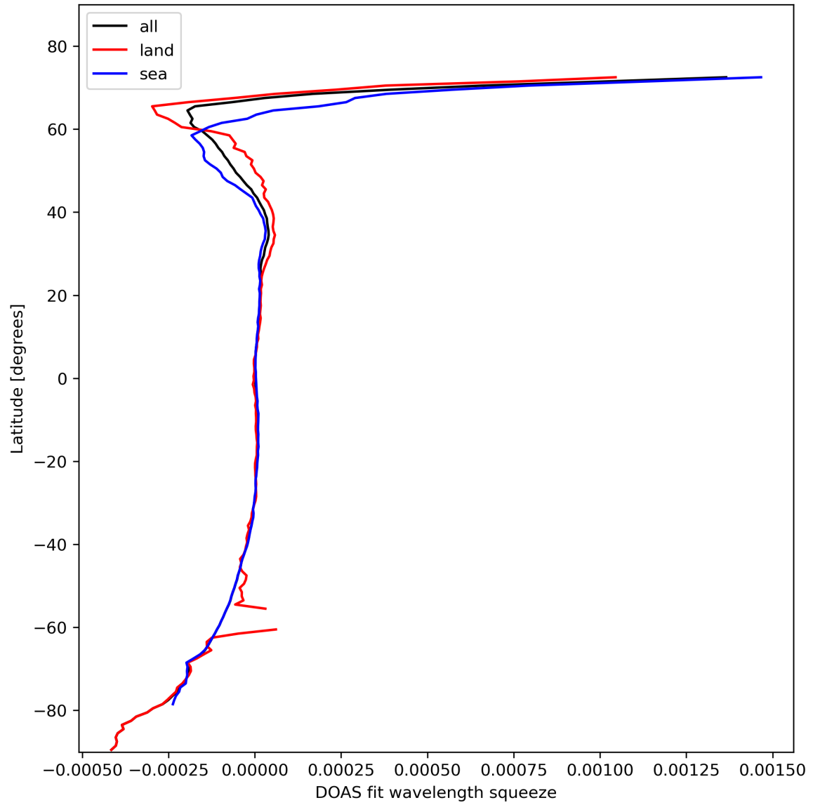
Figure 46: Zonal average of “DOAS fit wavelength squeeze” for 2024-02-16 to 2024-02-17.
