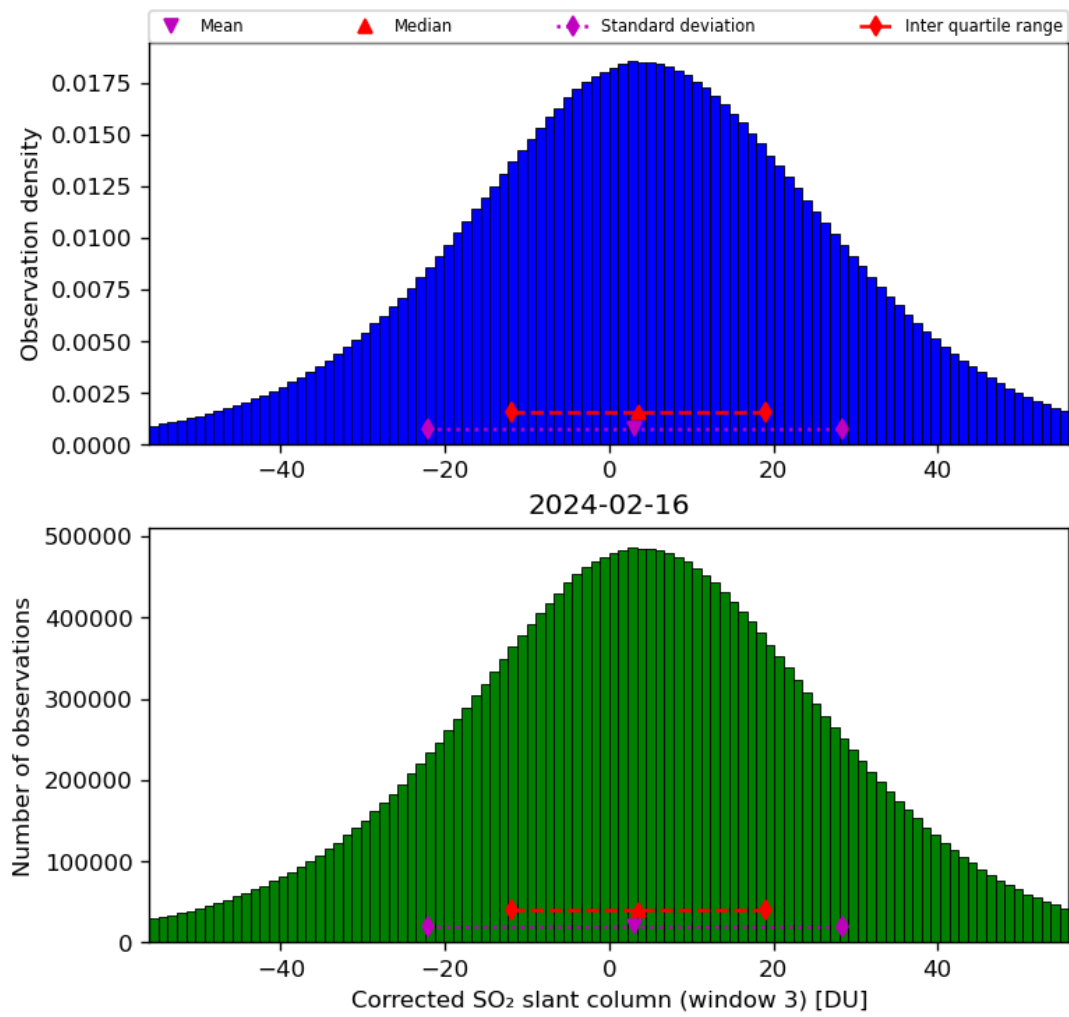
Figure 66: Histogram of “Corrected SO 2 slant column (window 3)” for 2024-02-16 to 2024-02-17
