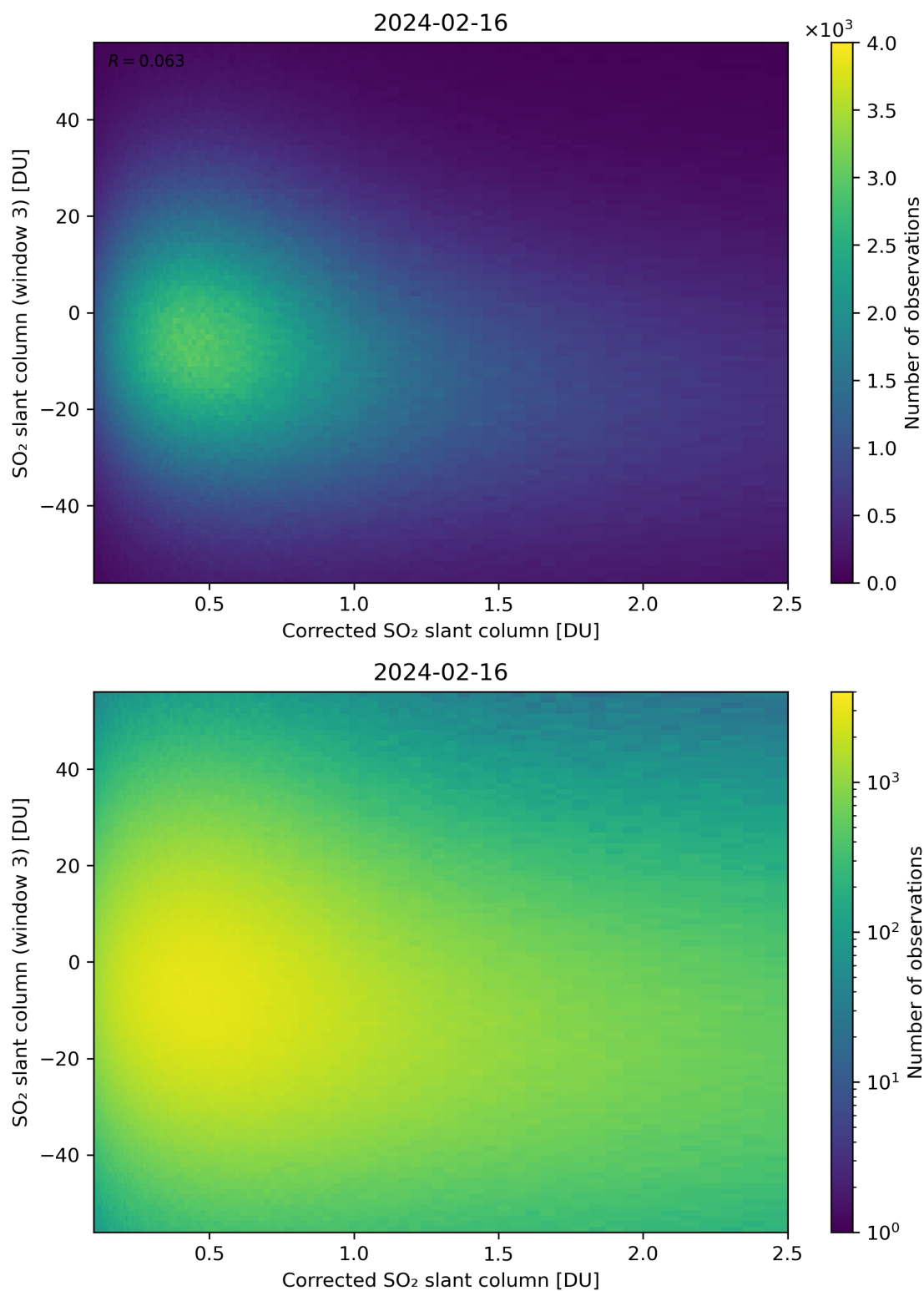
Figure 190: Scatter density plot of “Corrected SO 2 slant column” against “SO 2 slant column (window 3)” for 2024-02-16 to 2024-02-17.
