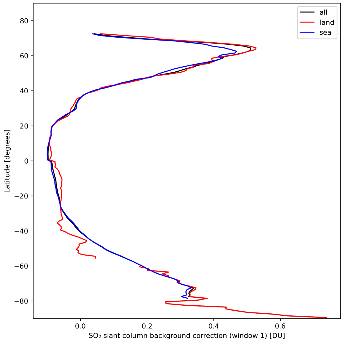
Figure 36: Zonal average of “SO 2 slant column background correction (window 1)” for 2024-02-16 to 2024-02-17.
