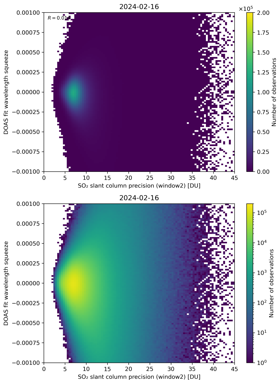
Figure 244: Scatter density plot of “SO 2 slant column precision (window2)” against “DOAS fit wavelength squeeze” for 2024-02-16 to 2024-02-17.
