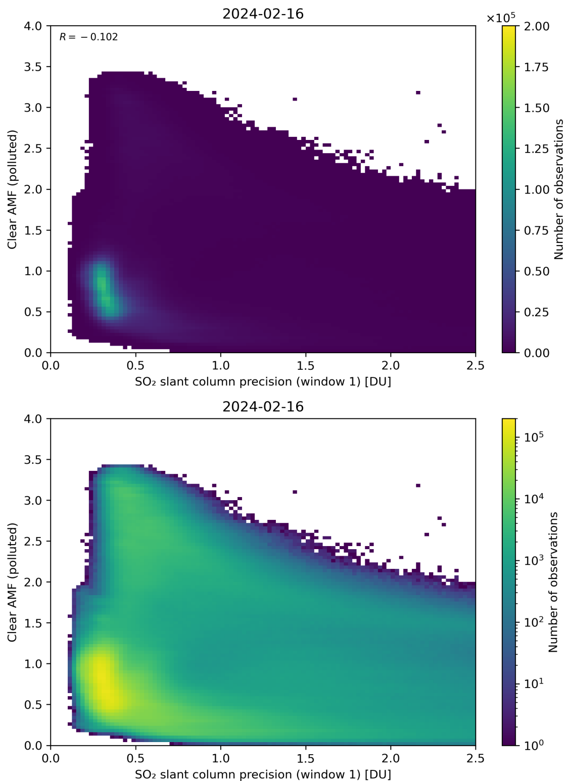
Figure 224: Scatter density plot of “SO 2 slant column precision (window 1)” against “Clear AMF (polluted)” for 2024-02-16 to 2024-02-17.
