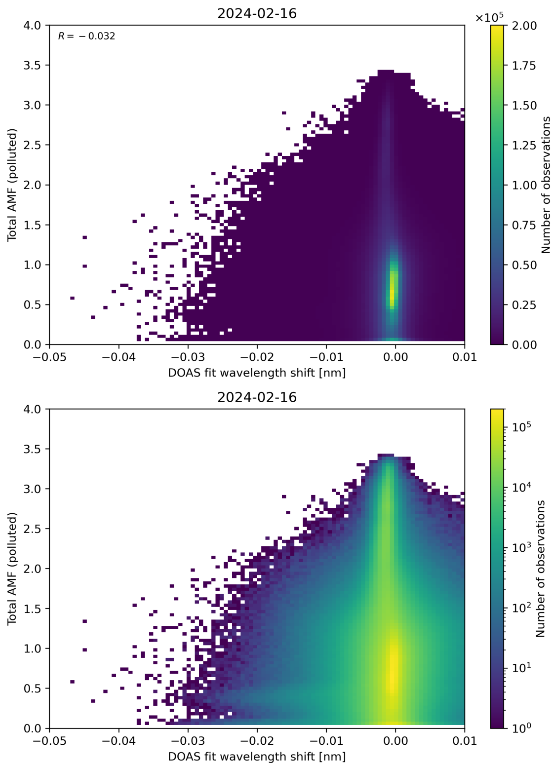
Figure 130: Scatter density plot of “DOAS fit wavelength shift” against “Total AMF (polluted)” for 2024-02-16 to 2024-02-17.
