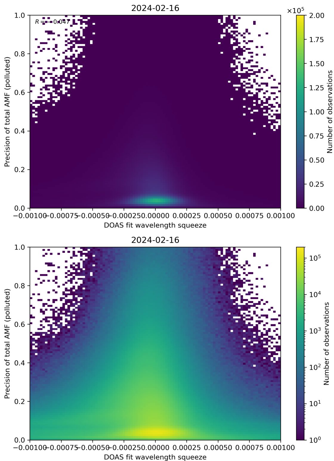
Figure 135: Scatter density plot of “DOAS fit wavelength squeeze” against “Precision of total AMF (polluted)” for 2024-02-16 to 2024-02-17.
