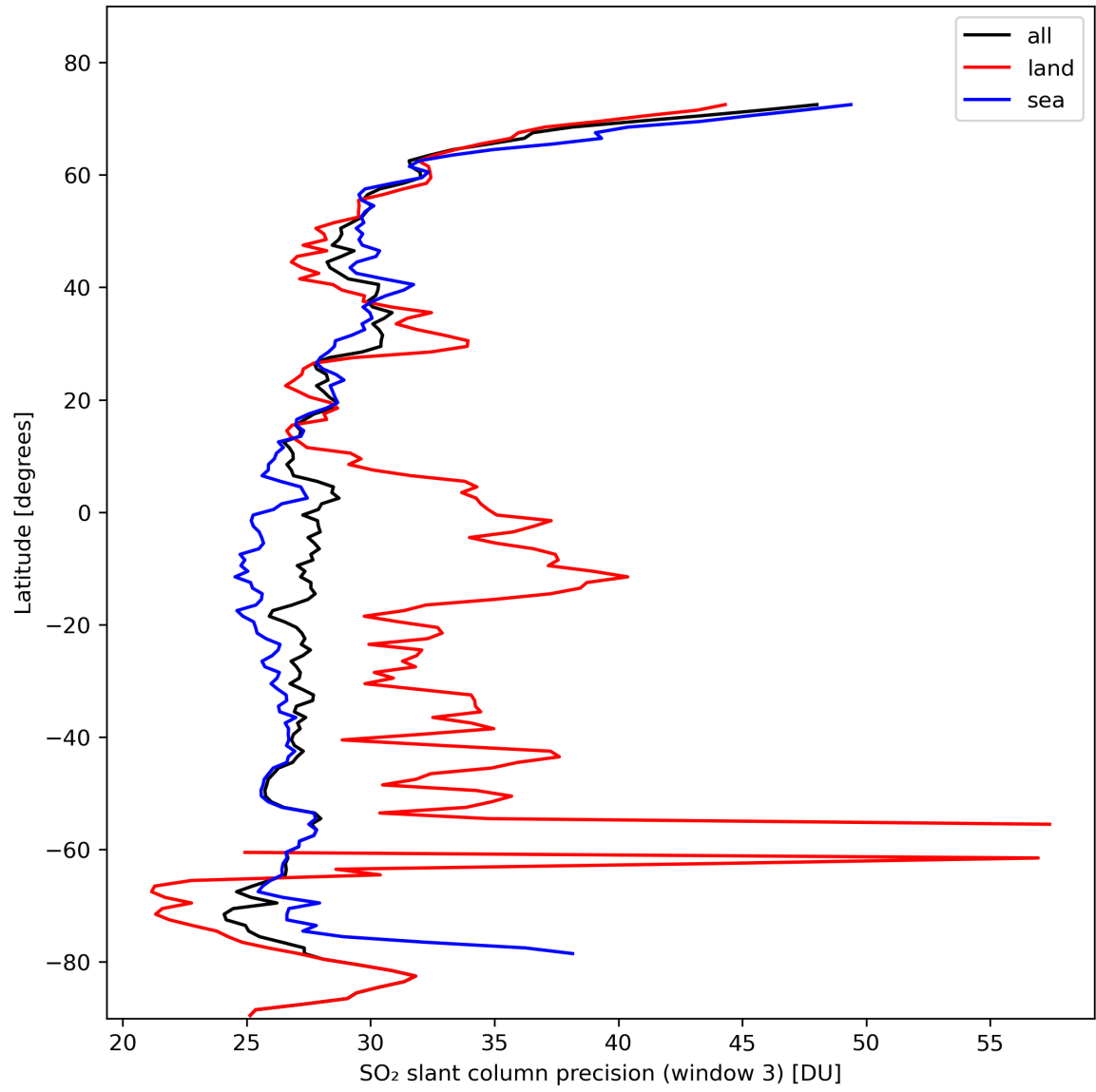
Figure 42: Zonal average of “SO 2 slant column precision (window 3)” for 2024-02-16 to 2024-02-17.
