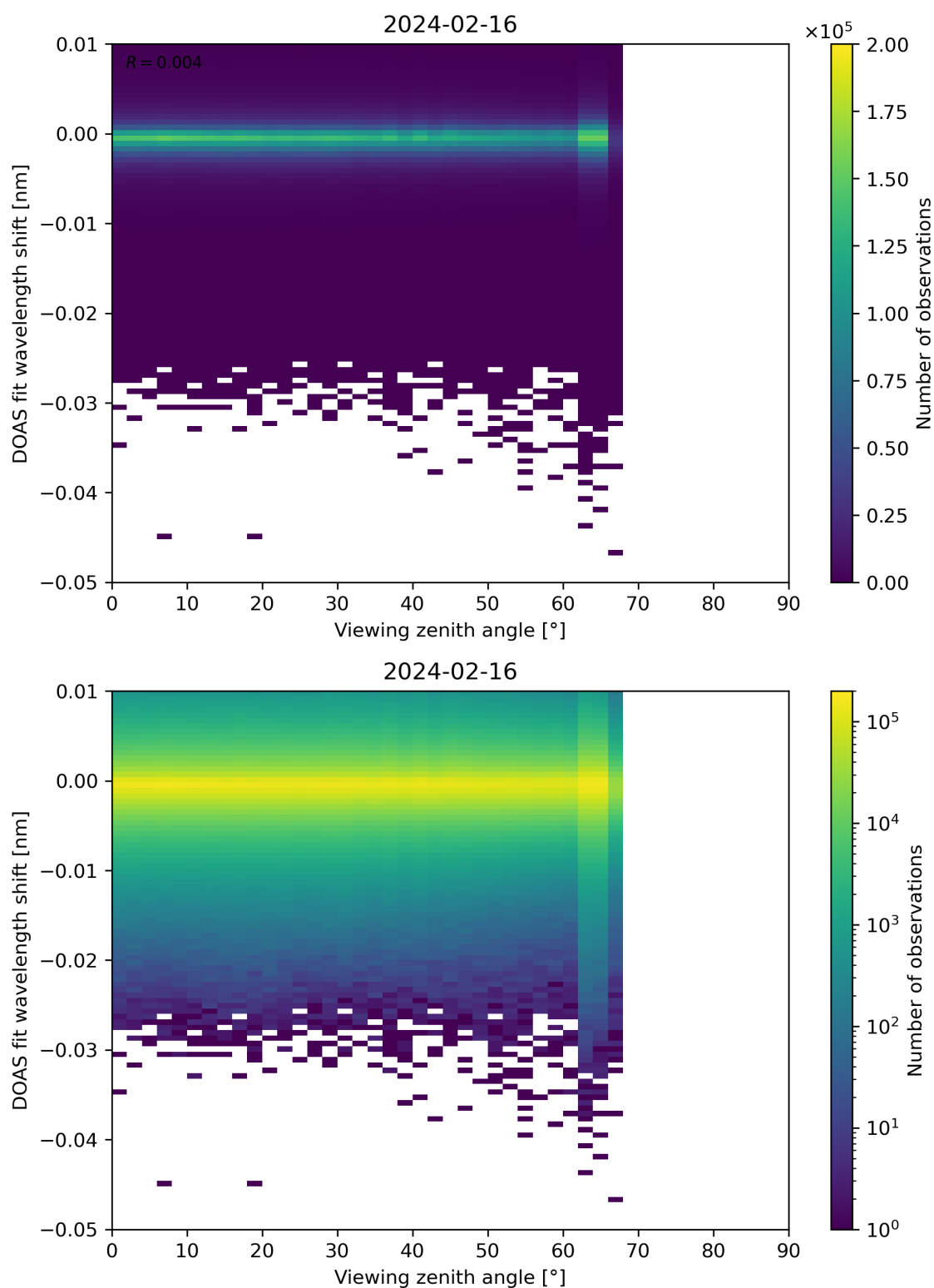
Figure 311: Scatter density plot of “Viewing zenith angle” against “DOAS fit wavelength shift” for 2024-02-16 to 2024-02-17.
