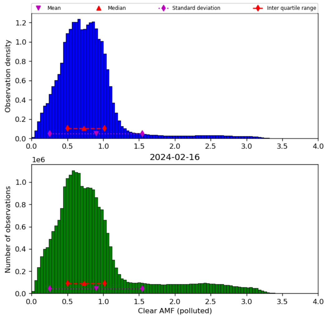
Figure 73: Histogram of “Clear AMF (polluted)” for 2024-02-16 to 2024-02-17
