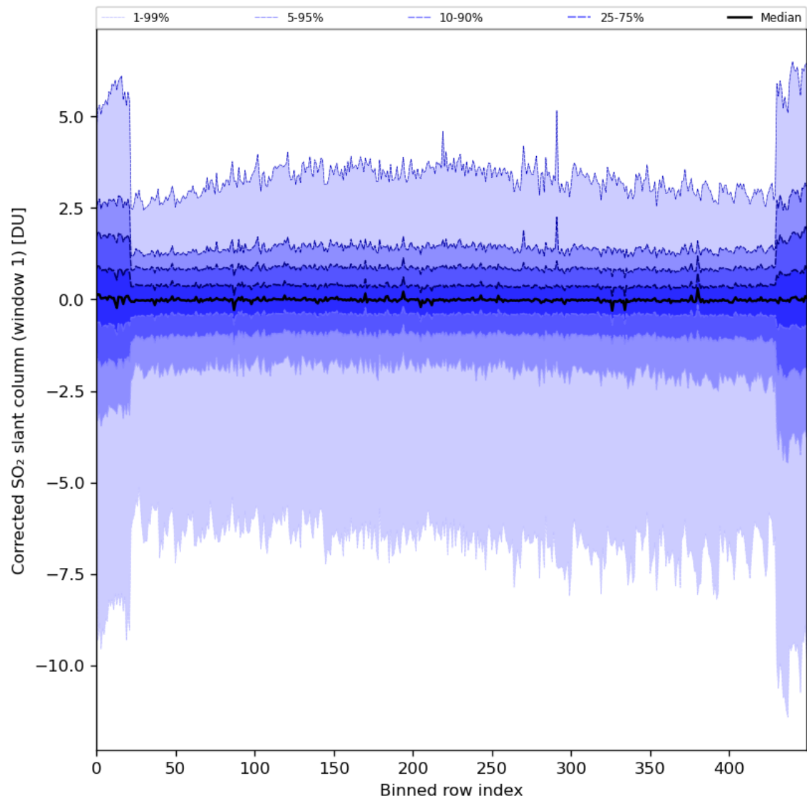
Figure 81: Along track statistics of “Corrected SO 2 slant column (window 1)” for 2024-02-16 to 2024-02-17
