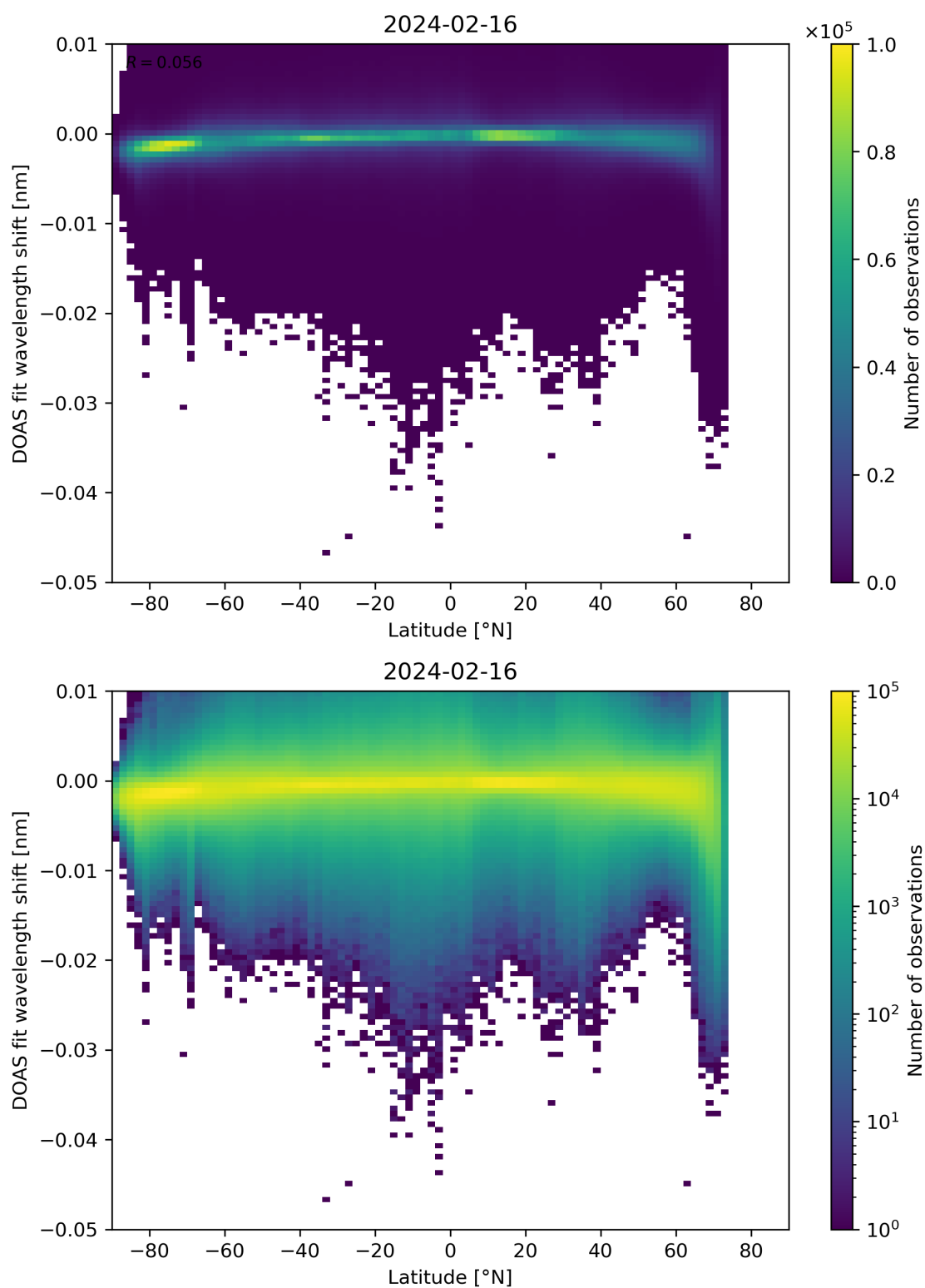
Figure 142: Scatter density plot of “Latitude” against “DOAS fit wavelength shift” for 2024-02-16 to 2024-02-17.
