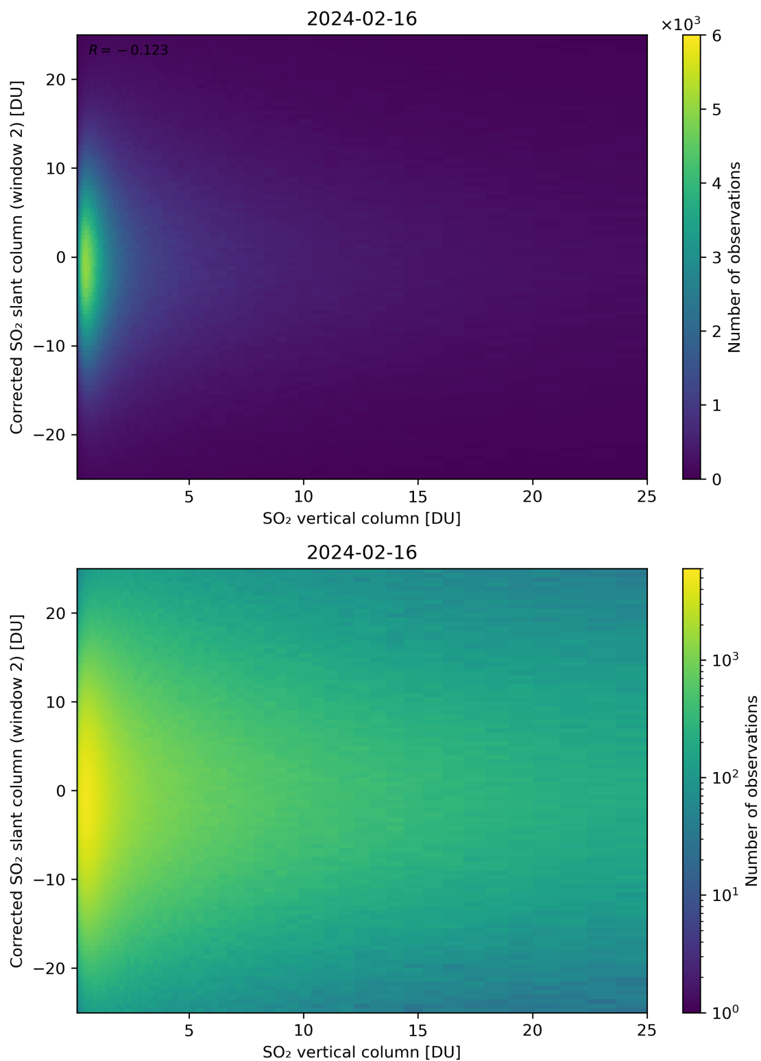
Figure 298: Scatter density plot of “SO 2 vertical column” against “Corrected SO 2 slant column (window 2)” for 2024-02-16 to 2024-02-17.
