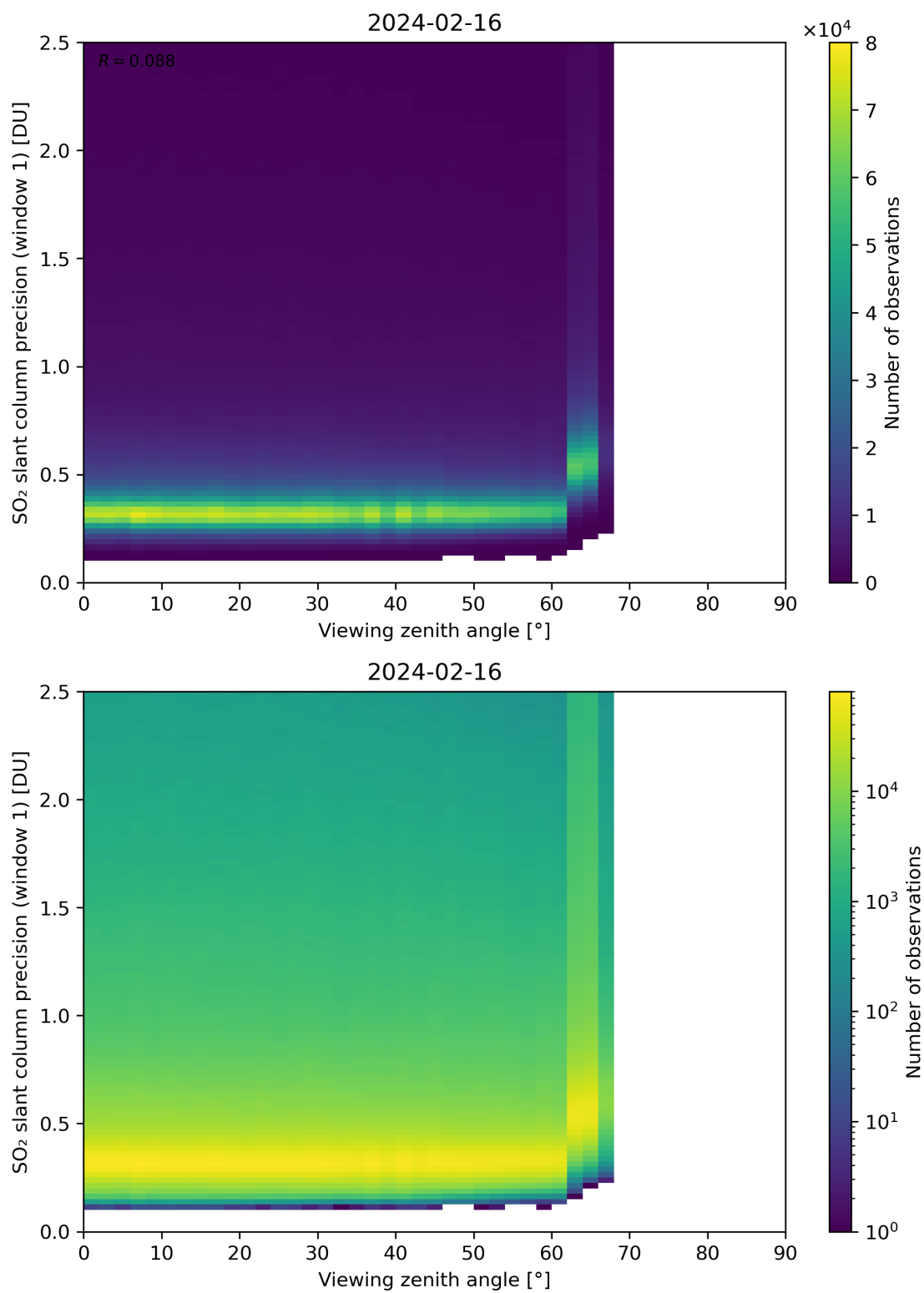
Figure 321: Scatter density plot of “Viewing zenith angle” against “SO 2 slant column precision (window 1)” for 2024-02-16 to 2024-02-17.
