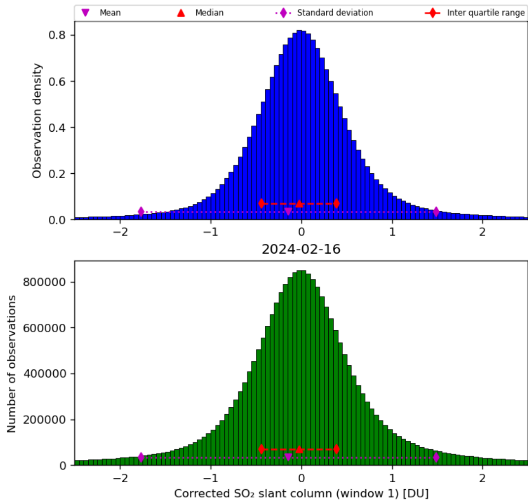
Figure 58: Histogram of “Corrected SO 2 slant column (window 1)” for 2024-02-16 to 2024-02-17
