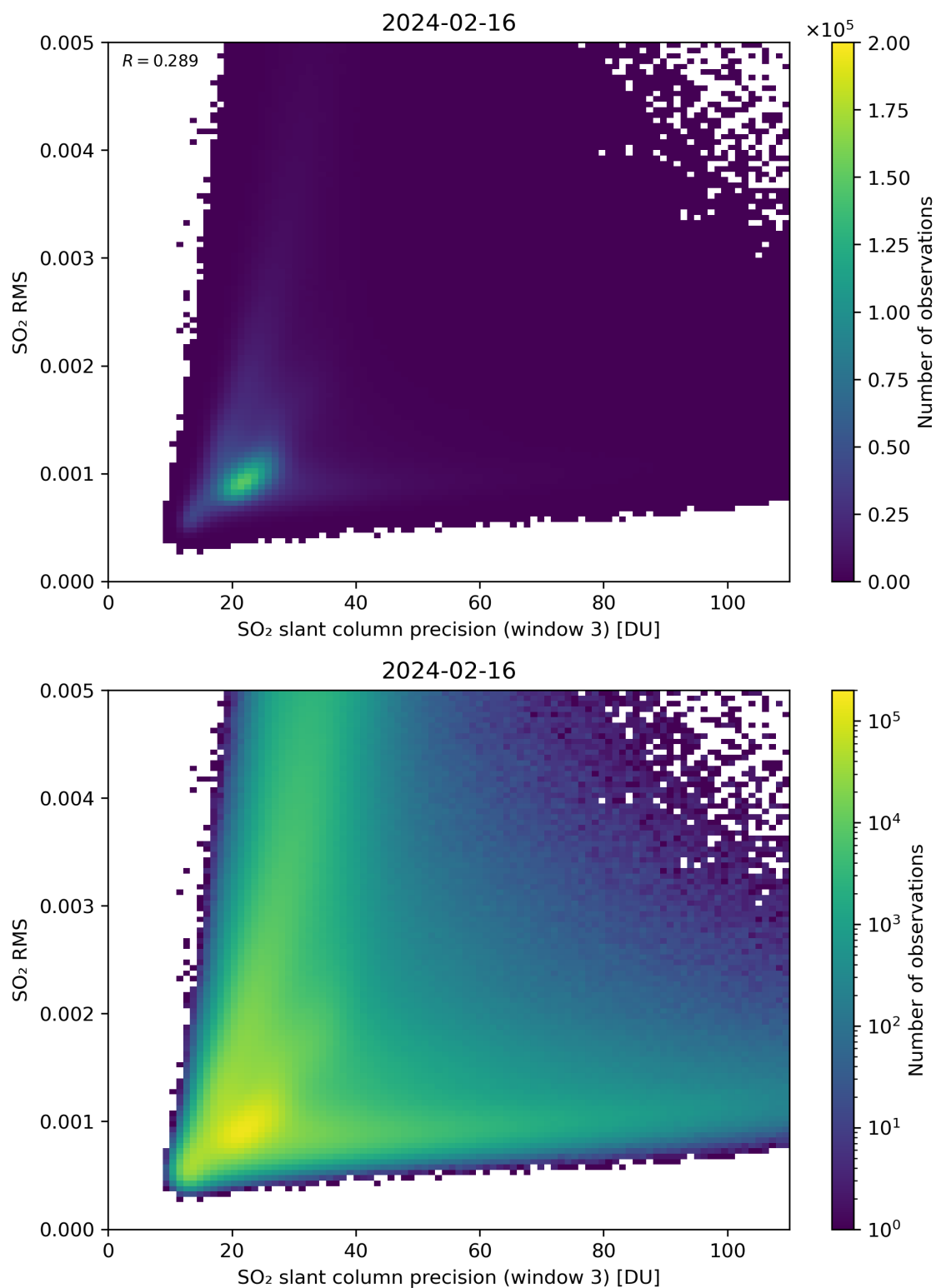
Figure 260: Scatter density plot of “SO 2 slant column precision (window 3)” against “SO 2 RMS” for 2024-02-16 to 2024-02-17.
