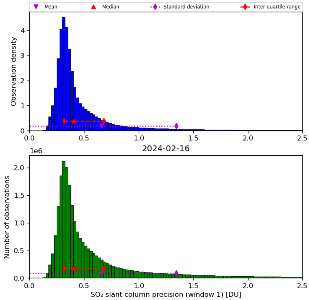
Figure 57: Histogram of “SO 2 slant column precision (window 1)” for 2024-02-16 to 2024-02-17
