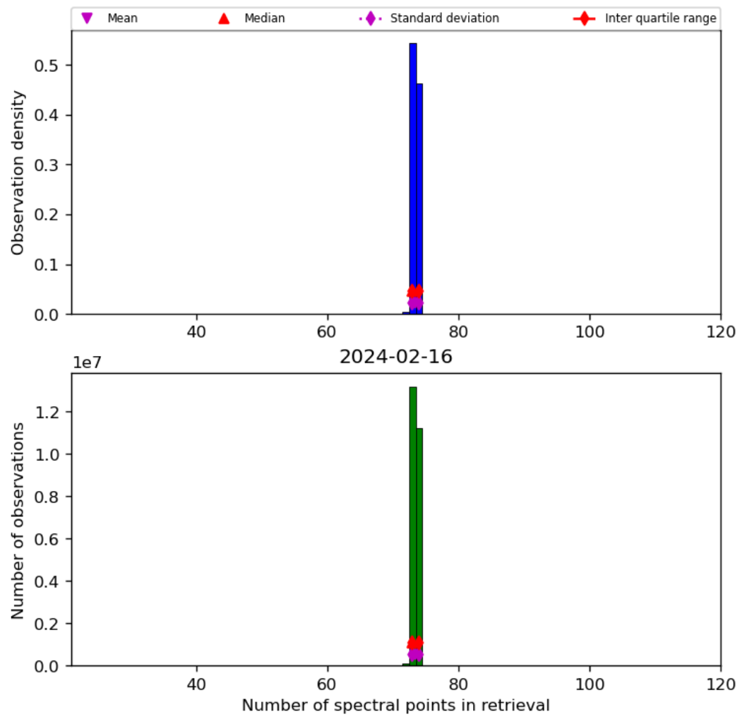
Figure 74: Histogram of “Number of spectral points in retrieval” for 2024-02-16 to 2024-02-17
