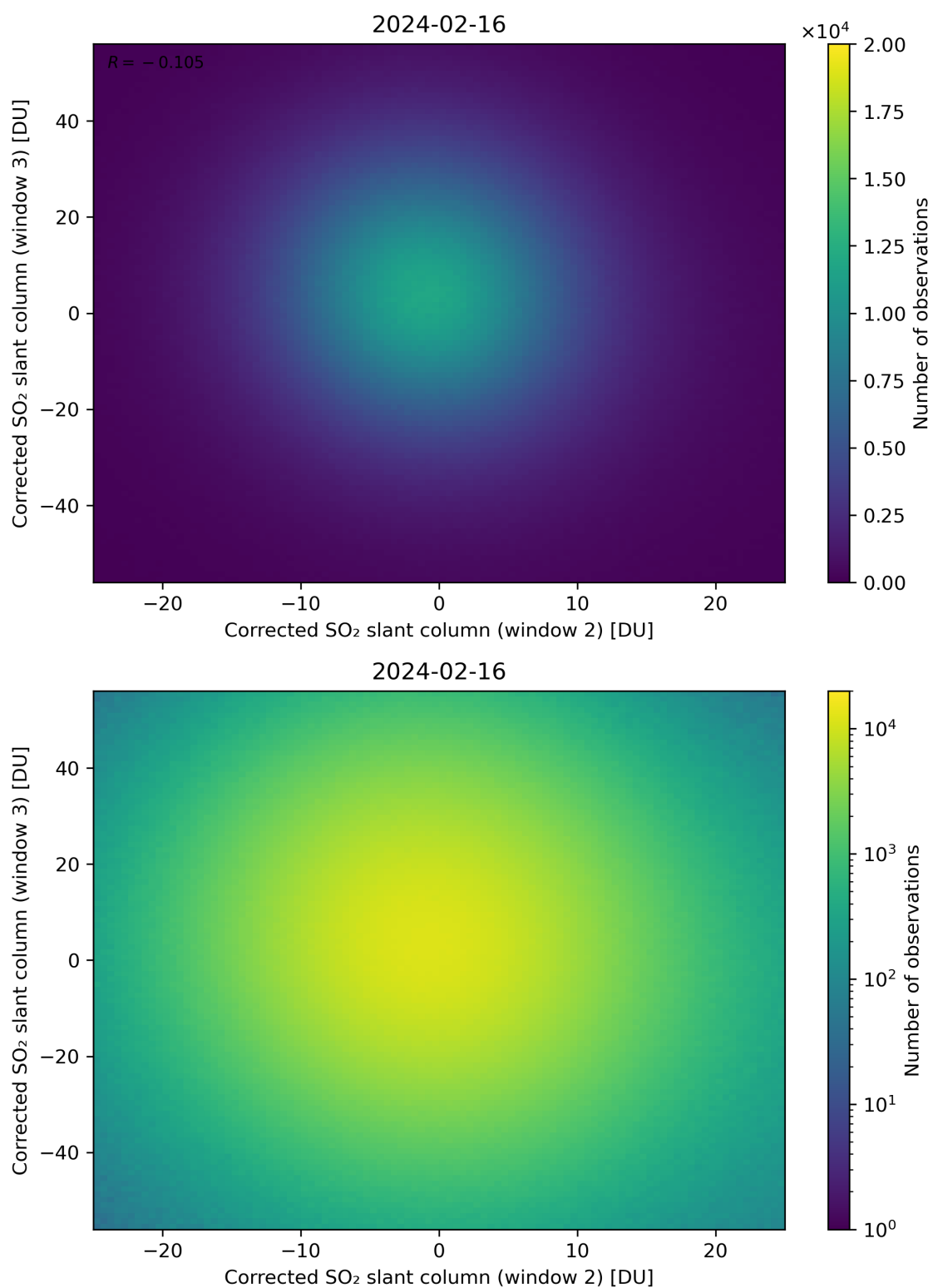
Figure 200: Scatter density plot of “Corrected SO 2 slant column (window 2)” against “Corrected SO 2 slant column (window 3)” for 2024-02-16 to 2024-02-17.
