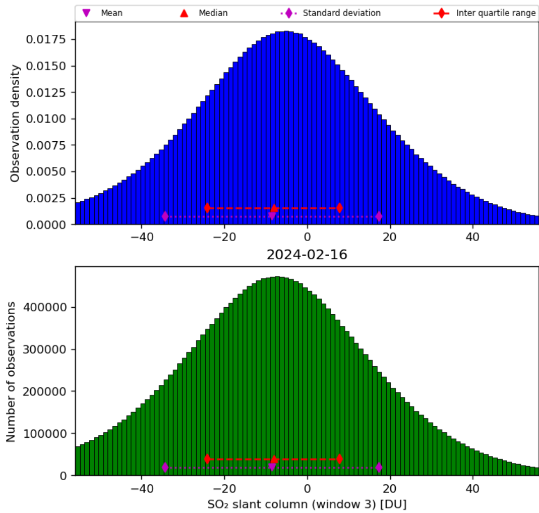
Figure 64: Histogram of “SO 2 slant column (window 3)” for 2024-02-16 to 2024-02-17
