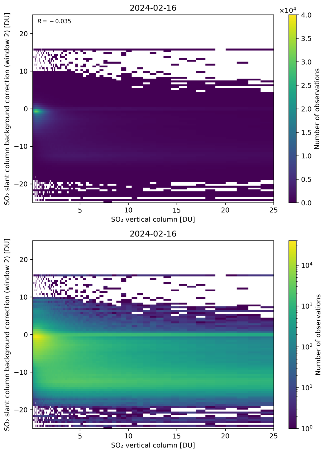
Figure 274: Scatter density plot of “SO 2 vertical column” against “SO 2 slant column background correction (window 2)” for 2024-02-16 to 2024-02-17.
