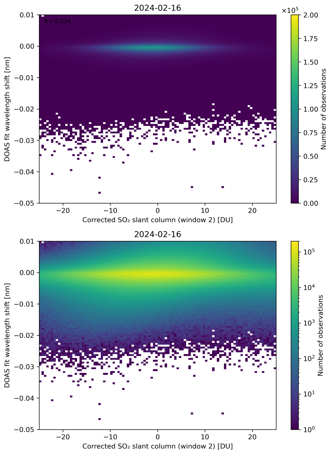
Figure 196: Scatter density plot of “Corrected SO 2 slant column (window 2)” against “DOAS fit wavelength shift” for 2024-02-16 to 2024-02-17.
