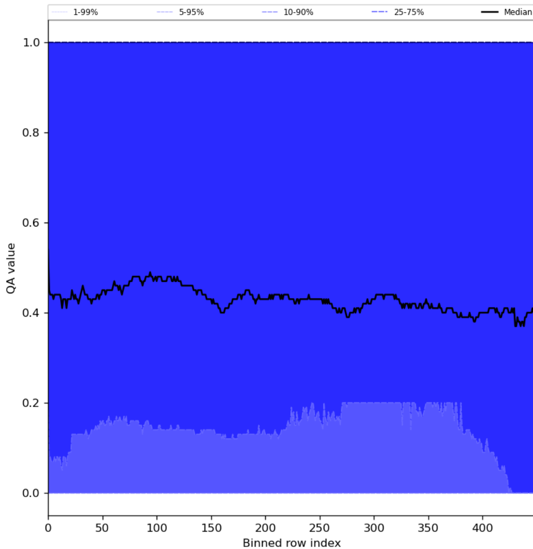
Figure 75: Along track statistics of “QA value” for 2024-02-16 to 2024-02-17
