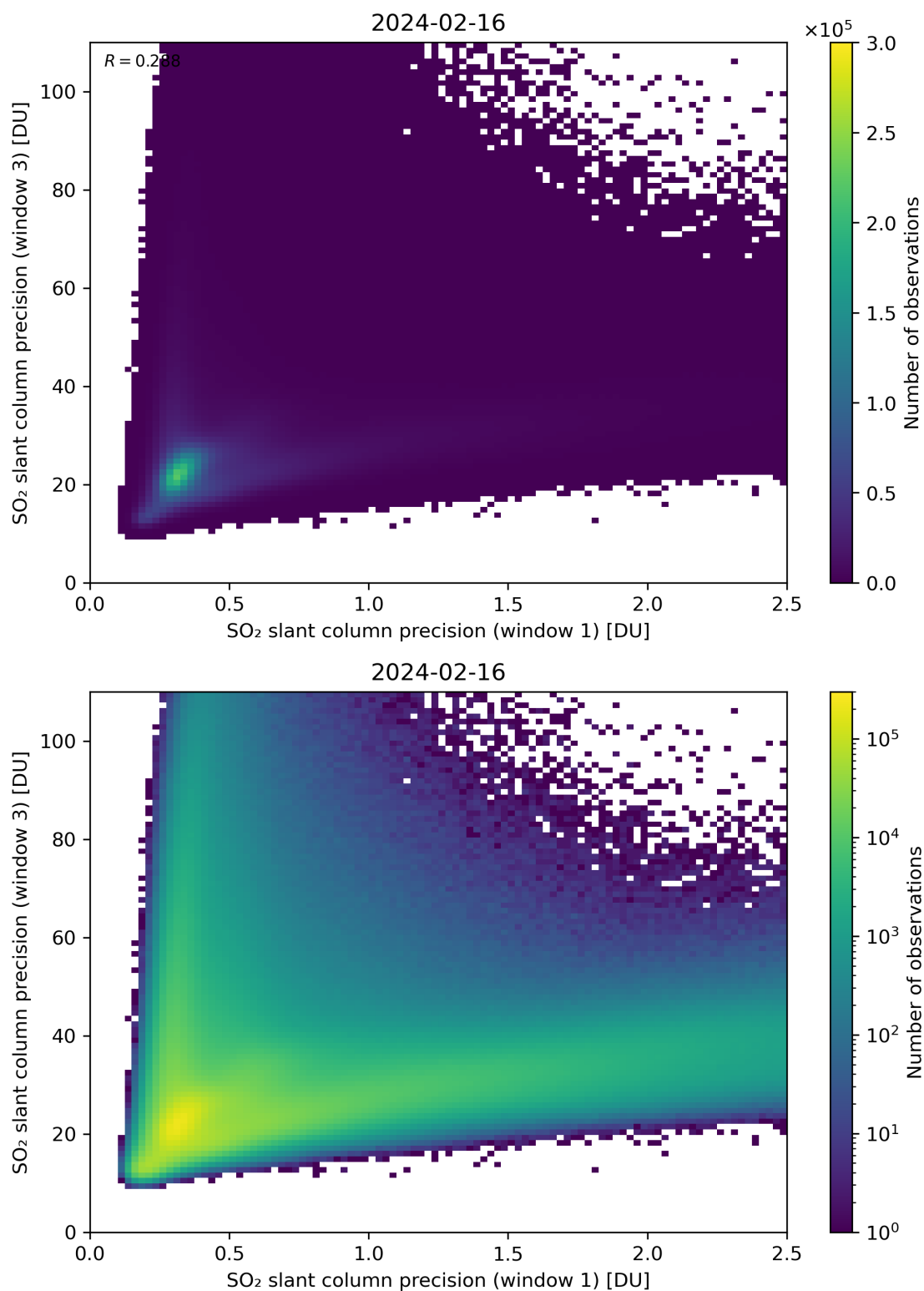
Figure 229: Scatter density plot of “SO 2 slant column precision (window 1)” against “SO 2 slant column precision (window 3)” for 2024-02-16 to 2024-02-17.
