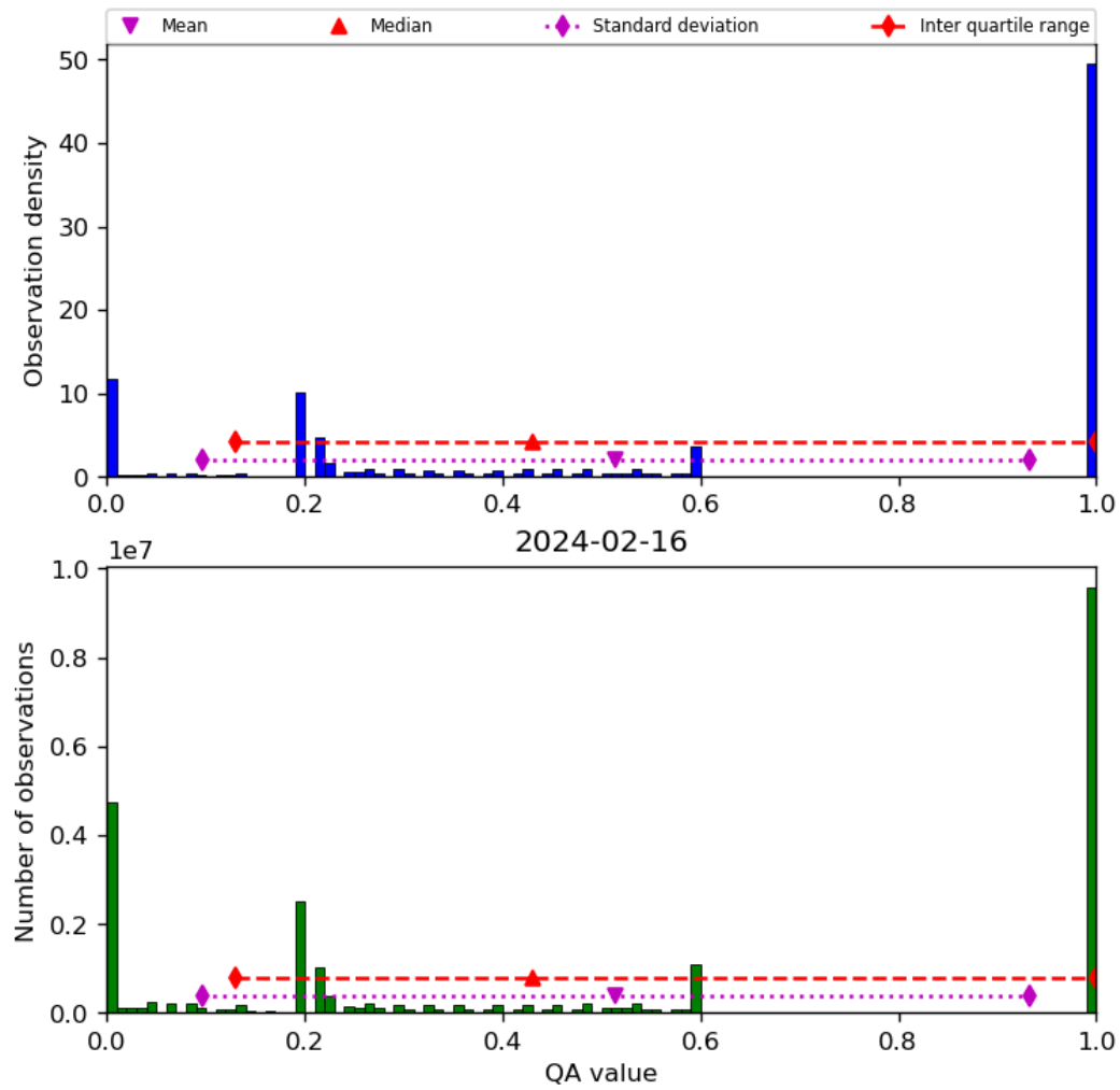
Figure 52: Histogram of “QA value” for 2024-02-16 to 2024-02-17
