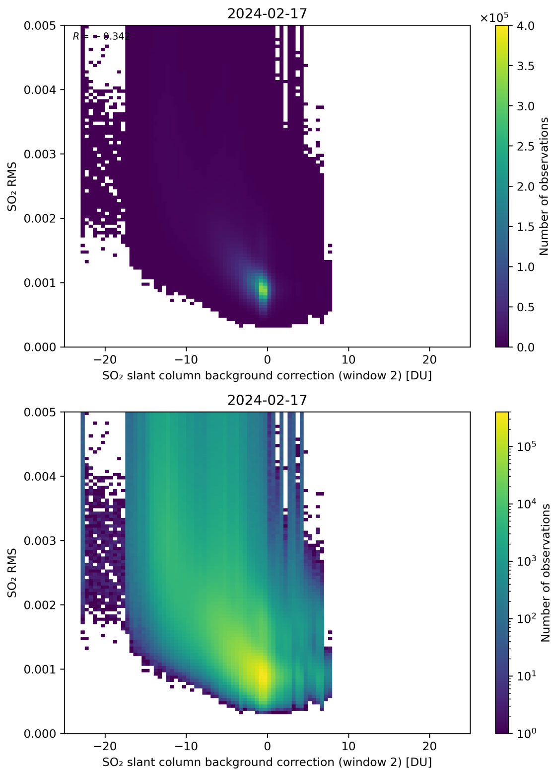
Figure 114: Scatter density plot of “SO 2 slant column background correction (window 2)” against “SO 2 RMS” for 2024-02-17 to 2024-02-18.
