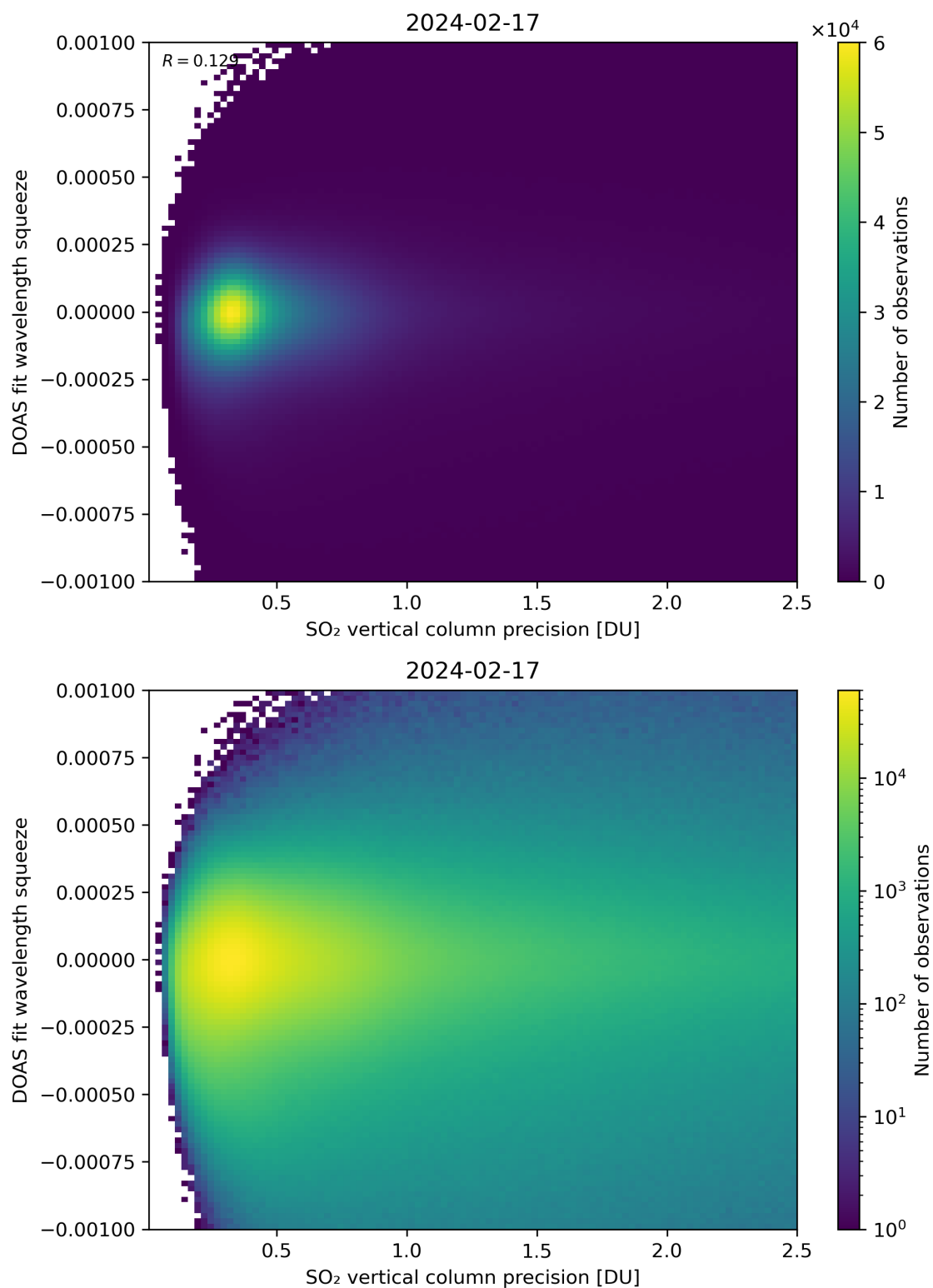
Figure 283: Scatter density plot of “SO 2 vertical column precision” against “DOAS fit wavelength squeeze” for 2024-02-17 to 2024-02-18.
