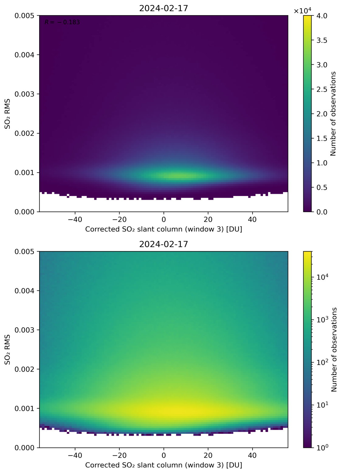
Figure 208: Scatter density plot of “Corrected SO 2 slant column (window 3)” against “SO 2 RMS” for 2024-02-17 to 2024-02-18.
