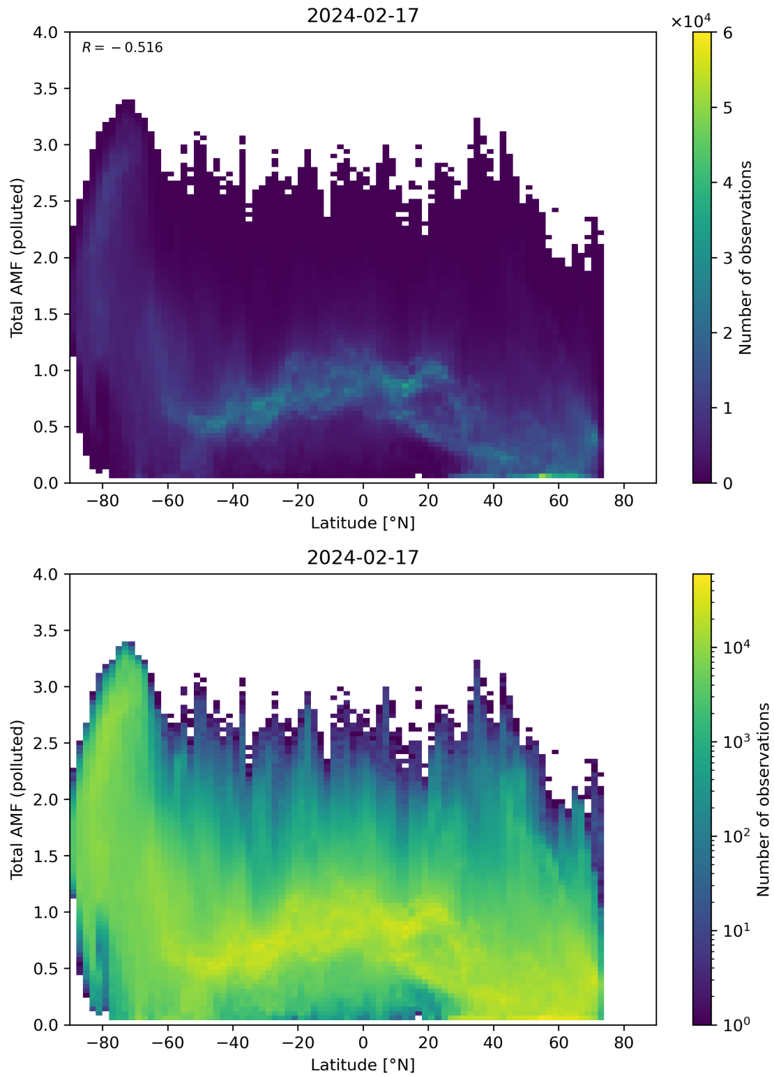
Figure 154: Scatter density plot of “Latitude” against “Total AMF (polluted)” for 2024-02-17 to 2024-02-18.
