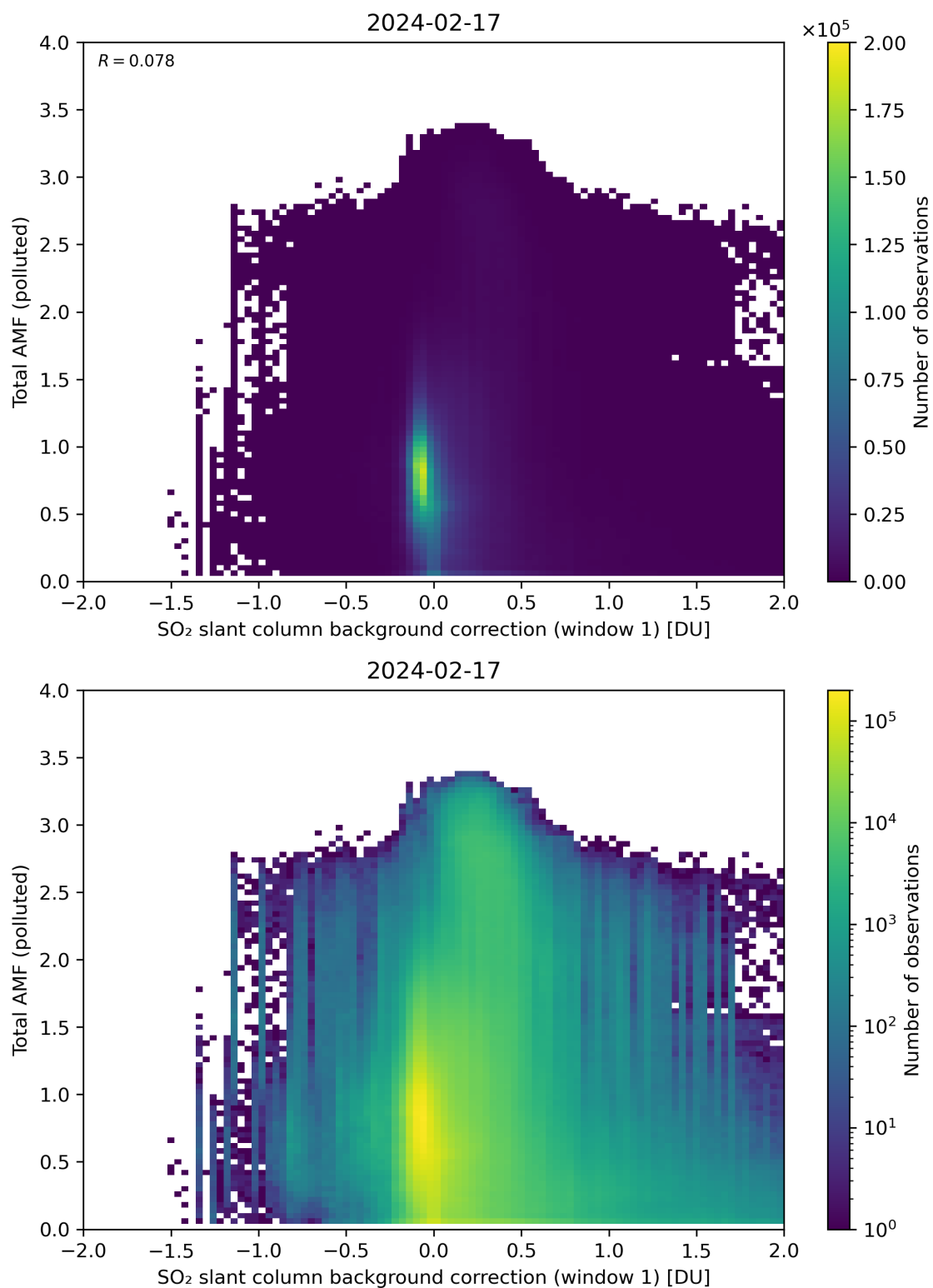
Figure 109: Scatter density plot of “SO 2 slant column background correction (window 1)” against “Total AMF (polluted)” for 2024-02-17 to 2024-02-18.
