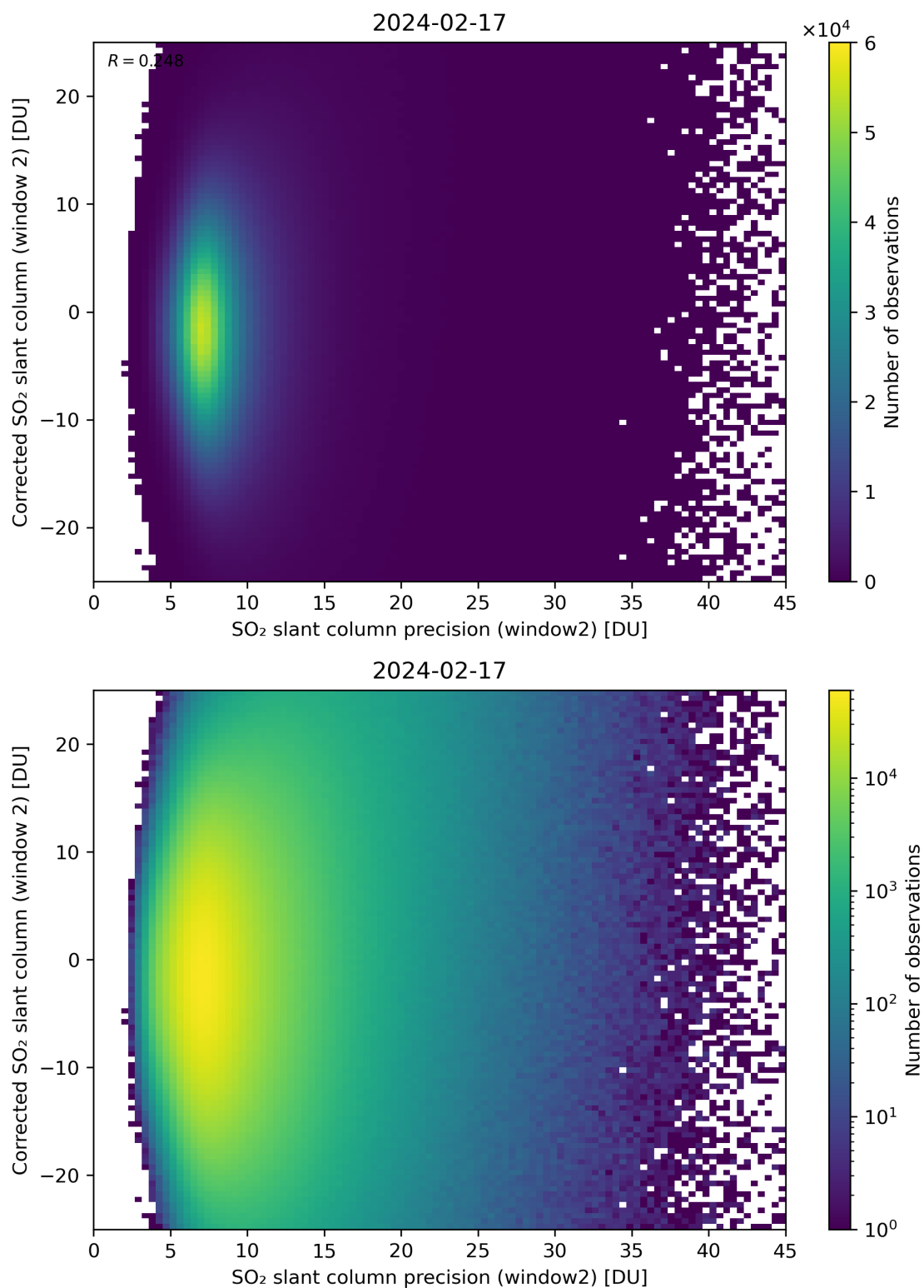
Figure 247: Scatter density plot of “SO 2 slant column precision (window2)” against “Corrected SO 2 slant column (window 2)” for 2024-02-17 to 2024-02-18.
