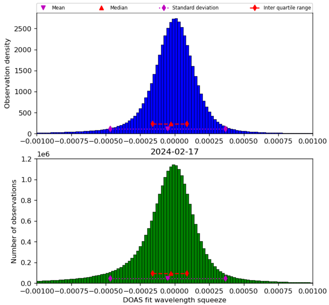
Figure 69: Histogram of “DOAS fit wavelength squeeze” for 2024-02-17 to 2024-02-18
