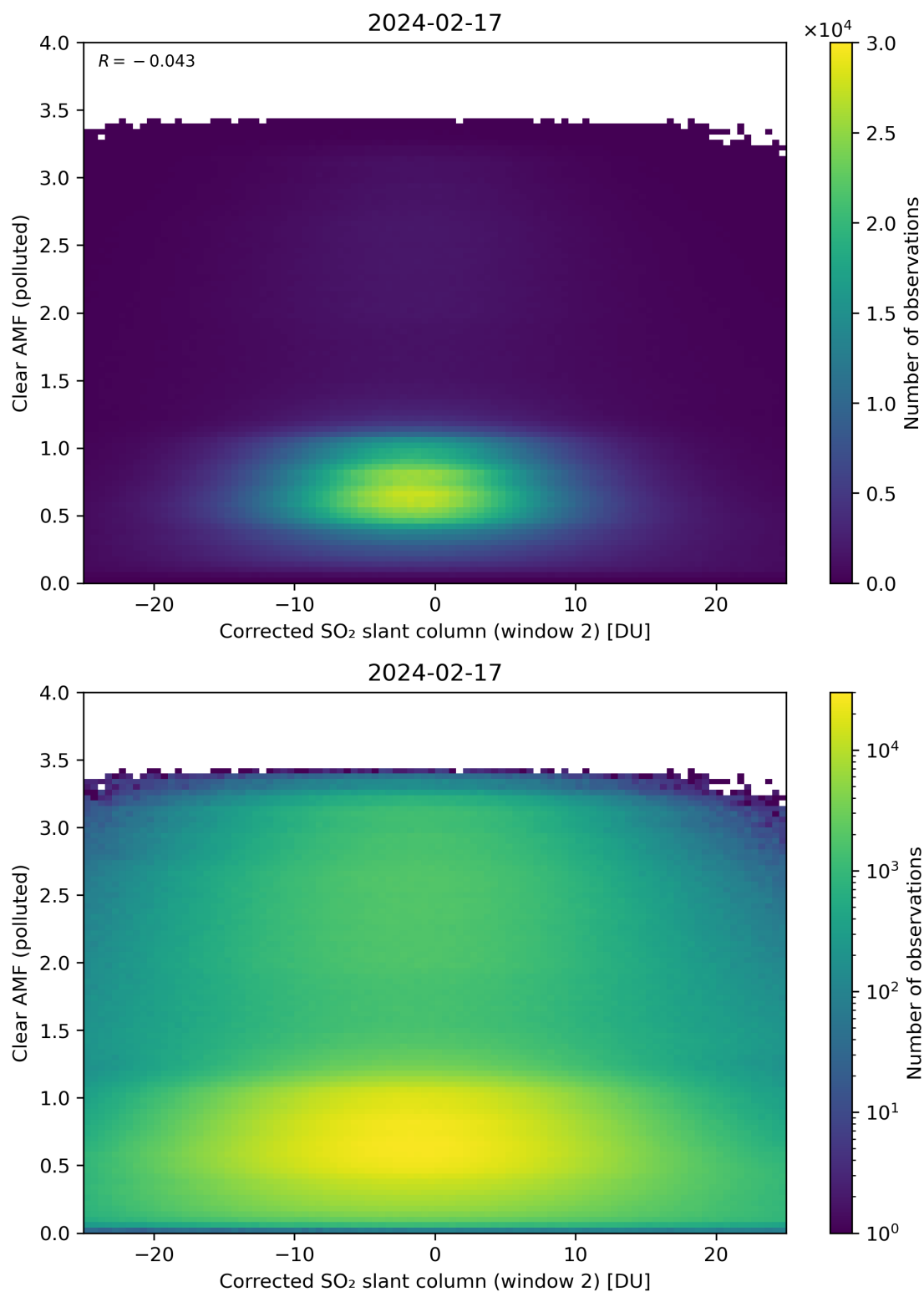
Figure 199: Scatter density plot of “Corrected SO 2 slant column (window 2)” against “Clear AMF (polluted)” for 2024-02-17 to 2024-02-18.
