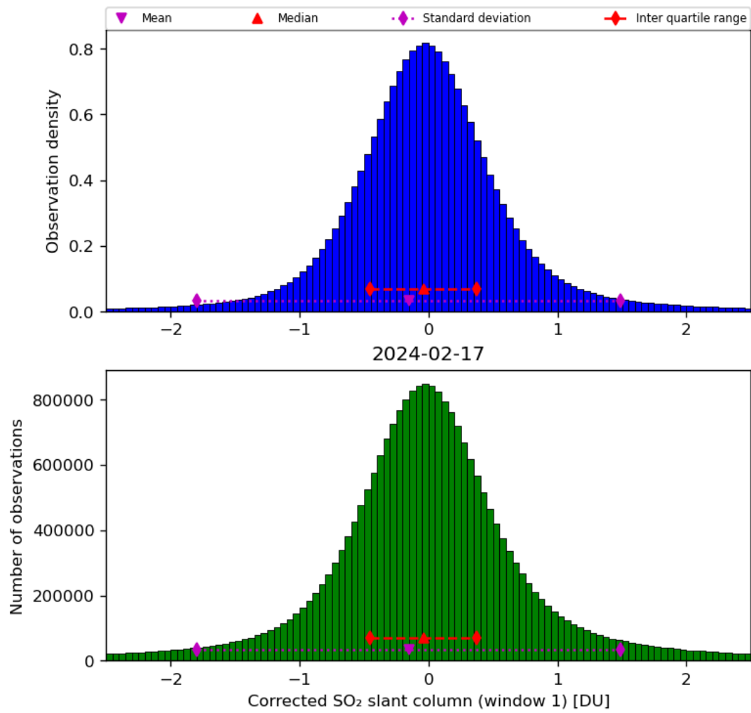
Figure 58: Histogram of “Corrected SO 2 slant column (window 1)” for 2024-02-17 to 2024-02-18
