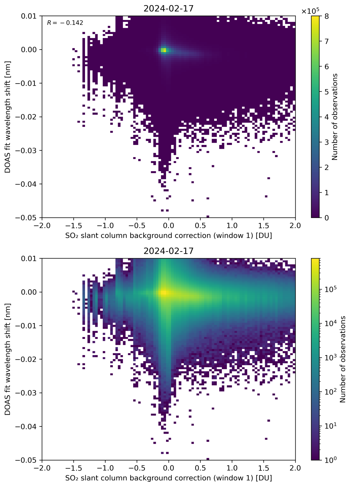
Figure 100: Scatter density plot of “SO 2 slant column background correction (window 1)” against “DOAS fit wavelength shift” for 2024-02-17 to 2024-02-18.
