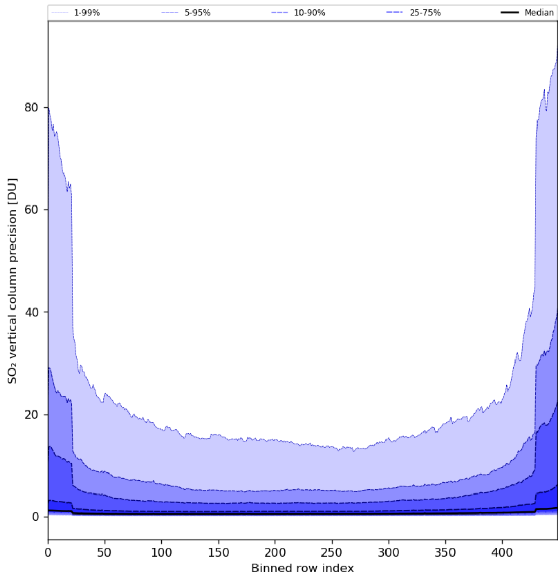
Figure 77: Along track statistics of “SO 2 vertical column precision” for 2024-02-17 to 2024-02-18
