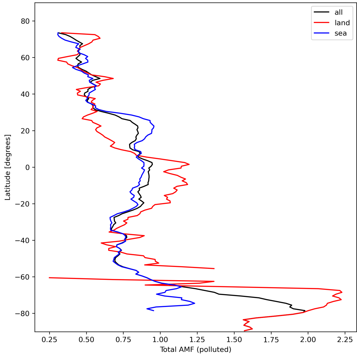
Figure 48: Zonal average of “Total AMF (polluted)” for 2024-02-17 to 2024-02-18.
