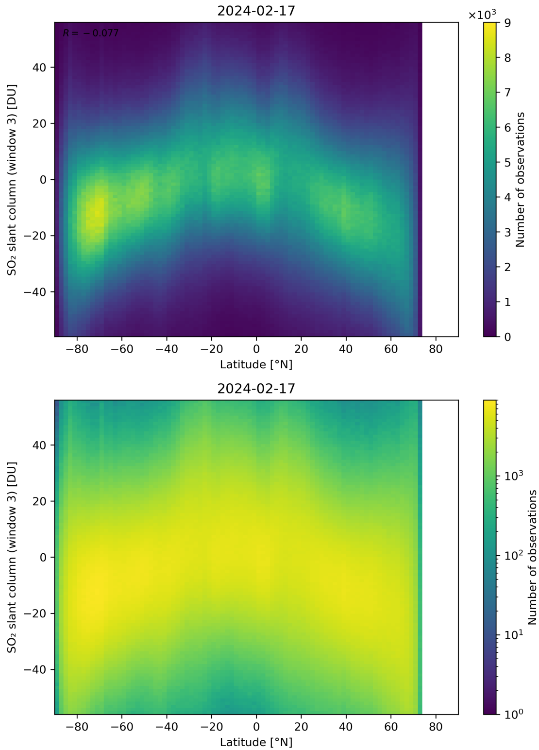
Figure 152: Scatter density plot of “Latitude” against “SO 2 slant column (window 3)” for 2024-02-17 to 2024-02-18.
