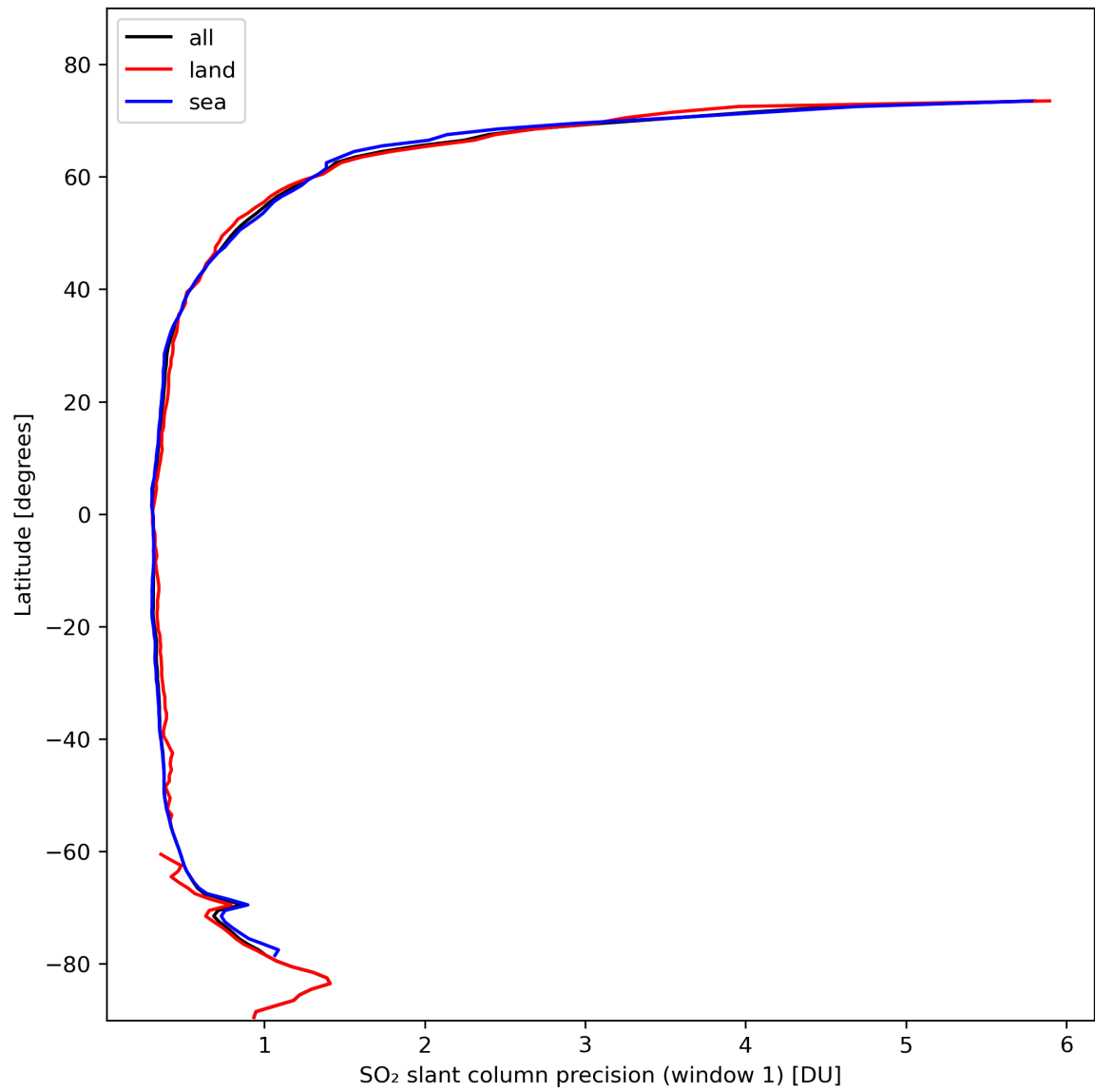
Figure 34: Zonal average of “SO 2 slant column precision (window 1)” for 2024-02-17 to 2024-02-18.
