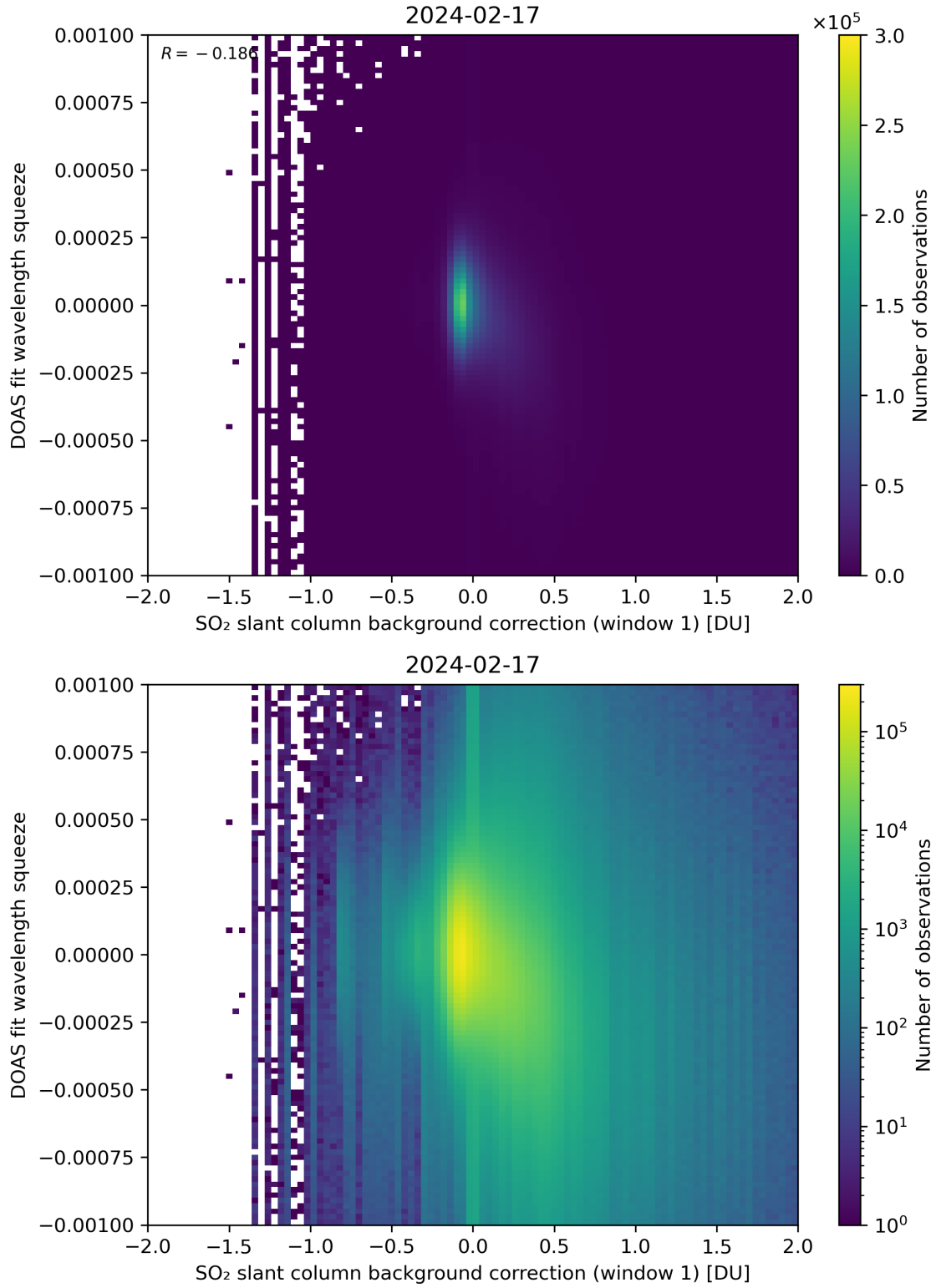
Figure 101: Scatter density plot of “SO 2 slant column background correction (window 1)” against “DOAS fit wavelength squeeze” for 2024-02-17 to 2024-02-18.
