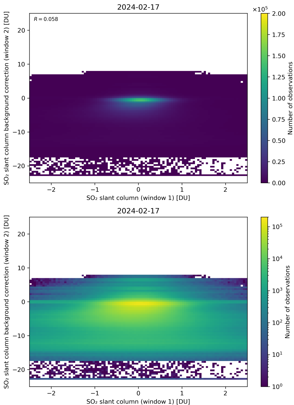
Figure 213: Scatter density plot of “SO 2 slant column (window 1)” against “SO 2 slant column background correction (window 2)” for 2024-02-17 to 2024-02-18.
