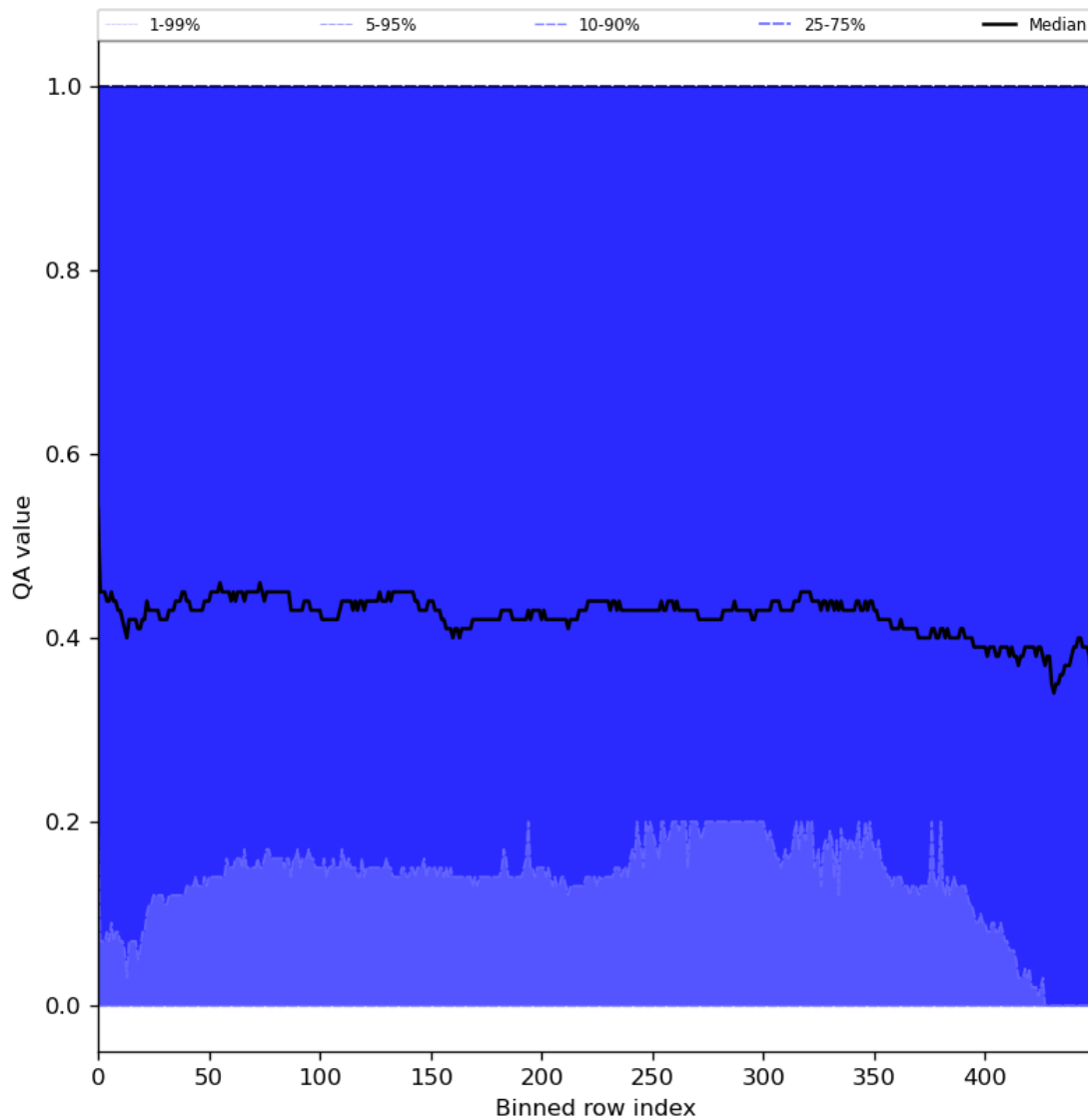
Figure 75: Along track statistics of “QA value” for 2024-02-17 to 2024-02-18
