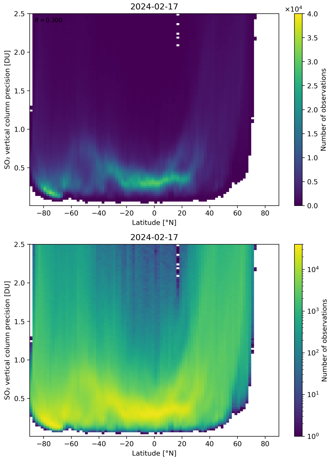
Figure 157: Scatter density plot of “Latitude” against “SO 2 vertical column precision” for 2024-02-17 to 2024-02-18.
