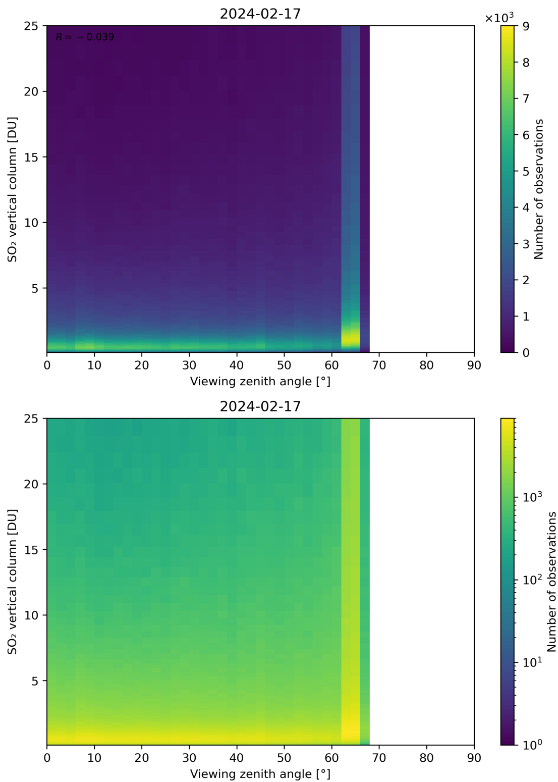
Figure 327: Scatter density plot of “Viewing zenith angle” against “SO 2 vertical column” for 2024-02-17 to 2024-02-18.
