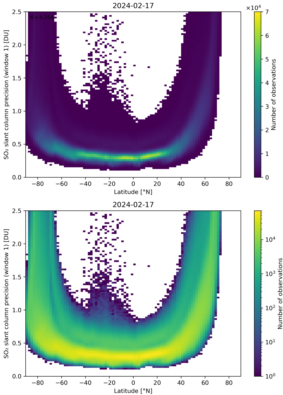
Figure 150: Scatter density plot of “Latitude” against “SO 2 slant column precision (window 1)” for 2024-02-17 to 2024-02-18.
