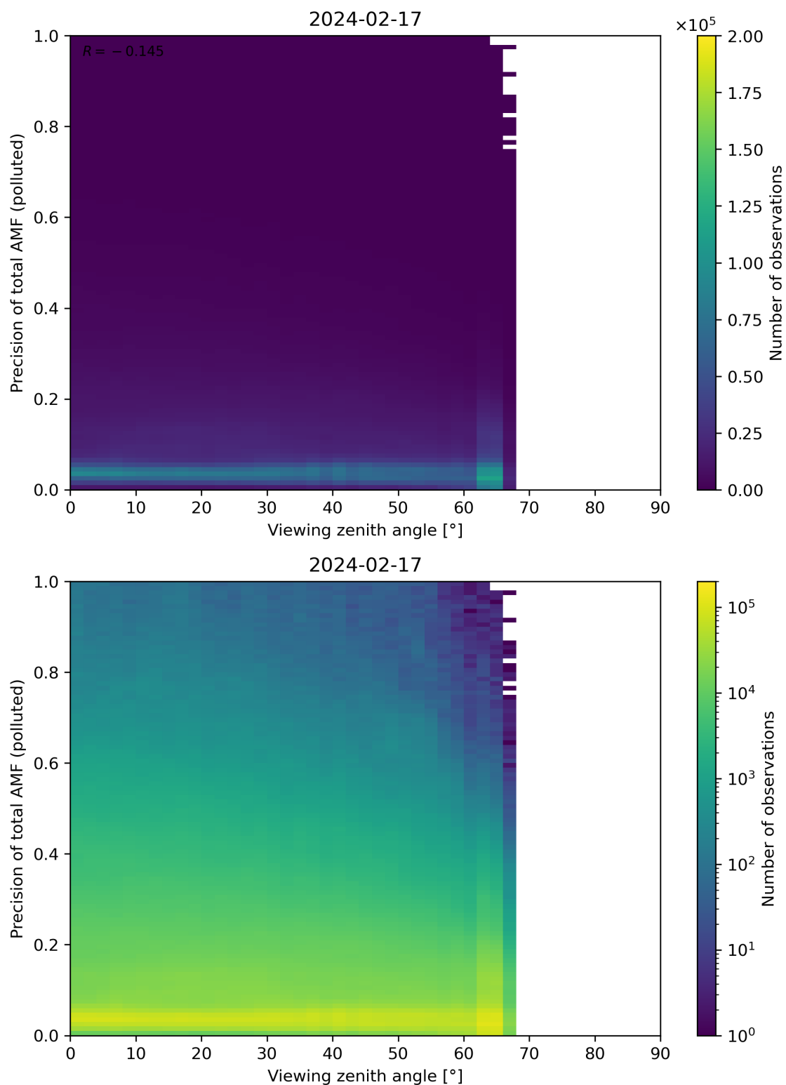
Figure 326: Scatter density plot of “Viewing zenith angle” against “Precision of total AMF (polluted)” for 2024-02-17 to 2024-02-18.
