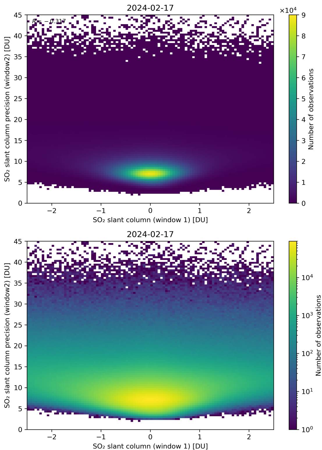
Figure 236: Scatter density plot of “SO 2 slant column (window 1)” against “SO 2 slant column precision (window2)” for 2024-02-17 to 2024-02-18.
