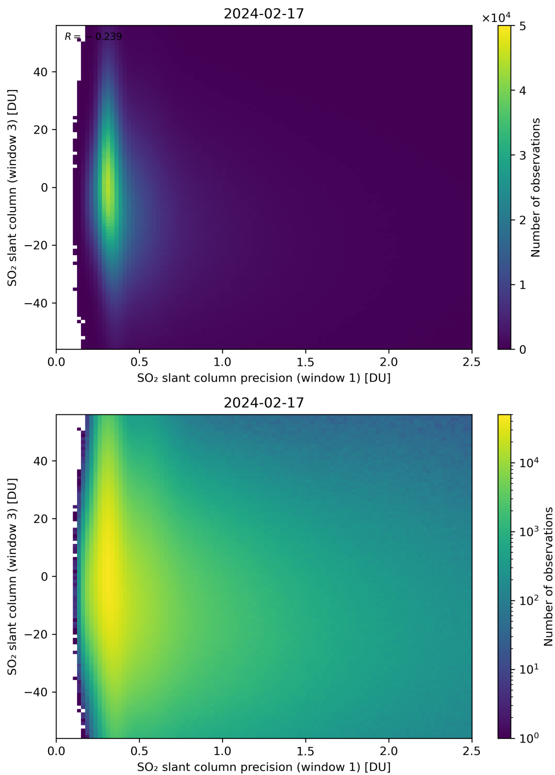
Figure 228: Scatter density plot of “SO 2 slant column precision (window 1)” against “SO 2 slant column (window 3)” for 2024-02-17 to 2024-02-18.
