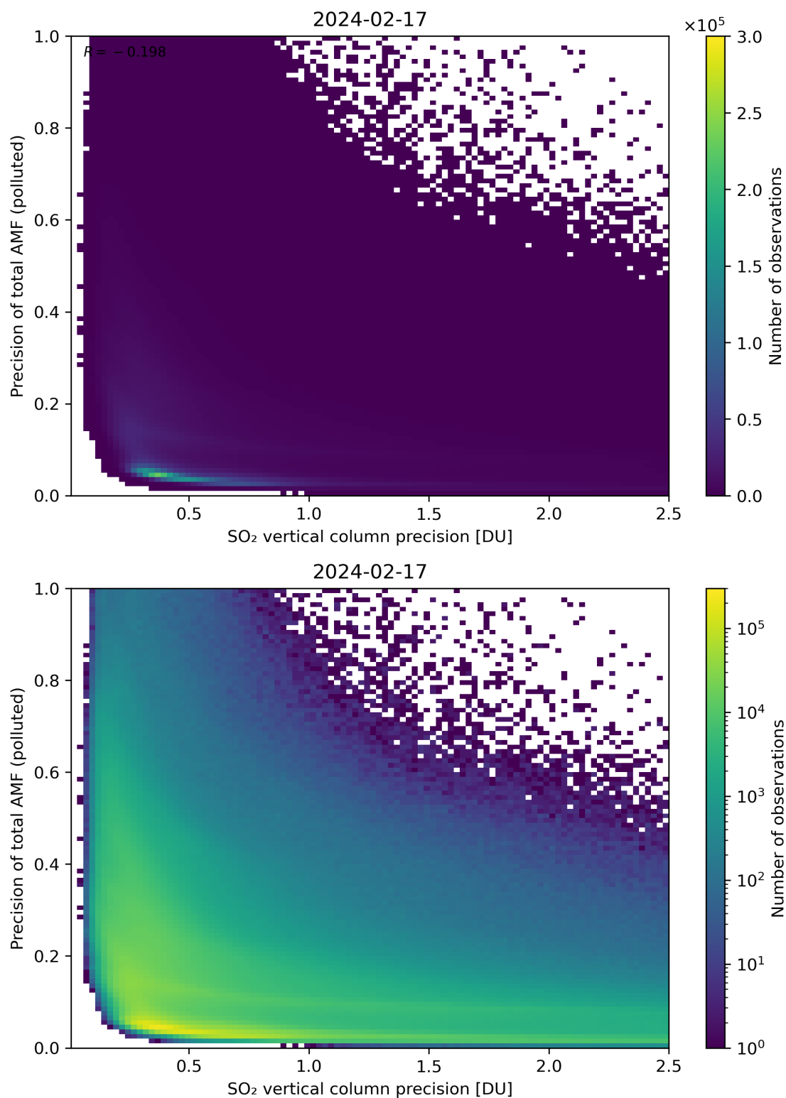
Figure 295: Scatter density plot of “SO 2 vertical column precision” against “Precision of total AMF (polluted)” for 2024-02-17 to 2024-02-18.
