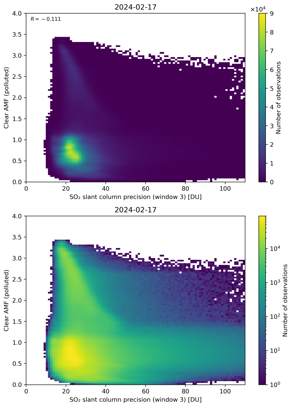
Figure 261: Scatter density plot of “SO 2 slant column precision (window 3)” against “Clear AMF (polluted)” for 2024-02-17 to 2024-02-18.
