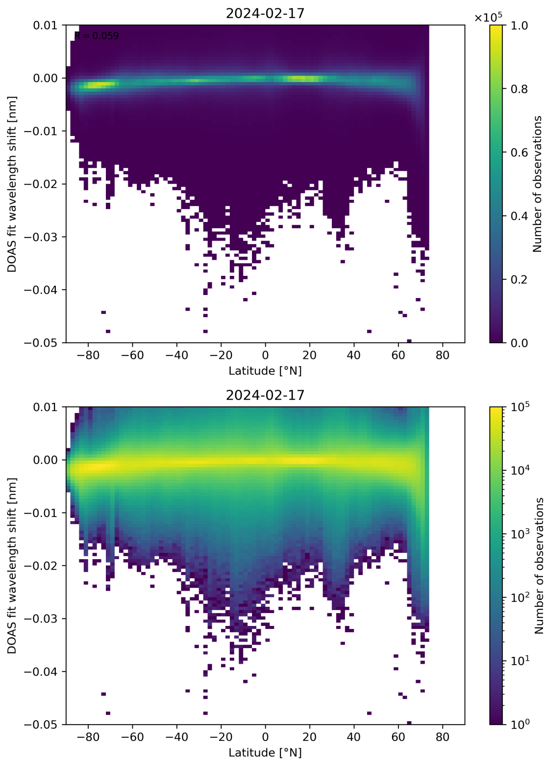
Figure 142: Scatter density plot of “Latitude” against “DOAS fit wavelength shift” for 2024-02-17 to 2024-02-18.
