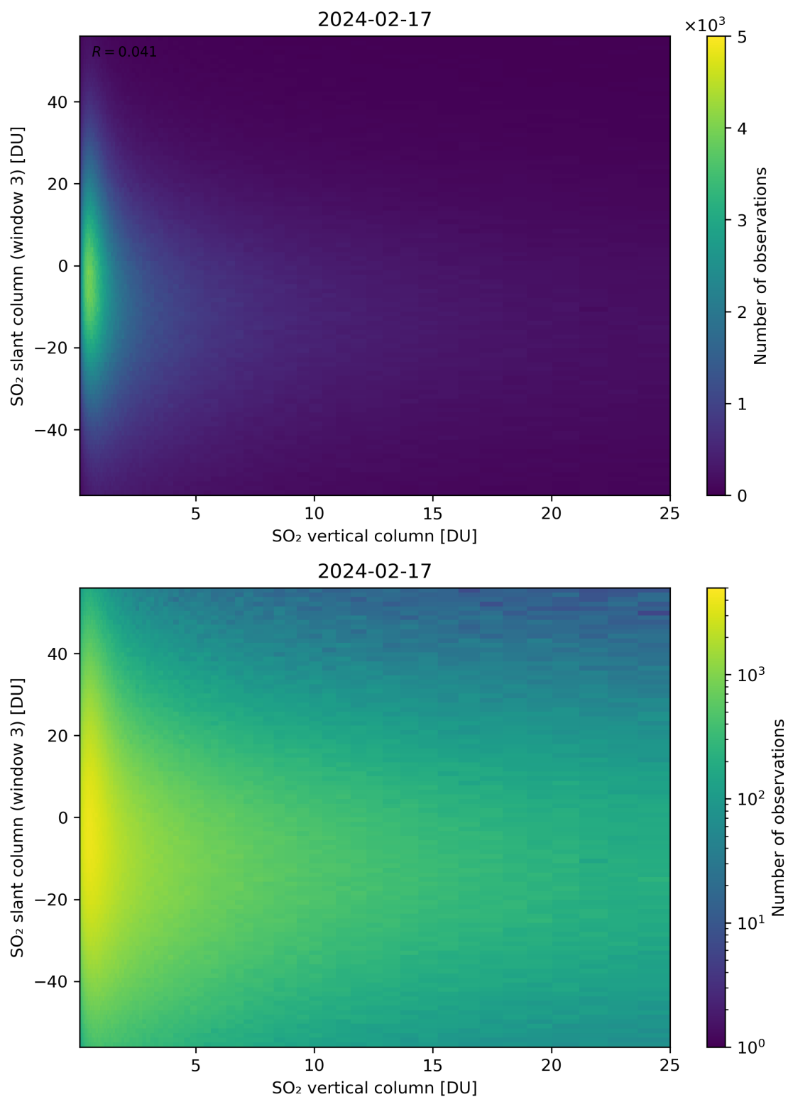
Figure 303: Scatter density plot of “SO 2 vertical column” against “SO 2 slant column (window 3)” for 2024-02-17 to 2024-02-18.
