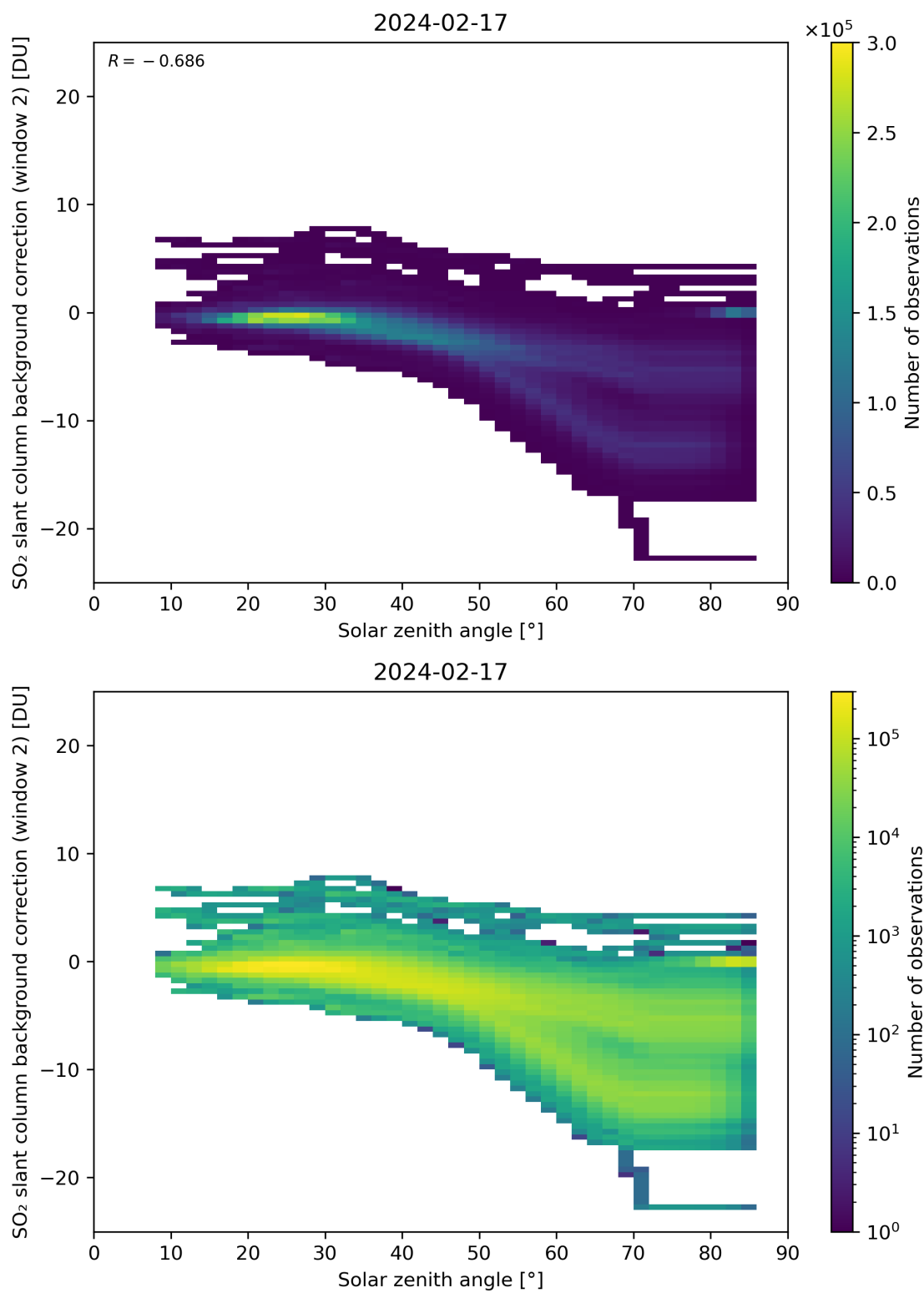
Figure 159: Scatter density plot of “Solar zenith angle” against “SO 2 slant column background correction (window 2)” for 2024-02-17 to 2024-02-18.
