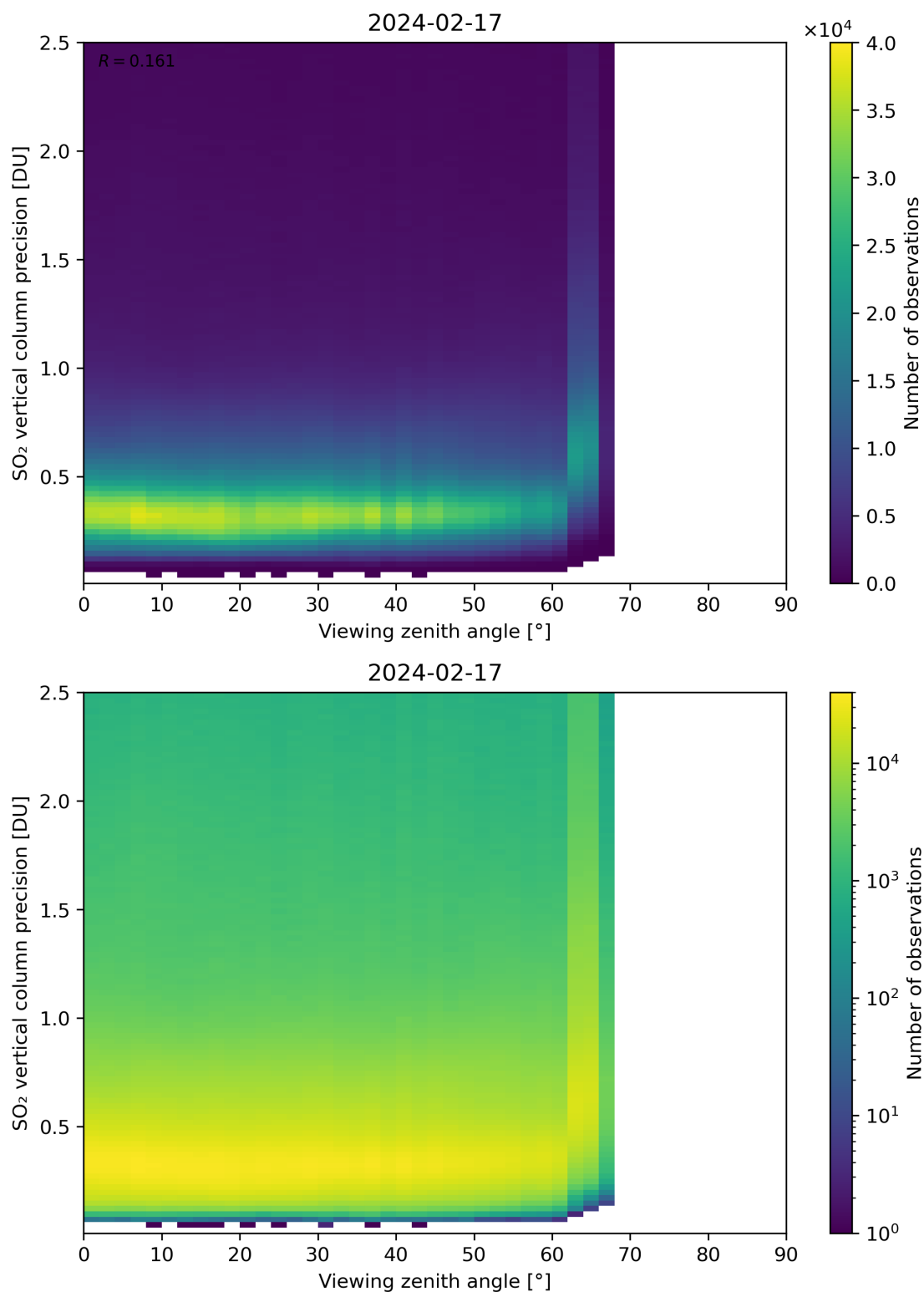
Figure 328: Scatter density plot of “Viewing zenith angle” against “SO 2 vertical column precision” for 2024-02-17 to 2024-02-18.
