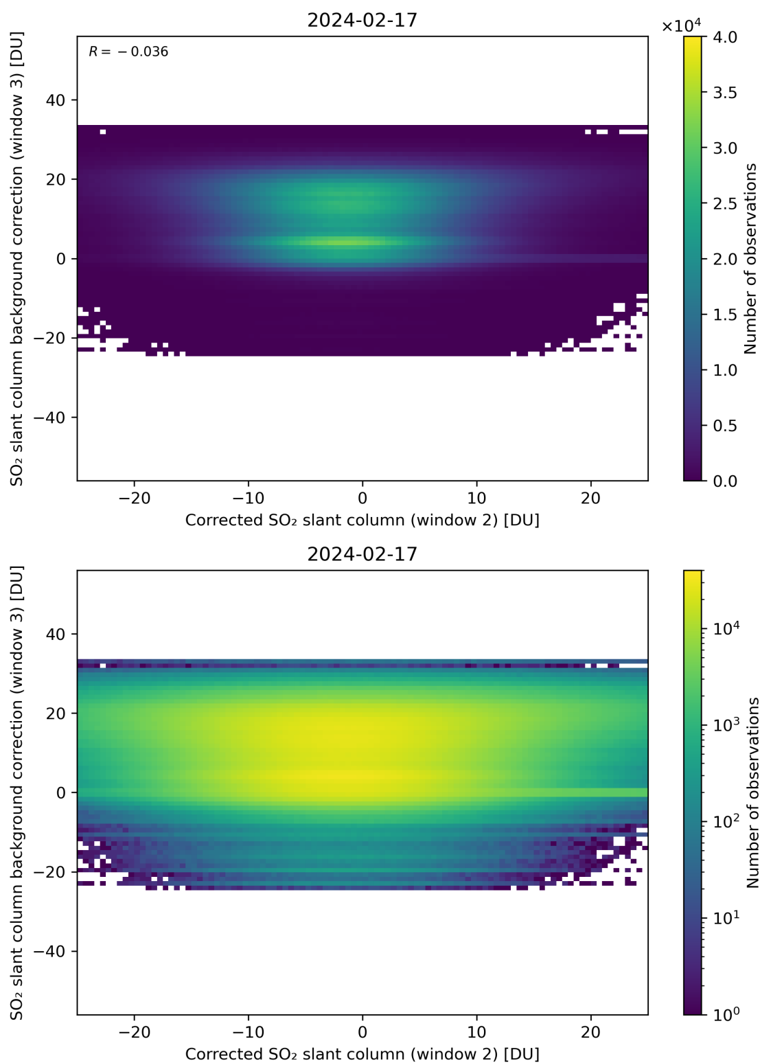
Figure 195: Scatter density plot of “Corrected SO 2 slant column (window 2)” against “SO 2 slant column background correction (window 3)” for 2024-02-17 to 2024-02-18.
