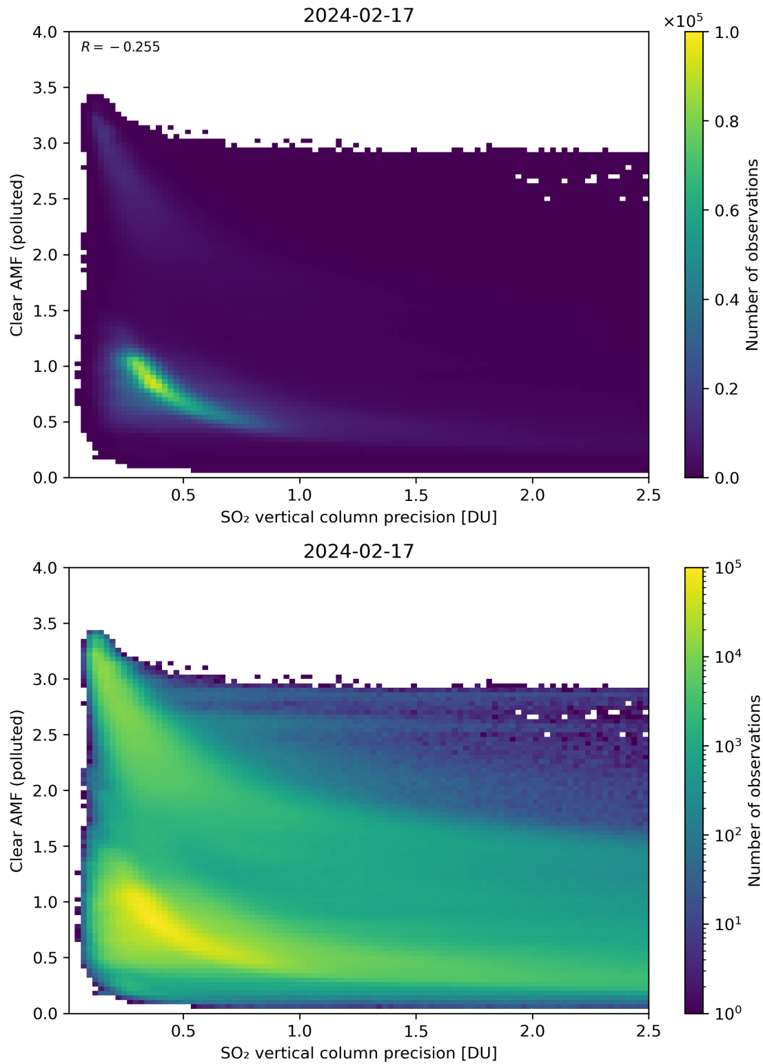
Figure 285: Scatter density plot of “SO 2 vertical column precision” against “Clear AMF (polluted)” for 2024-02-17 to 2024-02-18.
