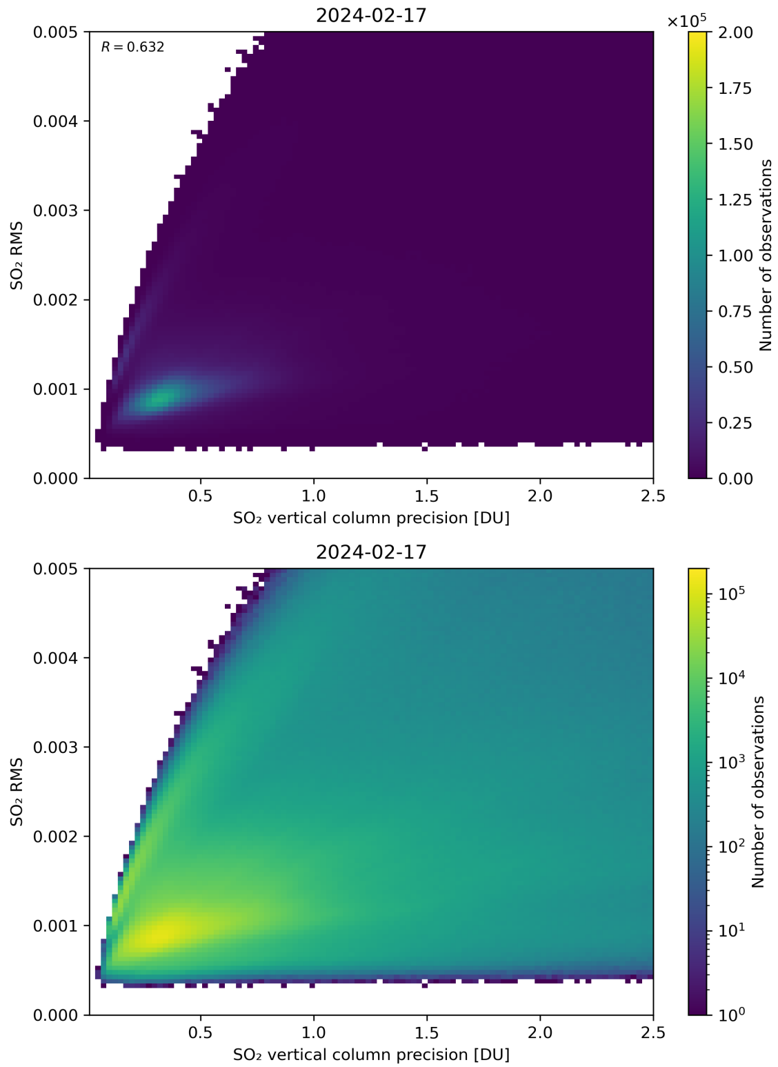
Figure 284: Scatter density plot of “SO 2 vertical column precision” against “SO 2 RMS” for 2024-02-17 to 2024-02-18.
