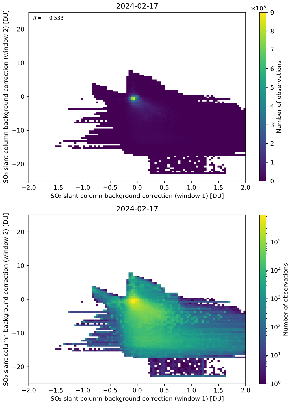
Figure 98: Scatter density plot of “SO 2 slant column background correction (window 1)” against “SO 2 slant column background correction (window 2)” for 2024-02-17 to 2024-02-18.
