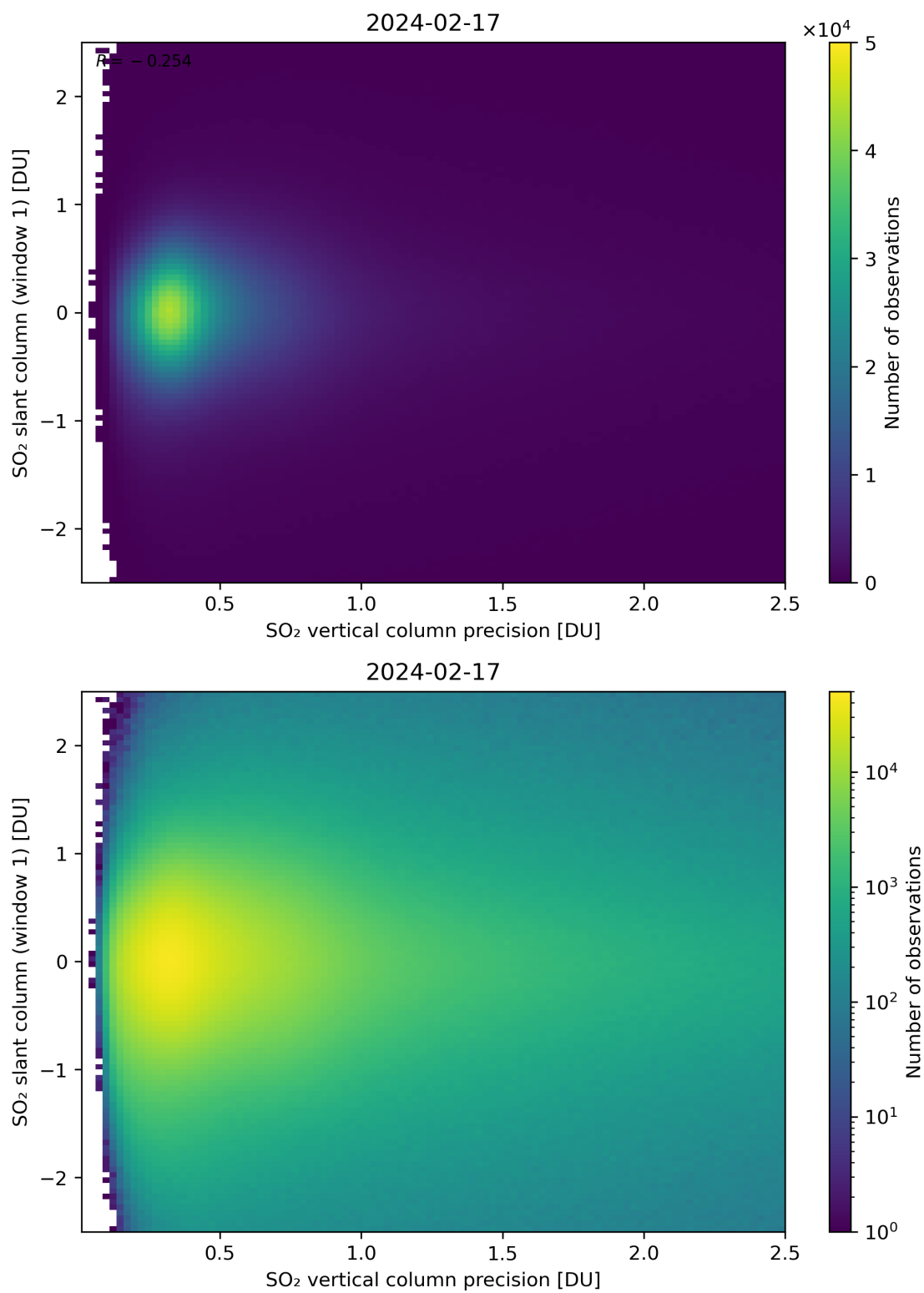
Figure 289: Scatter density plot of “SO 2 vertical column precision” against “SO 2 slant column (window 1)” for 2024-02-17 to 2024-02-18.
