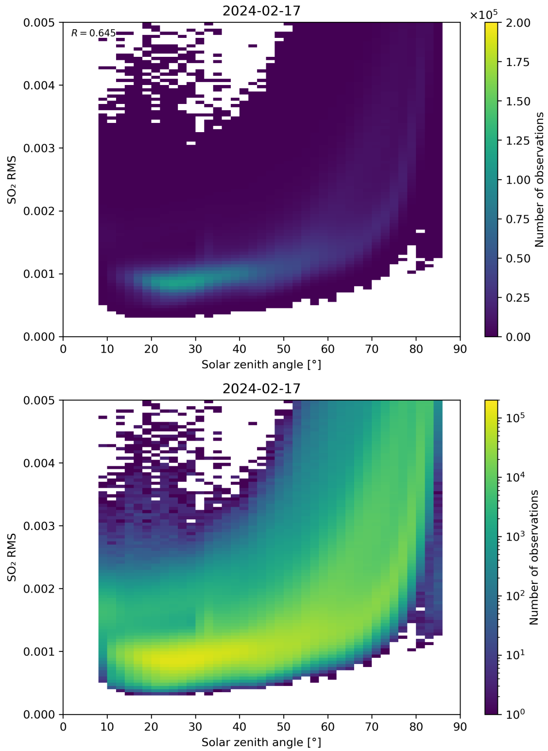
Figure 163: Scatter density plot of “Solar zenith angle” against “SO 2 RMS” for 2024-02-17 to 2024-02-18.
