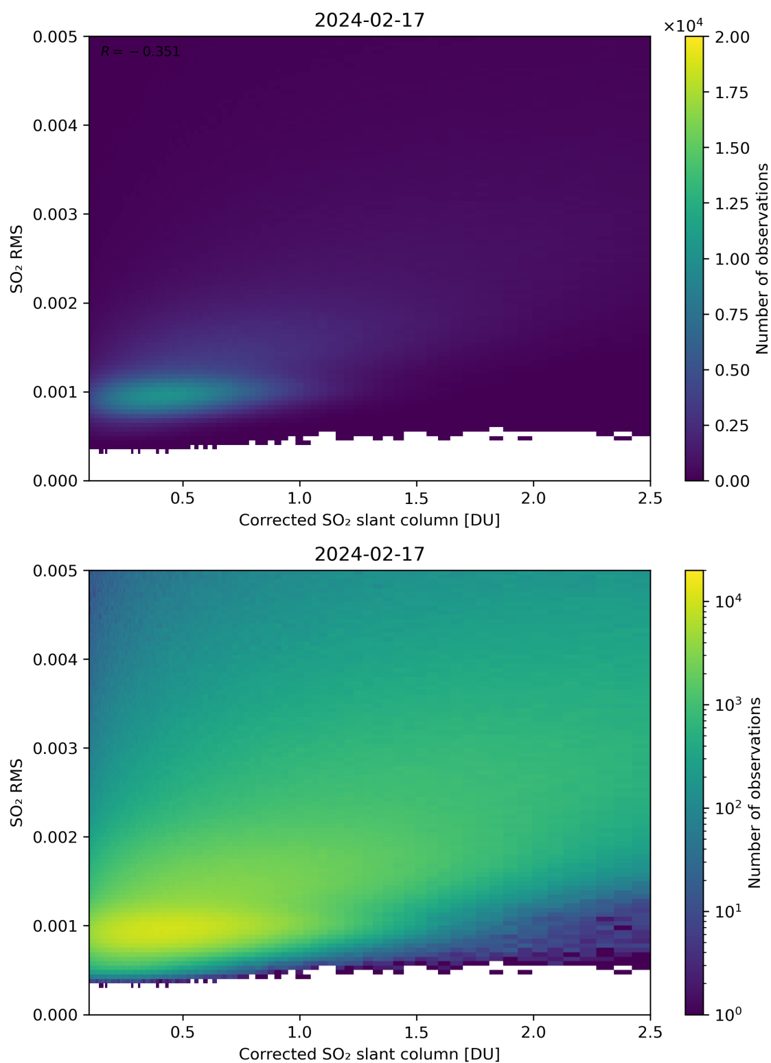
Figure 183: Scatter density plot of “Corrected SO 2 slant column” against “SO 2 RMS” for 2024-02-17 to 2024-02-18.
