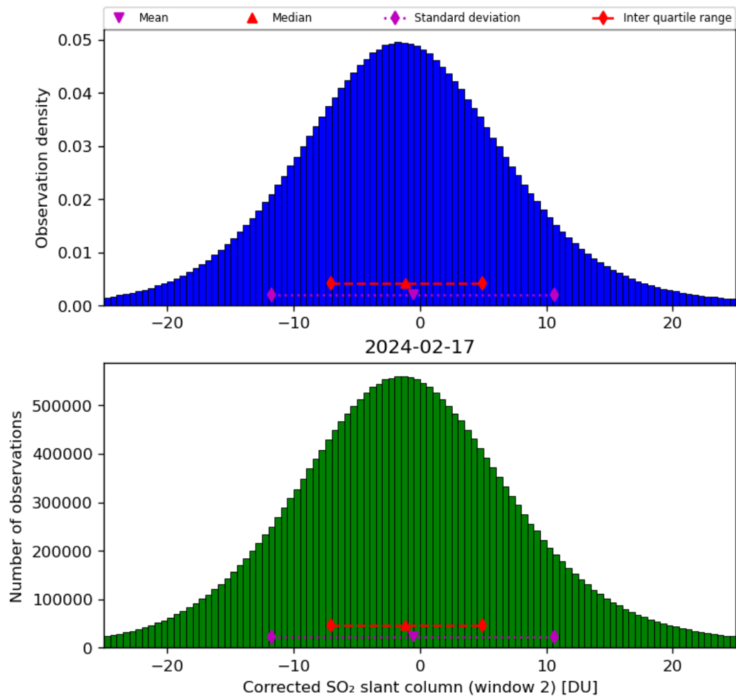
Figure 62: Histogram of “Corrected SO 2 slant column (window 2)” for 2024-02-17 to 2024-02-18
