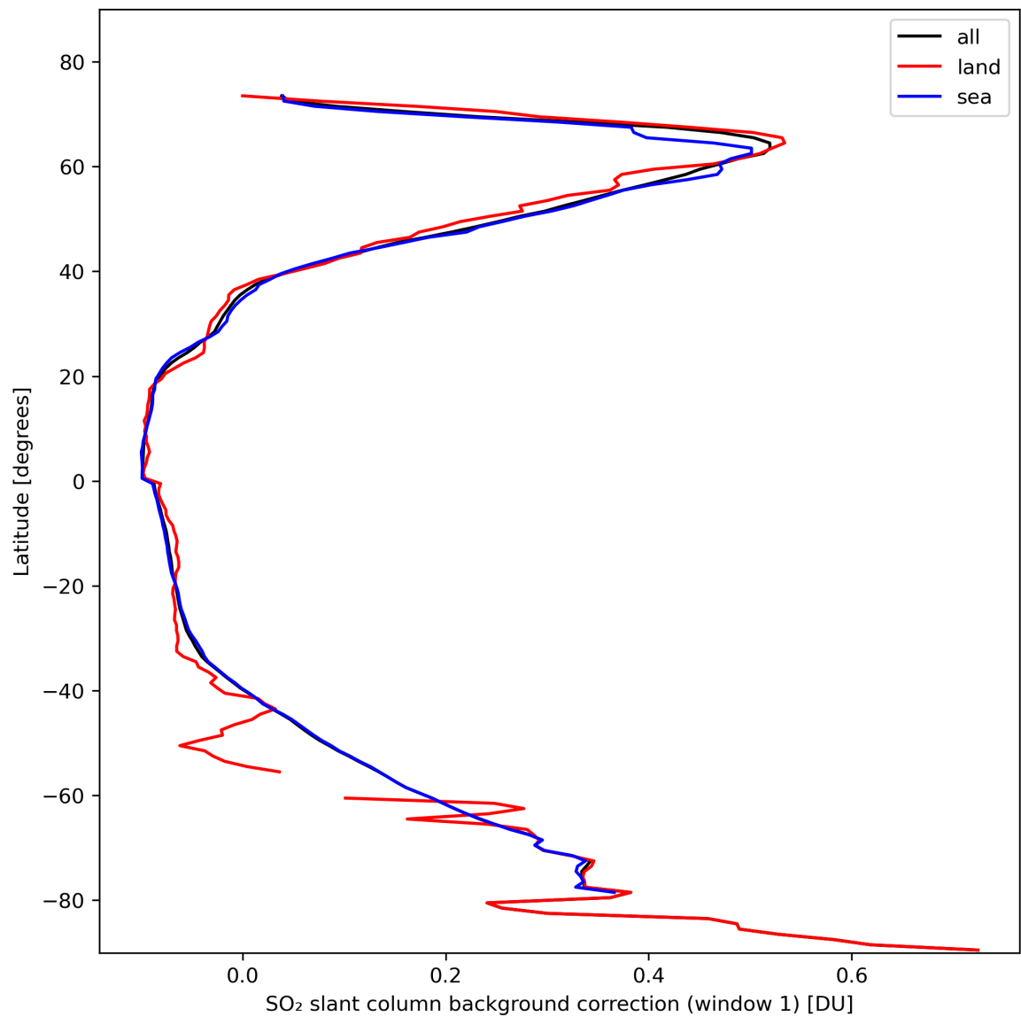
Figure 36: Zonal average of “SO 2 slant column background correction (window 1)” for 2024-02-17 to 2024-02-18.
