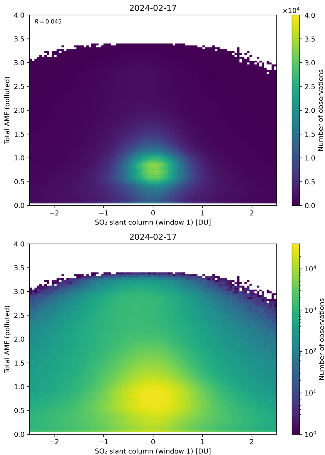
Figure 239: Scatter density plot of “SO 2 slant column (window 1)” against “Total AMF (polluted)” for 2024-02-17 to 2024-02-18.
