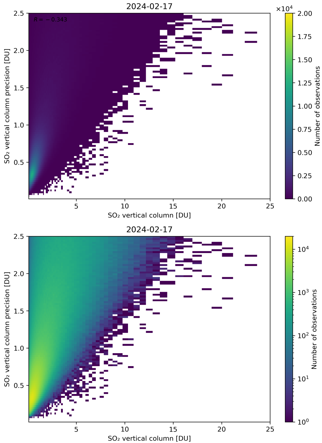
Figure 307: Scatter density plot of “SO 2 vertical column” against “SO 2 vertical column precision” for 2024-02-17 to 2024-02-18.
