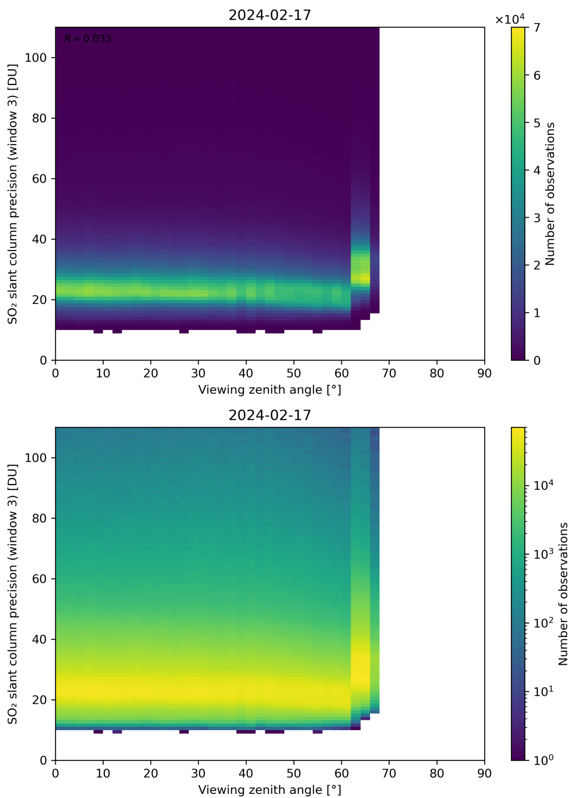
Figure 324: Scatter density plot of “Viewing zenith angle” against “SO 2 slant column precision (window 3)” for 2024-02-17 to 2024-02-18.
