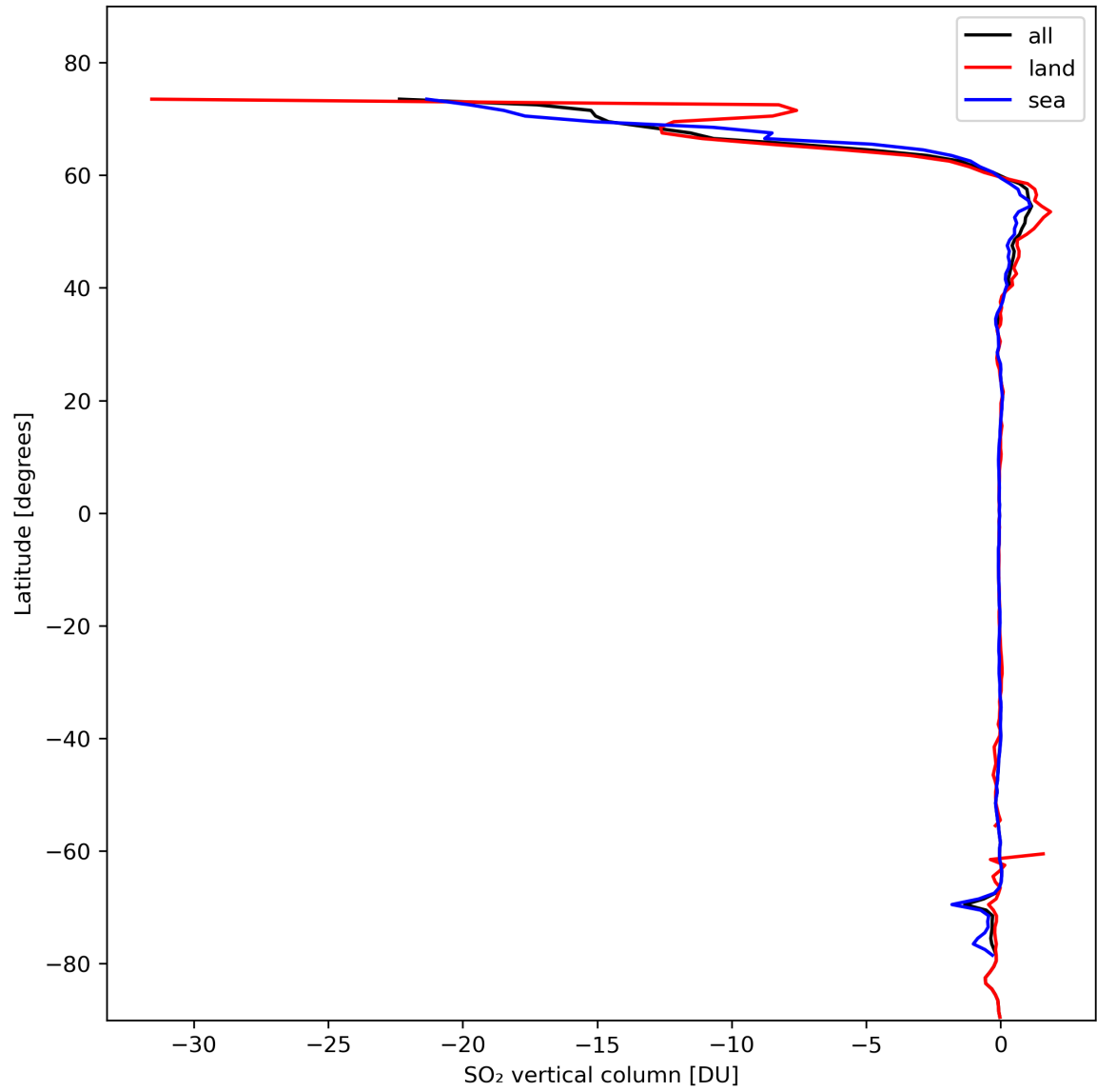
Figure 30: Zonal average of “SO 2 vertical column” for 2024-02-17 to 2024-02-18.
