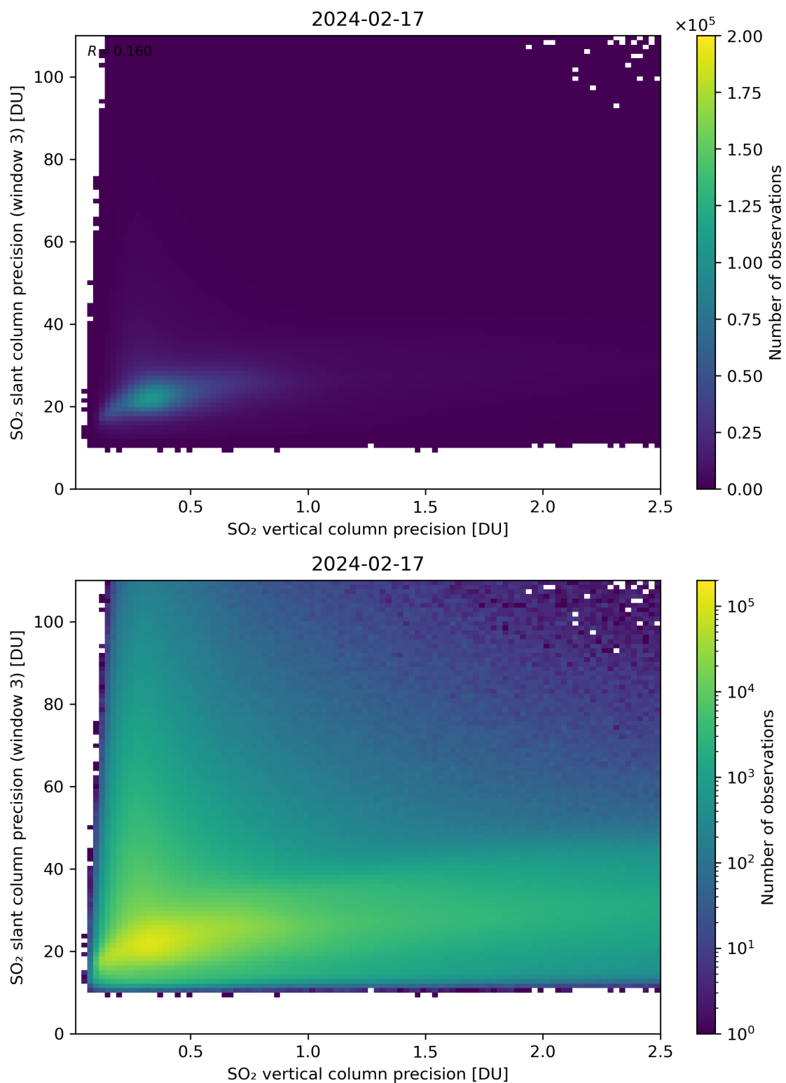
Figure 293: Scatter density plot of “SO 2 vertical column precision” against “SO 2 slant column precision (window 3)” for 2024-02-17 to 2024-02-18.
