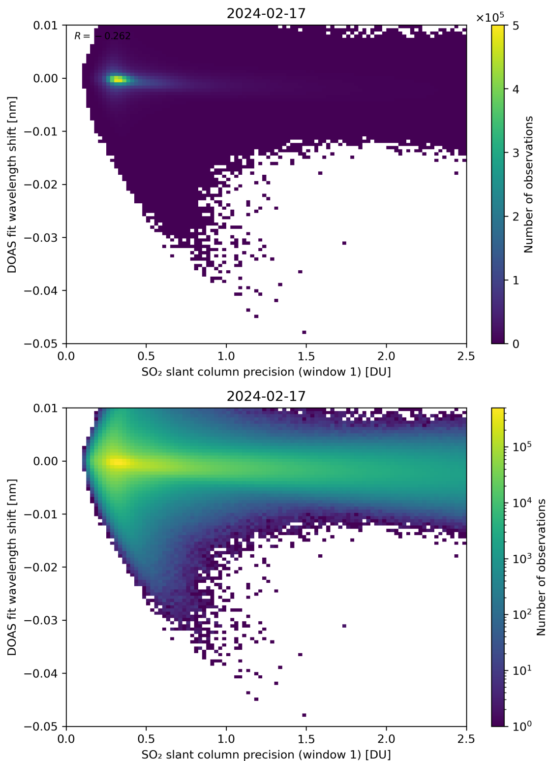
Figure 221: Scatter density plot of “SO 2 slant column precision (window 1)” against “DOAS fit wavelength shift” for 2024-02-17 to 2024-02-18.
