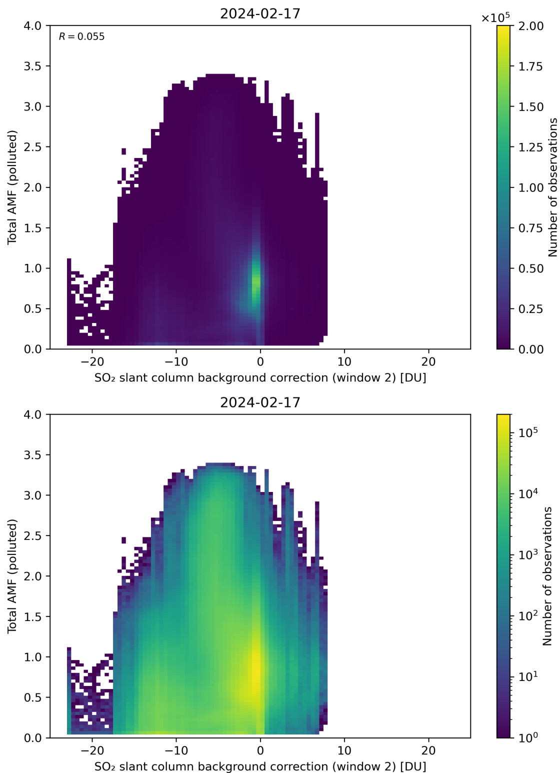
Figure 119: Scatter density plot of “SO 2 slant column background correction (window 2)” against “Total AMF (polluted)” for 2024-02-17 to 2024-02-18.
