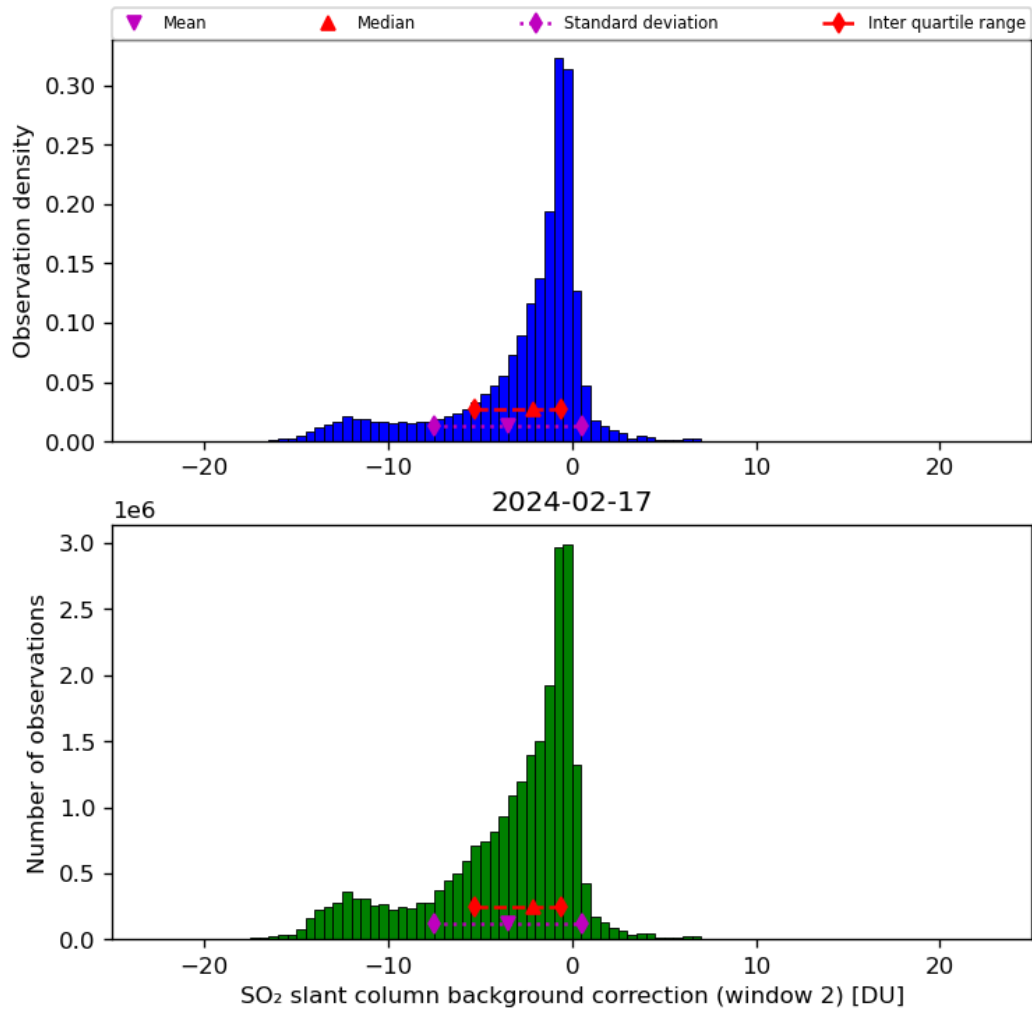
Figure 63: Histogram of “SO 2 slant column background correction (window 2)” for 2024-02-17 to 2024-02-18
