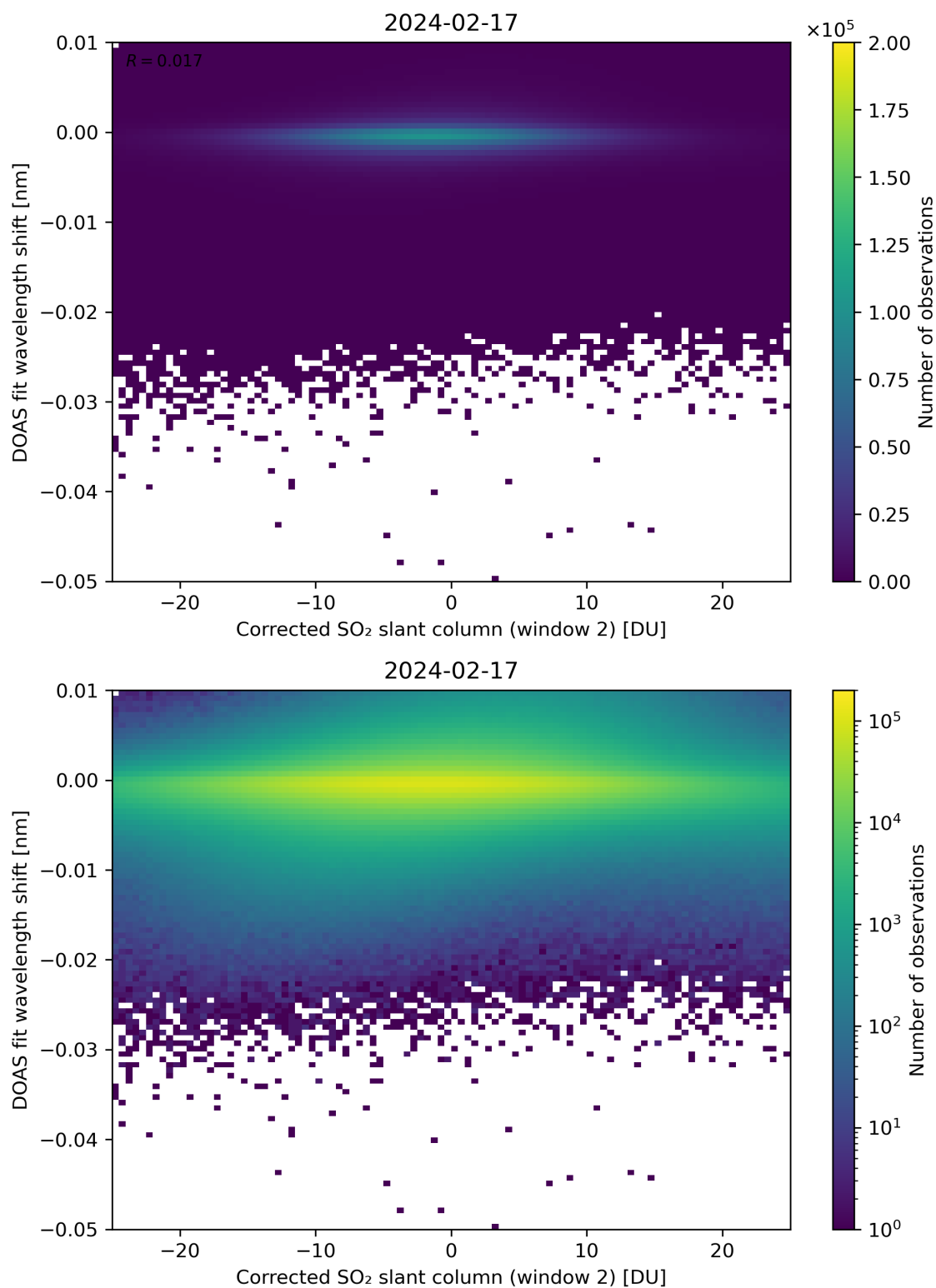
Figure 196: Scatter density plot of “Corrected SO 2 slant column (window 2)” against “DOAS fit wavelength shift” for 2024-02-17 to 2024-02-18.
