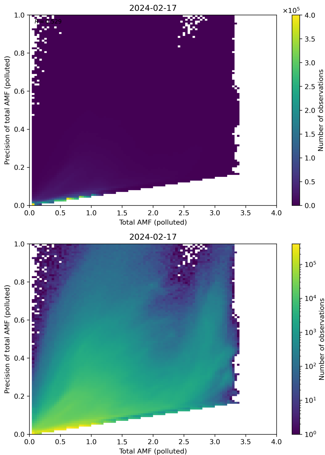
Figure 272: Scatter density plot of “Total AMF (polluted)” against “Precision of total AMF (polluted)” for 2024-02-17 to 2024-02-18.
