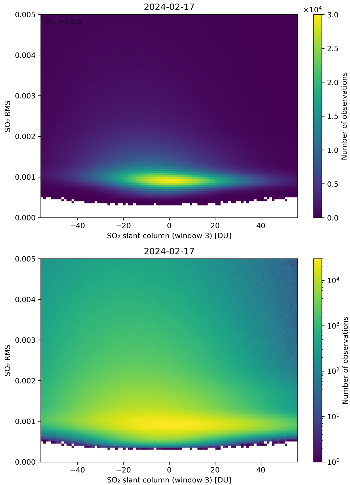
Figure 256: Scatter density plot of “SO 2 slant column (window 3)” against “SO 2 RMS” for 2024-02-17 to 2024-02-18.
