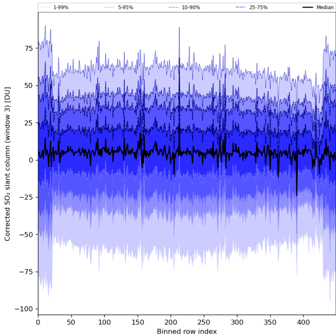
Figure 89: Along track statistics of “Corrected SO 2 slant column (window 3)” for 2024-02-17 to 2024-02-18
