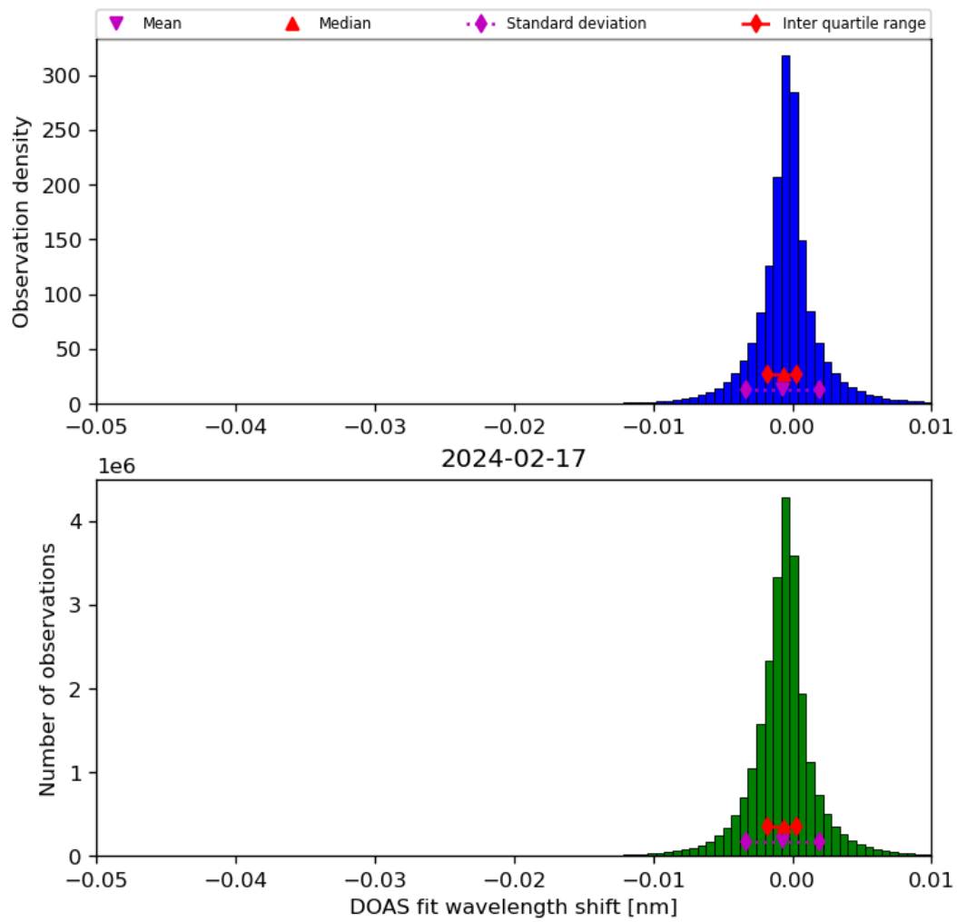
Figure 68: Histogram of “DOAS fit wavelength shift” for 2024-02-17 to 2024-02-18
