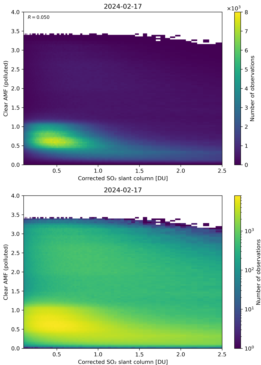
Figure 184: Scatter density plot of “Corrected SO 2 slant column” against “Clear AMF (polluted)” for 2024-02-17 to 2024-02-18.
