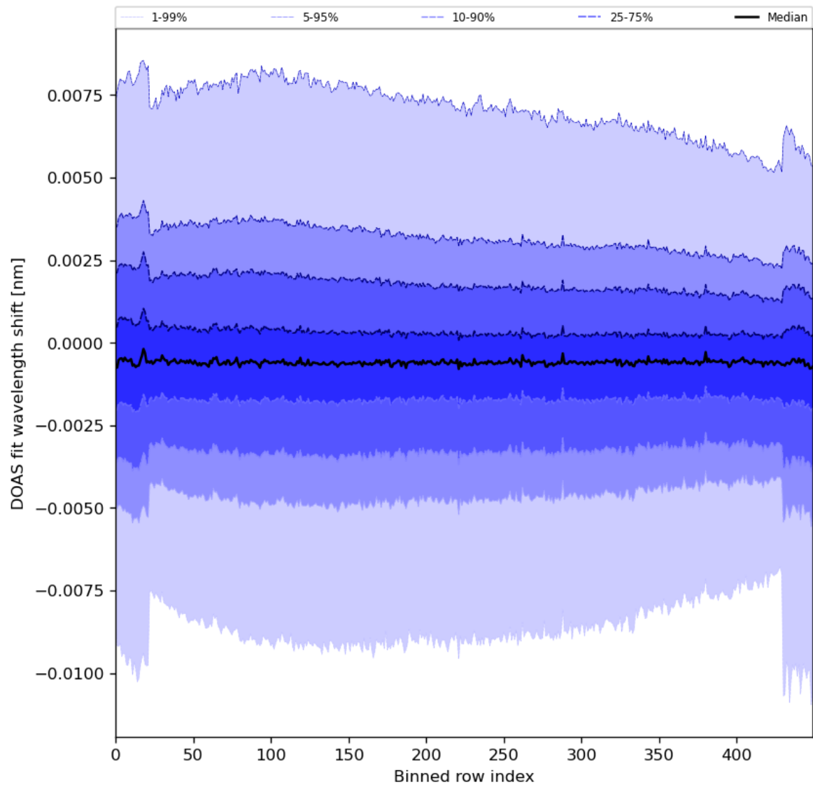
Figure 91: Along track statistics of “DOAS fit wavelength shift” for 2024-02-17 to 2024-02-18
