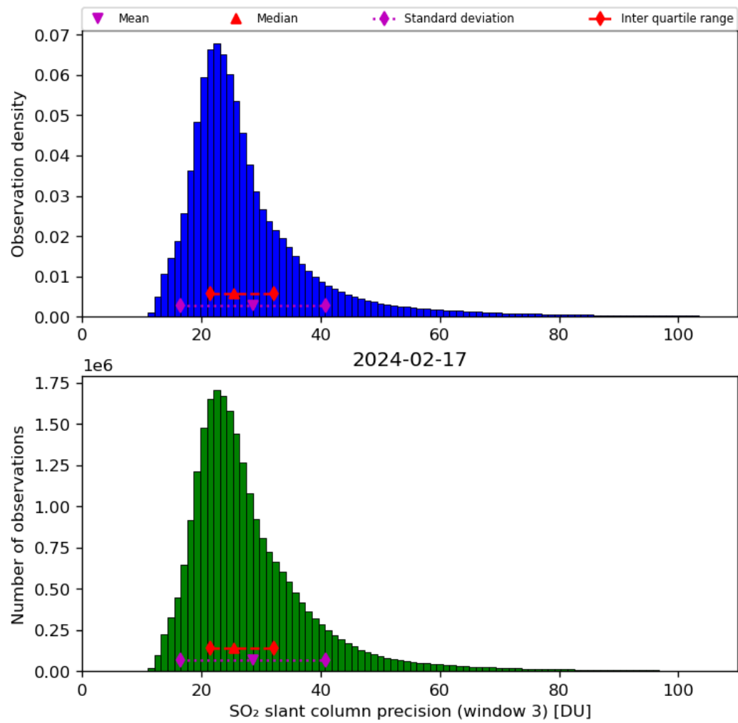
Figure 65: Histogram of “SO 2 slant column precision (window 3)” for 2024-02-17 to 2024-02-18
