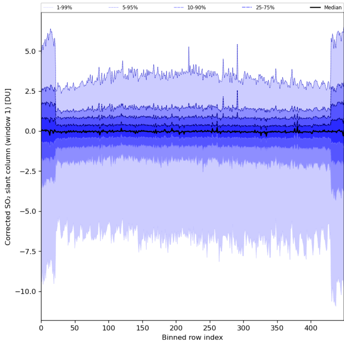
Figure 81: Along track statistics of “Corrected SO 2 slant column (window 1)” for 2024-02-17 to 2024-02-18
