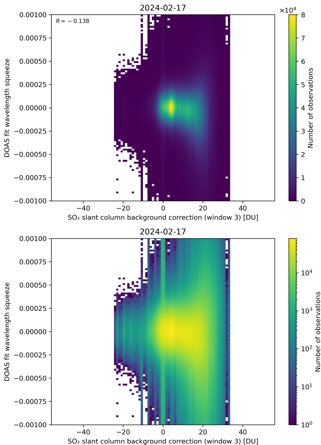
Figure 122: Scatter density plot of “SO 2 slant column background correction (window 3)” against “DOAS fit wavelength squeeze” for 2024-02-17 to 2024-02-18.
