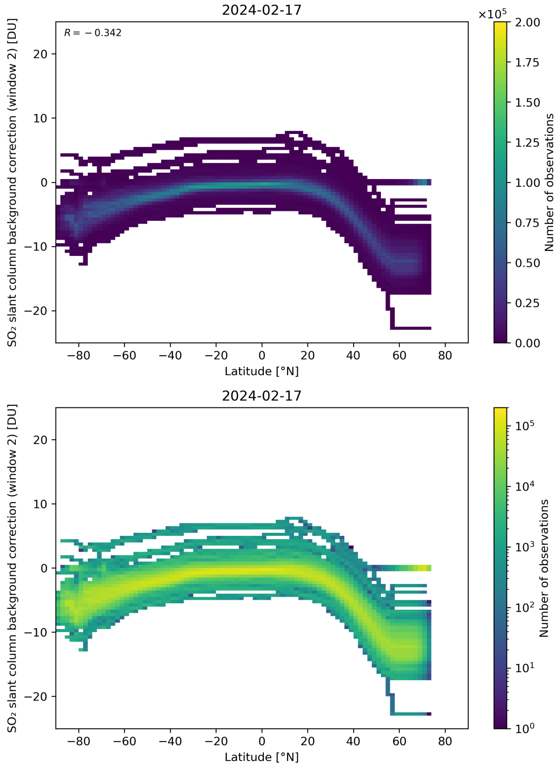
Figure 140: Scatter density plot of “Latitude” against “SO 2 slant column background correction (window 2)” for 2024-02-17 to 2024-02-18.
