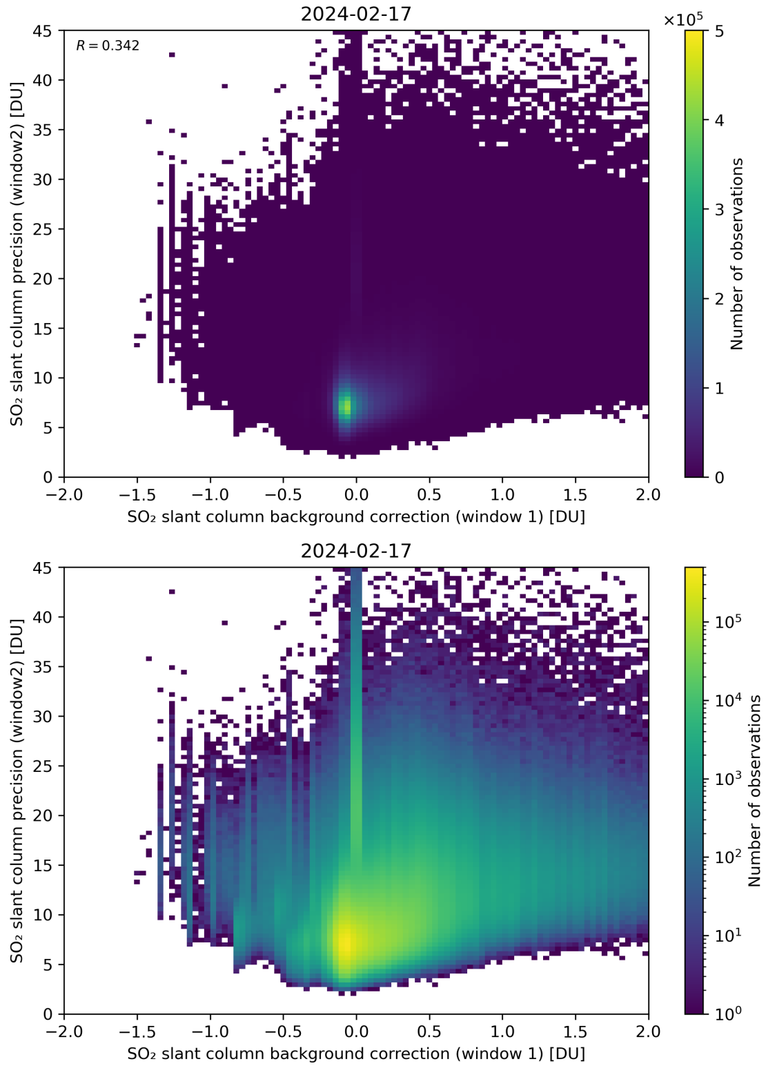
Figure 106: Scatter density plot of “SO 2 slant column background correction (window 1)” against “SO 2 slant column precision (window2)” for 2024-02-17 to 2024-02-18.
