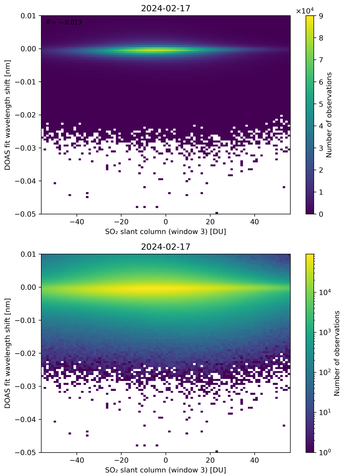
Figure 254: Scatter density plot of “SO 2 slant column (window 3)” against “DOAS fit wavelength shift” for 2024-02-17 to 2024-02-18.
