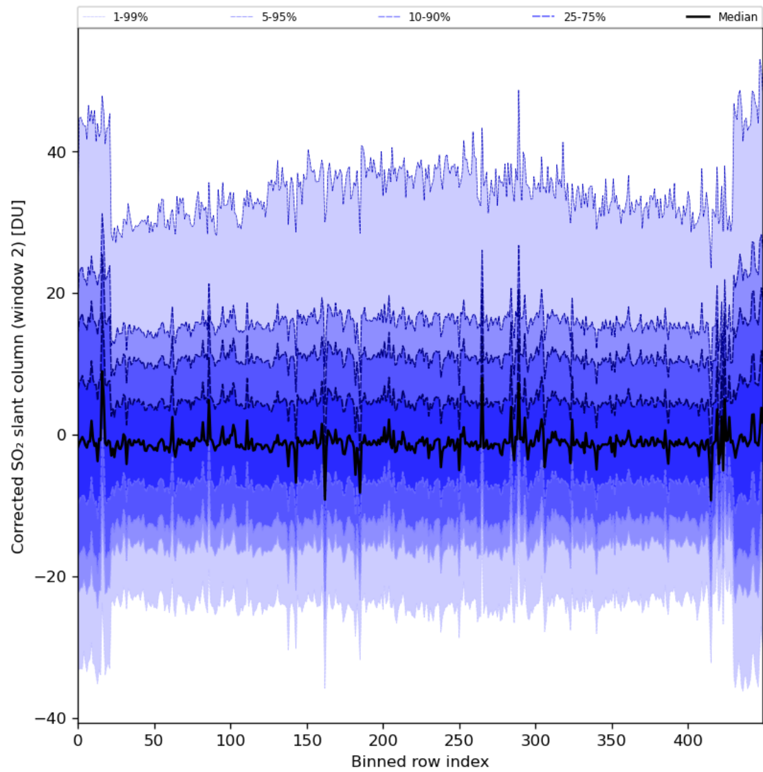
Figure 85: Along track statistics of “Corrected SO 2 slant column (window 2)” for 2024-02-17 to 2024-02-18
