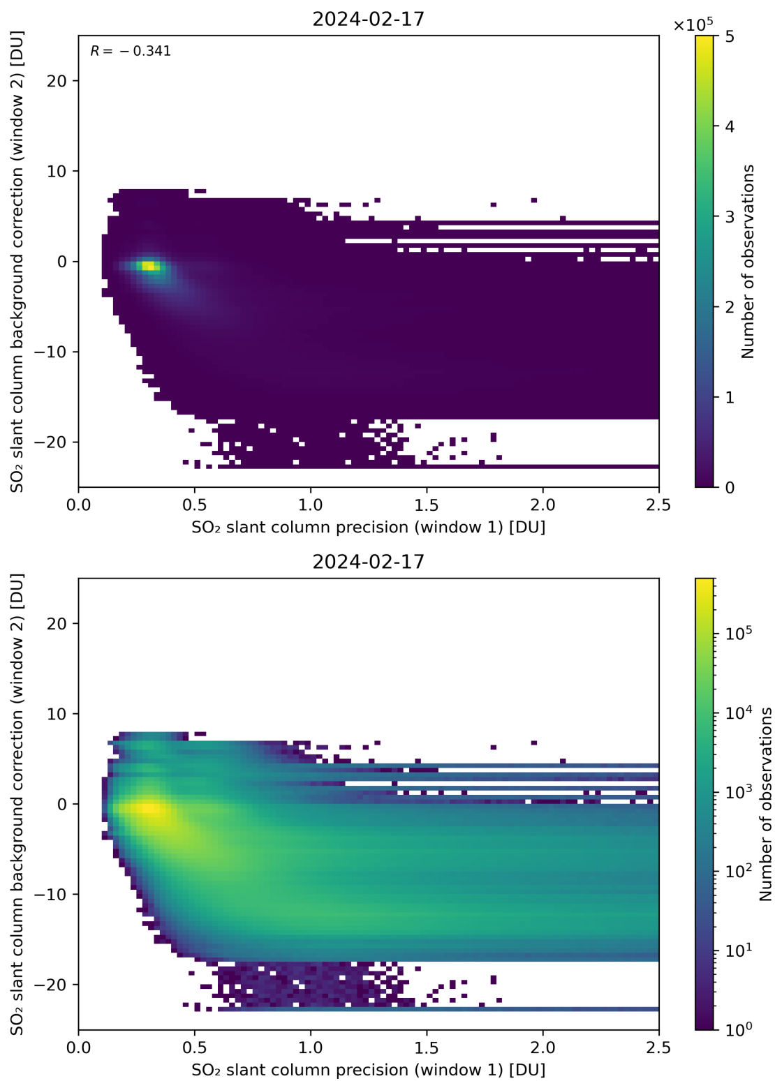
Figure 219: Scatter density plot of “SO 2 slant column precision (window 1)” against “SO 2 slant column background correction (window 2)” for 2024-02-17 to 2024-02-18.
