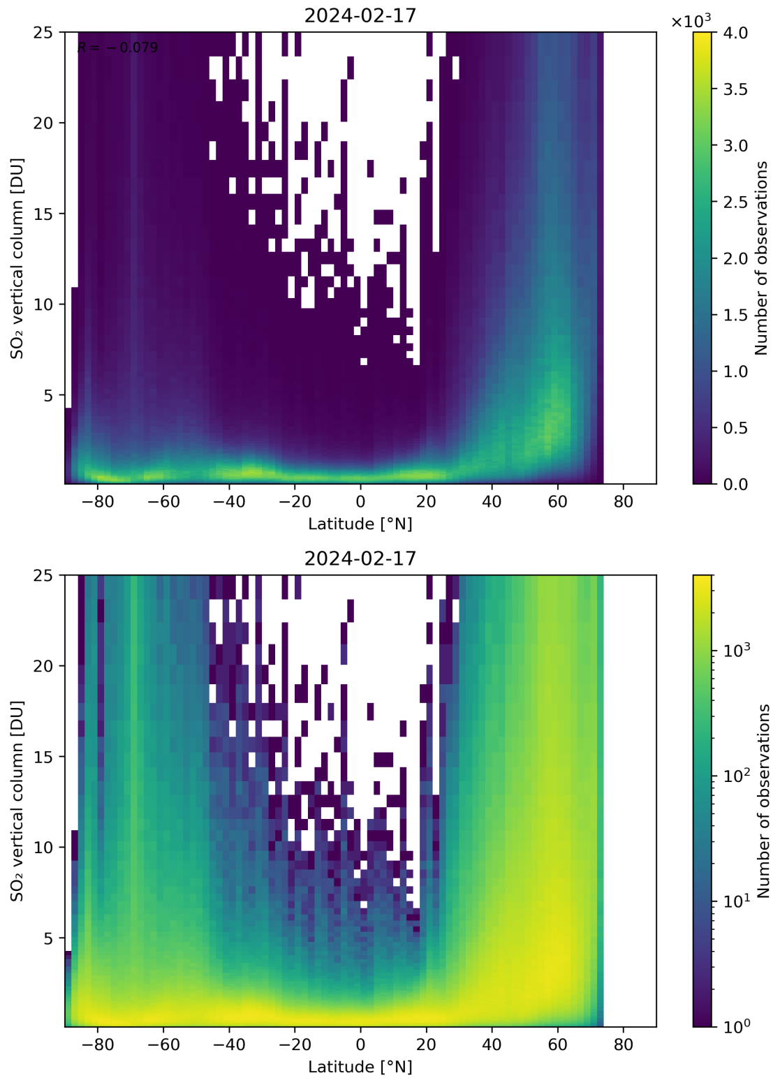
Figure 156: Scatter density plot of “Latitude” against “SO 2 vertical column” for 2024-02-17 to 2024-02-18.
