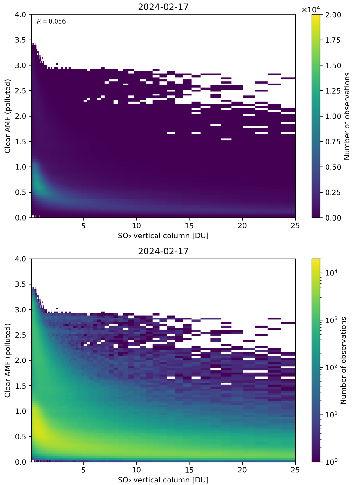
Figure 296: Scatter density plot of “SO 2 vertical column” against “Clear AMF (polluted)” for 2024-02-17 to 2024-02-18.
