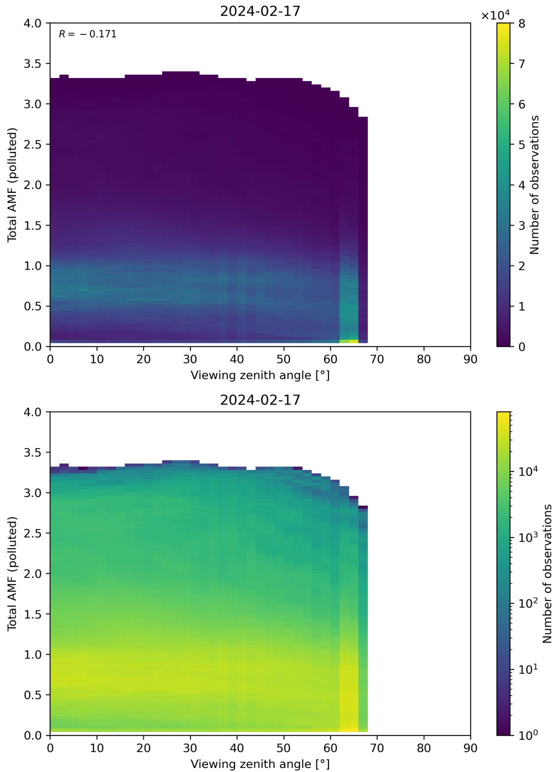
Figure 325: Scatter density plot of “Viewing zenith angle” against “Total AMF (polluted)” for 2024-02-17 to 2024-02-18.
