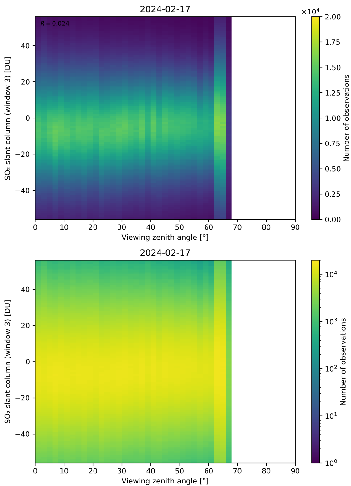
Figure 323: Scatter density plot of “Viewing zenith angle” against “SO 2 slant column (window 3)” for 2024-02-17 to 2024-02-18.
