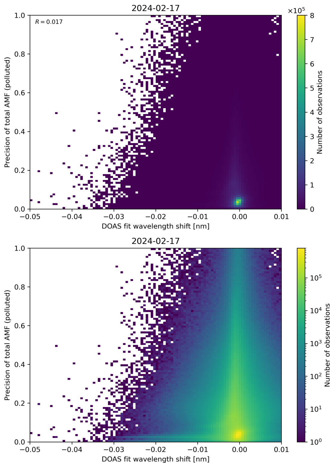
Figure 131: Scatter density plot of “DOAS fit wavelength shift” against “Precision of total AMF (polluted)” for 2024-02-17 to 2024-02-18.
