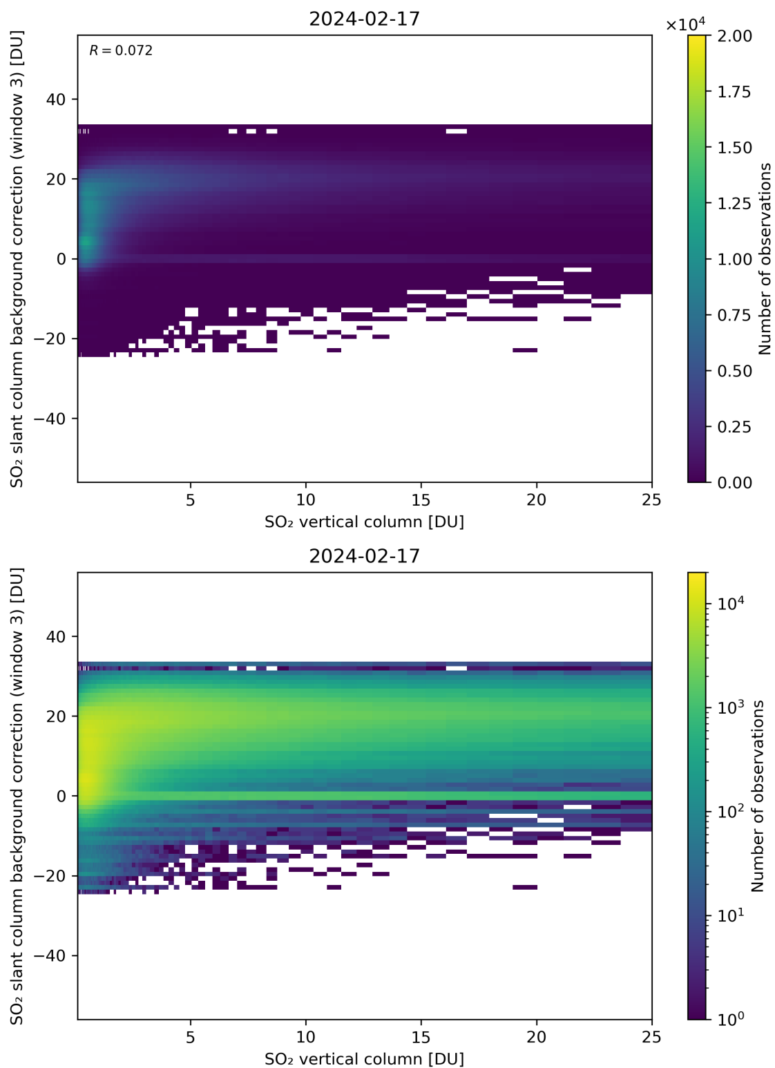
Figure 275: Scatter density plot of “SO 2 vertical column” against “SO 2 slant column background correction (window 3)” for 2024-02-17 to 2024-02-18.
