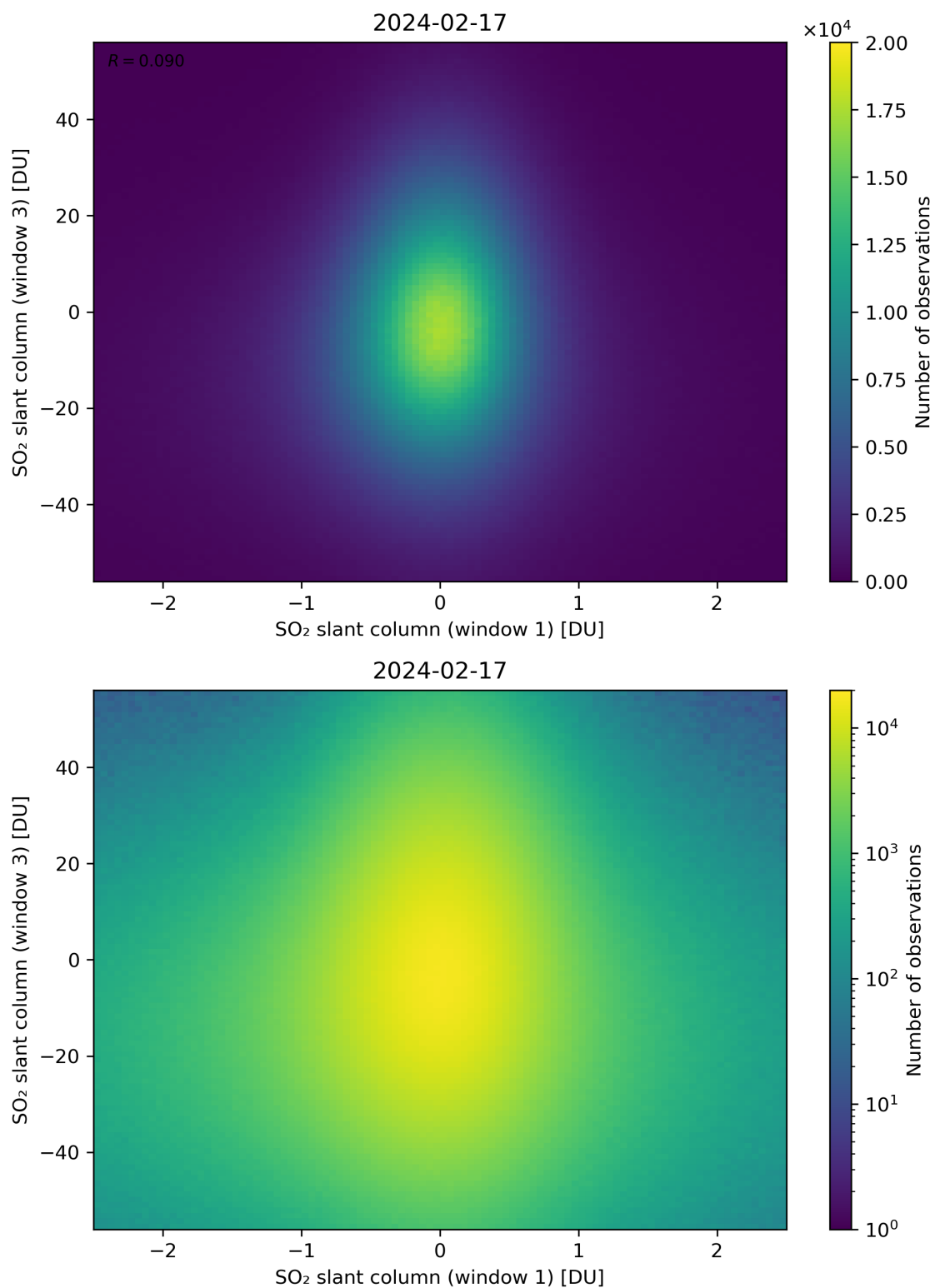
Figure 237: Scatter density plot of “SO 2 slant column (window 1)” against “SO 2 slant column (window 3)” for 2024-02-17 to 2024-02-18.
