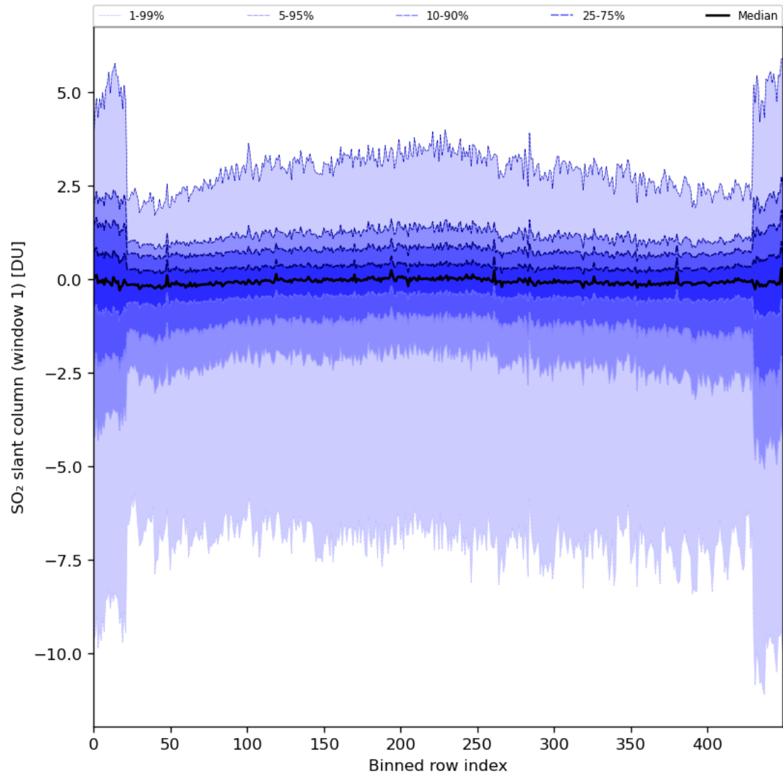
Figure 79: Along track statistics of “SO 2 slant column (window 1)” for 2024-02-17 to 2024-02-18
