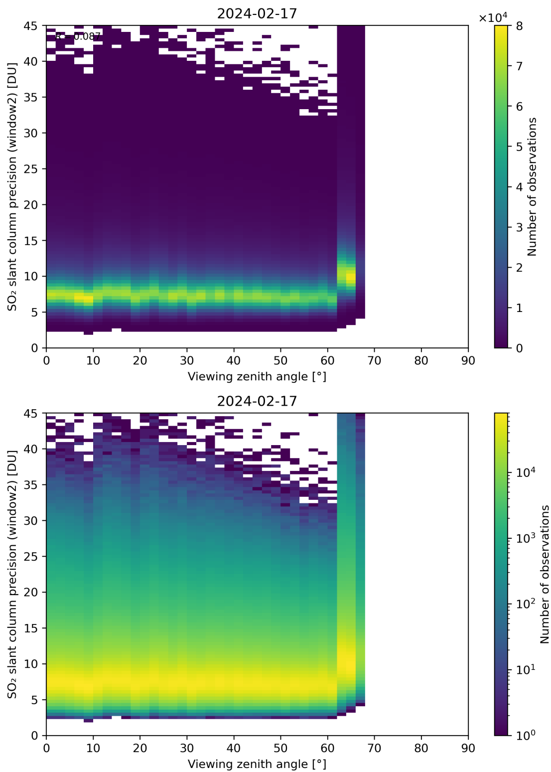
Figure 322: Scatter density plot of “Viewing zenith angle” against “SO 2 slant column precision (window2)” for 2024-02-17 to 2024-02-18.
