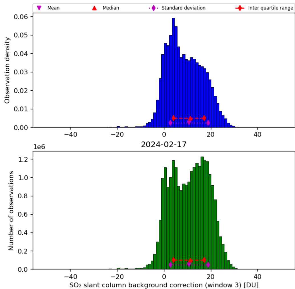
Figure 67: Histogram of “SO 2 slant column background correction (window 3)” for 2024-02-17 to 2024-02-18
