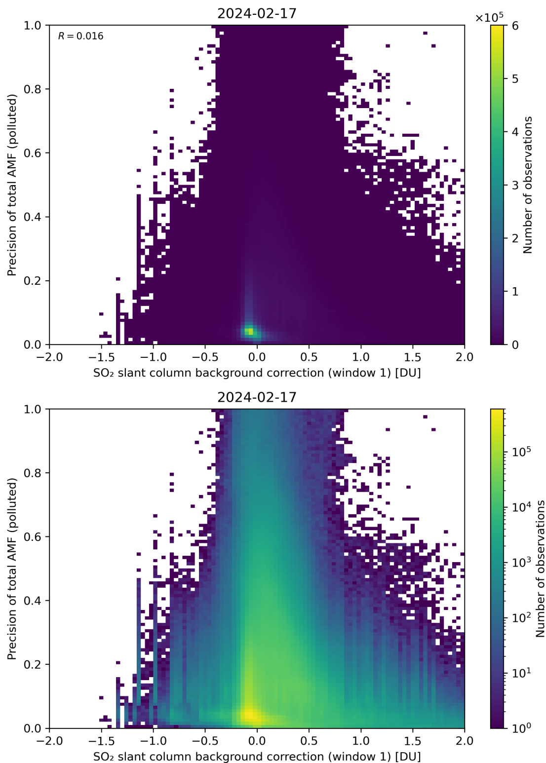
Figure 110: Scatter density plot of “SO 2 slant column background correction (window 1)” against “Precision of total AMF (polluted)” for 2024-02-17 to 2024-02-18.
