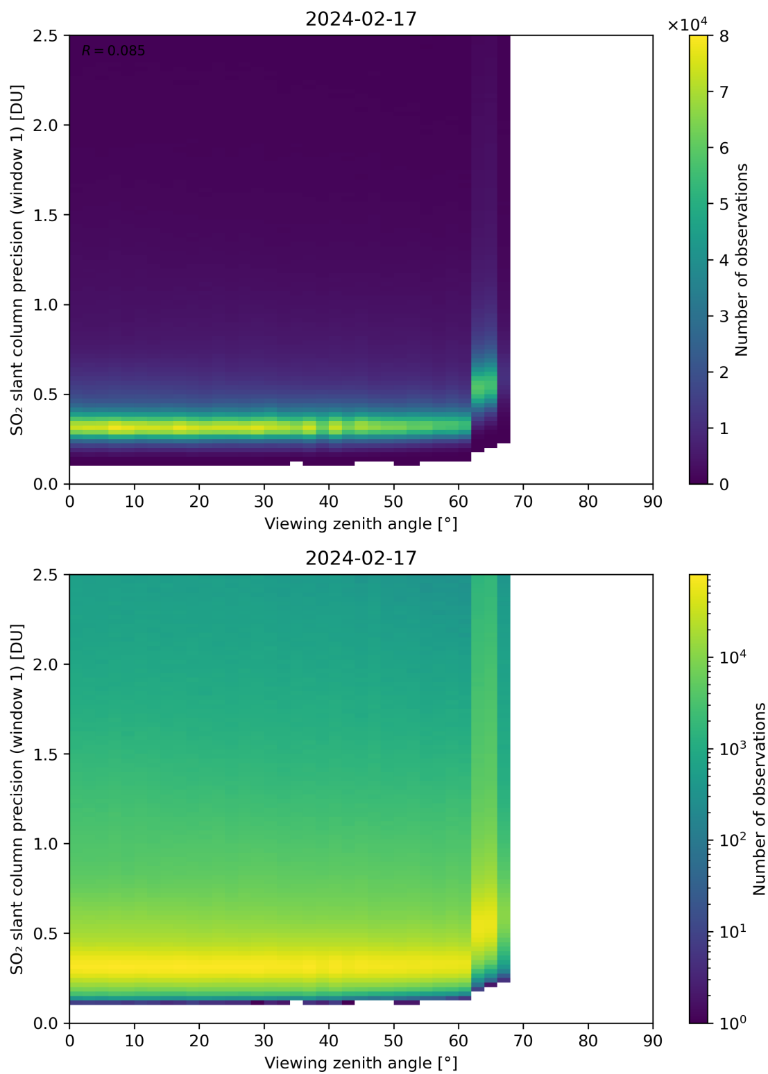
Figure 321: Scatter density plot of “Viewing zenith angle” against “SO 2 slant column precision (window 1)” for 2024-02-17 to 2024-02-18.
