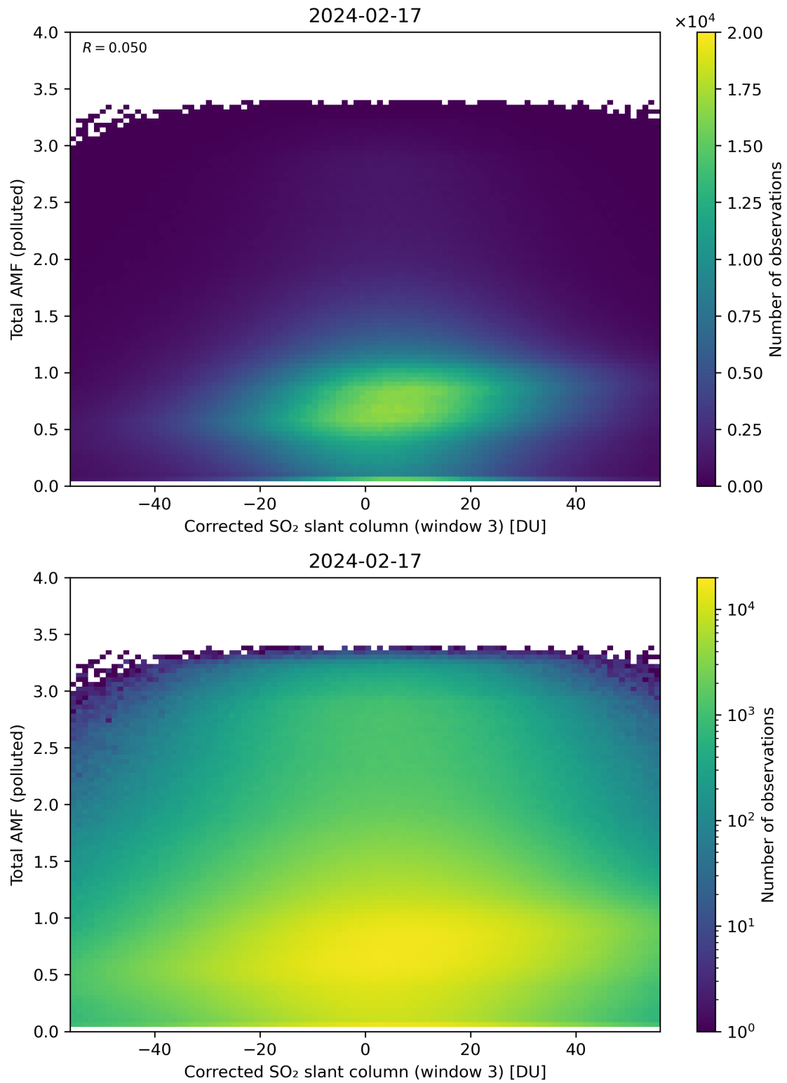
Figure 210: Scatter density plot of “Corrected SO 2 slant column (window 3)” against “Total AMF (polluted)” for 2024-02-17 to 2024-02-18.
