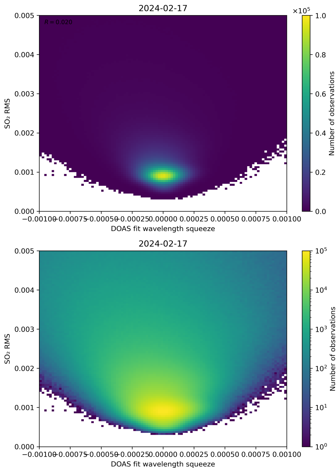
Figure 132: Scatter density plot of “DOAS fit wavelength squeeze” against “SO 2 RMS” for 2024-02-17 to 2024-02-18.
