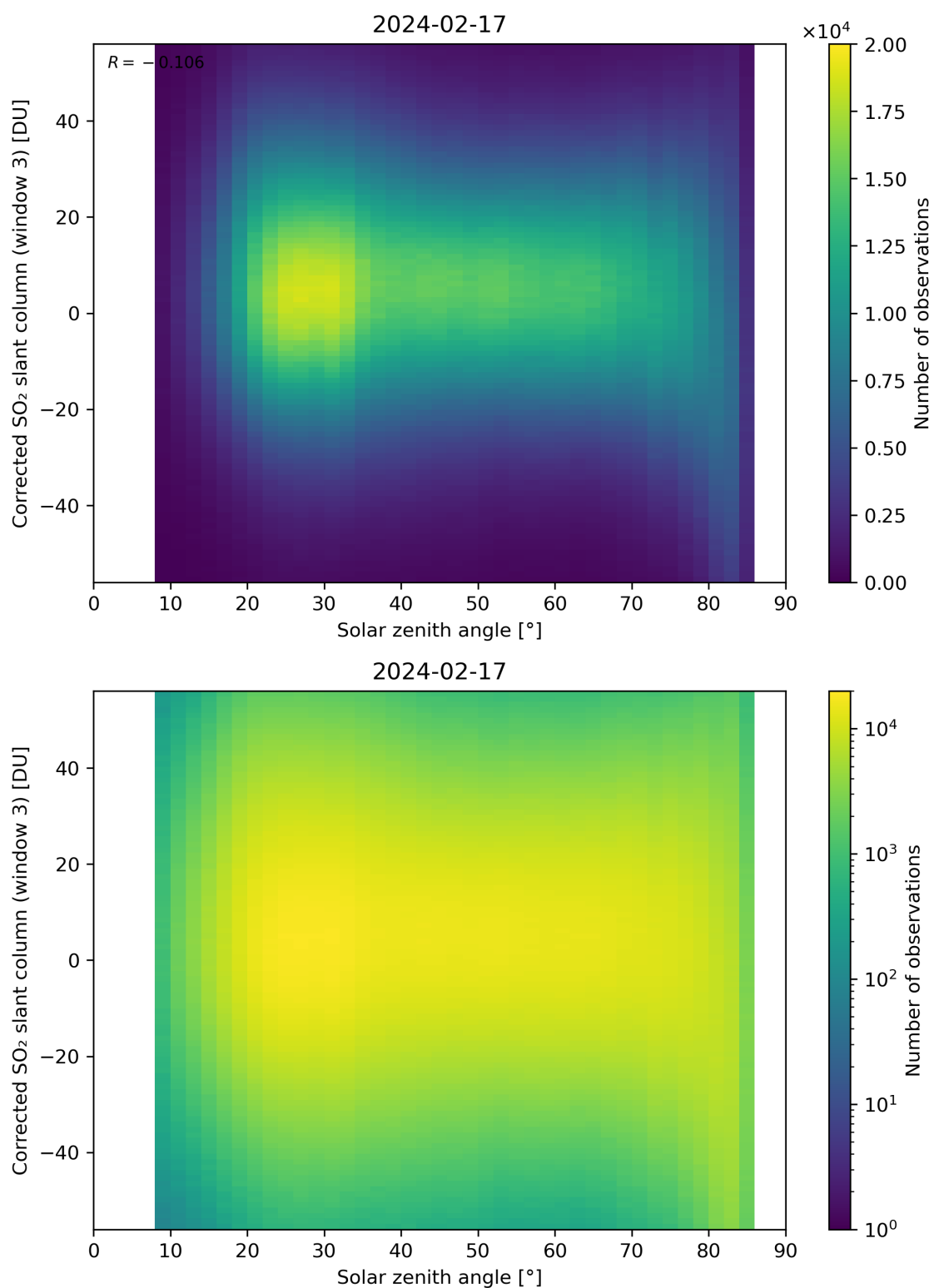
Figure 168: Scatter density plot of “Solar zenith angle” against “Corrected SO 2 slant column (window 3)” for 2024-02-17 to 2024-02-18.
