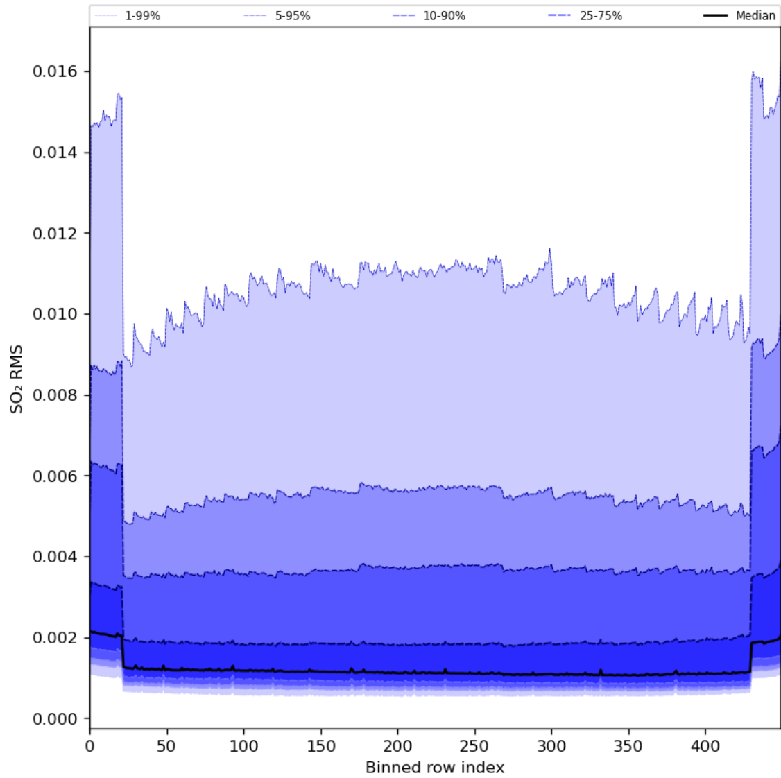
Figure 93: Along track statistics of “SO 2 RMS” for 2024-02-17 to 2024-02-18
