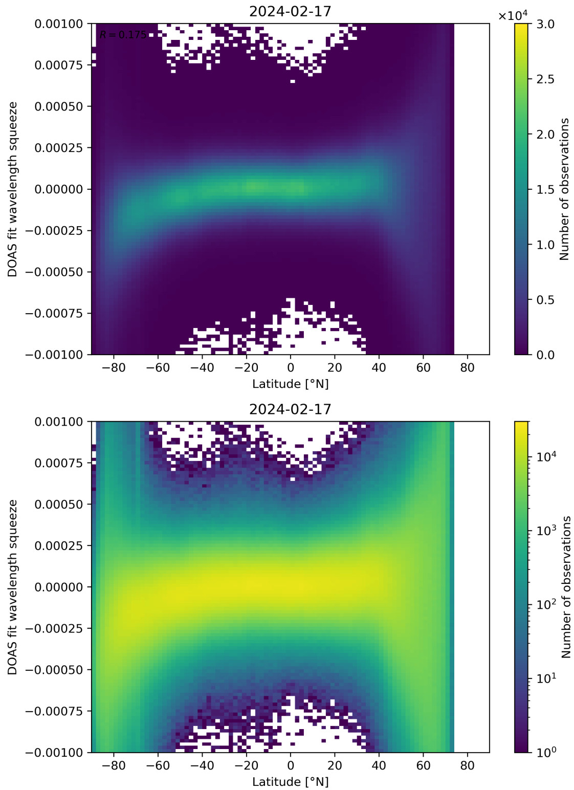
Figure 143: Scatter density plot of “Latitude” against “DOAS fit wavelength squeeze” for 2024-02-17 to 2024-02-18.
