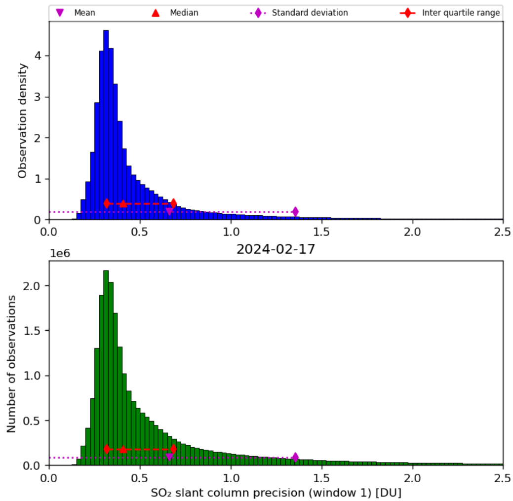
Figure 57: Histogram of “SO 2 slant column precision (window 1)” for 2024-02-17 to 2024-02-18
