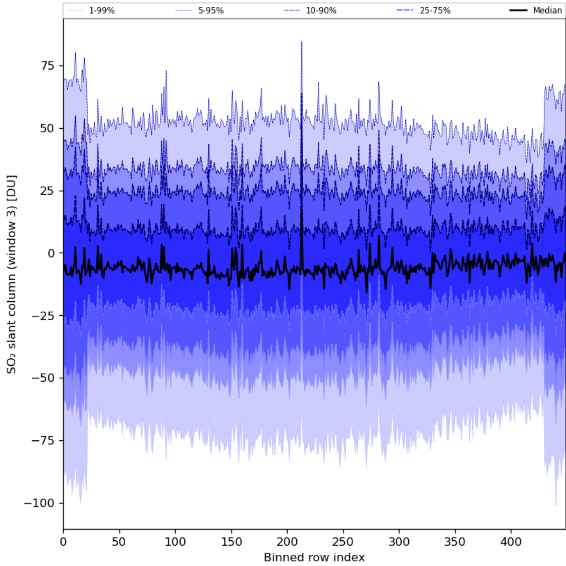
Figure 87: Along track statistics of “SO 2 slant column (window 3)” for 2024-02-17 to 2024-02-18
