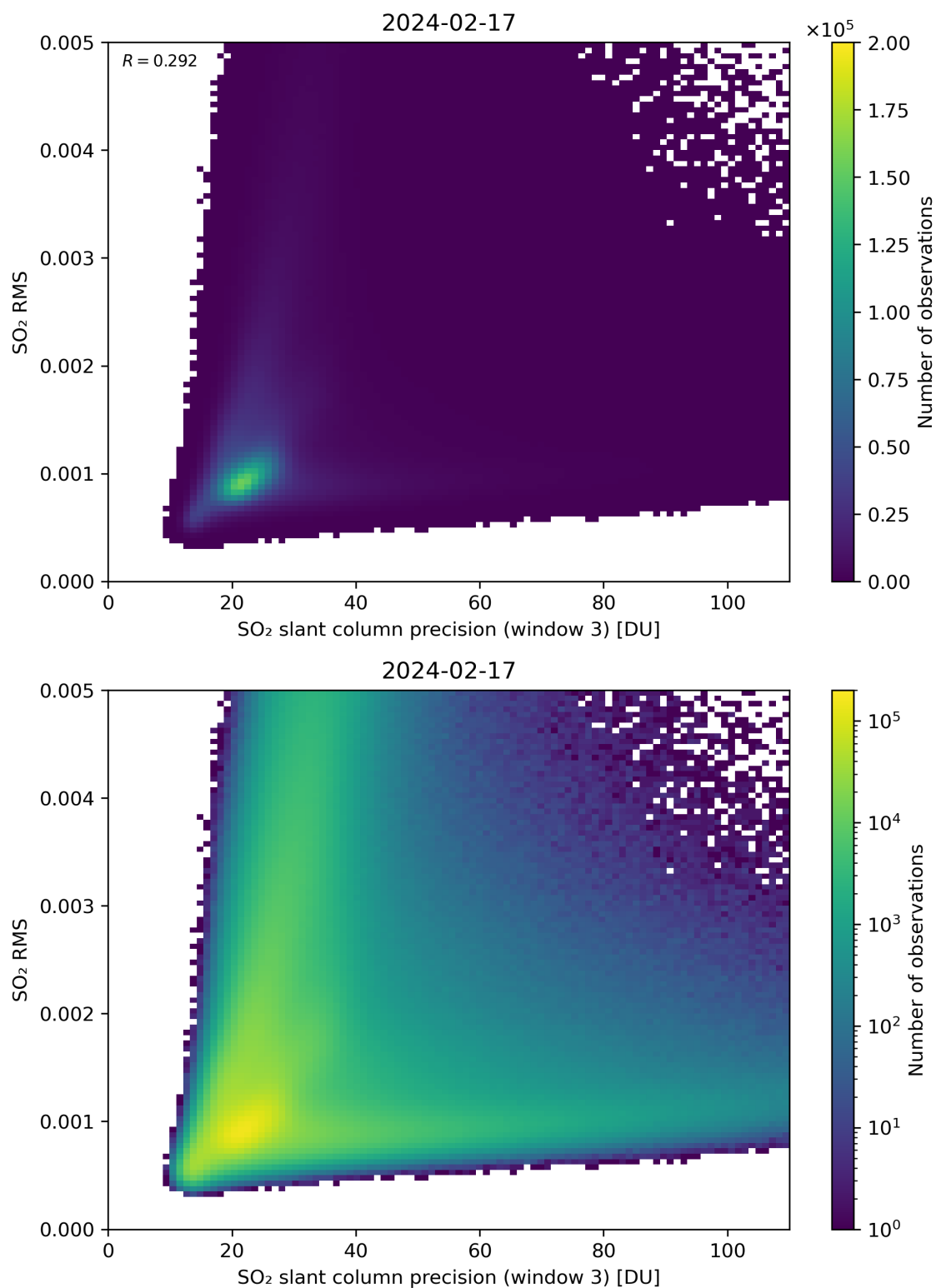
Figure 260: Scatter density plot of “SO 2 slant column precision (window 3)” against “SO 2 RMS” for 2024-02-17 to 2024-02-18.
