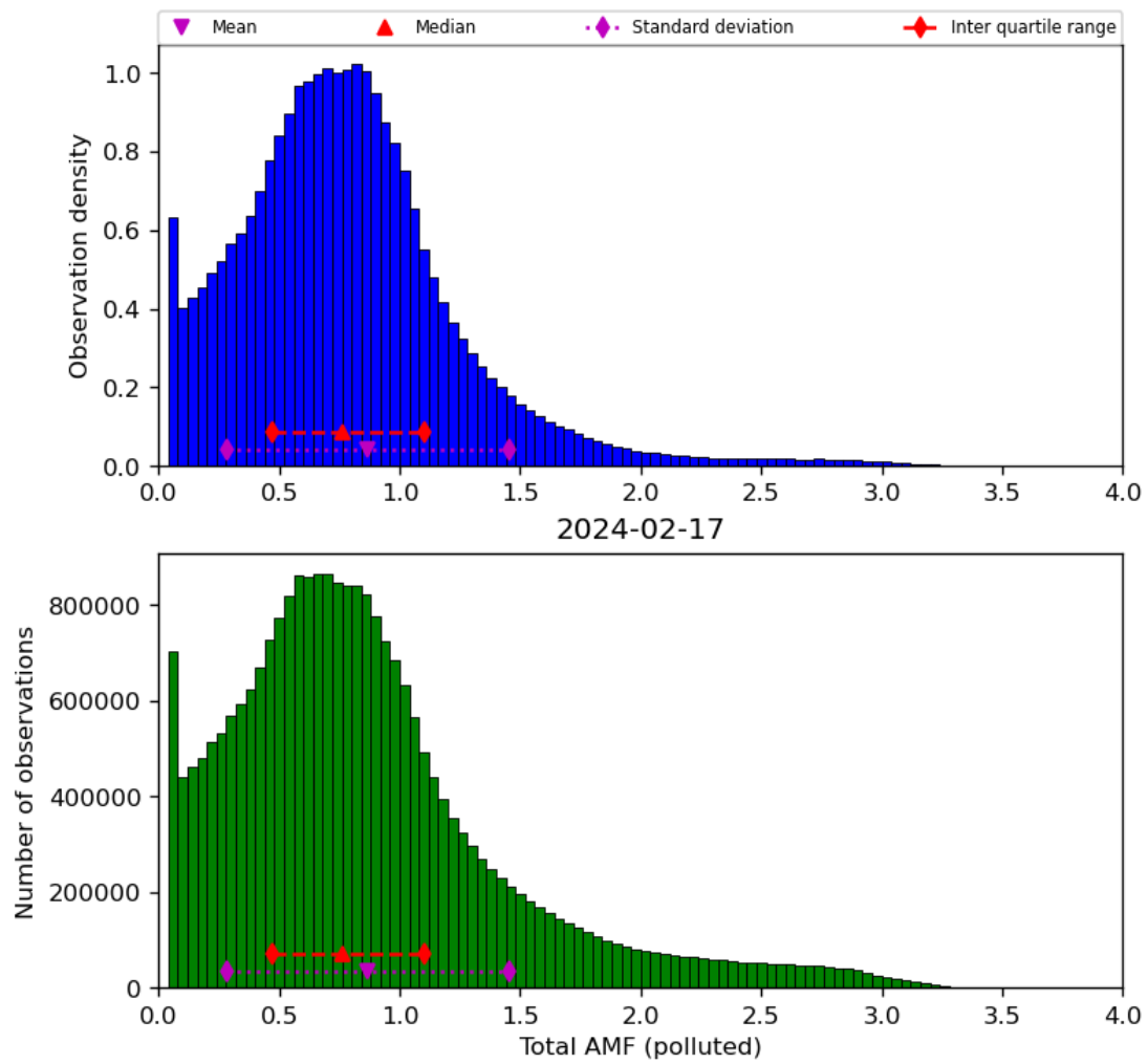
Figure 71: Histogram of “Total AMF (polluted)” for 2024-02-17 to 2024-02-18
