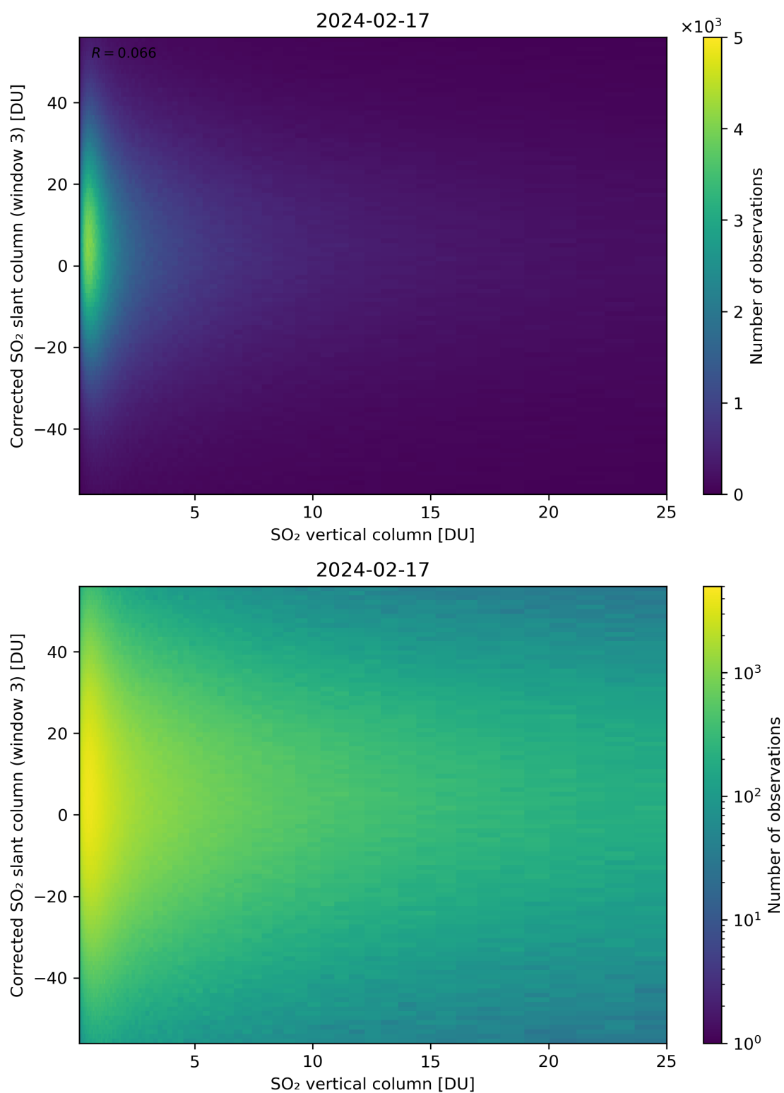
Figure 299: Scatter density plot of “SO 2 vertical column” against “Corrected SO 2 slant column (window 3)” for 2024-02-17 to 2024-02-18.
