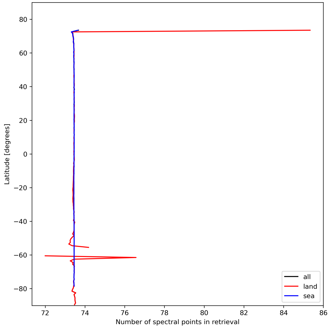
Figure 51: Zonal average of “Number of spectral points in retrieval” for 2024-02-17 to 2024-02-18.
