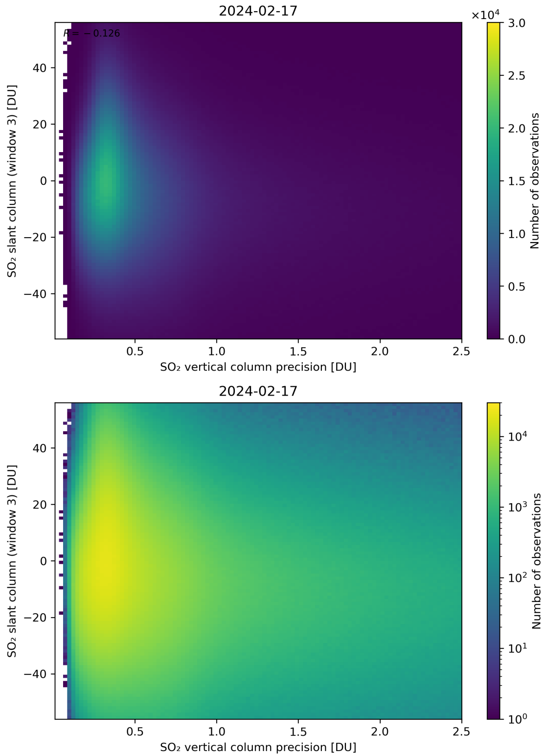
Figure 292: Scatter density plot of “SO 2 vertical column precision” against “SO 2 slant column (window 3)” for 2024-02-17 to 2024-02-18.
