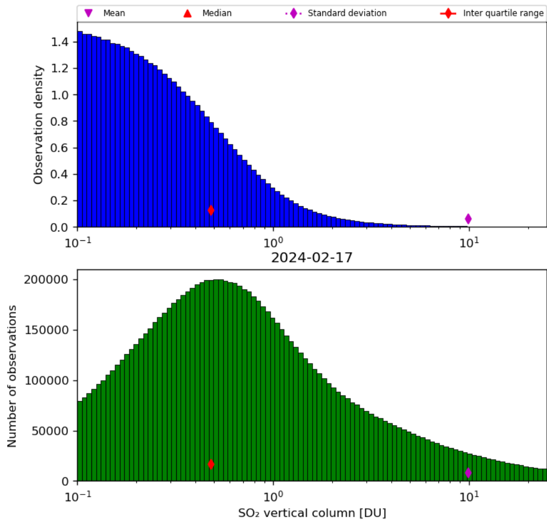
Figure 53: Histogram of “SO 2 vertical column” for 2024-02-17 to 2024-02-18
