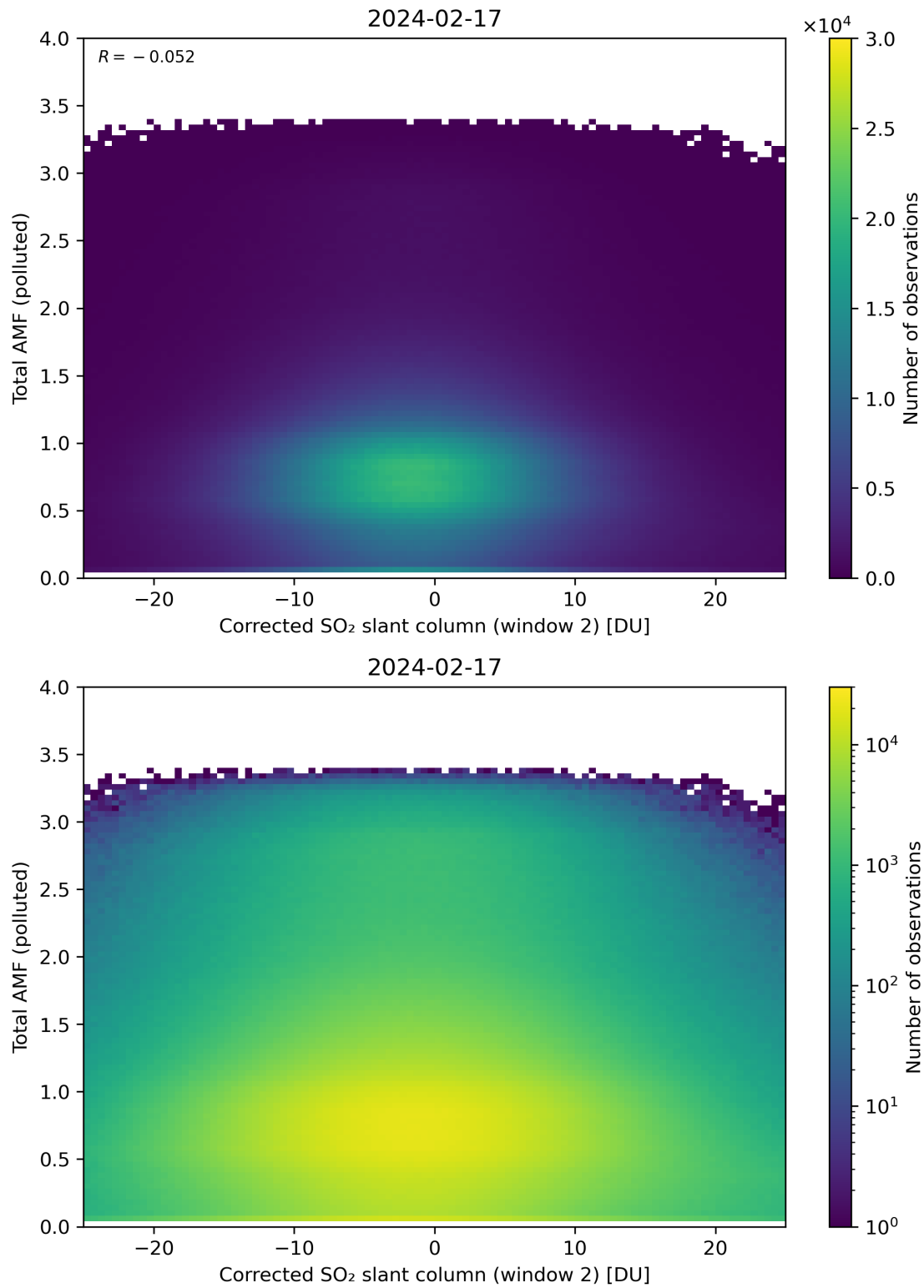
Figure 203: Scatter density plot of “Corrected SO 2 slant column (window 2)” against “Total AMF (polluted)” for 2024-02-17 to 2024-02-18.
