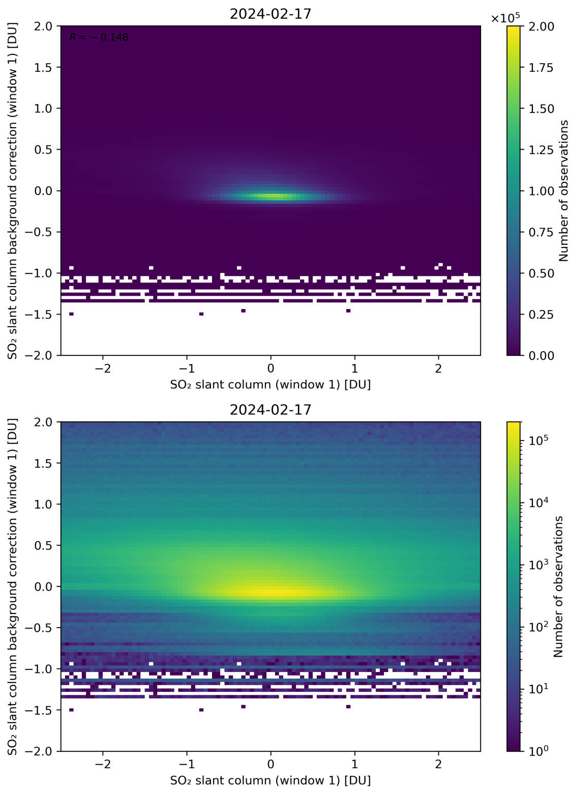
Figure 212: Scatter density plot of “SO 2 slant column (window 1)” against “SO 2 slant column background correction (window 1)” for 2024-02-17 to 2024-02-18.
