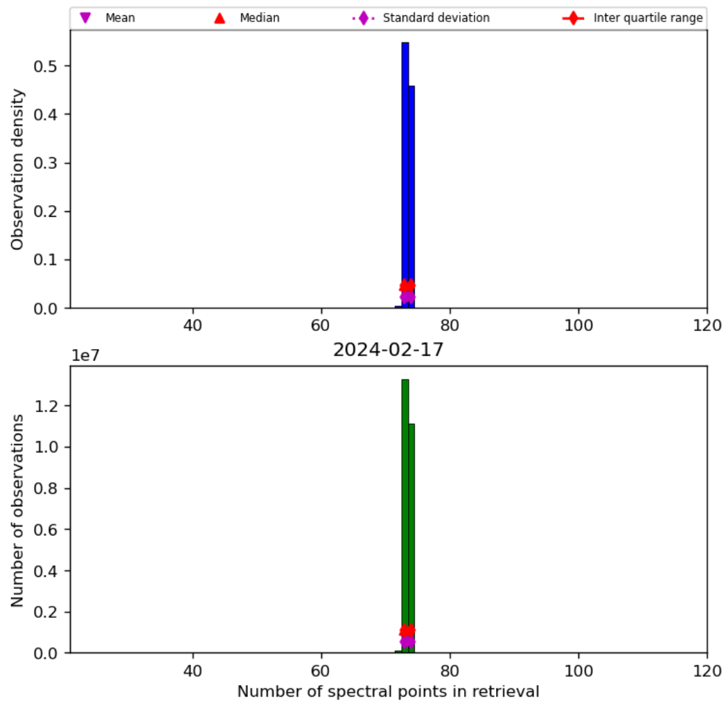
Figure 74: Histogram of “Number of spectral points in retrieval” for 2024-02-17 to 2024-02-18
