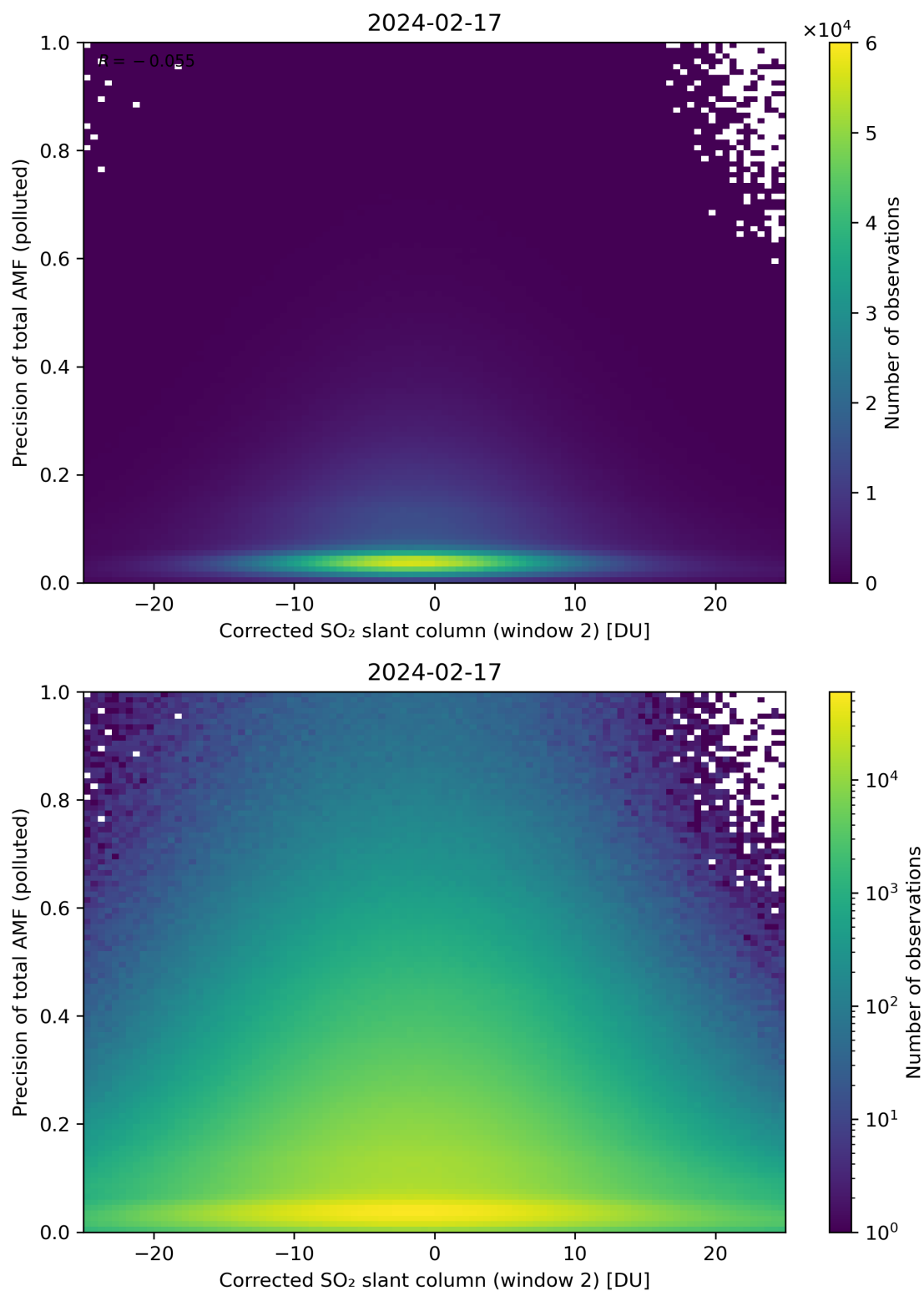
Figure 204: Scatter density plot of “Corrected SO 2 slant column (window 2)” against “Precision of total AMF (polluted)” for 2024-02-17 to 2024-02-18.
