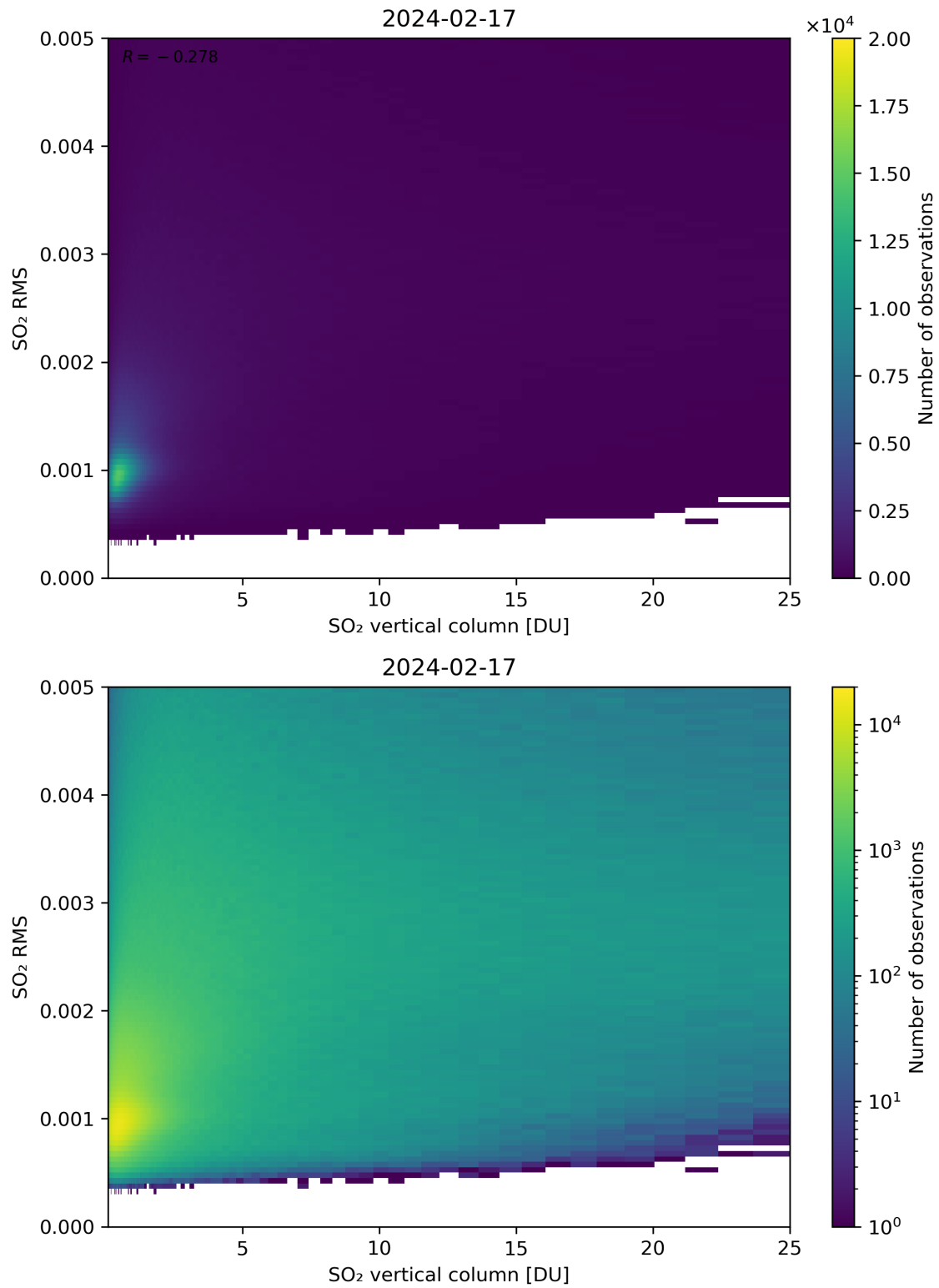
Figure 278: Scatter density plot of “SO 2 vertical column” against “SO 2 RMS” for 2024-02-17 to 2024-02-18.
