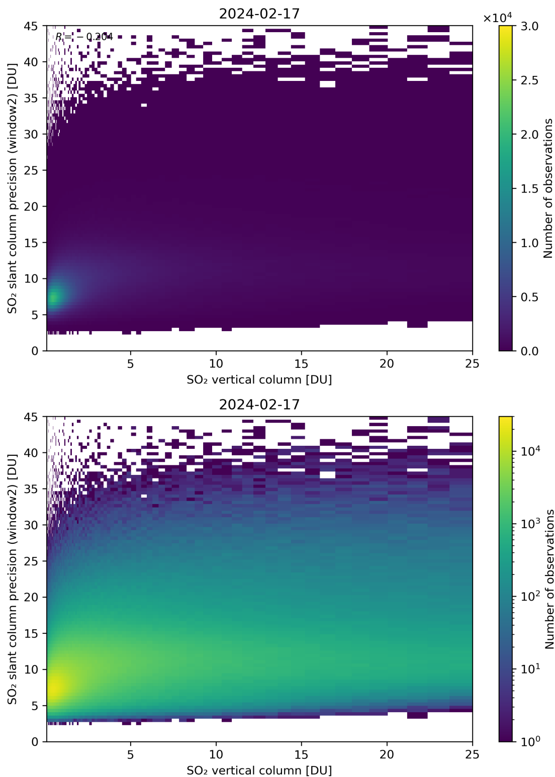
Figure 302: Scatter density plot of “SO 2 vertical column” against “SO 2 slant column precision (window2)” for 2024-02-17 to 2024-02-18.
