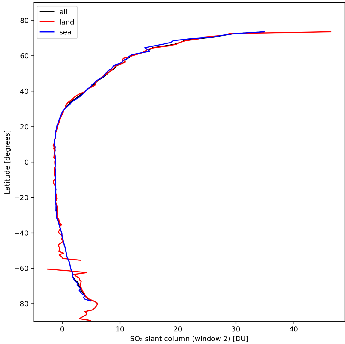
Figure 37: Zonal average of “SO 2 slant column (window 2)” for 2024-02-17 to 2024-02-18.
