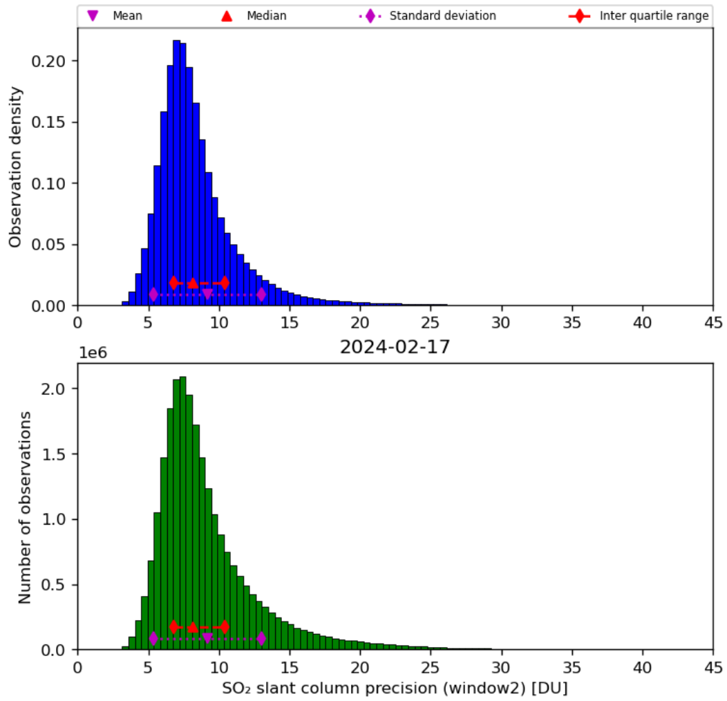
Figure 61: Histogram of “SO 2 slant column precision (window2)” for 2024-02-17 to 2024-02-18
