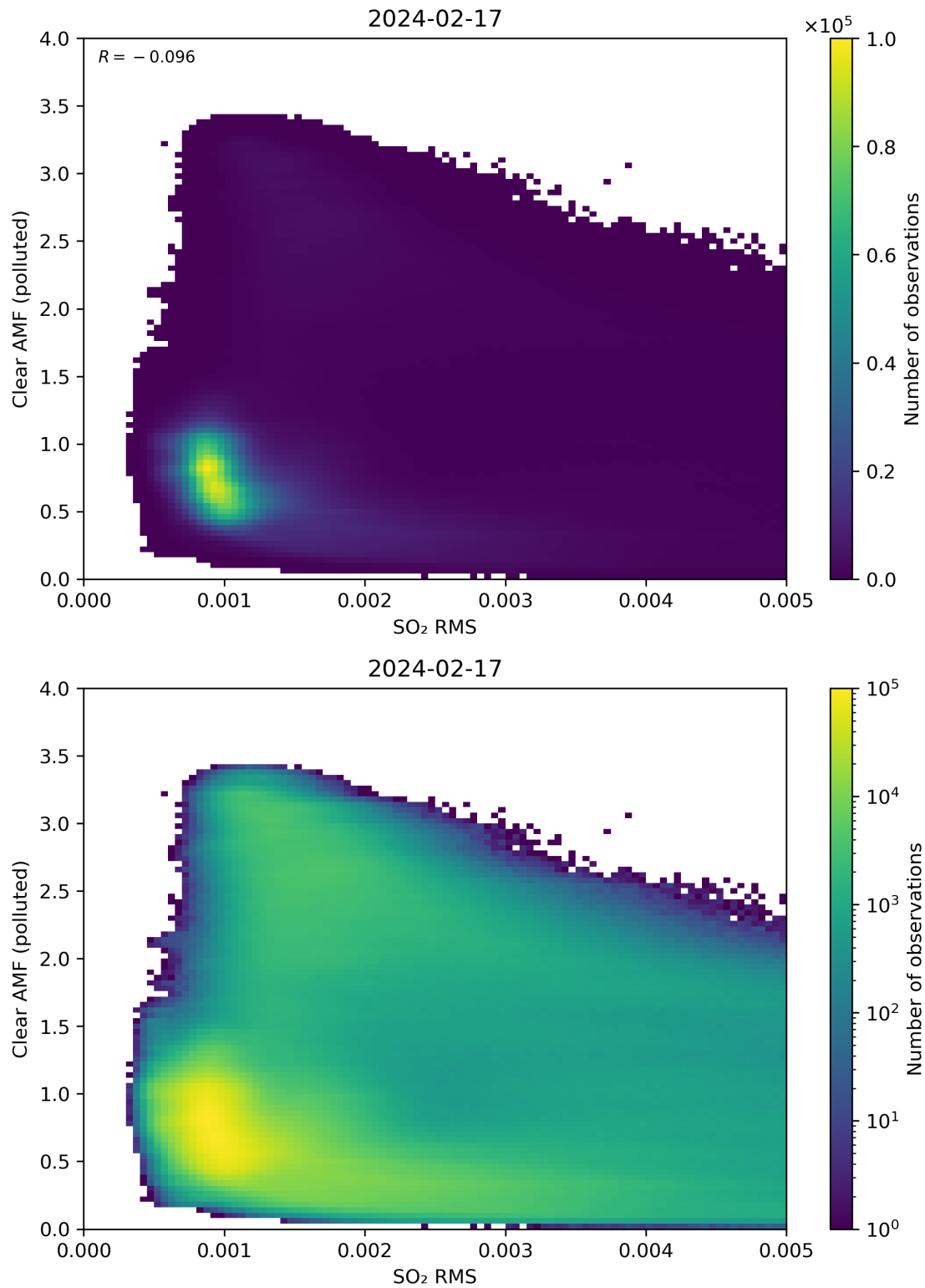
Figure 136: Scatter density plot of “SO 2 RMS” against “Clear AMF (polluted)” for 2024-02-17 to 2024-02-18.
