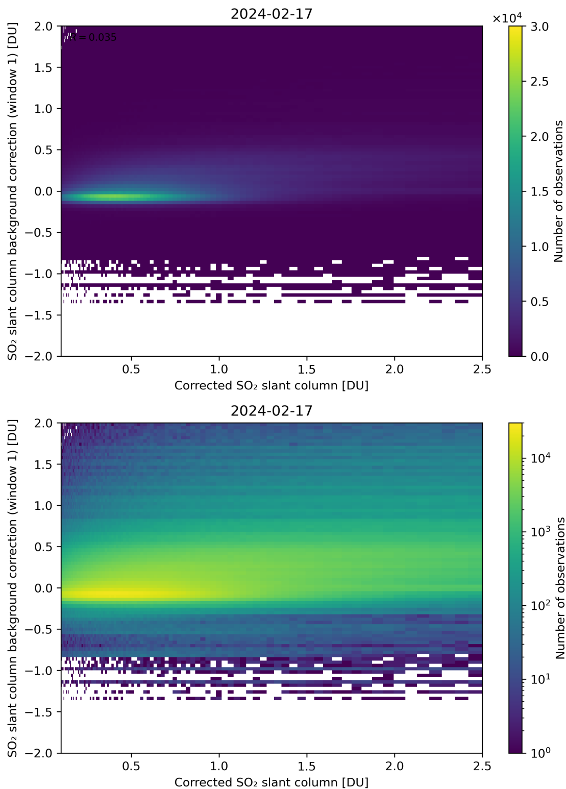
Figure 178: Scatter density plot of “Corrected SO 2 slant column” against “SO 2 slant column background correction (window 1)” for 2024-02-17 to 2024-02-18.
