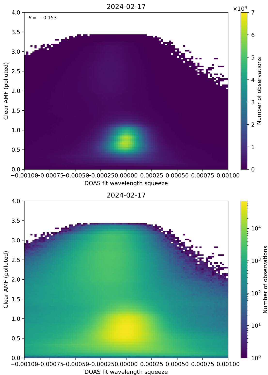
Figure 133: Scatter density plot of “DOAS fit wavelength squeeze” against “Clear AMF (polluted)” for 2024-02-17 to 2024-02-18.
