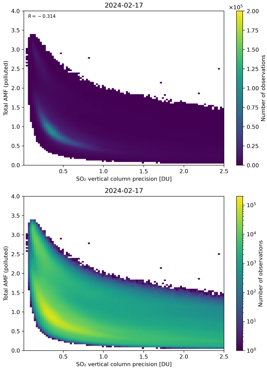
Figure 294: Scatter density plot of “SO 2 vertical column precision” against “Total AMF (polluted)” for 2024-02-17 to 2024-02-18.
