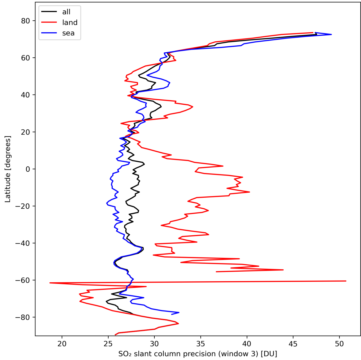
Figure 42: Zonal average of “SO 2 slant column precision (window 3)” for 2024-02-17 to 2024-02-18.
