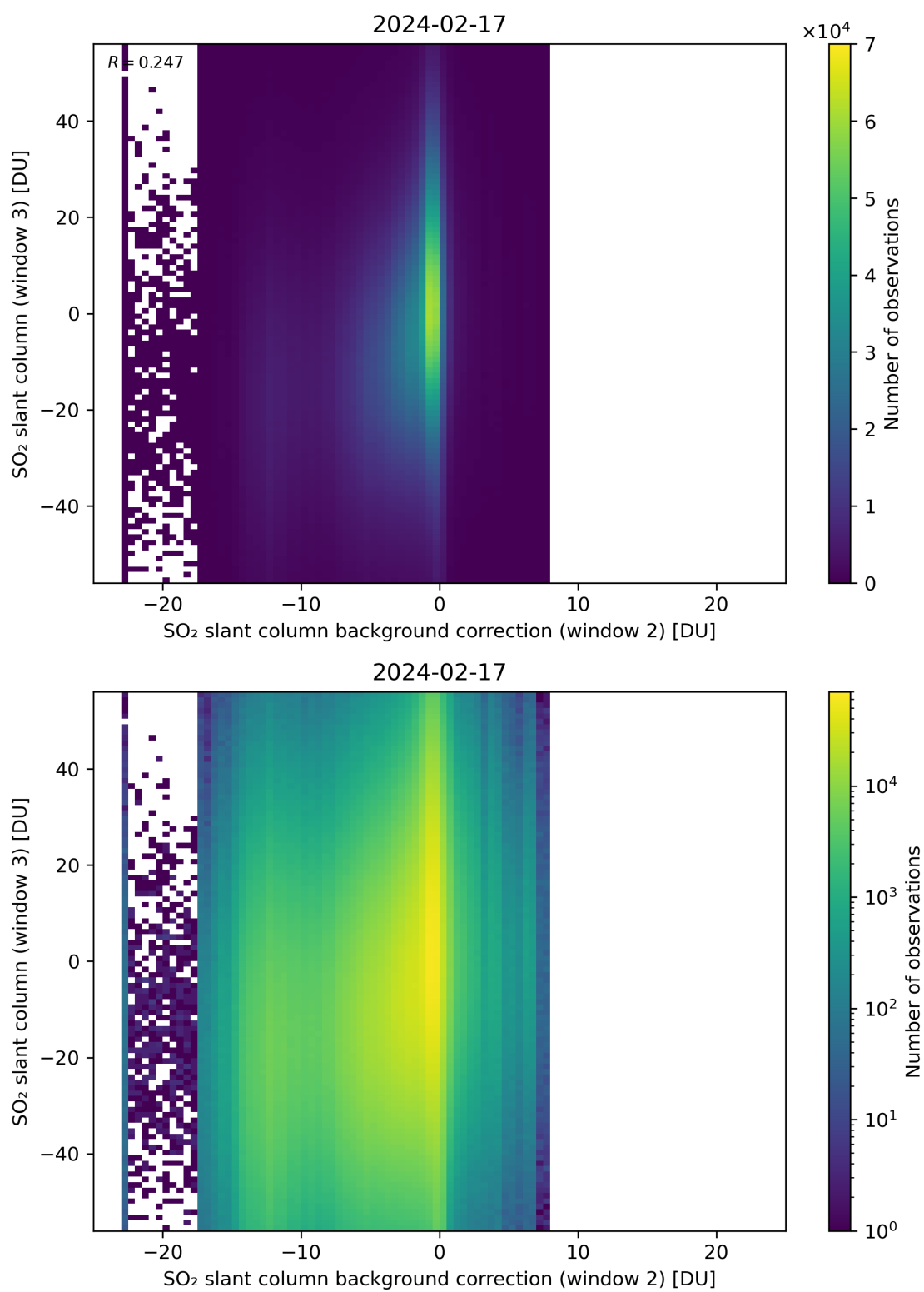
Figure 117: Scatter density plot of “SO 2 slant column background correction (window 2)” against “SO 2 slant column (window 3)” for 2024-02-17 to 2024-02-18.
