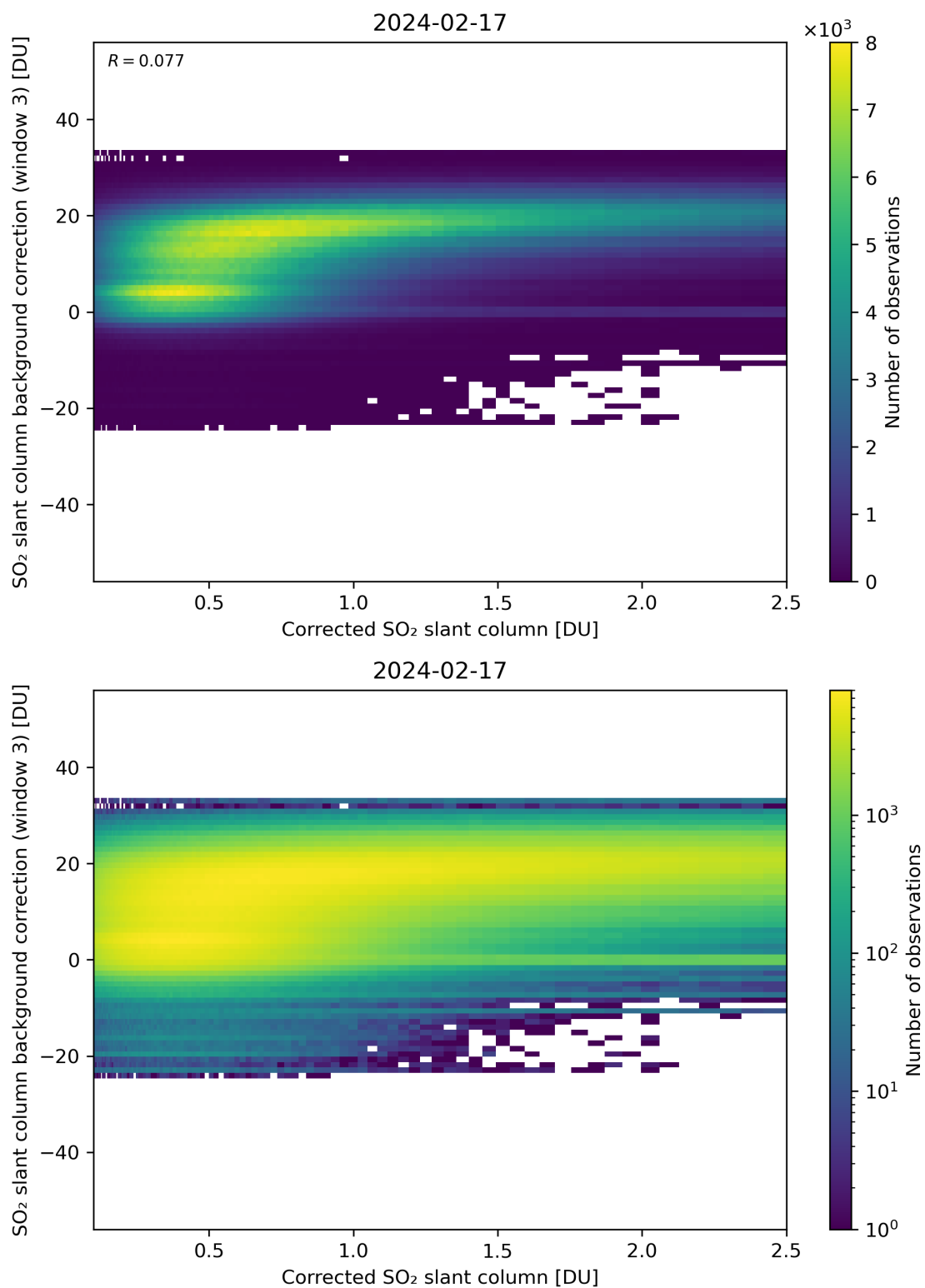
Figure 180: Scatter density plot of “Corrected SO 2 slant column” against “SO 2 slant column background correction (window 3)” for 2024-02-17 to 2024-02-18.
