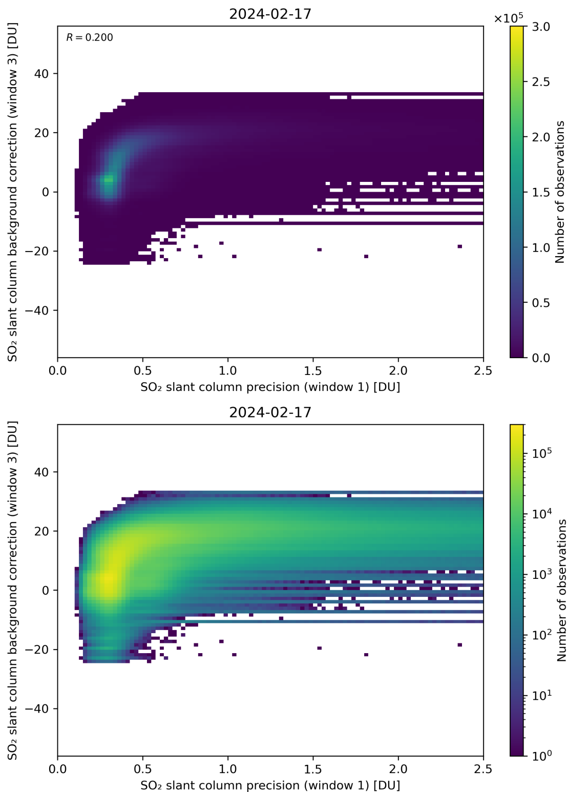
Figure 220: Scatter density plot of “SO 2 slant column precision (window 1)” against “SO 2 slant column background correction (window 3)” for 2024-02-17 to 2024-02-18.
