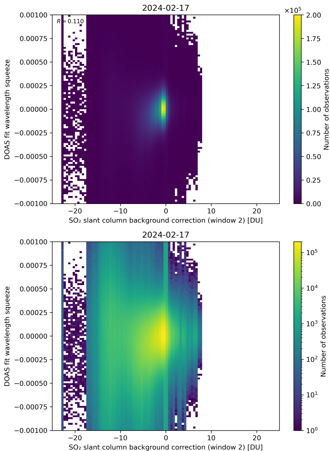
Figure 113: Scatter density plot of “SO 2 slant column background correction (window 2)” against “DOAS fit wavelength squeeze” for 2024-02-17 to 2024-02-18.
