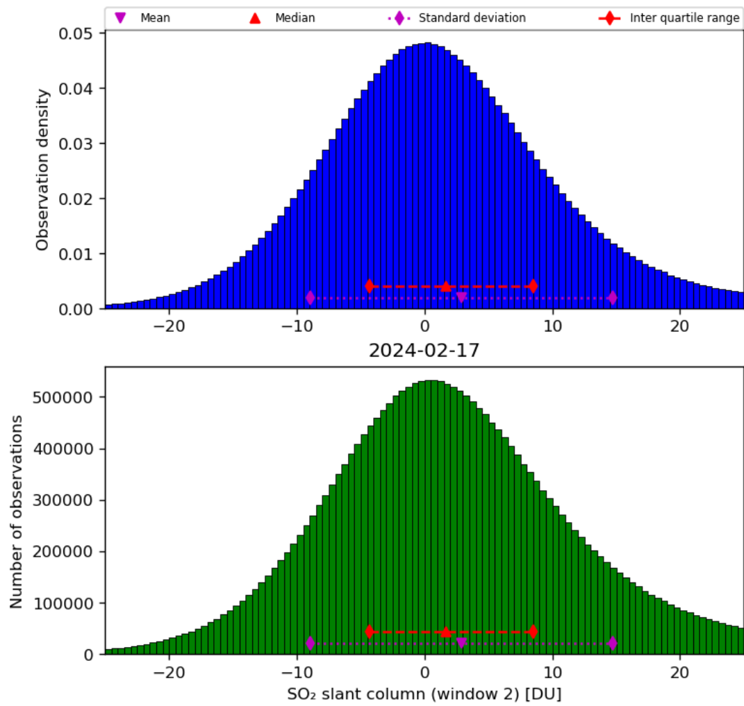
Figure 60: Histogram of “SO 2 slant column (window 2)” for 2024-02-17 to 2024-02-18
