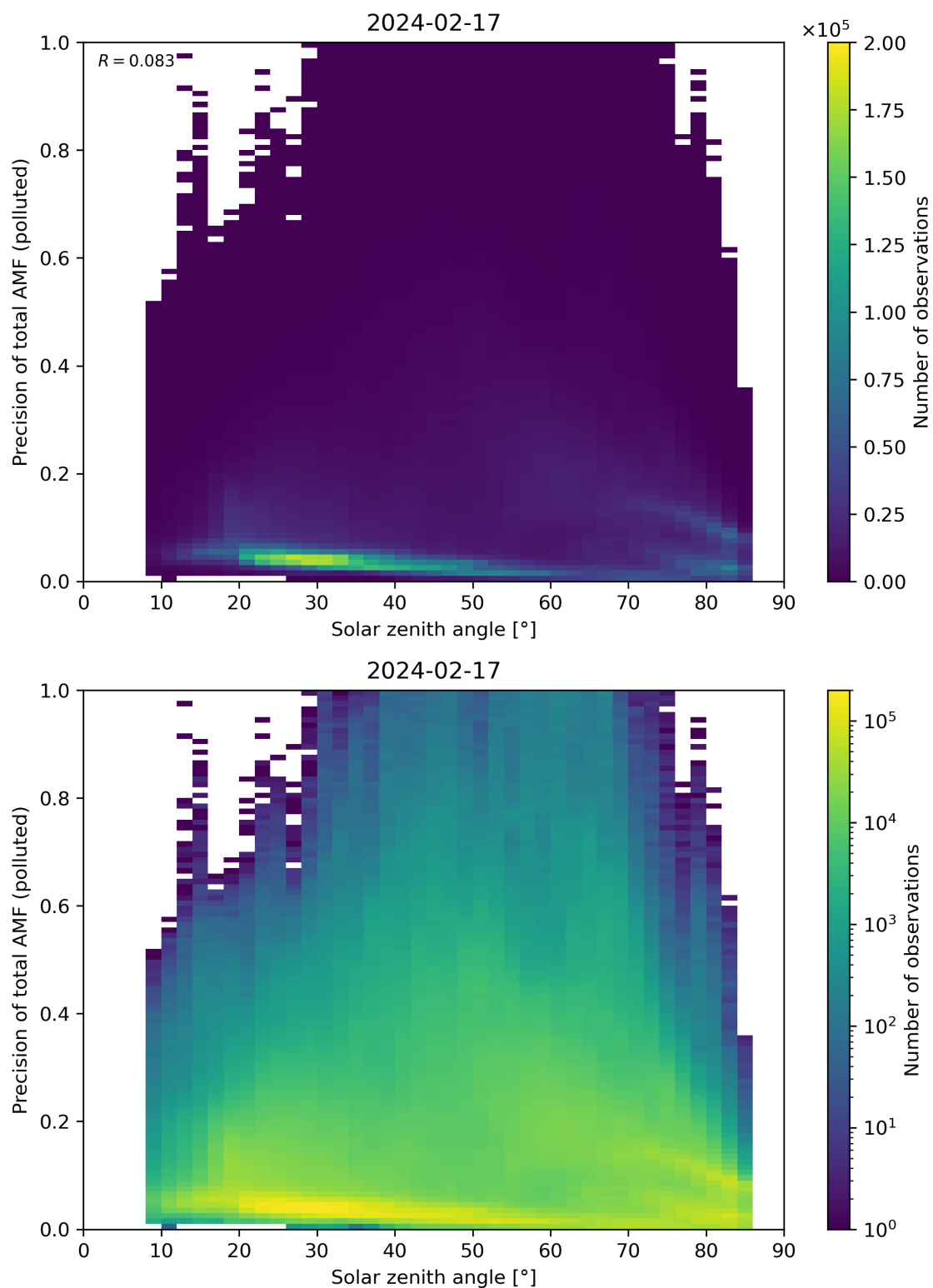
Figure 175: Scatter density plot of “Solar zenith angle” against “Precision of total AMF (polluted)” for 2024-02-17 to 2024-02-18.
