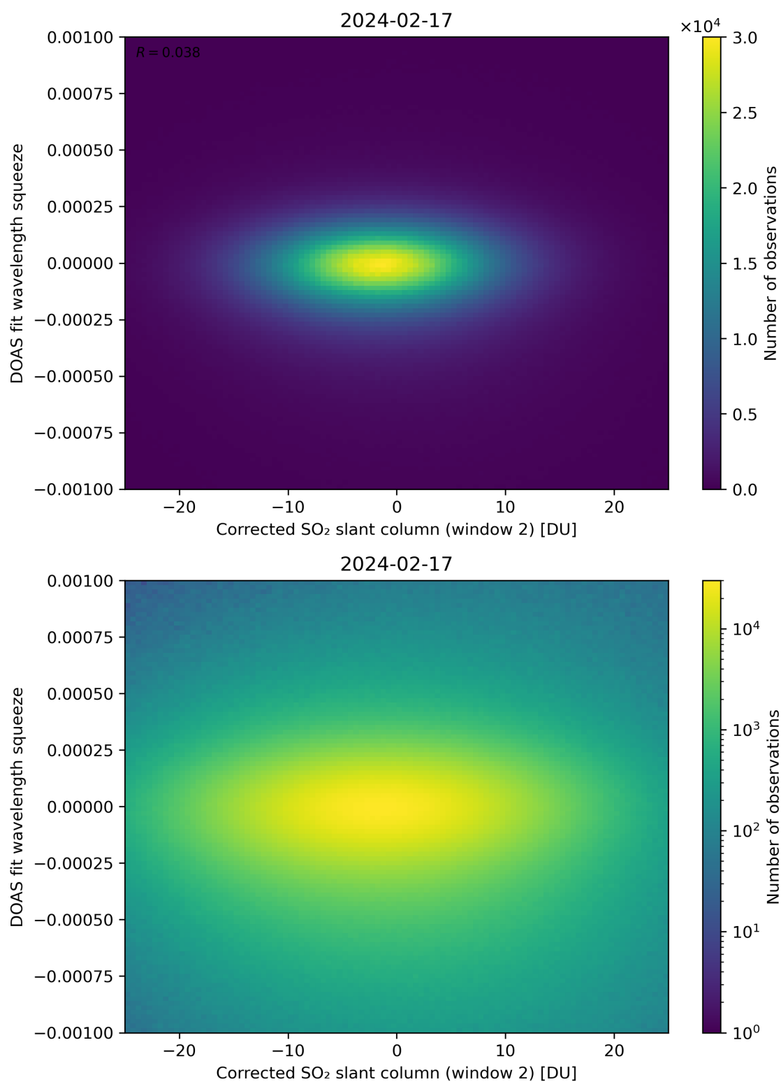
Figure 197: Scatter density plot of “Corrected SO 2 slant column (window 2)” against “DOAS fit wavelength squeeze” for 2024-02-17 to 2024-02-18.
