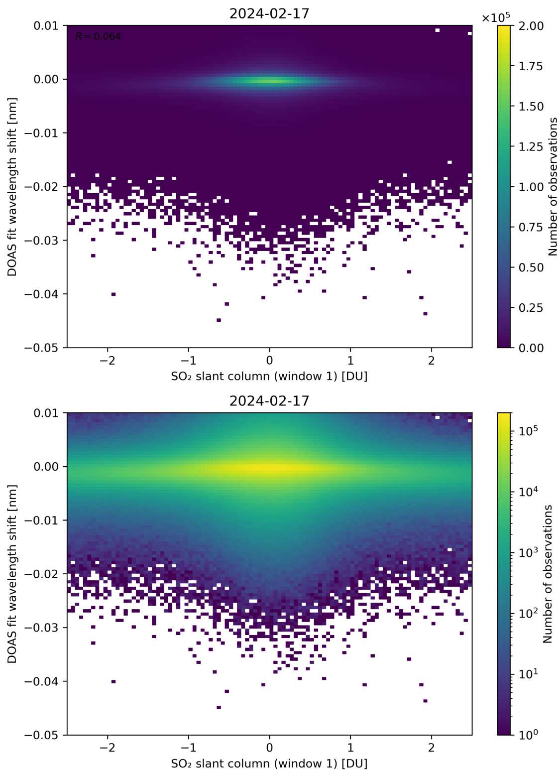
Figure 215: Scatter density plot of “SO 2 slant column (window 1)” against “DOAS fit wavelength shift” for 2024-02-17 to 2024-02-18.
