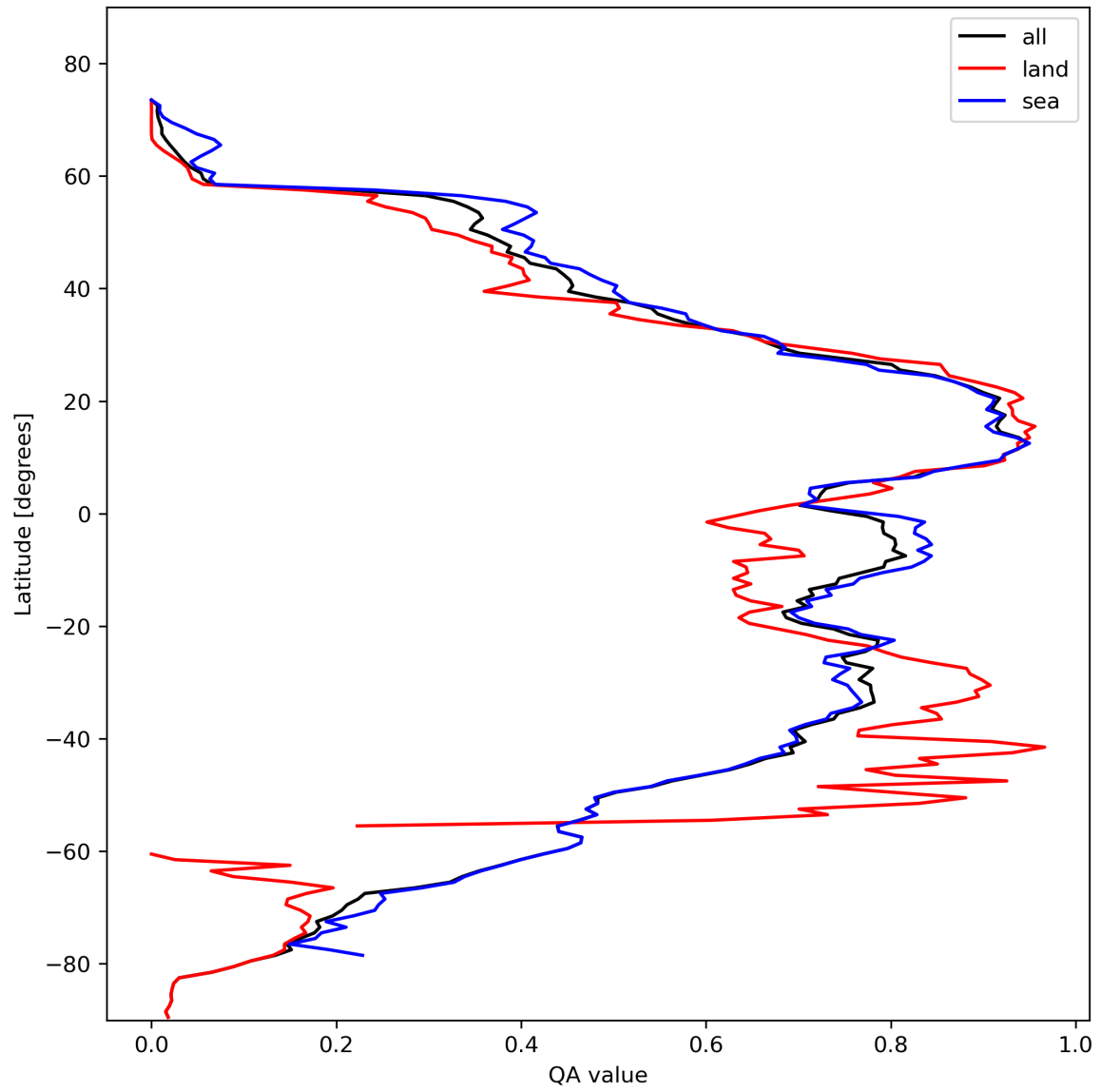
Figure 29: Zonal average of “QA value” for 2024-02-17 to 2024-02-18.
