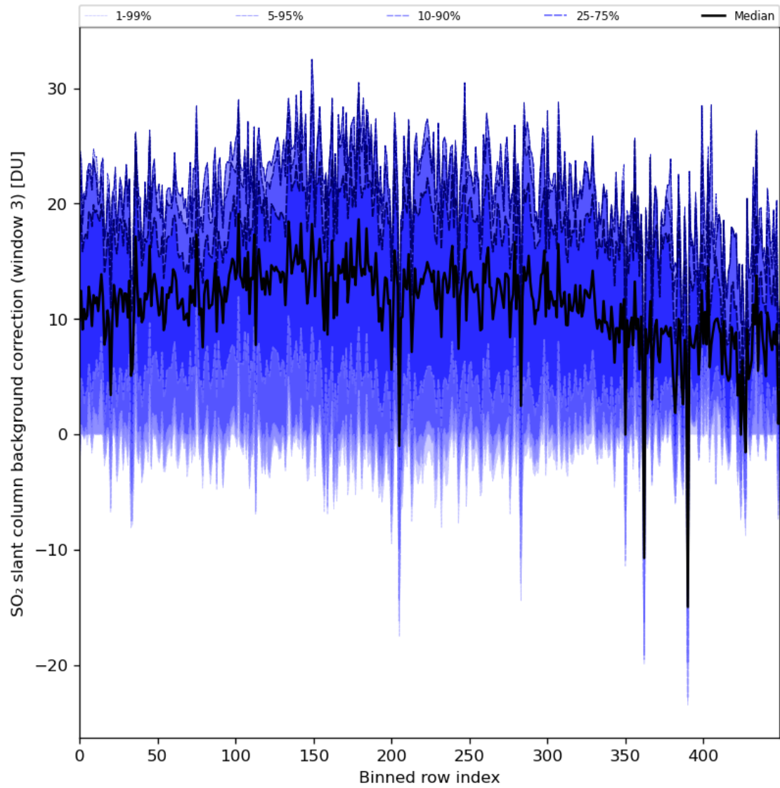
Figure 90: Along track statistics of “SO 2 slant column background correction (window 3)” for 2024-02-17 to 2024-02-18
