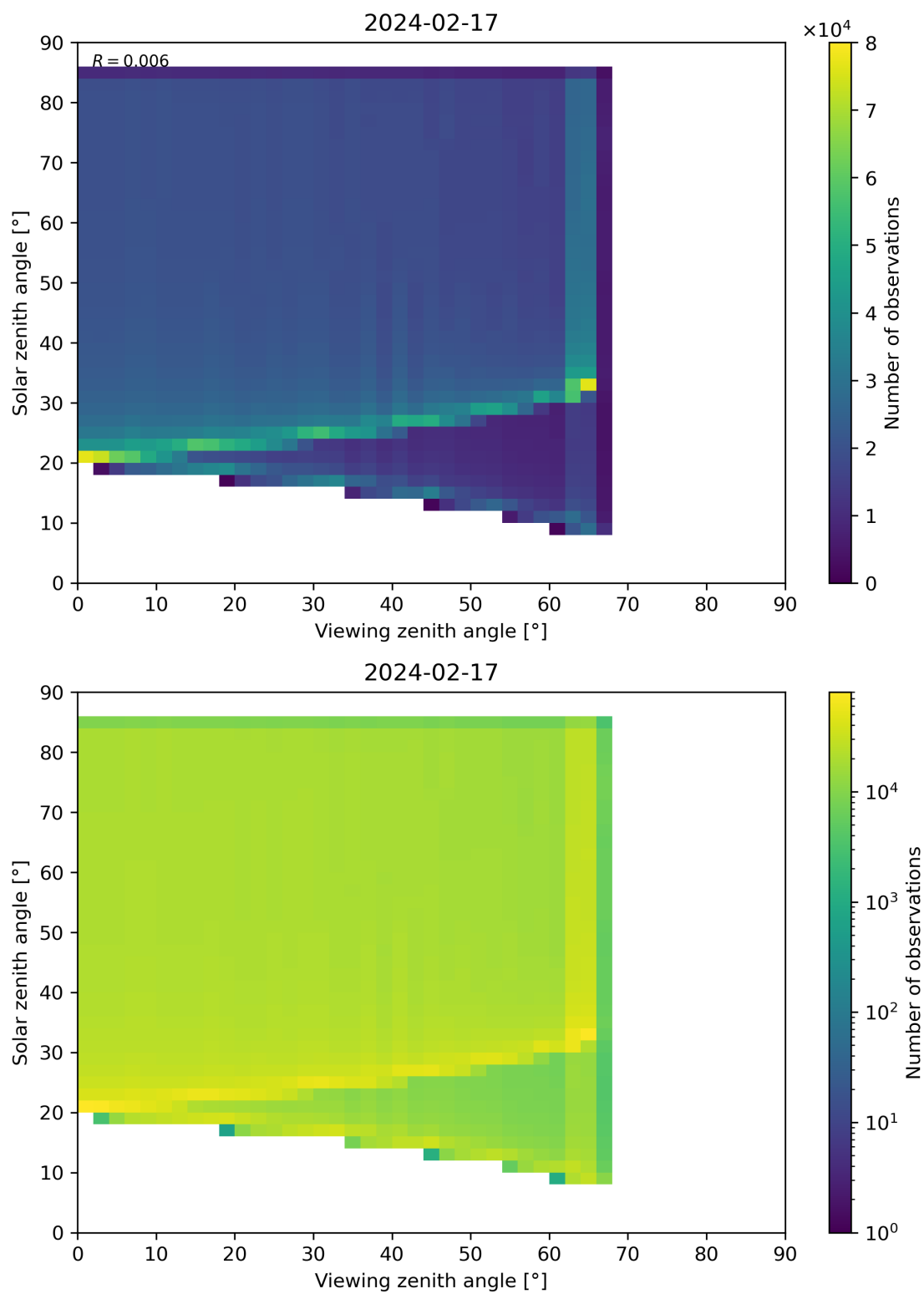
Figure 315: Scatter density plot of “Viewing zenith angle” against “Solar zenith angle” for 2024-02-17 to 2024-02-18.
