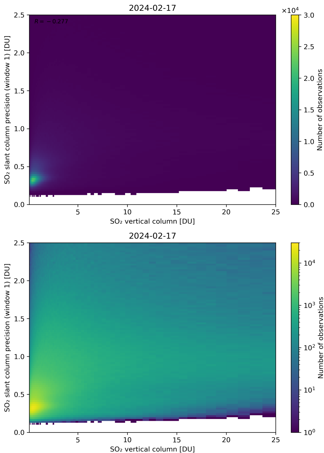
Figure 301: Scatter density plot of “SO 2 vertical column” against “SO 2 slant column precision (window 1)” for 2024-02-17 to 2024-02-18.
