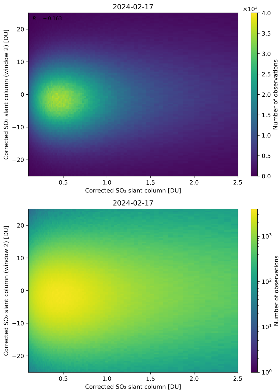
Figure 185: Scatter density plot of “Corrected SO 2 slant column” against “Corrected SO 2 slant column (window 2)” for 2024-02-17 to 2024-02-18.
