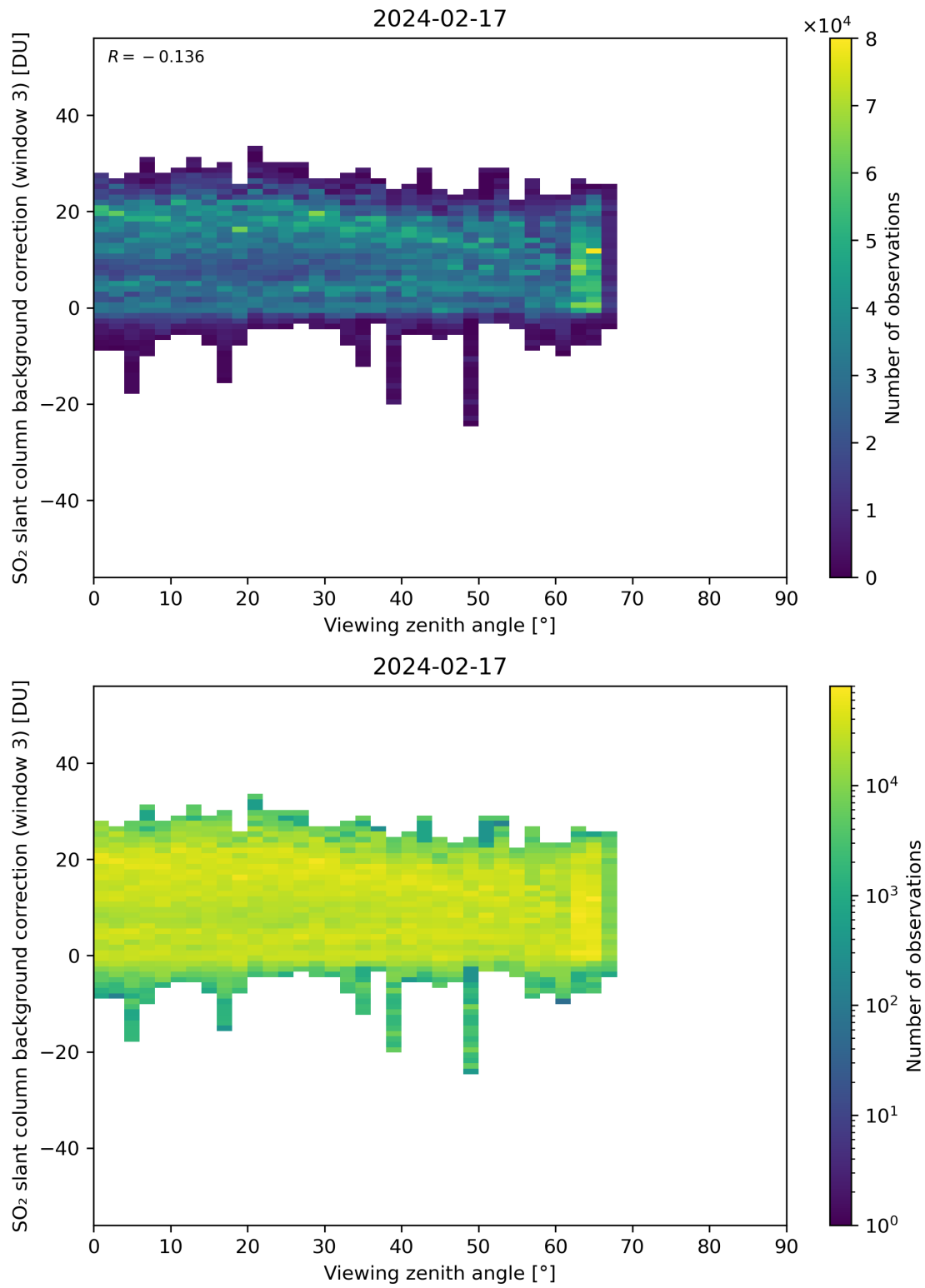
Figure 310: Scatter density plot of “Viewing zenith angle” against “SO 2 slant column background correction (window 3)” for 2024-02-17 to 2024-02-18.
