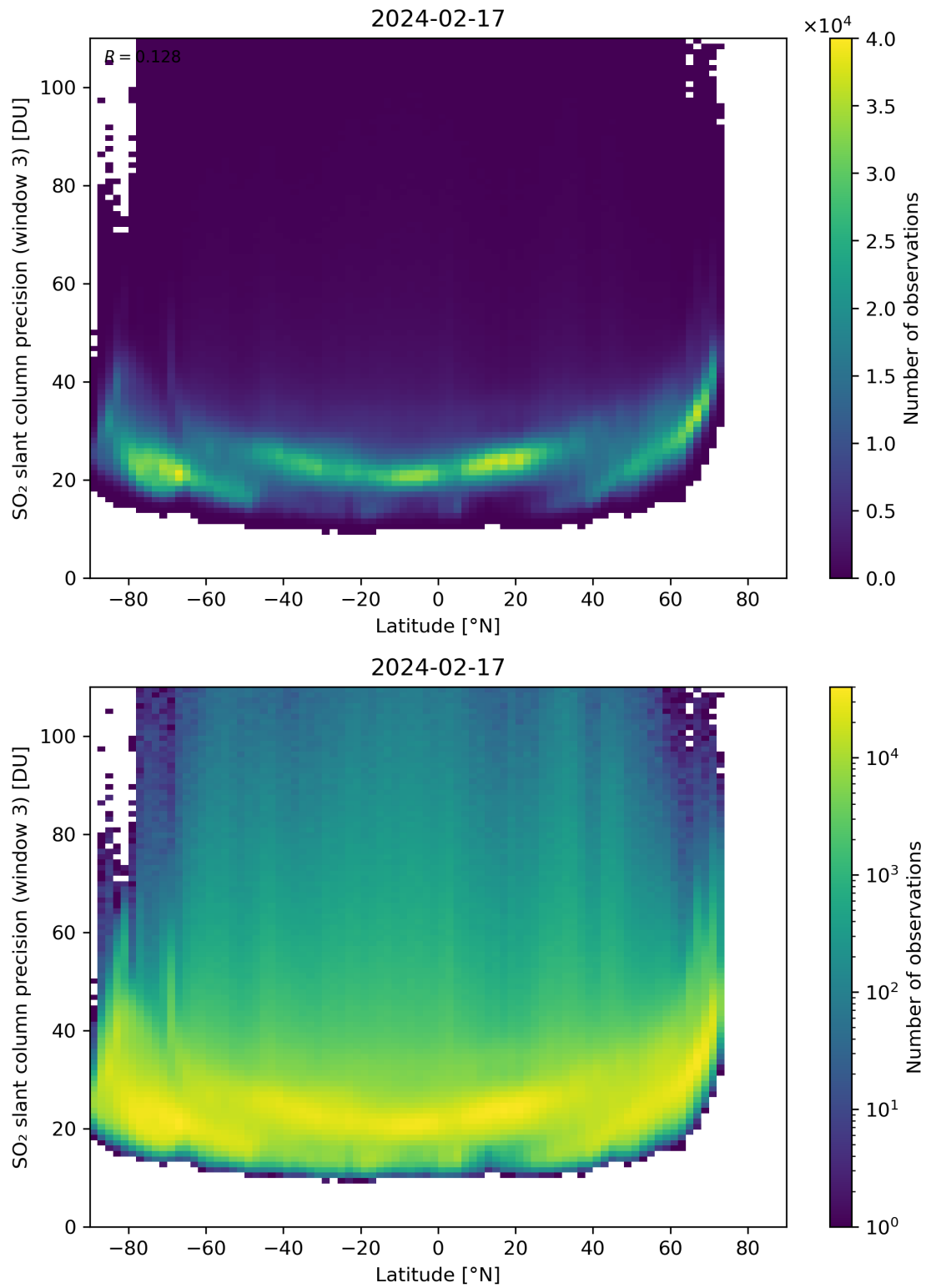
Figure 153: Scatter density plot of “Latitude” against “SO 2 slant column precision (window 3)” for 2024-02-17 to 2024-02-18.
