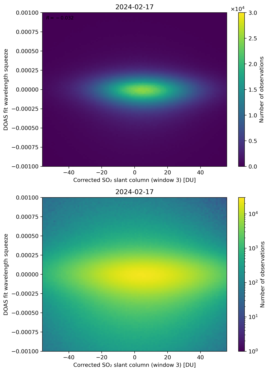
Figure 207: Scatter density plot of “Corrected SO 2 slant column (window 3)” against “DOAS fit wavelength squeeze” for 2024-02-17 to 2024-02-18.
