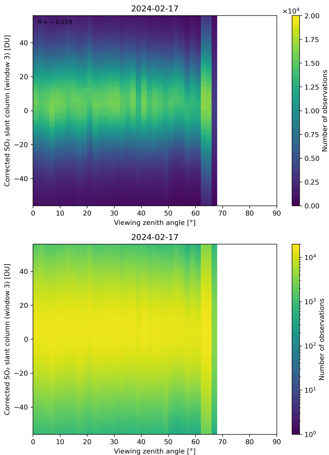
Figure 319: Scatter density plot of “Viewing zenith angle” against “Corrected SO 2 slant column (window 3)” for 2024-02-17 to 2024-02-18.
