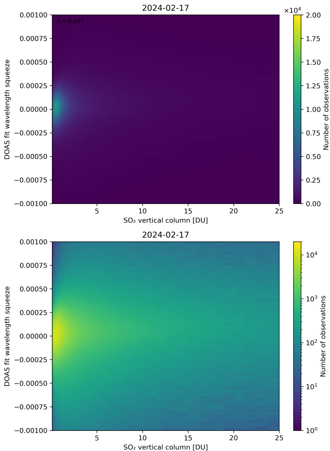
Figure 277: Scatter density plot of “SO 2 vertical column” against “DOAS fit wavelength squeeze” for 2024-02-17 to 2024-02-18.
