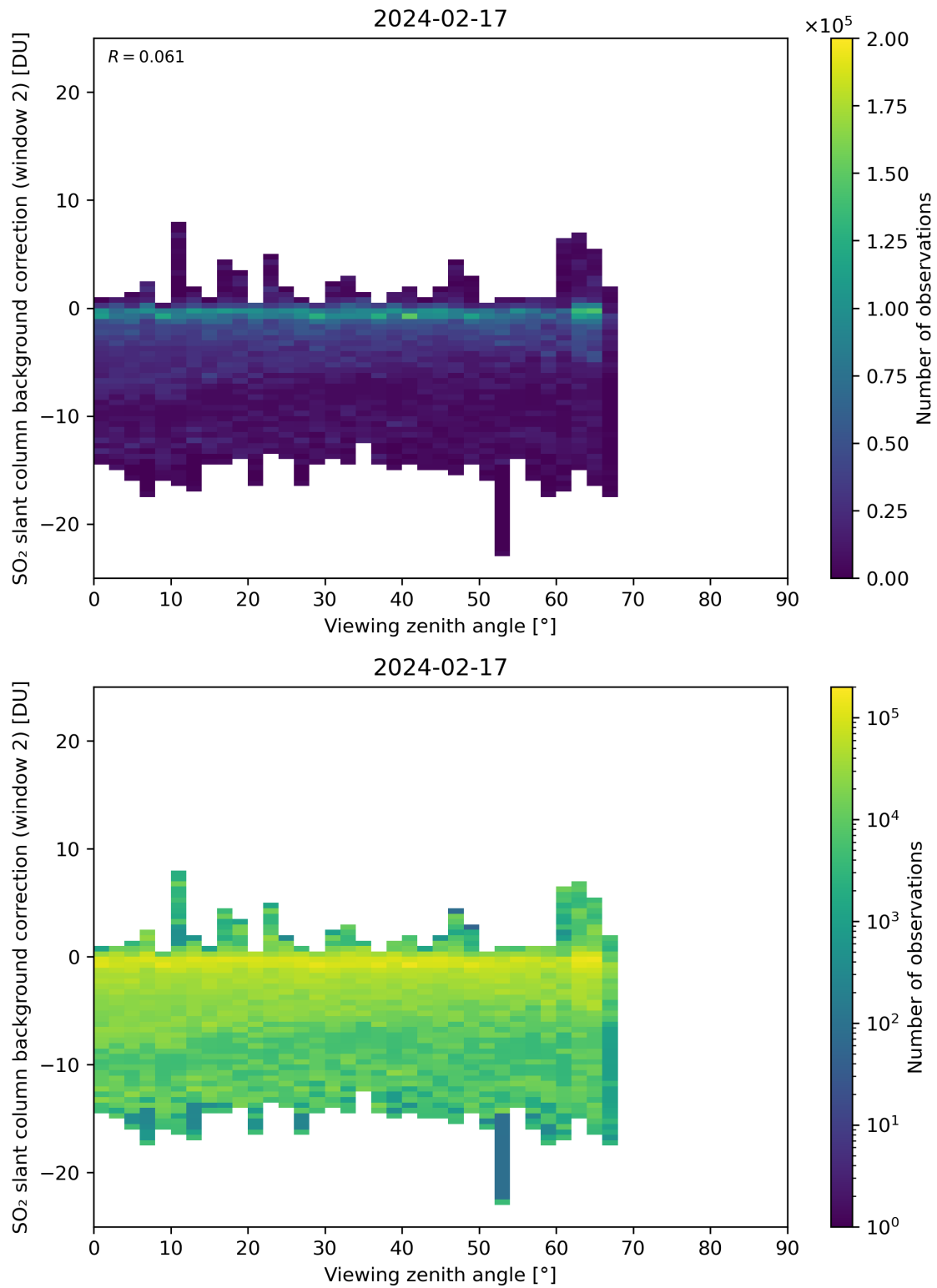
Figure 309: Scatter density plot of “Viewing zenith angle” against “SO 2 slant column background correction (window 2)” for 2024-02-17 to 2024-02-18.
