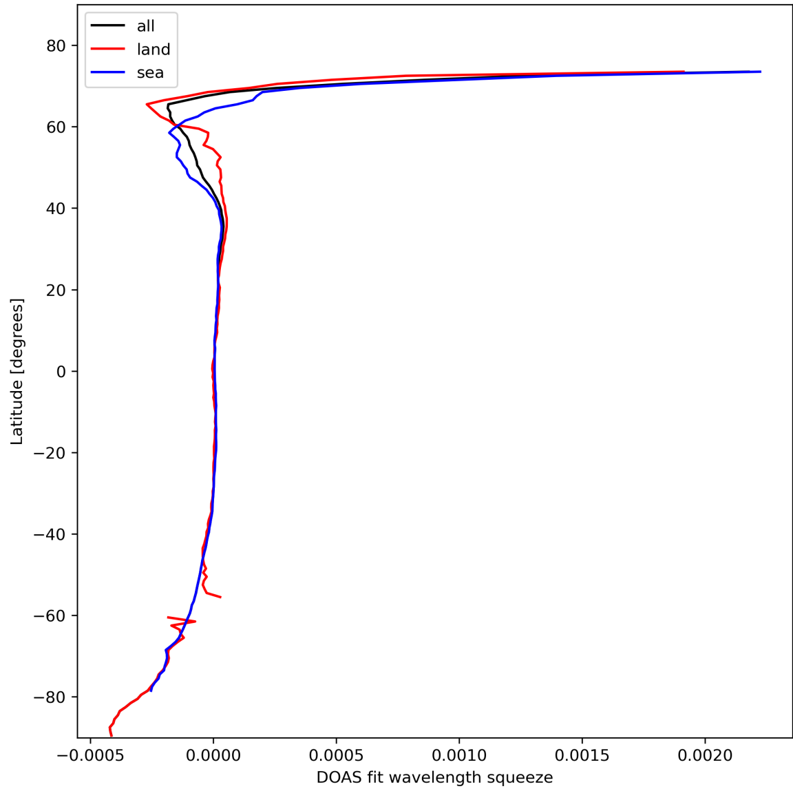
Figure 46: Zonal average of “DOAS fit wavelength squeeze” for 2024-02-17 to 2024-02-18.
