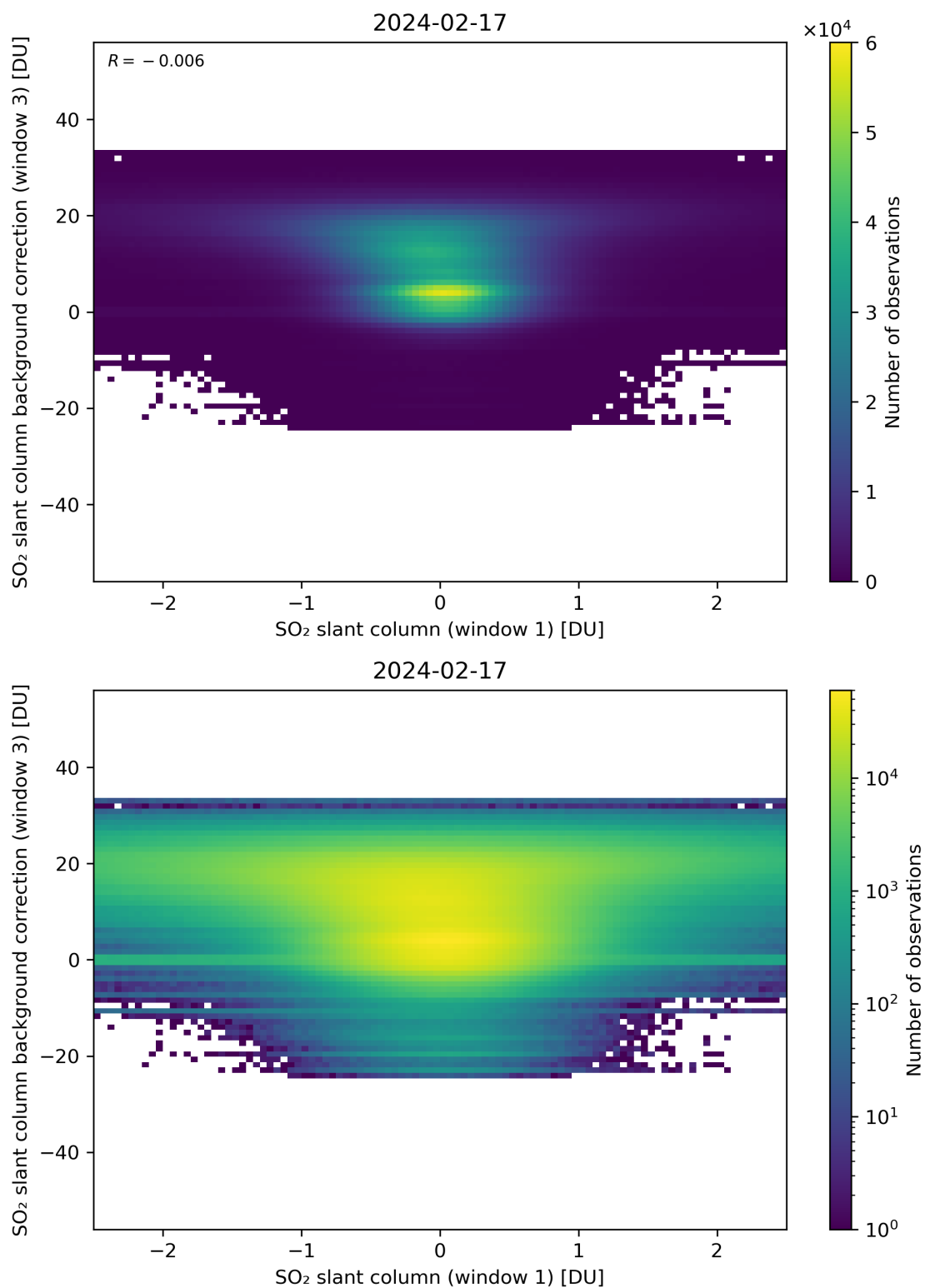
Figure 214: Scatter density plot of “SO 2 slant column (window 1)” against “SO 2 slant column background correction (window 3)” for 2024-02-17 to 2024-02-18.
