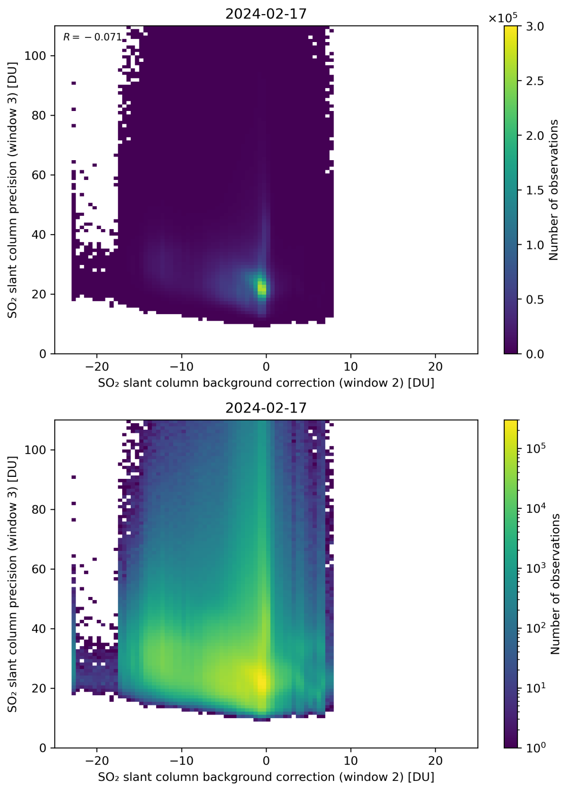
Figure 118: Scatter density plot of “SO 2 slant column background correction (window 2)” against “SO 2 slant column precision (window 3)” for 2024-02-17 to 2024-02-18.
