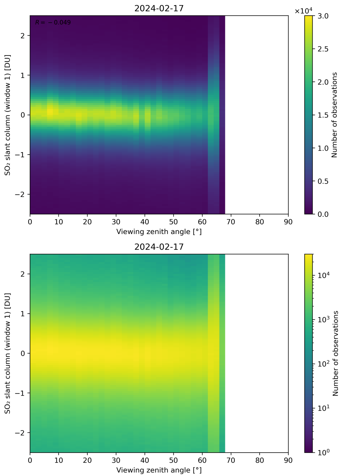
Figure 320: Scatter density plot of “Viewing zenith angle” against “SO 2 slant column (window 1)” for 2024-02-17 to 2024-02-18.
