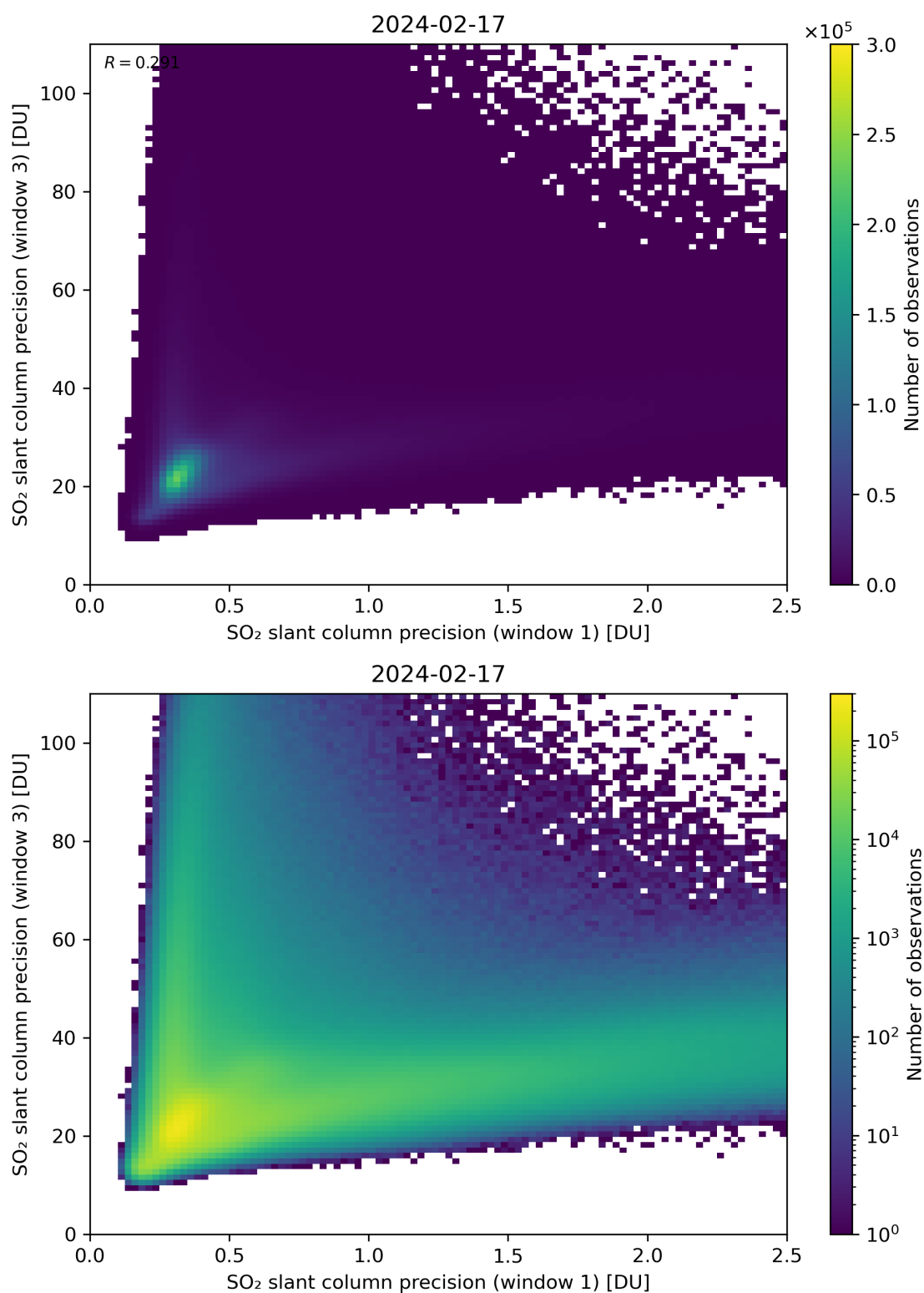
Figure 229: Scatter density plot of “SO 2 slant column precision (window 1)” against “SO 2 slant column precision (window 3)” for 2024-02-17 to 2024-02-18.
