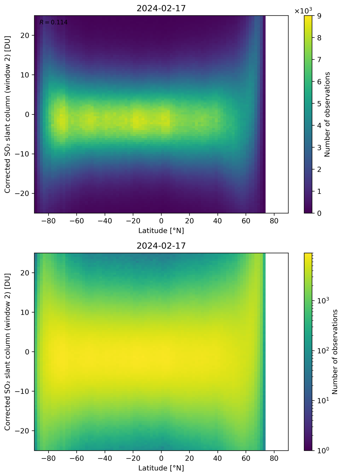
Figure 147: Scatter density plot of “Latitude” against “Corrected SO 2 slant column (window 2)” for 2024-02-17 to 2024-02-18.
