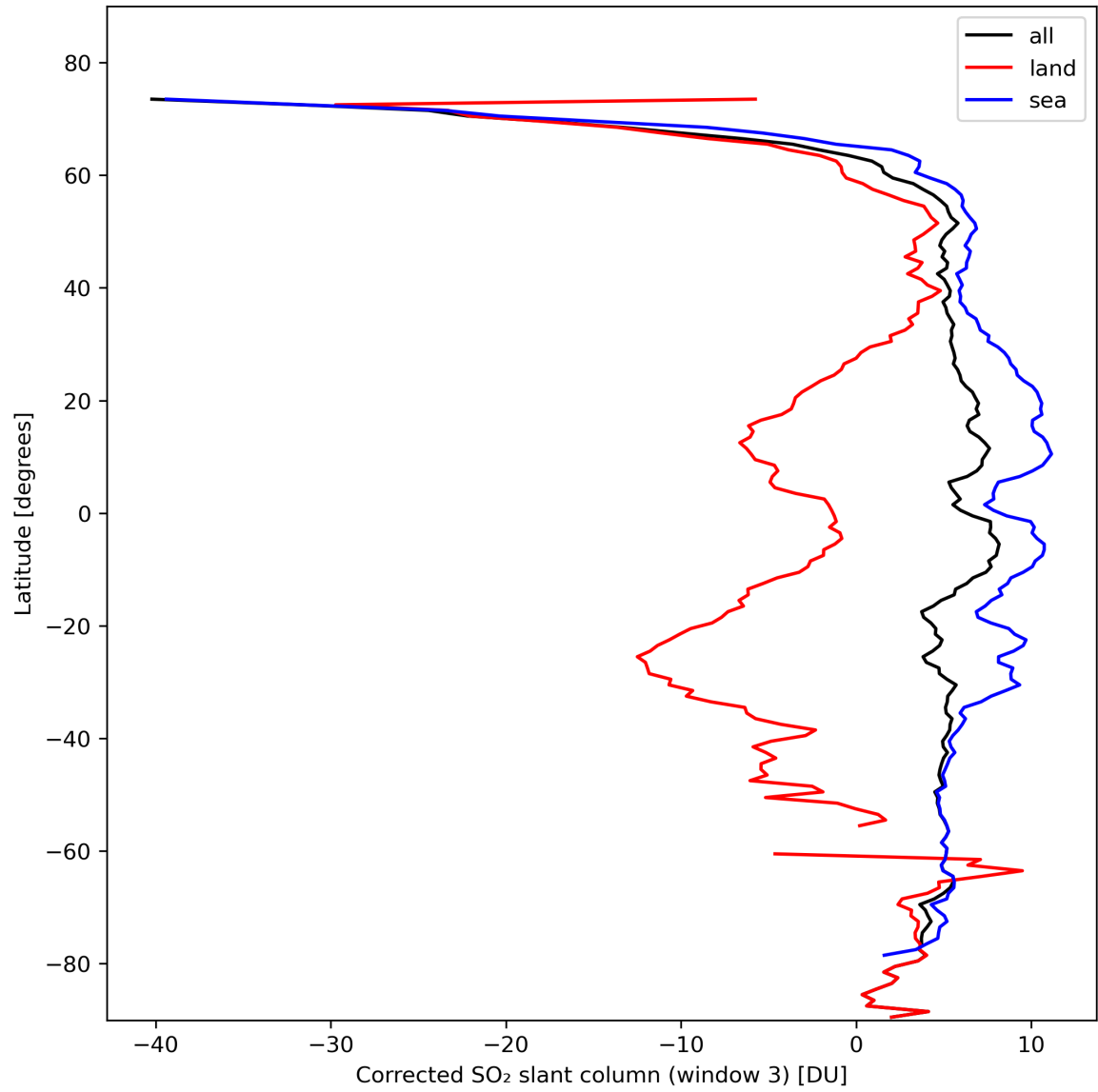
Figure 43: Zonal average of “Corrected SO 2 slant column (window 3)” for 2024-02-17 to 2024-02-18.
