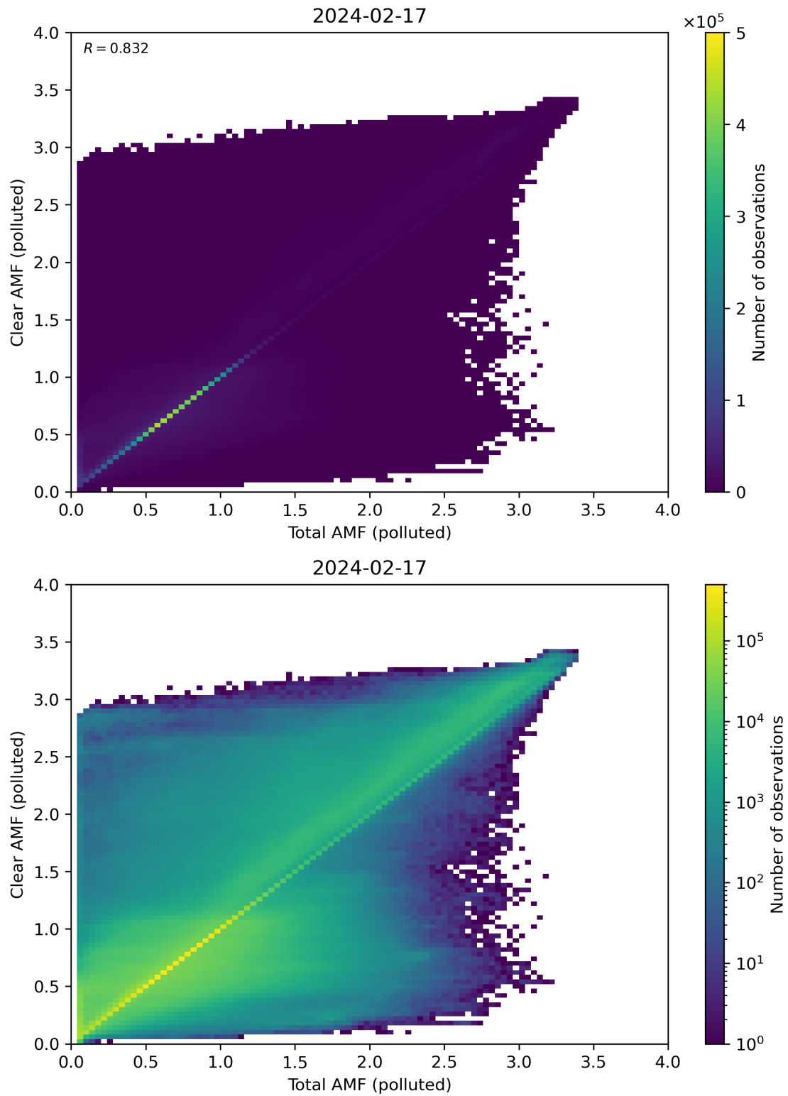
Figure 271: Scatter density plot of “Total AMF (polluted)” against “Clear AMF (polluted)” for 2024-02-17 to 2024-02-18.
