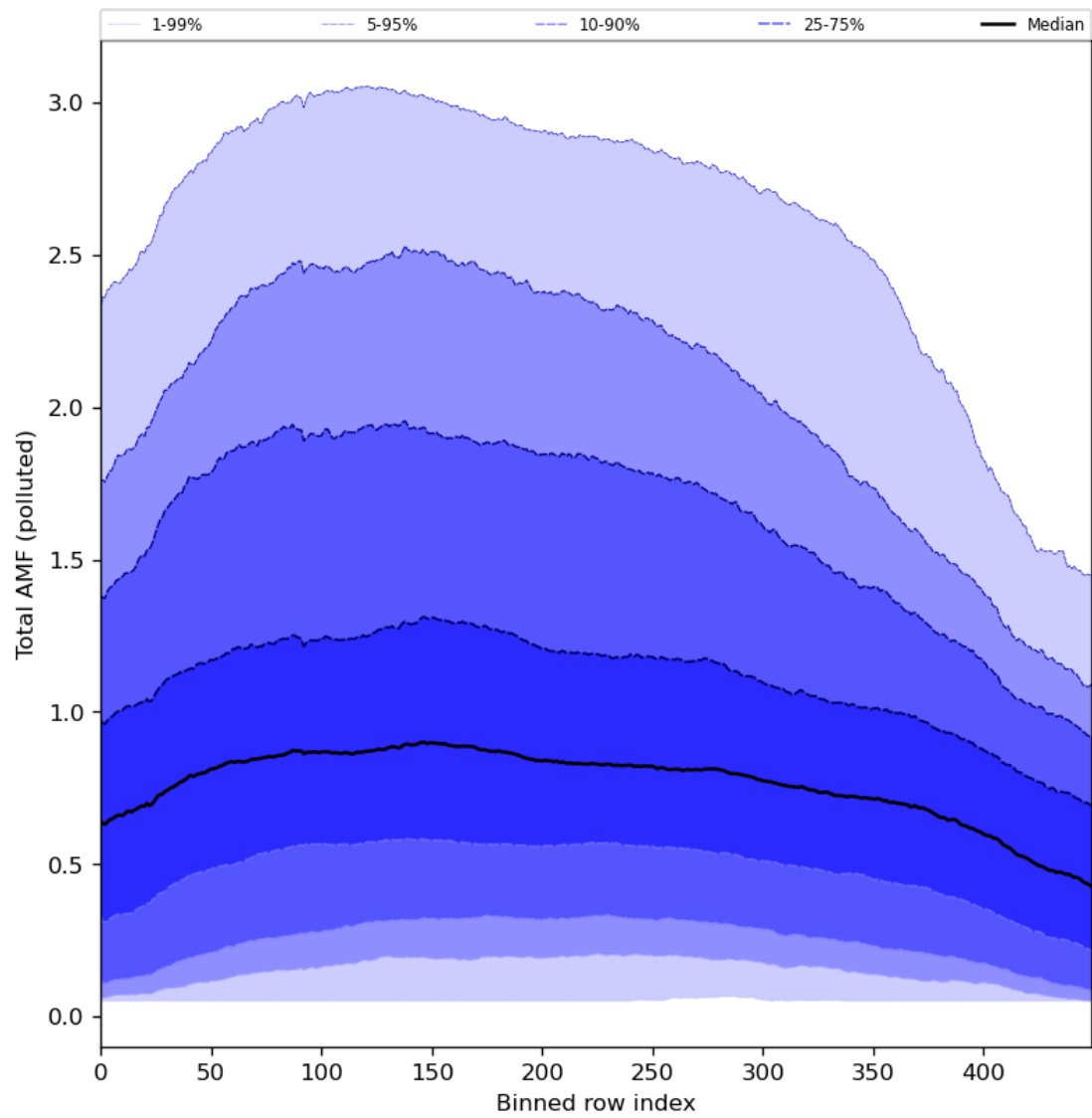
Figure 94: Along track statistics of “Total AMF (polluted)” for 2024-02-17 to 2024-02-18
