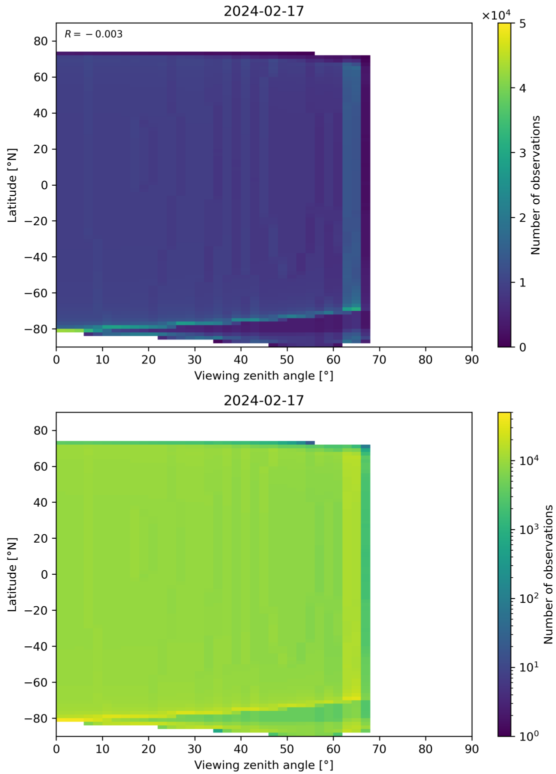
Figure 314: Scatter density plot of “Viewing zenith angle” against “Latitude” for 2024-02-17 to 2024-02-18.
