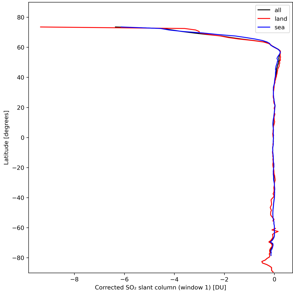
Figure 35: Zonal average of “Corrected SO 2 slant column (window 1)” for 2024-02-17 to 2024-02-18.
