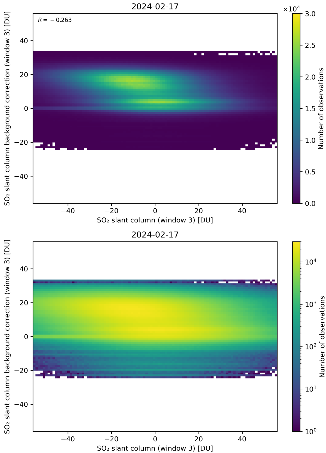
Figure 253: Scatter density plot of “SO 2 slant column (window 3)” against “SO 2 slant column background correction (window 3)” for 2024-02-17 to 2024-02-18.
