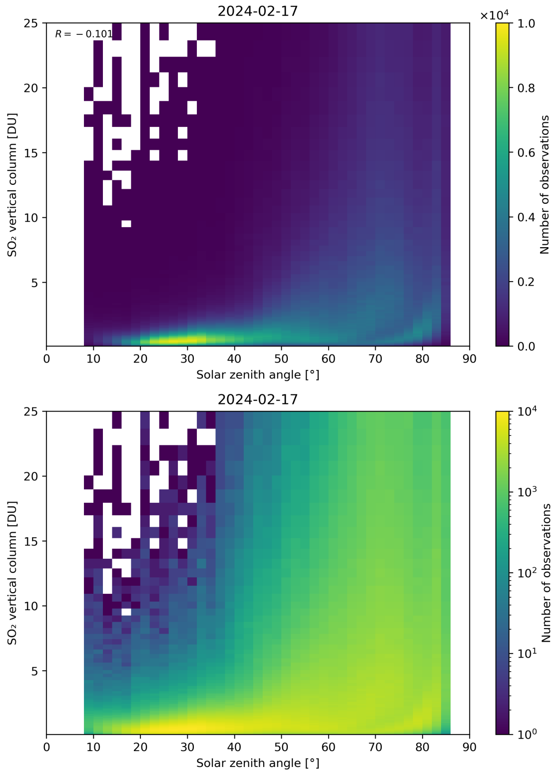
Figure 176: Scatter density plot of “Solar zenith angle” against “SO 2 vertical column” for 2024-02-17 to 2024-02-18.
