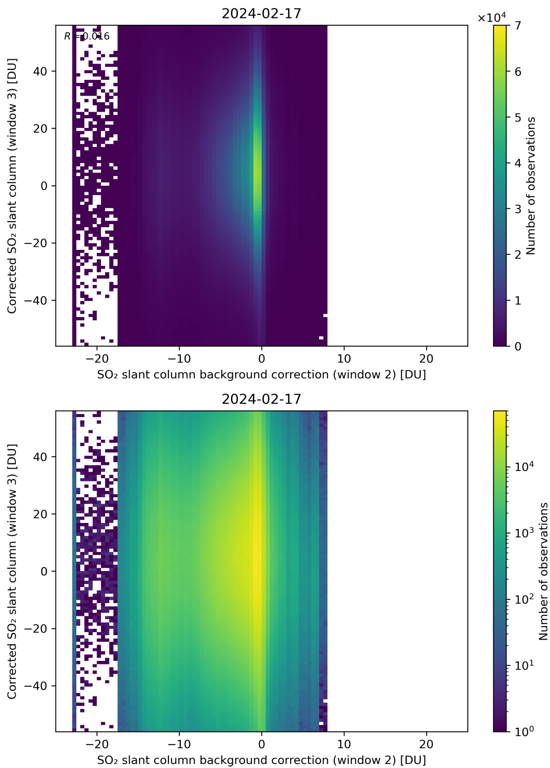
Figure 116: Scatter density plot of “SO 2 slant column background correction (window 2)” against “Corrected SO 2 slant column (window 3)” for 2024-02-17 to 2024-02-18.
