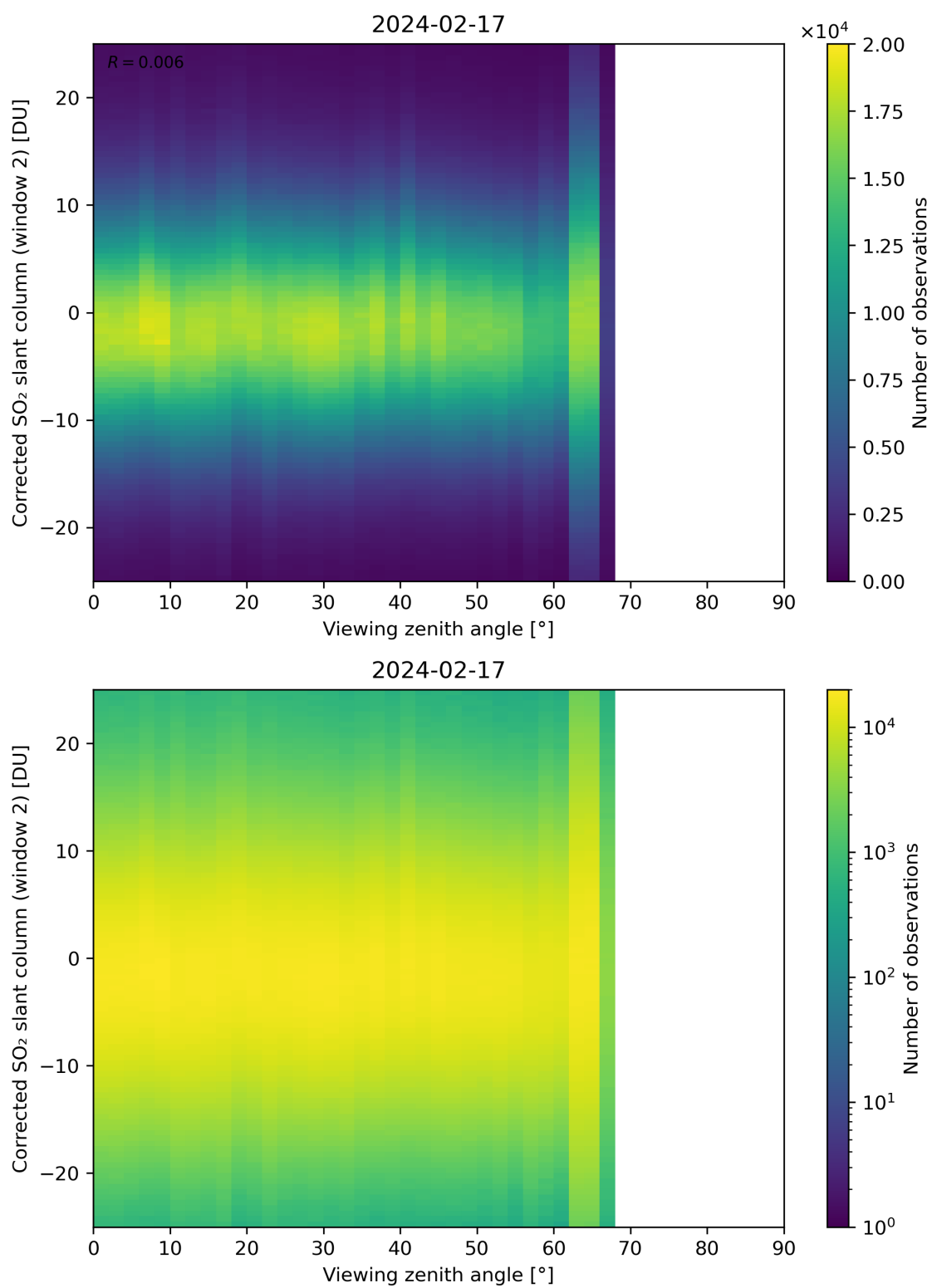
Figure 318: Scatter density plot of “Viewing zenith angle” against “Corrected SO 2 slant column (window 2)” for 2024-02-17 to 2024-02-18.
