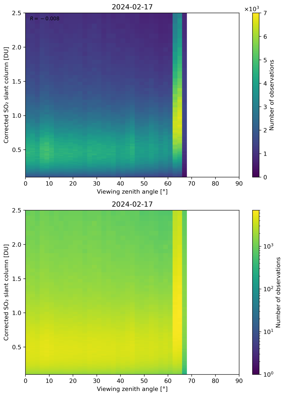
Figure 317: Scatter density plot of “Viewing zenith angle” against “Corrected SO 2 slant column” for 2024-02-17 to 2024-02-18.
