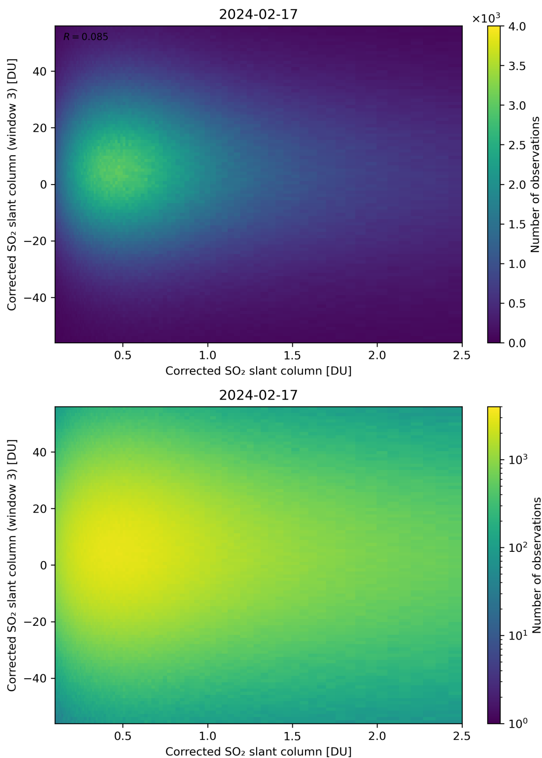
Figure 186: Scatter density plot of “Corrected SO 2 slant column” against “Corrected SO 2 slant column (window 3)” for 2024-02-17 to 2024-02-18.
