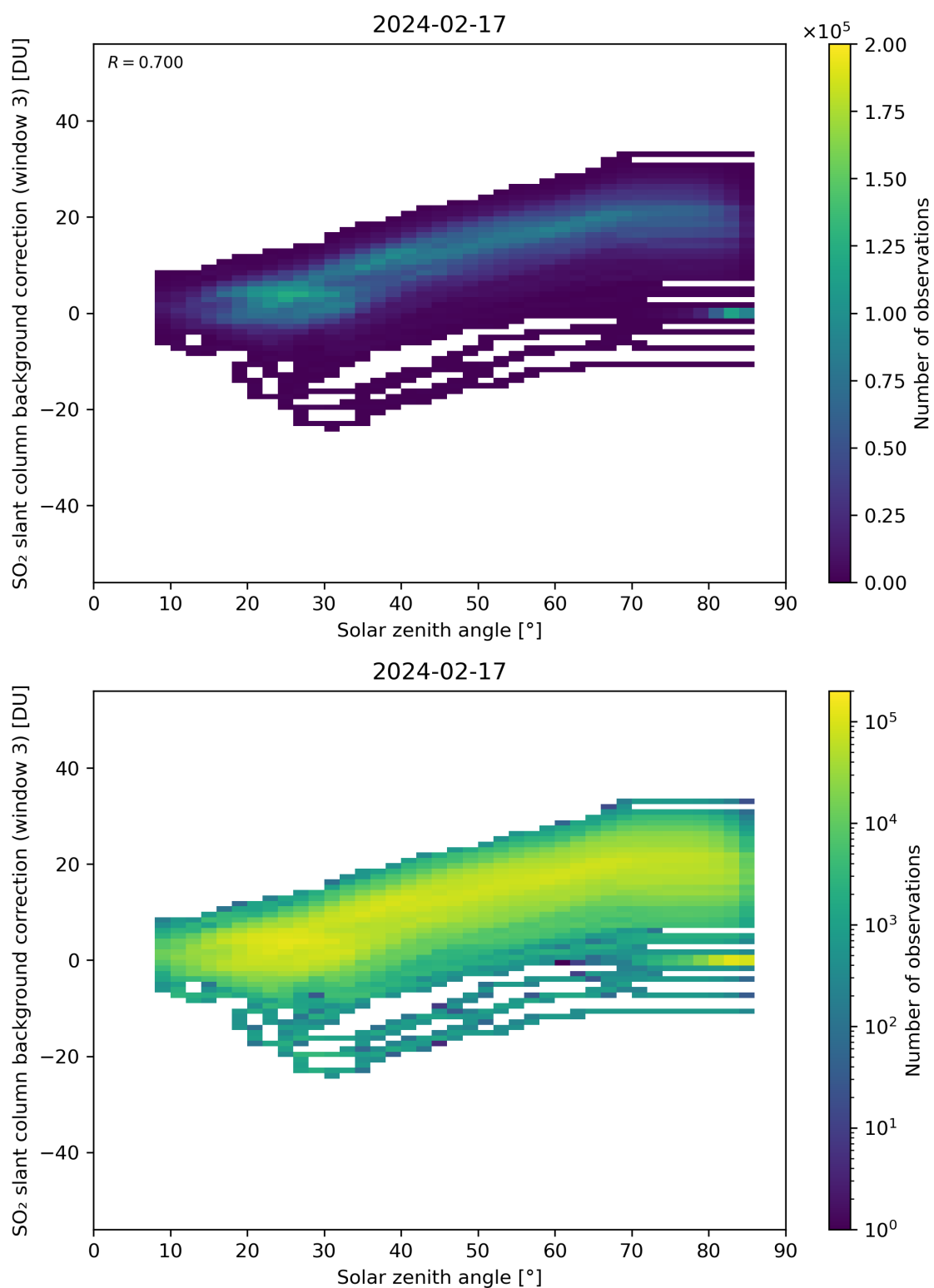
Figure 160: Scatter density plot of “Solar zenith angle” against “SO 2 slant column background correction (window 3)” for 2024-02-17 to 2024-02-18.
