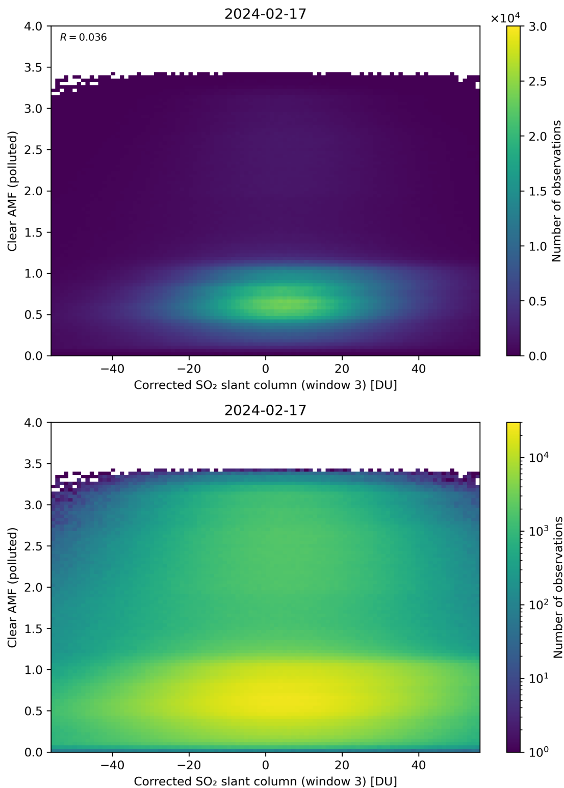
Figure 209: Scatter density plot of “Corrected SO 2 slant column (window 3)” against “Clear AMF (polluted)” for 2024-02-17 to 2024-02-18.
