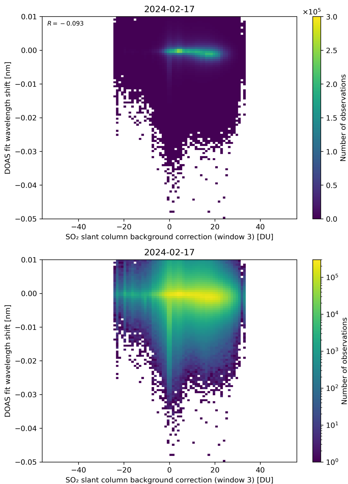
Figure 121: Scatter density plot of “SO 2 slant column background correction (window 3)” against “DOAS fit wavelength shift” for 2024-02-17 to 2024-02-18.
