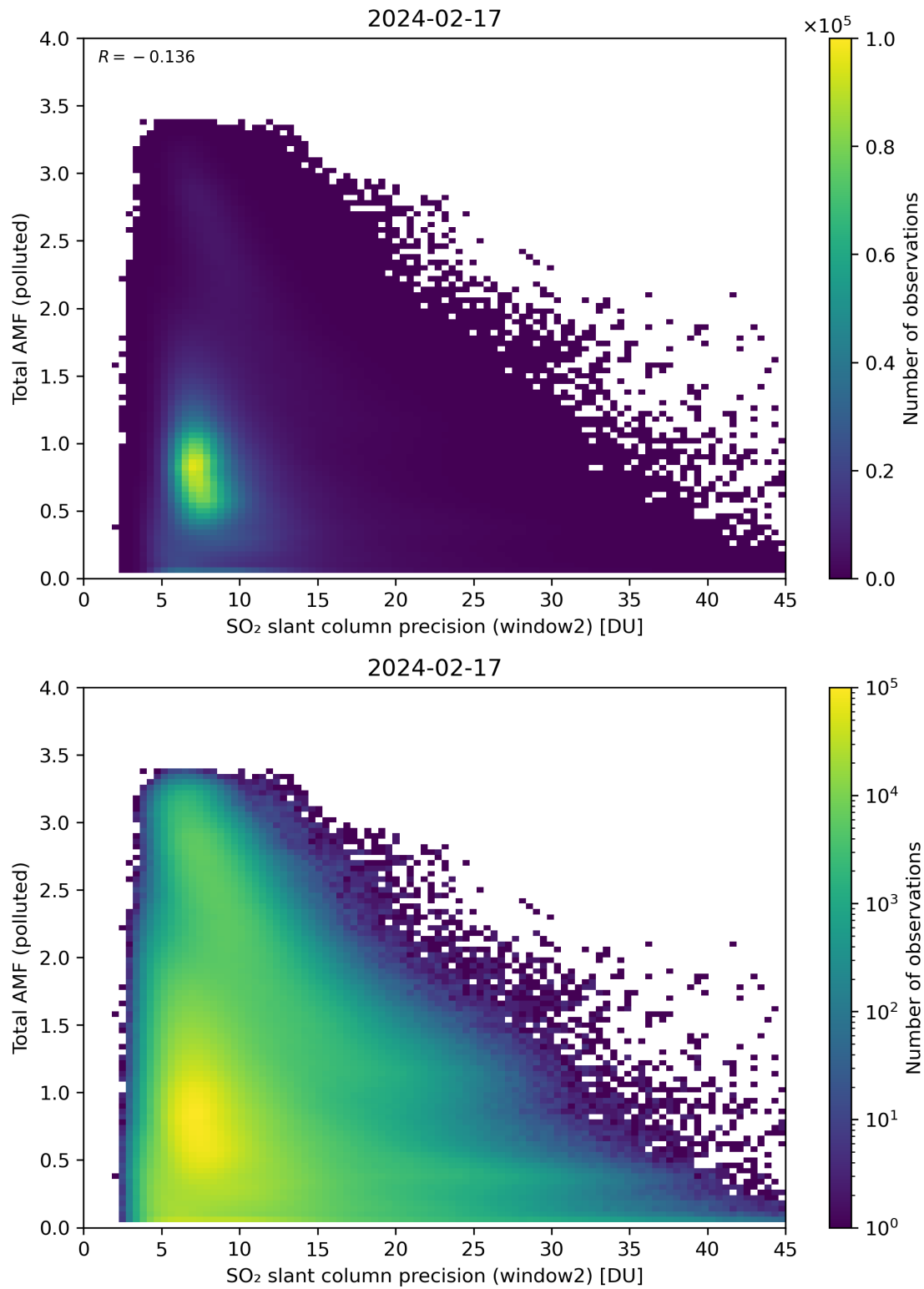
Figure 251: Scatter density plot of “SO 2 slant column precision (window2)” against “Total AMF (polluted)” for 2024-02-17 to 2024-02-18.
