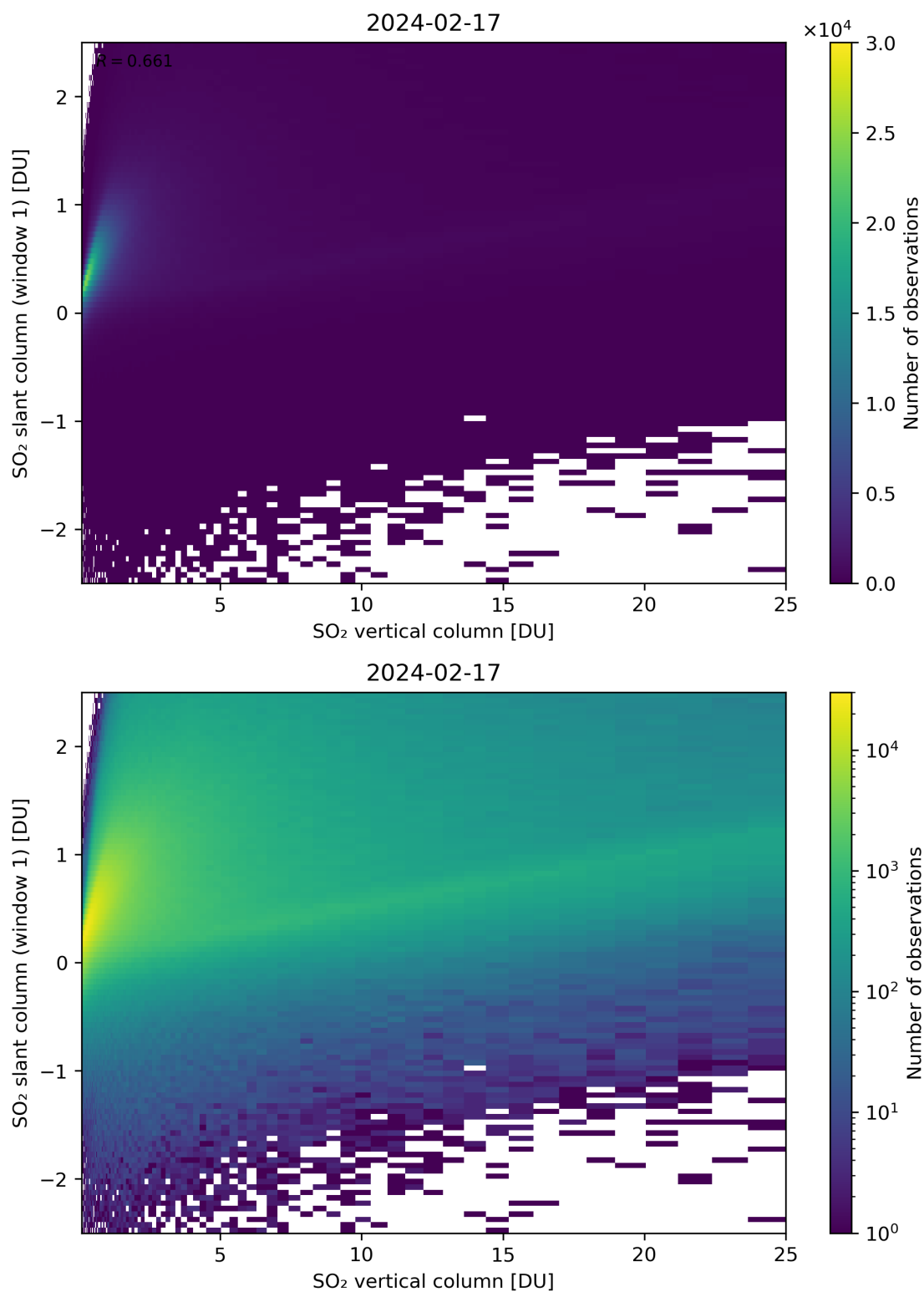
Figure 300: Scatter density plot of “SO 2 vertical column” against “SO 2 slant column (window 1)” for 2024-02-17 to 2024-02-18.
