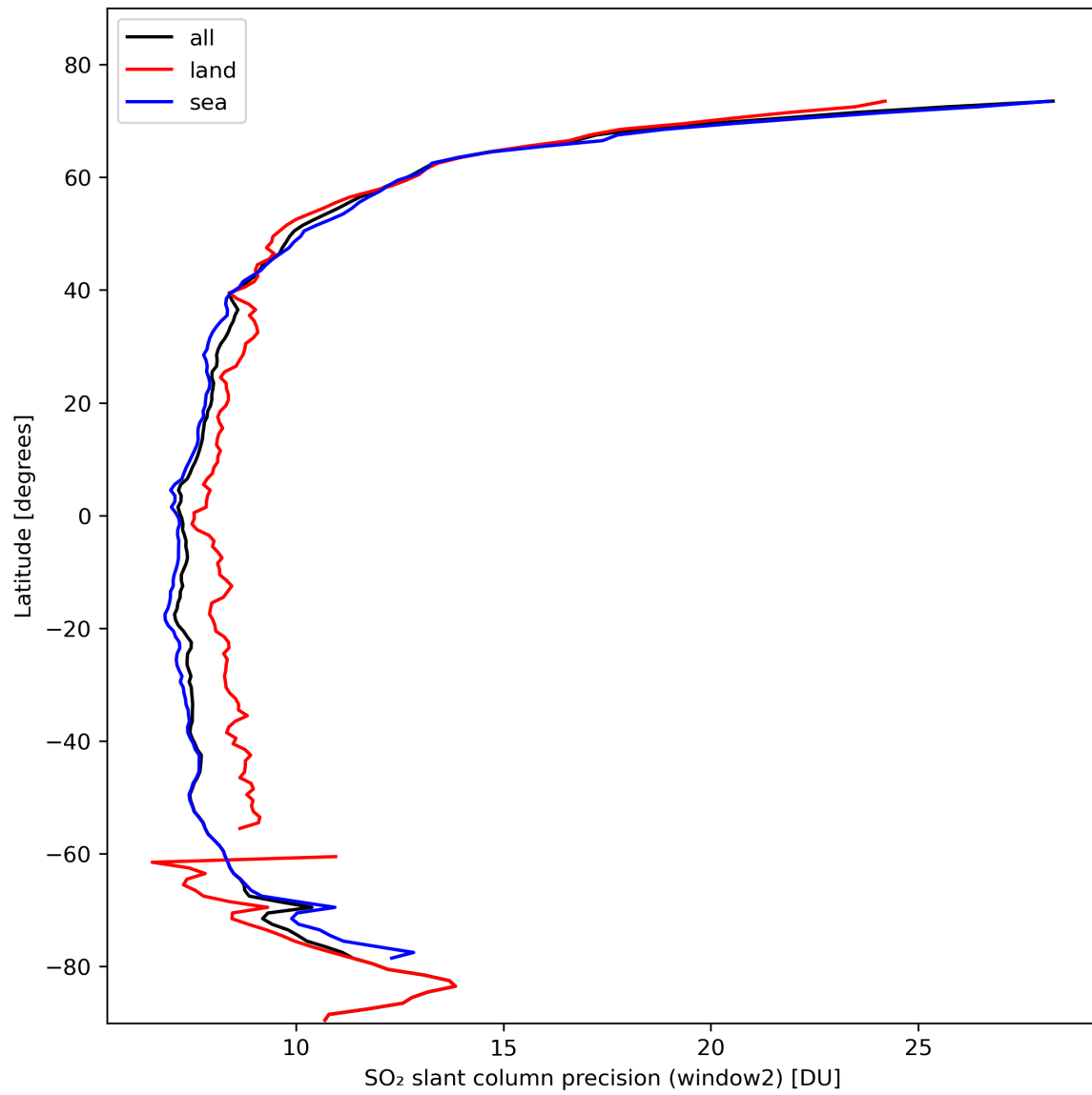
Figure 38: Zonal average of “SO 2 slant column precision (window2)” for 2024-02-17 to 2024-02-18.
