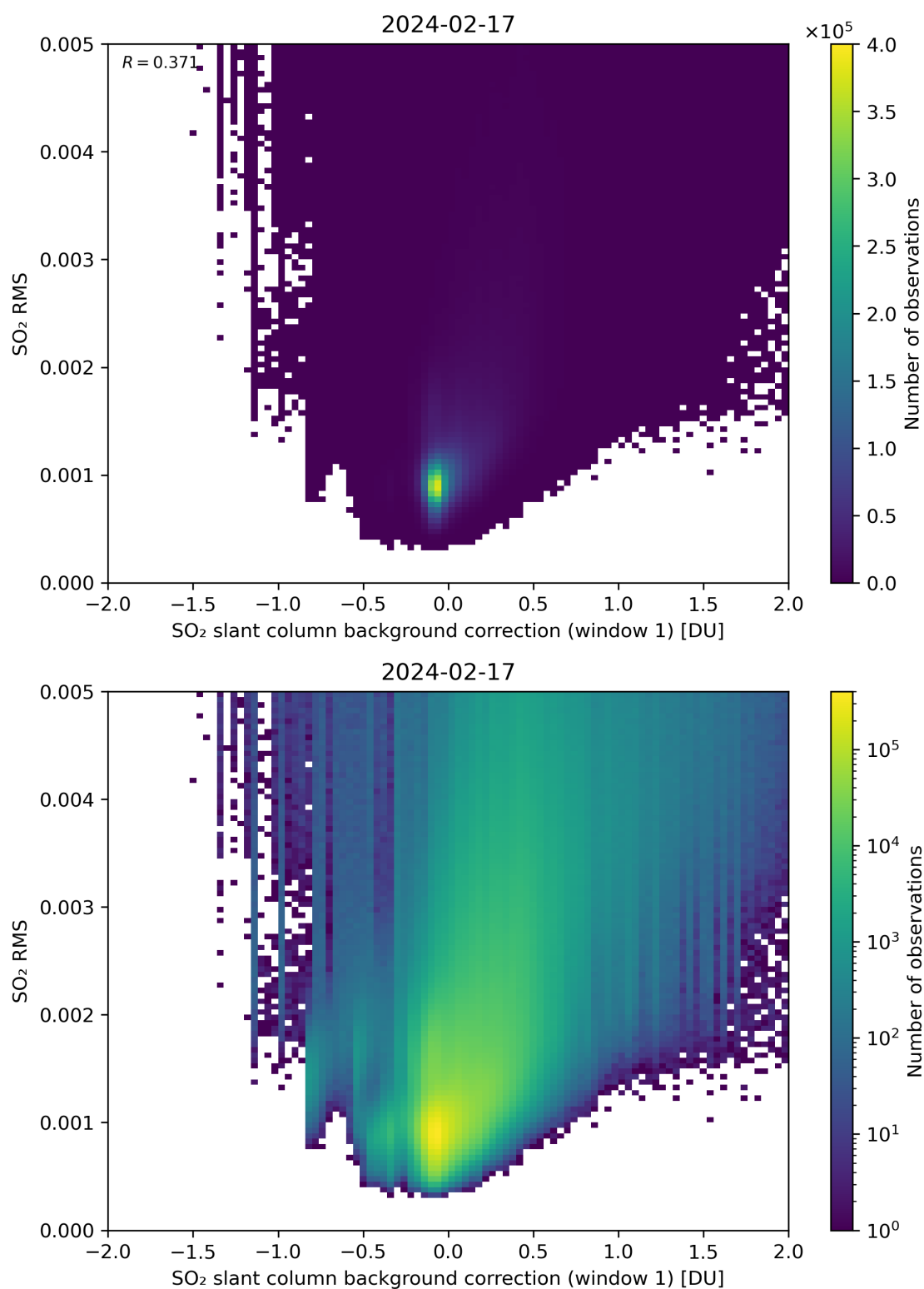
Figure 102: Scatter density plot of “SO 2 slant column background correction (window 1)” against “SO 2 RMS” for 2024-02-17 to 2024-02-18.
