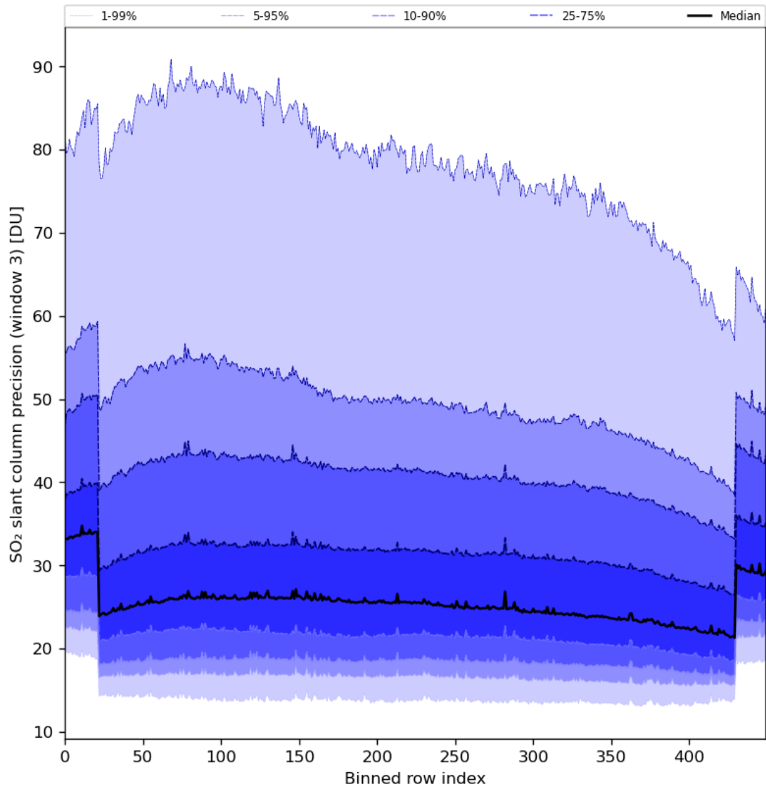
Figure 88: Along track statistics of “SO 2 slant column precision (window 3)” for 2024-02-17 to 2024-02-18
