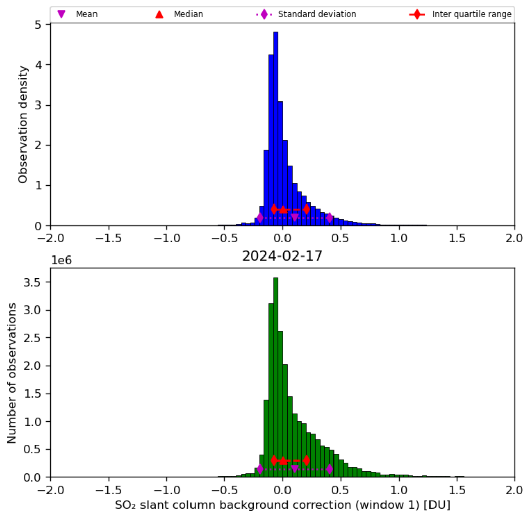
Figure 59: Histogram of “SO 2 slant column background correction (window 1)” for 2024-02-17 to 2024-02-18
