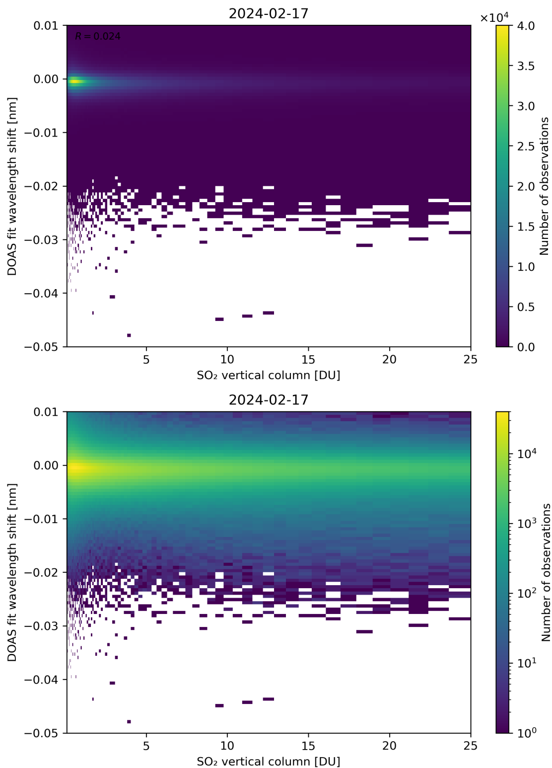
Figure 276: Scatter density plot of “SO 2 vertical column” against “DOAS fit wavelength shift” for 2024-02-17 to 2024-02-18.
