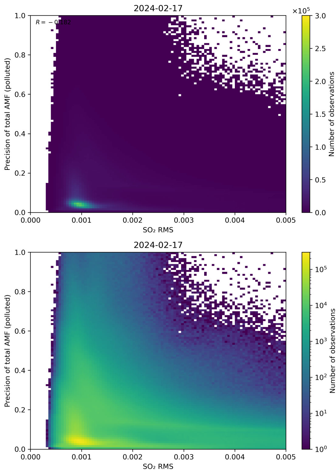
Figure 138: Scatter density plot of “SO 2 RMS” against “Precision of total AMF (polluted)” for 2024-02-17 to 2024-02-18.
