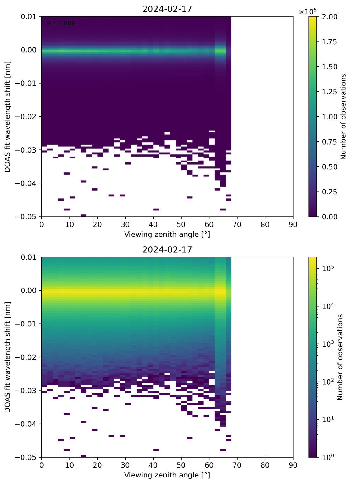
Figure 311: Scatter density plot of “Viewing zenith angle” against “DOAS fit wavelength shift” for 2024-02-17 to 2024-02-18.
