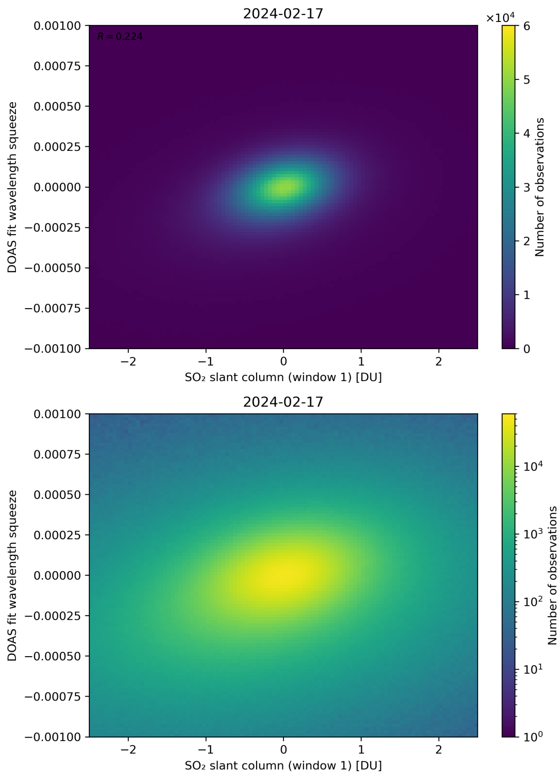
Figure 216: Scatter density plot of “SO 2 slant column (window 1)” against “DOAS fit wavelength squeeze” for 2024-02-17 to 2024-02-18.
