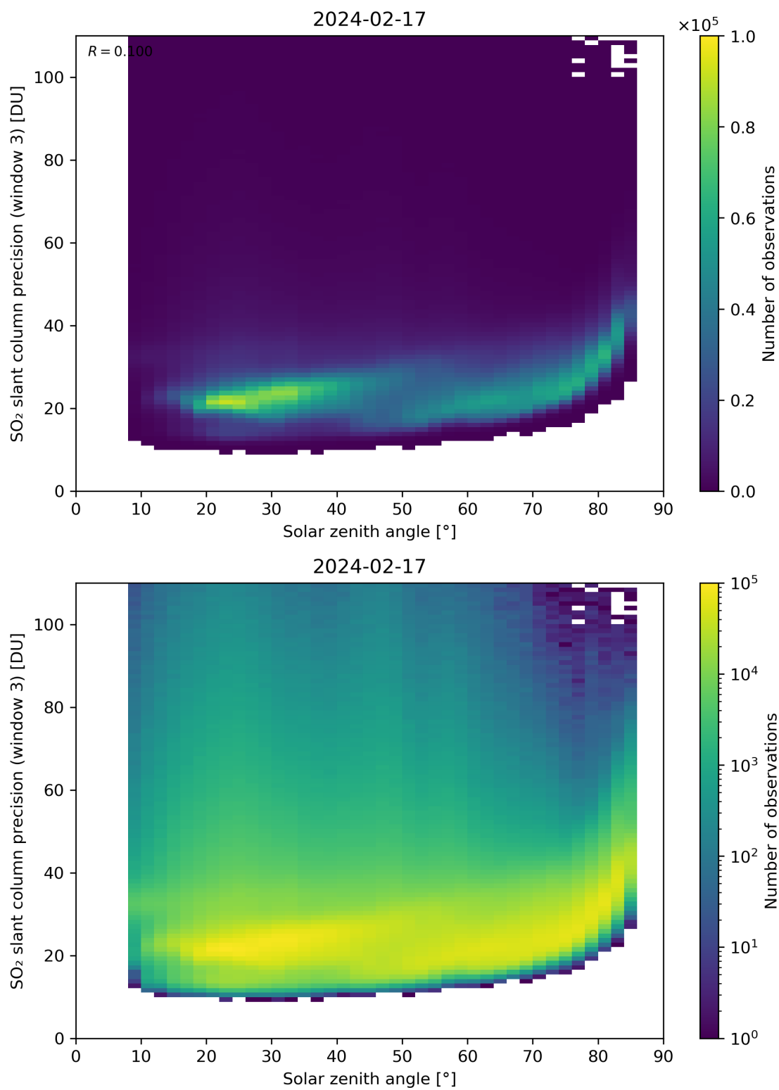
Figure 173: Scatter density plot of “Solar zenith angle” against “SO 2 slant column precision (window 3)” for 2024-02-17 to 2024-02-18.
