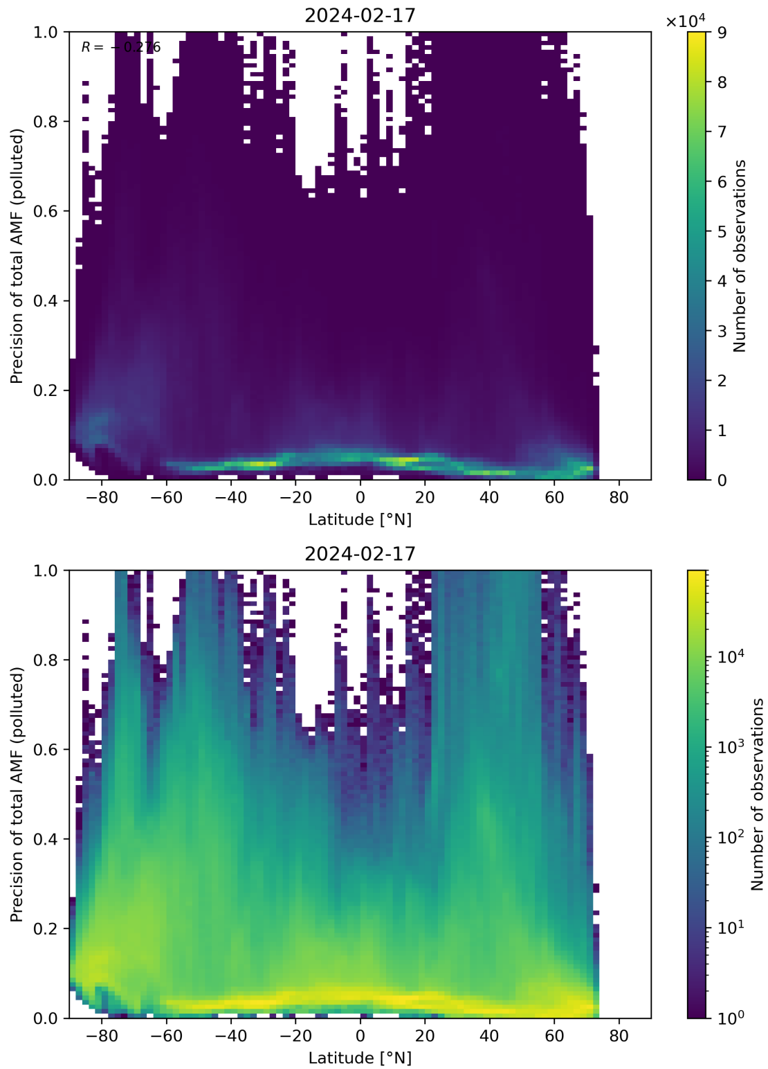
Figure 155: Scatter density plot of “Latitude” against “Precision of total AMF (polluted)” for 2024-02-17 to 2024-02-18.
