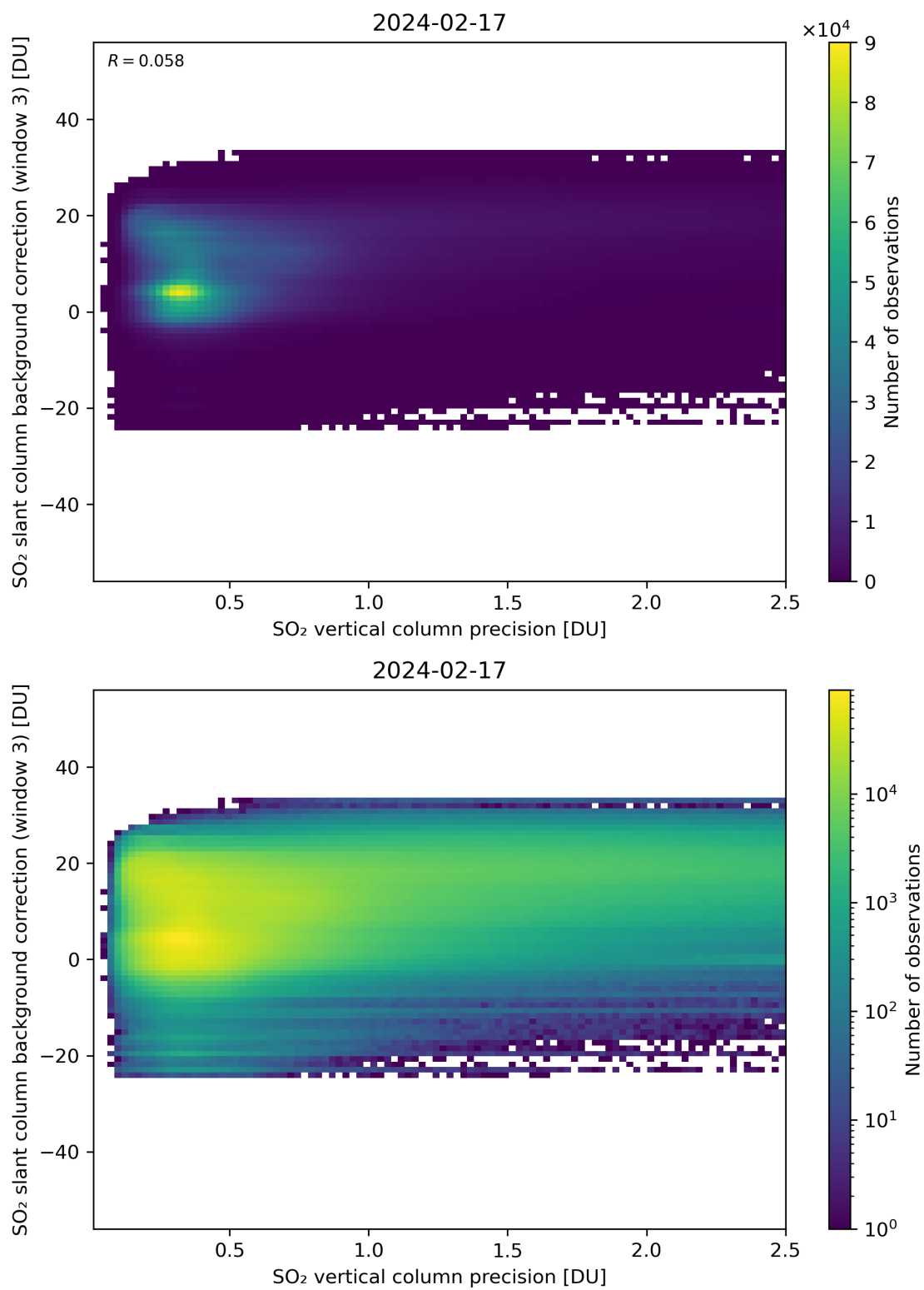
Figure 281: Scatter density plot of “SO 2 vertical column precision” against “SO 2 slant column background correction (window 3)” for 2024-02-17 to 2024-02-18.
