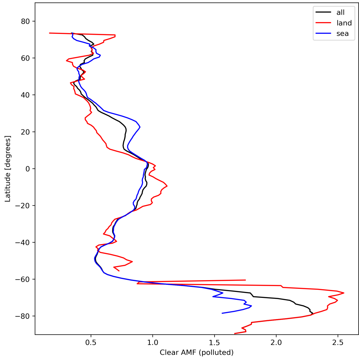
Figure 50: Zonal average of “Clear AMF (polluted)” for 2024-02-17 to 2024-02-18.
