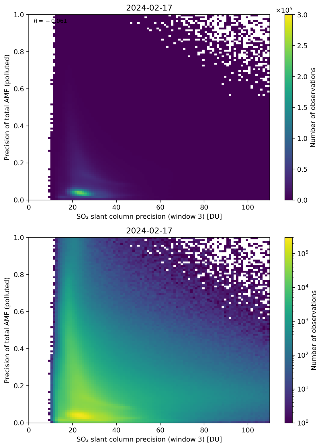
Figure 264: Scatter density plot of “SO 2 slant column precision (window 3)” against “Precision of total AMF (polluted)” for 2024-02-17 to 2024-02-18.
