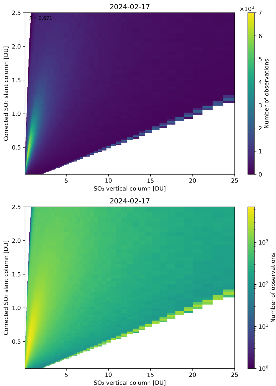
Figure 297: Scatter density plot of “SO 2 vertical column” against “Corrected SO 2 slant column” for 2024-02-17 to 2024-02-18.
