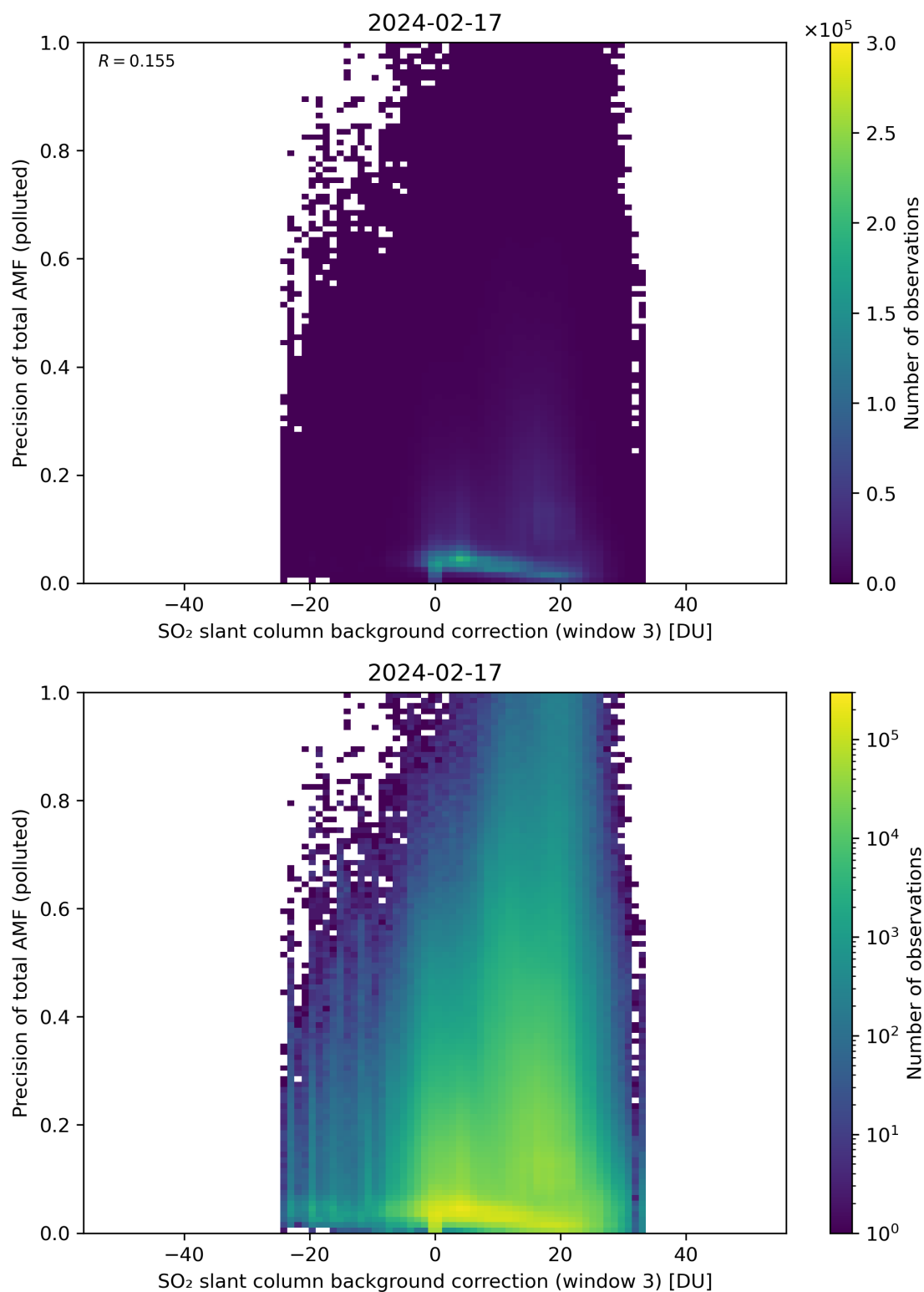
Figure 126: Scatter density plot of “SO 2 slant column background correction (window 3)” against “Precision of total AMF (polluted)” for 2024-02-17 to 2024-02-18.
