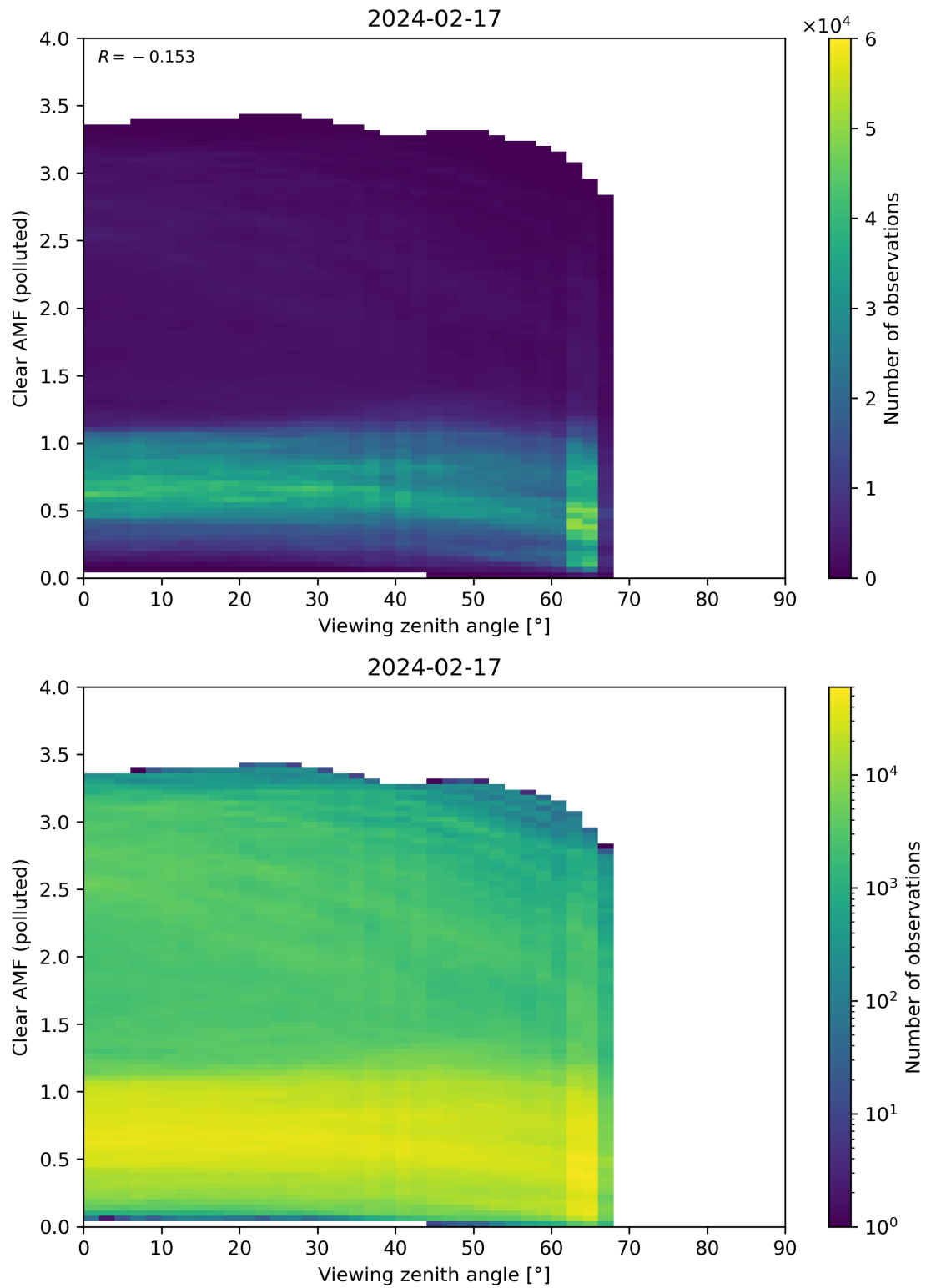
Figure 316: Scatter density plot of “Viewing zenith angle” against “Clear AMF (polluted)” for 2024-02-17 to 2024-02-18.
