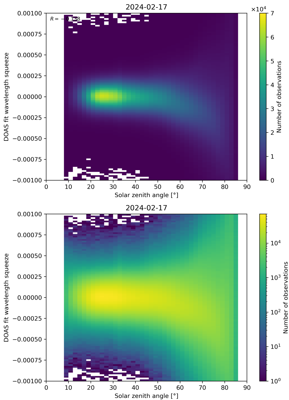
Figure 162: Scatter density plot of “Solar zenith angle” against “DOAS fit wavelength squeeze” for 2024-02-17 to 2024-02-18.
