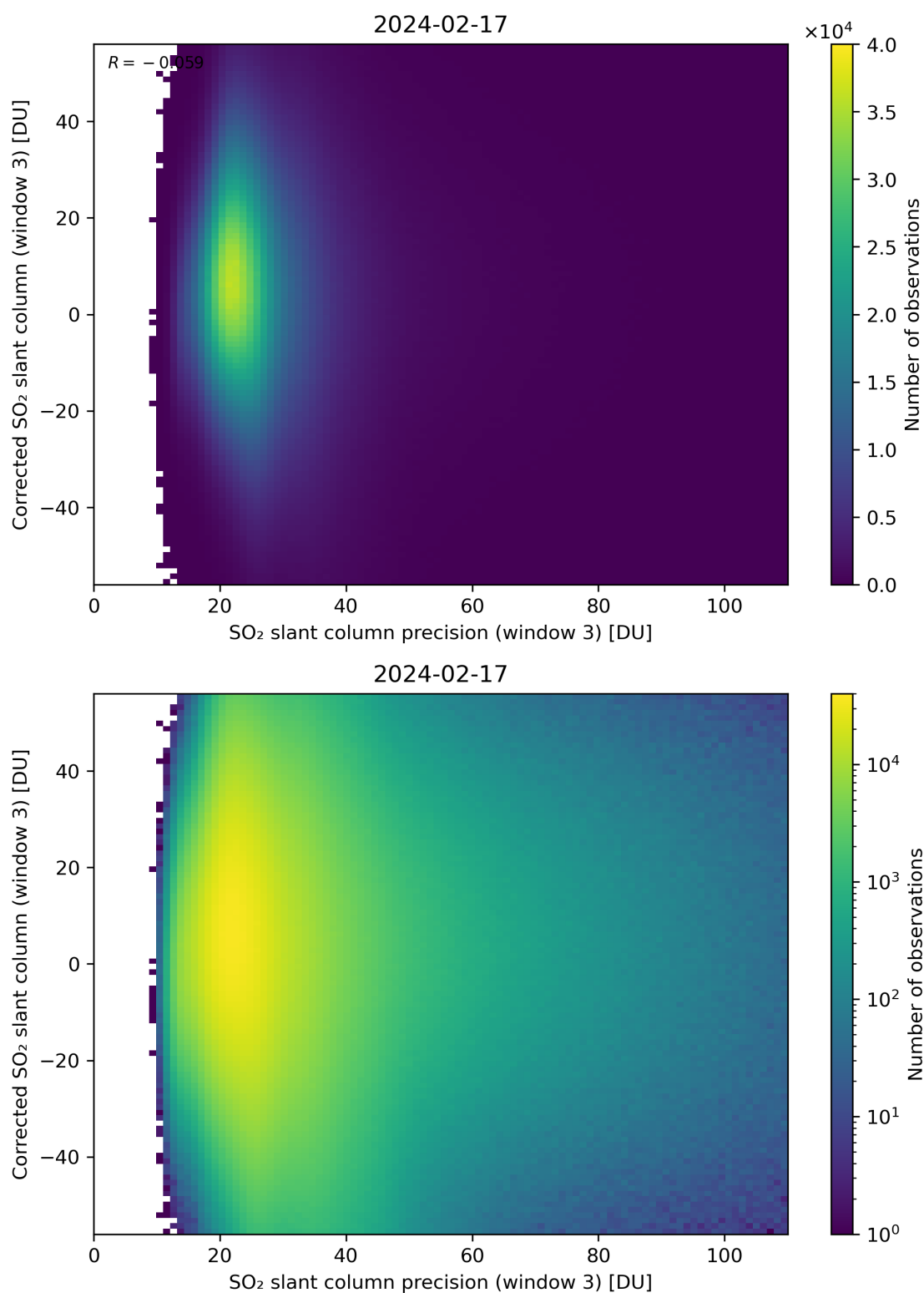
Figure 262: Scatter density plot of “SO 2 slant column precision (window 3)” against “Corrected SO 2 slant column (window 3)” for 2024-02-17 to 2024-02-18.
