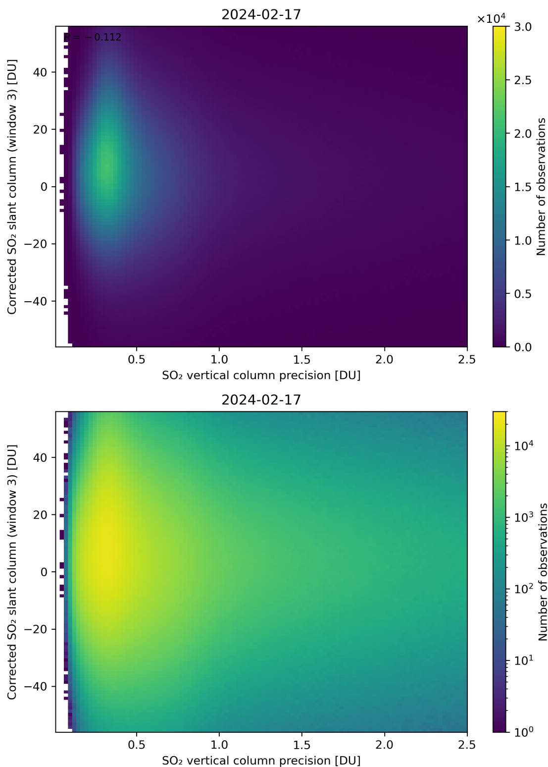
Figure 288: Scatter density plot of “SO 2 vertical column precision” against “Corrected SO 2 slant column (window 3)” for 2024-02-17 to 2024-02-18.
