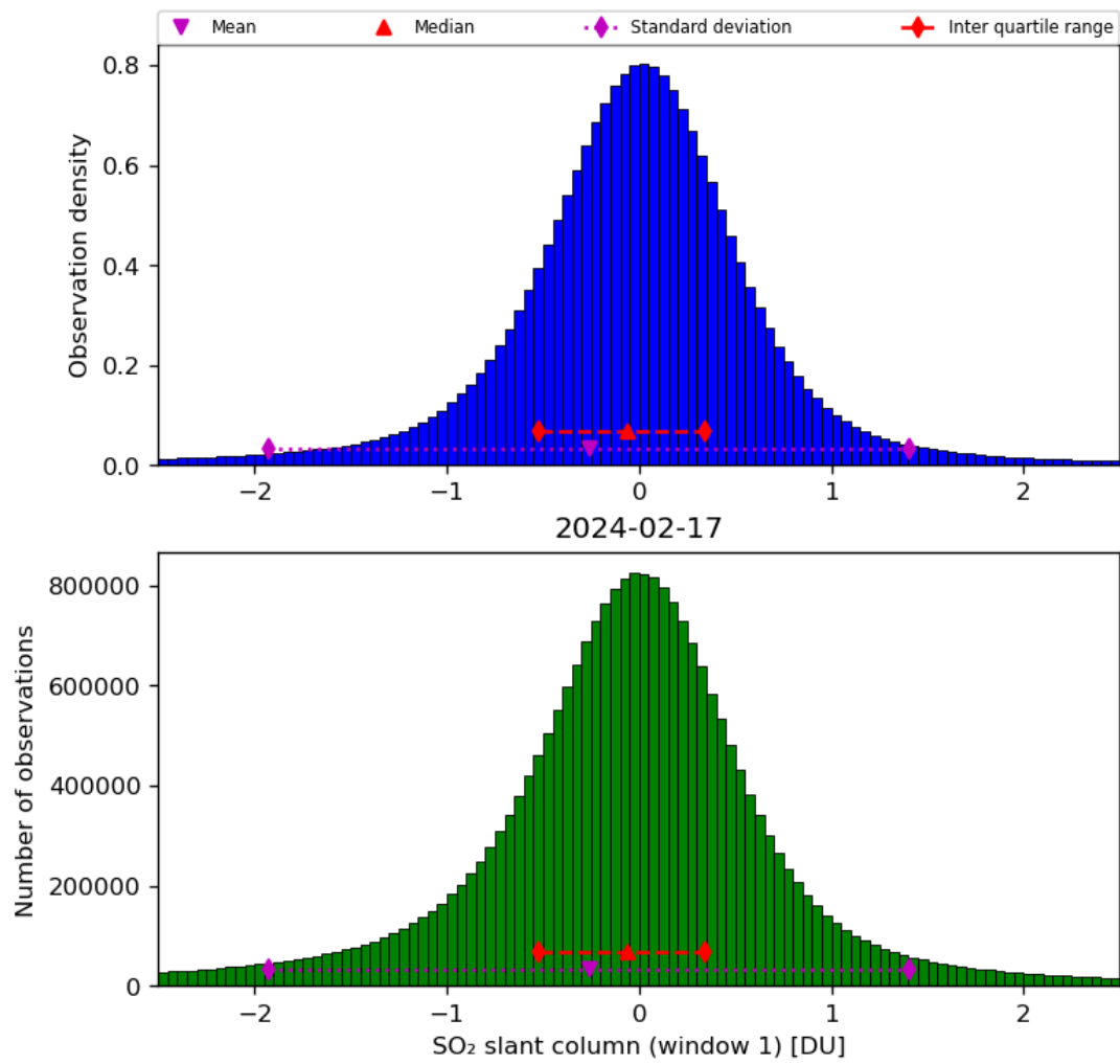
Figure 56: Histogram of “SO 2 slant column (window 1)” for 2024-02-17 to 2024-02-18
