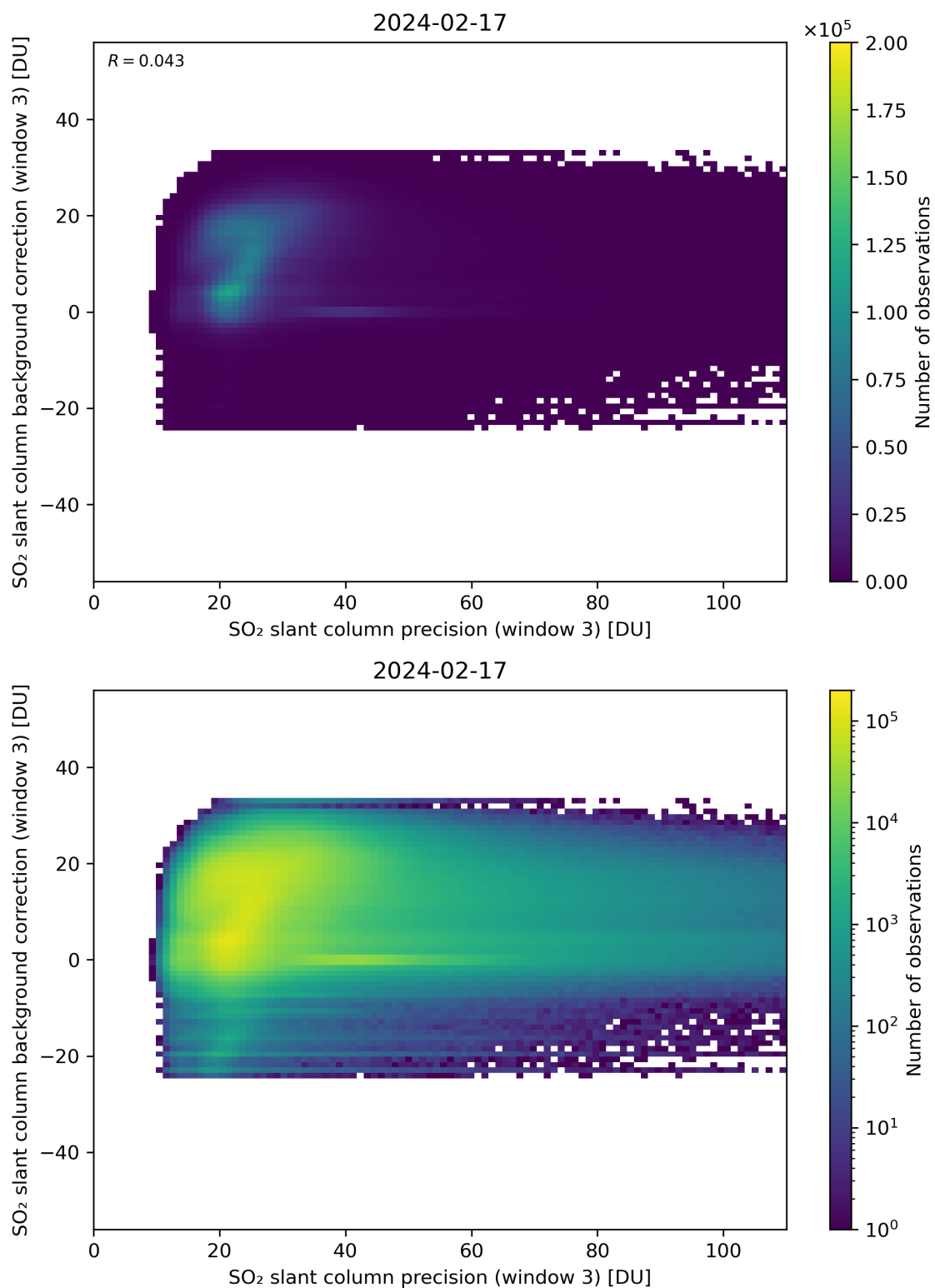
Figure 257: Scatter density plot of “SO 2 slant column precision (window 3)” against “SO 2 slant column background correction (window 3)” for 2024-02-17 to 2024-02-18.
