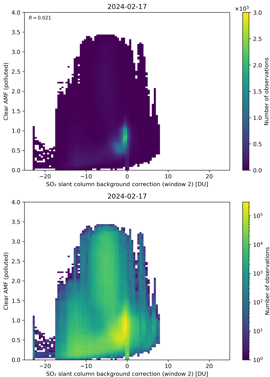
Figure 115: Scatter density plot of “SO 2 slant column background correction (window 2)” against “Clear AMF (polluted)” for 2024-02-17 to 2024-02-18.
