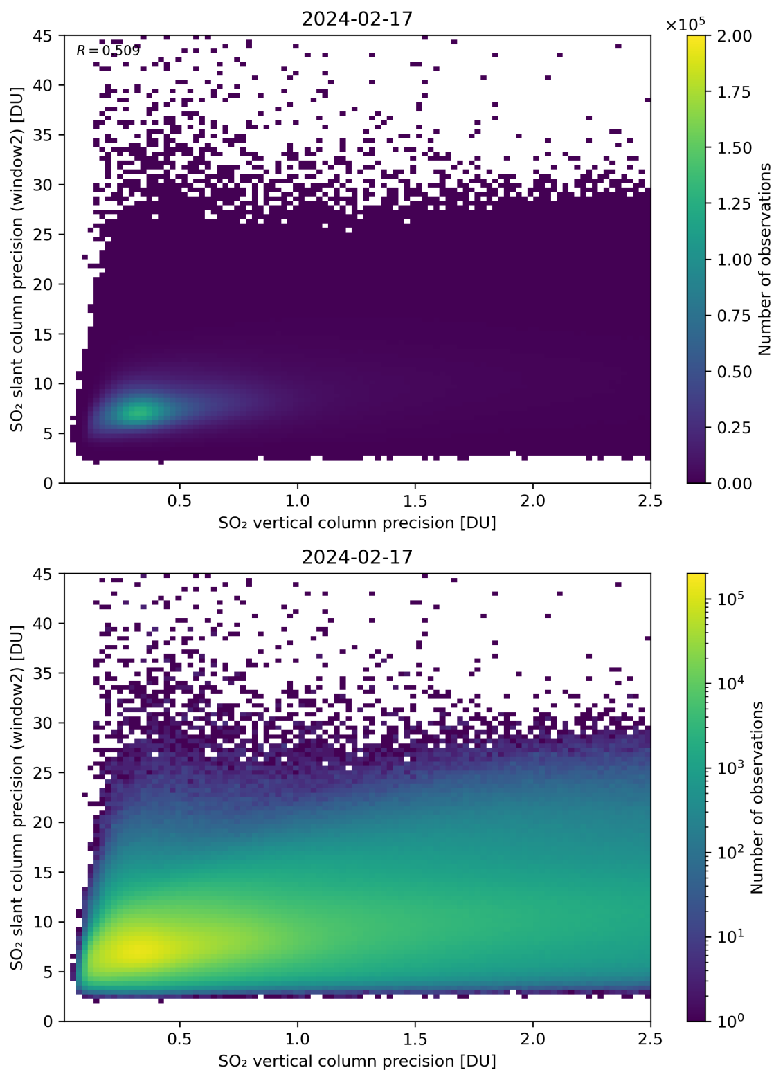
Figure 291: Scatter density plot of “SO 2 vertical column precision” against “SO 2 slant column precision (window2)” for 2024-02-17 to 2024-02-18.
