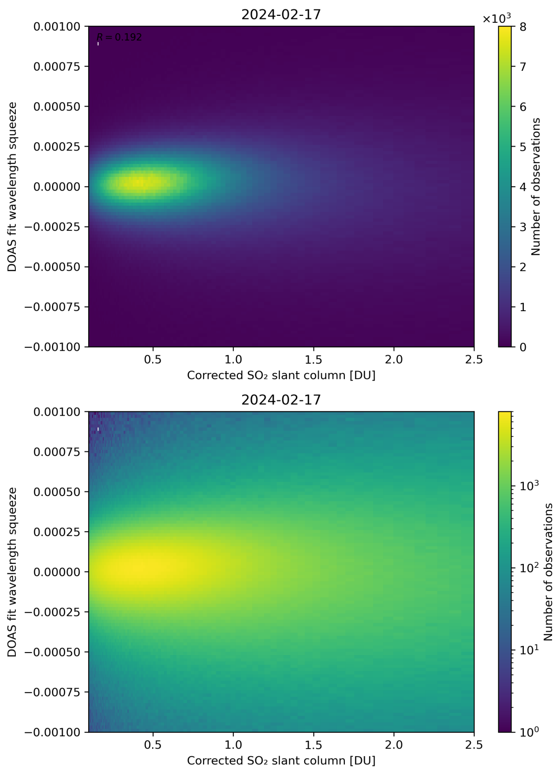
Figure 182: Scatter density plot of “Corrected SO 2 slant column” against “DOAS fit wavelength squeeze” for 2024-02-17 to 2024-02-18.
