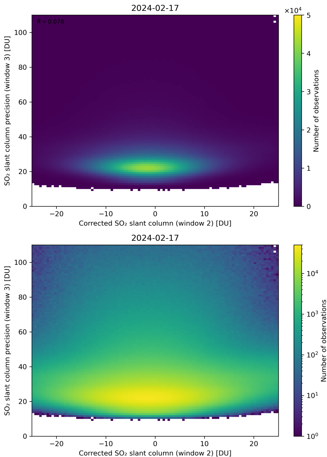
Figure 202: Scatter density plot of “Corrected SO 2 slant column (window 2)” against “SO 2 slant column precision (window 3)” for 2024-02-17 to 2024-02-18.
