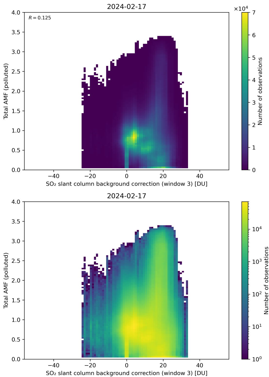
Figure 125: Scatter density plot of “SO 2 slant column background correction (window 3)” against “Total AMF (polluted)” for 2024-02-17 to 2024-02-18.
