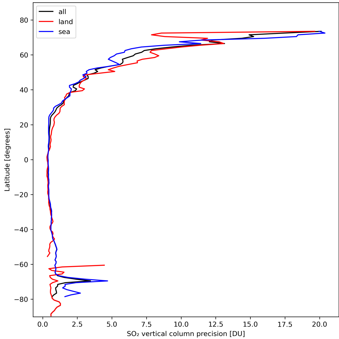
Figure 31: Zonal average of “SO 2 vertical column precision” for 2024-02-17 to 2024-02-18.
