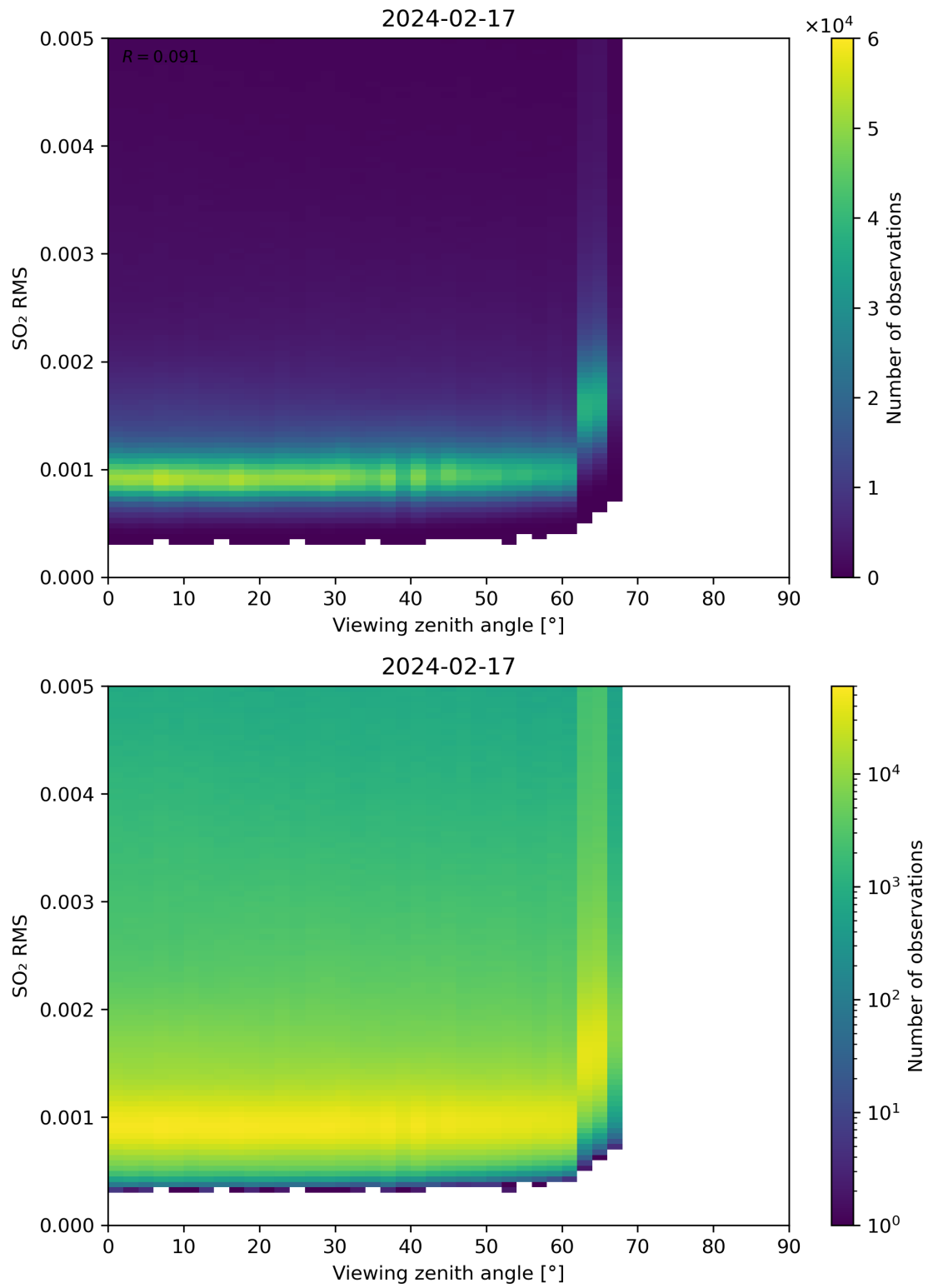
Figure 313: Scatter density plot of “Viewing zenith angle” against “SO 2 RMS” for 2024-02-17 to 2024-02-18.
