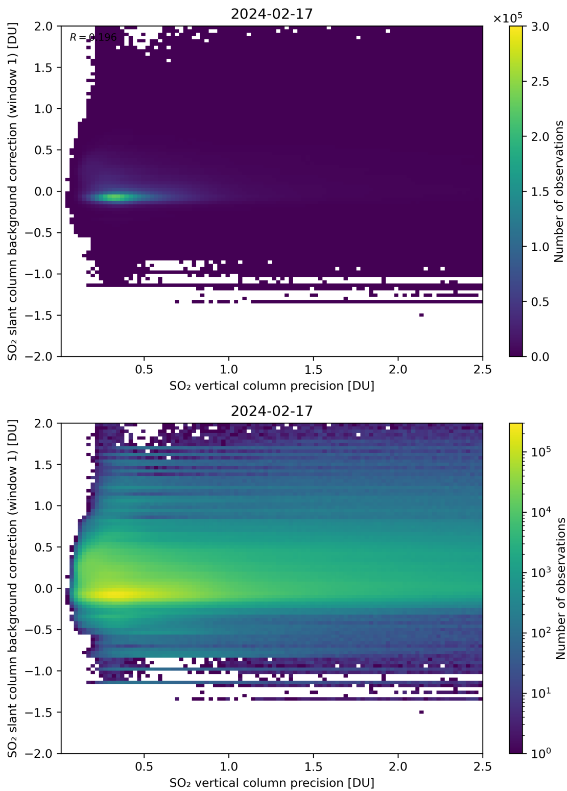
Figure 279: Scatter density plot of “SO 2 vertical column precision” against “SO 2 slant column background correction (window 1)” for 2024-02-17 to 2024-02-18.
