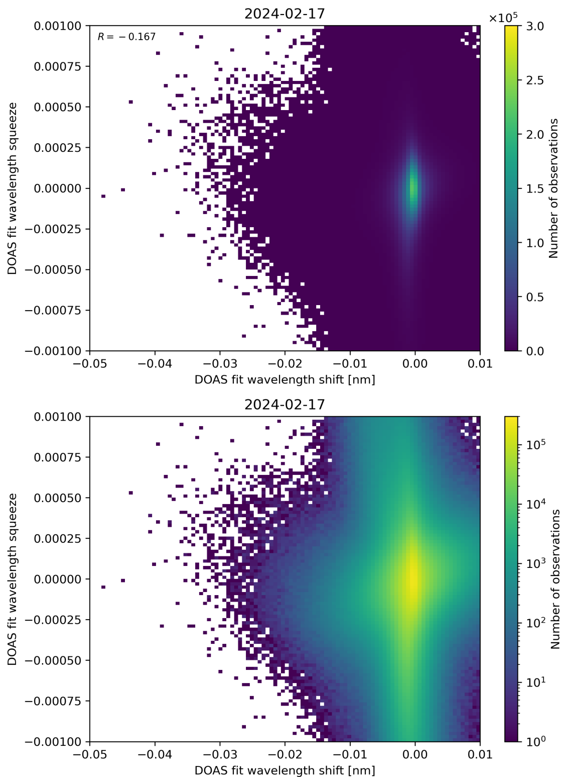
Figure 127: Scatter density plot of “DOAS fit wavelength shift” against “DOAS fit wavelength squeeze” for 2024-02-17 to 2024-02-18.
