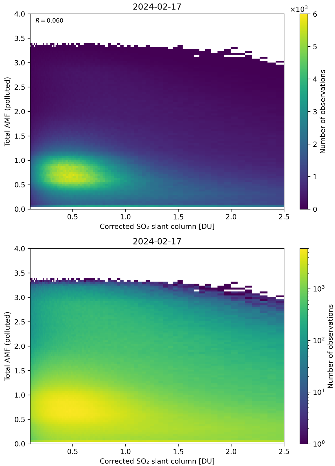
Figure 192: Scatter density plot of “Corrected SO 2 slant column” against “Total AMF (polluted)” for 2024-02-17 to 2024-02-18.
