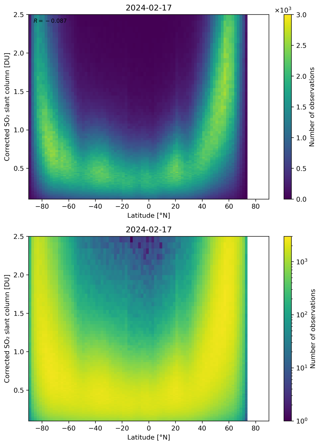
Figure 146: Scatter density plot of “Latitude” against “Corrected SO 2 slant column” for 2024-02-17 to 2024-02-18.
