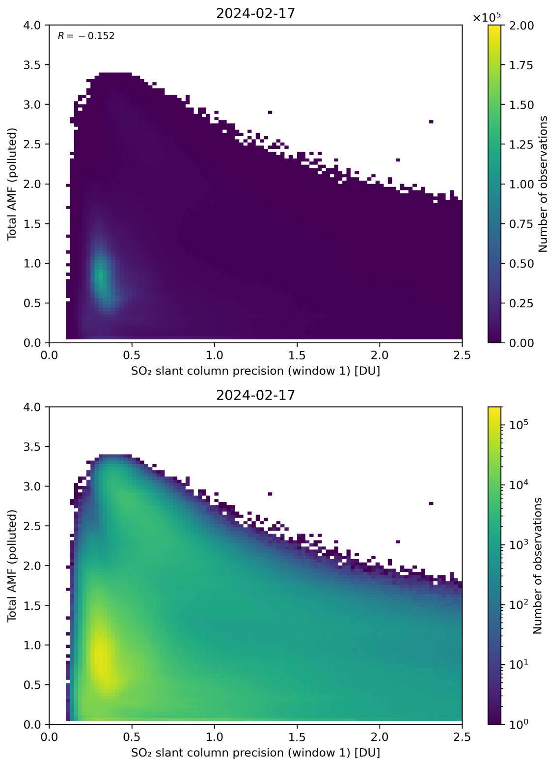
Figure 230: Scatter density plot of “SO 2 slant column precision (window 1)” against “Total AMF (polluted)” for 2024-02-17 to 2024-02-18.
