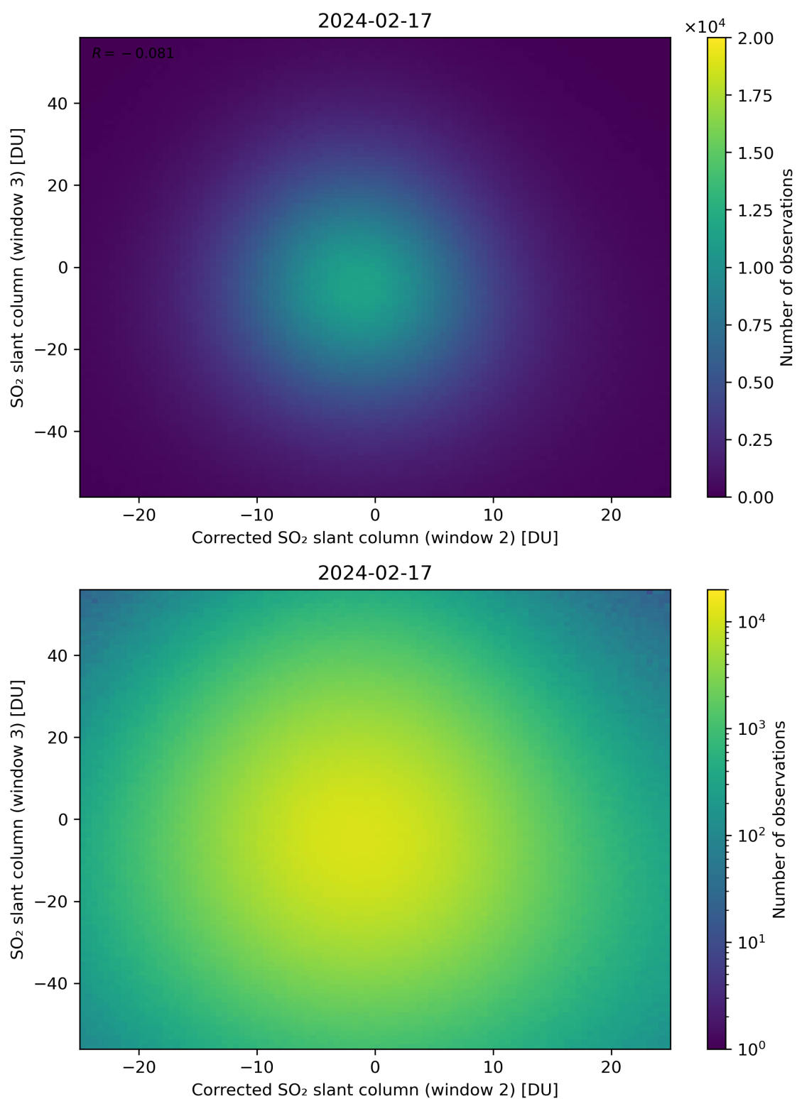
Figure 201: Scatter density plot of “Corrected SO 2 slant column (window 2)” against “SO 2 slant column (window 3)” for 2024-02-17 to 2024-02-18.
