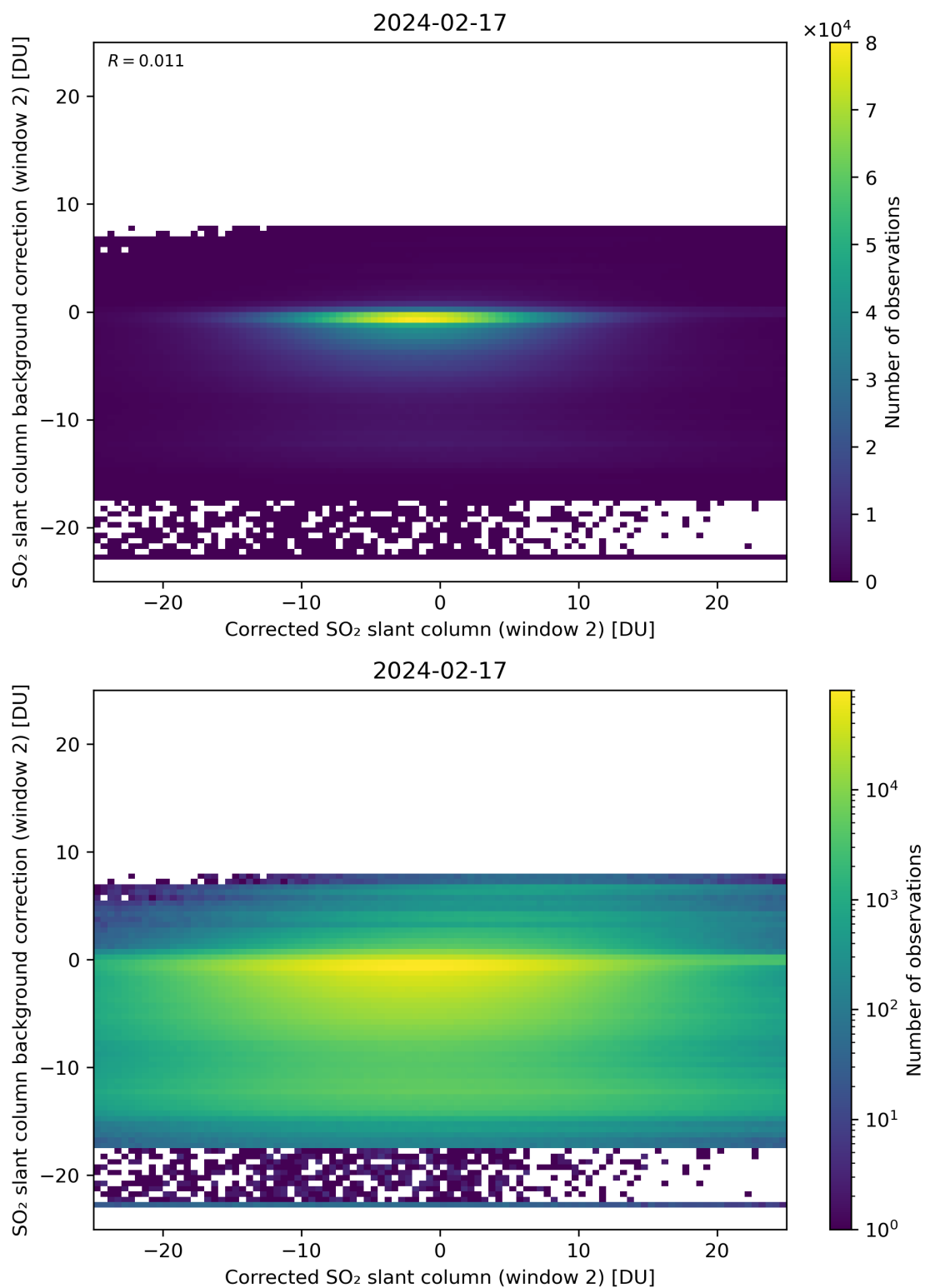
Figure 194: Scatter density plot of “Corrected SO 2 slant column (window 2)” against “SO 2 slant column background correction (window 2)” for 2024-02-17 to 2024-02-18.
