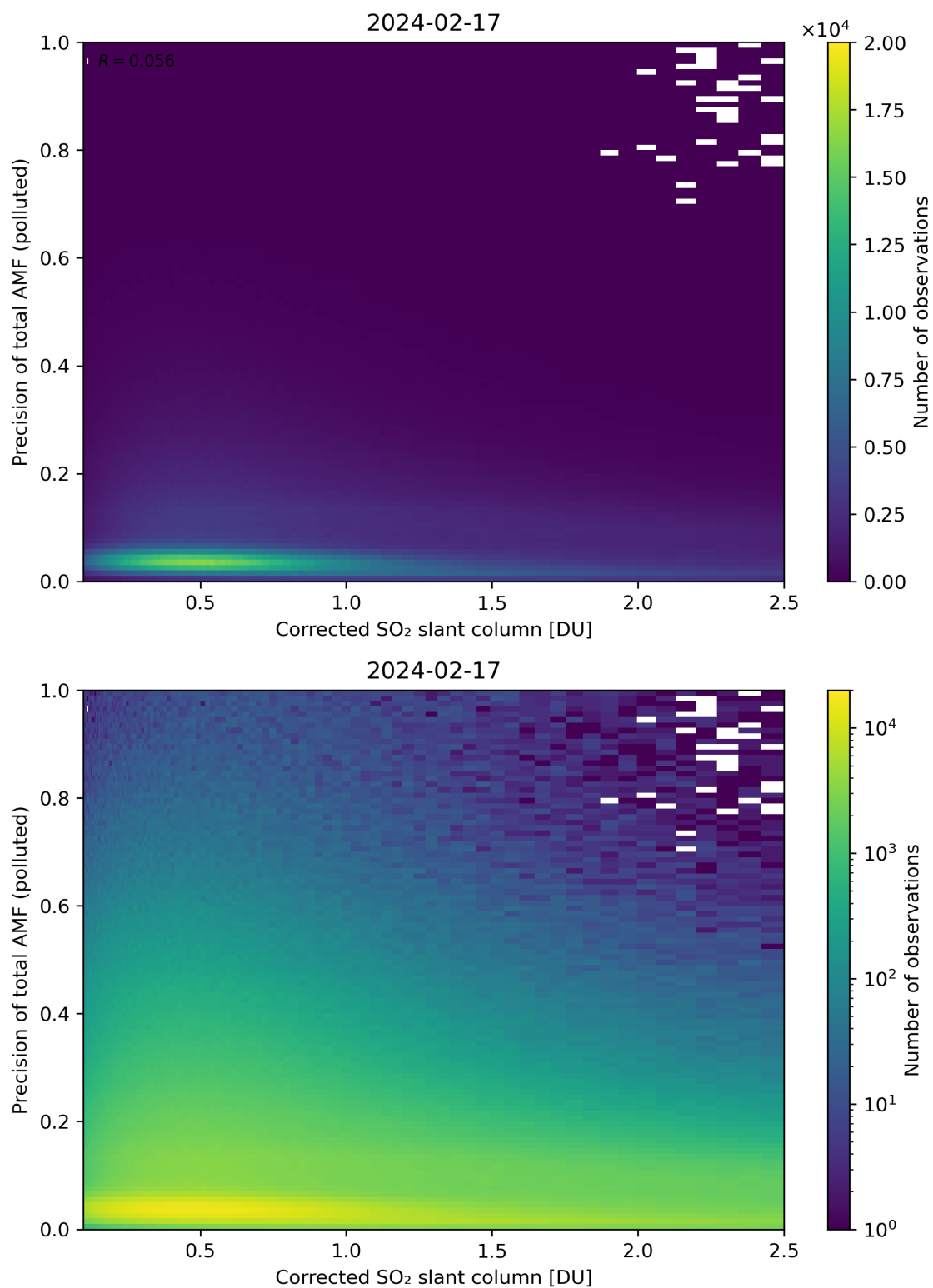
Figure 193: Scatter density plot of “Corrected SO 2 slant column” against “Precision of total AMF (polluted)” for 2024-02-17 to 2024-02-18.
