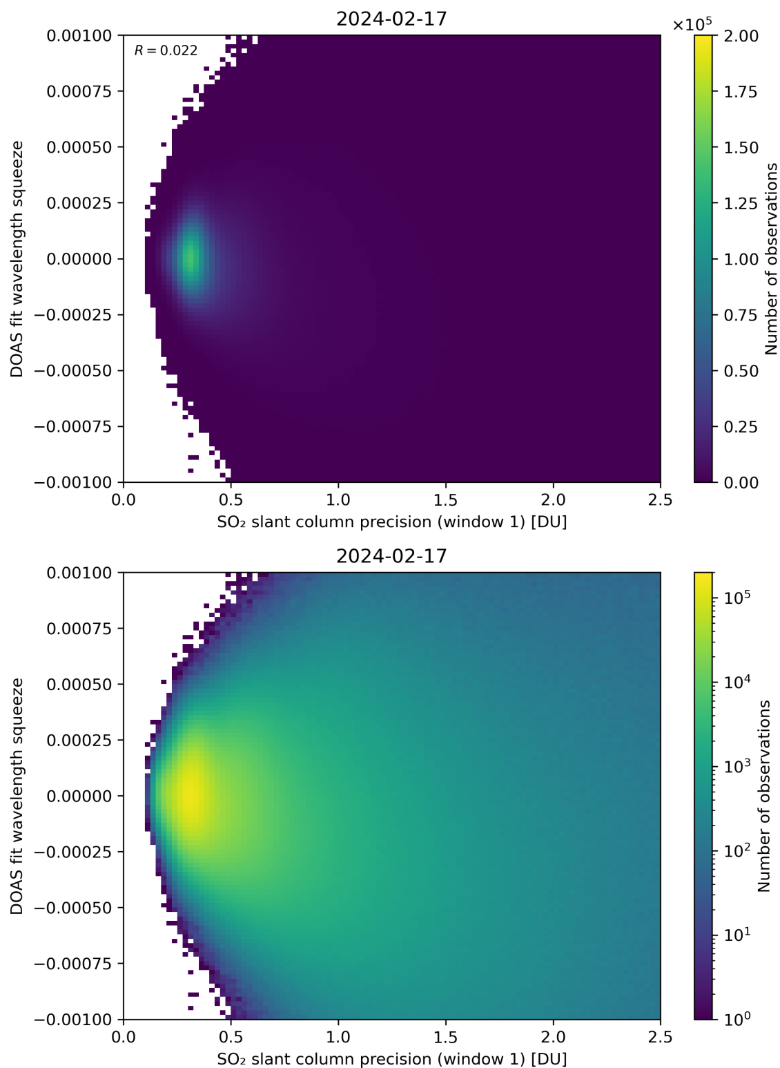
Figure 222: Scatter density plot of “SO 2 slant column precision (window 1)” against “DOAS fit wavelength squeeze” for 2024-02-17 to 2024-02-18.
