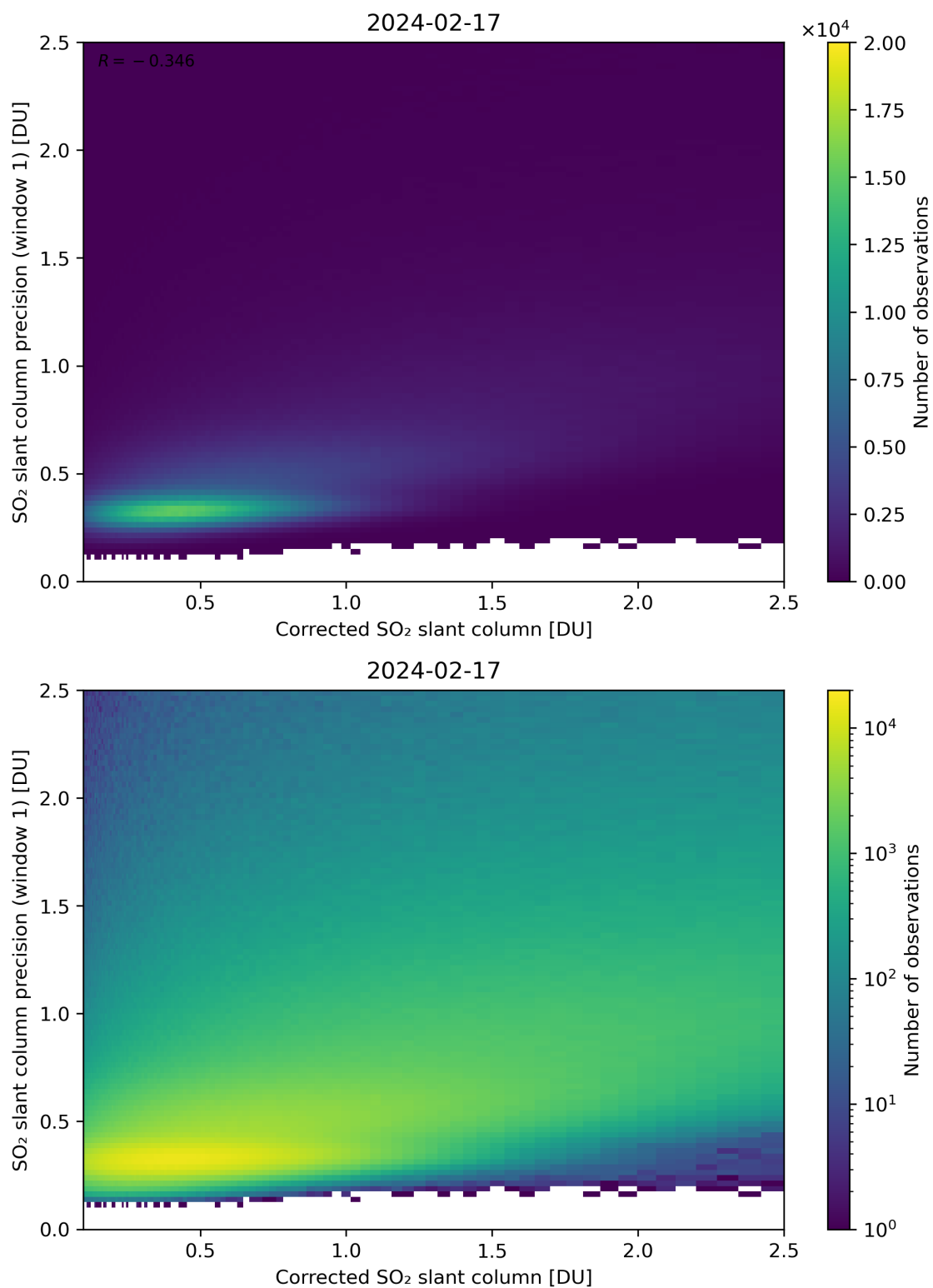
Figure 188: Scatter density plot of “Corrected SO 2 slant column” against “SO 2 slant column precision (window 1)” for 2024-02-17 to 2024-02-18.
