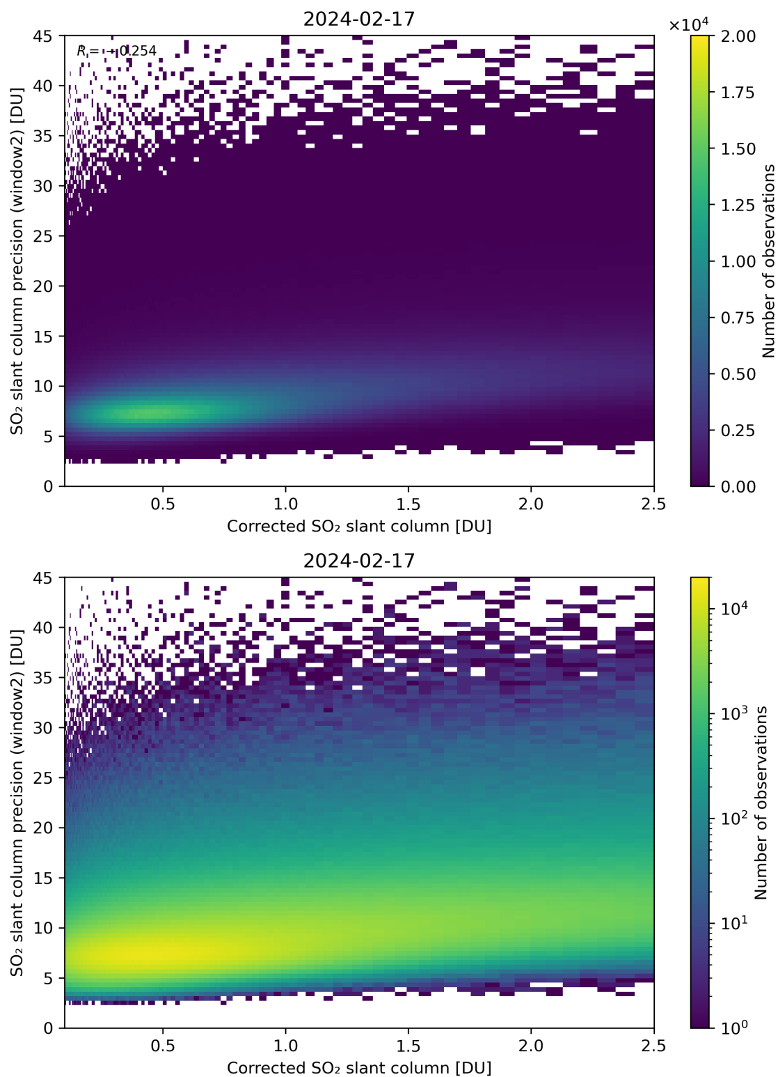
Figure 189: Scatter density plot of “Corrected SO 2 slant column” against “SO 2 slant column precision (window2)” for 2024-02-17 to 2024-02-18.
