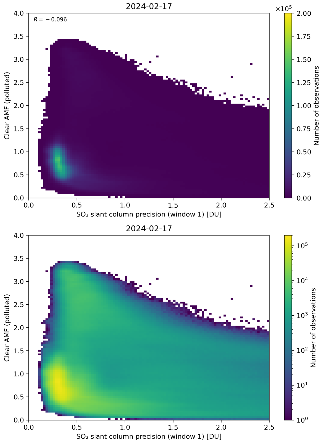
Figure 224: Scatter density plot of “SO 2 slant column precision (window 1)” against “Clear AMF (polluted)” for 2024-02-17 to 2024-02-18.
