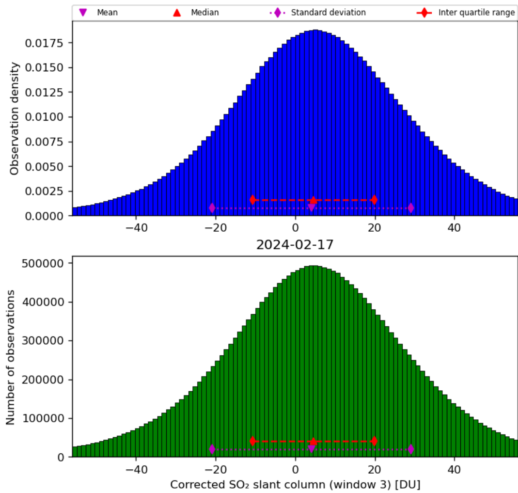
Figure 66: Histogram of “Corrected SO 2 slant column (window 3)” for 2024-02-17 to 2024-02-18
