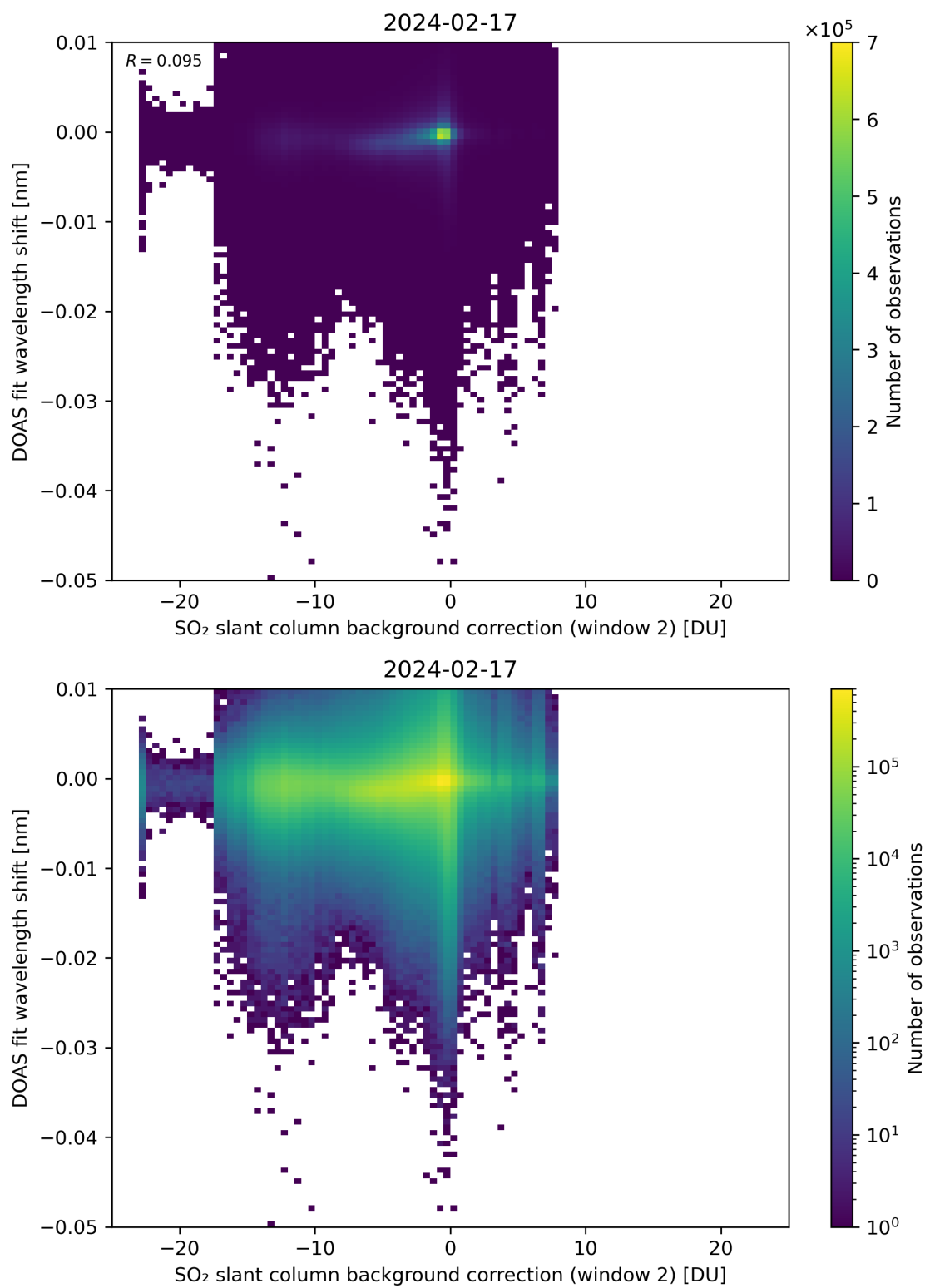
Figure 112: Scatter density plot of “SO 2 slant column background correction (window 2)” against “DOAS fit wavelength shift” for 2024-02-17 to 2024-02-18.
