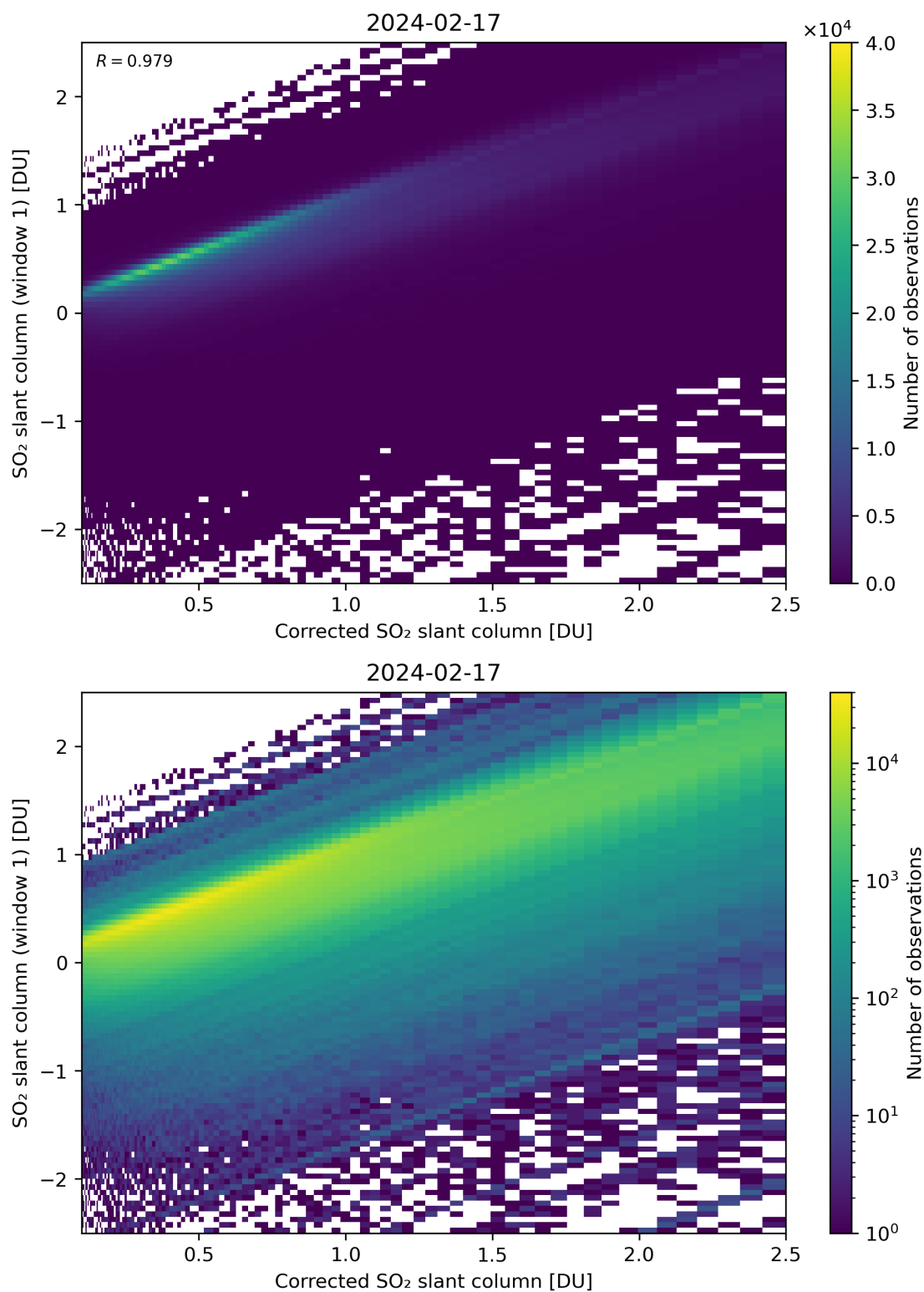
Figure 187: Scatter density plot of “Corrected SO 2 slant column” against “SO 2 slant column (window 1)” for 2024-02-17 to 2024-02-18.
