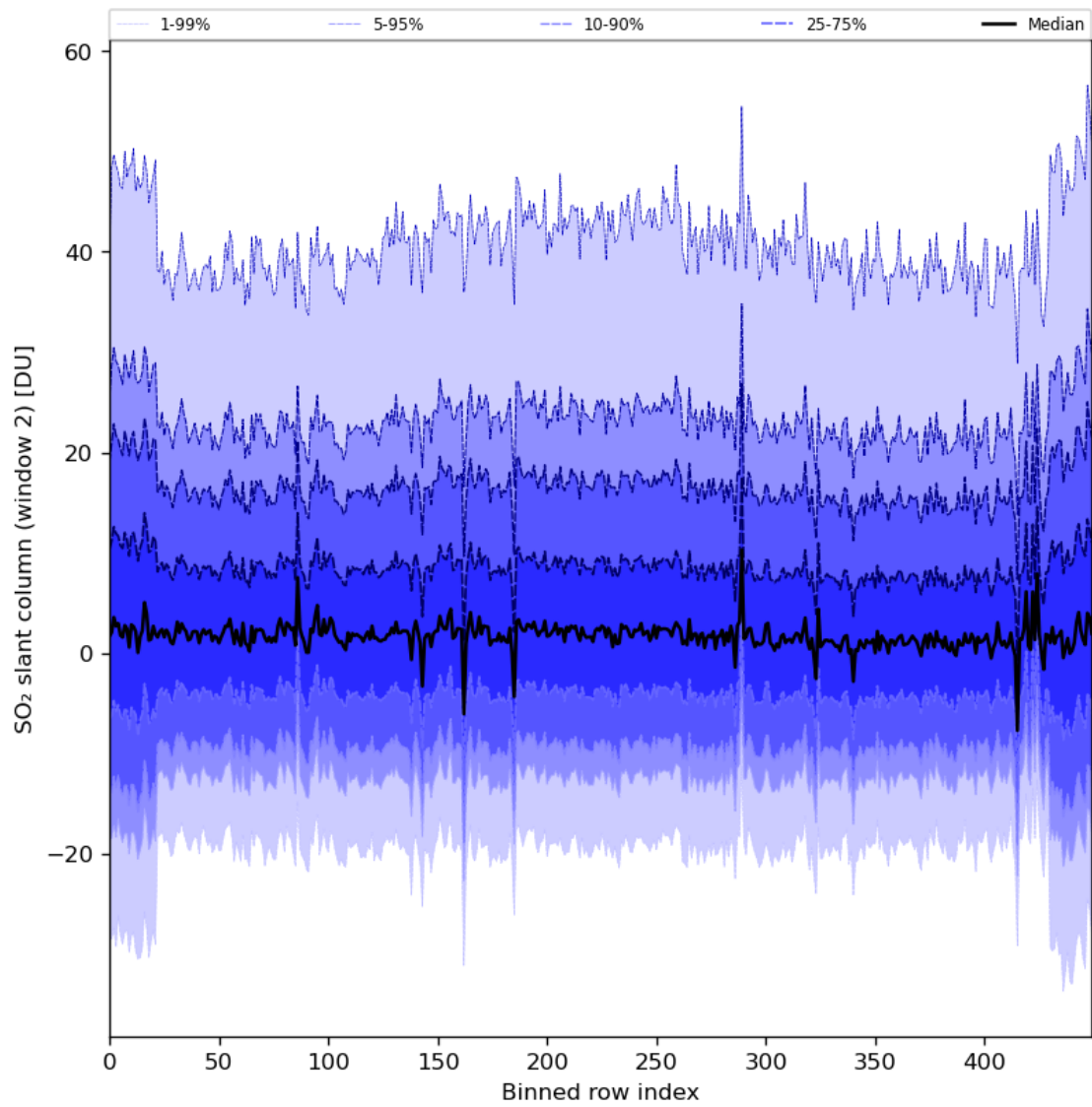
Figure 83: Along track statistics of “SO 2 slant column (window 2)” for 2024-02-17 to 2024-02-18
