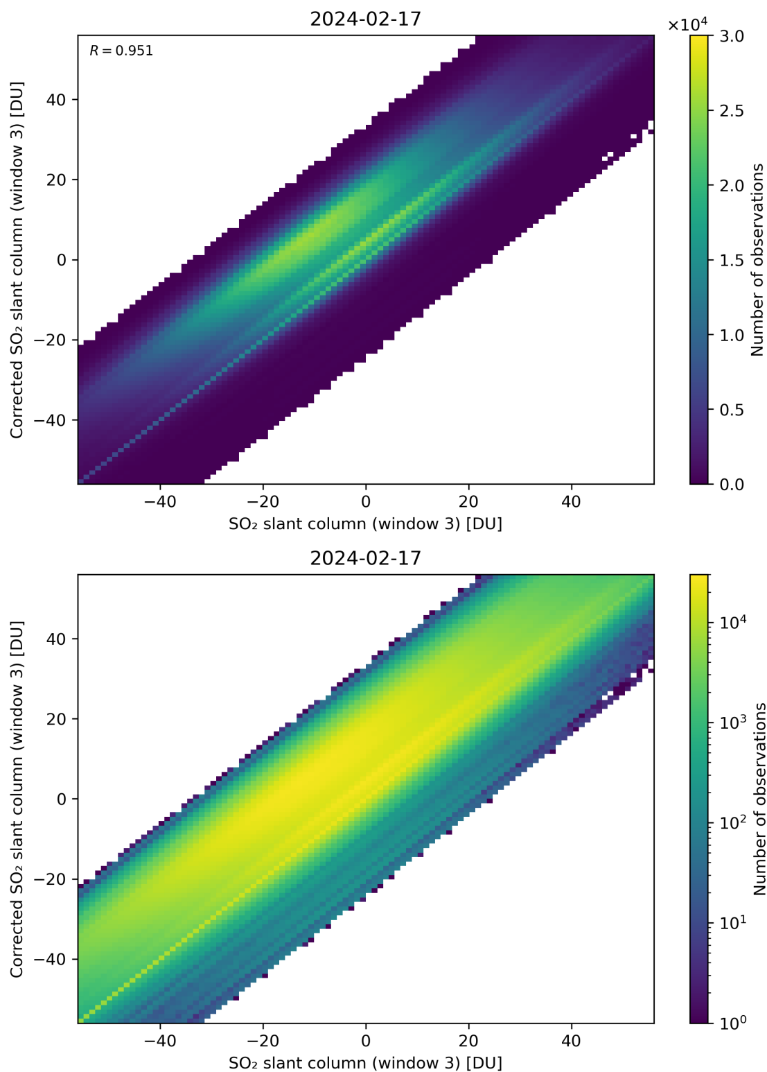
Figure 266: Scatter density plot of “SO 2 slant column (window 3)” against “Corrected SO 2 slant column (window 3)” for 2024-02-17 to 2024-02-18.
