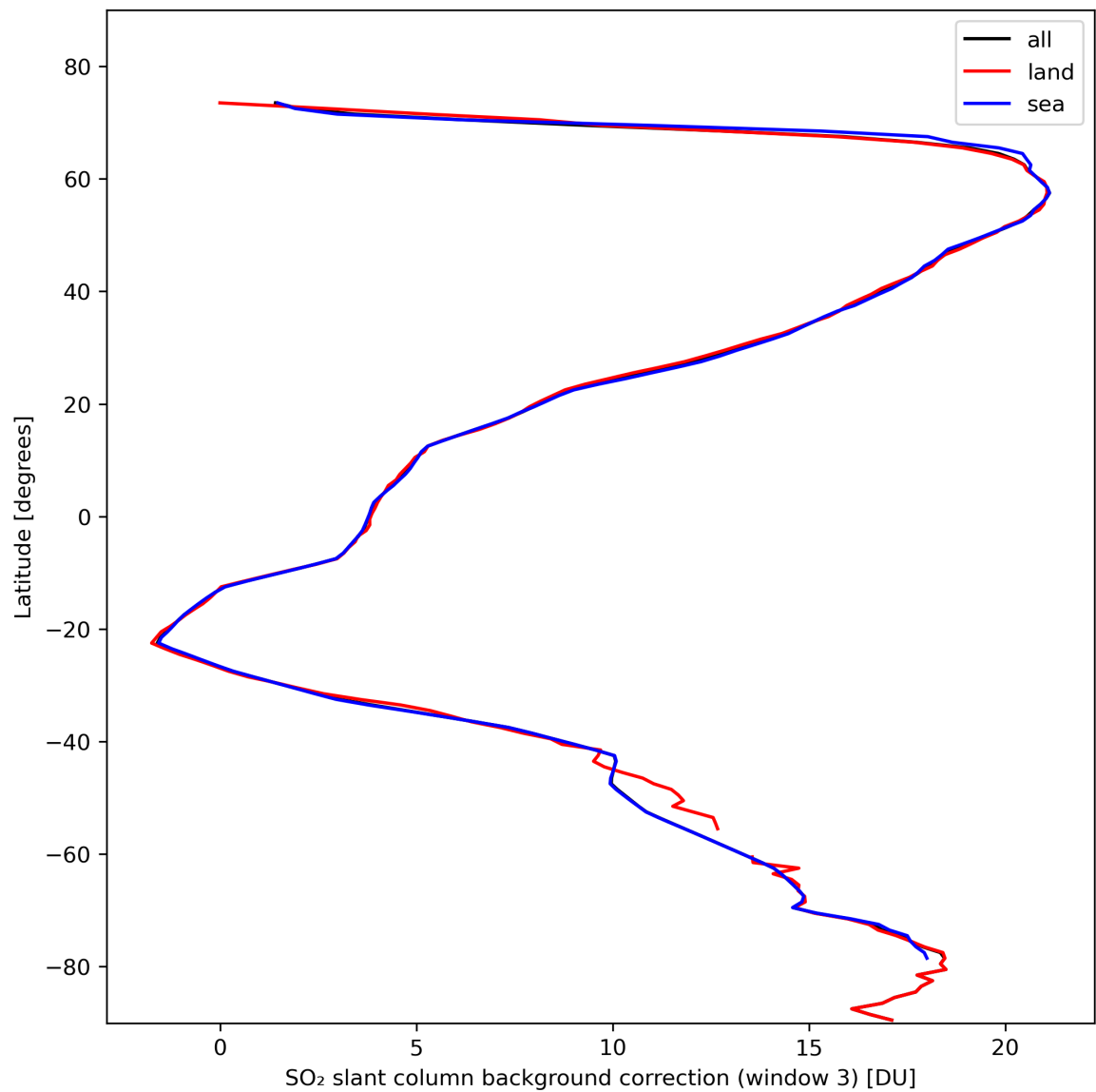
Figure 44: Zonal average of “SO 2 slant column background correction (window 3)” for 2024-02-17 to 2024-02-18.
