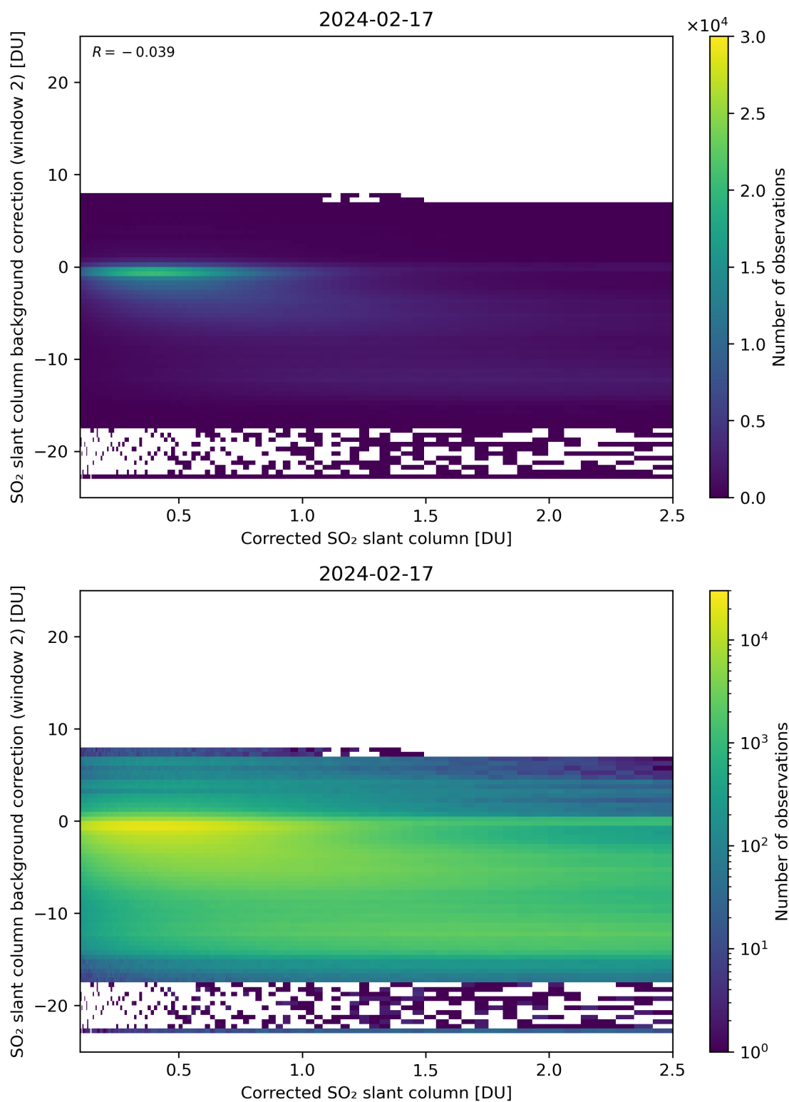
Figure 179: Scatter density plot of “Corrected SO 2 slant column” against “SO 2 slant column background correction (window 2)” for 2024-02-17 to 2024-02-18.
