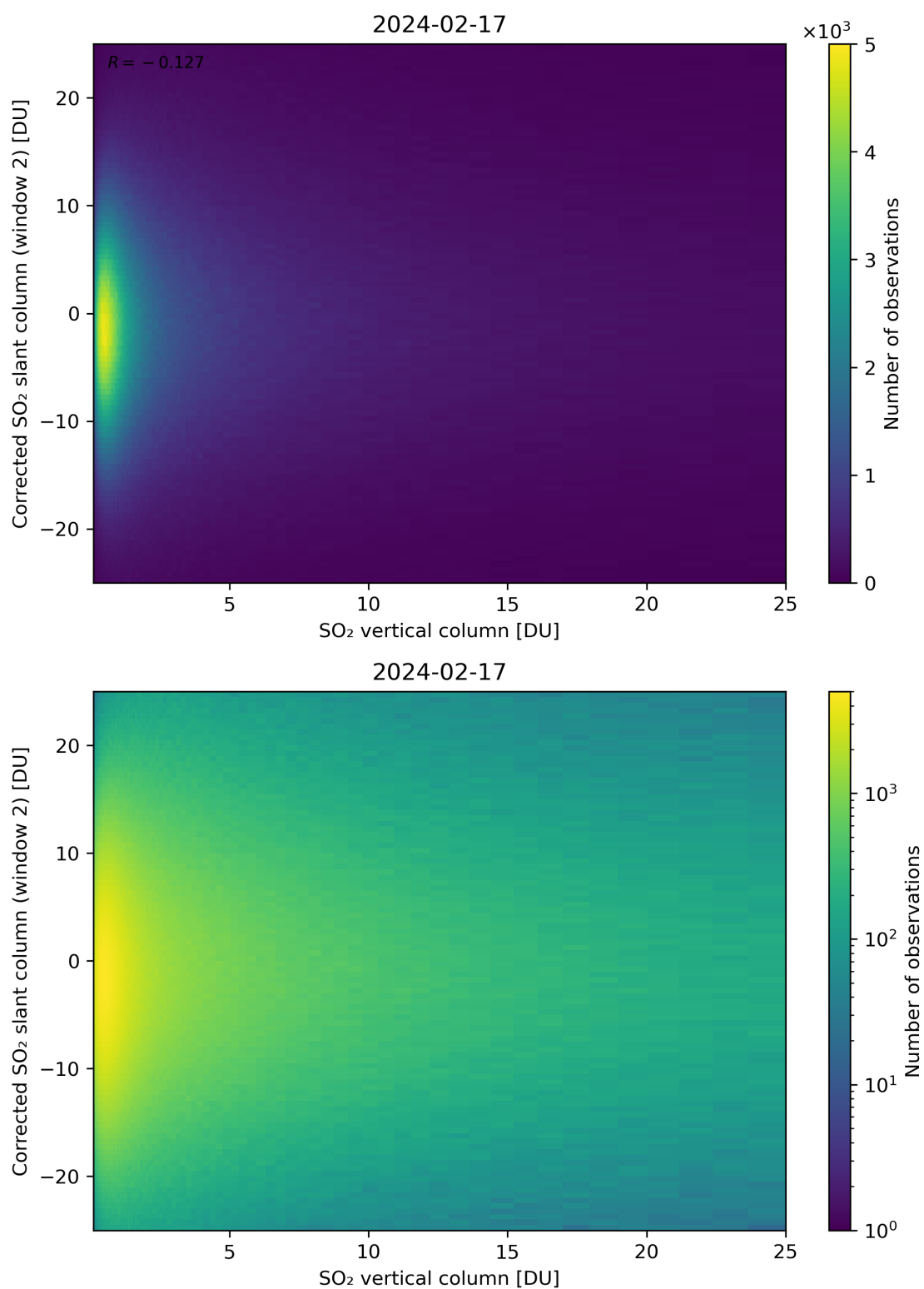
Figure 298: Scatter density plot of “SO 2 vertical column” against “Corrected SO 2 slant column (window 2)” for 2024-02-17 to 2024-02-18.
