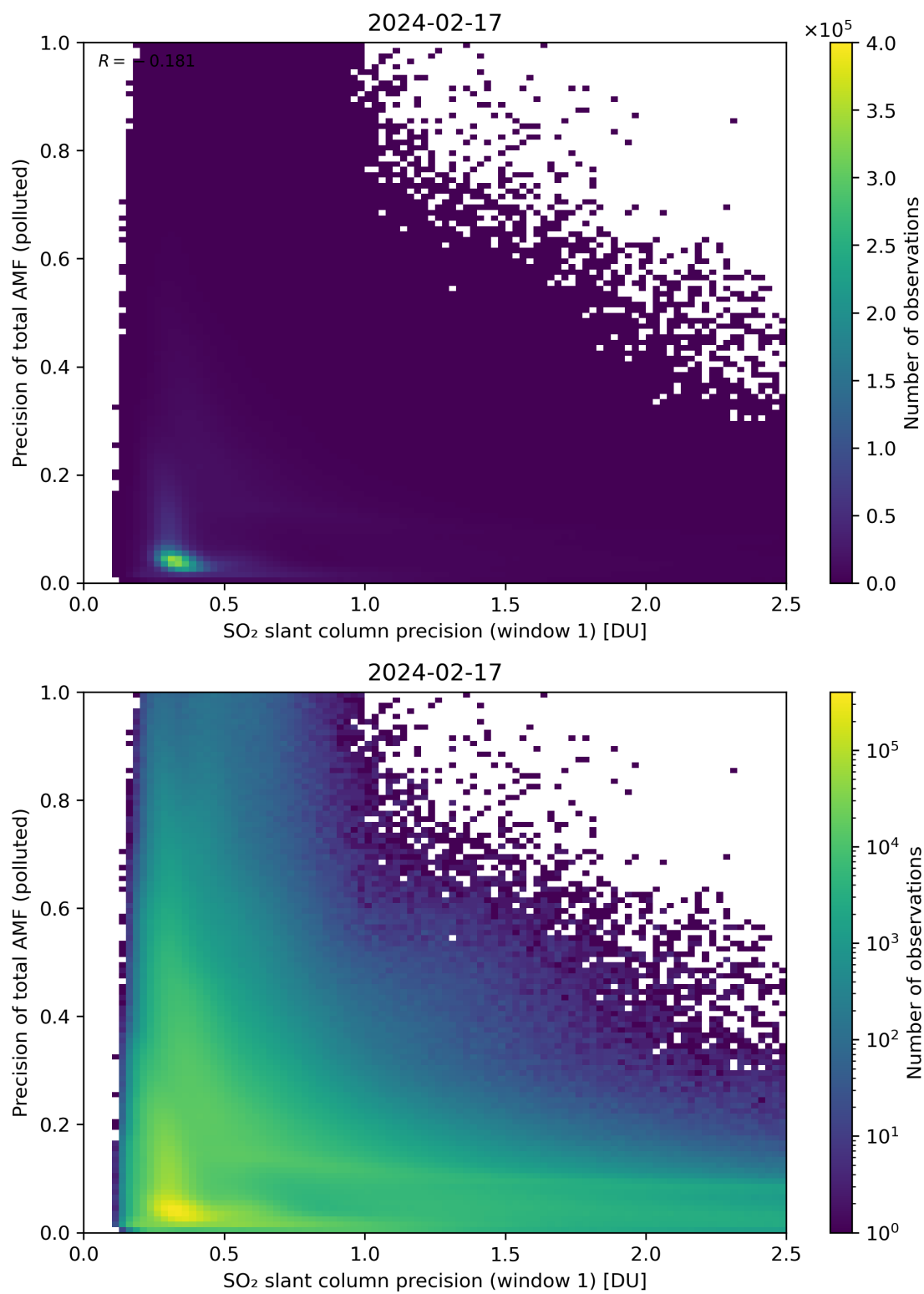
Figure 231: Scatter density plot of “SO 2 slant column precision (window 1)” against “Precision of total AMF (polluted)” for 2024-02-17 to 2024-02-18.
