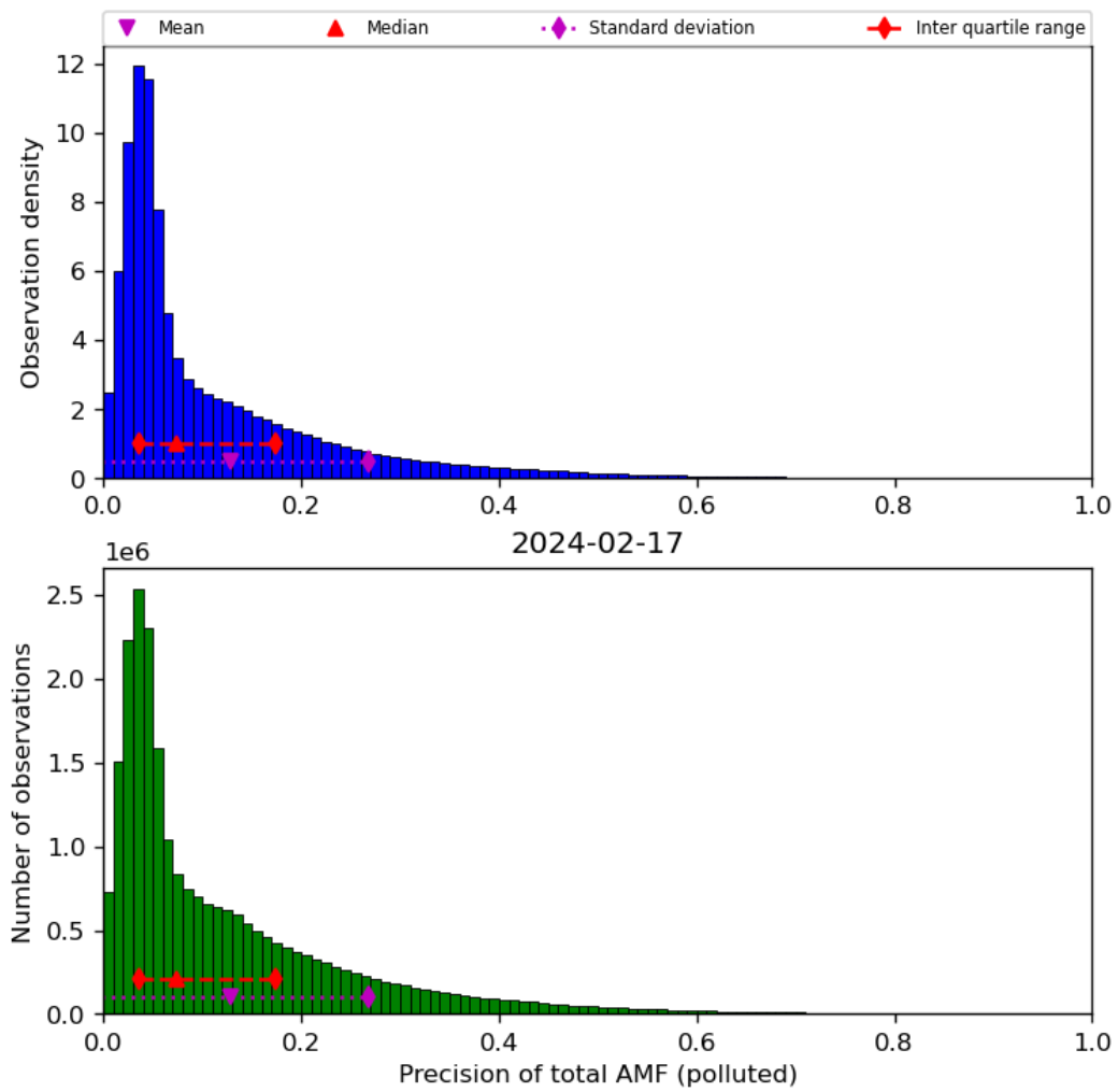
Figure 72: Histogram of “Precision of total AMF (polluted)” for 2024-02-17 to 2024-02-18
