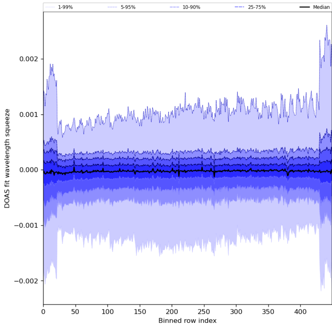
Figure 92: Along track statistics of “DOAS fit wavelength squeeze” for 2024-02-17 to 2024-02-18
