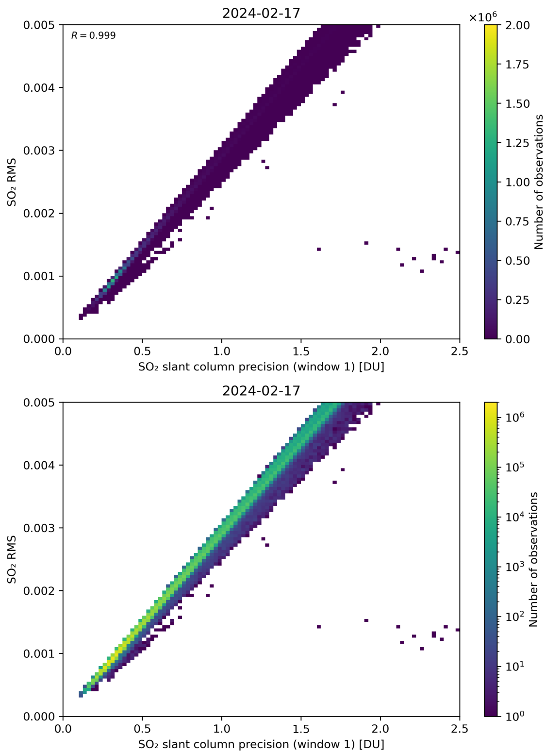
Figure 223: Scatter density plot of “SO 2 slant column precision (window 1)” against “SO 2 RMS” for 2024-02-17 to 2024-02-18.
