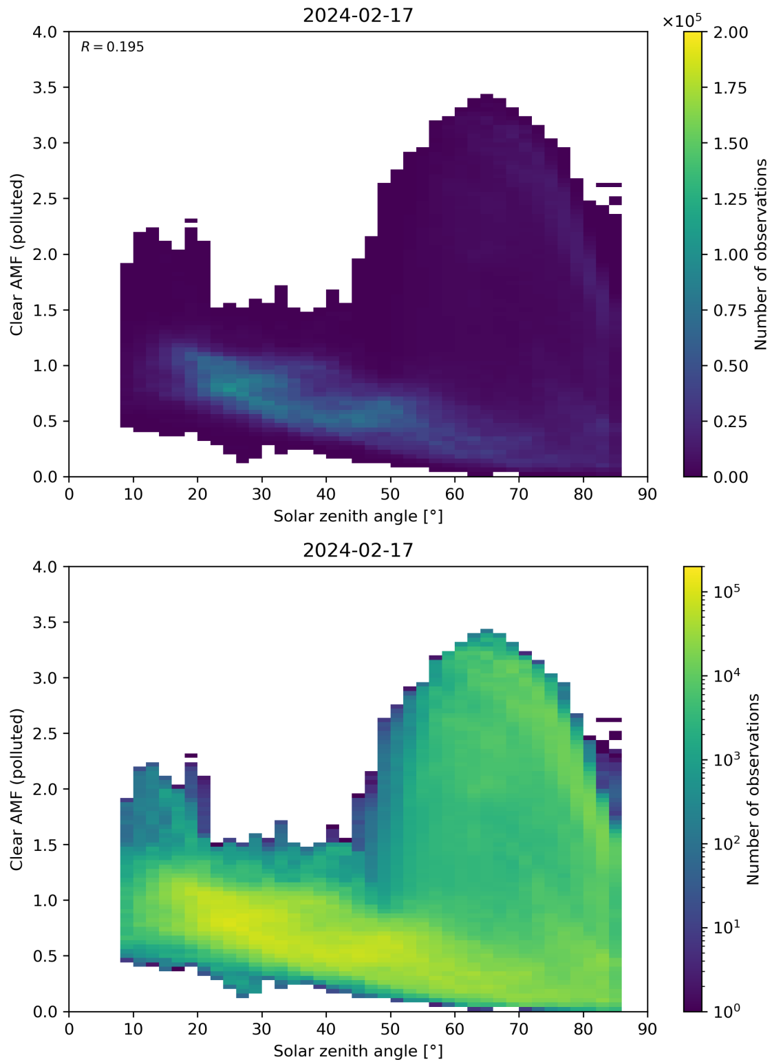
Figure 165: Scatter density plot of “Solar zenith angle” against “Clear AMF (polluted)” for 2024-02-17 to 2024-02-18.
