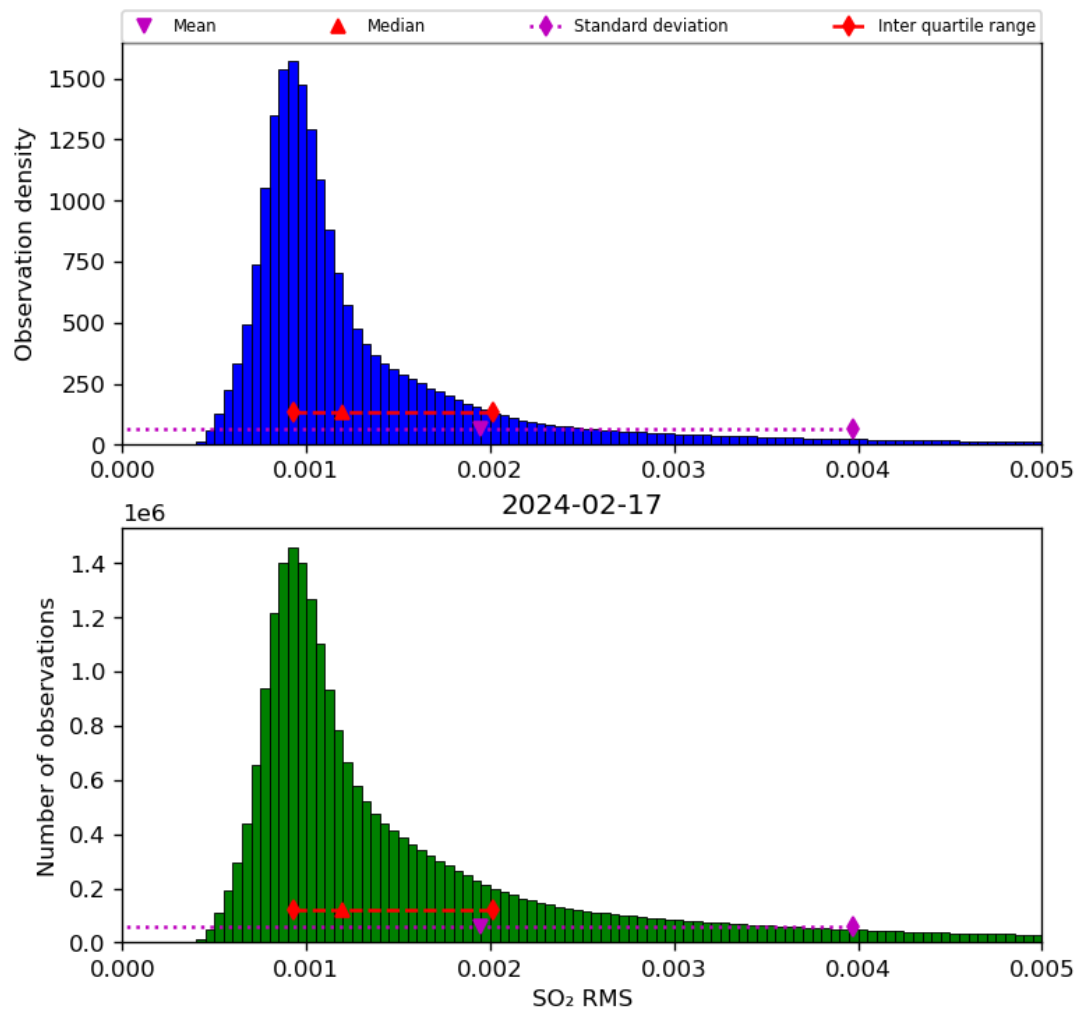
Figure 70: Histogram of “SO 2 RMS” for 2024-02-17 to 2024-02-18
