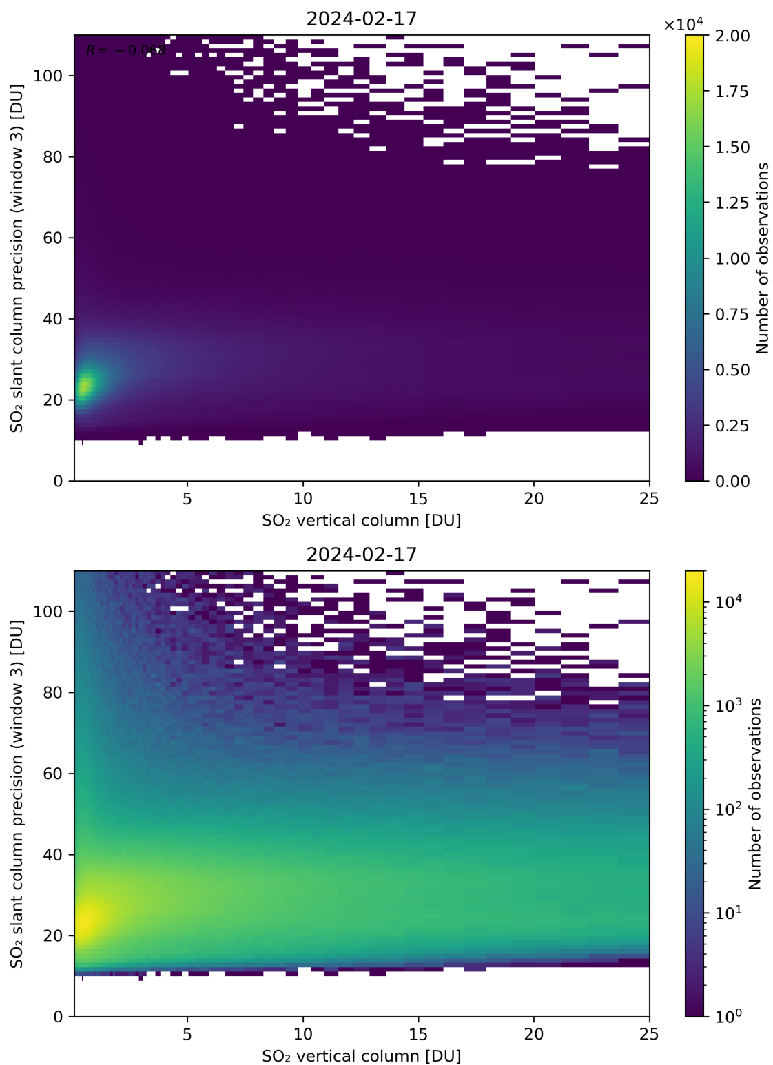
Figure 304: Scatter density plot of “SO 2 vertical column” against “SO 2 slant column precision (window 3)” for 2024-02-17 to 2024-02-18.
