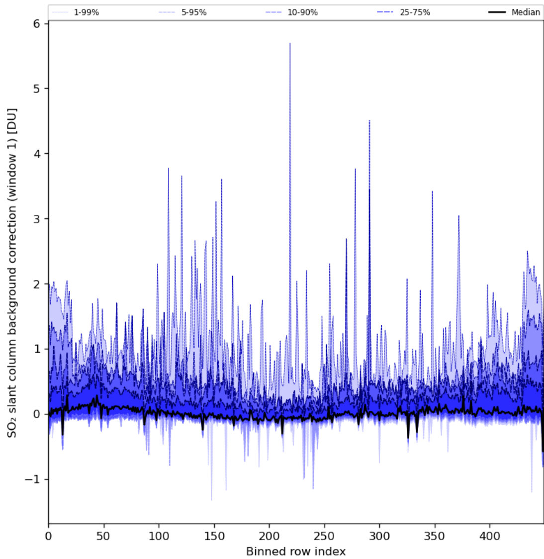
Figure 82: Along track statistics of “SO 2 slant column background correction (window 1)” for 2024-02-17 to 2024-02-18
