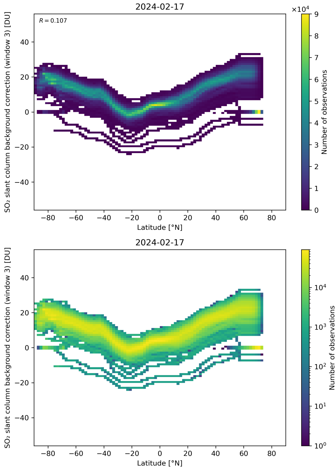
Figure 141: Scatter density plot of “Latitude” against “SO 2 slant column background correction (window 3)” for 2024-02-17 to 2024-02-18.
