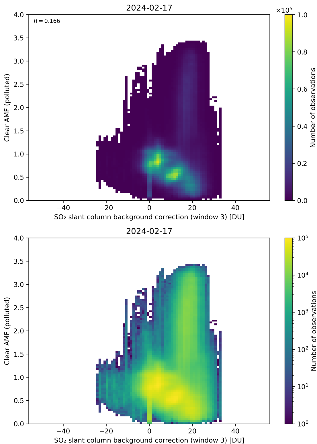
Figure 124: Scatter density plot of “SO 2 slant column background correction (window 3)” against “Clear AMF (polluted)” for 2024-02-17 to 2024-02-18.
