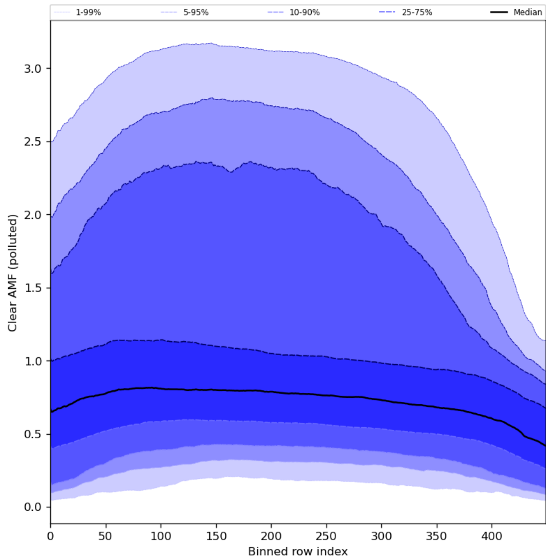
Figure 96: Along track statistics of “Clear AMF (polluted)” for 2024-02-17 to 2024-02-18
