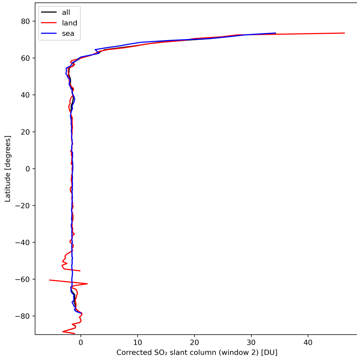
Figure 39: Zonal average of “Corrected SO 2 slant column (window 2)” for 2024-02-17 to 2024-02-18.
