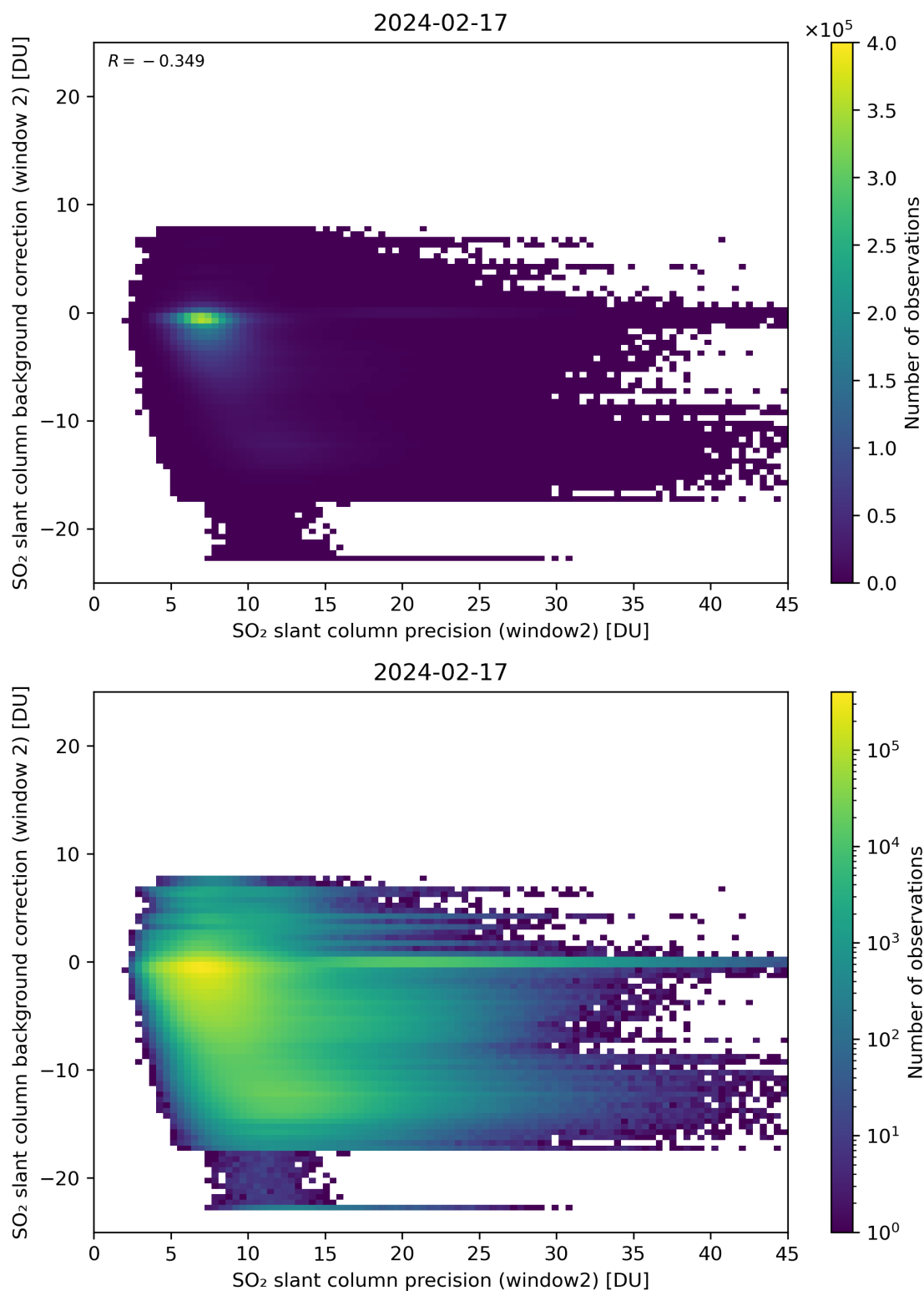
Figure 241: Scatter density plot of “SO 2 slant column precision (window2)” against “SO 2 slant column background correction (window 2)” for 2024-02-17 to 2024-02-18.
