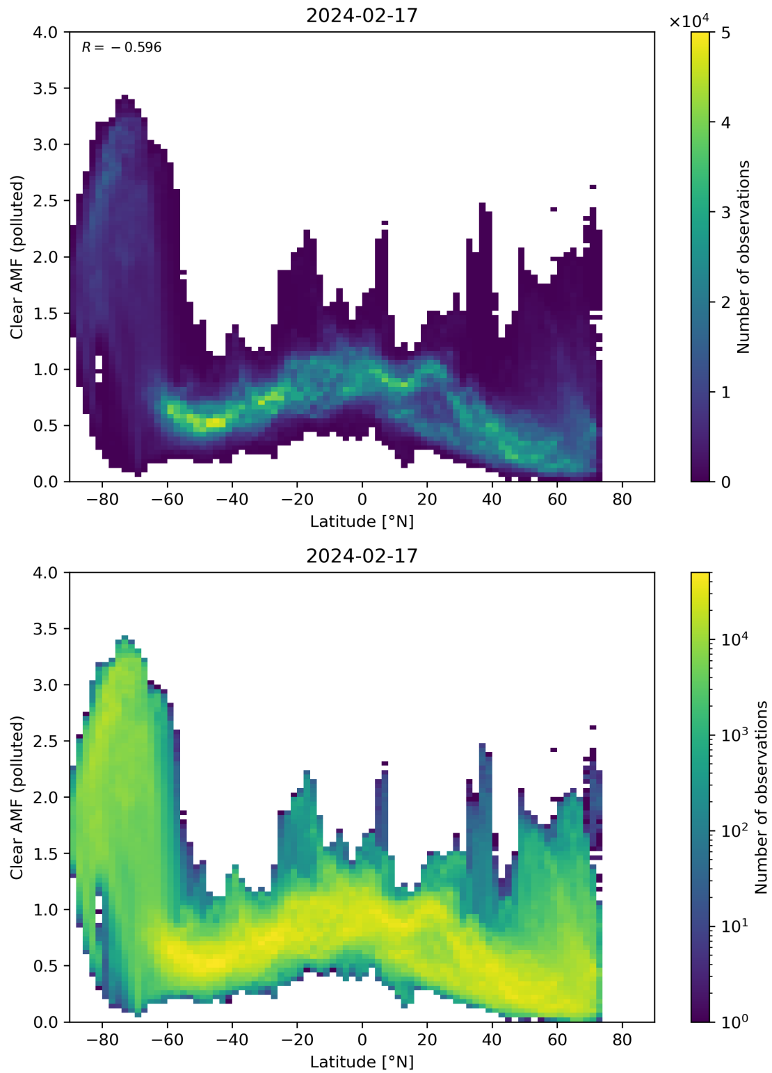
Figure 145: Scatter density plot of “Latitude” against “Clear AMF (polluted)” for 2024-02-17 to 2024-02-18.
