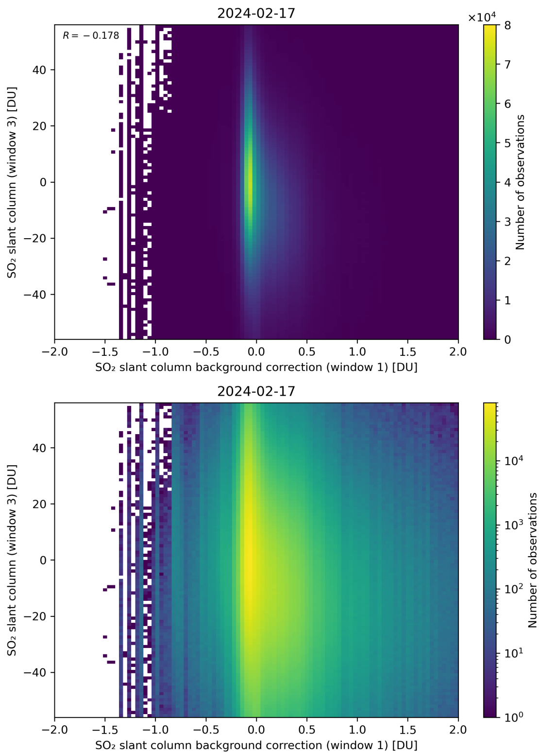
Figure 107: Scatter density plot of “SO 2 slant column background correction (window 1)” against “SO 2 slant column (window 3)” for 2024-02-17 to 2024-02-18.
