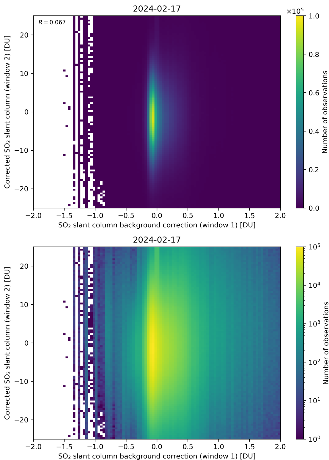
Figure 104: Scatter density plot of “SO 2 slant column background correction (window 1)” against “Corrected SO 2 slant column (window 2)” for 2024-02-17 to 2024-02-18.
