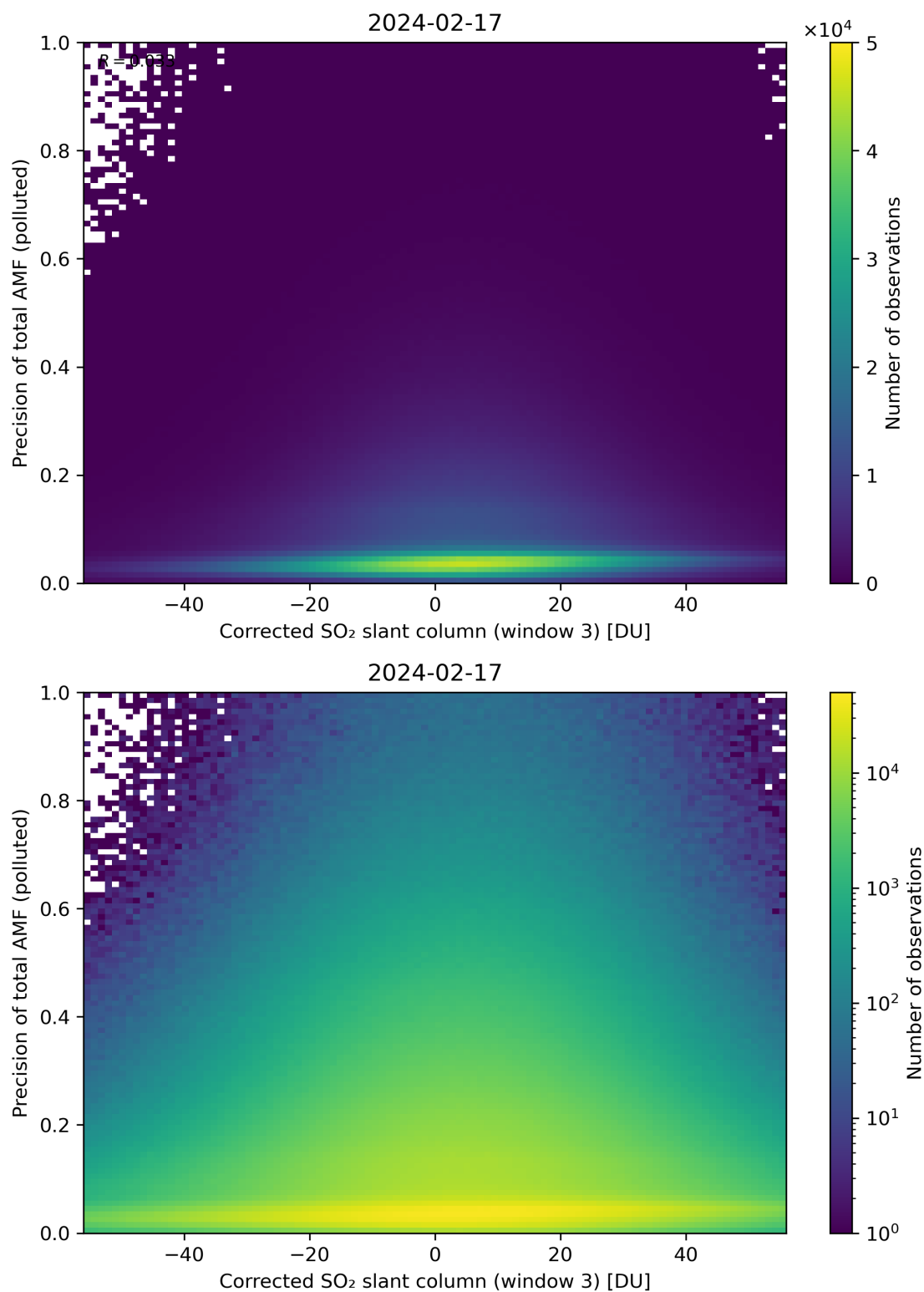
Figure 211: Scatter density plot of “Corrected SO 2 slant column (window 3)” against “Precision of total AMF (polluted)” for 2024-02-17 to 2024-02-18.
