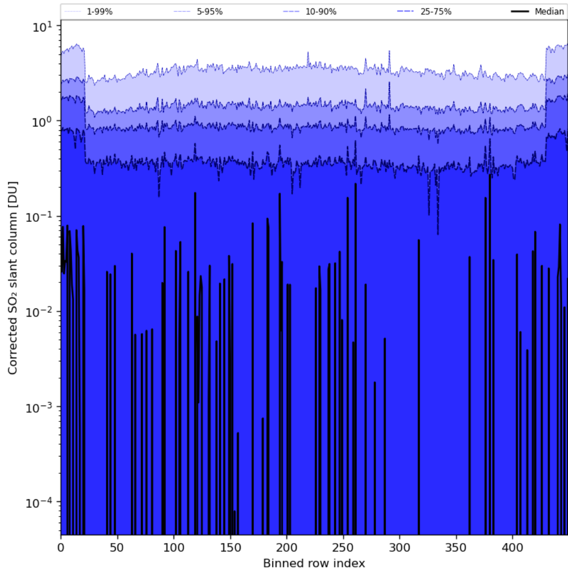
Figure 78: Along track statistics of “Corrected SO 2 slant column” for 2024-02-17 to 2024-02-18
