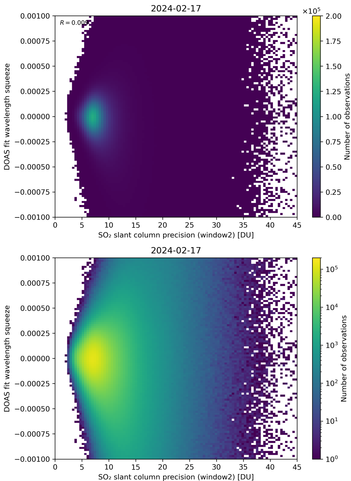
Figure 244: Scatter density plot of “SO 2 slant column precision (window2)” against “DOAS fit wavelength squeeze” for 2024-02-17 to 2024-02-18.
