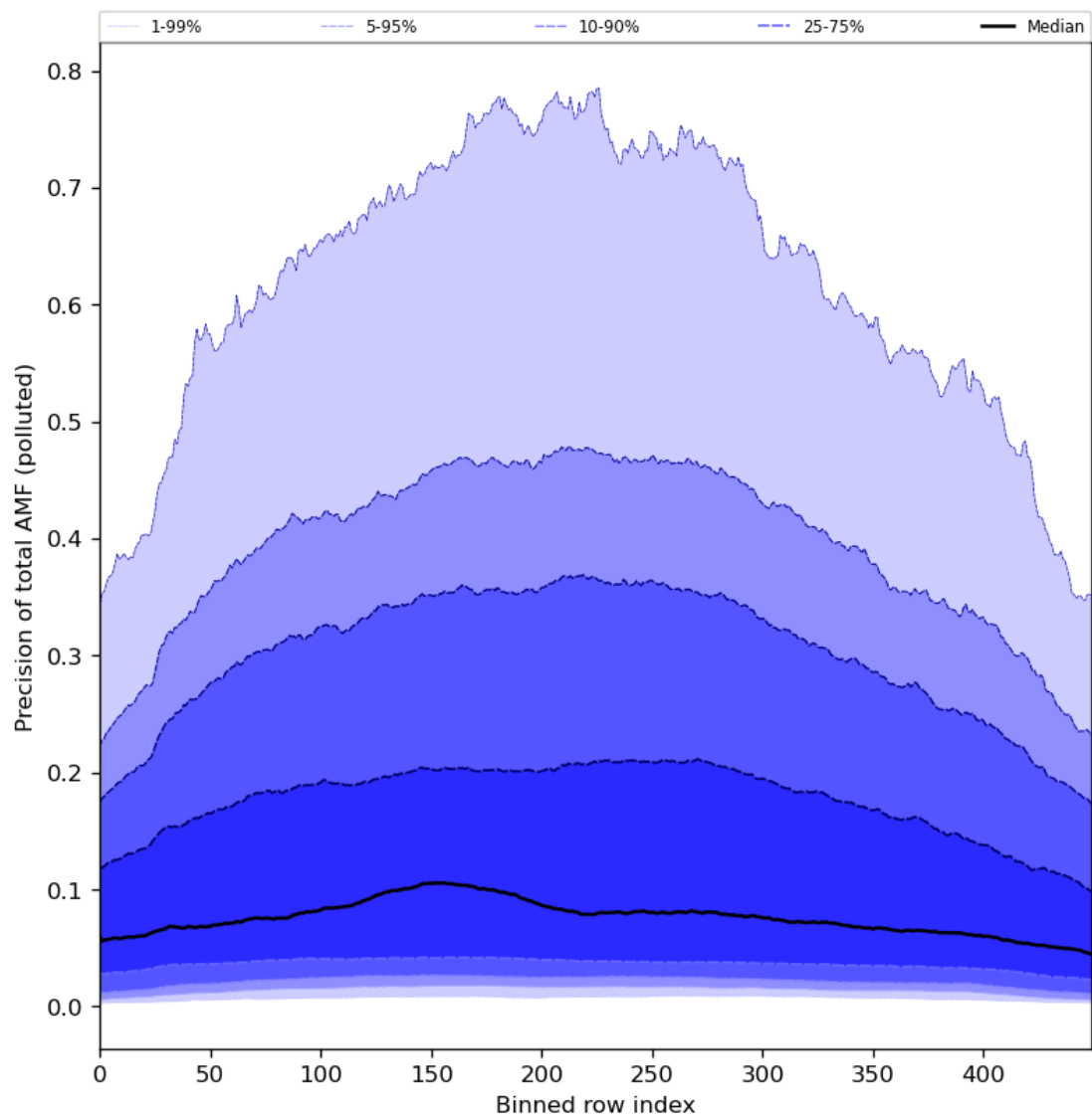
Figure 95: Along track statistics of “Precision of total AMF (polluted)” for 2024-02-17 to 2024-02-18
