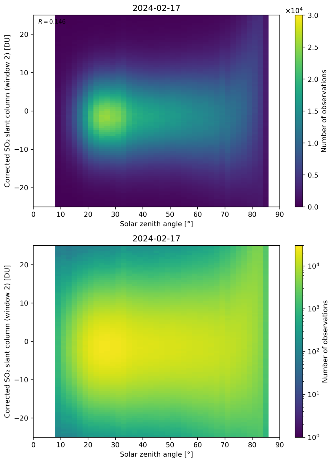
Figure 167: Scatter density plot of “Solar zenith angle” against “Corrected SO 2 slant column (window 2)” for 2024-02-17 to 2024-02-18.
