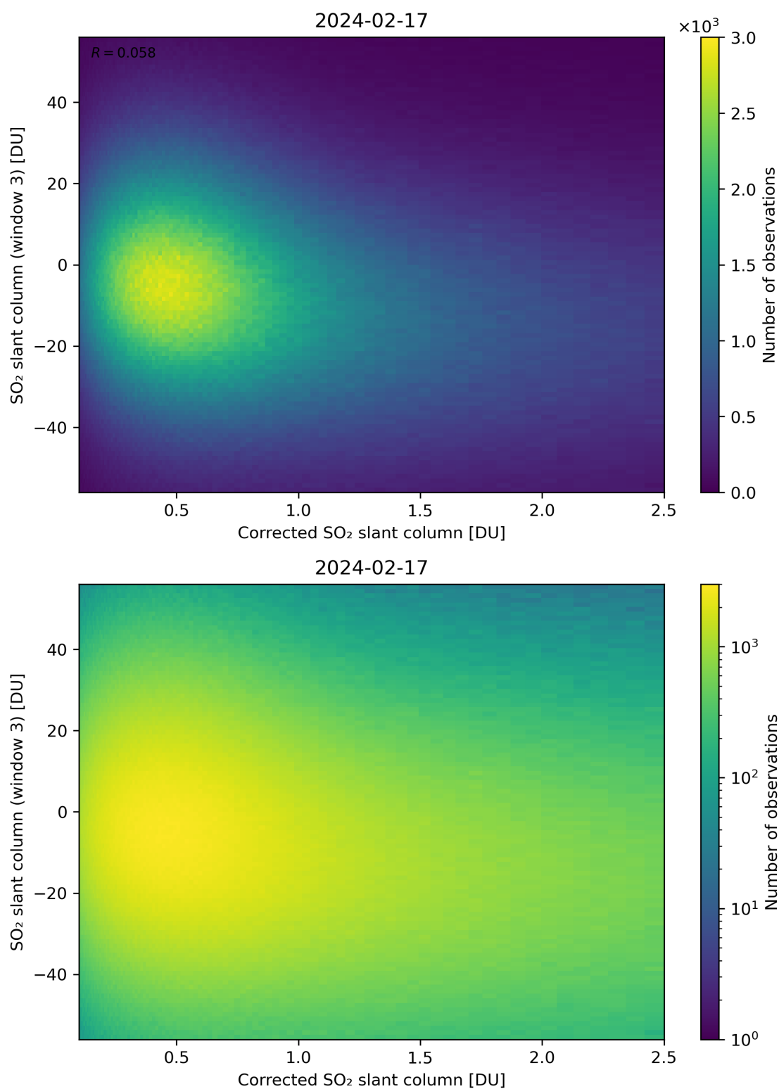
Figure 190: Scatter density plot of “Corrected SO 2 slant column” against “SO 2 slant column (window 3)” for 2024-02-17 to 2024-02-18.
