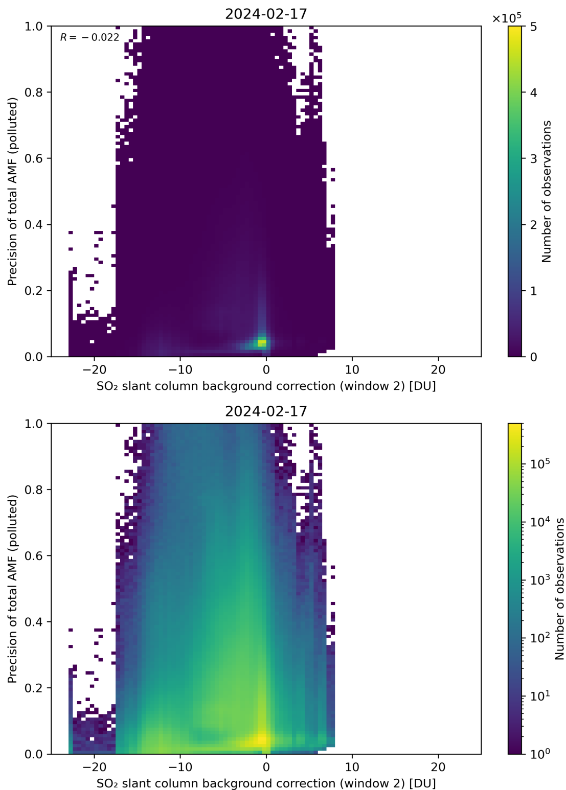
Figure 120: Scatter density plot of “SO 2 slant column background correction (window 2)” against “Precision of total AMF (polluted)” for 2024-02-17 to 2024-02-18.
