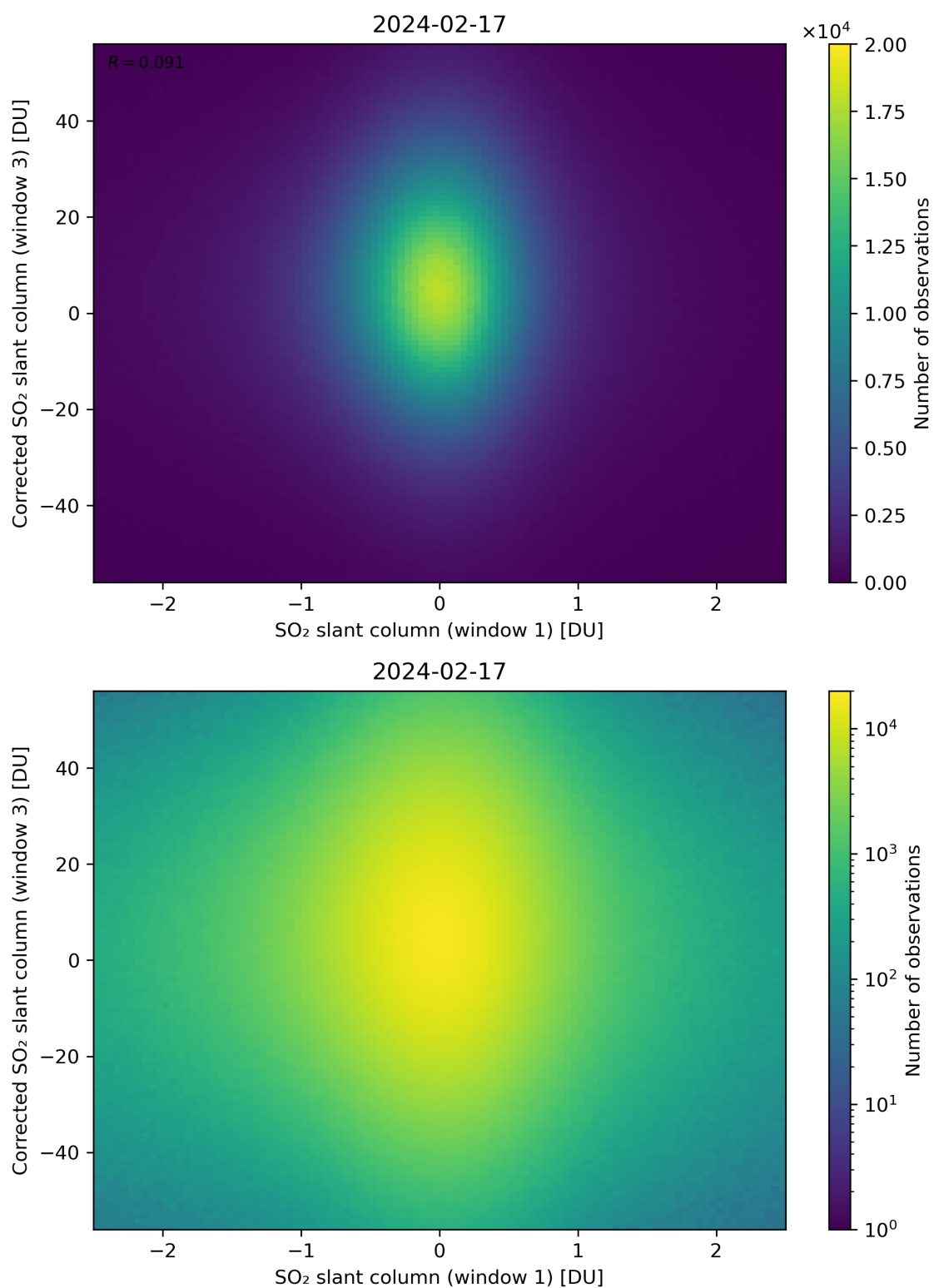
Figure 234: Scatter density plot of “SO 2 slant column (window 1)” against “Corrected SO 2 slant column (window 3)” for 2024-02-17 to 2024-02-18.
