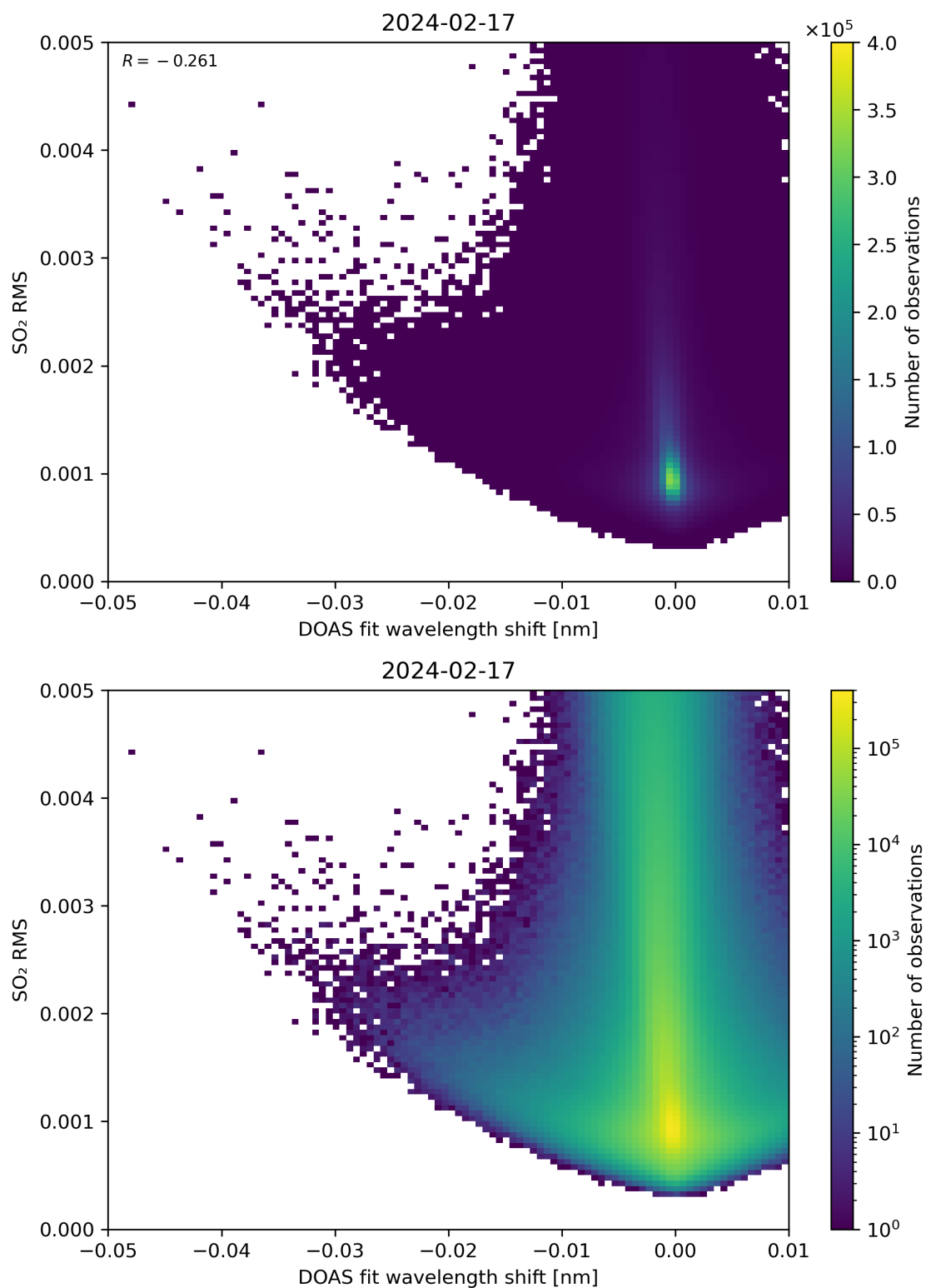
Figure 128: Scatter density plot of “DOAS fit wavelength shift” against “SO 2 RMS” for 2024-02-17 to 2024-02-18.
