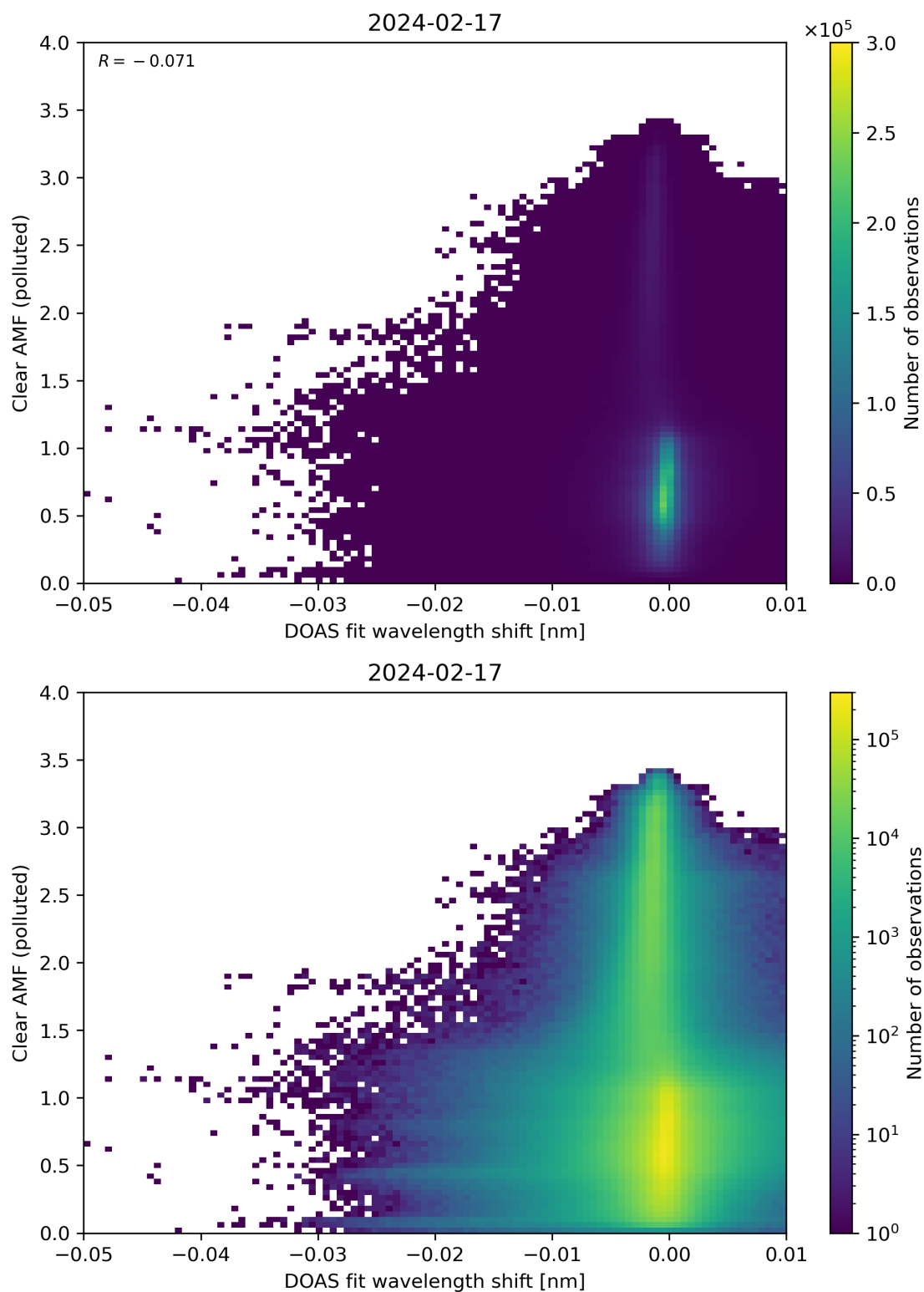
Figure 129: Scatter density plot of “DOAS fit wavelength shift” against “Clear AMF (polluted)” for 2024-02-17 to 2024-02-18.
