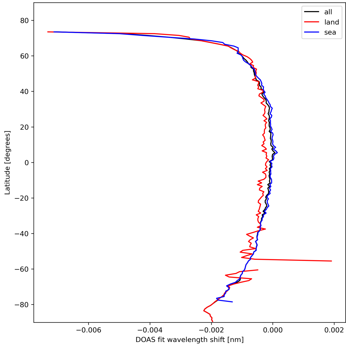
Figure 45: Zonal average of “DOAS fit wavelength shift” for 2024-02-17 to 2024-02-18.
