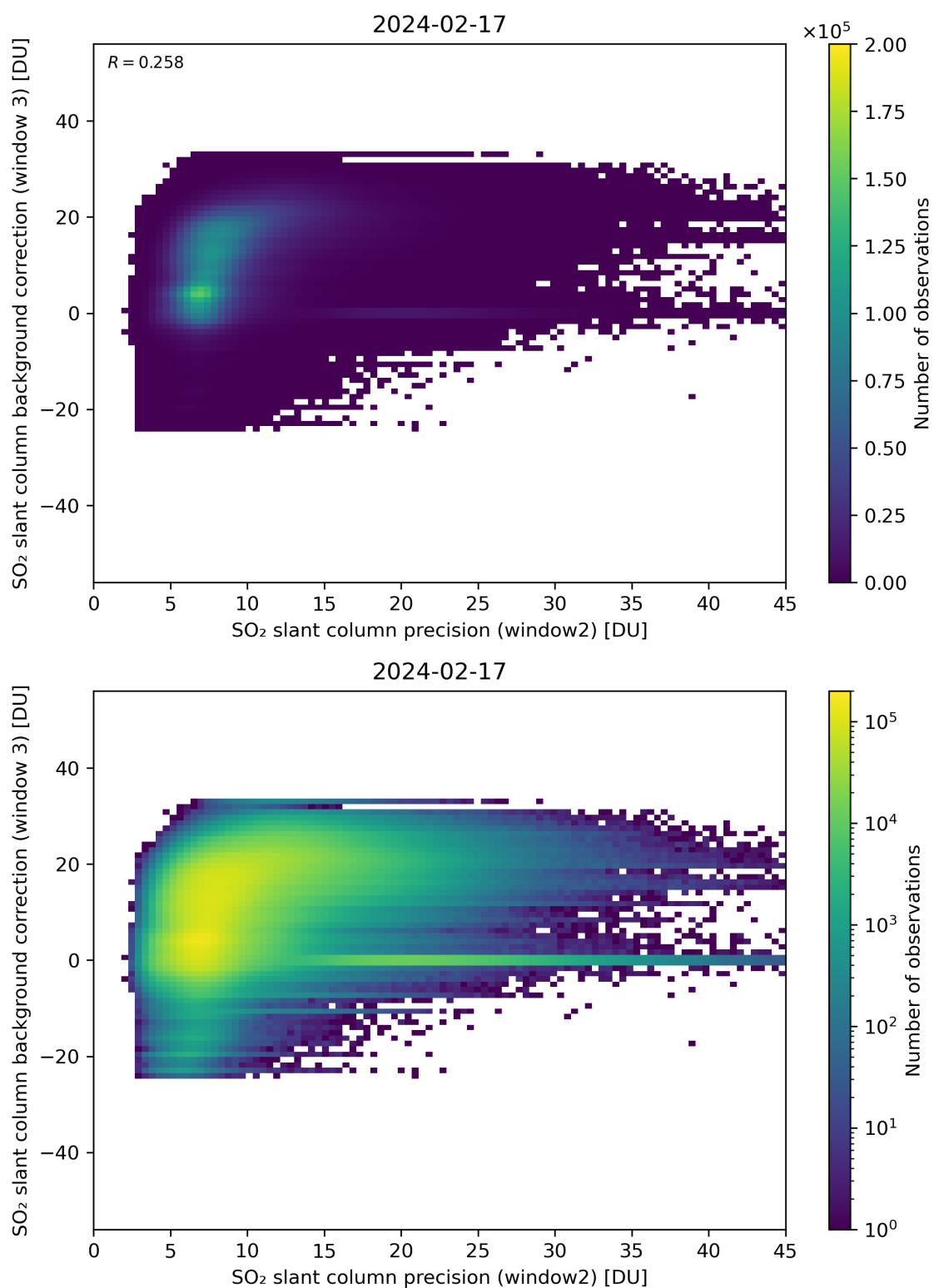
Figure 242: Scatter density plot of “SO 2 slant column precision (window2)” against “SO 2 slant column background correction (window 3)” for 2024-02-17 to 2024-02-18.
