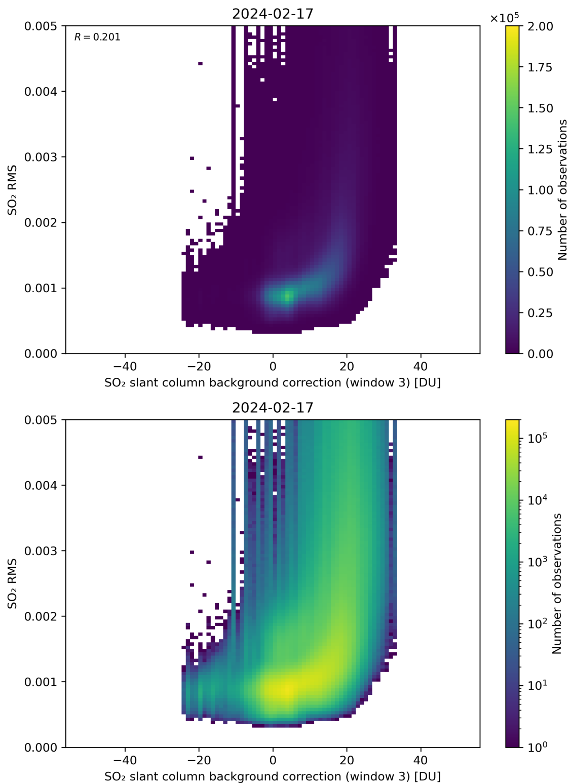
Figure 123: Scatter density plot of “SO 2 slant column background correction (window 3)” against “SO 2 RMS” for 2024-02-17 to 2024-02-18.
