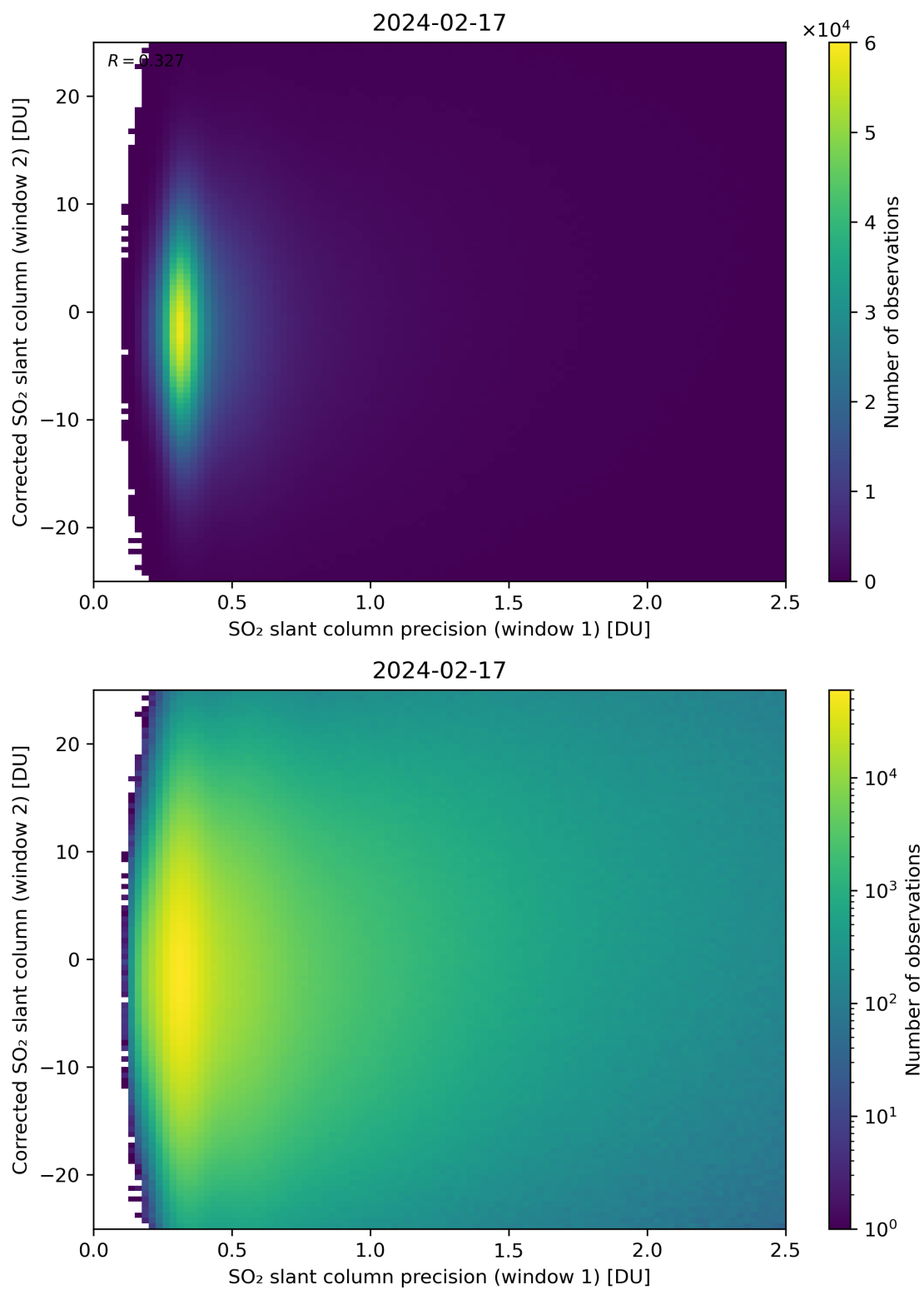
Figure 225: Scatter density plot of “SO 2 slant column precision (window 1)” against “Corrected SO 2 slant column (window 2)” for 2024-02-17 to 2024-02-18.
