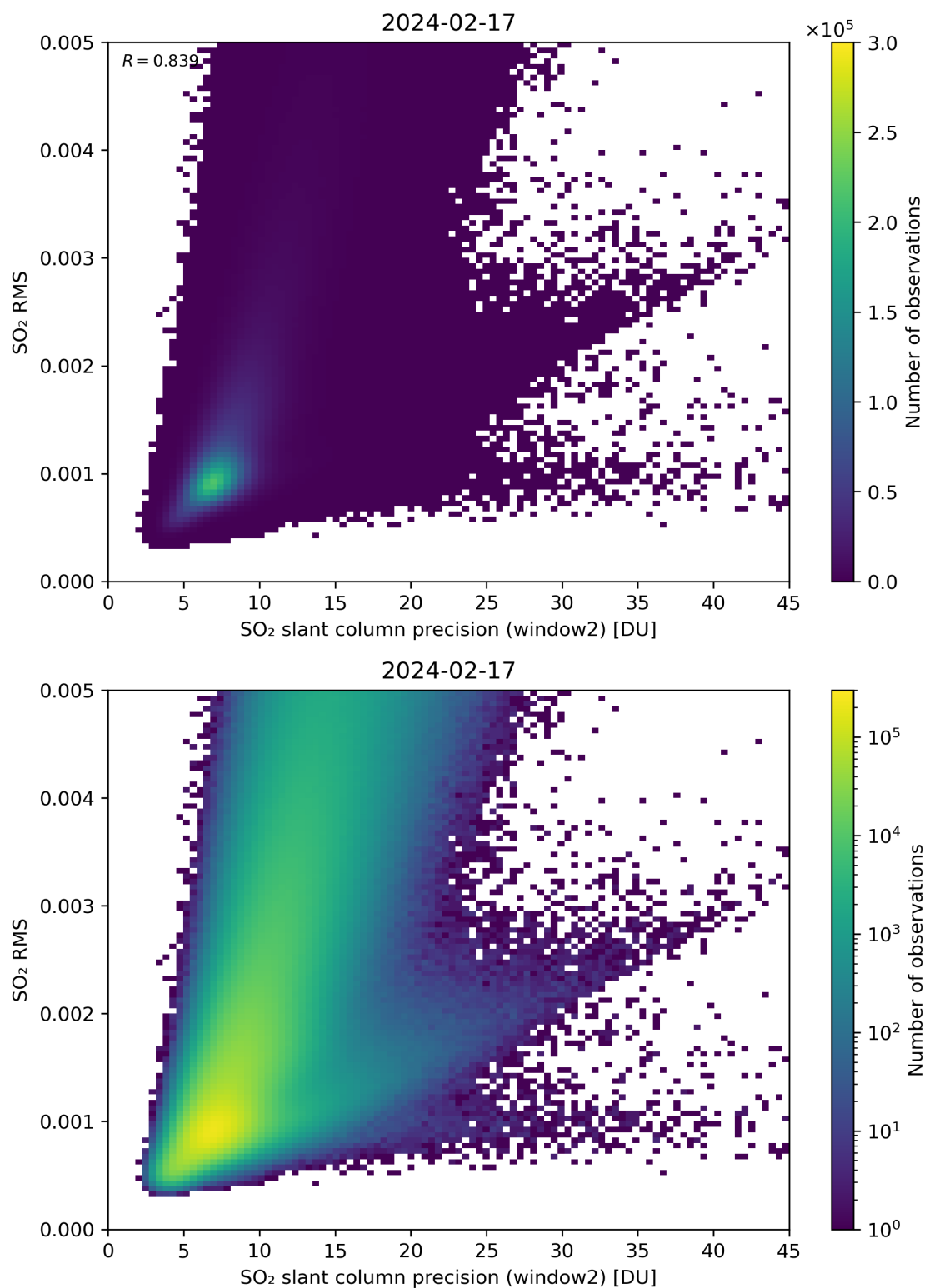
Figure 245: Scatter density plot of “SO 2 slant column precision (window2)” against “SO 2 RMS” for 2024-02-17 to 2024-02-18.
