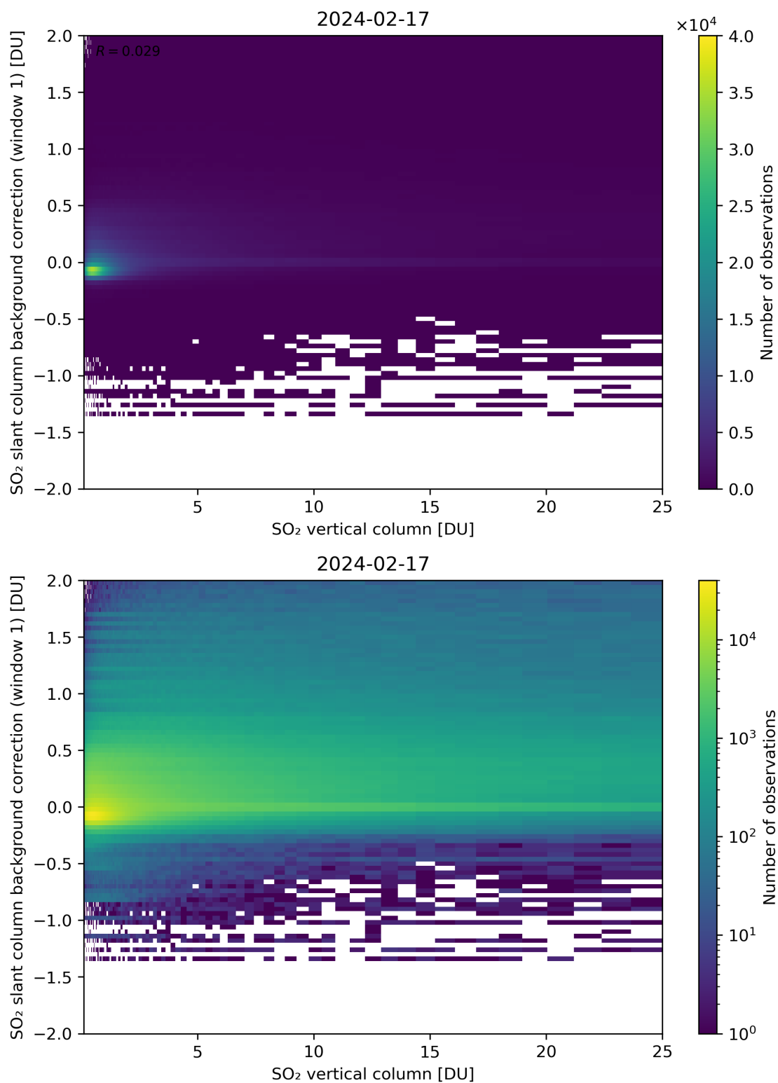
Figure 273: Scatter density plot of “SO 2 vertical column” against “SO 2 slant column background correction (window 1)” for 2024-02-17 to 2024-02-18.
