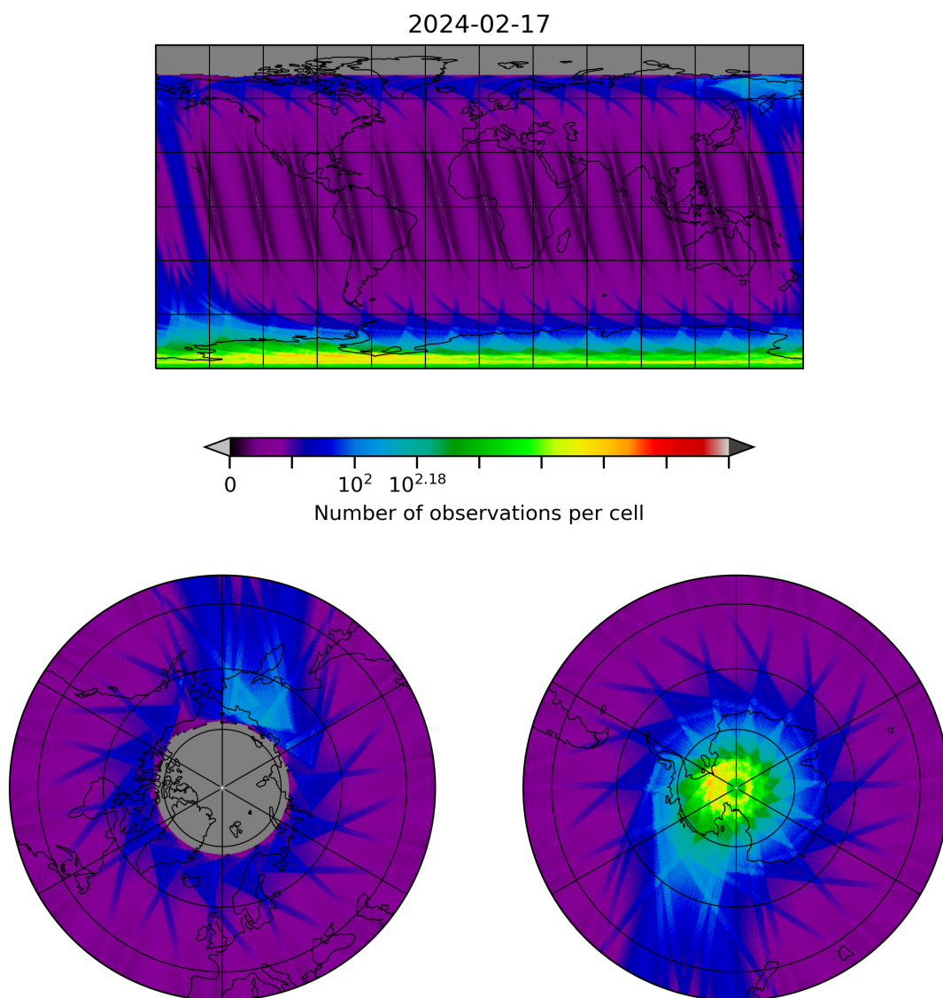
Figure 28: Map of the number of observations for 2024-02-17 to 2024-02-18
