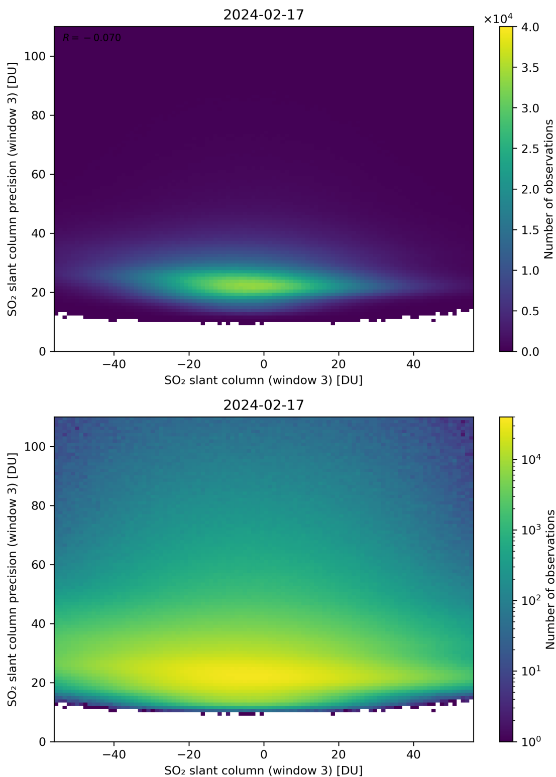
Figure 267: Scatter density plot of “SO 2 slant column (window 3)” against “SO 2 slant column precision (window 3)” for 2024-02-17 to 2024-02-18.
