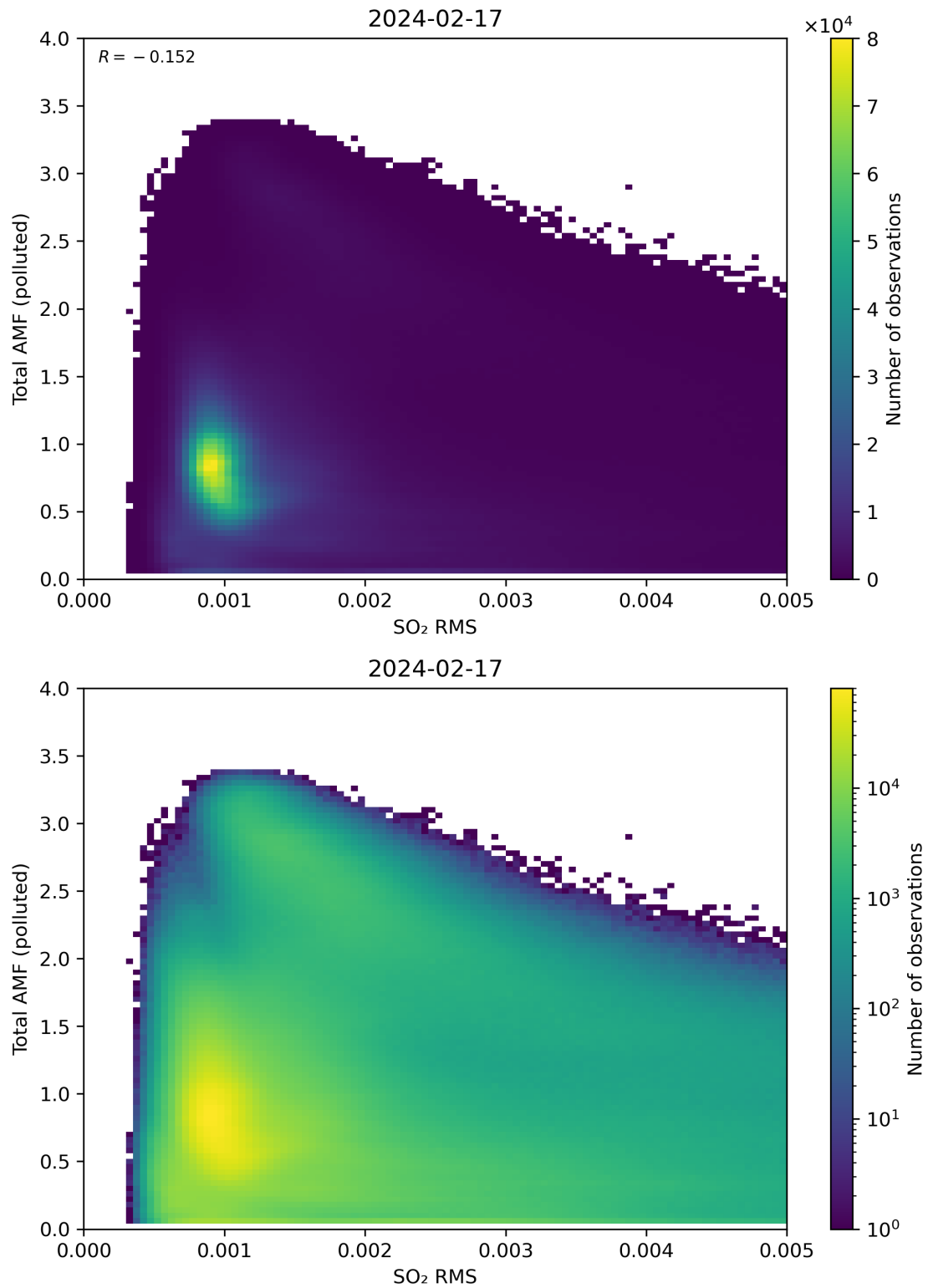
Figure 137: Scatter density plot of “SO 2 RMS” against “Total AMF (polluted)” for 2024-02-17 to 2024-02-18.
