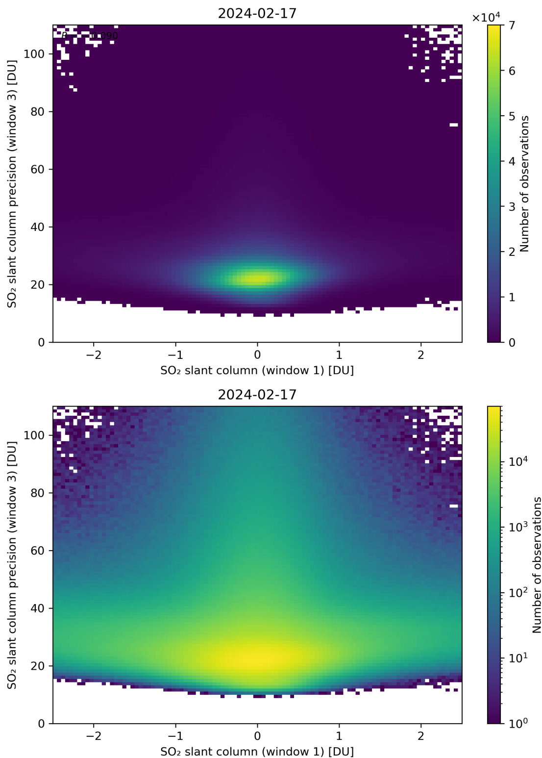
Figure 238: Scatter density plot of “SO 2 slant column (window 1)” against “SO 2 slant column precision (window 3)” for 2024-02-17 to 2024-02-18.
