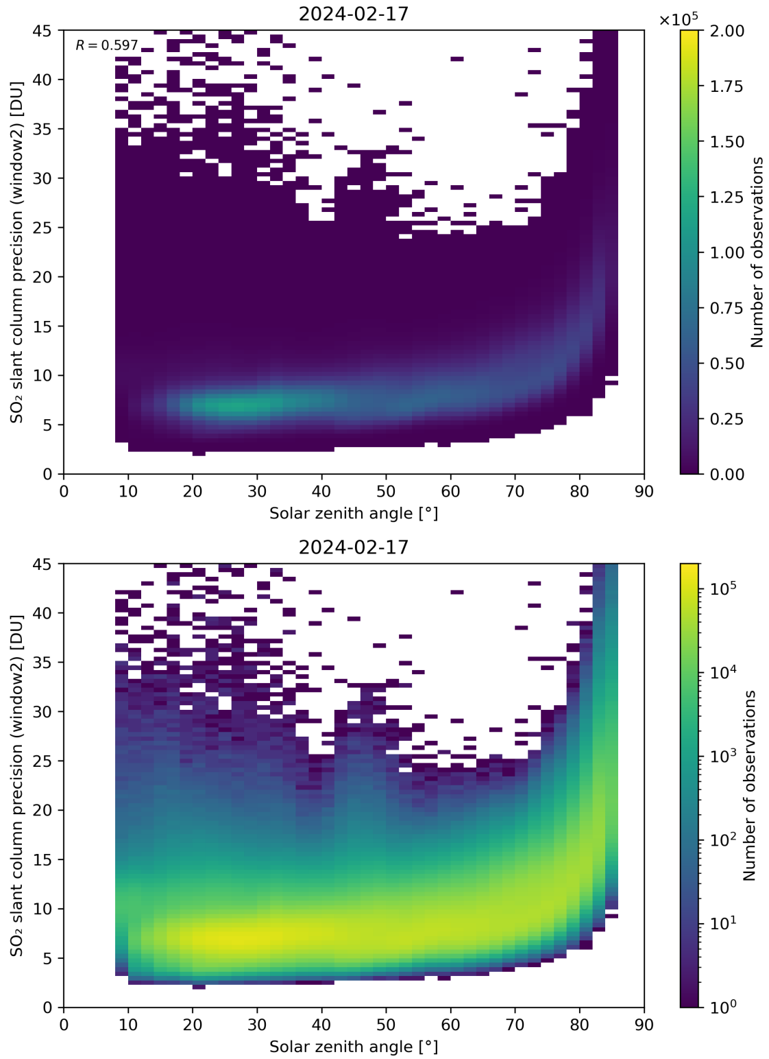
Figure 171: Scatter density plot of “Solar zenith angle” against “SO 2 slant column precision (window2)” for 2024-02-17 to 2024-02-18.
