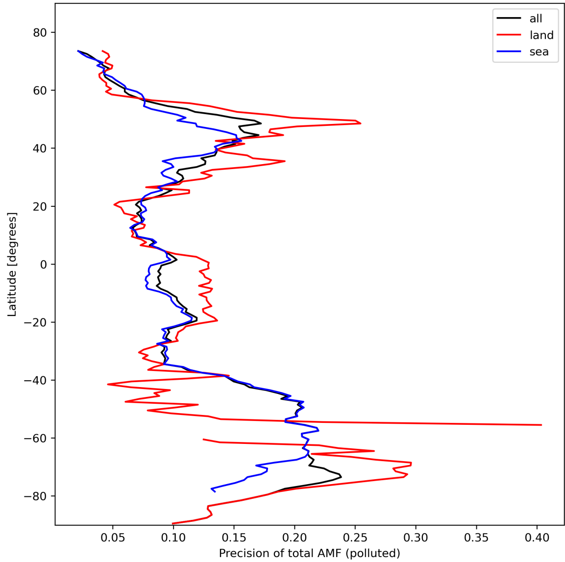
Figure 49: Zonal average of “Precision of total AMF (polluted)” for 2024-02-17 to 2024-02-18.
