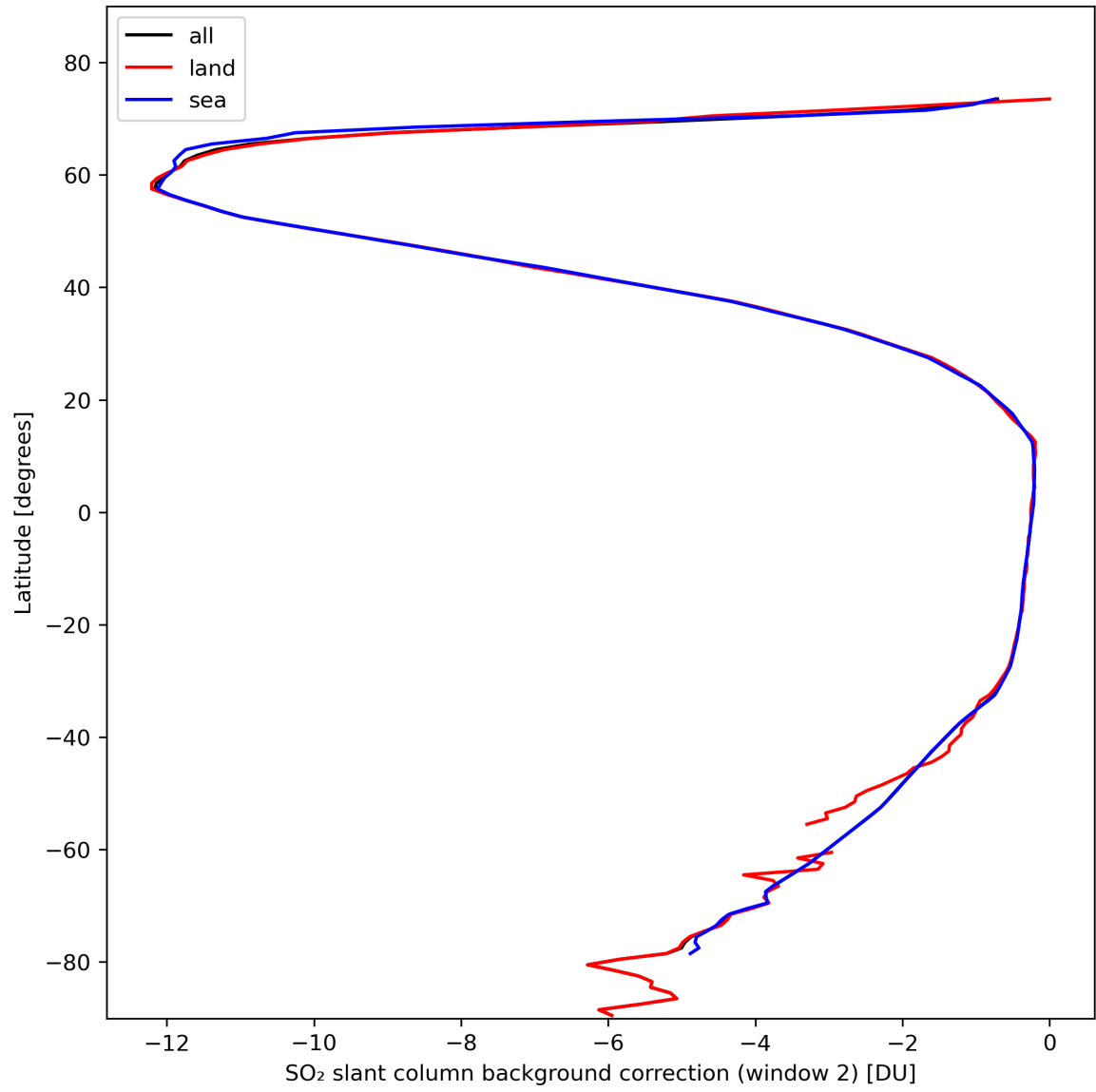
Figure 40: Zonal average of “SO 2 slant column background correction (window 2)” for 2024-02-17 to 2024-02-18.
