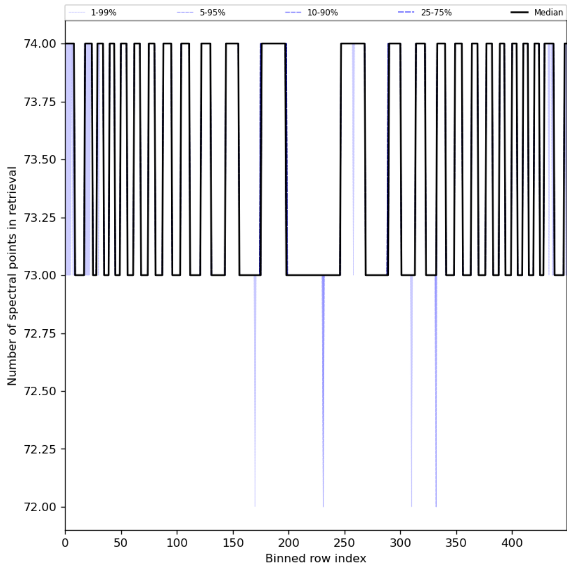
Figure 97: Along track statistics of “Number of spectral points in retrieval” for 2024-02-17 to 2024-02-18
