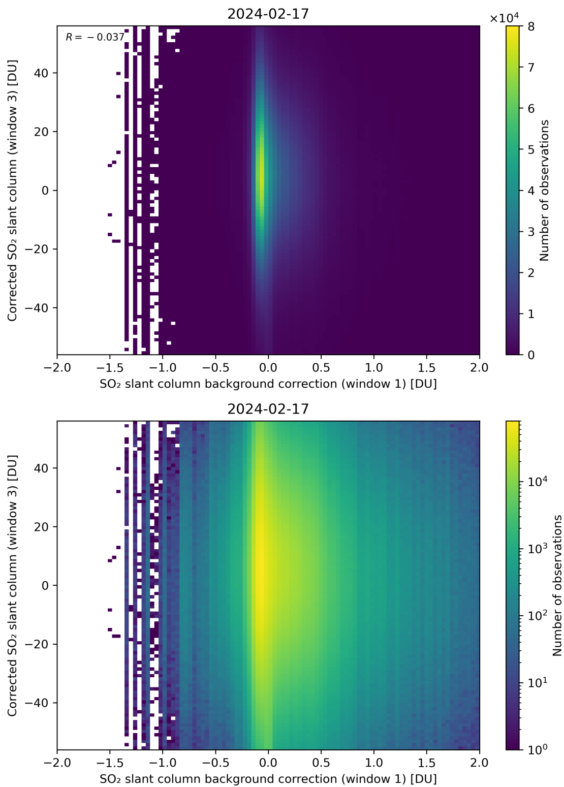
Figure 105: Scatter density plot of “SO 2 slant column background correction (window 1)” against “Corrected SO 2 slant column (window 3)” for 2024-02-17 to 2024-02-18.
