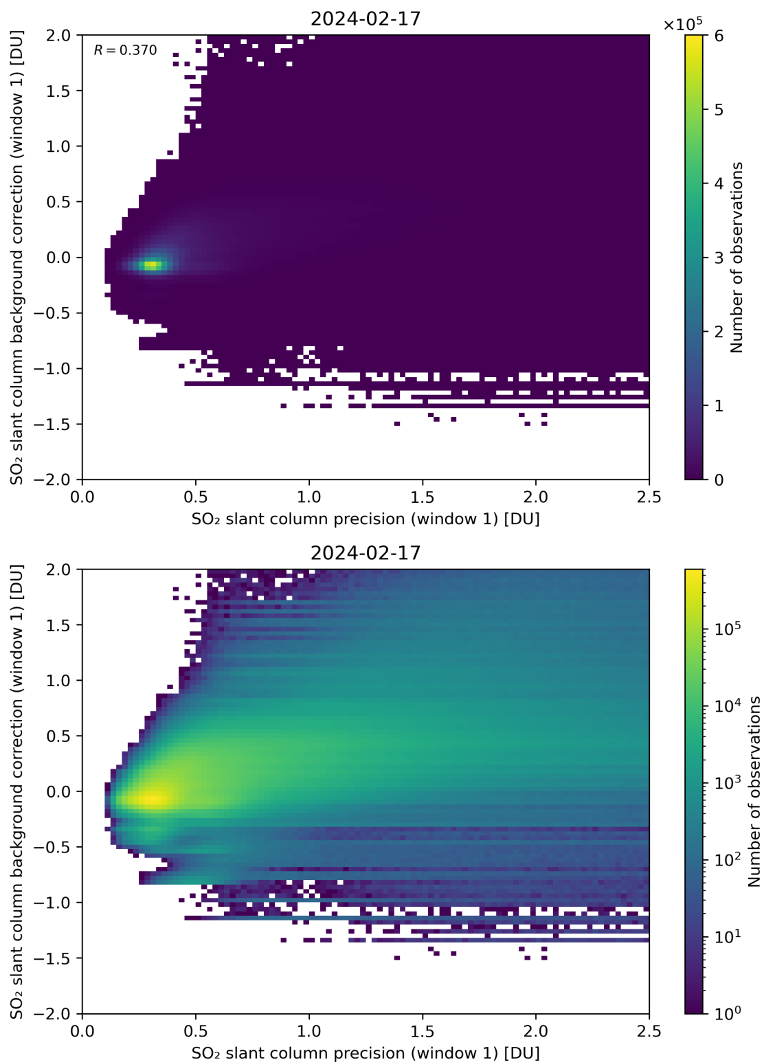
Figure 218: Scatter density plot of “SO 2 slant column precision (window 1)” against “SO 2 slant column background correction (window 1)” for 2024-02-17 to 2024-02-18.
