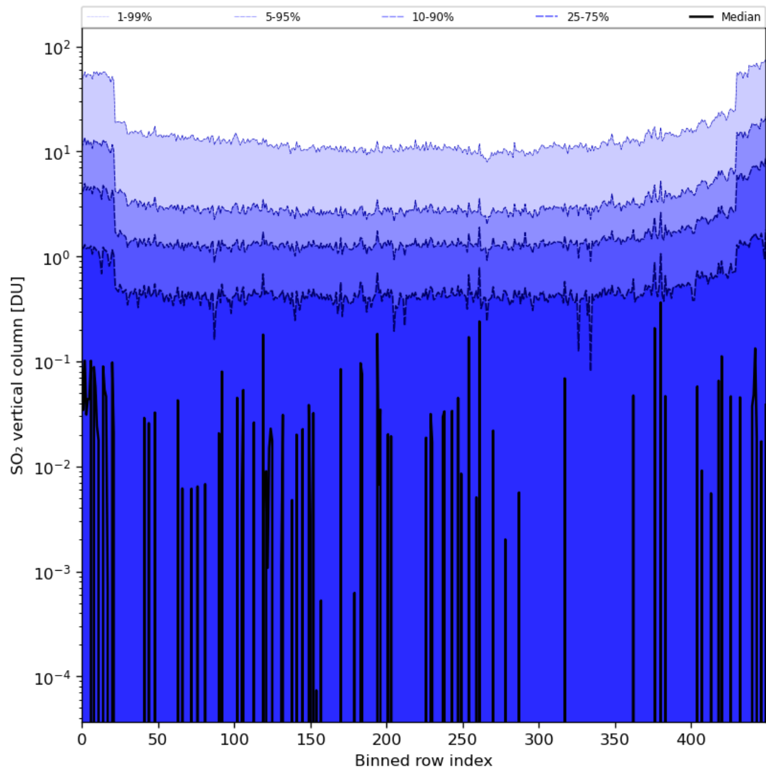
Figure 76: Along track statistics of “SO 2 vertical column” for 2024-02-17 to 2024-02-18
