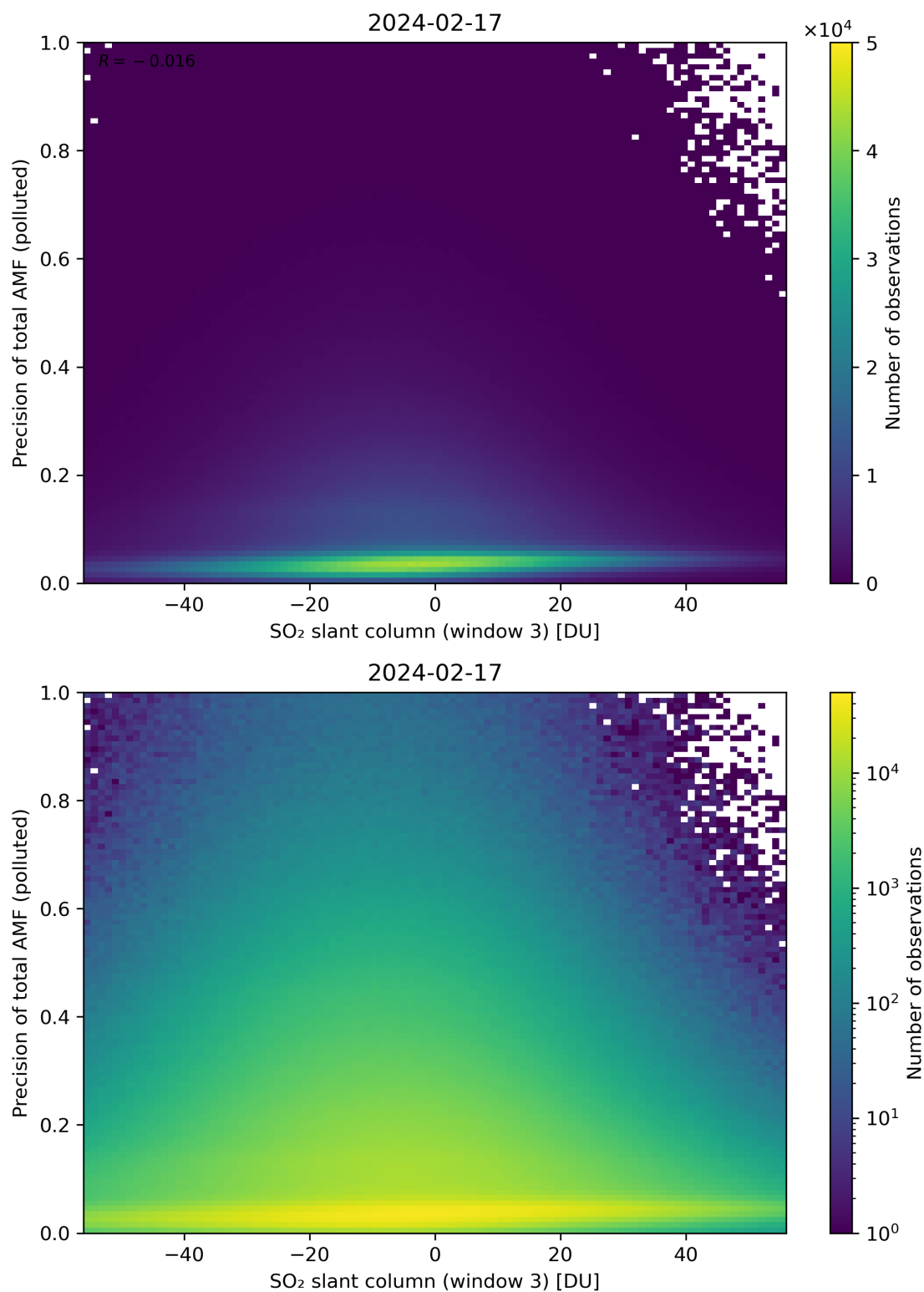
Figure 269: Scatter density plot of “SO 2 slant column (window 3)” against “Precision of total AMF (polluted)” for 2024-02-17 to 2024-02-18.
