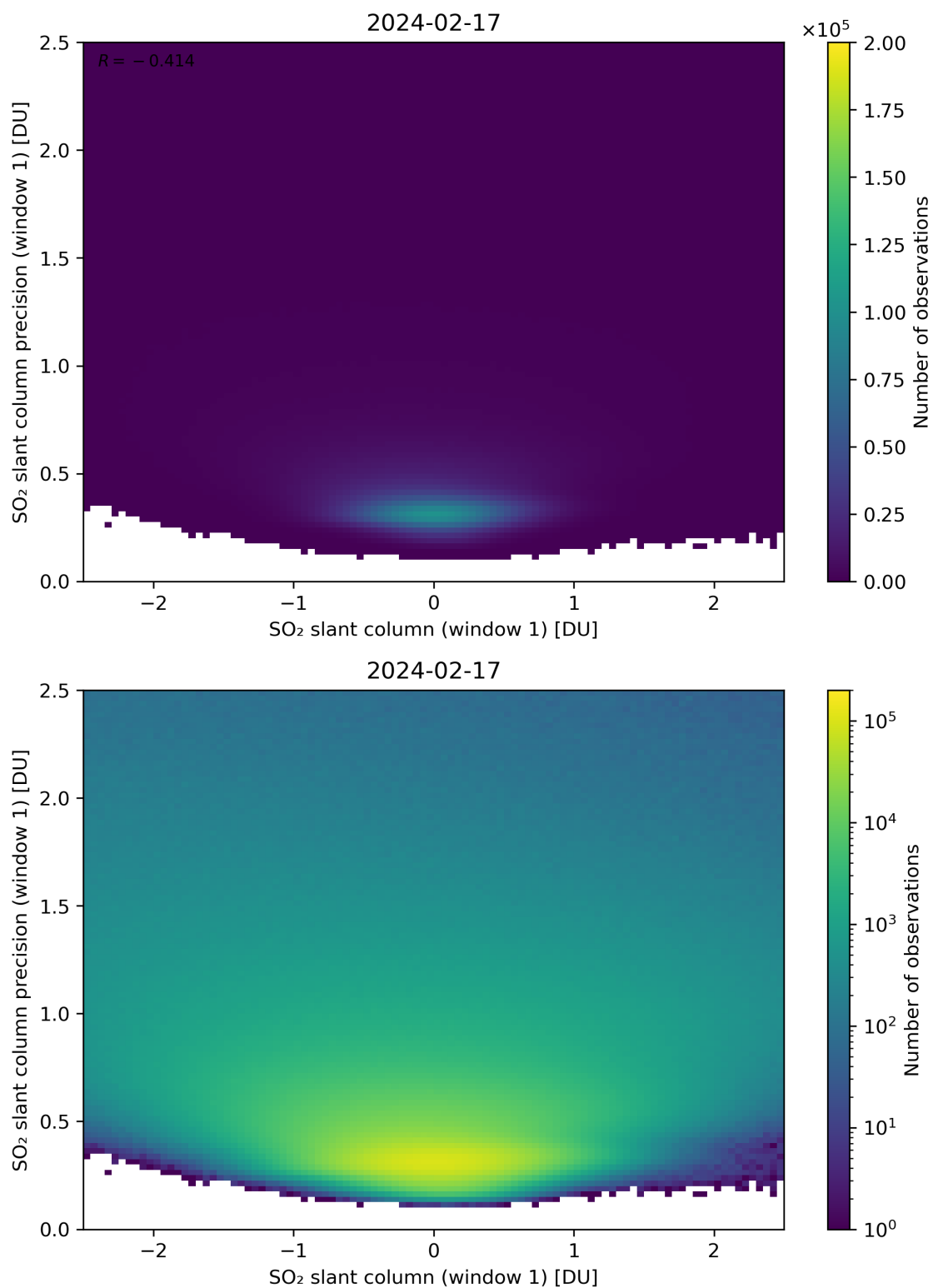
Figure 235: Scatter density plot of “SO 2 slant column (window 1)” against “SO 2 slant column precision (window 1)” for 2024-02-17 to 2024-02-18.
