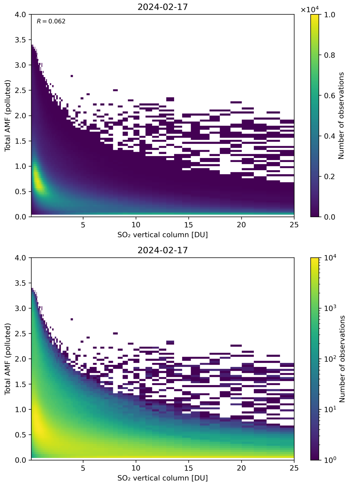
Figure 305: Scatter density plot of “SO 2 vertical column” against “Total AMF (polluted)” for 2024-02-17 to 2024-02-18.
