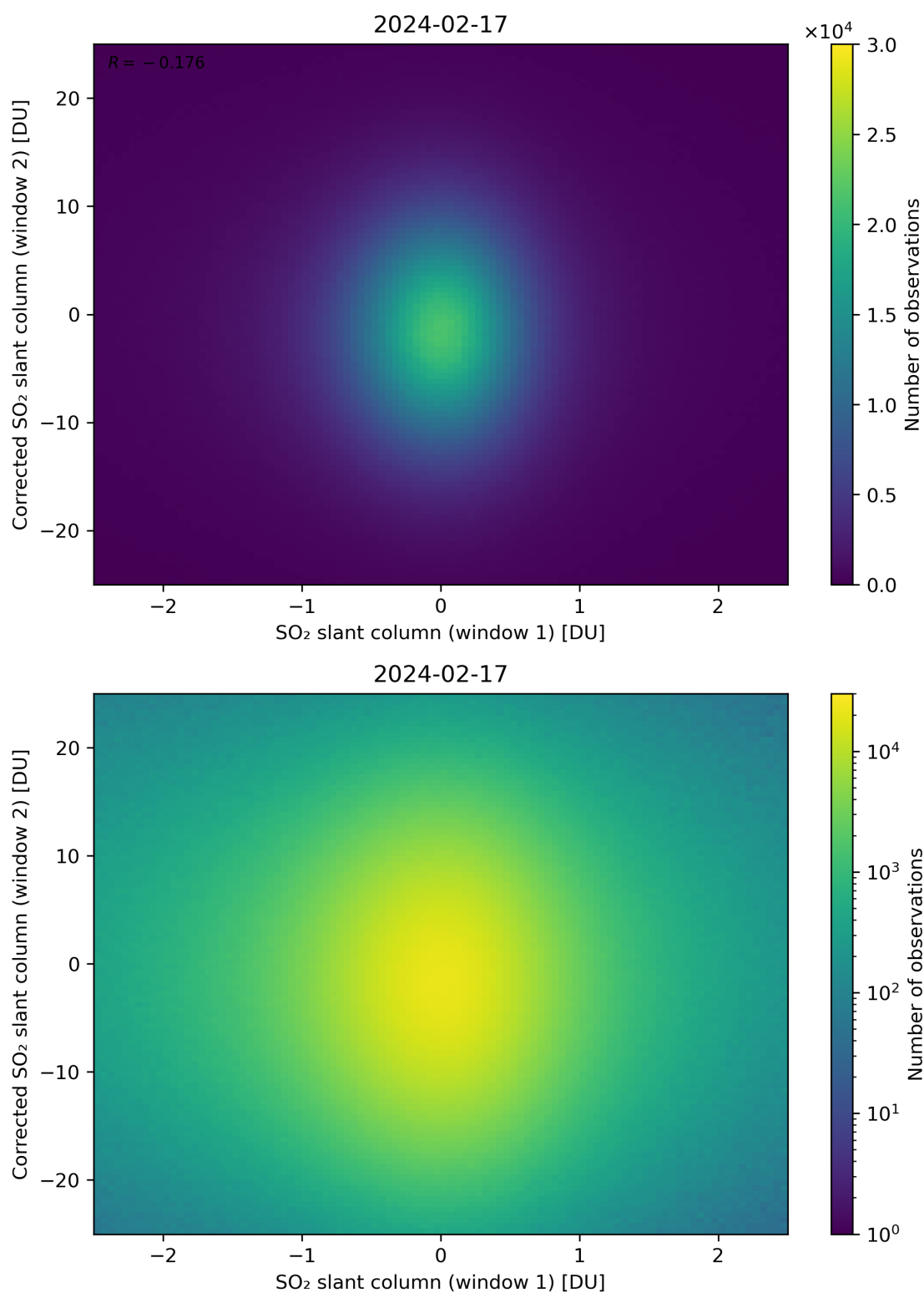
Figure 233: Scatter density plot of “SO 2 slant column (window 1)” against “Corrected SO 2 slant column (window 2)” for 2024-02-17 to 2024-02-18.
