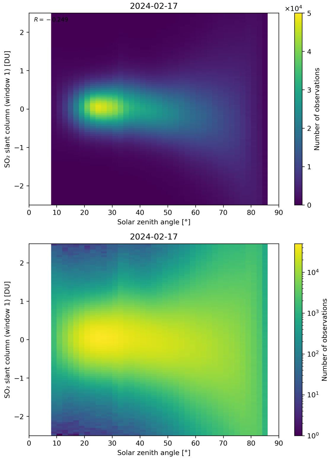
Figure 169: Scatter density plot of “Solar zenith angle” against “SO 2 slant column (window 1)” for 2024-02-17 to 2024-02-18.
