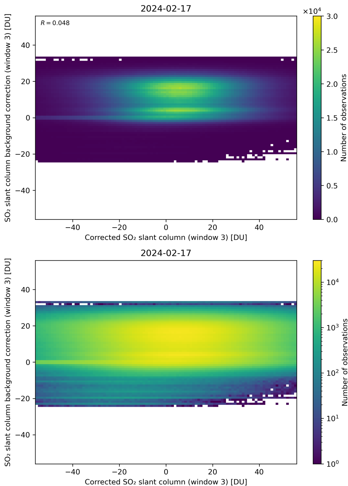
Figure 205: Scatter density plot of “Corrected SO 2 slant column (window 3)” against “SO 2 slant column background correction (window 3)” for 2024-02-17 to 2024-02-18.
