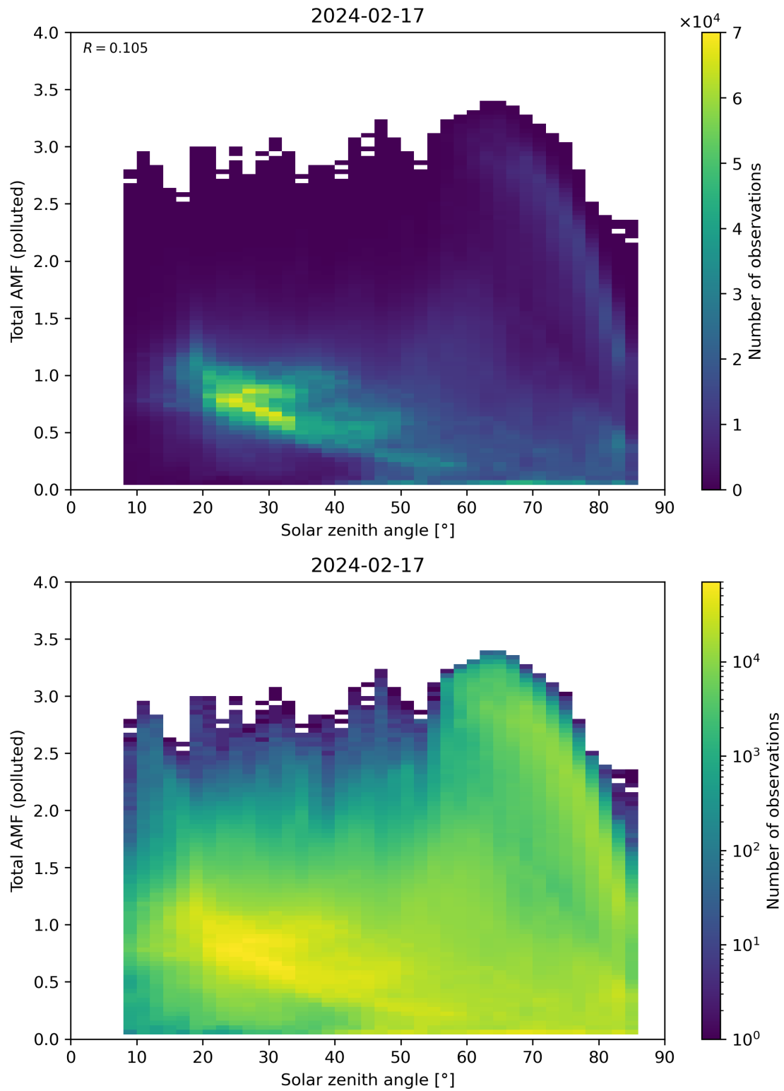
Figure 174: Scatter density plot of “Solar zenith angle” against “Total AMF (polluted)” for 2024-02-17 to 2024-02-18.
