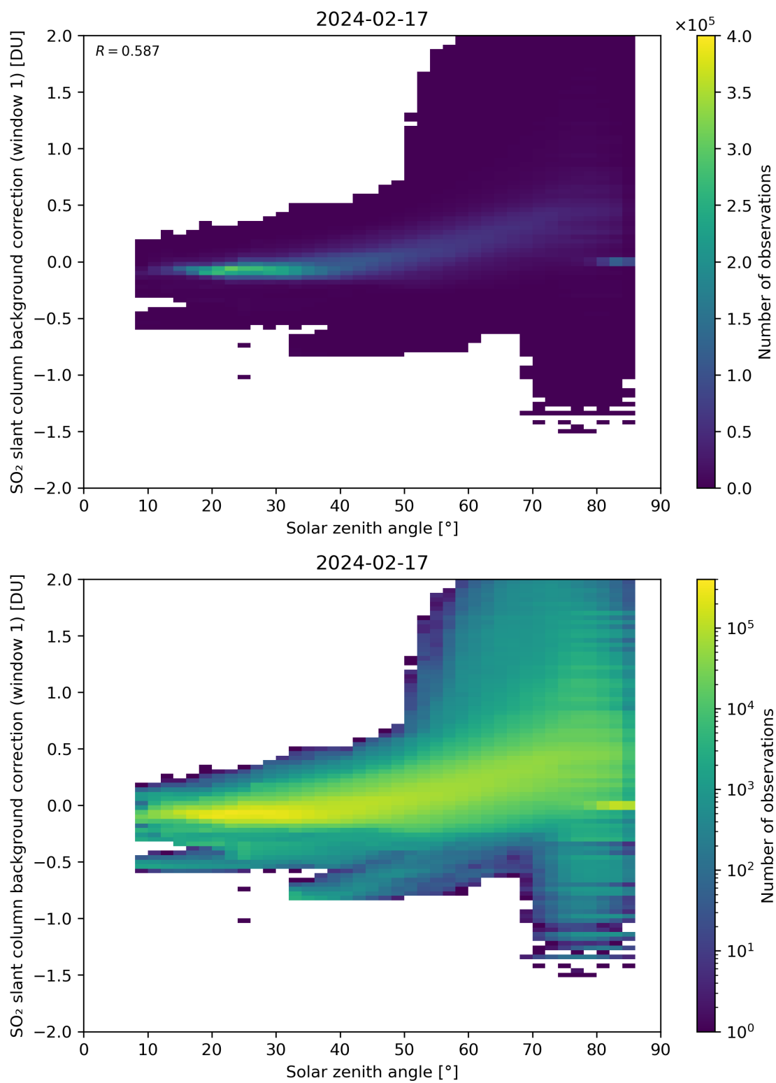
Figure 158: Scatter density plot of “Solar zenith angle” against “SO 2 slant column background correction (window 1)” for 2024-02-17 to 2024-02-18.
