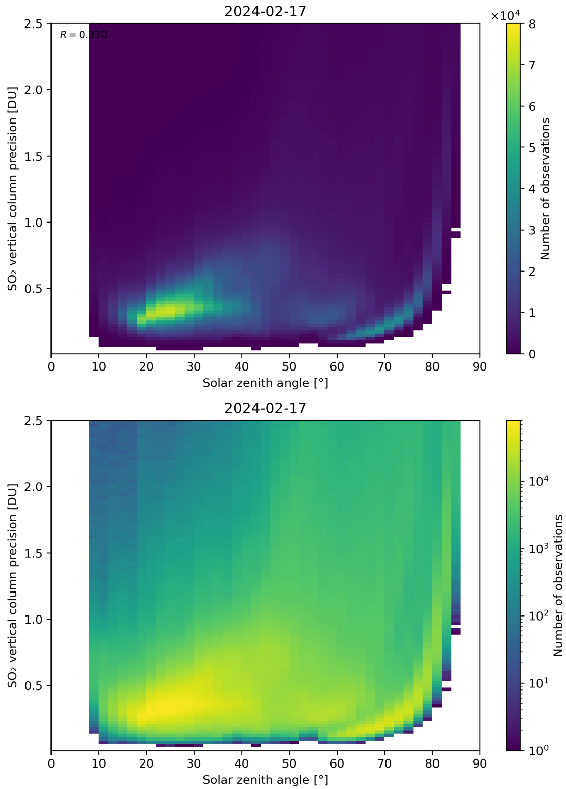
Figure 177: Scatter density plot of “Solar zenith angle” against “SO 2 vertical column precision” for 2024-02-17 to 2024-02-18.
