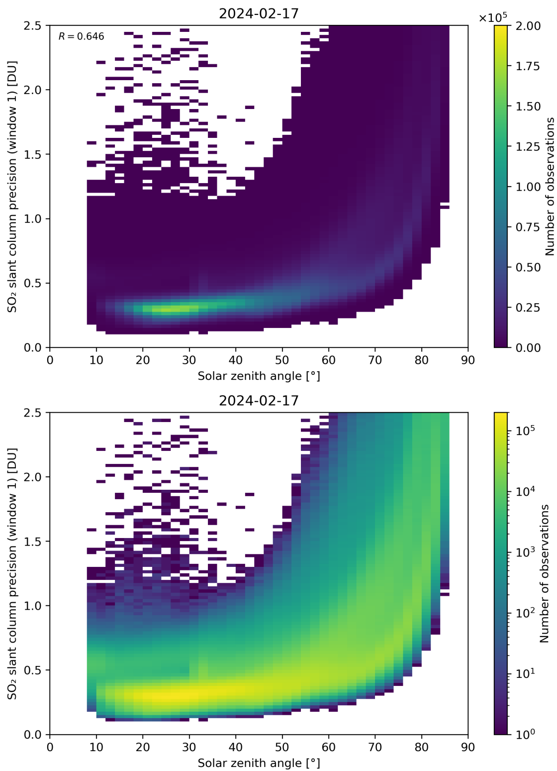
Figure 170: Scatter density plot of “Solar zenith angle” against “SO 2 slant column precision (window 1)” for 2024-02-17 to 2024-02-18.
