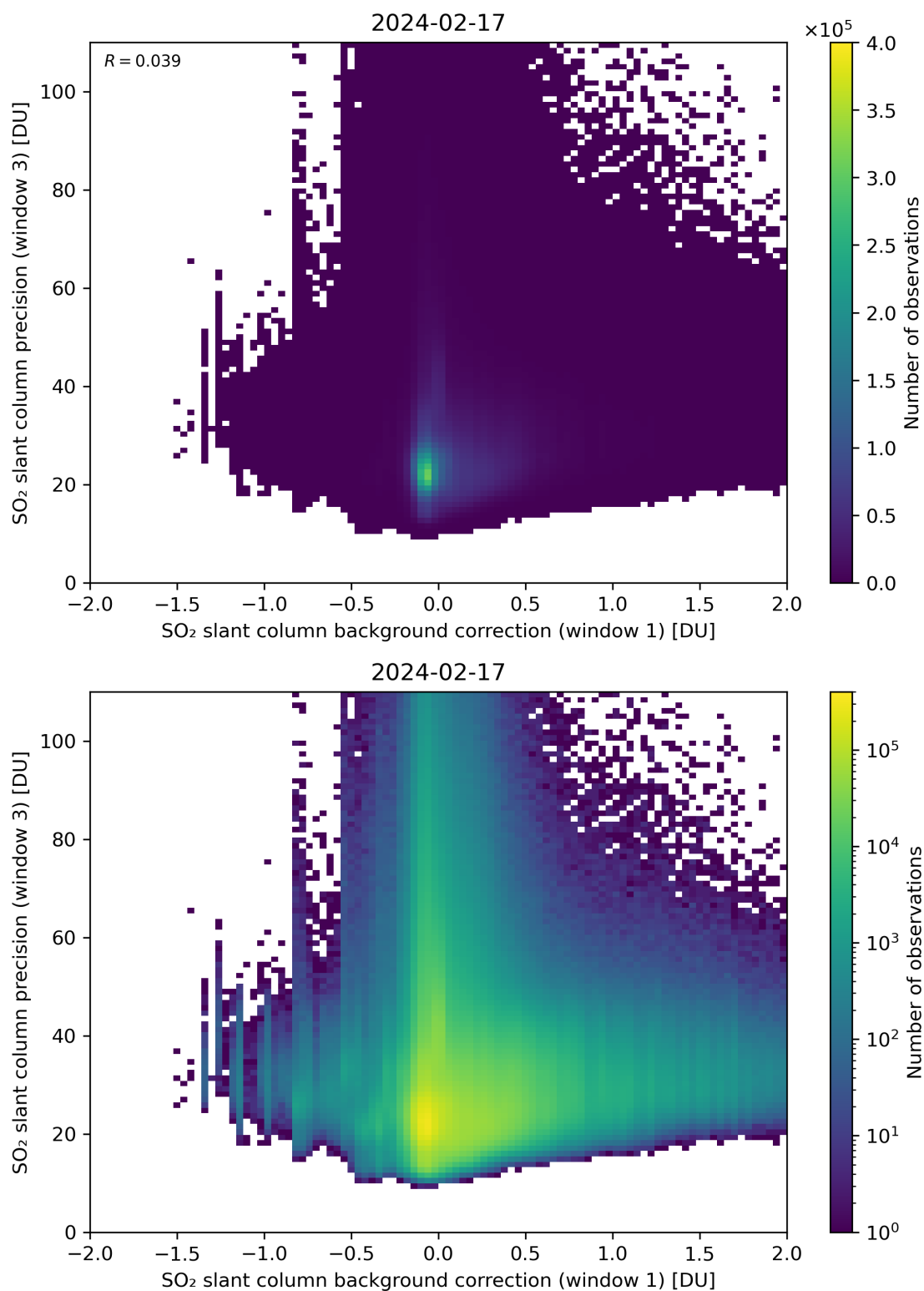
Figure 108: Scatter density plot of “SO 2 slant column background correction (window 1)” against “SO 2 slant column precision (window 3)” for 2024-02-17 to 2024-02-18.
