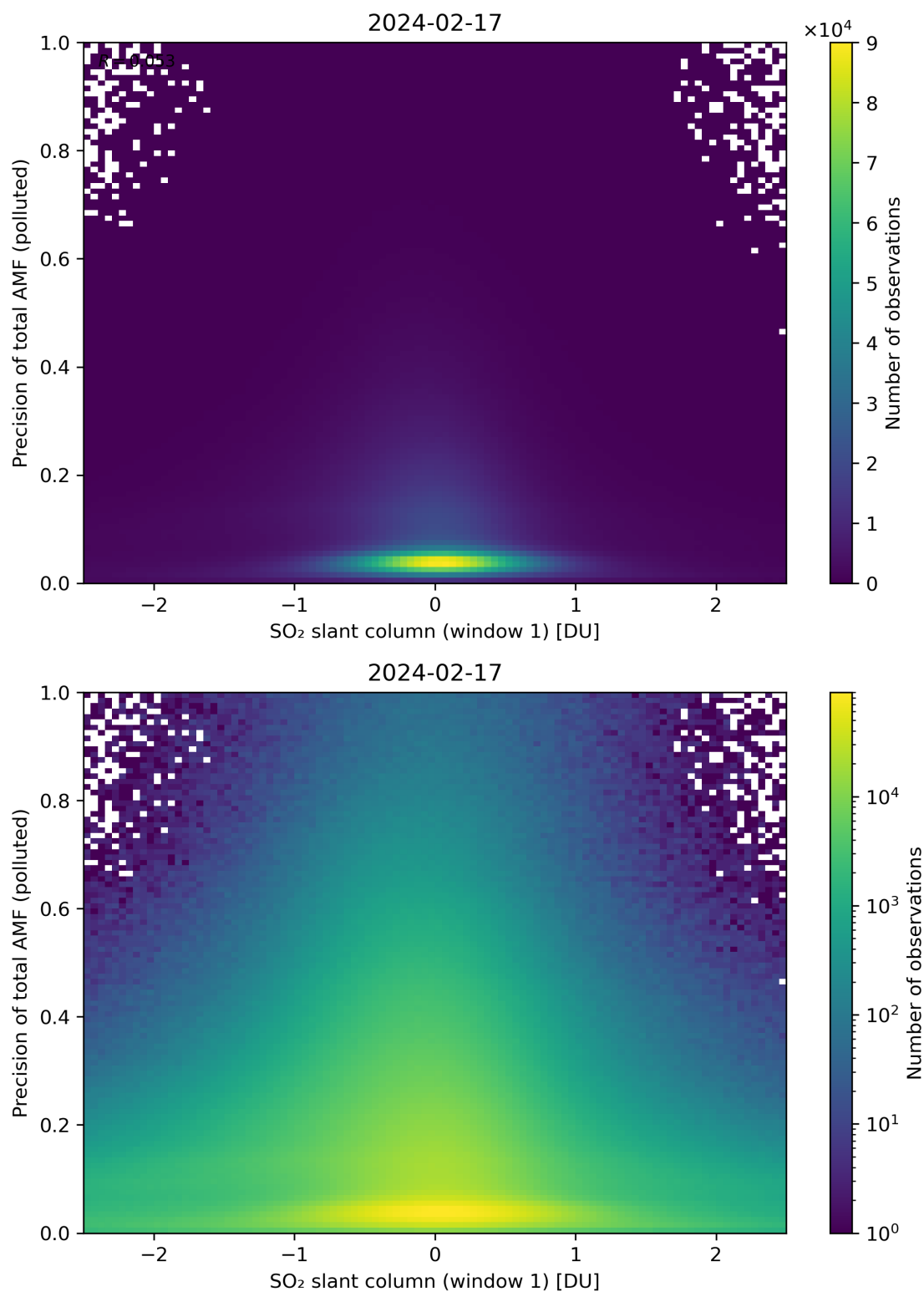
Figure 240: Scatter density plot of “SO 2 slant column (window 1)” against “Precision of total AMF (polluted)” for 2024-02-17 to 2024-02-18.
