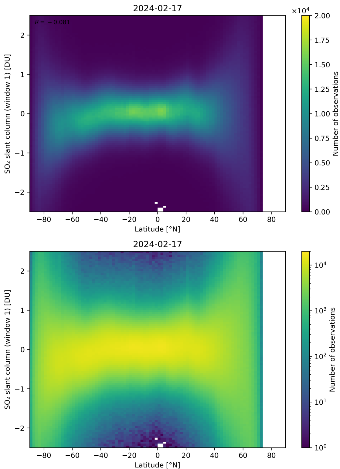
Figure 149: Scatter density plot of “Latitude” against “SO 2 slant column (window 1)” for 2024-02-17 to 2024-02-18.
