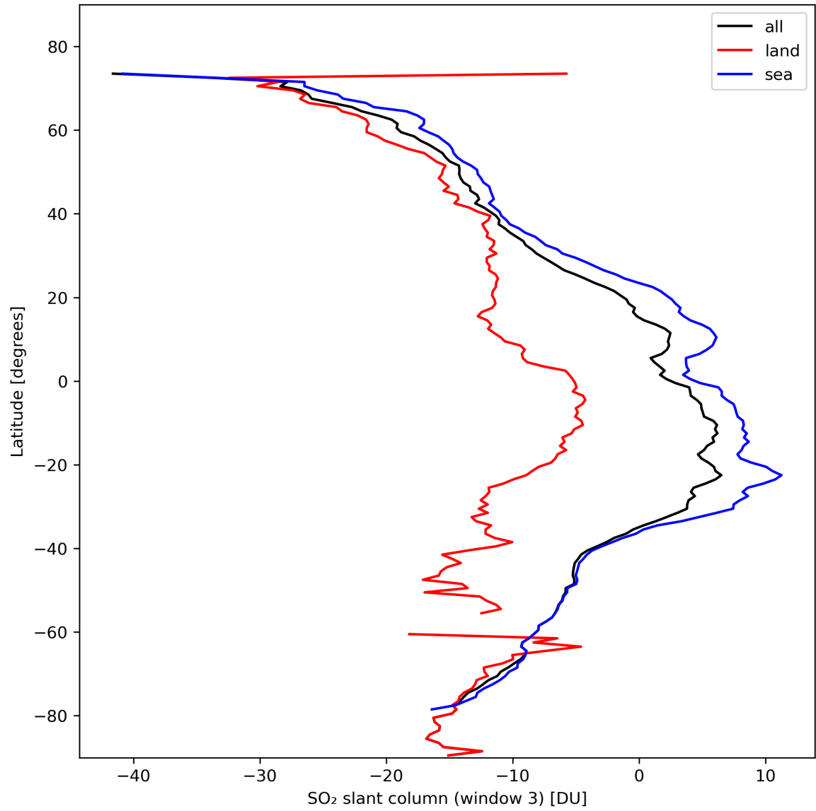
Figure 41: Zonal average of “SO 2 slant column (window 3)” for 2024-02-17 to 2024-02-18.
