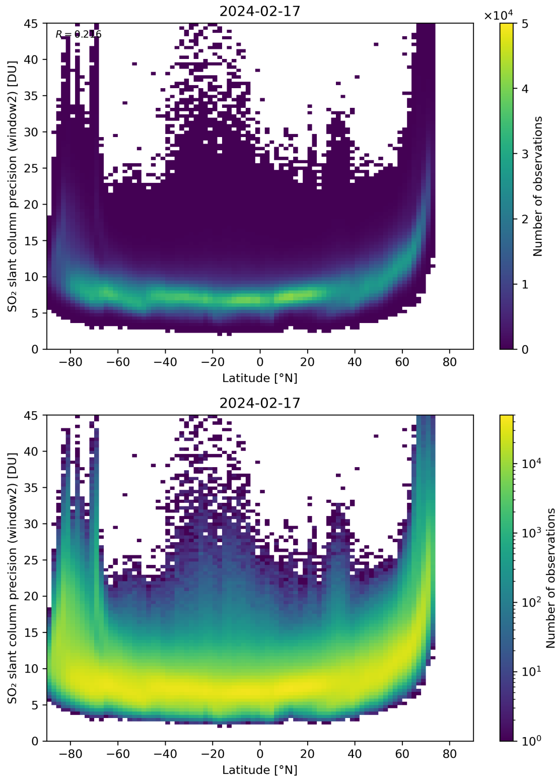
Figure 151: Scatter density plot of “Latitude” against “SO 2 slant column precision (window2)” for 2024-02-17 to 2024-02-18.
