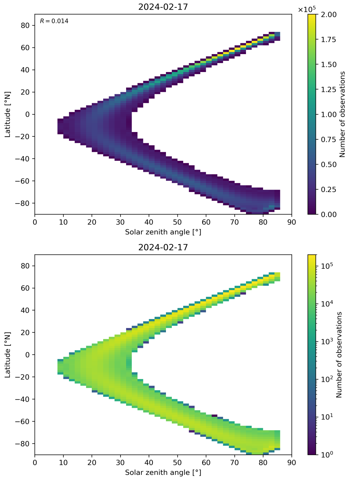
Figure 164: Scatter density plot of “Solar zenith angle” against “Latitude” for 2024-02-17 to 2024-02-18.
