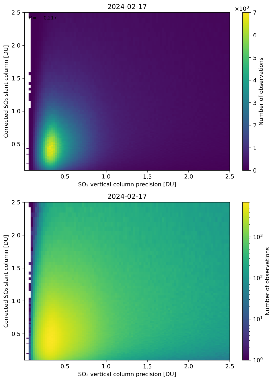
Figure 286: Scatter density plot of “SO 2 vertical column precision” against “Corrected SO 2 slant column” for 2024-02-17 to 2024-02-18.
