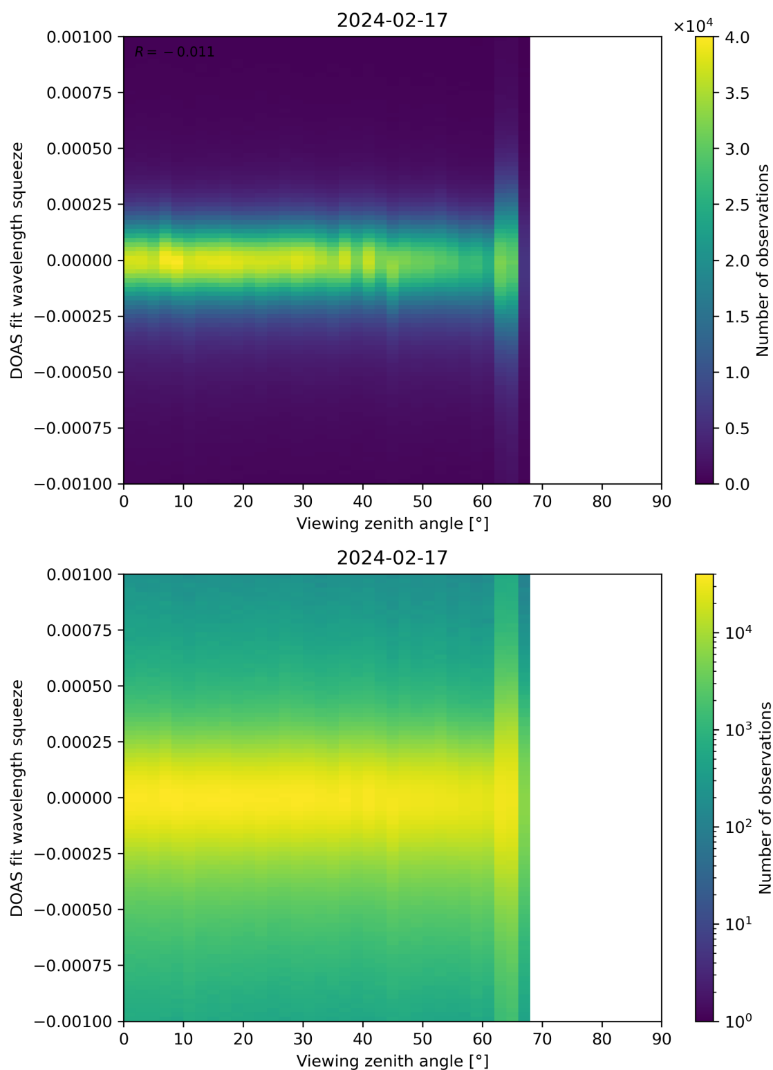
Figure 312: Scatter density plot of “Viewing zenith angle” against “DOAS fit wavelength squeeze” for 2024-02-17 to 2024-02-18.
