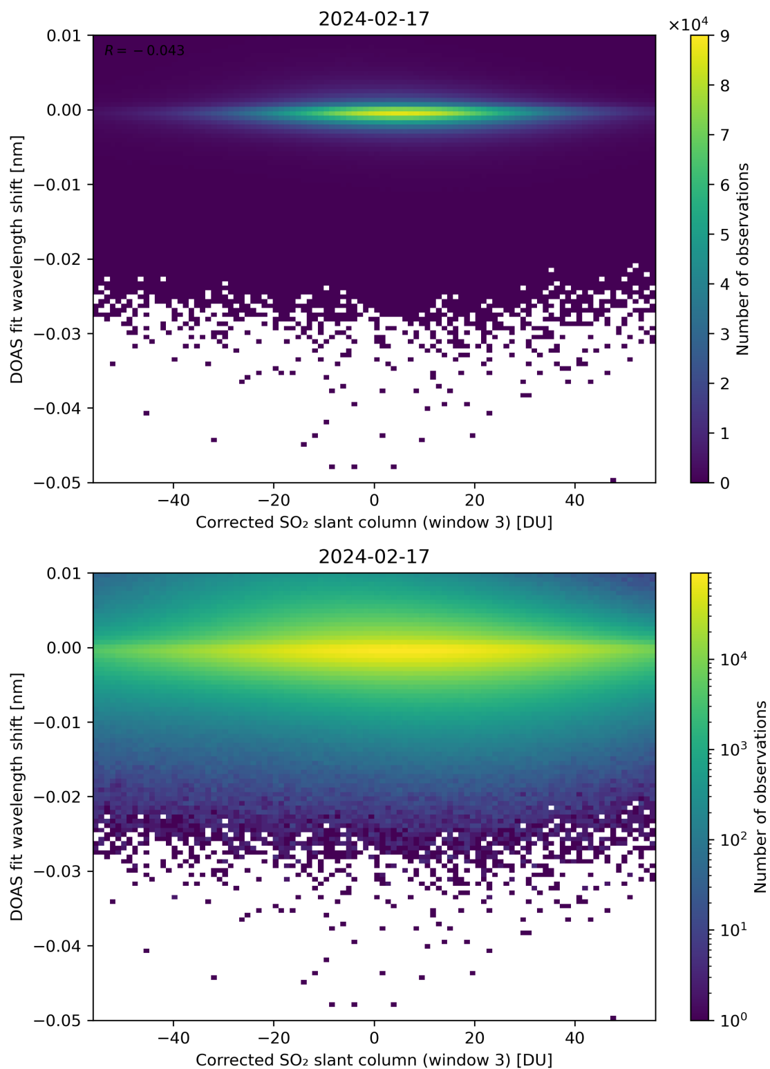
Figure 206: Scatter density plot of “Corrected SO 2 slant column (window 3)” against “DOAS fit wavelength shift” for 2024-02-17 to 2024-02-18.
