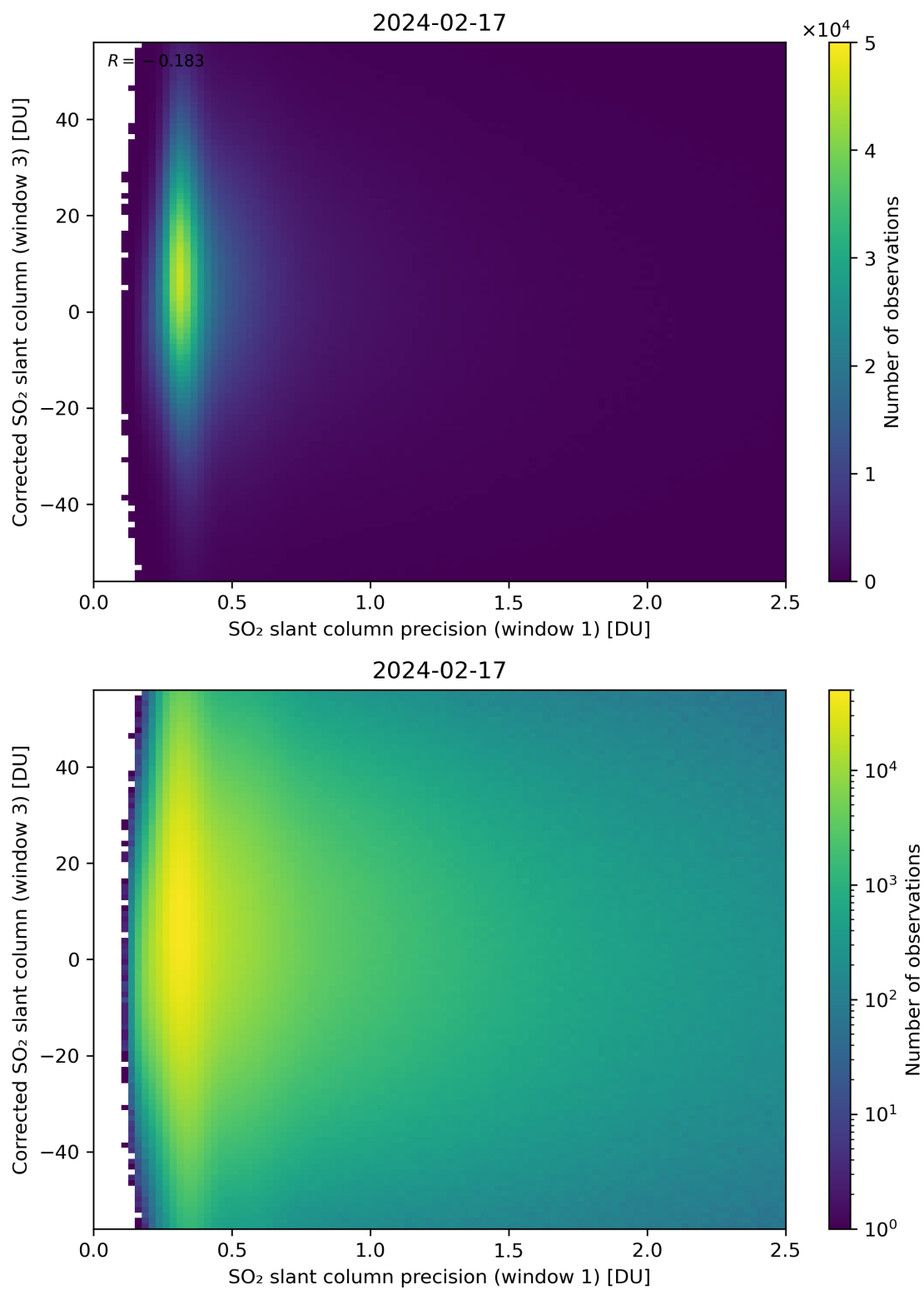
Figure 226: Scatter density plot of “SO 2 slant column precision (window 1)” against “Corrected SO 2 slant column (window 3)” for 2024-02-17 to 2024-02-18.
