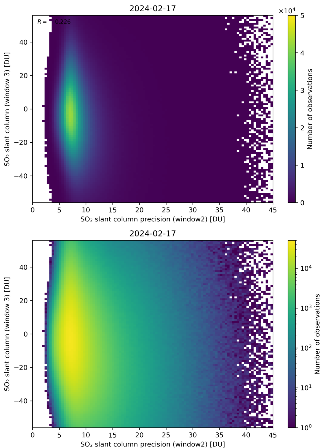
Figure 249: Scatter density plot of “SO 2 slant column precision (window2)” against “SO 2 slant column (window 3)” for 2024-02-17 to 2024-02-18.
