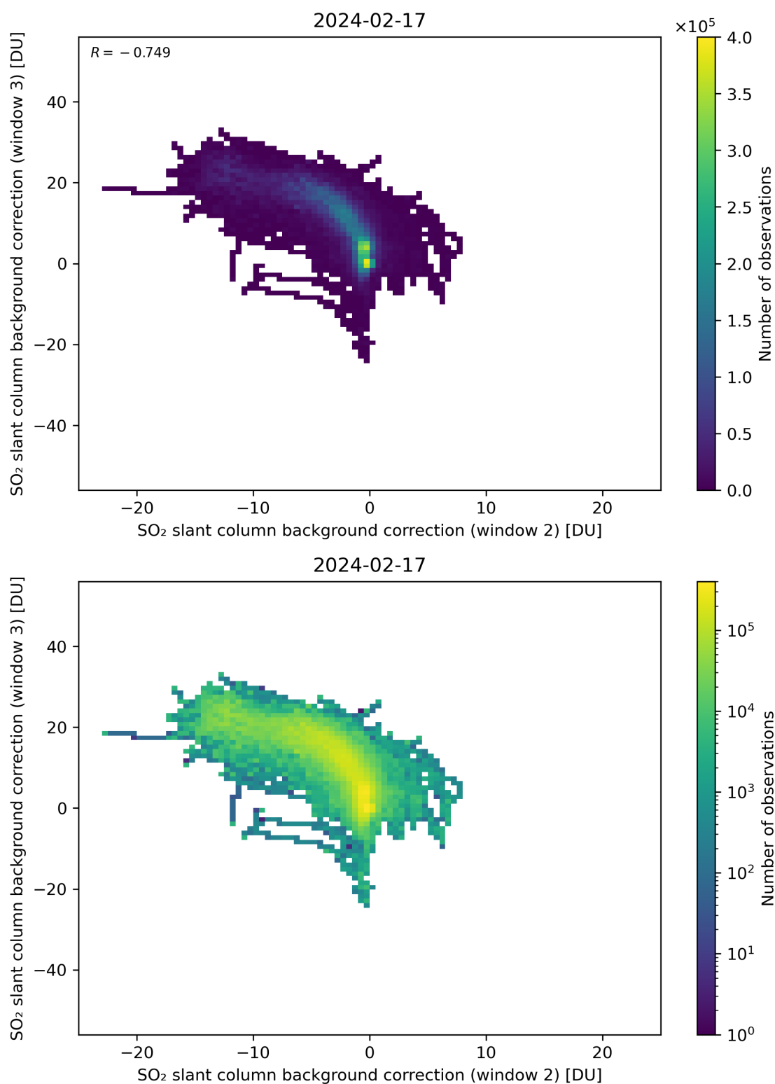
Figure 111: Scatter density plot of “SO 2 slant column background correction (window 2)” against “SO 2 slant column background correction (window 3)” for 2024-02-17 to 2024-02-18.
