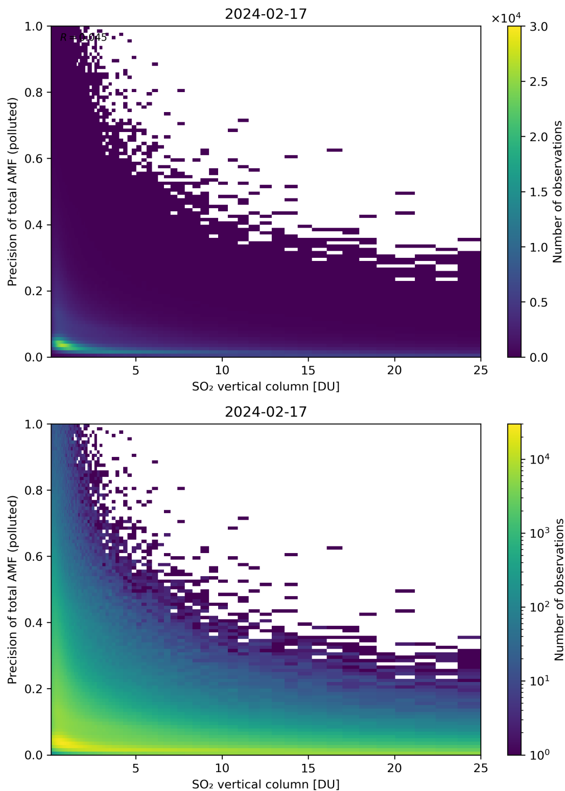
Figure 306: Scatter density plot of “SO 2 vertical column” against “Precision of total AMF (polluted)” for 2024-02-17 to 2024-02-18.
