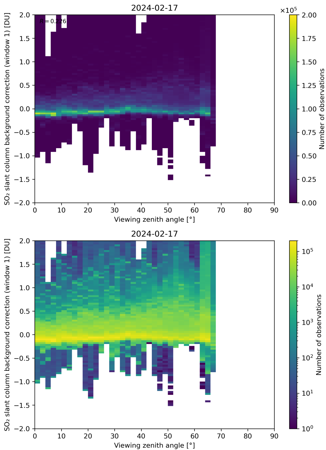
Figure 308: Scatter density plot of “Viewing zenith angle” against “SO 2 slant column background correction (window 1)” for 2024-02-17 to 2024-02-18.
