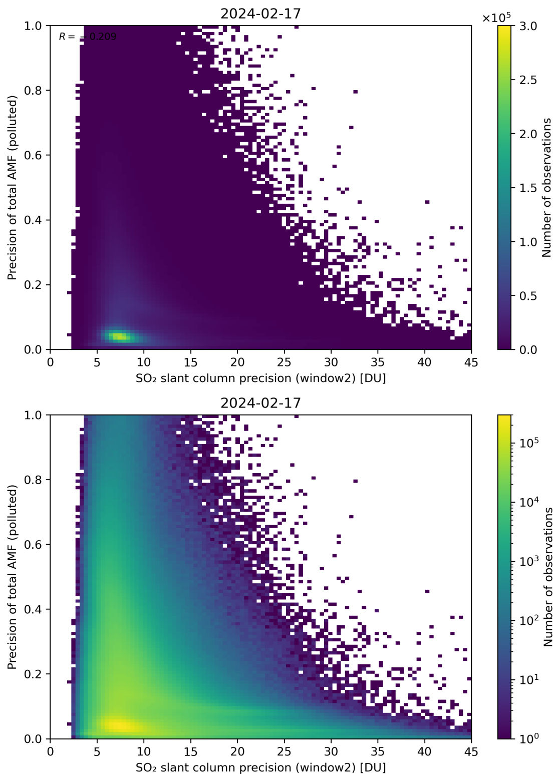
Figure 252: Scatter density plot of “SO 2 slant column precision (window2)” against “Precision of total AMF (polluted)” for 2024-02-17 to 2024-02-18.
