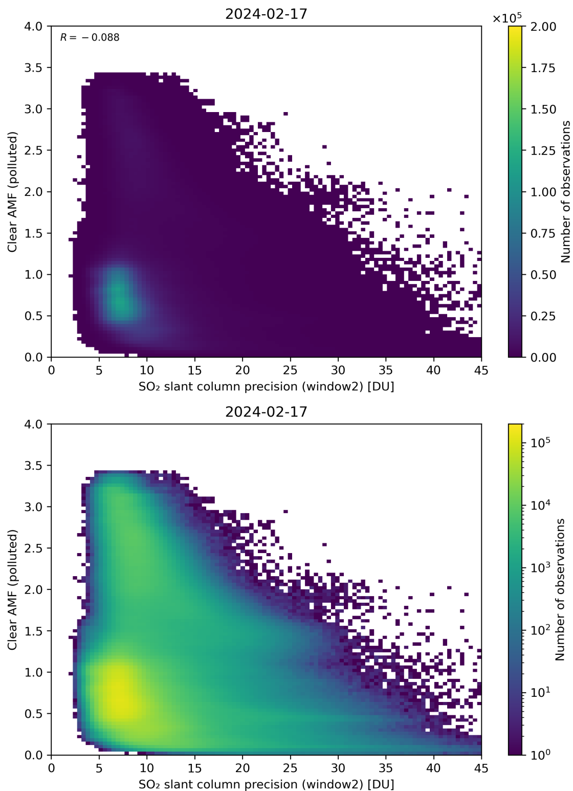
Figure 246: Scatter density plot of “SO 2 slant column precision (window2)” against “Clear AMF (polluted)” for 2024-02-17 to 2024-02-18.
