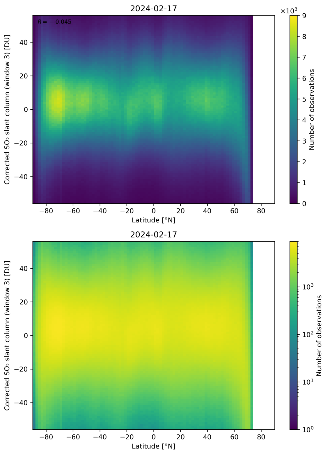
Figure 148: Scatter density plot of “Latitude” against “Corrected SO 2 slant column (window 3)” for 2024-02-17 to 2024-02-18.
