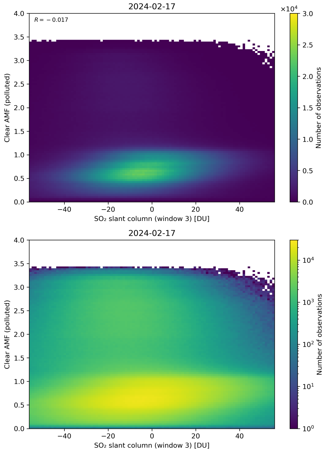
Figure 265: Scatter density plot of “SO 2 slant column (window 3)” against “Clear AMF (polluted)” for 2024-02-17 to 2024-02-18.
