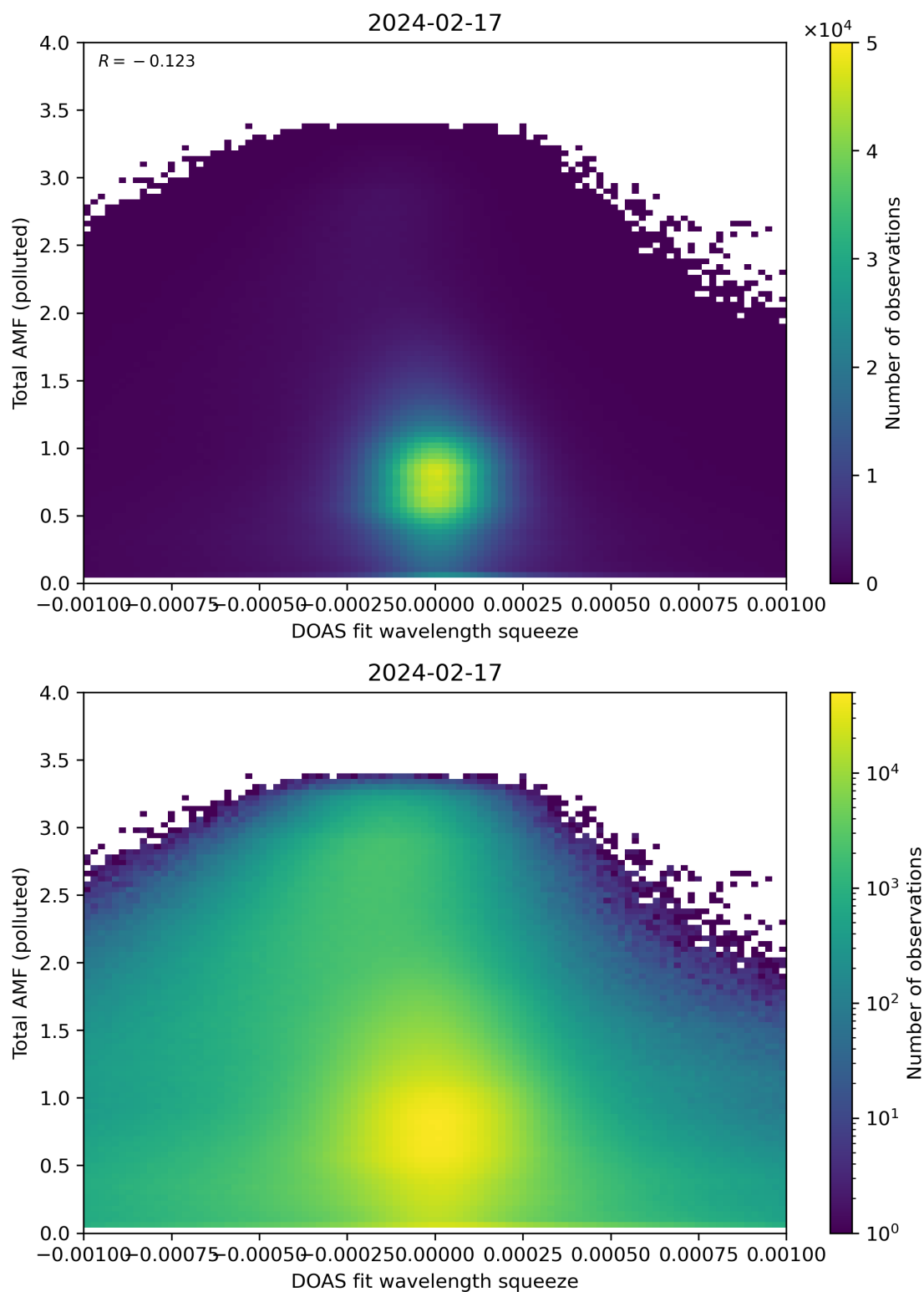
Figure 134: Scatter density plot of “DOAS fit wavelength squeeze” against “Total AMF (polluted)” for 2024-02-17 to 2024-02-18.
