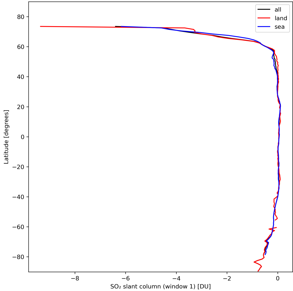
Figure 33: Zonal average of “SO 2 slant column (window 1)” for 2024-02-17 to 2024-02-18.
