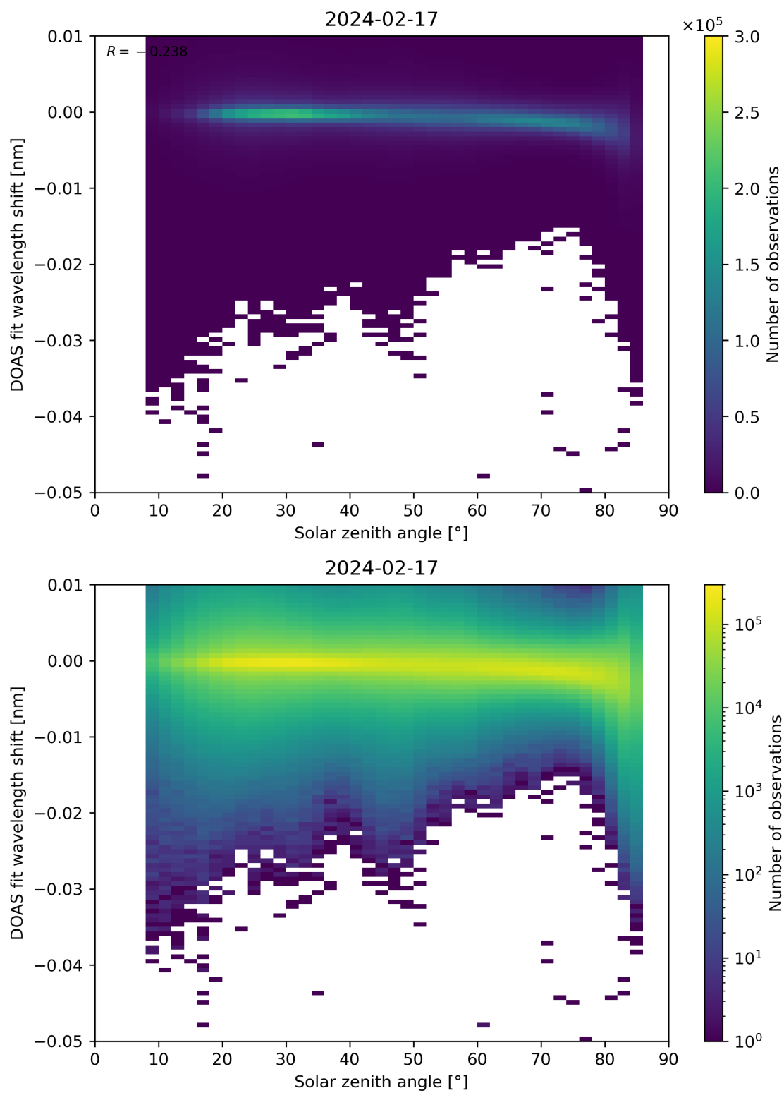
Figure 161: Scatter density plot of “Solar zenith angle” against “DOAS fit wavelength shift” for 2024-02-17 to 2024-02-18.
