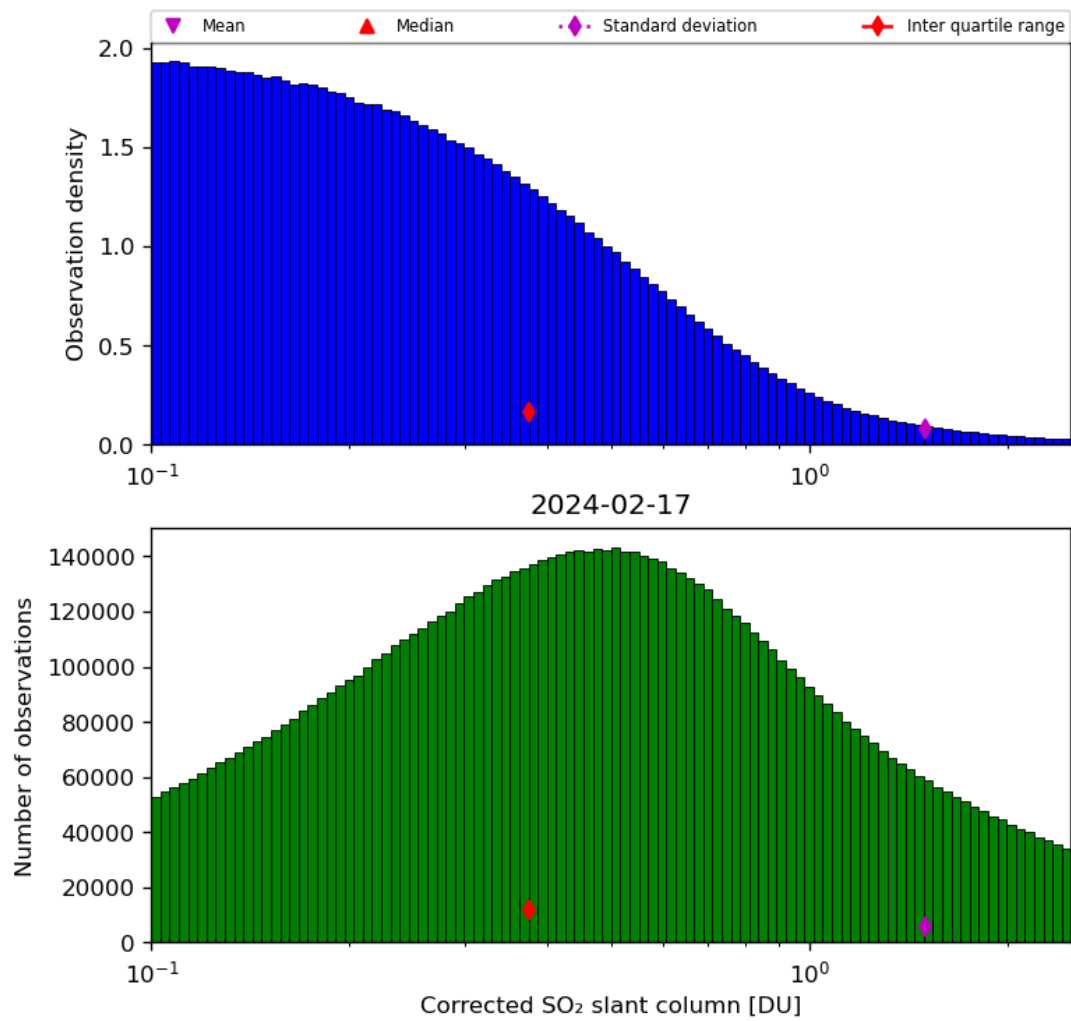
Figure 55: Histogram of “Corrected SO 2 slant column” for 2024-02-17 to 2024-02-18
