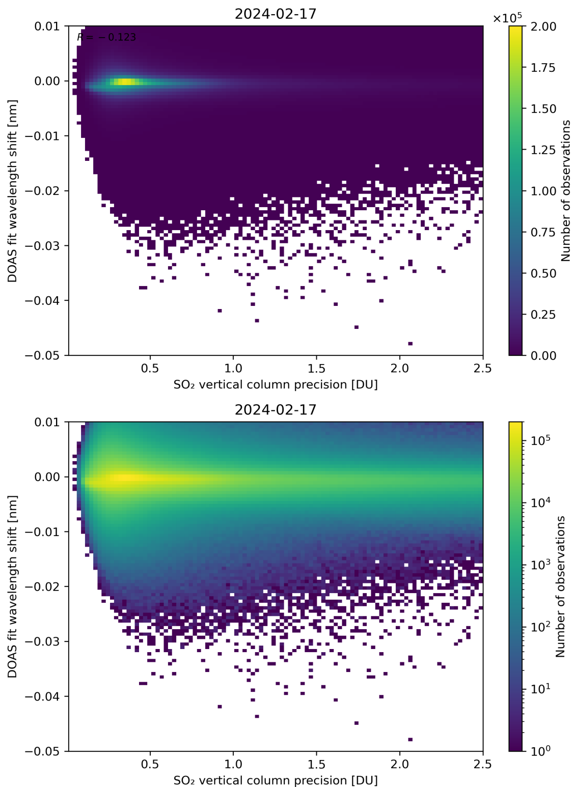
Figure 282: Scatter density plot of “SO 2 vertical column precision” against “DOAS fit wavelength shift” for 2024-02-17 to 2024-02-18.
