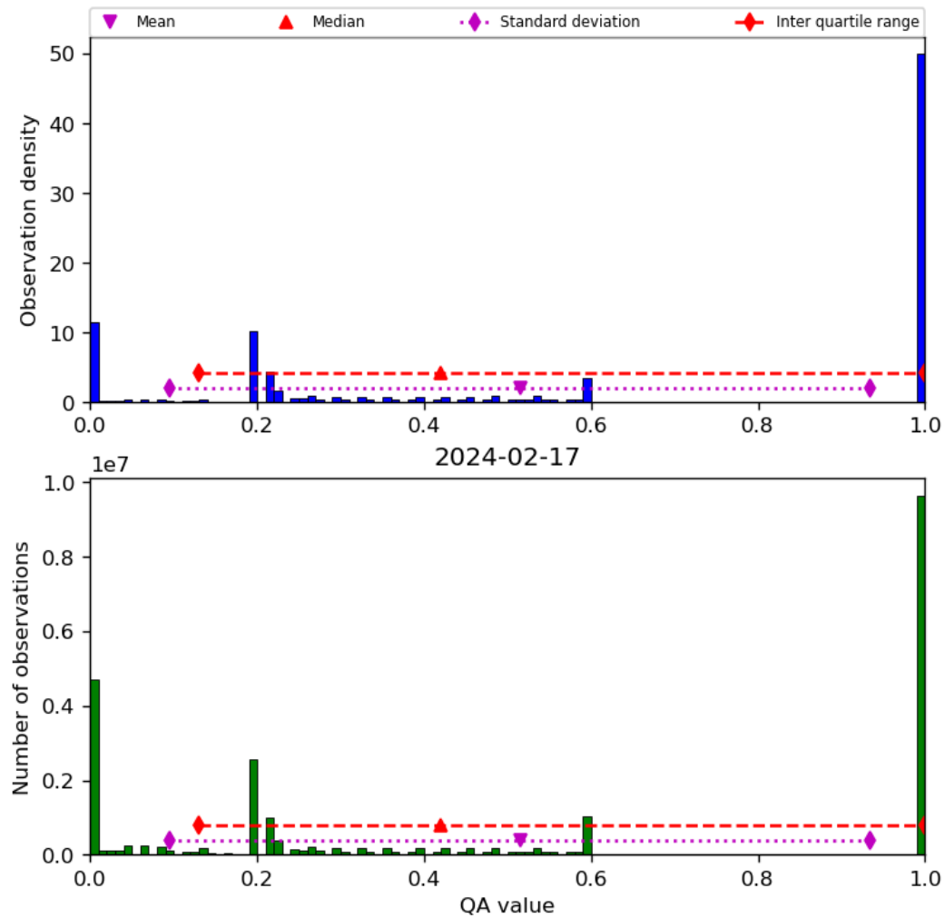
Figure 52: Histogram of “QA value” for 2024-02-17 to 2024-02-18
