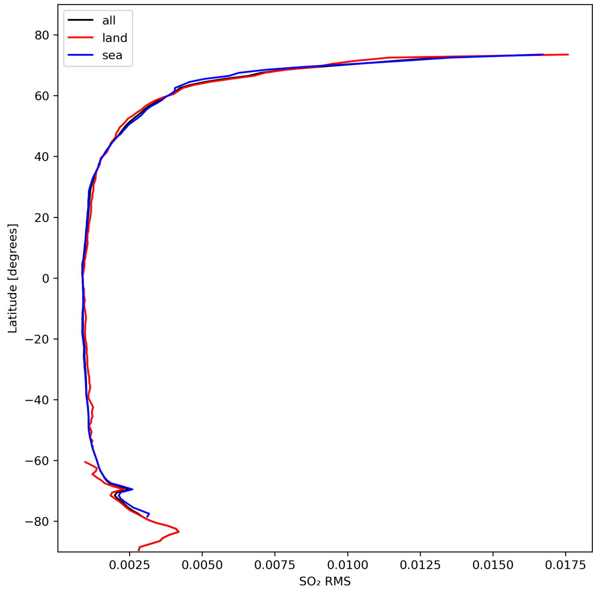
Figure 47: Zonal average of “SO 2 RMS” for 2024-02-17 to 2024-02-18.
