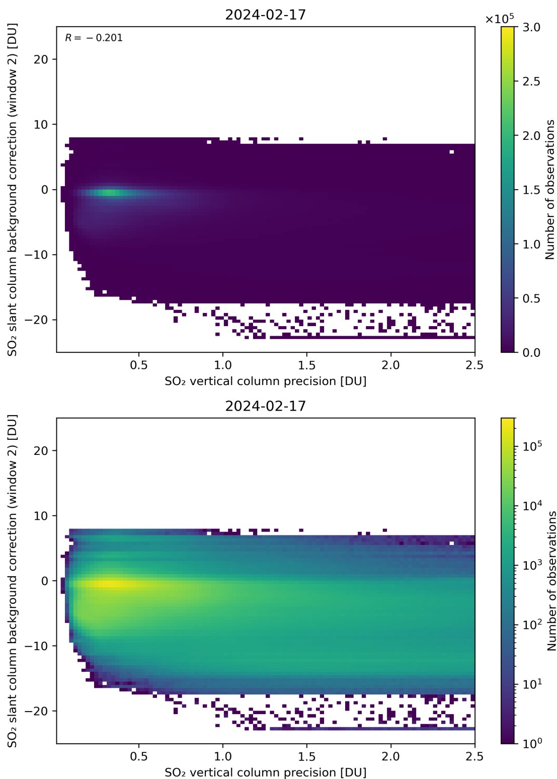
Figure 280: Scatter density plot of “SO 2 vertical column precision” against “SO 2 slant column background correction (window 2)” for 2024-02-17 to 2024-02-18.
