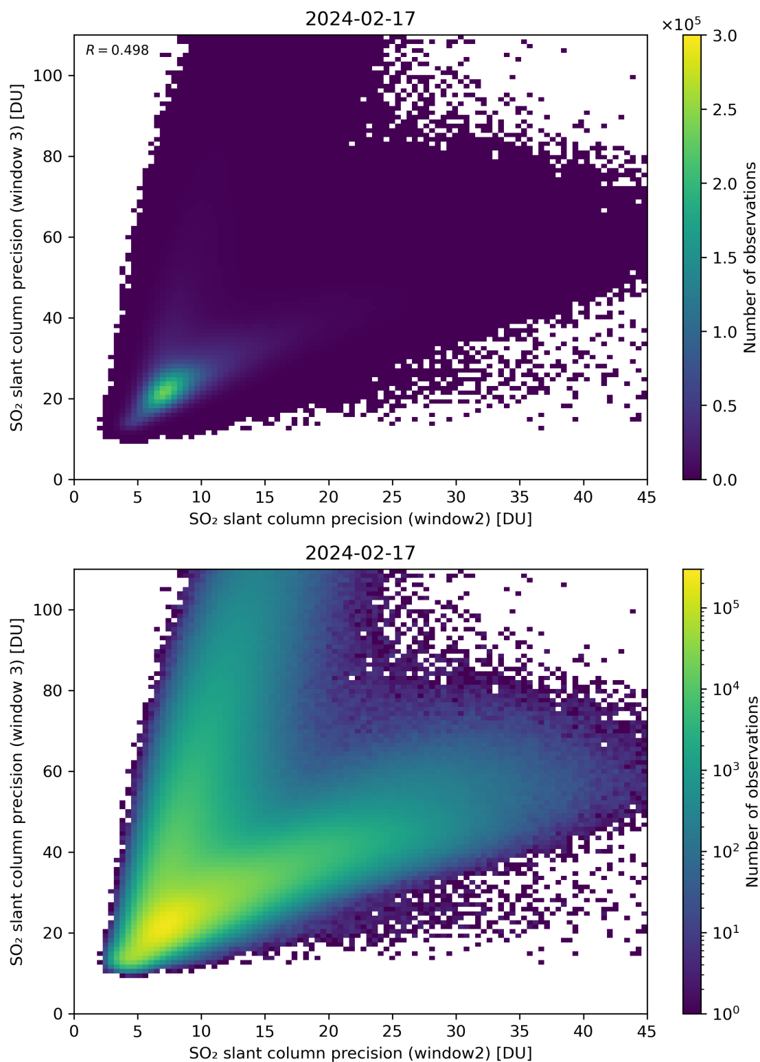
Figure 250: Scatter density plot of “SO 2 slant column precision (window2)” against “SO 2 slant column precision (window 3)” for 2024-02-17 to 2024-02-18.
