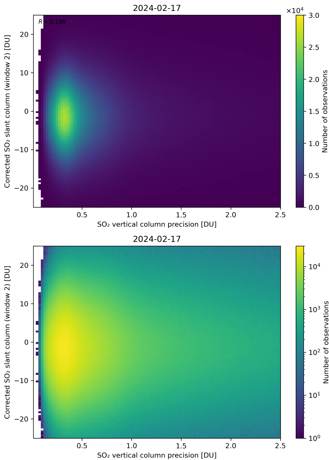
Figure 287: Scatter density plot of “SO 2 vertical column precision” against “Corrected SO 2 slant column (window 2)” for 2024-02-17 to 2024-02-18.
