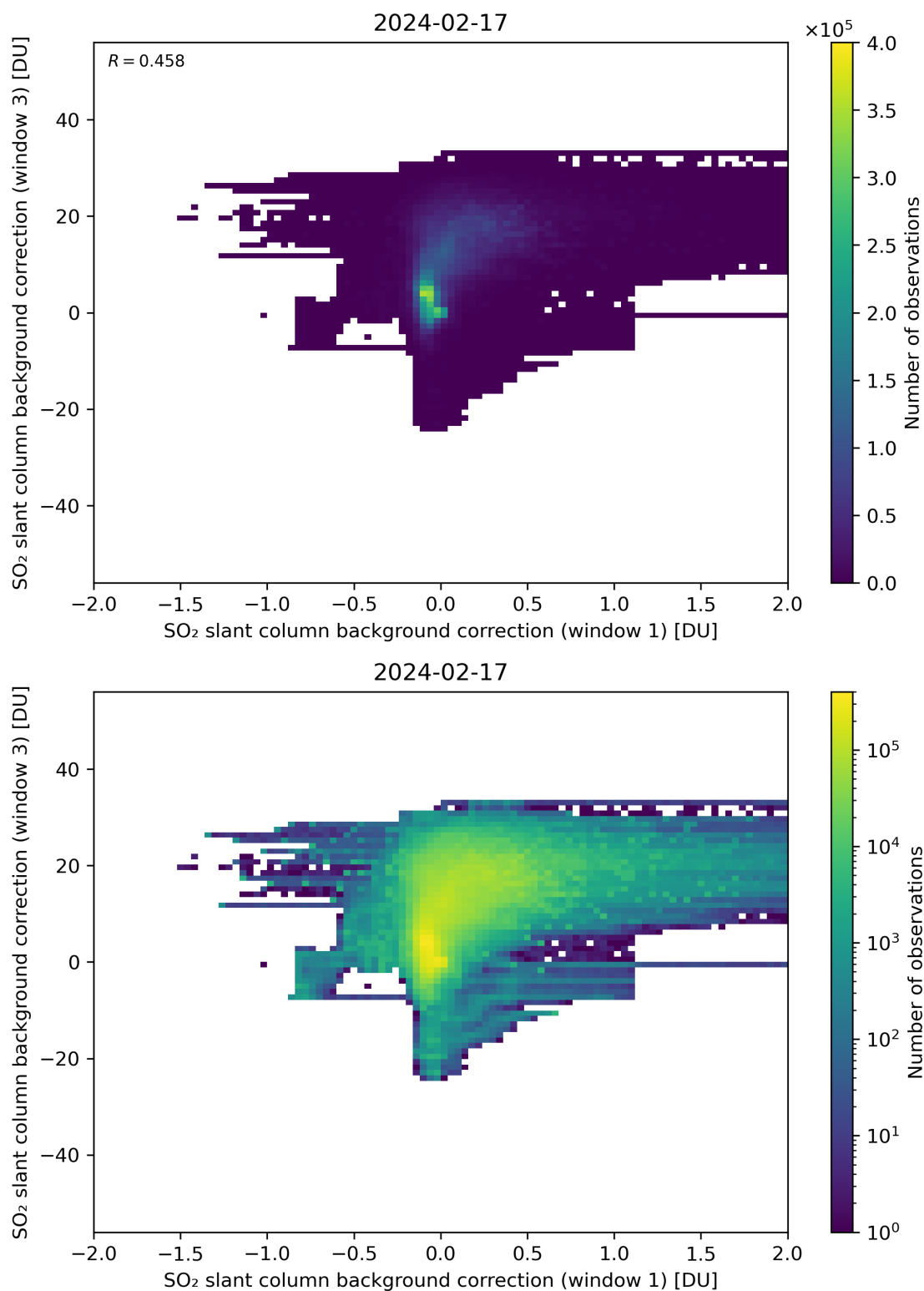
Figure 99: Scatter density plot of “SO 2 slant column background correction (window 1)” against “SO 2 slant column background correction (window 3)” for 2024-02-17 to 2024-02-18.
