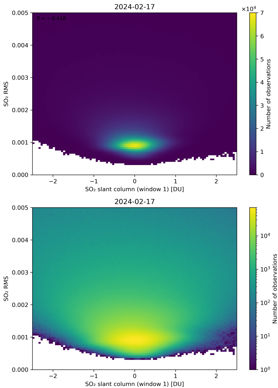
Figure 217: Scatter density plot of “SO 2 slant column (window 1)” against “SO 2 RMS” for 2024-02-17 to 2024-02-18.
