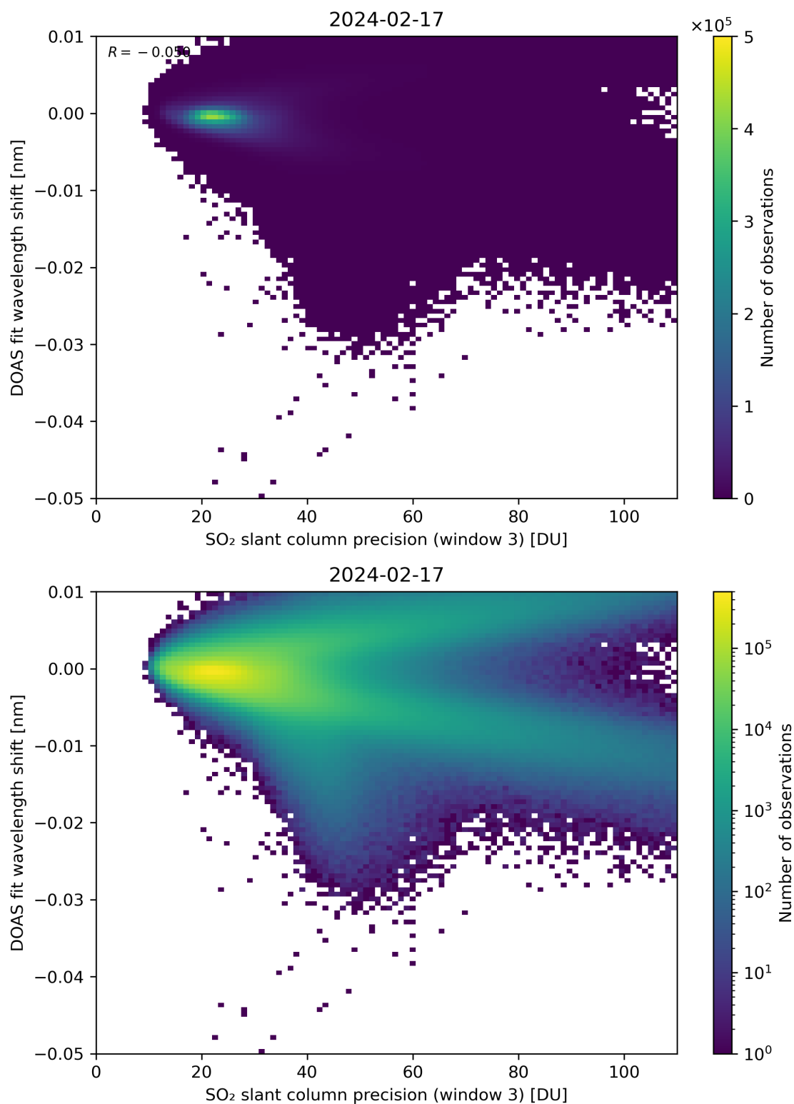
Figure 258: Scatter density plot of “SO 2 slant column precision (window 3)” against “DOAS fit wavelength shift” for 2024-02-17 to 2024-02-18.
