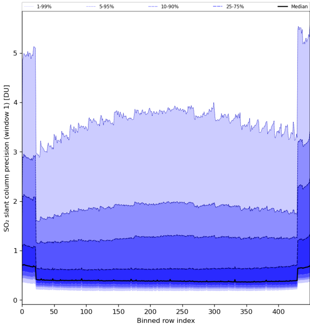
Figure 80: Along track statistics of “SO 2 slant column precision (window 1)” for 2024-02-17 to 2024-02-18
