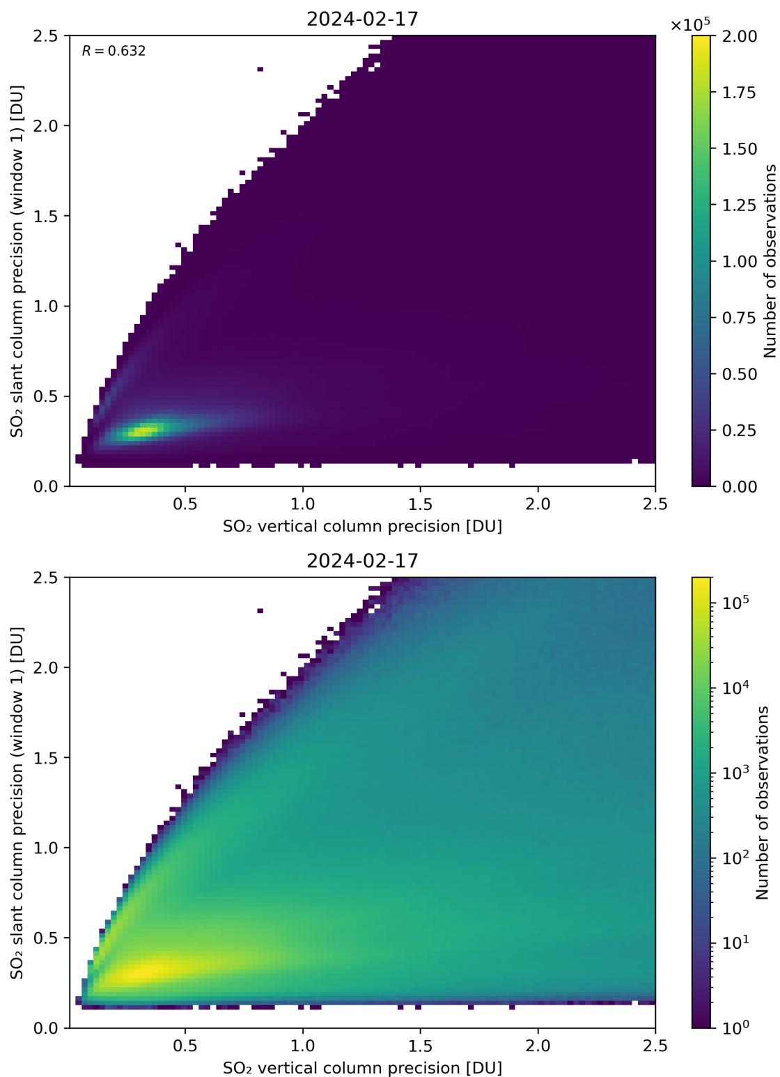
Figure 290: Scatter density plot of “SO 2 vertical column precision” against “SO 2 slant column precision (window 1)” for 2024-02-17 to 2024-02-18.
