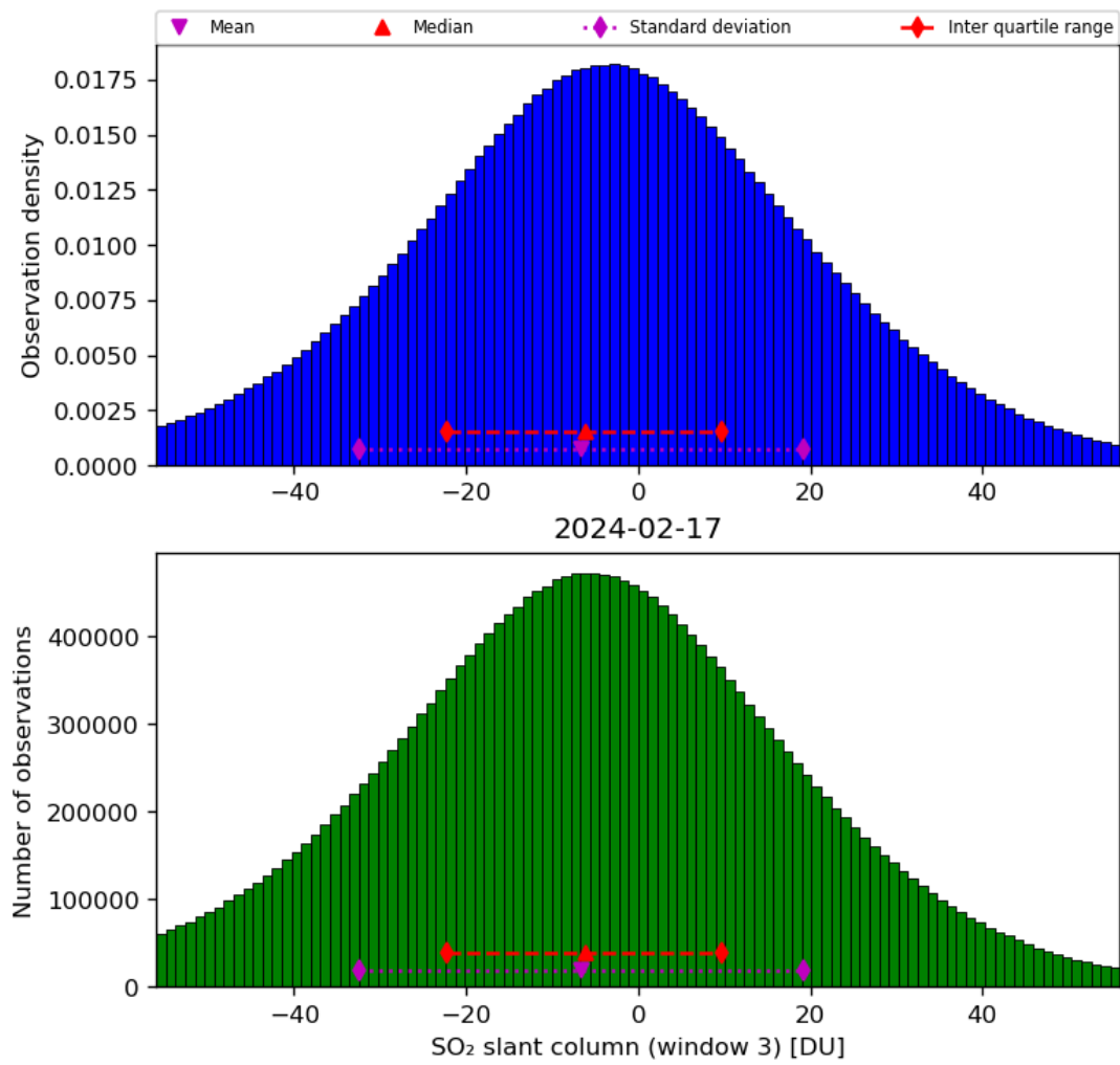
Figure 64: Histogram of “SO 2 slant column (window 3)” for 2024-02-17 to 2024-02-18
