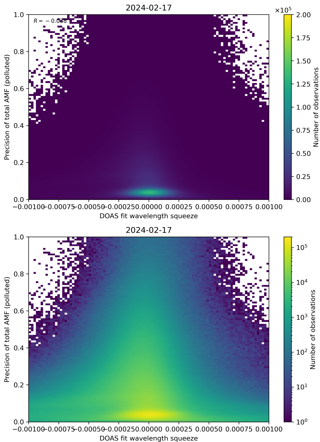
Figure 135: Scatter density plot of “DOAS fit wavelength squeeze” against “Precision of total AMF (polluted)” for 2024-02-17 to 2024-02-18.
