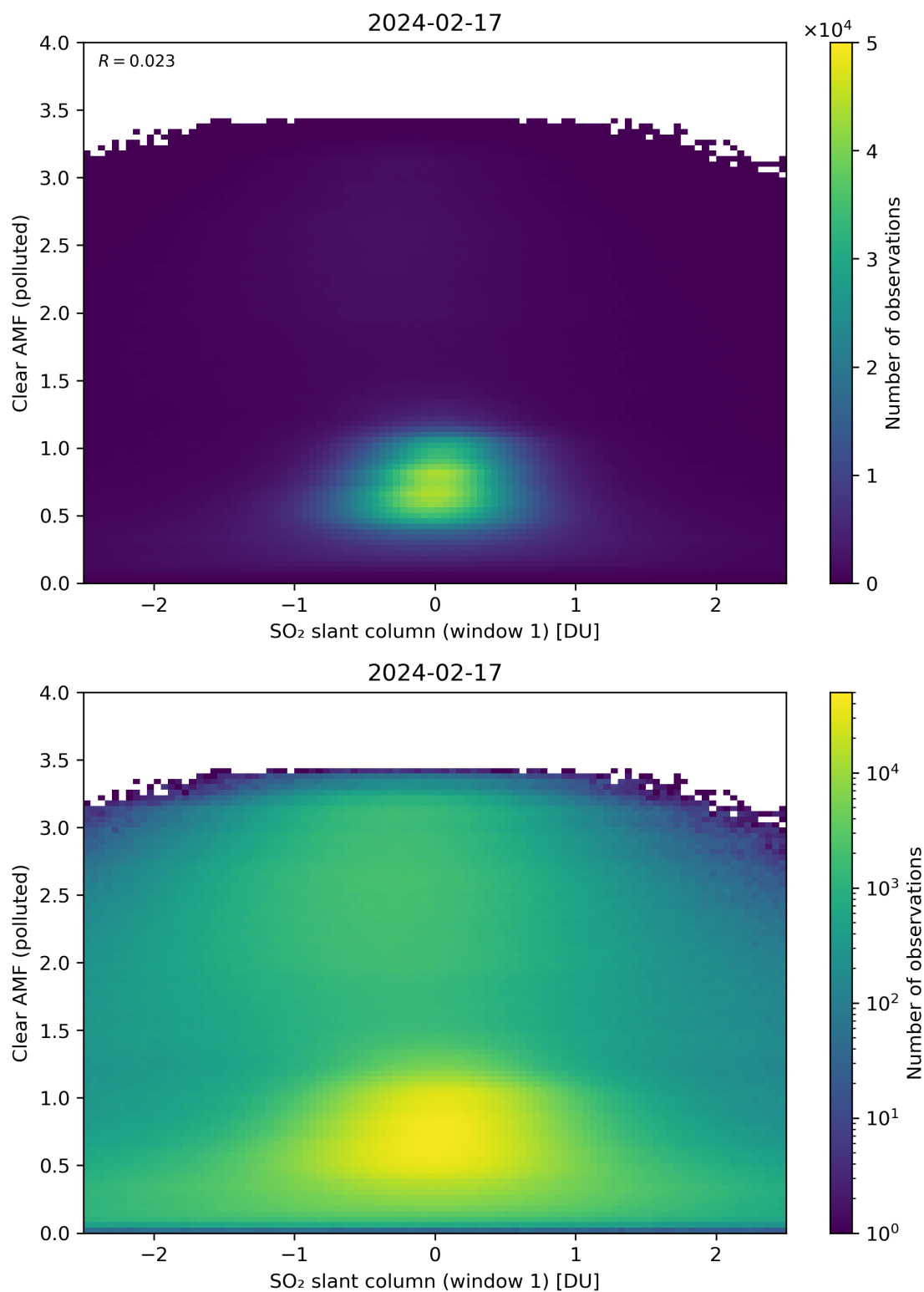
Figure 232: Scatter density plot of “SO 2 slant column (window 1)” against “Clear AMF (polluted)” for 2024-02-17 to 2024-02-18.
