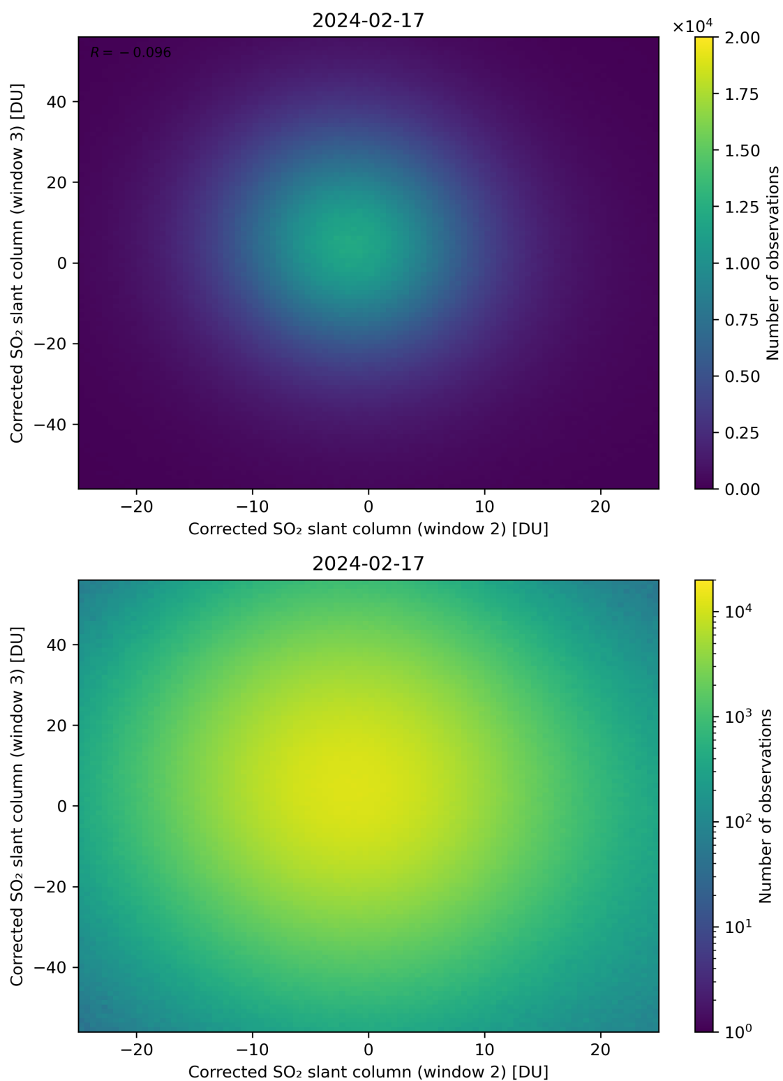
Figure 200: Scatter density plot of “Corrected SO 2 slant column (window 2)” against “Corrected SO 2 slant column (window 3)” for 2024-02-17 to 2024-02-18.
