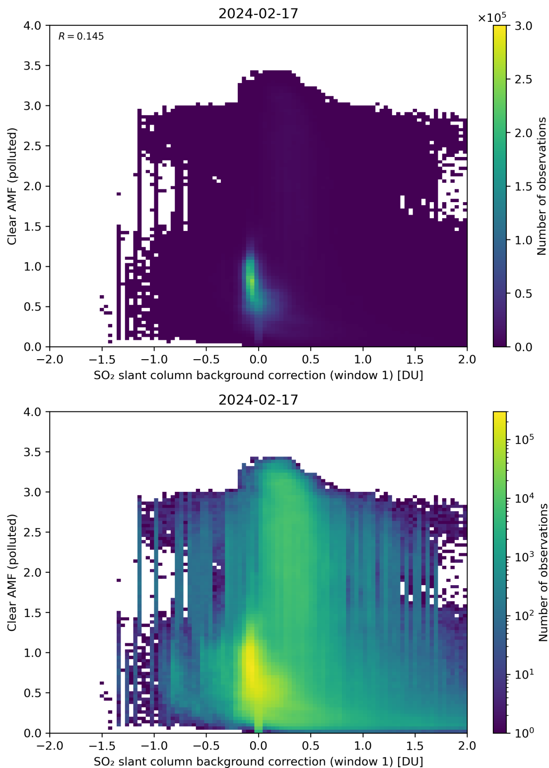
Figure 103: Scatter density plot of “SO 2 slant column background correction (window 1)” against “Clear AMF (polluted)” for 2024-02-17 to 2024-02-18.
