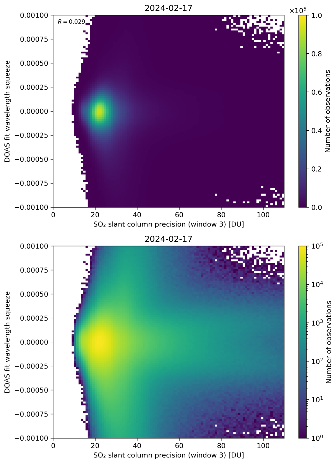
Figure 259: Scatter density plot of “SO 2 slant column precision (window 3)” against “DOAS fit wavelength squeeze” for 2024-02-17 to 2024-02-18.
