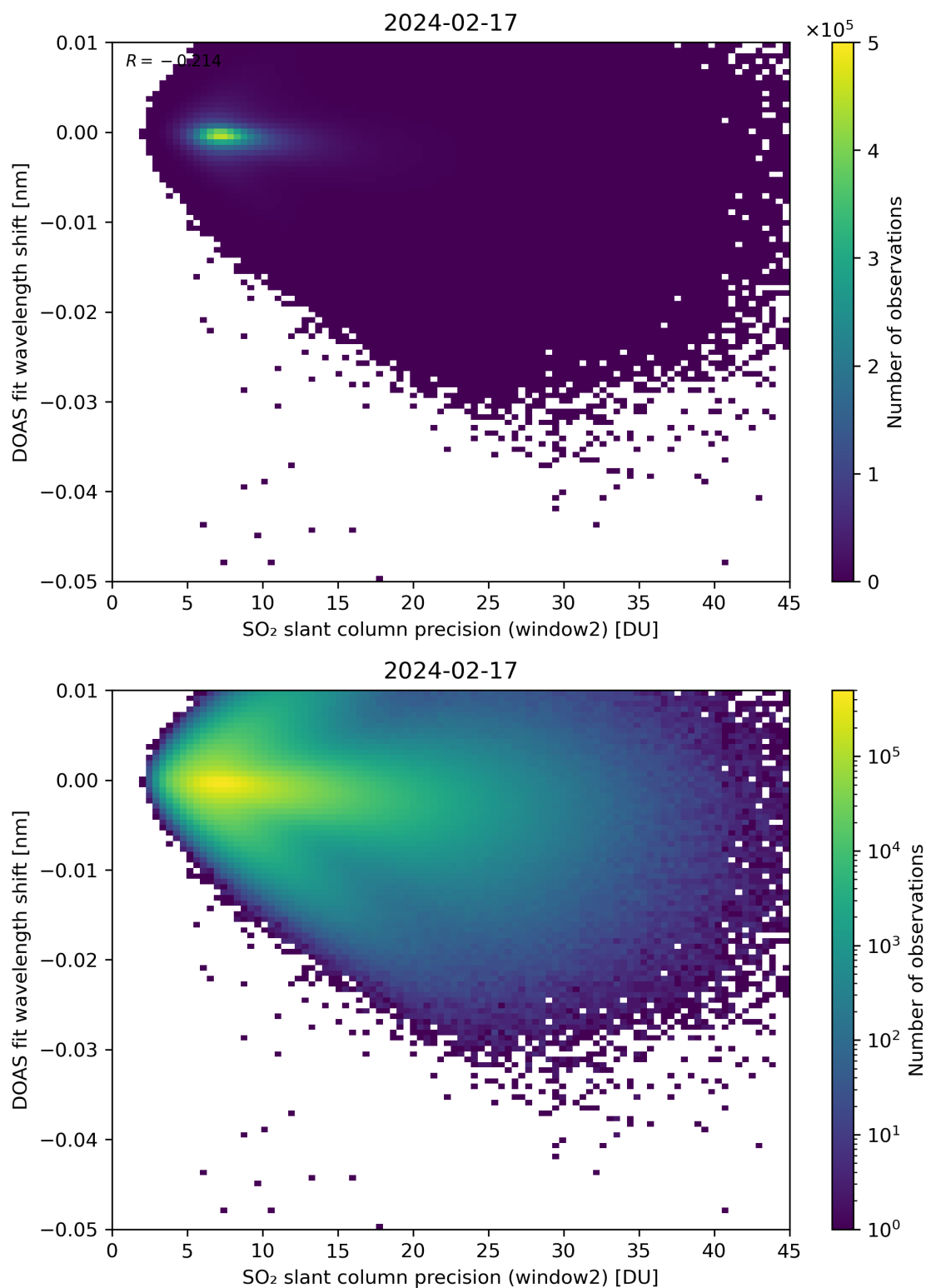
Figure 243: Scatter density plot of “SO 2 slant column precision (window2)” against “DOAS fit wavelength shift” for 2024-02-17 to 2024-02-18.
