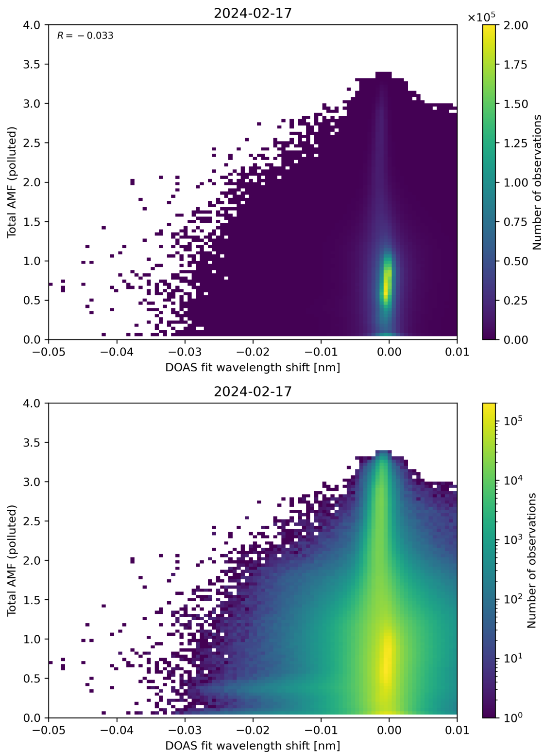
Figure 130: Scatter density plot of “DOAS fit wavelength shift” against “Total AMF (polluted)” for 2024-02-17 to 2024-02-18.
