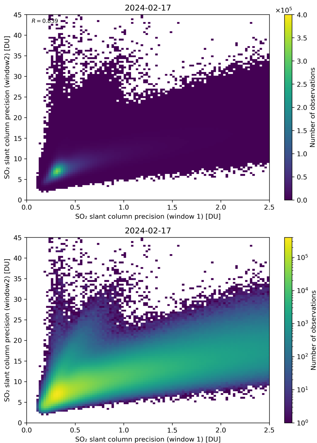
Figure 227: Scatter density plot of “SO 2 slant column precision (window 1)” against “SO 2 slant column precision (window 2)” for 2024-02-17 to 2024-02-18.
