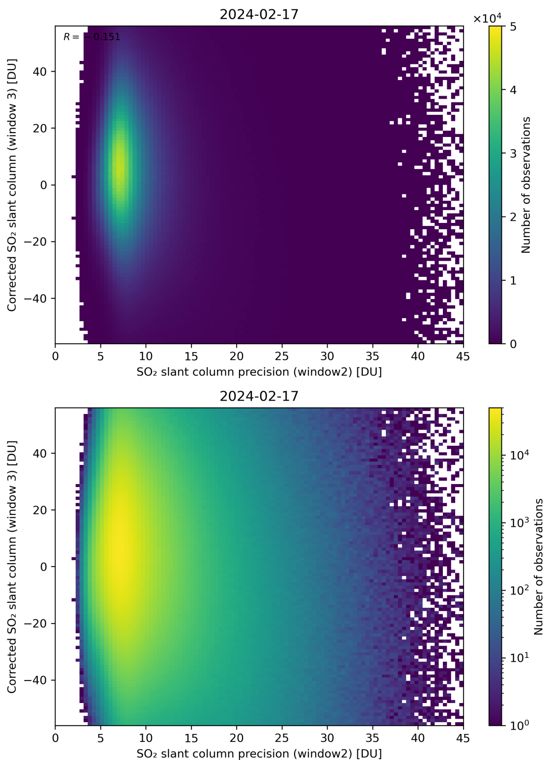
Figure 248: Scatter density plot of “SO 2 slant column precision (window2)” against “Corrected SO 2 slant column (window 3)” for 2024-02-17 to 2024-02-18.
