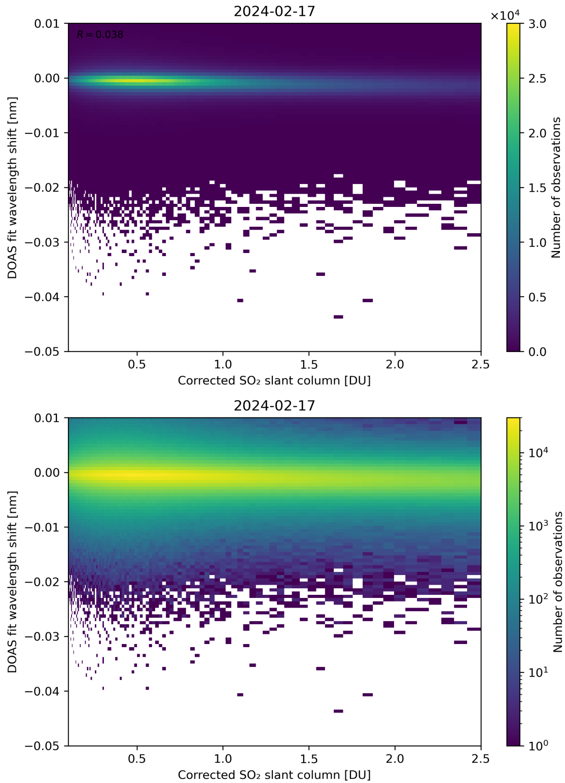
Figure 181: Scatter density plot of “Corrected SO 2 slant column” against “DOAS fit wavelength shift” for 2024-02-17 to 2024-02-18.
