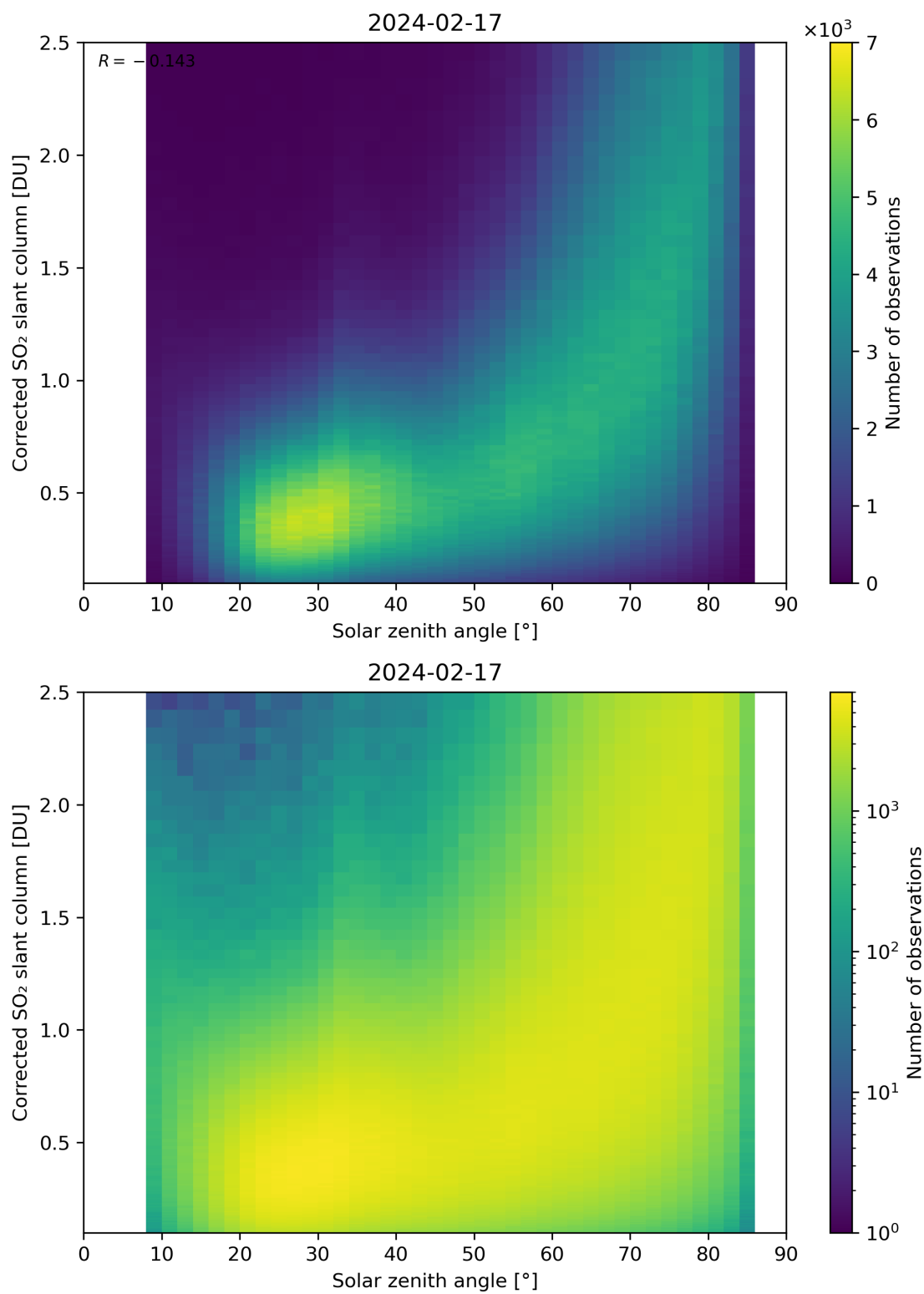
Figure 166: Scatter density plot of “Solar zenith angle” against “Corrected SO 2 slant column” for 2024-02-17 to 2024-02-18.
