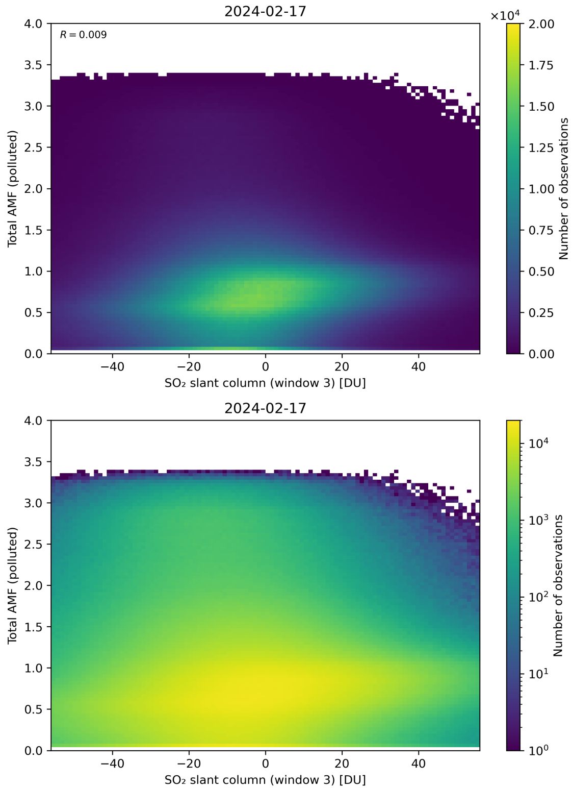
Figure 268: Scatter density plot of “SO 2 slant column (window 3)” against “Total AMF (polluted)” for 2024-02-17 to 2024-02-18.
