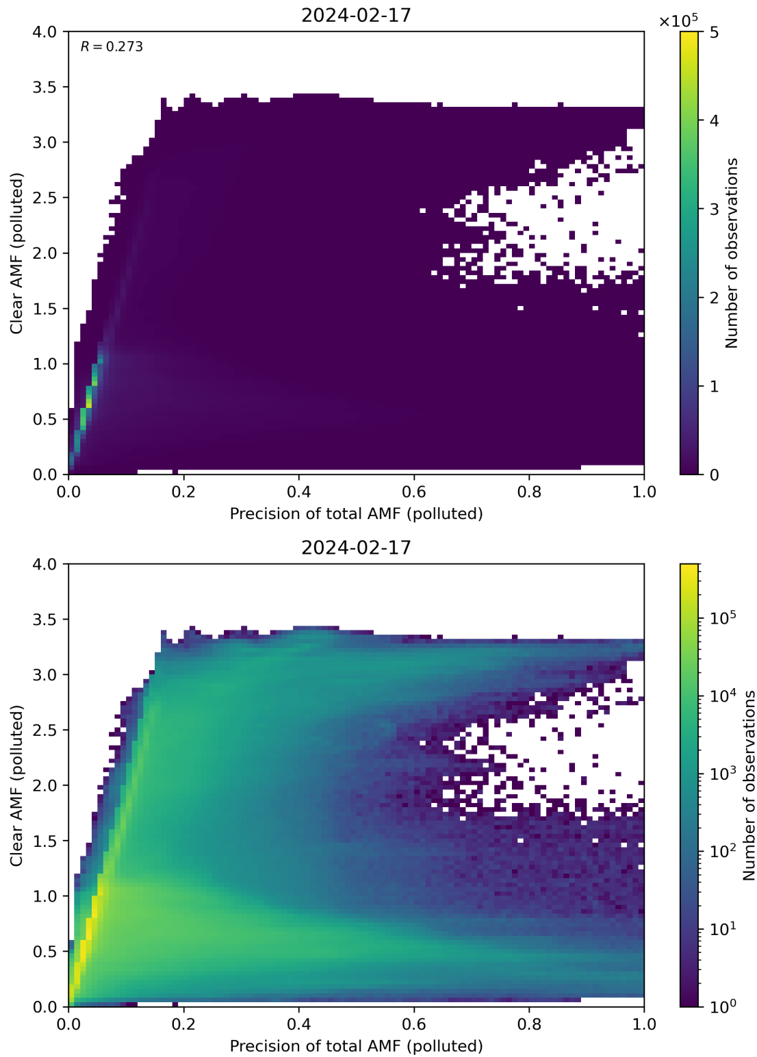
Figure 270: Scatter density plot of “Precision of total AMF (polluted)” against “Clear AMF (polluted)” for 2024-02-17 to 2024-02-18.
