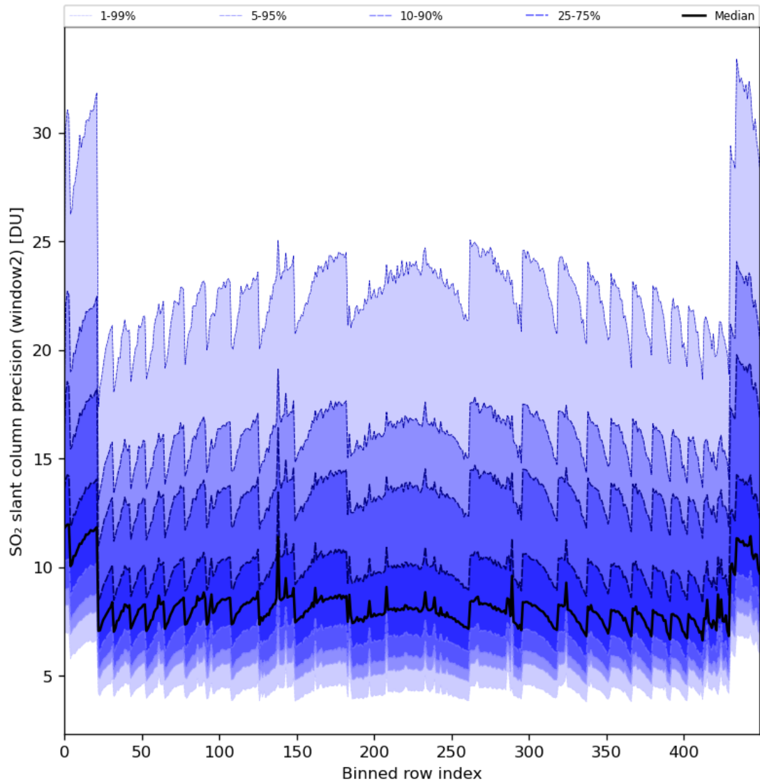
Figure 84: Along track statistics of “SO 2 slant column precision (window2)” for 2024-02-17 to 2024-02-18
