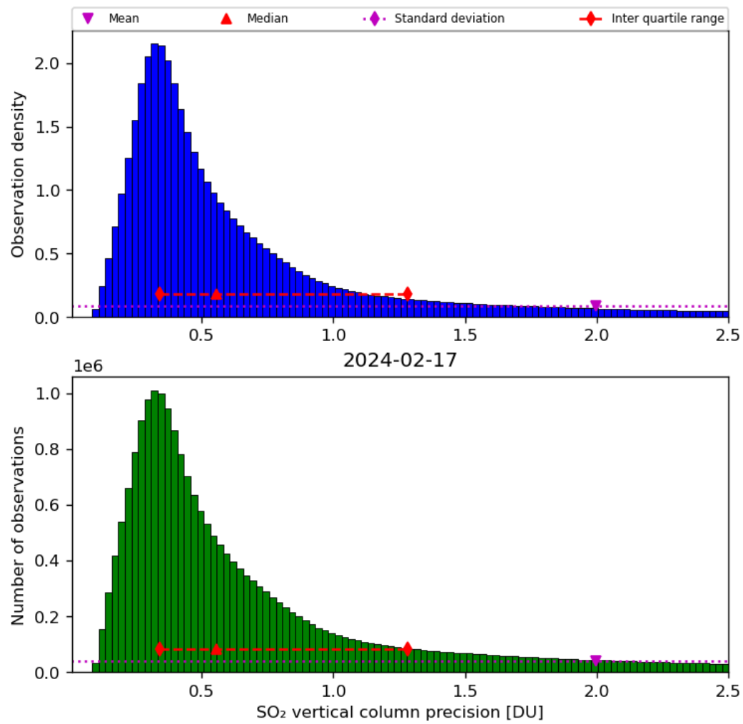
Figure 54: Histogram of “SO 2 vertical column precision” for 2024-02-17 to 2024-02-18
