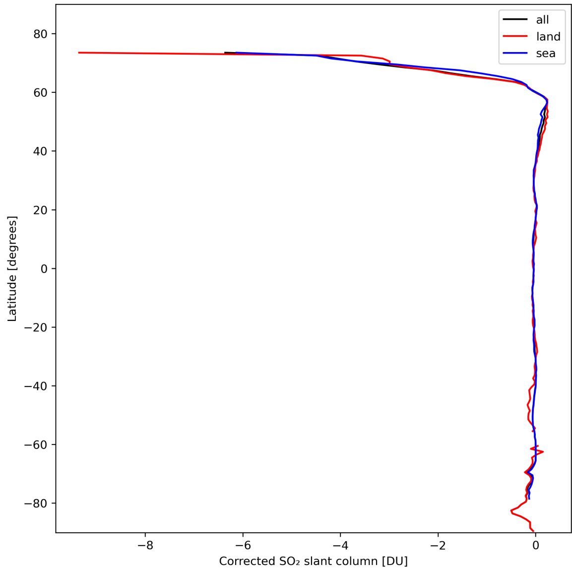
Figure 32: Zonal average of “Corrected SO 2 slant column” for 2024-02-17 to 2024-02-18.
