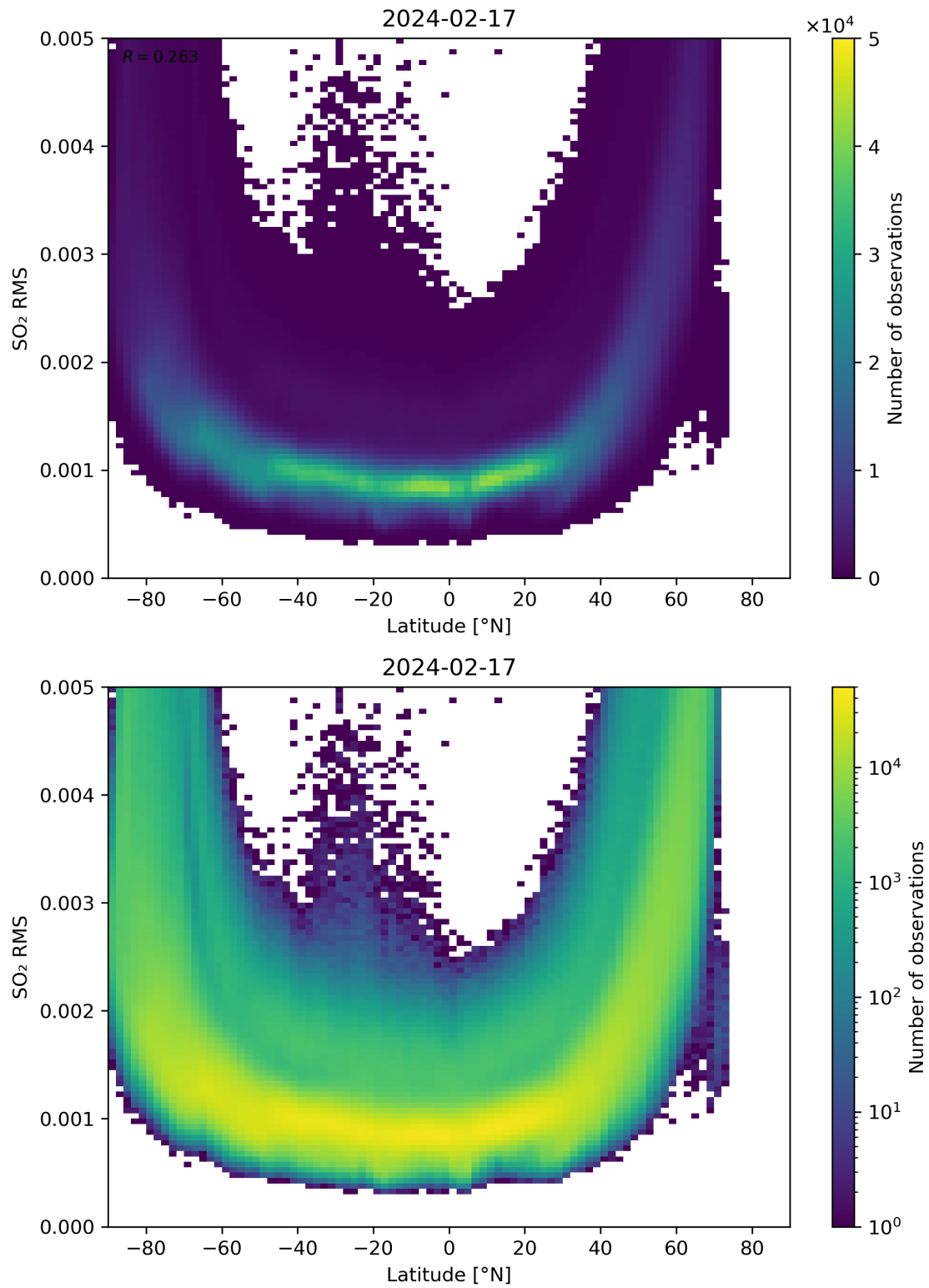
Figure 144: Scatter density plot of “Latitude” against “SO 2 RMS” for 2024-02-17 to 2024-02-18.
