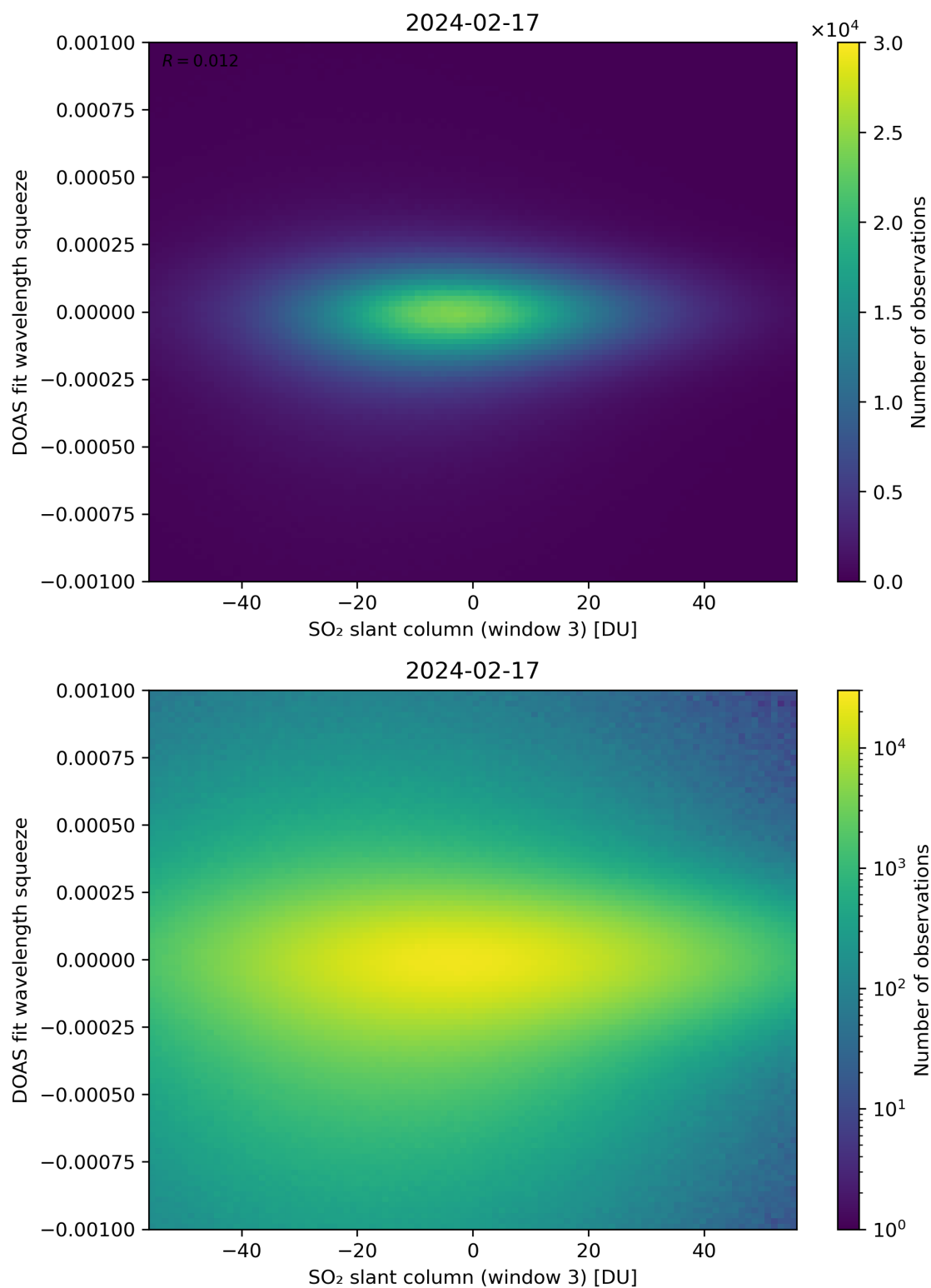
Figure 255: Scatter density plot of “SO 2 slant column (window 3)” against “DOAS fit wavelength squeeze” for 2024-02-17 to 2024-02-18.
