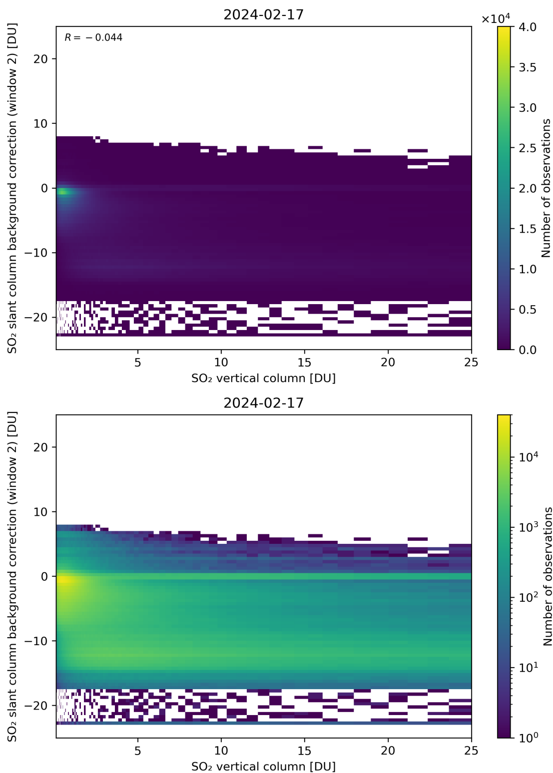
Figure 274: Scatter density plot of “SO 2 vertical column” against “SO 2 slant column background correction (window 2)” for 2024-02-17 to 2024-02-18.
