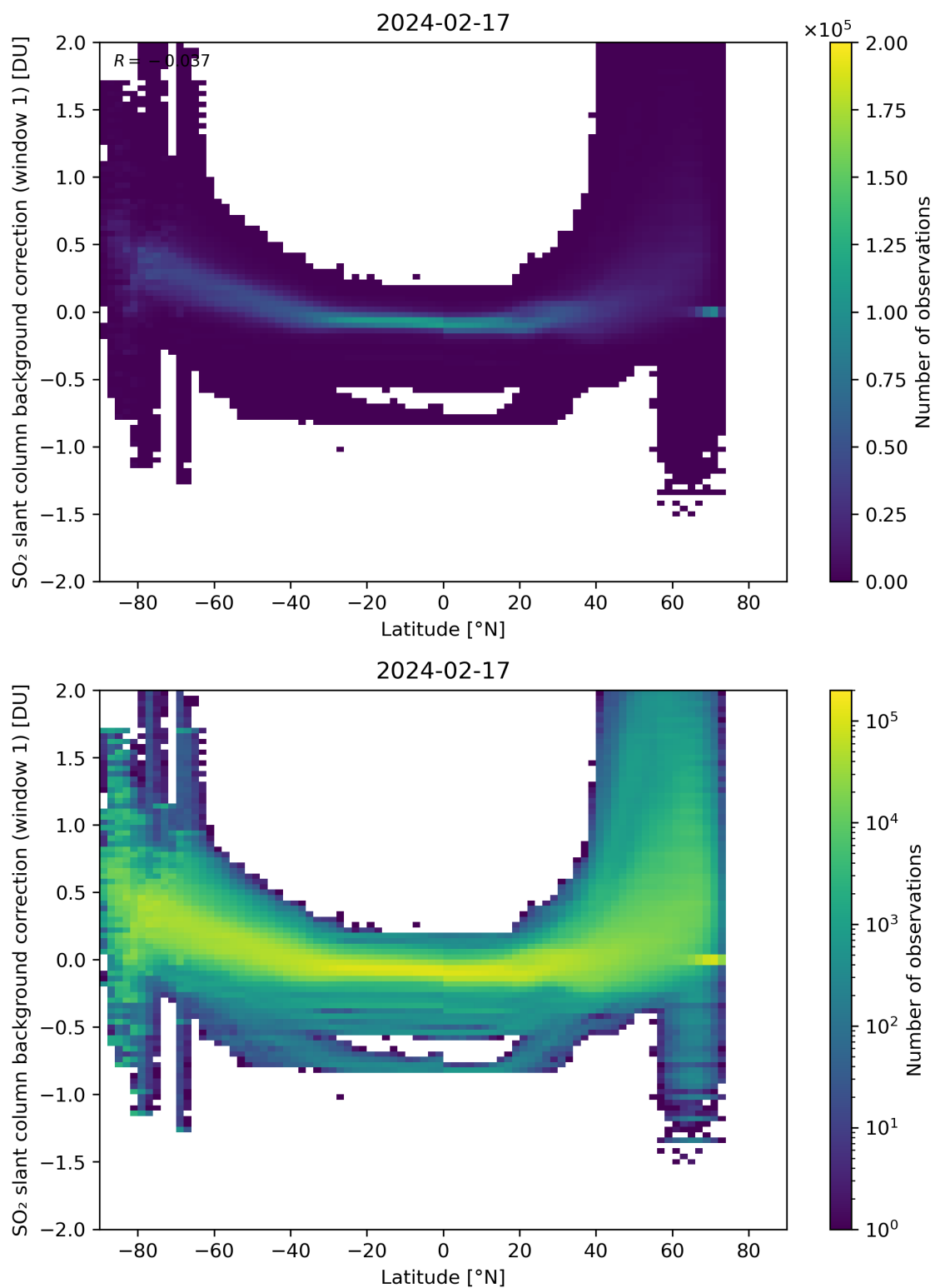
Figure 139: Scatter density plot of “Latitude” against “SO 2 slant column background correction (window 1)” for 2024-02-17 to 2024-02-18.
