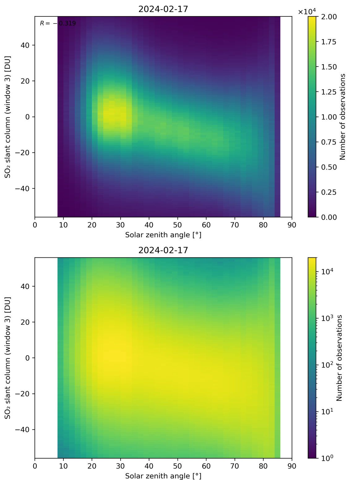
Figure 172: Scatter density plot of “Solar zenith angle” against “SO 2 slant column (window 3)” for 2024-02-17 to 2024-02-18.
