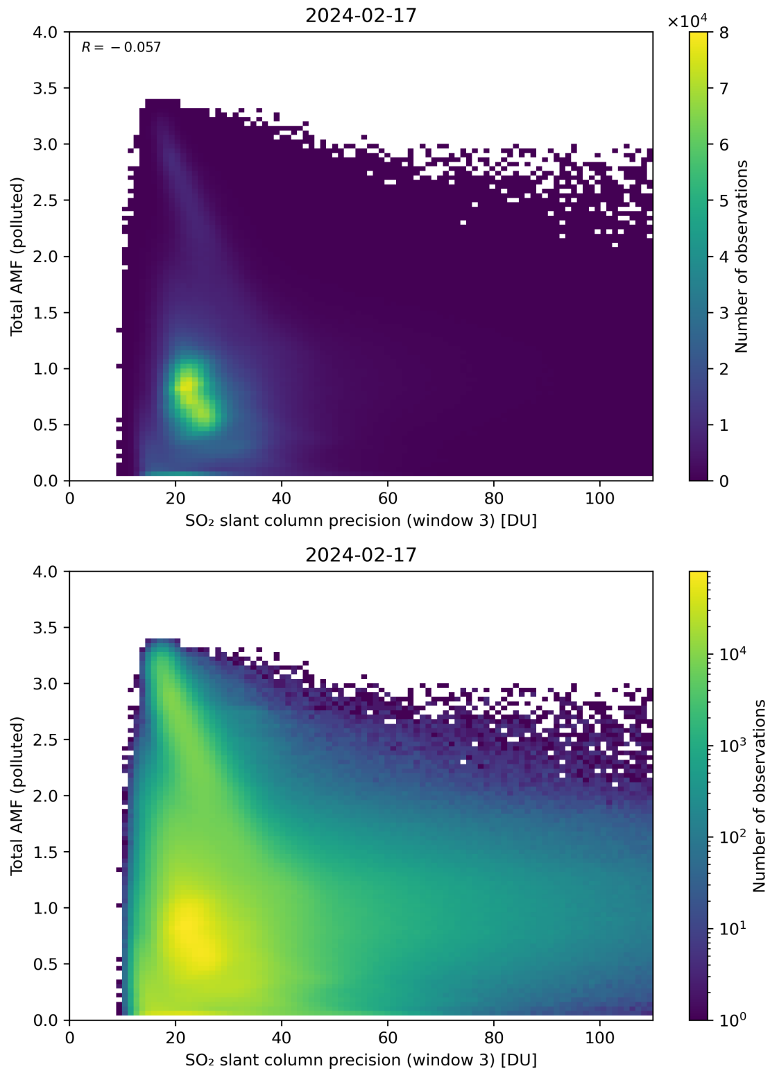
Figure 263: Scatter density plot of “SO 2 slant column precision (window 3)” against “Total AMF (polluted)” for 2024-02-17 to 2024-02-18.
