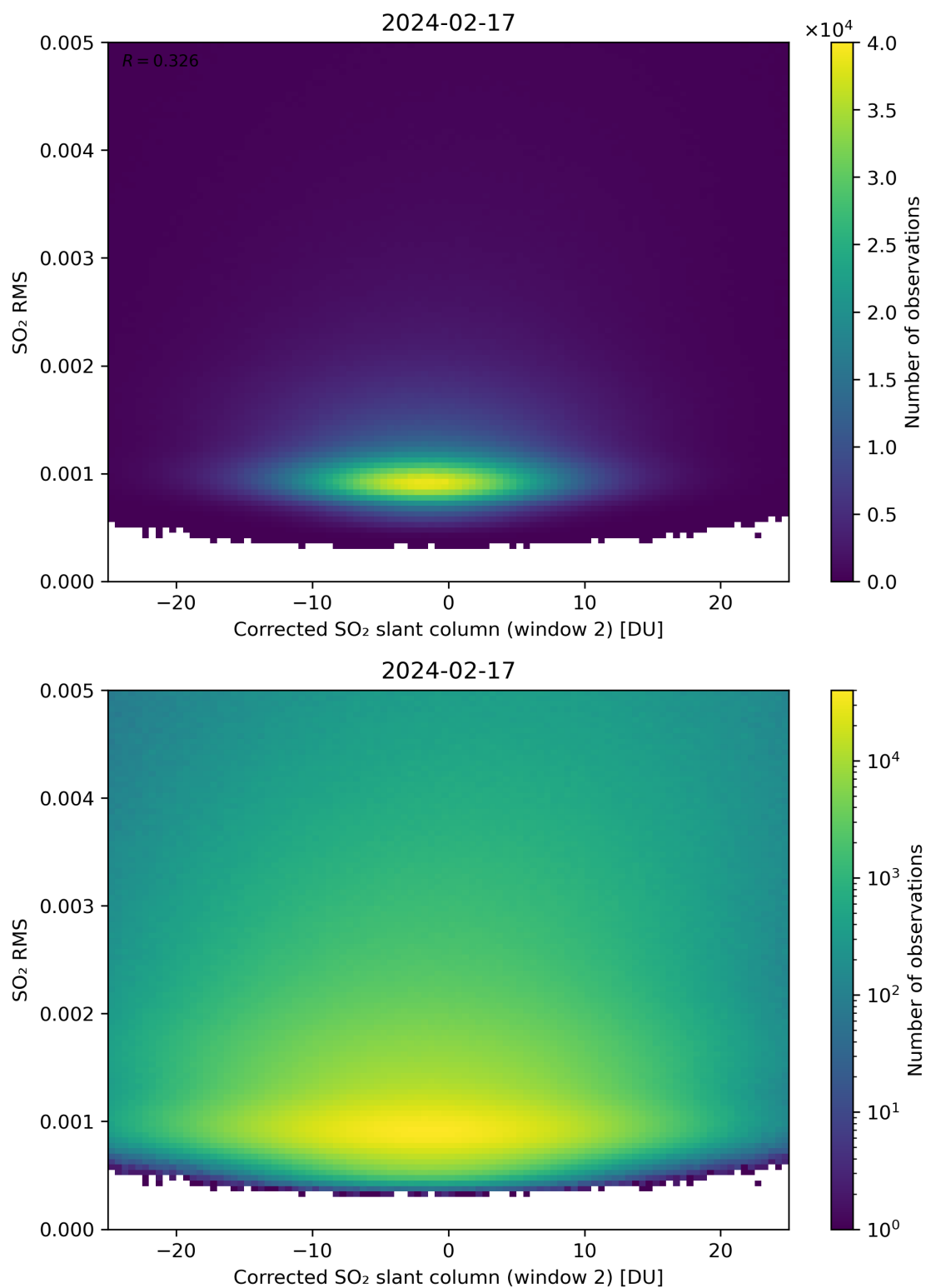
Figure 198: Scatter density plot of “Corrected SO 2 slant column (window 2)” against “SO 2 RMS” for 2024-02-17 to 2024-02-18.
