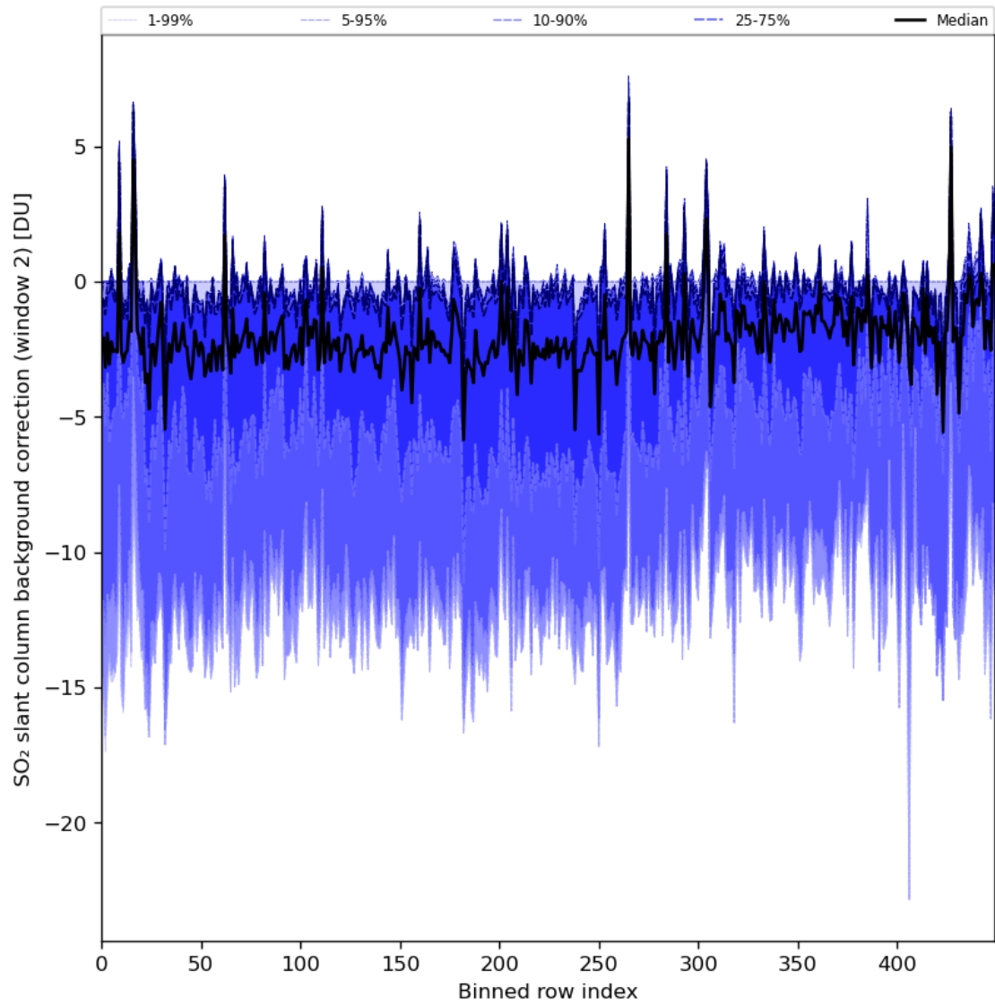
Figure 86: Along track statistics of “SO 2 slant column background correction (window 2)” for 2024-02-17 to 2024-02-18
