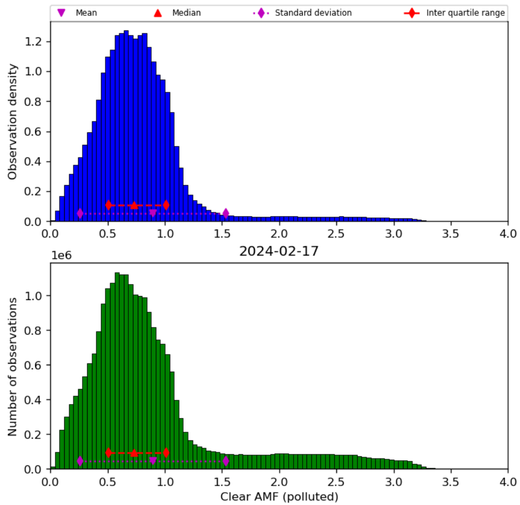
Figure 73: Histogram of “Clear AMF (polluted)” for 2024-02-17 to 2024-02-18
