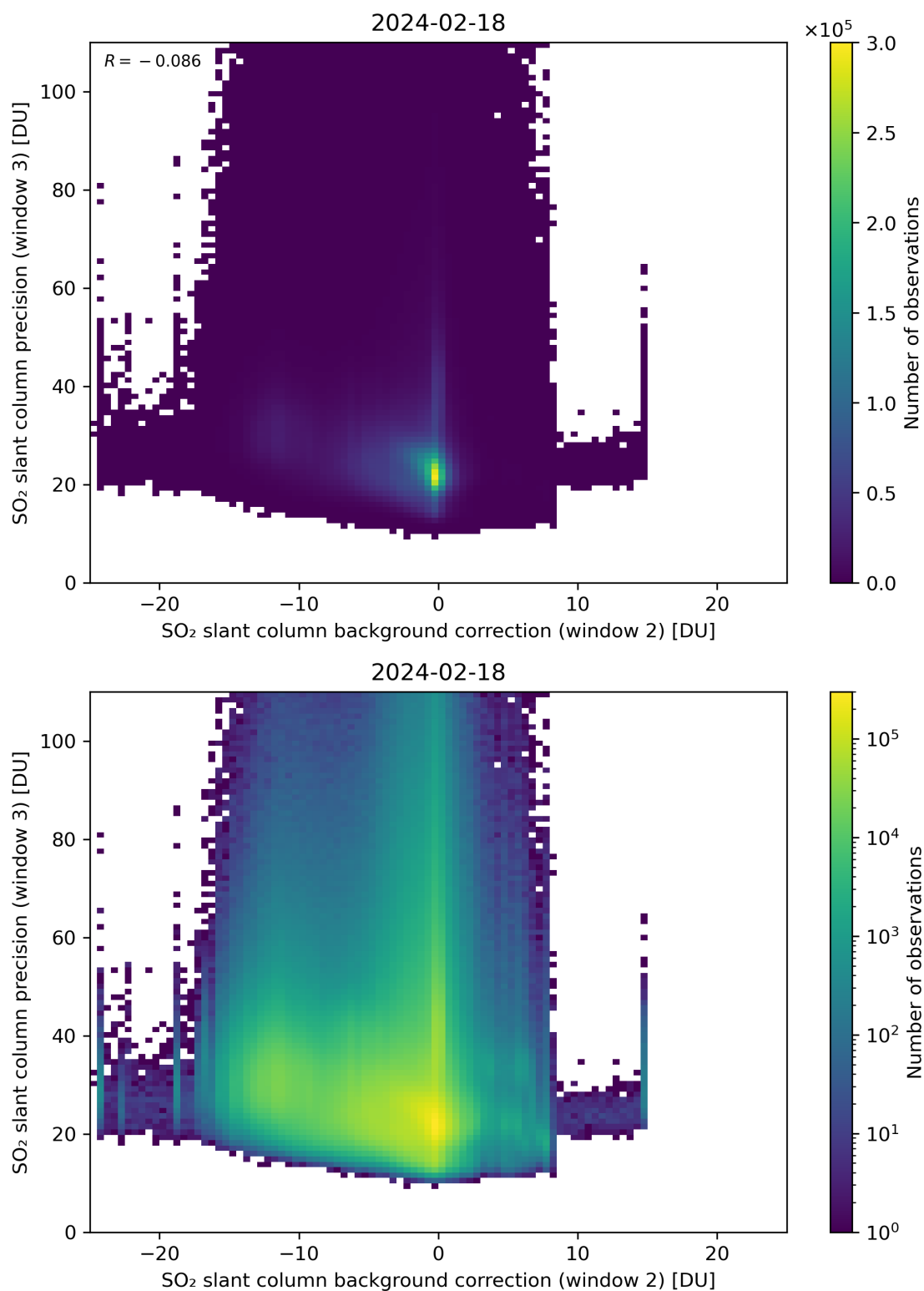
Figure 118: Scatter density plot of “SO 2 slant column background correction (window 2)” against “SO 2 slant column precision (window 3)” for 2024-02-17 to 2024-02-19.
