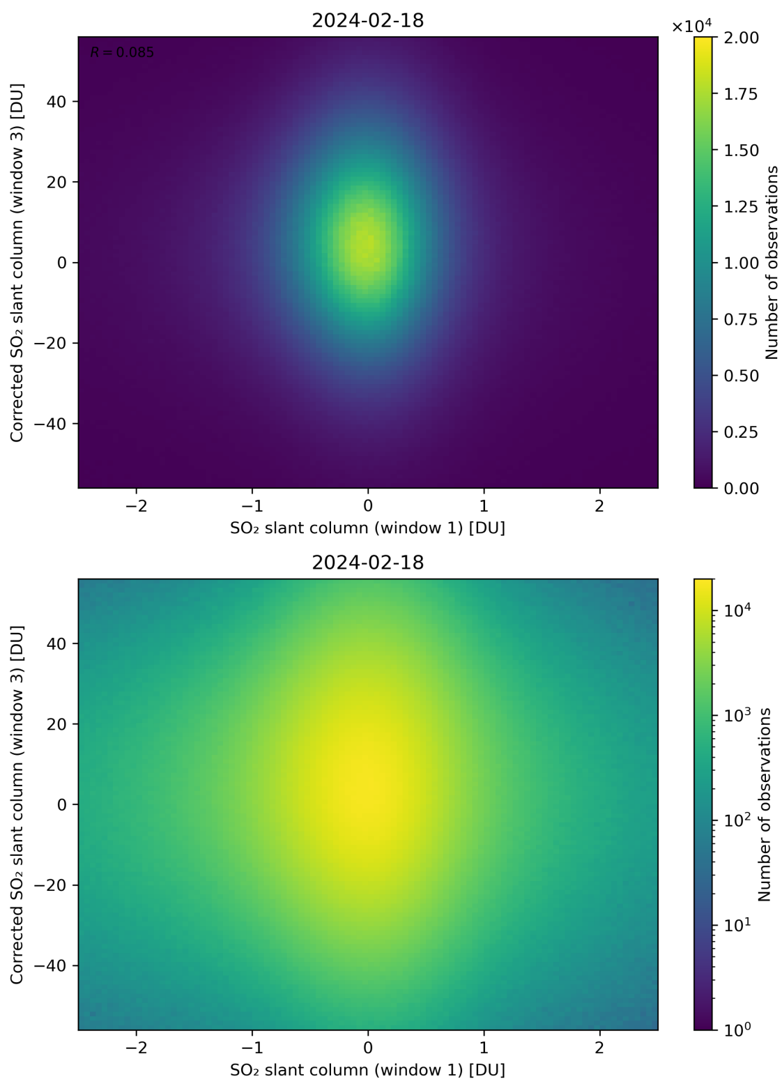
Figure 234: Scatter density plot of “SO 2 slant column (window 1)” against “Corrected SO 2 slant column (window 3)” for 2024-02-17 to 2024-02-19.
