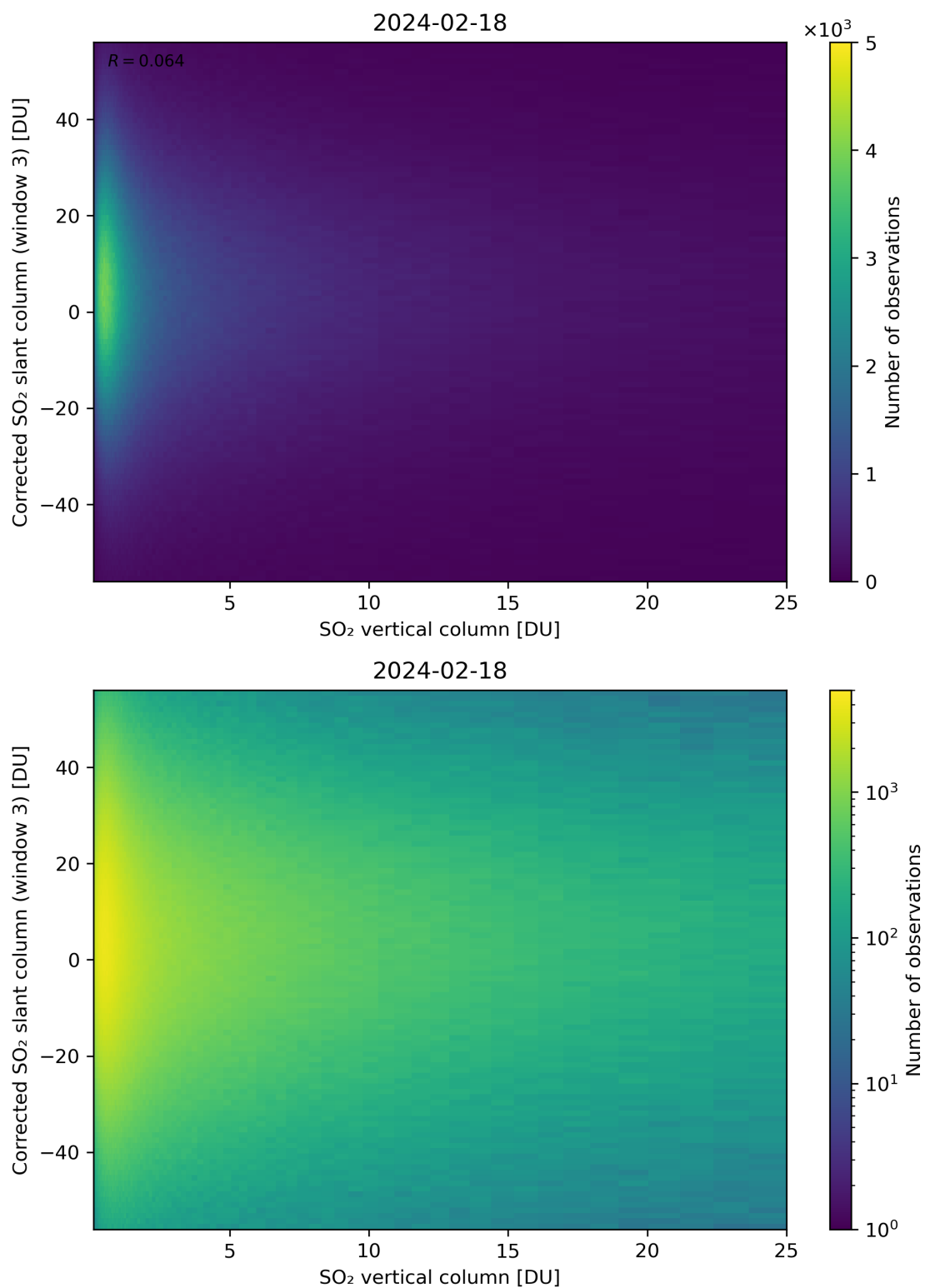
Figure 299: Scatter density plot of “SO 2 vertical column” against “Corrected SO 2 slant column (window 3)” for 2024-02-17 to 2024-02-19.
