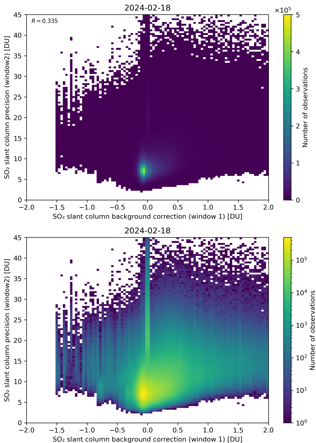
Figure 106: Scatter density plot of “SO 2 slant column background correction (window 1)” against “SO 2 slant column precision (window2)” for 2024-02-17 to 2024-02-19.
