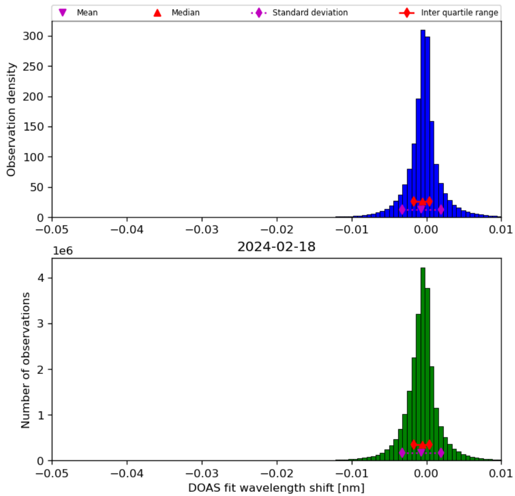
Figure 68: Histogram of “DOAS fit wavelength shift” for 2024-02-17 to 2024-02-19
