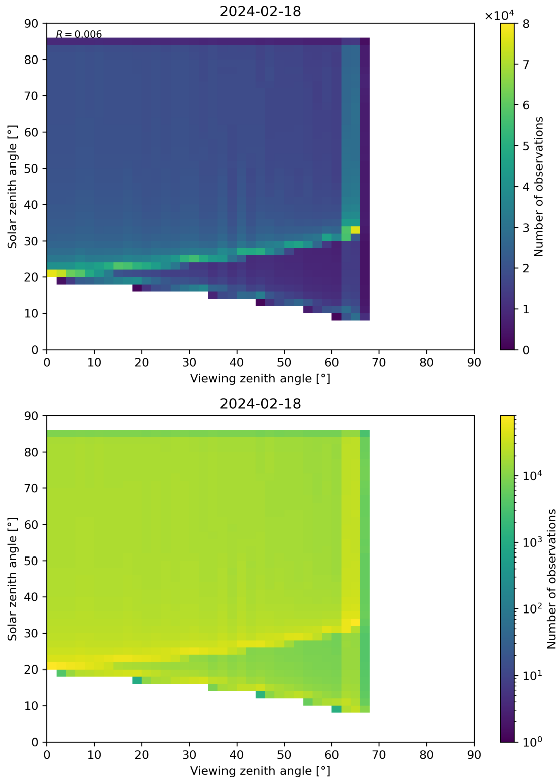
Figure 315: Scatter density plot of “Viewing zenith angle” against “Solar zenith angle” for 2024-02-17 to 2024-02-19.
