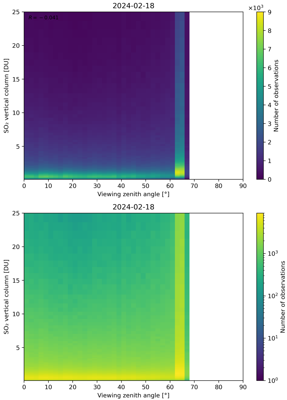
Figure 327: Scatter density plot of “Viewing zenith angle” against “SO 2 vertical column” for 2024-02-17 to 2024-02-19.
