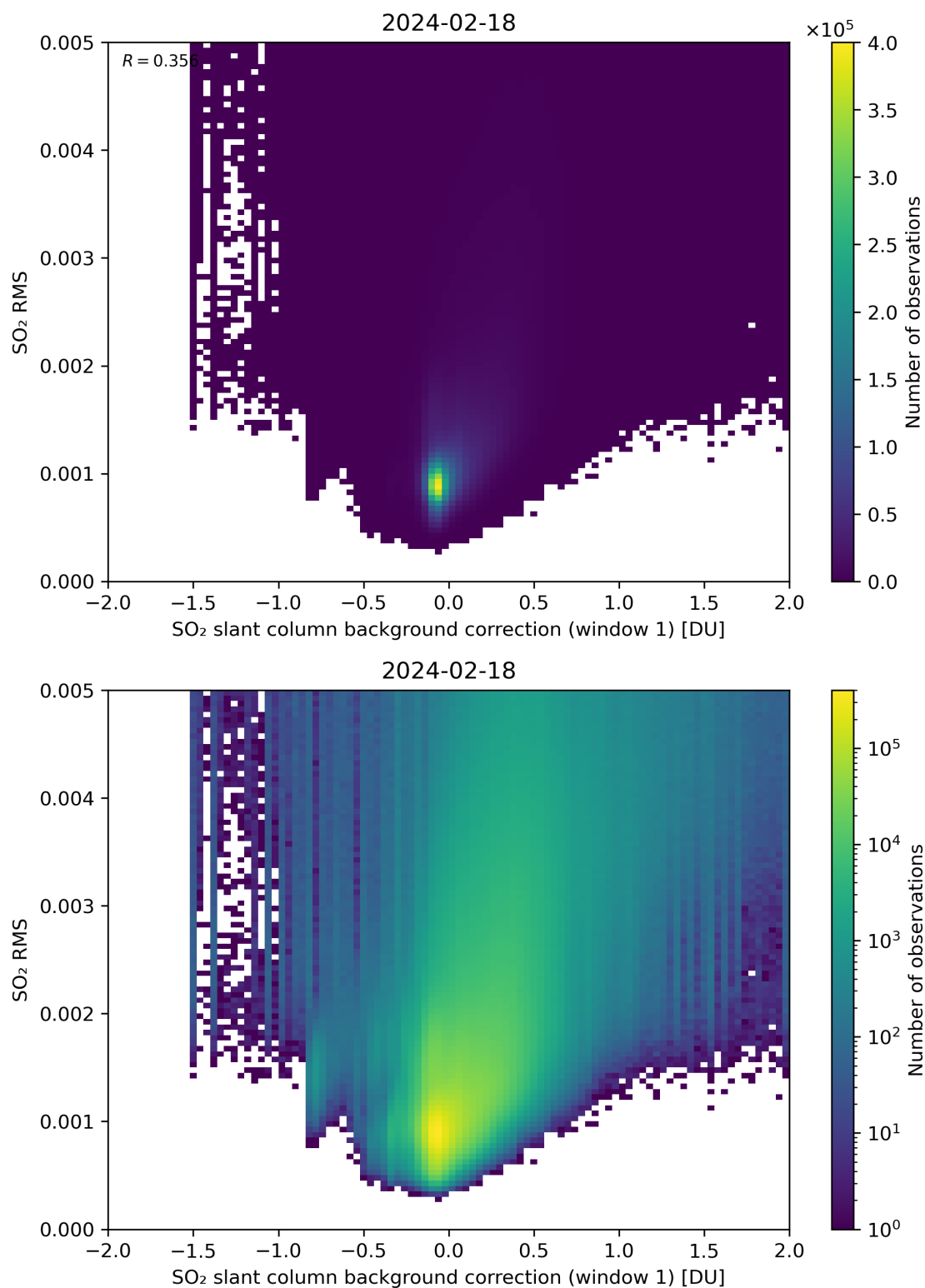
Figure 102: Scatter density plot of “SO 2 slant column background correction (window 1)” against “SO 2 RMS” for 2024-02-17 to 2024-02-19.
