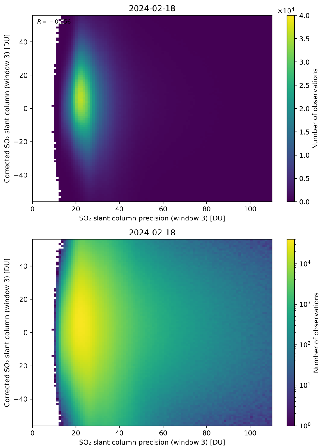
Figure 262: Scatter density plot of “SO 2 slant column precision (window 3)” against “Corrected SO 2 slant column (window 3)” for 2024-02-17 to 2024-02-19.
