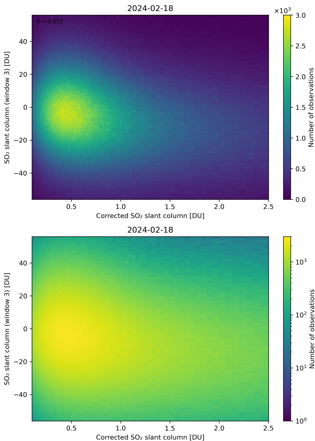
Figure 190: Scatter density plot of “Corrected SO 2 slant column” against “SO 2 slant column (window 3)” for 2024-02-17 to 2024-02-19.
