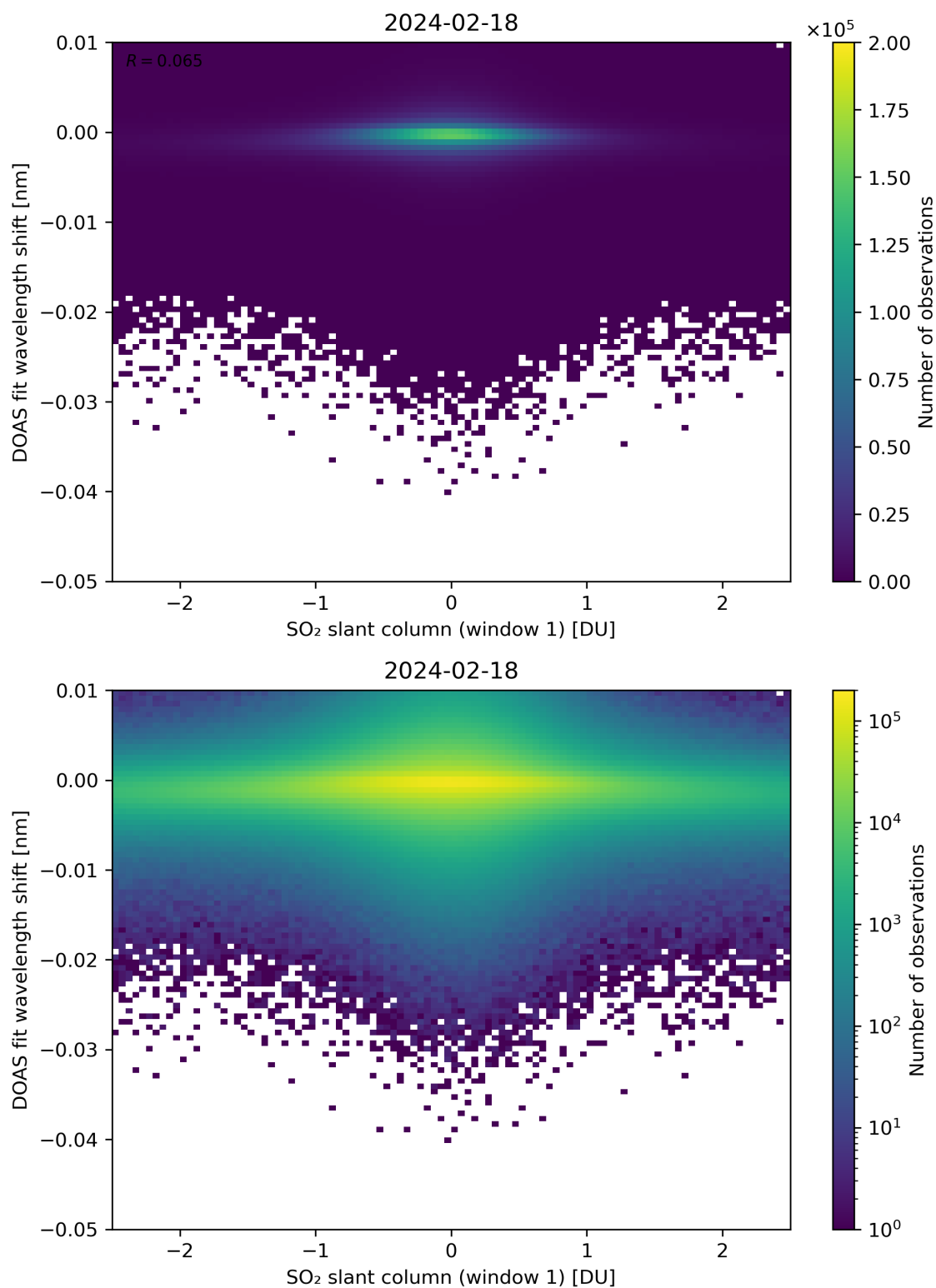
Figure 215: Scatter density plot of “SO 2 slant column (window 1)” against “DOAS fit wavelength shift” for 2024-02-17 to 2024-02-19.
