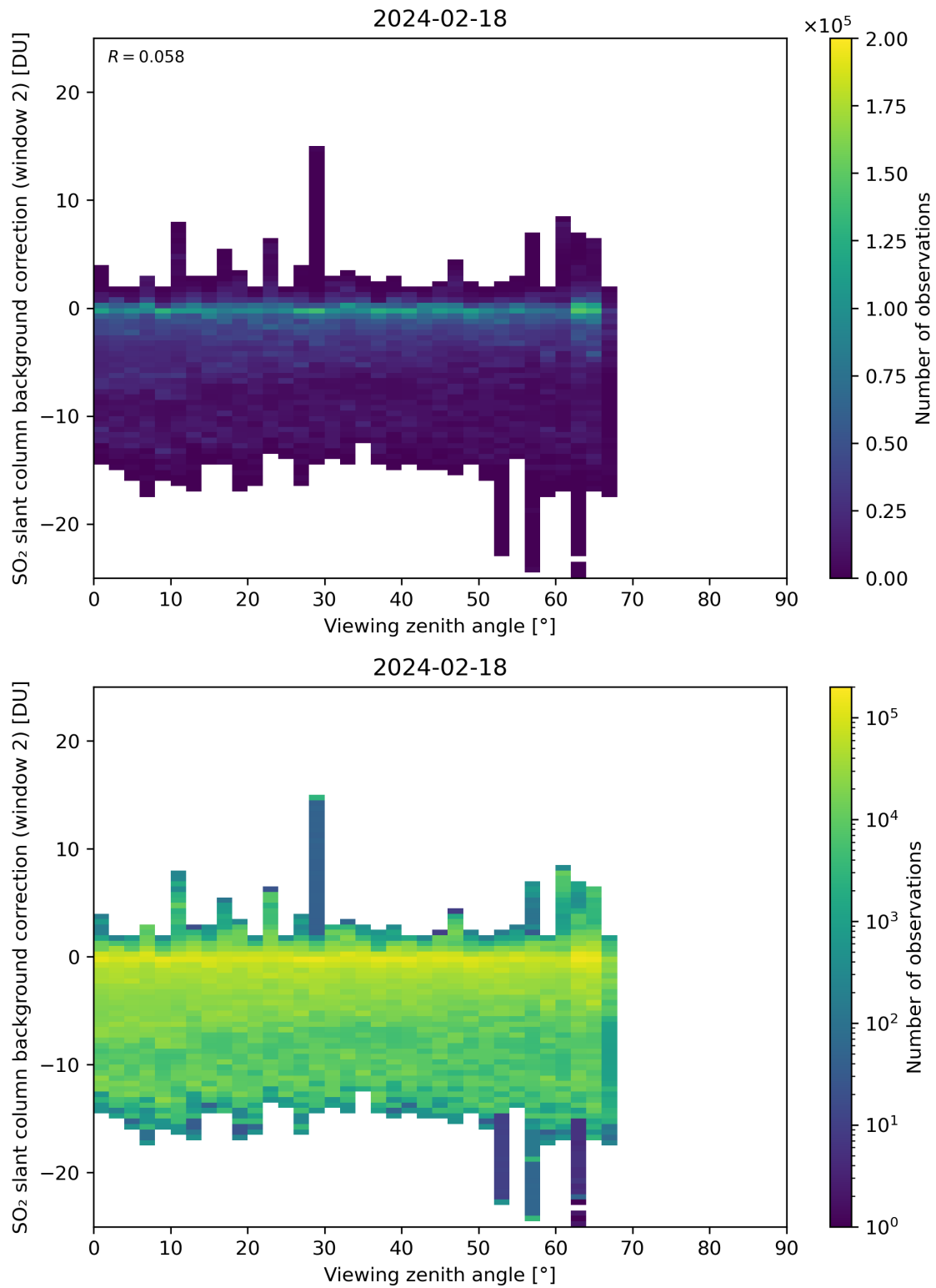
Figure 309: Scatter density plot of “Viewing zenith angle” against “SO 2 slant column background correction (window 2)” for 2024-02-17 to 2024-02-19.
