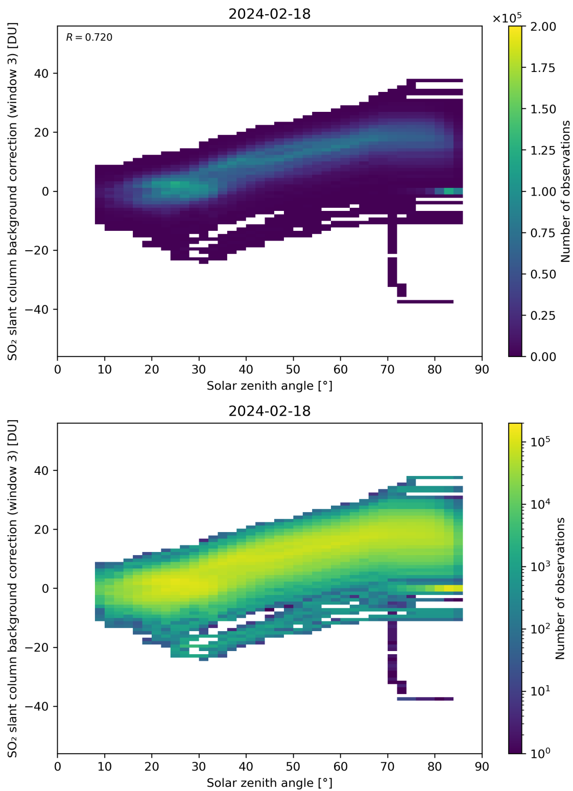
Figure 160: Scatter density plot of “Solar zenith angle” against “SO 2 slant column background correction (window 3)” for 2024-02-17 to 2024-02-19.
