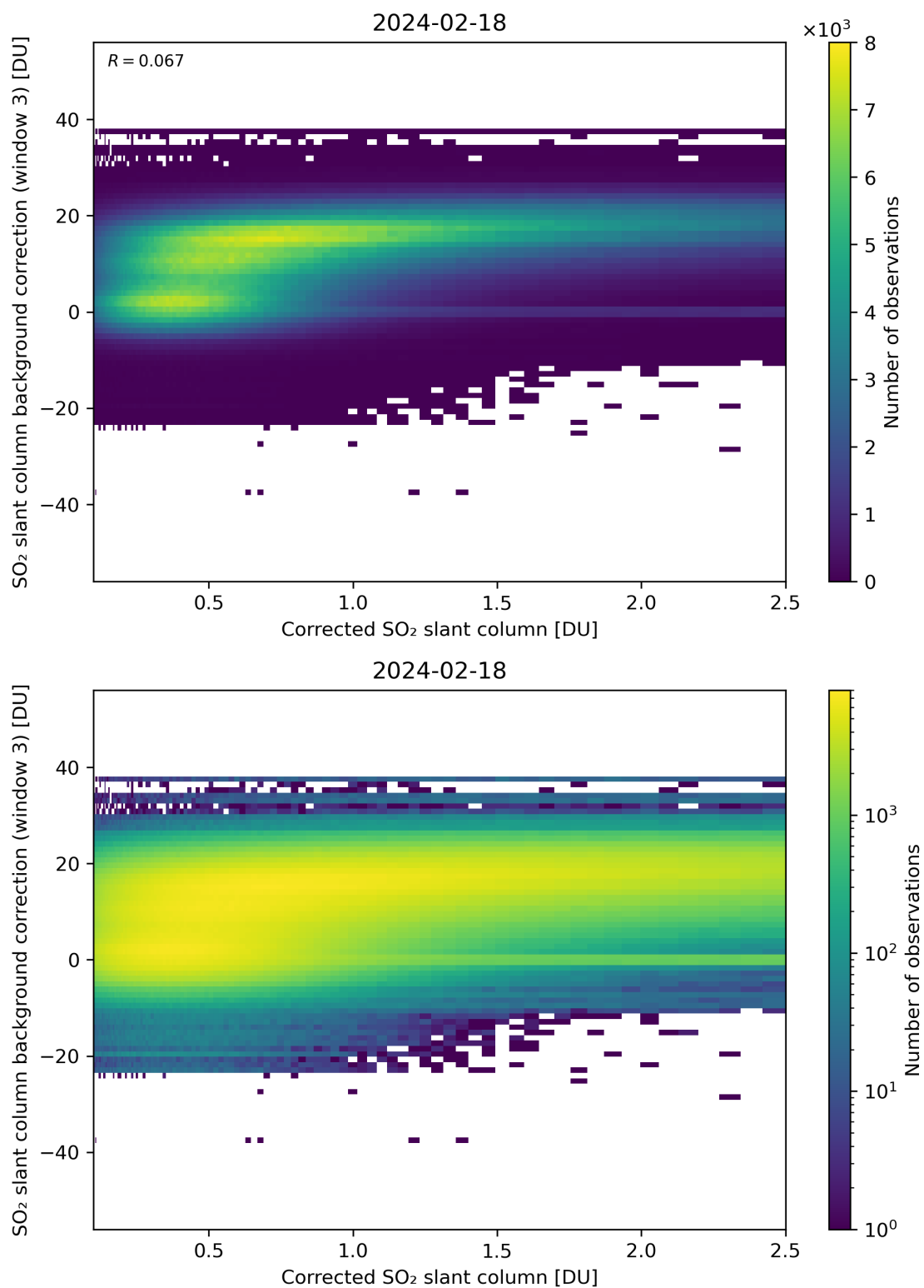
Figure 180: Scatter density plot of “Corrected SO 2 slant column” against “SO 2 slant column background correction (window 3)” for 2024-02-17 to 2024-02-19.
