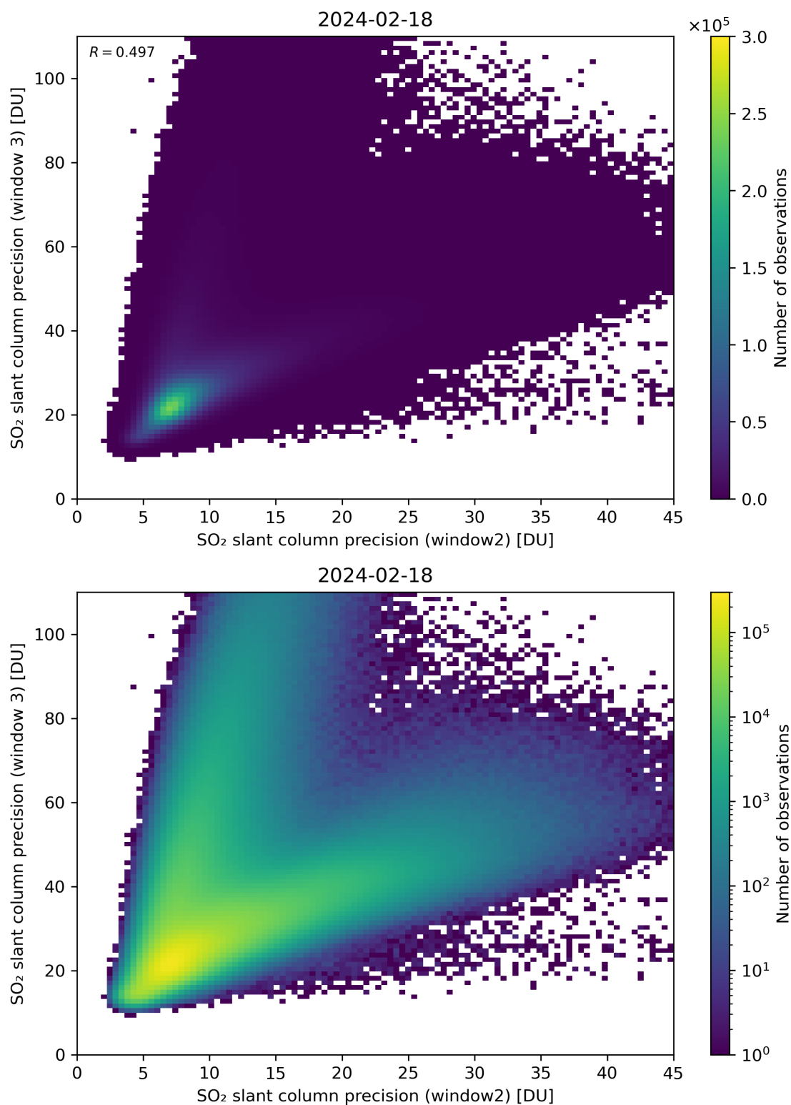
Figure 250: Scatter density plot of “SO 2 slant column precision (window2)” against “SO 2 slant column precision (window 3)” for 2024-02-17 to 2024-02-19.
