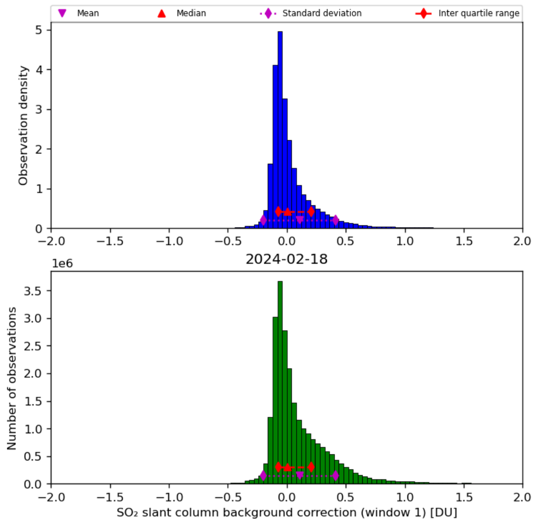
Figure 59: Histogram of “SO 2 slant column background correction (window 1)” for 2024-02-17 to 2024-02-19
