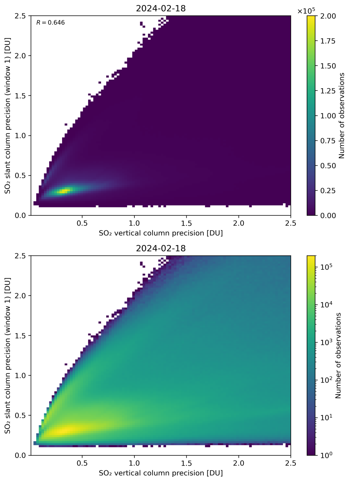
Figure 290: Scatter density plot of “SO 2 vertical column precision” against “SO 2 slant column precision (window 1)” for 2024-02-17 to 2024-02-19.
