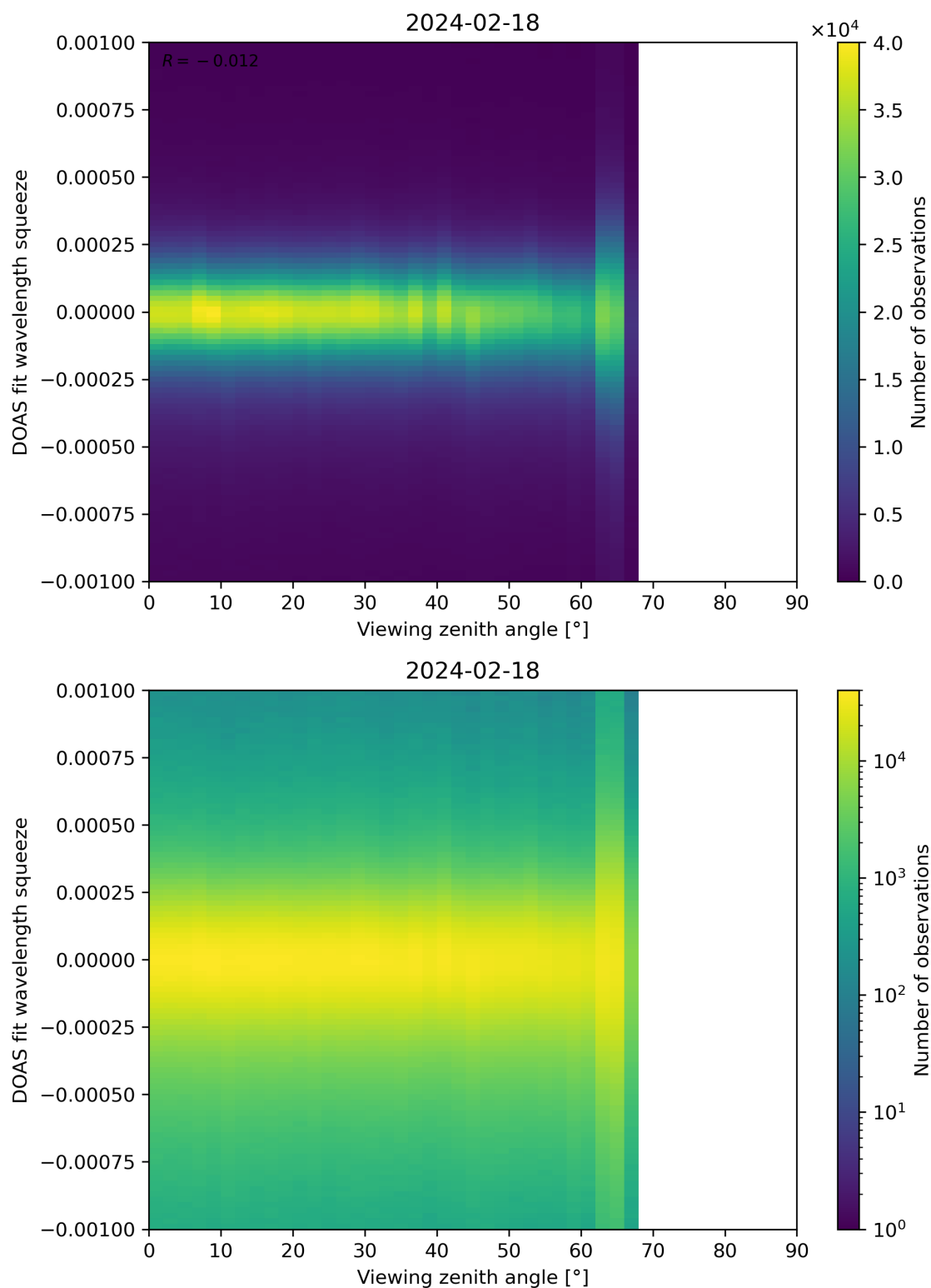
Figure 312: Scatter density plot of “Viewing zenith angle” against “DOAS fit wavelength squeeze” for 2024-02-17 to 2024-02-19.
