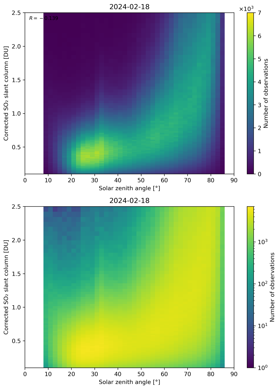
Figure 166: Scatter density plot of “Solar zenith angle” against “Corrected SO 2 slant column” for 2024-02-17 to 2024-02-19.
