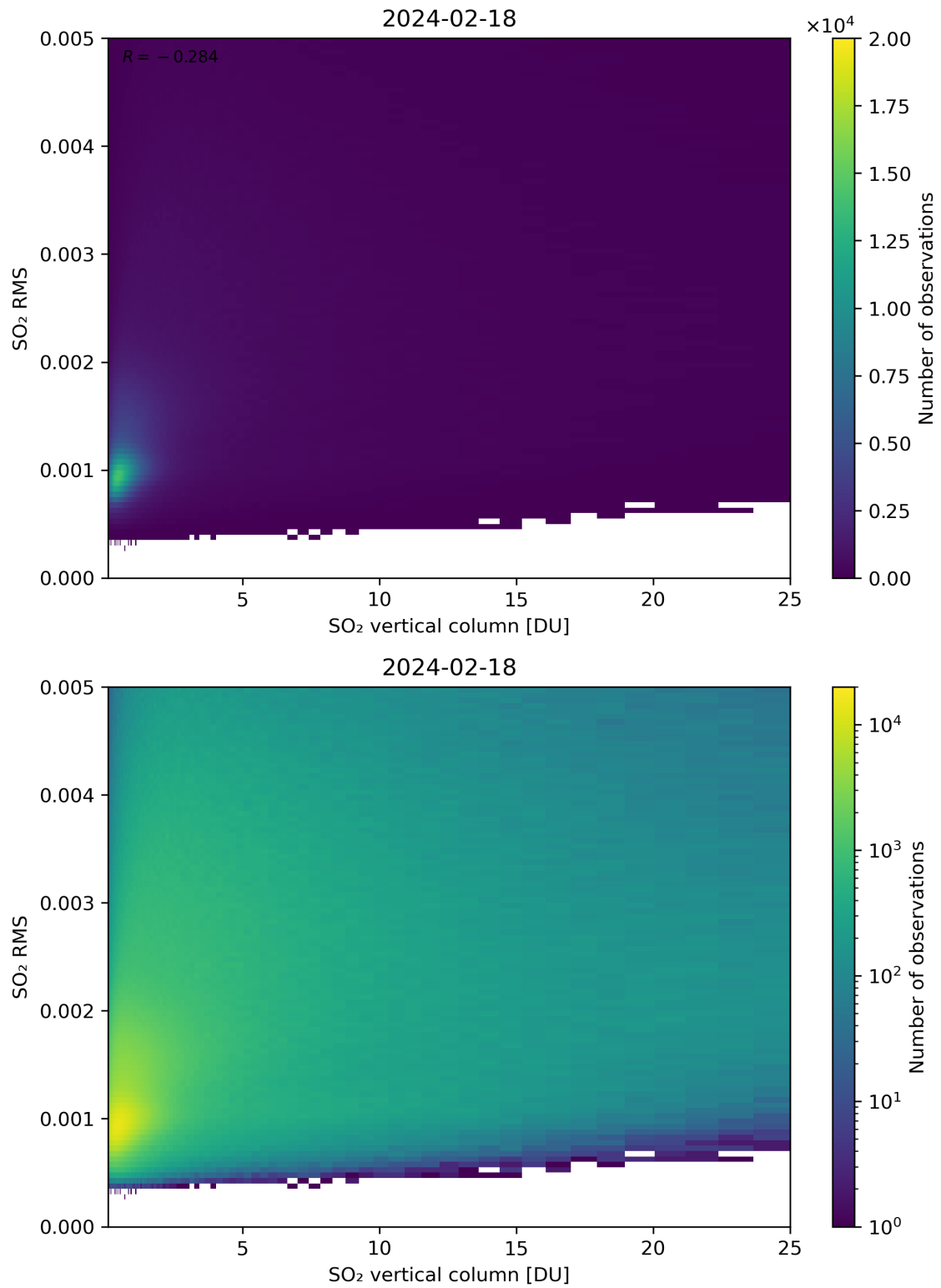
Figure 278: Scatter density plot of “SO 2 vertical column” against “SO 2 RMS” for 2024-02-17 to 2024-02-19.
