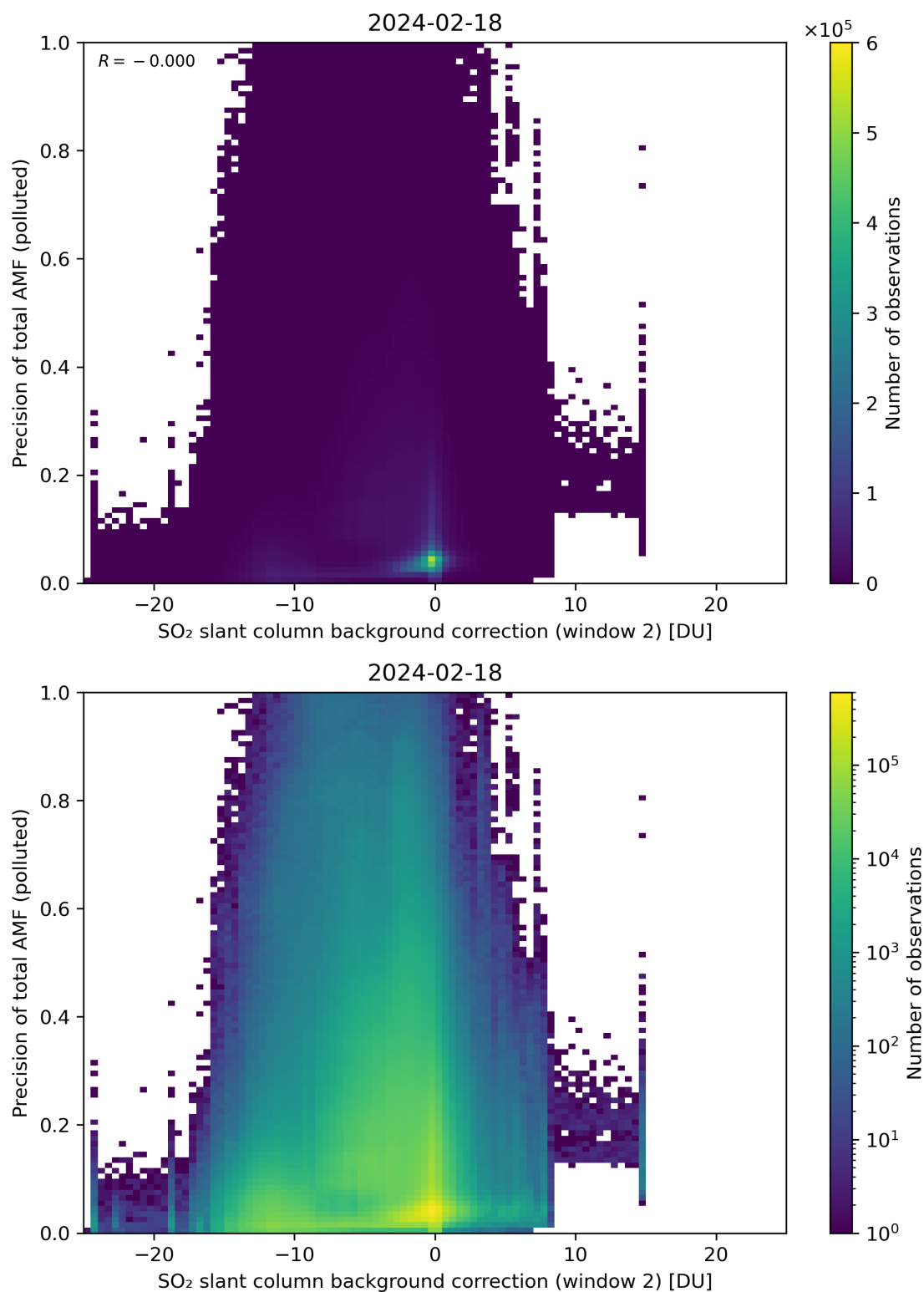
Figure 120: Scatter density plot of “SO 2 slant column background correction (window 2)” against “Precision of total AMF (polluted)” for 2024-02-17 to 2024-02-19.
