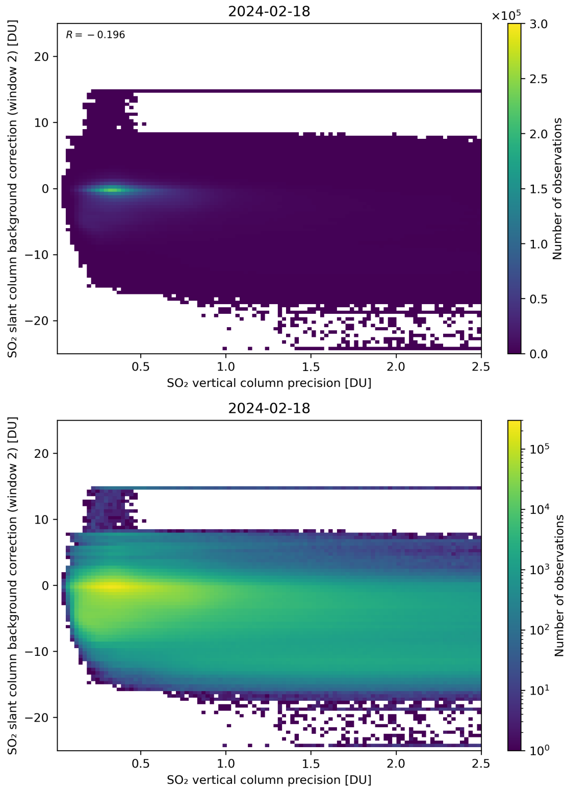
Figure 280: Scatter density plot of “SO 2 vertical column precision” against “SO 2 slant column background correction (window 2)” for 2024-02-17 to 2024-02-19.
