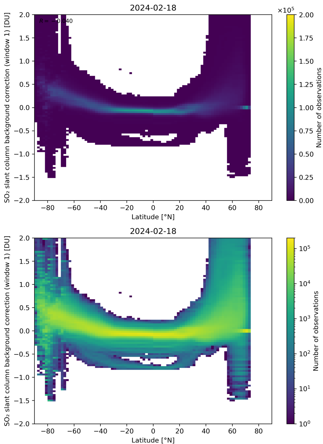
Figure 139: Scatter density plot of “Latitude” against “SO 2 slant column background correction (window 1)” for 2024-02-17 to 2024-02-19.
