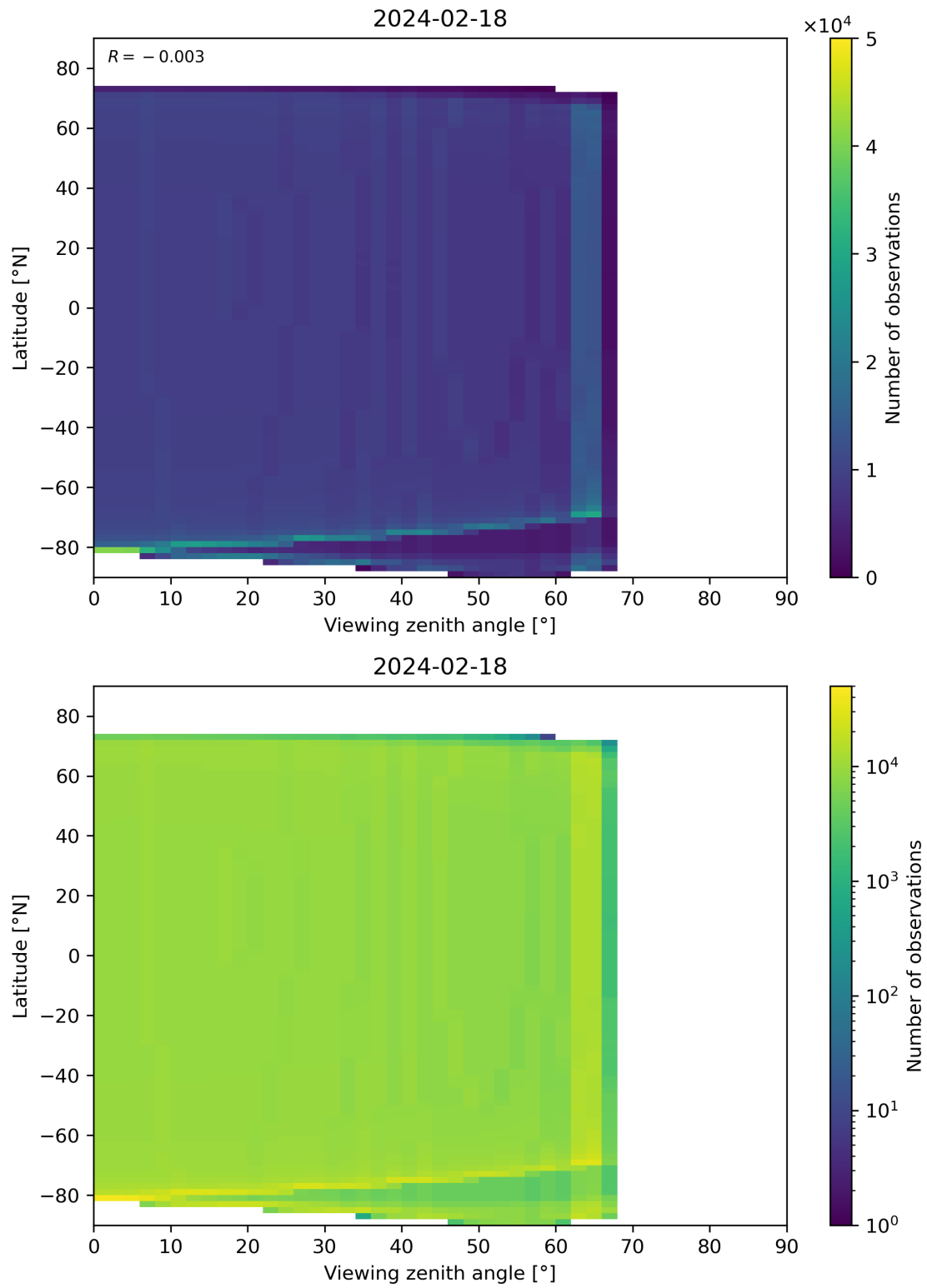
Figure 314: Scatter density plot of “Viewing zenith angle” against “Latitude” for 2024-02-17 to 2024-02-19.
