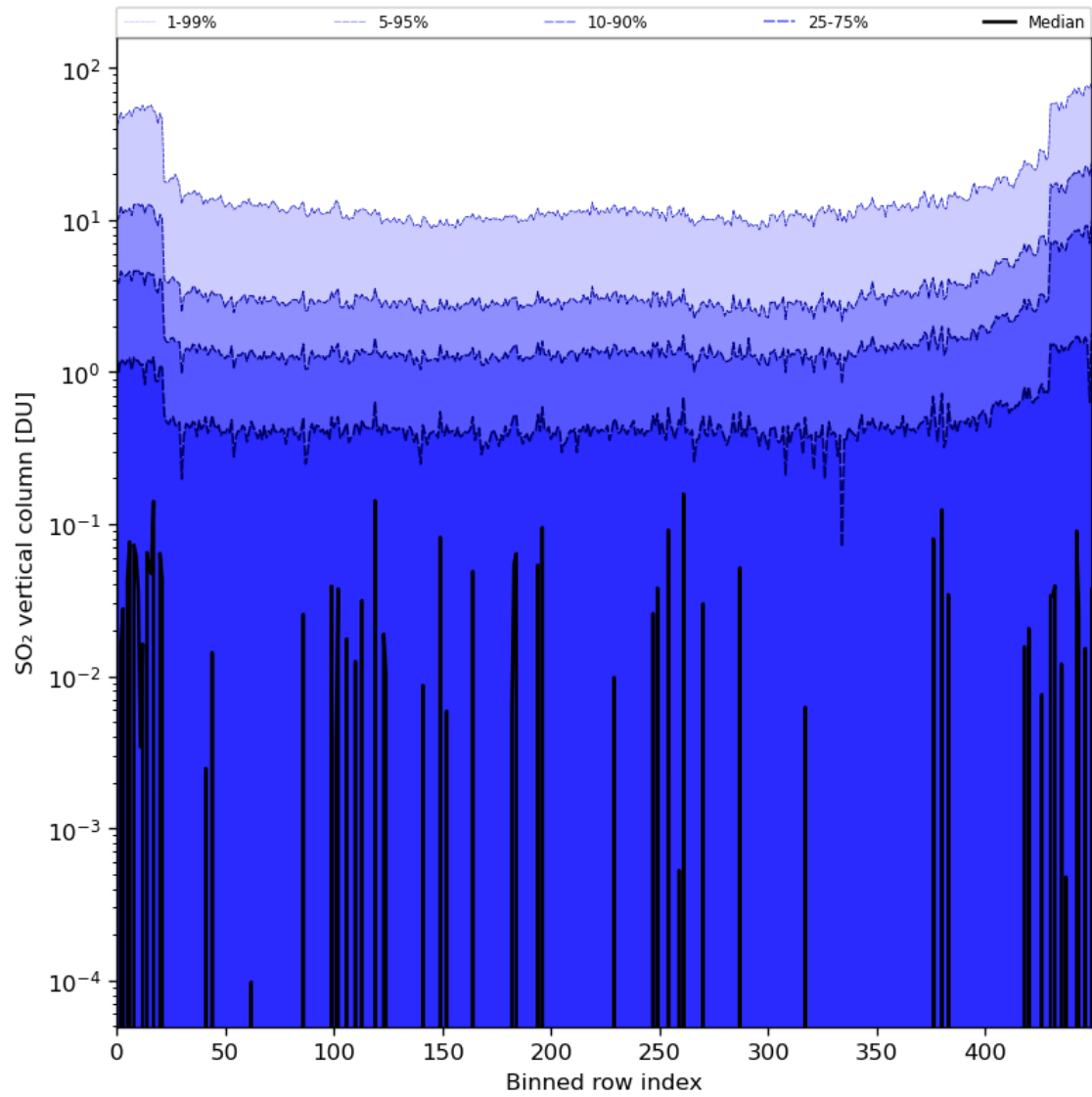
Figure 76: Along track statistics of “SO 2 vertical column” for 2024-02-17 to 2024-02-19
