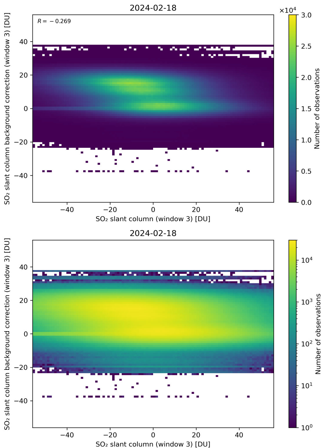
Figure 253: Scatter density plot of “SO 2 slant column (window 3)” against “SO 2 slant column background correction (window 3)” for 2024-02-17 to 2024-02-19.
