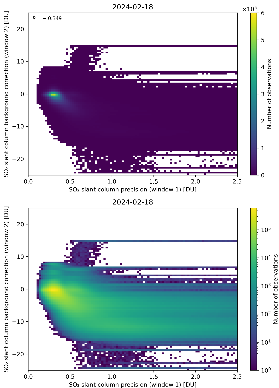
Figure 219: Scatter density plot of “SO 2 slant column precision (window 1)” against “SO 2 slant column background correction (window 2)” for 2024-02-17 to 2024-02-19.
