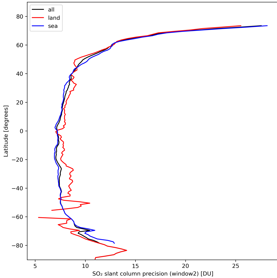
Figure 38: Zonal average of “SO 2 slant column precision (window2)” for 2024-02-17 to 2024-02-19.
