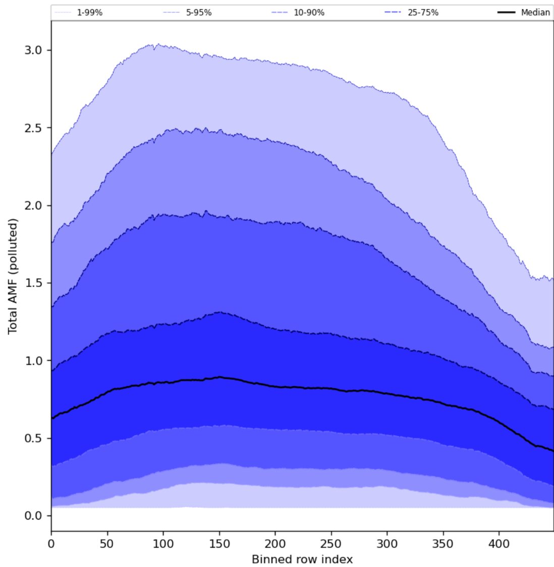
Figure 94: Along track statistics of “Total AMF (polluted)” for 2024-02-17 to 2024-02-19
