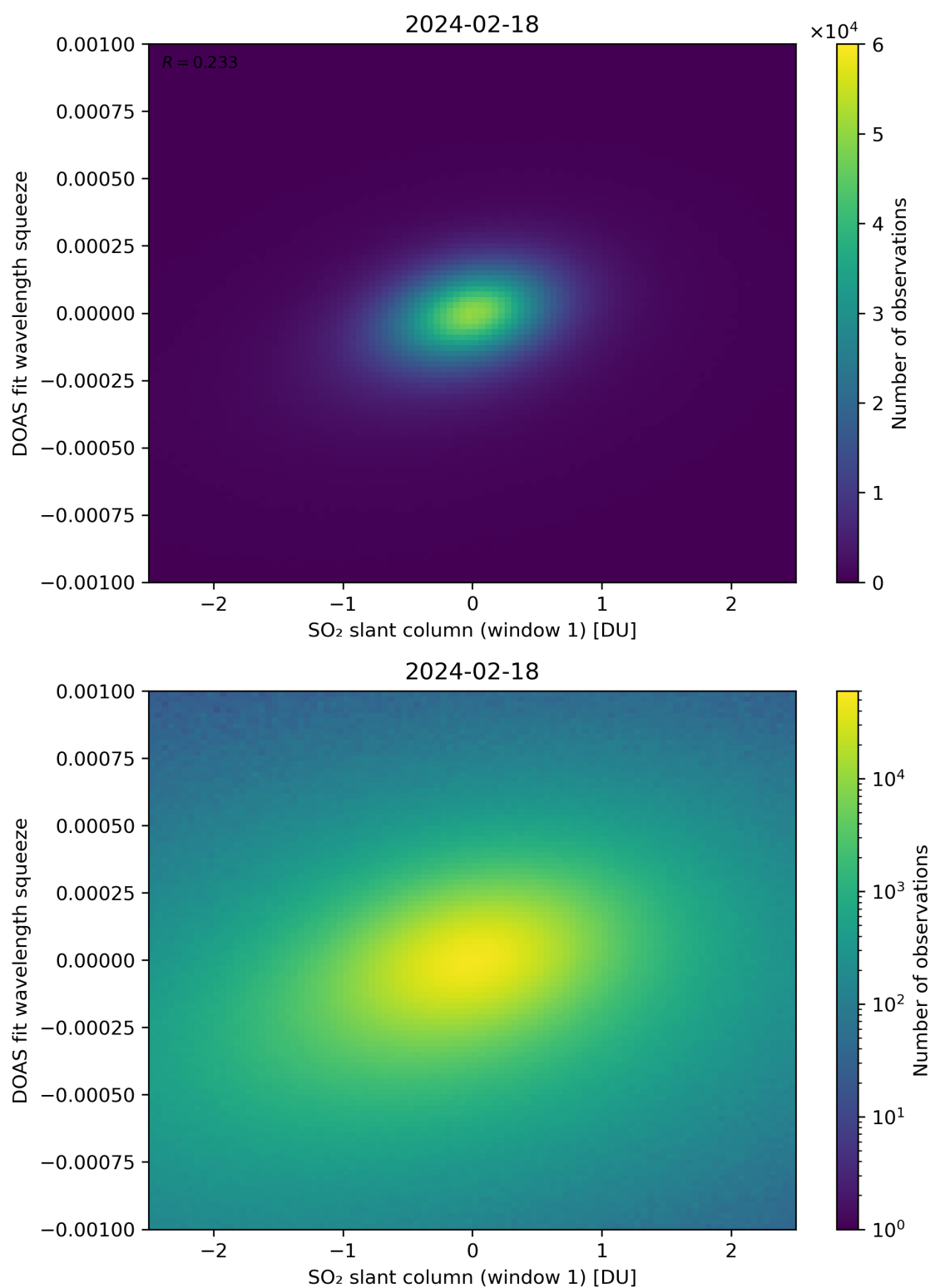
Figure 216: Scatter density plot of “SO 2 slant column (window 1)” against “DOAS fit wavelength squeeze” for 2024-02-17 to 2024-02-19.
