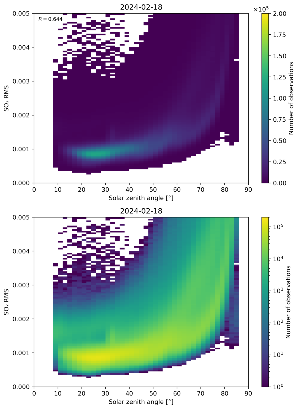
Figure 163: Scatter density plot of “Solar zenith angle” against “SO 2 RMS” for 2024-02-17 to 2024-02-19.
