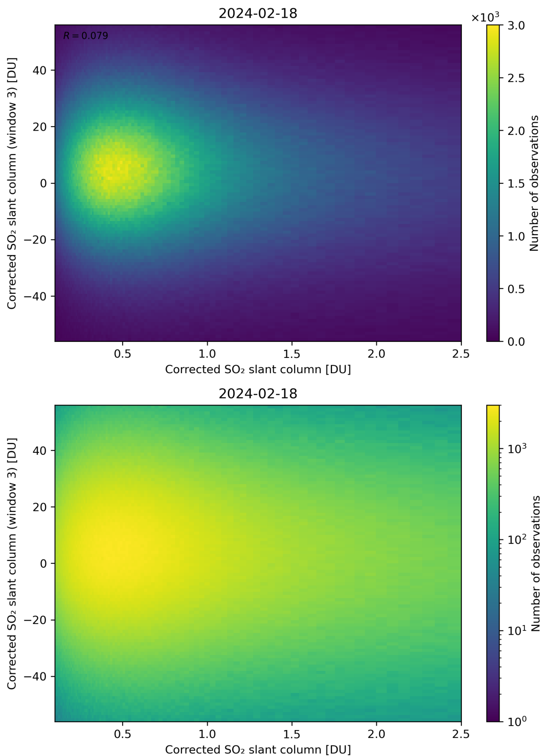
Figure 186: Scatter density plot of “Corrected SO 2 slant column” against “Corrected SO 2 slant column (window 3)” for 2024-02-17 to 2024-02-19.
