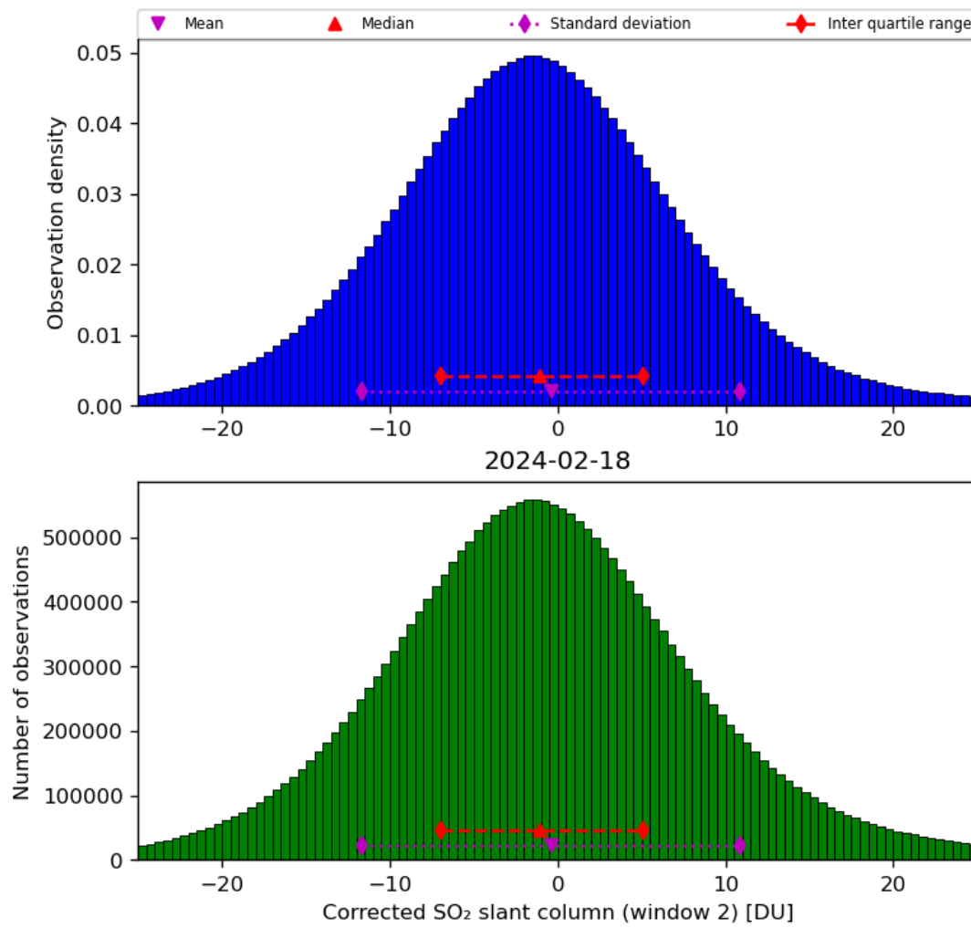
Figure 62: Histogram of “Corrected SO 2 slant column (window 2)” for 2024-02-17 to 2024-02-19
