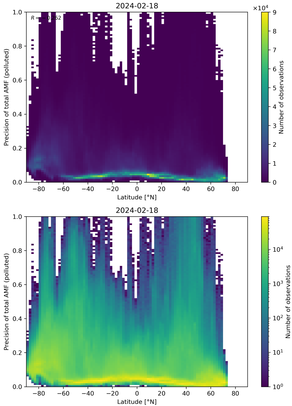
Figure 155: Scatter density plot of “Latitude” against “Precision of total AMF (polluted)” for 2024-02-17 to 2024-02-19.
