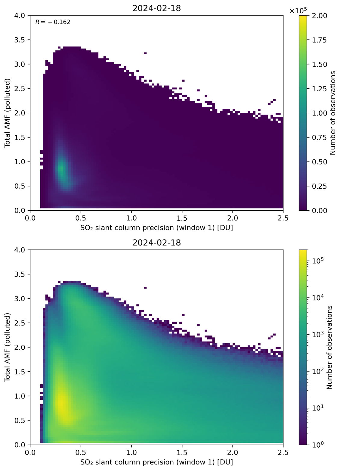
Figure 230: Scatter density plot of “SO 2 slant column precision (window 1)” against “Total AMF (polluted)” for 2024-02-17 to 2024-02-19.
