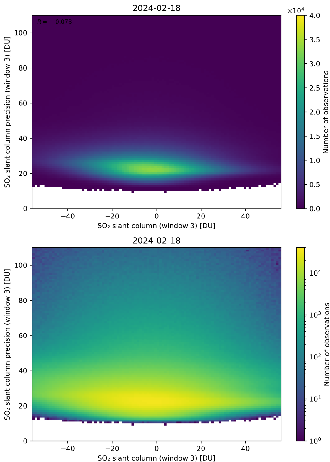
Figure 267: Scatter density plot of “SO 2 slant column (window 3)” against “SO 2 slant column precision (window 3)” for 2024-02-17 to 2024-02-19.
