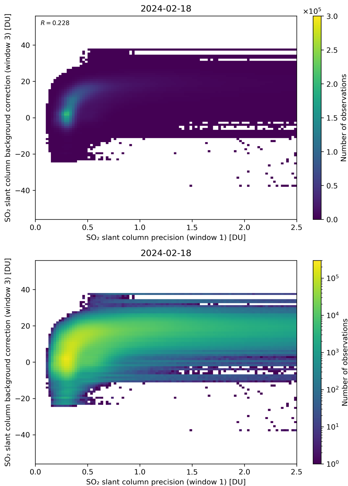
Figure 220: Scatter density plot of “SO 2 slant column precision (window 1)” against “SO 2 slant column background correction (window 3)” for 2024-02-17 to 2024-02-19.
