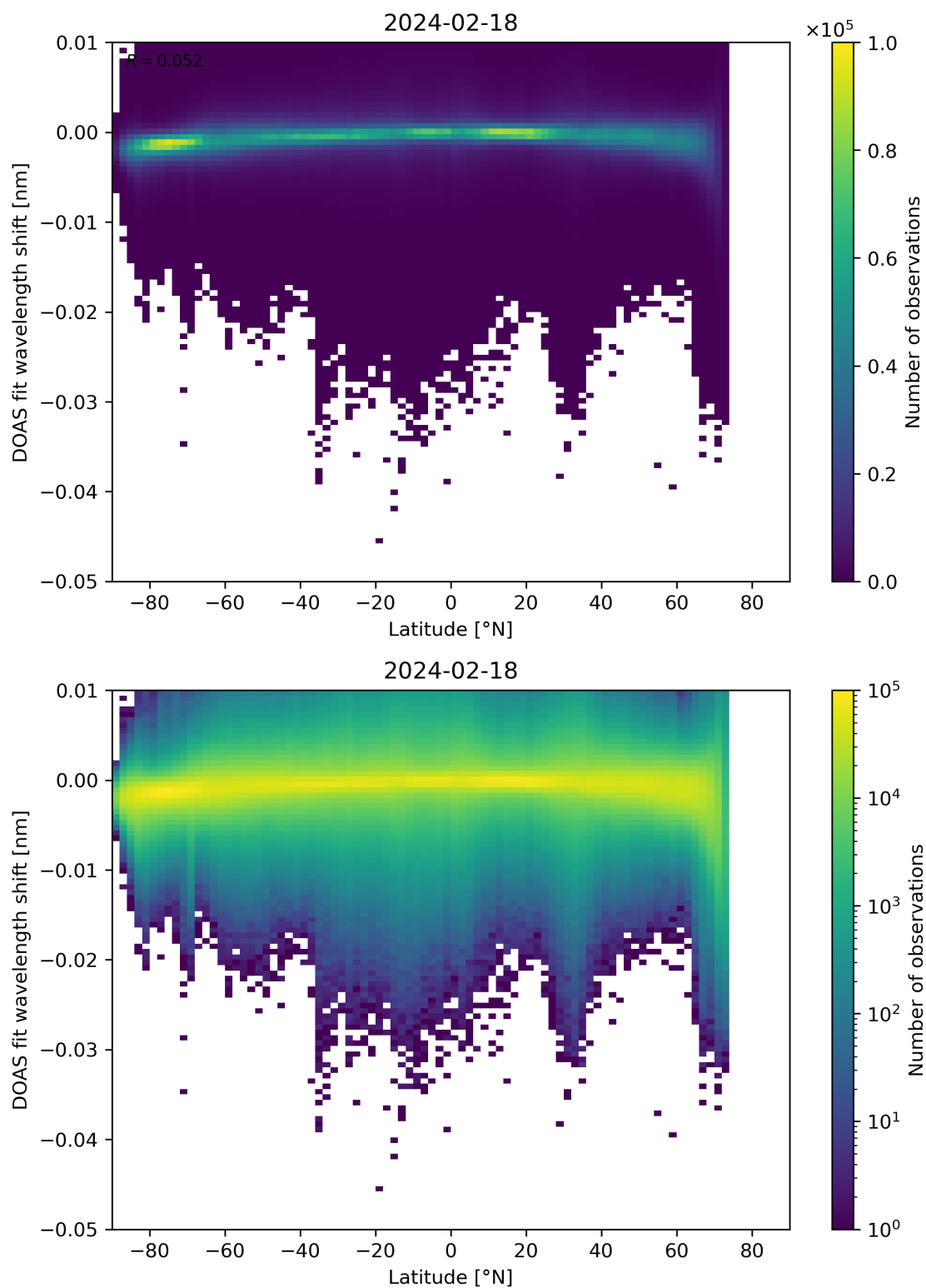
Figure 142: Scatter density plot of “Latitude” against “DOAS fit wavelength shift” for 2024-02-17 to 2024-02-19.
