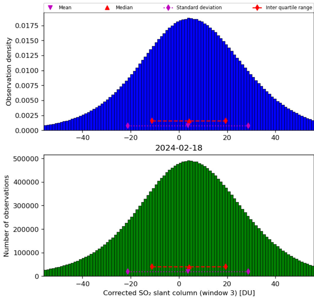
Figure 66: Histogram of "Corrected SO 2 slant column (window 3)" for 2024-02-17 to 2024-02-19
