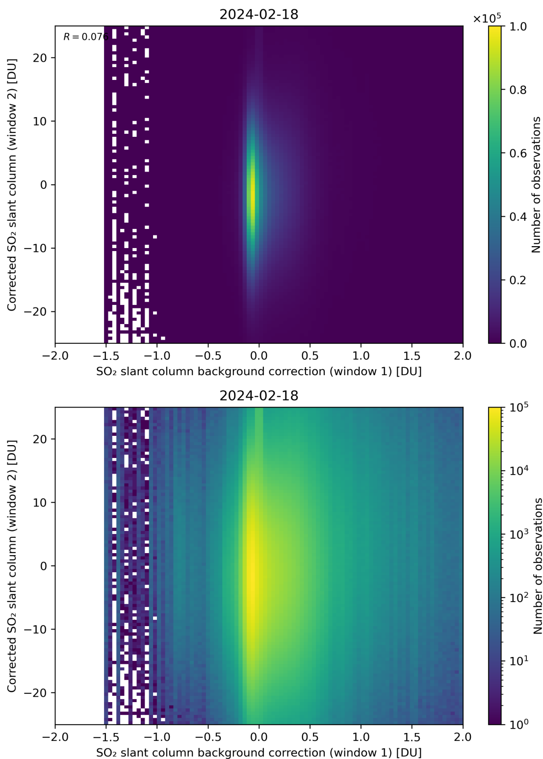
Figure 104: Scatter density plot of “SO 2 slant column background correction (window 1)” against “Corrected SO 2 slant column (window 2)” for 2024-02-17 to 2024-02-19.
