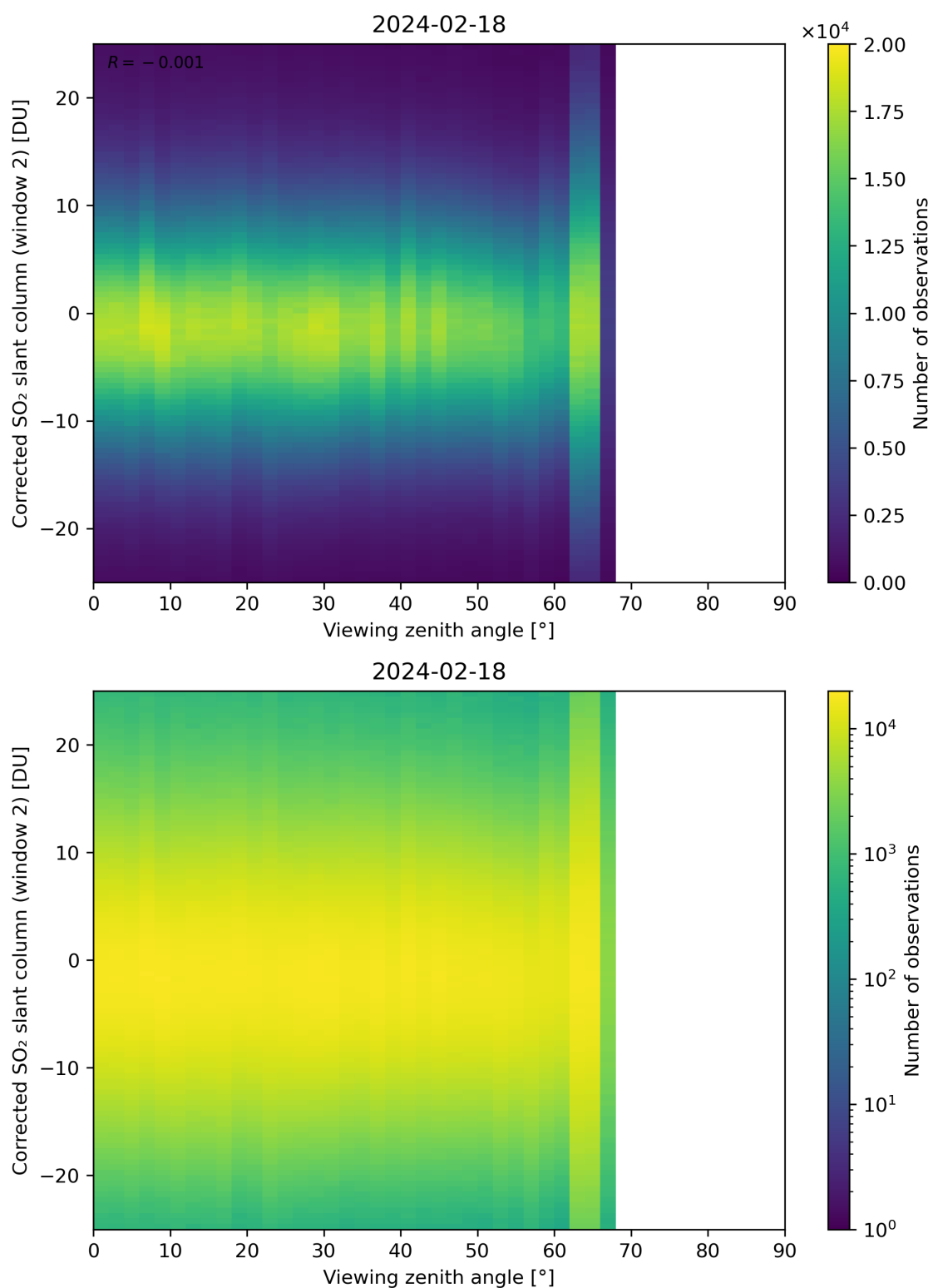
Figure 318: Scatter density plot of “Viewing zenith angle” against “Corrected SO 2 slant column (window 2)” for 2024-02-17 to 2024-02-19.
