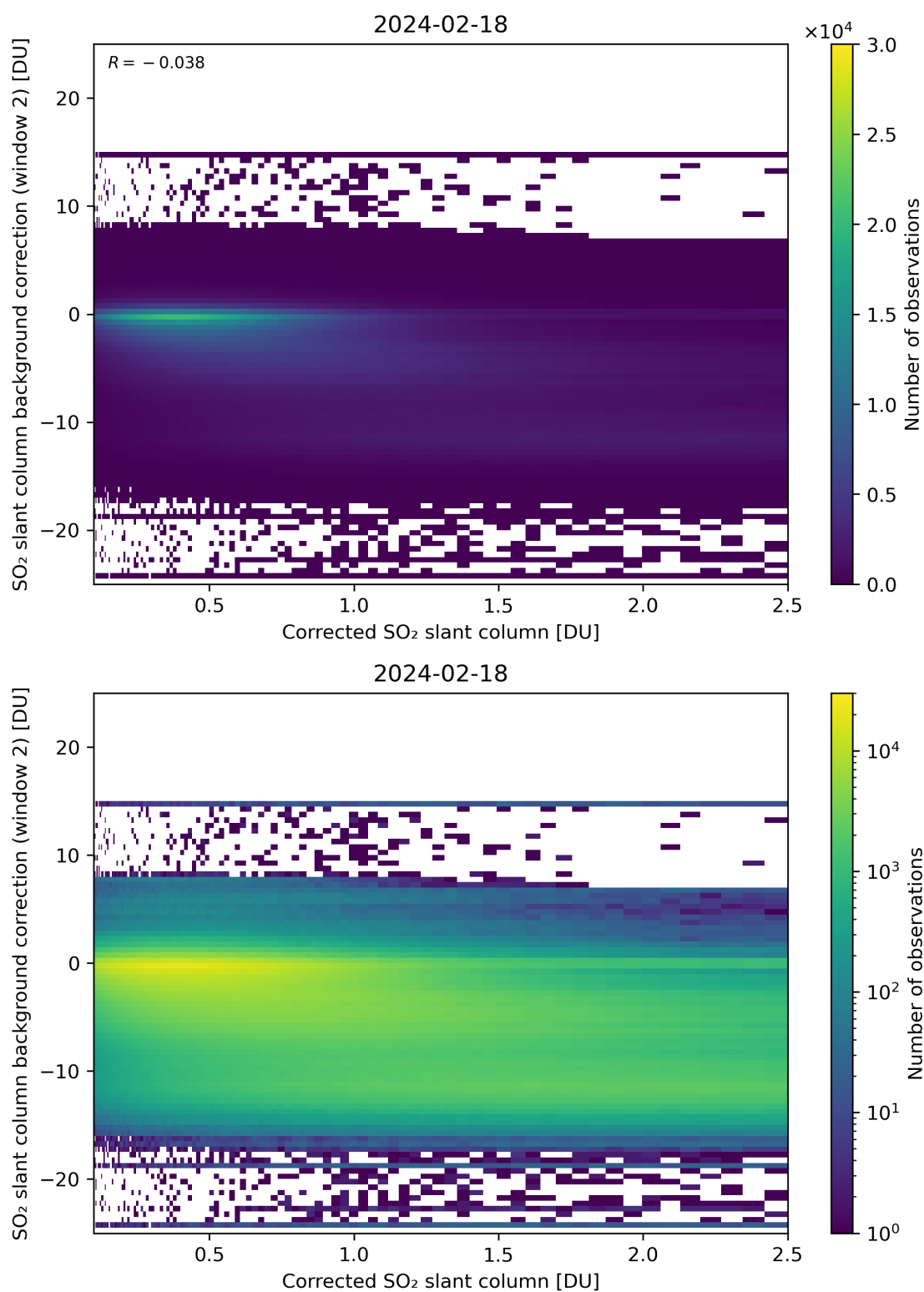
Figure 179: Scatter density plot of “Corrected SO 2 slant column” against “SO 2 slant column background correction (window 2)” for 2024-02-17 to 2024-02-19.
