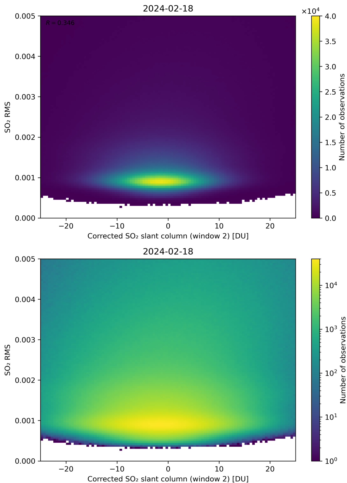
Figure 198: Scatter density plot of “Corrected SO 2 slant column (window 2)” against “SO 2 RMS” for 2024-02-17 to 2024-02-19.
