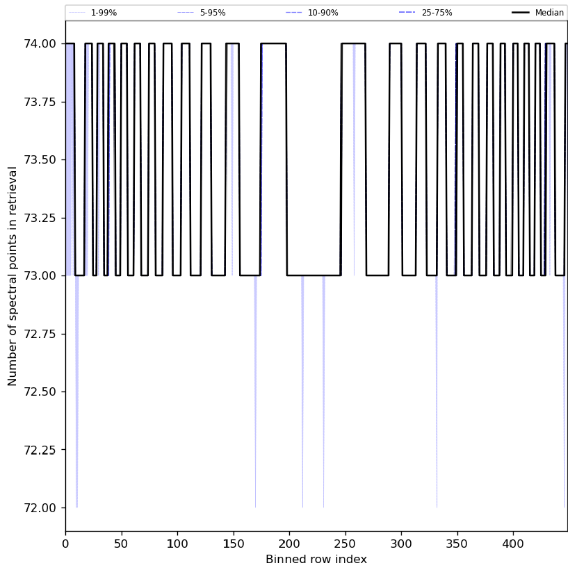
Figure 97: Along track statistics of “Number of spectral points in retrieval” for 2024-02-17 to 2024-02-19
