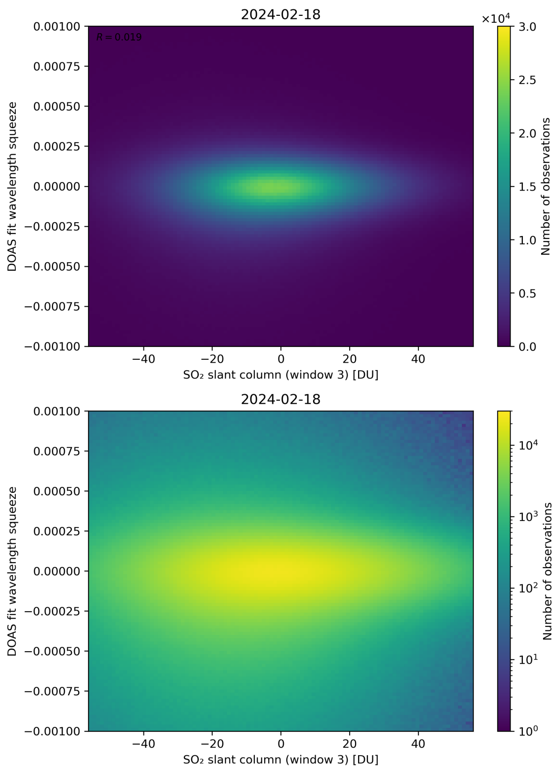
Figure 255: Scatter density plot of “SO 2 slant column (window 3)” against “DOAS fit wavelength squeeze” for 2024-02-17 to 2024-02-19.
