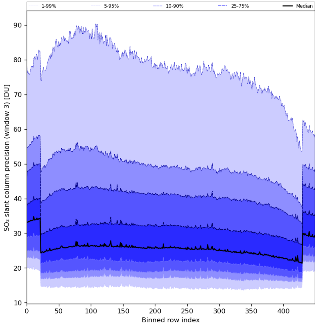
Figure 88: Along track statistics of “SO 2 slant column precision (window 3)” for 2024-02-17 to 2024-02-19
