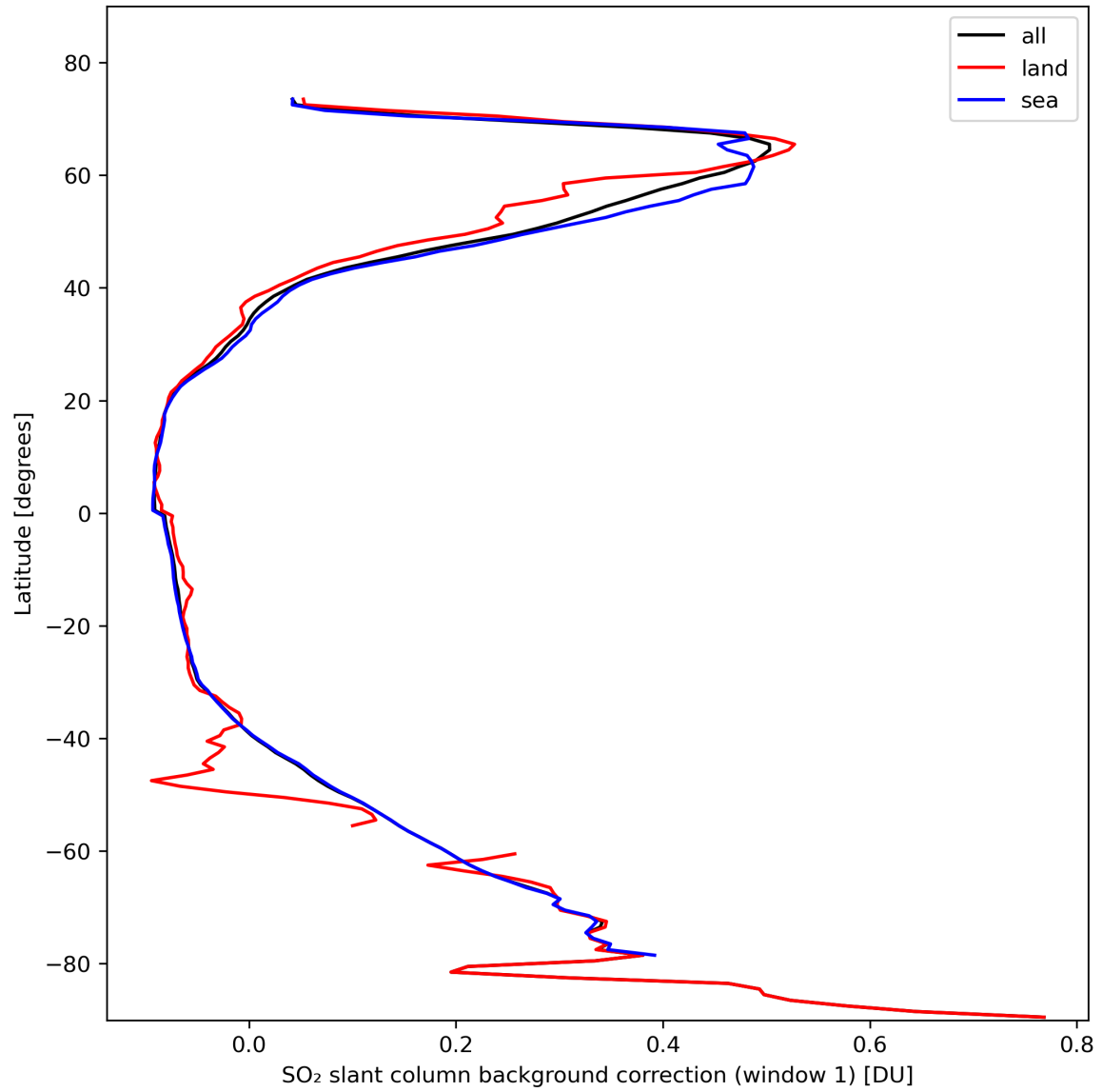
Figure 36: Zonal average of “SO 2 slant column background correction (window 1)” for 2024-02-17 to 2024-02-19.
