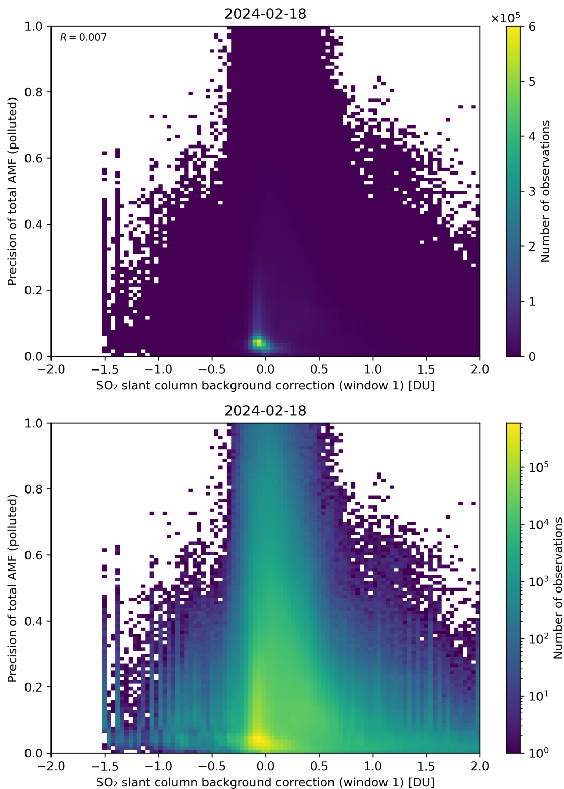
Figure 110: Scatter density plot of “SO 2 slant column background correction (window 1)” against “Precision of total AMF (polluted)” for 2024-02-17 to 2024-02-19.
