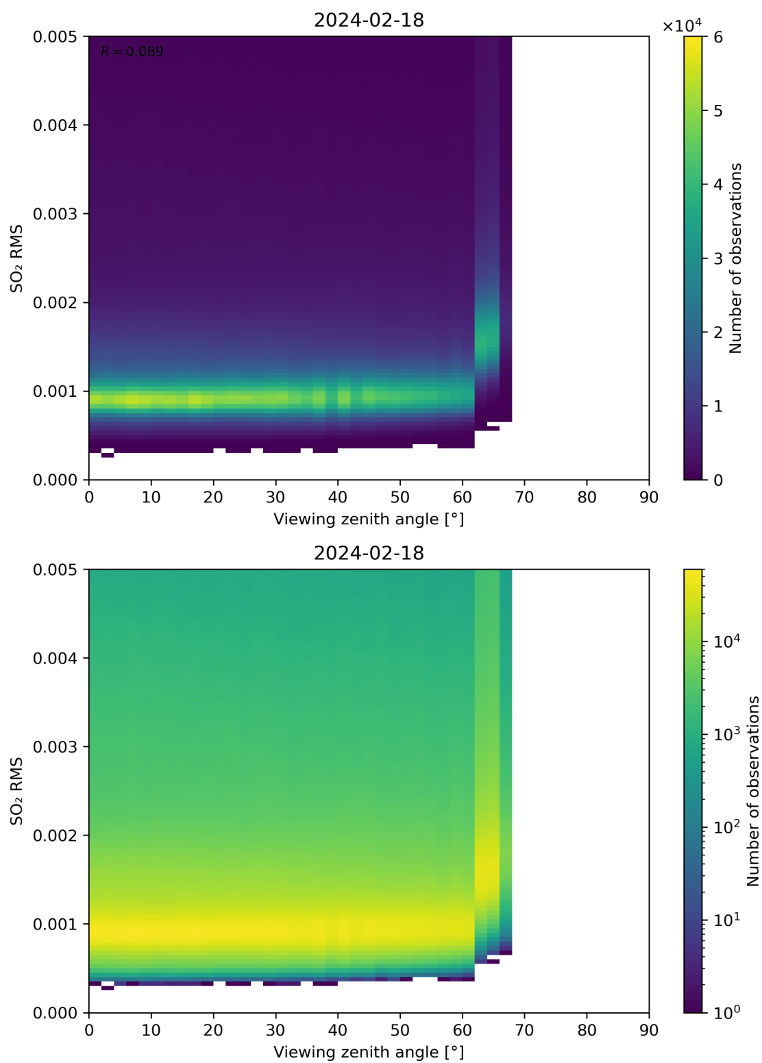
Figure 313: Scatter density plot of “Viewing zenith angle” against “SO 2 RMS” for 2024-02-17 to 2024-02-19.
