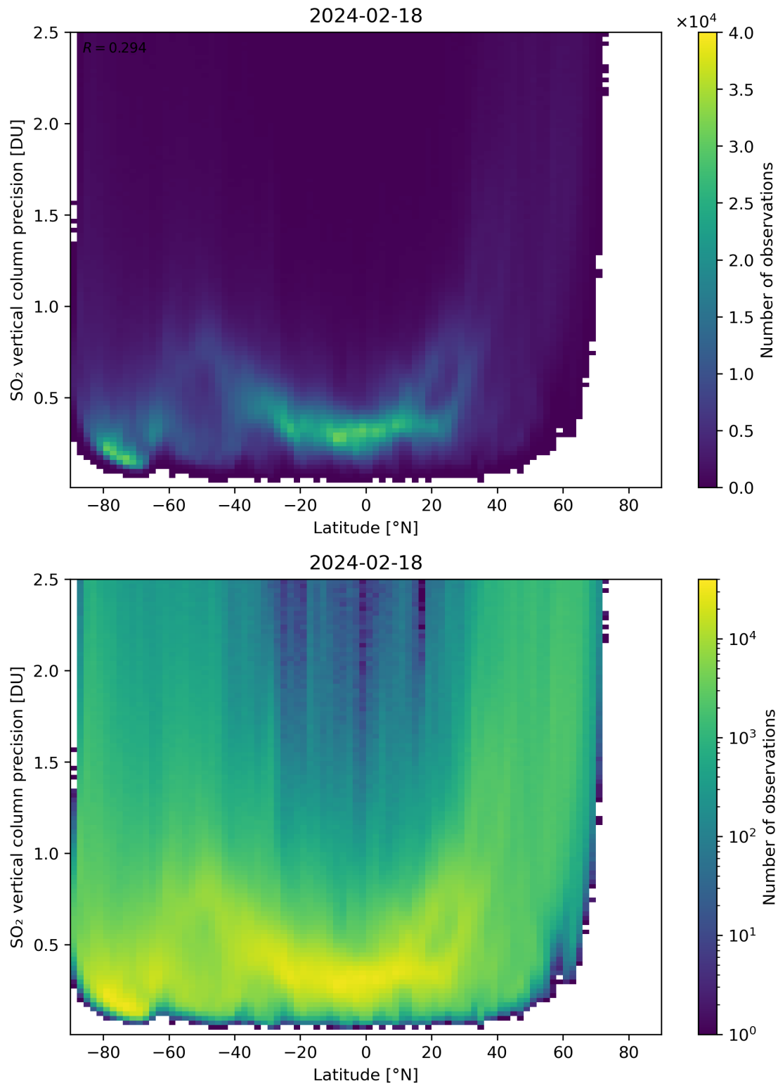
Figure 157: Scatter density plot of “Latitude” against “SO 2 vertical column precision” for 2024-02-17 to 2024-02-19.
