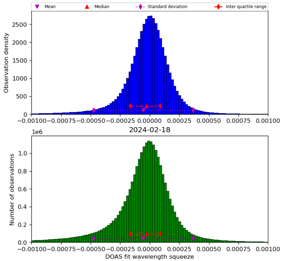
Figure 69: Histogram of “DOAS fit wavelength squeeze” for 2024-02-17 to 2024-02-19
