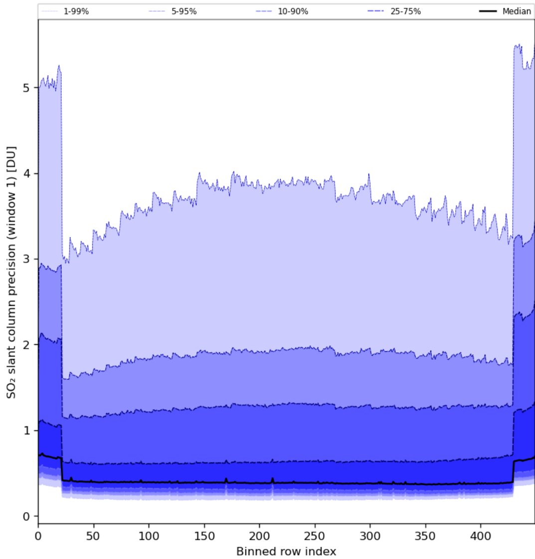
Figure 80: Along track statistics of “SO 2 slant column precision (window 1)” for 2024-02-17 to 2024-02-19
