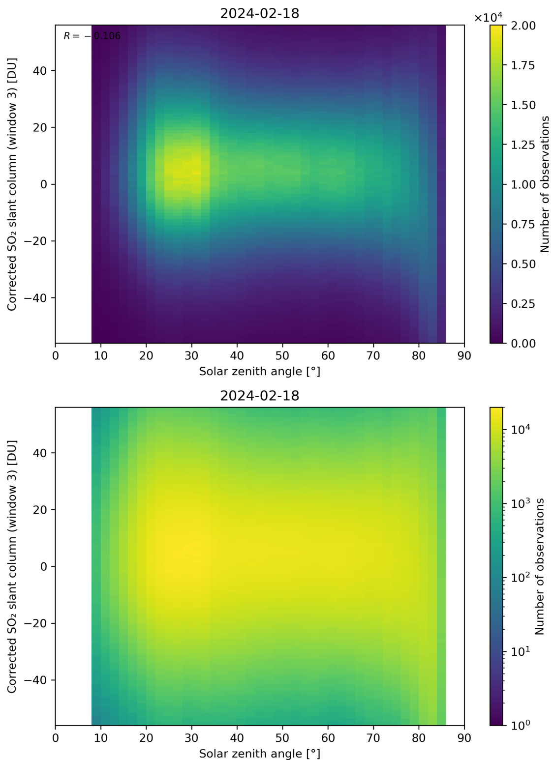
Figure 168: Scatter density plot of “Solar zenith angle” against “Corrected SO 2 slant column (window 3)” for 2024-02-17 to 2024-02-19.
