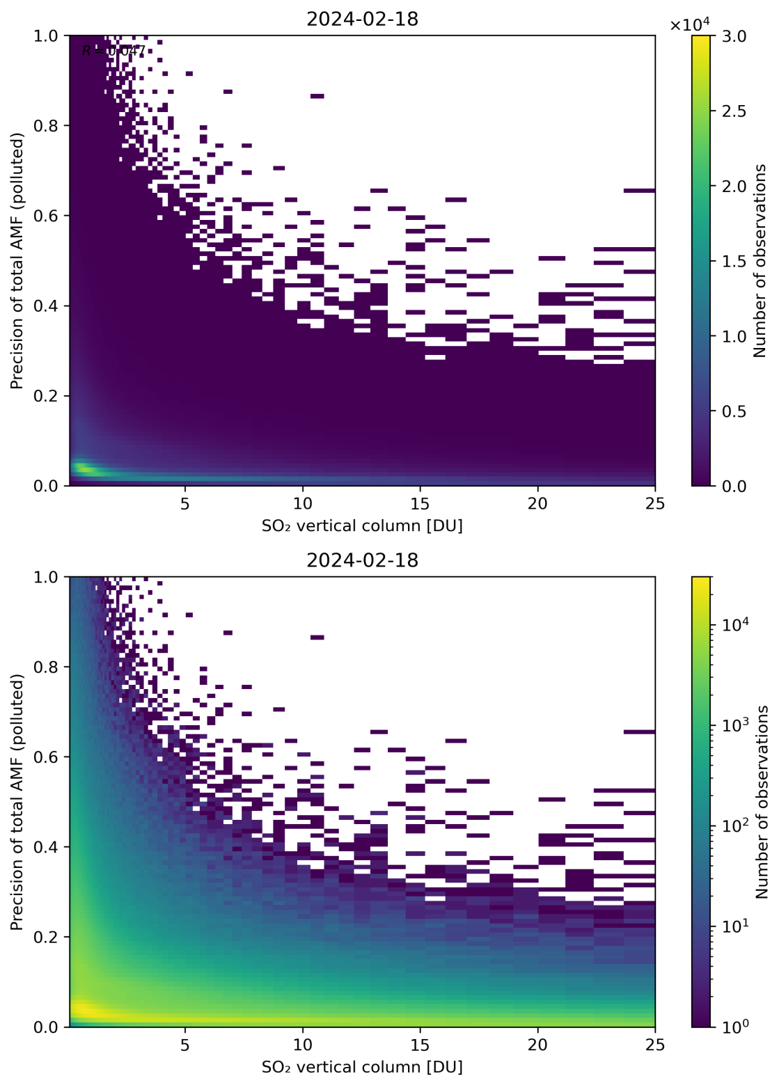
Figure 306: Scatter density plot of “SO 2 vertical column” against “Precision of total AMF (polluted)” for 2024-02-17 to 2024-02-19.
