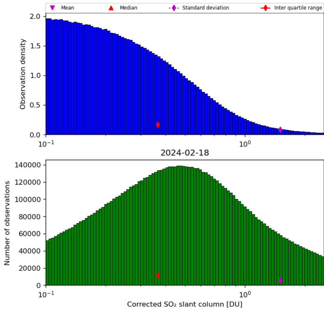
Figure 55: Histogram of “Corrected SO 2 slant column” for 2024-02-17 to 2024-02-19
