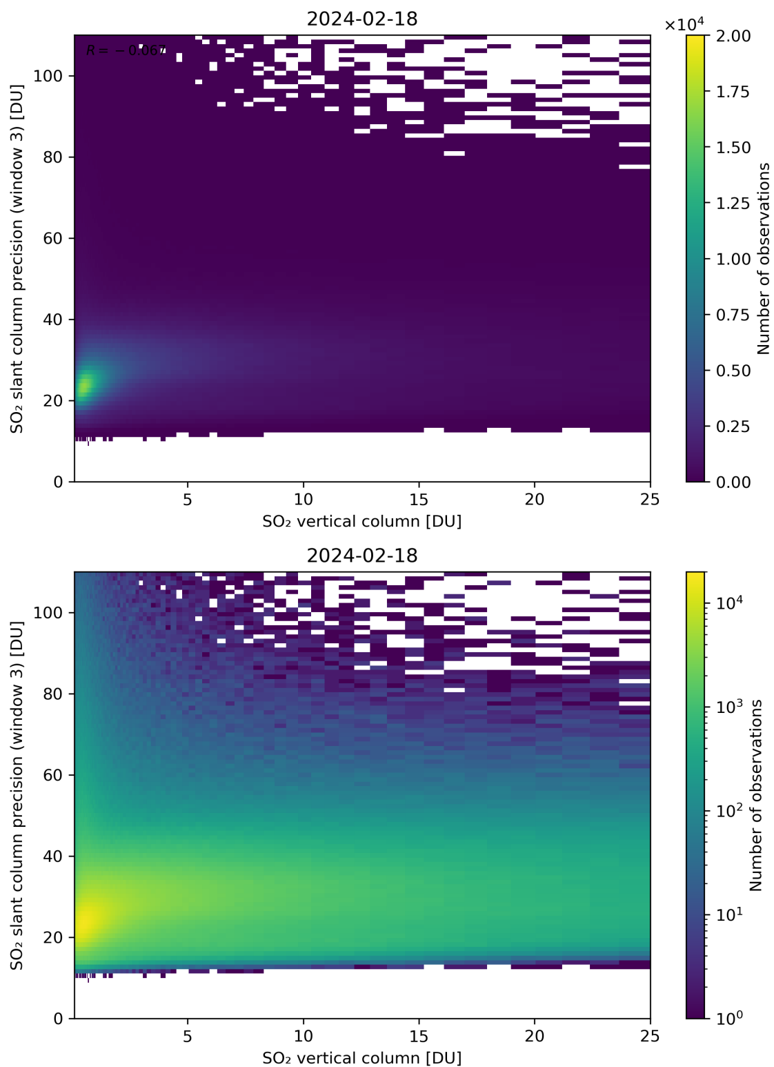
Figure 304: Scatter density plot of “SO 2 vertical column” against “SO 2 slant column precision (window 3)” for 2024-02-17 to 2024-02-19.
