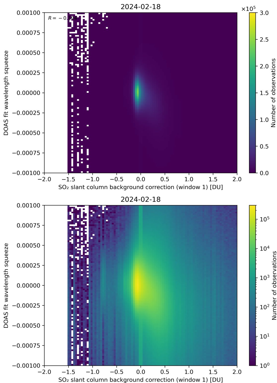
Figure 101: Scatter density plot of “SO 2 slant column background correction (window 1)” against “DOAS fit wavelength squeeze” for 2024-02-17 to 2024-02-19.
