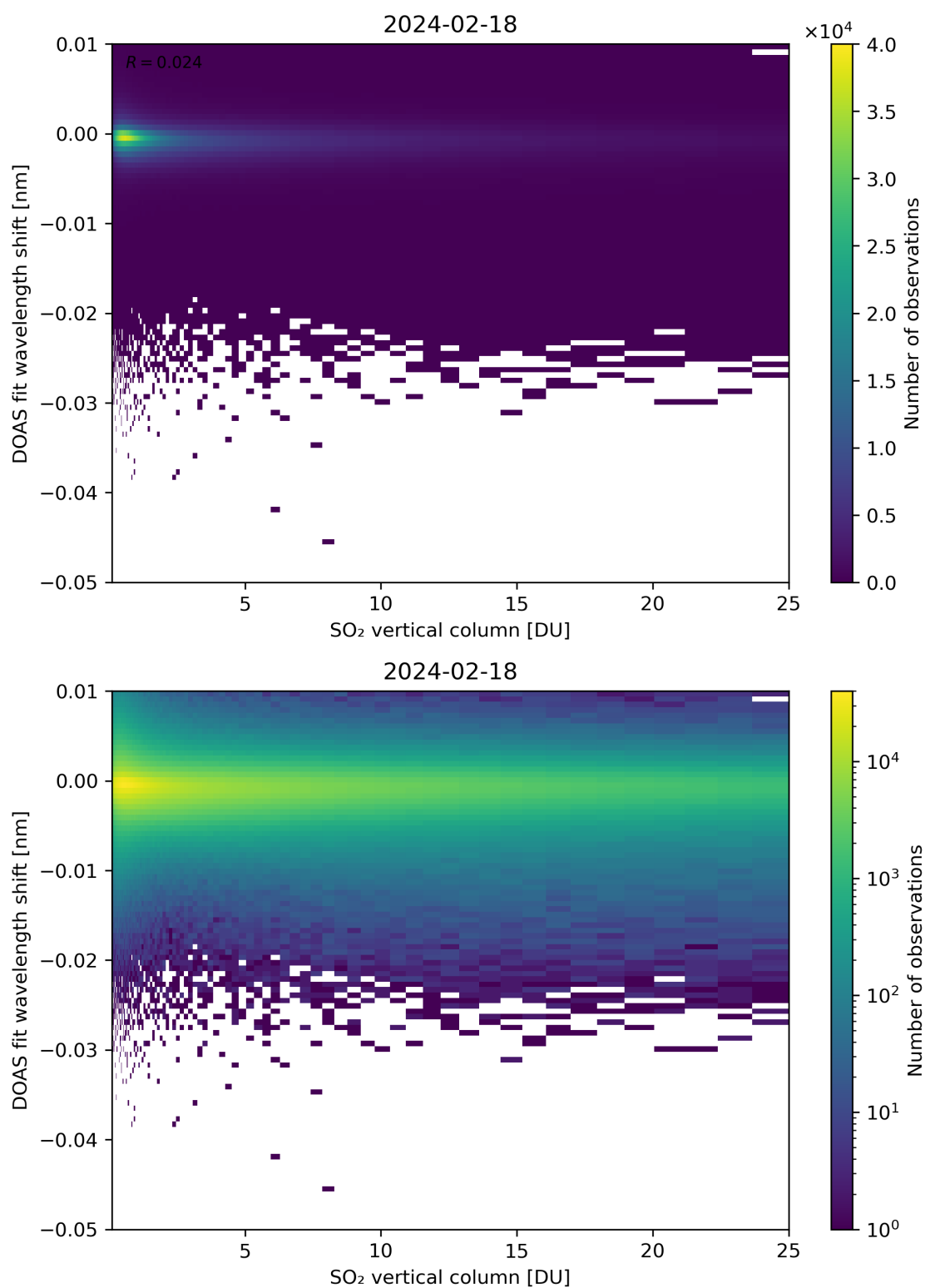
Figure 276: Scatter density plot of “SO 2 vertical column” against “DOAS fit wavelength shift” for 2024-02-17 to 2024-02-19.
