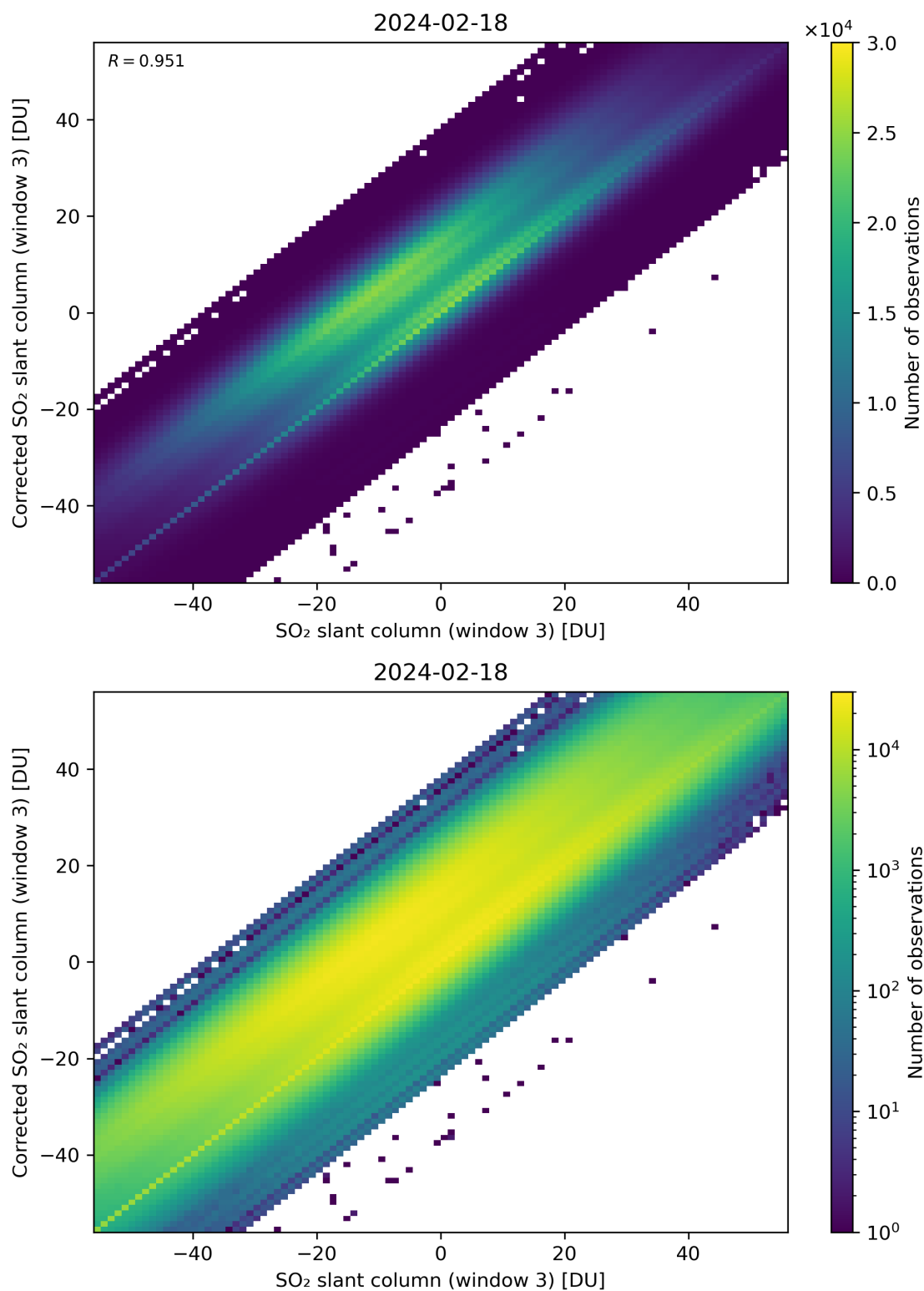
Figure 266: Scatter density plot of “SO 2 slant column (window 3)” against “Corrected SO 2 slant column (window 3)” for 2024-02-17 to 2024-02-19.
