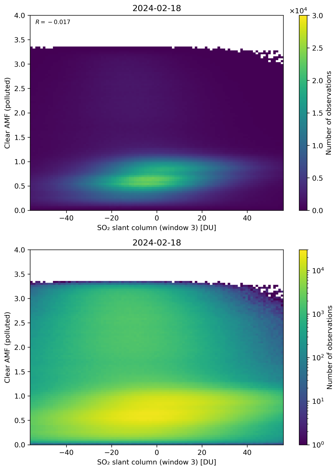
Figure 265: Scatter density plot of “SO 2 slant column (window 3)” against “Clear AMF (polluted)” for 2024-02-17 to 2024-02-19.
