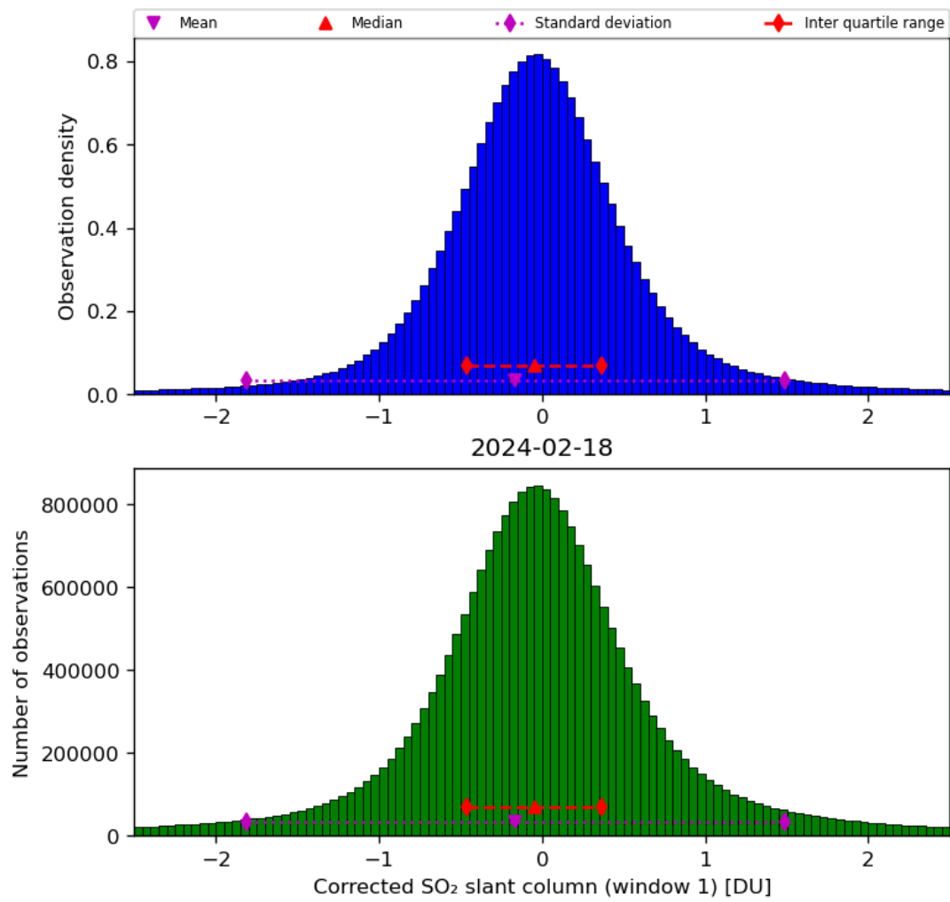
Figure 58: Histogram of “Corrected SO 2 slant column (window 1)” for 2024-02-17 to 2024-02-19
