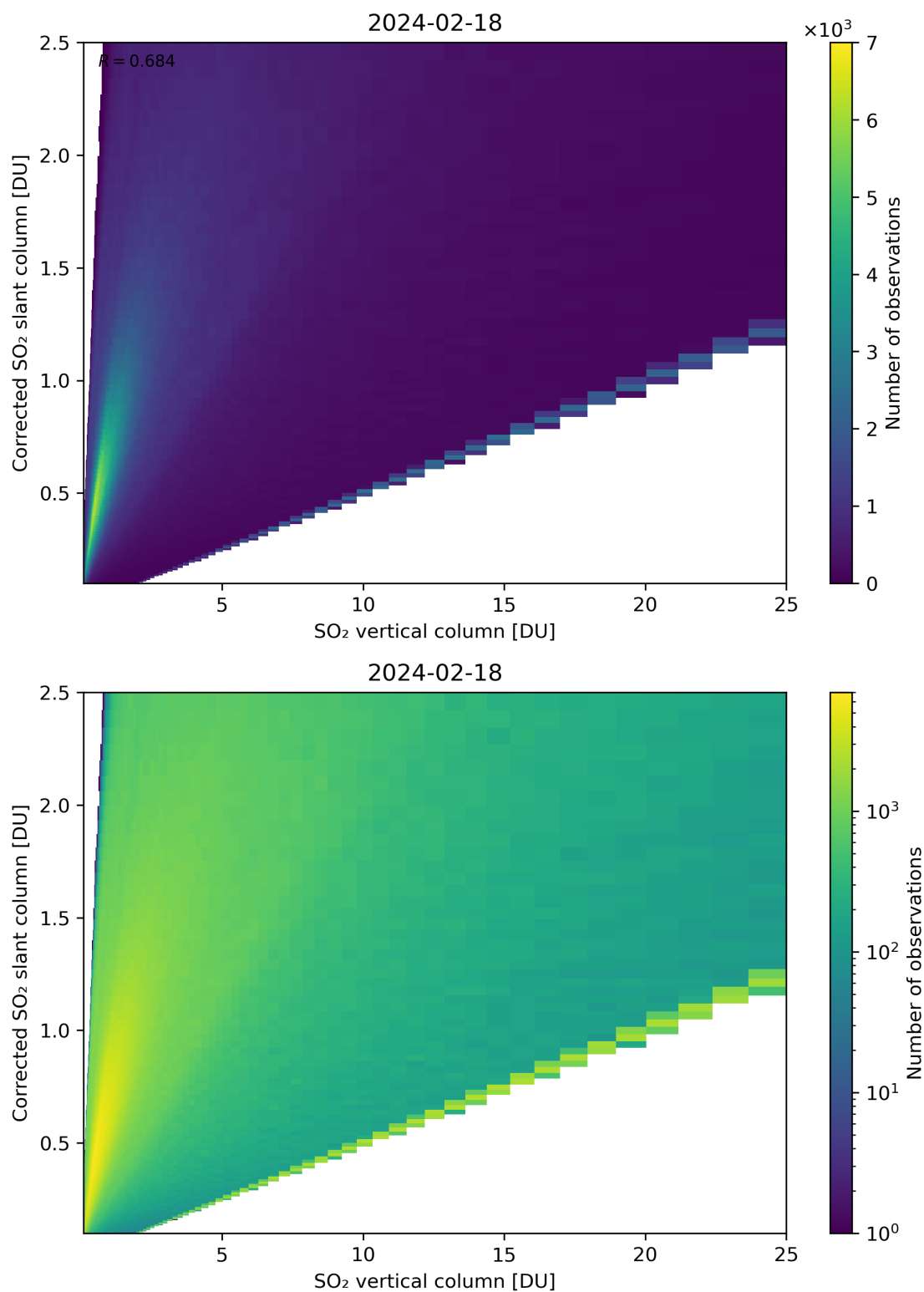
Figure 297: Scatter density plot of “SO 2 vertical column” against “Corrected SO 2 slant column” for 2024-02-17 to 2024-02-19.
