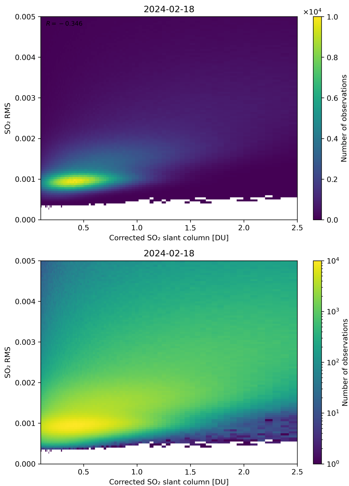
Figure 183: Scatter density plot of “Corrected SO 2 slant column” against “SO 2 RMS” for 2024-02-17 to 2024-02-19.
