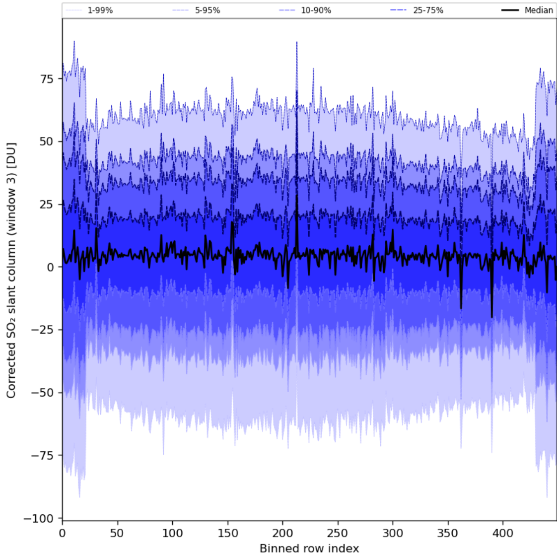
Figure 89: Along track statistics of “Corrected SO 2 slant column (window 3)” for 2024-02-17 to 2024-02-19
