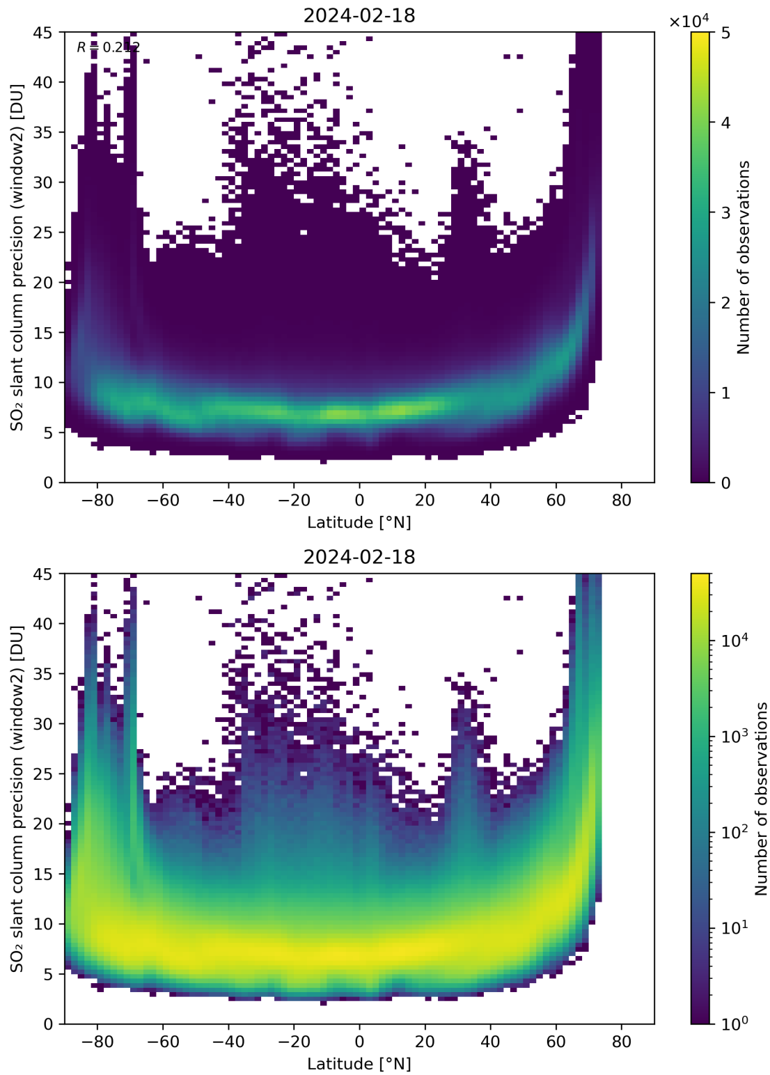
Figure 151: Scatter density plot of “Latitude” against “SO 2 slant column precision (window2)” for 2024-02-17 to 2024-02-19.
