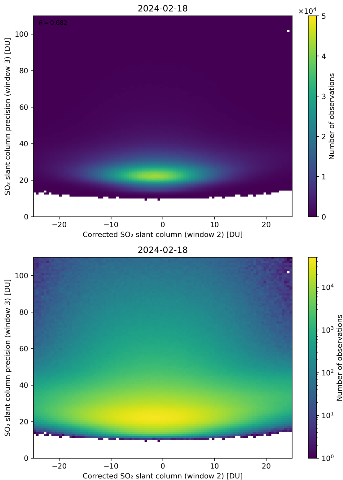
Figure 202: Scatter density plot of “Corrected SO 2 slant column (window 2)” against “SO 2 slant column precision (window 3)” for 2024-02-17 to 2024-02-19.
