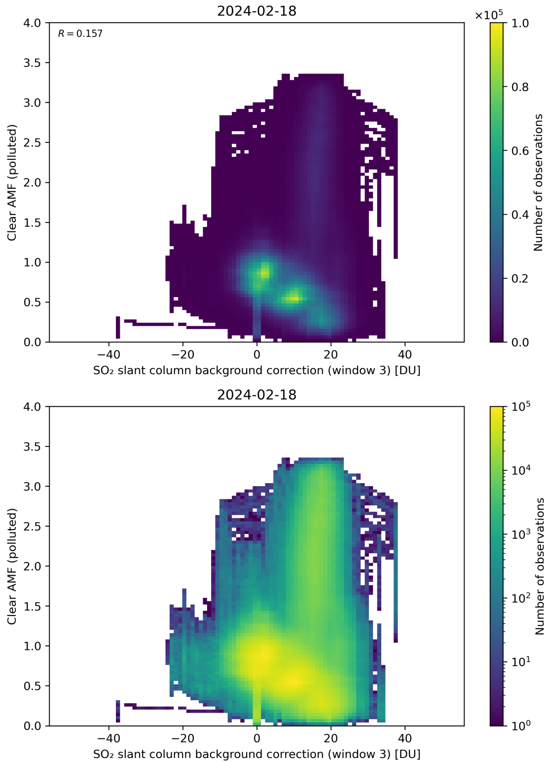
Figure 124: Scatter density plot of “SO 2 slant column background correction (window 3)” against “Clear AMF (polluted)” for 2024-02-17 to 2024-02-19.
