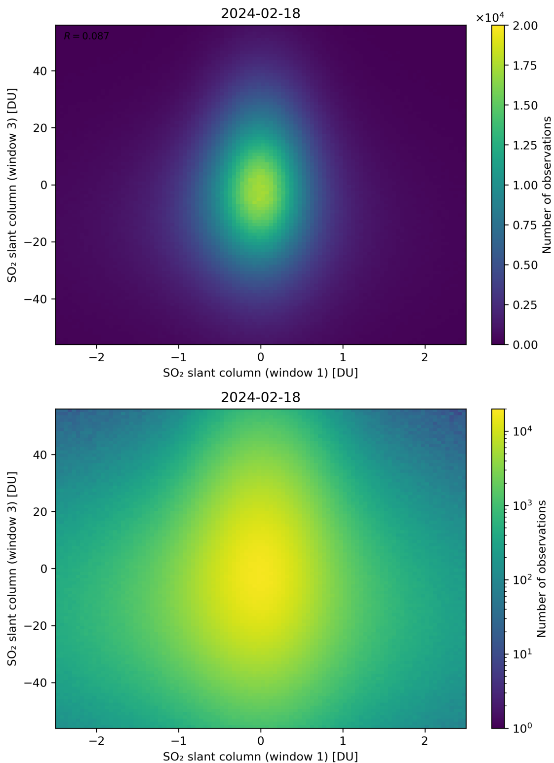
Figure 237: Scatter density plot of “SO 2 slant column (window 1)” against “SO 2 slant column (window 3)” for 2024-02-17 to 2024-02-19.
