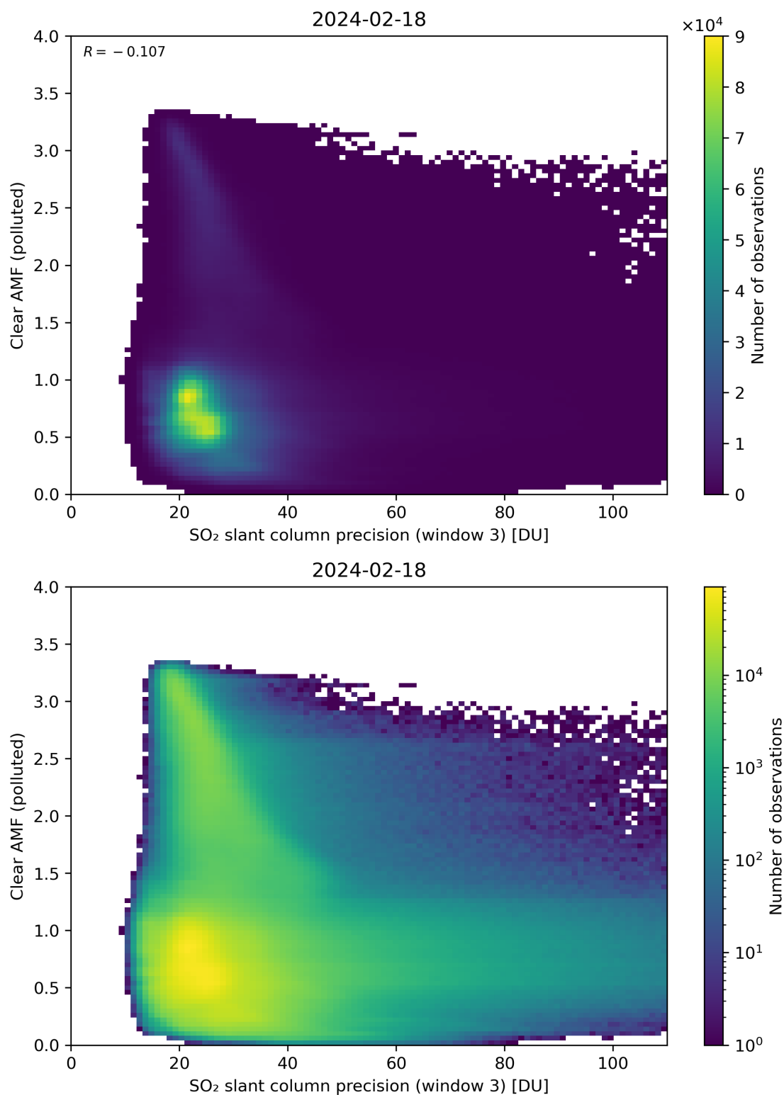
Figure 261: Scatter density plot of “SO 2 slant column precision (window 3)” against “Clear AMF (polluted)” for 2024-02-17 to 2024-02-19.
