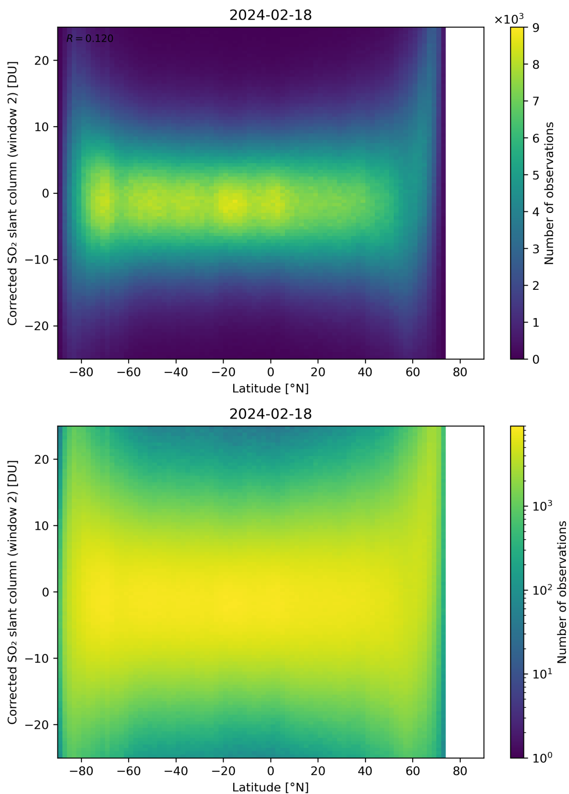
Figure 147: Scatter density plot of “Latitude” against “Corrected SO 2 slant column (window 2)” for 2024-02-17 to 2024-02-19.
