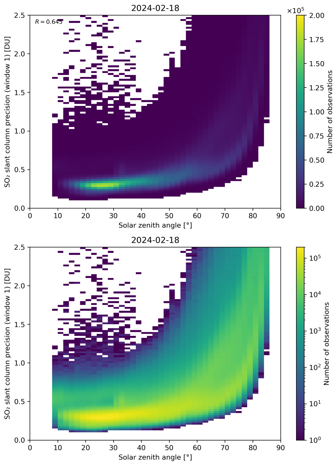
Figure 170: Scatter density plot of “Solar zenith angle” against “SO 2 slant column precision (window 1)” for 2024-02-17 to 2024-02-19.
