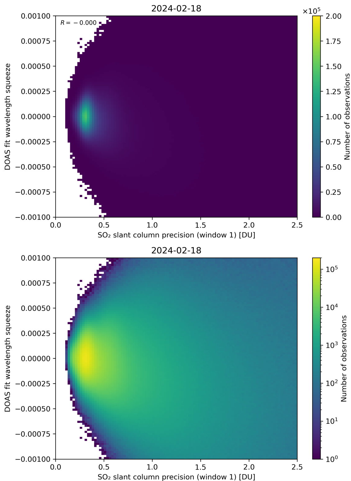
Figure 222: Scatter density plot of “SO 2 slant column precision (window 1)” against “DOAS fit wavelength squeeze” for 2024-02-17 to 2024-02-19.
