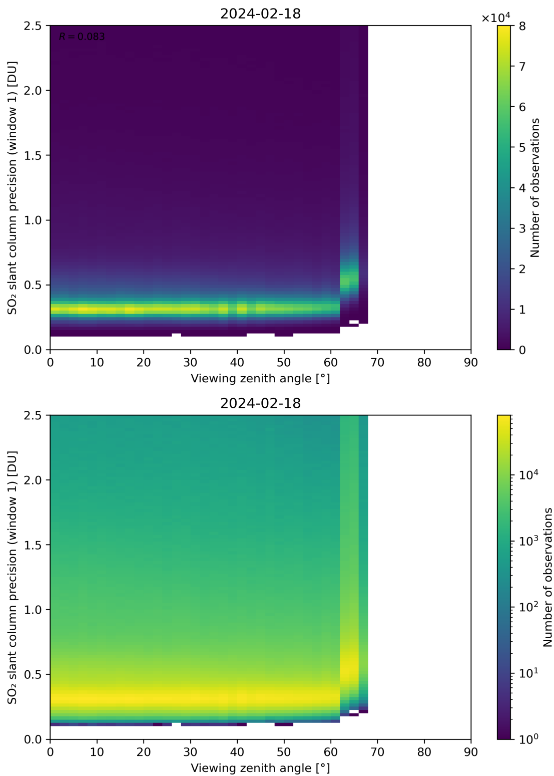
Figure 321: Scatter density plot of “Viewing zenith angle” against “SO 2 slant column precision (window 1)” for 2024-02-17 to 2024-02-19.
