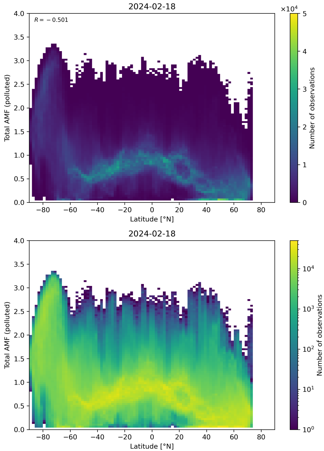
Figure 154: Scatter density plot of “Latitude” against “Total AMF (polluted)” for 2024-02-17 to 2024-02-19.
