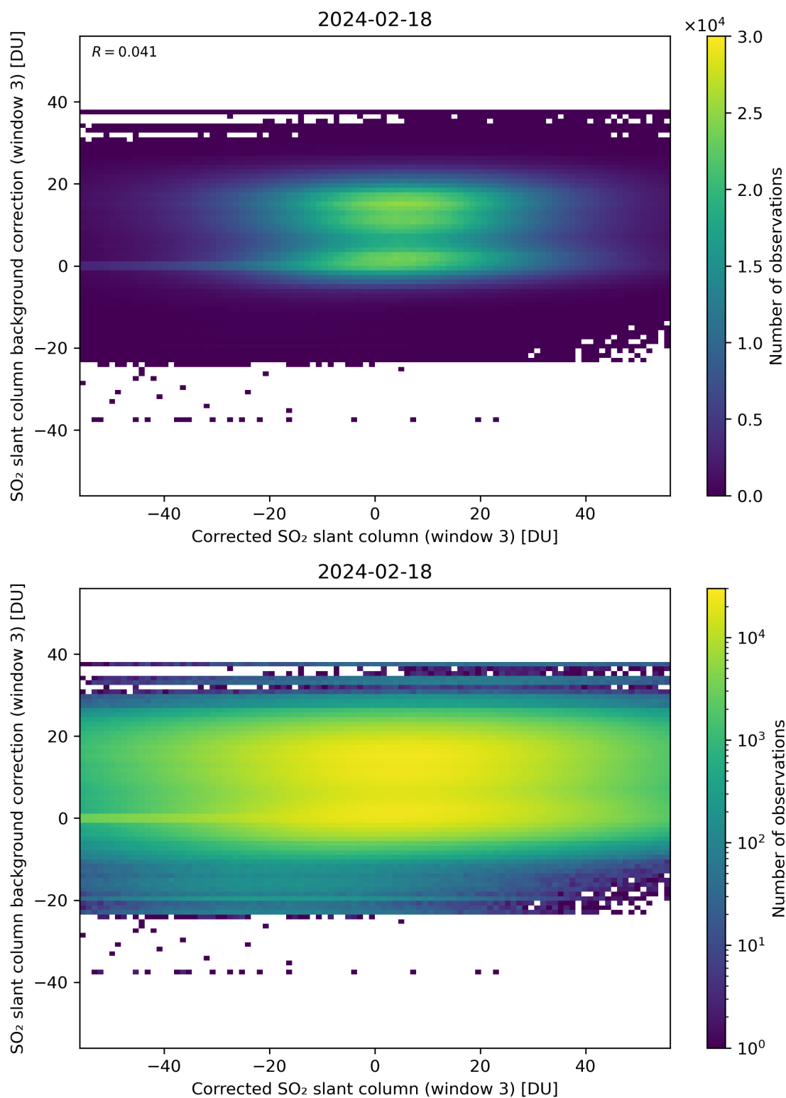
Figure 205: Scatter density plot of “Corrected SO 2 slant column (window 3)” against “SO 2 slant column background correction (window 3)” for 2024-02-17 to 2024-02-19.
