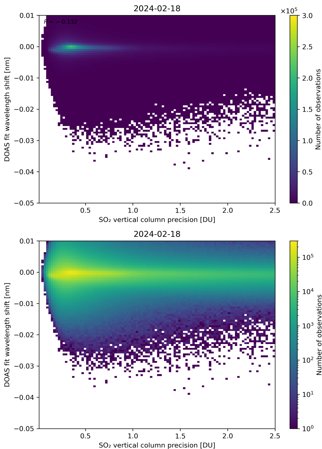
Figure 282: Scatter density plot of “SO 2 vertical column precision” against “DOAS fit wavelength shift” for 2024-02-17 to 2024-02-19.
