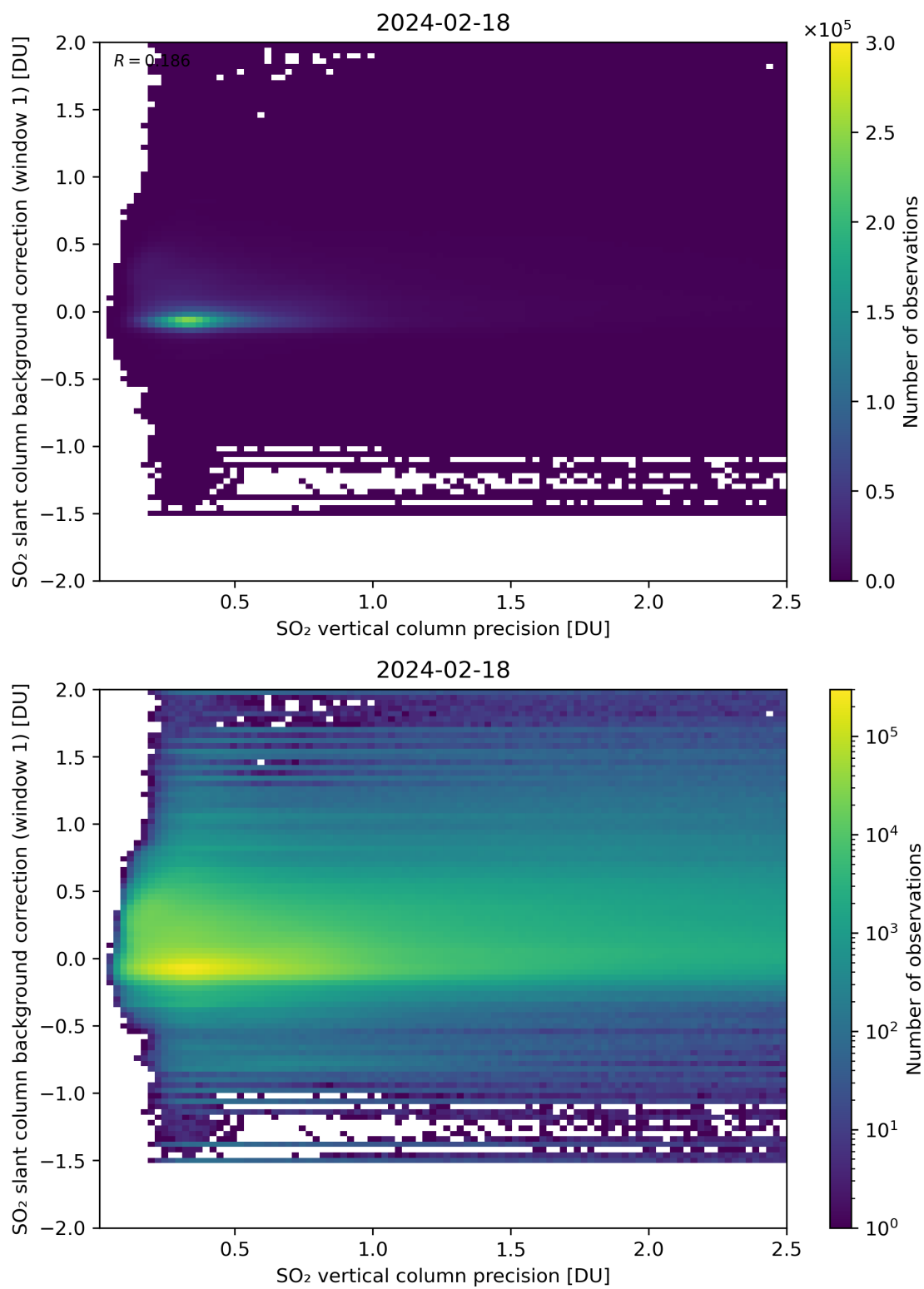
Figure 279: Scatter density plot of “SO 2 vertical column precision” against “SO 2 slant column background correction (window 1)” for 2024-02-17 to 2024-02-19.
