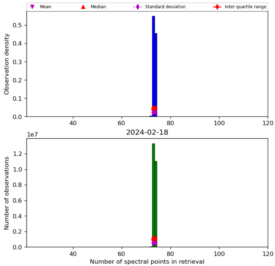
Figure 74: Histogram of “Number of spectral points in retrieval” for 2024-02-17 to 2024-02-19
