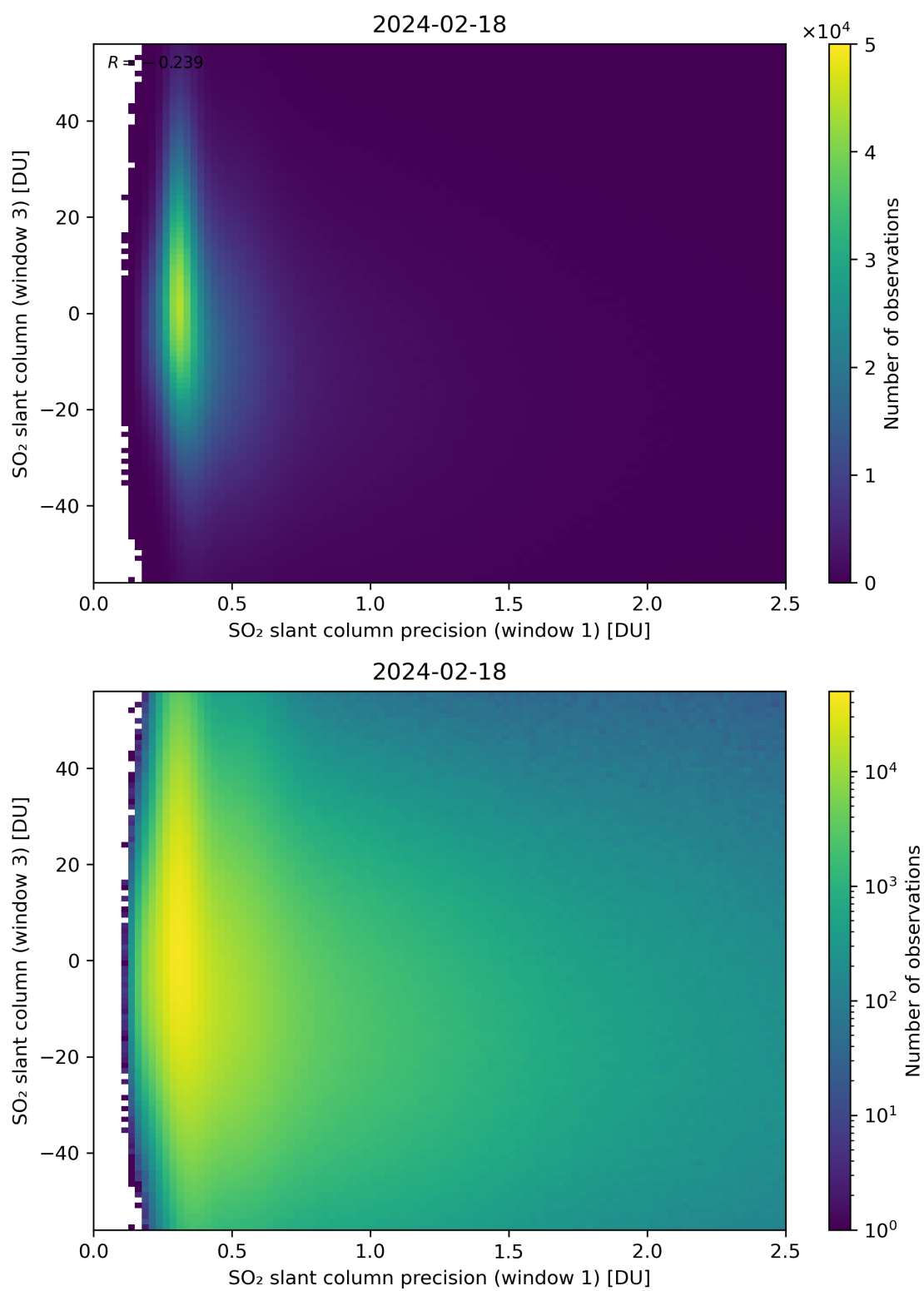
Figure 228: Scatter density plot of “SO 2 slant column precision (window 1)” against “SO 2 slant column (window 3)” for 2024-02-17 to 2024-02-19.
