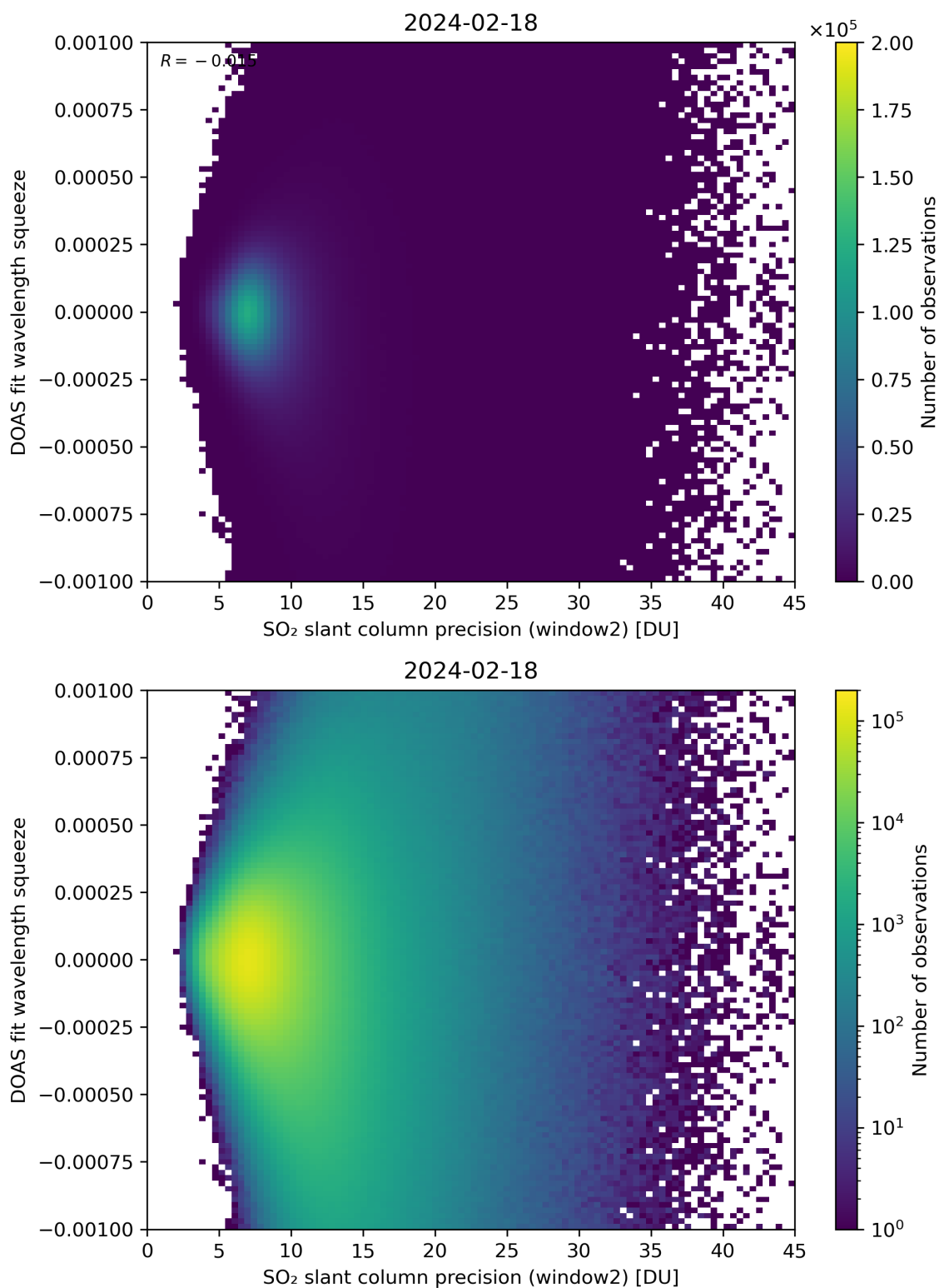
Figure 244: Scatter density plot of “SO 2 slant column precision (window2)” against “DOAS fit wavelength squeeze” for 2024-02-17 to 2024-02-19.
