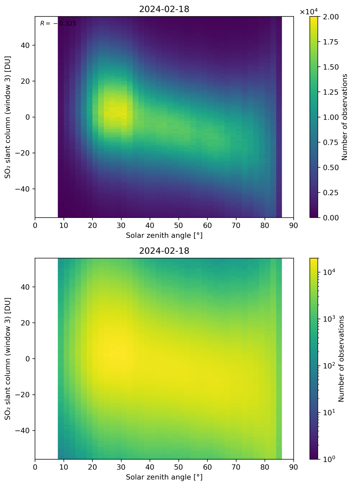
Figure 172: Scatter density plot of “Solar zenith angle” against “SO 2 slant column (window 3)” for 2024-02-17 to 2024-02-19.
