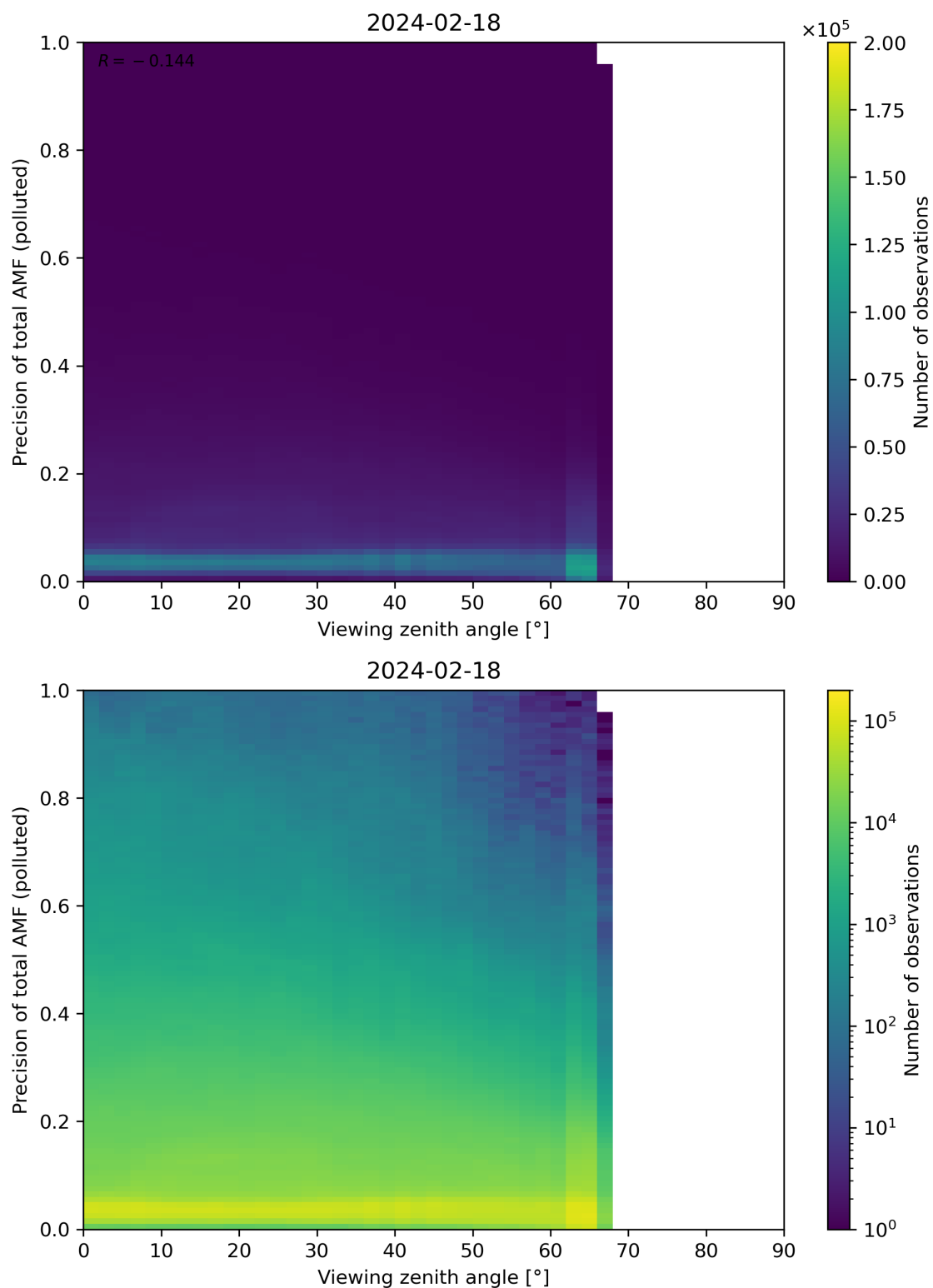
Figure 326: Scatter density plot of “Viewing zenith angle” against “Precision of total AMF (polluted)” for 2024-02-17 to 2024-02-19.
