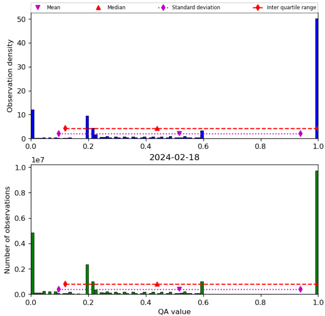
Figure 52: Histogram of “QA value” for 2024-02-17 to 2024-02-19
