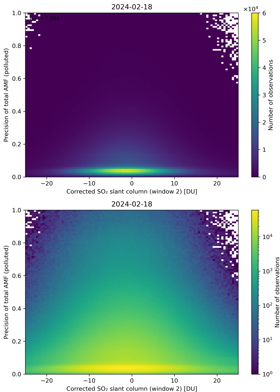
Figure 204: Scatter density plot of “Corrected SO 2 slant column (window 2)” against “Precision of total AMF (polluted)” for 2024-02-17 to 2024-02-19.
