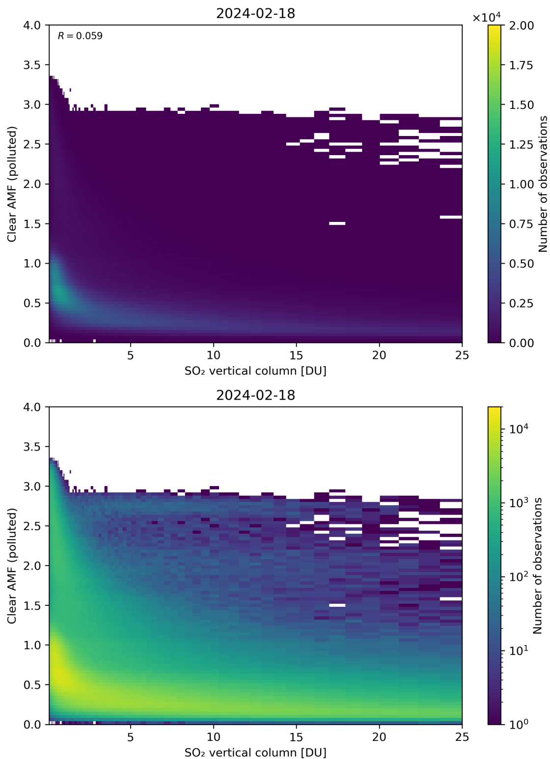
Figure 296: Scatter density plot of “SO 2 vertical column” against “Clear AMF (polluted)” for 2024-02-17 to 2024-02-19.
