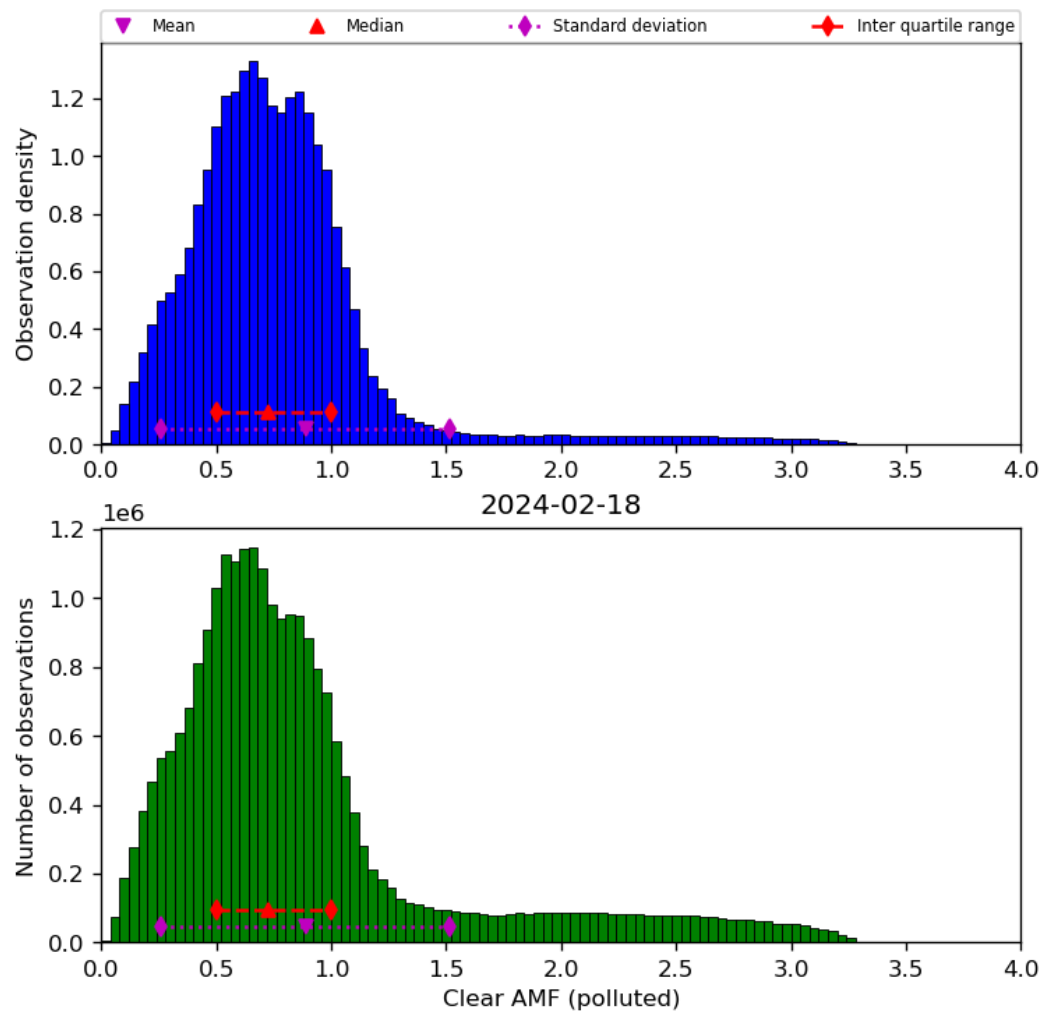
Figure 73: Histogram of “Clear AMF (polluted)” for 2024-02-17 to 2024-02-19
