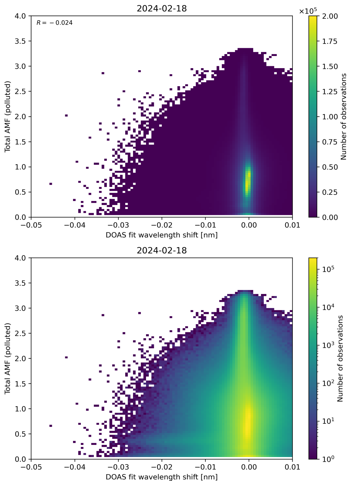
Figure 130: Scatter density plot of “DOAS fit wavelength shift” against “Total AMF (polluted)” for 2024-02-17 to 2024-02-19.
