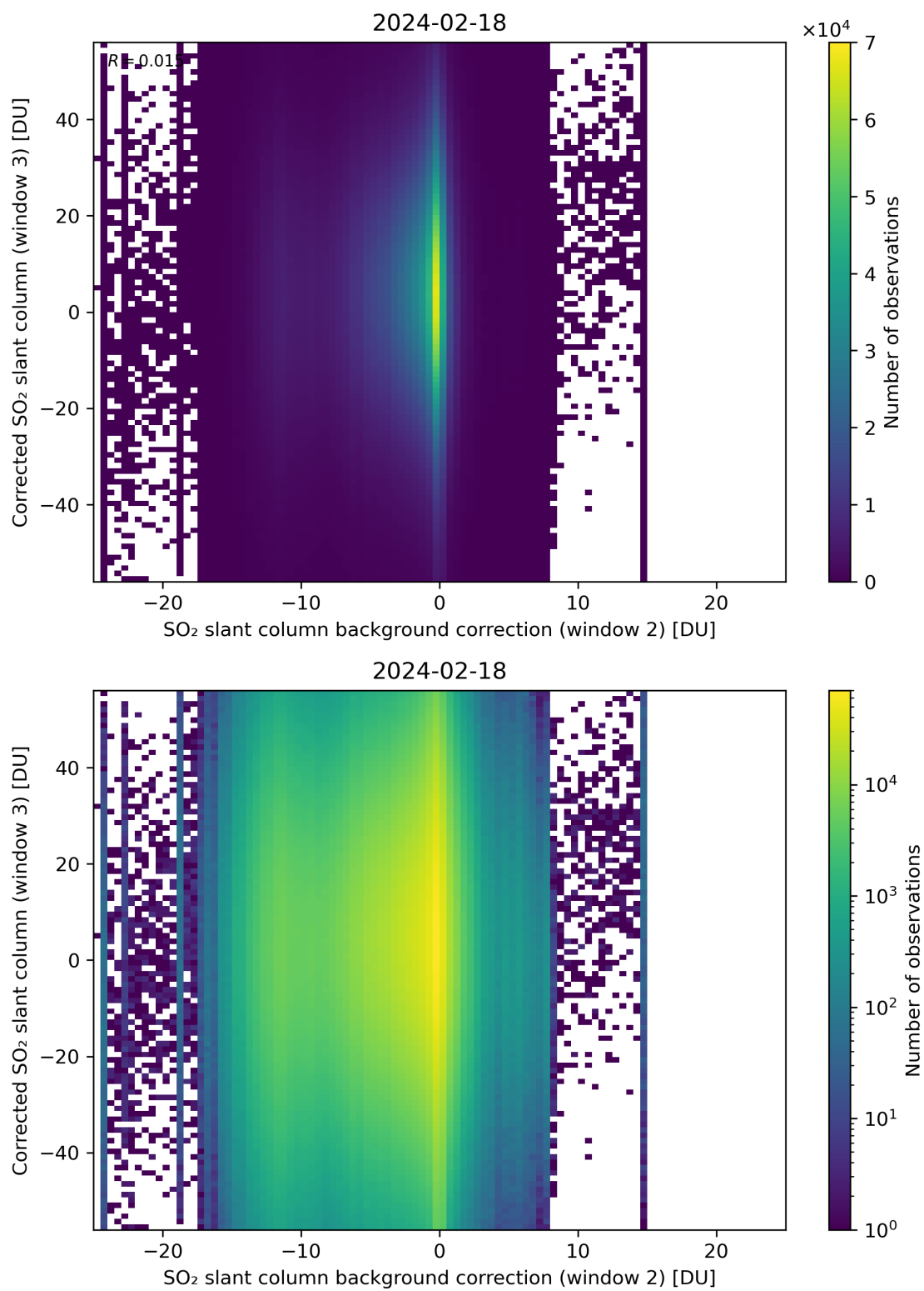
Figure 116: Scatter density plot of “SO 2 slant column background correction (window 2)” against “Corrected SO 2 slant column (window 3)” for 2024-02-17 to 2024-02-19.
