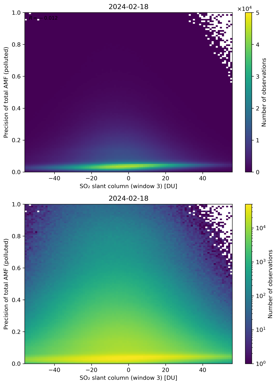
Figure 269: Scatter density plot of “SO 2 slant column (window 3)” against “Precision of total AMF (polluted)” for 2024-02-17 to 2024-02-19.
