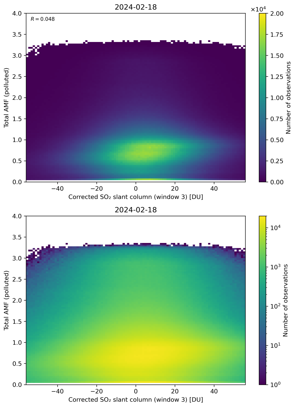
Figure 210: Scatter density plot of “Corrected SO 2 slant column (window 3)” against “Total AMF (polluted)” for 2024-02-17 to 2024-02-19.
