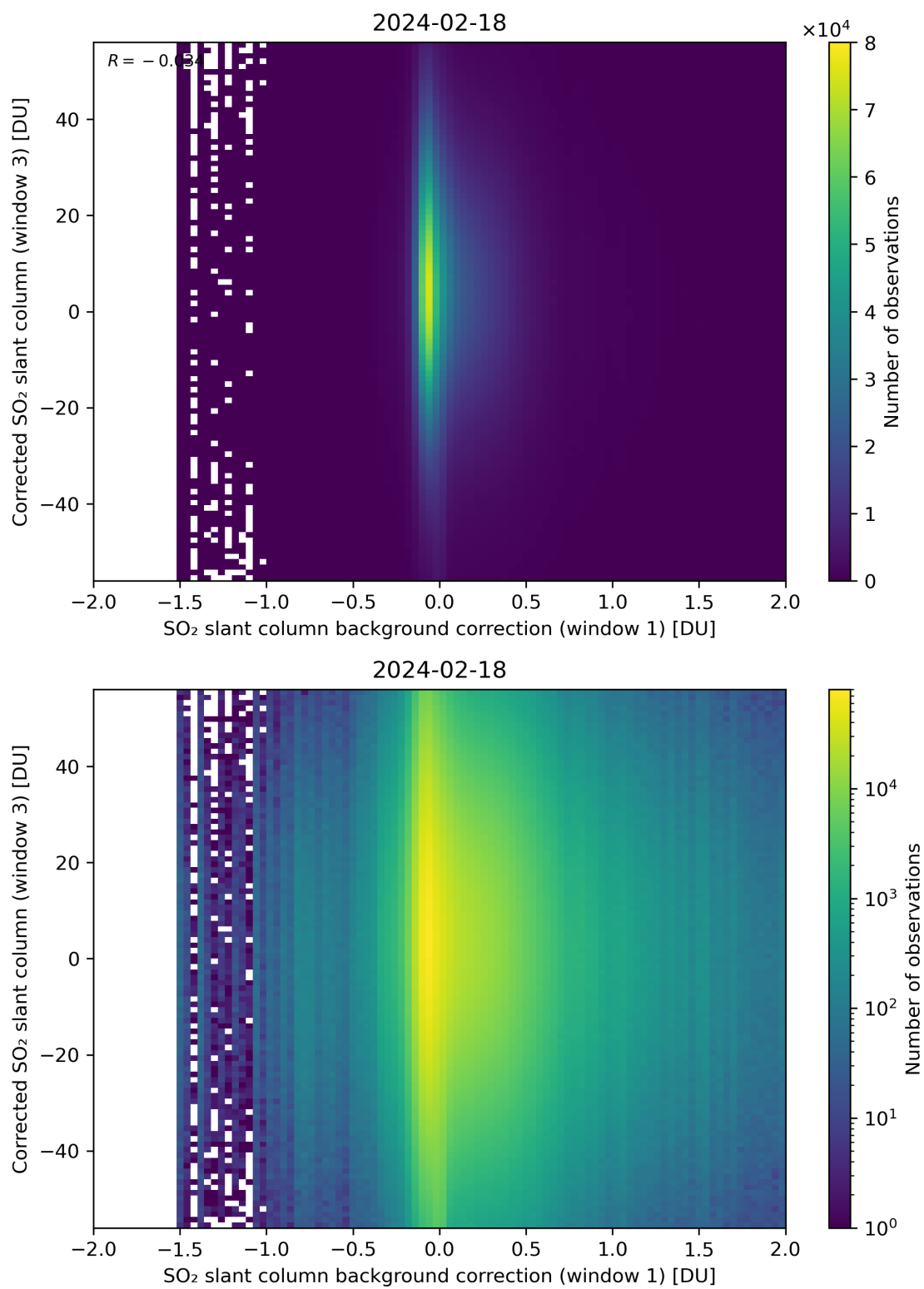
Figure 105: Scatter density plot of “SO 2 slant column background correction (window 1)” against “Corrected SO 2 slant column (window 3)” for 2024-02-17 to 2024-02-19.
