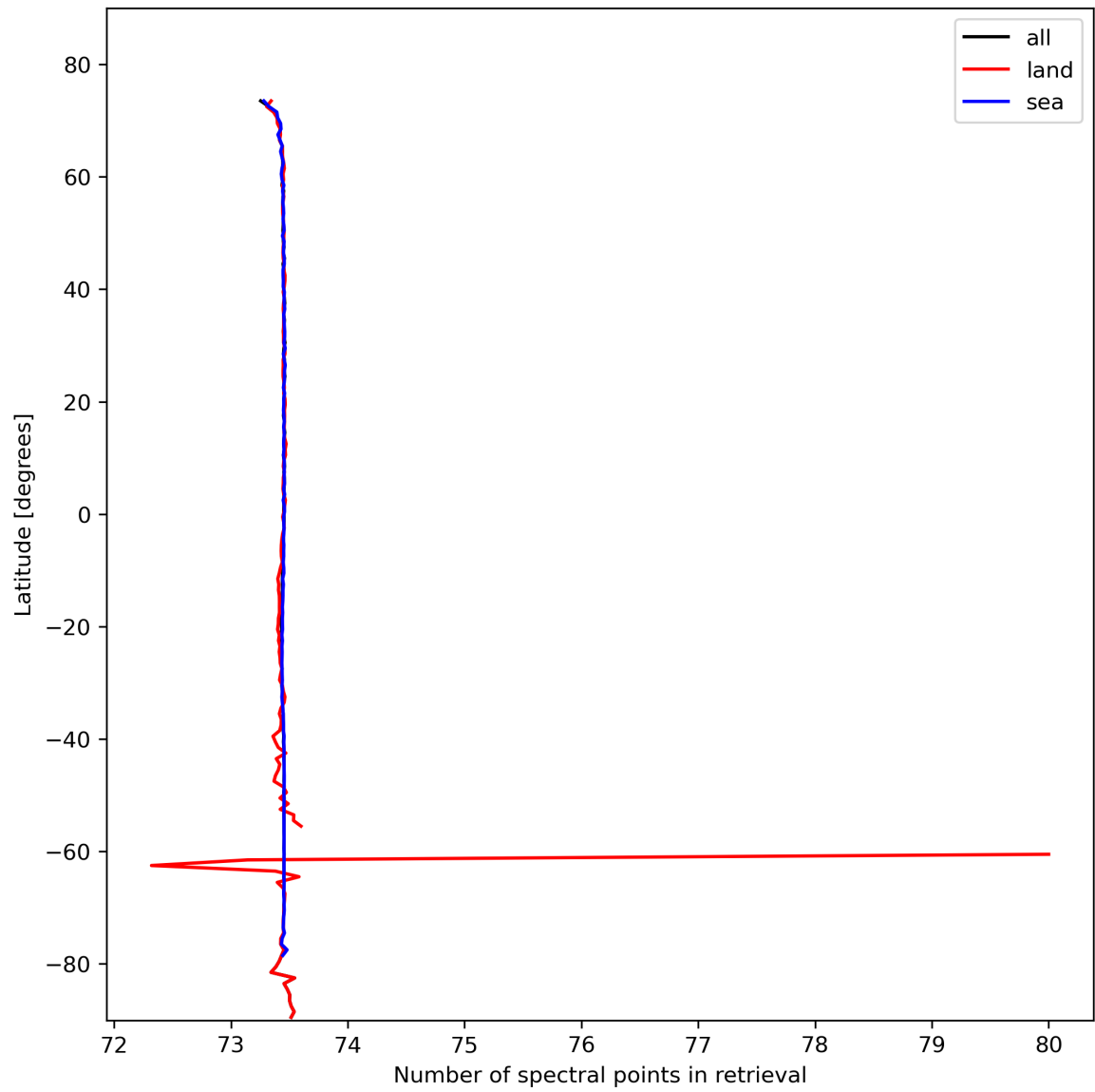
Figure 51: Zonal average of “Number of spectral points in retrieval” for 2024-02-17 to 2024-02-19.
