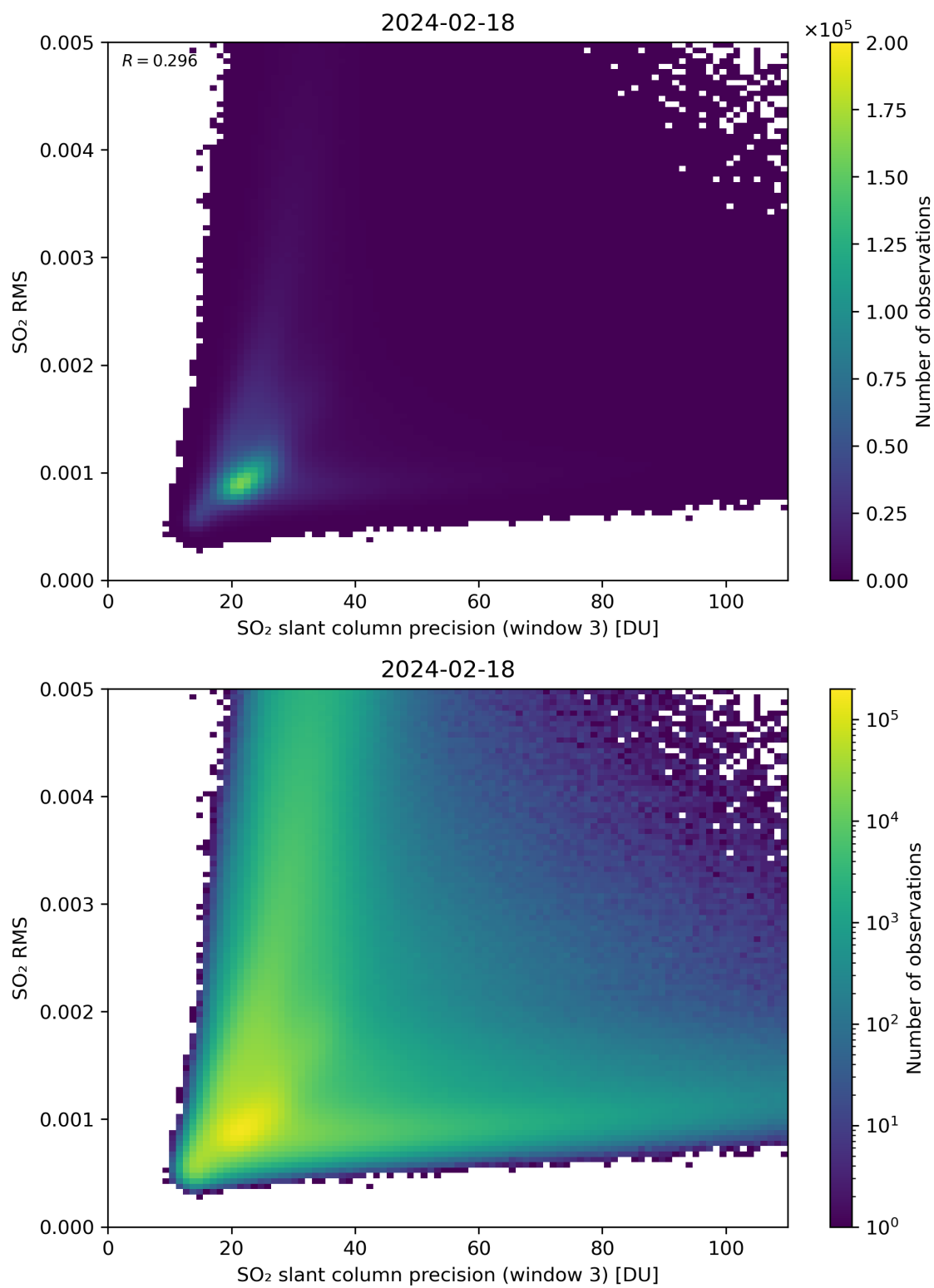
Figure 260: Scatter density plot of “SO 2 slant column precision (window 3)” against “SO 2 RMS” for 2024-02-17 to 2024-02-19.
