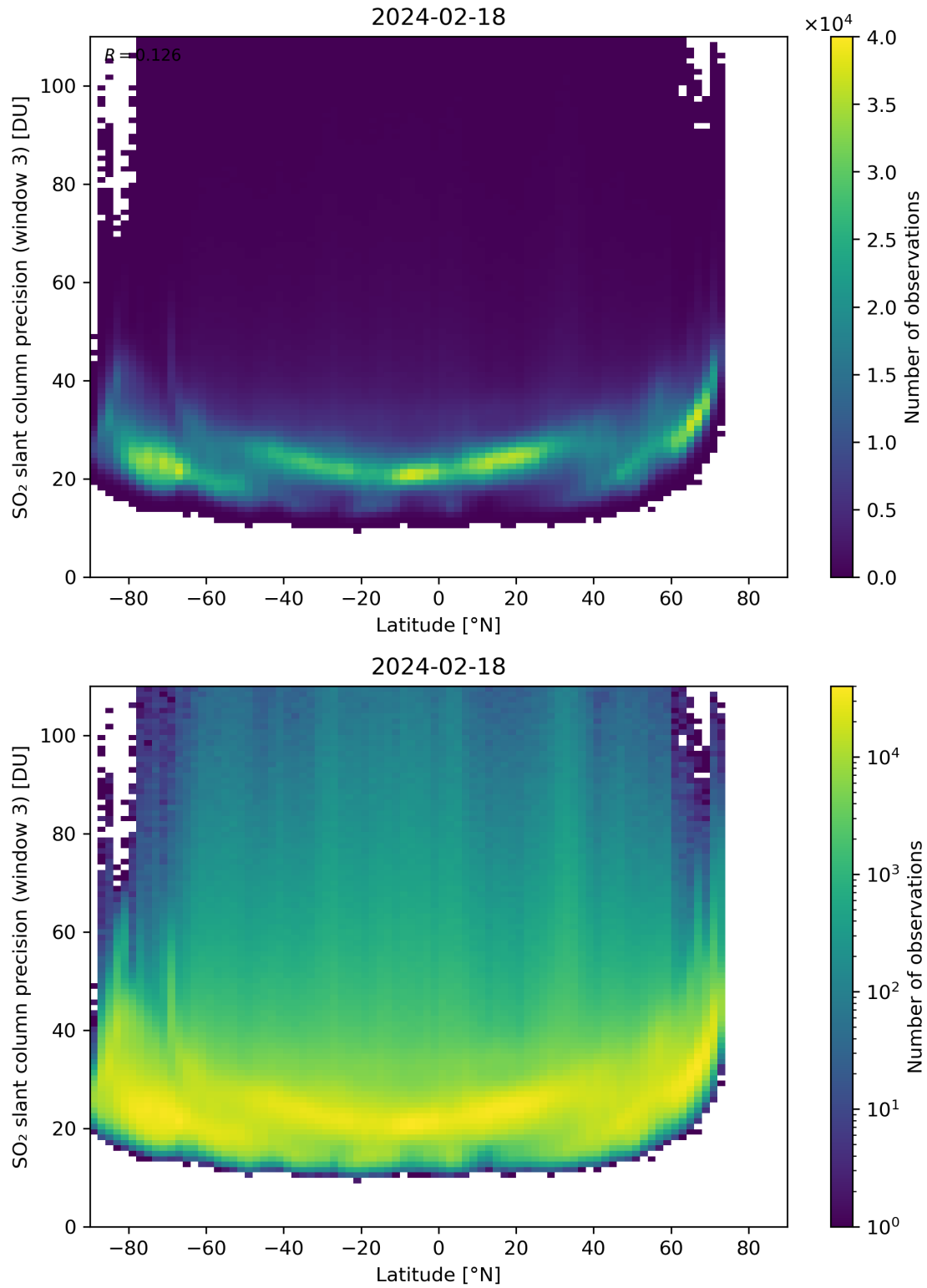
Figure 153: Scatter density plot of “Latitude” against “SO 2 slant column precision (window 3)” for 2024-02-17 to 2024-02-19.
