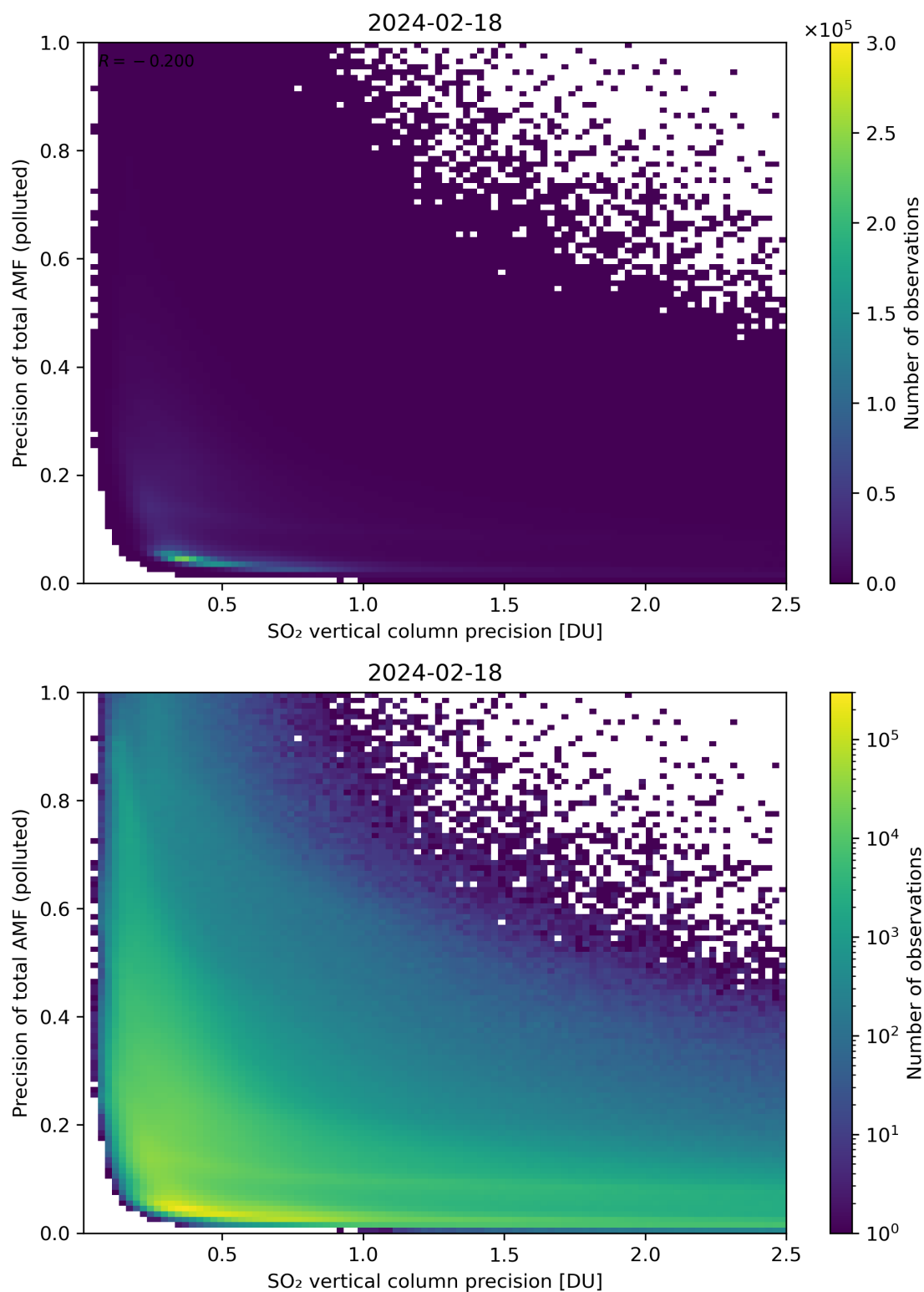
Figure 295: Scatter density plot of “SO 2 vertical column precision” against “Precision of total AMF (polluted)” for 2024-02-17 to 2024-02-19.
