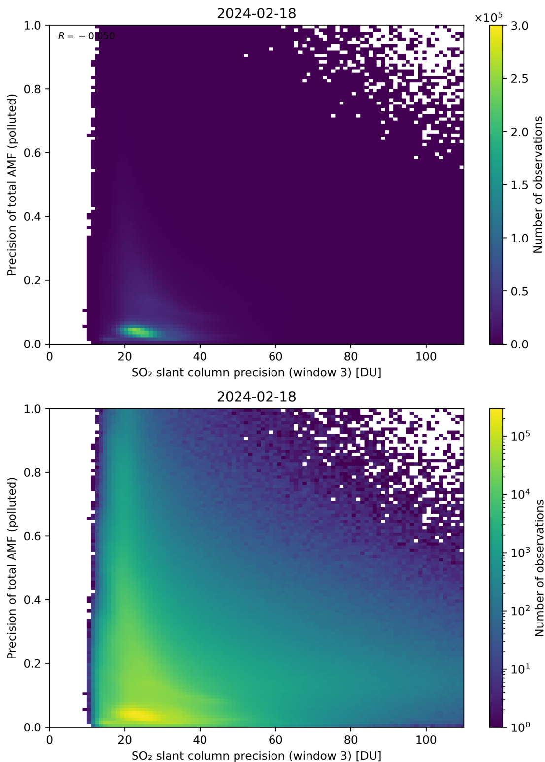
Figure 264: Scatter density plot of “SO 2 slant column precision (window 3)” against “Precision of total AMF (polluted)” for 2024-02-17 to 2024-02-19.
