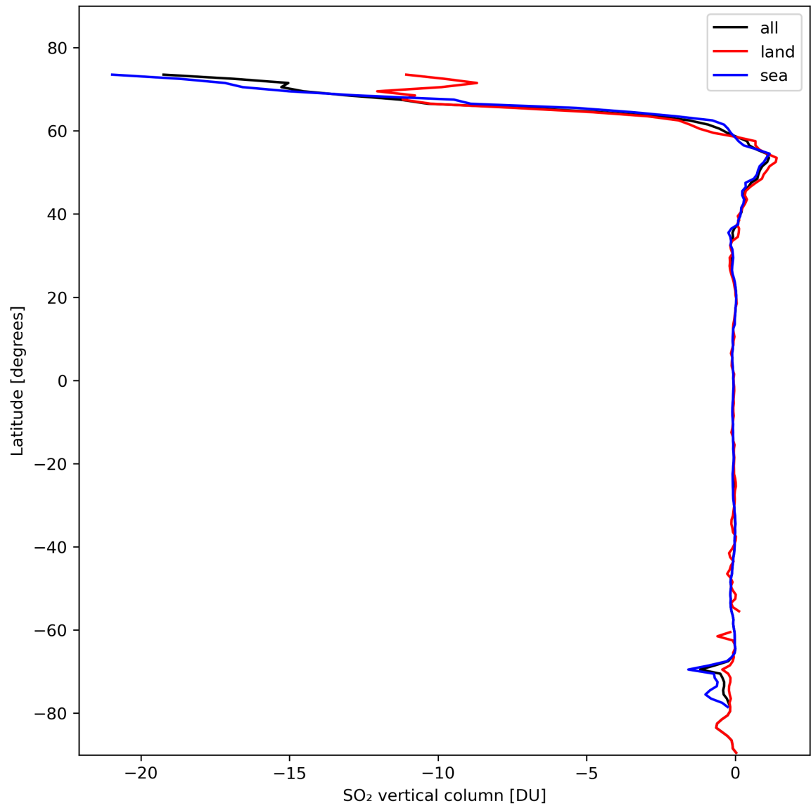
Figure 30: Zonal average of “SO 2 vertical column” for 2024-02-17 to 2024-02-19.
