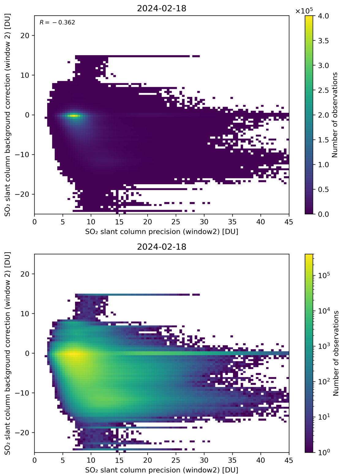
Figure 241: Scatter density plot of “SO 2 slant column precision (window2)” against “SO 2 slant column background correction (window 2)” for 2024-02-17 to 2024-02-19.
