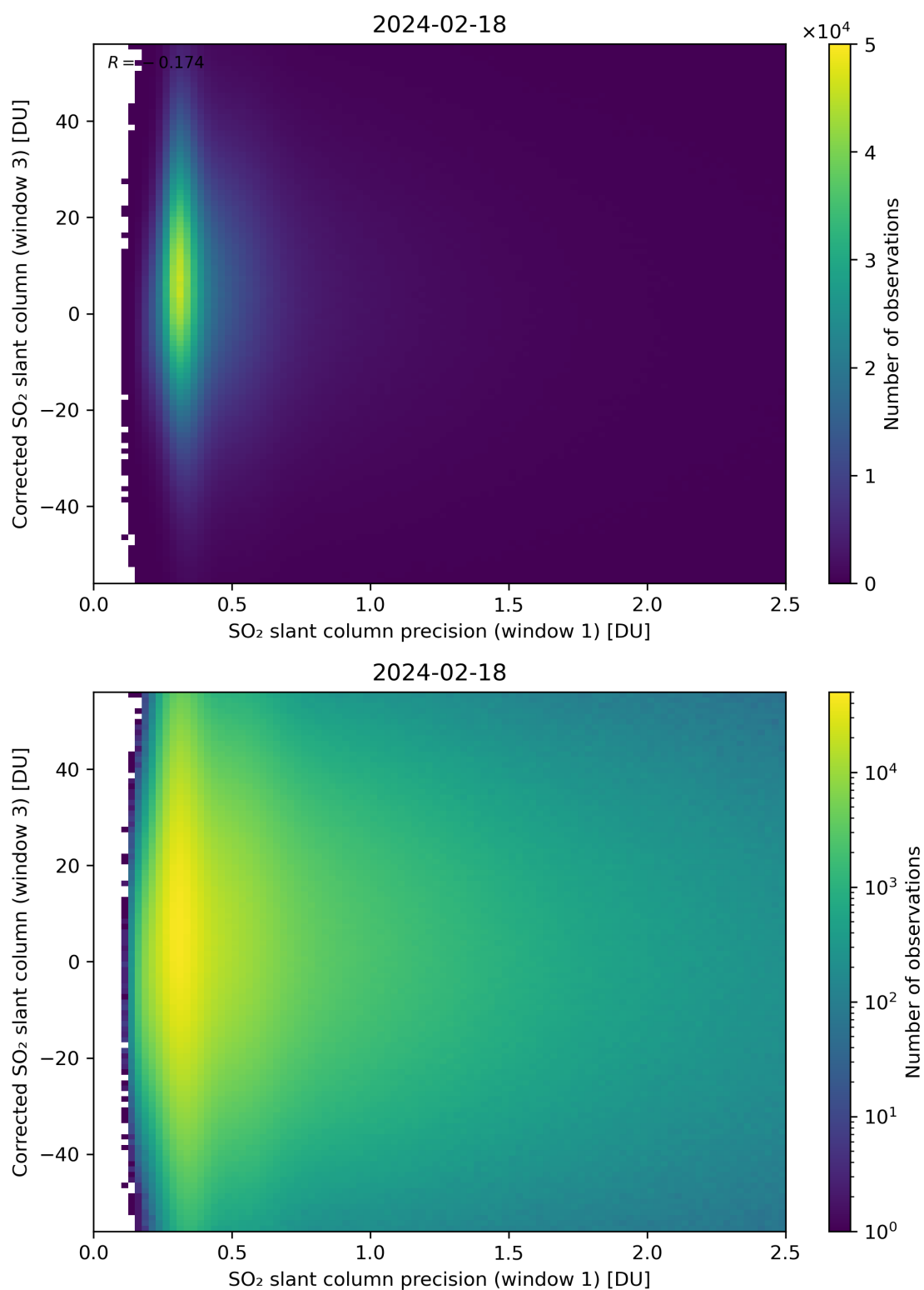
Figure 226: Scatter density plot of “SO 2 slant column precision (window 1)” against “Corrected SO 2 slant column (window 3)” for 2024-02-17 to 2024-02-19.
