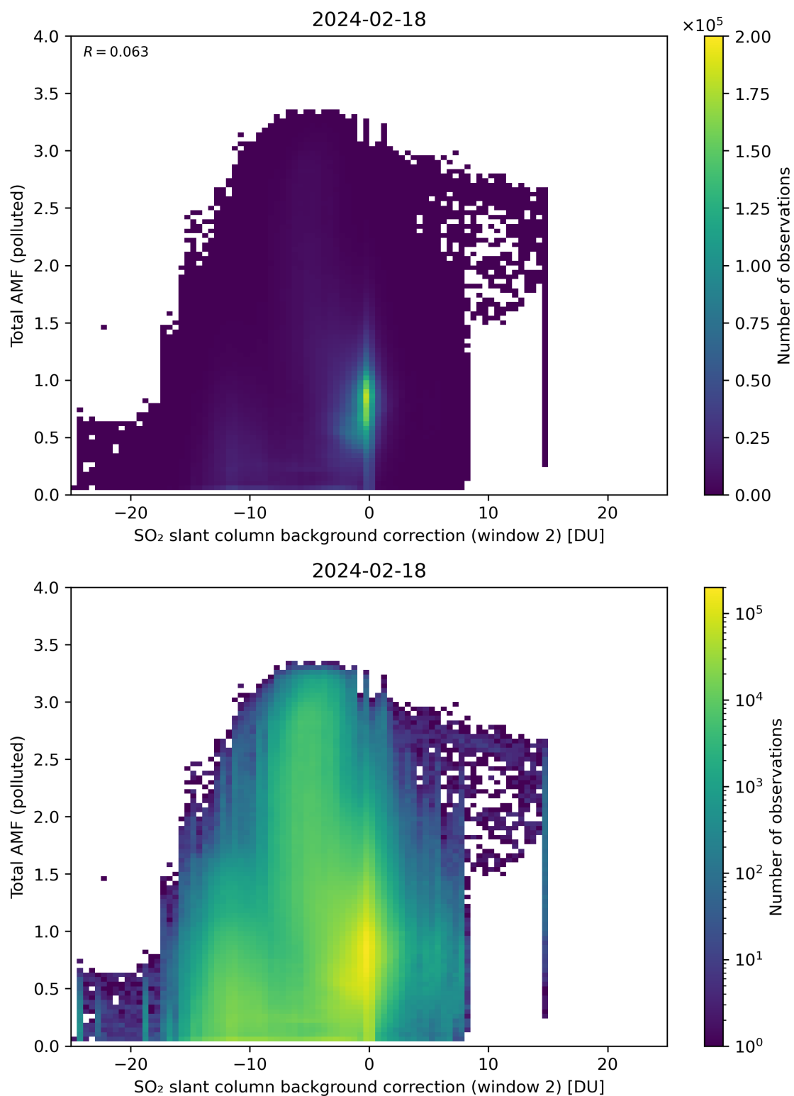
Figure 119: Scatter density plot of “SO 2 slant column background correction (window 2)” against “Total AMF (polluted)” for 2024-02-17 to 2024-02-19.
