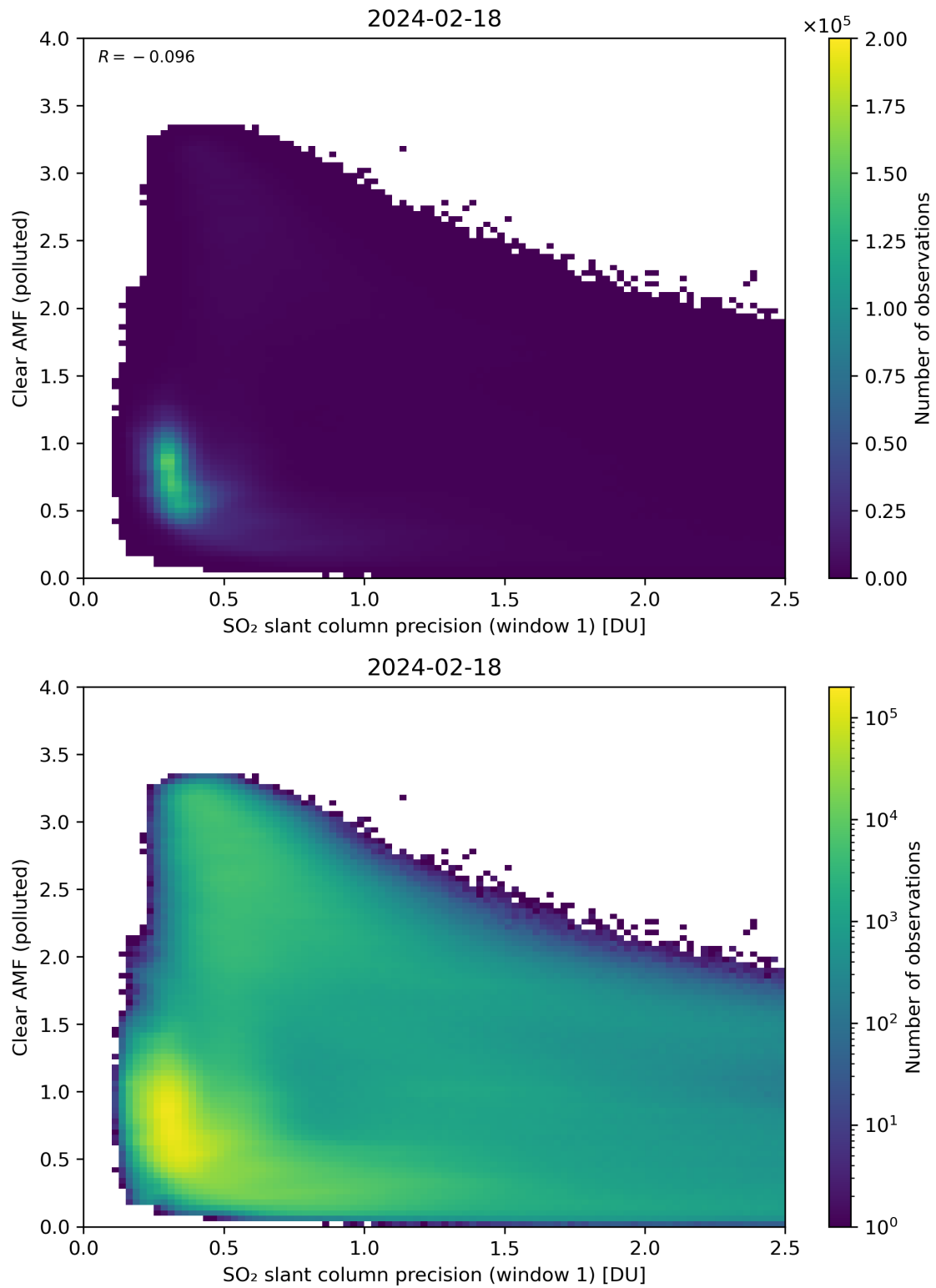
Figure 224: Scatter density plot of “SO 2 slant column precision (window 1)” against “Clear AMF (polluted)” for 2024-02-17 to 2024-02-19.
