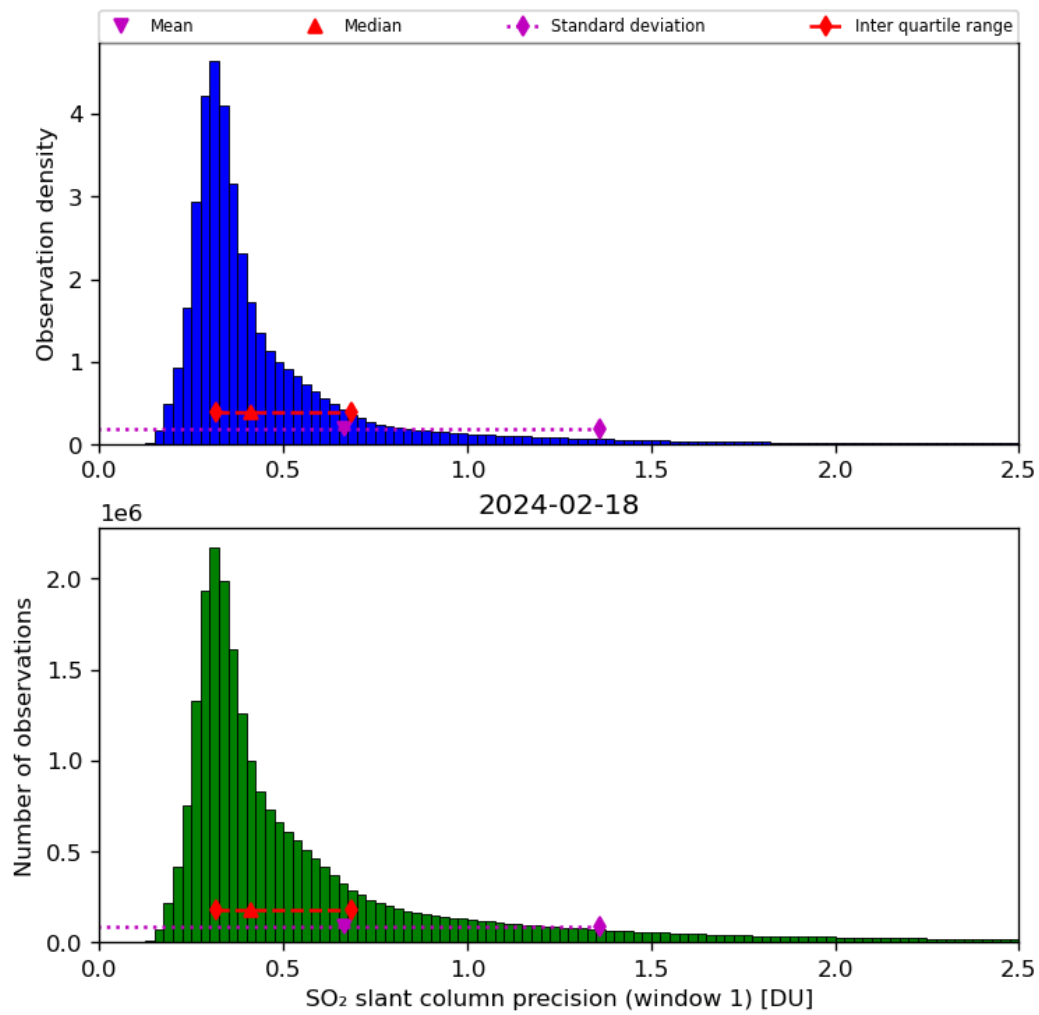
Figure 57: Histogram of “SO 2 slant column precision (window 1)” for 2024-02-17 to 2024-02-19
