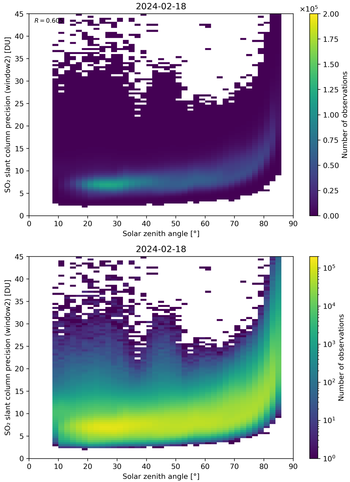
Figure 171: Scatter density plot of “Solar zenith angle” against “SO 2 slant column precision (window2)” for 2024-02-17 to 2024-02-19.
