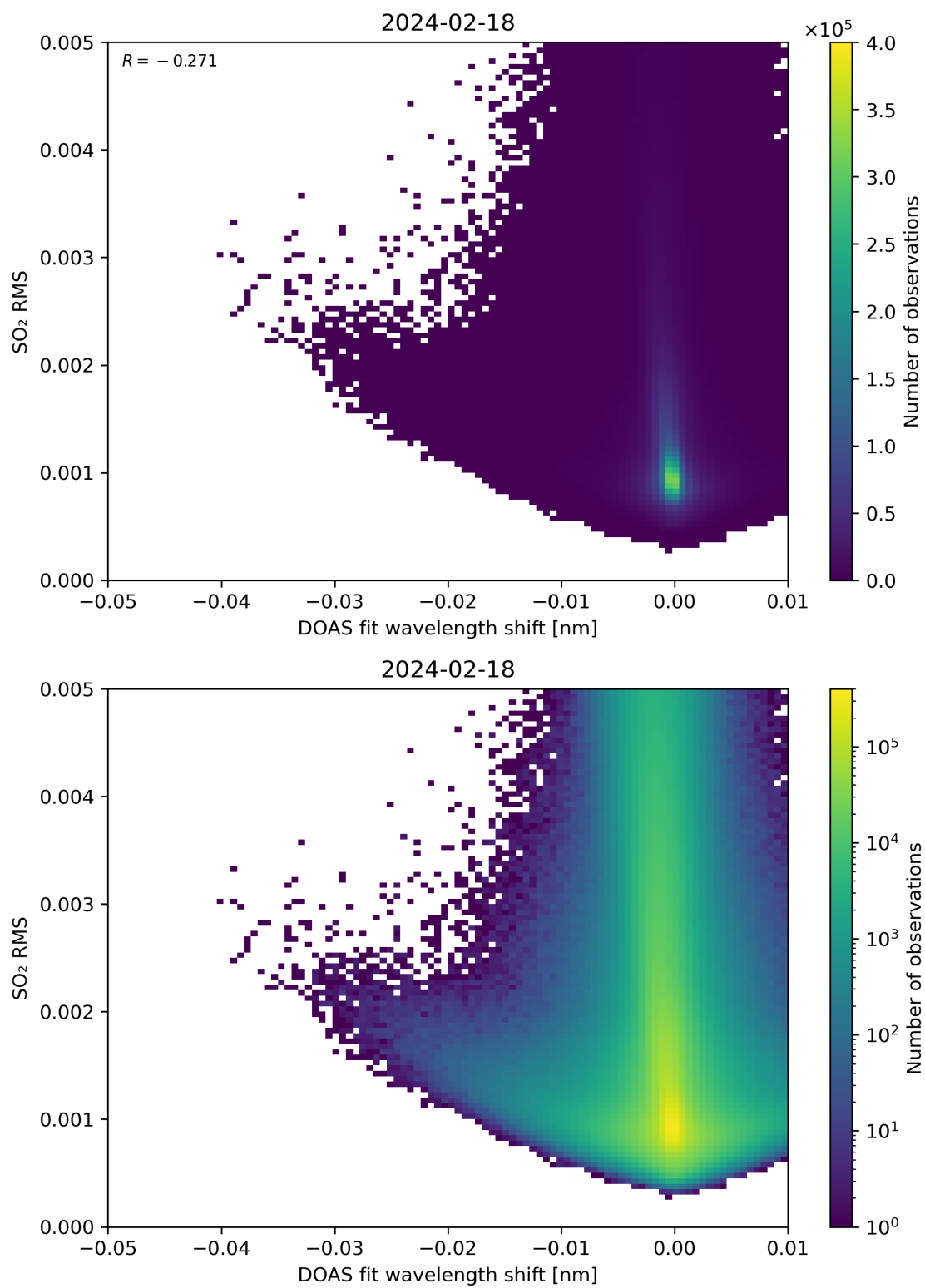
Figure 128: Scatter density plot of “DOAS fit wavelength shift” against “SO 2 RMS” for 2024-02-17 to 2024-02-19.
