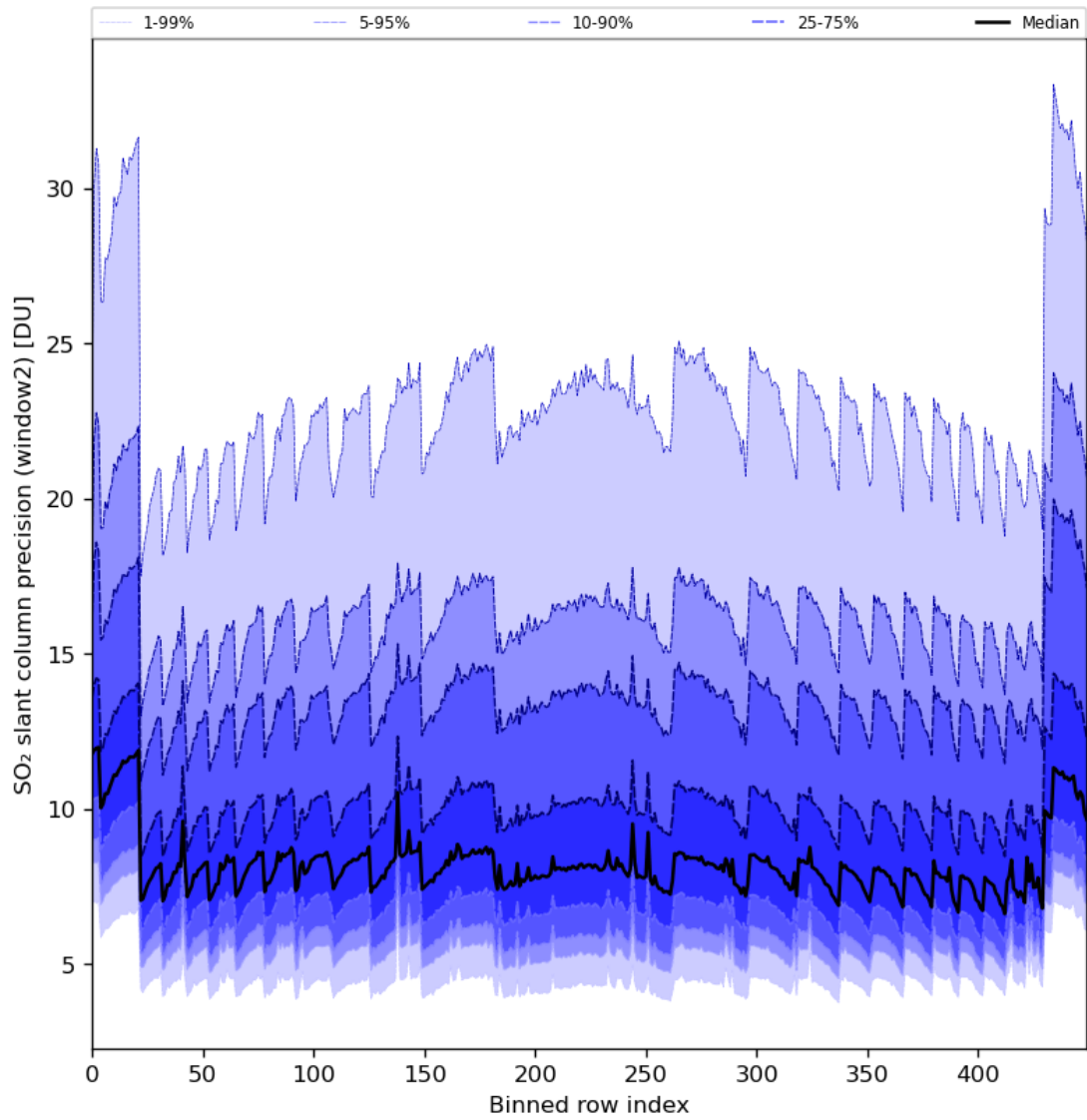
Figure 84: Along track statistics of “SO 2 slant column precision (window2)” for 2024-02-17 to 2024-02-19
