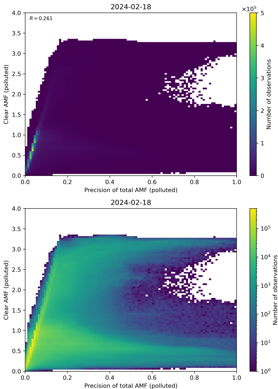
Figure 270: Scatter density plot of “Precision of total AMF (polluted)” against “Clear AMF (polluted)” for 2024-02-17 to 2024-02-19.
