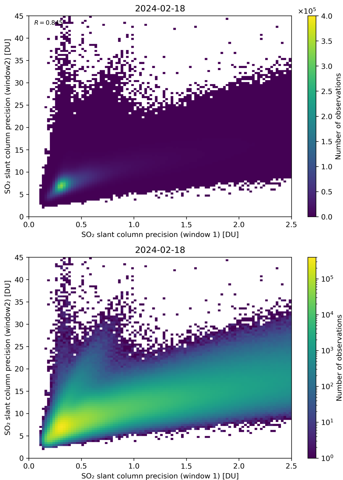
Figure 227: Scatter density plot of “SO 2 slant column precision (window 1)” against “SO 2 slant column precision (window 2)” for 2024-02-17 to 2024-02-19.
