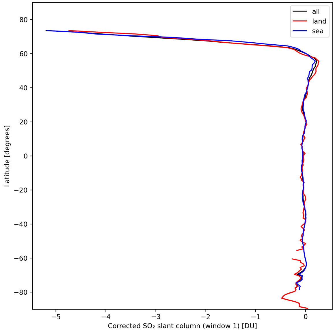
Figure 35: Zonal average of “Corrected SO 2 slant column (window 1)” for 2024-02-17 to 2024-02-19.
