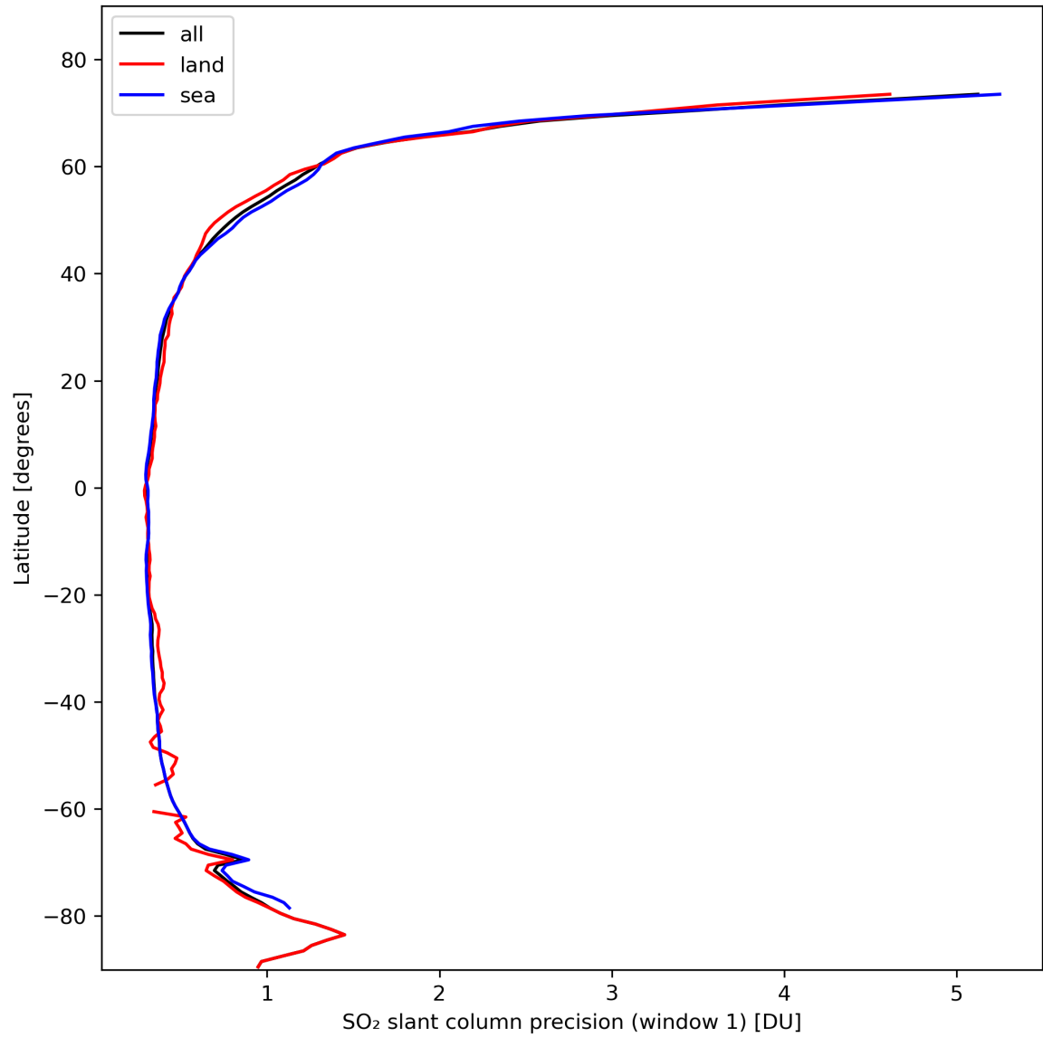
Figure 34: Zonal average of “SO 2 slant column precision (window 1)” for 2024-02-17 to 2024-02-19.
