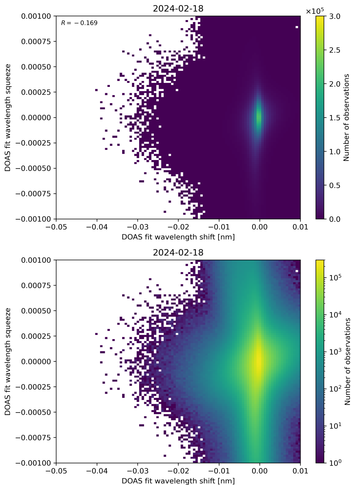
Figure 127: Scatter density plot of “DOAS fit wavelength shift” against “DOAS fit wavelength squeeze” for 2024-02-17 to 2024-02-19.
