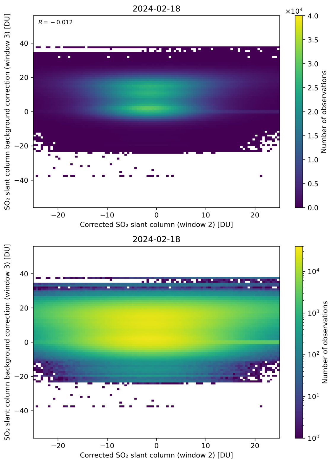
Figure 195: Scatter density plot of “Corrected SO 2 slant column (window 2)” against “SO 2 slant column background correction (window 3)” for 2024-02-17 to 2024-02-19.
