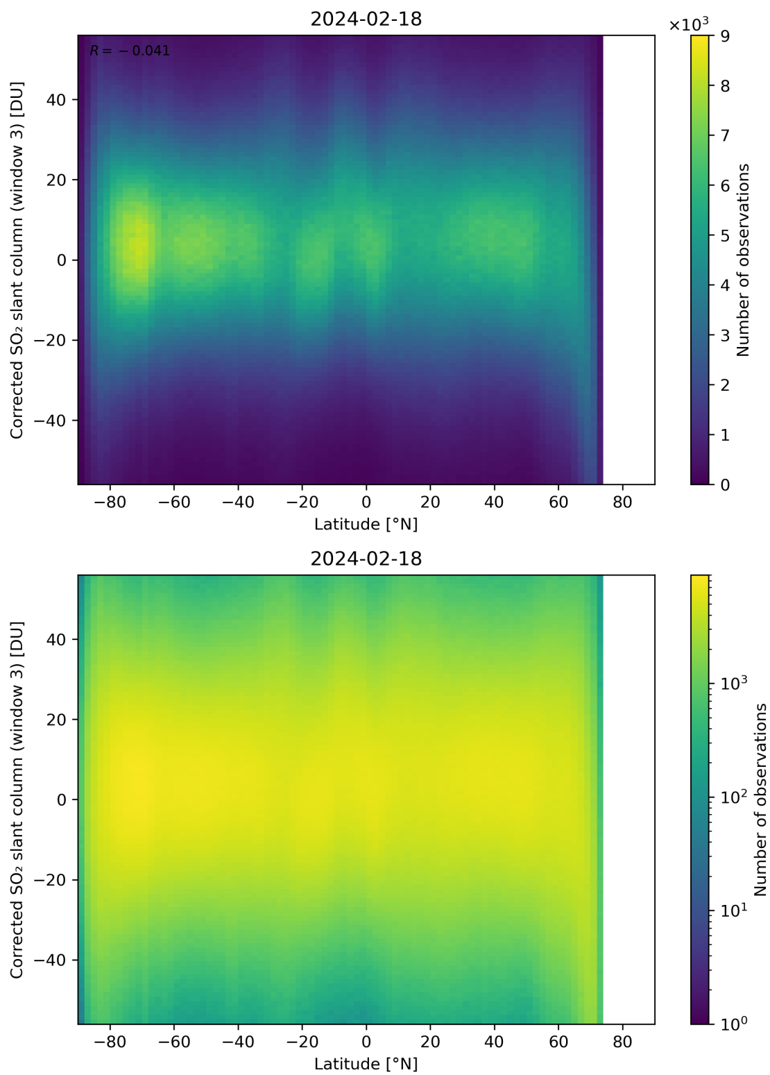
Figure 148: Scatter density plot of “Latitude” against “Corrected SO 2 slant column (window 3)” for 2024-02-17 to 2024-02-19.
