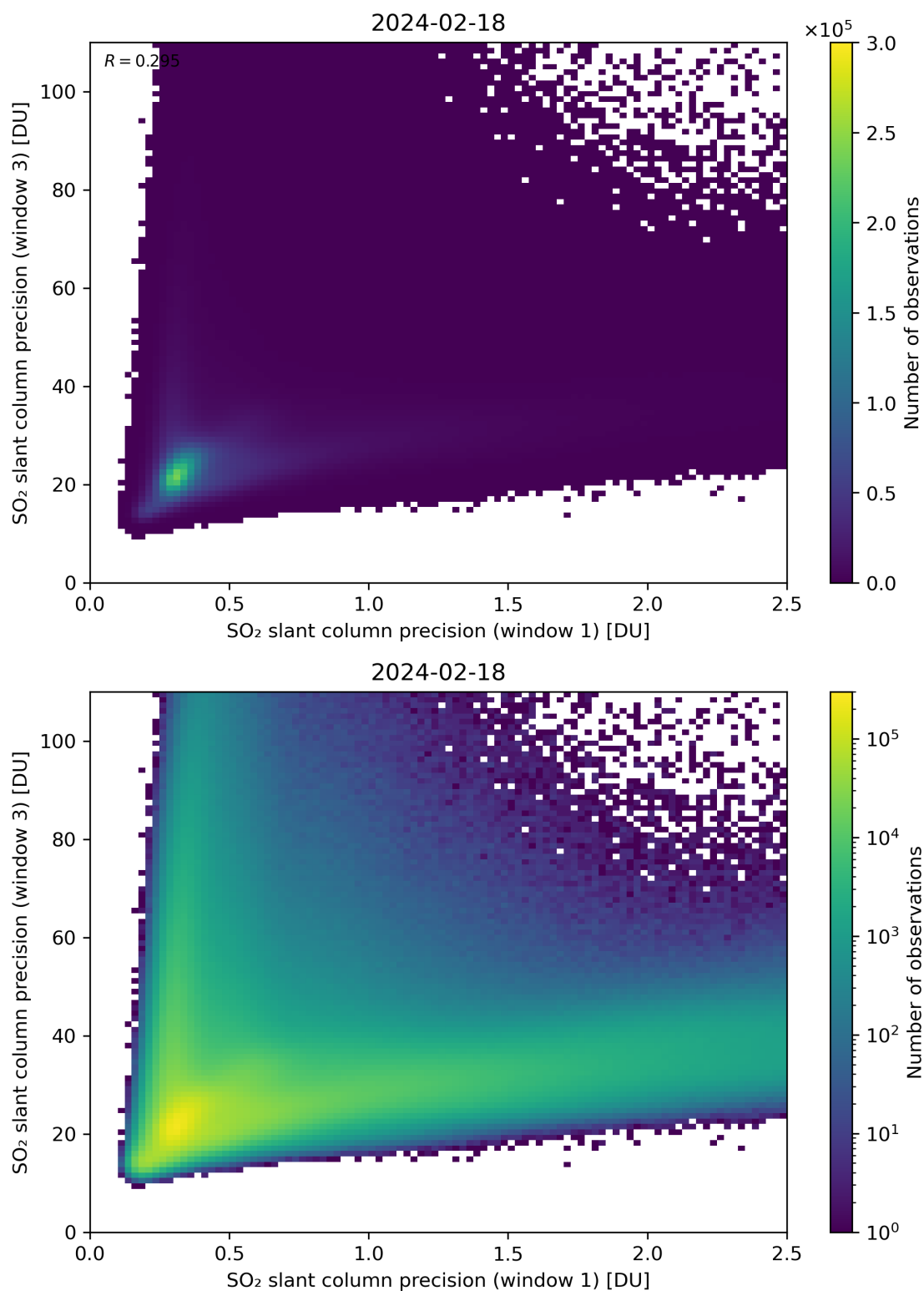
Figure 229: Scatter density plot of “SO 2 slant column precision (window 1)” against “SO 2 slant column precision (window 3)” for 2024-02-17 to 2024-02-19.
