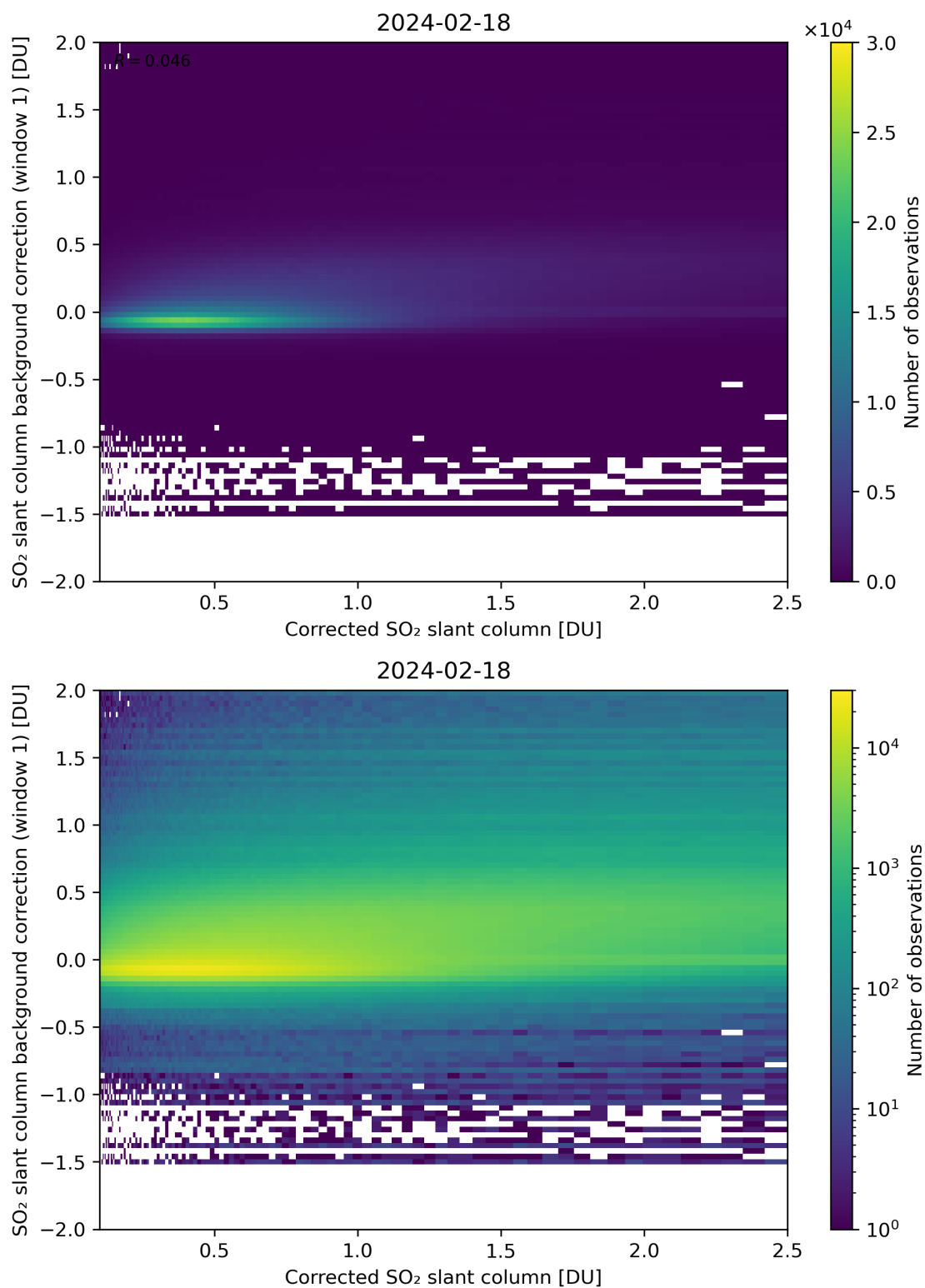
Figure 178: Scatter density plot of “Corrected SO 2 slant column” against “SO 2 slant column background correction (window 1)” for 2024-02-17 to 2024-02-19.
