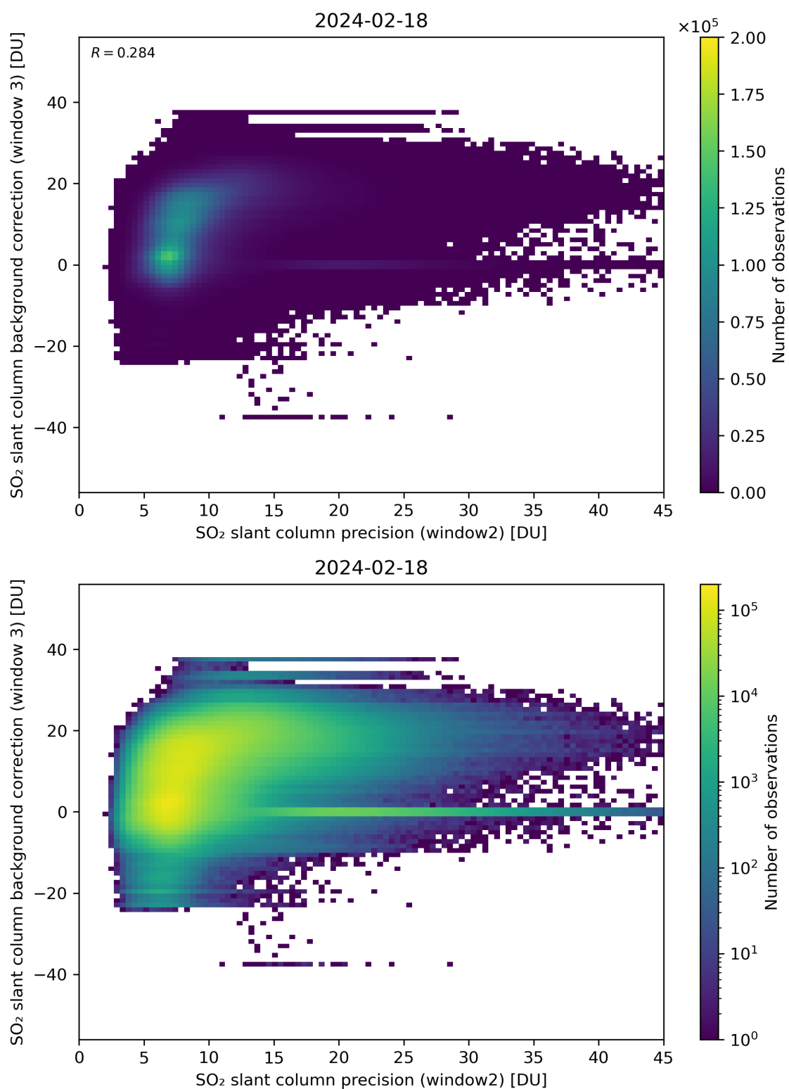
Figure 242: Scatter density plot of “SO 2 slant column precision (window2)” against “SO 2 slant column background correction (window 3)” for 2024-02-17 to 2024-02-19.
