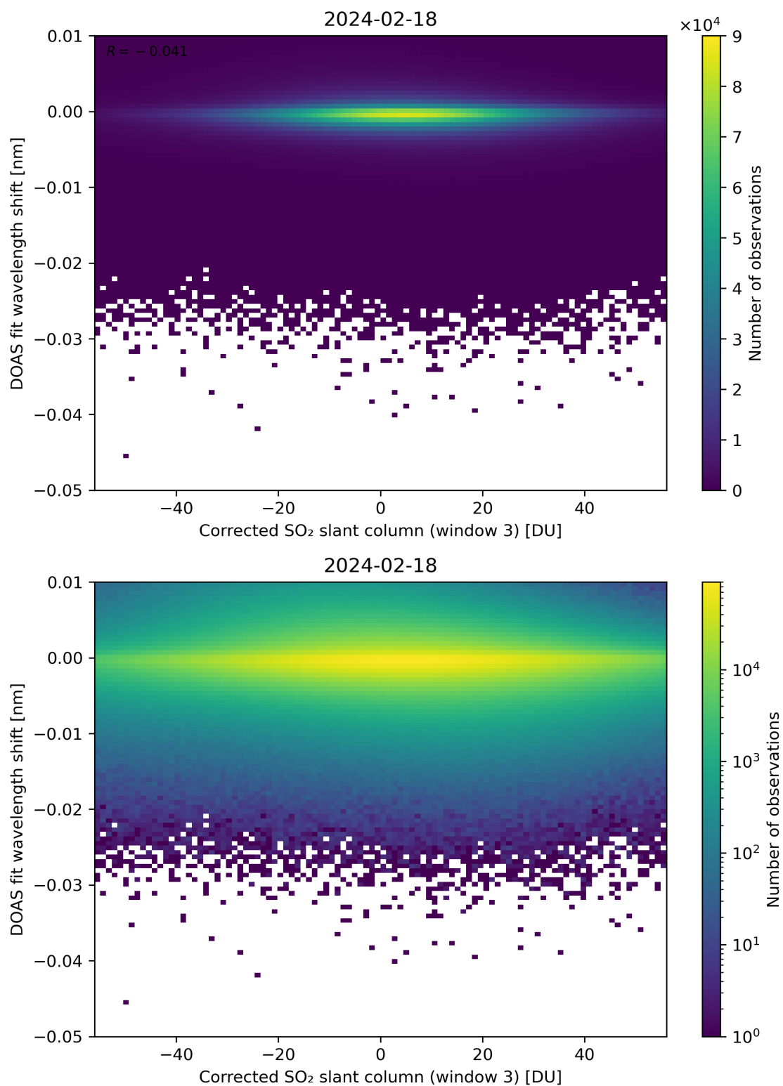
Figure 206: Scatter density plot of “Corrected SO 2 slant column (window 3)” against “DOAS fit wavelength shift” for 2024-02-17 to 2024-02-19.
