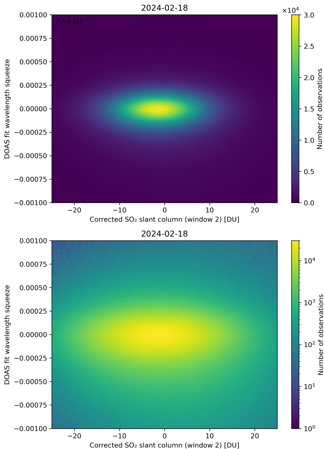
Figure 197: Scatter density plot of “Corrected SO 2 slant column (window 2)” against “DOAS fit wavelength squeeze” for 2024-02-17 to 2024-02-19.
