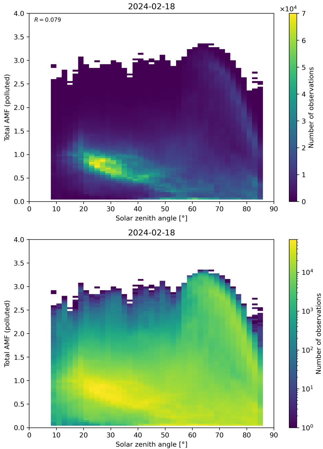
Figure 174: Scatter density plot of “Solar zenith angle” against “Total AMF (polluted)” for 2024-02-17 to 2024-02-19.
