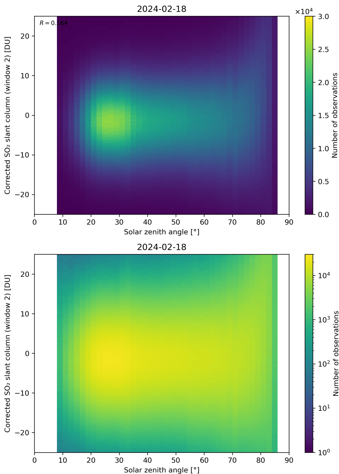
Figure 167: Scatter density plot of “Solar zenith angle” against “Corrected SO 2 slant column (window 2)” for 2024-02-17 to 2024-02-19.
