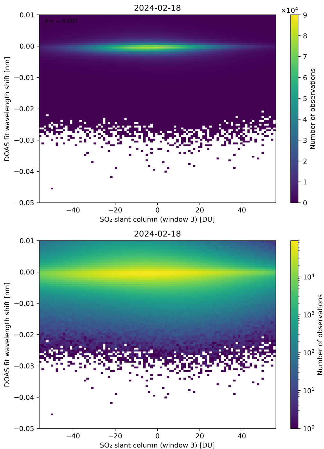
Figure 254: Scatter density plot of “SO 2 slant column (window 3)” against “DOAS fit wavelength shift” for 2024-02-17 to 2024-02-19.
