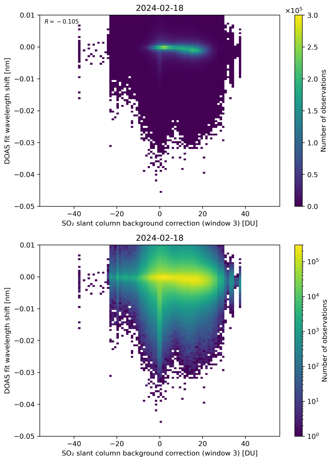
Figure 121: Scatter density plot of “SO 2 slant column background correction (window 3)” against “DOAS fit wavelength shift” for 2024-02-17 to 2024-02-19.
