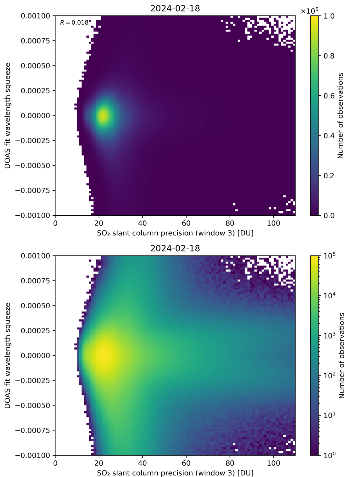
Figure 259: Scatter density plot of “SO 2 slant column precision (window 3)” against “DOAS fit wavelength squeeze” for 2024-02-17 to 2024-02-19.
