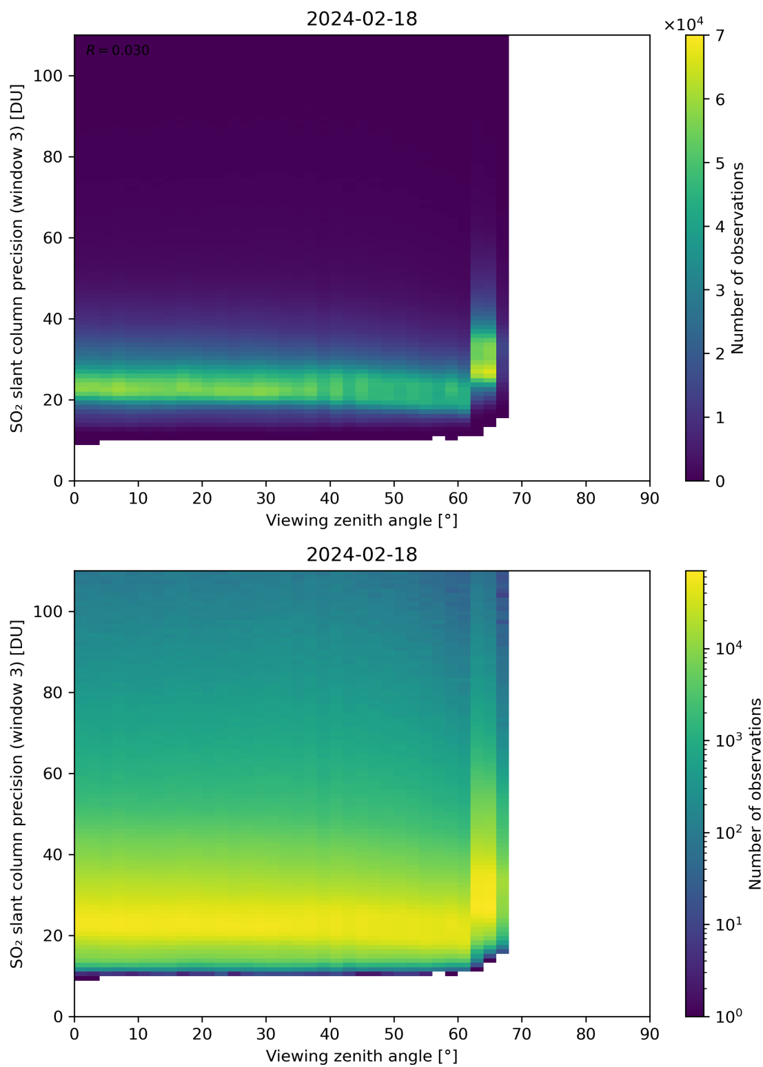
Figure 324: Scatter density plot of “Viewing zenith angle” against “SO 2 slant column precision (window 3)” for 2024-02-17 to 2024-02-19.
