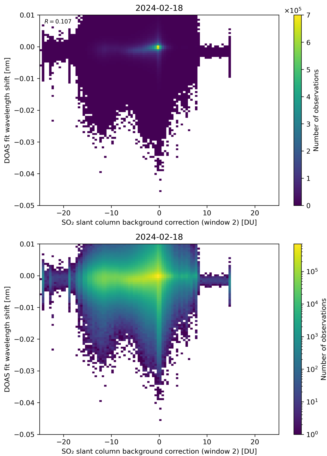
Figure 112: Scatter density plot of “SO 2 slant column background correction (window 2)” against “DOAS fit wavelength shift” for 2024-02-17 to 2024-02-19.
