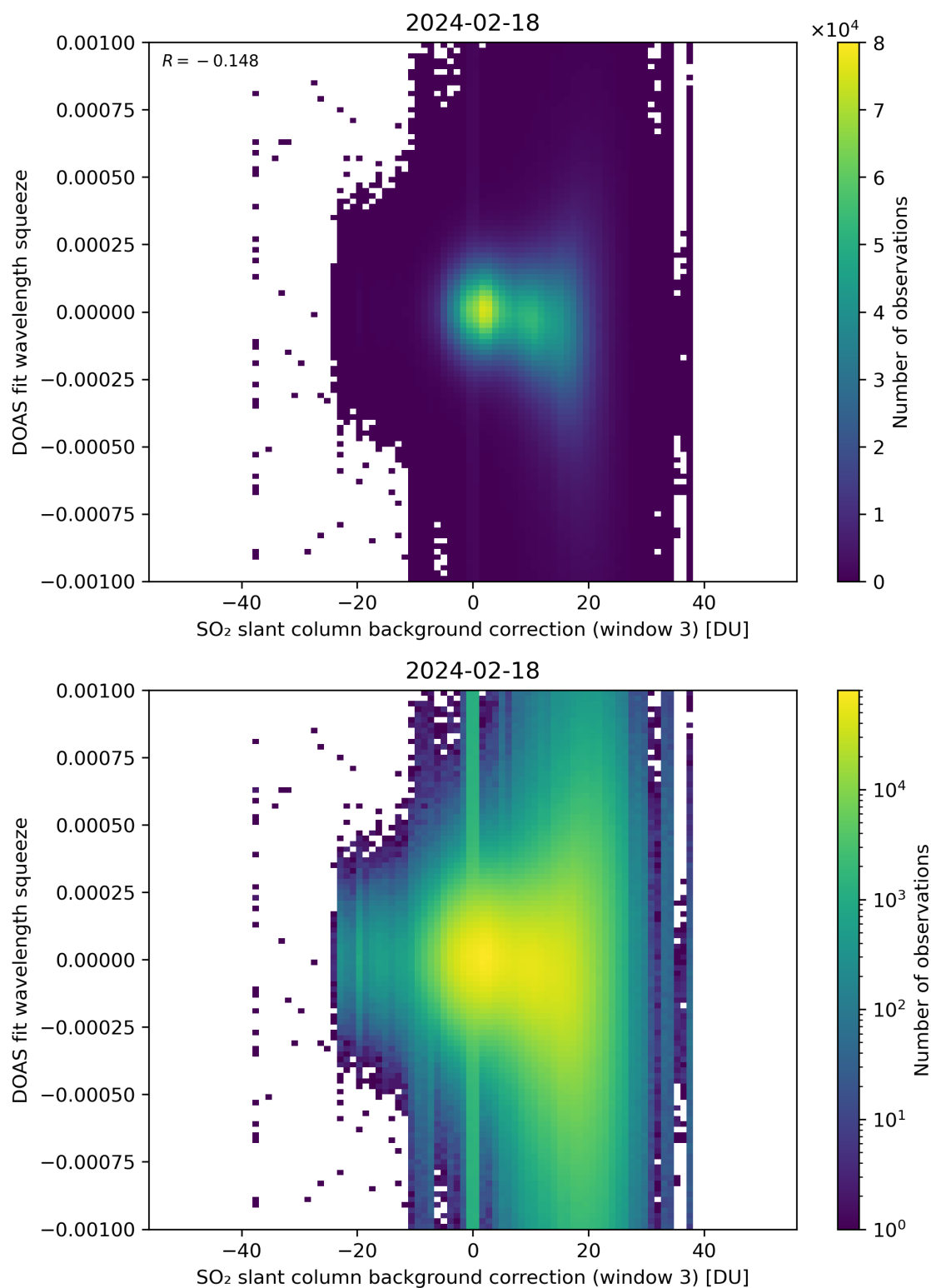
Figure 122: Scatter density plot of “SO 2 slant column background correction (window 3)” against “DOAS fit wavelength squeeze” for 2024-02-17 to 2024-02-19.
