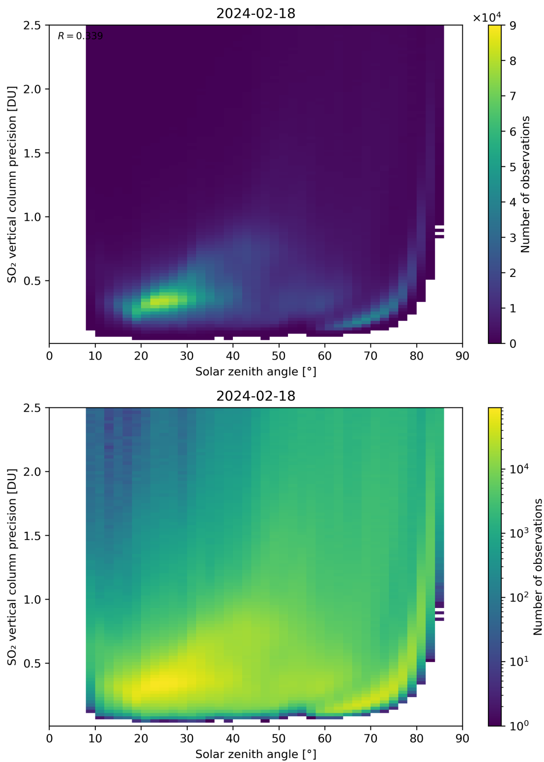
Figure 177: Scatter density plot of “Solar zenith angle” against “SO 2 vertical column precision” for 2024-02-17 to 2024-02-19.
