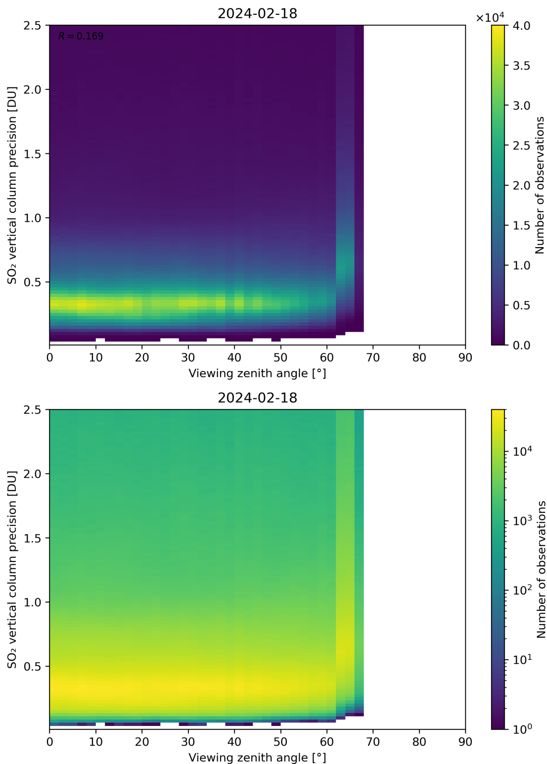
Figure 328: Scatter density plot of “Viewing zenith angle” against “SO 2 vertical column precision” for 2024-02-17 to 2024-02-19.
