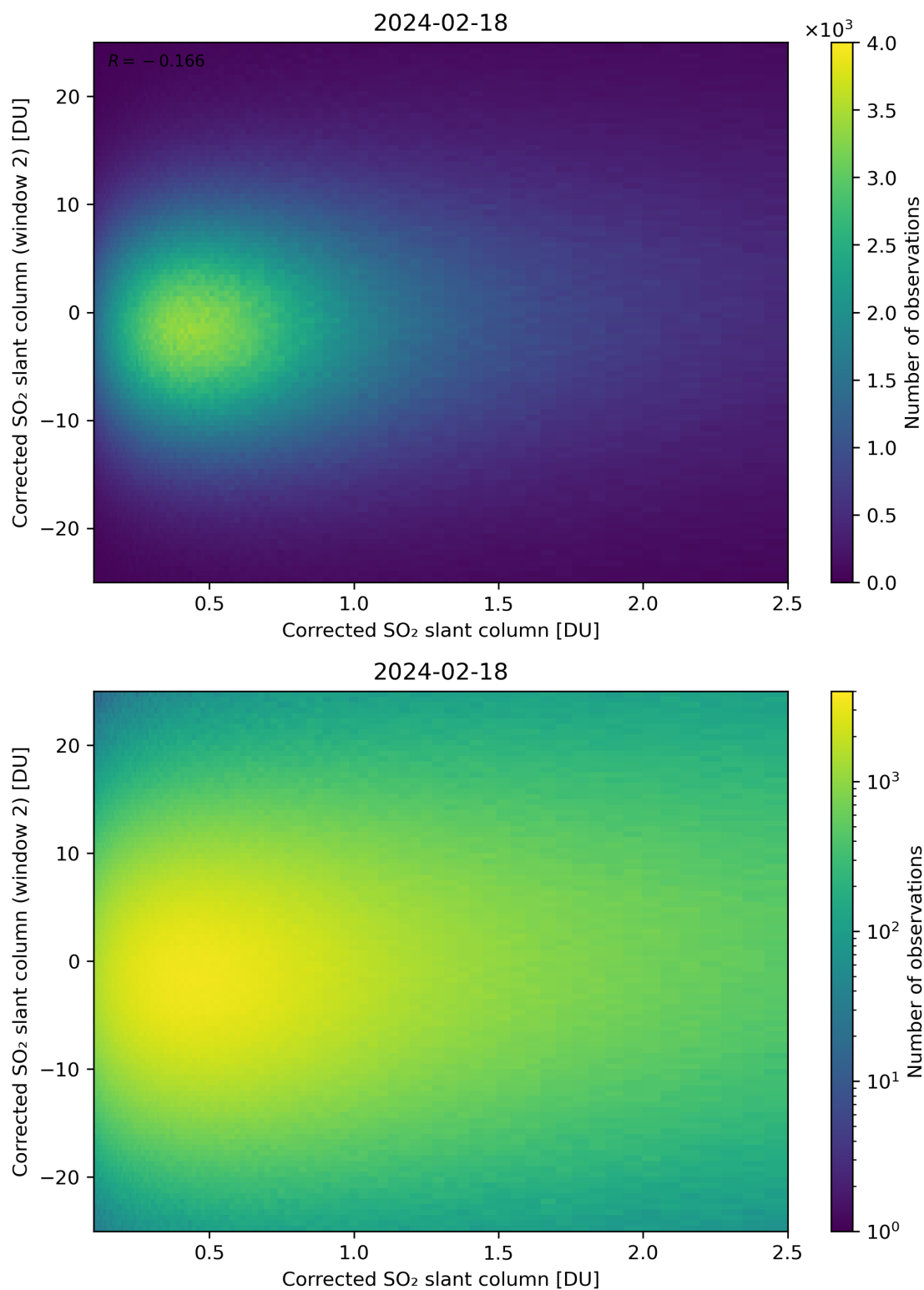
Figure 185: Scatter density plot of “Corrected SO 2 slant column” against “Corrected SO 2 slant column (window 2)” for 2024-02-17 to 2024-02-19.
