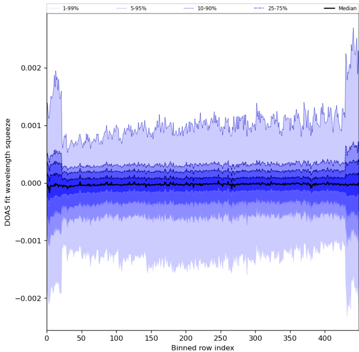
Figure 92: Along track statistics of “DOAS fit wavelength squeeze” for 2024-02-17 to 2024-02-19
