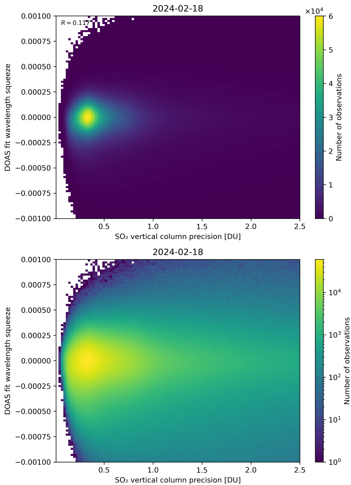
Figure 283: Scatter density plot of “SO 2 vertical column precision” against “DOAS fit wavelength squeeze” for 2024-02-17 to 2024-02-19.
