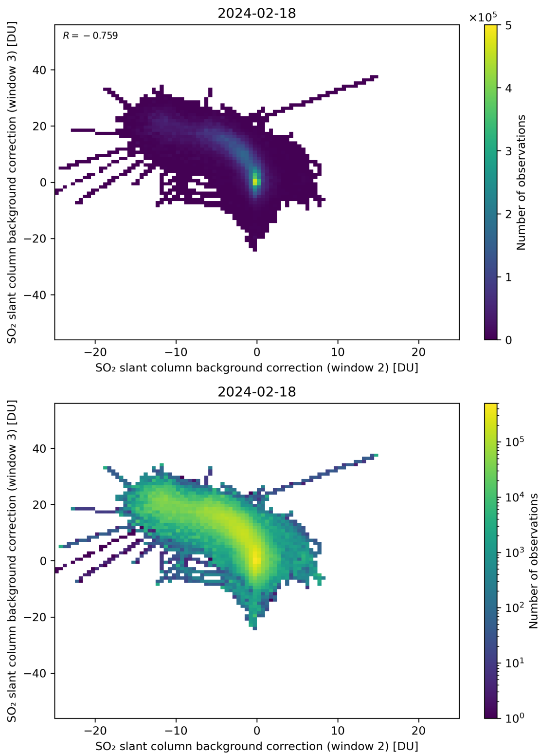
Figure 111: Scatter density plot of “SO 2 slant column background correction (window 2)” against “SO 2 slant column background correction (window 3)” for 2024-02-17 to 2024-02-19.
