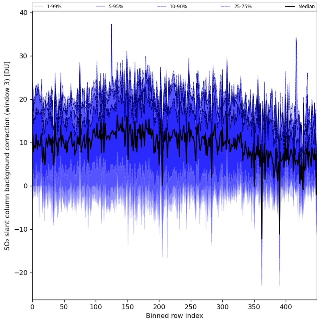
Figure 90: Along track statistics of “SO 2 slant column background correction (window 3)” for 2024-02-17 to 2024-02-19
