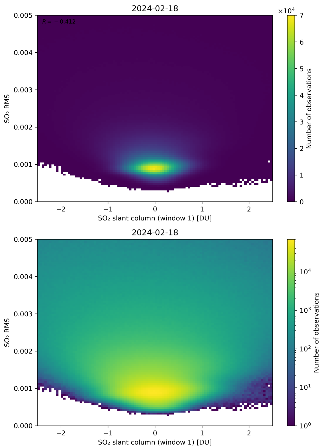
Figure 217: Scatter density plot of “SO 2 slant column (window 1)” against “SO 2 RMS” for 2024-02-17 to 2024-02-19.
