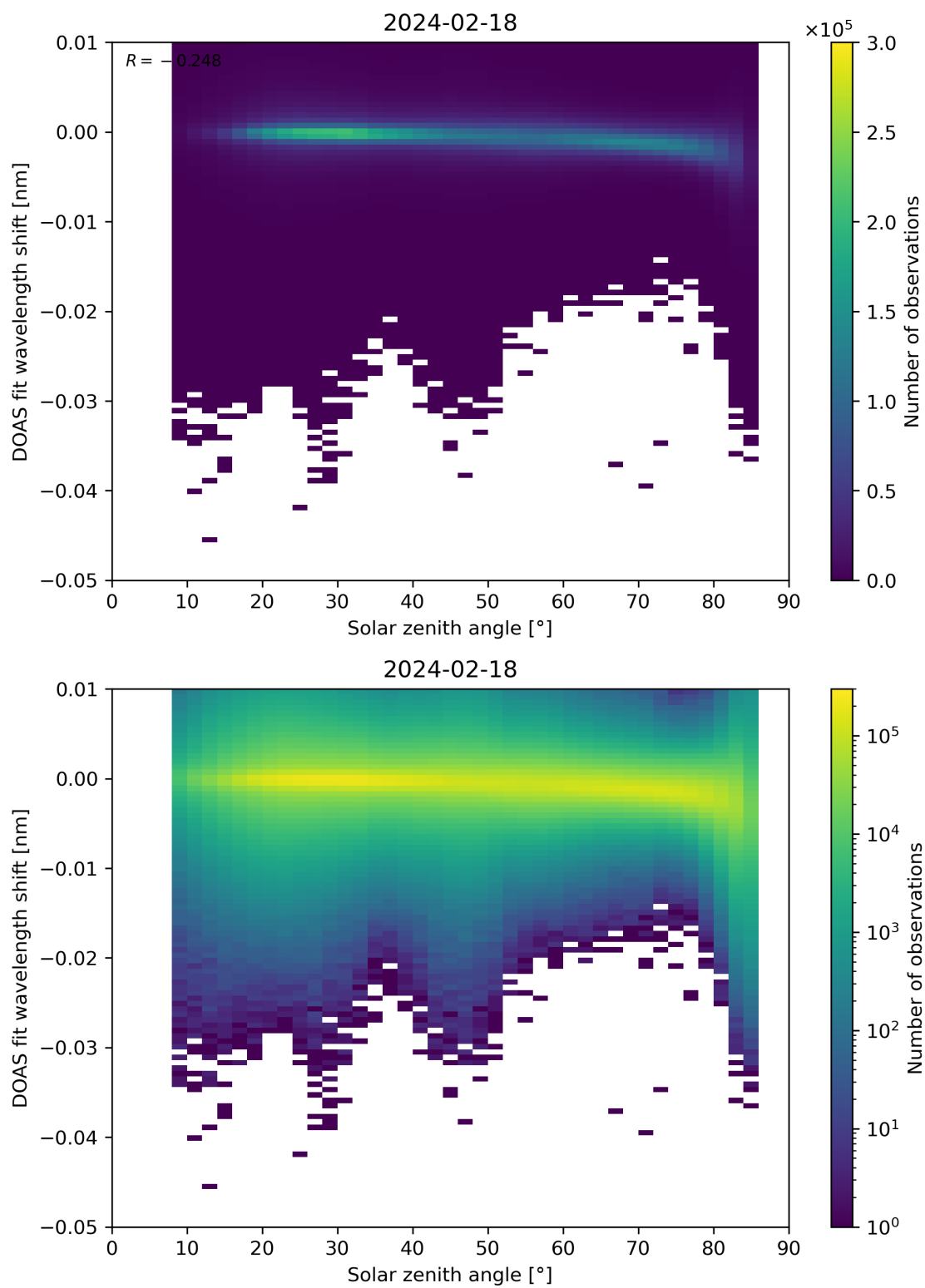
Figure 161: Scatter density plot of “Solar zenith angle” against “DOAS fit wavelength shift” for 2024-02-17 to 2024-02-19.
