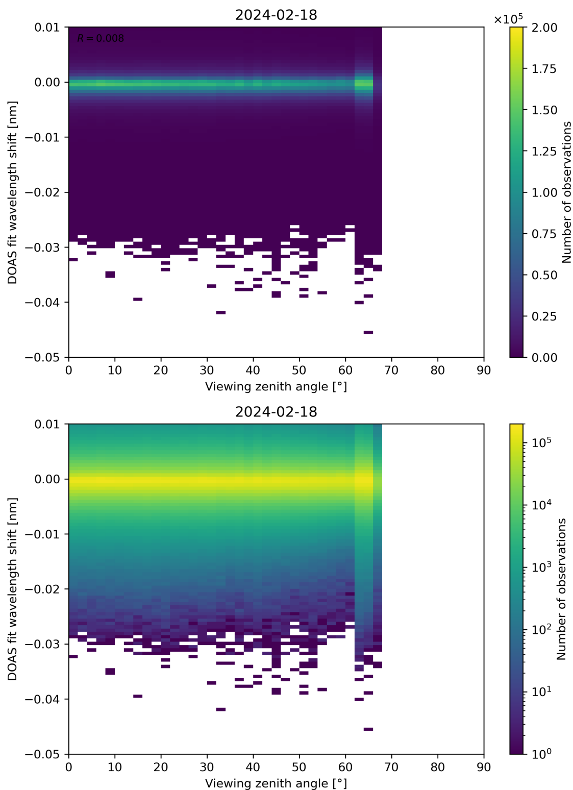
Figure 311: Scatter density plot of “Viewing zenith angle” against “DOAS fit wavelength shift” for 2024-02-17 to 2024-02-19.
