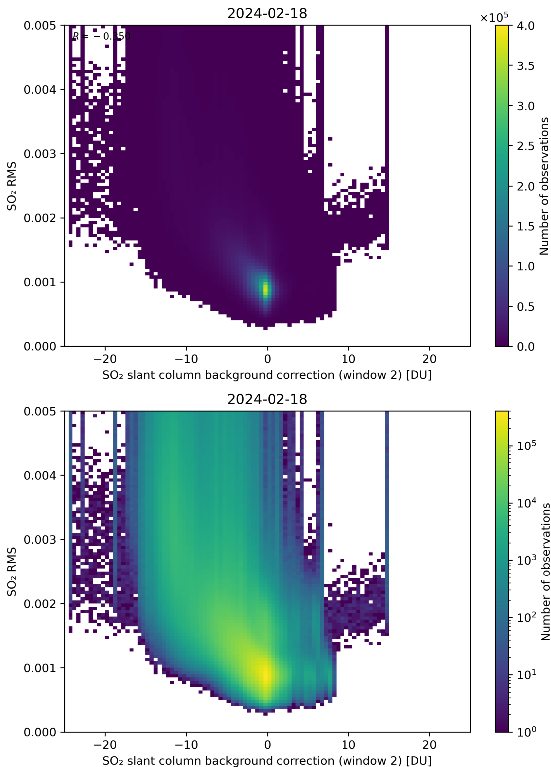
Figure 114: Scatter density plot of “SO 2 slant column background correction (window 2)” against “SO 2 RMS” for 2024-02-17 to 2024-02-19.
