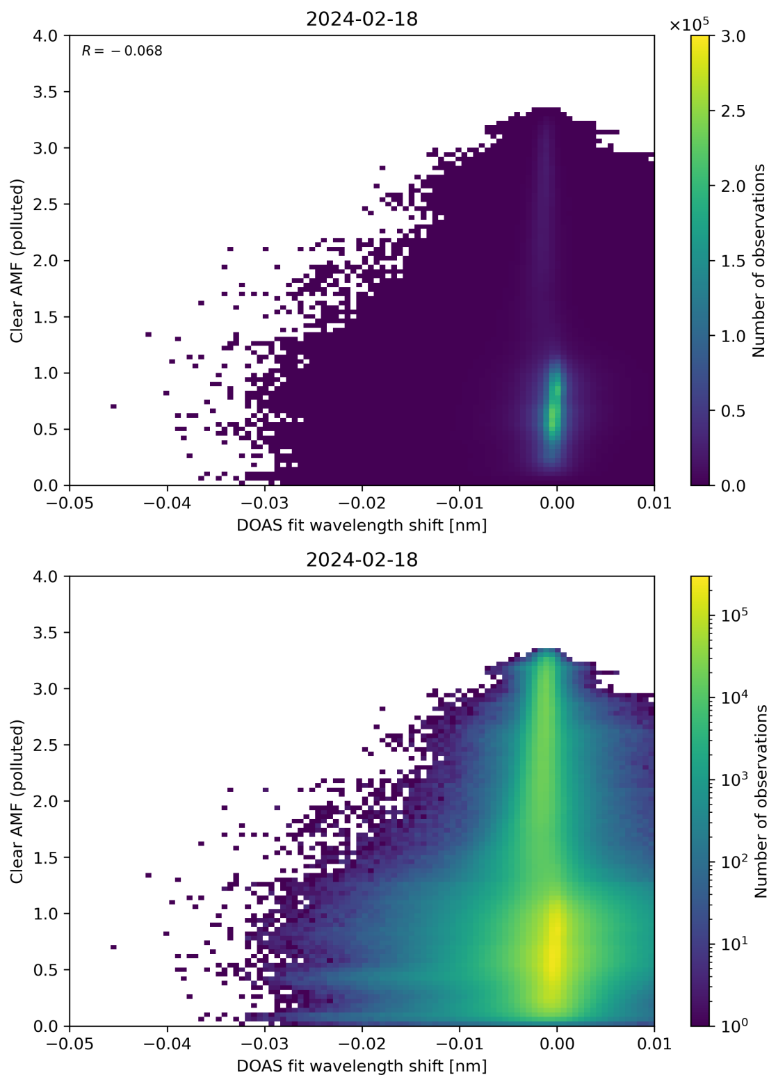
Figure 129: Scatter density plot of “DOAS fit wavelength shift” against “Clear AMF (polluted)” for 2024-02-17 to 2024-02-19.
