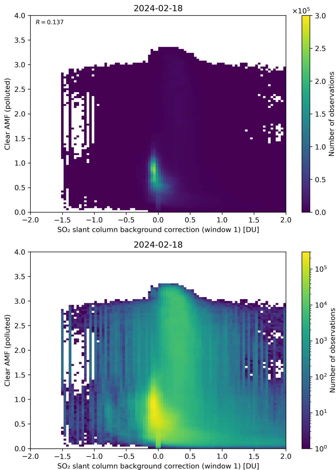
Figure 103: Scatter density plot of “SO 2 slant column background correction (window 1)” against “Clear AMF (polluted)” for 2024-02-17 to 2024-02-19.
