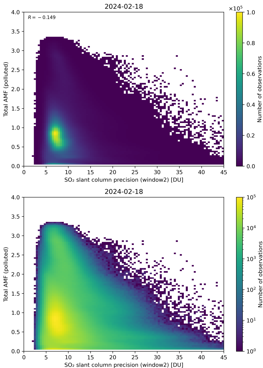
Figure 251: Scatter density plot of “SO 2 slant column precision (window2)” against “Total AMF (polluted)” for 2024-02-17 to 2024-02-19.
