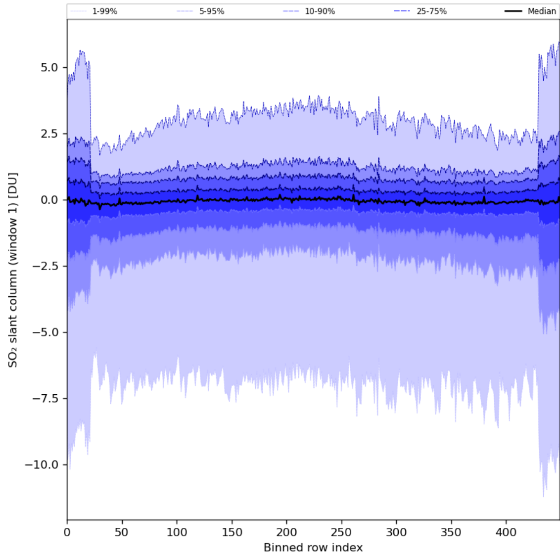
Figure 79: Along track statistics of “SO 2 slant column (window 1)” for 2024-02-17 to 2024-02-19
