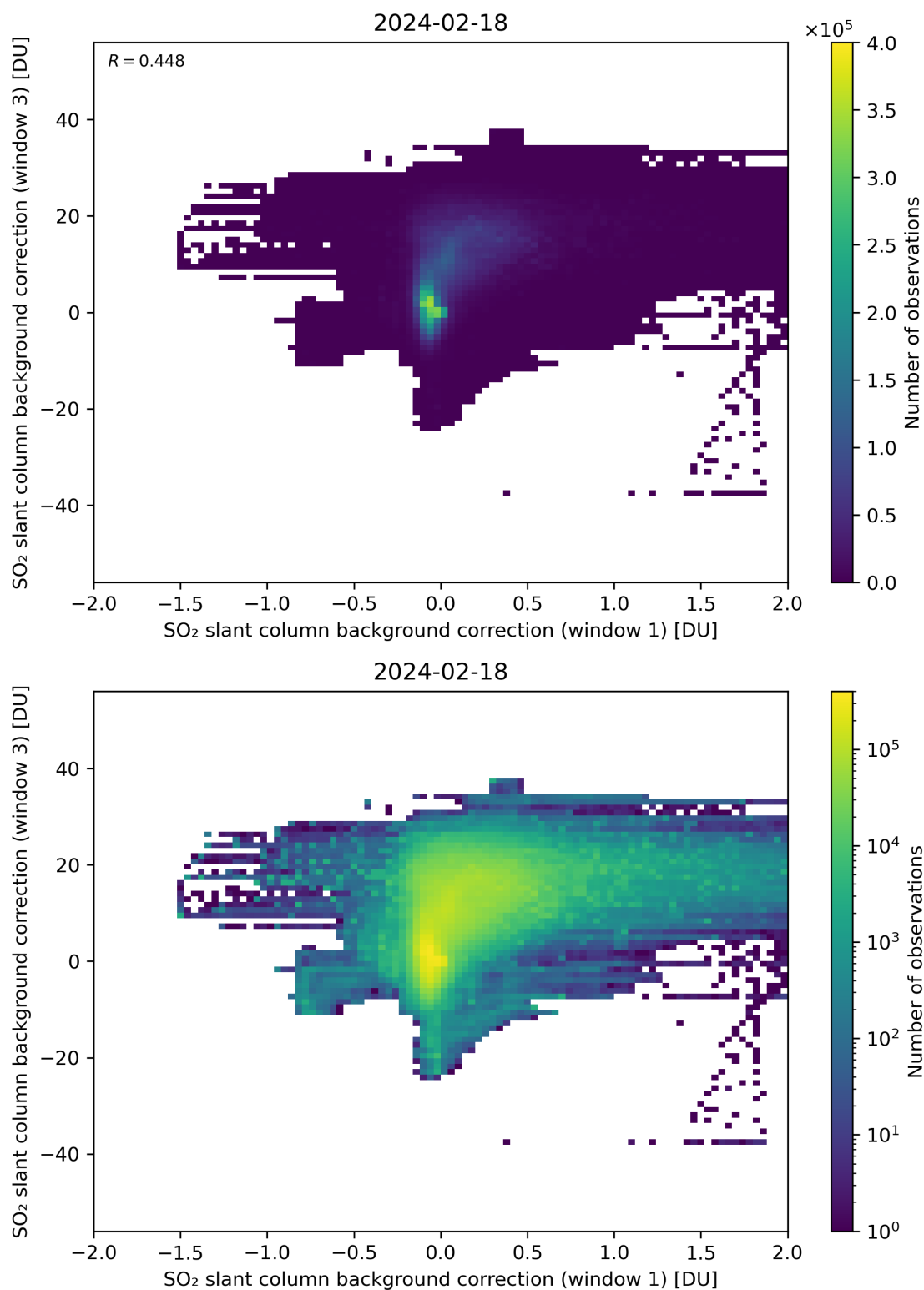
Figure 99: Scatter density plot of “SO 2 slant column background correction (window 1)” against “SO 2 slant column background correction (window 3)” for 2024-02-17 to 2024-02-19.
