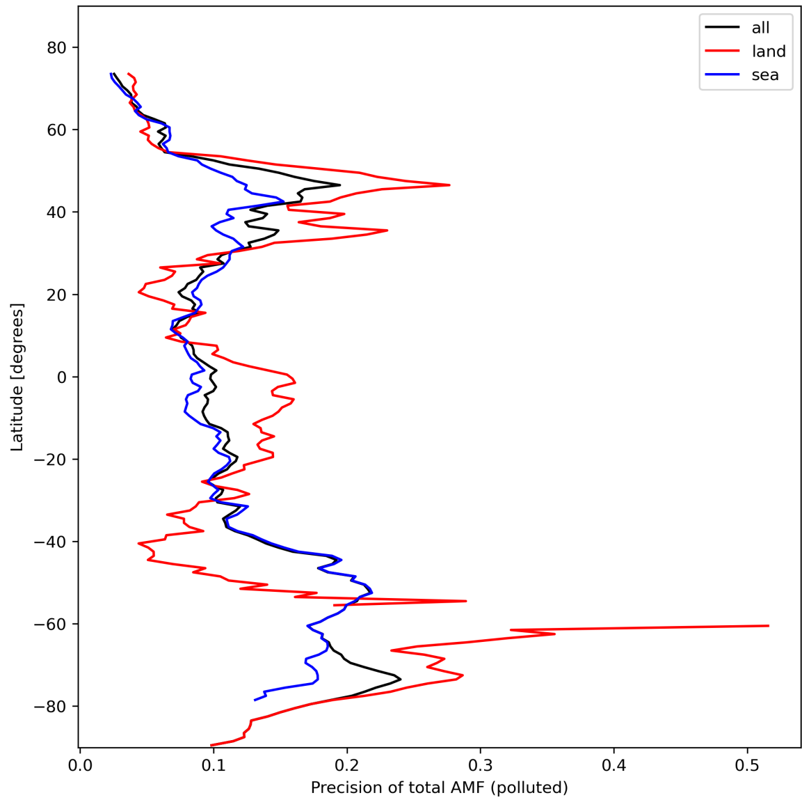
Figure 49: Zonal average of “Precision of total AMF (polluted)” for 2024-02-17 to 2024-02-19.
