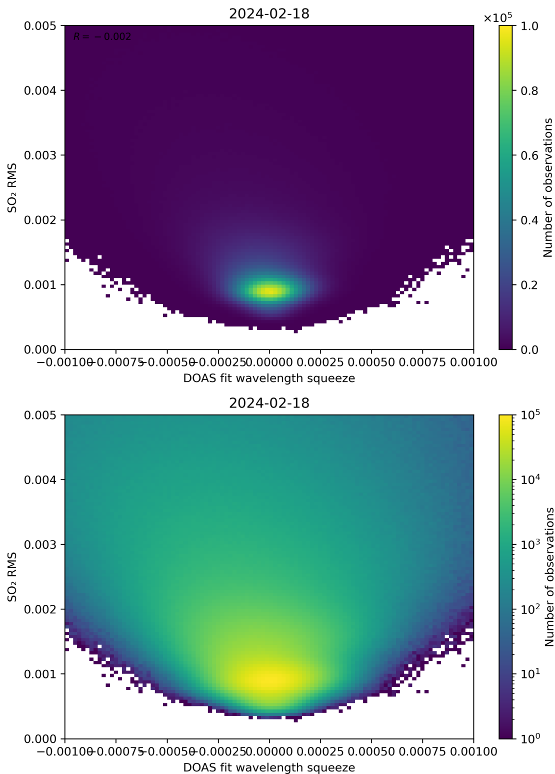
Figure 132: Scatter density plot of “DOAS fit wavelength squeeze” against “SO 2 RMS” for 2024-02-17 to 2024-02-19.
