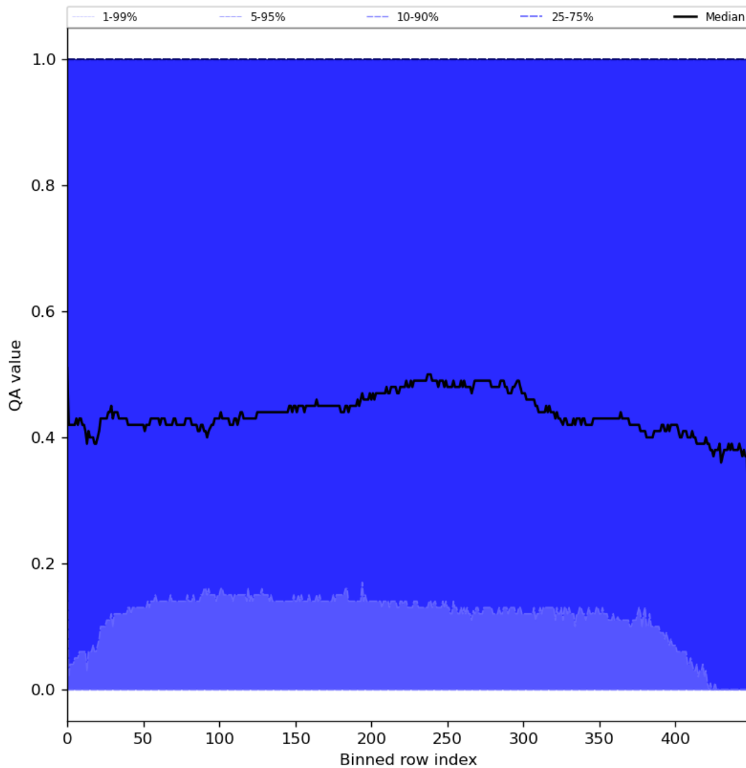
Figure 75: Along track statistics of “QA value” for 2024-02-17 to 2024-02-19
