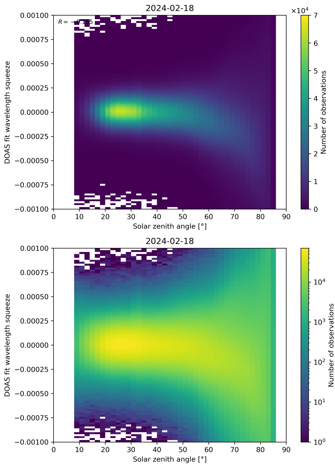
Figure 162: Scatter density plot of “Solar zenith angle” against “DOAS fit wavelength squeeze” for 2024-02-17 to 2024-02-19.
