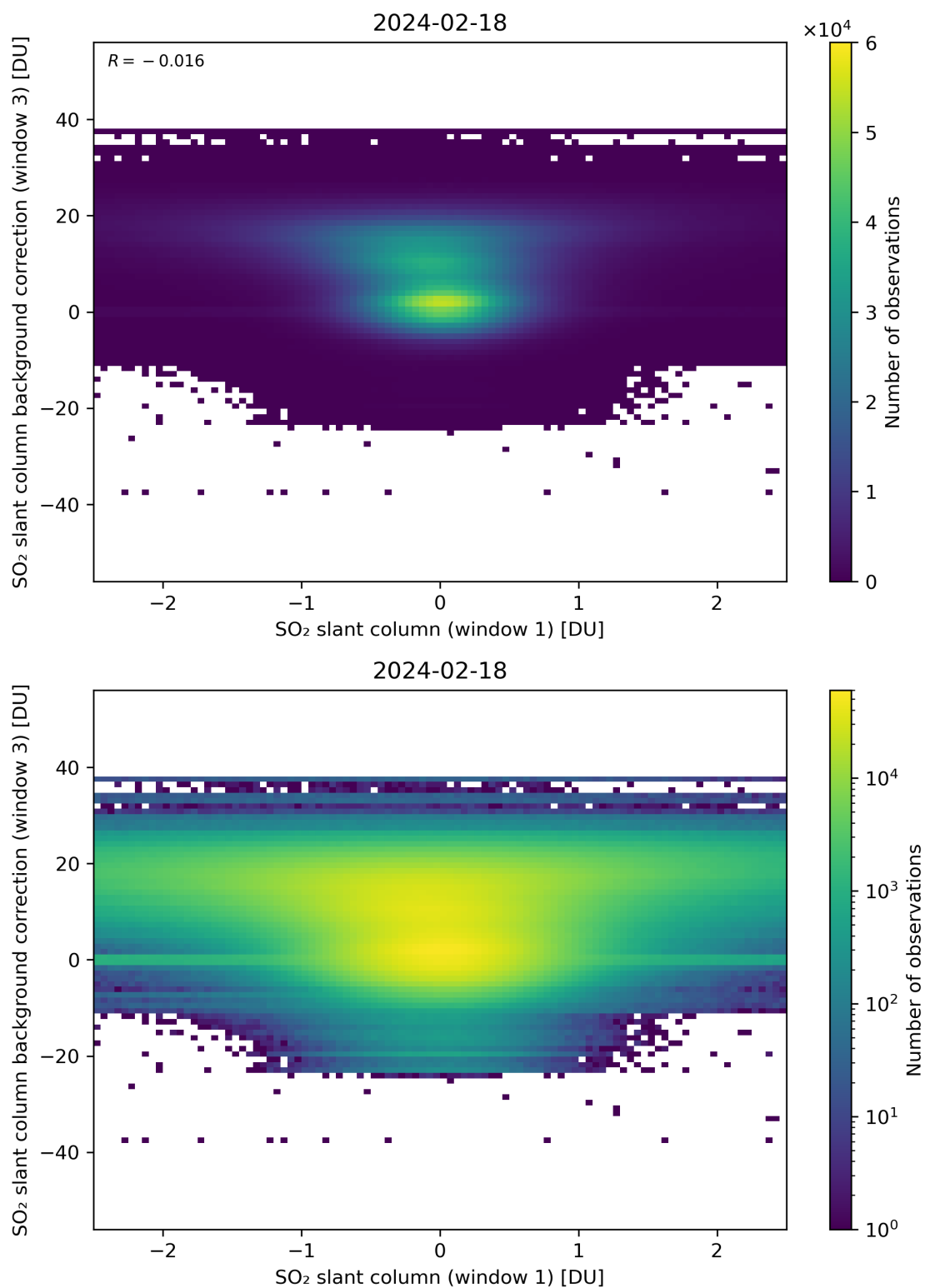
Figure 214: Scatter density plot of “SO 2 slant column (window 1)” against “SO 2 slant column background correction (window 3)” for 2024-02-17 to 2024-02-19.
