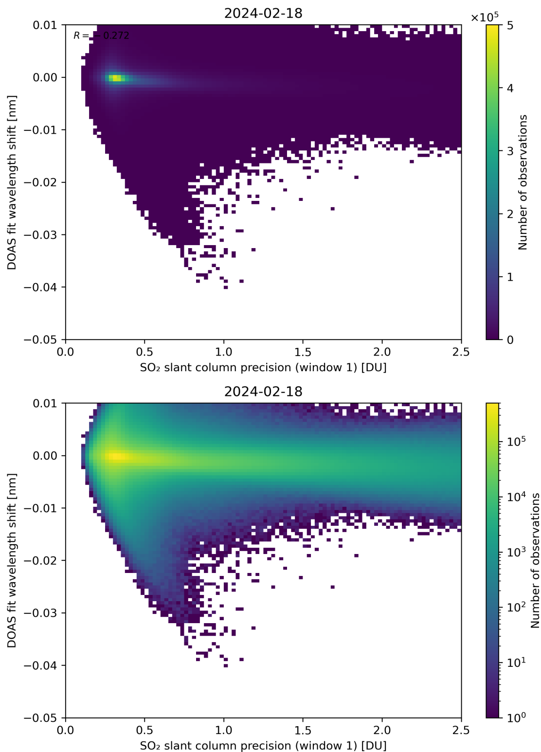
Figure 221: Scatter density plot of “SO 2 slant column precision (window 1)” against “DOAS fit wavelength shift” for 2024-02-17 to 2024-02-19.
