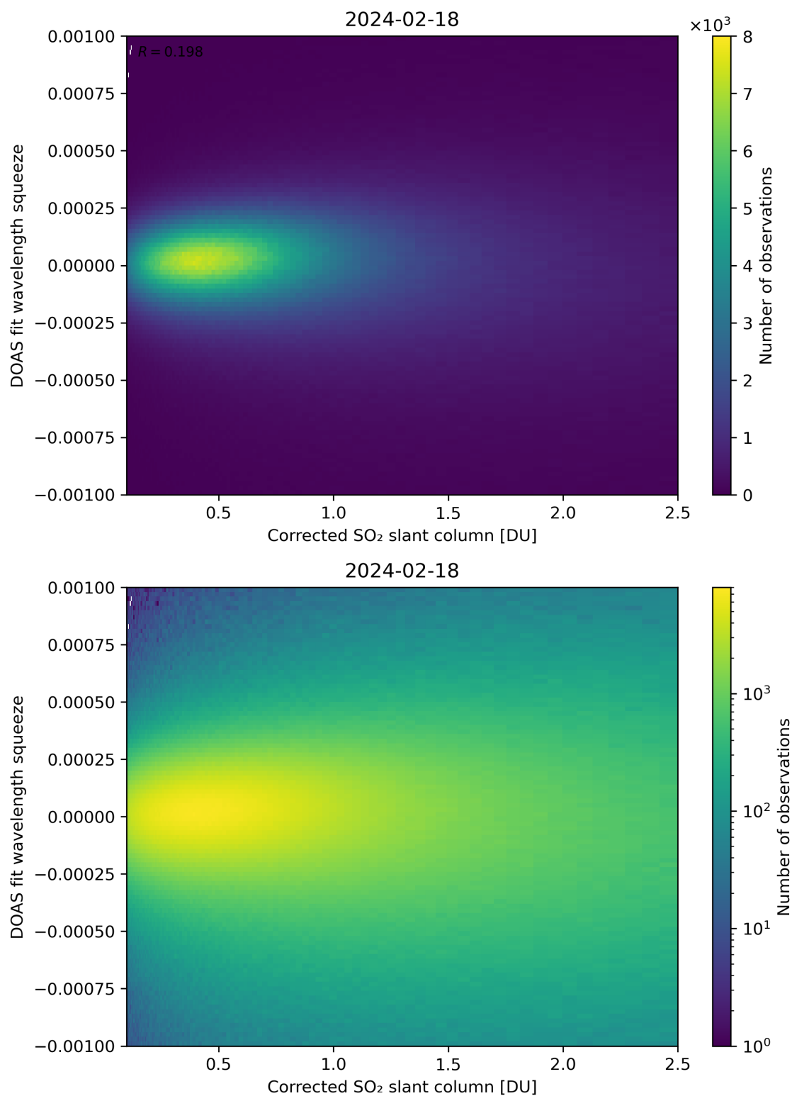
Figure 182: Scatter density plot of “Corrected SO 2 slant column” against “DOAS fit wavelength squeeze” for 2024-02-17 to 2024-02-19.
