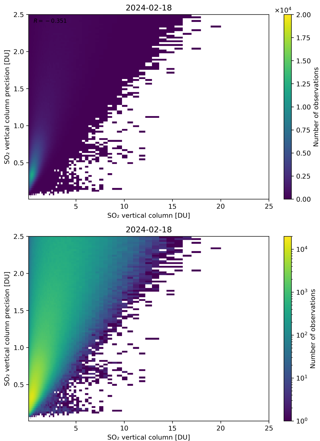
Figure 307: Scatter density plot of “SO 2 vertical column” against “SO 2 vertical column precision” for 2024-02-17 to 2024-02-19.
