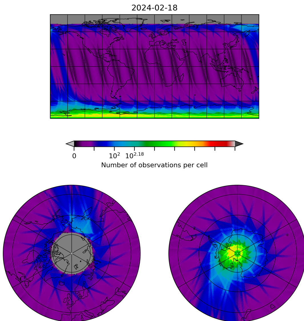
Figure 28: Map of the number of observations for 2024-02-17 to 2024-02-19
