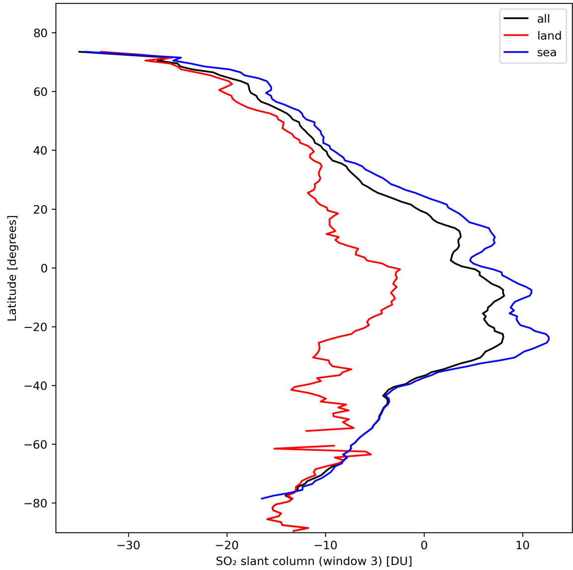
Figure 41: Zonal average of “SO 2 slant column (window 3)” for 2024-02-17 to 2024-02-19.
