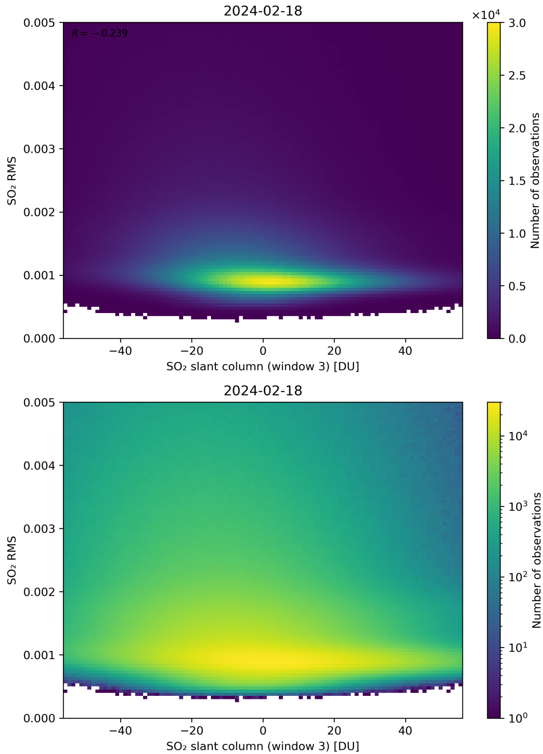
Figure 256: Scatter density plot of “SO 2 slant column (window 3)” against “SO 2 RMS” for 2024-02-17 to 2024-02-19.
