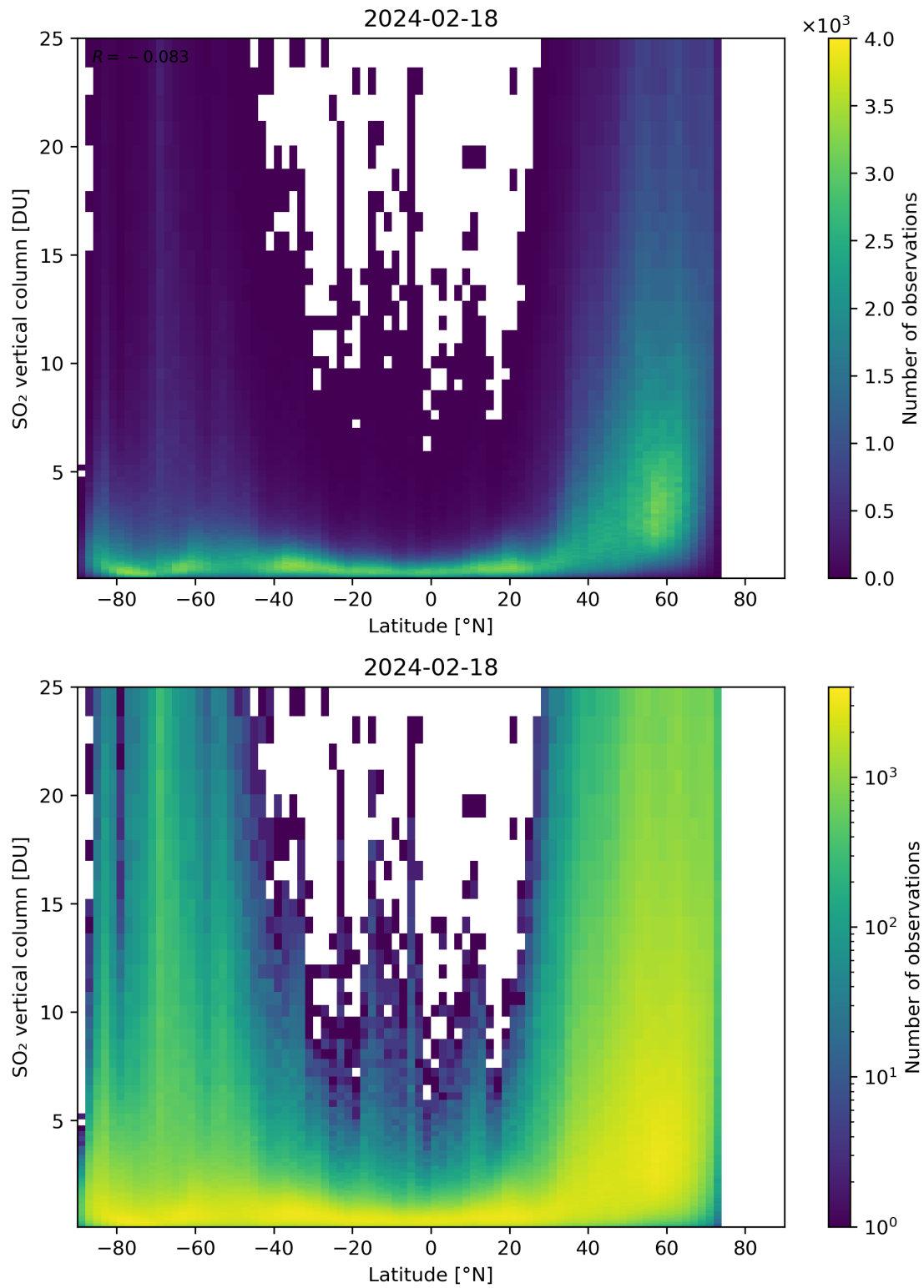
Figure 156: Scatter density plot of “Latitude” against “SO 2 vertical column” for 2024-02-17 to 2024-02-19.
