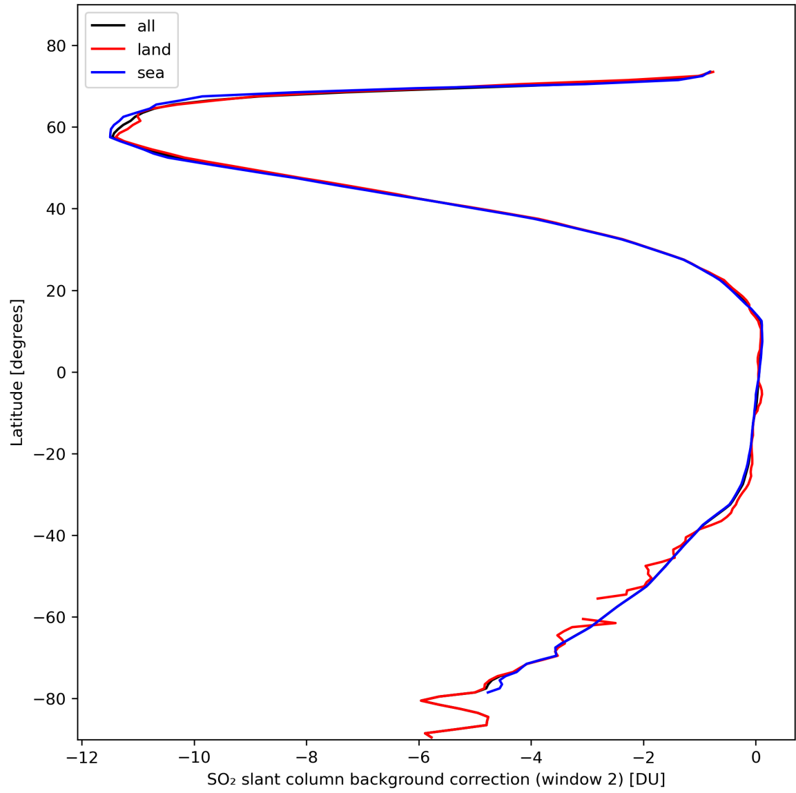
Figure 40: Zonal average of "SO 2 slant column background correction (window 2)" for 2024-02-17 to 2024-02-19.
