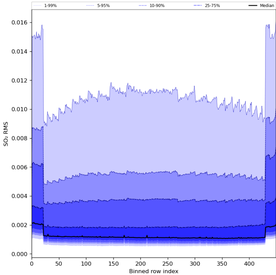
Figure 93: Along track statistics of “SO 2 RMS” for 2024-02-17 to 2024-02-19
