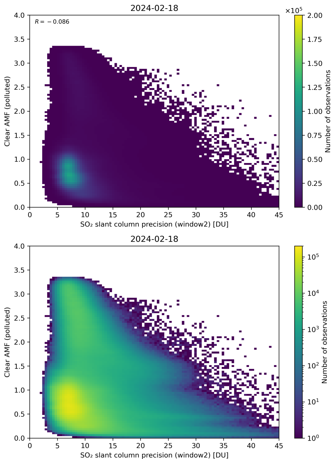
Figure 246: Scatter density plot of “SO 2 slant column precision (window2)” against “Clear AMF (polluted)” for 2024-02-17 to 2024-02-19.
