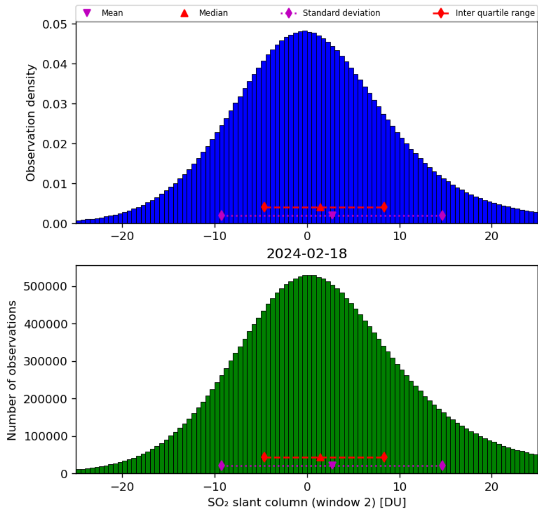
Figure 60: Histogram of “SO 2 slant column (window 2)” for 2024-02-17 to 2024-02-19
