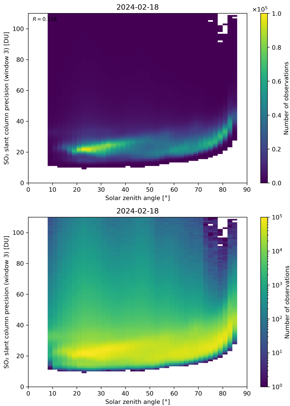
Figure 173: Scatter density plot of “Solar zenith angle” against “SO 2 slant column precision (window 3)” for 2024-02-17 to 2024-02-19.
