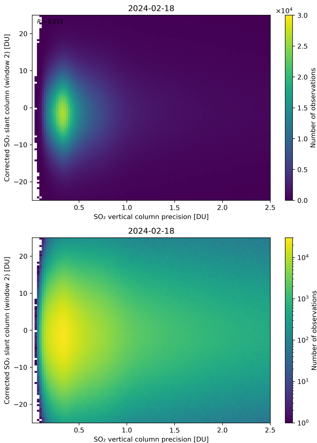
Figure 287: Scatter density plot of “SO 2 vertical column precision” against “Corrected SO 2 slant column (window 2)” for 2024-02-17 to 2024-02-19.
