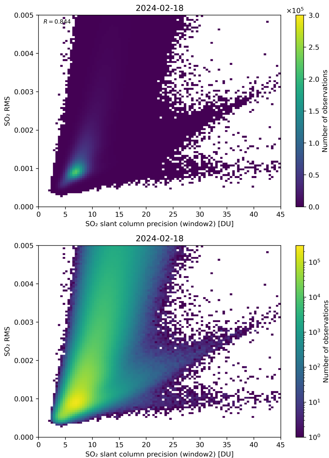
Figure 245: Scatter density plot of “SO 2 slant column precision (window2)” against “SO 2 RMS” for 2024-02-17 to 2024-02-19.
