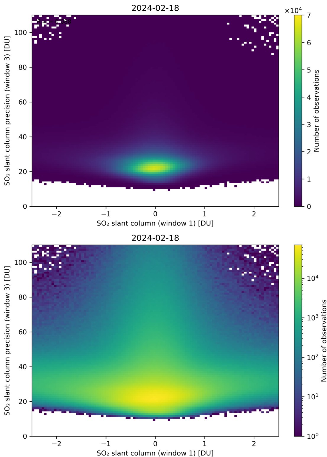
Figure 238: Scatter density plot of “SO 2 slant column (window 1)” against “SO 2 slant column precision (window 3)” for 2024-02-17 to 2024-02-19.
