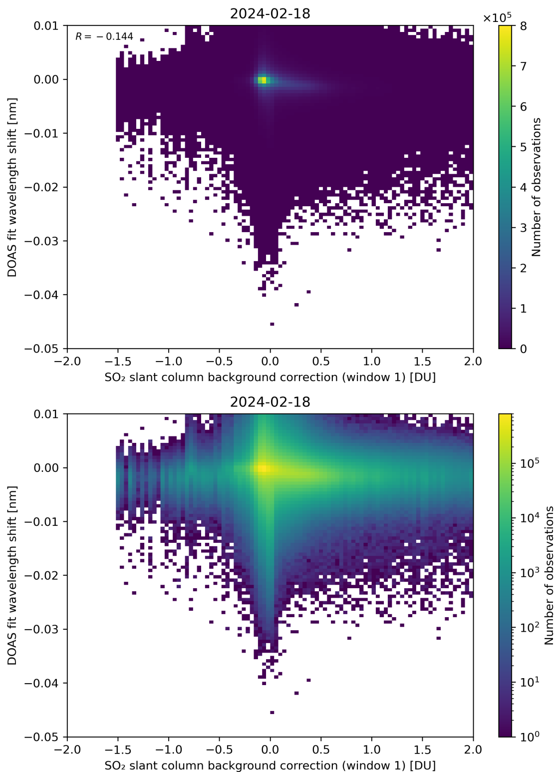
Figure 100: Scatter density plot of “SO 2 slant column background correction (window 1)” against “DOAS fit wavelength shift” for 2024-02-17 to 2024-02-19.
