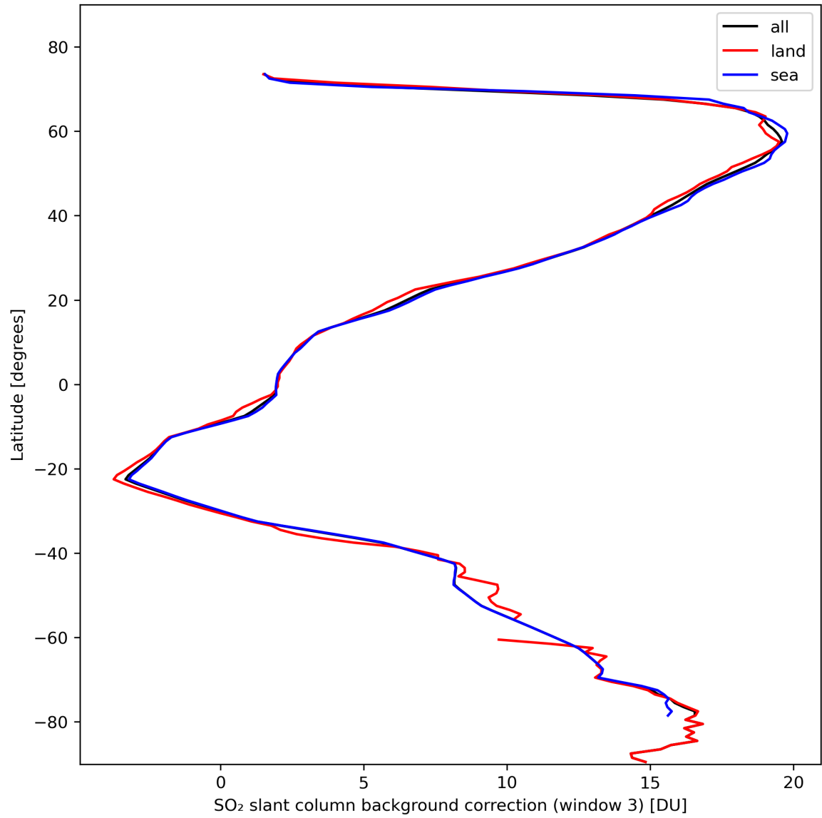
Figure 44: Zonal average of “SO 2 slant column background correction (window 3)” for 2024-02-17 to 2024-02-19.
