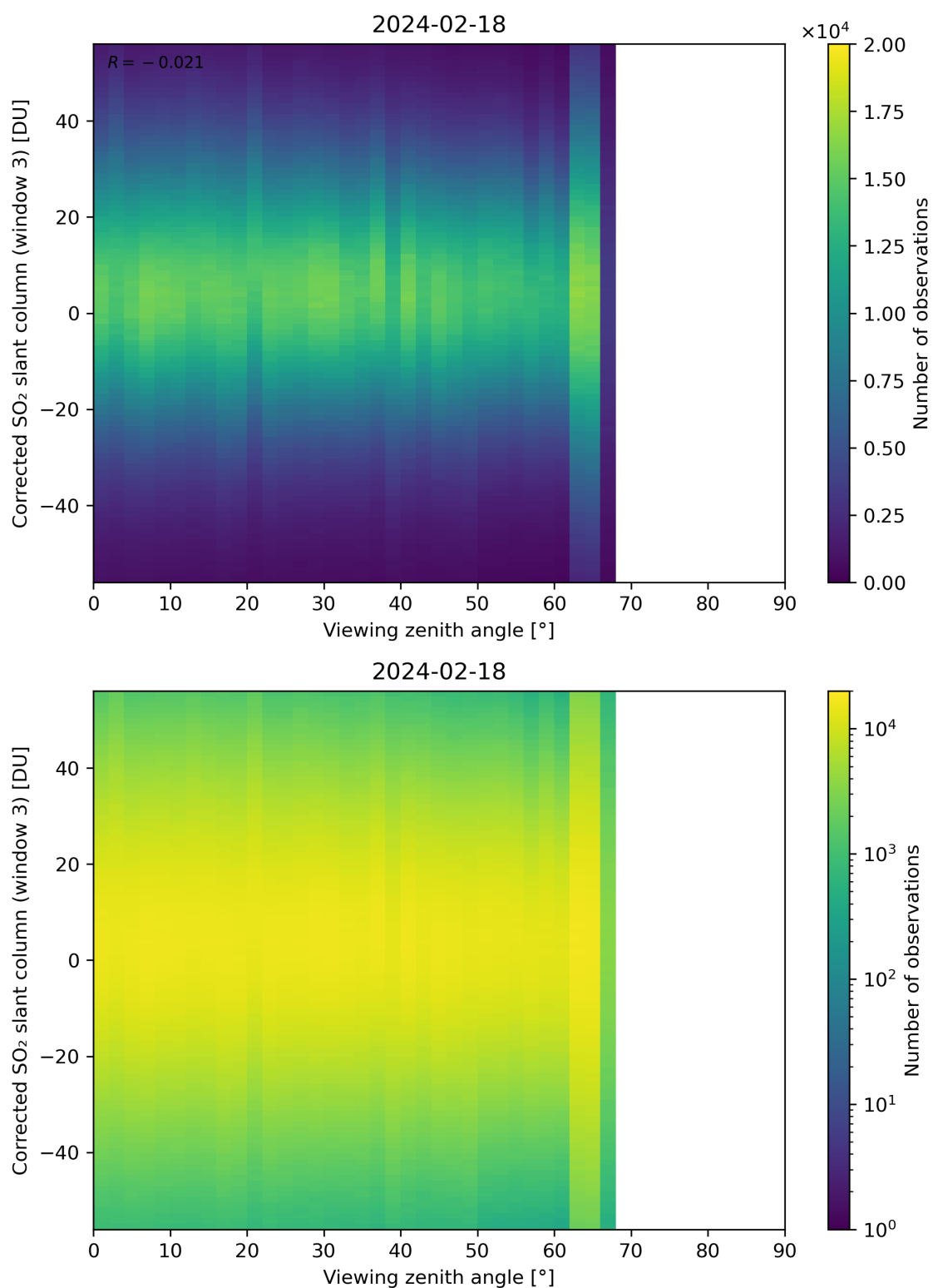
Figure 319: Scatter density plot of “Viewing zenith angle” against “Corrected SO 2 slant column (window 3)” for 2024-02-17 to 2024-02-19.
