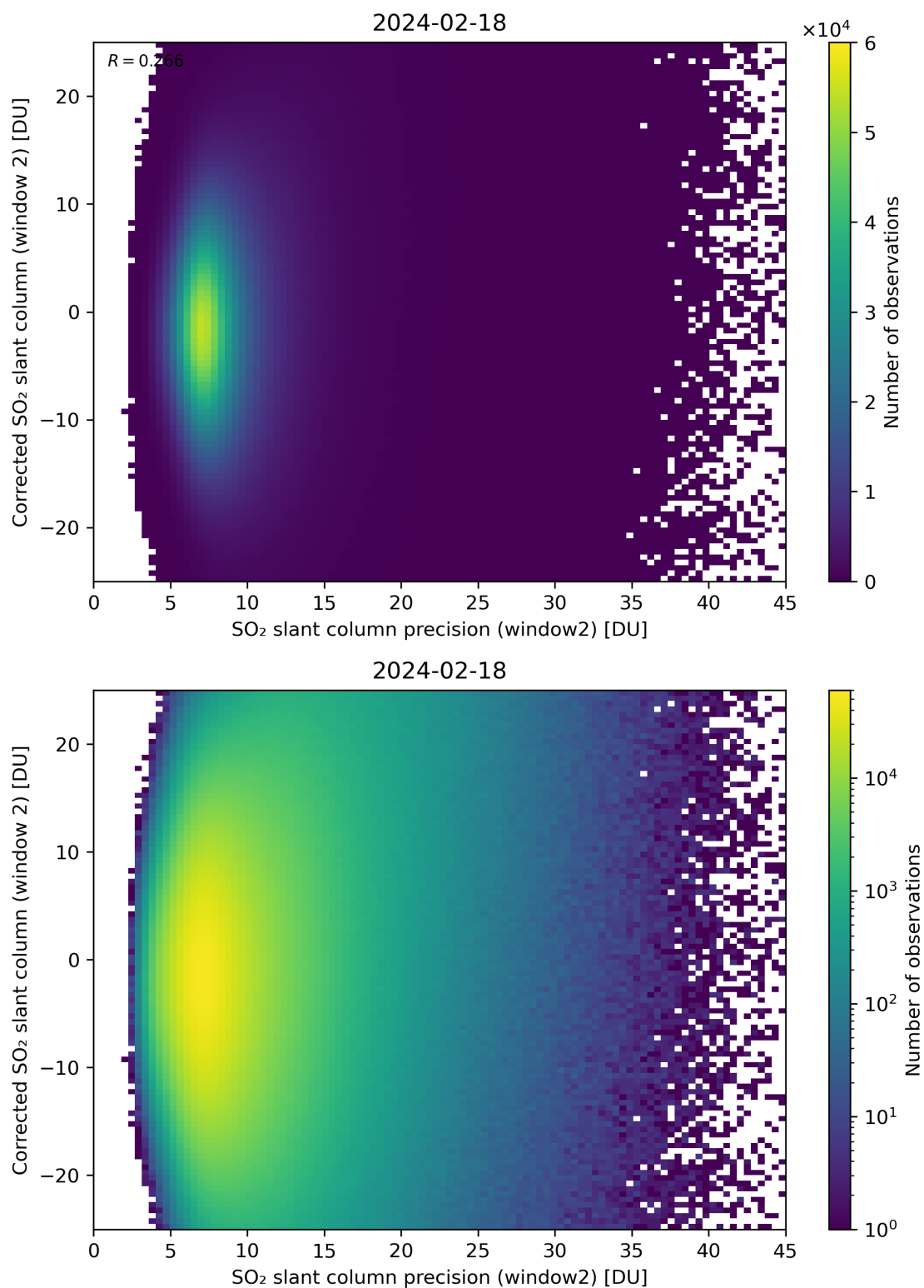
Figure 247: Scatter density plot of “SO 2 slant column precision (window2)” against “Corrected SO 2 slant column (window 2)” for 2024-02-17 to 2024-02-19.
