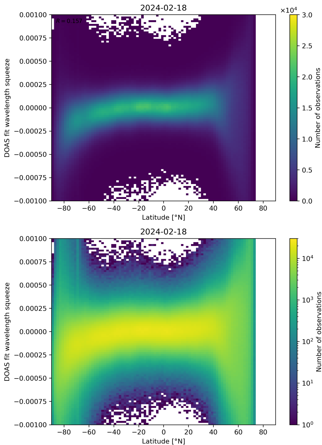
Figure 143: Scatter density plot of “Latitude” against “DOAS fit wavelength squeeze” for 2024-02-17 to 2024-02-19.
