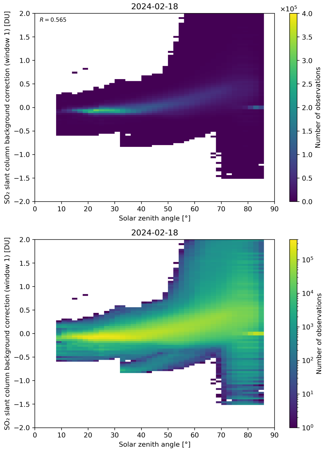
Figure 158: Scatter density plot of “Solar zenith angle” against “SO 2 slant column background correction (window 1)” for 2024-02-17 to 2024-02-19.
