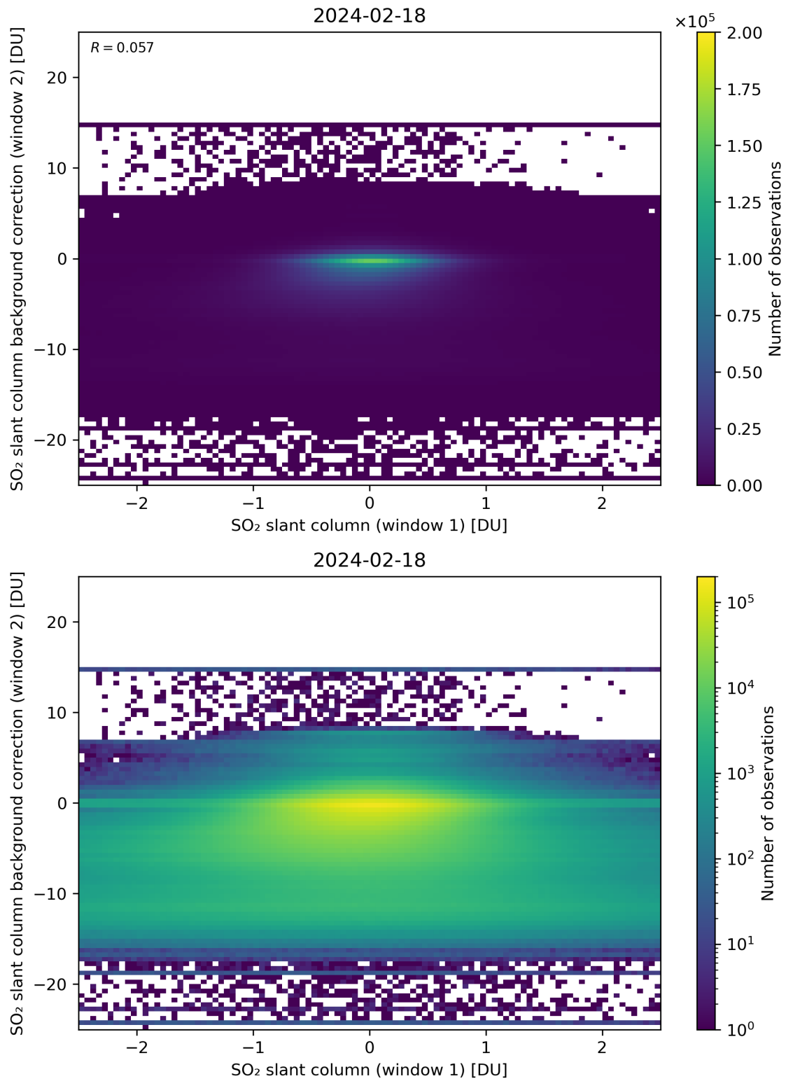
Figure 213: Scatter density plot of “SO 2 slant column (window 1)” against “SO 2 slant column background correction (window 2)” for 2024-02-17 to 2024-02-19.
