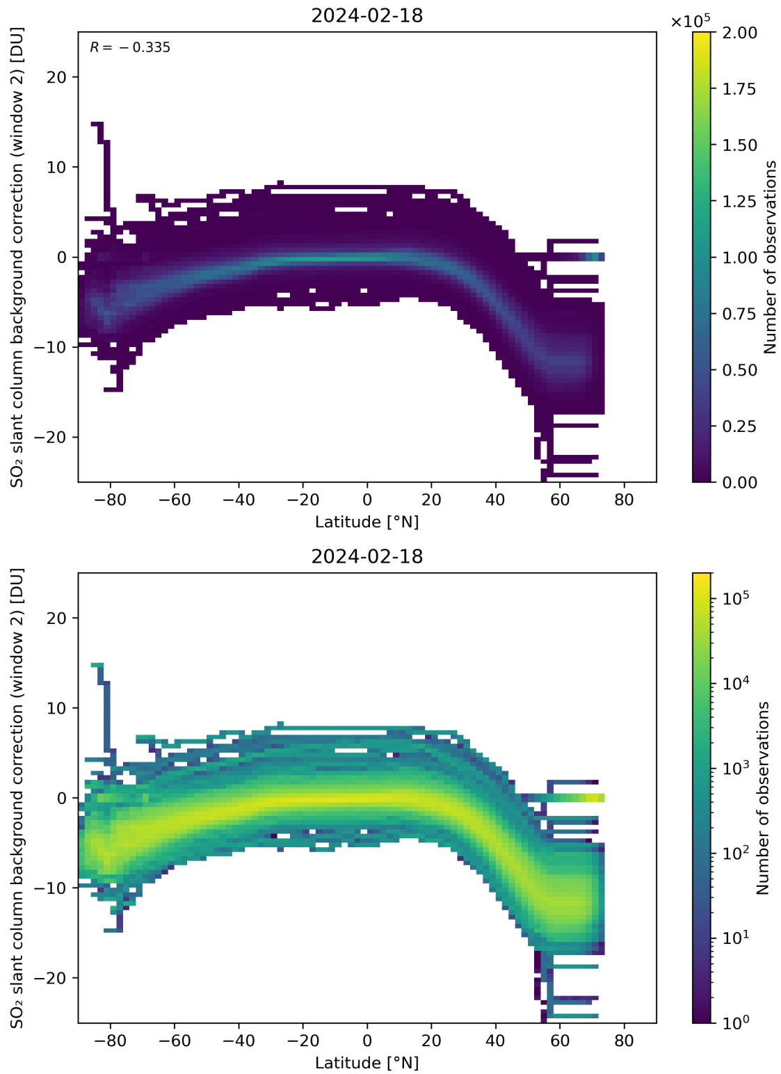
Figure 140: Scatter density plot of “Latitude” against “SO 2 slant column background correction (window 2)” for 2024-02-17 to 2024-02-19.
