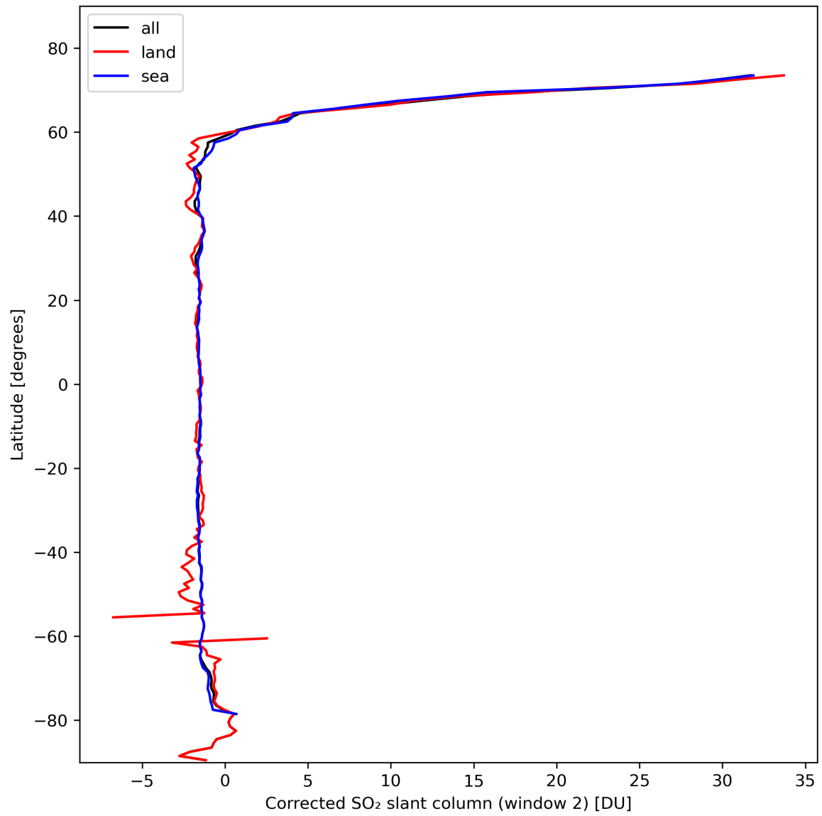
Figure 39: Zonal average of “Corrected SO 2 slant column (window 2)” for 2024-02-17 to 2024-02-19.
