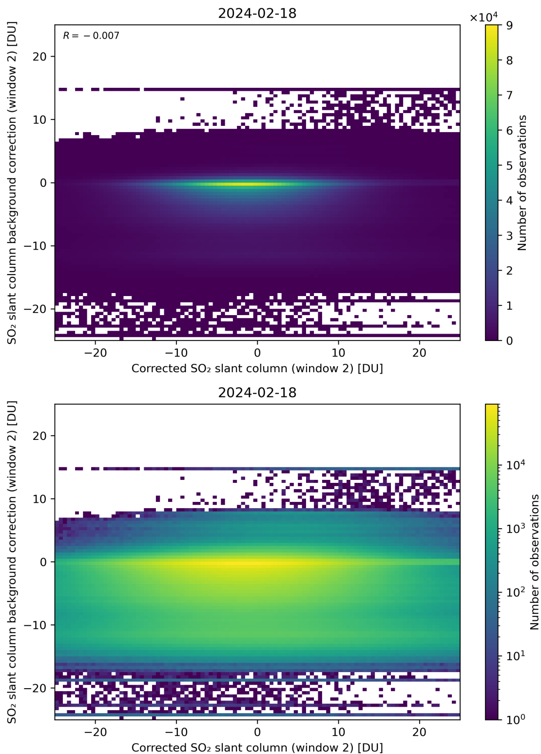
Figure 194: Scatter density plot of “Corrected SO 2 slant column (window 2)” against “SO 2 slant column background correction (window 2)” for 2024-02-17 to 2024-02-19.
