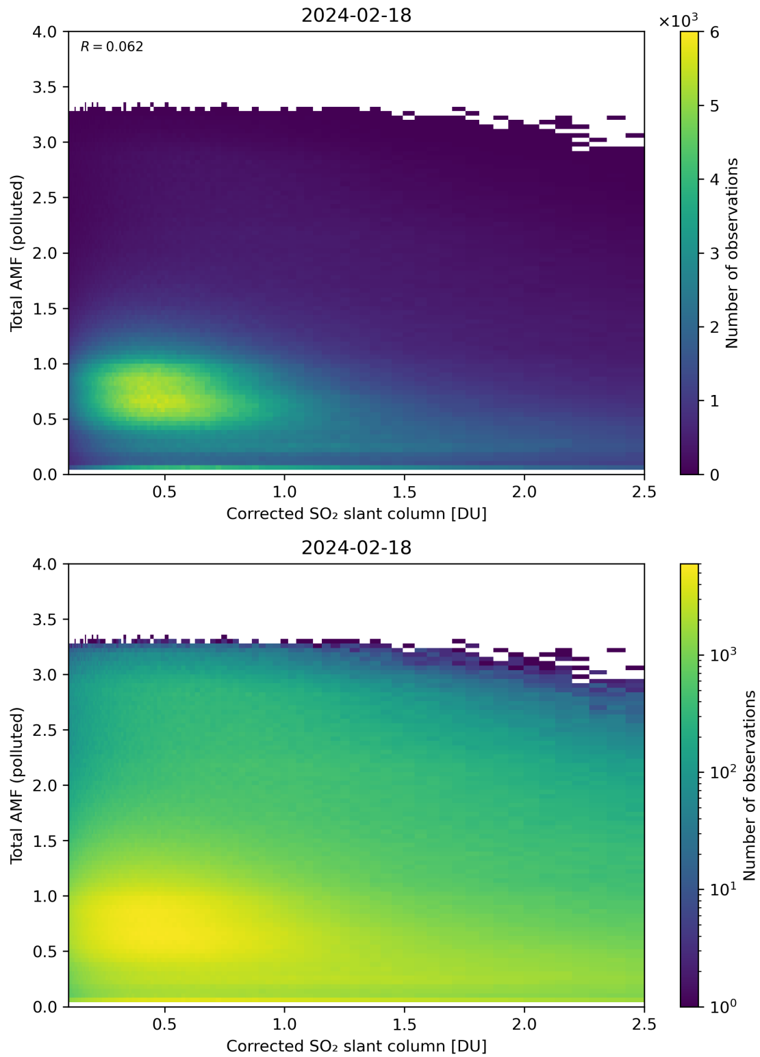
Figure 192: Scatter density plot of “Corrected SO 2 slant column” against “Total AMF (polluted)” for 2024-02-17 to 2024-02-19.
