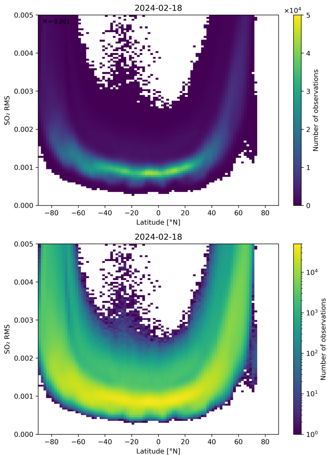
Figure 144: Scatter density plot of “Latitude” against “SO 2 RMS” for 2024-02-17 to 2024-02-19.
