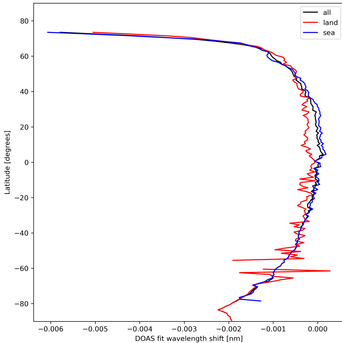
Figure 45: Zonal average of “DOAS fit wavelength shift” for 2024-02-17 to 2024-02-19.
