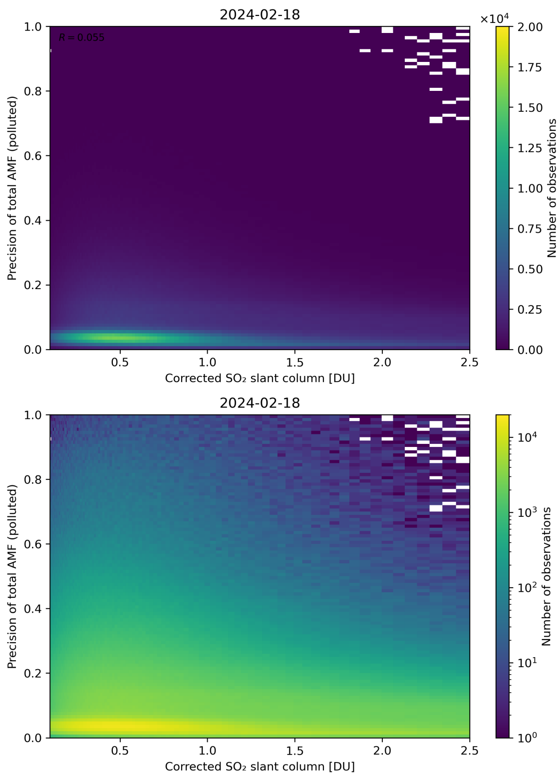
Figure 193: Scatter density plot of “Corrected SO 2 slant column” against “Precision of total AMF (polluted)” for 2024-02-17 to 2024-02-19.
