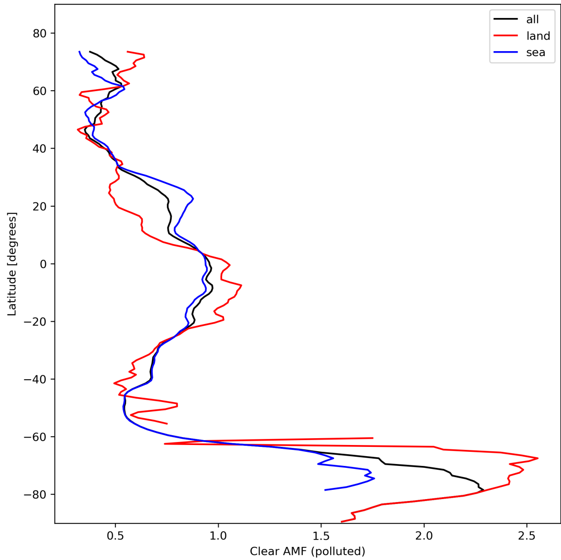
Figure 50: Zonal average of “Clear AMF (polluted)” for 2024-02-17 to 2024-02-19.
