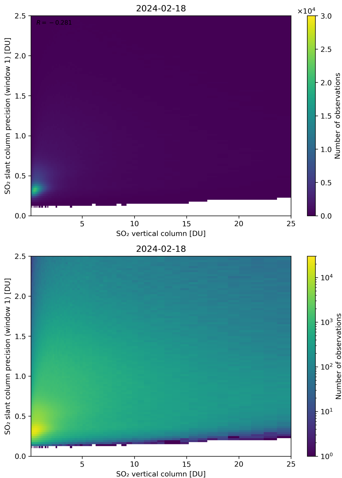
Figure 301: Scatter density plot of “SO 2 vertical column” against “SO 2 slant column precision (window 1)” for 2024-02-17 to 2024-02-19.
