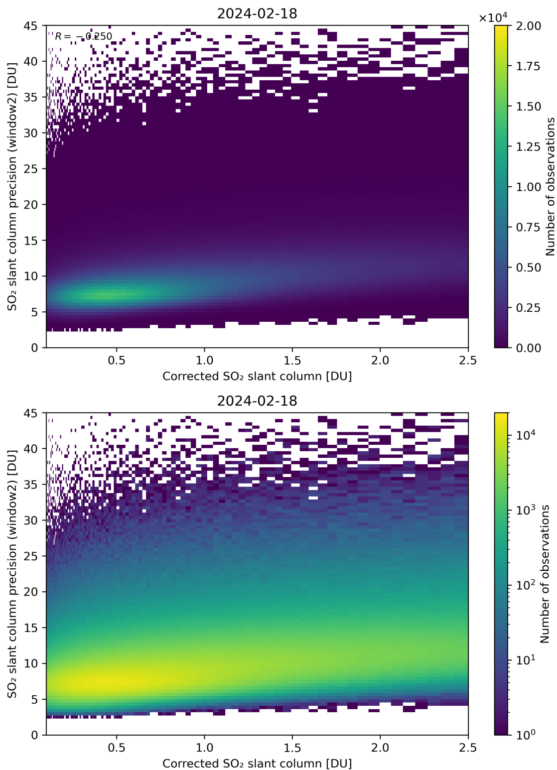
Figure 189: Scatter density plot of “Corrected SO 2 slant column” against “SO 2 slant column precision (window2)” for 2024-02-17 to 2024-02-19.
