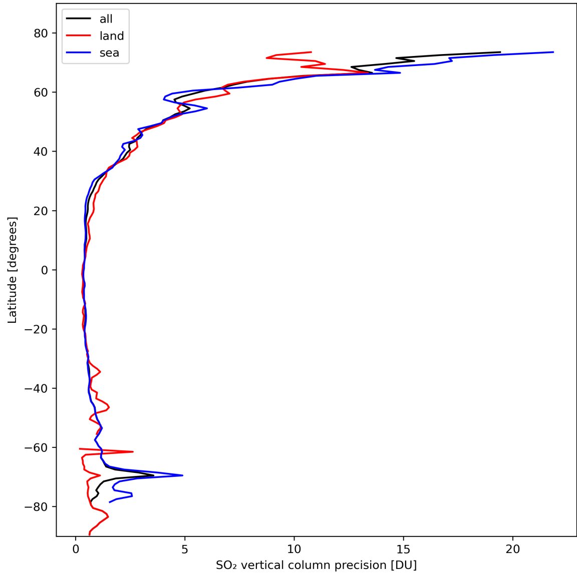
Figure 31: Zonal average of “SO 2 vertical column precision” for 2024-02-17 to 2024-02-19.
