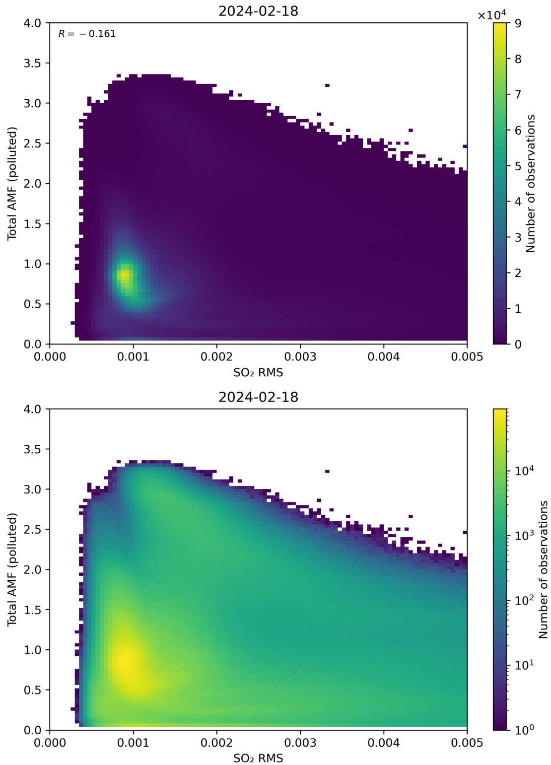
Figure 137: Scatter density plot of “SO 2 RMS” against “Total AMF (polluted)” for 2024-02-17 to 2024-02-19.
