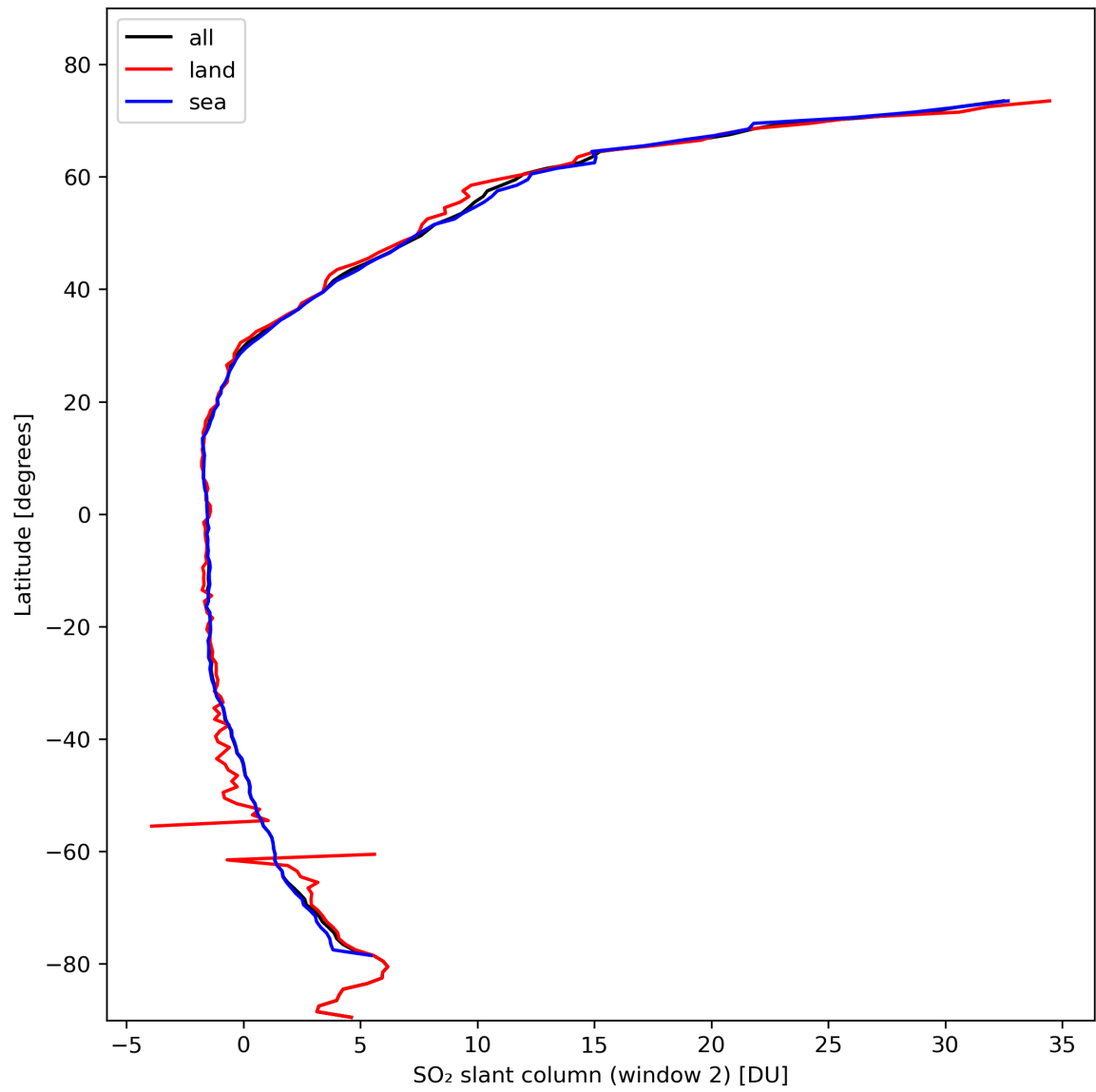
Figure 37: Zonal average of “SO 2 slant column (window 2)” for 2024-02-17 to 2024-02-19.
