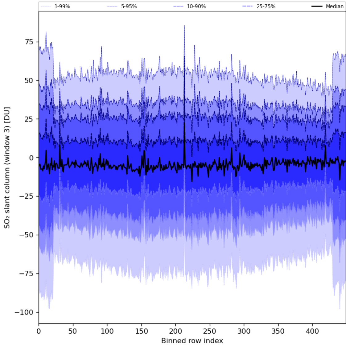
Figure 87: Along track statistics of “SO 2 slant column (window 3)” for 2024-02-17 to 2024-02-19
