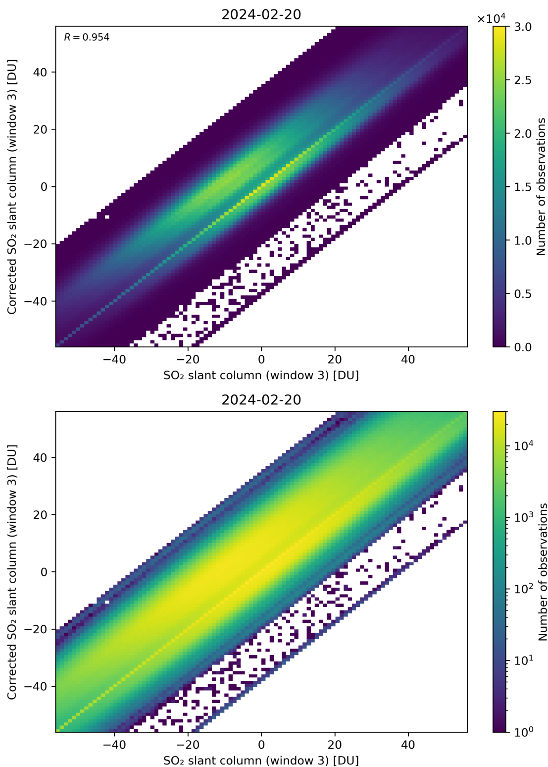
Figure 266: Scatter density plot of “SO 2 slant column (window 3)” against “Corrected SO 2 slant column (window 3)” for 2024-02-19 to 2024-02-21.
