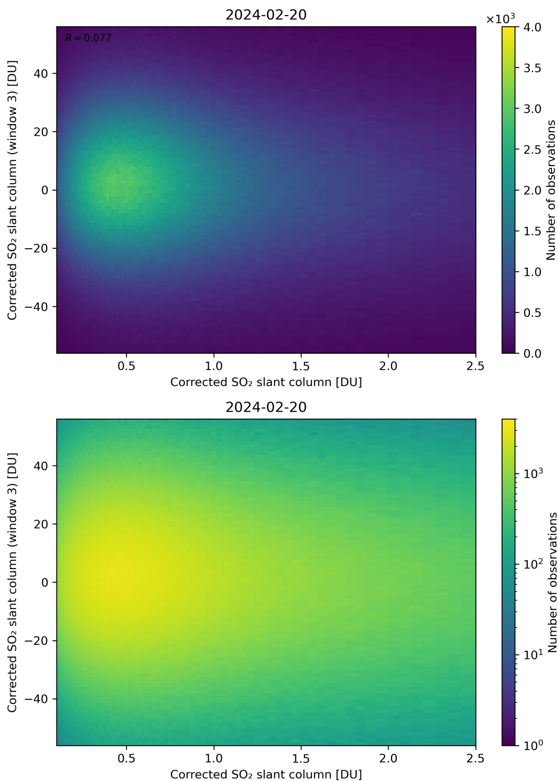
Figure 186: Scatter density plot of “Corrected SO 2 slant column” against “Corrected SO 2 slant column (window 3)” for 2024-02-19 to 2024-02-21.
