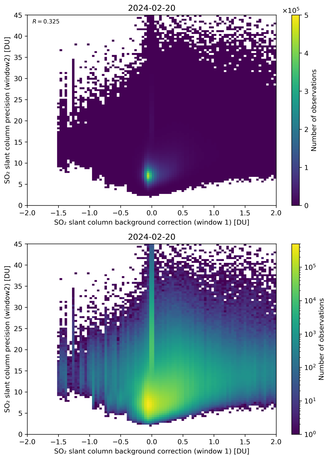
Figure 106: Scatter density plot of “SO 2 slant column background correction (window 1)” against “SO 2 slant column precision (window2)” for 2024-02-19 to 2024-02-21.
