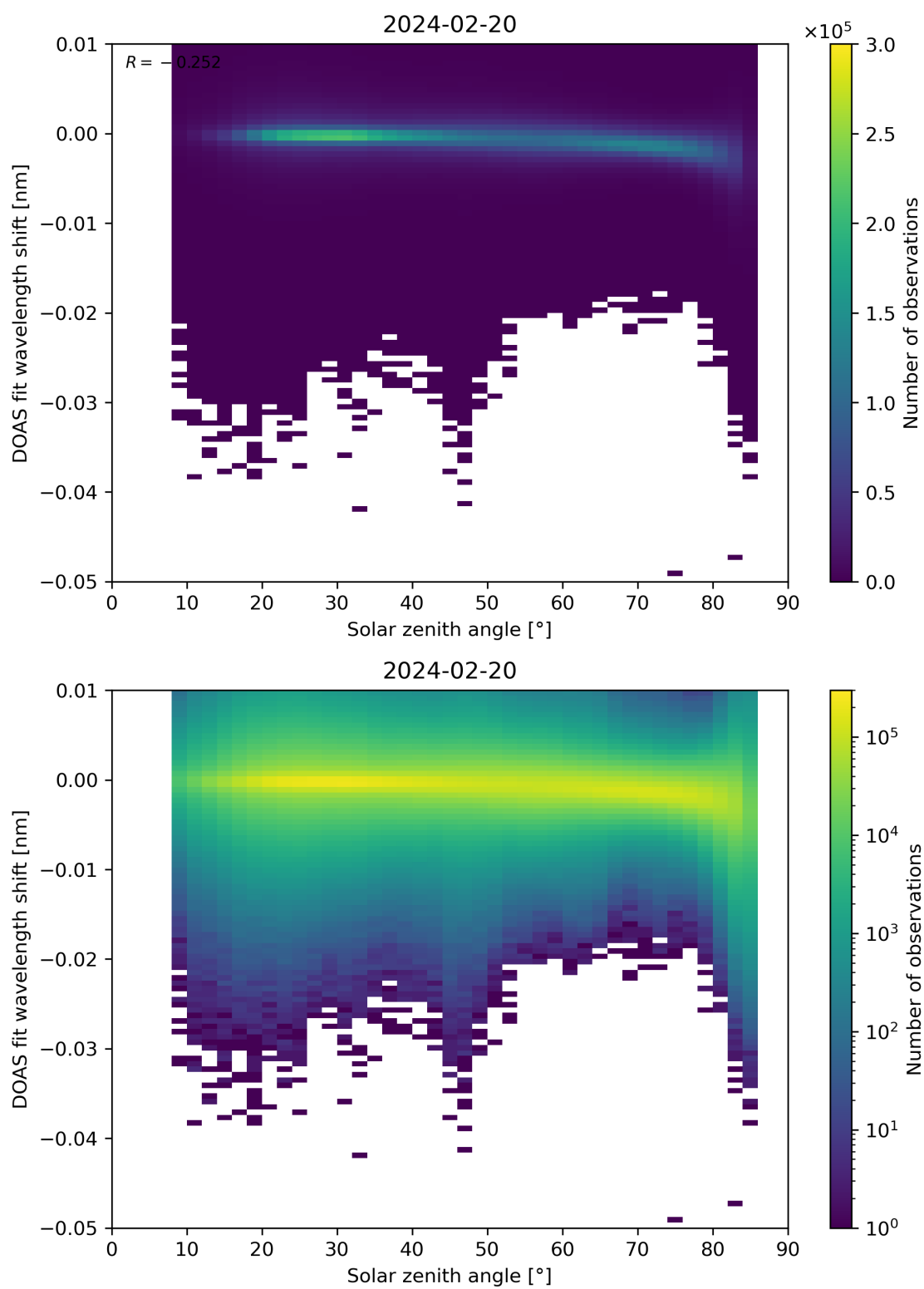
Figure 161: Scatter density plot of “Solar zenith angle” against “DOAS fit wavelength shift” for 2024-02-19 to 2024-02-21.
