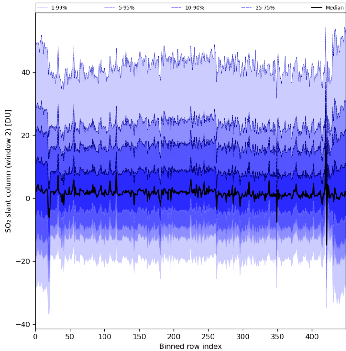
Figure 83: Along track statistics of “SO 2 slant column (window 2)” for 2024-02-19 to 2024-02-21
