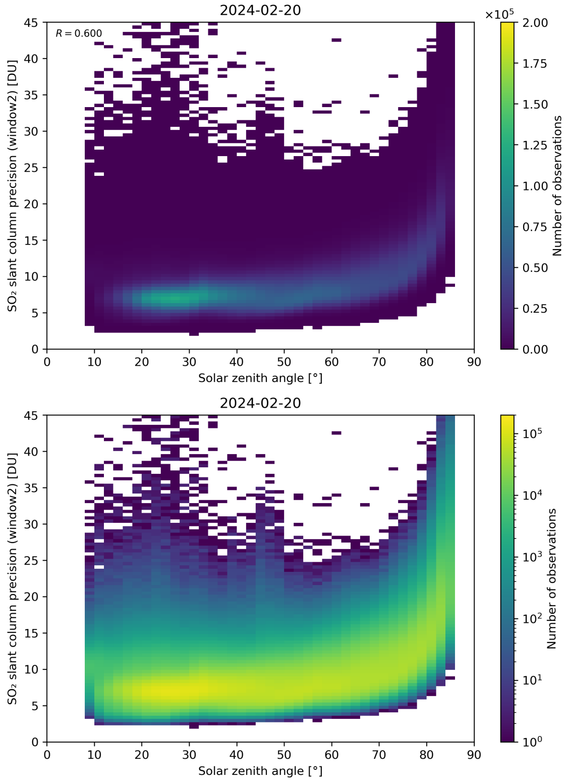
Figure 171: Scatter density plot of “Solar zenith angle” against “SO 2 slant column precision (window2)” for 2024-02-19 to 2024-02-21.
