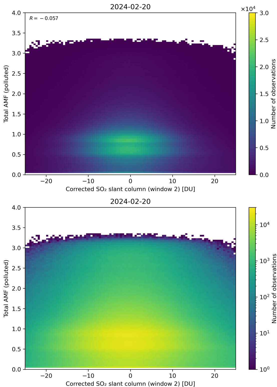
Figure 203: Scatter density plot of “Corrected SO 2 slant column (window 2)” against “Total AMF (polluted)” for 2024-02-19 to 2024-02-21.
