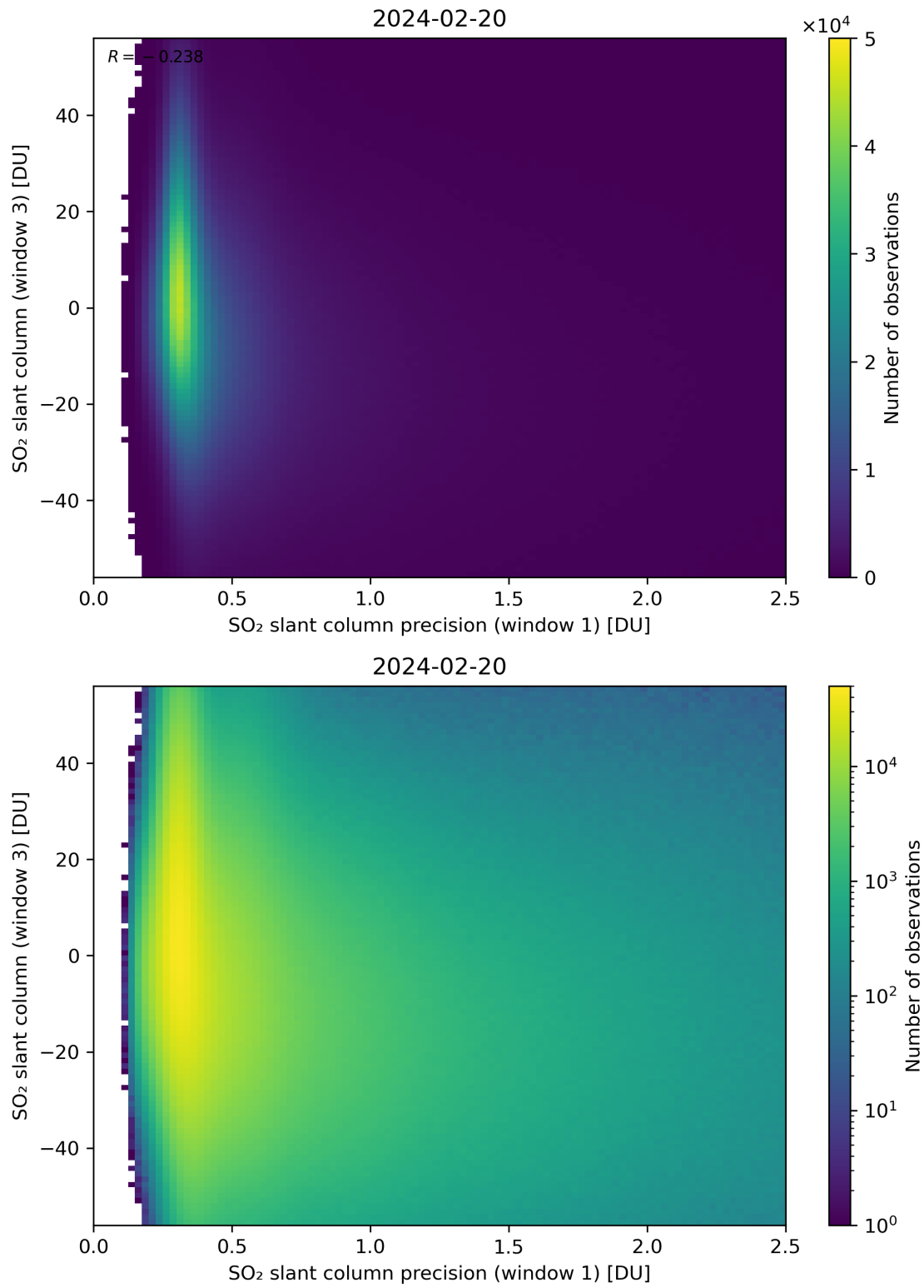
Figure 228: Scatter density plot of “SO 2 slant column precision (window 1)” against “SO 2 slant column (window 3)” for 2024-02-19 to 2024-02-21.
