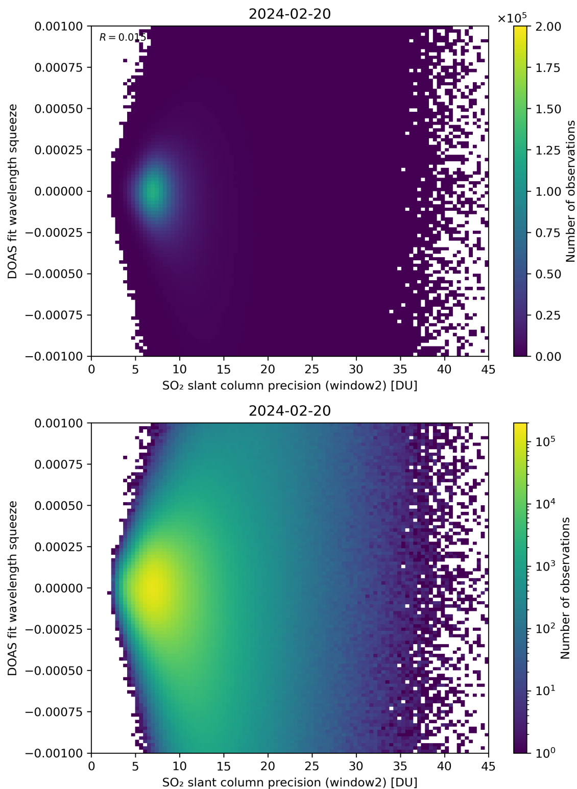
Figure 244: Scatter density plot of “SO 2 slant column precision (window2)” against “DOAS fit wavelength squeeze” for 2024-02-19 to 2024-02-21.
