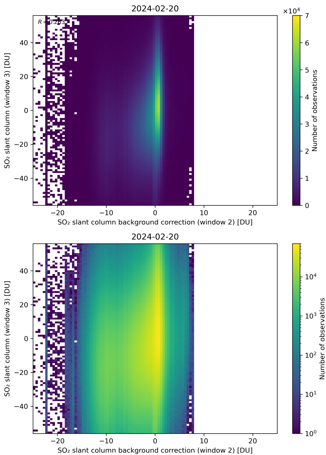
Figure 117: Scatter density plot of “SO 2 slant column background correction (window 2)” against “SO 2 slant column (window 3)” for 2024-02-19 to 2024-02-21.
