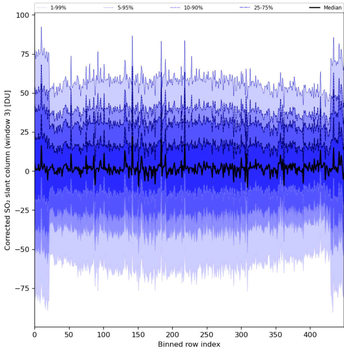
Figure 89: Along track statistics of “Corrected SO 2 slant column (window 3)” for 2024-02-19 to 2024-02-21
