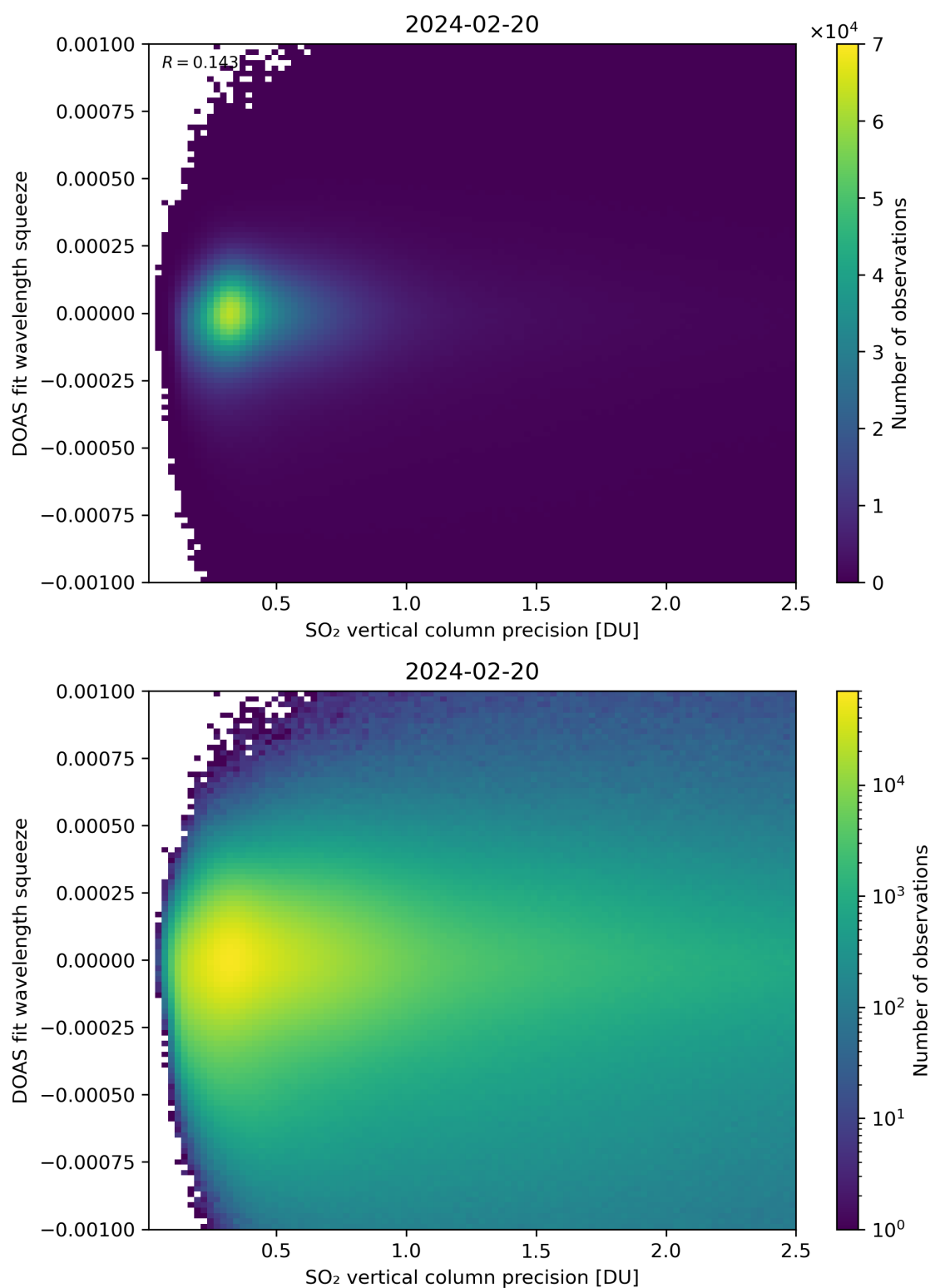
Figure 283: Scatter density plot of “SO 2 vertical column precision” against “DOAS fit wavelength squeeze” for 2024-02-19 to 2024-02-21.
