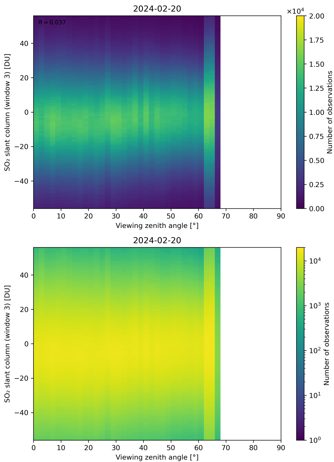
Figure 323: Scatter density plot of “Viewing zenith angle” against “SO 2 slant column (window 3)” for 2024-02-19 to 2024-02-21.
