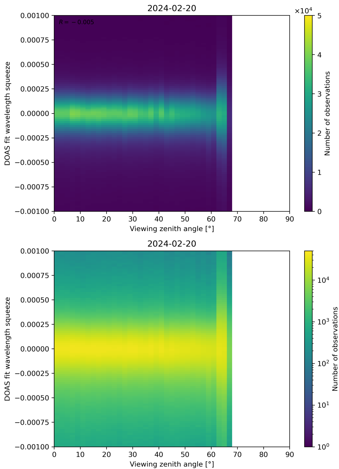
Figure 312: Scatter density plot of “Viewing zenith angle” against “DOAS fit wavelength squeeze” for 2024-02-19 to 2024-02-21.
