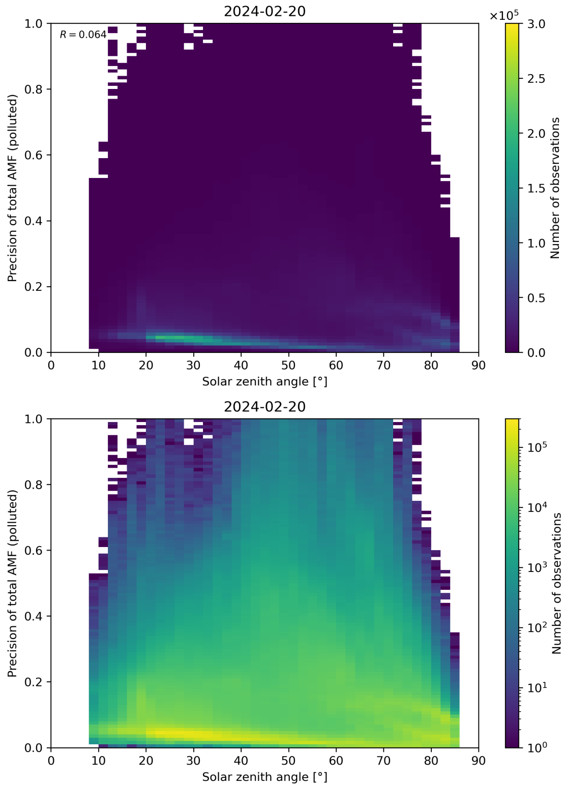
Figure 175: Scatter density plot of “Solar zenith angle” against “Precision of total AMF (polluted)” for 2024-02-19 to 2024-02-21.
