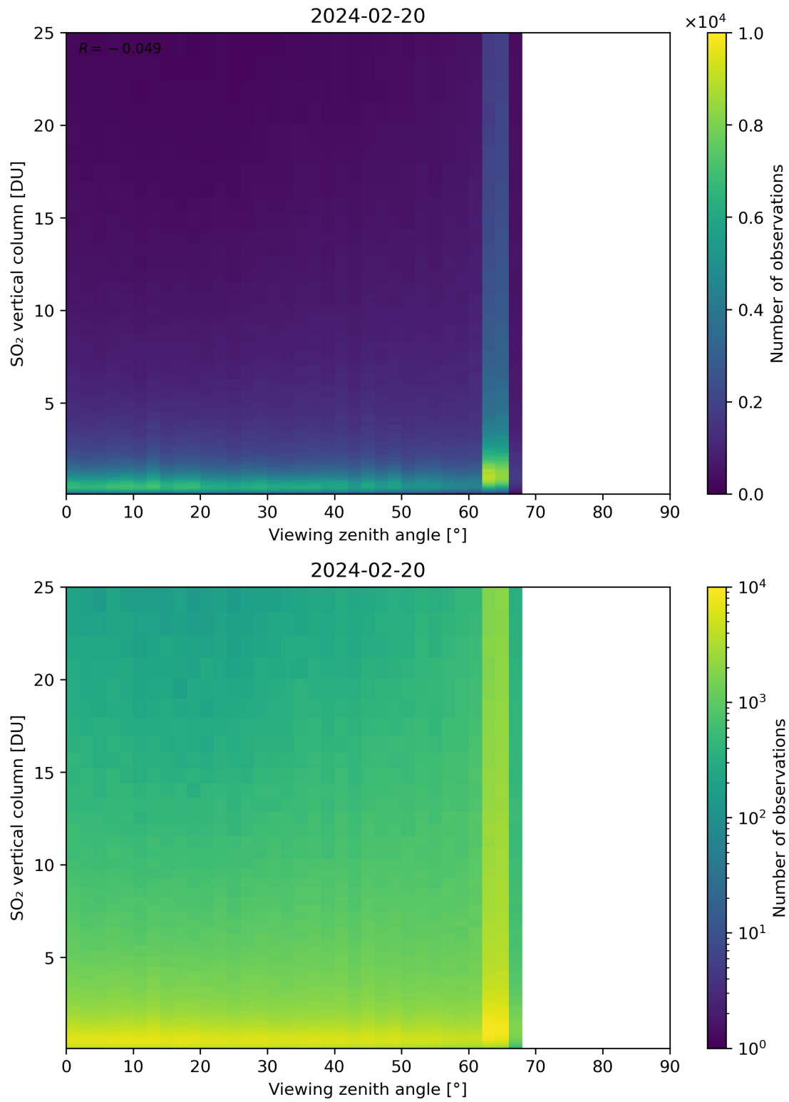
Figure 327: Scatter density plot of “Viewing zenith angle” against “SO 2 vertical column” for 2024-02-19 to 2024-02-21.
