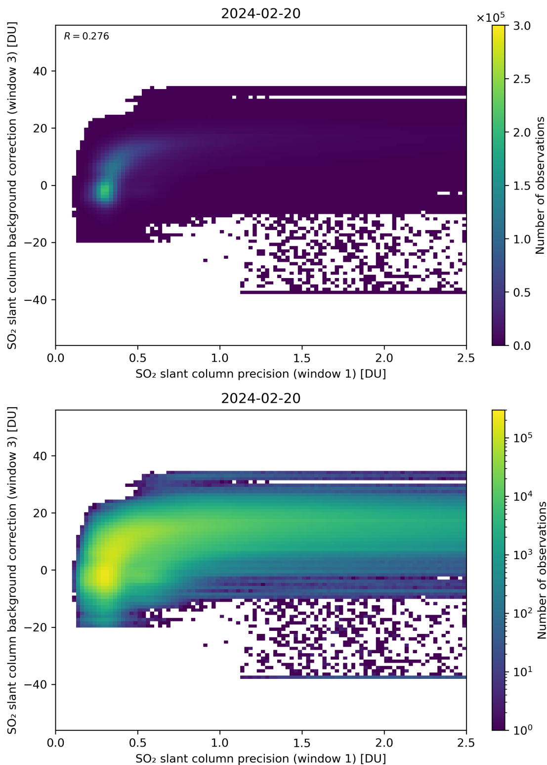
Figure 220: Scatter density plot of “SO 2 slant column precision (window 1)” against “SO 2 slant column background correction (window 3)” for 2024-02-19 to 2024-02-21.
