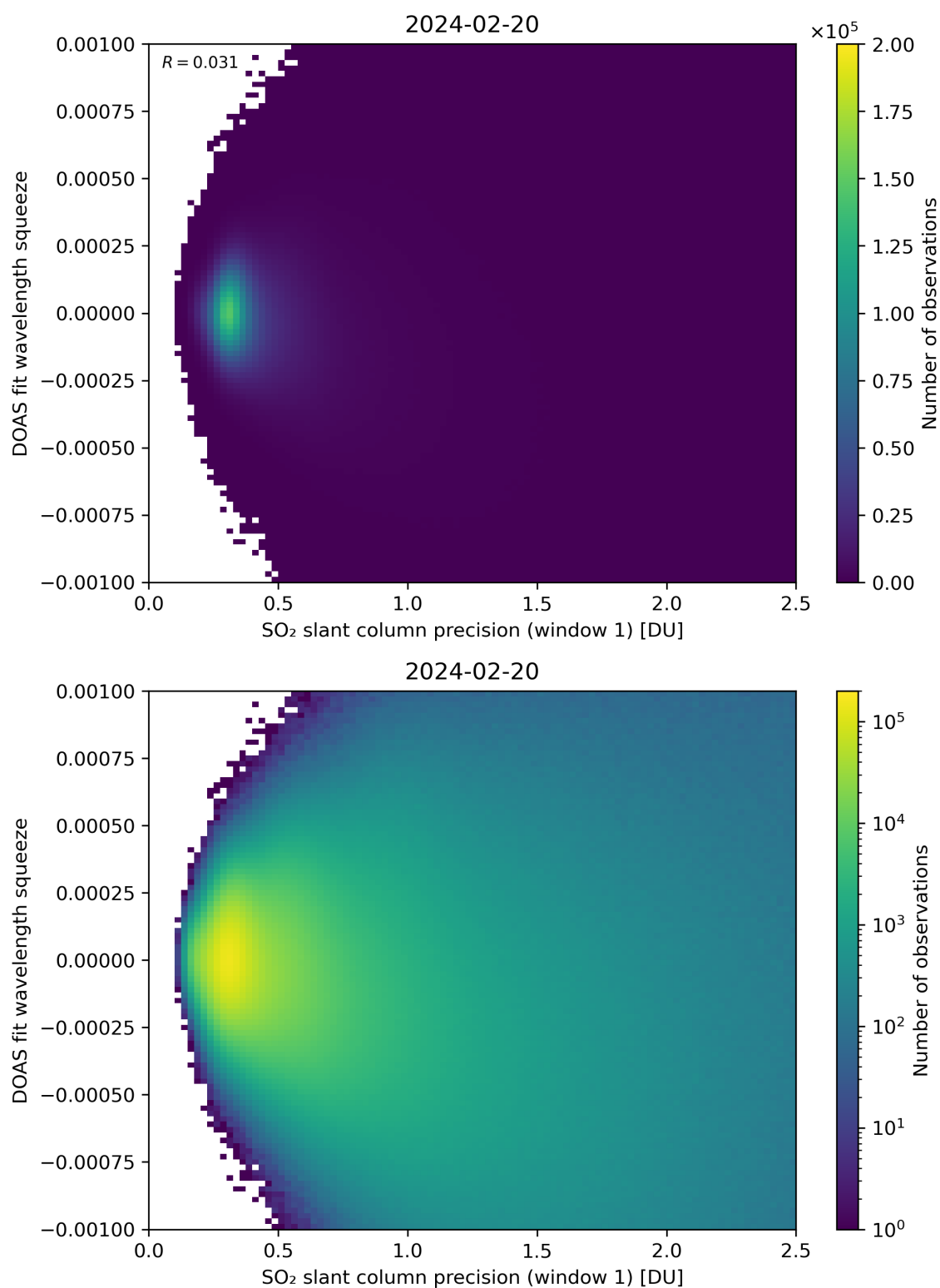
Figure 222: Scatter density plot of “SO 2 slant column precision (window 1)” against “DOAS fit wavelength squeeze” for 2024-02-19 to 2024-02-21.
