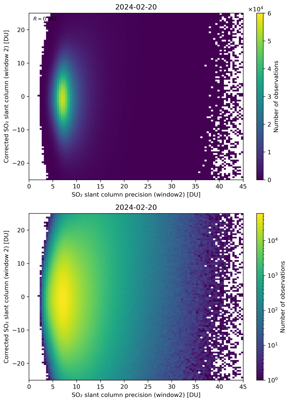
Figure 247: Scatter density plot of “SO 2 slant column precision (window2)” against “Corrected SO 2 slant column (window 2)” for 2024-02-19 to 2024-02-21.
