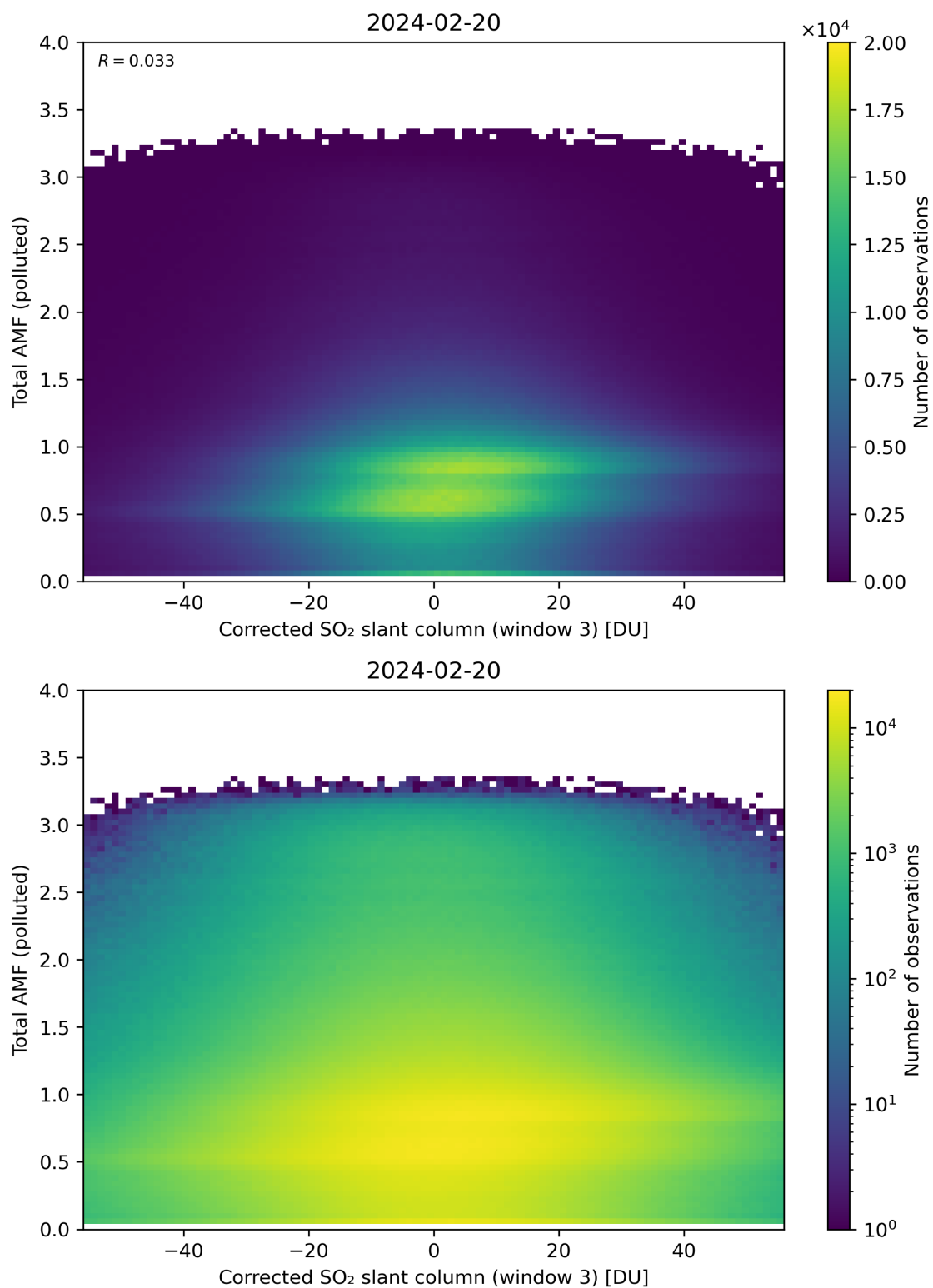
Figure 210: Scatter density plot of “Corrected SO 2 slant column (window 3)” against “Total AMF (polluted)” for 2024-02-19 to 2024-02-21.
