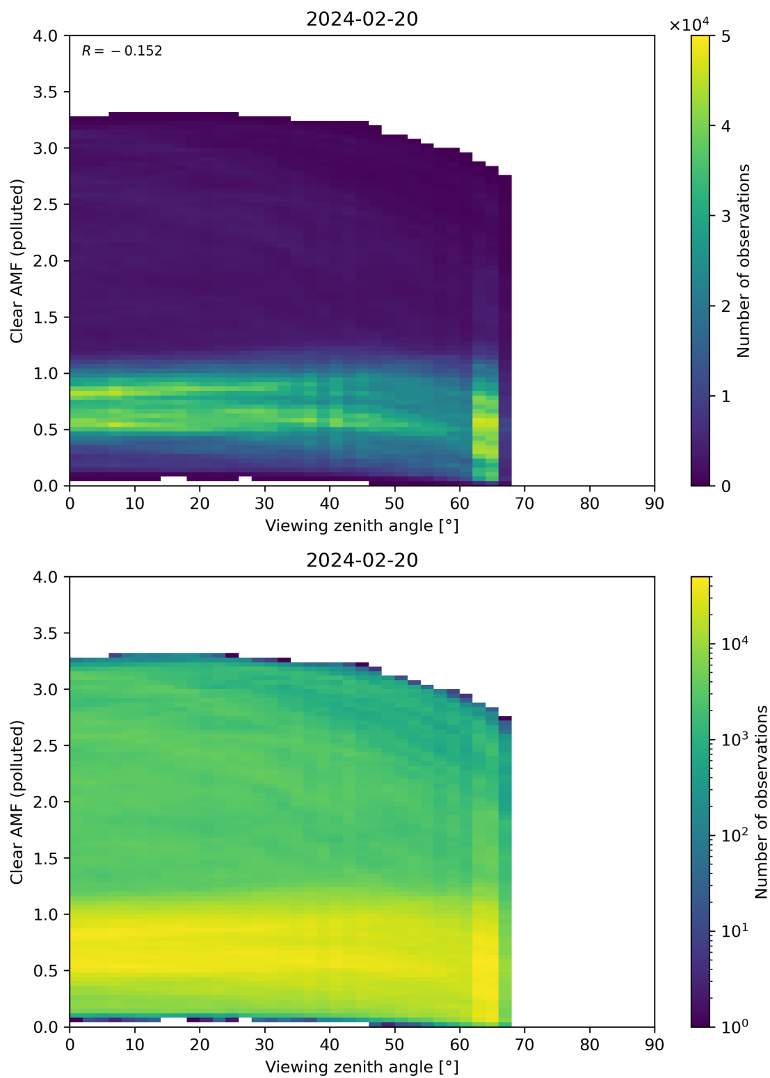
Figure 316: Scatter density plot of “Viewing zenith angle” against “Clear AMF (polluted)” for 2024-02-19 to 2024-02-21.
