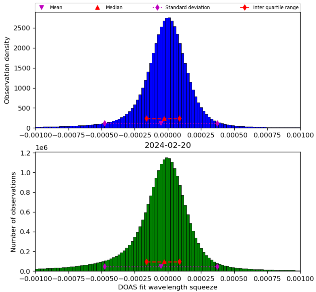
Figure 69: Histogram of “DOAS fit wavelength squeeze” for 2024-02-19 to 2024-02-21
