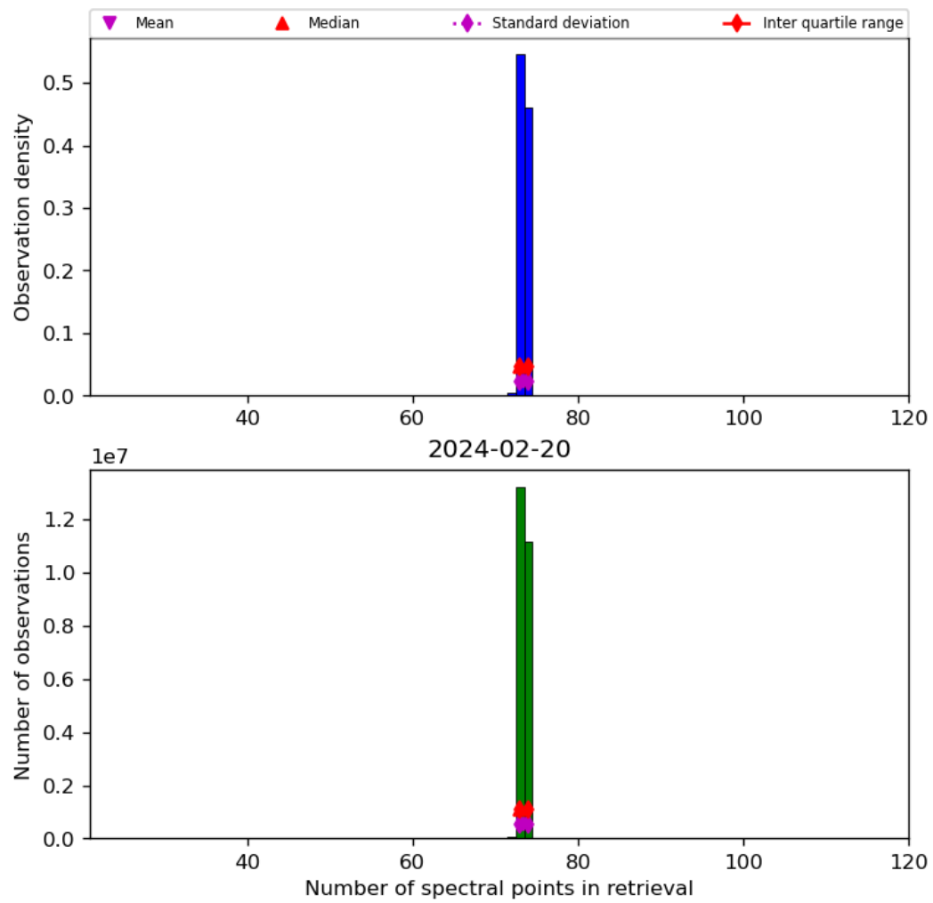
Figure 74: Histogram of “Number of spectral points in retrieval” for 2024-02-19 to 2024-02-21
