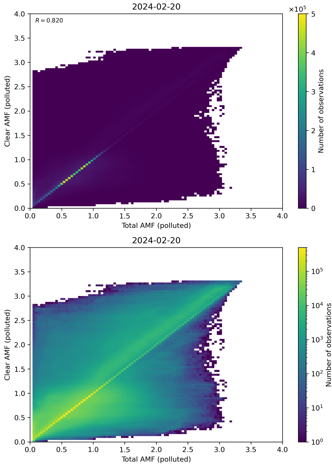
Figure 271: Scatter density plot of “Total AMF (polluted)” against “Clear AMF (polluted)” for 2024-02-19 to 2024-02-21.
