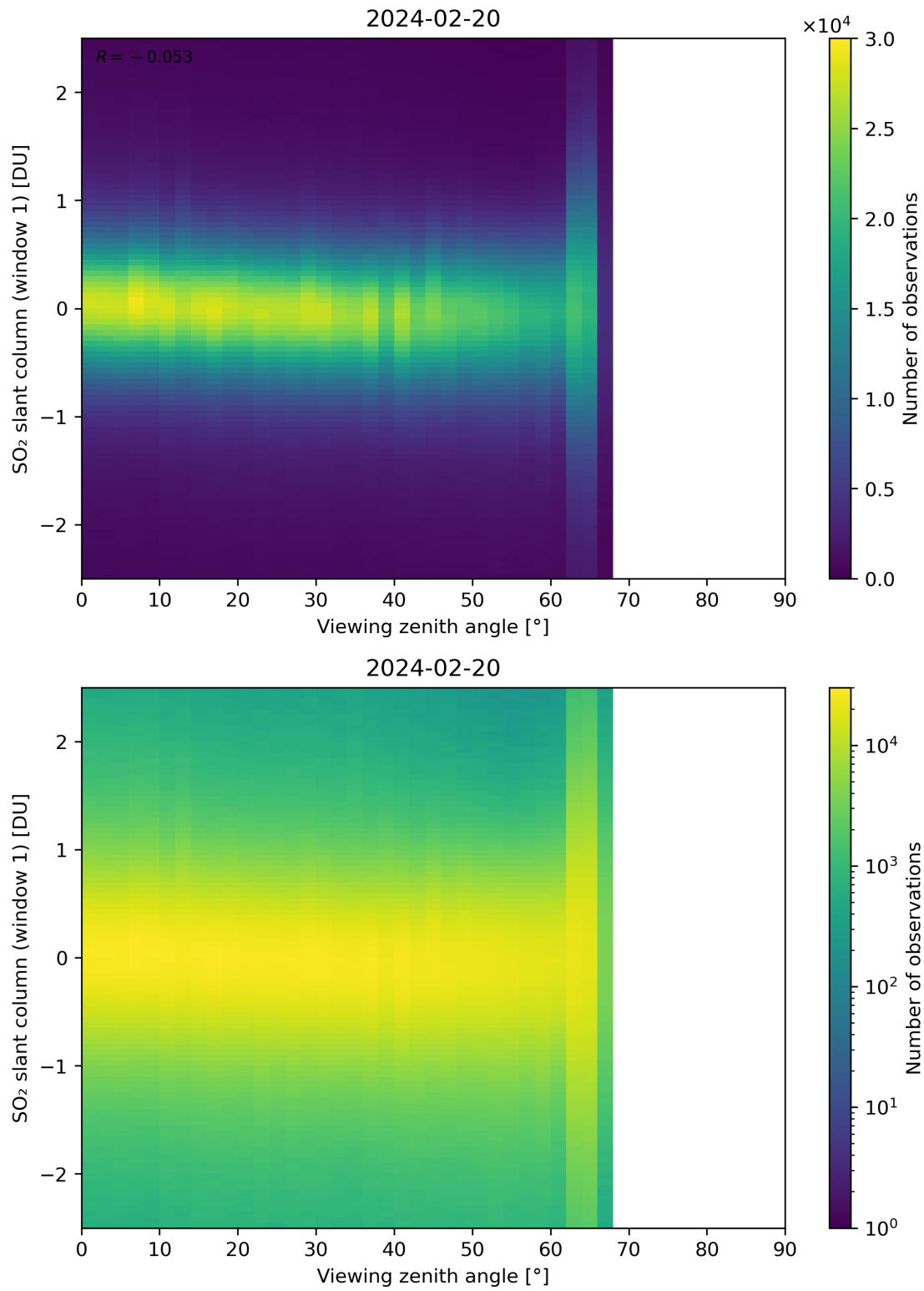
Figure 320: Scatter density plot of “Viewing zenith angle” against “SO 2 slant column (window 1)” for 2024-02-19 to 2024-02-21.
