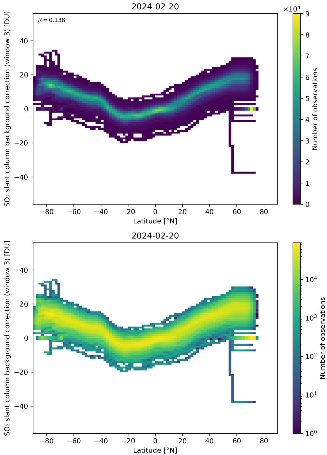
Figure 141: Scatter density plot of “Latitude” against “SO 2 slant column background correction (window 3)” for 2024-02-19 to 2024-02-21.
