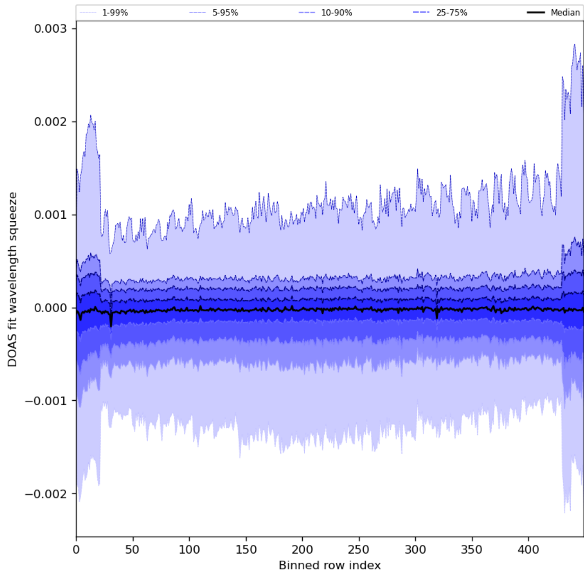
Figure 92: Along track statistics of “DOAS fit wavelength squeeze” for 2024-02-19 to 2024-02-21
