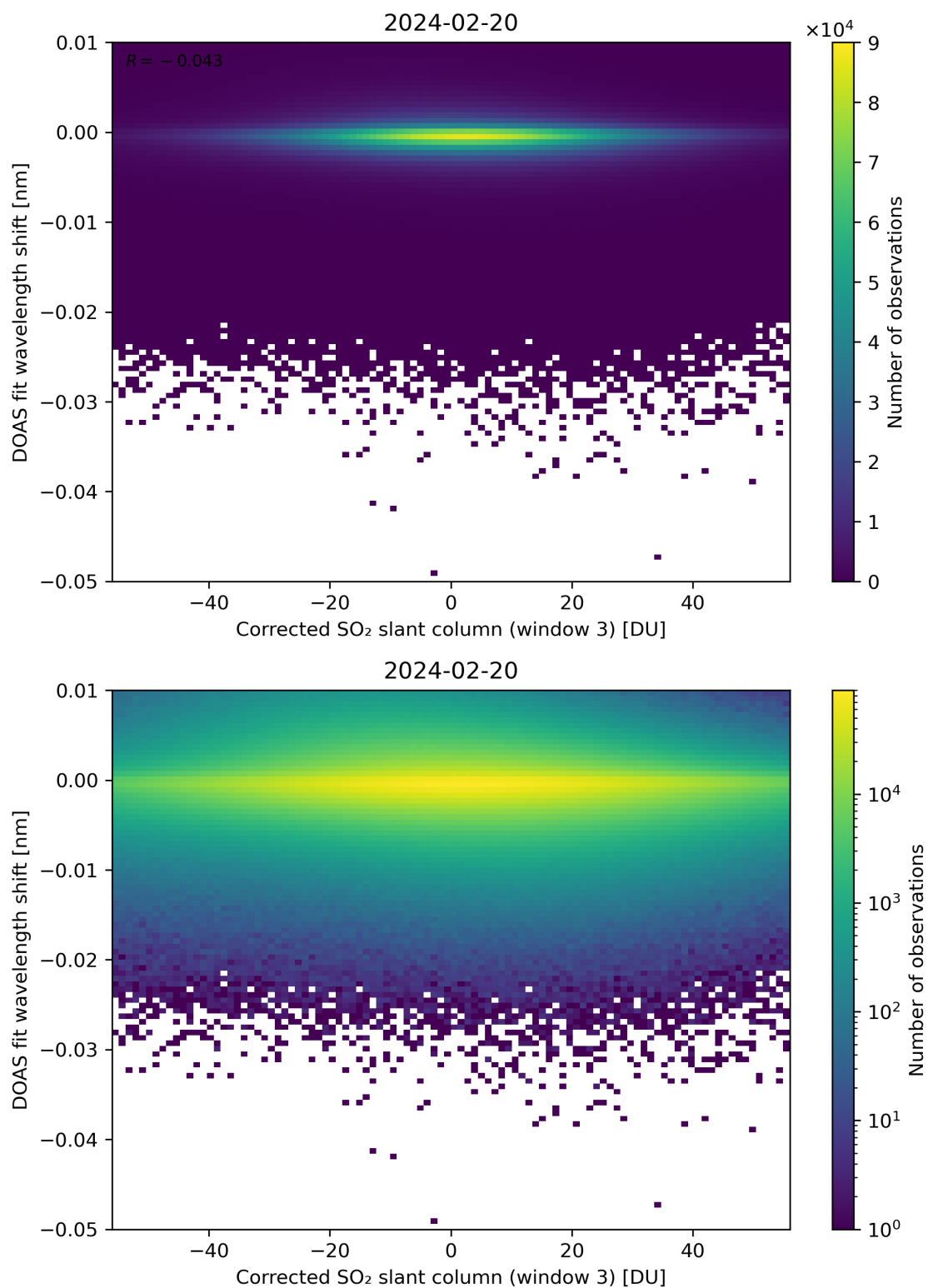
Figure 206: Scatter density plot of “Corrected SO 2 slant column (window 3)” against “DOAS fit wavelength shift” for 2024-02-19 to 2024-02-21.
