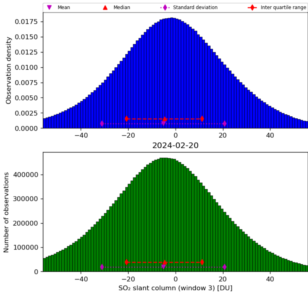
Figure 64: Histogram of “SO 2 slant column (window 3)” for 2024-02-19 to 2024-02-21
