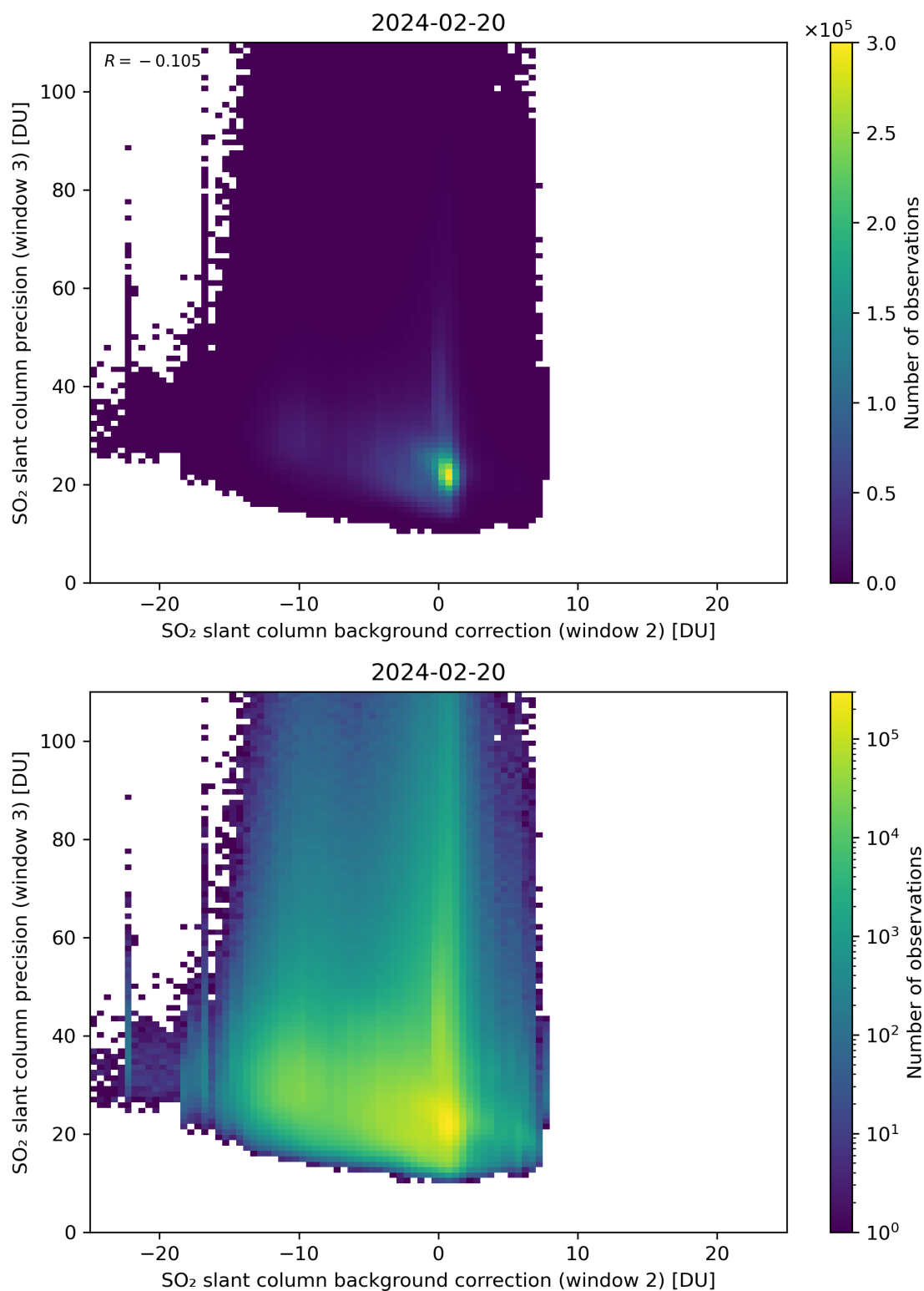
Figure 118: Scatter density plot of “SO 2 slant column background correction (window 2)” against “SO 2 slant column precision (window 3)” for 2024-02-19 to 2024-02-21.
