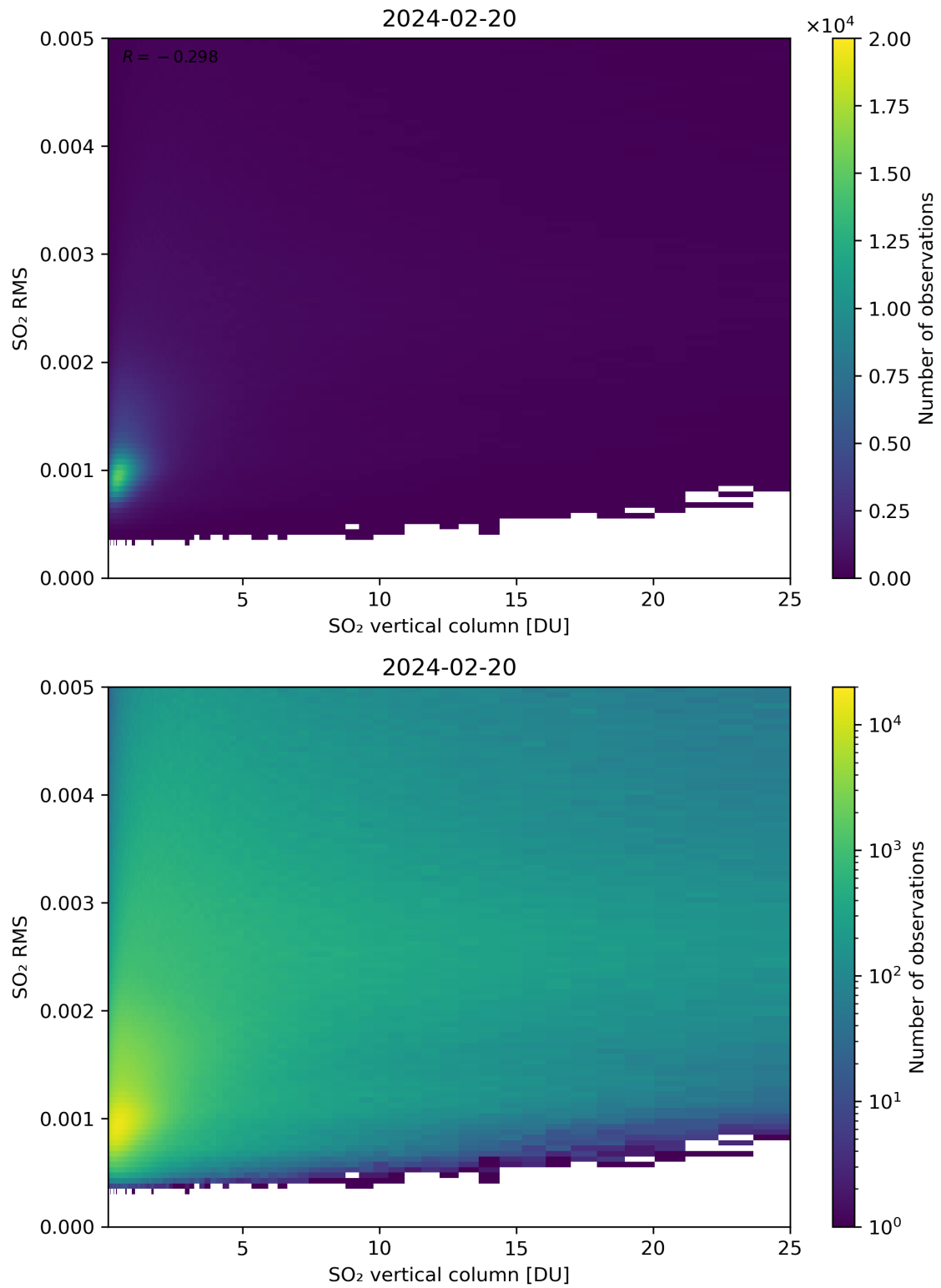
Figure 278: Scatter density plot of “SO 2 vertical column” against “SO 2 RMS” for 2024-02-19 to 2024-02-21.
