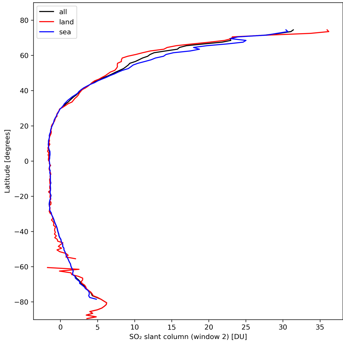
Figure 37: Zonal average of “SO 2 slant column (window 2)” for 2024-02-19 to 2024-02-21.
