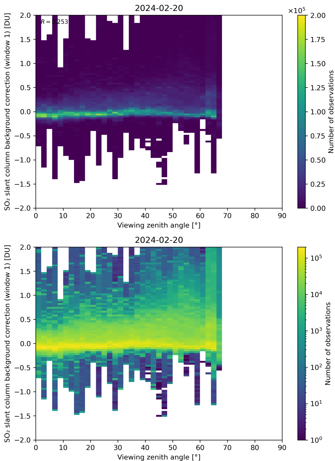
Figure 308: Scatter density plot of “Viewing zenith angle” against “SO 2 slant column background correction (window 1)” for 2024-02-19 to 2024-02-21.
