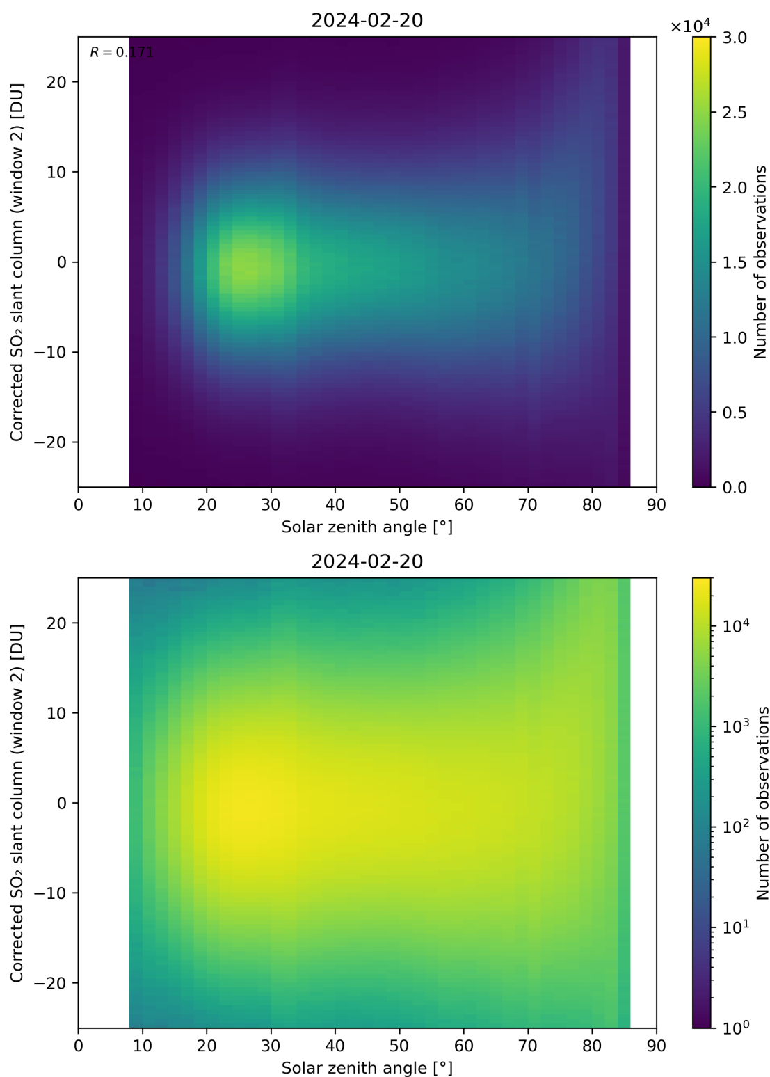
Figure 167: Scatter density plot of “Solar zenith angle” against “Corrected SO 2 slant column (window 2)” for 2024-02-19 to 2024-02-21.
