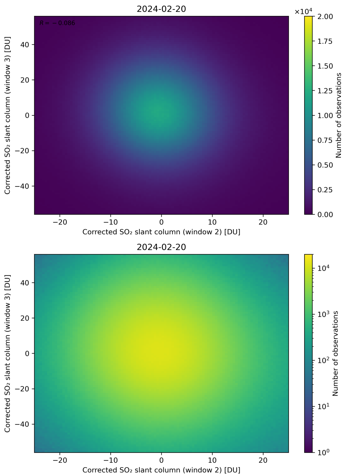
Figure 200: Scatter density plot of “Corrected SO 2 slant column (window 2)” against “Corrected SO 2 slant column (window 3)” for 2024-02-19 to 2024-02-21.
