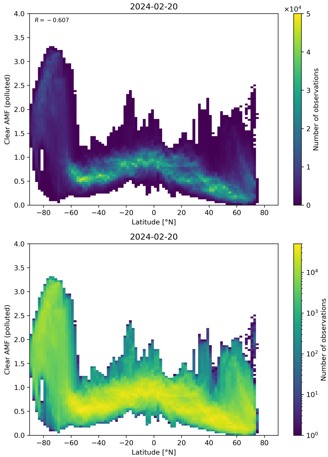
Figure 145: Scatter density plot of “Latitude” against “Clear AMF (polluted)” for 2024-02-19 to 2024-02-21.
