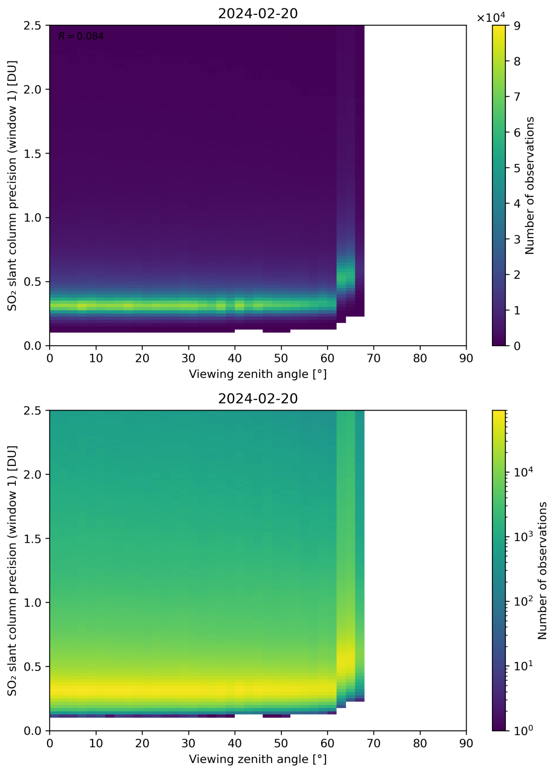
Figure 321: Scatter density plot of “Viewing zenith angle” against “SO 2 slant column precision (window 1)” for 2024-02-19 to 2024-02-21.
