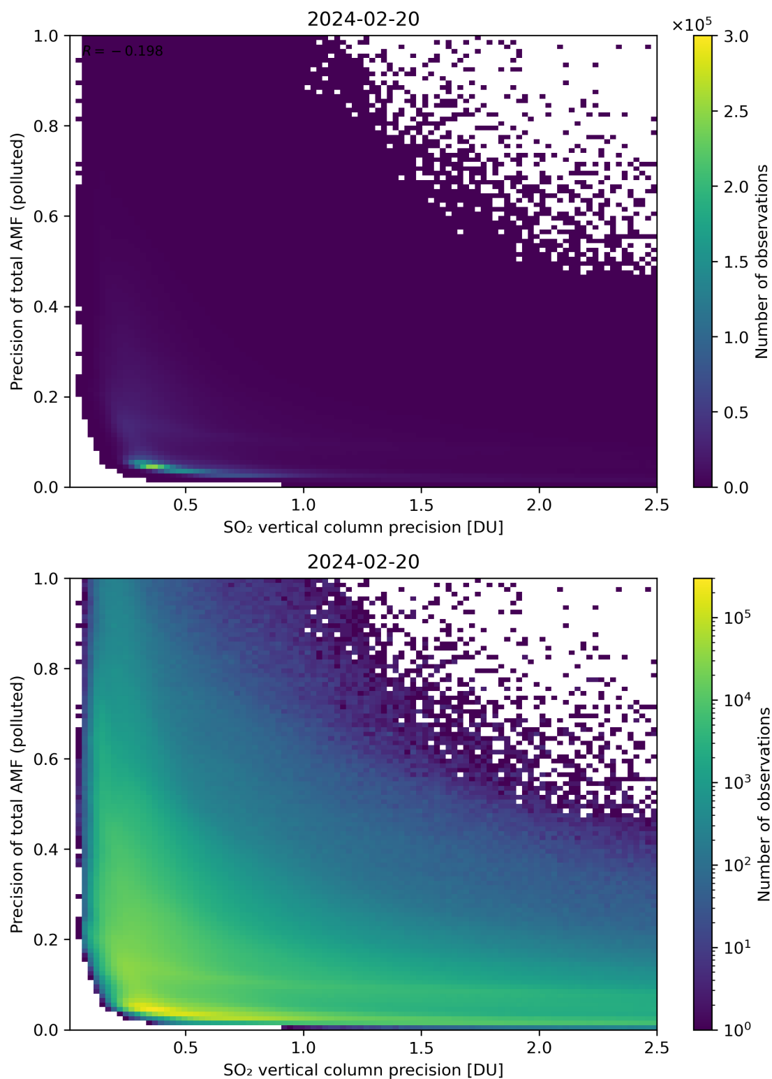
Figure 295: Scatter density plot of “SO 2 vertical column precision” against “Precision of total AMF (polluted)” for 2024-02-19 to 2024-02-21.
