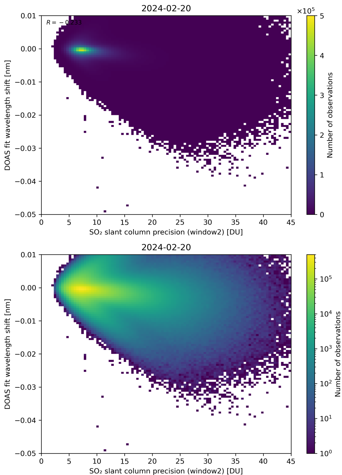
Figure 243: Scatter density plot of “SO 2 slant column precision (window2)” against “DOAS fit wavelength shift” for 2024-02-19 to 2024-02-21.
