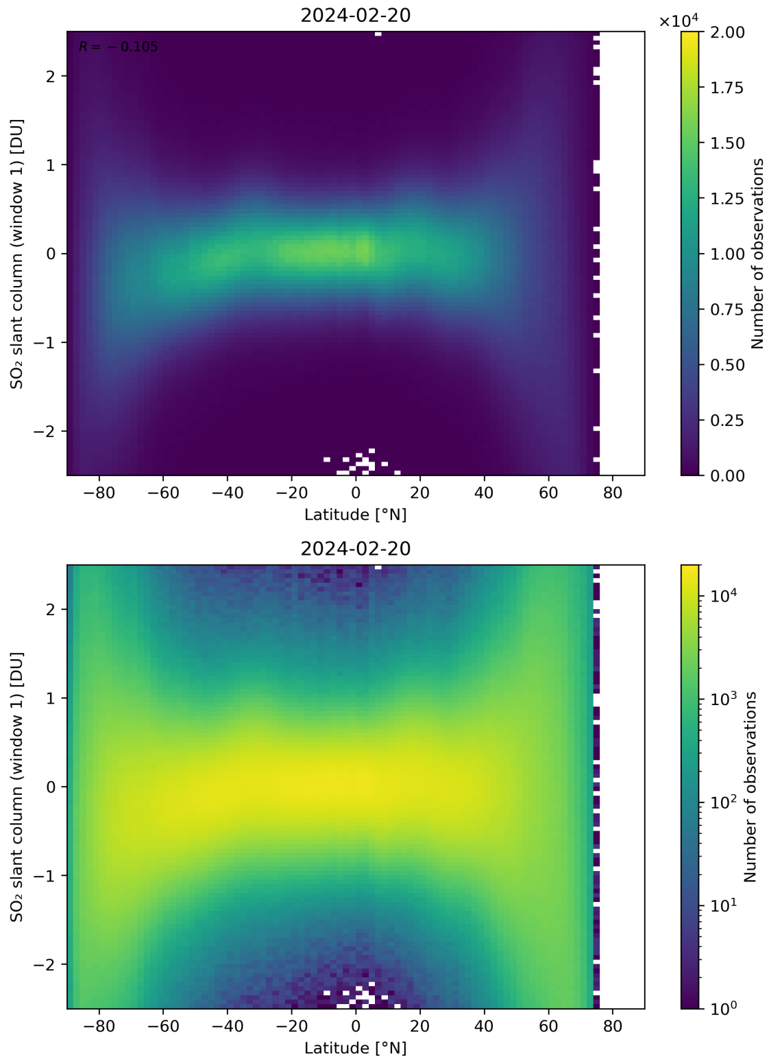
Figure 149: Scatter density plot of “Latitude” against “SO 2 slant column (window 1)” for 2024-02-19 to 2024-02-21.
