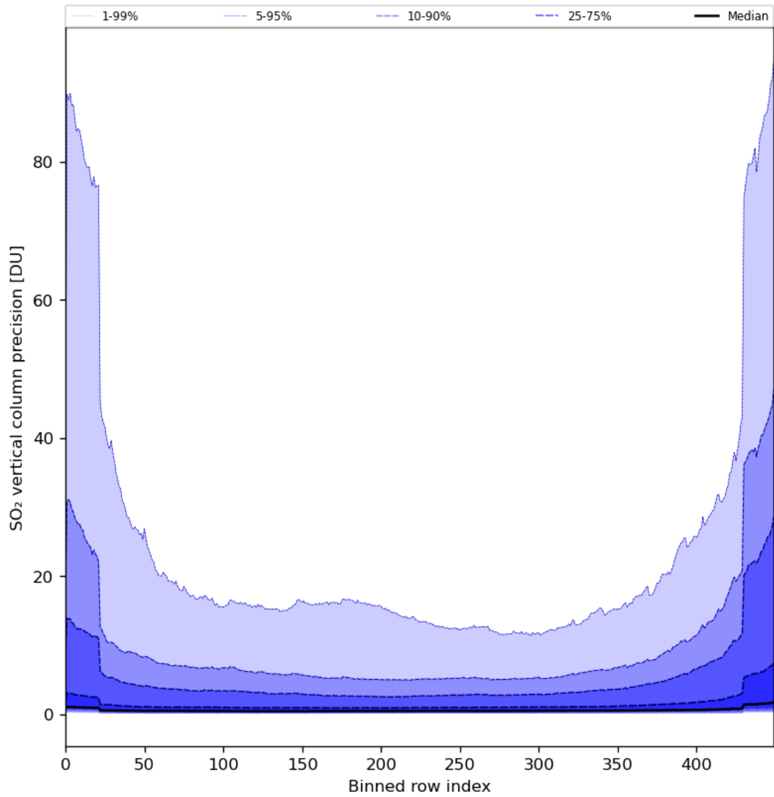
Figure 77: Along track statistics of “SO 2 vertical column precision” for 2024-02-19 to 2024-02-21
