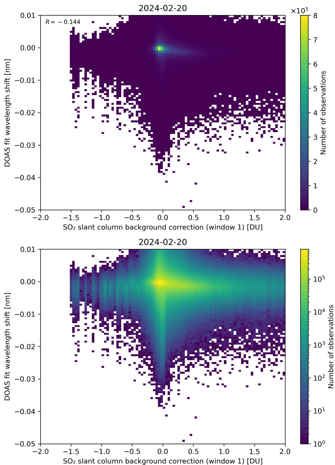
Figure 100: Scatter density plot of “SO 2 slant column background correction (window 1)” against “DOAS fit wavelength shift” for 2024-02-19 to 2024-02-21.
