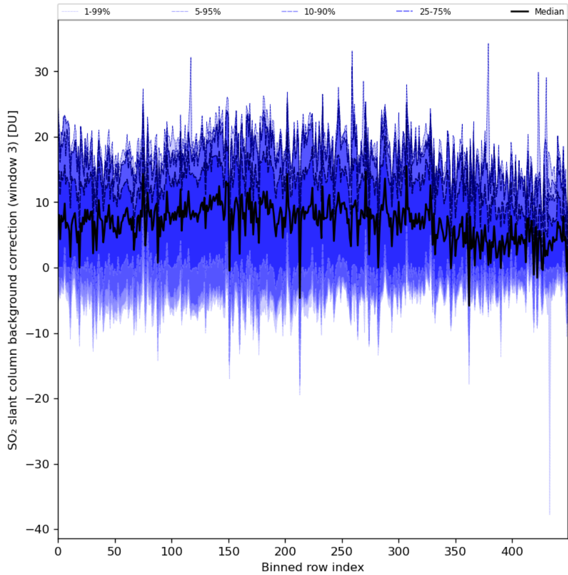
Figure 90: Along track statistics of “SO 2 slant column background correction (window 3)” for 2024-02-19 to 2024-02-21
