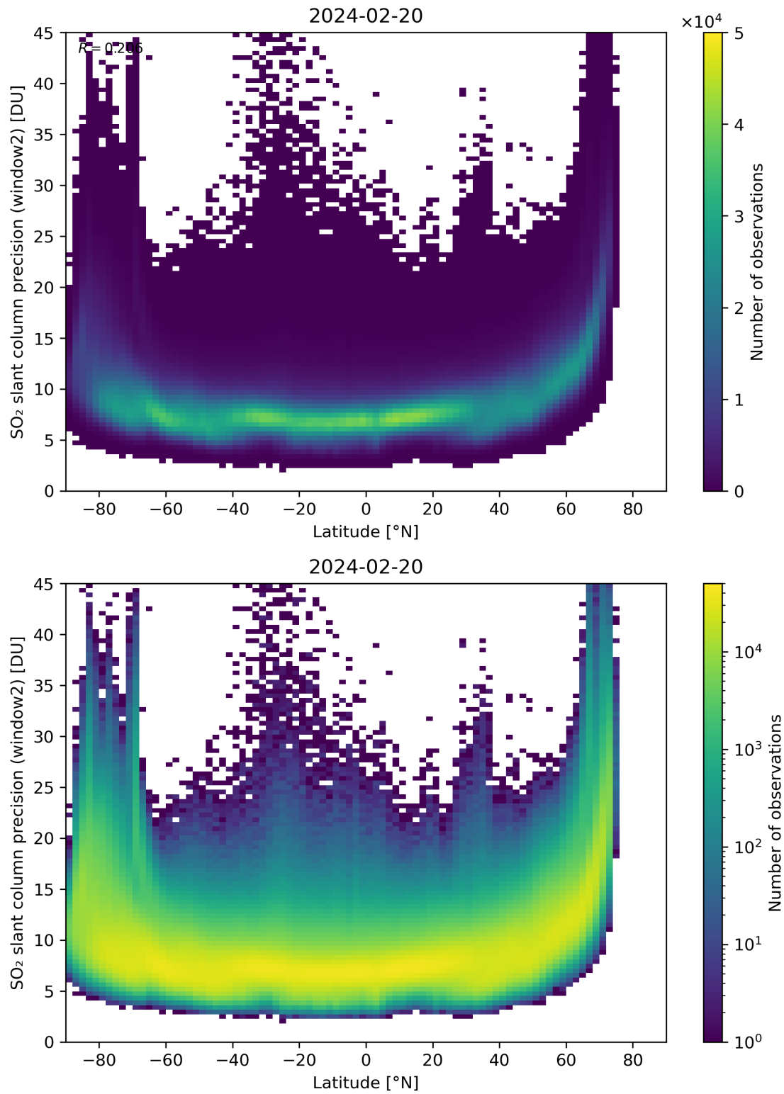
Figure 151: Scatter density plot of “Latitude” against “SO 2 slant column precision (window2)” for 2024-02-19 to 2024-02-21.
