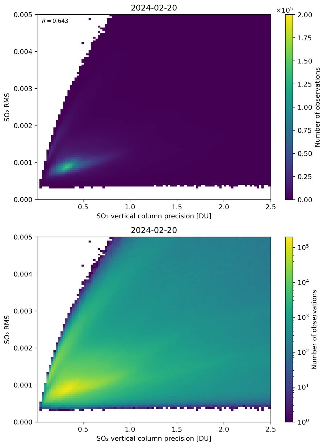
Figure 284: Scatter density plot of “SO 2 vertical column precision” against “SO 2 RMS” for 2024-02-19 to 2024-02-21.
