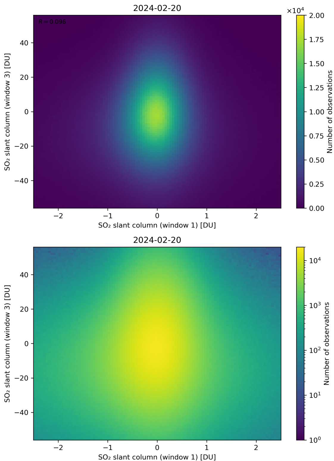
Figure 237: Scatter density plot of “SO 2 slant column (window 1)” against “SO 2 slant column (window 3)” for 2024-02-19 to 2024-02-21.
