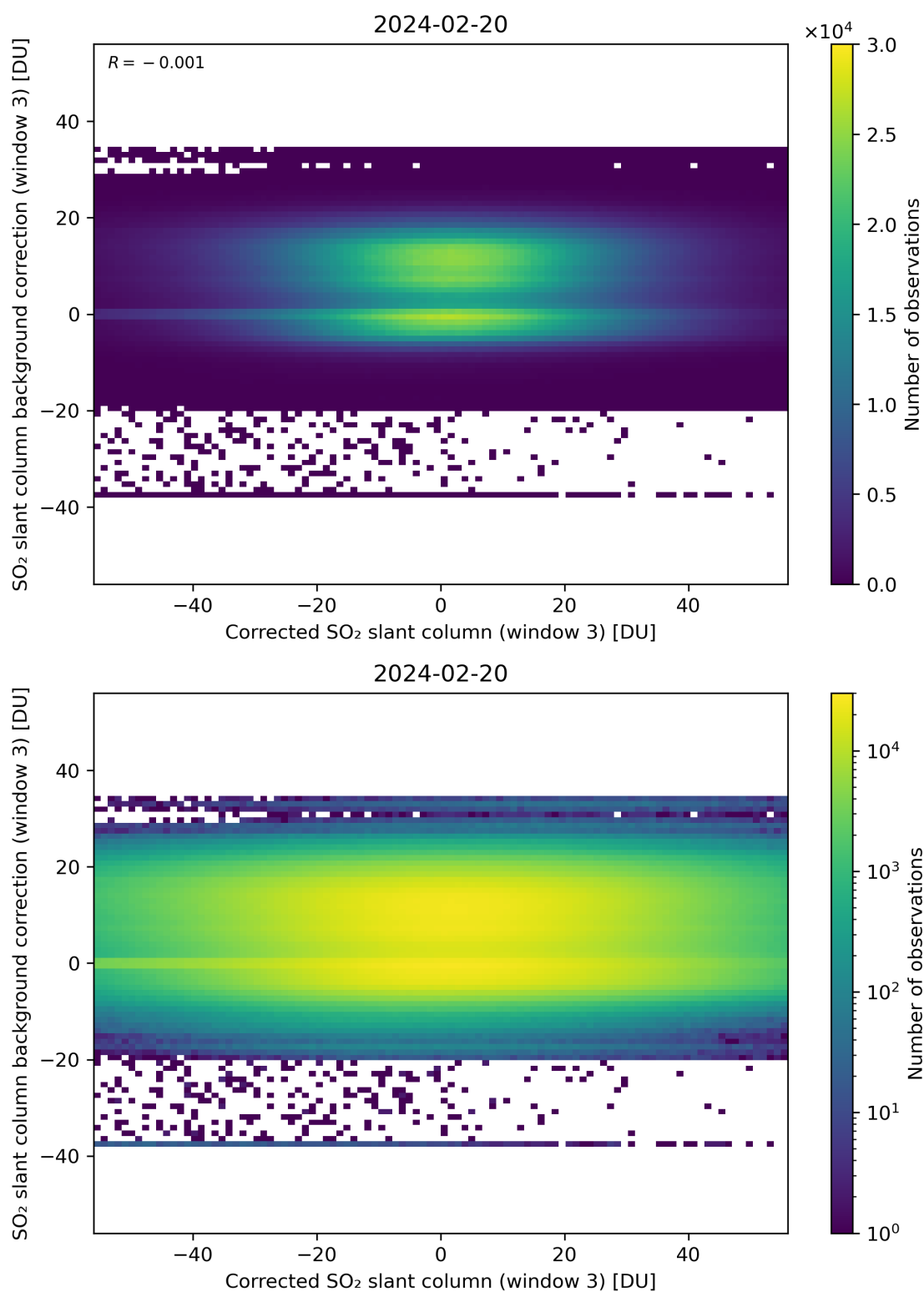
Figure 205: Scatter density plot of “Corrected SO 2 slant column (window 3)” against “SO 2 slant column background correction (window 3)” for 2024-02-19 to 2024-02-21.
