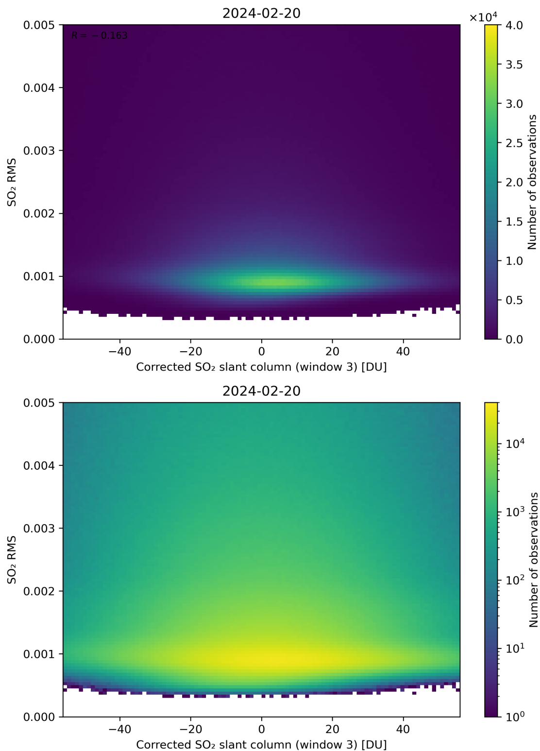
Figure 208: Scatter density plot of “Corrected SO 2 slant column (window 3)” against “SO 2 RMS” for 2024-02-19 to 2024-02-21.
