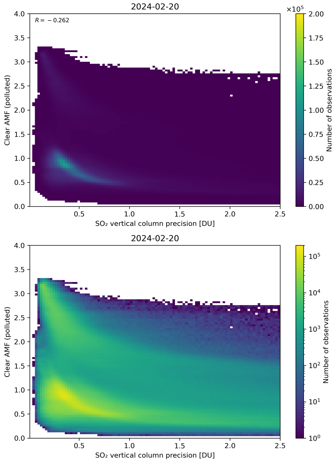
Figure 285: Scatter density plot of “SO 2 vertical column precision” against “Clear AMF (polluted)” for 2024-02-19 to 2024-02-21.
