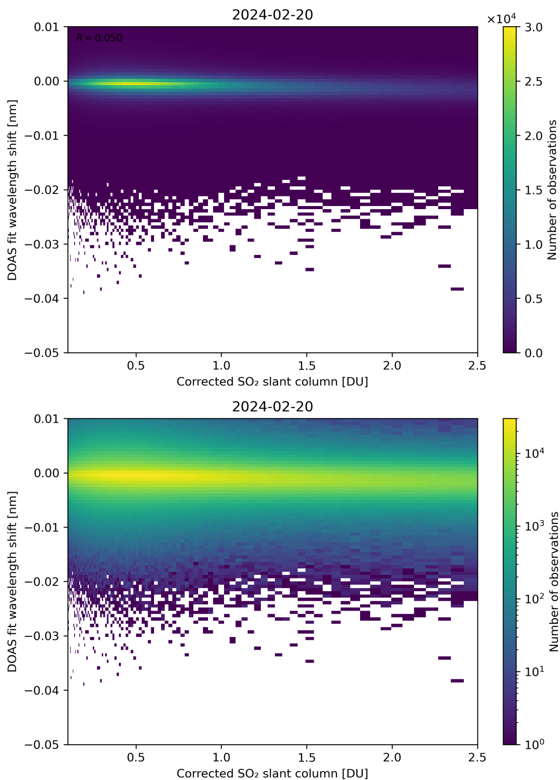
Figure 181: Scatter density plot of “Corrected SO 2 slant column” against “DOAS fit wavelength shift” for 2024-02-19 to 2024-02-21.
