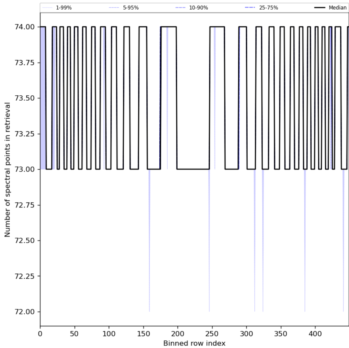
Figure 97: Along track statistics of “Number of spectral points in retrieval” for 2024-02-19 to 2024-02-21
