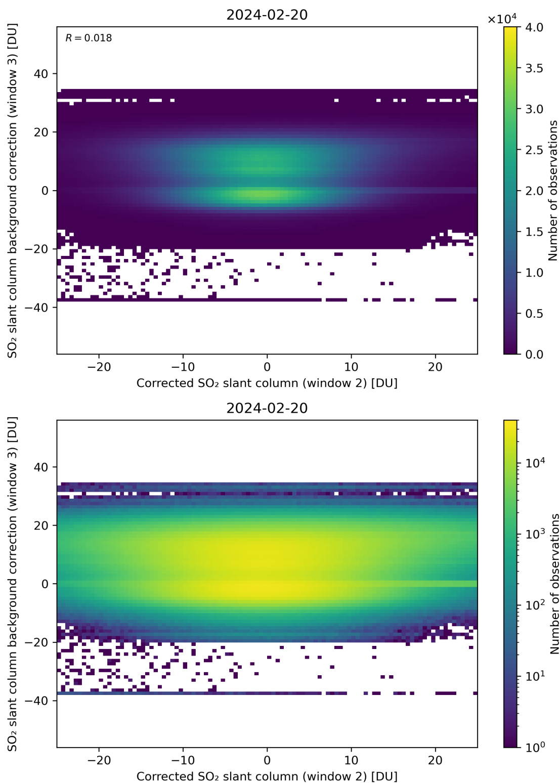
Figure 195: Scatter density plot of “Corrected SO 2 slant column (window 2)” against “SO 2 slant column background correction (window 3)” for 2024-02-19 to 2024-02-21.
