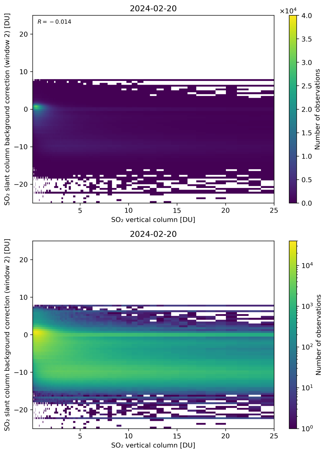
Figure 274: Scatter density plot of “SO 2 vertical column” against “SO 2 slant column background correction (window 2)” for 2024-02-19 to 2024-02-21.
