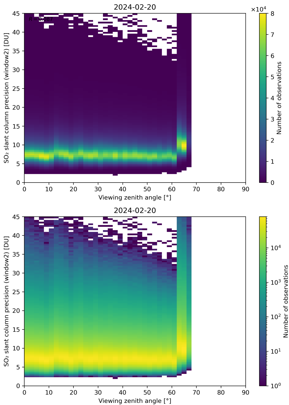
Figure 322: Scatter density plot of “Viewing zenith angle” against “SO 2 slant column precision (window2)” for 2024-02-19 to 2024-02-21.
