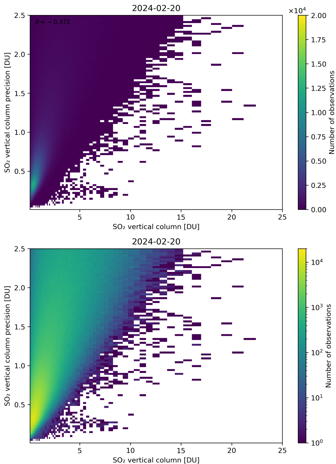
Figure 307: Scatter density plot of “SO 2 vertical column” against “SO 2 vertical column precision” for 2024-02-19 to 2024-02-21.
