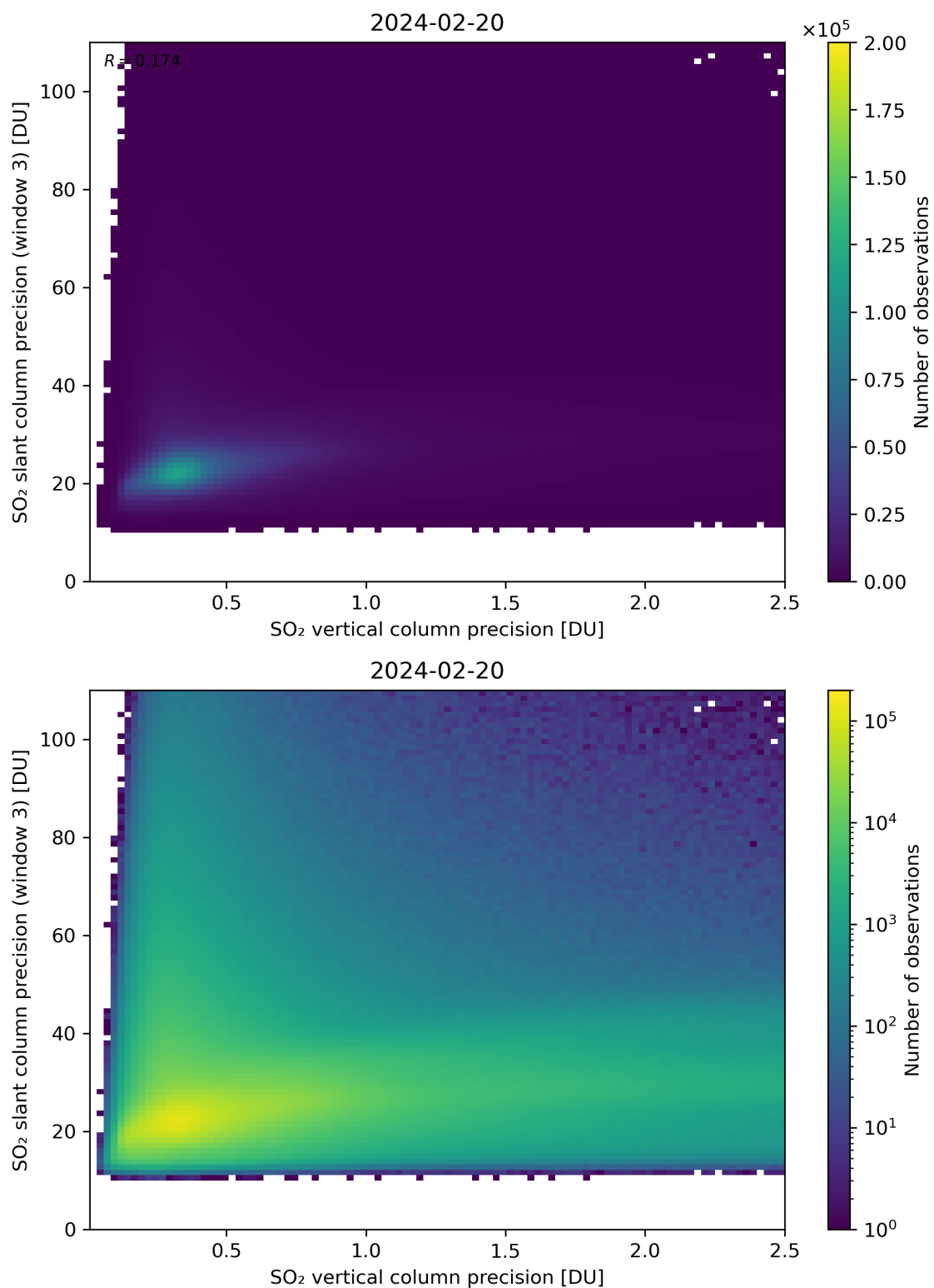
Figure 293: Scatter density plot of “SO 2 vertical column precision” against “SO 2 slant column precision (window 3)” for 2024-02-19 to 2024-02-21.
