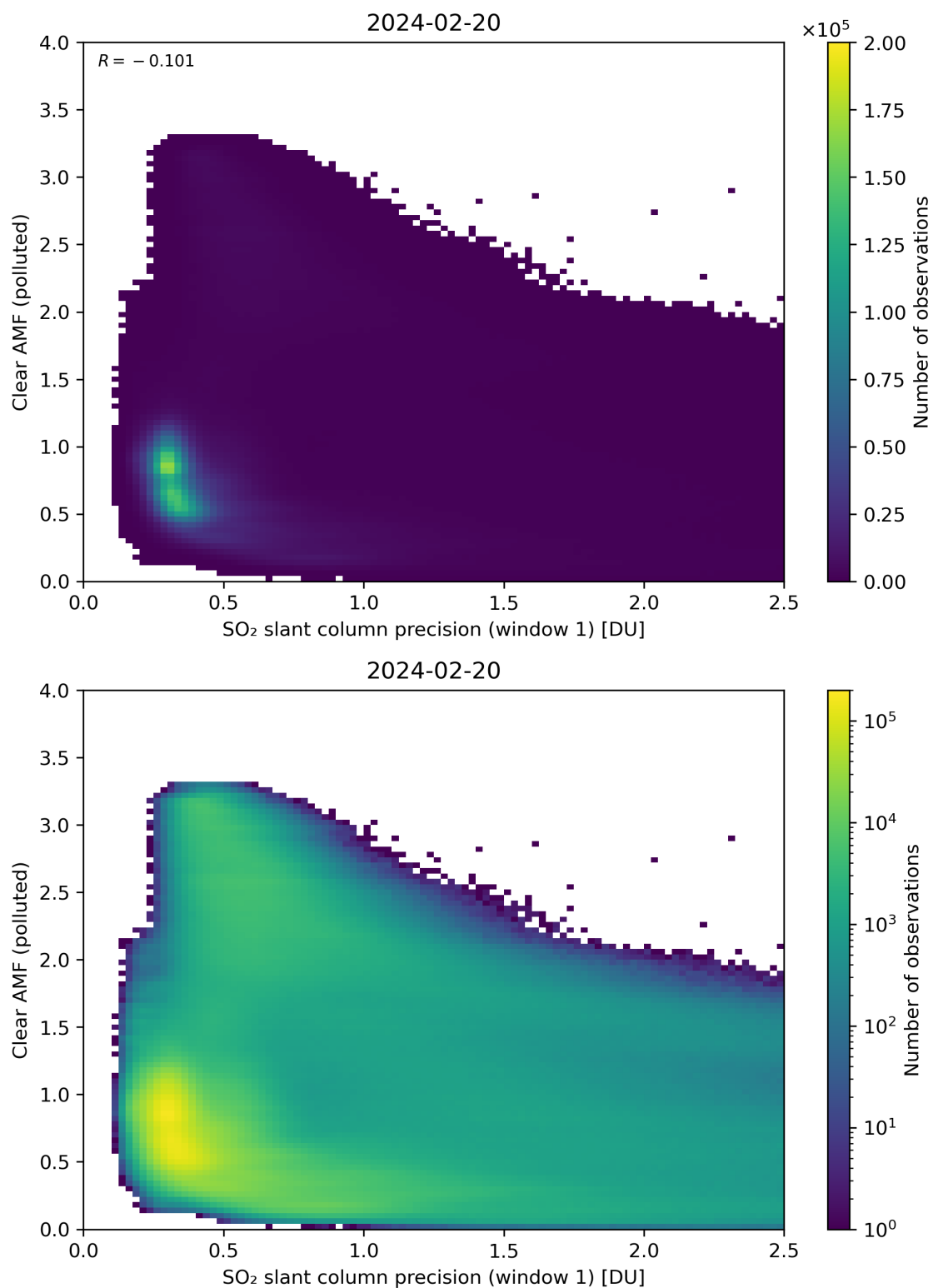
Figure 224: Scatter density plot of “SO 2 slant column precision (window 1)” against “Clear AMF (polluted)” for 2024-02-19 to 2024-02-21.
