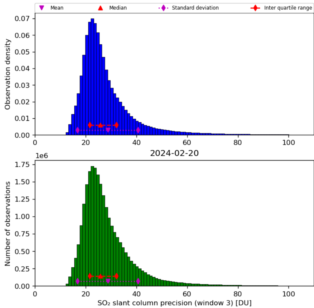
Figure 65: Histogram of “SO 2 slant column precision (window 3)” for 2024-02-19 to 2024-02-21
