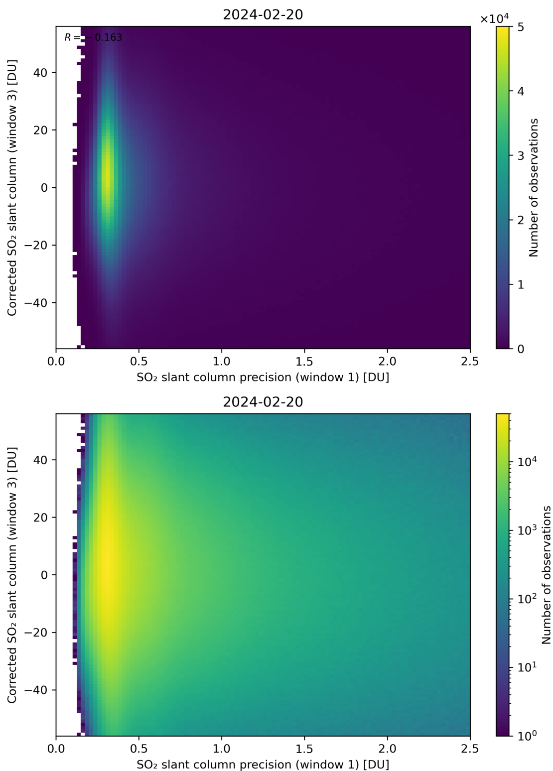
Figure 226: Scatter density plot of “SO 2 slant column precision (window 1)” against “Corrected SO 2 slant column (window 3)” for 2024-02-19 to 2024-02-21.
