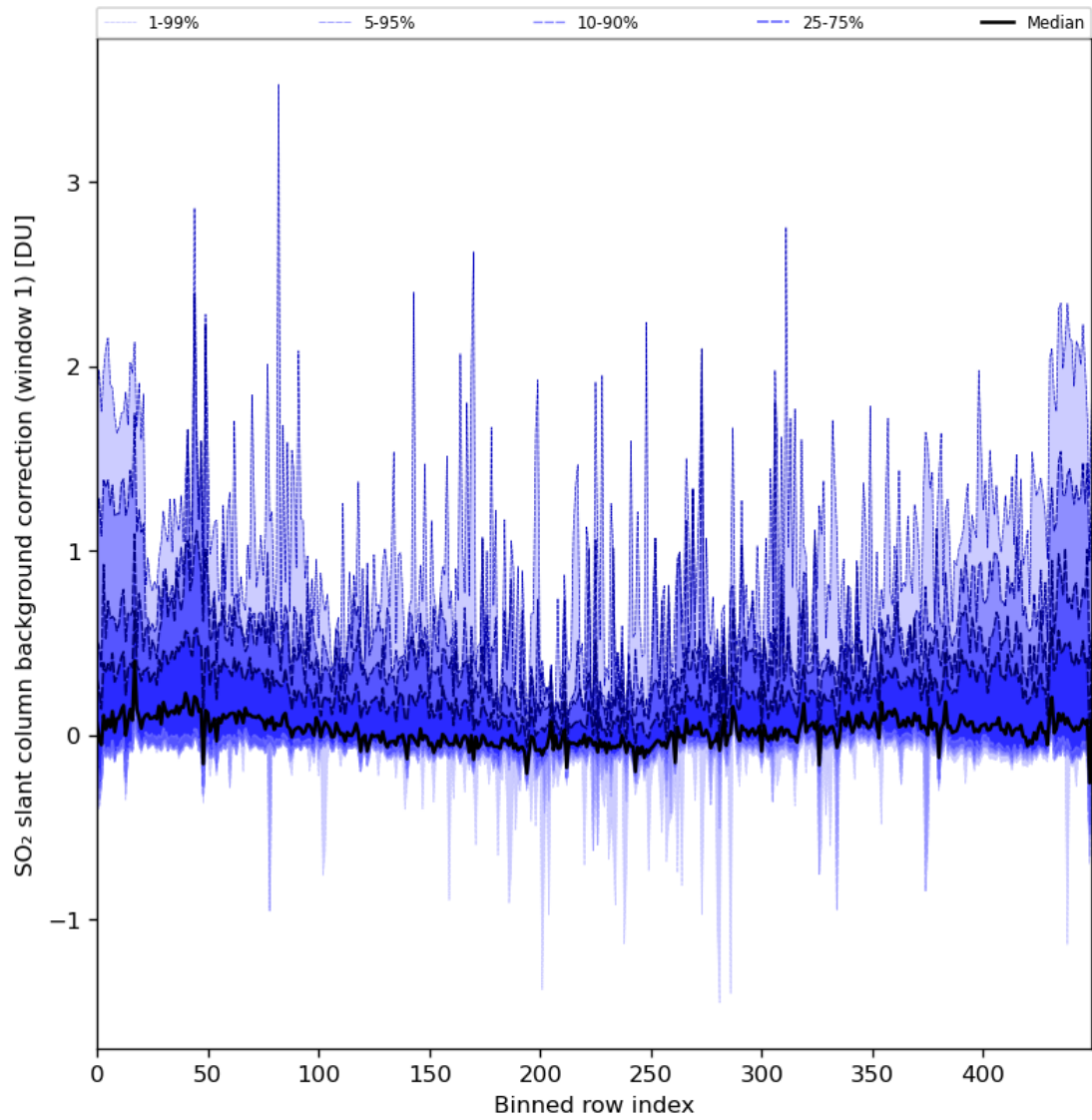
Figure 82: Along track statistics of “SO 2 slant column background correction (window 1)” for 2024-02-19 to 2024-02-21
