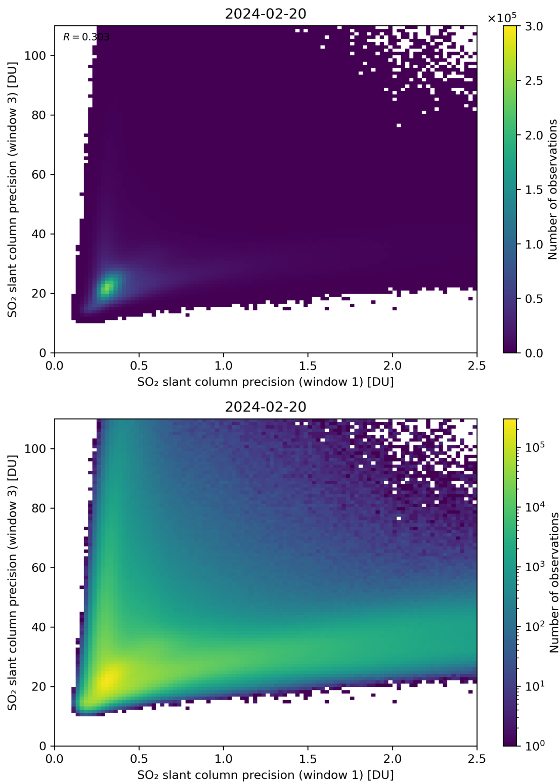
Figure 229: Scatter density plot of “SO 2 slant column precision (window 1)” against “SO 2 slant column precision (window 3)” for 2024-02-19 to 2024-02-21.
