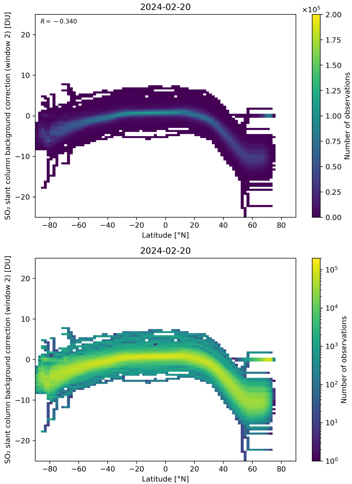
Figure 140: Scatter density plot of “Latitude” against “SO 2 slant column background correction (window 2)” for 2024-02-19 to 2024-02-21.
