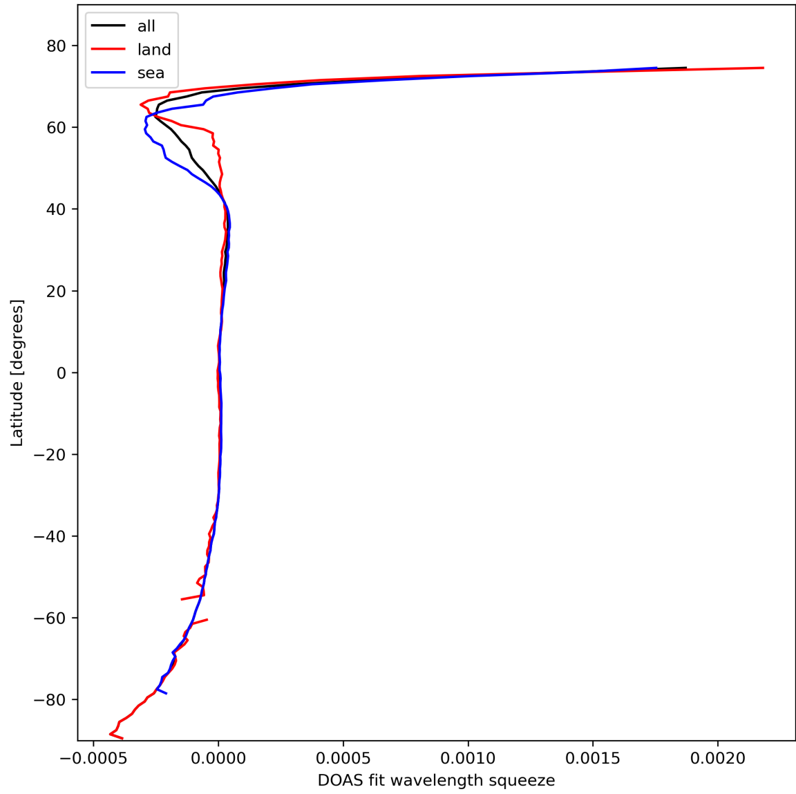
Figure 46: Zonal average of “DOAS fit wavelength squeeze” for 2024-02-19 to 2024-02-21.
