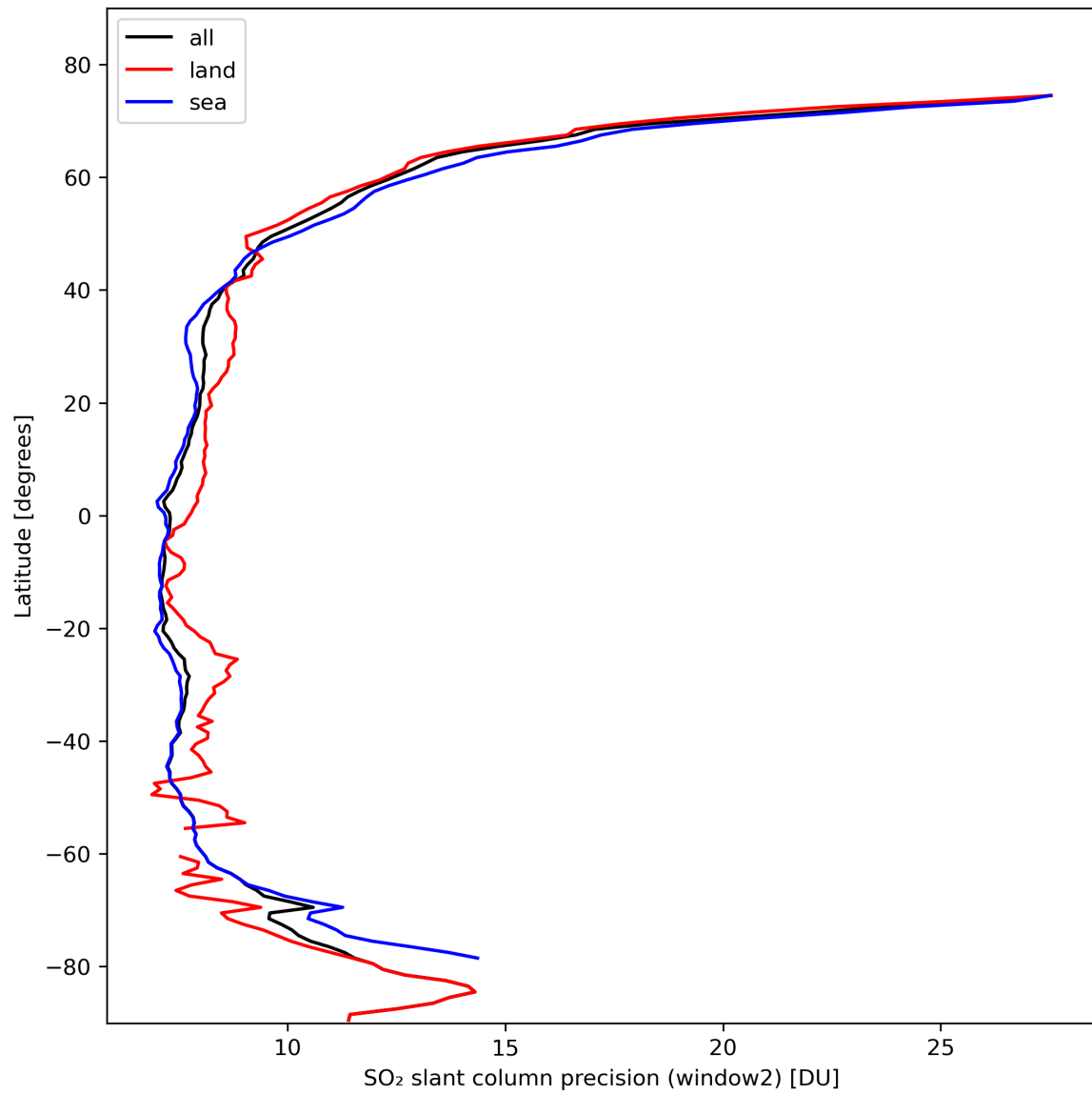
Figure 38: Zonal average of “SO 2 slant column precision (window2)” for 2024-02-19 to 2024-02-21.
