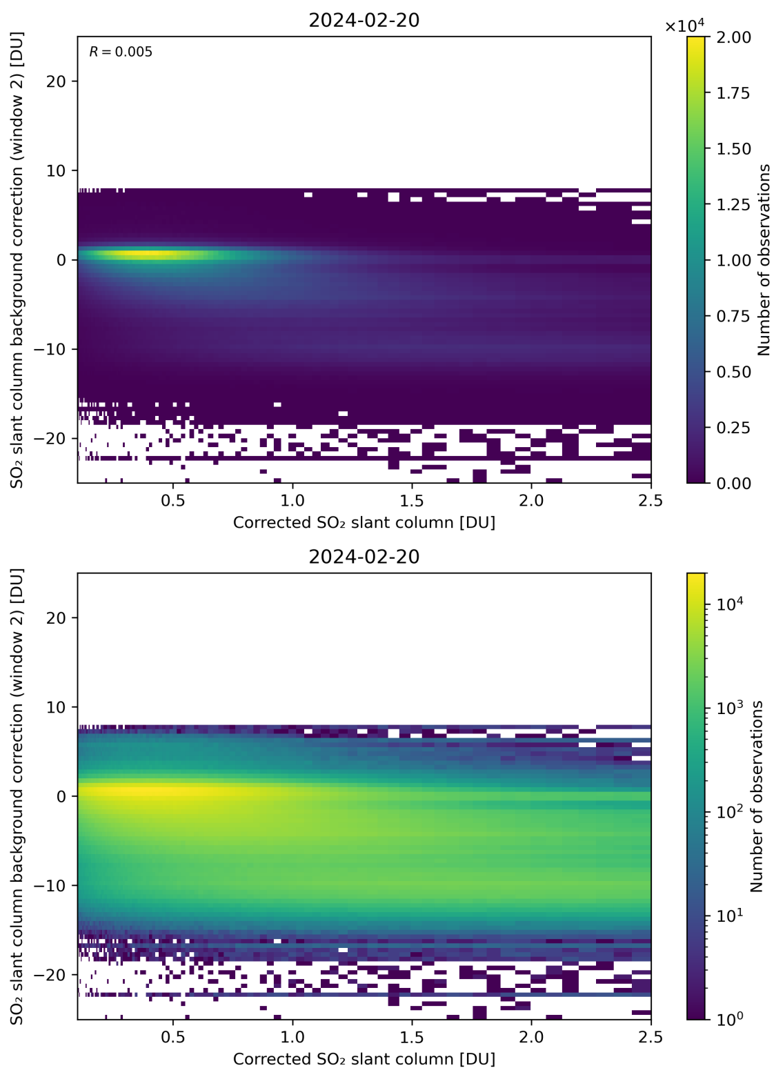
Figure 179: Scatter density plot of “Corrected SO 2 slant column” against “SO 2 slant column background correction (window 2)” for 2024-02-19 to 2024-02-21.
