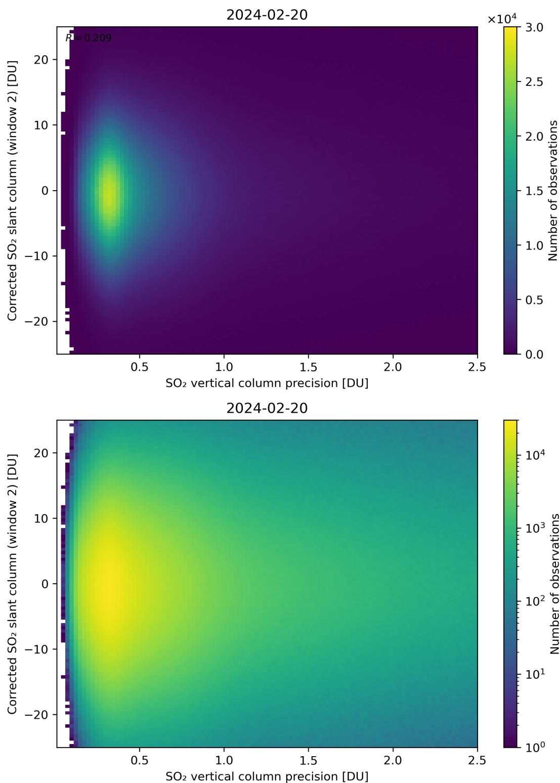
Figure 287: Scatter density plot of “SO 2 vertical column precision” against “Corrected SO 2 slant column (window 2)” for 2024-02-19 to 2024-02-21.
