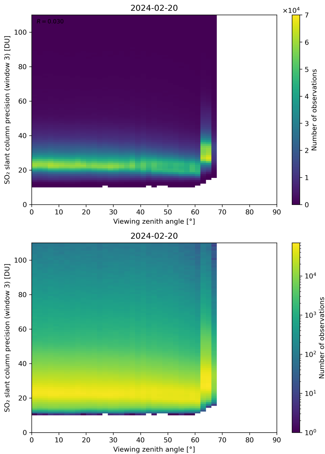
Figure 324: Scatter density plot of “Viewing zenith angle” against “SO 2 slant column precision (window 3)” for 2024-02-19 to 2024-02-21.
