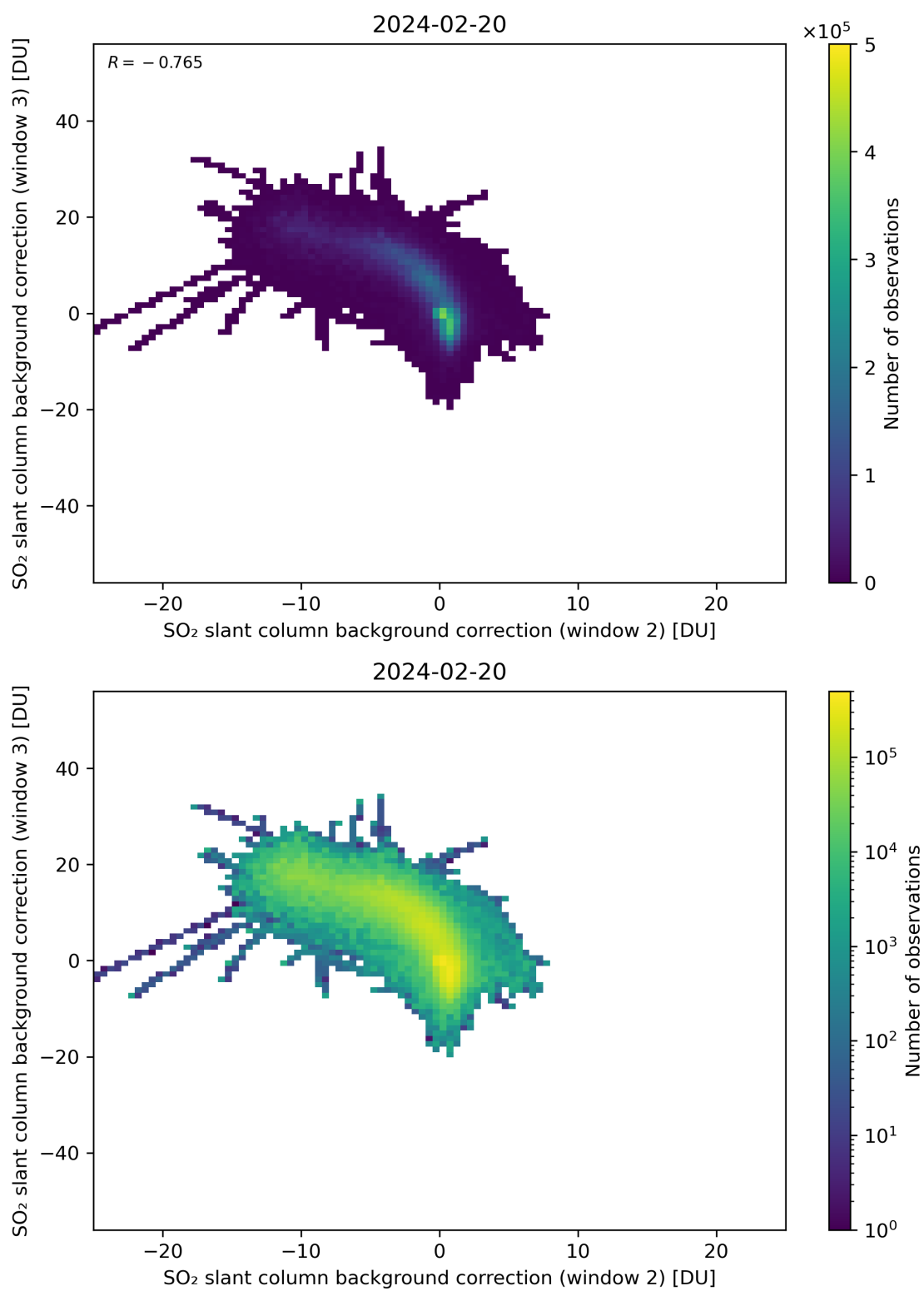
Figure 111: Scatter density plot of “SO 2 slant column background correction (window 2)” against “SO 2 slant column background correction (window 3)” for 2024-02-19 to 2024-02-21.
