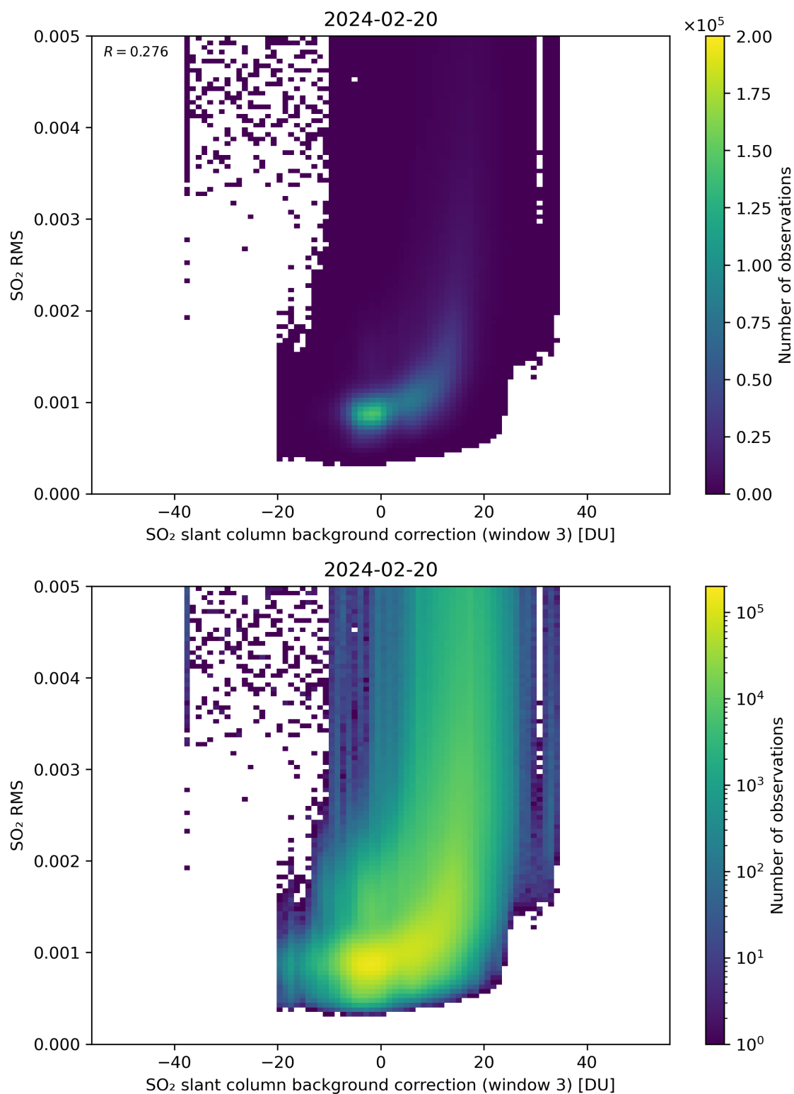
Figure 123: Scatter density plot of “SO 2 slant column background correction (window 3)” against “SO 2 RMS” for 2024-02-19 to 2024-02-21.
