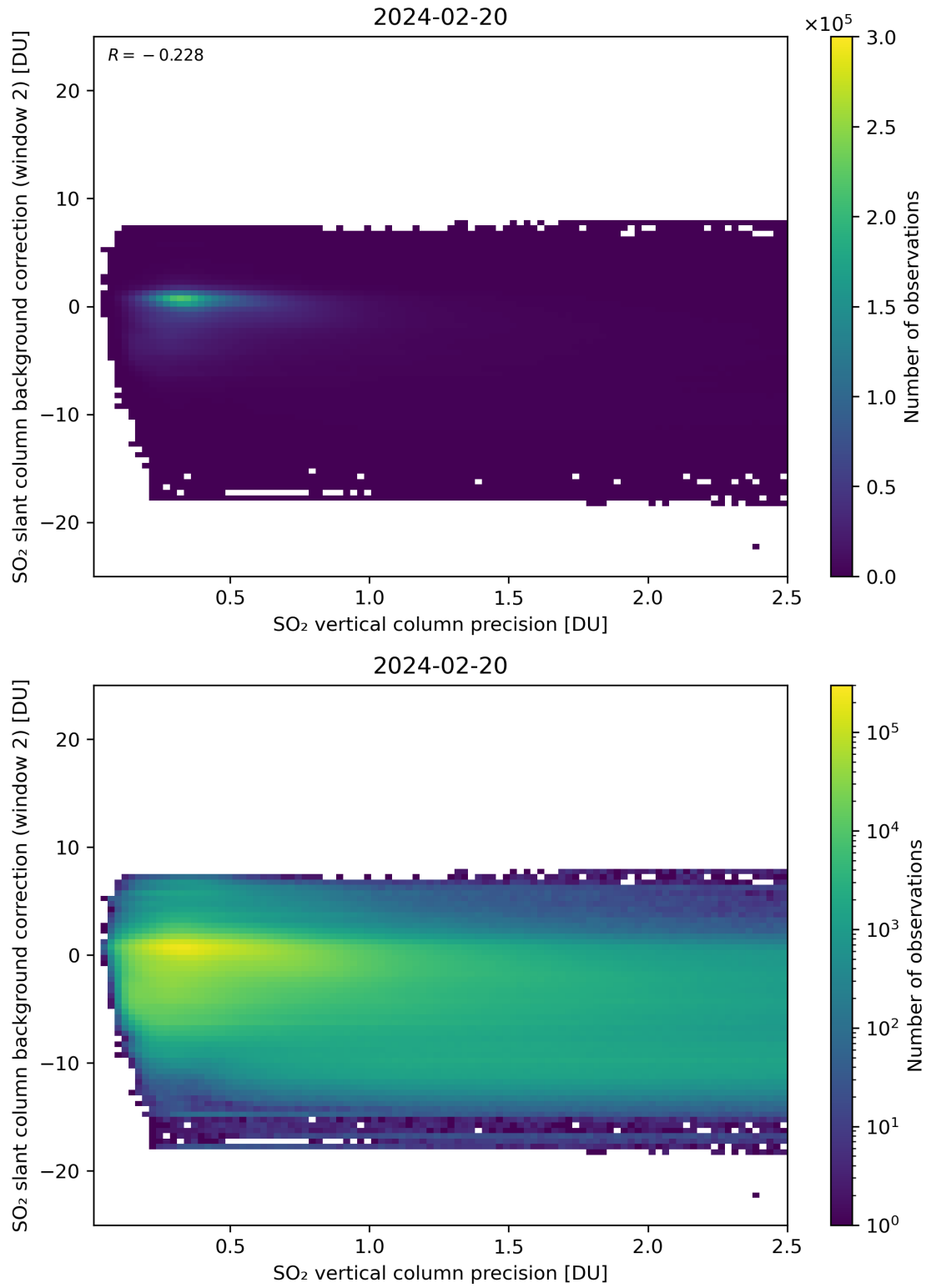
Figure 280: Scatter density plot of “SO 2 vertical column precision” against “SO 2 slant column background correction (window 2)” for 2024-02-19 to 2024-02-21.
