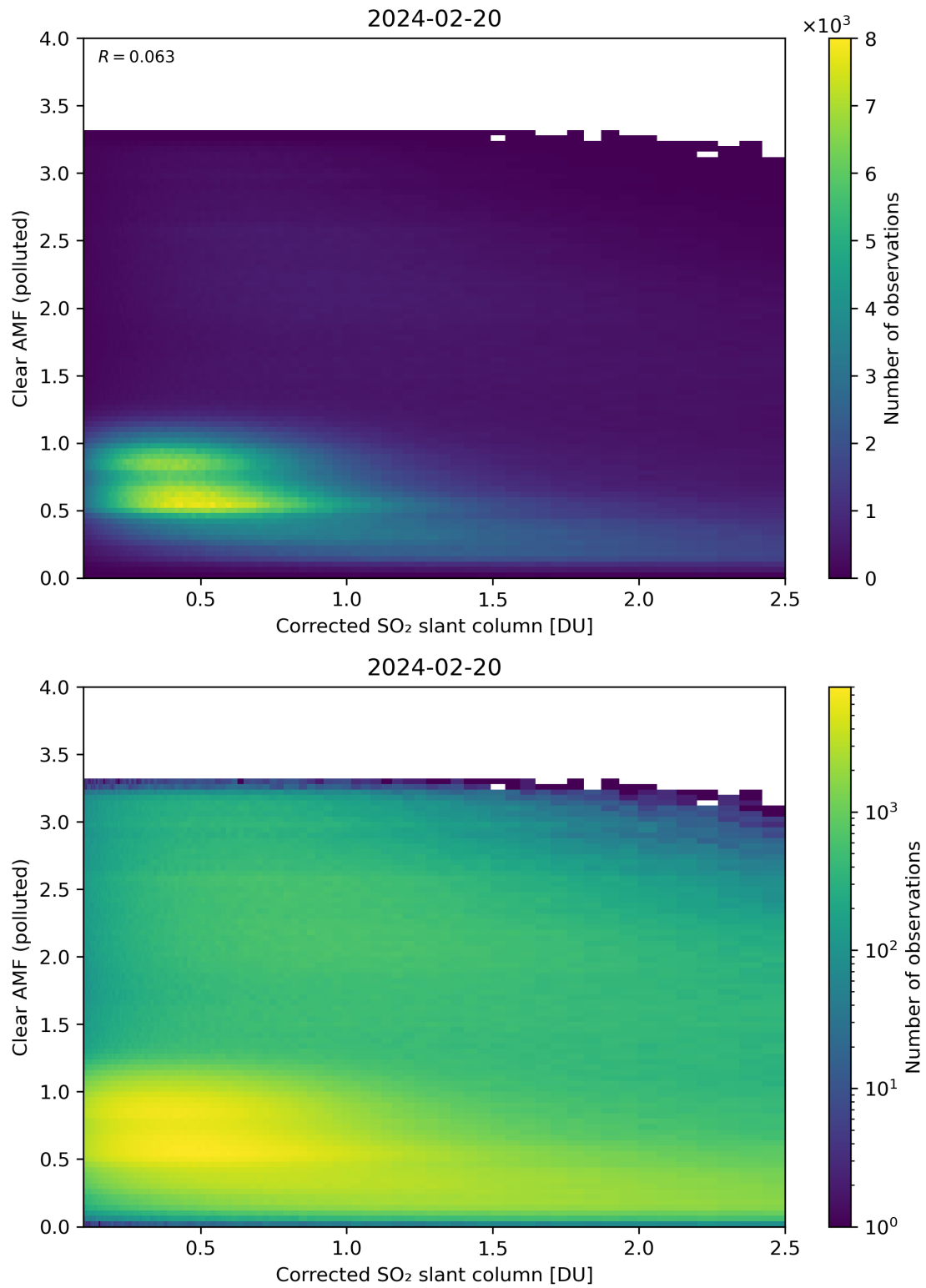
Figure 184: Scatter density plot of “Corrected SO 2 slant column” against “Clear AMF (polluted)” for 2024-02-19 to 2024-02-21.
