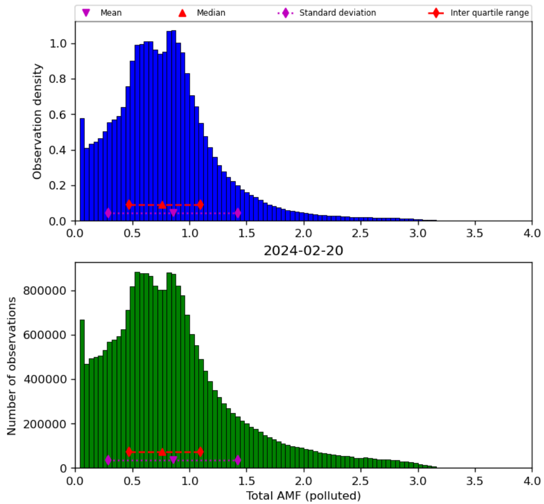
Figure 71: Histogram of “Total AMF (polluted)” for 2024-02-19 to 2024-02-21
