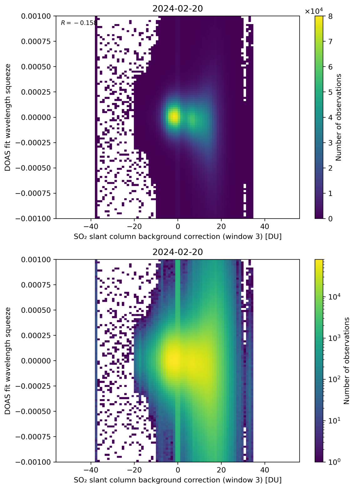
Figure 122: Scatter density plot of “SO 2 slant column background correction (window 3)” against “DOAS fit wavelength squeeze” for 2024-02-19 to 2024-02-21.
