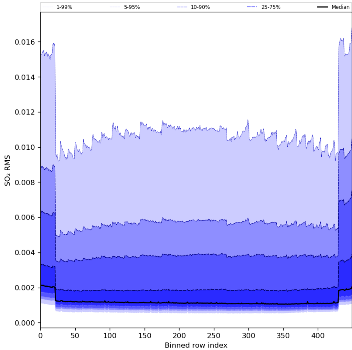
Figure 93: Along track statistics of “SO 2 RMS” for 2024-02-19 to 2024-02-21
