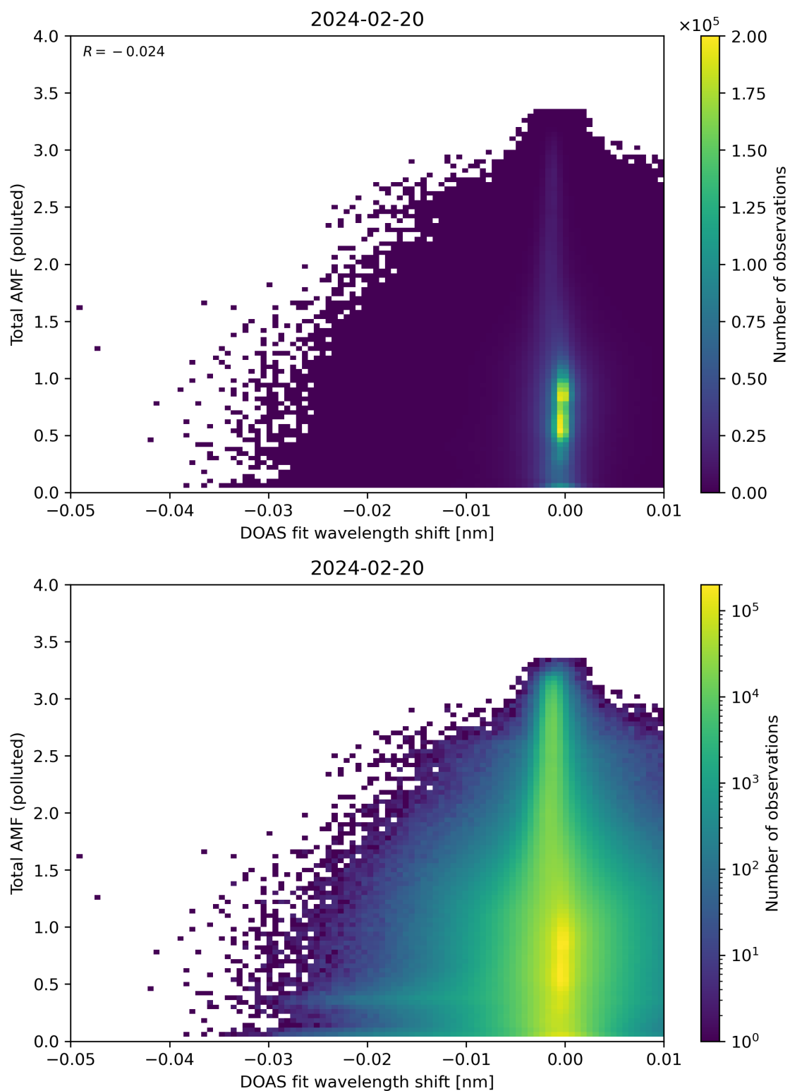
Figure 130: Scatter density plot of “DOAS fit wavelength shift” against “Total AMF (polluted)” for 2024-02-19 to 2024-02-21.
