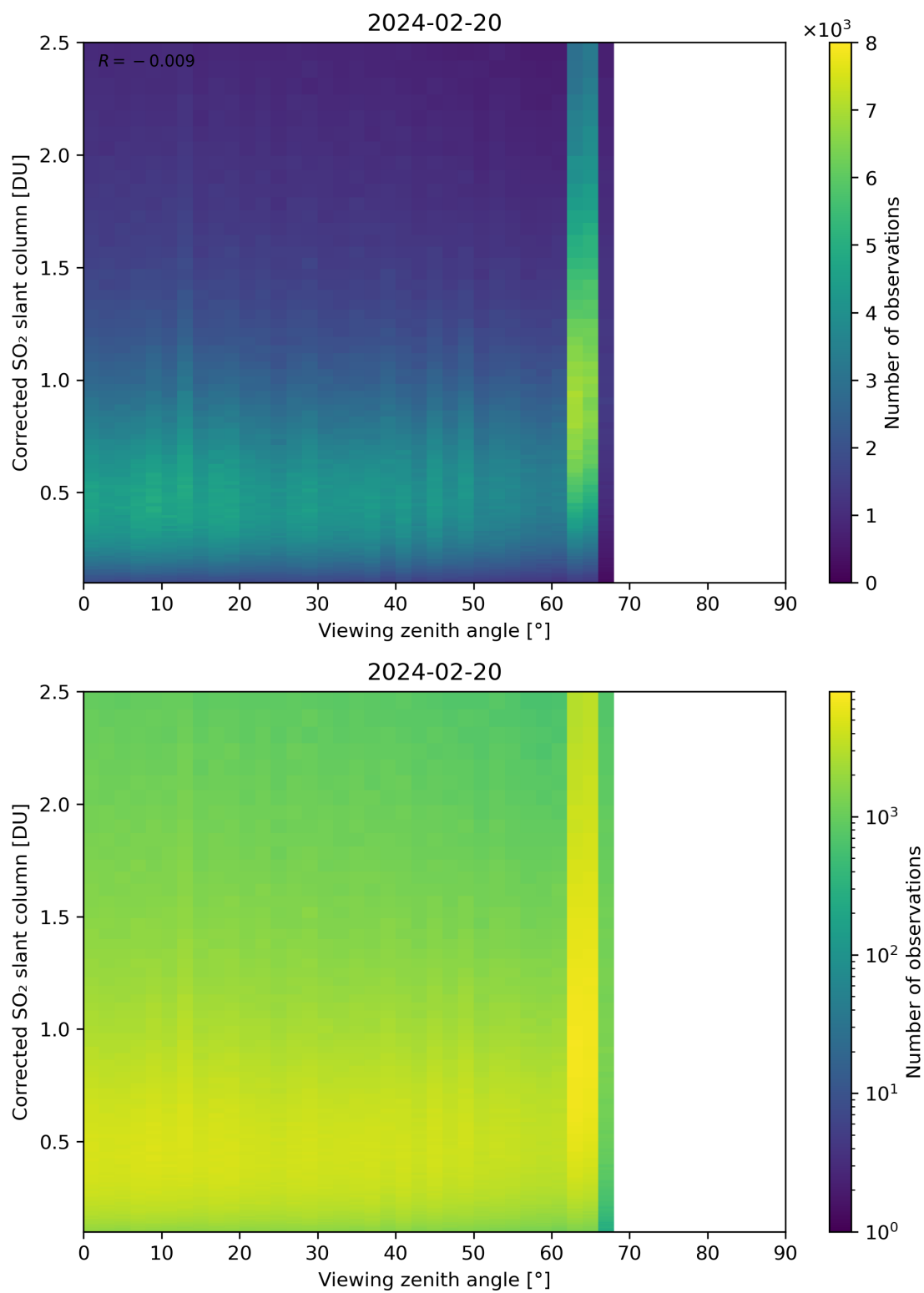
Figure 317: Scatter density plot of “Viewing zenith angle” against “Corrected SO 2 slant column” for 2024-02-19 to 2024-02-21.
