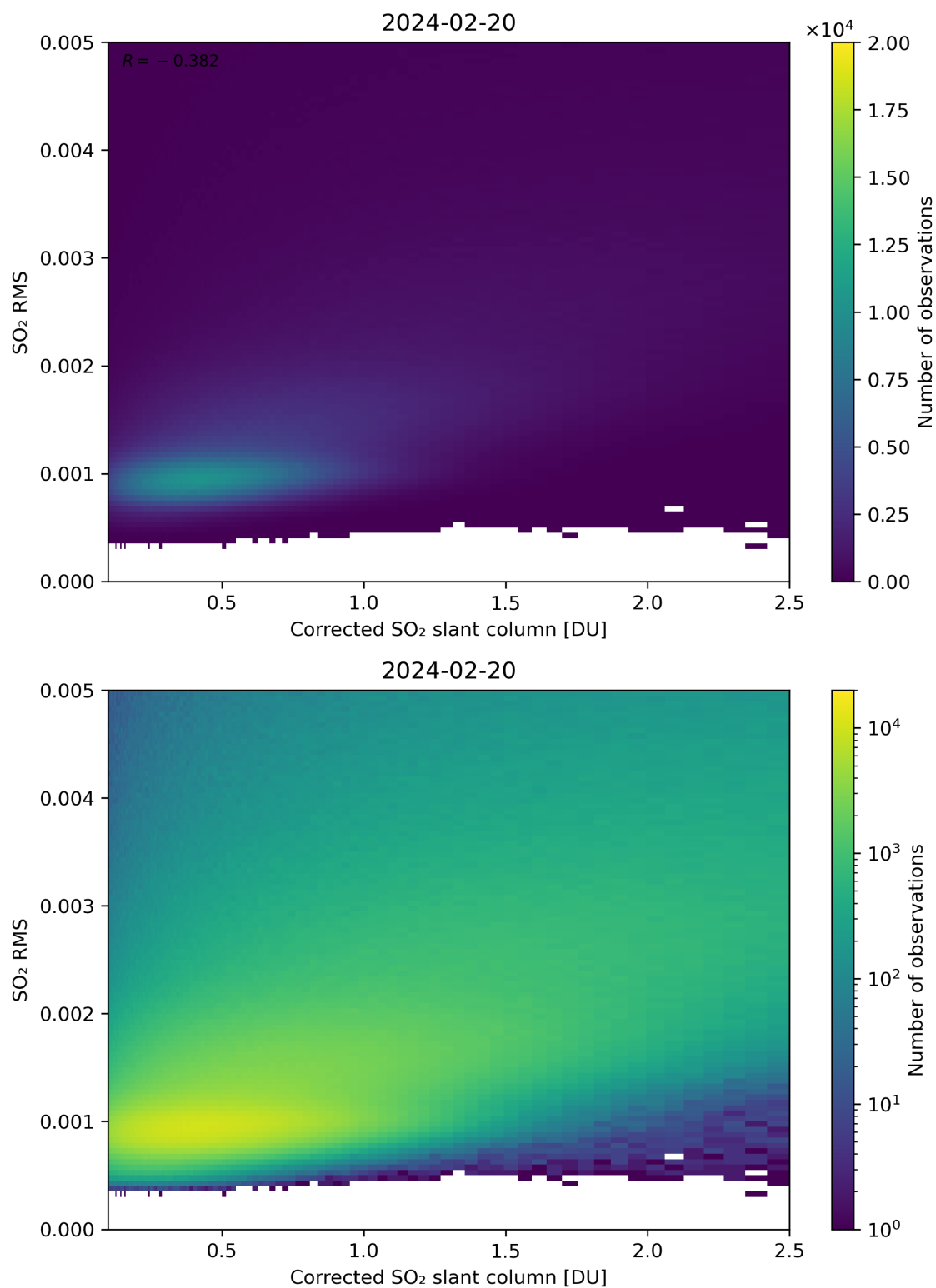
Figure 183: Scatter density plot of “Corrected SO 2 slant column” against “SO 2 RMS” for 2024-02-19 to 2024-02-21.
