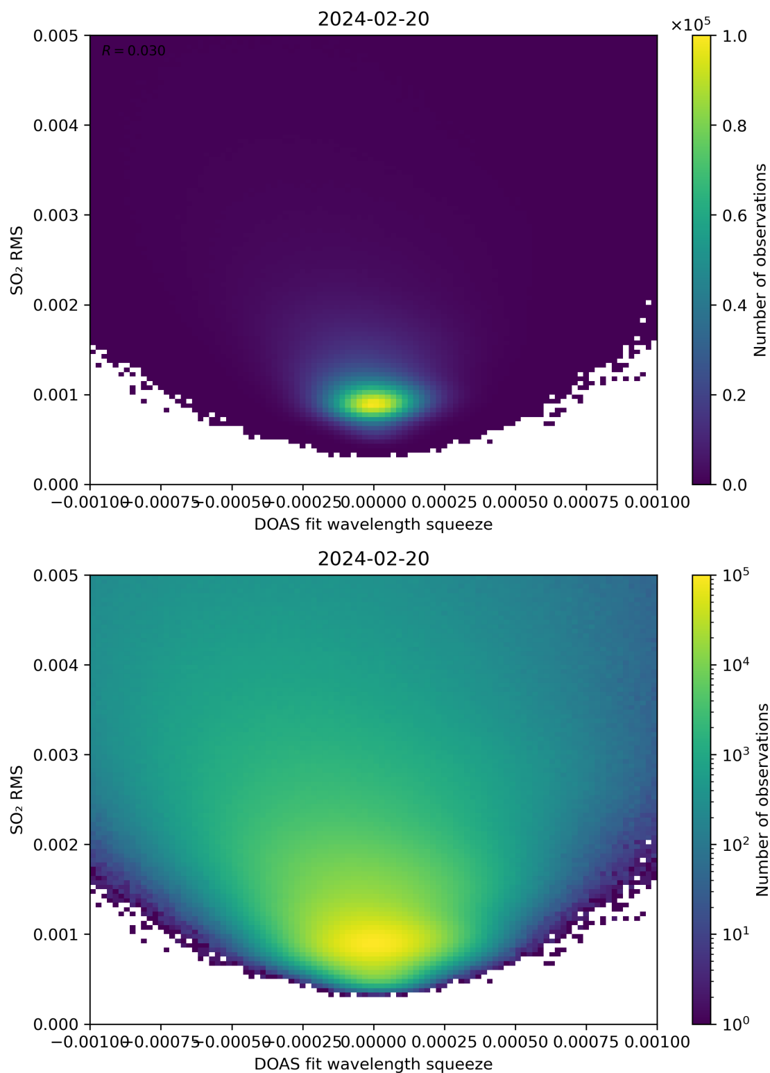
Figure 132: Scatter density plot of “DOAS fit wavelength squeeze” against “SO 2 RMS” for 2024-02-19 to 2024-02-21.
