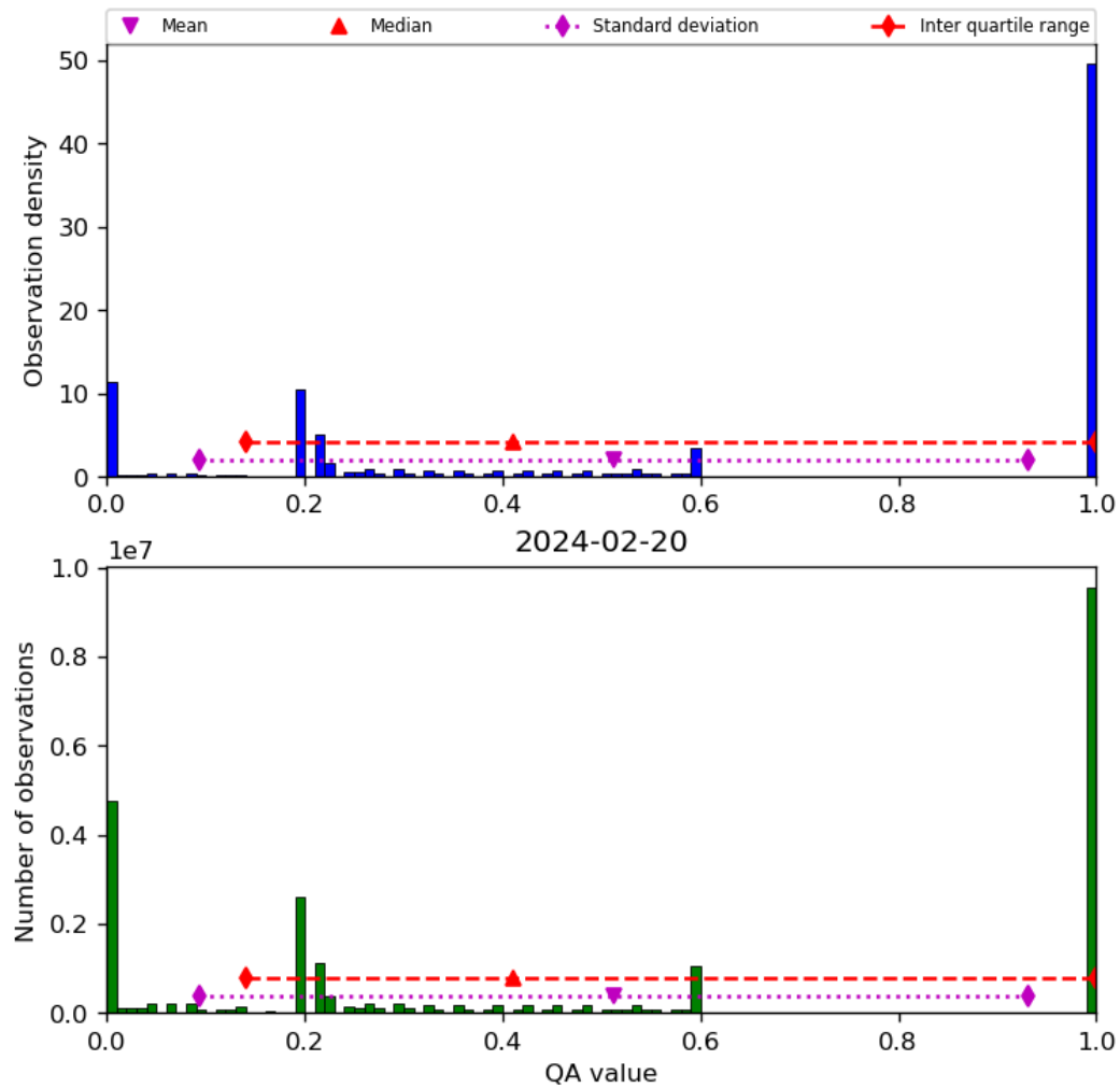
Figure 52: Histogram of “QA value” for 2024-02-19 to 2024-02-21
