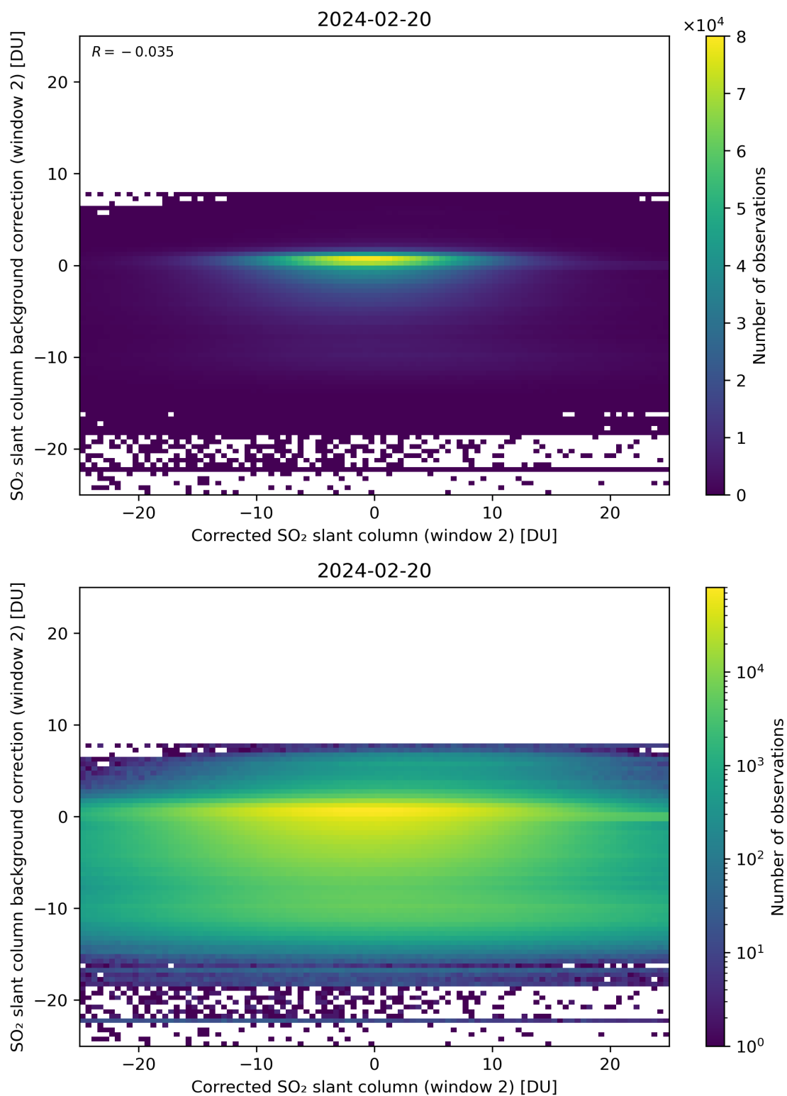
Figure 194: Scatter density plot of “Corrected SO 2 slant column (window 2)” against “SO 2 slant column background correction (window 2)” for 2024-02-19 to 2024-02-21.
