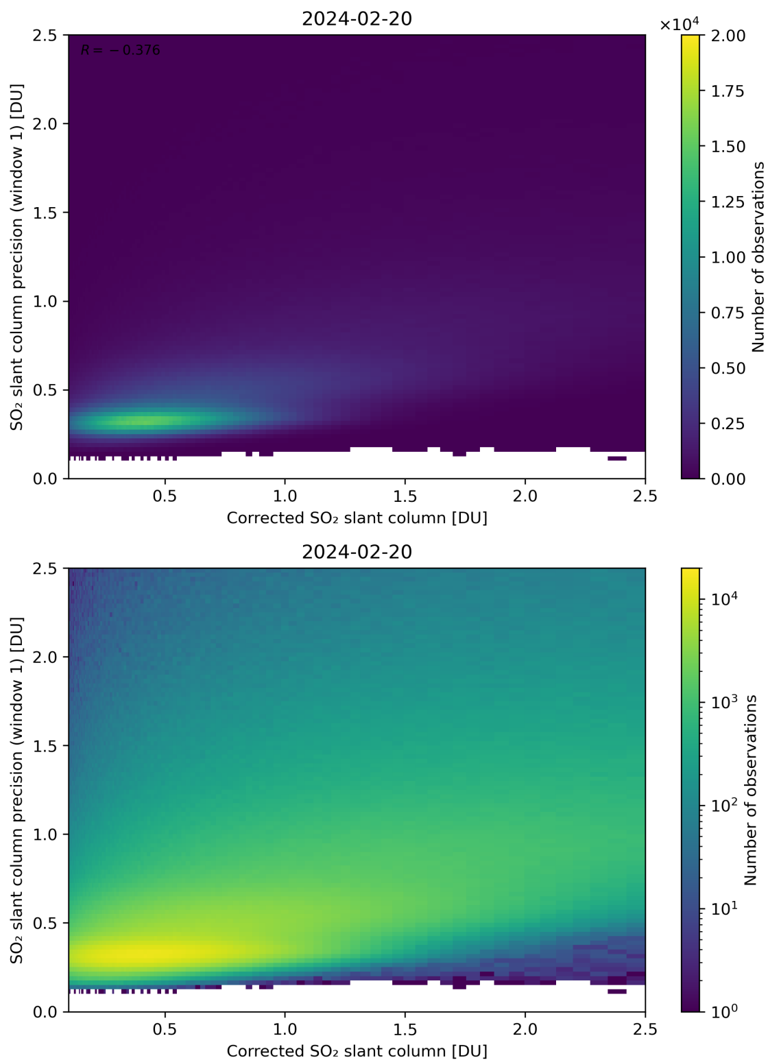
Figure 188: Scatter density plot of “Corrected SO 2 slant column” against “SO 2 slant column precision (window 1)” for 2024-02-19 to 2024-02-21.
