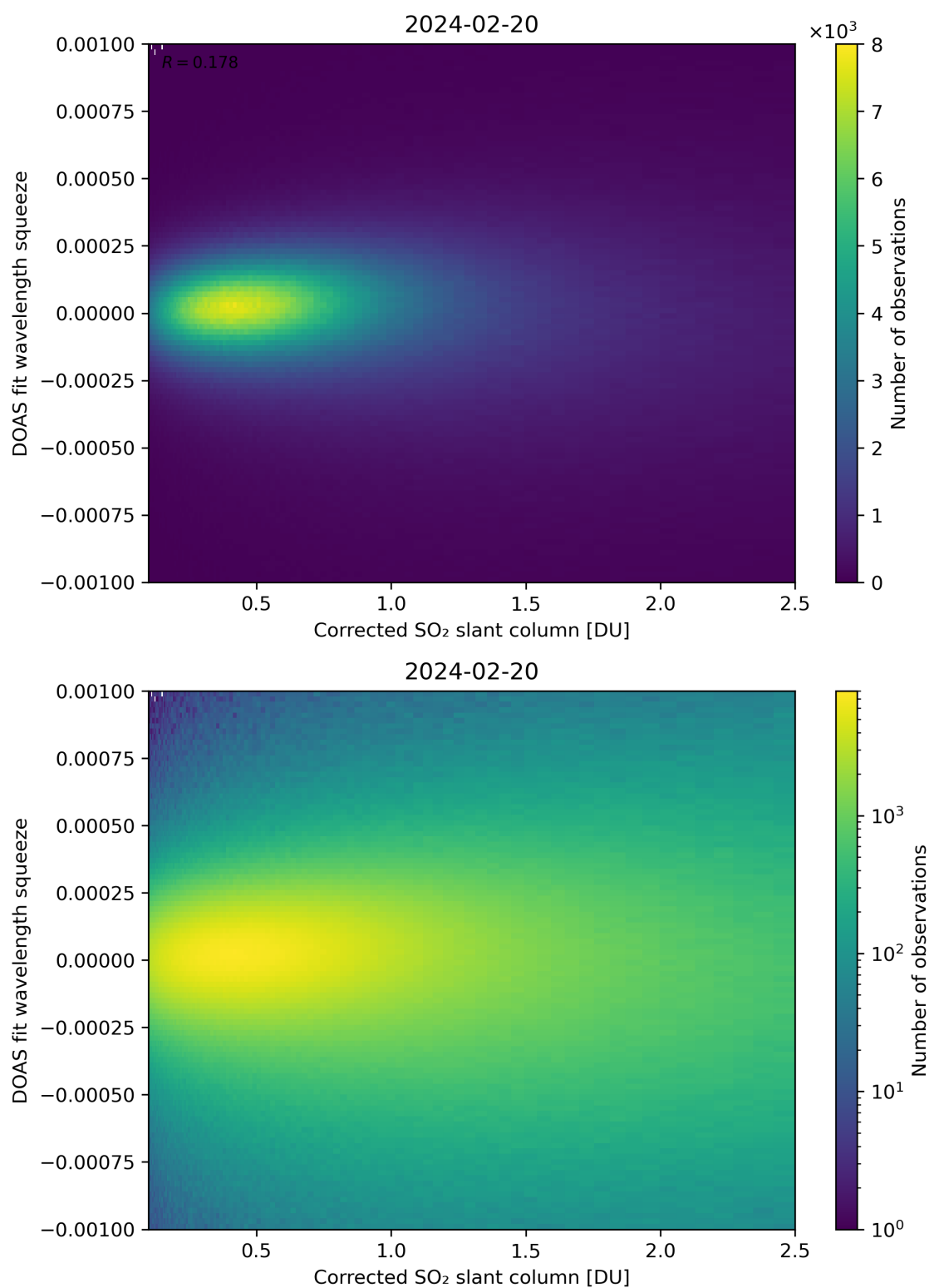
Figure 182: Scatter density plot of “Corrected SO 2 slant column” against “DOAS fit wavelength squeeze” for 2024-02-19 to 2024-02-21.
