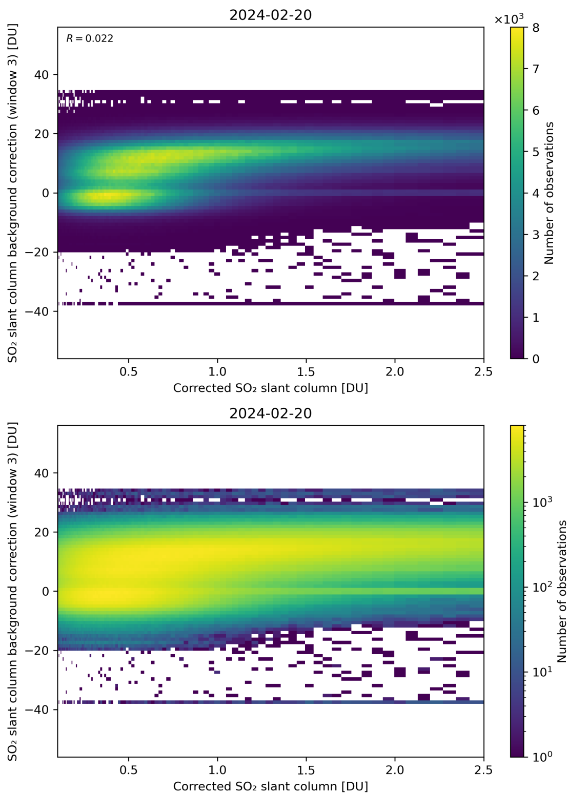
Figure 180: Scatter density plot of “Corrected SO 2 slant column” against “SO 2 slant column background correction (window 3)” for 2024-02-19 to 2024-02-21.
