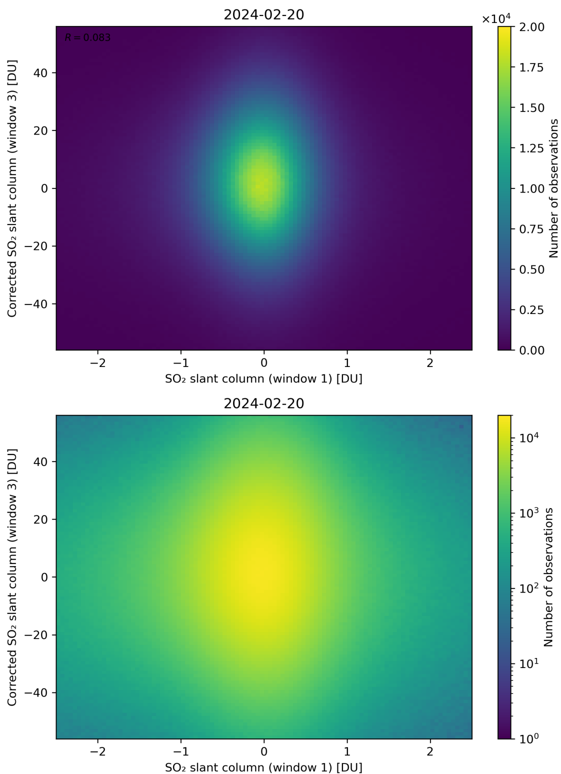
Figure 234: Scatter density plot of “SO 2 slant column (window 1)” against “Corrected SO 2 slant column (window 3)” for 2024-02-19 to 2024-02-21.
