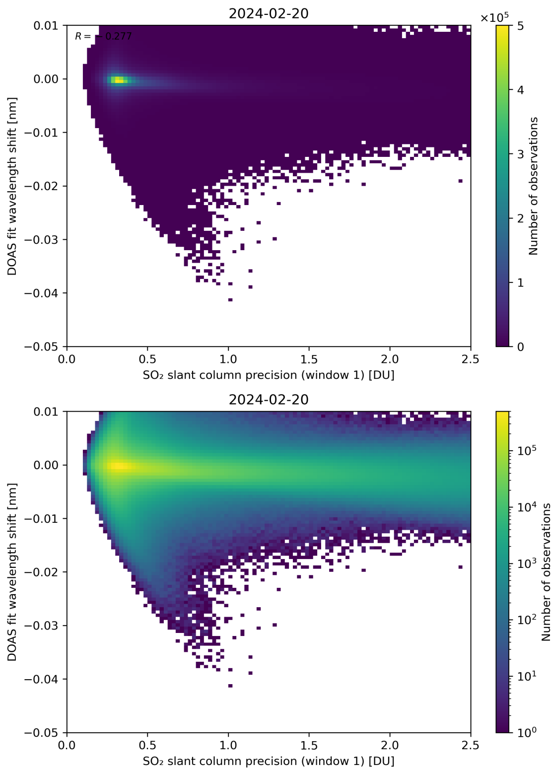
Figure 221: Scatter density plot of “SO 2 slant column precision (window 1)” against “DOAS fit wavelength shift” for 2024-02-19 to 2024-02-21.
