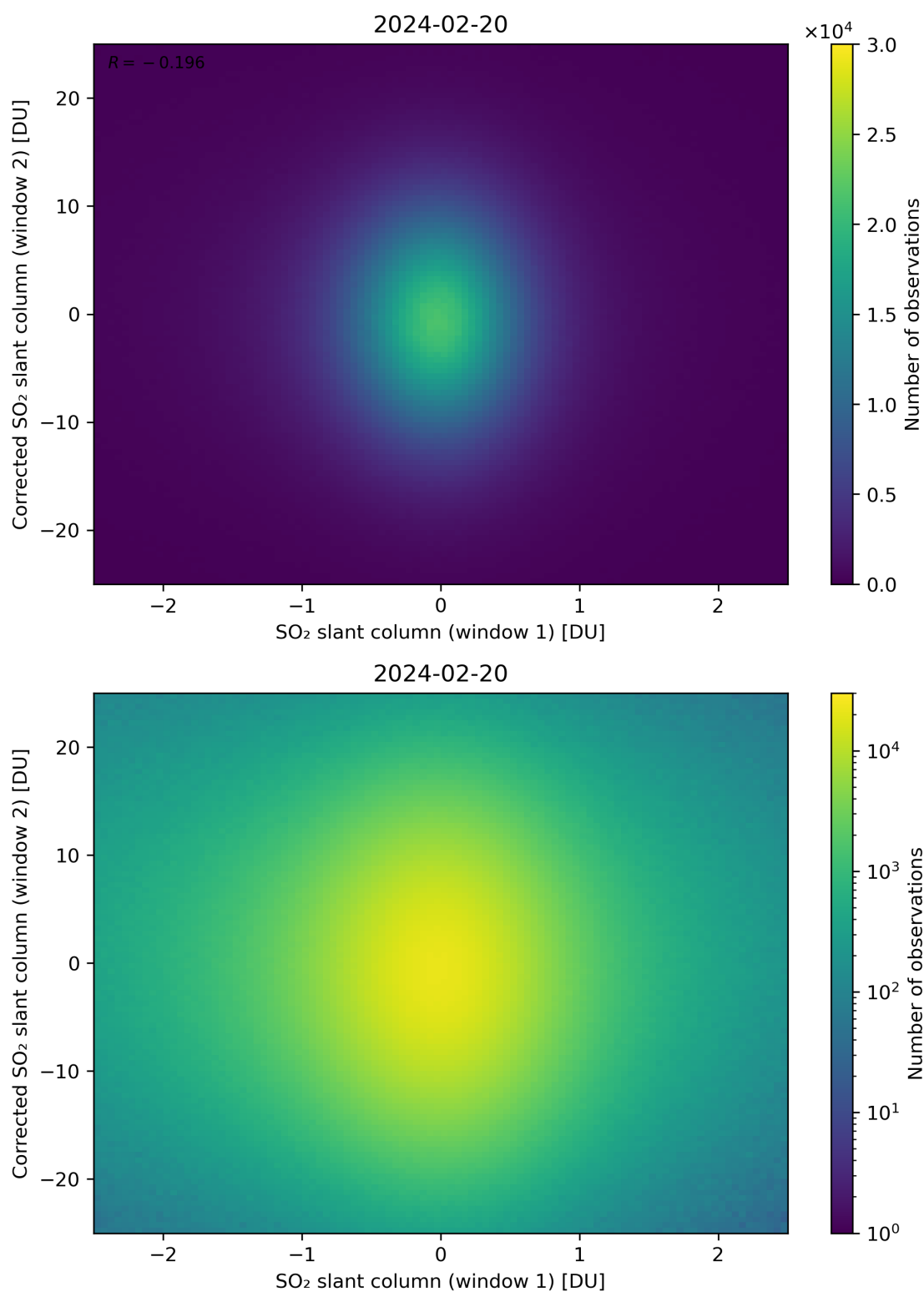
Figure 233: Scatter density plot of “SO 2 slant column (window 1)” against “Corrected SO 2 slant column (window 2)” for 2024-02-19 to 2024-02-21.
