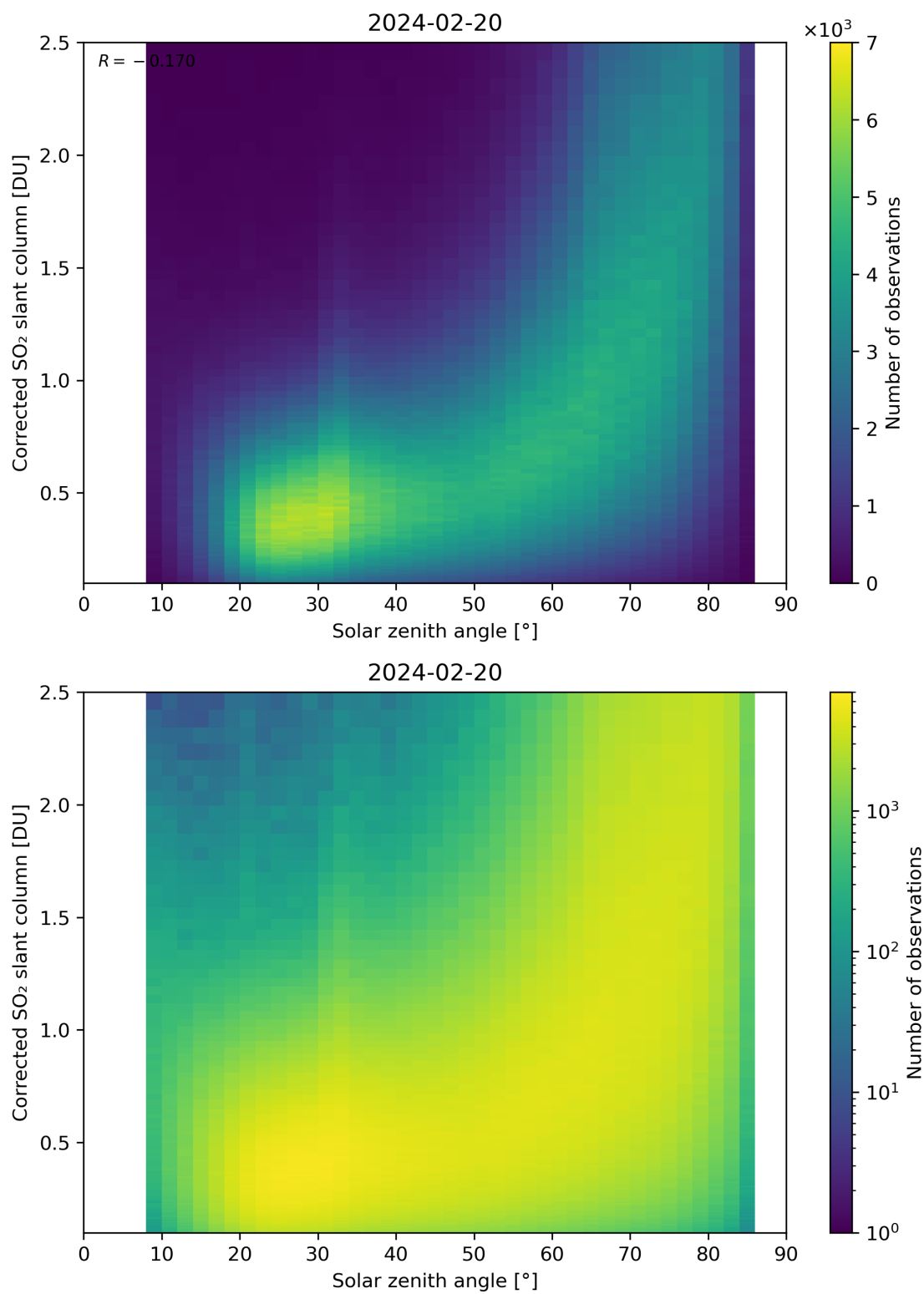
Figure 166: Scatter density plot of “Solar zenith angle” against “Corrected SO 2 slant column” for 2024-02-19 to 2024-02-21.
