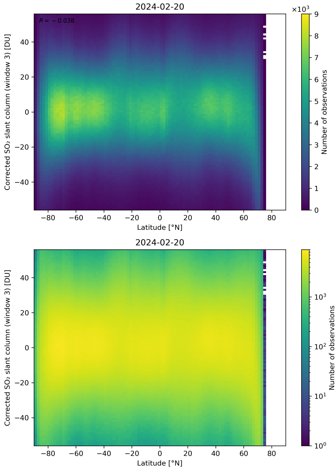
Figure 148: Scatter density plot of “Latitude” against “Corrected SO 2 slant column (window 3)” for 2024-02-19 to 2024-02-21.
