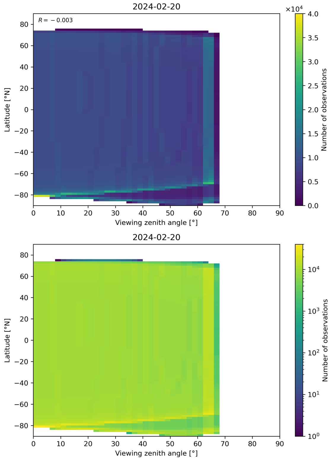
Figure 314: Scatter density plot of “Viewing zenith angle” against “Latitude” for 2024-02-19 to 2024-02-21.
