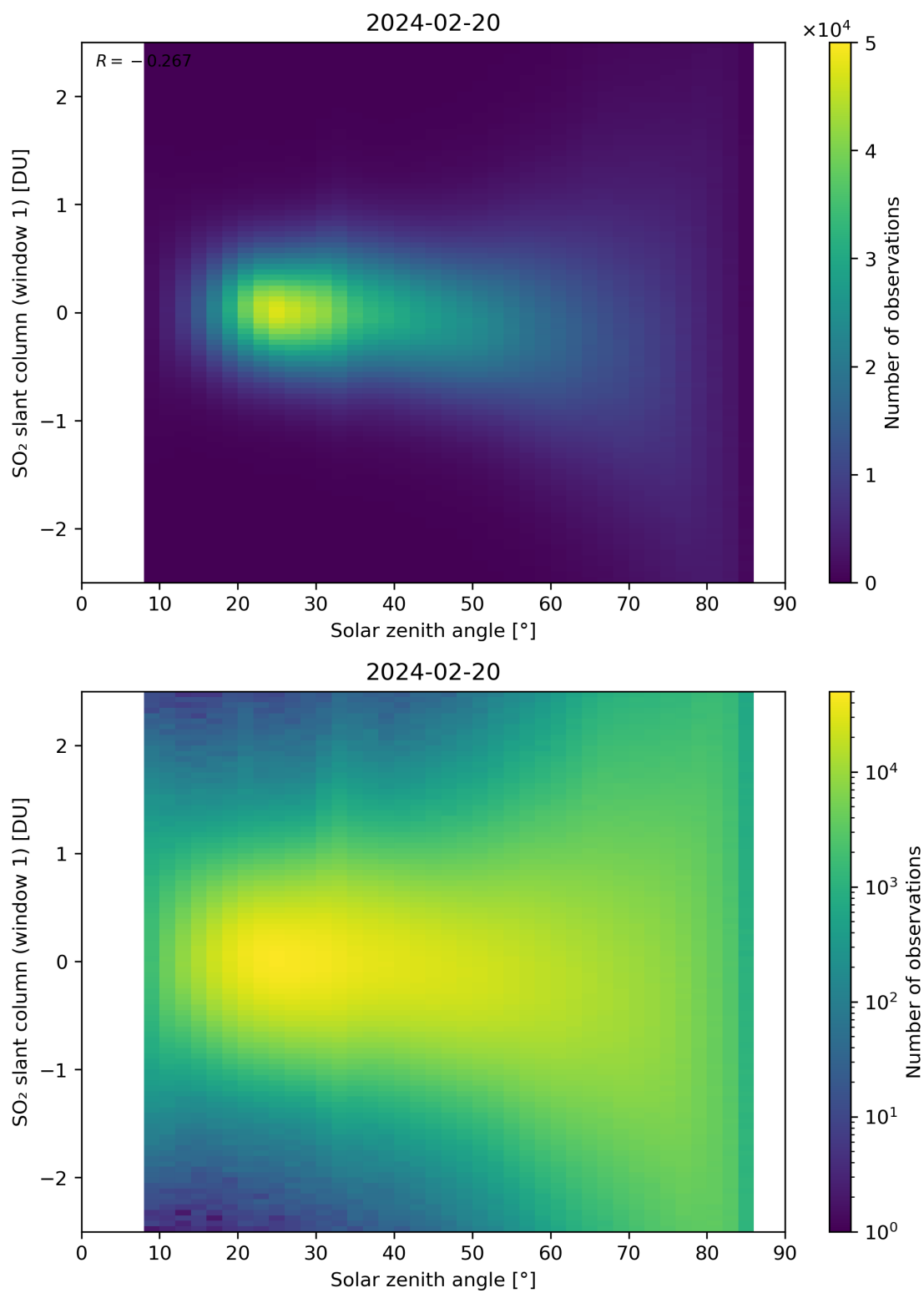
Figure 169: Scatter density plot of “Solar zenith angle” against “SO 2 slant column (window 1)” for 2024-02-19 to 2024-02-21.
