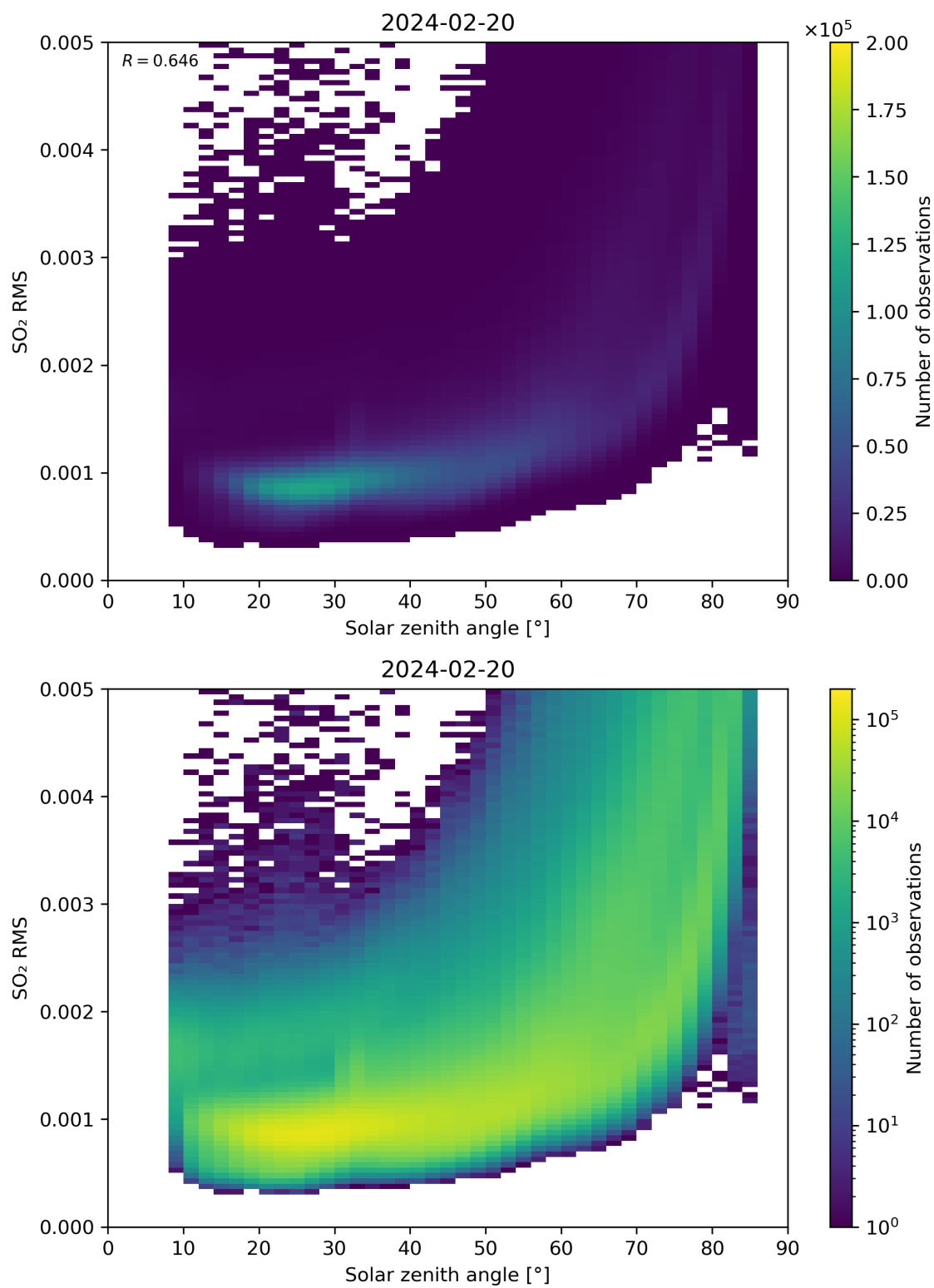
Figure 163: Scatter density plot of “Solar zenith angle” against “SO 2 RMS” for 2024-02-19 to 2024-02-21.
