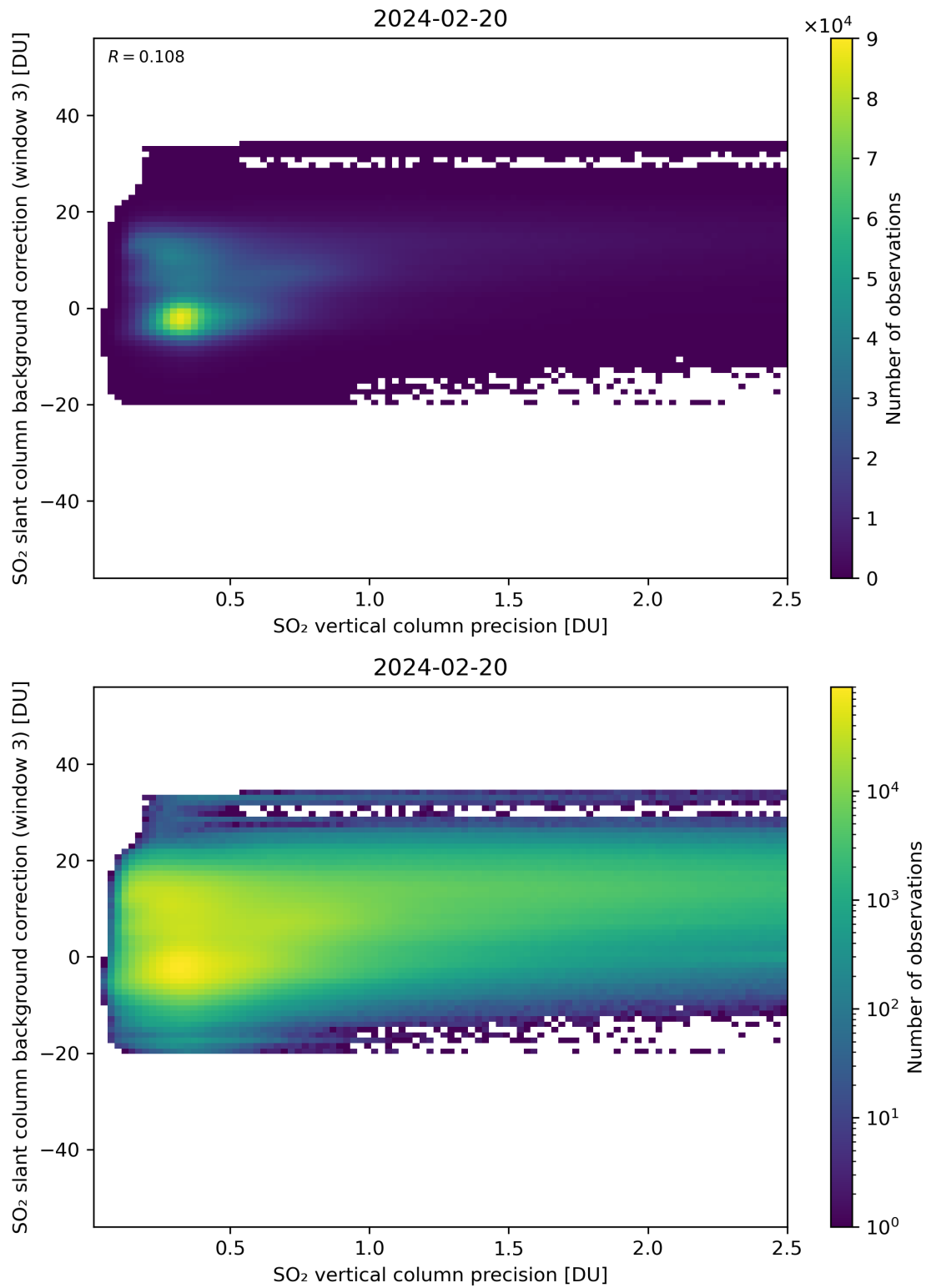
Figure 281: Scatter density plot of “SO 2 vertical column precision” against “SO 2 slant column background correction (window 3)” for 2024-02-19 to 2024-02-21.
