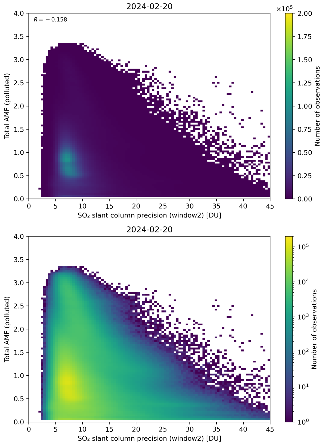
Figure 251: Scatter density plot of “SO 2 slant column precision (window2)” against “Total AMF (polluted)” for 2024-02-19 to 2024-02-21.
