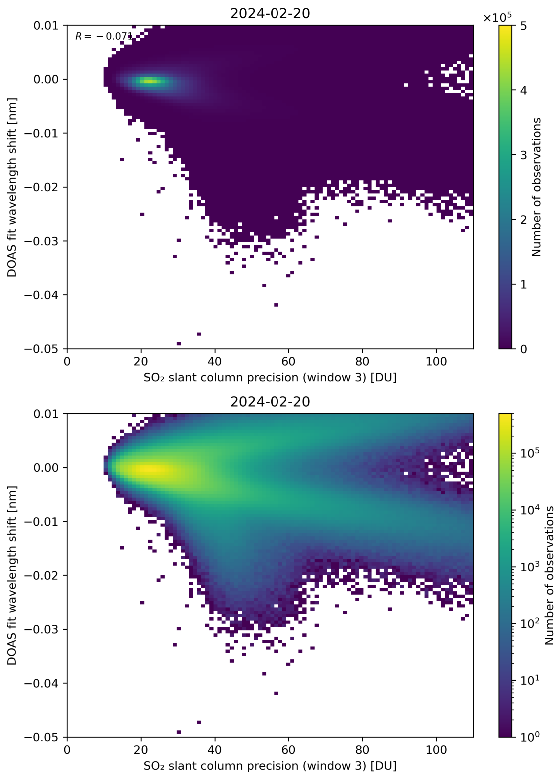
Figure 258: Scatter density plot of “SO 2 slant column precision (window 3)” against “DOAS fit wavelength shift” for 2024-02-19 to 2024-02-21.
