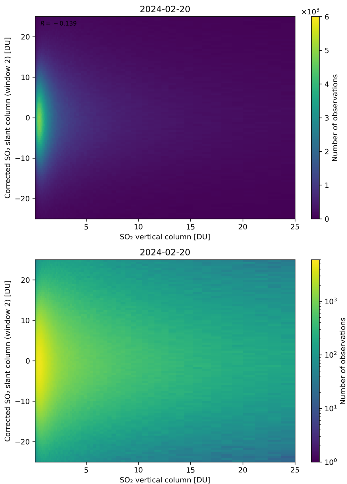
Figure 298: Scatter density plot of “SO 2 vertical column” against “Corrected SO 2 slant column (window 2)” for 2024-02-19 to 2024-02-21.
