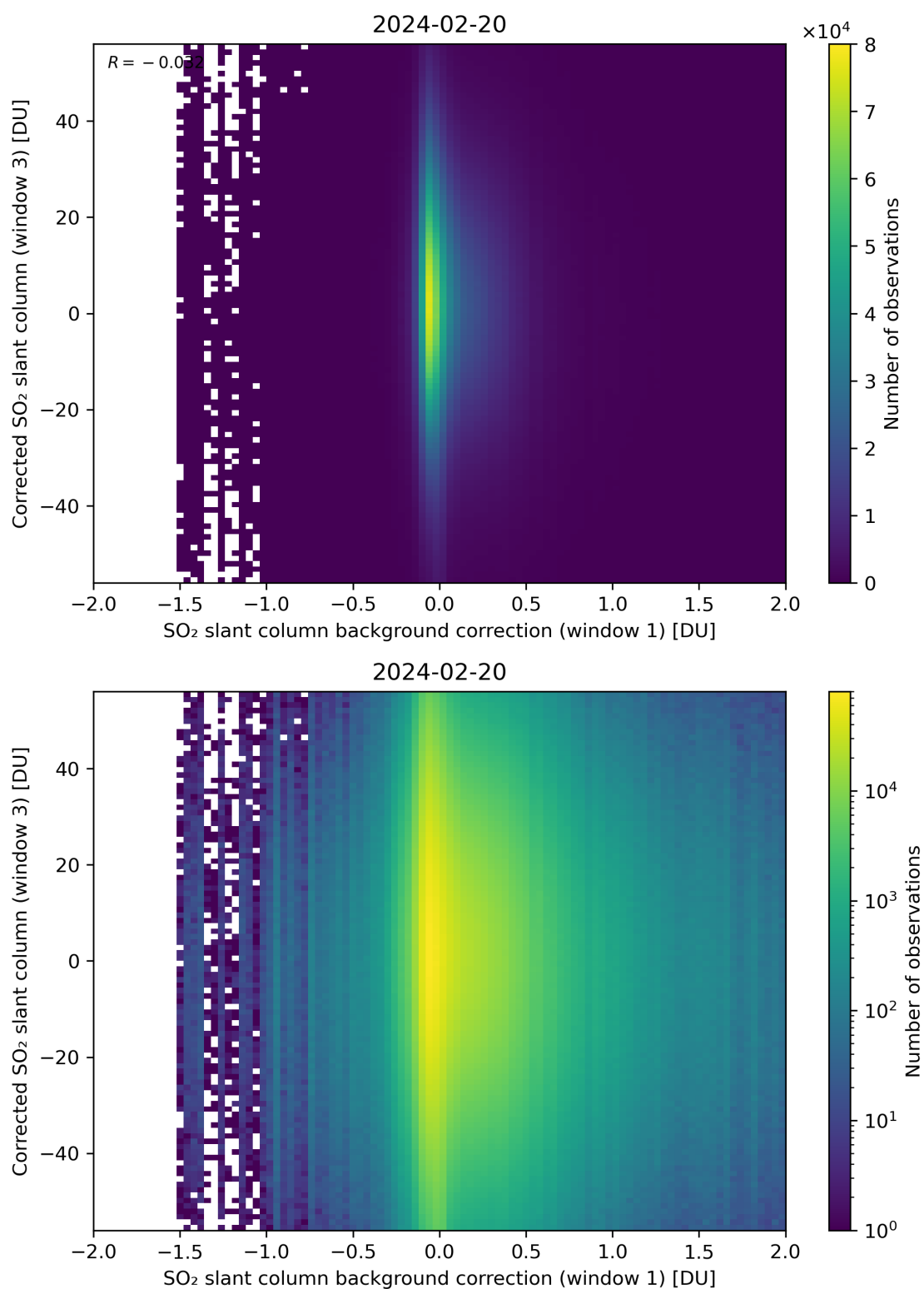
Figure 105: Scatter density plot of “SO 2 slant column background correction (window 1)” against “Corrected SO 2 slant column (window 3)” for 2024-02-19 to 2024-02-21.
