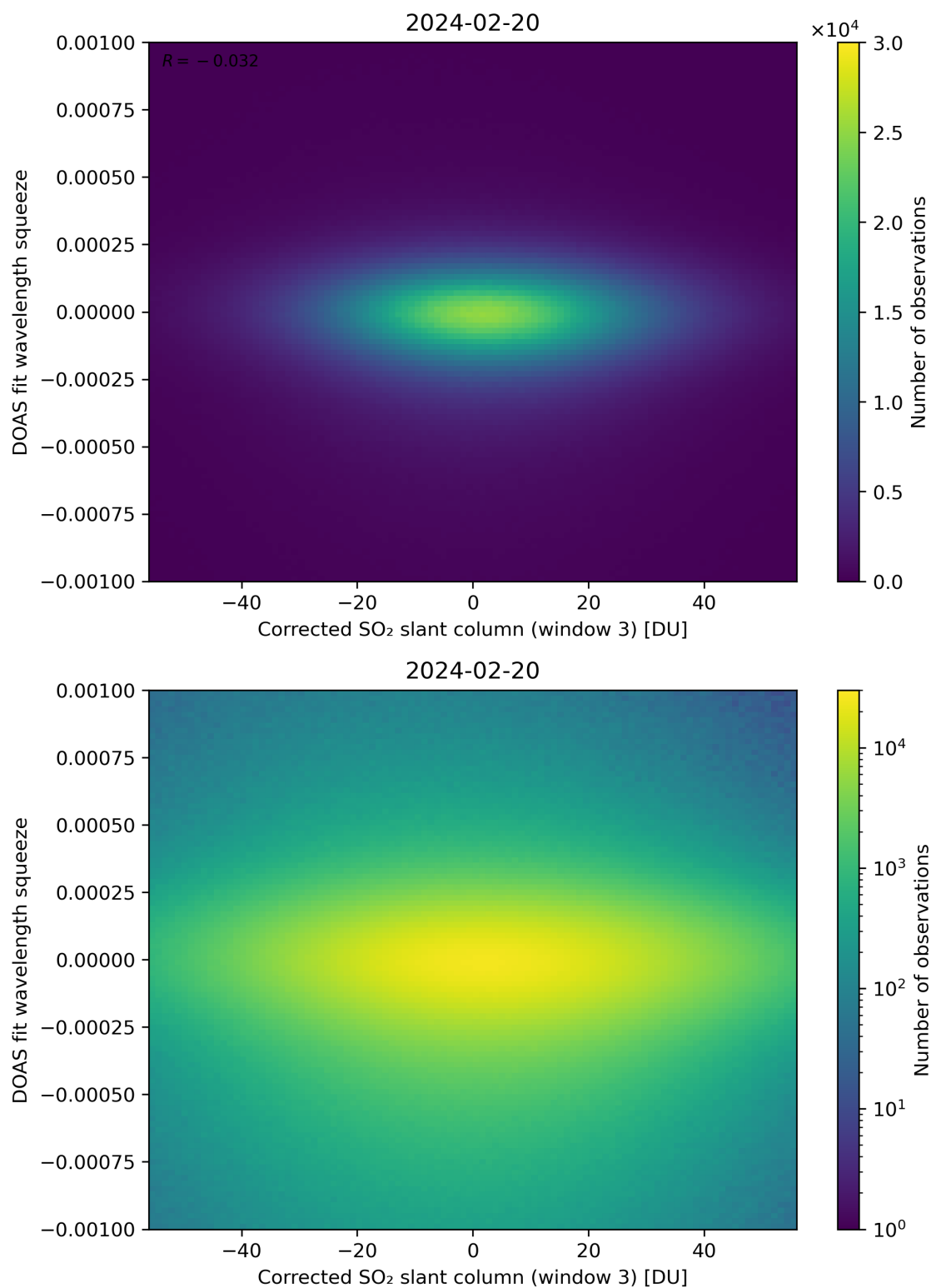
Figure 207: Scatter density plot of “Corrected SO 2 slant column (window 3)” against “DOAS fit wavelength squeeze” for 2024-02-19 to 2024-02-21.
