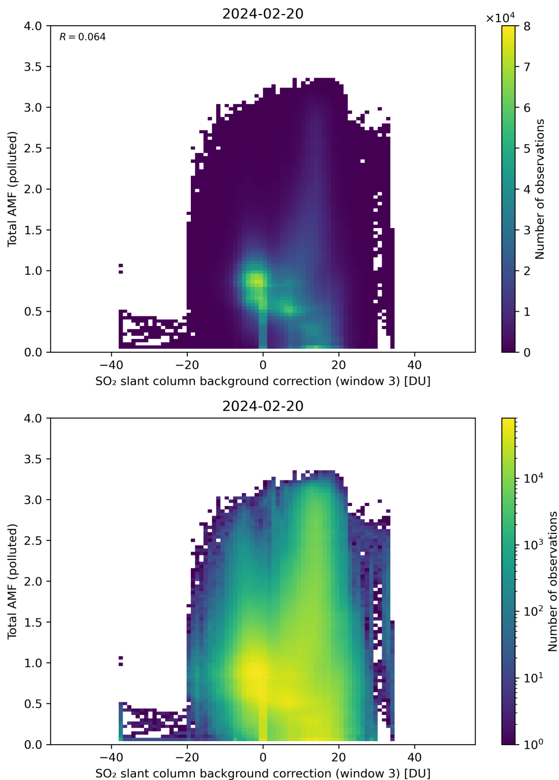
Figure 125: Scatter density plot of “SO 2 slant column background correction (window 3)” against “Total AMF (polluted)” for 2024-02-19 to 2024-02-21.
