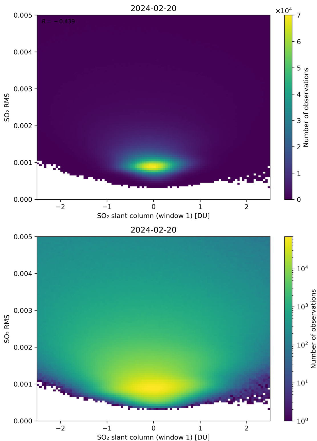
Figure 217: Scatter density plot of “SO 2 slant column (window 1)” against “SO 2 RMS” for 2024-02-19 to 2024-02-21.
