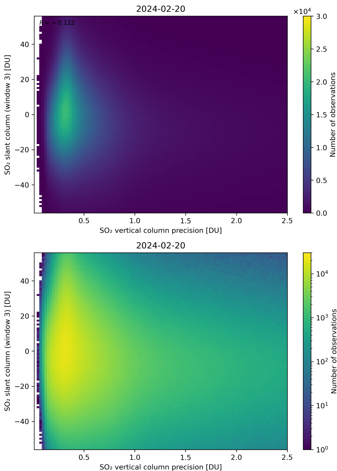
Figure 292: Scatter density plot of “SO 2 vertical column precision” against “SO 2 slant column (window 3)” for 2024-02-19 to 2024-02-21.
