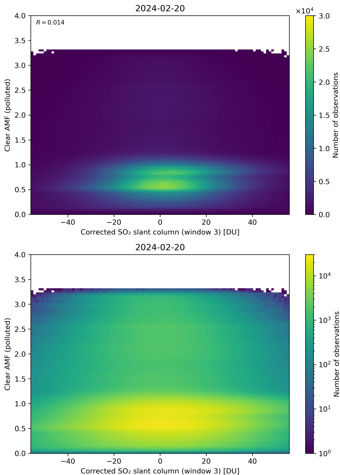
Figure 209: Scatter density plot of “Corrected SO 2 slant column (window 3)” against “Clear AMF (polluted)” for 2024-02-19 to 2024-02-21.
