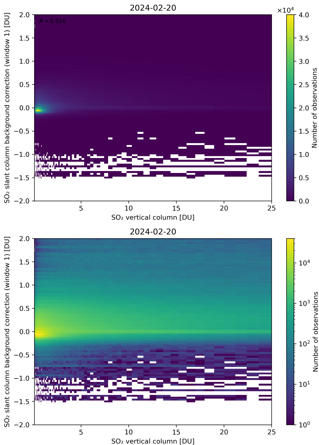
Figure 273: Scatter density plot of “SO 2 vertical column” against “SO 2 slant column background correction (window 1)” for 2024-02-19 to 2024-02-21.
