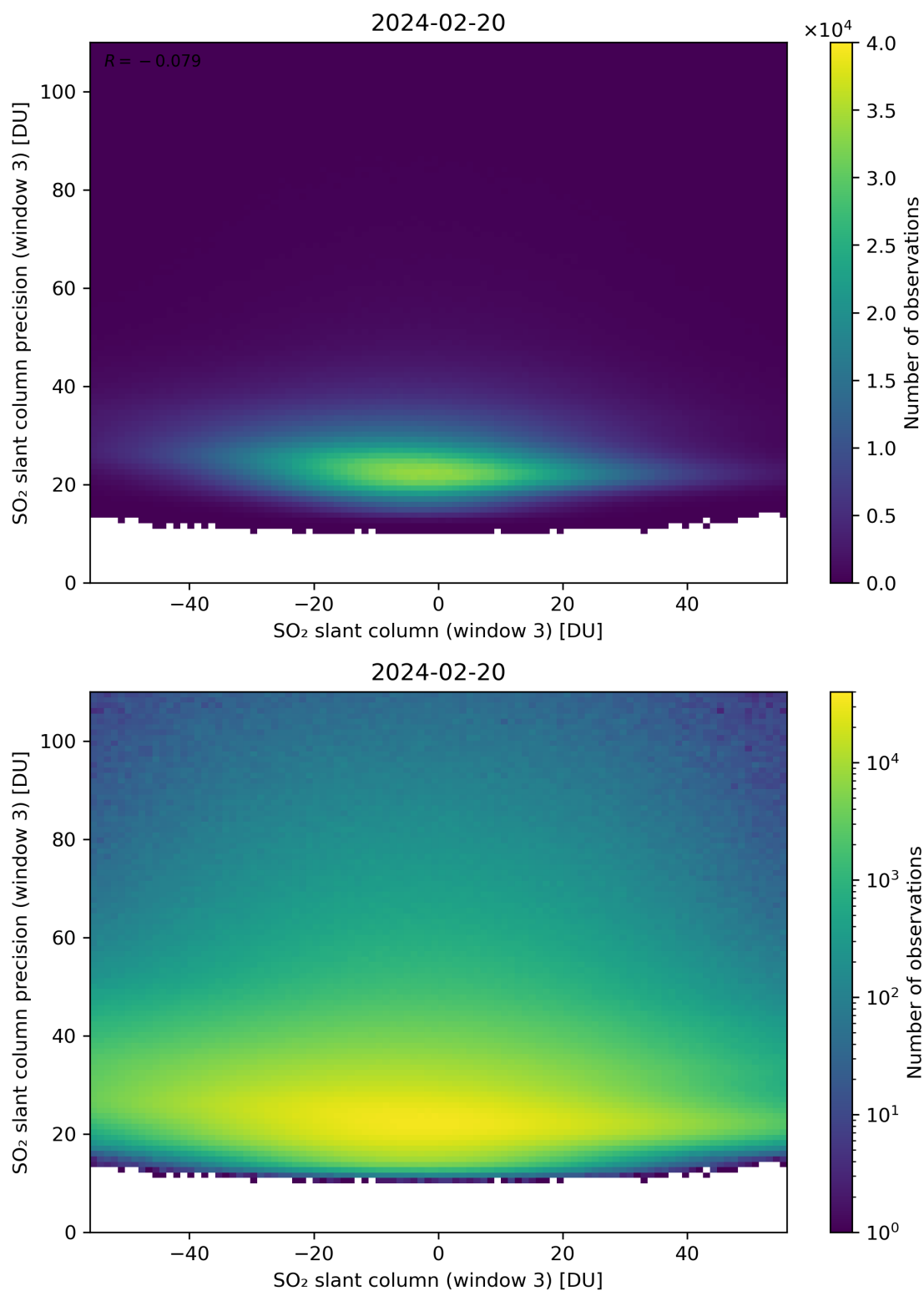
Figure 267: Scatter density plot of “SO 2 slant column (window 3)” against “SO 2 slant column precision (window 3)” for 2024-02-19 to 2024-02-21.
