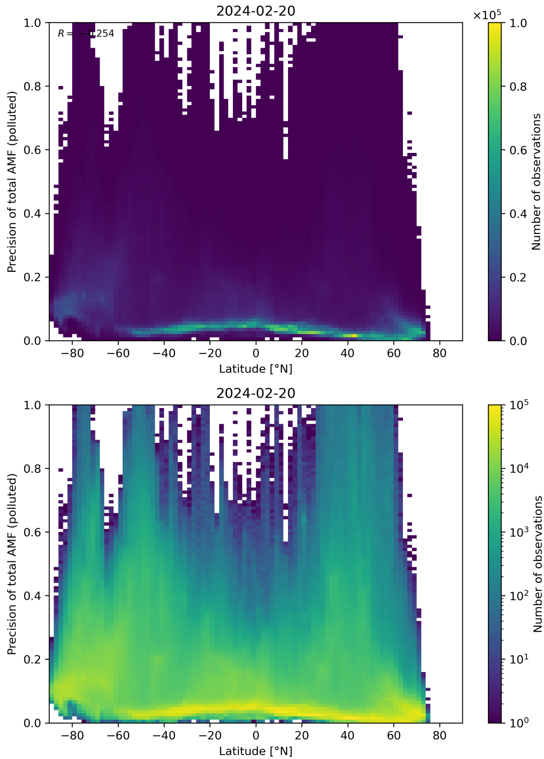
Figure 155: Scatter density plot of “Latitude” against “Precision of total AMF (polluted)” for 2024-02-19 to 2024-02-21.
