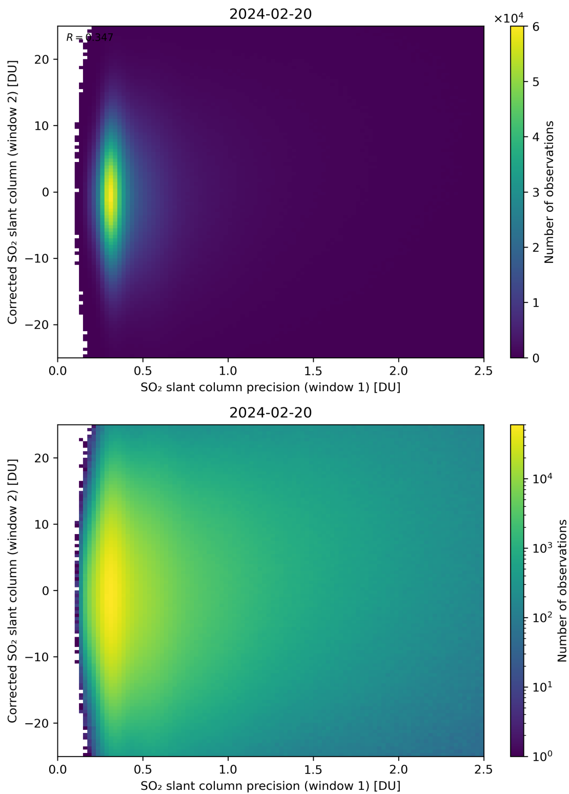
Figure 225: Scatter density plot of “SO 2 slant column precision (window 1)” against “Corrected SO 2 slant column (window 2)” for 2024-02-19 to 2024-02-21.
