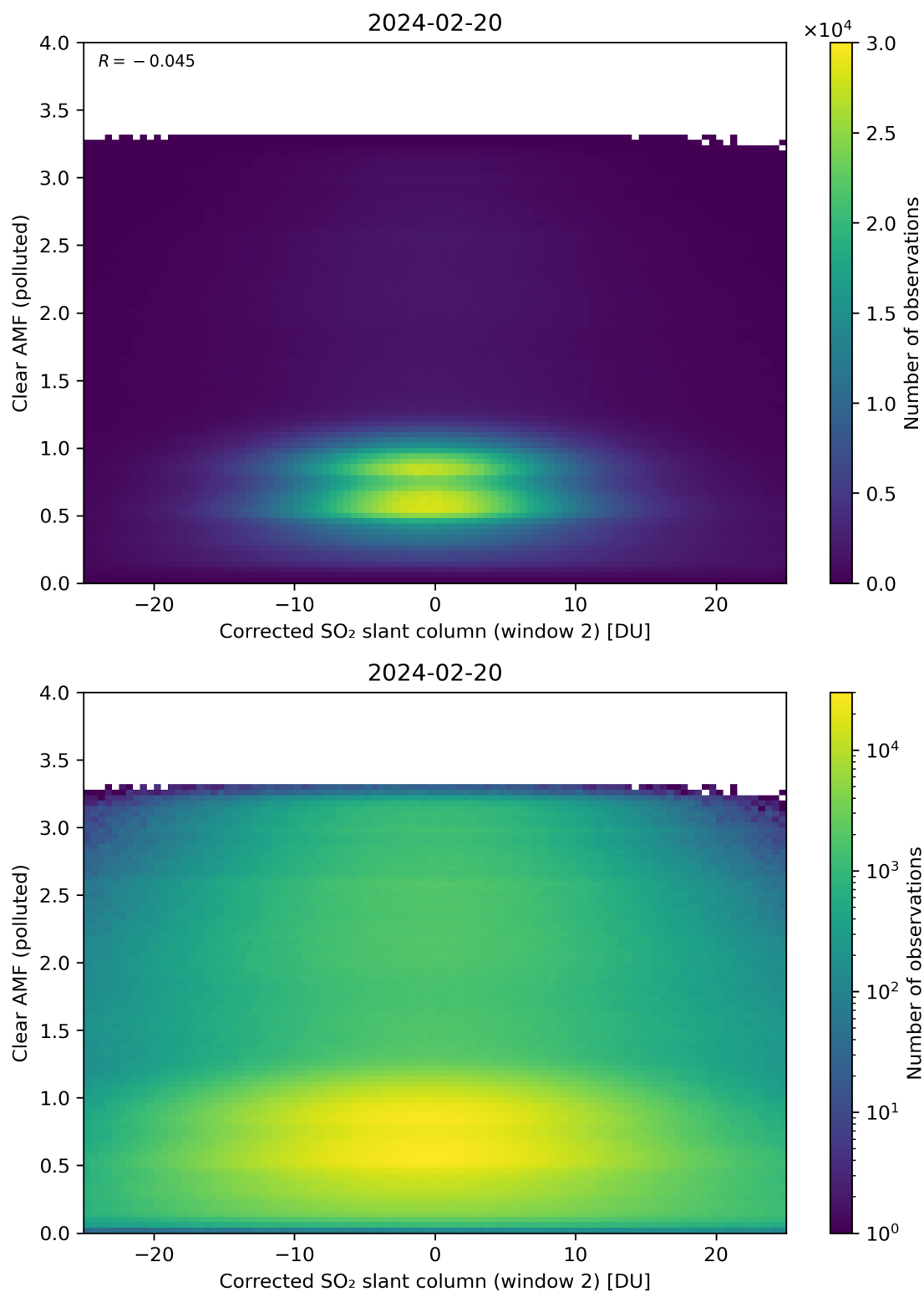
Figure 199: Scatter density plot of “Corrected SO 2 slant column (window 2)” against “Clear AMF (polluted)” for 2024-02-19 to 2024-02-21.
