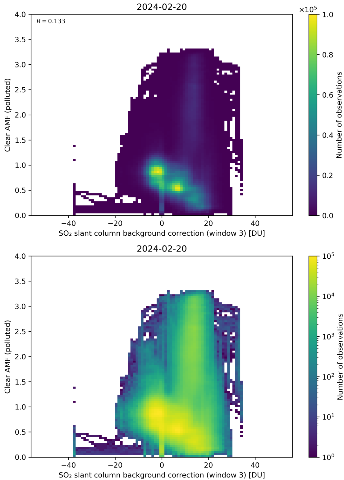
Figure 124: Scatter density plot of “SO 2 slant column background correction (window 3)” against “Clear AMF (polluted)” for 2024-02-19 to 2024-02-21.
