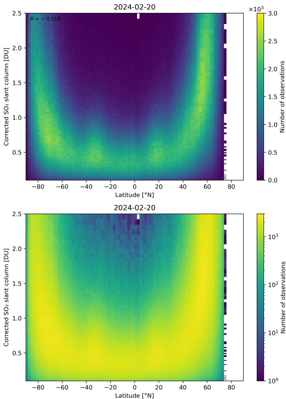
Figure 146: Scatter density plot of “Latitude” against “Corrected SO 2 slant column” for 2024-02-19 to 2024-02-21.
