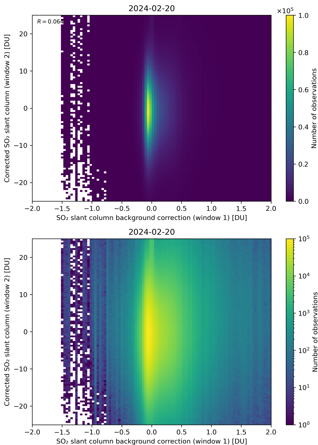
Figure 104: Scatter density plot of “SO 2 slant column background correction (window 1)” against “Corrected SO 2 slant column (window 2)” for 2024-02-19 to 2024-02-21.
