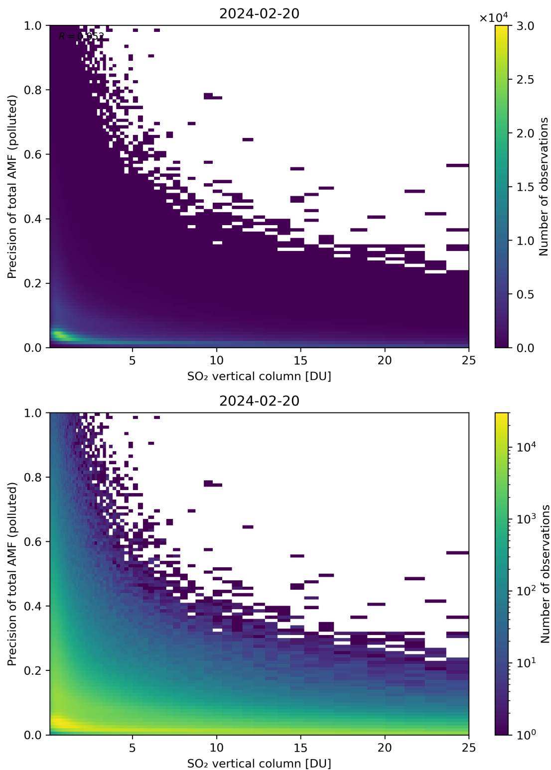
Figure 306: Scatter density plot of “SO 2 vertical column” against “Precision of total AMF (polluted)” for 2024-02-19 to 2024-02-21.
