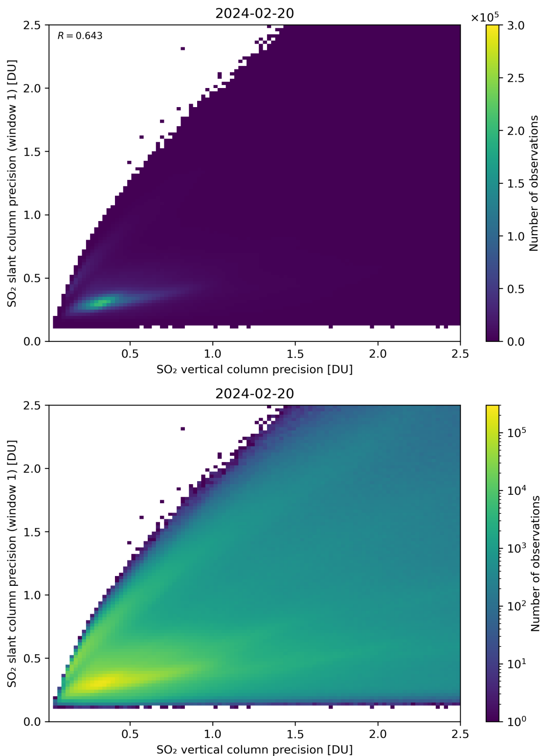
Figure 290: Scatter density plot of “SO 2 vertical column precision” against “SO 2 slant column precision (window 1)” for 2024-02-19 to 2024-02-21.
