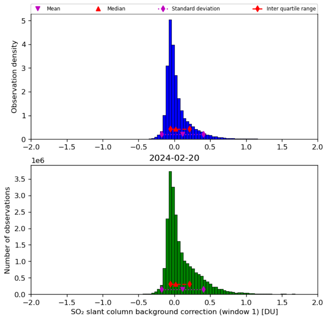
Figure 59: Histogram of “SO 2 slant column background correction (window 1)” for 2024-02-19 to 2024-02-21
