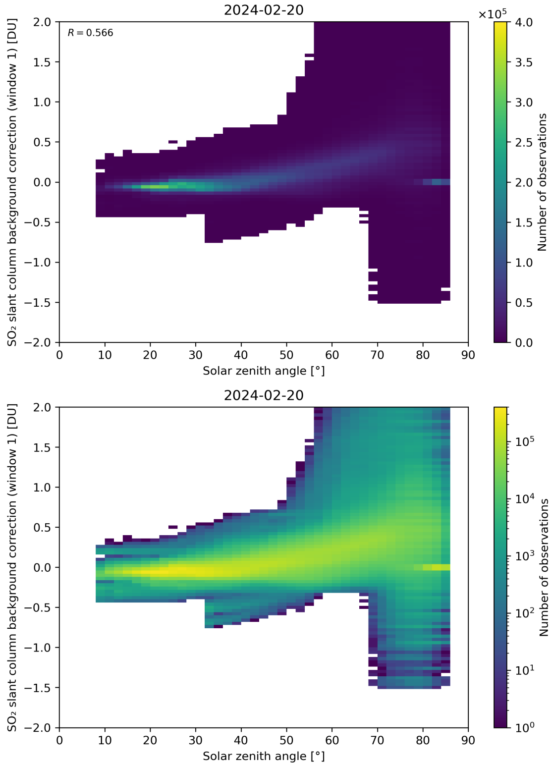
Figure 158: Scatter density plot of “Solar zenith angle” against “SO 2 slant column background correction (window 1)” for 2024-02-19 to 2024-02-21.
