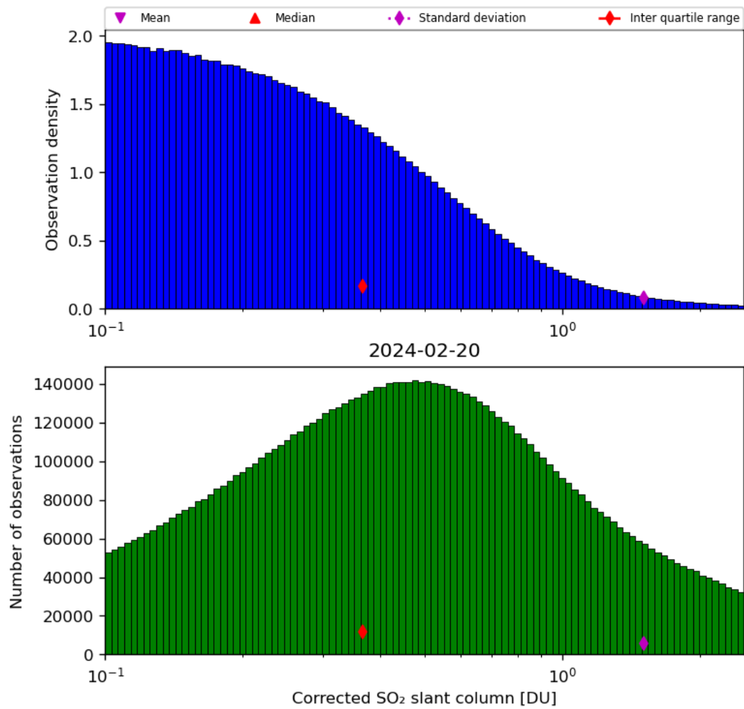
Figure 55: Histogram of “Corrected SO 2 slant column” for 2024-02-19 to 2024-02-21
