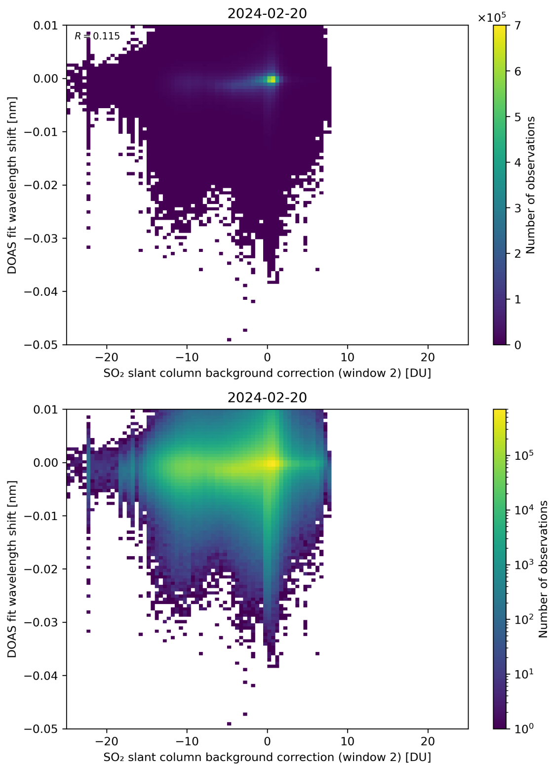
Figure 112: Scatter density plot of “SO 2 slant column background correction (window 2)” against “DOAS fit wavelength shift” for 2024-02-19 to 2024-02-21.
