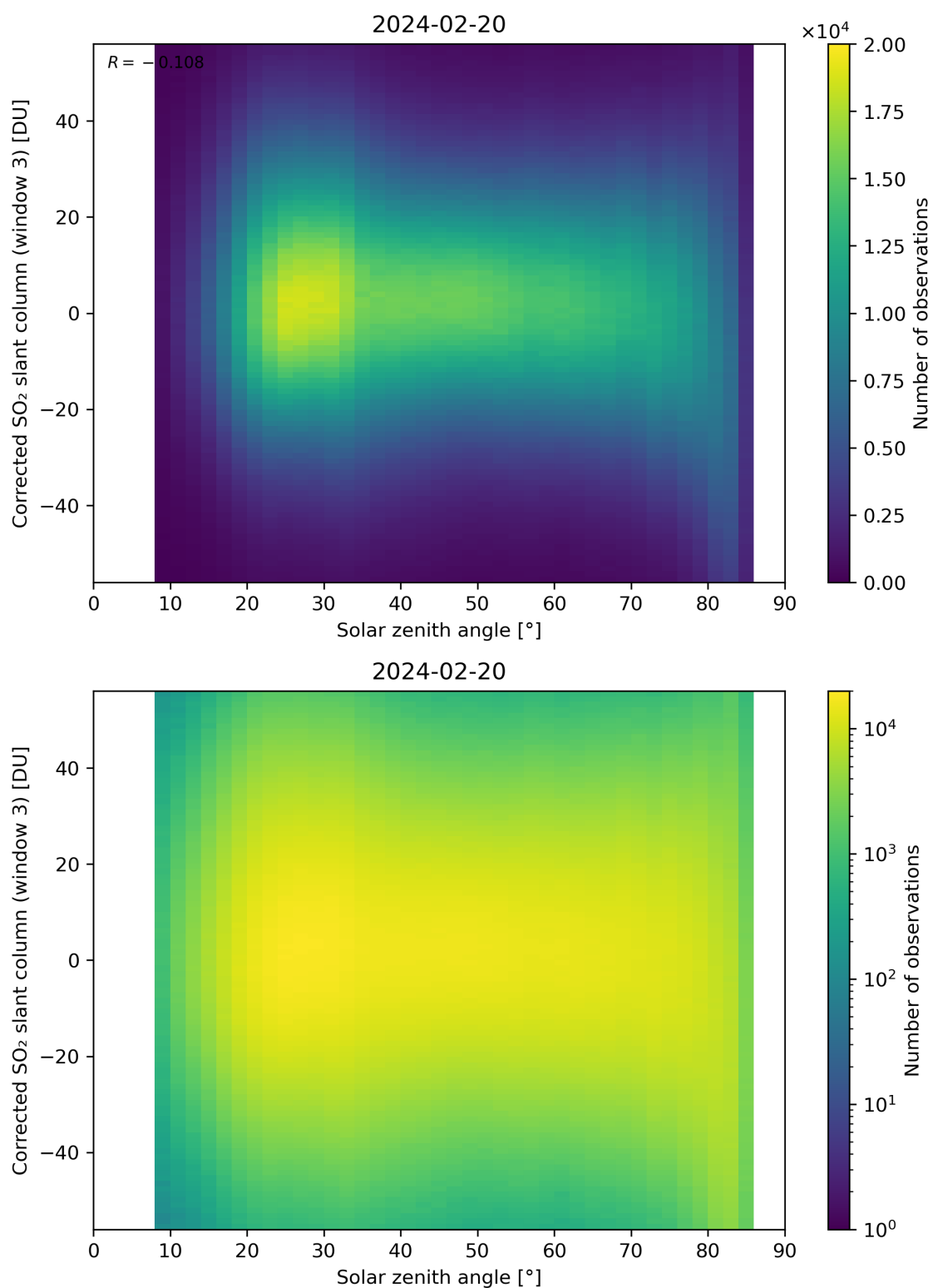
Figure 168: Scatter density plot of “Solar zenith angle” against “Corrected SO 2 slant column (window 3)” for 2024-02-19 to 2024-02-21.
