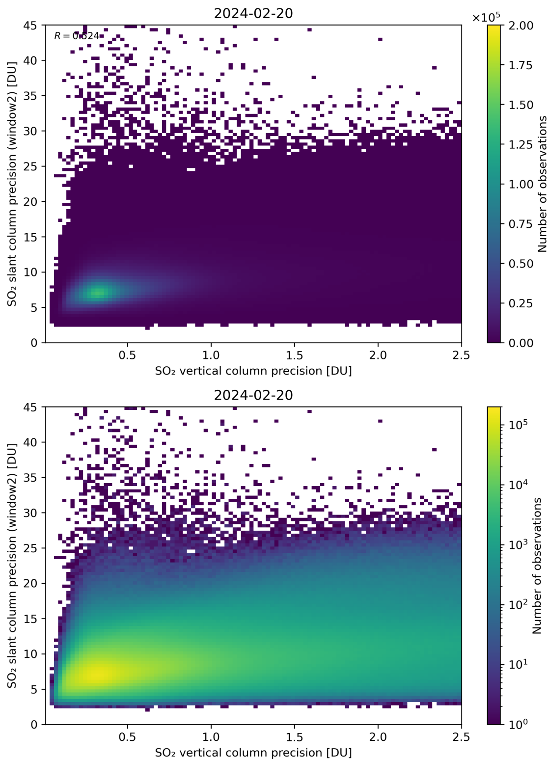
Figure 291: Scatter density plot of “SO 2 vertical column precision” against “SO 2 slant column precision (window2)” for 2024-02-19 to 2024-02-21.
