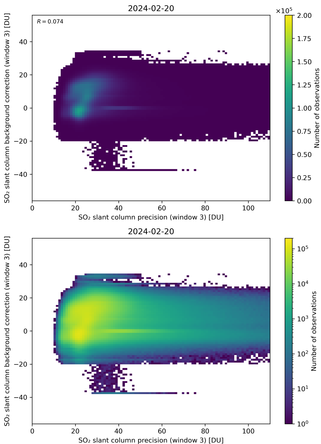
Figure 257: Scatter density plot of “SO 2 slant column precision (window 3)” against “SO 2 slant column background correction (window 3)” for 2024-02-19 to 2024-02-21.
