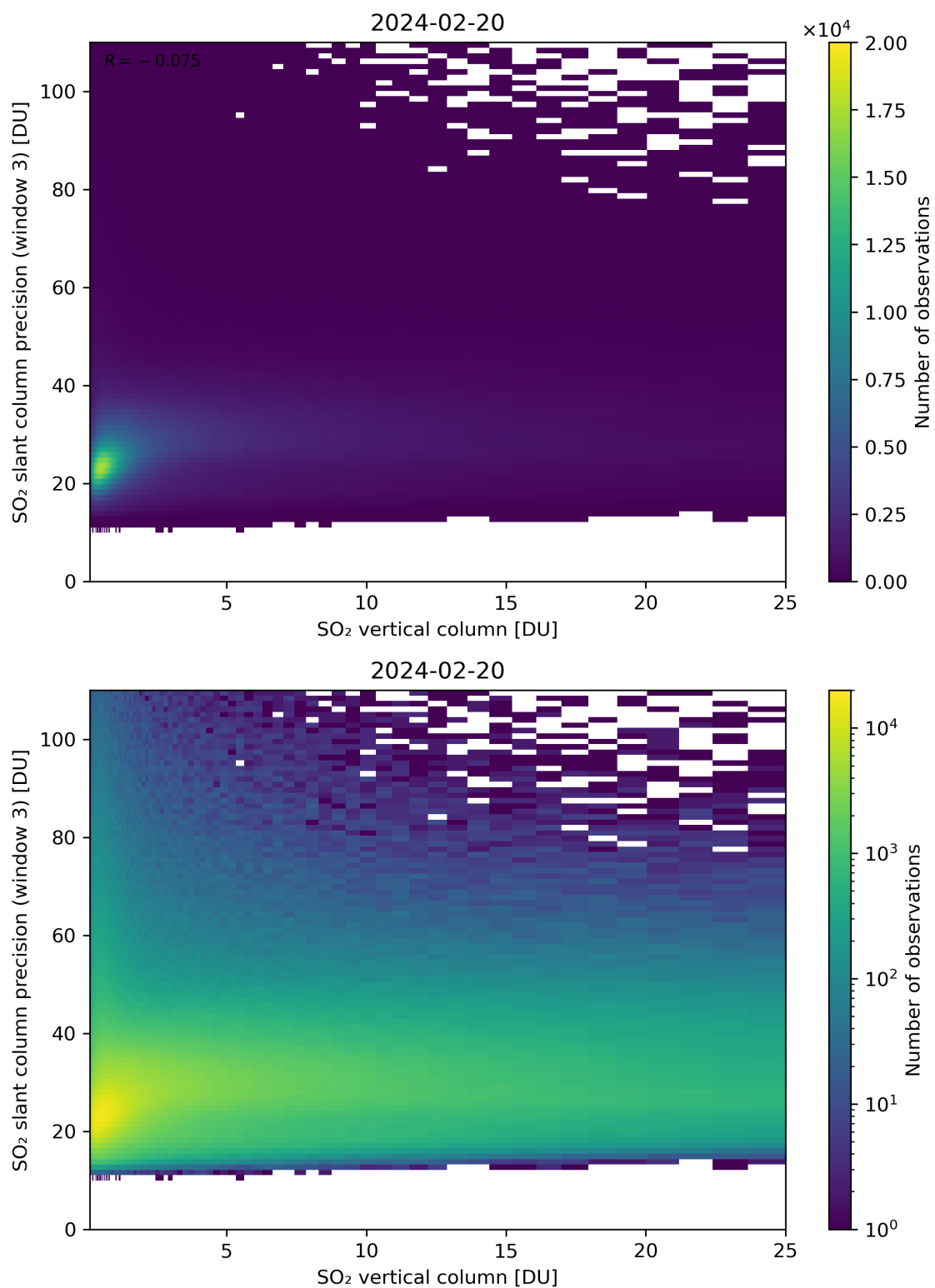
Figure 304: Scatter density plot of “SO 2 vertical column” against “SO 2 slant column precision (window 3)” for 2024-02-19 to 2024-02-21.
