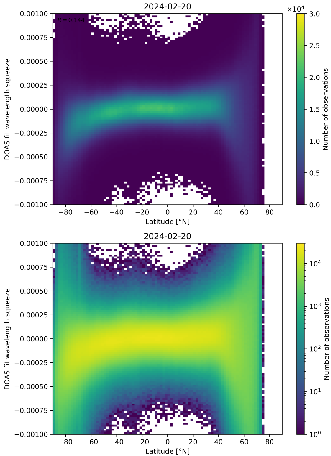
Figure 143: Scatter density plot of “Latitude” against “DOAS fit wavelength squeeze” for 2024-02-19 to 2024-02-21.
