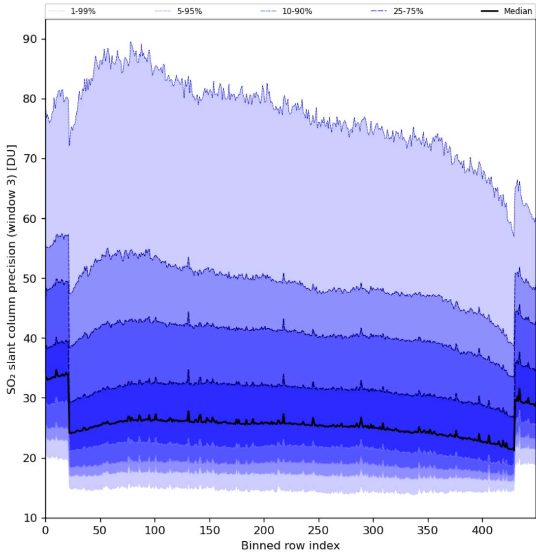
Figure 88: Along track statistics of “SO 2 slant column precision (window 3)” for 2024-02-19 to 2024-02-21
