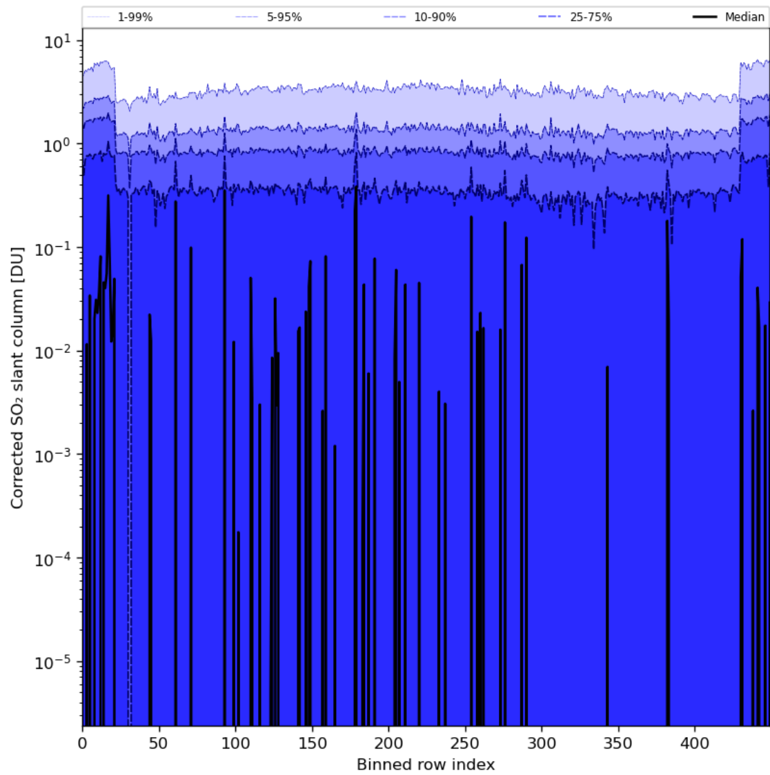
Figure 78: Along track statistics of “Corrected SO 2 slant column” for 2024-02-19 to 2024-02-21
