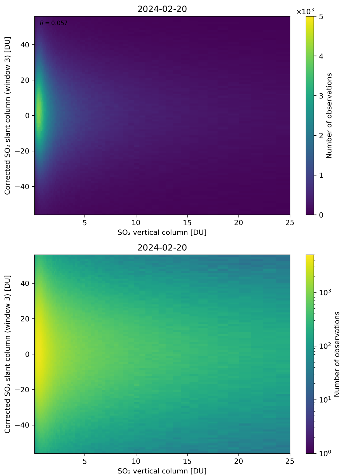
Figure 299: Scatter density plot of “SO 2 vertical column” against “Corrected SO 2 slant column (window 3)” for 2024-02-19 to 2024-02-21.
