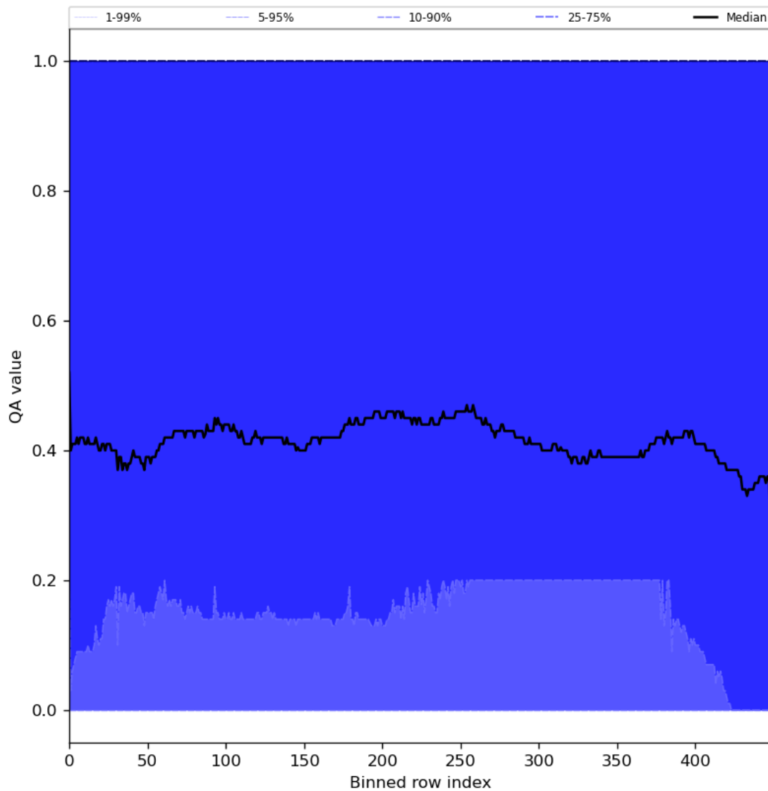
Figure 75: Along track statistics of “QA value” for 2024-02-19 to 2024-02-21
