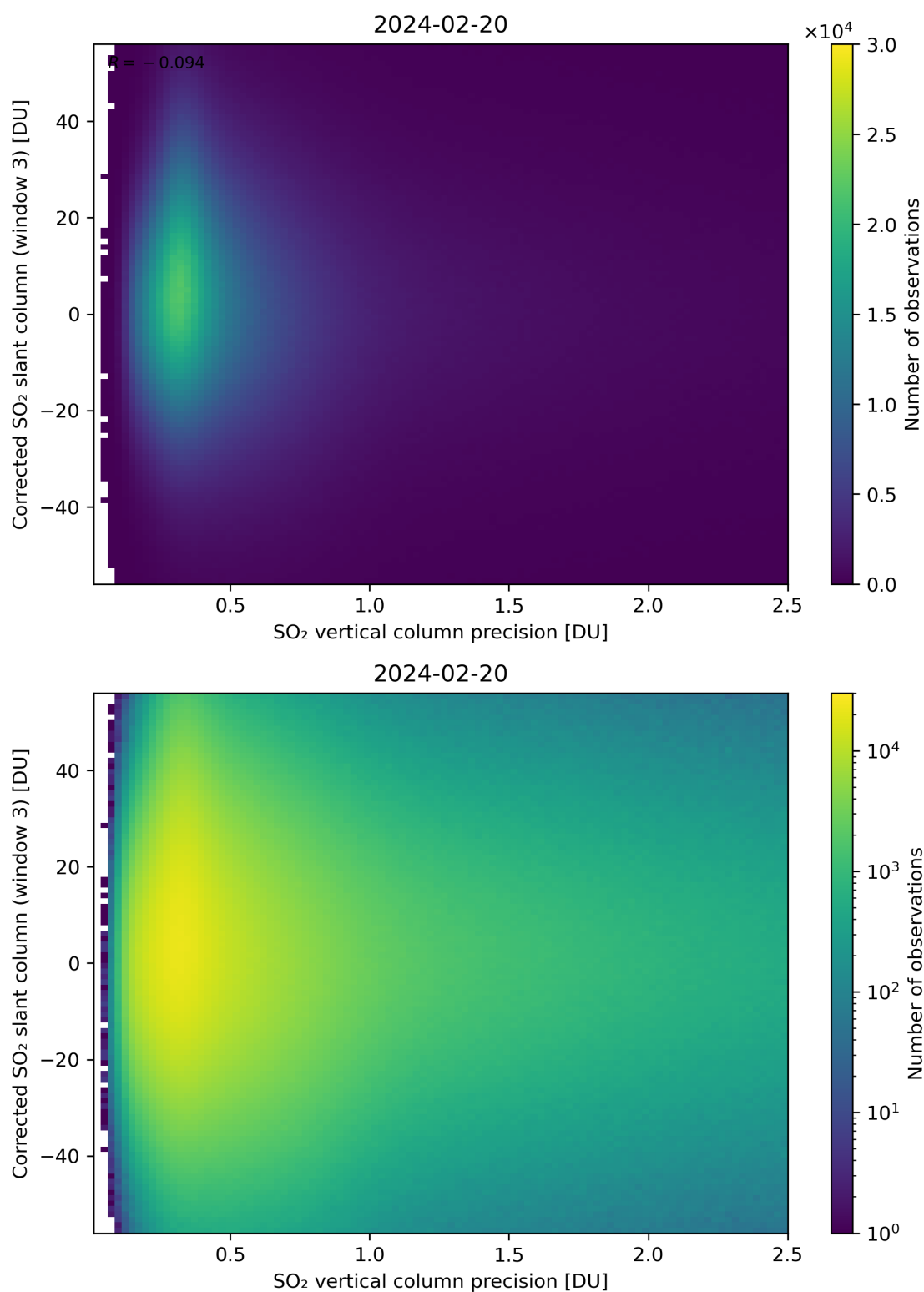
Figure 288: Scatter density plot of “SO 2 vertical column precision” against “Corrected SO 2 slant column (window 3)” for 2024-02-19 to 2024-02-21.
