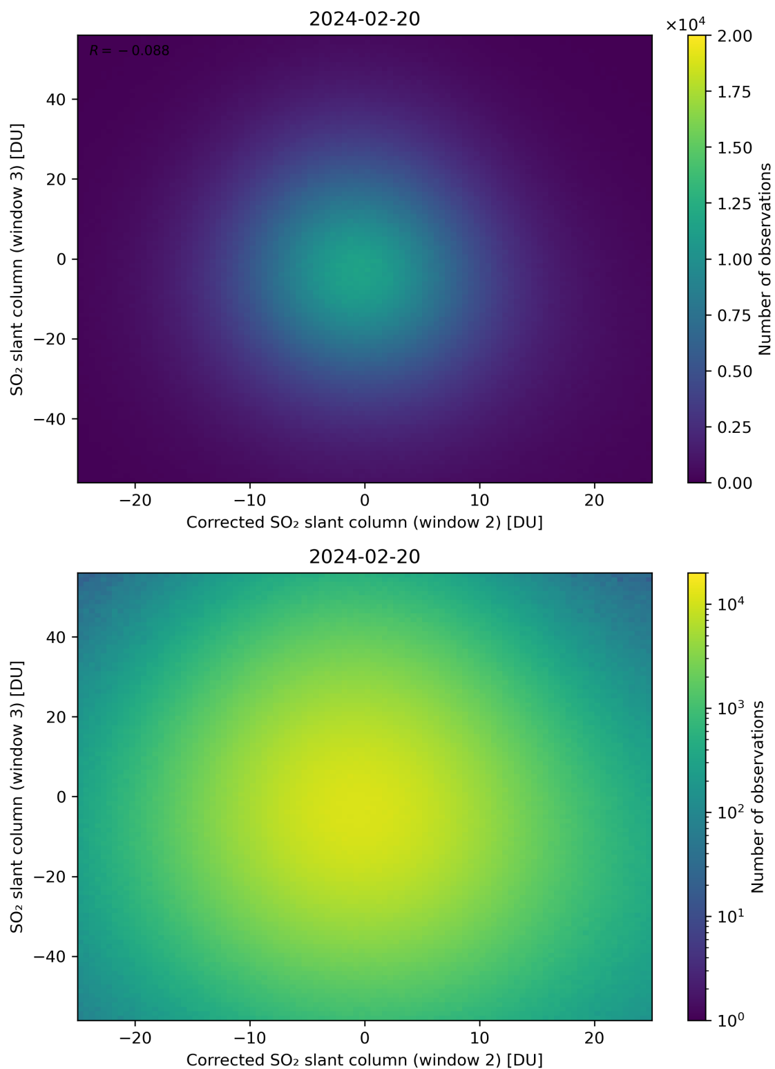
Figure 201: Scatter density plot of “Corrected SO 2 slant column (window 2)” against “SO 2 slant column (window 3)” for 2024-02-19 to 2024-02-21.
