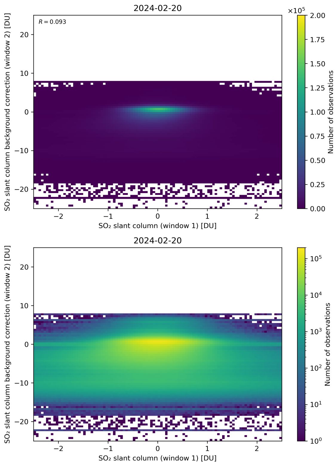
Figure 213: Scatter density plot of “SO 2 slant column (window 1)” against “SO 2 slant column background correction (window 2)” for 2024-02-19 to 2024-02-21.
