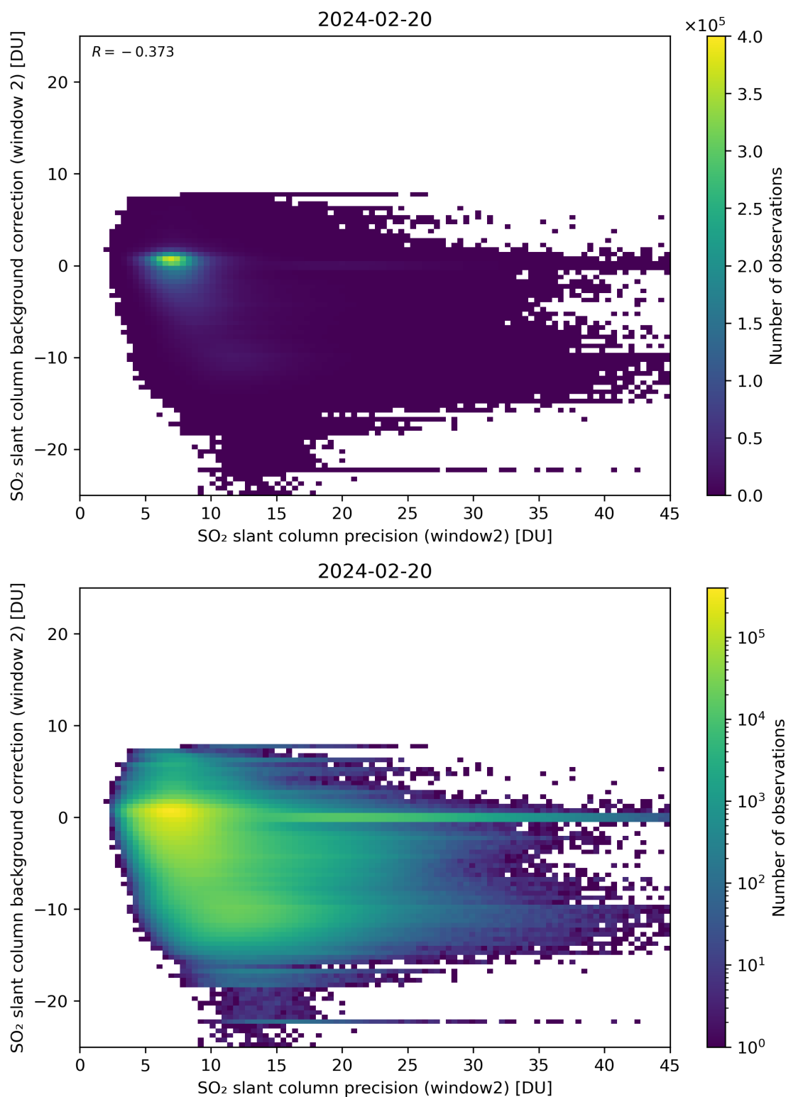
Figure 241: Scatter density plot of “SO 2 slant column precision (window2)” against “SO 2 slant column background correction (window 2)” for 2024-02-19 to 2024-02-21.
