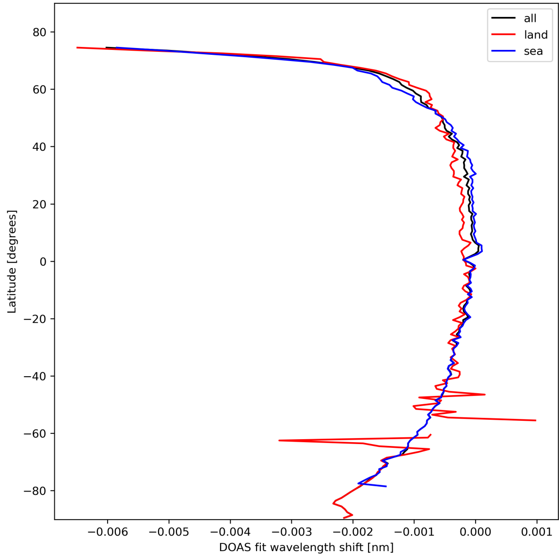
Figure 45: Zonal average of “DOAS fit wavelength shift” for 2024-02-19 to 2024-02-21.
