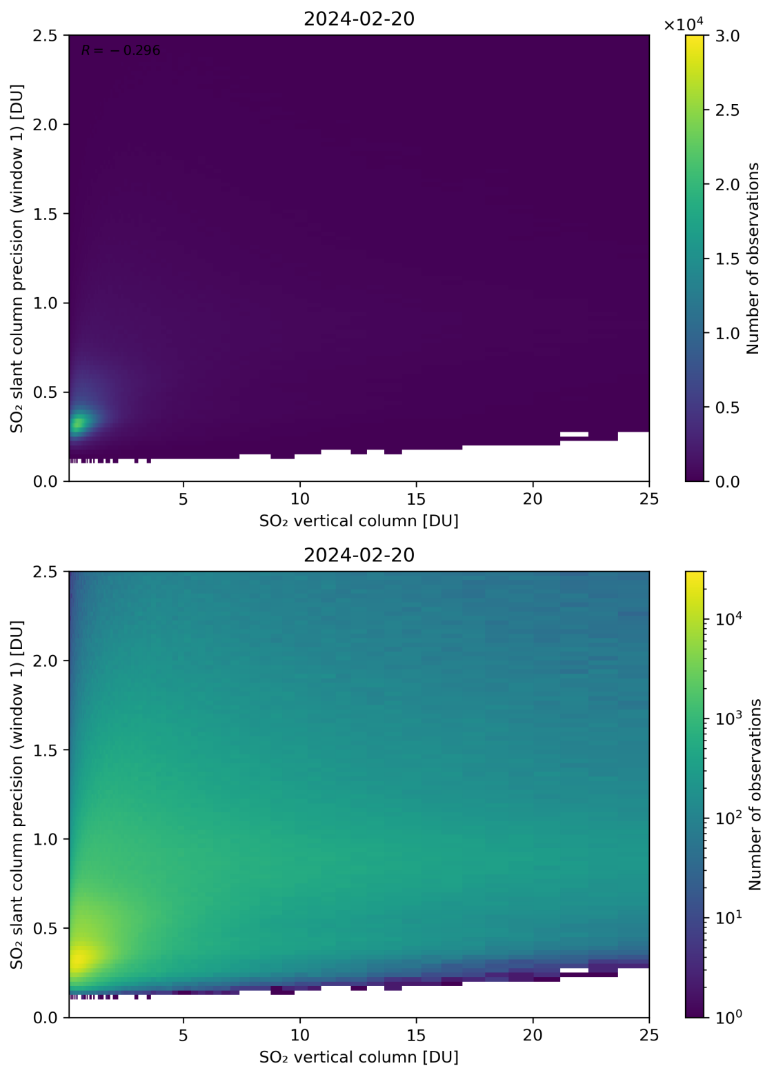
Figure 301: Scatter density plot of “SO 2 vertical column” against “SO 2 slant column precision (window 1)” for 2024-02-19 to 2024-02-21.
