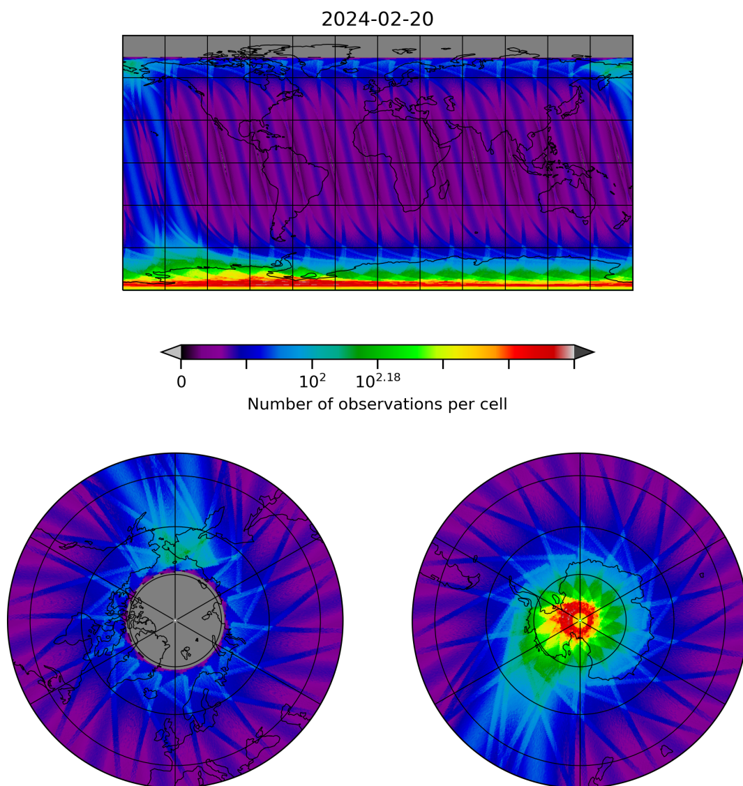
Figure 28: Map of the number of observations for 2024-02-19 to 2024-02-21
