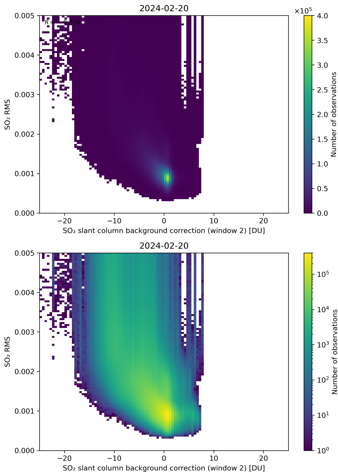
Figure 114: Scatter density plot of “SO 2 slant column background correction (window 2)” against “SO 2 RMS” for 2024-02-19 to 2024-02-21.
