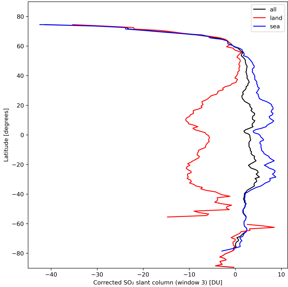
Figure 43: Zonal average of “Corrected SO 2 slant column (window 3)” for 2024-02-19 to 2024-02-21.
