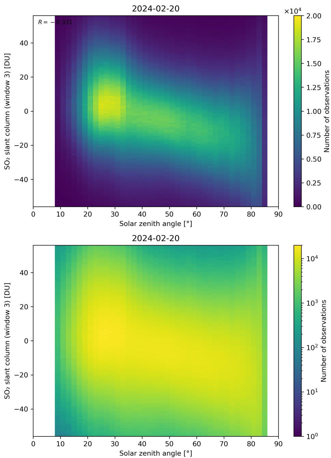
Figure 172: Scatter density plot of “Solar zenith angle” against “SO 2 slant column (window 3)” for 2024-02-19 to 2024-02-21.
