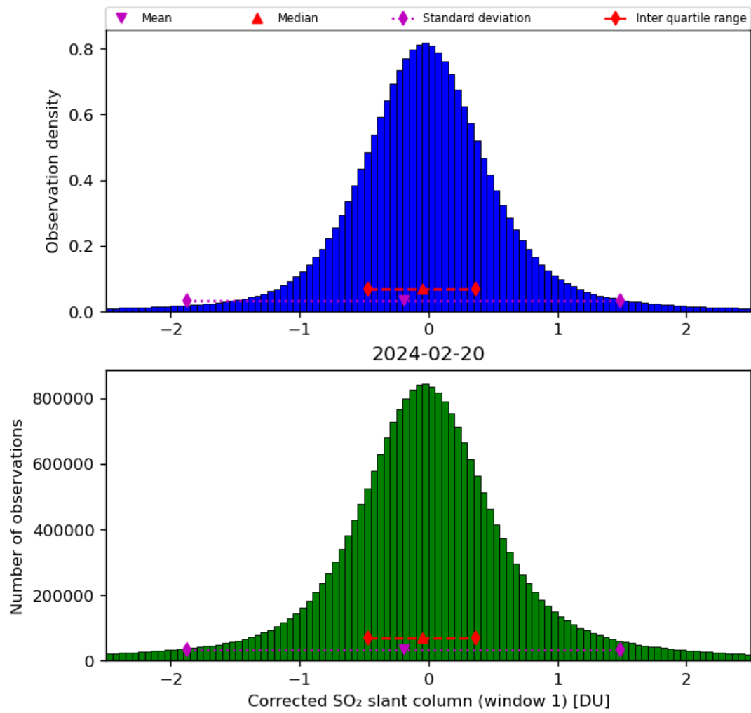
Figure 58: Histogram of “Corrected SO 2 slant column (window 1)” for 2024-02-19 to 2024-02-21
