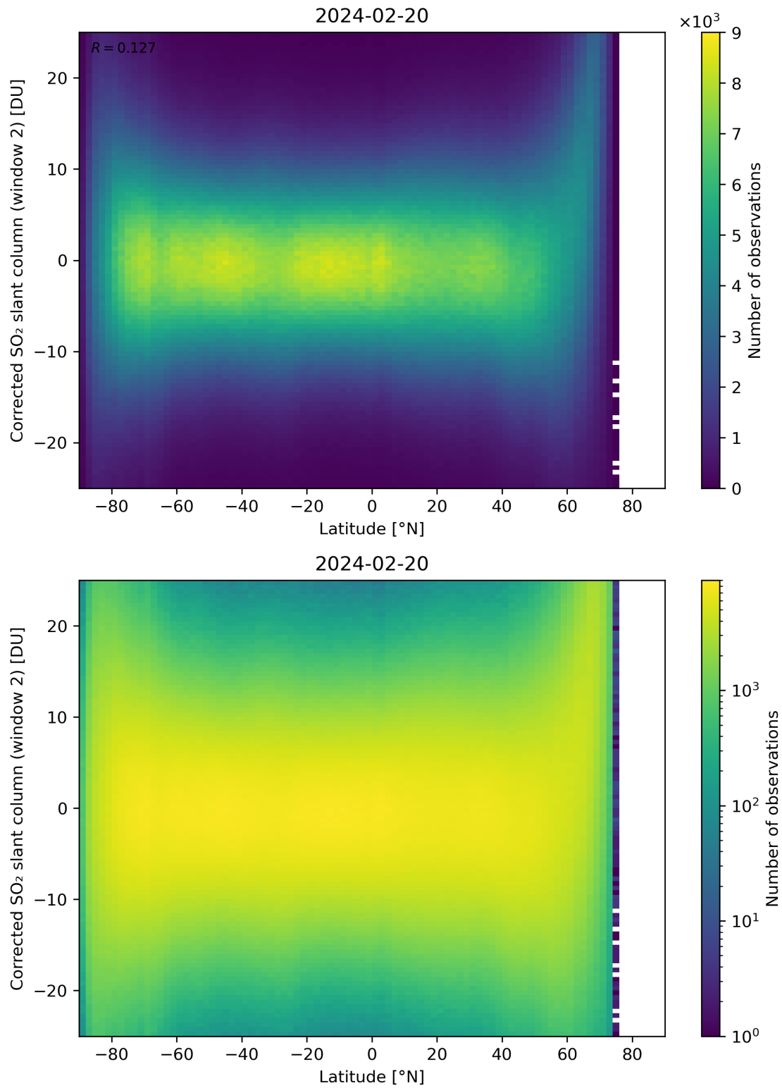
Figure 147: Scatter density plot of “Latitude” against “Corrected SO 2 slant column (window 2)” for 2024-02-19 to 2024-02-21.
