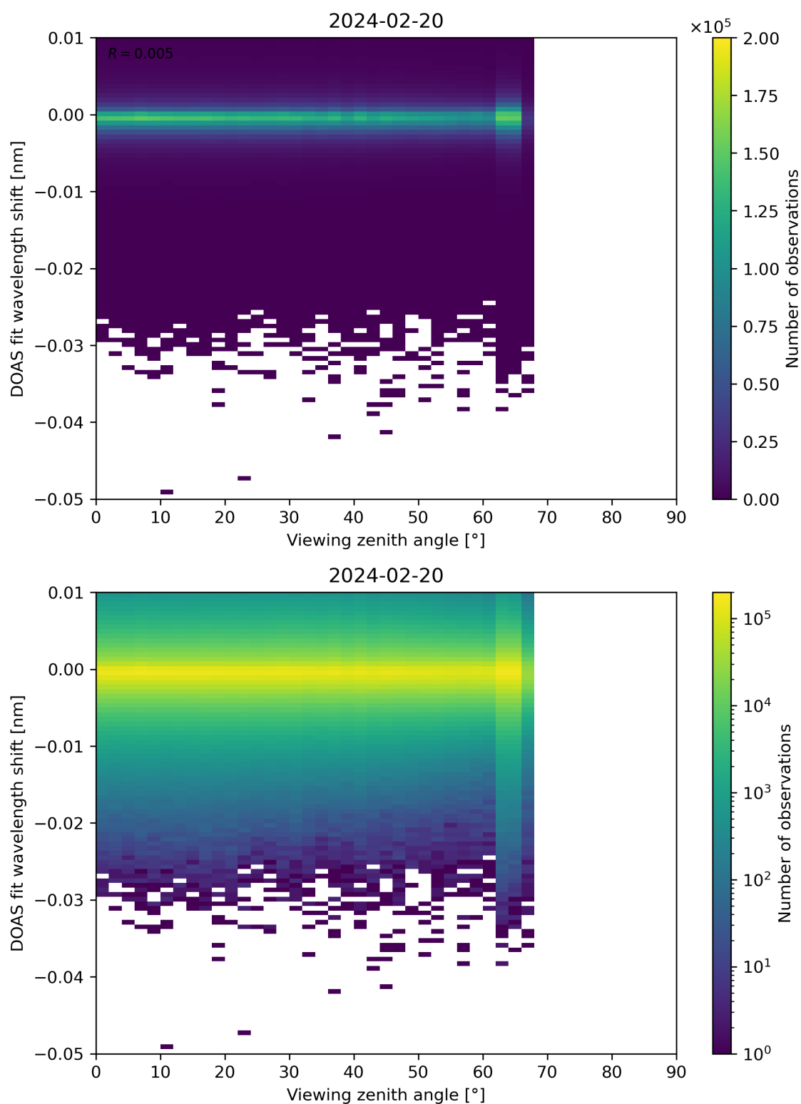
Figure 311: Scatter density plot of “Viewing zenith angle” against “DOAS fit wavelength shift” for 2024-02-19 to 2024-02-21.
