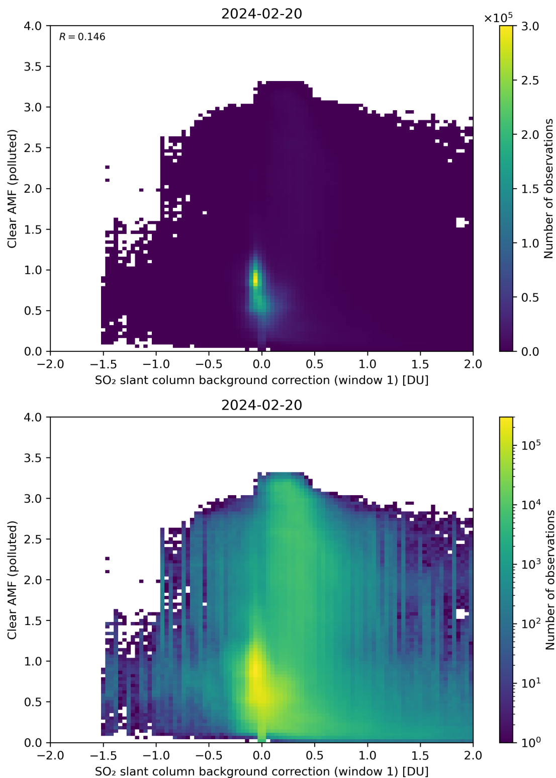
Figure 103: Scatter density plot of “SO 2 slant column background correction (window 1)” against “Clear AMF (polluted)” for 2024-02-19 to 2024-02-21.
