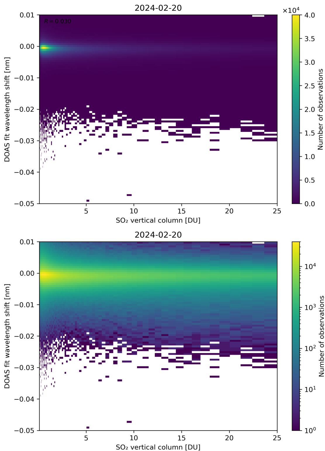
Figure 276: Scatter density plot of “SO 2 vertical column” against “DOAS fit wavelength shift” for 2024-02-19 to 2024-02-21.
