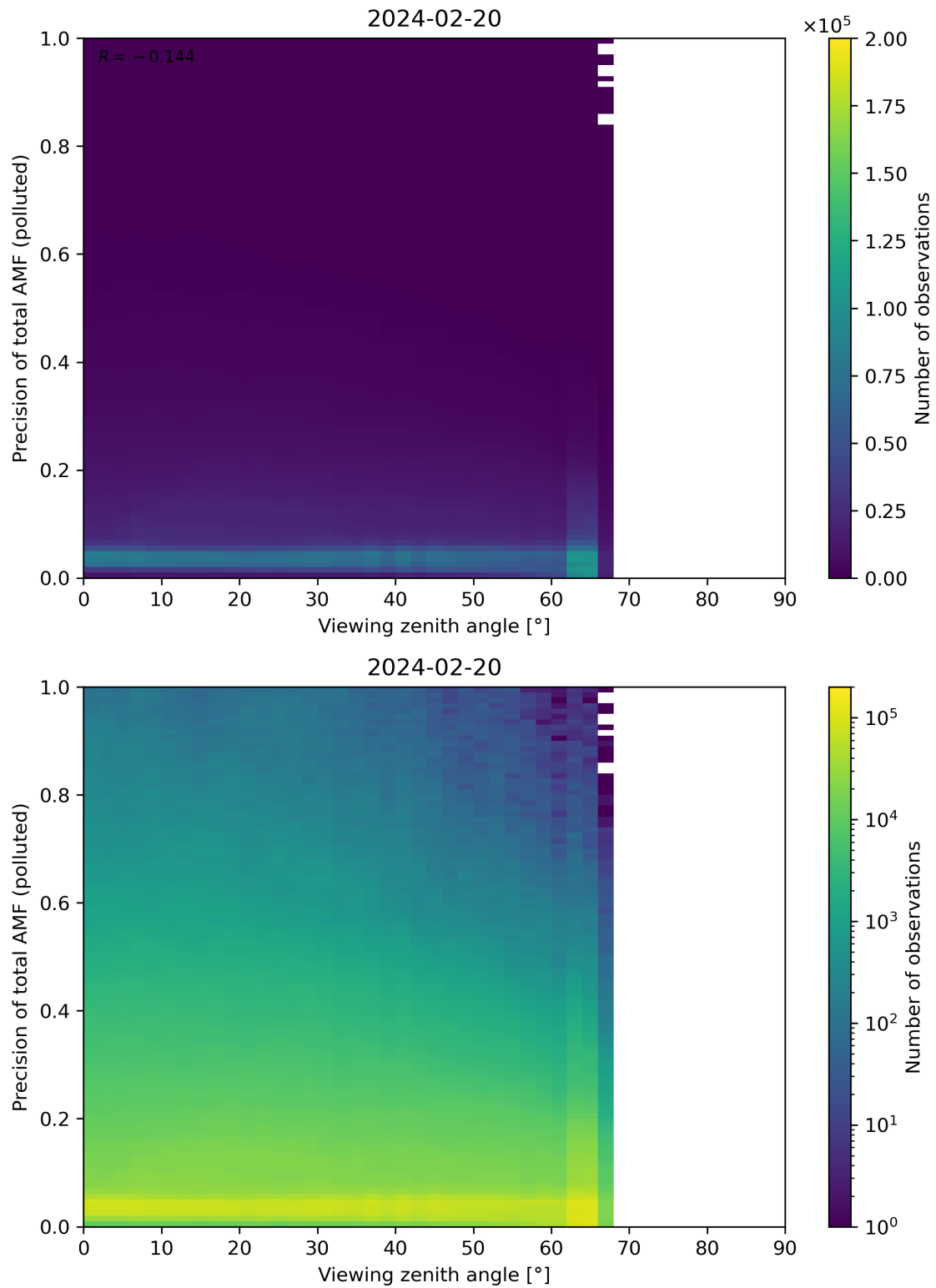
Figure 326: Scatter density plot of “Viewing zenith angle” against “Precision of total AMF (polluted)” for 2024-02-19 to 2024-02-21.
