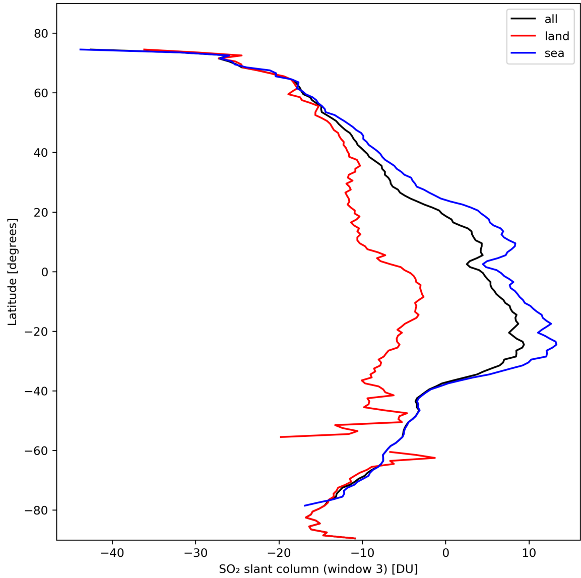
Figure 41: Zonal average of “SO 2 slant column (window 3)” for 2024-02-19 to 2024-02-21.
