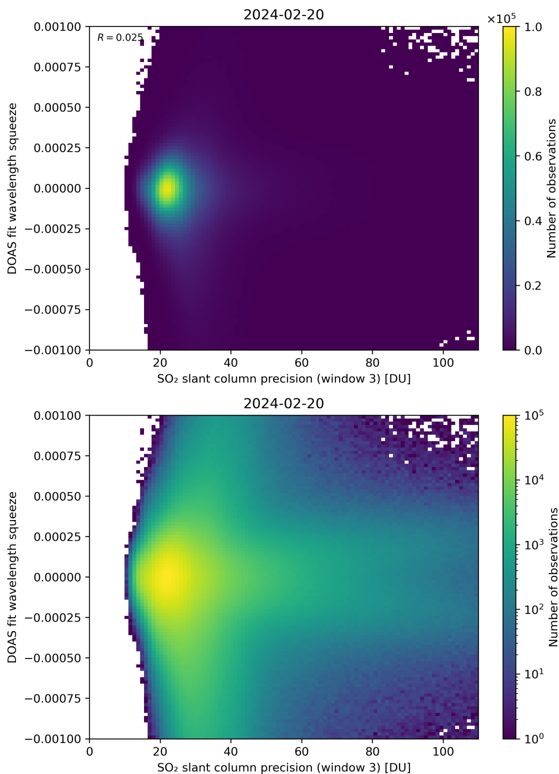
Figure 259: Scatter density plot of “SO 2 slant column precision (window 3)” against “DOAS fit wavelength squeeze” for 2024-02-19 to 2024-02-21.
