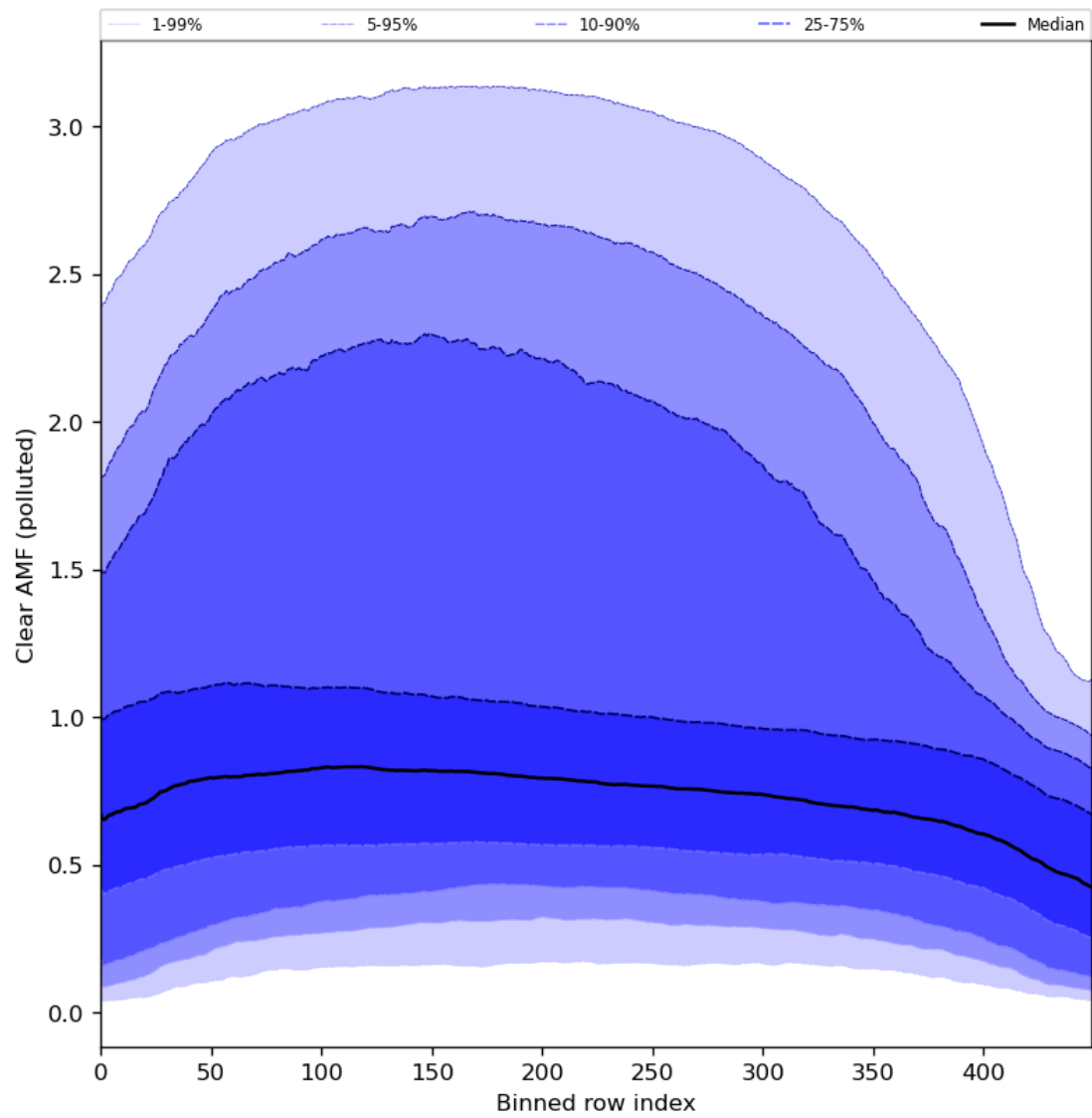
Figure 96: Along track statistics of “Clear AMF (polluted)” for 2024-02-19 to 2024-02-21
