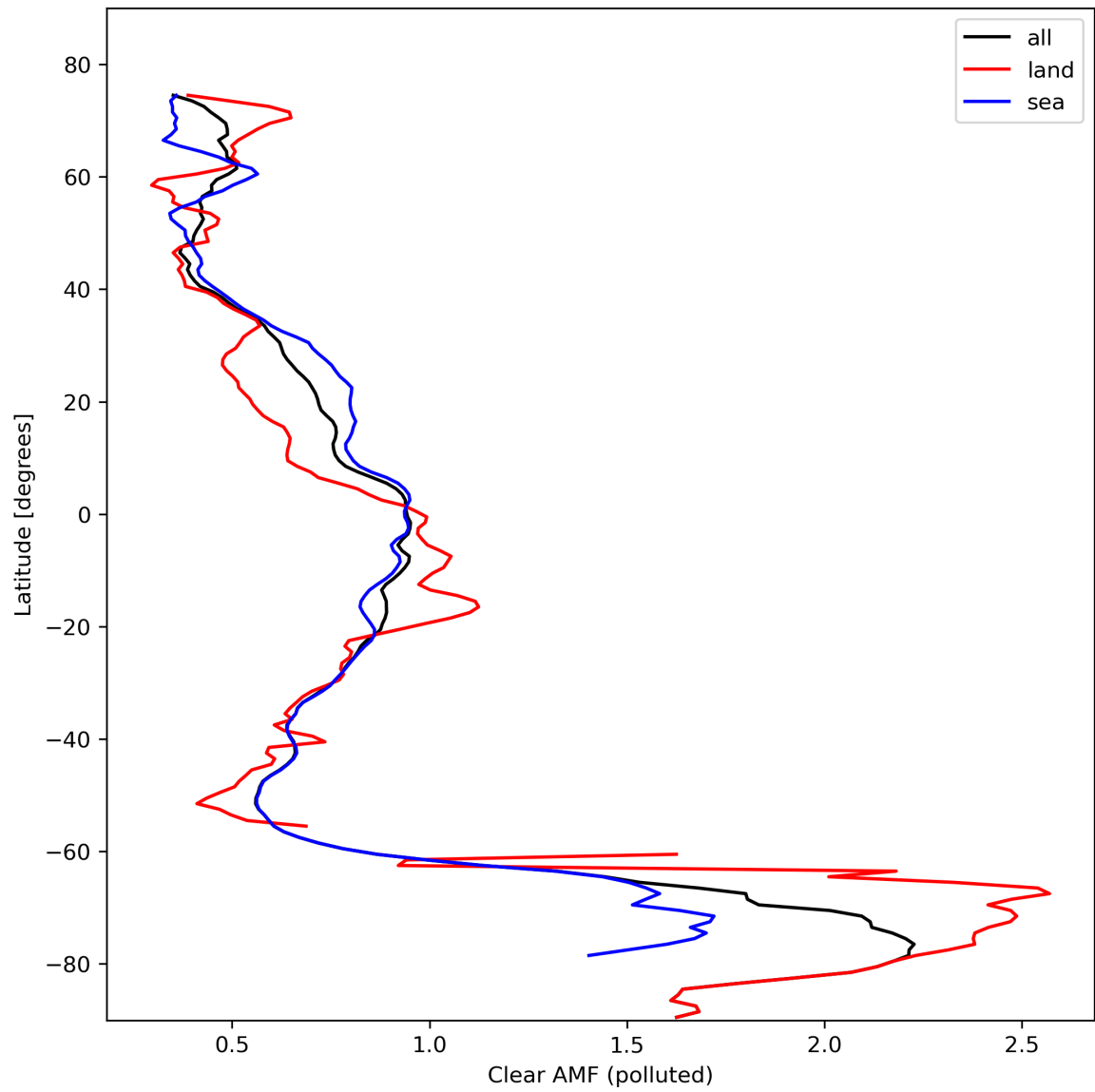
Figure 50: Zonal average of “Clear AMF (polluted)” for 2024-02-19 to 2024-02-21.
