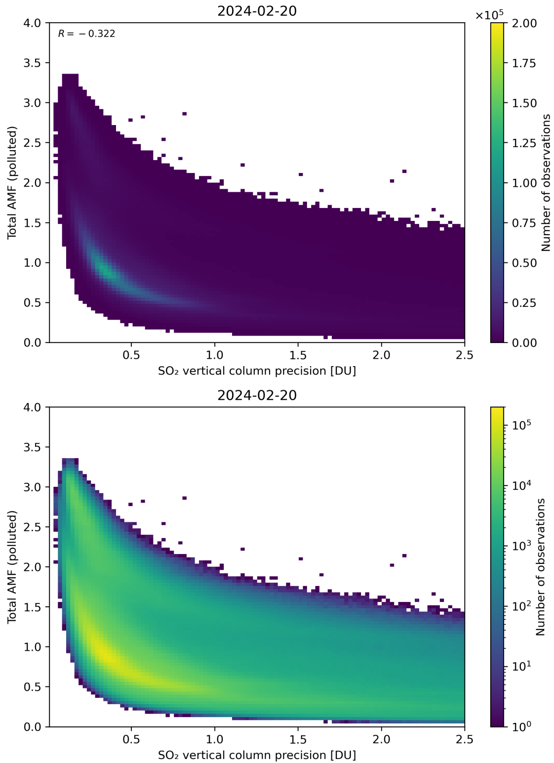
Figure 294: Scatter density plot of “SO 2 vertical column precision” against “Total AMF (polluted)” for 2024-02-19 to 2024-02-21.
