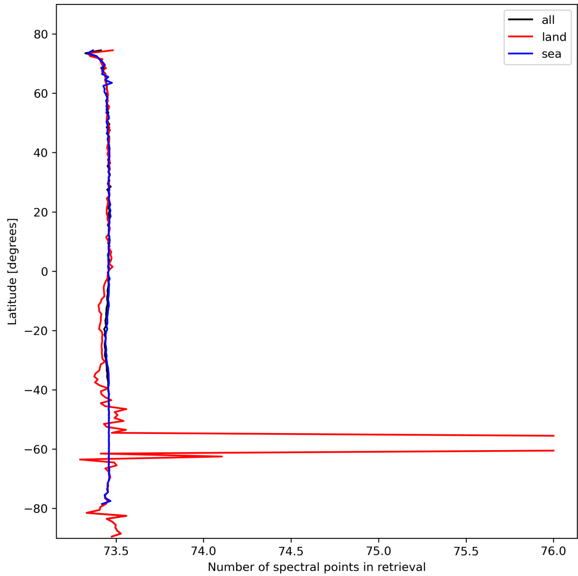
Figure 51: Zonal average of “Number of spectral points in retrieval” for 2024-02-19 to 2024-02-21.
