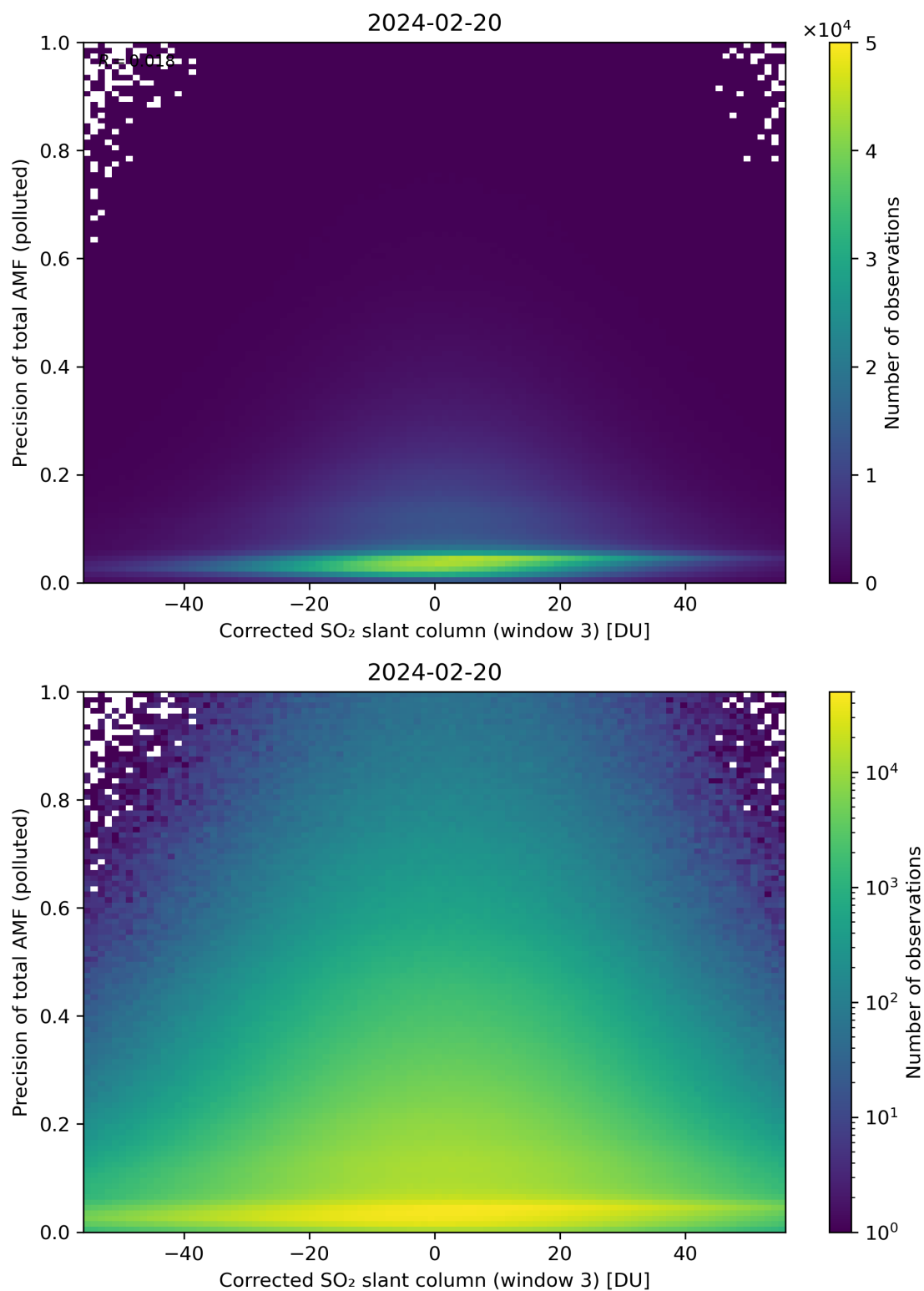
Figure 211: Scatter density plot of “Corrected SO 2 slant column (window 3)” against “Precision of total AMF (polluted)” for 2024-02-19 to 2024-02-21.
