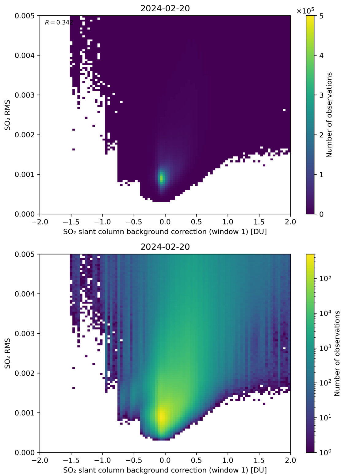
Figure 102: Scatter density plot of “SO 2 slant column background correction (window 1)” against “SO 2 RMS” for 2024-02-19 to 2024-02-21.
