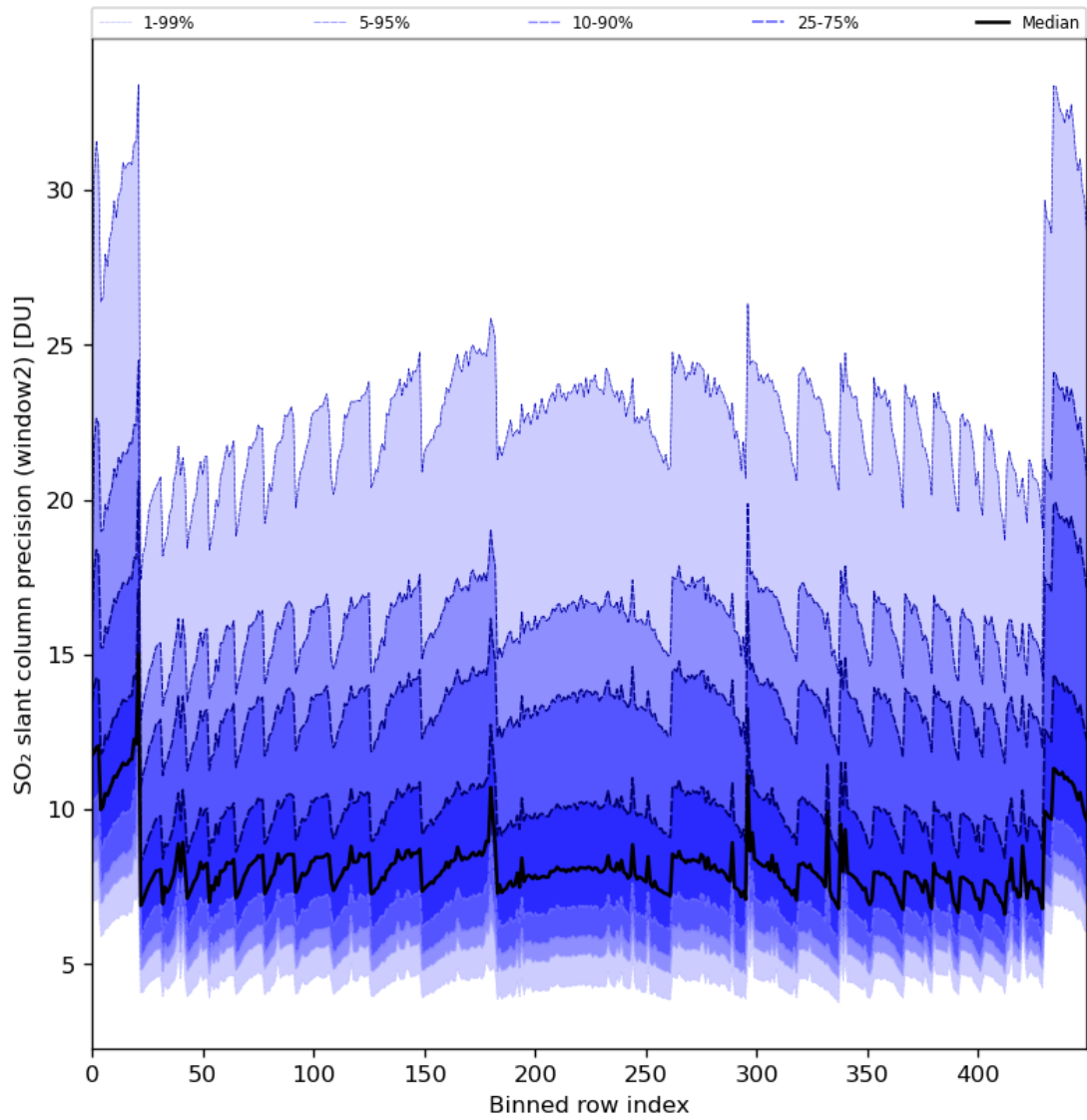
Figure 84: Along track statistics of “SO 2 slant column precision (window2)” for 2024-02-19 to 2024-02-21
