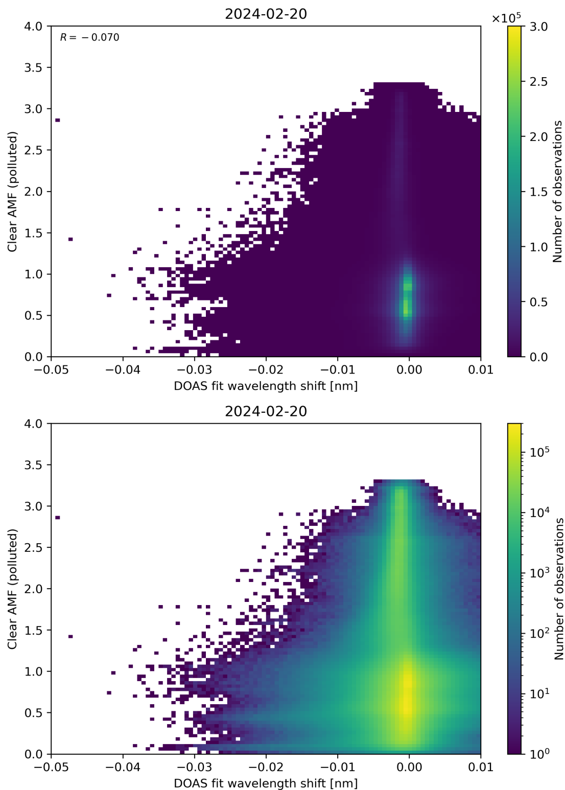
Figure 129: Scatter density plot of “DOAS fit wavelength shift” against “Clear AMF (polluted)” for 2024-02-19 to 2024-02-21.
