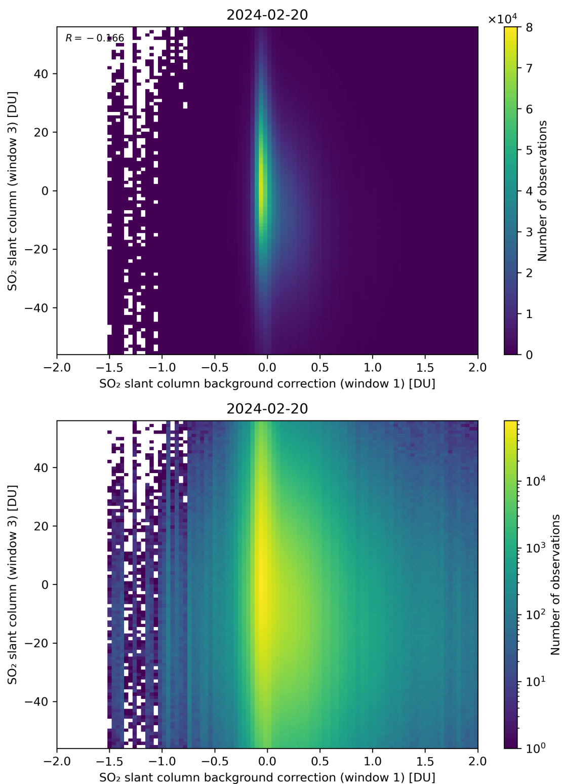
Figure 107: Scatter density plot of “SO 2 slant column background correction (window 1)” against “SO 2 slant column (window 3)” for 2024-02-19 to 2024-02-21.
