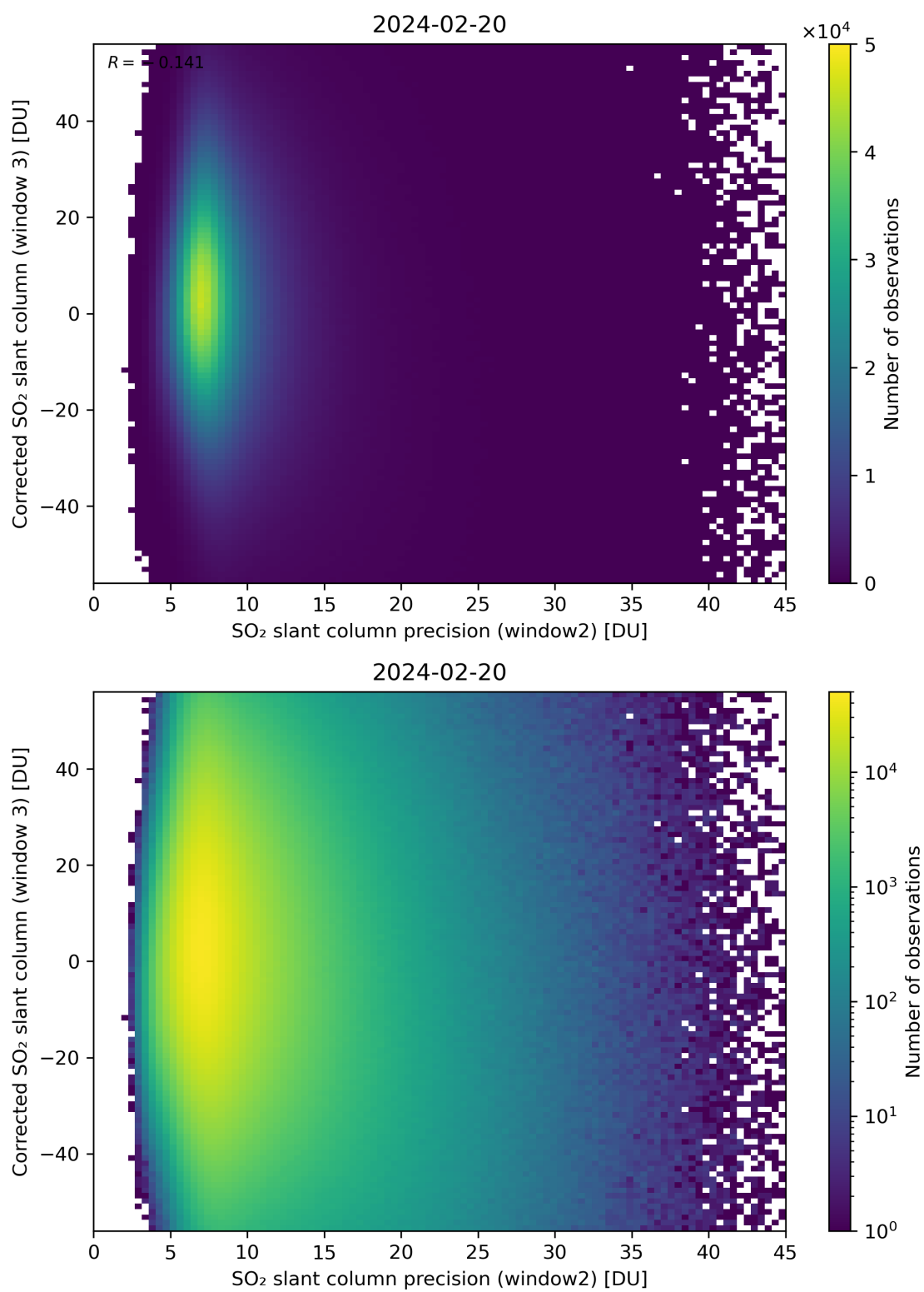
Figure 248: Scatter density plot of “SO 2 slant column precision (window2)” against “Corrected SO 2 slant column (window 3)” for 2024-02-19 to 2024-02-21.
