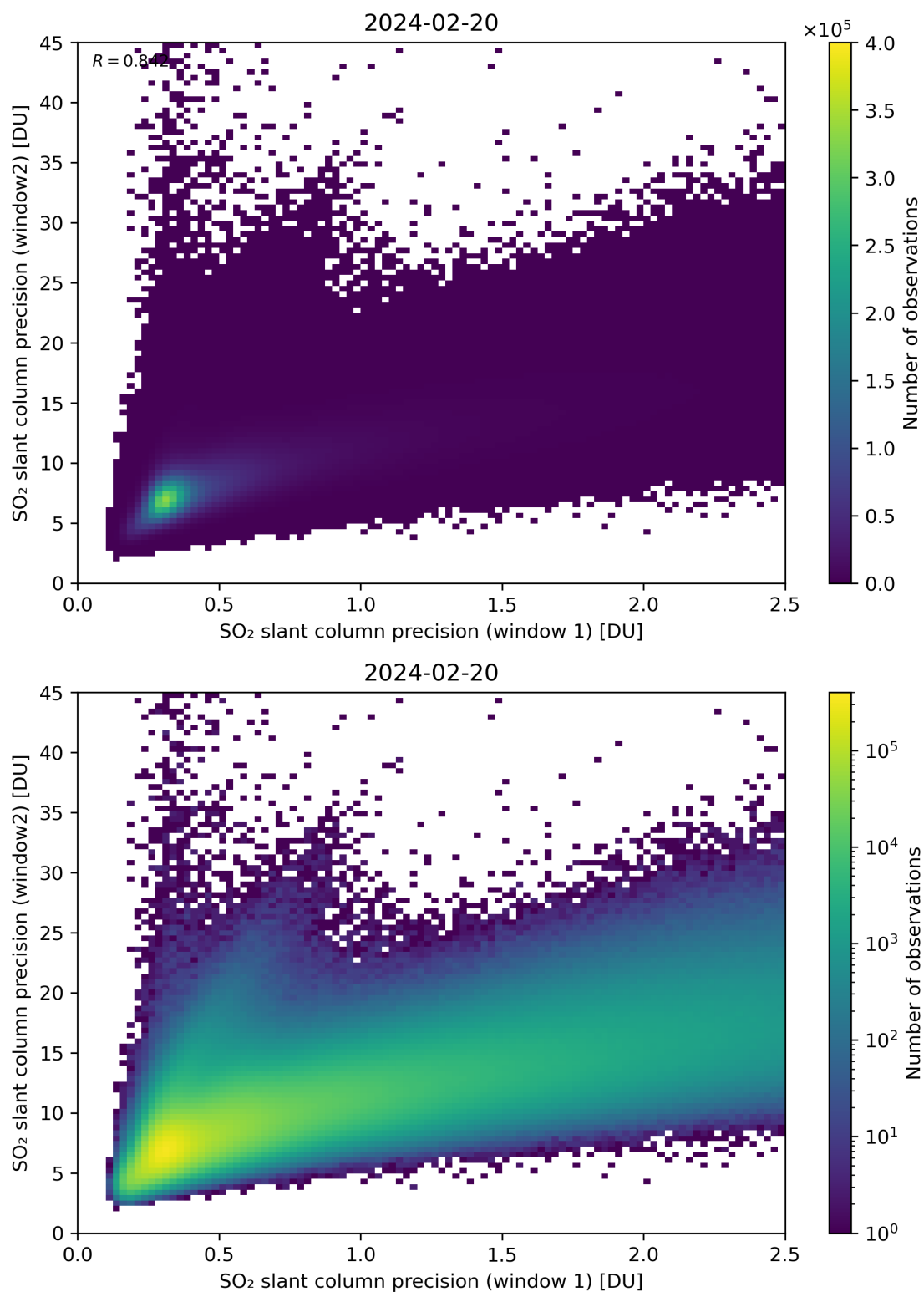
Figure 227: Scatter density plot of “SO 2 slant column precision (window 1)” against “SO 2 slant column precision (window2)” for 2024-02-19 to 2024-02-21.
