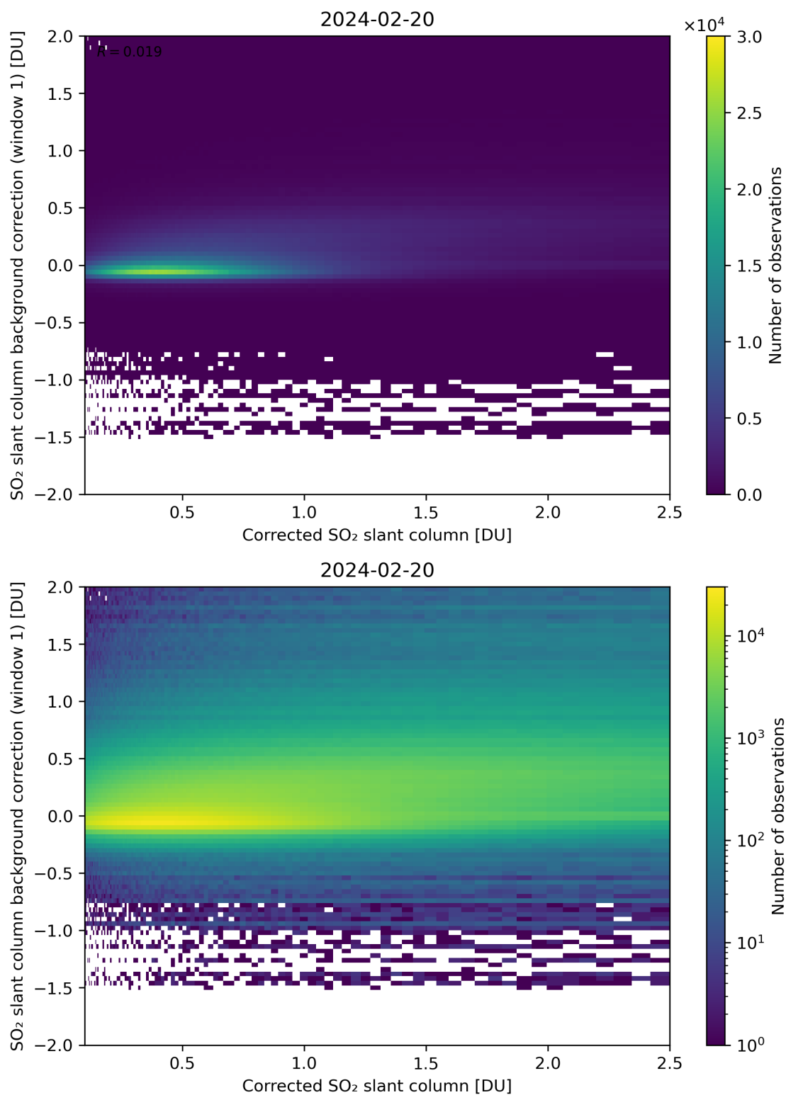
Figure 178: Scatter density plot of “Corrected SO 2 slant column” against “SO 2 slant column background correction (window 1)” for 2024-02-19 to 2024-02-21.
