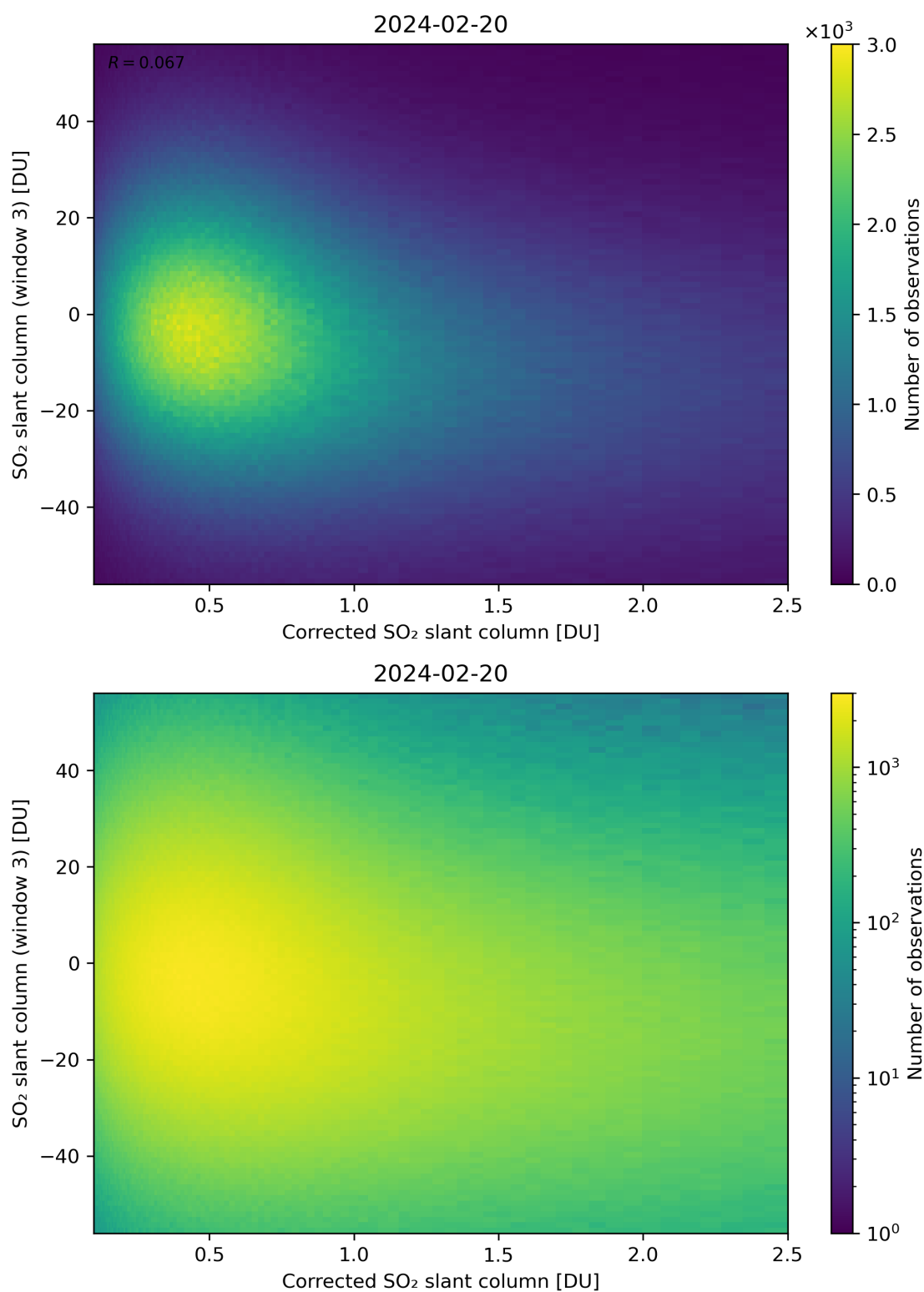
Figure 190: Scatter density plot of “Corrected SO 2 slant column” against “SO 2 slant column (window 3)” for 2024-02-19 to 2024-02-21.
