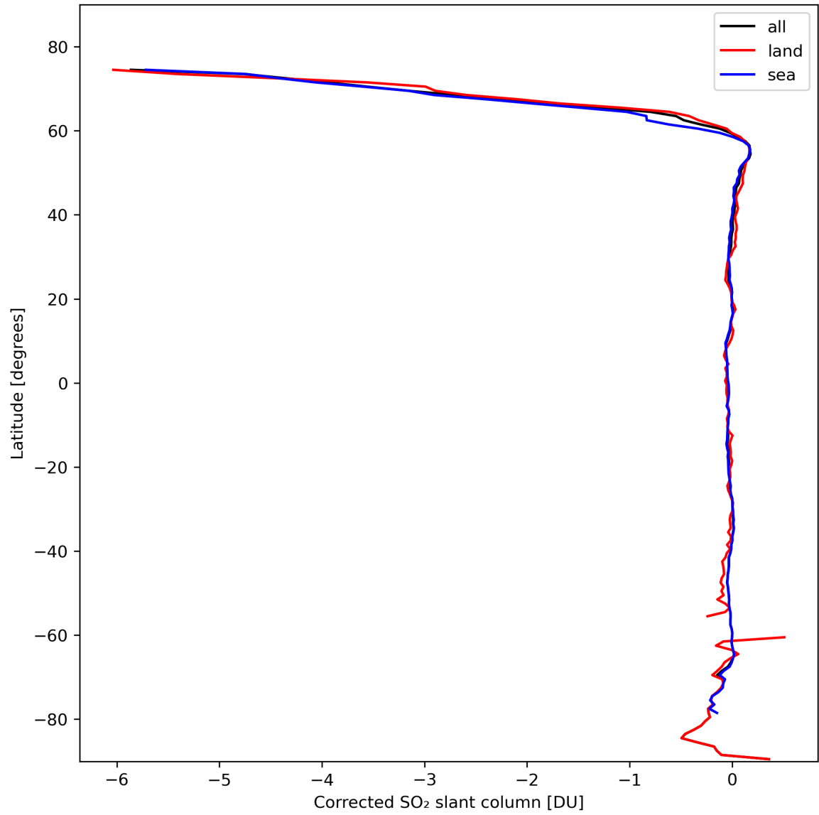
Figure 32: Zonal average of “Corrected SO 2 slant column” for 2024-02-19 to 2024-02-21.
