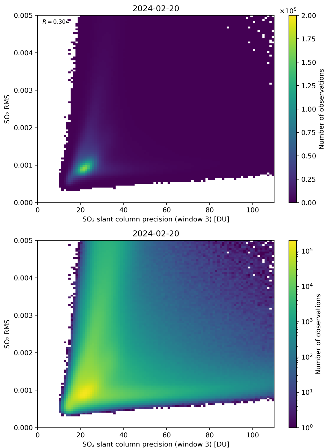
Figure 260: Scatter density plot of “SO 2 slant column precision (window 3)” against “SO 2 RMS” for 2024-02-19 to 2024-02-21.
