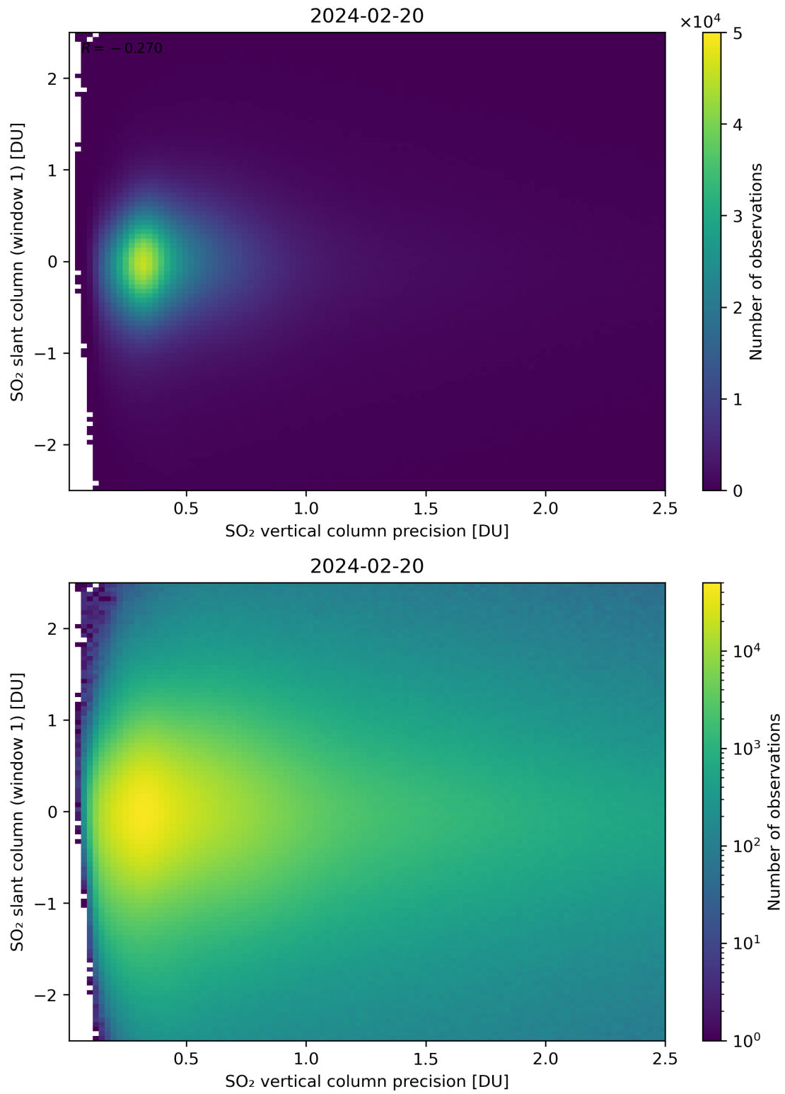
Figure 289: Scatter density plot of “SO 2 vertical column precision” against “SO 2 slant column (window 1)” for 2024-02-19 to 2024-02-21.
