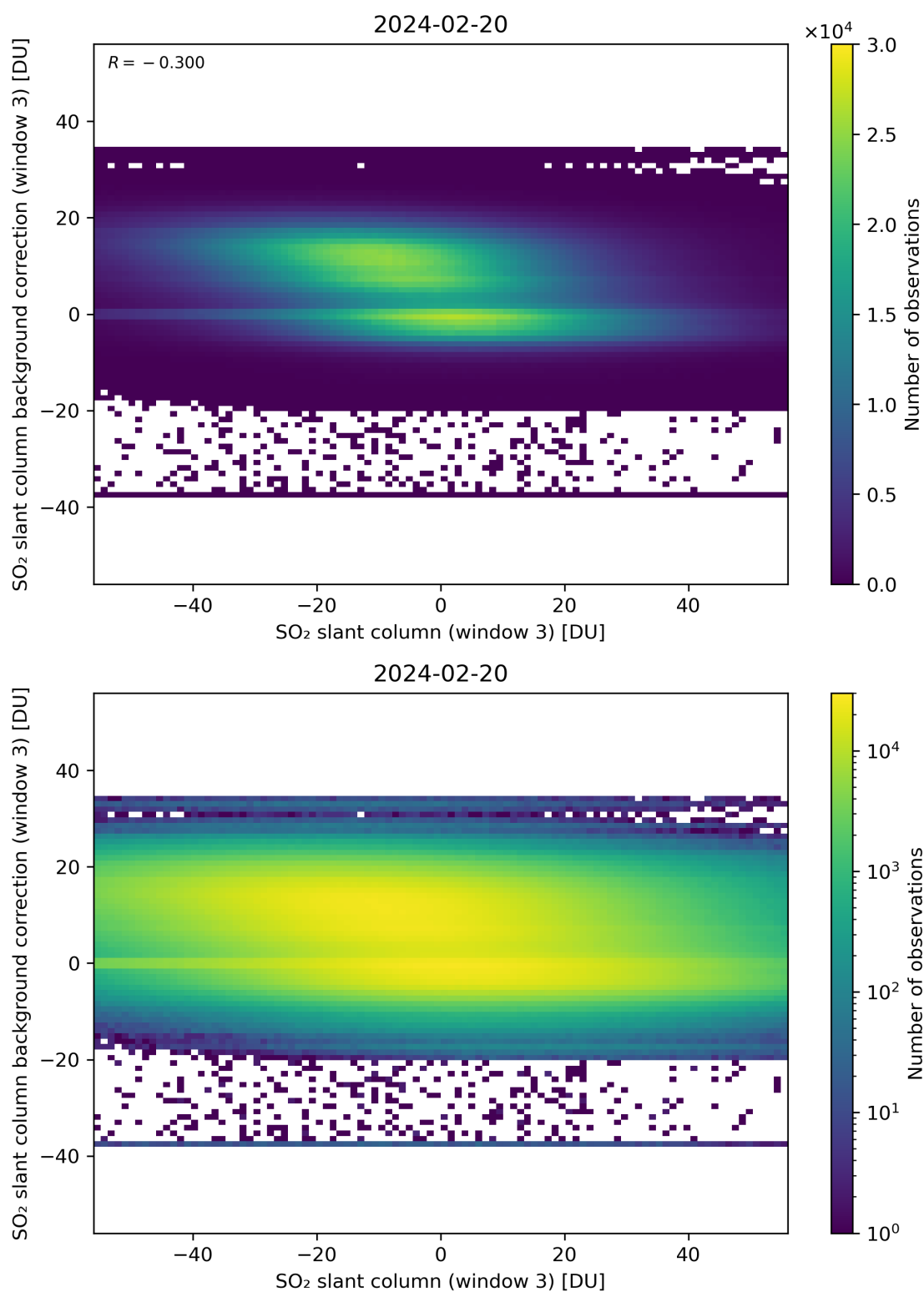
Figure 253: Scatter density plot of “SO 2 slant column (window 3)” against “SO 2 slant column background correction (window 3)” for 2024-02-19 to 2024-02-21.
