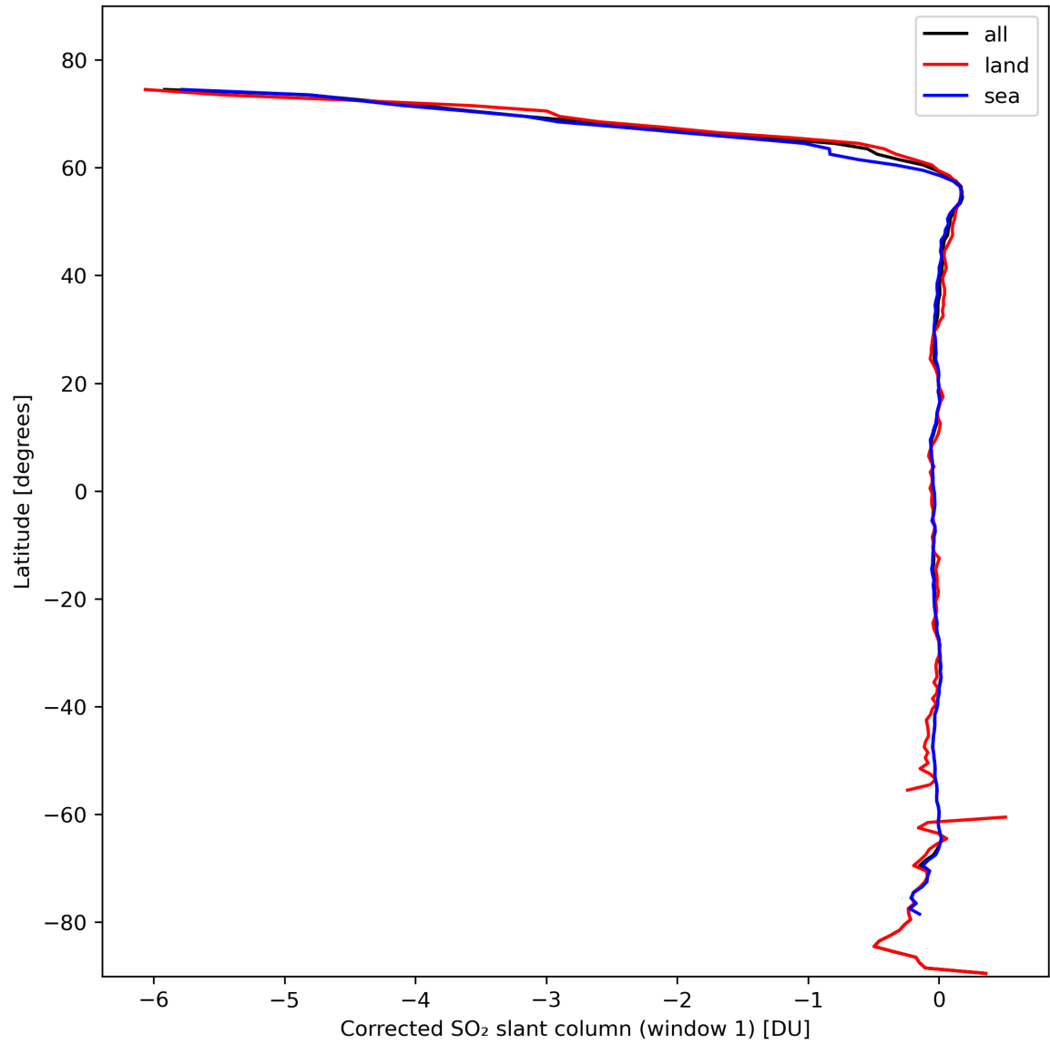
Figure 35: Zonal average of “Corrected SO 2 slant column (window 1)” for 2024-02-19 to 2024-02-21.
