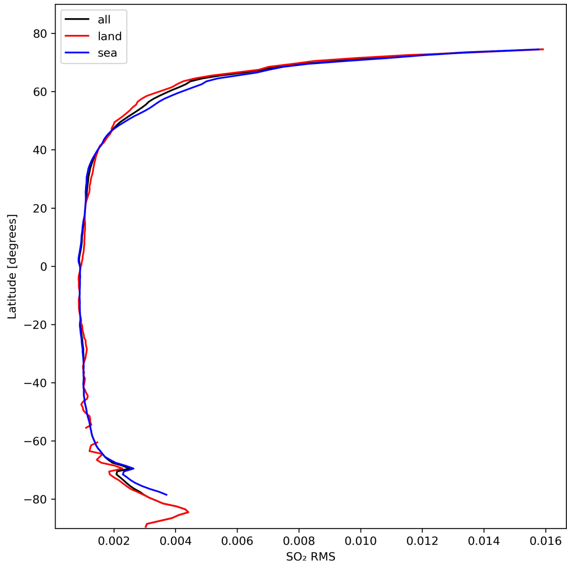
Figure 47: Zonal average of “SO 2 RMS” for 2024-02-19 to 2024-02-21.
