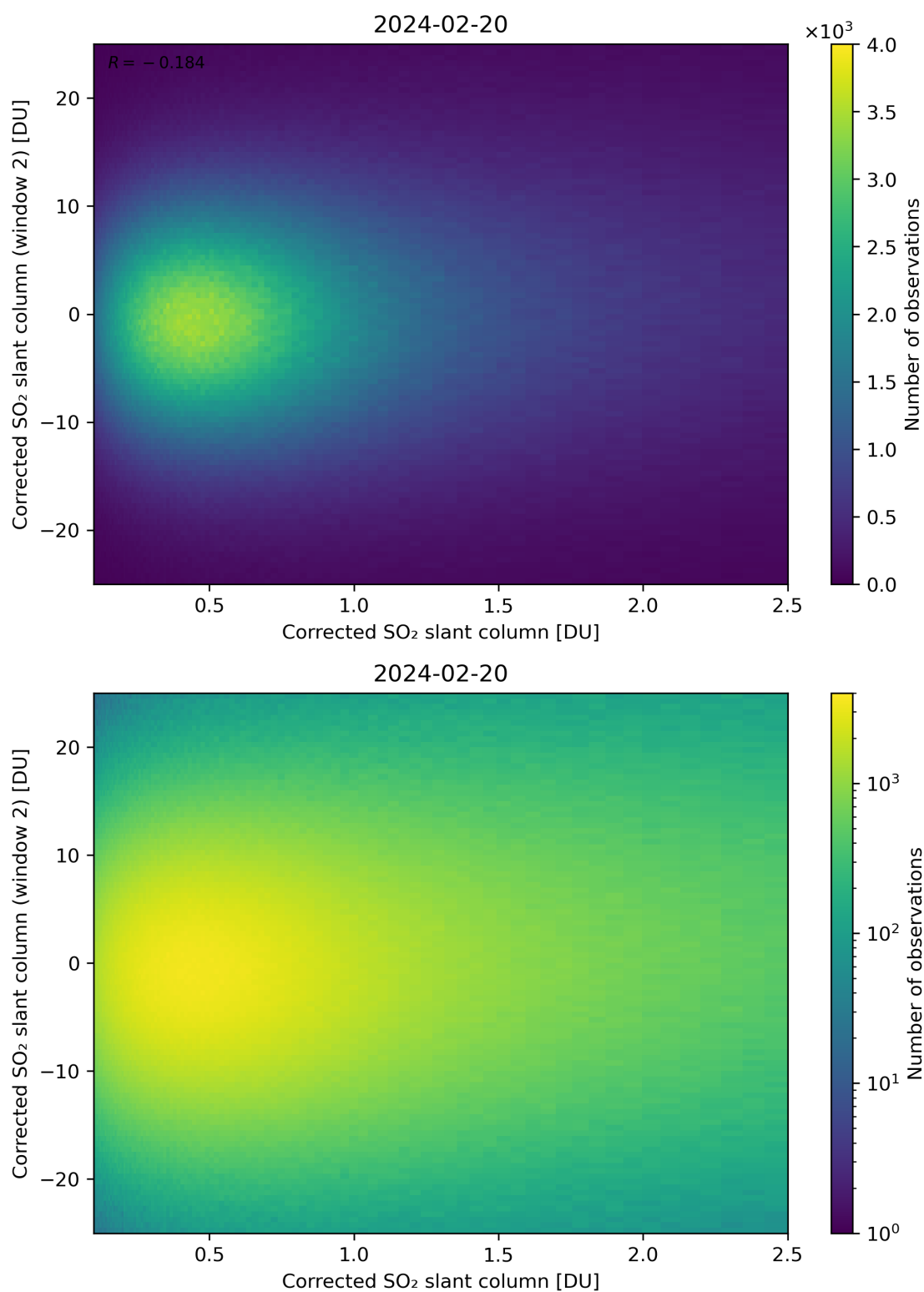
Figure 185: Scatter density plot of “Corrected SO 2 slant column” against “Corrected SO 2 slant column (window 2)” for 2024-02-19 to 2024-02-21.
