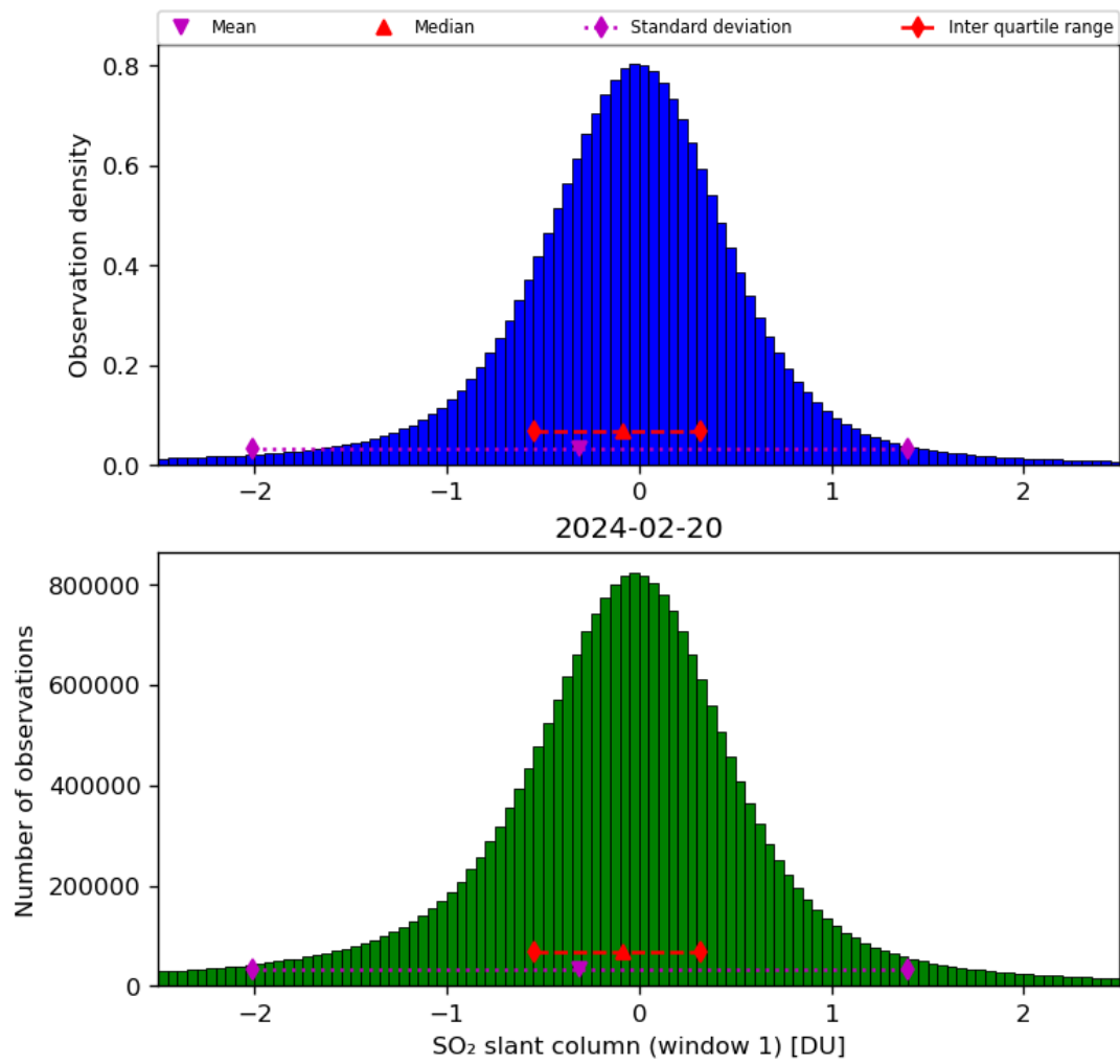
Figure 56: Histogram of “SO 2 slant column (window 1)” for 2024-02-19 to 2024-02-21
