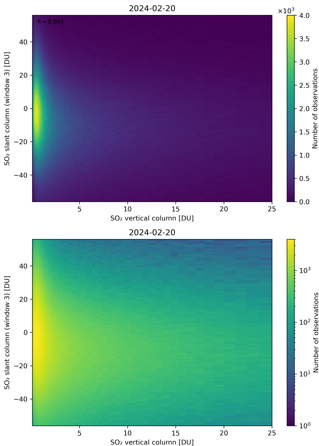
Figure 303: Scatter density plot of “SO 2 vertical column” against “SO 2 slant column (window 3)” for 2024-02-19 to 2024-02-21.
