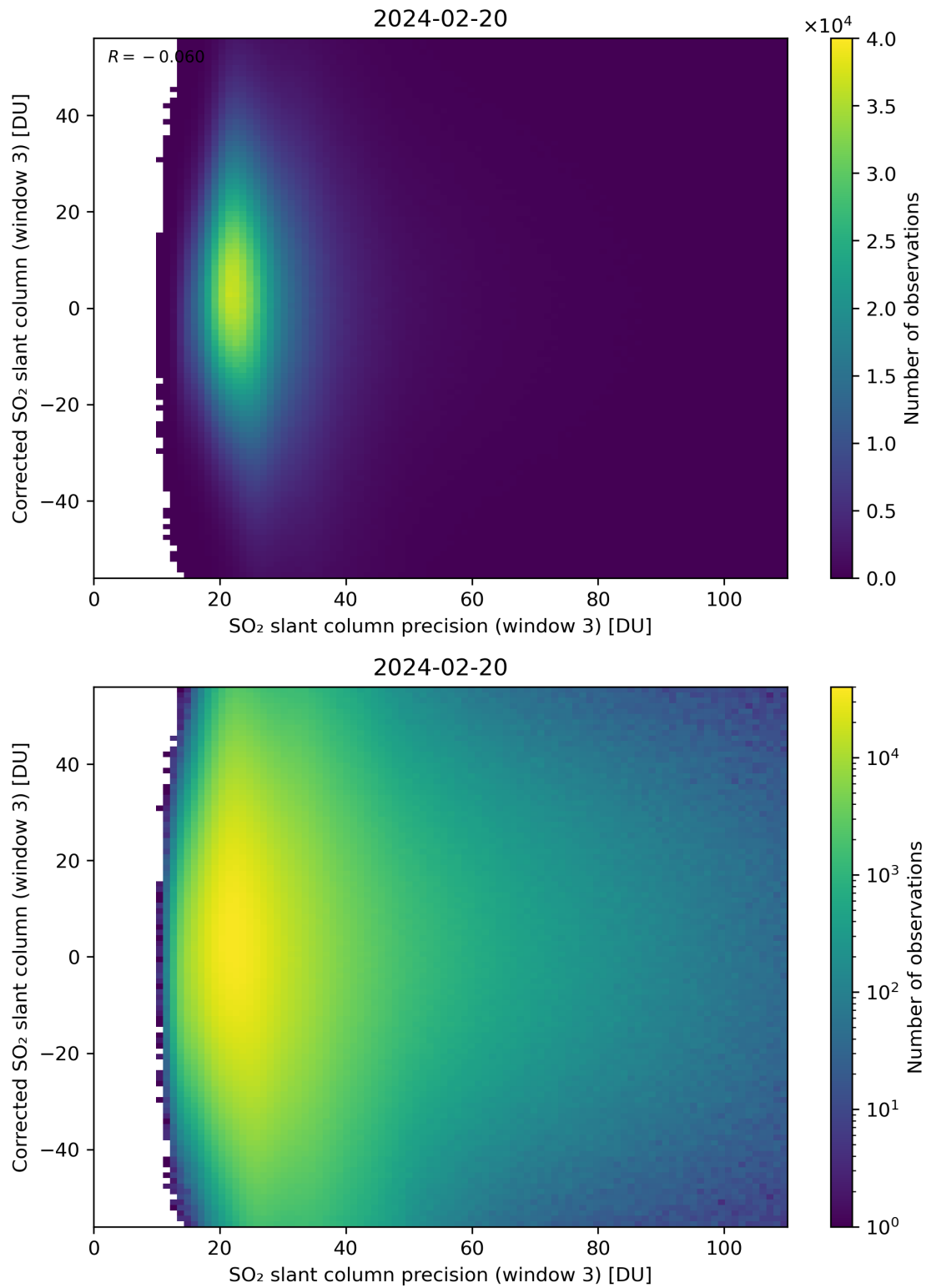
Figure 262: Scatter density plot of “SO 2 slant column precision (window 3)” against “Corrected SO 2 slant column (window 3)” for 2024-02-19 to 2024-02-21.
