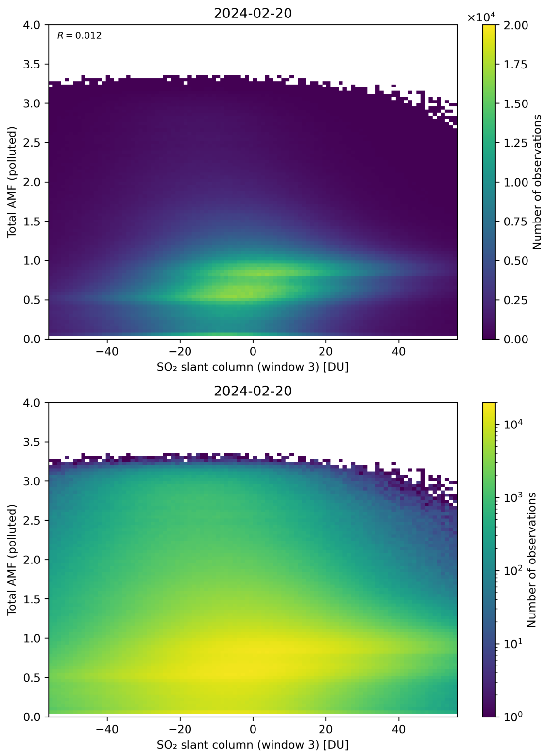
Figure 268: Scatter density plot of “SO 2 slant column (window 3)” against “Total AMF (polluted)” for 2024-02-19 to 2024-02-21.
