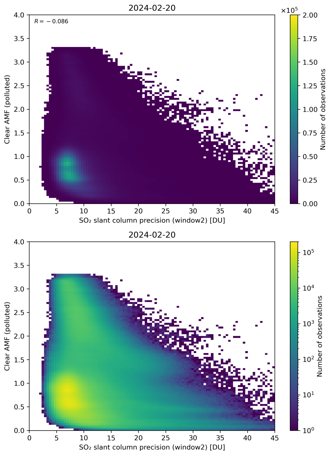
Figure 246: Scatter density plot of “SO 2 slant column precision (window2)” against “Clear AMF (polluted)” for 2024-02-19 to 2024-02-21.
