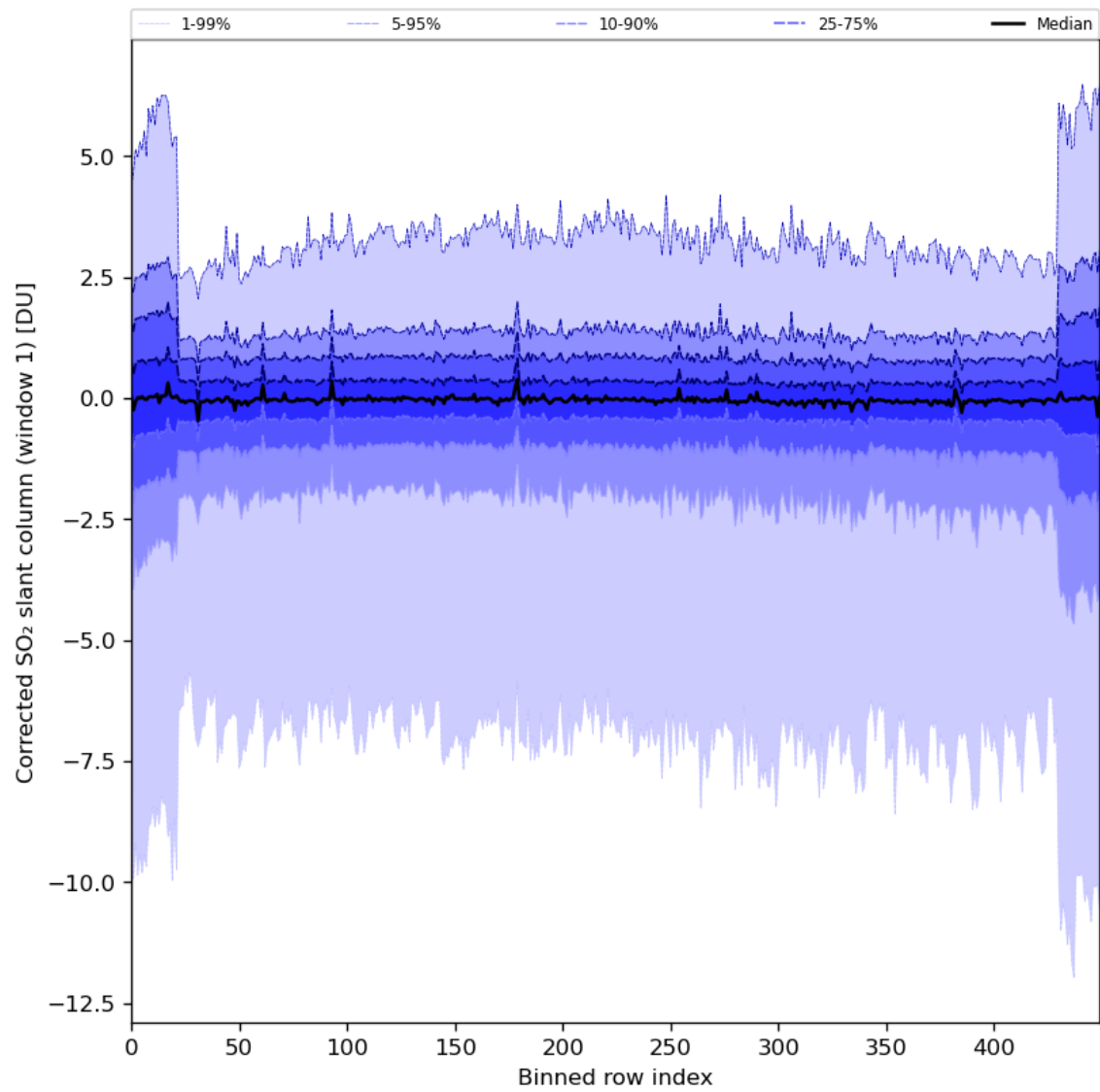
Figure 81: Along track statistics of “Corrected SO 2 slant column (window 1)” for 2024-02-19 to 2024-02-21
