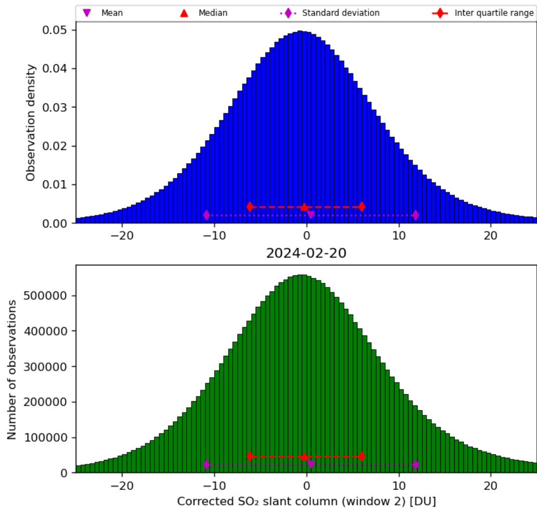
Figure 62: Histogram of “Corrected SO 2 slant column (window 2)” for 2024-02-19 to 2024-02-21
