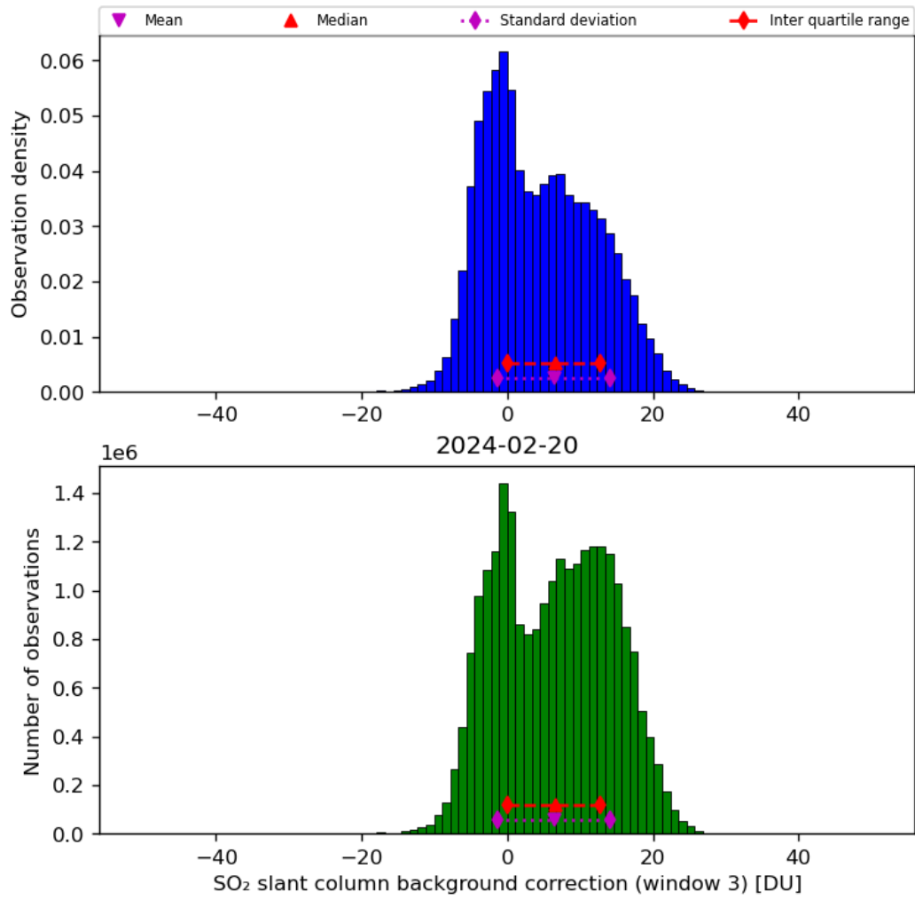
Figure 67: Histogram of “SO 2 slant column background correction (window 3)” for 2024-02-19 to 2024-02-21
