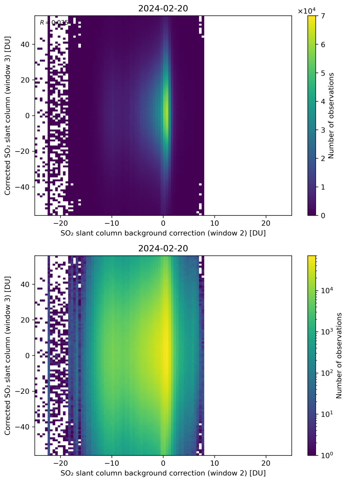
Figure 116: Scatter density plot of “SO 2 slant column background correction (window 2)” against “Corrected SO 2 slant column (window 3)” for 2024-02-19 to 2024-02-21.
