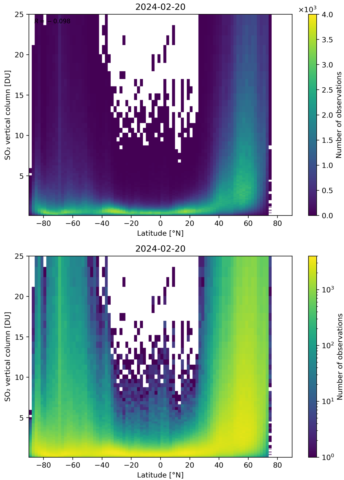
Figure 156: Scatter density plot of “Latitude” against “SO 2 vertical column” for 2024-02-19 to 2024-02-21.
