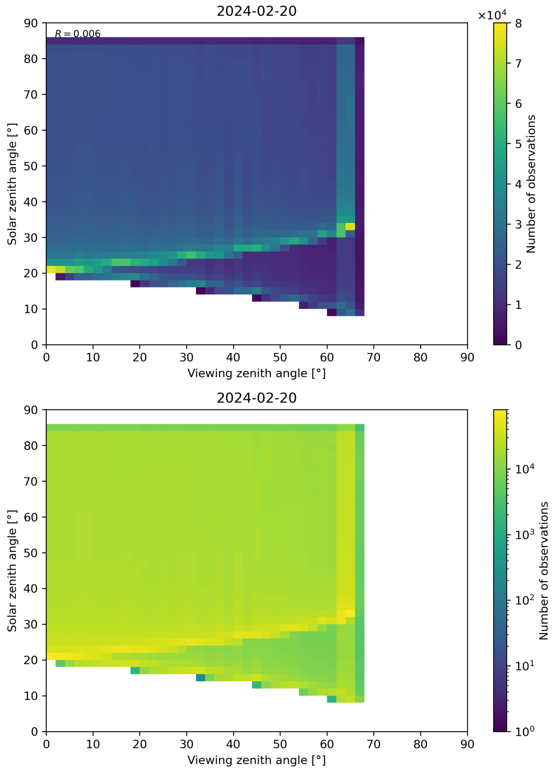
Figure 315: Scatter density plot of “Viewing zenith angle” against “Solar zenith angle” for 2024-02-19 to 2024-02-21.
