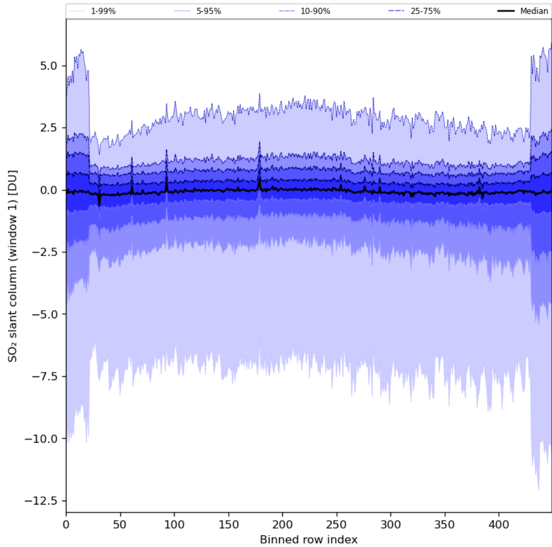
Figure 79: Along track statistics of “SO 2 slant column (window 1)” for 2024-02-19 to 2024-02-21
