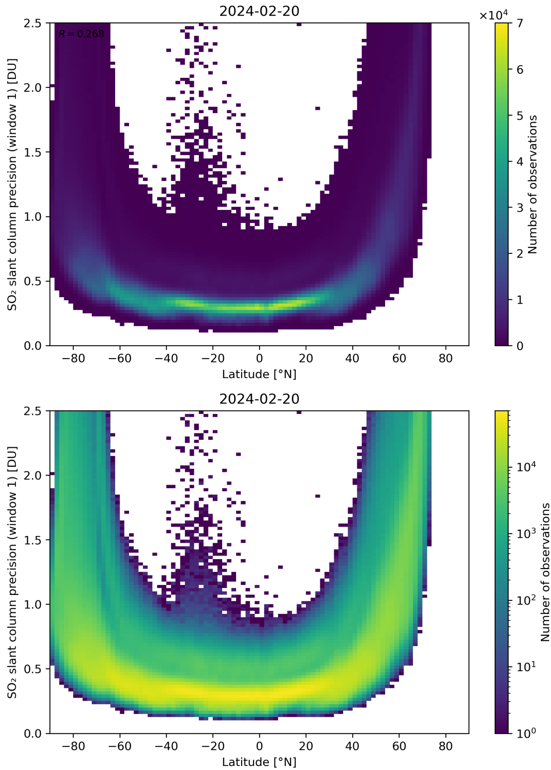
Figure 150: Scatter density plot of “Latitude” against “SO 2 slant column precision (window 1)” for 2024-02-19 to 2024-02-21.
