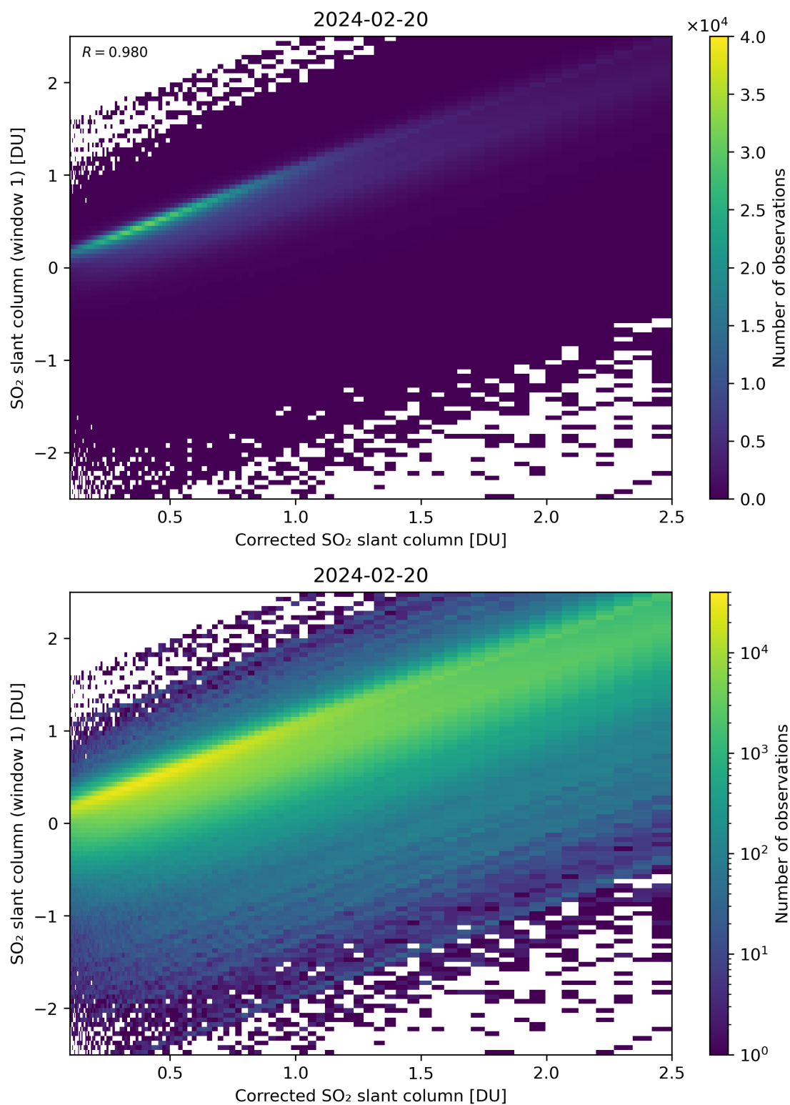
Figure 187: Scatter density plot of “Corrected SO 2 slant column” against “SO 2 slant column (window 1)” for 2024-02-19 to 2024-02-21.
