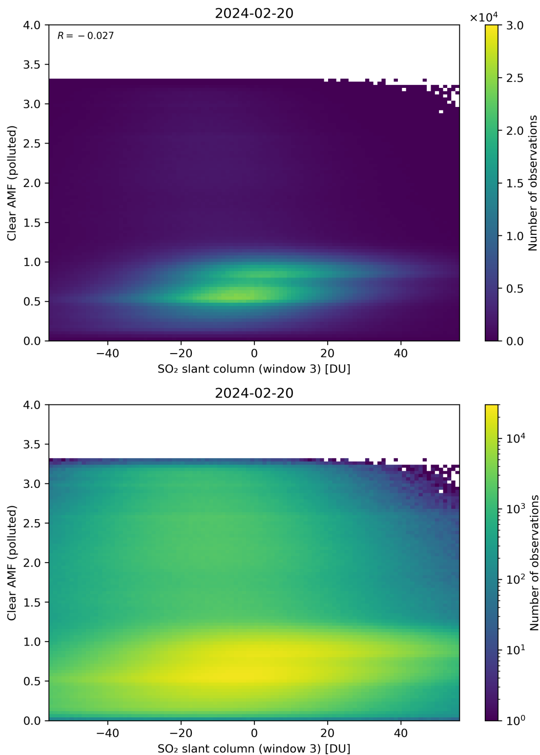
Figure 265: Scatter density plot of “SO 2 slant column (window 3)” against “Clear AMF (polluted)” for 2024-02-19 to 2024-02-21.
