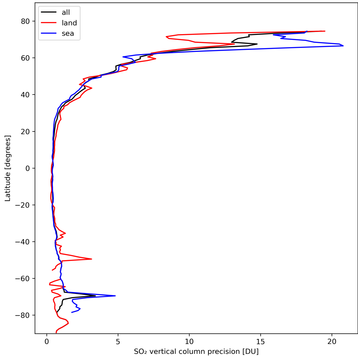
Figure 31: Zonal average of “SO 2 vertical column precision” for 2024-02-19 to 2024-02-21.
