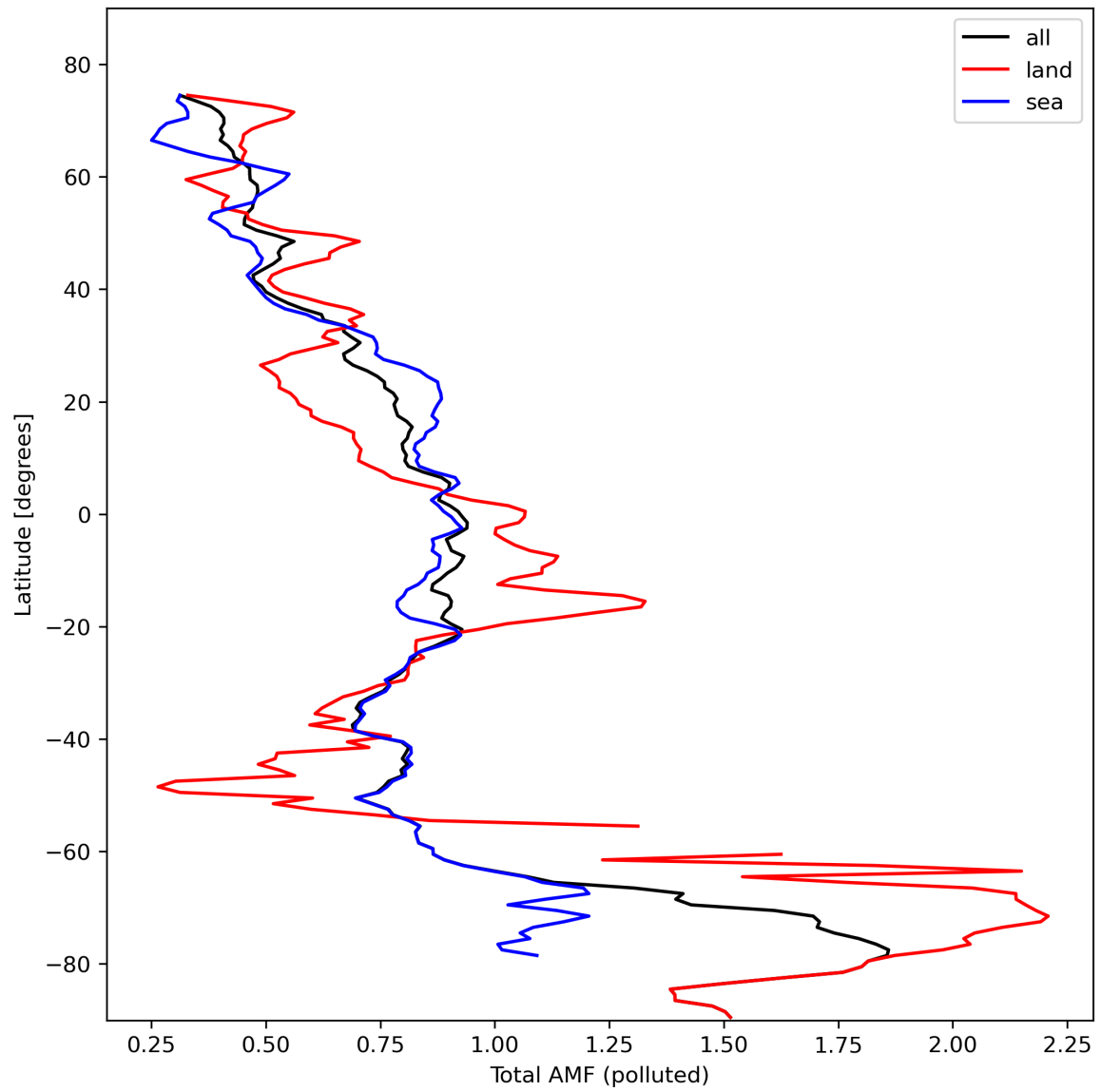
Figure 48: Zonal average of “Total AMF (polluted)” for 2024-02-19 to 2024-02-21.
