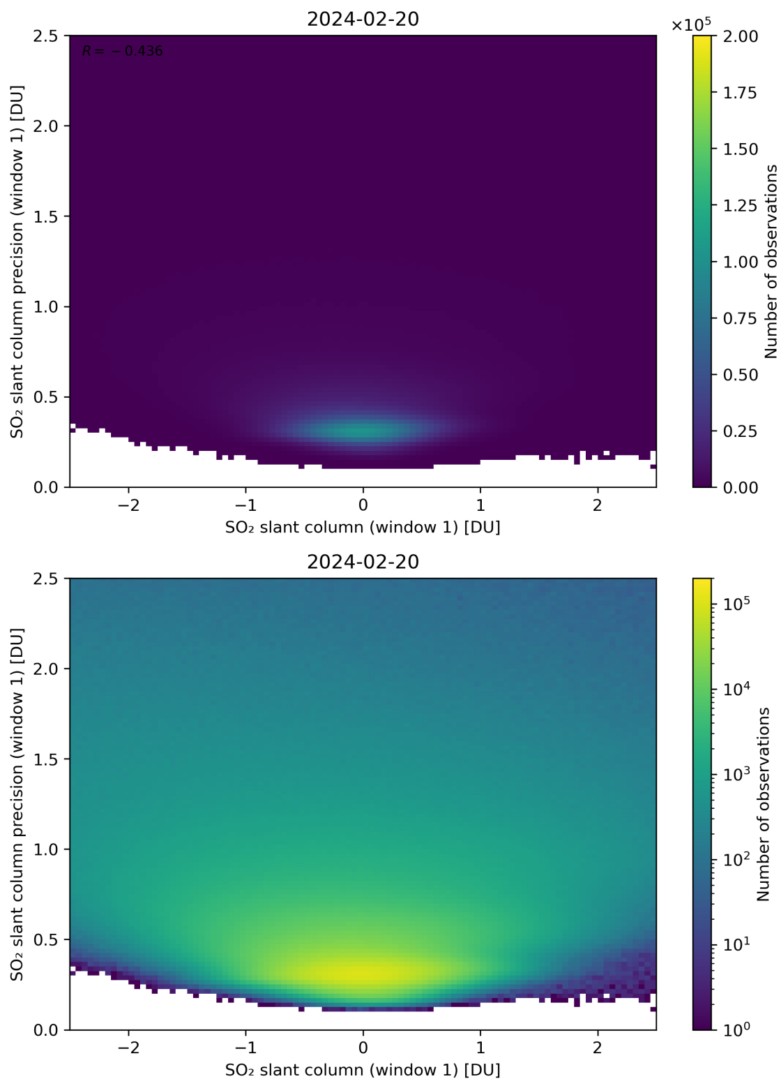
Figure 235: Scatter density plot of “SO 2 slant column (window 1)” against “SO 2 slant column precision (window 1)” for 2024-02-19 to 2024-02-21.
