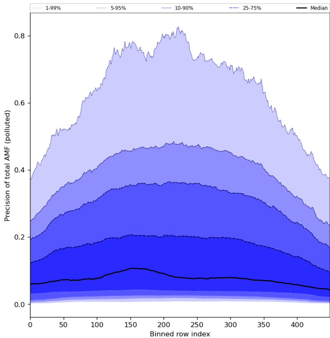
Figure 95: Along track statistics of “Precision of total AMF (polluted)” for 2024-02-19 to 2024-02-21
