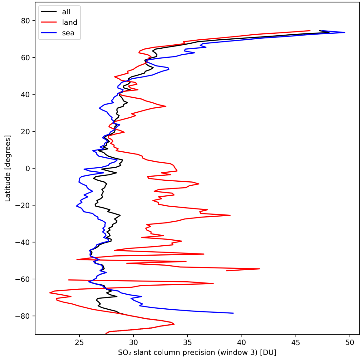
Figure 42: Zonal average of “SO 2 slant column precision (window 3)” for 2024-02-19 to 2024-02-21.
