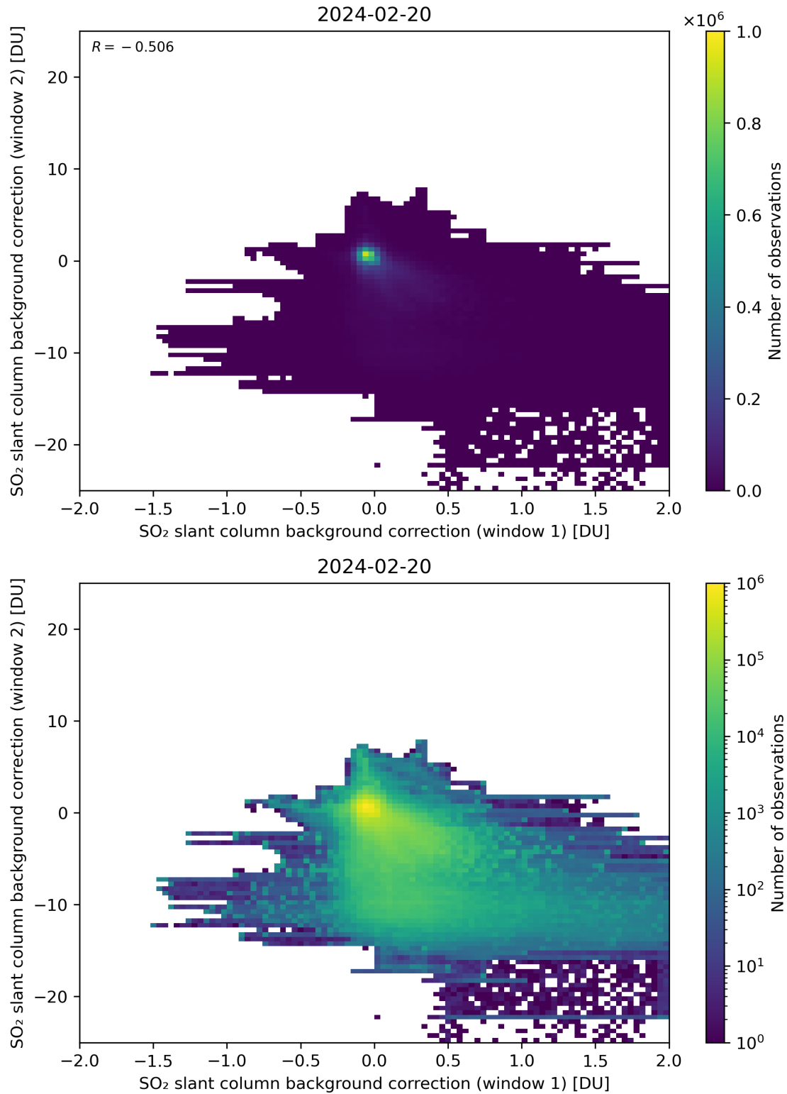
Figure 98: Scatter density plot of “SO 2 slant column background correction (window 1)” against “SO 2 slant column background correction (window 2)” for 2024-02-19 to 2024-02-21.
