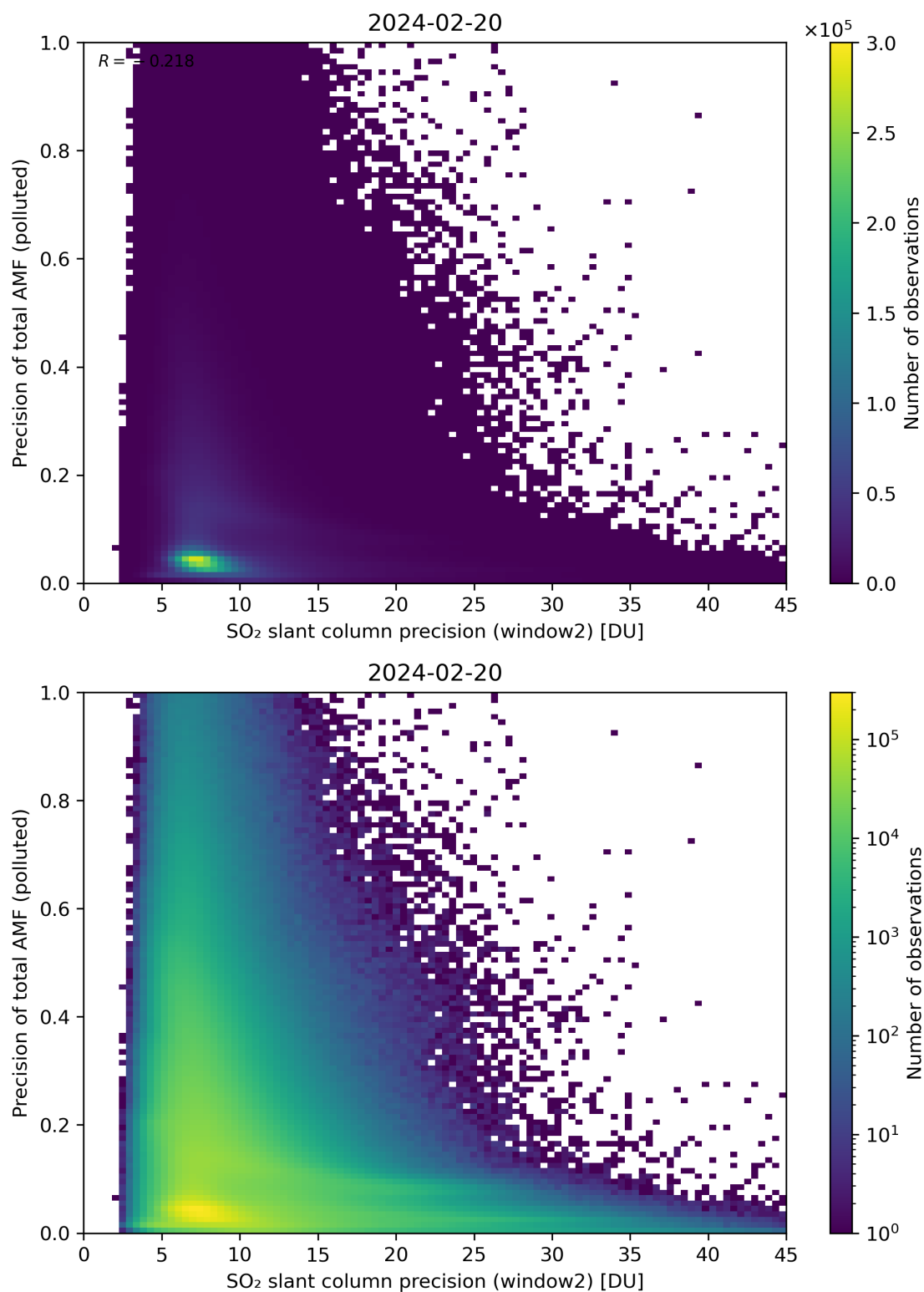
Figure 252: Scatter density plot of “SO 2 slant column precision (window2)” against “Precision of total AMF (polluted)” for 2024-02-19 to 2024-02-21.
