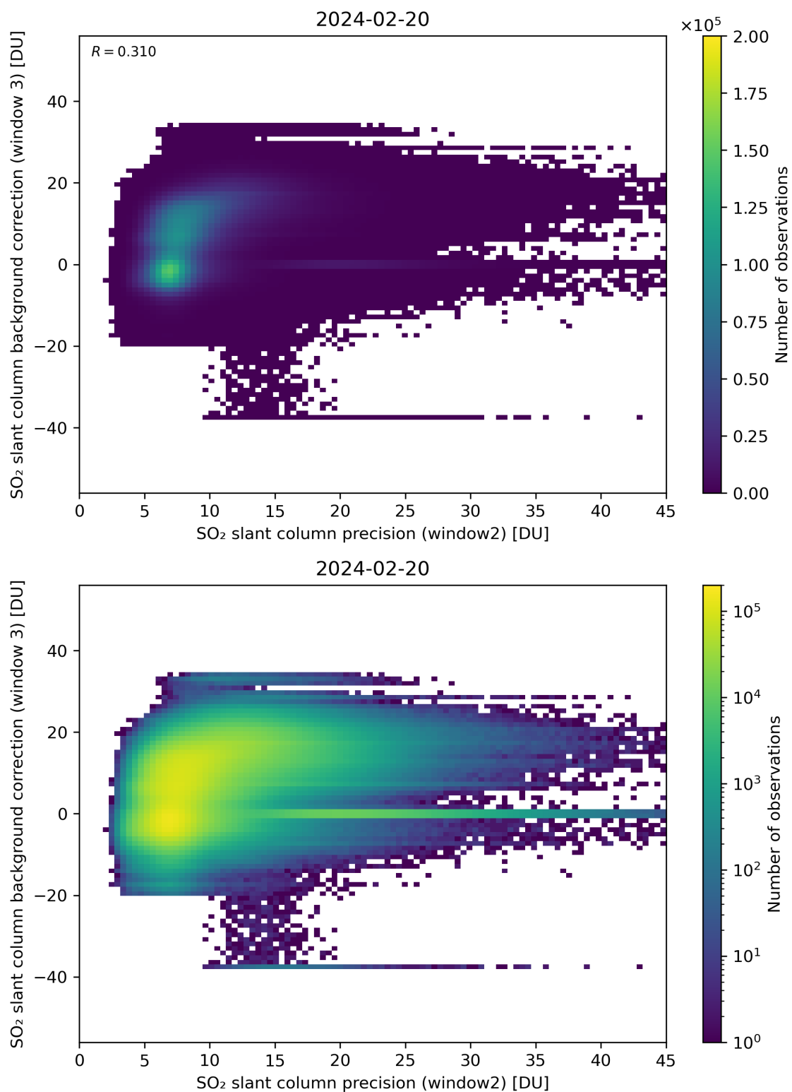
Figure 242: Scatter density plot of “SO 2 slant column precision (window2)” against “SO 2 slant column background correction (window 3)” for 2024-02-19 to 2024-02-21.
