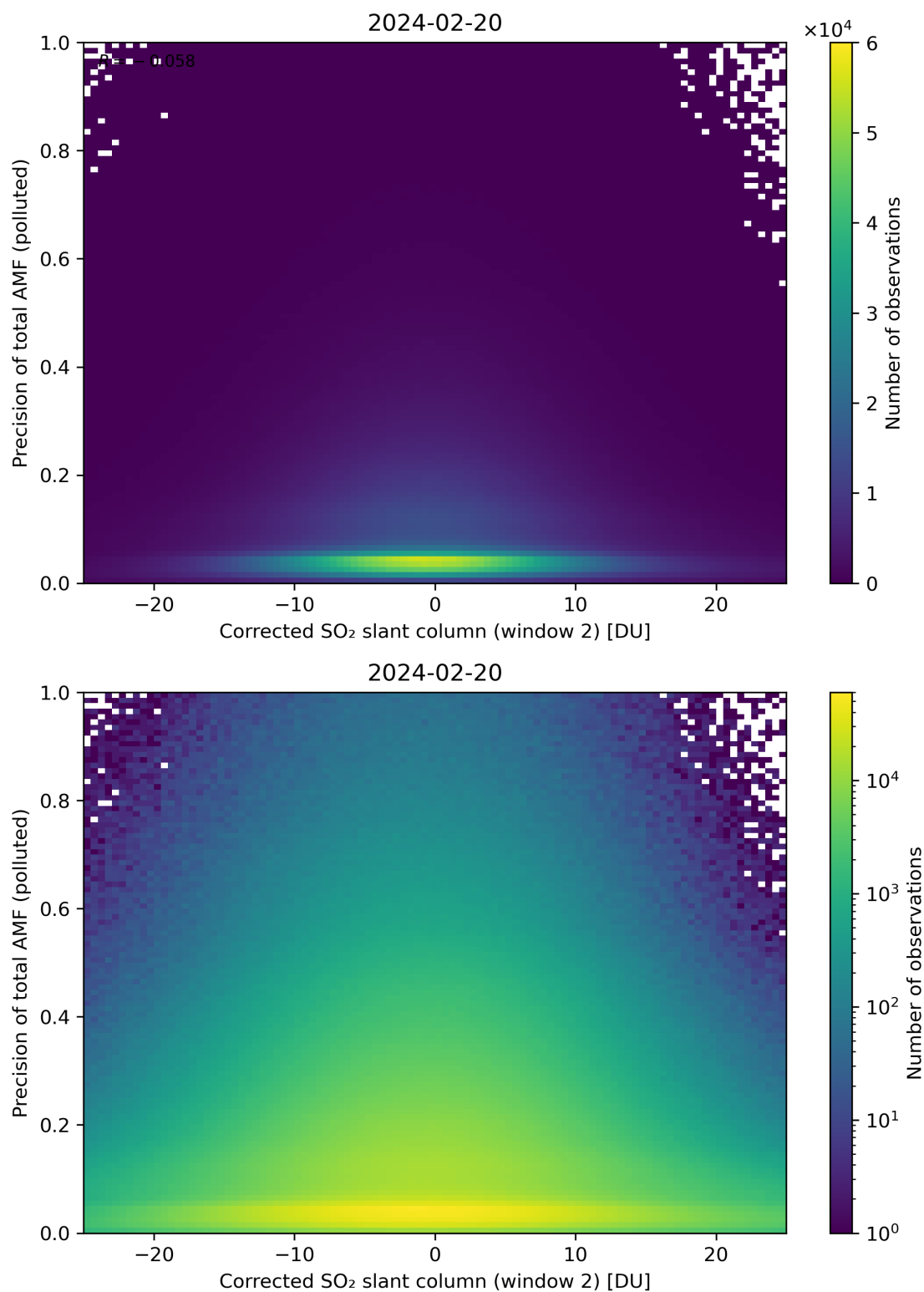
Figure 204: Scatter density plot of “Corrected SO 2 slant column (window 2)” against “Precision of total AMF (polluted)” for 2024-02-19 to 2024-02-21.
