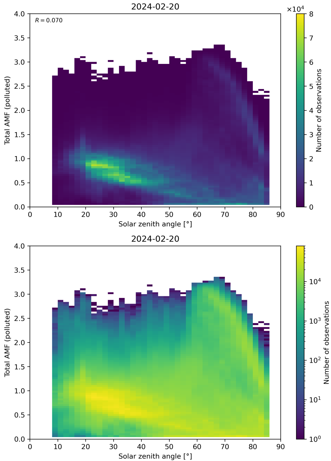
Figure 174: Scatter density plot of “Solar zenith angle” against “Total AMF (polluted)” for 2024-02-19 to 2024-02-21.
