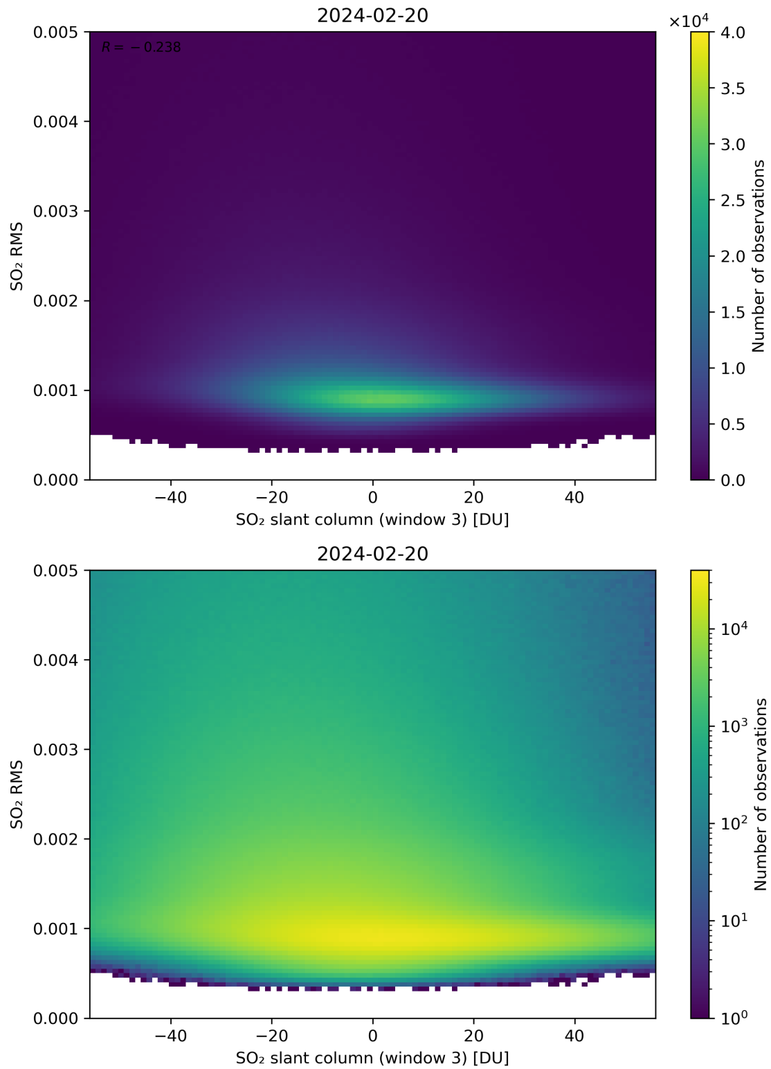
Figure 256: Scatter density plot of “SO 2 slant column (window 3)” against “SO 2 RMS” for 2024-02-19 to 2024-02-21.
