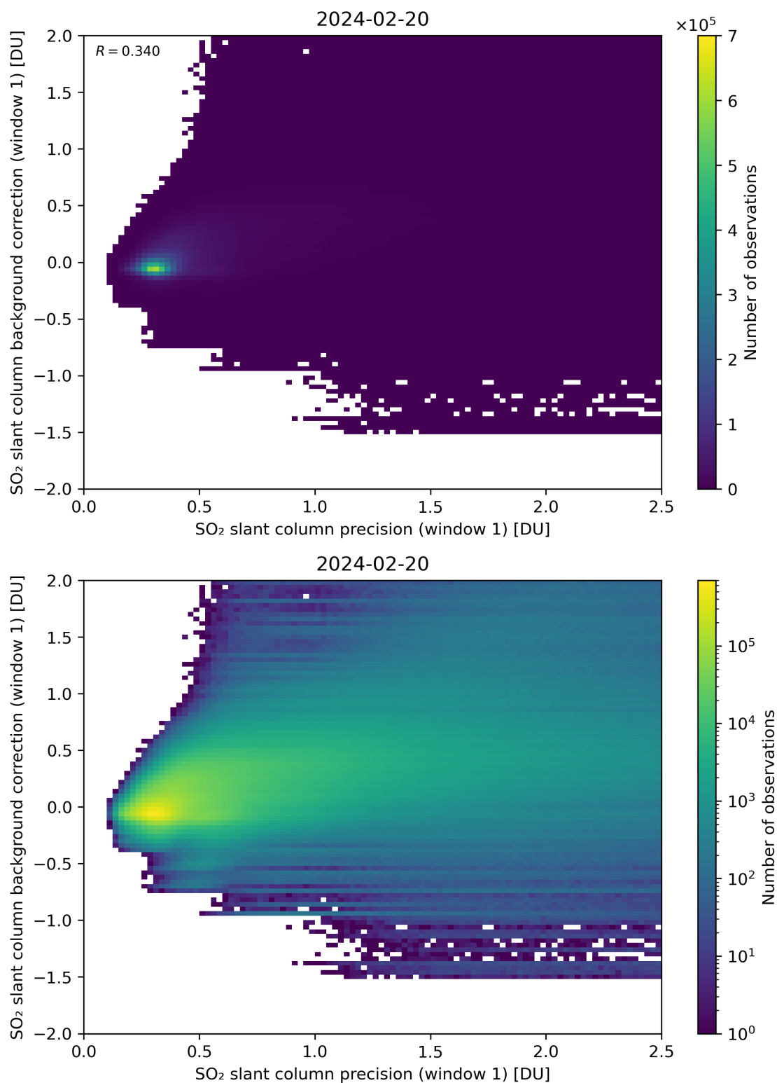
Figure 218: Scatter density plot of “SO 2 slant column precision (window 1)” against “SO 2 slant column background correction (window 1)” for 2024-02-19 to 2024-02-21.
