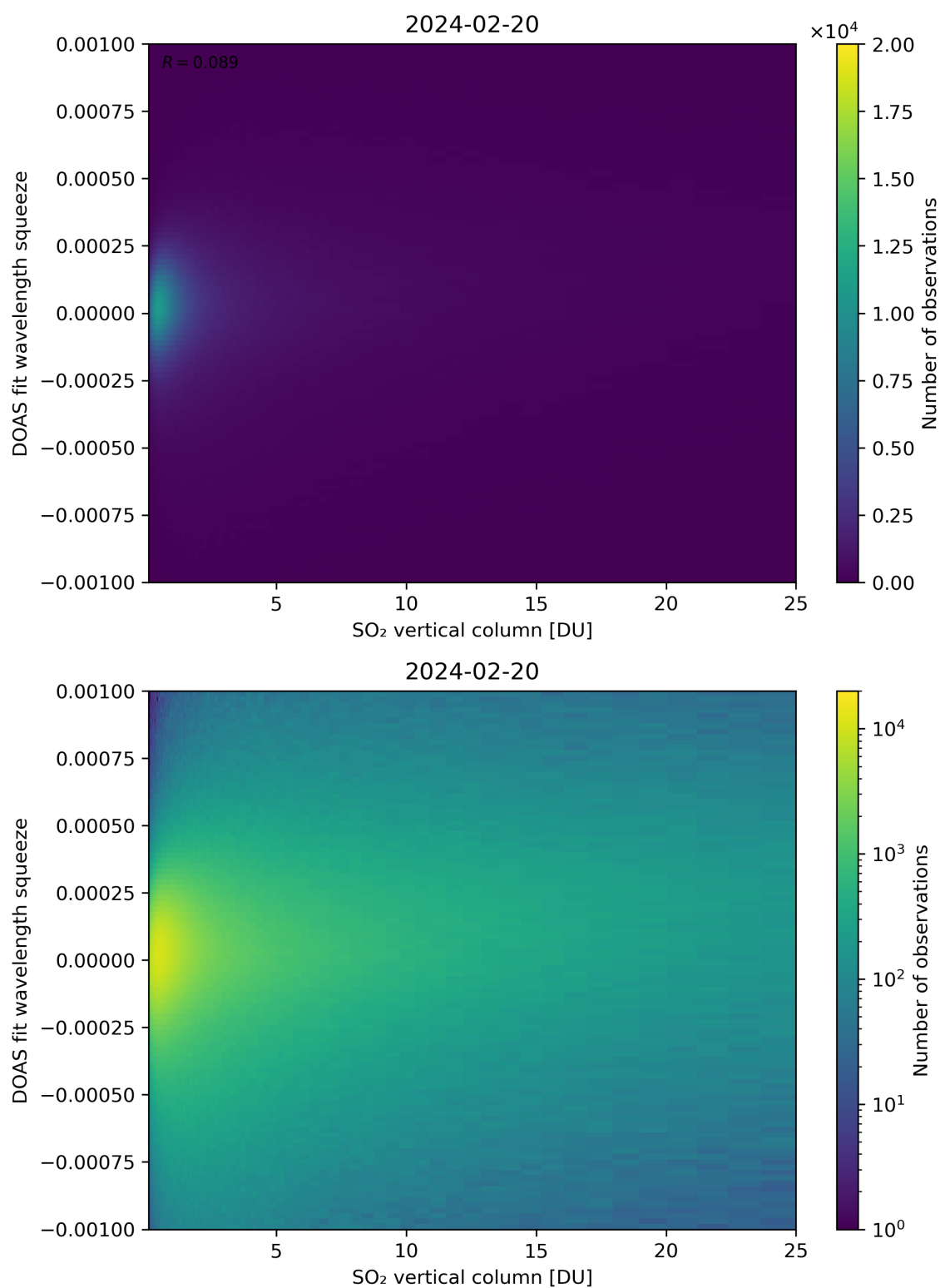
Figure 277: Scatter density plot of “SO 2 vertical column” against “DOAS fit wavelength squeeze” for 2024-02-19 to 2024-02-21.
