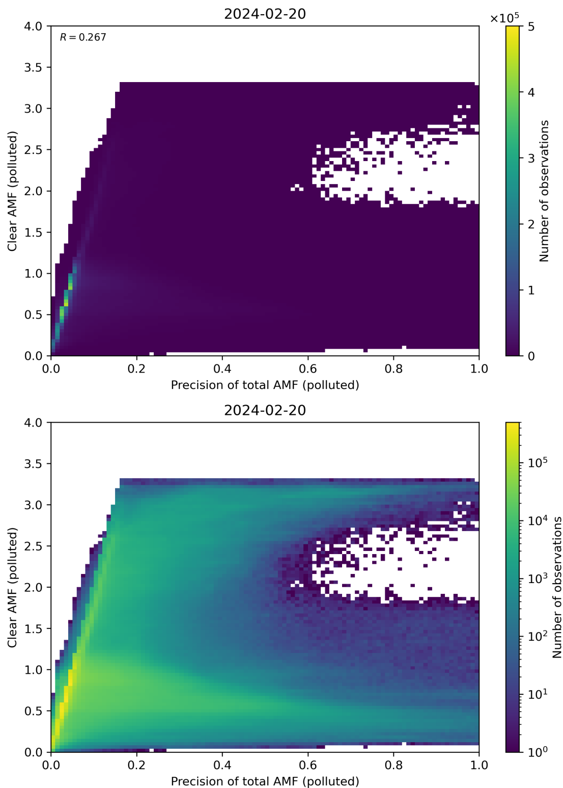
Figure 270: Scatter density plot of “Precision of total AMF (polluted)” against “Clear AMF (polluted)” for 2024-02-19 to 2024-02-21.
