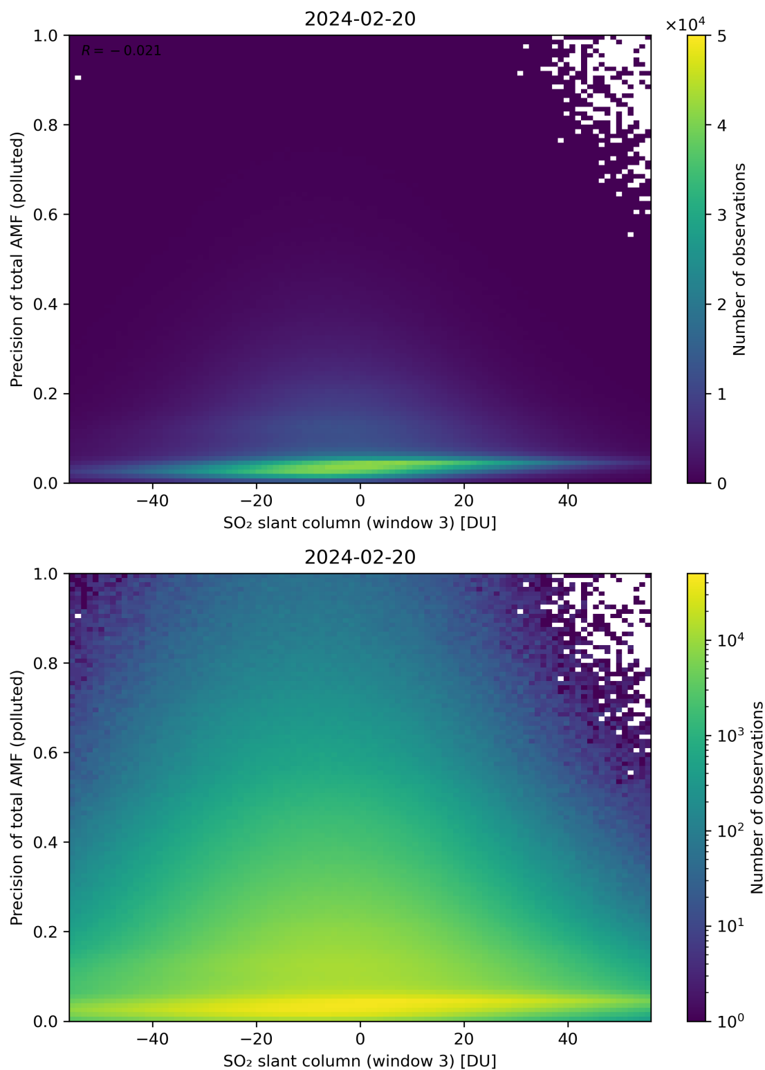
Figure 269: Scatter density plot of “SO 2 slant column (window 3)” against “Precision of total AMF (polluted)” for 2024-02-19 to 2024-02-21.
