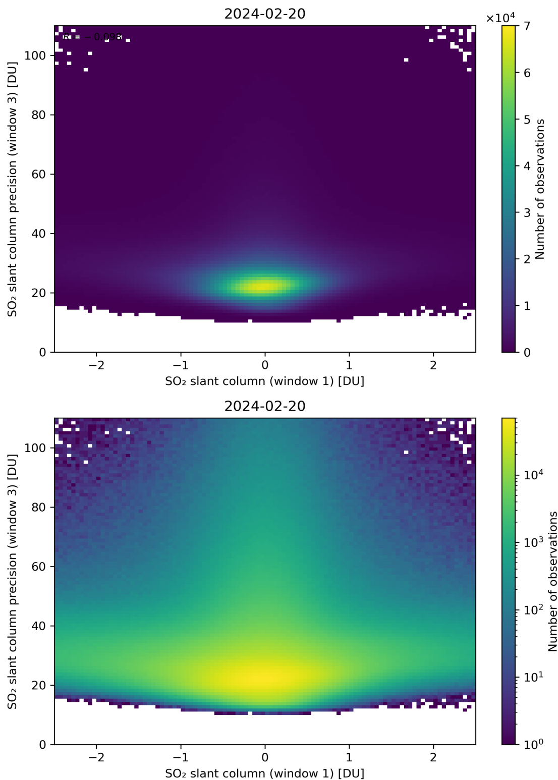
Figure 238: Scatter density plot of “SO 2 slant column (window 1)” against “SO 2 slant column precision (window 3)” for 2024-02-19 to 2024-02-21.
