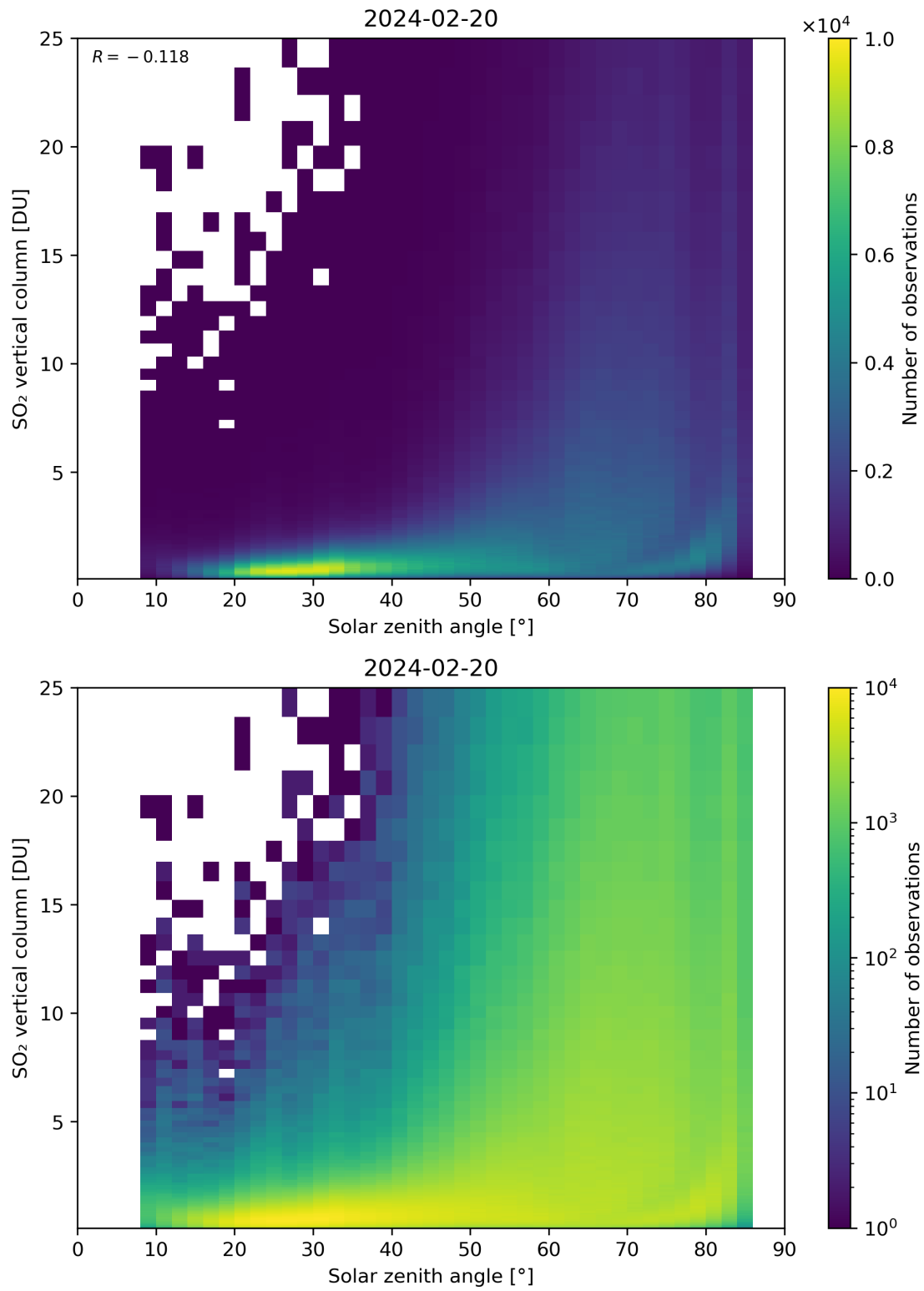
Figure 176: Scatter density plot of “Solar zenith angle” against “SO 2 vertical column” for 2024-02-19 to 2024-02-21.
