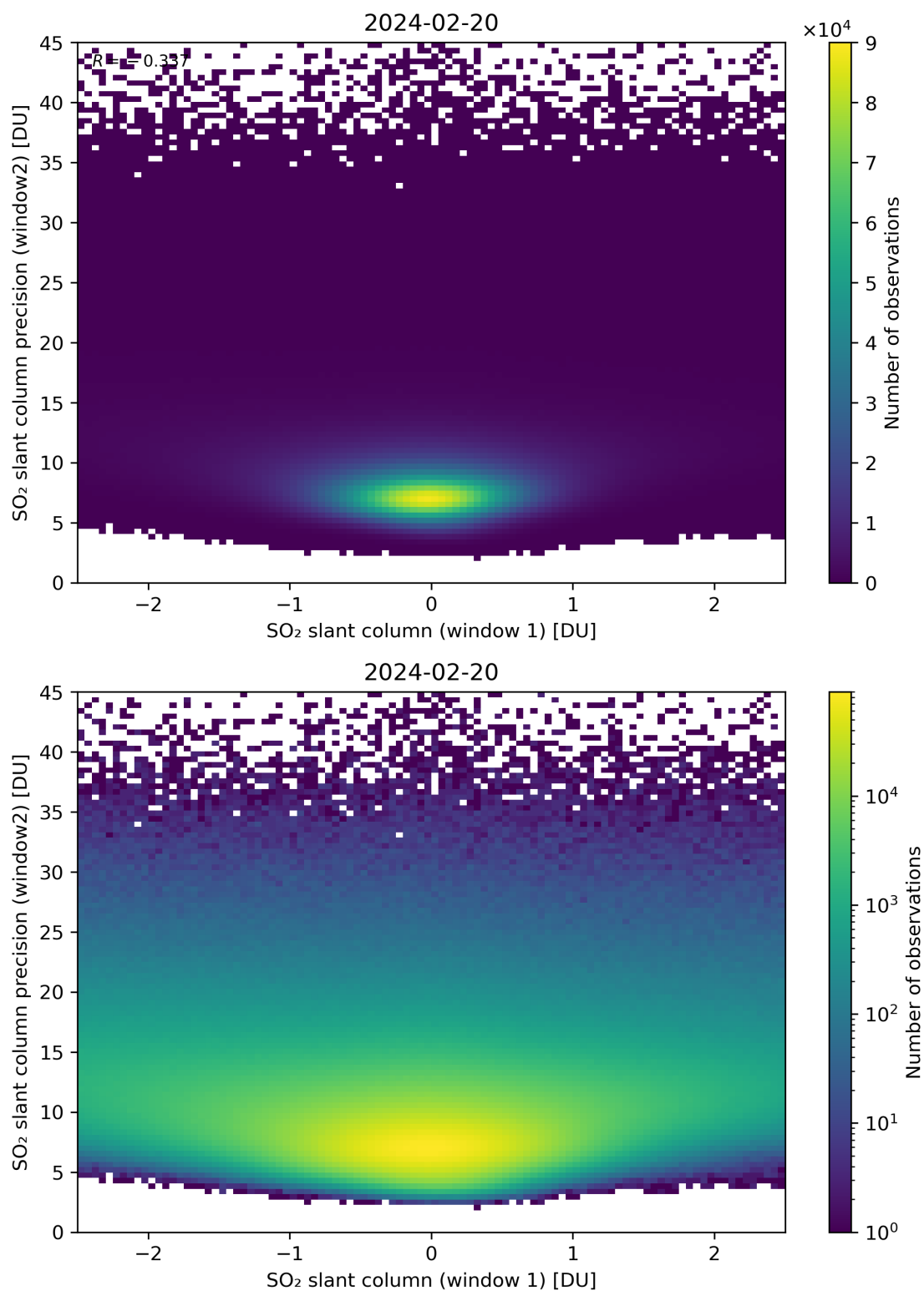
Figure 236: Scatter density plot of “SO 2 slant column (window 1)” against “SO 2 slant column precision (window2)” for 2024-02-19 to 2024-02-21.
