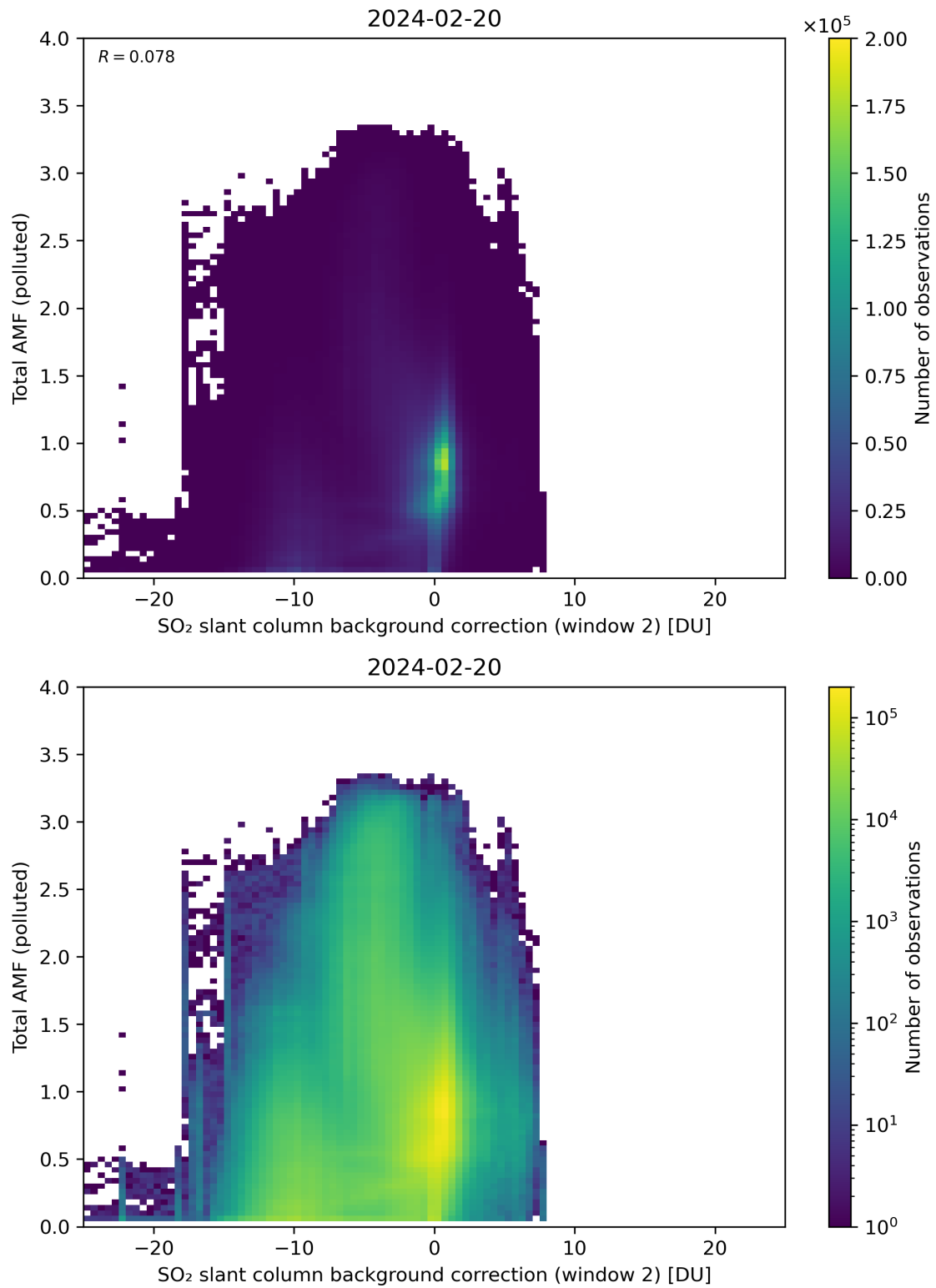
Figure 119: Scatter density plot of “SO 2 slant column background correction (window 2)” against “Total AMF (polluted)” for 2024-02-19 to 2024-02-21.
