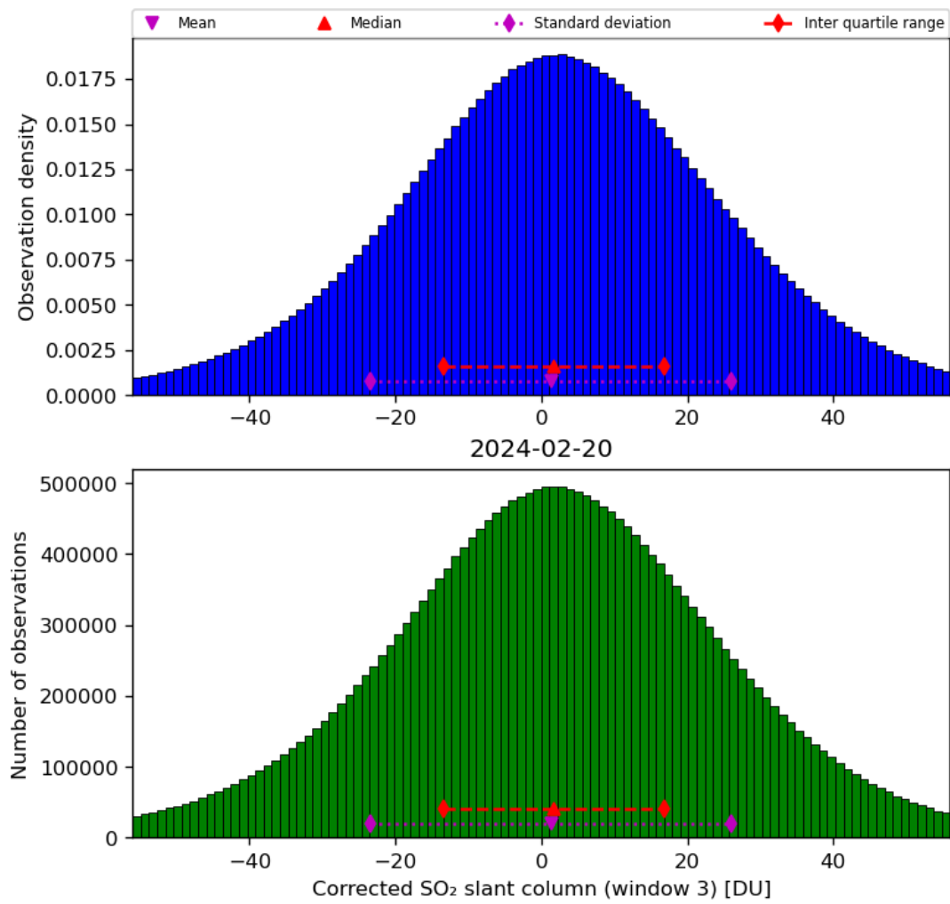
Figure 66: Histogram of “Corrected SO 2 slant column (window 3)” for 2024-02-19 to 2024-02-21
