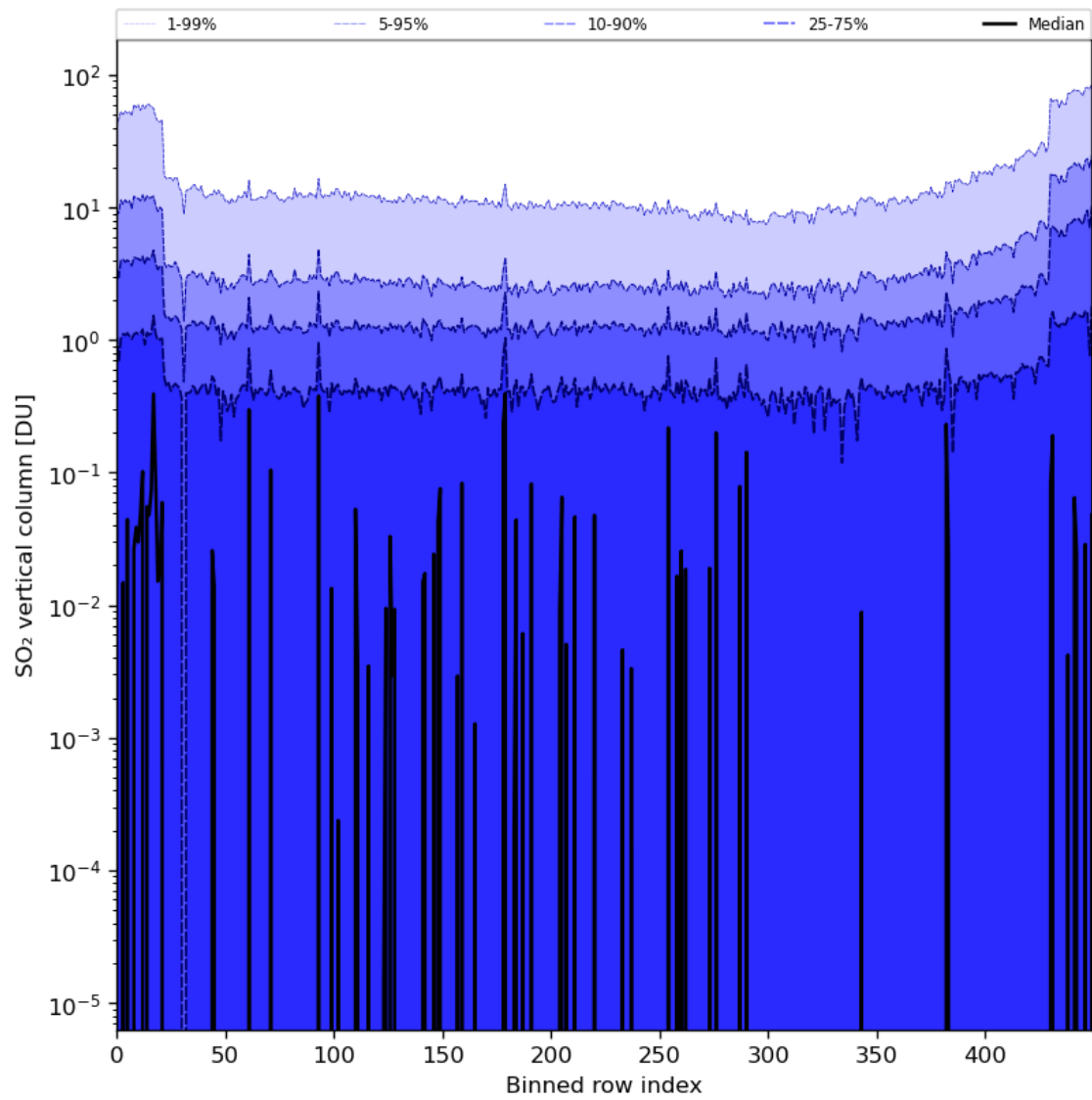
Figure 76: Along track statistics of “SO 2 vertical column” for 2024-02-19 to 2024-02-21
