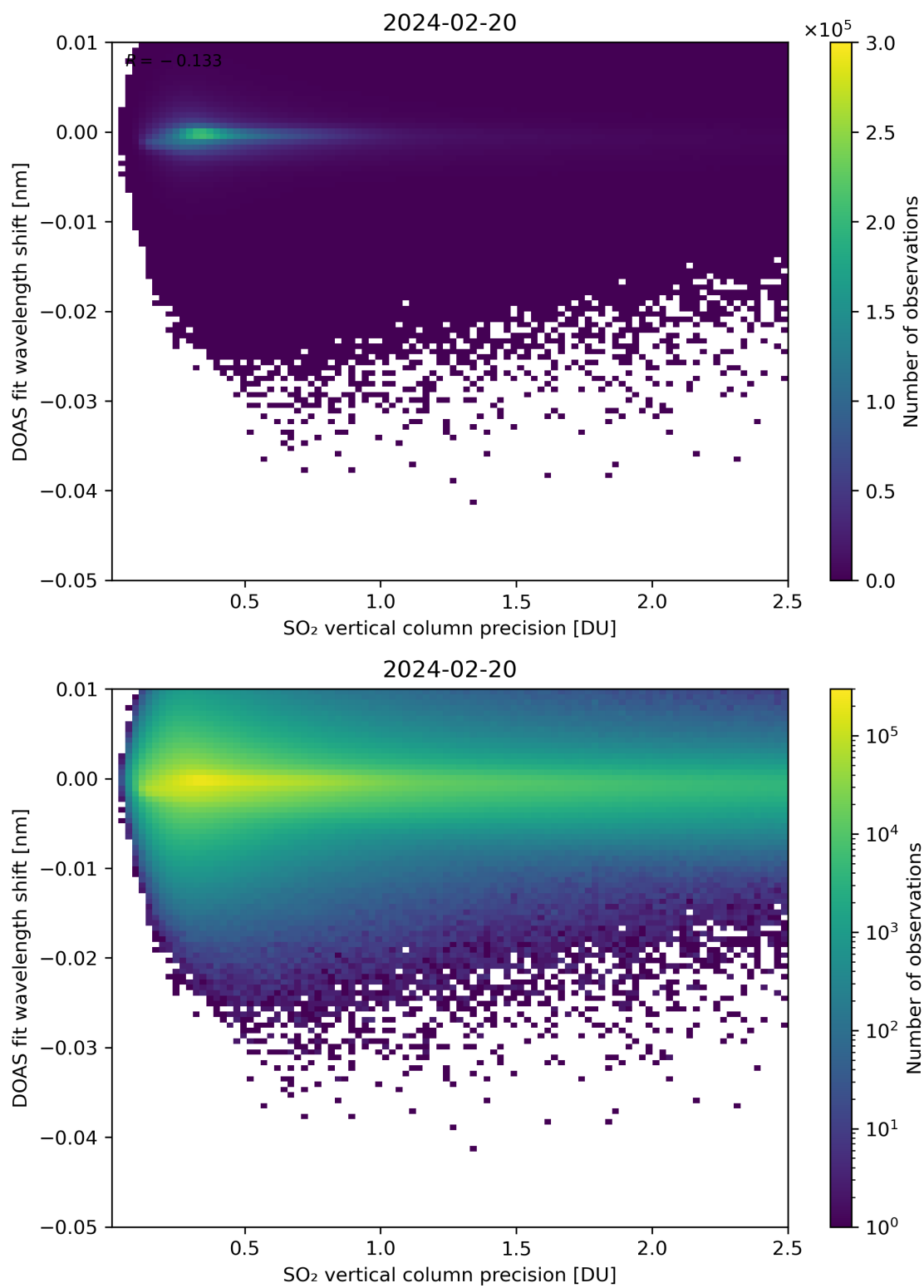
Figure 282: Scatter density plot of “SO 2 vertical column precision” against “DOAS fit wavelength shift” for 2024-02-19 to 2024-02-21.
