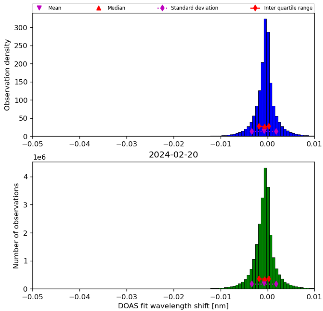
Figure 68: Histogram of “DOAS fit wavelength shift” for 2024-02-19 to 2024-02-21
