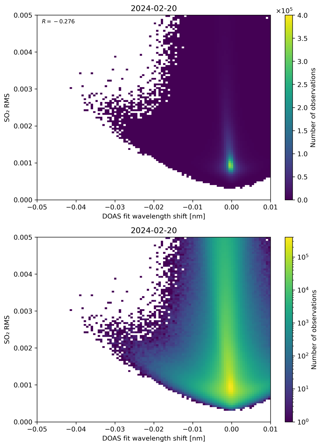
Figure 128: Scatter density plot of “DOAS fit wavelength shift” against “SO 2 RMS” for 2024-02-19 to 2024-02-21.
