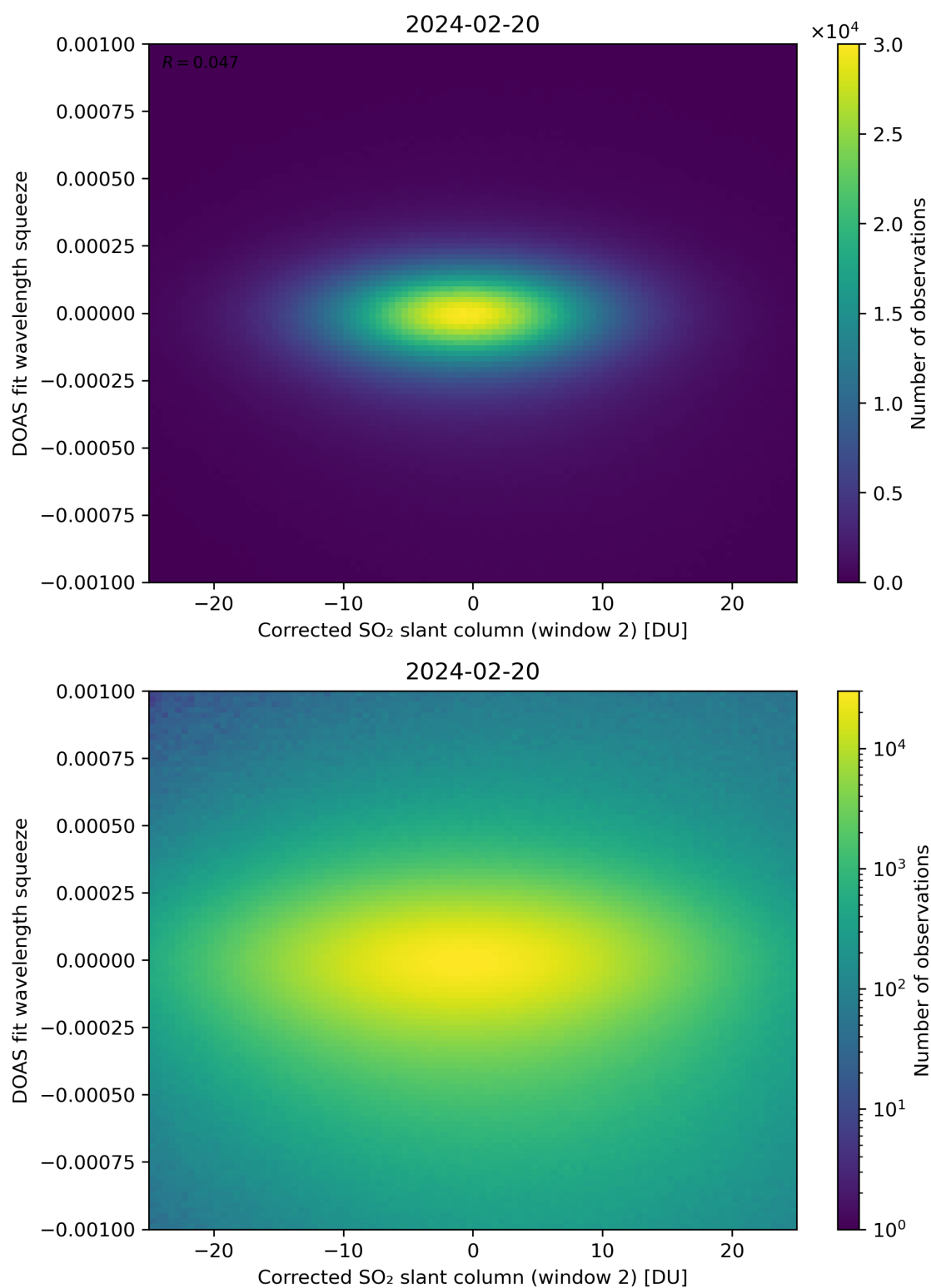
Figure 197: Scatter density plot of “Corrected SO 2 slant column (window 2)” against “DOAS fit wavelength squeeze” for 2024-02-19 to 2024-02-21.
