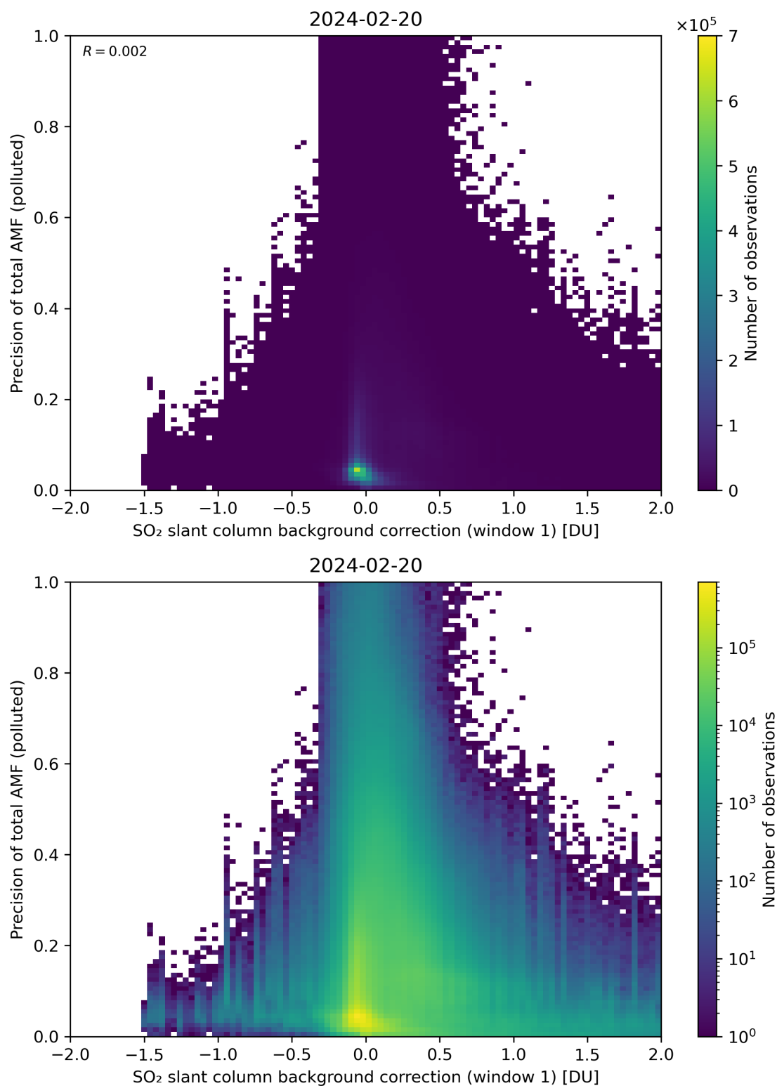
Figure 110: Scatter density plot of “SO 2 slant column background correction (window 1)” against “Precision of total AMF (polluted)” for 2024-02-19 to 2024-02-21.
