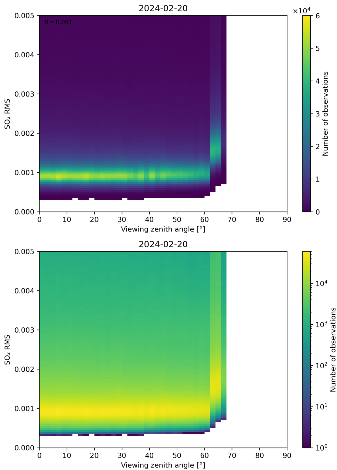
Figure 313: Scatter density plot of “Viewing zenith angle” against “SO 2 RMS” for 2024-02-19 to 2024-02-21.
