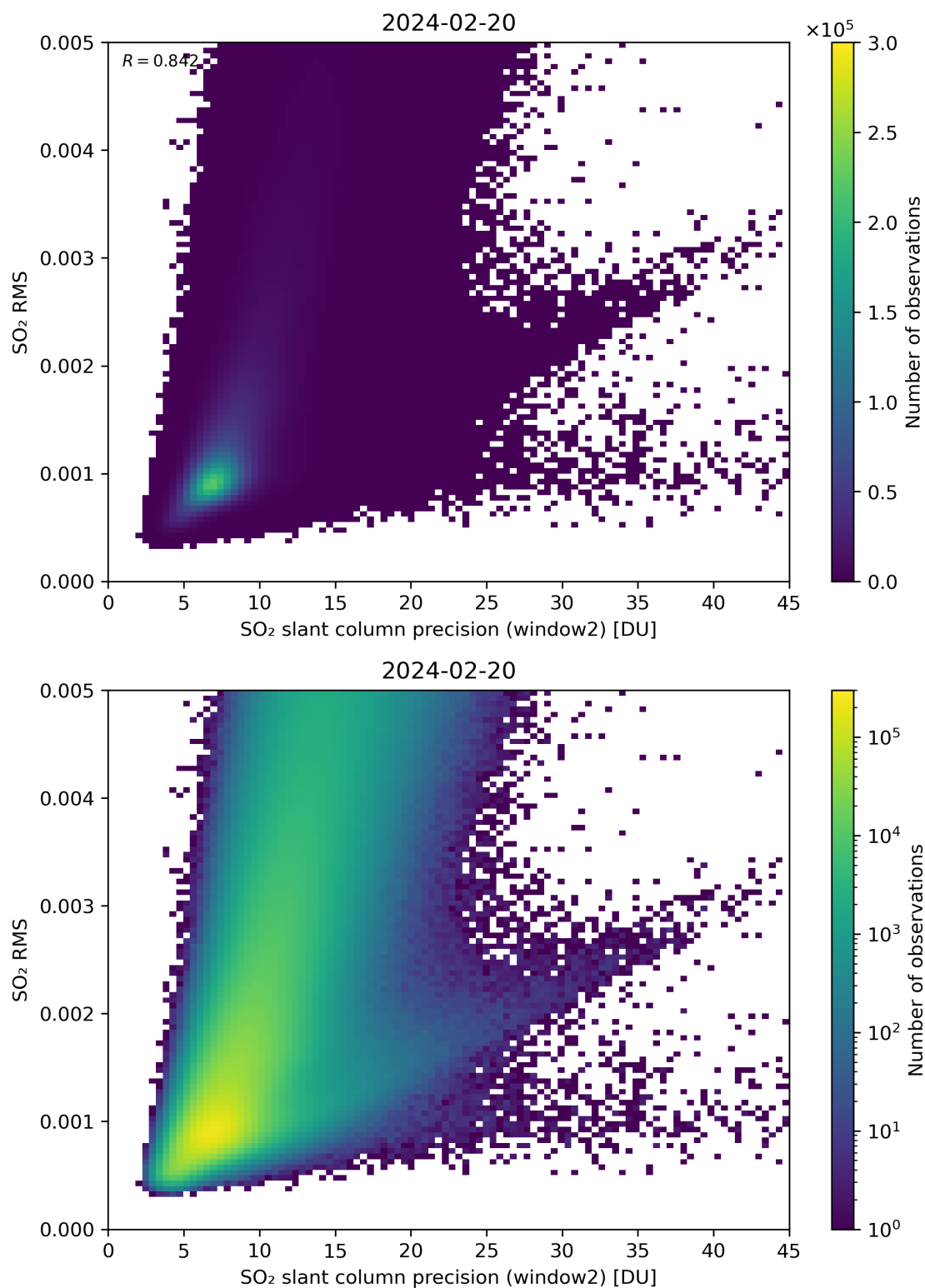
Figure 245: Scatter density plot of “SO 2 slant column precision (window2)” against “SO 2 RMS” for 2024-02-19 to 2024-02-21.
