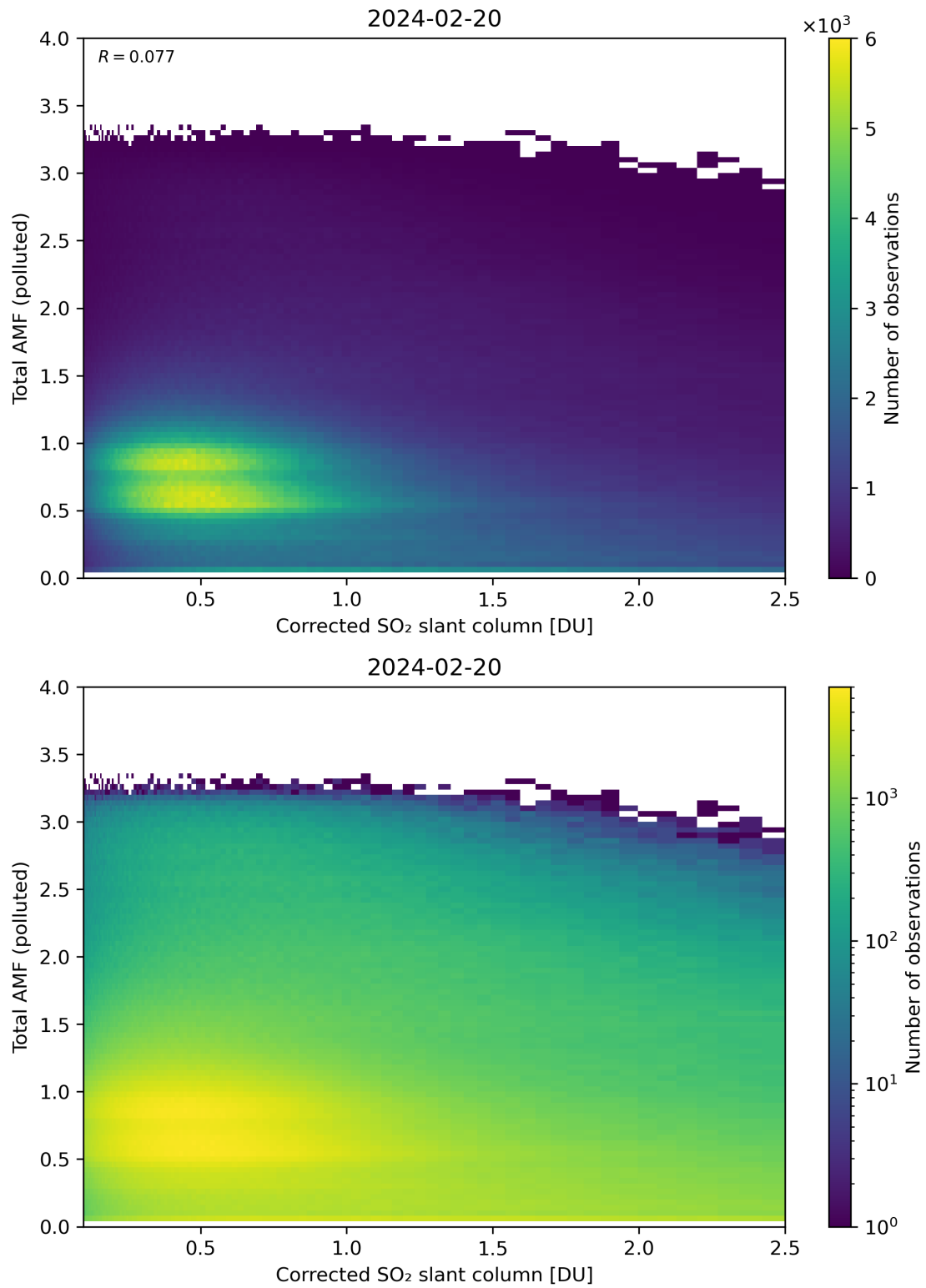
Figure 192: Scatter density plot of “Corrected SO 2 slant column” against “Total AMF (polluted)” for 2024-02-19 to 2024-02-21.
