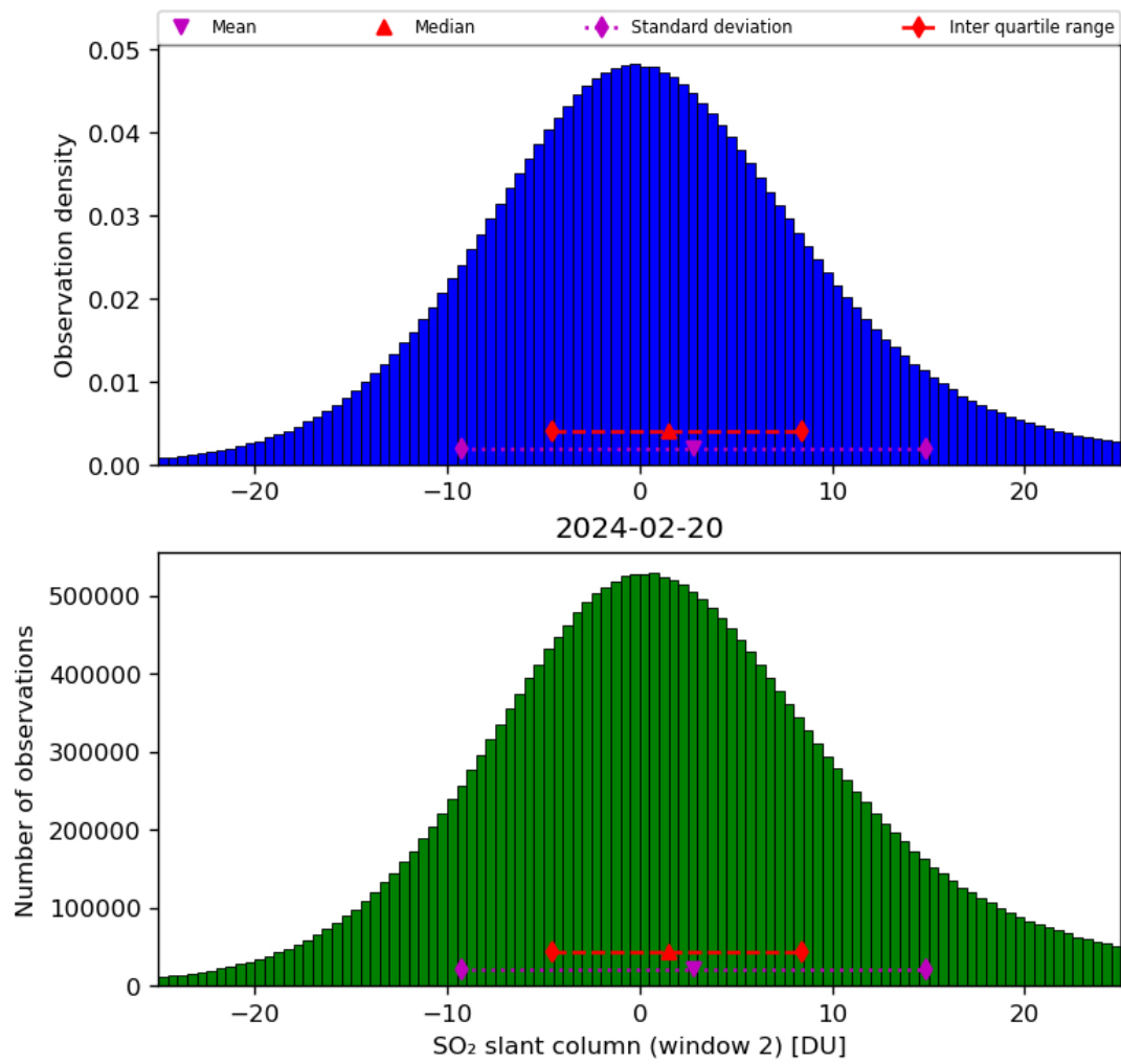
Figure 60: Histogram of “SO 2 slant column (window 2)” for 2024-02-19 to 2024-02-21
