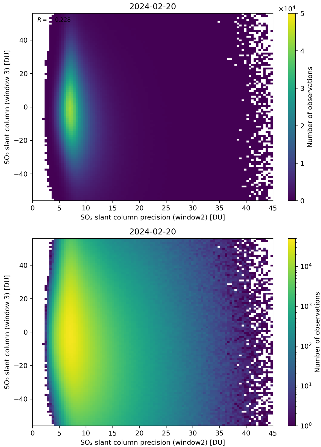
Figure 249: Scatter density plot of “SO 2 slant column precision (window2)” against “SO 2 slant column (window 3)” for 2024-02-19 to 2024-02-21.
