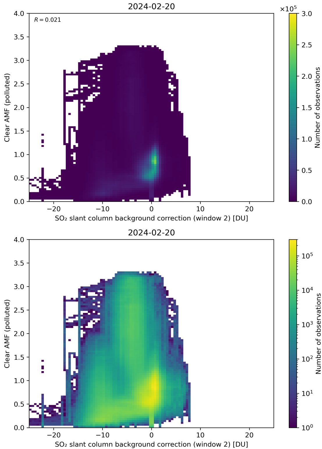
Figure 115: Scatter density plot of “SO 2 slant column background correction (window 2)” against “Clear AMF (polluted)” for 2024-02-19 to 2024-02-21.
