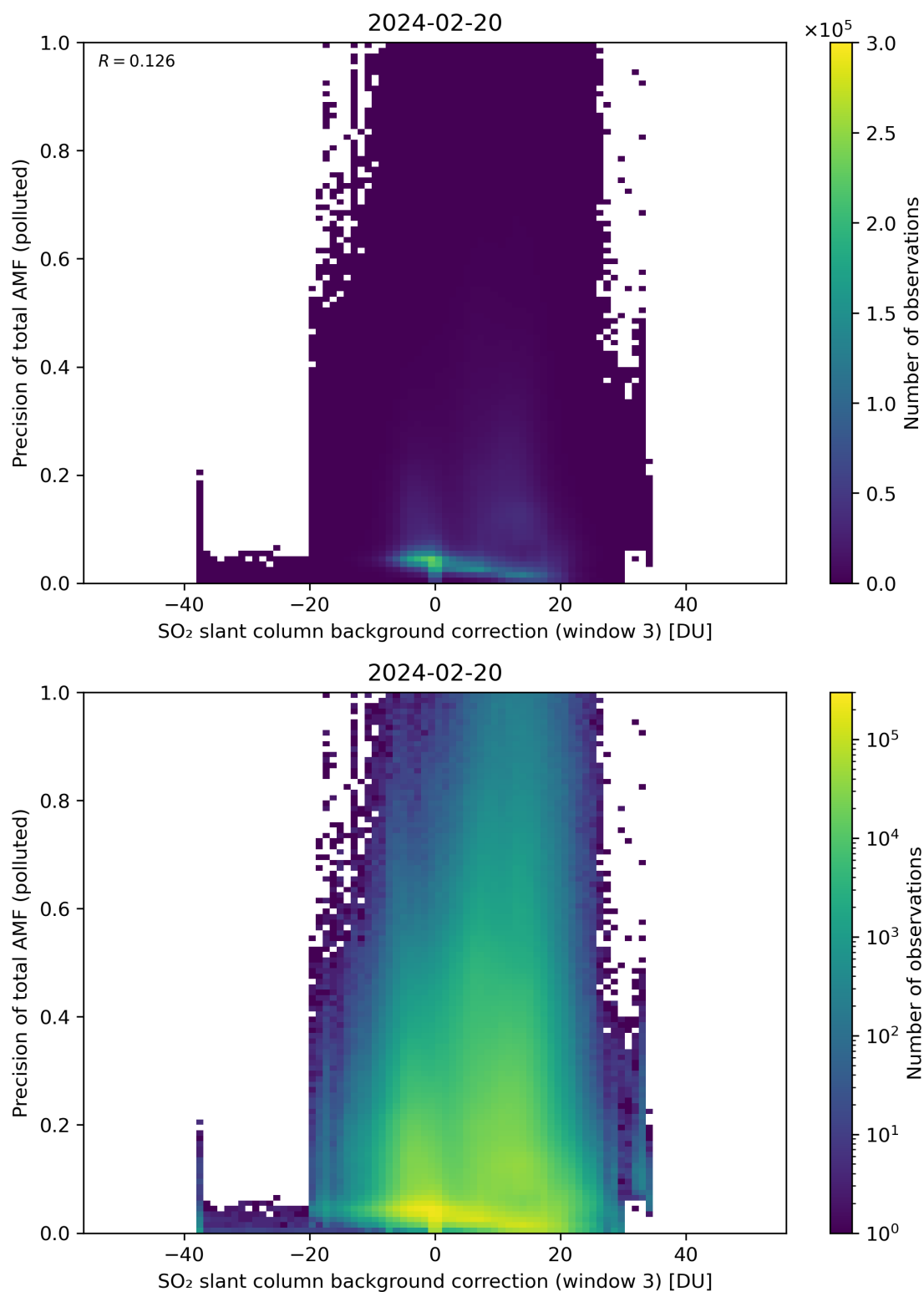
Figure 126: Scatter density plot of “SO 2 slant column background correction (window 3)” against “Precision of total AMF (polluted)” for 2024-02-19 to 2024-02-21.
