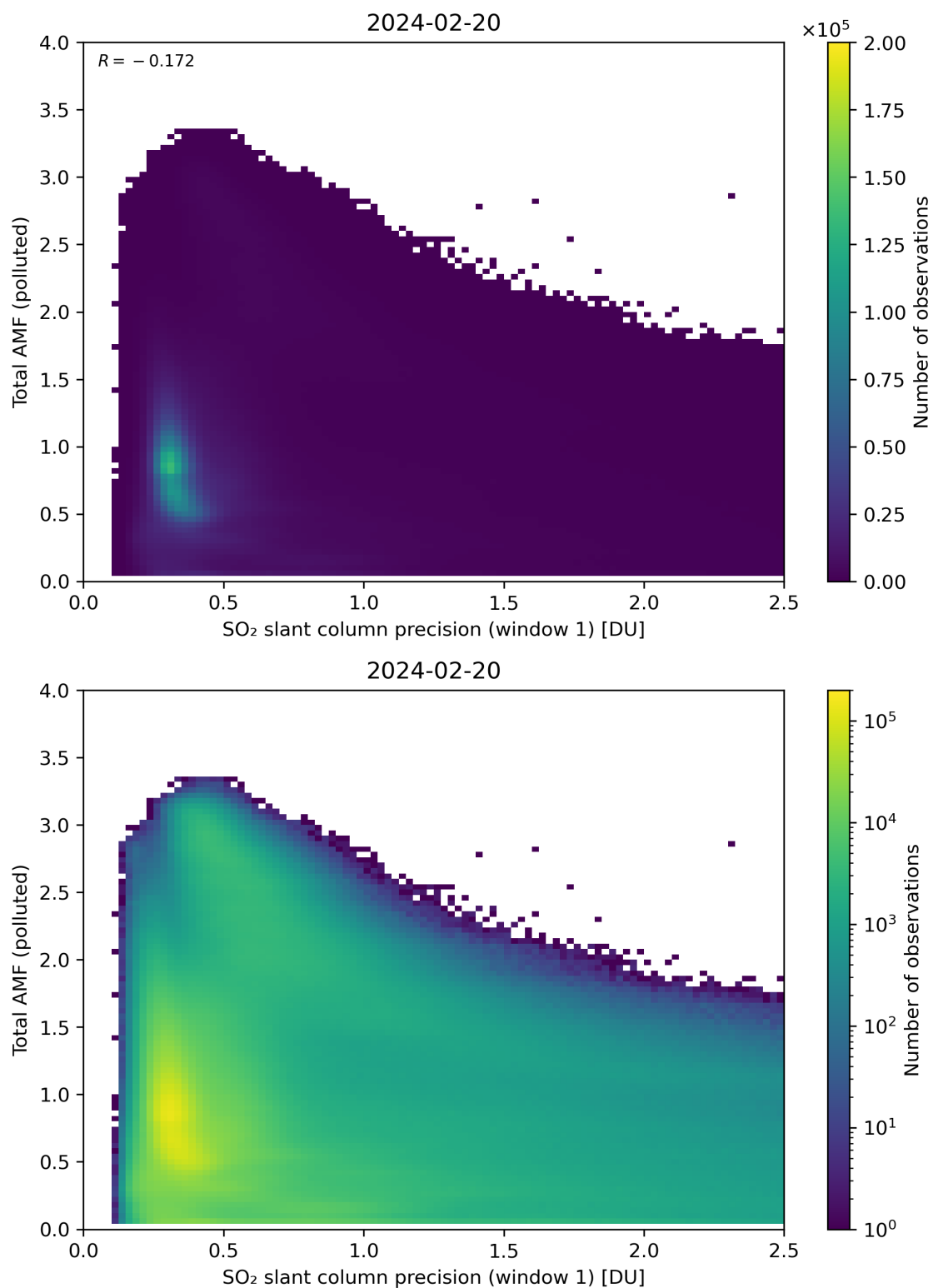
Figure 230: Scatter density plot of “SO 2 slant column precision (window 1)” against “Total AMF (polluted)” for 2024-02-19 to 2024-02-21.
