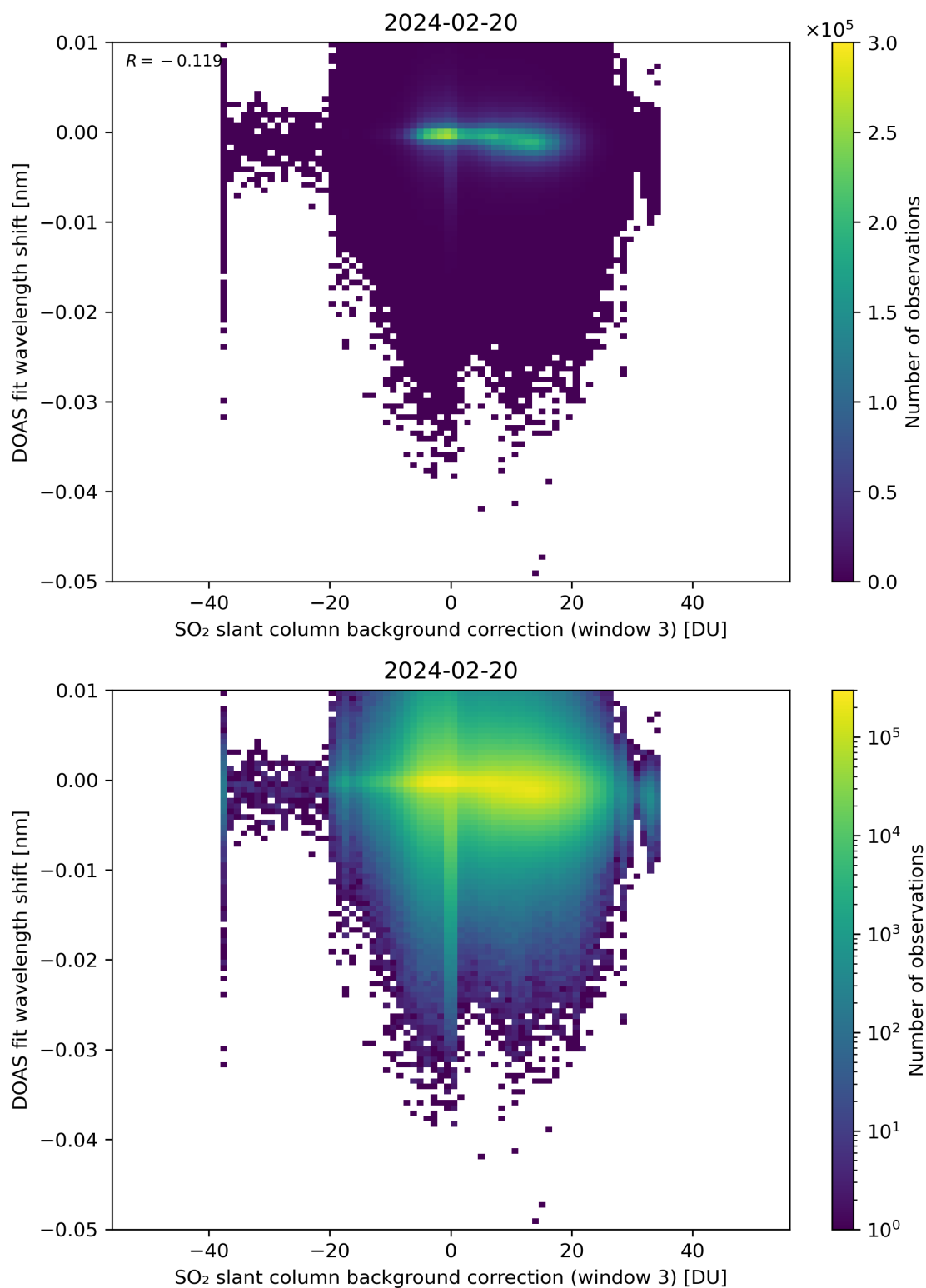
Figure 121: Scatter density plot of “SO 2 slant column background correction (window 3)” against “DOAS fit wavelength shift” for 2024-02-19 to 2024-02-21.
