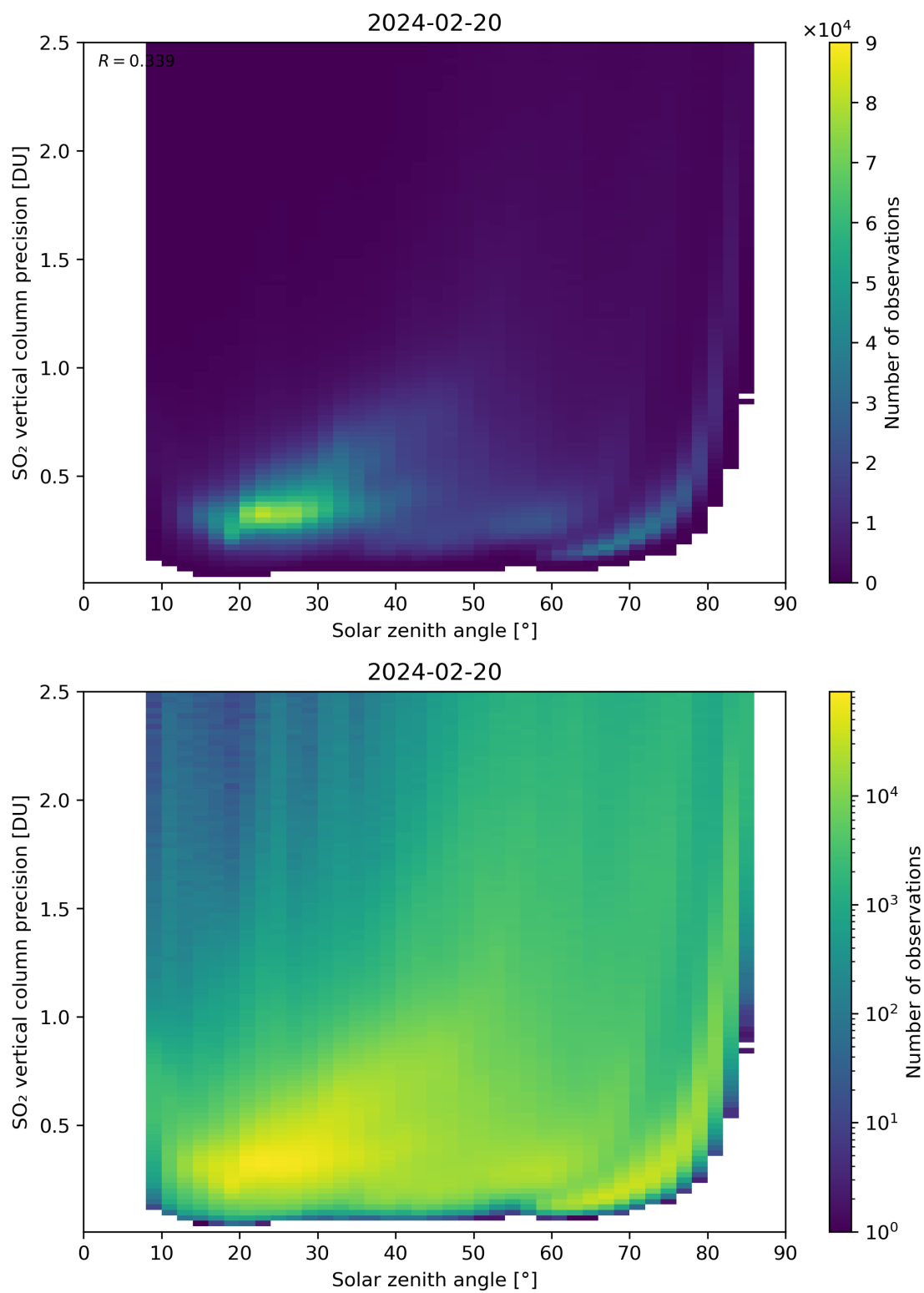
Figure 177: Scatter density plot of “Solar zenith angle” against “SO 2 vertical column precision” for 2024-02-19 to 2024-02-21.
