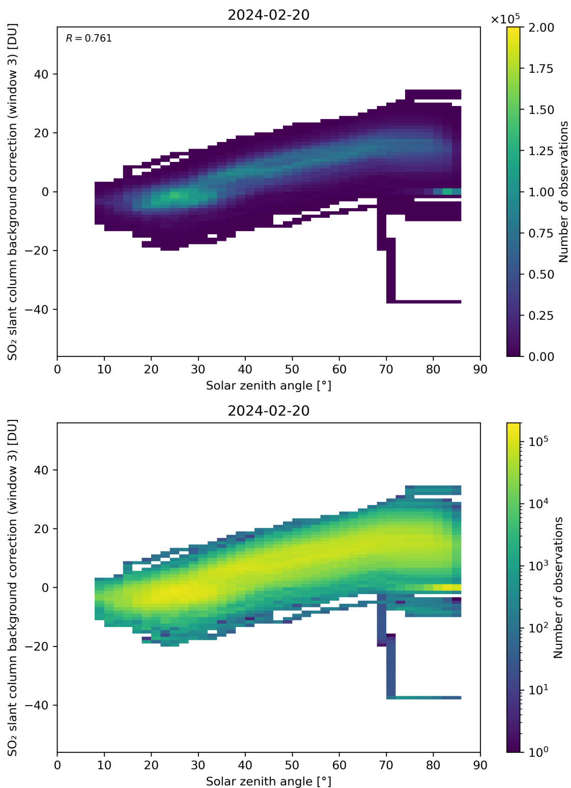
Figure 160: Scatter density plot of “Solar zenith angle” against “SO 2 slant column background correction (window 3)” for 2024-02-19 to 2024-02-21.
