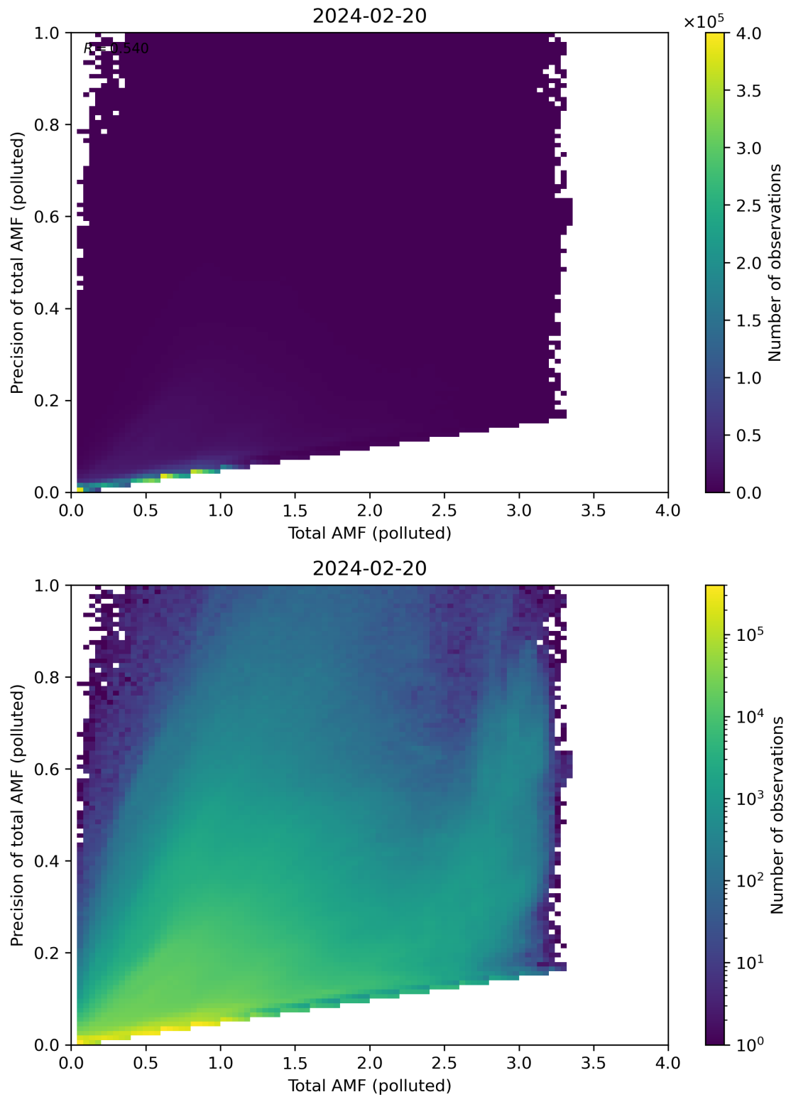
Figure 272: Scatter density plot of “Total AMF (polluted)” against “Precision of total AMF (polluted)” for 2024-02-19 to 2024-02-21.
