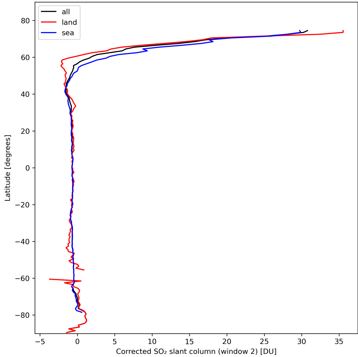
Figure 39: Zonal average of “Corrected SO 2 slant column (window 2)” for 2024-02-19 to 2024-02-21.
