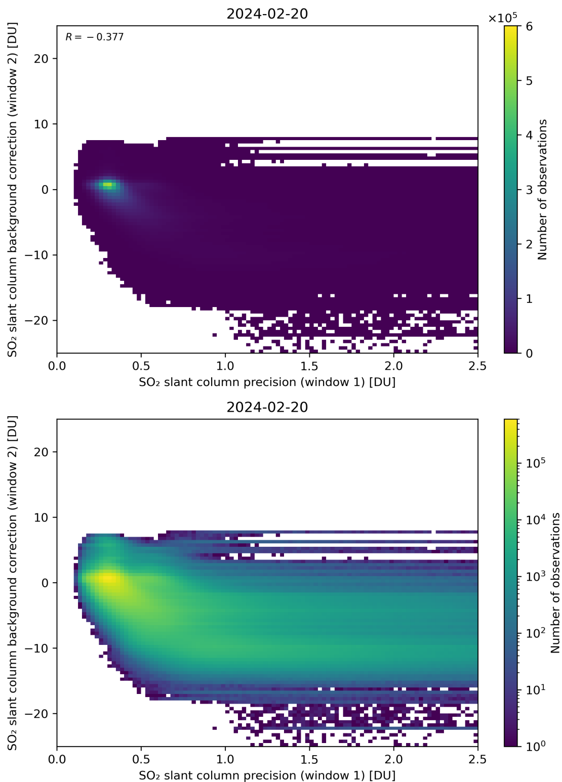
Figure 219: Scatter density plot of “SO 2 slant column precision (window 1)” against “SO 2 slant column background correction (window 2)” for 2024-02-19 to 2024-02-21.
