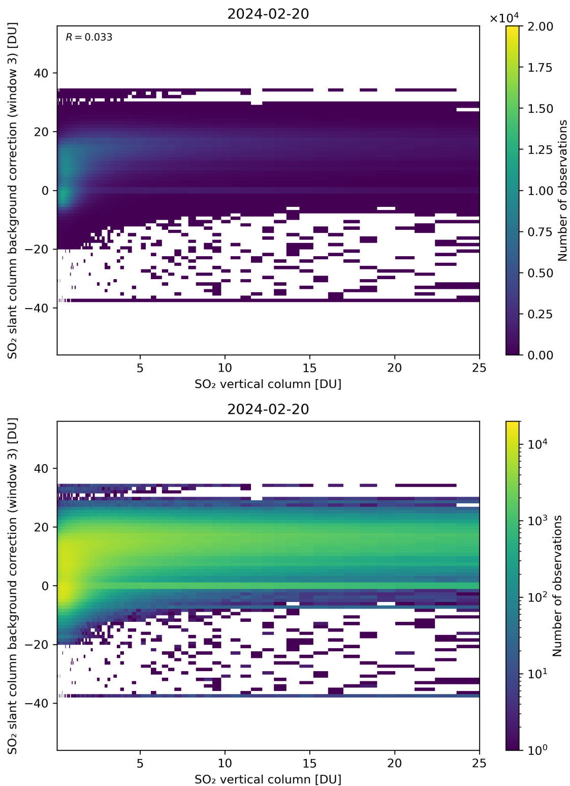
Figure 275: Scatter density plot of “SO 2 vertical column” against “SO 2 slant column background correction (window 3)” for 2024-02-19 to 2024-02-21.
