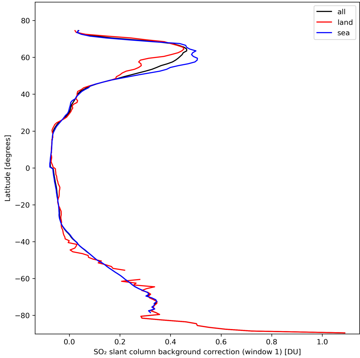
Figure 36: Zonal average of “SO 2 slant column background correction (window 1)” for 2024-02-19 to 2024-02-21.
