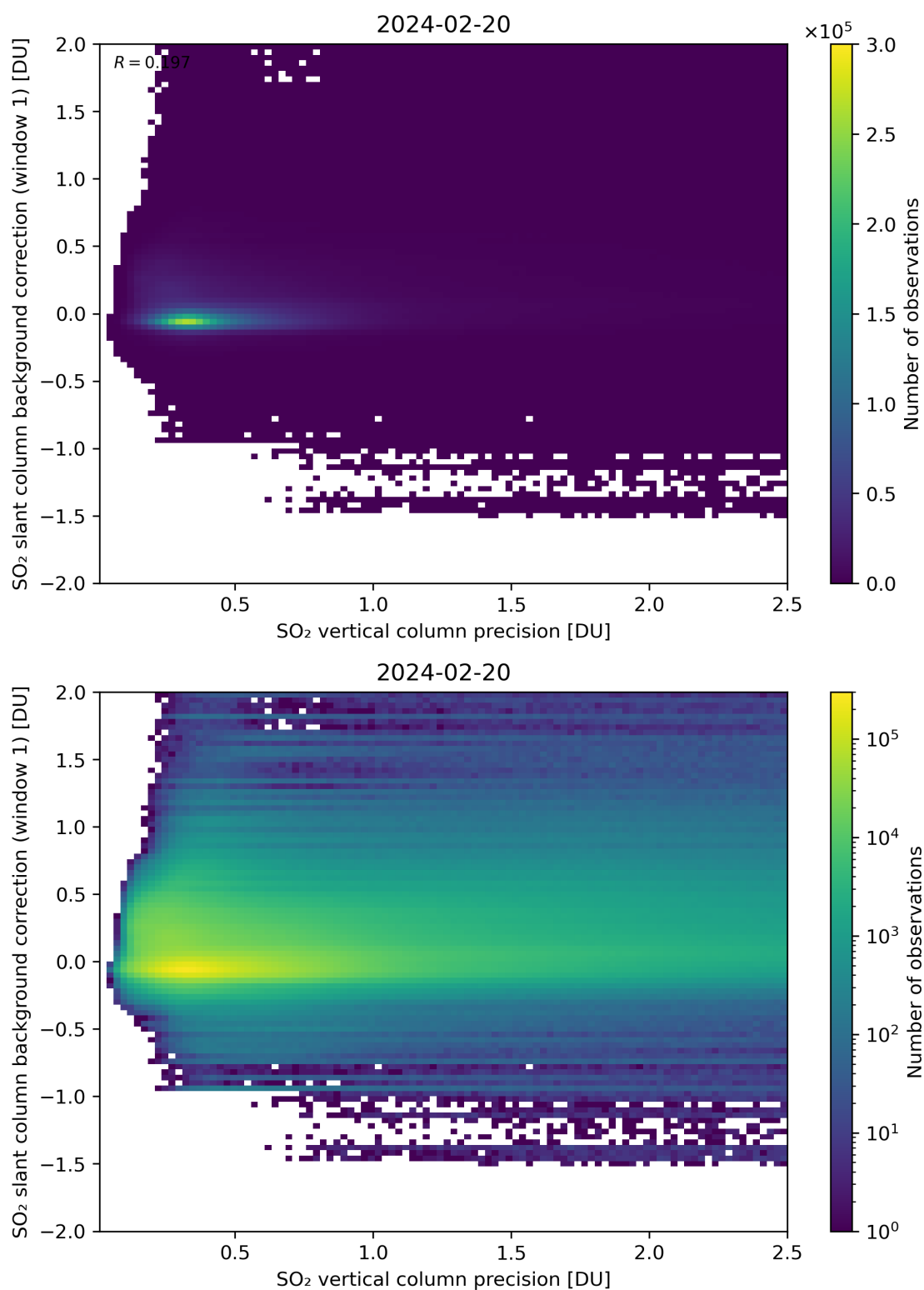
Figure 279: Scatter density plot of “SO 2 vertical column precision” against “SO 2 slant column background correction (window 1)” for 2024-02-19 to 2024-02-21.
