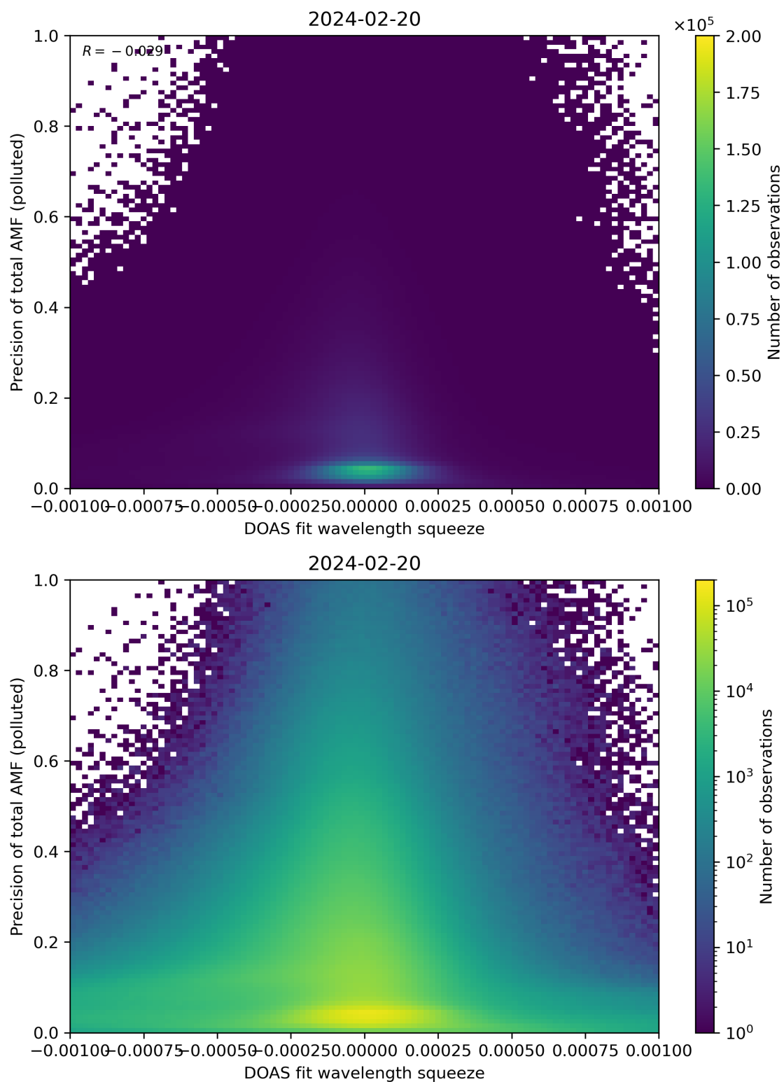
Figure 135: Scatter density plot of “DOAS fit wavelength squeeze” against “Precision of total AMF (polluted)” for 2024-02-19 to 2024-02-21.
