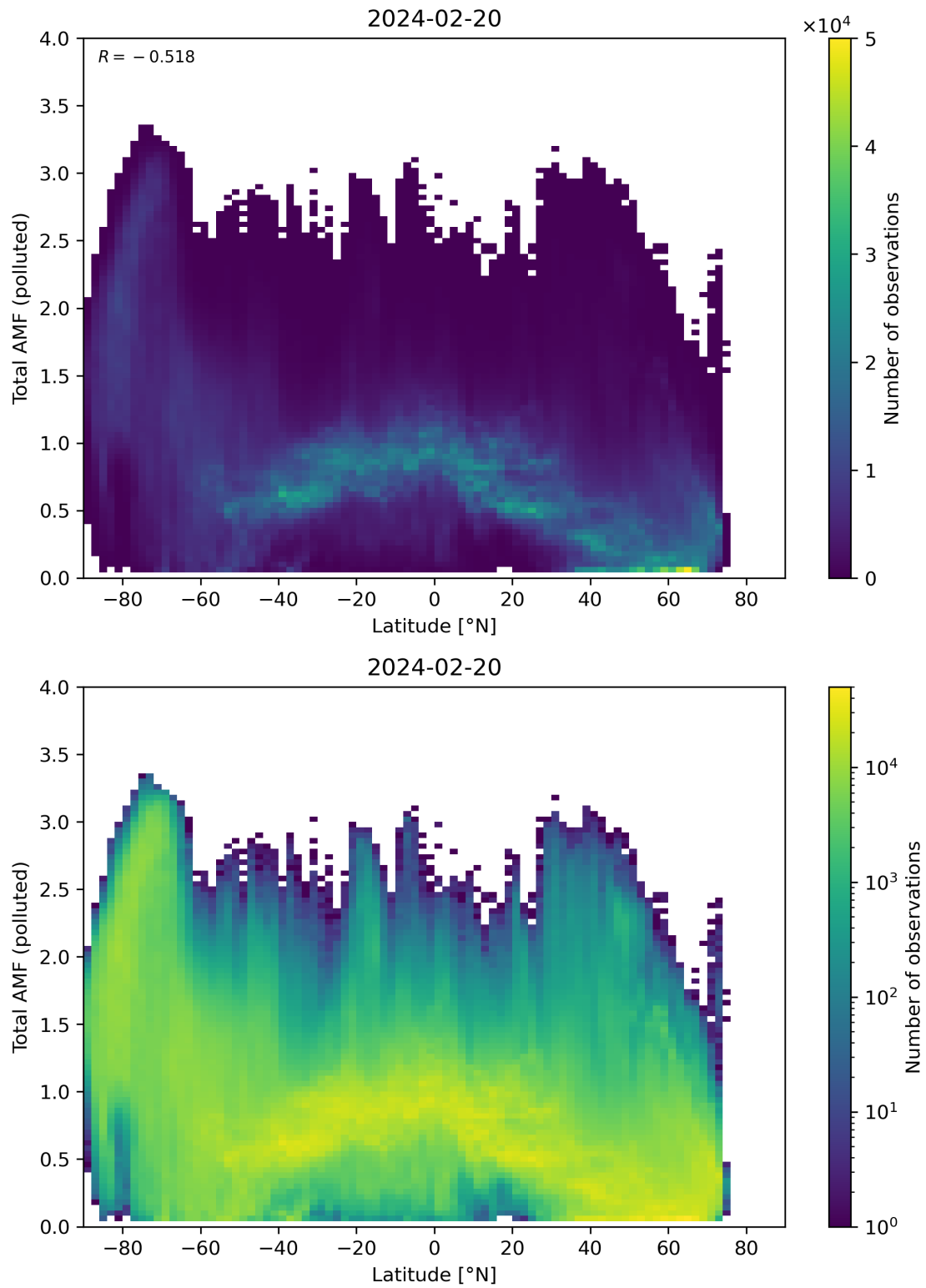
Figure 154: Scatter density plot of “Latitude” against “Total AMF (polluted)” for 2024-02-19 to 2024-02-21.
