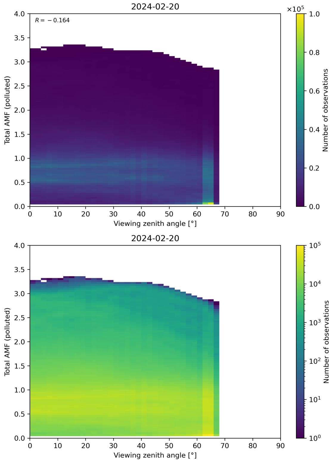
Figure 325: Scatter density plot of “Viewing zenith angle” against “Total AMF (polluted)” for 2024-02-19 to 2024-02-21.
