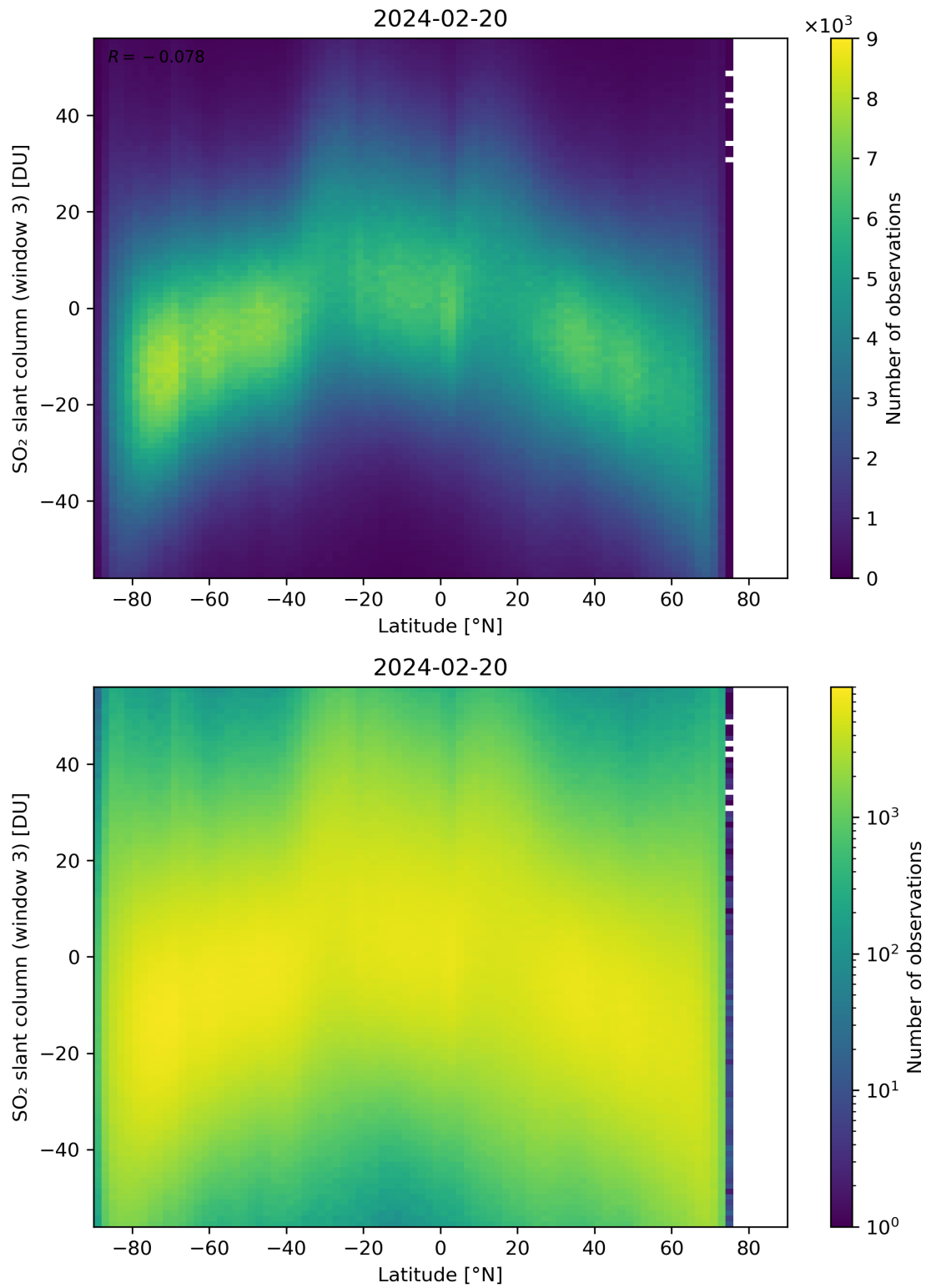
Figure 152: Scatter density plot of “Latitude” against “SO 2 slant column (window 3)” for 2024-02-19 to 2024-02-21.
