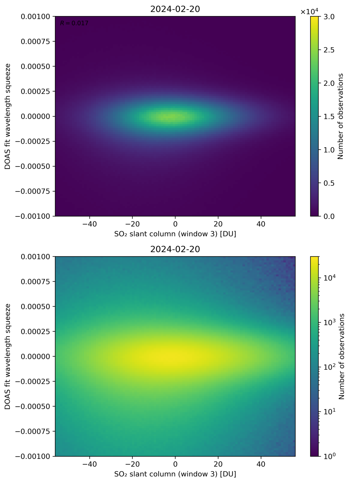
Figure 255: Scatter density plot of “SO 2 slant column (window 3)” against “DOAS fit wavelength squeeze” for 2024-02-19 to 2024-02-21.
