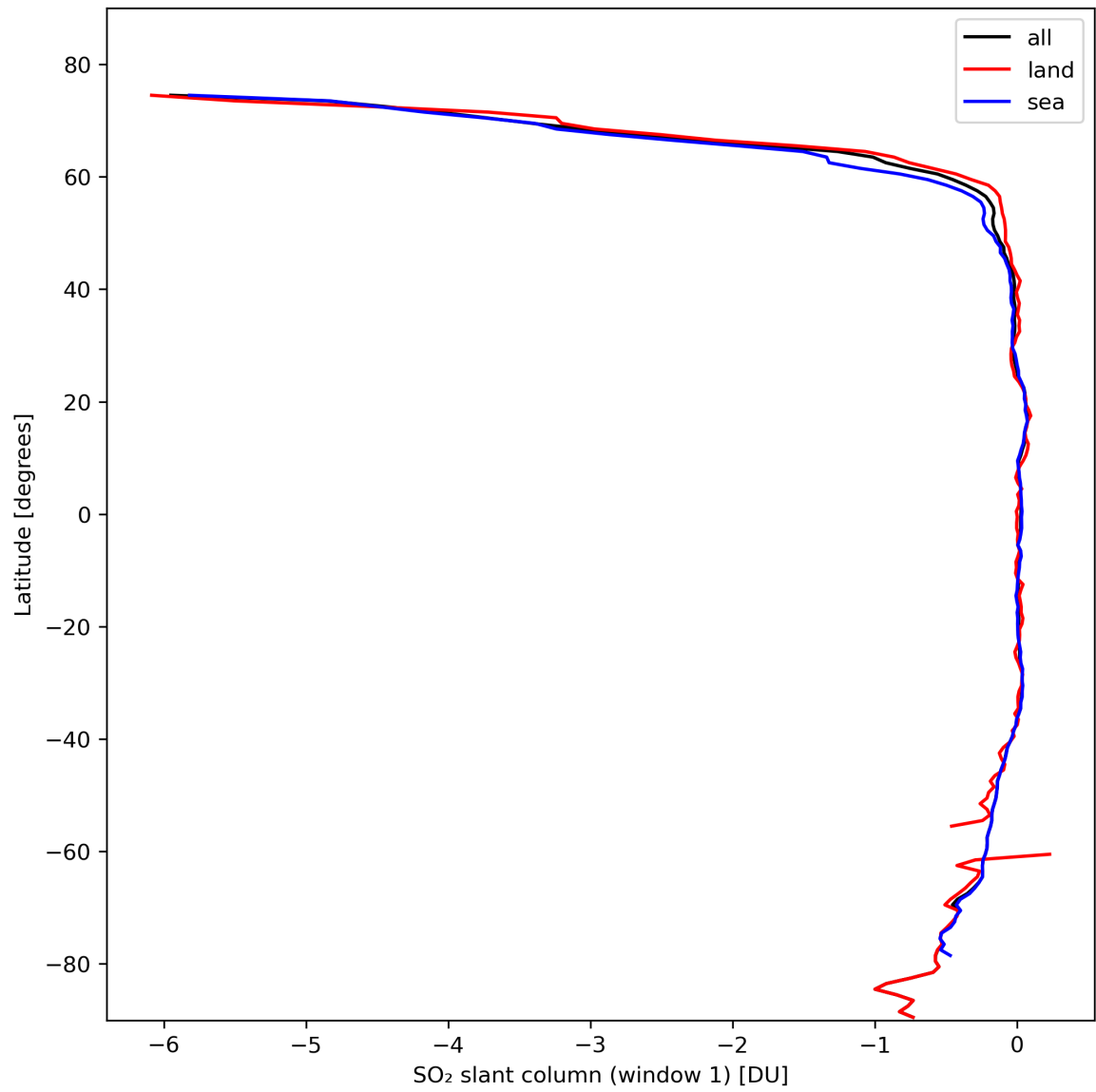
Figure 33: Zonal average of “SO 2 slant column (window 1)” for 2024-02-19 to 2024-02-21.
