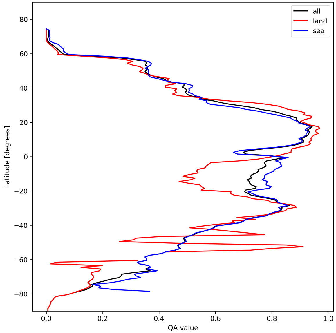
Figure 29: Zonal average of “QA value” for 2024-02-19 to 2024-02-21.
