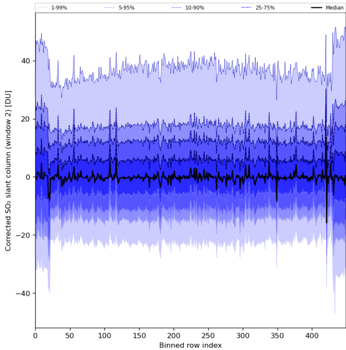
Figure 85: Along track statistics of “Corrected SO 2 slant column (window 2)” for 2024-02-19 to 2024-02-21
