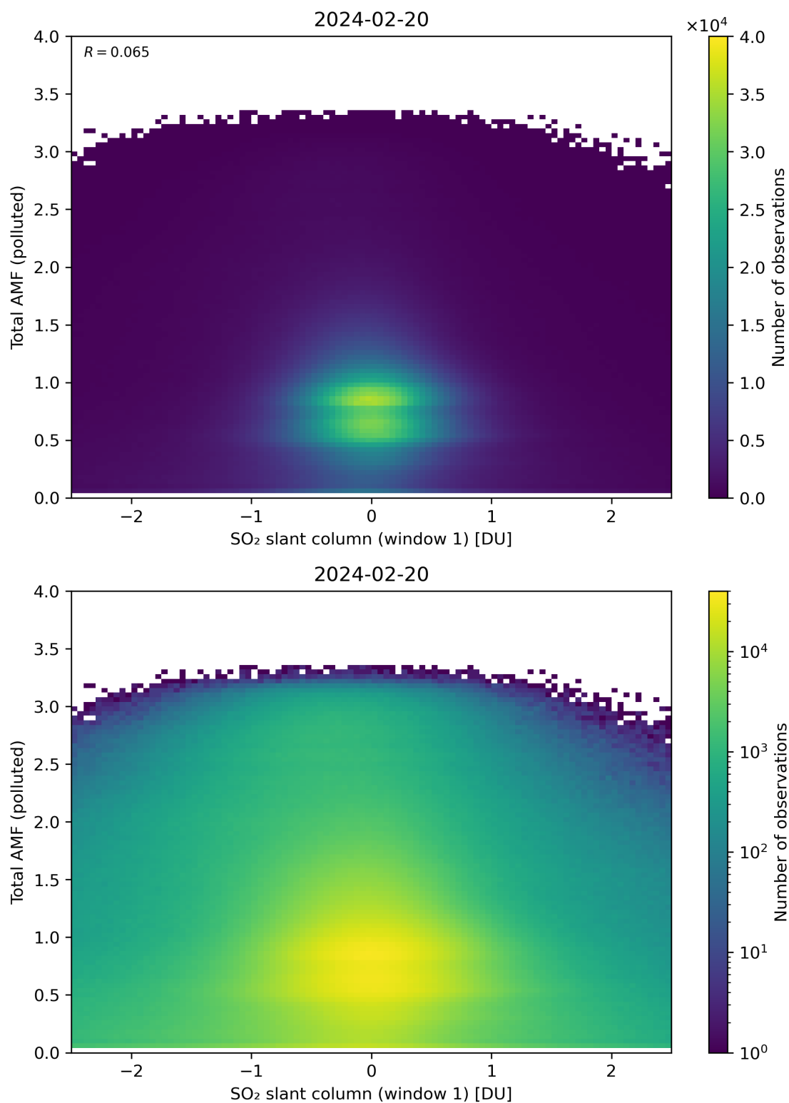
Figure 239: Scatter density plot of “SO 2 slant column (window 1)” against “Total AMF (polluted)” for 2024-02-19 to 2024-02-21.
