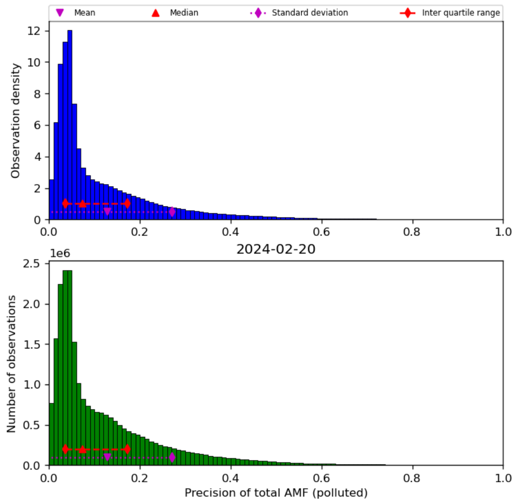
Figure 72: Histogram of “Precision of total AMF (polluted)” for 2024-02-19 to 2024-02-21
