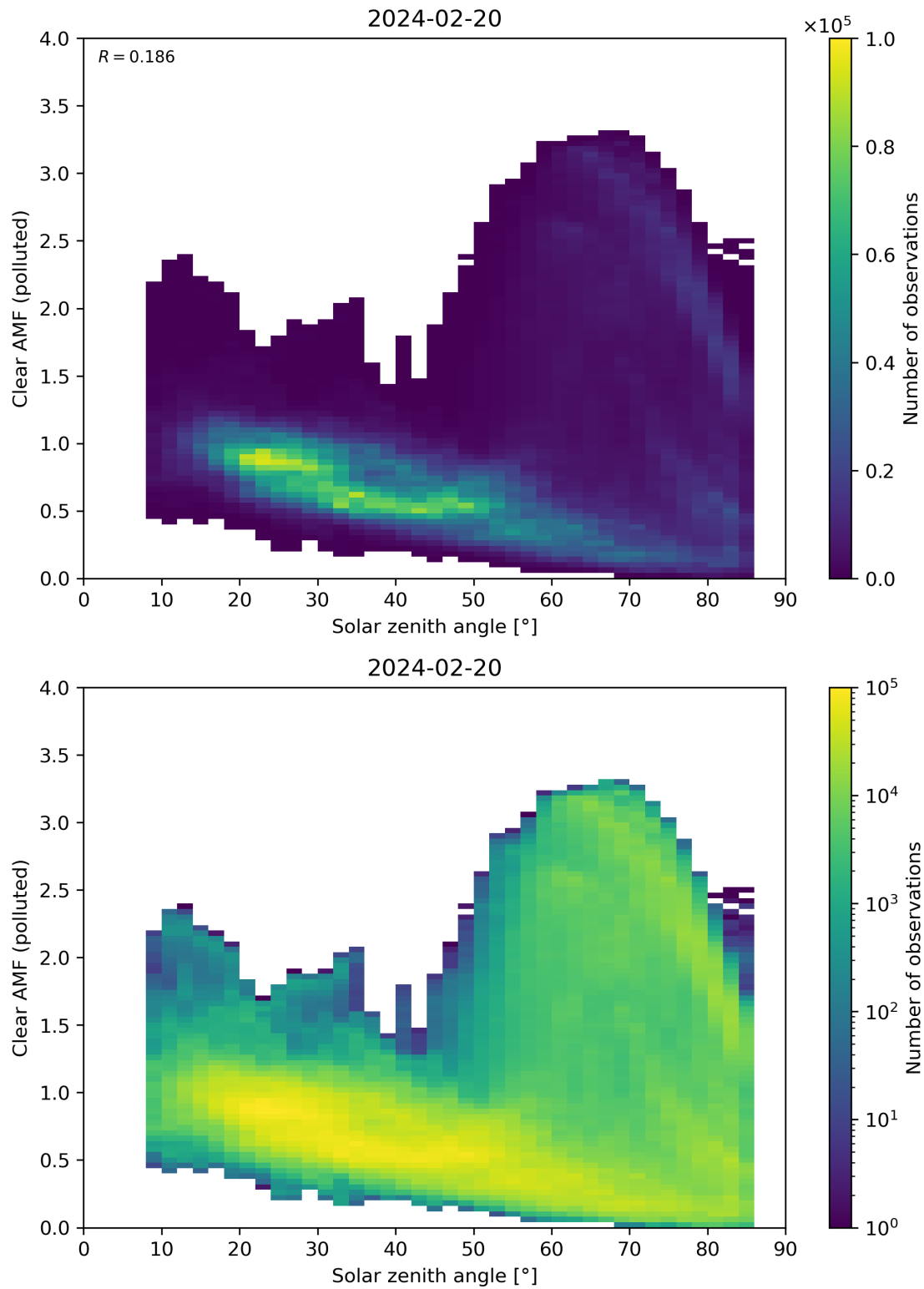
Figure 165: Scatter density plot of “Solar zenith angle” against “Clear AMF (polluted)” for 2024-02-19 to 2024-02-21.
