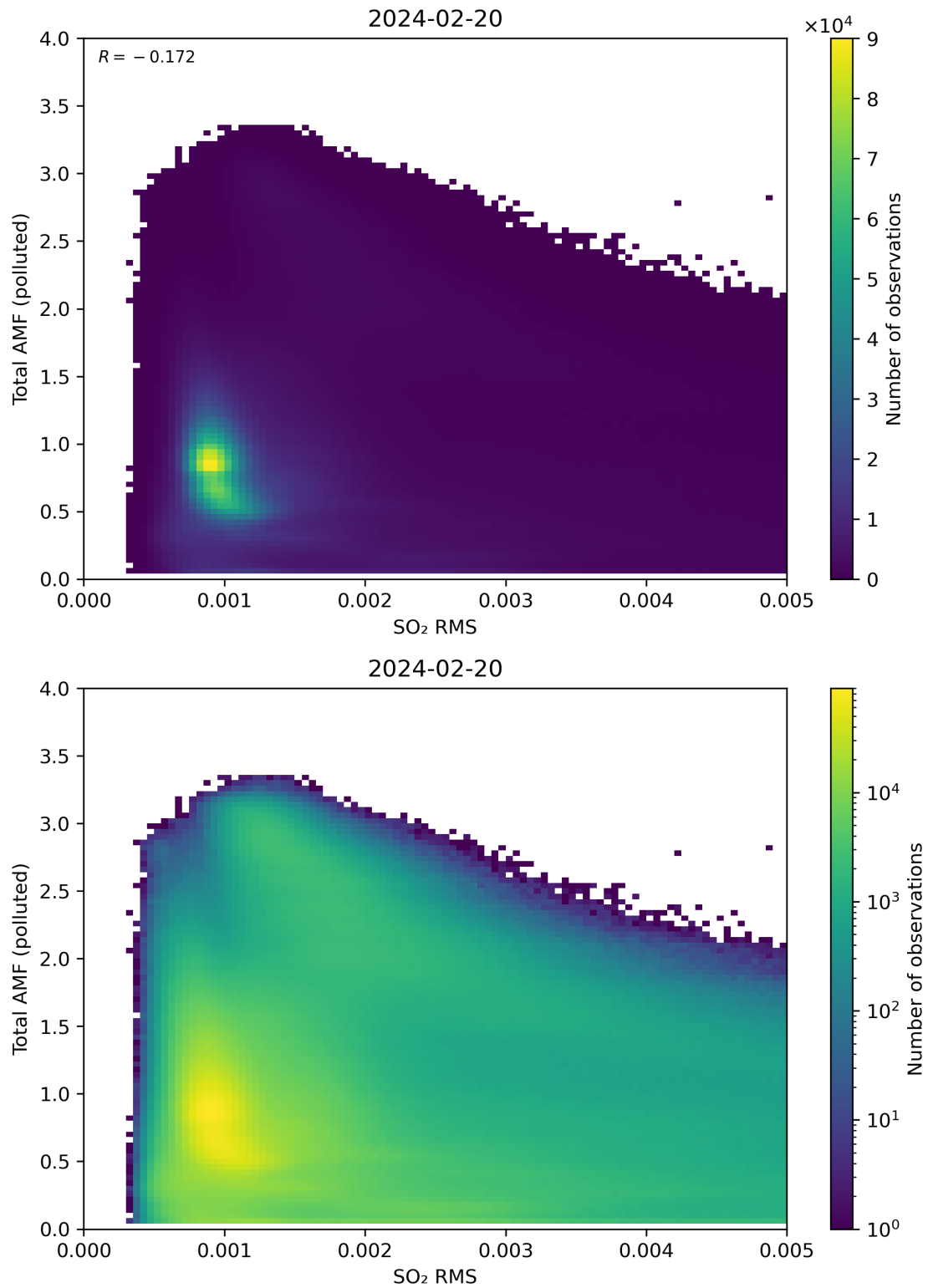
Figure 137: Scatter density plot of “SO 2 RMS” against “Total AMF (polluted)” for 2024-02-19 to 2024-02-21.
