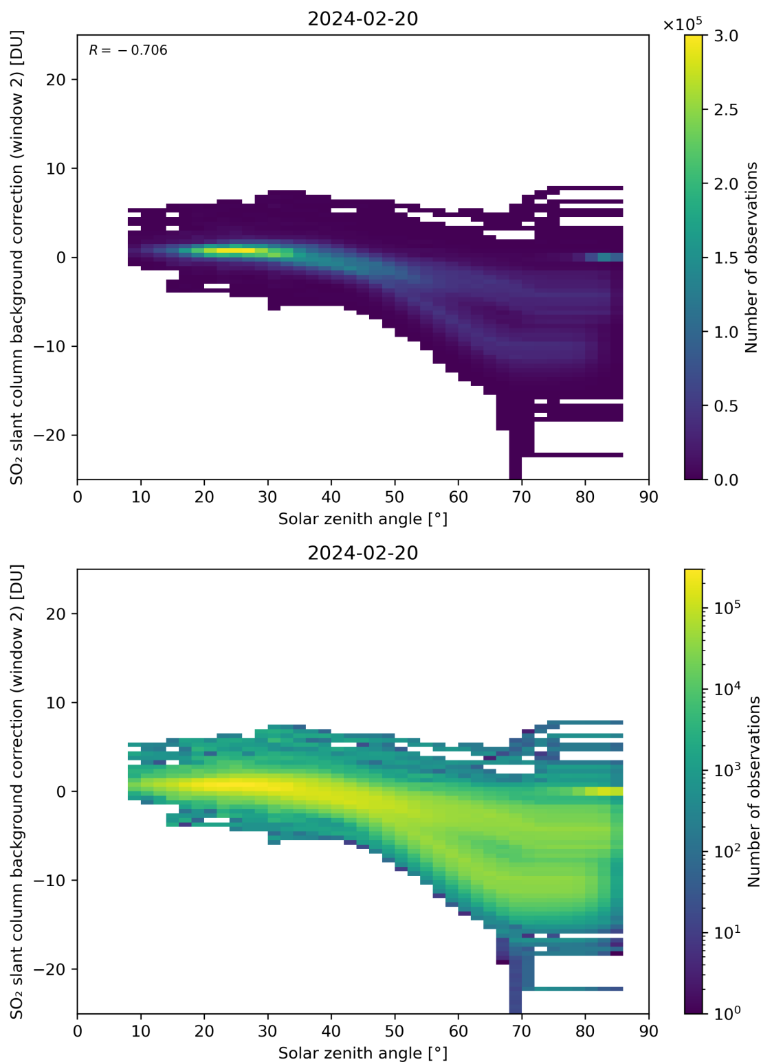
Figure 159: Scatter density plot of “Solar zenith angle” against “SO 2 slant column background correction (window 2)” for 2024-02-19 to 2024-02-21.
