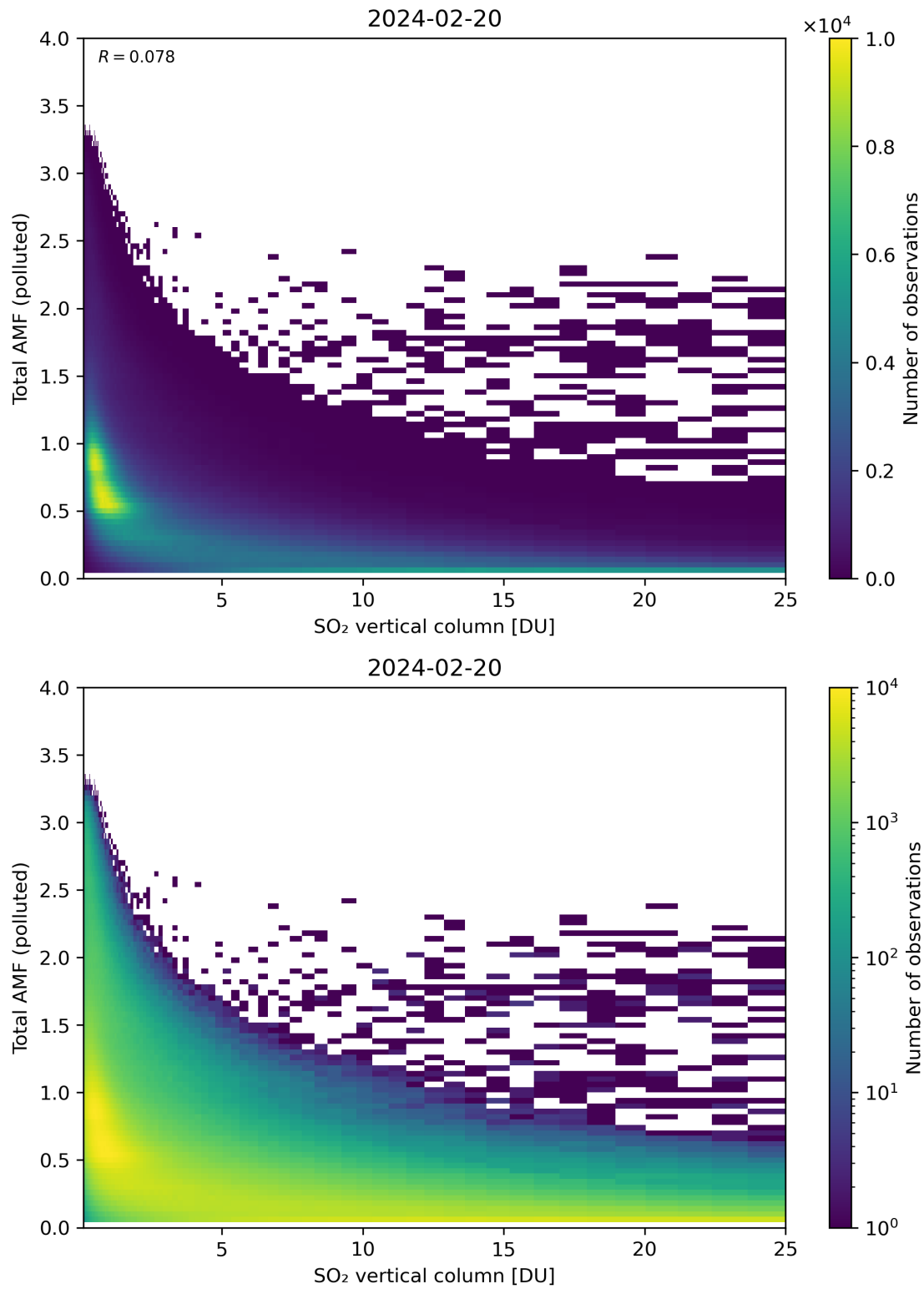
Figure 305: Scatter density plot of “SO 2 vertical column” against “Total AMF (polluted)” for 2024-02-19 to 2024-02-21.
