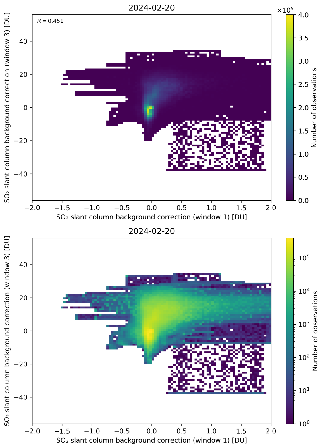
Figure 99: Scatter density plot of “SO 2 slant column background correction (window 1)” against “SO 2 slant column background correction (window 3)” for 2024-02-19 to 2024-02-21.
