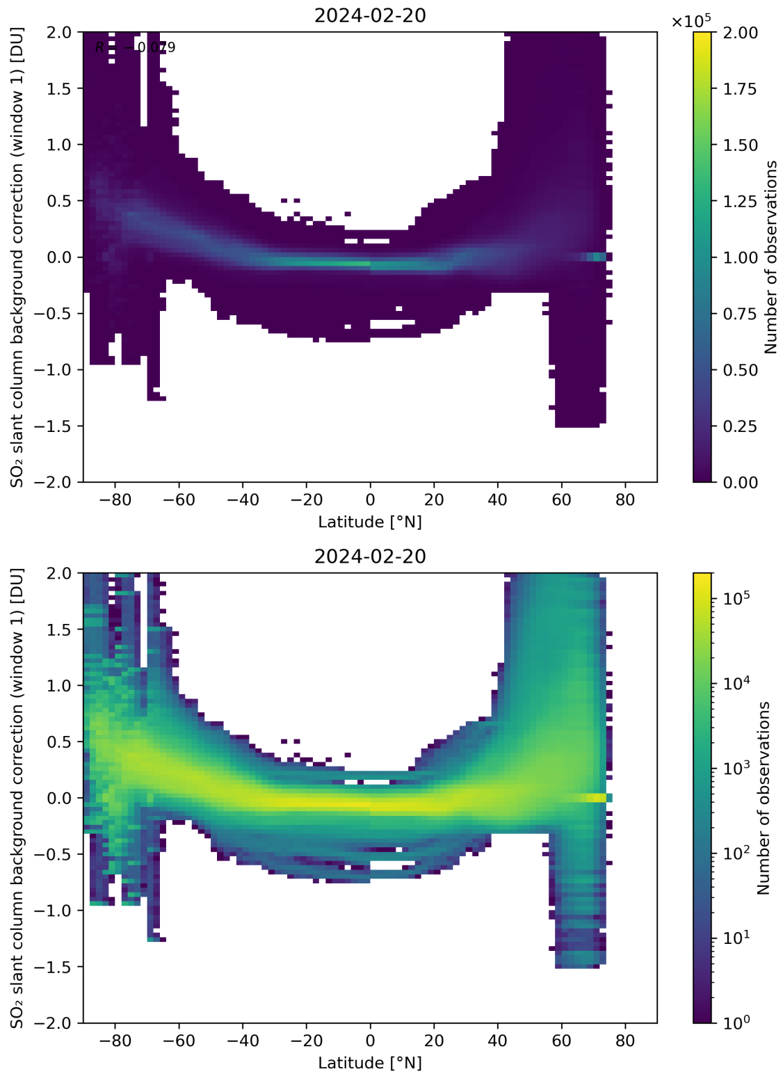
Figure 139: Scatter density plot of “Latitude” against “SO 2 slant column background correction (window 1)” for 2024-02-19 to 2024-02-21.
