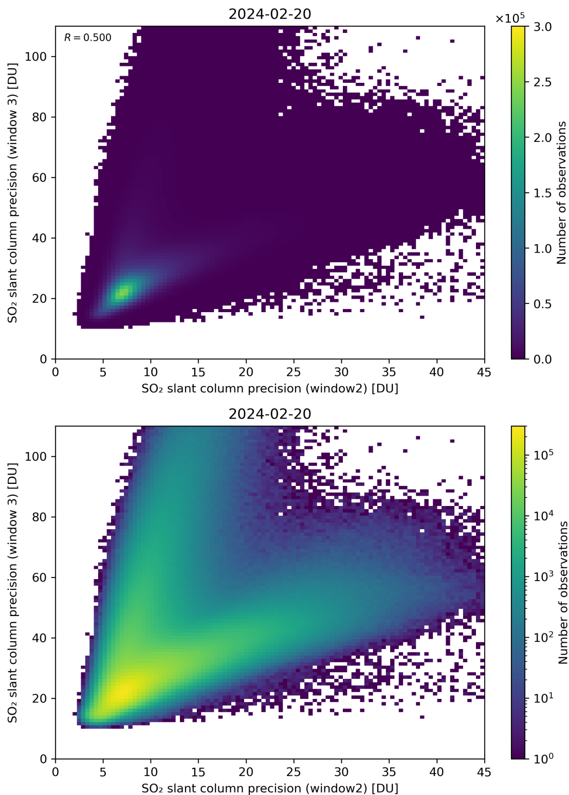
Figure 250: Scatter density plot of “SO 2 slant column precision (window2)” against “SO 2 slant column precision (window 3)” for 2024-02-19 to 2024-02-21.
