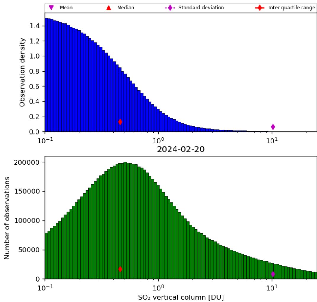
Figure 53: Histogram of “SO 2 vertical column” for 2024-02-19 to 2024-02-21
