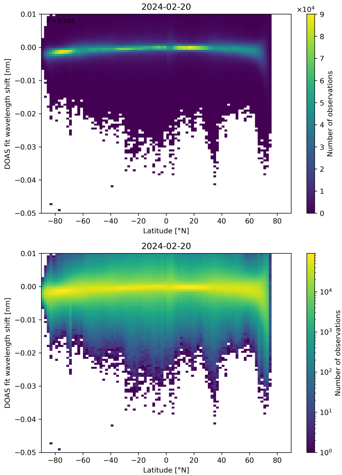
Figure 142: Scatter density plot of “Latitude” against “DOAS fit wavelength shift” for 2024-02-19 to 2024-02-21.
