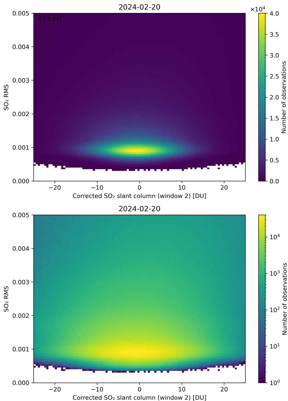
Figure 198: Scatter density plot of “Corrected SO 2 slant column (window 2)” against “SO 2 RMS” for 2024-02-19 to 2024-02-21.
