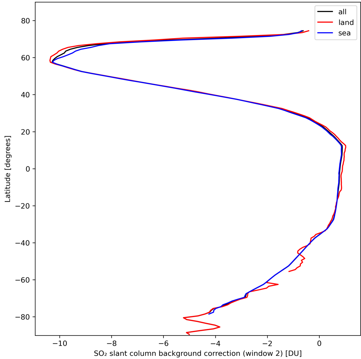
Figure 40: Zonal average of “SO 2 slant column background correction (window 2)” for 2024-02-19 to 2024-02-21.
