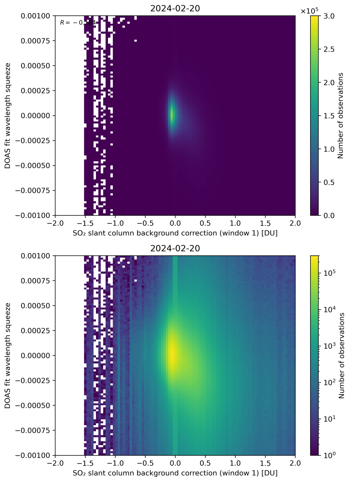
Figure 101: Scatter density plot of “SO 2 slant column background correction (window 1)” against “DOAS fit wavelength squeeze” for 2024-02-19 to 2024-02-21.
