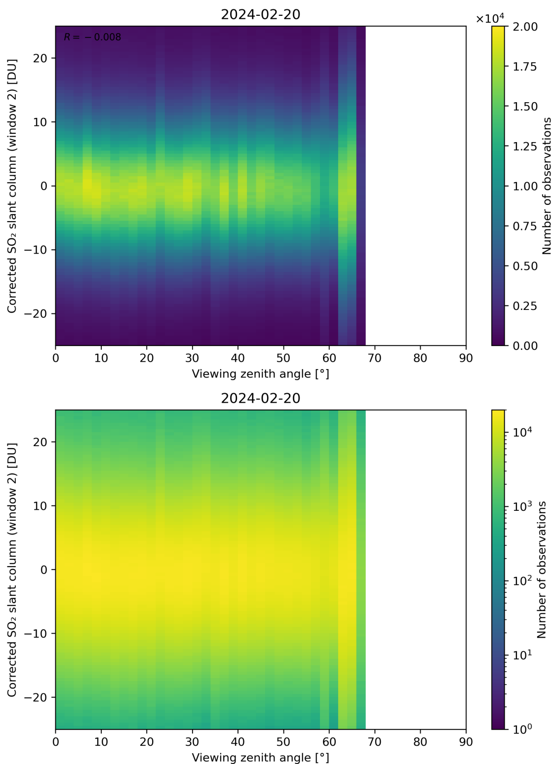
Figure 318: Scatter density plot of “Viewing zenith angle” against “Corrected SO 2 slant column (window 2)” for 2024-02-19 to 2024-02-21.
