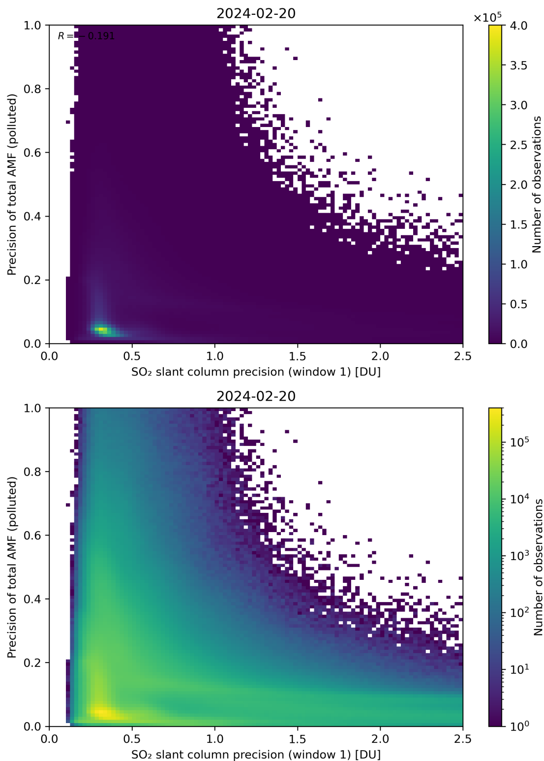
Figure 231: Scatter density plot of “SO 2 slant column precision (window 1)” against “Precision of total AMF (polluted)” for 2024-02-19 to 2024-02-21.
