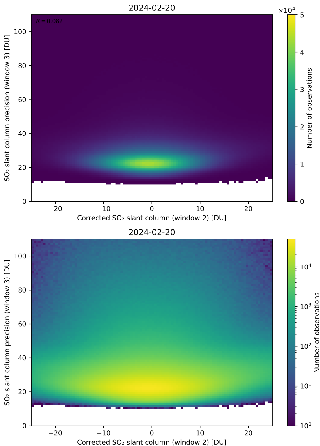
Figure 202: Scatter density plot of “Corrected SO 2 slant column (window 2)” against “SO 2 slant column precision (window 3)” for 2024-02-19 to 2024-02-21.
