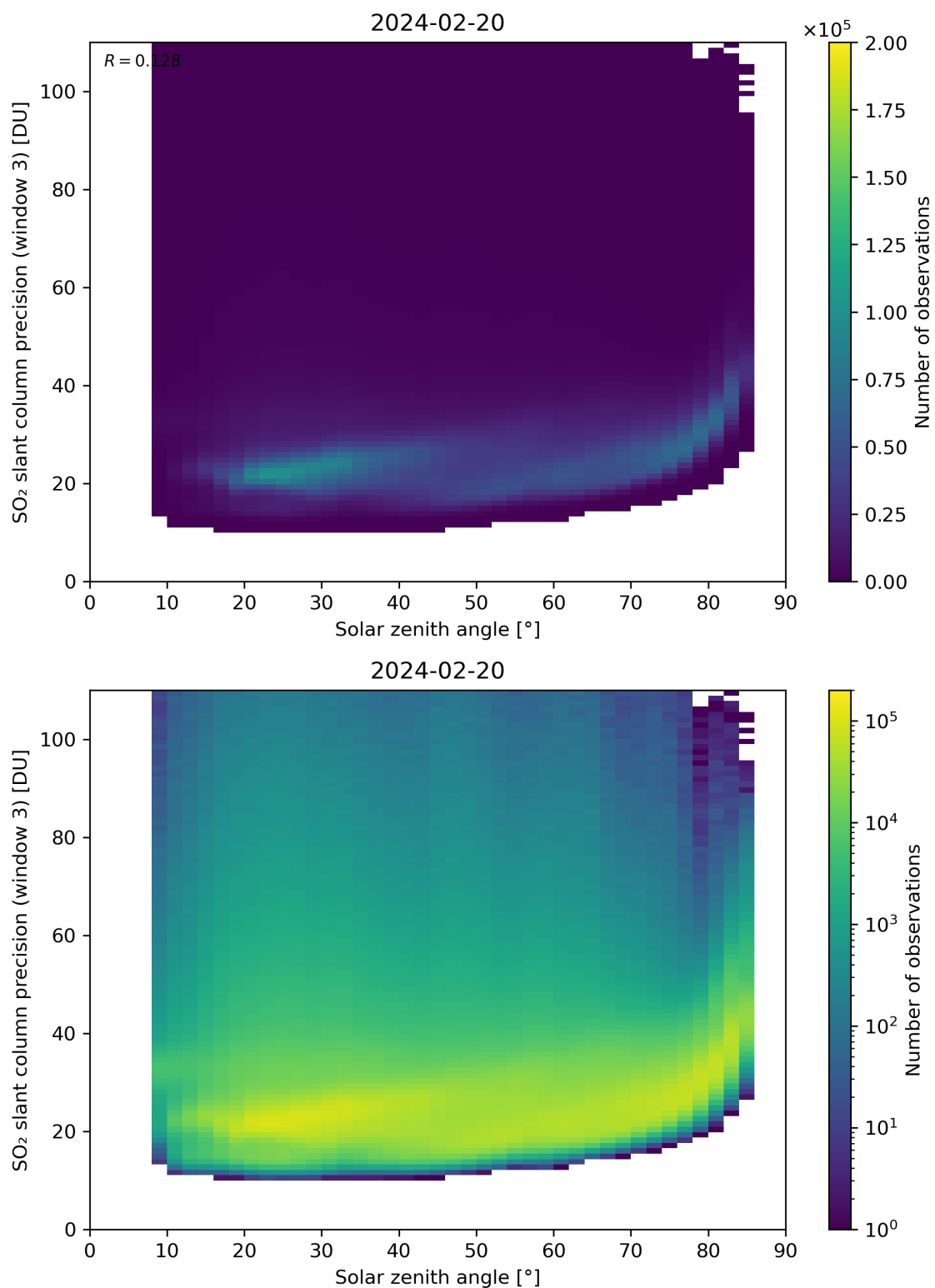
Figure 173: Scatter density plot of “Solar zenith angle” against “SO 2 slant column precision (window 3)” for 2024-02-19 to 2024-02-21.
