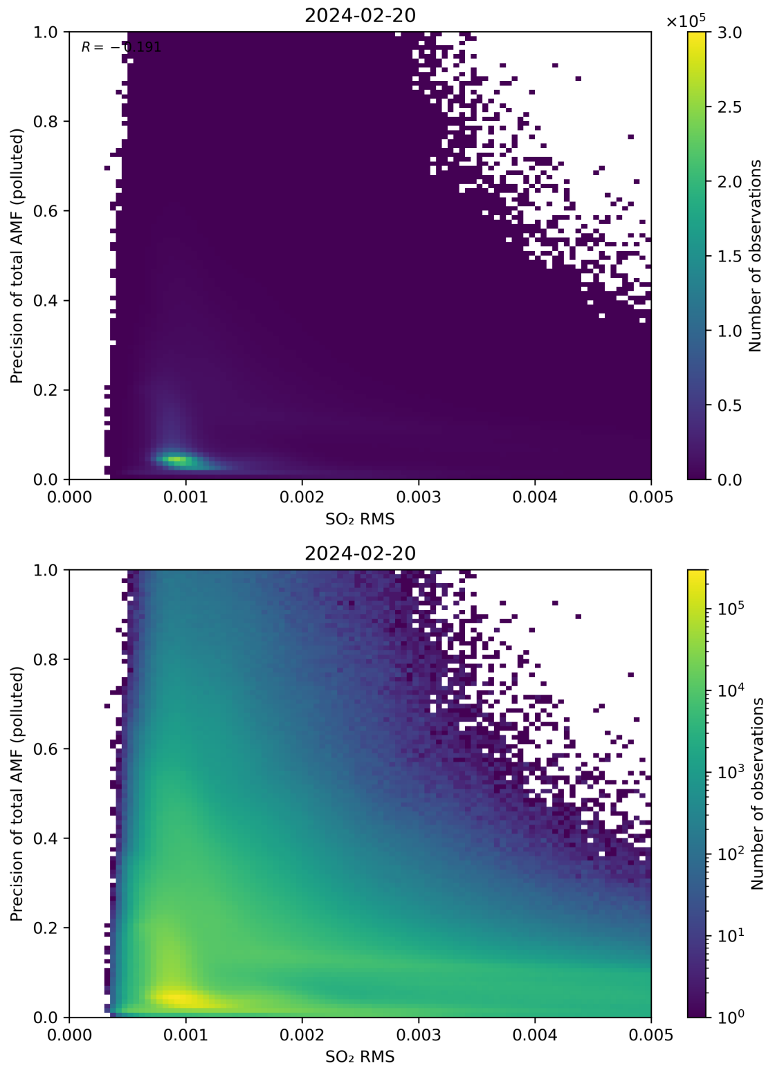
Figure 138: Scatter density plot of “SO 2 RMS” against “Precision of total AMF (polluted)” for 2024-02-19 to 2024-02-21.
