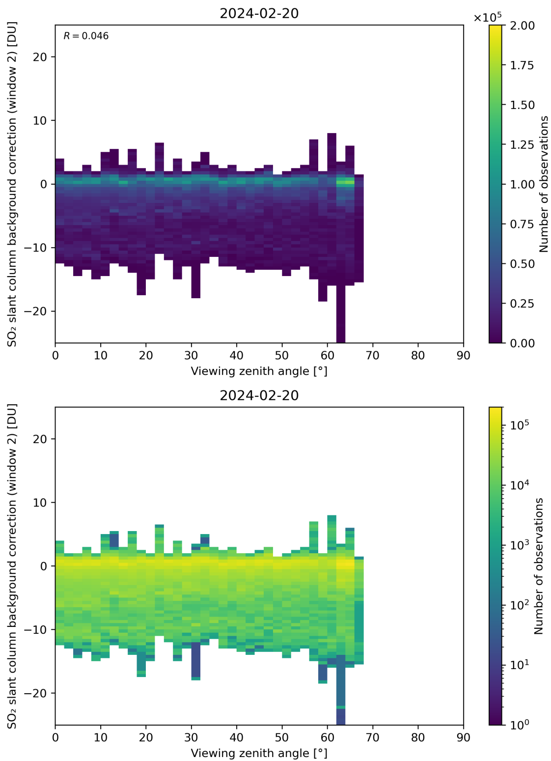
Figure 309: Scatter density plot of “Viewing zenith angle” against “SO 2 slant column background correction (window 2)” for 2024-02-19 to 2024-02-21.
