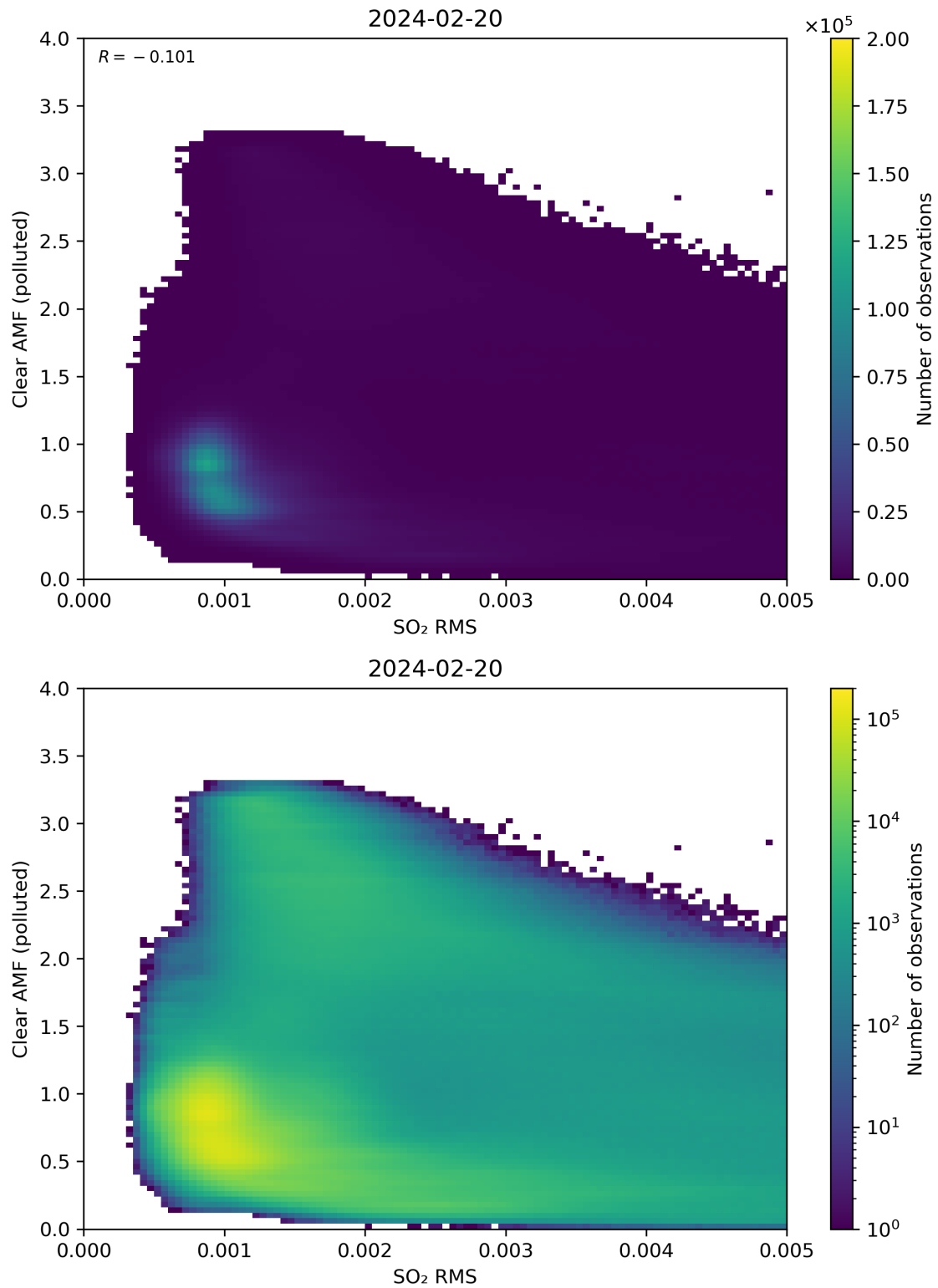
Figure 136: Scatter density plot of “SO 2 RMS” against “Clear AMF (polluted)” for 2024-02-19 to 2024-02-21.
