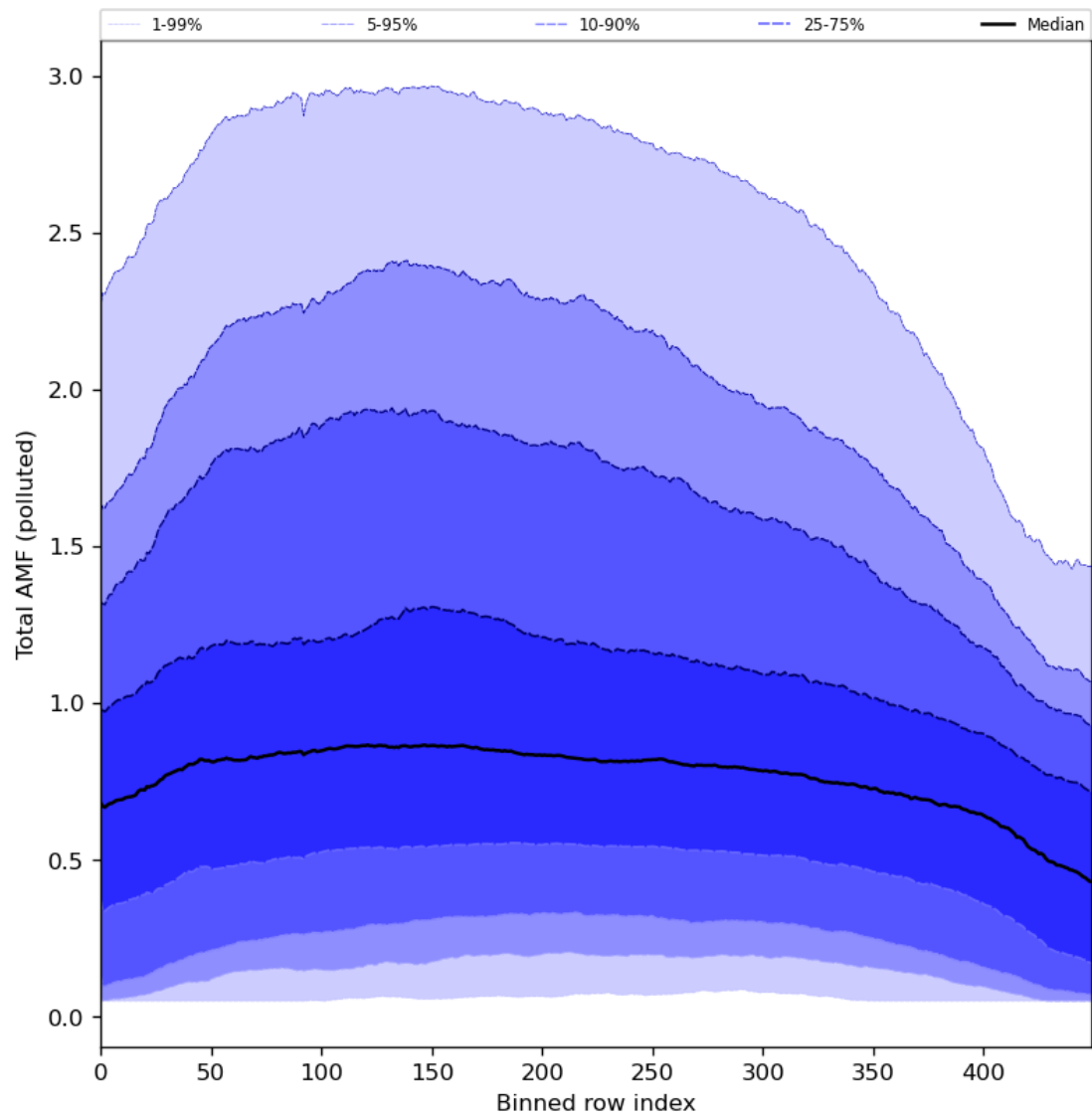
Figure 94: Along track statistics of “Total AMF (polluted)” for 2024-02-19 to 2024-02-21
