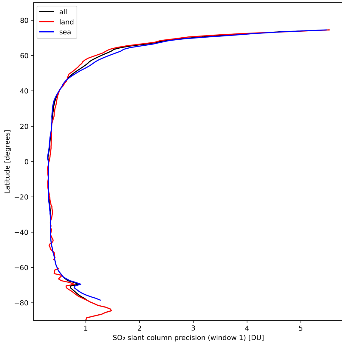
Figure 34: Zonal average of “SO 2 slant column precision (window 1)” for 2024-02-19 to 2024-02-21.
