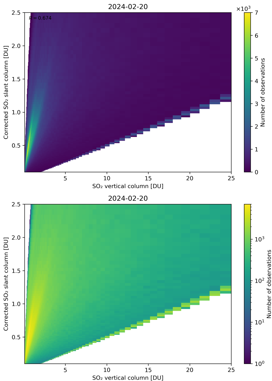
Figure 297: Scatter density plot of “SO 2 vertical column” against “Corrected SO 2 slant column” for 2024-02-19 to 2024-02-21.
