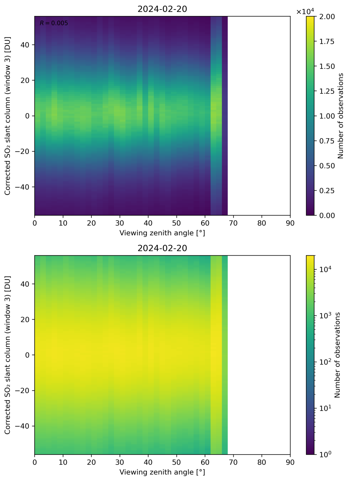
Figure 319: Scatter density plot of “Viewing zenith angle” against “Corrected SO 2 slant column (window 3)” for 2024-02-19 to 2024-02-21.
