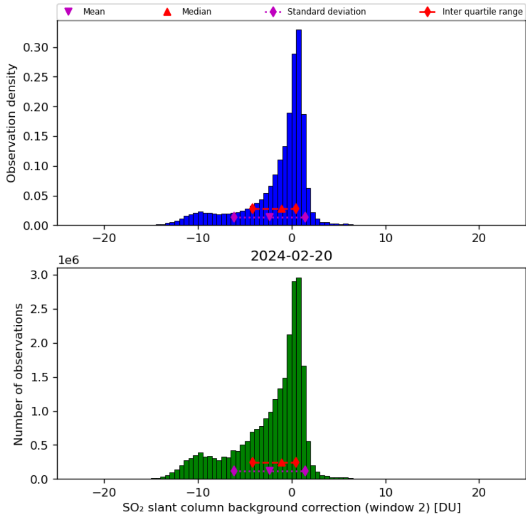
Figure 63: Histogram of “SO 2 slant column background correction (window 2)” for 2024-02-19 to 2024-02-21
