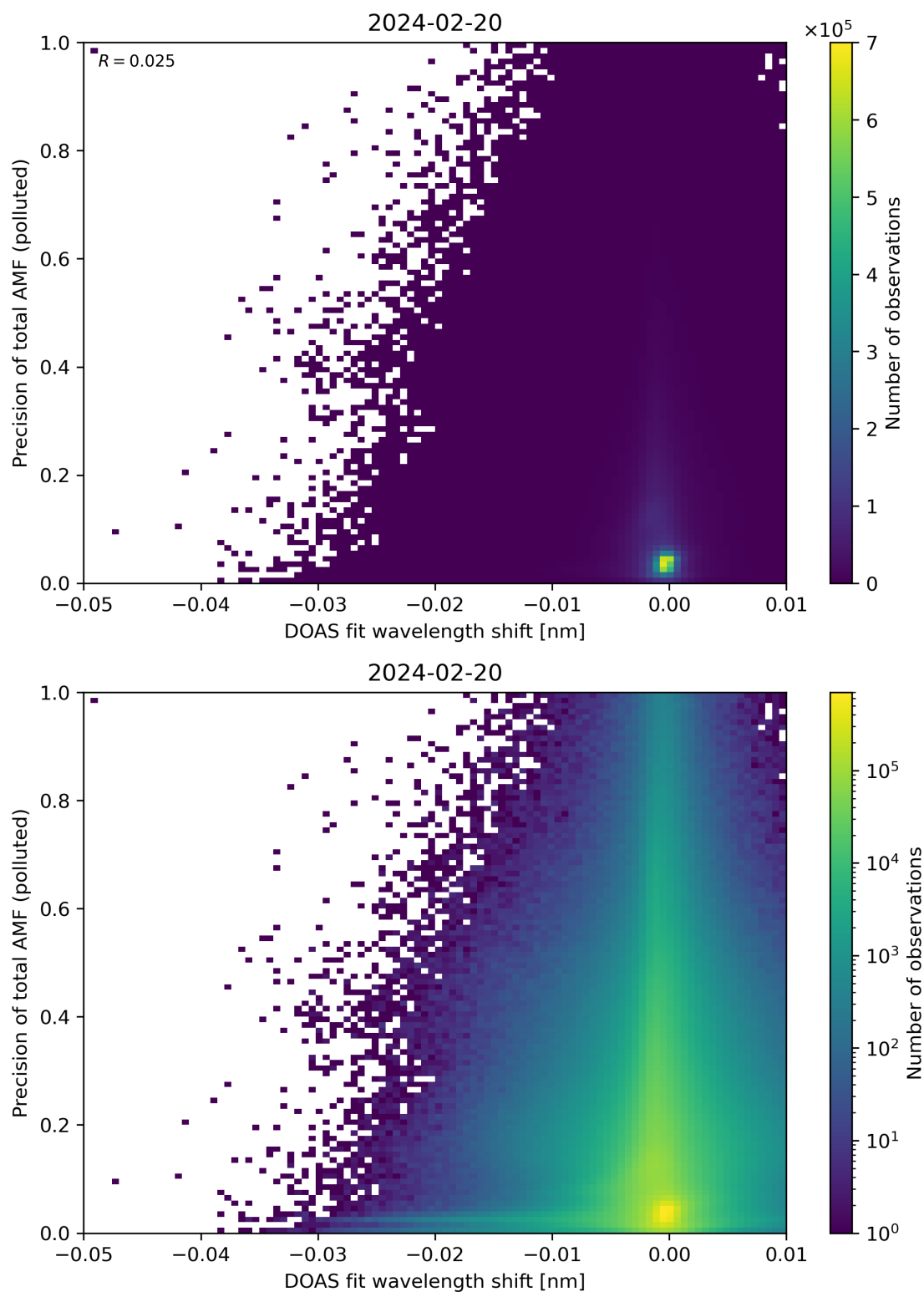
Figure 131: Scatter density plot of “DOAS fit wavelength shift” against “Precision of total AMF (polluted)” for 2024-02-19 to 2024-02-21.
