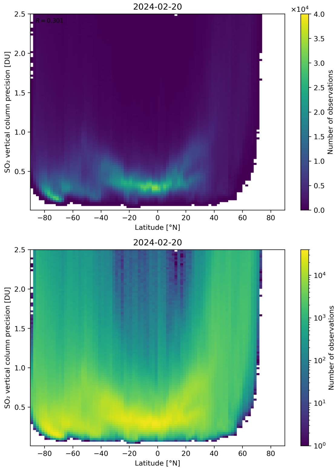
Figure 157: Scatter density plot of “Latitude” against “SO 2 vertical column precision” for 2024-02-19 to 2024-02-21.
