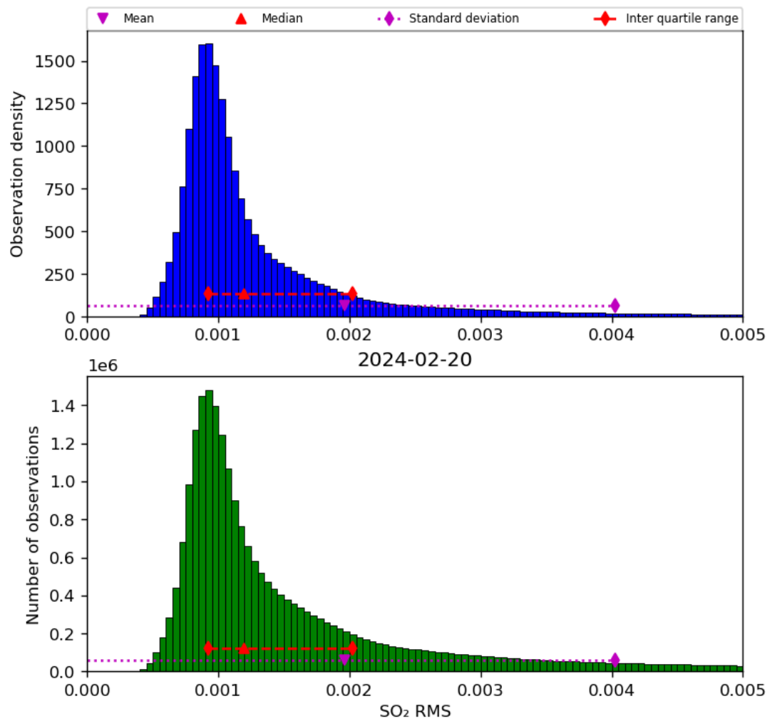
Figure 70: Histogram of “SO 2 RMS” for 2024-02-19 to 2024-02-21
