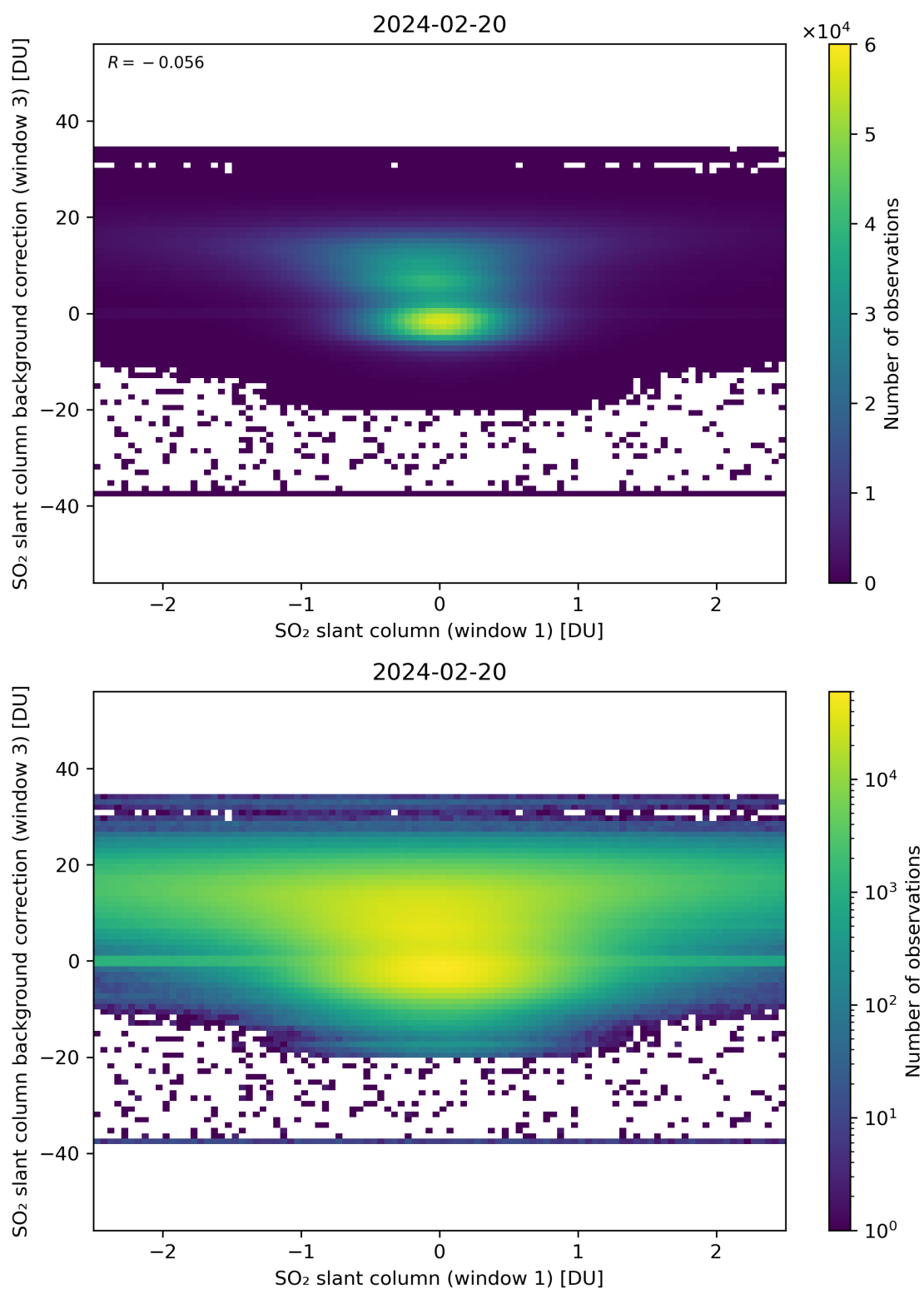
Figure 214: Scatter density plot of “SO 2 slant column (window 1)” against “SO 2 slant column background correction (window 3)” for 2024-02-19 to 2024-02-21.
