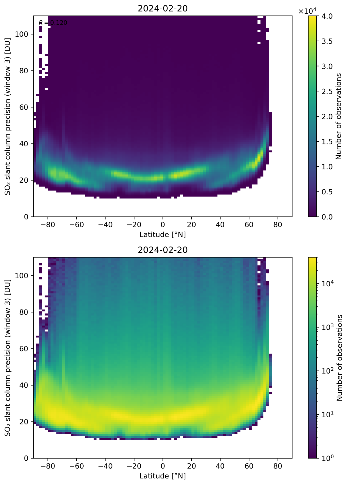
Figure 153: Scatter density plot of “Latitude” against “SO 2 slant column precision (window 3)” for 2024-02-19 to 2024-02-21.
