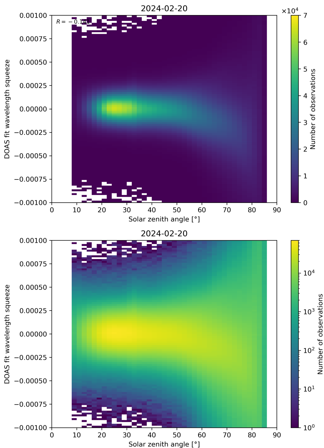
Figure 162: Scatter density plot of “Solar zenith angle” against “DOAS fit wavelength squeeze” for 2024-02-19 to 2024-02-21.
