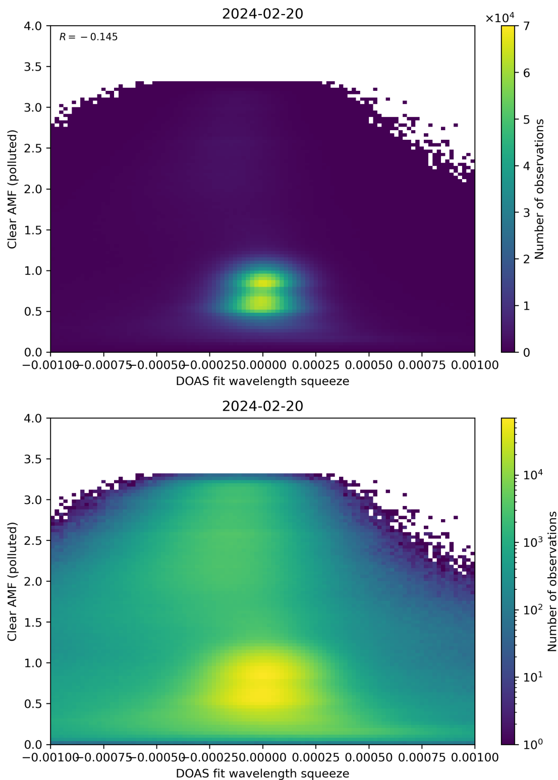
Figure 133: Scatter density plot of “DOAS fit wavelength squeeze” against “Clear AMF (polluted)” for 2024-02-19 to 2024-02-21.
