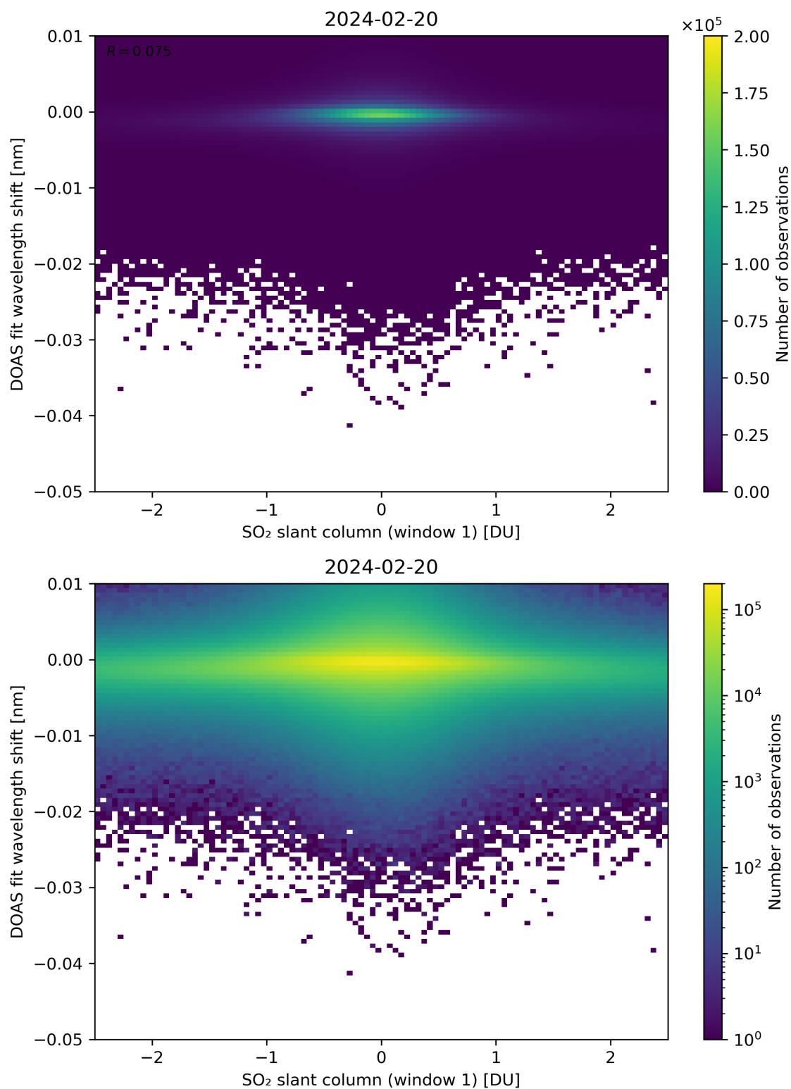
Figure 215: Scatter density plot of “SO 2 slant column (window 1)” against “DOAS fit wavelength shift” for 2024-02-19 to 2024-02-21.
