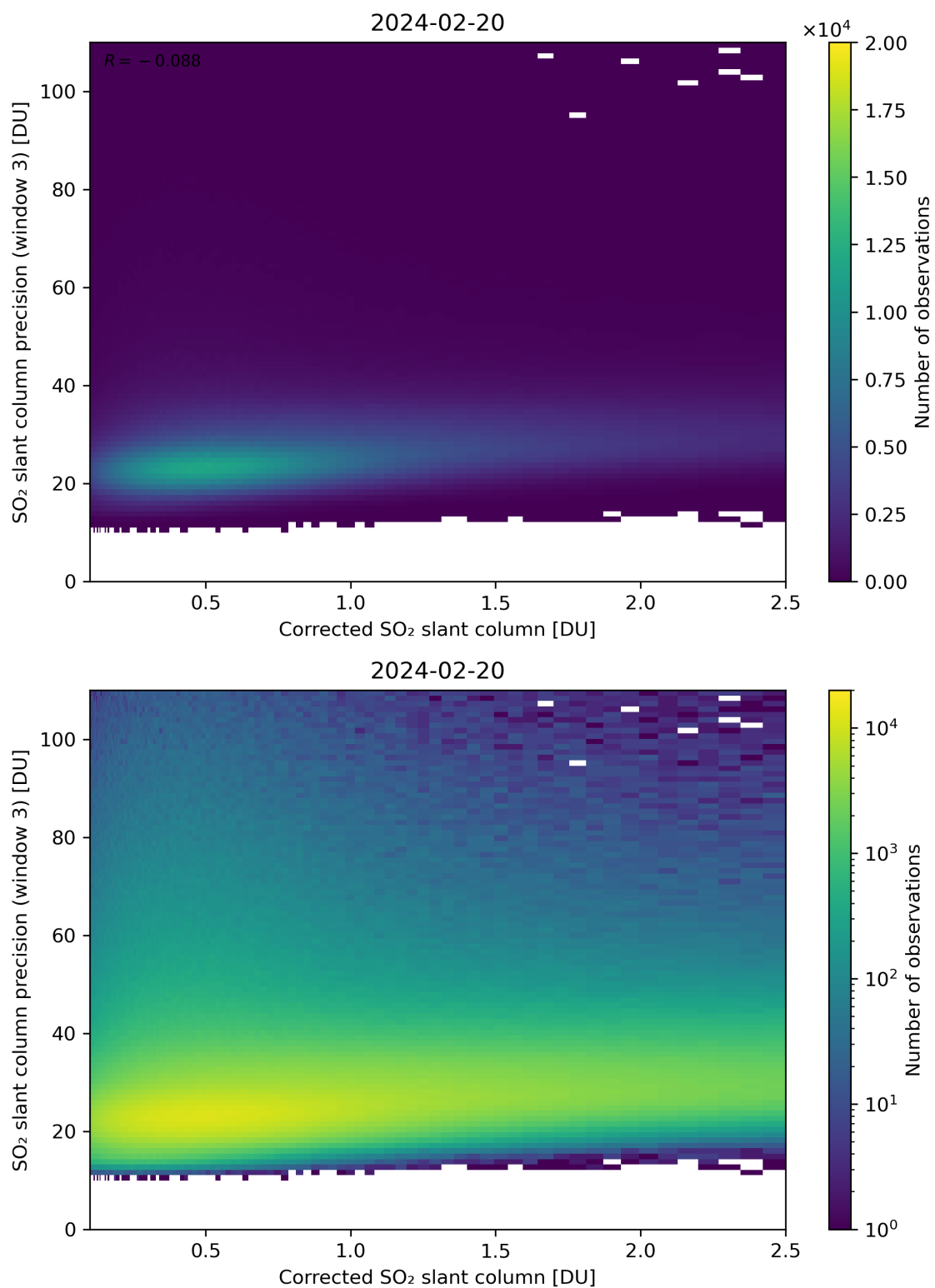
Figure 191: Scatter density plot of “Corrected SO 2 slant column” against “SO 2 slant column precision (window 3)” for 2024-02-19 to 2024-02-21.
