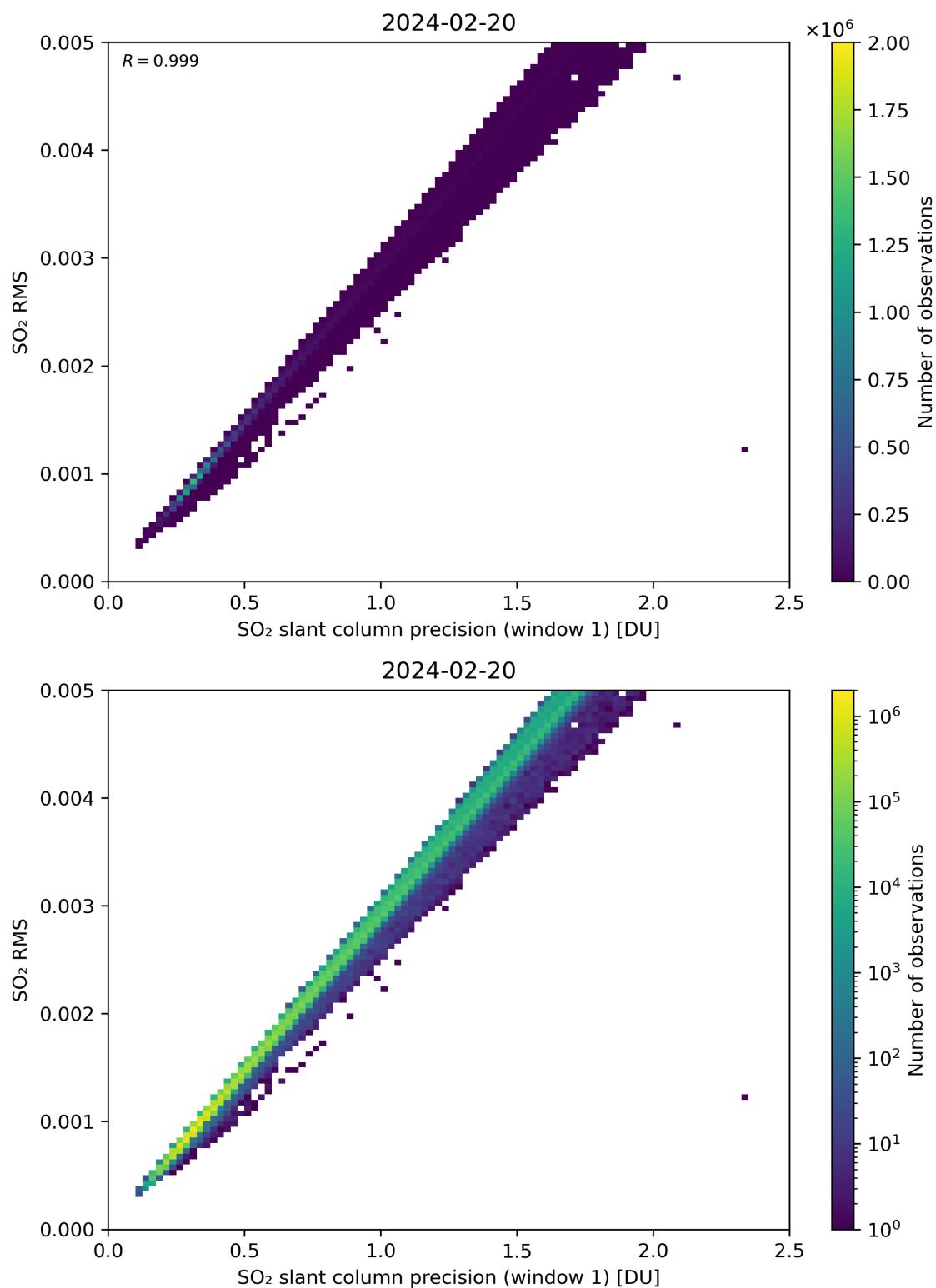
Figure 223: Scatter density plot of “SO 2 slant column precision (window 1)” against “SO 2 RMS” for 2024-02-19 to 2024-02-21.
