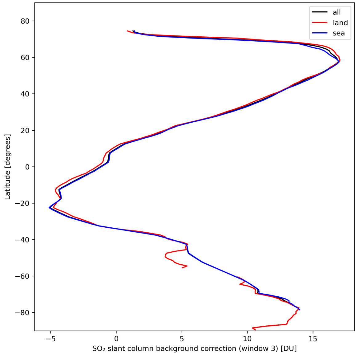
Figure 44: Zonal average of “SO 2 slant column background correction (window 3)” for 2024-02-19 to 2024-02-21.
