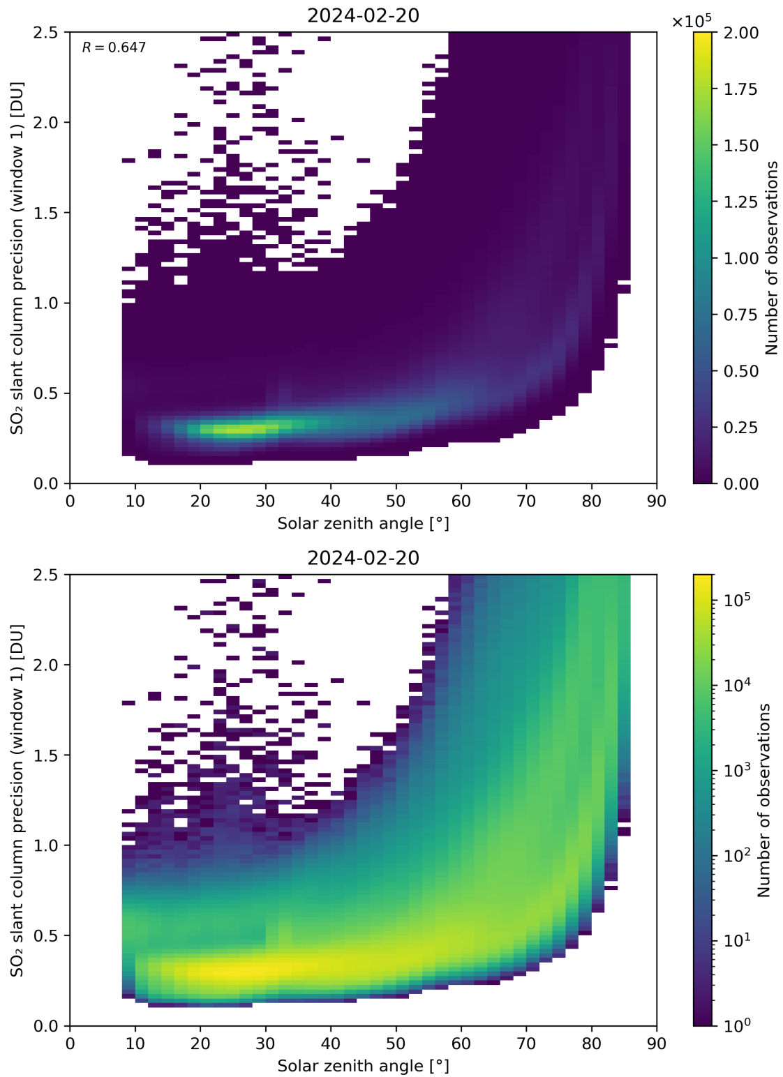
Figure 170: Scatter density plot of “Solar zenith angle” against “SO 2 slant column precision (window 1)” for 2024-02-19 to 2024-02-21.
