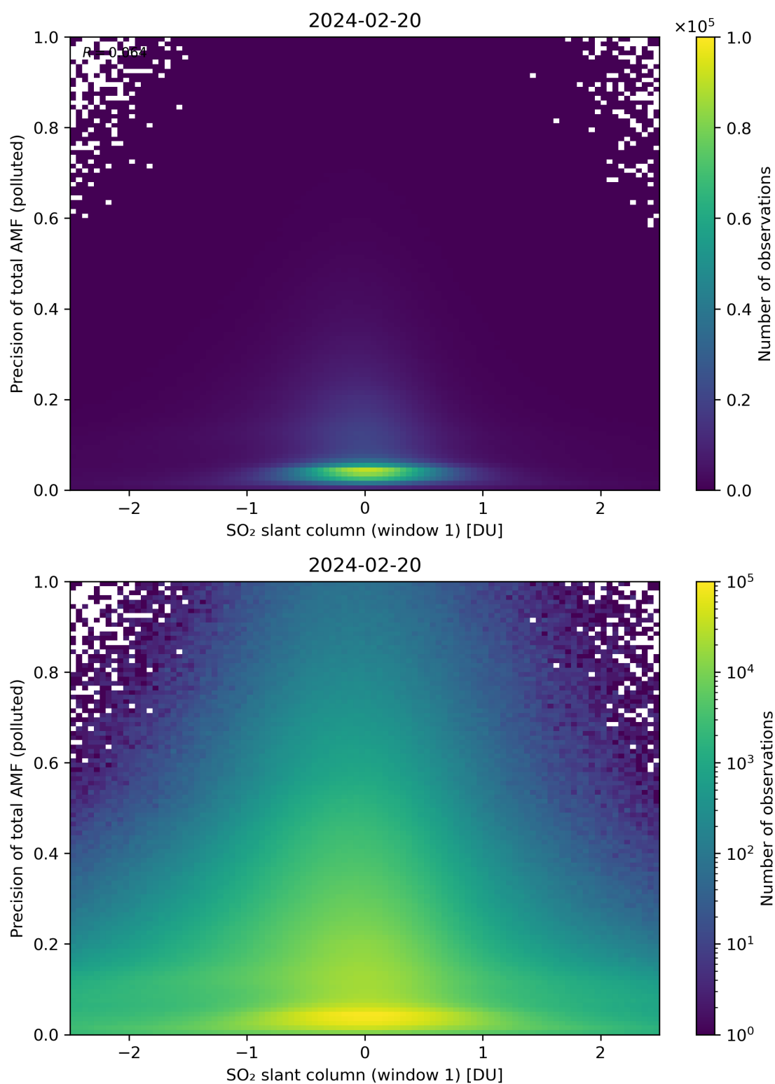
Figure 240: Scatter density plot of “SO 2 slant column (window 1)” against “Precision of total AMF (polluted)” for 2024-02-19 to 2024-02-21.
