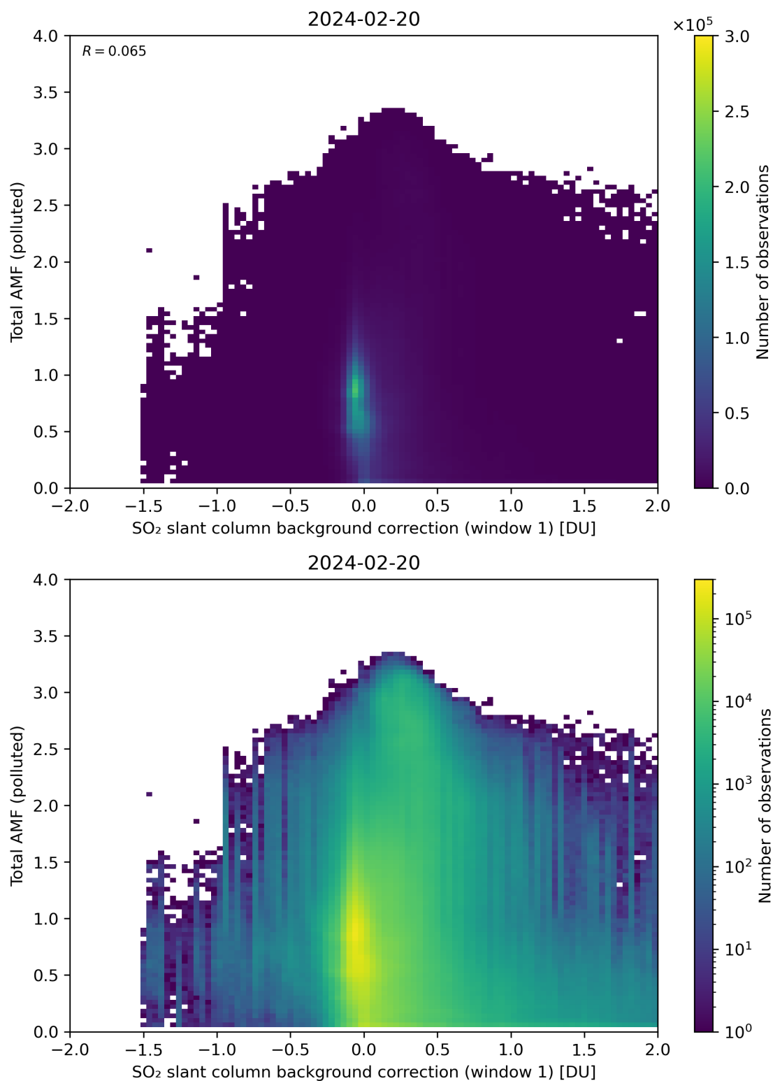
Figure 109: Scatter density plot of “SO 2 slant column background correction (window 1)” against “Total AMF (polluted)” for 2024-02-19 to 2024-02-21.
