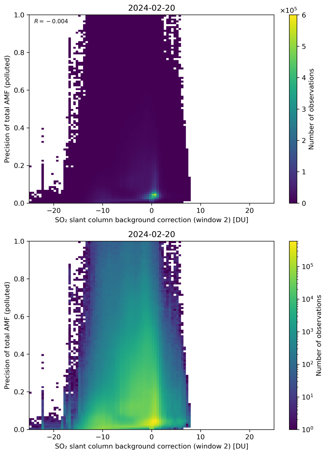
Figure 120: Scatter density plot of “SO 2 slant column background correction (window 2)” against “Precision of total AMF (polluted)” for 2024-02-19 to 2024-02-21.
