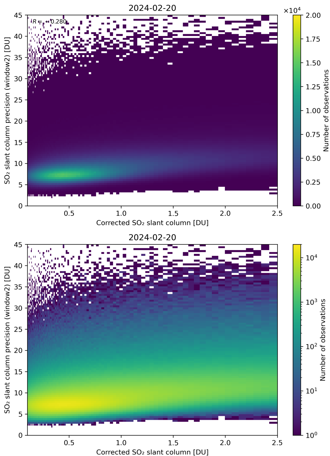
Figure 189: Scatter density plot of “Corrected SO 2 slant column” against “SO 2 slant column precision (window2)” for 2024-02-19 to 2024-02-21.
