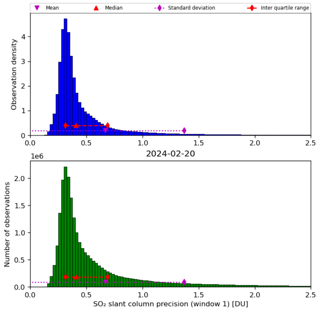
Figure 57: Histogram of “SO 2 slant column precision (window 1)” for 2024-02-19 to 2024-02-21
