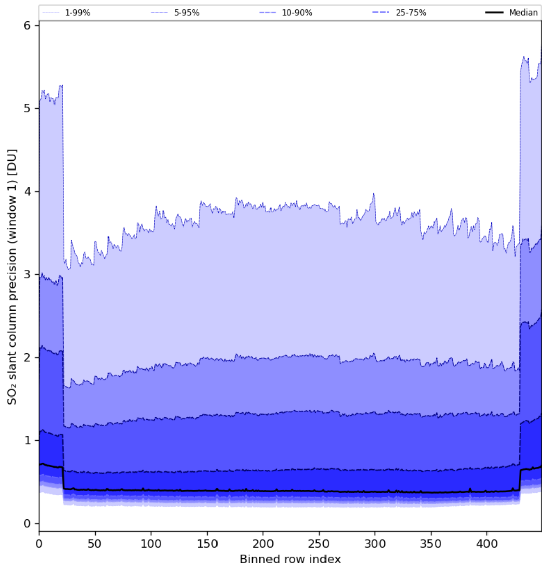
Figure 80: Along track statistics of “SO 2 slant column precision (window 1)” for 2024-02-19 to 2024-02-21
