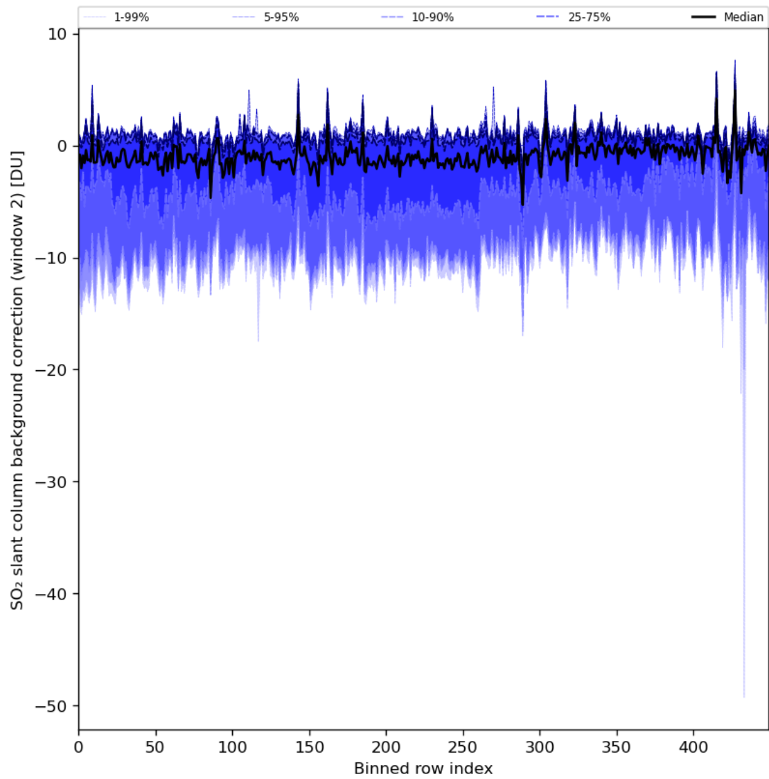
Figure 86: Along track statistics of “SO 2 slant column background correction (window 2)” for 2024-02-19 to 2024-02-21
