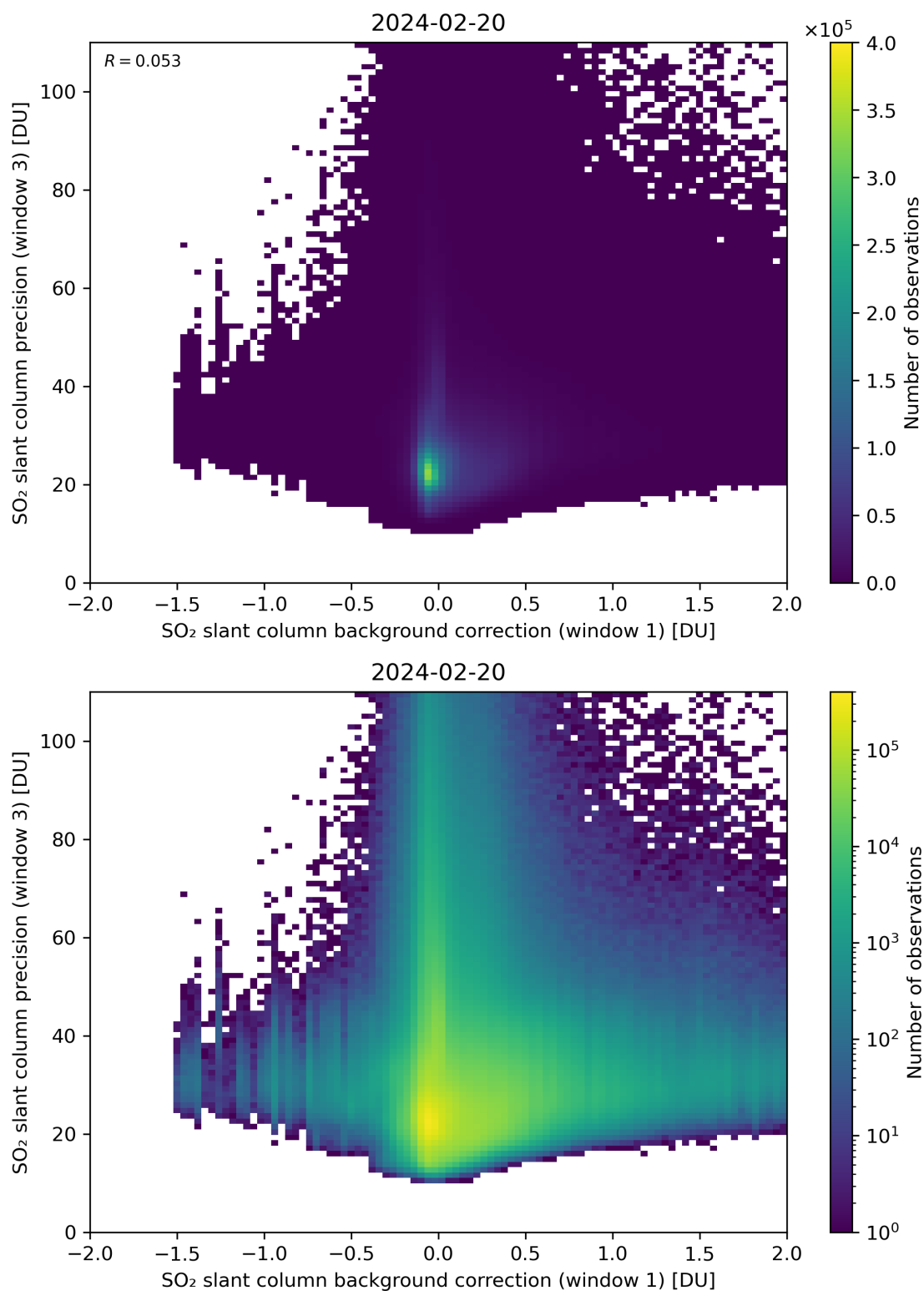
Figure 108: Scatter density plot of “SO 2 slant column background correction (window 1)” against “SO 2 slant column precision (window 3)” for 2024-02-19 to 2024-02-21.
