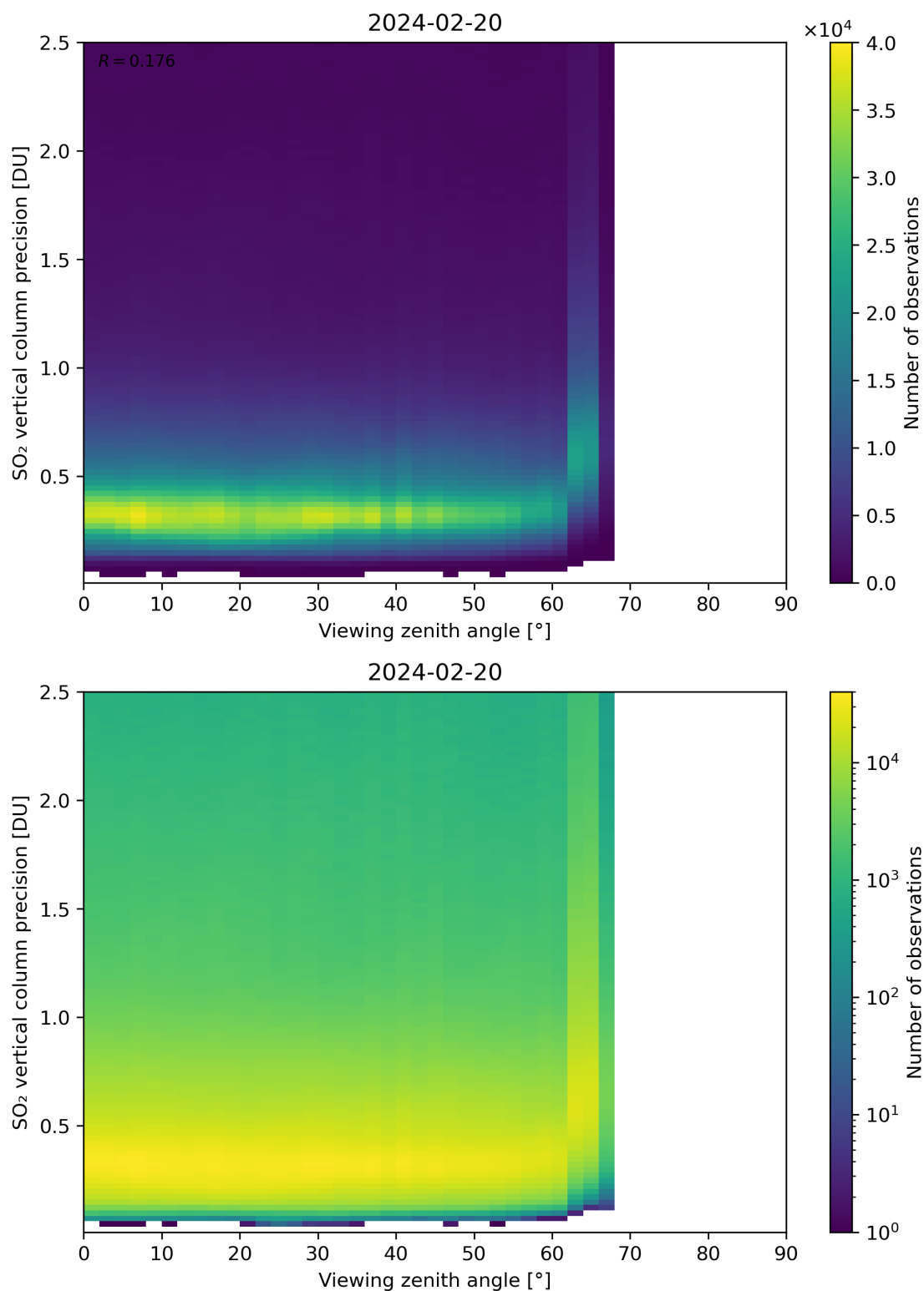
Figure 328: Scatter density plot of “Viewing zenith angle” against “SO 2 vertical column precision” for 2024-02-19 to 2024-02-21.
