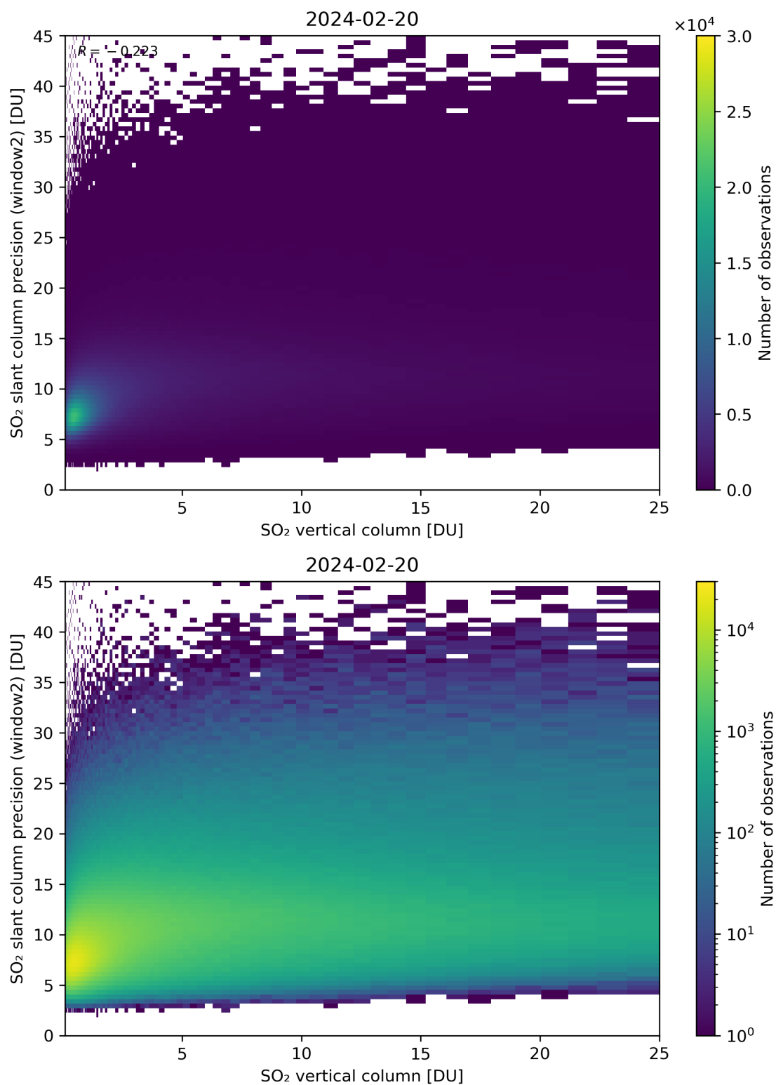
Figure 302: Scatter density plot of “SO 2 vertical column” against “SO 2 slant column precision (window2)” for 2024-02-19 to 2024-02-21.
