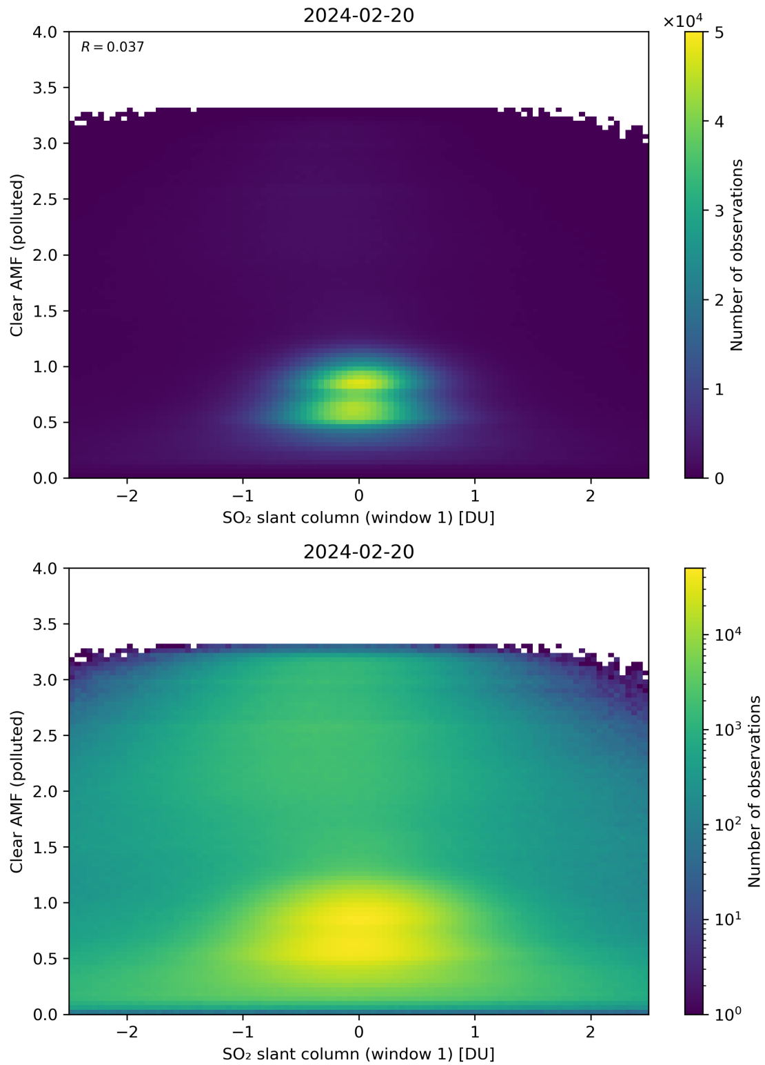
Figure 232: Scatter density plot of “SO 2 slant column (window 1)” against “Clear AMF (polluted)” for 2024-02-19 to 2024-02-21.
