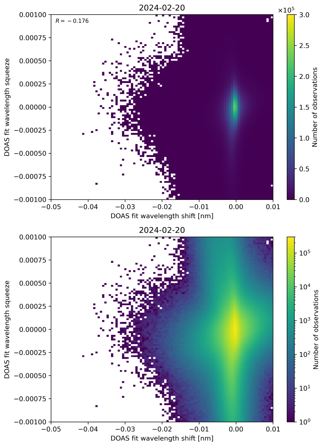
Figure 127: Scatter density plot of “DOAS fit wavelength shift” against “DOAS fit wavelength squeeze” for 2024-02-19 to 2024-02-21.
