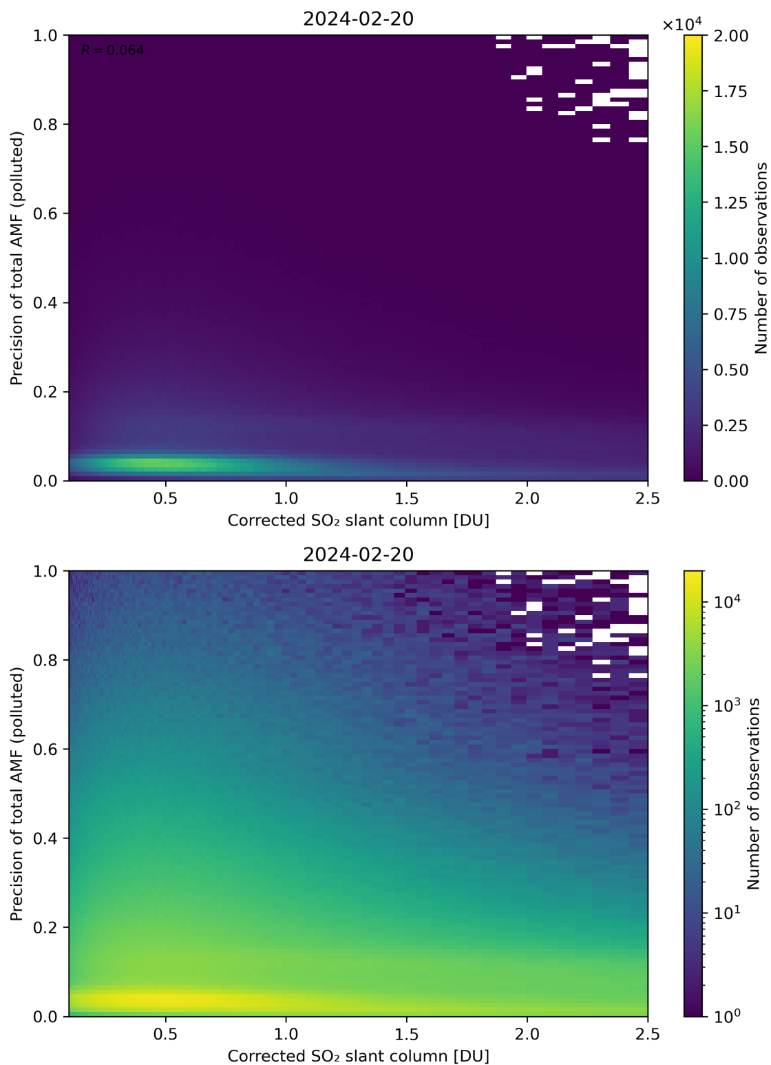
Figure 193: Scatter density plot of “Corrected SO 2 slant column” against “Precision of total AMF (polluted)” for 2024-02-19 to 2024-02-21.
