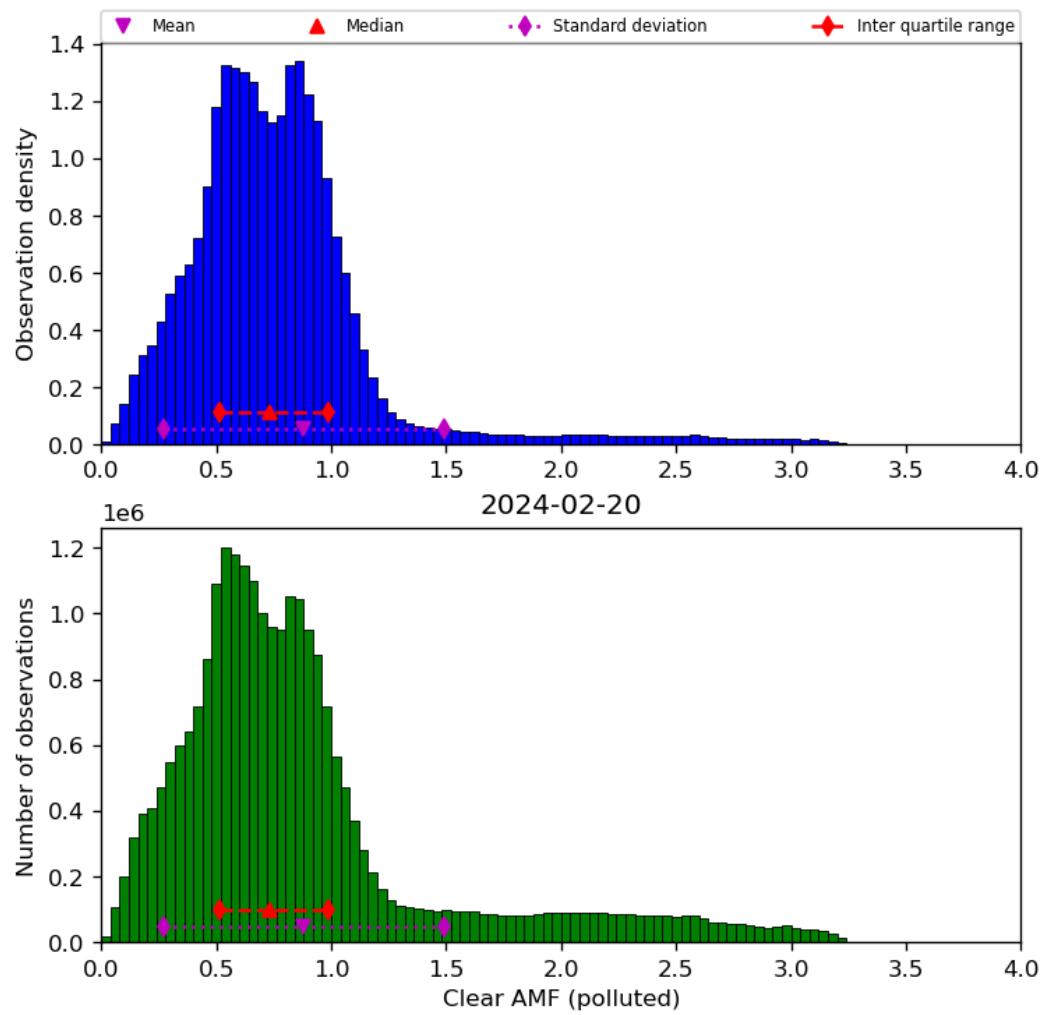
Figure 73: Histogram of “Clear AMF (polluted)” for 2024-02-19 to 2024-02-21
