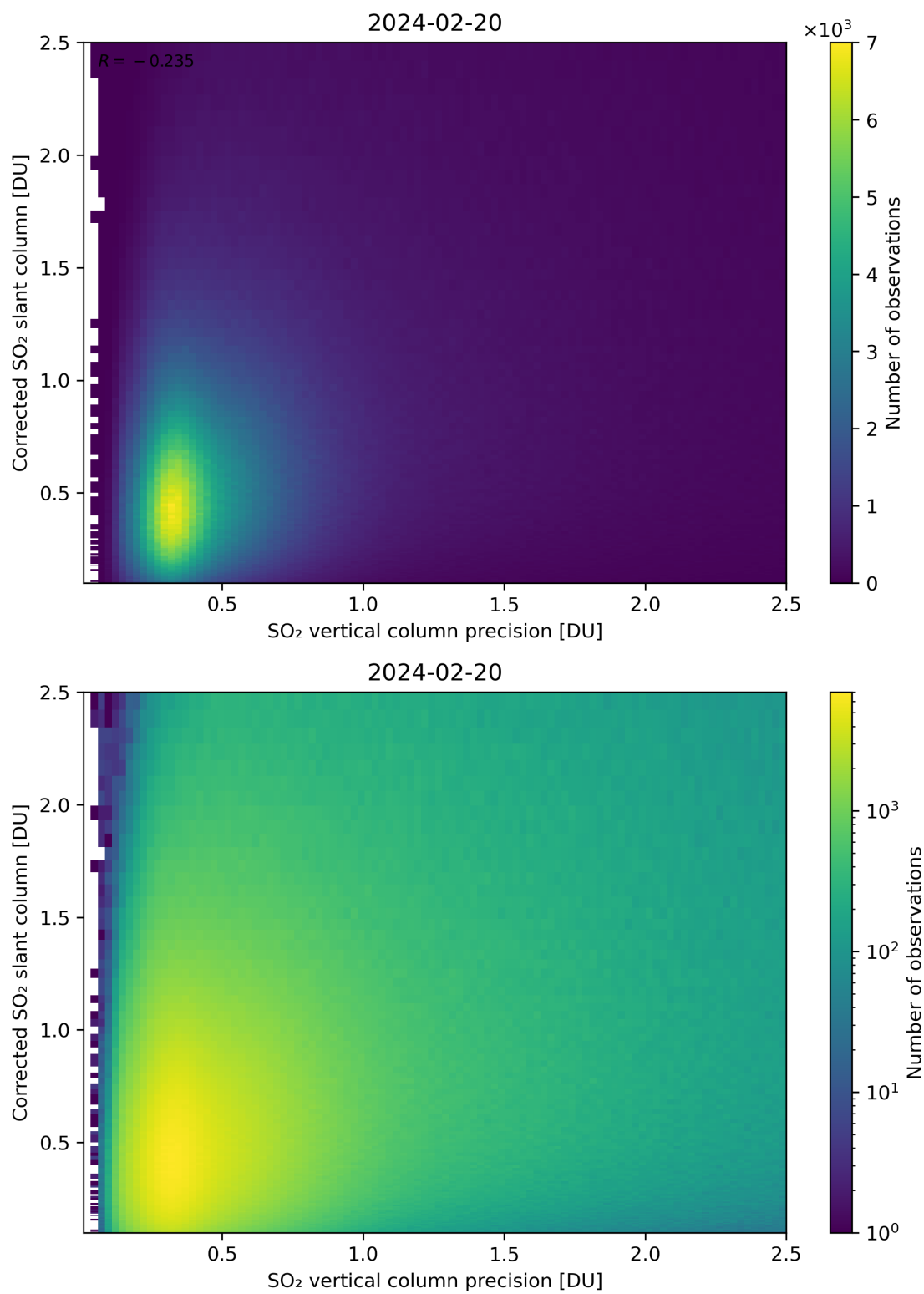
Figure 286: Scatter density plot of “SO 2 vertical column precision” against “Corrected SO 2 slant column” for 2024-02-19 to 2024-02-21.
