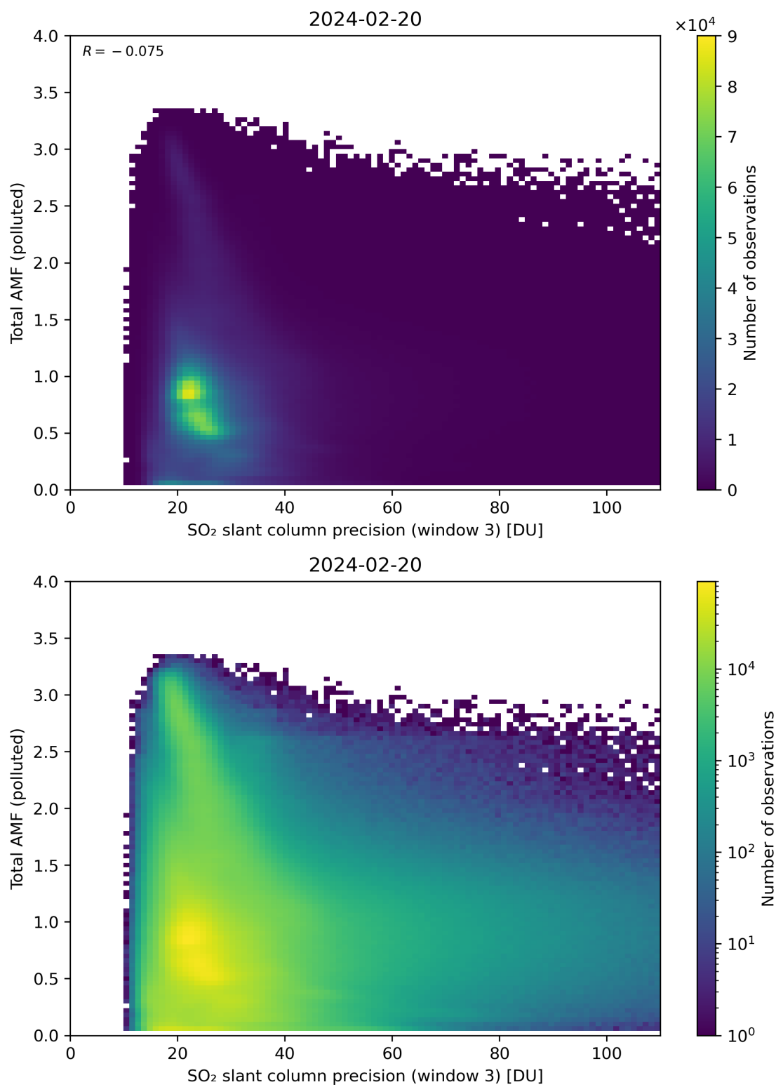
Figure 263: Scatter density plot of “SO 2 slant column precision (window 3)” against “Total AMF (polluted)” for 2024-02-19 to 2024-02-21.
