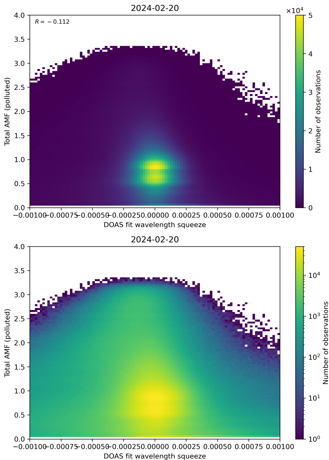
Figure 134: Scatter density plot of “DOAS fit wavelength squeeze” against “Total AMF (polluted)” for 2024-02-19 to 2024-02-21.
