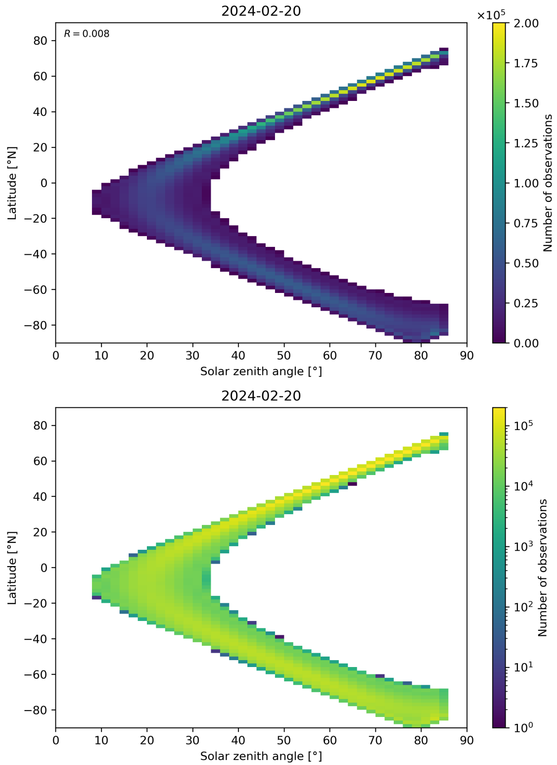
Figure 164: Scatter density plot of “Solar zenith angle” against “Latitude” for 2024-02-19 to 2024-02-21.
