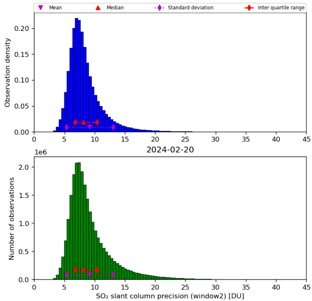
Figure 61: Histogram of “SO 2 slant column precision (window2)” for 2024-02-19 to 2024-02-21
