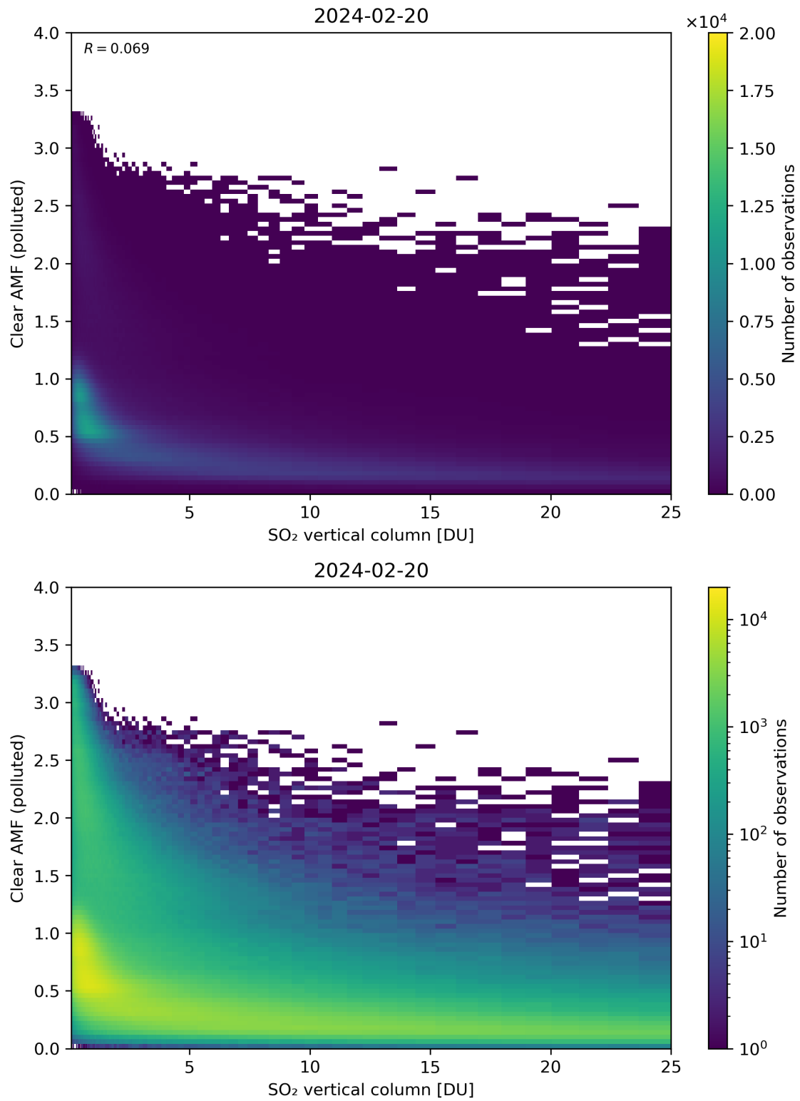
Figure 296: Scatter density plot of “SO 2 vertical column” against “Clear AMF (polluted)” for 2024-02-19 to 2024-02-21.
