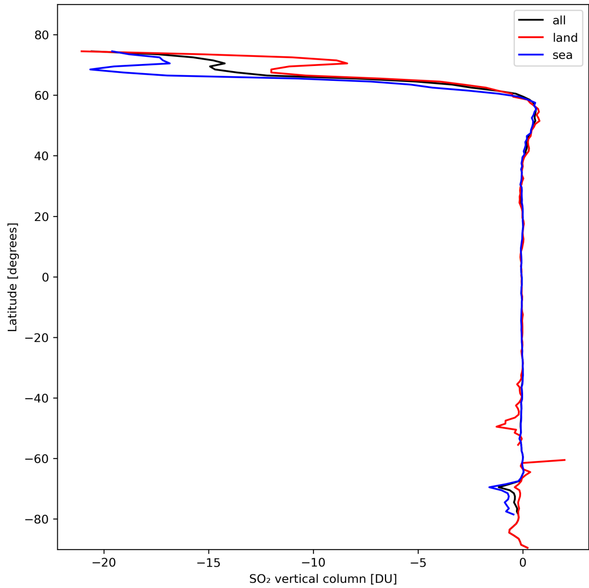
Figure 30: Zonal average of “SO 2 vertical column” for 2024-02-19 to 2024-02-21.
