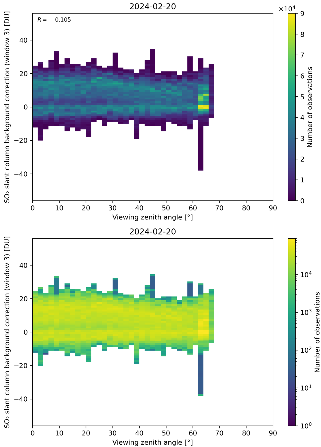
Figure 310: Scatter density plot of “Viewing zenith angle” against “SO 2 slant column background correction (window 3)” for 2024-02-19 to 2024-02-21.
