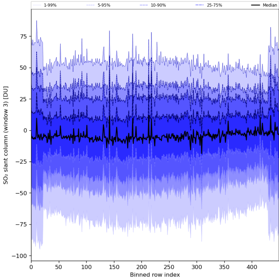
Figure 87: Along track statistics of "SO 2 slant column (window 3)" for 2024-02-19 to 2024-02-21
