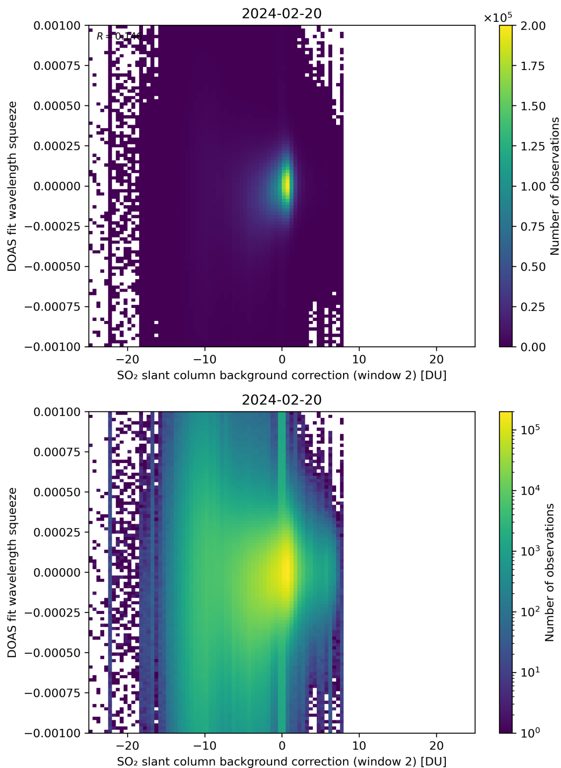
Figure 113: Scatter density plot of “SO 2 slant column background correction (window 2)” against “DOAS fit wavelength squeeze” for 2024-02-19 to 2024-02-21.
