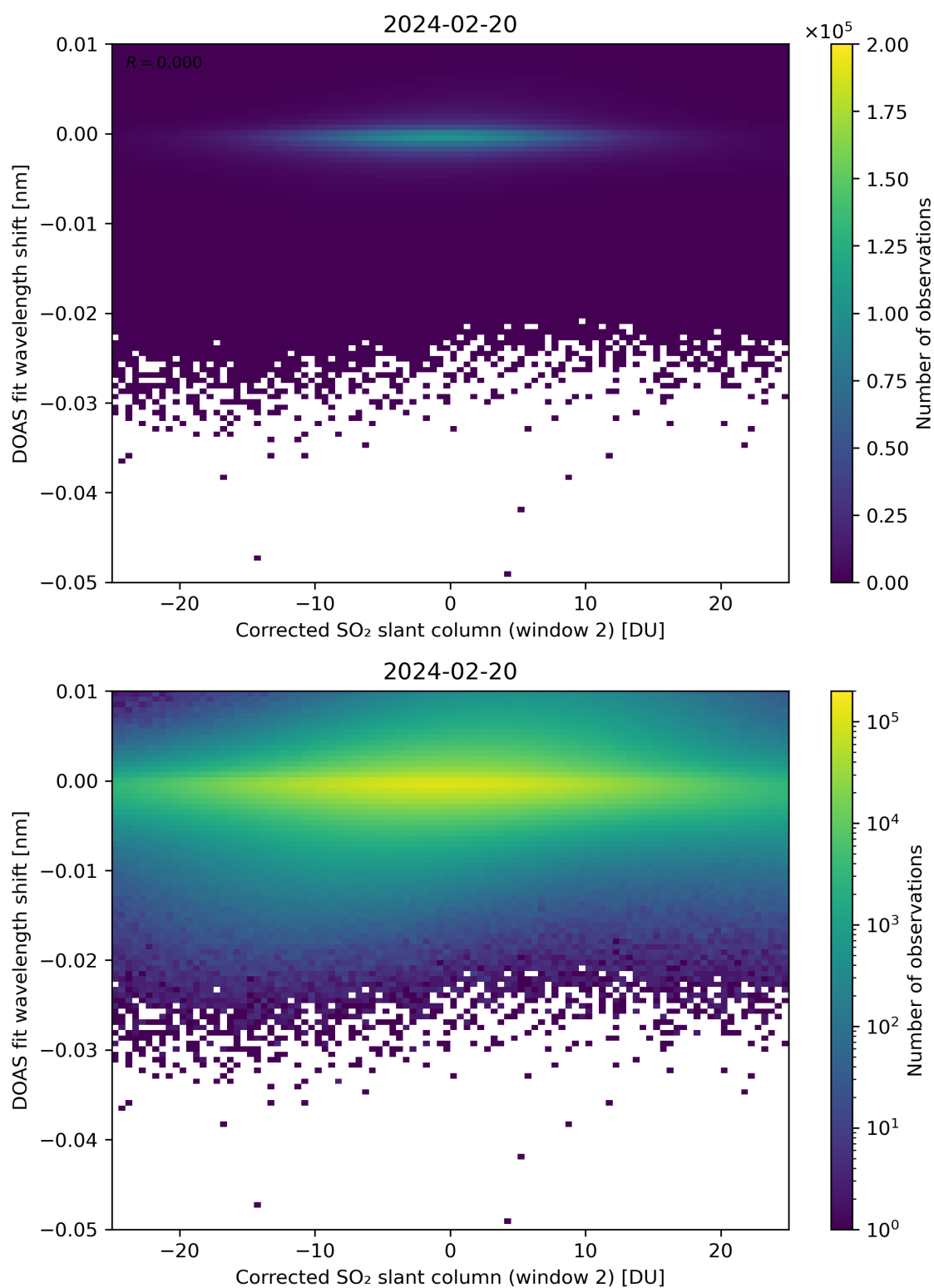
Figure 196: Scatter density plot of “Corrected SO 2 slant column (window 2)” against “DOAS fit wavelength shift” for 2024-02-19 to 2024-02-21.
