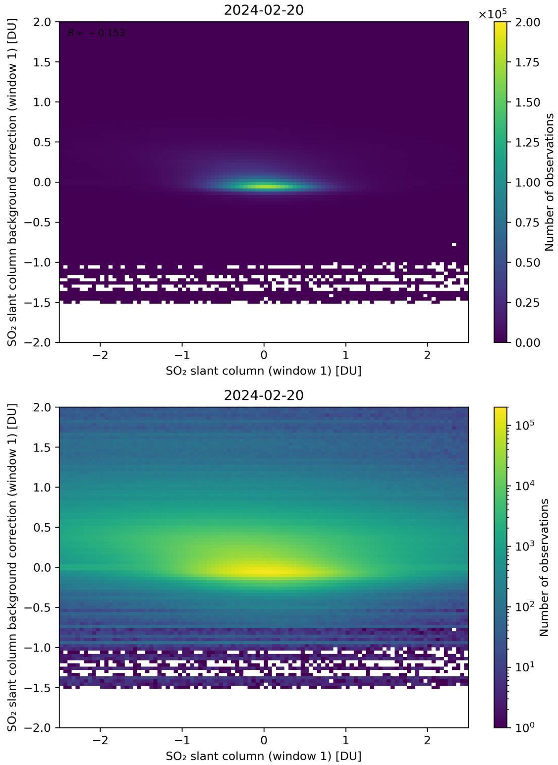
Figure 212: Scatter density plot of “SO 2 slant column (window 1)” against “SO 2 slant column background correction (window 1)” for 2024-02-19 to 2024-02-21.
