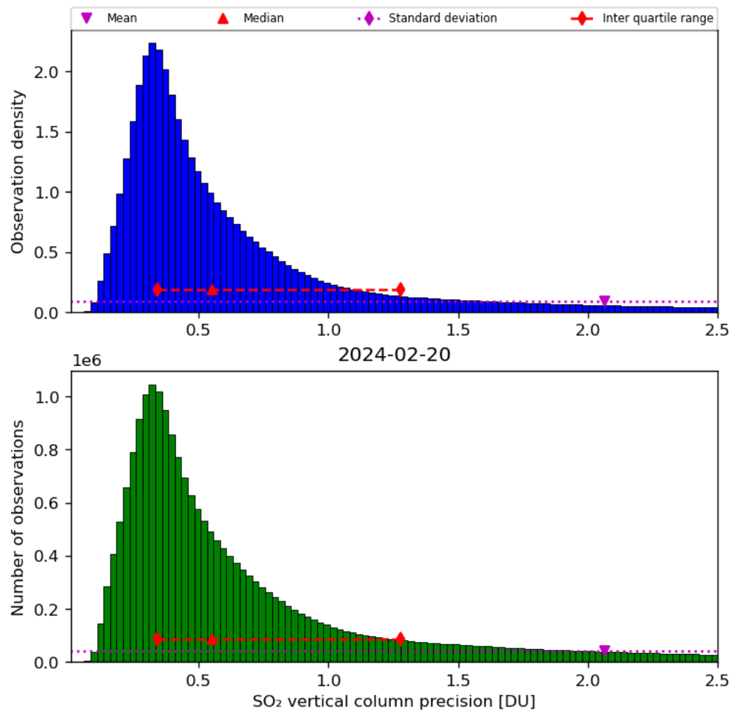
Figure 54: Histogram of “SO 2 vertical column precision” for 2024-02-19 to 2024-02-21
