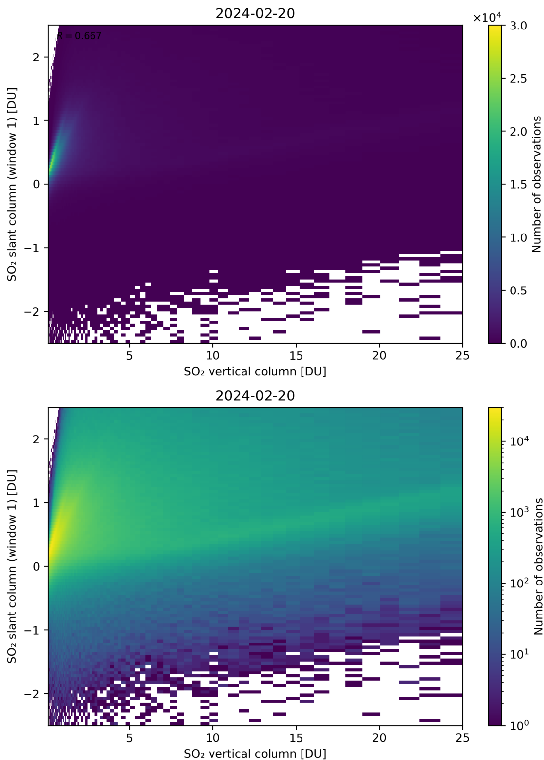
Figure 300: Scatter density plot of “SO 2 vertical column” against “SO 2 slant column (window 1)” for 2024-02-19 to 2024-02-21.
