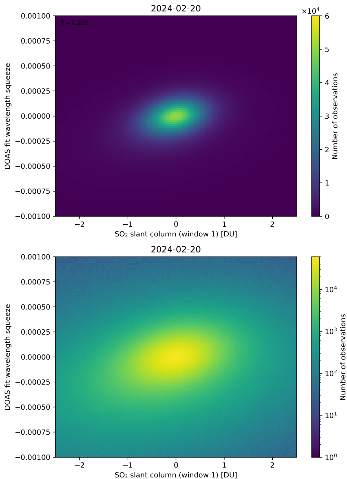
Figure 216: Scatter density plot of “SO 2 slant column (window 1)” against “DOAS fit wavelength squeeze” for 2024-02-19 to 2024-02-21.
