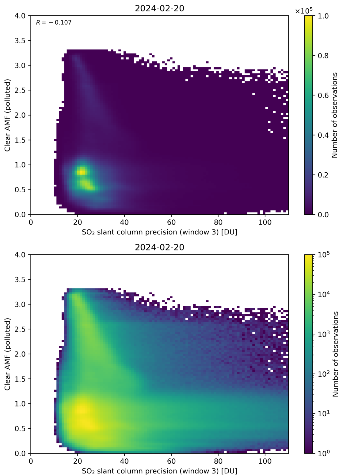
Figure 261: Scatter density plot of “SO 2 slant column precision (window 3)” against “Clear AMF (polluted)” for 2024-02-19 to 2024-02-21.
