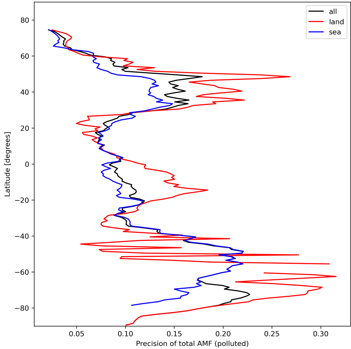
Figure 49: Zonal average of “Precision of total AMF (polluted)” for 2024-02-19 to 2024-02-21.
