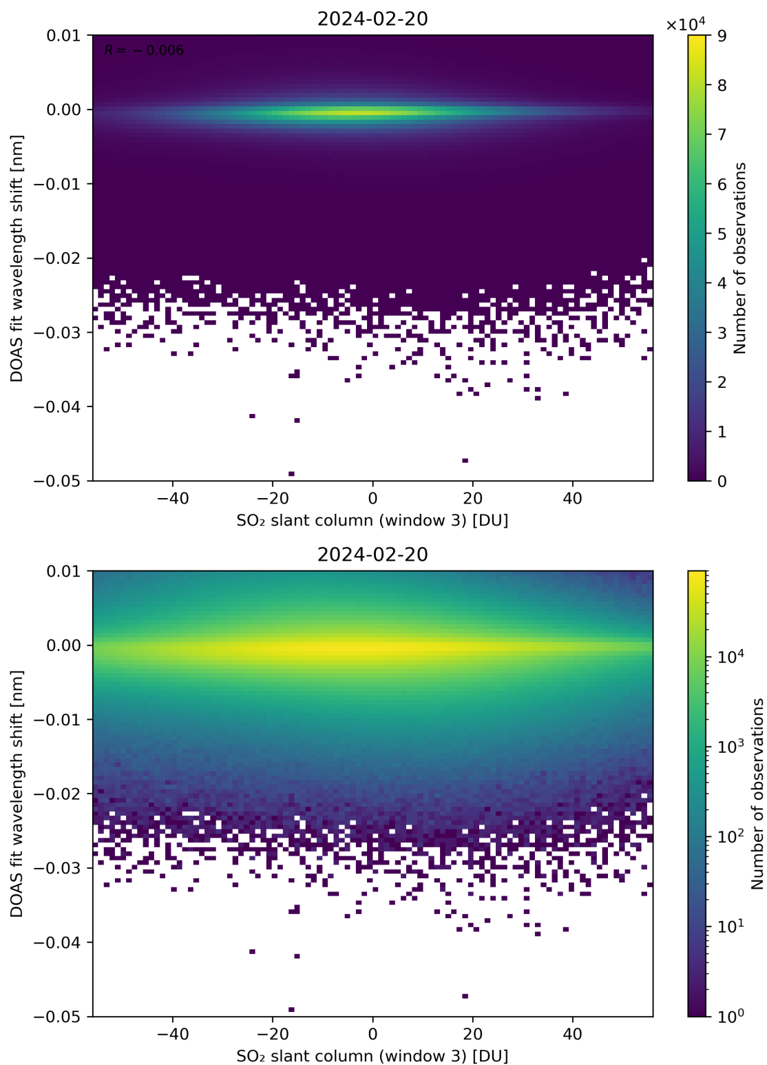
Figure 254: Scatter density plot of “SO 2 slant column (window 3)” against “DOAS fit wavelength shift” for 2024-02-19 to 2024-02-21.
