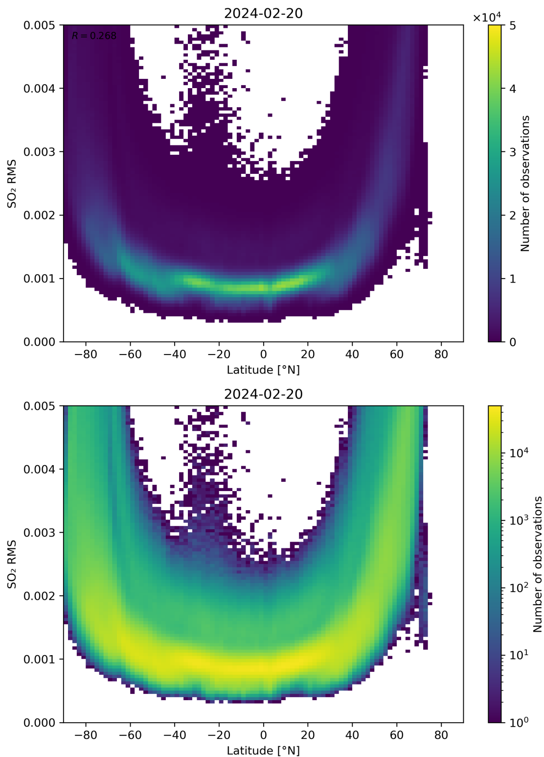
Figure 144: Scatter density plot of “Latitude” against “SO 2 RMS” for 2024-02-19 to 2024-02-21.
