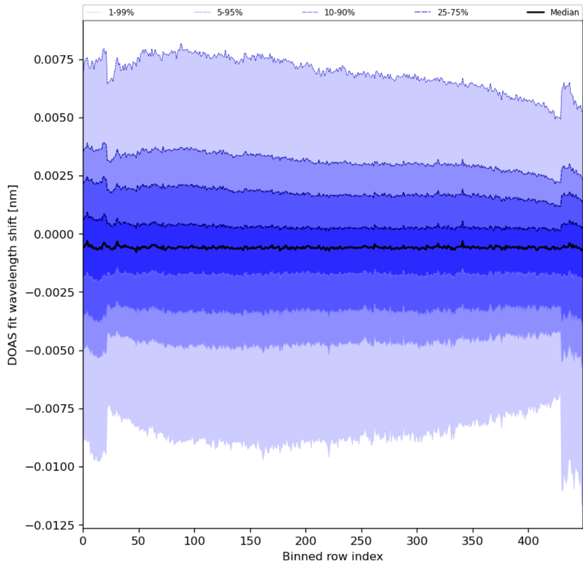
Figure 91: Along track statistics of “DOAS fit wavelength shift” for 2024-02-19 to 2024-02-21
