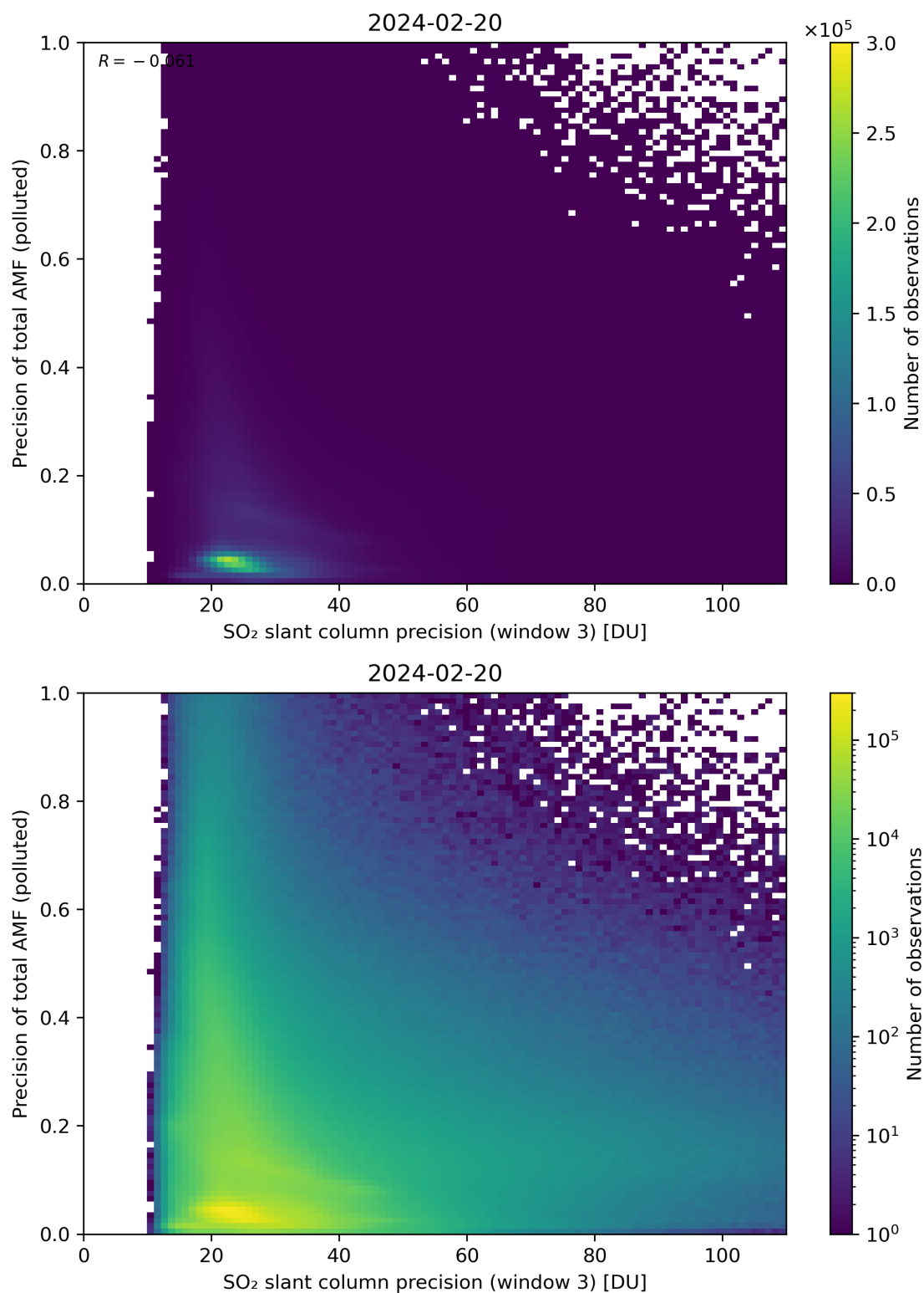
Figure 264: Scatter density plot of “SO 2 slant column precision (window 3)” against “Precision of total AMF (polluted)” for 2024-02-19 to 2024-02-21.
