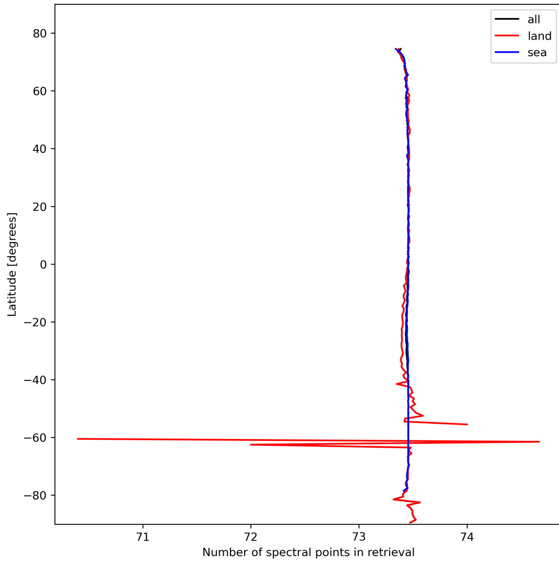
Figure 51: Zonal average of “Number of spectral points in retrieval” for 2024-02-20 to 2024-02-22.
