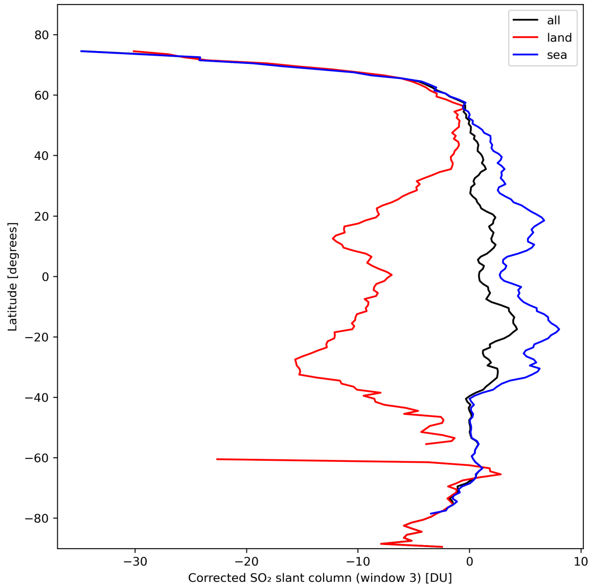
Figure 43: Zonal average of “Corrected SO 2 slant column (window 3)” for 2024-02-20 to 2024-02-22.
