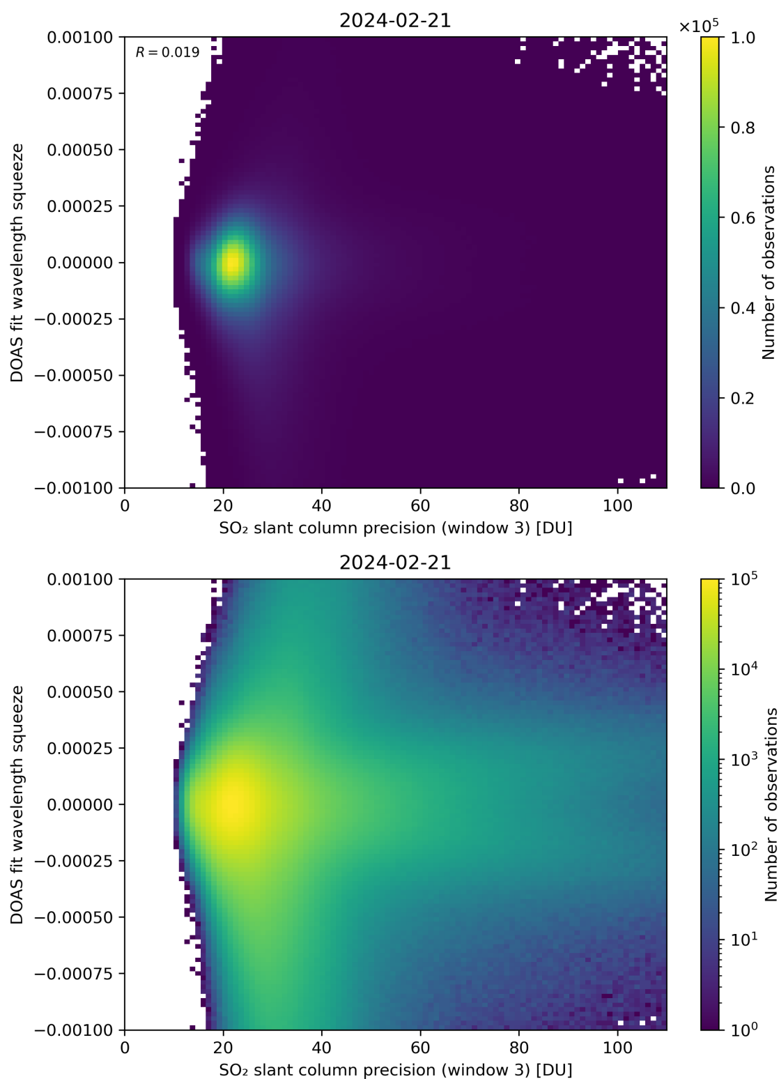
Figure 259: Scatter density plot of “SO 2 slant column precision (window 3)” against “DOAS fit wavelength squeeze” for 2024-02-20 to 2024-02-22.
