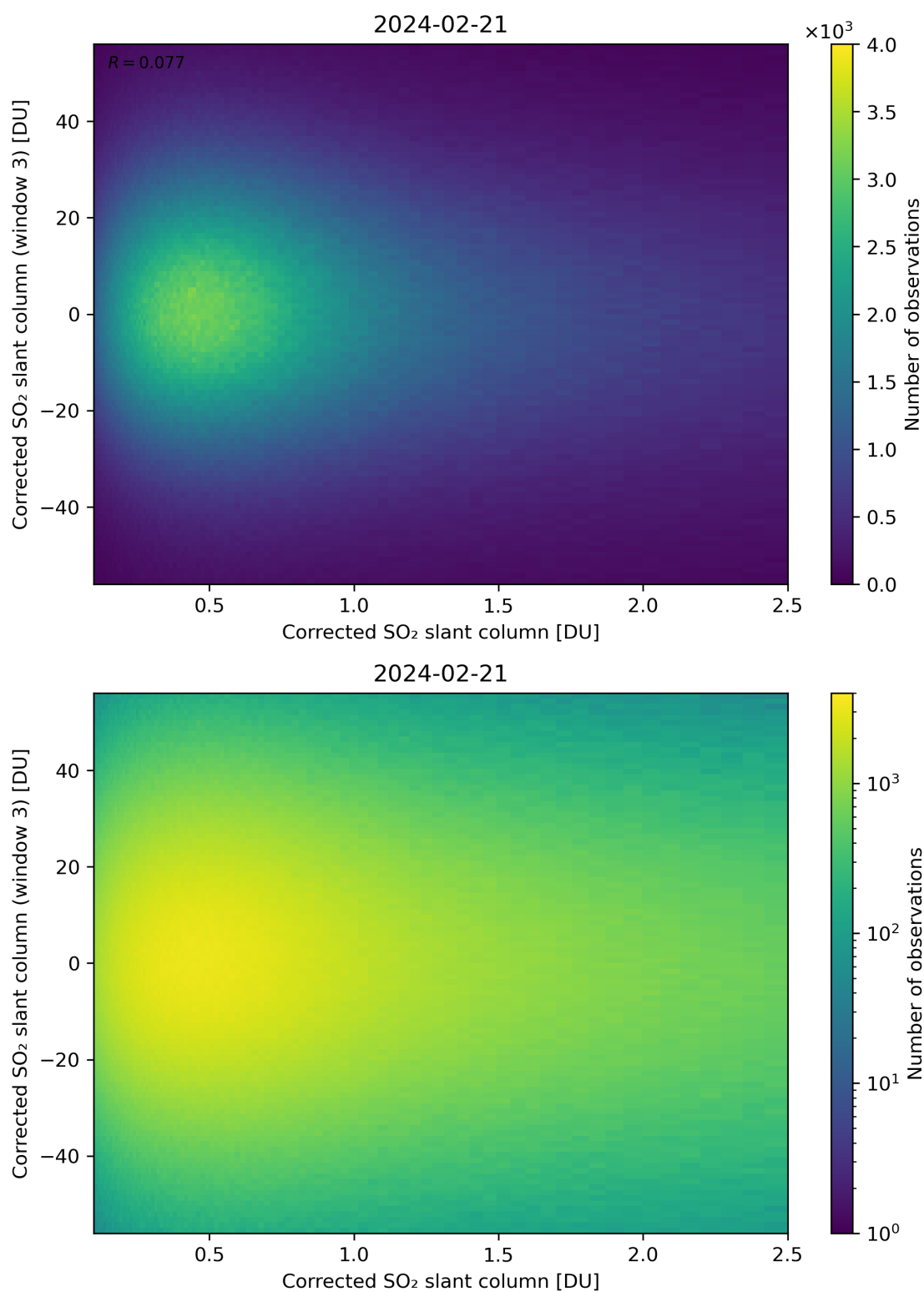
Figure 186: Scatter density plot of “Corrected SO 2 slant column” against “Corrected SO 2 slant column (window 3)” for 2024-02-20 to 2024-02-22.
