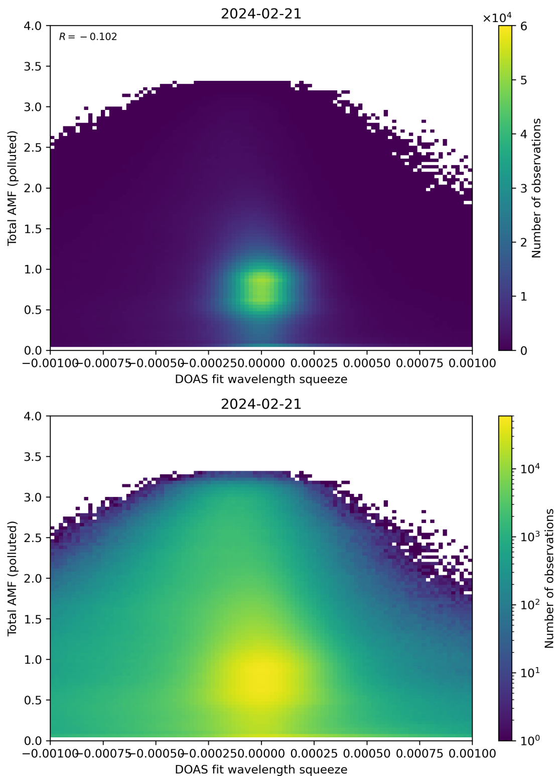
Figure 134: Scatter density plot of “DOAS fit wavelength squeeze” against “Total AMF (polluted)” for 2024-02-20 to 2024-02-22.
