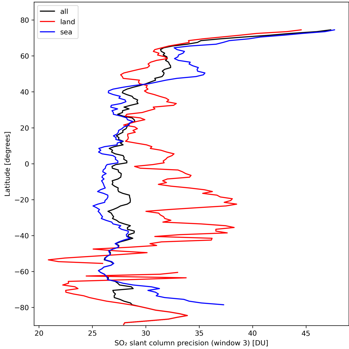
Figure 42: Zonal average of “SO 2 slant column precision (window 3)” for 2024-02-20 to 2024-02-22.
