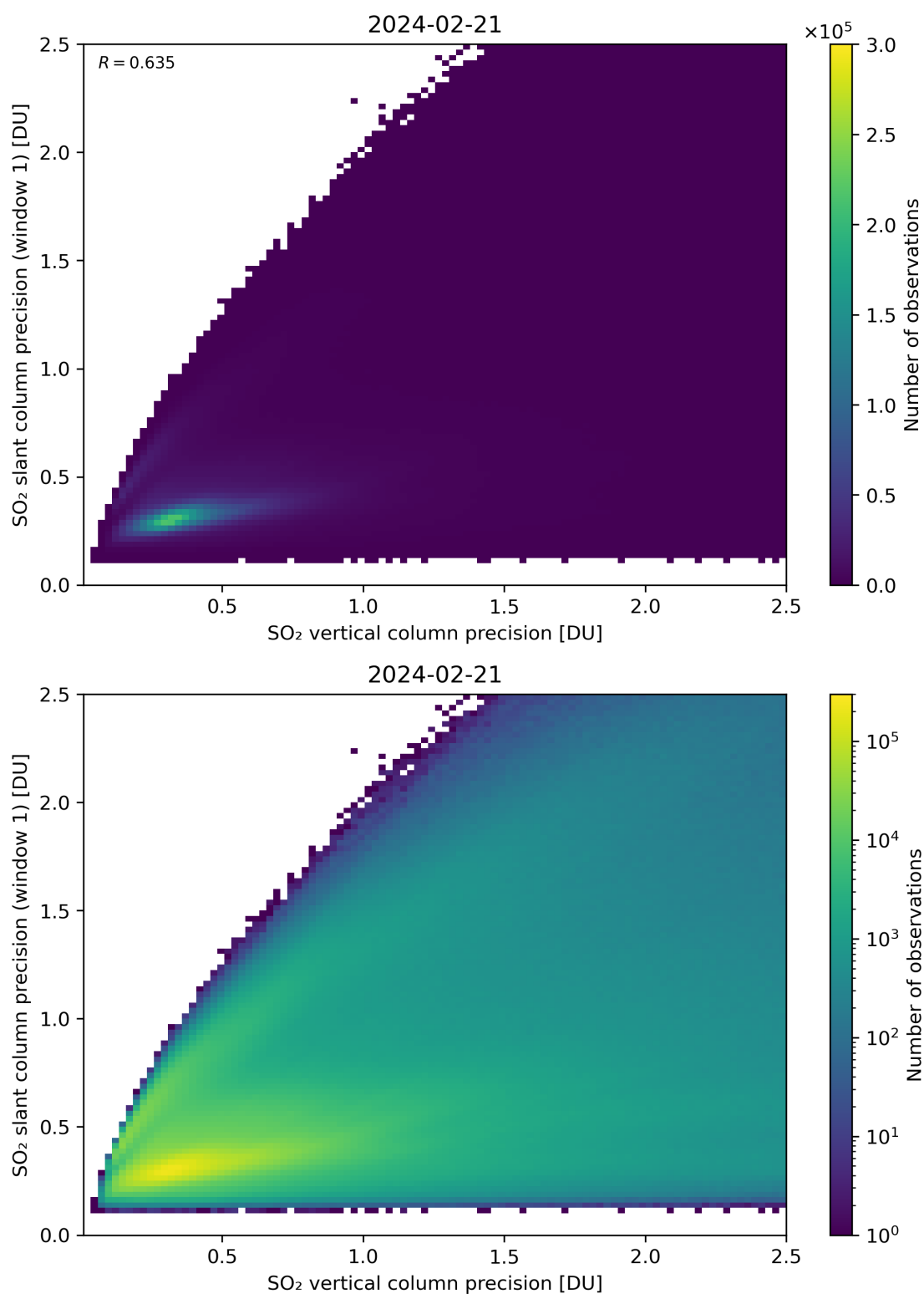
Figure 290: Scatter density plot of “SO 2 vertical column precision” against “SO 2 slant column precision (window 1)” for 2024-02-20 to 2024-02-22.
