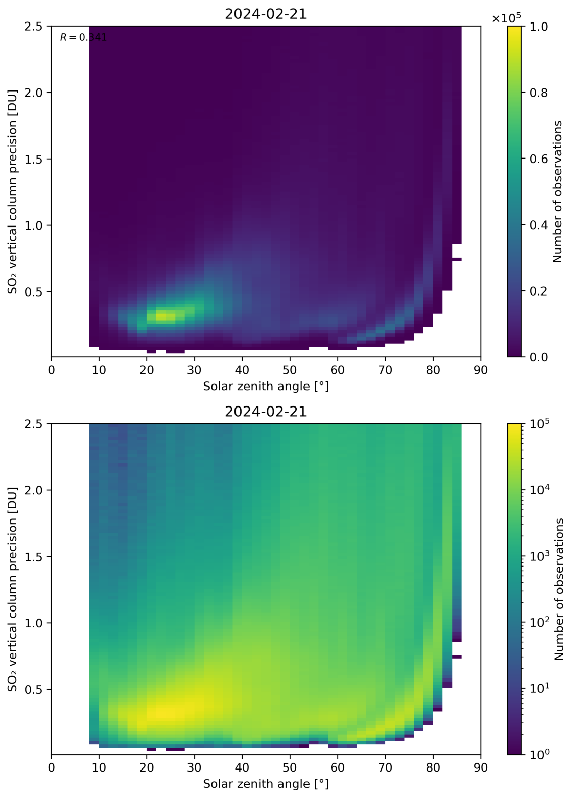
Figure 177: Scatter density plot of “Solar zenith angle” against “SO 2 vertical column precision” for 2024-02-20 to 2024-02-22.
