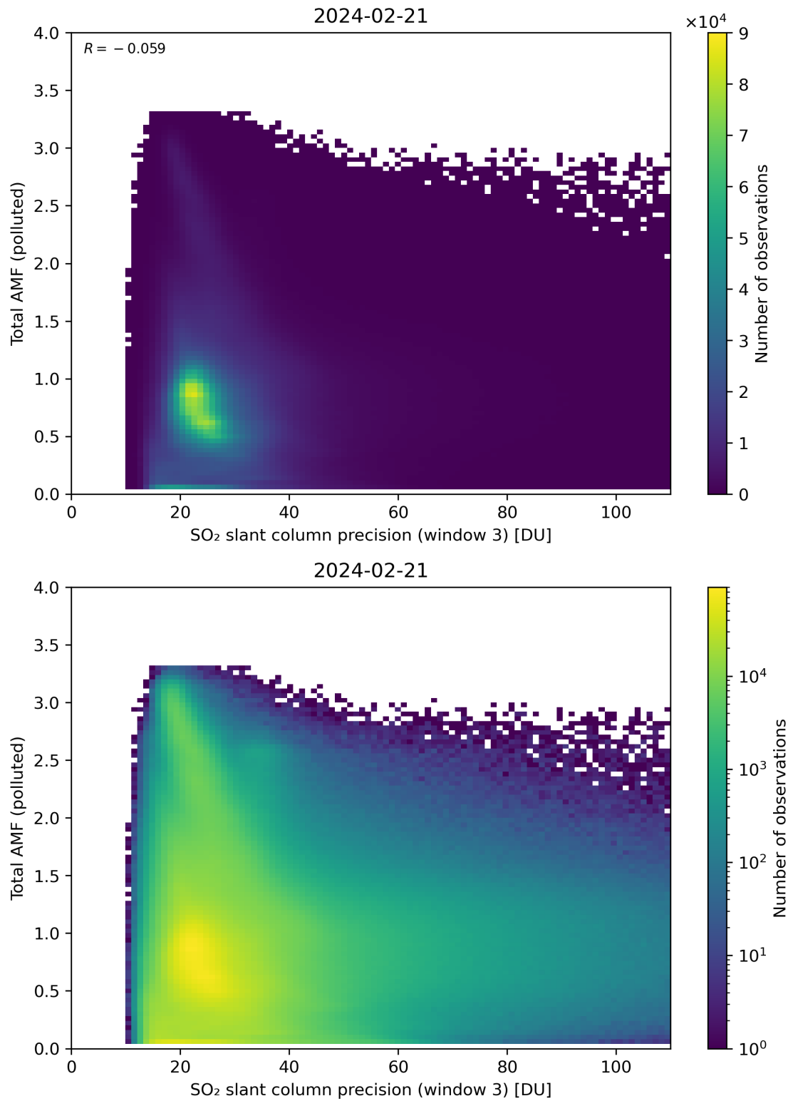
Figure 263: Scatter density plot of “SO 2 slant column precision (window 3)” against “Total AMF (polluted)” for 2024-02-20 to 2024-02-22.
