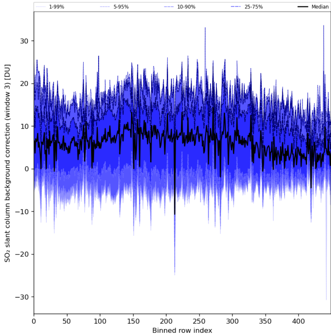
Figure 90: Along track statistics of “SO 2 slant column background correction (window 3)” for 2024-02-20 to 2024-02-22
