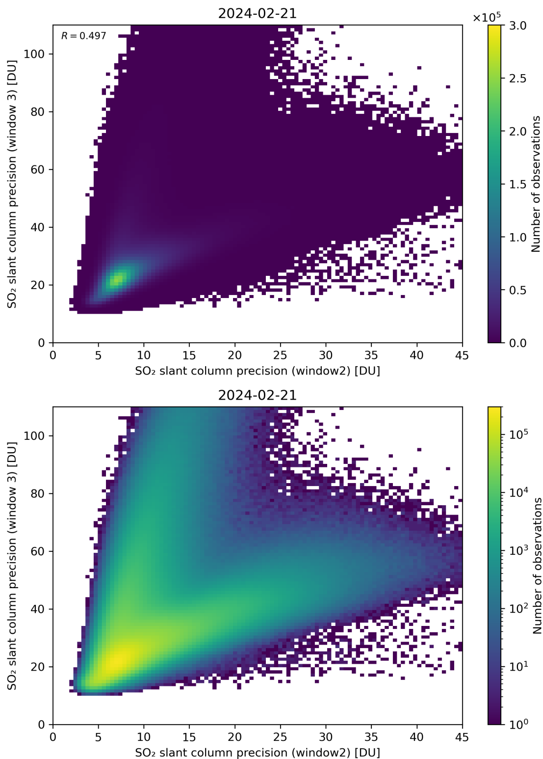
Figure 250: Scatter density plot of “SO 2 slant column precision (window2)” against “SO 2 slant column precision (window 3)” for 2024-02-20 to 2024-02-22.
