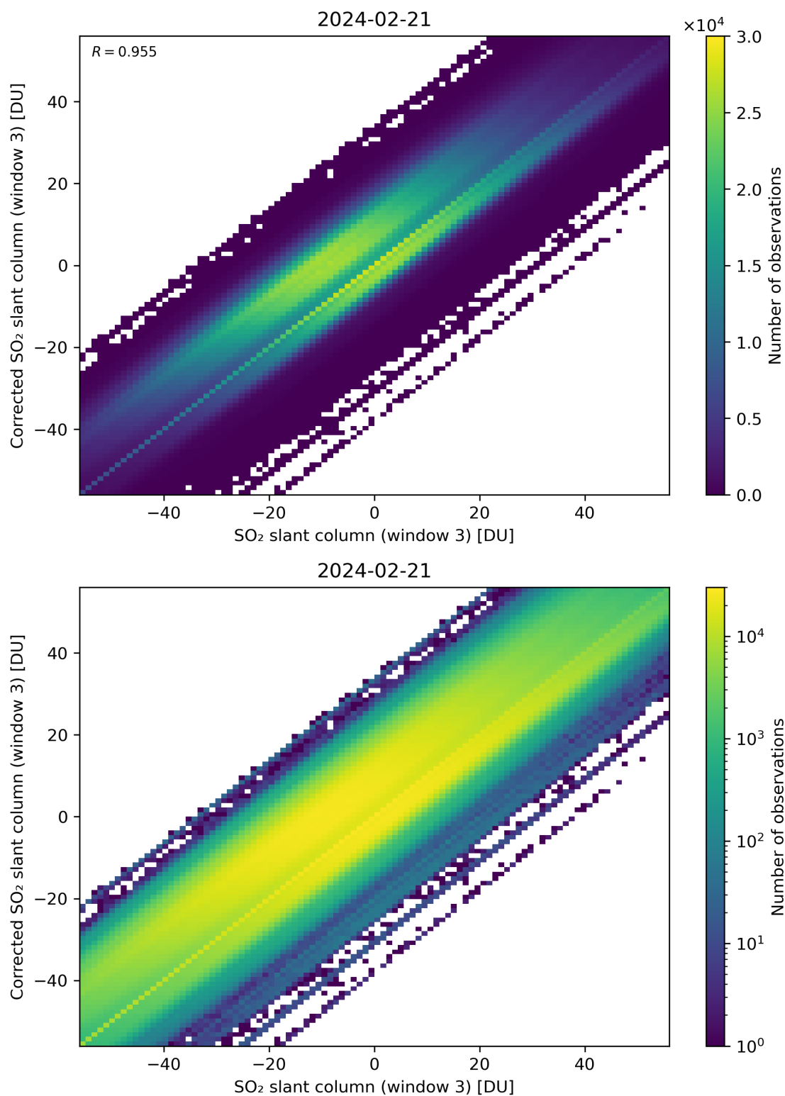
Figure 266: Scatter density plot of “SO 2 slant column (window 3)” against “Corrected SO 2 slant column (window 3)” for 2024-02-20 to 2024-02-22.
