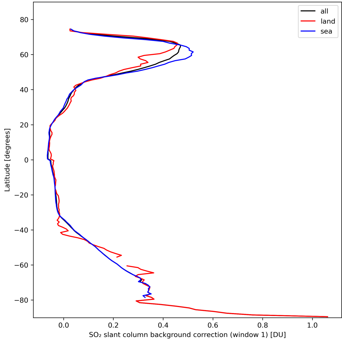
Figure 36: Zonal average of “SO 2 slant column background correction (window 1)” for 2024-02-20 to 2024-02-22.
