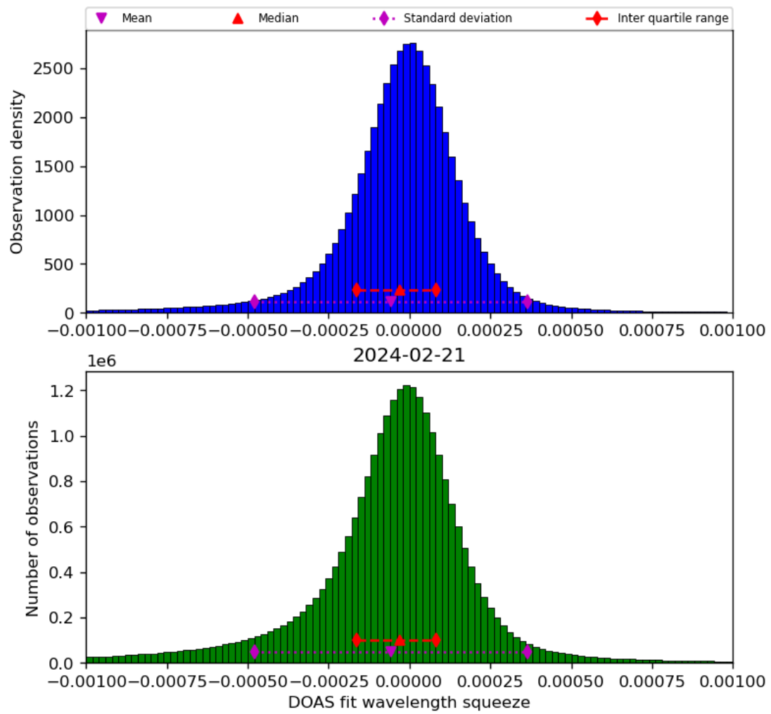
Figure 69: Histogram of “DOAS fit wavelength squeeze” for 2024-02-20 to 2024-02-22
