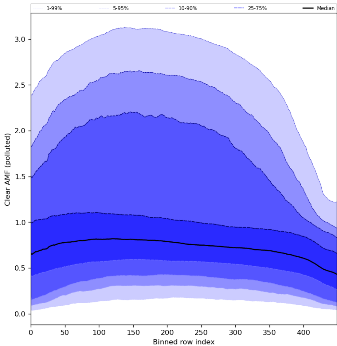
Figure 96: Along track statistics of “Clear AMF (polluted)” for 2024-02-20 to 2024-02-22
