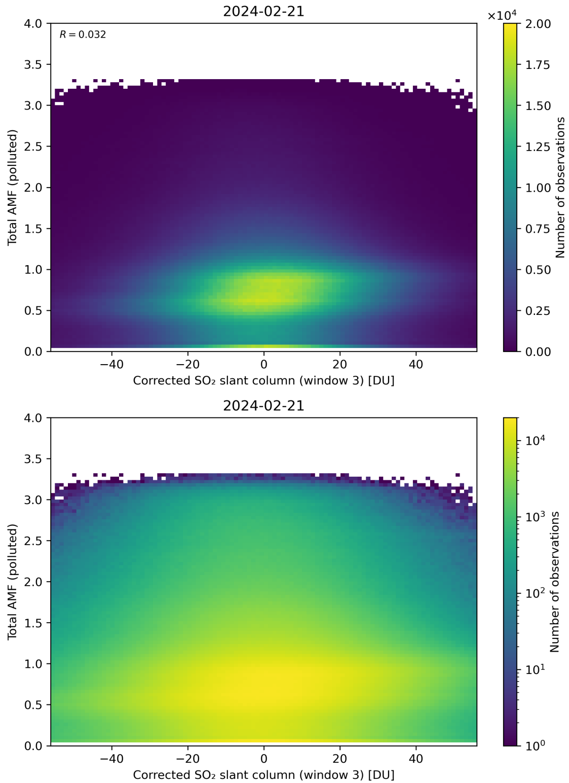
Figure 210: Scatter density plot of “Corrected SO 2 slant column (window 3)” against “Total AMF (polluted)” for 2024-02-20 to 2024-02-22.
