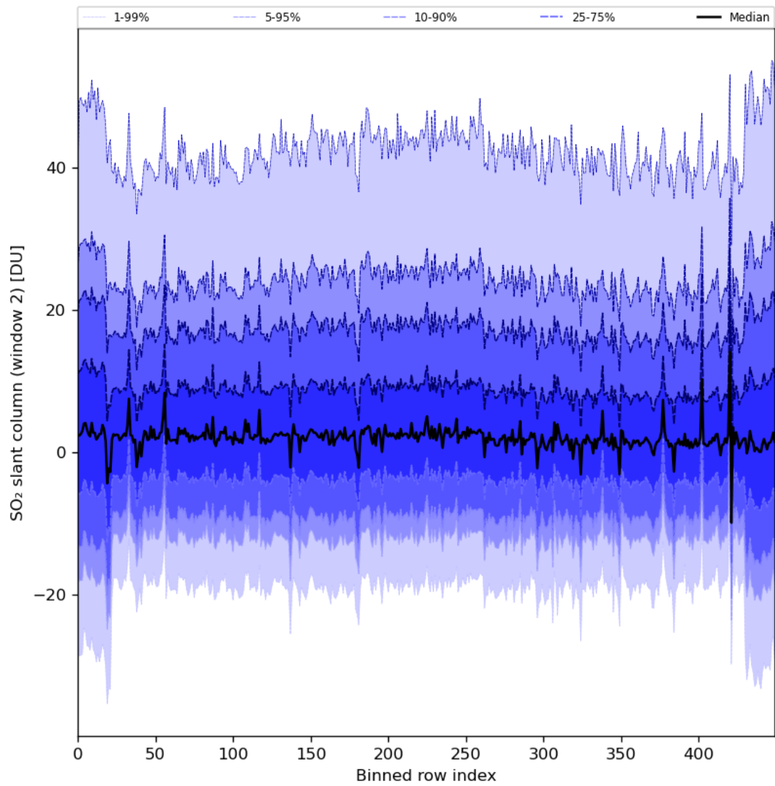
Figure 83: Along track statistics of “SO 2 slant column (window 2)” for 2024-02-20 to 2024-02-22
