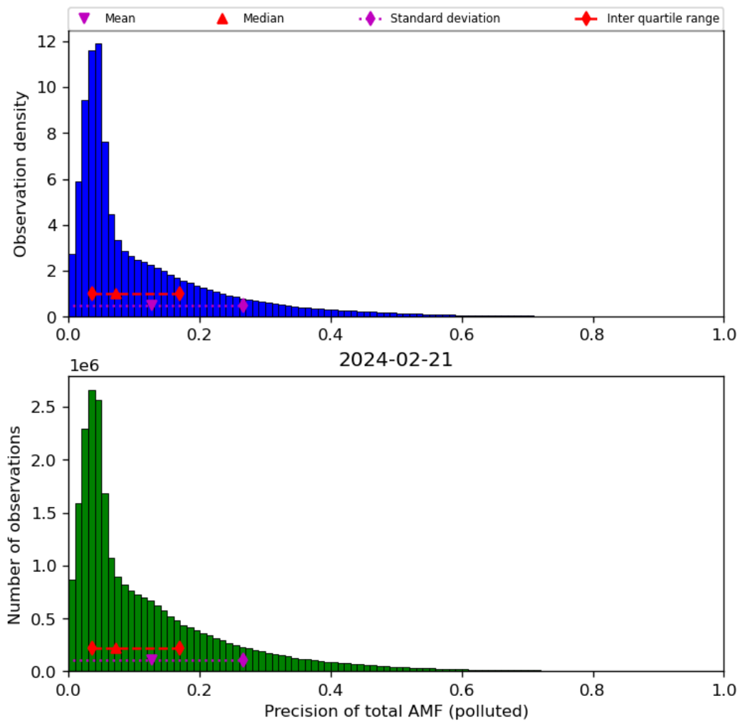
Figure 72: Histogram of “Precision of total AMF (polluted)” for 2024-02-20 to 2024-02-22
