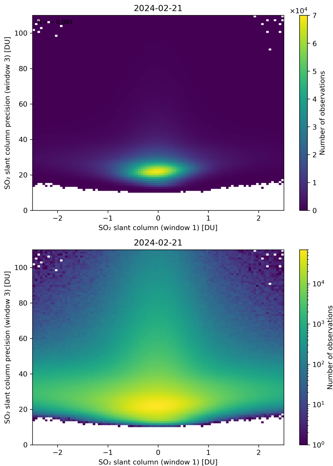
Figure 238: Scatter density plot of “SO 2 slant column (window 1)” against “SO 2 slant column precision (window 3)” for 2024-02-20 to 2024-02-22.
