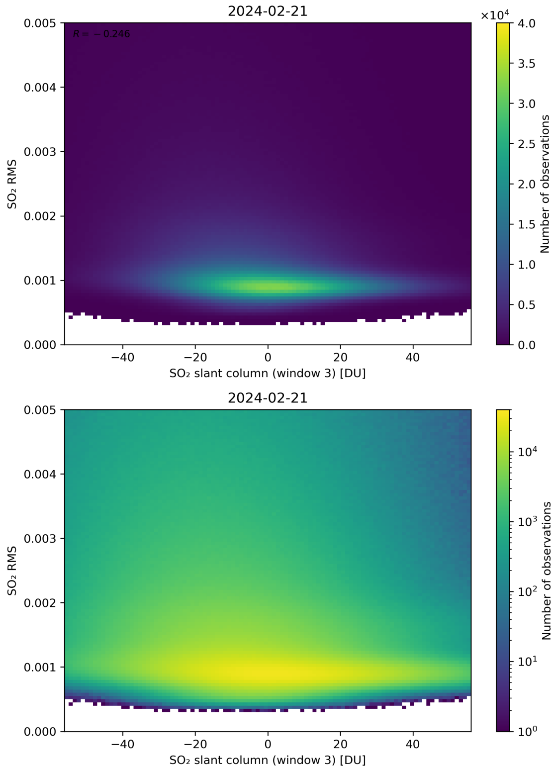
Figure 256: Scatter density plot of “SO 2 slant column (window 3)” against “SO 2 RMS” for 2024-02-20 to 2024-02-22.
