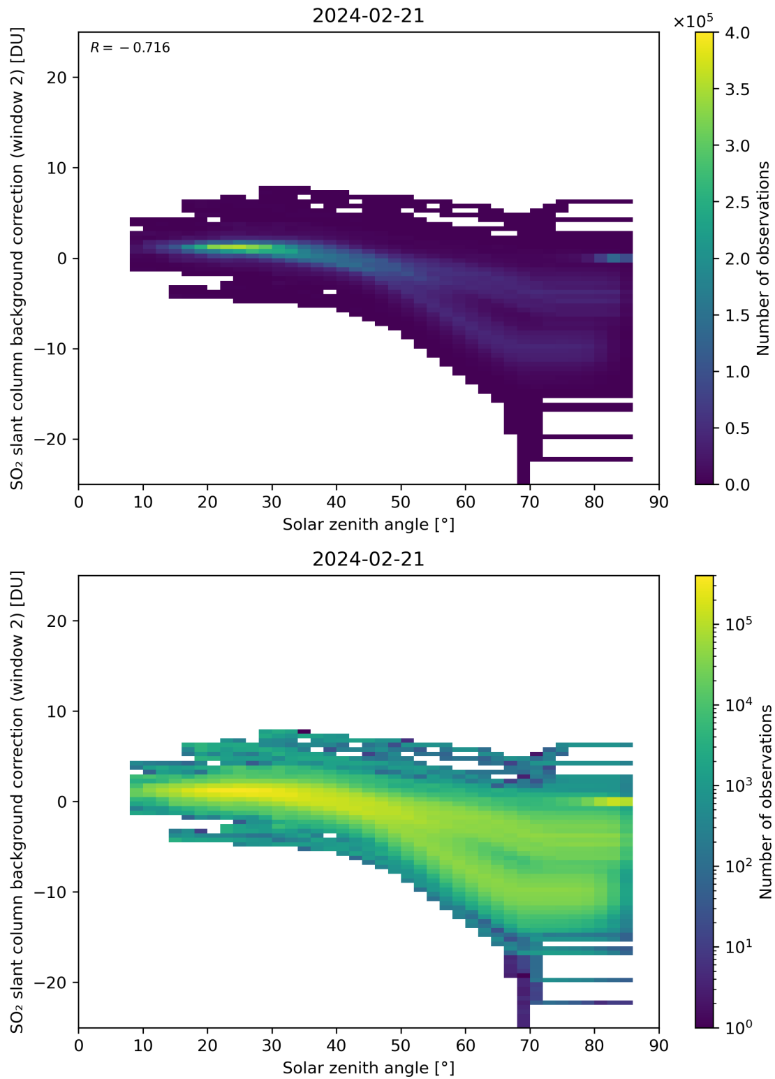
Figure 159: Scatter density plot of “Solar zenith angle” against “SO 2 slant column background correction (window 2)” for 2024-02-20 to 2024-02-22.
