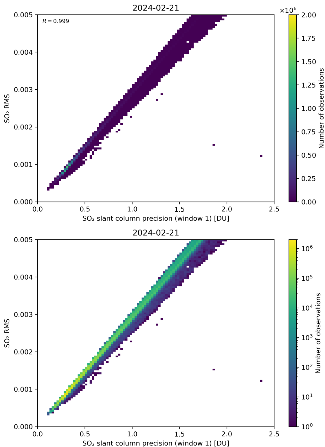
Figure 223: Scatter density plot of “SO 2 slant column precision (window 1)” against “SO 2 RMS” for 2024-02-20 to 2024-02-22.
