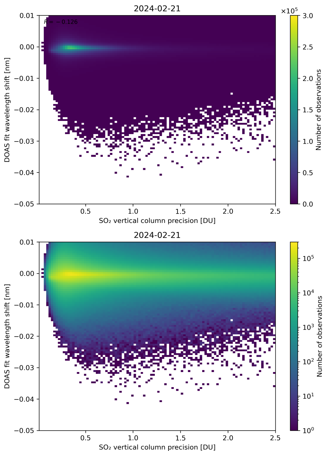
Figure 282: Scatter density plot of “SO 2 vertical column precision” against “DOAS fit wavelength shift” for 2024-02-20 to 2024-02-22.
