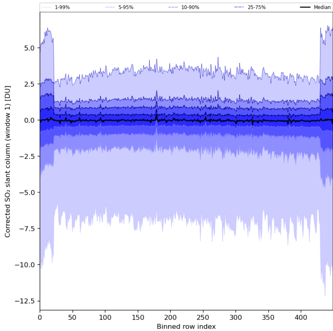
Figure 81: Along track statistics of "Corrected SO 2 slant column (window 1)" for 2024-02-20 to 2024-02-22
