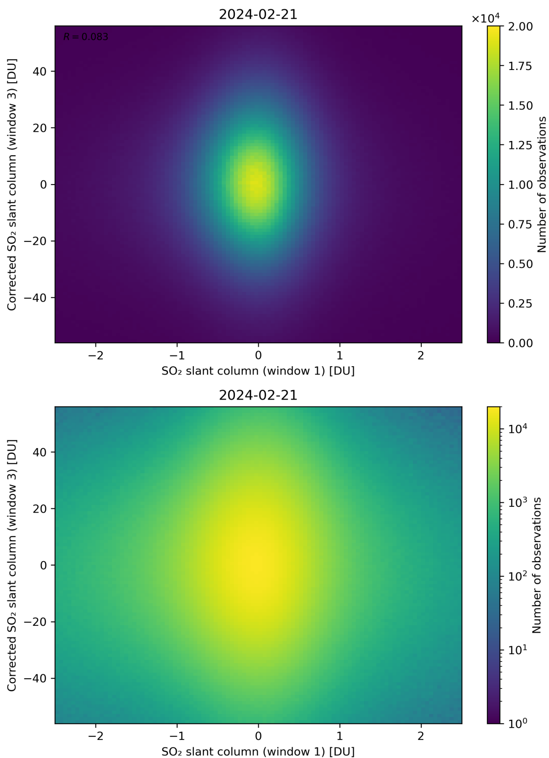
Figure 234: Scatter density plot of “SO 2 slant column (window 1)” against “Corrected SO 2 slant column (window 3)” for 2024-02-20 to 2024-02-22.
