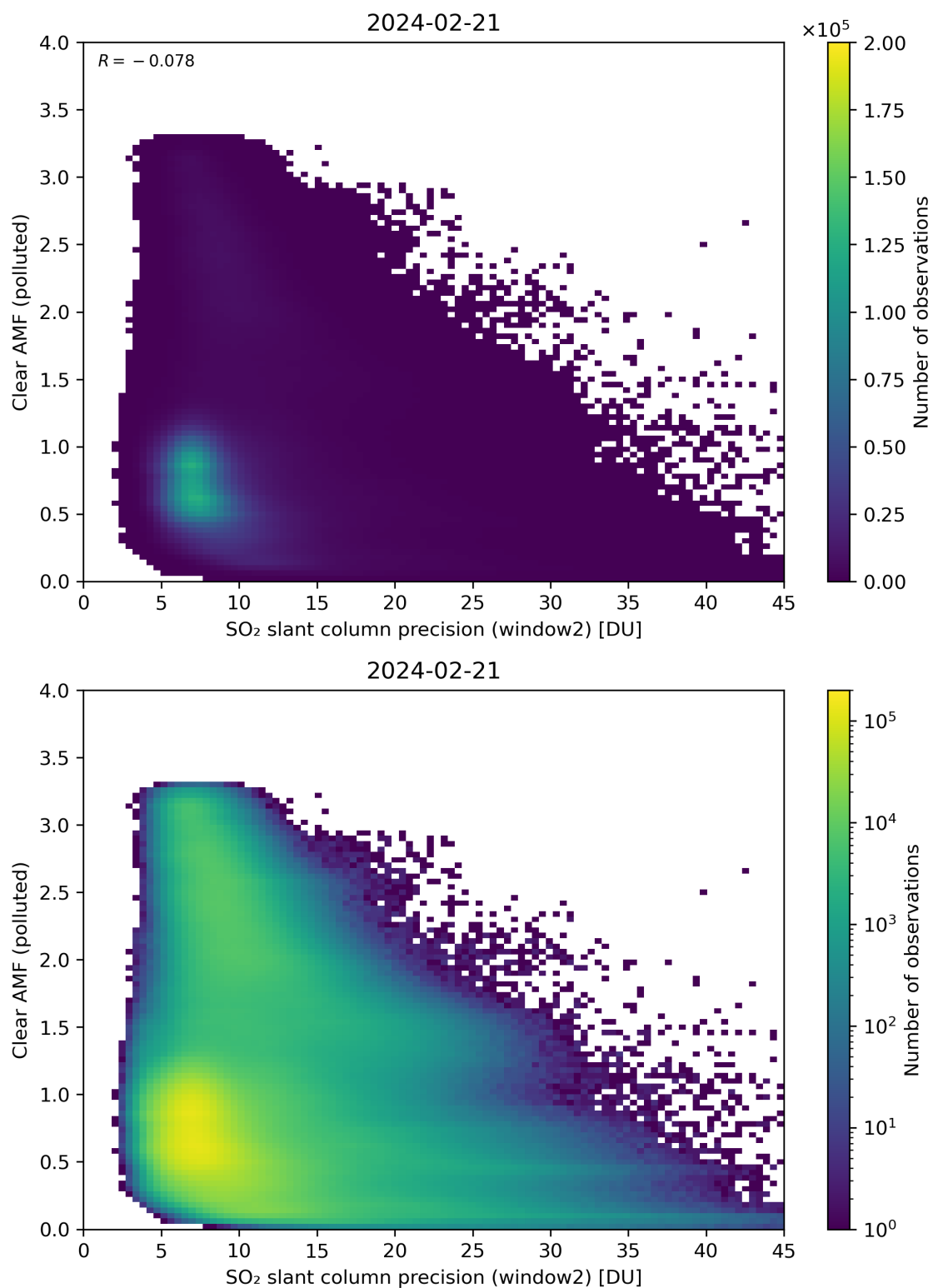
Figure 246: Scatter density plot of “SO 2 slant column precision (window2)” against “Clear AMF (polluted)” for 2024-02-20 to 2024-02-22.
