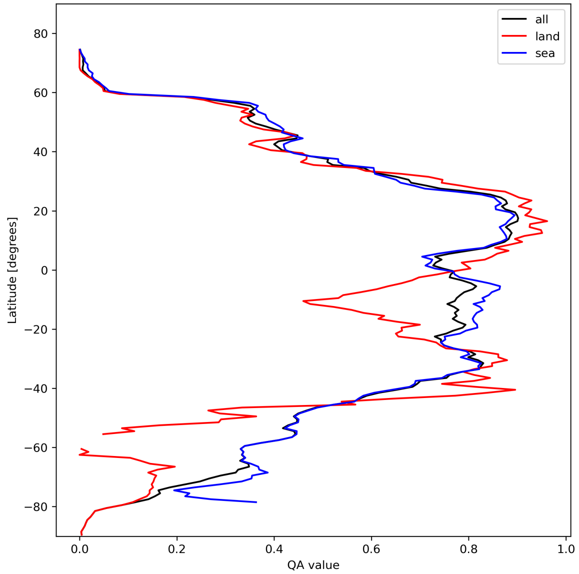
Figure 29: Zonal average of “QA value” for 2024-02-20 to 2024-02-22.
