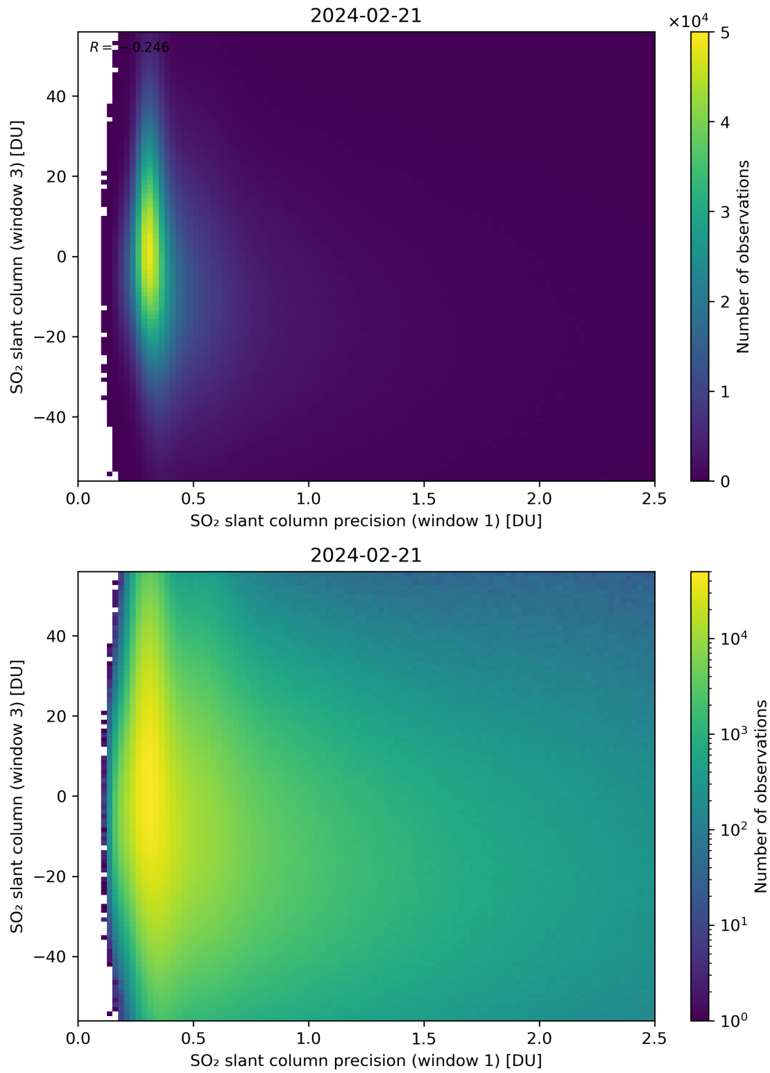
Figure 228: Scatter density plot of “SO 2 slant column precision (window 1)” against “SO 2 slant column (window 3)” for 2024-02-20 to 2024-02-22.
