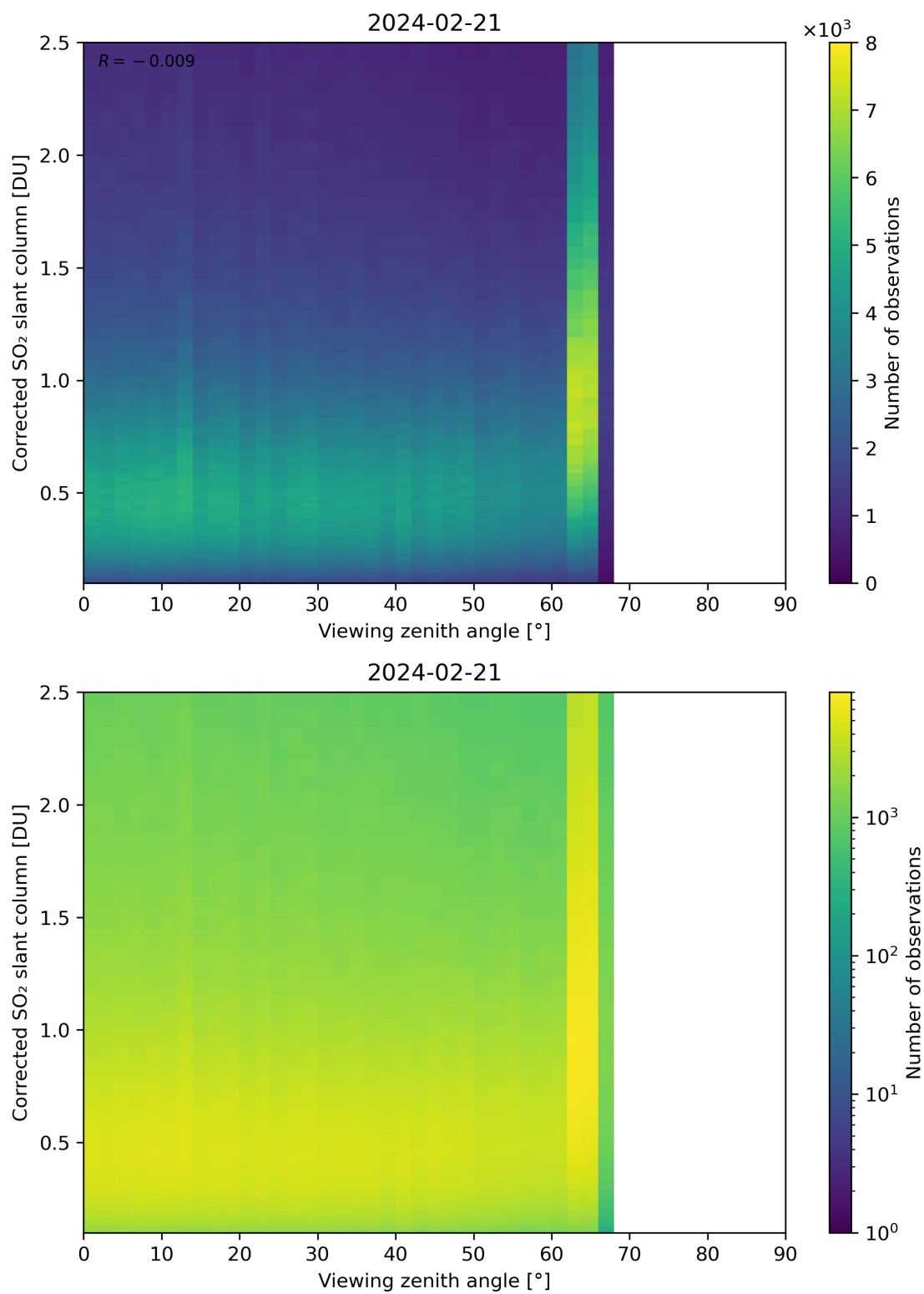
Figure 317: Scatter density plot of “Viewing zenith angle” against “Corrected SO 2 slant column” for 2024-02-20 to 2024-02-22.
