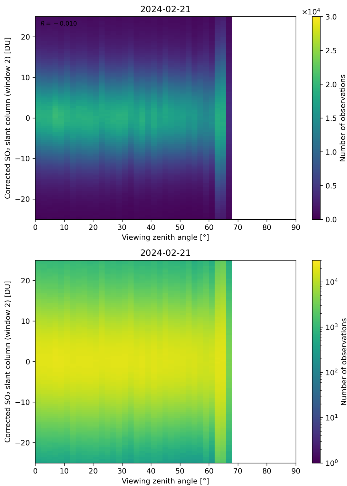
Figure 318: Scatter density plot of “Viewing zenith angle” against “Corrected SO 2 slant column (window 2)” for 2024-02-20 to 2024-02-22.
