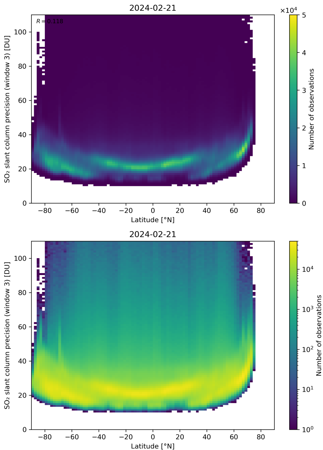
Figure 153: Scatter density plot of “Latitude” against “SO 2 slant column precision (window 3)” for 2024-02-20 to 2024-02-22.
