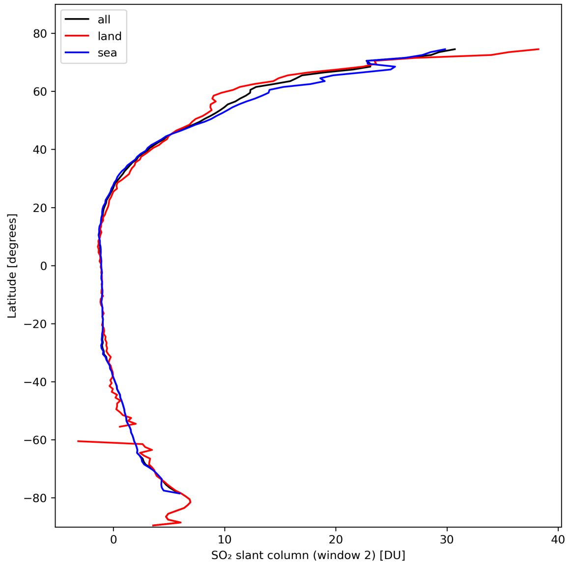
Figure 37: Zonal average of “SO 2 slant column (window 2)” for 2024-02-20 to 2024-02-22.
