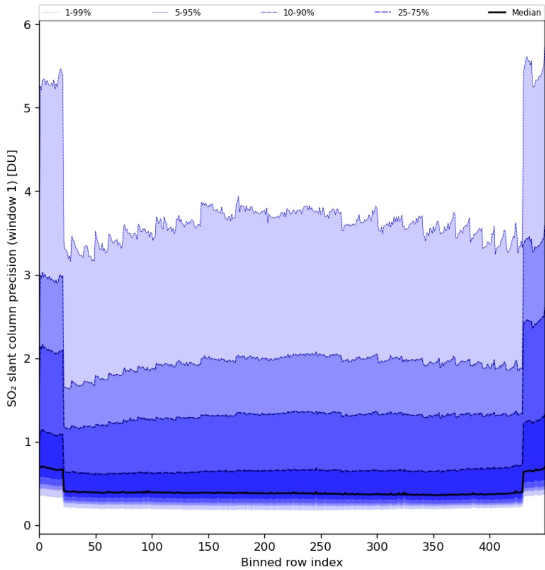
Figure 80: Along track statistics of “SO 2 slant column precision (window 1)” for 2024-02-20 to 2024-02-22
