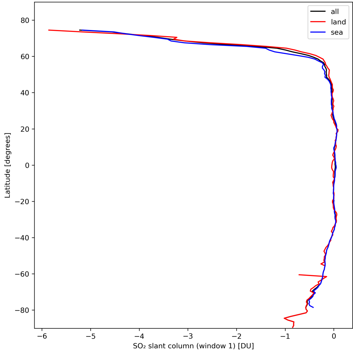
Figure 33: Zonal average of “SO 2 slant column (window 1)” for 2024-02-20 to 2024-02-22.
