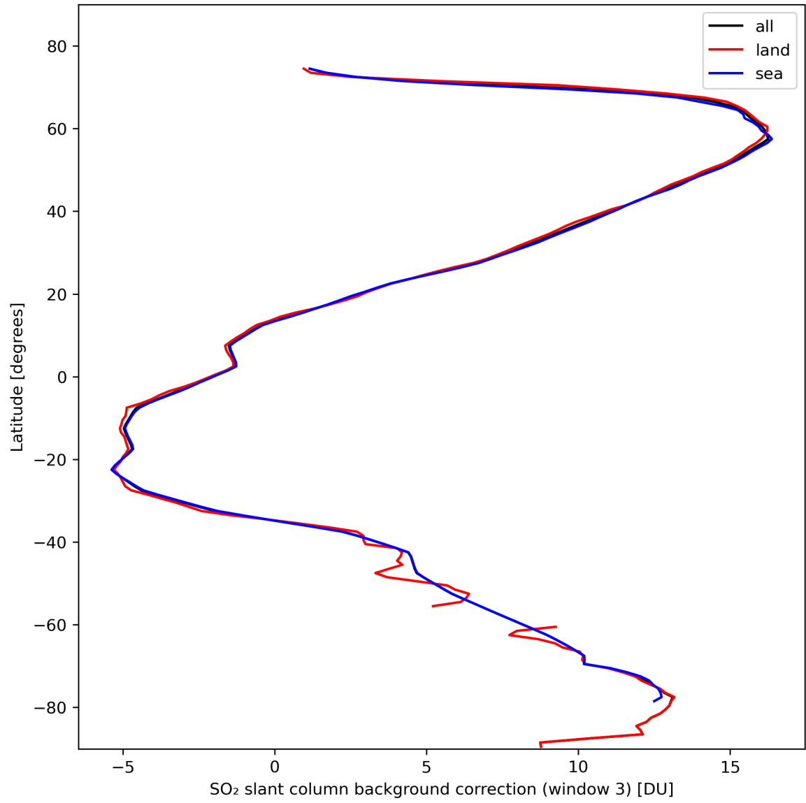
Figure 44: Zonal average of “SO 2 slant column background correction (window 3)” for 2024-02-20 to 2024-02-22.
