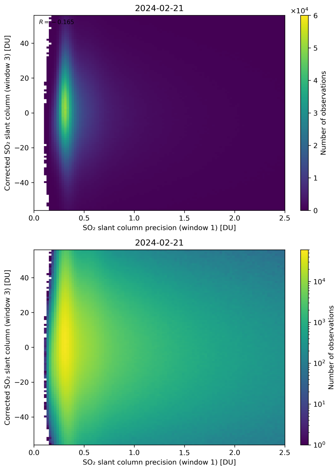
Figure 226: Scatter density plot of “SO 2 slant column precision (window 1)” against “Corrected SO 2 slant column (window 3)” for 2024-02-20 to 2024-02-22.
