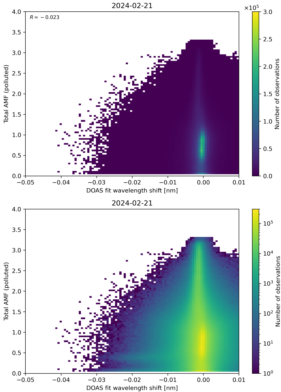
Figure 130: Scatter density plot of “DOAS fit wavelength shift” against “Total AMF (polluted)” for 2024-02-20 to 2024-02-22.
