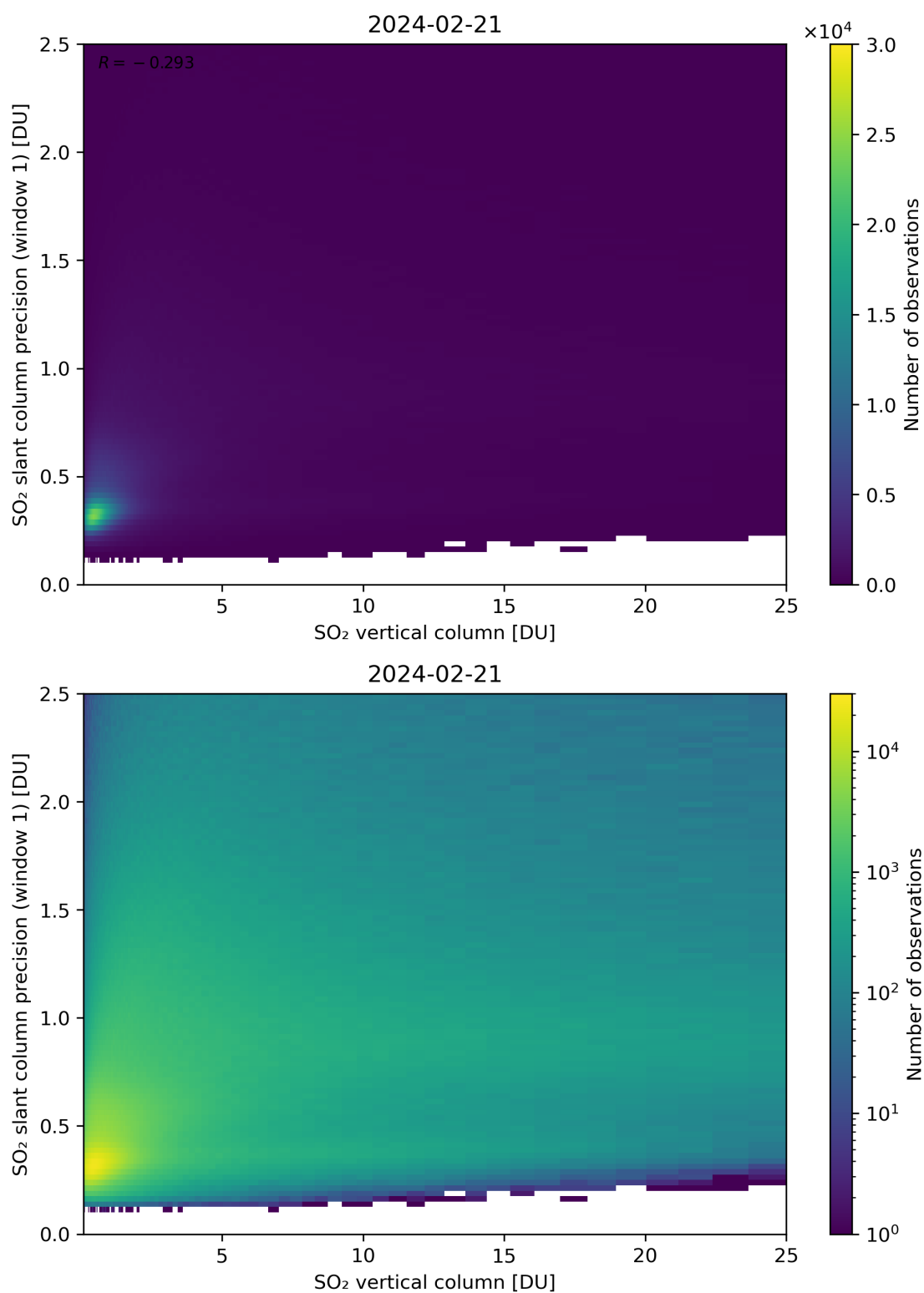
Figure 301: Scatter density plot of “SO 2 vertical column” against “SO 2 slant column precision (window 1)” for 2024-02-20 to 2024-02-22.
