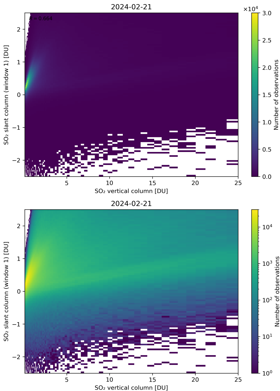
Figure 300: Scatter density plot of “SO 2 vertical column” against “SO 2 slant column (window 1)” for 2024-02-20 to 2024-02-22.
