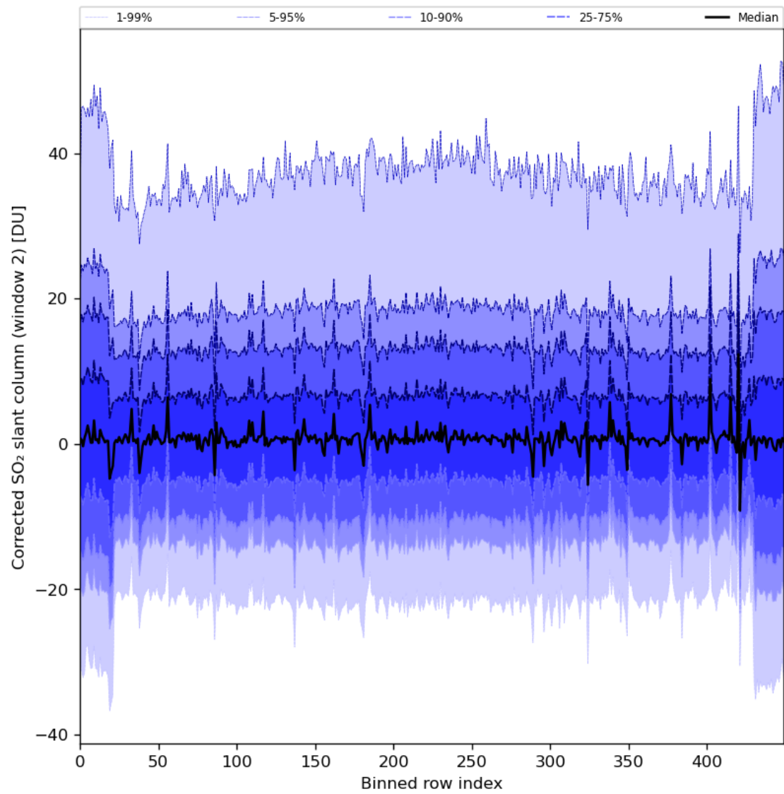
Figure 85: Along track statistics of “Corrected SO 2 slant column (window 2)” for 2024-02-20 to 2024-02-22
