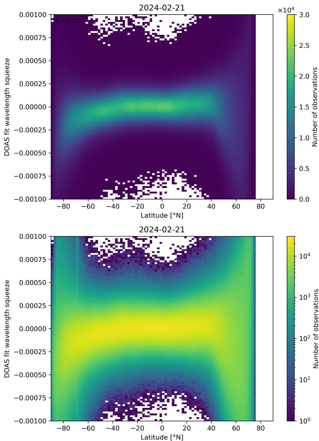
Figure 143: Scatter density plot of “Latitude” against “DOAS fit wavelength squeeze” for 2024-02-20 to 2024-02-22.
