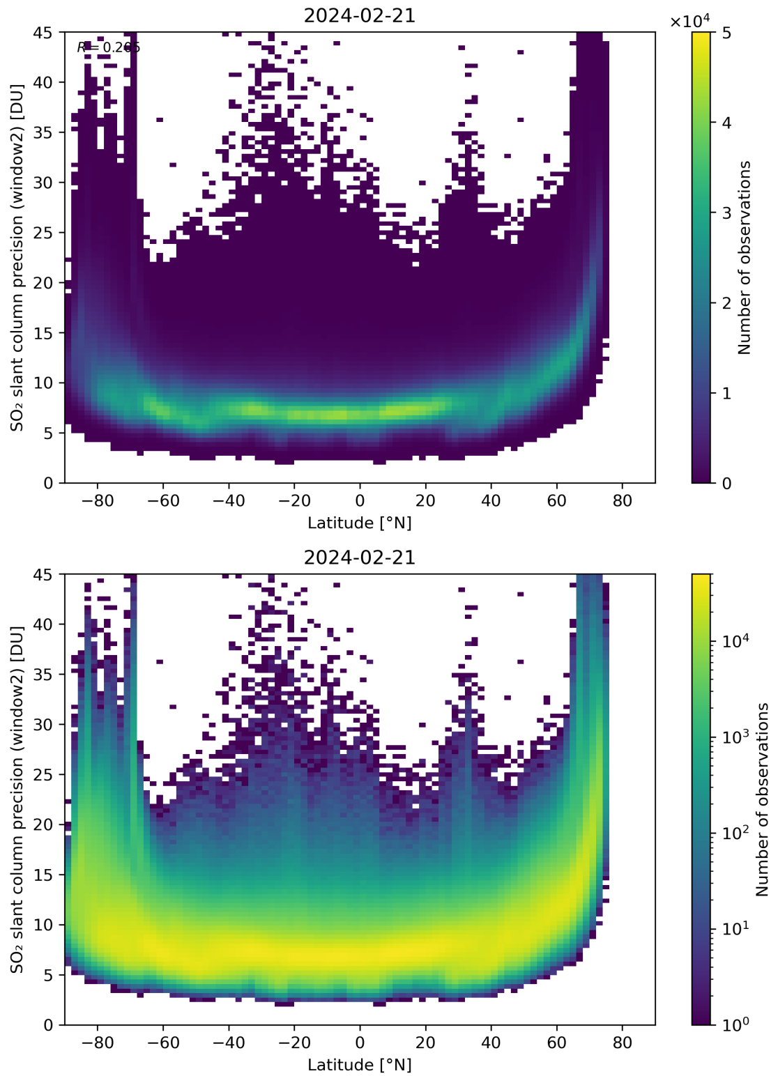
Figure 151: Scatter density plot of “Latitude” against “SO 2 slant column precision (window2)” for 2024-02-20 to 2024-02-22.
