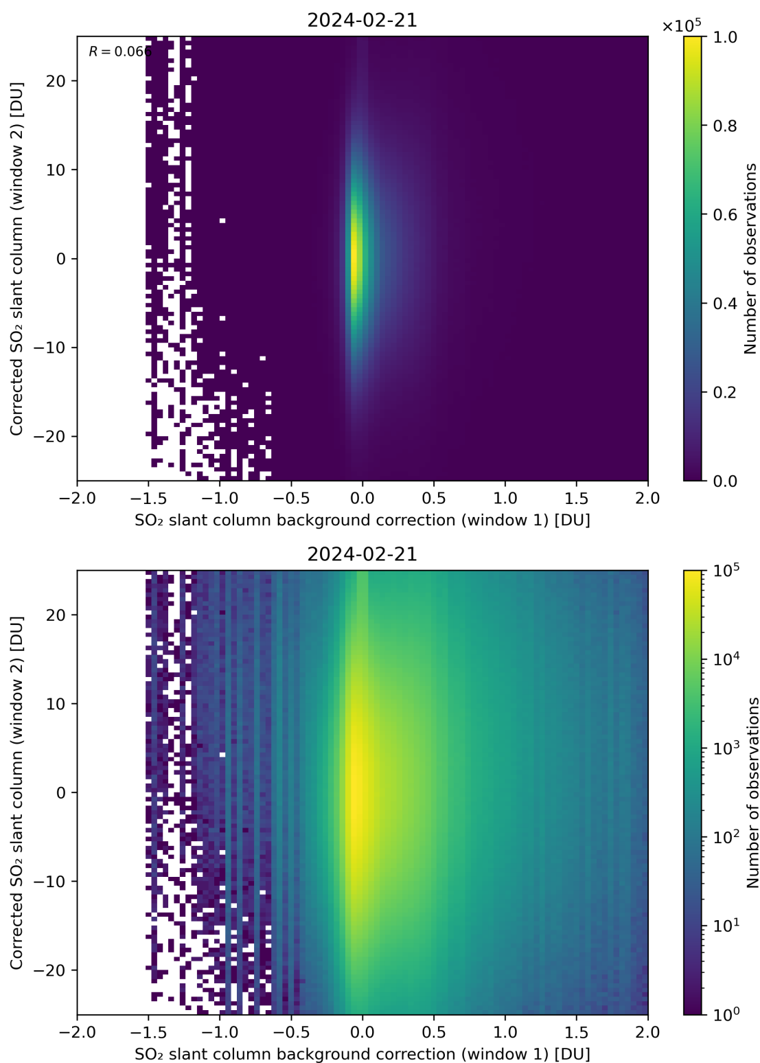
Figure 104: Scatter density plot of “SO 2 slant column background correction (window 1)” against “Corrected SO 2 slant column (window 2)” for 2024-02-20 to 2024-02-22.
