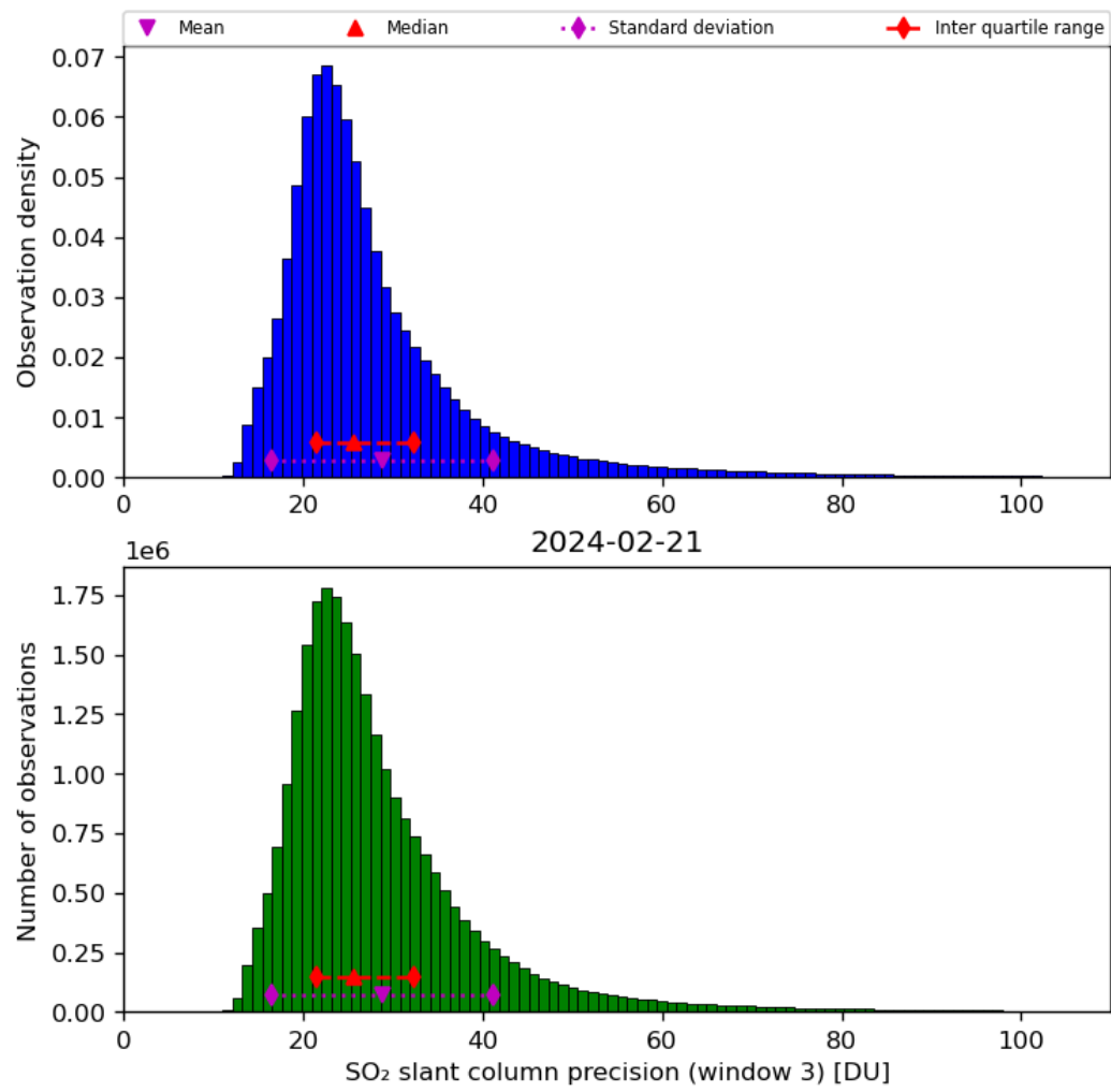
Figure 65: Histogram of “SO 2 slant column precision (window 3)” for 2024-02-20 to 2024-02-22
