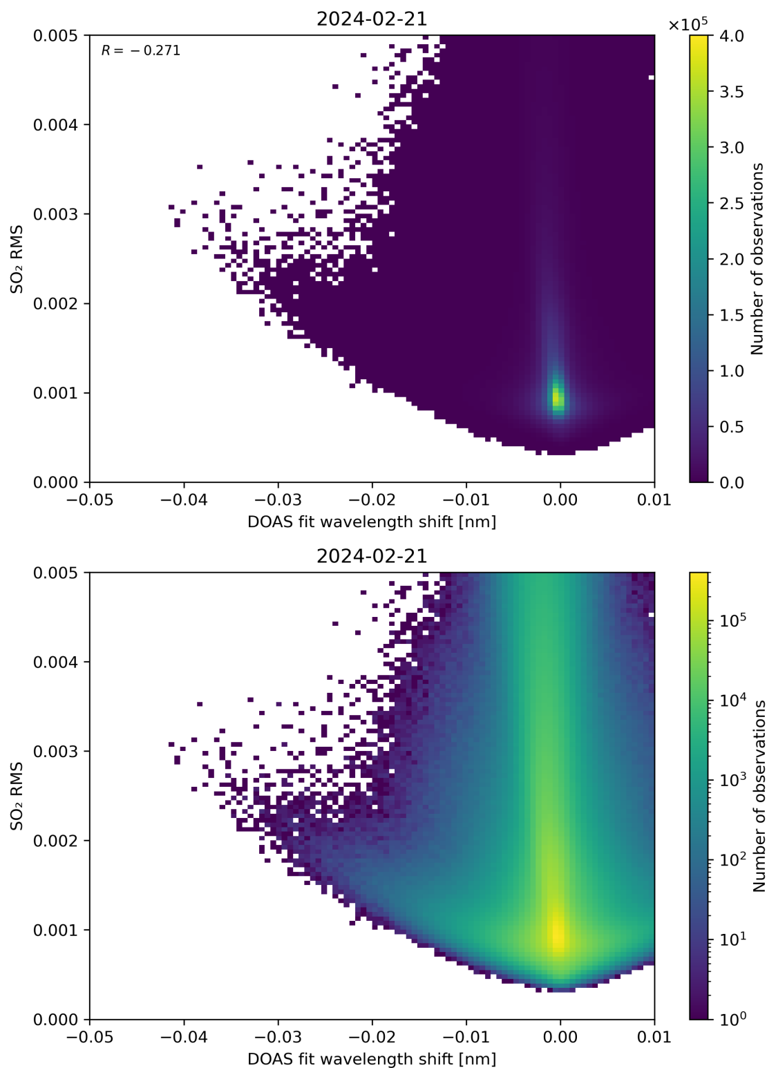
Figure 128: Scatter density plot of “DOAS fit wavelength shift” against “SO 2 RMS” for 2024-02-20 to 2024-02-22.
