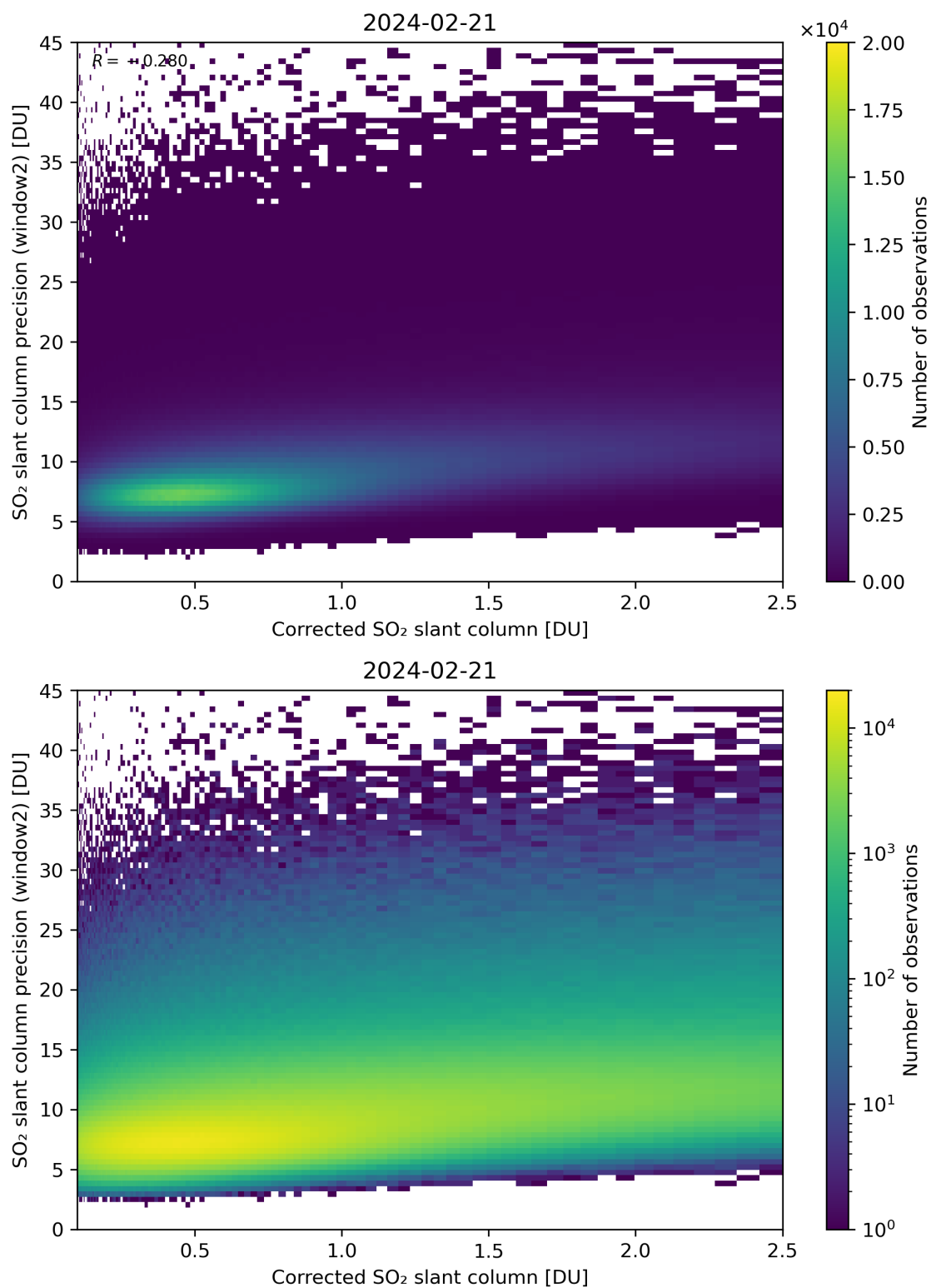
Figure 189: Scatter density plot of “Corrected SO 2 slant column” against “SO 2 slant column precision (window2)” for 2024-02-20 to 2024-02-22.
