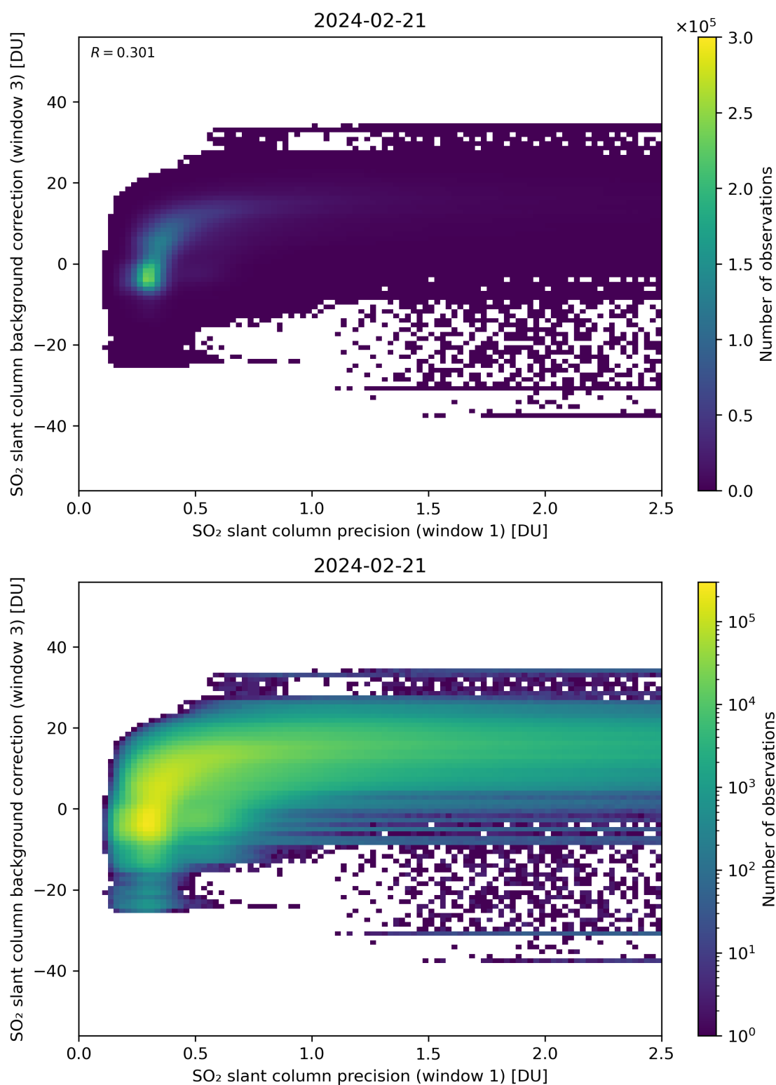
Figure 220: Scatter density plot of “SO 2 slant column precision (window 1)” against “SO 2 slant column background correction (window 3)” for 2024-02-20 to 2024-02-22.
