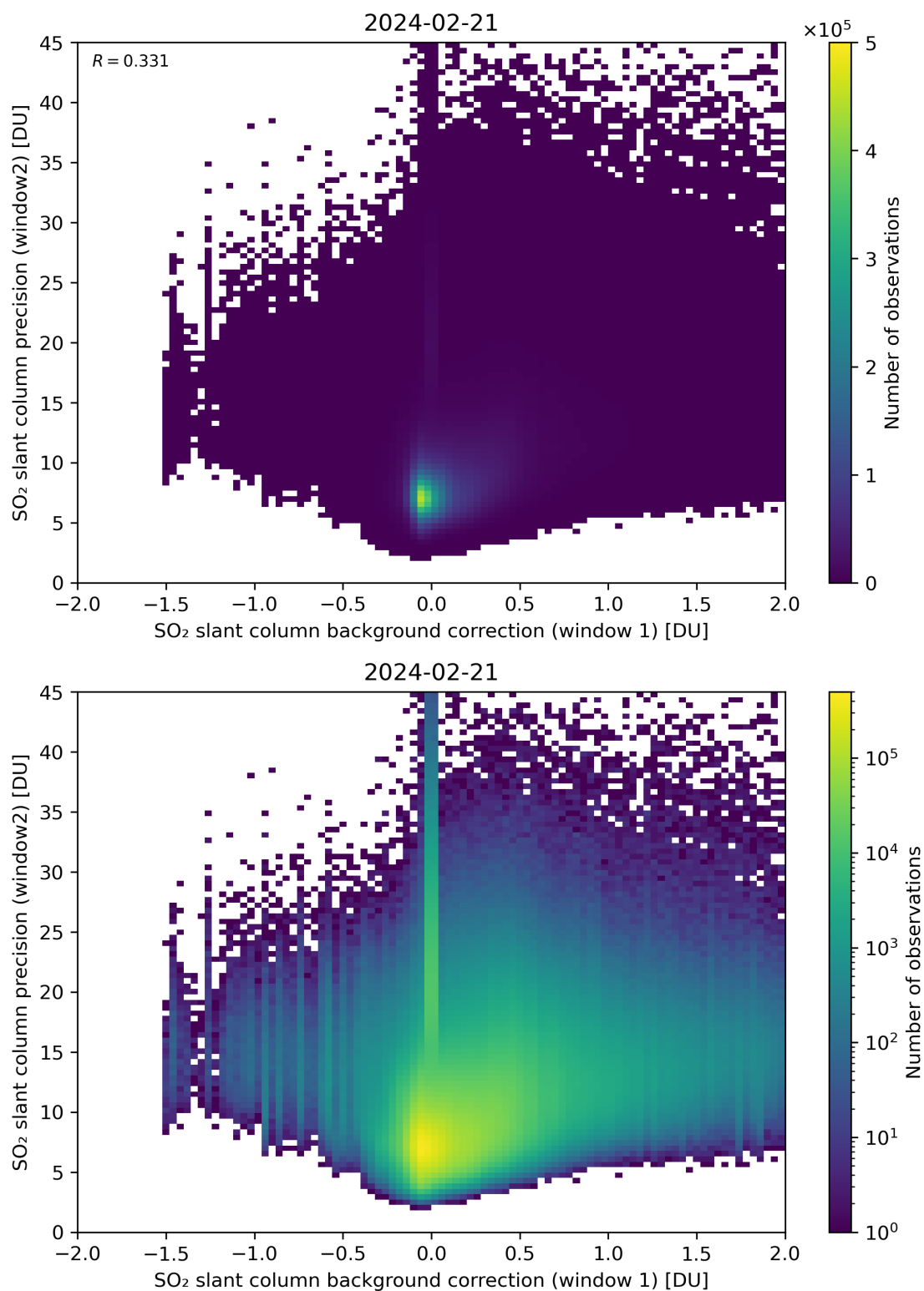
Figure 106: Scatter density plot of “SO 2 slant column background correction (window 1)” against “SO 2 slant column precision (window2)” for 2024-02-20 to 2024-02-22.
