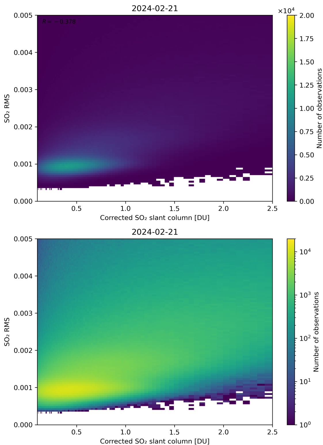
Figure 183: Scatter density plot of “Corrected SO 2 slant column” against “SO 2 RMS” for 2024-02-20 to 2024-02-22.
