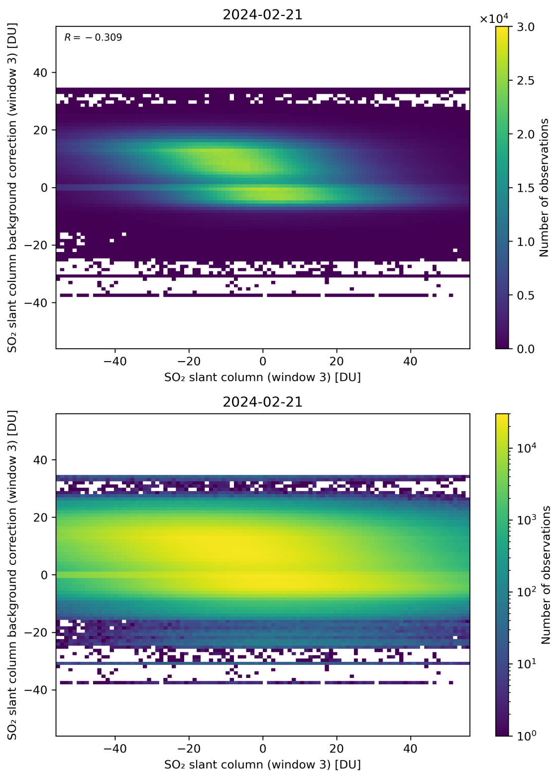
Figure 253: Scatter density plot of “SO 2 slant column (window 3)” against “SO 2 slant column background correction (window 3)” for 2024-02-20 to 2024-02-22.
