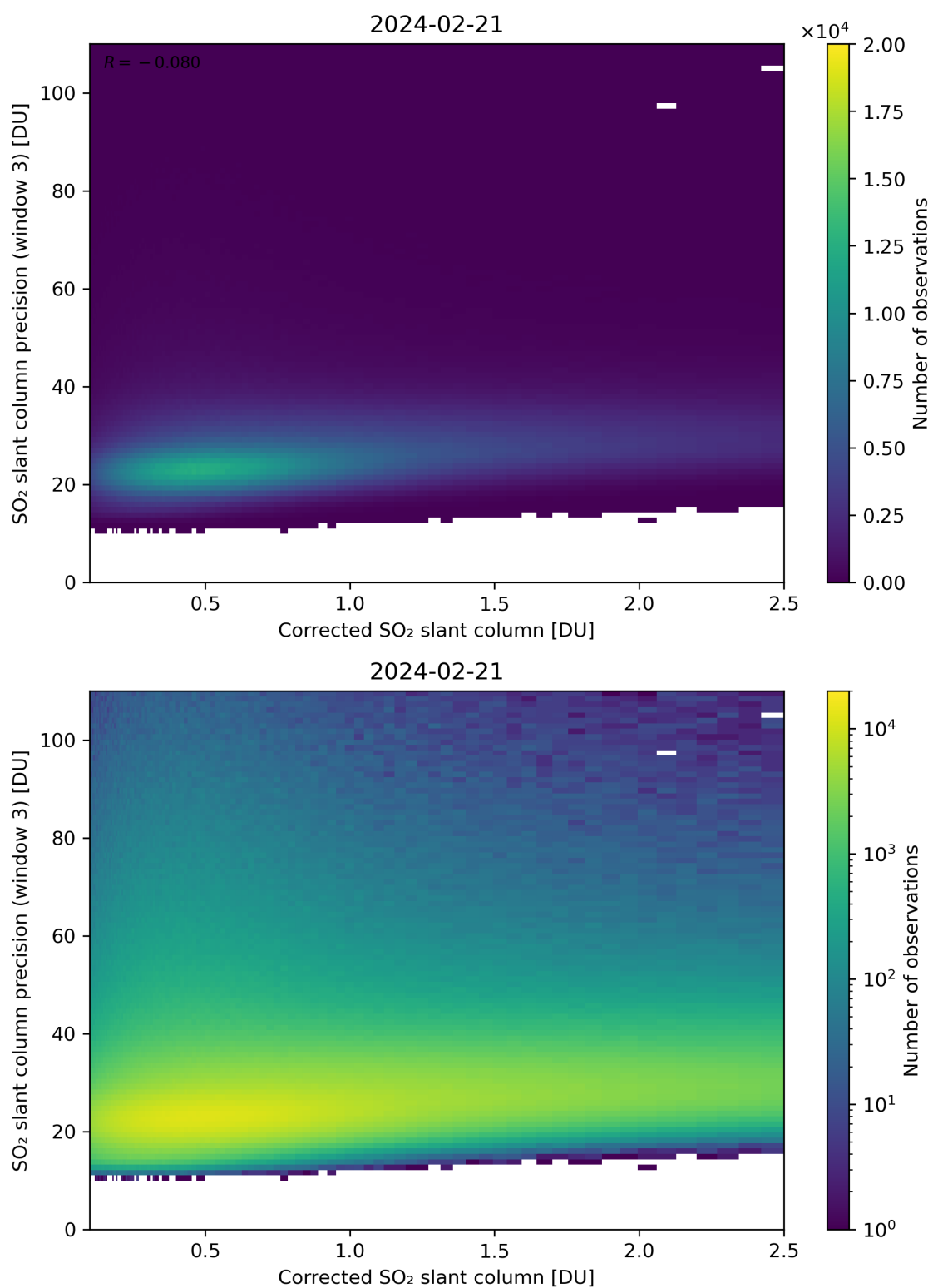
Figure 191: Scatter density plot of “Corrected SO 2 slant column” against “SO 2 slant column precision (window 3)” for 2024-02-20 to 2024-02-22.
