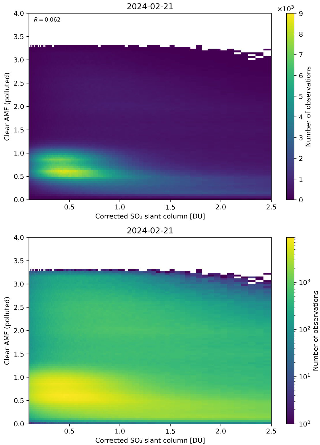
Figure 184: Scatter density plot of “Corrected SO 2 slant column” against “Clear AMF (polluted)” for 2024-02-20 to 2024-02-22.
