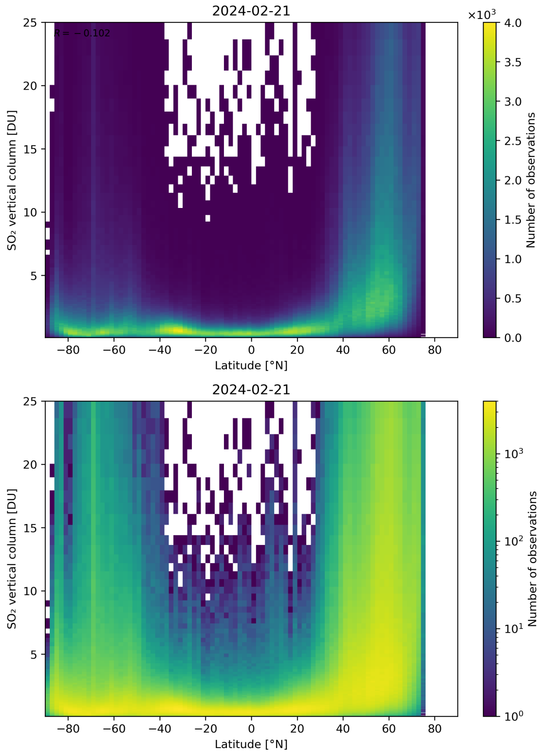
Figure 156: Scatter density plot of “Latitude” against “SO 2 vertical column” for 2024-02-20 to 2024-02-22.
