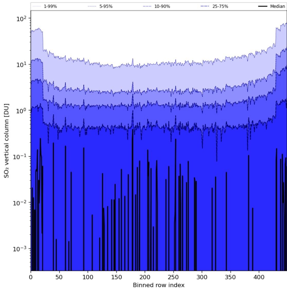
Figure 76: Along track statistics of “SO 2 vertical column” for 2024-02-20 to 2024-02-22
