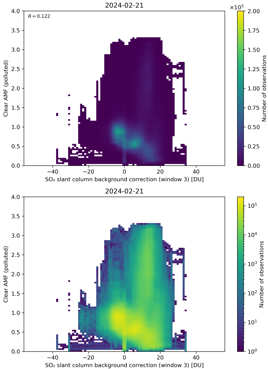
Figure 124: Scatter density plot of “SO 2 slant column background correction (window 3)” against “Clear AMF (polluted)” for 2024-02-20 to 2024-02-22.
