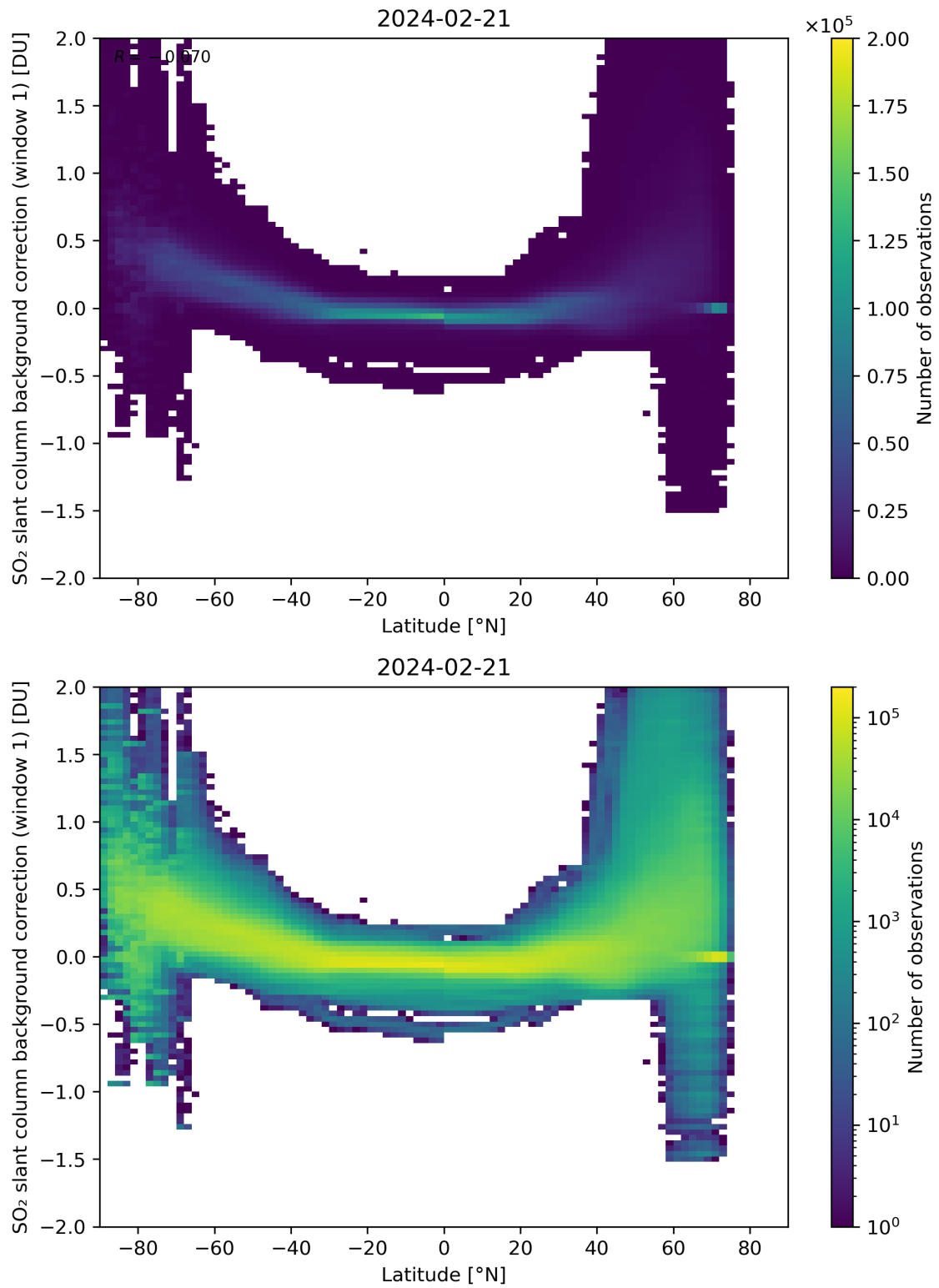
Figure 139: Scatter density plot of “Latitude” against “SO 2 slant column background correction (window 1)” for 2024-02-20 to 2024-02-22.
