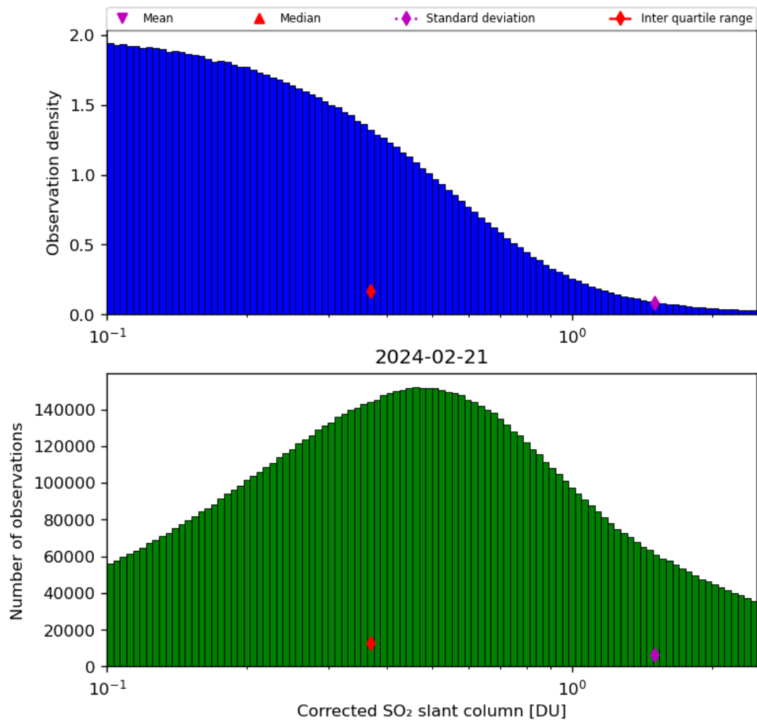
Figure 55: Histogram of “Corrected SO 2 slant column” for 2024-02-20 to 2024-02-22
