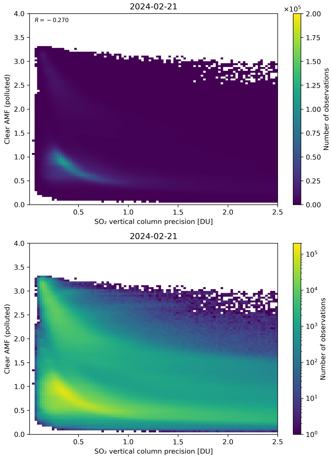
Figure 285: Scatter density plot of “SO 2 vertical column precision” against “Clear AMF (polluted)” for 2024-02-20 to 2024-02-22.
