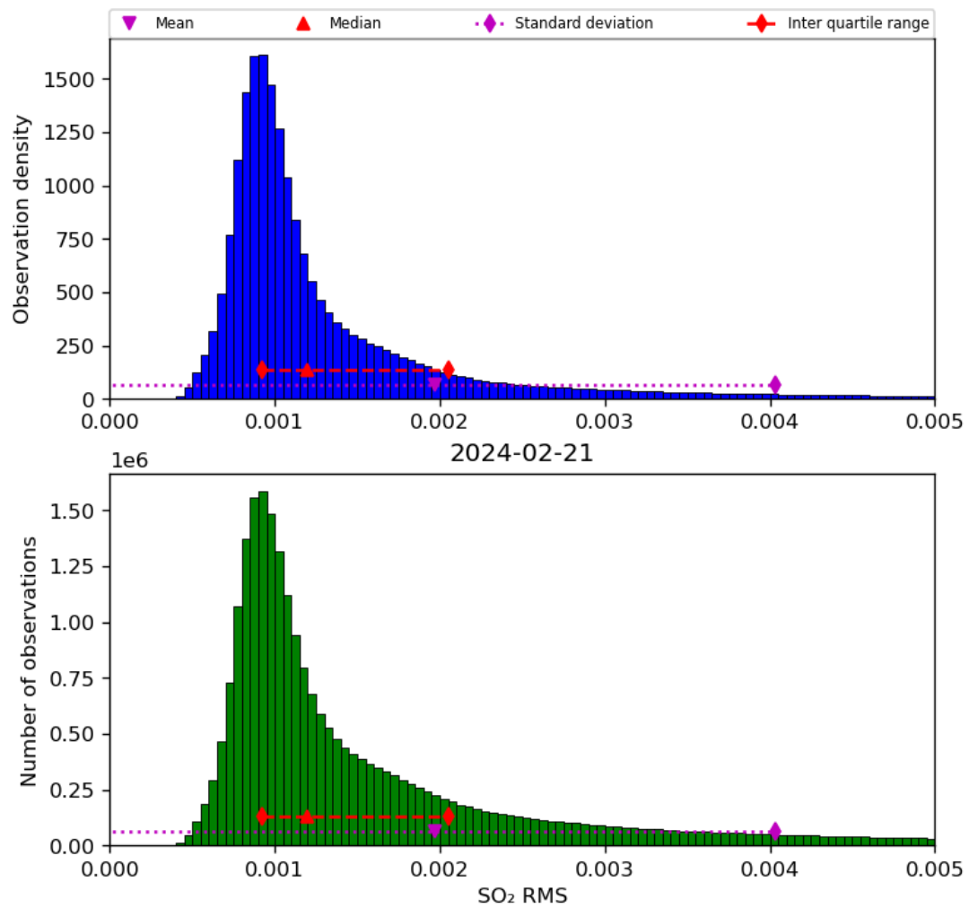
Figure 70: Histogram of “SO 2 RMS” for 2024-02-20 to 2024-02-22
