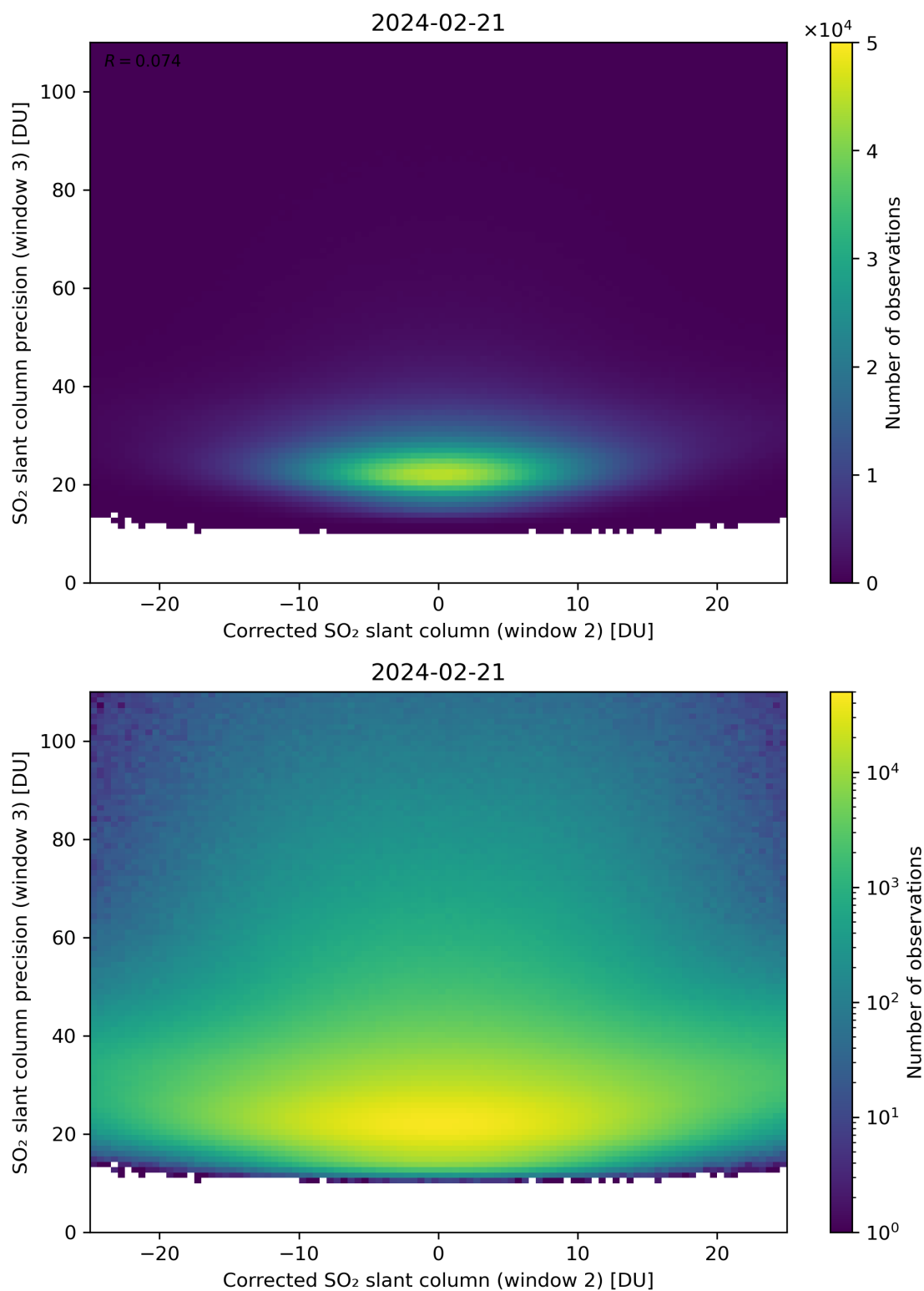
Figure 202: Scatter density plot of “Corrected SO 2 slant column (window 2)” against “SO 2 slant column precision (window 3)” for 2024-02-20 to 2024-02-22.
