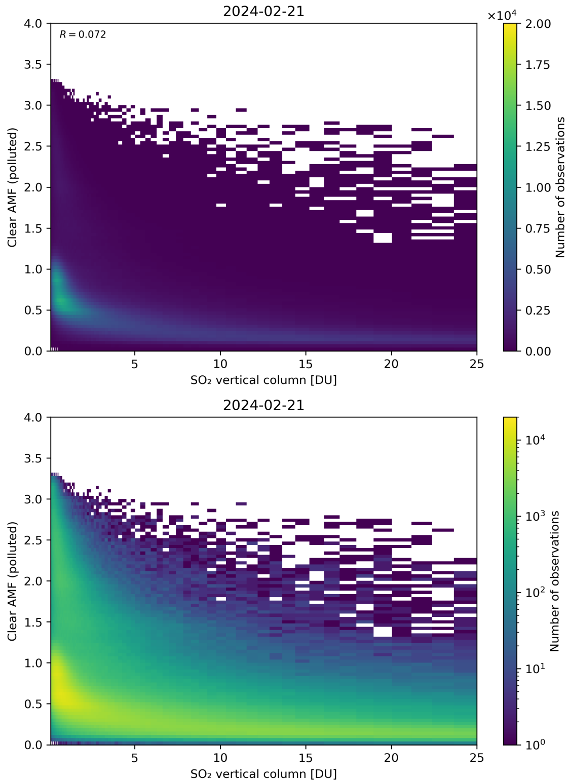
Figure 296: Scatter density plot of “SO 2 vertical column” against “Clear AMF (polluted)” for 2024-02-20 to 2024-02-22.
