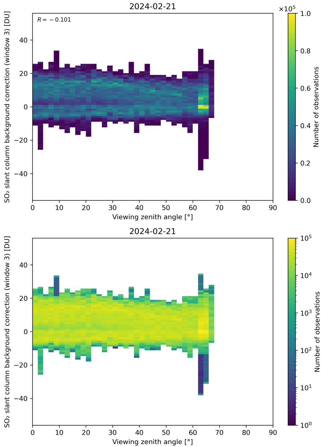
Figure 310: Scatter density plot of “Viewing zenith angle” against “SO 2 slant column background correction (window 3)” for 2024-02-20 to 2024-02-22.
