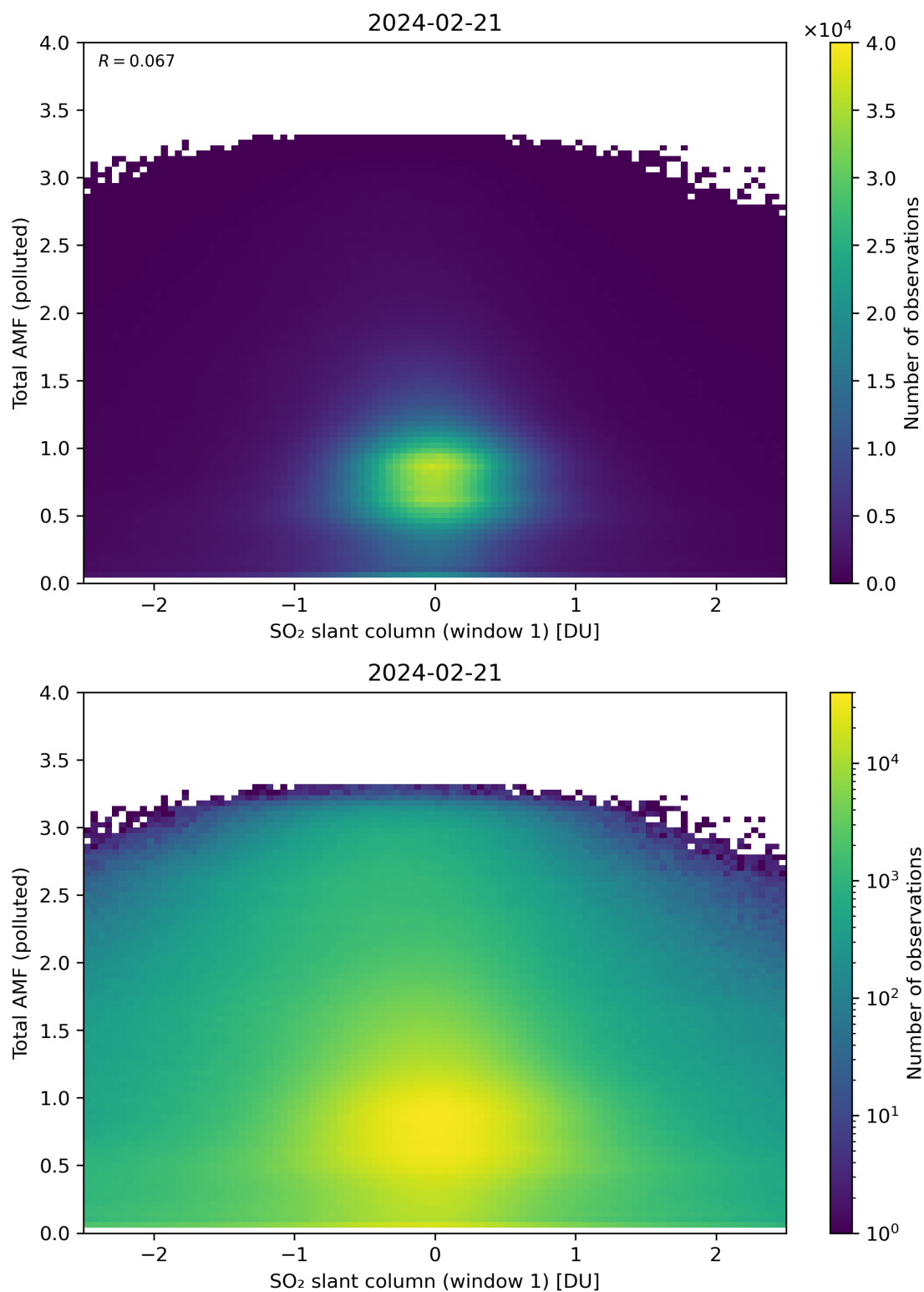
Figure 239: Scatter density plot of “SO 2 slant column (window 1)” against “Total AMF (polluted)” for 2024-02-20 to 2024-02-22.
