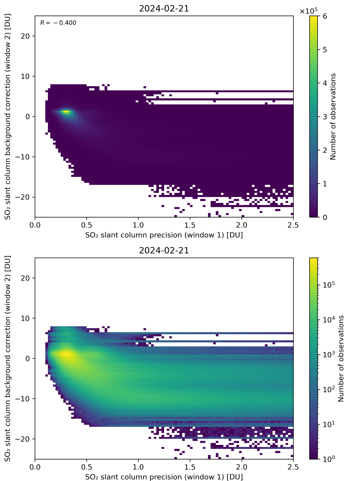
Figure 219: Scatter density plot of “SO 2 slant column precision (window 1)” against “SO 2 slant column background correction (window 2)” for 2024-02-20 to 2024-02-22.
