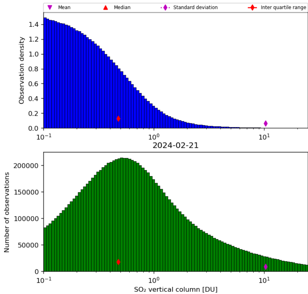
Figure 53: Histogram of “SO 2 vertical column” for 2024-02-20 to 2024-02-22
