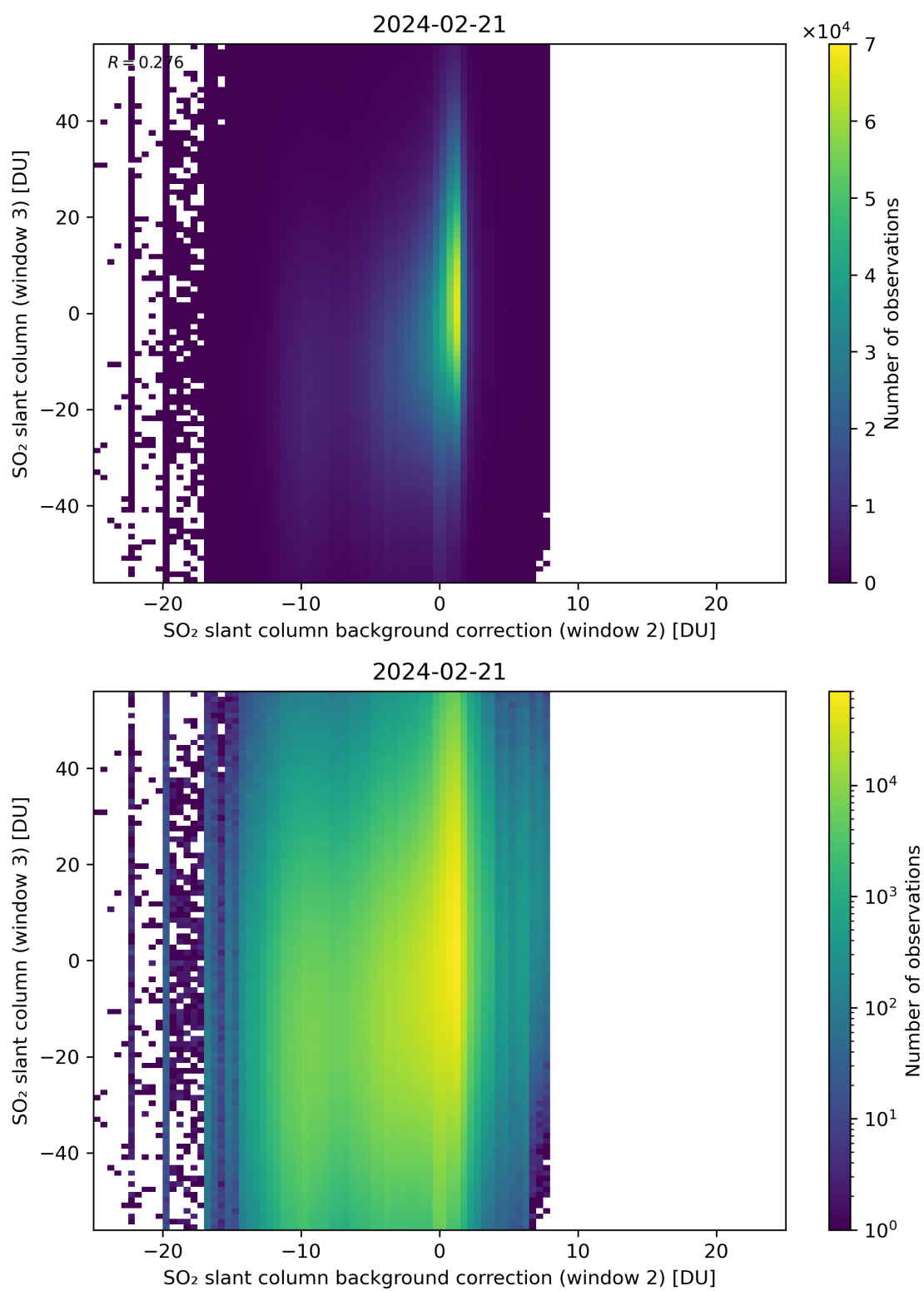
Figure 117: Scatter density plot of “SO 2 slant column background correction (window 2)” against “SO 2 slant column (window 3)” for 2024-02-20 to 2024-02-22.
