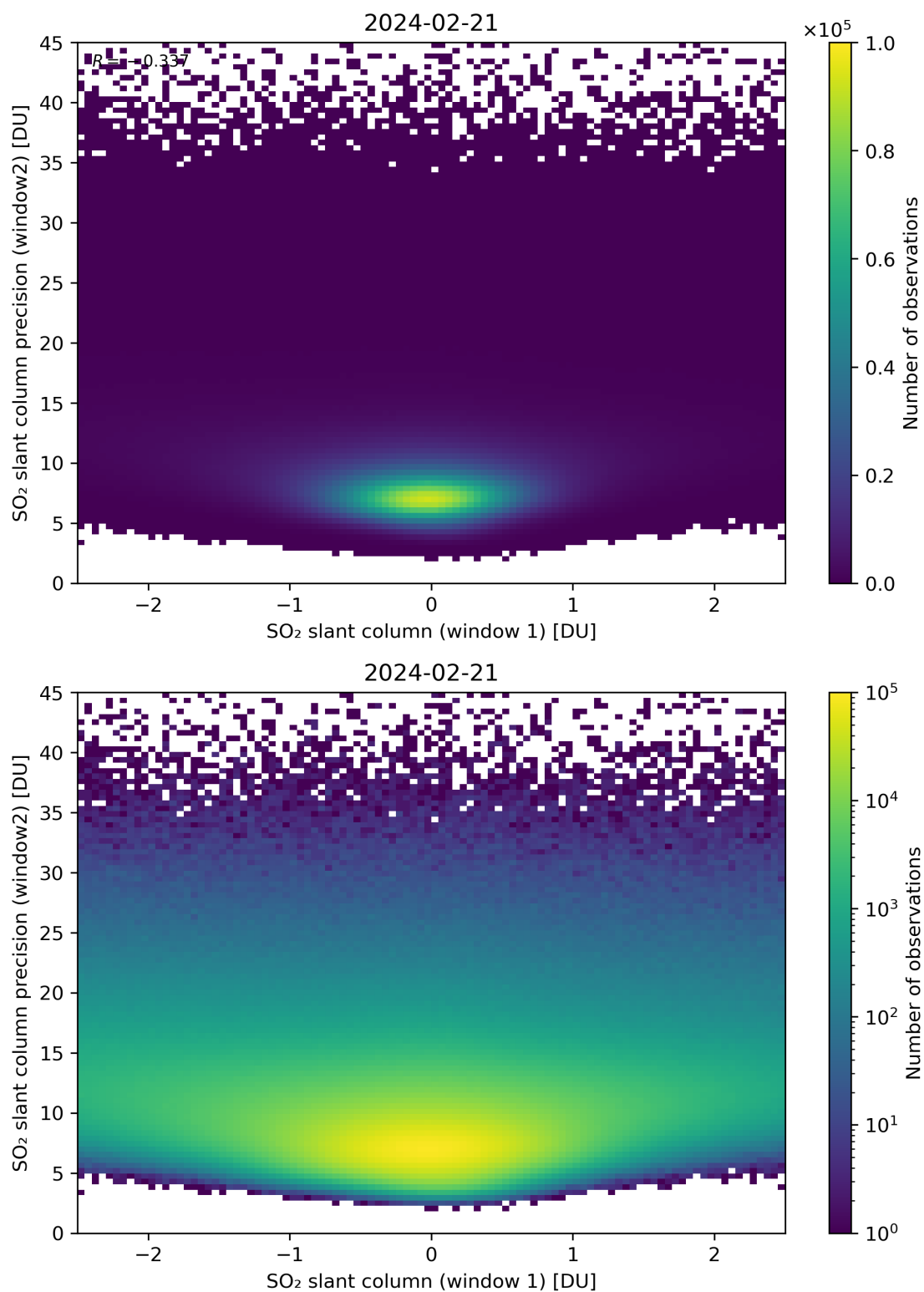
Figure 236: Scatter density plot of “SO 2 slant column (window 1)” against “SO 2 slant column precision (window2)” for 2024-02-20 to 2024-02-22.
