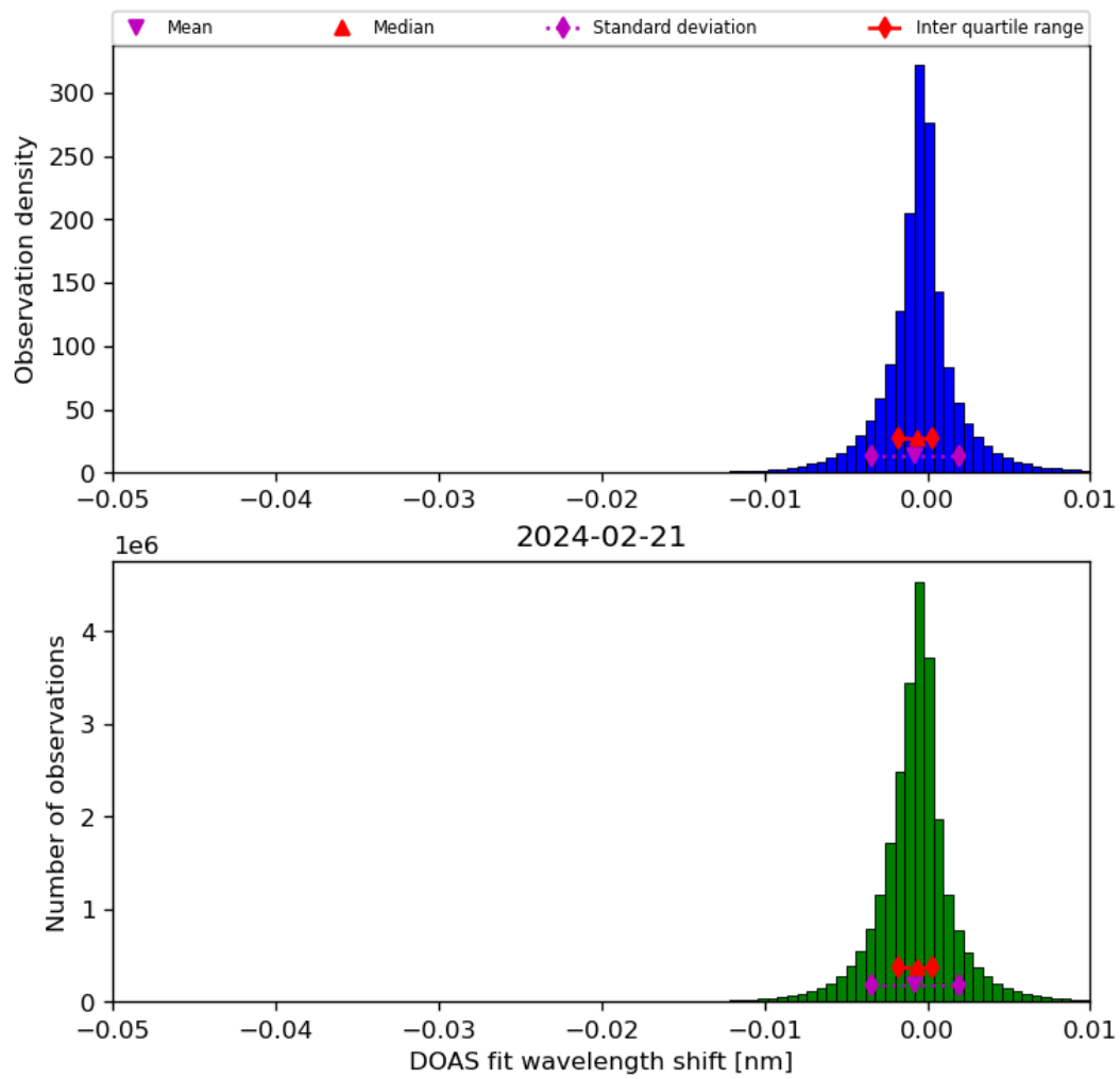
Figure 68: Histogram of “DOAS fit wavelength shift” for 2024-02-20 to 2024-02-22
