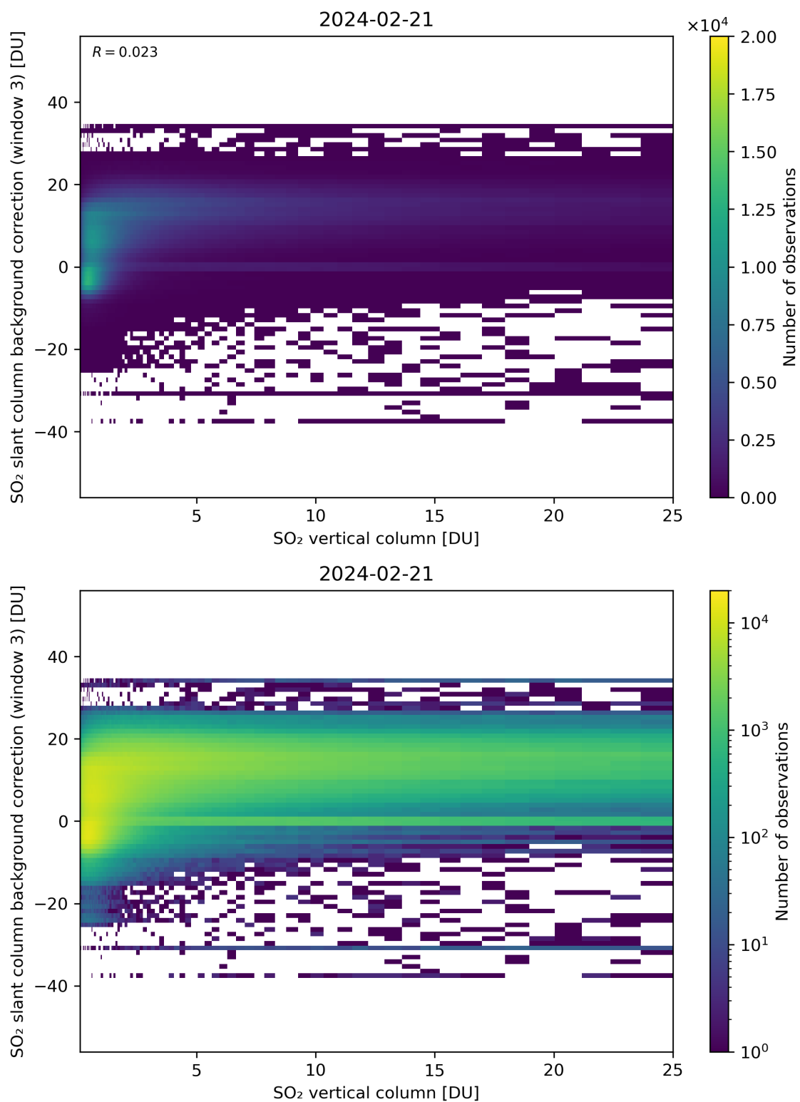
Figure 275: Scatter density plot of “SO 2 vertical column” against “SO 2 slant column background correction (window 3)” for 2024-02-20 to 2024-02-22.
