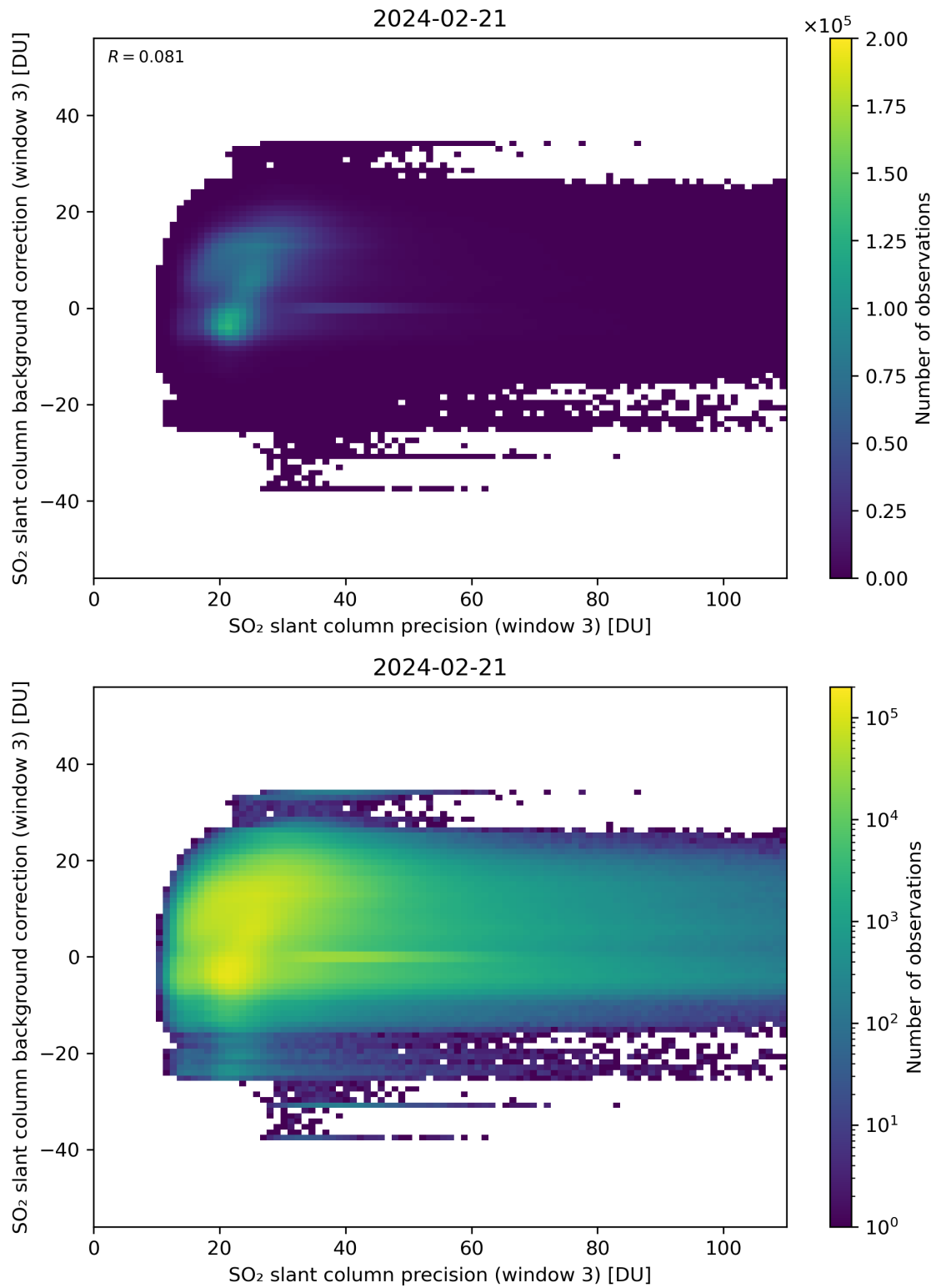
Figure 257: Scatter density plot of “SO 2 slant column precision (window 3)” against “SO 2 slant column background correction (window 3)” for 2024-02-20 to 2024-02-22.
