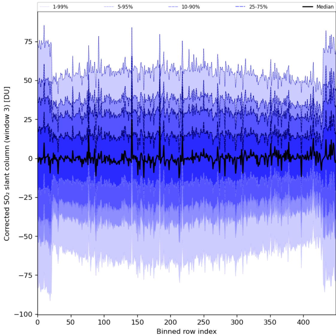
Figure 89: Along track statistics of “Corrected SO 2 slant column (window 3)” for 2024-02-20 to 2024-02-22
