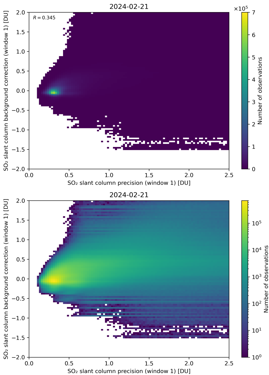
Figure 218: Scatter density plot of “SO 2 slant column precision (window 1)” against “SO 2 slant column background correction (window 1)” for 2024-02-20 to 2024-02-22.
