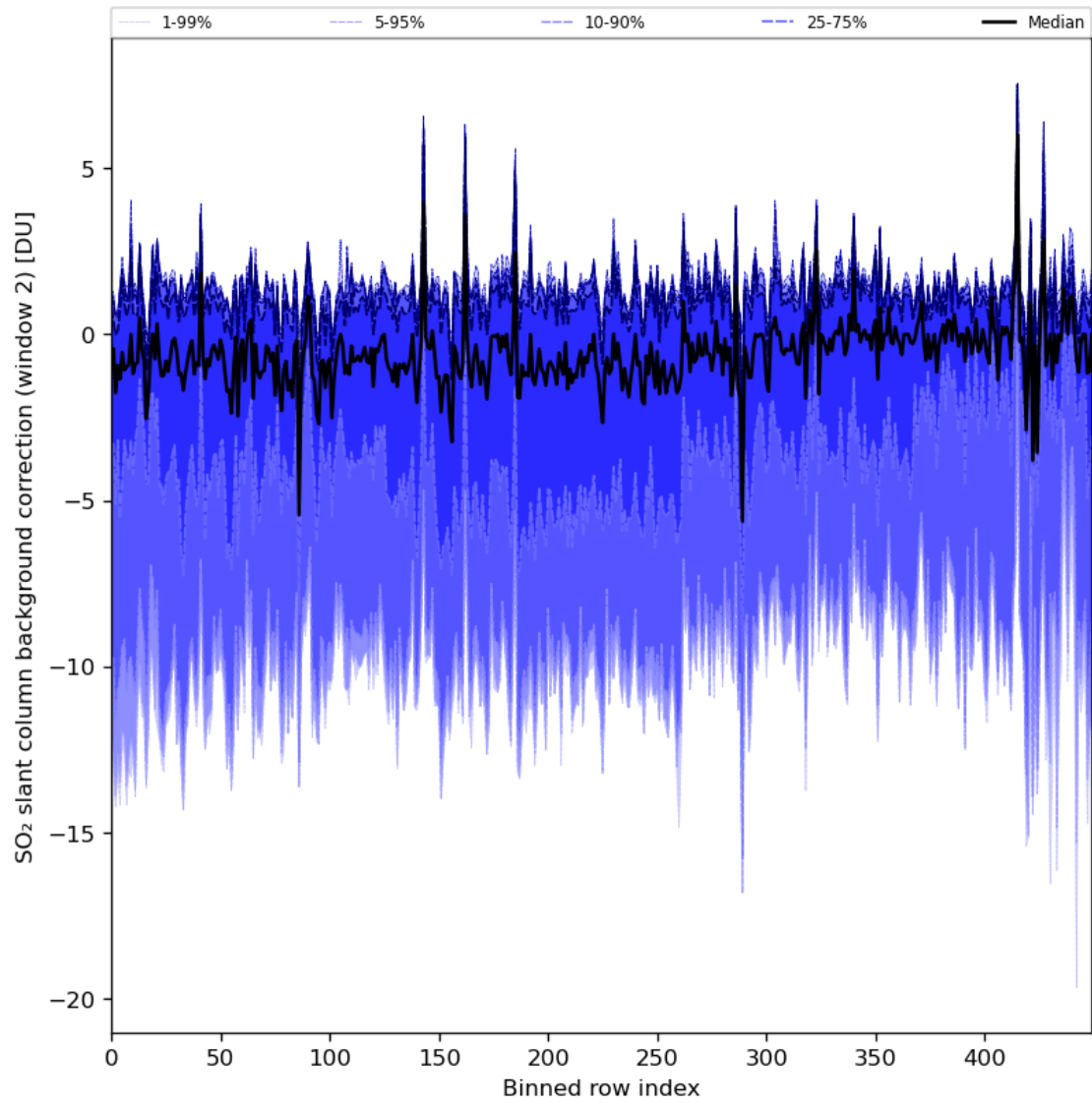
Figure 86: Along track statistics of “SO 2 slant column background correction (window 2)” for 2024-02-20 to 2024-02-22
