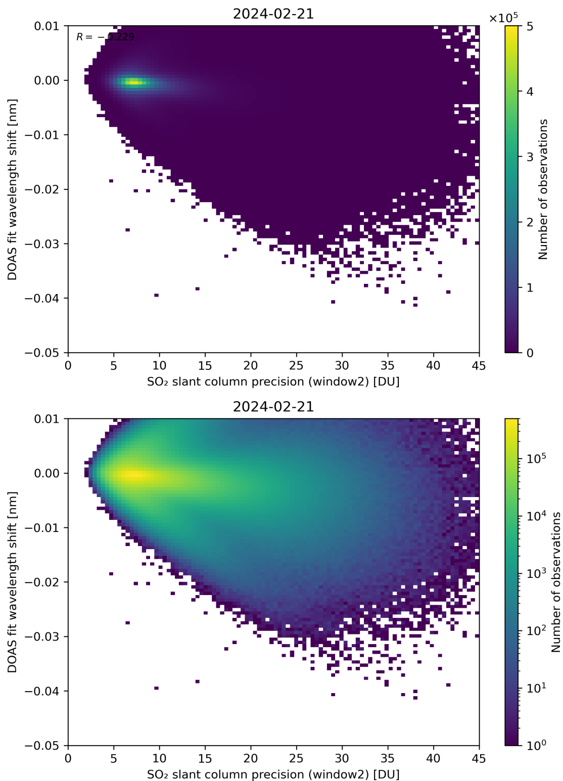
Figure 243: Scatter density plot of “SO 2 slant column precision (window2)” against “DOAS fit wavelength shift” for 2024-02-20 to 2024-02-22.
