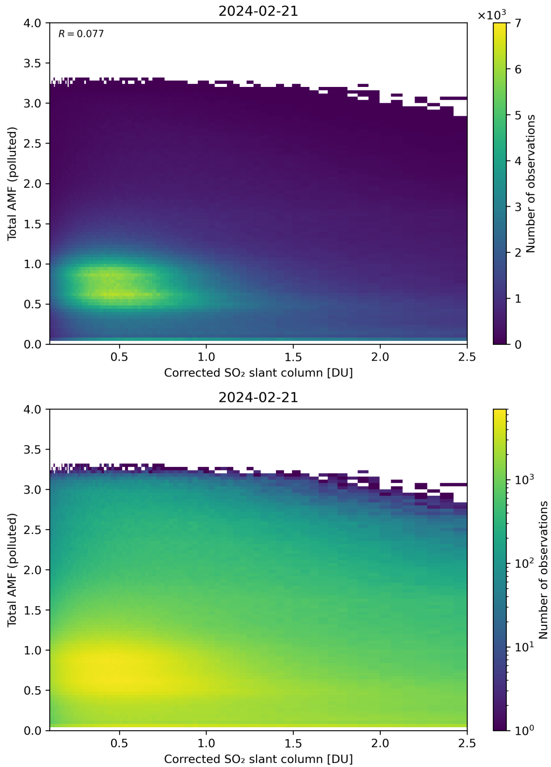
Figure 192: Scatter density plot of “Corrected SO 2 slant column” against “Total AMF (polluted)” for 2024-02-20 to 2024-02-22.
