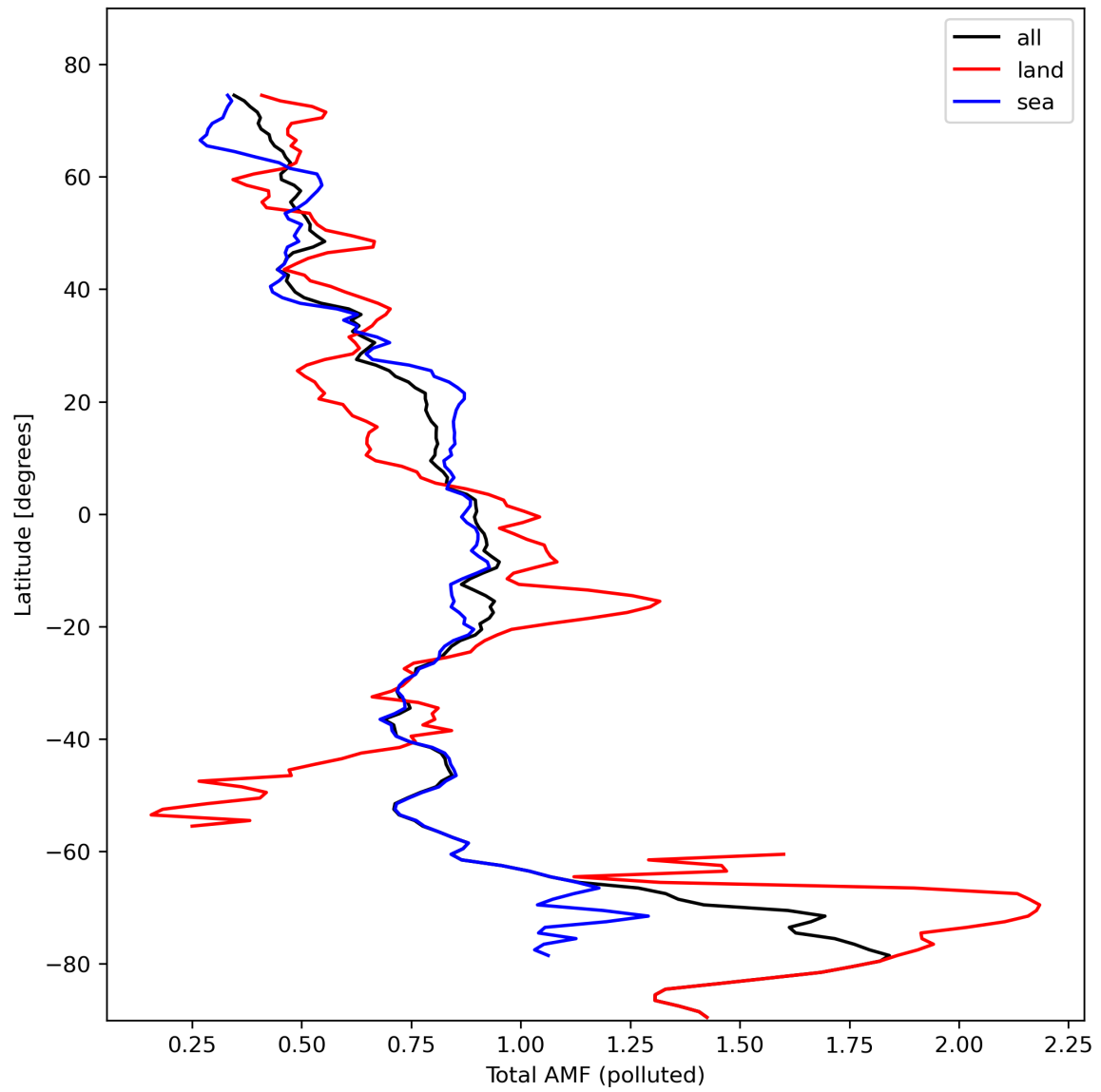
Figure 48: Zonal average of “Total AMF (polluted)” for 2024-02-20 to 2024-02-22.
