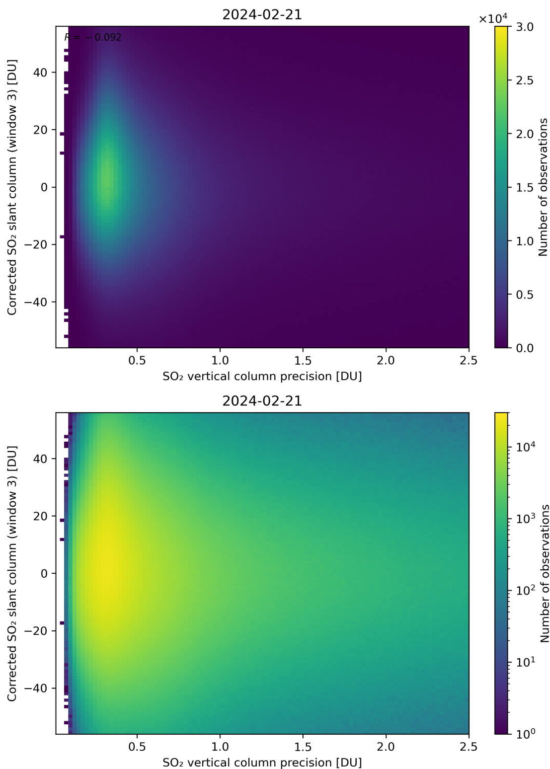
Figure 288: Scatter density plot of “SO 2 vertical column precision” against “Corrected SO 2 slant column (window 3)” for 2024-02-20 to 2024-02-22.
