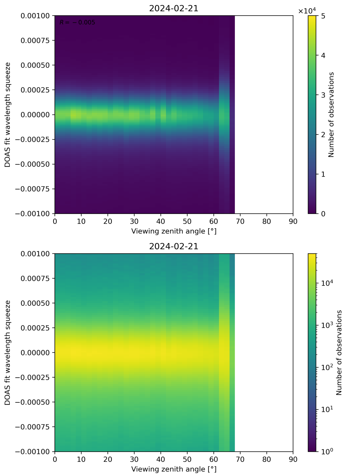
Figure 312: Scatter density plot of “Viewing zenith angle” against “DOAS fit wavelength squeeze” for 2024-02-20 to 2024-02-22.
