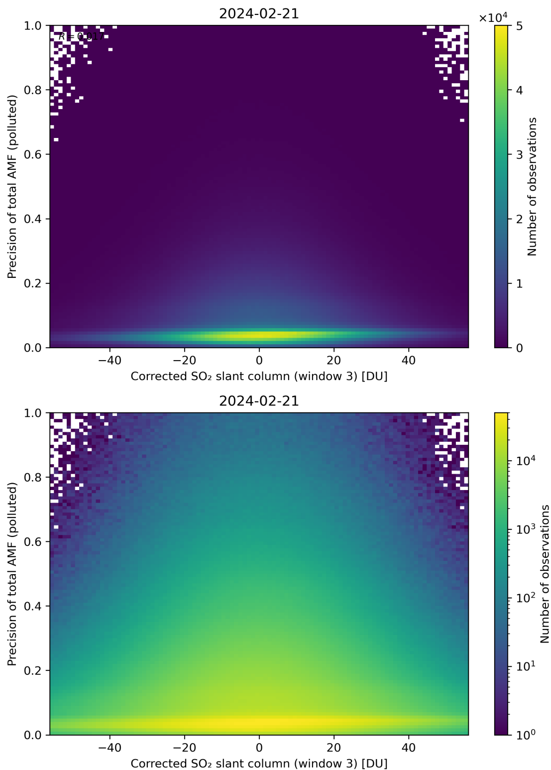
Figure 211: Scatter density plot of “Corrected SO 2 slant column (window 3)” against “Precision of total AMF (polluted)” for 2024-02-20 to 2024-02-22.
