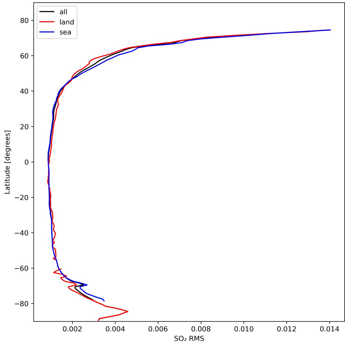
Figure 47: Zonal average of “SO 2 RMS” for 2024-02-20 to 2024-02-22.
