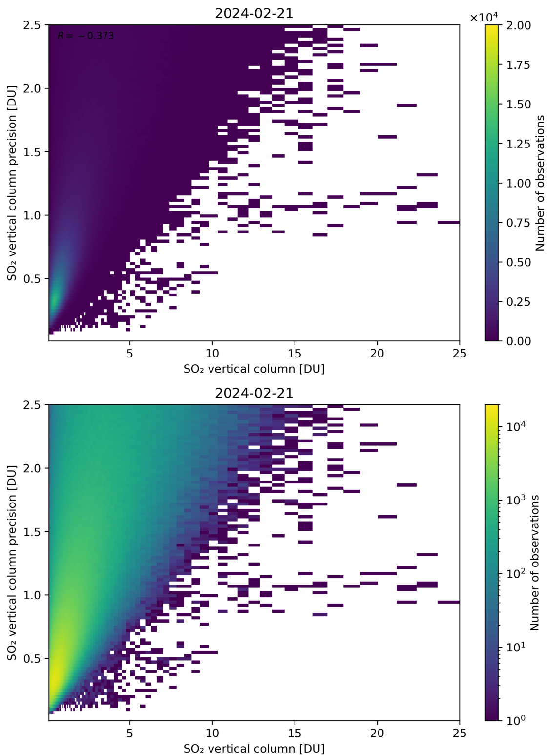
Figure 307: Scatter density plot of “SO 2 vertical column” against “SO 2 vertical column precision” for 2024-02-20 to 2024-02-22.
