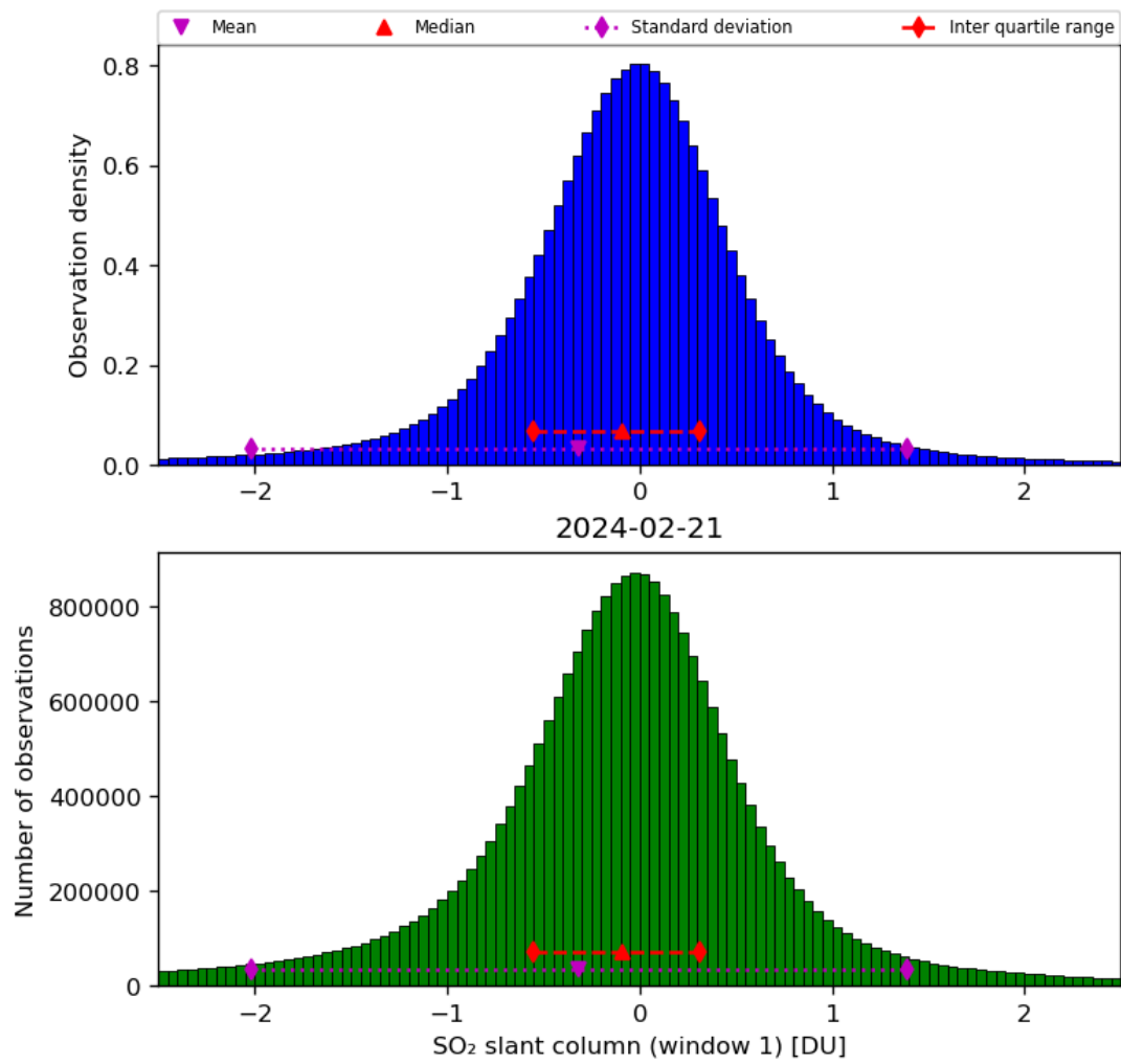
Figure 56: Histogram of “SO 2 slant column (window 1)” for 2024-02-20 to 2024-02-22
