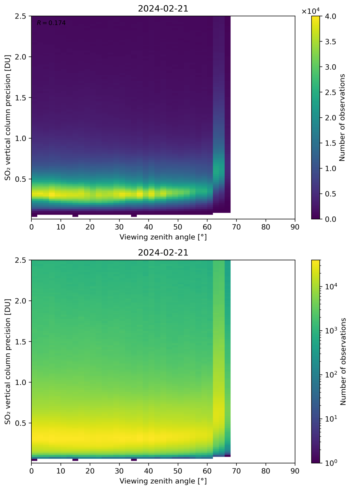
Figure 328: Scatter density plot of “Viewing zenith angle” against “SO 2 vertical column precision” for 2024-02-20 to 2024-02-22.
