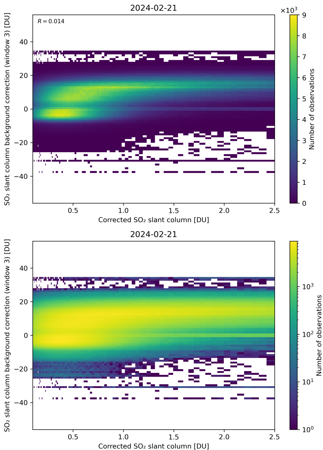
Figure 180: Scatter density plot of “Corrected SO 2 slant column” against “SO 2 slant column background correction (window 3)” for 2024-02-20 to 2024-02-22.
