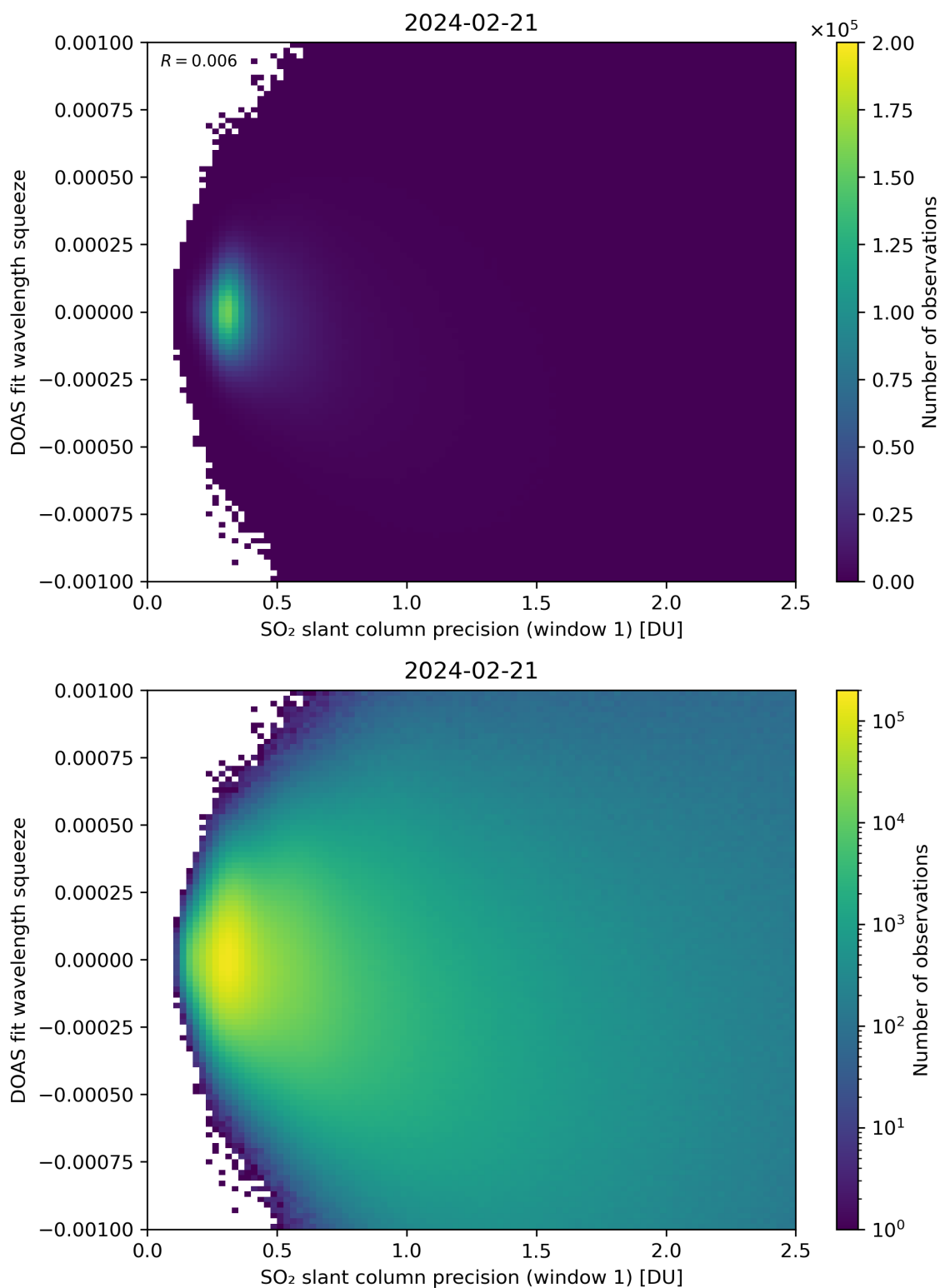
Figure 222: Scatter density plot of “SO 2 slant column precision (window 1)” against “DOAS fit wavelength squeeze” for 2024-02-20 to 2024-02-22.
