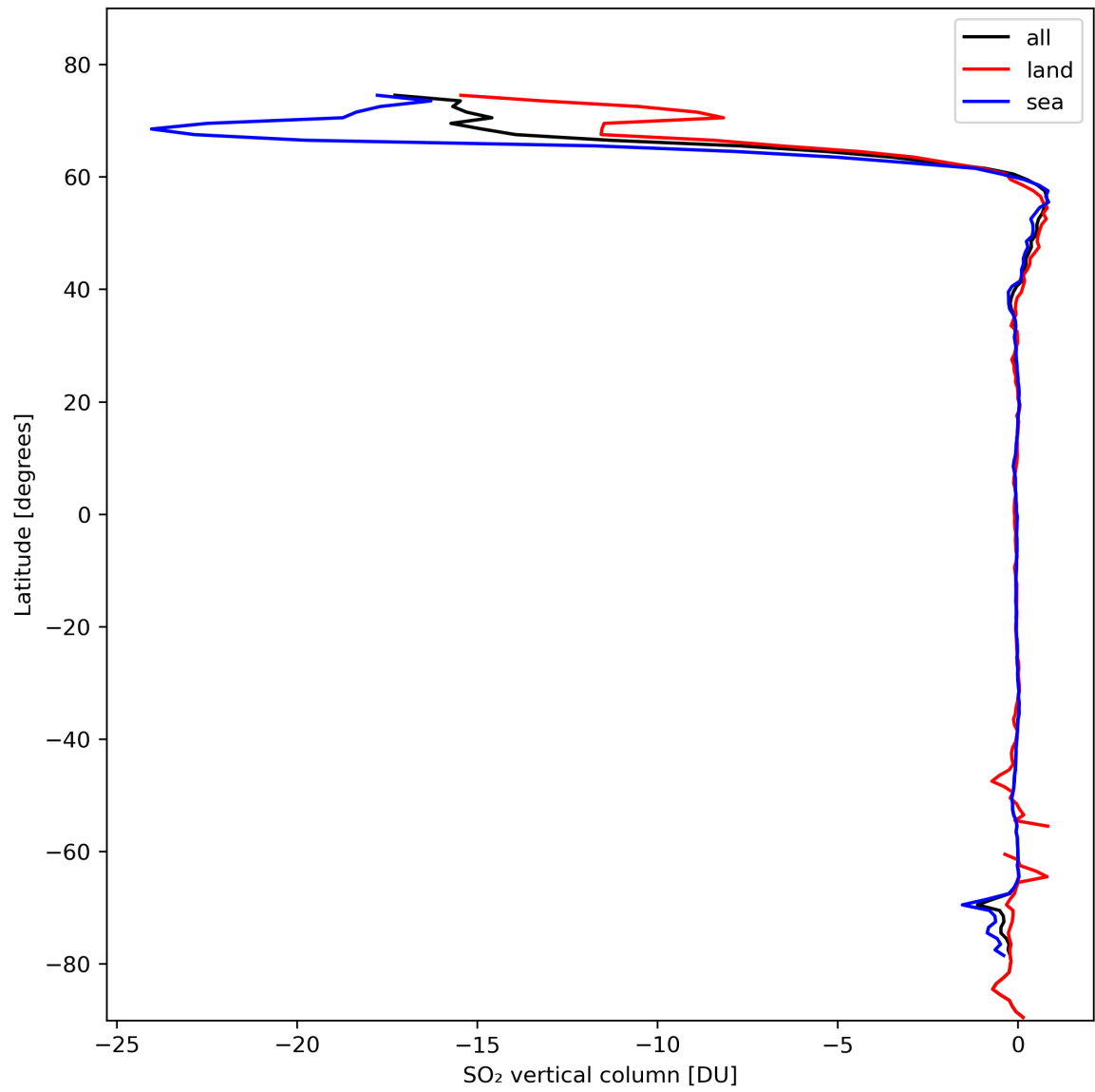
Figure 30: Zonal average of “SO 2 vertical column” for 2024-02-20 to 2024-02-22.
