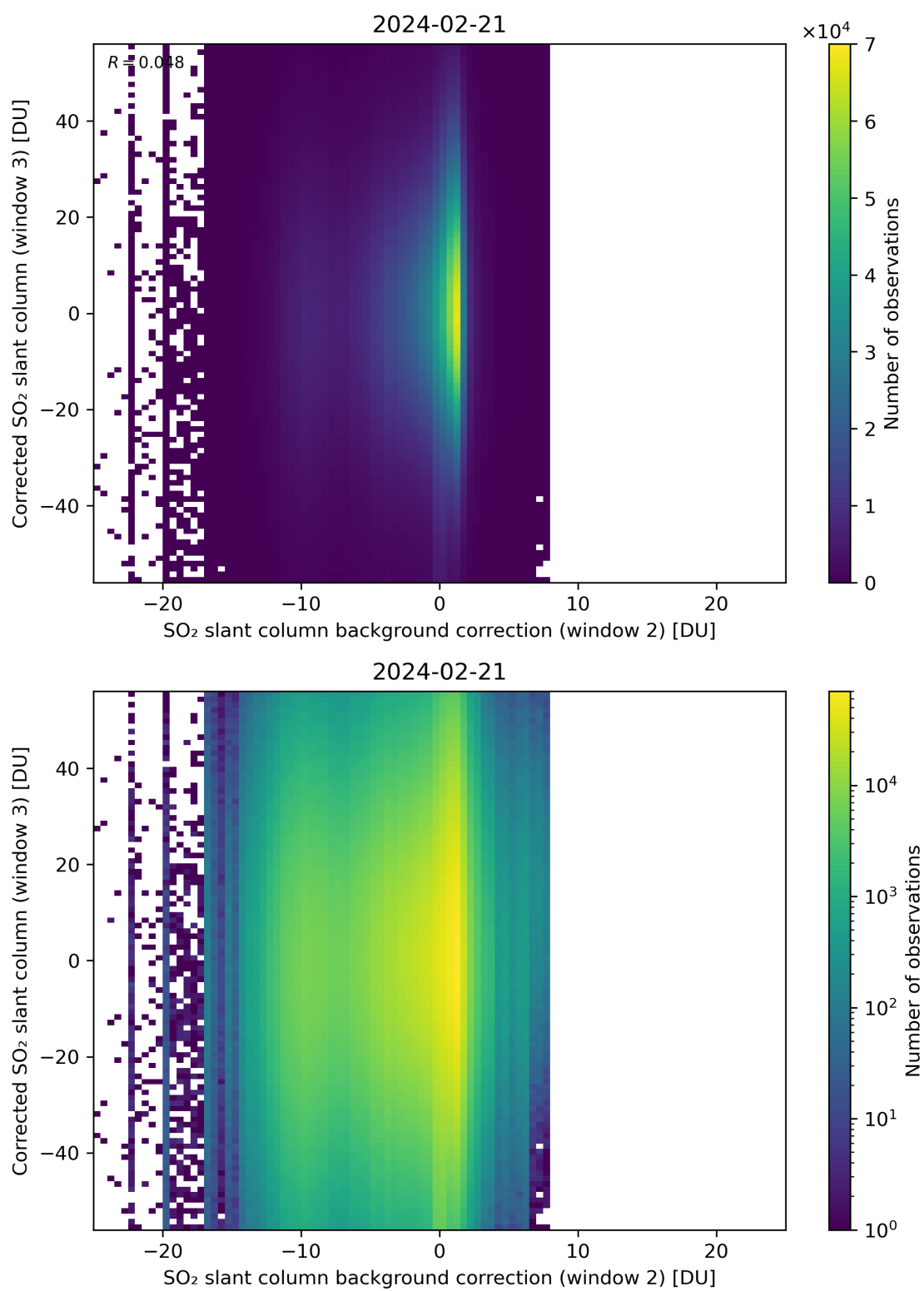
Figure 116: Scatter density plot of “SO 2 slant column background correction (window 2)” against “Corrected SO 2 slant column (window 3)” for 2024-02-20 to 2024-02-22.
