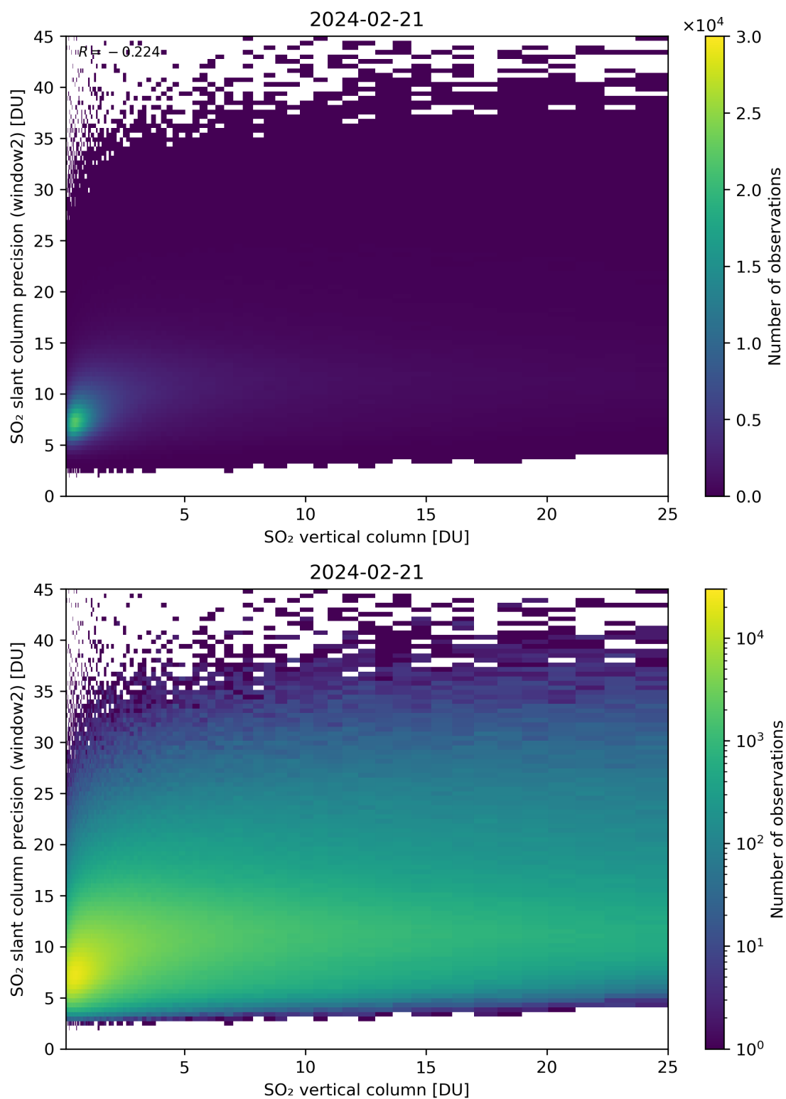
Figure 302: Scatter density plot of “SO 2 vertical column” against “SO 2 slant column precision (window2)” for 2024-02-20 to 2024-02-22.
