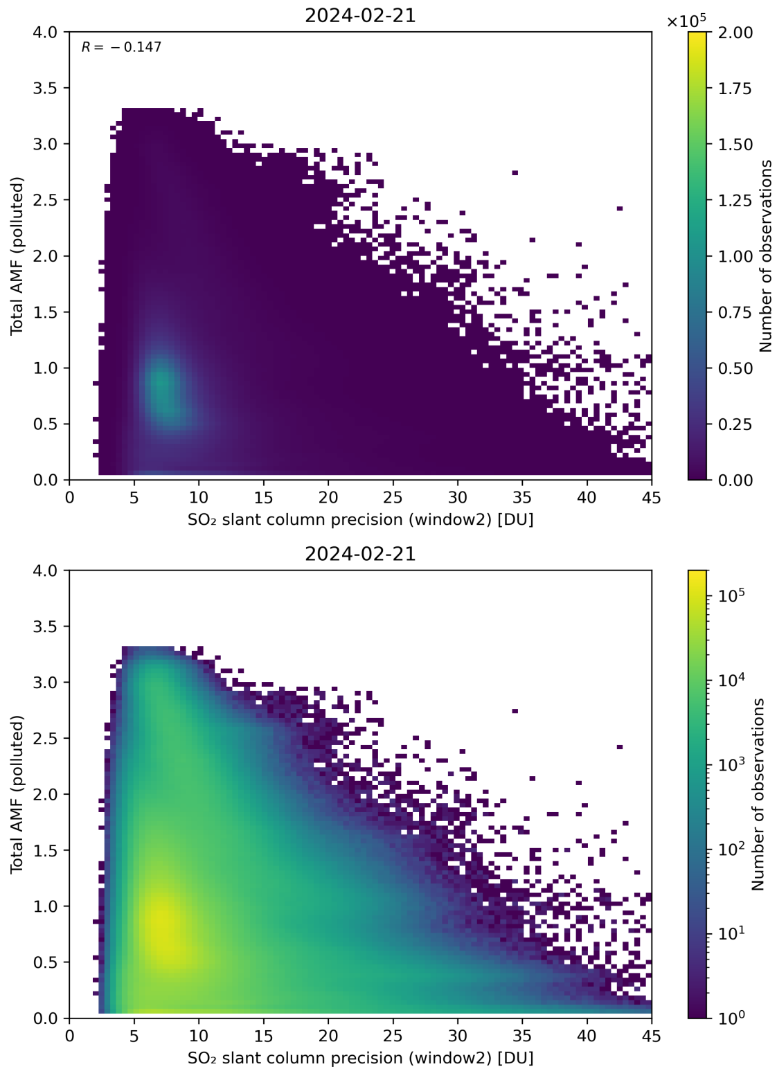
Figure 251: Scatter density plot of “SO 2 slant column precision (window2)” against “Total AMF (polluted)” for 2024-02-20 to 2024-02-22.
