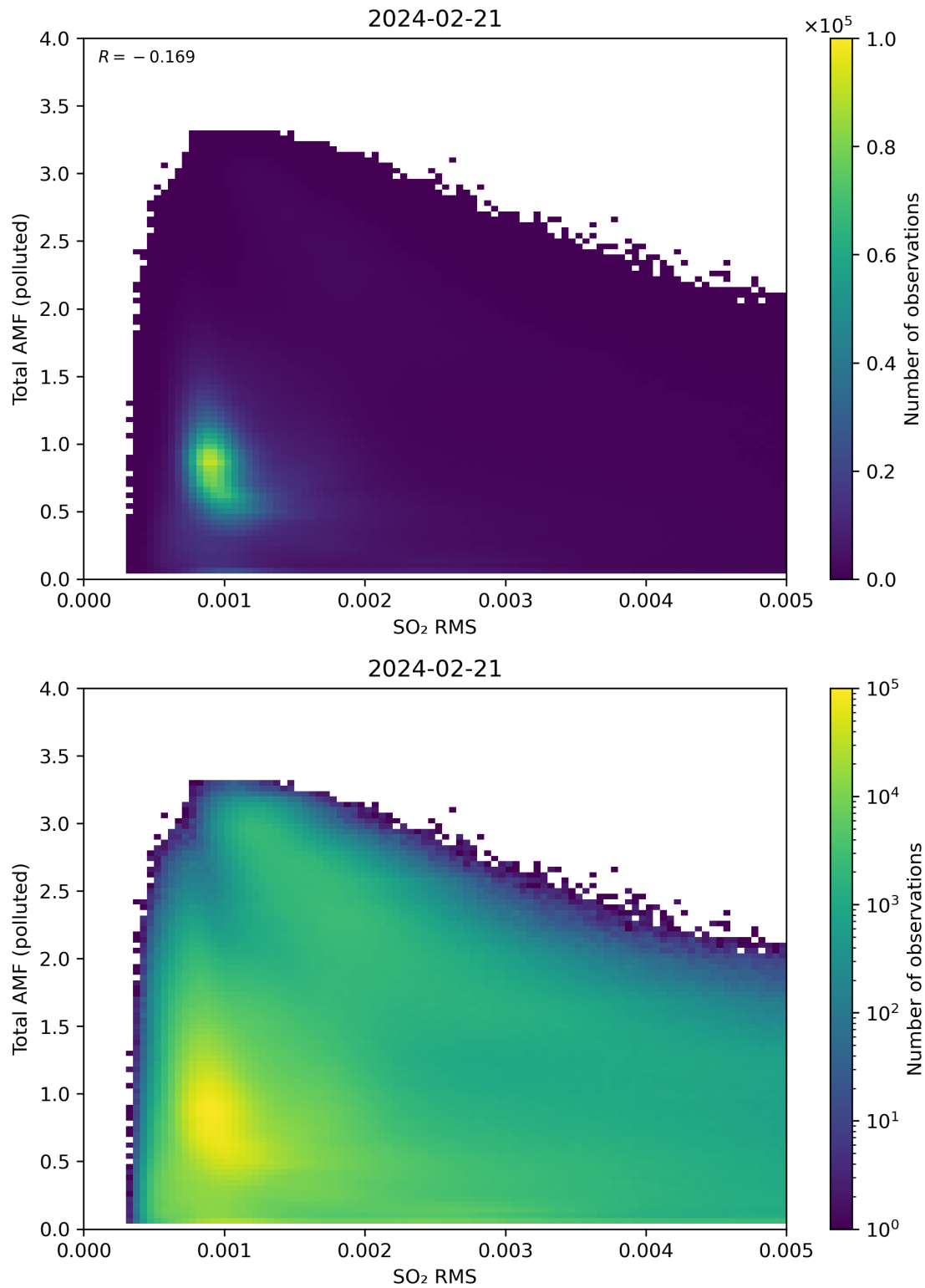
Figure 137: Scatter density plot of “SO 2 RMS” against “Total AMF (polluted)” for 2024-02-20 to 2024-02-22.
