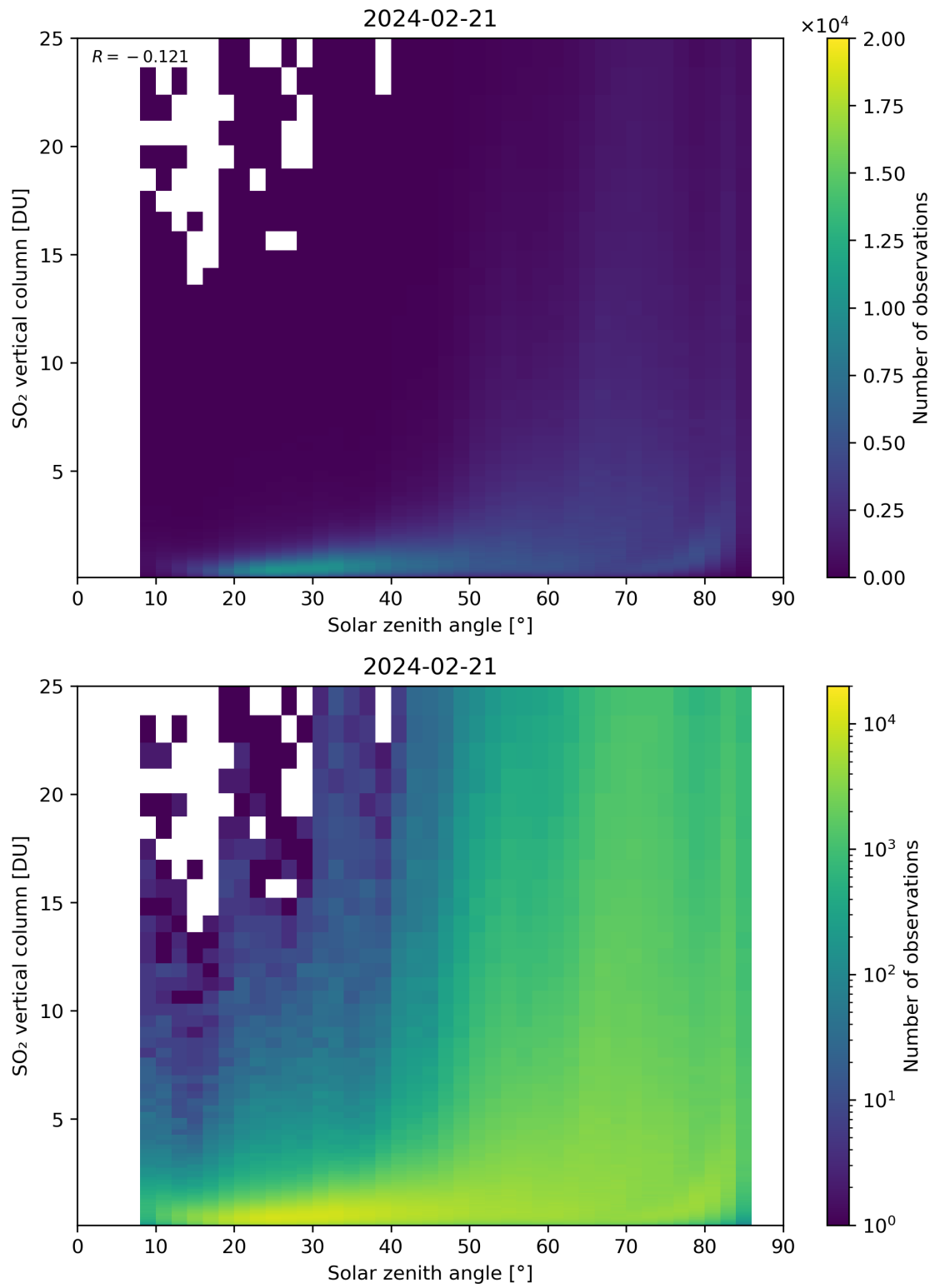
Figure 176: Scatter density plot of “Solar zenith angle” against “SO 2 vertical column” for 2024-02-20 to 2024-02-22.
