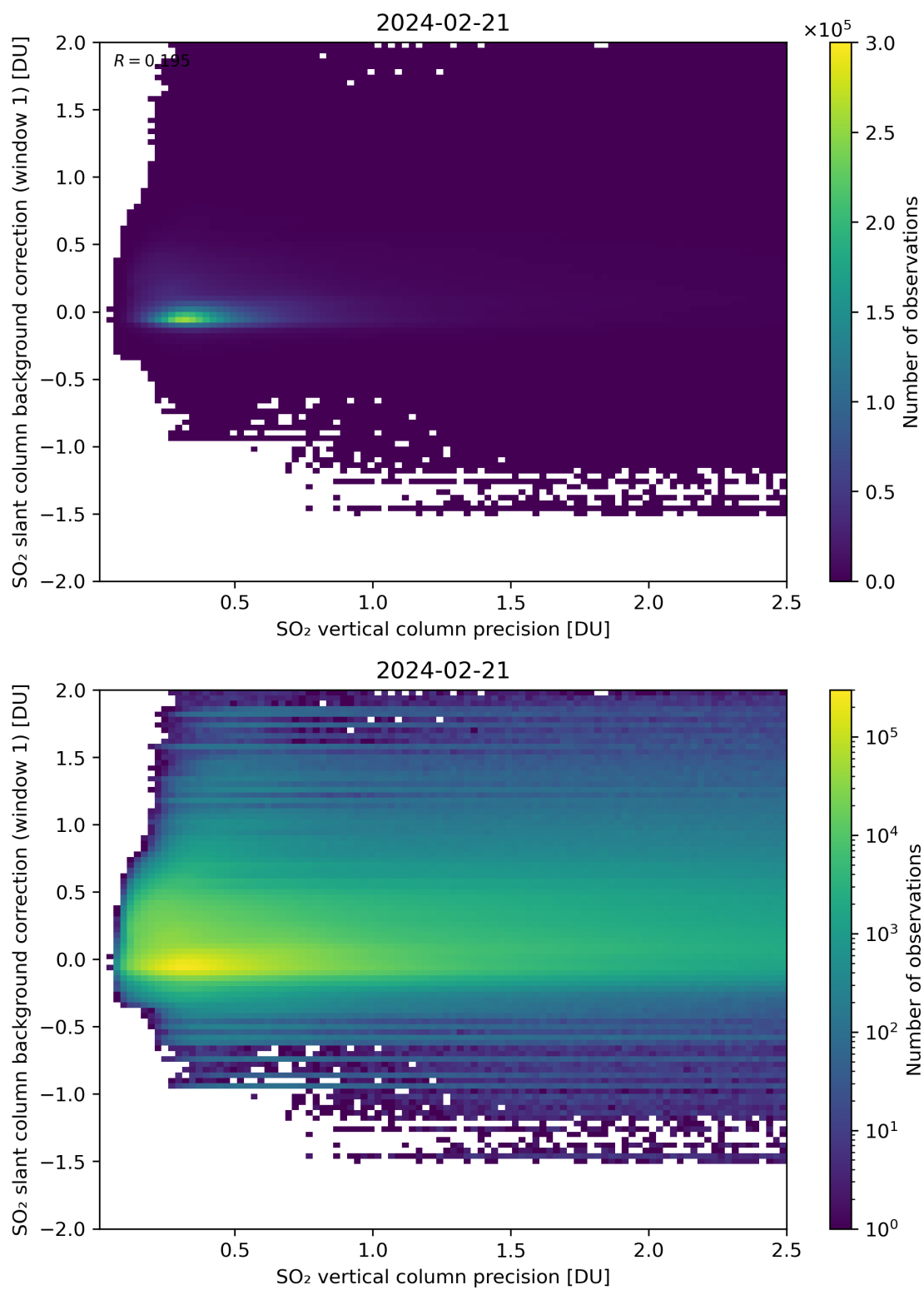
Figure 279: Scatter density plot of “SO 2 vertical column precision” against “SO 2 slant column background correction (window 1)” for 2024-02-20 to 2024-02-22.
