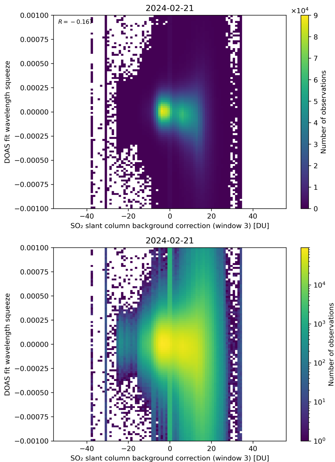
Figure 122: Scatter density plot of “SO 2 slant column background correction (window 3)” against “DOAS fit wavelength squeeze” for 2024-02-20 to 2024-02-22.
