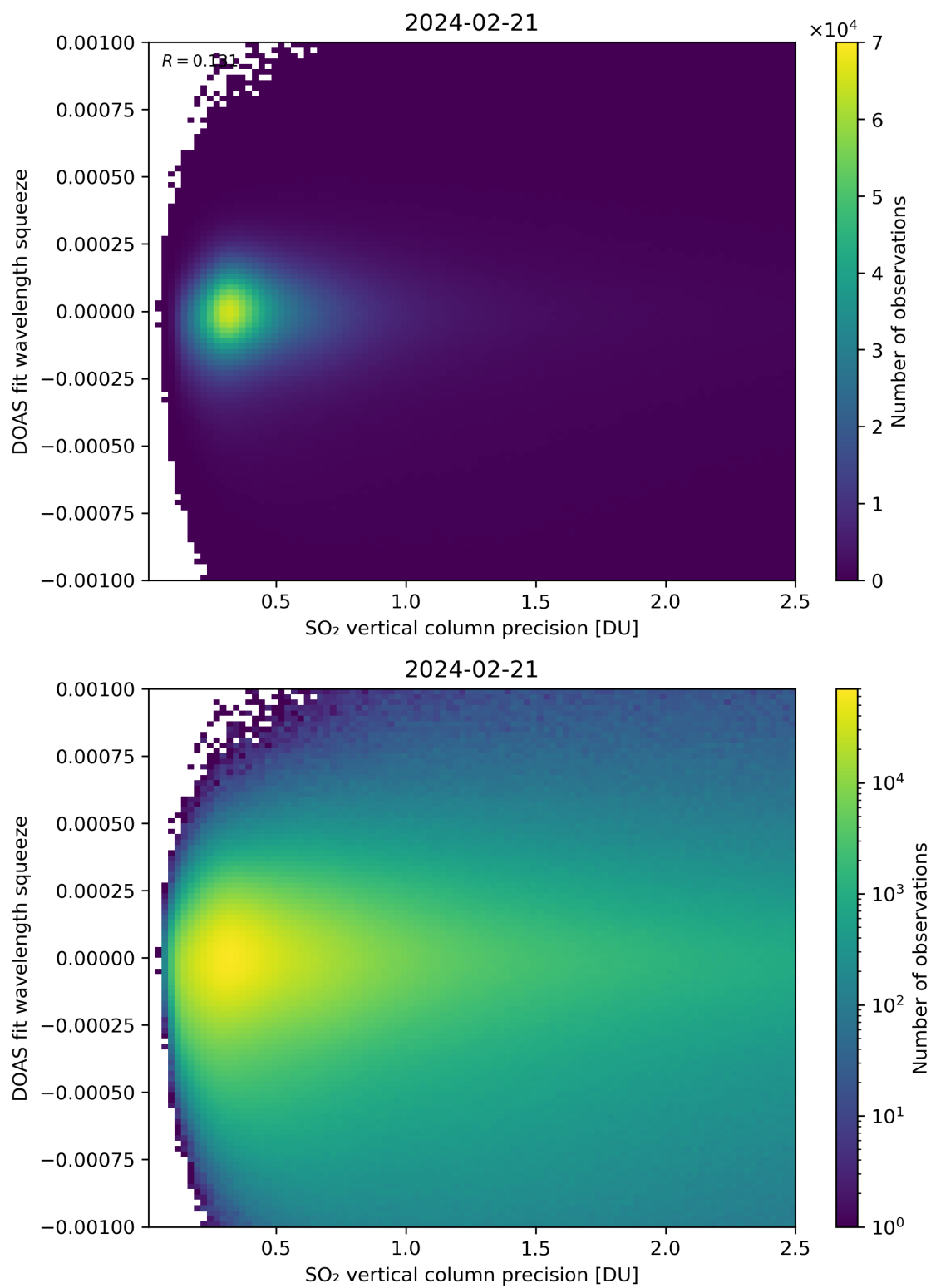
Figure 283: Scatter density plot of “SO 2 vertical column precision” against “DOAS fit wavelength squeeze” for 2024-02-20 to 2024-02-22.
