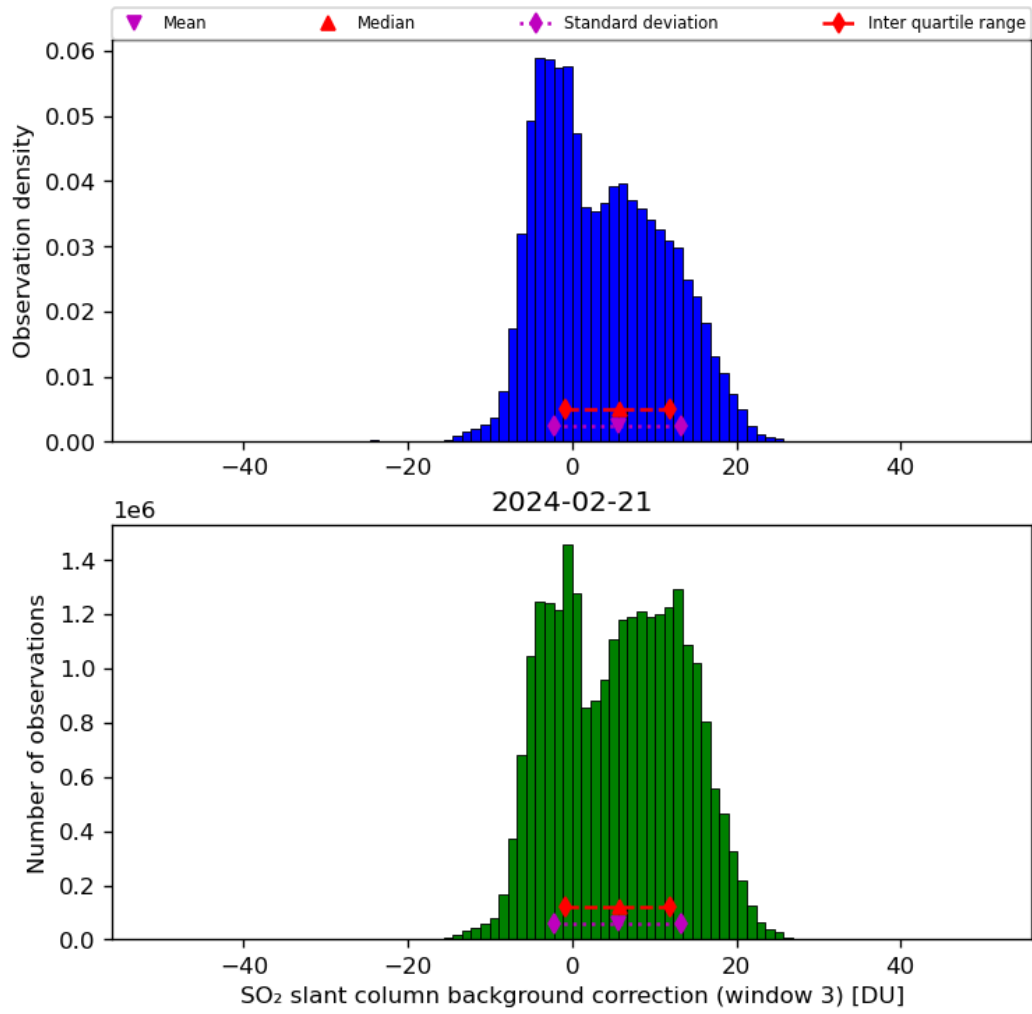
Figure 67: Histogram of “SO 2 slant column background correction (window 3)” for 2024-02-20 to 2024-02-22
