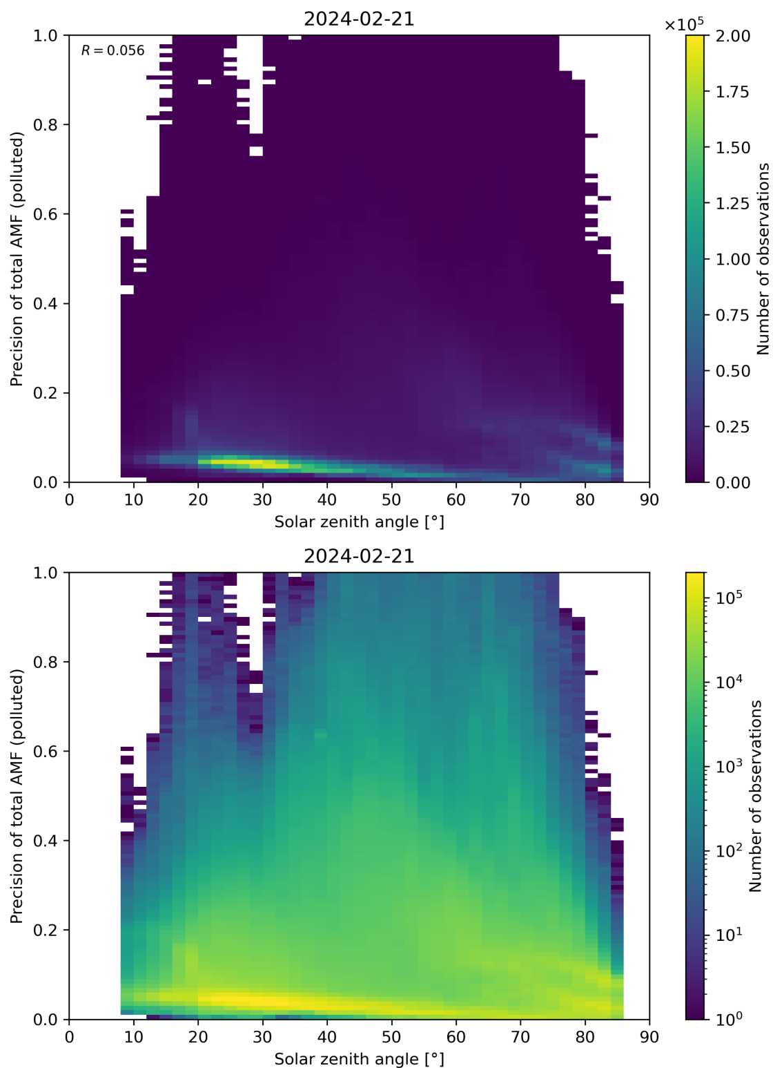
Figure 175: Scatter density plot of “Solar zenith angle” against “Precision of total AMF (polluted)” for 2024-02-20 to 2024-02-22.
