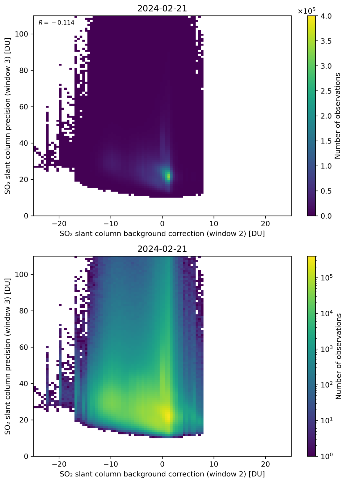
Figure 118: Scatter density plot of “SO 2 slant column background correction (window 2)” against “SO 2 slant column precision (window 3)” for 2024-02-20 to 2024-02-22.
