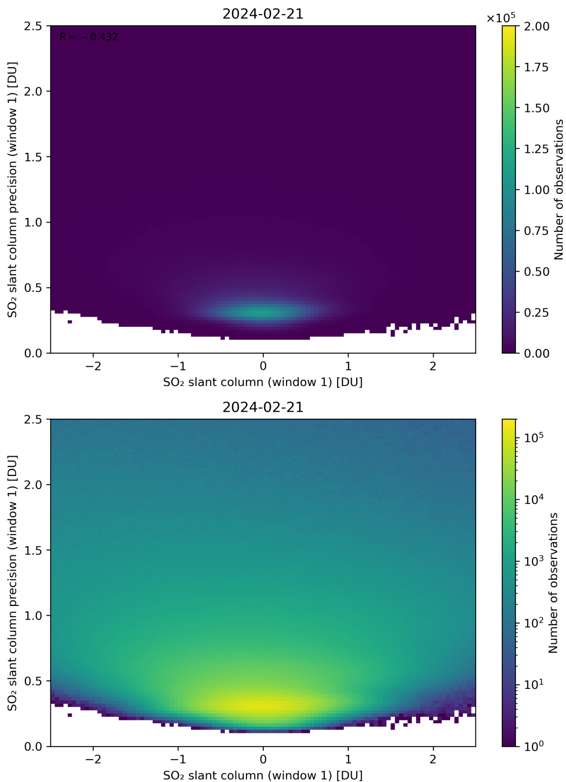
Figure 235: Scatter density plot of “SO 2 slant column (window 1)” against “SO 2 slant column precision (window 1)” for 2024-02-20 to 2024-02-22.
