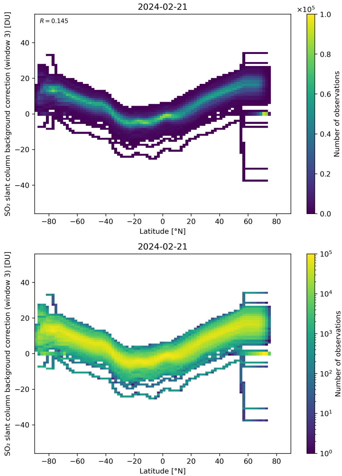
Figure 141: Scatter density plot of “Latitude” against “SO 2 slant column background correction (window 3)” for 2024-02-20 to 2024-02-22.
