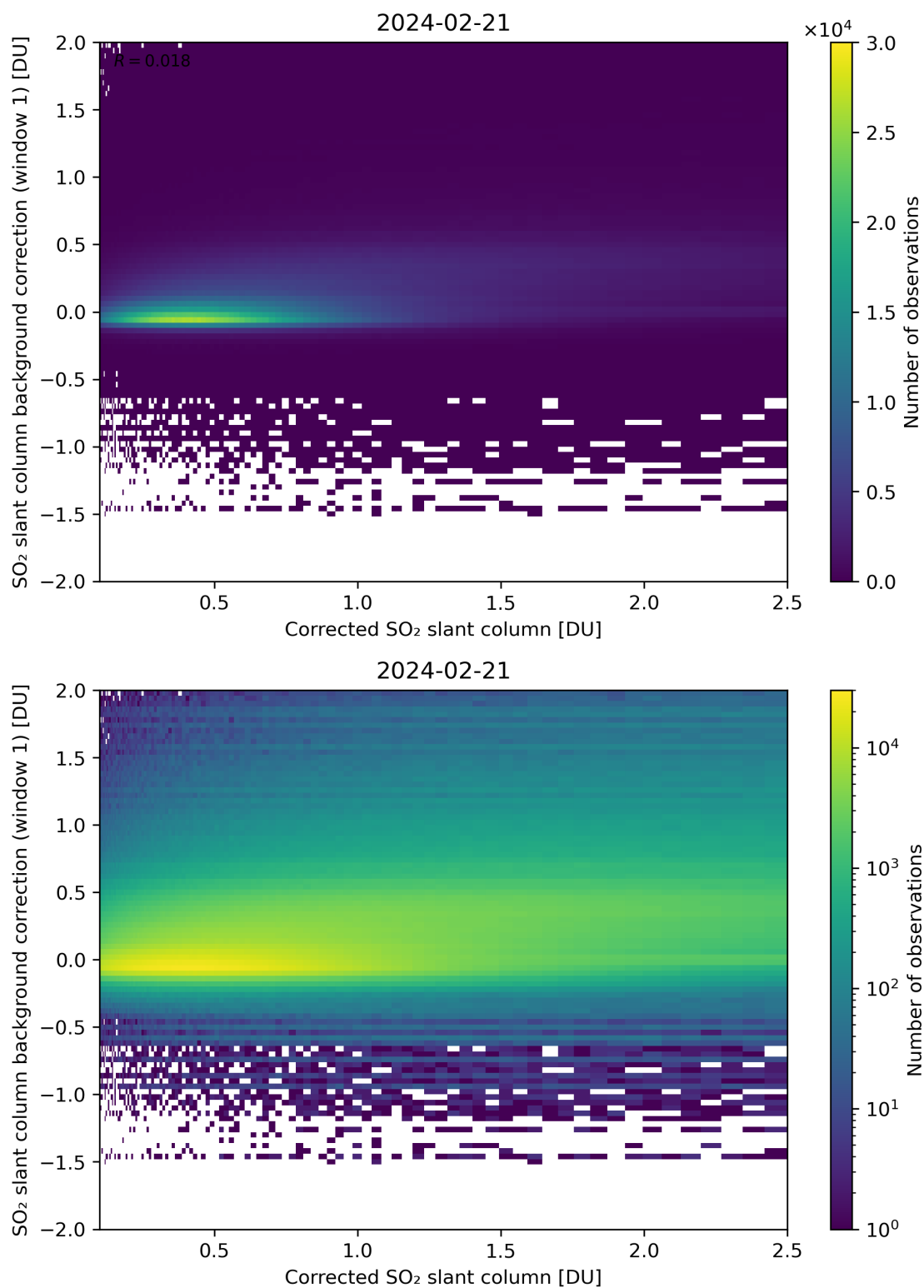
Figure 178: Scatter density plot of “Corrected SO 2 slant column” against “SO 2 slant column background correction (window 1)” for 2024-02-20 to 2024-02-22.
