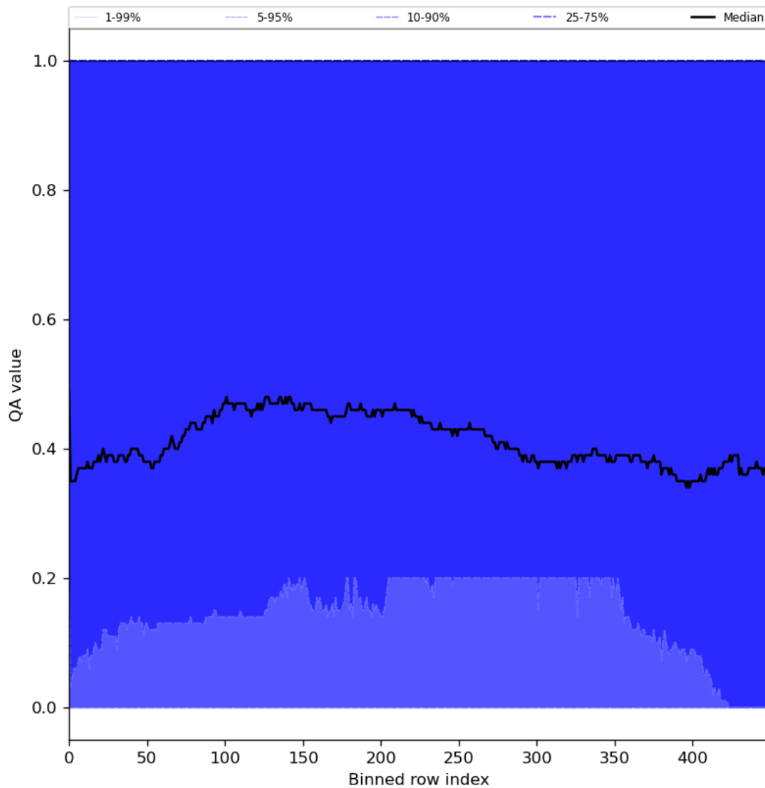
Figure 75: Along track statistics of “QA value” for 2024-02-20 to 2024-02-22
