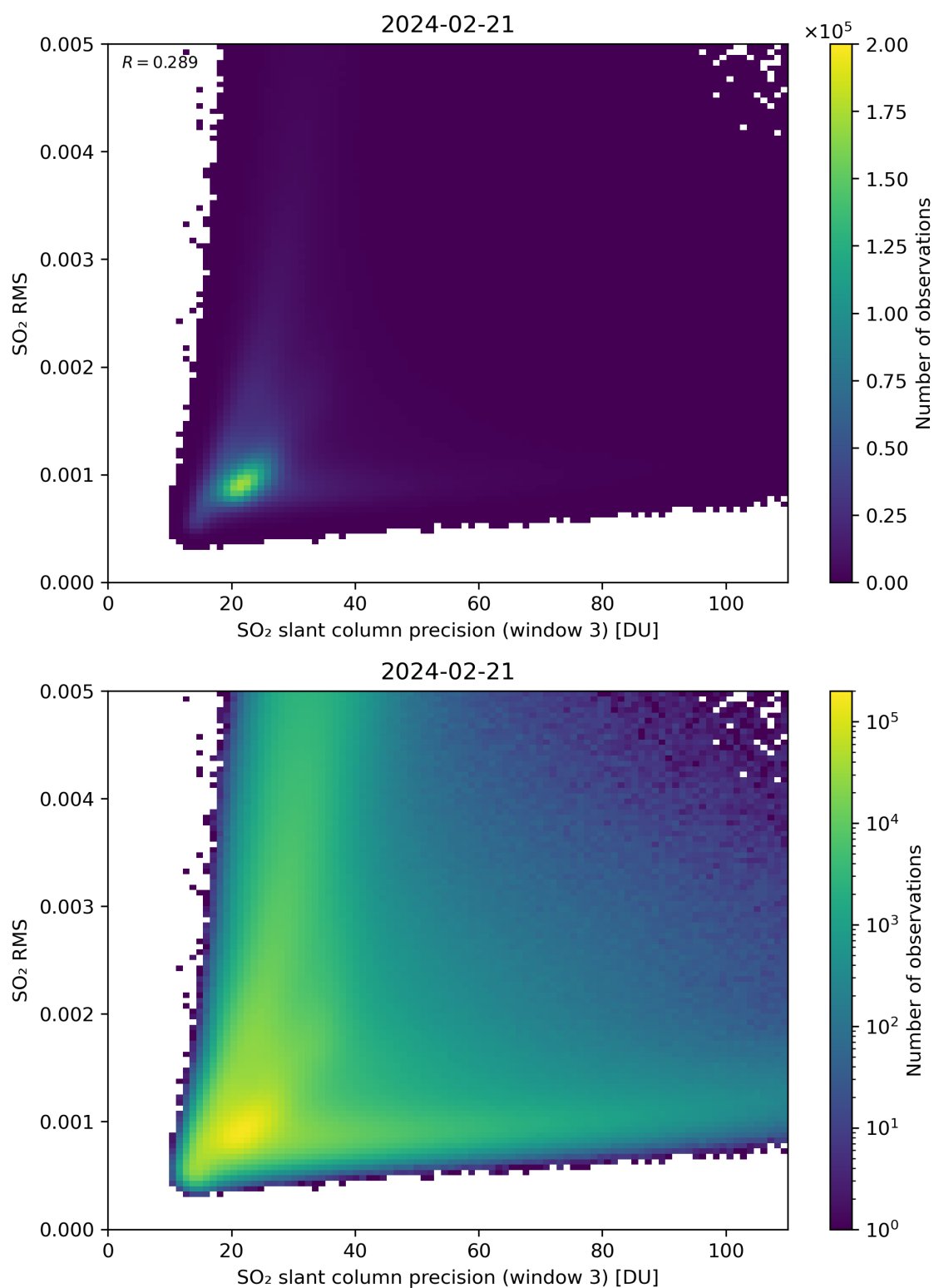
Figure 260: Scatter density plot of “SO 2 slant column precision (window 3)” against “SO 2 RMS” for 2024-02-20 to 2024-02-22.
