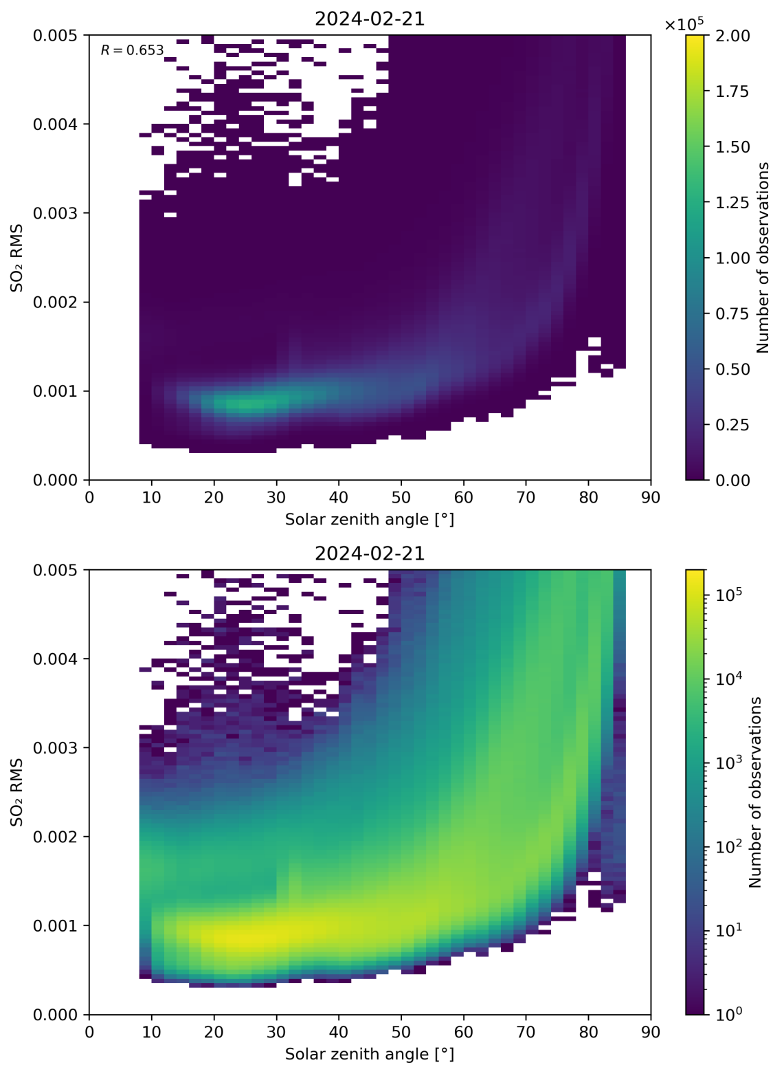
Figure 163: Scatter density plot of “Solar zenith angle” against “SO 2 RMS” for 2024-02-20 to 2024-02-22.
