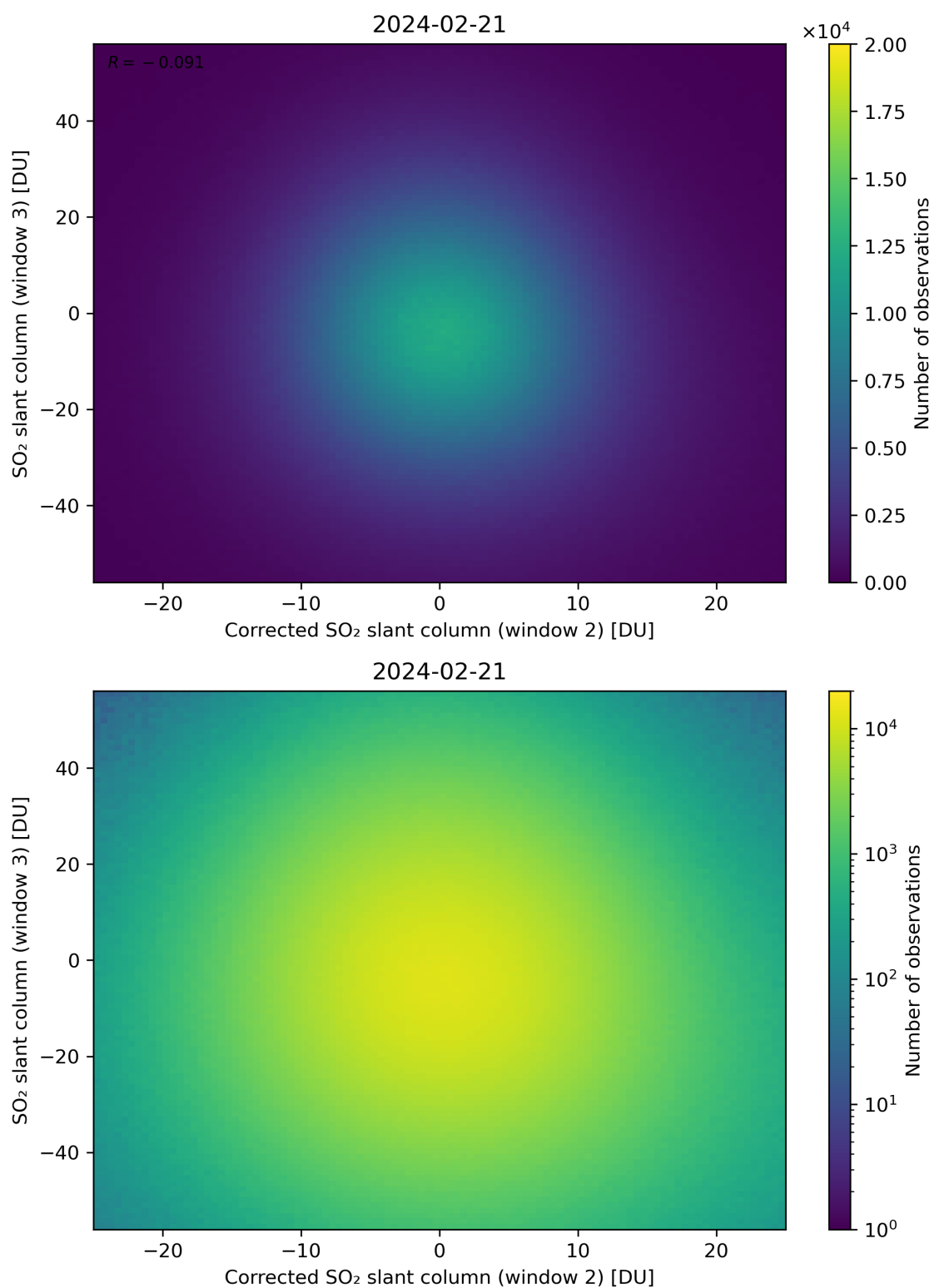
Figure 201: Scatter density plot of “Corrected SO 2 slant column (window 2)” against “SO 2 slant column (window 3)” for 2024-02-20 to 2024-02-22.
