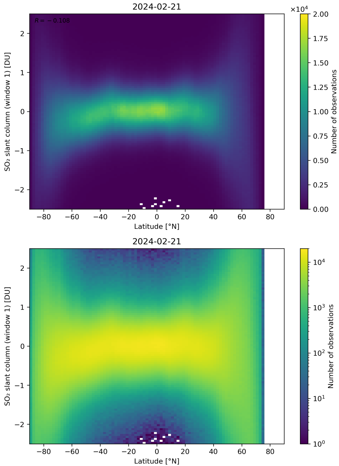
Figure 149: Scatter density plot of “Latitude” against “SO 2 slant column (window 1)” for 2024-02-20 to 2024-02-22.
