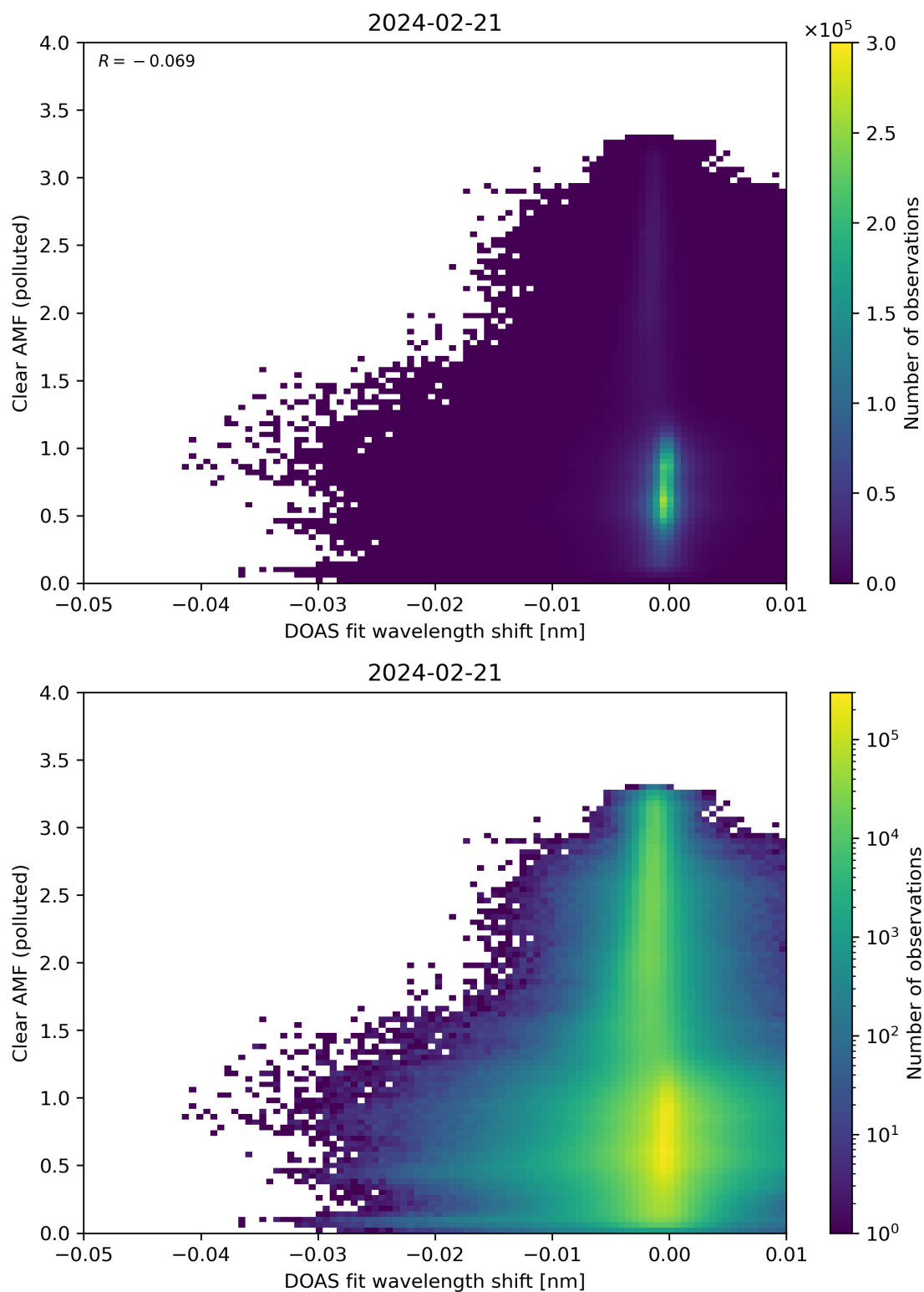
Figure 129: Scatter density plot of “DOAS fit wavelength shift” against “Clear AMF (polluted)” for 2024-02-20 to 2024-02-22.
