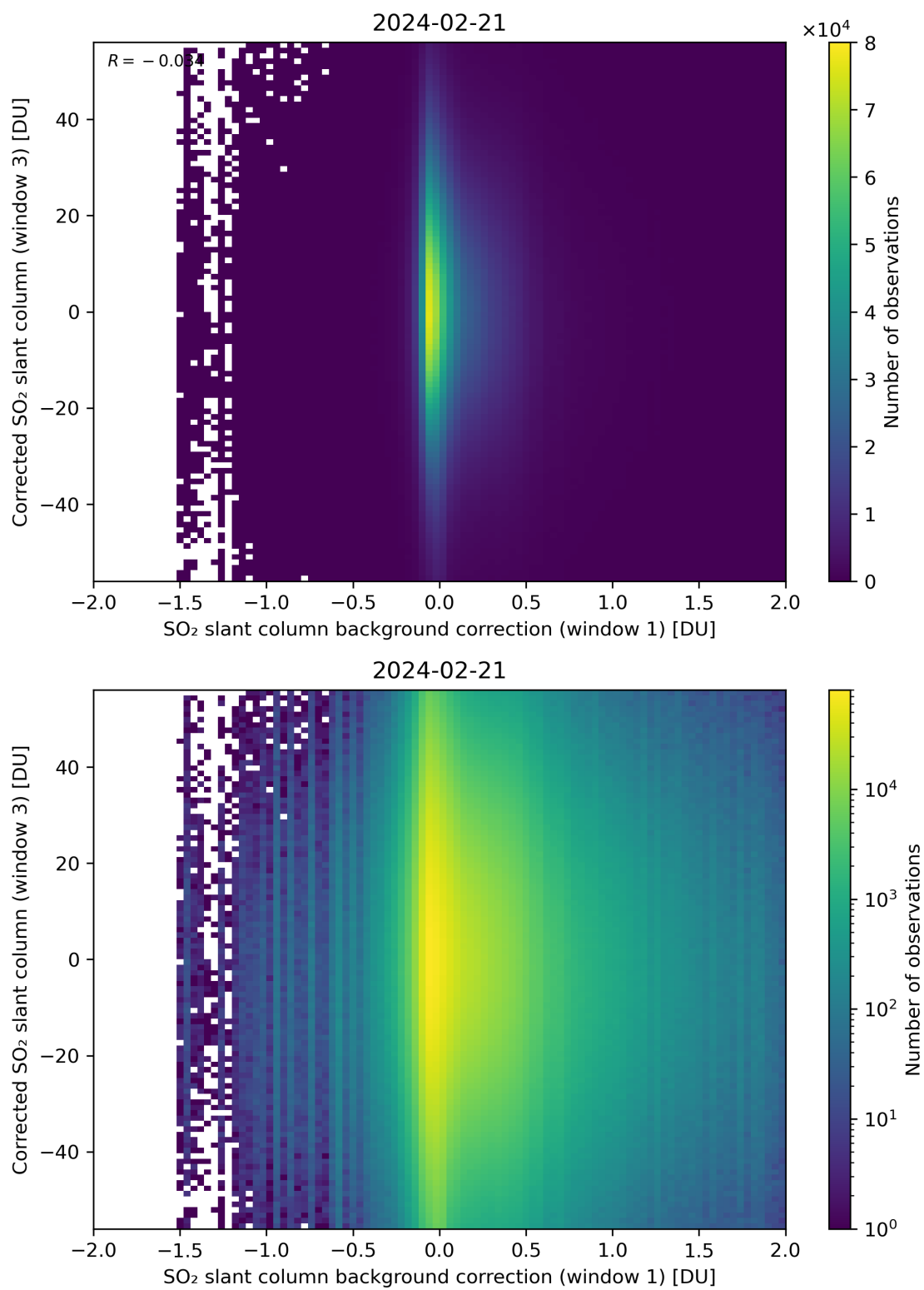
Figure 105: Scatter density plot of “SO 2 slant column background correction (window 1)” against “Corrected SO 2 slant column (window 3)” for 2024-02-20 to 2024-02-22.
