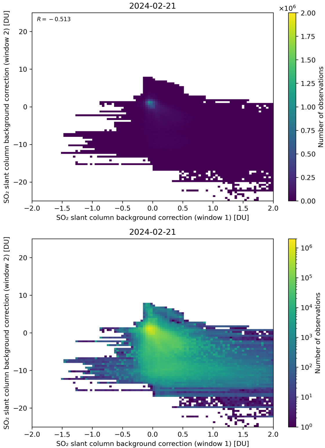
Figure 98: Scatter density plot of “SO 2 slant column background correction (window 1)” against “SO 2 slant column background correction (window 2)” for 2024-02-20 to 2024-02-22.
