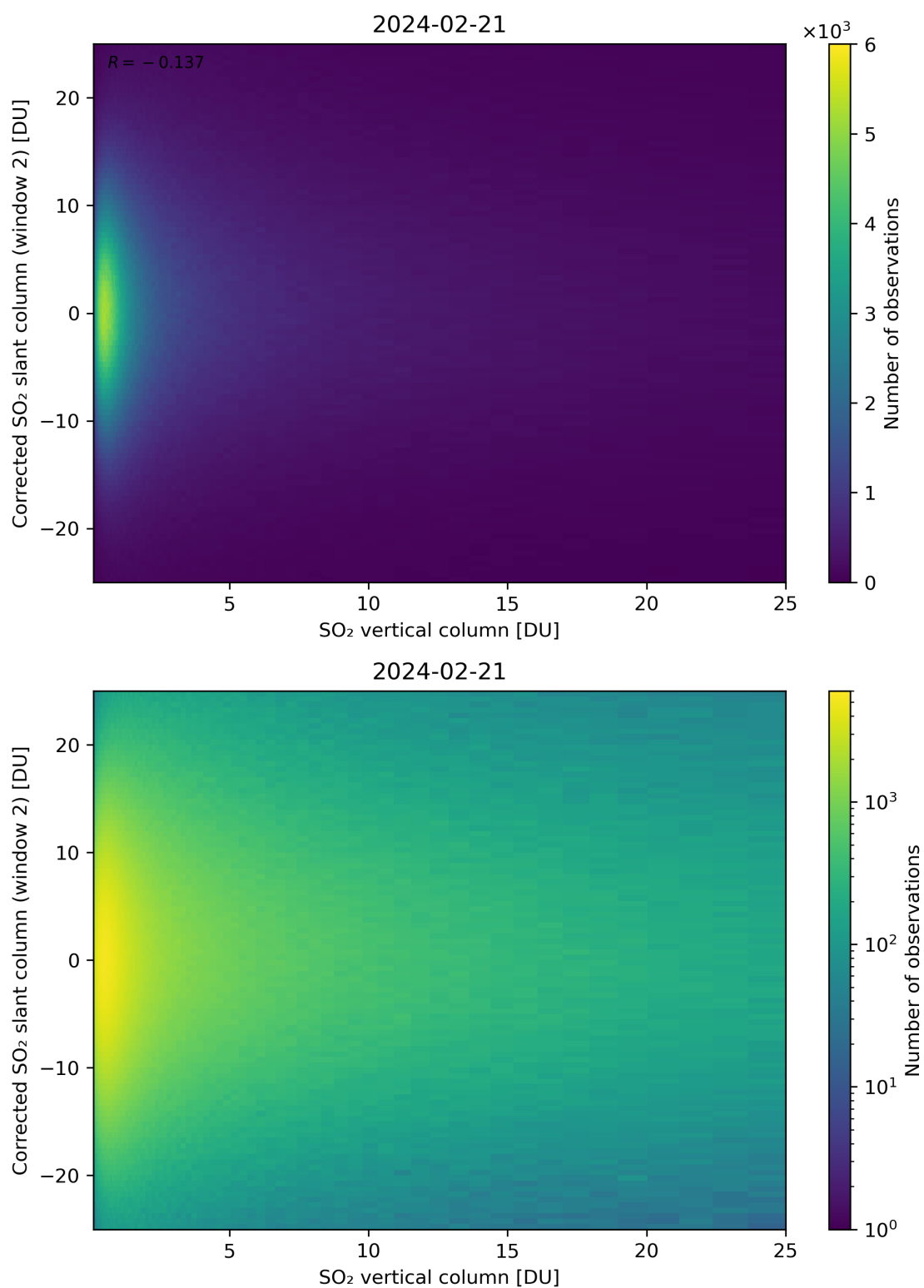
Figure 298: Scatter density plot of “SO 2 vertical column” against “Corrected SO 2 slant column (window 2)” for 2024-02-20 to 2024-02-22.
