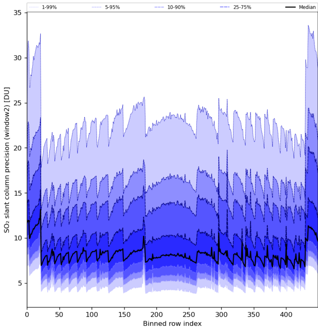
Figure 84: Along track statistics of “SO 2 slant column precision (window2)” for 2024-02-20 to 2024-02-22
