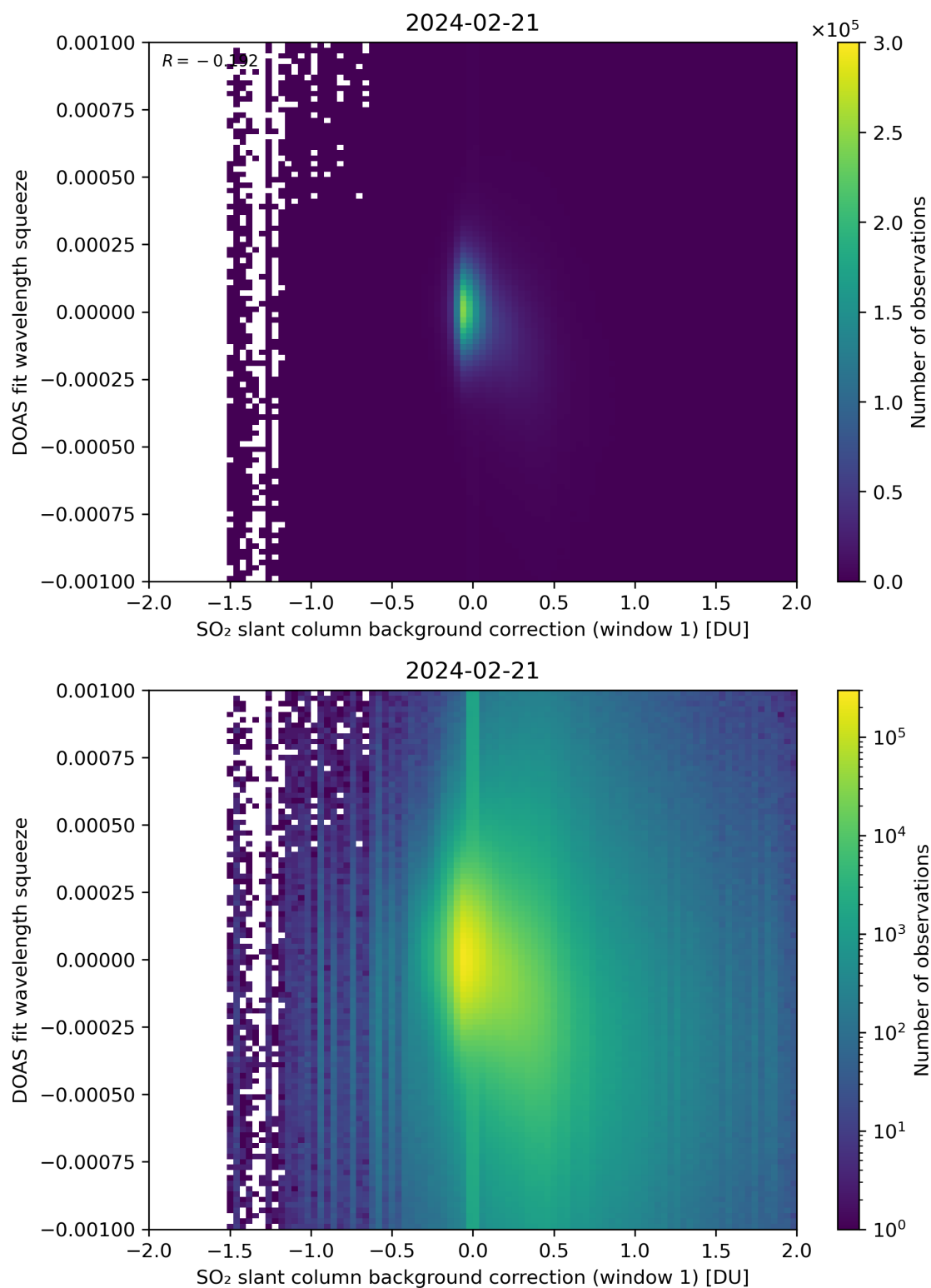
Figure 101: Scatter density plot of “SO 2 slant column background correction (window 1)” against “DOAS fit wavelength squeeze” for 2024-02-20 to 2024-02-22.
