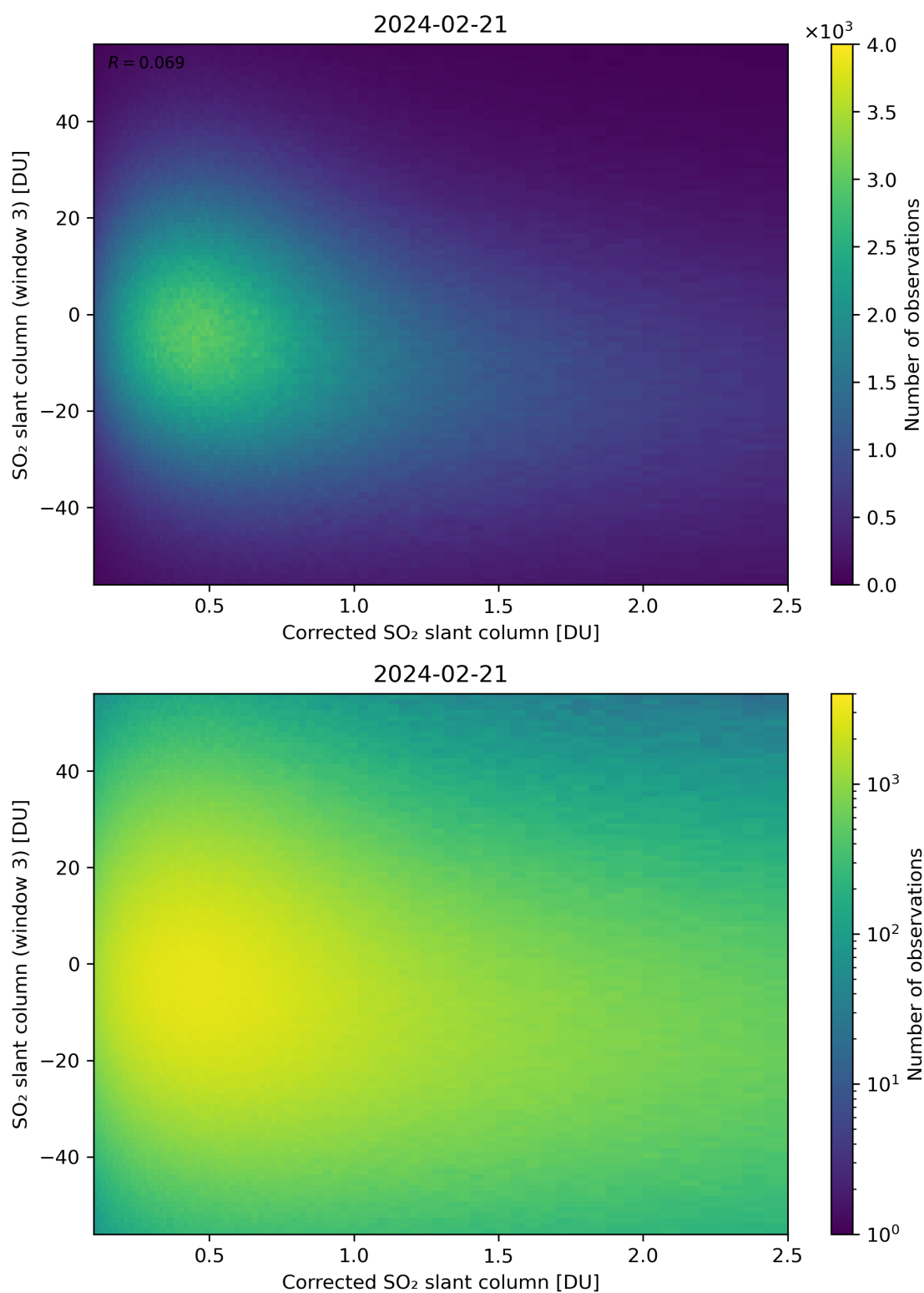
Figure 190: Scatter density plot of “Corrected SO 2 slant column” against “SO 2 slant column (window 3)” for 2024-02-20 to 2024-02-22.
