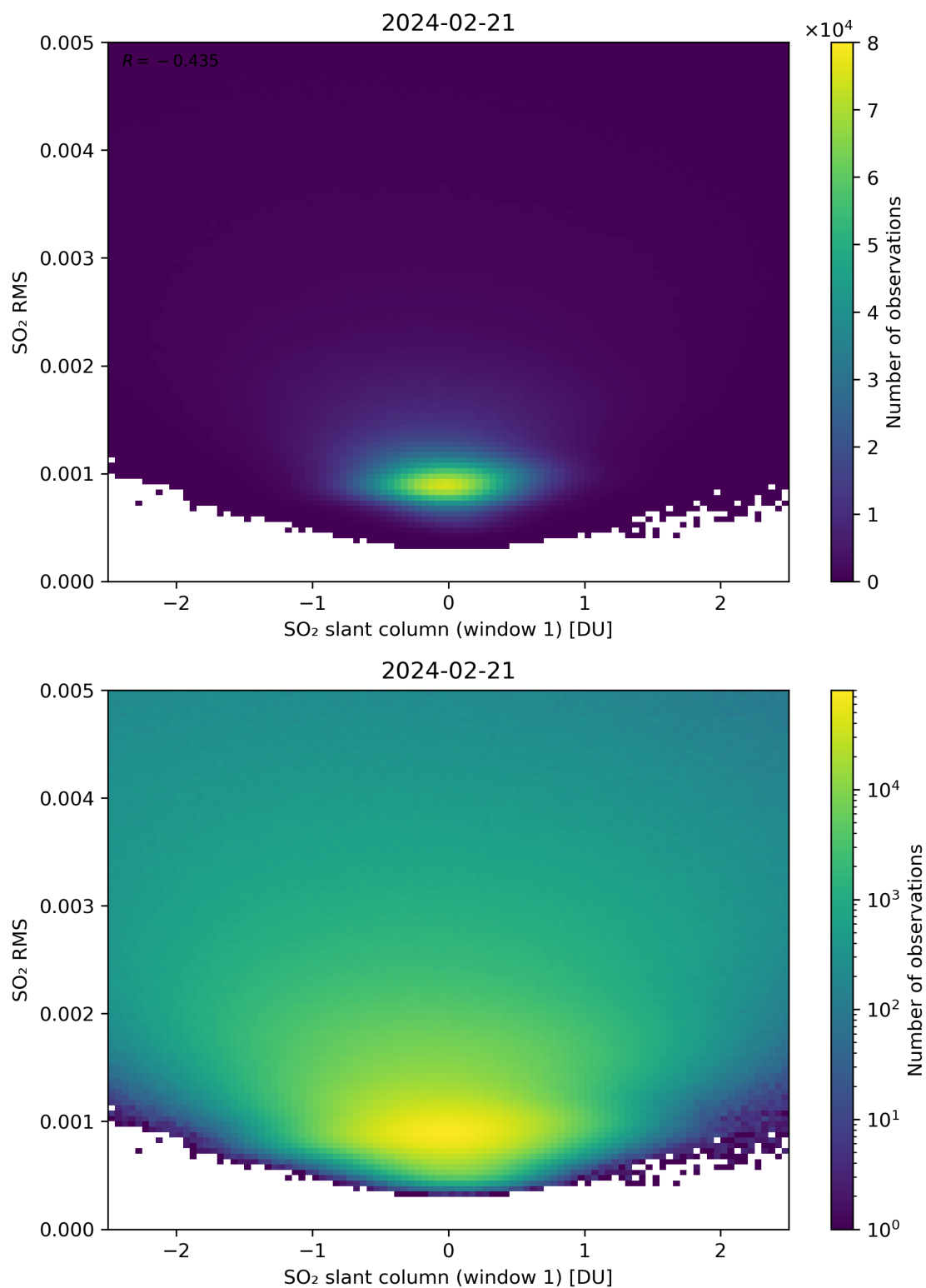
Figure 217: Scatter density plot of “SO 2 slant column (window 1)” against “SO 2 RMS” for 2024-02-20 to 2024-02-22.
