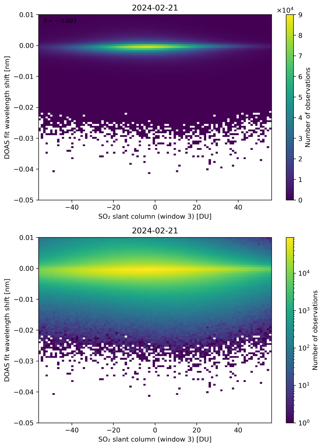
Figure 254: Scatter density plot of “SO 2 slant column (window 3)” against “DOAS fit wavelength shift” for 2024-02-20 to 2024-02-22.
