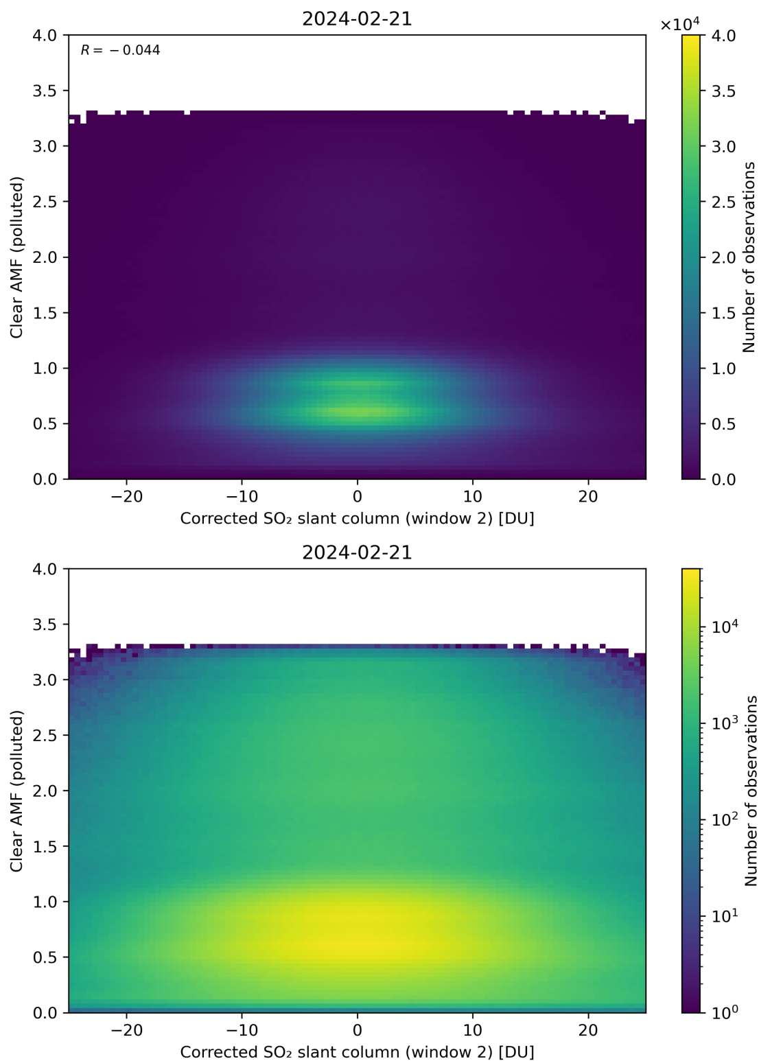
Figure 199: Scatter density plot of “Corrected SO 2 slant column (window 2)” against “Clear AMF (polluted)” for 2024-02-20 to 2024-02-22.
