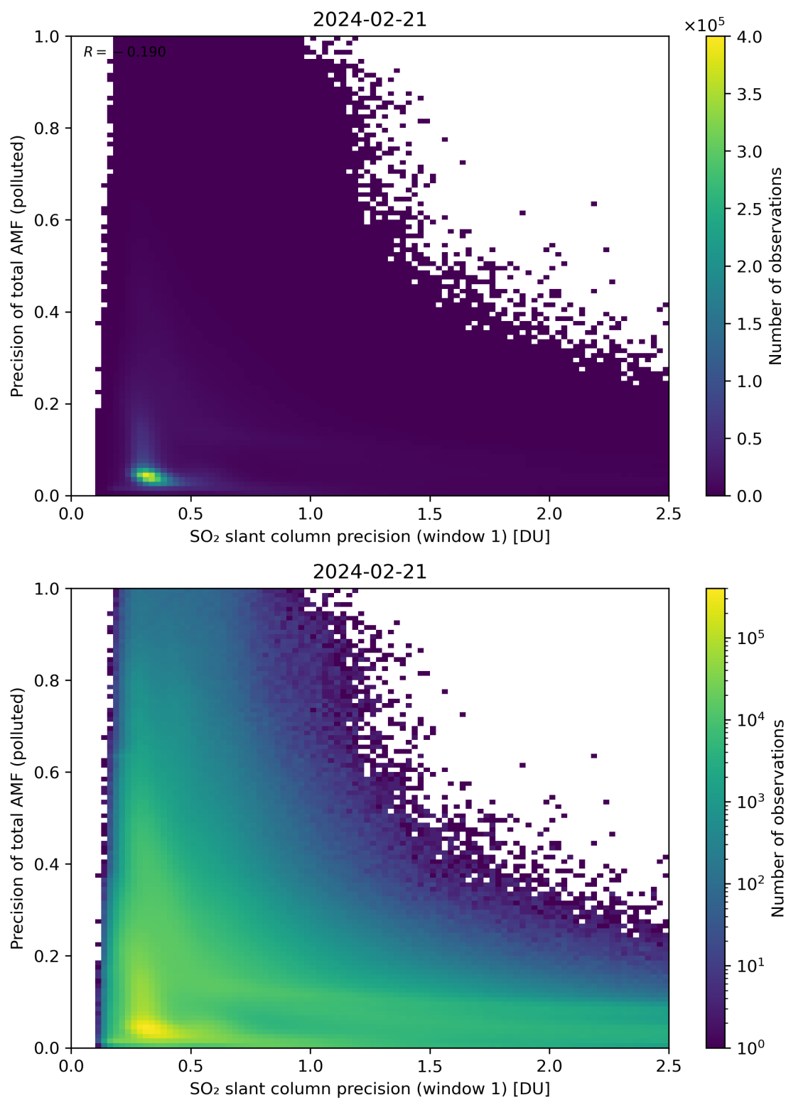
Figure 231: Scatter density plot of “SO 2 slant column precision (window 1)” against “Precision of total AMF (polluted)” for 2024-02-20 to 2024-02-22.
