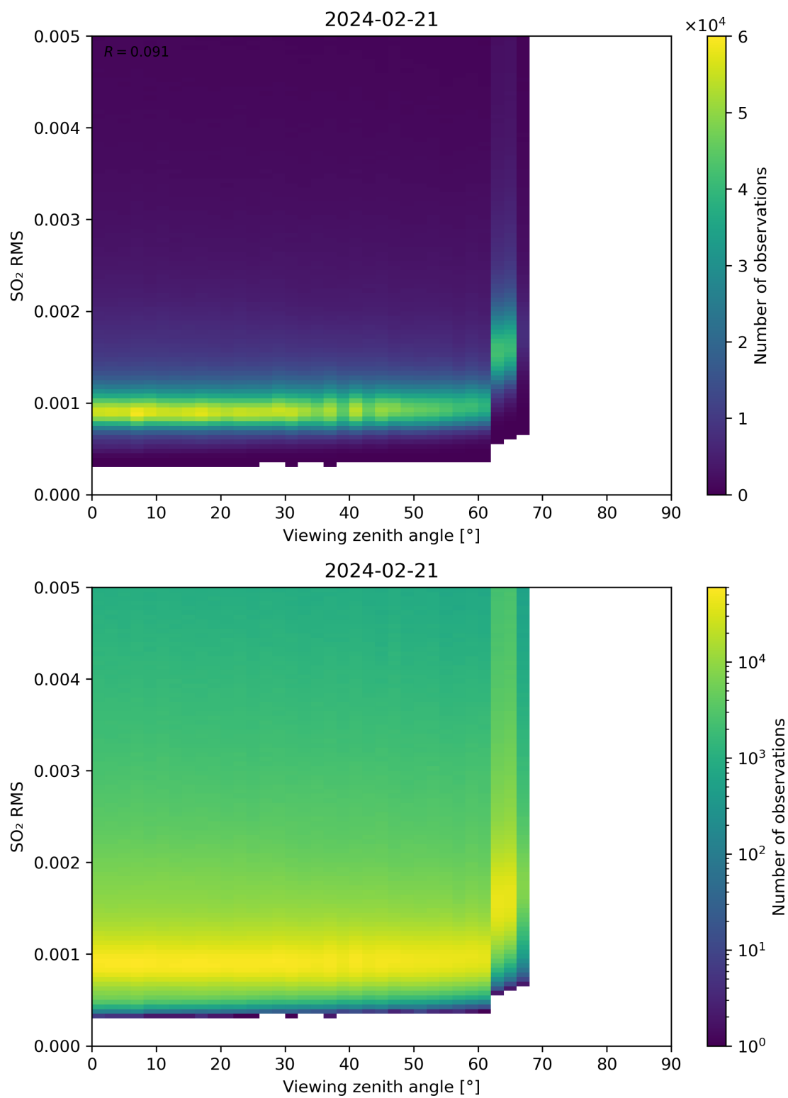
Figure 313: Scatter density plot of “Viewing zenith angle” against “SO 2 RMS” for 2024-02-20 to 2024-02-22.
