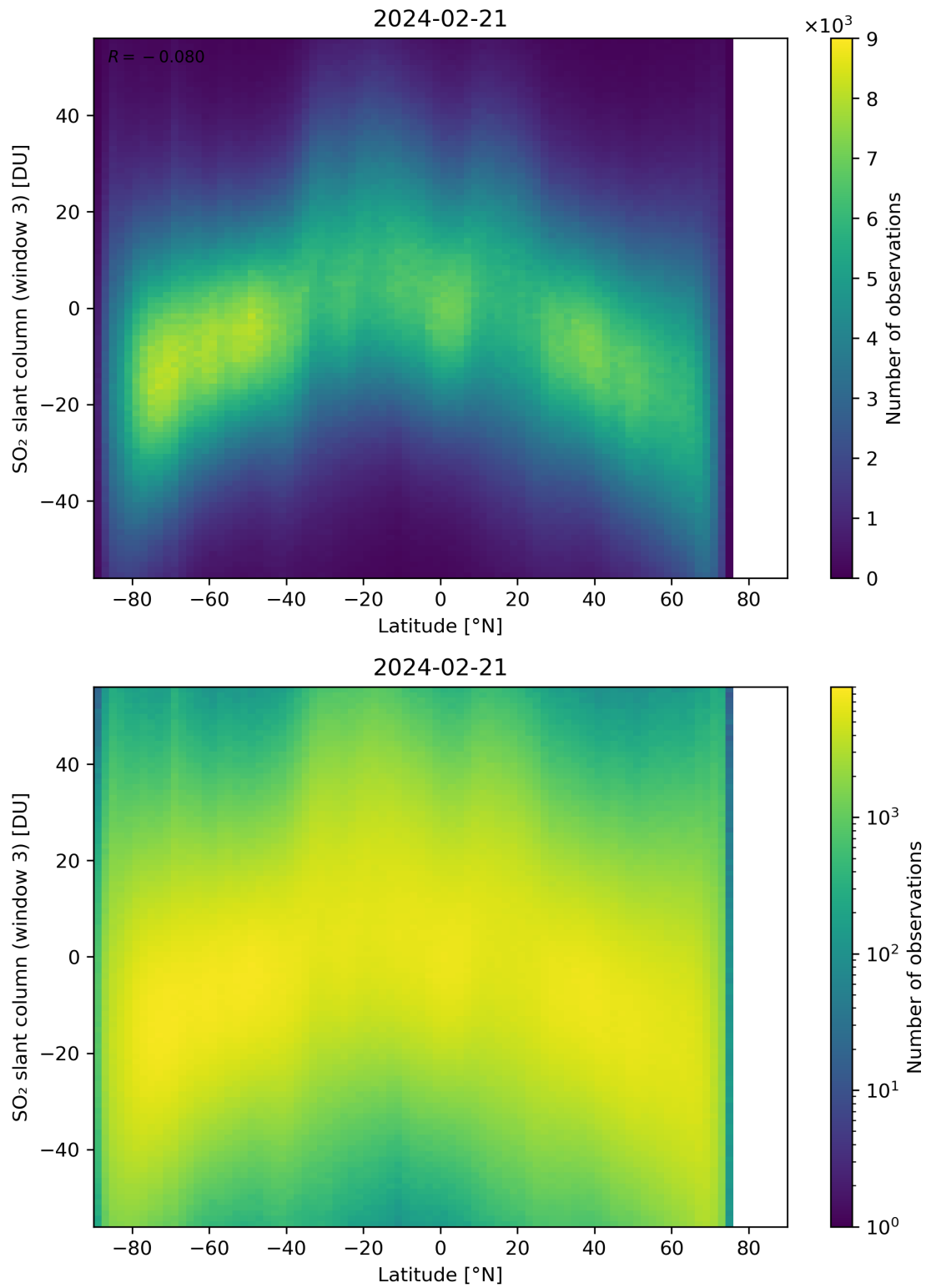
Figure 152: Scatter density plot of “Latitude” against “SO 2 slant column (window 3)” for 2024-02-20 to 2024-02-22.
