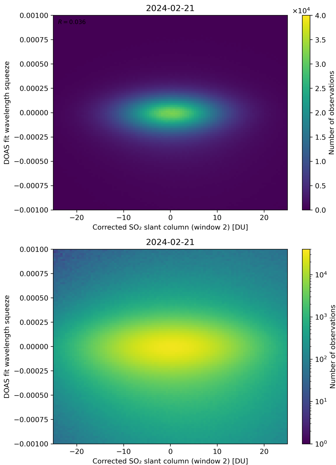
Figure 197: Scatter density plot of “Corrected SO 2 slant column (window 2)” against “DOAS fit wavelength squeeze” for 2024-02-20 to 2024-02-22.
