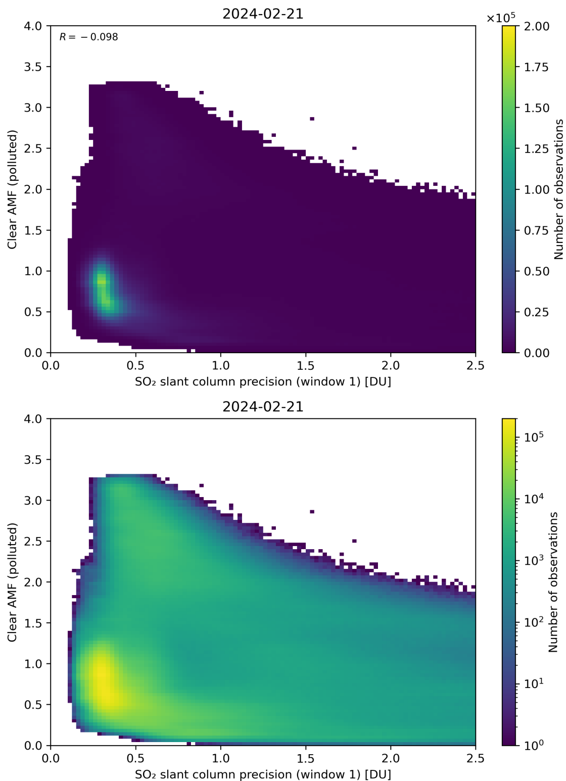
Figure 224: Scatter density plot of “SO 2 slant column precision (window 1)” against “Clear AMF (polluted)” for 2024-02-20 to 2024-02-22.
