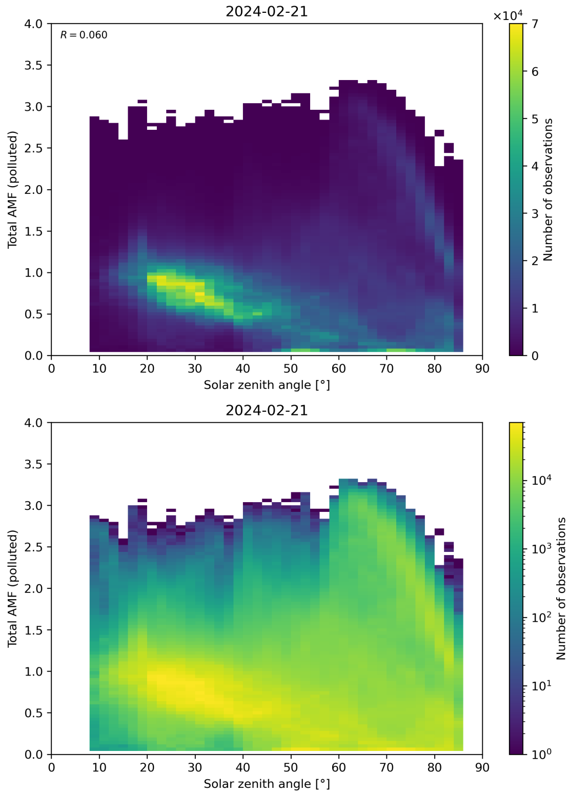
Figure 174: Scatter density plot of “Solar zenith angle” against “Total AMF (polluted)” for 2024-02-20 to 2024-02-22.
