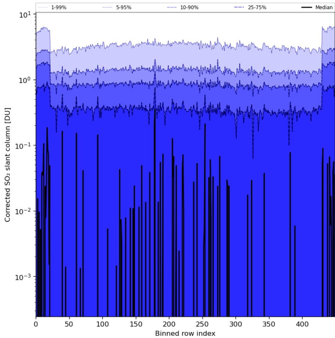
Figure 78: Along track statistics of “Corrected SO 2 slant column” for 2024-02-20 to 2024-02-22
