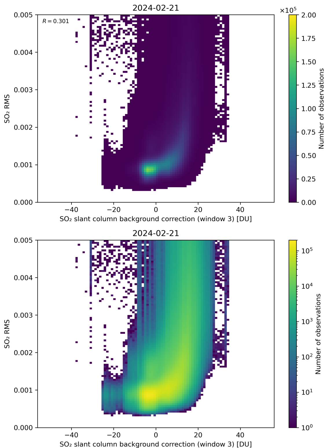
Figure 123: Scatter density plot of “SO 2 slant column background correction (window 3)” against “SO 2 RMS” for 2024-02-20 to 2024-02-22.
