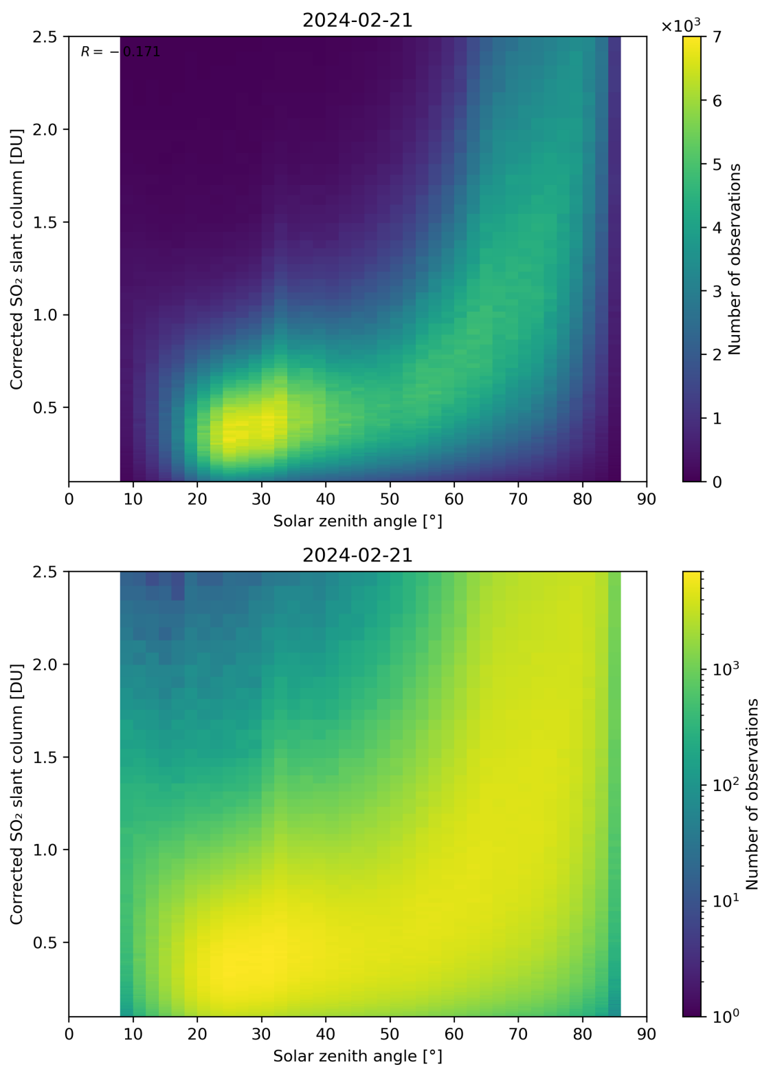
Figure 166: Scatter density plot of “Solar zenith angle” against “Corrected SO 2 slant column” for 2024-02-20 to 2024-02-22.
