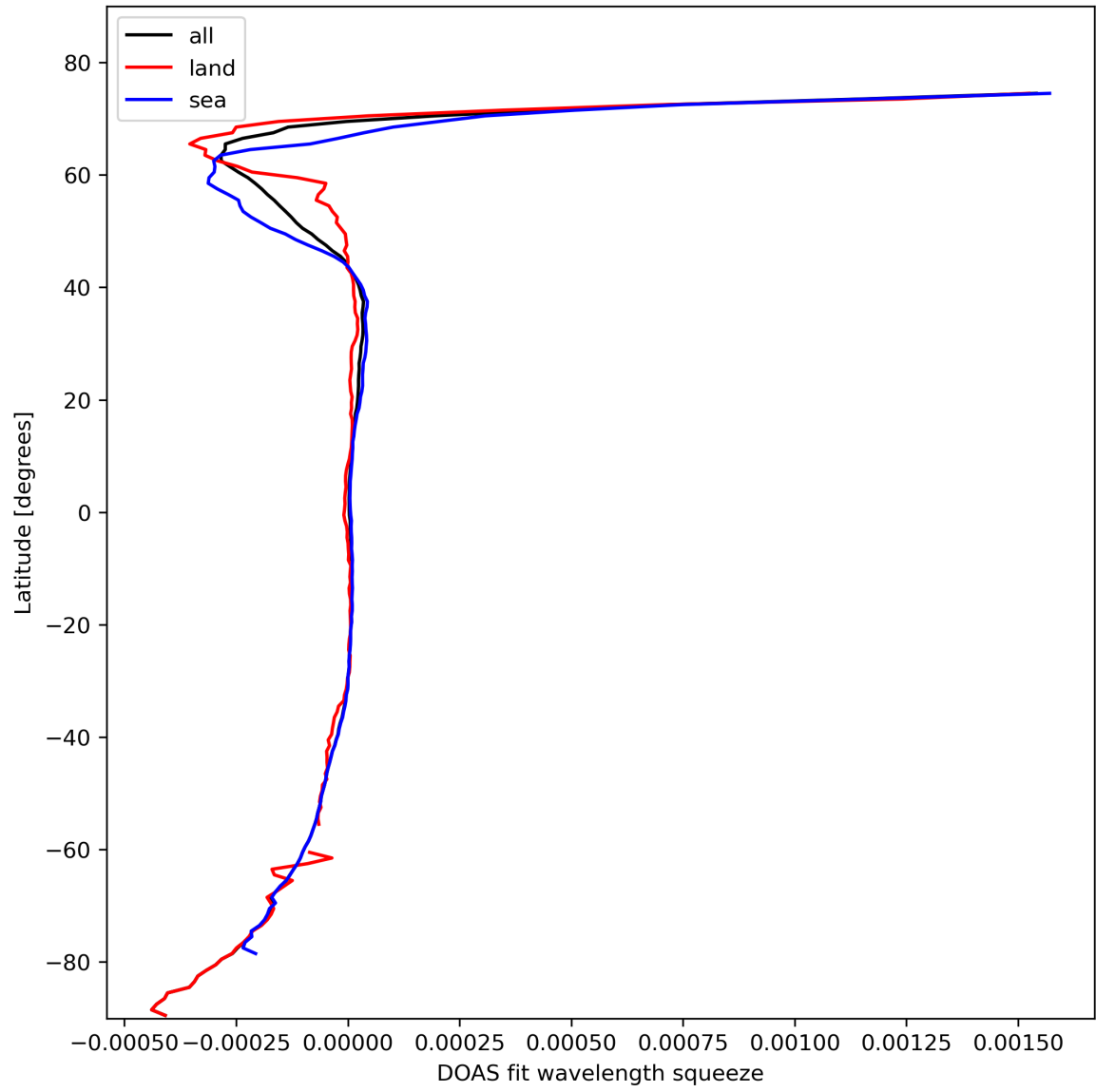
Figure 46: Zonal average of “DOAS fit wavelength squeeze” for 2024-02-20 to 2024-02-22.
