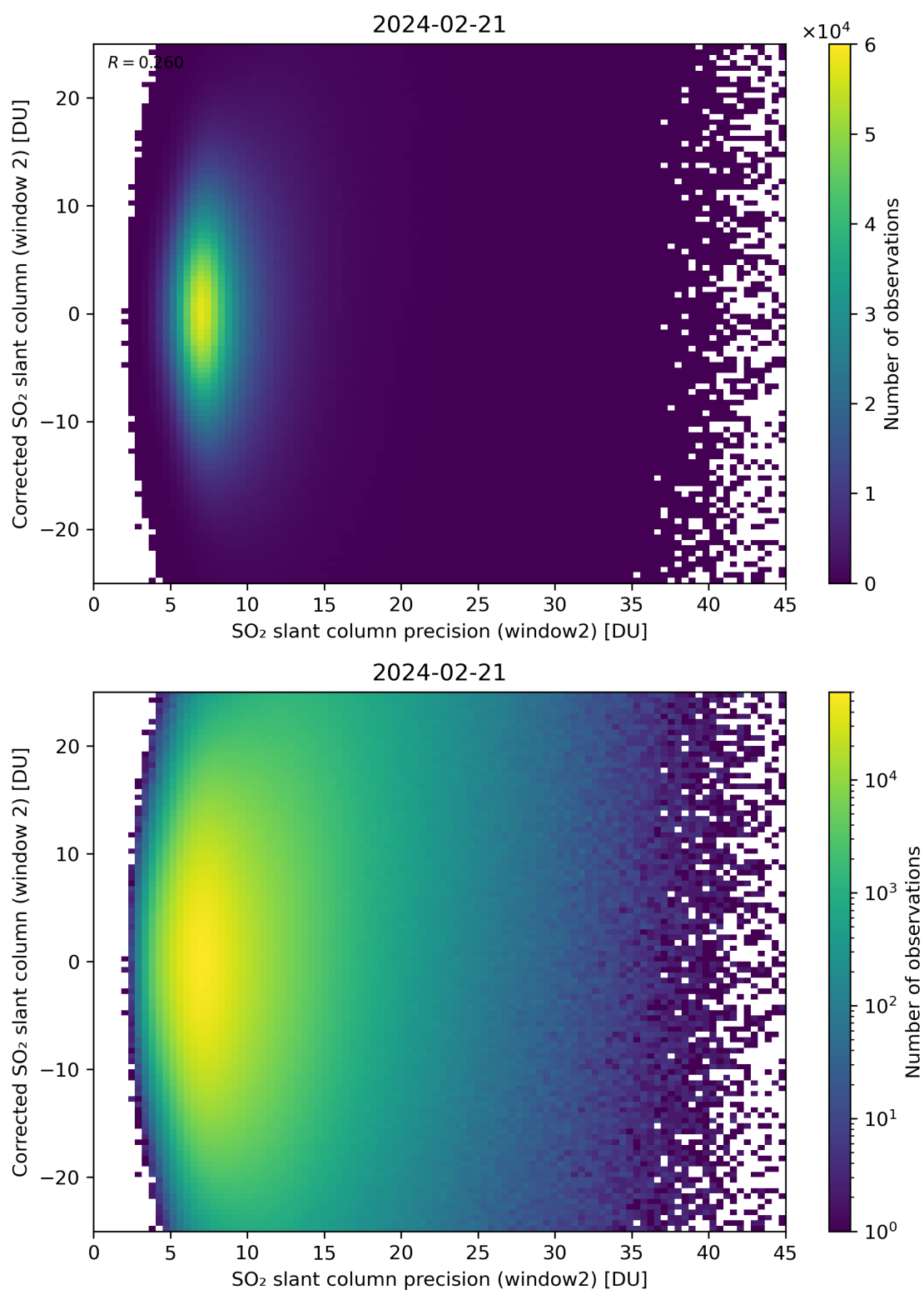
Figure 247: Scatter density plot of “SO 2 slant column precision (window2)” against “Corrected SO 2 slant column (window 2)” for 2024-02-20 to 2024-02-22.
