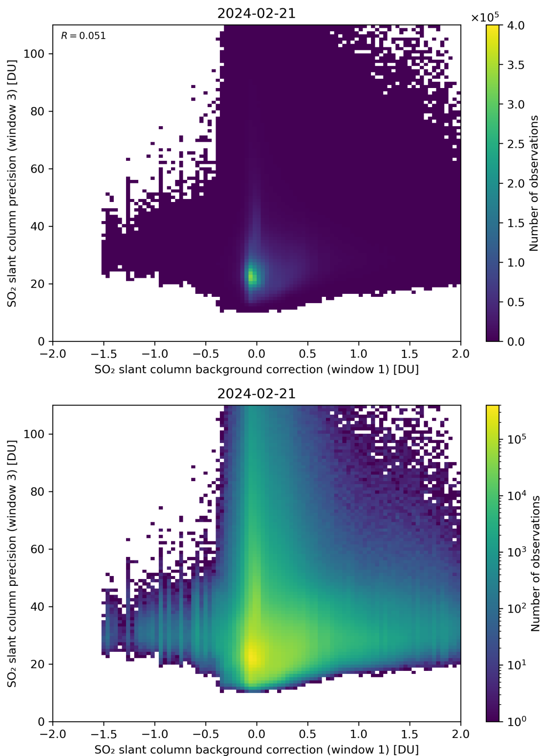
Figure 108: Scatter density plot of “SO 2 slant column background correction (window 1)” against “SO 2 slant column precision (window 3)” for 2024-02-20 to 2024-02-22.
