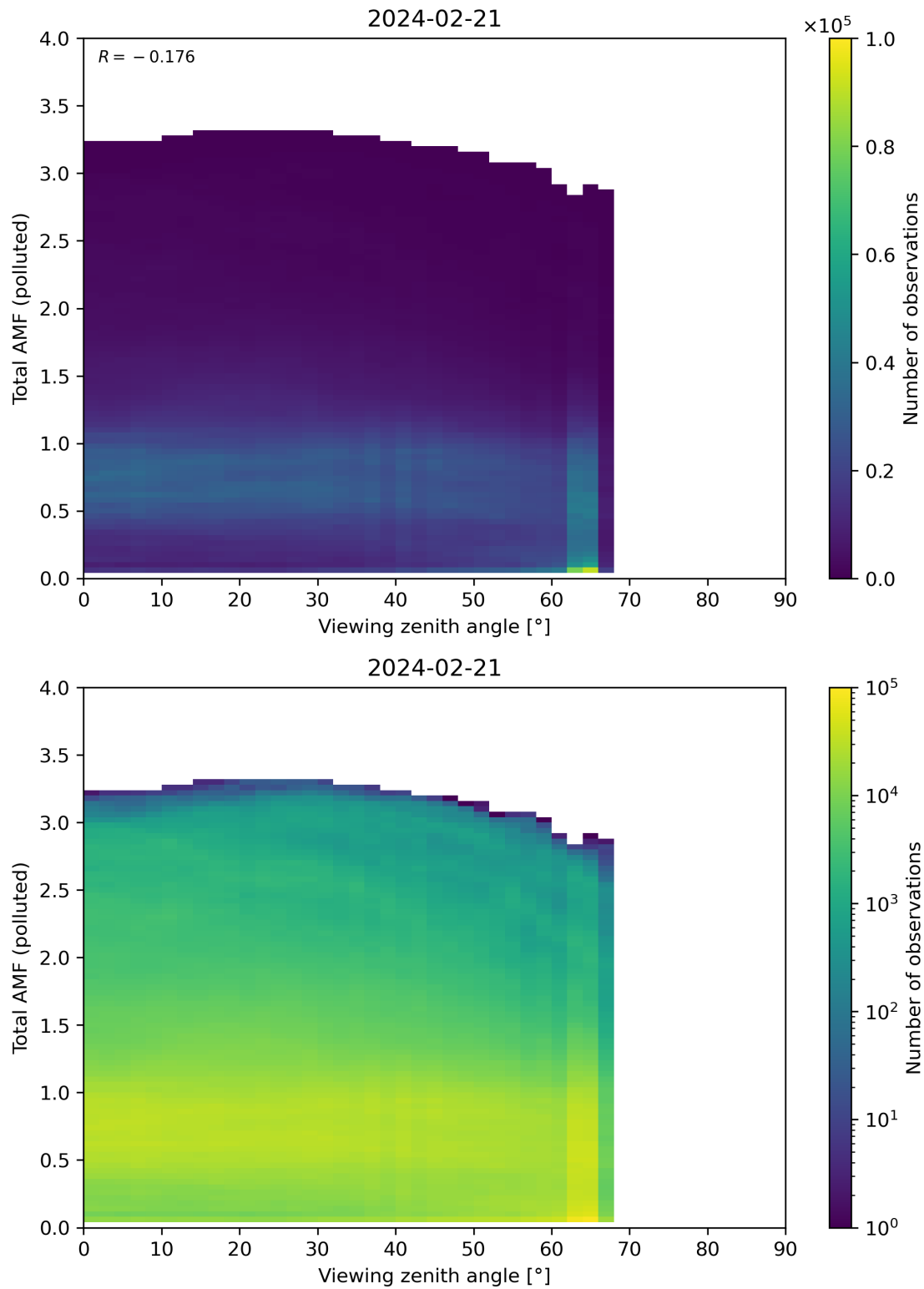
Figure 325: Scatter density plot of “Viewing zenith angle” against “Total AMF (polluted)” for 2024-02-20 to 2024-02-22.
