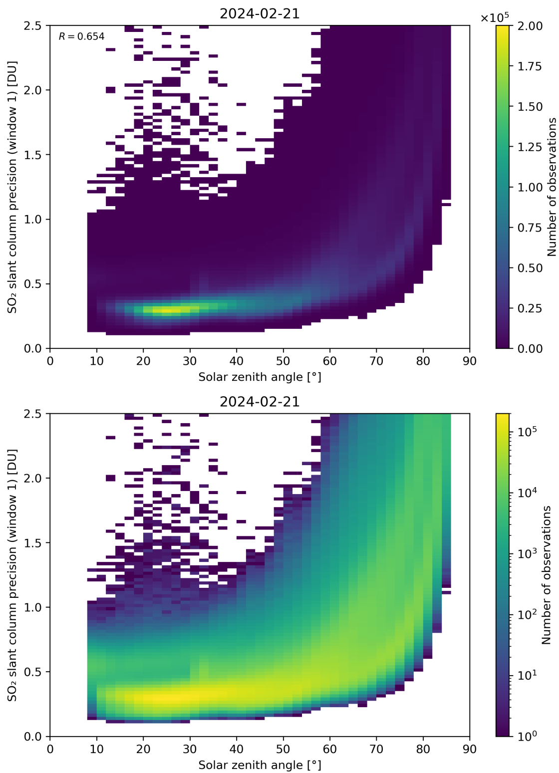
Figure 170: Scatter density plot of “Solar zenith angle” against “SO 2 slant column precision (window 1)” for 2024-02-20 to 2024-02-22.
