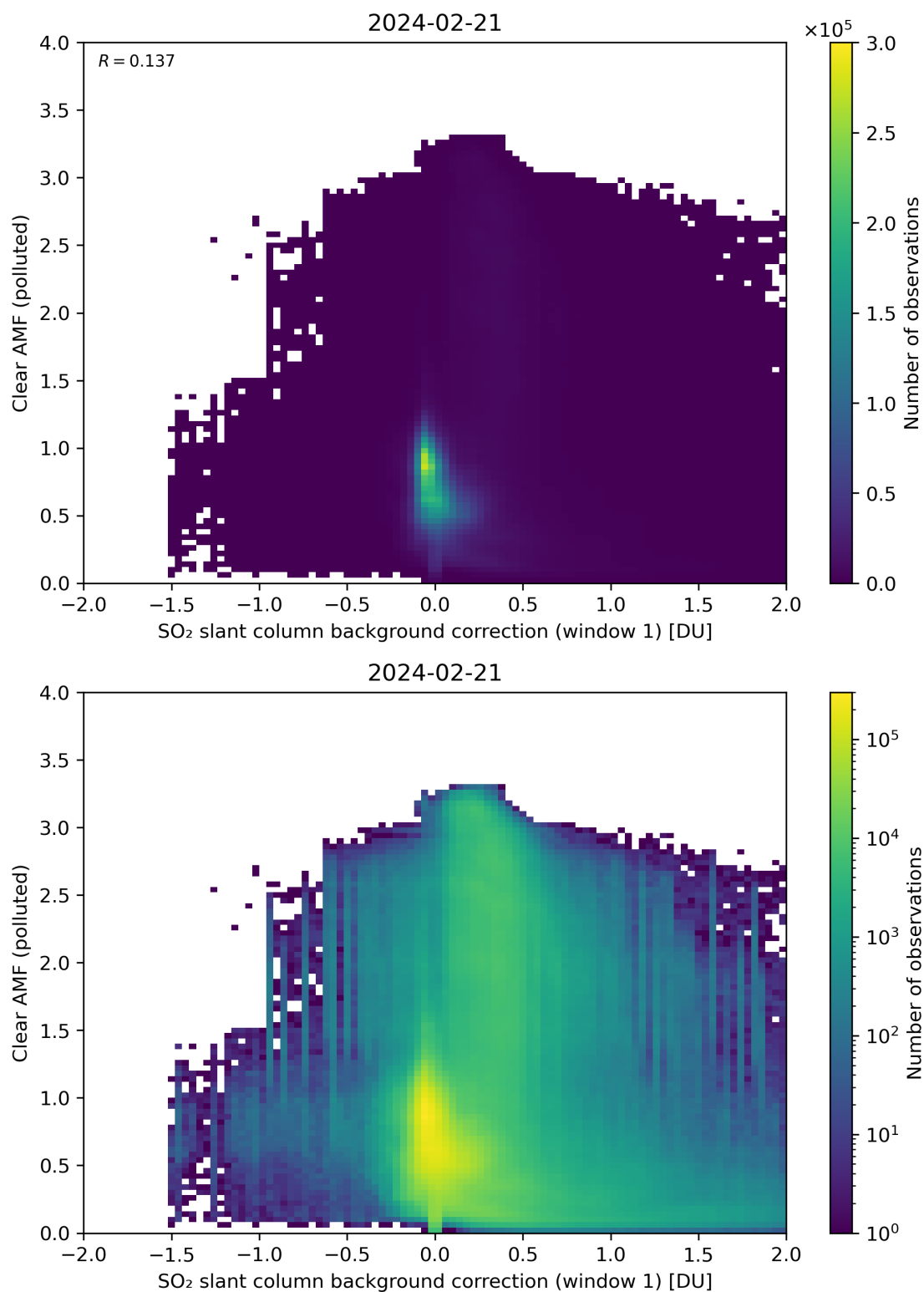
Figure 103: Scatter density plot of “SO 2 slant column background correction (window 1)” against “Clear AMF (polluted)” for 2024-02-20 to 2024-02-22.
