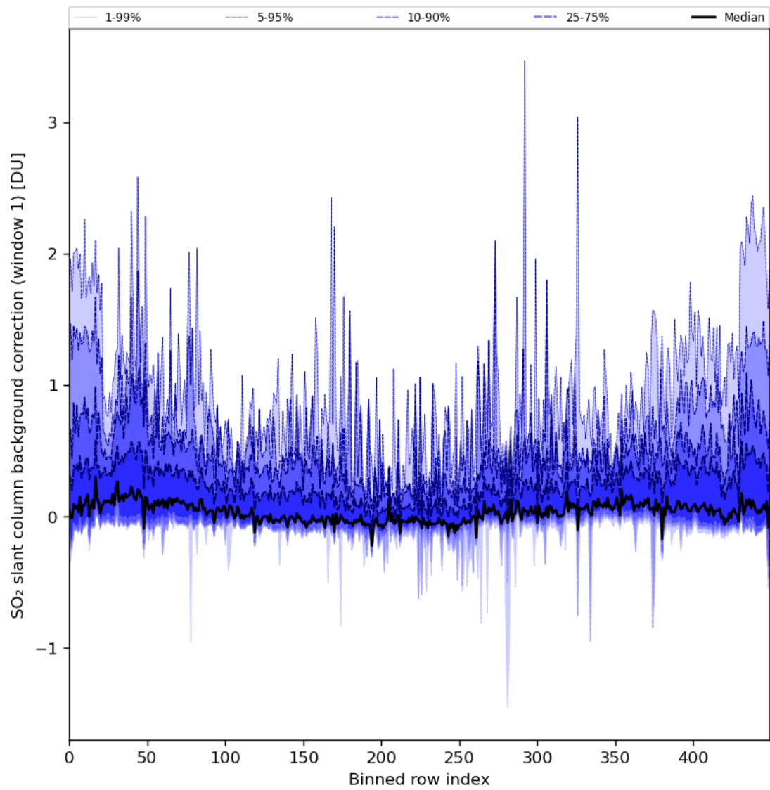
Figure 82: Along track statistics of “SO 2 slant column background correction (window 1)” for 2024-02-20 to 2024-02-22
