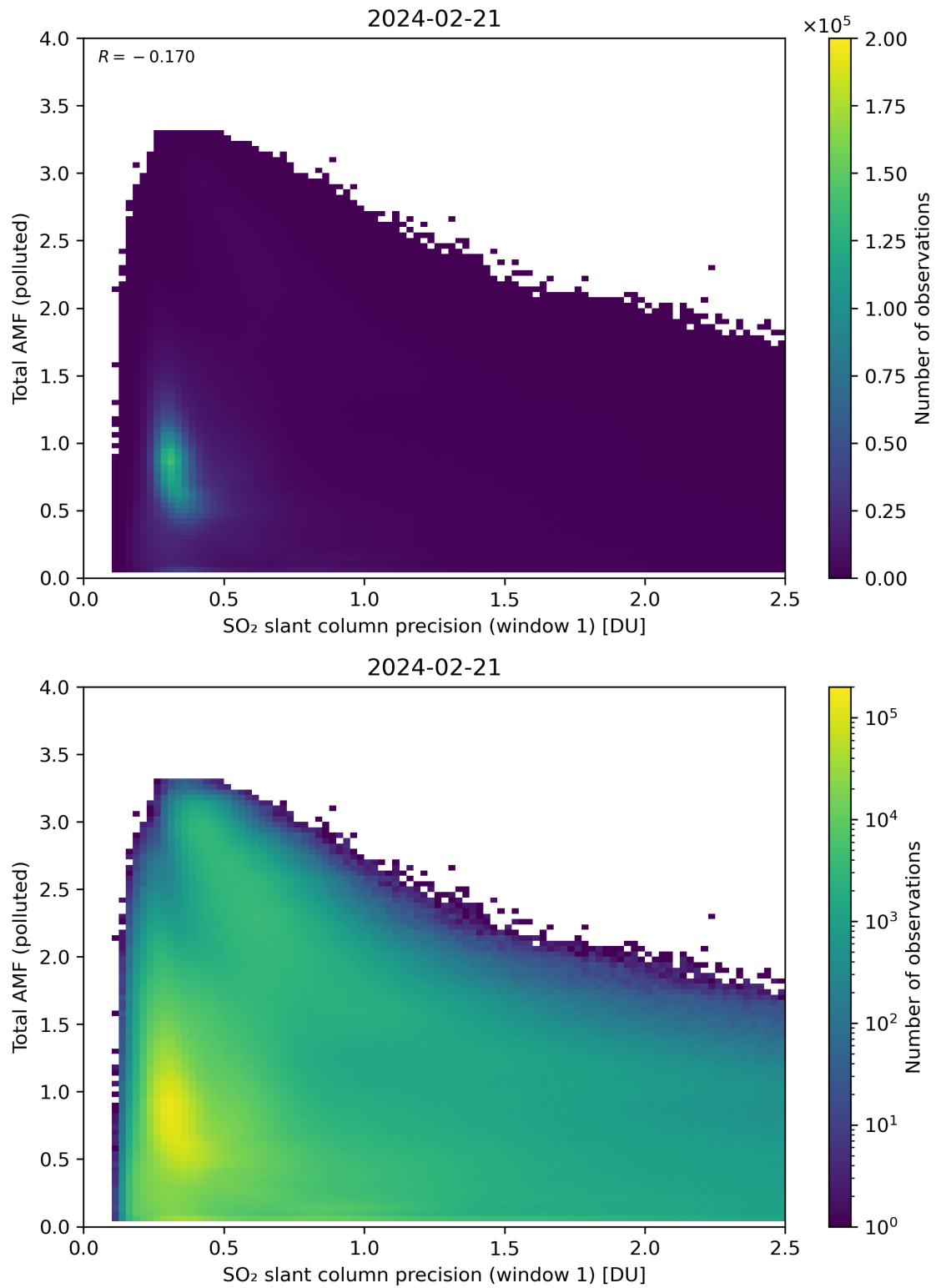
Figure 230: Scatter density plot of “SO 2 slant column precision (window 1)” against “Total AMF (polluted)” for 2024-02-20 to 2024-02-22.
