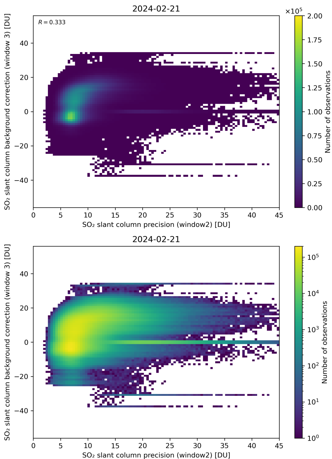
Figure 242: Scatter density plot of “SO 2 slant column precision (window2)” against “SO 2 slant column background correction (window 3)” for 2024-02-20 to 2024-02-22.
