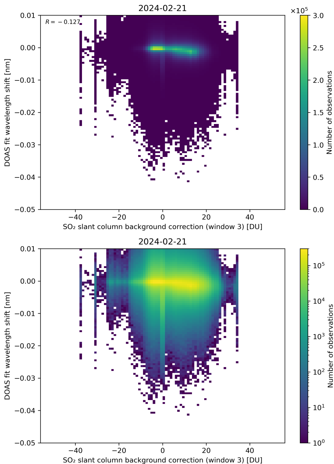
Figure 121: Scatter density plot of “SO 2 slant column background correction (window 3)” against “DOAS fit wavelength shift” for 2024-02-20 to 2024-02-22.
