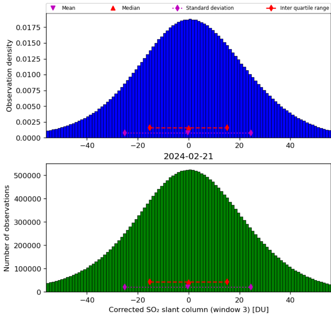
Figure 66: Histogram of “Corrected SO 2 slant column (window 3)” for 2024-02-20 to 2024-02-22
