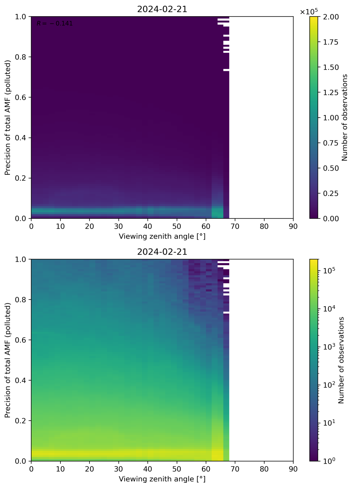
Figure 326: Scatter density plot of “Viewing zenith angle” against “Precision of total AMF (polluted)” for 2024-02-20 to 2024-02-22.
