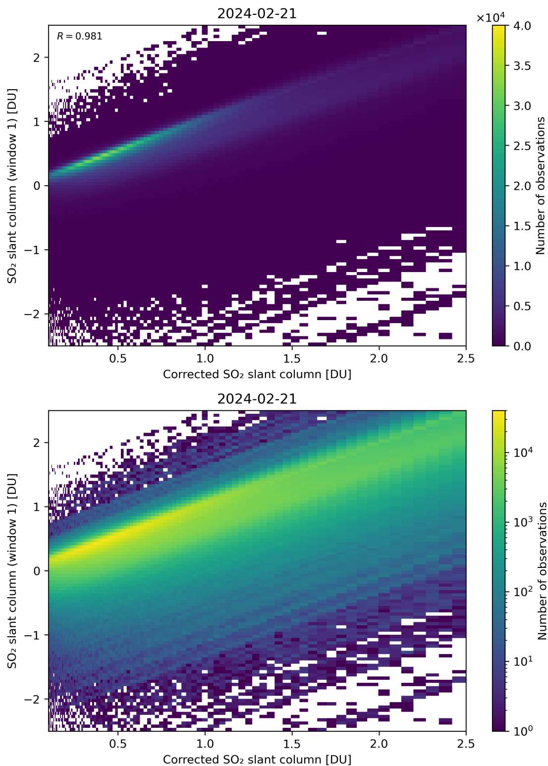
Figure 187: Scatter density plot of “Corrected SO 2 slant column” against “SO 2 slant column (window 1)” for 2024-02-20 to 2024-02-22.
