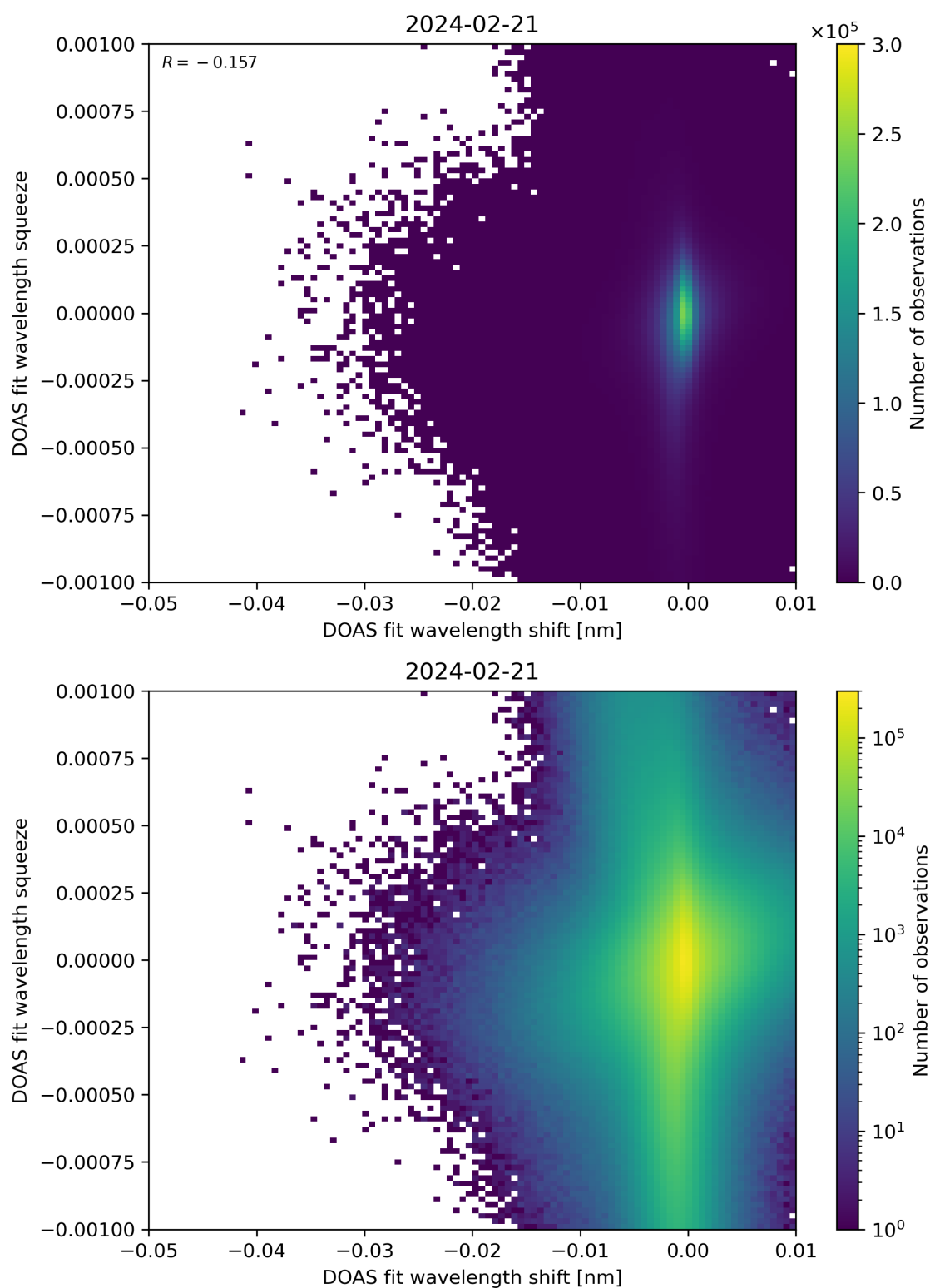
Figure 127: Scatter density plot of “DOAS fit wavelength shift” against “DOAS fit wavelength squeeze” for 2024-02-20 to 2024-02-22.
