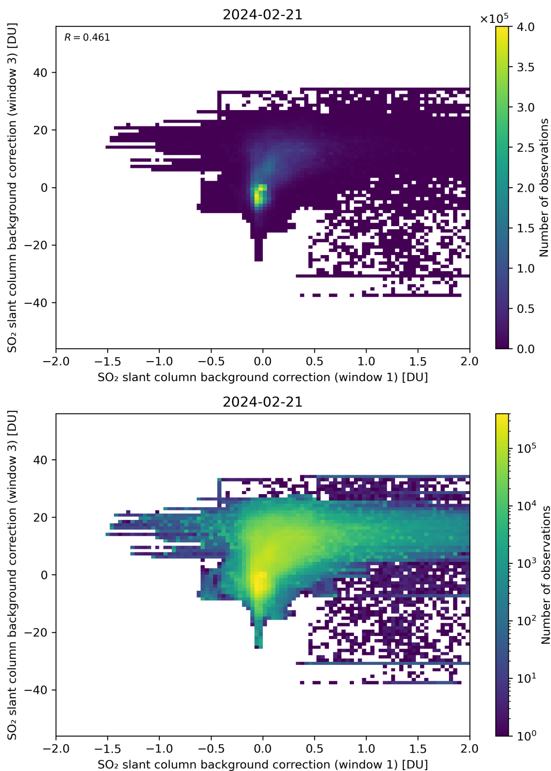
Figure 99: Scatter density plot of “SO 2 slant column background correction (window 1)” against “SO 2 slant column background correction (window 3)” for 2024-02-20 to 2024-02-22.
