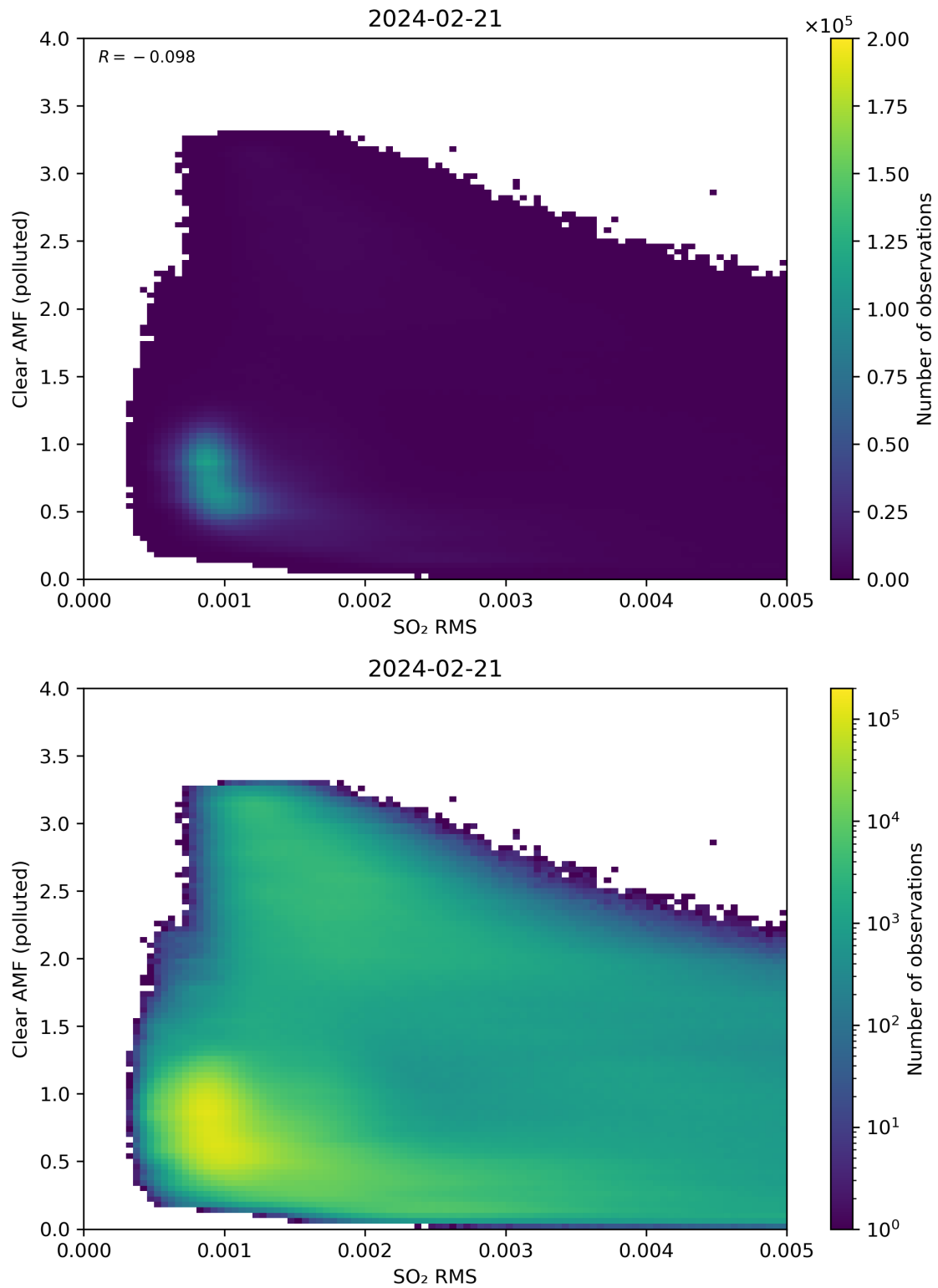
Figure 136: Scatter density plot of “SO 2 RMS” against “Clear AMF (polluted)” for 2024-02-20 to 2024-02-22.
