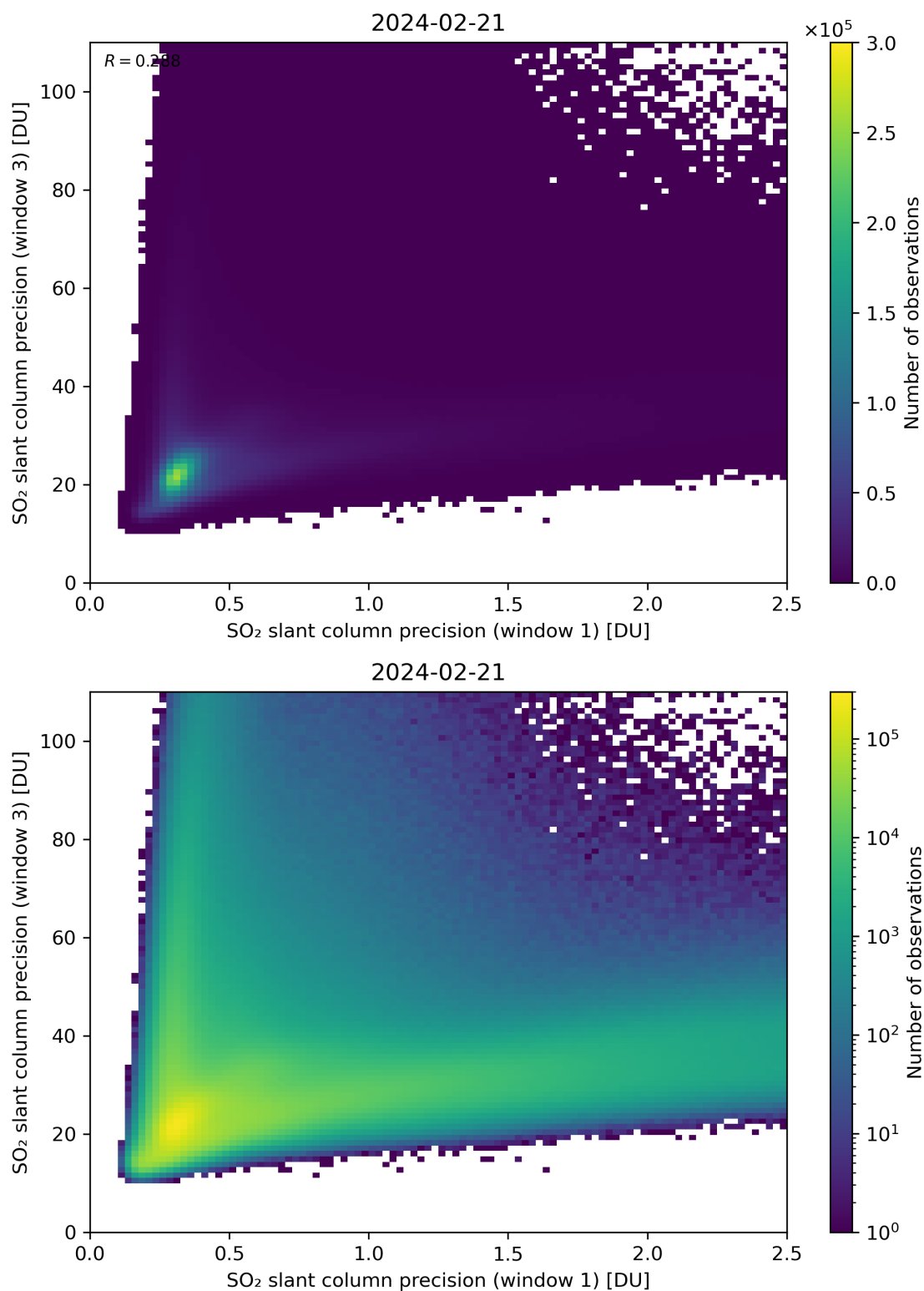
Figure 229: Scatter density plot of “SO 2 slant column precision (window 1)” against “SO 2 slant column precision (window 3)” for 2024-02-20 to 2024-02-22.
