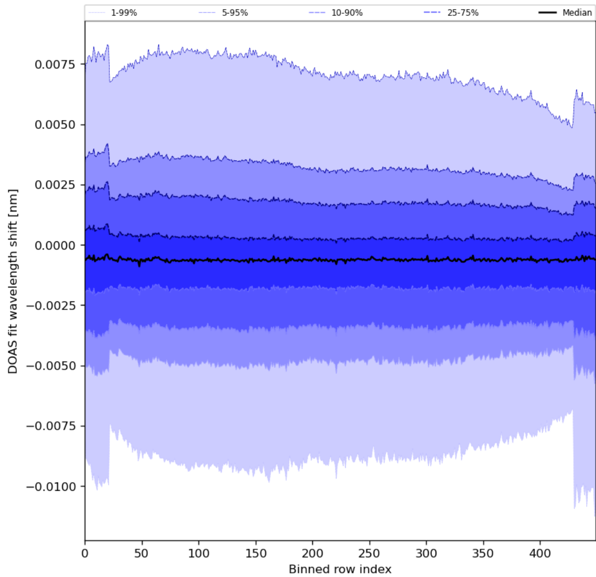
Figure 91: Along track statistics of “DOAS fit wavelength shift” for 2024-02-20 to 2024-02-22
