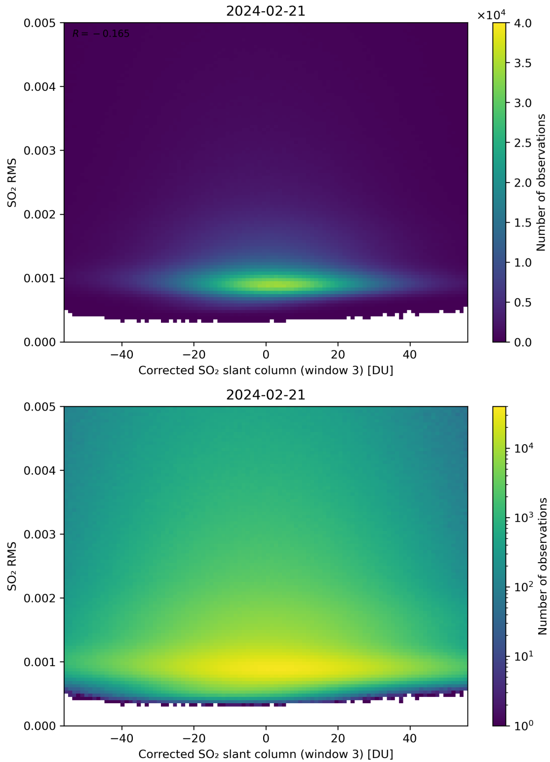
Figure 208: Scatter density plot of “Corrected SO 2 slant column (window 3)” against “SO 2 RMS” for 2024-02-20 to 2024-02-22.
