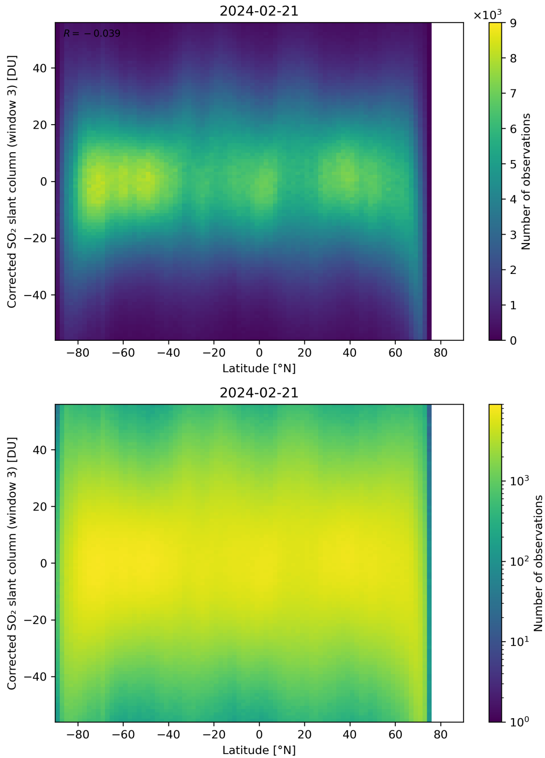
Figure 148: Scatter density plot of “Latitude” against “Corrected SO 2 slant column (window 3)” for 2024-02-20 to 2024-02-22.
