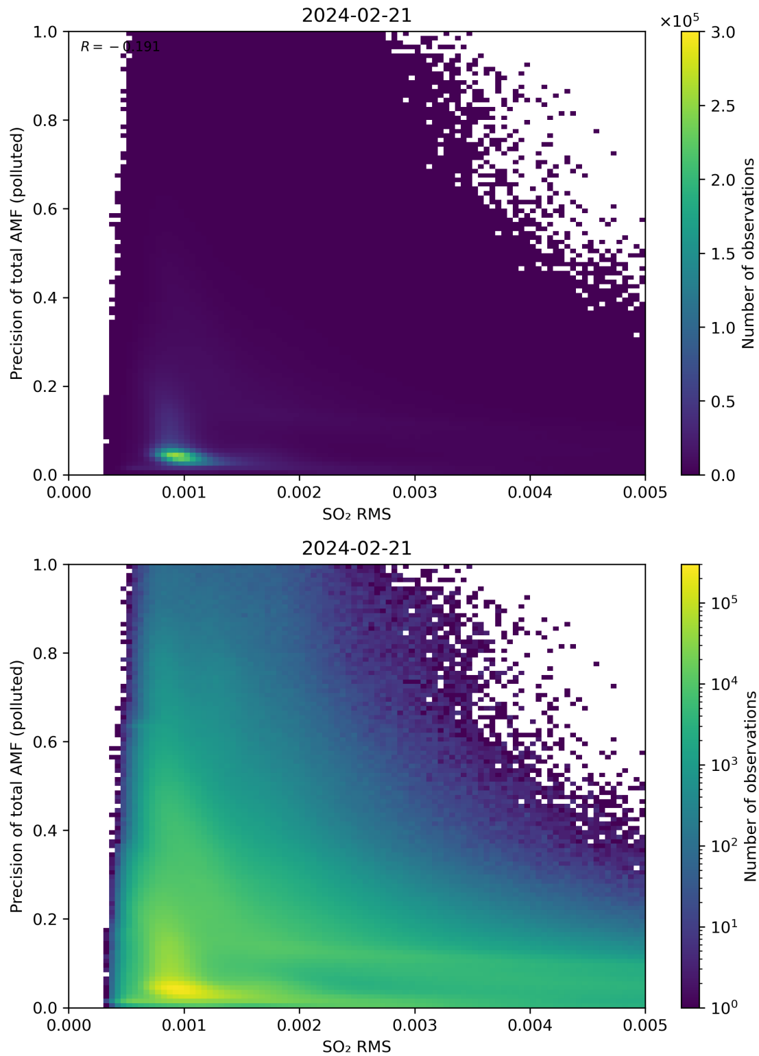
Figure 138: Scatter density plot of “SO 2 RMS” against “Precision of total AMF (polluted)” for 2024-02-20 to 2024-02-22.
