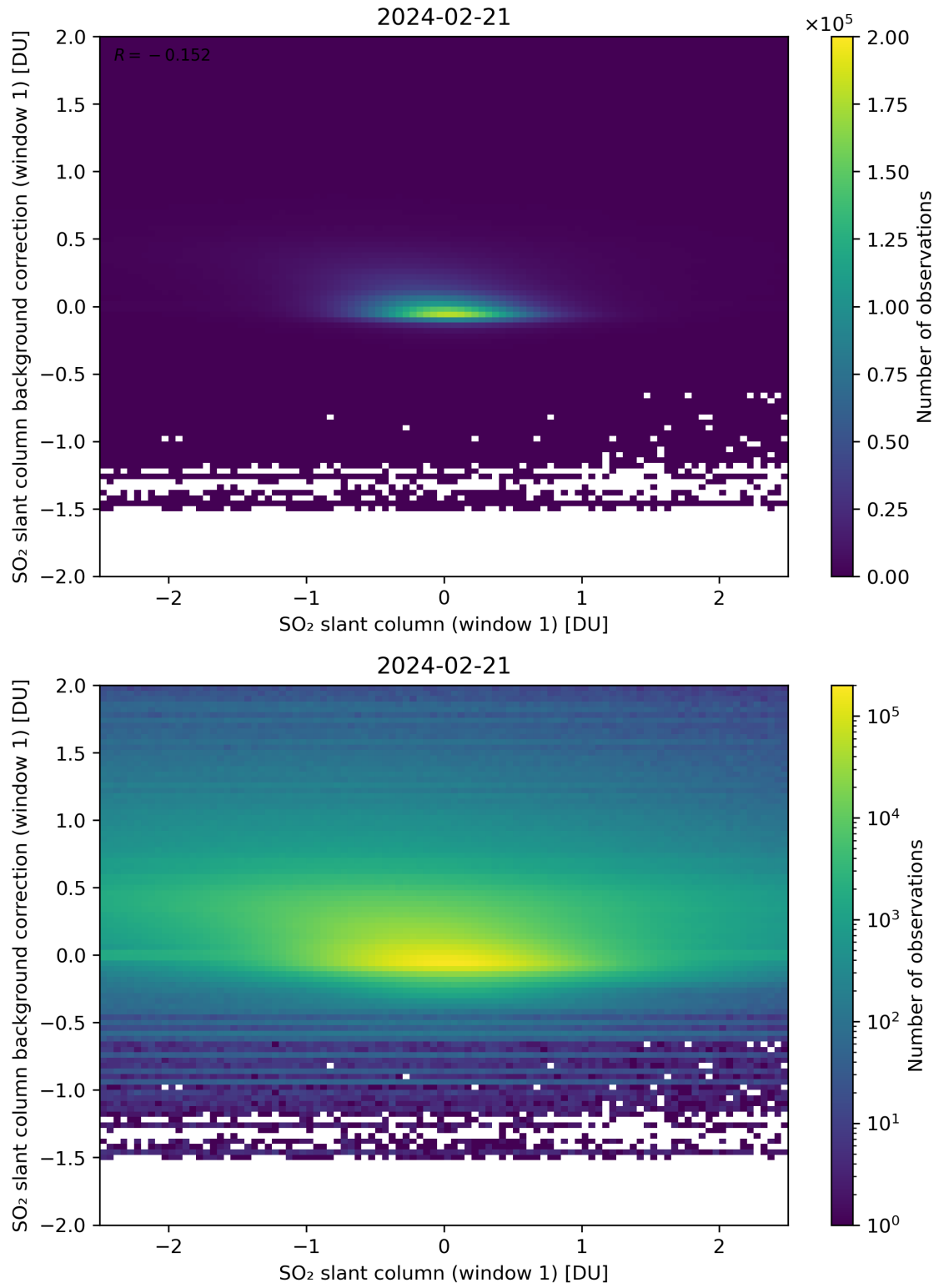
Figure 212: Scatter density plot of “SO 2 slant column (window 1)” against “SO 2 slant column background correction (window 1)” for 2024-02-20 to 2024-02-22.
