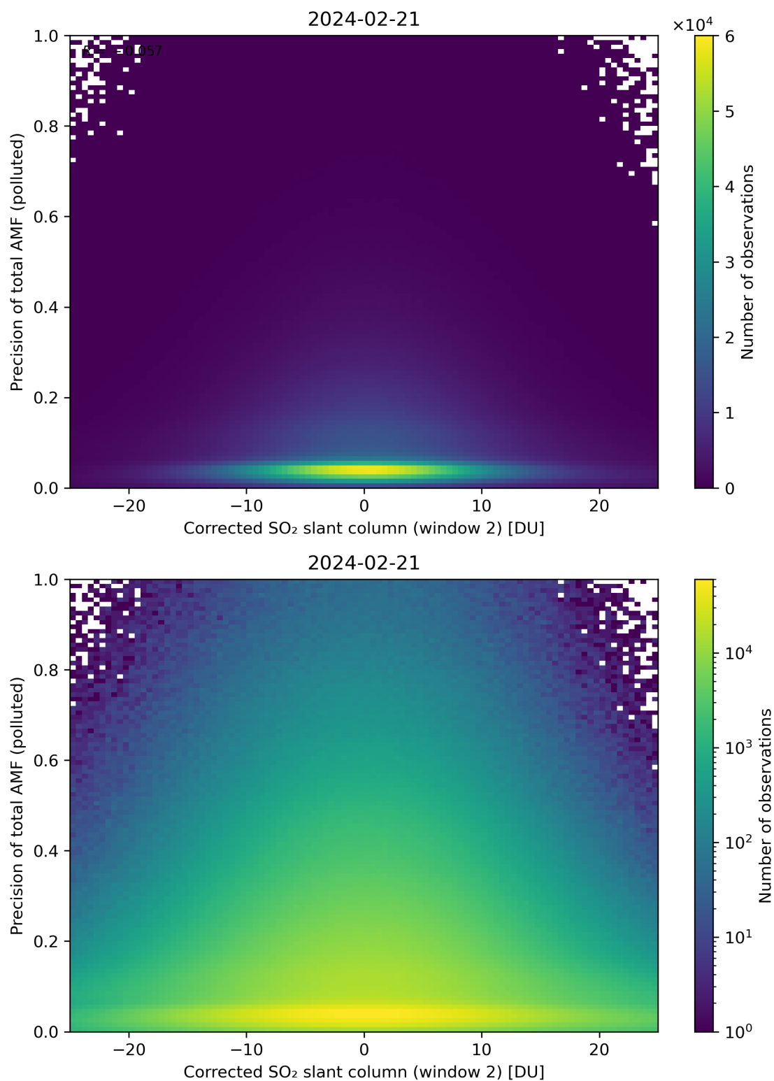
Figure 204: Scatter density plot of “Corrected SO 2 slant column (window 2)” against “Precision of total AMF (polluted)” for 2024-02-20 to 2024-02-22.
