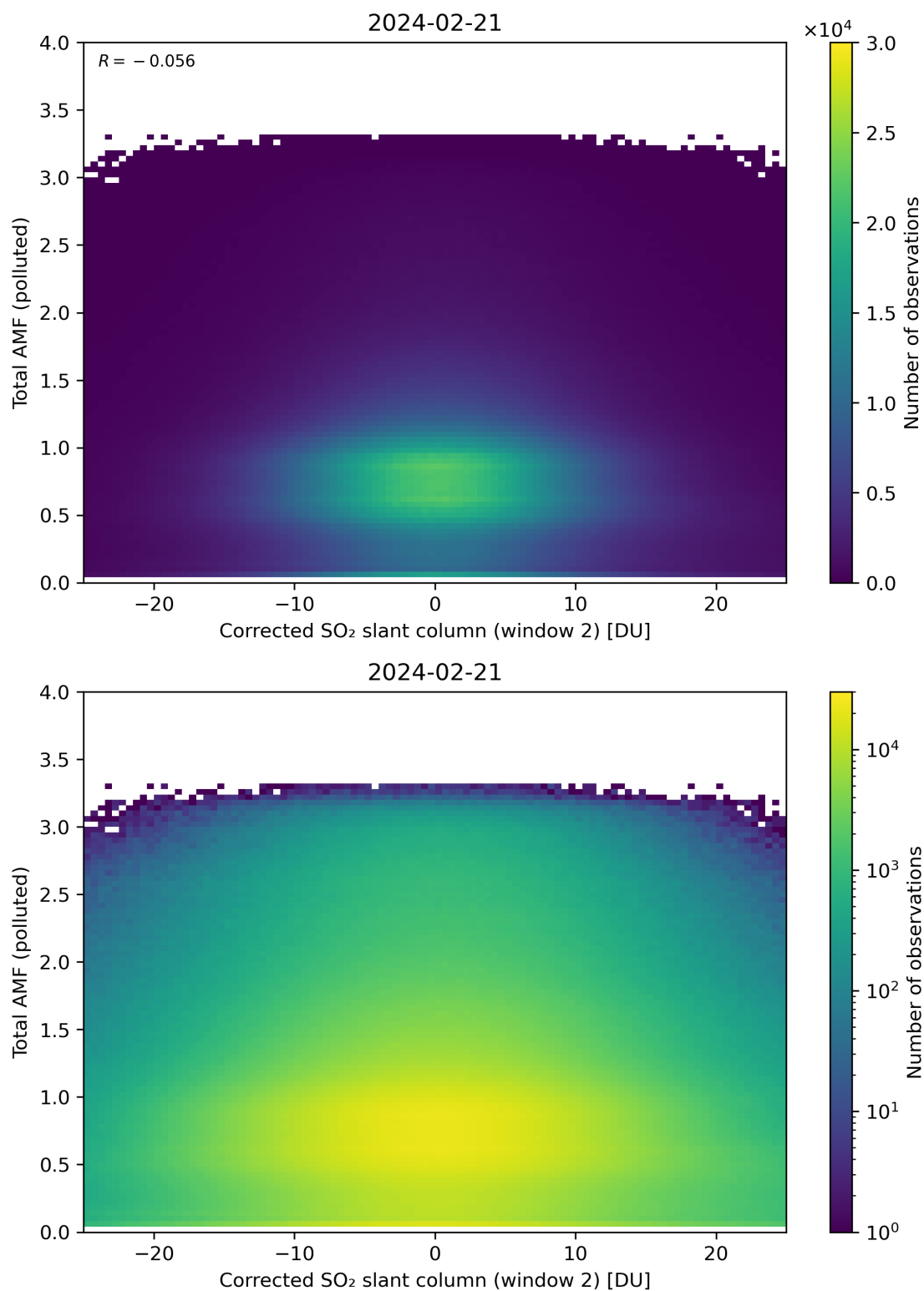
Figure 203: Scatter density plot of “Corrected SO 2 slant column (window 2)” against “Total AMF (polluted)” for 2024-02-20 to 2024-02-22.
