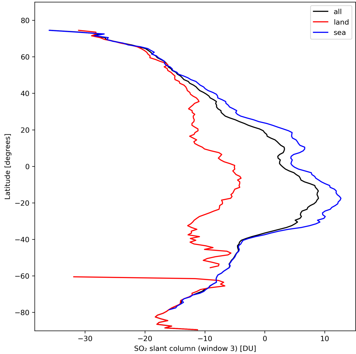
Figure 41: Zonal average of “SO 2 slant column (window 3)” for 2024-02-20 to 2024-02-22.
