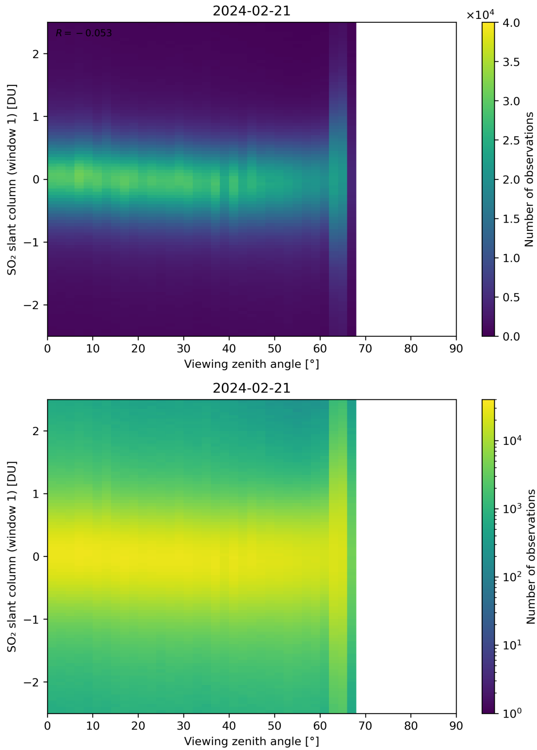
Figure 320: Scatter density plot of “Viewing zenith angle” against “SO 2 slant column (window 1)” for 2024-02-20 to 2024-02-22.
