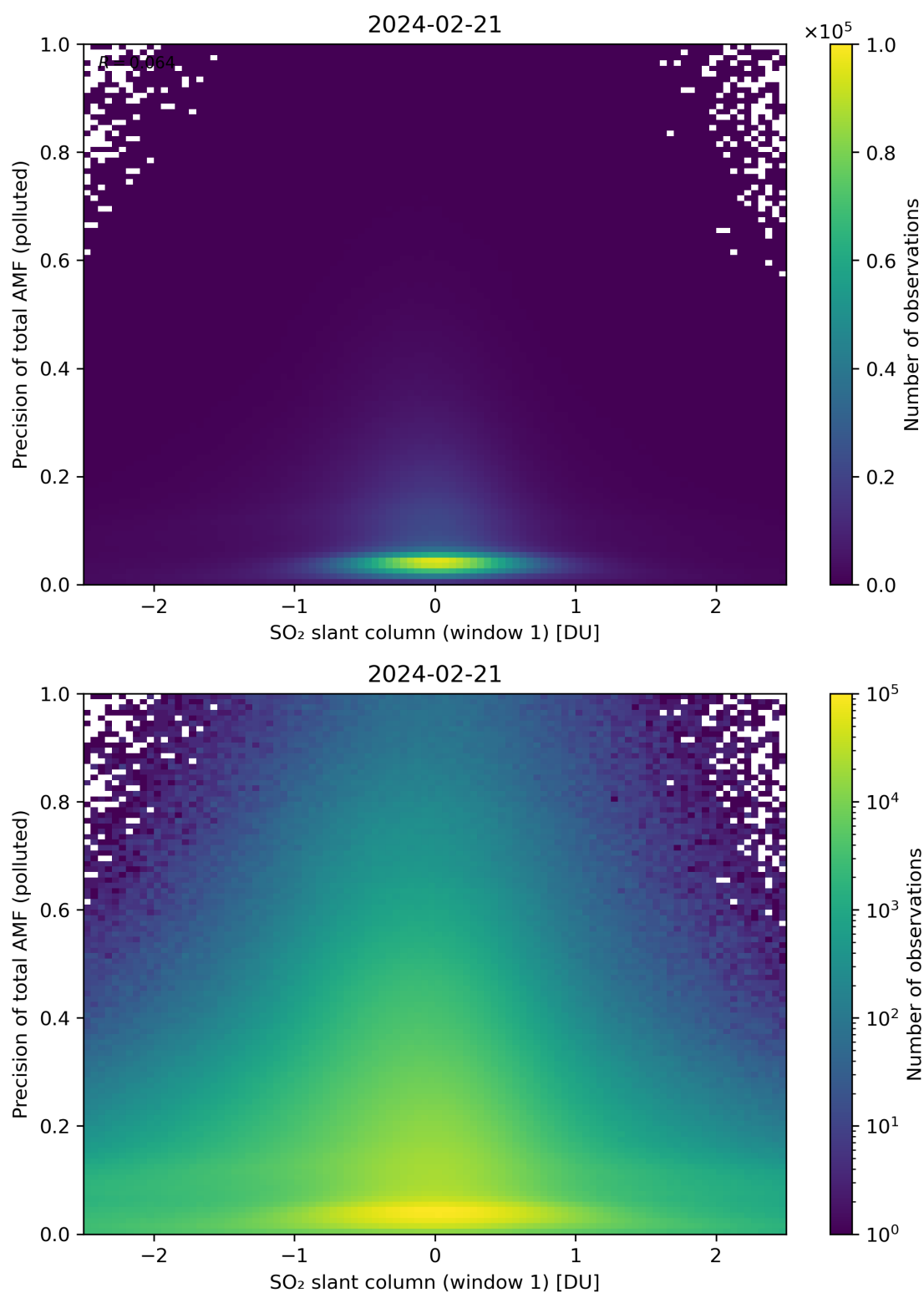
Figure 240: Scatter density plot of “SO 2 slant column (window 1)” against “Precision of total AMF (polluted)” for 2024-02-20 to 2024-02-22.
