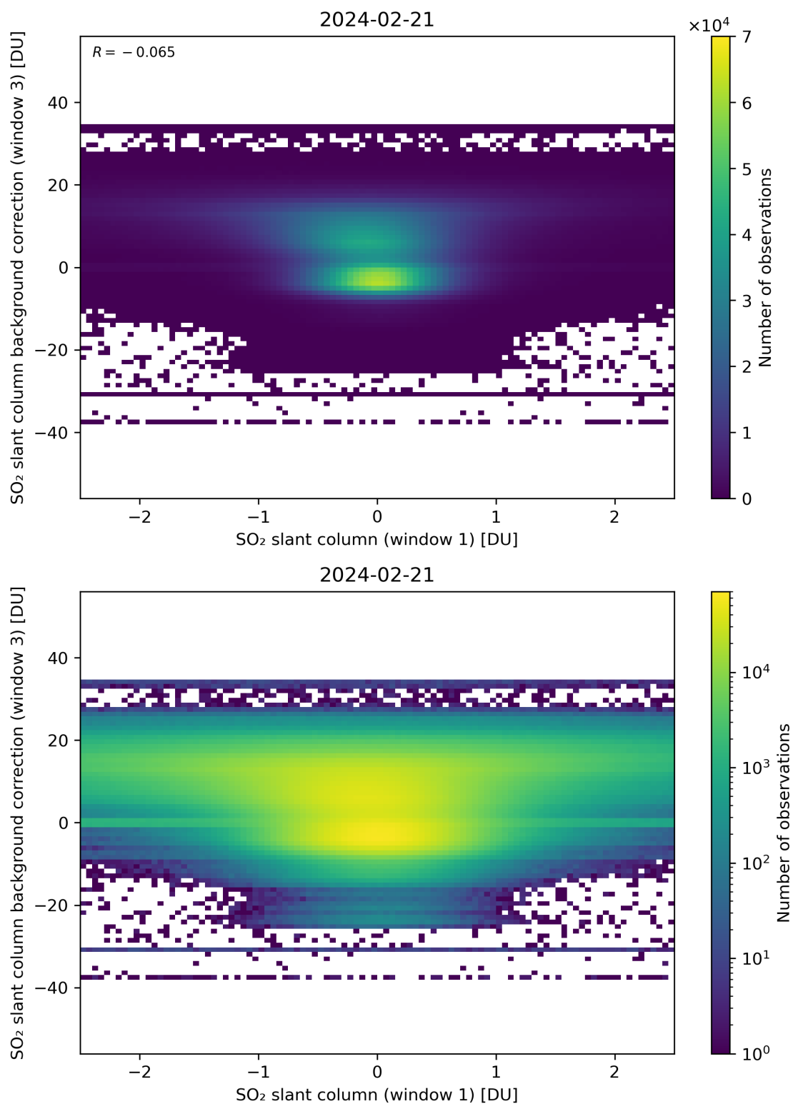
Figure 214: Scatter density plot of “SO 2 slant column (window 1)” against “SO 2 slant column background correction (window 3)” for 2024-02-20 to 2024-02-22.
