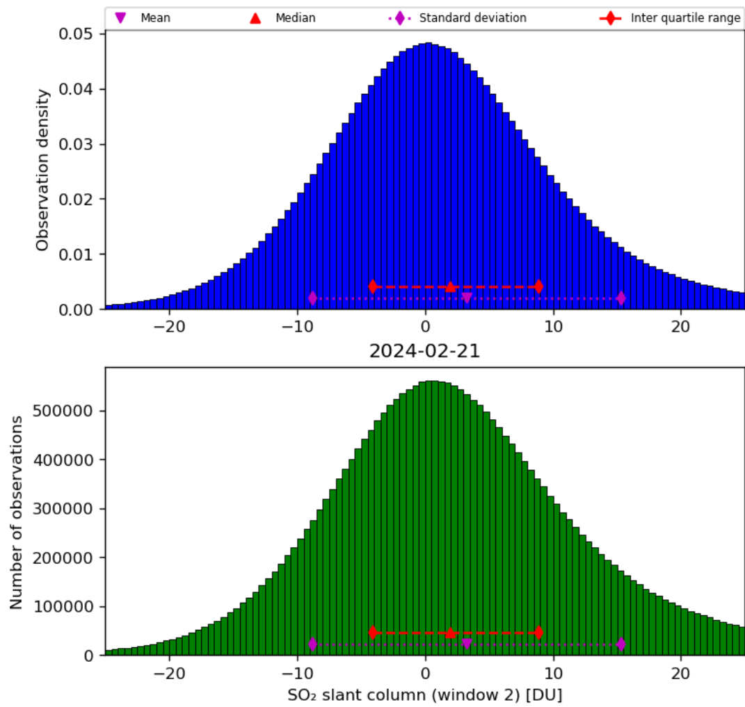
Figure 60: Histogram of “SO 2 slant column (window 2)” for 2024-02-20 to 2024-02-22
