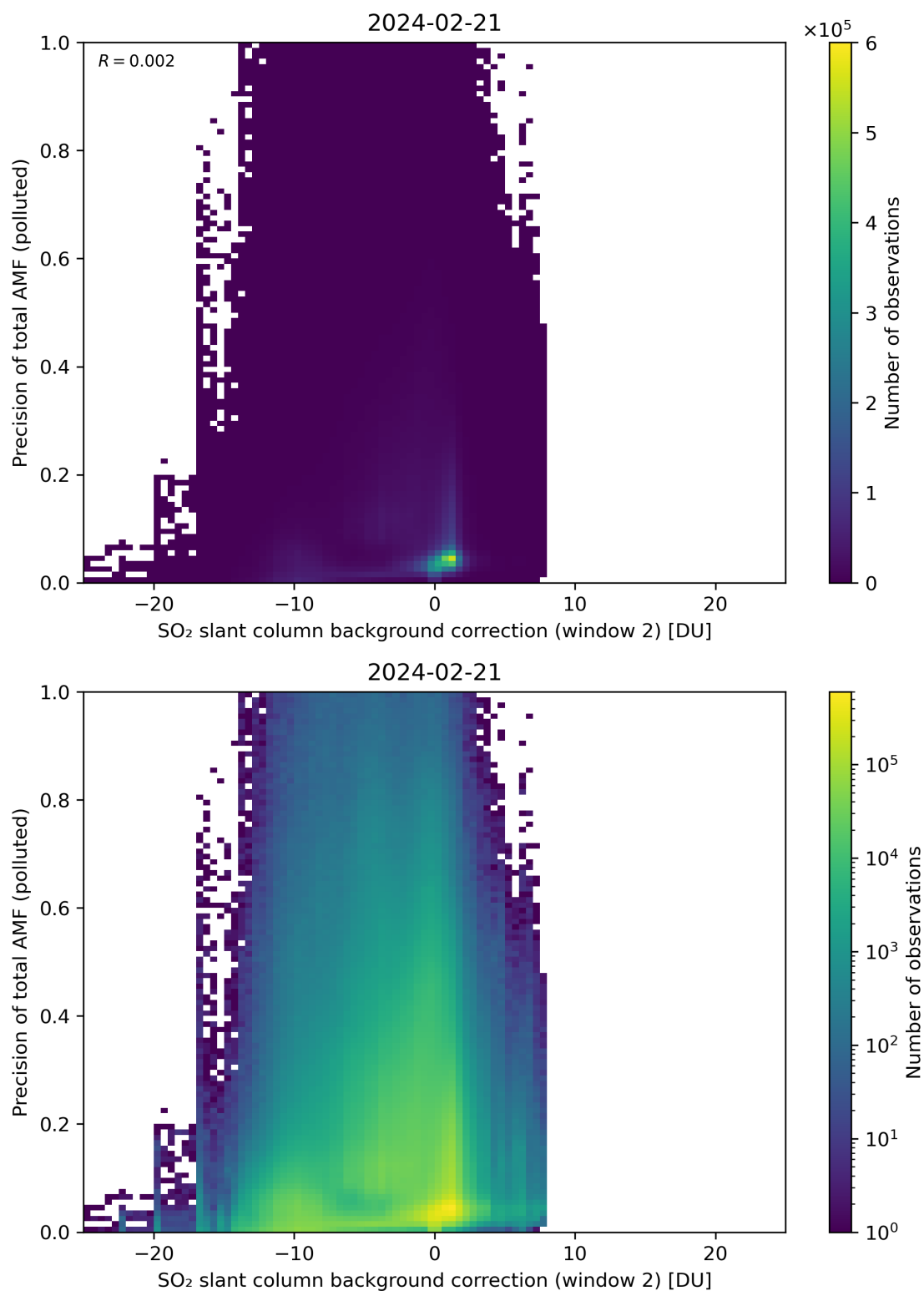
Figure 120: Scatter density plot of “SO 2 slant column background correction (window 2)” against “Precision of total AMF (polluted)” for 2024-02-20 to 2024-02-22.
