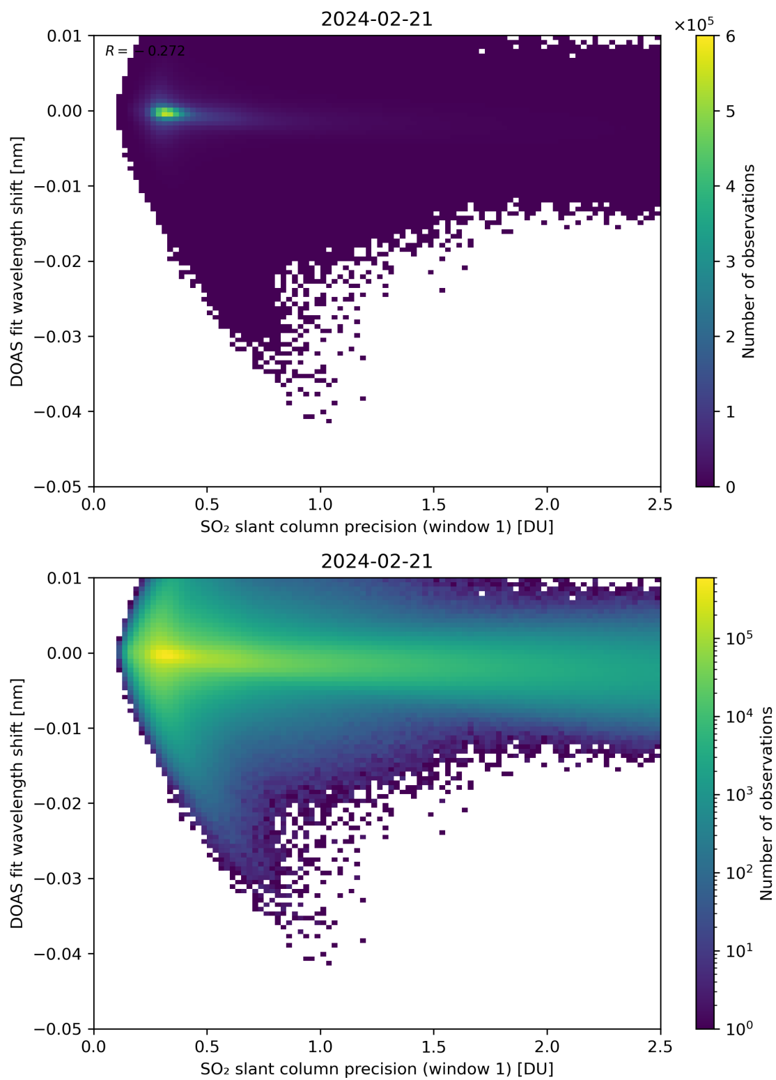
Figure 221: Scatter density plot of “SO 2 slant column precision (window 1)” against “DOAS fit wavelength shift” for 2024-02-20 to 2024-02-22.
