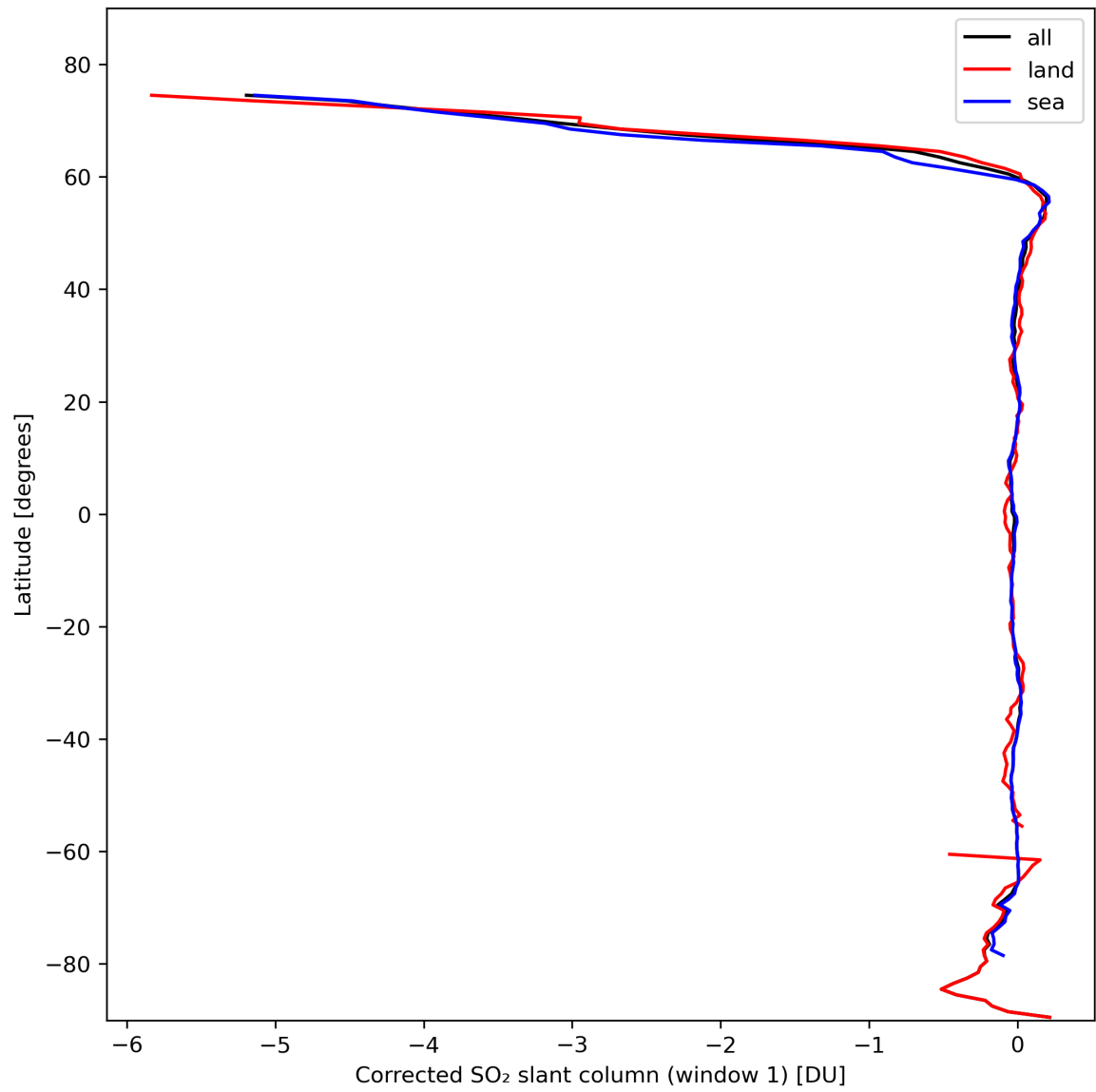
Figure 35: Zonal average of “Corrected SO 2 slant column (window 1)” for 2024-02-20 to 2024-02-22.
