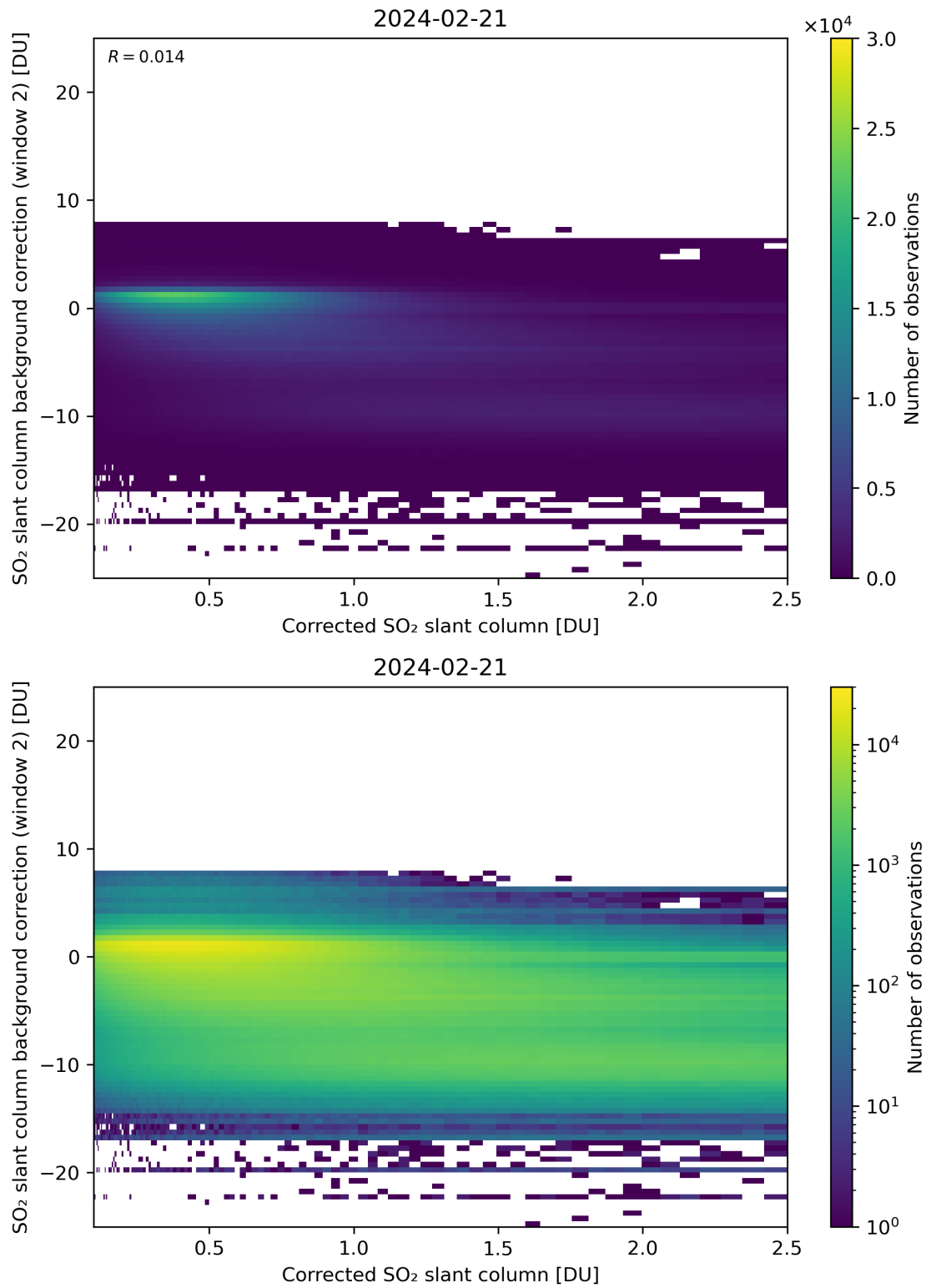
Figure 179: Scatter density plot of “Corrected SO 2 slant column” against “SO 2 slant column background correction (window 2)” for 2024-02-20 to 2024-02-22.
