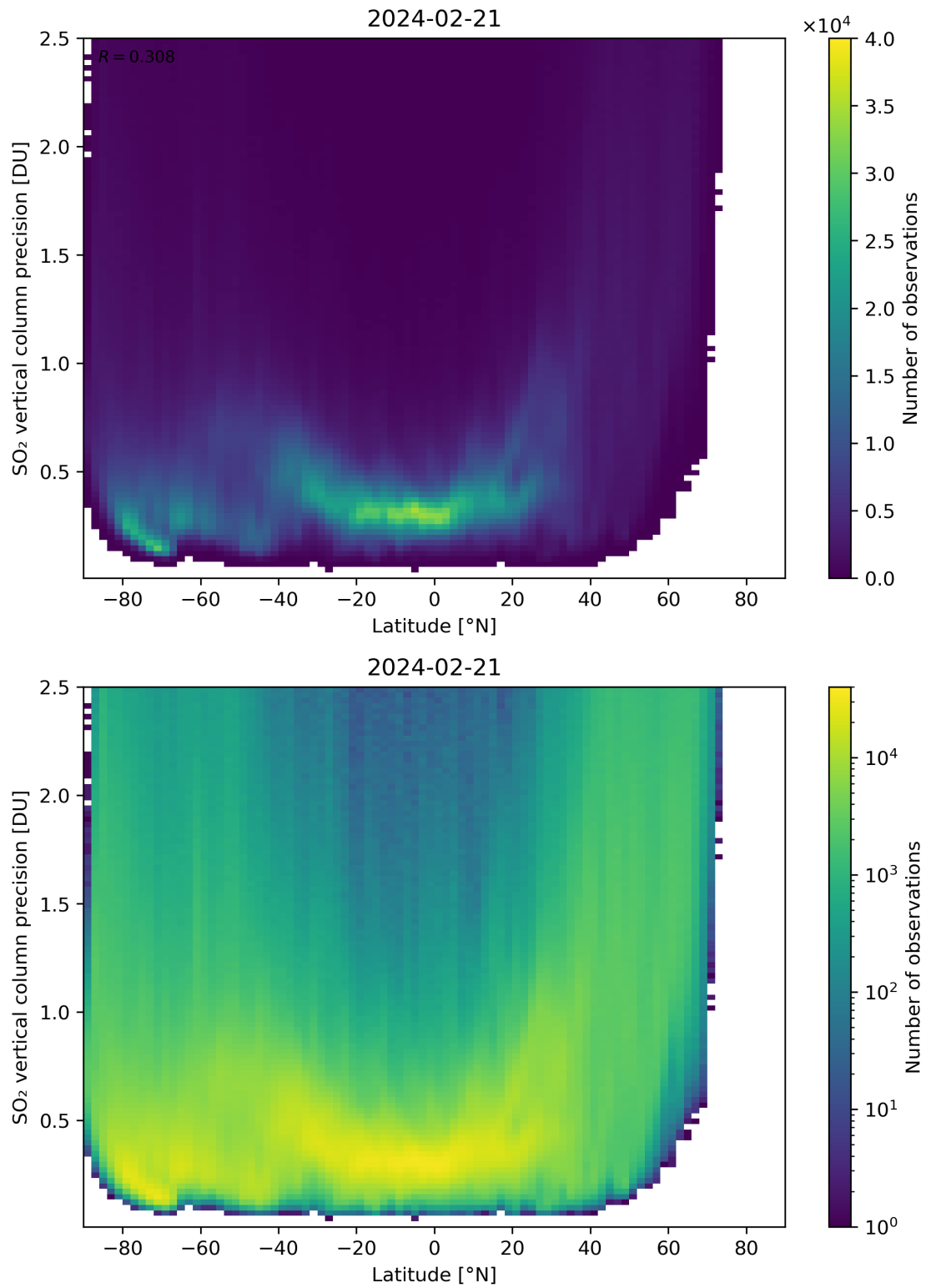
Figure 157: Scatter density plot of “Latitude” against “SO 2 vertical column precision” for 2024-02-20 to 2024-02-22.
