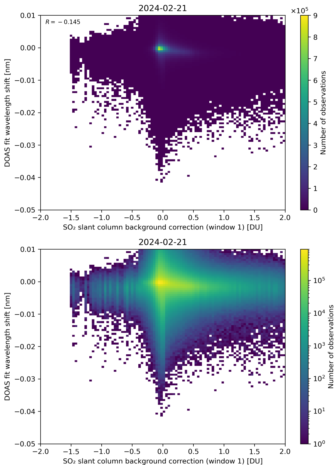
Figure 100: Scatter density plot of “SO 2 slant column background correction (window 1)” against “DOAS fit wavelength shift” for 2024-02-20 to 2024-02-22.
