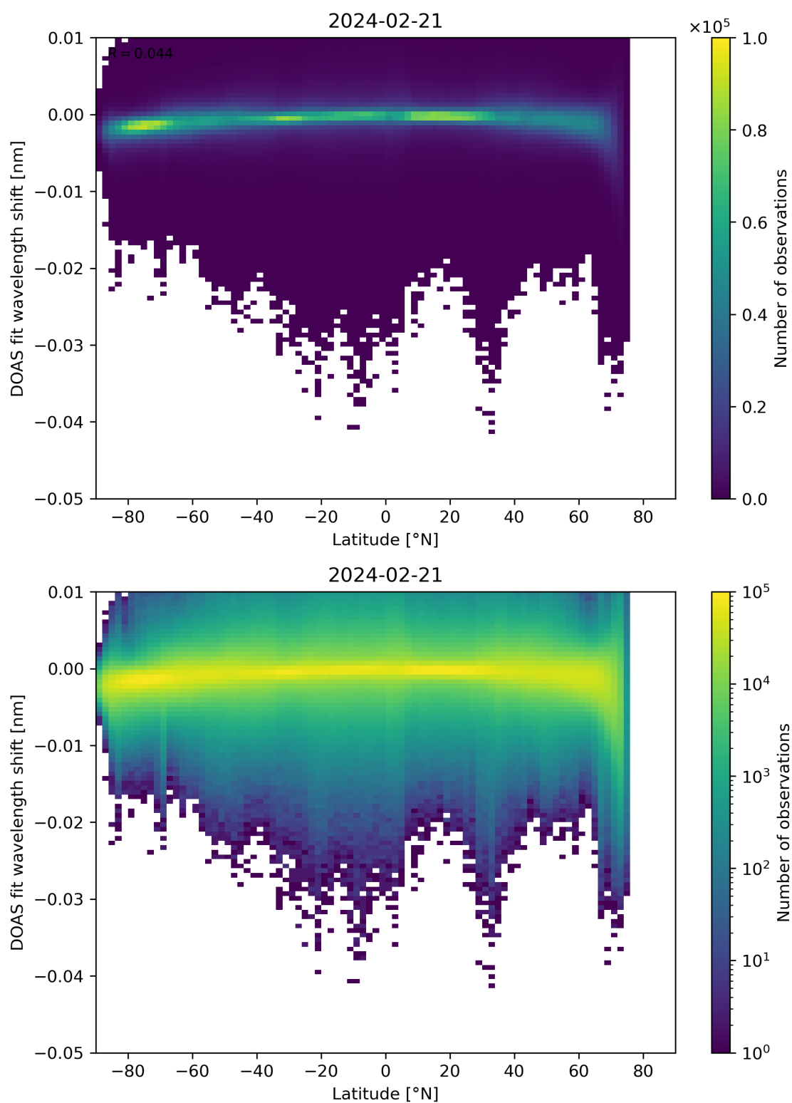
Figure 142: Scatter density plot of “Latitude” against “DOAS fit wavelength shift” for 2024-02-20 to 2024-02-22.
