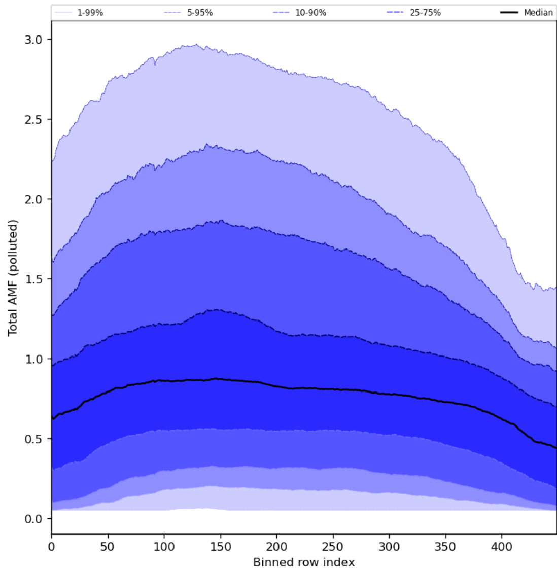
Figure 94: Along track statistics of “Total AMF (polluted)” for 2024-02-20 to 2024-02-22
