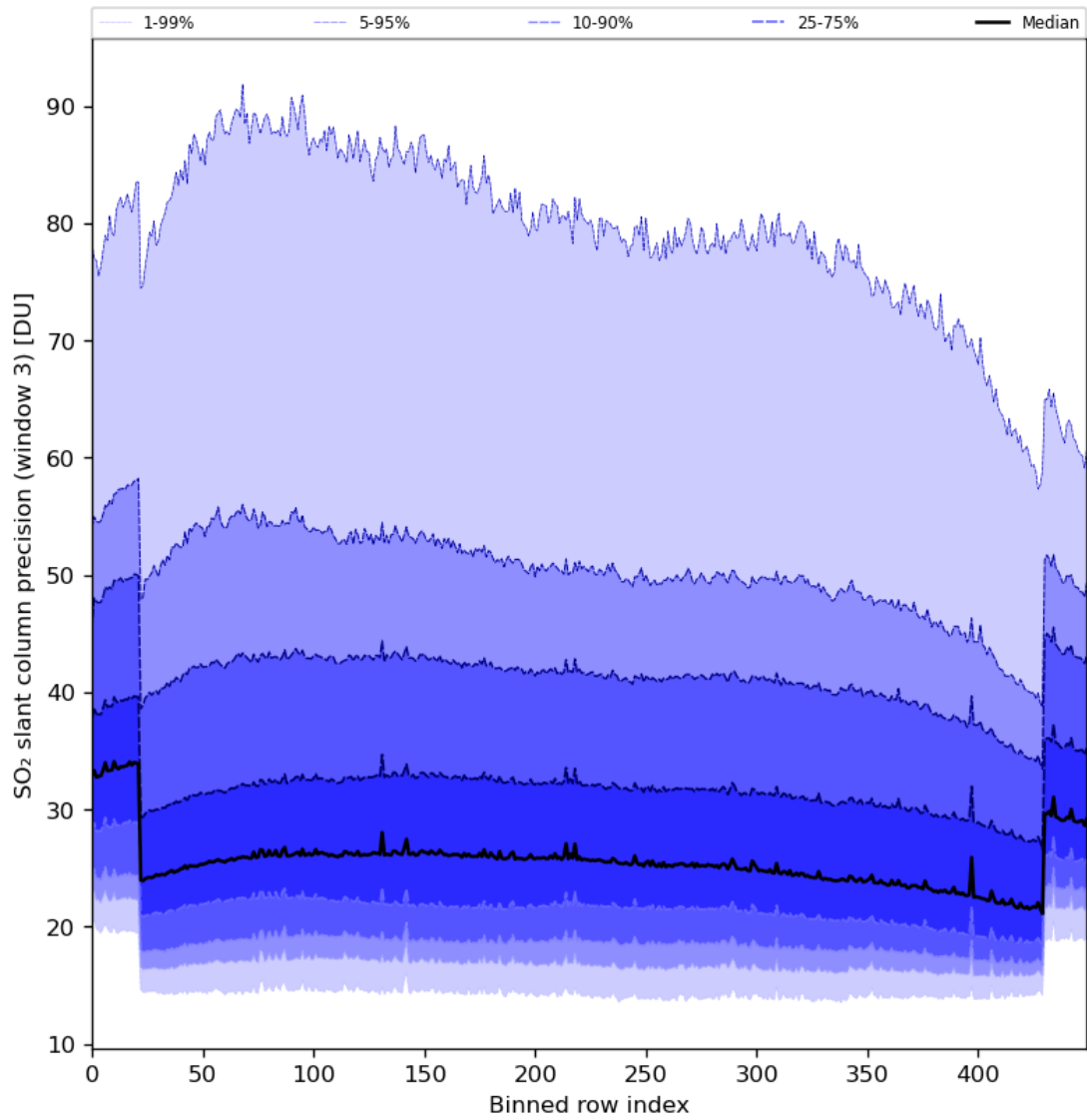
Figure 88: Along track statistics of “SO 2 slant column precision (window 3)” for 2024-02-20 to 2024-02-22
