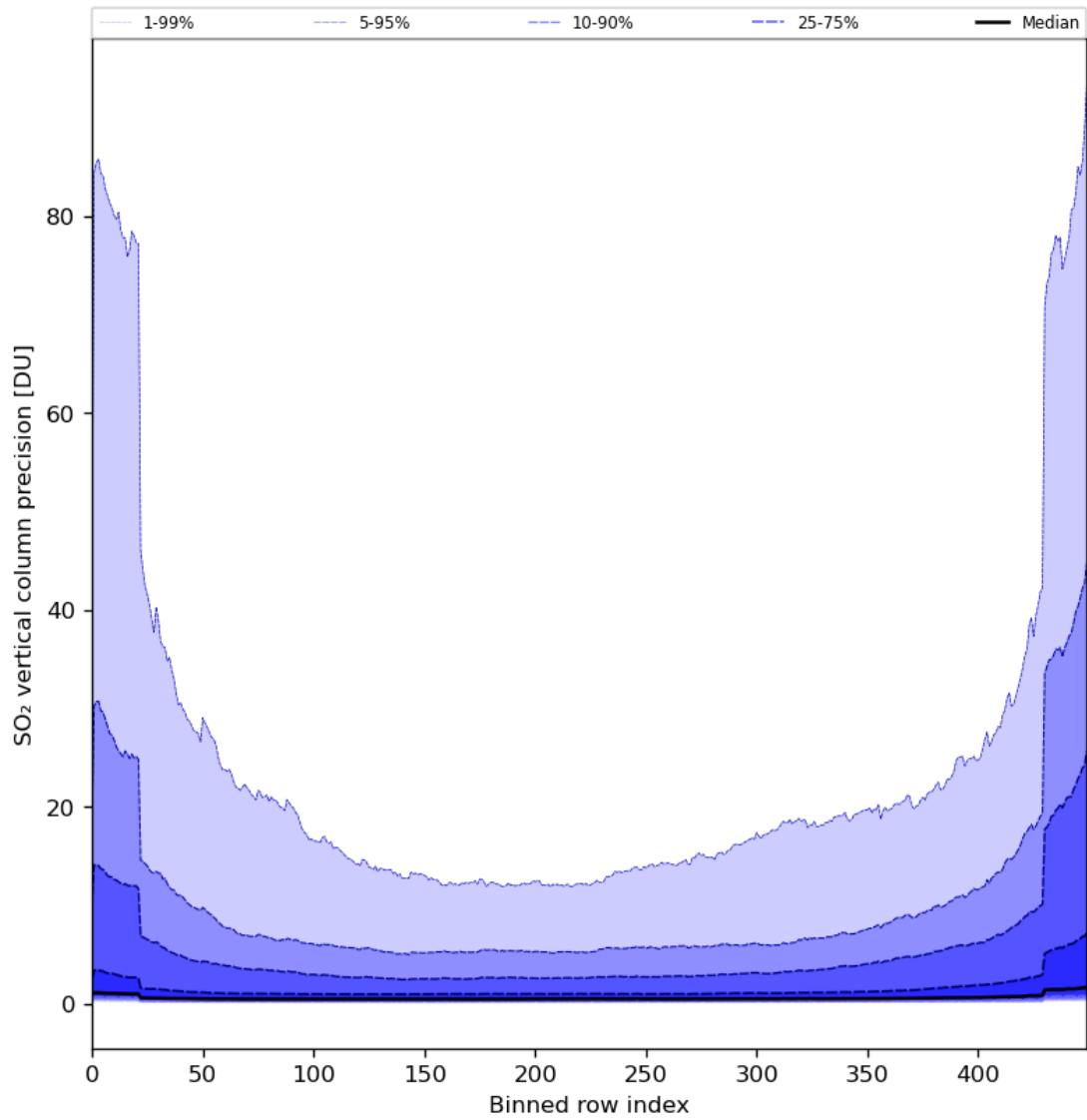
Figure 77: Along track statistics of “SO 2 vertical column precision” for 2024-02-20 to 2024-02-22
