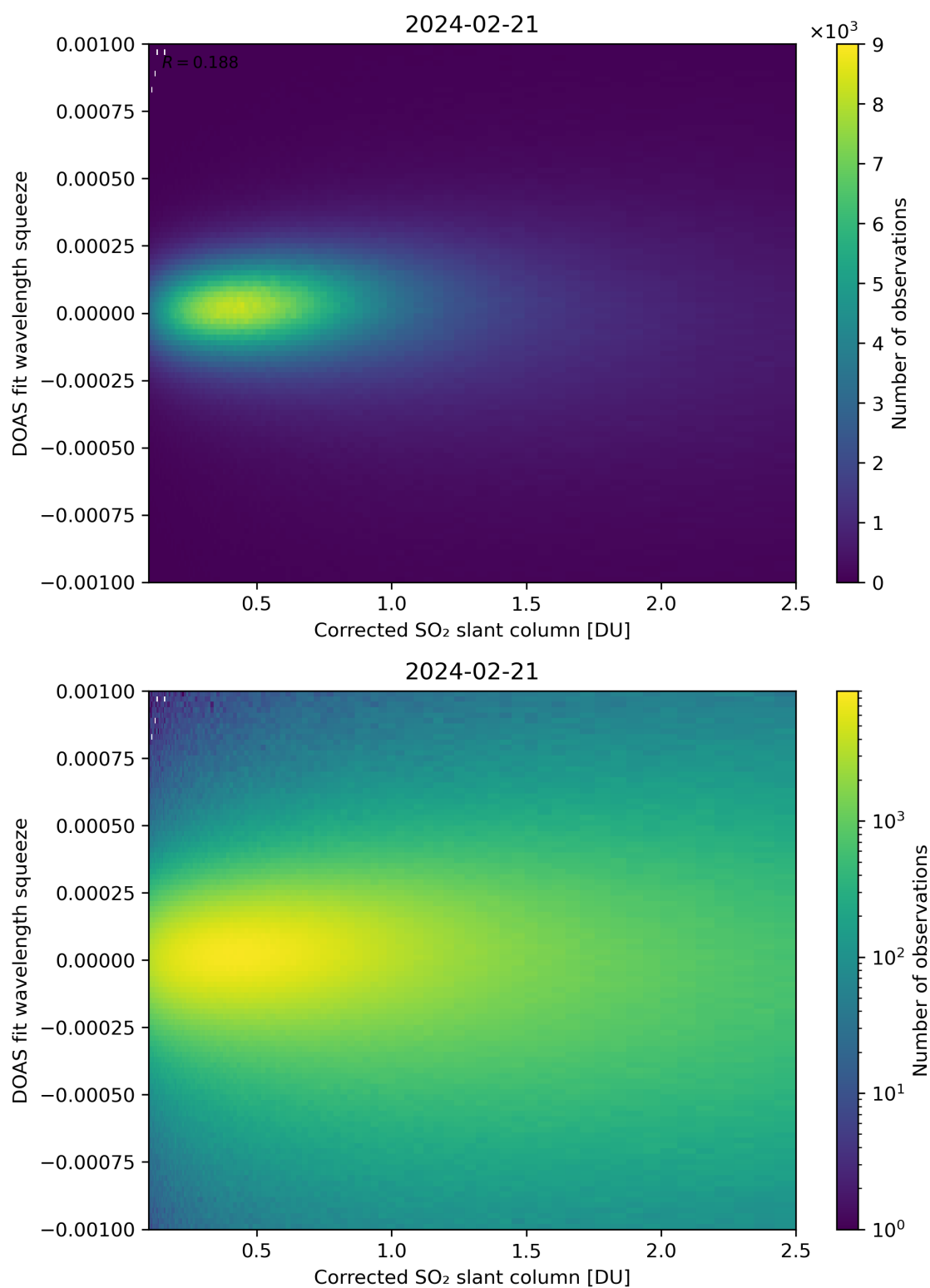
Figure 182: Scatter density plot of “Corrected SO 2 slant column” against “DOAS fit wavelength squeeze” for 2024-02-20 to 2024-02-22.
