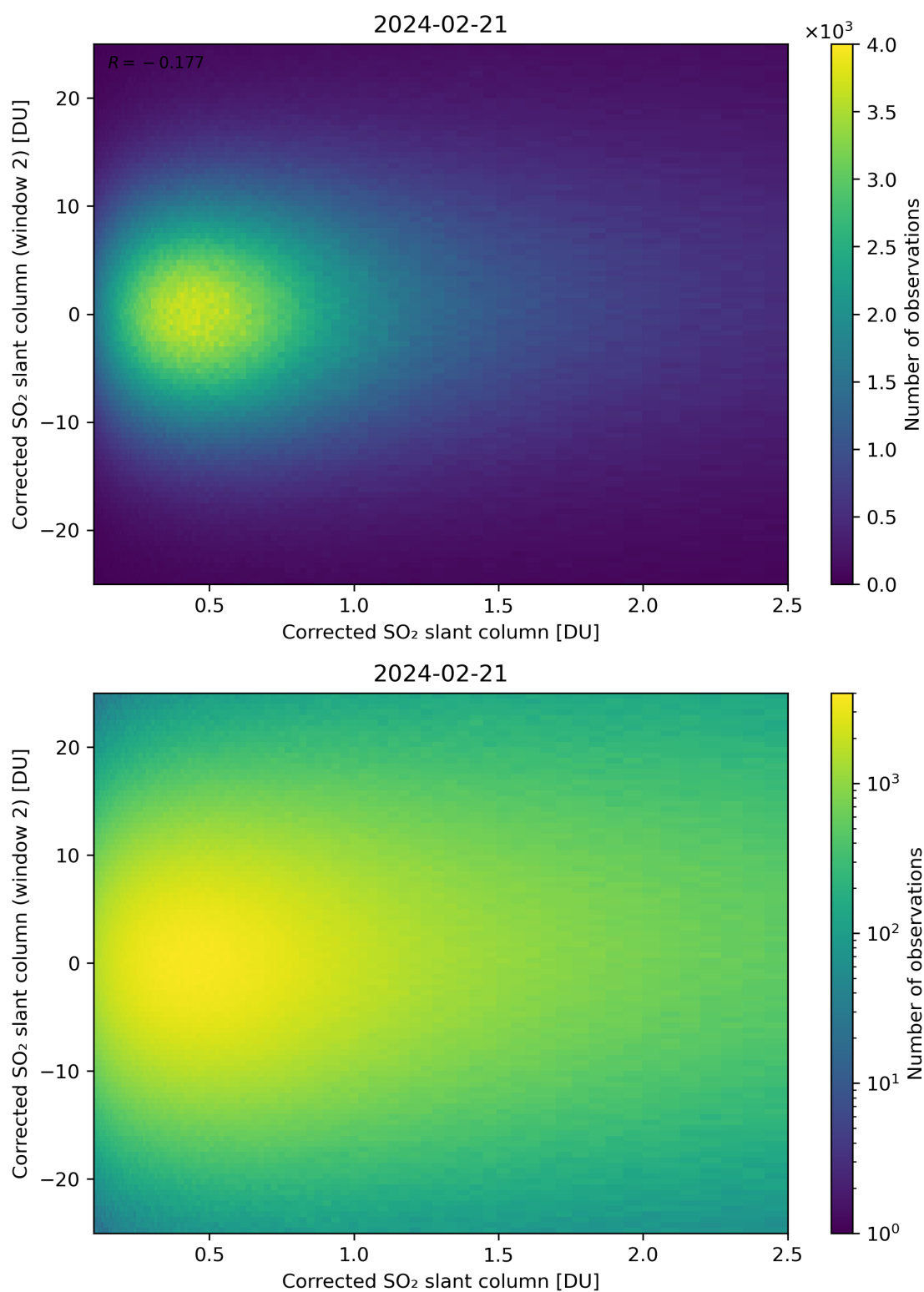
Figure 185: Scatter density plot of “Corrected SO 2 slant column” against “Corrected SO 2 slant column (window 2)” for 2024-02-20 to 2024-02-22.
