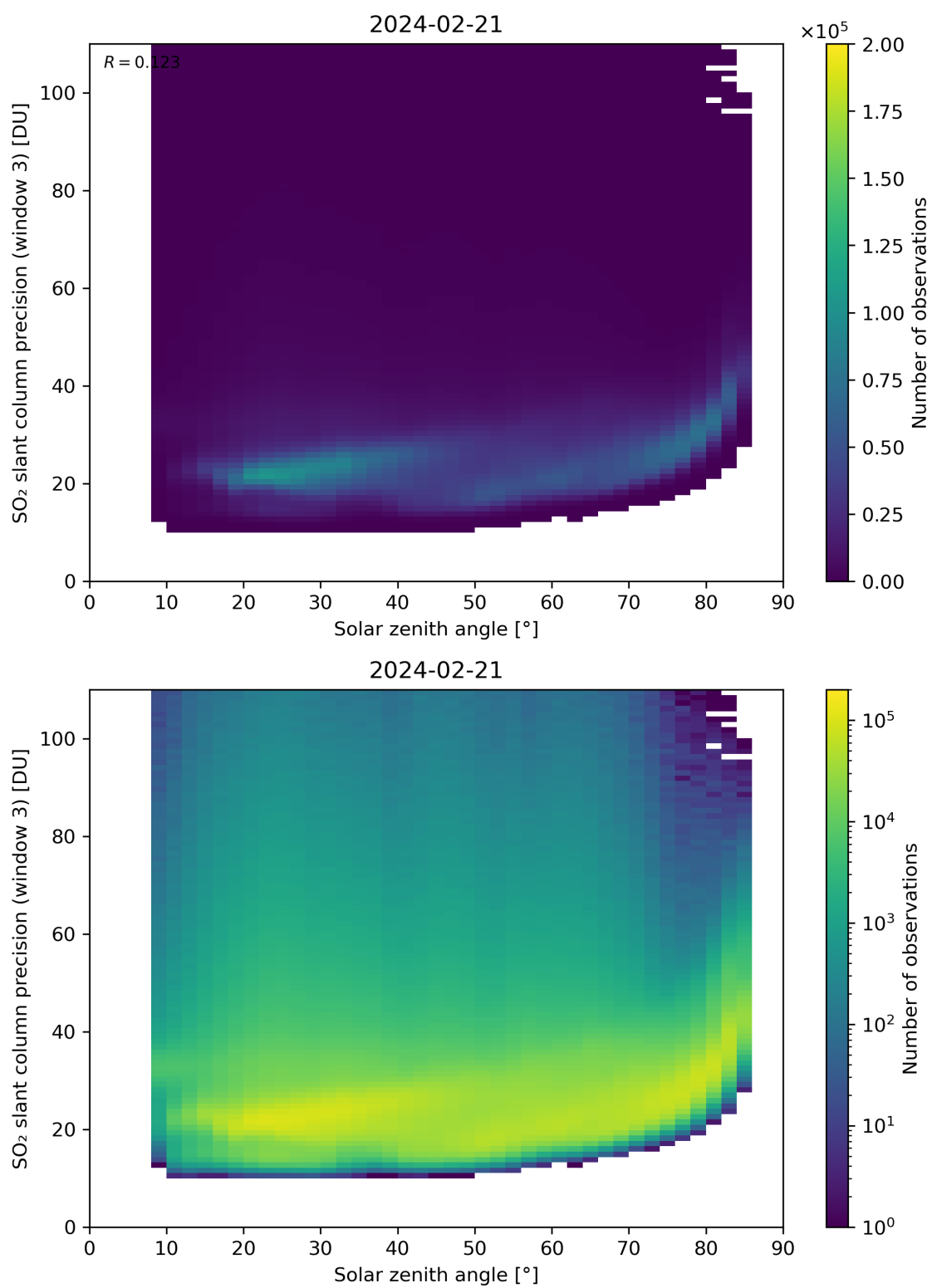
Figure 173: Scatter density plot of “Solar zenith angle” against “SO 2 slant column precision (window 3)” for 2024-02-20 to 2024-02-22.
