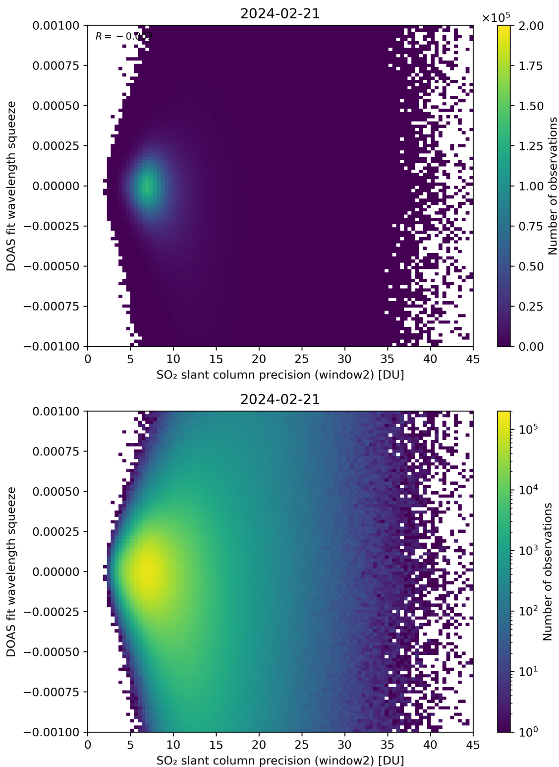
Figure 244: Scatter density plot of “SO 2 slant column precision (window2)” against “DOAS fit wavelength squeeze” for 2024-02-20 to 2024-02-22.
