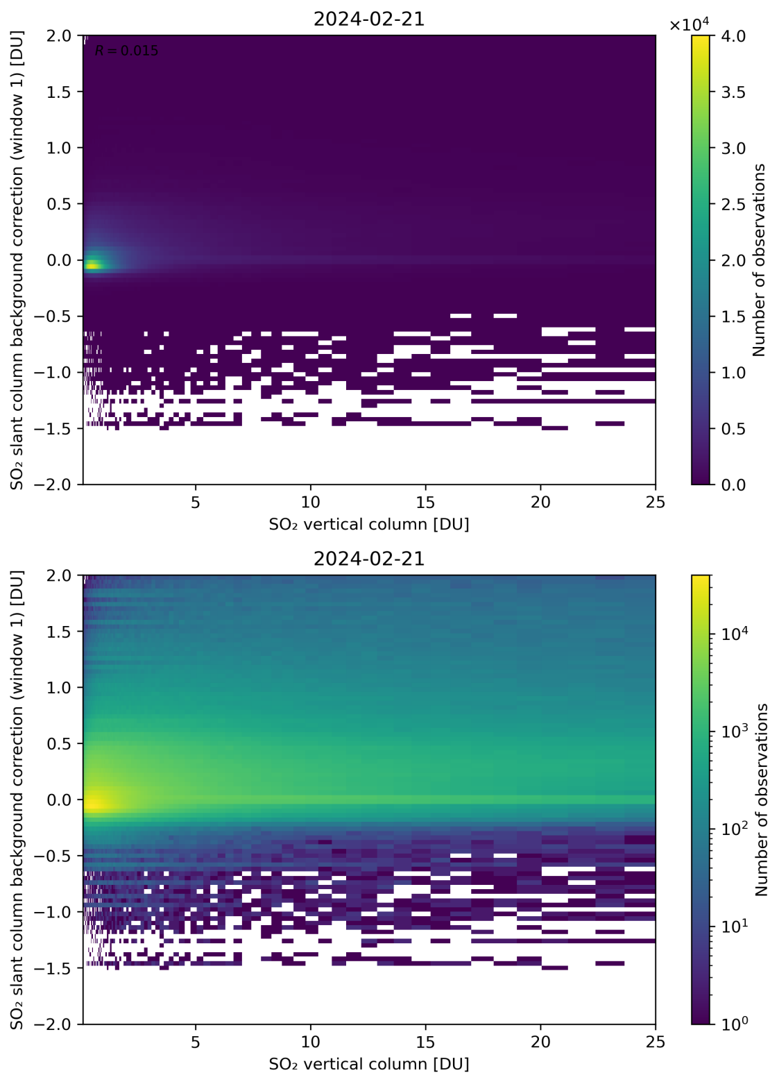
Figure 273: Scatter density plot of “SO 2 vertical column” against “SO 2 slant column background correction (window 1)” for 2024-02-20 to 2024-02-22.
