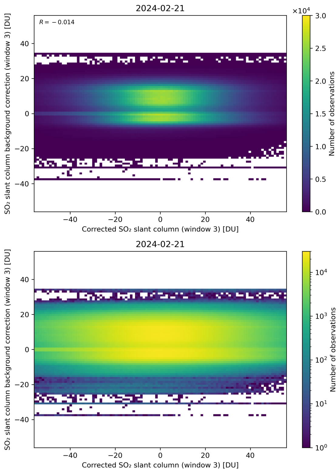
Figure 205: Scatter density plot of “Corrected SO 2 slant column (window 3)” against “SO 2 slant column background correction (window 3)” for 2024-02-20 to 2024-02-22.
