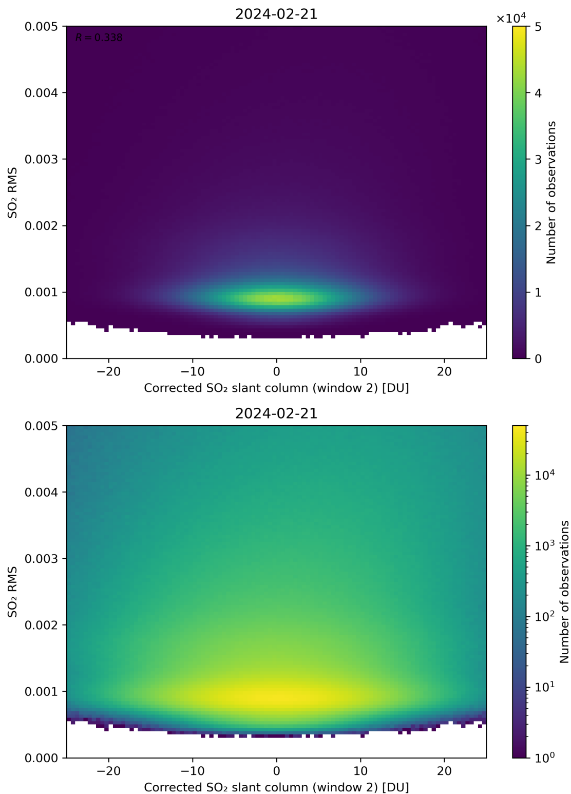
Figure 198: Scatter density plot of “Corrected SO 2 slant column (window 2)” against “SO 2 RMS” for 2024-02-20 to 2024-02-22.
