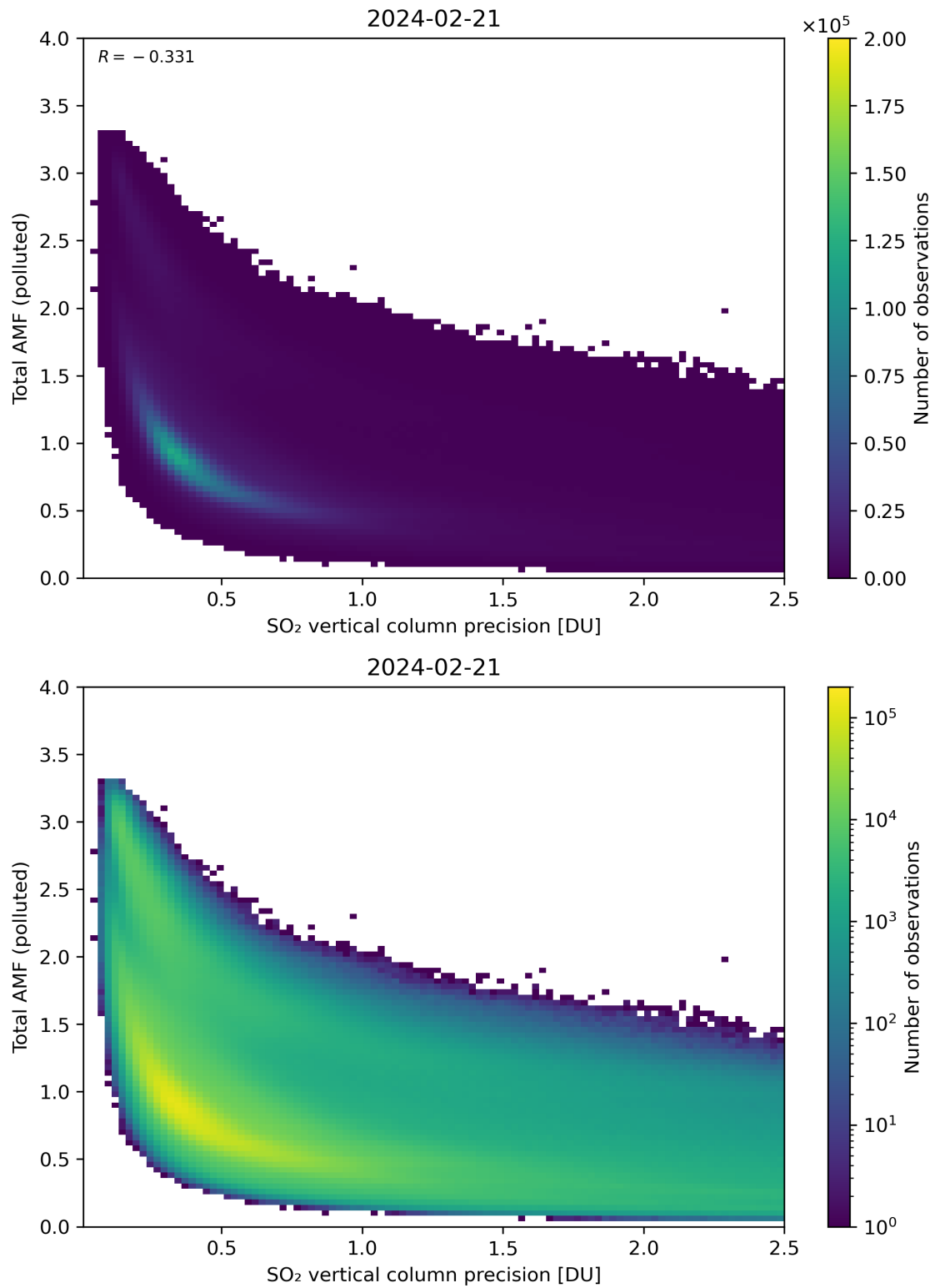
Figure 294: Scatter density plot of “SO 2 vertical column precision” against “Total AMF (polluted)” for 2024-02-20 to 2024-02-22.
