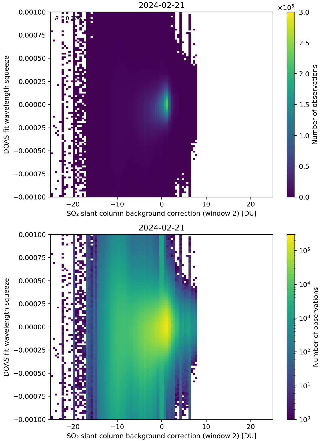
Figure 113: Scatter density plot of “SO 2 slant column background correction (window 2)” against “DOAS fit wavelength squeeze” for 2024-02-20 to 2024-02-22.
