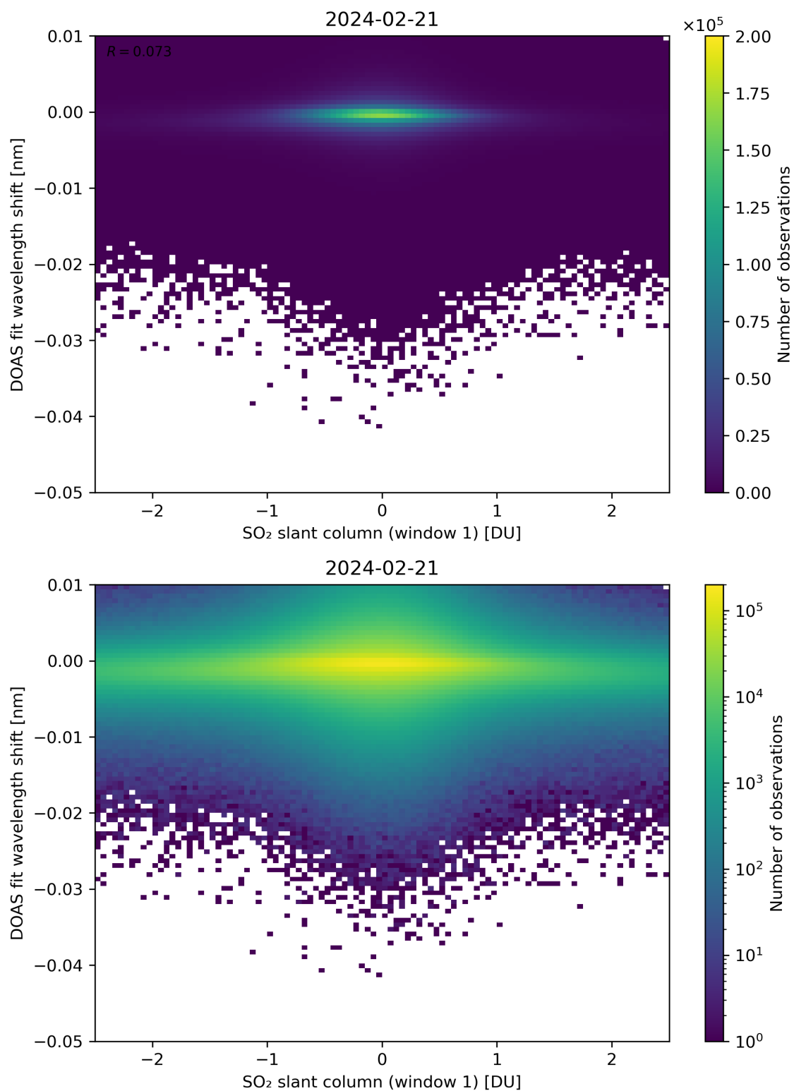
Figure 215: Scatter density plot of “SO 2 slant column (window 1)” against “DOAS fit wavelength shift” for 2024-02-20 to 2024-02-22.
