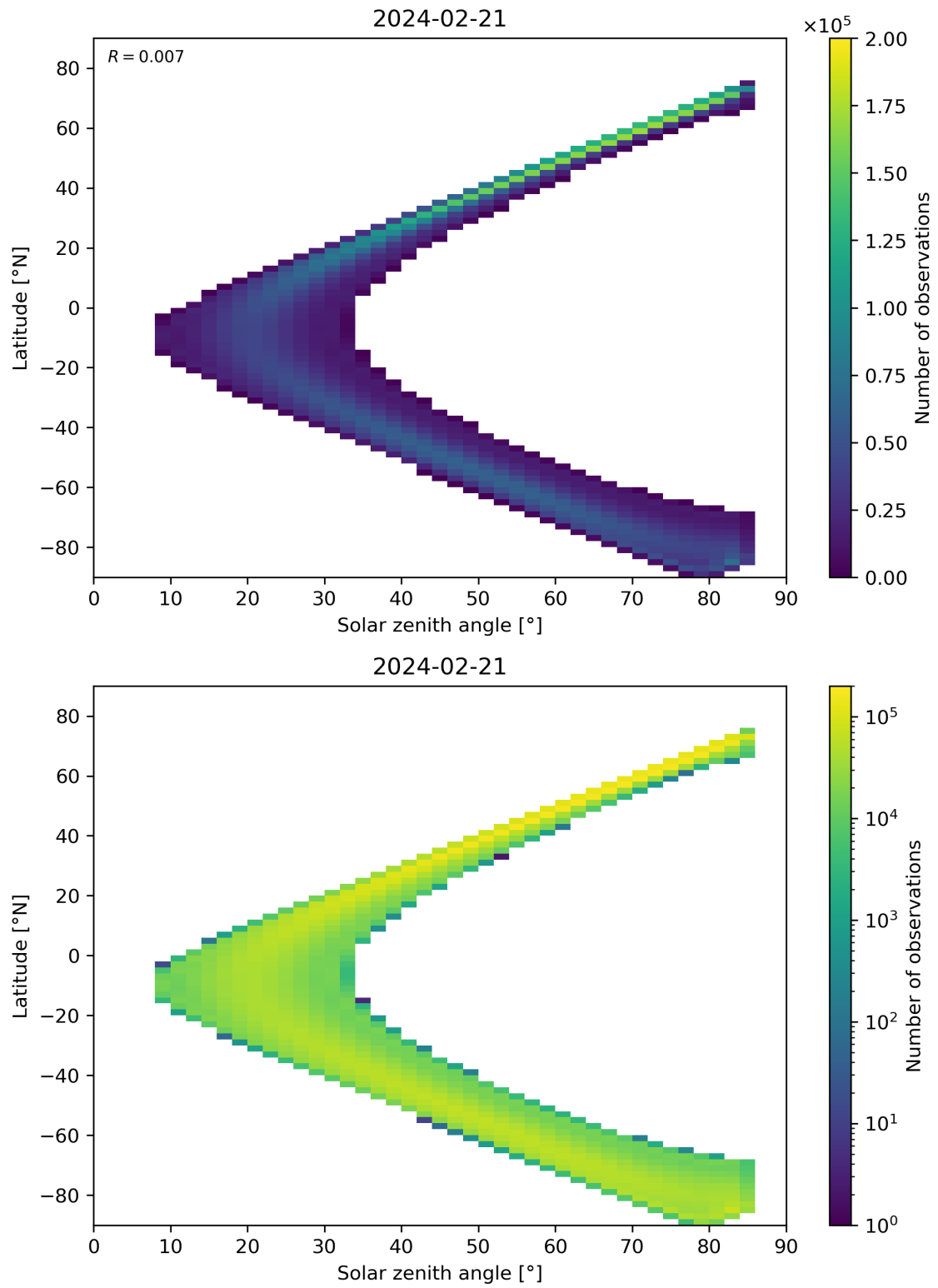
Figure 164: Scatter density plot of “Solar zenith angle” against “Latitude” for 2024-02-20 to 2024-02-22.
