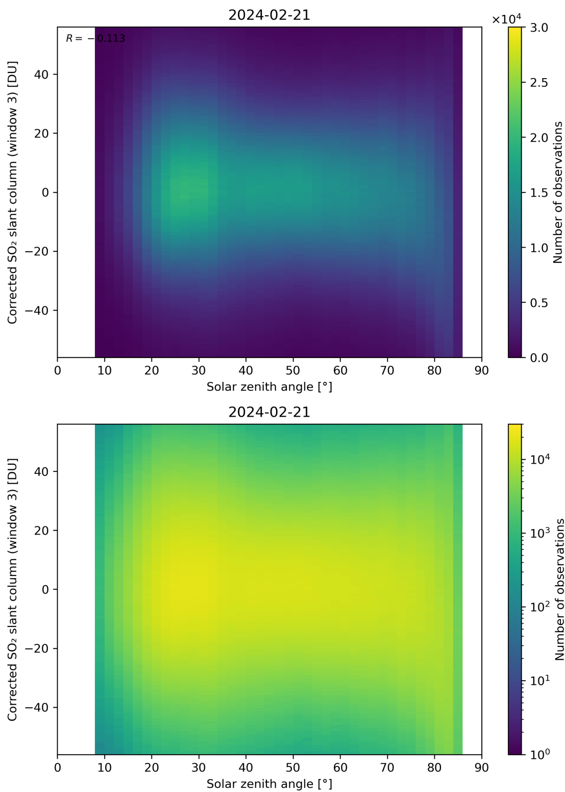
Figure 168: Scatter density plot of “Solar zenith angle” against “Corrected SO 2 slant column (window 3)” for 2024-02-20 to 2024-02-22.
