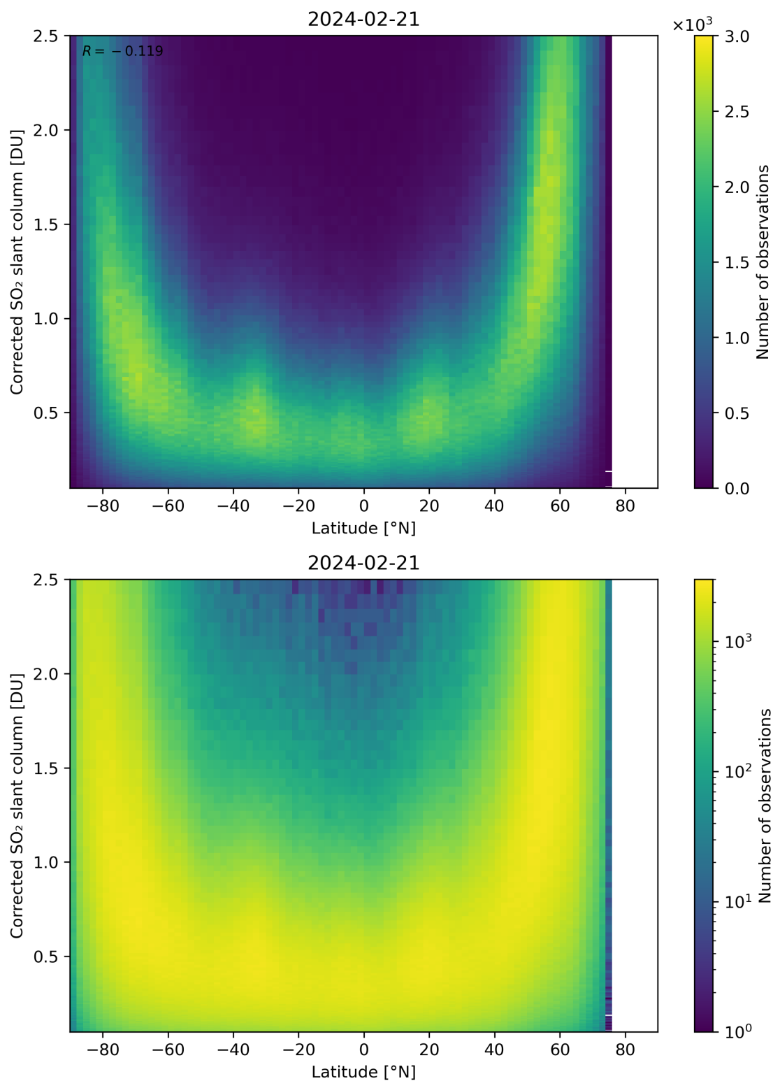
Figure 146: Scatter density plot of “Latitude” against “Corrected SO 2 slant column” for 2024-02-20 to 2024-02-22.
