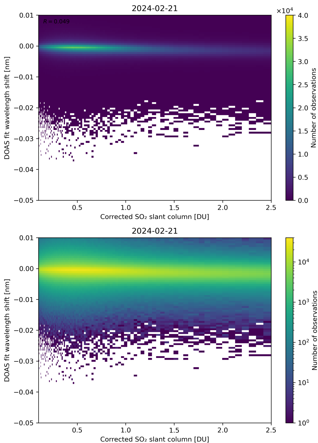
Figure 181: Scatter density plot of “Corrected SO 2 slant column” against “DOAS fit wavelength shift” for 2024-02-20 to 2024-02-22.
