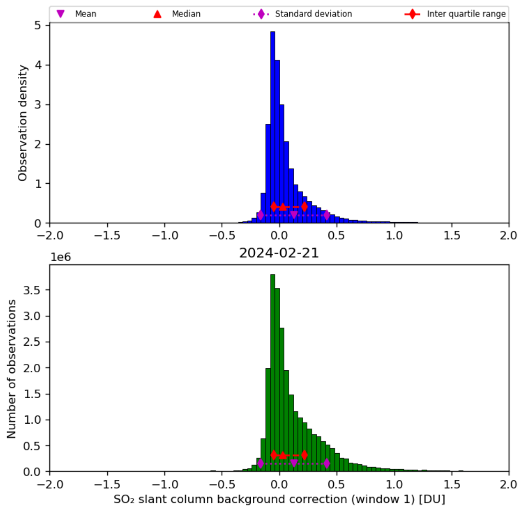
Figure 59: Histogram of “SO 2 slant column background correction (window 1)” for 2024-02-20 to 2024-02-22
