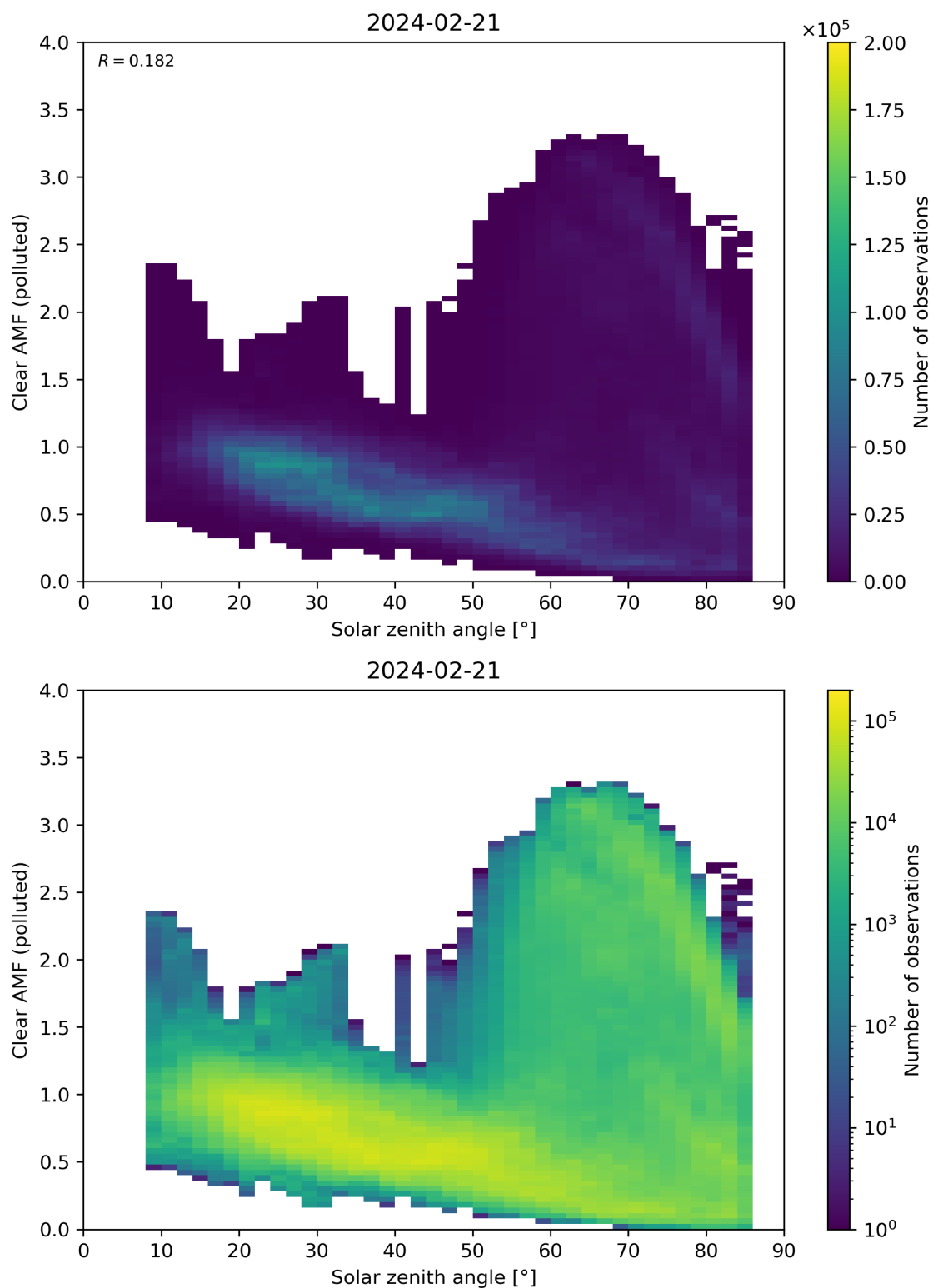
Figure 165: Scatter density plot of “Solar zenith angle” against “Clear AMF (polluted)” for 2024-02-20 to 2024-02-22.
