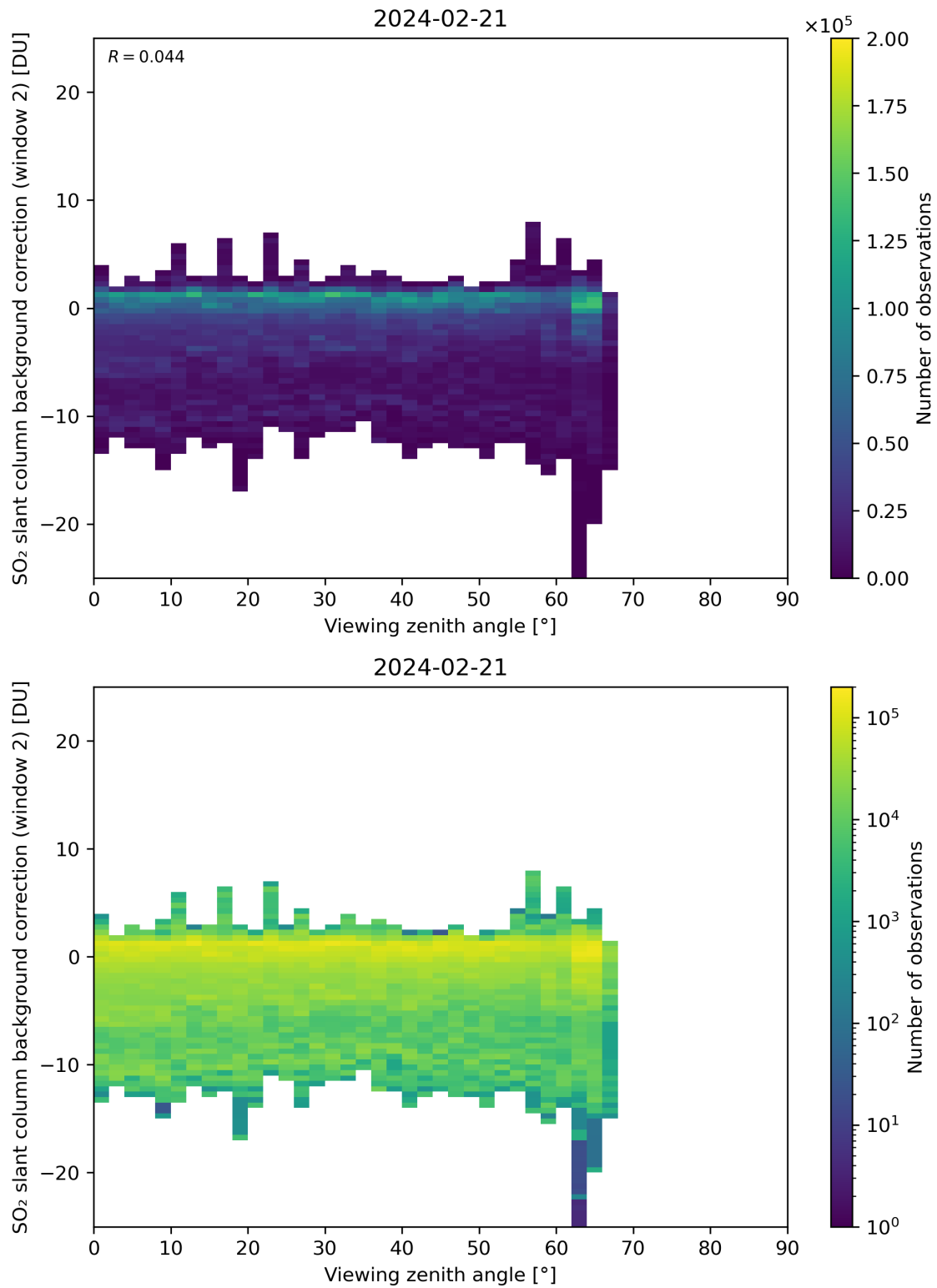
Figure 309: Scatter density plot of “Viewing zenith angle” against “SO 2 slant column background correction (window 2)” for 2024-02-20 to 2024-02-22.
