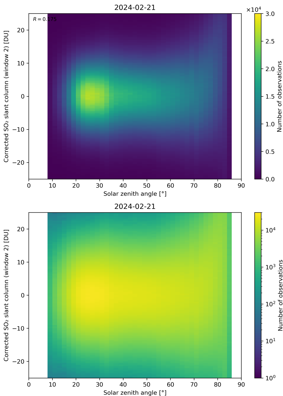
Figure 167: Scatter density plot of “Solar zenith angle” against “Corrected SO 2 slant column (window 2)” for 2024-02-20 to 2024-02-22.
