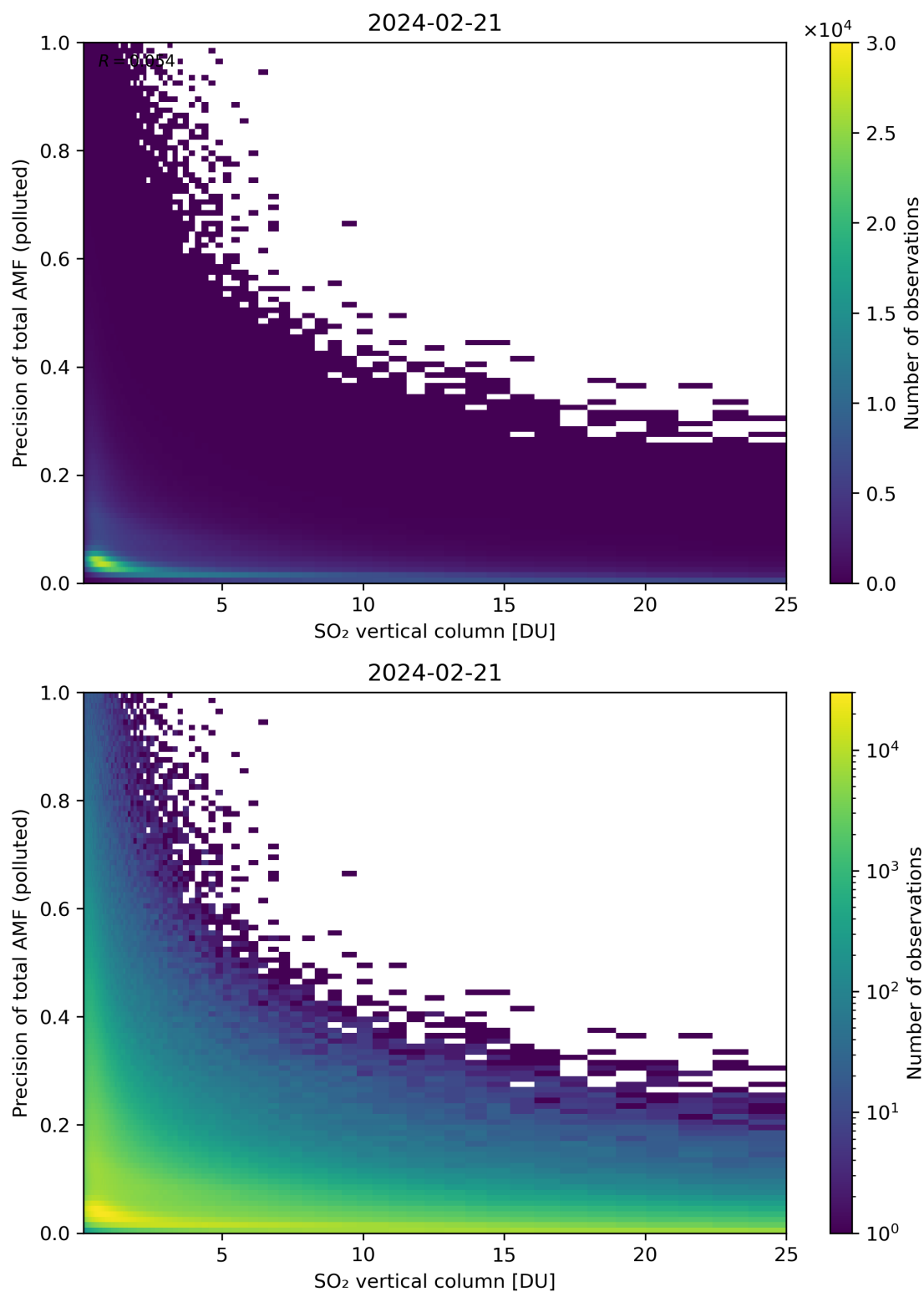
Figure 306: Scatter density plot of “SO 2 vertical column” against “Precision of total AMF (polluted)” for 2024-02-20 to 2024-02-22.
