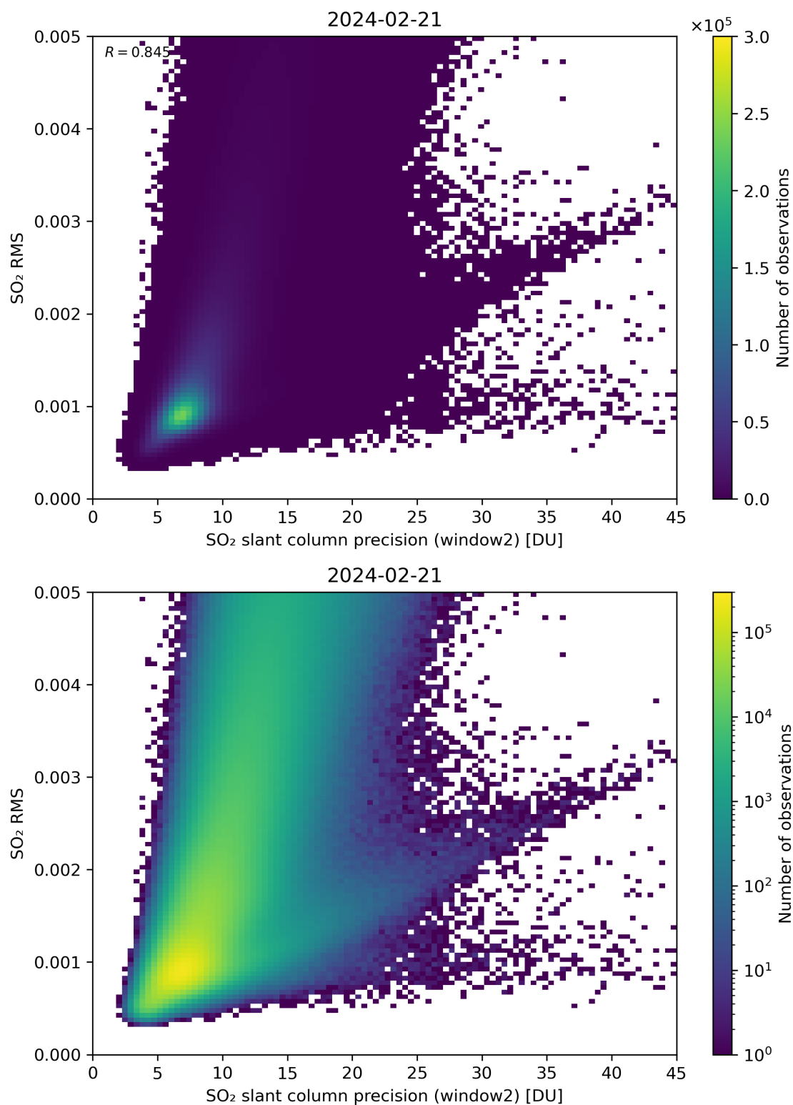
Figure 245: Scatter density plot of “SO 2 slant column precision (window2)” against “SO 2 RMS” for 2024-02-20 to 2024-02-22.
