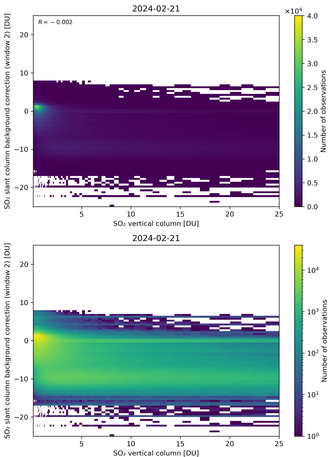
Figure 274: Scatter density plot of “SO 2 vertical column” against “SO 2 slant column background correction (window 2)” for 2024-02-20 to 2024-02-22.
