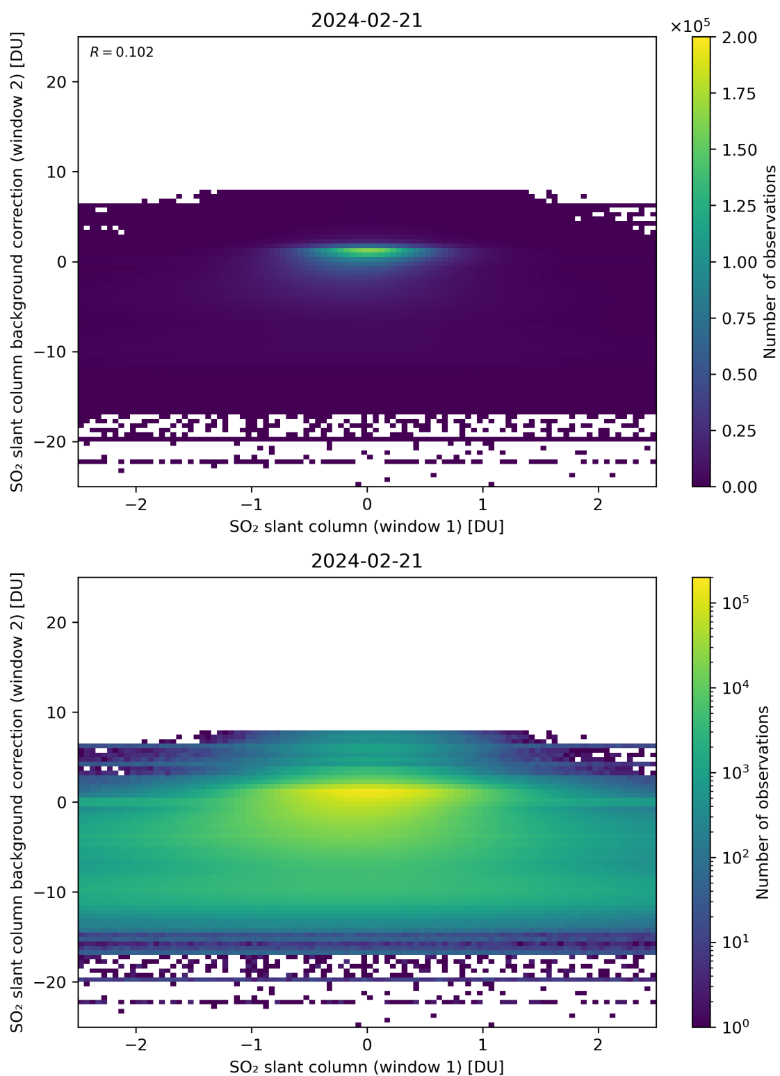
Figure 213: Scatter density plot of “SO 2 slant column (window 1)” against “SO 2 slant column background correction (window 2)” for 2024-02-20 to 2024-02-22.
