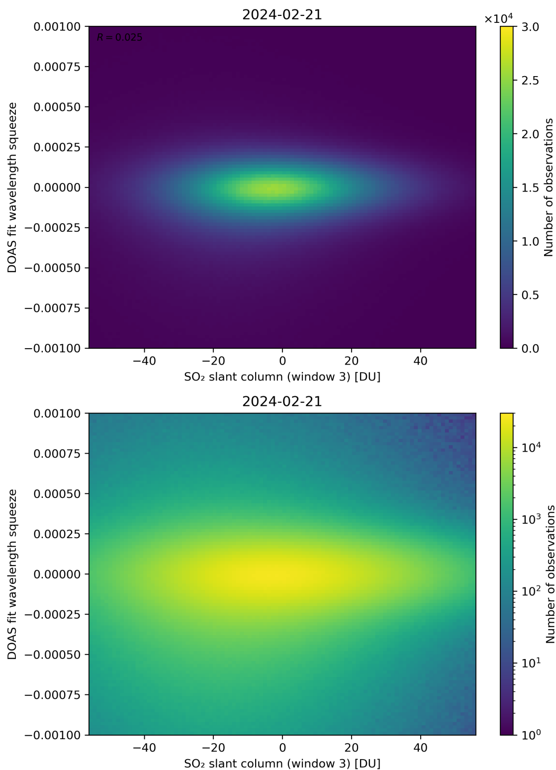
Figure 255: Scatter density plot of “SO 2 slant column (window 3)” against “DOAS fit wavelength squeeze” for 2024-02-20 to 2024-02-22.
