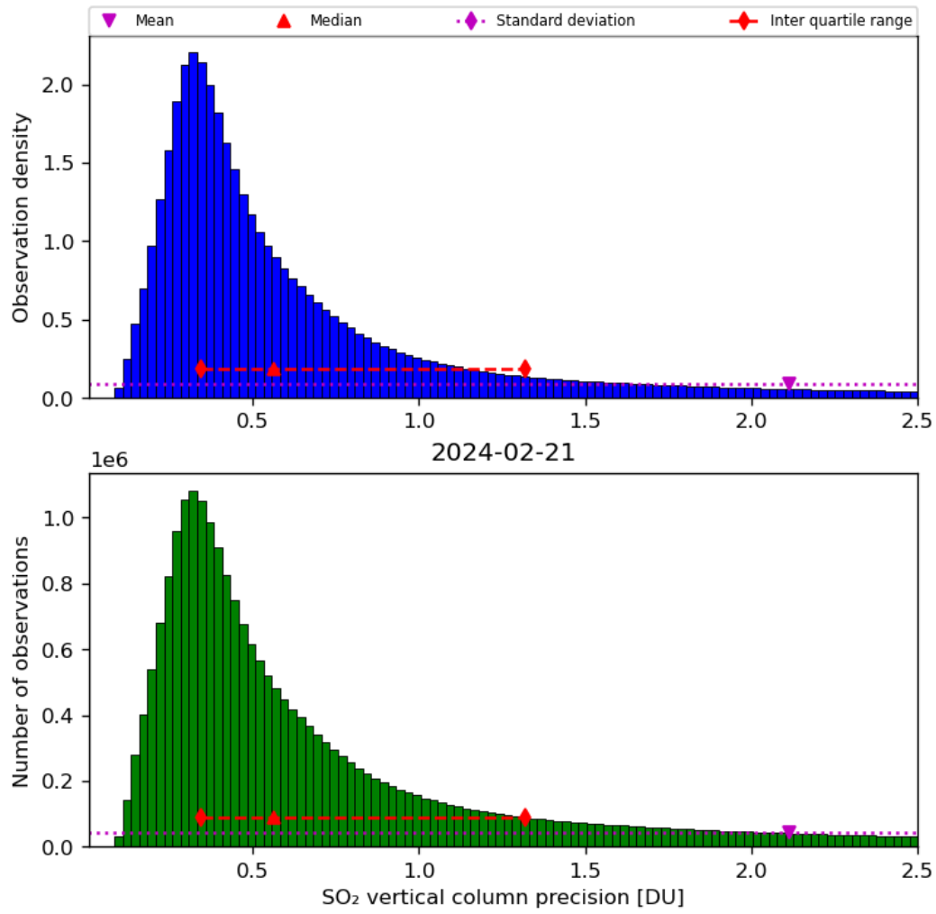
Figure 54: Histogram of “SO 2 vertical column precision” for 2024-02-20 to 2024-02-22
