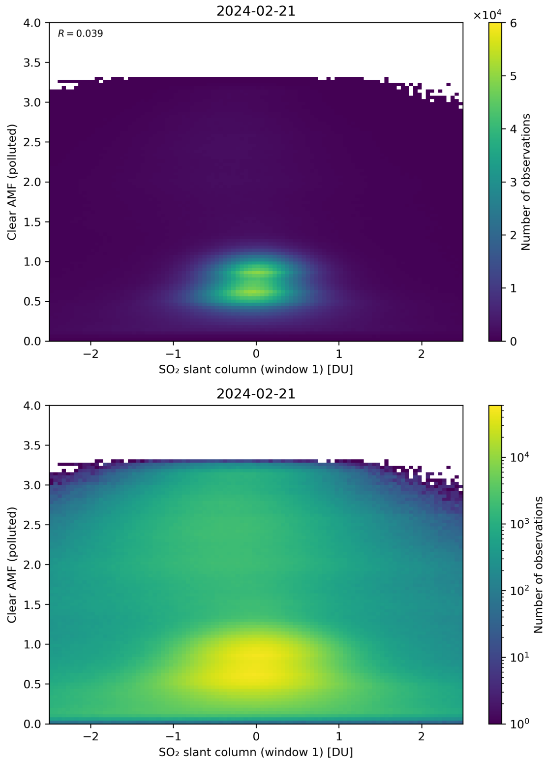
Figure 232: Scatter density plot of “SO 2 slant column (window 1)” against “Clear AMF (polluted)” for 2024-02-20 to 2024-02-22.
