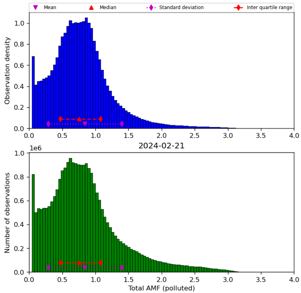
Figure 71: Histogram of “Total AMF (polluted)” for 2024-02-20 to 2024-02-22
