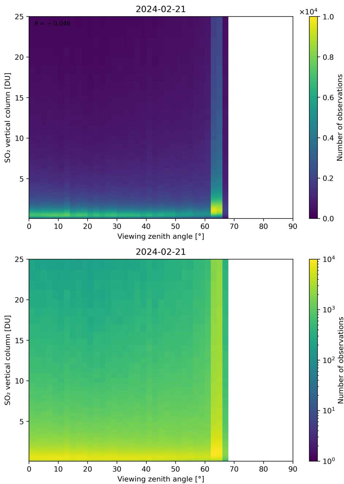
Figure 327: Scatter density plot of “Viewing zenith angle” against “SO 2 vertical column” for 2024-02-20 to 2024-02-22.
