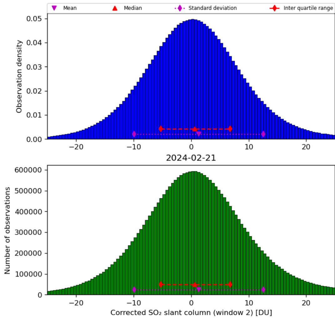
Figure 62: Histogram of “Corrected SO 2 slant column (window 2)” for 2024-02-20 to 2024-02-22
