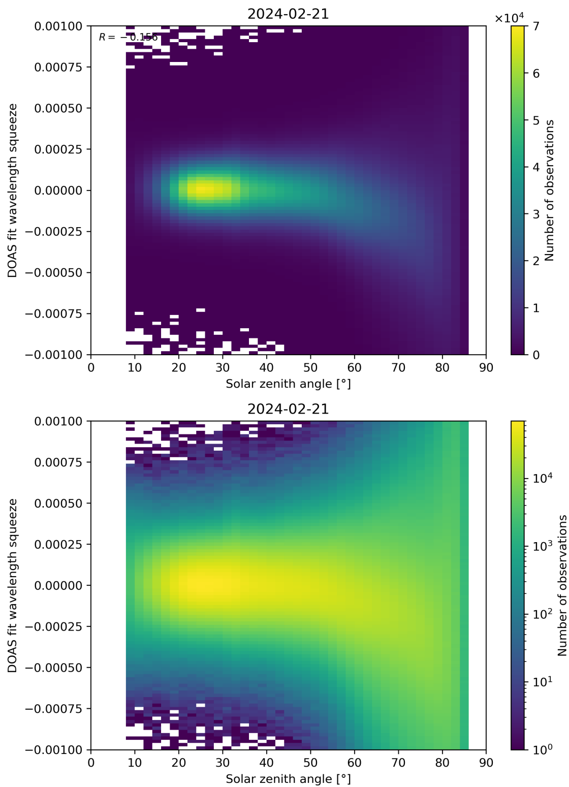
Figure 162: Scatter density plot of “Solar zenith angle” against “DOAS fit wavelength squeeze” for 2024-02-20 to 2024-02-22.
