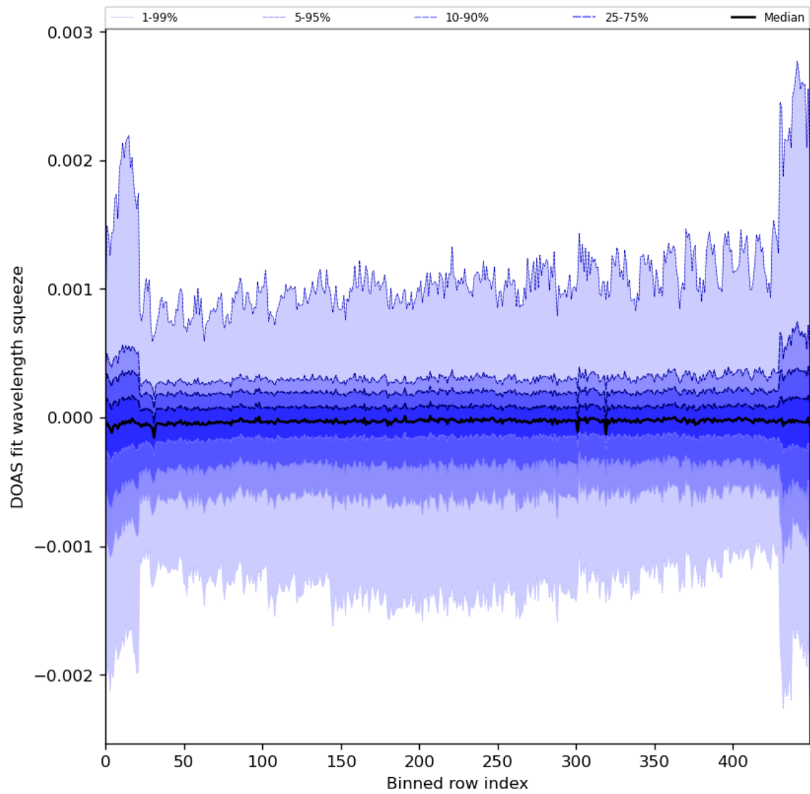
Figure 92: Along track statistics of “DOAS fit wavelength squeeze” for 2024-02-20 to 2024-02-22
