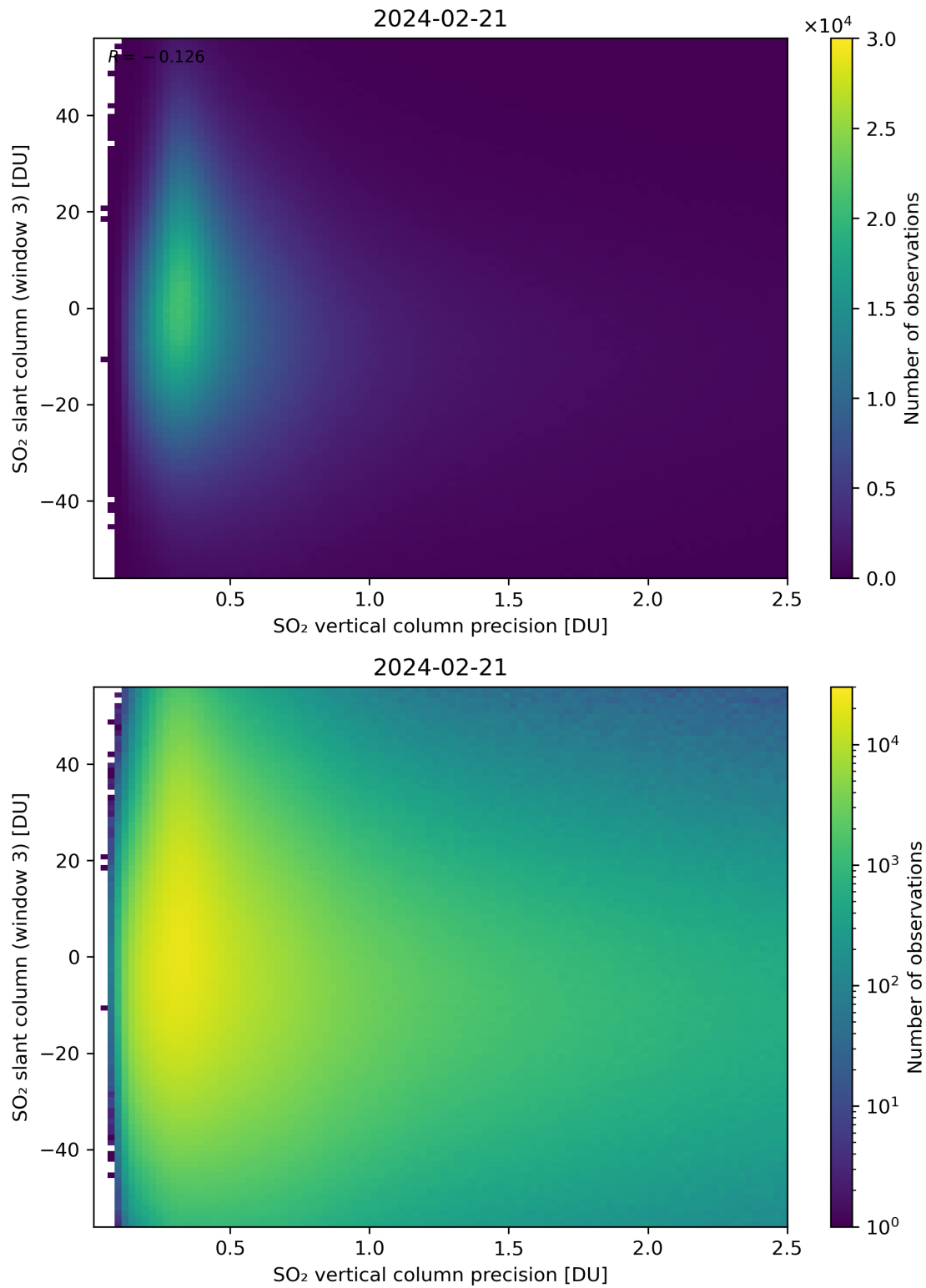
Figure 292: Scatter density plot of “SO 2 vertical column precision” against “SO 2 slant column (window 3)” for 2024-02-20 to 2024-02-22.
