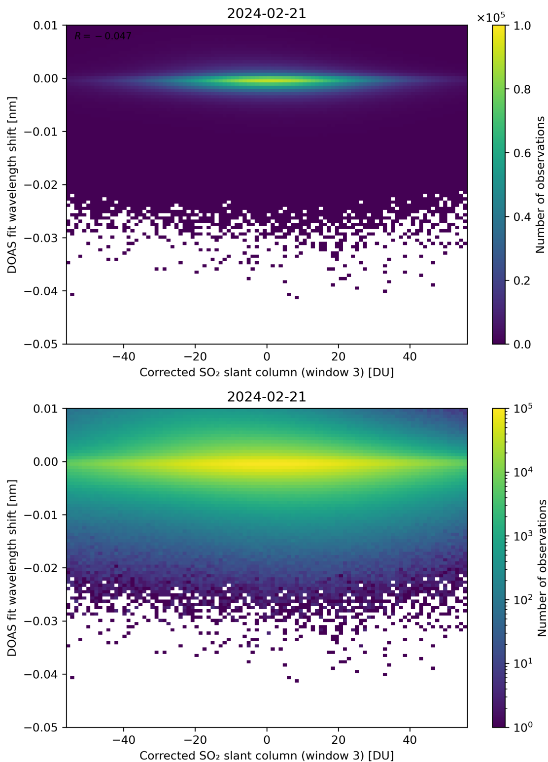
Figure 206: Scatter density plot of “Corrected SO 2 slant column (window 3)” against “DOAS fit wavelength shift” for 2024-02-20 to 2024-02-22.
