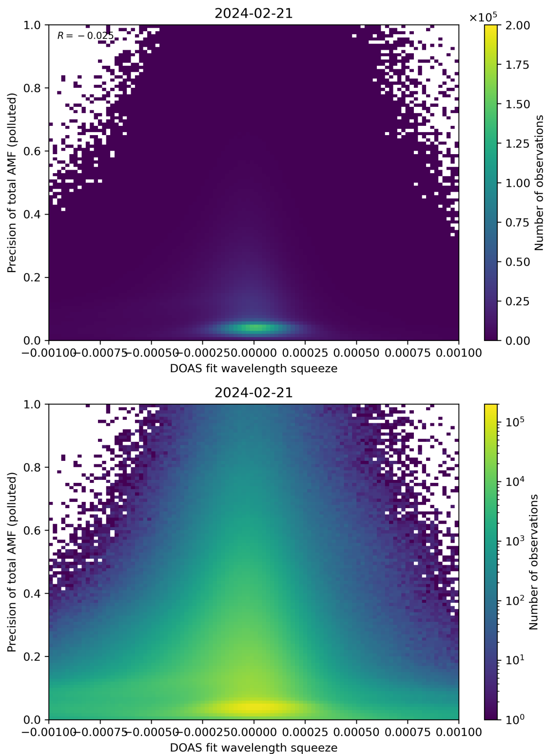
Figure 135: Scatter density plot of “DOAS fit wavelength squeeze” against “Precision of total AMF (polluted)” for 2024-02-20 to 2024-02-22.
