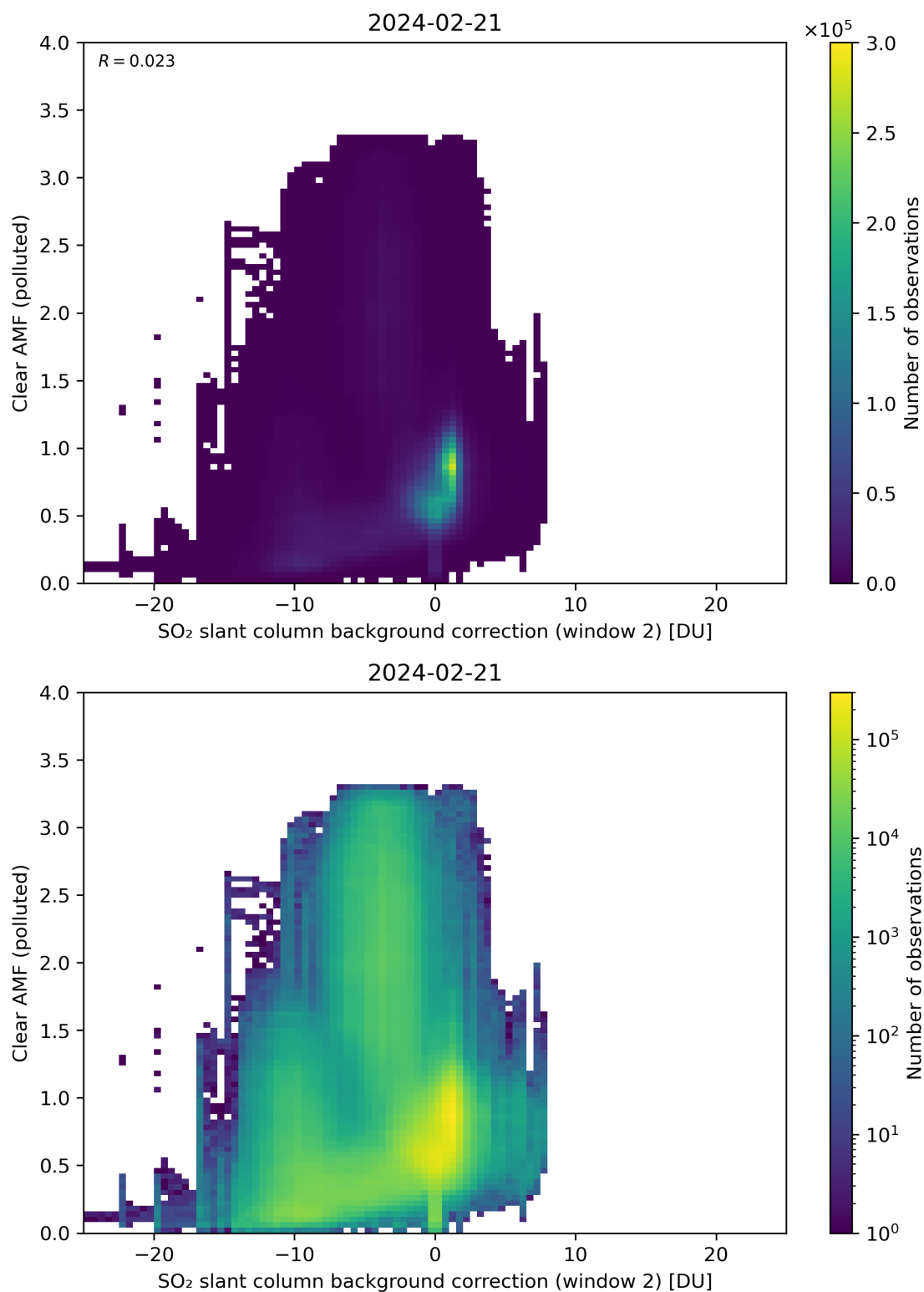
Figure 115: Scatter density plot of “SO 2 slant column background correction (window 2)” against “Clear AMF (polluted)” for 2024-02-20 to 2024-02-22.
