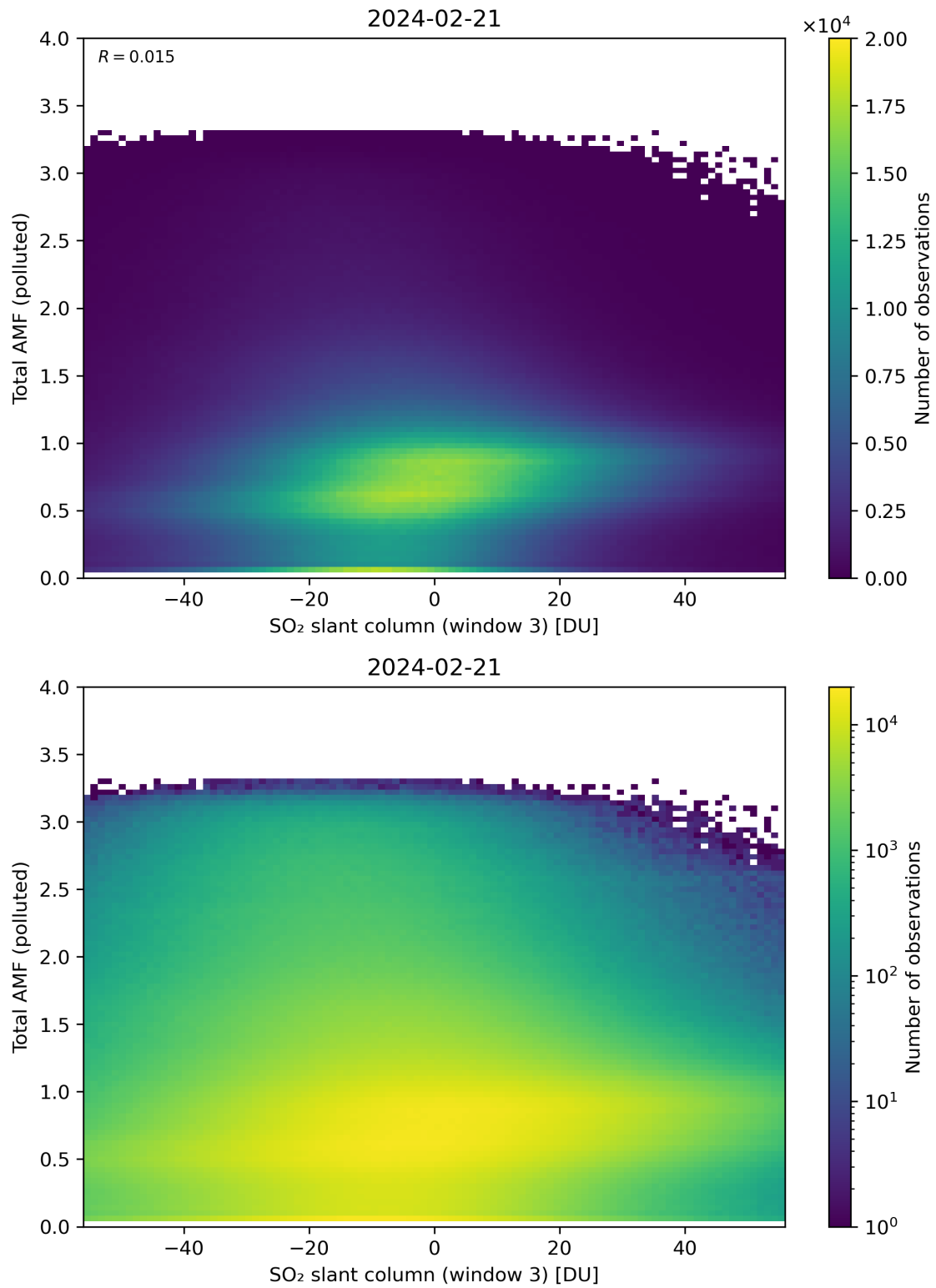
Figure 268: Scatter density plot of “SO 2 slant column (window 3)” against “Total AMF (polluted)” for 2024-02-20 to 2024-02-22.
