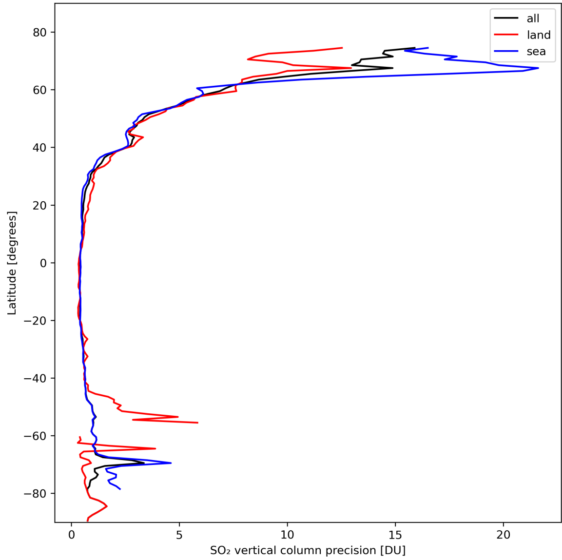
Figure 31: Zonal average of “SO 2 vertical column precision” for 2024-02-20 to 2024-02-22.
