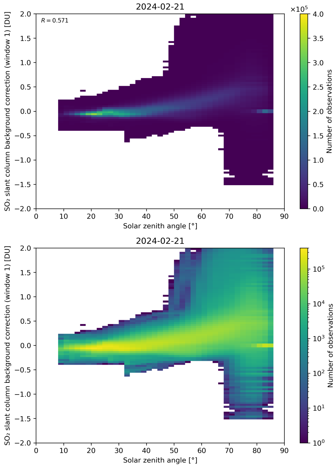
Figure 158: Scatter density plot of “Solar zenith angle” against “SO 2 slant column background correction (window 1)” for 2024-02-20 to 2024-02-22.
