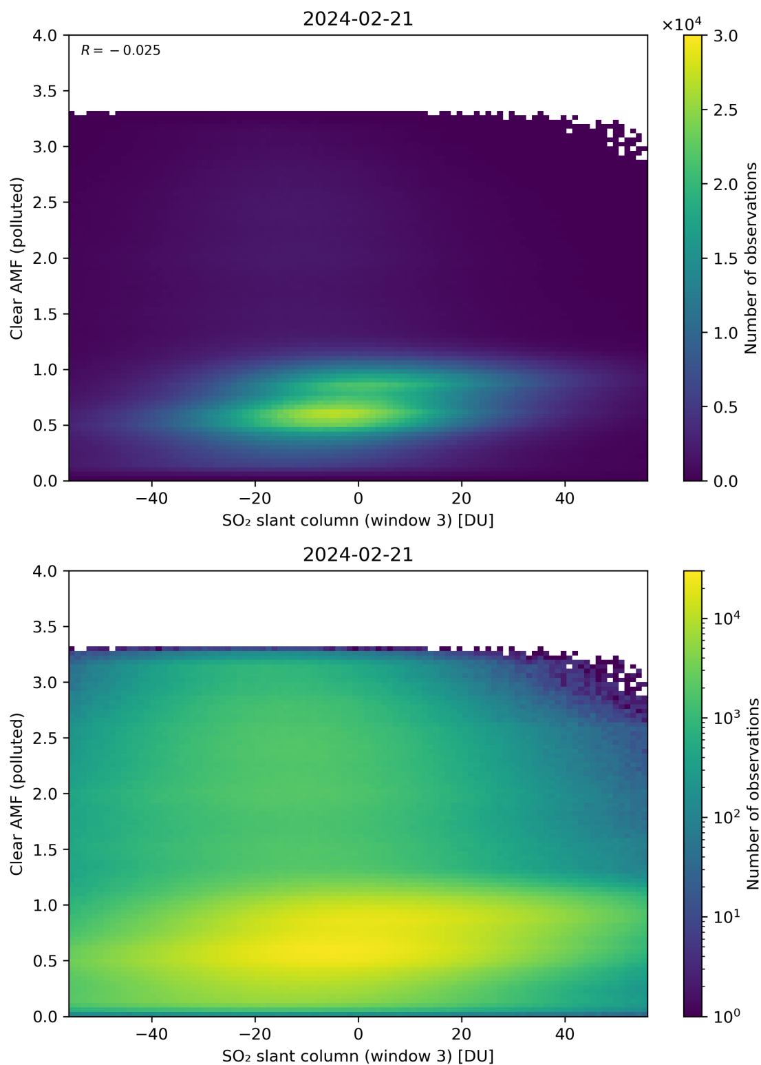
Figure 265: Scatter density plot of “SO 2 slant column (window 3)” against “Clear AMF (polluted)” for 2024-02-20 to 2024-02-22.
