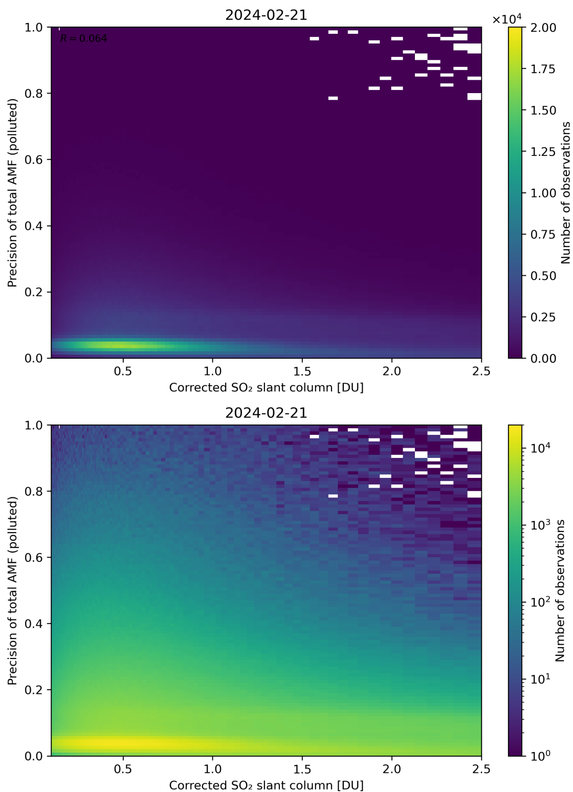
Figure 193: Scatter density plot of “Corrected SO 2 slant column” against “Precision of total AMF (polluted)” for 2024-02-20 to 2024-02-22.
