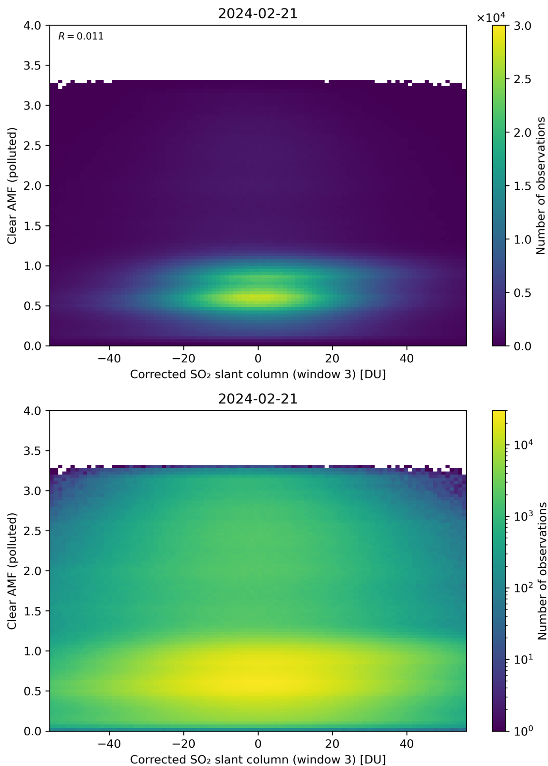
Figure 209: Scatter density plot of “Corrected SO 2 slant column (window 3)” against “Clear AMF (polluted)” for 2024-02-20 to 2024-02-22.
