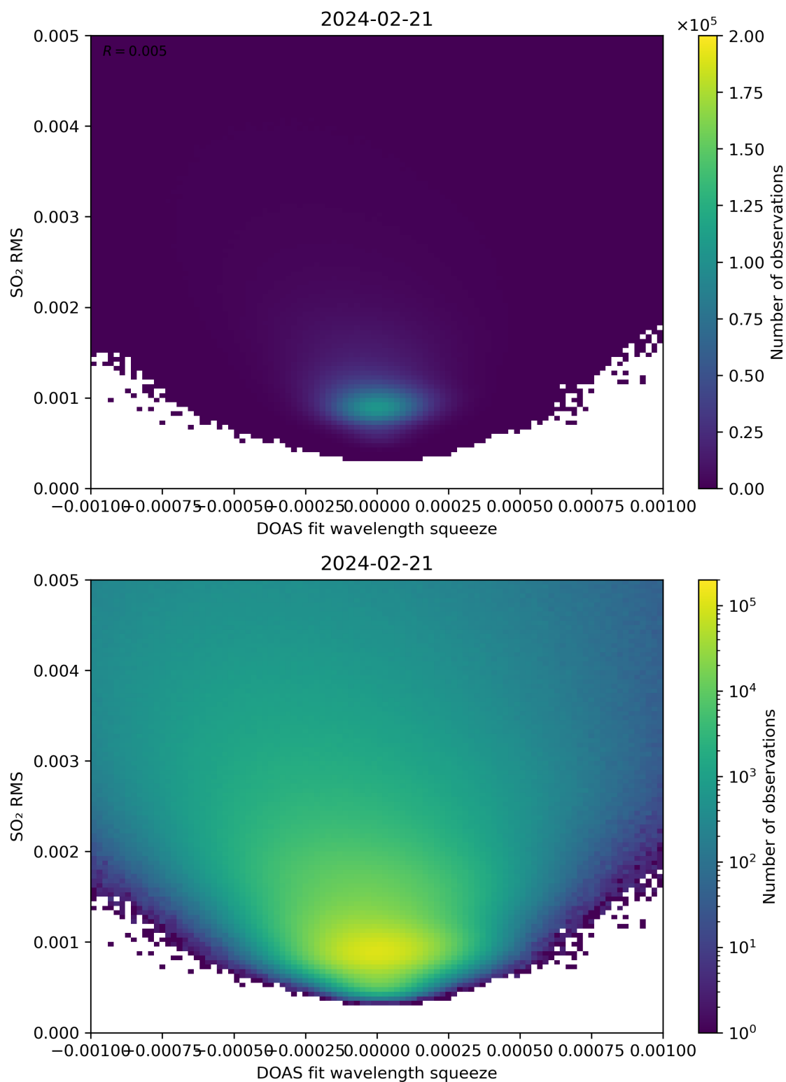
Figure 132: Scatter density plot of “DOAS fit wavelength squeeze” against “SO 2 RMS” for 2024-02-20 to 2024-02-22.
