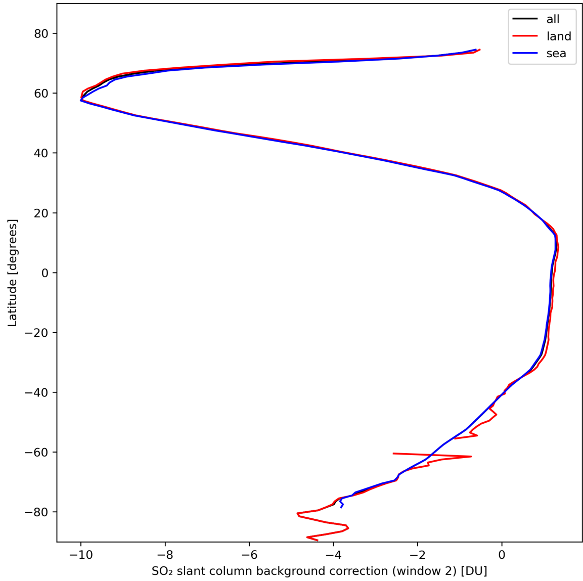
Figure 40: Zonal average of “SO 2 slant column background correction (window 2)” for 2024-02-20 to 2024-02-22.
