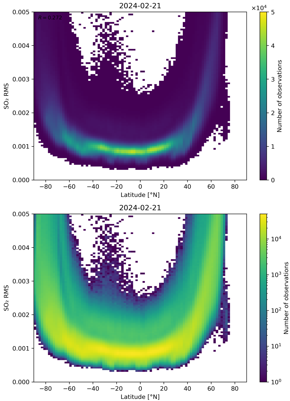
Figure 144: Scatter density plot of “Latitude” against “SO 2 RMS” for 2024-02-20 to 2024-02-22.
