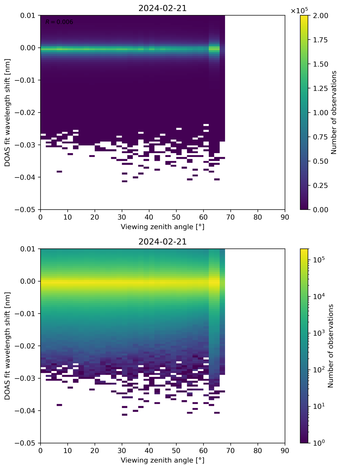
Figure 311: Scatter density plot of “Viewing zenith angle” against “DOAS fit wavelength shift” for 2024-02-20 to 2024-02-22.
