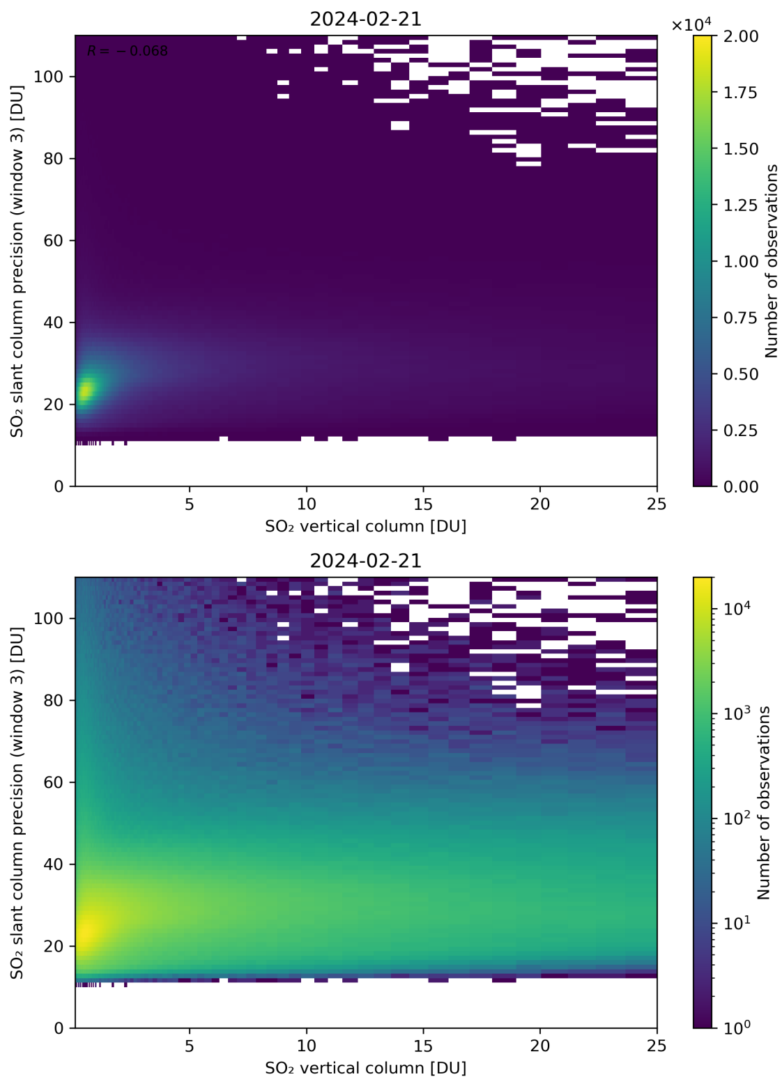
Figure 304: Scatter density plot of “SO 2 vertical column” against “SO 2 slant column precision (window 3)” for 2024-02-20 to 2024-02-22.
