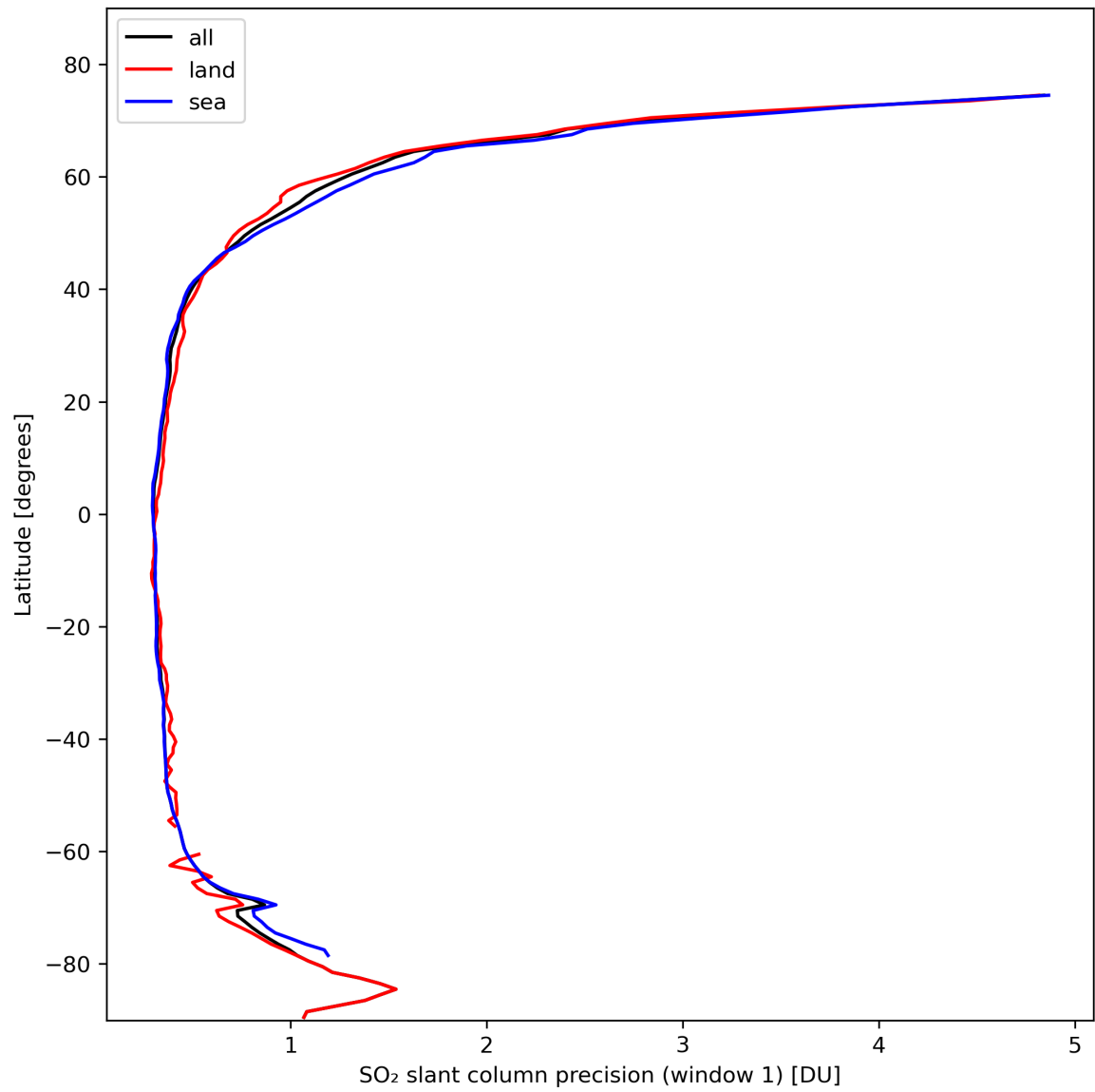
Figure 34: Zonal average of “SO 2 slant column precision (window 1)” for 2024-02-20 to 2024-02-22.
