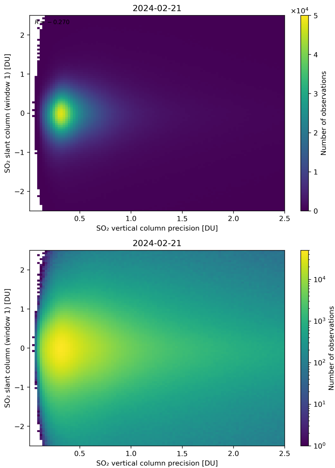
Figure 289: Scatter density plot of “SO 2 vertical column precision” against “SO 2 slant column (window 1)” for 2024-02-20 to 2024-02-22.
