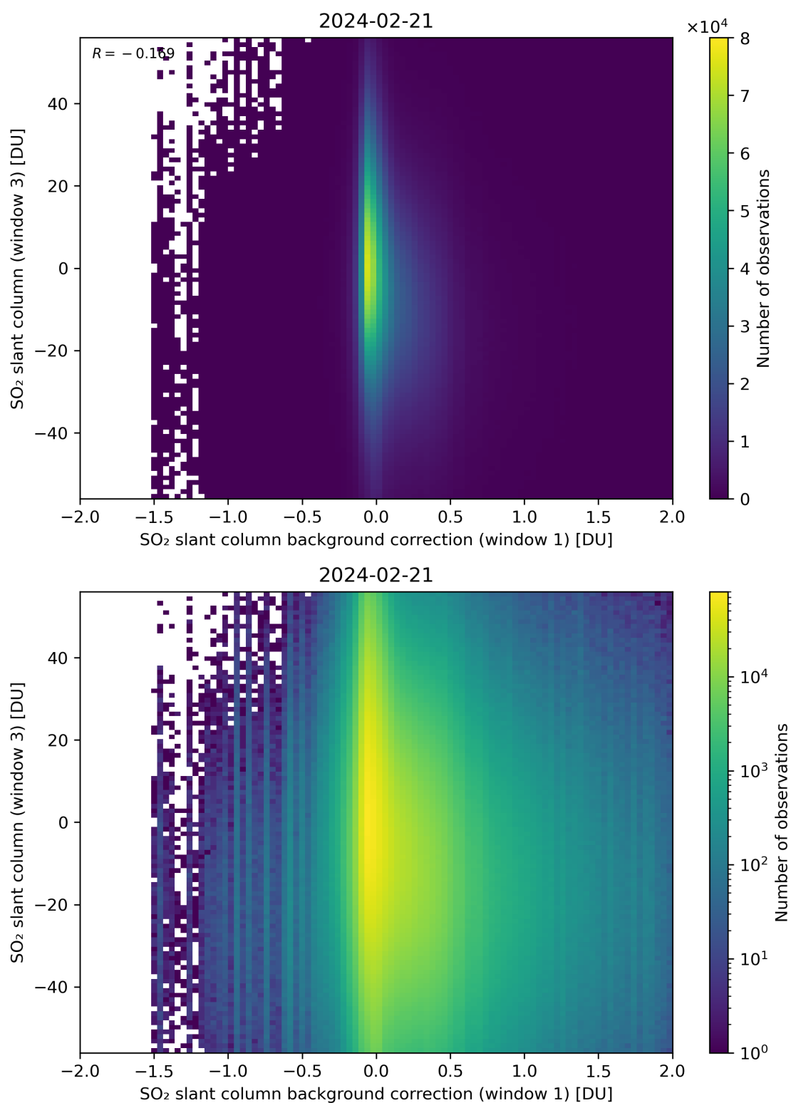
Figure 107: Scatter density plot of “SO 2 slant column background correction (window 1)” against “SO 2 slant column (window 3)” for 2024-02-20 to 2024-02-22.
