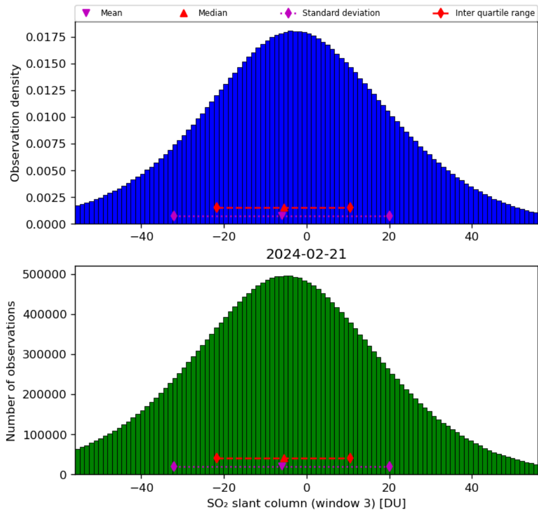
Figure 64: Histogram of “SO 2 slant column (window 3)” for 2024-02-20 to 2024-02-22
