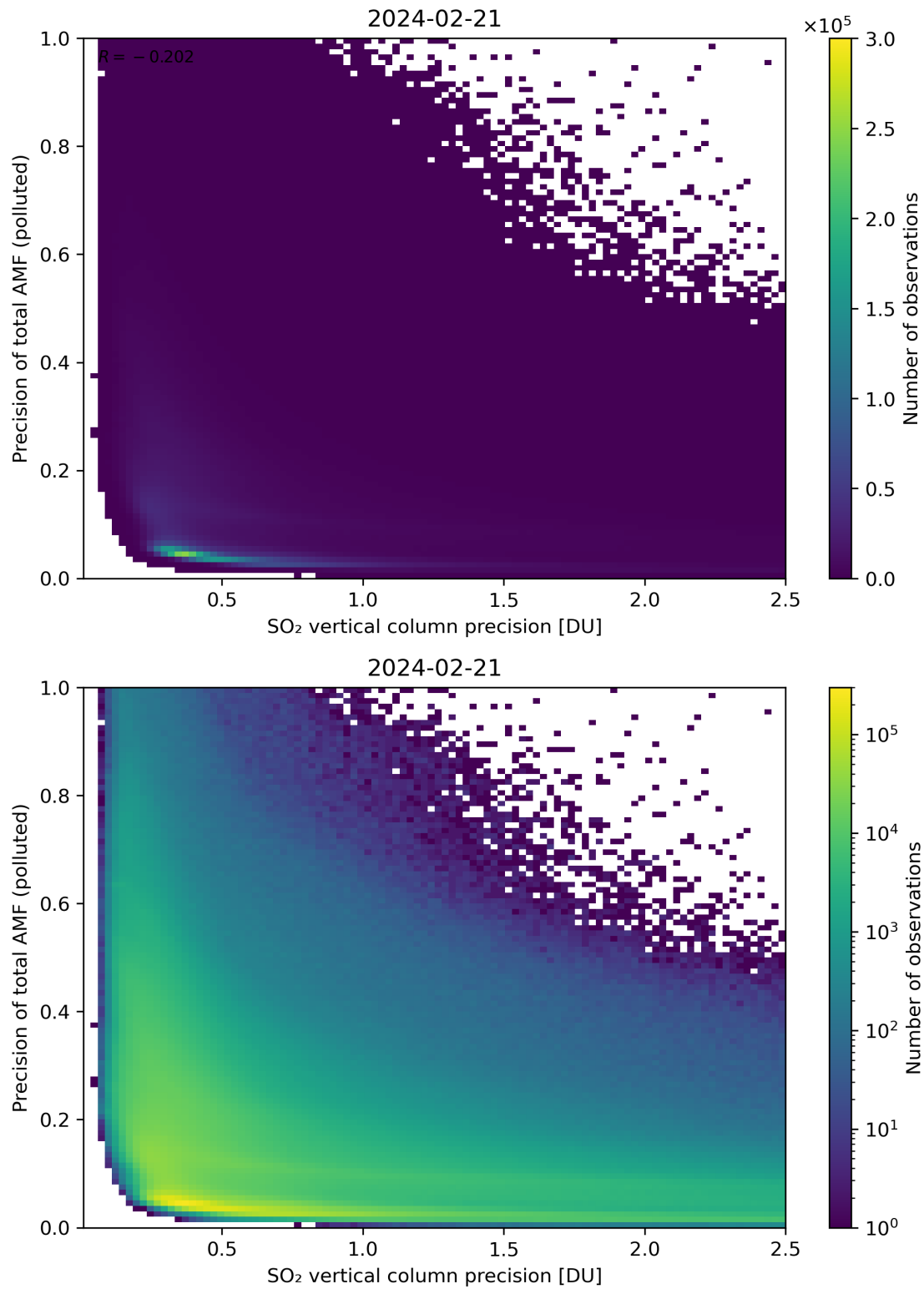
Figure 295: Scatter density plot of “SO 2 vertical column precision” against “Precision of total AMF (polluted)” for 2024-02-20 to 2024-02-22.
