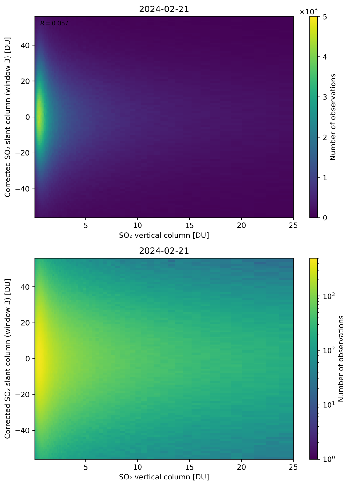
Figure 299: Scatter density plot of “SO 2 vertical column” against “Corrected SO 2 slant column (window 3)” for 2024-02-20 to 2024-02-22.
