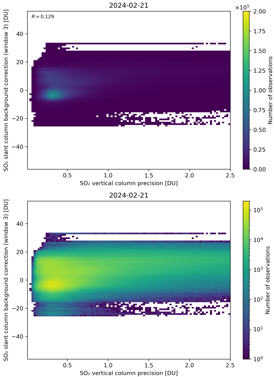
Figure 281: Scatter density plot of “SO 2 vertical column precision” against “SO 2 slant column background correction (window 3)” for 2024-02-20 to 2024-02-22.
