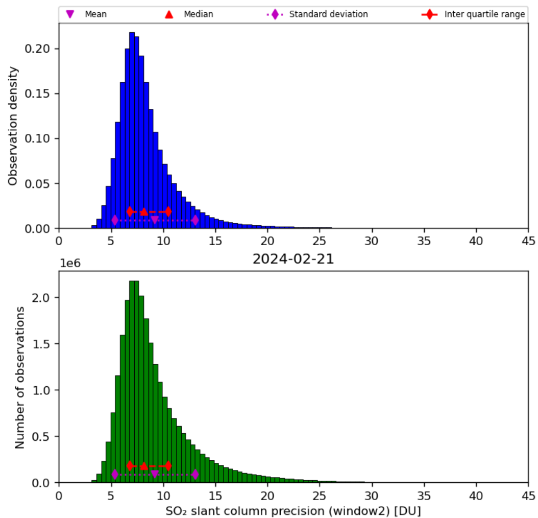
Figure 61: Histogram of “SO 2 slant column precision (window2)” for 2024-02-20 to 2024-02-22
