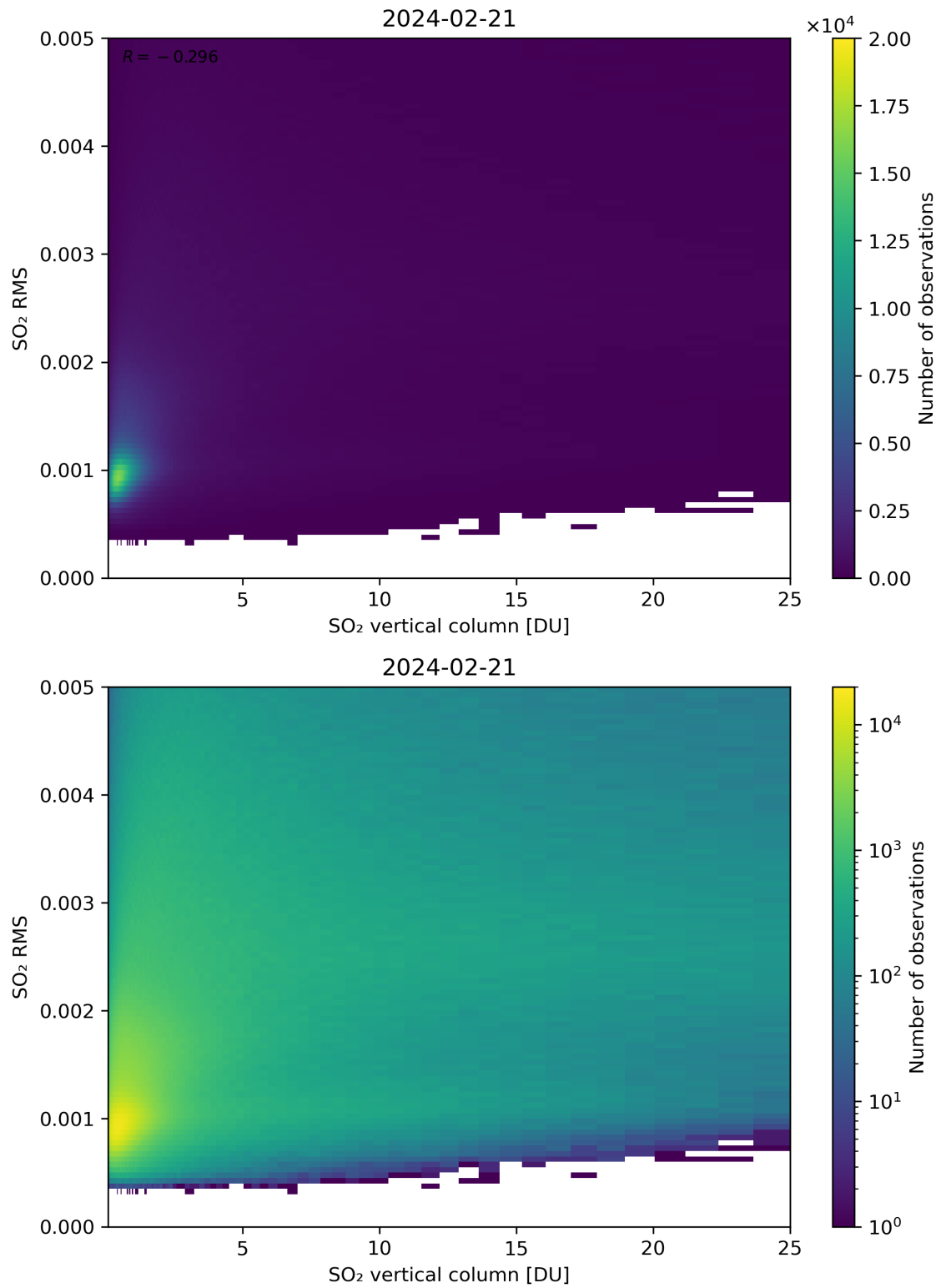
Figure 278: Scatter density plot of “SO 2 vertical column” against “SO 2 RMS” for 2024-02-20 to 2024-02-22.
