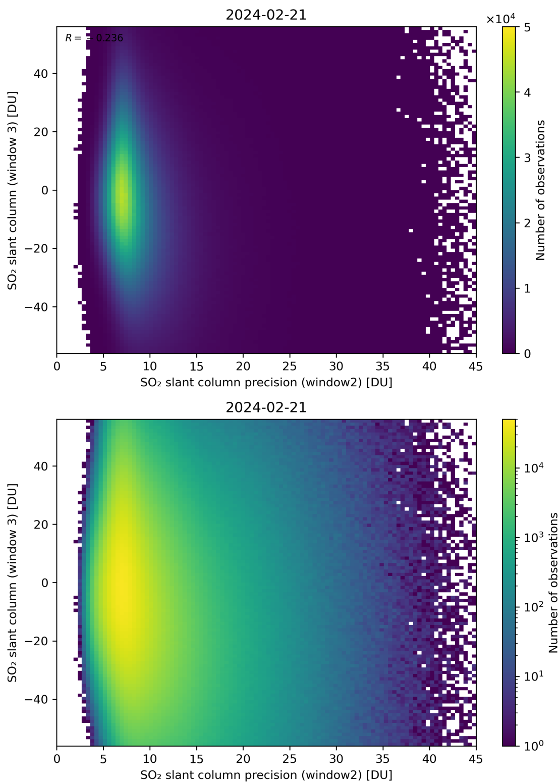
Figure 249: Scatter density plot of “SO 2 slant column precision (window2)” against “SO 2 slant column (window 3)” for 2024-02-20 to 2024-02-22.
