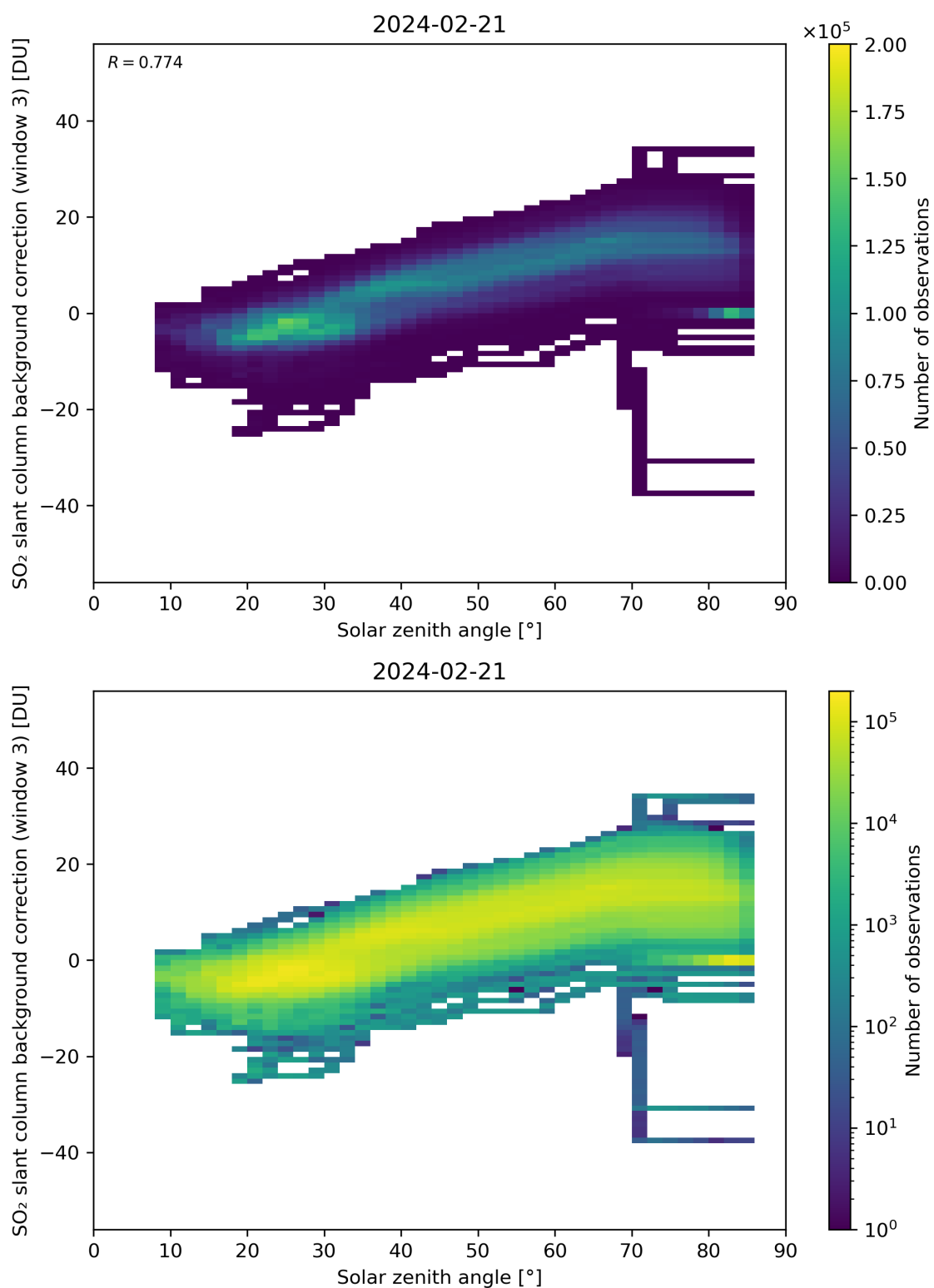
Figure 160: Scatter density plot of “Solar zenith angle” against “SO 2 slant column background correction (window 3)” for 2024-02-20 to 2024-02-22.
