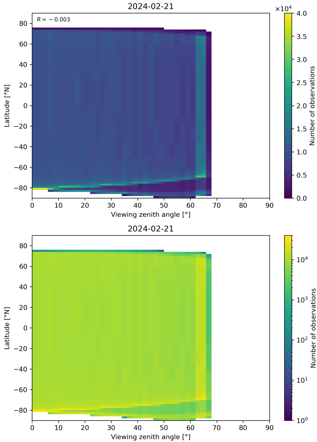
Figure 314: Scatter density plot of “Viewing zenith angle” against “Latitude” for 2024-02-20 to 2024-02-22.
