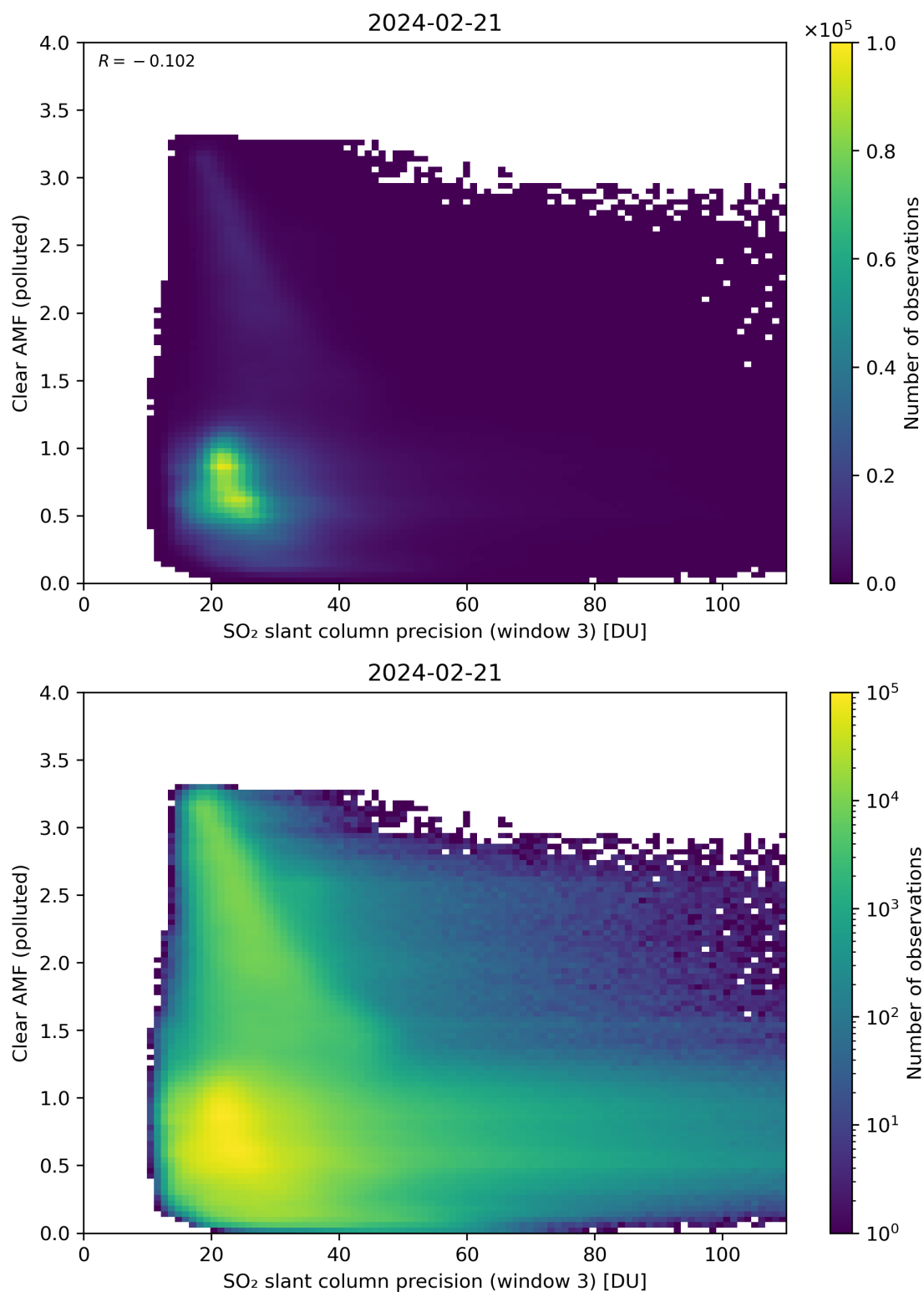
Figure 261: Scatter density plot of “SO 2 slant column precision (window 3)” against “Clear AMF (polluted)” for 2024-02-20 to 2024-02-22.
