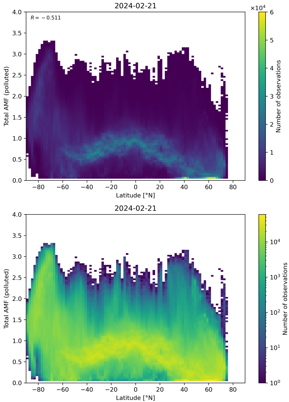
Figure 154: Scatter density plot of “Latitude” against “Total AMF (polluted)” for 2024-02-20 to 2024-02-22.
