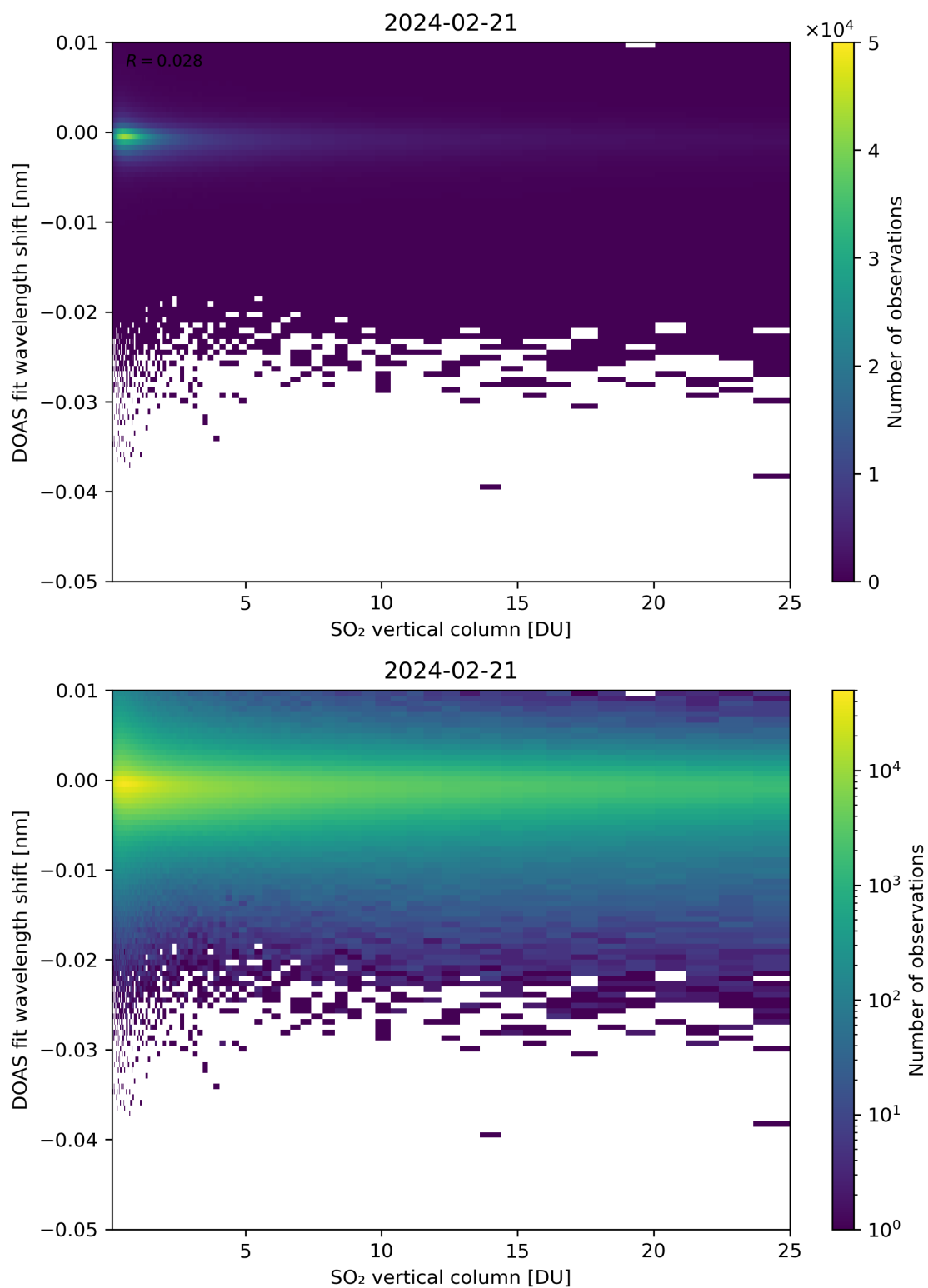
Figure 276: Scatter density plot of “SO 2 vertical column” against “DOAS fit wavelength shift” for 2024-02-20 to 2024-02-22.
