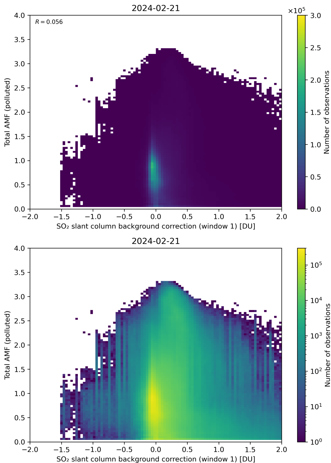
Figure 109: Scatter density plot of “SO 2 slant column background correction (window 1)” against “Total AMF (polluted)” for 2024-02-20 to 2024-02-22.
