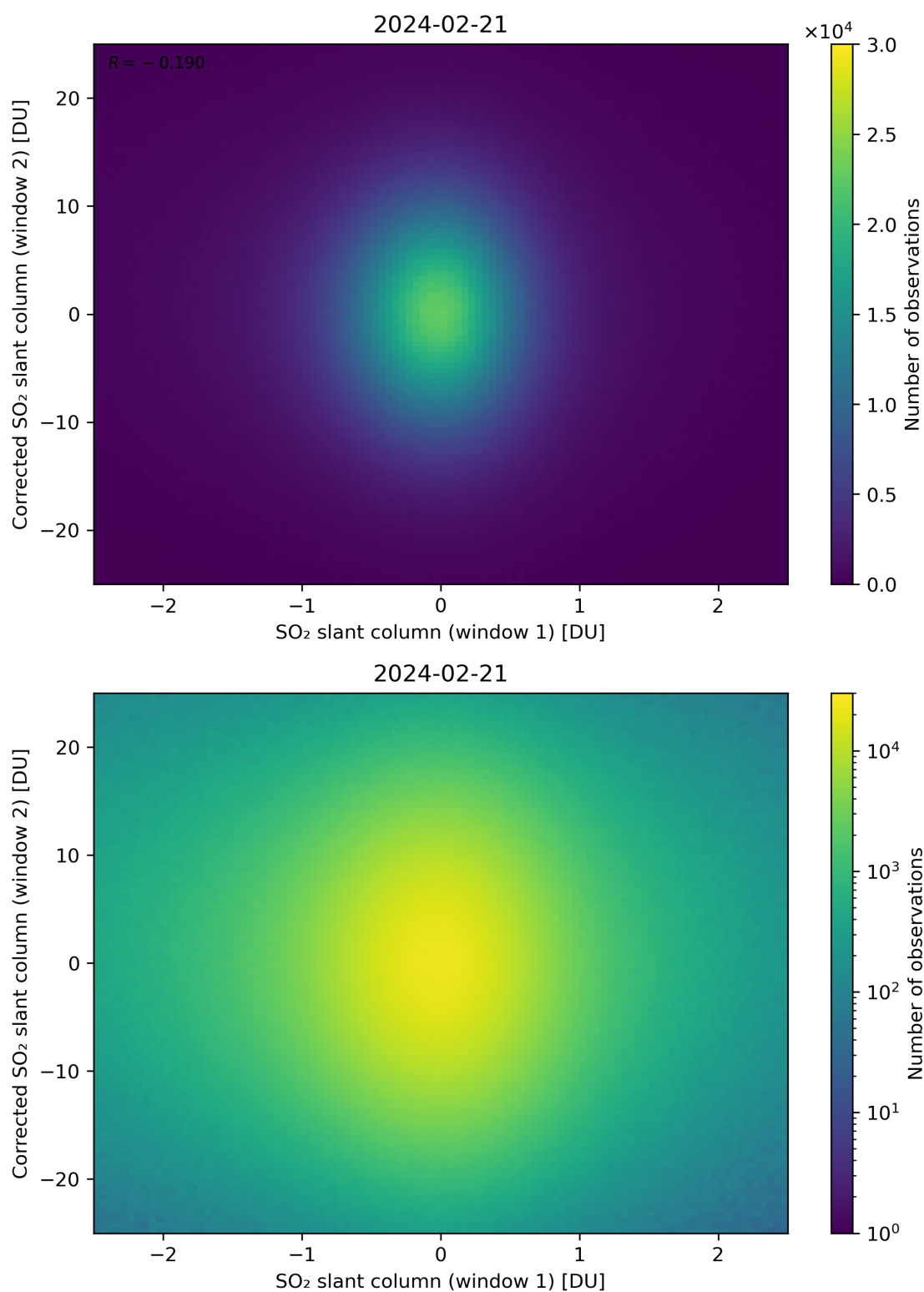
Figure 233: Scatter density plot of “SO 2 slant column (window 1)” against “Corrected SO 2 slant column (window 2)” for 2024-02-20 to 2024-02-22.
