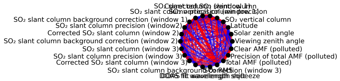
Figure 1: Map of correlation graph for 2024-02-20 to 2024-02-22.
