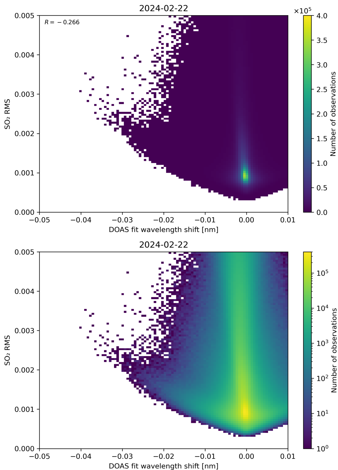
Figure 128: Scatter density plot of “DOAS fit wavelength shift” against “SO 2 RMS” for 2024-02-22 to 2024-02-23.
