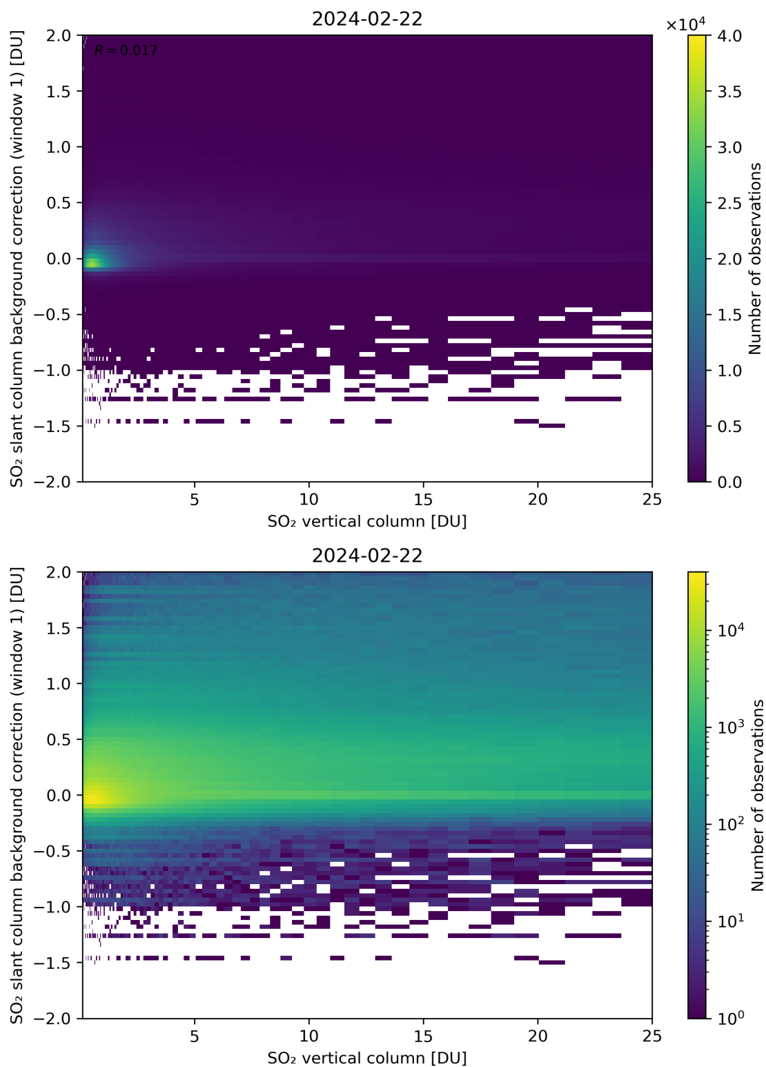
Figure 273: Scatter density plot of “SO 2 vertical column” against “SO 2 slant column background correction (window 1)” for 2024-02-22 to 2024-02-23.
