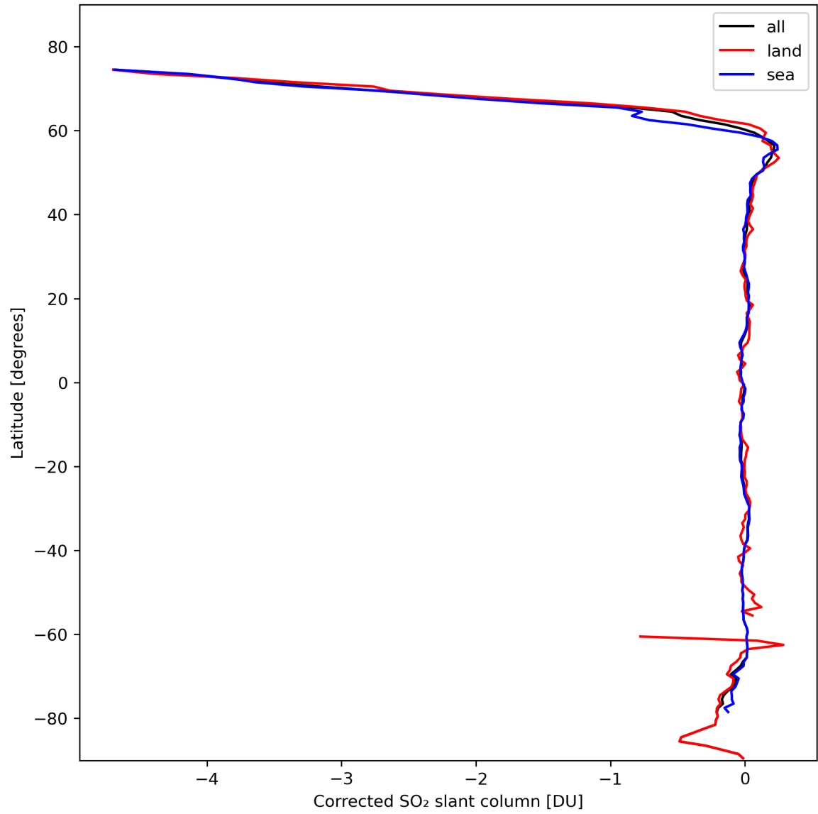
Figure 32: Zonal average of “Corrected SO 2 slant column” for 2024-02-22 to 2024-02-23.
