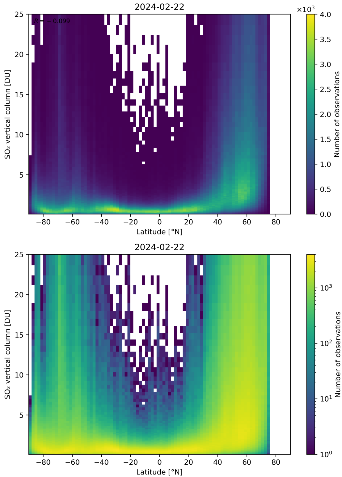
Figure 156: Scatter density plot of “Latitude” against “SO 2 vertical column” for 2024-02-22 to 2024-02-23.
