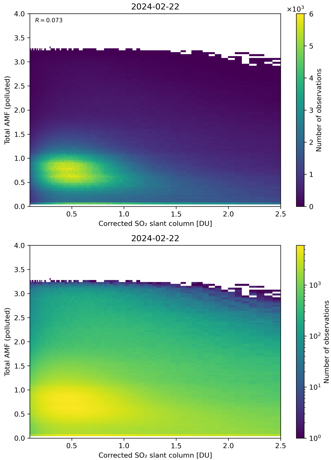
Figure 192: Scatter density plot of “Corrected SO 2 slant column” against “Total AMF (polluted)” for 2024-02-22 to 2024-02-23.
