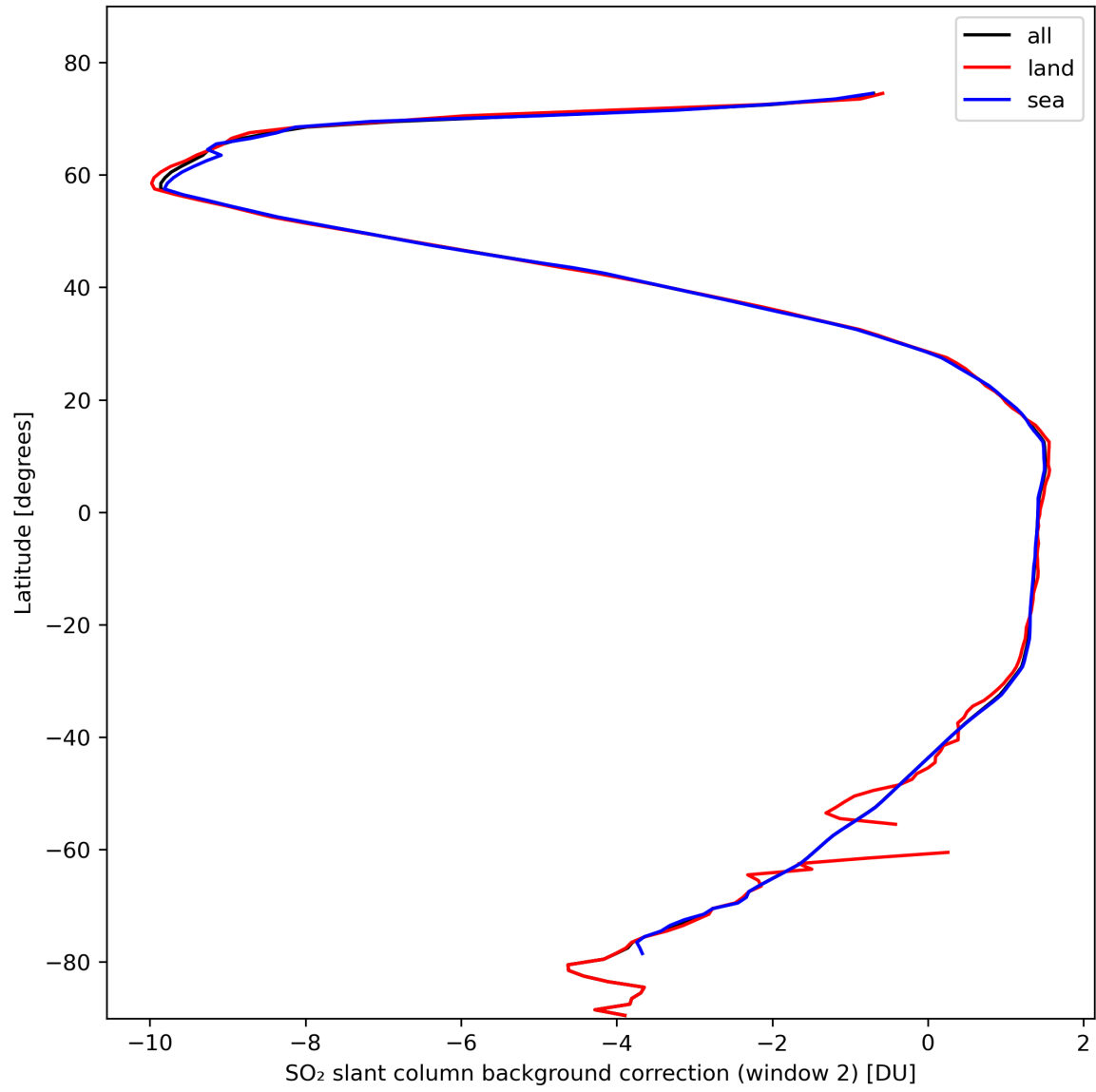
Figure 40: Zonal average of “SO 2 slant column background correction (window 2)” for 2024-02-22 to 2024-02-23.
