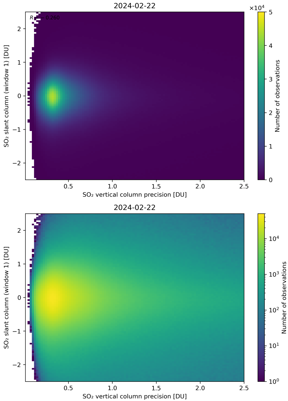
Figure 289: Scatter density plot of “SO 2 vertical column precision” against “SO 2 slant column (window 1)” for 2024-02-22 to 2024-02-23.
