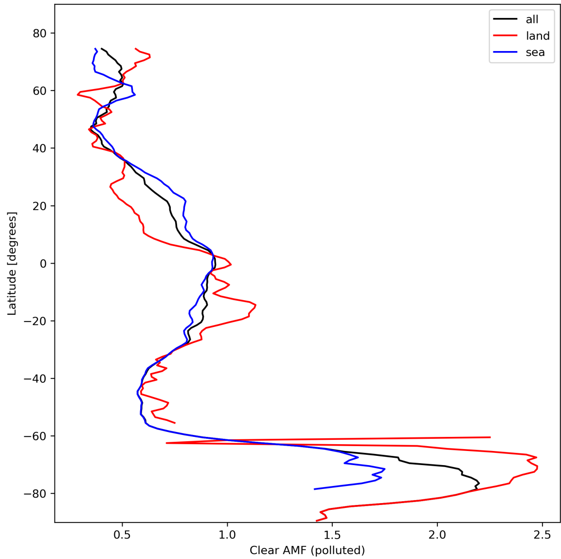
Figure 50: Zonal average of “Clear AMF (polluted)” for 2024-02-22 to 2024-02-23.
