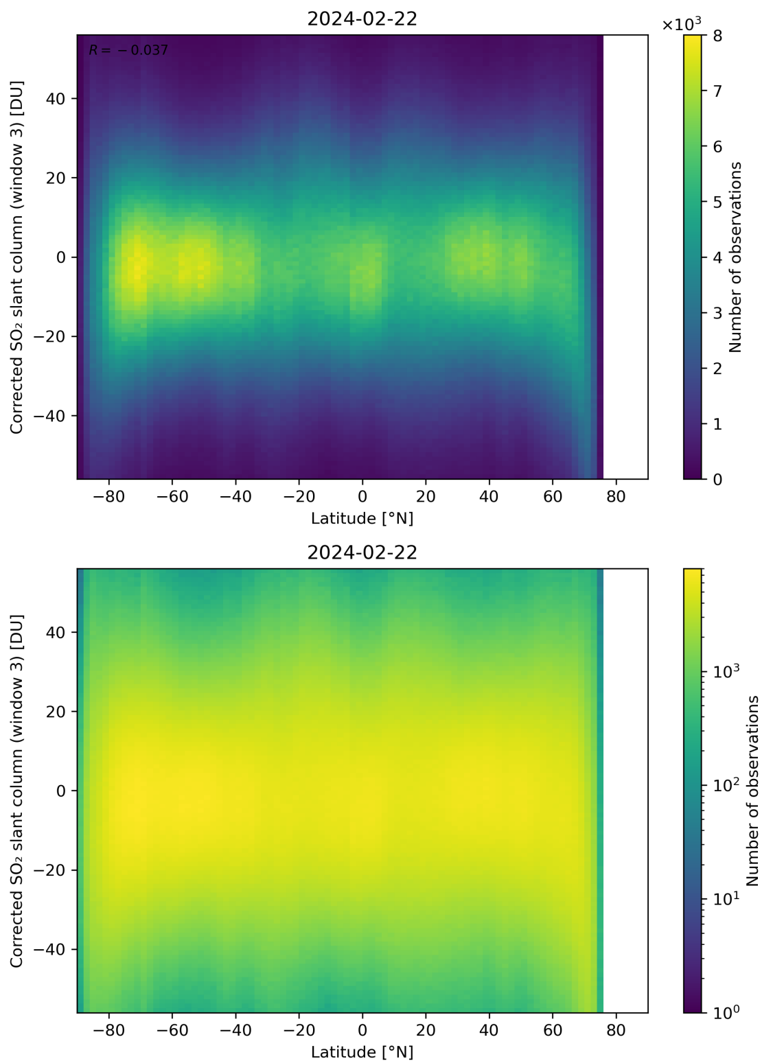
Figure 148: Scatter density plot of “Latitude” against “Corrected SO 2 slant column (window 3)” for 2024-02-22 to 2024-02-23.
