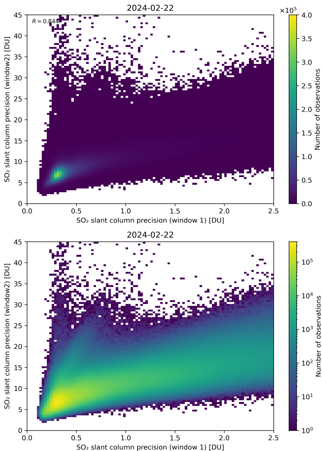
Figure 227: Scatter density plot of “SO 2 slant column precision (window 1)” against “SO 2 slant column precision (window2)” for 2024-02-22 to 2024-02-23.
