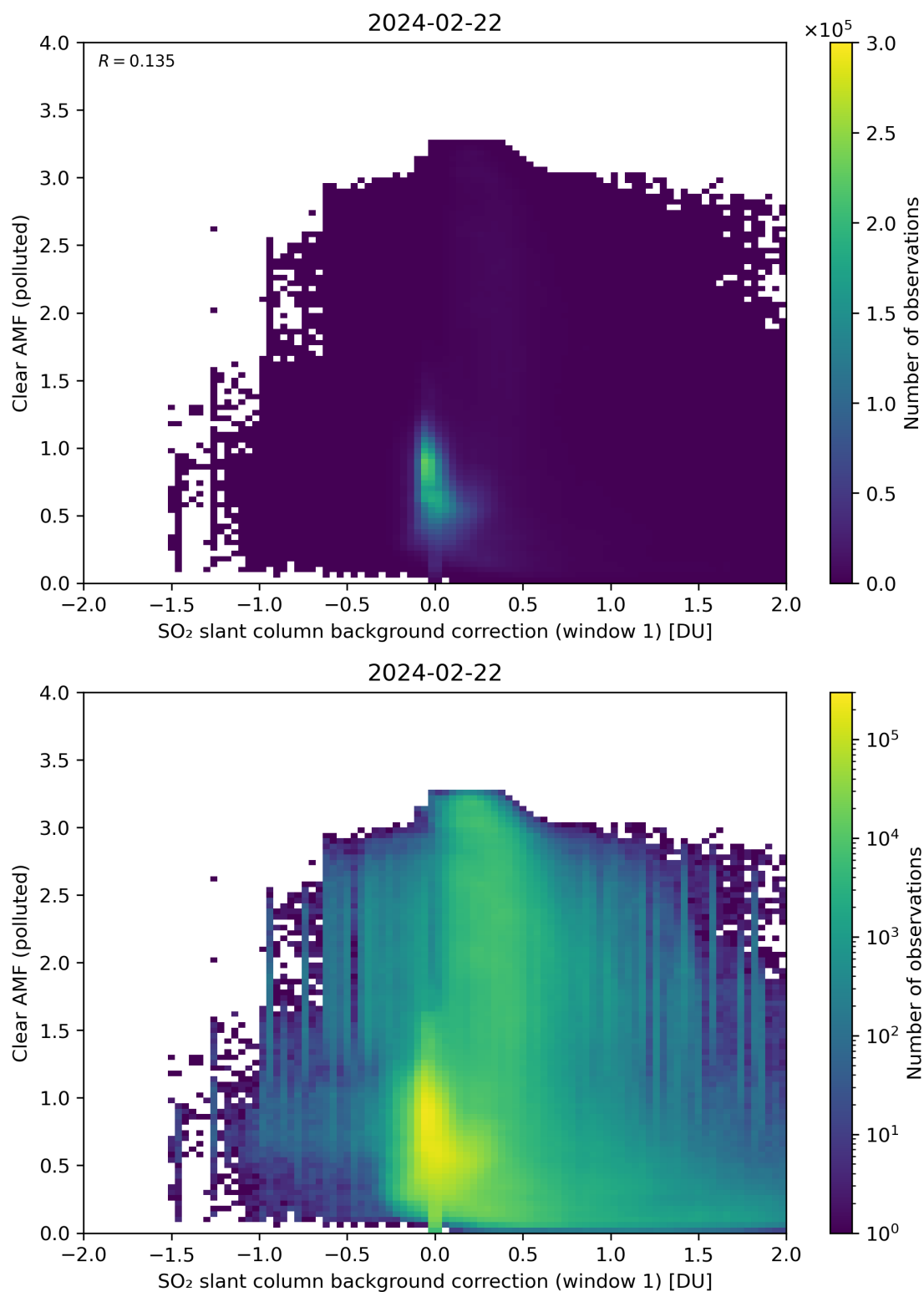
Figure 103: Scatter density plot of “SO 2 slant column background correction (window 1)” against “Clear AMF (polluted)” for 2024-02-22 to 2024-02-23.
