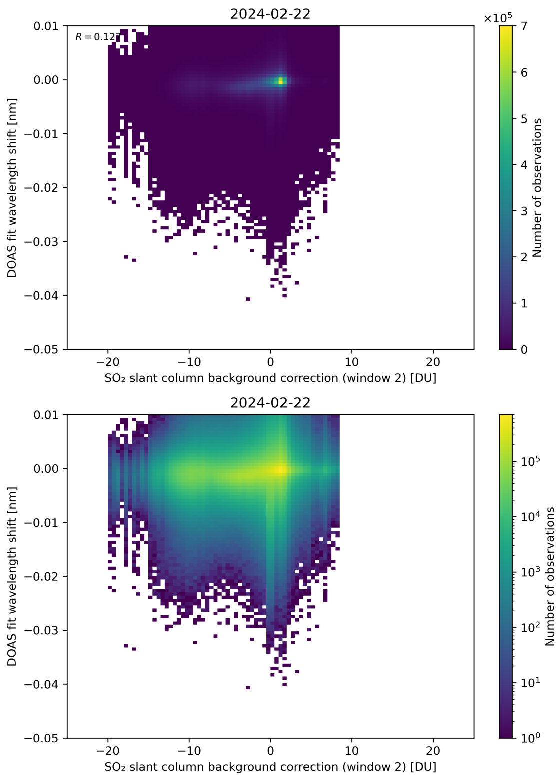
Figure 112: Scatter density plot of “SO 2 slant column background correction (window 2)” against “DOAS fit wavelength shift” for 2024-02-22 to 2024-02-23.
