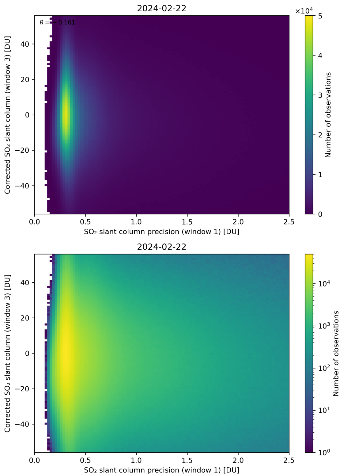
Figure 226: Scatter density plot of “SO 2 slant column precision (window 1)” against “Corrected SO 2 slant column (window 3)” for 2024-02-22 to 2024-02-23.
