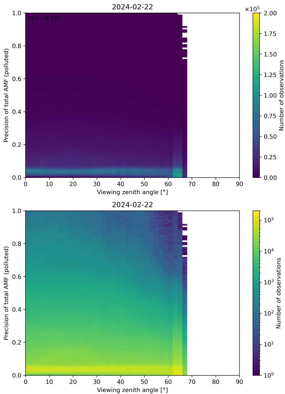
Figure 326: Scatter density plot of “Viewing zenith angle” against “Precision of total AMF (polluted)” for 2024-02-22 to 2024-02-23.
