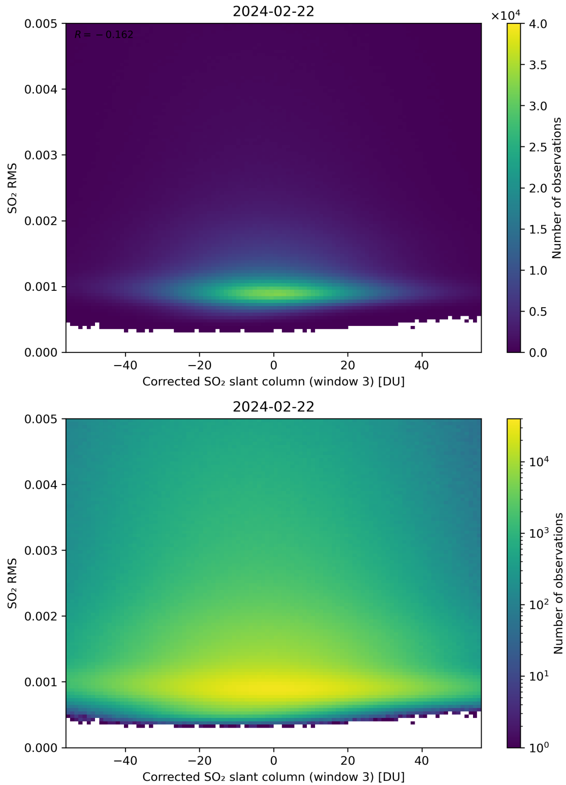
Figure 208: Scatter density plot of “Corrected SO 2 slant column (window 3)” against “SO 2 RMS” for 2024-02-22 to 2024-02-23.
