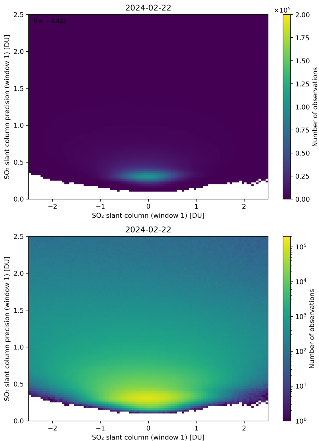
Figure 235: Scatter density plot of “SO 2 slant column (window 1)” against “SO 2 slant column precision (window 1)” for 2024-02-22 to 2024-02-23.
