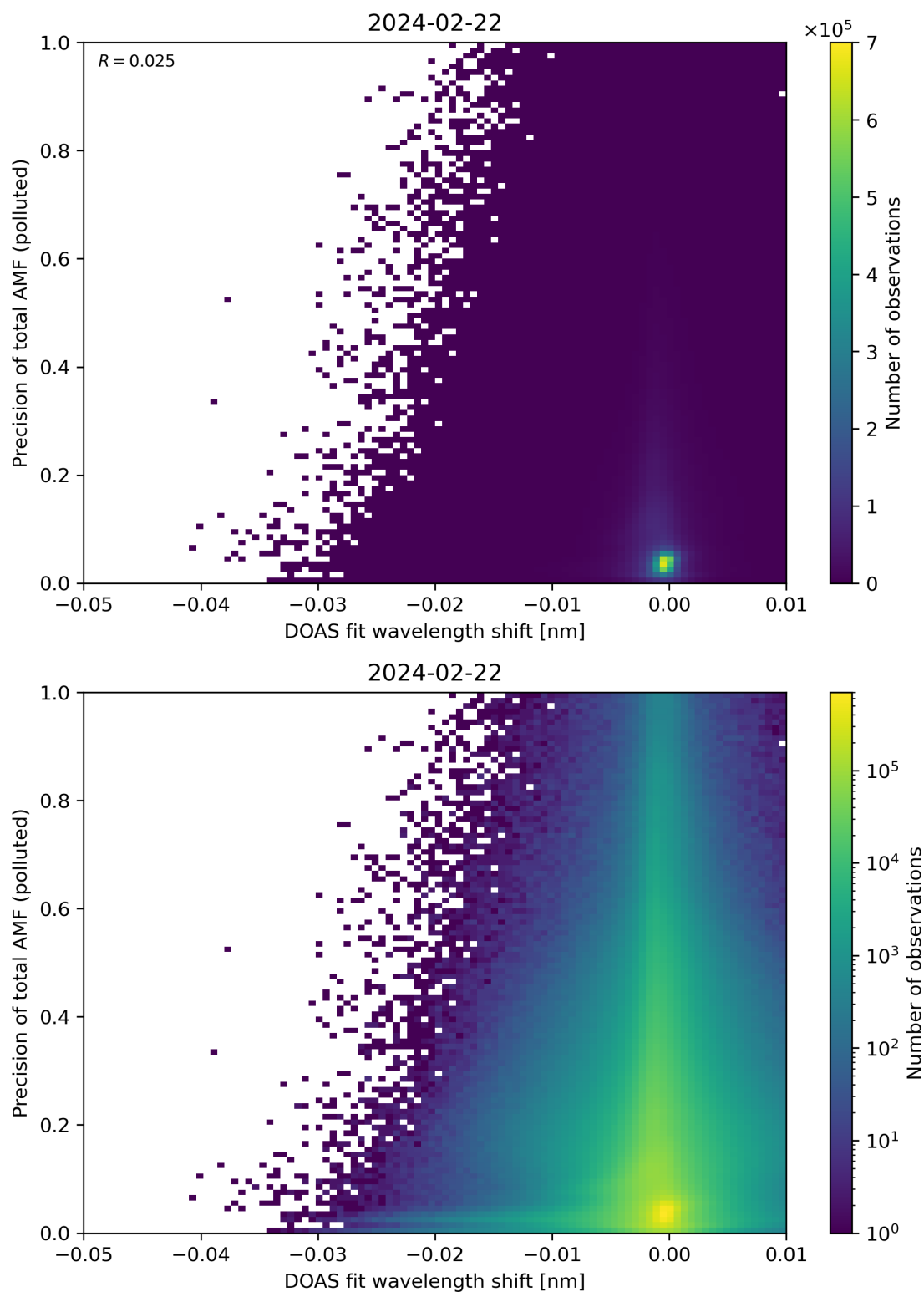
Figure 131: Scatter density plot of “DOAS fit wavelength shift” against “Precision of total AMF (polluted)” for 2024-02-22 to 2024-02-23.
