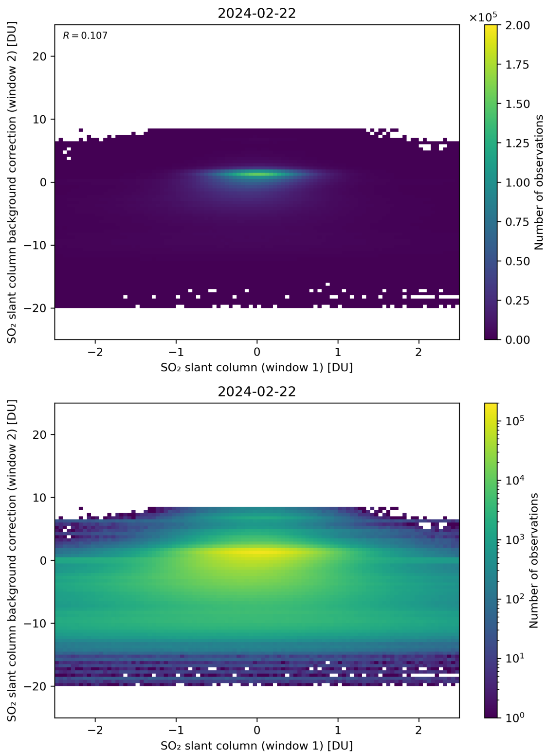
Figure 213: Scatter density plot of “SO 2 slant column (window 1)” against “SO 2 slant column background correction (window 2)” for 2024-02-22 to 2024-02-23.
