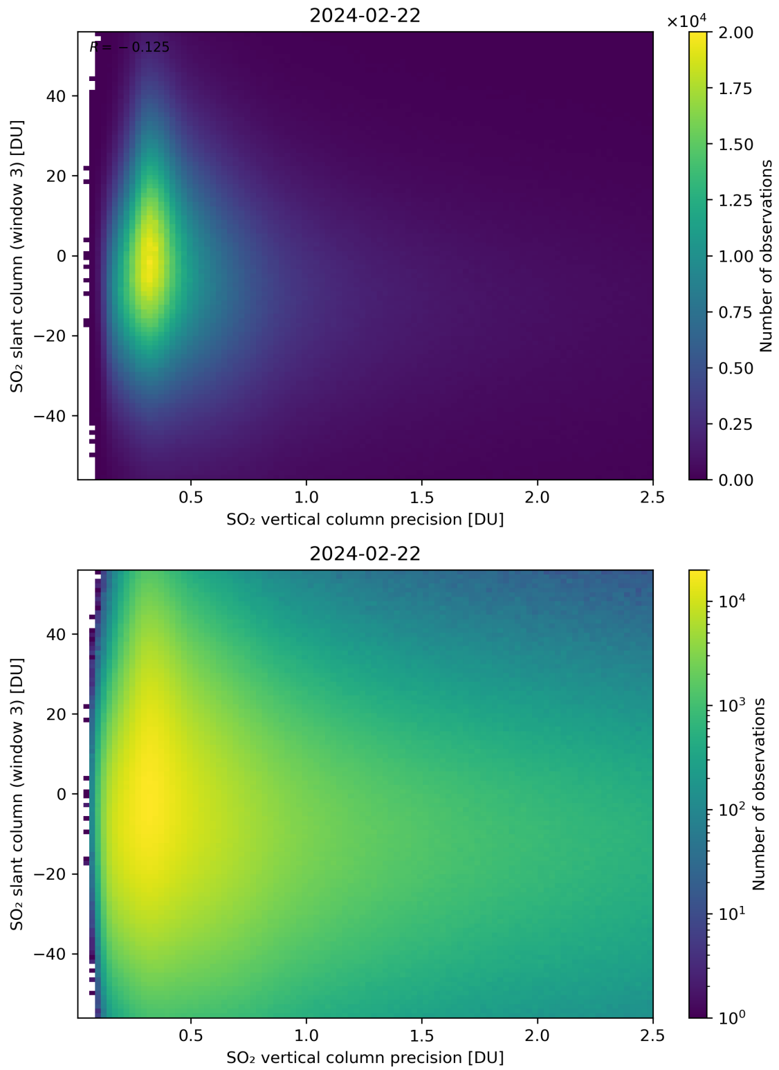
Figure 292: Scatter density plot of “SO 2 vertical column precision” against “SO 2 slant column (window 3)” for 2024-02-22 to 2024-02-23.
