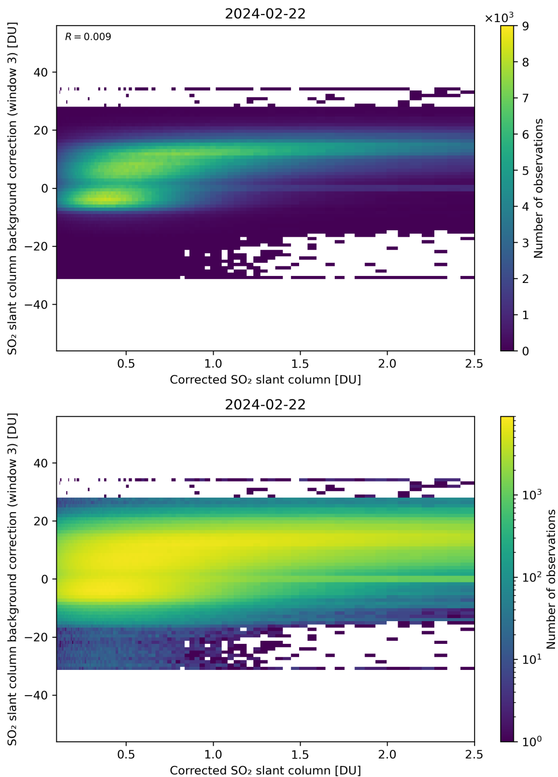
Figure 180: Scatter density plot of “Corrected SO 2 slant column” against “SO 2 slant column background correction (window 3)” for 2024-02-22 to 2024-02-23.
