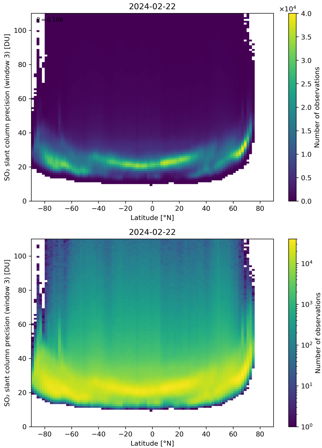
Figure 153: Scatter density plot of “Latitude” against “SO 2 slant column precision (window 3)” for 2024-02-22 to 2024-02-23.
