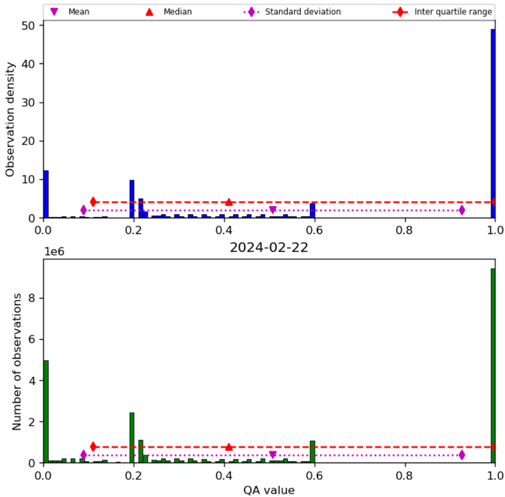
Figure 52: Histogram of “QA value” for 2024-02-22 to 2024-02-23
