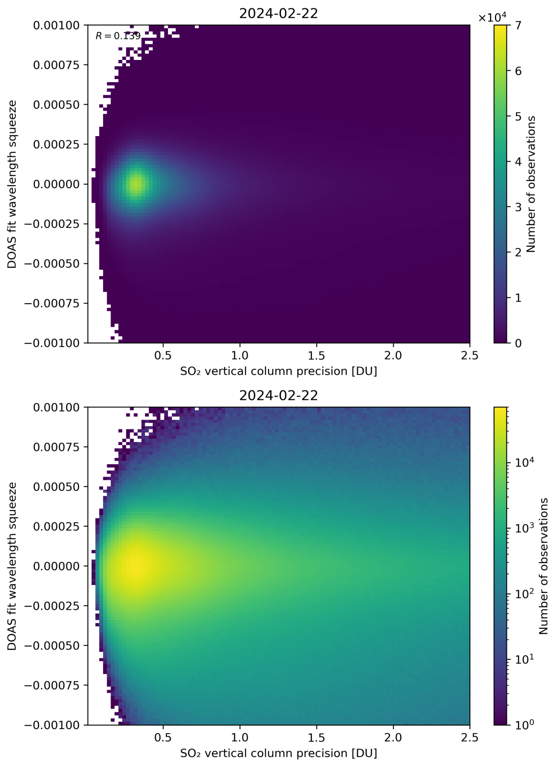
Figure 283: Scatter density plot of “SO 2 vertical column precision” against “DOAS fit wavelength squeeze” for 2024-02-22 to 2024-02-23.
