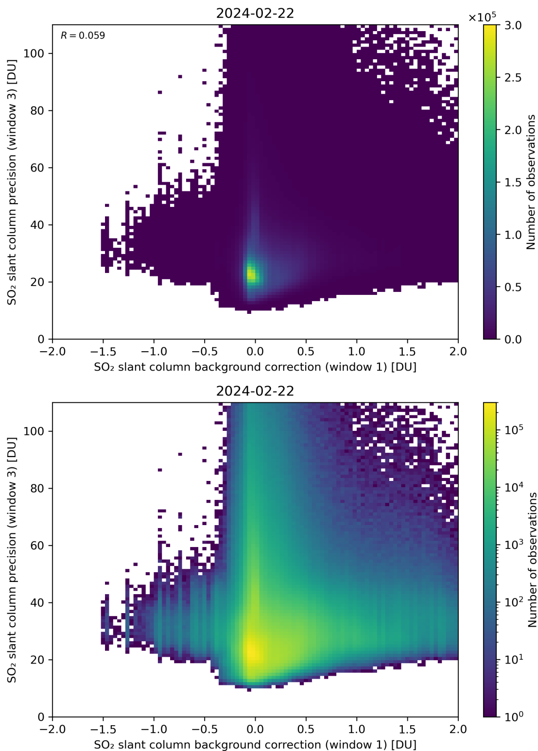
Figure 108: Scatter density plot of “SO 2 slant column background correction (window 1)” against “SO 2 slant column precision (window 3)” for 2024-02-22 to 2024-02-23.
