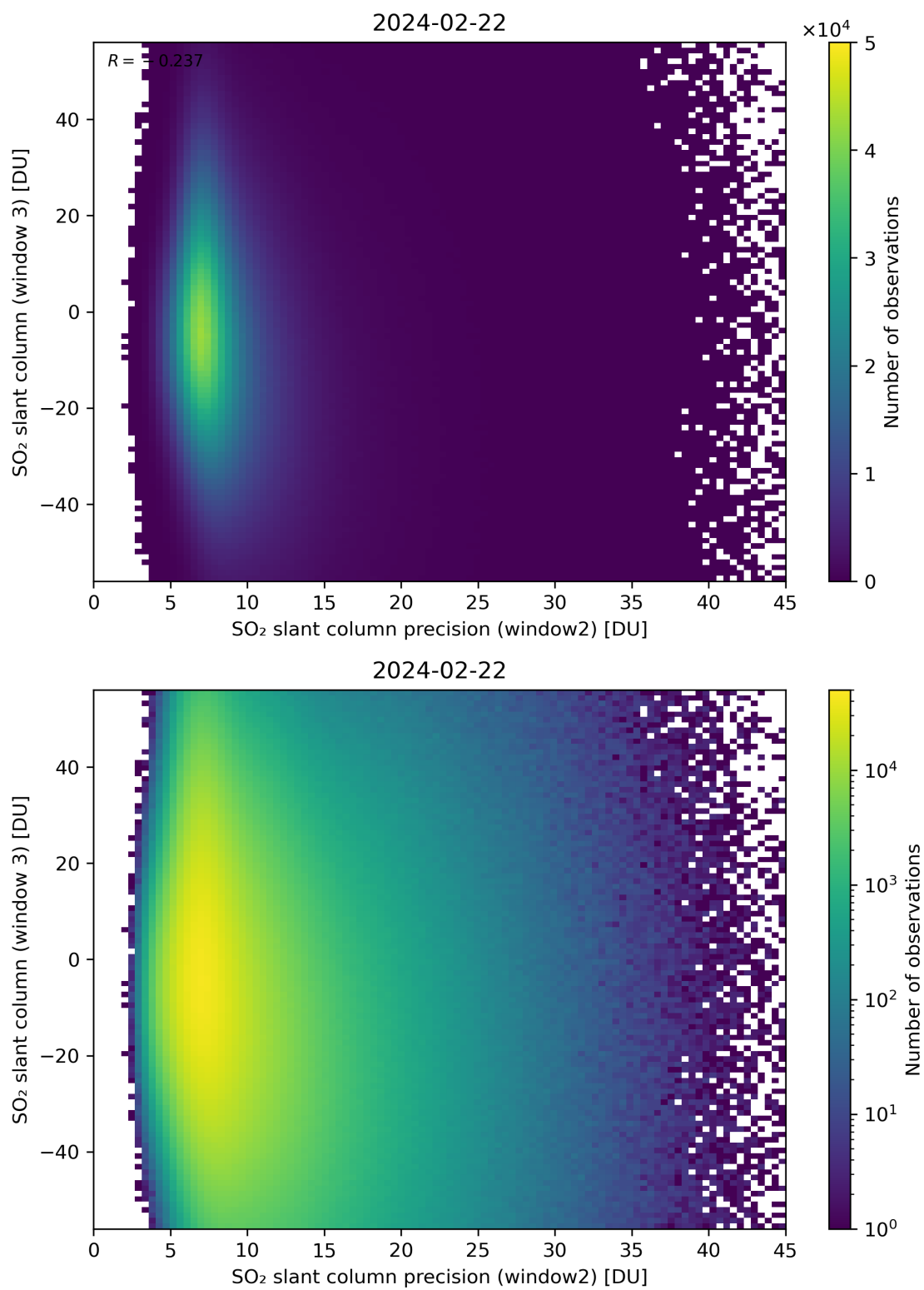
Figure 249: Scatter density plot of “SO 2 slant column precision (window2)” against “SO 2 slant column (window 3)” for 2024-02-22 to 2024-02-23.
