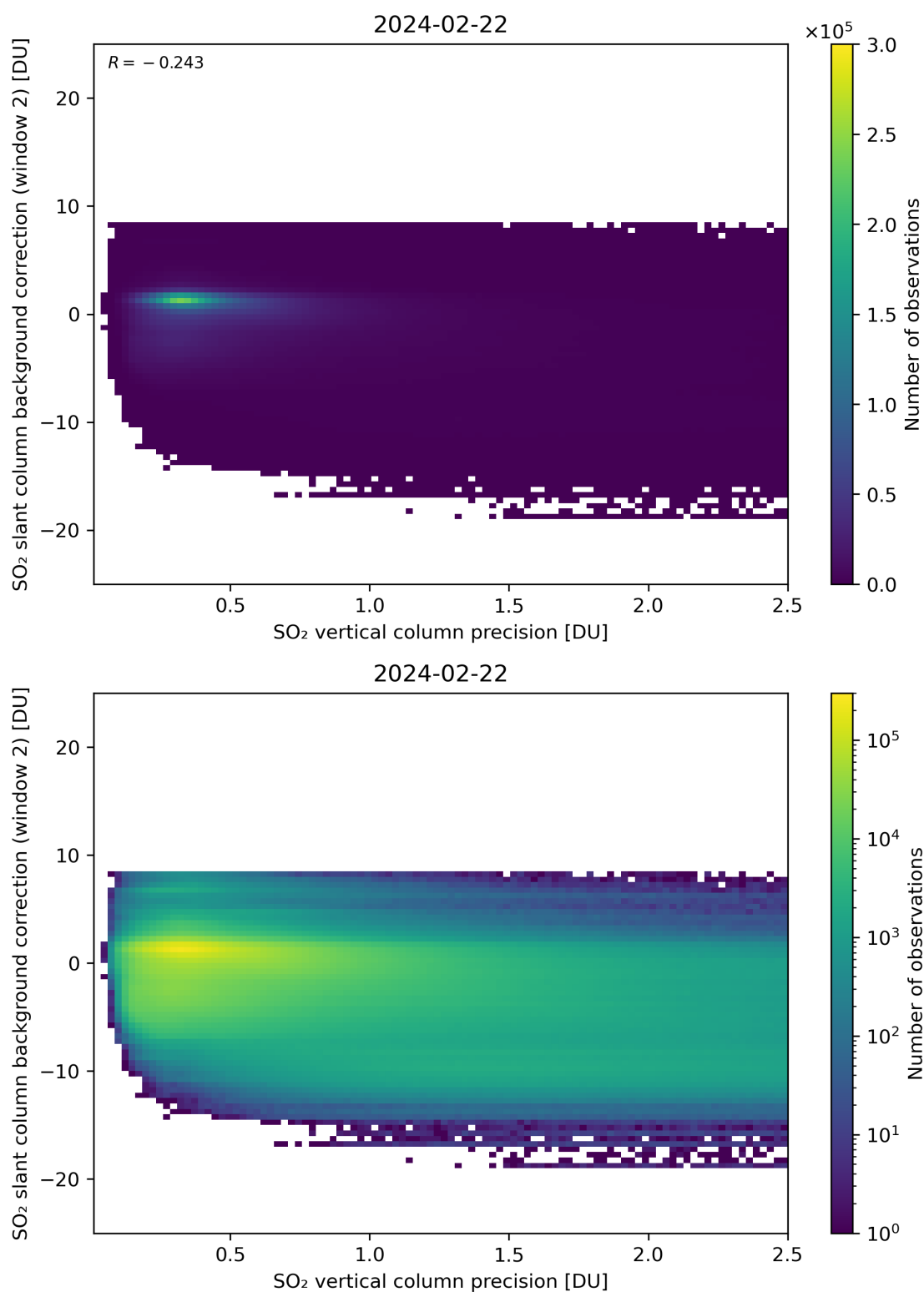
Figure 280: Scatter density plot of “SO 2 vertical column precision” against “SO 2 slant column background correction (window 2)” for 2024-02-22 to 2024-02-23.
