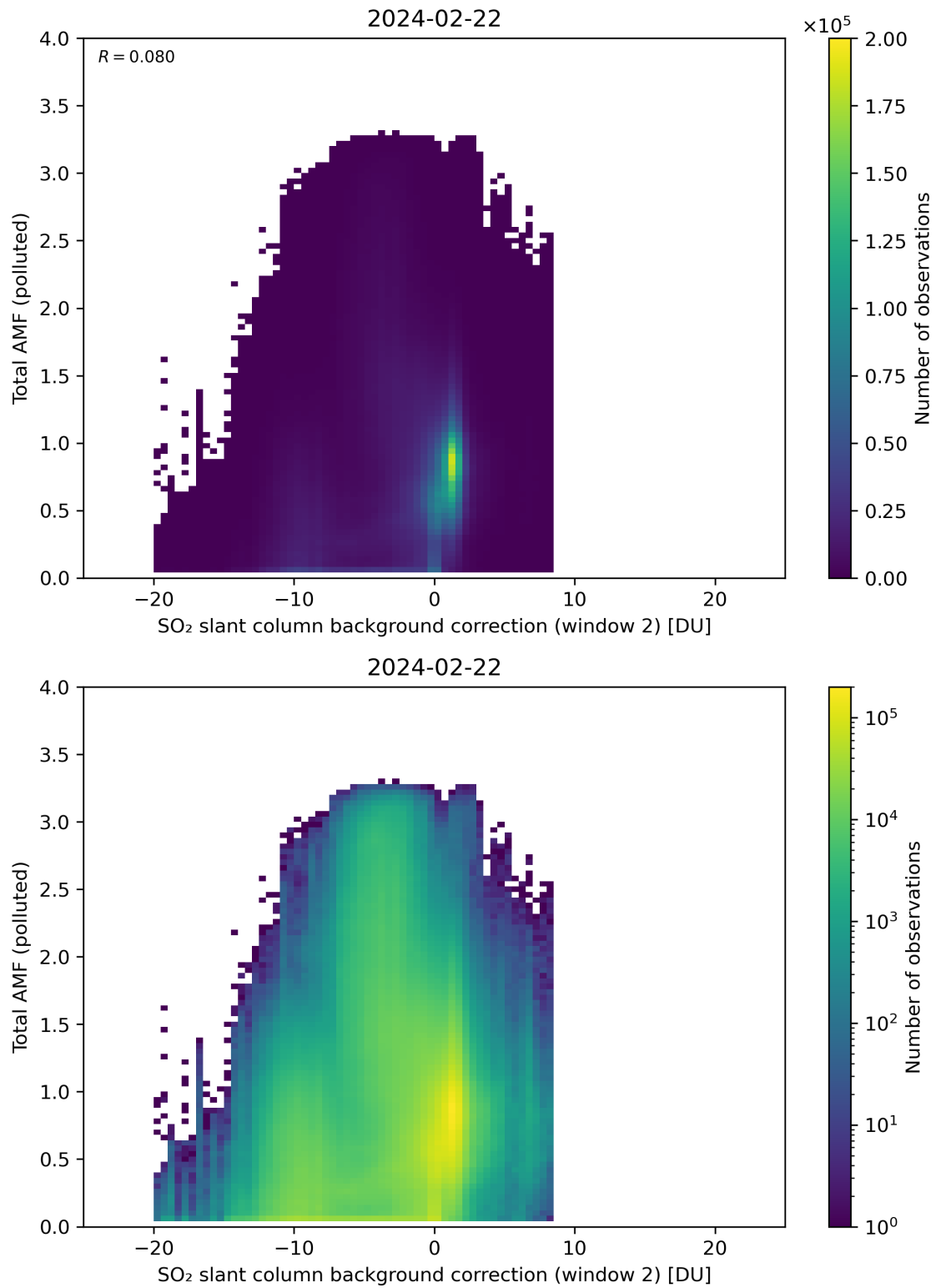
Figure 119: Scatter density plot of “SO 2 slant column background correction (window 2)” against “Total AMF (polluted)” for 2024-02-22 to 2024-02-23.
