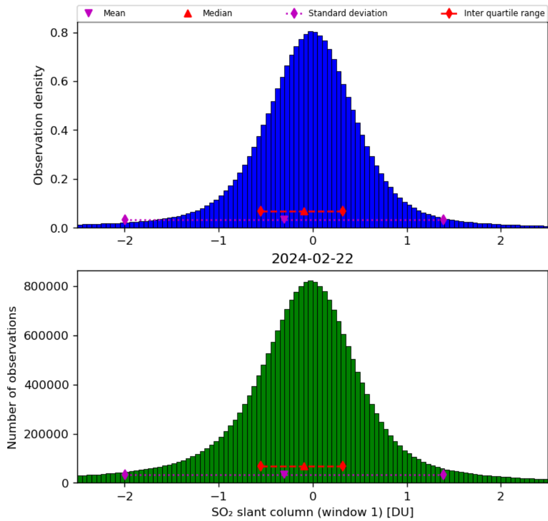
Figure 56: Histogram of “SO 2 slant column (window 1)” for 2024-02-22 to 2024-02-23
