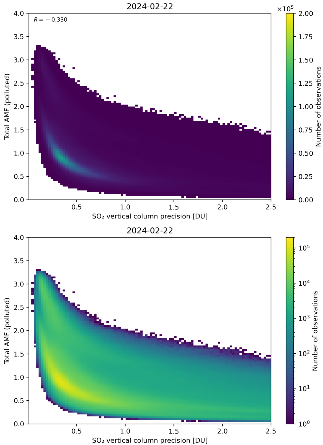
Figure 294: Scatter density plot of “SO 2 vertical column precision” against “Total AMF (polluted)” for 2024-02-22 to 2024-02-23.
