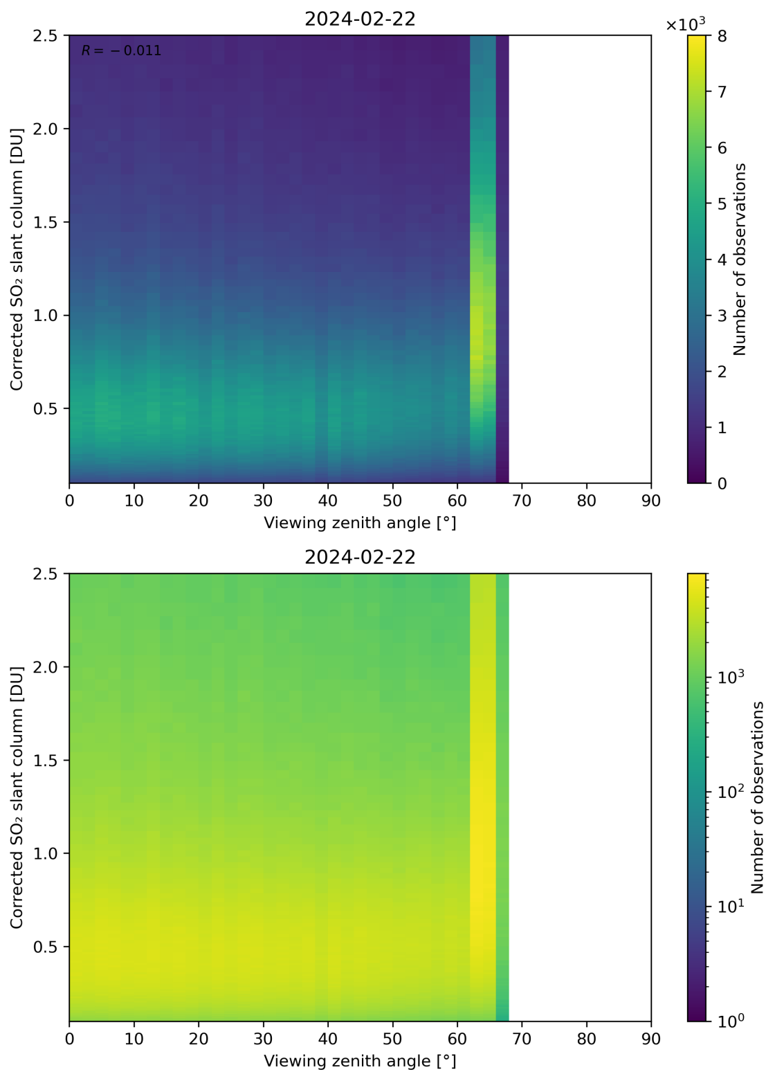
Figure 317: Scatter density plot of “Viewing zenith angle” against “Corrected SO 2 slant column” for 2024-02-22 to 2024-02-23.
