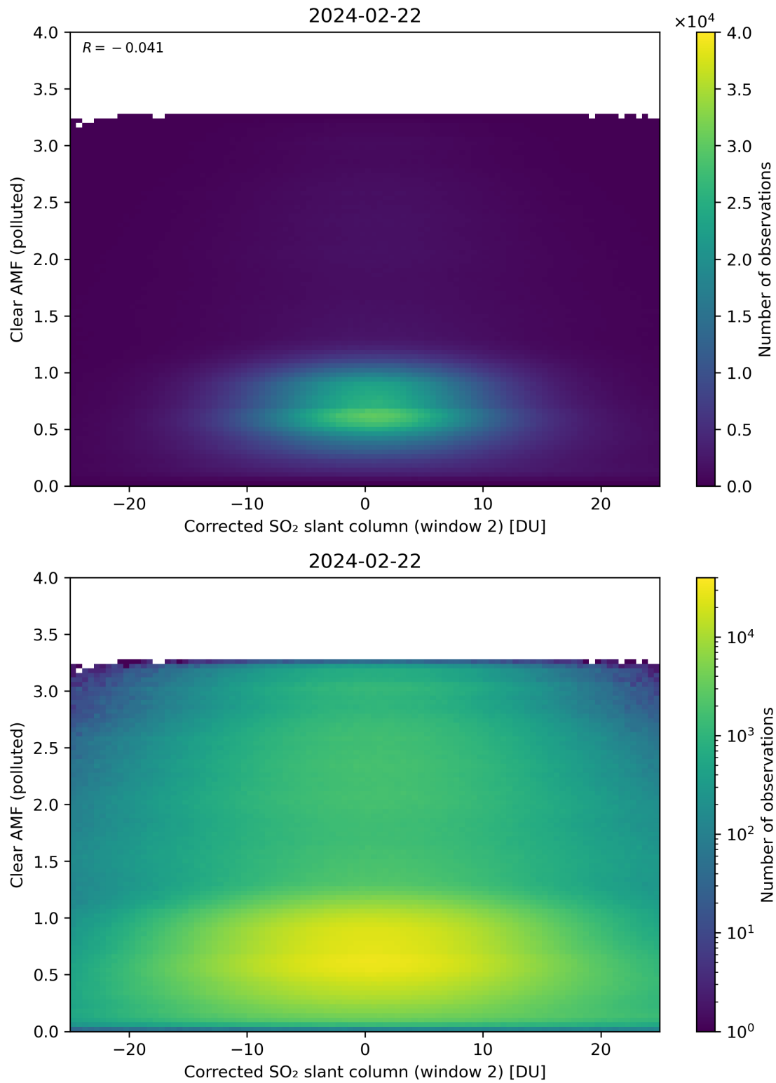
Figure 199: Scatter density plot of “Corrected SO 2 slant column (window 2)” against “Clear AMF (polluted)” for 2024-02-22 to 2024-02-23.
