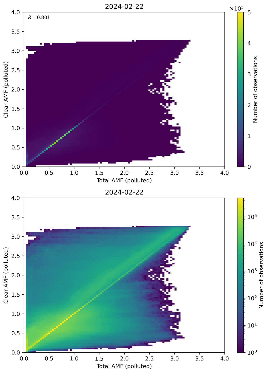
Figure 271: Scatter density plot of “Total AMF (polluted)” against “Clear AMF (polluted)” for 2024-02-22 to 2024-02-23.
