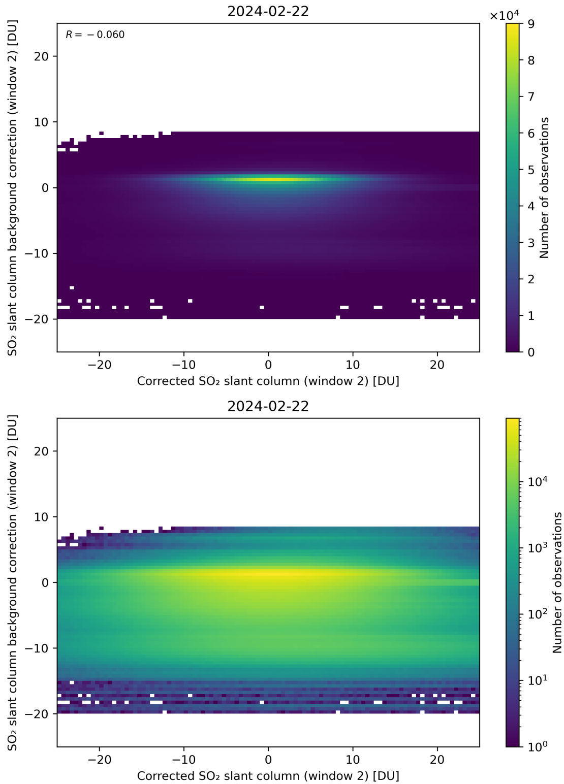
Figure 194: Scatter density plot of “Corrected SO 2 slant column (window 2)” against “SO 2 slant column background correction (window 2)” for 2024-02-22 to 2024-02-23.
