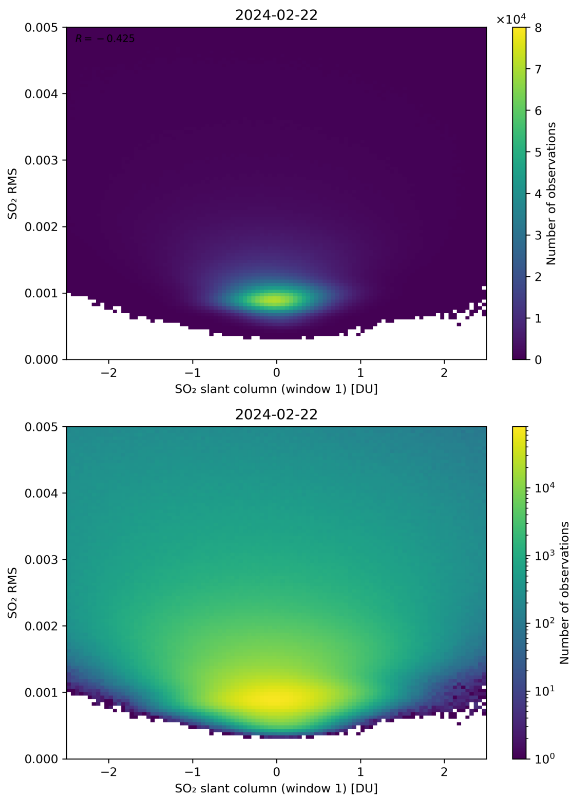
Figure 217: Scatter density plot of “SO 2 slant column (window 1)” against “SO 2 RMS” for 2024-02-22 to 2024-02-23.
