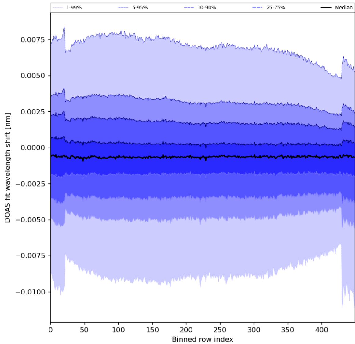
Figure 91: Along track statistics of “DOAS fit wavelength shift” for 2024-02-22 to 2024-02-23
