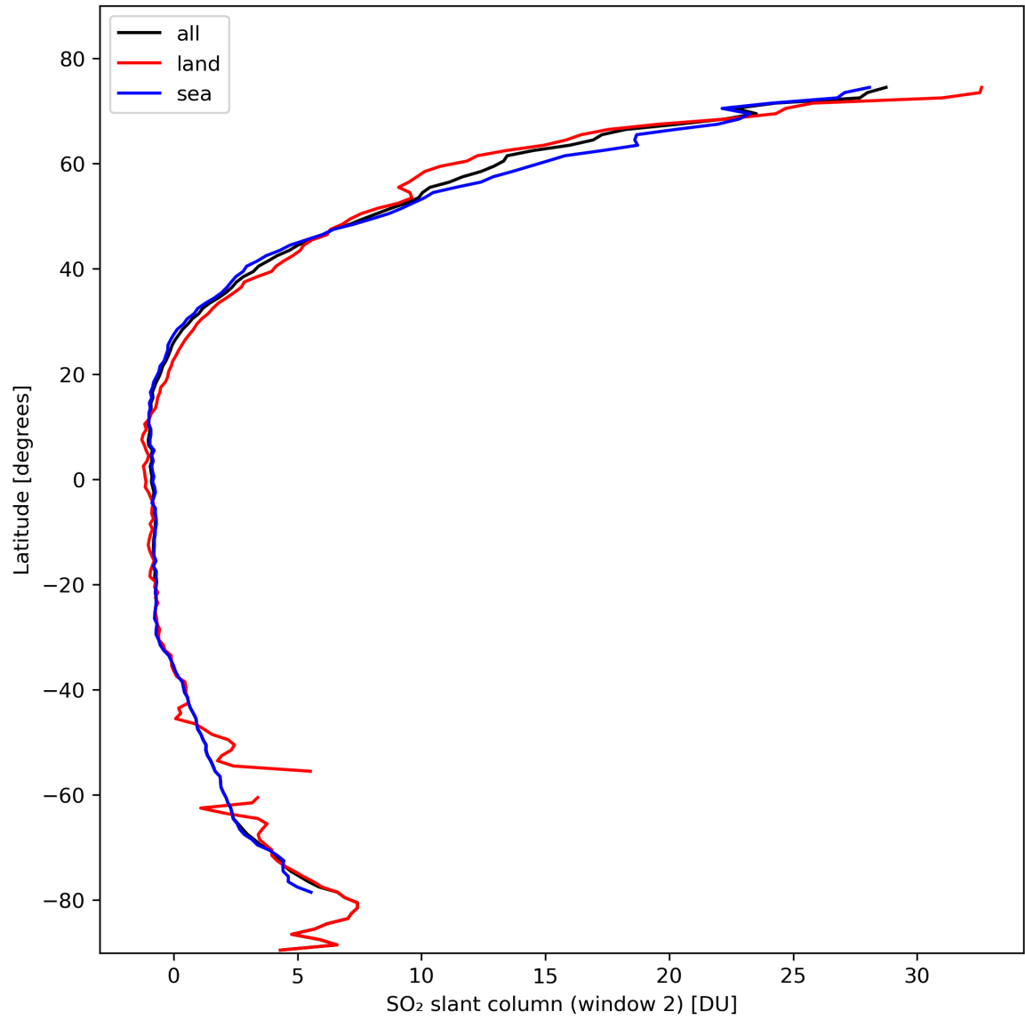
Figure 37: Zonal average of “SO 2 slant column (window 2)” for 2024-02-22 to 2024-02-23.
