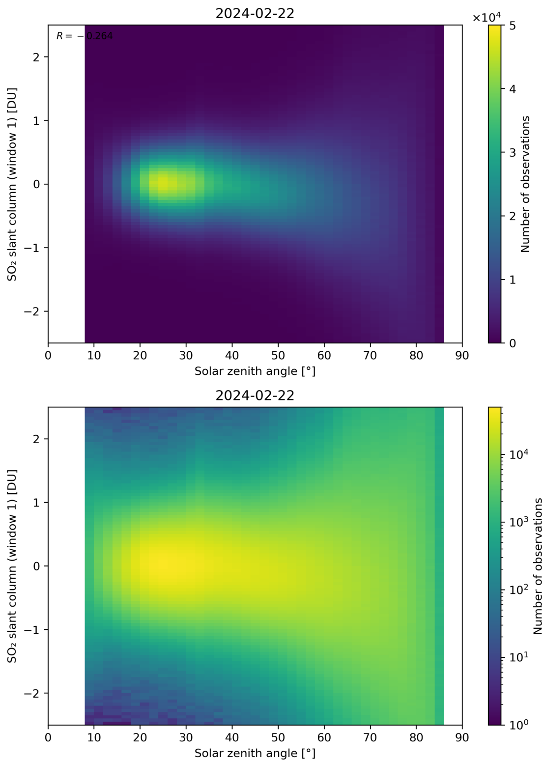
Figure 169: Scatter density plot of “Solar zenith angle” against “SO 2 slant column (window 1)” for 2024-02-22 to 2024-02-23.
