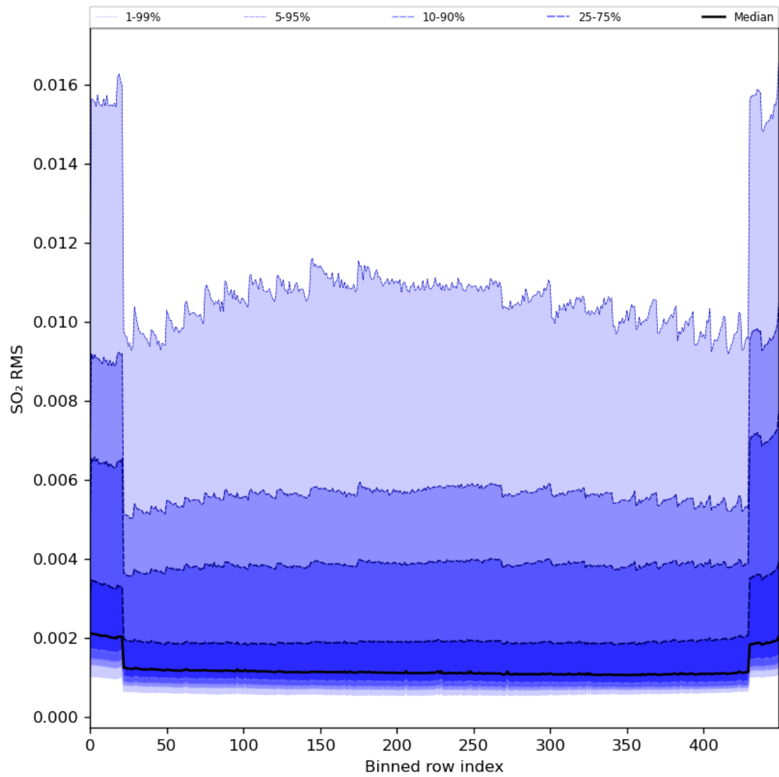
Figure 93: Along track statistics of “SO 2 RMS” for 2024-02-22 to 2024-02-23
