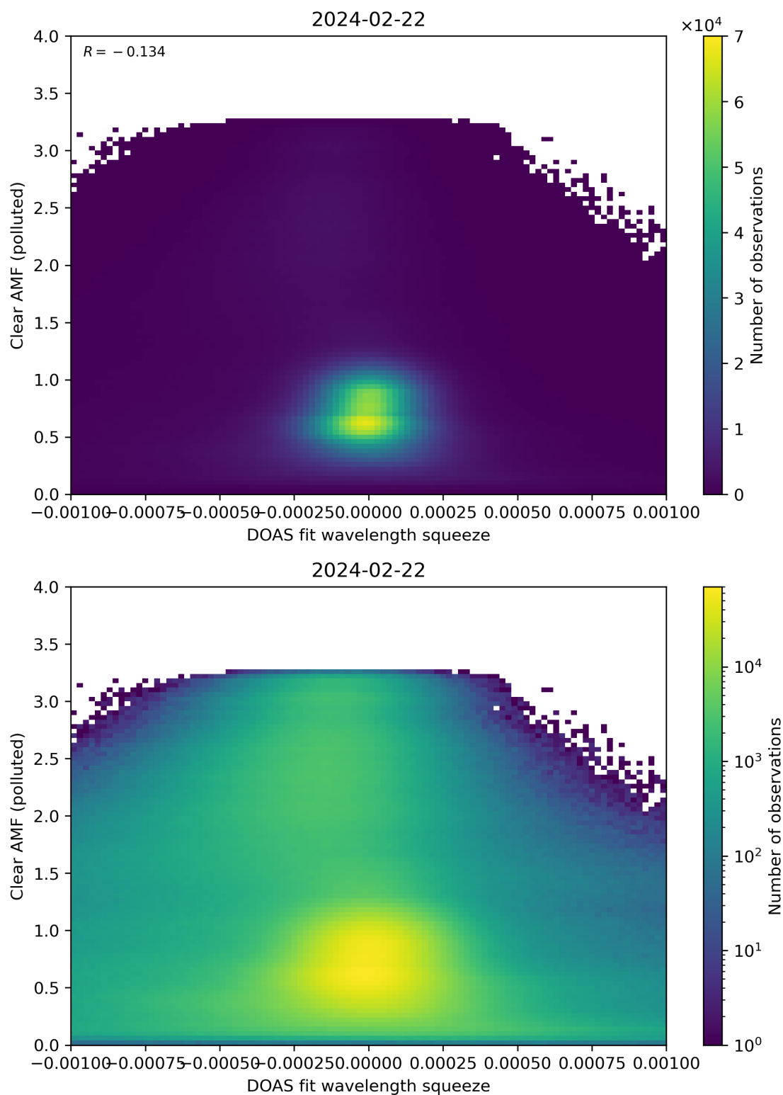
Figure 133: Scatter density plot of “DOAS fit wavelength squeeze” against “Clear AMF (polluted)” for 2024-02-22 to 2024-02-23.
