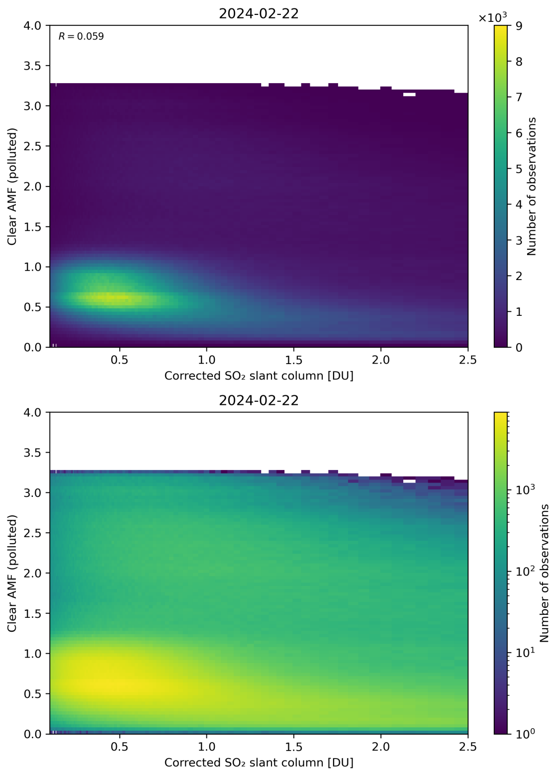
Figure 184: Scatter density plot of “Corrected SO 2 slant column” against “Clear AMF (polluted)” for 2024-02-22 to 2024-02-23.
