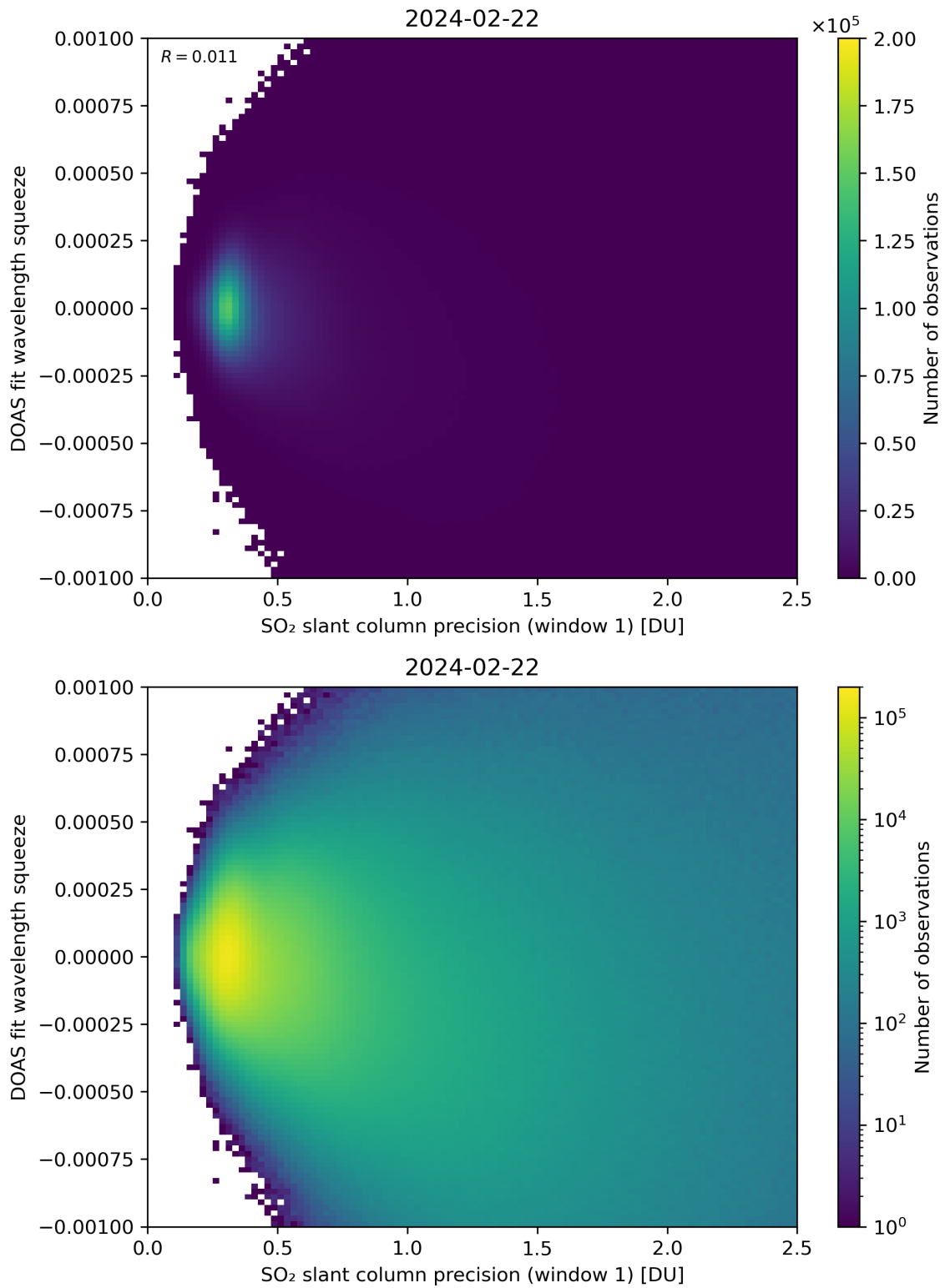
Figure 222: Scatter density plot of “SO 2 slant column precision (window 1)” against “DOAS fit wavelength squeeze” for 2024-02-22 to 2024-02-23.
