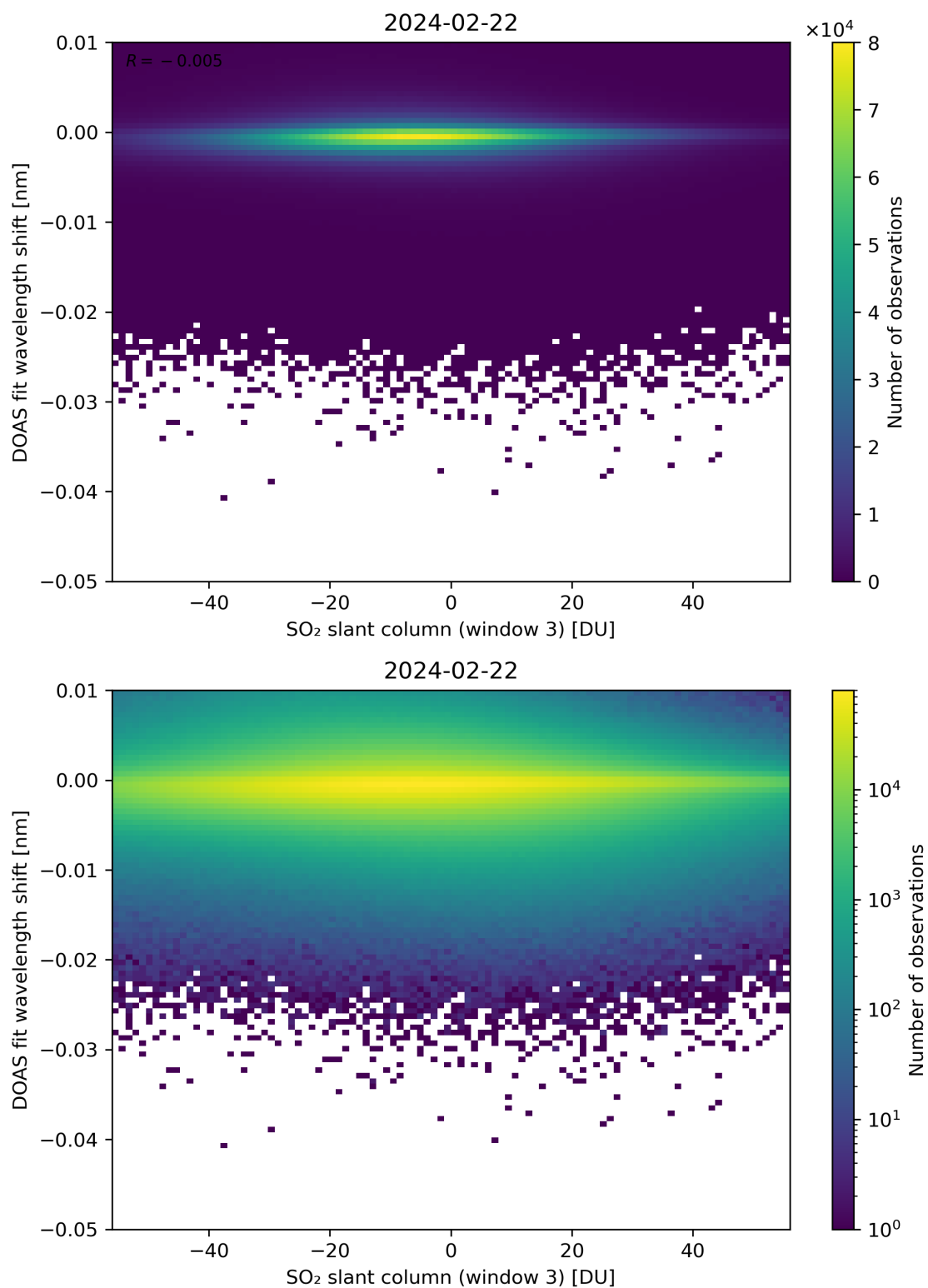
Figure 254: Scatter density plot of “SO 2 slant column (window 3)” against “DOAS fit wavelength shift” for 2024-02-22 to 2024-02-23.
