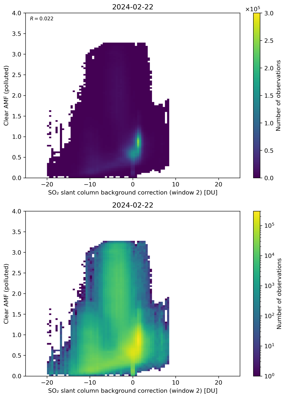
Figure 115: Scatter density plot of “SO 2 slant column background correction (window 2)” against “Clear AMF (polluted)” for 2024-02-22 to 2024-02-23.
