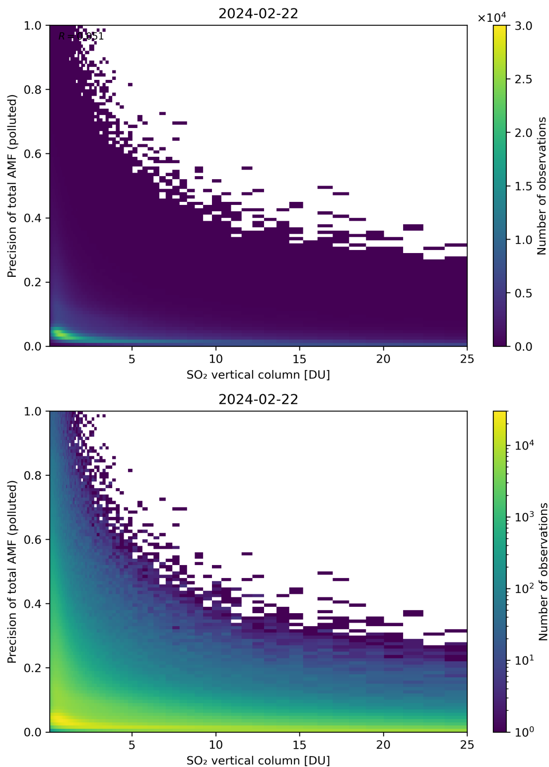
Figure 306: Scatter density plot of “SO 2 vertical column” against “Precision of total AMF (polluted)” for 2024-02-22 to 2024-02-23.
