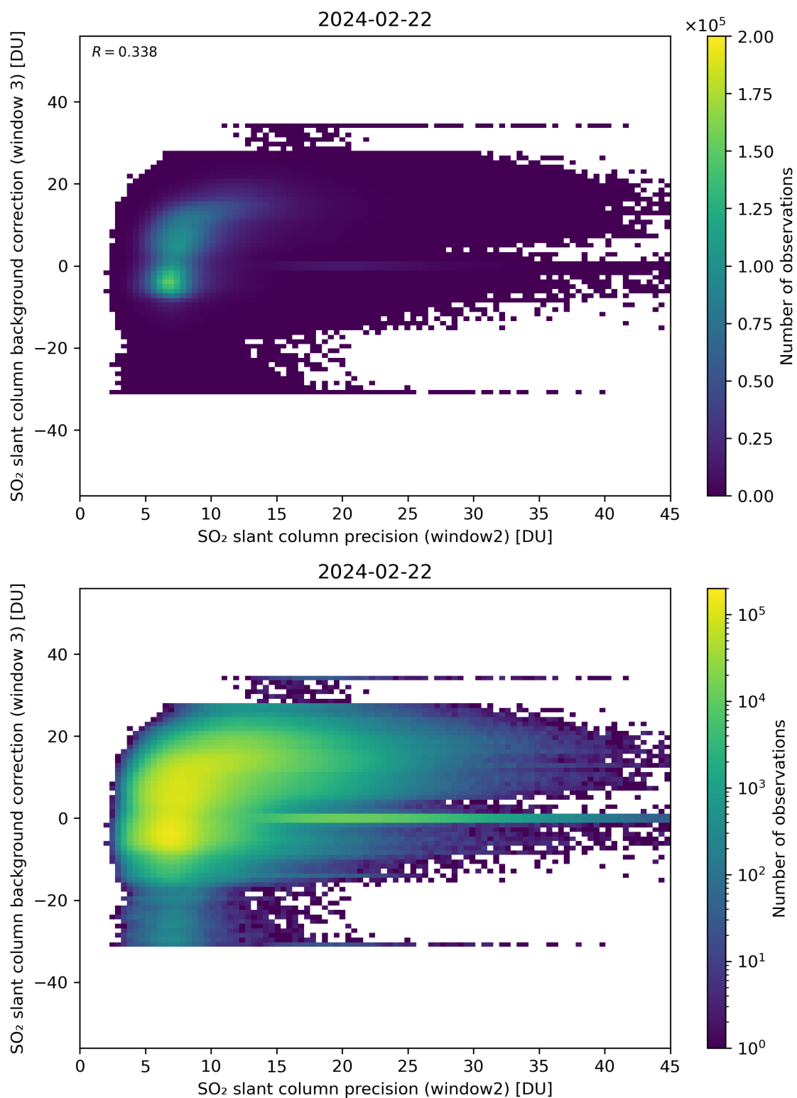
Figure 242: Scatter density plot of “SO 2 slant column precision (window2)” against “SO 2 slant column background correction (window 3)” for 2024-02-22 to 2024-02-23.
