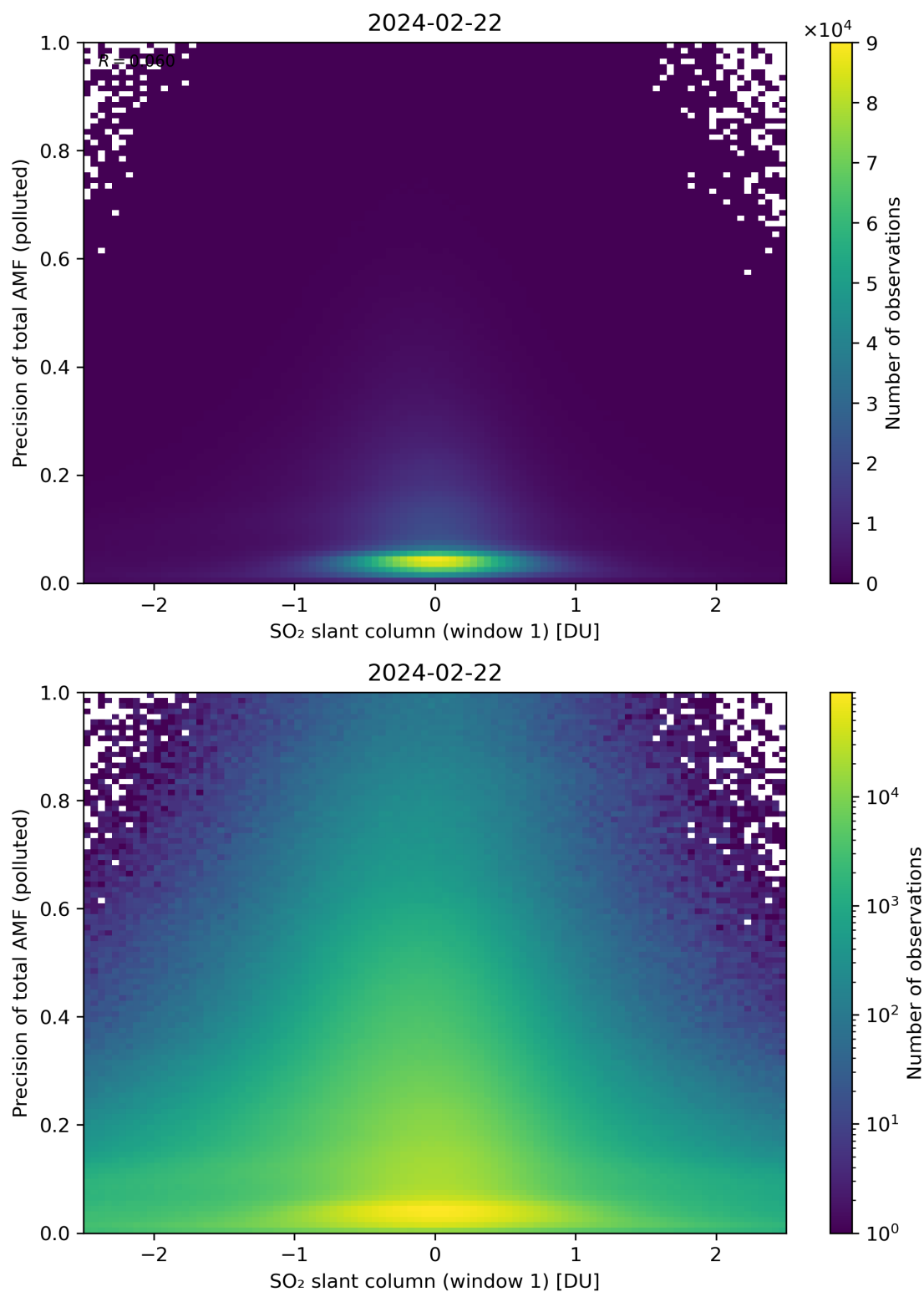
Figure 240: Scatter density plot of “SO 2 slant column (window 1)” against “Precision of total AMF (polluted)” for 2024-02-22 to 2024-02-23.
