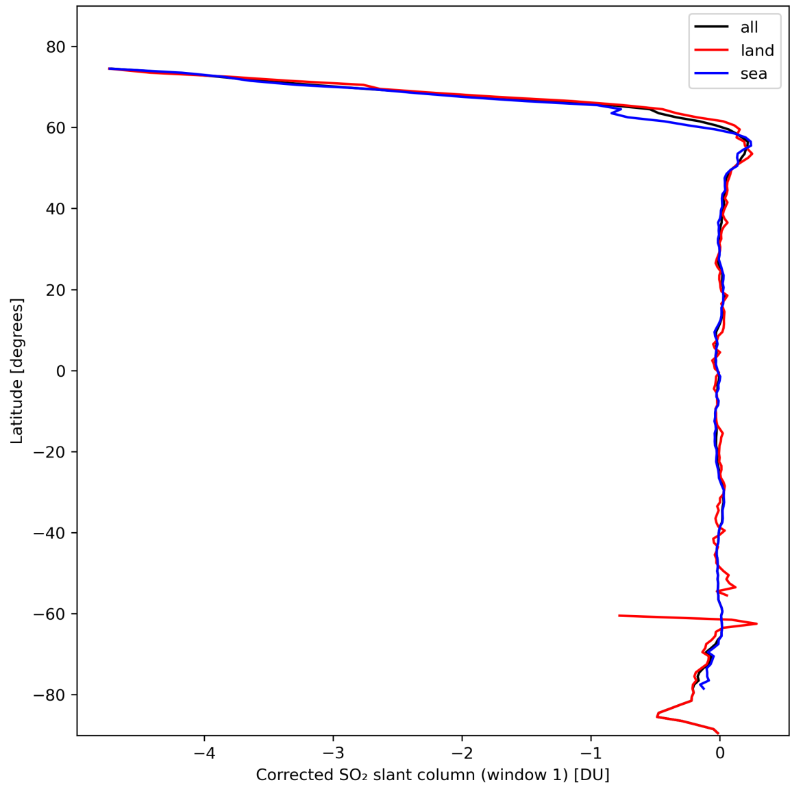
Figure 35: Zonal average of “Corrected SO 2 slant column (window 1)” for 2024-02-22 to 2024-02-23.
