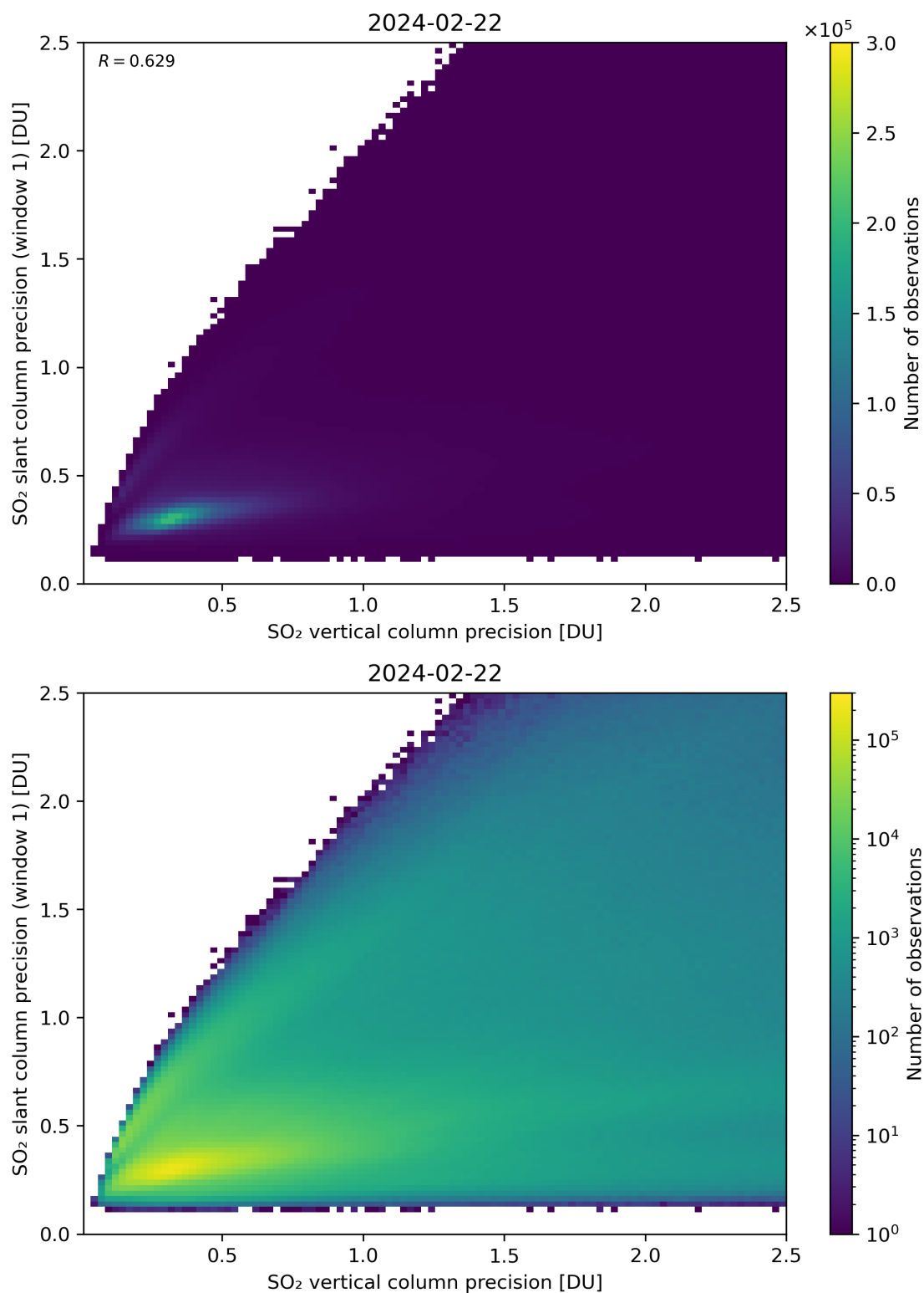
Figure 290: Scatter density plot of “SO 2 vertical column precision” against “SO 2 slant column precision (window 1)” for 2024-02-22 to 2024-02-23.
