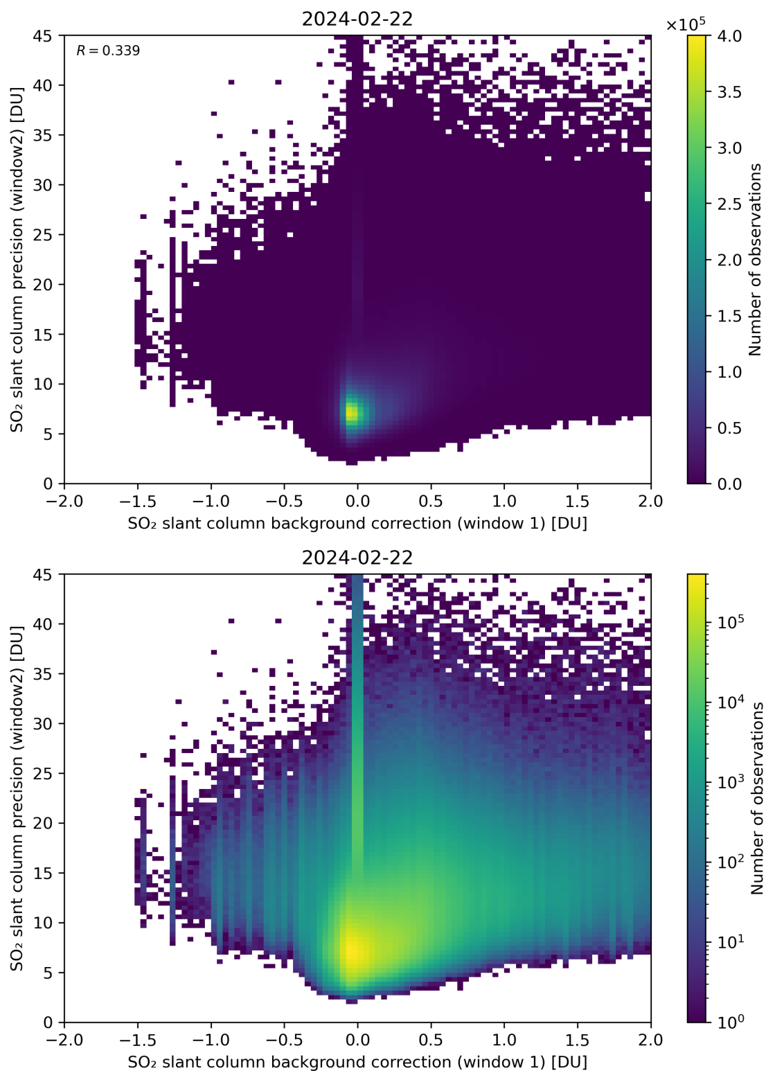
Figure 106: Scatter density plot of “SO 2 slant column background correction (window 1)” against “SO 2 slant column precision (window2)” for 2024-02-22 to 2024-02-23.
