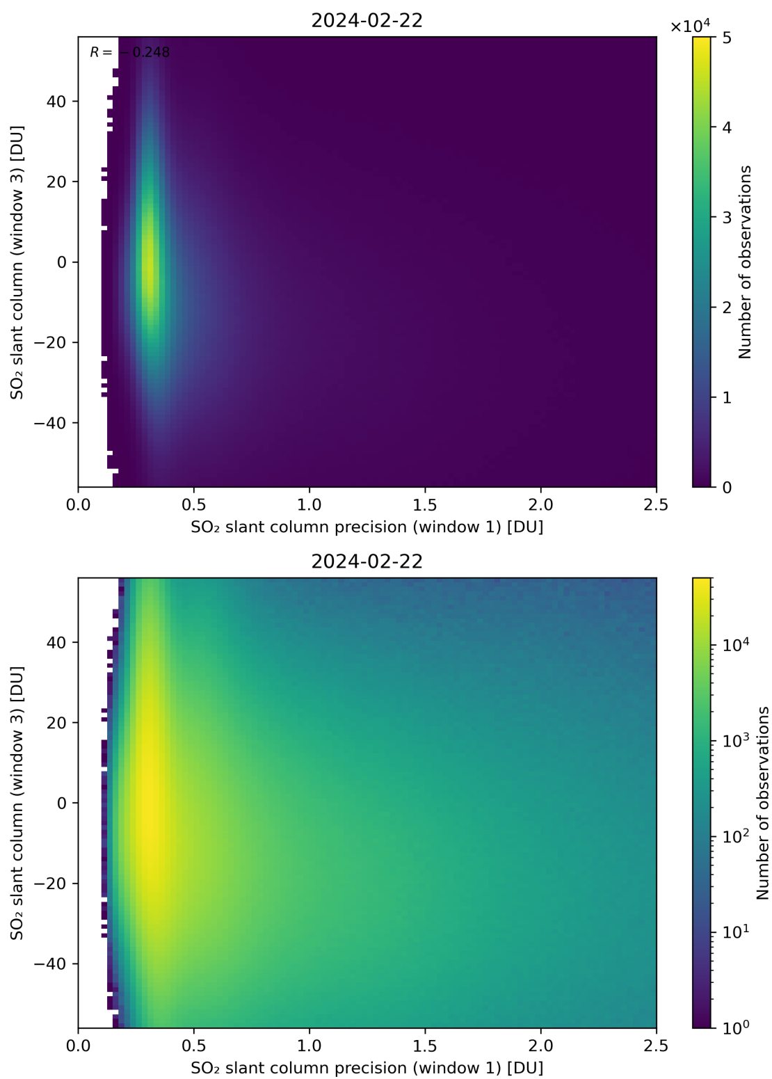
Figure 228: Scatter density plot of “SO 2 slant column precision (window 1)” against “SO 2 slant column (window 3)” for 2024-02-22 to 2024-02-23.
