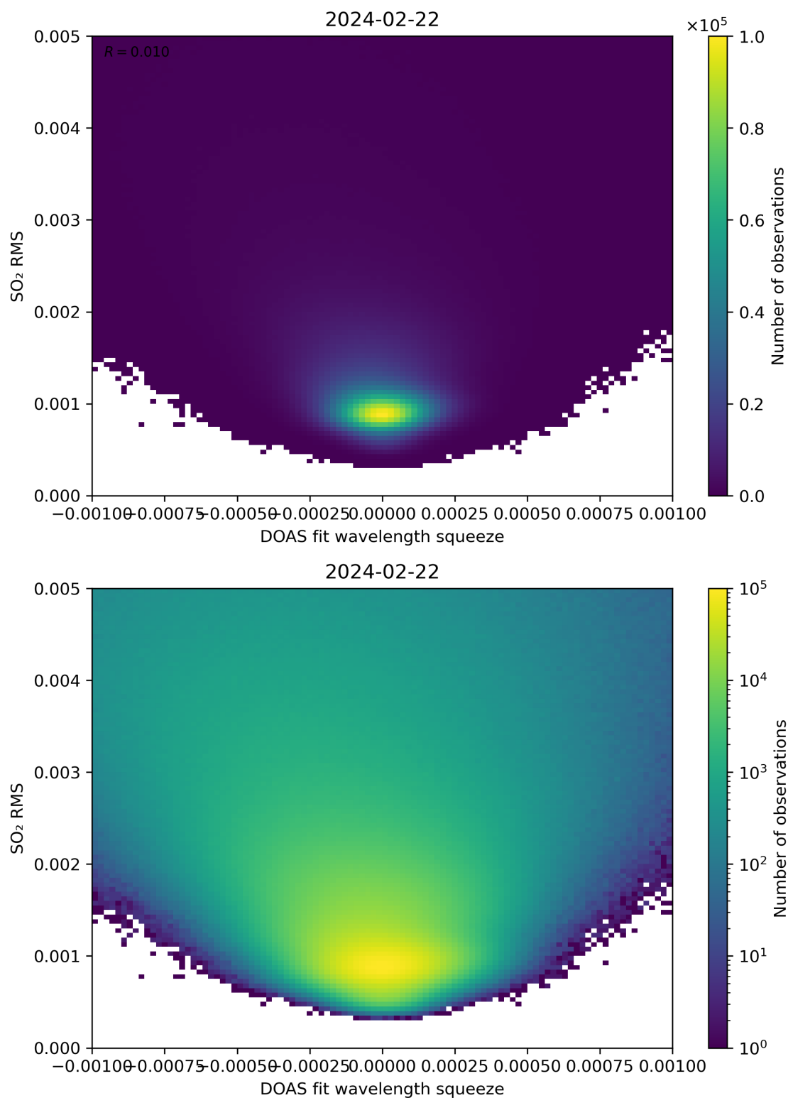
Figure 132: Scatter density plot of “DOAS fit wavelength squeeze” against “SO 2 RMS” for 2024-02-22 to 2024-02-23.
