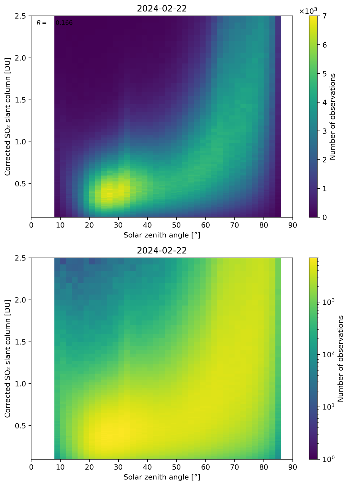
Figure 166: Scatter density plot of “Solar zenith angle” against “Corrected SO 2 slant column” for 2024-02-22 to 2024-02-23.
