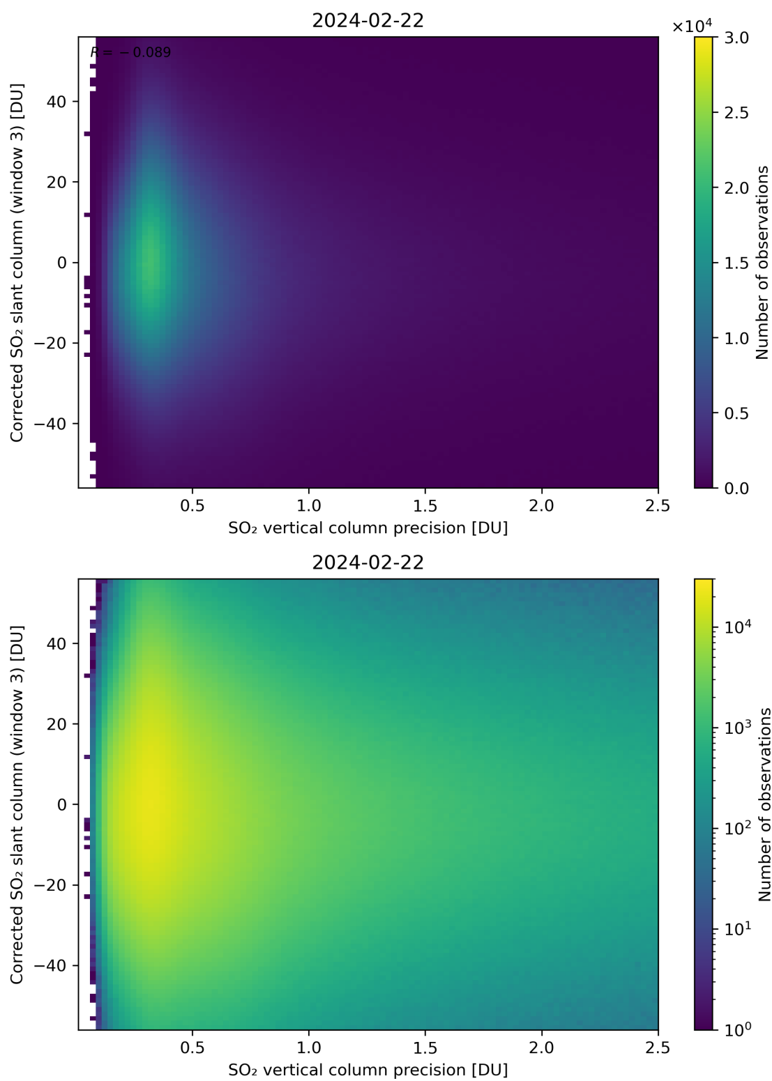
Figure 288: Scatter density plot of “SO 2 vertical column precision” against “Corrected SO 2 slant column (window 3)” for 2024-02-22 to 2024-02-23.
