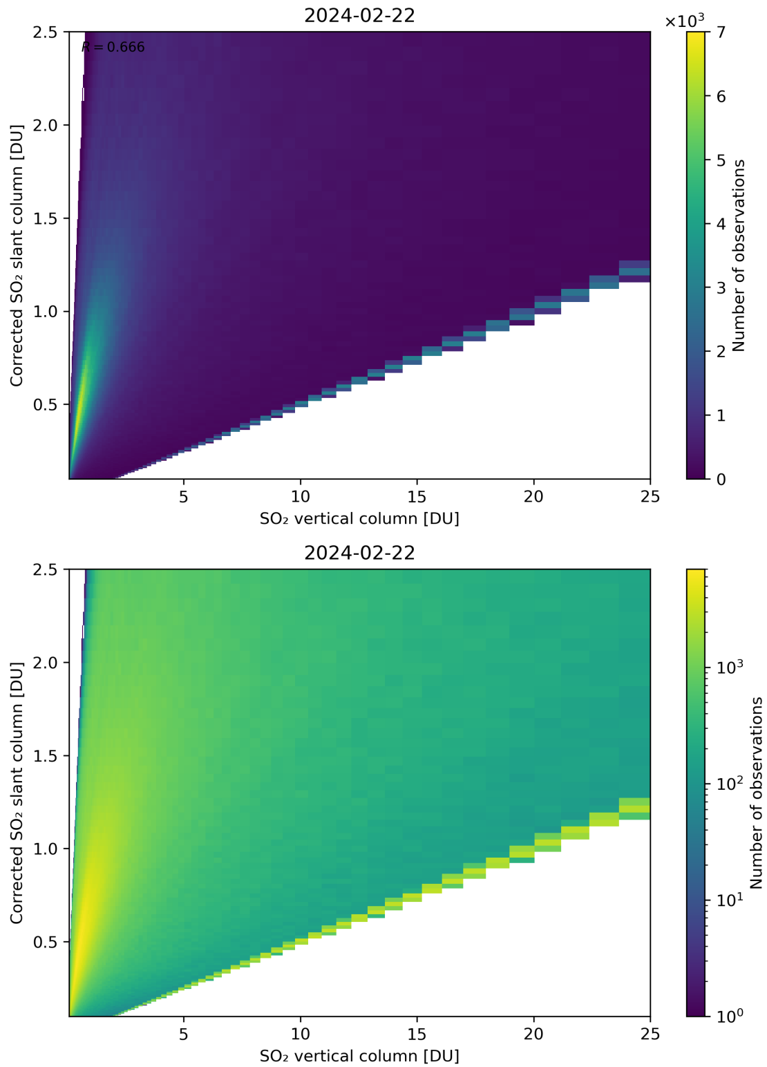
Figure 297: Scatter density plot of “SO 2 vertical column” against “Corrected SO 2 slant column” for 2024-02-22 to 2024-02-23.
