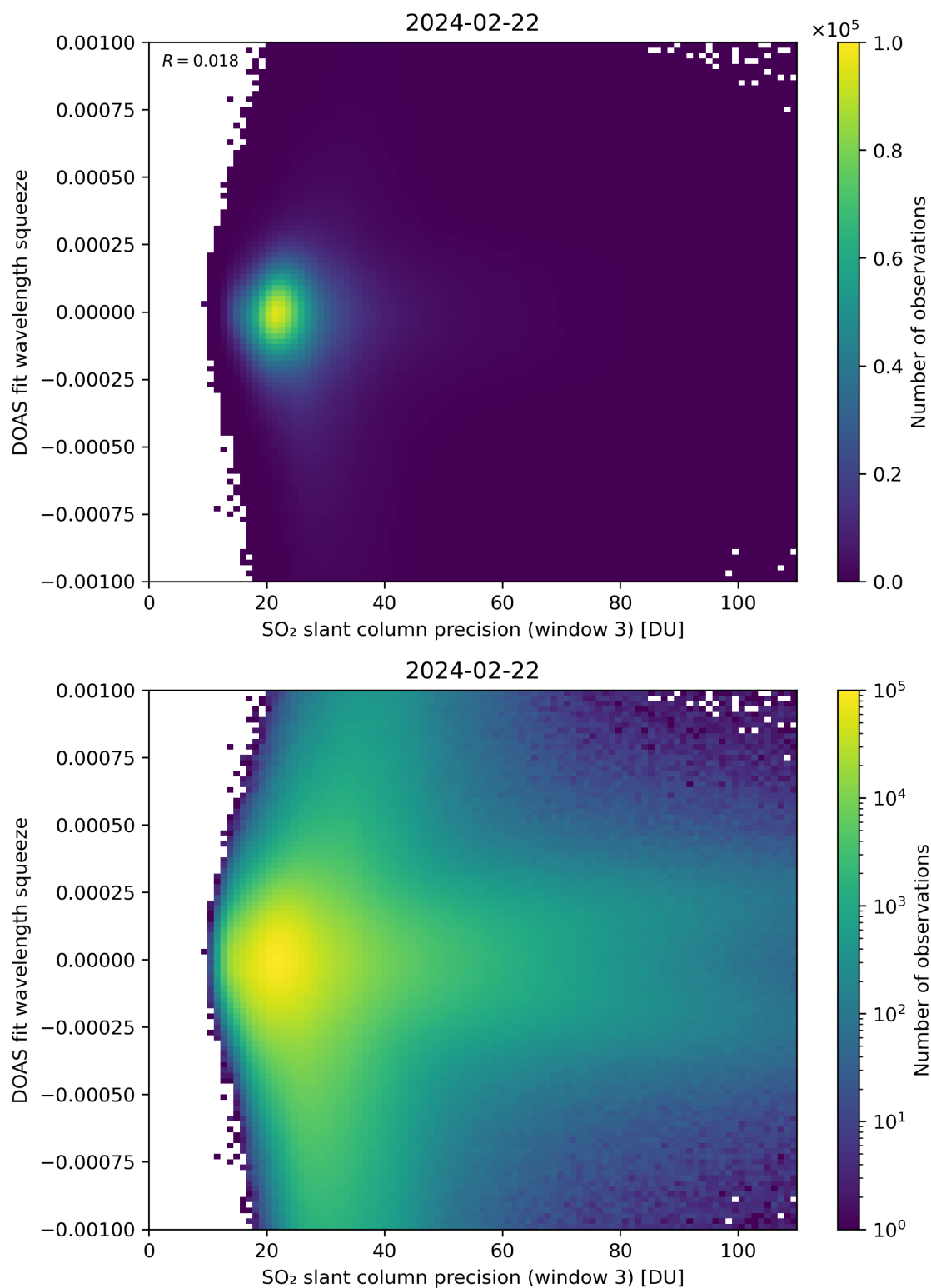
Figure 259: Scatter density plot of “SO 2 slant column precision (window 3)” against “DOAS fit wavelength squeeze” for 2024-02-22 to 2024-02-23.
