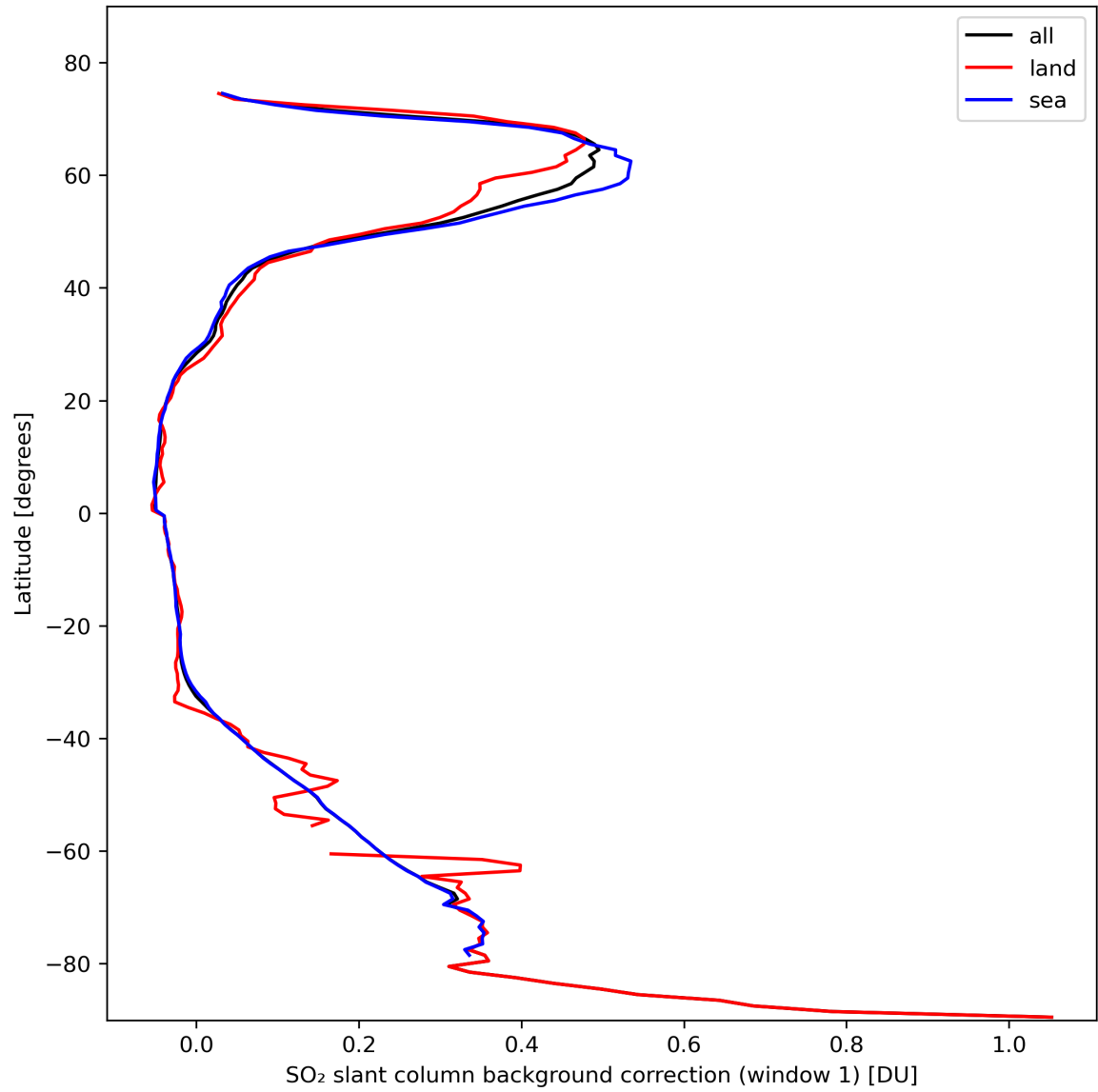
Figure 36: Zonal average of “SO 2 slant column background correction (window 1)” for 2024-02-22 to 2024-02-23.
