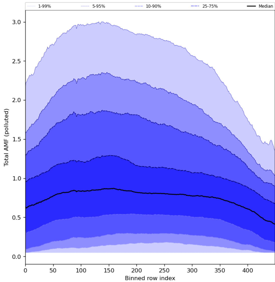
Figure 94: Along track statistics of “Total AMF (polluted)” for 2024-02-22 to 2024-02-23
