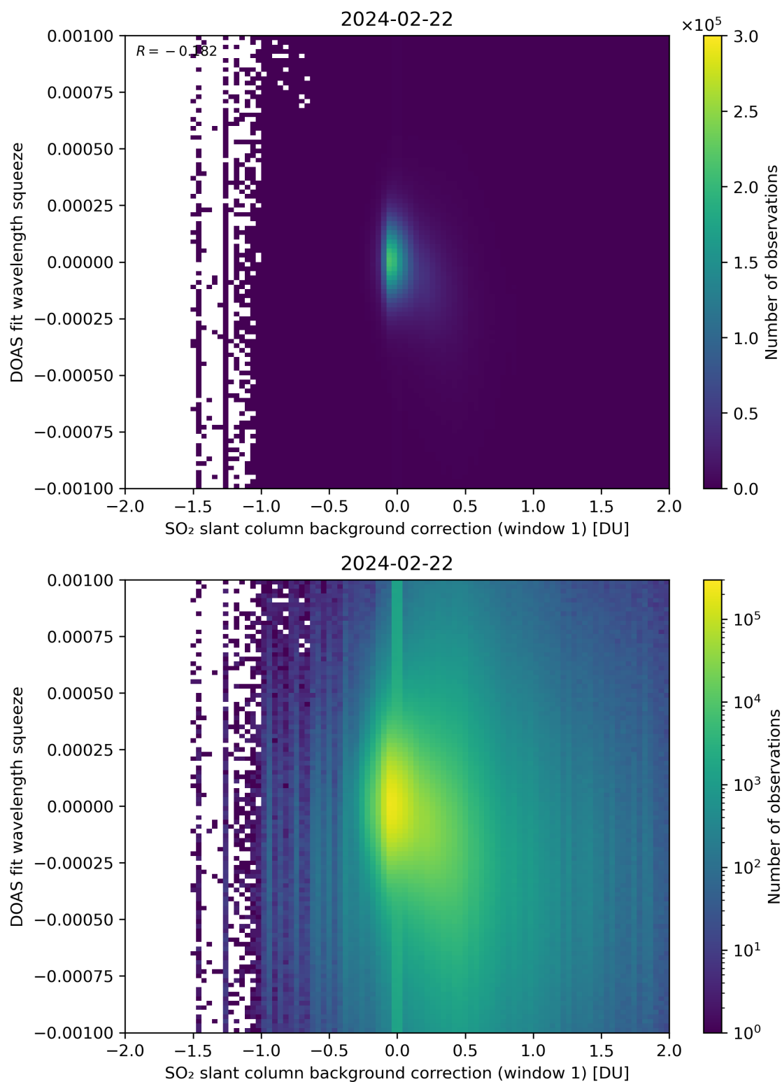
Figure 101: Scatter density plot of “SO 2 slant column background correction (window 1)” against “DOAS fit wavelength squeeze” for 2024-02-22 to 2024-02-23.
