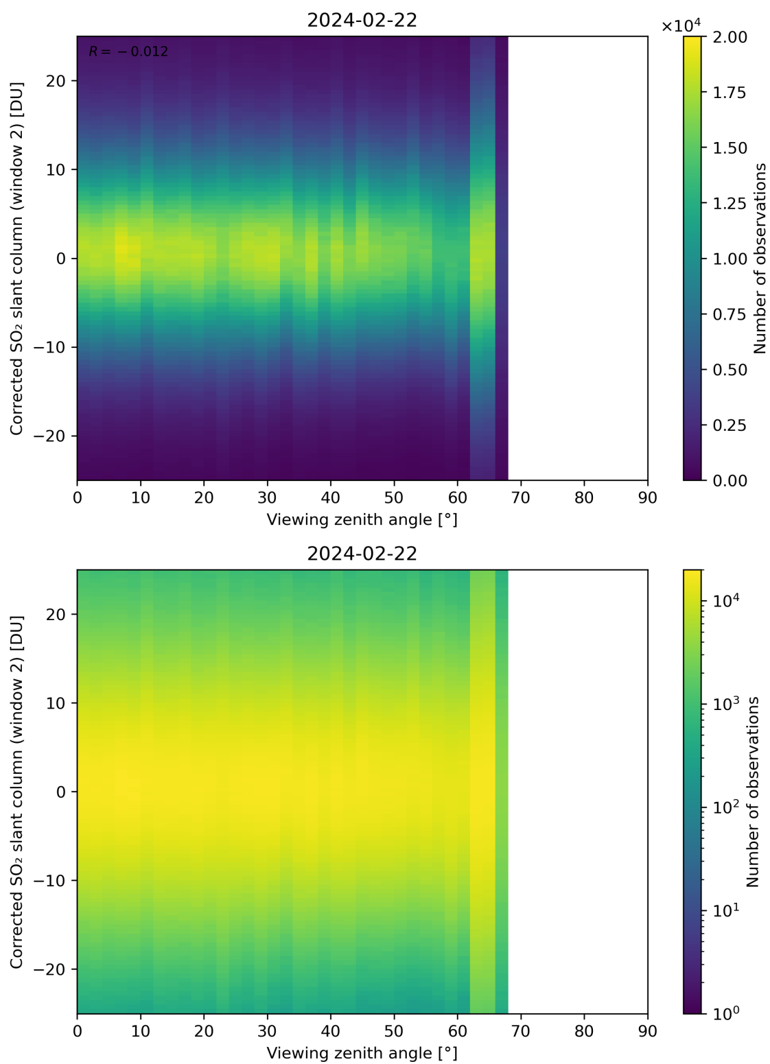
Figure 318: Scatter density plot of “Viewing zenith angle” against “Corrected SO 2 slant column (window 2)” for 2024-02-22 to 2024-02-23.
