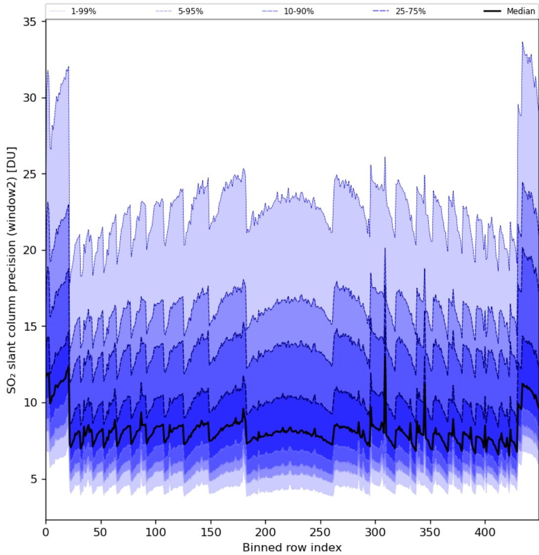
Figure 84: Along track statistics of “SO 2 slant column precision (window2)” for 2024-02-22 to 2024-02-23
