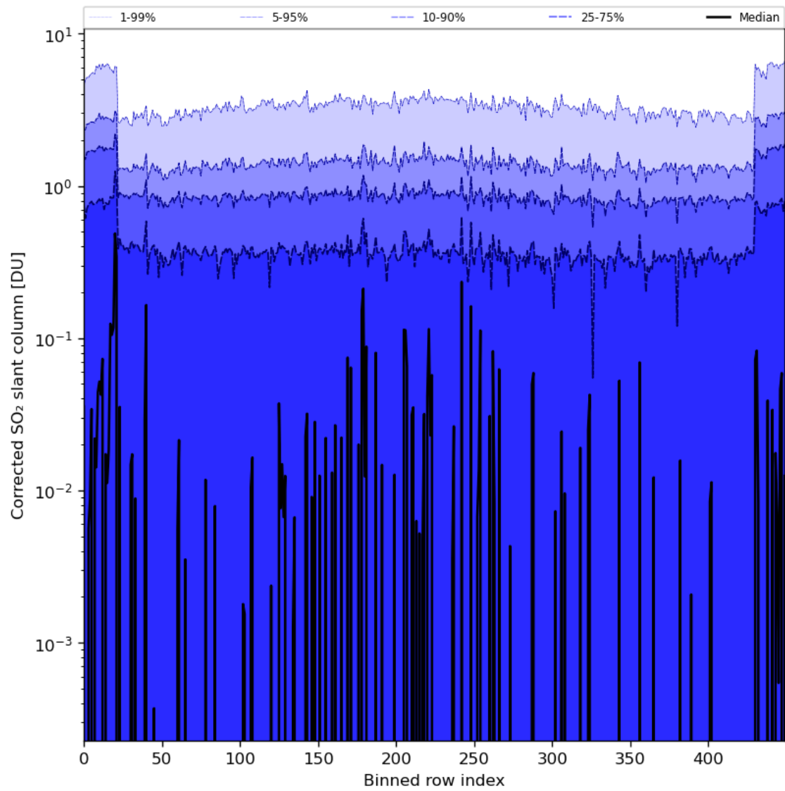
Figure 78: Along track statistics of “Corrected SO 2 slant column” for 2024-02-22 to 2024-02-23
