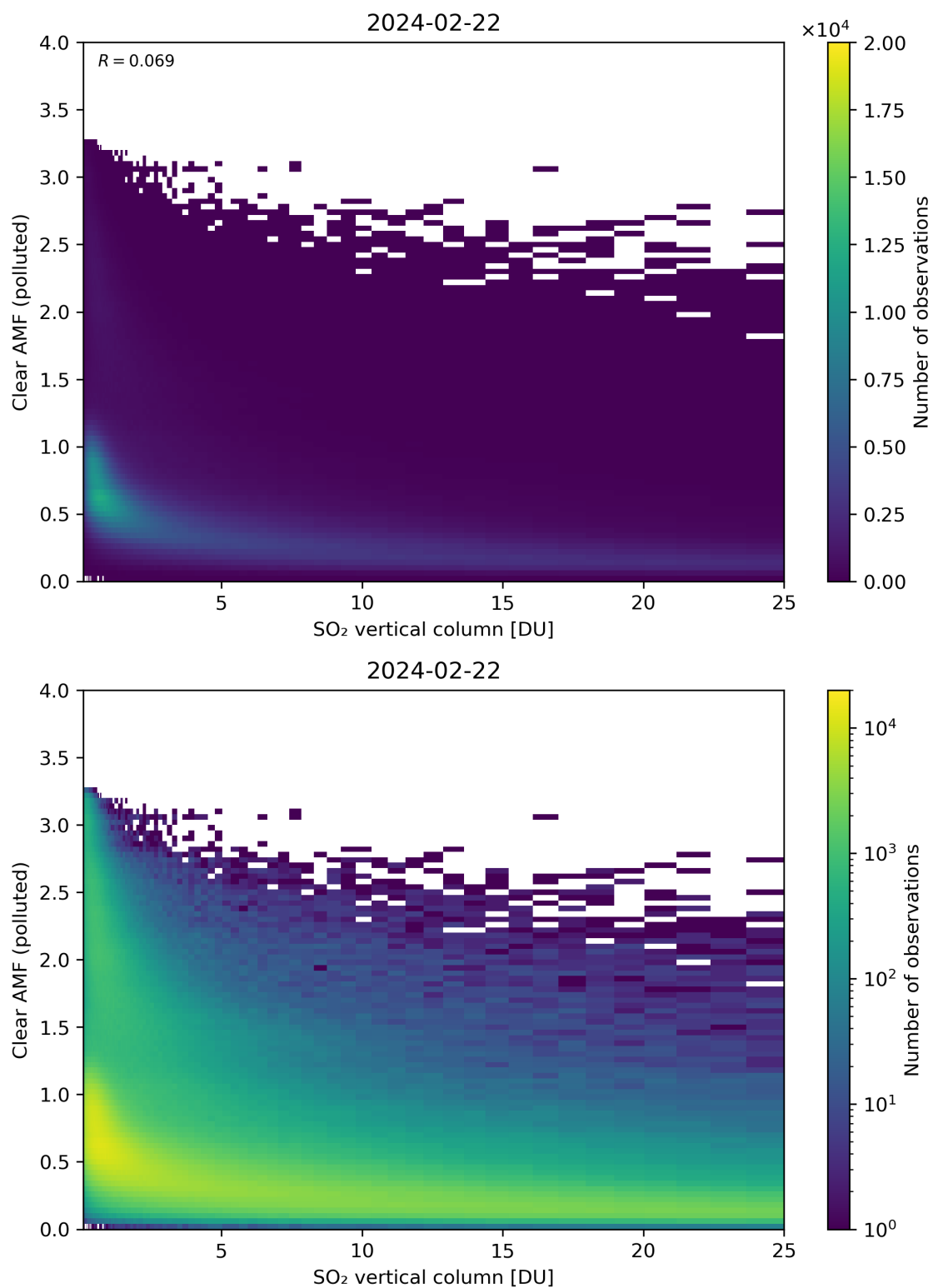
Figure 296: Scatter density plot of “SO 2 vertical column” against “Clear AMF (polluted)” for 2024-02-22 to 2024-02-23.
