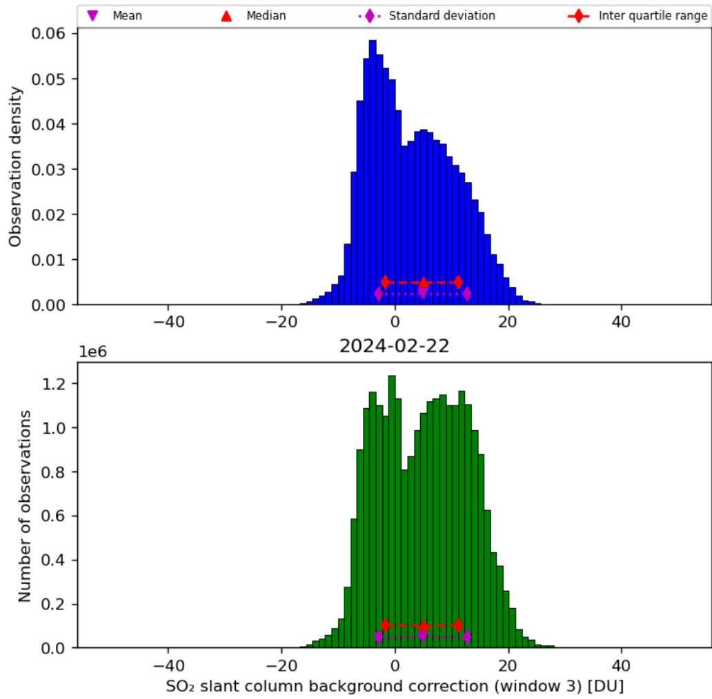
Figure 67: Histogram of “SO 2 slant column background correction (window 3)” for 2024-02-22 to 2024-02-23
