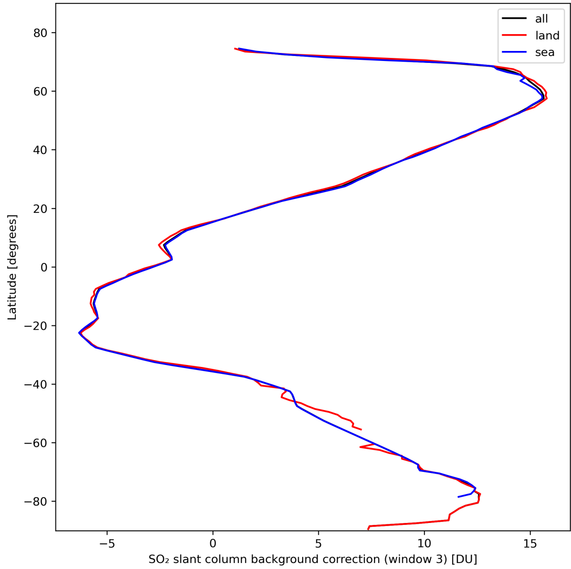
Figure 44: Zonal average of “SO 2 slant column background correction (window 3)” for 2024-02-22 to 2024-02-23.
