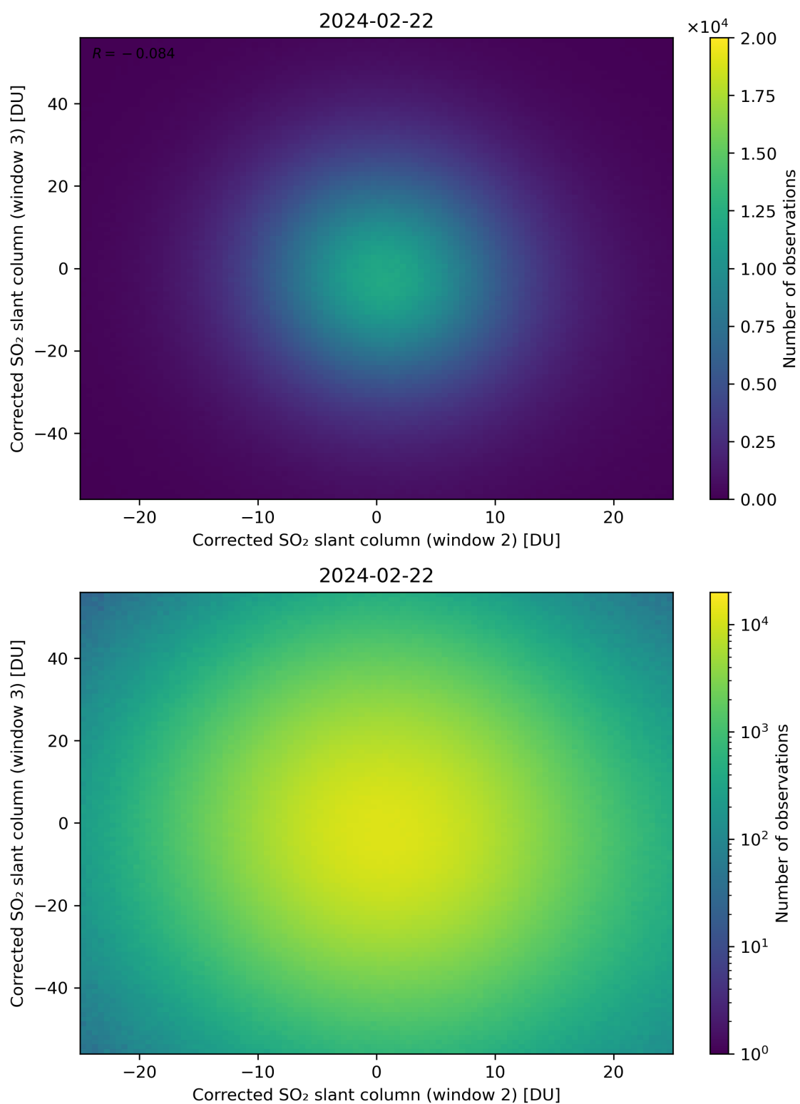
Figure 200: Scatter density plot of “Corrected SO 2 slant column (window 2)” against “Corrected SO 2 slant column (window 3)” for 2024-02-22 to 2024-02-23.
