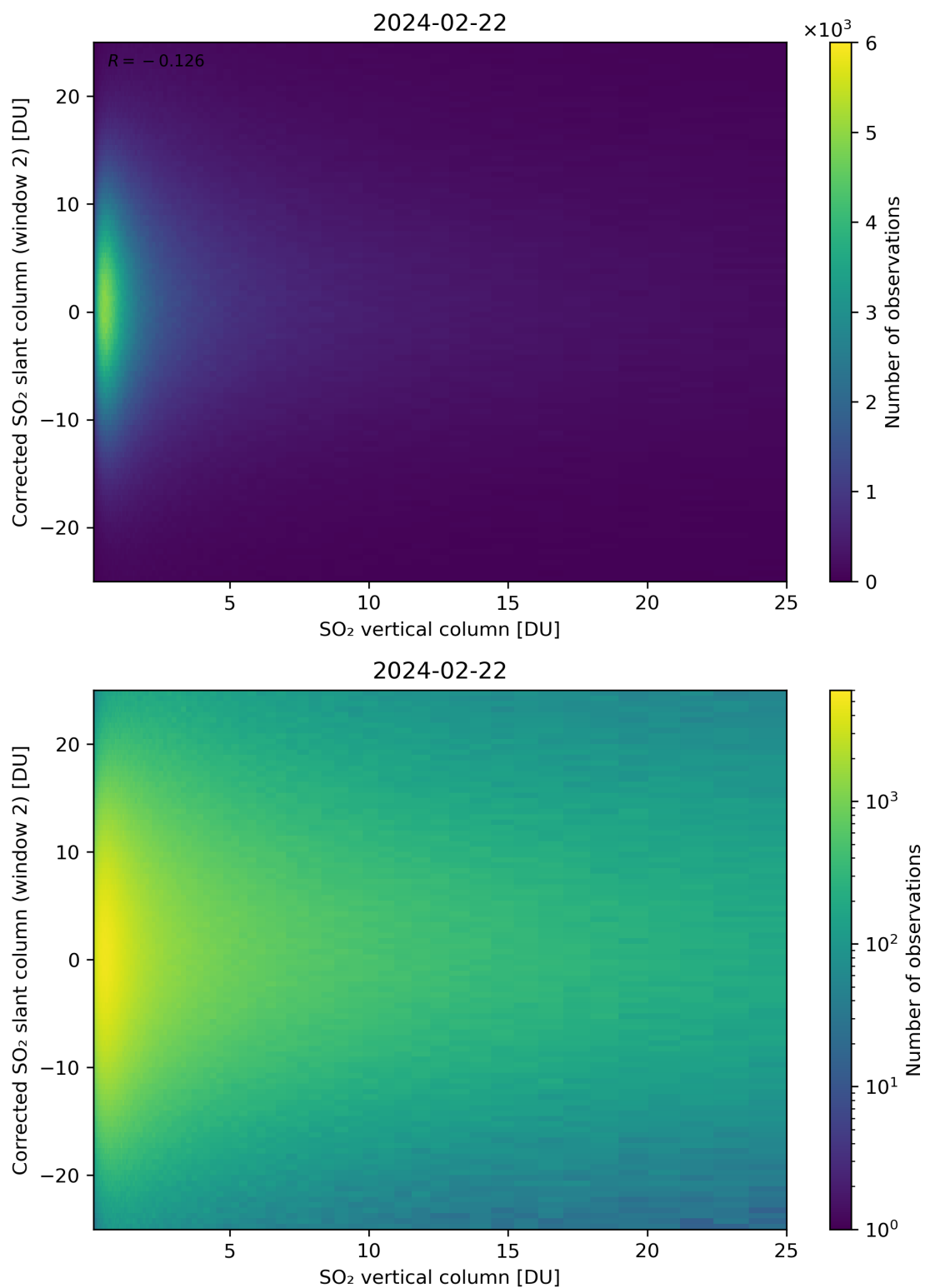
Figure 298: Scatter density plot of “SO 2 vertical column” against “Corrected SO 2 slant column (window 2)” for 2024-02-22 to 2024-02-23.
