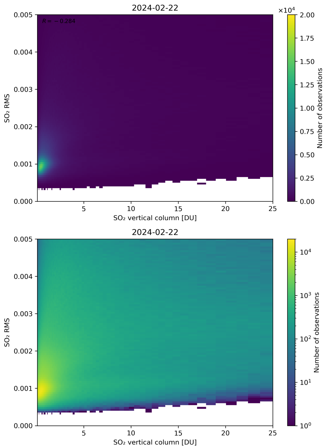
Figure 278: Scatter density plot of “SO 2 vertical column” against “SO 2 RMS” for 2024-02-22 to 2024-02-23.
