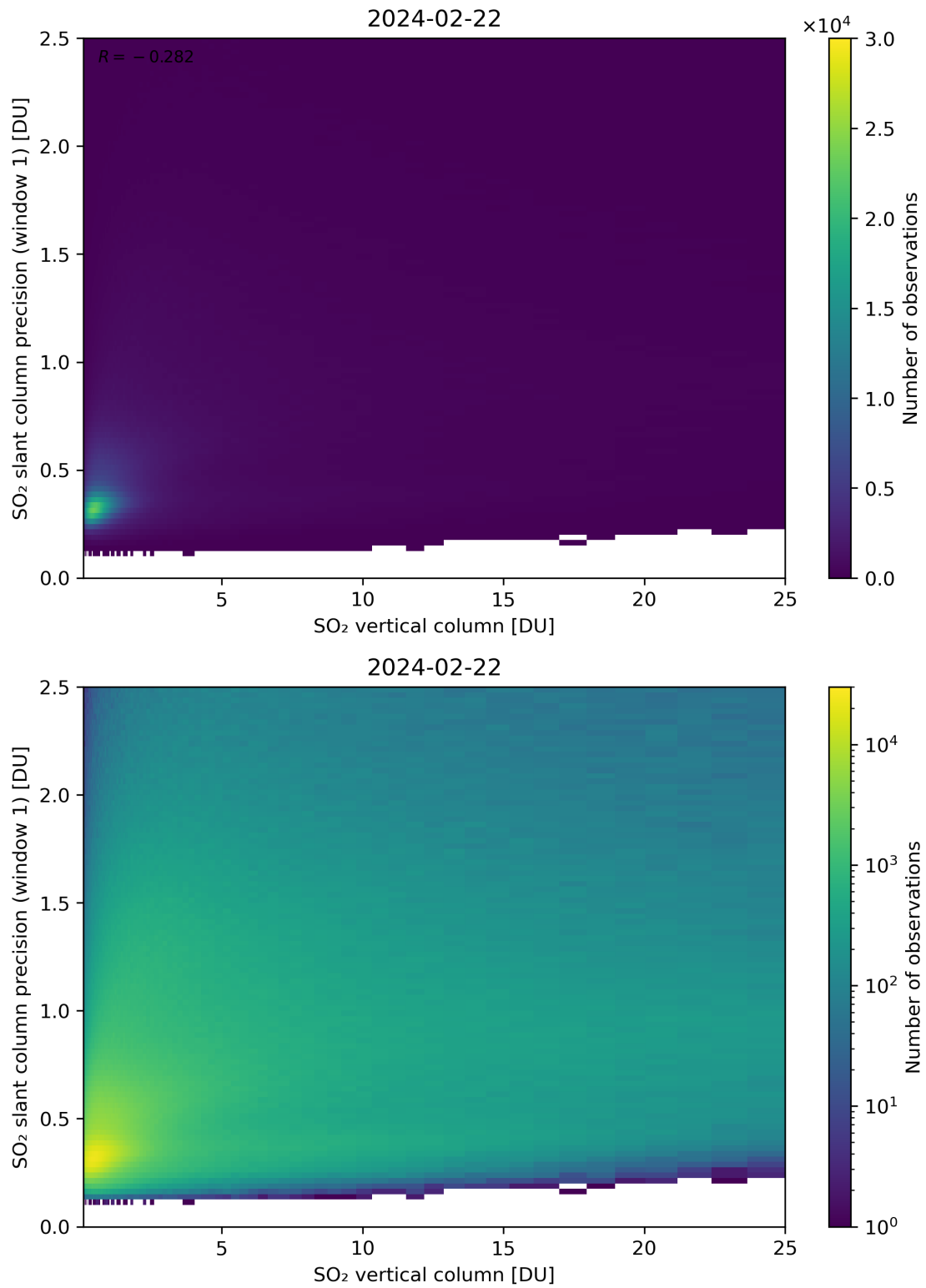
Figure 301: Scatter density plot of “SO 2 vertical column” against “SO 2 slant column precision (window 1)” for 2024-02-22 to 2024-02-23.
