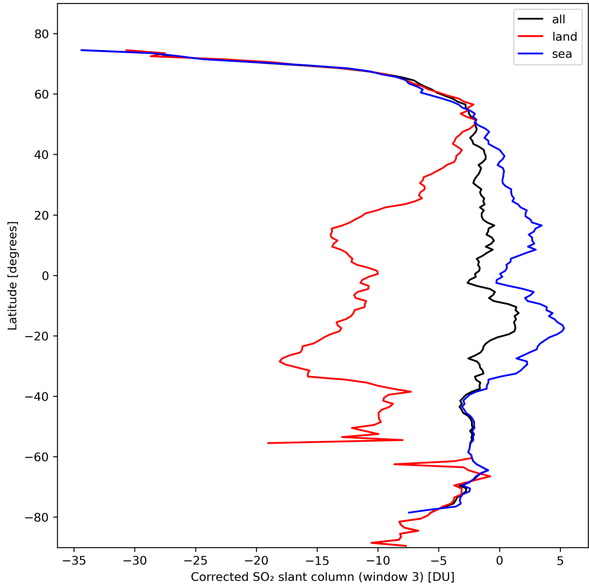
Figure 43: Zonal average of “Corrected SO 2 slant column (window 3)” for 2024-02-22 to 2024-02-23.
