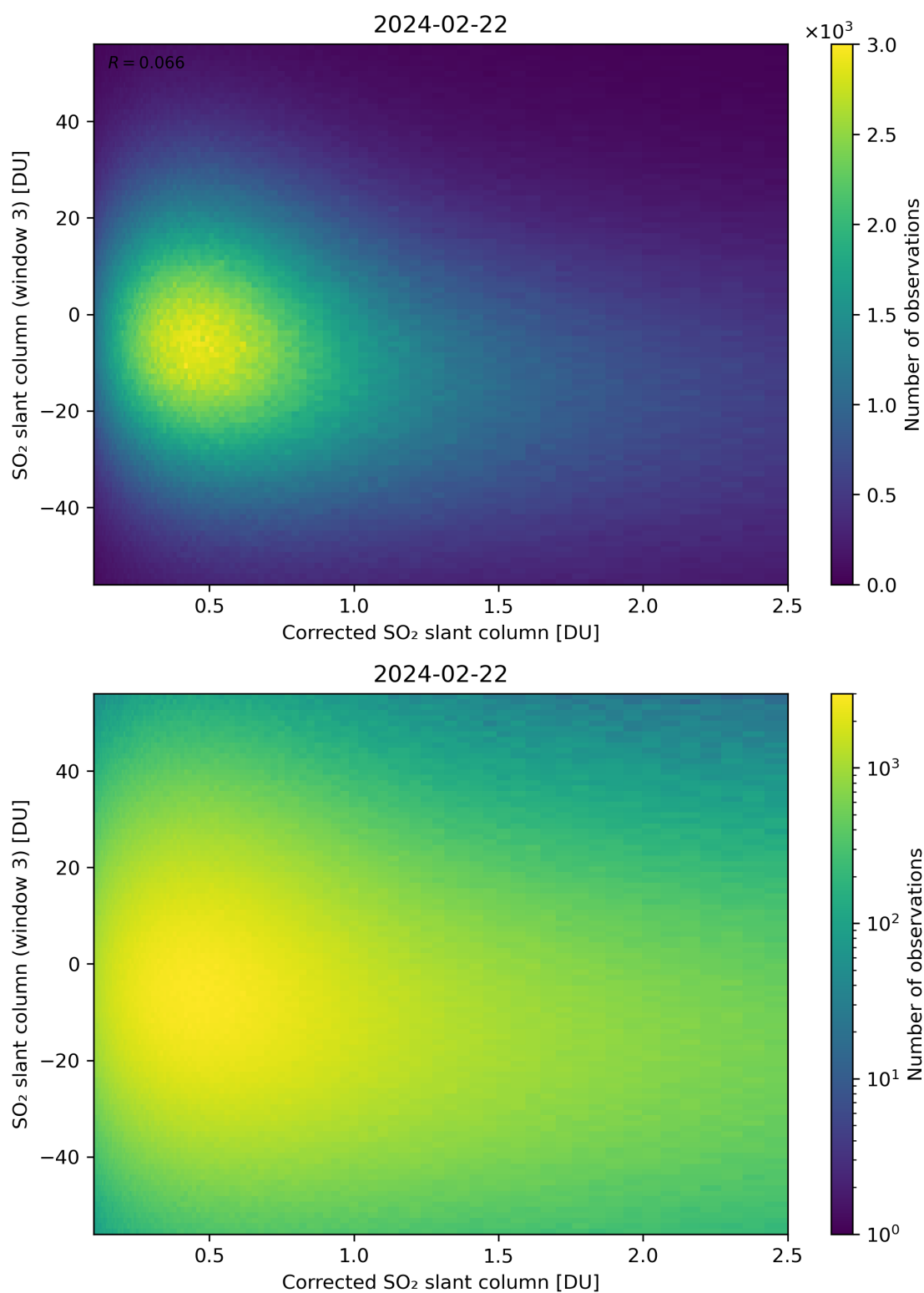
Figure 190: Scatter density plot of “Corrected SO 2 slant column” against “SO 2 slant column (window 3)” for 2024-02-22 to 2024-02-23.
