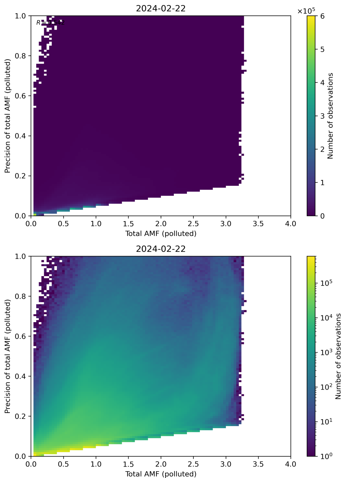
Figure 272: Scatter density plot of “Total AMF (polluted)” against “Precision of total AMF (polluted)” for 2024-02-22 to 2024-02-23.
