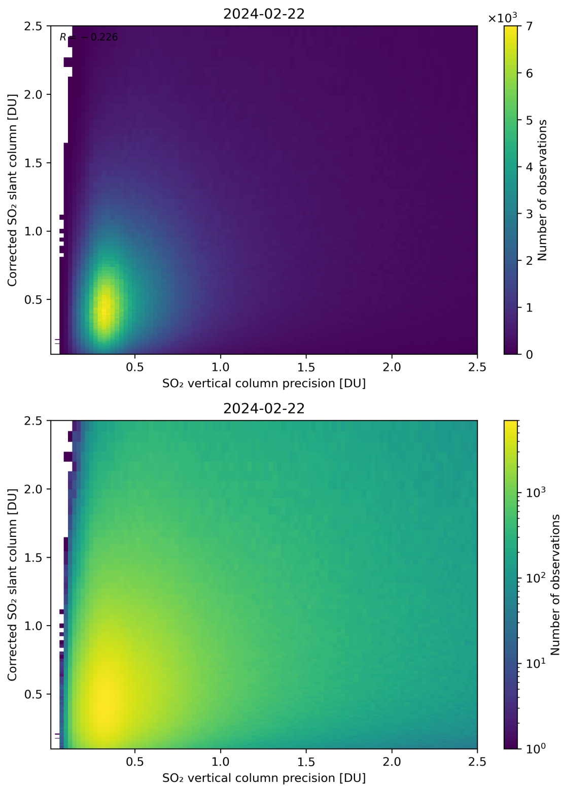
Figure 286: Scatter density plot of “SO 2 vertical column precision” against “Corrected SO 2 slant column” for 2024-02-22 to 2024-02-23.
