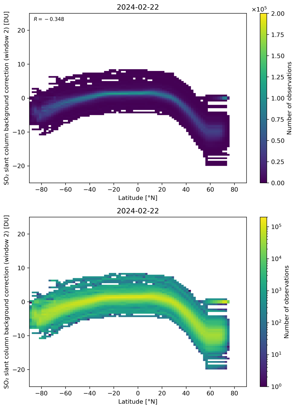
Figure 140: Scatter density plot of “Latitude” against “SO 2 slant column background correction (window 2)” for 2024-02-22 to 2024-02-23.
