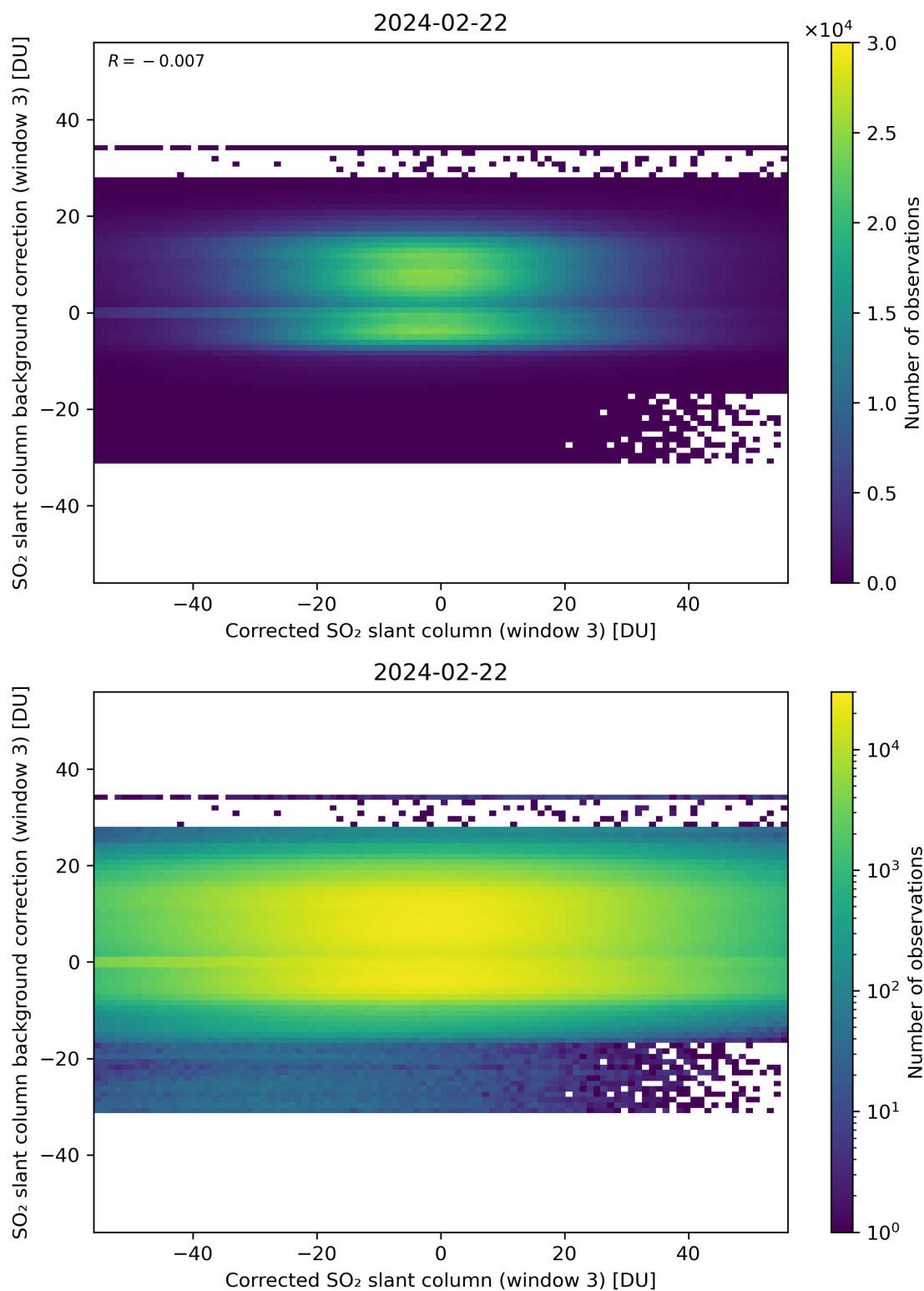
Figure 205: Scatter density plot of “Corrected SO 2 slant column (window 3)” against “SO 2 slant column background correction (window 3)” for 2024-02-22 to 2024-02-23.
