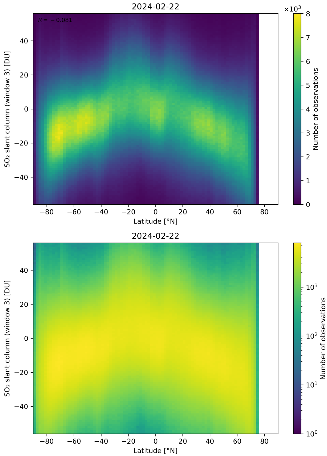
Figure 152: Scatter density plot of “Latitude” against “SO 2 slant column (window 3)” for 2024-02-22 to 2024-02-23.
