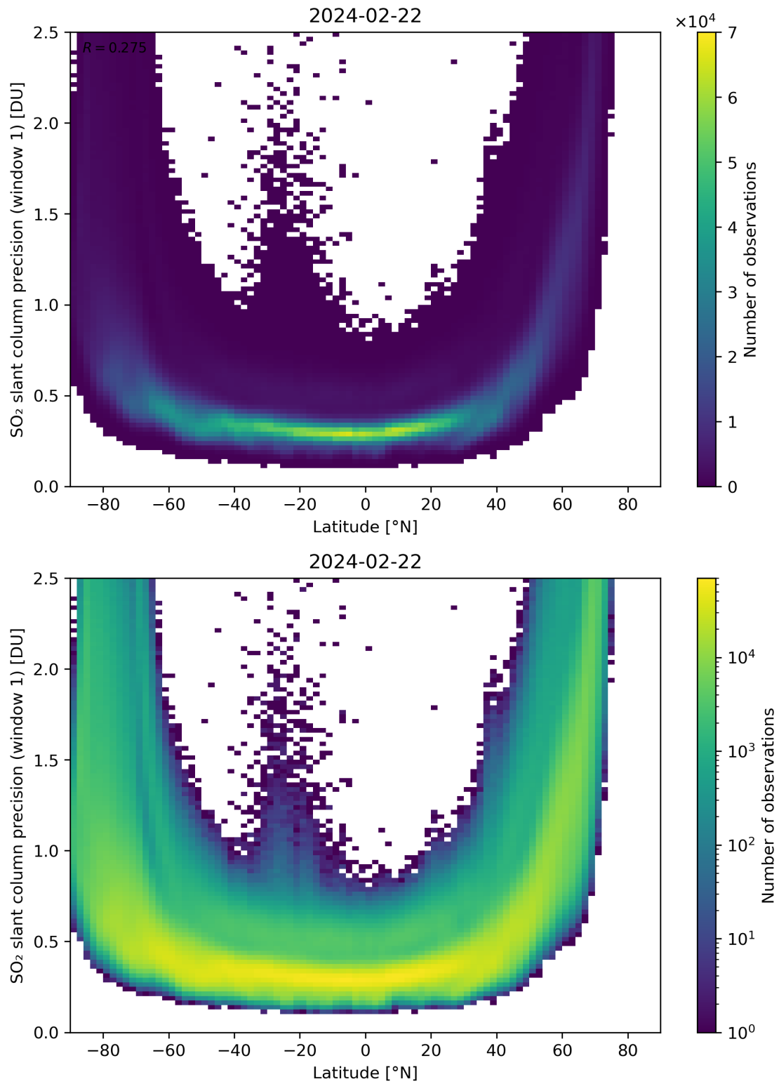
Figure 150: Scatter density plot of “Latitude” against “SO 2 slant column precision (window 1)” for 2024-02-22 to 2024-02-23.
