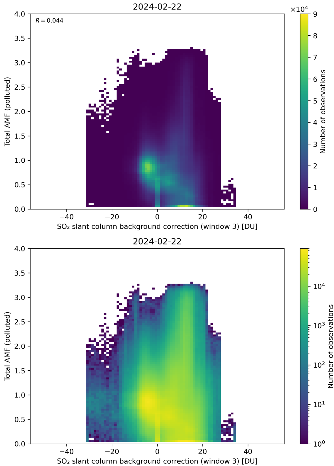
Figure 125: Scatter density plot of “SO 2 slant column background correction (window 3)” against “Total AMF (polluted)” for 2024-02-22 to 2024-02-23.
