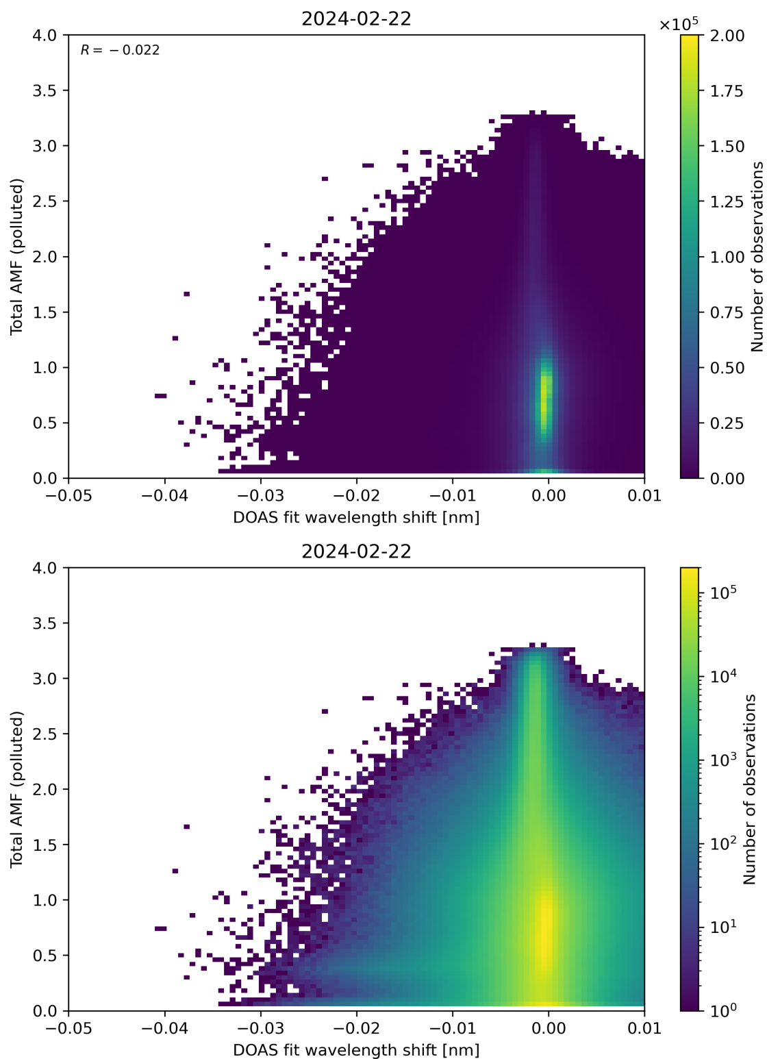
Figure 130: Scatter density plot of “DOAS fit wavelength shift” against “Total AMF (polluted)” for 2024-02-22 to 2024-02-23.
