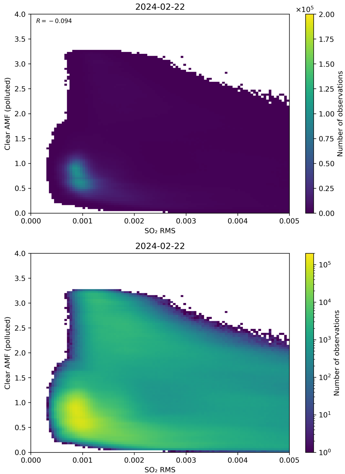
Figure 136: Scatter density plot of “SO 2 RMS” against “Clear AMF (polluted)” for 2024-02-22 to 2024-02-23.
