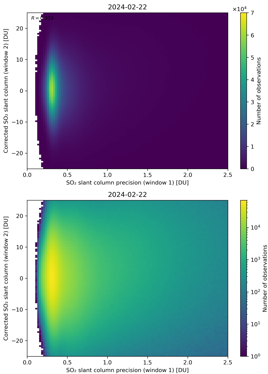
Figure 225: Scatter density plot of “SO 2 slant column precision (window 1)” against “Corrected SO 2 slant column (window 2)” for 2024-02-22 to 2024-02-23.
