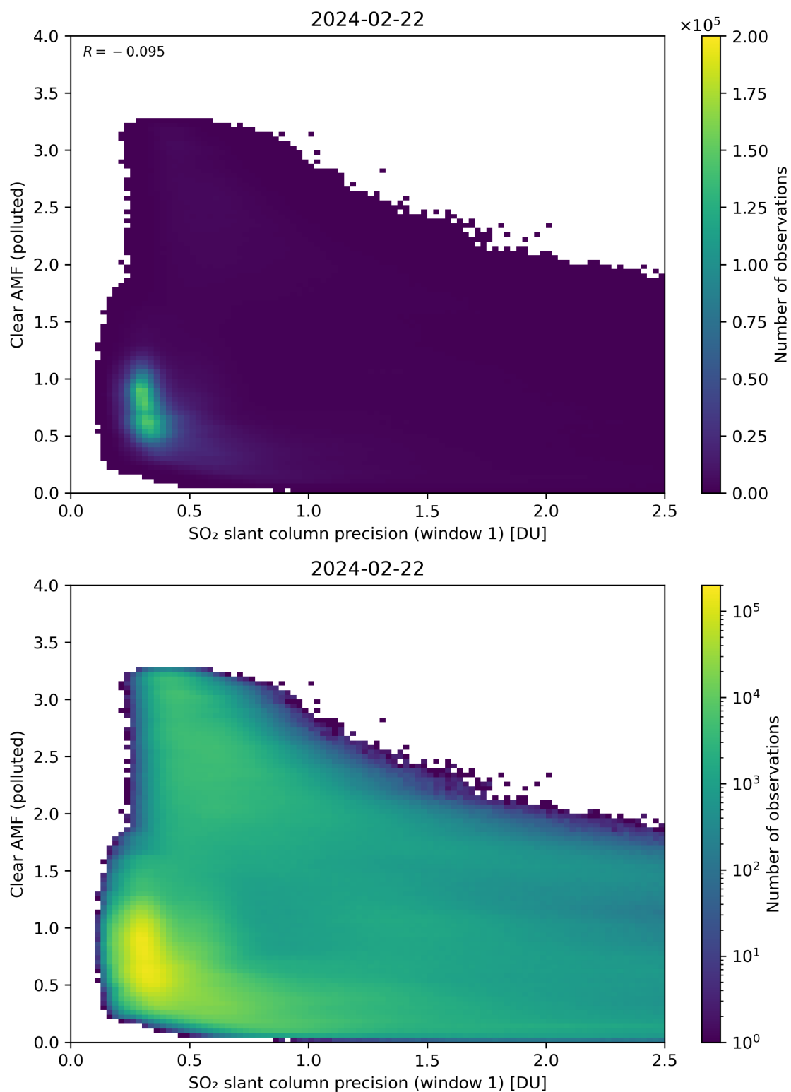
Figure 224: Scatter density plot of “SO 2 slant column precision (window 1)” against “Clear AMF (polluted)” for 2024-02-22 to 2024-02-23.
