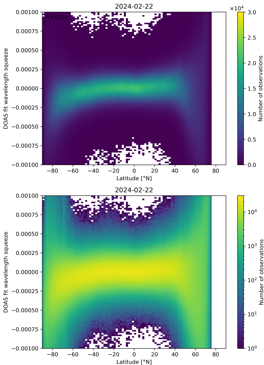
Figure 143: Scatter density plot of “Latitude” against “DOAS fit wavelength squeeze” for 2024-02-22 to 2024-02-23.
