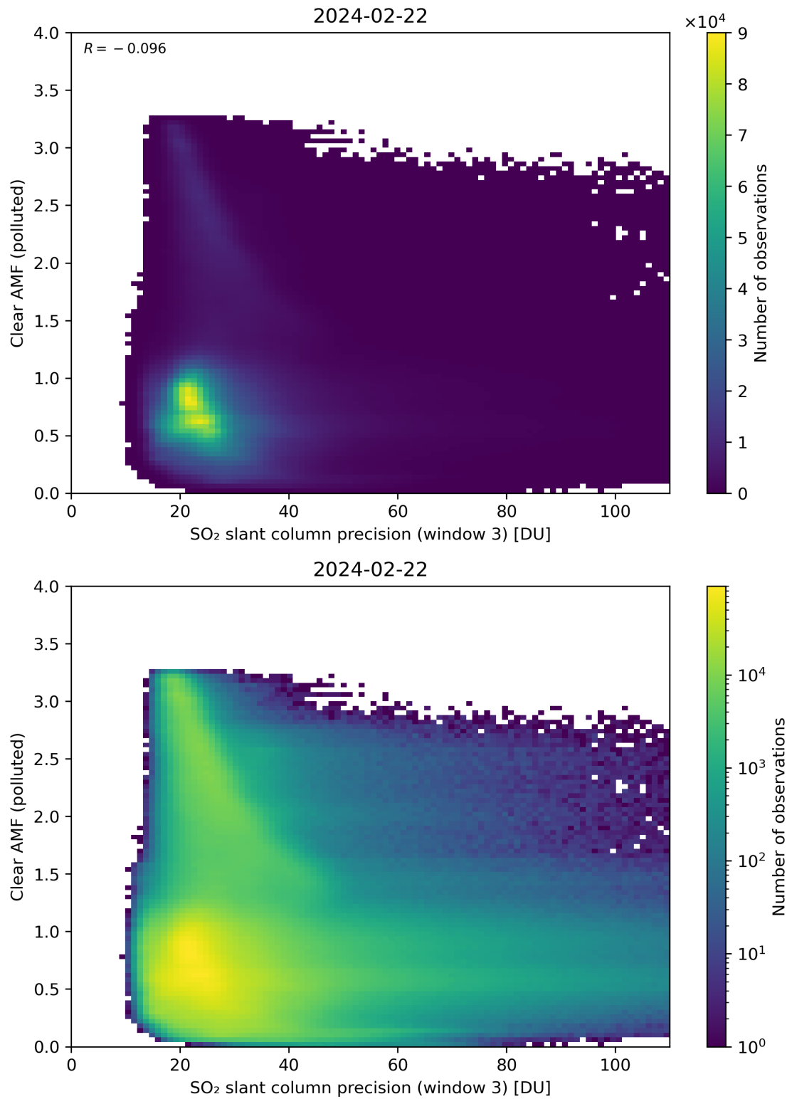
Figure 261: Scatter density plot of “SO 2 slant column precision (window 3)” against “Clear AMF (polluted)” for 2024-02-22 to 2024-02-23.
