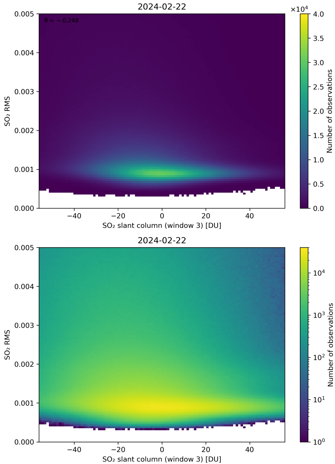
Figure 256: Scatter density plot of “SO 2 slant column (window 3)” against “SO 2 RMS” for 2024-02-22 to 2024-02-23.
