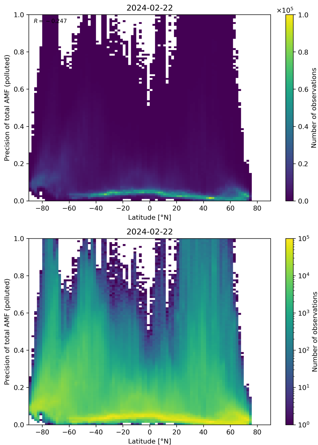
Figure 155: Scatter density plot of “Latitude” against “Precision of total AMF (polluted)” for 2024-02-22 to 2024-02-23.
