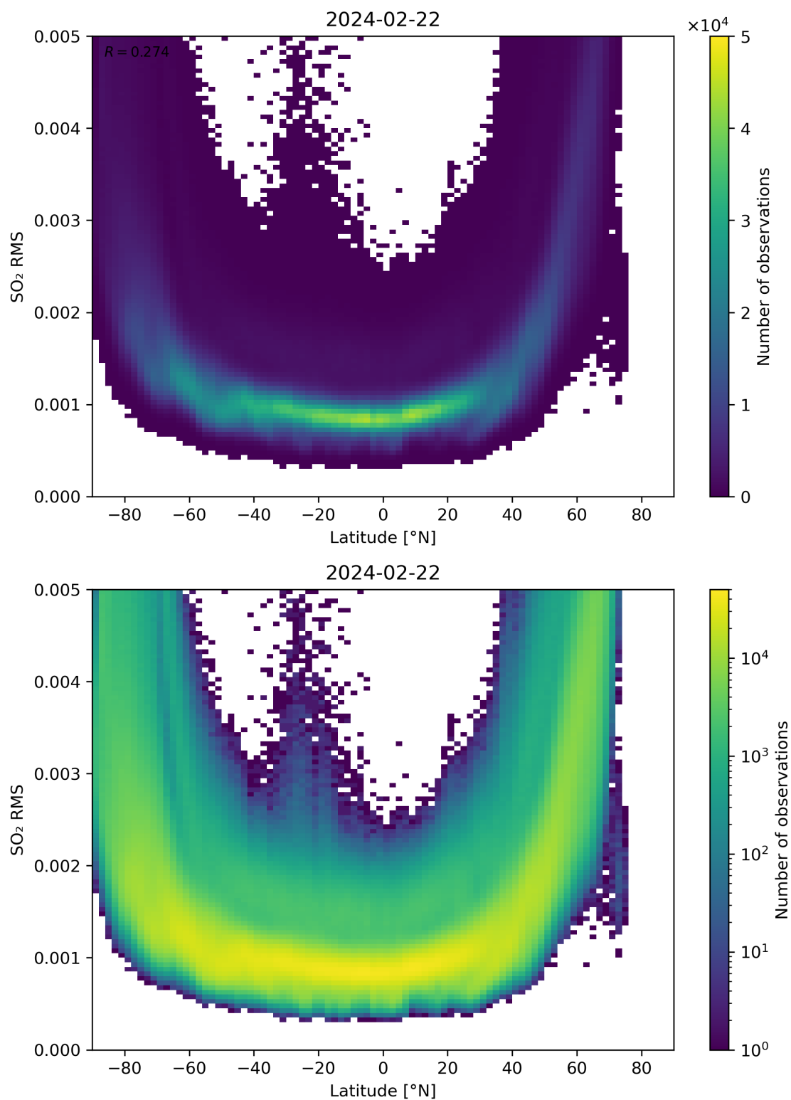
Figure 144: Scatter density plot of “Latitude” against “SO 2 RMS” for 2024-02-22 to 2024-02-23.
