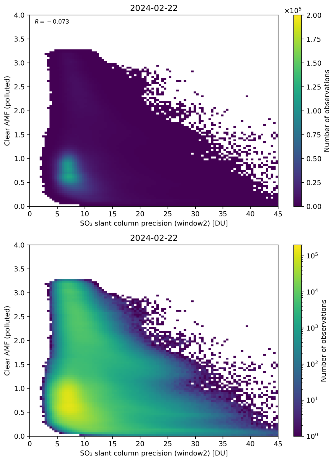
Figure 246: Scatter density plot of “SO 2 slant column precision (window2)” against “Clear AMF (polluted)” for 2024-02-22 to 2024-02-23.
