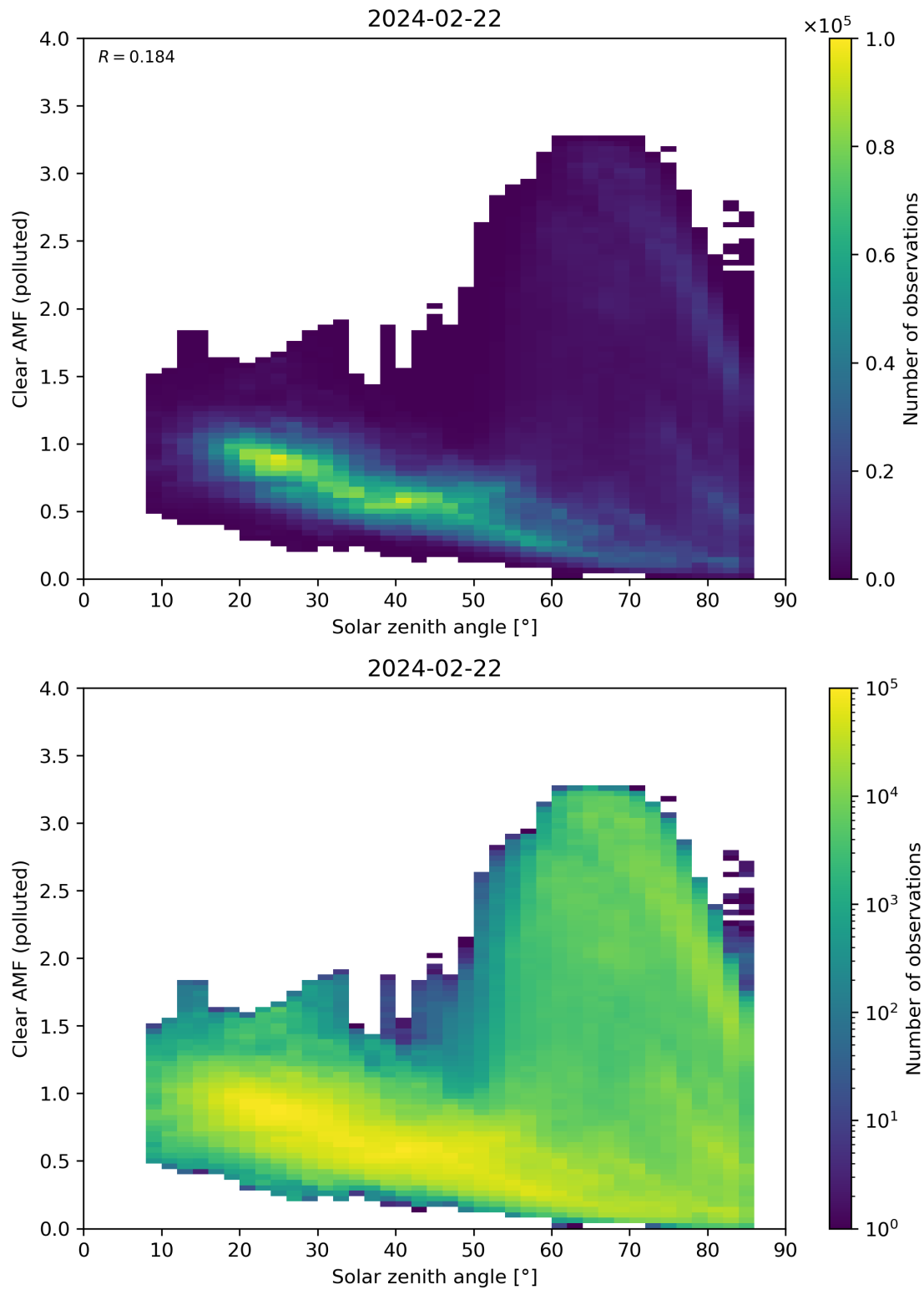
Figure 165: Scatter density plot of “Solar zenith angle” against “Clear AMF (polluted)” for 2024-02-22 to 2024-02-23.
