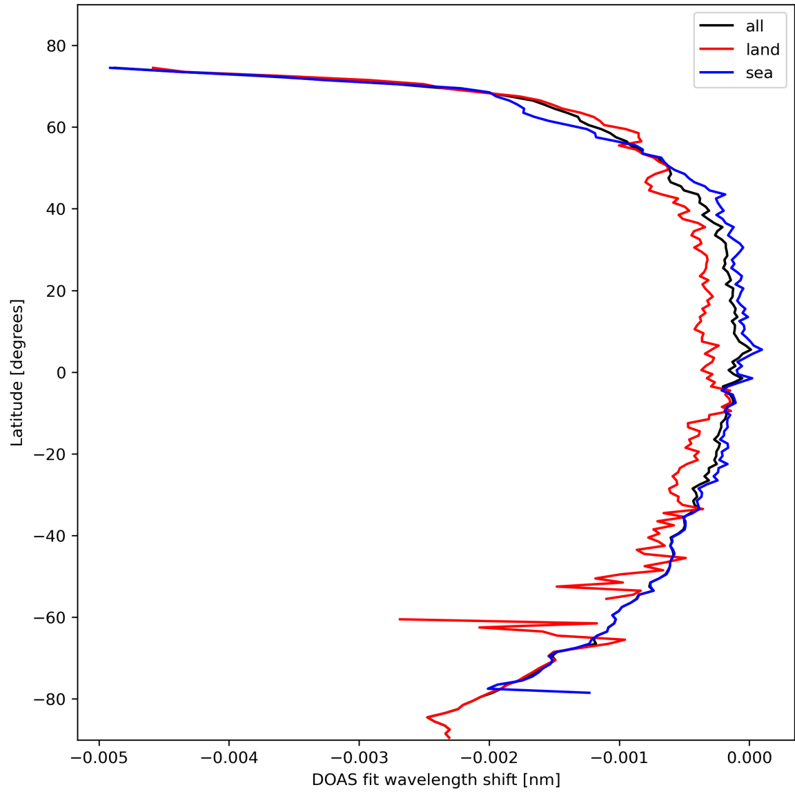
Figure 45: Zonal average of “DOAS fit wavelength shift” for 2024-02-22 to 2024-02-23.
