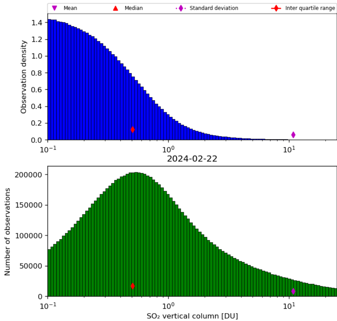
Figure 53: Histogram of “SO 2 vertical column” for 2024-02-22 to 2024-02-23
