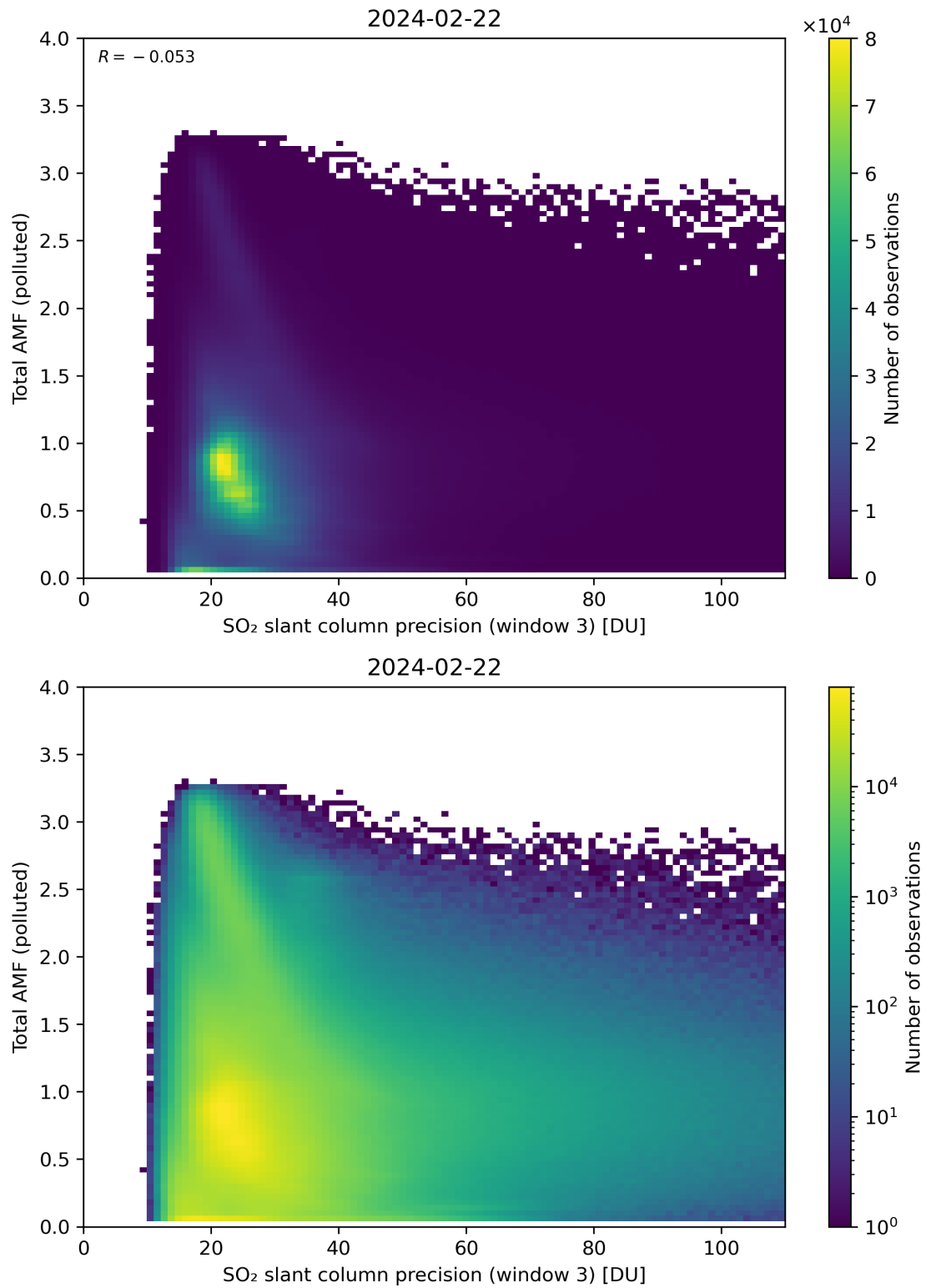
Figure 263: Scatter density plot of “SO 2 slant column precision (window 3)” against “Total AMF (polluted)” for 2024-02-22 to 2024-02-23.
