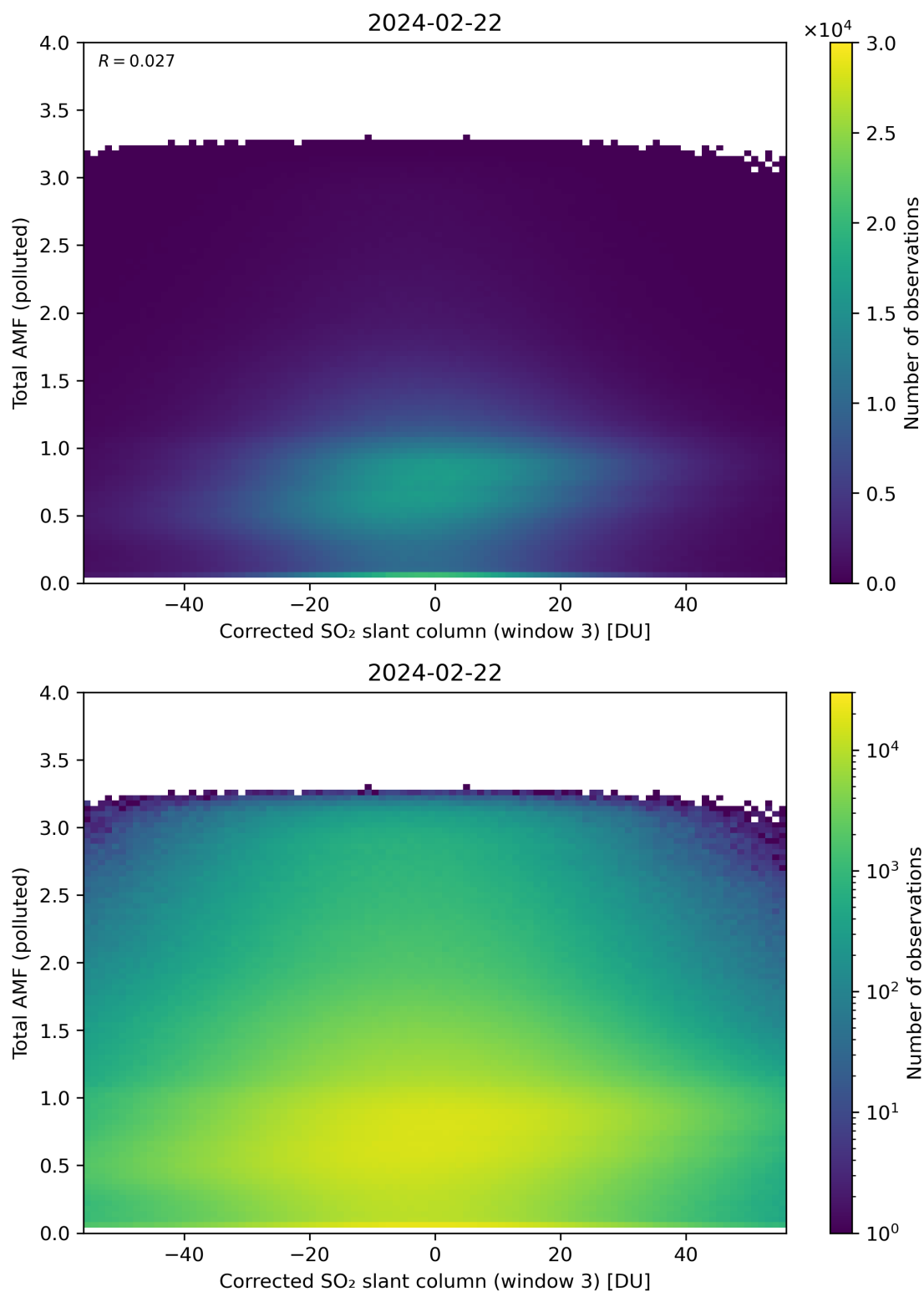
Figure 210: Scatter density plot of “Corrected SO 2 slant column (window 3)” against “Total AMF (polluted)” for 2024-02-22 to 2024-02-23.
