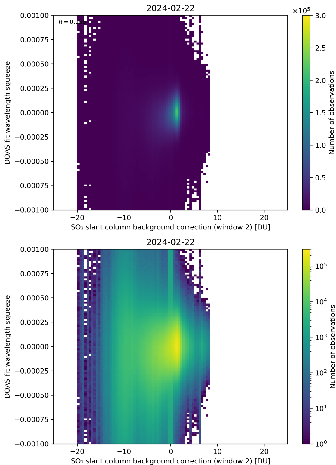
Figure 113: Scatter density plot of “SO 2 slant column background correction (window 2)” against “DOAS fit wavelength squeeze” for 2024-02-22 to 2024-02-23.
