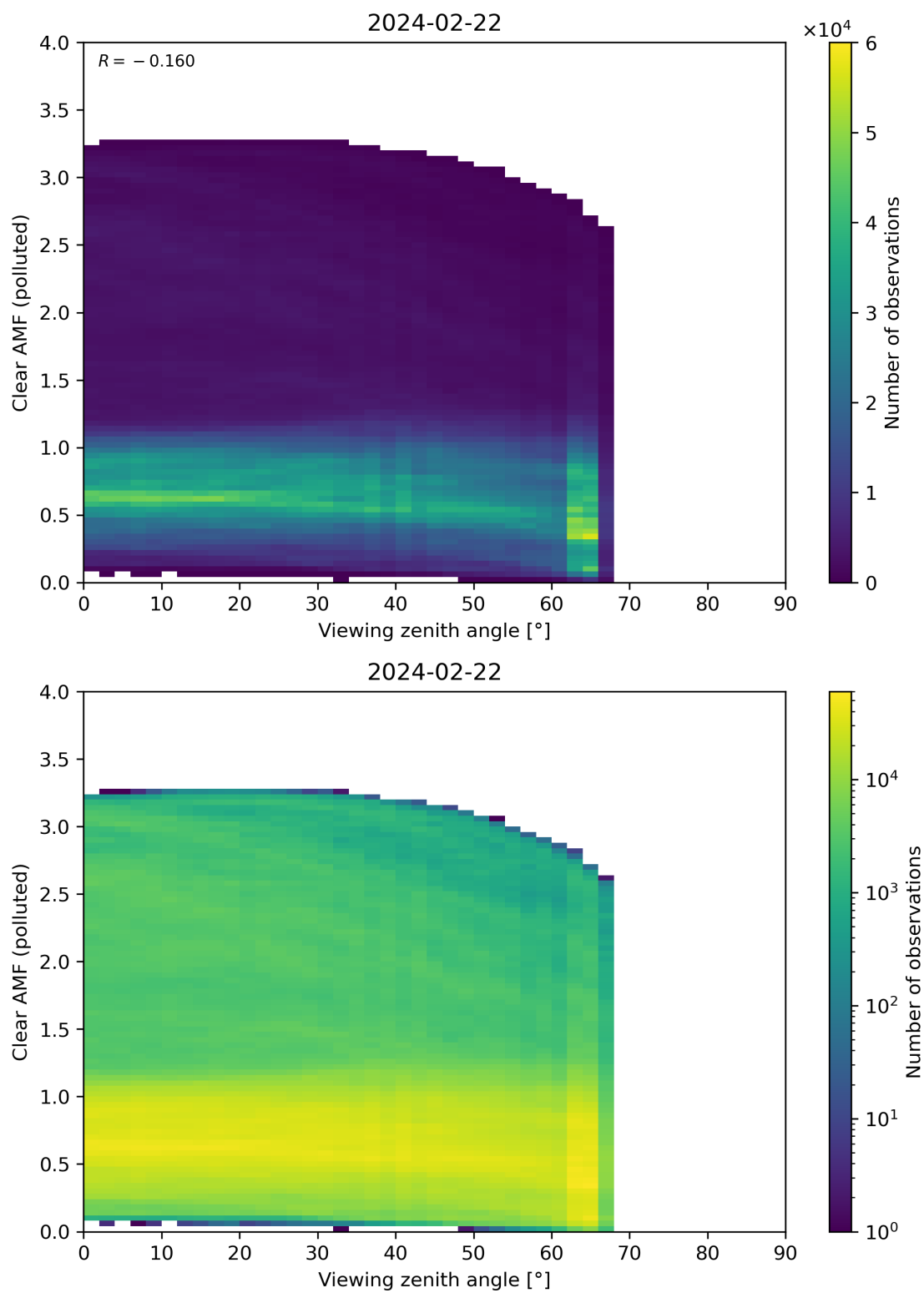
Figure 316: Scatter density plot of “Viewing zenith angle” against “Clear AMF (polluted)” for 2024-02-22 to 2024-02-23.
