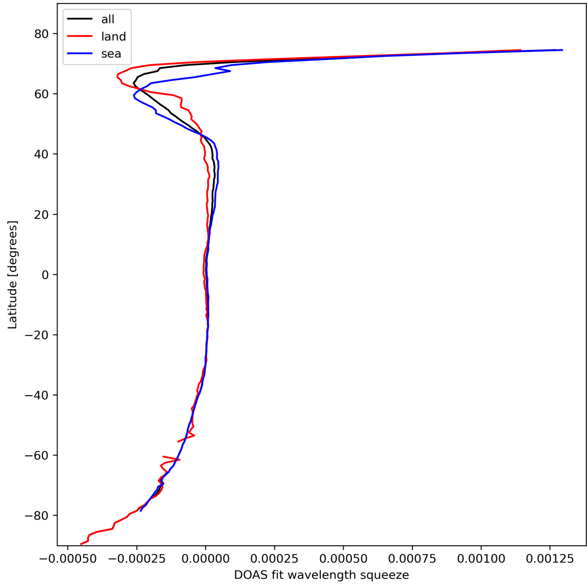
Figure 46: Zonal average of “DOAS fit wavelength squeeze” for 2024-02-22 to 2024-02-23.
