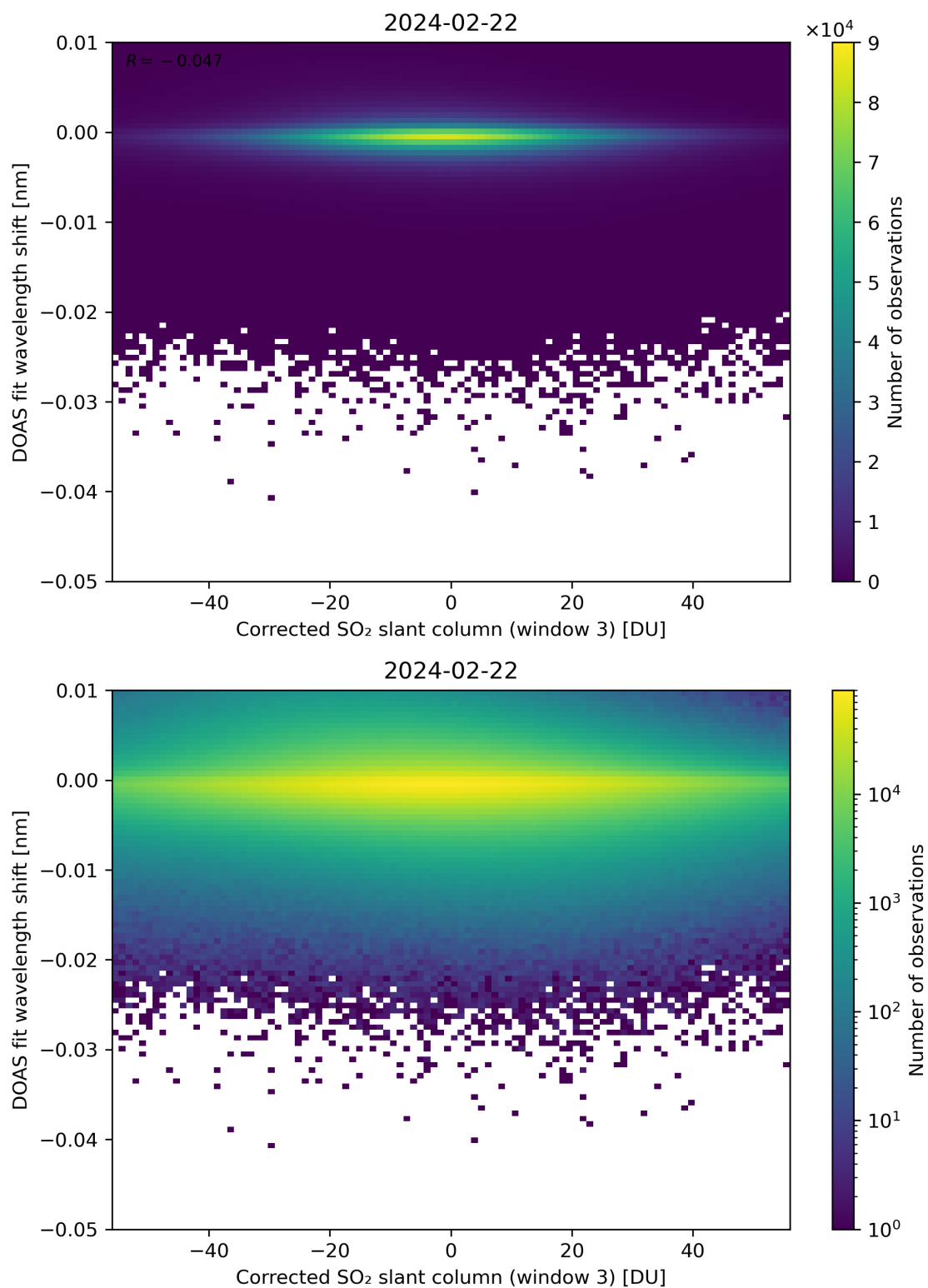
Figure 206: Scatter density plot of “Corrected SO 2 slant column (window 3)” against “DOAS fit wavelength shift” for 2024-02-22 to 2024-02-23.
