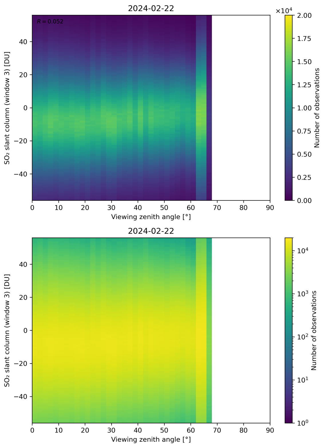
Figure 323: Scatter density plot of “Viewing zenith angle” against “SO 2 slant column (window 3)” for 2024-02-22 to 2024-02-23.
