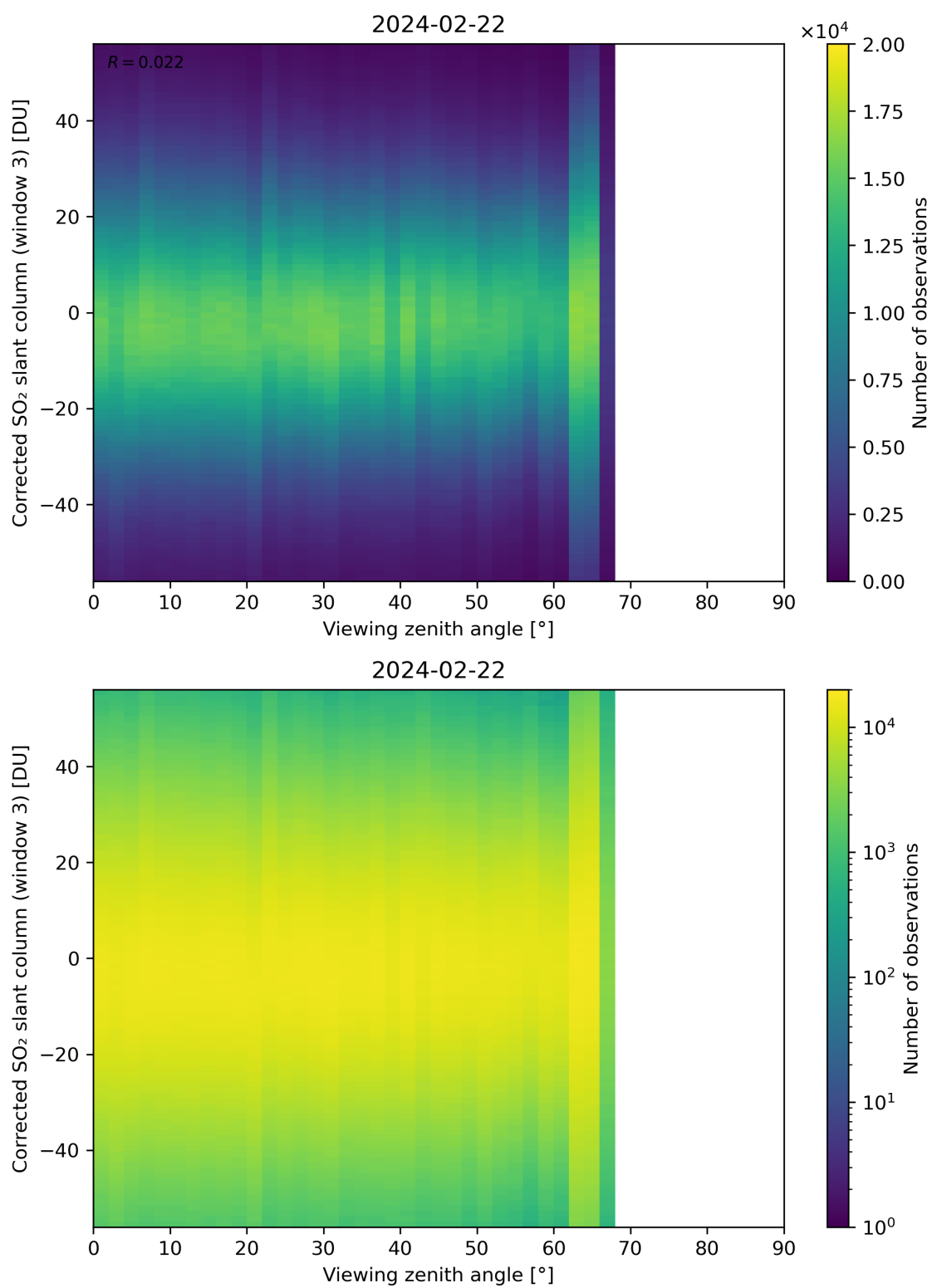
Figure 319: Scatter density plot of “Viewing zenith angle” against “Corrected SO 2 slant column (window 3)” for 2024-02-22 to 2024-02-23.
