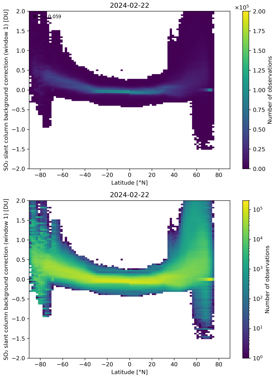
Figure 139: Scatter density plot of “Latitude” against “SO 2 slant column background correction (window 1)” for 2024-02-22 to 2024-02-23.
