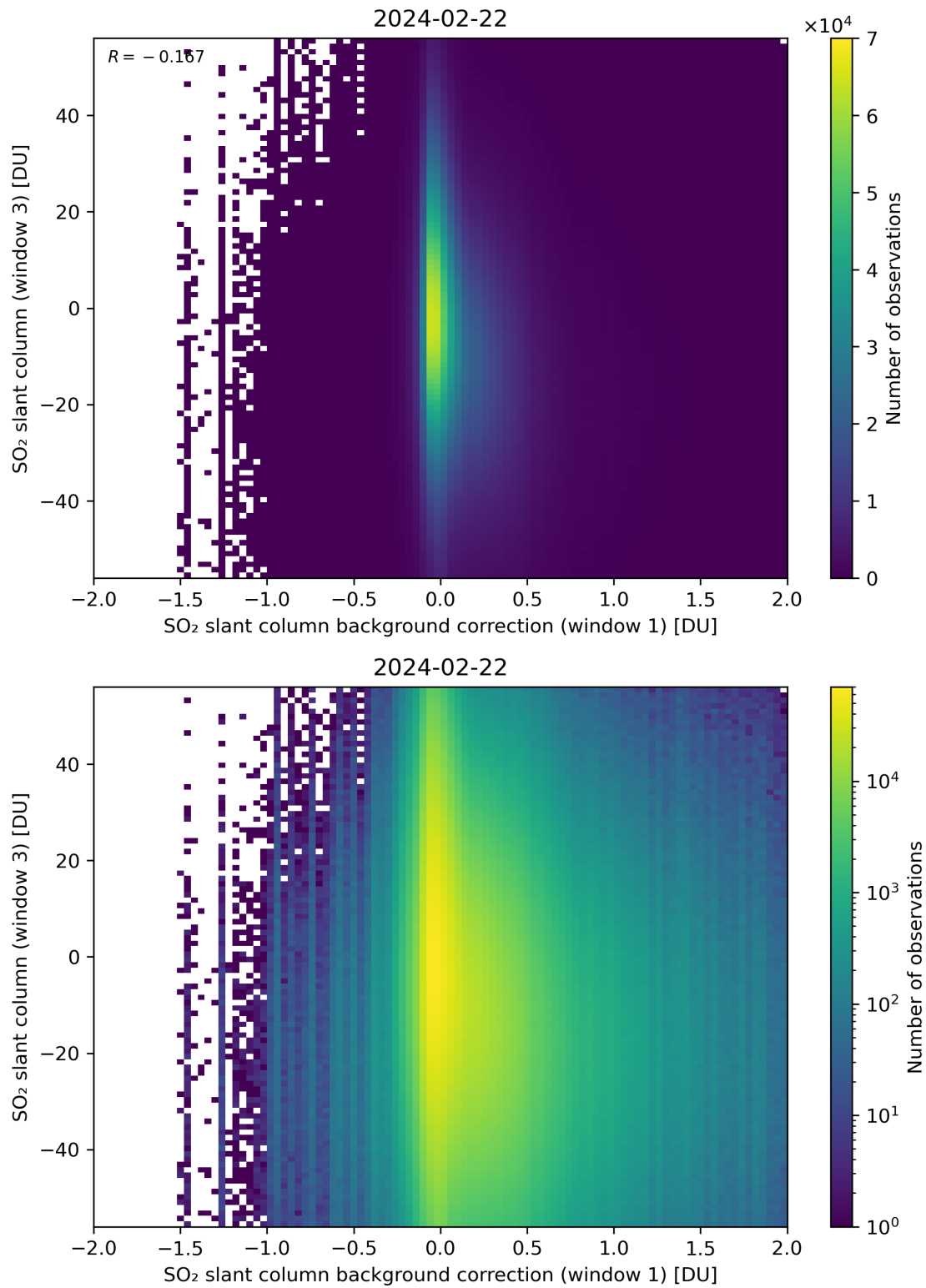
Figure 107: Scatter density plot of “SO 2 slant column background correction (window 1)” against “SO 2 slant column (window 3)” for 2024-02-22 to 2024-02-23.
