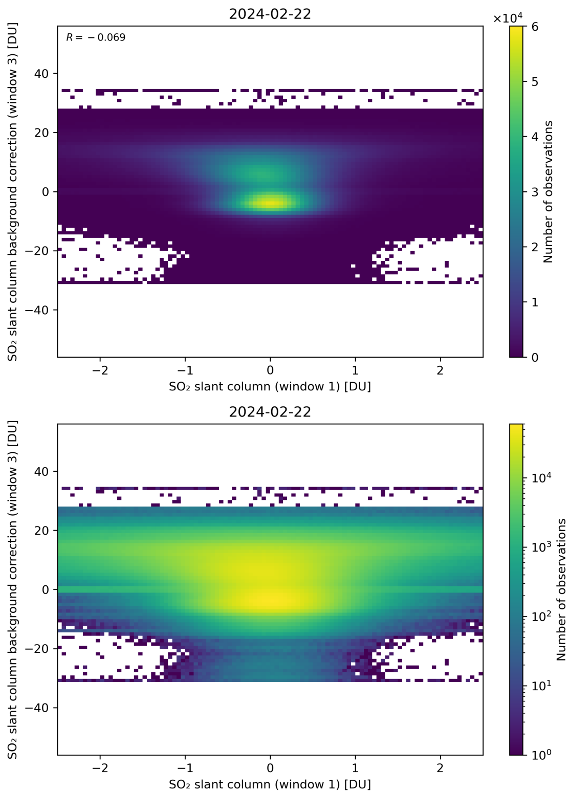
Figure 214: Scatter density plot of “SO 2 slant column (window 1)” against “SO 2 slant column background correction (window 3)” for 2024-02-22 to 2024-02-23.
