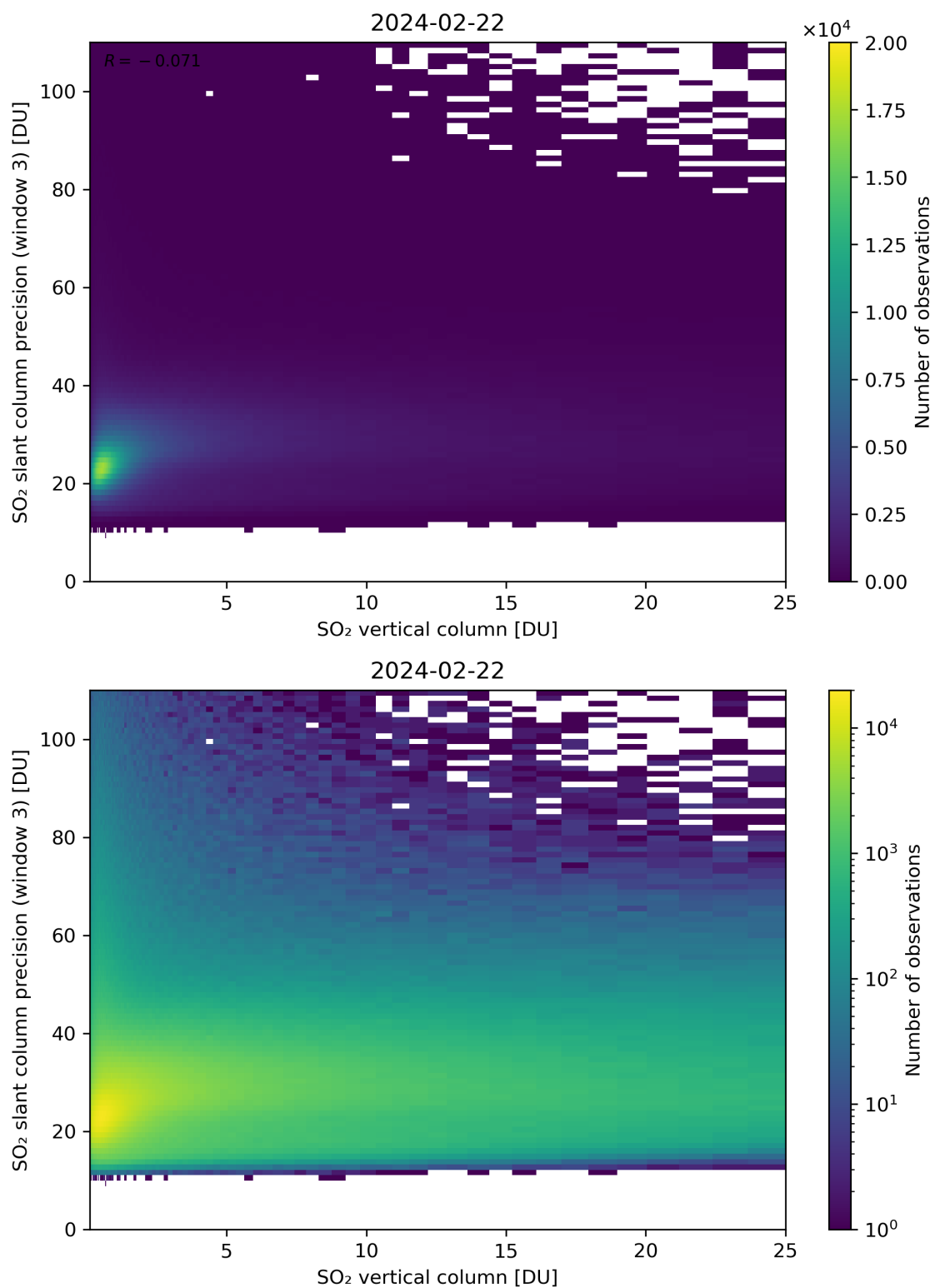
Figure 304: Scatter density plot of “SO 2 vertical column” against “SO 2 slant column precision (window 3)” for 2024-02-22 to 2024-02-23.
