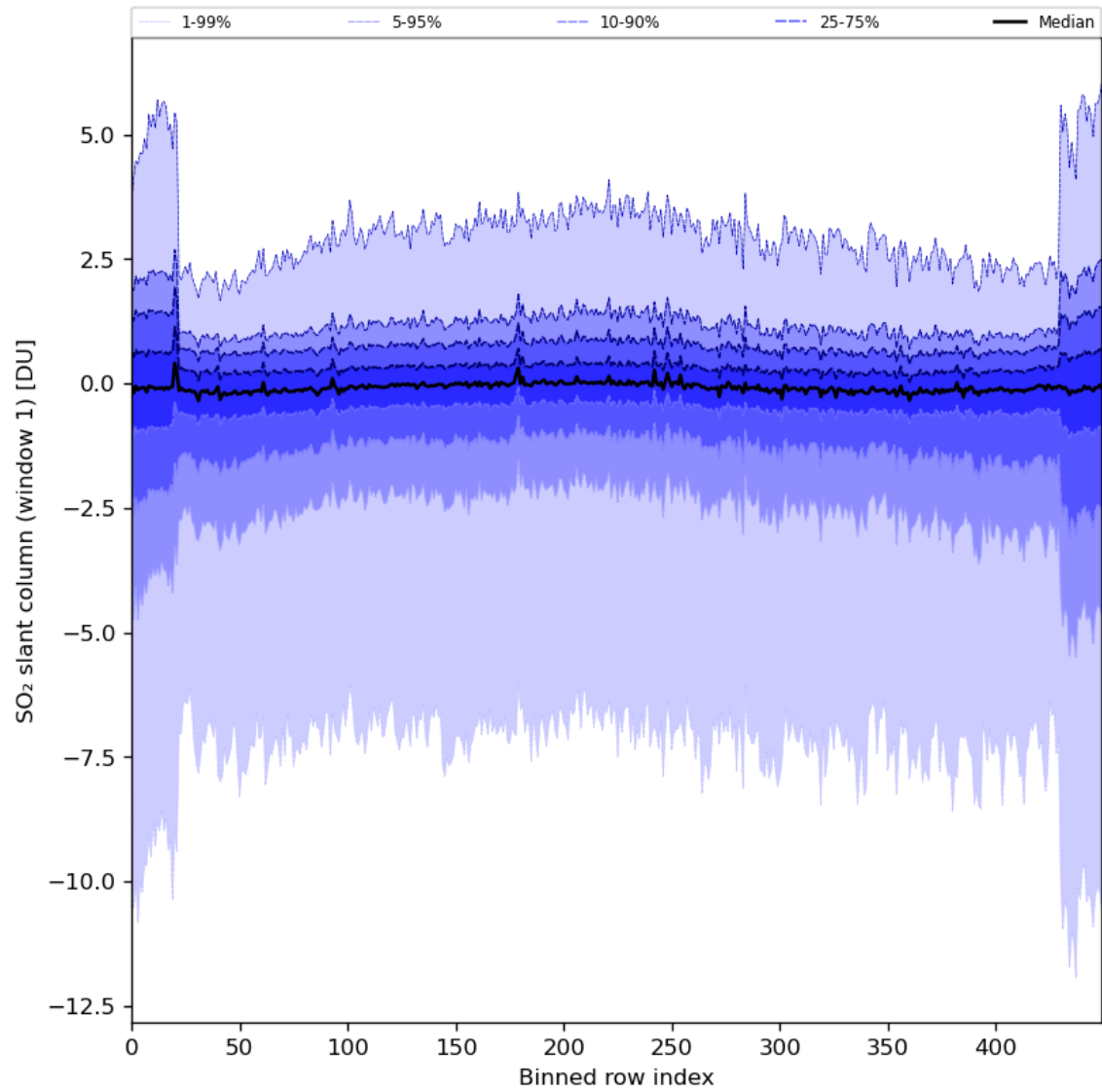
Figure 79: Along track statistics of “SO 2 slant column (window 1)” for 2024-02-22 to 2024-02-23
