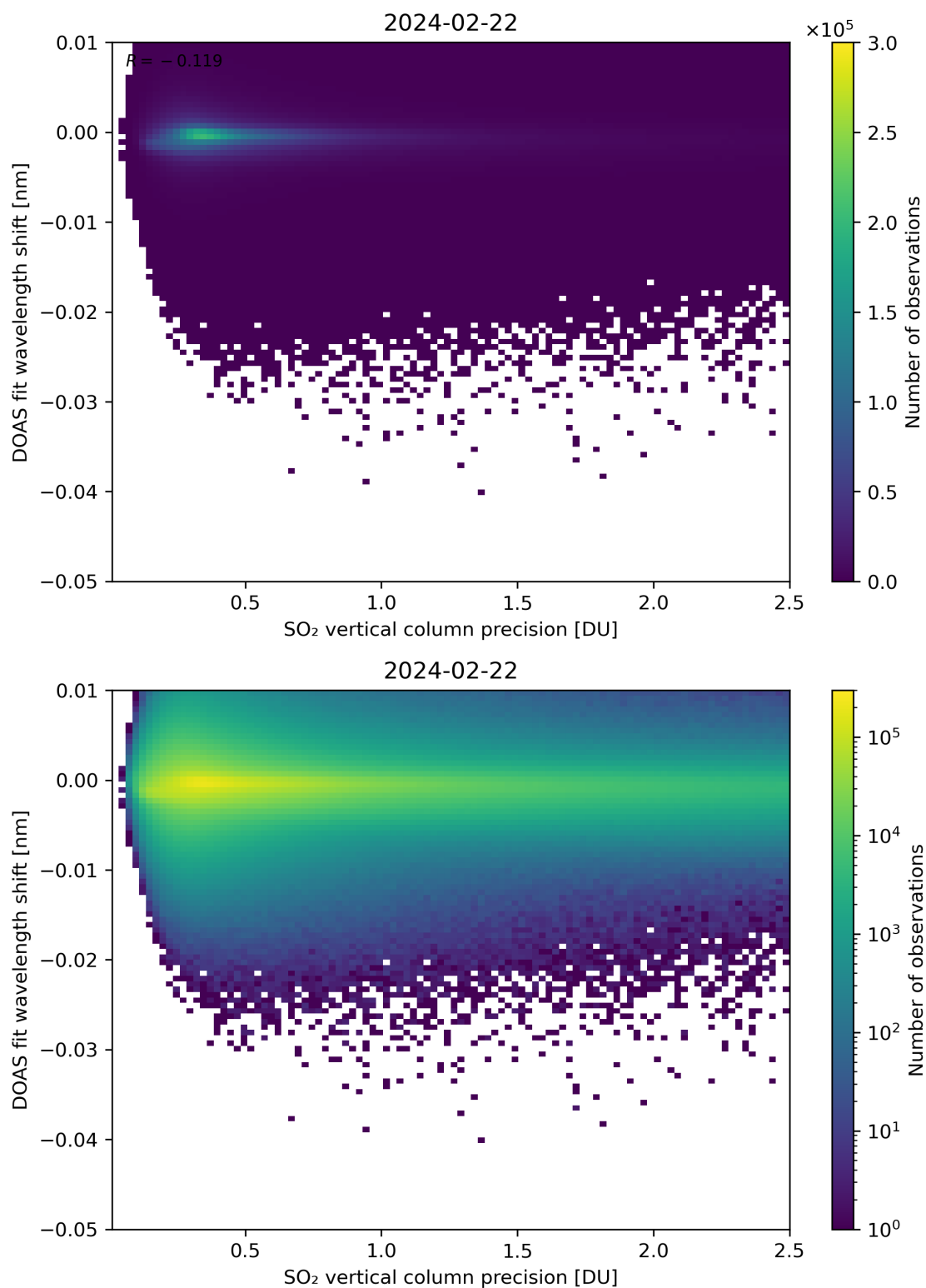
Figure 282: Scatter density plot of “SO 2 vertical column precision” against “DOAS fit wavelength shift” for 2024-02-22 to 2024-02-23.
