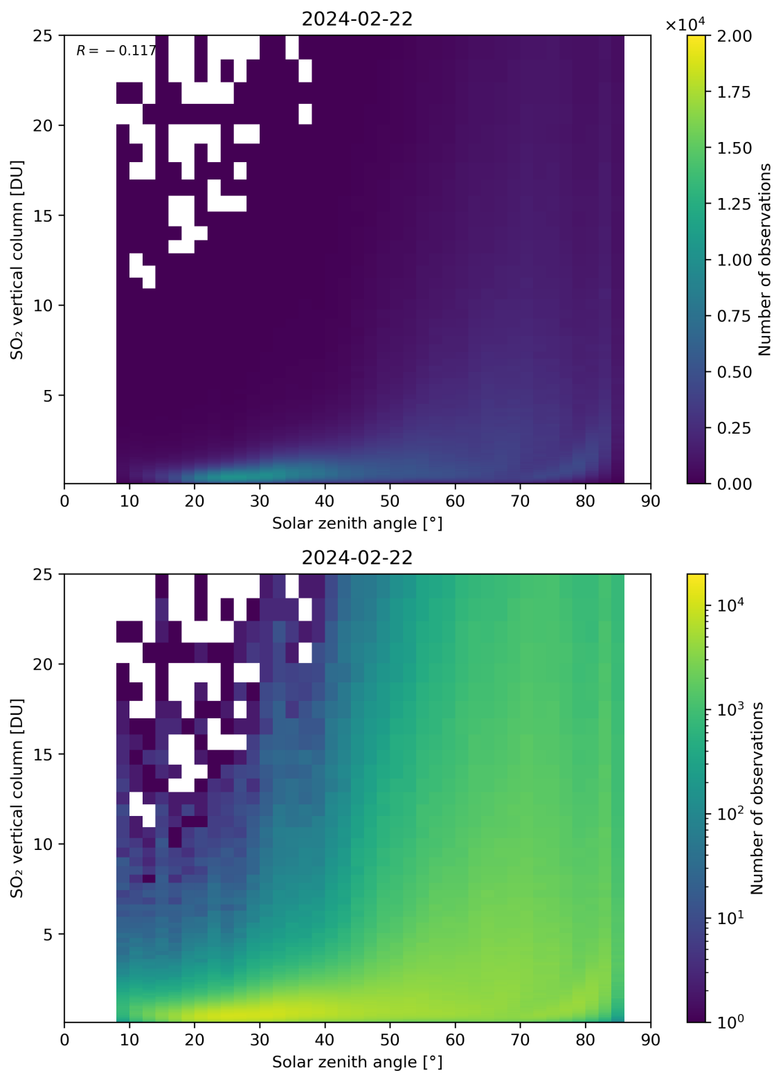
Figure 176: Scatter density plot of “Solar zenith angle” against “SO 2 vertical column” for 2024-02-22 to 2024-02-23.
