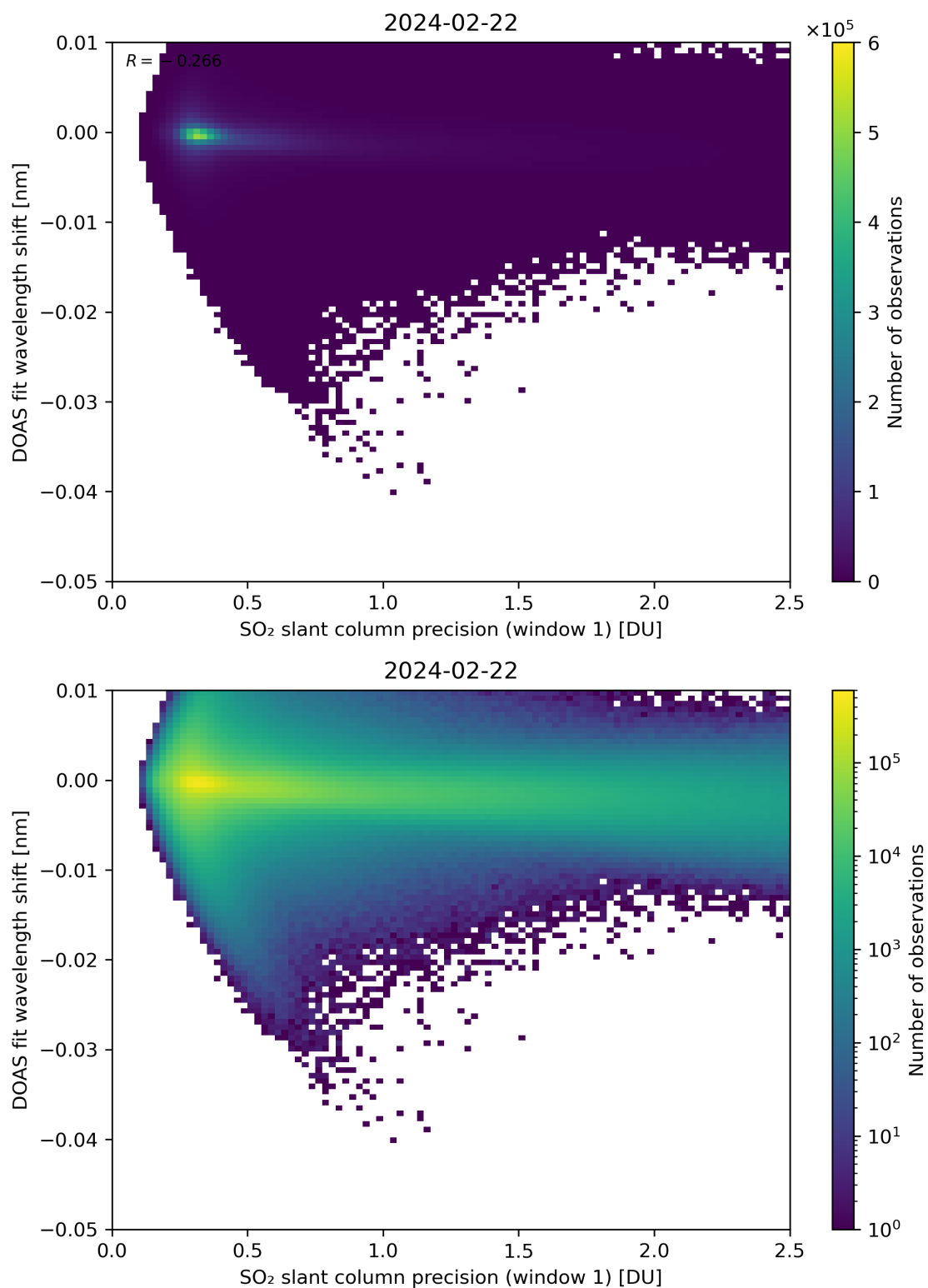
Figure 221: Scatter density plot of “SO 2 slant column precision (window 1)” against “DOAS fit wavelength shift” for 2024-02-22 to 2024-02-23.
