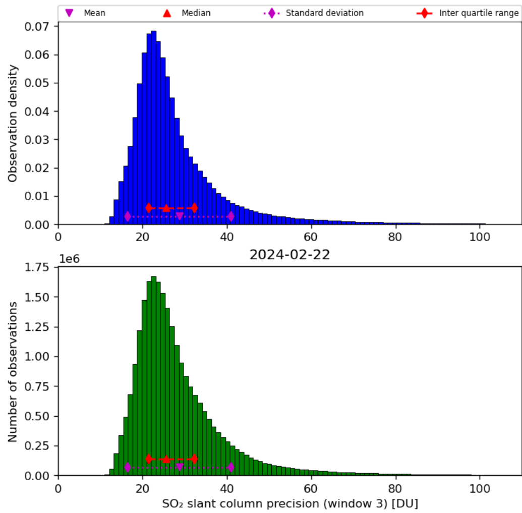
Figure 65: Histogram of “SO 2 slant column precision (window 3)” for 2024-02-22 to 2024-02-23
