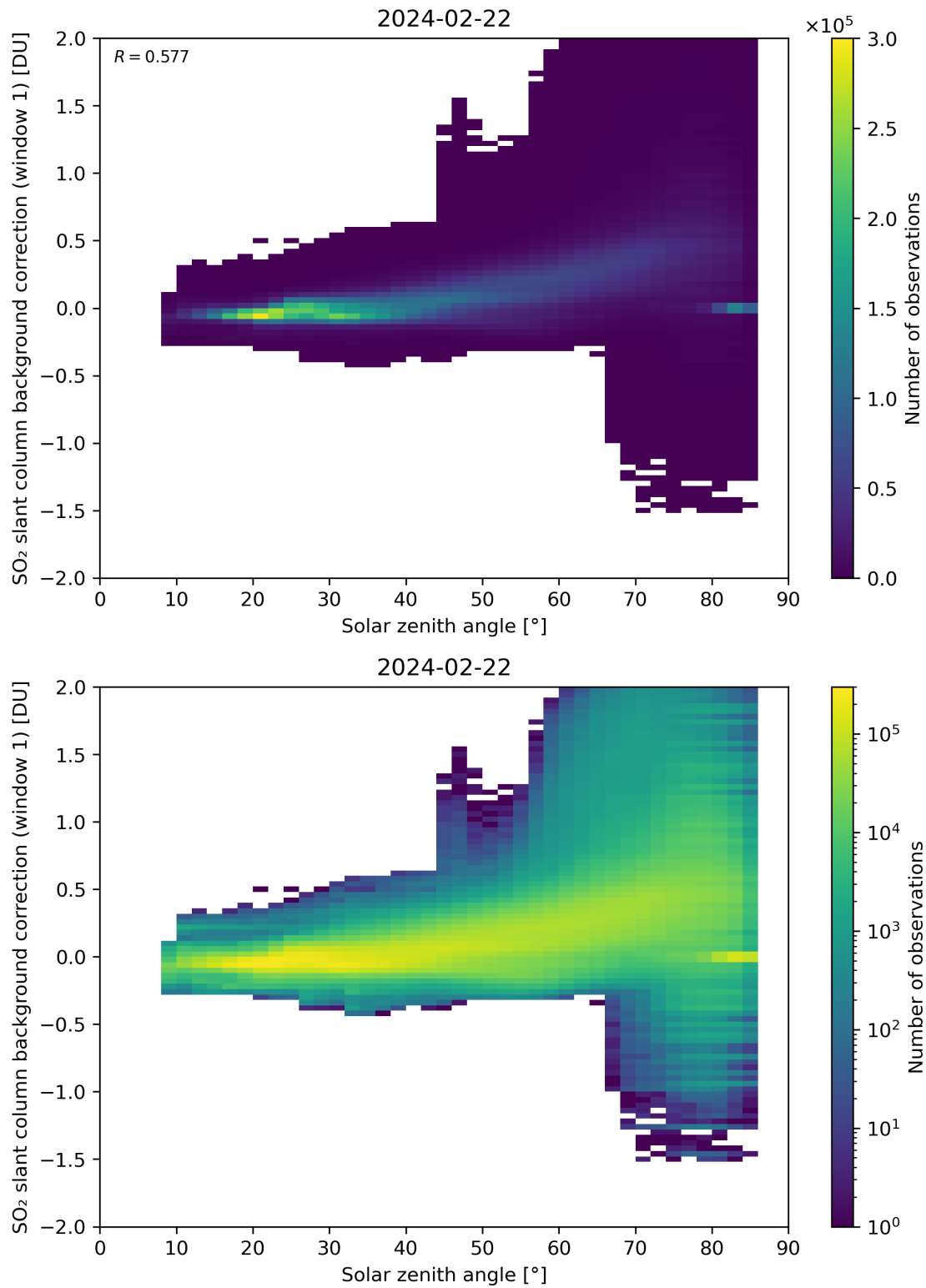
Figure 158: Scatter density plot of “Solar zenith angle” against “SO 2 slant column background correction (window 1)” for 2024-02-22 to 2024-02-23.
