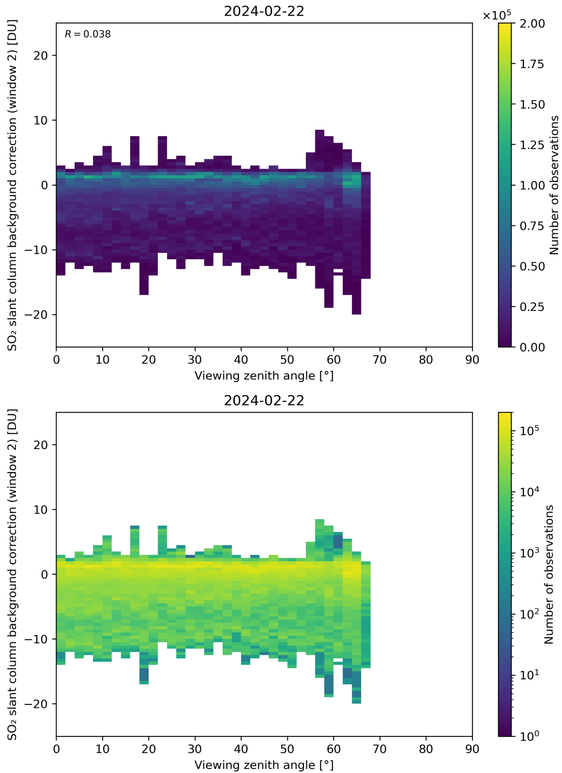
Figure 309: Scatter density plot of “Viewing zenith angle” against “SO 2 slant column background correction (window 2)” for 2024-02-22 to 2024-02-23.
