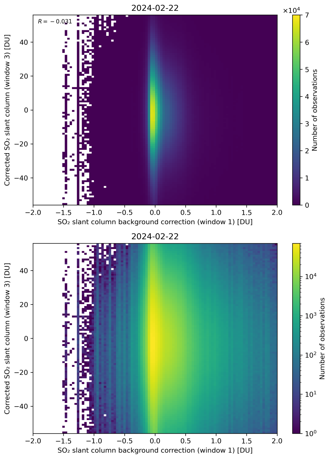
Figure 105: Scatter density plot of “SO 2 slant column background correction (window 1)” against “Corrected SO 2 slant column (window 3)” for 2024-02-22 to 2024-02-23.
