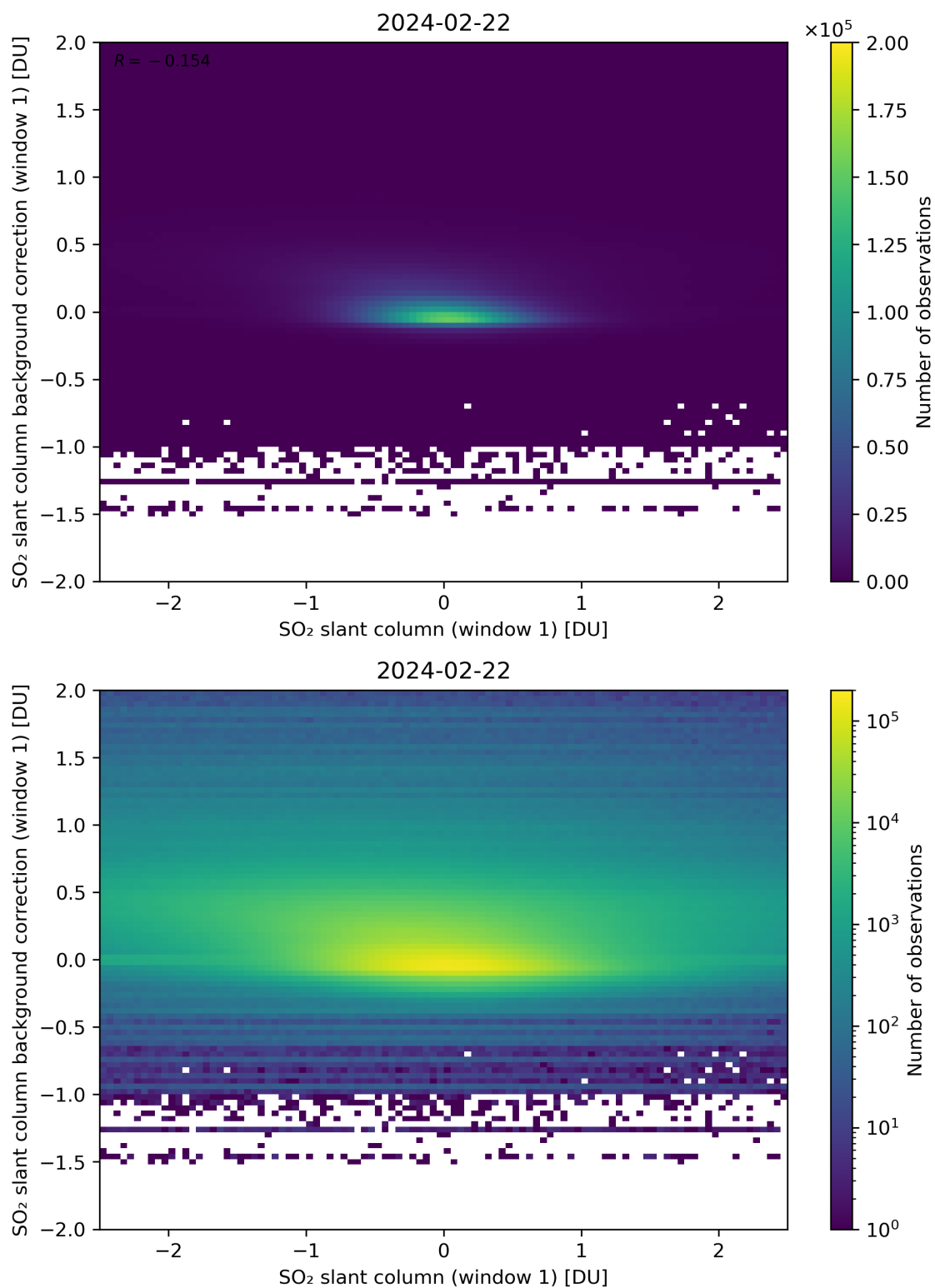
Figure 212: Scatter density plot of “SO 2 slant column (window 1)” against “SO 2 slant column background correction (window 1)” for 2024-02-22 to 2024-02-23.
