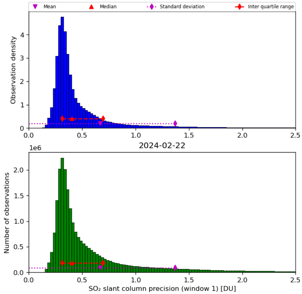
Figure 57: Histogram of “SO 2 slant column precision (window 1)” for 2024-02-22 to 2024-02-23
