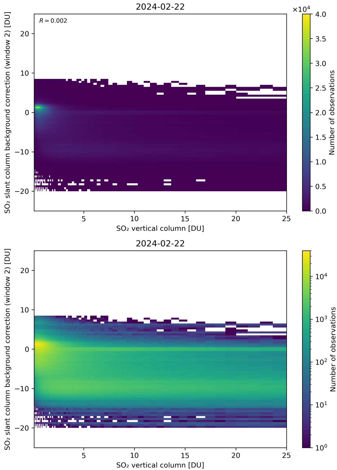
Figure 274: Scatter density plot of “SO 2 vertical column” against “SO 2 slant column background correction (window 2)” for 2024-02-22 to 2024-02-23.
