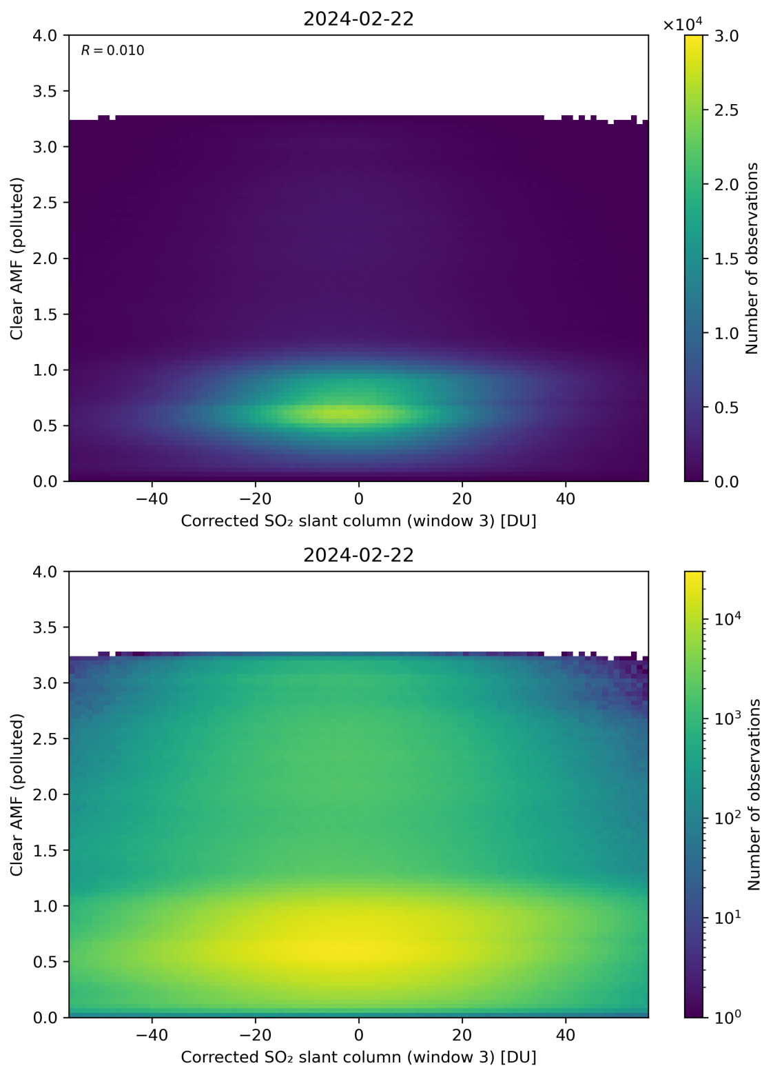
Figure 209: Scatter density plot of “Corrected SO 2 slant column (window 3)” against “Clear AMF (polluted)” for 2024-02-22 to 2024-02-23.
