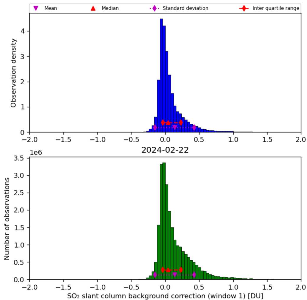
Figure 59: Histogram of “SO 2 slant column background correction (window 1)” for 2024-02-22 to 2024-02-23
