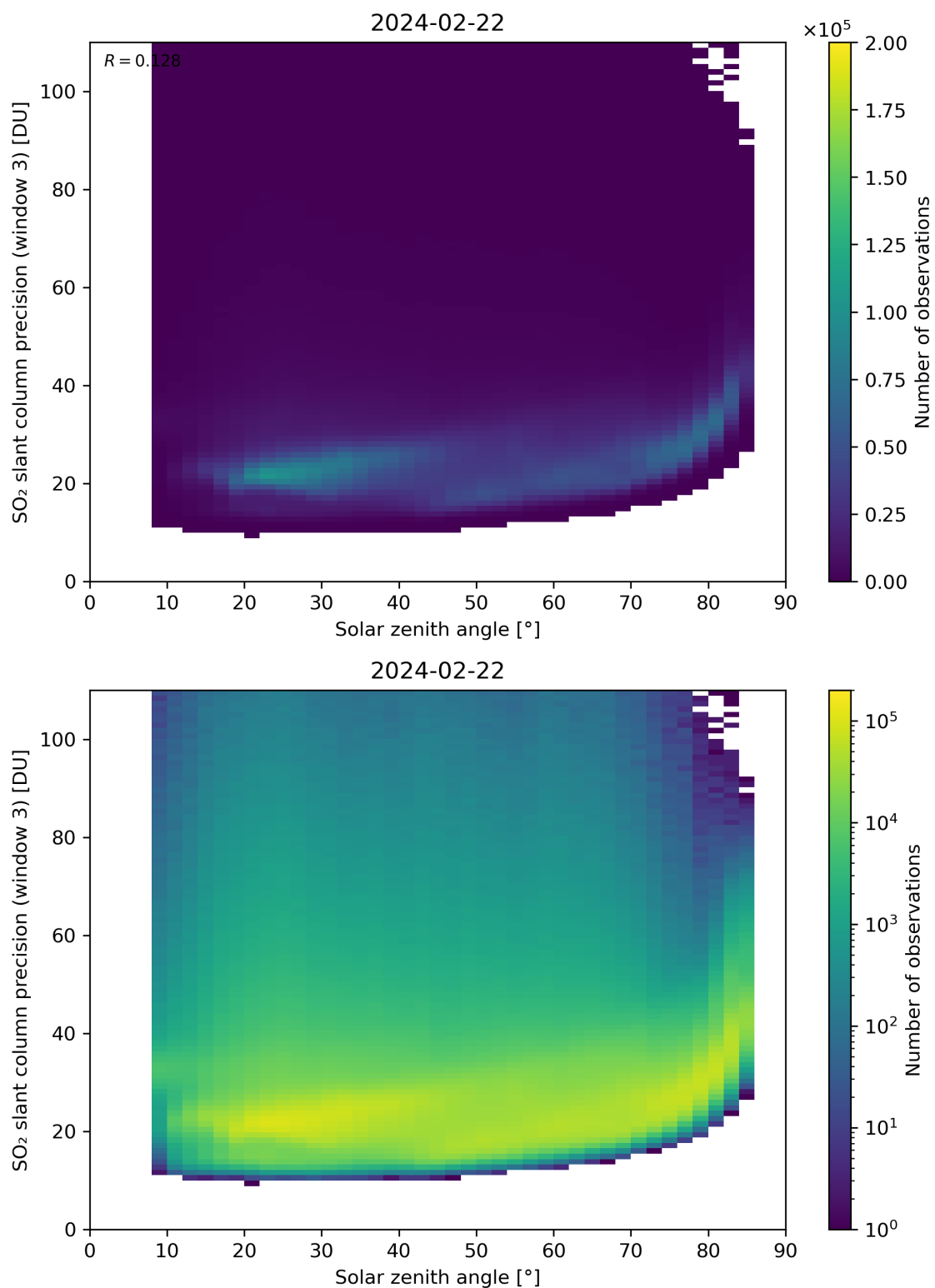
Figure 173: Scatter density plot of “Solar zenith angle” against “SO 2 slant column precision (window 3)” for 2024-02-22 to 2024-02-23.
