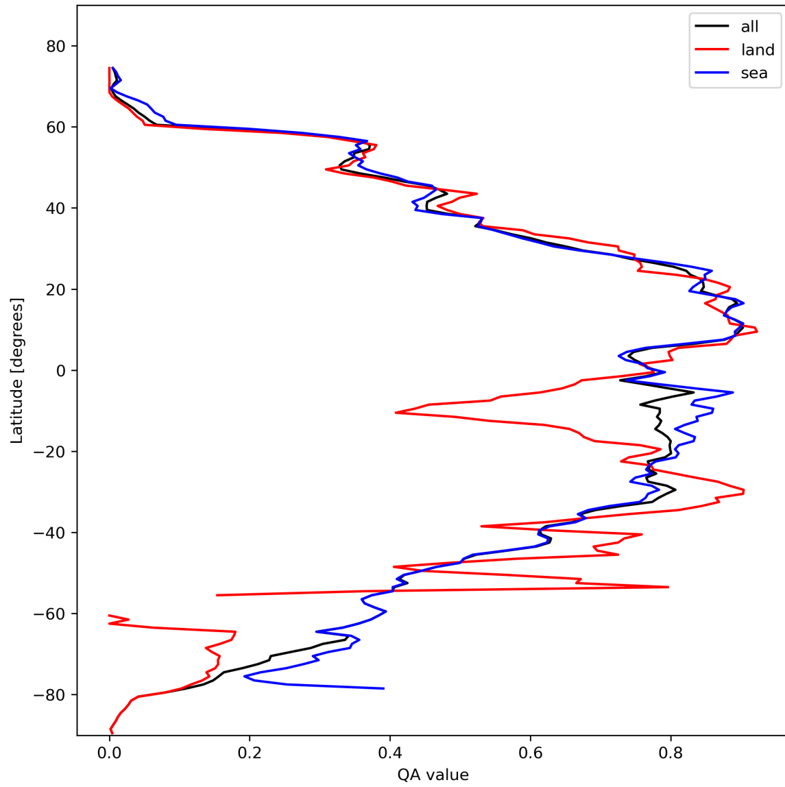
Figure 29: Zonal average of “QA value” for 2024-02-22 to 2024-02-23.
