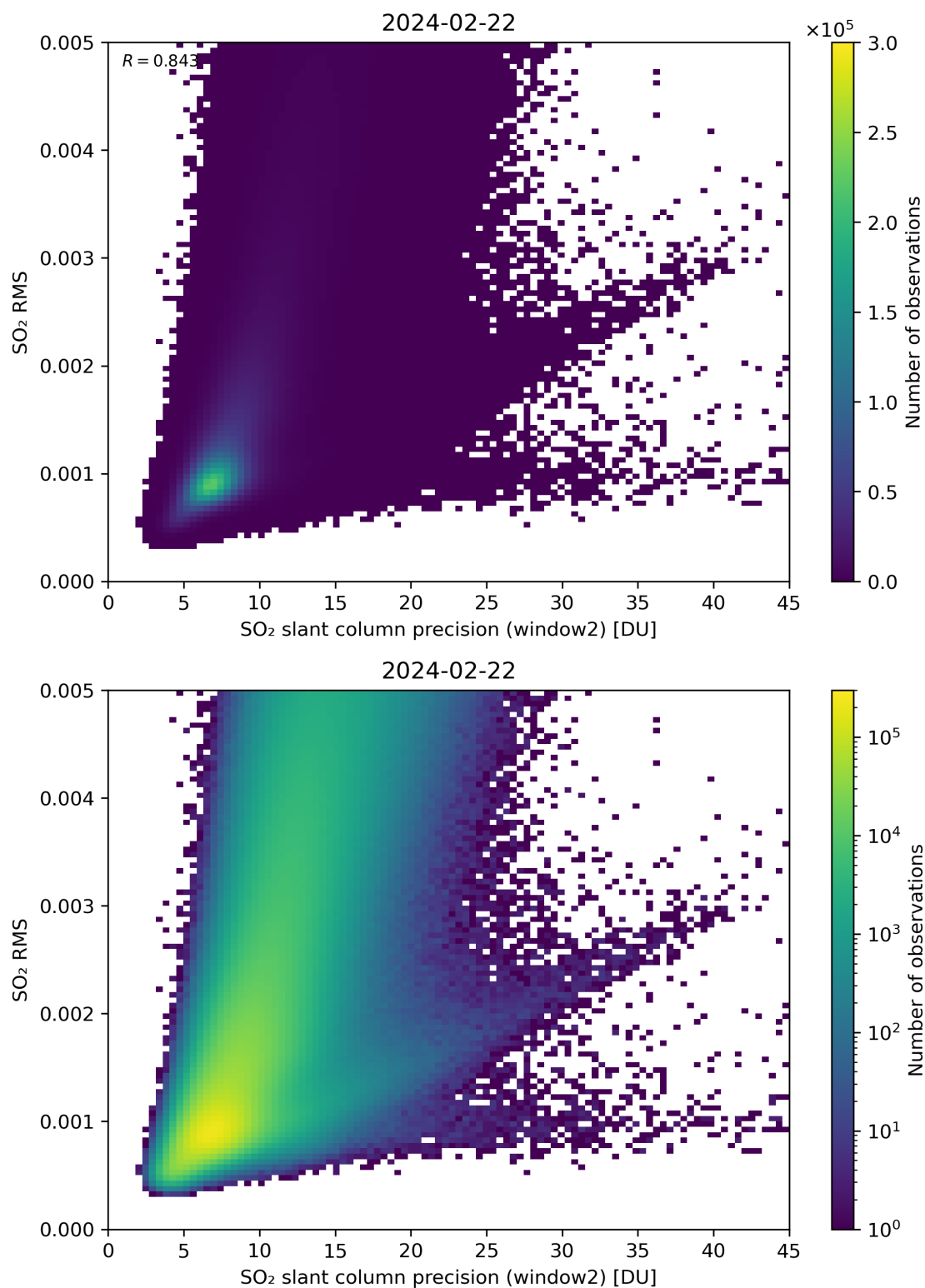
Figure 245: Scatter density plot of “SO 2 slant column precision (window2)” against “SO 2 RMS” for 2024-02-22 to 2024-02-23.
