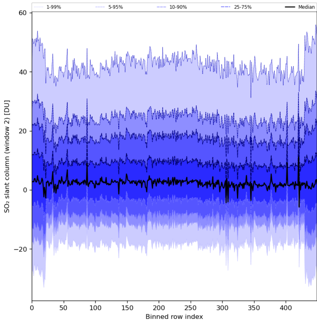
Figure 83: Along track statistics of “SO 2 slant column (window 2)” for 2024-02-22 to 2024-02-23
