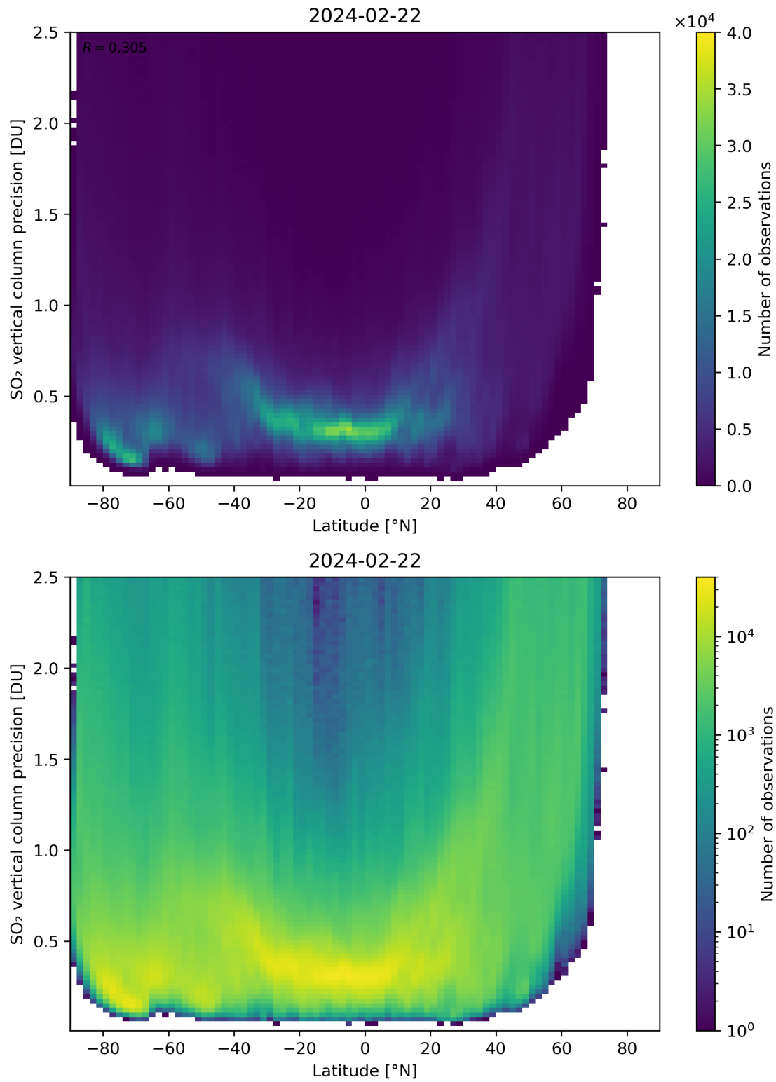
Figure 157: Scatter density plot of “Latitude” against “SO 2 vertical column precision” for 2024-02-22 to 2024-02-23.
