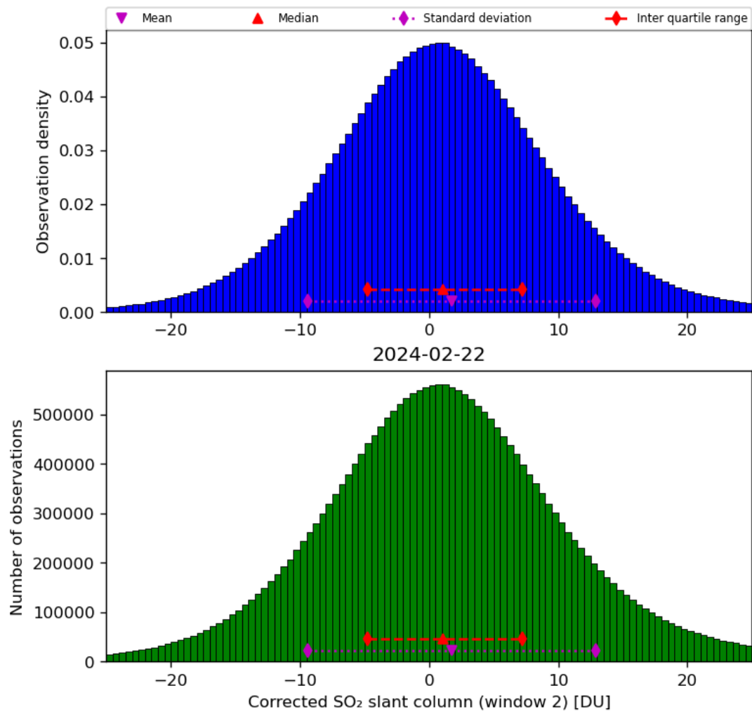
Figure 62: Histogram of “Corrected SO 2 slant column (window 2)” for 2024-02-22 to 2024-02-23
