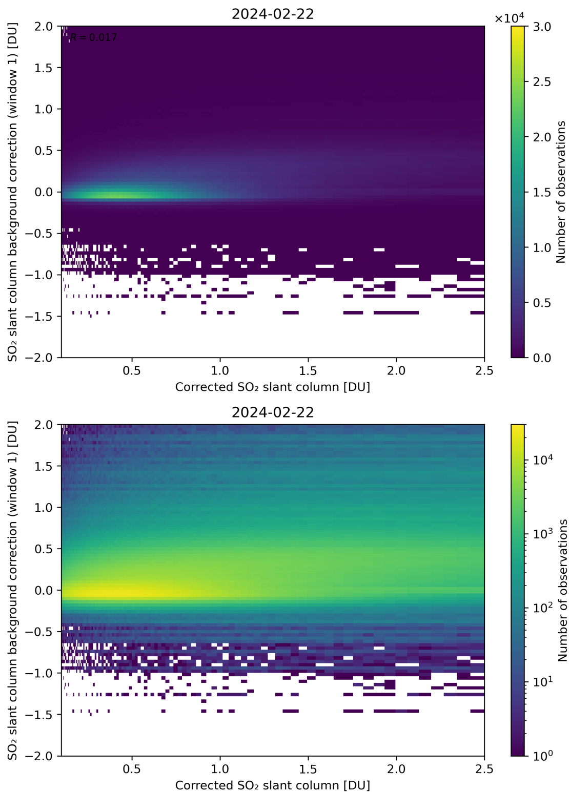
Figure 178: Scatter density plot of “Corrected SO 2 slant column” against “SO 2 slant column background correction (window 1)” for 2024-02-22 to 2024-02-23.
