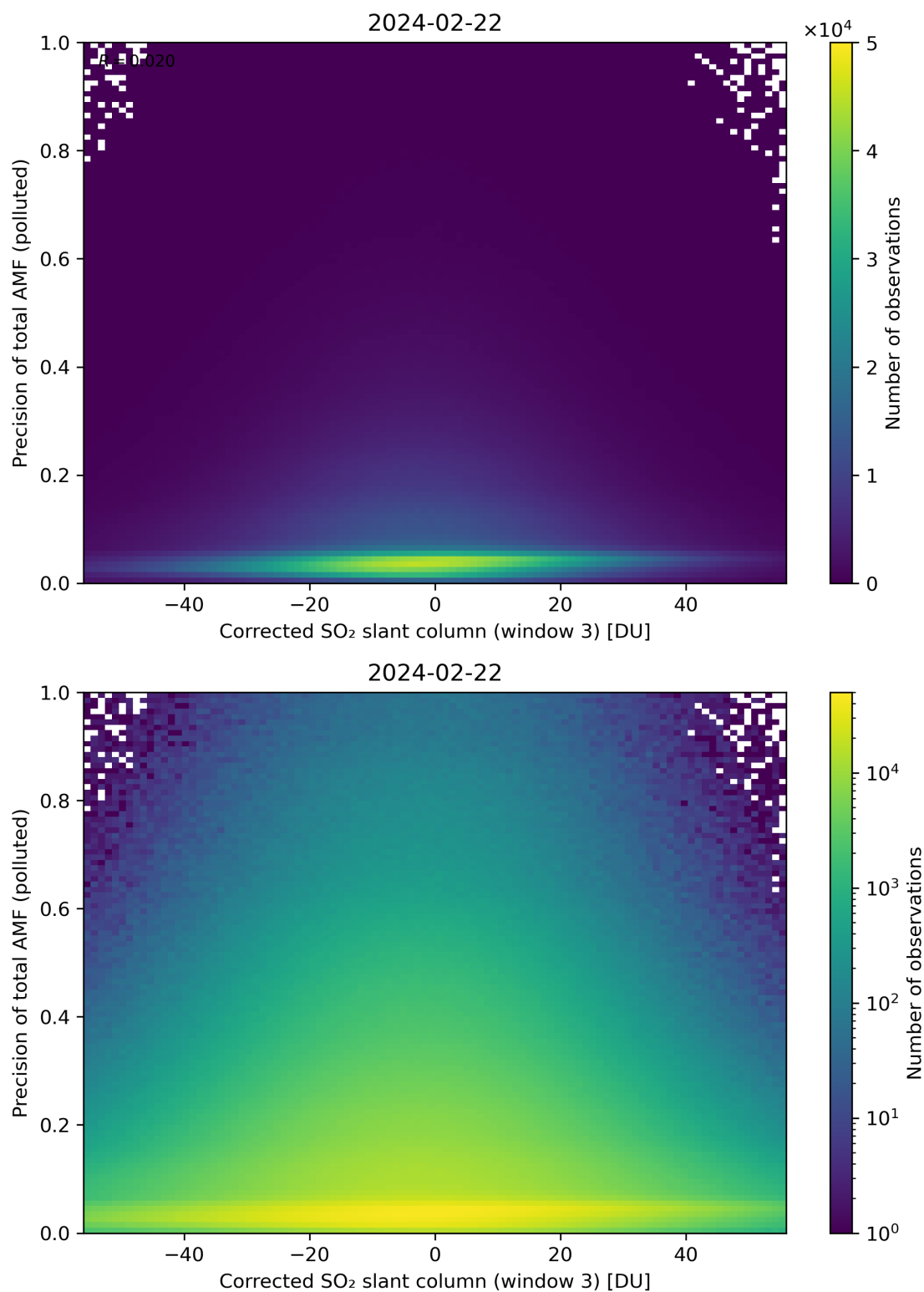
Figure 211: Scatter density plot of “Corrected SO 2 slant column (window 3)” against “Precision of total AMF (polluted)” for 2024-02-22 to 2024-02-23.
