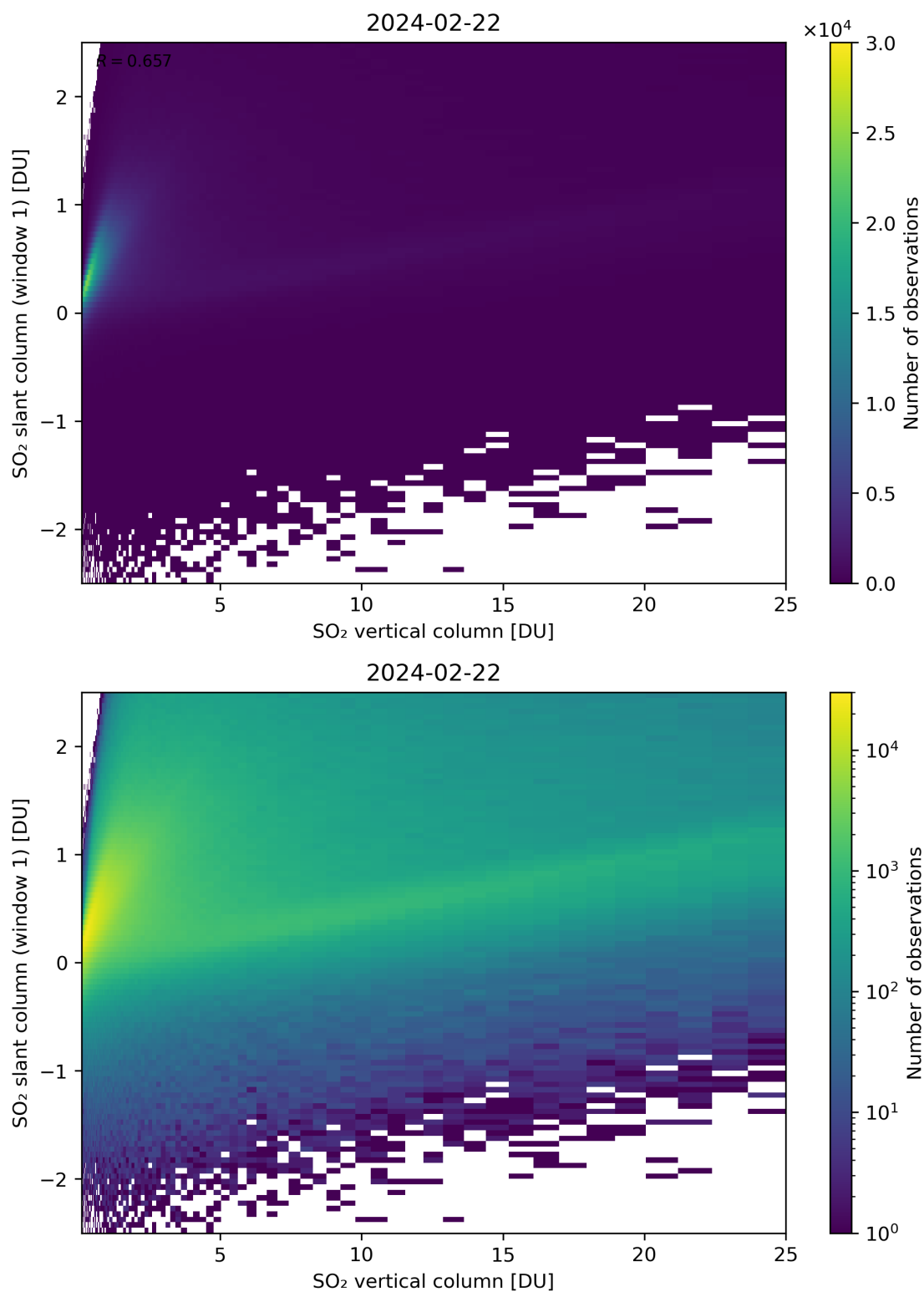
Figure 300: Scatter density plot of “SO 2 vertical column” against “SO 2 slant column (window 1)” for 2024-02-22 to 2024-02-23.
