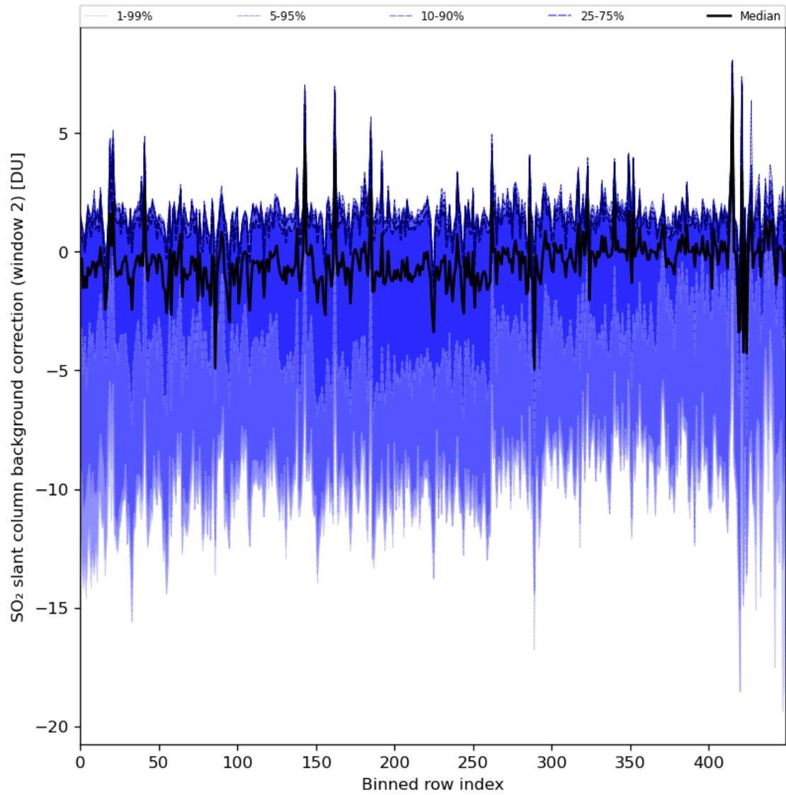
Figure 86: Along track statistics of “SO 2 slant column background correction (window 2)” for 2024-02-22 to 2024-02-23
