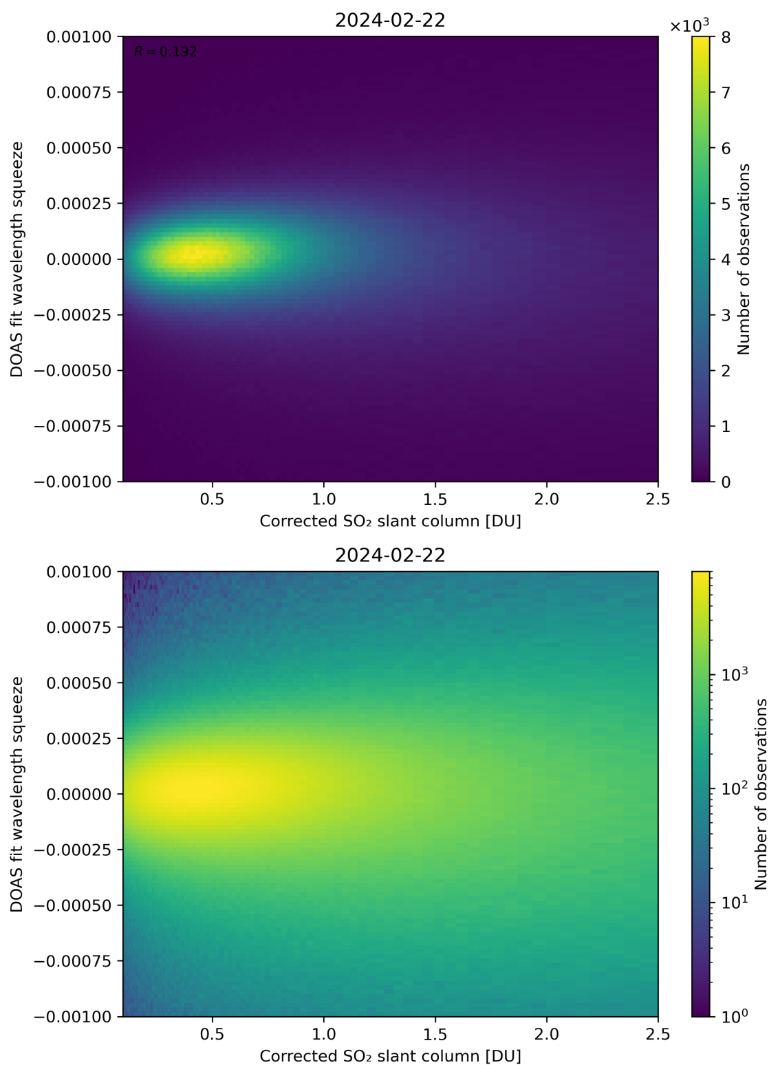
Figure 182: Scatter density plot of “Corrected SO 2 slant column” against “DOAS fit wavelength squeeze” for 2024-02-22 to 2024-02-23.
