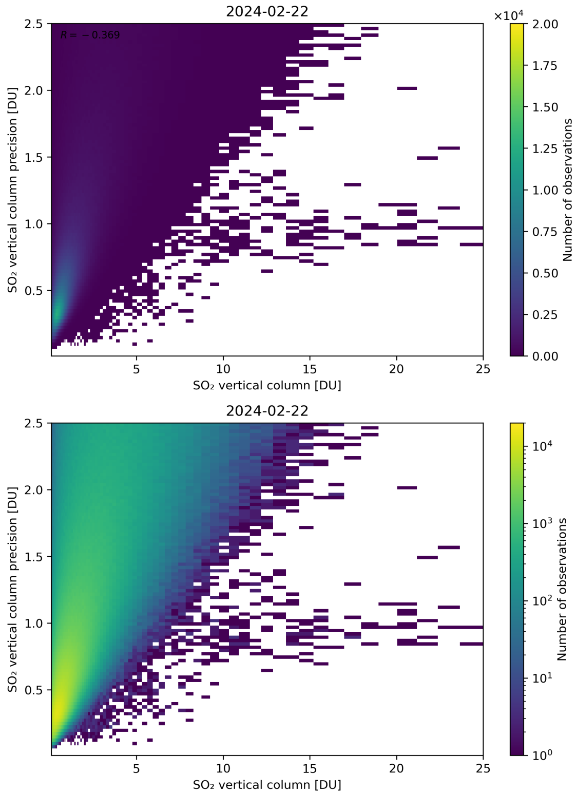
Figure 307: Scatter density plot of “SO 2 vertical column” against “SO 2 vertical column precision” for 2024-02-22 to 2024-02-23.
