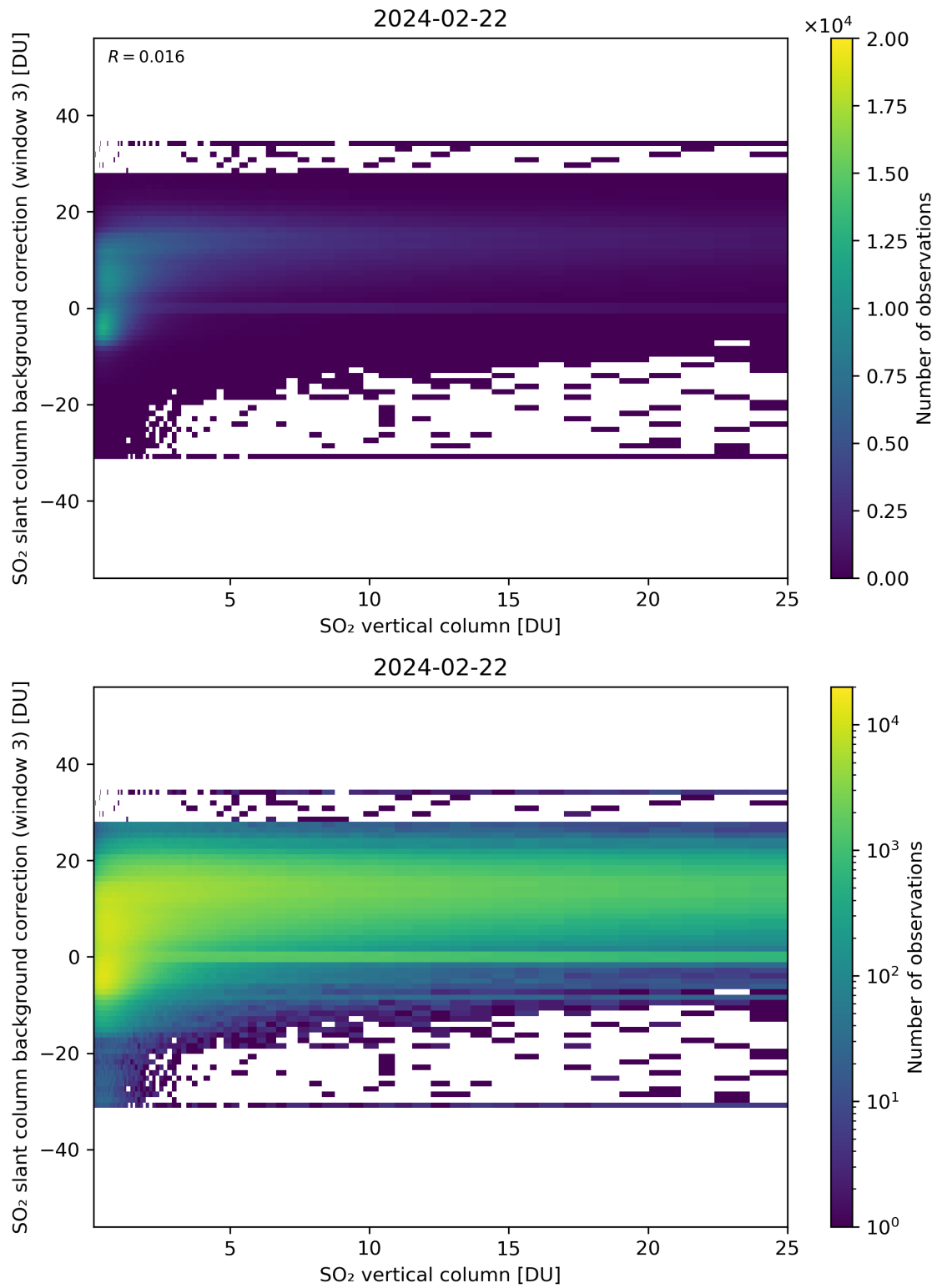
Figure 275: Scatter density plot of “SO 2 vertical column” against “SO 2 slant column background correction (window 3)” for 2024-02-22 to 2024-02-23.
