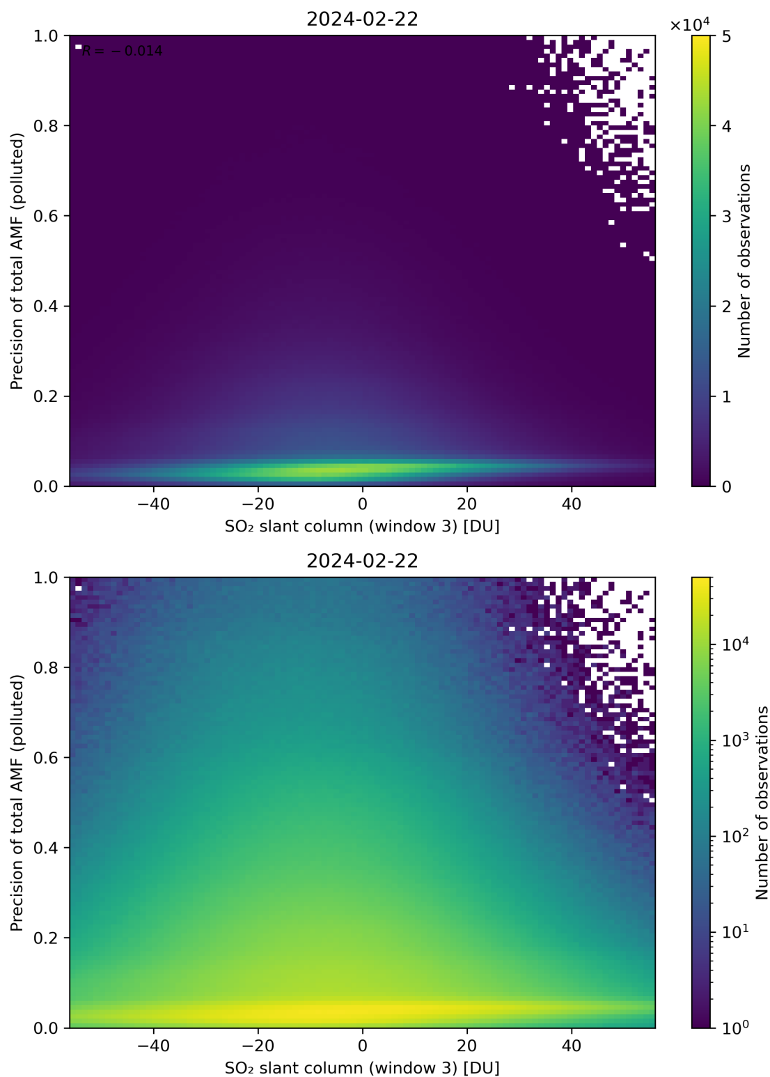
Figure 269: Scatter density plot of “SO 2 slant column (window 3)” against “Precision of total AMF (polluted)” for 2024-02-22 to 2024-02-23.
