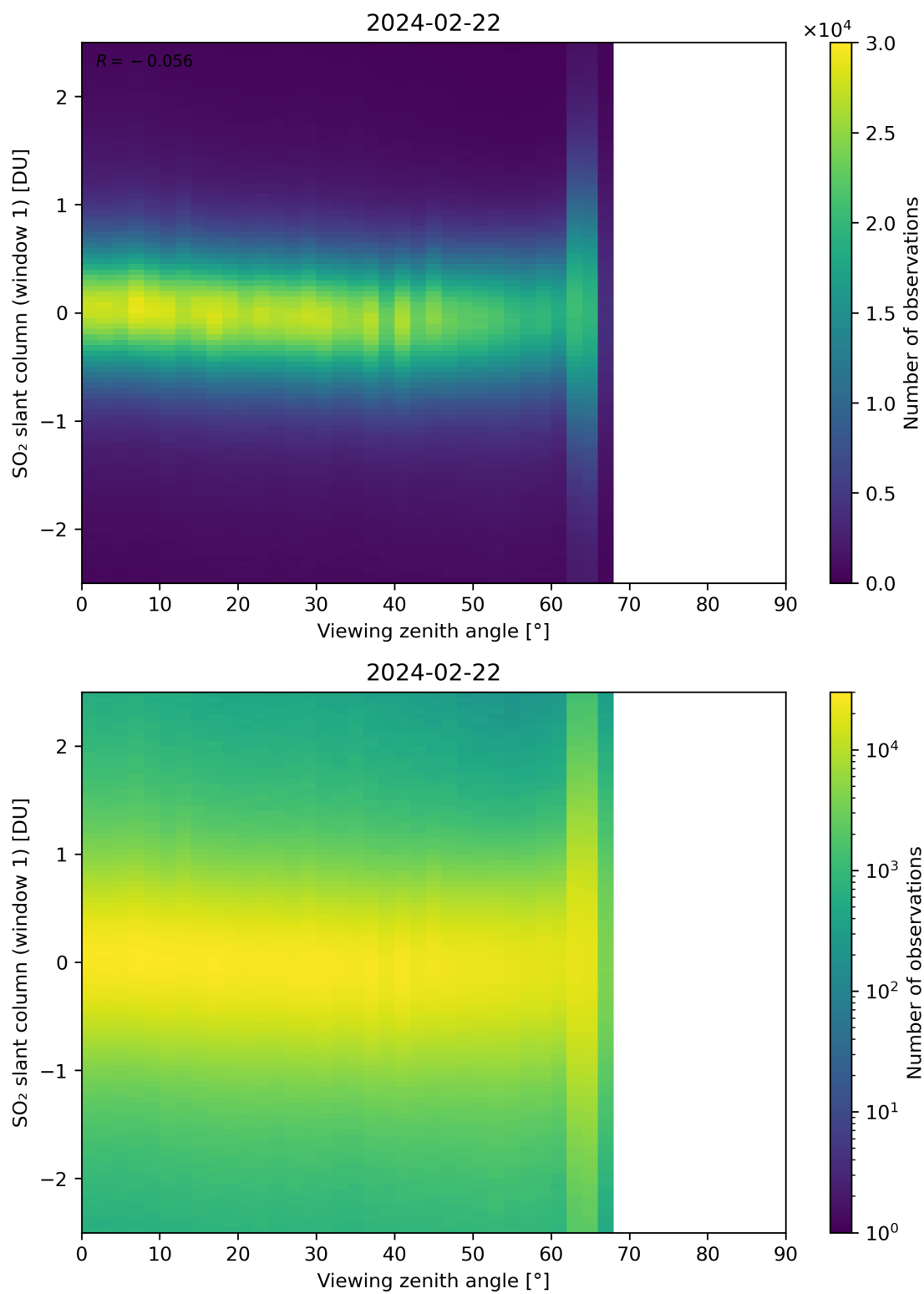
Figure 320: Scatter density plot of “Viewing zenith angle” against “SO 2 slant column (window 1)” for 2024-02-22 to 2024-02-23.
