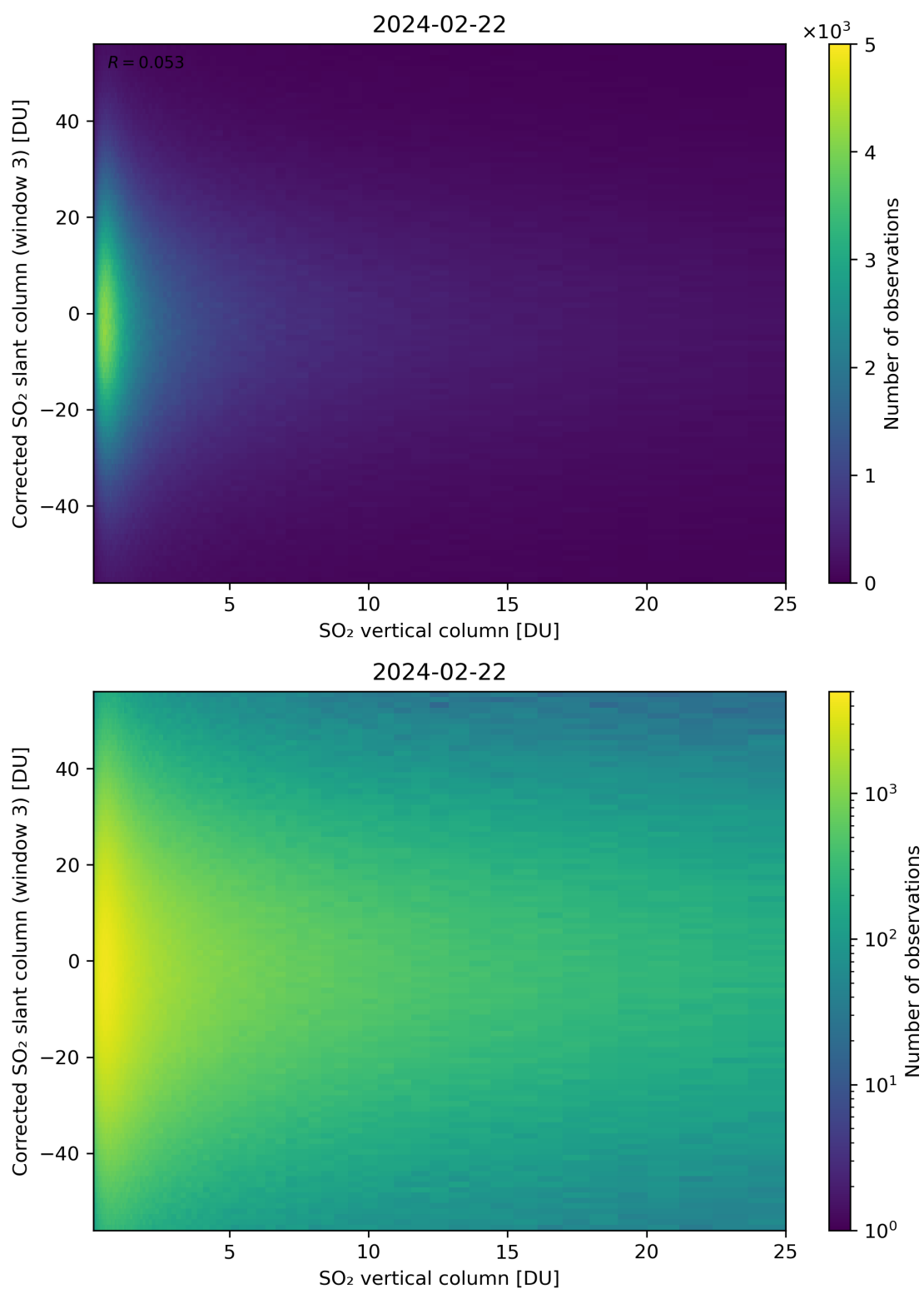
Figure 299: Scatter density plot of “SO 2 vertical column” against “Corrected SO 2 slant column (window 3)” for 2024-02-22 to 2024-02-23.
