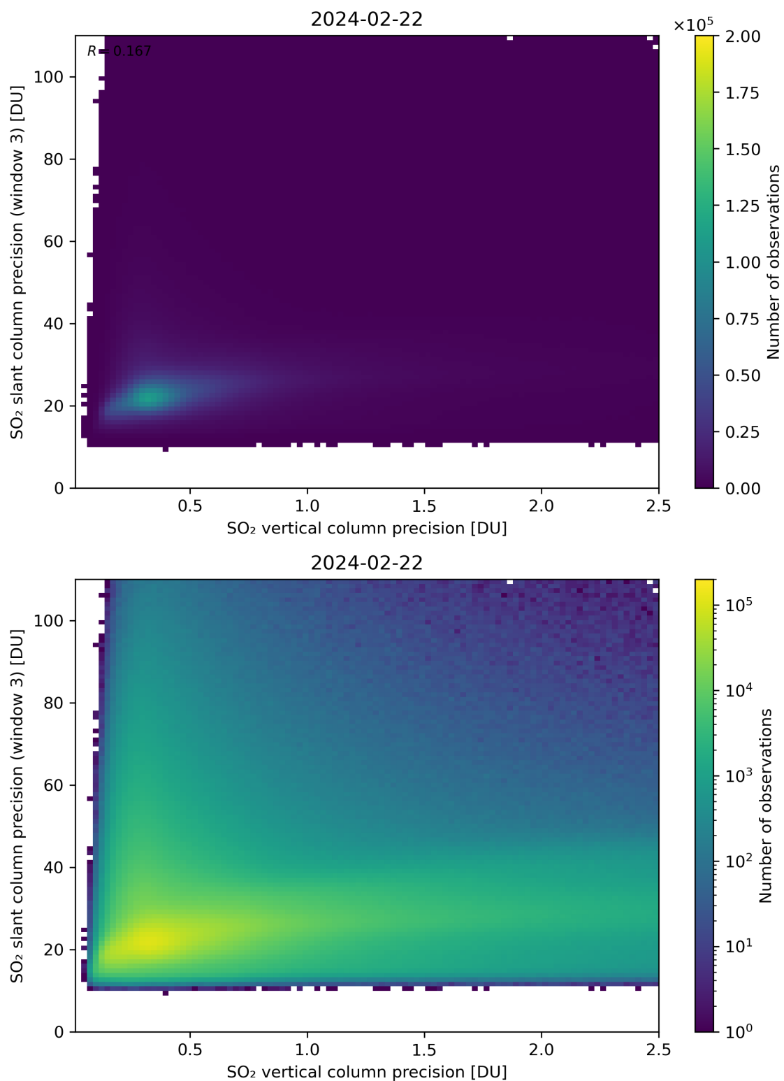
Figure 293: Scatter density plot of “SO 2 vertical column precision” against “SO 2 slant column precision (window 3)” for 2024-02-22 to 2024-02-23.
