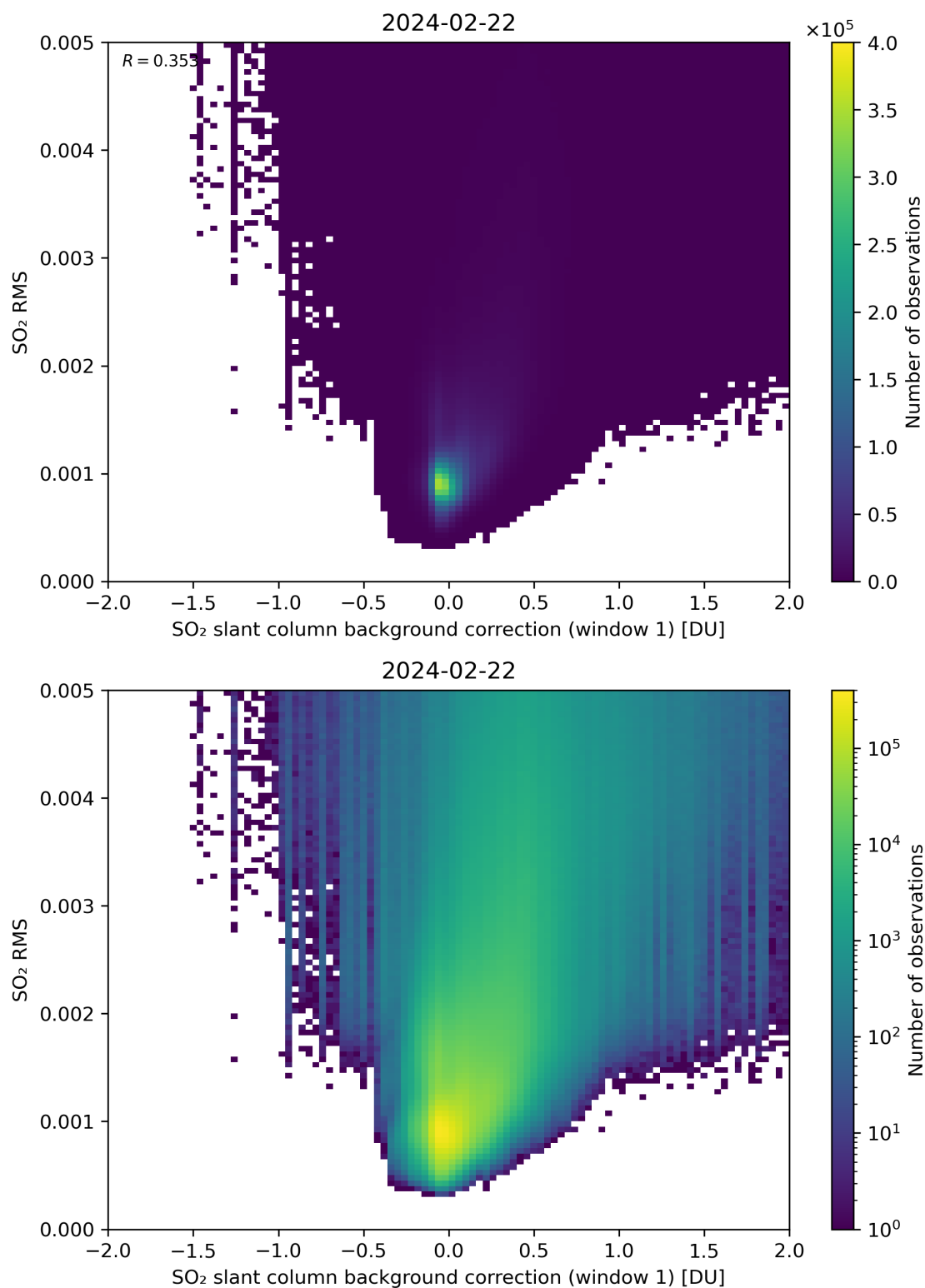
Figure 102: Scatter density plot of “SO 2 slant column background correction (window 1)” against “SO 2 RMS” for 2024-02-22 to 2024-02-23.
