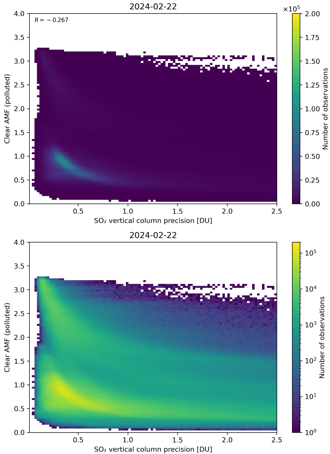
Figure 285: Scatter density plot of “SO 2 vertical column precision” against “Clear AMF (polluted)” for 2024-02-22 to 2024-02-23.
