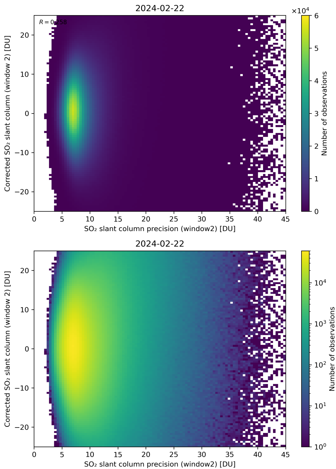
Figure 247: Scatter density plot of “SO 2 slant column precision (window2)” against “Corrected SO 2 slant column (window 2)” for 2024-02-22 to 2024-02-23.
