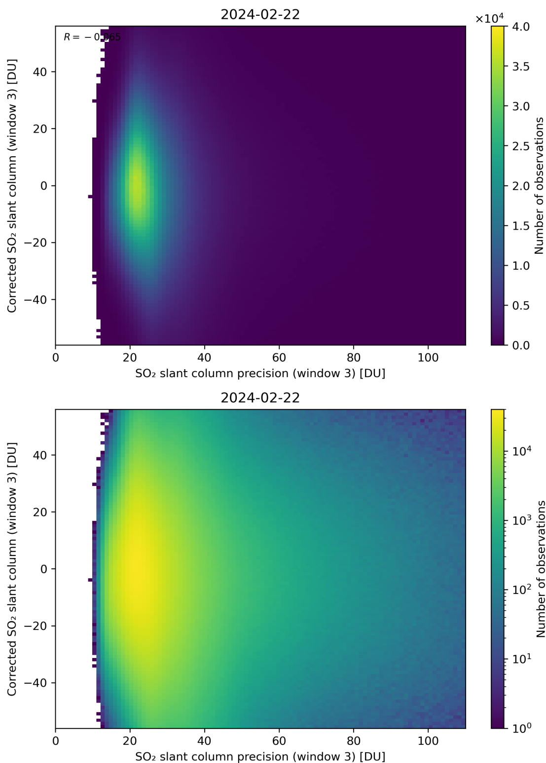
Figure 262: Scatter density plot of “SO 2 slant column precision (window 3)” against “Corrected SO 2 slant column (window 3)” for 2024-02-22 to 2024-02-23.
