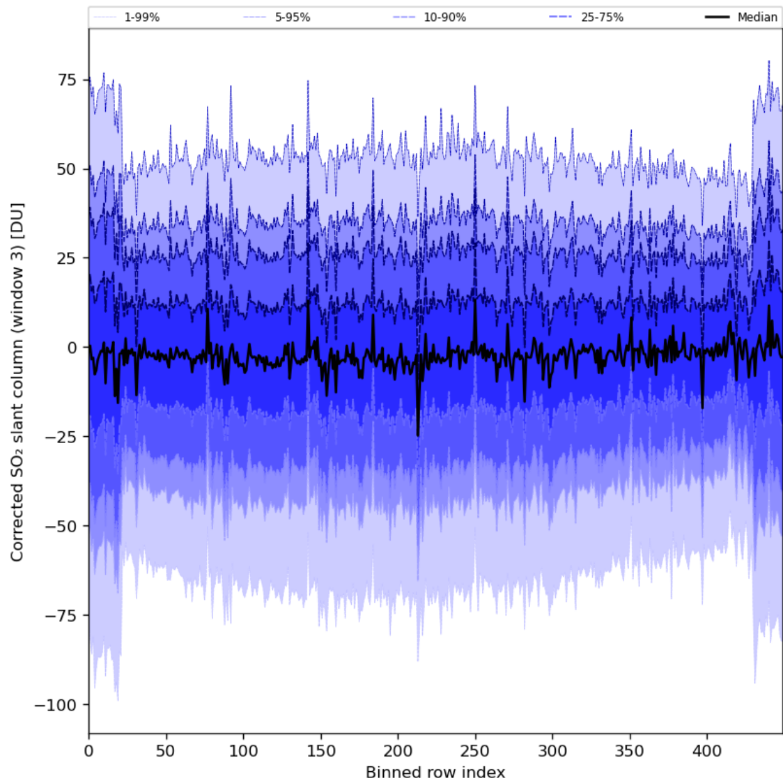
Figure 89: Along track statistics of “Corrected SO 2 slant column (window 3)” for 2024-02-22 to 2024-02-23
