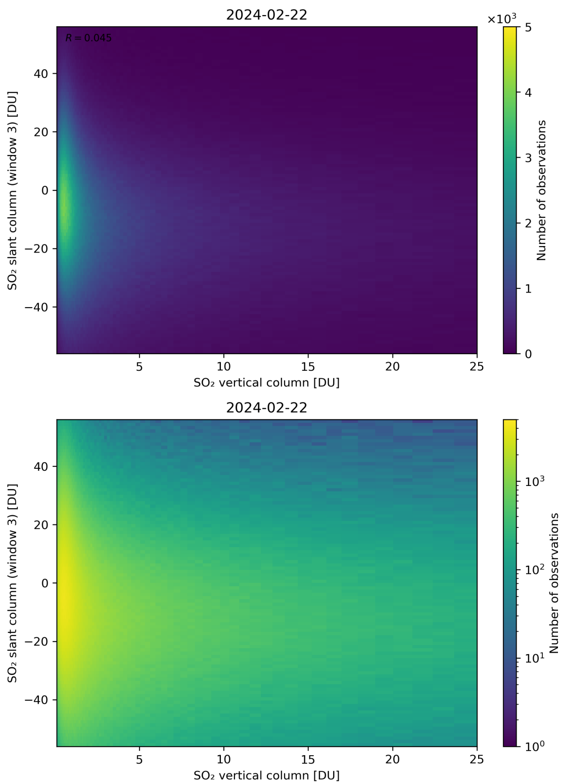
Figure 303: Scatter density plot of “SO 2 vertical column” against “SO 2 slant column (window 3)” for 2024-02-22 to 2024-02-23.
