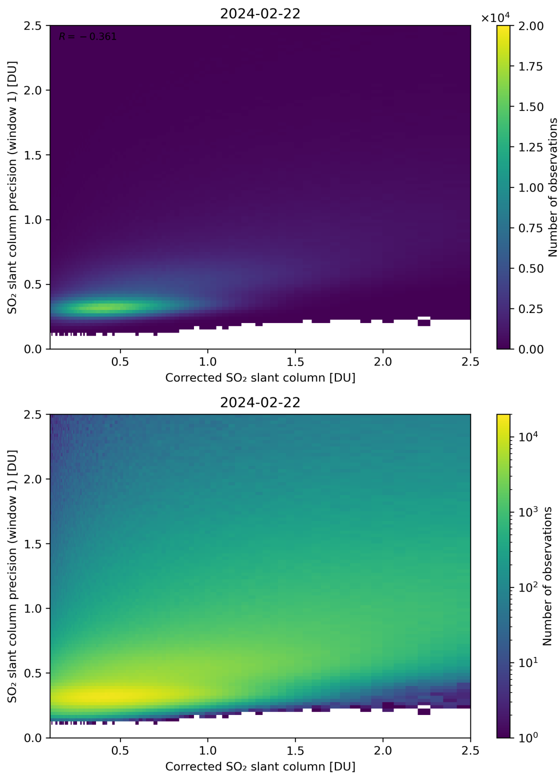
Figure 188: Scatter density plot of “Corrected SO 2 slant column” against “SO 2 slant column precision (window 1)” for 2024-02-22 to 2024-02-23.
