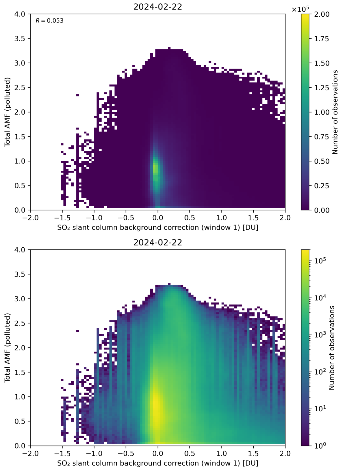
Figure 109: Scatter density plot of “SO 2 slant column background correction (window 1)” against “Total AMF (polluted)” for 2024-02-22 to 2024-02-23.
