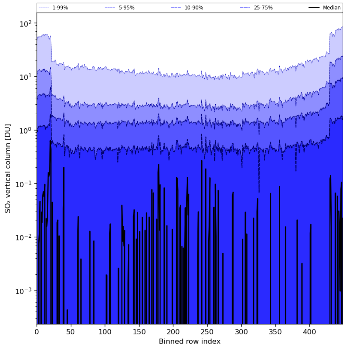
Figure 76: Along track statistics of “SO 2 vertical column” for 2024-02-22 to 2024-02-23
