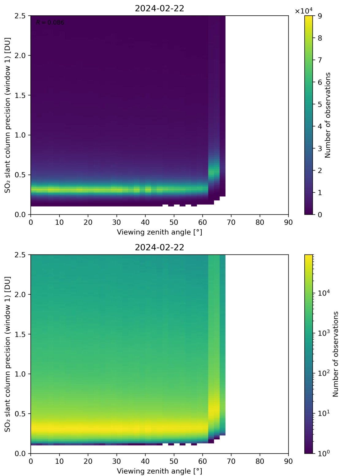
Figure 321: Scatter density plot of “Viewing zenith angle” against “SO 2 slant column precision (window 1)” for 2024-02-22 to 2024-02-23.
