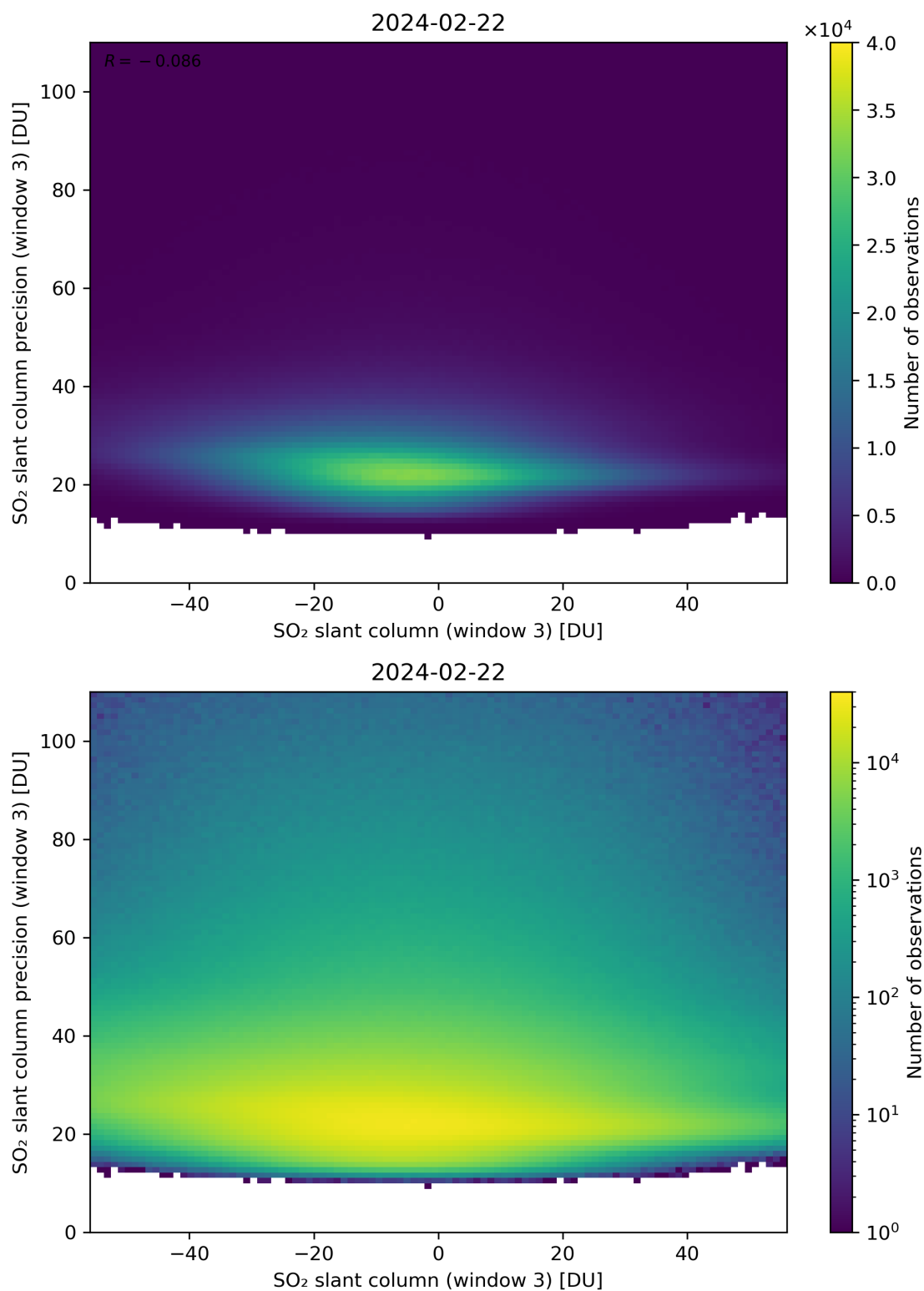
Figure 267: Scatter density plot of “SO 2 slant column (window 3)” against “SO 2 slant column precision (window 3)” for 2024-02-22 to 2024-02-23.
