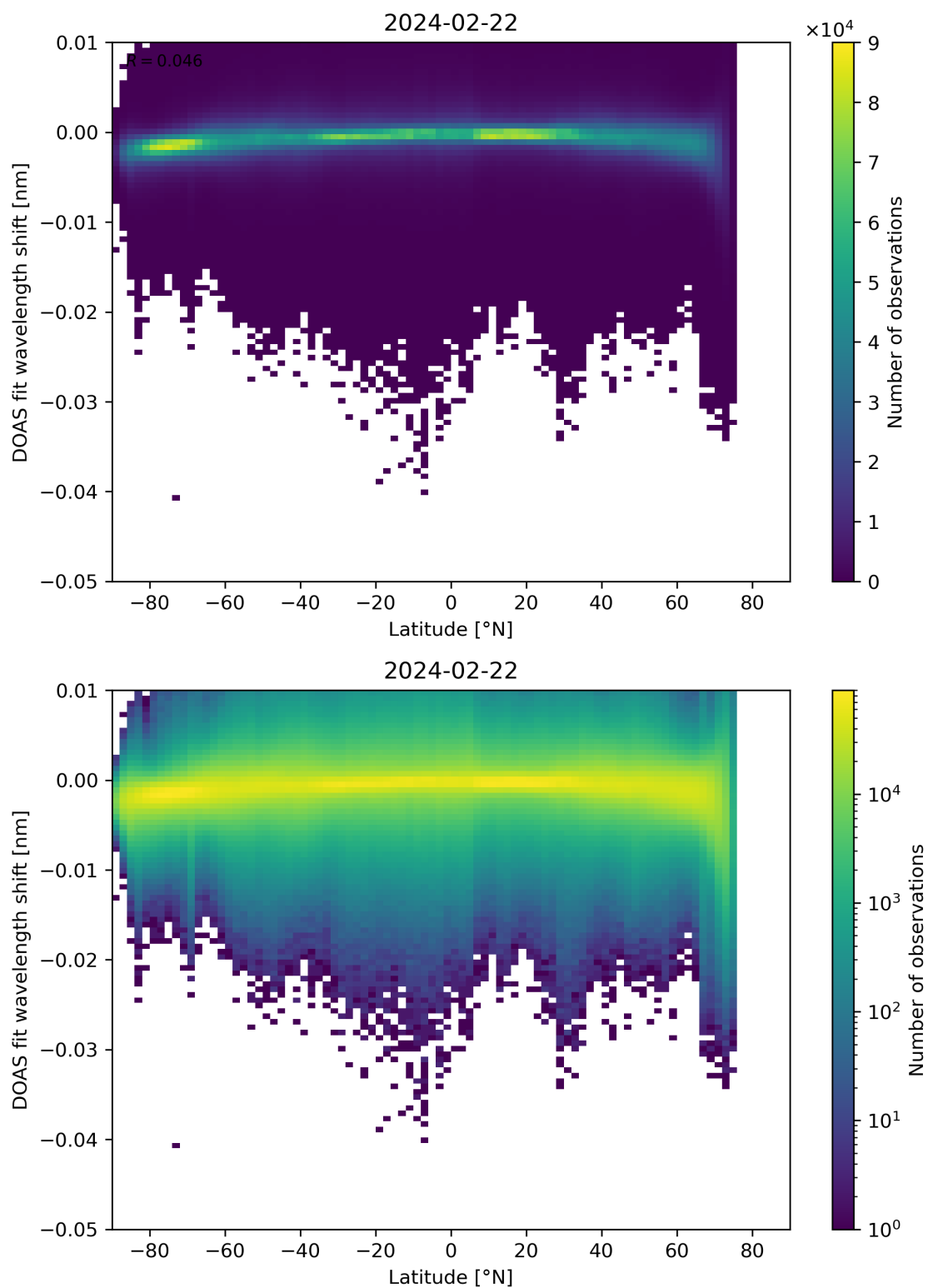
Figure 142: Scatter density plot of “Latitude” against “DOAS fit wavelength shift” for 2024-02-22 to 2024-02-23.
