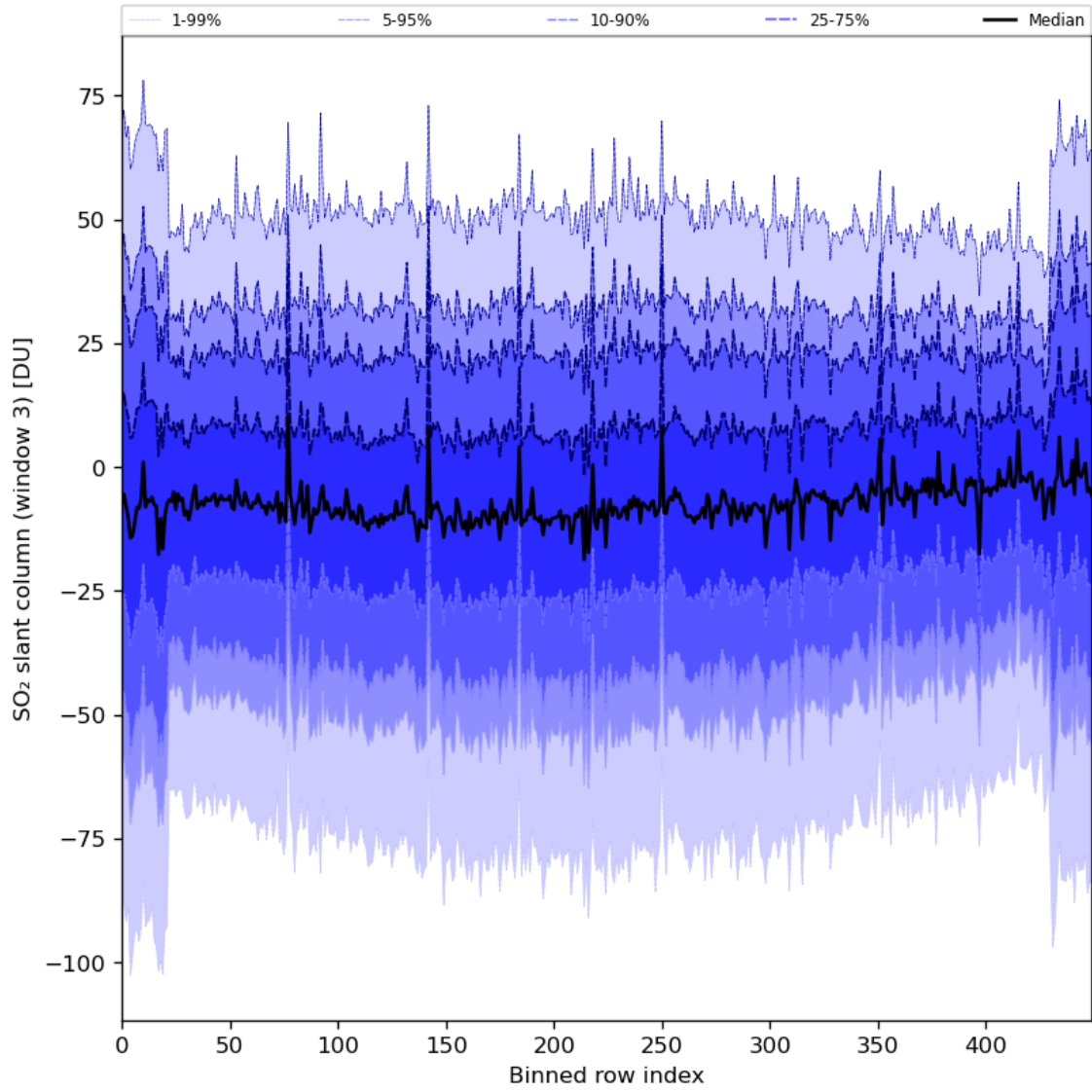
Figure 87: Along track statistics of “SO 2 slant column (window 3)” for 2024-02-22 to 2024-02-23
