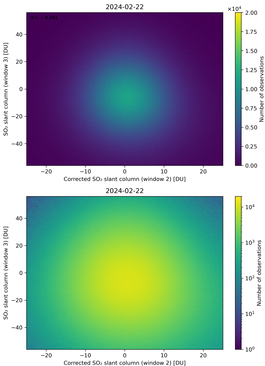
Figure 201: Scatter density plot of “Corrected SO 2 slant column (window 2)” against “SO 2 slant column (window 3)” for 2024-02-22 to 2024-02-23.
