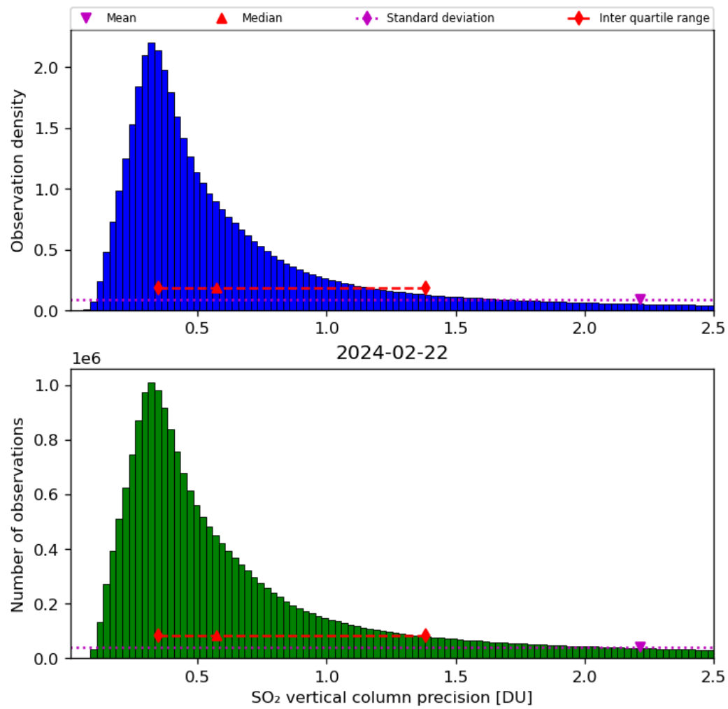
Figure 54: Histogram of “SO 2 vertical column precision” for 2024-02-22 to 2024-02-23
