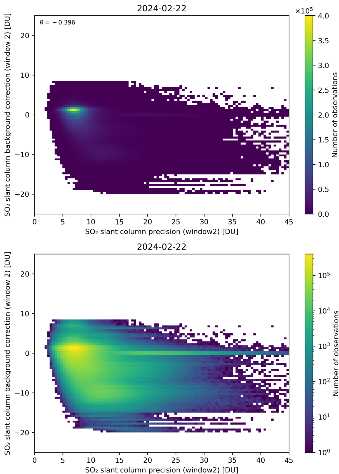
Figure 241: Scatter density plot of “SO 2 slant column precision (window2)” against “SO 2 slant column background correction (window 2)” for 2024-02-22 to 2024-02-23.
