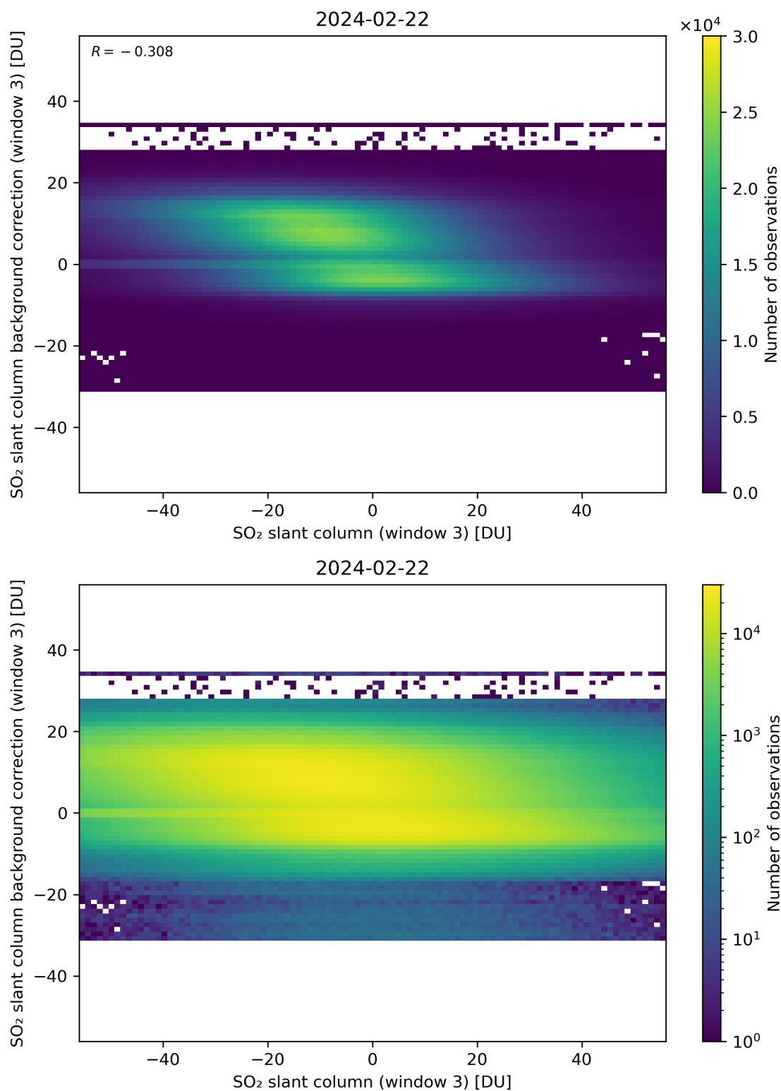
Figure 253: Scatter density plot of “SO 2 slant column (window 3)” against “SO 2 slant column background correction (window 3)” for 2024-02-22 to 2024-02-23.
