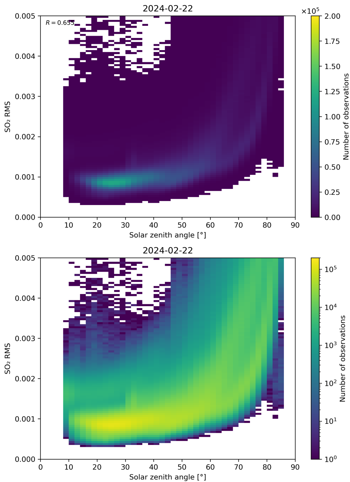
Figure 163: Scatter density plot of “Solar zenith angle” against “SO 2 RMS” for 2024-02-22 to 2024-02-23.
