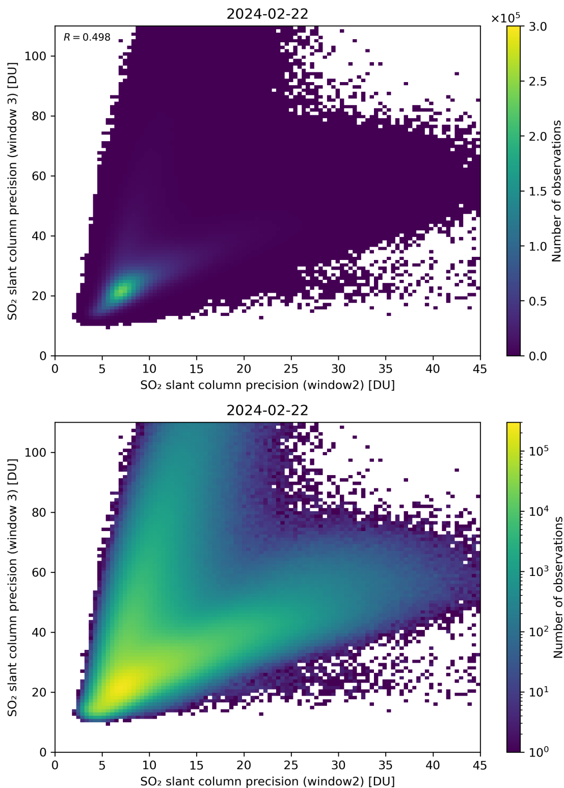
Figure 250: Scatter density plot of “SO 2 slant column precision (window2)” against “SO 2 slant column precision (window 3)” for 2024-02-22 to 2024-02-23.
