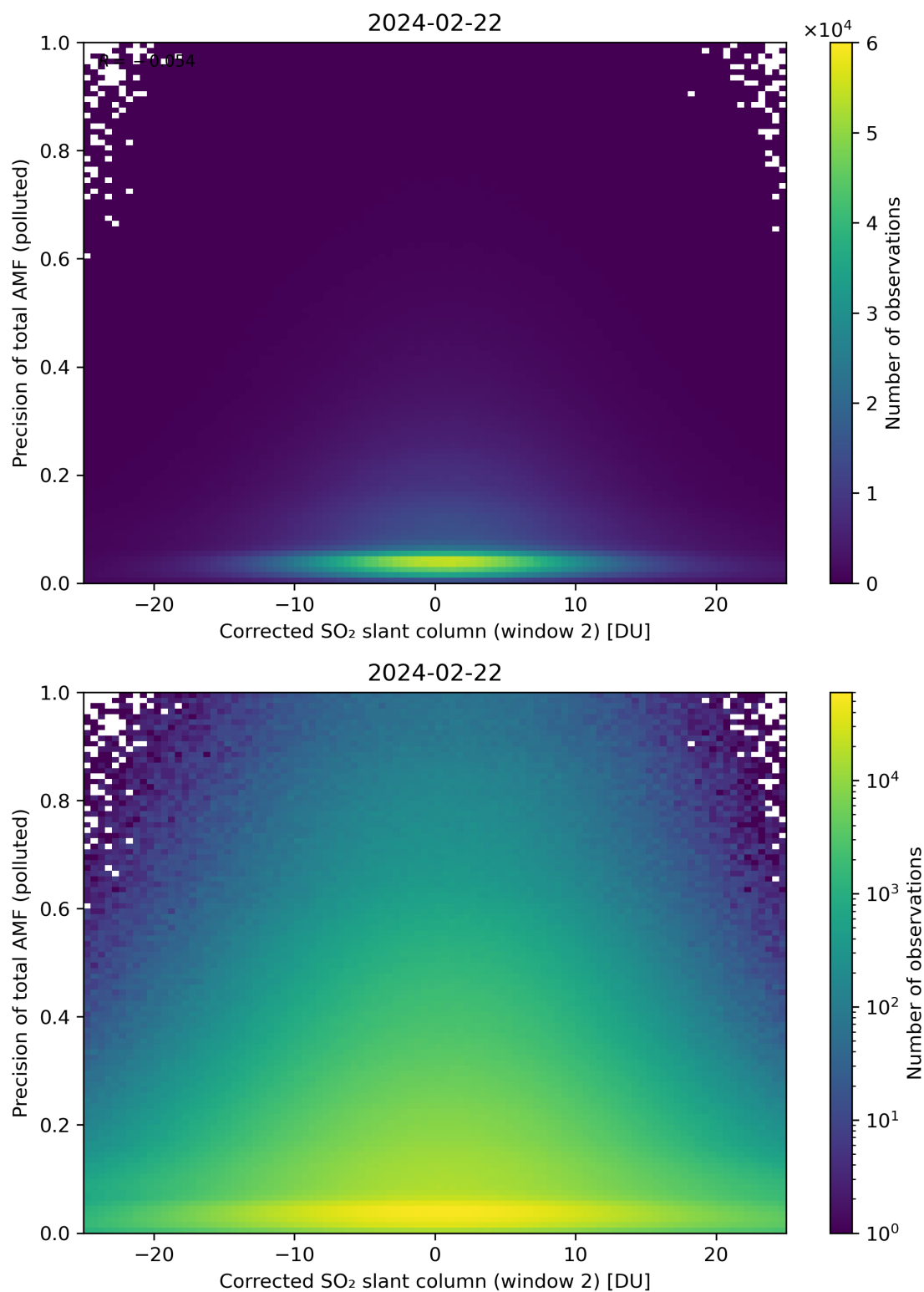
Figure 204: Scatter density plot of “Corrected SO 2 slant column (window 2)” against “Precision of total AMF (polluted)” for 2024-02-22 to 2024-02-23.
