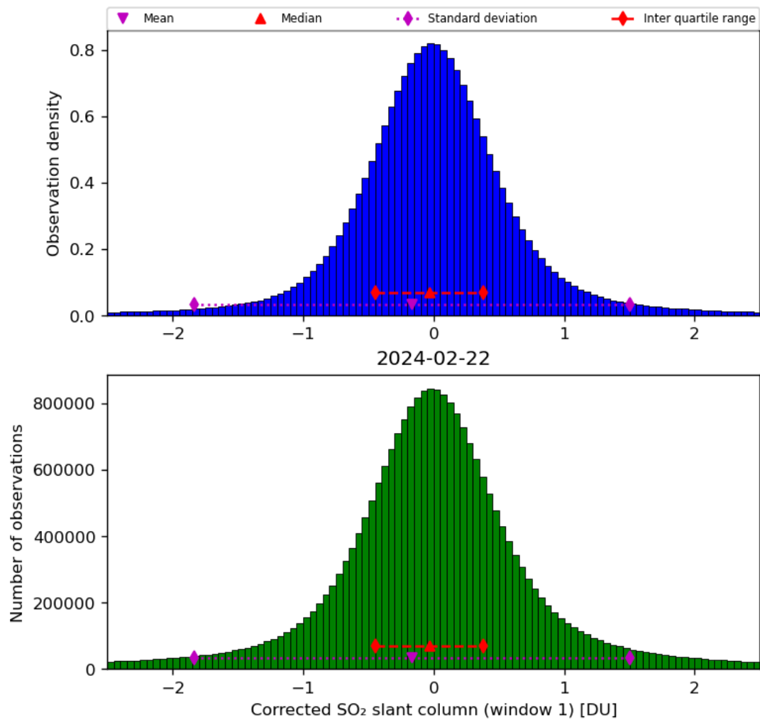
Figure 58: Histogram of “Corrected SO 2 slant column (window 1)” for 2024-02-22 to 2024-02-23
