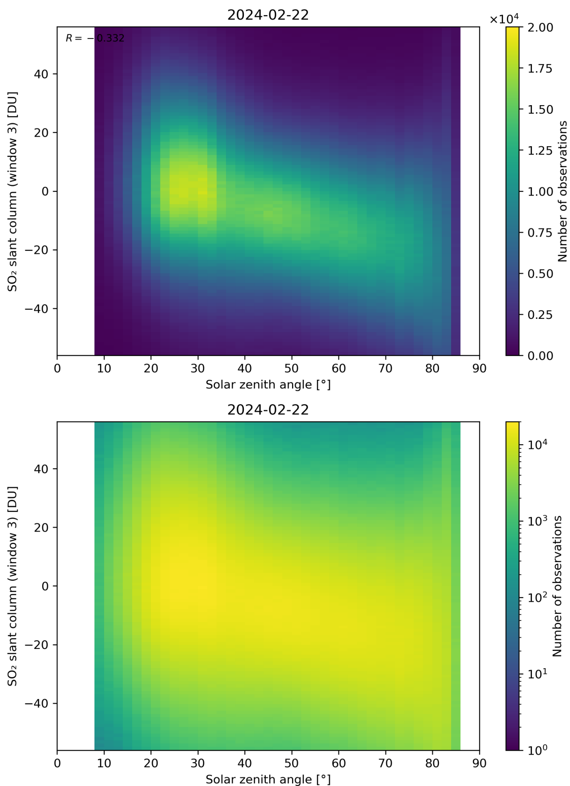
Figure 172: Scatter density plot of “Solar zenith angle” against “SO 2 slant column (window 3)” for 2024-02-22 to 2024-02-23.
