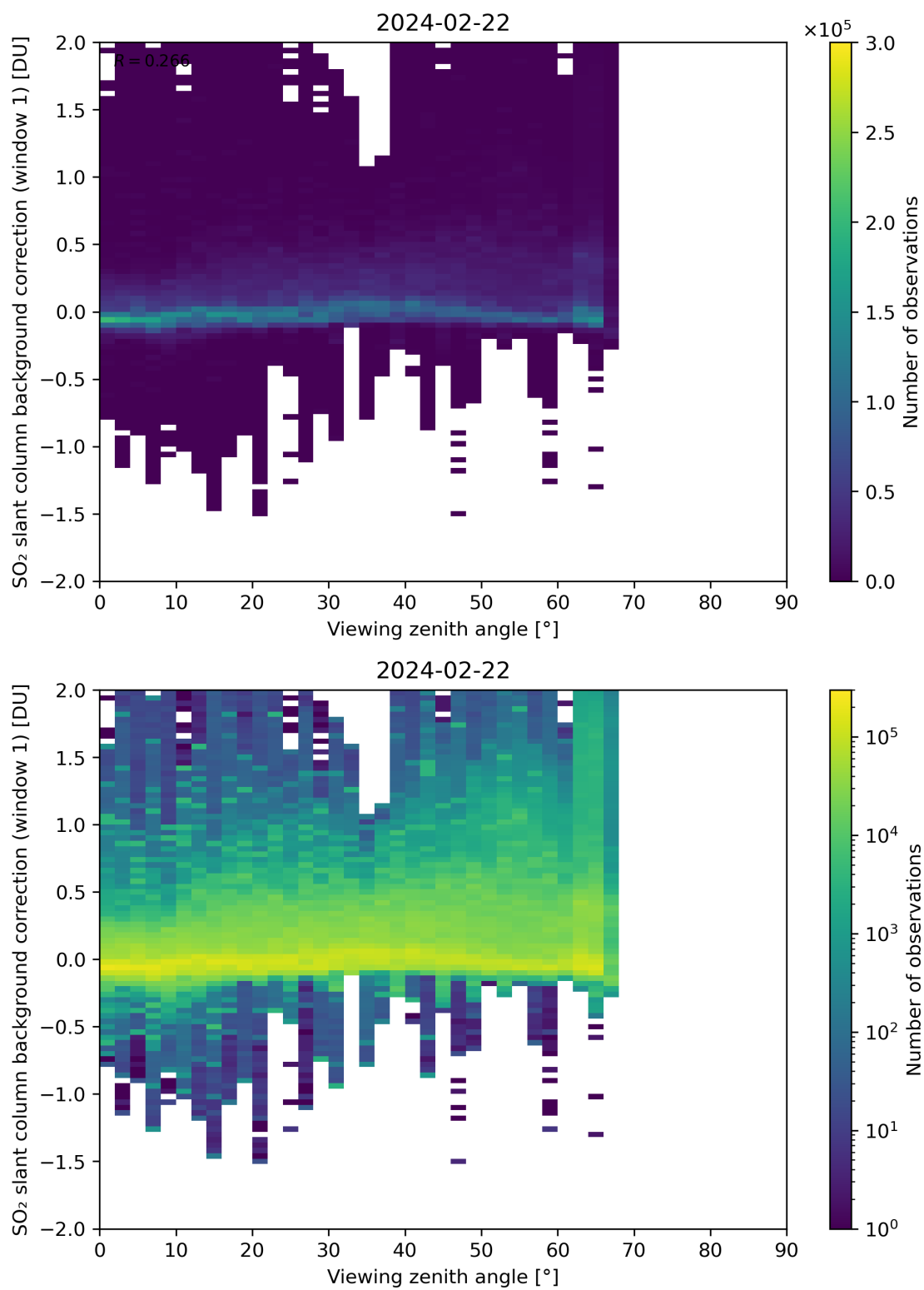
Figure 308: Scatter density plot of “Viewing zenith angle” against “SO 2 slant column background correction (window 1)” for 2024-02-22 to 2024-02-23.
