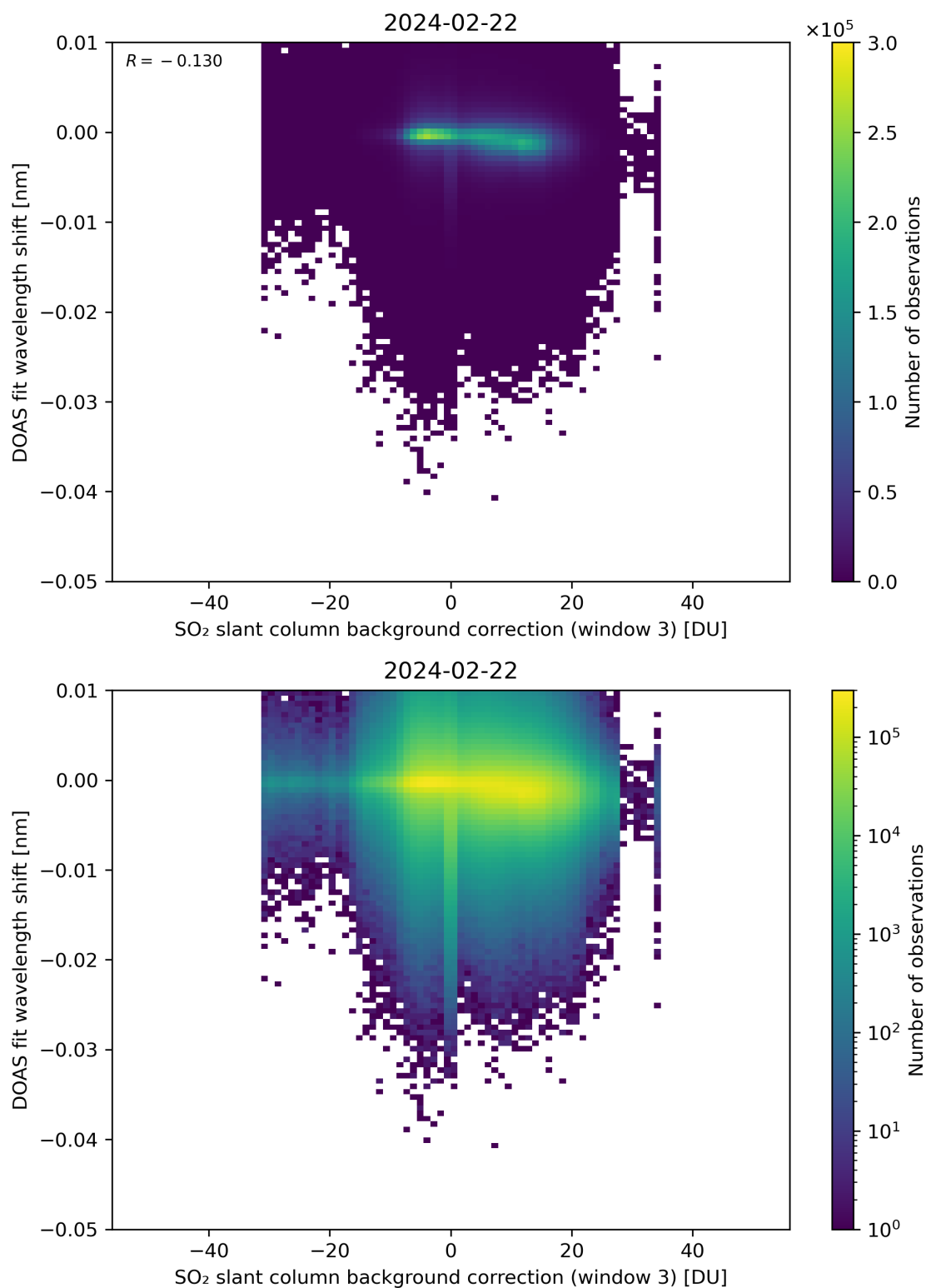
Figure 121: Scatter density plot of “SO 2 slant column background correction (window 3)” against “DOAS fit wavelength shift” for 2024-02-22 to 2024-02-23.
