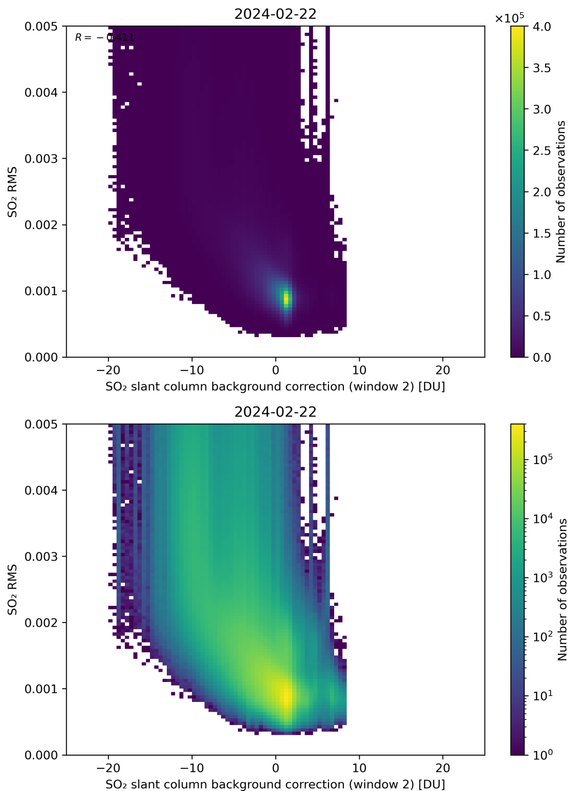
Figure 114: Scatter density plot of “SO 2 slant column background correction (window 2)” against “SO 2 RMS” for 2024-02-22 to 2024-02-23.
