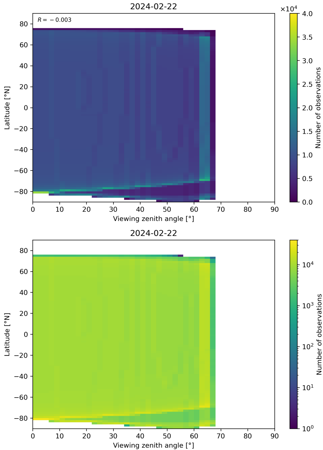
Figure 314: Scatter density plot of “Viewing zenith angle” against “Latitude” for 2024-02-22 to 2024-02-23.
