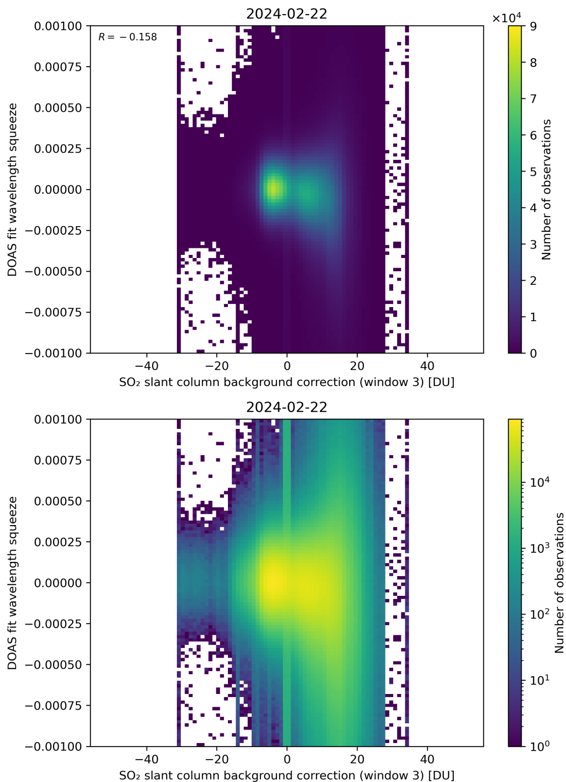
Figure 122: Scatter density plot of “SO 2 slant column background correction (window 3)” against “DOAS fit wavelength squeeze” for 2024-02-22 to 2024-02-23.
