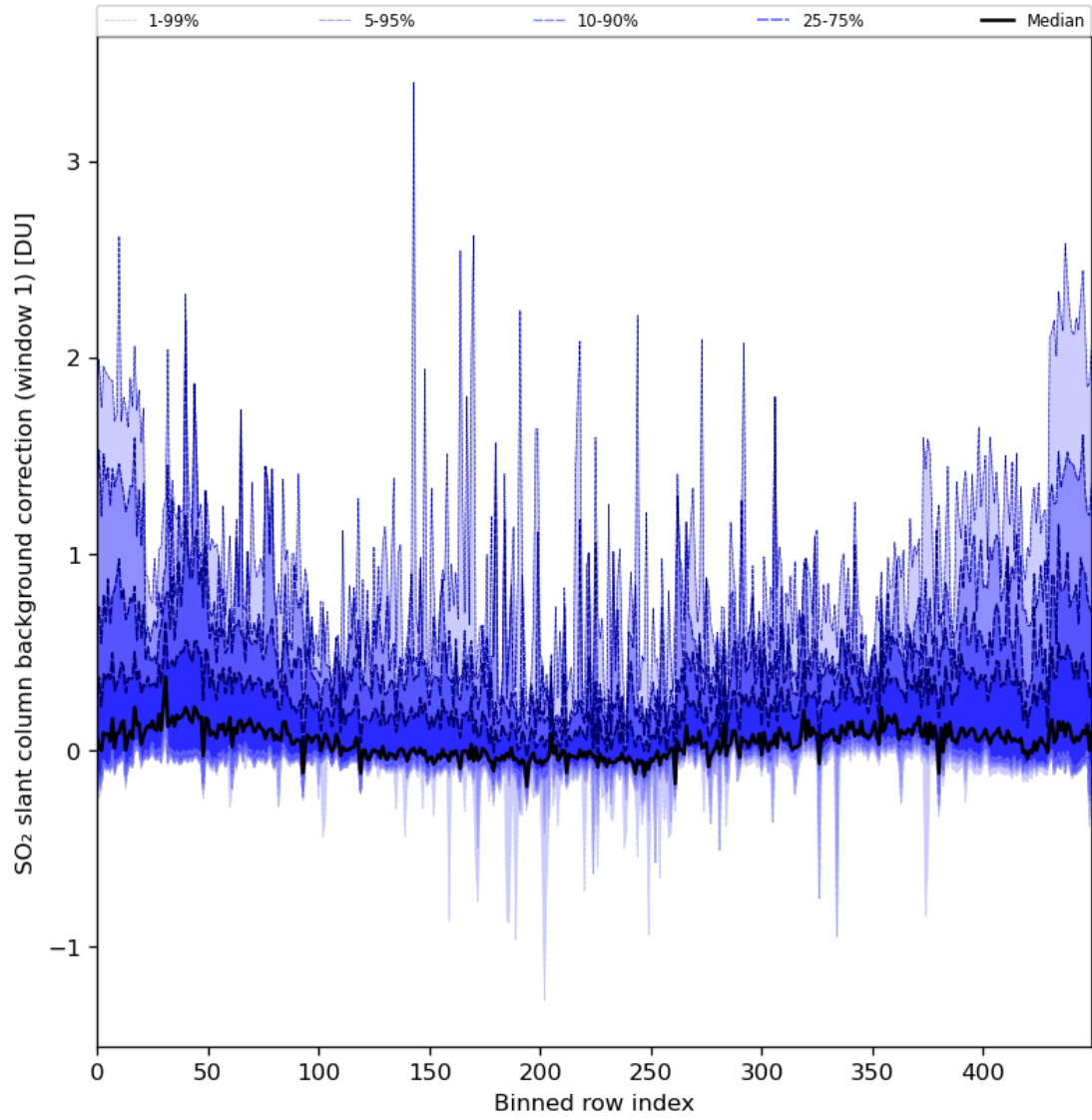
Figure 82: Along track statistics of “SO 2 slant column background correction (window 1)” for 2024-02-22 to 2024-02-23
