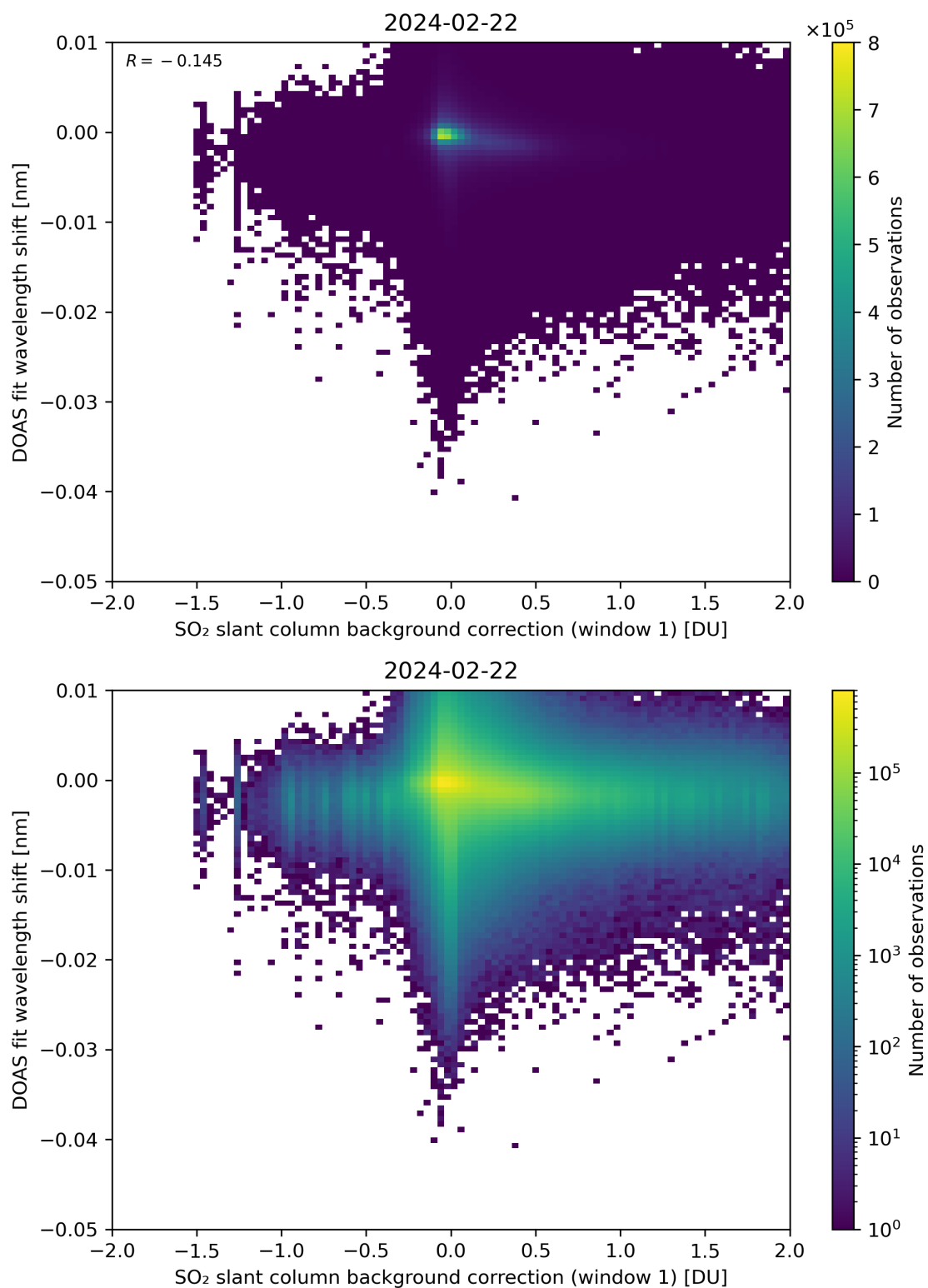
Figure 100: Scatter density plot of “SO 2 slant column background correction (window 1)” against “DOAS fit wavelength shift” for 2024-02-22 to 2024-02-23.
