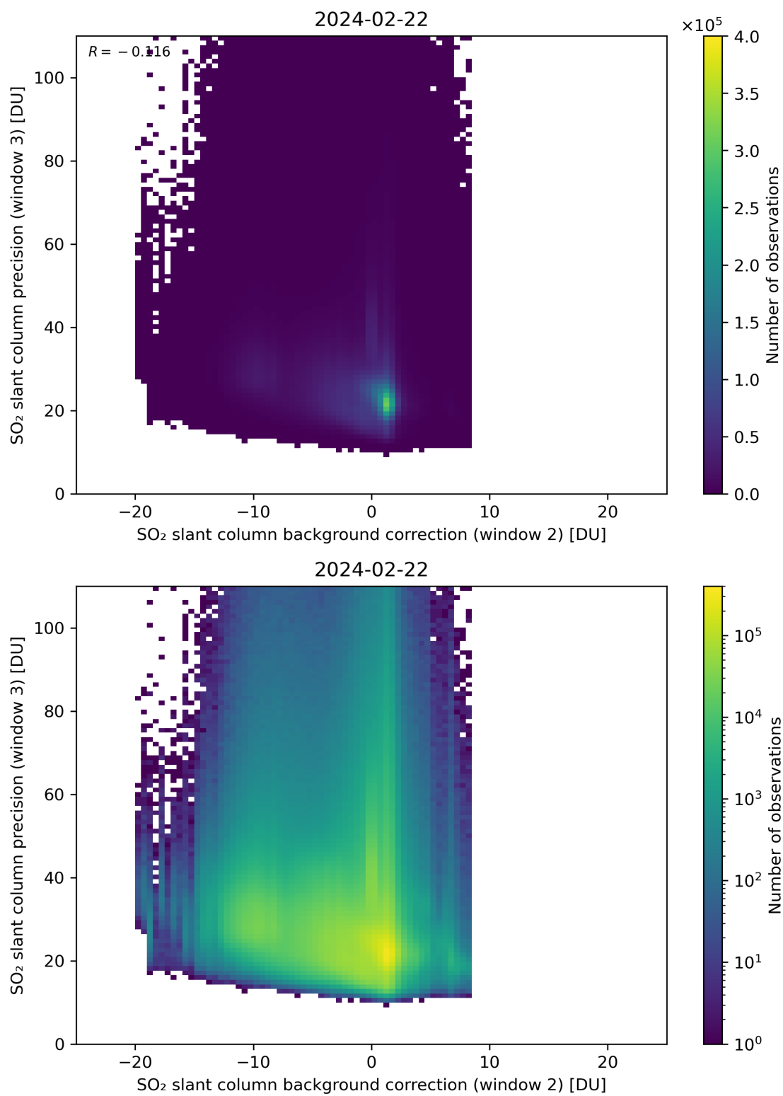
Figure 118: Scatter density plot of “SO 2 slant column background correction (window 2)” against “SO 2 slant column precision (window 3)” for 2024-02-22 to 2024-02-23.
