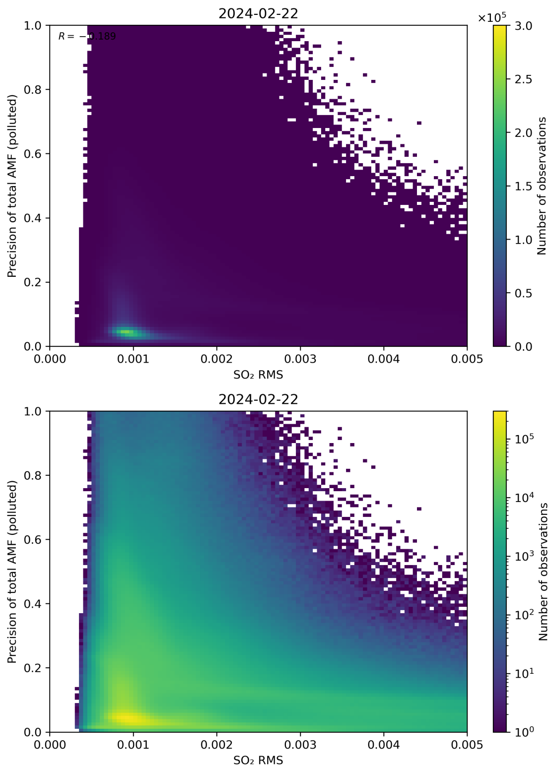
Figure 138: Scatter density plot of “SO 2 RMS” against “Precision of total AMF (polluted)” for 2024-02-22 to 2024-02-23.
