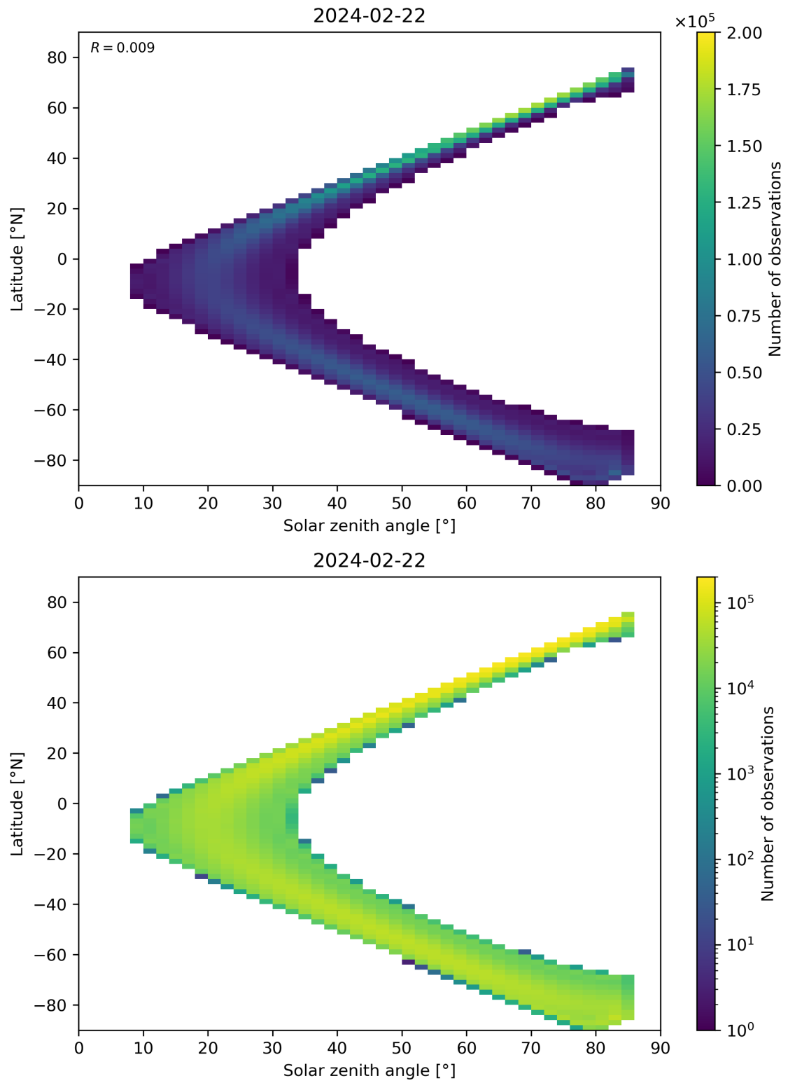
Figure 164: Scatter density plot of “Solar zenith angle” against “Latitude” for 2024-02-22 to 2024-02-23.
