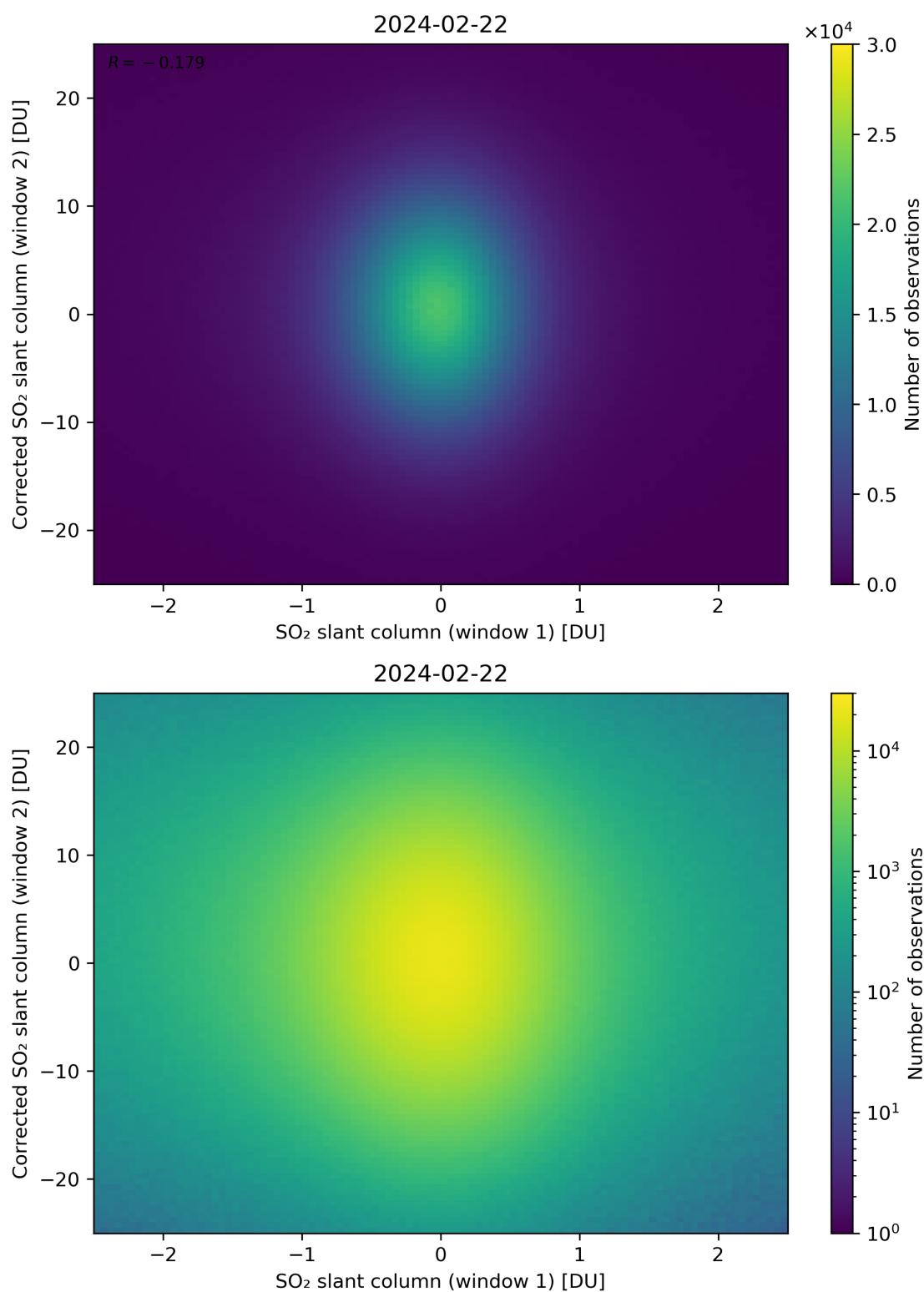
Figure 233: Scatter density plot of “SO 2 slant column (window 1)” against “Corrected SO 2 slant column (window 2)” for 2024-02-22 to 2024-02-23.
