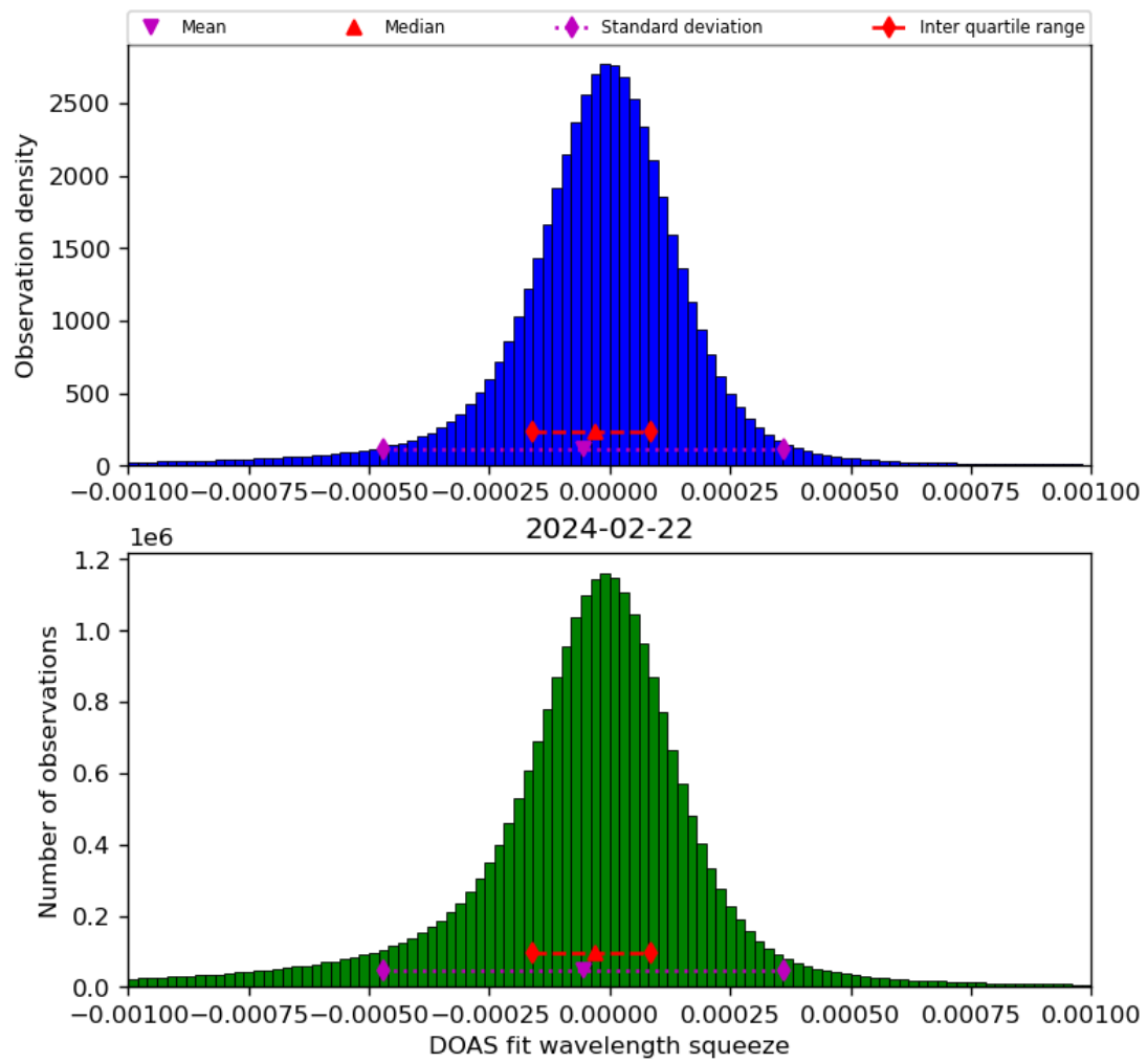
Figure 69: Histogram of “DOAS fit wavelength squeeze” for 2024-02-22 to 2024-02-23
