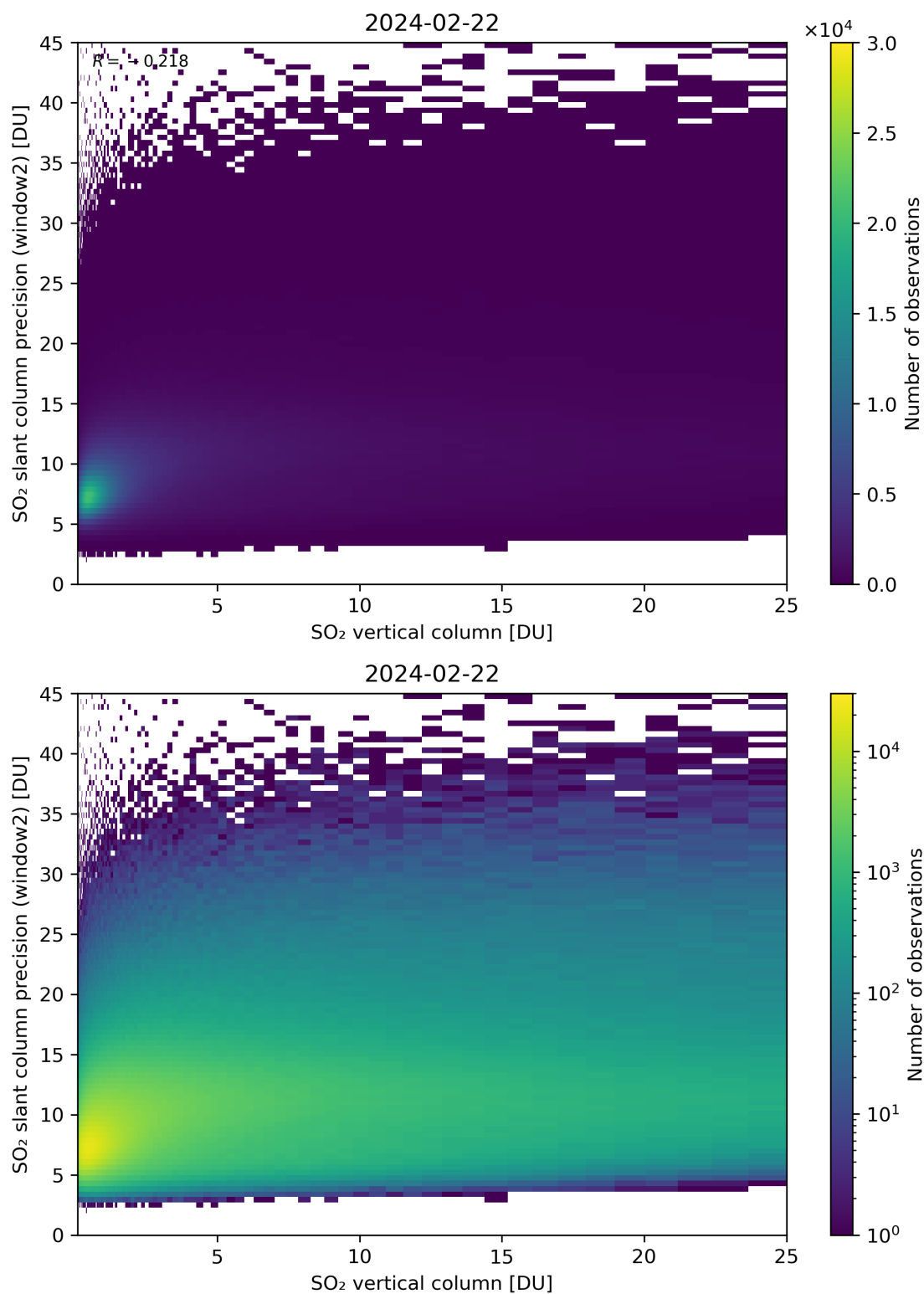
Figure 302: Scatter density plot of “SO 2 vertical column” against “SO 2 slant column precision (window2)” for 2024-02-22 to 2024-02-23.
