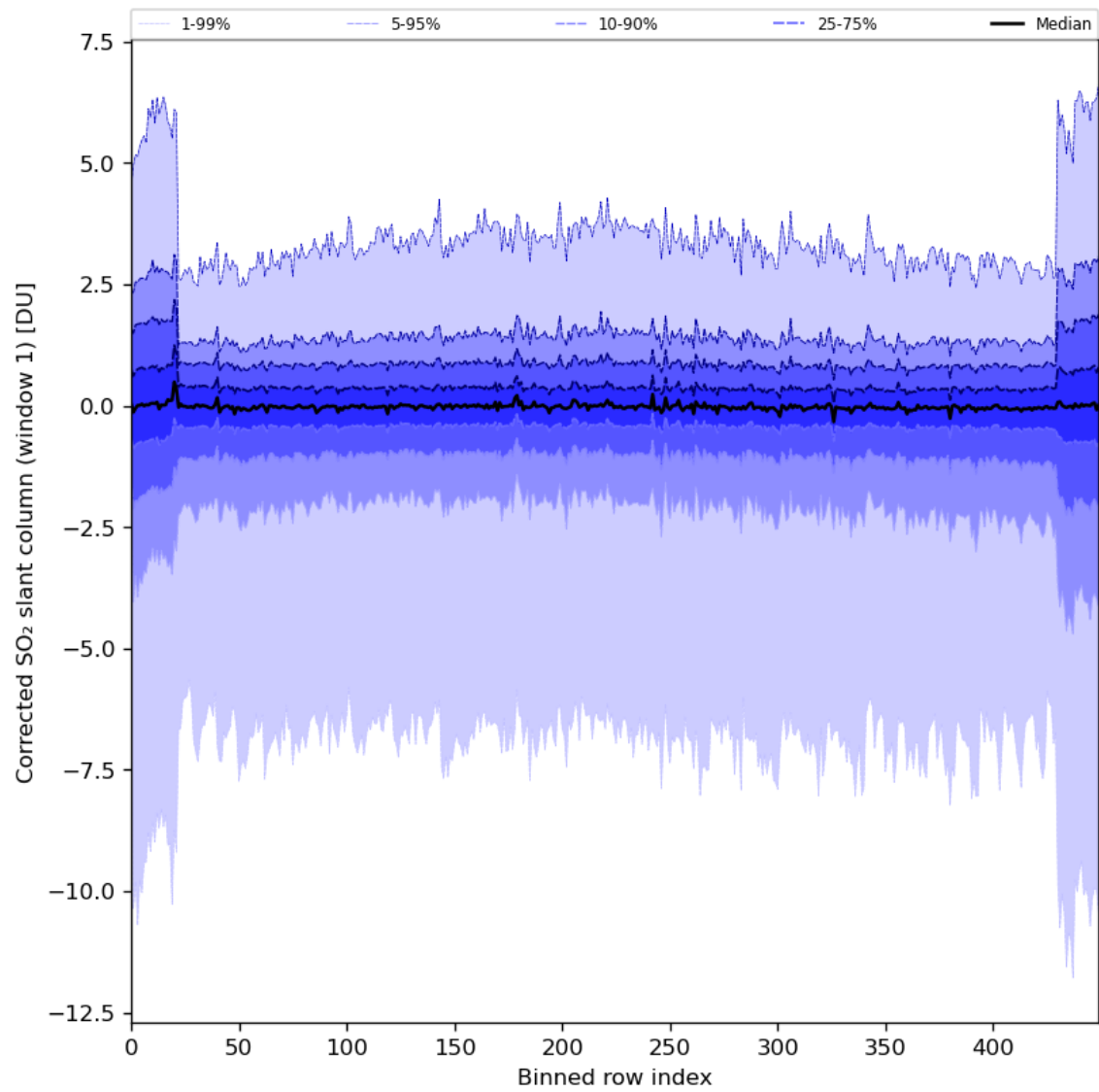
Figure 81: Along track statistics of “Corrected SO 2 slant column (window 1)” for 2024-02-22 to 2024-02-23
