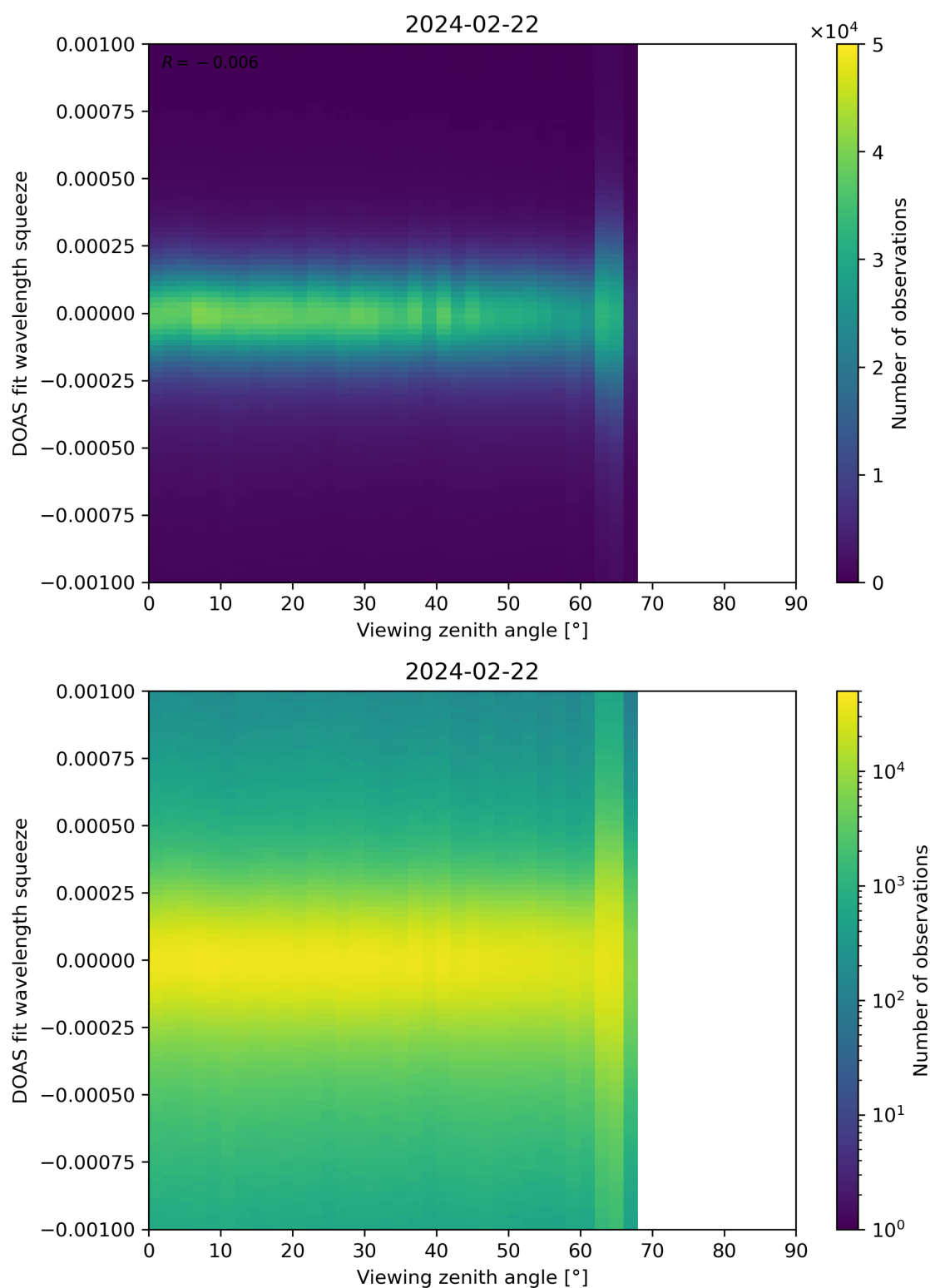
Figure 312: Scatter density plot of “Viewing zenith angle” against “DOAS fit wavelength squeeze” for 2024-02-22 to 2024-02-23.
