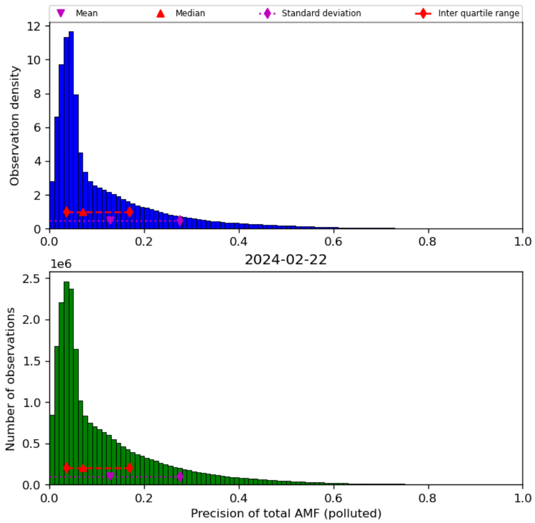
Figure 72: Histogram of “Precision of total AMF (polluted)” for 2024-02-22 to 2024-02-23
