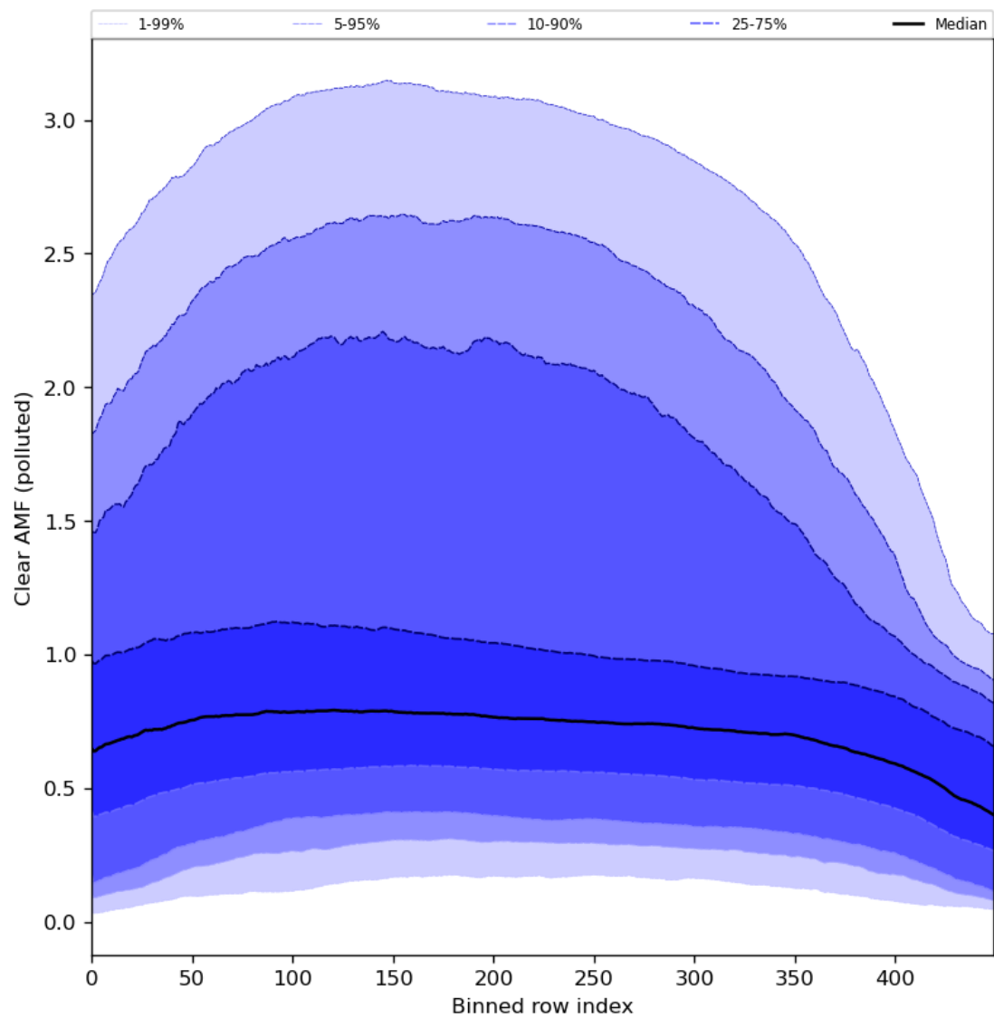
Figure 96: Along track statistics of “Clear AMF (polluted)” for 2024-02-22 to 2024-02-23
