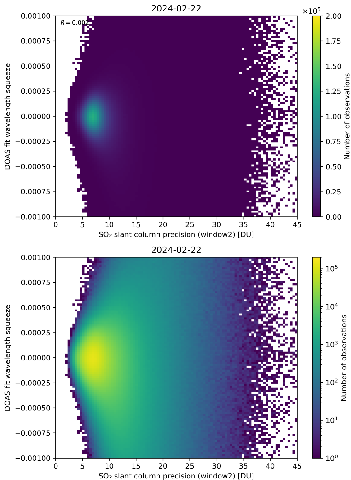
Figure 244: Scatter density plot of “SO 2 slant column precision (window2)” against “DOAS fit wavelength squeeze” for 2024-02-22 to 2024-02-23.
