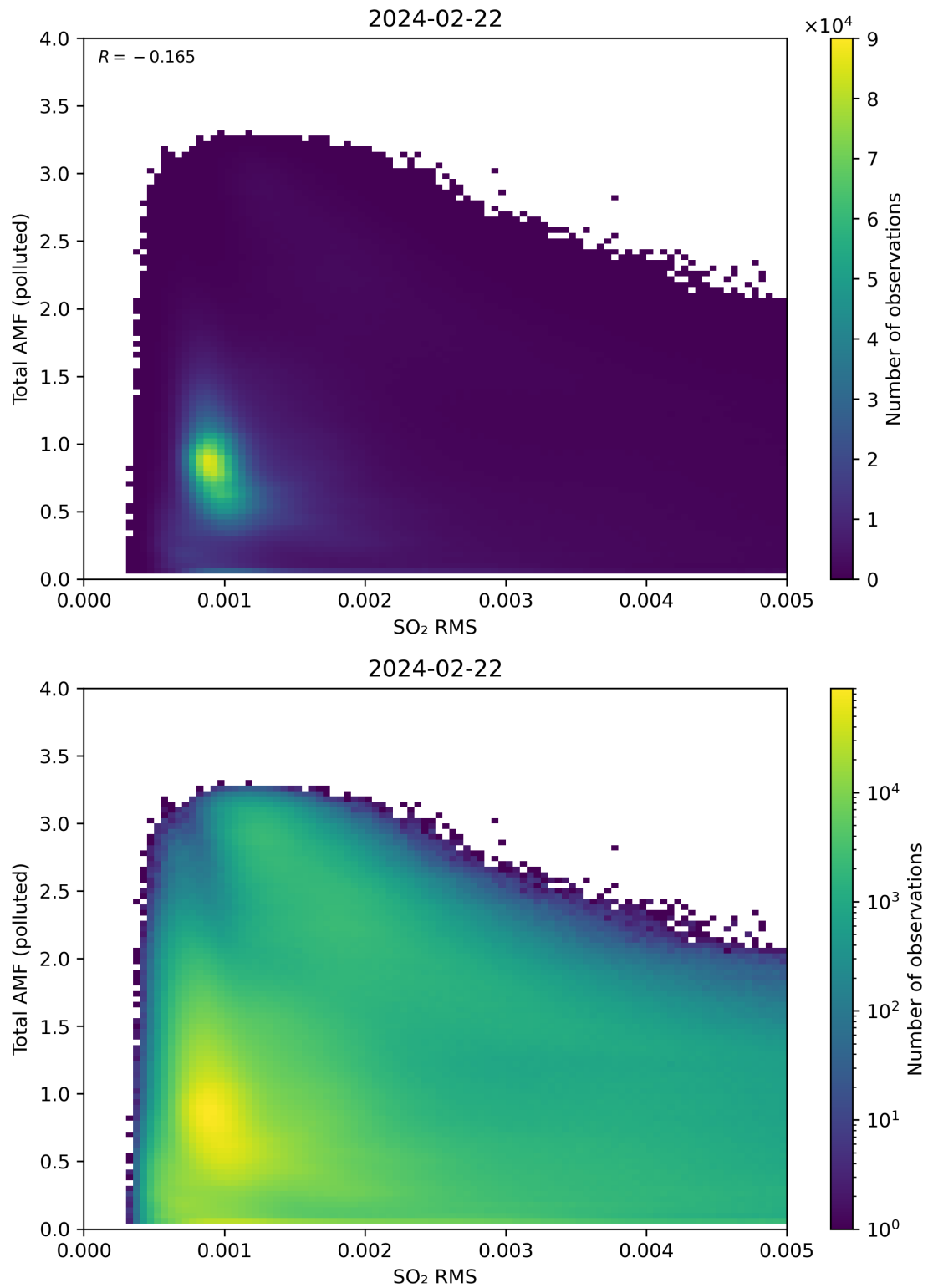
Figure 137: Scatter density plot of “SO 2 RMS” against “Total AMF (polluted)” for 2024-02-22 to 2024-02-23.
