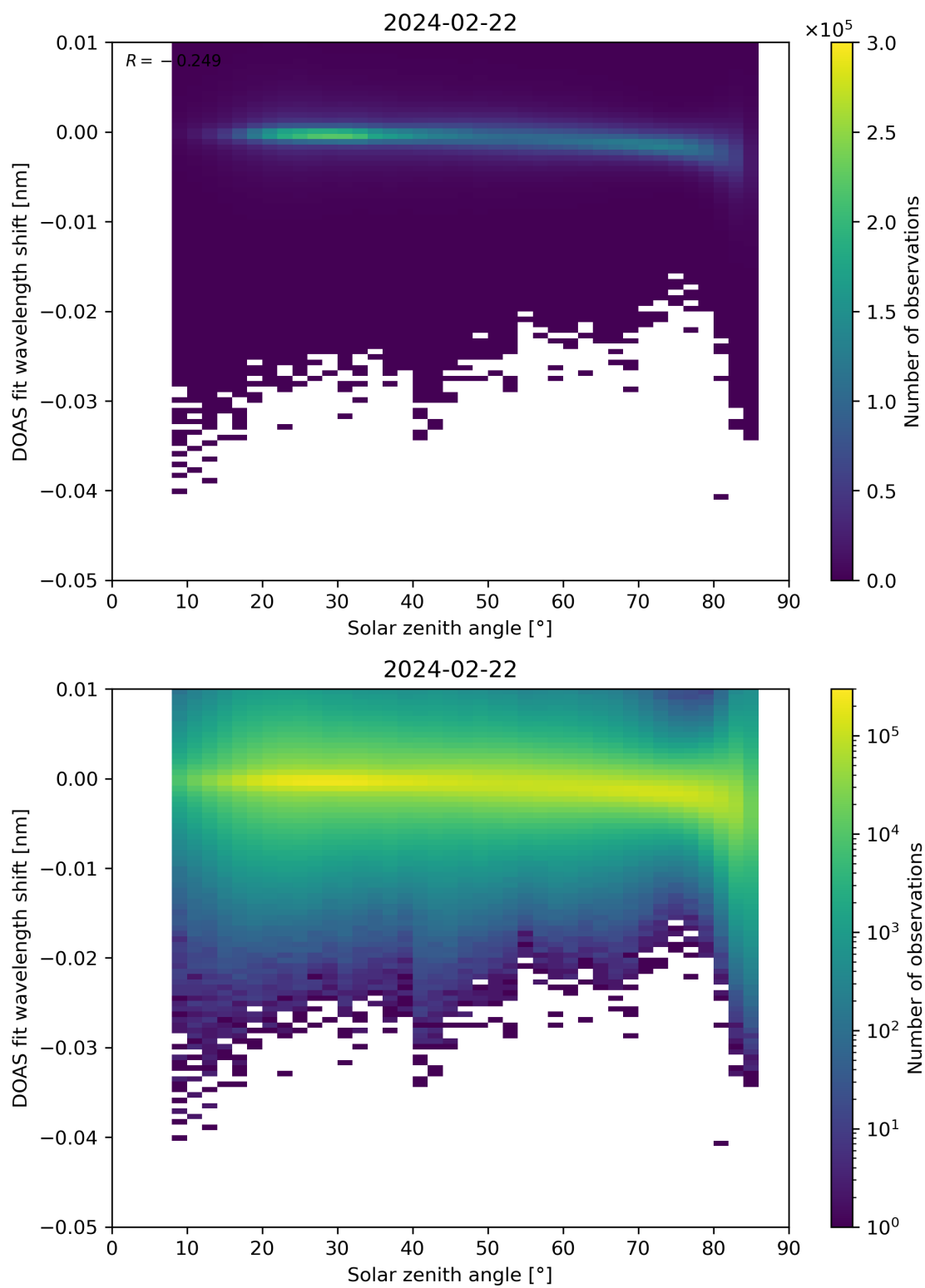
Figure 161: Scatter density plot of “Solar zenith angle” against “DOAS fit wavelength shift” for 2024-02-22 to 2024-02-23.
