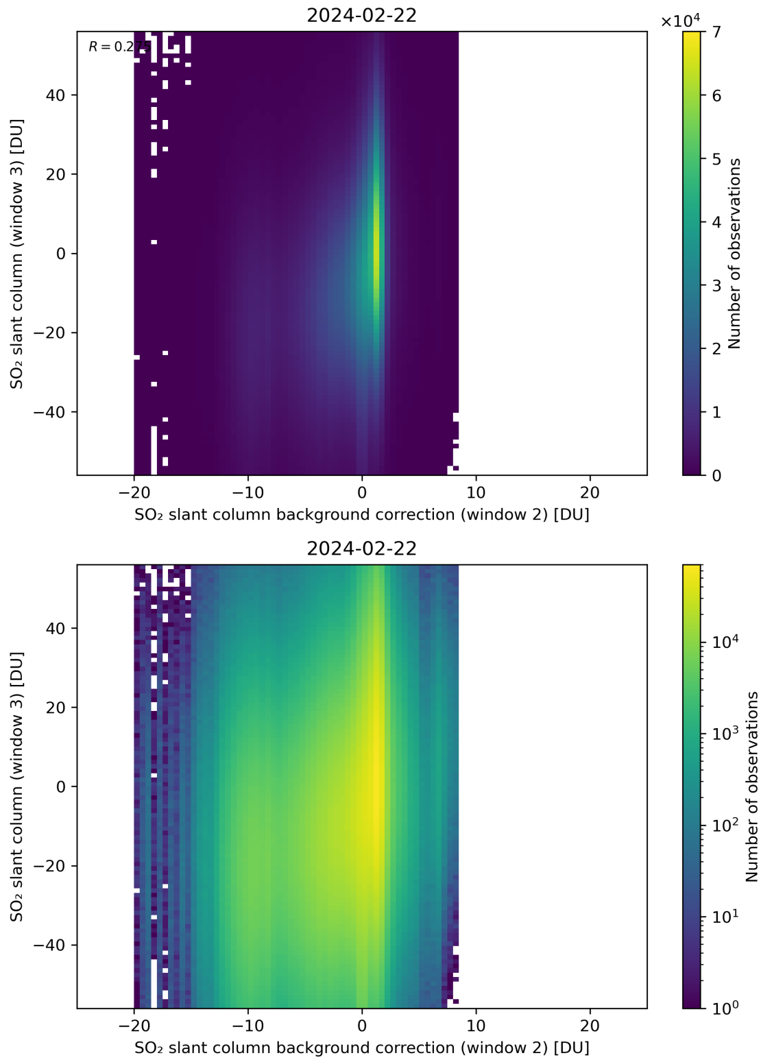
Figure 117: Scatter density plot of “SO 2 slant column background correction (window 2)” against “SO 2 slant column (window 3)” for 2024-02-22 to 2024-02-23.
