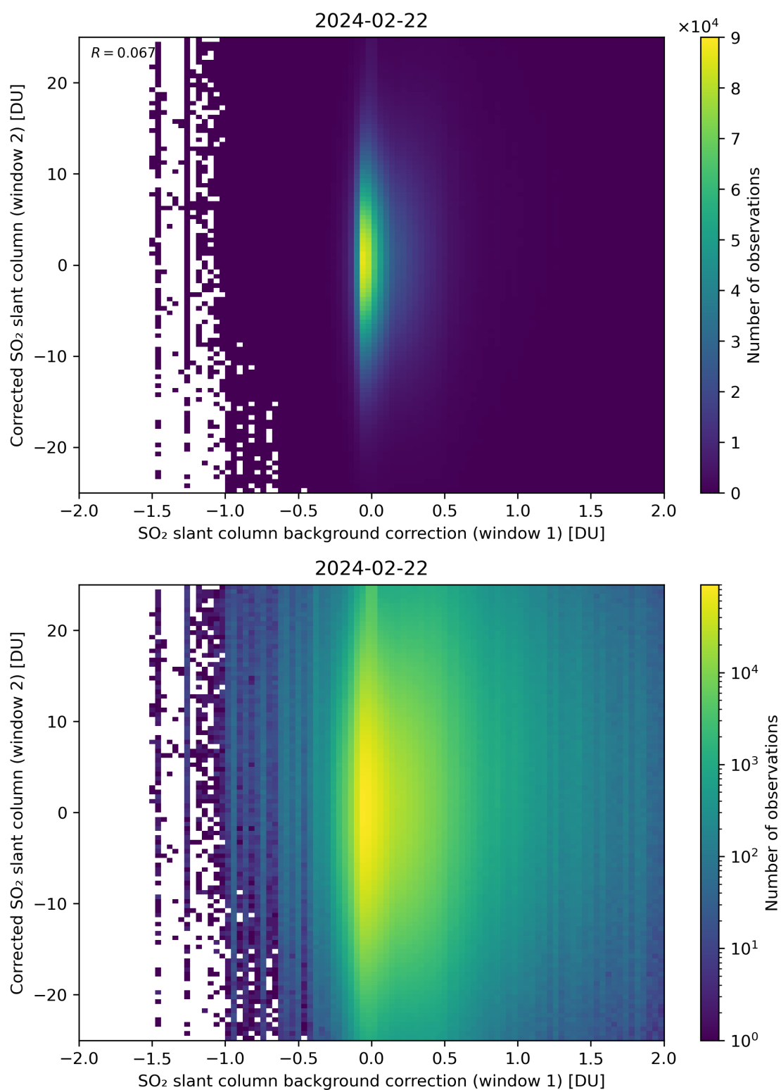
Figure 104: Scatter density plot of “SO 2 slant column background correction (window 1)” against “Corrected SO 2 slant column (window 2)” for 2024-02-22 to 2024-02-23.
