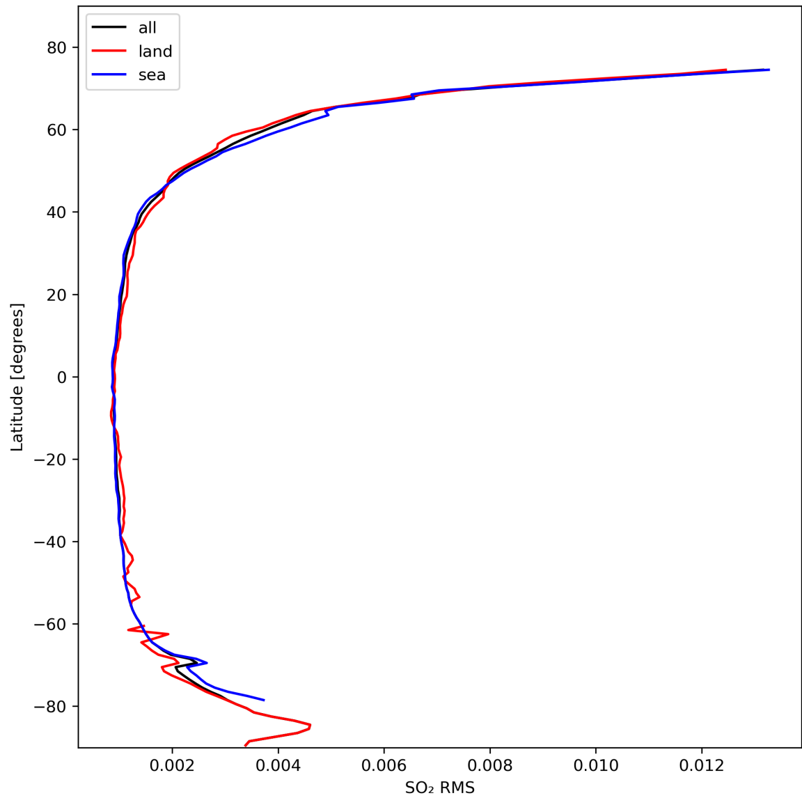
Figure 47: Zonal average of “SO 2 RMS” for 2024-02-22 to 2024-02-23.
