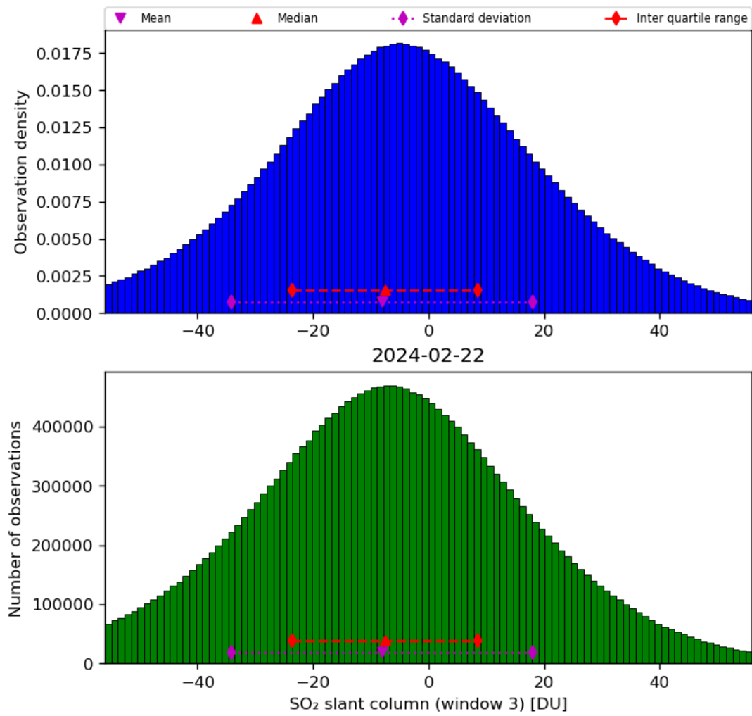
Figure 64: Histogram of “SO 2 slant column (window 3)” for 2024-02-22 to 2024-02-23
