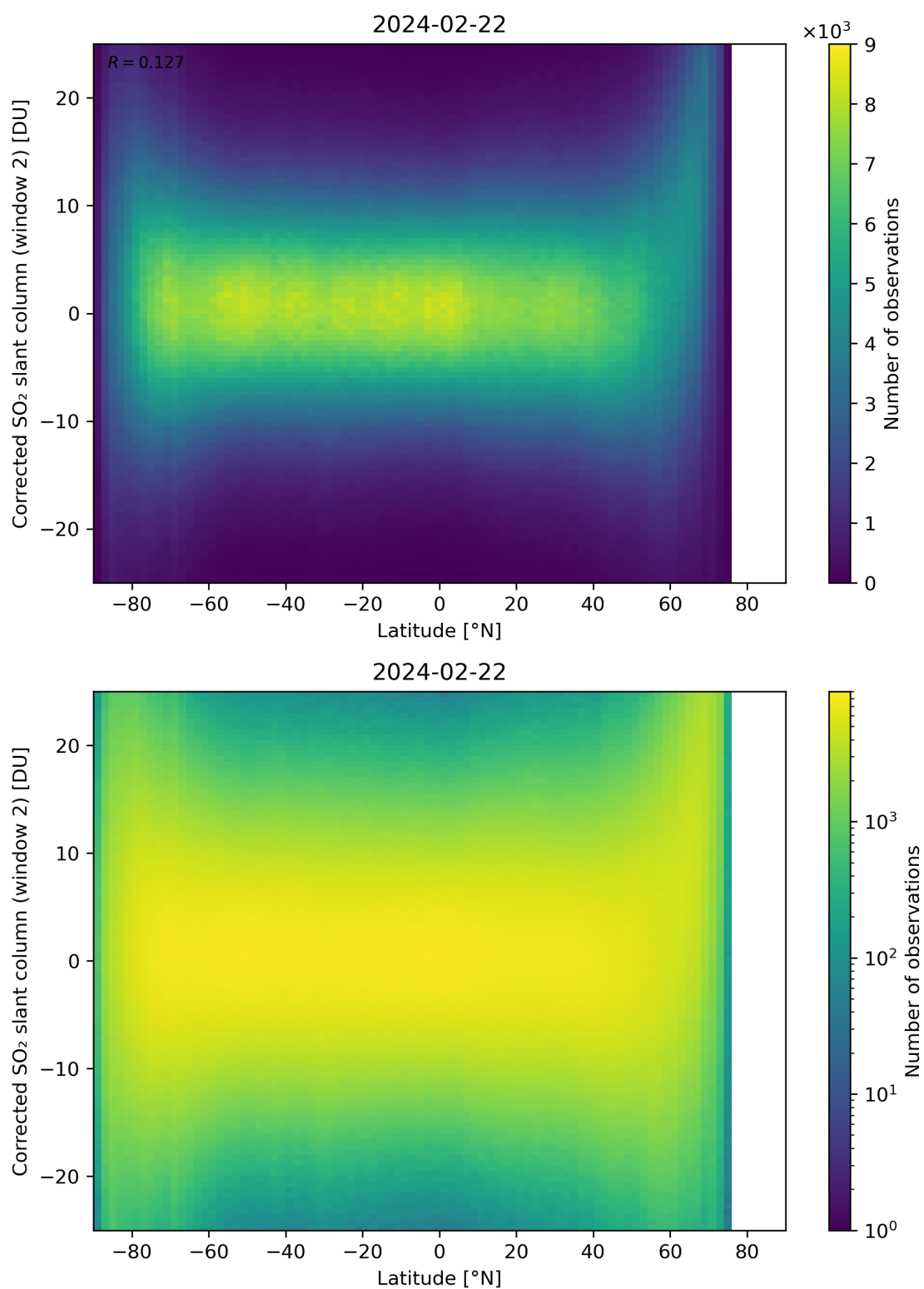
Figure 147: Scatter density plot of “Latitude” against “Corrected SO 2 slant column (window 2)” for 2024-02-22 to 2024-02-23.
