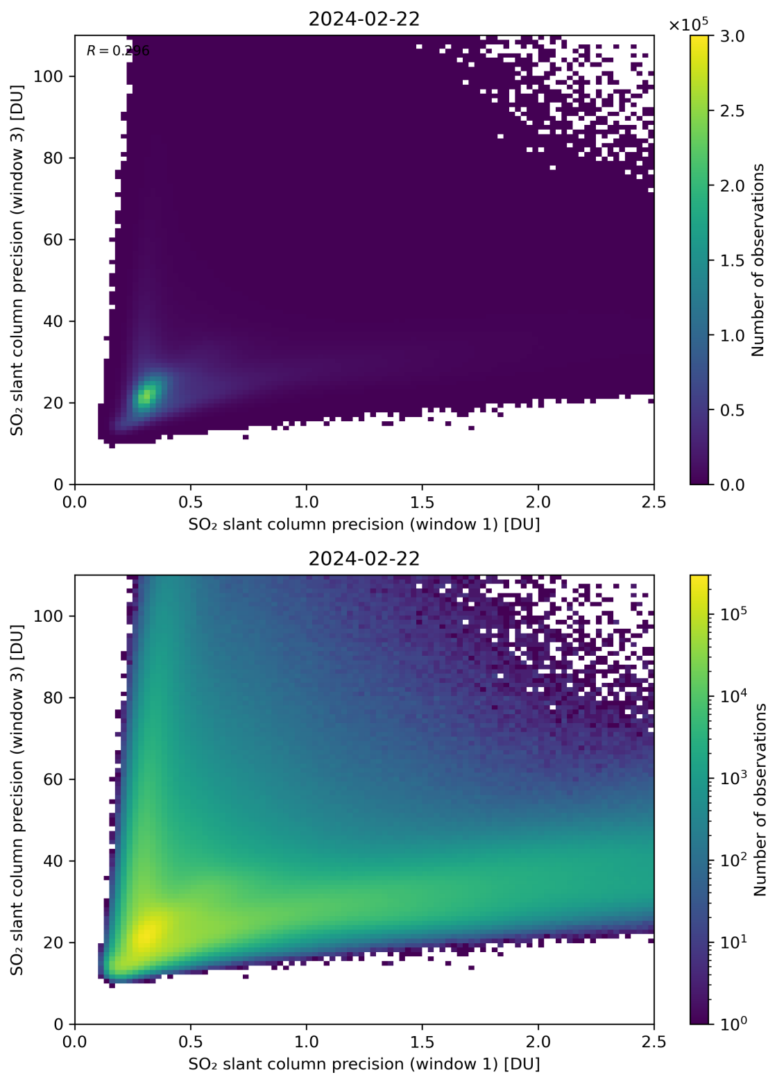
Figure 229: Scatter density plot of “SO 2 slant column precision (window 1)” against “SO 2 slant column precision (window 3)” for 2024-02-22 to 2024-02-23.
