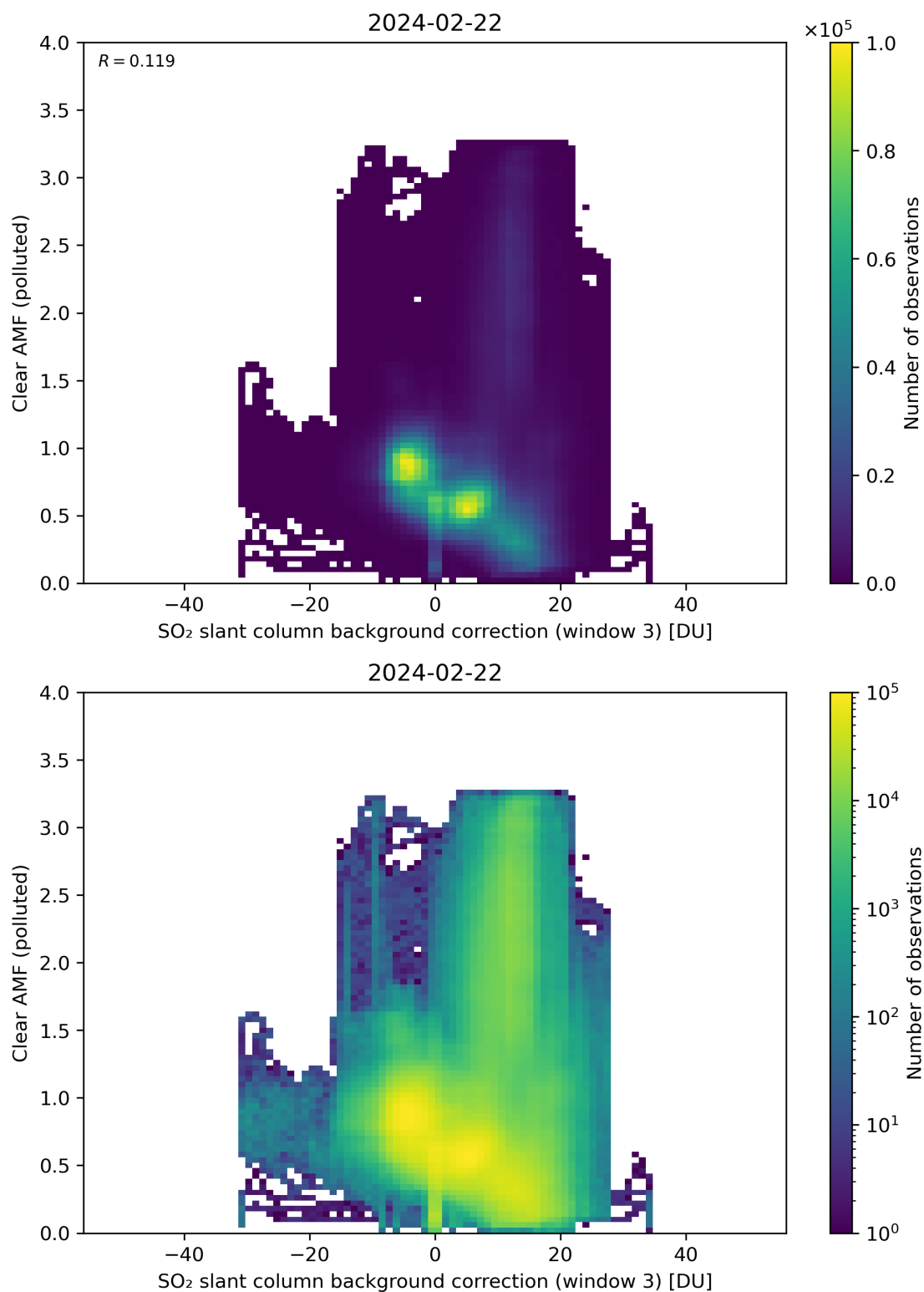
Figure 124: Scatter density plot of “SO 2 slant column background correction (window 3)” against “Clear AMF (polluted)” for 2024-02-22 to 2024-02-23.
