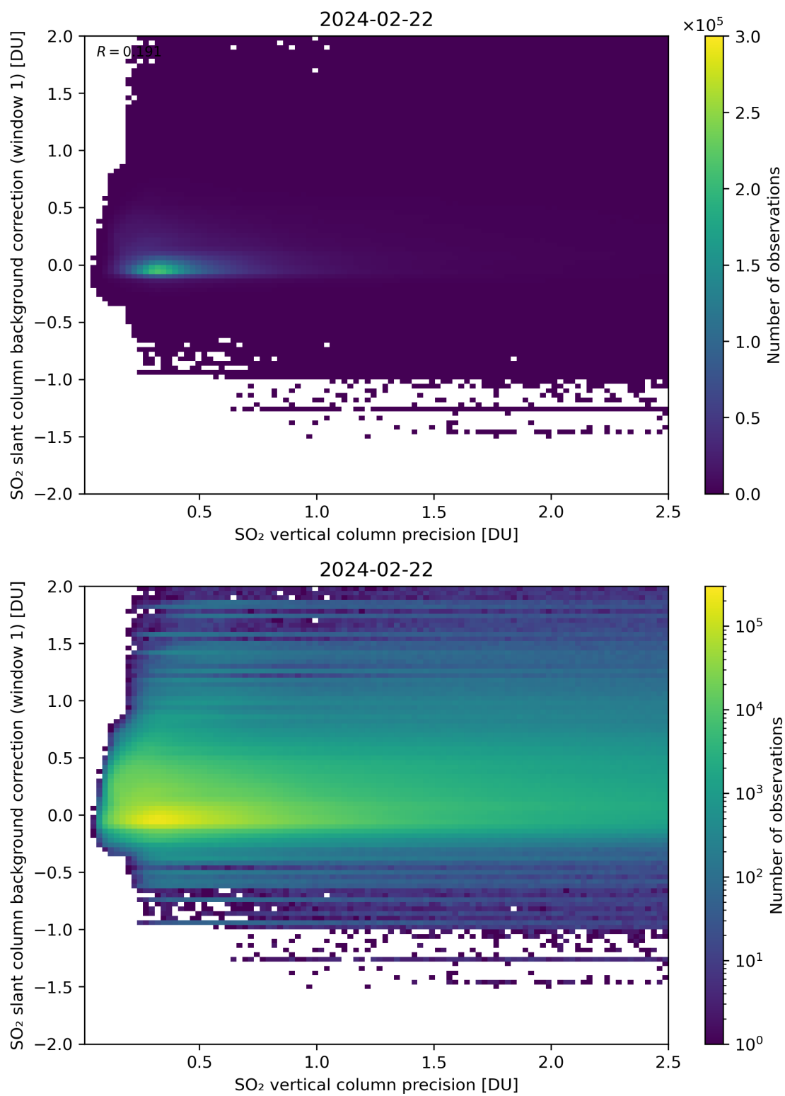
Figure 279: Scatter density plot of “SO 2 vertical column precision” against “SO 2 slant column background correction (window 1)” for 2024-02-22 to 2024-02-23.
