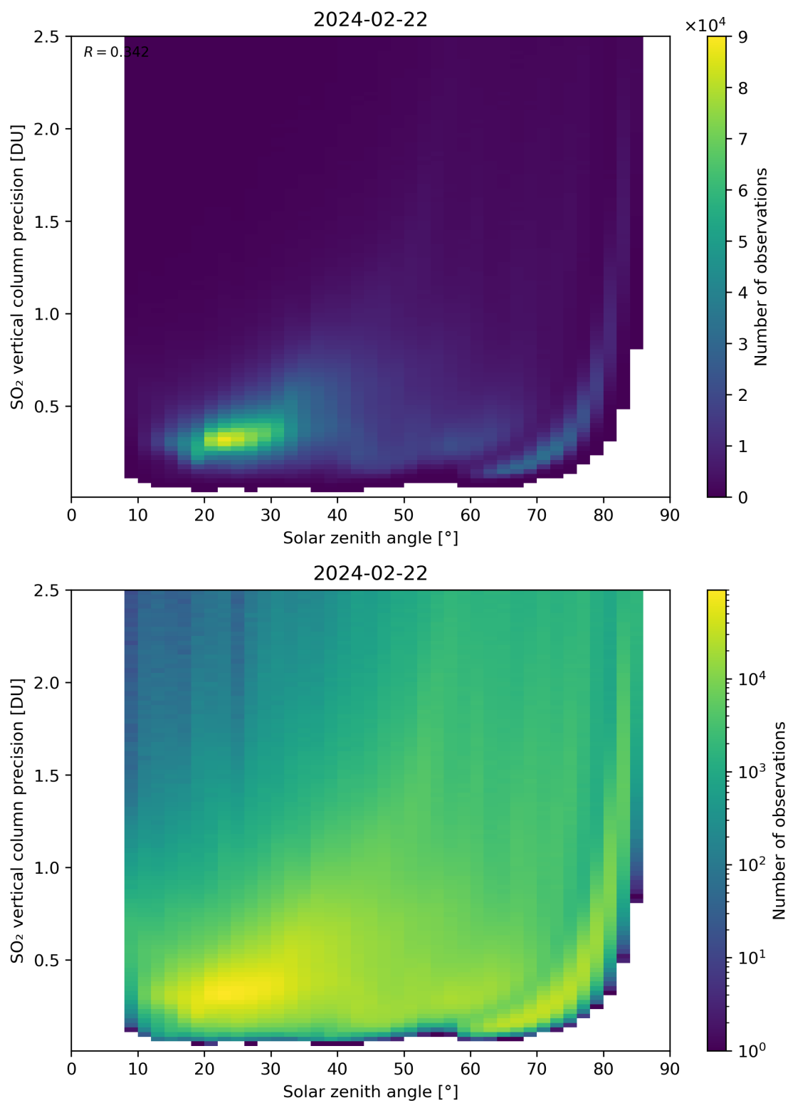
Figure 177: Scatter density plot of “Solar zenith angle” against “SO 2 vertical column precision” for 2024-02-22 to 2024-02-23.
