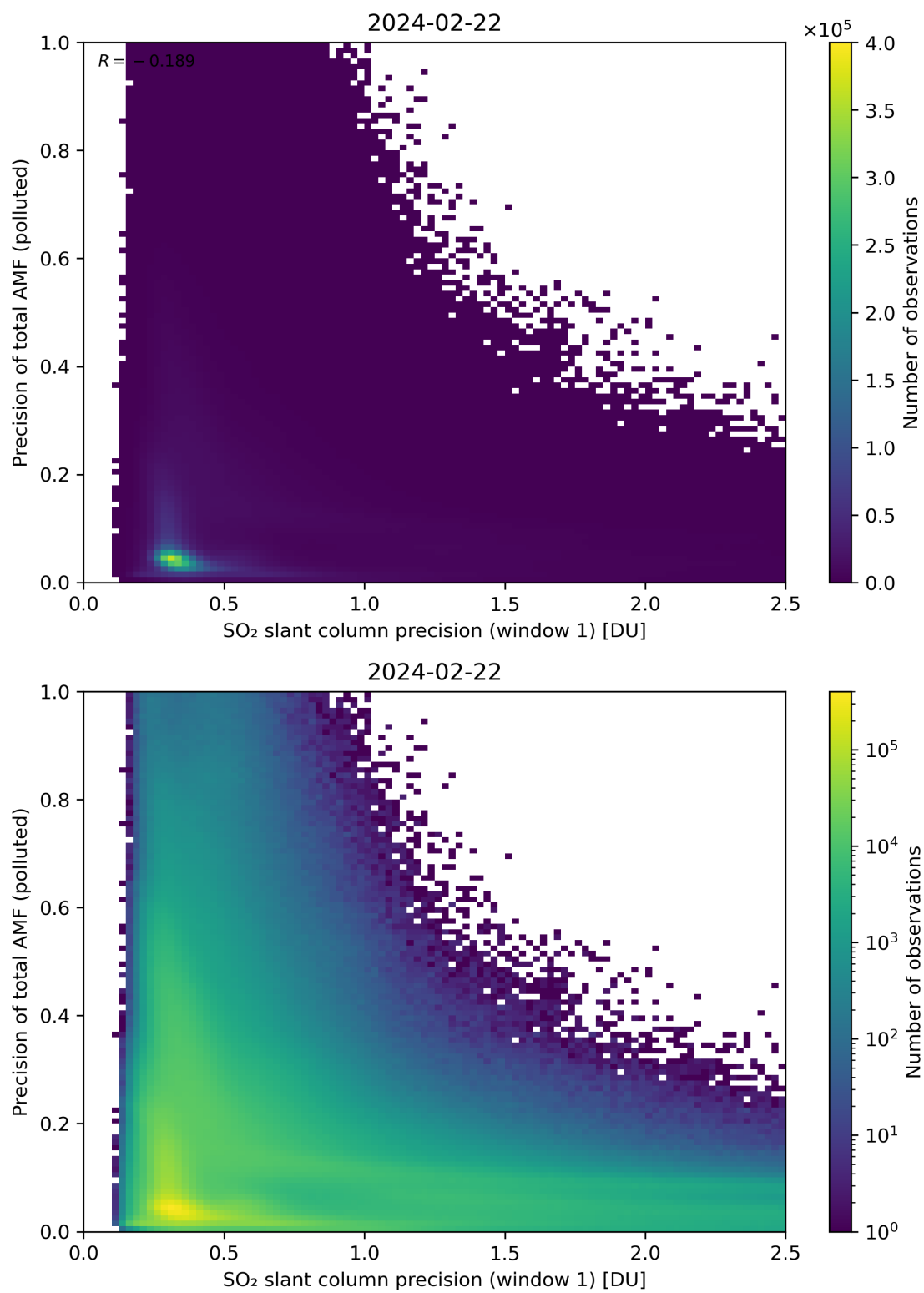
Figure 231: Scatter density plot of “SO 2 slant column precision (window 1)” against “Precision of total AMF (polluted)” for 2024-02-22 to 2024-02-23.
