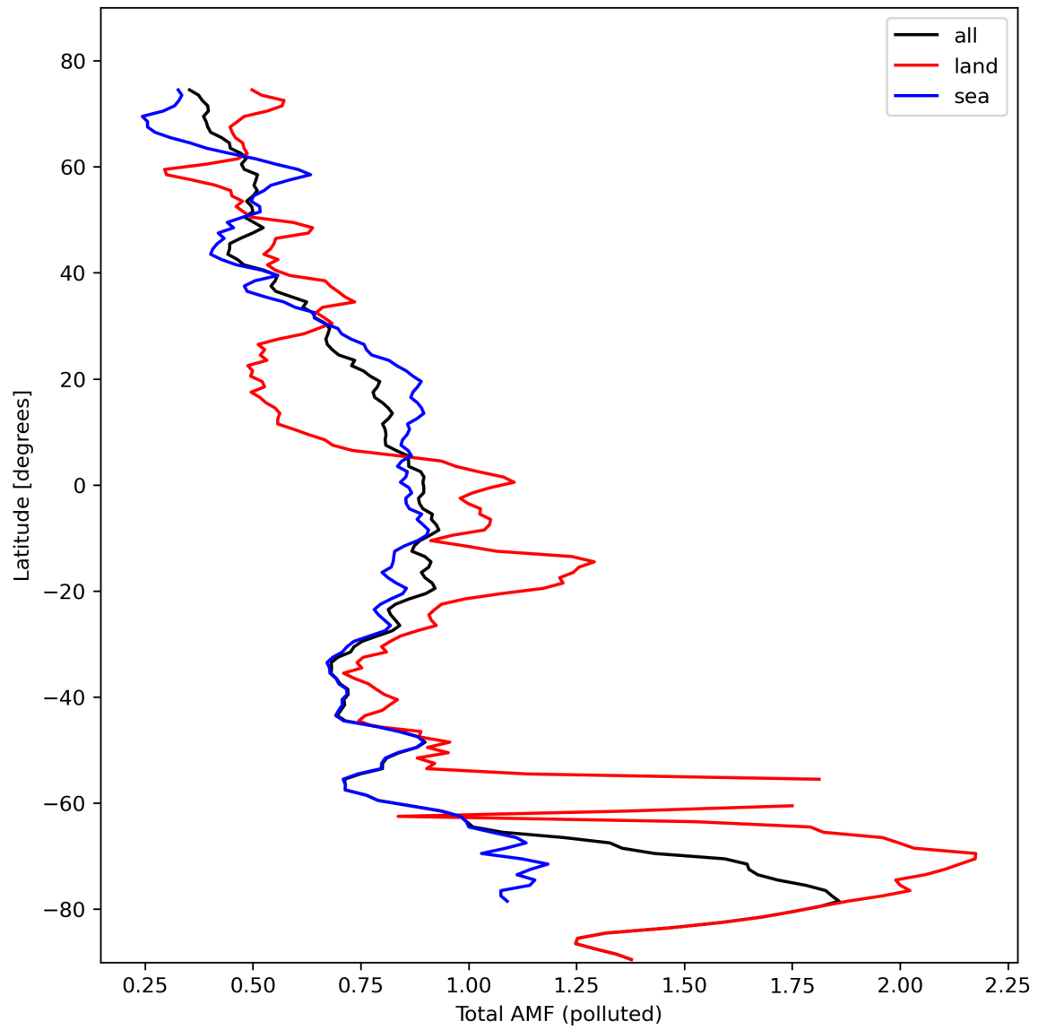
Figure 48: Zonal average of “Total AMF (polluted)” for 2024-02-22 to 2024-02-23.
