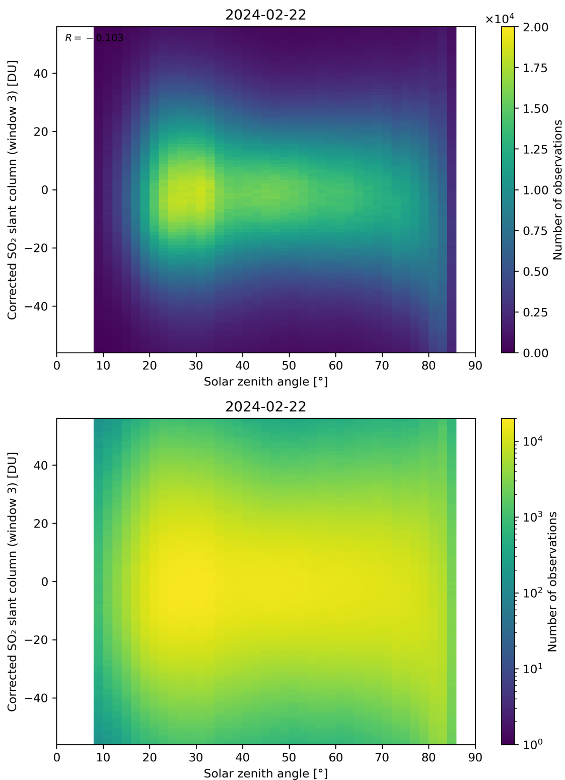
Figure 168: Scatter density plot of “Solar zenith angle” against “Corrected SO 2 slant column (window 3)” for 2024-02-22 to 2024-02-23.
