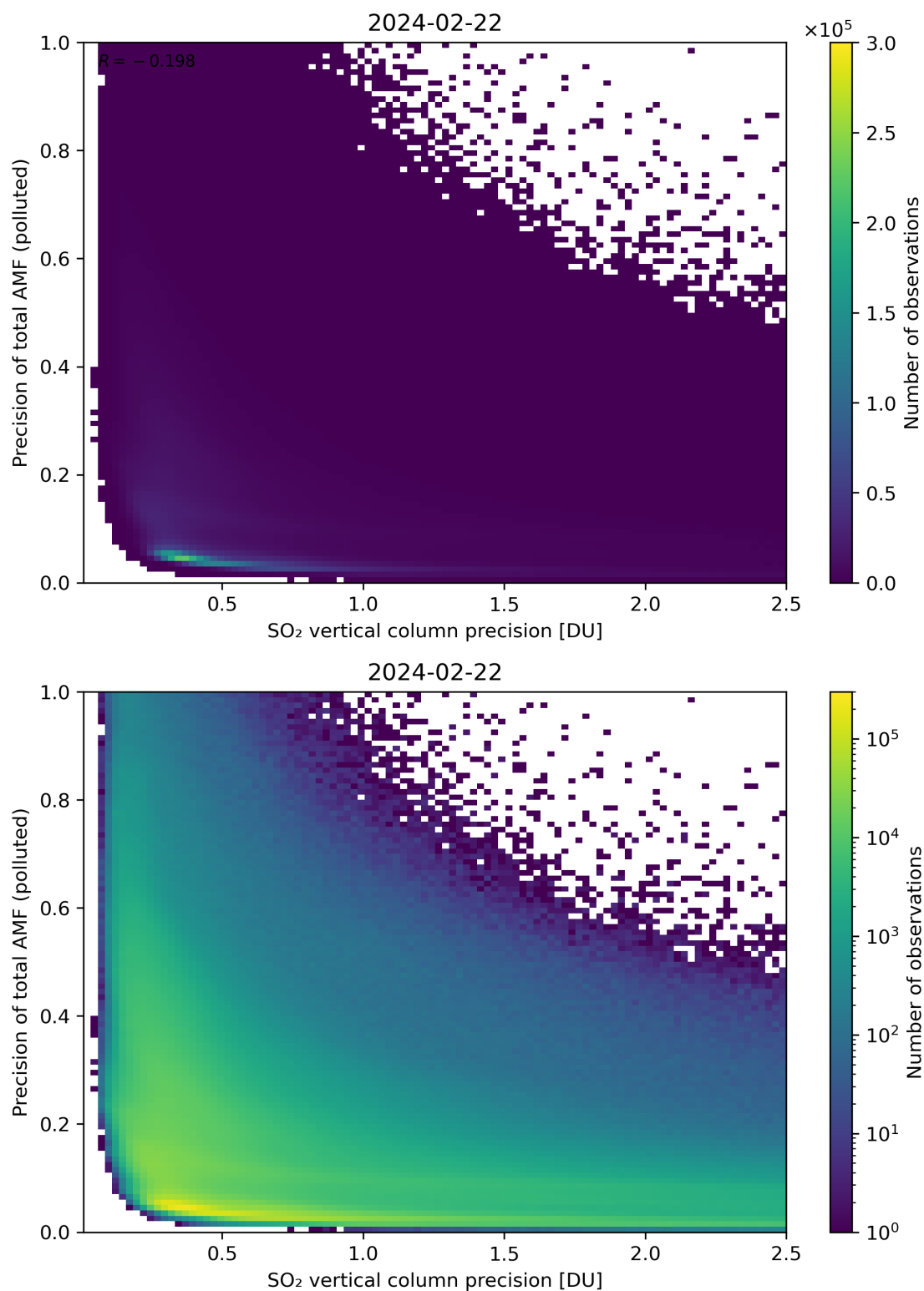
Figure 295: Scatter density plot of “SO 2 vertical column precision” against “Precision of total AMF (polluted)” for 2024-02-22 to 2024-02-23.
