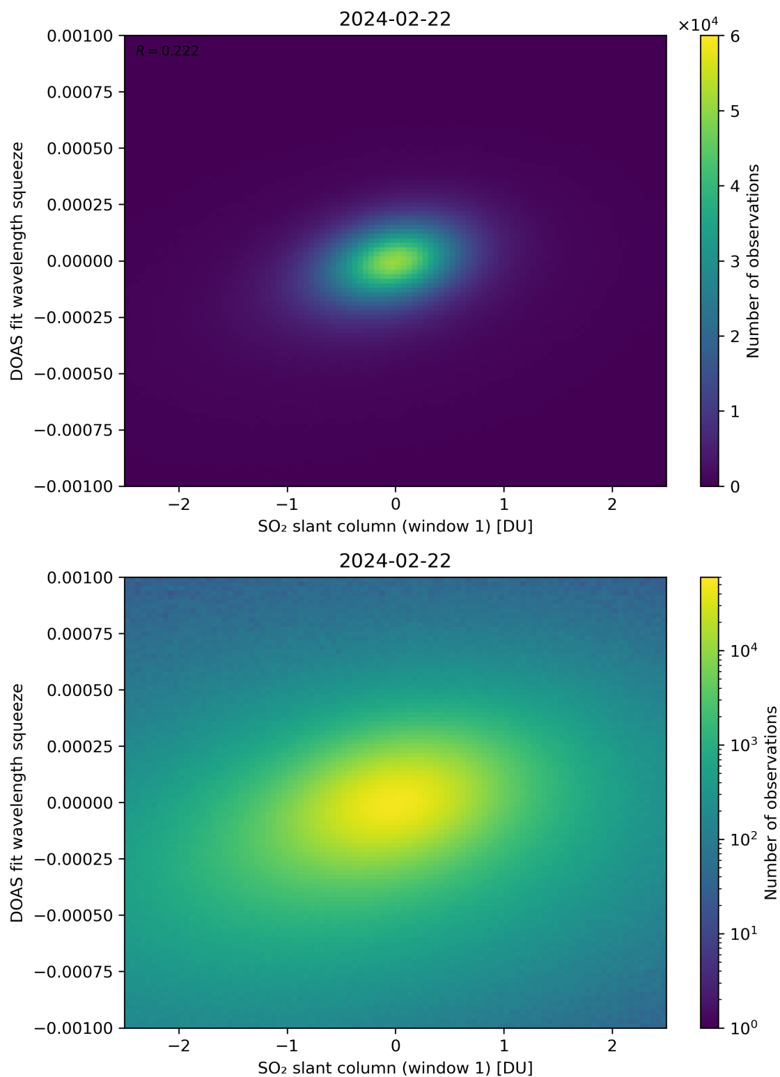
Figure 216: Scatter density plot of “SO 2 slant column (window 1)” against “DOAS fit wavelength squeeze” for 2024-02-22 to 2024-02-23.
