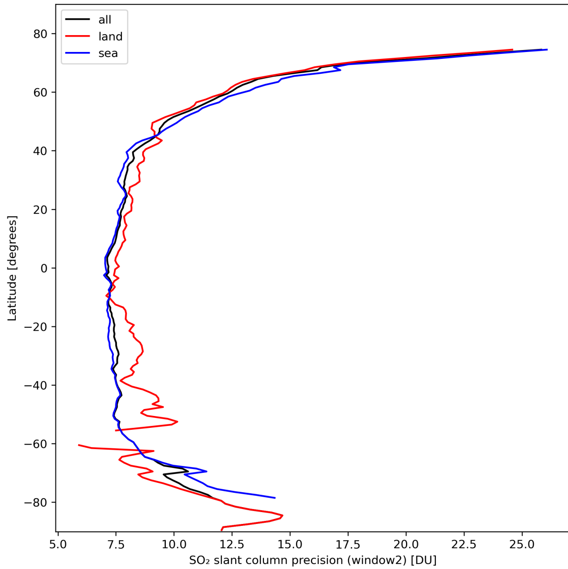
Figure 38: Zonal average of “SO 2 slant column precision (window2)” for 2024-02-22 to 2024-02-23.
