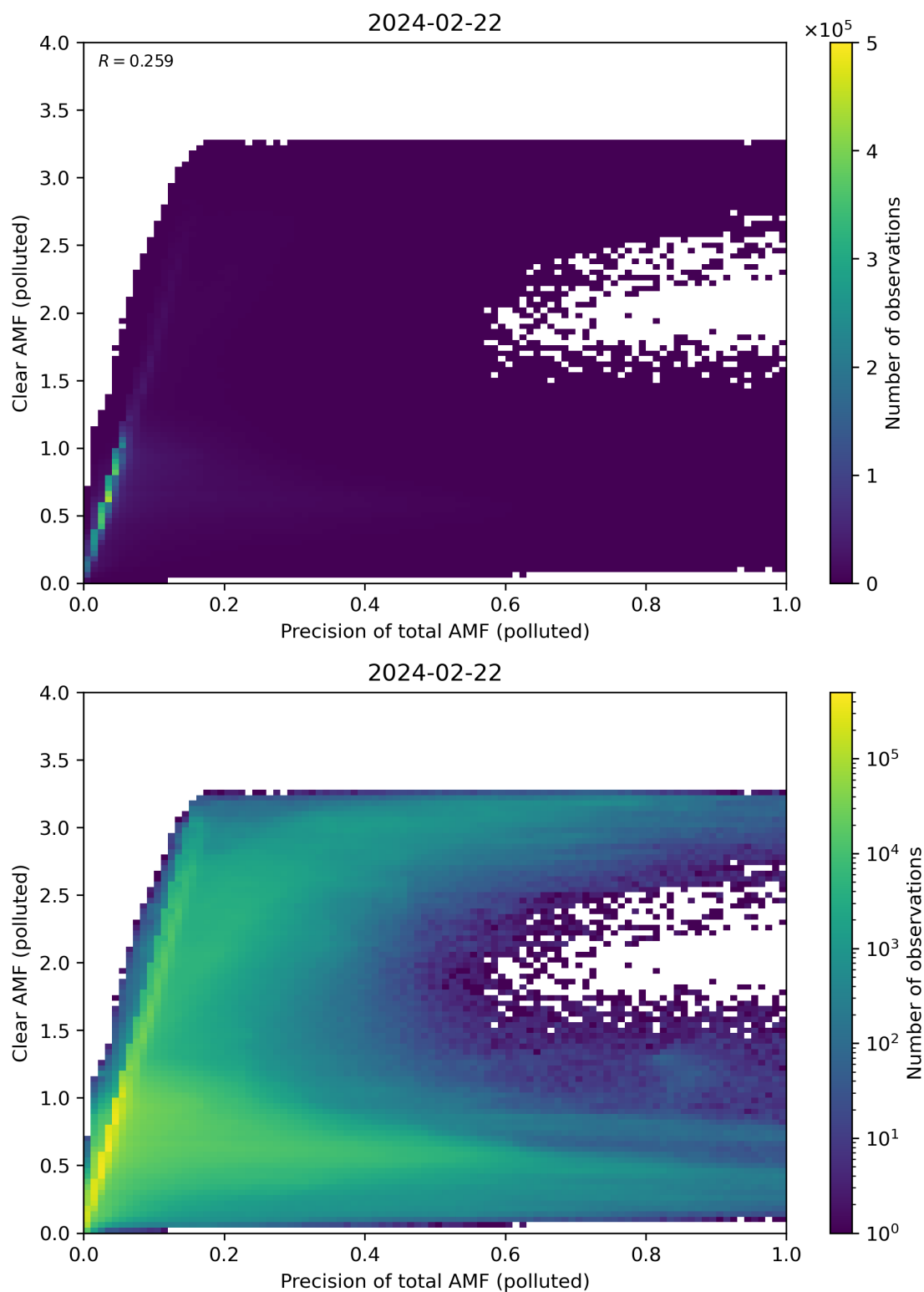
Figure 270: Scatter density plot of “Precision of total AMF (polluted)” against “Clear AMF (polluted)” for 2024-02-22 to 2024-02-23.
