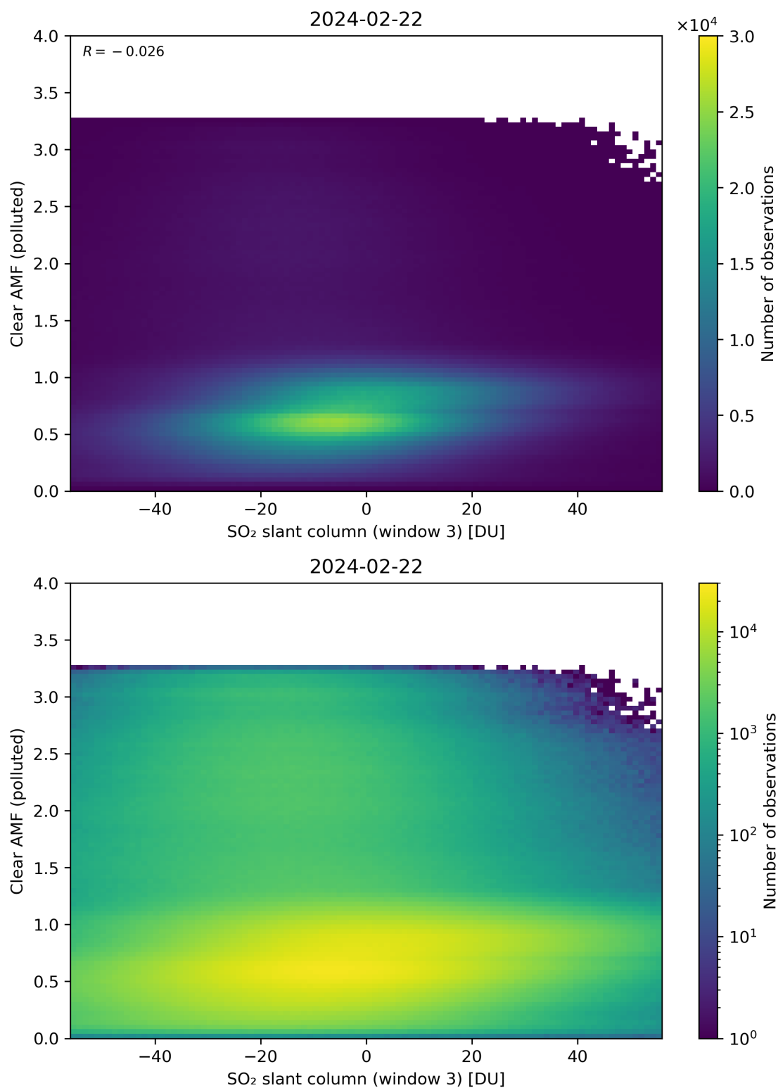
Figure 265: Scatter density plot of “SO 2 slant column (window 3)” against “Clear AMF (polluted)” for 2024-02-22 to 2024-02-23.
