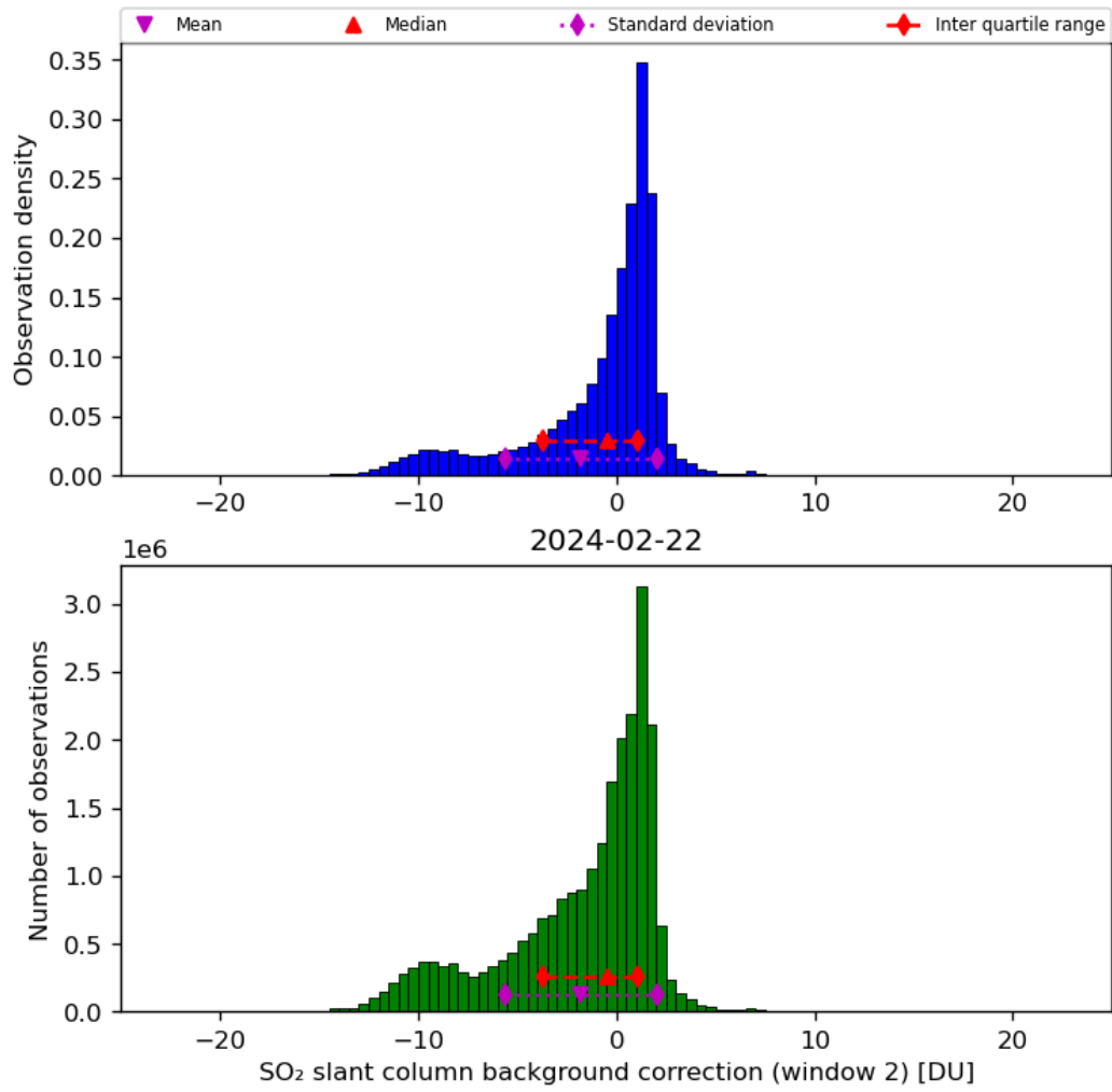
Figure 63: Histogram of “SO 2 slant column background correction (window 2)” for 2024-02-22 to 2024-02-23
