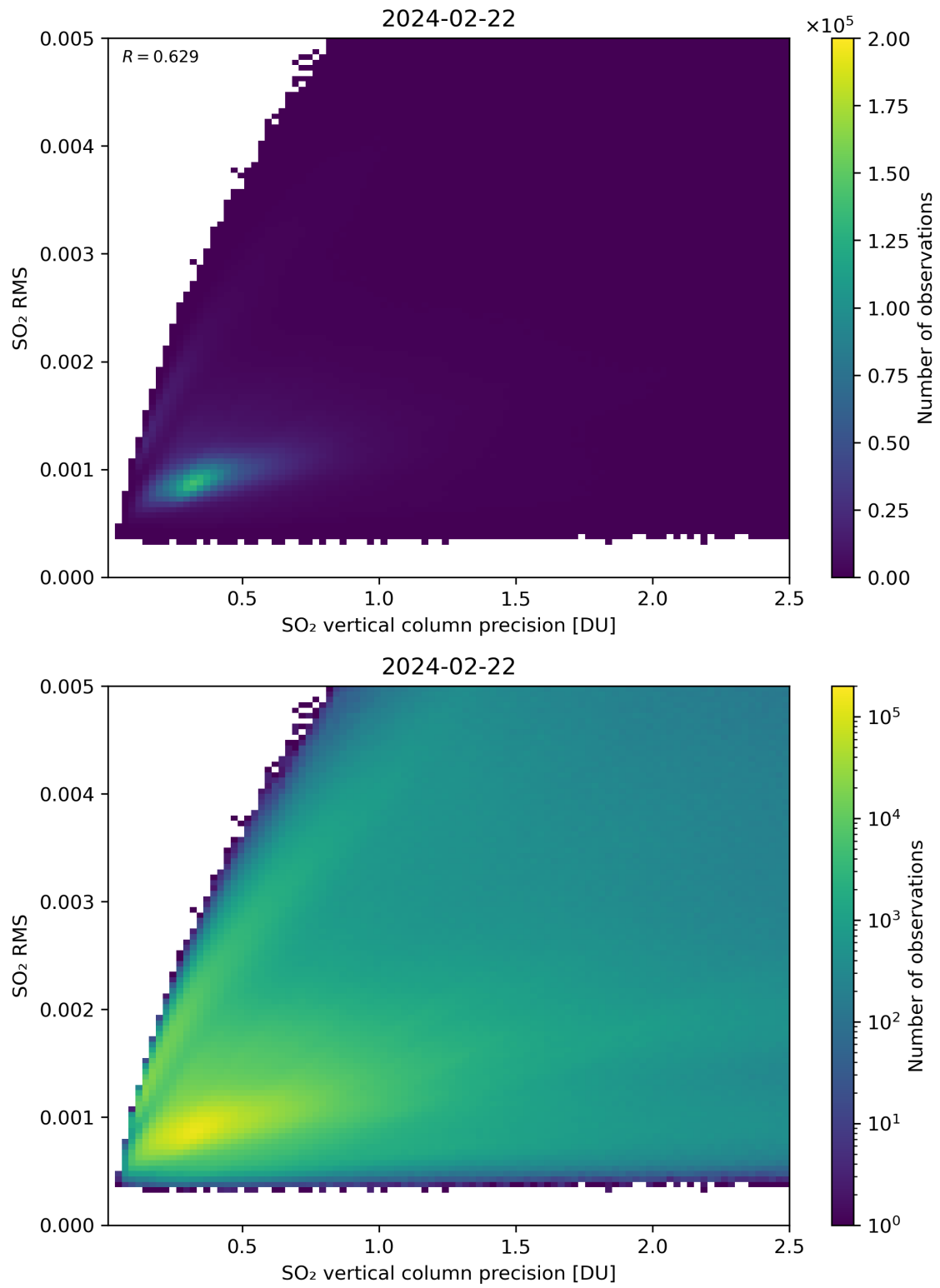
Figure 284: Scatter density plot of “SO 2 vertical column precision” against “SO 2 RMS” for 2024-02-22 to 2024-02-23.
