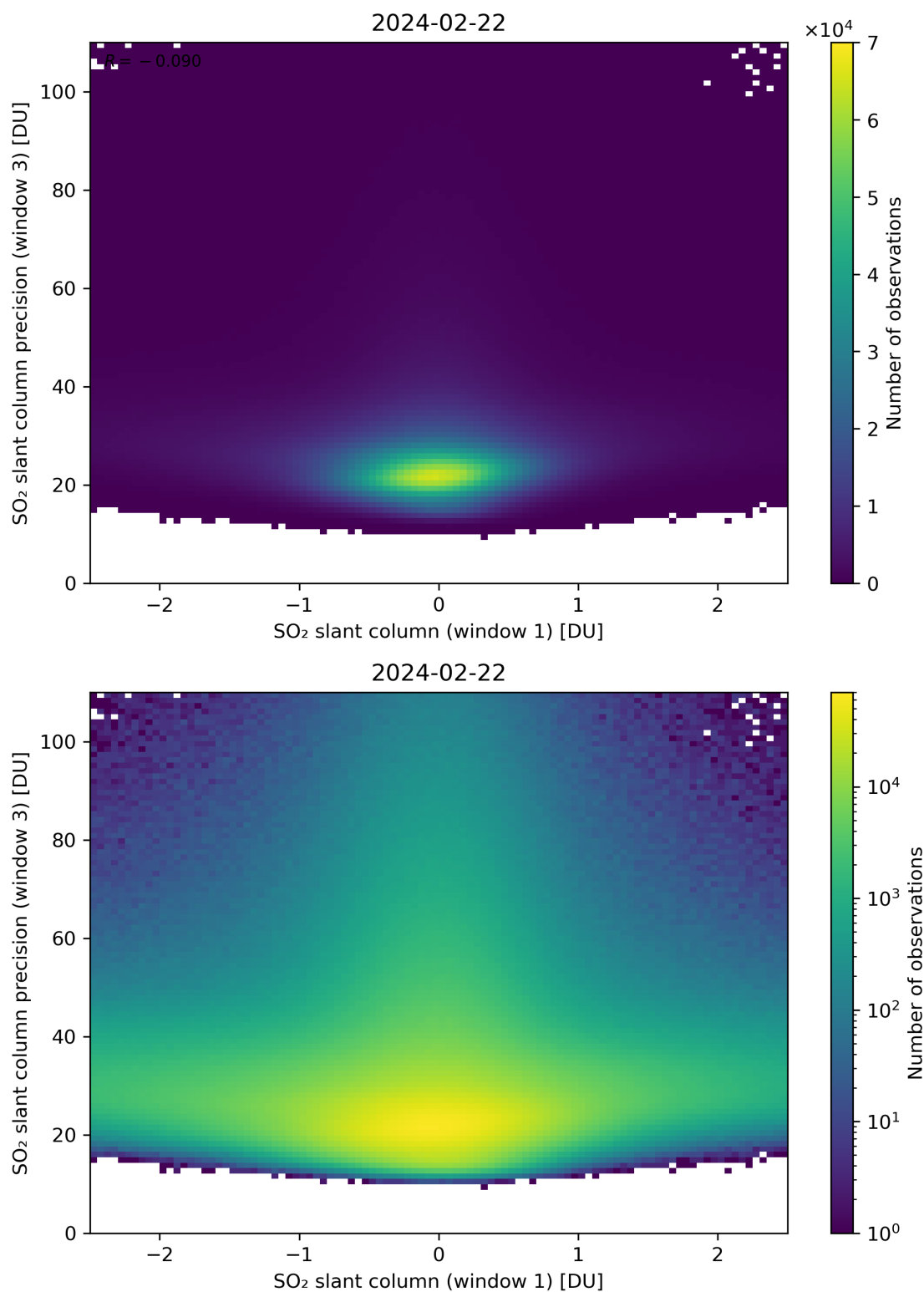
Figure 238: Scatter density plot of “SO 2 slant column (window 1)” against “SO 2 slant column precision (window 3)” for 2024-02-22 to 2024-02-23.
