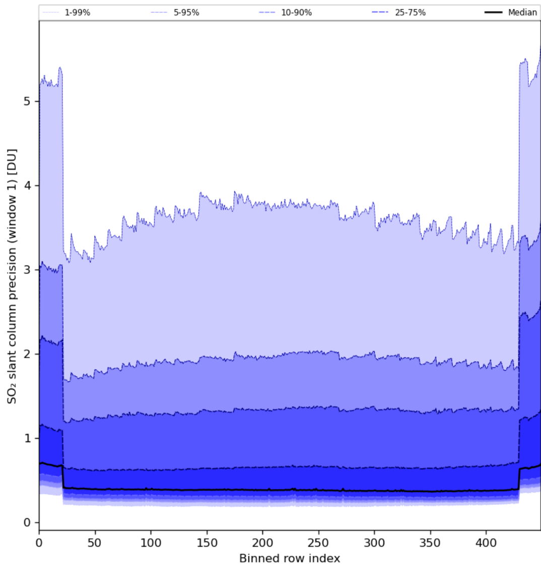
Figure 80: Along track statistics of “SO 2 slant column precision (window 1)” for 2024-02-22 to 2024-02-23
