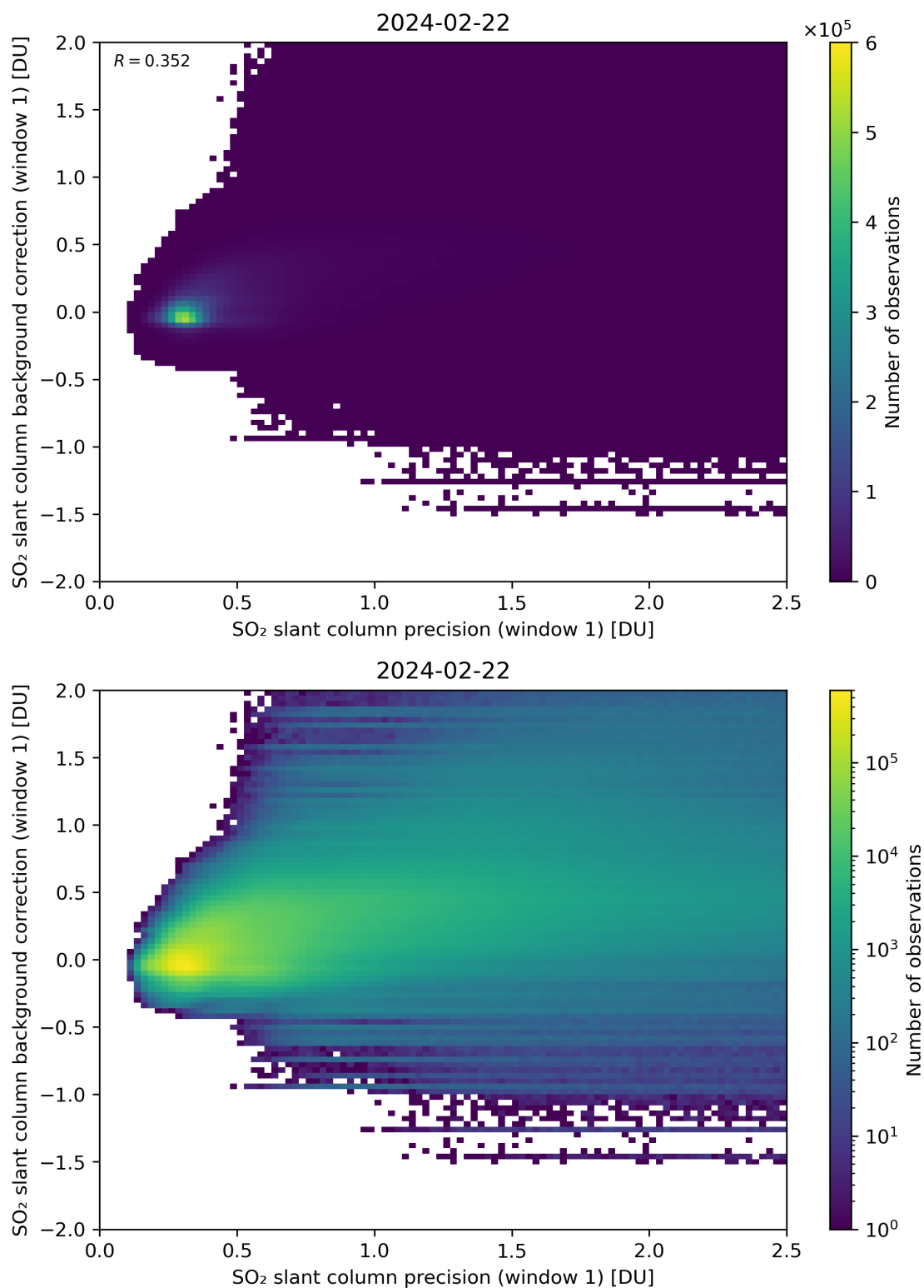
Figure 218: Scatter density plot of “SO 2 slant column precision (window 1)” against “SO 2 slant column background correction (window 1)” for 2024-02-22 to 2024-02-23.
