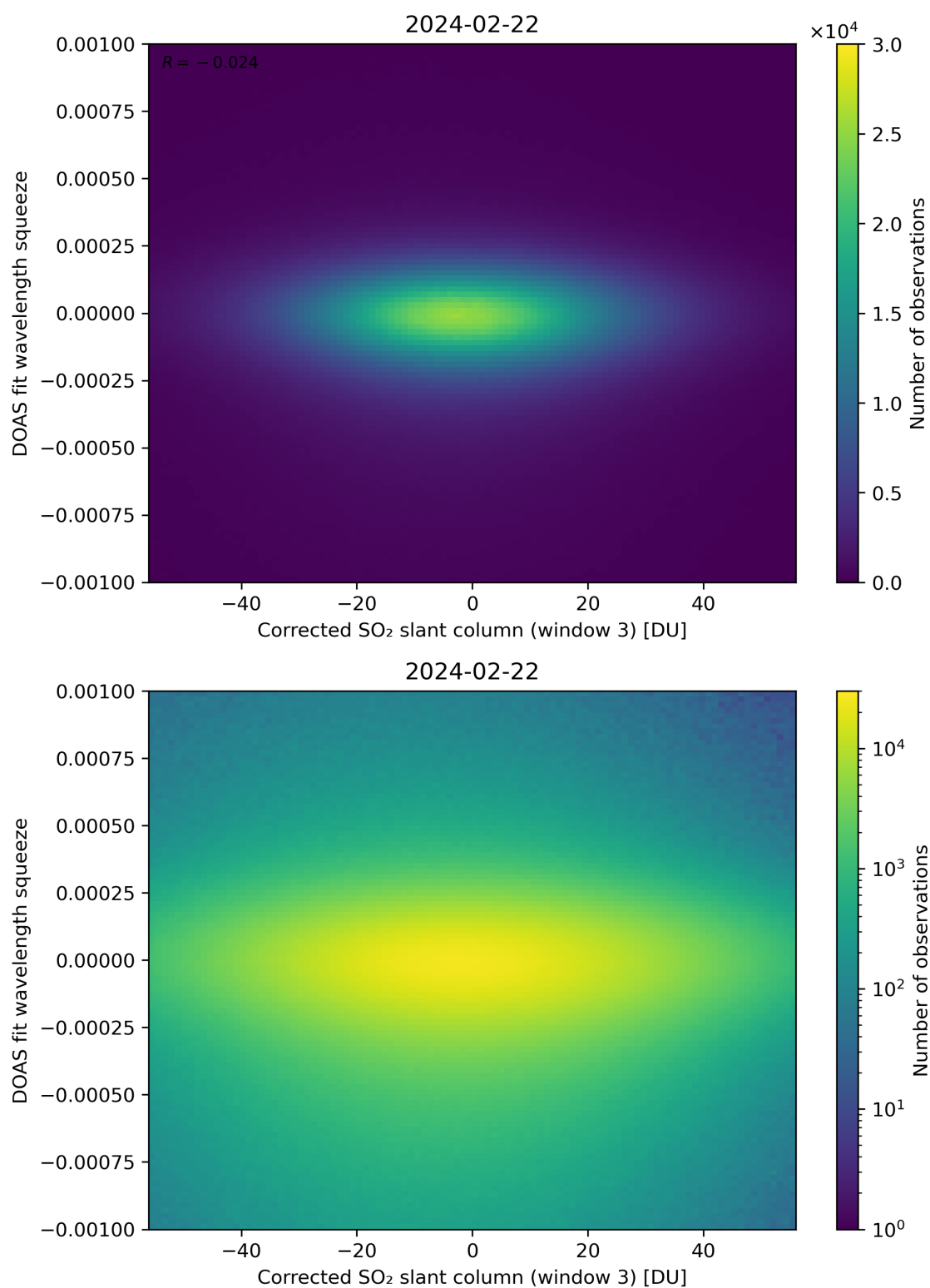
Figure 207: Scatter density plot of “Corrected SO 2 slant column (window 3)” against “DOAS fit wavelength squeeze” for 2024-02-22 to 2024-02-23.
