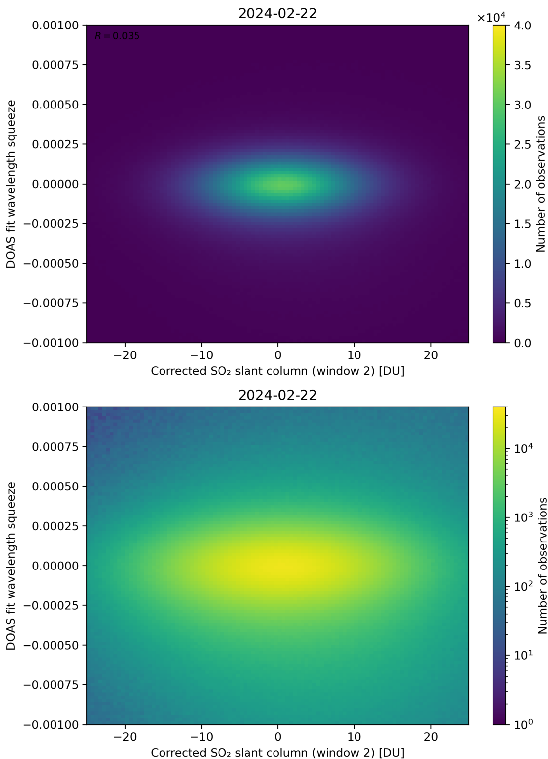
Figure 197: Scatter density plot of “Corrected SO 2 slant column (window 2)” against “DOAS fit wavelength squeeze” for 2024-02-22 to 2024-02-23.
