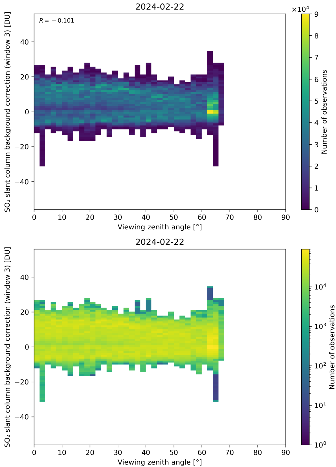
Figure 310: Scatter density plot of “Viewing zenith angle” against “SO 2 slant column background correction (window 3)” for 2024-02-22 to 2024-02-23.
