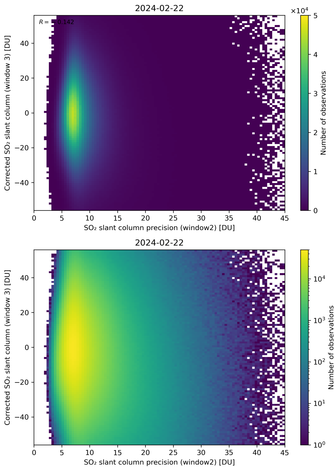
Figure 248: Scatter density plot of “SO 2 slant column precision (window2)” against “Corrected SO 2 slant column (window 3)” for 2024-02-22 to 2024-02-23.
