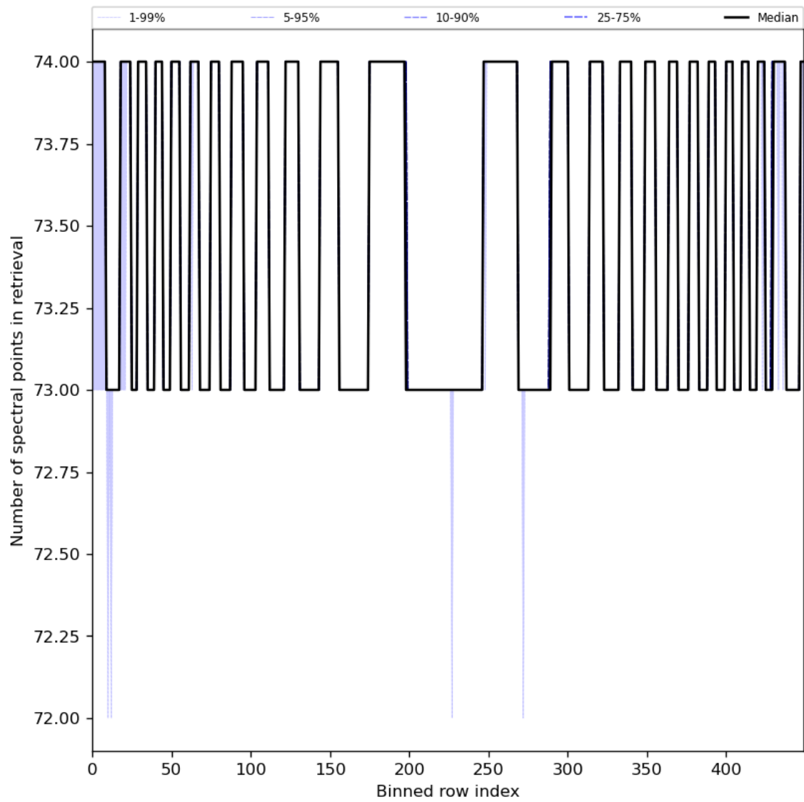
Figure 97: Along track statistics of “Number of spectral points in retrieval” for 2024-02-22 to 2024-02-23
