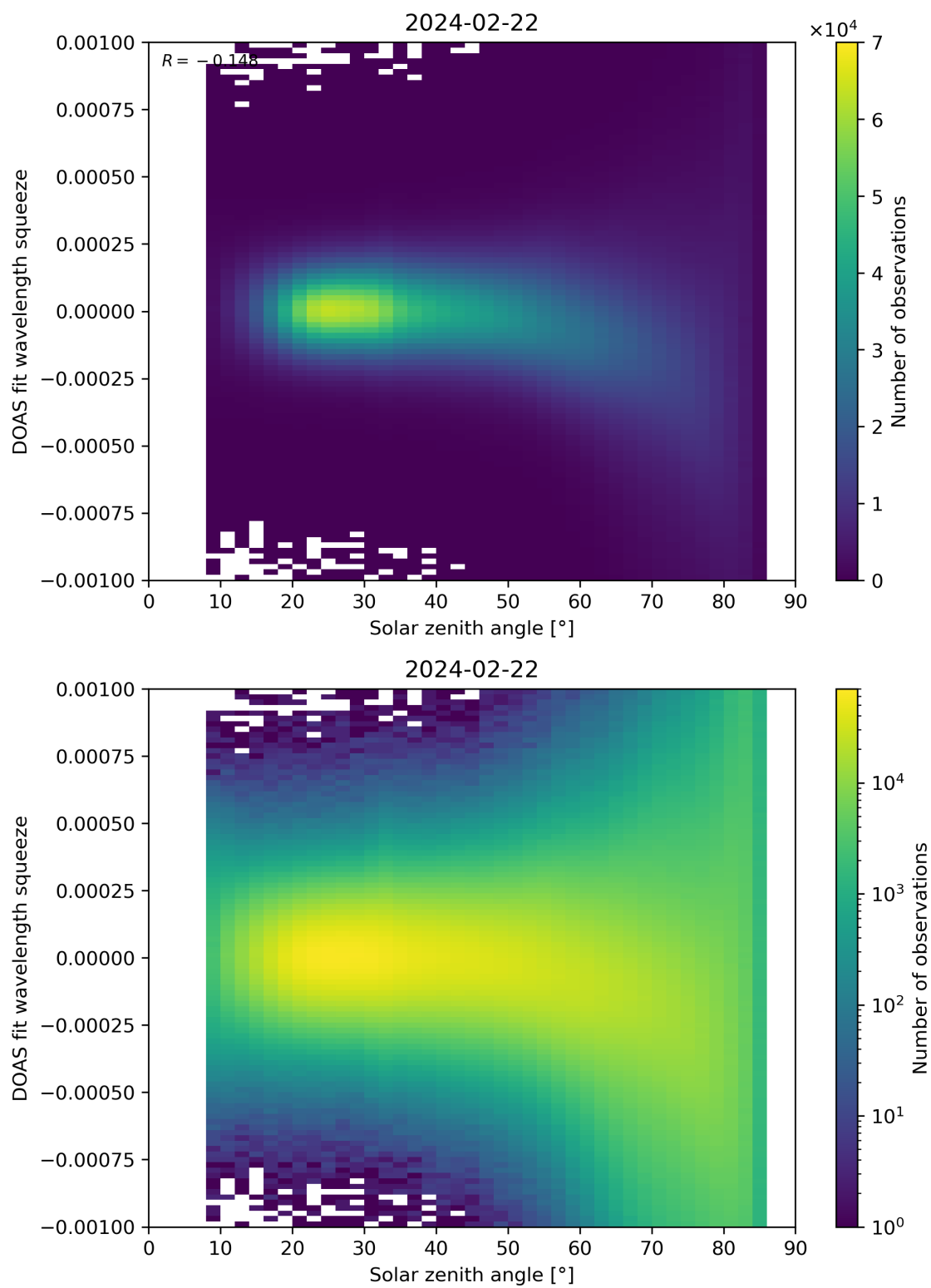
Figure 162: Scatter density plot of “Solar zenith angle” against “DOAS fit wavelength squeeze” for 2024-02-22 to 2024-02-23.
