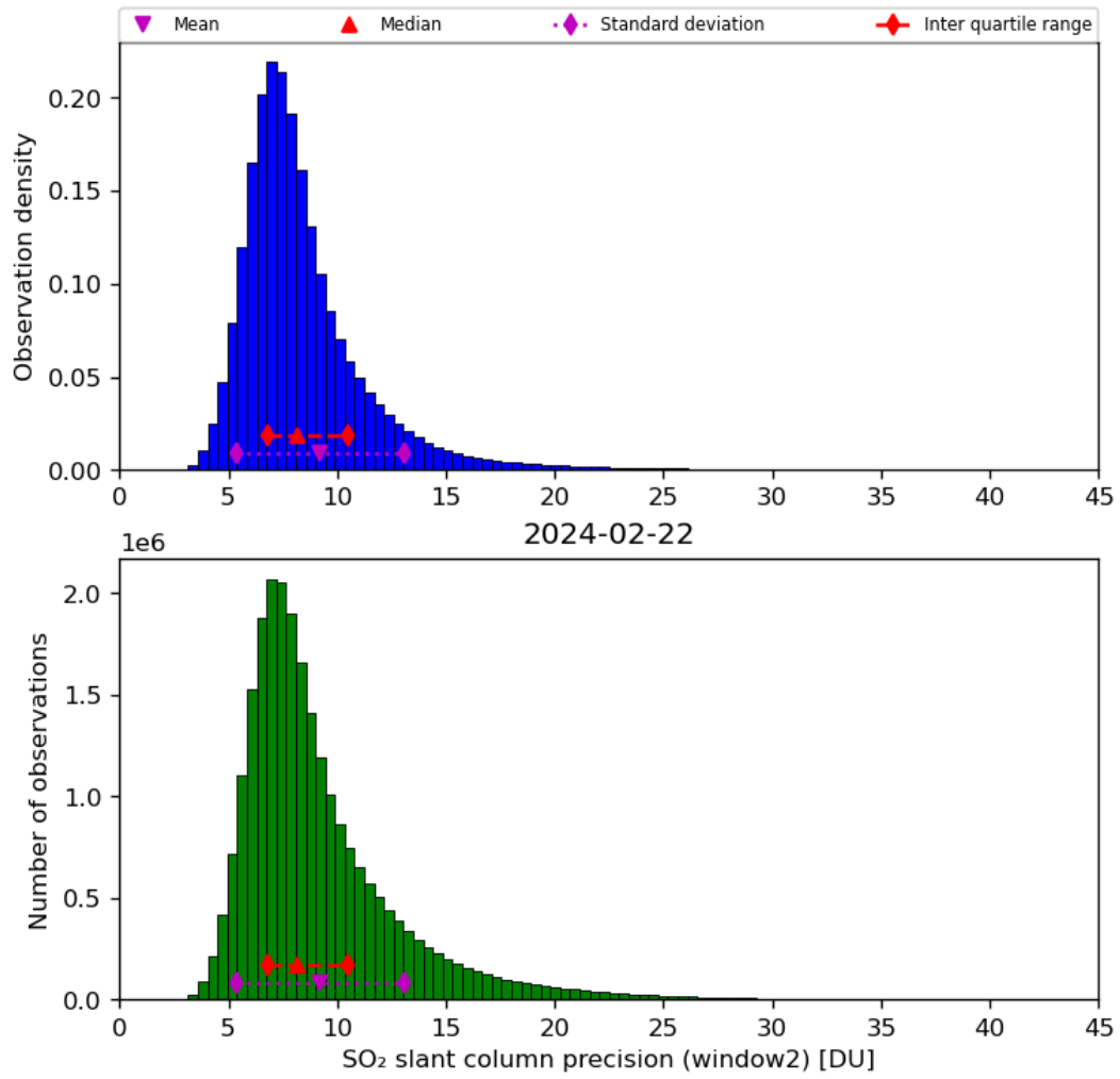
Figure 61: Histogram of “SO 2 slant column precision (window2)” for 2024-02-22 to 2024-02-23
