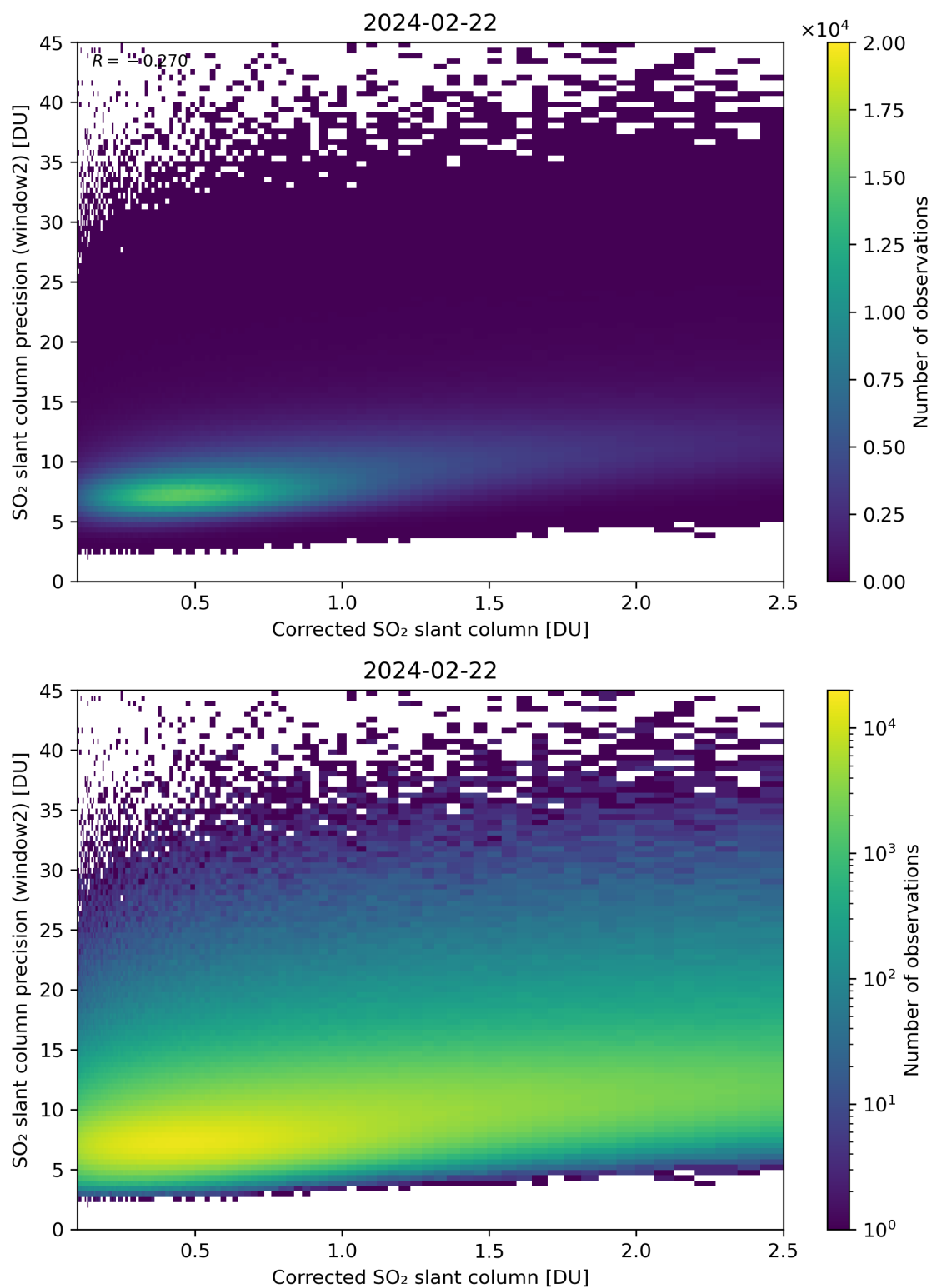
Figure 189: Scatter density plot of “Corrected SO 2 slant column” against “SO 2 slant column precision (window2)” for 2024-02-22 to 2024-02-23.
