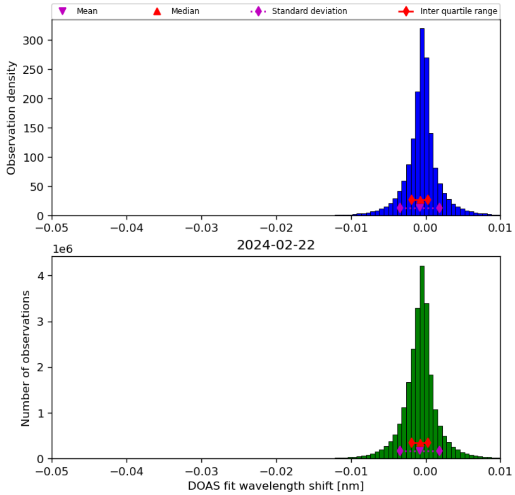
Figure 68: Histogram of “DOAS fit wavelength shift” for 2024-02-22 to 2024-02-23
