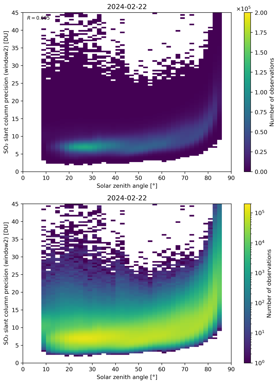
Figure 171: Scatter density plot of “Solar zenith angle” against “SO 2 slant column precision (window2)” for 2024-02-22 to 2024-02-23.
