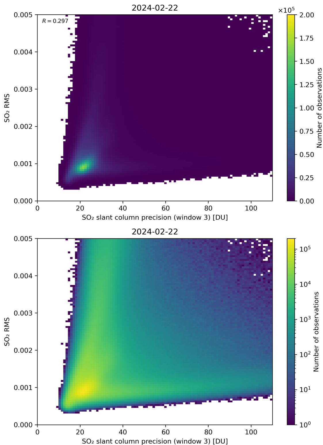
Figure 260: Scatter density plot of “SO 2 slant column precision (window 3)” against “SO 2 RMS” for 2024-02-22 to 2024-02-23.
