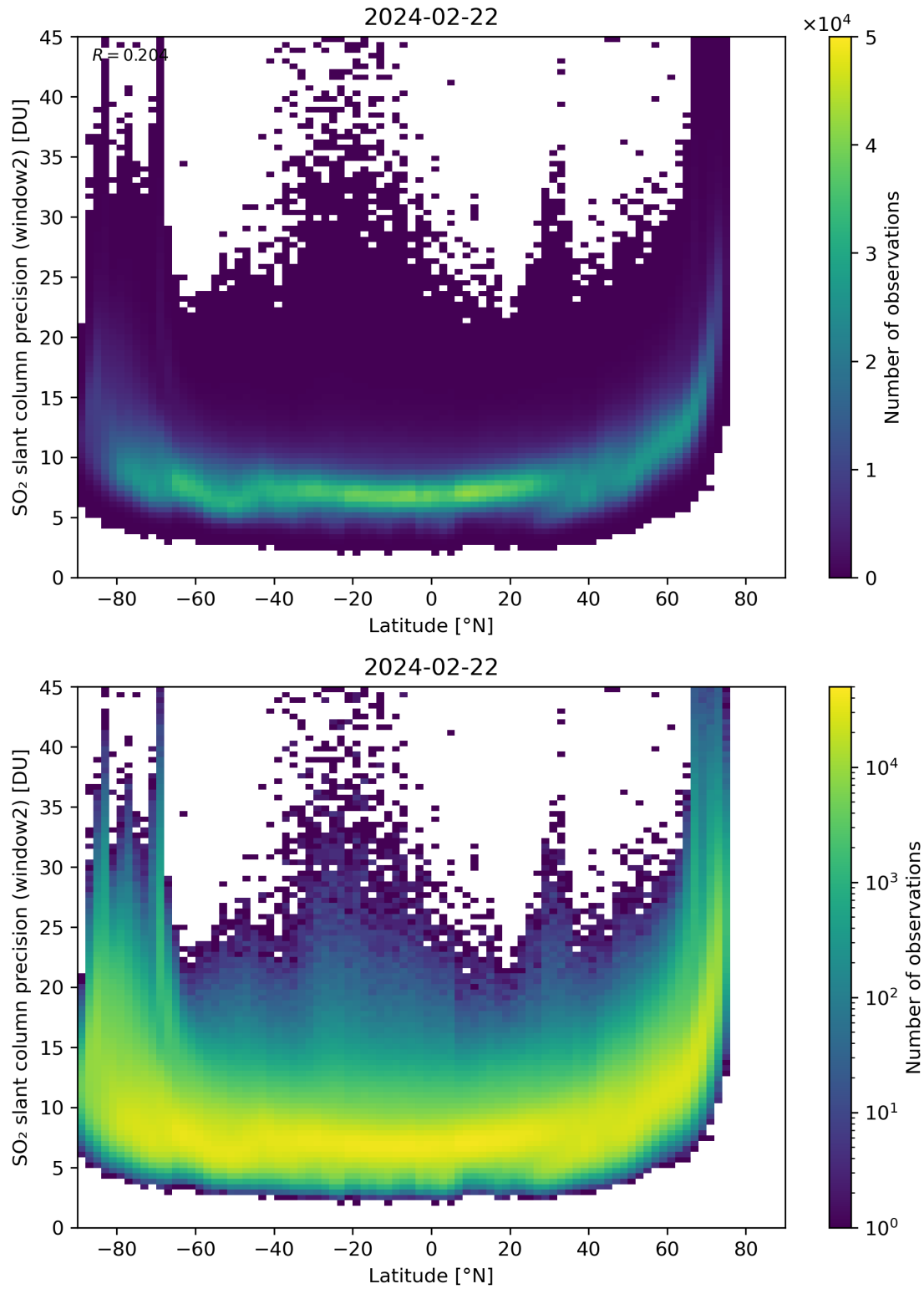
Figure 151: Scatter density plot of “Latitude” against “SO 2 slant column precision (window2)” for 2024-02-22 to 2024-02-23.
