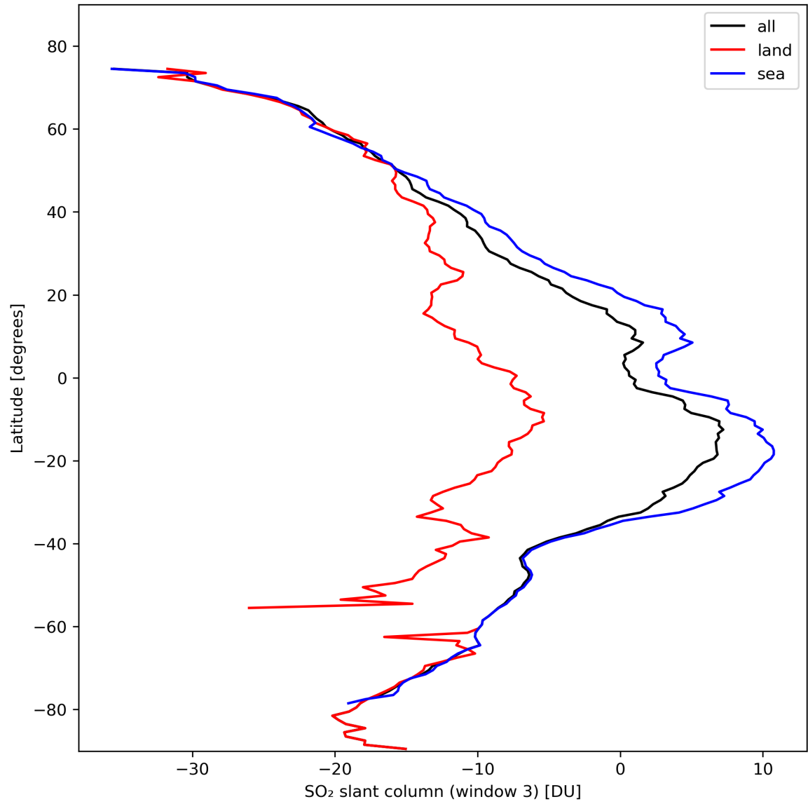
Figure 41: Zonal average of “SO 2 slant column (window 3)” for 2024-02-22 to 2024-02-23.
