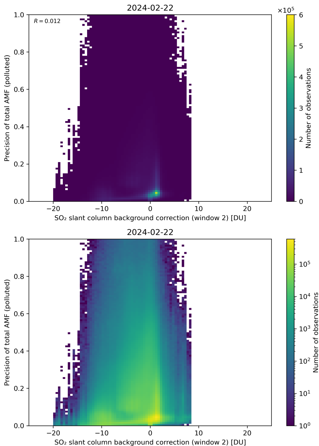
Figure 120: Scatter density plot of “SO 2 slant column background correction (window 2)” against “Precision of total AMF (polluted)” for 2024-02-22 to 2024-02-23.
