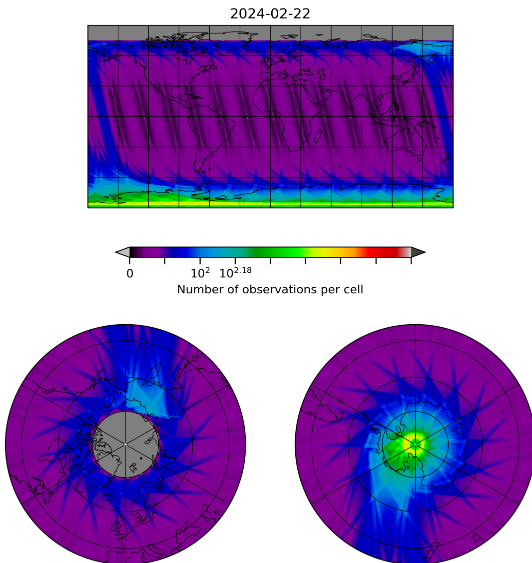
Figure 28: Map of the number of observations for 2024-02-22 to 2024-02-23
