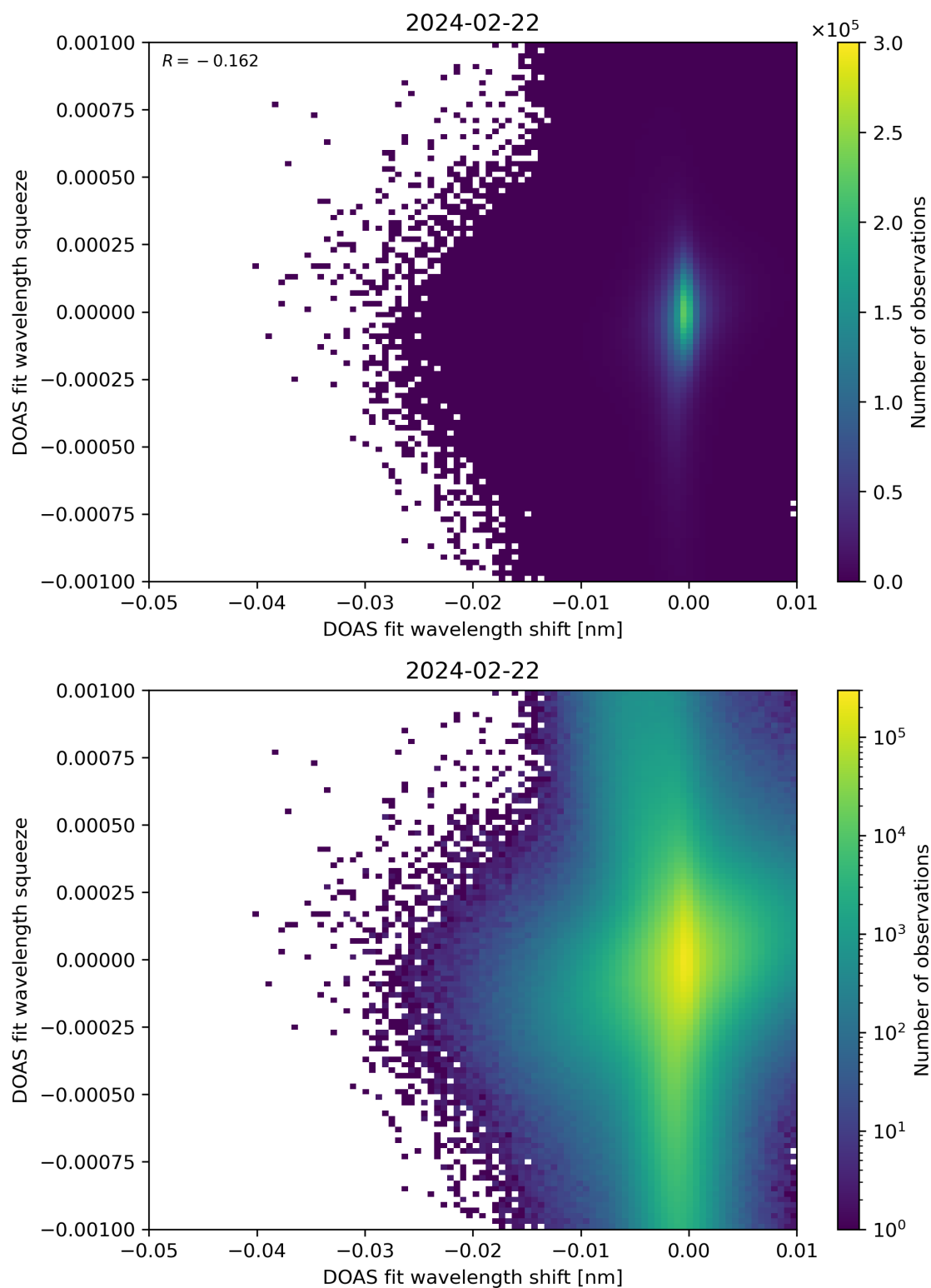
Figure 127: Scatter density plot of “DOAS fit wavelength shift” against “DOAS fit wavelength squeeze” for 2024-02-22 to 2024-02-23.
