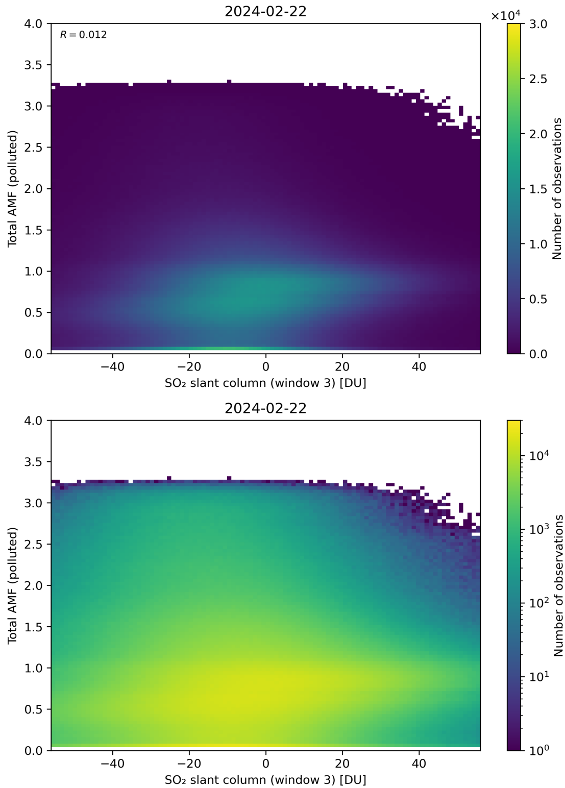
Figure 268: Scatter density plot of “SO 2 slant column (window 3)” against “Total AMF (polluted)” for 2024-02-22 to 2024-02-23.
