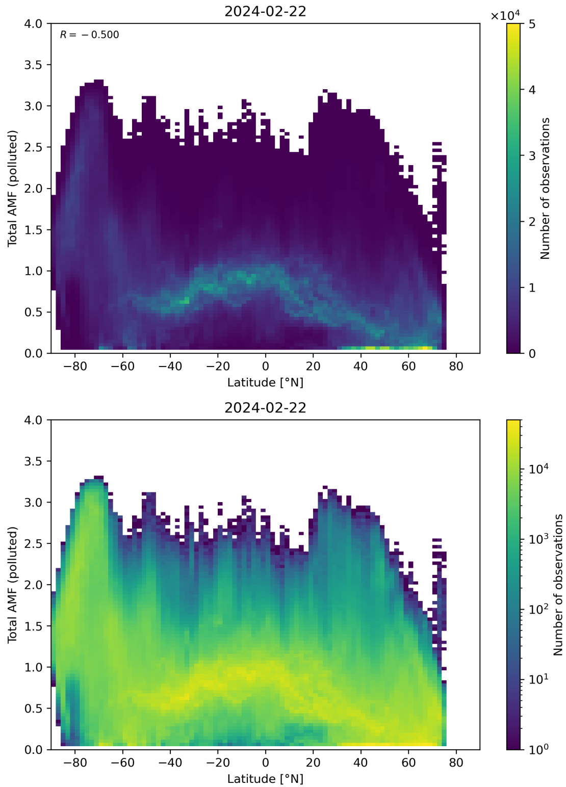
Figure 154: Scatter density plot of “Latitude” against “Total AMF (polluted)” for 2024-02-22 to 2024-02-23.
