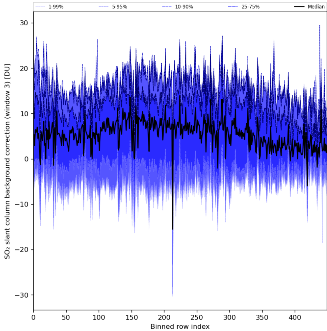
Figure 90: Along track statistics of “SO 2 slant column background correction (window 3)” for 2024-02-22 to 2024-02-23
