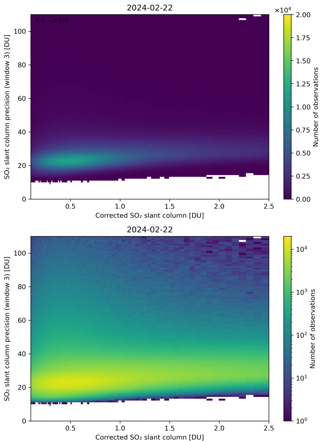
Figure 191: Scatter density plot of “Corrected SO 2 slant column” against “SO 2 slant column precision (window 3)” for 2024-02-22 to 2024-02-23.
