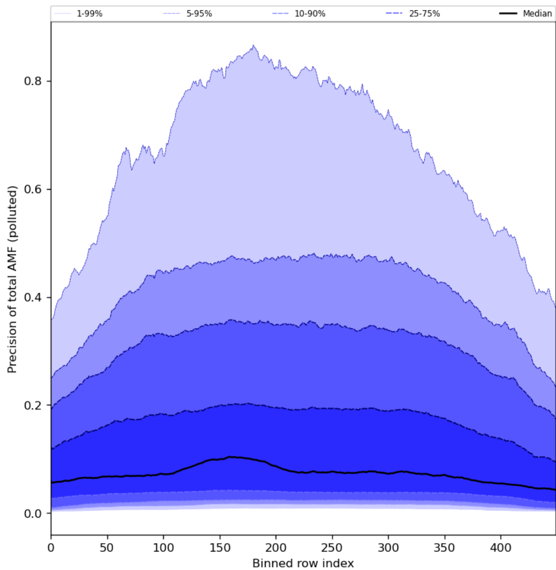
Figure 95: Along track statistics of “Precision of total AMF (polluted)” for 2024-02-22 to 2024-02-23
