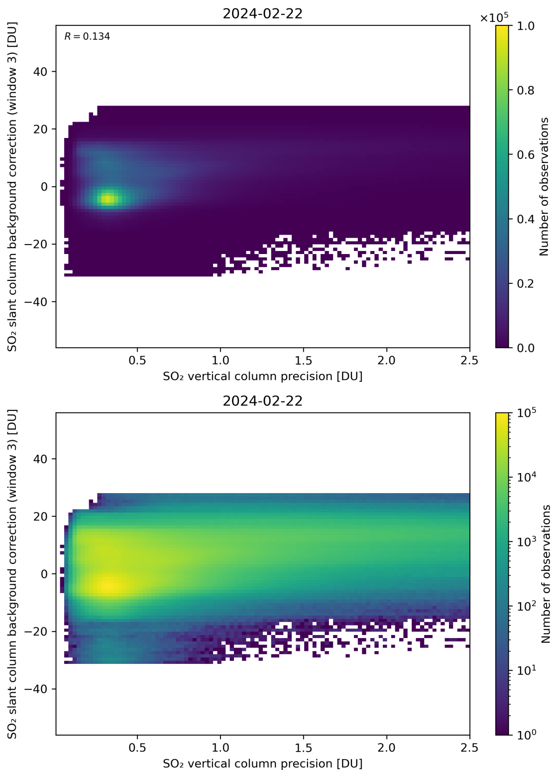
Figure 281: Scatter density plot of “SO 2 vertical column precision” against “SO 2 slant column background correction (window 3)” for 2024-02-22 to 2024-02-23.
