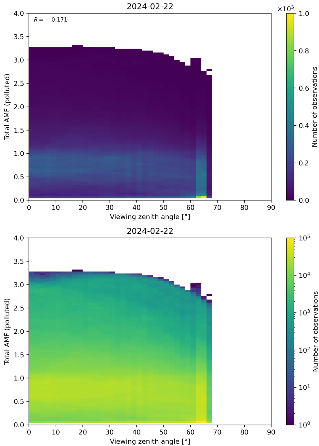
Figure 325: Scatter density plot of “Viewing zenith angle” against “Total AMF (polluted)” for 2024-02-22 to 2024-02-23.
