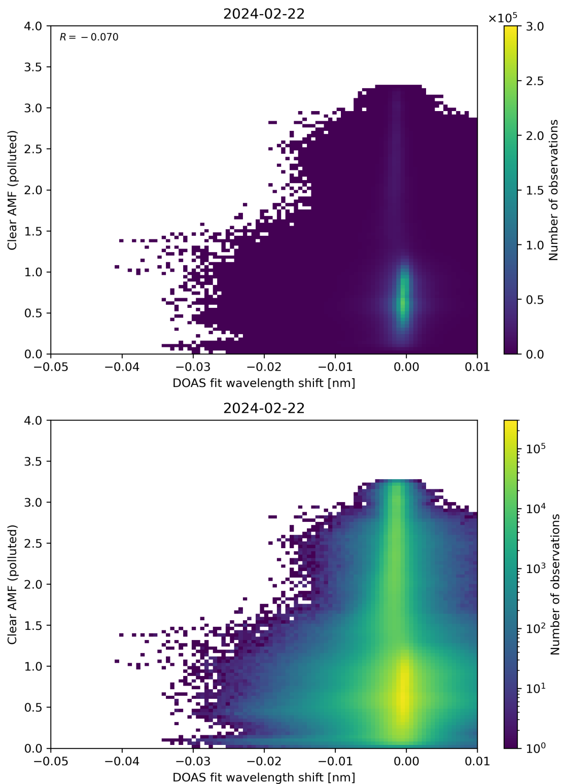
Figure 129: Scatter density plot of “DOAS fit wavelength shift” against “Clear AMF (polluted)” for 2024-02-22 to 2024-02-23.
