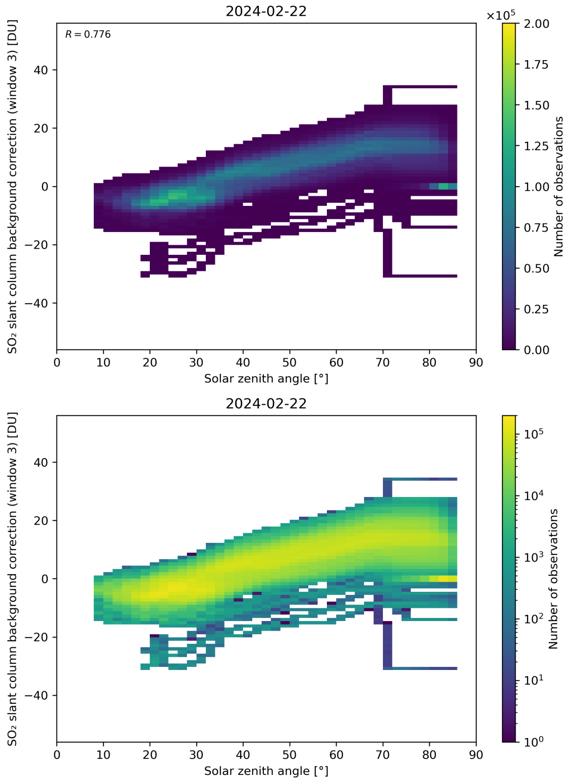
Figure 160: Scatter density plot of “Solar zenith angle” against “SO 2 slant column background correction (window 3)” for 2024-02-22 to 2024-02-23.
