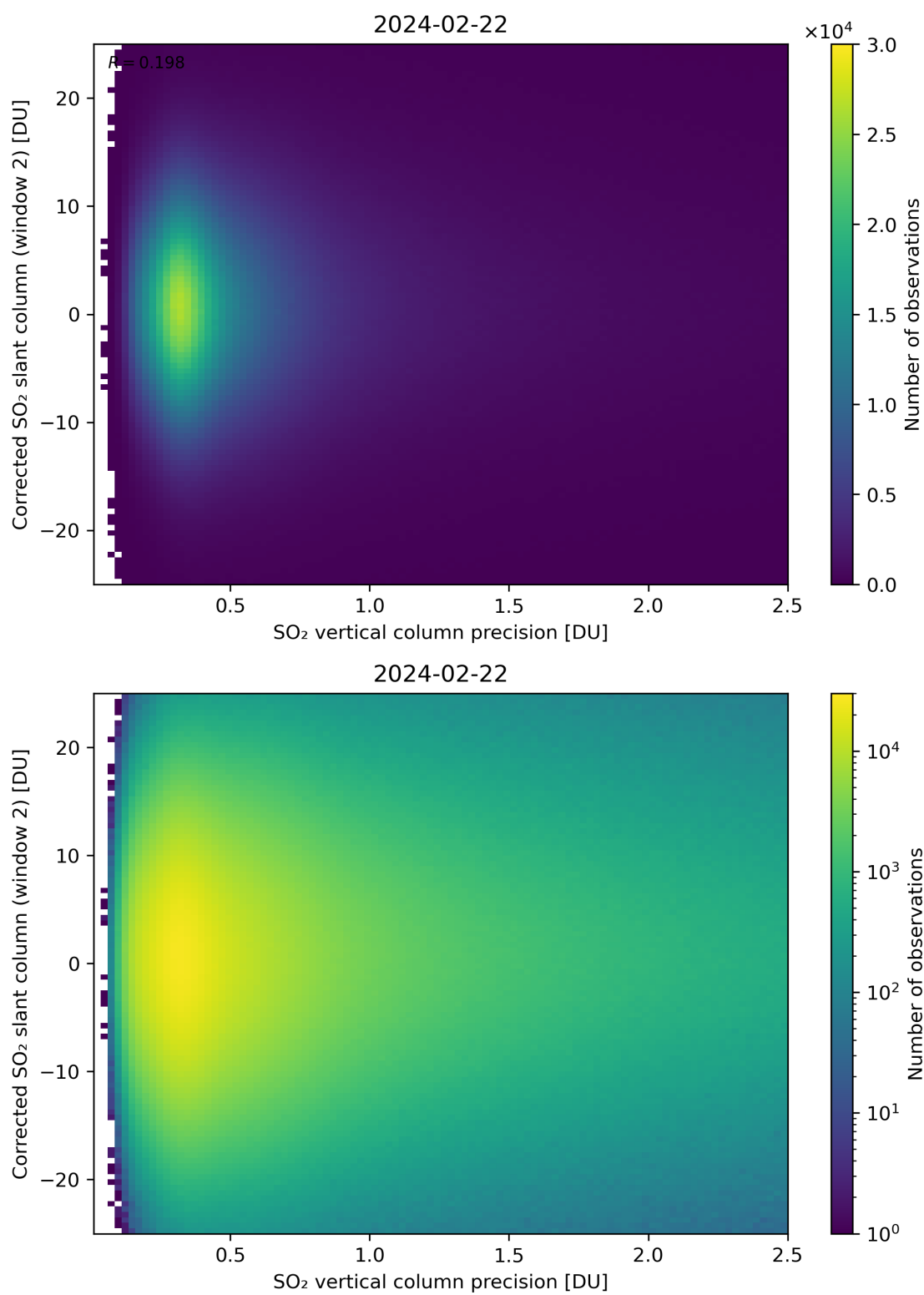
Figure 287: Scatter density plot of “SO 2 vertical column precision” against “Corrected SO 2 slant column (window 2)” for 2024-02-22 to 2024-02-23.
