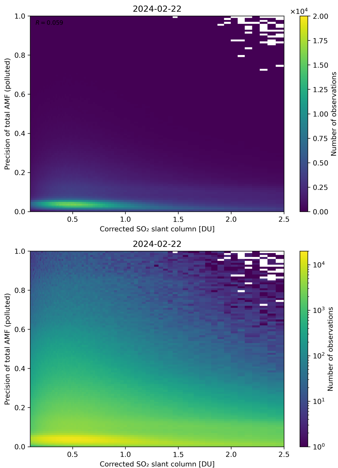
Figure 193: Scatter density plot of “Corrected SO 2 slant column” against “Precision of total AMF (polluted)” for 2024-02-22 to 2024-02-23.
