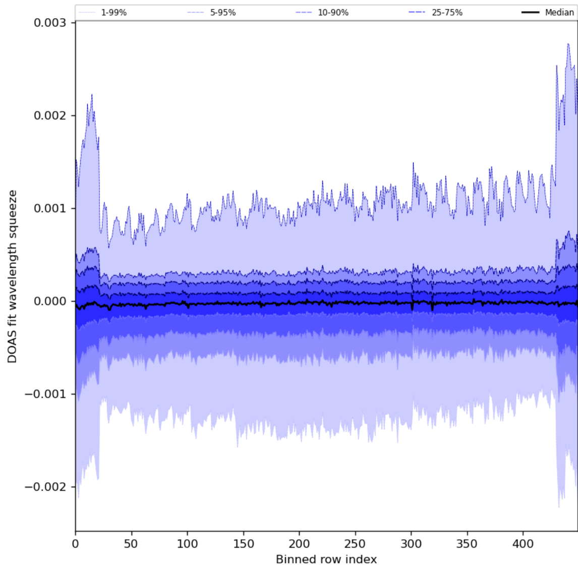
Figure 92: Along track statistics of “DOAS fit wavelength squeeze” for 2024-02-22 to 2024-02-23
