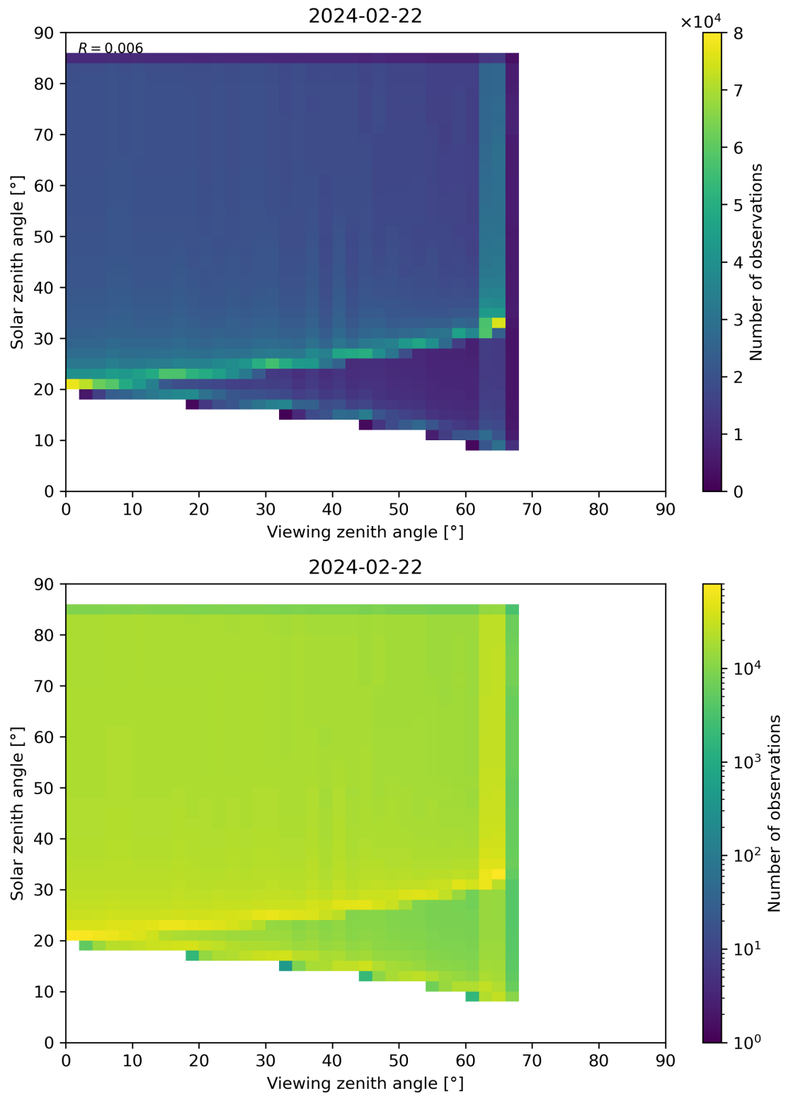
Figure 315: Scatter density plot of “Viewing zenith angle” against “Solar zenith angle” for 2024-02-22 to 2024-02-23.
