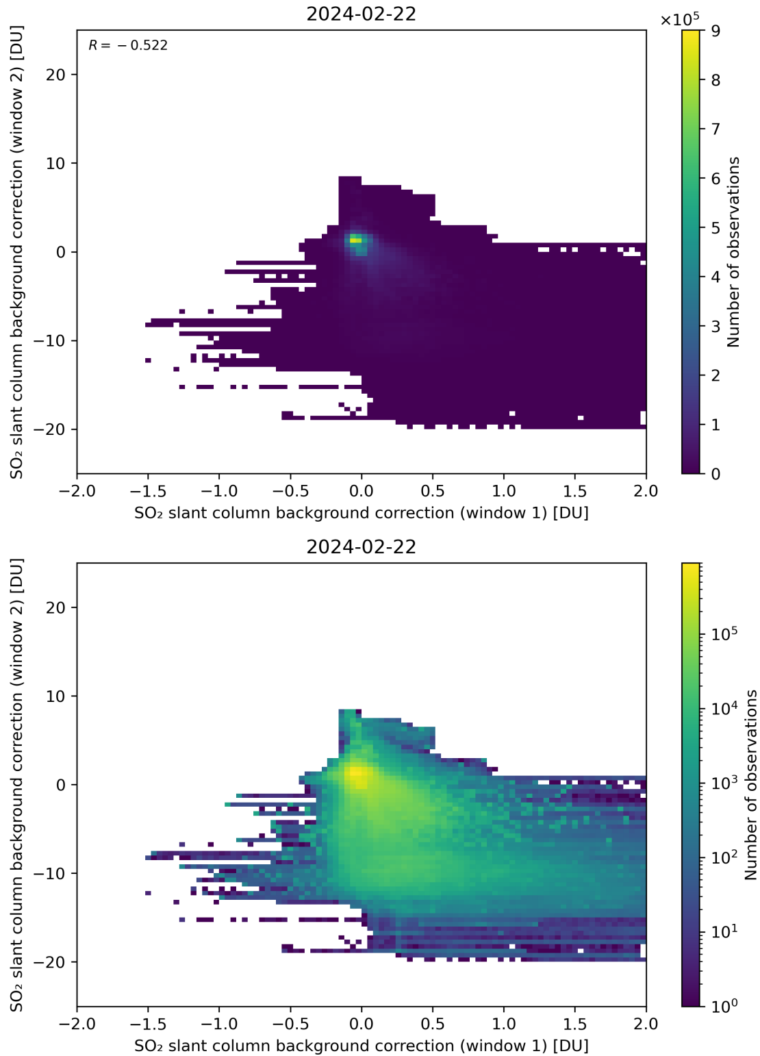
Figure 98: Scatter density plot of “SO 2 slant column background correction (window 1)” against “SO 2 slant column background correction (window 2)” for 2024-02-22 to 2024-02-23.
