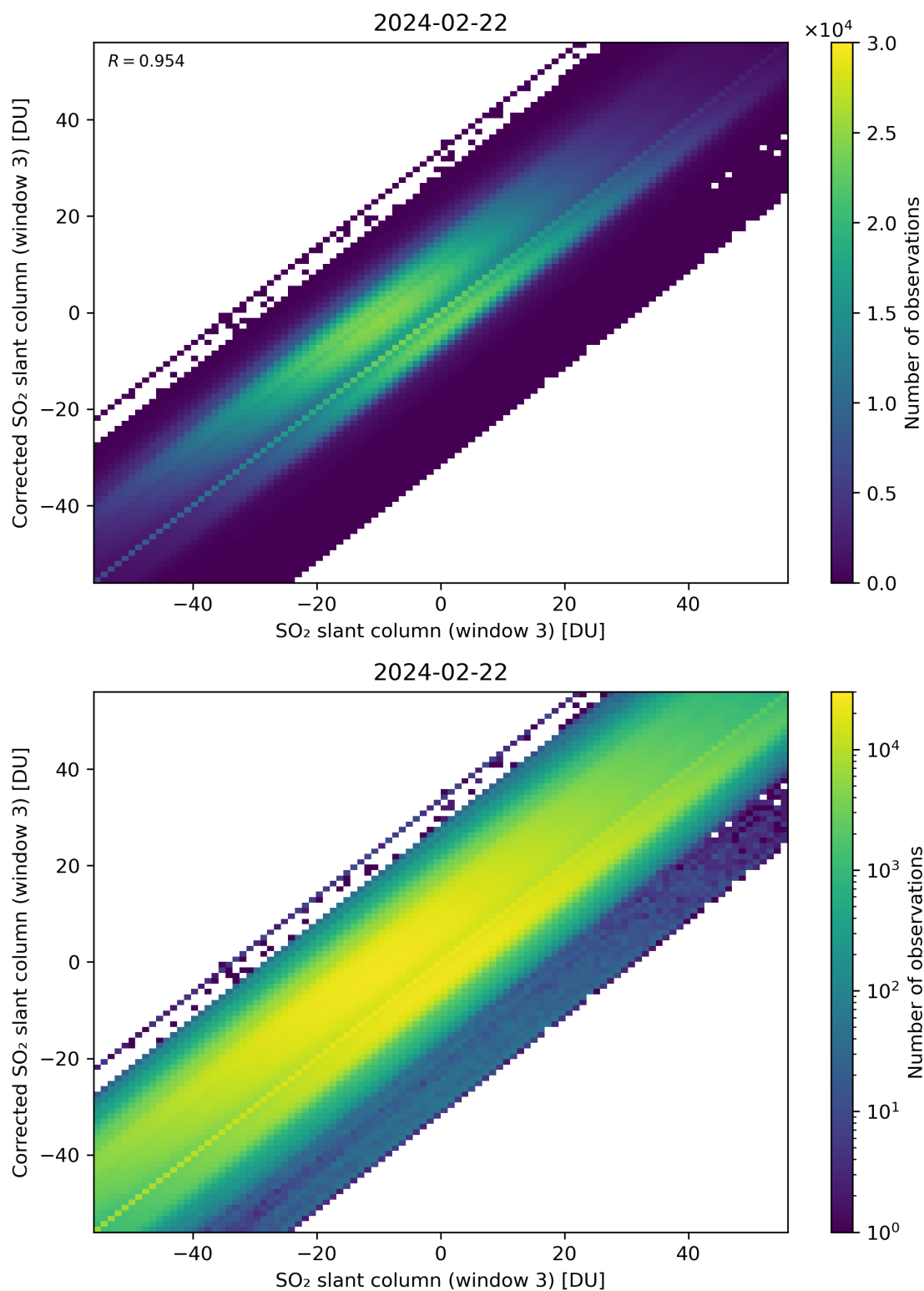
Figure 266: Scatter density plot of “SO 2 slant column (window 3)” against “Corrected SO 2 slant column (window 3)” for 2024-02-22 to 2024-02-23.
