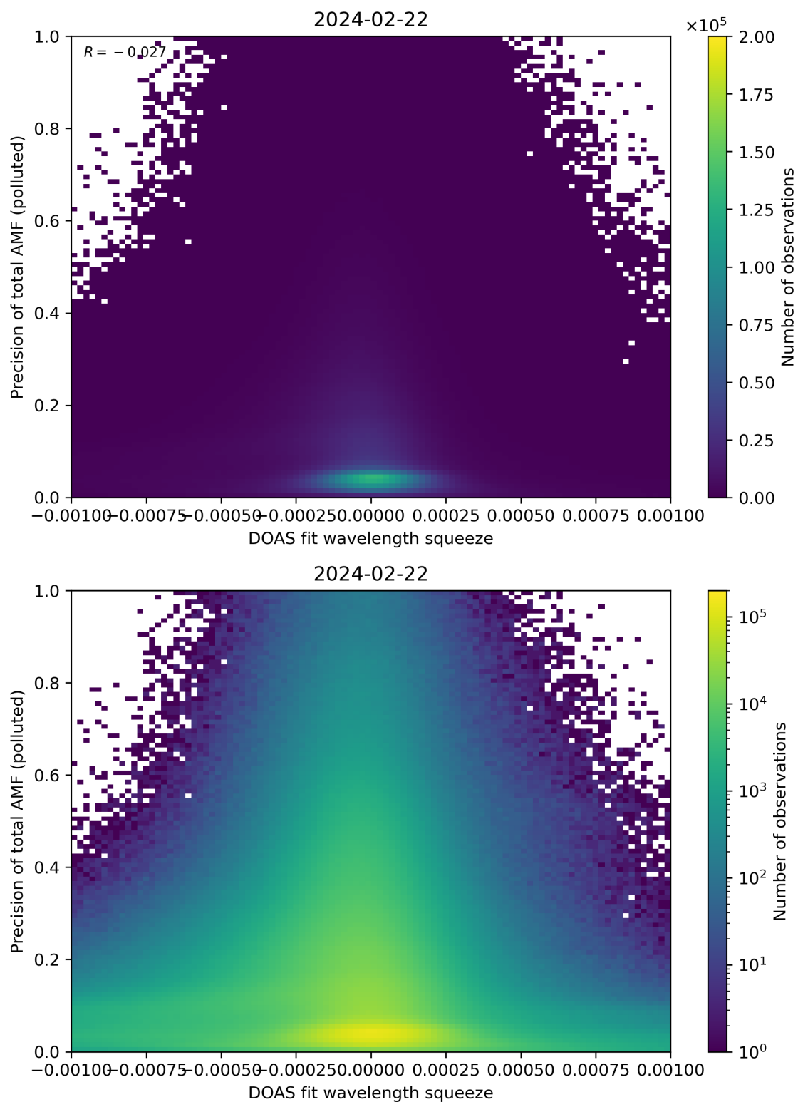
Figure 135: Scatter density plot of “DOAS fit wavelength squeeze” against “Precision of total AMF (polluted)” for 2024-02-22 to 2024-02-23.
