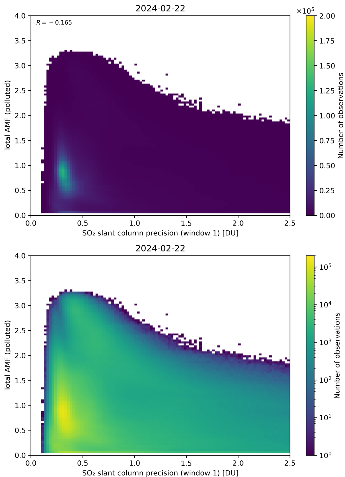
Figure 230: Scatter density plot of “SO 2 slant column precision (window 1)” against “Total AMF (polluted)” for 2024-02-22 to 2024-02-23.
