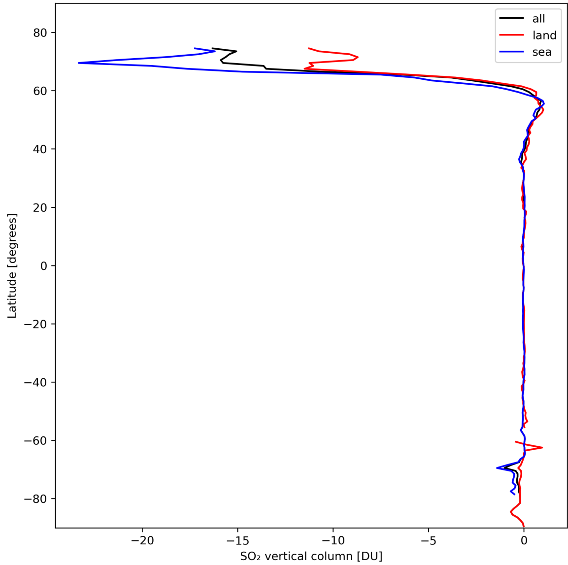
Figure 30: Zonal average of “SO 2 vertical column” for 2024-02-22 to 2024-02-23.
