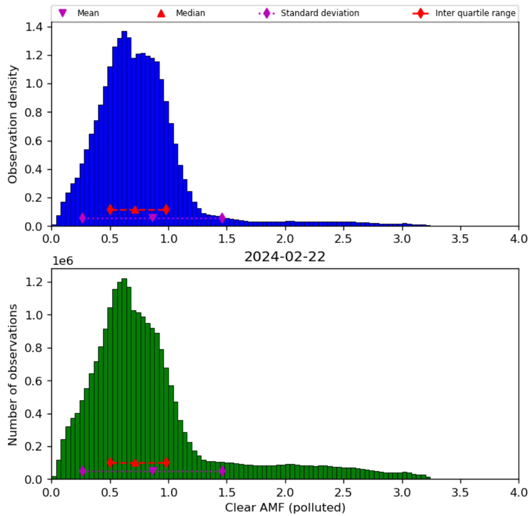
Figure 73: Histogram of “Clear AMF (polluted)” for 2024-02-22 to 2024-02-23
