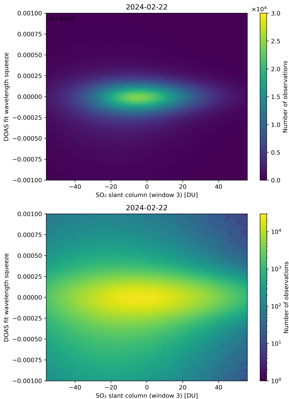
Figure 255: Scatter density plot of “SO 2 slant column (window 3)” against “DOAS fit wavelength squeeze” for 2024-02-22 to 2024-02-23.
