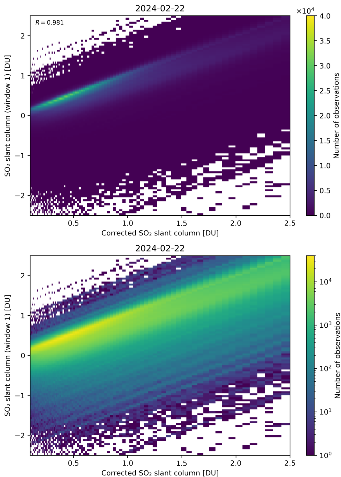
Figure 187: Scatter density plot of “Corrected SO 2 slant column” against “SO 2 slant column (window 1)” for 2024-02-22 to 2024-02-23.
