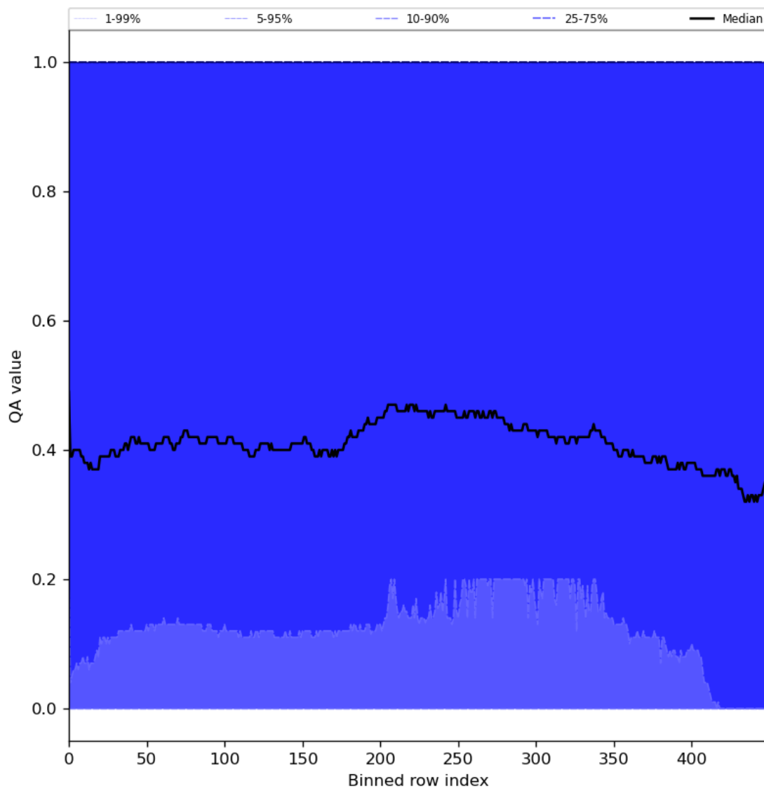
Figure 75: Along track statistics of “QA value” for 2024-02-22 to 2024-02-23
