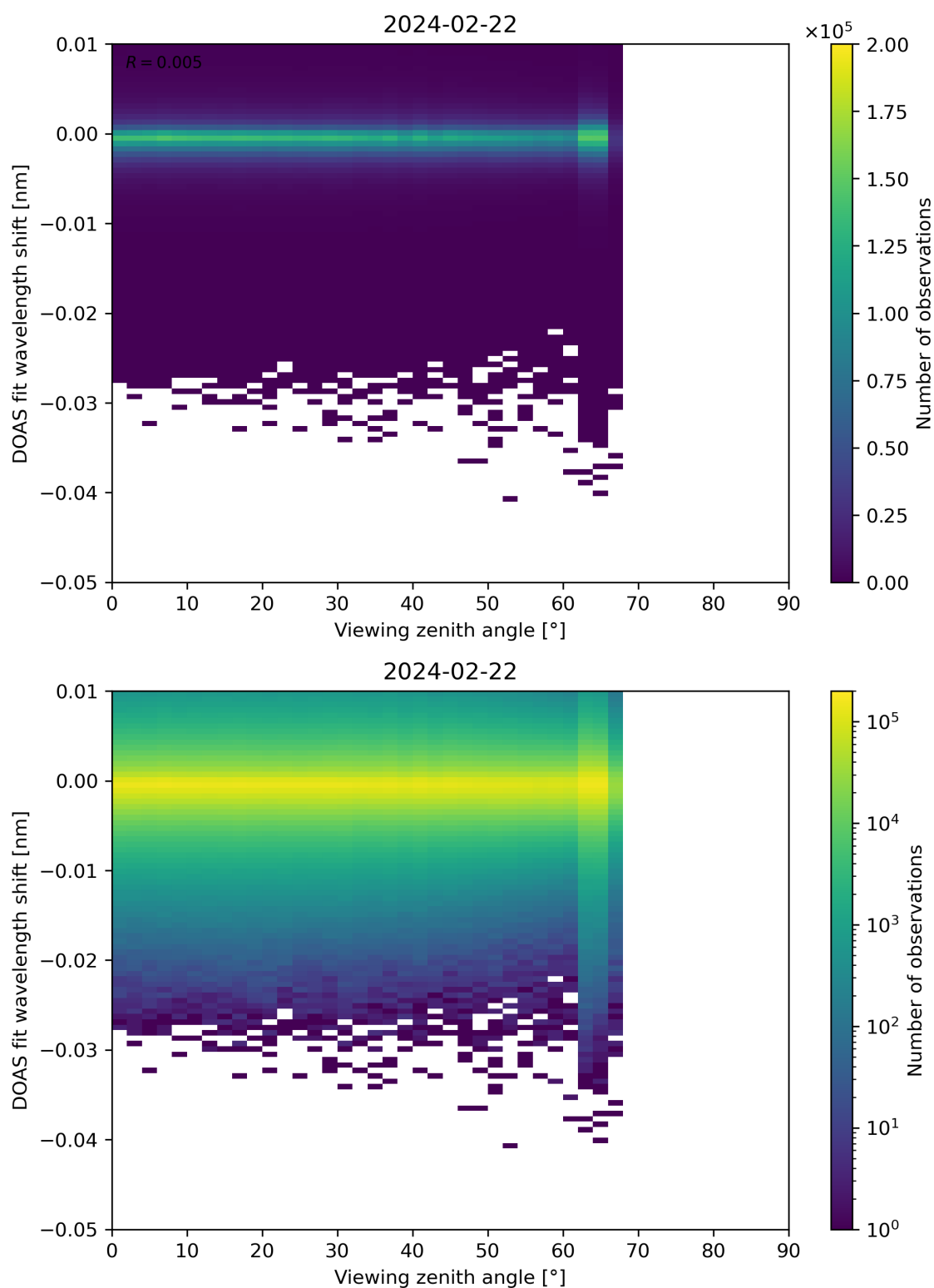
Figure 311: Scatter density plot of “Viewing zenith angle” against “DOAS fit wavelength shift” for 2024-02-22 to 2024-02-23.
