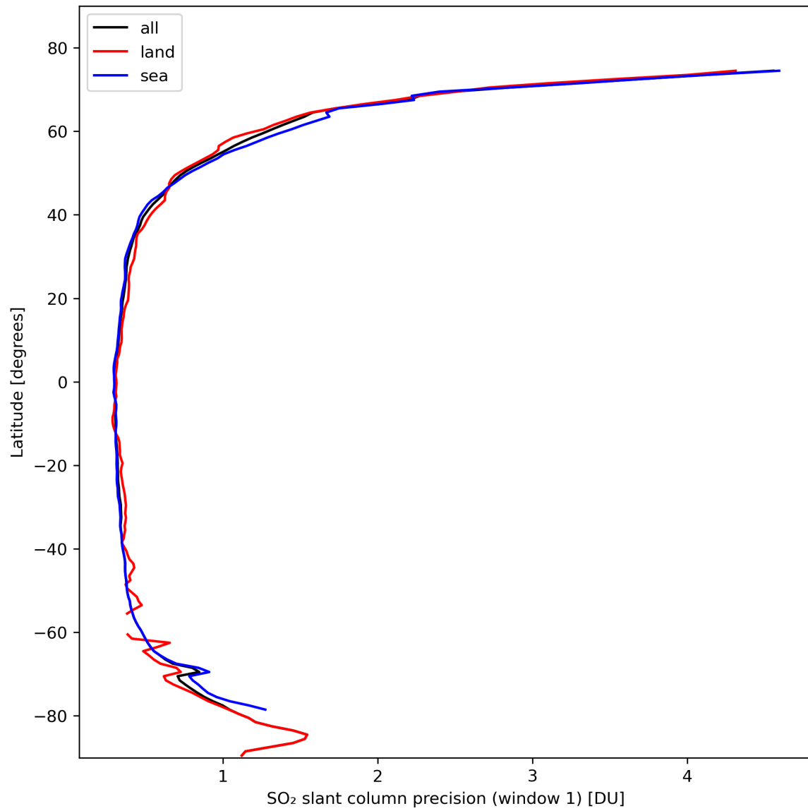
Figure 34: Zonal average of “SO 2 slant column precision (window 1)” for 2024-02-22 to 2024-02-23.
