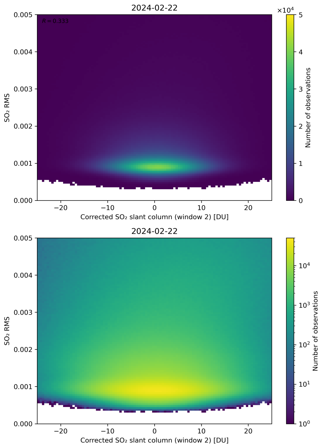
Figure 198: Scatter density plot of “Corrected SO 2 slant column (window 2)” against “SO 2 RMS” for 2024-02-22 to 2024-02-23.
