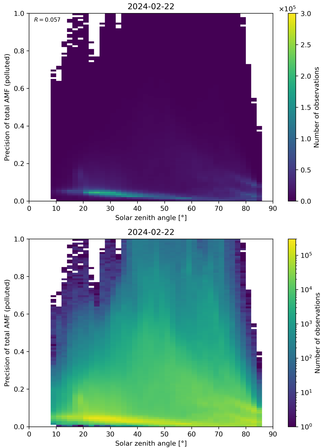
Figure 175: Scatter density plot of “Solar zenith angle” against “Precision of total AMF (polluted)” for 2024-02-22 to 2024-02-23.
