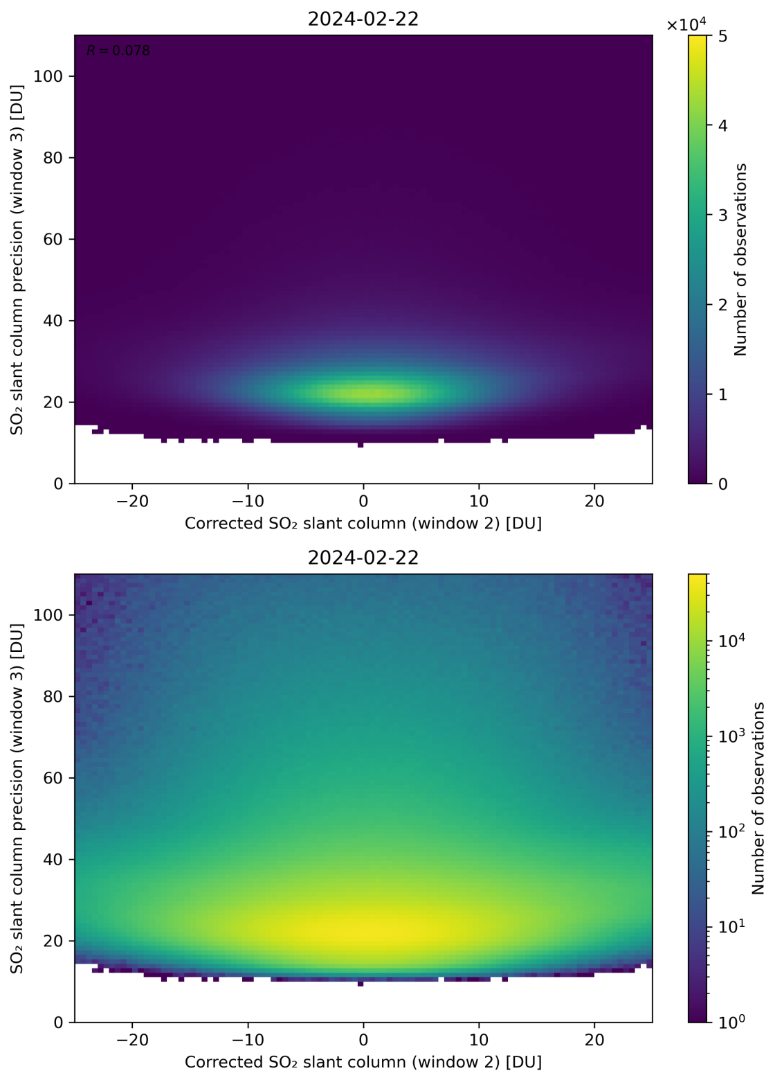
Figure 202: Scatter density plot of “Corrected SO 2 slant column (window 2)” against “SO 2 slant column precision (window 3)” for 2024-02-22 to 2024-02-23.
