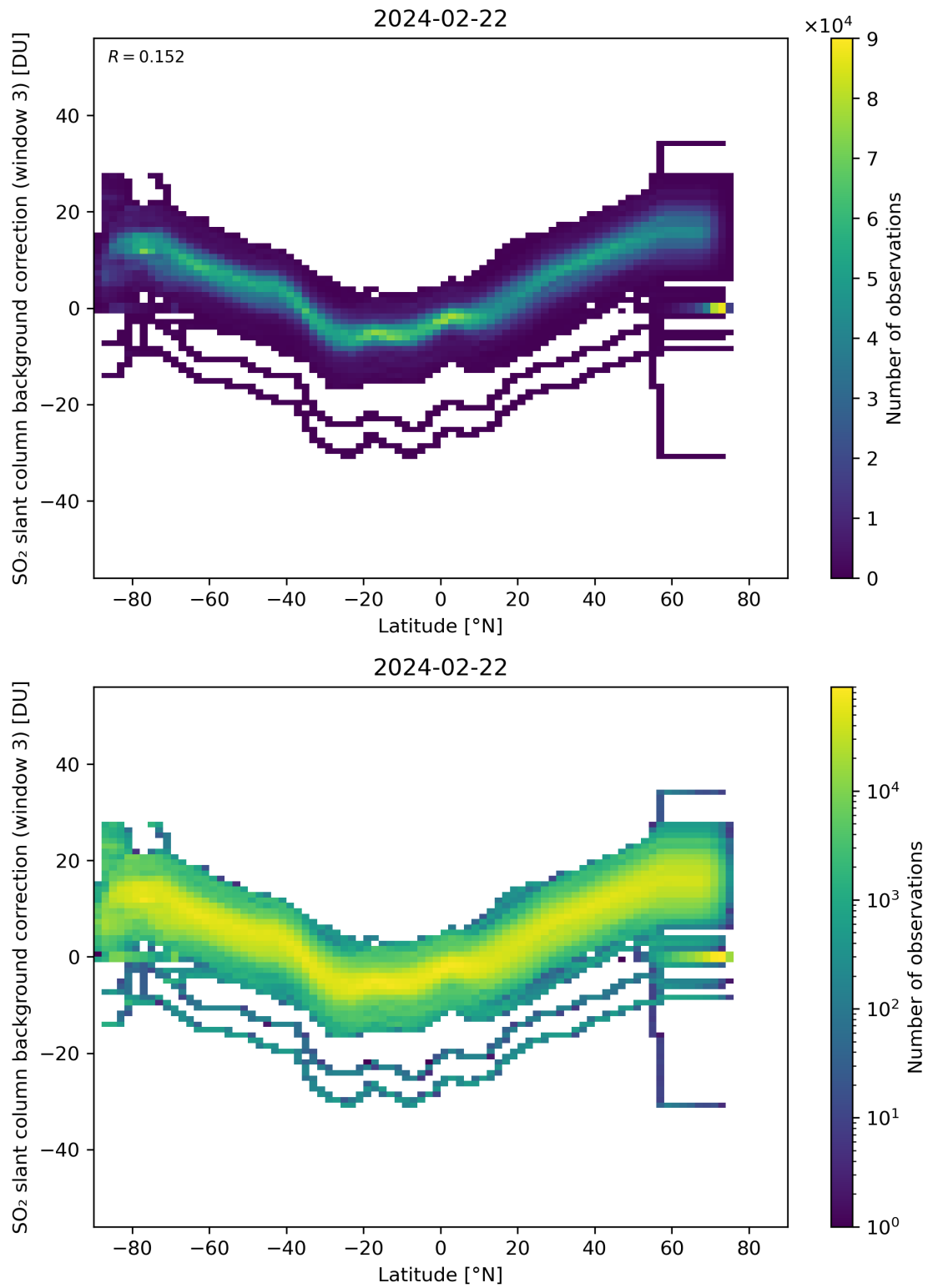
Figure 141: Scatter density plot of “Latitude” against “SO 2 slant column background correction (window 3)” for 2024-02-22 to 2024-02-23.
