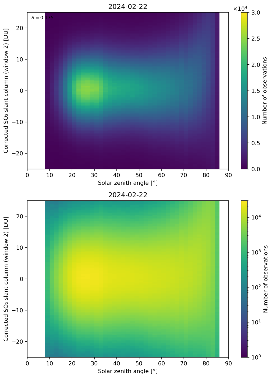
Figure 167: Scatter density plot of “Solar zenith angle” against “Corrected SO 2 slant column (window 2)” for 2024-02-22 to 2024-02-23.
