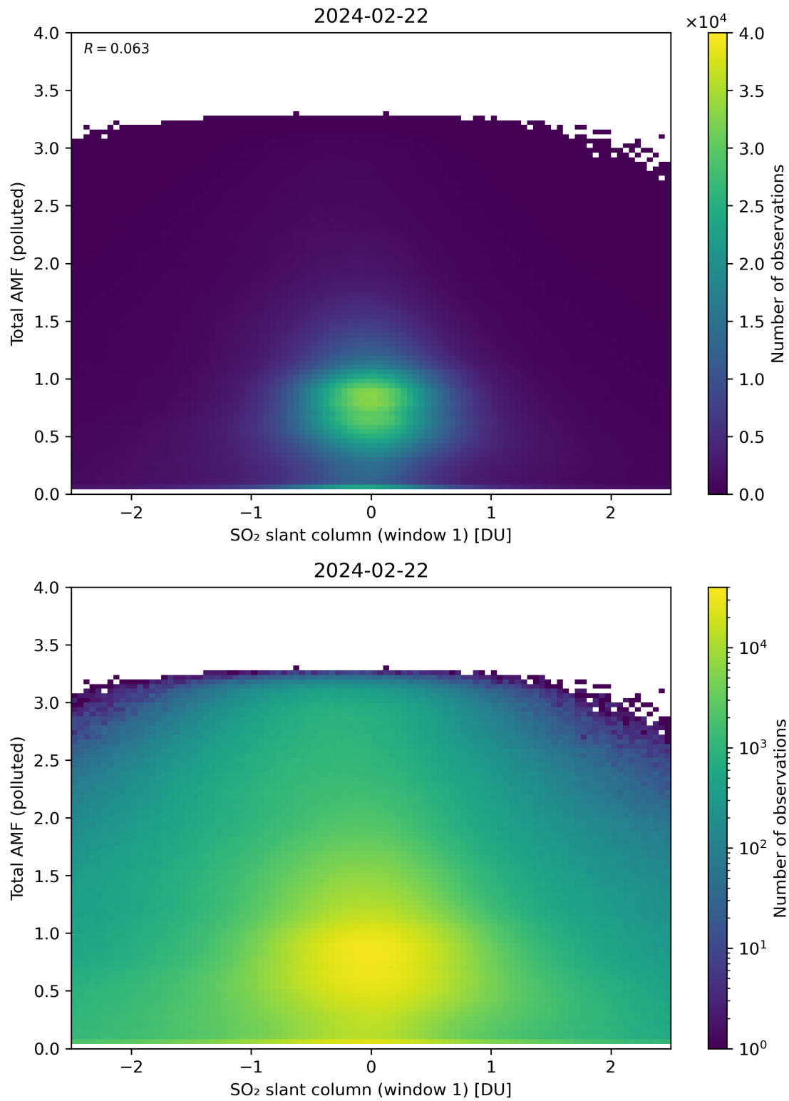
Figure 239: Scatter density plot of “SO 2 slant column (window 1)” against “Total AMF (polluted)” for 2024-02-22 to 2024-02-23.
