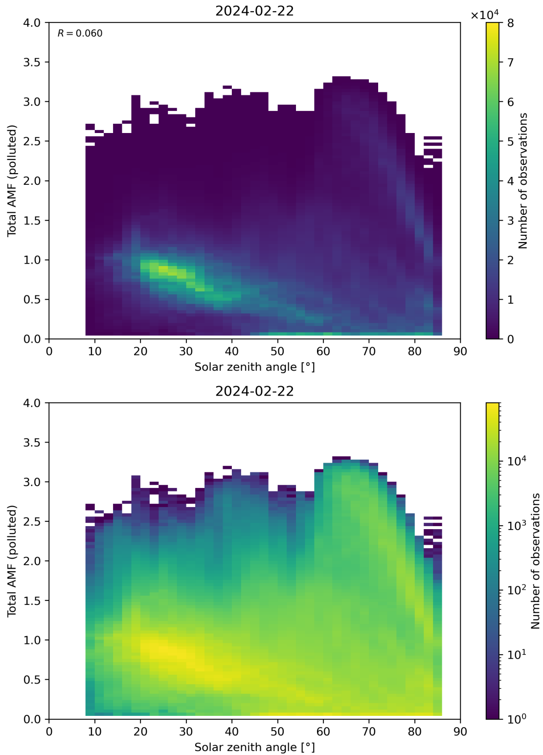
Figure 174: Scatter density plot of “Solar zenith angle” against “Total AMF (polluted)” for 2024-02-22 to 2024-02-23.
