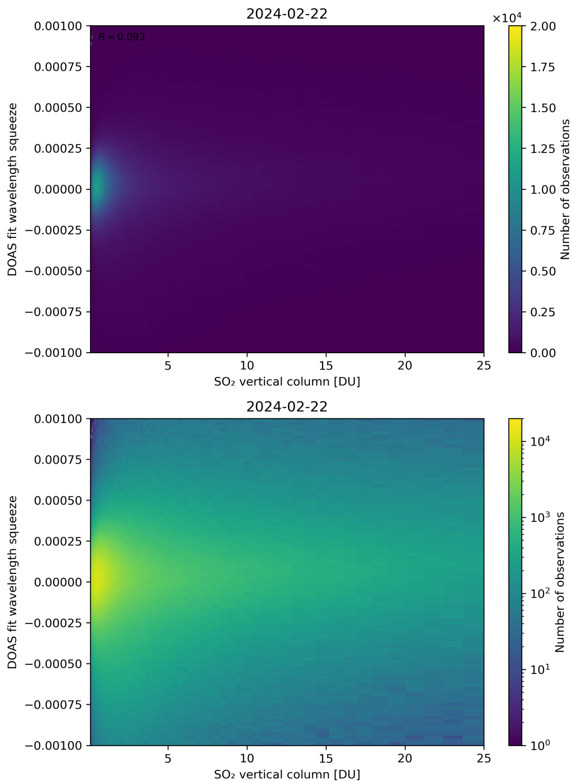
Figure 277: Scatter density plot of “SO 2 vertical column” against “DOAS fit wavelength squeeze” for 2024-02-22 to 2024-02-23.
