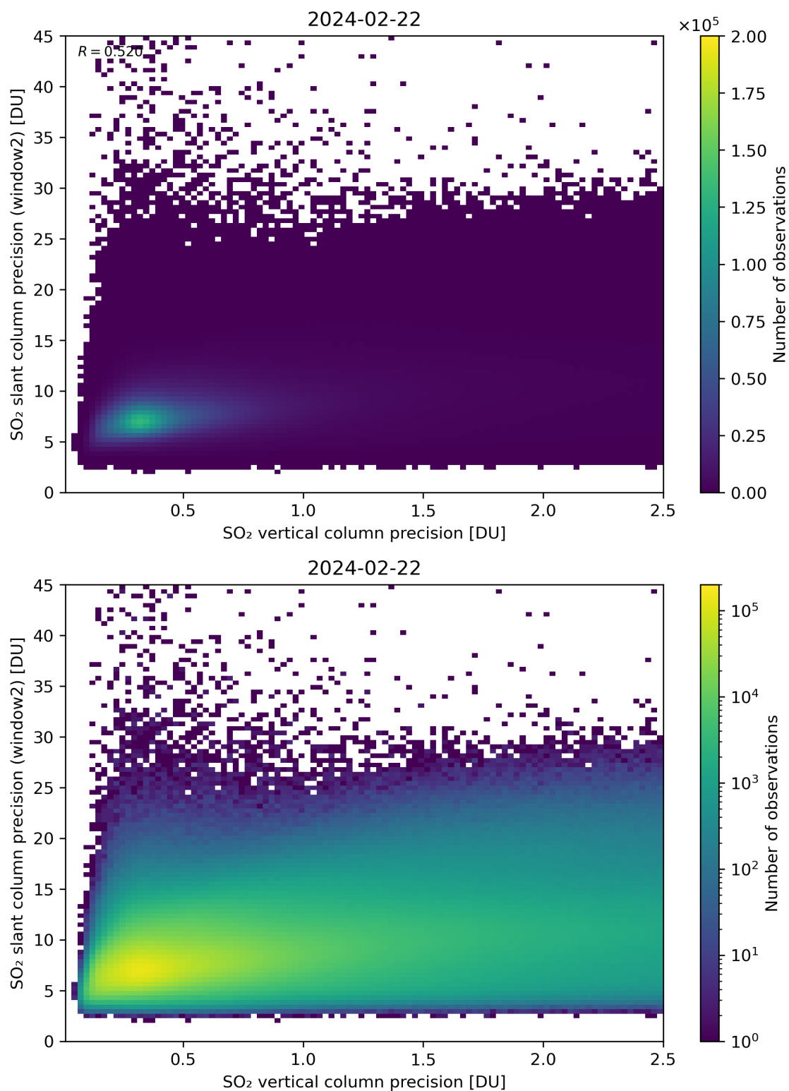
Figure 291: Scatter density plot of “SO 2 vertical column precision” against “SO 2 slant column precision (window2)” for 2024-02-22 to 2024-02-23.
