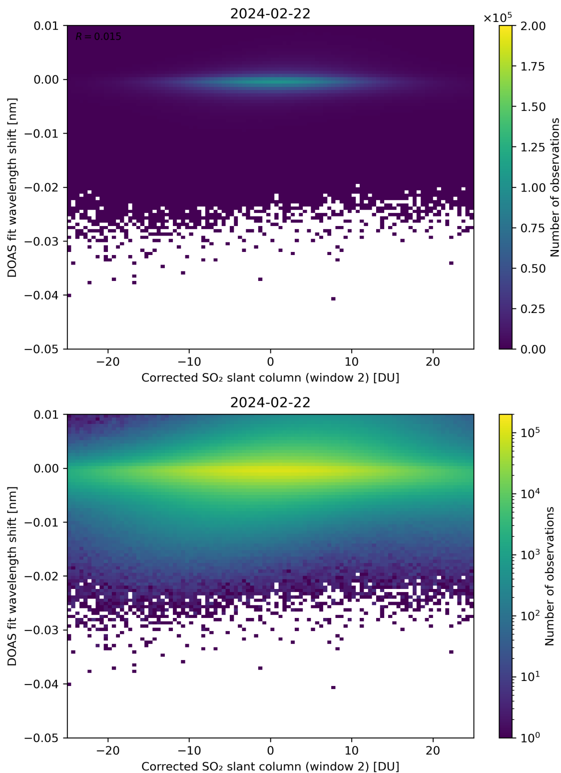
Figure 196: Scatter density plot of “Corrected SO 2 slant column (window 2)” against “DOAS fit wavelength shift” for 2024-02-22 to 2024-02-23.
