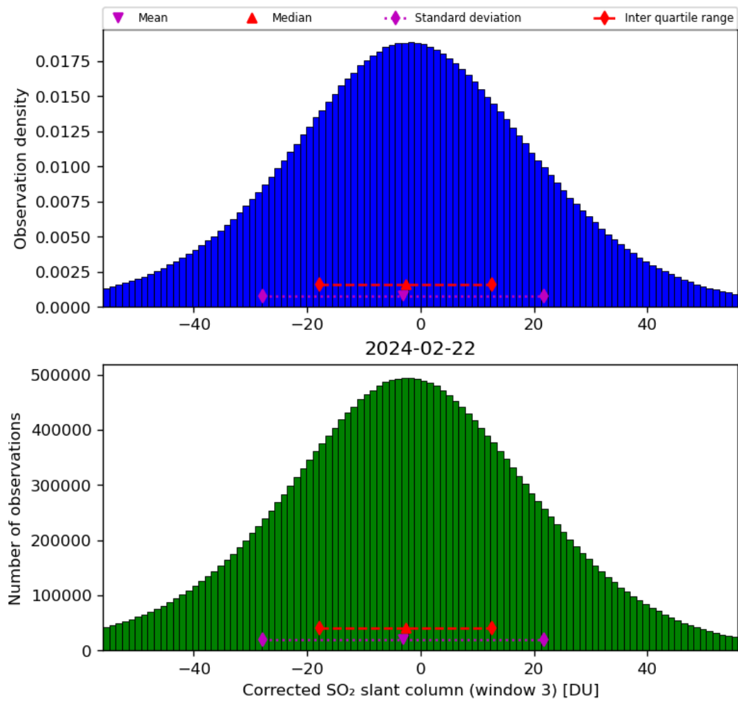
Figure 66: Histogram of “Corrected SO 2 slant column (window 3)” for 2024-02-22 to 2024-02-23
