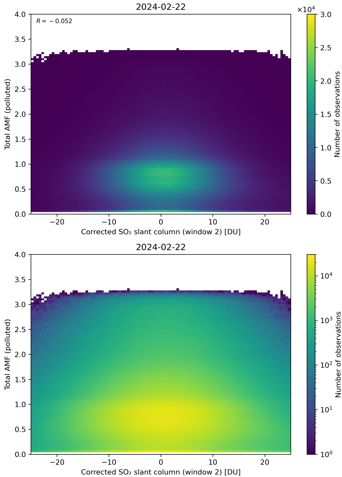
Figure 203: Scatter density plot of “Corrected SO 2 slant column (window 2)” against “Total AMF (polluted)” for 2024-02-22 to 2024-02-23.
