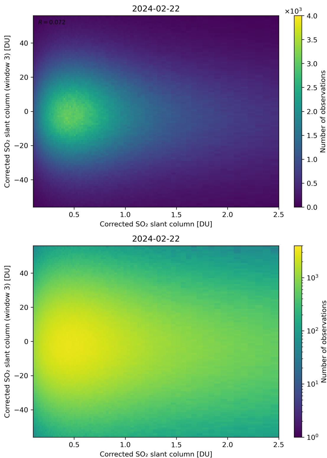
Figure 186: Scatter density plot of “Corrected SO 2 slant column” against “Corrected SO 2 slant column (window 3)” for 2024-02-22 to 2024-02-23.
