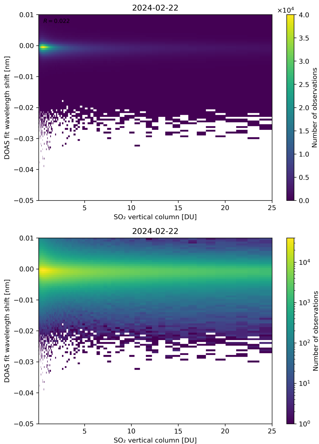
Figure 276: Scatter density plot of “SO 2 vertical column” against “DOAS fit wavelength shift” for 2024-02-22 to 2024-02-23.
