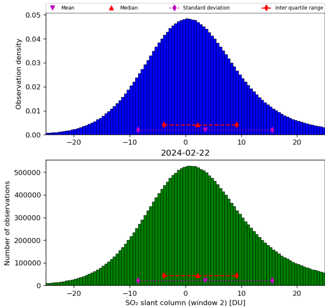
Figure 60: Histogram of “SO 2 slant column (window 2)” for 2024-02-22 to 2024-02-23
