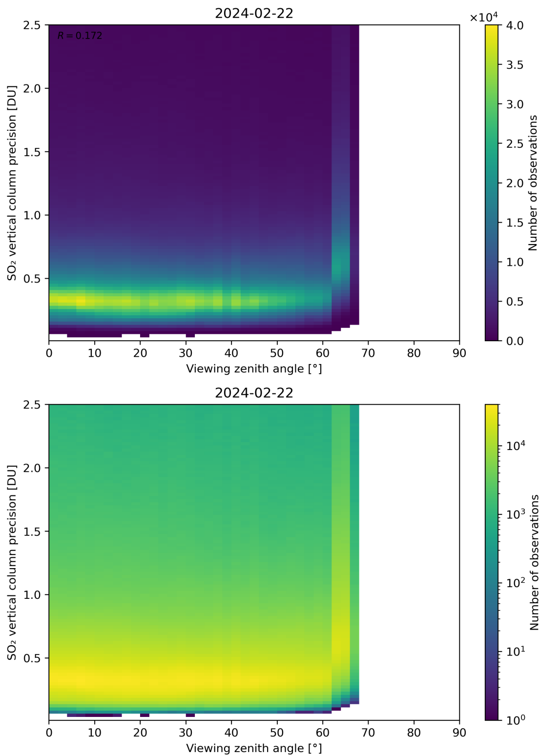
Figure 328: Scatter density plot of “Viewing zenith angle” against “SO 2 vertical column precision” for 2024-02-22 to 2024-02-23.
