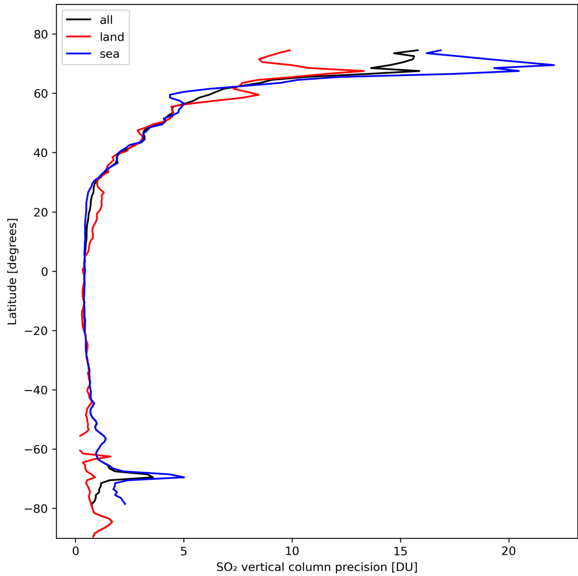
Figure 31: Zonal average of “SO 2 vertical column precision” for 2024-02-22 to 2024-02-23.
