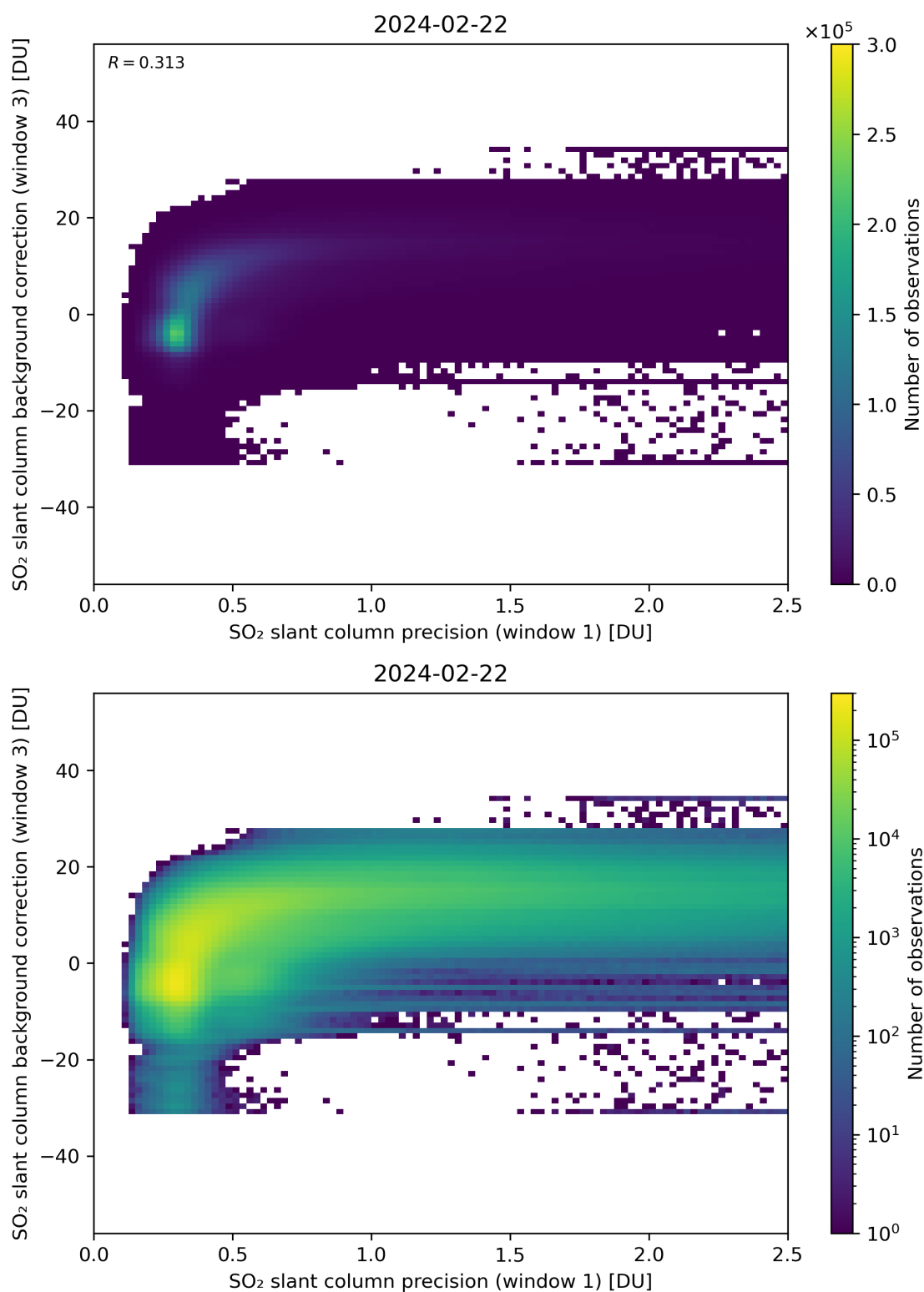
Figure 220: Scatter density plot of “SO 2 slant column precision (window 1)” against “SO 2 slant column background correction (window 3)” for 2024-02-22 to 2024-02-23.
