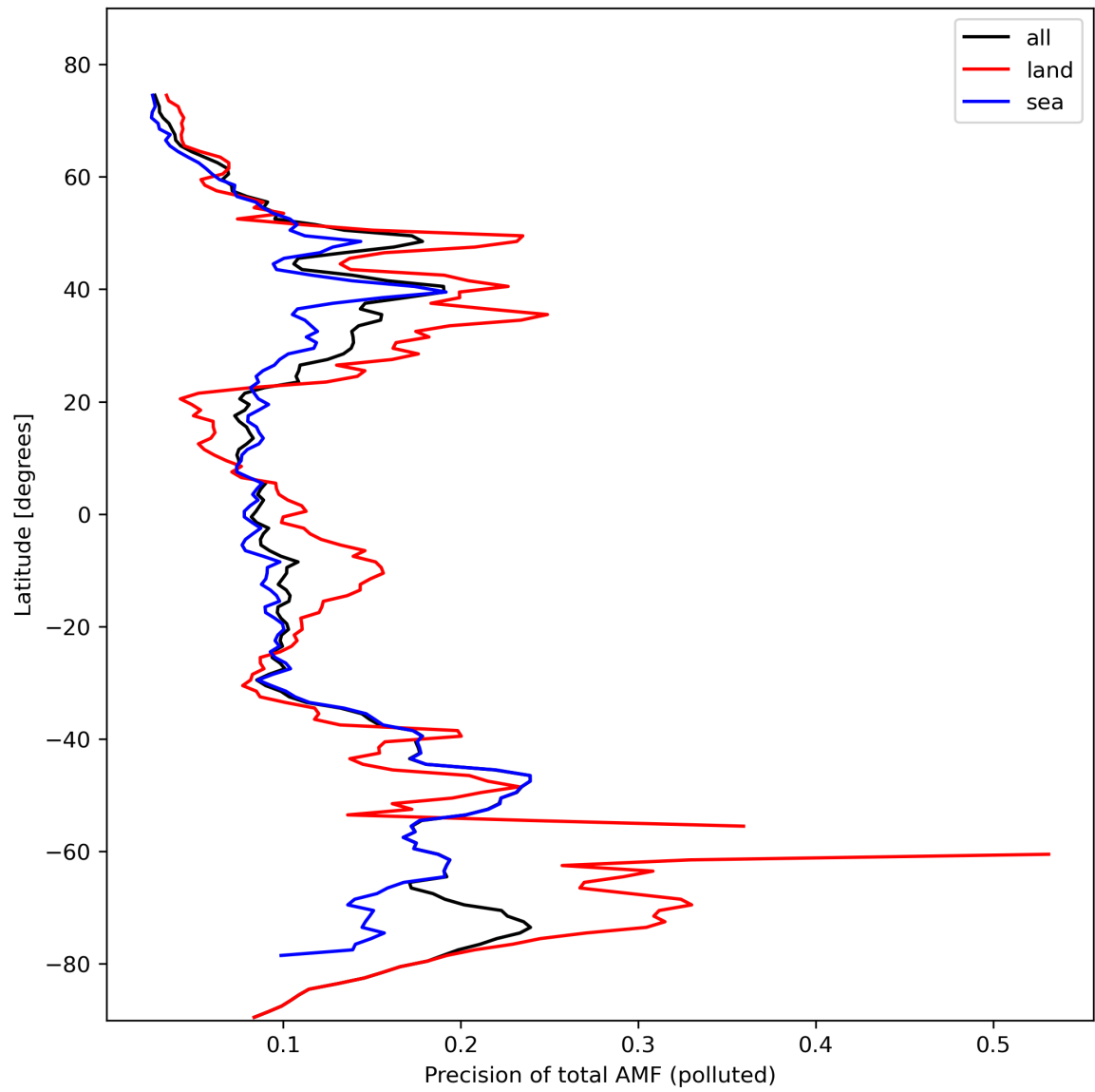
Figure 49: Zonal average of “Precision of total AMF (polluted)” for 2024-02-22 to 2024-02-23.
