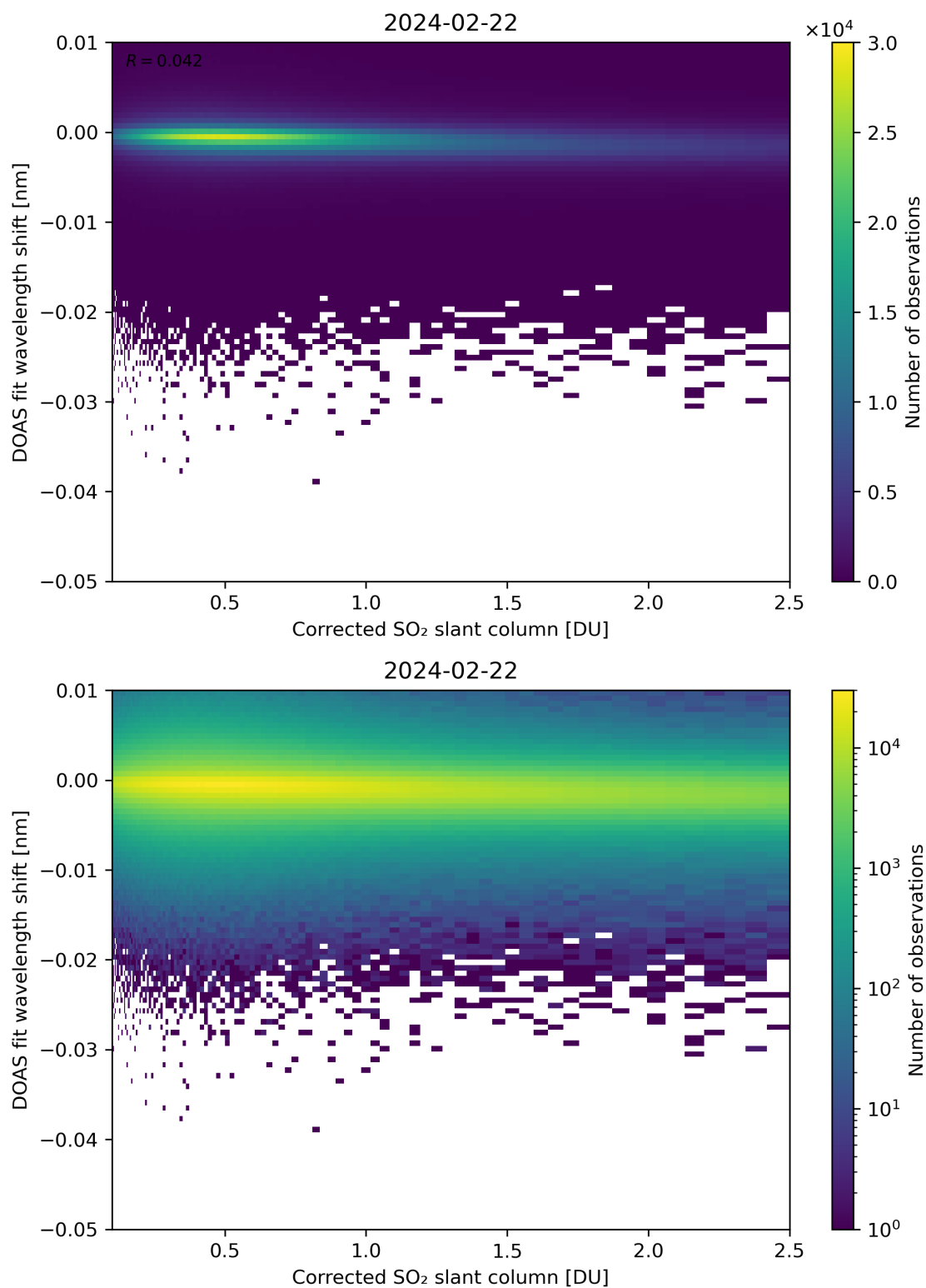
Figure 181: Scatter density plot of “Corrected SO 2 slant column” against “DOAS fit wavelength shift” for 2024-02-22 to 2024-02-23.
