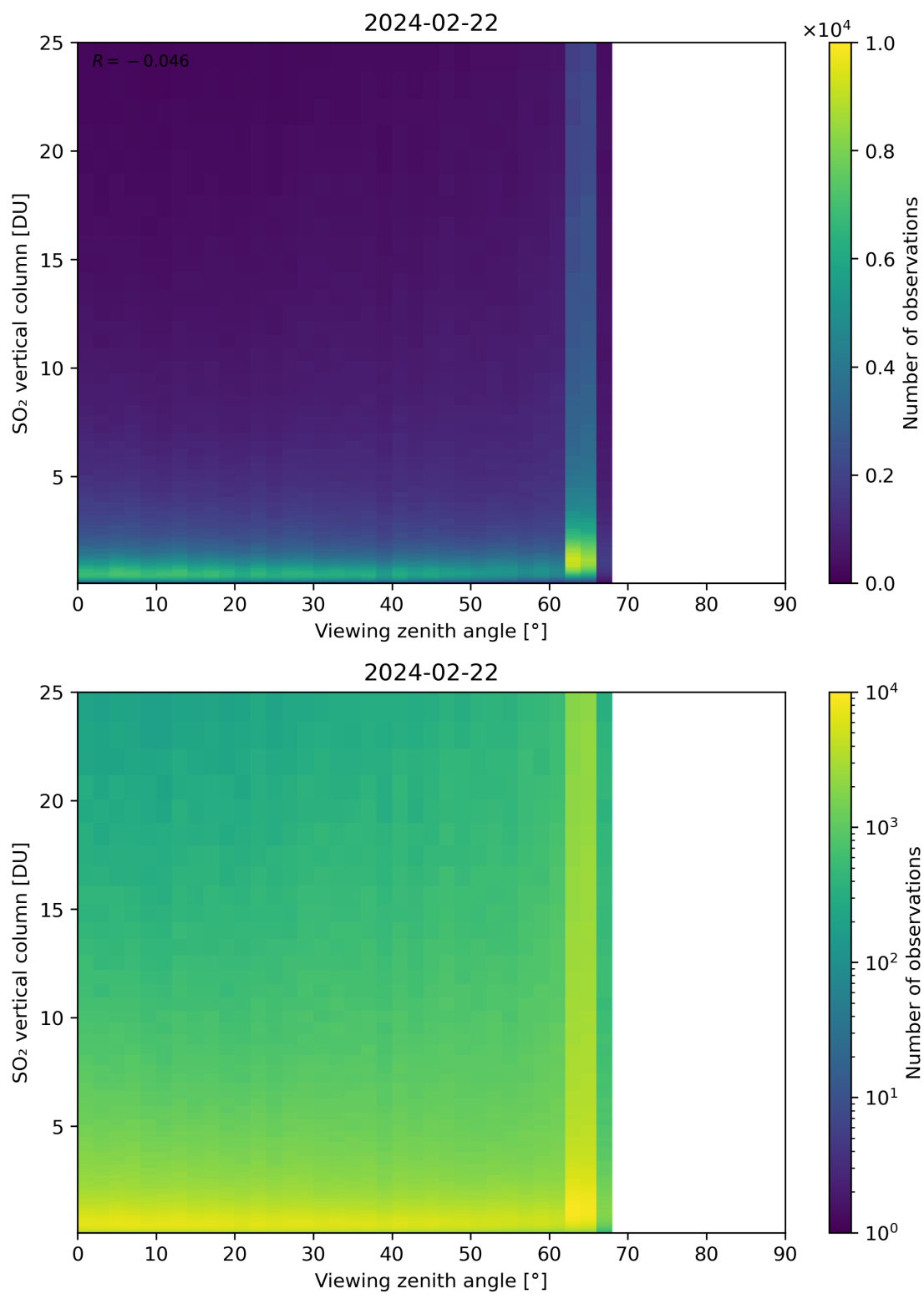
Figure 327: Scatter density plot of “Viewing zenith angle” against “SO 2 vertical column” for 2024-02-22 to 2024-02-23.
