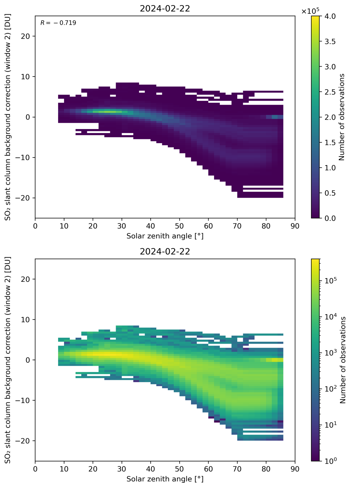
Figure 159: Scatter density plot of “Solar zenith angle” against “SO 2 slant column background correction (window 2)” for 2024-02-22 to 2024-02-23.
