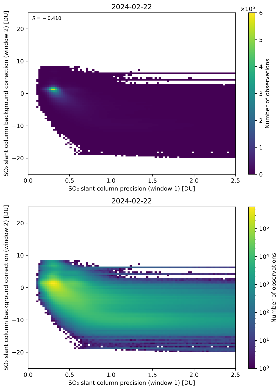
Figure 219: Scatter density plot of “SO 2 slant column precision (window 1)” against “SO 2 slant column background correction (window 2)” for 2024-02-22 to 2024-02-23.
