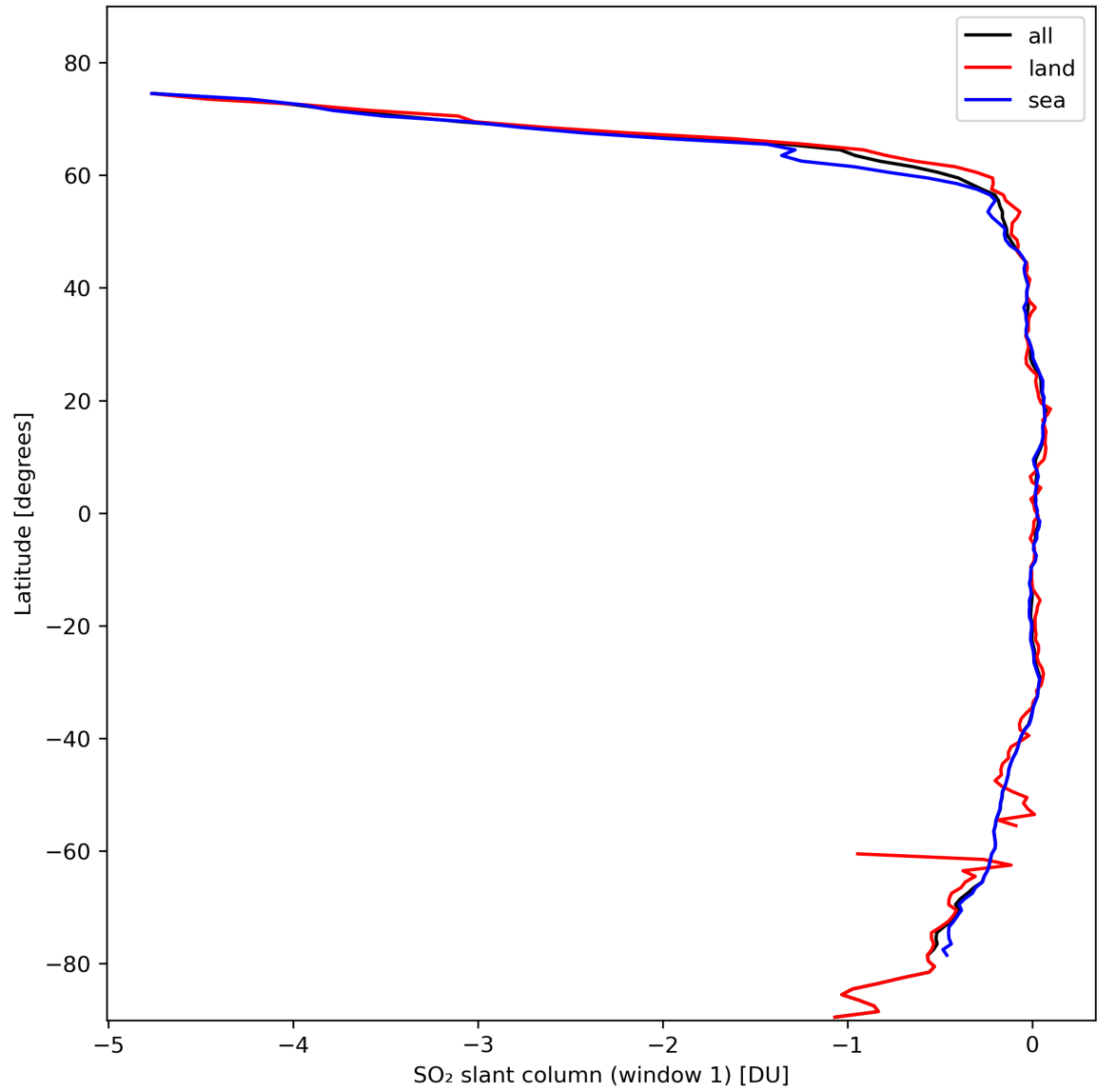
Figure 33: Zonal average of “SO 2 slant column (window 1)” for 2024-02-22 to 2024-02-23.
