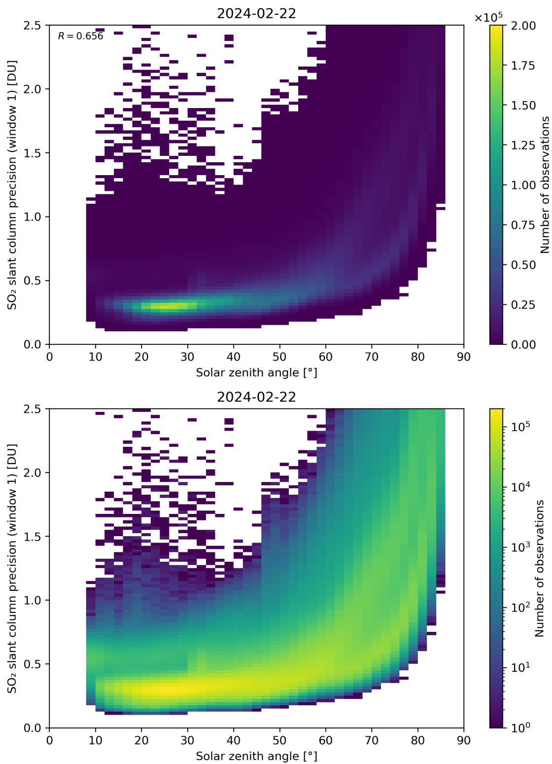
Figure 170: Scatter density plot of “Solar zenith angle” against “SO 2 slant column precision (window 1)” for 2024-02-22 to 2024-02-23.
