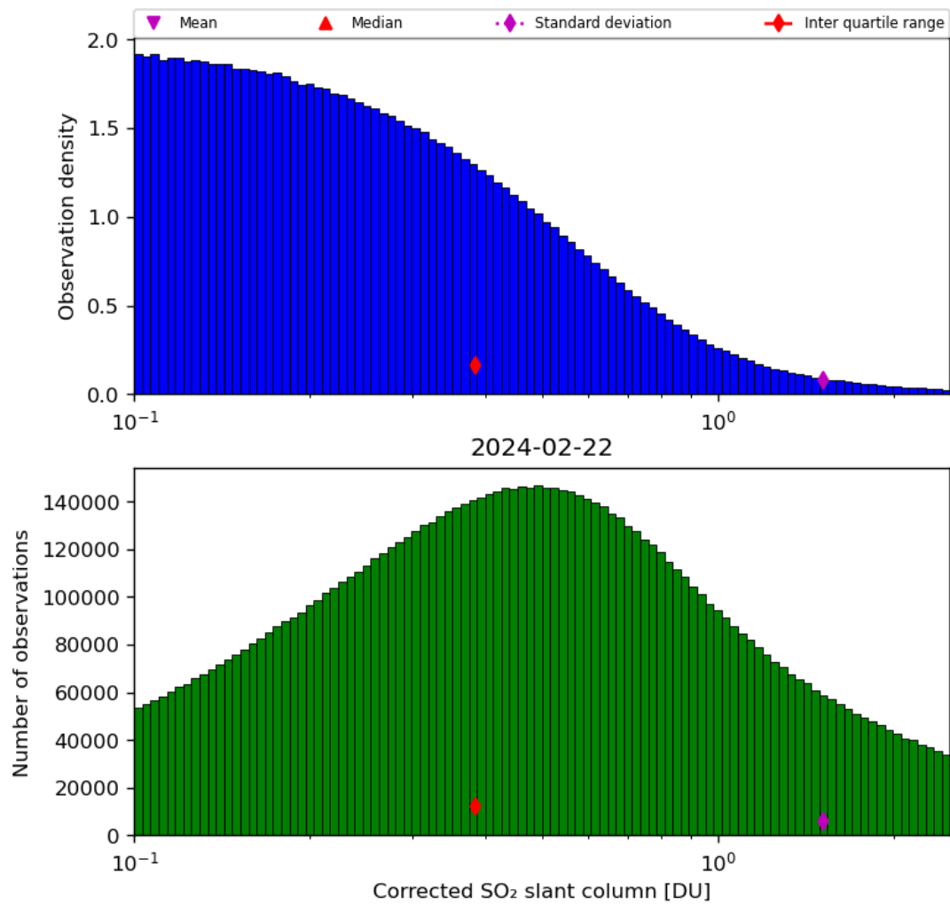
Figure 55: Histogram of “Corrected SO 2 slant column” for 2024-02-22 to 2024-02-23
