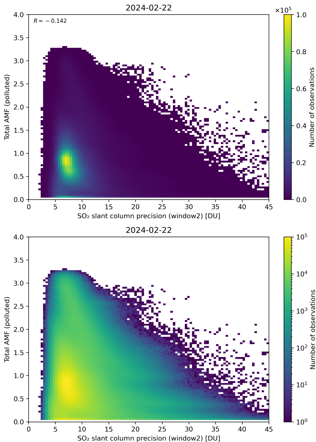
Figure 251: Scatter density plot of “SO 2 slant column precision (window2)” against “Total AMF (polluted)” for 2024-02-22 to 2024-02-23.
