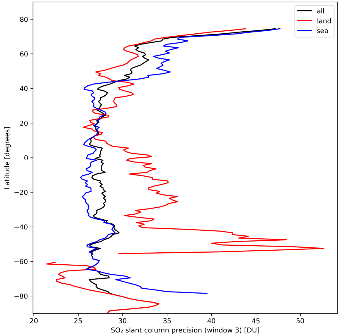
Figure 42: Zonal average of “SO 2 slant column precision (window 3)” for 2024-02-22 to 2024-02-23.
