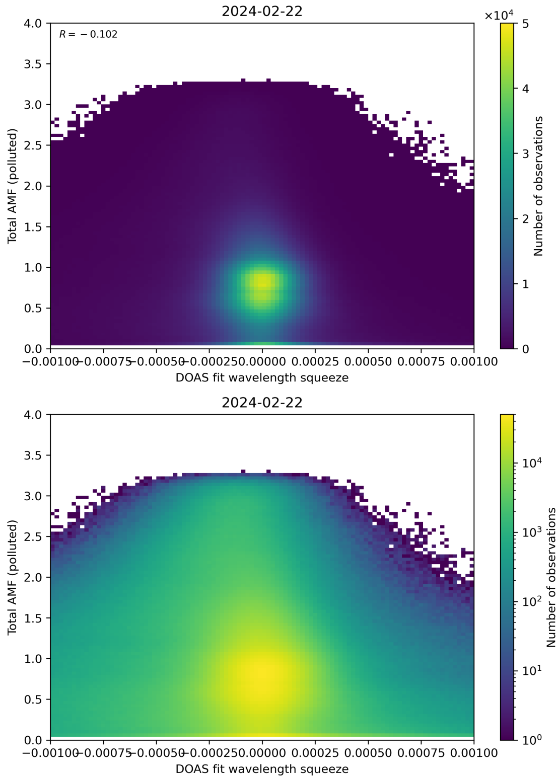
Figure 134: Scatter density plot of “DOAS fit wavelength squeeze” against “Total AMF (polluted)” for 2024-02-22 to 2024-02-23.
