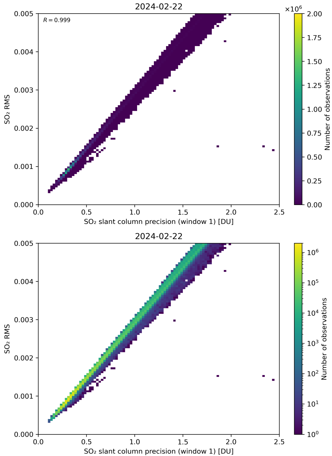
Figure 223: Scatter density plot of “SO 2 slant column precision (window 1)” against “SO 2 RMS” for 2024-02-22 to 2024-02-23.
