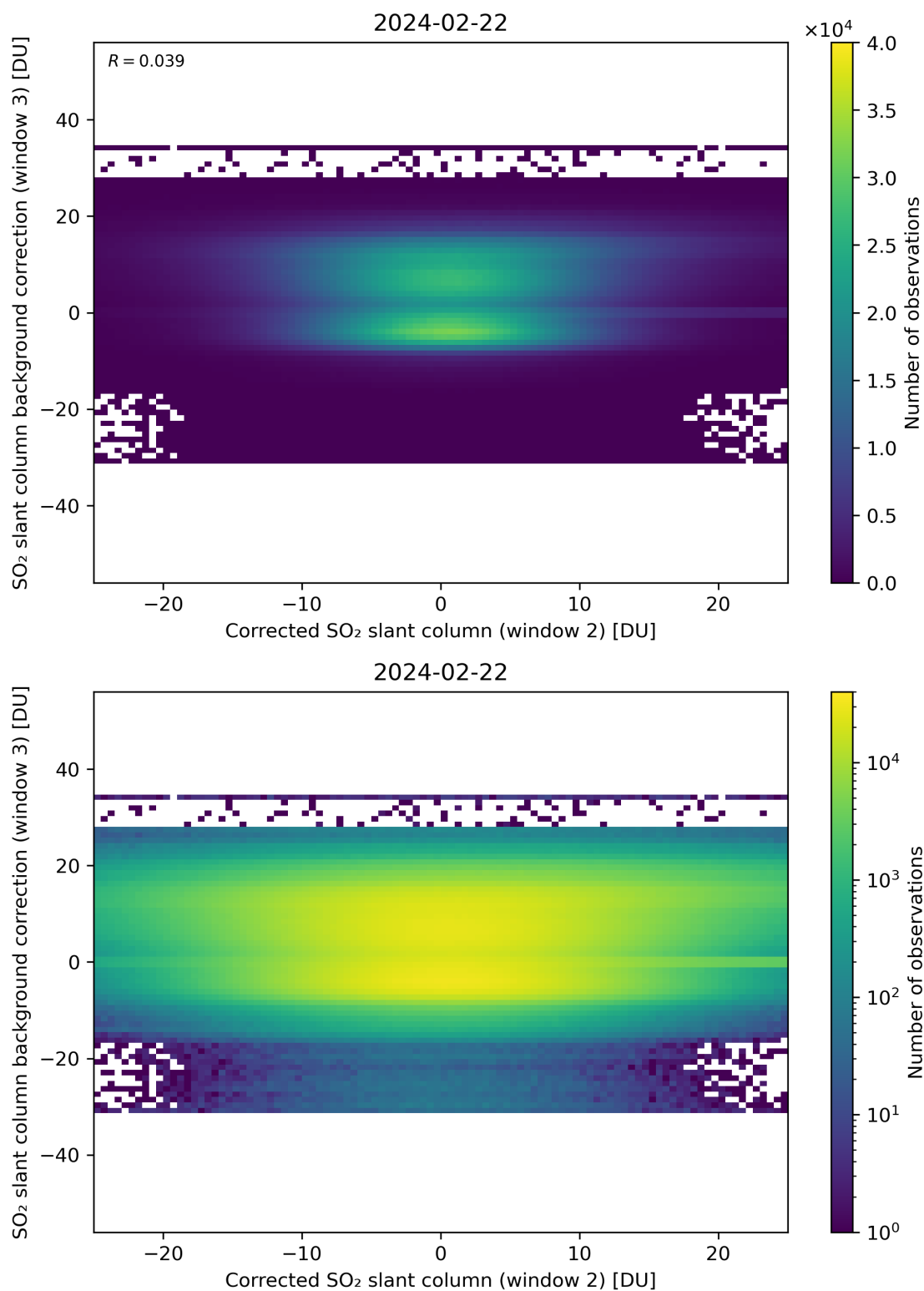
Figure 195: Scatter density plot of “Corrected SO 2 slant column (window 2)” against “SO 2 slant column background correction (window 3)” for 2024-02-22 to 2024-02-23.
