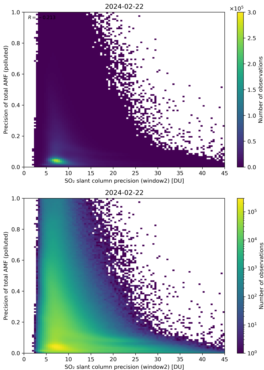
Figure 252: Scatter density plot of “SO 2 slant column precision (window2)” against “Precision of total AMF (polluted)” for 2024-02-22 to 2024-02-23.
