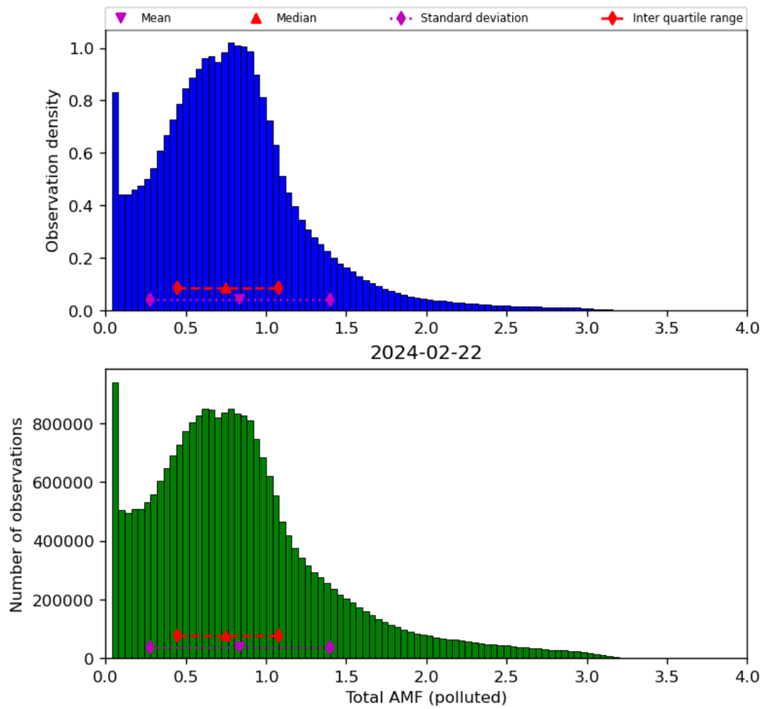
Figure 71: Histogram of “Total AMF (polluted)” for 2024-02-22 to 2024-02-23
