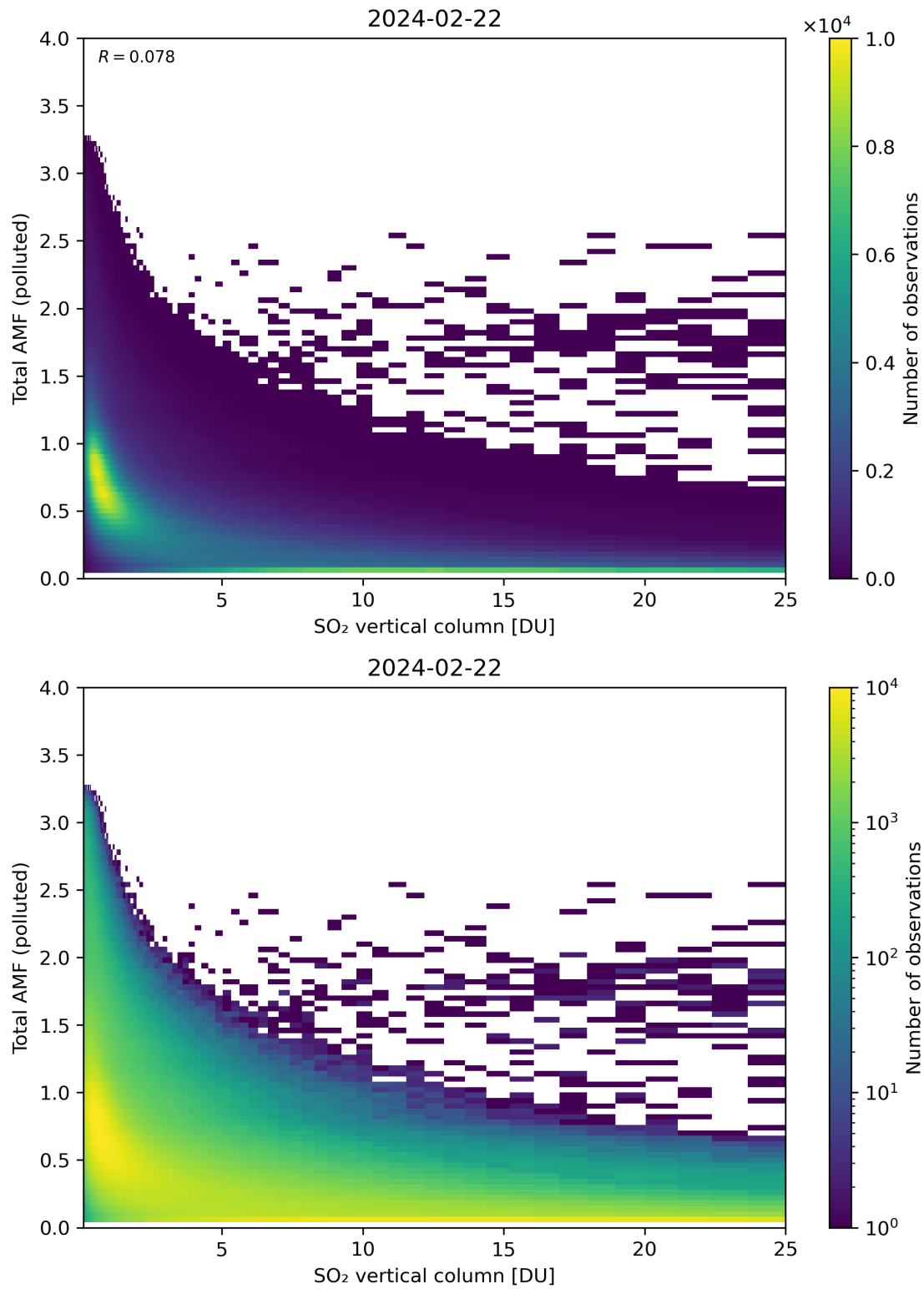
Figure 305: Scatter density plot of “SO 2 vertical column” against “Total AMF (polluted)” for 2024-02-22 to 2024-02-23.
