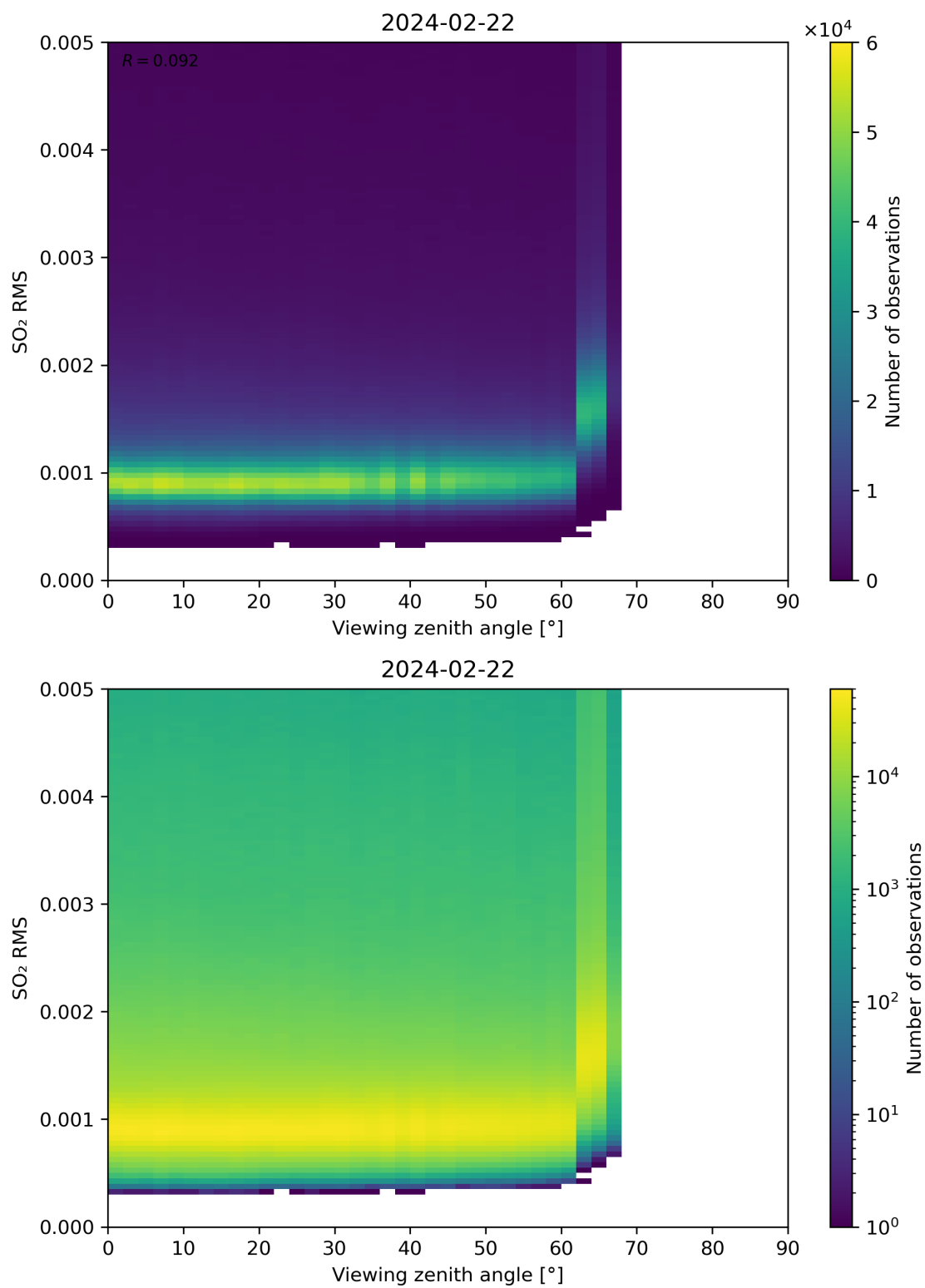
Figure 313: Scatter density plot of “Viewing zenith angle” against “SO 2 RMS” for 2024-02-22 to 2024-02-23.
