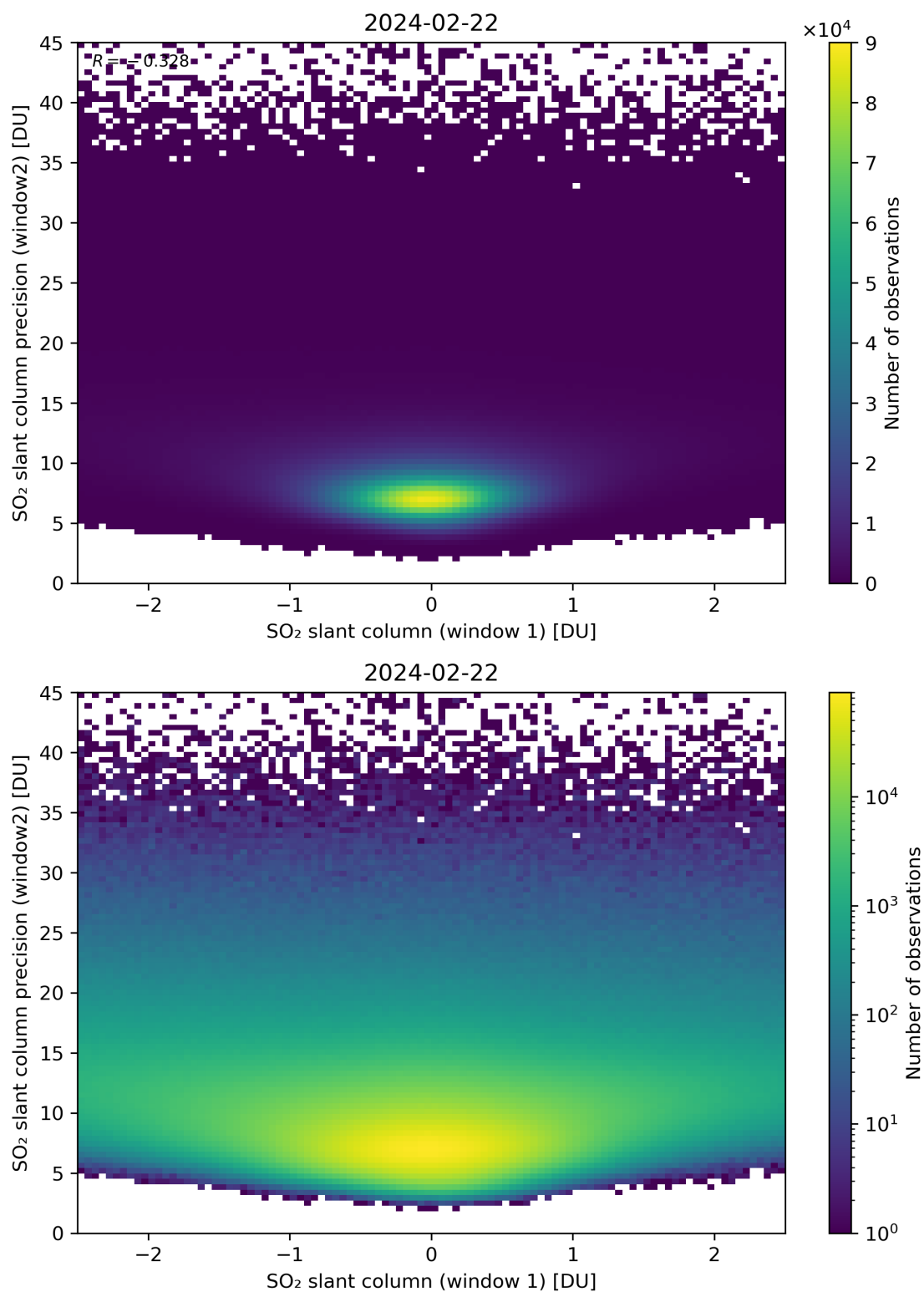
Figure 236: Scatter density plot of “SO 2 slant column (window 1)” against “SO 2 slant column precision (window2)” for 2024-02-22 to 2024-02-23.
