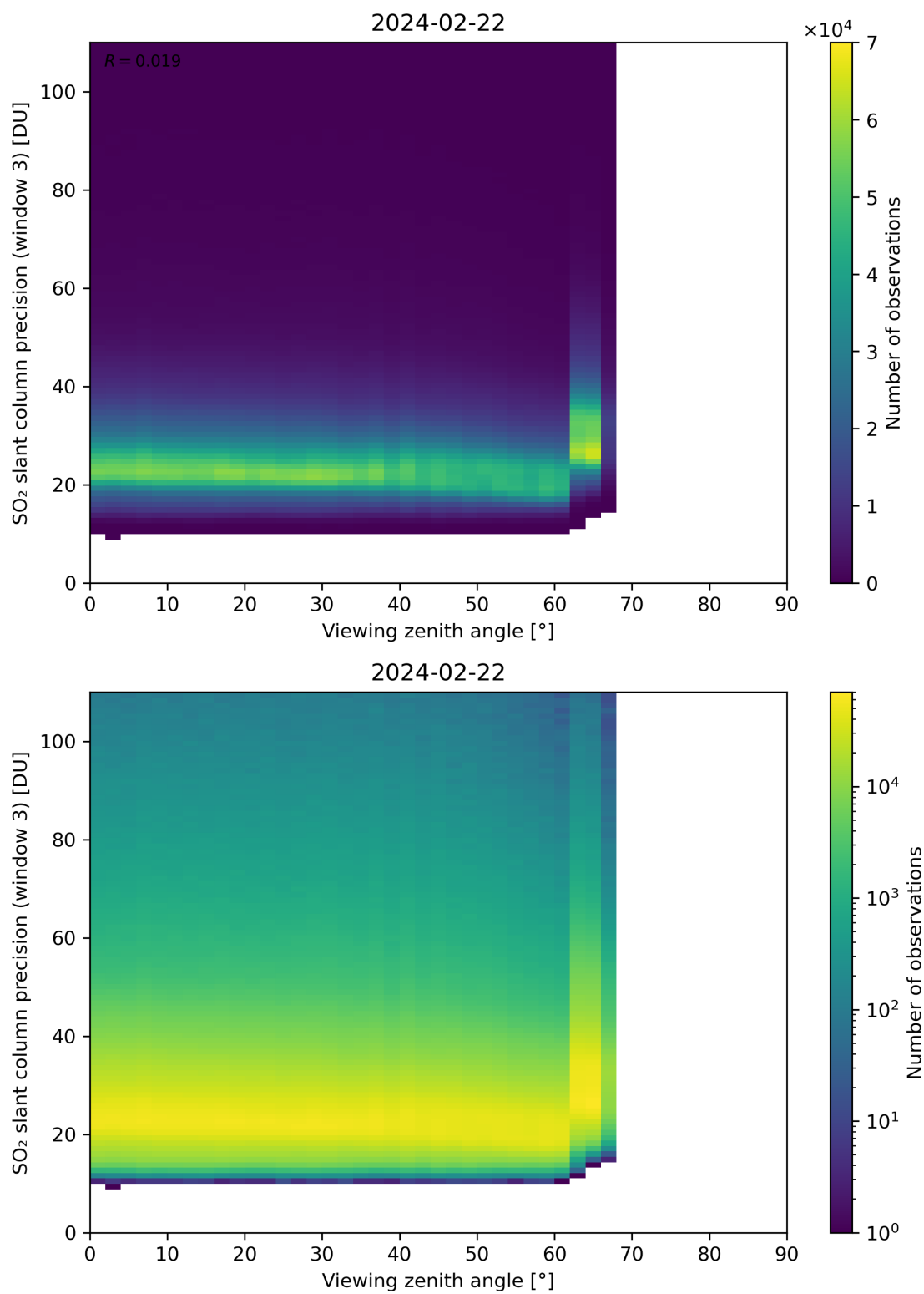
Figure 324: Scatter density plot of “Viewing zenith angle” against “SO 2 slant column precision (window 3)” for 2024-02-22 to 2024-02-23.
