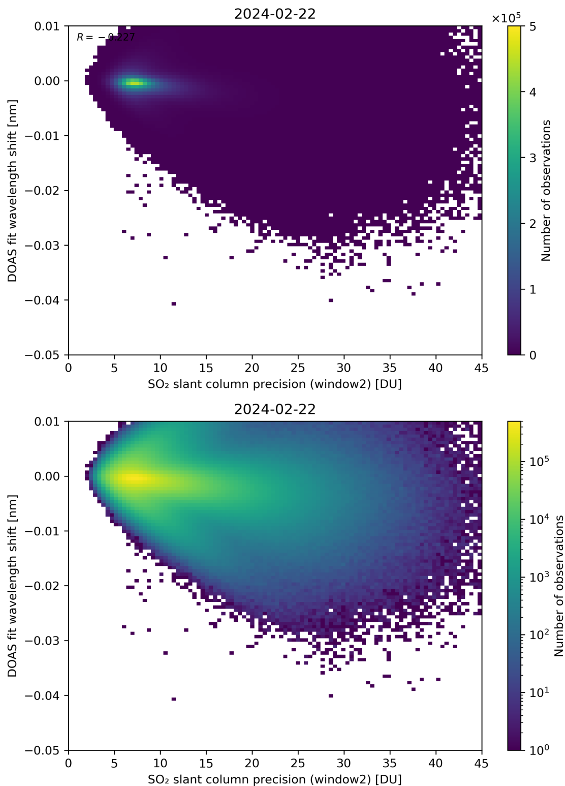
Figure 243: Scatter density plot of “SO 2 slant column precision (window2)” against “DOAS fit wavelength shift” for 2024-02-22 to 2024-02-23.
