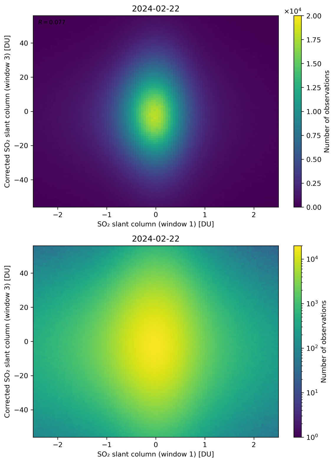
Figure 234: Scatter density plot of “SO 2 slant column (window 1)” against “Corrected SO 2 slant column (window 3)” for 2024-02-22 to 2024-02-23.
