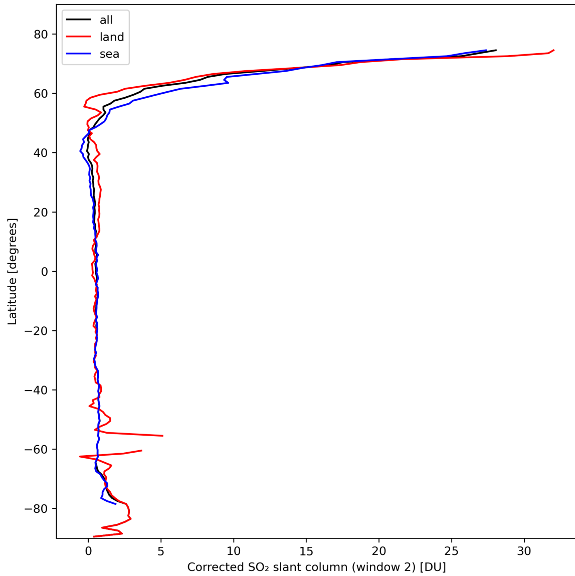
Figure 39: Zonal average of “Corrected SO 2 slant column (window 2)” for 2024-02-22 to 2024-02-23.
