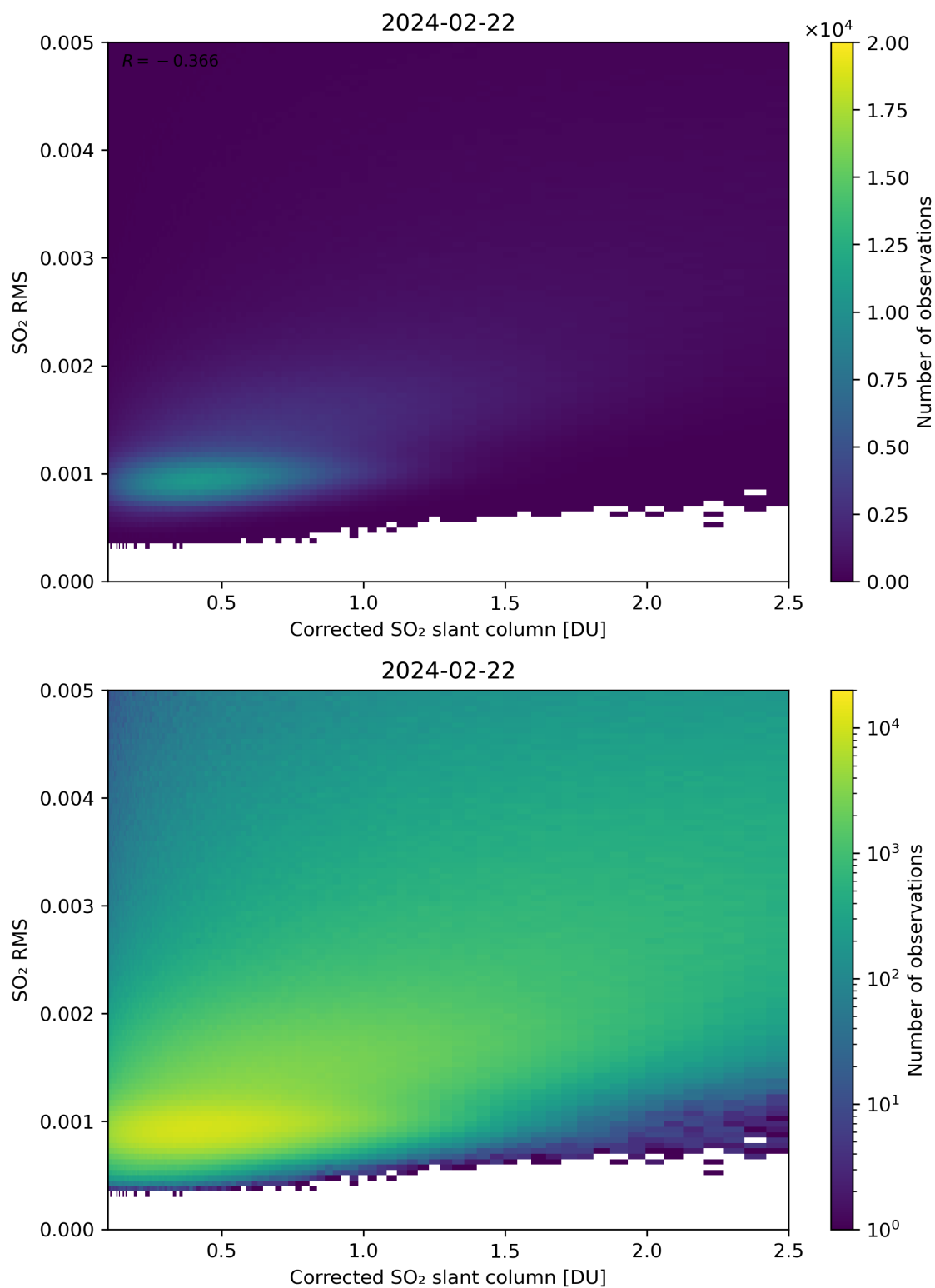
Figure 183: Scatter density plot of “Corrected SO 2 slant column” against “SO 2 RMS” for 2024-02-22 to 2024-02-23.
