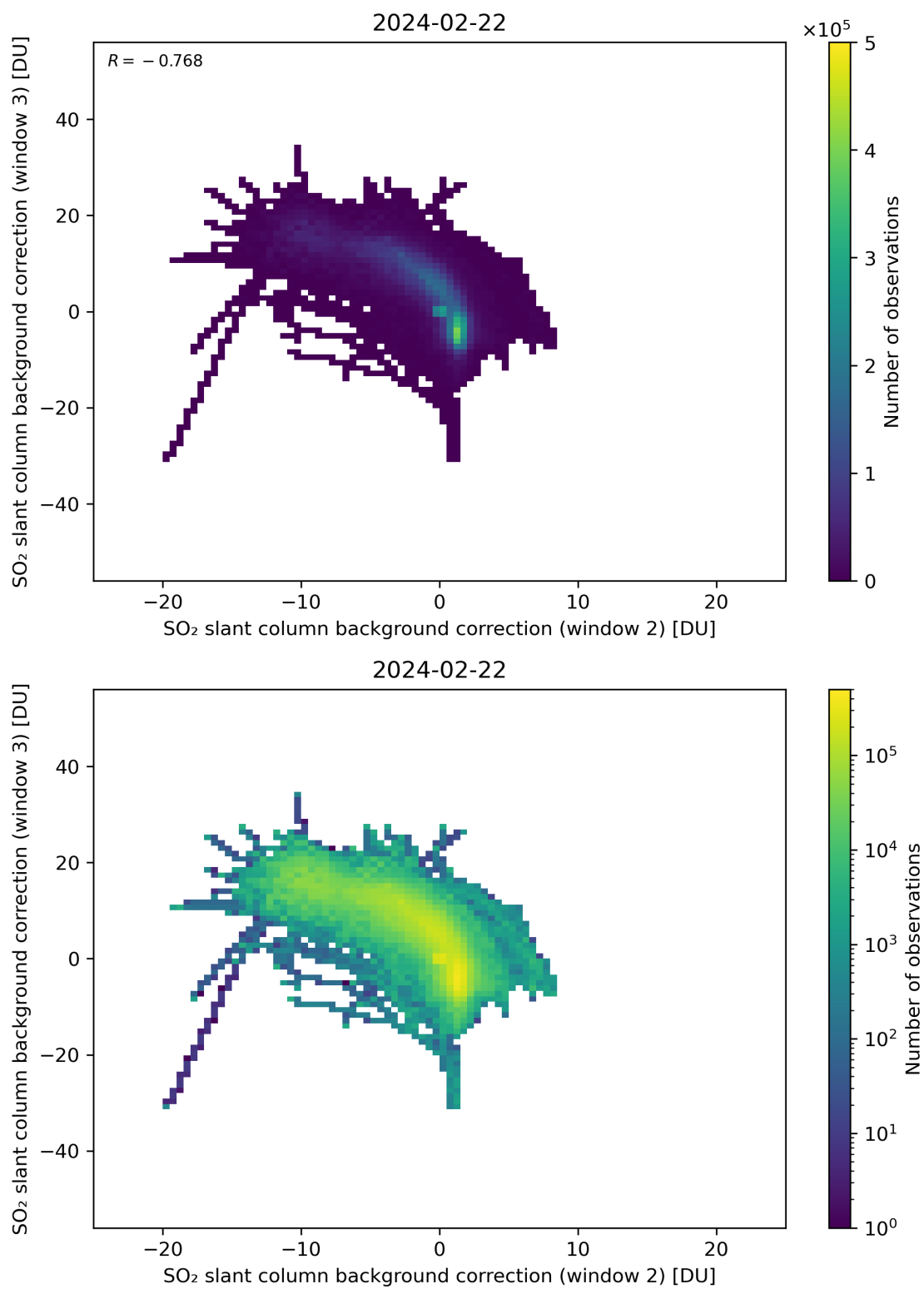
Figure 111: Scatter density plot of “SO 2 slant column background correction (window 2)” against “SO 2 slant column background correction (window 3)” for 2024-02-22 to 2024-02-23.
