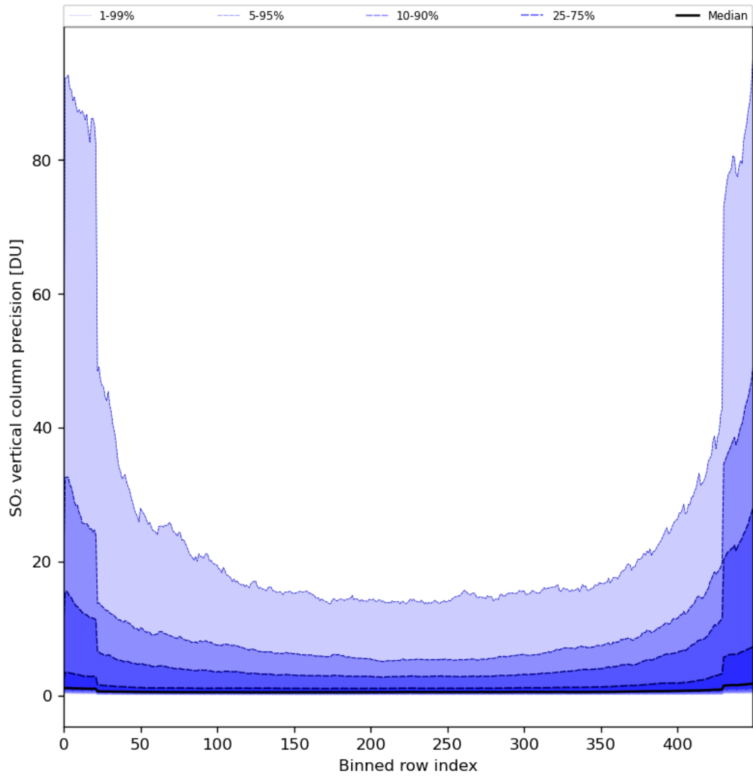
Figure 77: Along track statistics of “SO 2 vertical column precision” for 2024-02-22 to 2024-02-23
