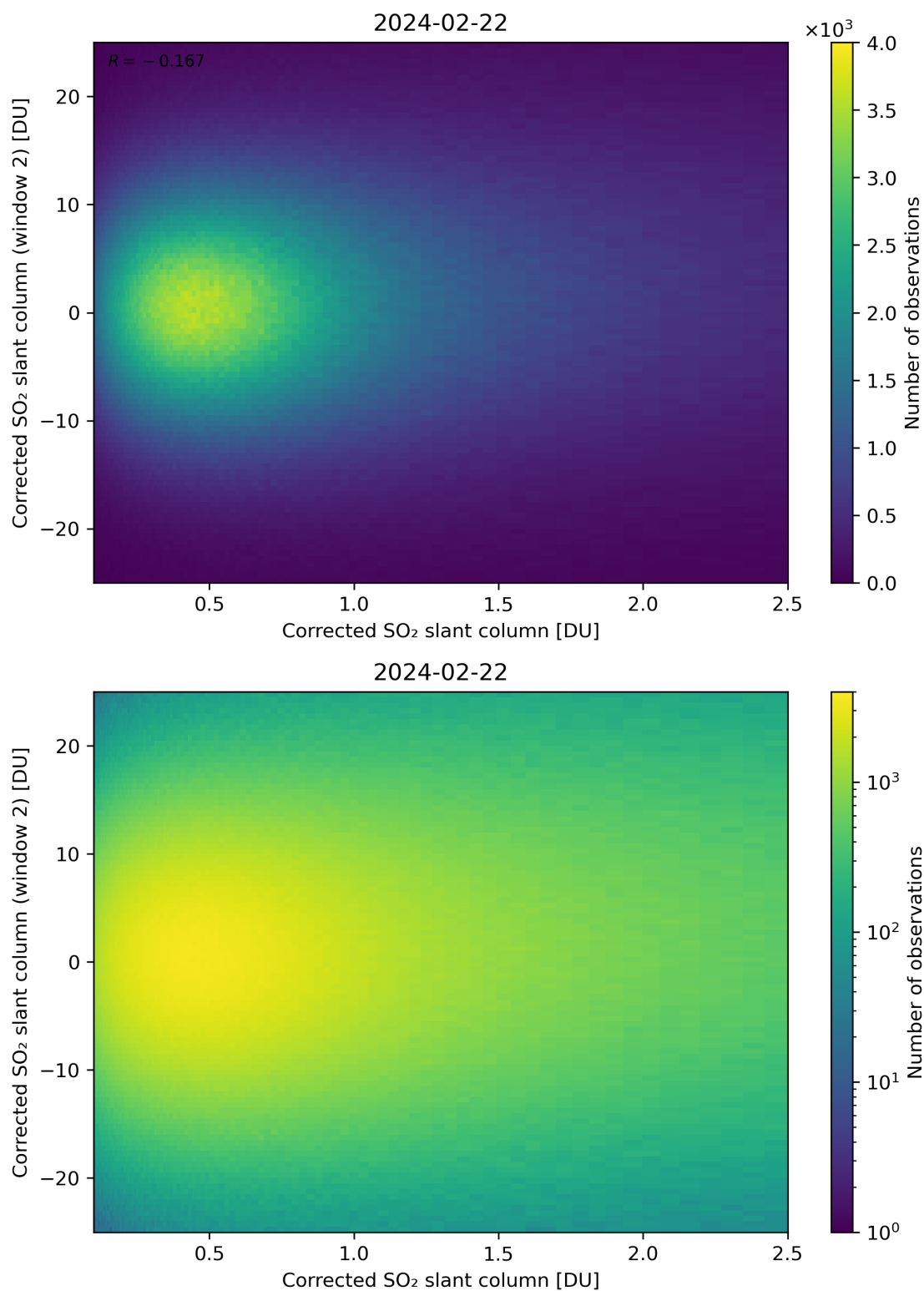
Figure 185: Scatter density plot of “Corrected SO 2 slant column” against “Corrected SO 2 slant column (window 2)” for 2024-02-22 to 2024-02-23.
