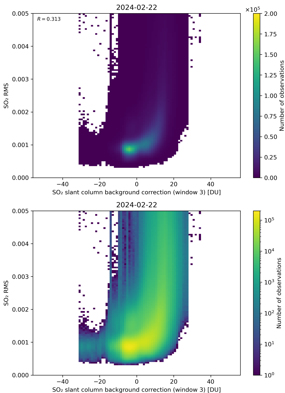
Figure 123: Scatter density plot of “SO 2 slant column background correction (window 3)” against “SO 2 RMS” for 2024-02-22 to 2024-02-23.
