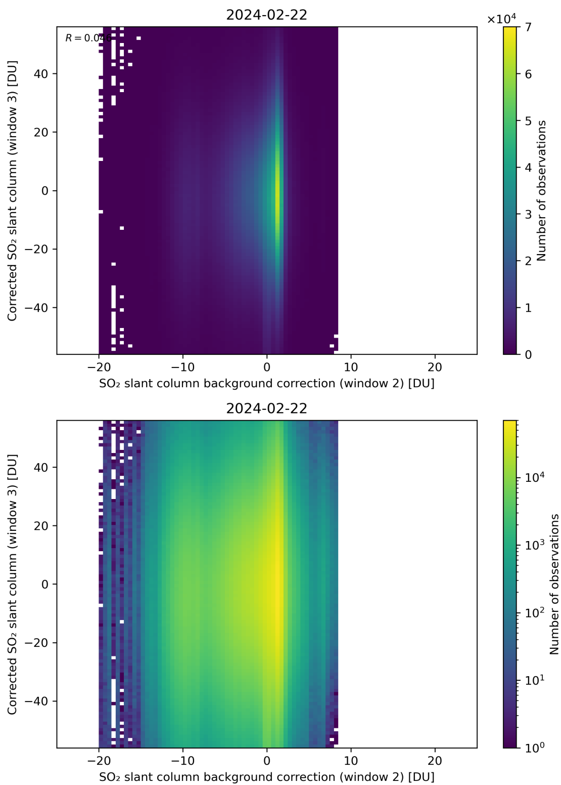
Figure 116: Scatter density plot of “SO 2 slant column background correction (window 2)” against “Corrected SO 2 slant column (window 3)” for 2024-02-22 to 2024-02-23.
