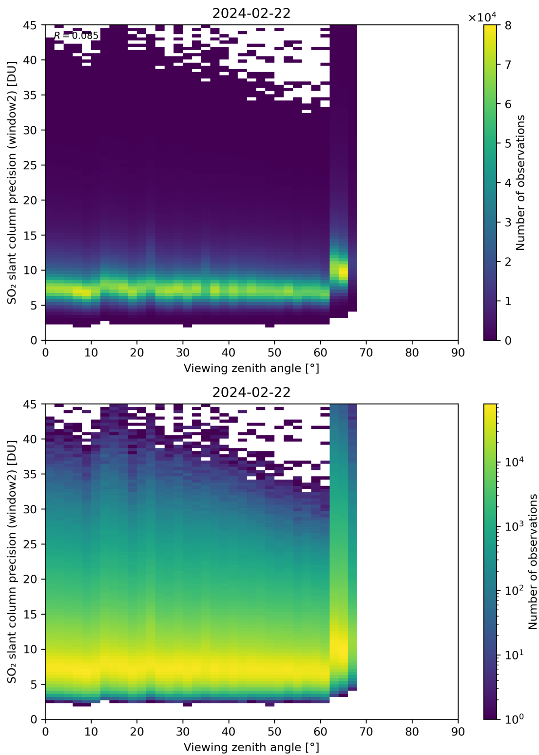
Figure 322: Scatter density plot of “Viewing zenith angle” against “SO 2 slant column precision (window2)” for 2024-02-22 to 2024-02-23.
