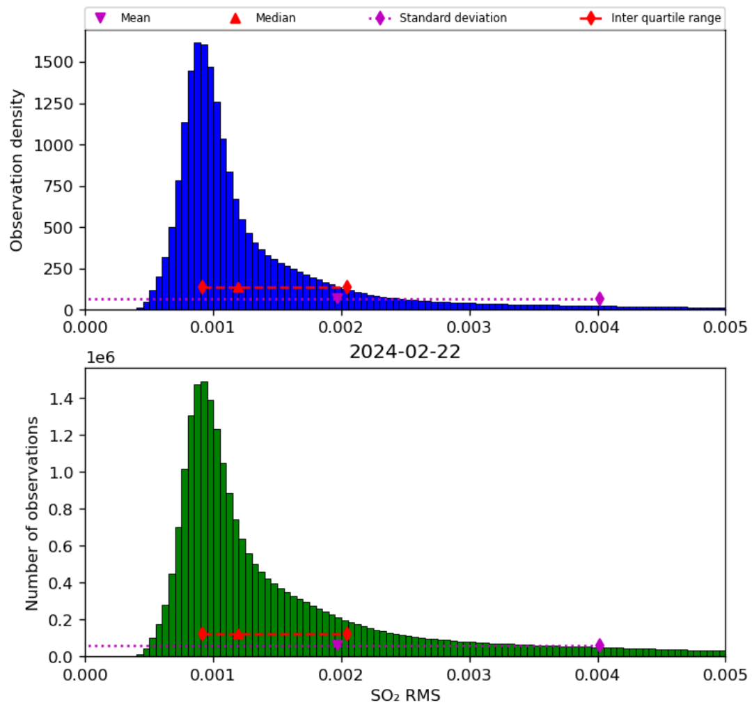
Figure 70: Histogram of “SO 2 RMS” for 2024-02-22 to 2024-02-23
