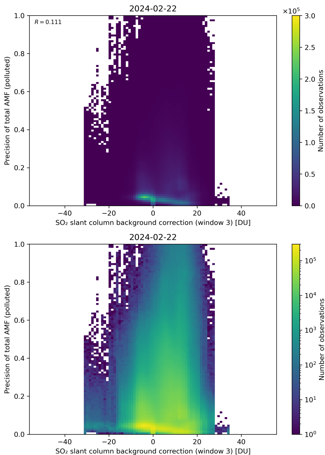
Figure 126: Scatter density plot of “SO 2 slant column background correction (window 3)” against “Precision of total AMF (polluted)” for 2024-02-22 to 2024-02-23.
