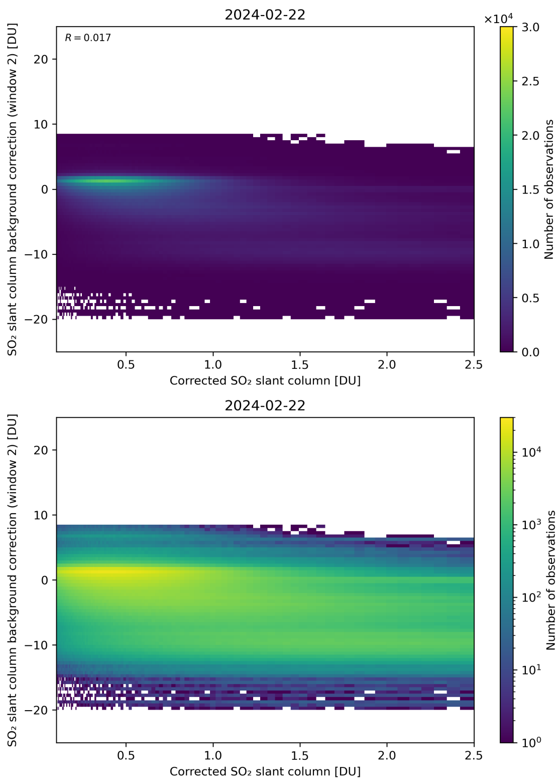
Figure 179: Scatter density plot of “Corrected SO 2 slant column” against “SO 2 slant column background correction (window 2)” for 2024-02-22 to 2024-02-23.
