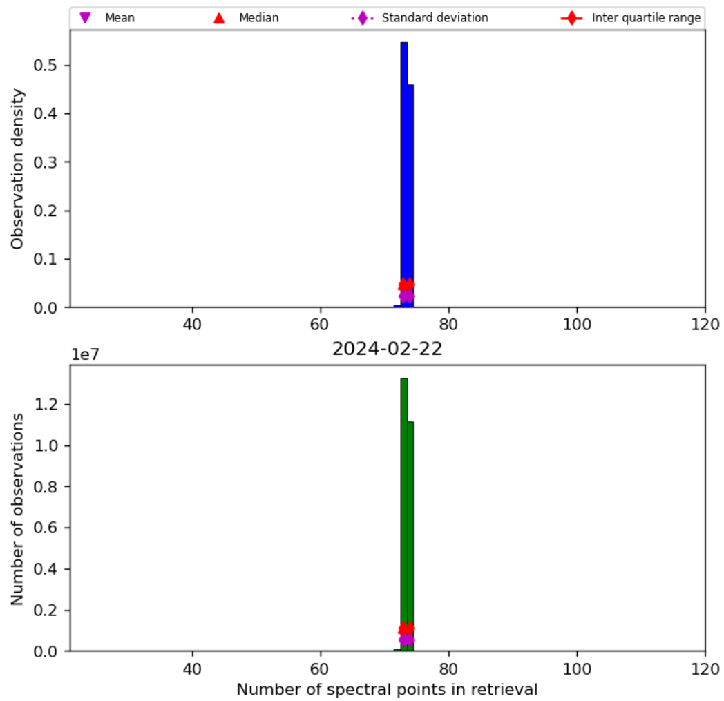
Figure 74: Histogram of “Number of spectral points in retrieval” for 2024-02-22 to 2024-02-23
