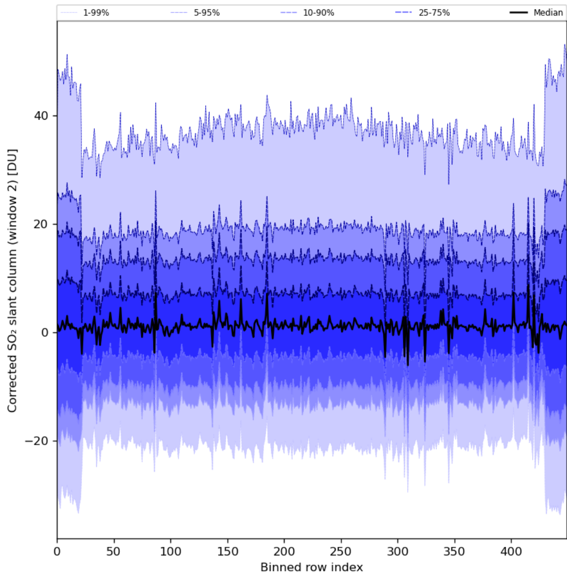
Figure 85: Along track statistics of “Corrected SO 2 slant column (window 2)” for 2024-02-22 to 2024-02-23
