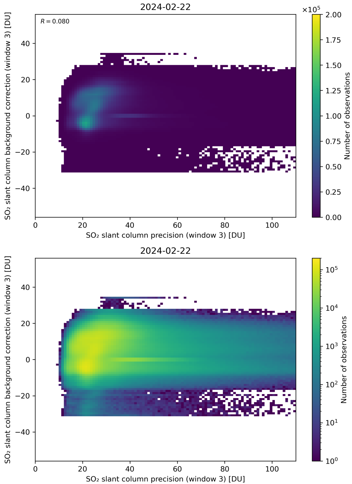
Figure 257: Scatter density plot of “SO 2 slant column precision (window 3)” against “SO 2 slant column background correction (window 3)” for 2024-02-22 to 2024-02-23.
