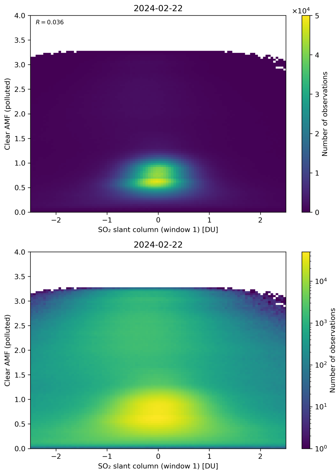
Figure 232: Scatter density plot of “SO 2 slant column (window 1)” against “Clear AMF (polluted)” for 2024-02-22 to 2024-02-23.
