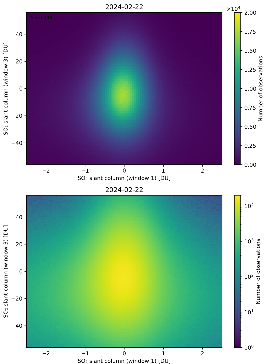
Figure 237: Scatter density plot of “SO 2 slant column (window 1)” against “SO 2 slant column (window 3)” for 2024-02-22 to 2024-02-23.
