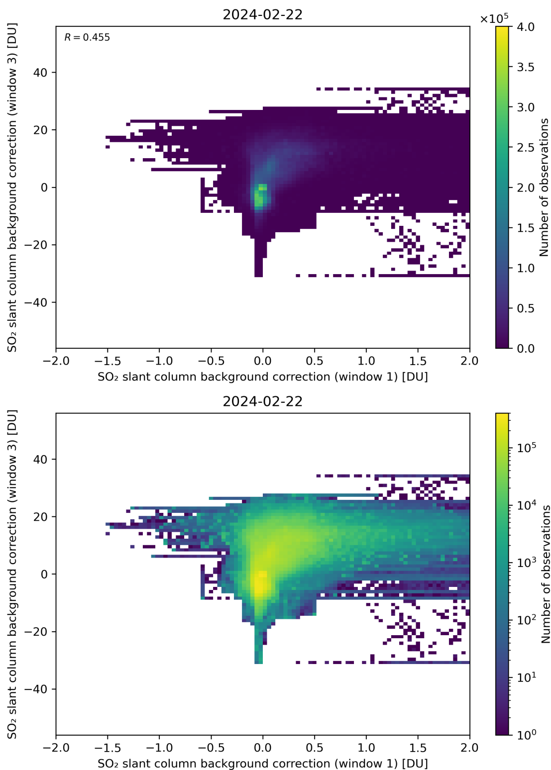
Figure 99: Scatter density plot of “SO 2 slant column background correction (window 1)” against “SO 2 slant column background correction (window 3)” for 2024-02-22 to 2024-02-23.
