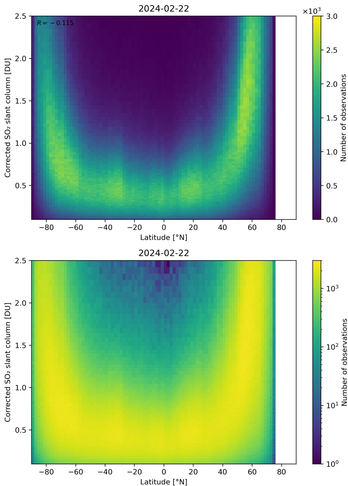
Figure 146: Scatter density plot of “Latitude” against “Corrected SO 2 slant column” for 2024-02-22 to 2024-02-23.
