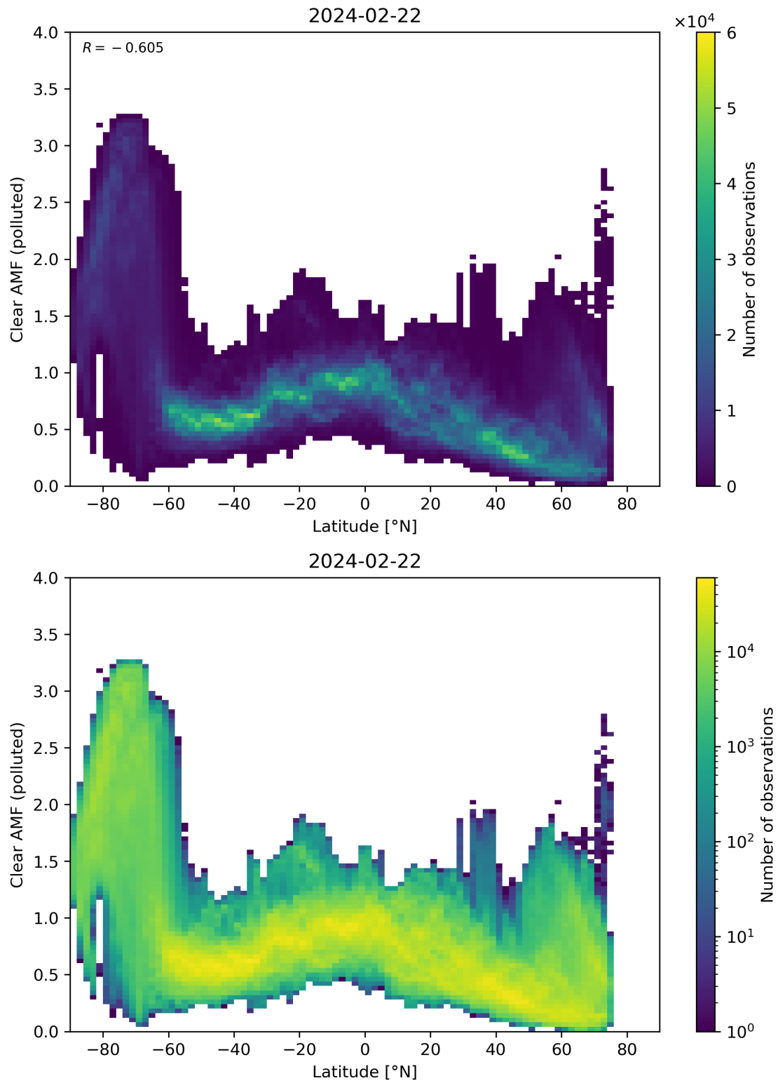
Figure 145: Scatter density plot of “Latitude” against “Clear AMF (polluted)” for 2024-02-22 to 2024-02-23.
