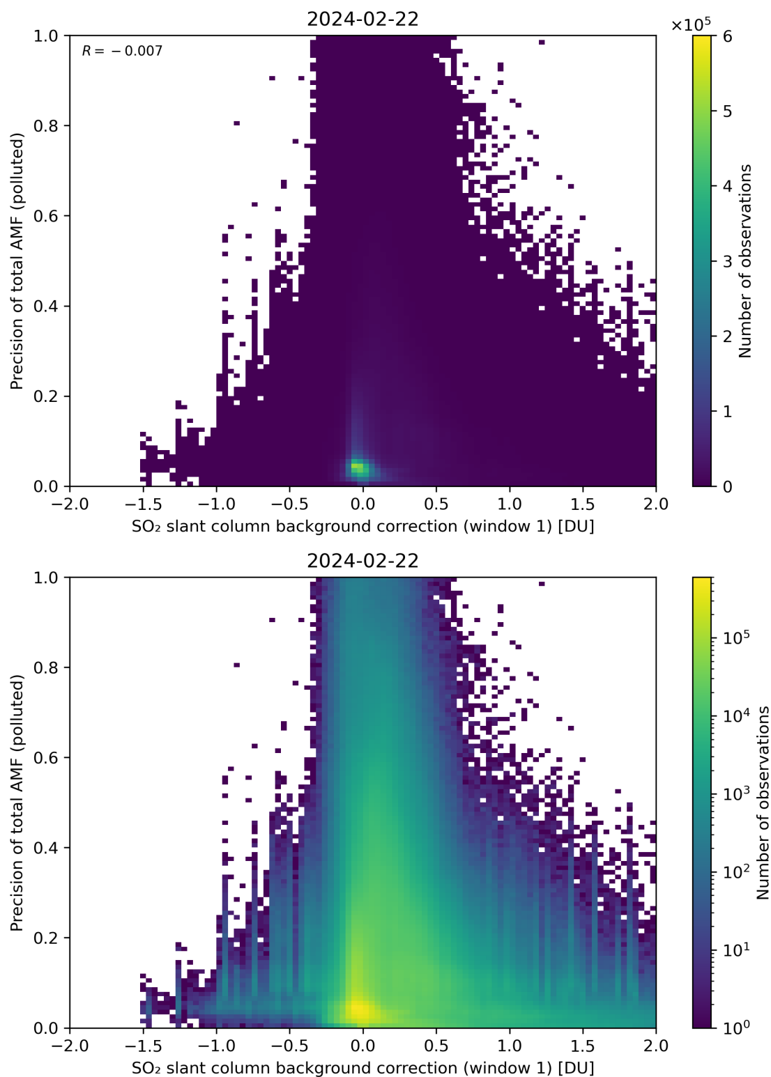
Figure 110: Scatter density plot of “SO 2 slant column background correction (window 1)” against “Precision of total AMF (polluted)” for 2024-02-22 to 2024-02-23.
