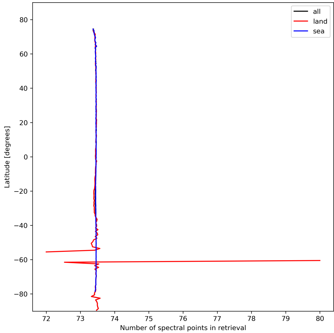
Figure 51: Zonal average of “Number of spectral points in retrieval” for 2024-02-22 to 2024-02-23.
