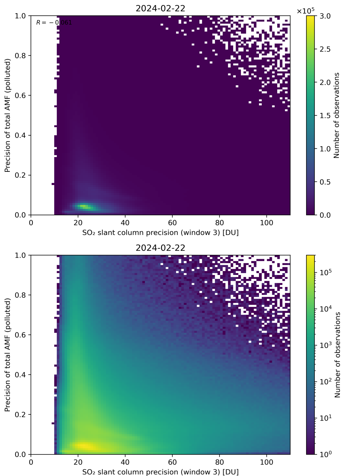
Figure 264: Scatter density plot of “SO 2 slant column precision (window 3)” against “Precision of total AMF (polluted)” for 2024-02-22 to 2024-02-23.
