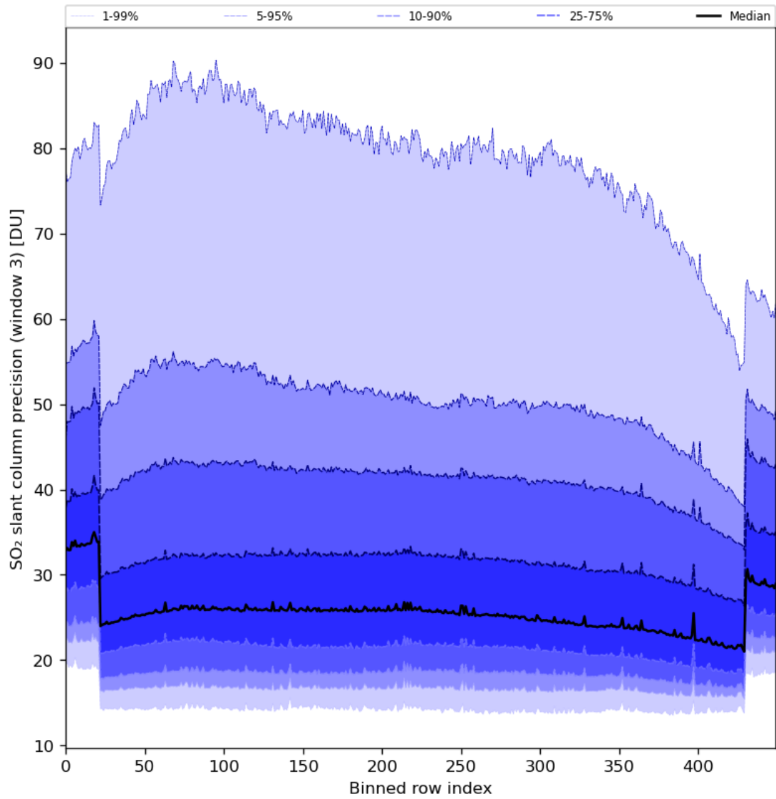
Figure 88: Along track statistics of “SO 2 slant column precision (window 3)” for 2024-02-22 to 2024-02-23
