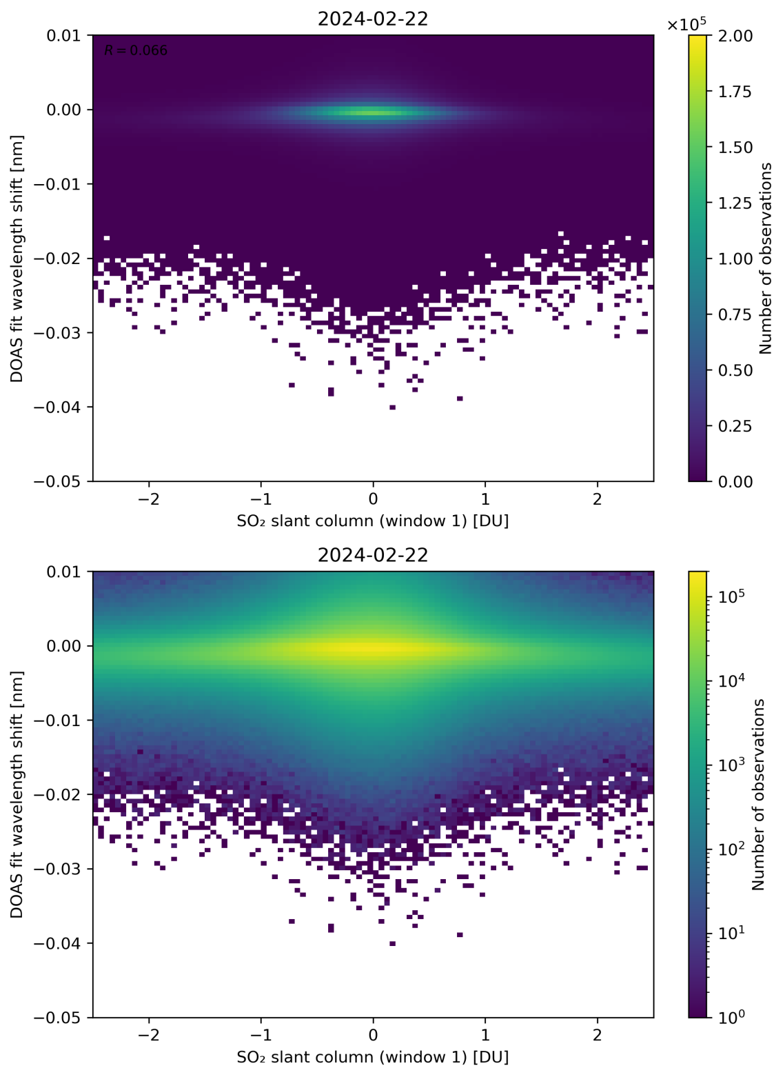
Figure 215: Scatter density plot of “SO 2 slant column (window 1)” against “DOAS fit wavelength shift” for 2024-02-22 to 2024-02-23.
