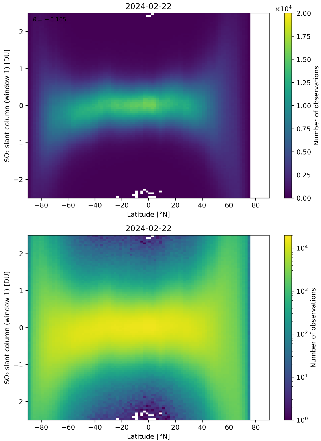
Figure 149: Scatter density plot of “Latitude” against “SO 2 slant column (window 1)” for 2024-02-22 to 2024-02-23.
