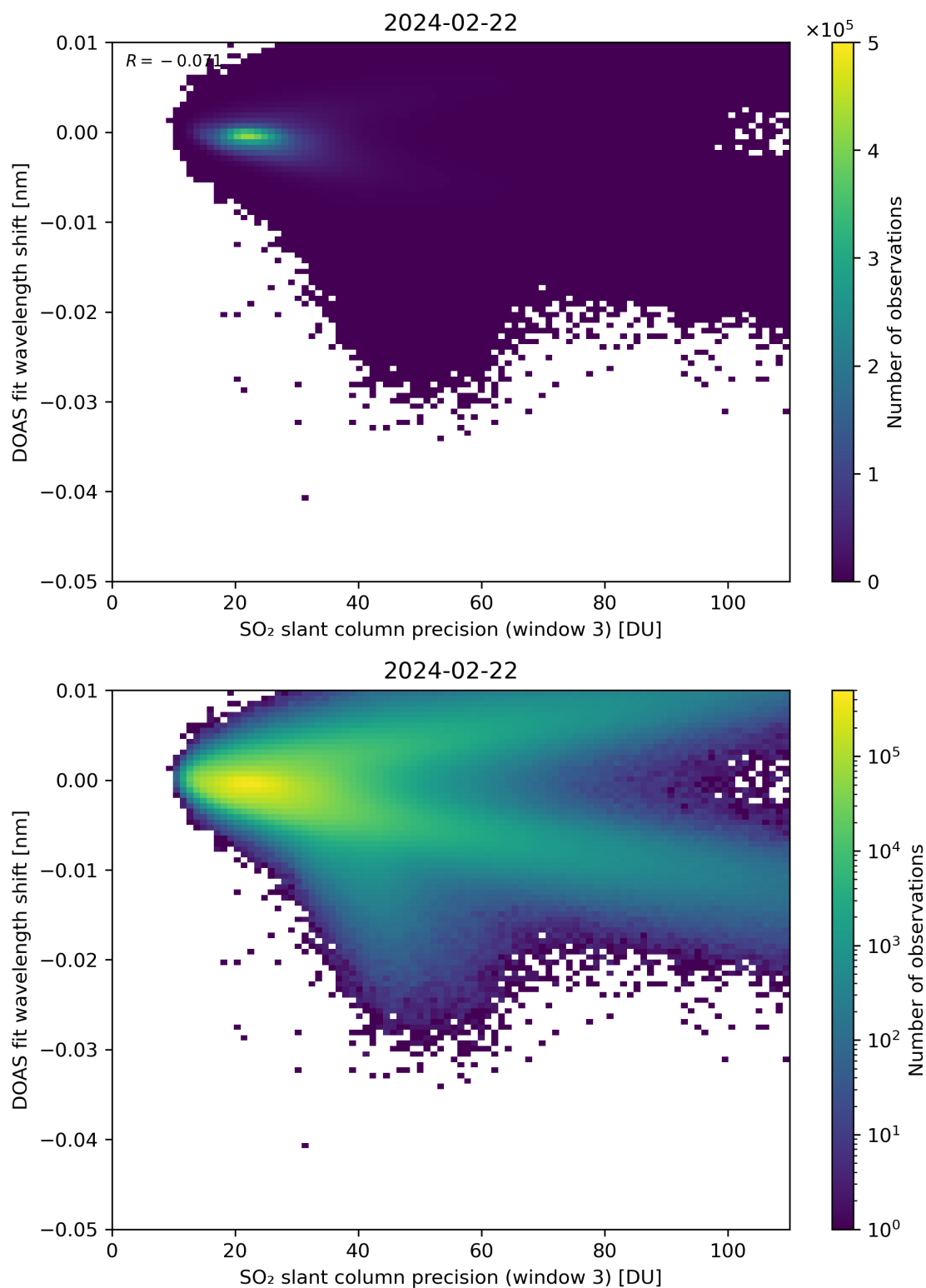
Figure 258: Scatter density plot of “SO 2 slant column precision (window 3)” against “DOAS fit wavelength shift” for 2024-02-22 to 2024-02-23.
