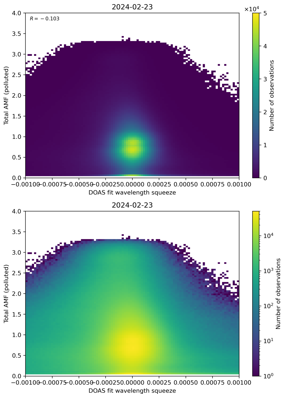
Figure 134: Scatter density plot of “DOAS fit wavelength squeeze” against “Total AMF (polluted)” for 2024-02-22 to 2024-02-24.
