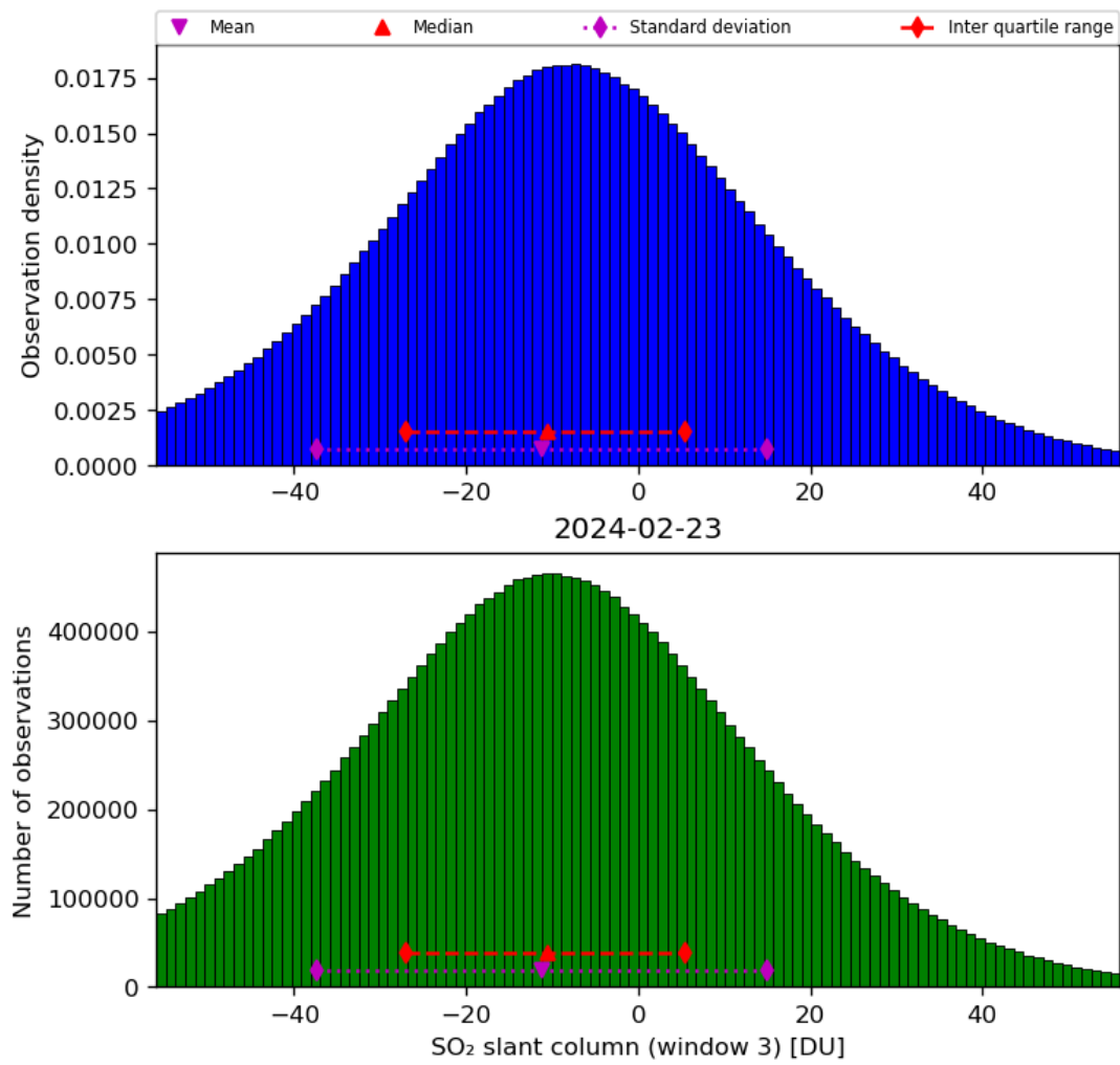
Figure 64: Histogram of “SO 2 slant column (window 3)” for 2024-02-22 to 2024-02-24
