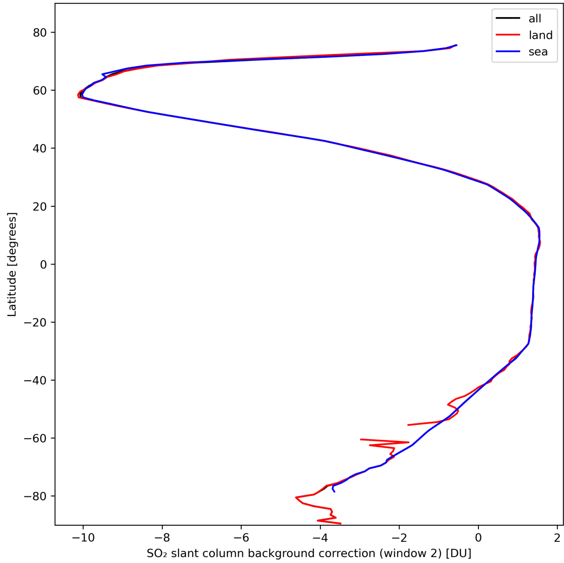
Figure 40: Zonal average of “SO 2 slant column background correction (window 2)” for 2024-02-22 to 2024-02-24.
