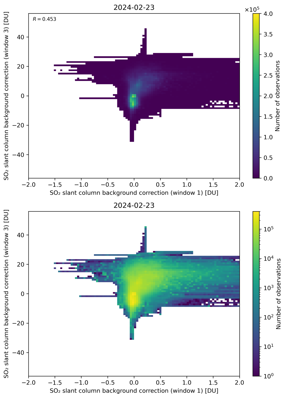
Figure 99: Scatter density plot of “SO 2 slant column background correction (window 1)” against “SO 2 slant column background correction (window 3)” for 2024-02-22 to 2024-02-24.
