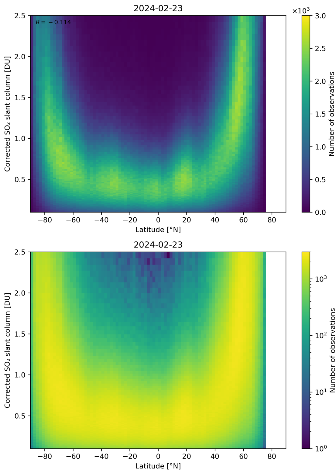
Figure 146: Scatter density plot of “Latitude” against “Corrected SO 2 slant column” for 2024-02-22 to 2024-02-24.
