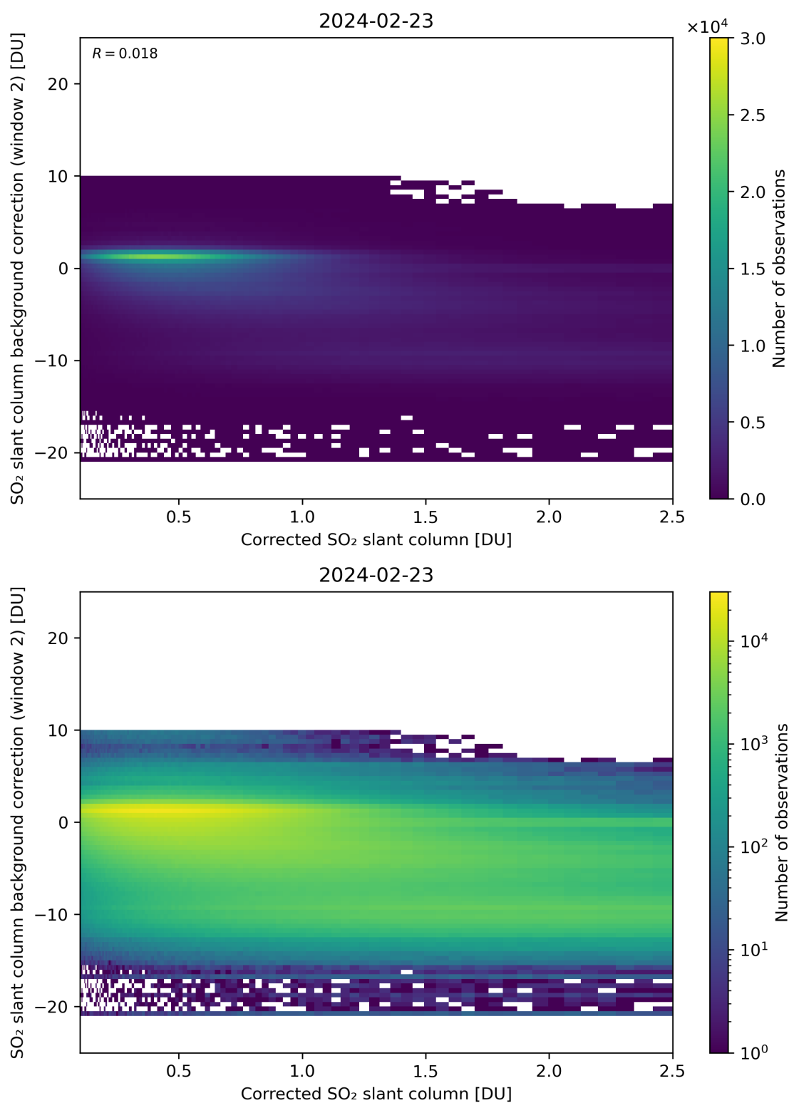
Figure 179: Scatter density plot of “Corrected SO 2 slant column” against “SO 2 slant column background correction (window 2)” for 2024-02-22 to 2024-02-24.
