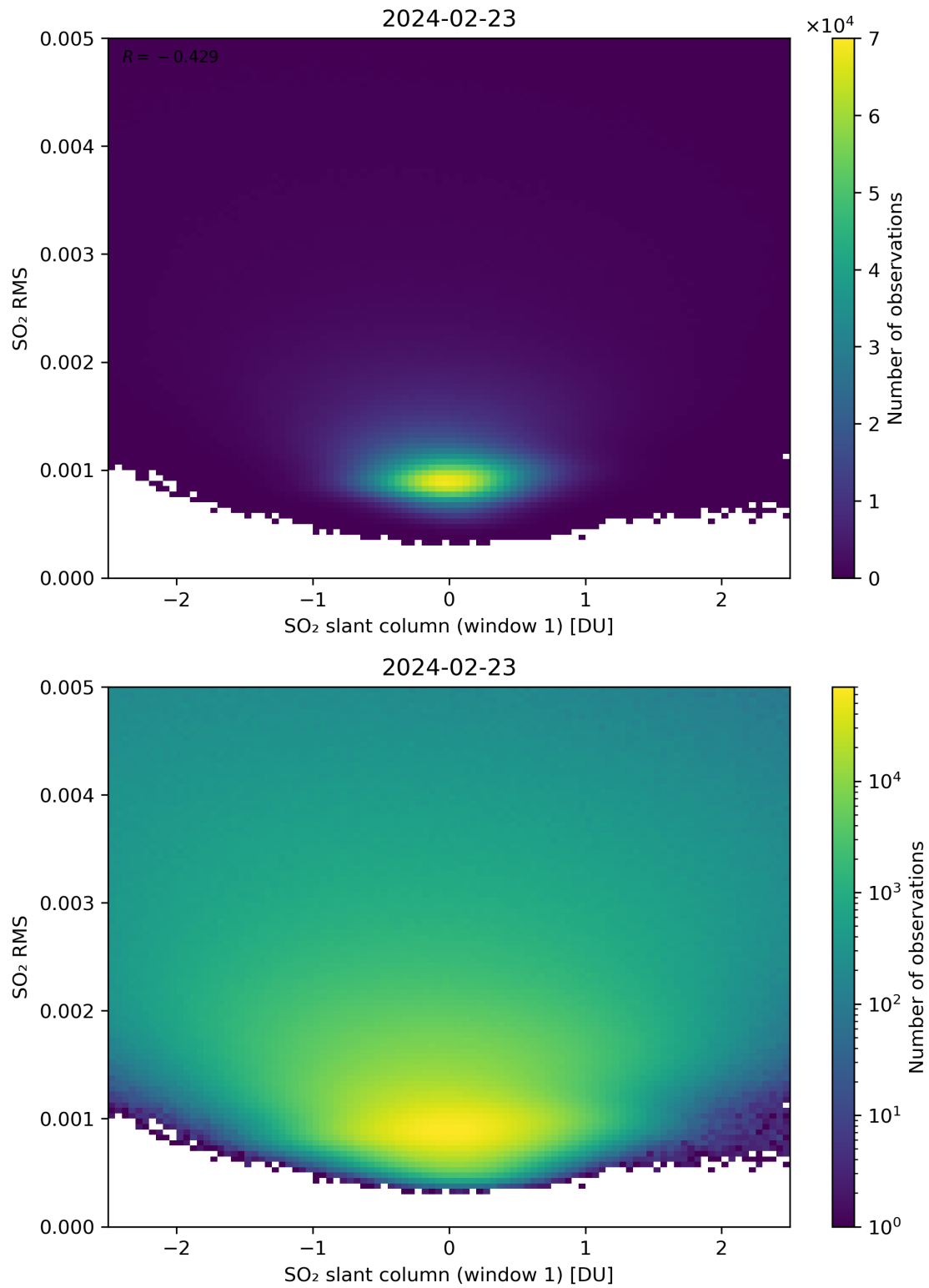
Figure 217: Scatter density plot of “SO 2 slant column (window 1)” against “SO 2 RMS” for 2024-02-22 to 2024-02-24.
