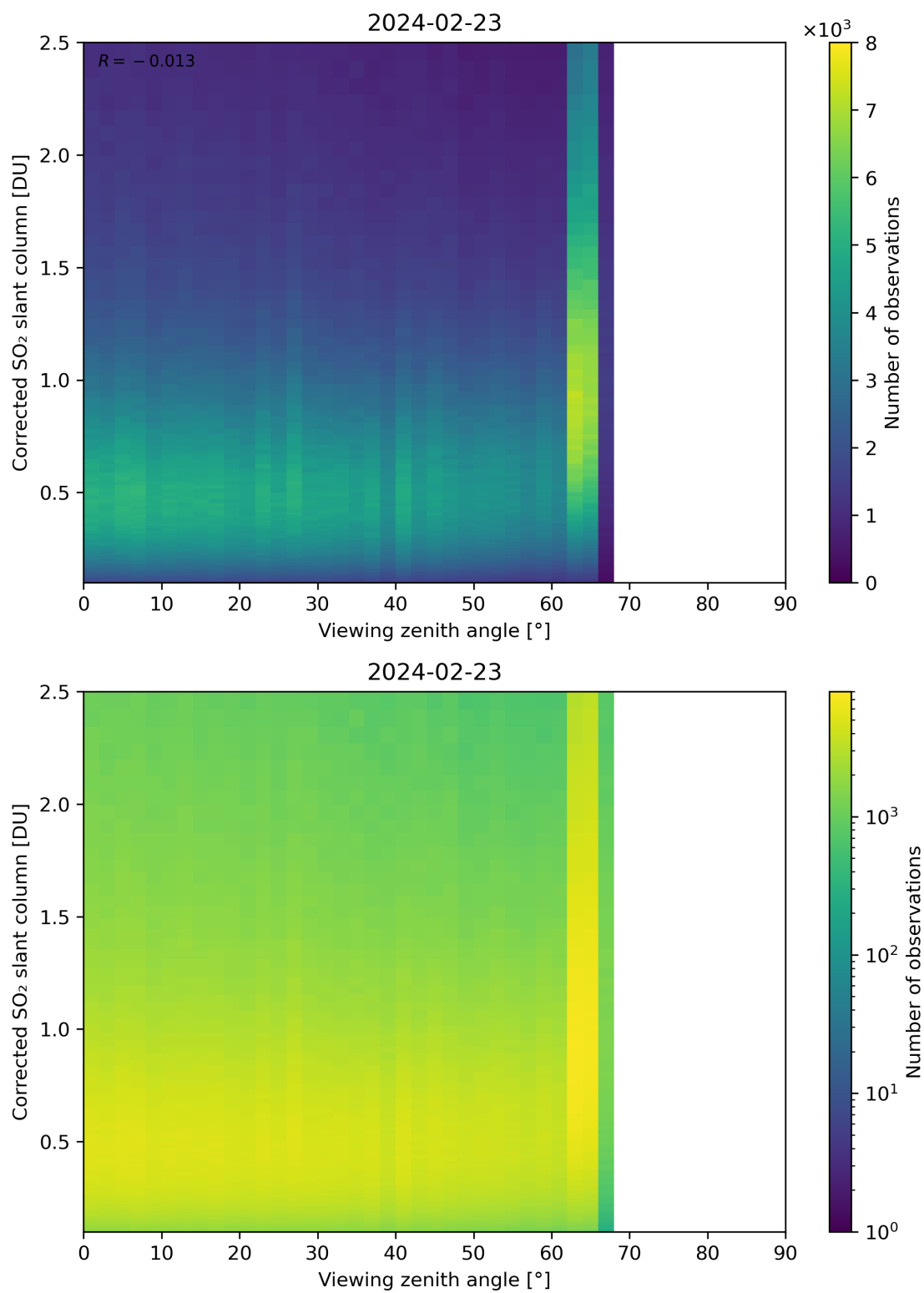
Figure 317: Scatter density plot of “Viewing zenith angle” against “Corrected SO 2 slant column” for 2024-02-22 to 2024-02-24.
