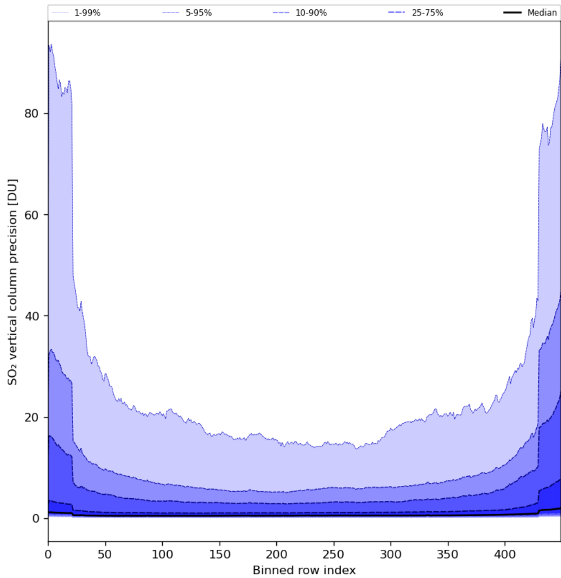
Figure 77: Along track statistics of “SO 2 vertical column precision” for 2024-02-22 to 2024-02-24
