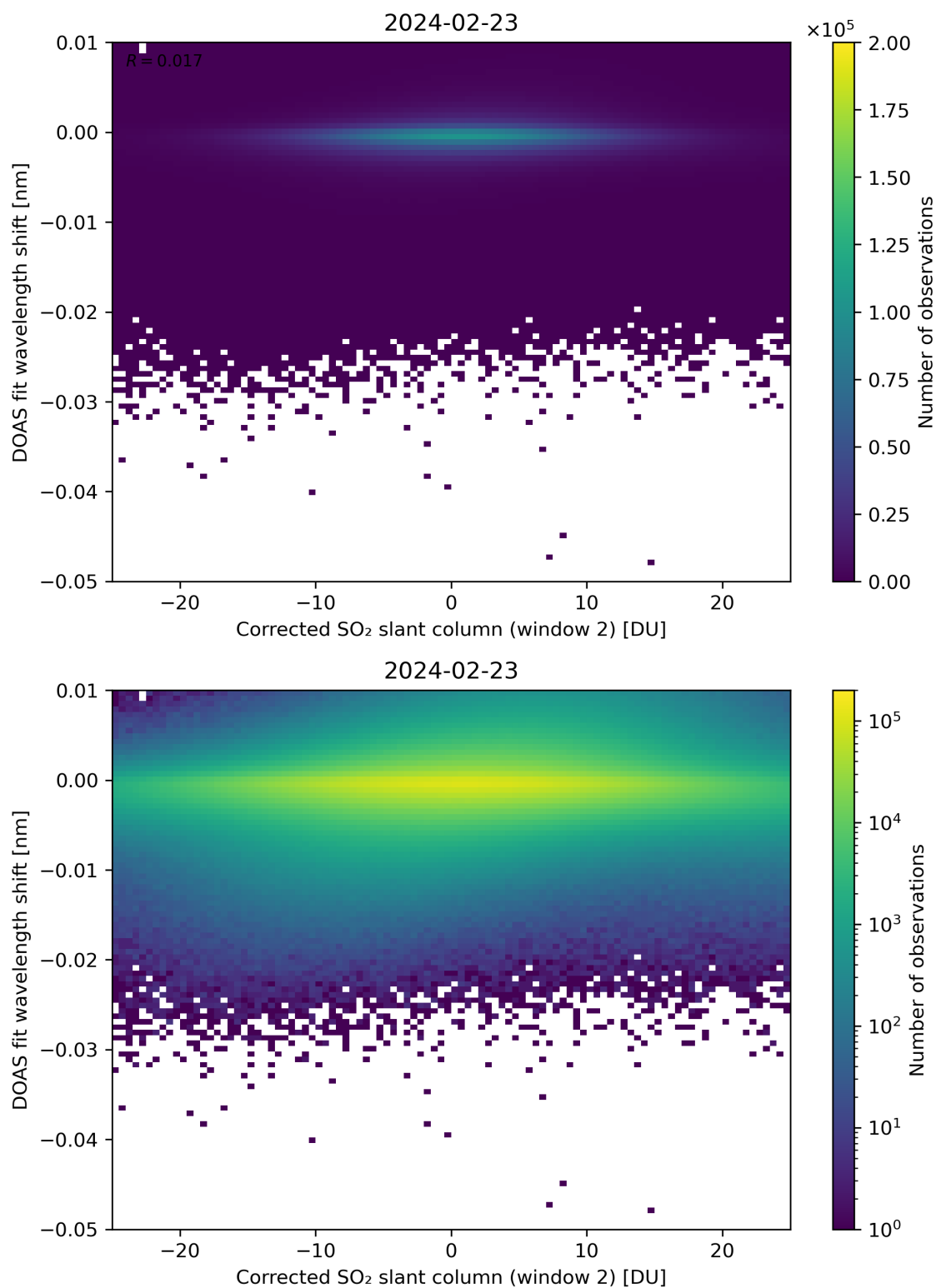
Figure 196: Scatter density plot of “Corrected SO 2 slant column (window 2)” against “DOAS fit wavelength shift” for 2024-02-22 to 2024-02-24.
