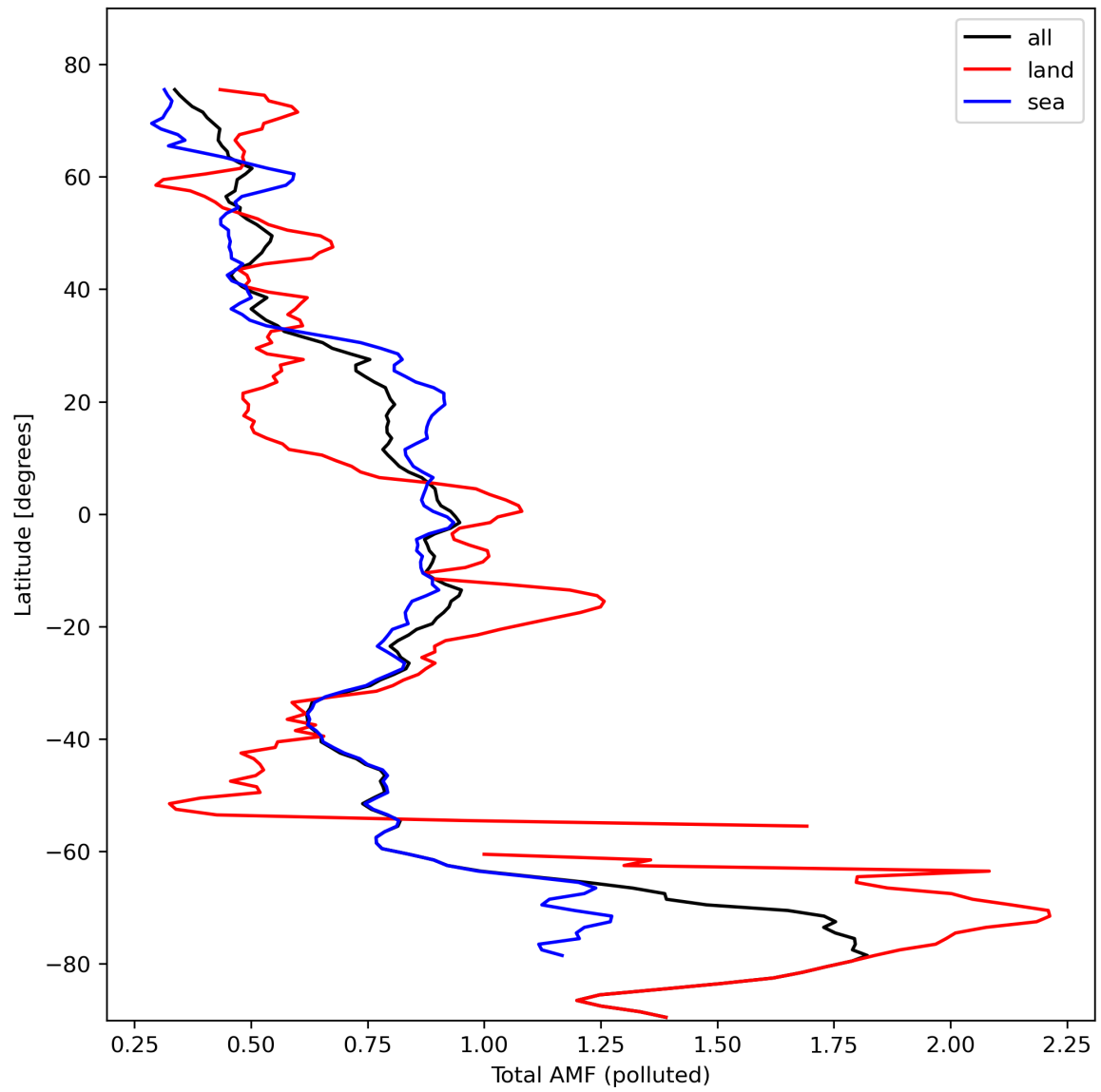
Figure 48: Zonal average of “Total AMF (polluted)” for 2024-02-22 to 2024-02-24.
