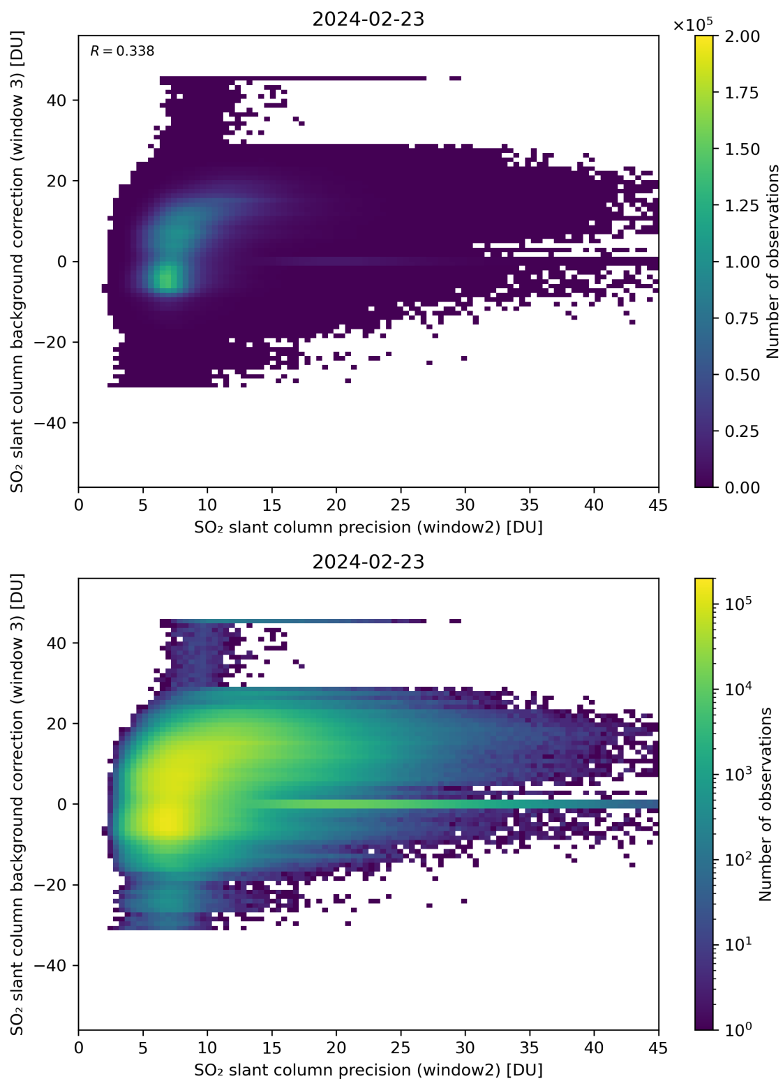
Figure 242: Scatter density plot of “SO 2 slant column precision (window2)” against “SO 2 slant column background correction (window 3)” for 2024-02-22 to 2024-02-24.
