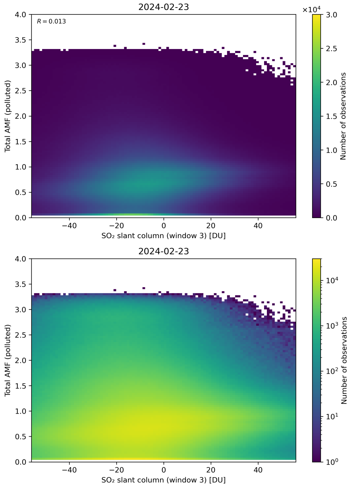
Figure 268: Scatter density plot of “SO 2 slant column (window 3)” against “Total AMF (polluted)” for 2024-02-22 to 2024-02-24.
