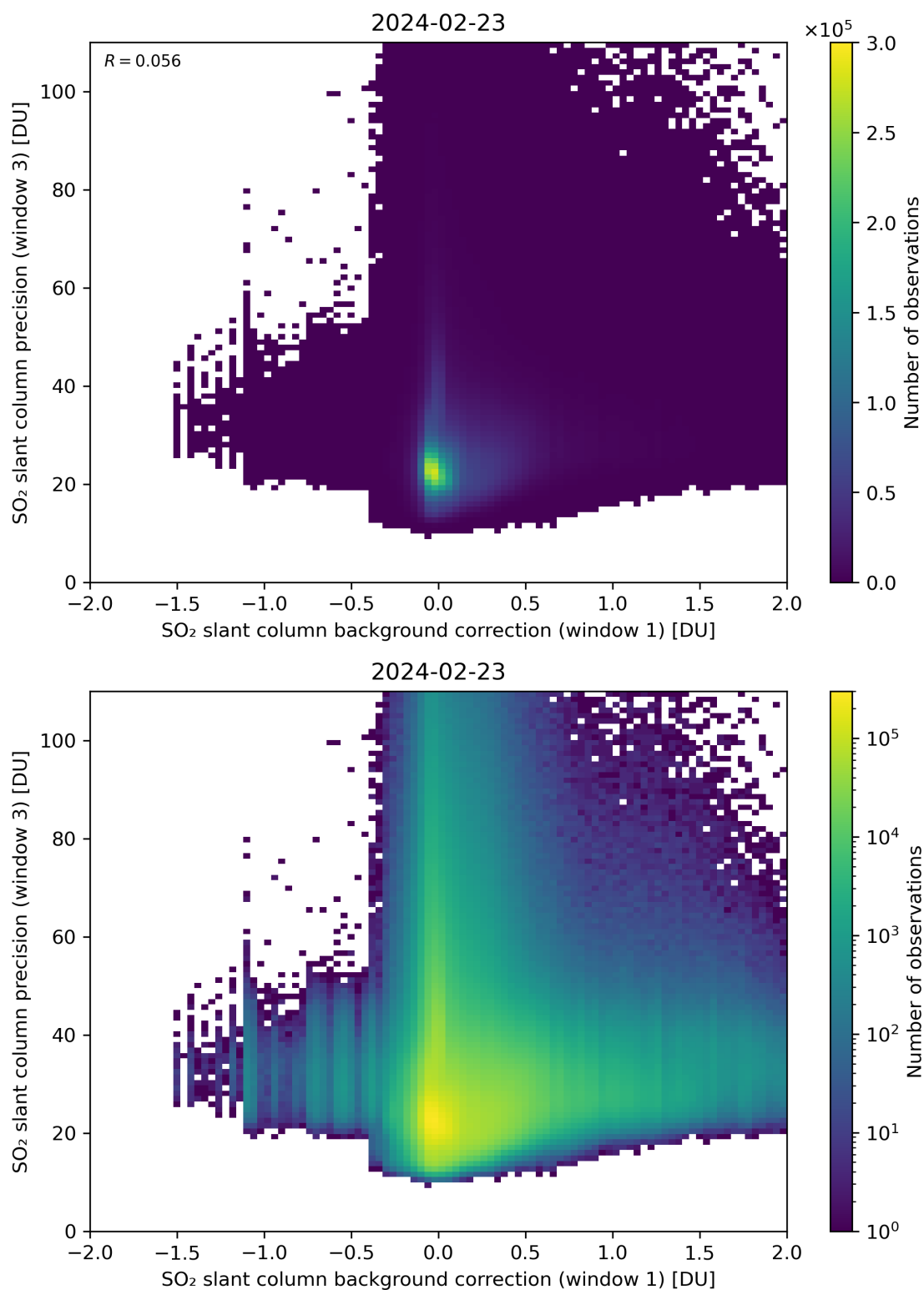
Figure 108: Scatter density plot of “SO 2 slant column background correction (window 1)” against “SO 2 slant column precision (window 3)” for 2024-02-22 to 2024-02-24.
