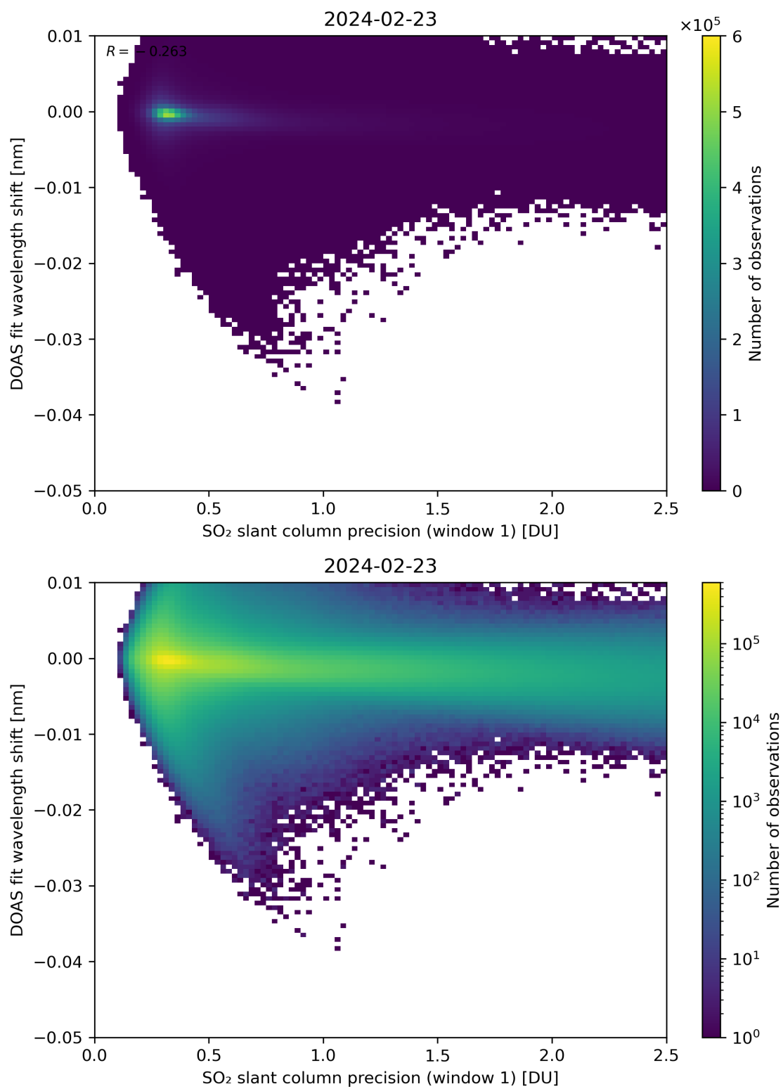
Figure 221: Scatter density plot of “SO 2 slant column precision (window 1)” against “DOAS fit wavelength shift” for 2024-02-22 to 2024-02-24.
