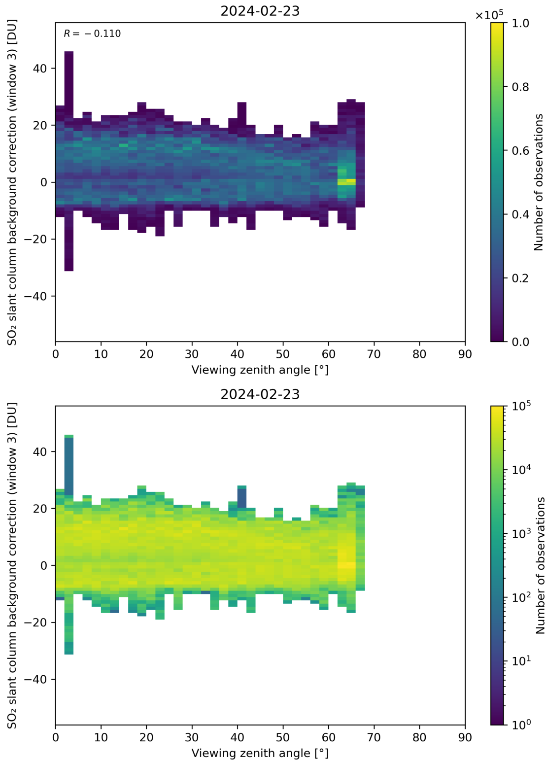
Figure 310: Scatter density plot of “Viewing zenith angle” against “SO 2 slant column background correction (window 3)” for 2024-02-22 to 2024-02-24.
