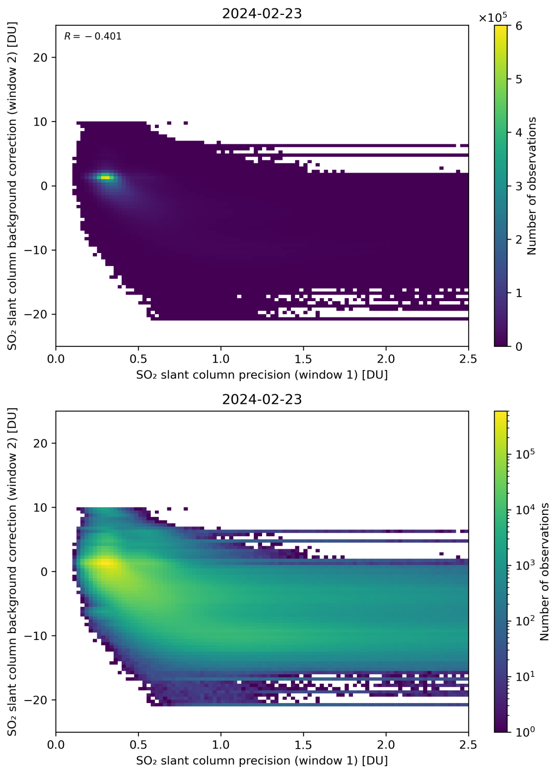
Figure 219: Scatter density plot of “SO 2 slant column precision (window 1)” against “SO 2 slant column background correction (window 2)” for 2024-02-22 to 2024-02-24.
