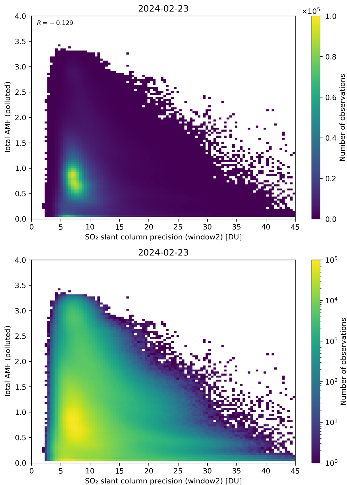
Figure 251: Scatter density plot of “SO 2 slant column precision (window2)” against “Total AMF (polluted)” for 2024-02-22 to 2024-02-24.
