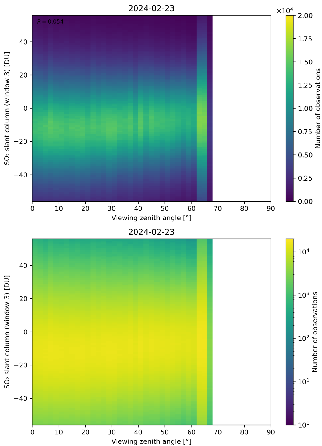
Figure 323: Scatter density plot of “Viewing zenith angle” against “SO 2 slant column (window 3)” for 2024-02-22 to 2024-02-24.
