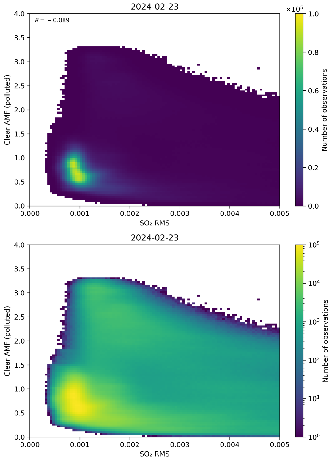
Figure 136: Scatter density plot of “SO 2 RMS” against “Clear AMF (polluted)” for 2024-02-22 to 2024-02-24.
