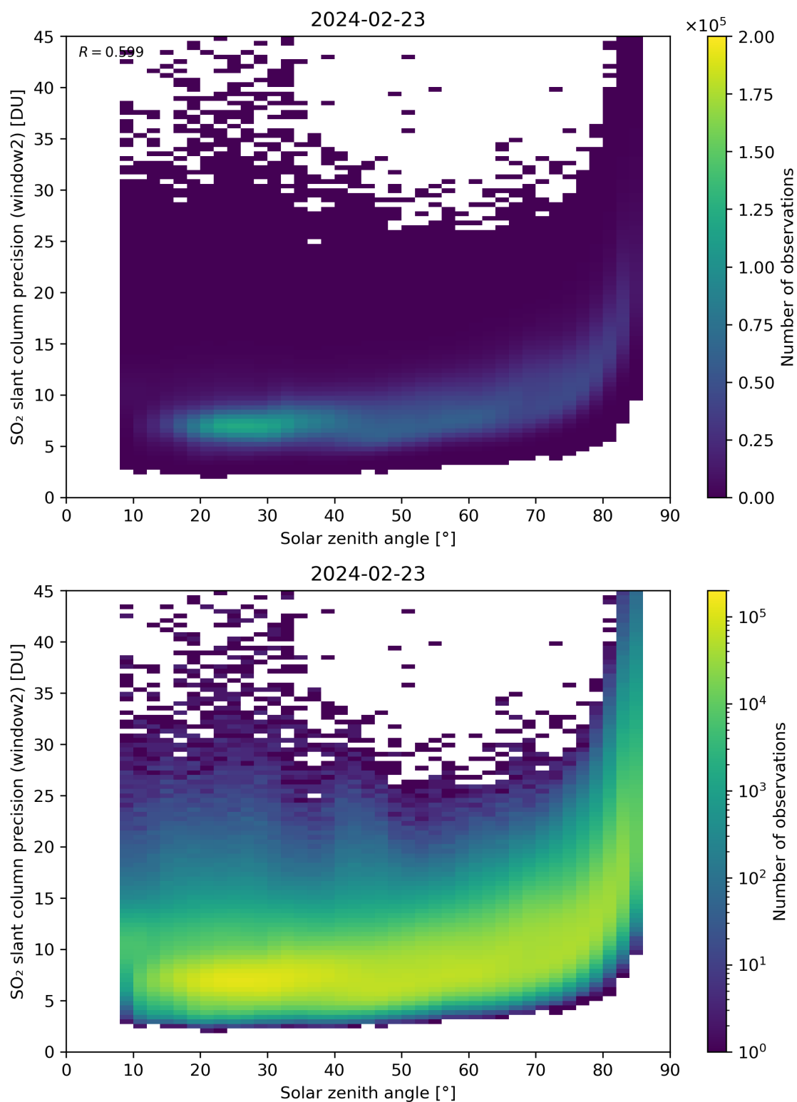
Figure 171: Scatter density plot of “Solar zenith angle” against “SO 2 slant column precision (window2)” for 2024-02-22 to 2024-02-24.
