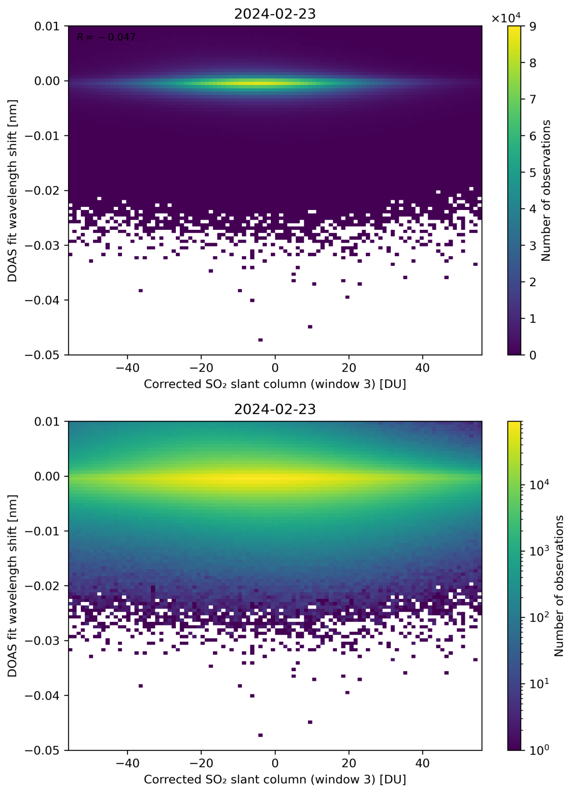
Figure 206: Scatter density plot of “Corrected SO 2 slant column (window 3)” against “DOAS fit wavelength shift” for 2024-02-22 to 2024-02-24.
