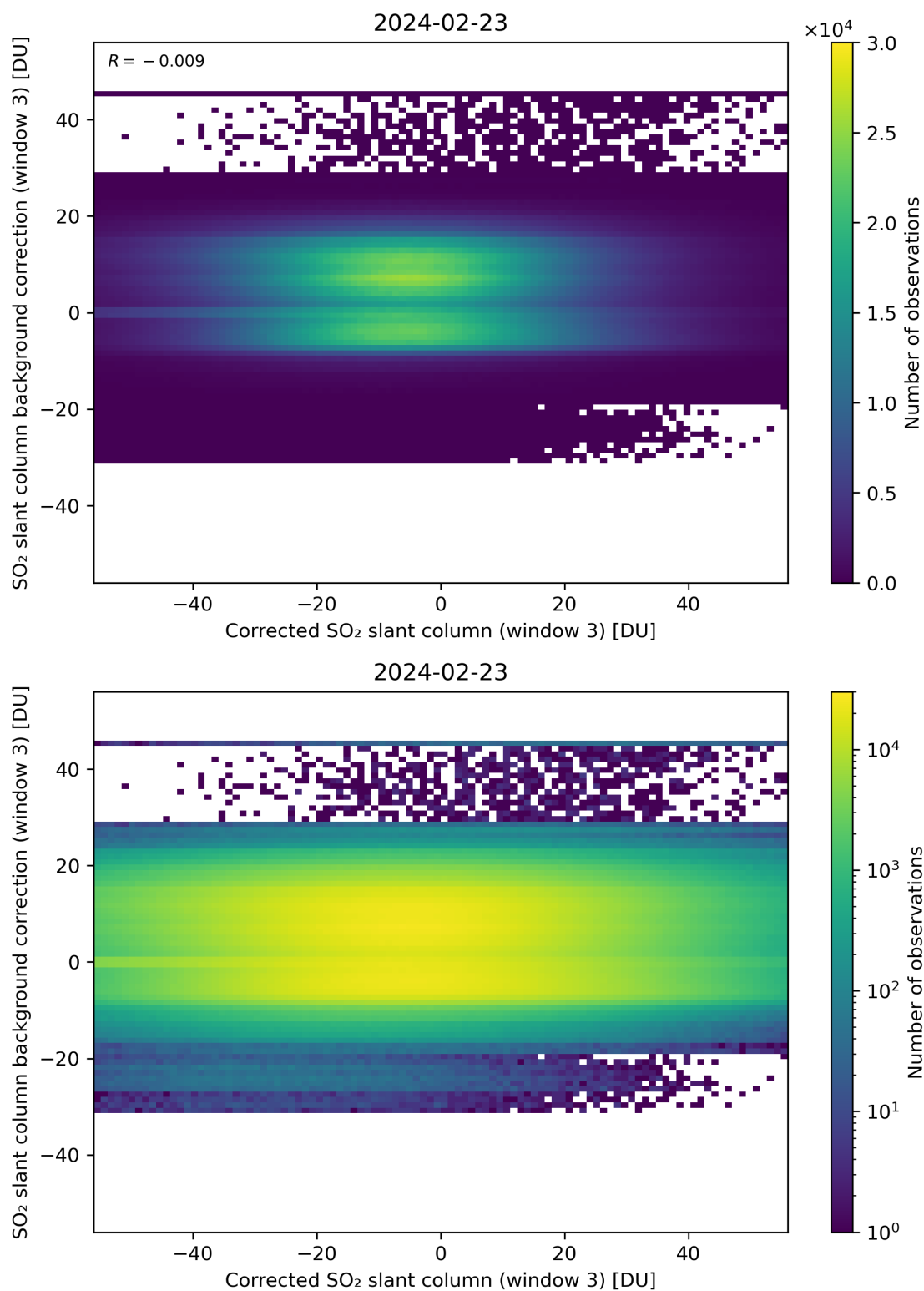
Figure 205: Scatter density plot of “Corrected SO 2 slant column (window 3)” against “SO 2 slant column background correction (window 3)” for 2024-02-22 to 2024-02-24.
