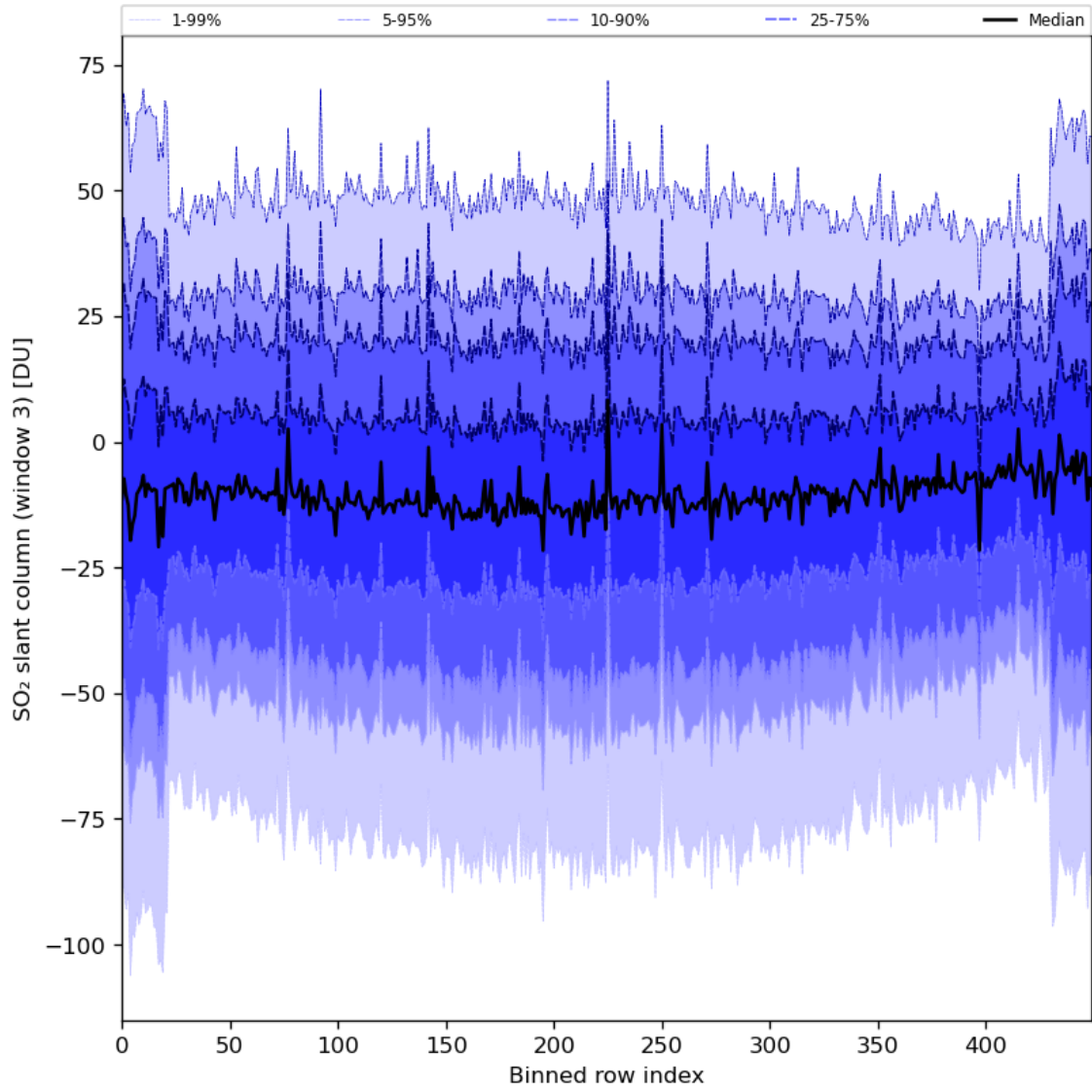
Figure 87: Along track statistics of “SO 2 slant column (window 3)” for 2024-02-22 to 2024-02-24
