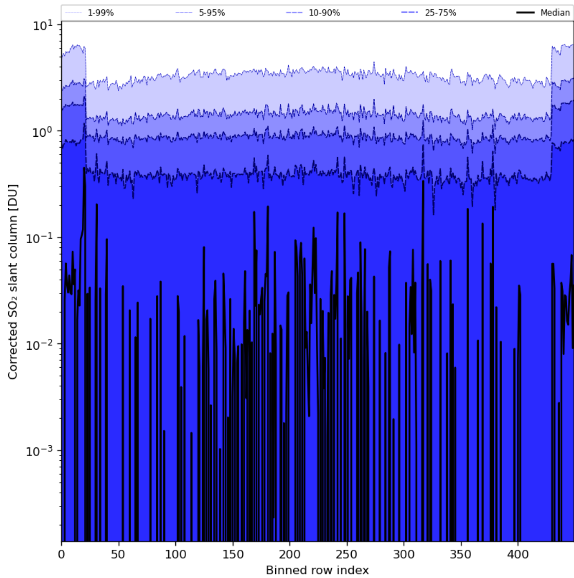
Figure 78: Along track statistics of “Corrected SO 2 slant column” for 2024-02-22 to 2024-02-24
