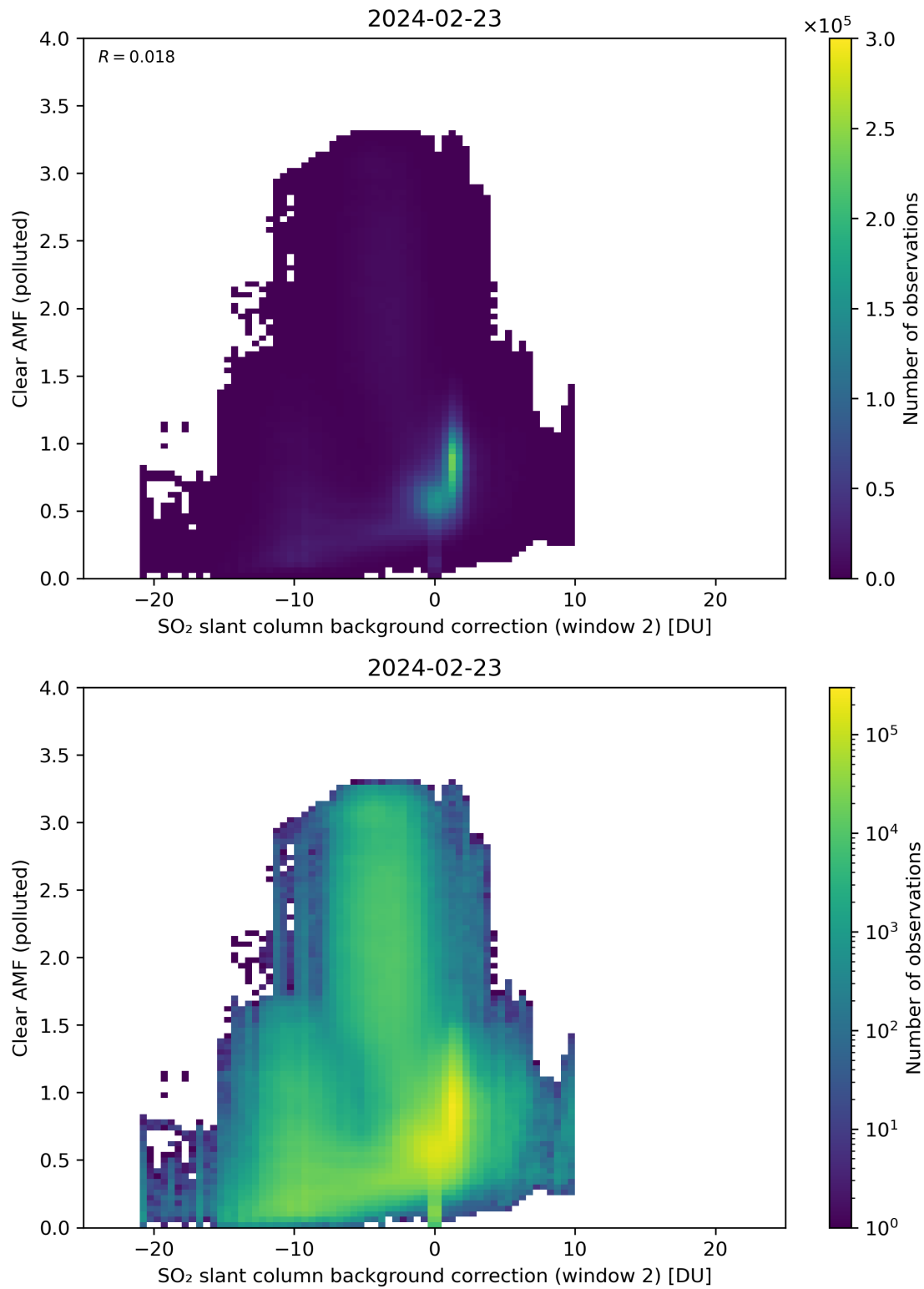
Figure 115: Scatter density plot of “SO 2 slant column background correction (window 2)” against “Clear AMF (polluted)” for 2024-02-22 to 2024-02-24.
