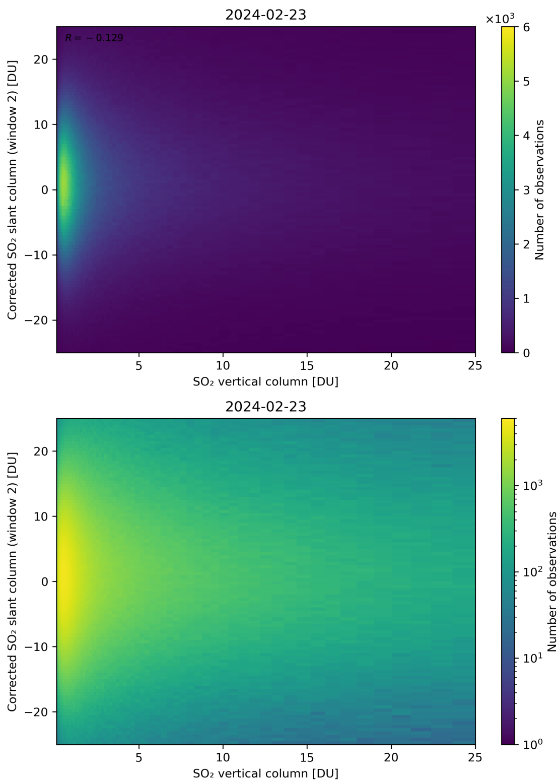
Figure 298: Scatter density plot of “SO 2 vertical column” against “Corrected SO 2 slant column (window 2)” for 2024-02-22 to 2024-02-24.
