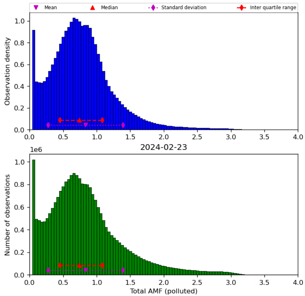
Figure 71: Histogram of “Total AMF (polluted)” for 2024-02-22 to 2024-02-24
