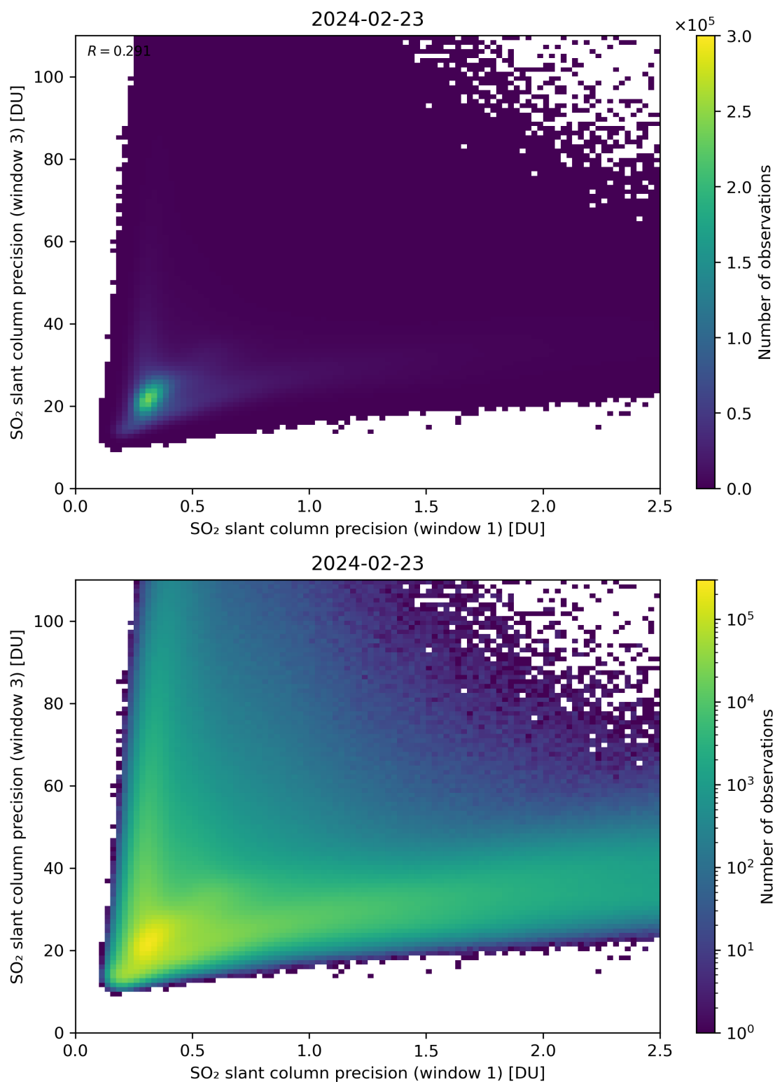
Figure 229: Scatter density plot of “SO 2 slant column precision (window 1)” against “SO 2 slant column precision (window 3)” for 2024-02-22 to 2024-02-24.
