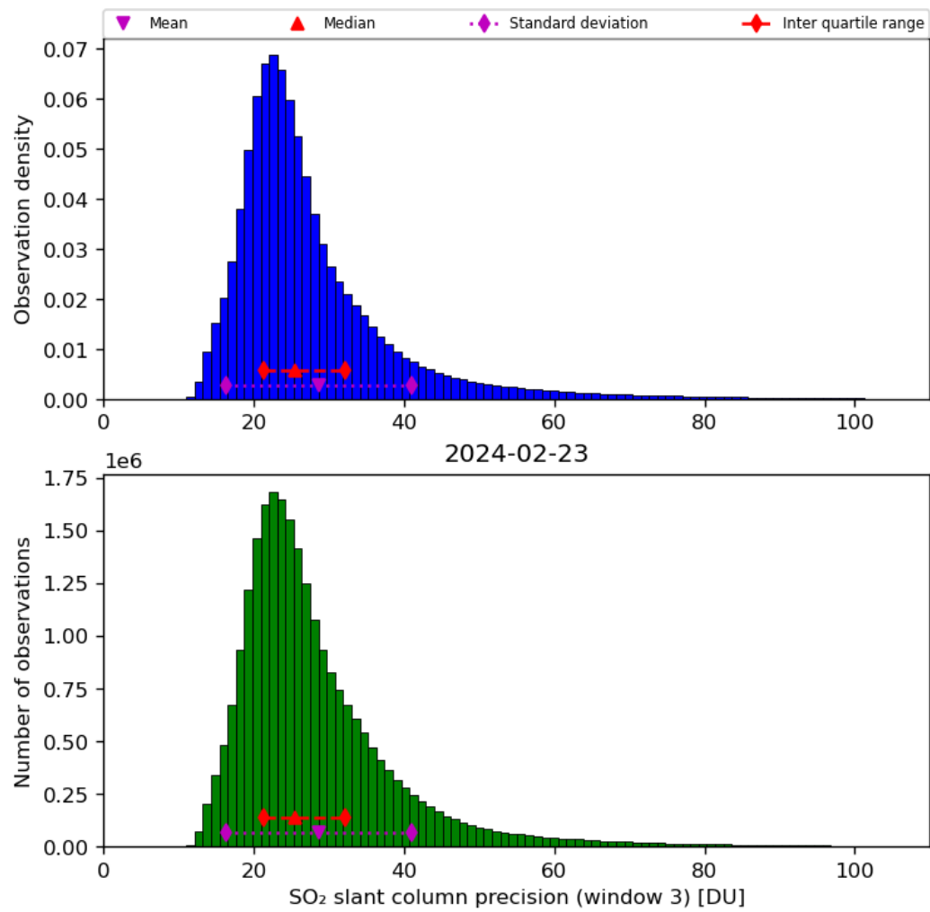
Figure 65: Histogram of “SO 2 slant column precision (window 3)” for 2024-02-22 to 2024-02-24
