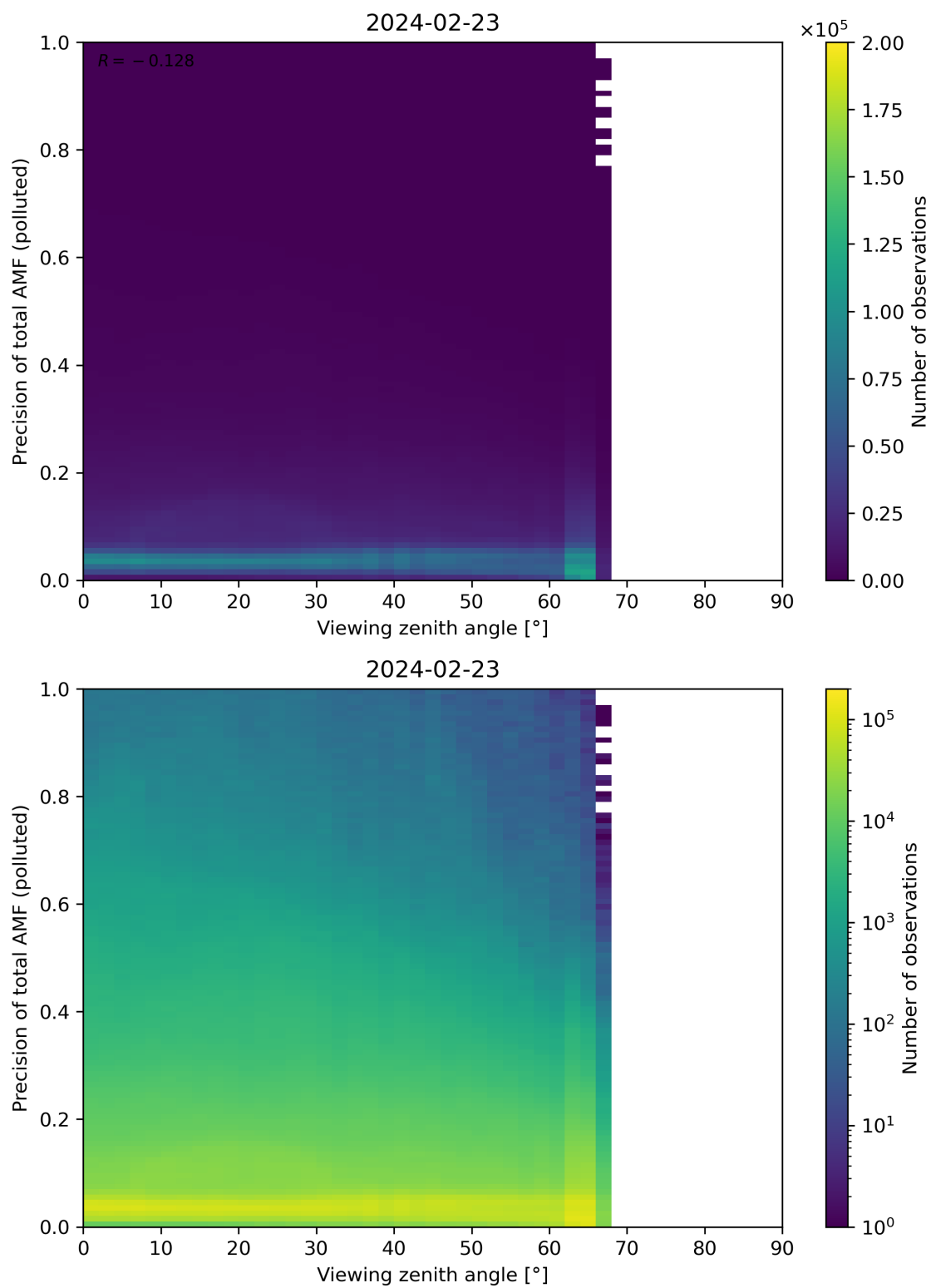
Figure 326: Scatter density plot of “Viewing zenith angle” against “Precision of total AMF (polluted)” for 2024-02-22 to 2024-02-24.
