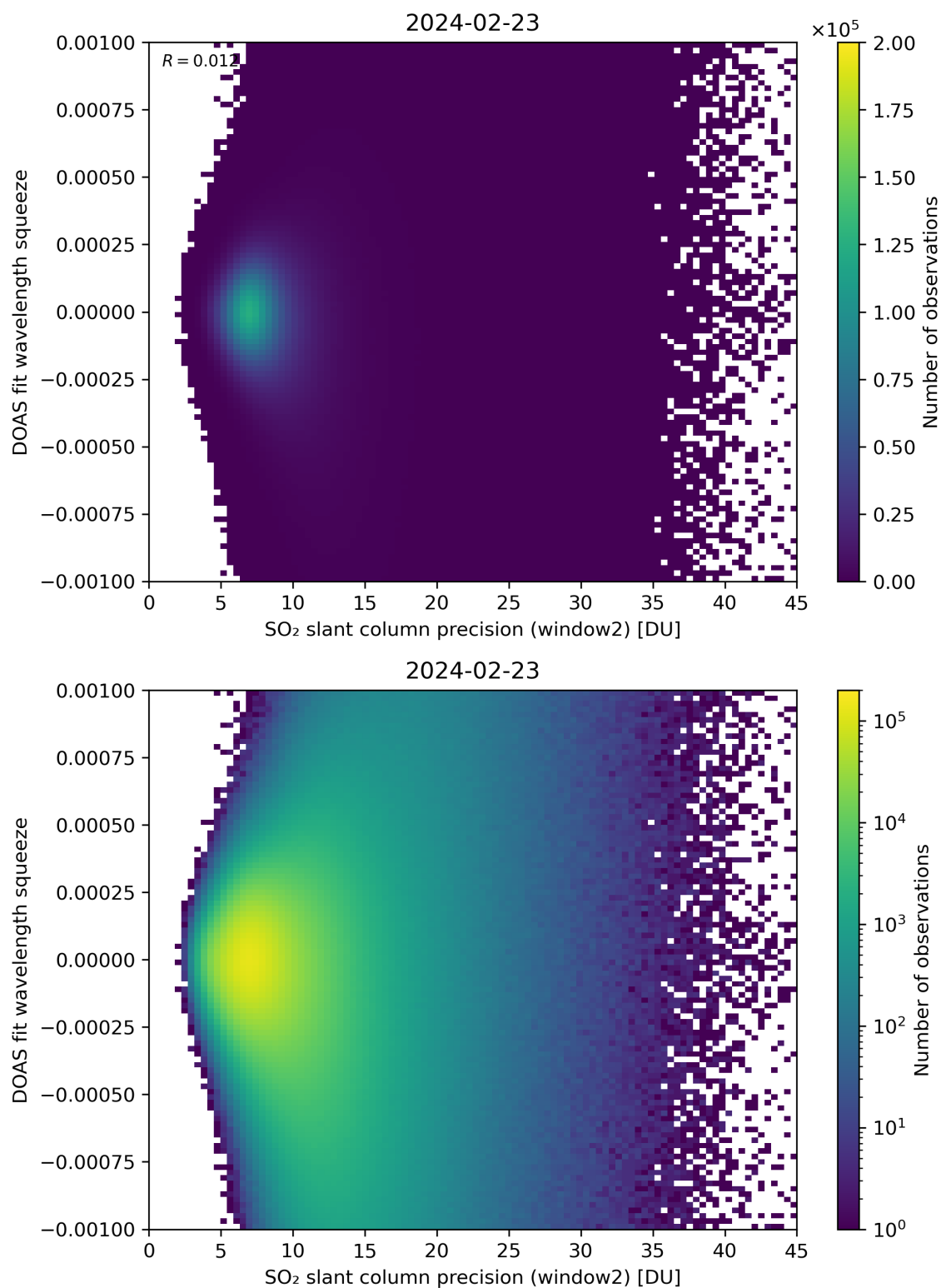
Figure 244: Scatter density plot of “SO 2 slant column precision (window2)” against “DOAS fit wavelength squeeze” for 2024-02-22 to 2024-02-24.
