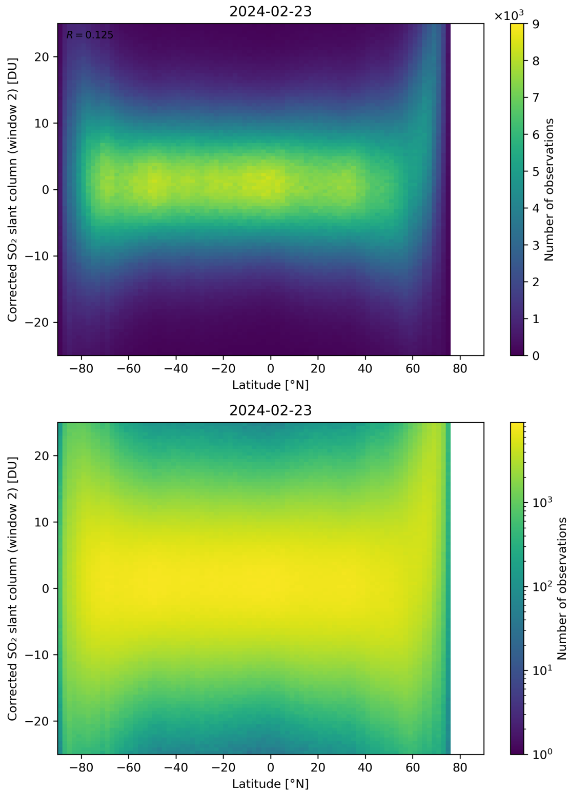
Figure 147: Scatter density plot of “Latitude” against “Corrected SO 2 slant column (window 2)” for 2024-02-22 to 2024-02-24.
