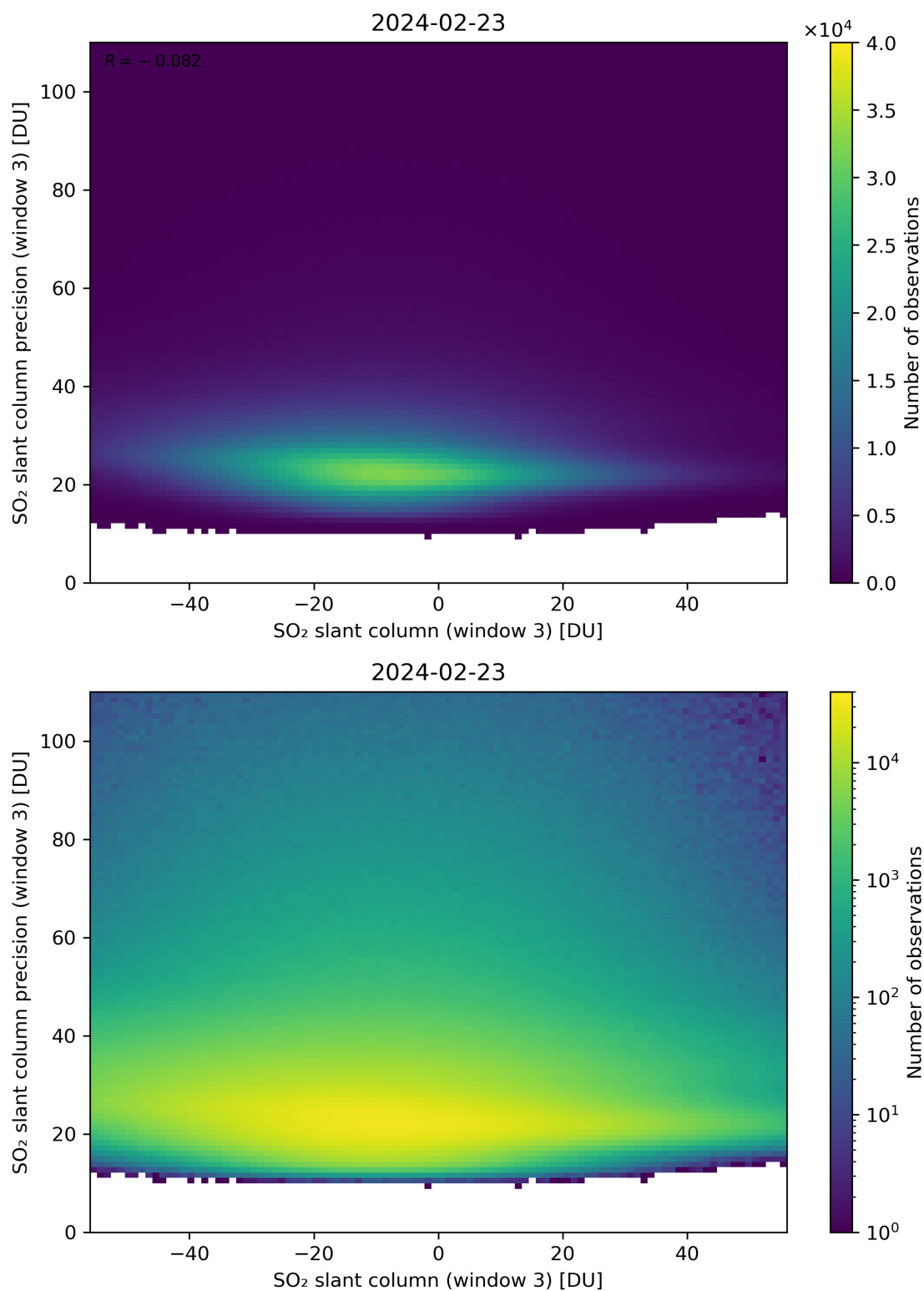
Figure 267: Scatter density plot of “SO 2 slant column (window 3)” against “SO 2 slant column precision (window 3)” for 2024-02-22 to 2024-02-24.
