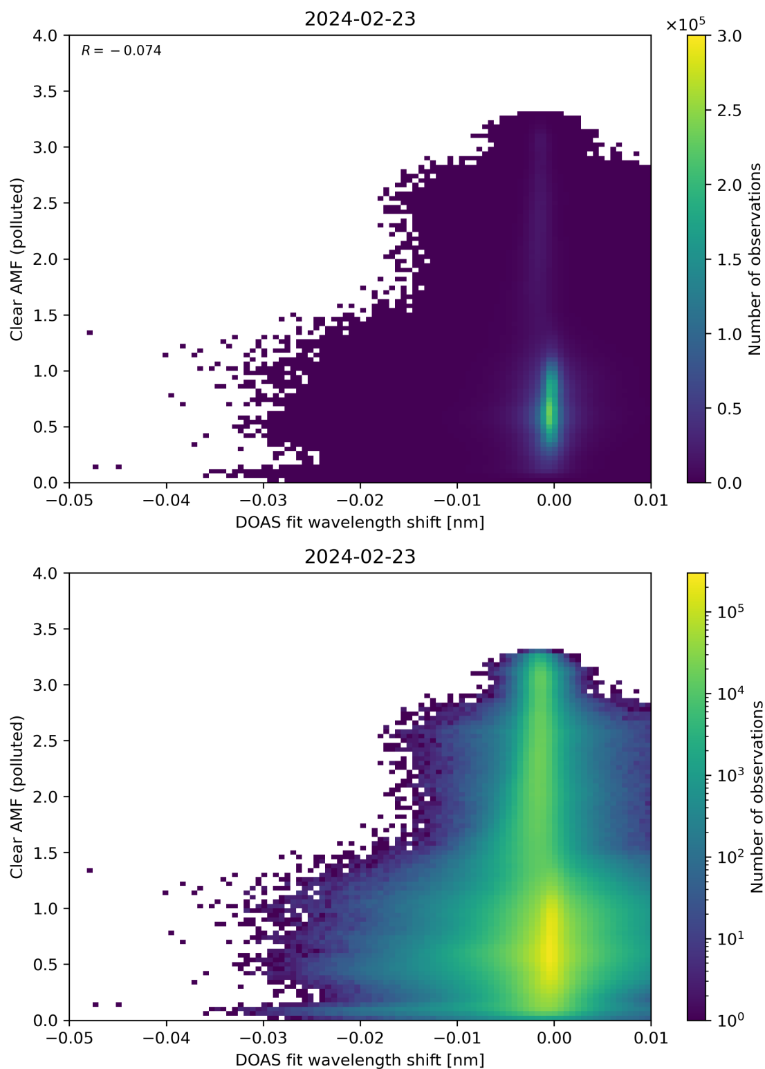
Figure 129: Scatter density plot of “DOAS fit wavelength shift” against “Clear AMF (polluted)” for 2024-02-22 to 2024-02-24.
