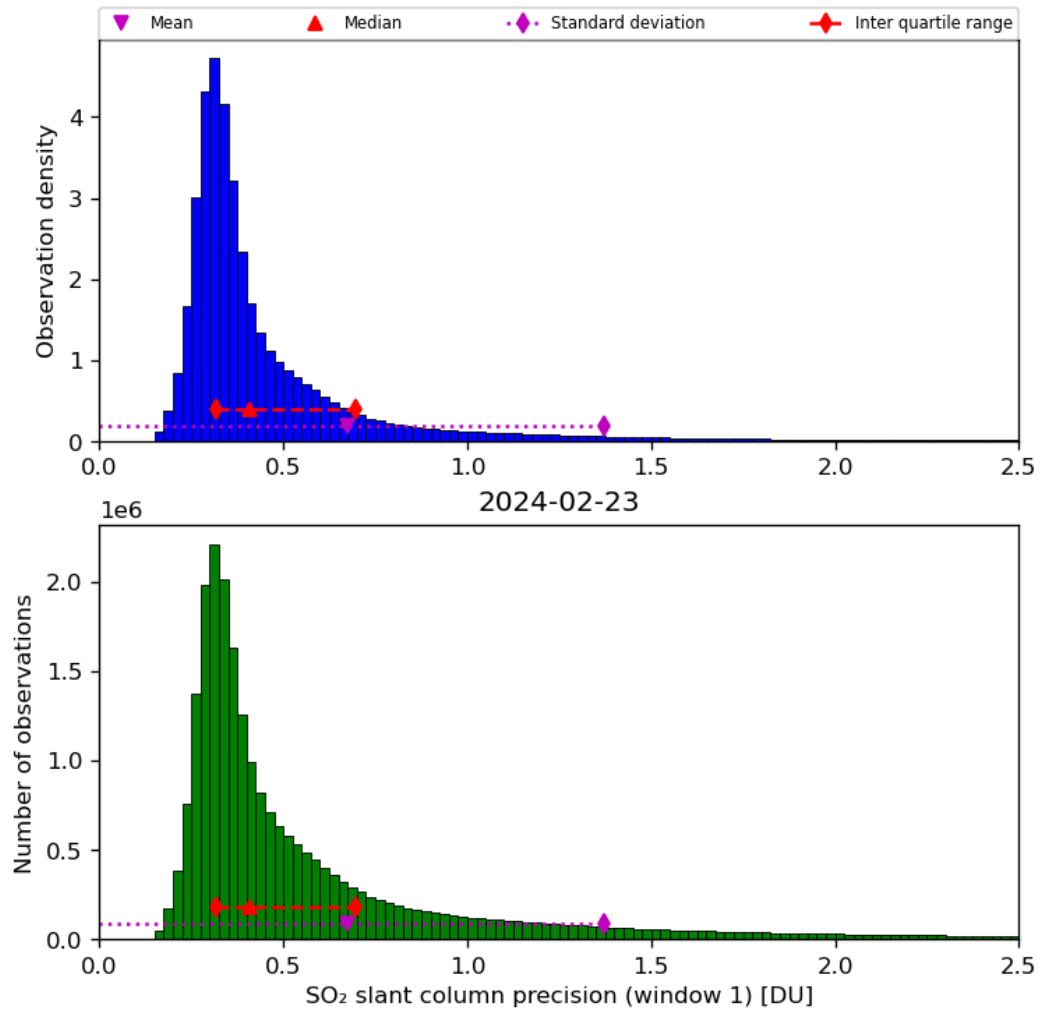
Figure 57: Histogram of “SO 2 slant column precision (window 1)” for 2024-02-22 to 2024-02-24
