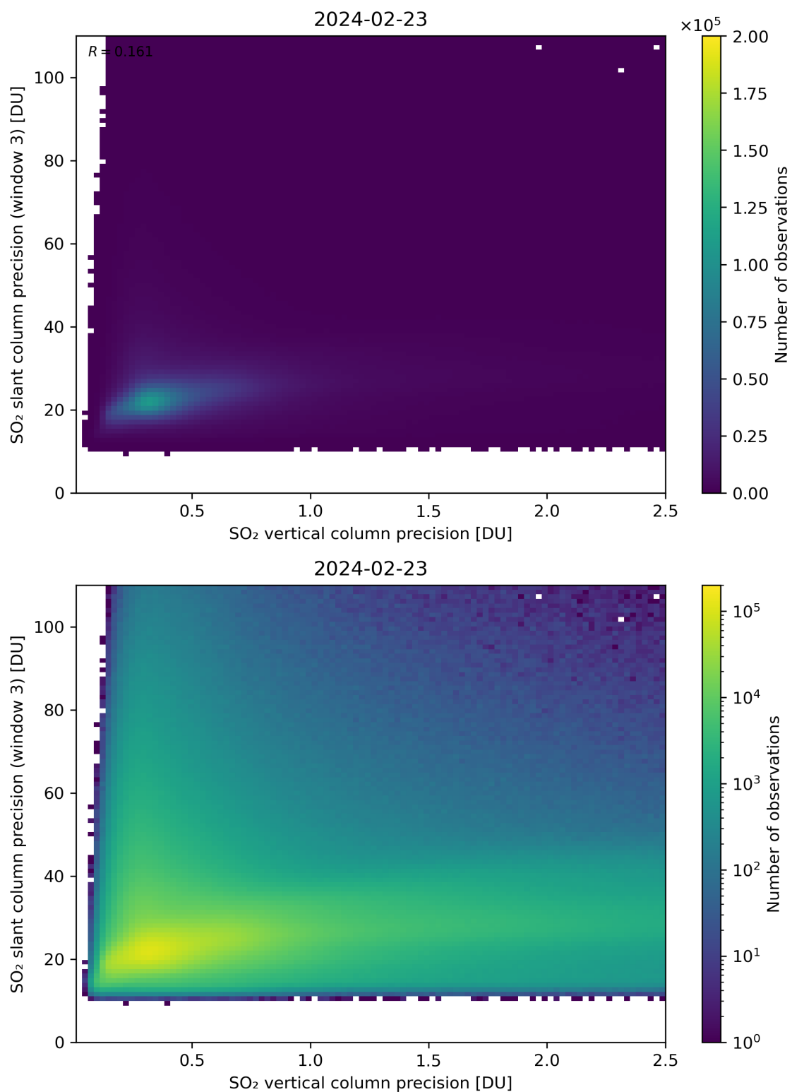
Figure 293: Scatter density plot of “SO 2 vertical column precision” against “SO 2 slant column precision (window 3)” for 2024-02-22 to 2024-02-24.
