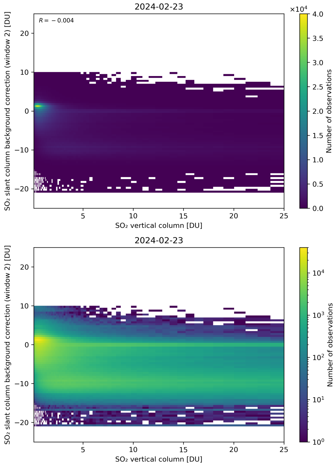
Figure 274: Scatter density plot of “SO 2 vertical column” against “SO 2 slant column background correction (window 2)” for 2024-02-22 to 2024-02-24.
