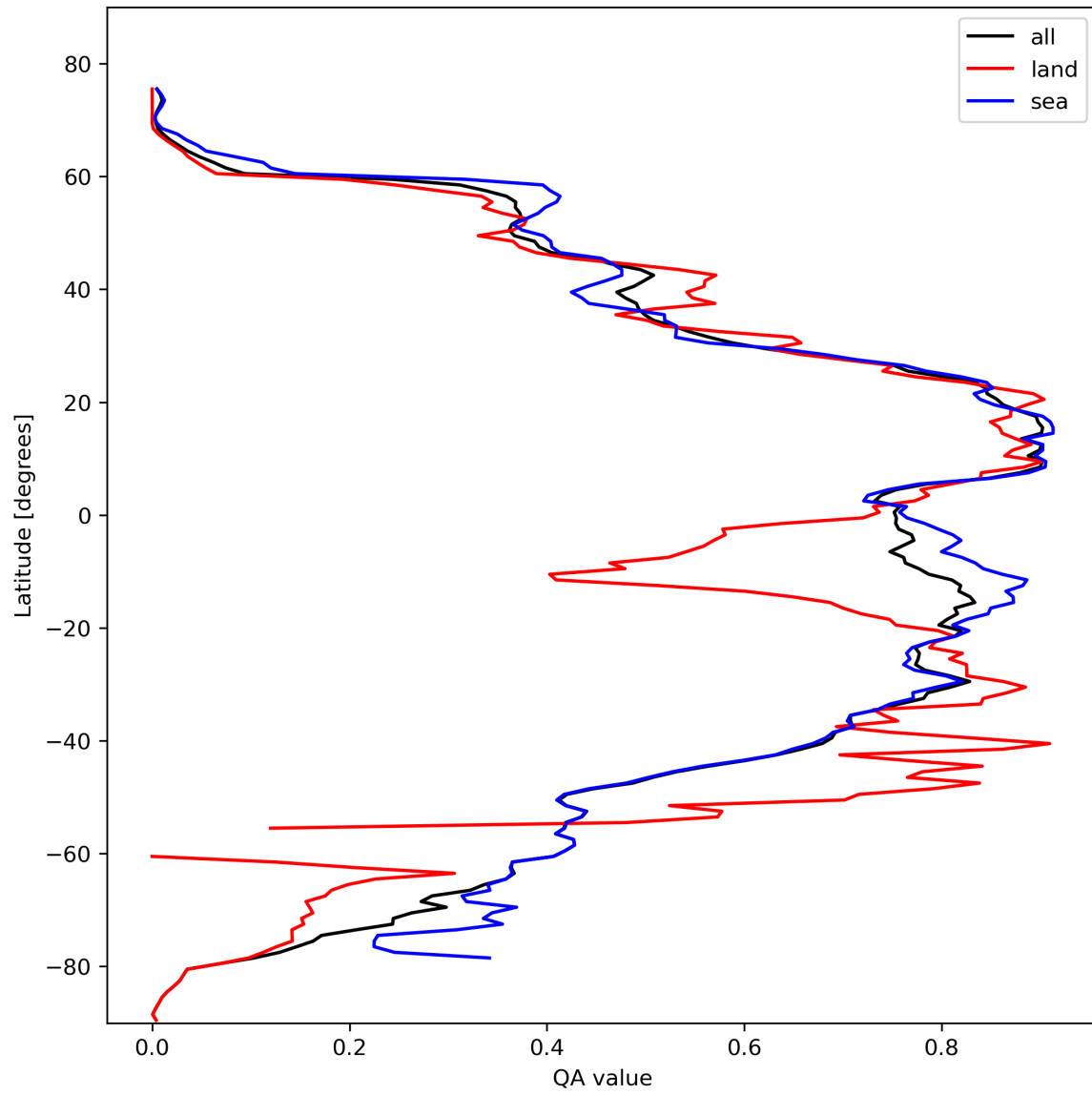
Figure 29: Zonal average of “QA value” for 2024-02-22 to 2024-02-24.
