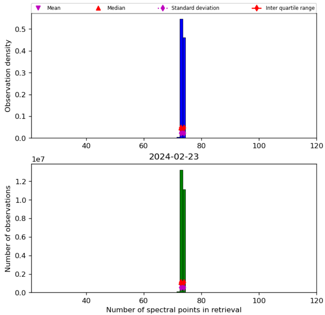
Figure 74: Histogram of “Number of spectral points in retrieval” for 2024-02-22 to 2024-02-24
