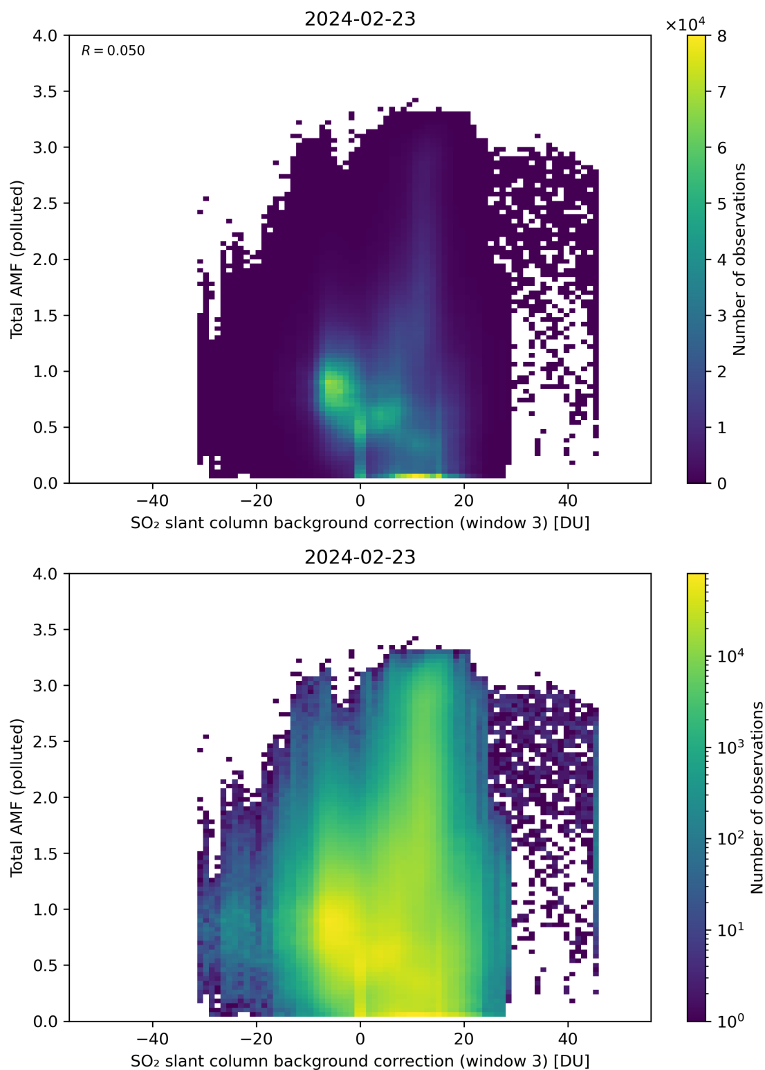
Figure 125: Scatter density plot of “SO 2 slant column background correction (window 3)” against “Total AMF (polluted)” for 2024-02-22 to 2024-02-24.
