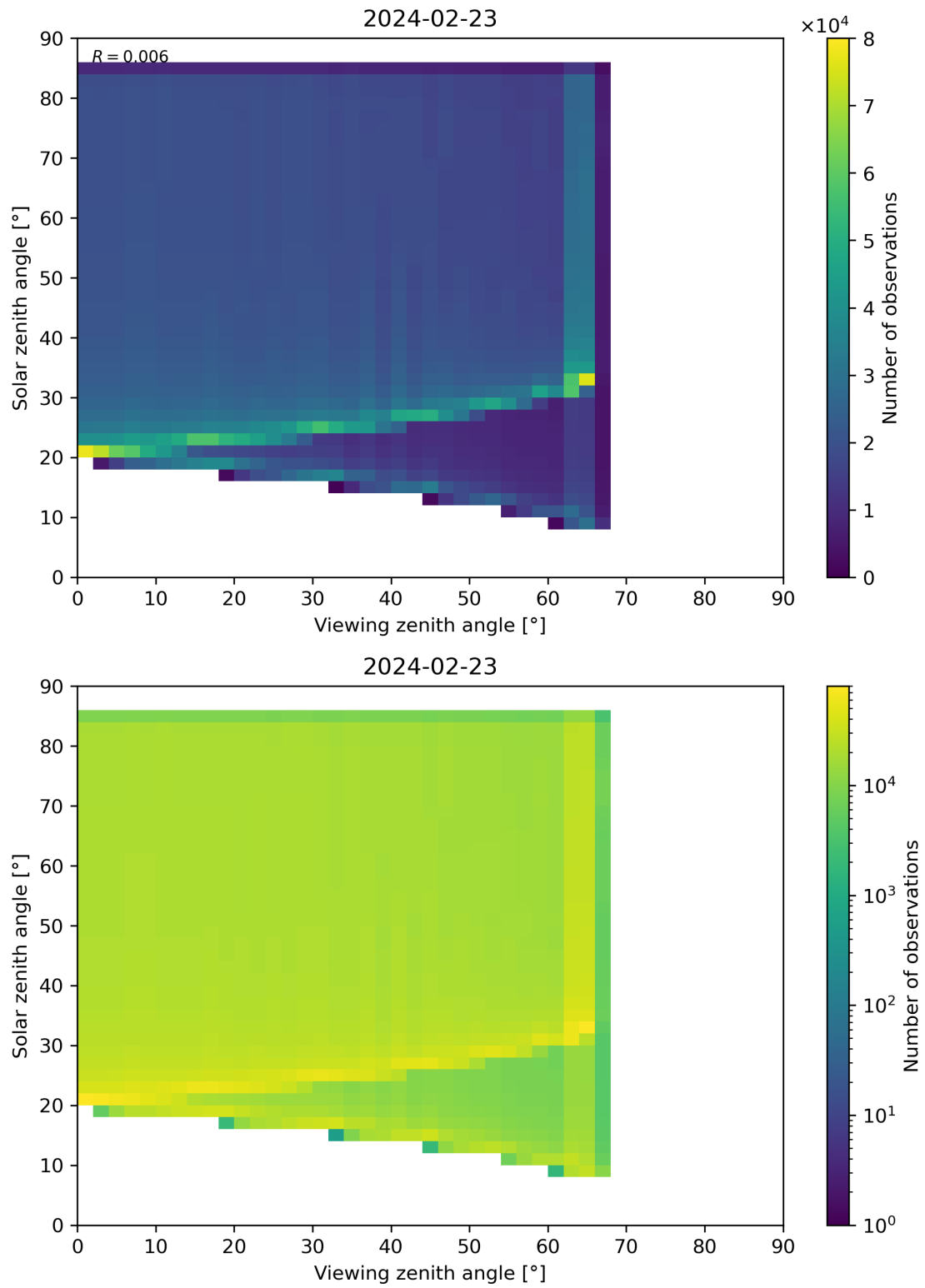
Figure 315: Scatter density plot of “Viewing zenith angle” against “Solar zenith angle” for 2024-02-22 to 2024-02-24.
