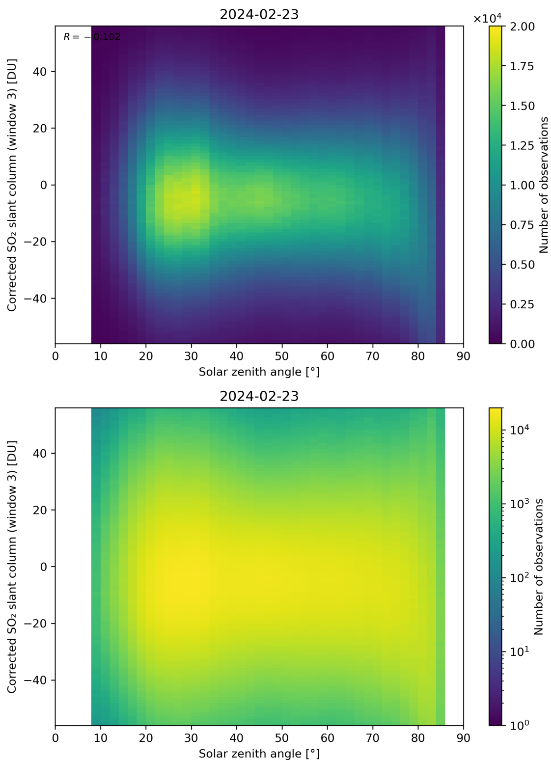
Figure 168: Scatter density plot of “Solar zenith angle” against “Corrected SO 2 slant column (window 3)” for 2024-02-22 to 2024-02-24.
