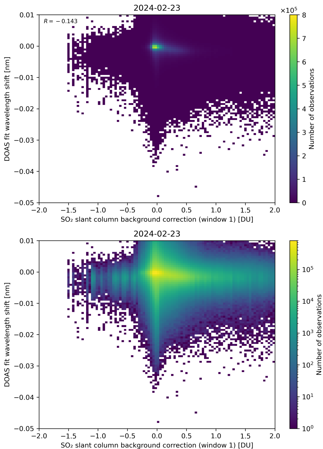
Figure 100: Scatter density plot of “SO 2 slant column background correction (window 1)” against “DOAS fit wavelength shift” for 2024-02-22 to 2024-02-24.
