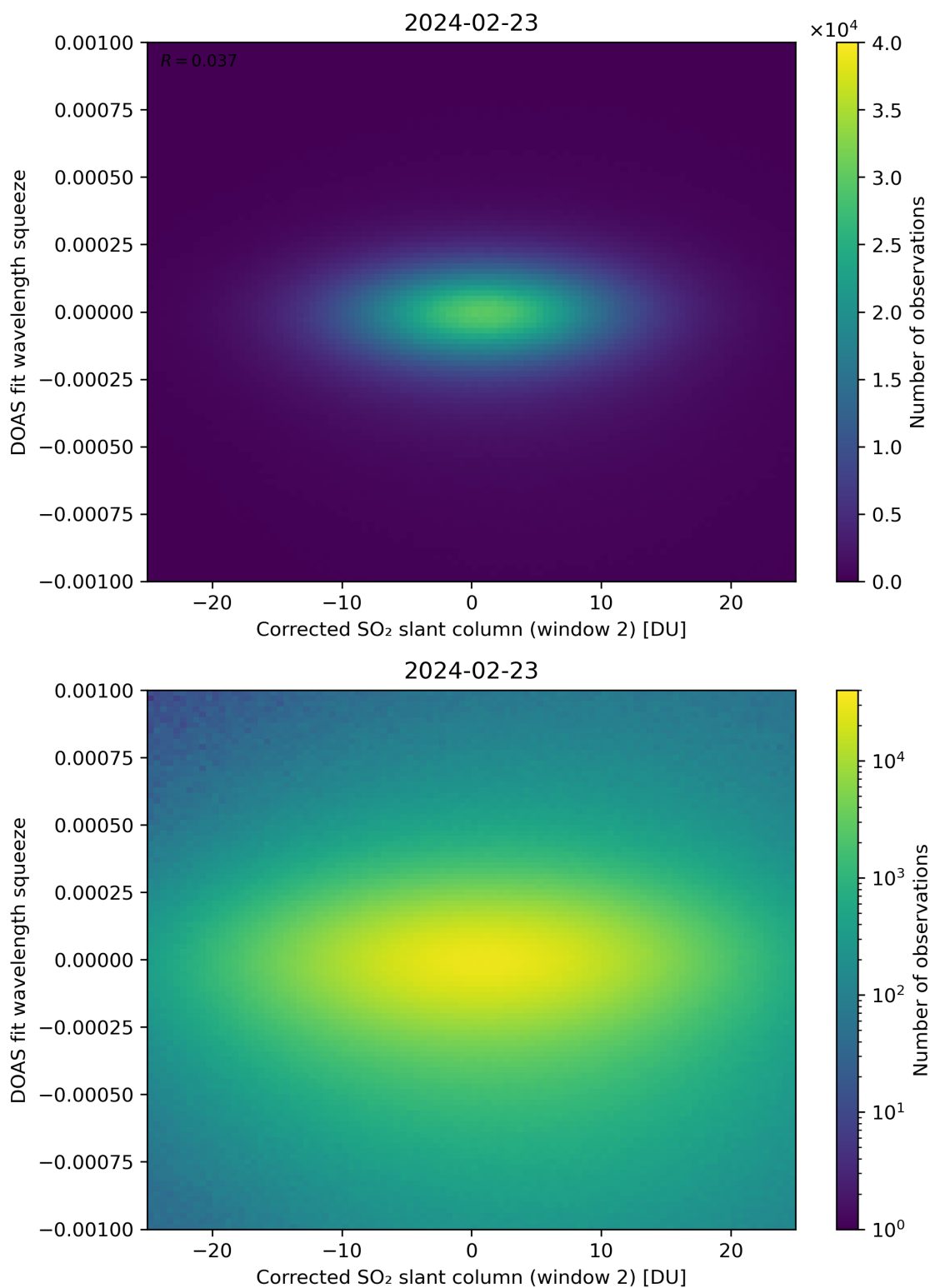
Figure 197: Scatter density plot of “Corrected SO 2 slant column (window 2)” against “DOAS fit wavelength squeeze” for 2024-02-22 to 2024-02-24.
