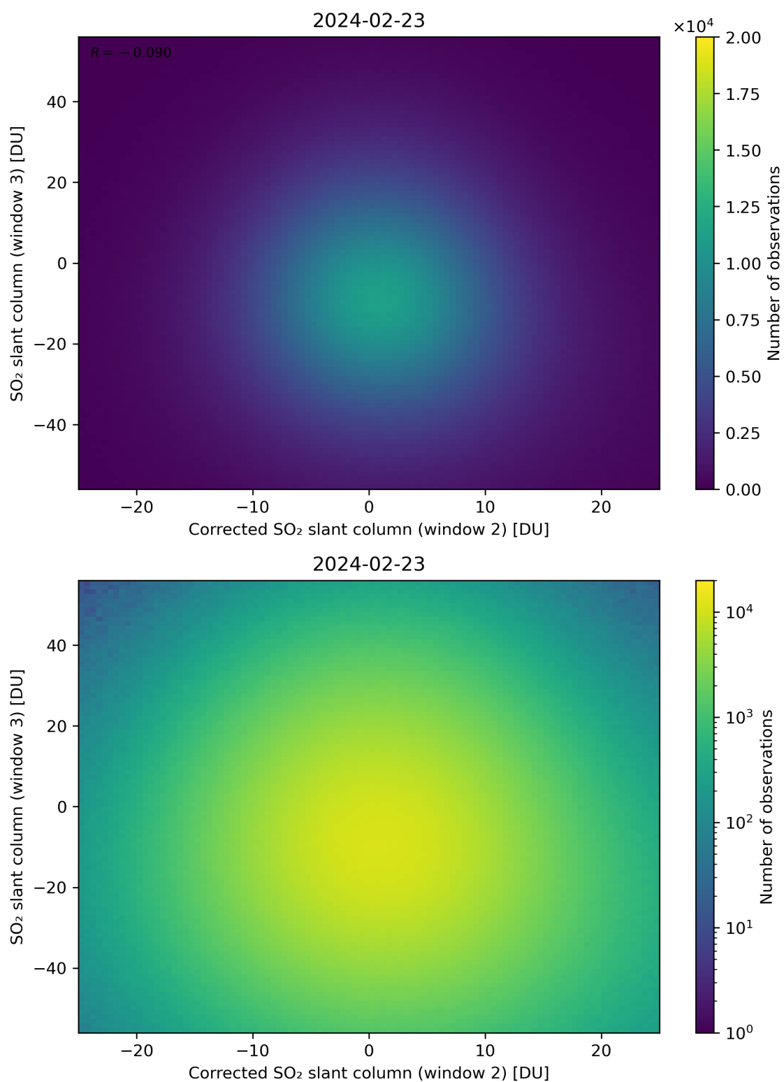
Figure 201: Scatter density plot of “Corrected SO 2 slant column (window 2)” against “SO 2 slant column (window 3)” for 2024-02-22 to 2024-02-24.
