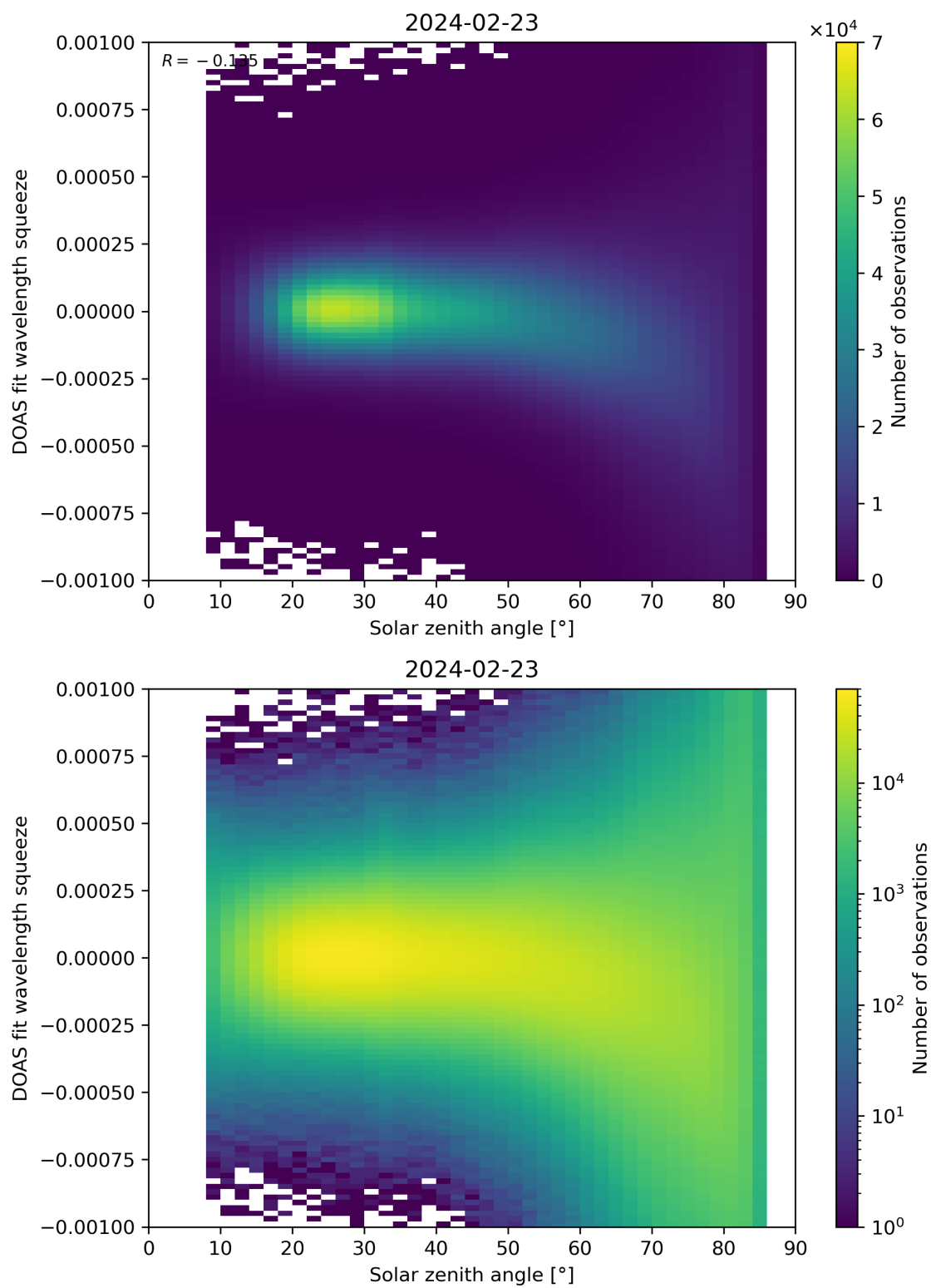
Figure 162: Scatter density plot of “Solar zenith angle” against “DOAS fit wavelength squeeze” for 2024-02-22 to 2024-02-24.
