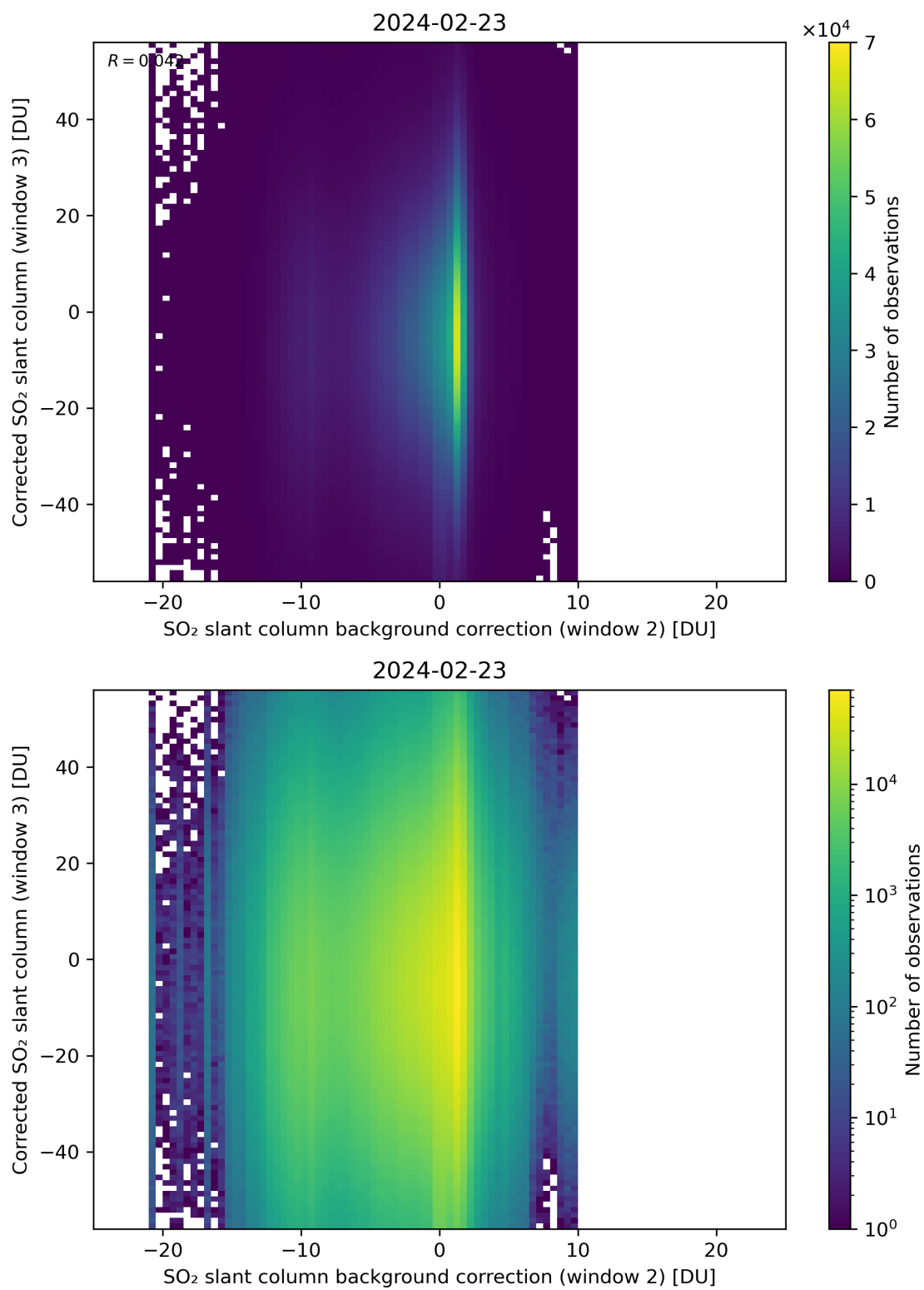
Figure 116: Scatter density plot of “SO 2 slant column background correction (window 2)” against “Corrected SO 2 slant column (window 3)” for 2024-02-22 to 2024-02-24.
