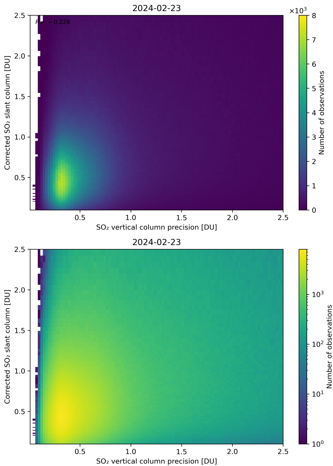
Figure 286: Scatter density plot of “SO 2 vertical column precision” against “Corrected SO 2 slant column” for 2024-02-22 to 2024-02-24.
