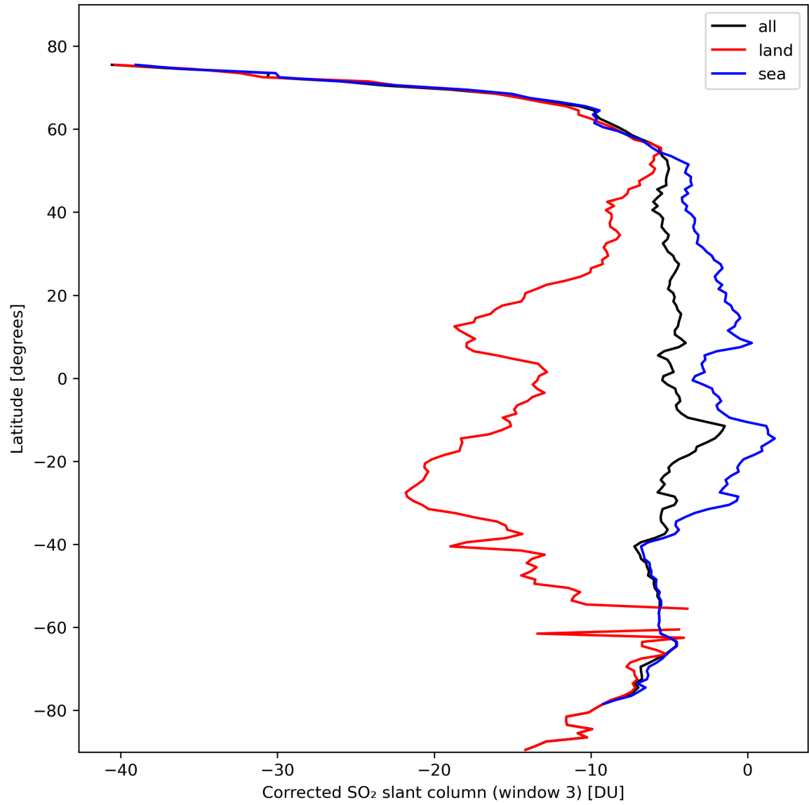
Figure 43: Zonal average of “Corrected SO 2 slant column (window 3)” for 2024-02-22 to 2024-02-24.
