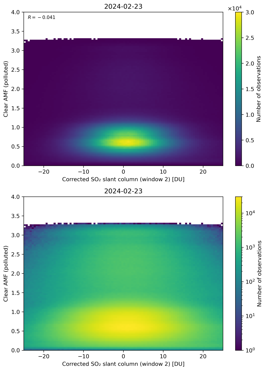
Figure 199: Scatter density plot of “Corrected SO 2 slant column (window 2)” against “Clear AMF (polluted)” for 2024-02-22 to 2024-02-24.
