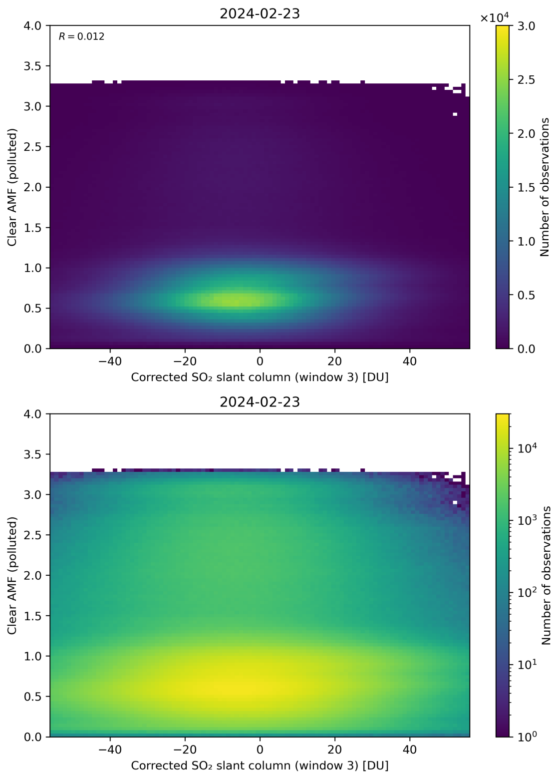
Figure 209: Scatter density plot of “Corrected SO 2 slant column (window 3)” against “Clear AMF (polluted)” for 2024-02-22 to 2024-02-24.
