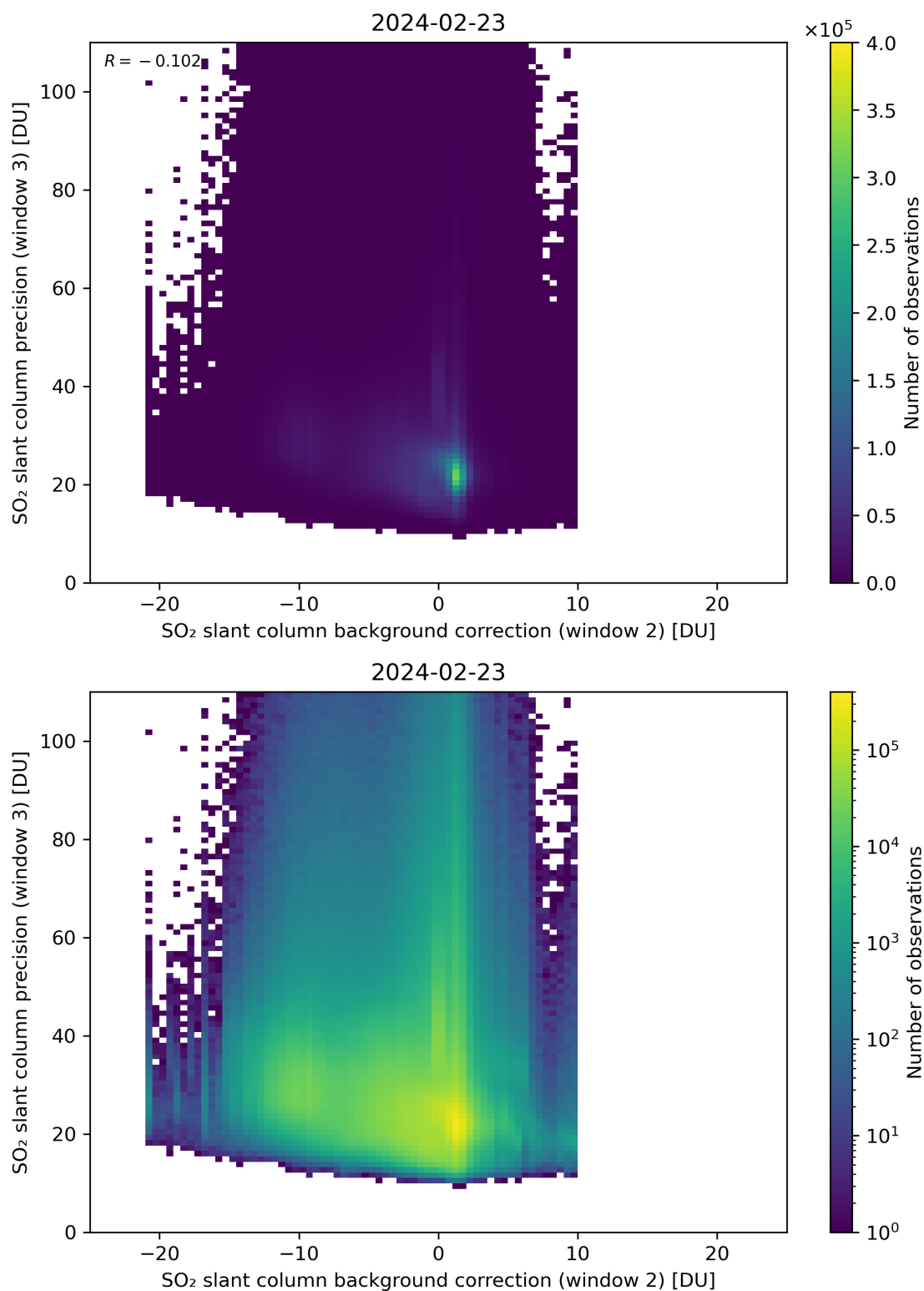
Figure 118: Scatter density plot of “SO 2 slant column background correction (window 2)” against “SO 2 slant column precision (window 3)” for 2024-02-22 to 2024-02-24.
