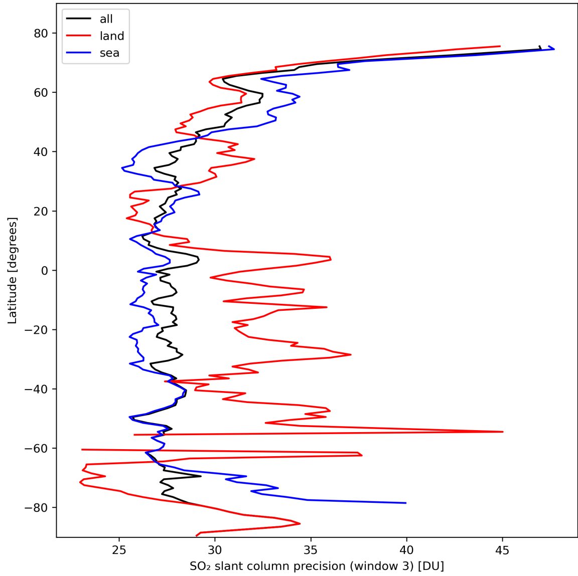
Figure 42: Zonal average of “SO 2 slant column precision (window 3)” for 2024-02-22 to 2024-02-24.
