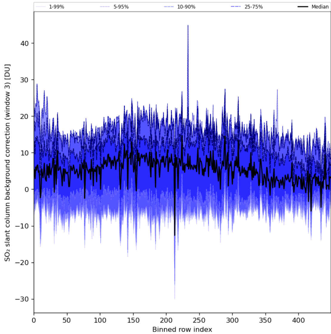
Figure 90: Along track statistics of “SO 2 slant column background correction (window 3)” for 2024-02-22 to 2024-02-24
