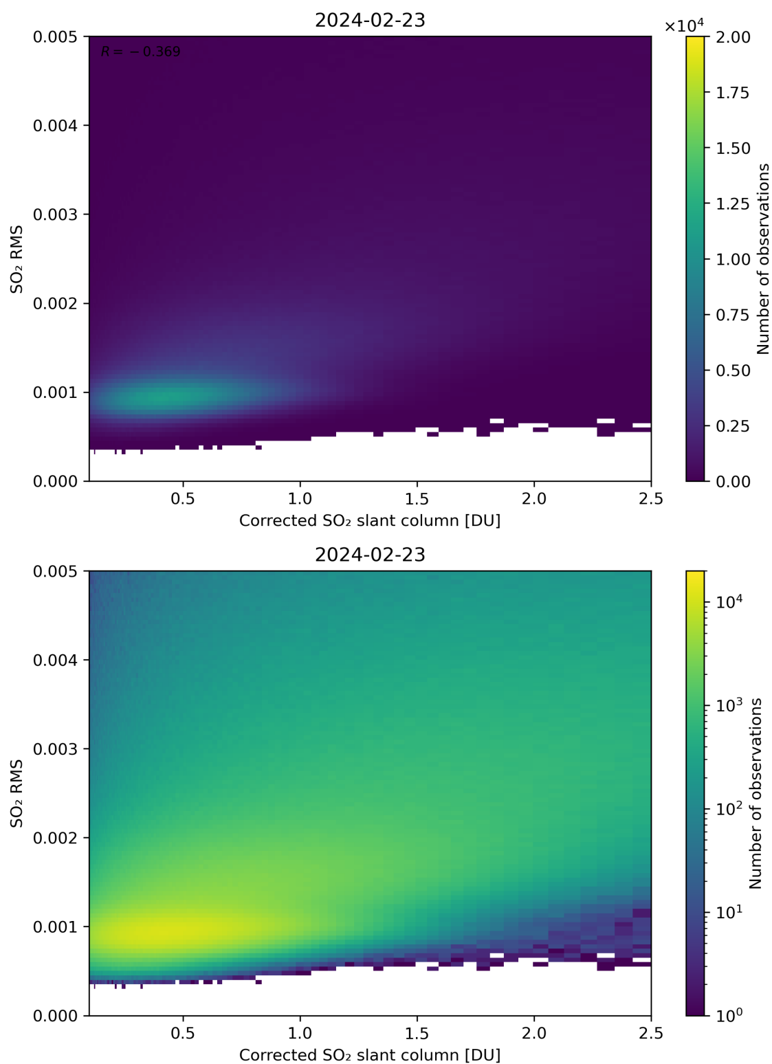
Figure 183: Scatter density plot of “Corrected SO 2 slant column” against “SO 2 RMS” for 2024-02-22 to 2024-02-24.
