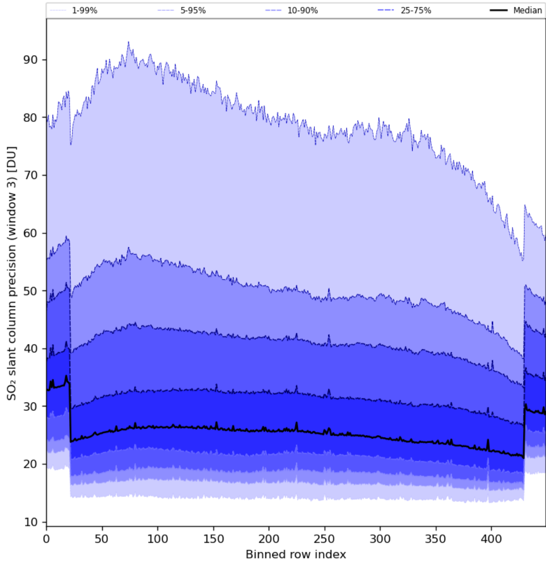
Figure 88: Along track statistics of “SO 2 slant column precision (window 3)” for 2024-02-22 to 2024-02-24
