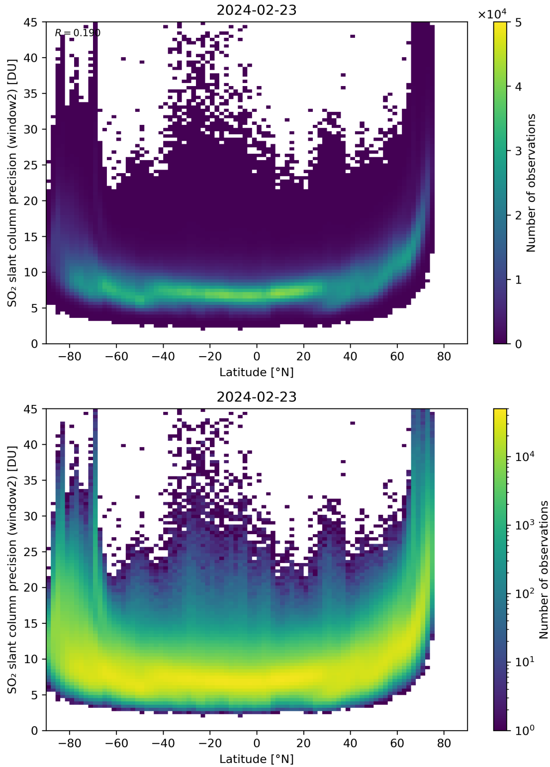
Figure 151: Scatter density plot of “Latitude” against “SO 2 slant column precision (window2)” for 2024-02-22 to 2024-02-24.
