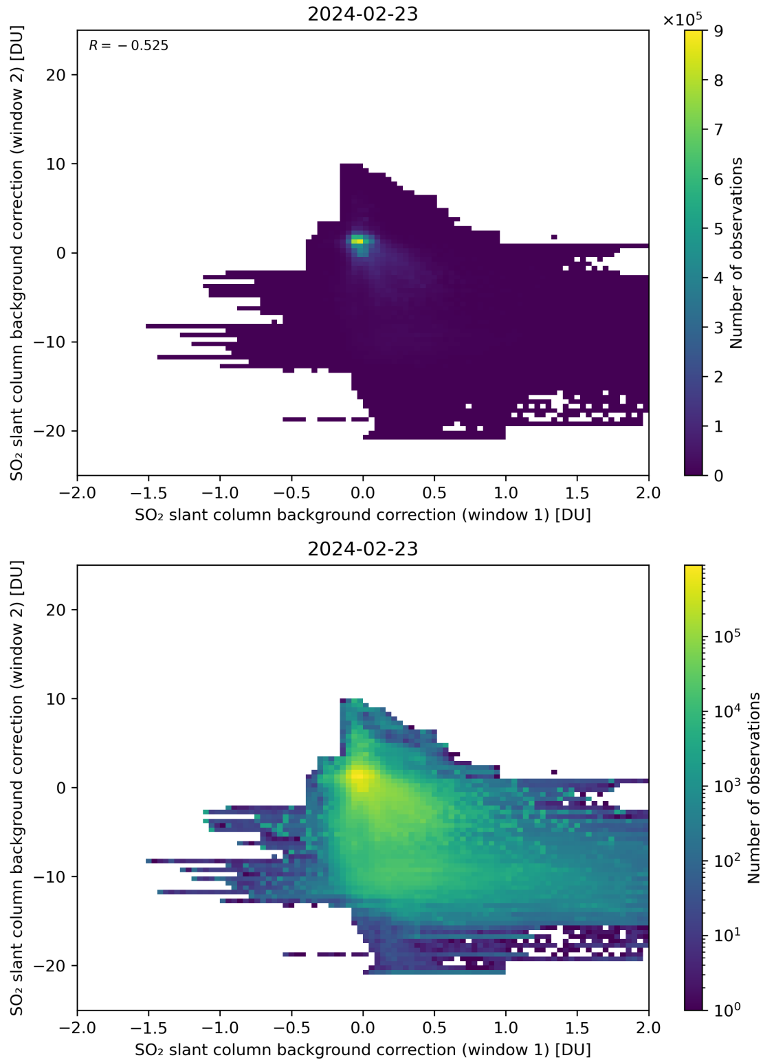
Figure 98: Scatter density plot of “SO 2 slant column background correction (window 1)” against “SO 2 slant column background correction (window 2)” for 2024-02-22 to 2024-02-24.
