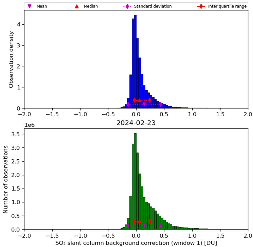
Figure 59: Histogram of “SO 2 slant column background correction (window 1)” for 2024-02-22 to 2024-02-24
