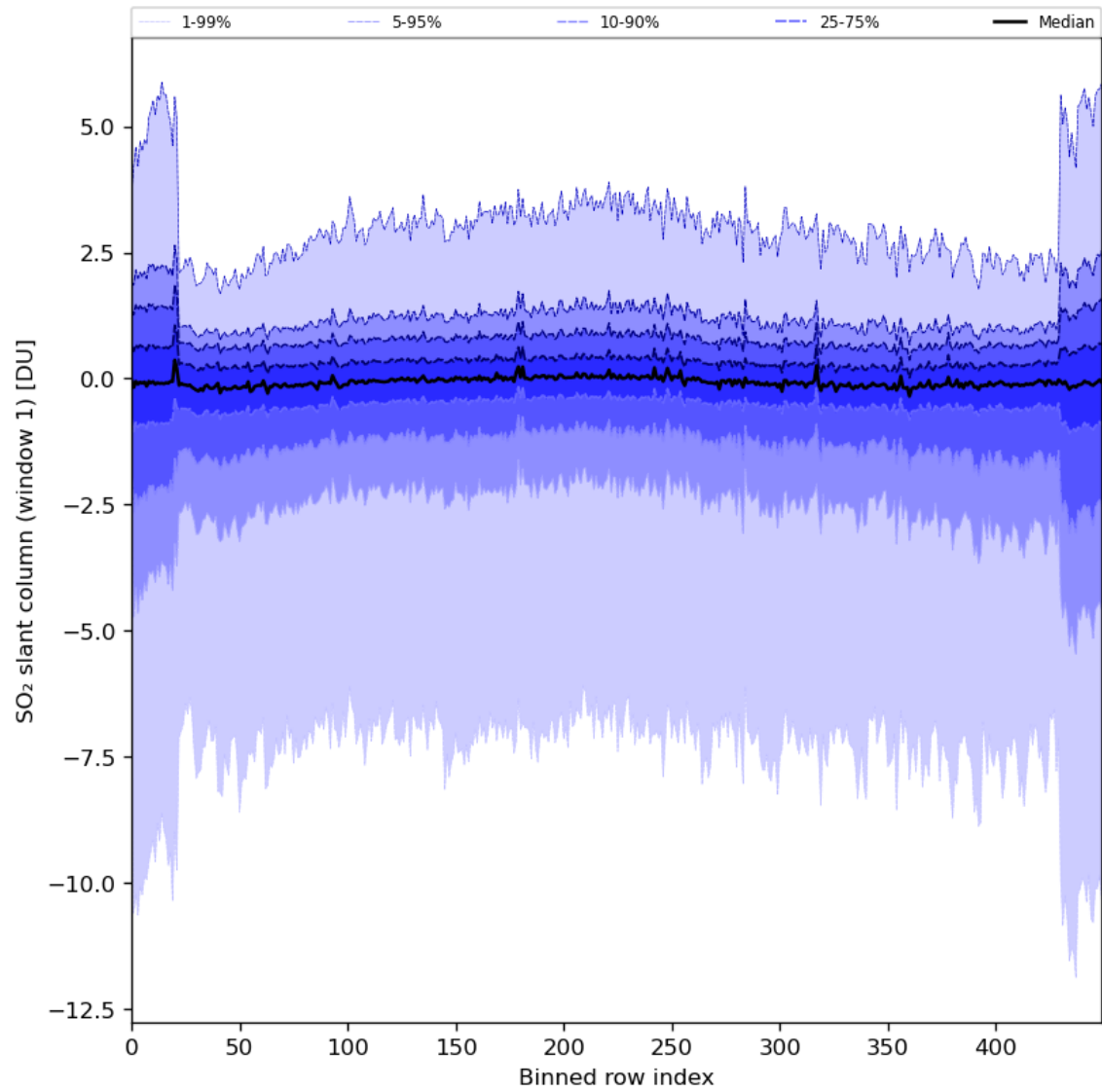
Figure 79: Along track statistics of “SO 2 slant column (window 1)” for 2024-02-22 to 2024-02-24
