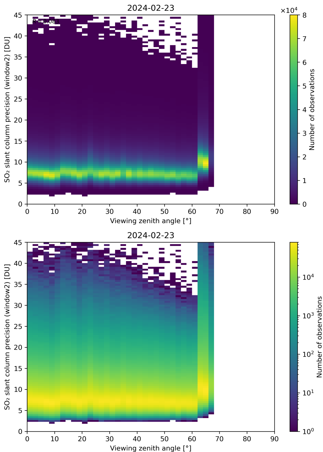
Figure 322: Scatter density plot of “Viewing zenith angle” against “SO 2 slant column precision (window2)” for 2024-02-22 to 2024-02-24.
