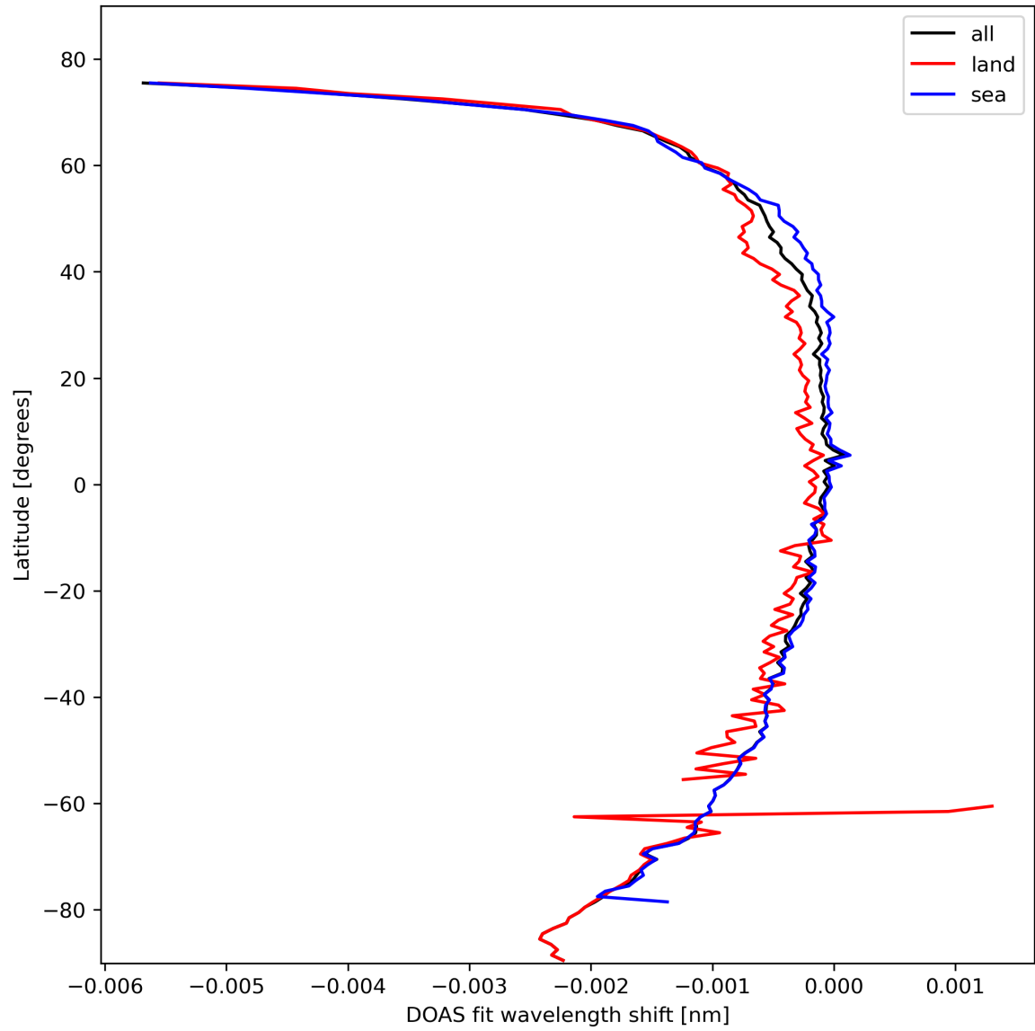
Figure 45: Zonal average of “DOAS fit wavelength shift” for 2024-02-22 to 2024-02-24.
