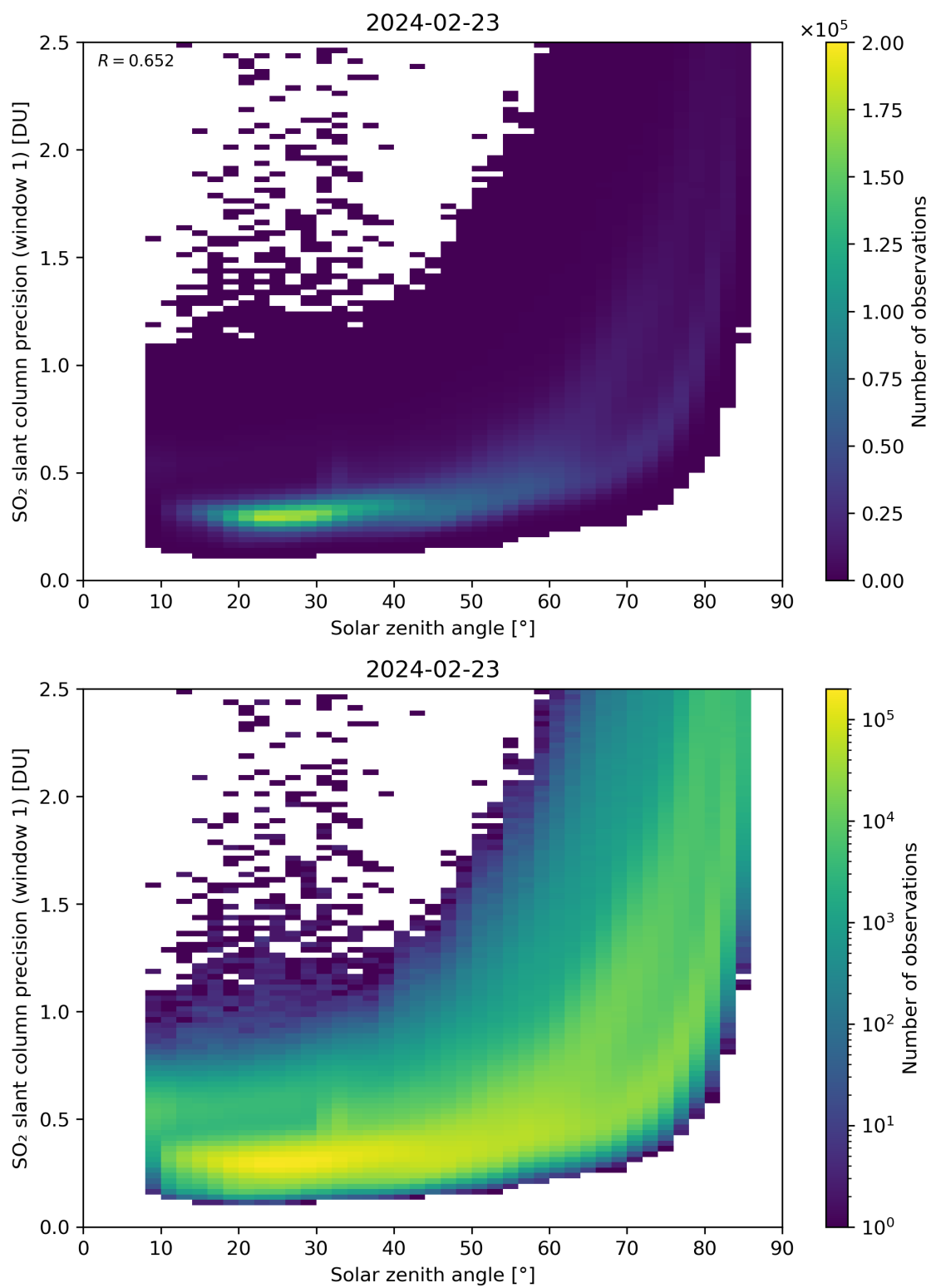
Figure 170: Scatter density plot of “Solar zenith angle” against “SO 2 slant column precision (window 1)” for 2024-02-22 to 2024-02-24.
