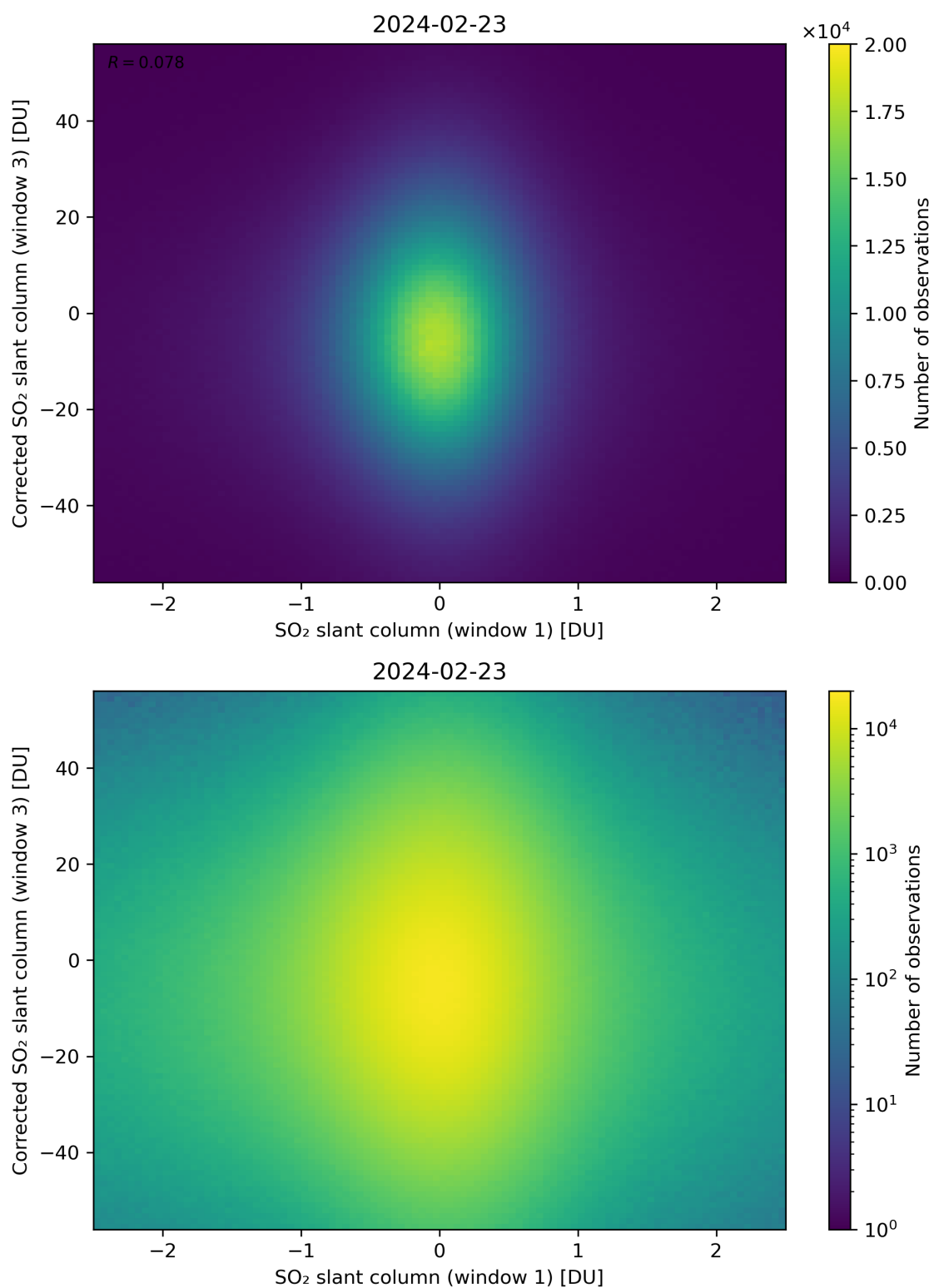
Figure 234: Scatter density plot of “SO 2 slant column (window 1)” against “Corrected SO 2 slant column (window 3)” for 2024-02-22 to 2024-02-24.
