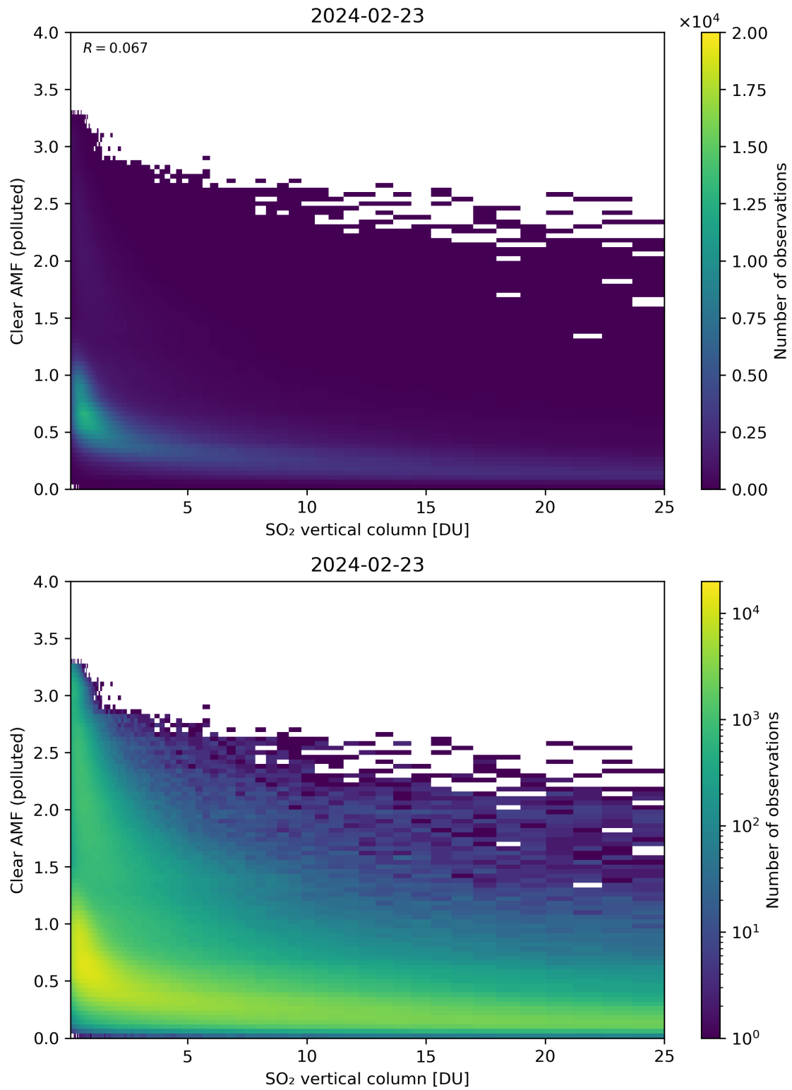
Figure 296: Scatter density plot of “SO 2 vertical column” against “Clear AMF (polluted)” for 2024-02-22 to 2024-02-24.
