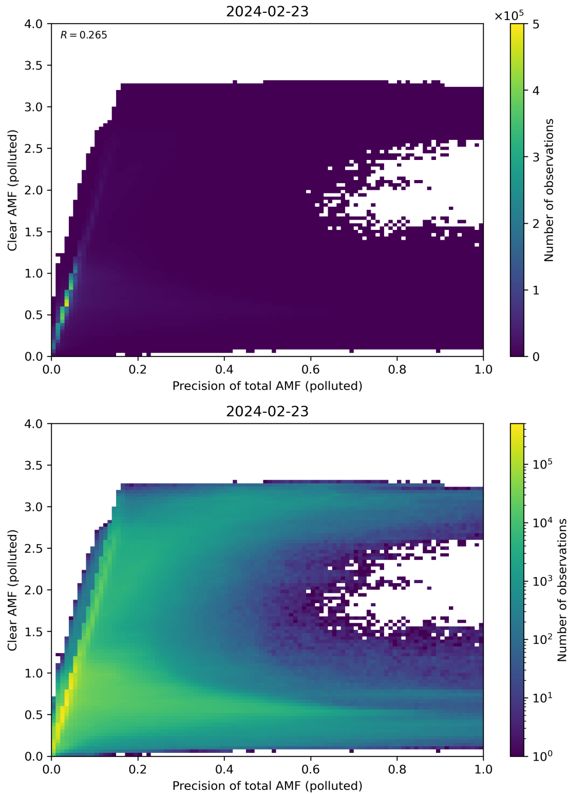
Figure 270: Scatter density plot of “Precision of total AMF (polluted)” against “Clear AMF (polluted)” for 2024-02-22 to 2024-02-24.
