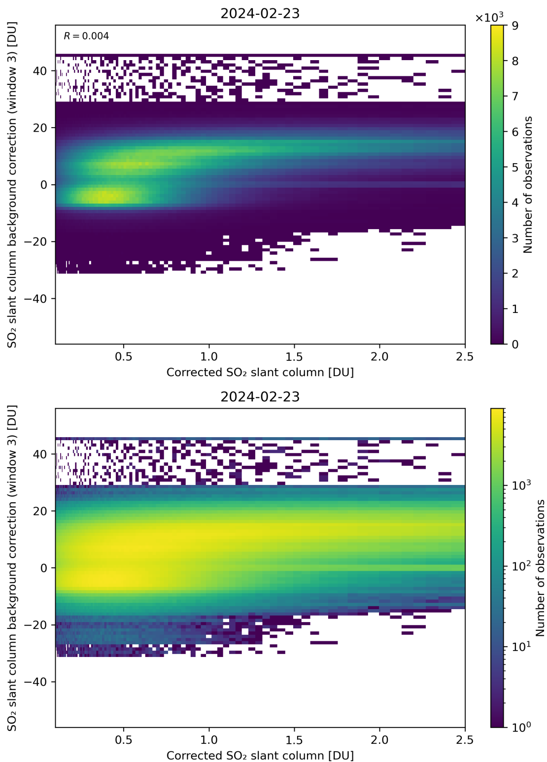
Figure 180: Scatter density plot of “Corrected SO 2 slant column” against “SO 2 slant column background correction (window 3)” for 2024-02-22 to 2024-02-24.
