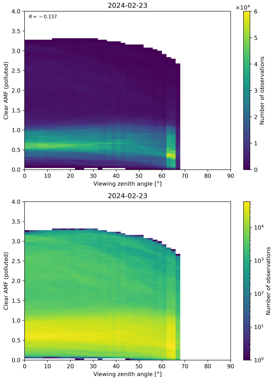
Figure 316: Scatter density plot of “Viewing zenith angle” against “Clear AMF (polluted)” for 2024-02-22 to 2024-02-24.
