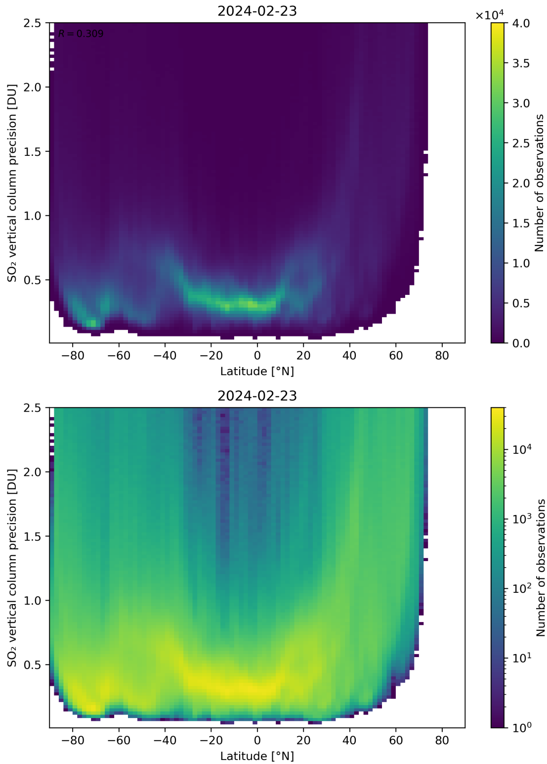
Figure 157: Scatter density plot of “Latitude” against “SO 2 vertical column precision” for 2024-02-22 to 2024-02-24.
