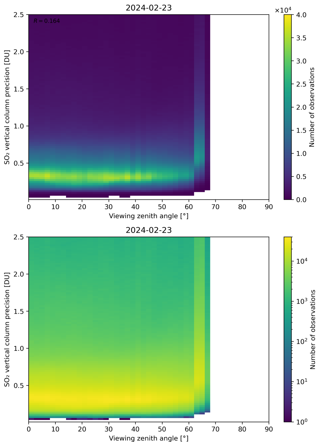
Figure 328: Scatter density plot of “Viewing zenith angle” against “SO 2 vertical column precision” for 2024-02-22 to 2024-02-24.
