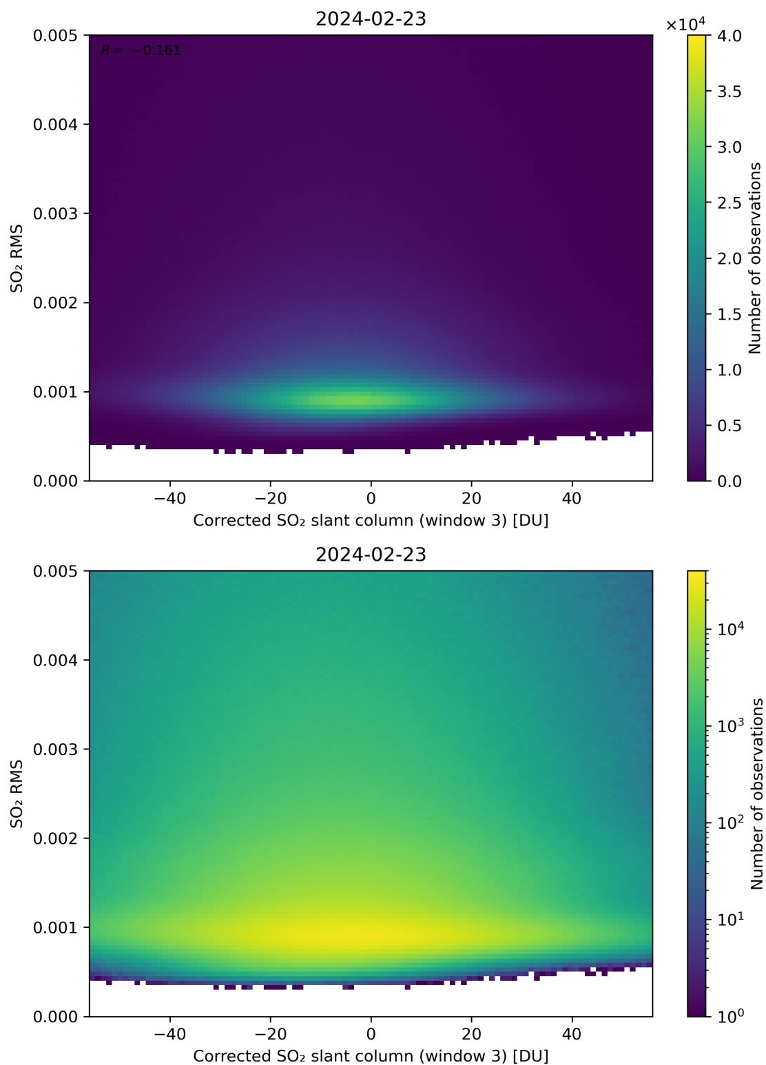
Figure 208: Scatter density plot of “Corrected SO 2 slant column (window 3)” against “SO 2 RMS” for 2024-02-22 to 2024-02-24.
