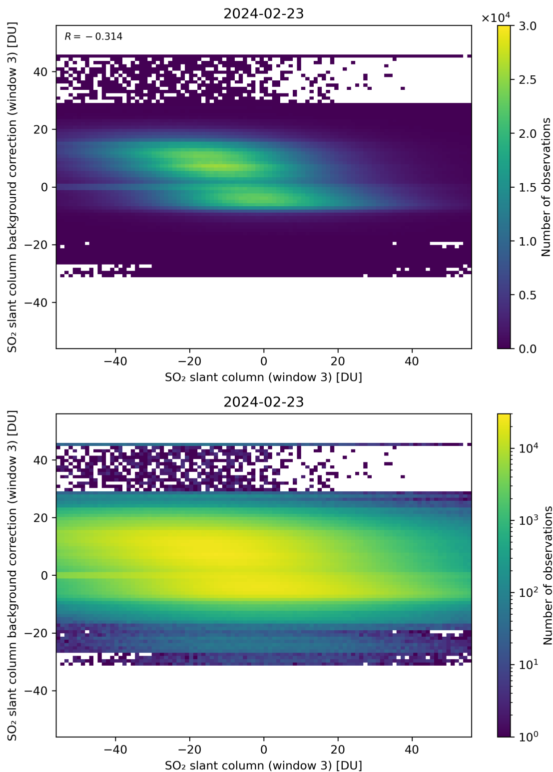
Figure 253: Scatter density plot of “SO 2 slant column (window 3)” against “SO 2 slant column background correction (window 3)” for 2024-02-22 to 2024-02-24.
