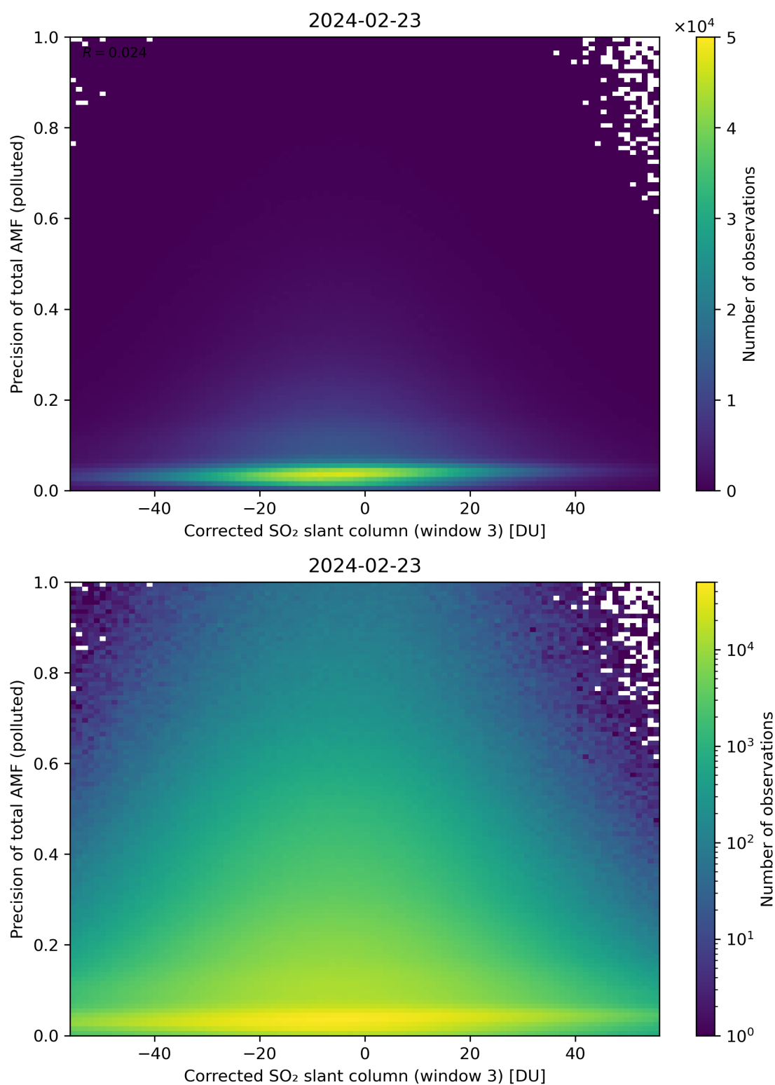
Figure 211: Scatter density plot of “Corrected SO 2 slant column (window 3)” against “Precision of total AMF (polluted)” for 2024-02-22 to 2024-02-24.
