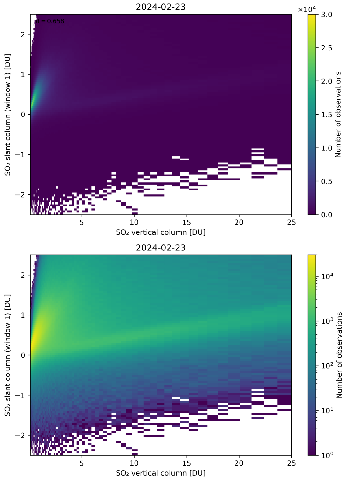
Figure 300: Scatter density plot of “SO 2 vertical column” against “SO 2 slant column (window 1)” for 2024-02-22 to 2024-02-24.
