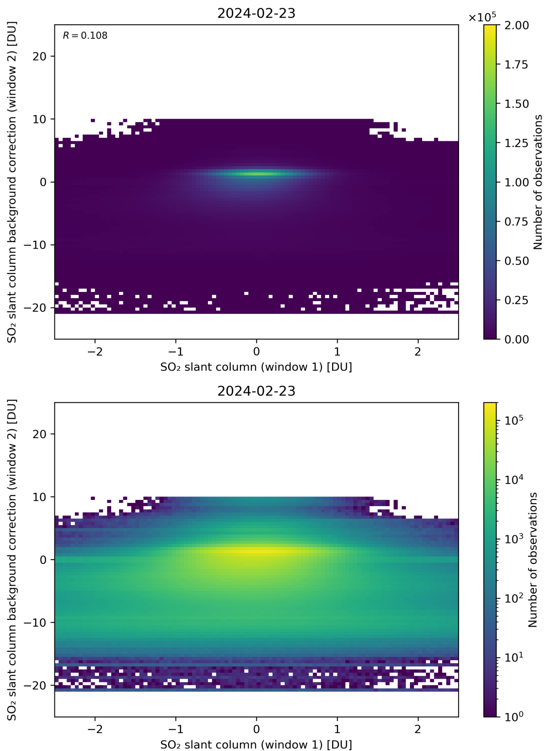
Figure 213: Scatter density plot of “SO 2 slant column (window 1)” against “SO 2 slant column background correction (window 2)” for 2024-02-22 to 2024-02-24.
