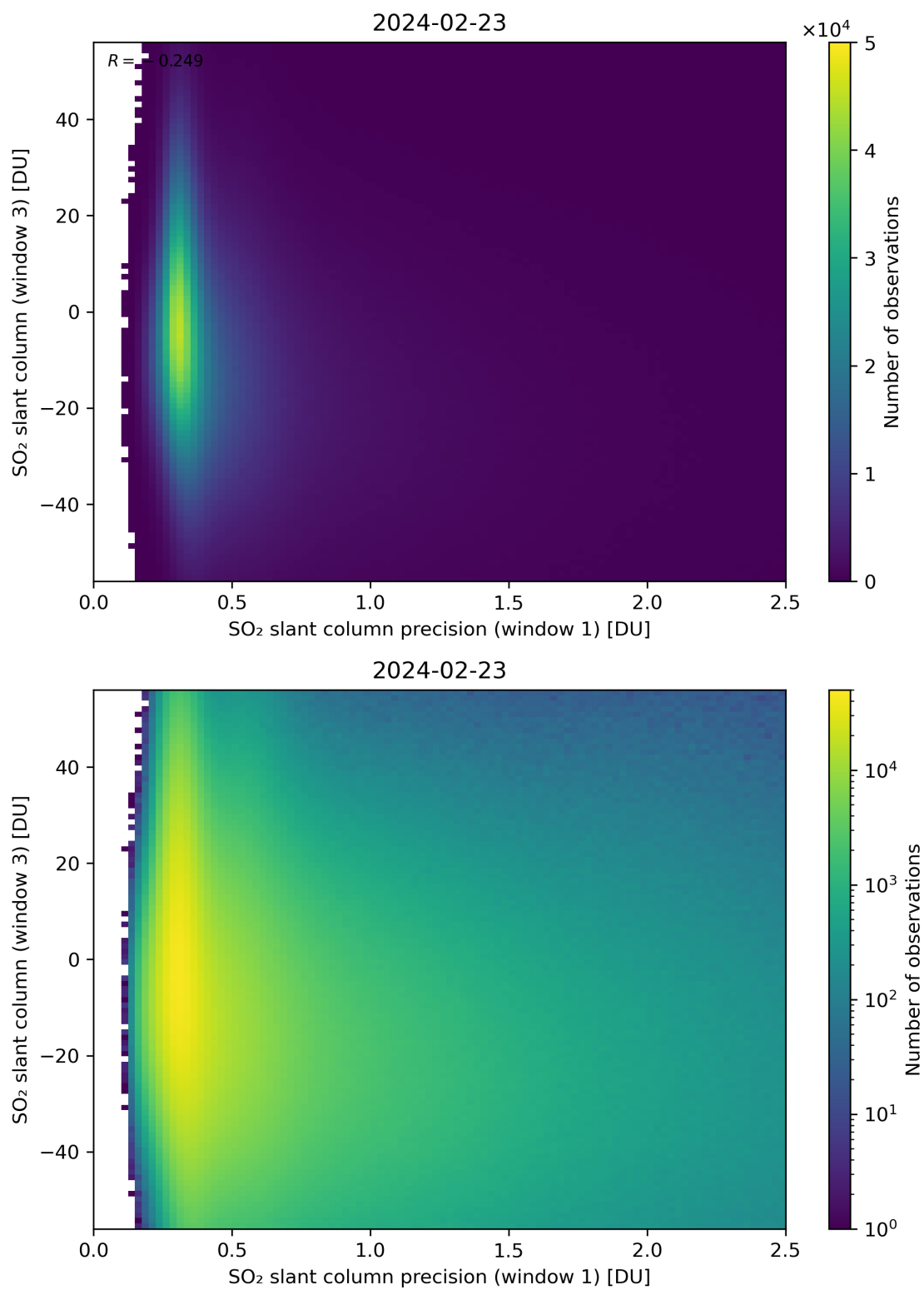
Figure 228: Scatter density plot of “SO 2 slant column precision (window 1)” against “SO 2 slant column (window 3)” for 2024-02-22 to 2024-02-24.
