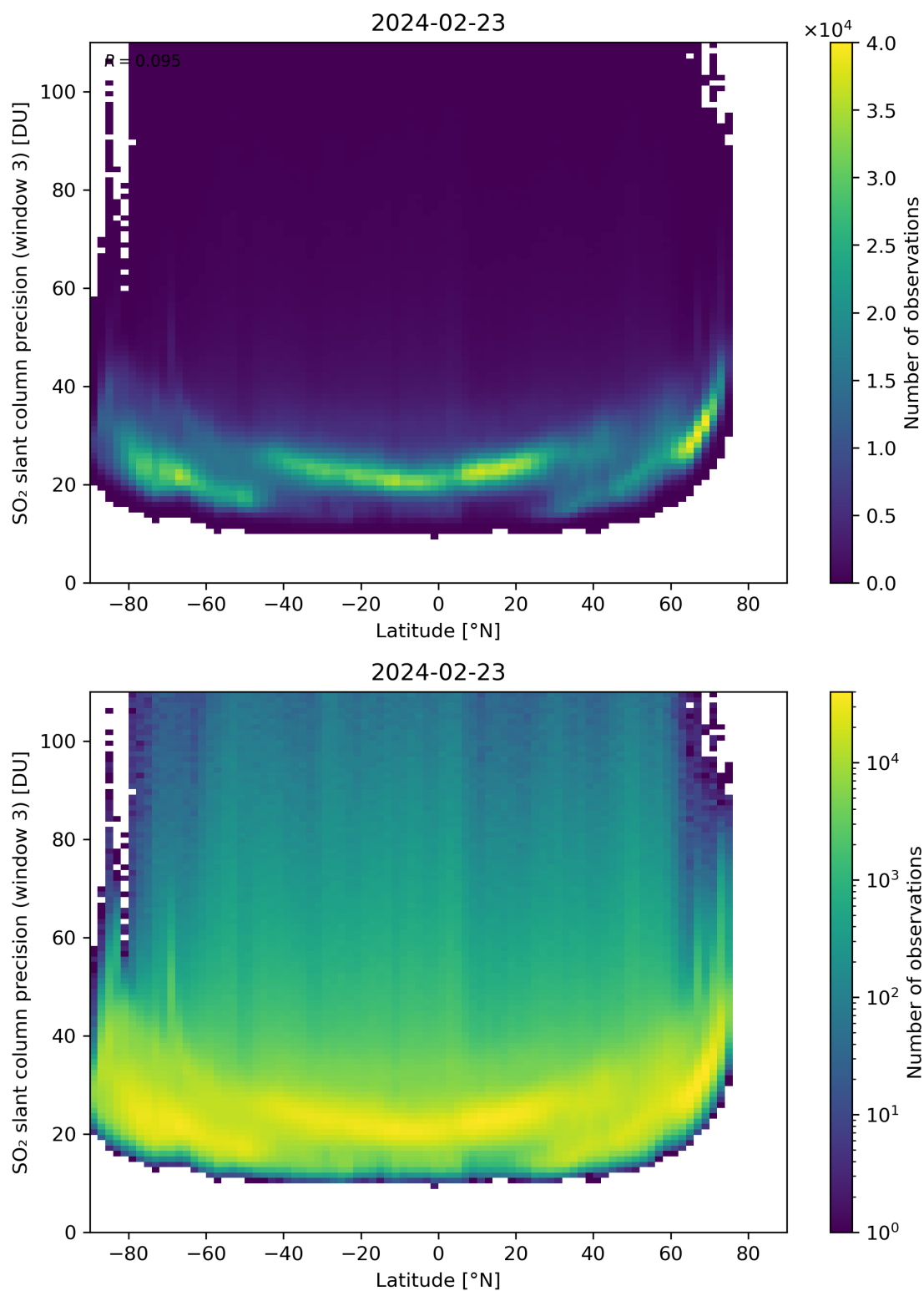
Figure 153: Scatter density plot of “Latitude” against “SO 2 slant column precision (window 3)” for 2024-02-22 to 2024-02-24.
