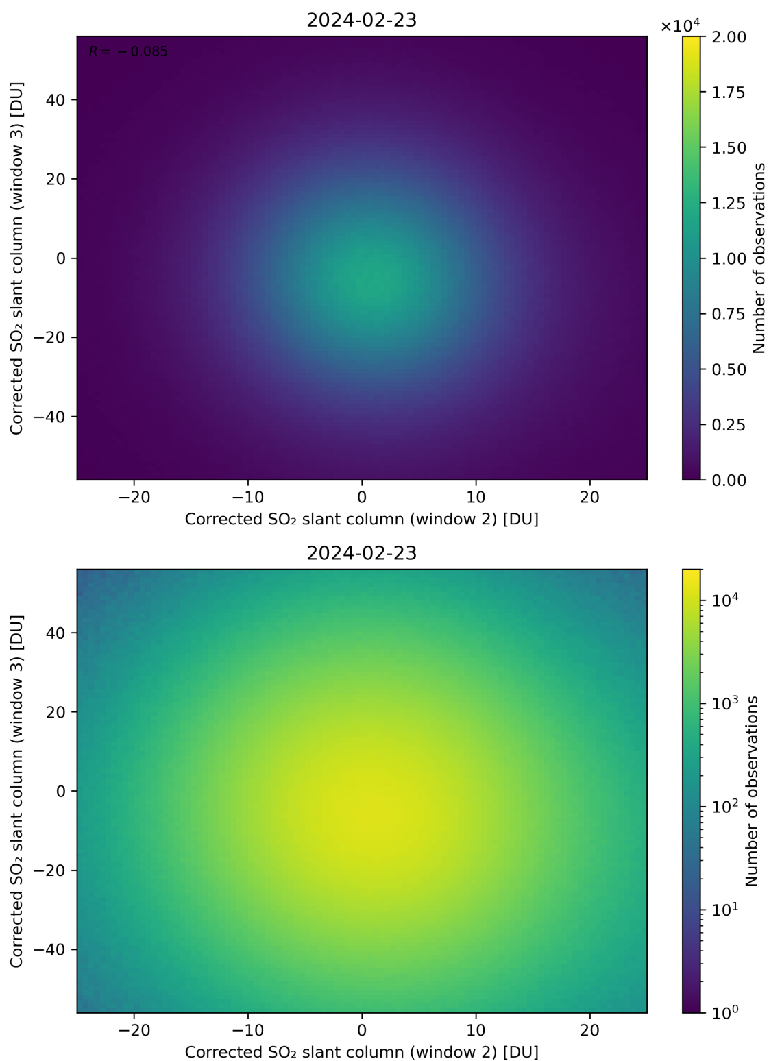
Figure 200: Scatter density plot of “Corrected SO 2 slant column (window 2)” against “Corrected SO 2 slant column (window 3)” for 2024-02-22 to 2024-02-24.
