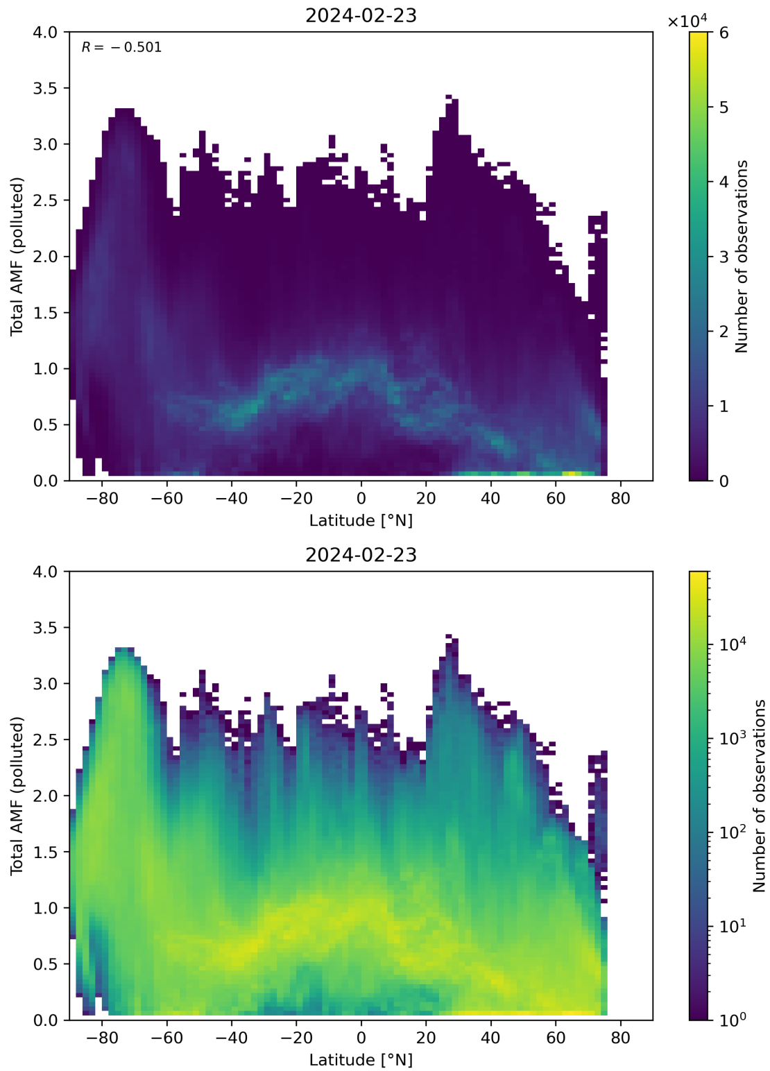
Figure 154: Scatter density plot of “Latitude” against “Total AMF (polluted)” for 2024-02-22 to 2024-02-24.
