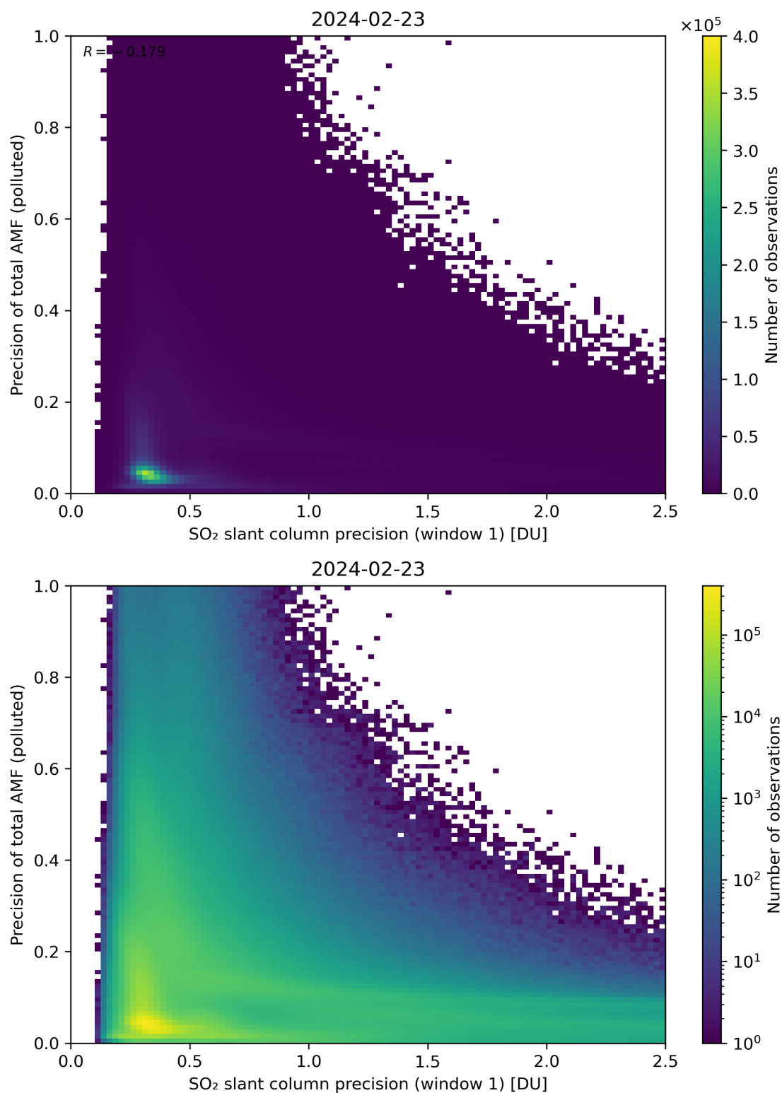
Figure 231: Scatter density plot of “SO 2 slant column precision (window 1)” against “Precision of total AMF (polluted)” for 2024-02-22 to 2024-02-24.
