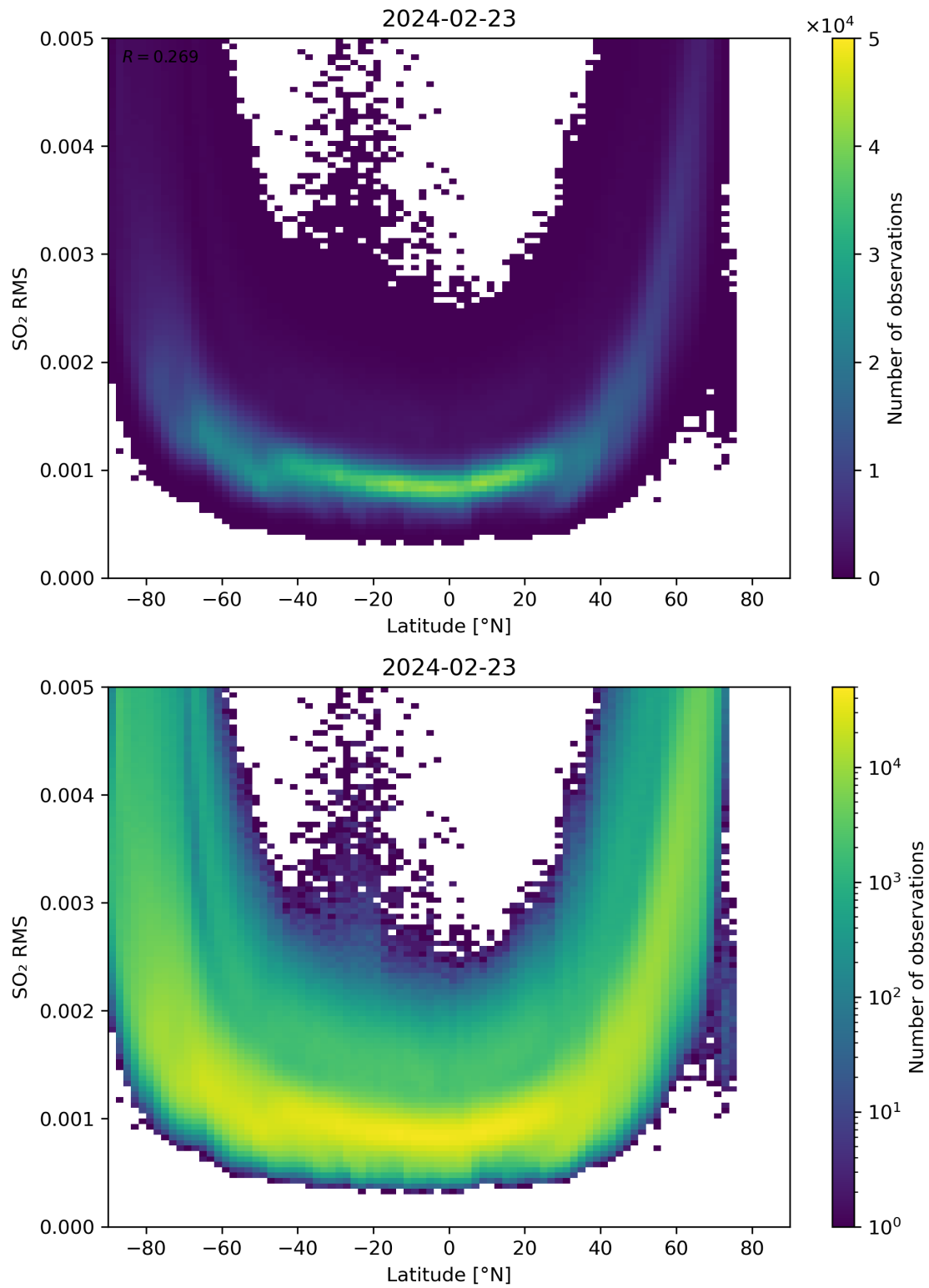
Figure 144: Scatter density plot of “Latitude” against “SO 2 RMS” for 2024-02-22 to 2024-02-24.
