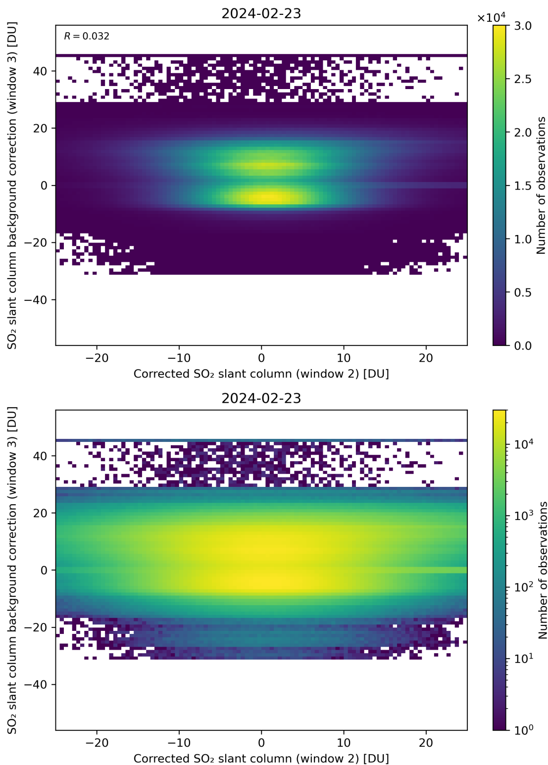
Figure 195: Scatter density plot of “Corrected SO 2 slant column (window 2)” against “SO 2 slant column background correction (window 3)” for 2024-02-22 to 2024-02-24.
