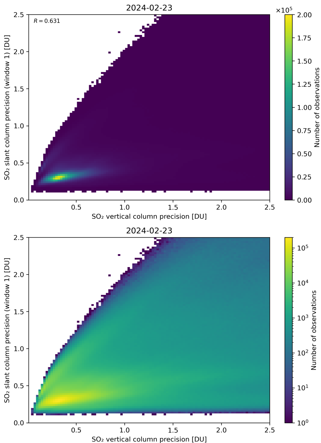
Figure 290: Scatter density plot of “SO 2 vertical column precision” against “SO 2 slant column precision (window 1)” for 2024-02-22 to 2024-02-24.
