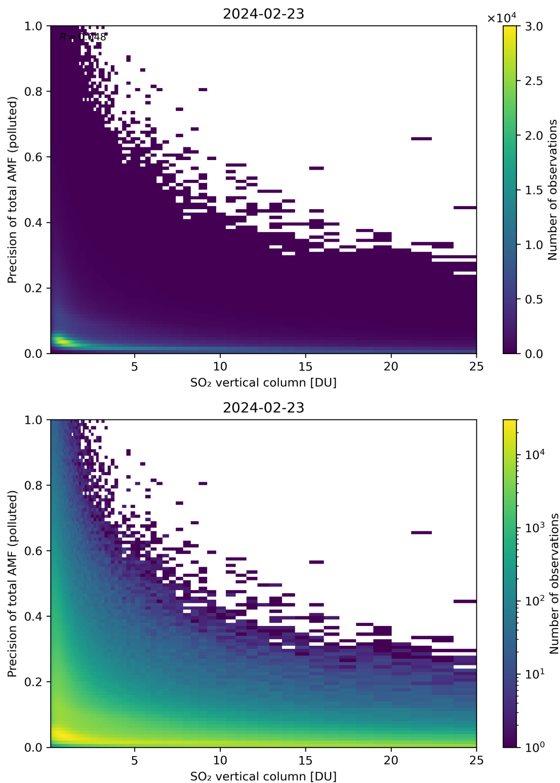
Figure 306: Scatter density plot of “SO 2 vertical column” against “Precision of total AMF (polluted)” for 2024-02-22 to 2024-02-24.
