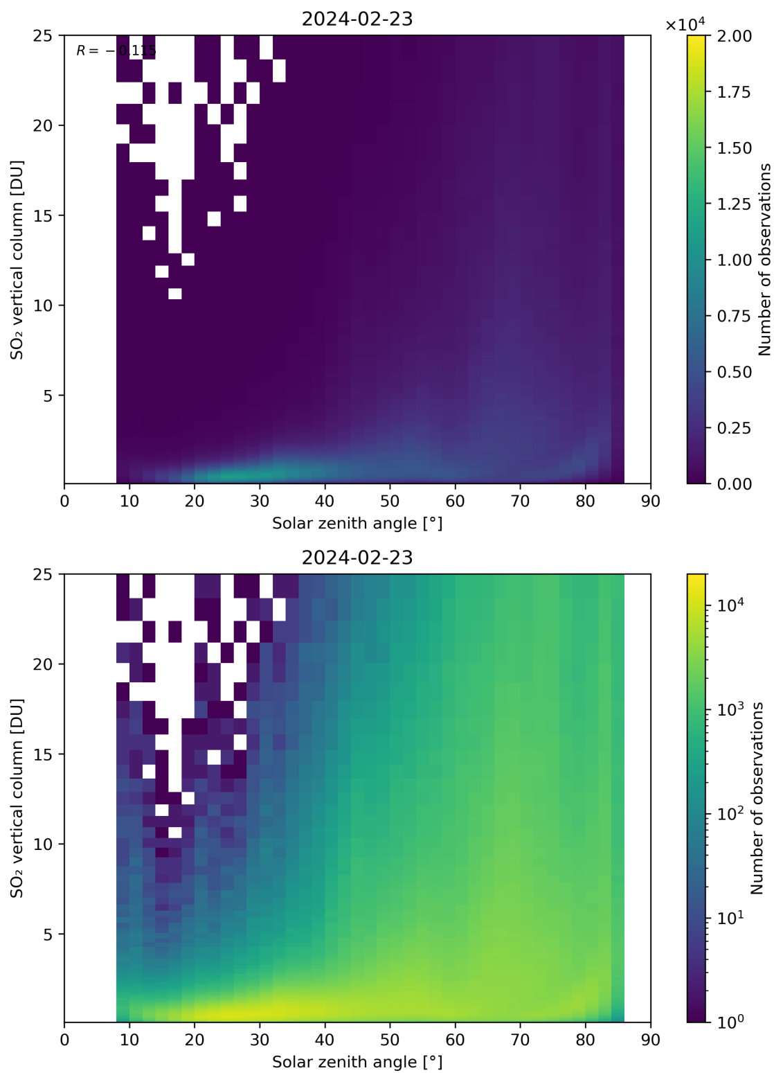
Figure 176: Scatter density plot of “Solar zenith angle” against “SO 2 vertical column” for 2024-02-22 to 2024-02-24.
