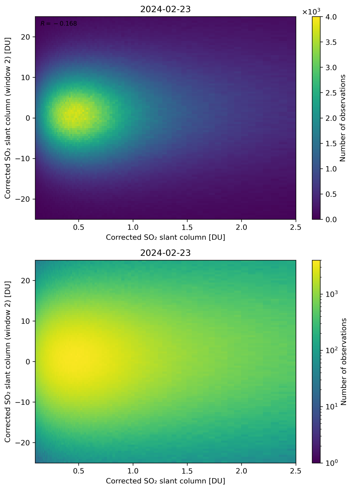
Figure 185: Scatter density plot of “Corrected SO 2 slant column” against “Corrected SO 2 slant column (window 2)” for 2024-02-22 to 2024-02-24.
