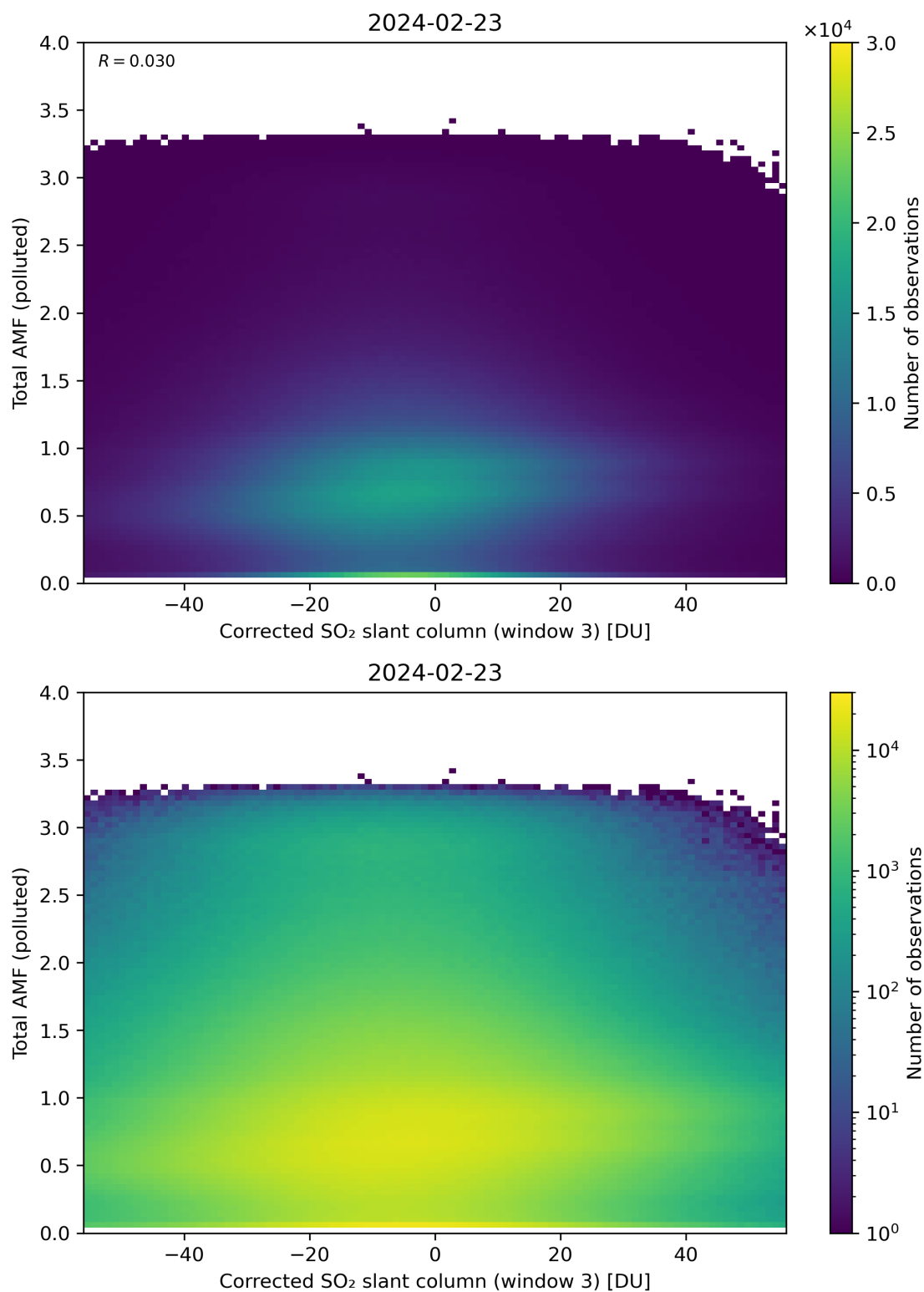
Figure 210: Scatter density plot of “Corrected SO 2 slant column (window 3)” against “Total AMF (polluted)” for 2024-02-22 to 2024-02-24.
