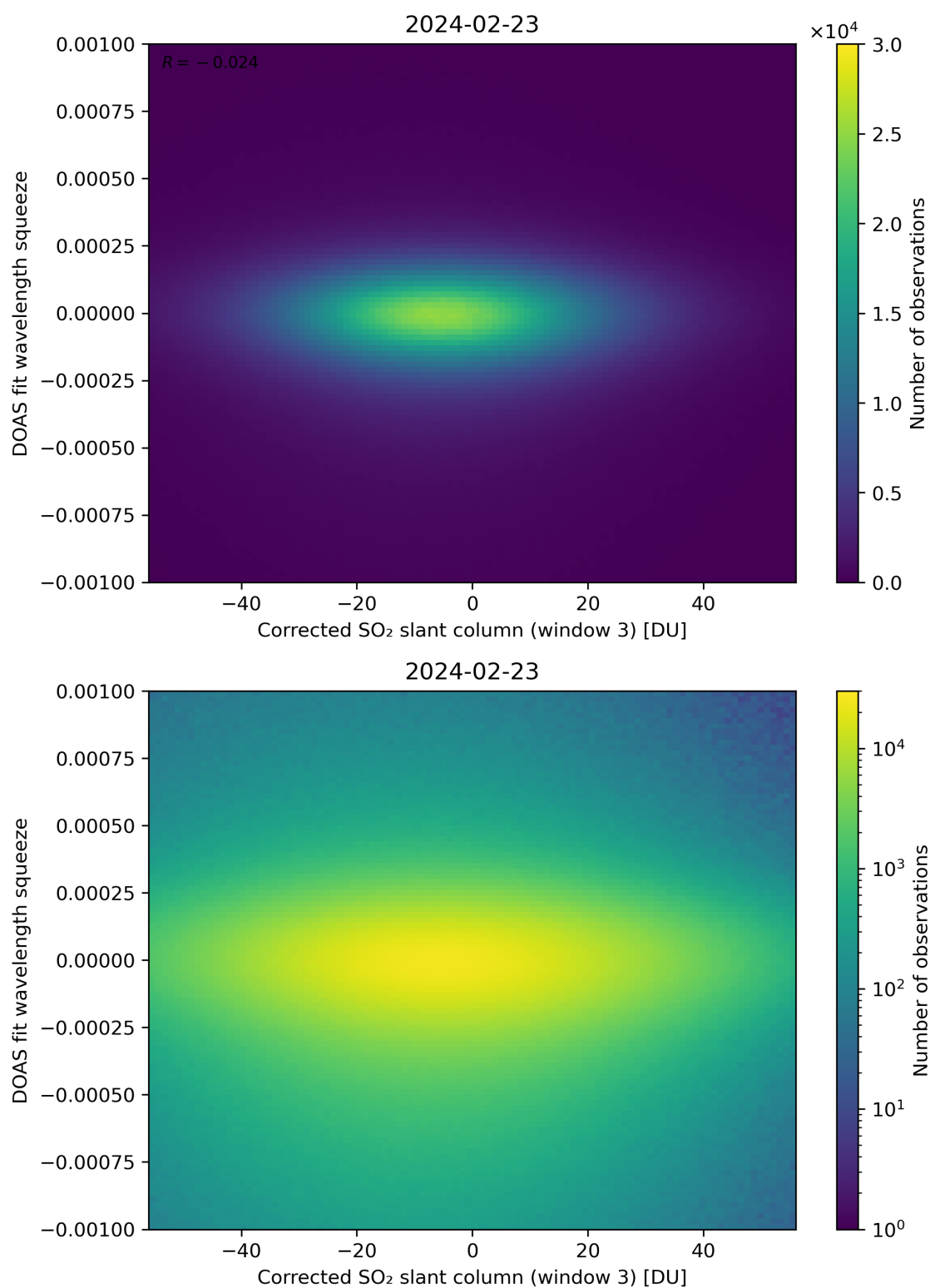
Figure 207: Scatter density plot of “Corrected SO 2 slant column (window 3)” against “DOAS fit wavelength squeeze” for 2024-02-22 to 2024-02-24.
