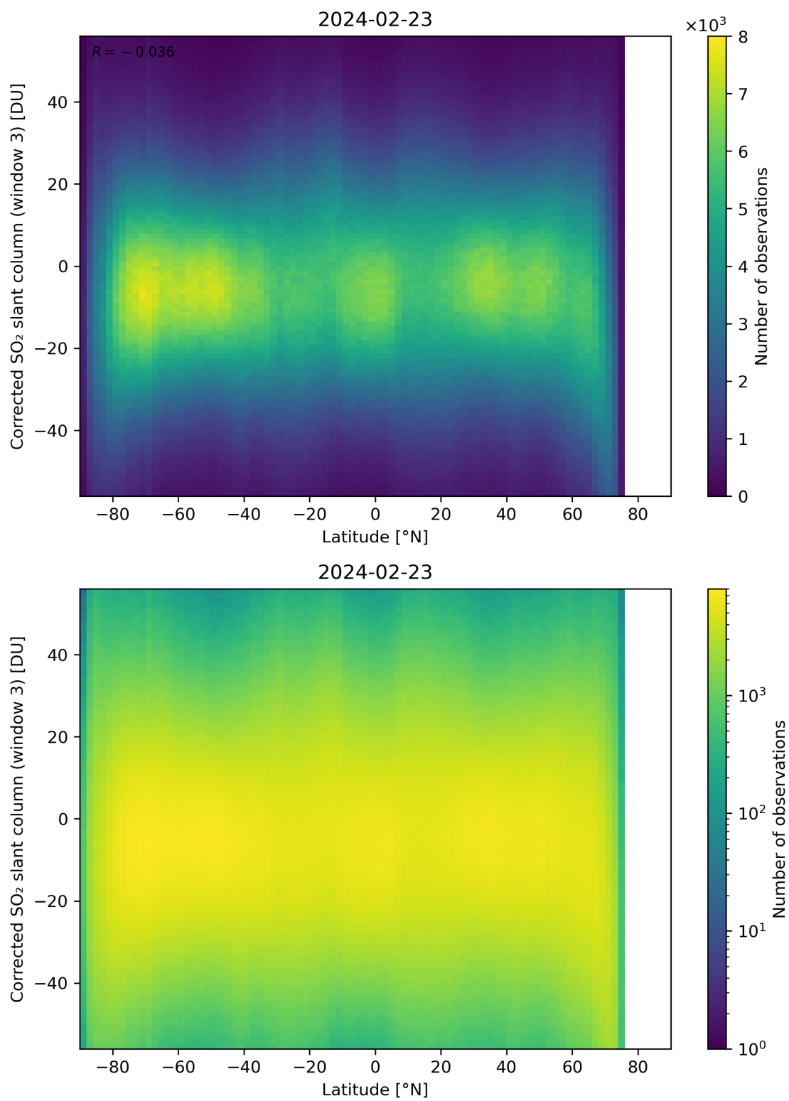
Figure 148: Scatter density plot of “Latitude” against “Corrected SO 2 slant column (window 3)” for 2024-02-22 to 2024-02-24.
