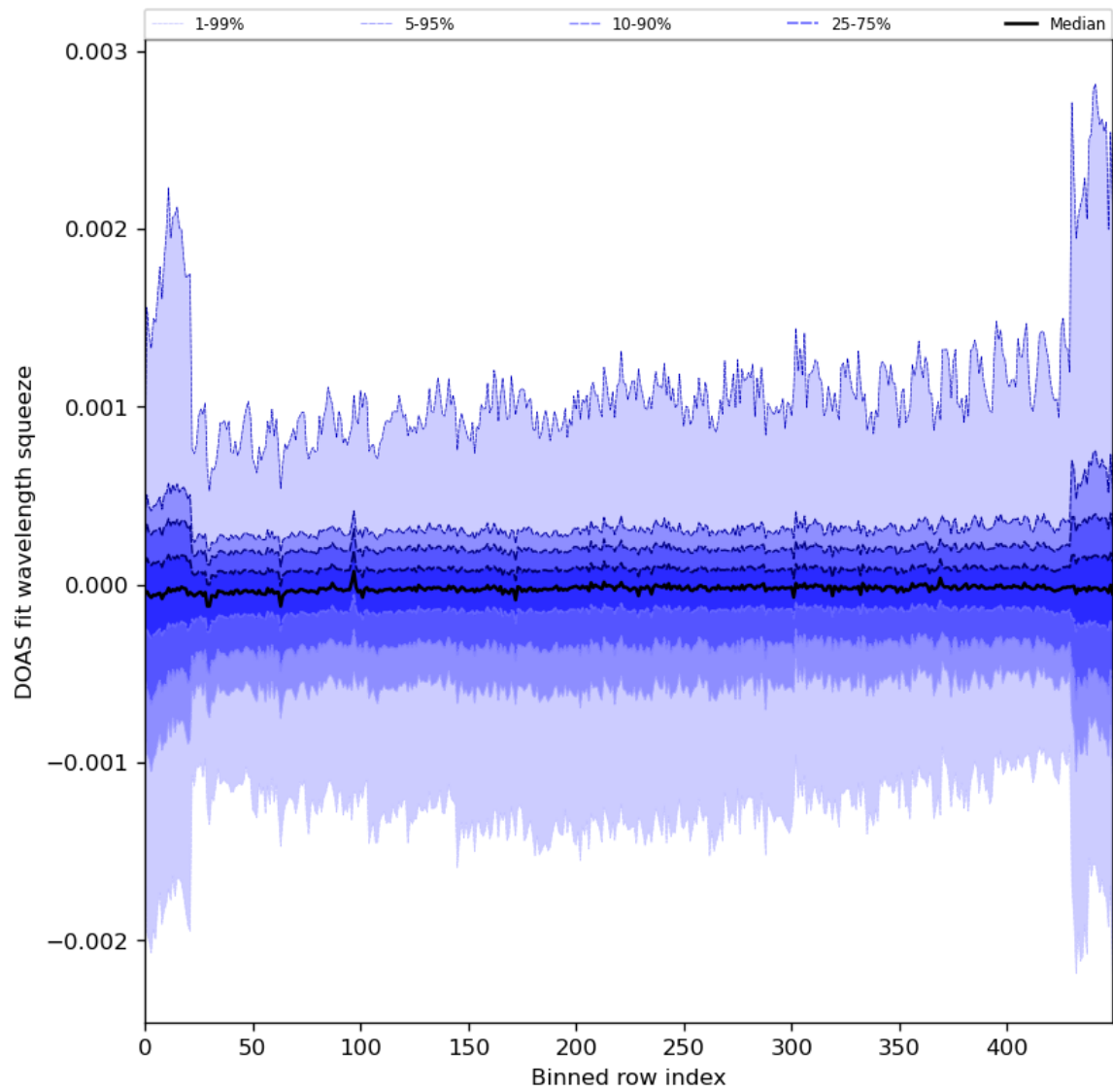
Figure 92: Along track statistics of “DOAS fit wavelength squeeze” for 2024-02-22 to 2024-02-24
