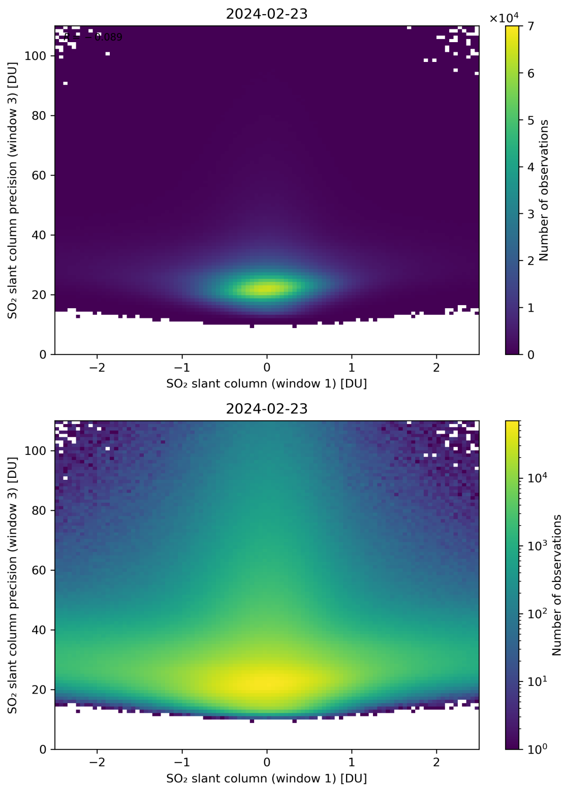
Figure 238: Scatter density plot of “SO 2 slant column (window 1)” against “SO 2 slant column precision (window 3)” for 2024-02-22 to 2024-02-24.
