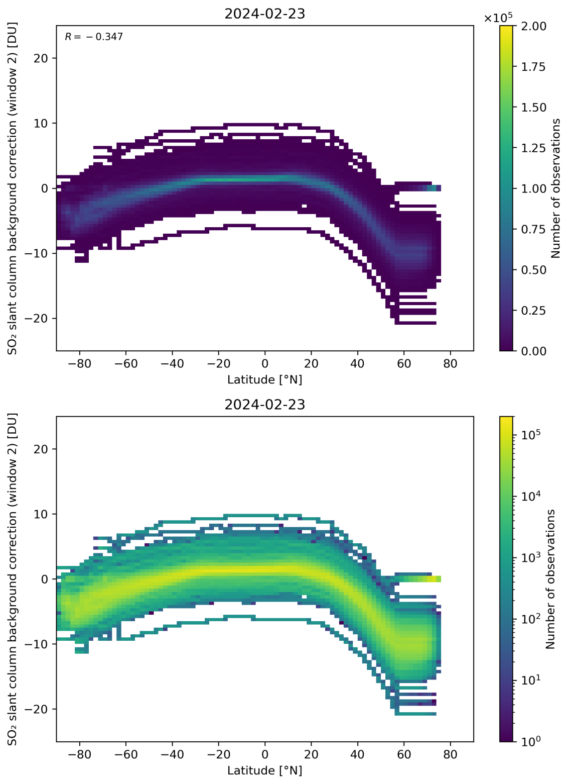
Figure 140: Scatter density plot of “Latitude” against “SO 2 slant column background correction (window 2)” for 2024-02-22 to 2024-02-24.
