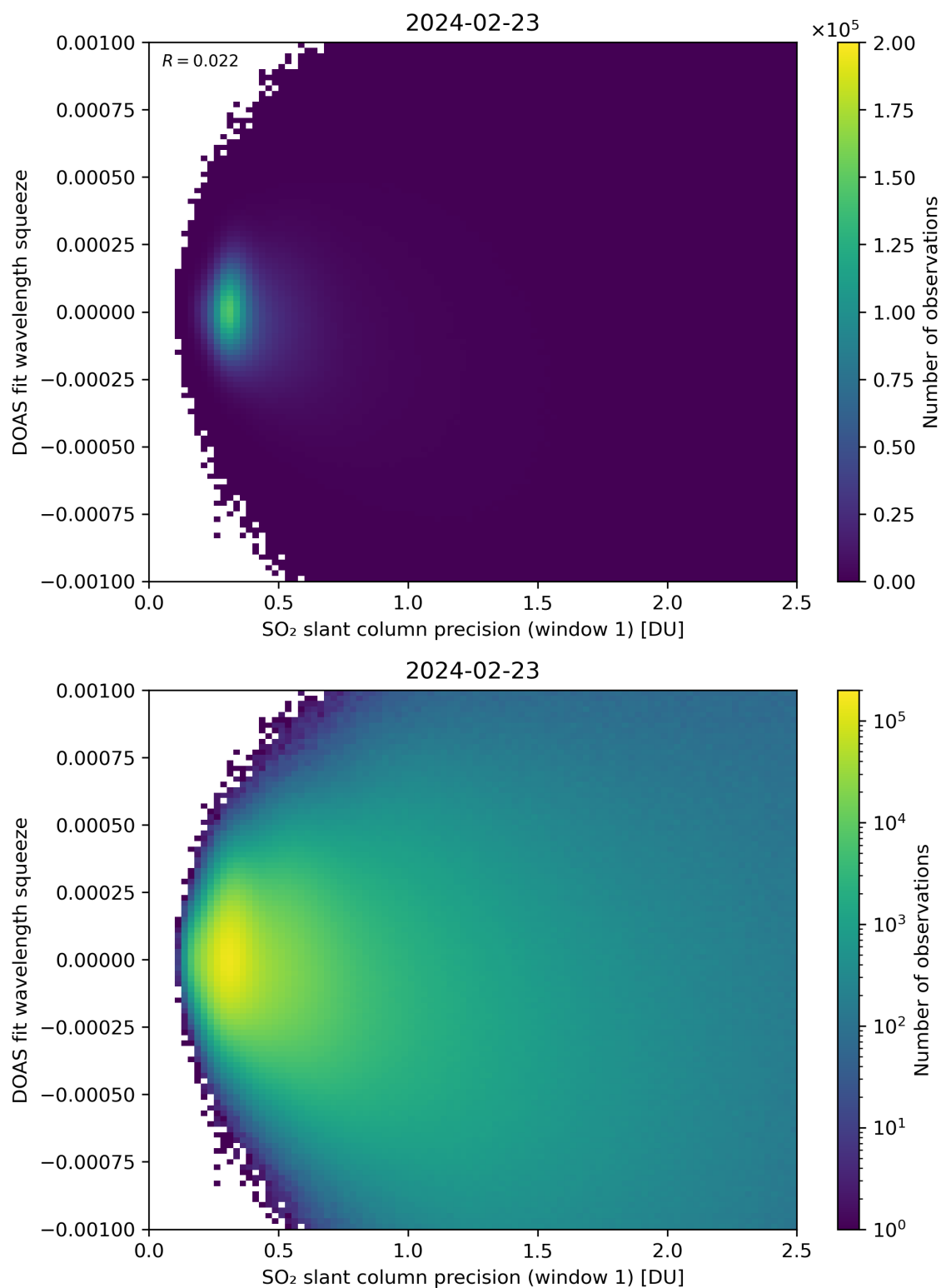
Figure 222: Scatter density plot of “SO 2 slant column precision (window 1)” against “DOAS fit wavelength squeeze” for 2024-02-22 to 2024-02-24.
