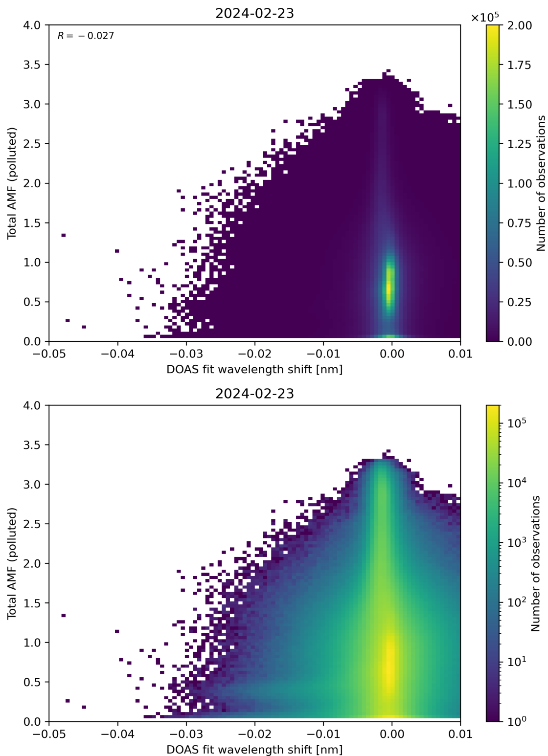
Figure 130: Scatter density plot of “DOAS fit wavelength shift” against “Total AMF (polluted)” for 2024-02-22 to 2024-02-24.
