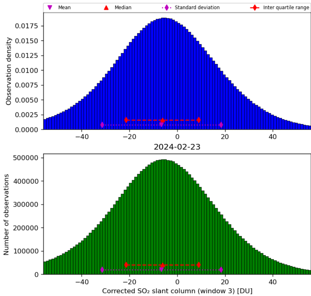
Figure 66: Histogram of "Corrected SO 2 slant column (window 3)" for 2024-02-22 to 2024-02-24
