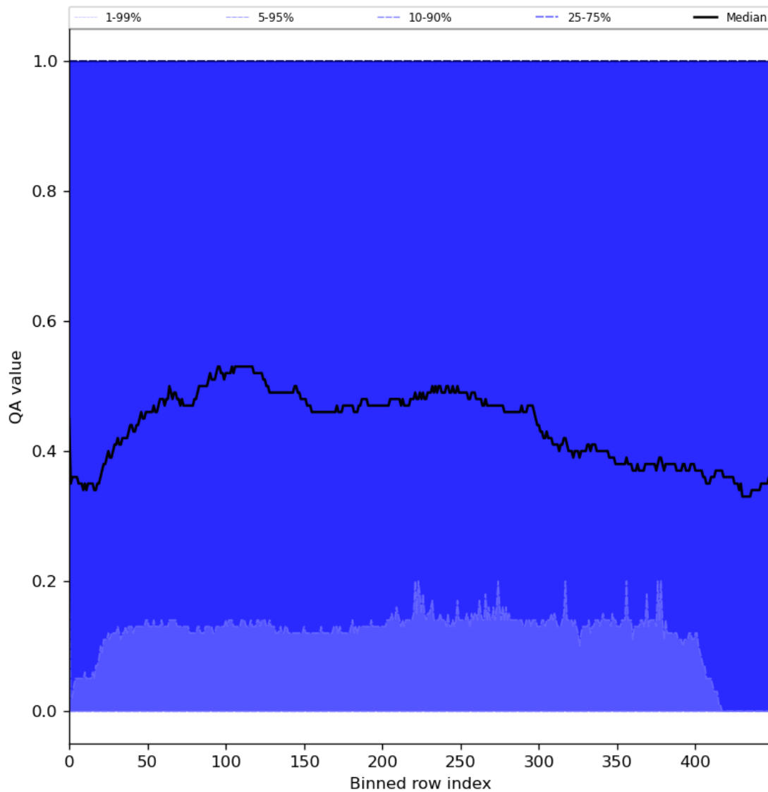
Figure 75: Along track statistics of “QA value” for 2024-02-22 to 2024-02-24
