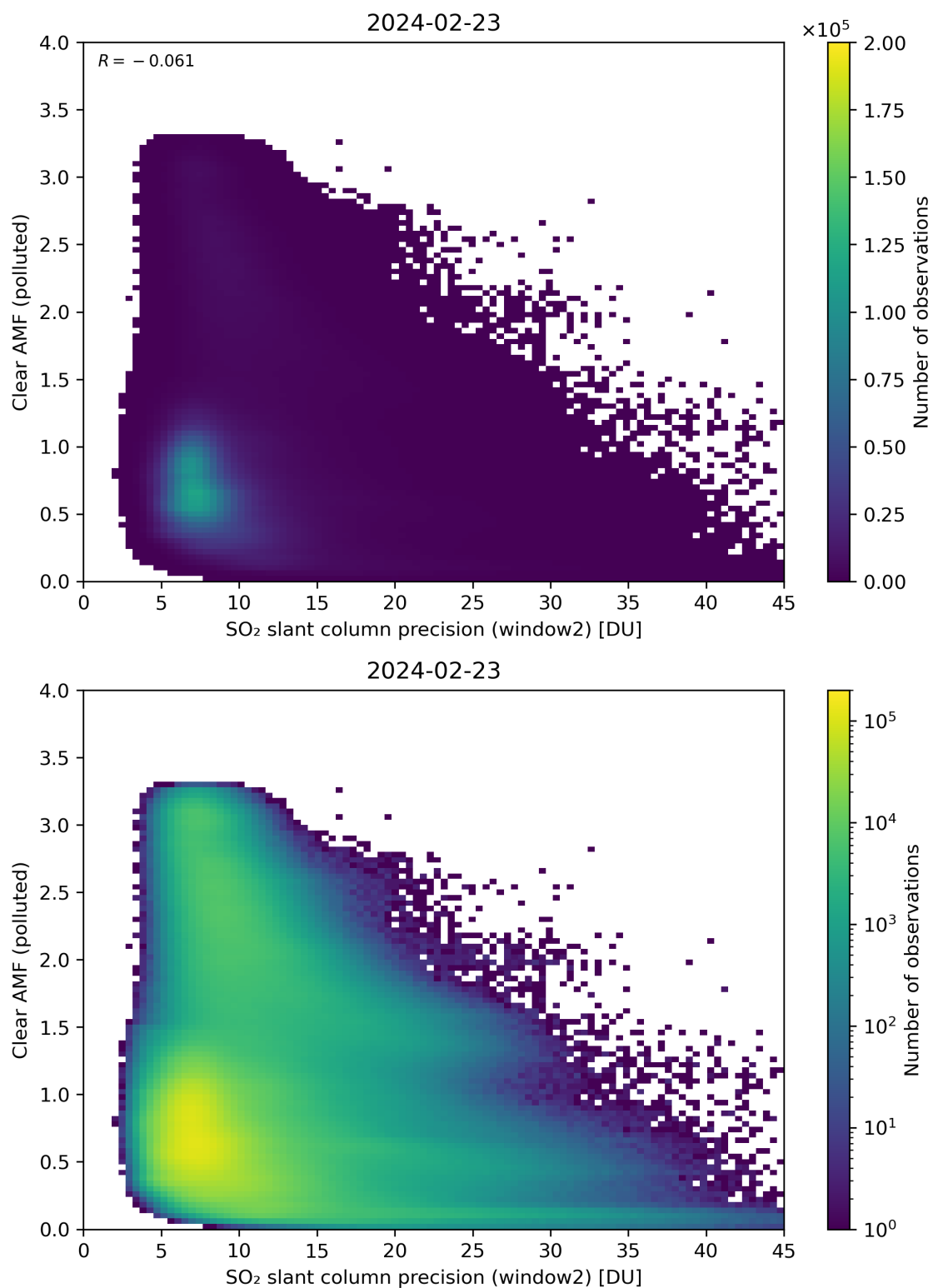
Figure 246: Scatter density plot of “SO 2 slant column precision (window2)” against “Clear AMF (polluted)” for 2024-02-22 to 2024-02-24.
