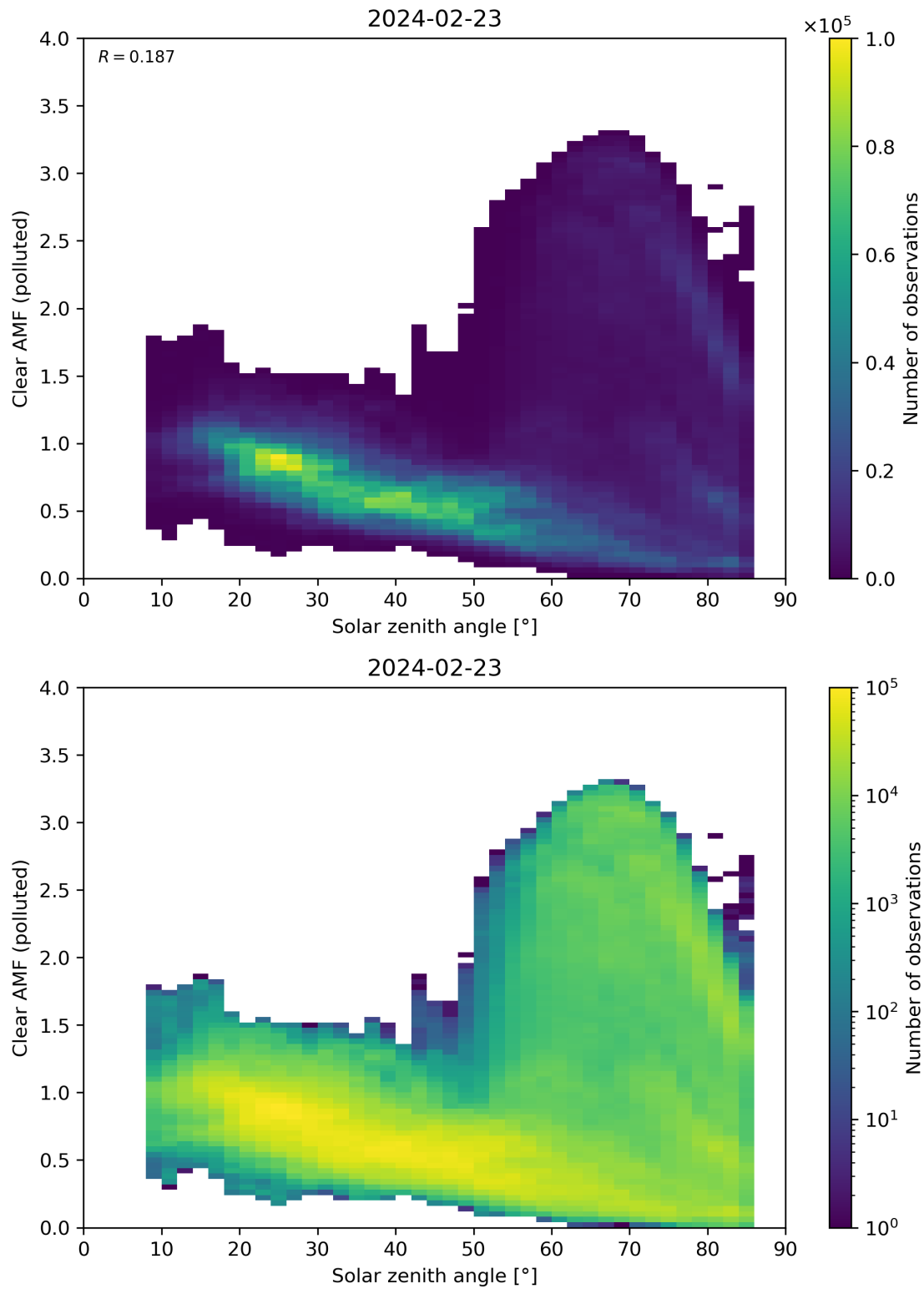
Figure 165: Scatter density plot of “Solar zenith angle” against “Clear AMF (polluted)” for 2024-02-22 to 2024-02-24.
