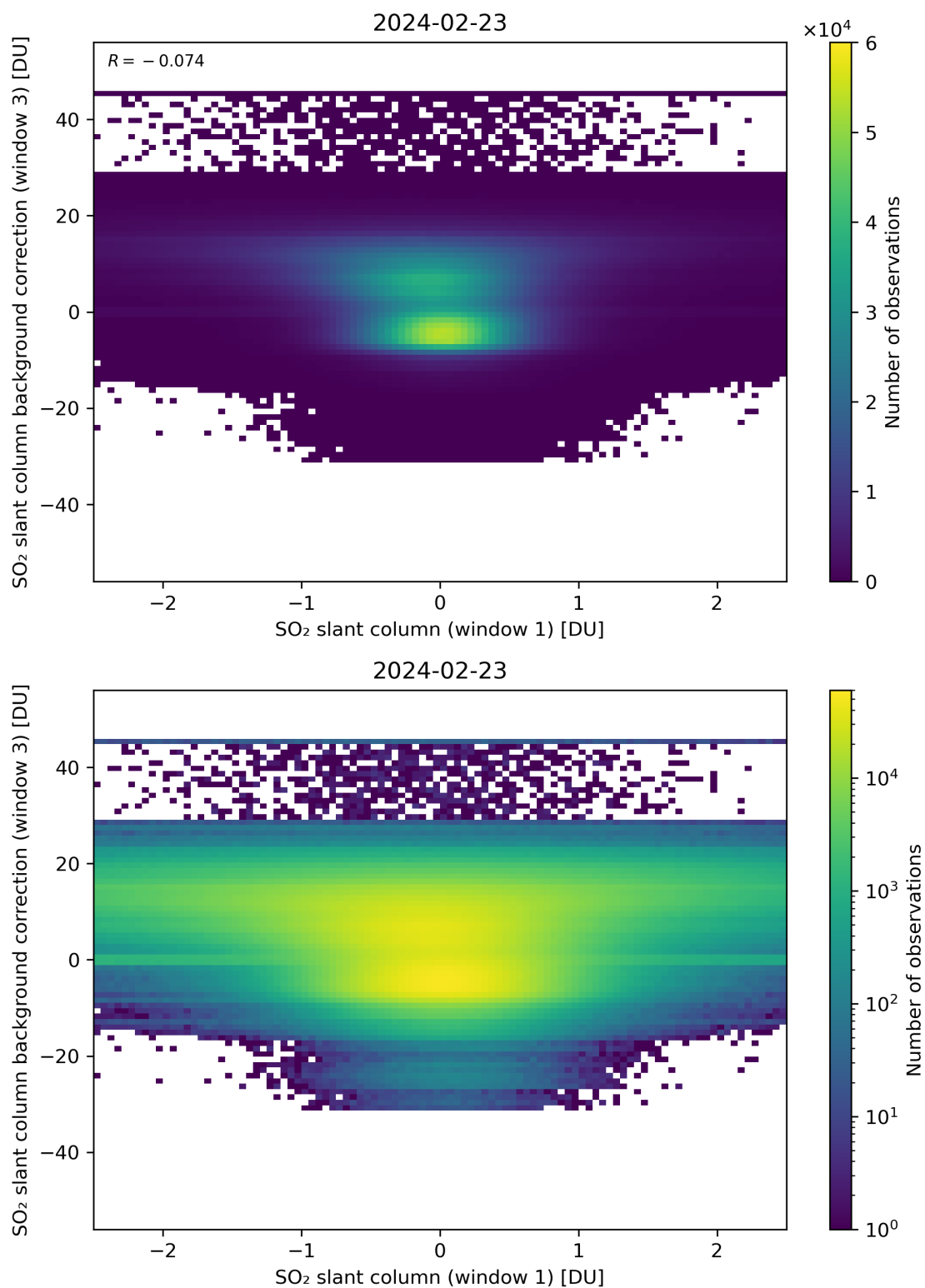
Figure 214: Scatter density plot of “SO 2 slant column (window 1)” against “SO 2 slant column background correction (window 3)” for 2024-02-22 to 2024-02-24.
