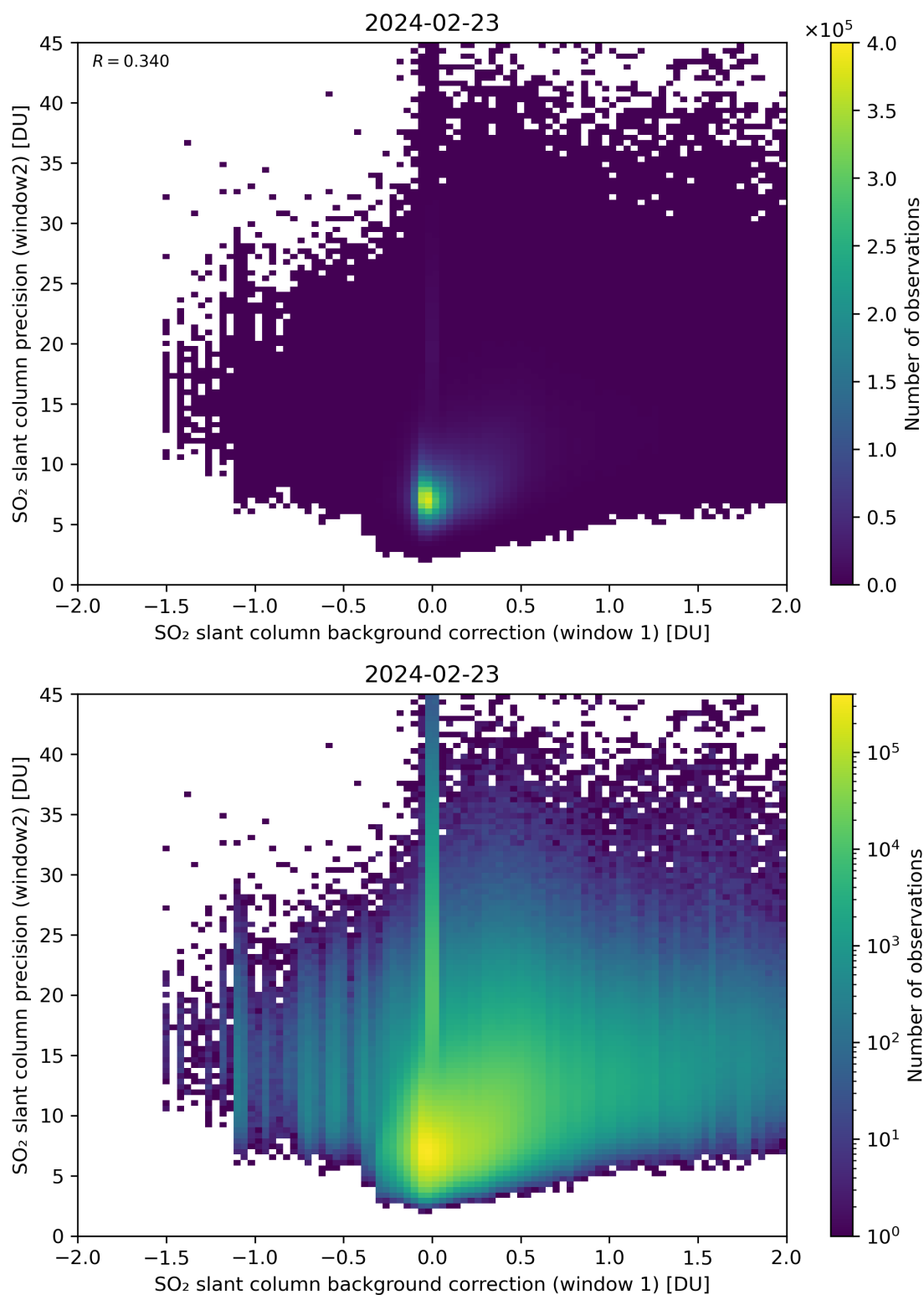
Figure 106: Scatter density plot of “SO 2 slant column background correction (window 1)” against “SO 2 slant column precision (window2)” for 2024-02-22 to 2024-02-24.
