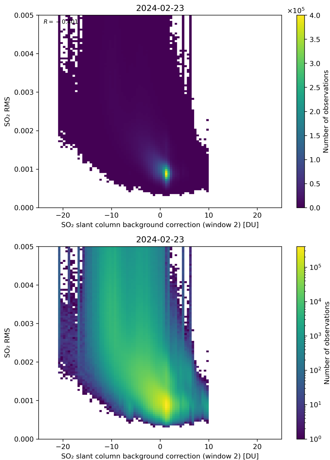
Figure 114: Scatter density plot of “SO 2 slant column background correction (window 2)” against “SO 2 RMS” for 2024-02-22 to 2024-02-24.
