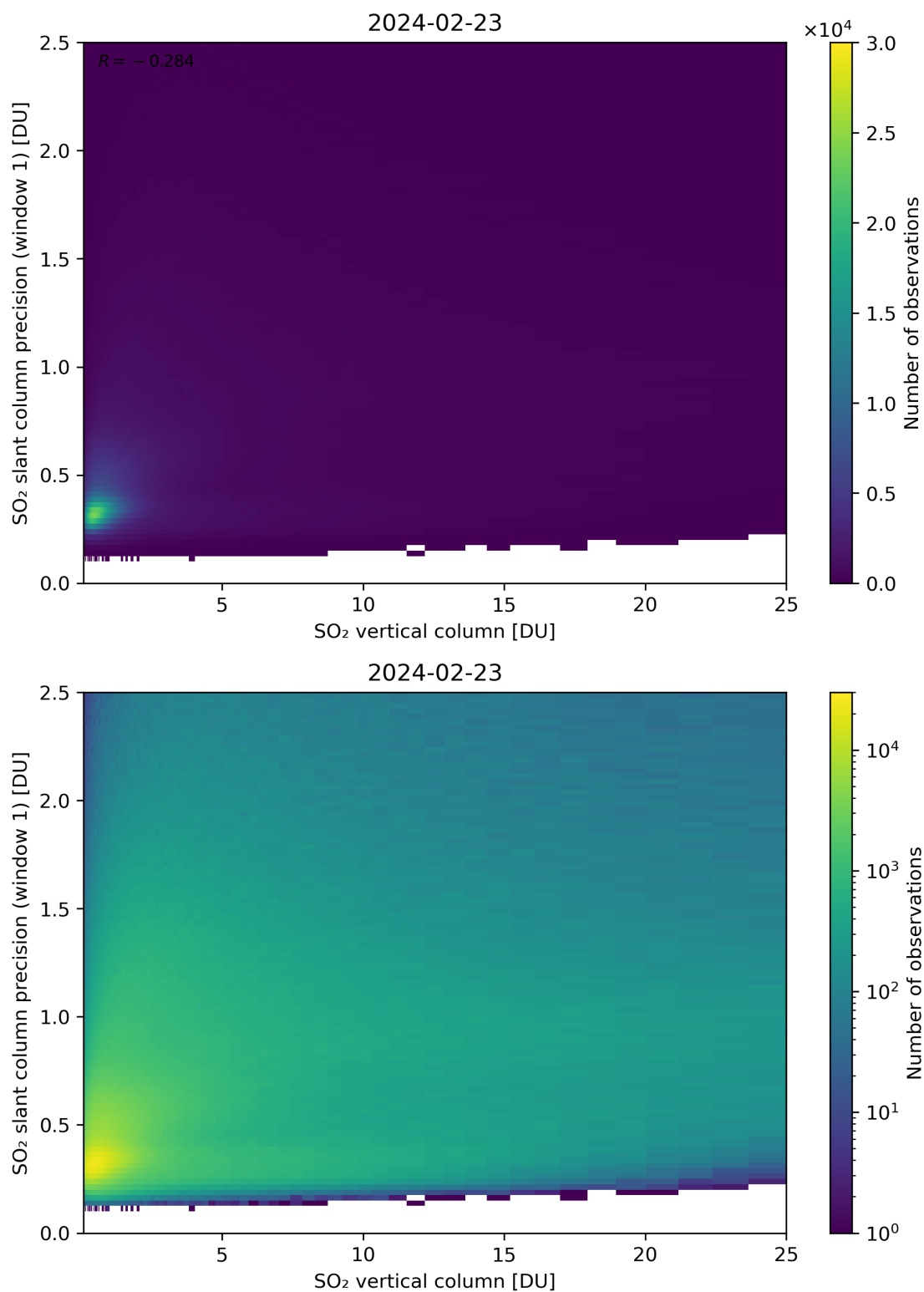
Figure 301: Scatter density plot of “SO 2 vertical column” against “SO 2 slant column precision (window 1)” for 2024-02-22 to 2024-02-24.
