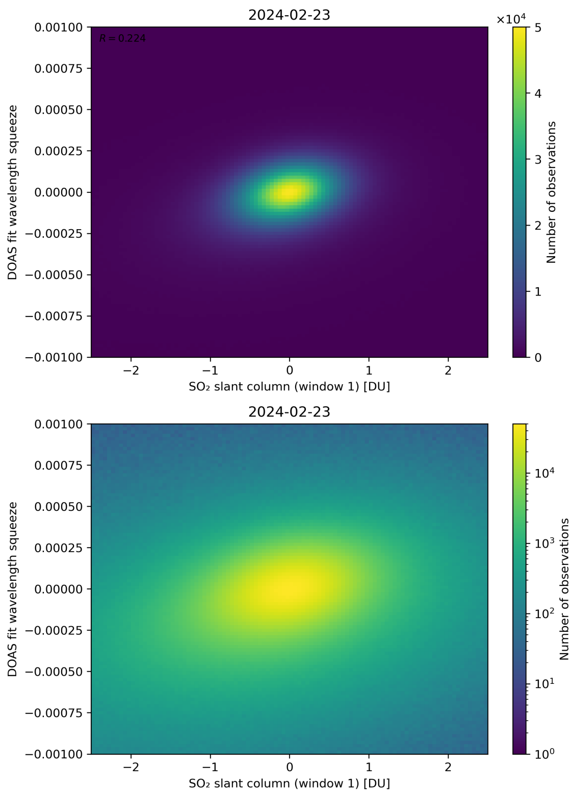
Figure 216: Scatter density plot of “SO 2 slant column (window 1)” against “DOAS fit wavelength squeeze” for 2024-02-22 to 2024-02-24.
