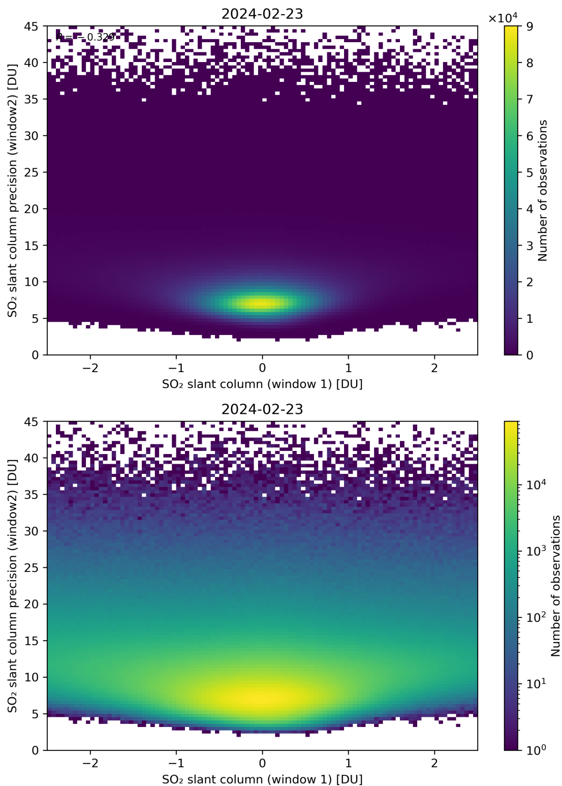
Figure 236: Scatter density plot of “SO 2 slant column (window 1)” against “SO 2 slant column precision (window2)” for 2024-02-22 to 2024-02-24.
