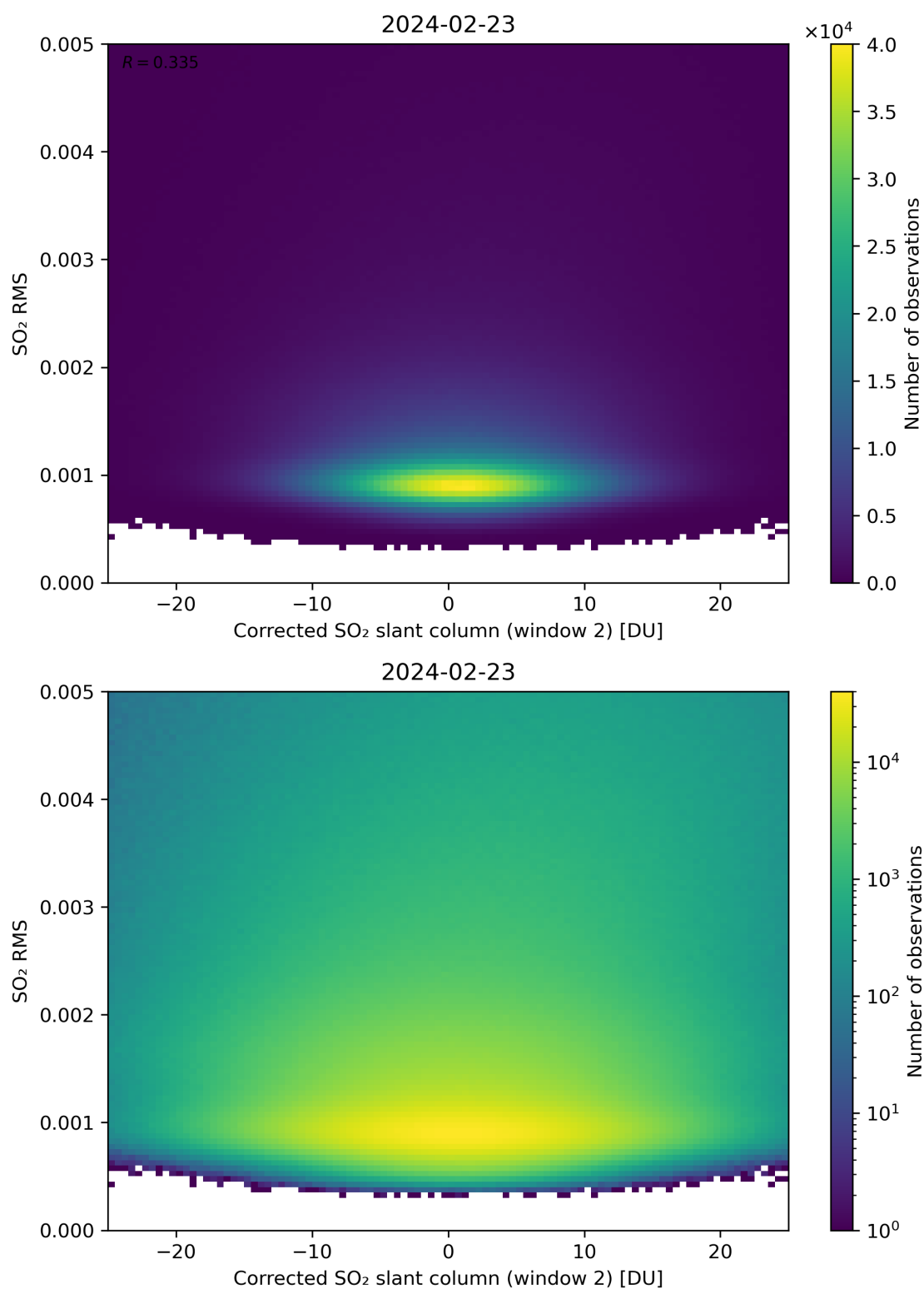
Figure 198: Scatter density plot of “Corrected SO 2 slant column (window 2)” against “SO 2 RMS” for 2024-02-22 to 2024-02-24.
