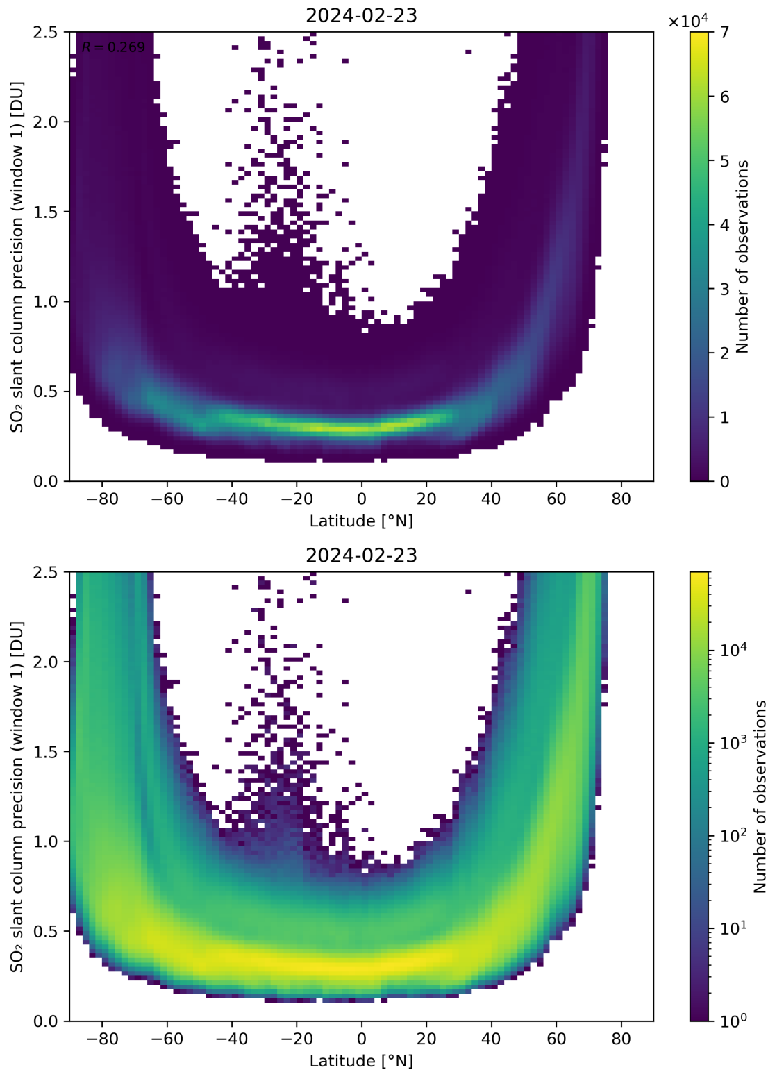
Figure 150: Scatter density plot of “Latitude” against “SO 2 slant column precision (window 1)” for 2024-02-22 to 2024-02-24.
