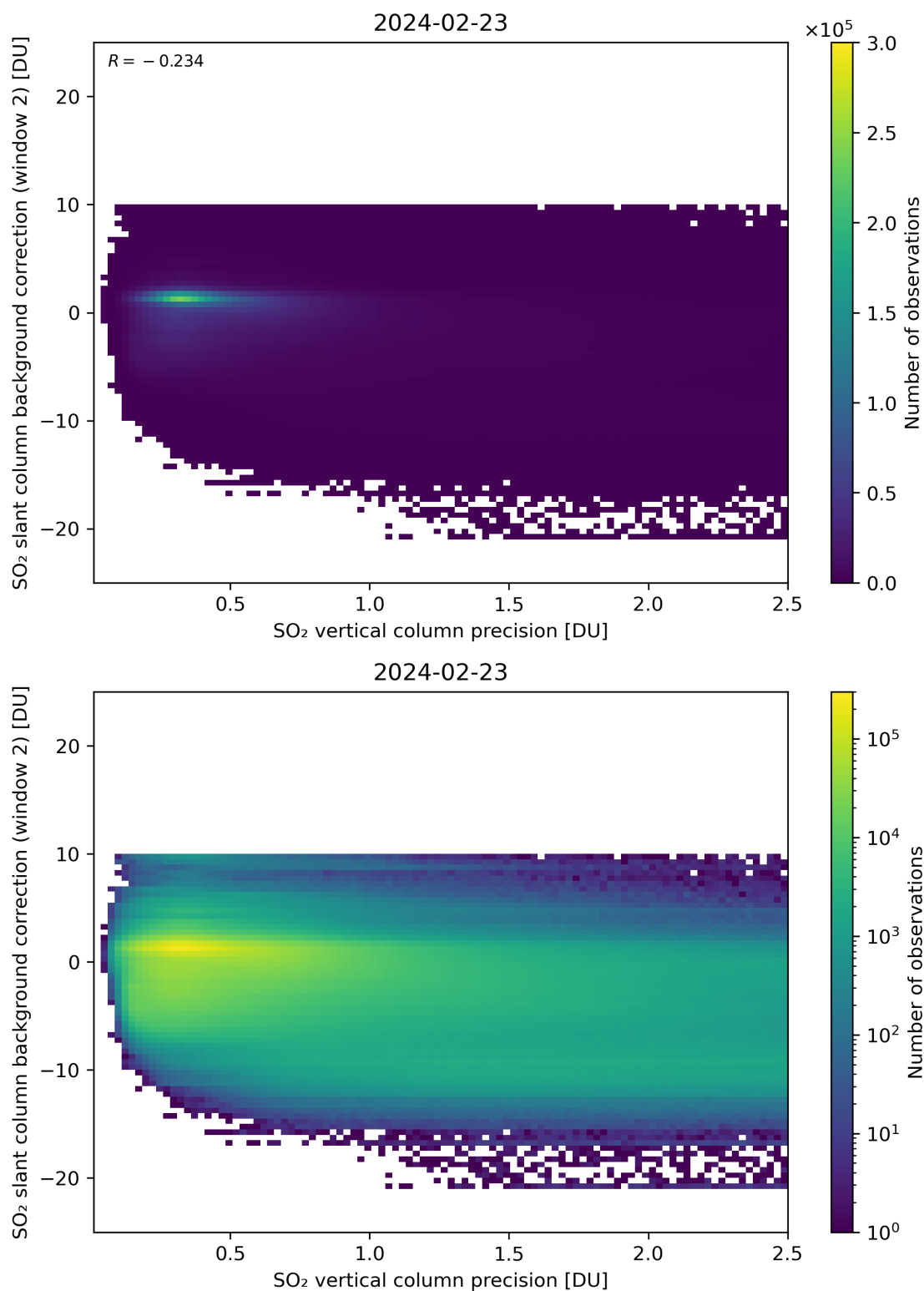
Figure 280: Scatter density plot of “SO 2 vertical column precision” against “SO 2 slant column background correction (window 2)” for 2024-02-22 to 2024-02-24.
