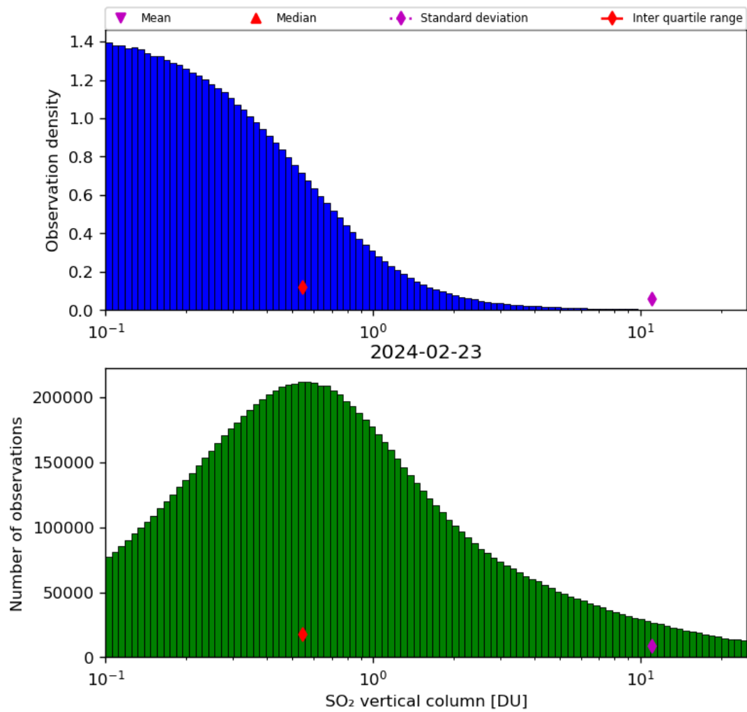
Figure 53: Histogram of “SO 2 vertical column” for 2024-02-22 to 2024-02-24
