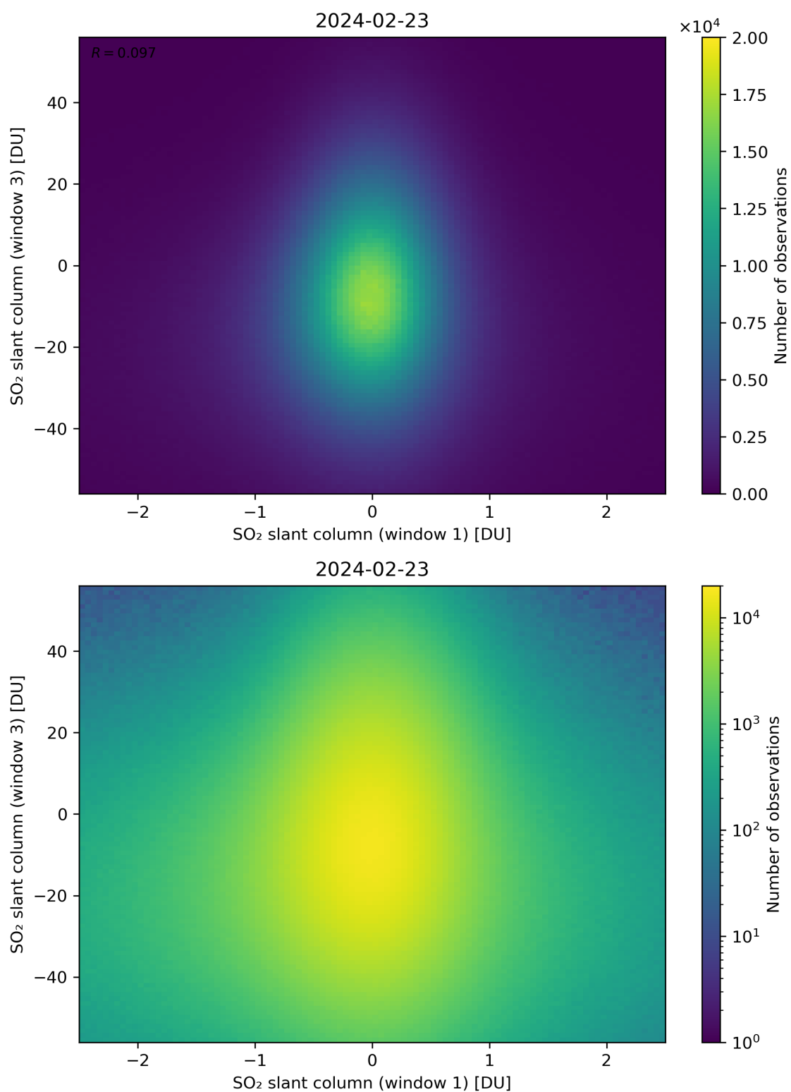
Figure 237: Scatter density plot of “SO 2 slant column (window 1)” against “SO 2 slant column (window 3)” for 2024-02-22 to 2024-02-24.
