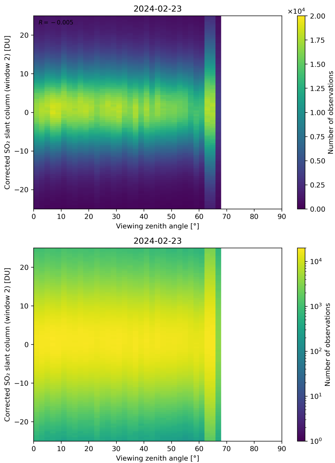
Figure 318: Scatter density plot of “Viewing zenith angle” against “Corrected SO 2 slant column (window 2)” for 2024-02-22 to 2024-02-24.
