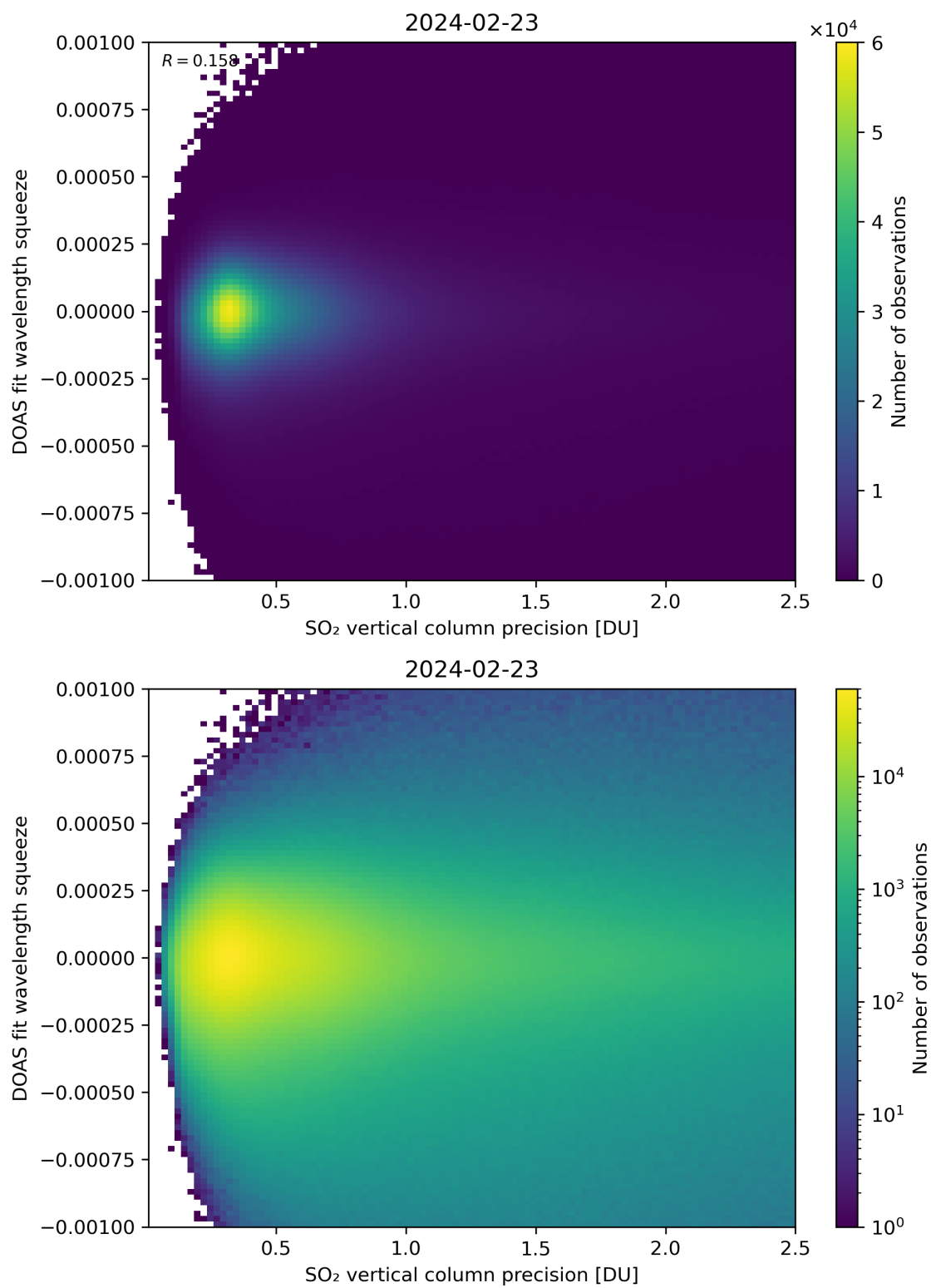
Figure 283: Scatter density plot of “SO 2 vertical column precision” against “DOAS fit wavelength squeeze” for 2024-02-22 to 2024-02-24.
