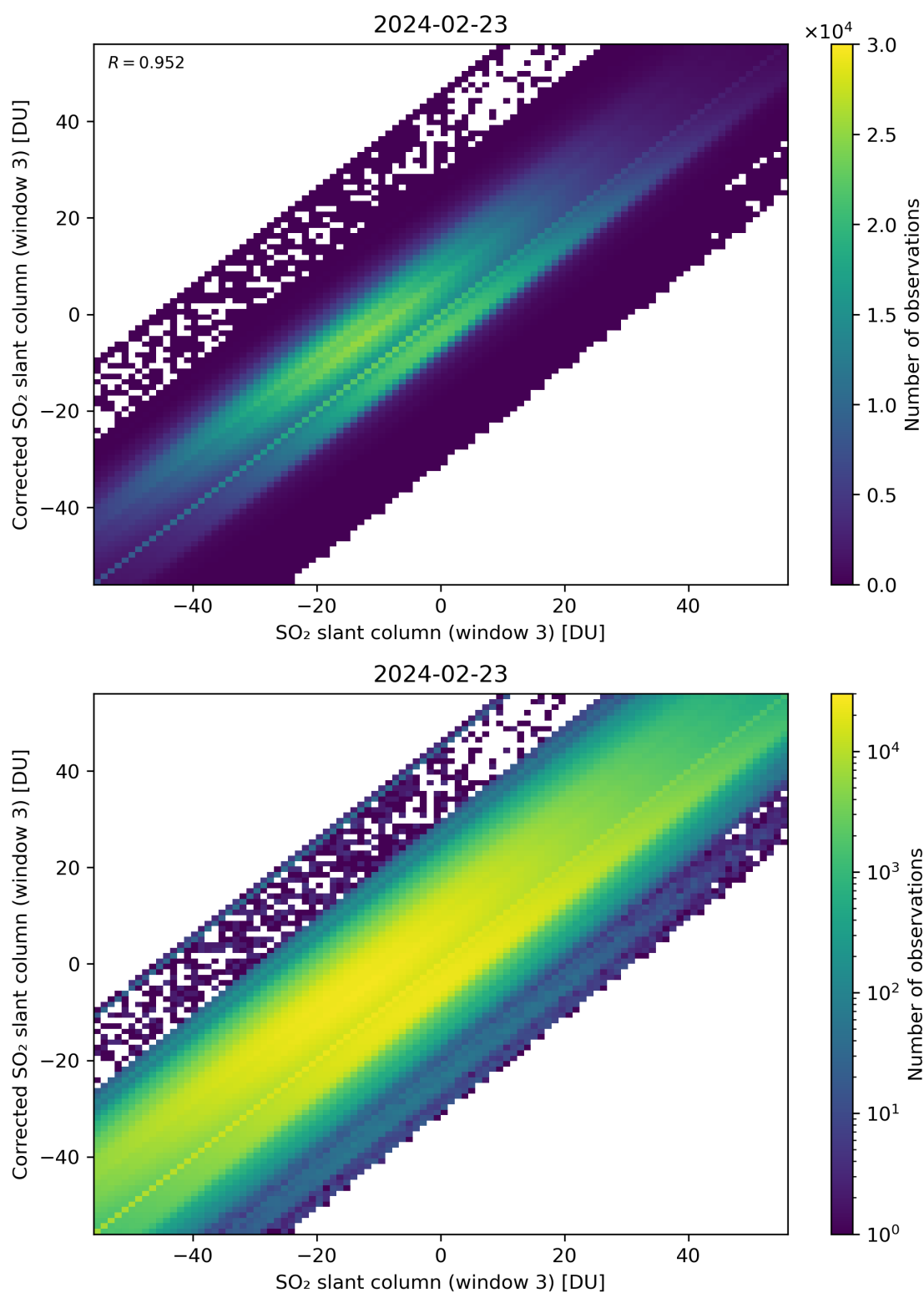
Figure 266: Scatter density plot of “SO 2 slant column (window 3)” against “Corrected SO 2 slant column (window 3)” for 2024-02-22 to 2024-02-24.
