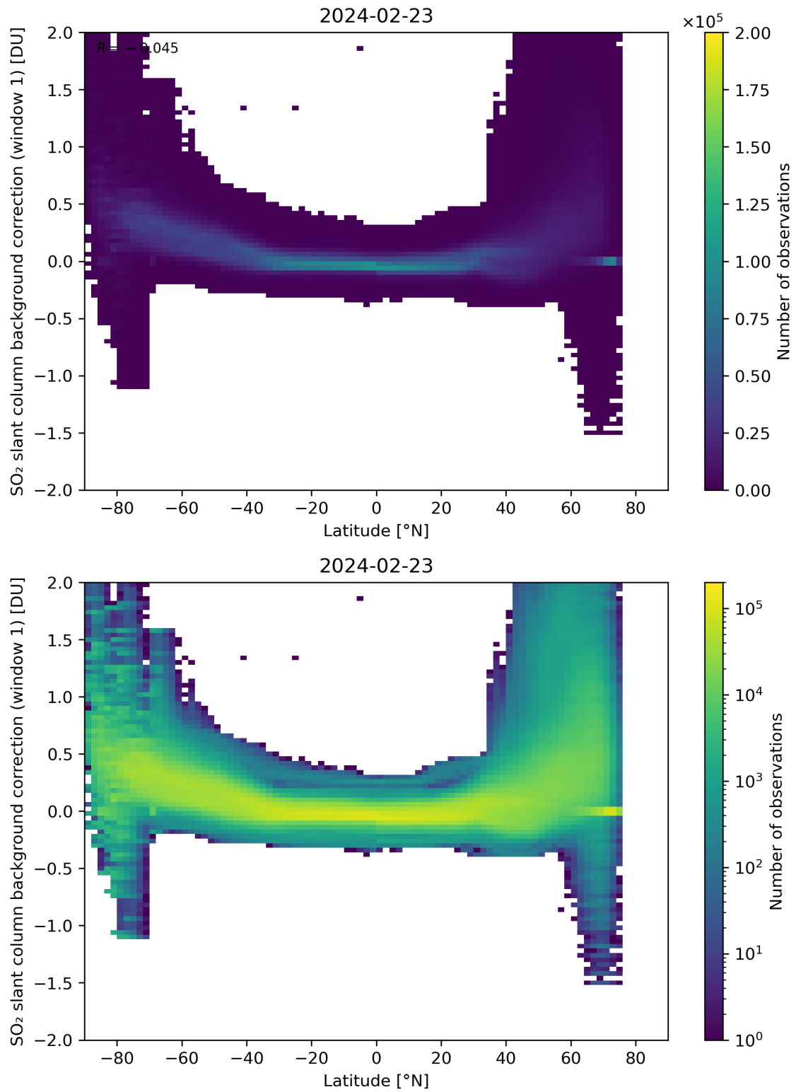
Figure 139: Scatter density plot of “Latitude” against “SO 2 slant column background correction (window 1)” for 2024-02-22 to 2024-02-24.
