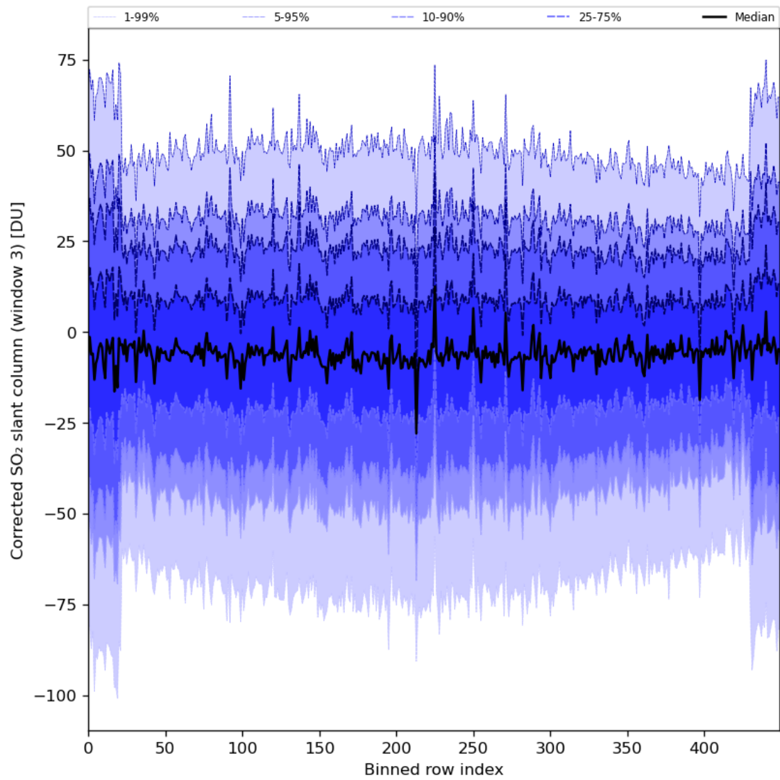
Figure 89: Along track statistics of “Corrected SO 2 slant column (window 3)” for 2024-02-22 to 2024-02-24
