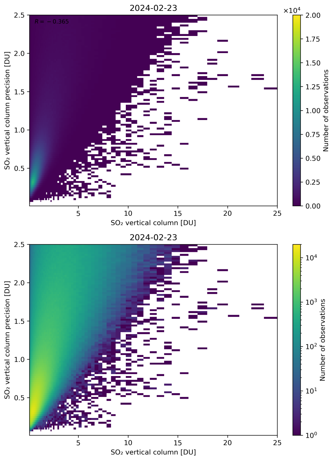
Figure 307: Scatter density plot of “SO 2 vertical column” against “SO 2 vertical column precision” for 2024-02-22 to 2024-02-24.
