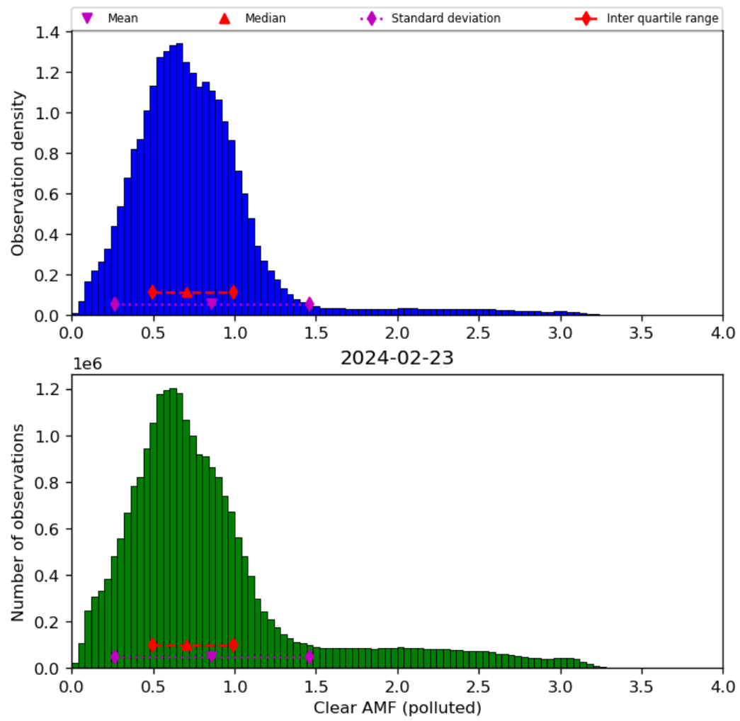
Figure 73: Histogram of “Clear AMF (polluted)” for 2024-02-22 to 2024-02-24
