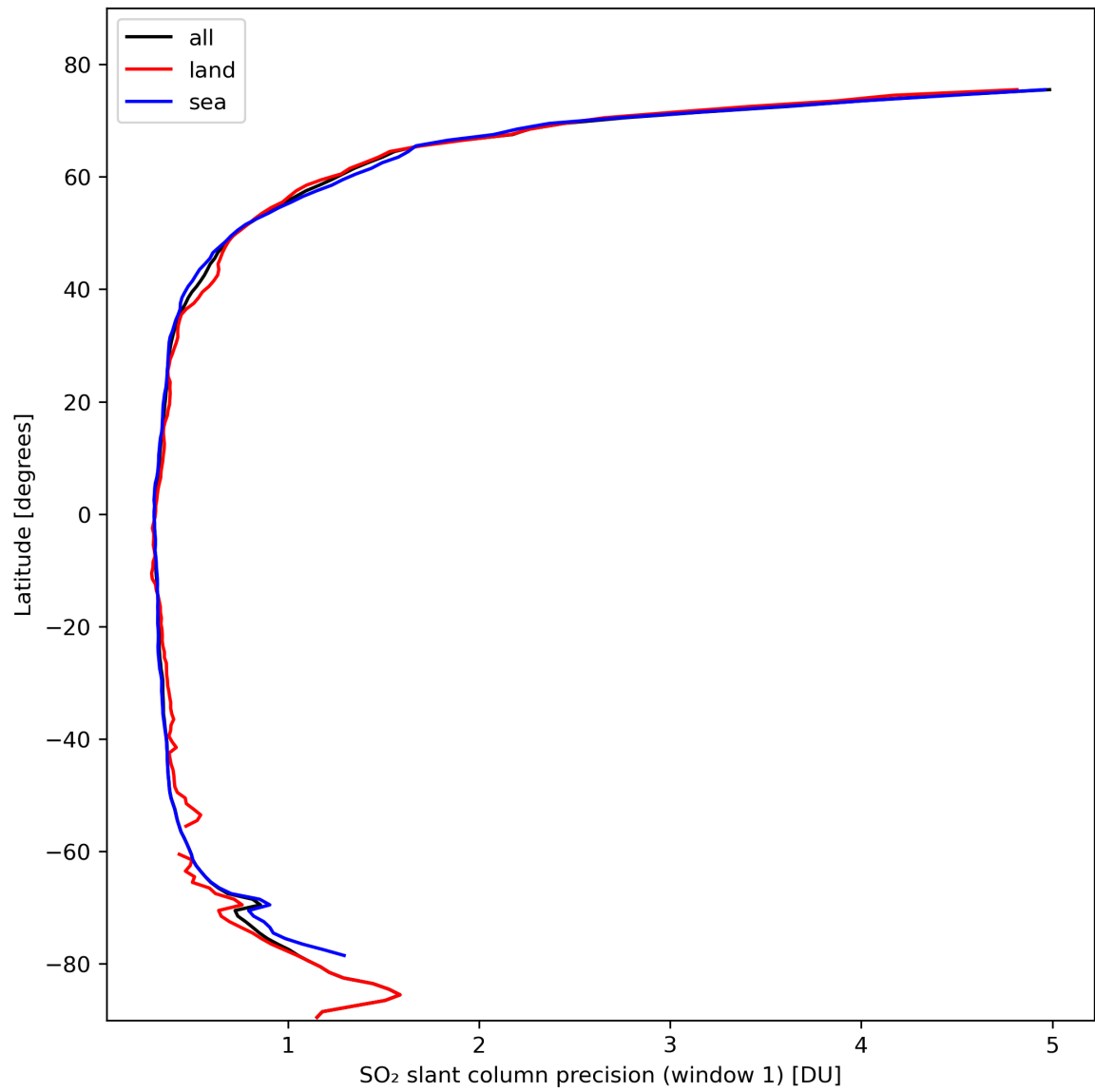
Figure 34: Zonal average of “SO 2 slant column precision (window 1)” for 2024-02-22 to 2024-02-24.
