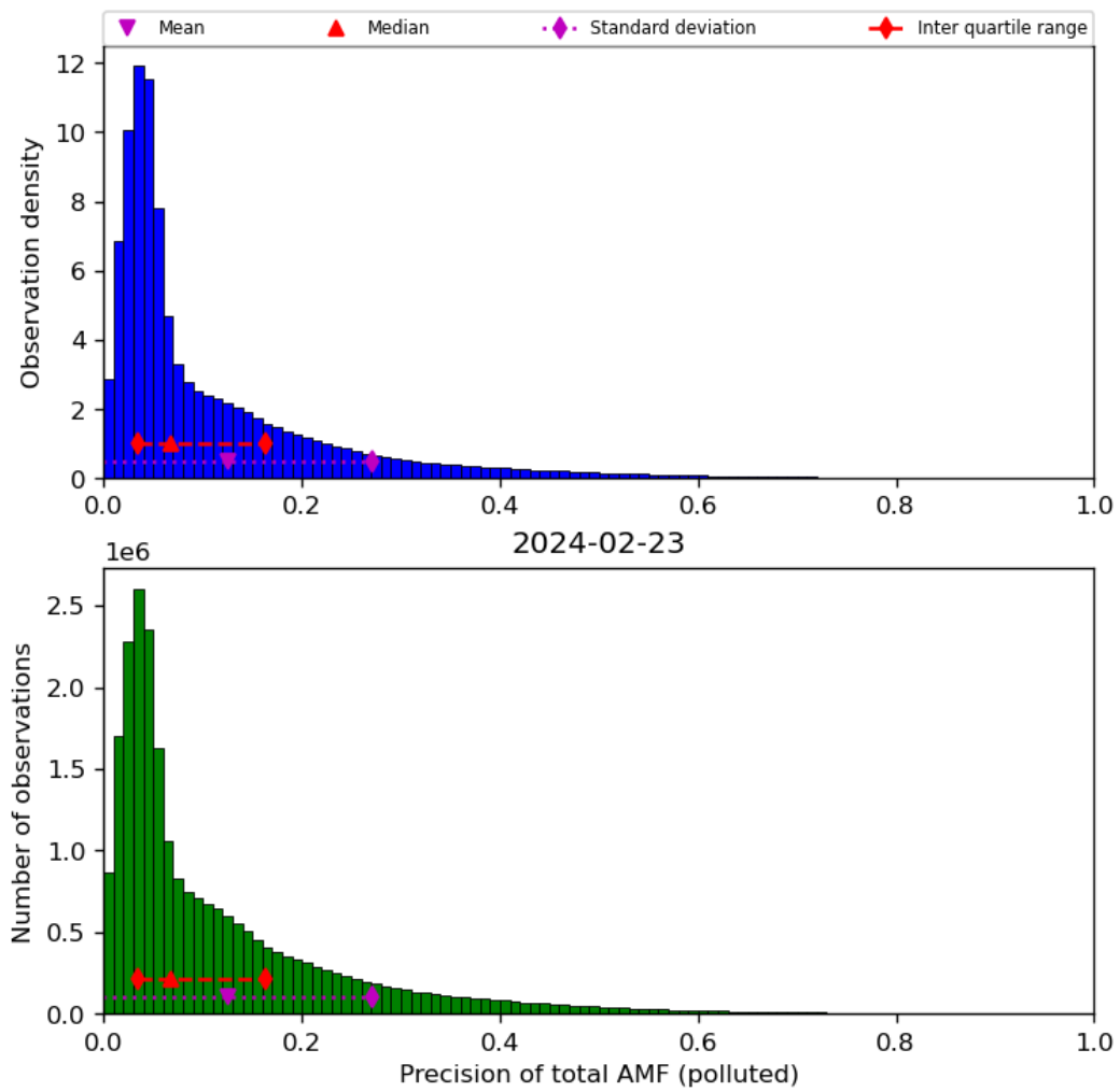
Figure 72: Histogram of “Precision of total AMF (polluted)” for 2024-02-22 to 2024-02-24
