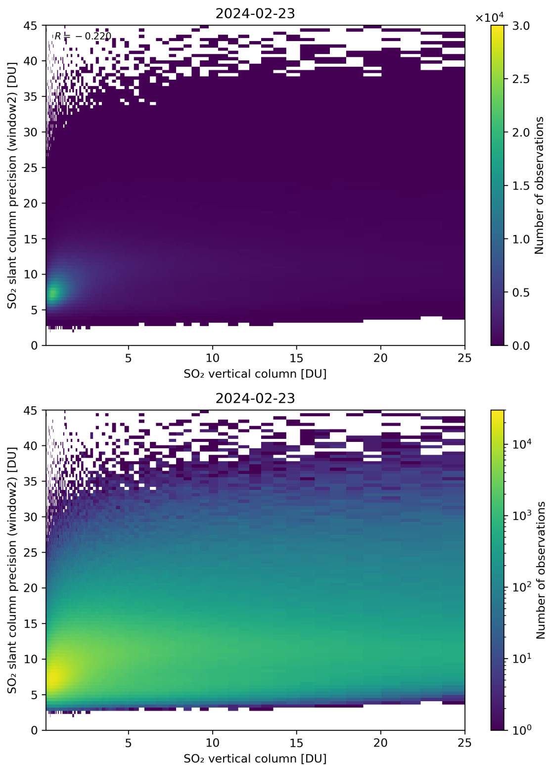
Figure 302: Scatter density plot of “SO 2 vertical column” against “SO 2 slant column precision (window2)” for 2024-02-22 to 2024-02-24.
