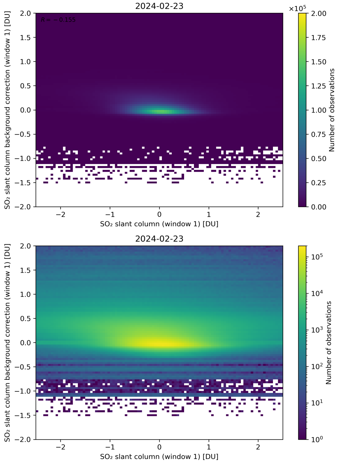
Figure 212: Scatter density plot of “SO 2 slant column (window 1)” against “SO 2 slant column background correction (window 1)” for 2024-02-22 to 2024-02-24.
