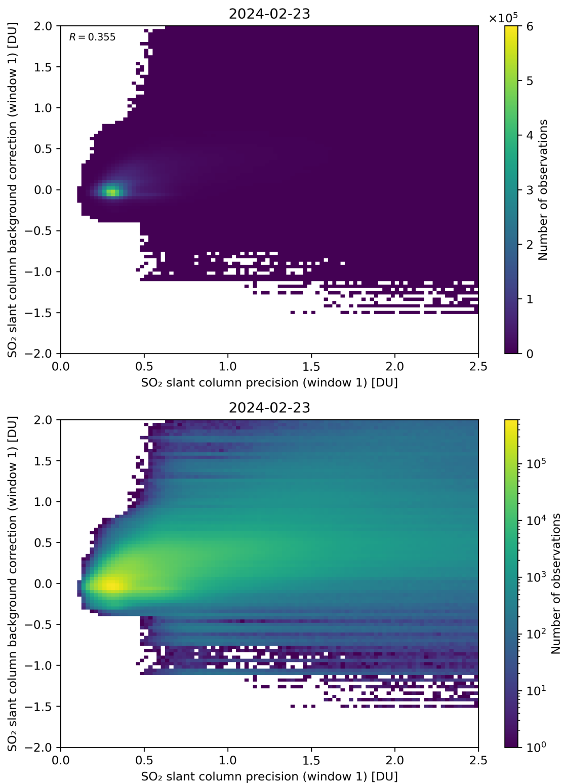
Figure 218: Scatter density plot of “SO 2 slant column precision (window 1)” against “SO 2 slant column background correction (window 1)” for 2024-02-22 to 2024-02-24.
