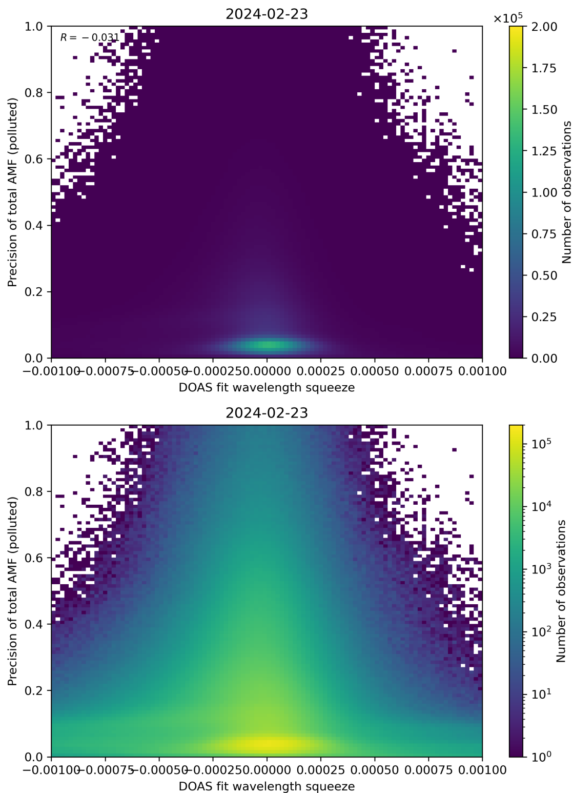
Figure 135: Scatter density plot of “DOAS fit wavelength squeeze” against “Precision of total AMF (polluted)” for 2024-02-22 to 2024-02-24.
