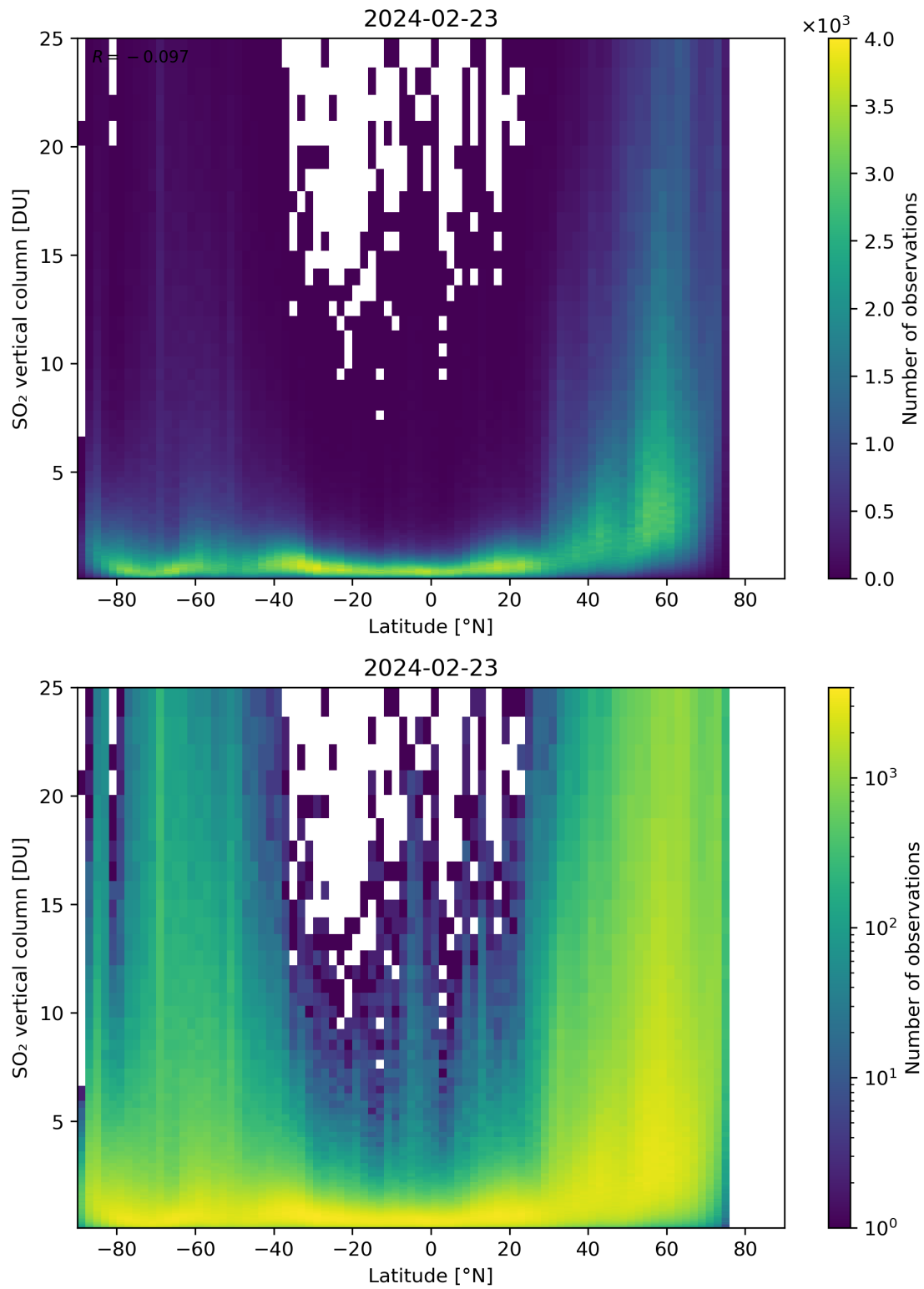
Figure 156: Scatter density plot of “Latitude” against “SO 2 vertical column” for 2024-02-22 to 2024-02-24.
