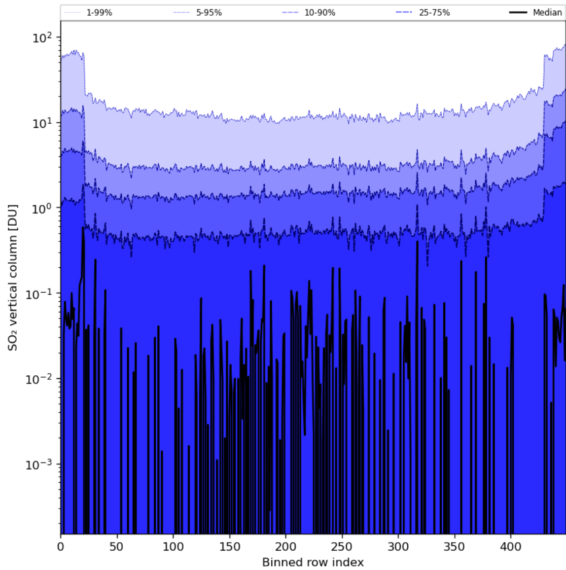
Figure 76: Along track statistics of “SO 2 vertical column” for 2024-02-22 to 2024-02-24
