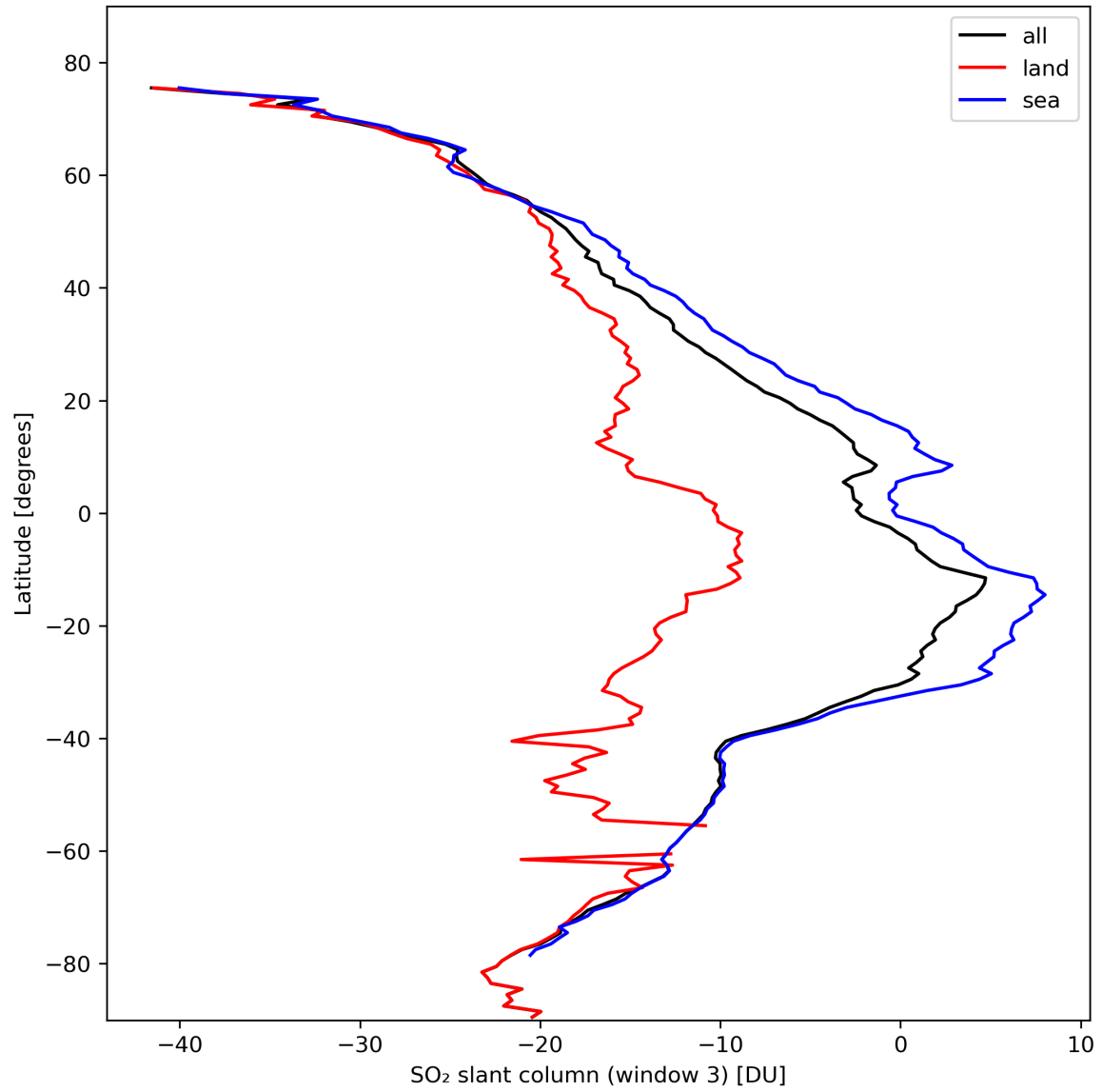
Figure 41: Zonal average of “SO 2 slant column (window 3)” for 2024-02-22 to 2024-02-24.
