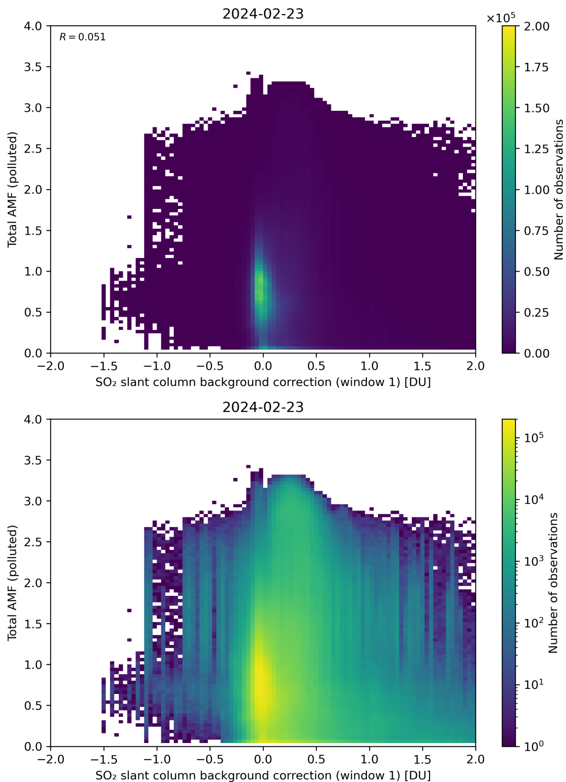
Figure 109: Scatter density plot of “SO 2 slant column background correction (window 1)” against “Total AMF (polluted)” for 2024-02-22 to 2024-02-24.
