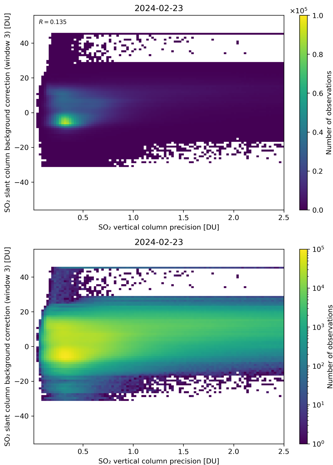
Figure 281: Scatter density plot of “SO 2 vertical column precision” against “SO 2 slant column background correction (window 3)” for 2024-02-22 to 2024-02-24.
