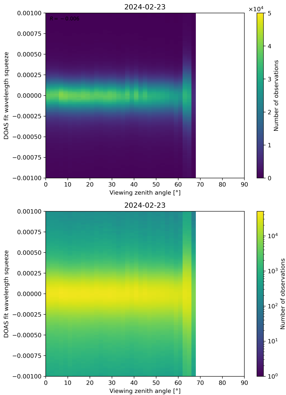
Figure 312: Scatter density plot of “Viewing zenith angle” against “DOAS fit wavelength squeeze” for 2024-02-22 to 2024-02-24.
