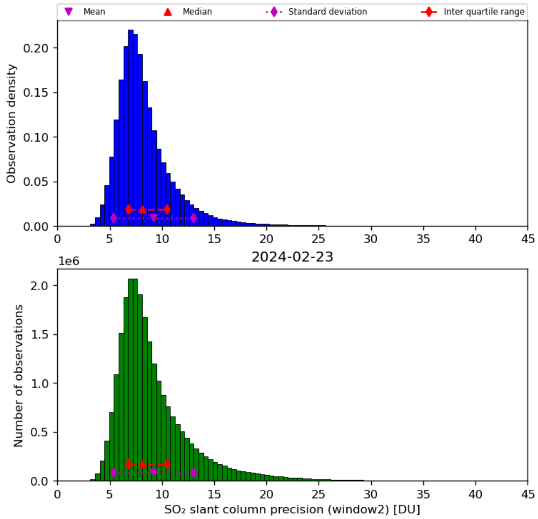
Figure 61: Histogram of “SO 2 slant column precision (window2)” for 2024-02-22 to 2024-02-24
