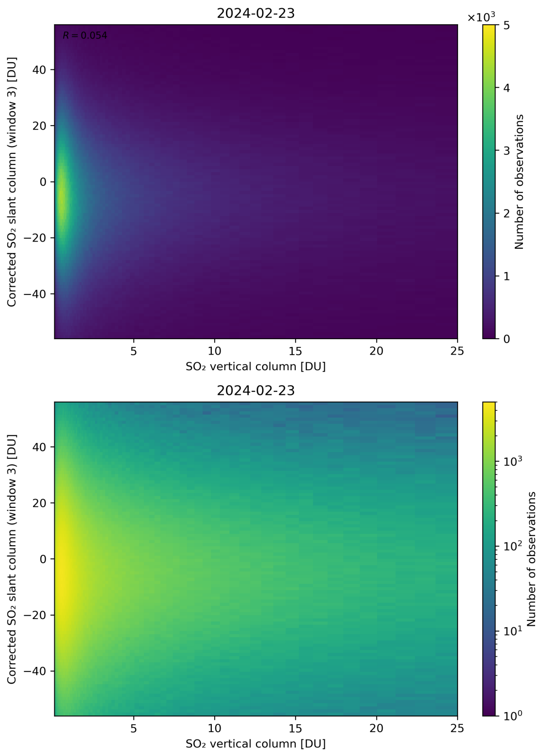
Figure 299: Scatter density plot of “SO 2 vertical column” against “Corrected SO 2 slant column (window 3)” for 2024-02-22 to 2024-02-24.
