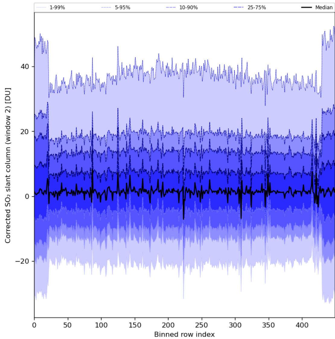
Figure 85: Along track statistics of “Corrected SO 2 slant column (window 2)” for 2024-02-22 to 2024-02-24
