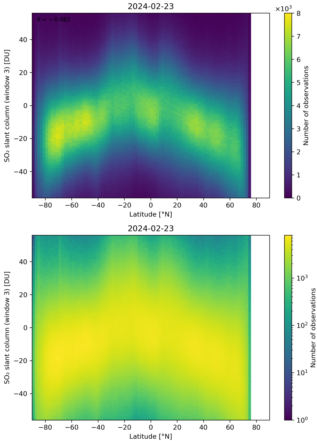
Figure 152: Scatter density plot of “Latitude” against “SO 2 slant column (window 3)” for 2024-02-22 to 2024-02-24.
