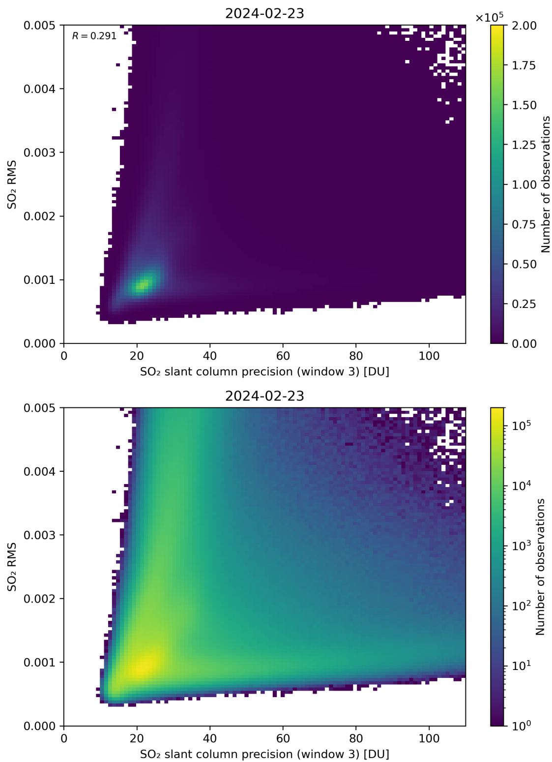
Figure 260: Scatter density plot of “SO 2 slant column precision (window 3)” against “SO 2 RMS” for 2024-02-22 to 2024-02-24.
