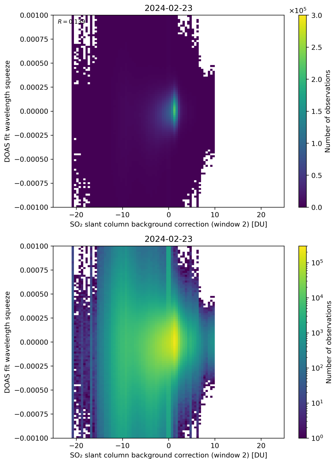
Figure 113: Scatter density plot of “SO 2 slant column background correction (window 2)” against “DOAS fit wavelength squeeze” for 2024-02-22 to 2024-02-24.
