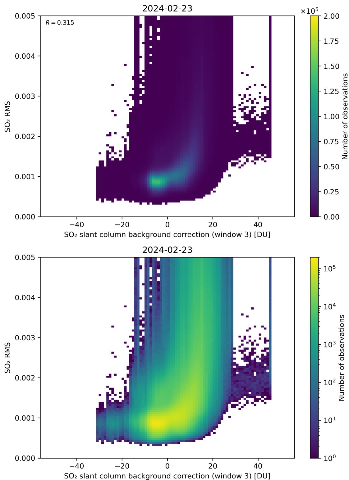
Figure 123: Scatter density plot of “SO 2 slant column background correction (window 3)” against “SO 2 RMS” for 2024-02-22 to 2024-02-24.
