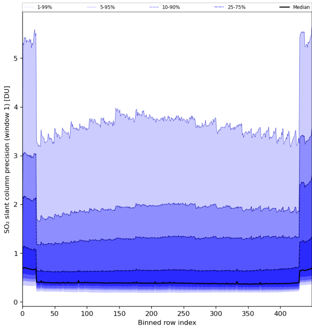
Figure 80: Along track statistics of “SO 2 slant column precision (window 1)” for 2024-02-22 to 2024-02-24
