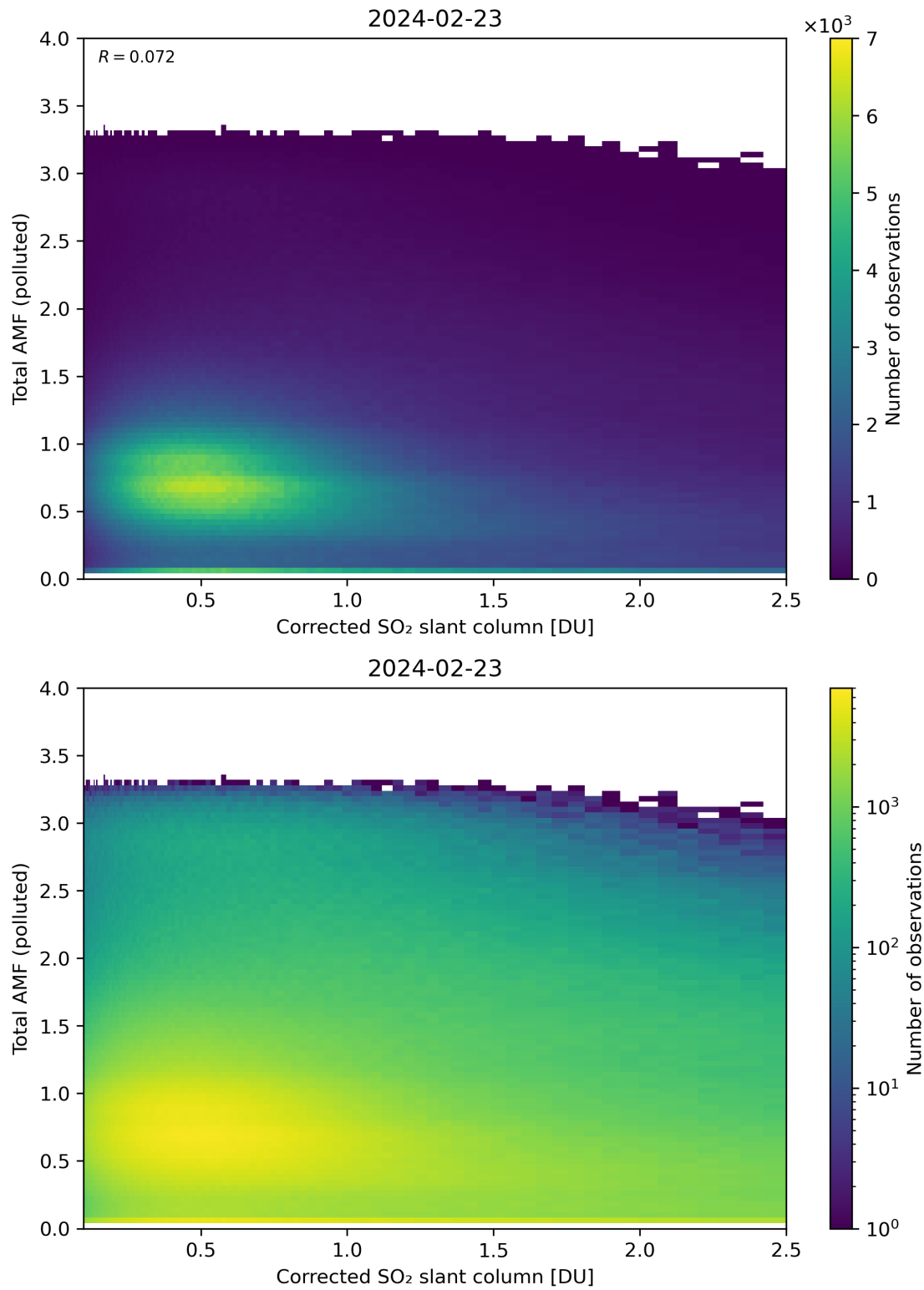
Figure 192: Scatter density plot of “Corrected SO 2 slant column” against “Total AMF (polluted)” for 2024-02-22 to 2024-02-24.
