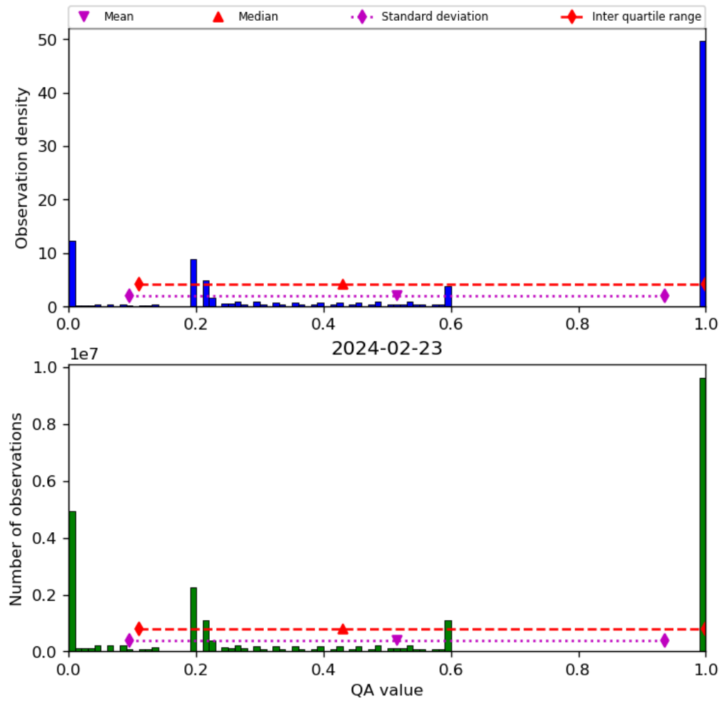
Figure 52: Histogram of “QA value” for 2024-02-22 to 2024-02-24
