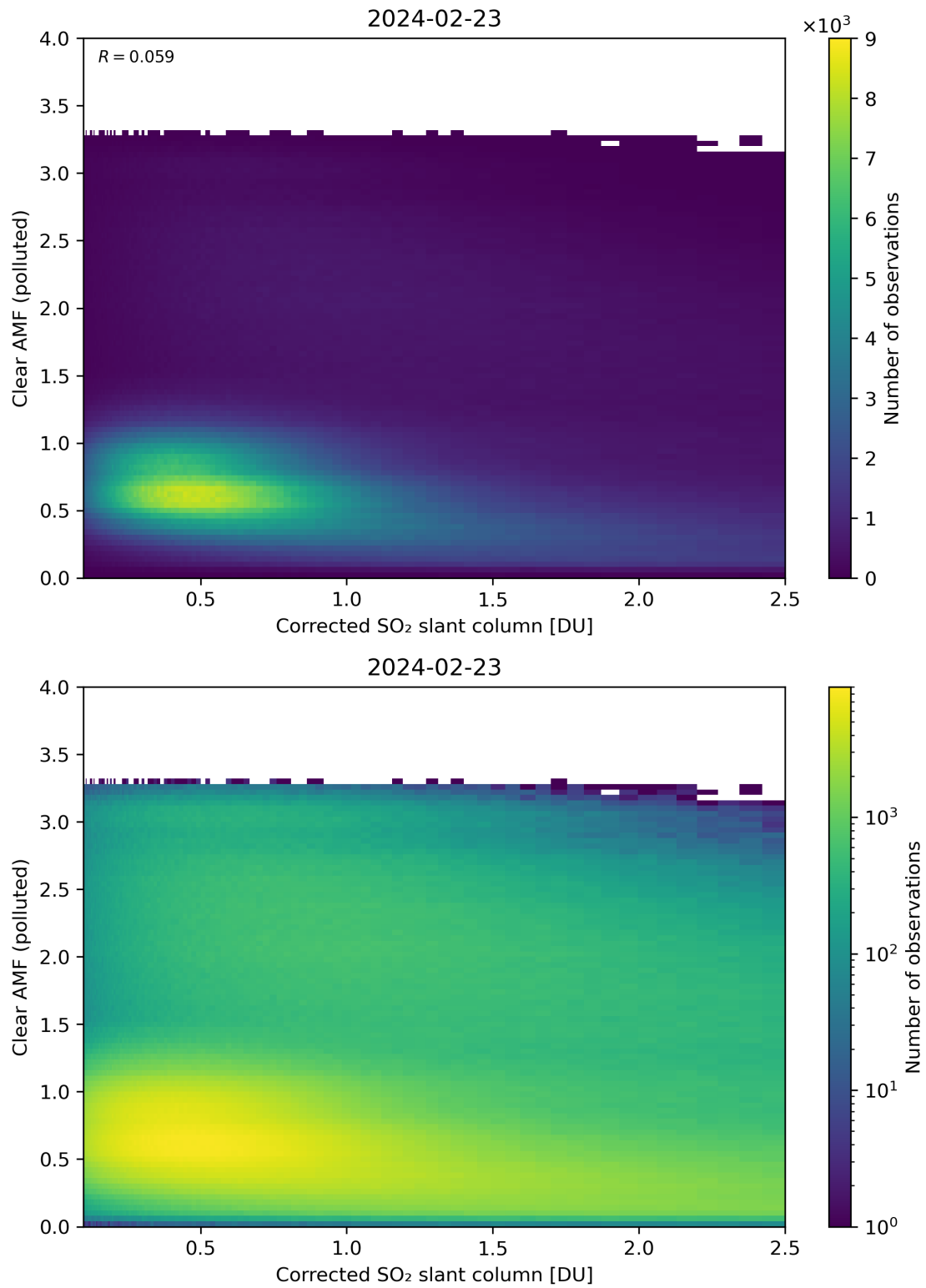
Figure 184: Scatter density plot of “Corrected SO 2 slant column” against “Clear AMF (polluted)” for 2024-02-22 to 2024-02-24.
