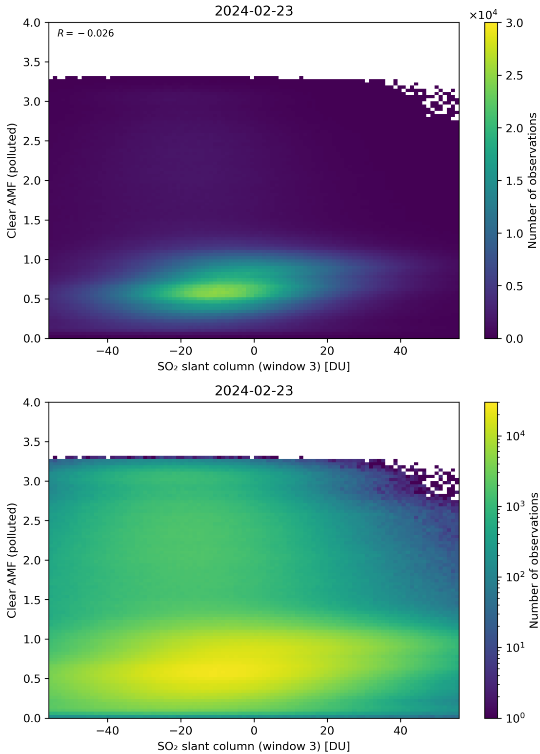
Figure 265: Scatter density plot of “SO 2 slant column (window 3)” against “Clear AMF (polluted)” for 2024-02-22 to 2024-02-24.
