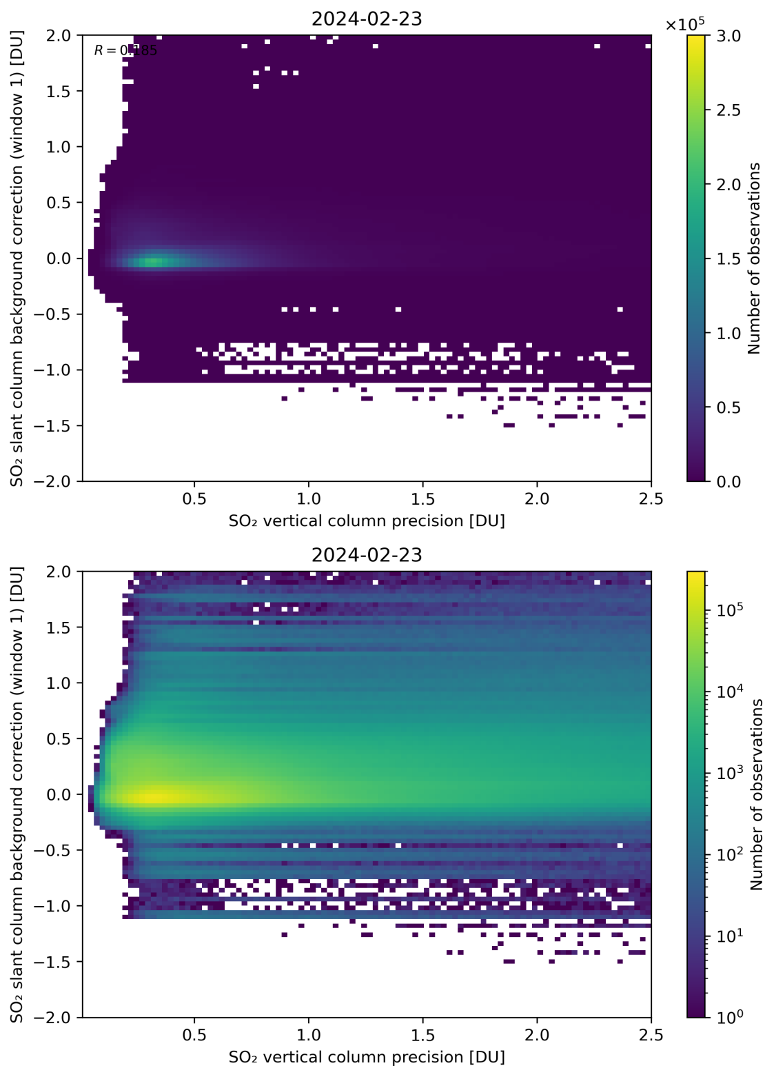
Figure 279: Scatter density plot of “SO 2 vertical column precision” against “SO 2 slant column background correction (window 1)” for 2024-02-22 to 2024-02-24.
