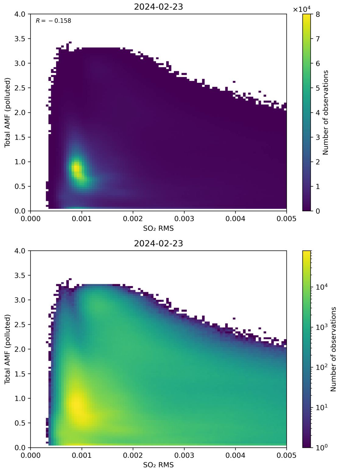
Figure 137: Scatter density plot of “SO 2 RMS” against “Total AMF (polluted)” for 2024-02-22 to 2024-02-24.
