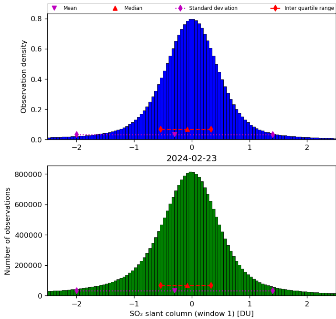
Figure 56: Histogram of “SO 2 slant column (window 1)” for 2024-02-22 to 2024-02-24
