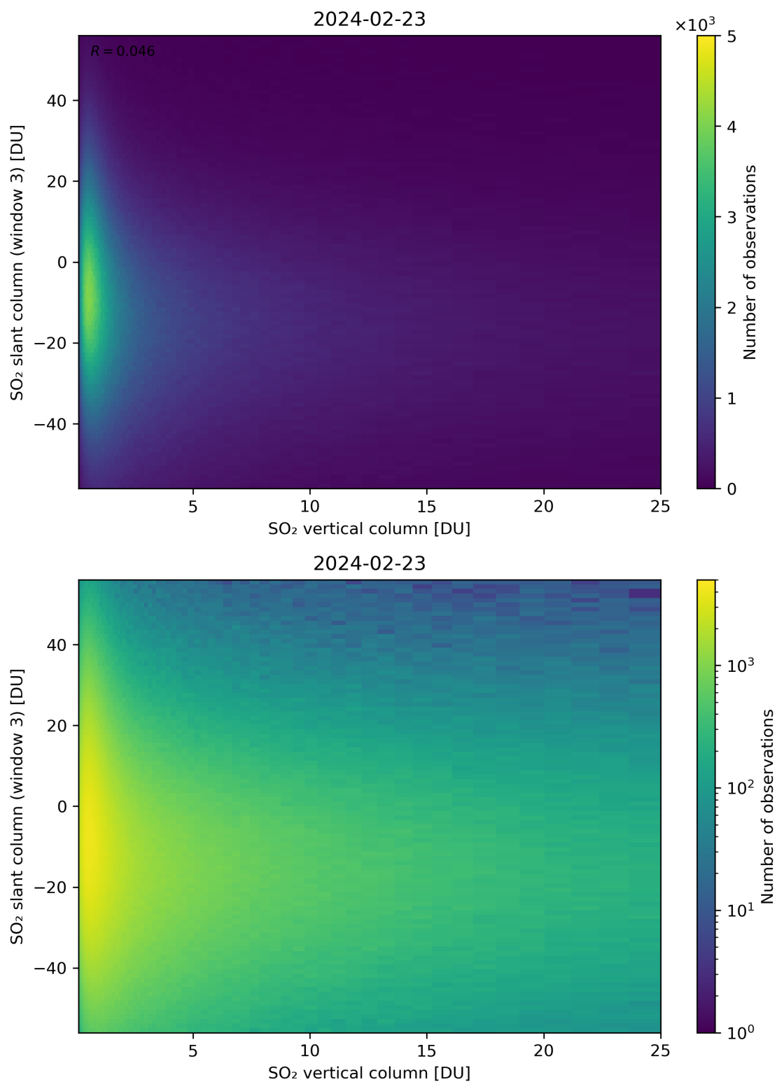
Figure 303: Scatter density plot of “SO 2 vertical column” against “SO 2 slant column (window 3)” for 2024-02-22 to 2024-02-24.
