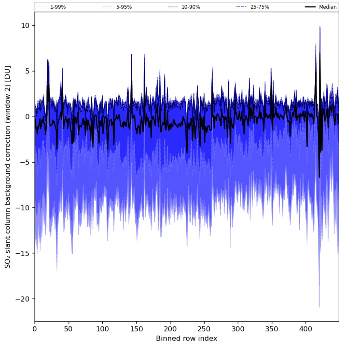
Figure 86: Along track statistics of “SO 2 slant column background correction (window 2)” for 2024-02-22 to 2024-02-24
