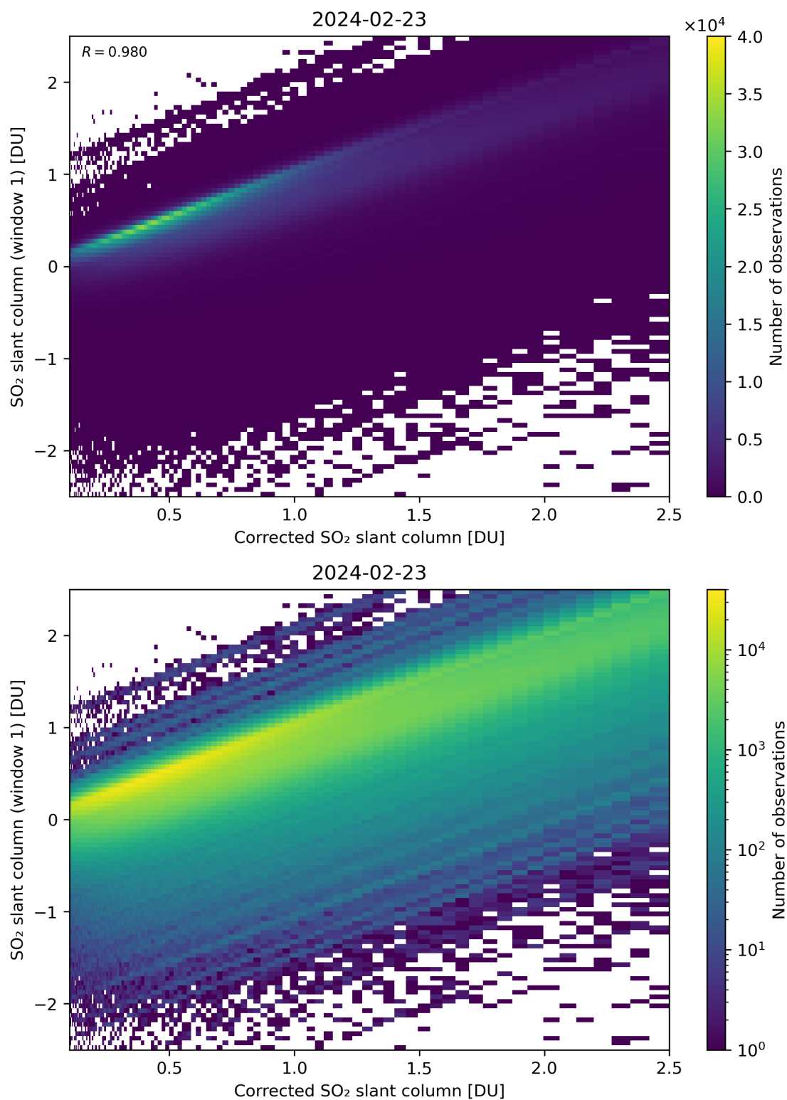
Figure 187: Scatter density plot of “Corrected SO 2 slant column” against “SO 2 slant column (window 1)” for 2024-02-22 to 2024-02-24.
