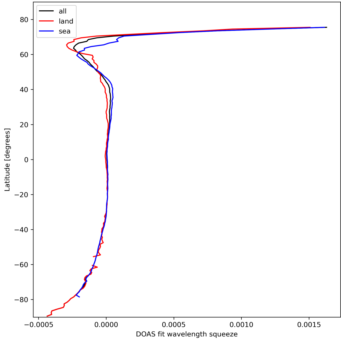
Figure 46: Zonal average of “DOAS fit wavelength squeeze” for 2024-02-22 to 2024-02-24.
