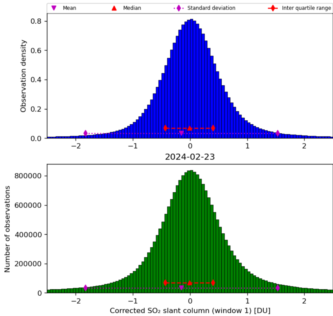
Figure 58: Histogram of “Corrected SO 2 slant column (window 1)” for 2024-02-22 to 2024-02-24
