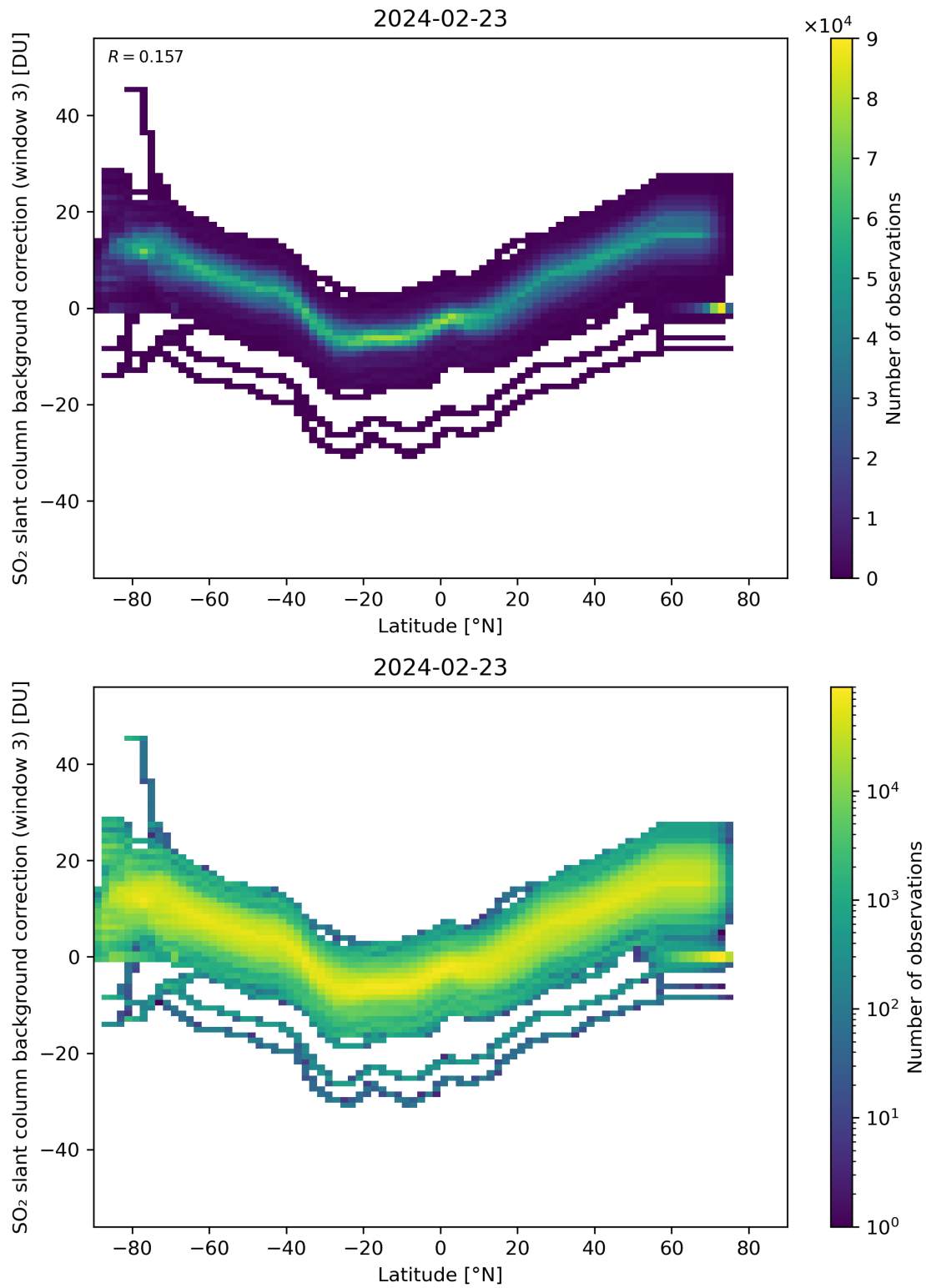
Figure 141: Scatter density plot of “Latitude” against “SO 2 slant column background correction (window 3)” for 2024-02-22 to 2024-02-24.
