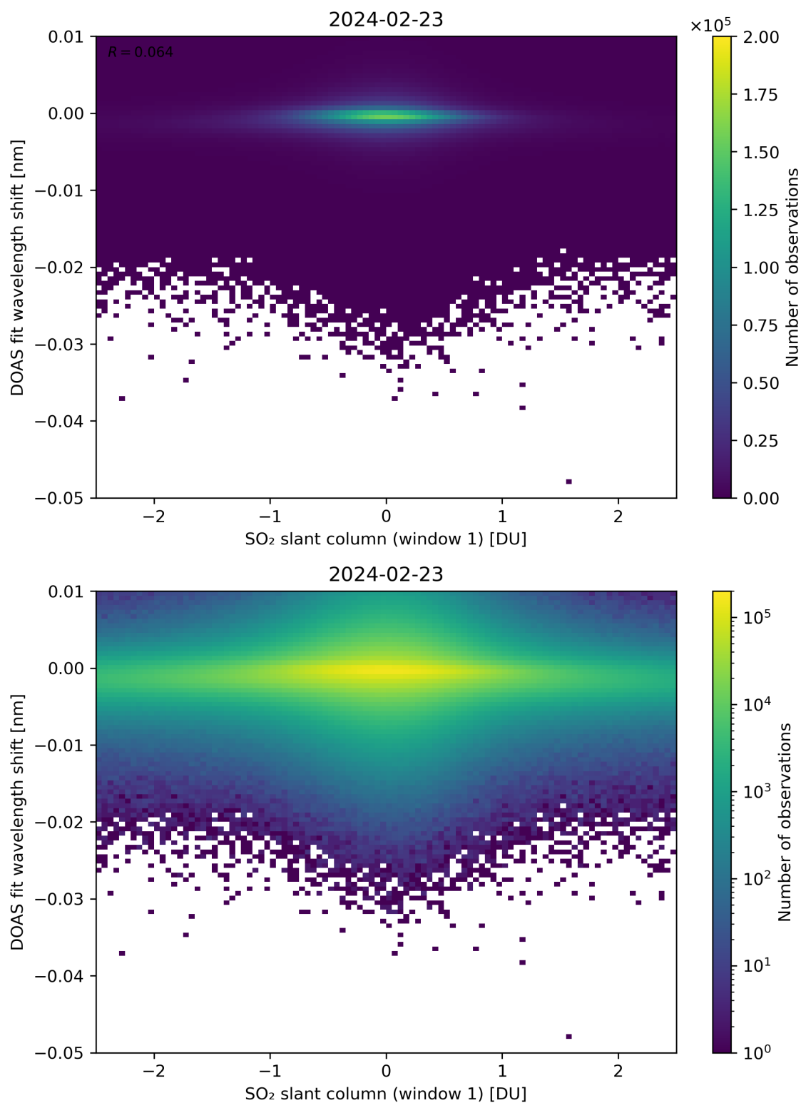
Figure 215: Scatter density plot of “SO 2 slant column (window 1)” against “DOAS fit wavelength shift” for 2024-02-22 to 2024-02-24.
