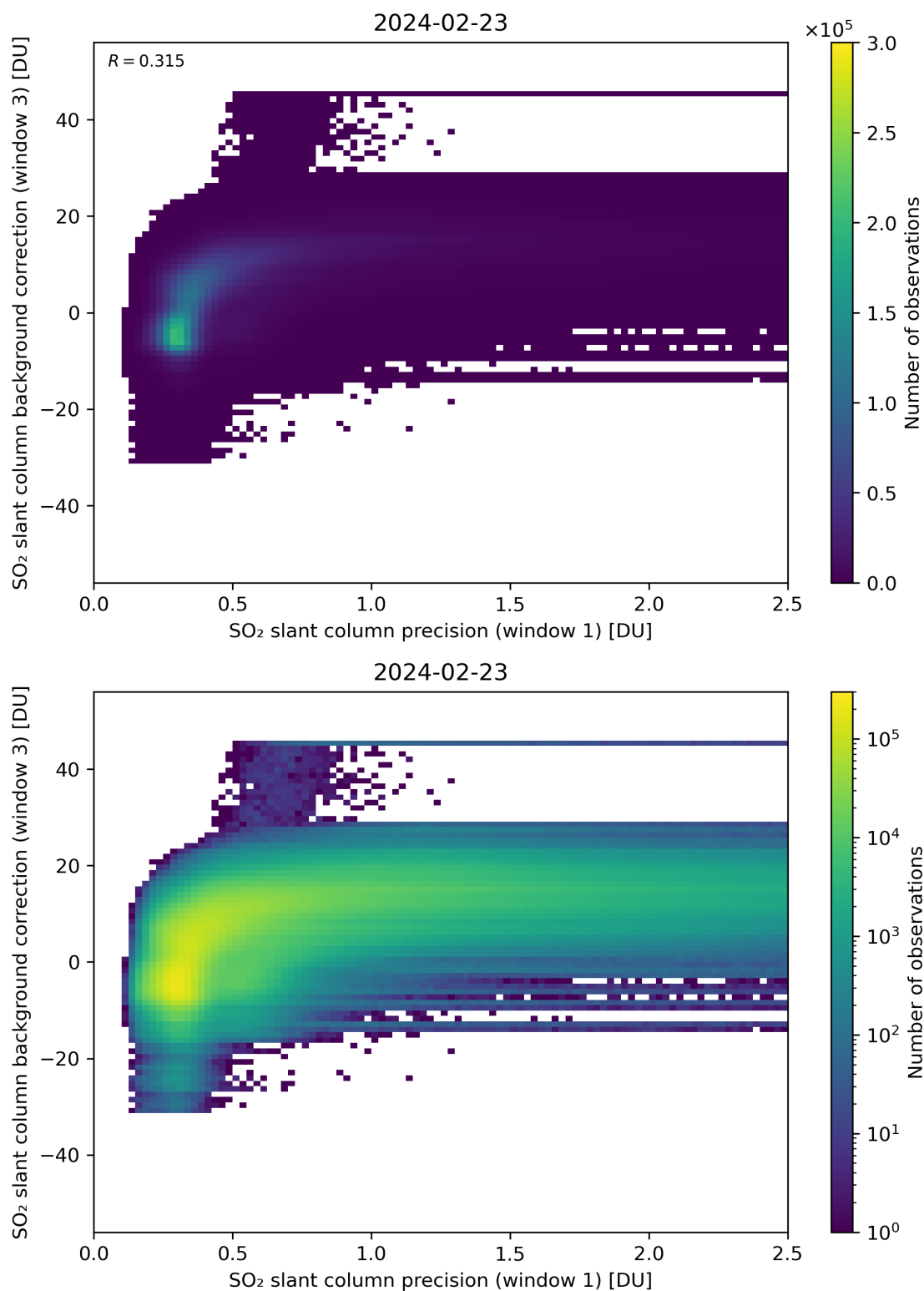
Figure 220: Scatter density plot of “SO 2 slant column precision (window 1)” against “SO 2 slant column background correction (window 3)” for 2024-02-22 to 2024-02-24.
