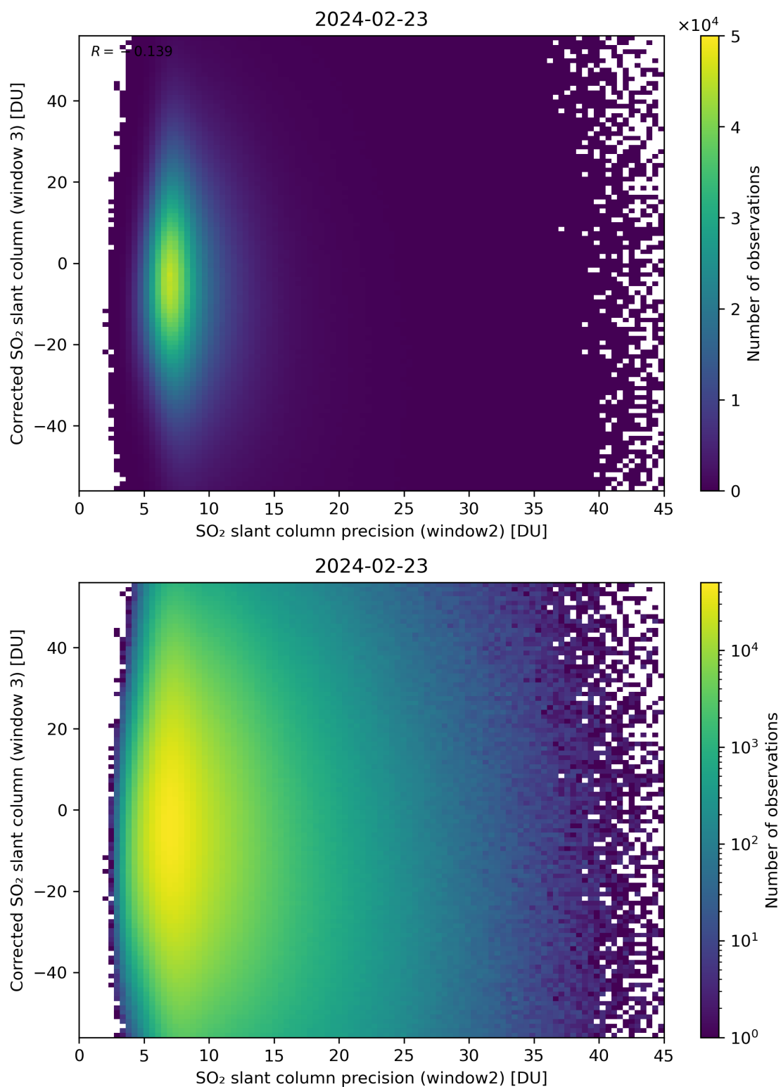
Figure 248: Scatter density plot of “SO 2 slant column precision (window2)” against “Corrected SO 2 slant column (window 3)” for 2024-02-22 to 2024-02-24.
