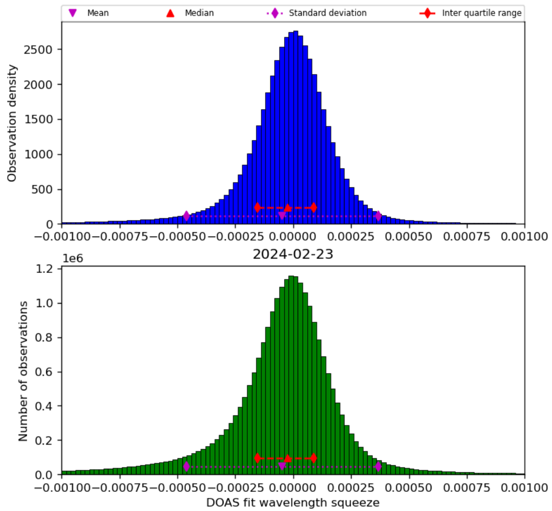
Figure 69: Histogram of “DOAS fit wavelength squeeze” for 2024-02-22 to 2024-02-24
