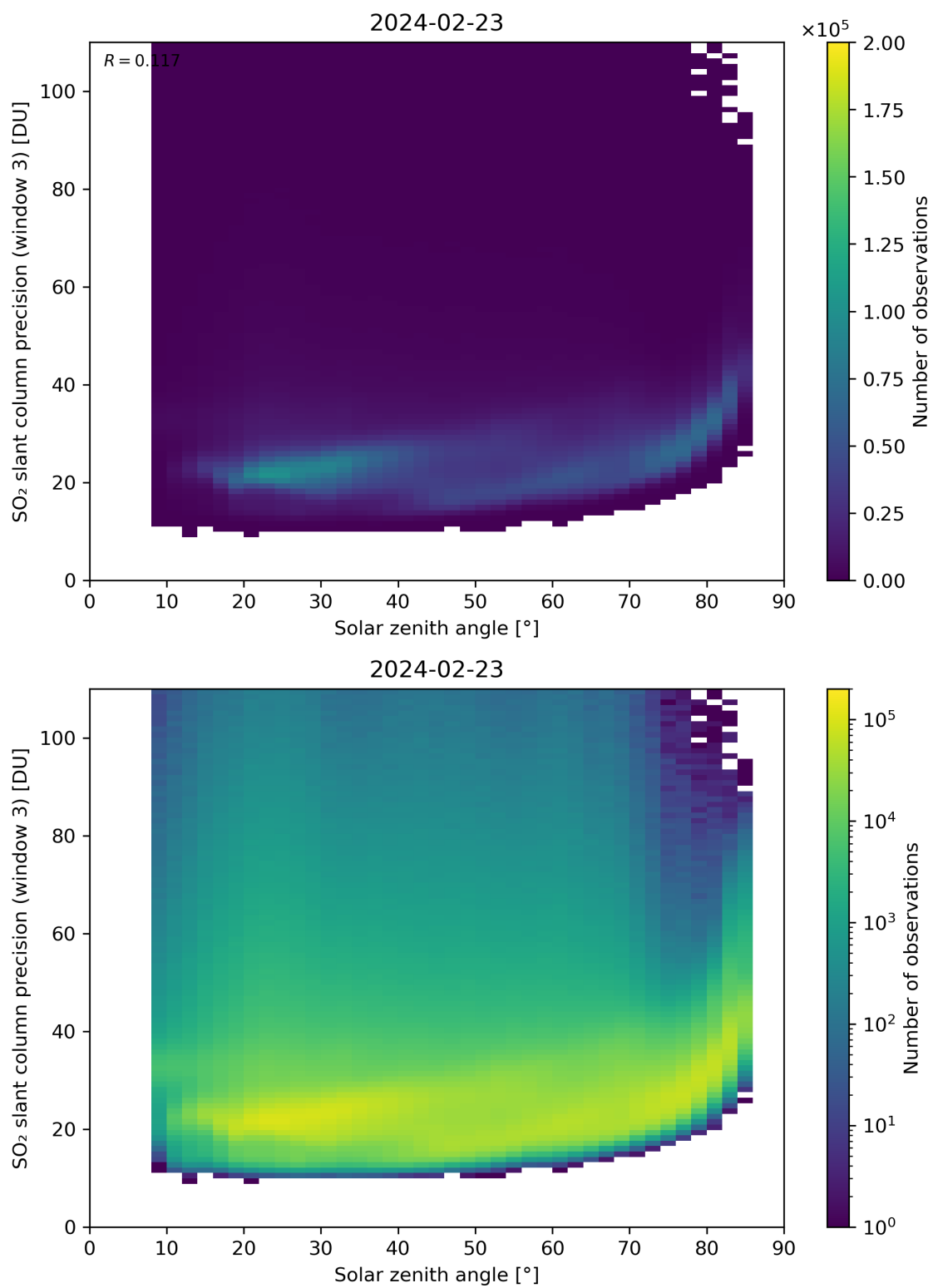
Figure 173: Scatter density plot of “Solar zenith angle” against “SO 2 slant column precision (window 3)” for 2024-02-22 to 2024-02-24.
