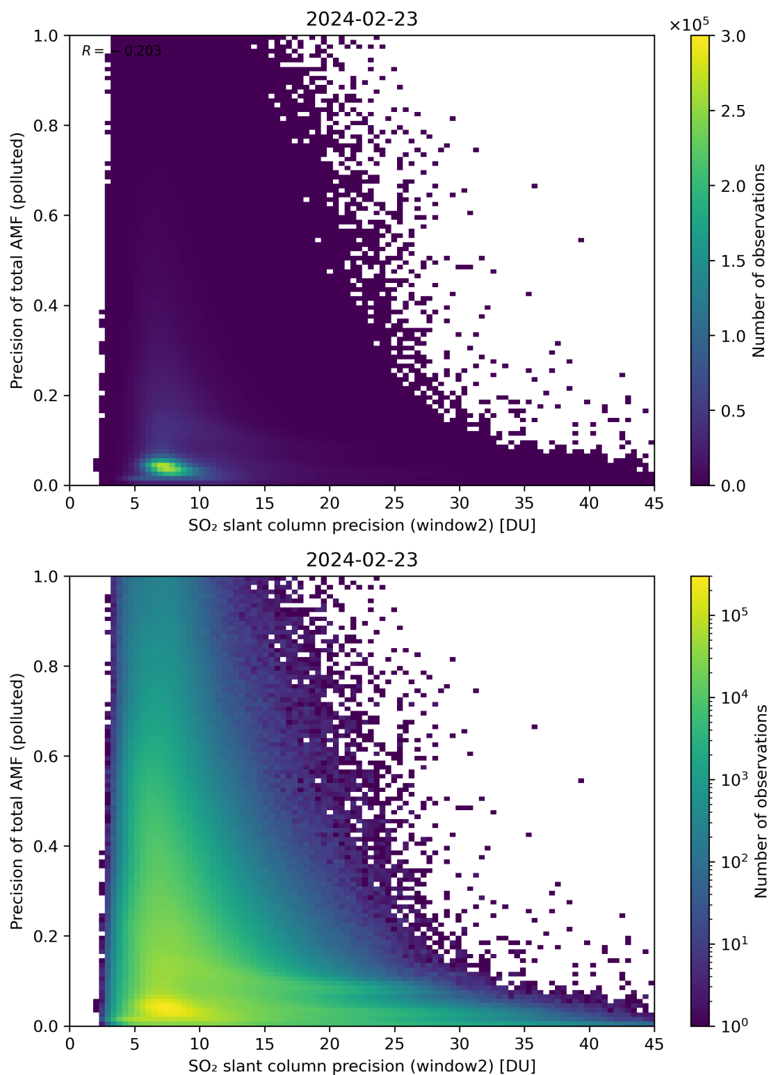
Figure 252: Scatter density plot of “SO 2 slant column precision (window2)” against “Precision of total AMF (polluted)” for 2024-02-22 to 2024-02-24.
