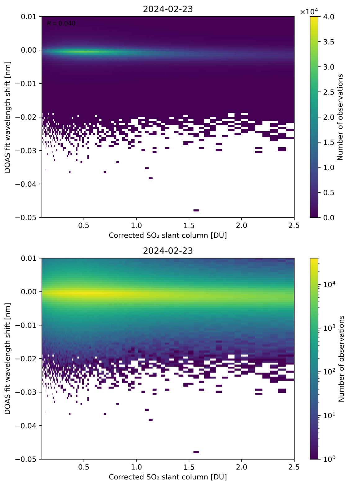
Figure 181: Scatter density plot of “Corrected SO 2 slant column” against “DOAS fit wavelength shift” for 2024-02-22 to 2024-02-24.
