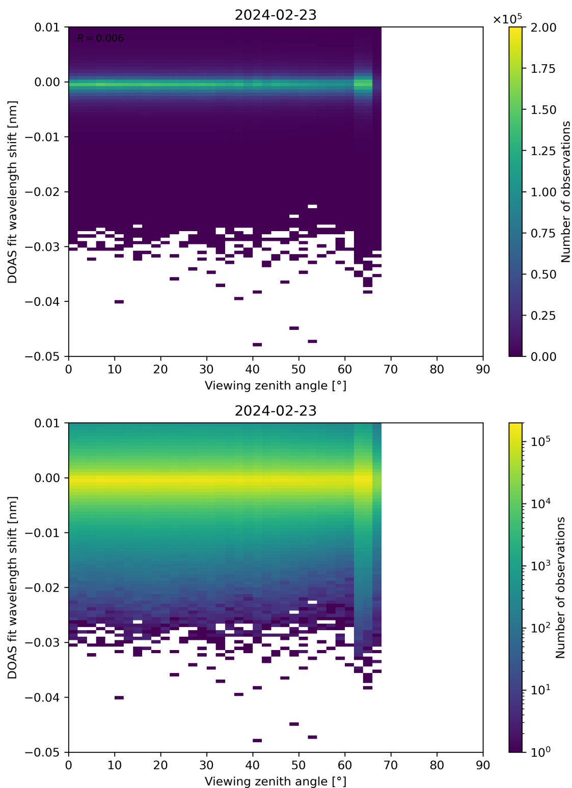
Figure 311: Scatter density plot of “Viewing zenith angle” against “DOAS fit wavelength shift” for 2024-02-22 to 2024-02-24.
