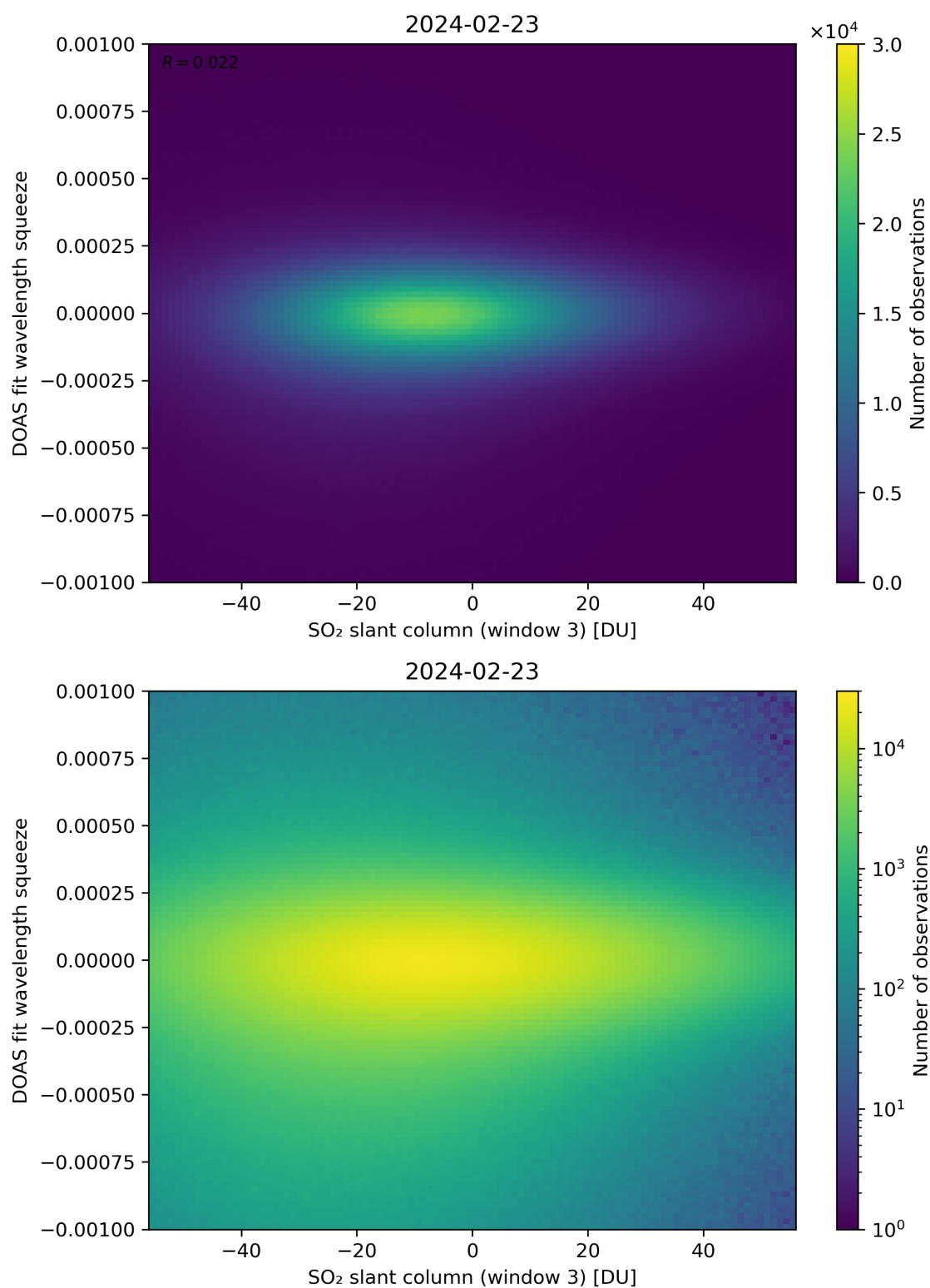
Figure 255: Scatter density plot of “SO 2 slant column (window 3)” against “DOAS fit wavelength squeeze” for 2024-02-22 to 2024-02-24.
