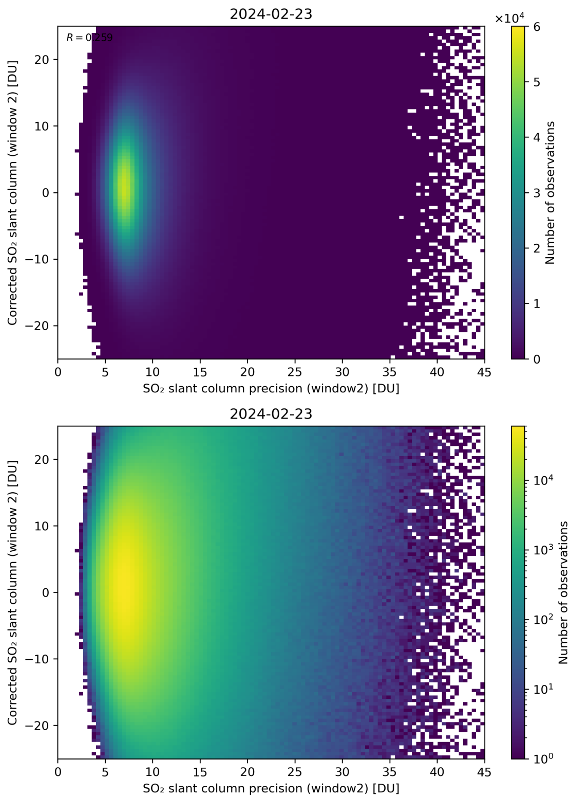
Figure 247: Scatter density plot of “SO 2 slant column precision (window2)” against “Corrected SO 2 slant column (window 2)” for 2024-02-22 to 2024-02-24.
