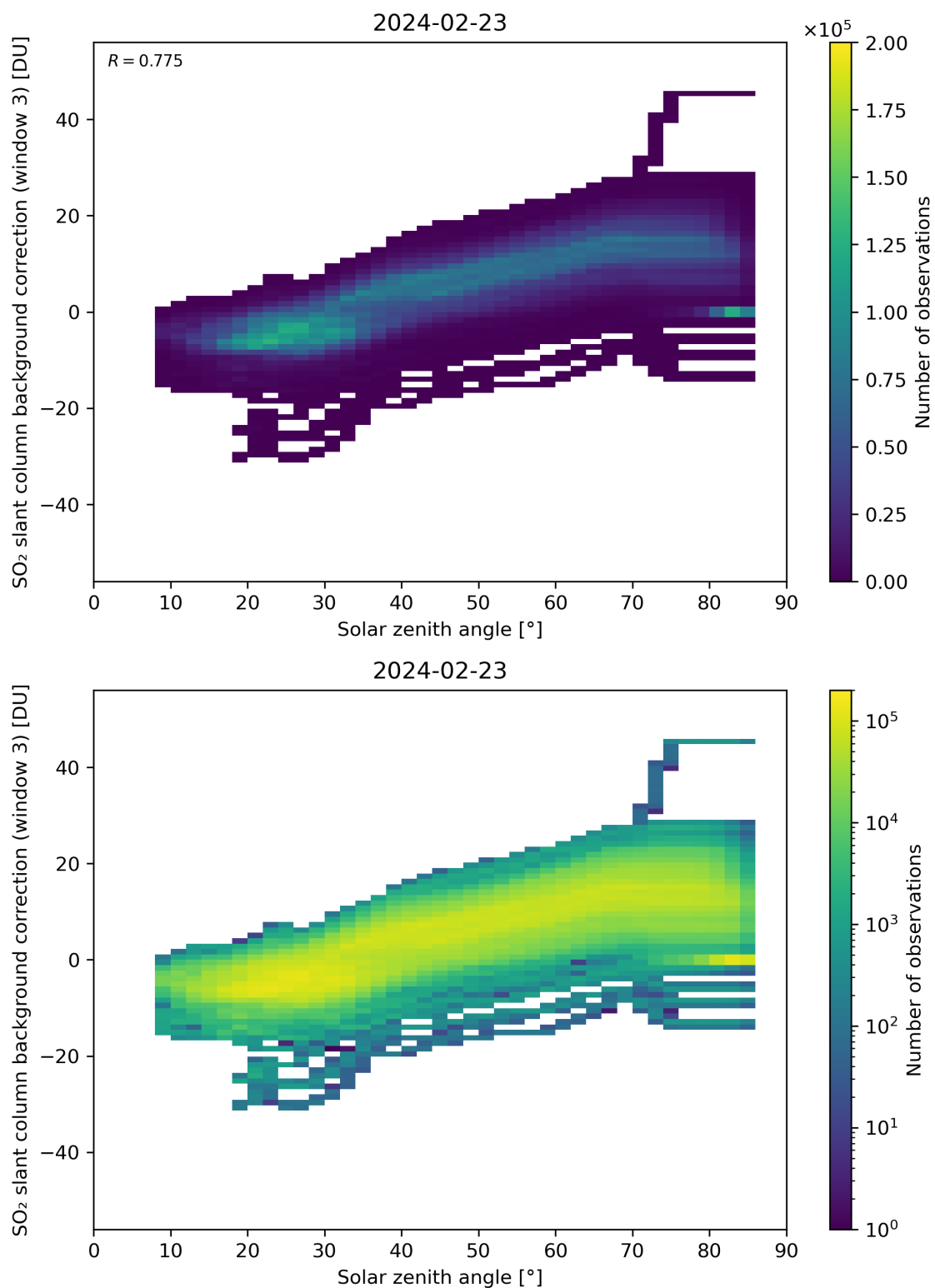
Figure 160: Scatter density plot of “Solar zenith angle” against “SO 2 slant column background correction (window 3)” for 2024-02-22 to 2024-02-24.
