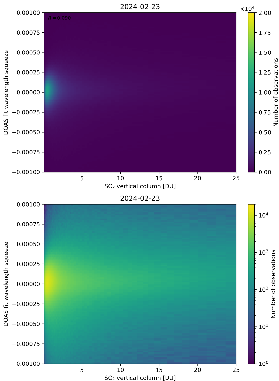
Figure 277: Scatter density plot of “SO 2 vertical column” against “DOAS fit wavelength squeeze” for 2024-02-22 to 2024-02-24.
