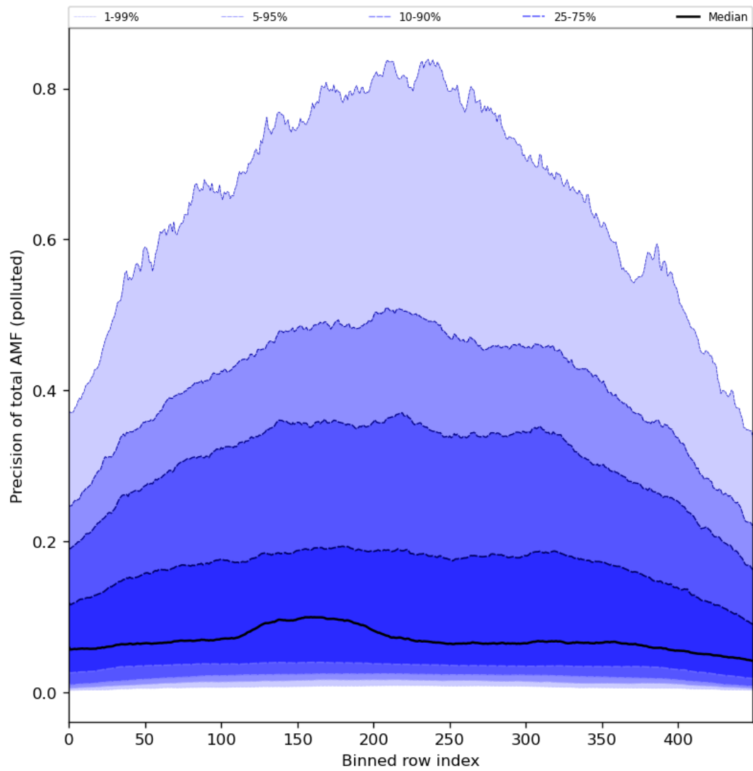
Figure 95: Along track statistics of “Precision of total AMF (polluted)” for 2024-02-22 to 2024-02-24
