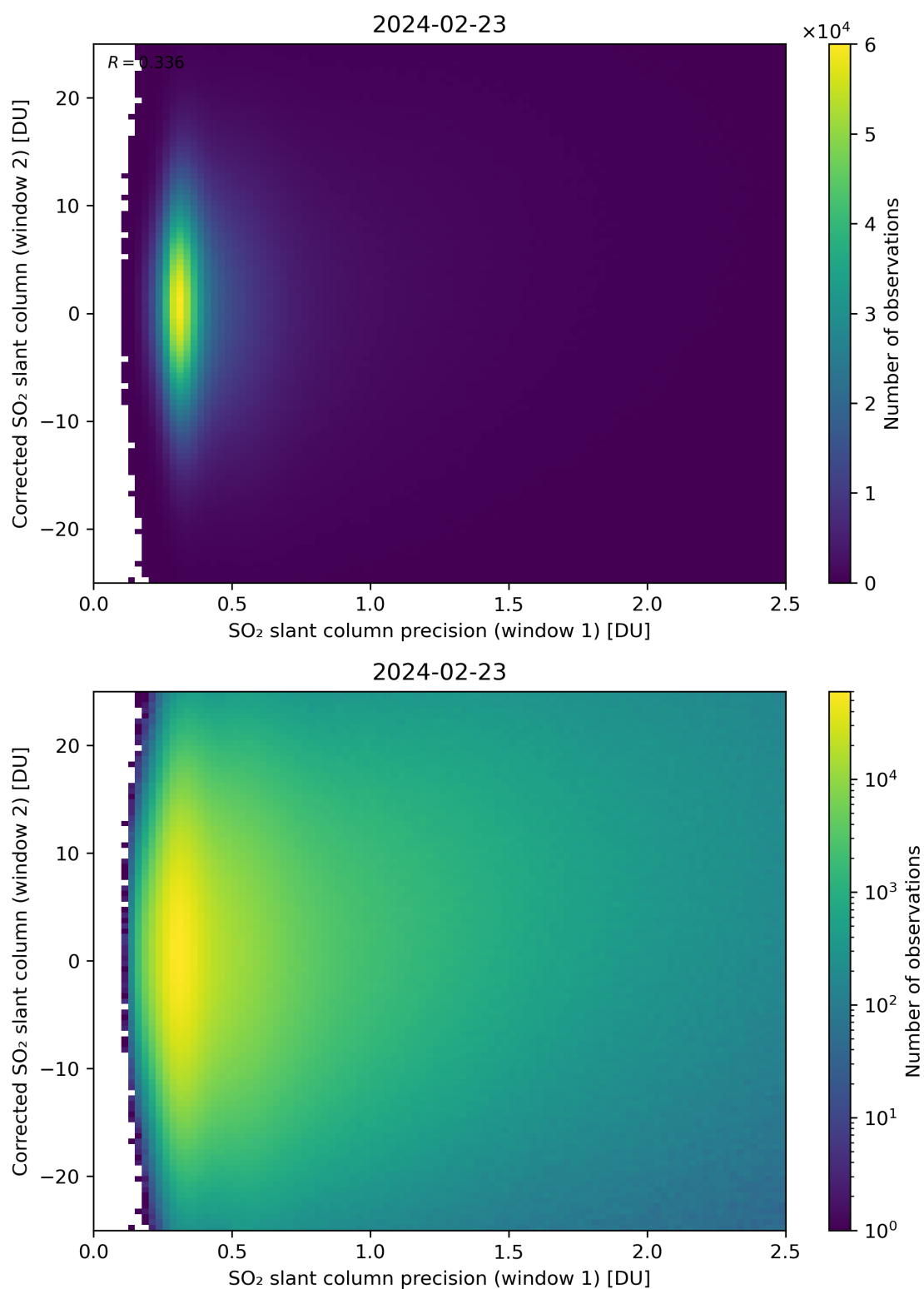
Figure 225: Scatter density plot of “SO 2 slant column precision (window 1)” against “Corrected SO 2 slant column (window 2)” for 2024-02-22 to 2024-02-24.
