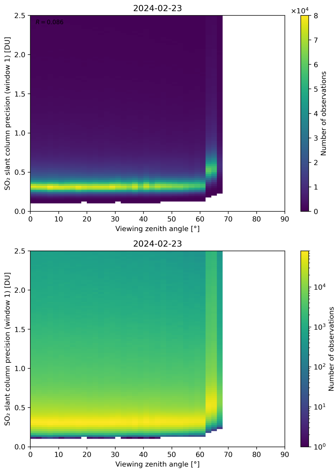
Figure 321: Scatter density plot of “Viewing zenith angle” against “SO 2 slant column precision (window 1)” for 2024-02-22 to 2024-02-24.
