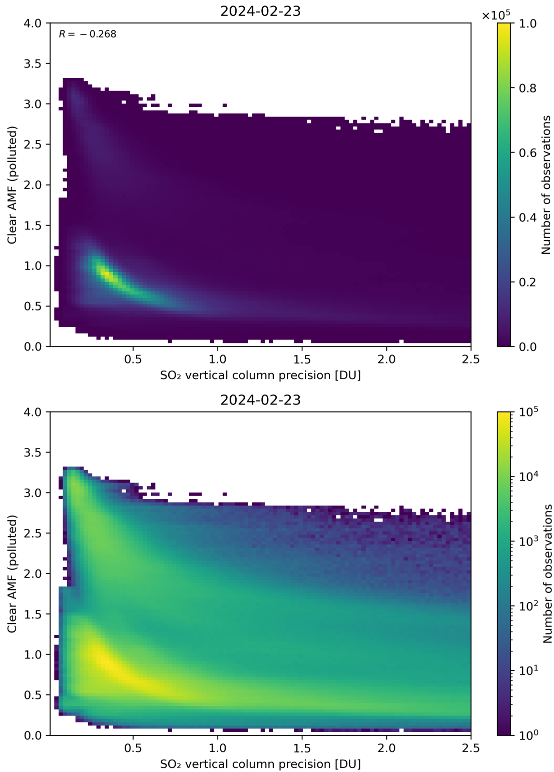
Figure 285: Scatter density plot of “SO 2 vertical column precision” against “Clear AMF (polluted)” for 2024-02-22 to 2024-02-24.
