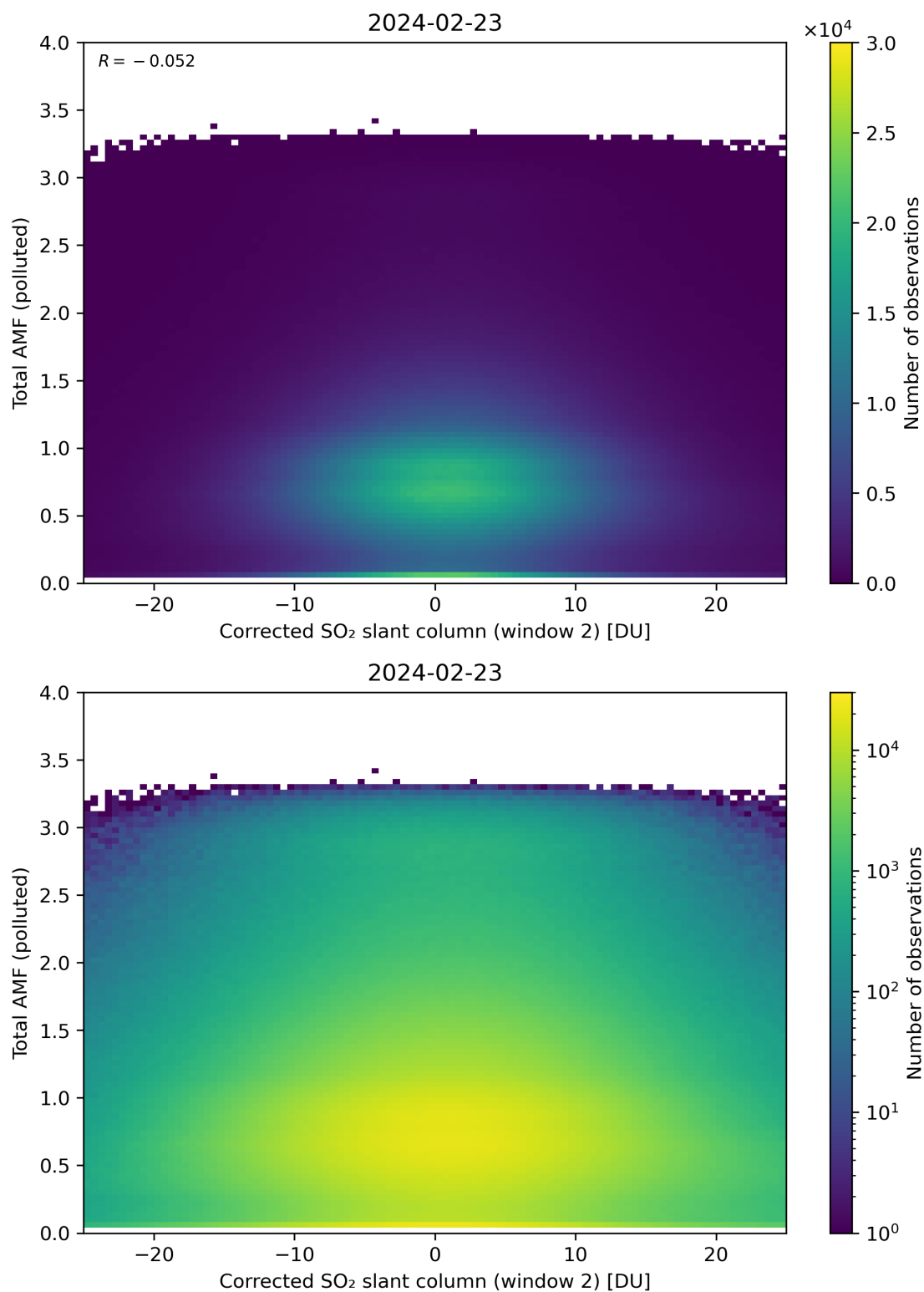
Figure 203: Scatter density plot of “Corrected SO 2 slant column (window 2)” against “Total AMF (polluted)” for 2024-02-22 to 2024-02-24.
