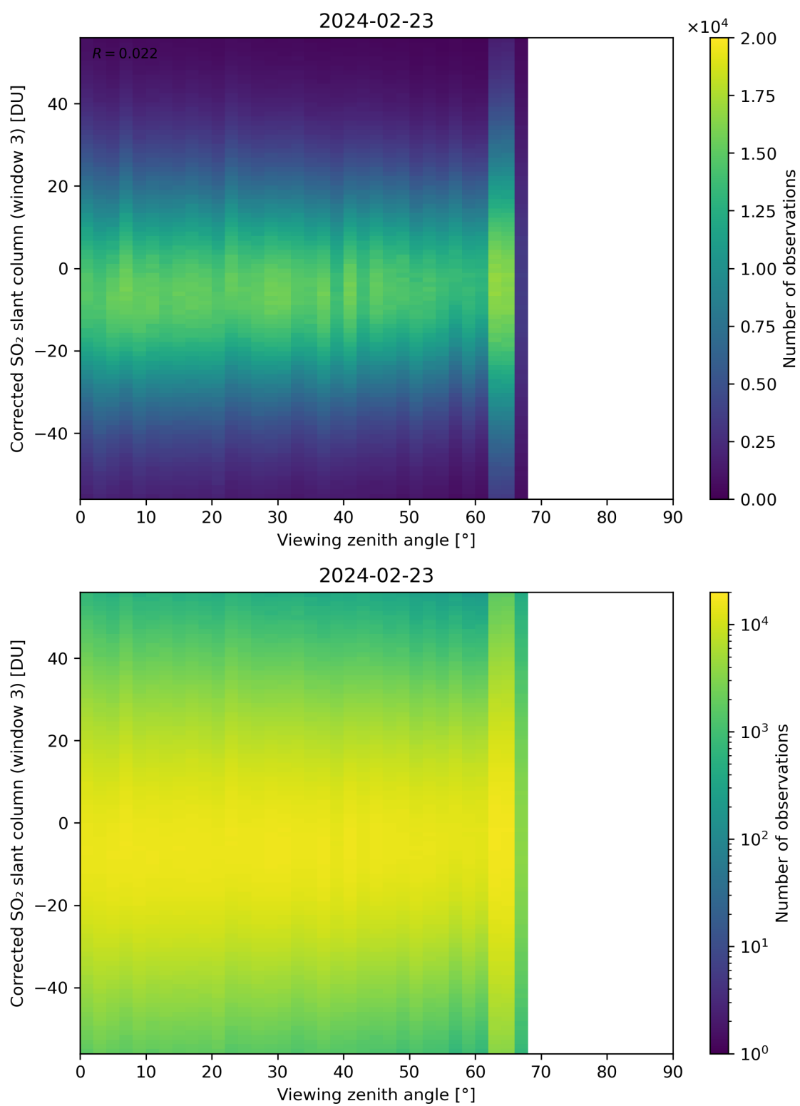
Figure 319: Scatter density plot of “Viewing zenith angle” against “Corrected SO 2 slant column (window 3)” for 2024-02-22 to 2024-02-24.
