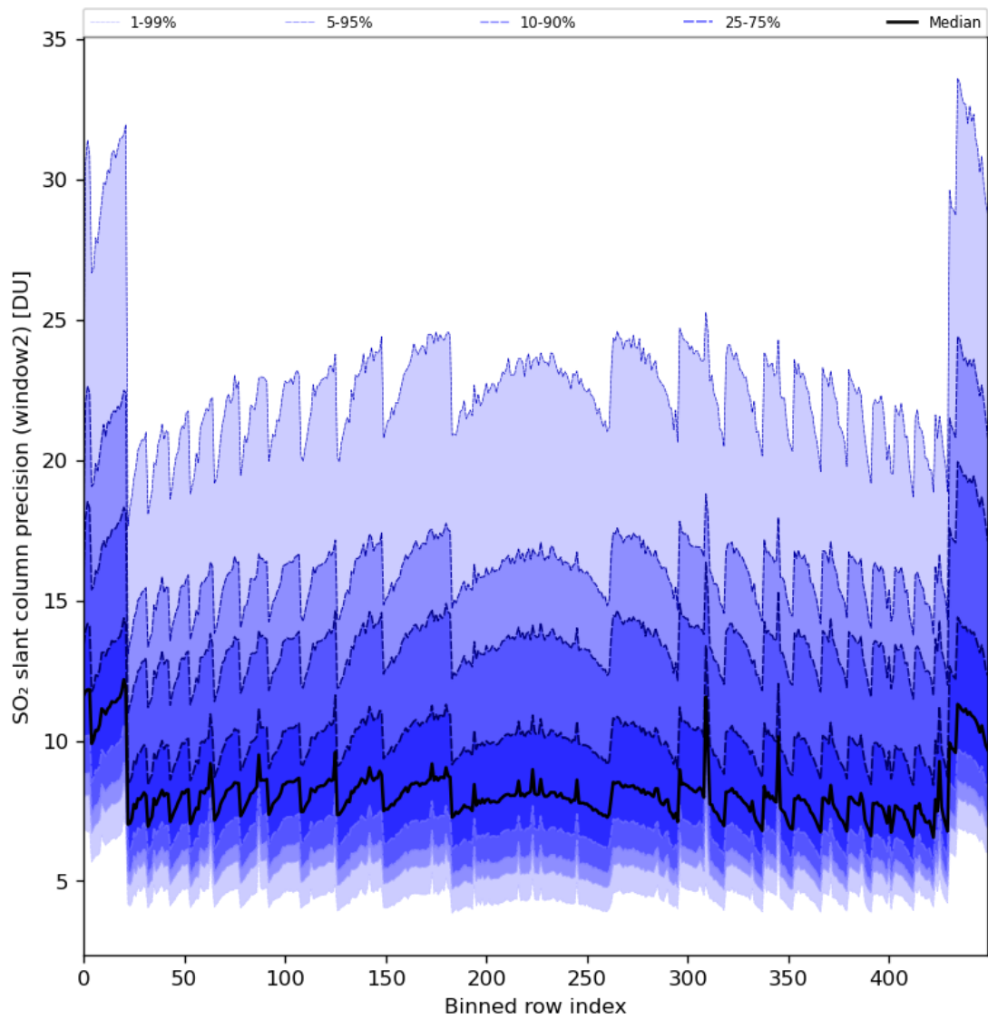
Figure 84: Along track statistics of “SO 2 slant column precision (window2)” for 2024-02-22 to 2024-02-24
