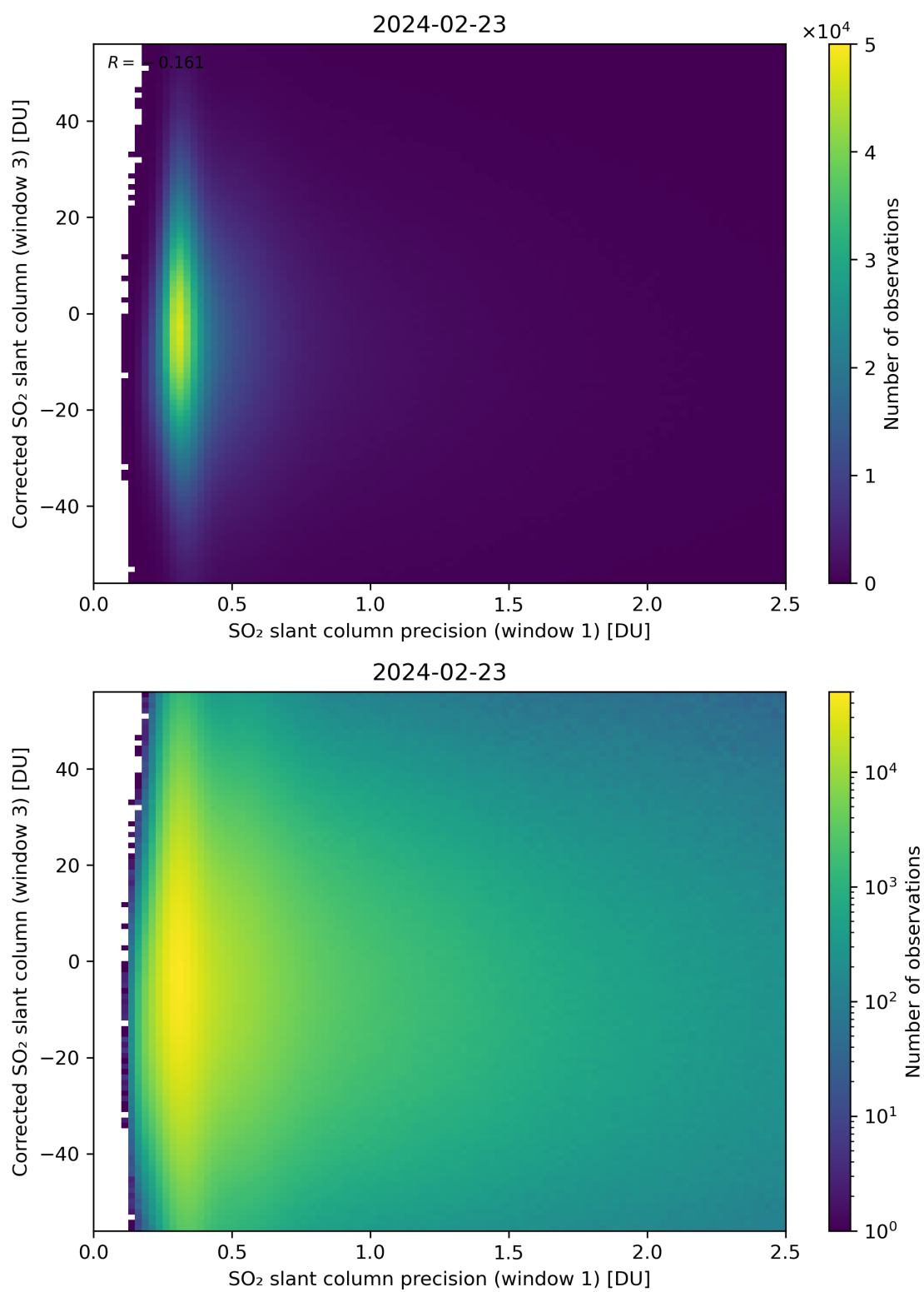
Figure 226: Scatter density plot of “SO 2 slant column precision (window 1)” against “Corrected SO 2 slant column (window 3)” for 2024-02-22 to 2024-02-24.
