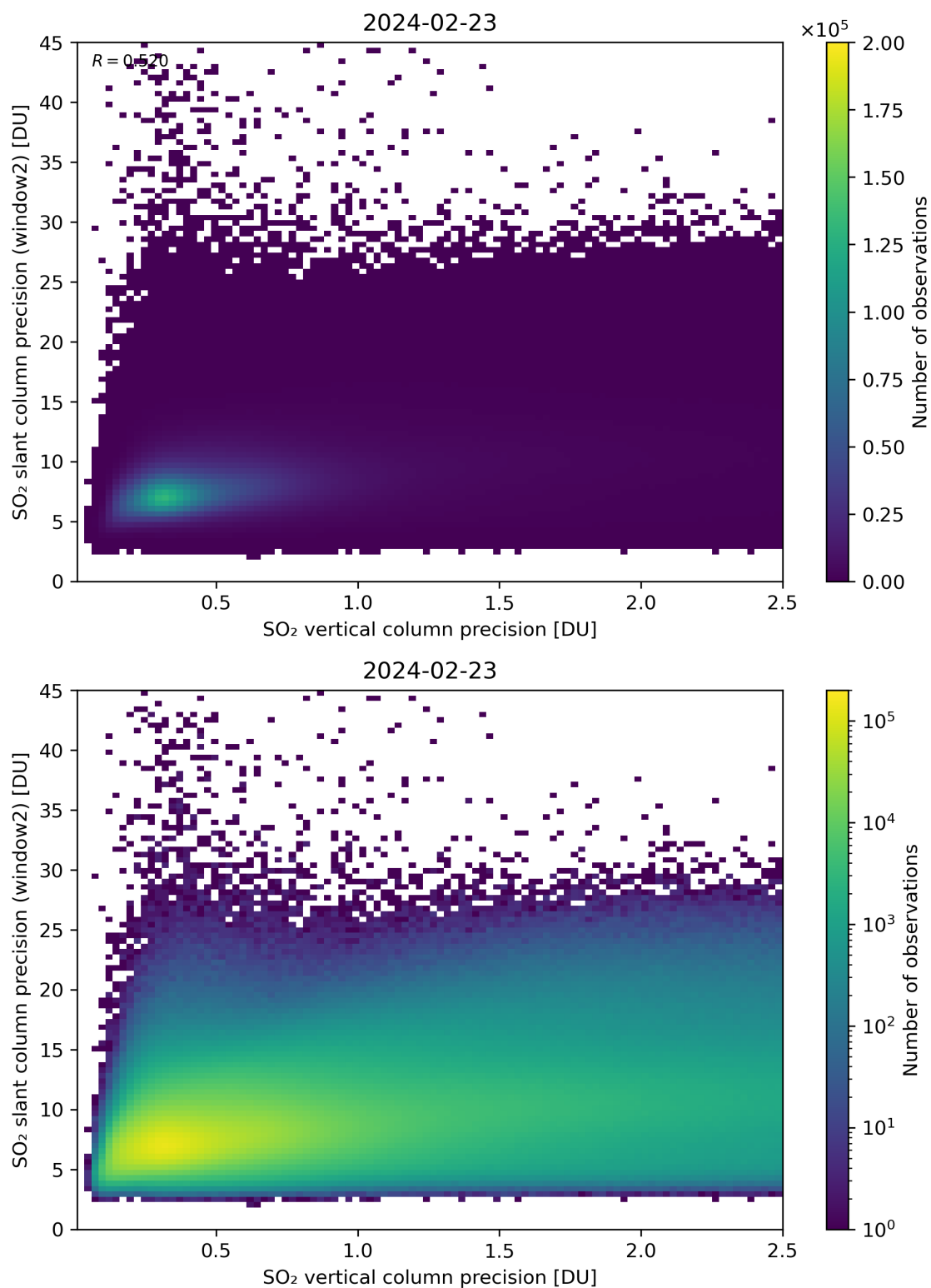
Figure 291: Scatter density plot of “SO 2 vertical column precision” against “SO 2 slant column precision (window2)” for 2024-02-22 to 2024-02-24.
