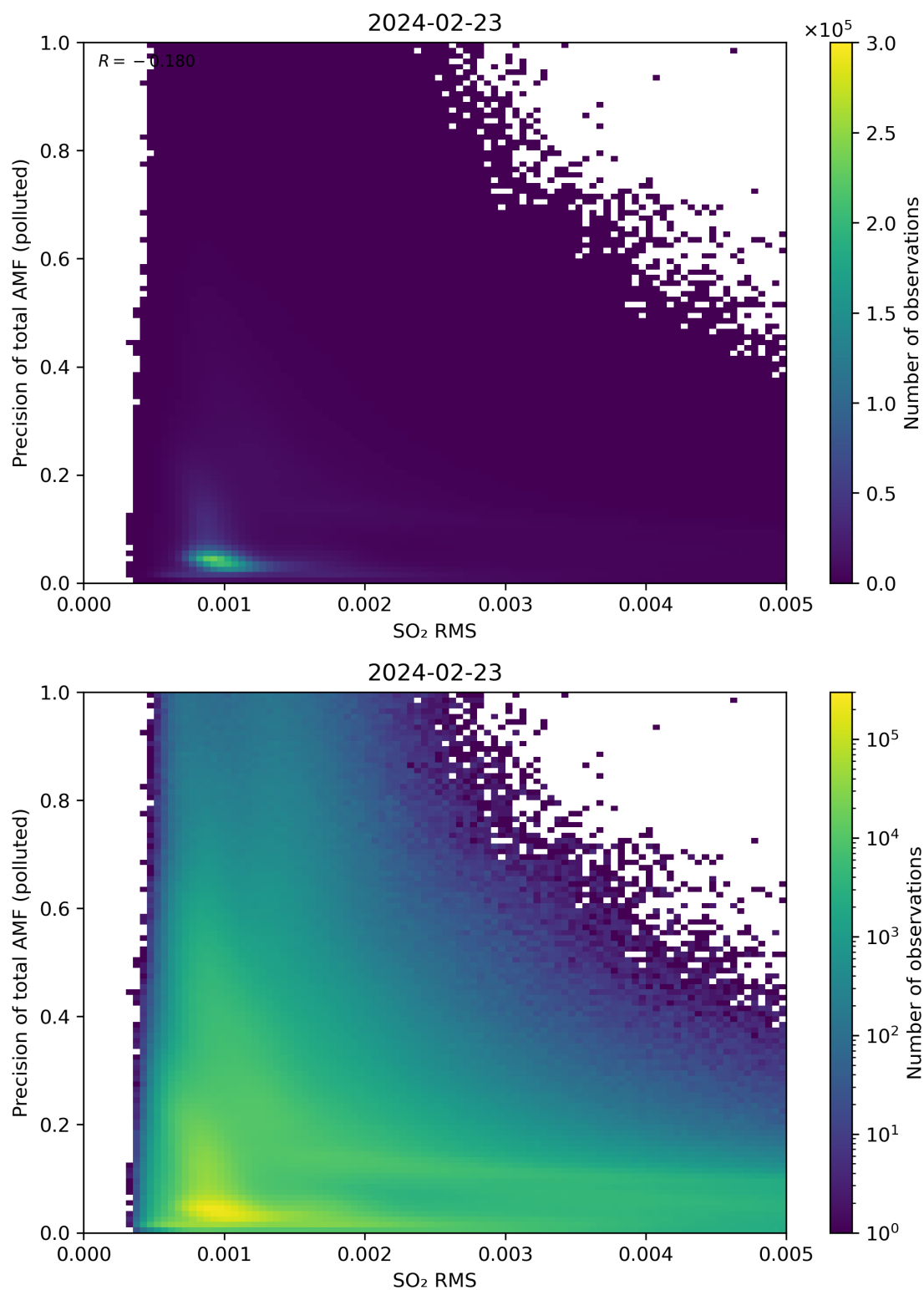
Figure 138: Scatter density plot of “SO 2 RMS” against “Precision of total AMF (polluted)” for 2024-02-22 to 2024-02-24.
