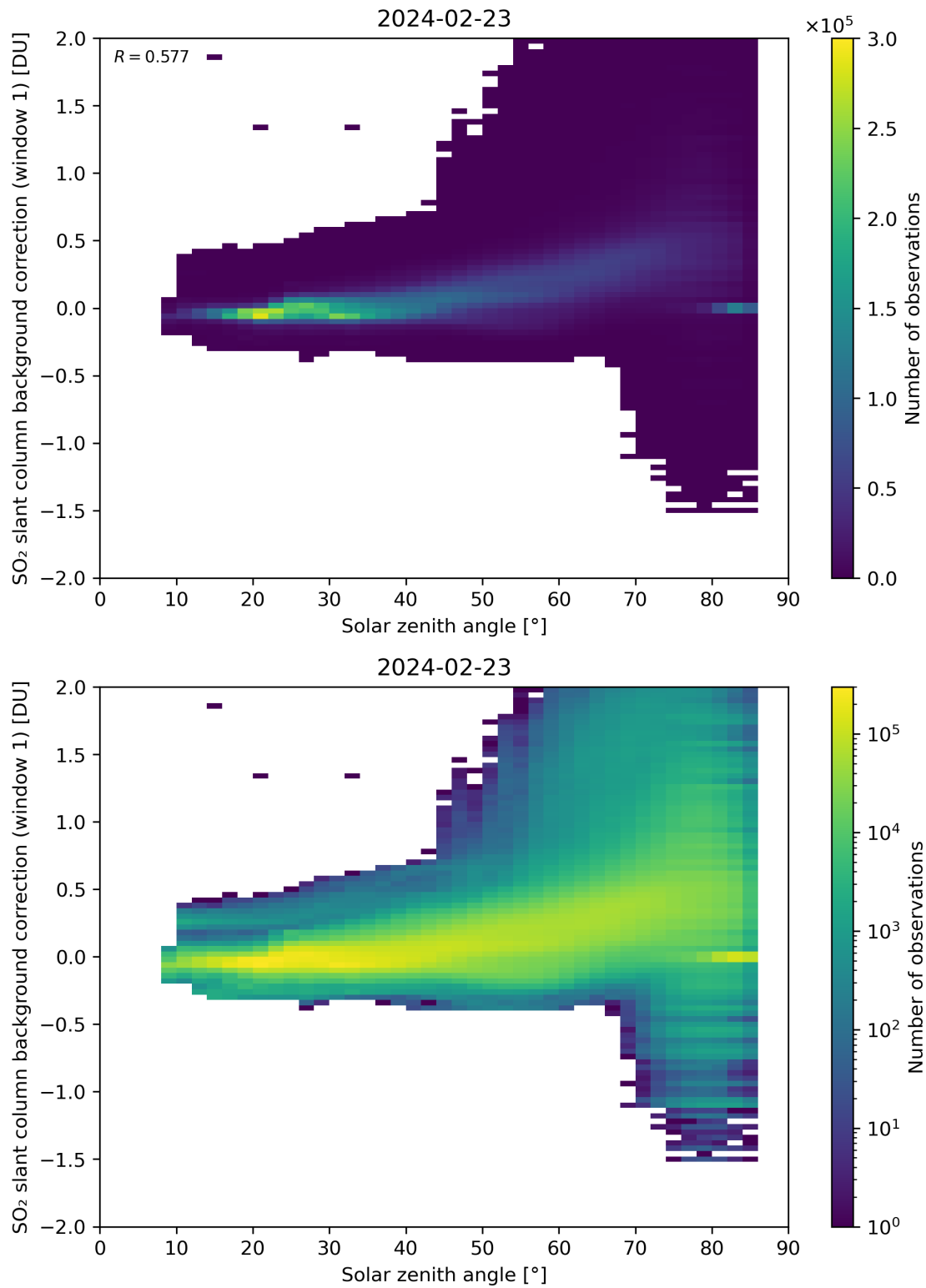
Figure 158: Scatter density plot of “Solar zenith angle” against “SO 2 slant column background correction (window 1)” for 2024-02-22 to 2024-02-24.
