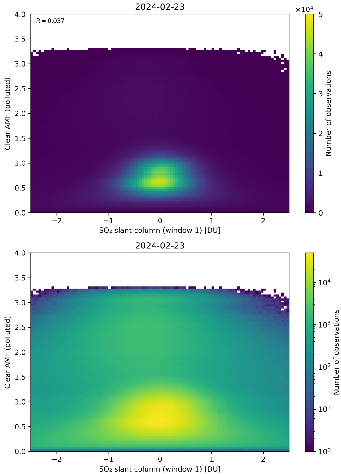
Figure 232: Scatter density plot of “SO 2 slant column (window 1)” against “Clear AMF (polluted)” for 2024-02-22 to 2024-02-24.
