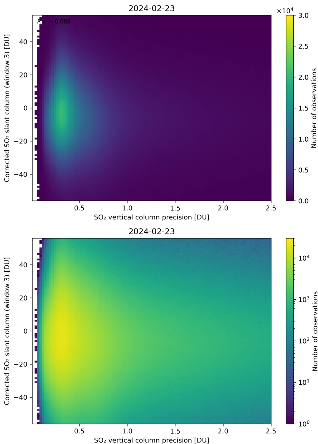
Figure 288: Scatter density plot of “SO 2 vertical column precision” against “Corrected SO 2 slant column (window 3)” for 2024-02-22 to 2024-02-24.
