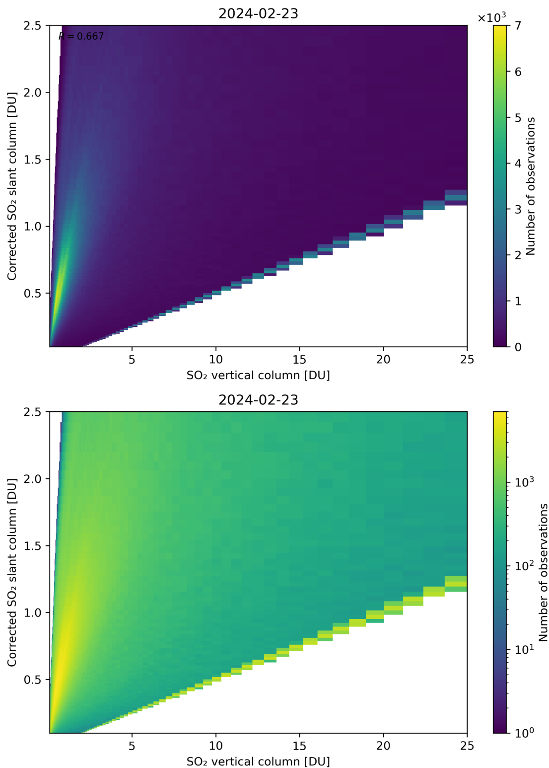
Figure 297: Scatter density plot of “SO 2 vertical column” against “Corrected SO 2 slant column” for 2024-02-22 to 2024-02-24.
