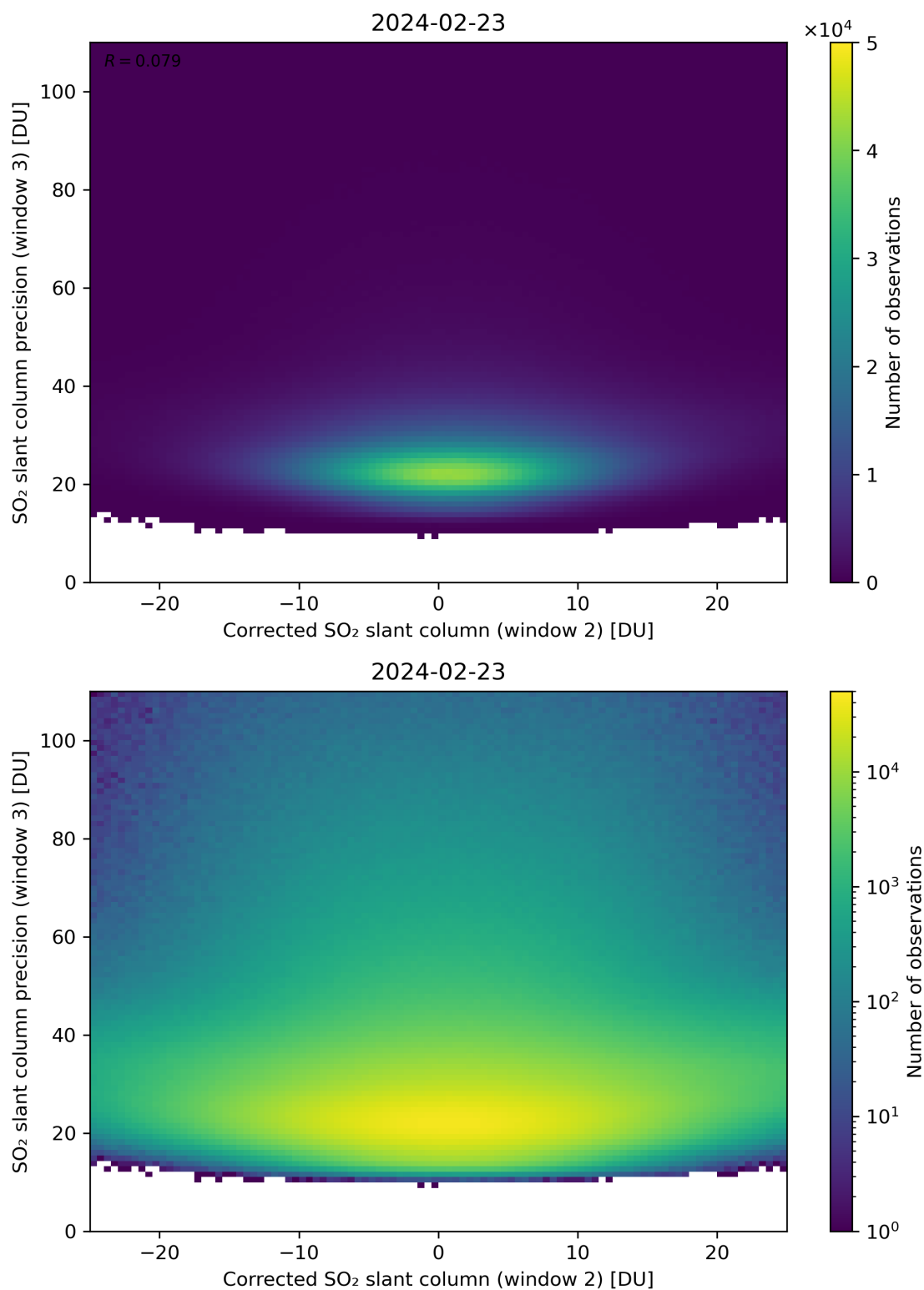
Figure 202: Scatter density plot of “Corrected SO 2 slant column (window 2)” against “SO 2 slant column precision (window 3)” for 2024-02-22 to 2024-02-24.
