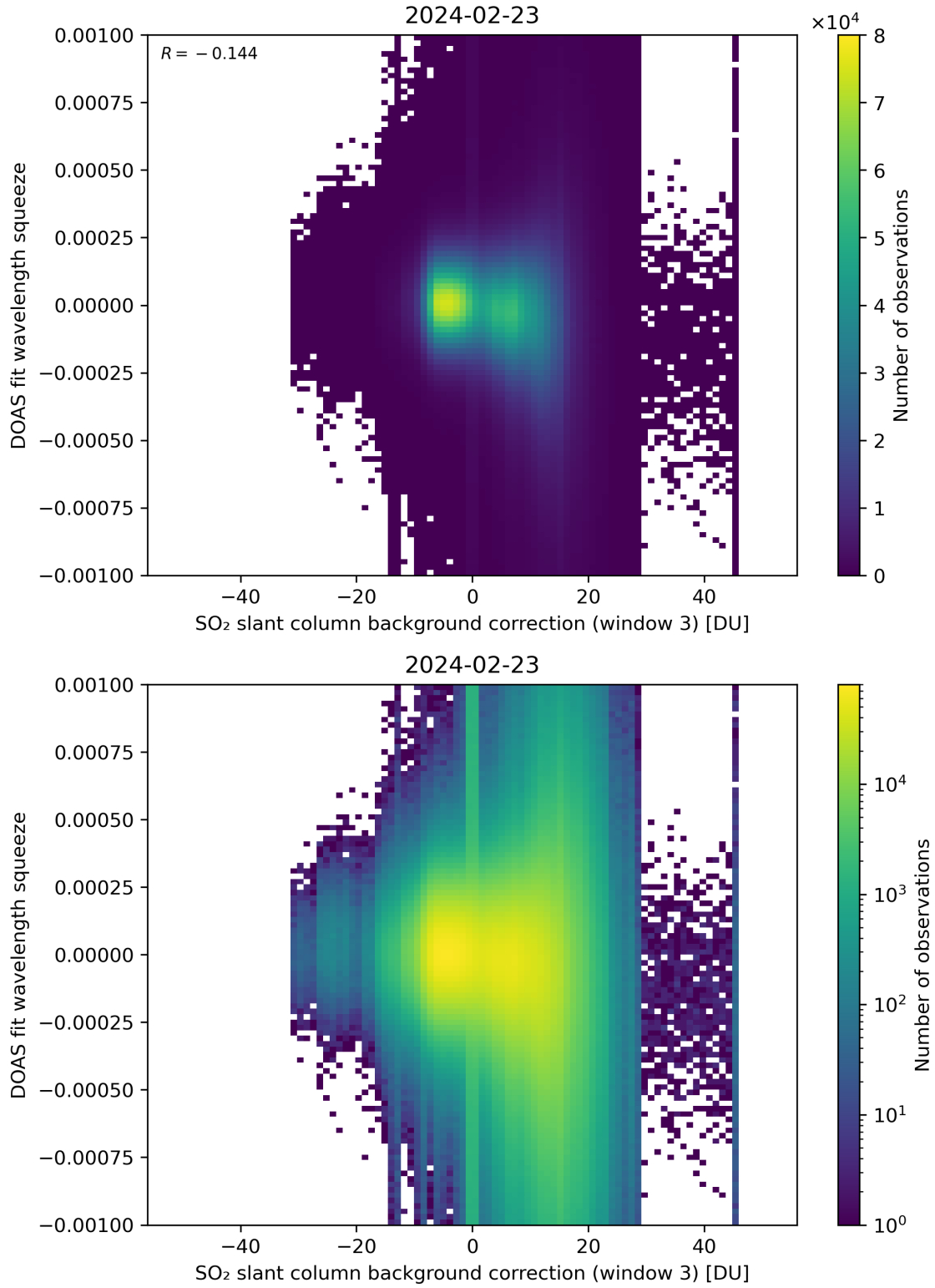
Figure 122: Scatter density plot of “SO 2 slant column background correction (window 3)” against “DOAS fit wavelength squeeze” for 2024-02-22 to 2024-02-24.
