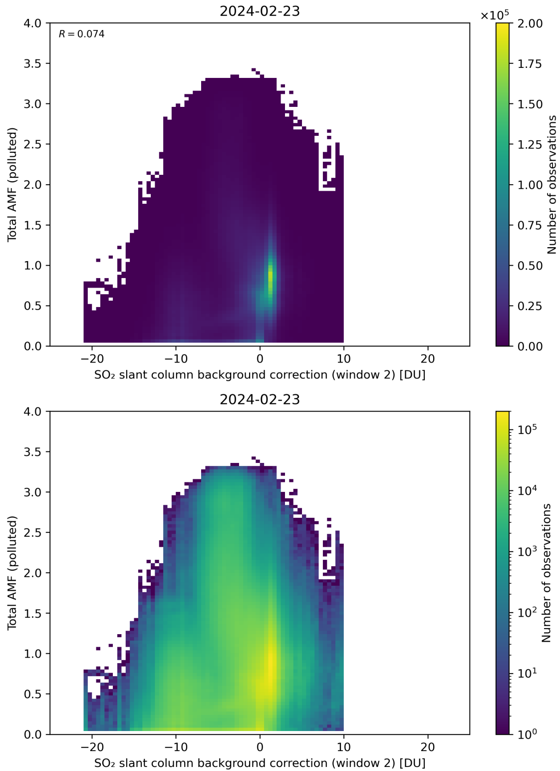
Figure 119: Scatter density plot of “SO 2 slant column background correction (window 2)” against “Total AMF (polluted)” for 2024-02-22 to 2024-02-24.
