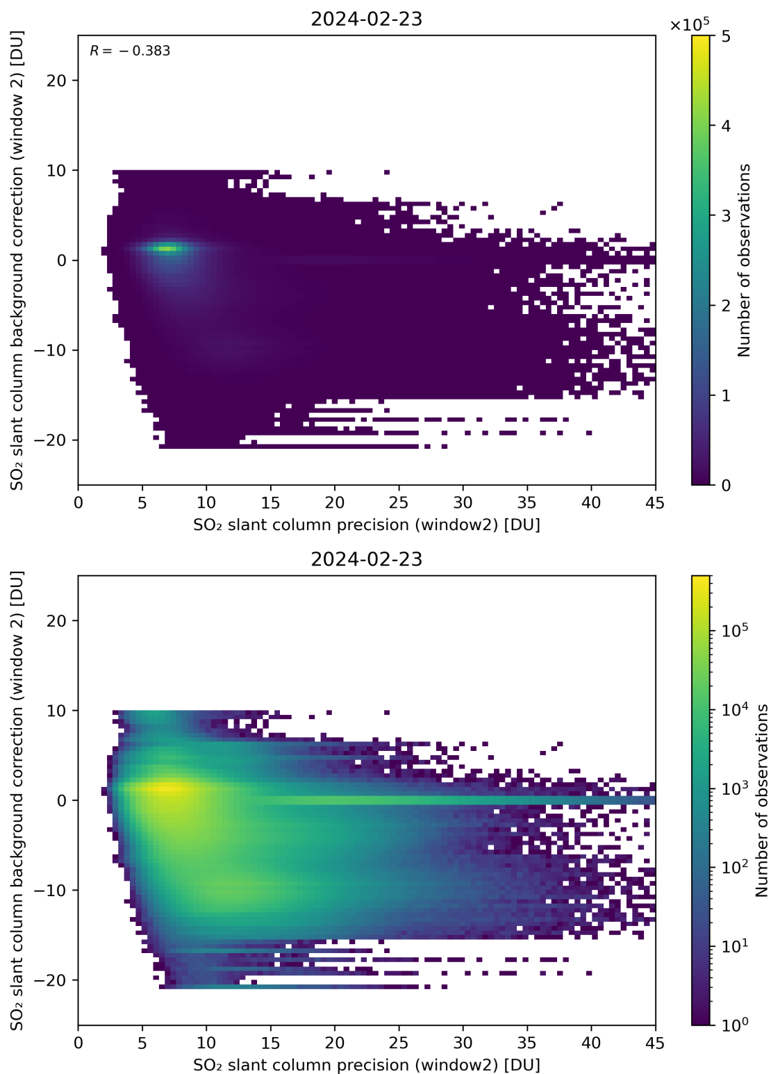
Figure 241: Scatter density plot of “SO 2 slant column precision (window2)” against “SO 2 slant column background correction (window 2)” for 2024-02-22 to 2024-02-24.
