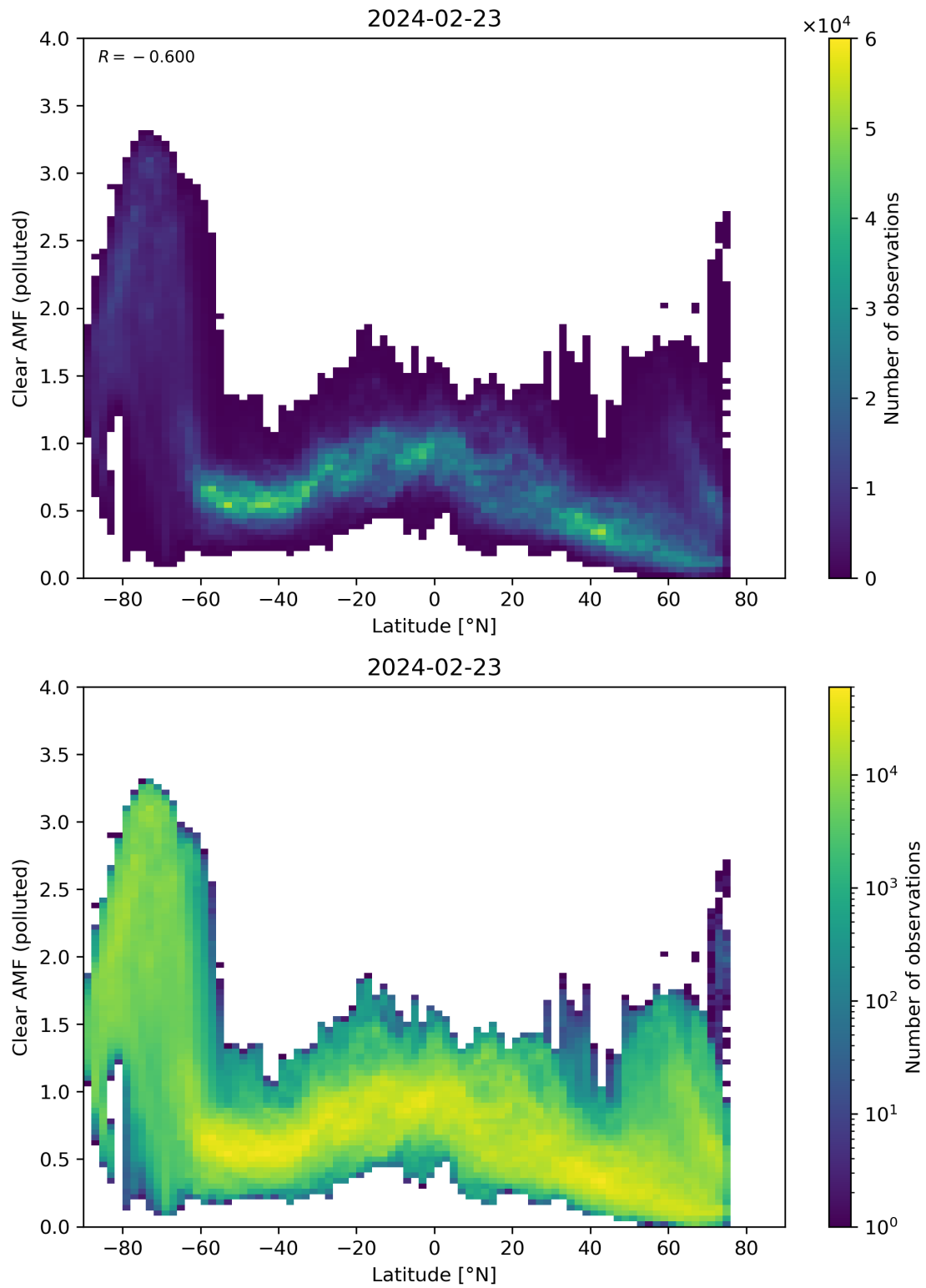
Figure 145: Scatter density plot of “Latitude” against “Clear AMF (polluted)” for 2024-02-22 to 2024-02-24.
