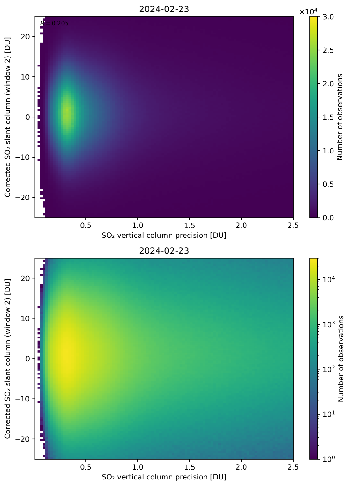
Figure 287: Scatter density plot of “SO 2 vertical column precision” against “Corrected SO 2 slant column (window 2)” for 2024-02-22 to 2024-02-24.
