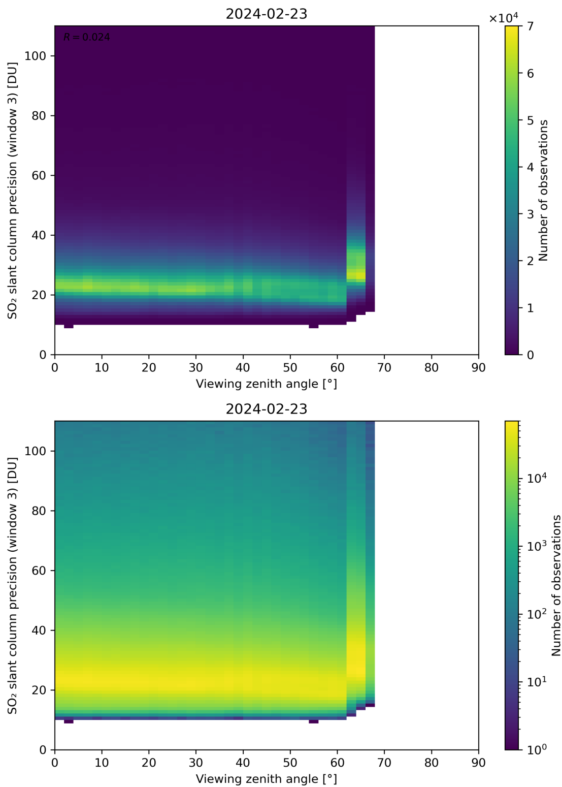
Figure 324: Scatter density plot of “Viewing zenith angle” against “SO 2 slant column precision (window 3)” for 2024-02-22 to 2024-02-24.
