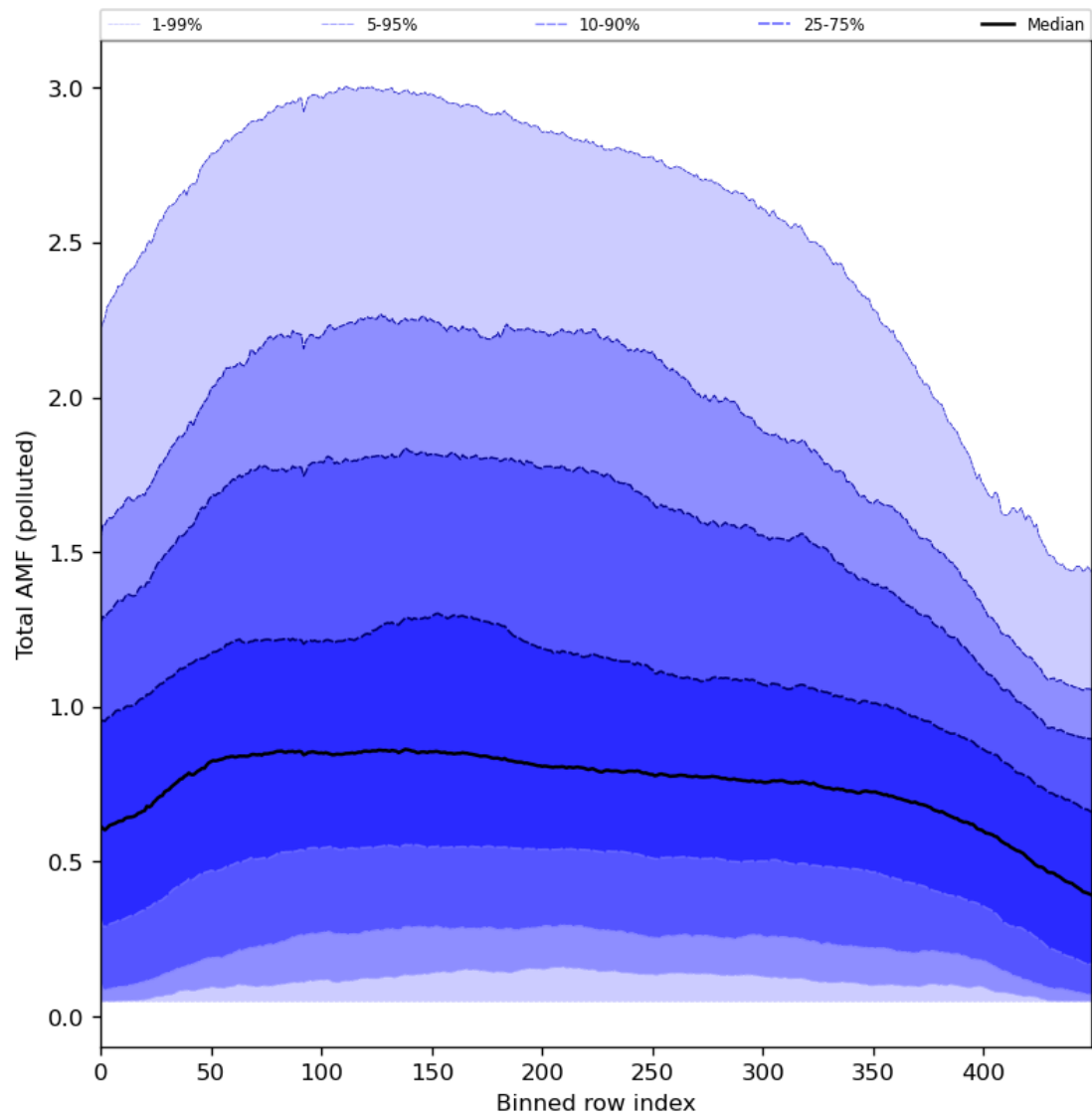
Figure 94: Along track statistics of “Total AMF (polluted)” for 2024-02-22 to 2024-02-24
