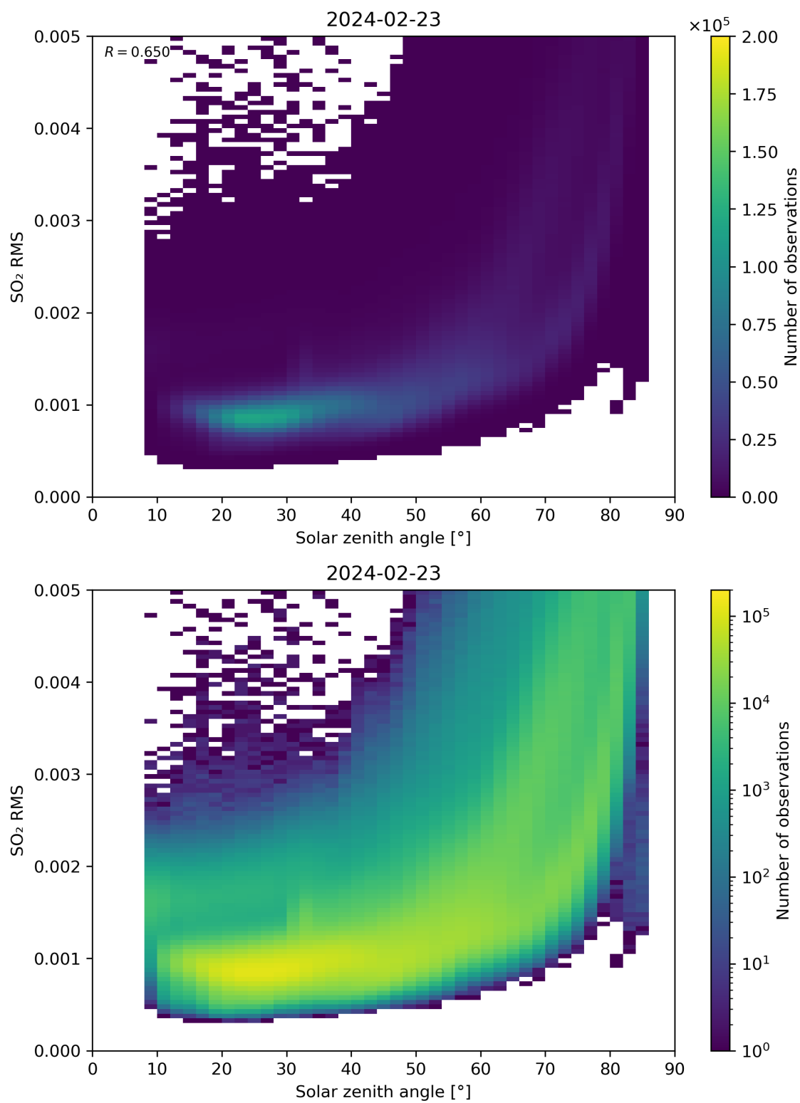
Figure 163: Scatter density plot of “Solar zenith angle” against “SO 2 RMS” for 2024-02-22 to 2024-02-24.
