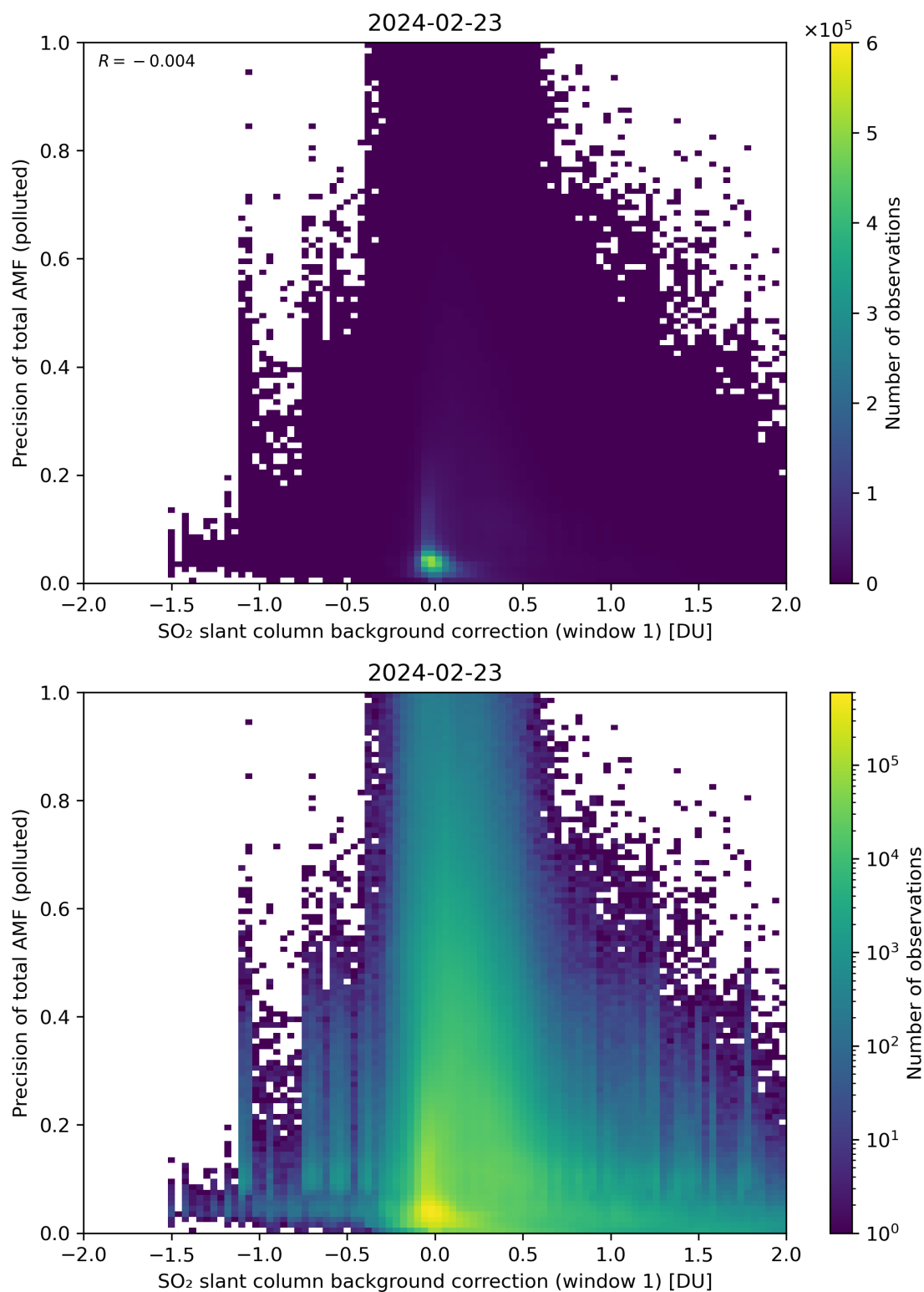
Figure 110: Scatter density plot of “SO 2 slant column background correction (window 1)” against “Precision of total AMF (polluted)” for 2024-02-22 to 2024-02-24.
