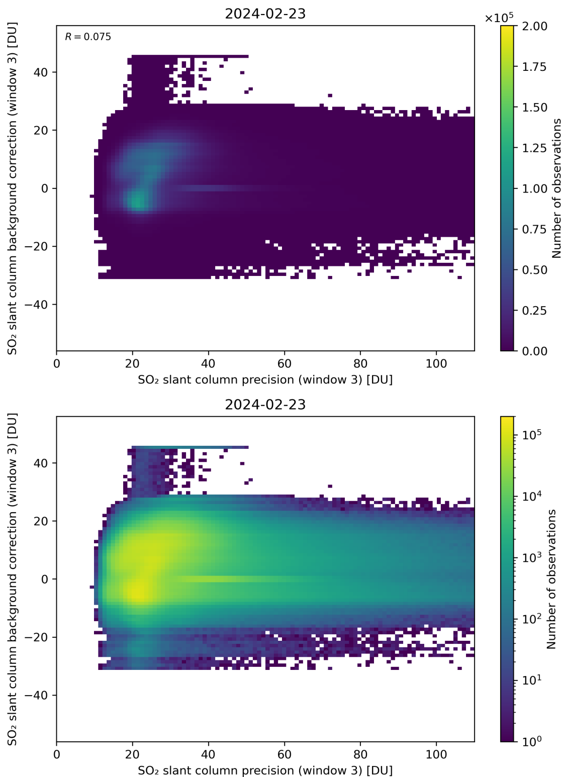
Figure 257: Scatter density plot of “SO 2 slant column precision (window 3)” against “SO 2 slant column background correction (window 3)” for 2024-02-22 to 2024-02-24.
