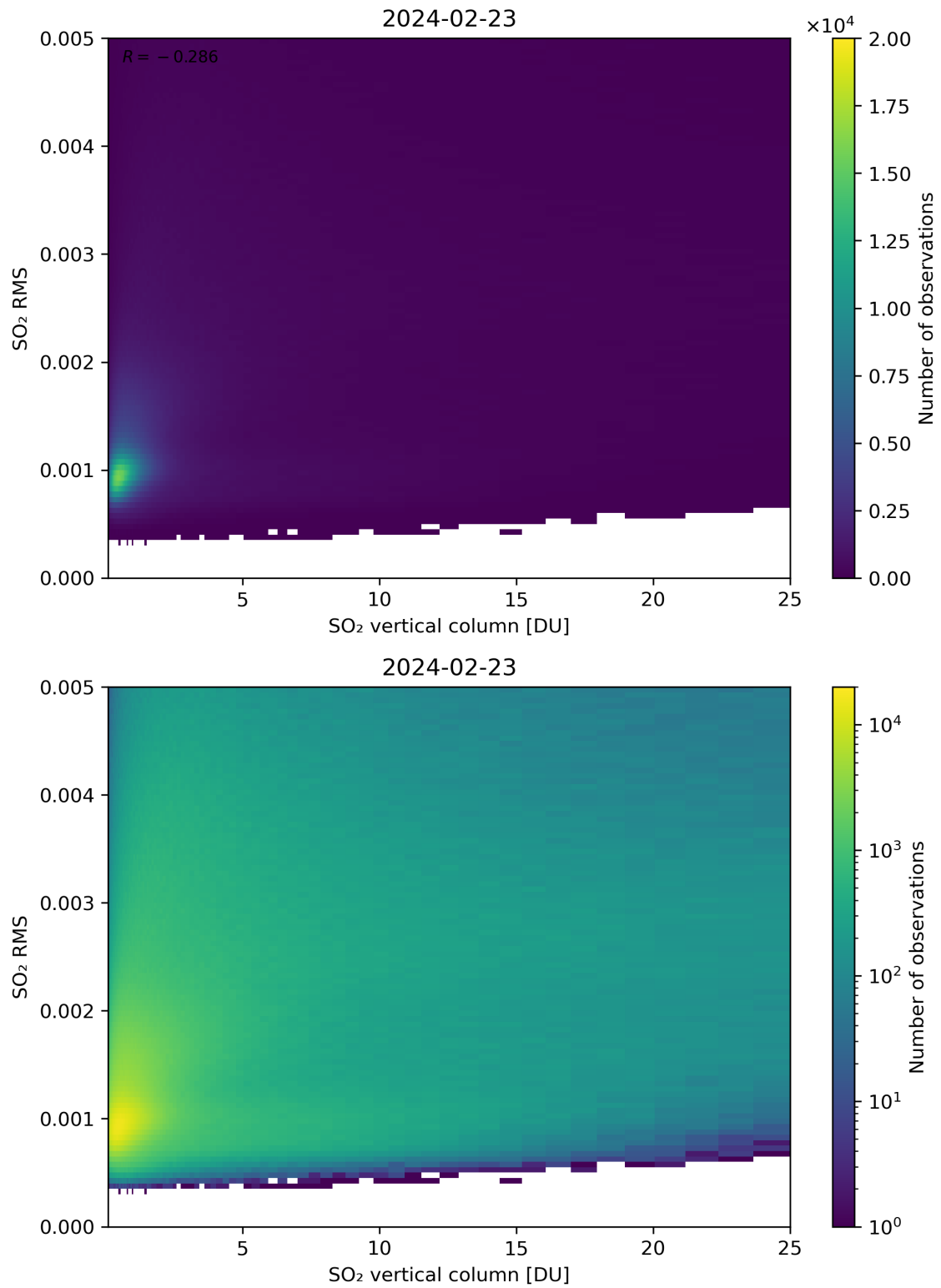
Figure 278: Scatter density plot of “SO 2 vertical column” against “SO 2 RMS” for 2024-02-22 to 2024-02-24.
