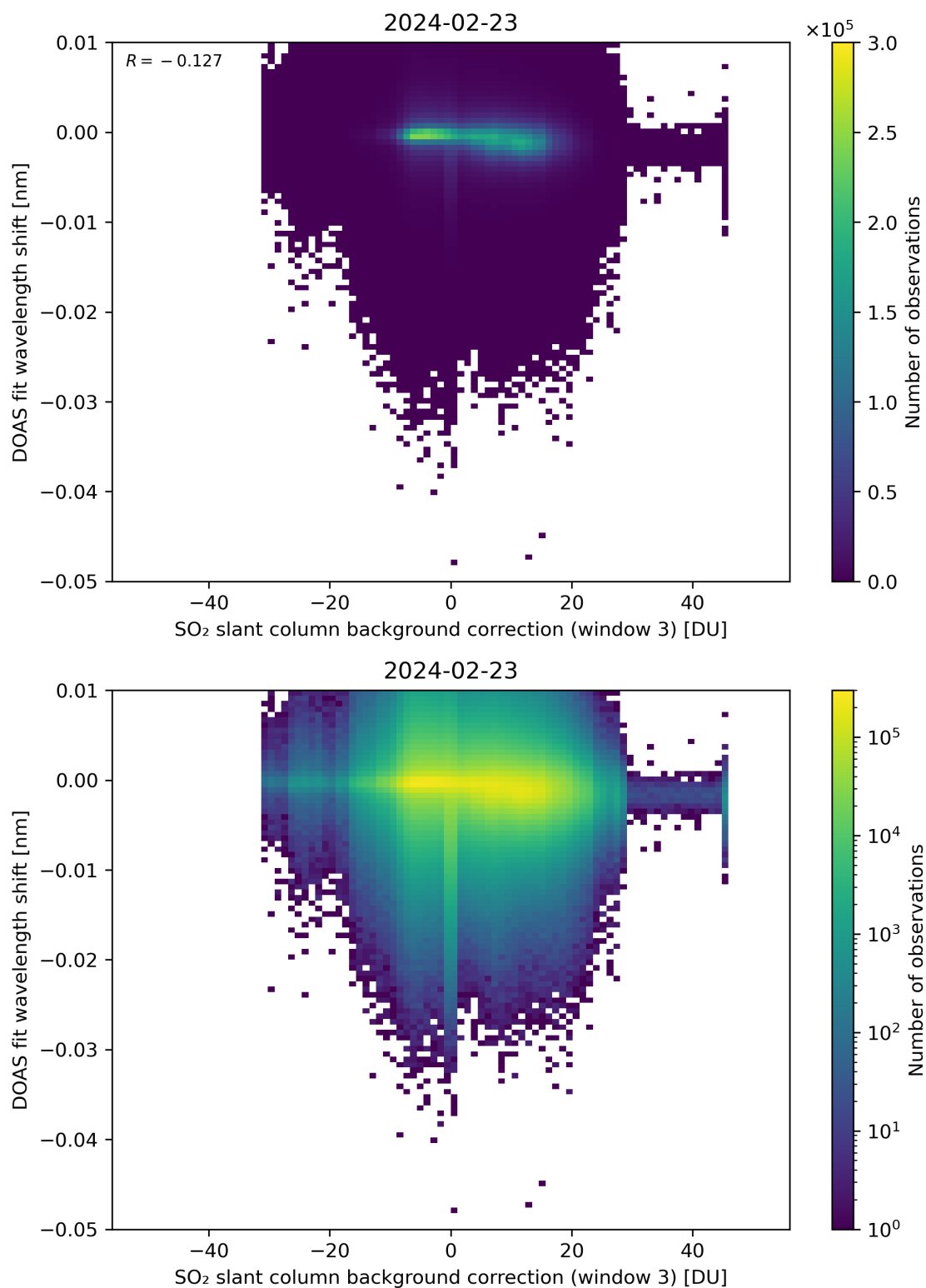
Figure 121: Scatter density plot of “SO 2 slant column background correction (window 3)” against “DOAS fit wavelength shift” for 2024-02-22 to 2024-02-24.
