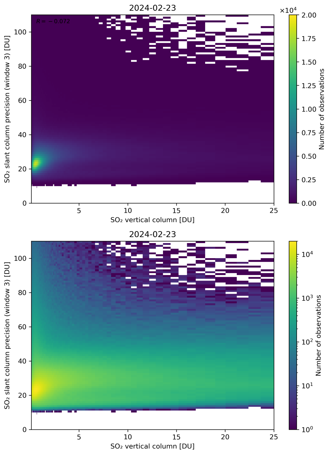
Figure 304: Scatter density plot of “SO 2 vertical column” against “SO 2 slant column precision (window 3)” for 2024-02-22 to 2024-02-24.
