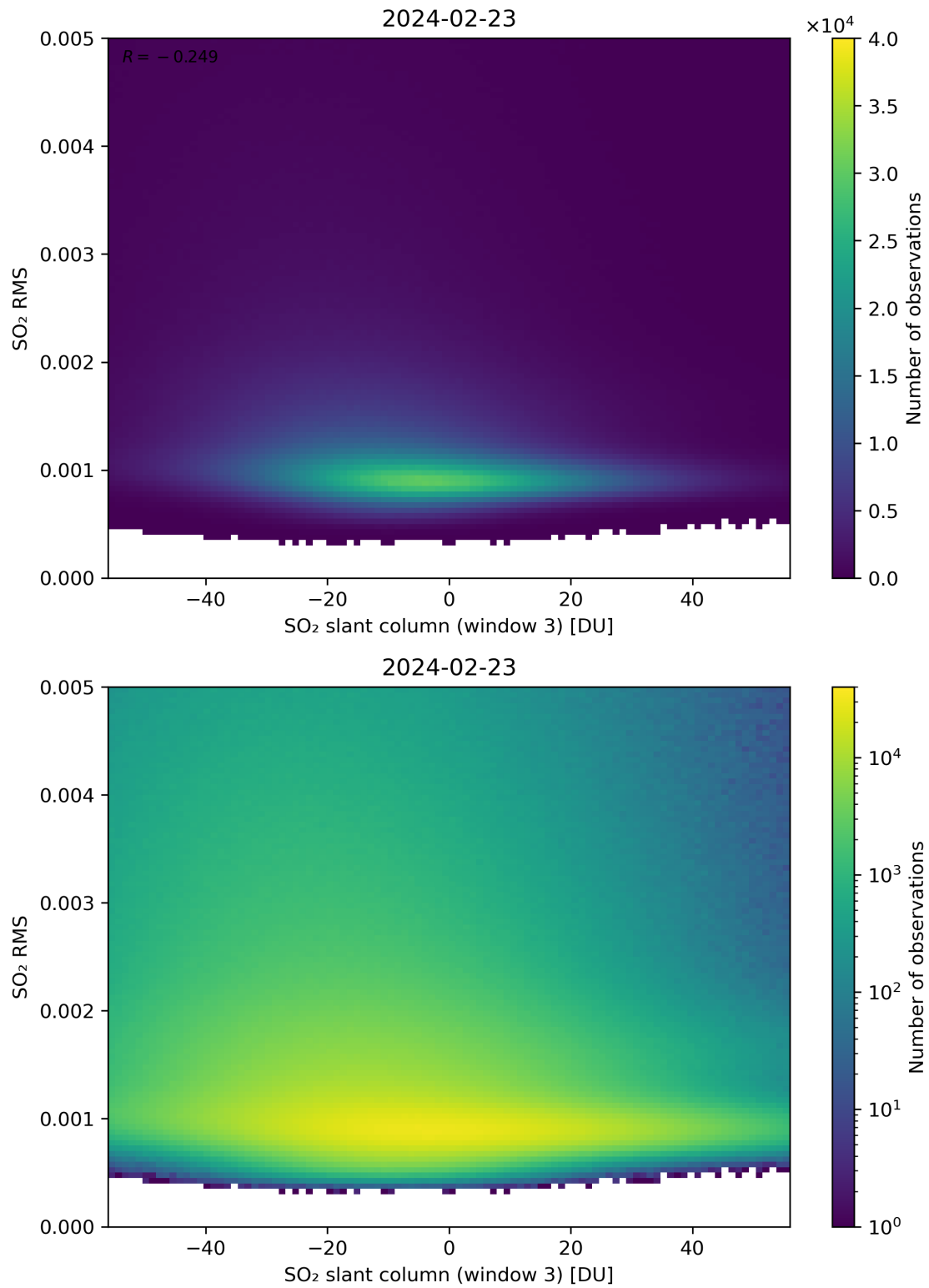
Figure 256: Scatter density plot of “SO 2 slant column (window 3)” against “SO 2 RMS” for 2024-02-22 to 2024-02-24.
