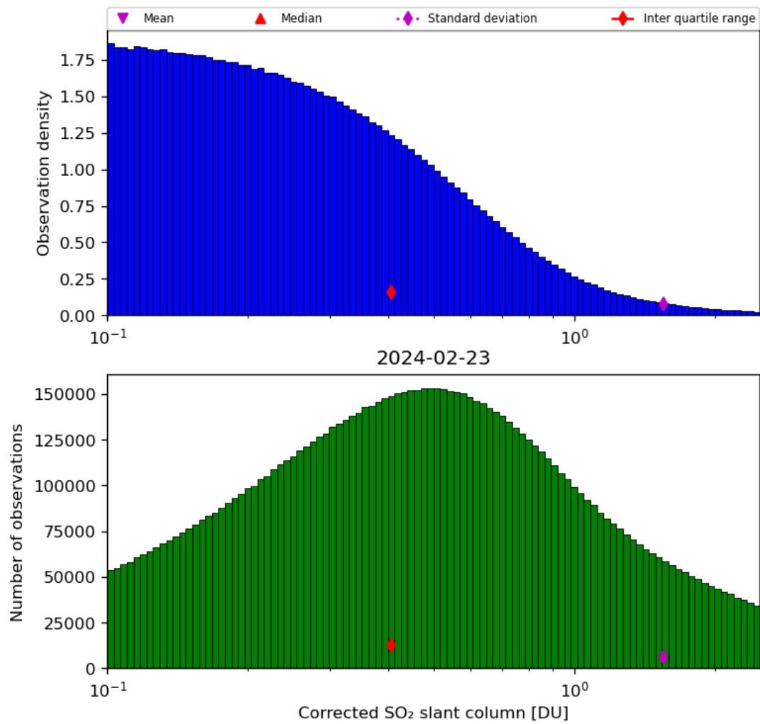
Figure 55: Histogram of “Corrected SO 2 slant column” for 2024-02-22 to 2024-02-24
