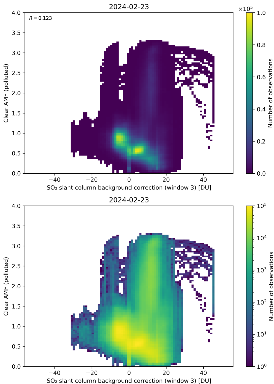
Figure 124: Scatter density plot of “SO 2 slant column background correction (window 3)” against “Clear AMF (polluted)” for 2024-02-22 to 2024-02-24.
