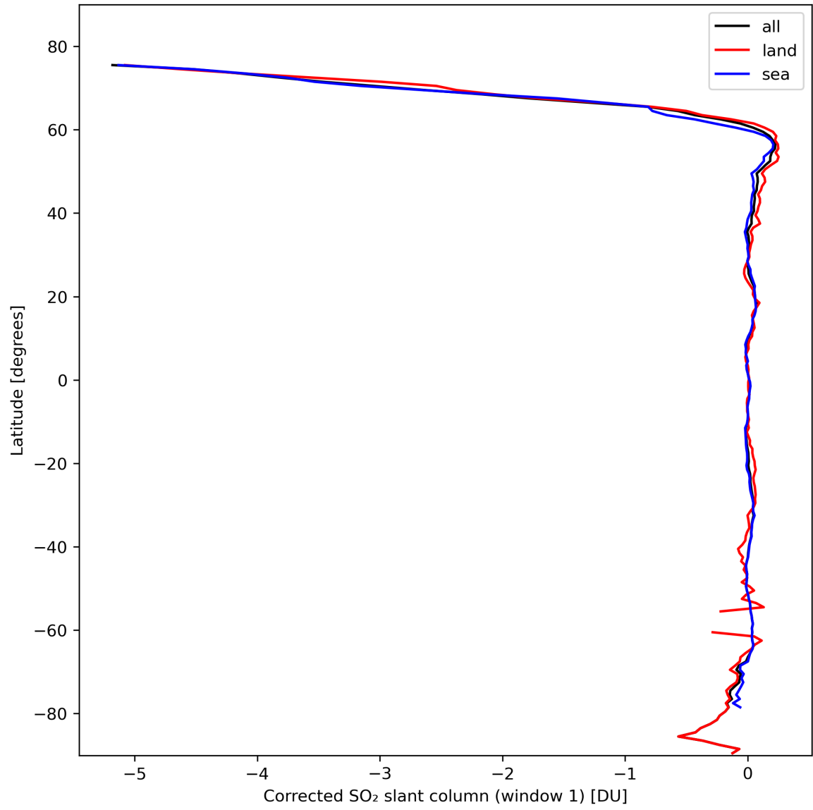
Figure 35: Zonal average of “Corrected SO 2 slant column (window 1)” for 2024-02-22 to 2024-02-24.
