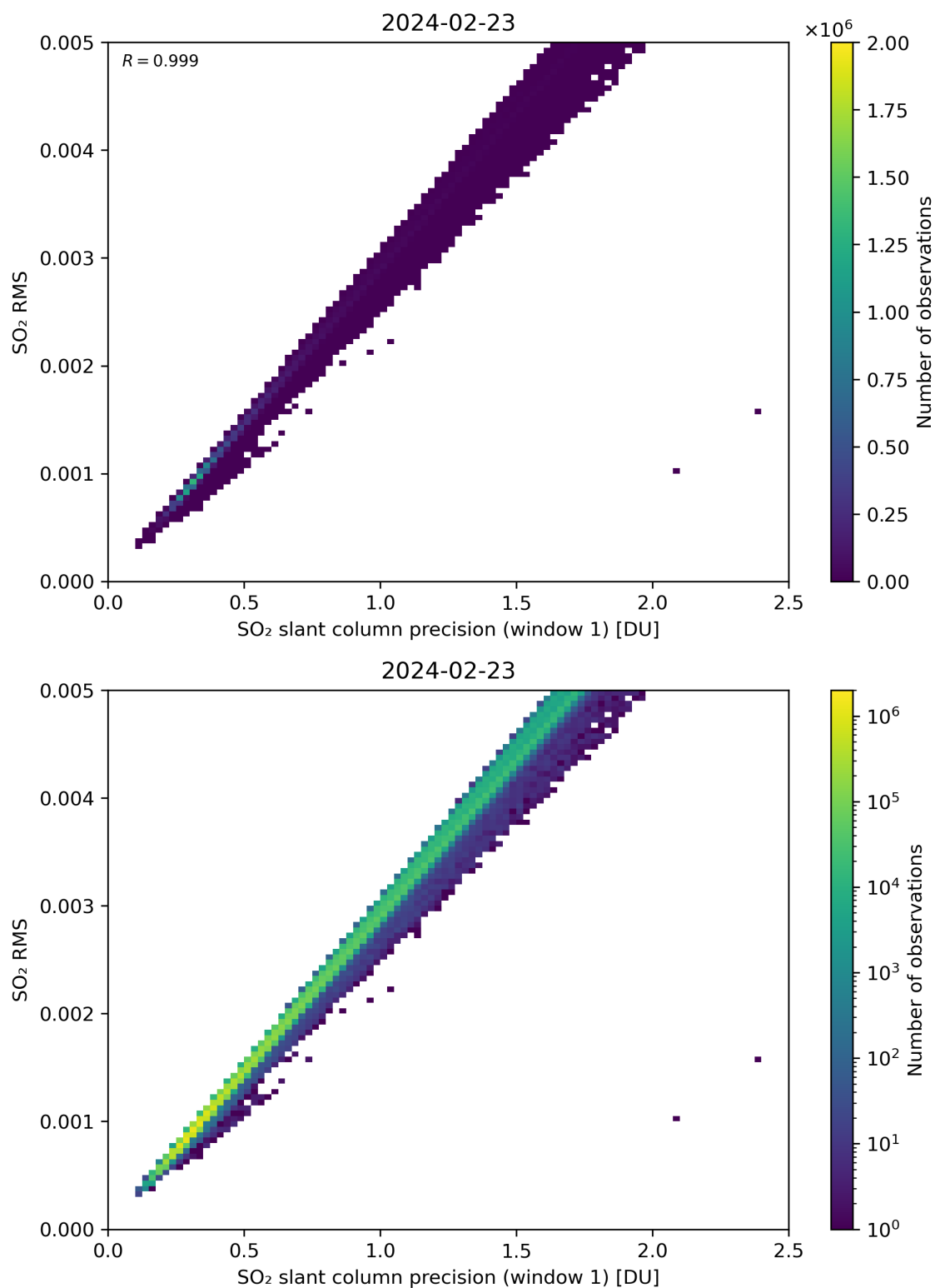
Figure 223: Scatter density plot of “SO 2 slant column precision (window 1)” against “SO 2 RMS” for 2024-02-22 to 2024-02-24.
