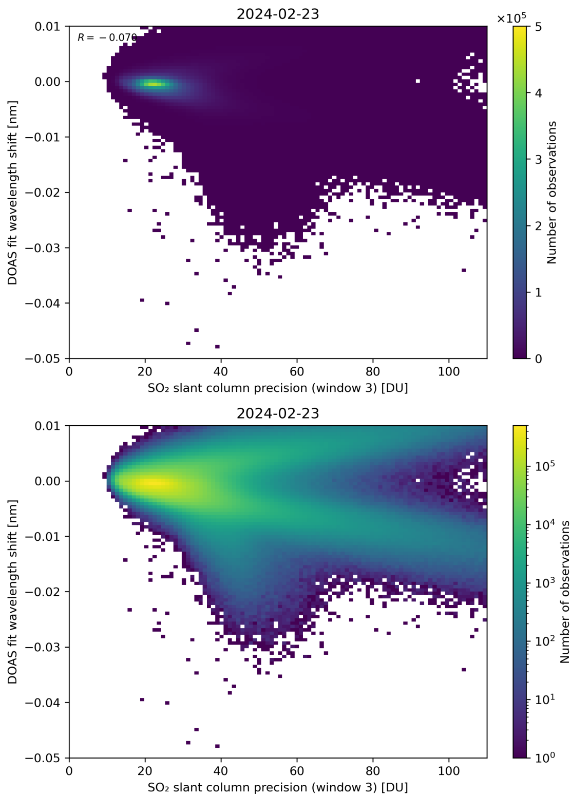
Figure 258: Scatter density plot of “SO 2 slant column precision (window 3)” against “DOAS fit wavelength shift” for 2024-02-22 to 2024-02-24.
