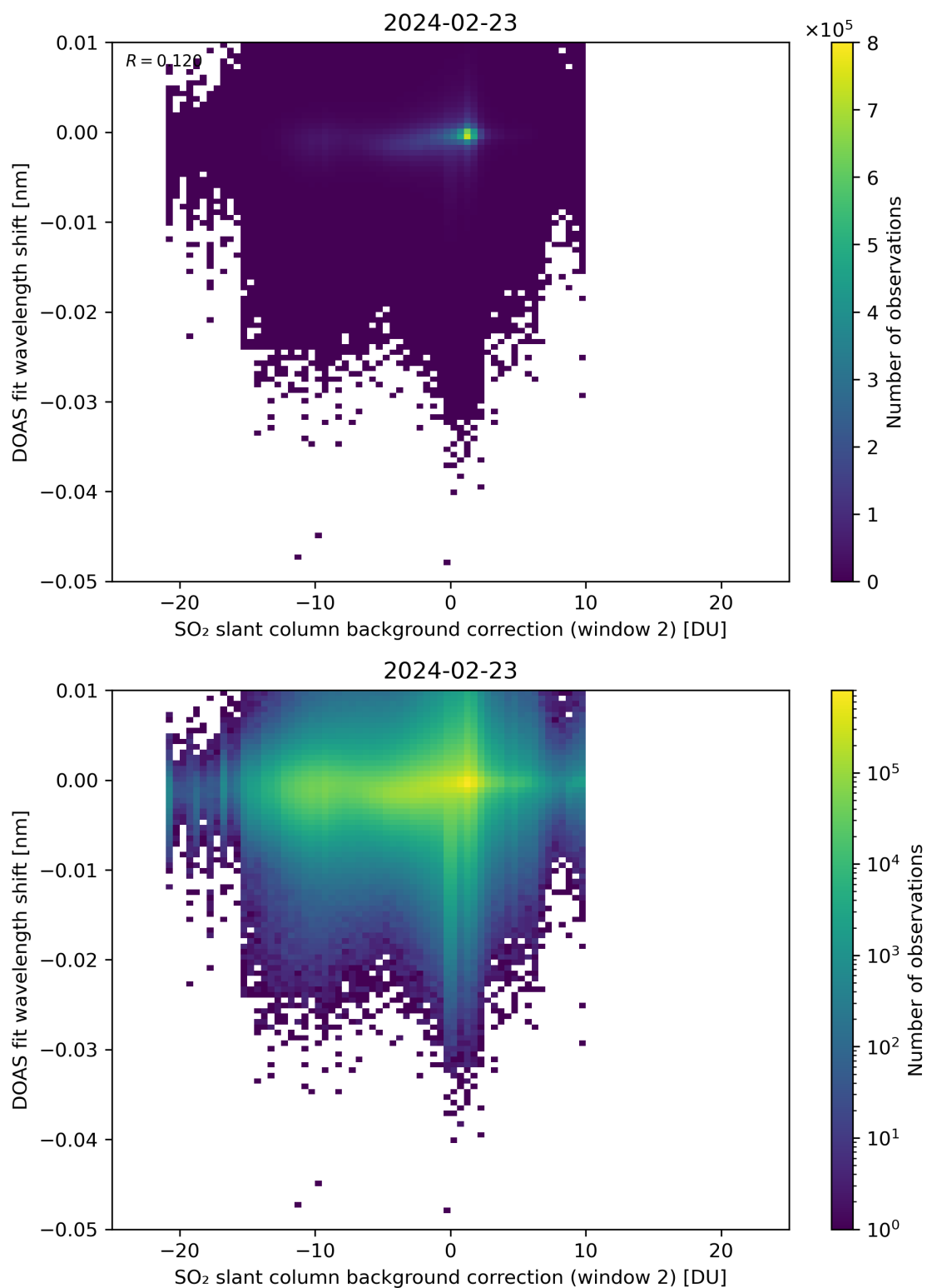
Figure 112: Scatter density plot of “SO 2 slant column background correction (window 2)” against “DOAS fit wavelength shift” for 2024-02-22 to 2024-02-24.
