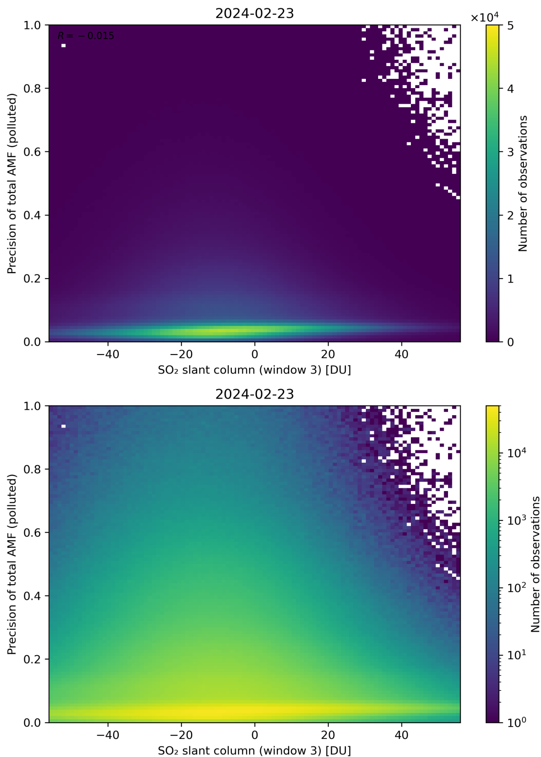
Figure 269: Scatter density plot of “SO 2 slant column (window 3)” against “Precision of total AMF (polluted)” for 2024-02-22 to 2024-02-24.
