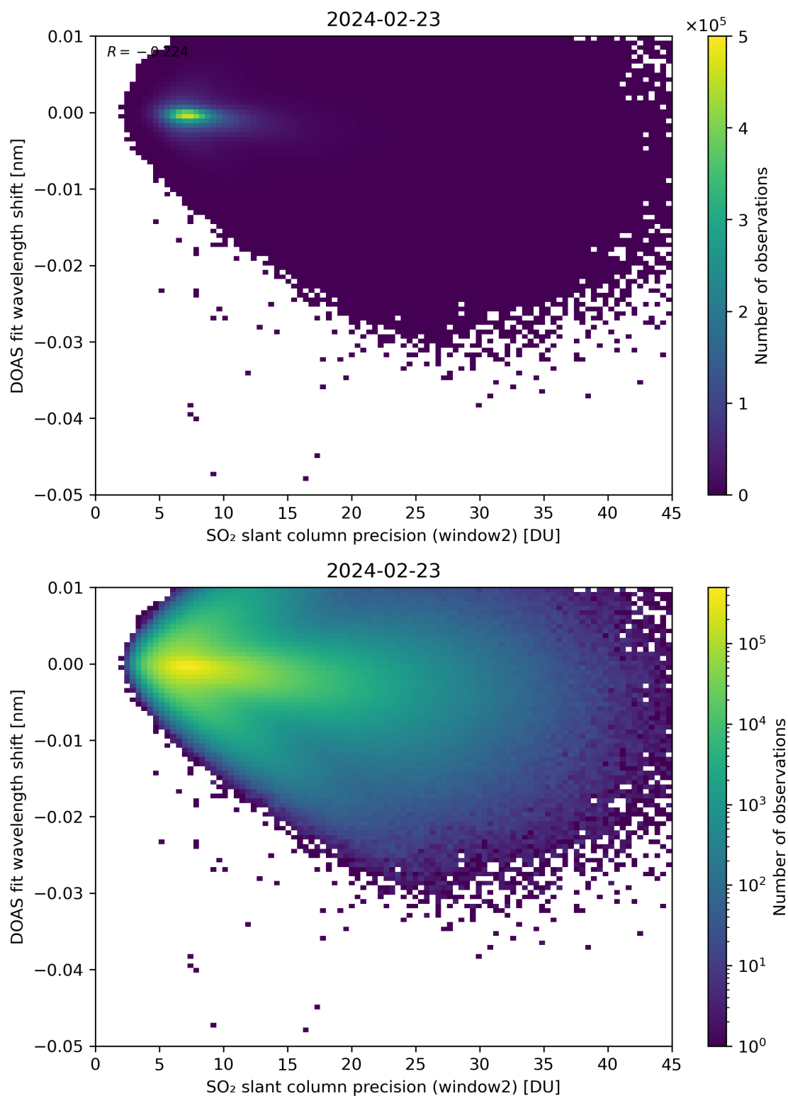
Figure 243: Scatter density plot of “SO 2 slant column precision (window2)” against “DOAS fit wavelength shift” for 2024-02-22 to 2024-02-24.
