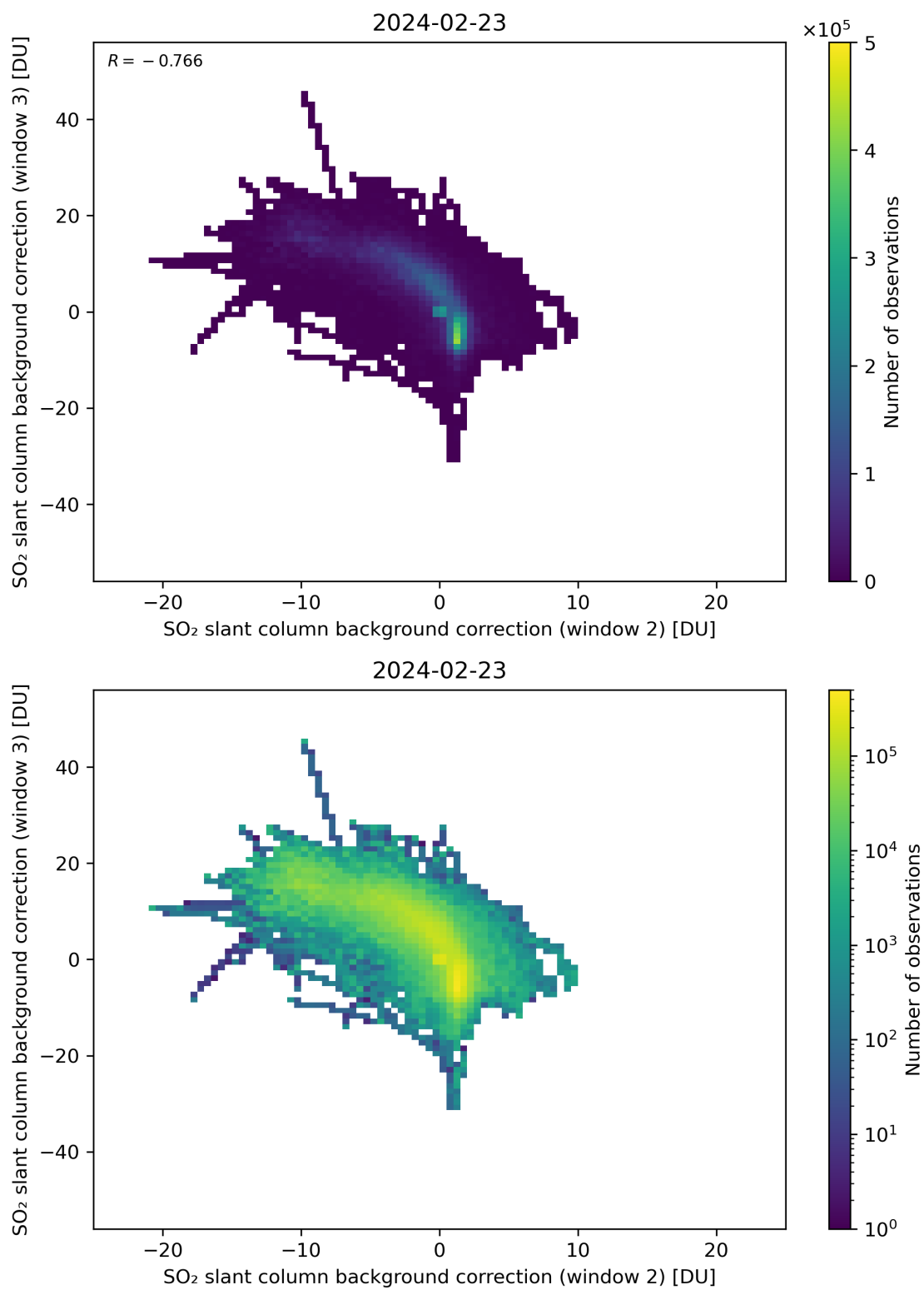
Figure 111: Scatter density plot of “SO 2 slant column background correction (window 2)” against “SO 2 slant column background correction (window 3)” for 2024-02-22 to 2024-02-24.
