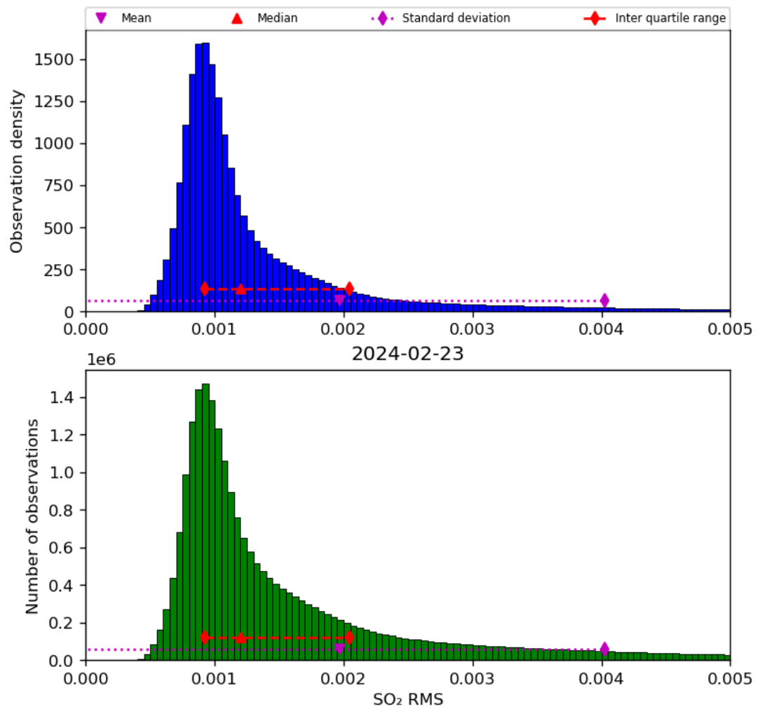
Figure 70: Histogram of “SO 2 RMS” for 2024-02-22 to 2024-02-24
