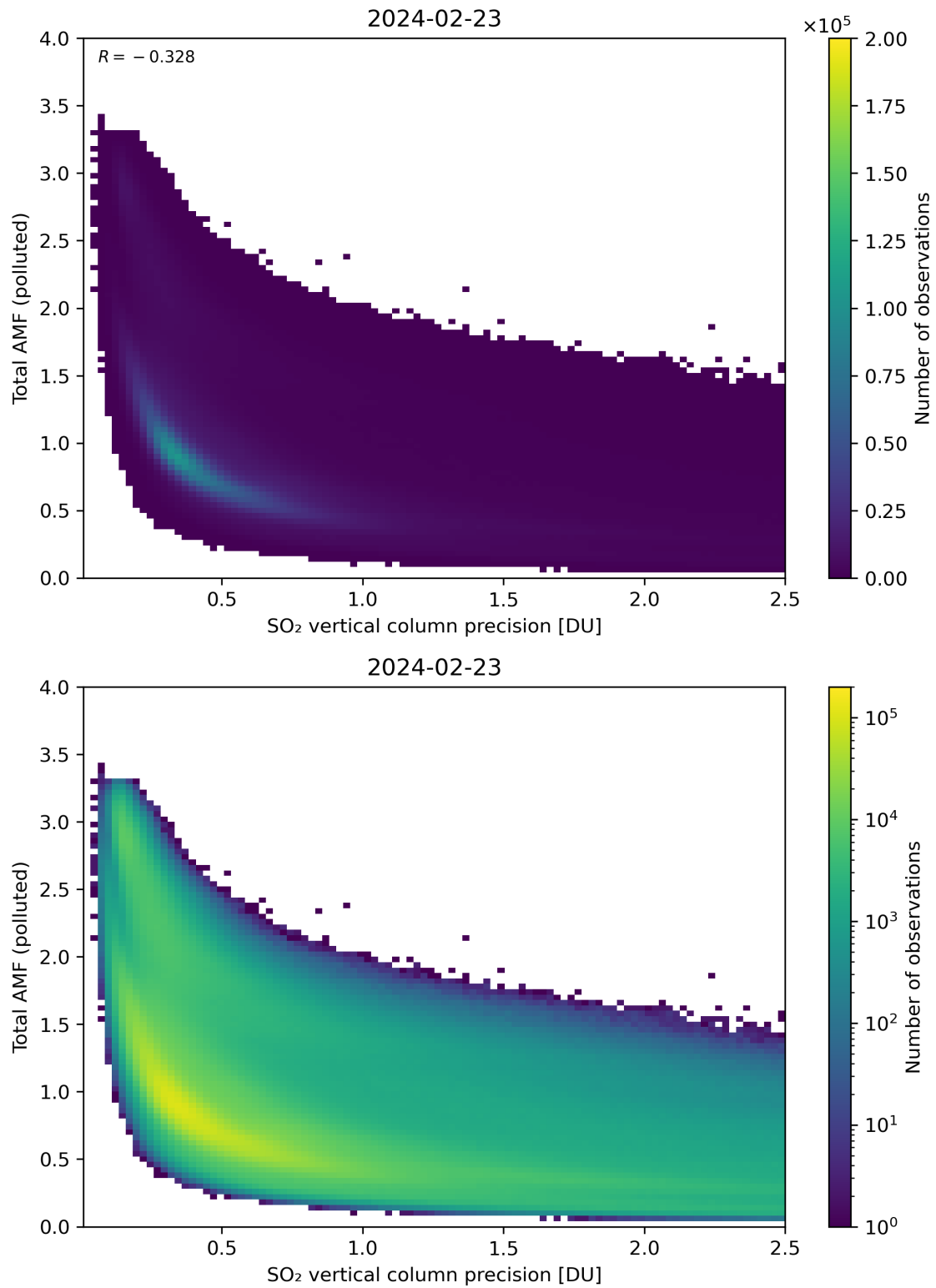
Figure 294: Scatter density plot of “SO 2 vertical column precision” against “Total AMF (polluted)” for 2024-02-22 to 2024-02-24.
