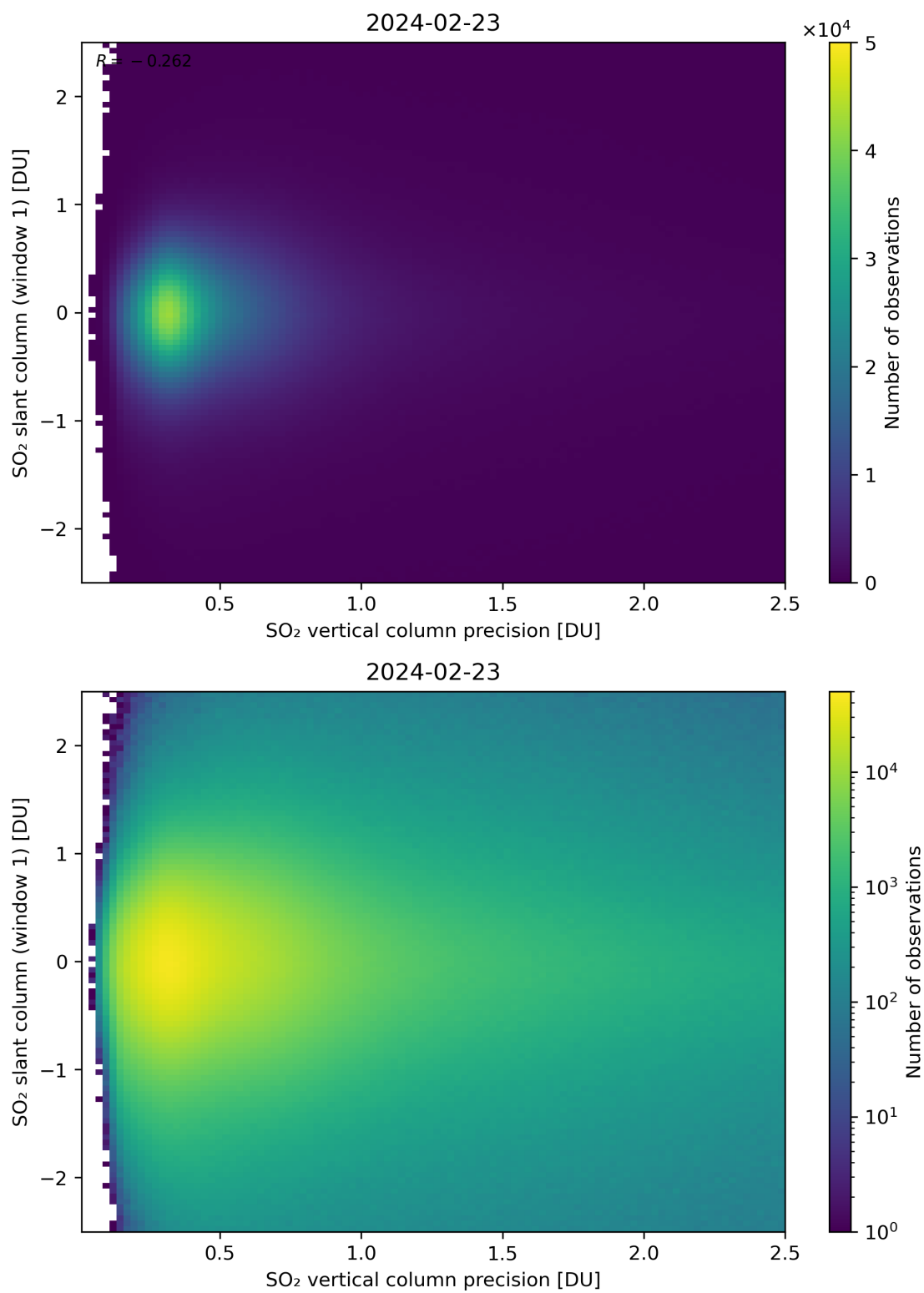
Figure 289: Scatter density plot of “SO 2 vertical column precision” against “SO 2 slant column (window 1)” for 2024-02-22 to 2024-02-24.
