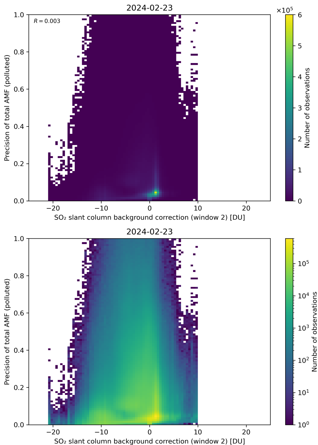
Figure 120: Scatter density plot of “SO 2 slant column background correction (window 2)” against “Precision of total AMF (polluted)” for 2024-02-22 to 2024-02-24.
