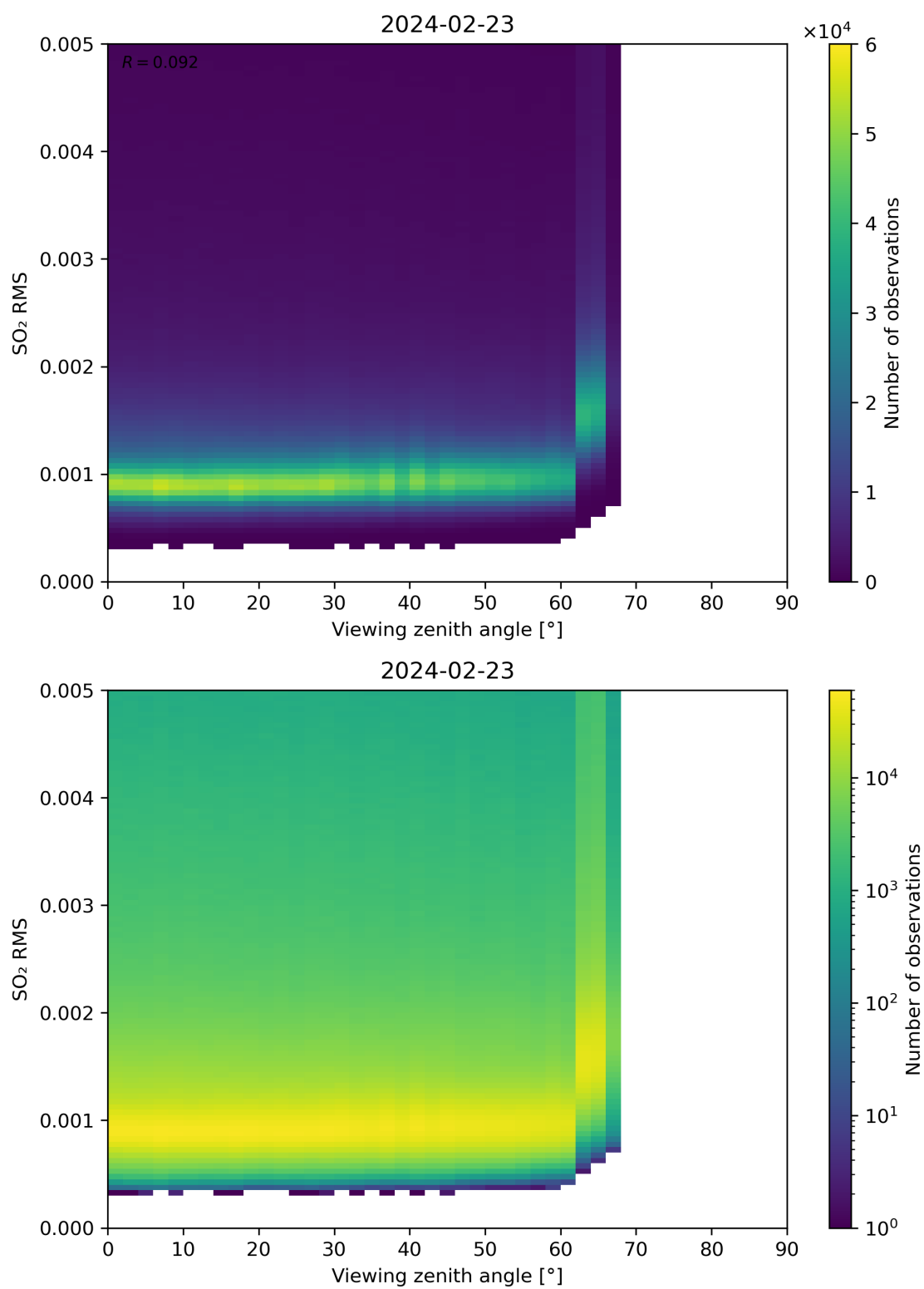
Figure 313: Scatter density plot of “Viewing zenith angle” against “SO 2 RMS” for 2024-02-22 to 2024-02-24.
