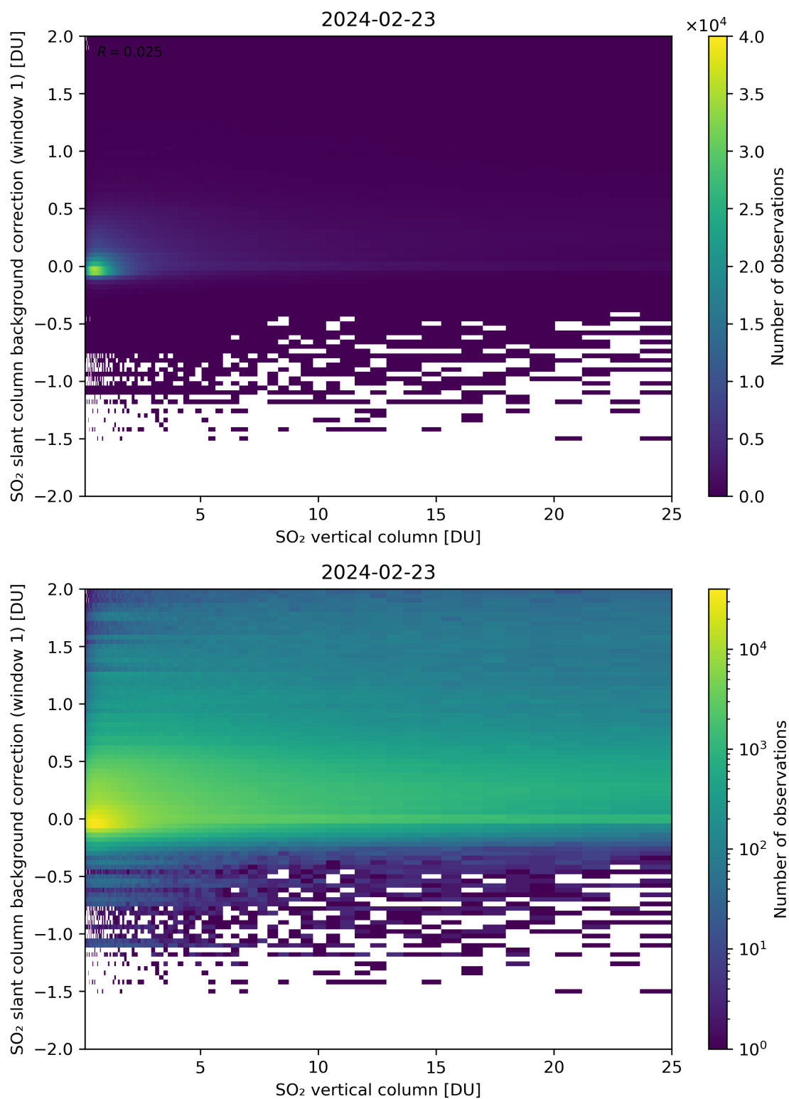
Figure 273: Scatter density plot of “SO 2 vertical column” against “SO 2 slant column background correction (window 1)” for 2024-02-22 to 2024-02-24.
