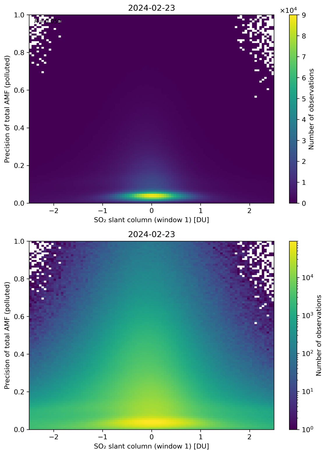
Figure 240: Scatter density plot of “SO 2 slant column (window 1)” against “Precision of total AMF (polluted)” for 2024-02-22 to 2024-02-24.
