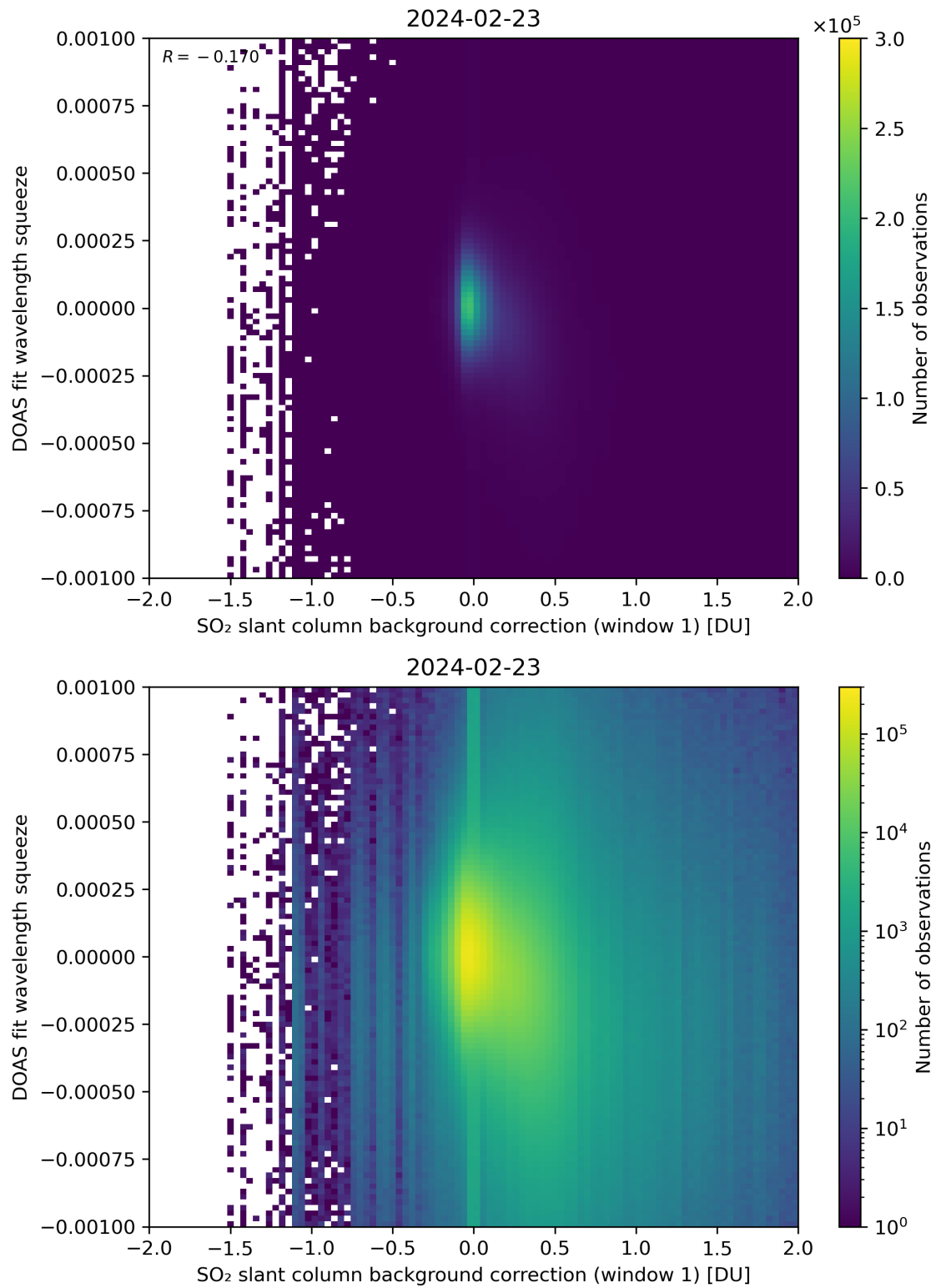
Figure 101: Scatter density plot of “SO 2 slant column background correction (window 1)” against “DOAS fit wavelength squeeze” for 2024-02-22 to 2024-02-24.
