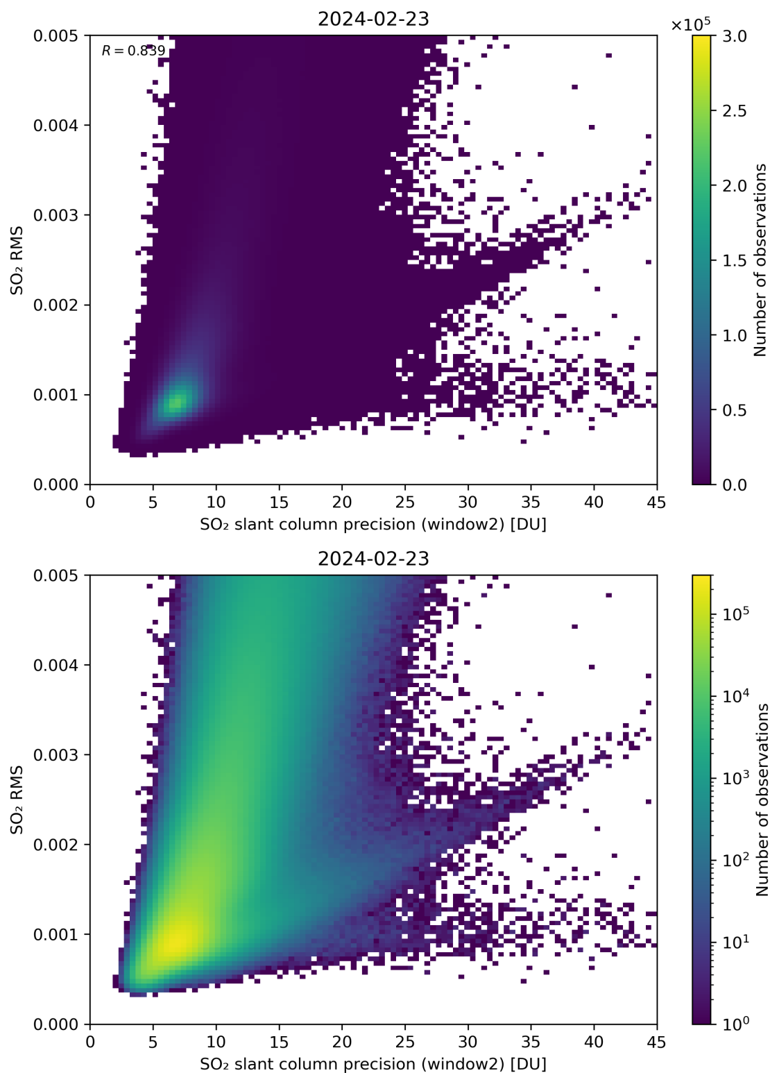
Figure 245: Scatter density plot of “SO 2 slant column precision (window2)” against “SO 2 RMS” for 2024-02-22 to 2024-02-24.
