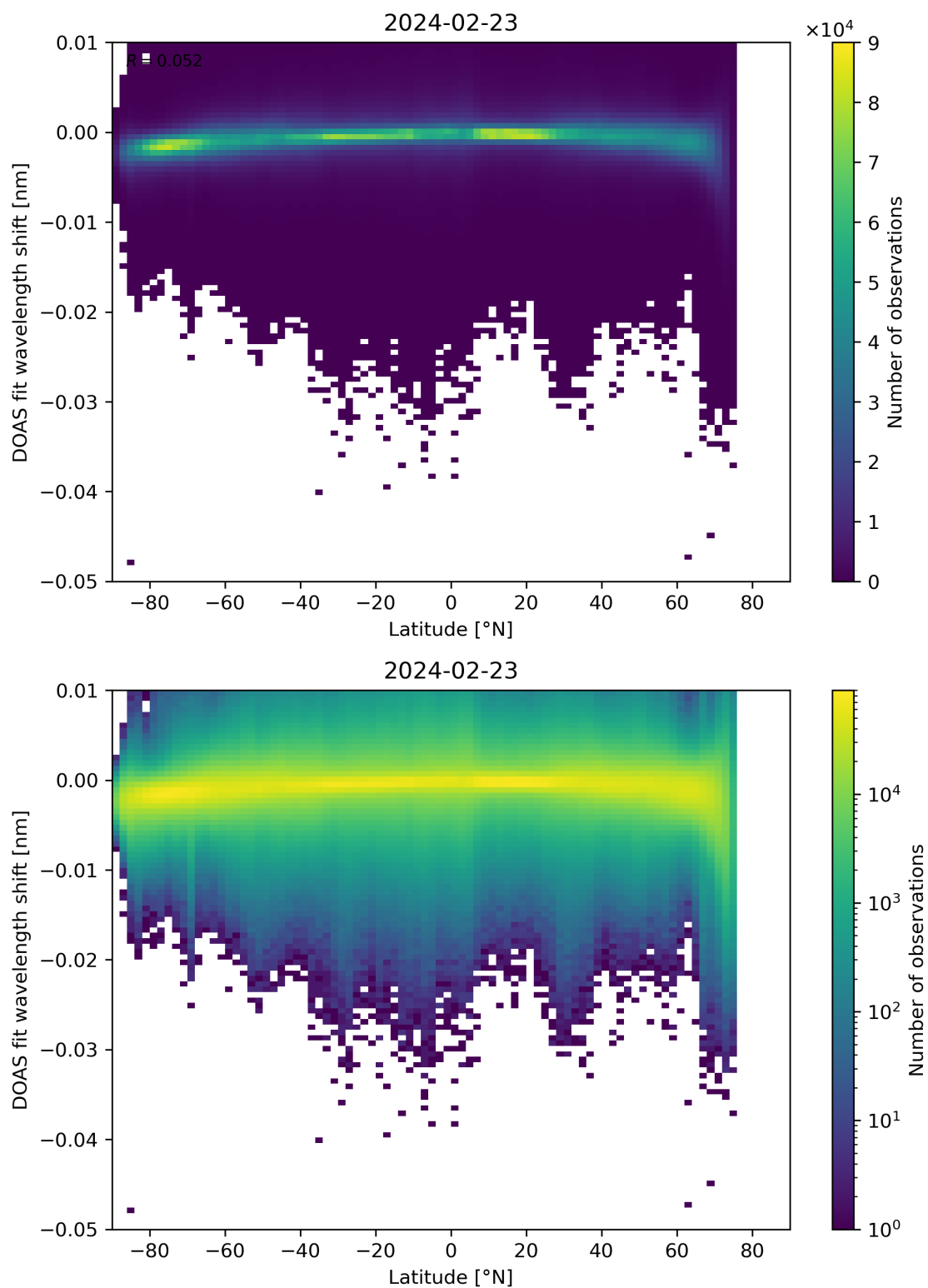
Figure 142: Scatter density plot of “Latitude” against “DOAS fit wavelength shift” for 2024-02-22 to 2024-02-24.
