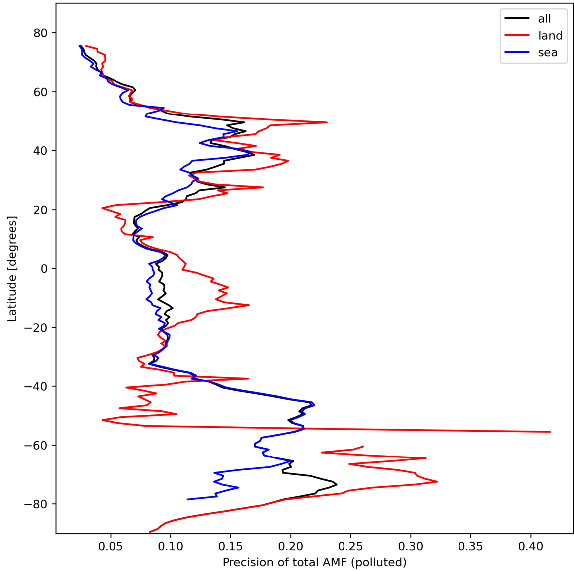
Figure 49: Zonal average of “Precision of total AMF (polluted)” for 2024-02-22 to 2024-02-24.
