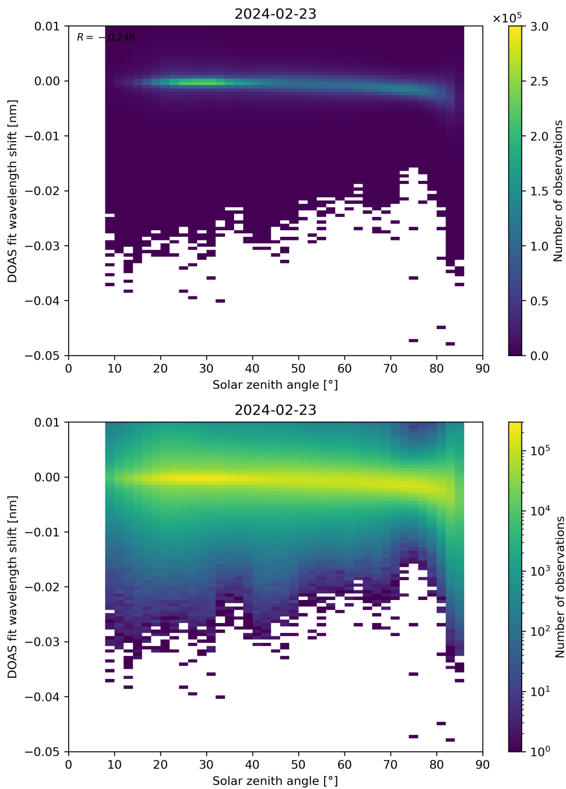
Figure 161: Scatter density plot of “Solar zenith angle” against “DOAS fit wavelength shift” for 2024-02-22 to 2024-02-24.
