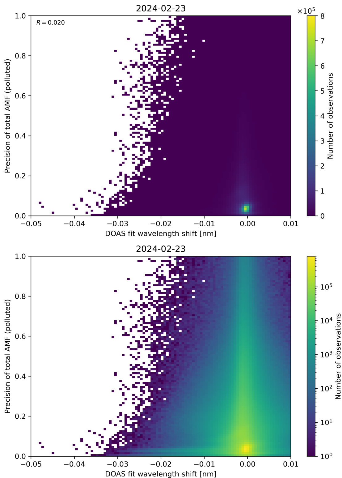
Figure 131: Scatter density plot of “DOAS fit wavelength shift” against “Precision of total AMF (polluted)” for 2024-02-22 to 2024-02-24.
