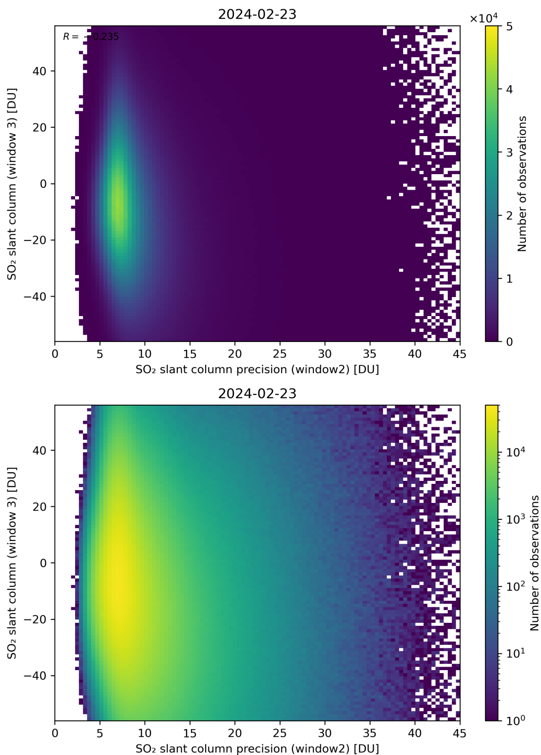
Figure 249: Scatter density plot of “SO 2 slant column precision (window2)” against “SO 2 slant column (window 3)” for 2024-02-22 to 2024-02-24.
