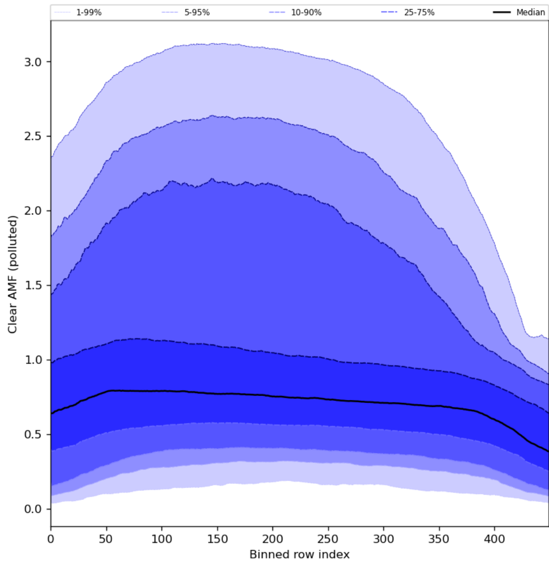
Figure 96: Along track statistics of “Clear AMF (polluted)” for 2024-02-22 to 2024-02-24
