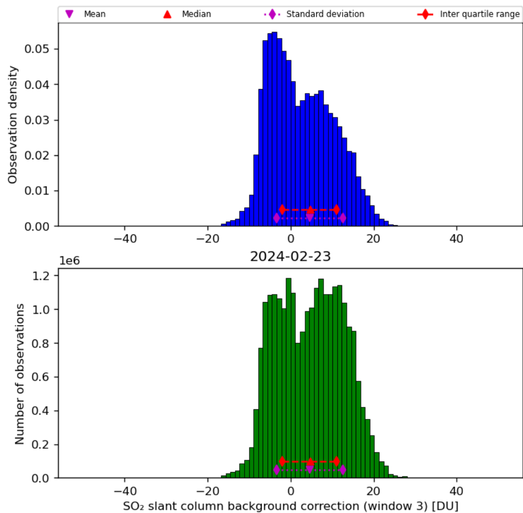
Figure 67: Histogram of “SO 2 slant column background correction (window 3)” for 2024-02-22 to 2024-02-24
