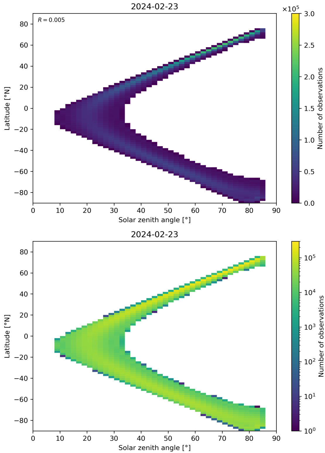
Figure 164: Scatter density plot of “Solar zenith angle” against “Latitude” for 2024-02-22 to 2024-02-24.
