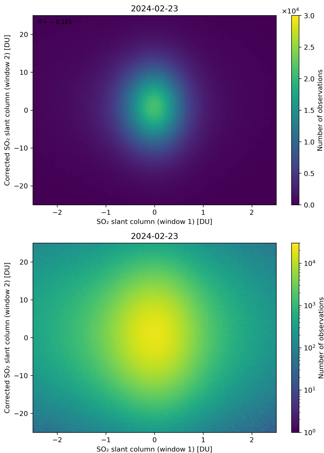
Figure 233: Scatter density plot of “SO 2 slant column (window 1)” against “Corrected SO 2 slant column (window 2)” for 2024-02-22 to 2024-02-24.
