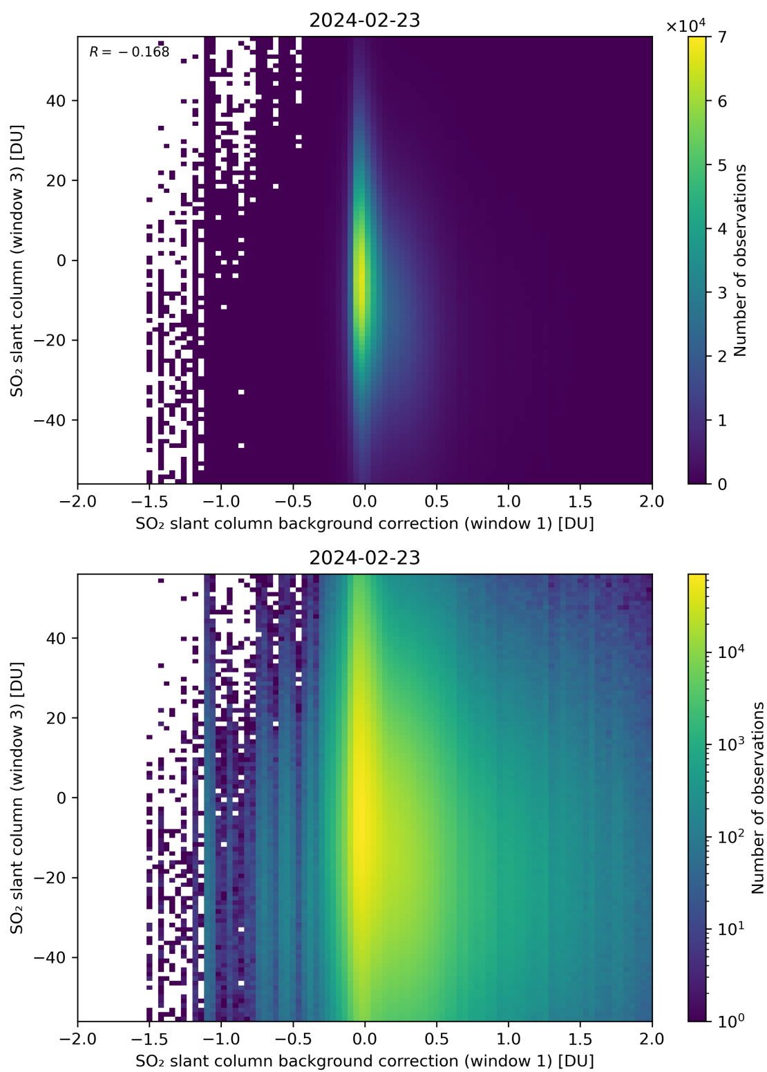
Figure 107: Scatter density plot of “SO 2 slant column background correction (window 1)” against “SO 2 slant column (window 3)” for 2024-02-22 to 2024-02-24.
