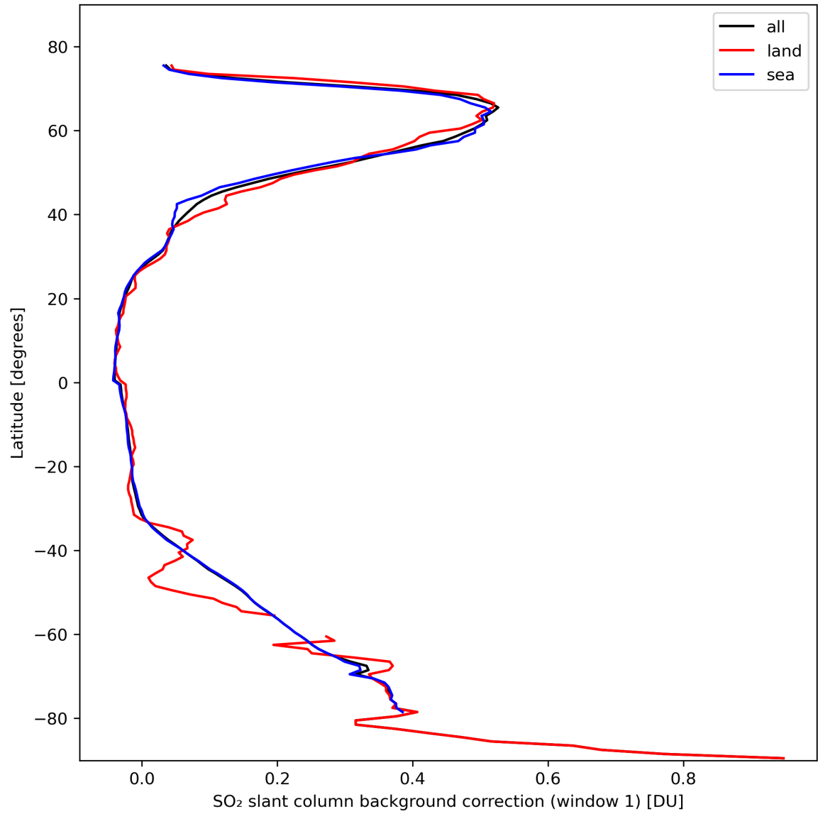
Figure 36: Zonal average of “SO 2 slant column background correction (window 1)” for 2024-02-22 to 2024-02-24.
