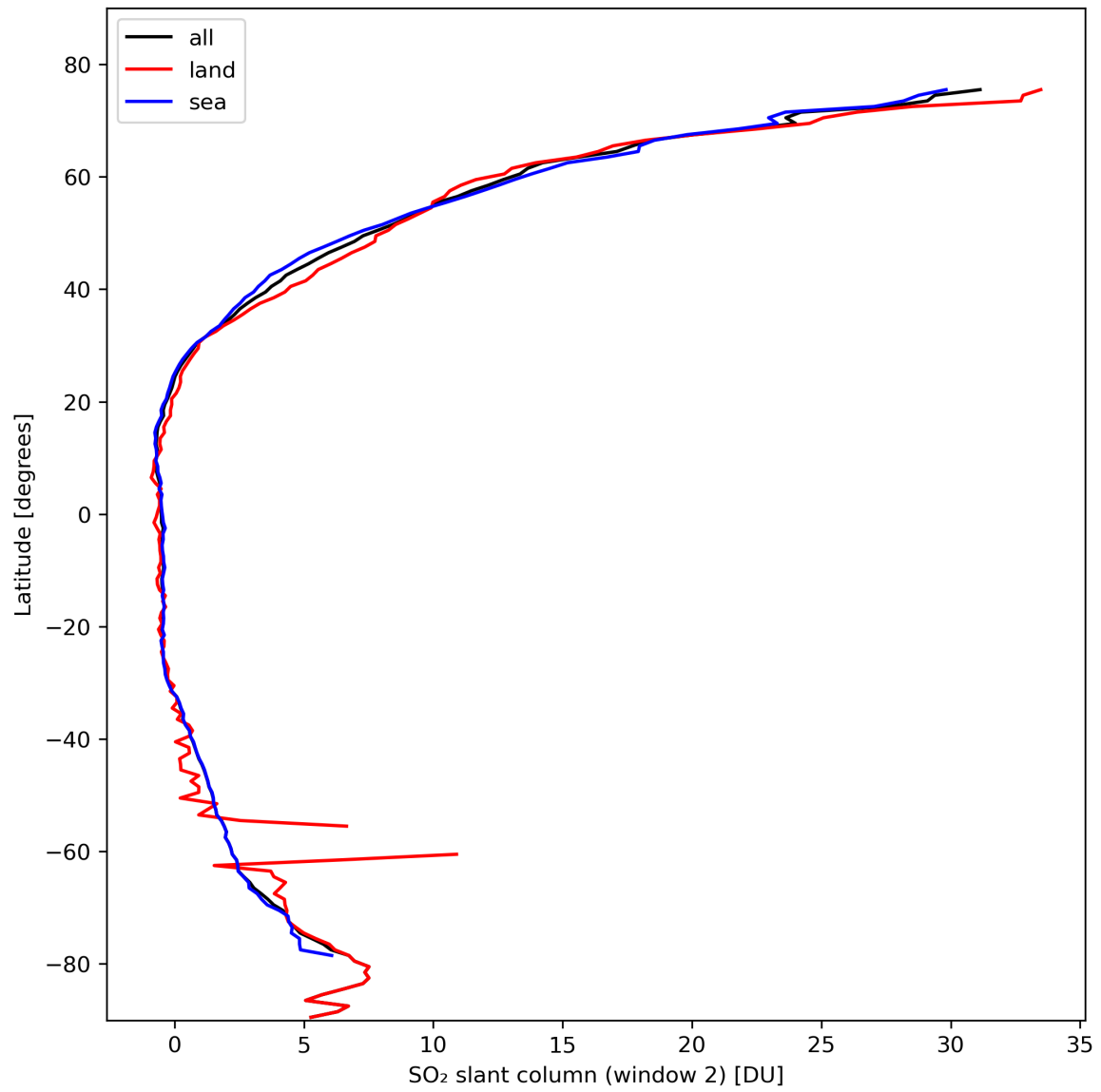
Figure 37: Zonal average of “SO 2 slant column (window 2)” for 2024-02-22 to 2024-02-24.
