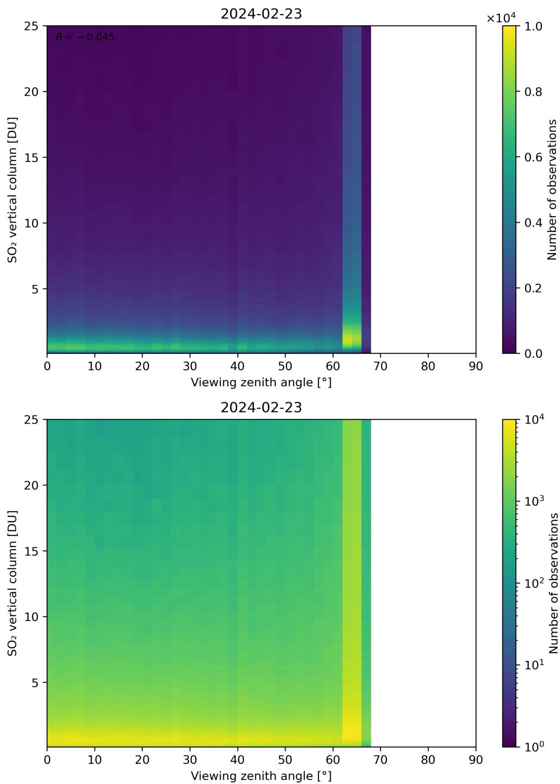
Figure 327: Scatter density plot of “Viewing zenith angle” against “SO 2 vertical column” for 2024-02-22 to 2024-02-24.
