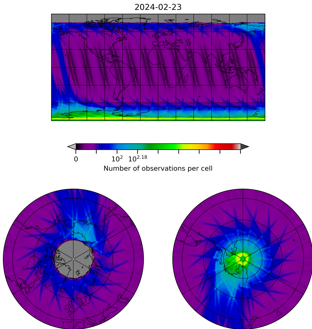
Figure 28: Map of the number of observations for 2024-02-22 to 2024-02-24
