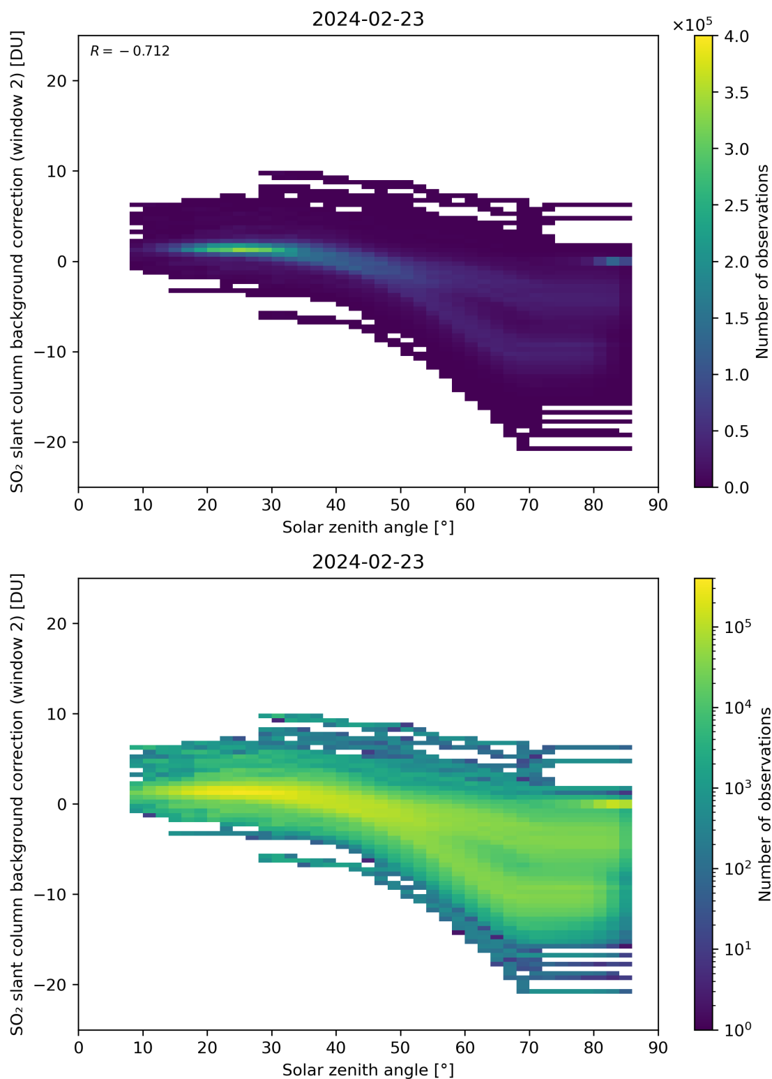
Figure 159: Scatter density plot of “Solar zenith angle” against “SO 2 slant column background correction (window 2)” for 2024-02-22 to 2024-02-24.
