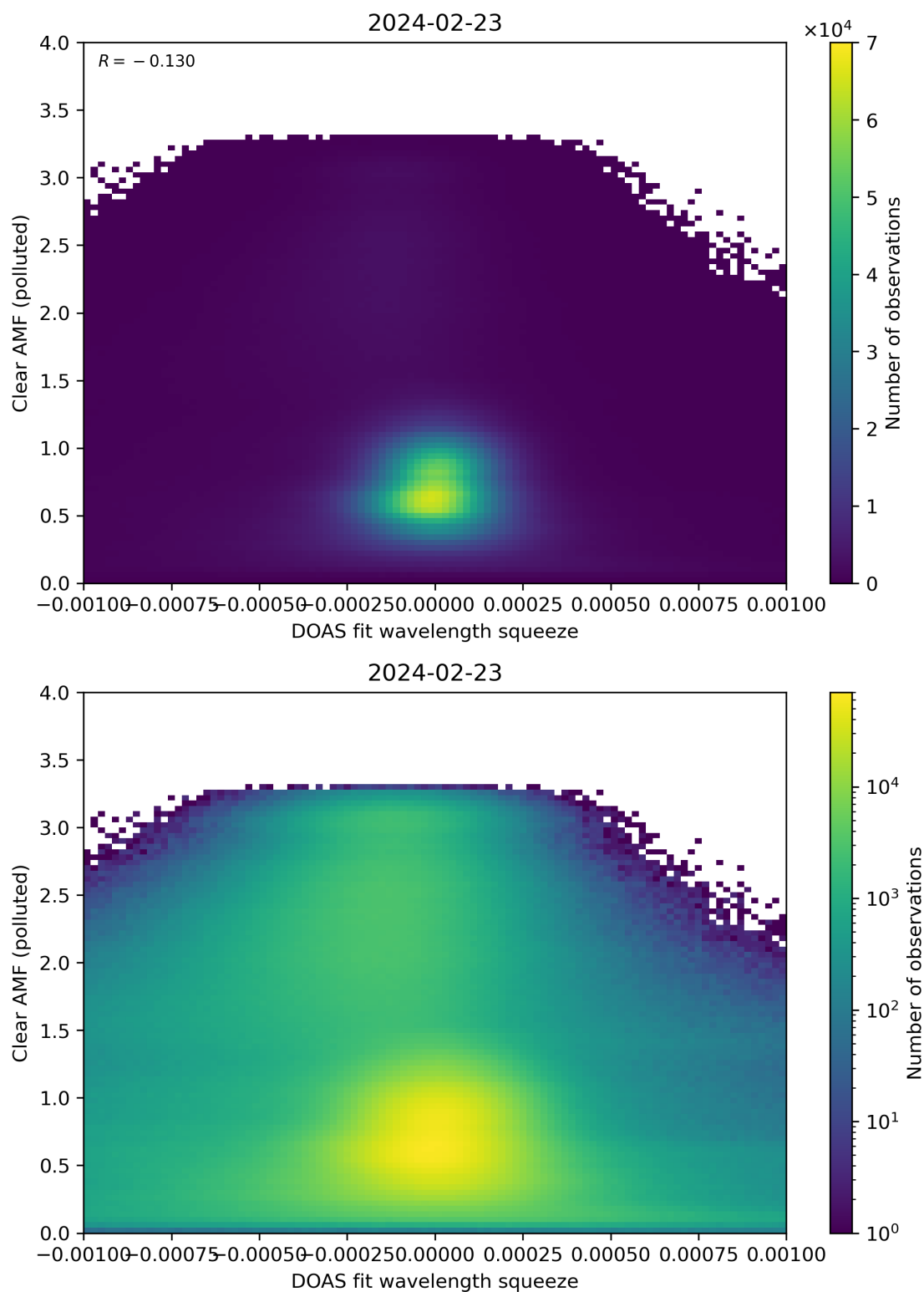
Figure 133: Scatter density plot of “DOAS fit wavelength squeeze” against “Clear AMF (polluted)” for 2024-02-22 to 2024-02-24.
