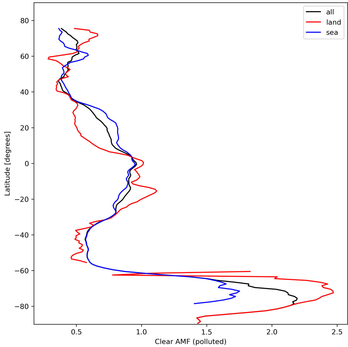
Figure 50: Zonal average of “Clear AMF (polluted)” for 2024-02-22 to 2024-02-24.
