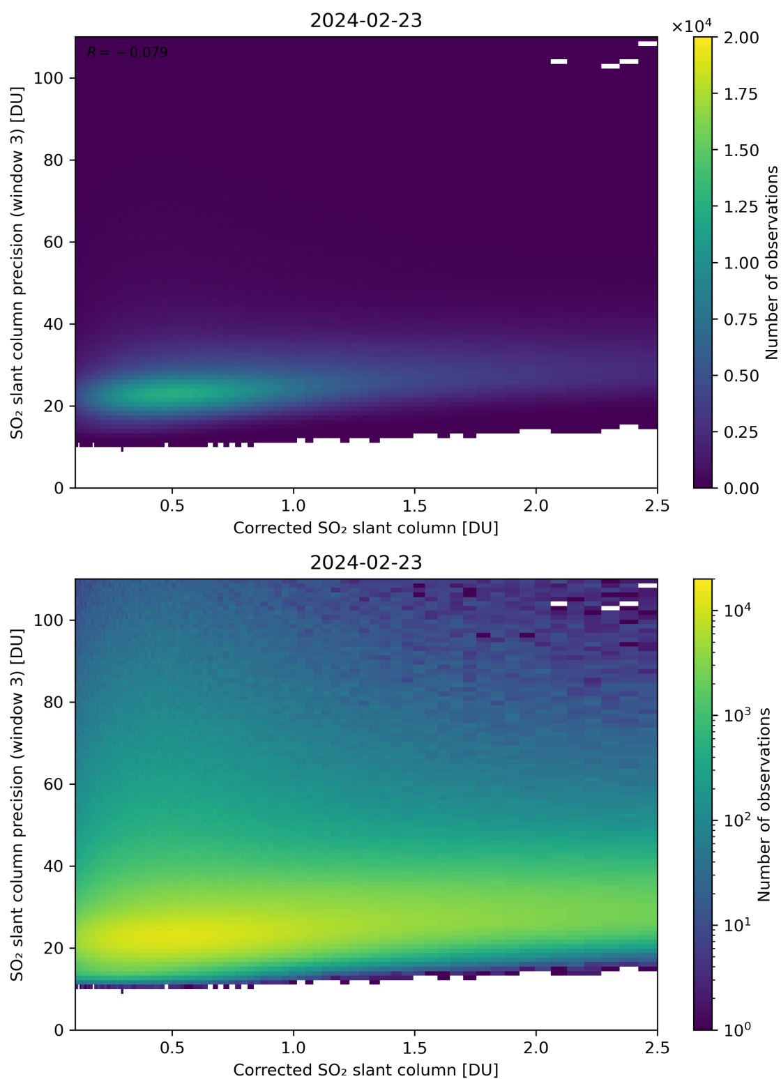
Figure 191: Scatter density plot of “Corrected SO 2 slant column” against “SO 2 slant column precision (window 3)” for 2024-02-22 to 2024-02-24.
