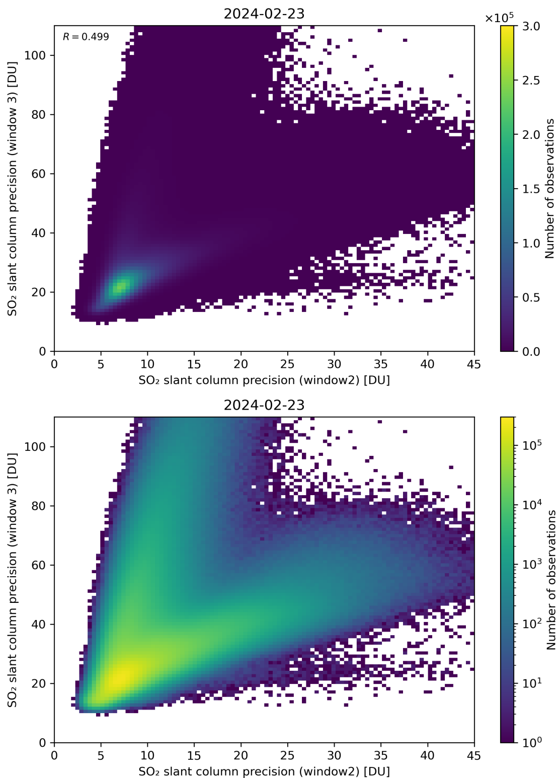
Figure 250: Scatter density plot of “SO 2 slant column precision (window2)” against “SO 2 slant column precision (window 3)” for 2024-02-22 to 2024-02-24.
