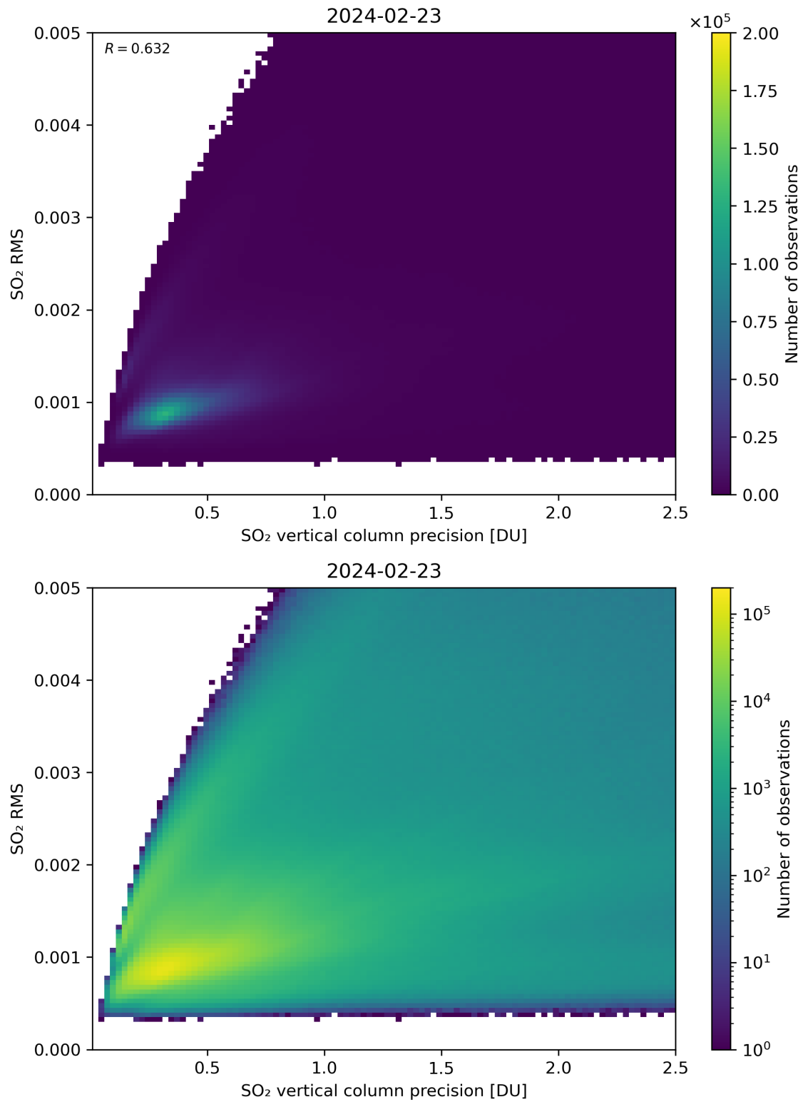
Figure 284: Scatter density plot of “SO 2 vertical column precision” against “SO 2 RMS” for 2024-02-22 to 2024-02-24.
