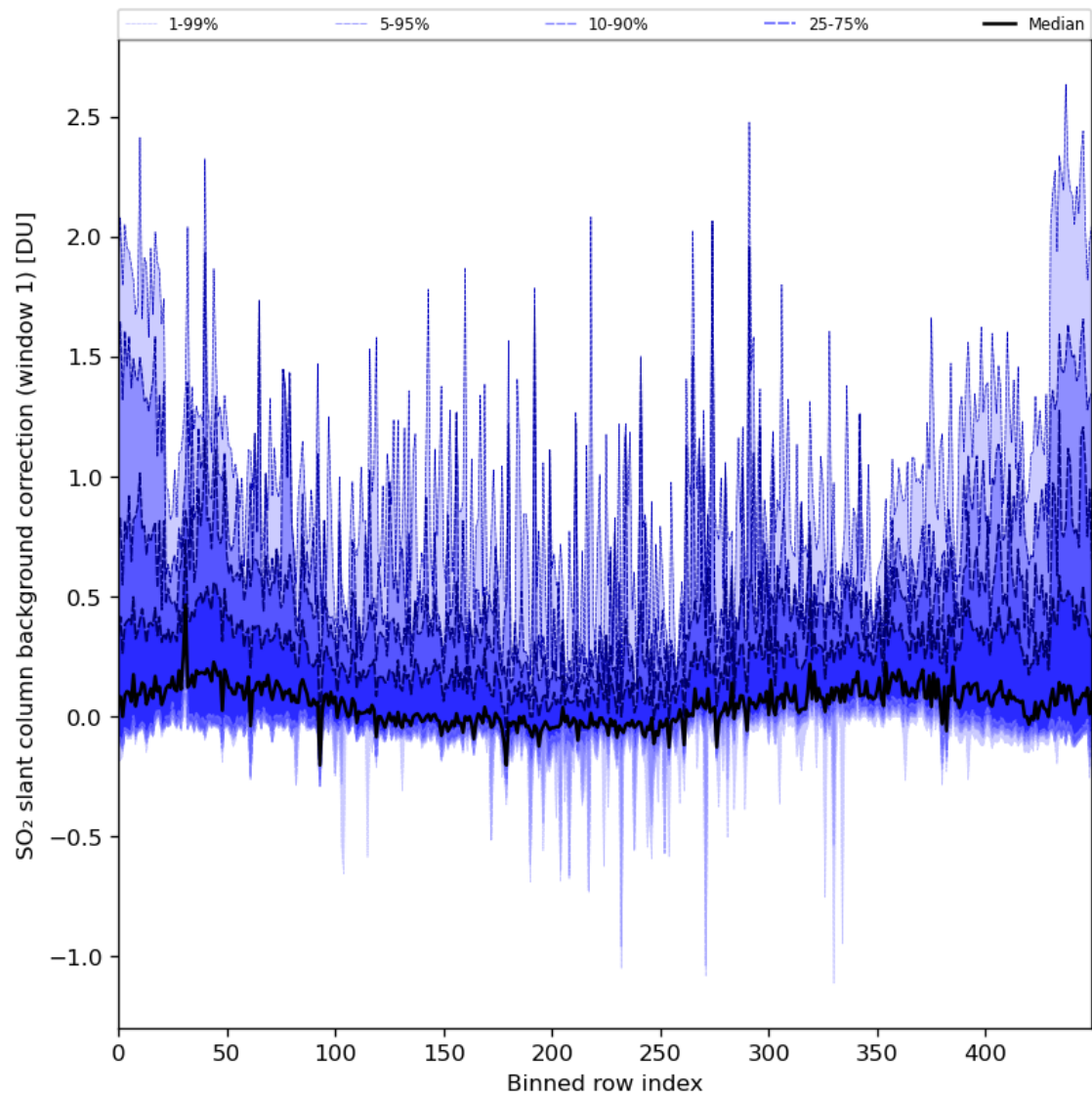
Figure 82: Along track statistics of “SO 2 slant column background correction (window 1)” for 2024-02-22 to 2024-02-24
