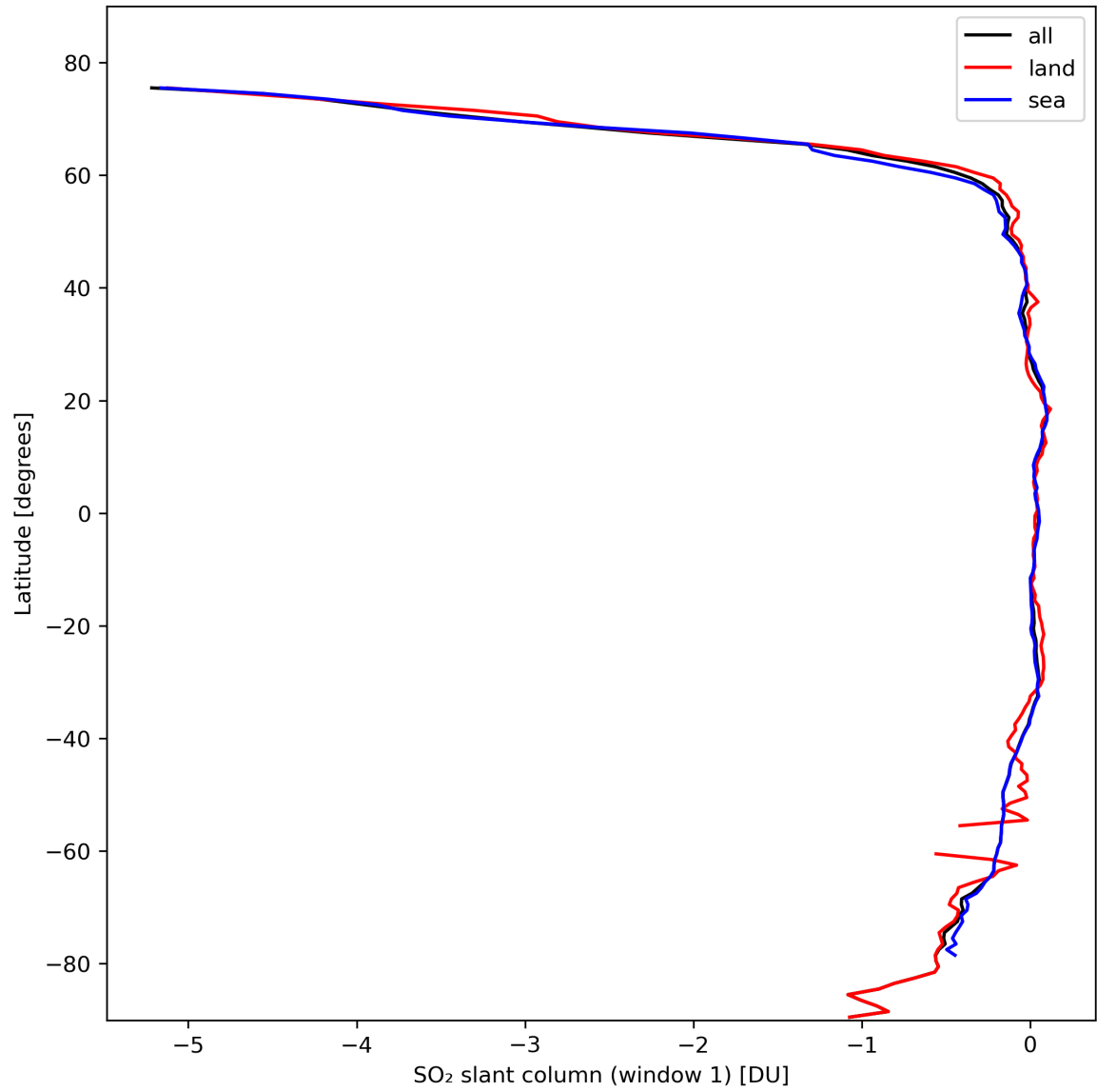
Figure 33: Zonal average of “SO 2 slant column (window 1)” for 2024-02-22 to 2024-02-24.
