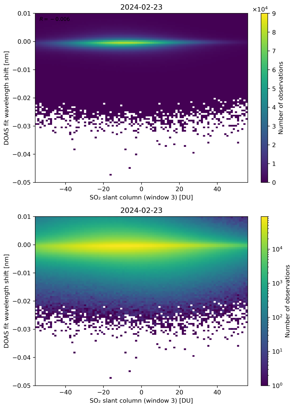
Figure 254: Scatter density plot of “SO 2 slant column (window 3)” against “DOAS fit wavelength shift” for 2024-02-22 to 2024-02-24.
