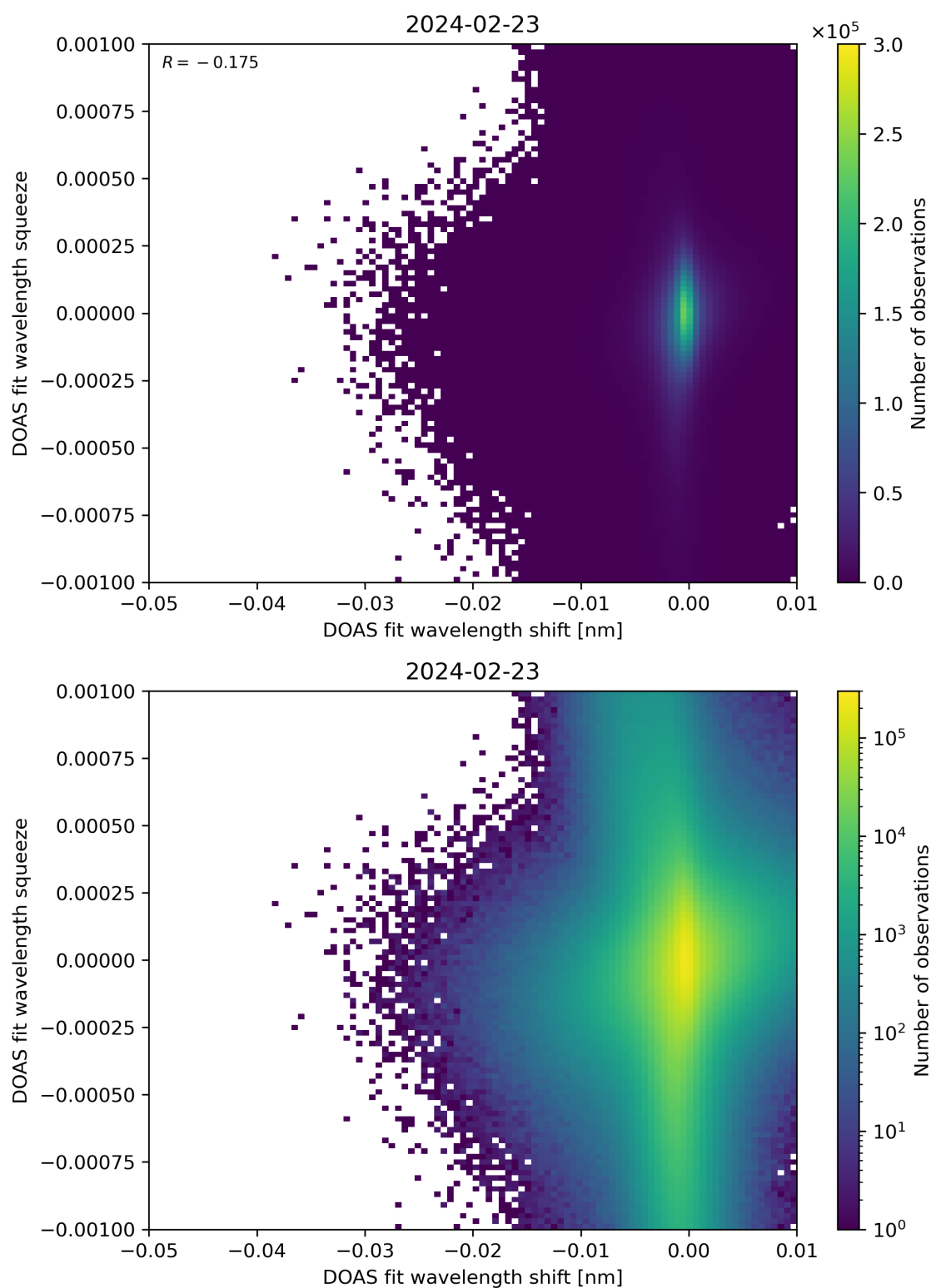
Figure 127: Scatter density plot of “DOAS fit wavelength shift” against “DOAS fit wavelength squeeze” for 2024-02-22 to 2024-02-24.
