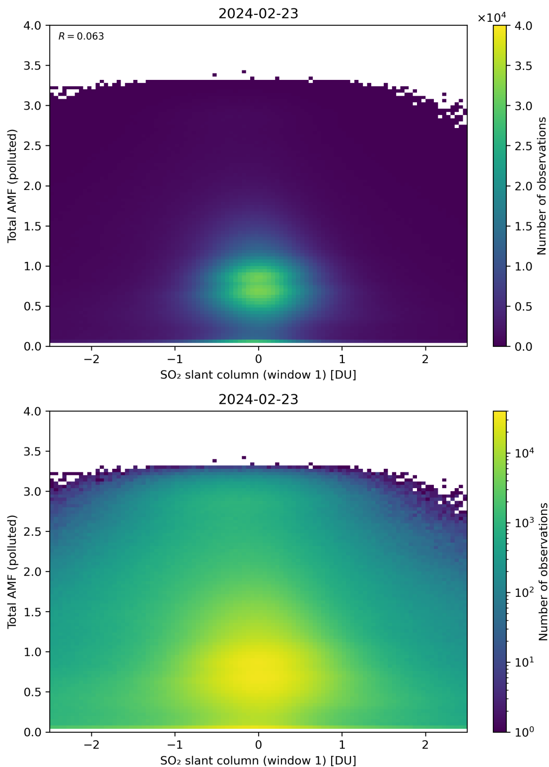
Figure 239: Scatter density plot of “SO 2 slant column (window 1)” against “Total AMF (polluted)” for 2024-02-22 to 2024-02-24.
