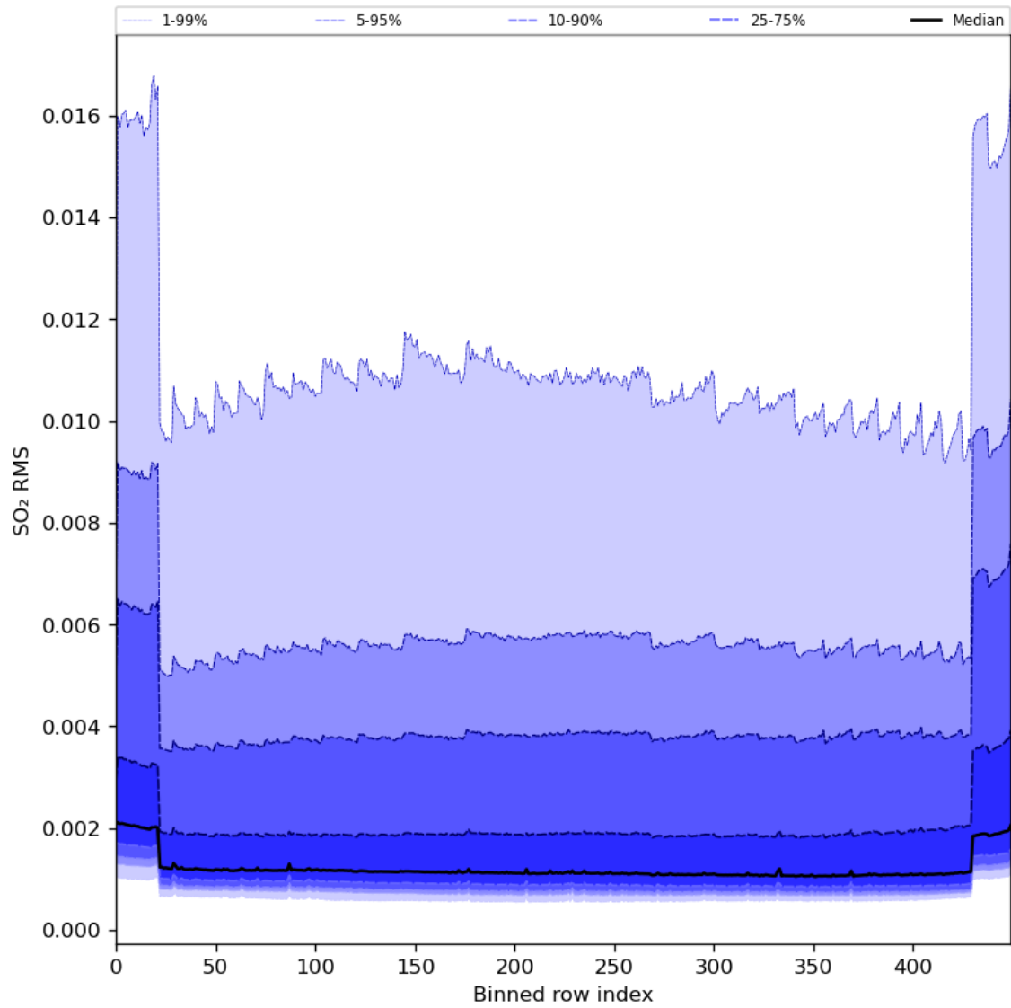
Figure 93: Along track statistics of "SO 2 RMS" for 2024-02-22 to 2024-02-24
