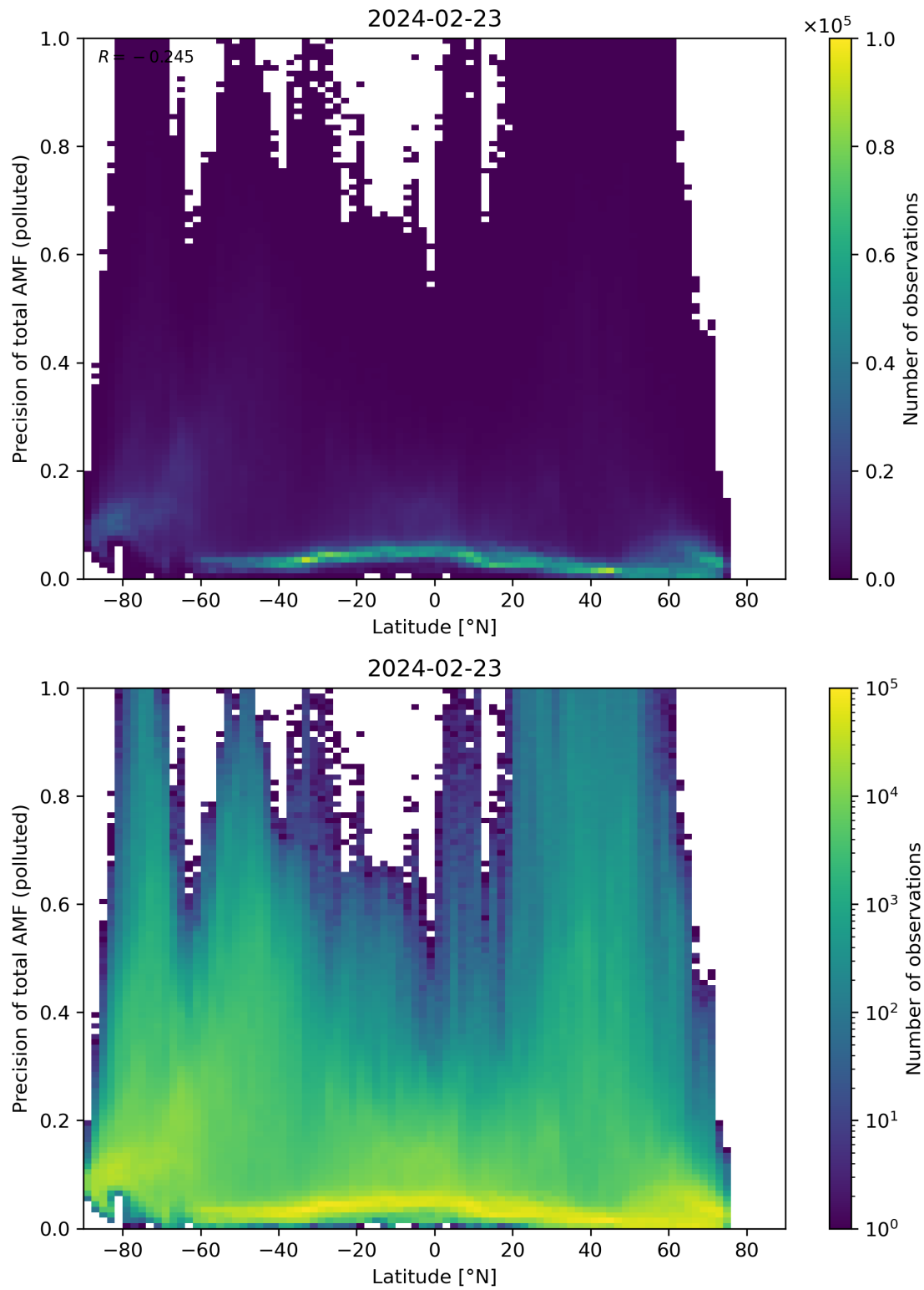
Figure 155: Scatter density plot of “Latitude” against “Precision of total AMF (polluted)” for 2024-02-22 to 2024-02-24.
