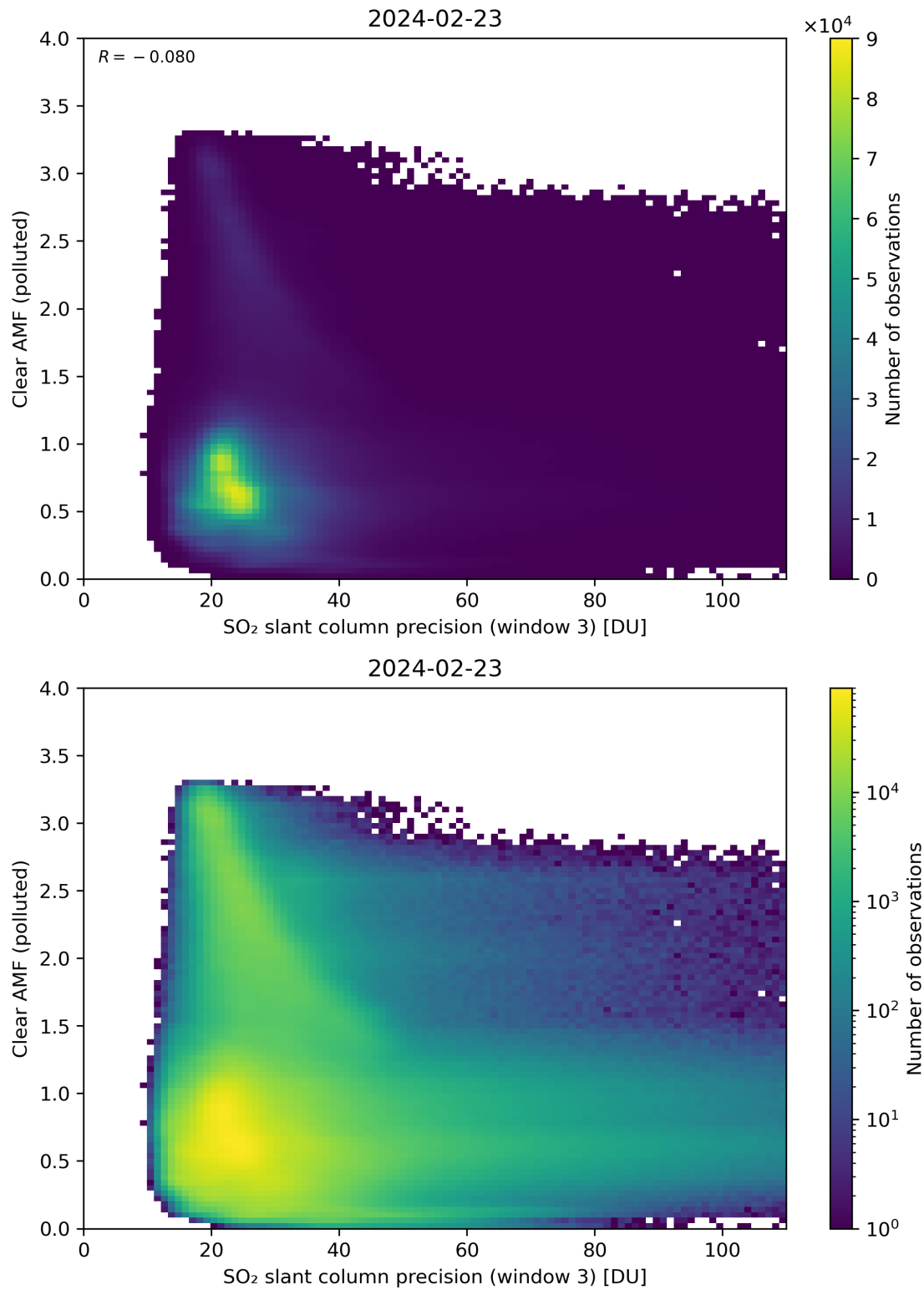
Figure 261: Scatter density plot of “SO 2 slant column precision (window 3)” against “Clear AMF (polluted)” for 2024-02-22 to 2024-02-24.
