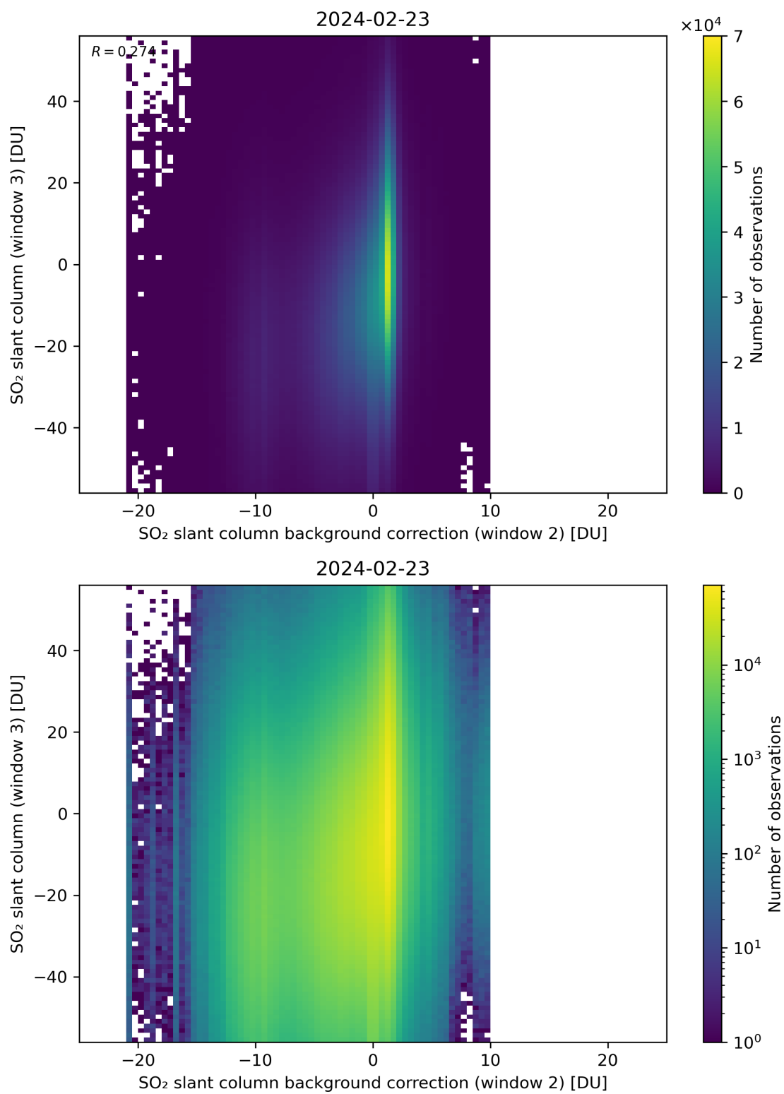
Figure 117: Scatter density plot of “SO 2 slant column background correction (window 2)” against “SO 2 slant column (window 3)” for 2024-02-22 to 2024-02-24.
