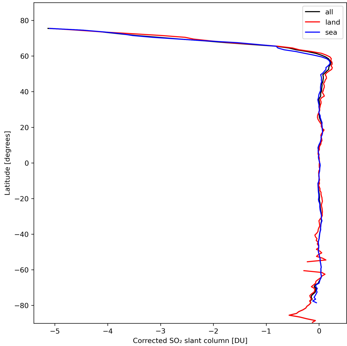
Figure 32: Zonal average of “Corrected SO 2 slant column” for 2024-02-22 to 2024-02-24.
