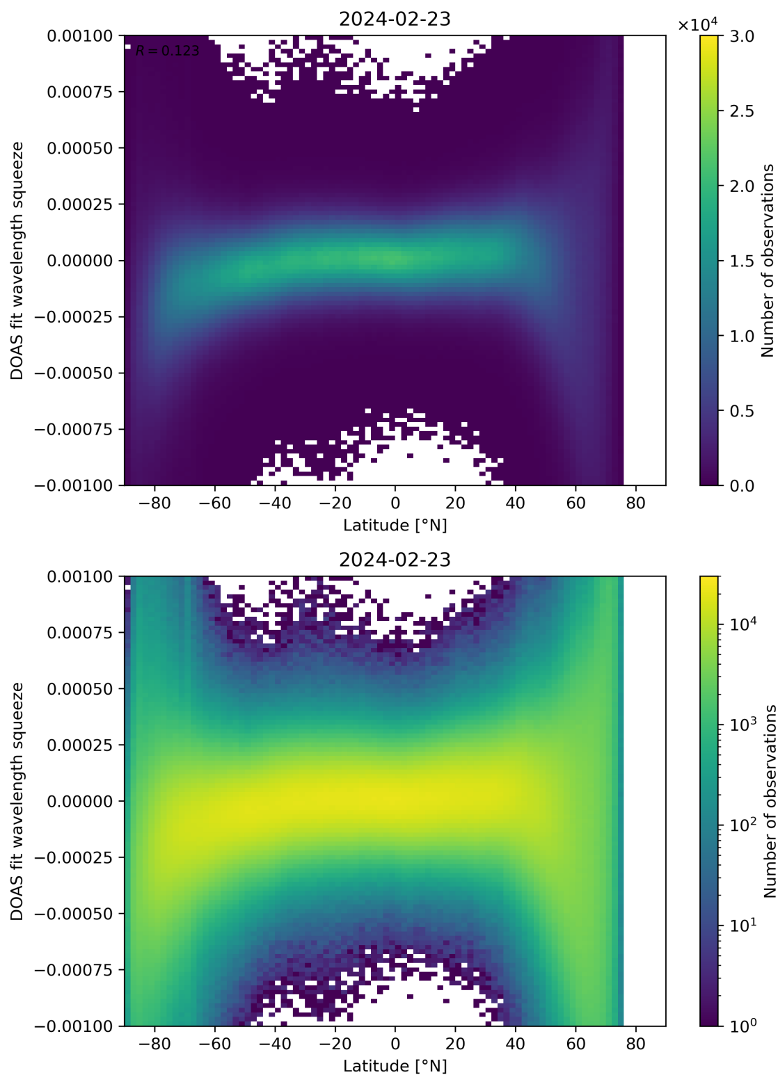
Figure 143: Scatter density plot of “Latitude” against “DOAS fit wavelength squeeze” for 2024-02-22 to 2024-02-24.
