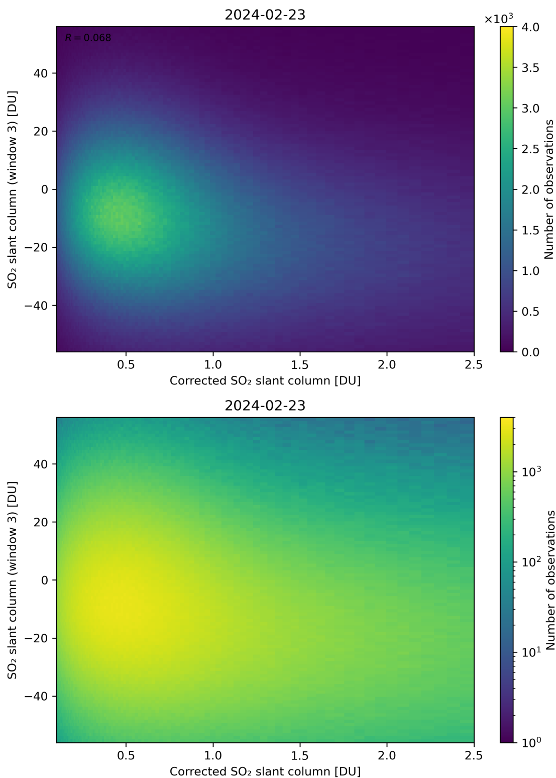
Figure 190: Scatter density plot of “Corrected SO 2 slant column” against “SO 2 slant column (window 3)” for 2024-02-22 to 2024-02-24.
