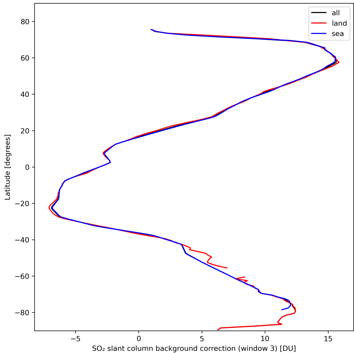
Figure 44: Zonal average of “SO 2 slant column background correction (window 3)” for 2024-02-22 to 2024-02-24.
