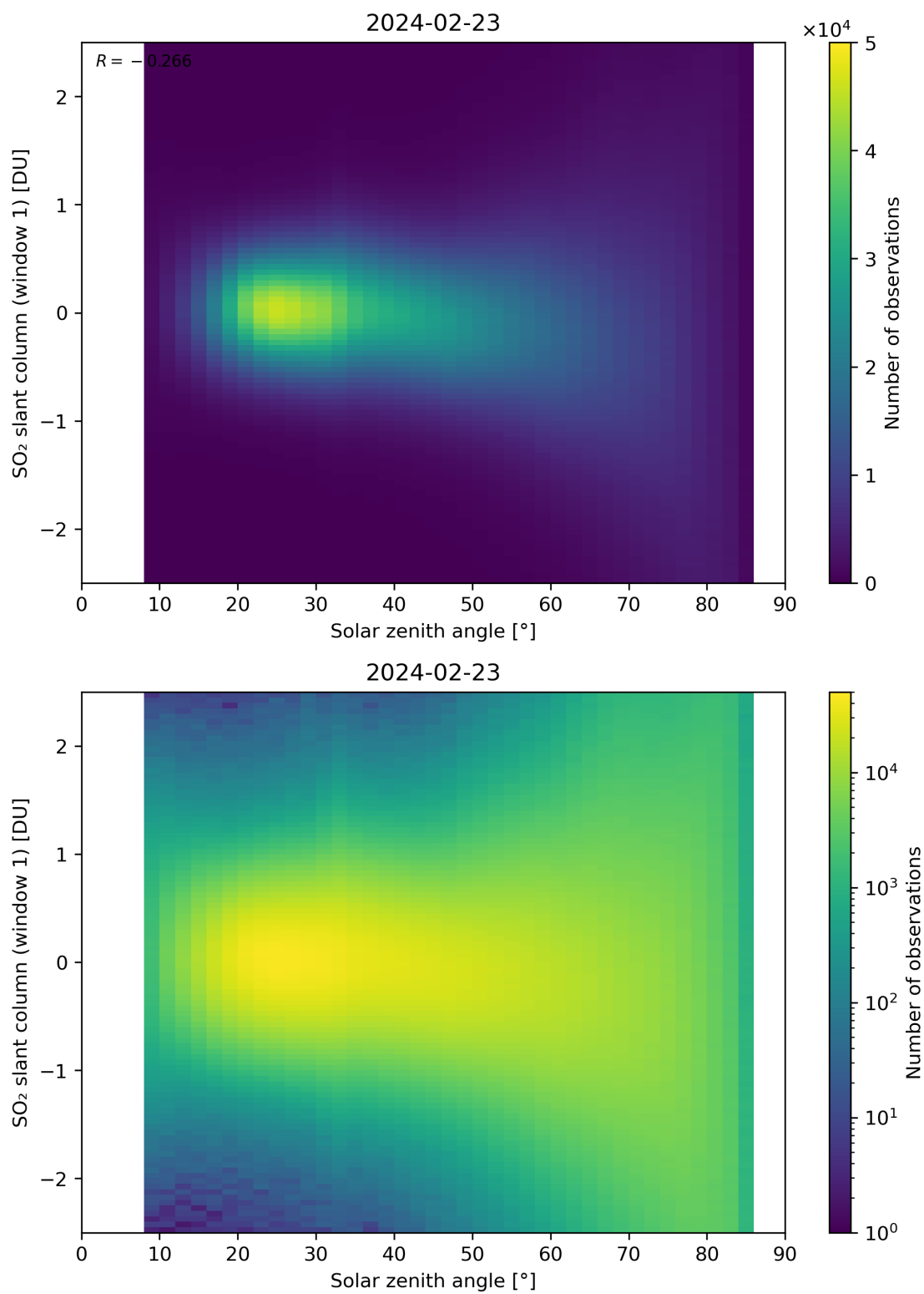
Figure 169: Scatter density plot of “Solar zenith angle” against “SO 2 slant column (window 1)” for 2024-02-22 to 2024-02-24.
