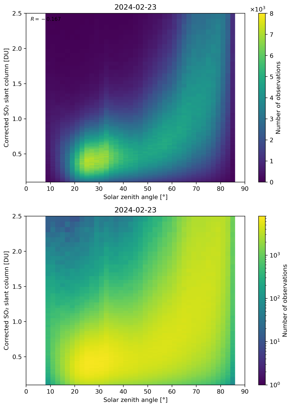
Figure 166: Scatter density plot of “Solar zenith angle” against “Corrected SO 2 slant column” for 2024-02-22 to 2024-02-24.
