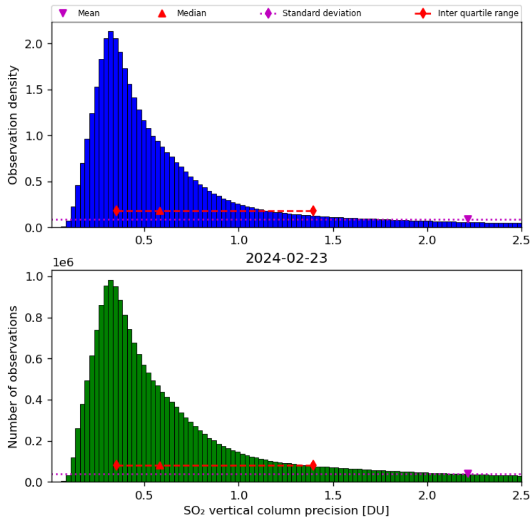
Figure 54: Histogram of “SO 2 vertical column precision” for 2024-02-22 to 2024-02-24
