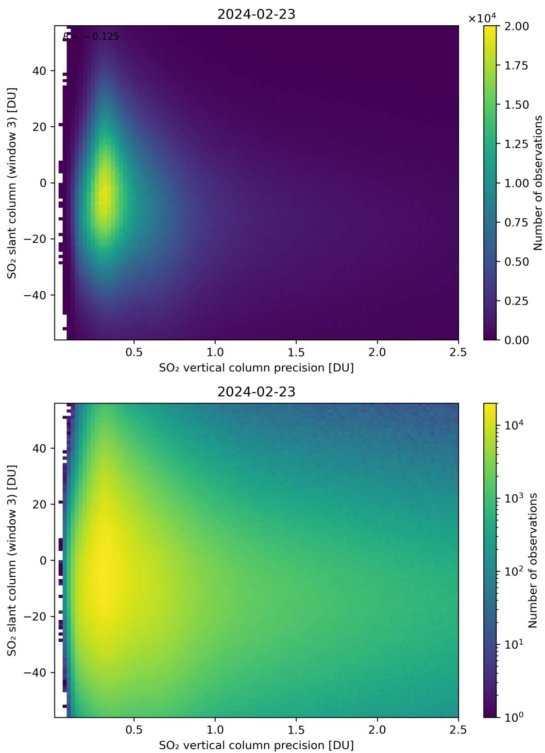
Figure 292: Scatter density plot of “SO 2 vertical column precision” against “SO 2 slant column (window 3)” for 2024-02-22 to 2024-02-24.
