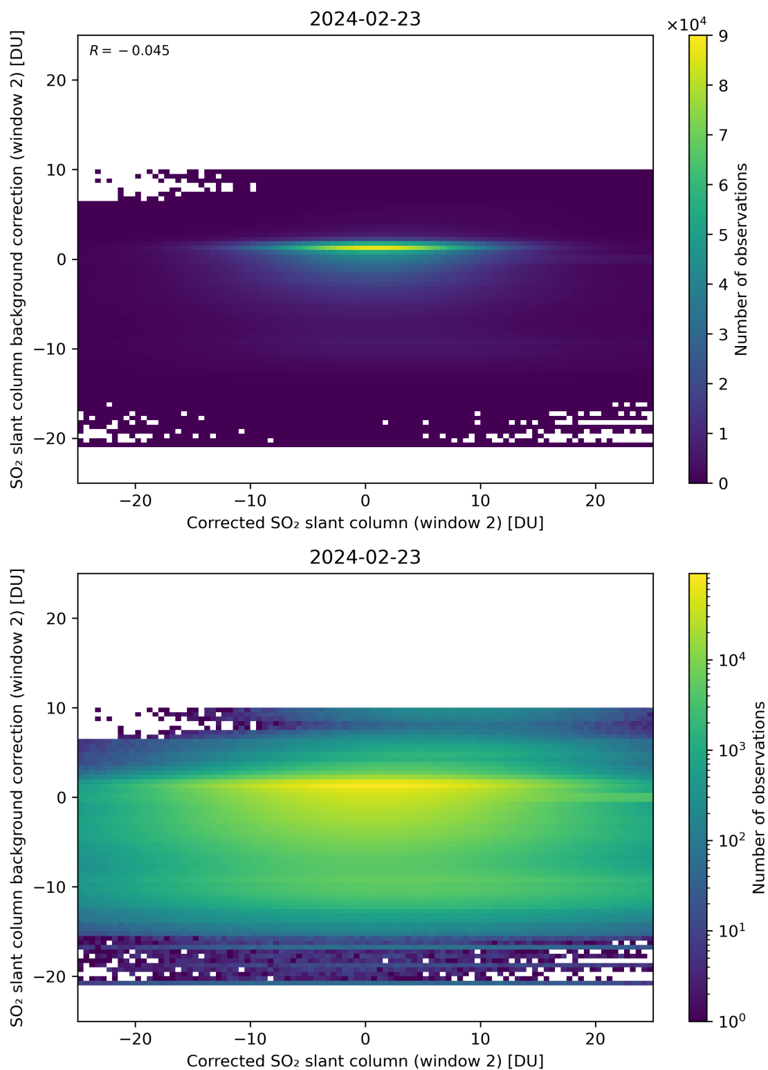
Figure 194: Scatter density plot of “Corrected SO 2 slant column (window 2)” against “SO 2 slant column background correction (window 2)” for 2024-02-22 to 2024-02-24.
