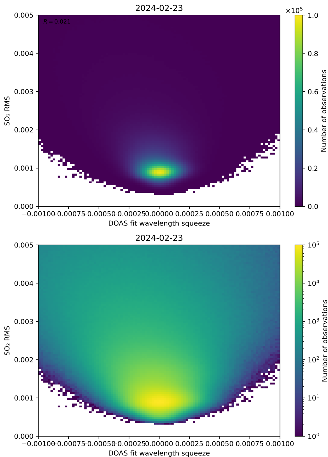
Figure 132: Scatter density plot of “DOAS fit wavelength squeeze” against “SO 2 RMS” for 2024-02-22 to 2024-02-24.
