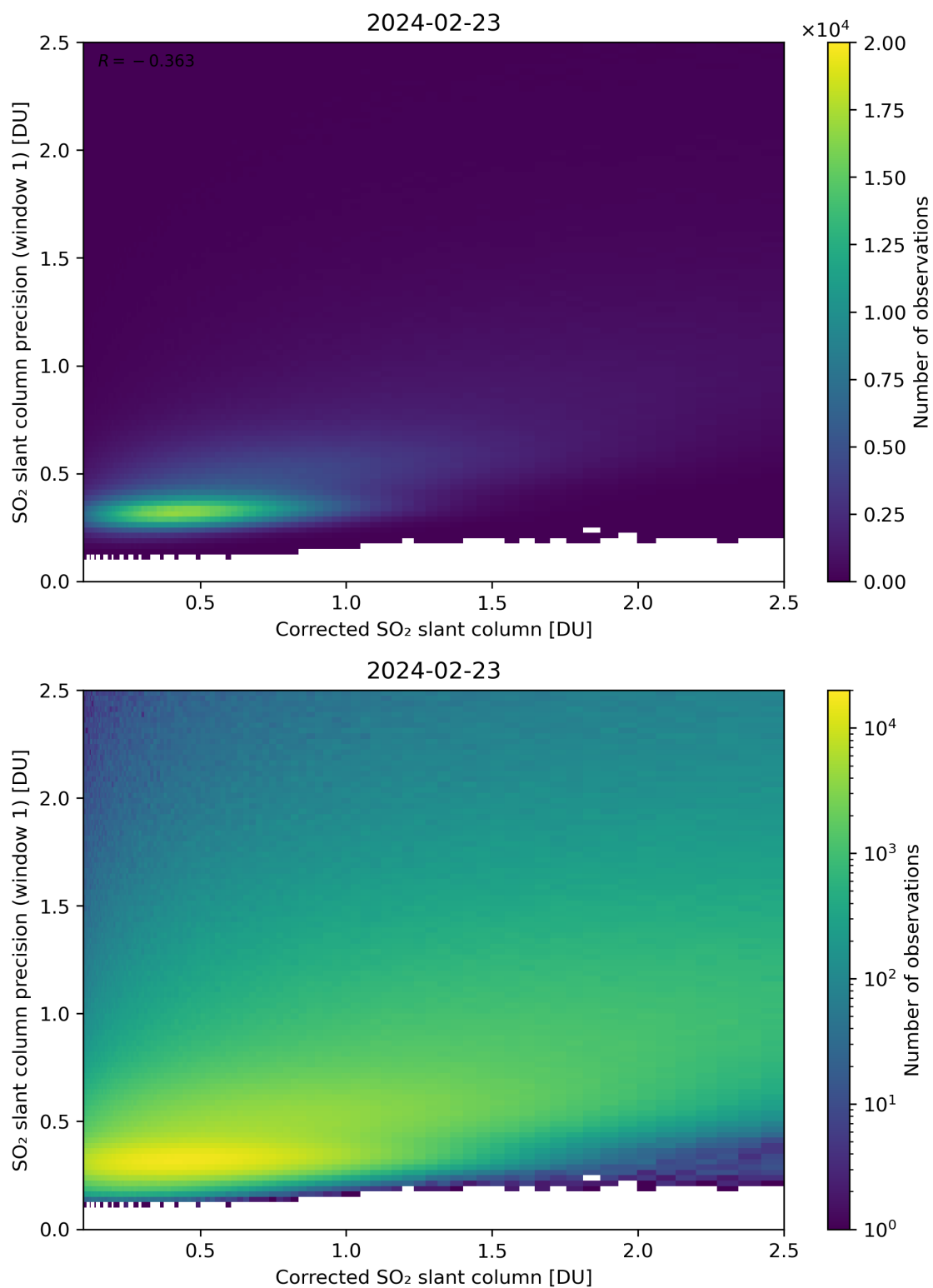
Figure 188: Scatter density plot of “Corrected SO 2 slant column” against “SO 2 slant column precision (window 1)” for 2024-02-22 to 2024-02-24.
