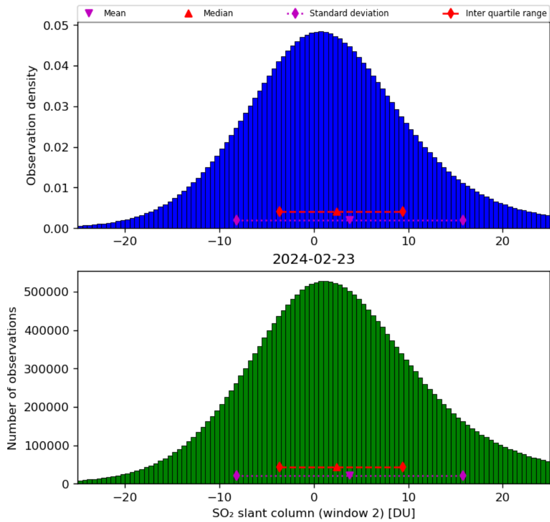
Figure 60: Histogram of “SO 2 slant column (window 2)” for 2024-02-22 to 2024-02-24
