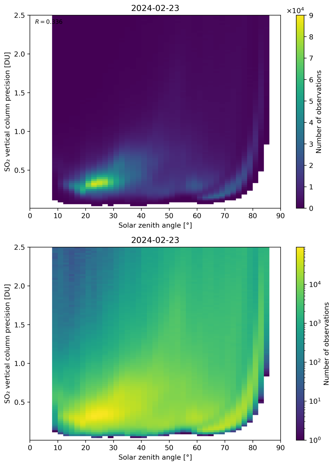
Figure 177: Scatter density plot of “Solar zenith angle” against “SO 2 vertical column precision” for 2024-02-22 to 2024-02-24.
