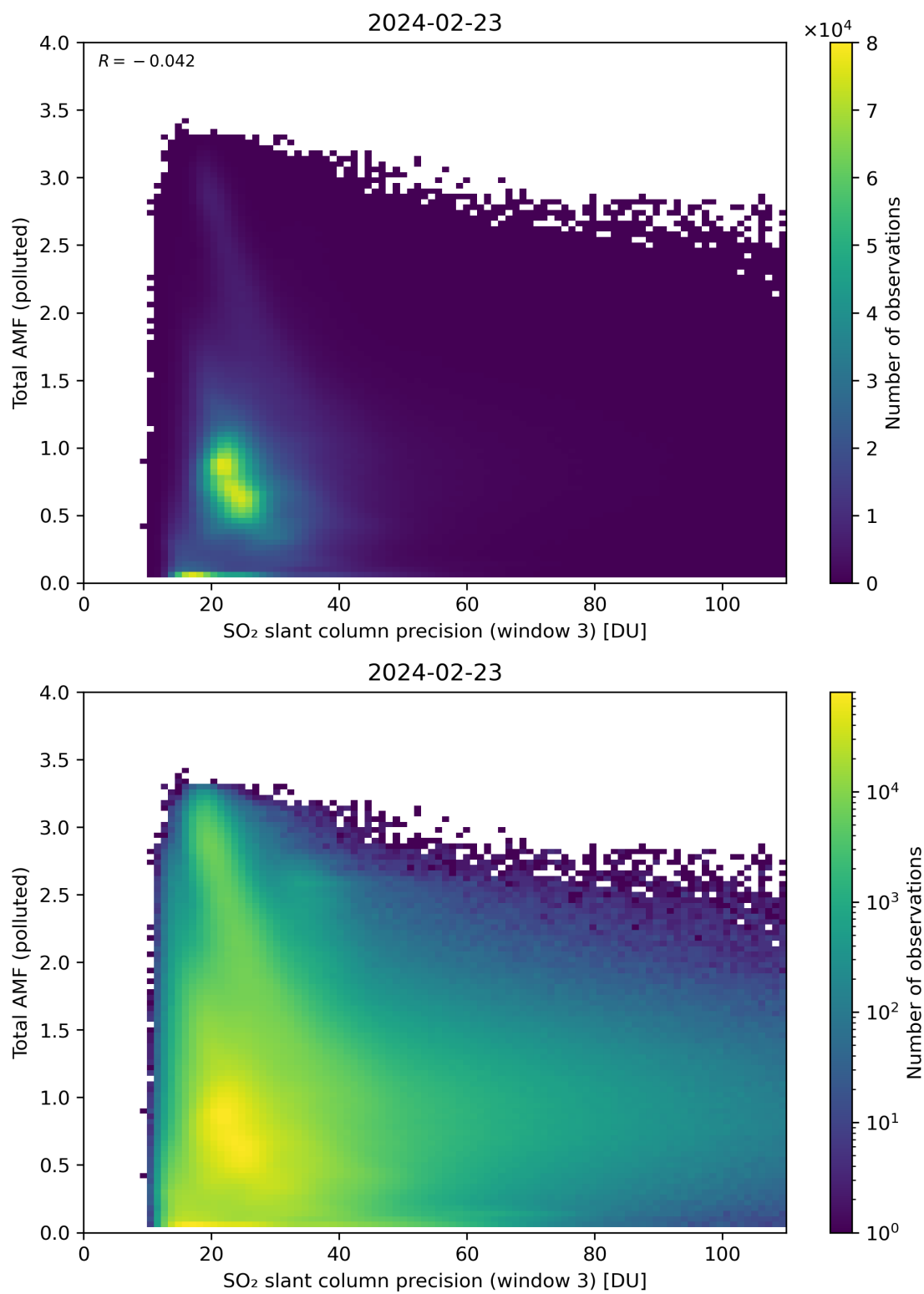
Figure 263: Scatter density plot of “SO 2 slant column precision (window 3)” against “Total AMF (polluted)” for 2024-02-22 to 2024-02-24.
