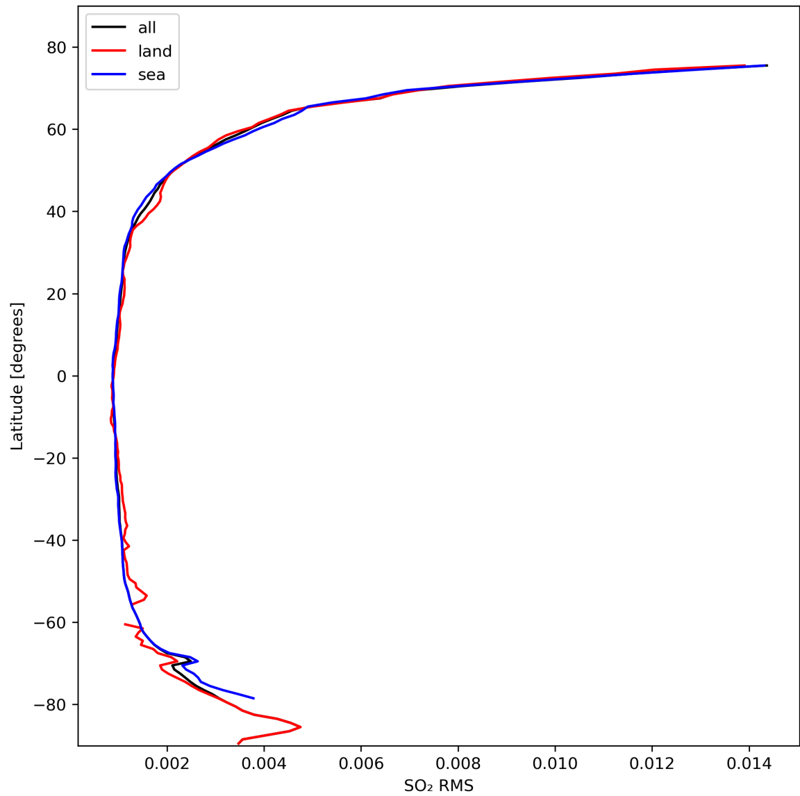
Figure 47: Zonal average of “SO 2 RMS” for 2024-02-22 to 2024-02-24.
