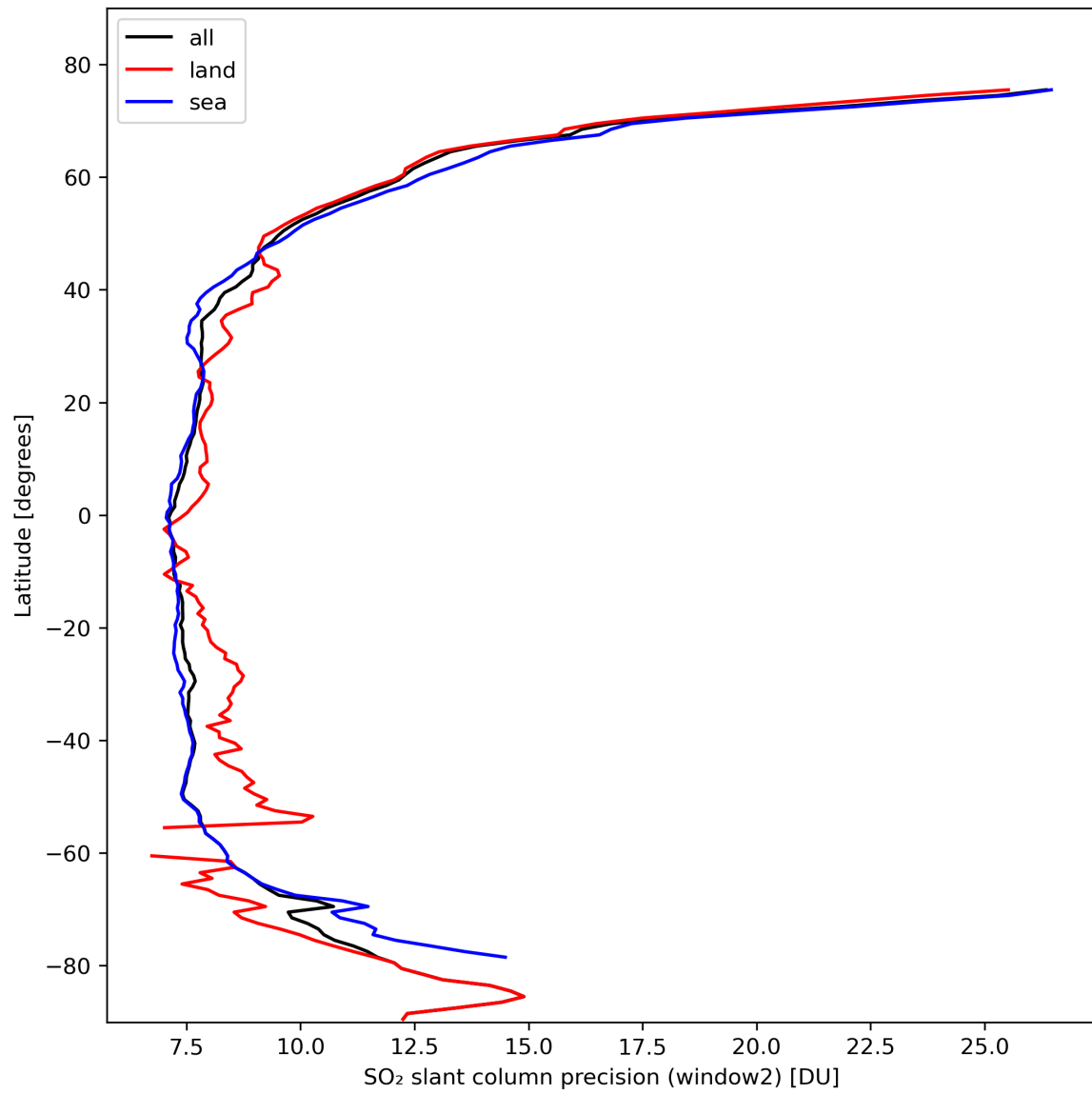
Figure 38: Zonal average of “SO 2 slant column precision (window2)” for 2024-02-22 to 2024-02-24.
