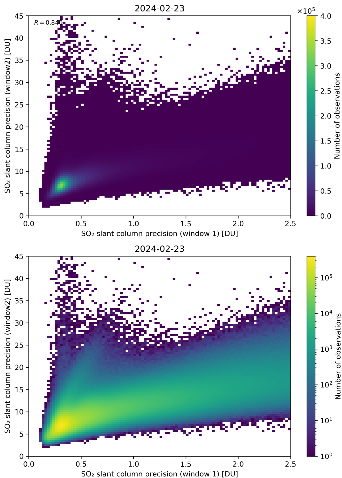
Figure 227: Scatter density plot of “SO 2 slant column precision (window 1)” against “SO 2 slant column precision (window2)” for 2024-02-22 to 2024-02-24.
