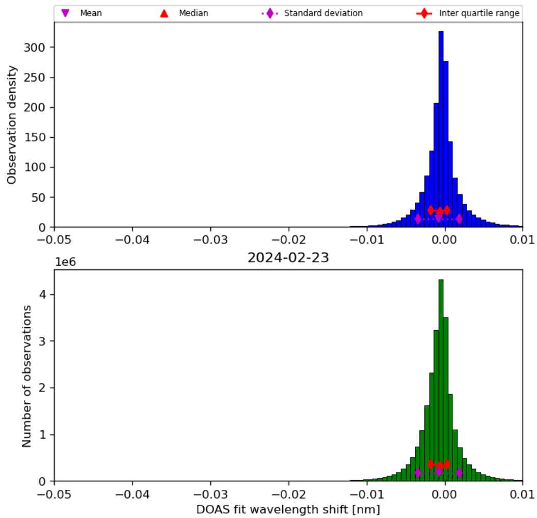
Figure 68: Histogram of “DOAS fit wavelength shift” for 2024-02-22 to 2024-02-24
