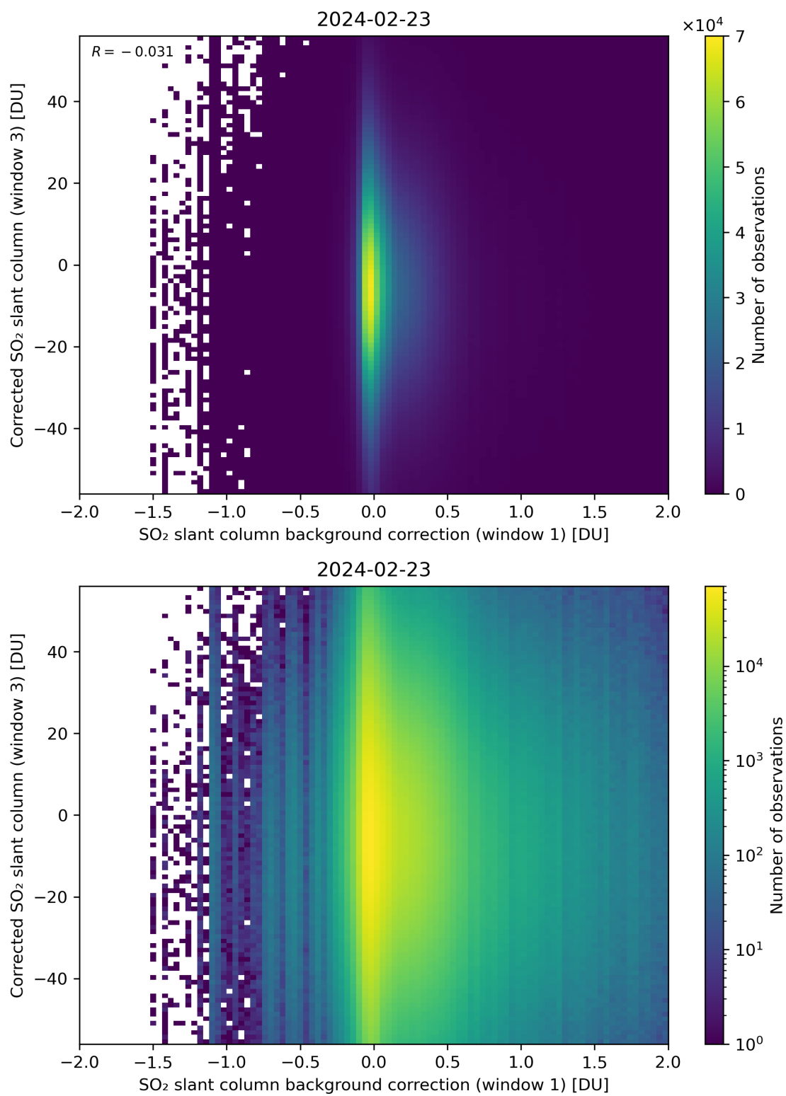
Figure 105: Scatter density plot of “SO 2 slant column background correction (window 1)” against “Corrected SO 2 slant column (window 3)” for 2024-02-22 to 2024-02-24.
