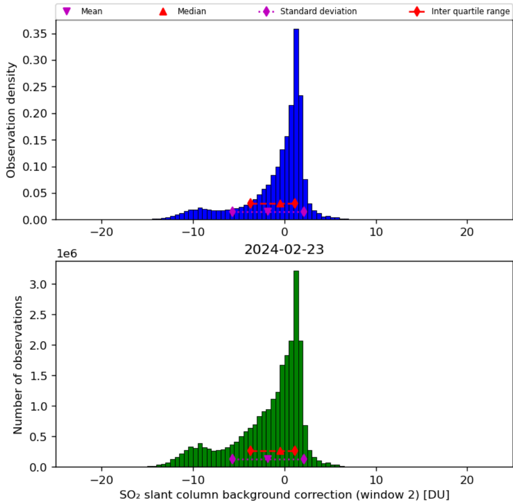
Figure 63: Histogram of “SO 2 slant column background correction (window 2)” for 2024-02-22 to 2024-02-24
