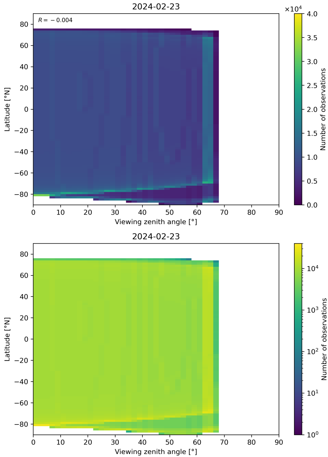
Figure 314: Scatter density plot of “Viewing zenith angle” against “Latitude” for 2024-02-22 to 2024-02-24.
