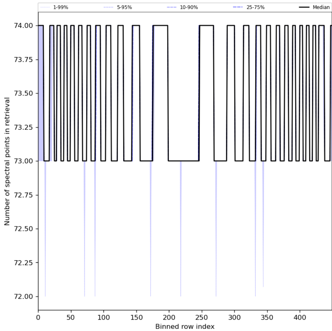
Figure 97: Along track statistics of “Number of spectral points in retrieval” for 2024-02-22 to 2024-02-24
