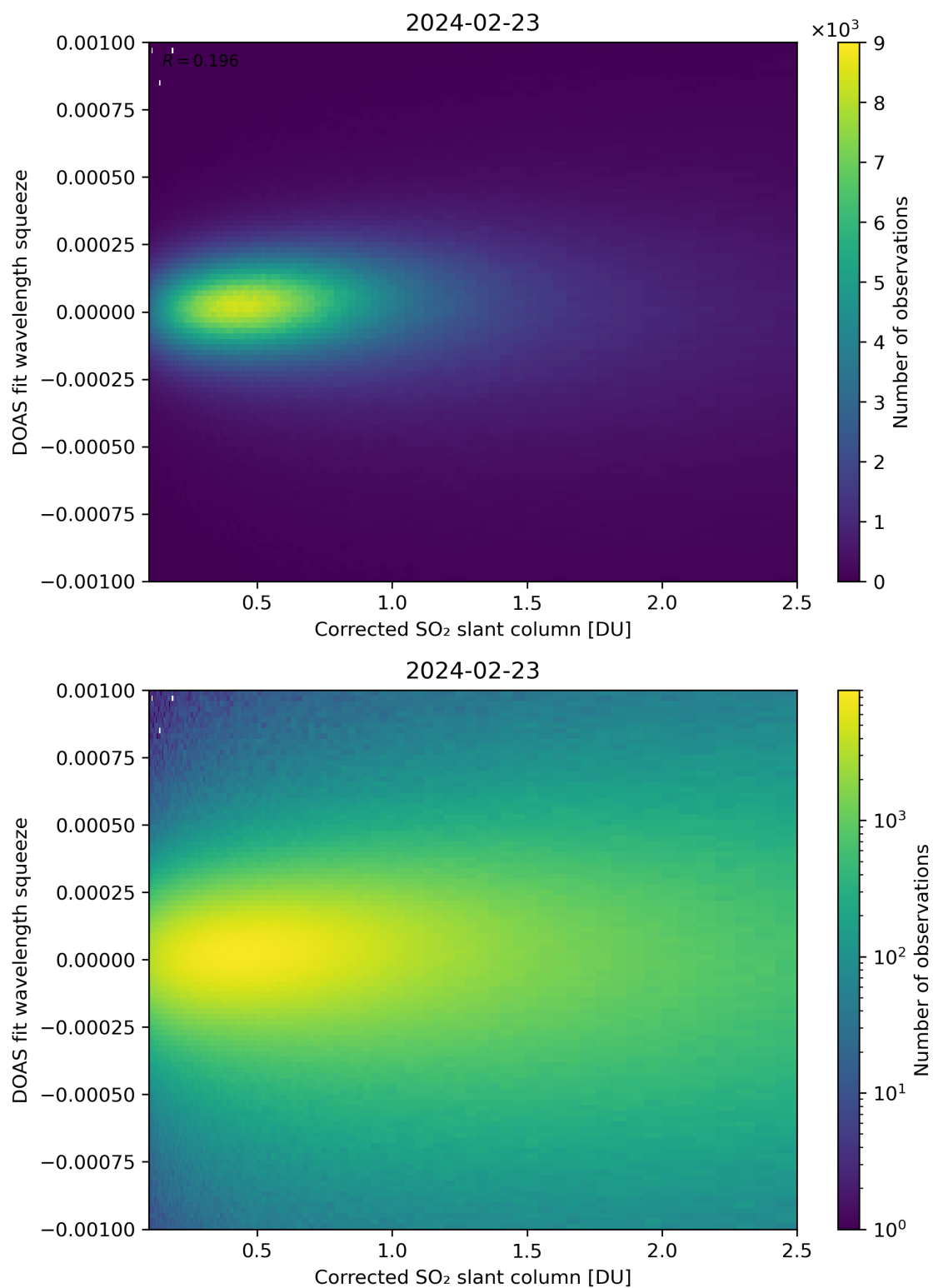
Figure 182: Scatter density plot of “Corrected SO 2 slant column” against “DOAS fit wavelength squeeze” for 2024-02-22 to 2024-02-24.
