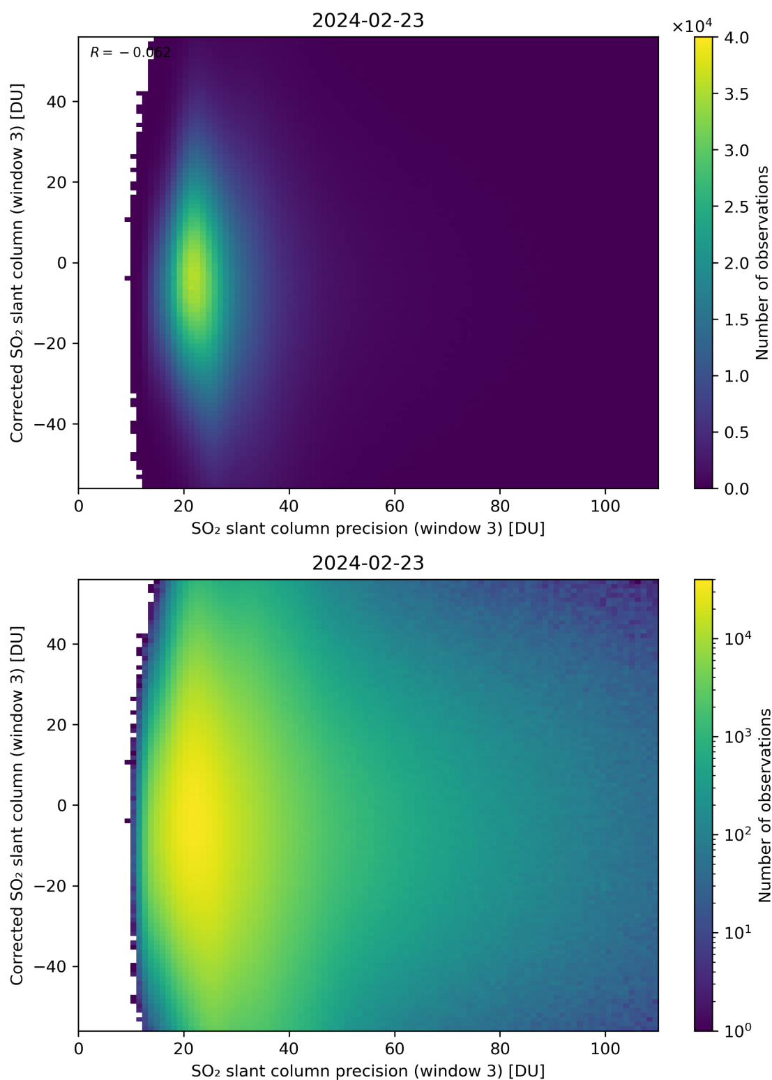
Figure 262: Scatter density plot of “SO 2 slant column precision (window 3)” against “Corrected SO 2 slant column (window 3)” for 2024-02-22 to 2024-02-24.
