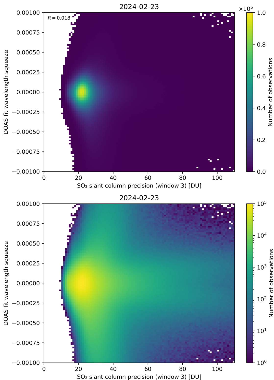
Figure 259: Scatter density plot of “SO 2 slant column precision (window 3)” against “DOAS fit wavelength squeeze” for 2024-02-22 to 2024-02-24.
