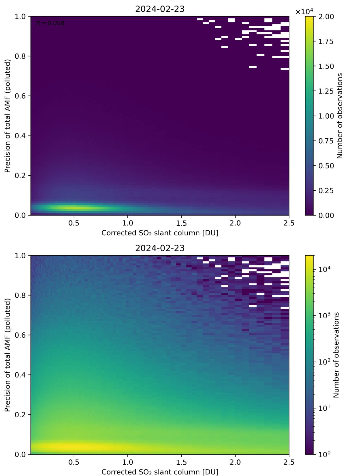
Figure 193: Scatter density plot of “Corrected SO 2 slant column” against “Precision of total AMF (polluted)” for 2024-02-22 to 2024-02-24.
