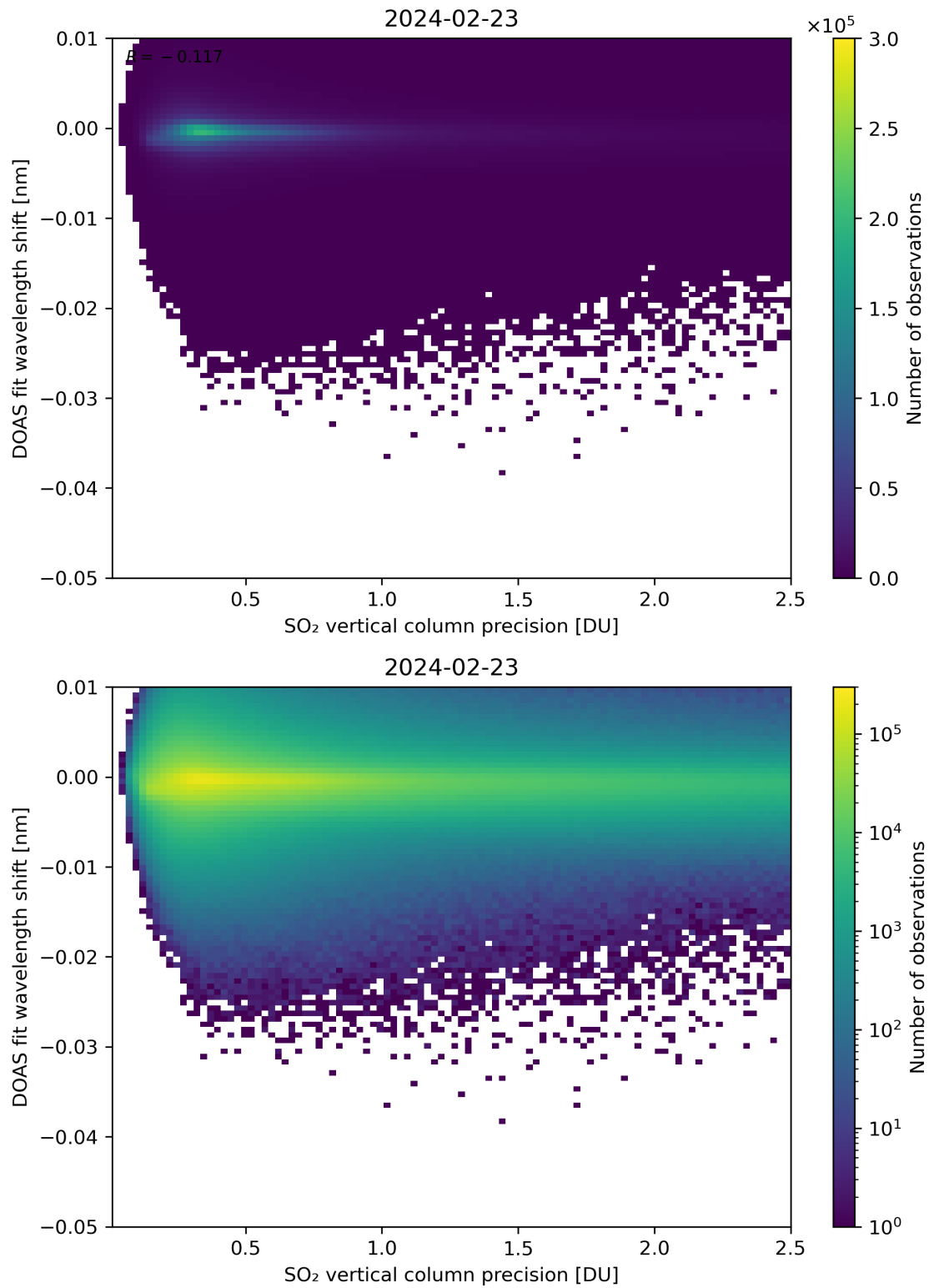
Figure 282: Scatter density plot of “SO 2 vertical column precision” against “DOAS fit wavelength shift” for 2024-02-22 to 2024-02-24.
