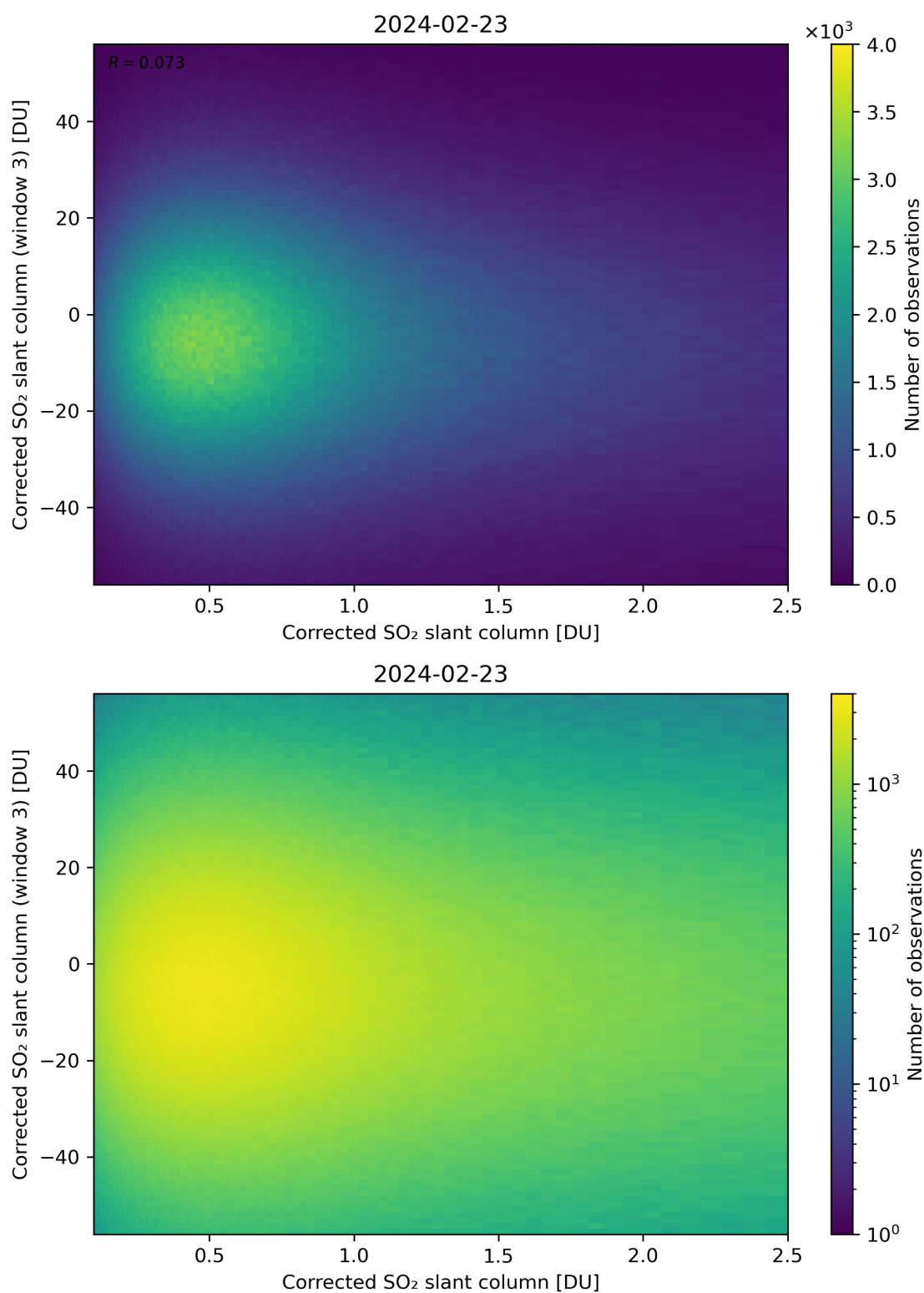
Figure 186: Scatter density plot of “Corrected SO 2 slant column” against “Corrected SO 2 slant column (window 3)” for 2024-02-22 to 2024-02-24.
