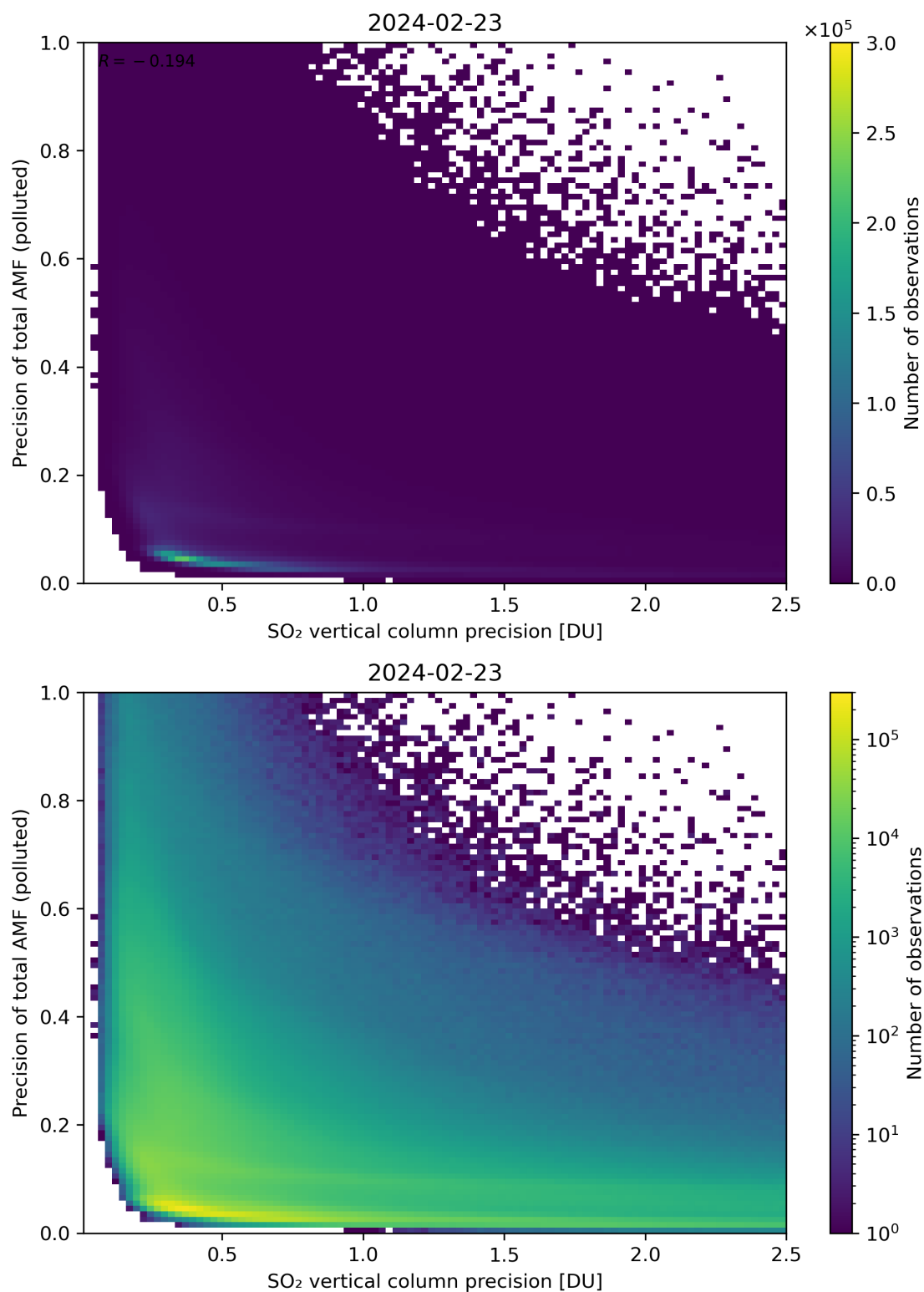
Figure 295: Scatter density plot of “SO 2 vertical column precision” against “Precision of total AMF (polluted)” for 2024-02-22 to 2024-02-24.
