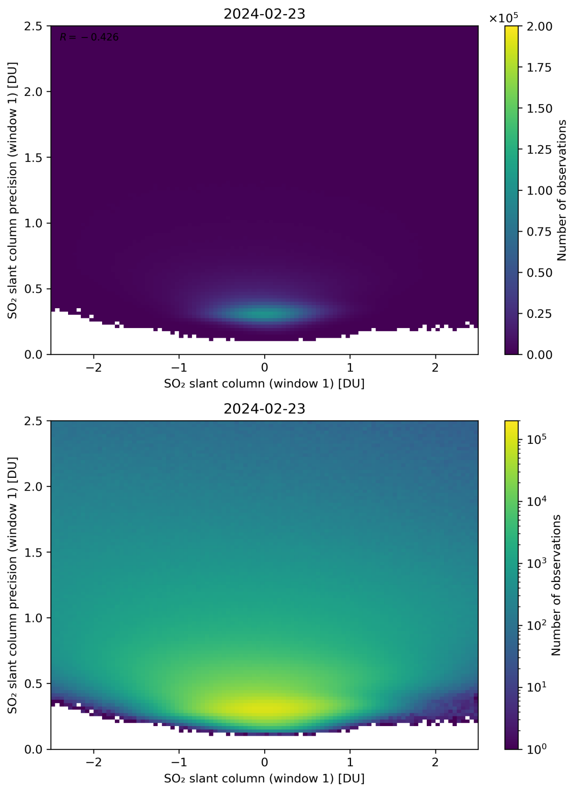
Figure 235: Scatter density plot of “SO 2 slant column (window 1)” against “SO 2 slant column precision (window 1)” for 2024-02-22 to 2024-02-24.
