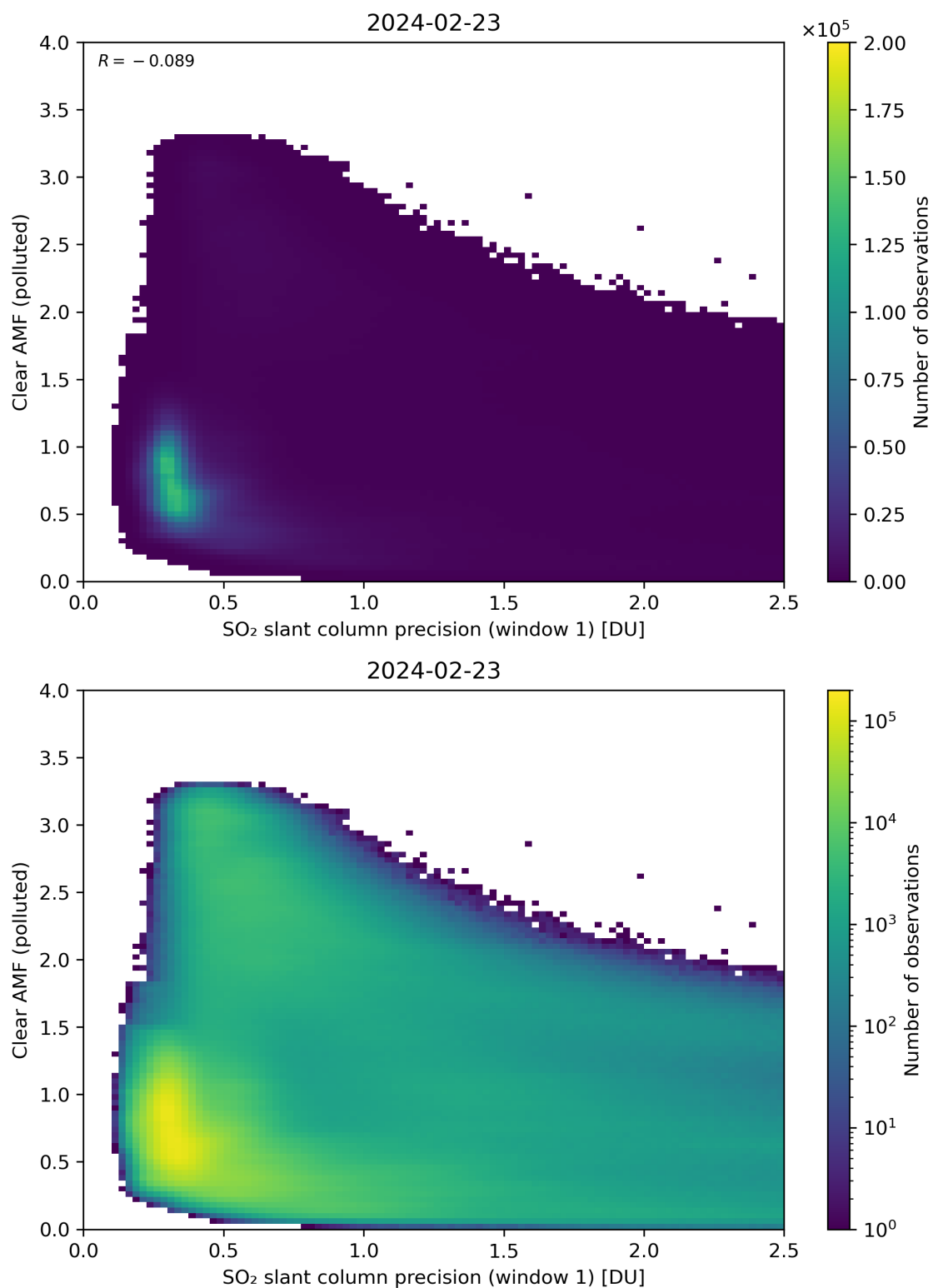
Figure 224: Scatter density plot of “SO 2 slant column precision (window 1)” against “Clear AMF (polluted)” for 2024-02-22 to 2024-02-24.
