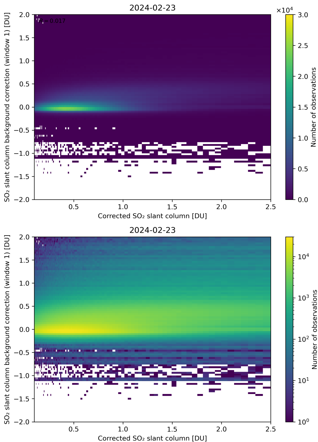
Figure 178: Scatter density plot of “Corrected SO 2 slant column” against “SO 2 slant column background correction (window 1)” for 2024-02-22 to 2024-02-24.
