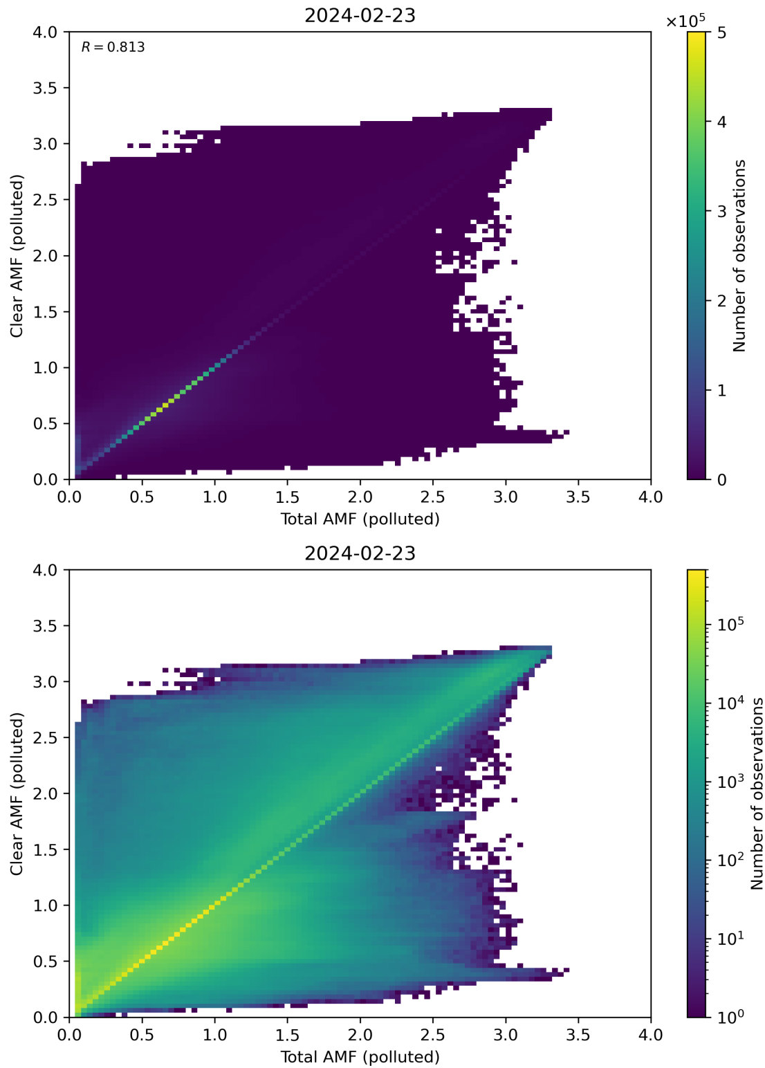
Figure 271: Scatter density plot of “Total AMF (polluted)” against “Clear AMF (polluted)” for 2024-02-22 to 2024-02-24.
