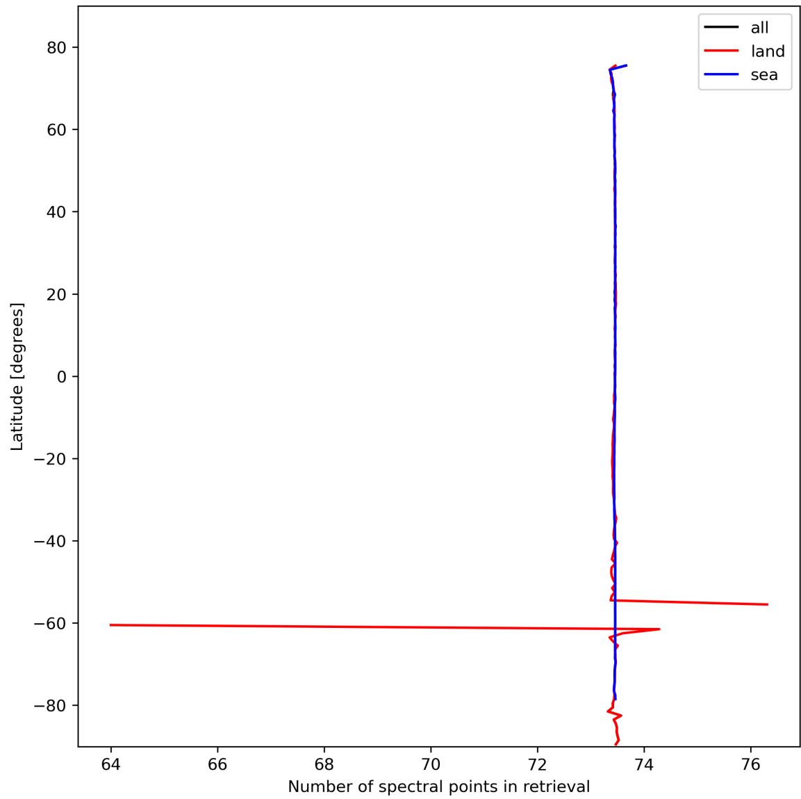
Figure 51: Zonal average of “Number of spectral points in retrieval” for 2024-02-22 to 2024-02-24.
