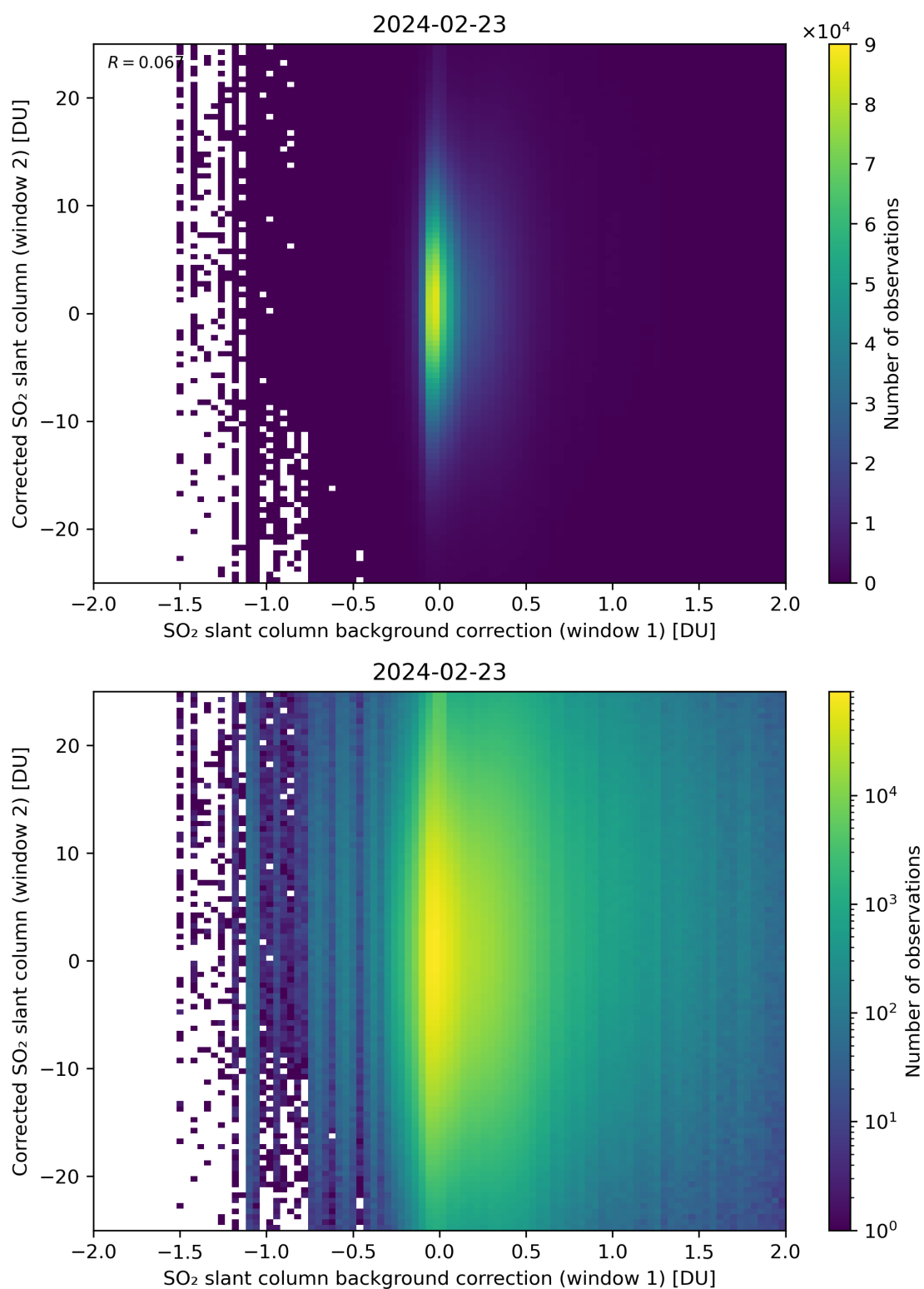
Figure 104: Scatter density plot of “SO 2 slant column background correction (window 1)” against “Corrected SO 2 slant column (window 2)” for 2024-02-22 to 2024-02-24.
