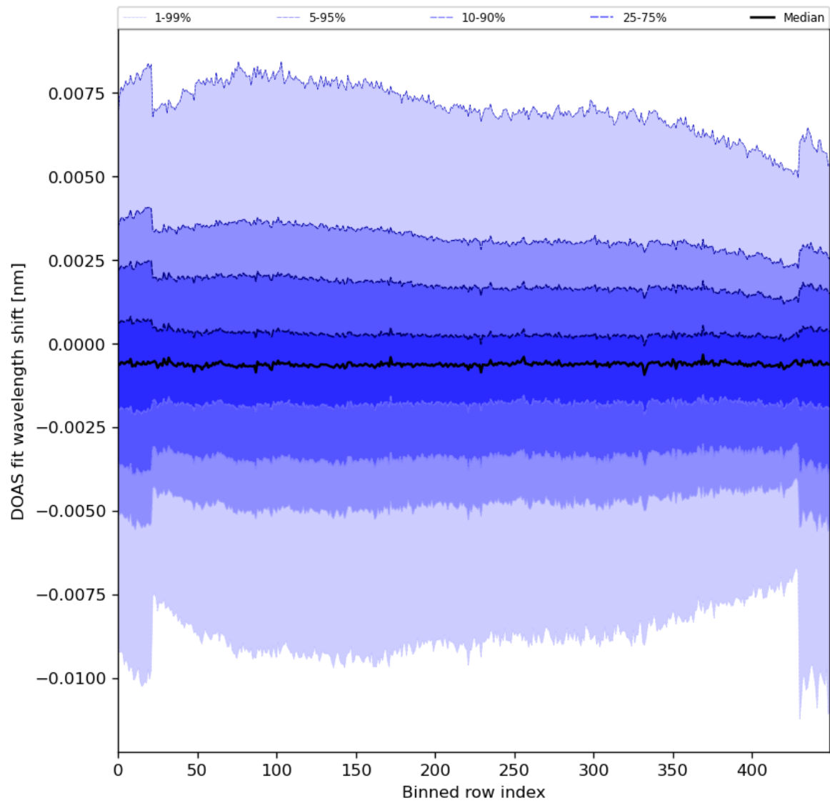
Figure 91: Along track statistics of “DOAS fit wavelength shift” for 2024-02-22 to 2024-02-24
