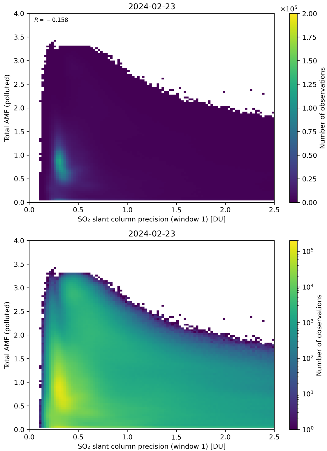
Figure 230: Scatter density plot of “SO 2 slant column precision (window 1)” against “Total AMF (polluted)” for 2024-02-22 to 2024-02-24.
