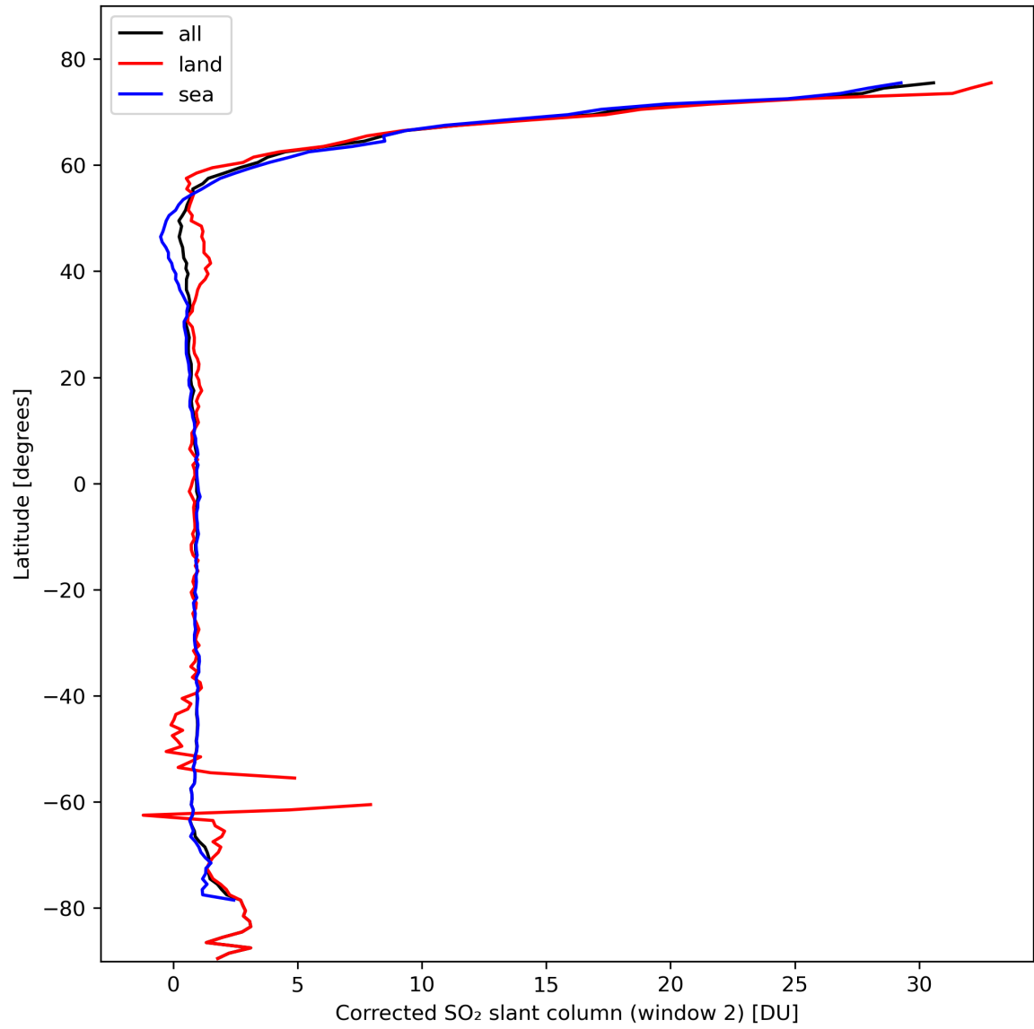
Figure 39: Zonal average of “Corrected SO 2 slant column (window 2)” for 2024-02-22 to 2024-02-24.
