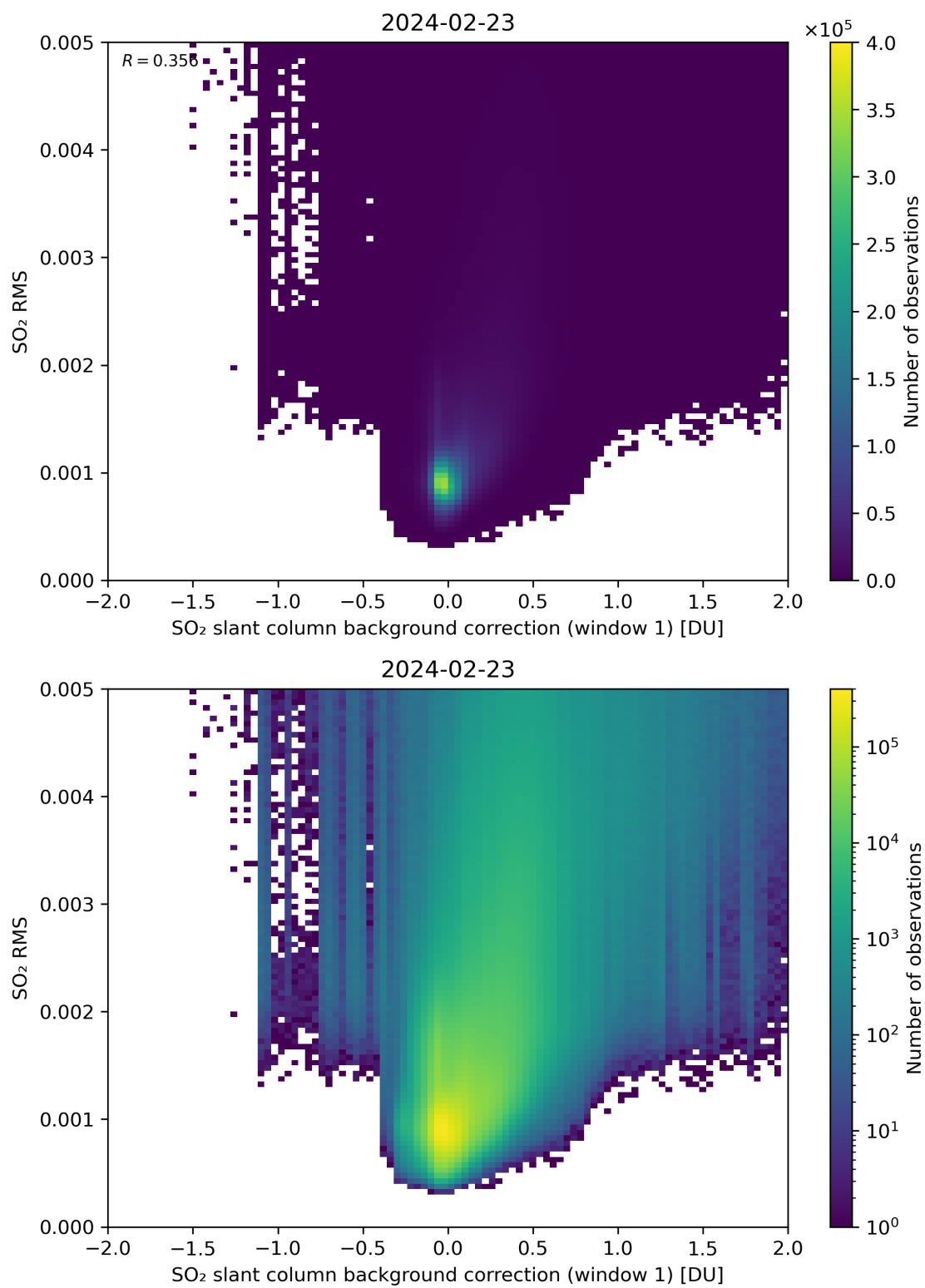
Figure 102: Scatter density plot of “SO 2 slant column background correction (window 1)” against “SO 2 RMS” for 2024-02-22 to 2024-02-24.
