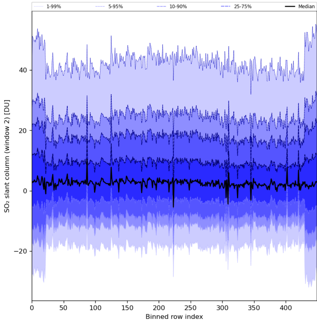
Figure 83: Along track statistics of “SO 2 slant column (window 2)” for 2024-02-22 to 2024-02-24
