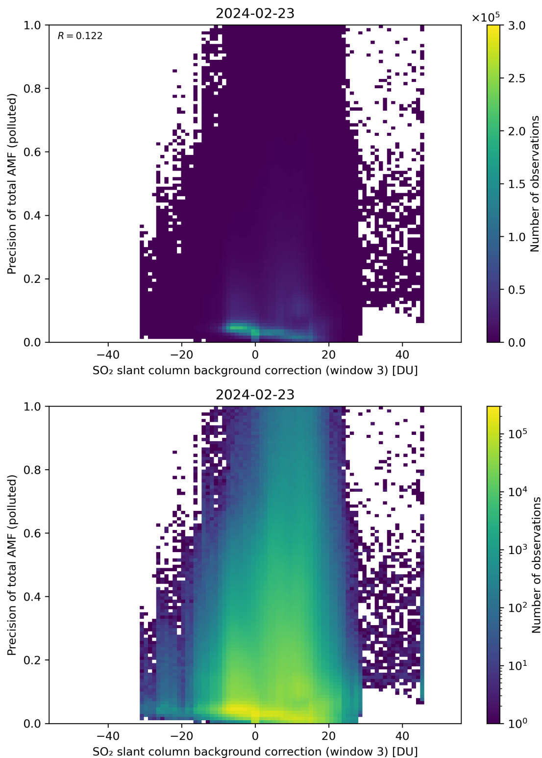
Figure 126: Scatter density plot of “SO 2 slant column background correction (window 3)” against “Precision of total AMF (polluted)” for 2024-02-22 to 2024-02-24.
