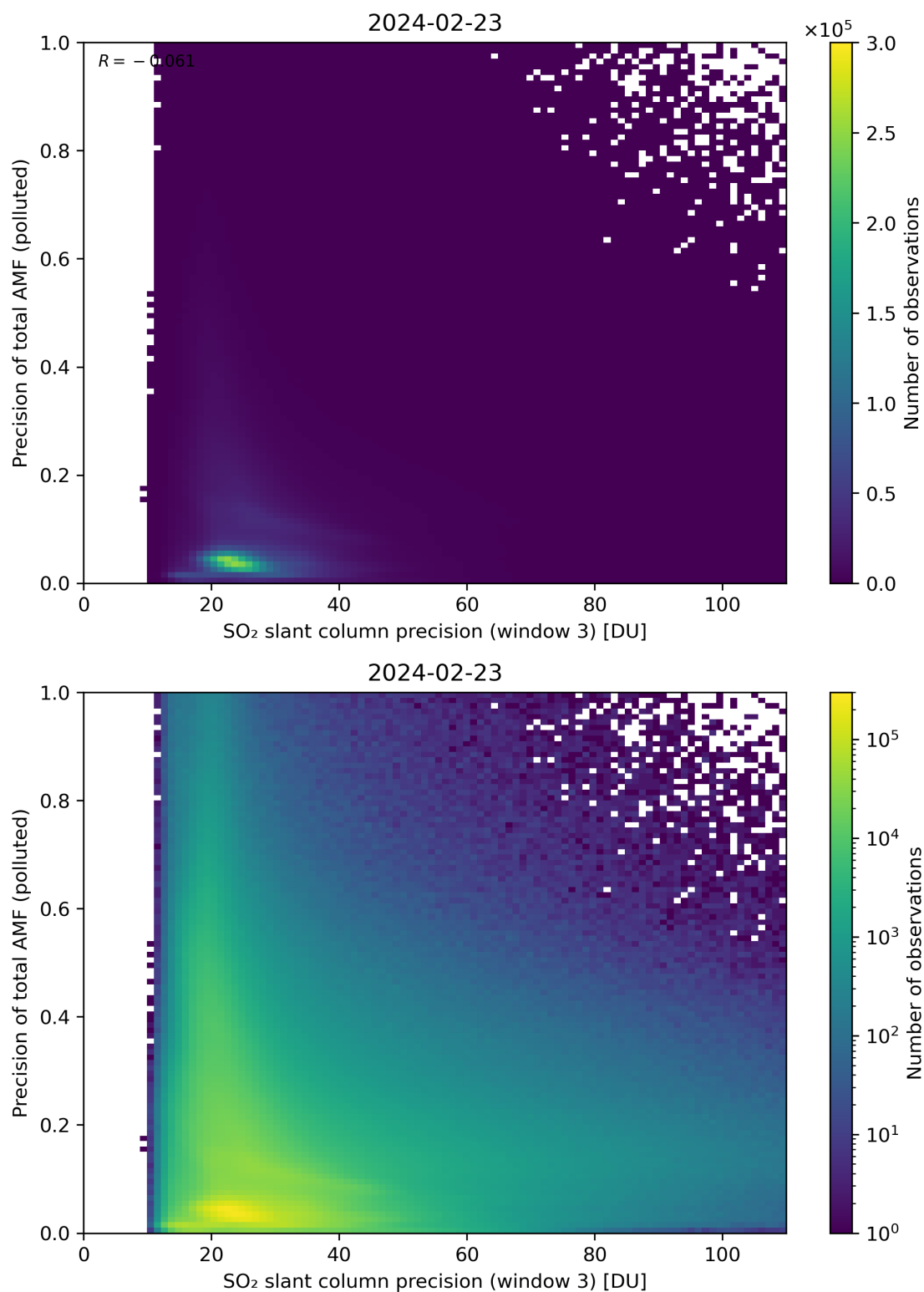
Figure 264: Scatter density plot of “SO 2 slant column precision (window 3)” against “Precision of total AMF (polluted)” for 2024-02-22 to 2024-02-24.
