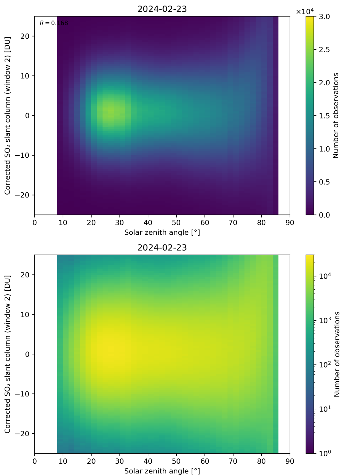
Figure 167: Scatter density plot of “Solar zenith angle” against “Corrected SO 2 slant column (window 2)” for 2024-02-22 to 2024-02-24.
