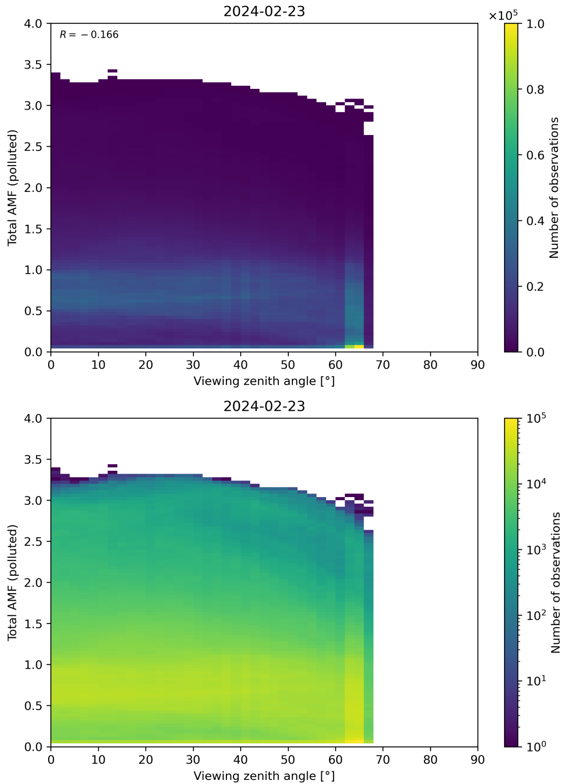
Figure 325: Scatter density plot of “Viewing zenith angle” against “Total AMF (polluted)” for 2024-02-22 to 2024-02-24.
