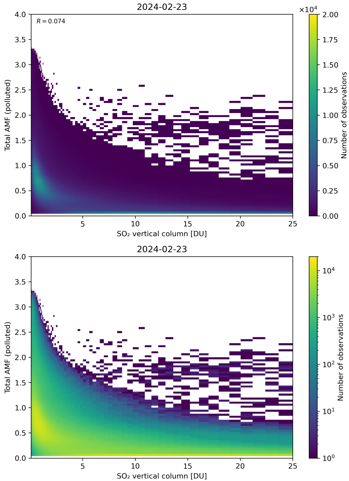
Figure 305: Scatter density plot of “SO 2 vertical column” against “Total AMF (polluted)” for 2024-02-22 to 2024-02-24.
