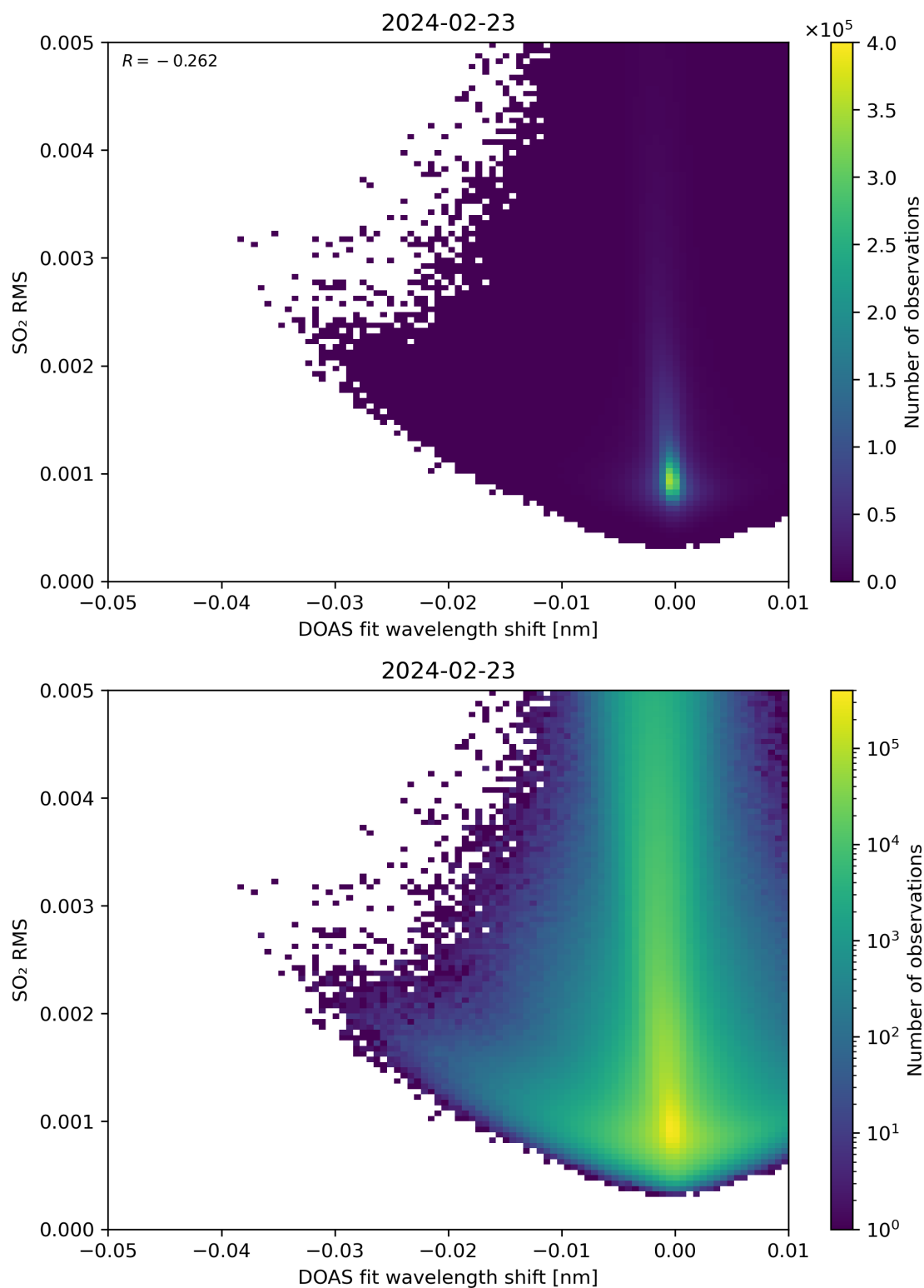
Figure 128: Scatter density plot of “DOAS fit wavelength shift” against “SO 2 RMS” for 2024-02-22 to 2024-02-24.
