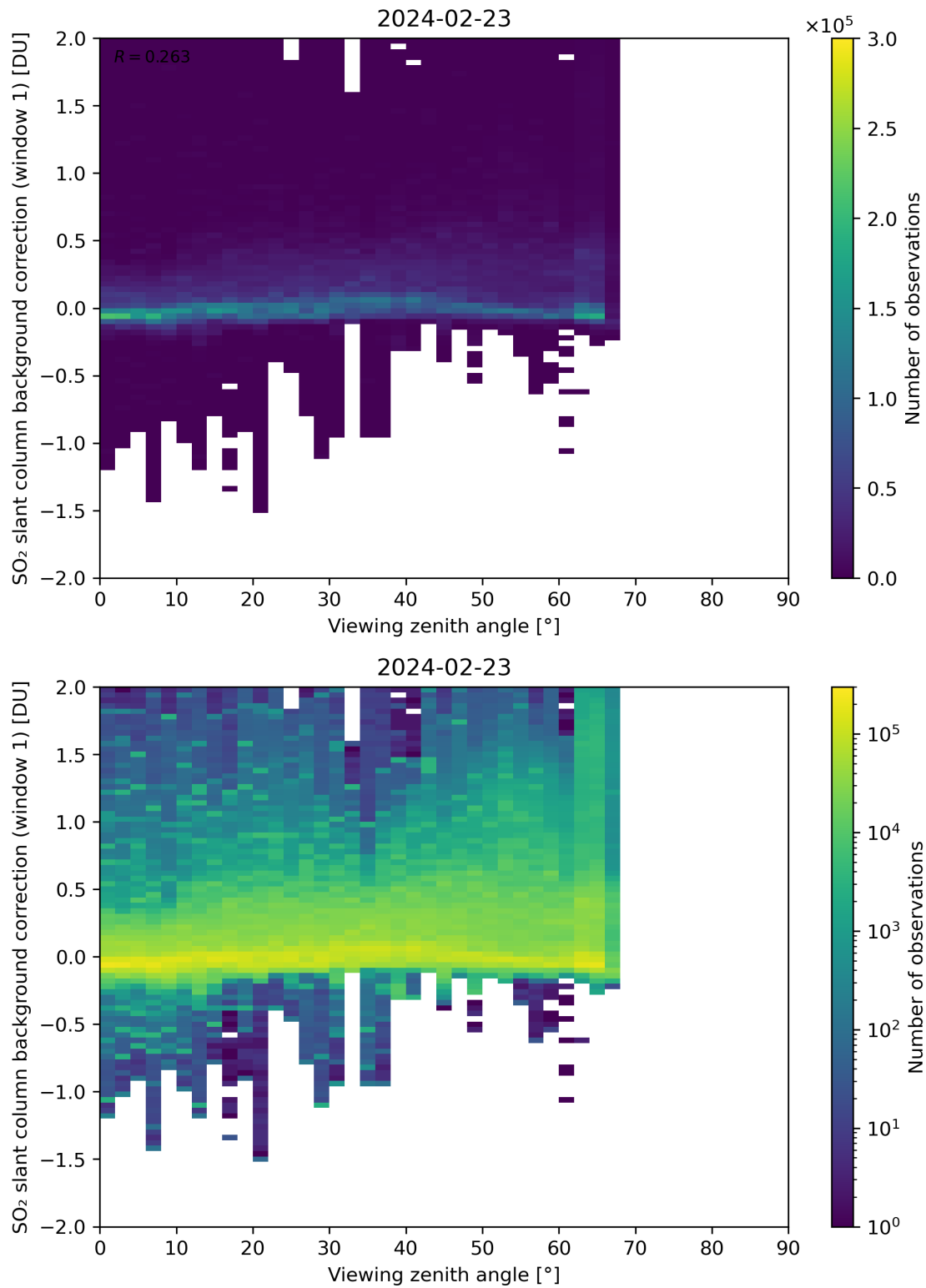
Figure 308: Scatter density plot of “Viewing zenith angle” against “SO 2 slant column background correction (window 1)” for 2024-02-22 to 2024-02-24.
