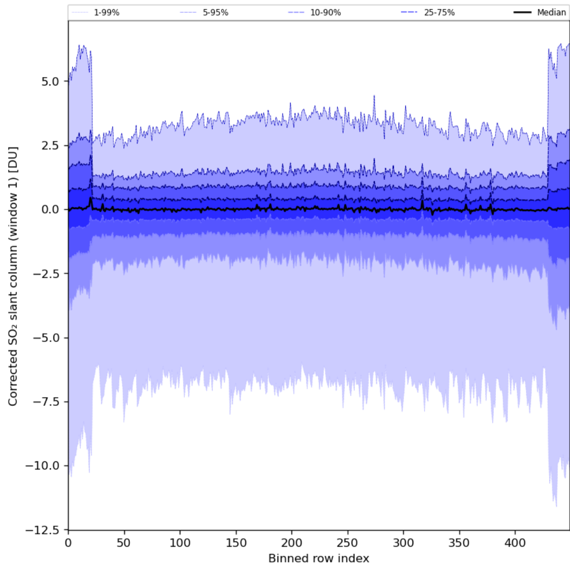
Figure 81: Along track statistics of “Corrected SO 2 slant column (window 1)” for 2024-02-22 to 2024-02-24
