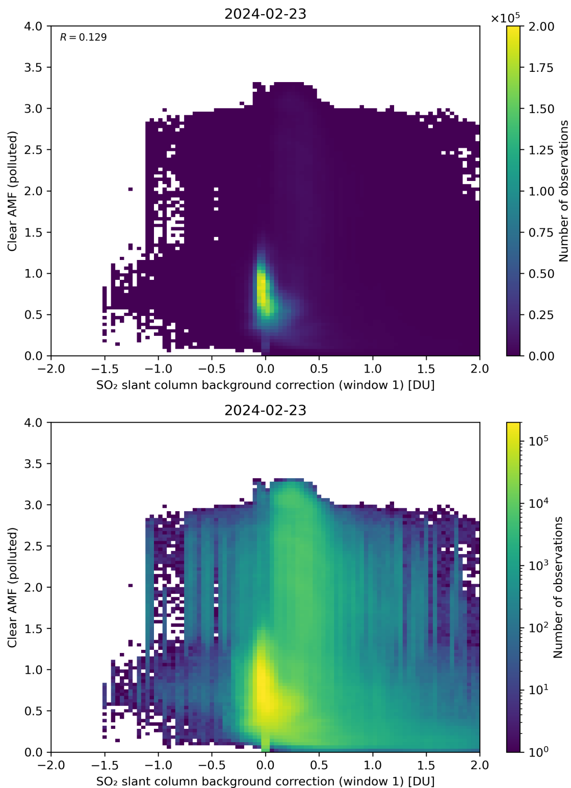
Figure 103: Scatter density plot of “SO 2 slant column background correction (window 1)” against “Clear AMF (polluted)” for 2024-02-22 to 2024-02-24.
