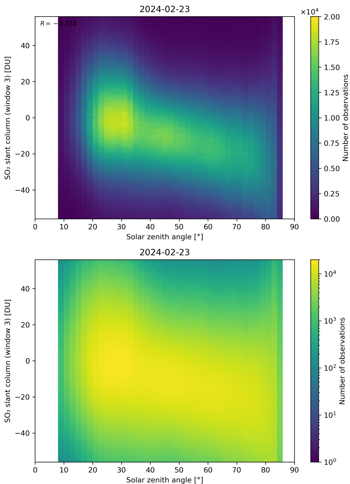
Figure 172: Scatter density plot of “Solar zenith angle” against “SO 2 slant column (window 3)” for 2024-02-22 to 2024-02-24.
