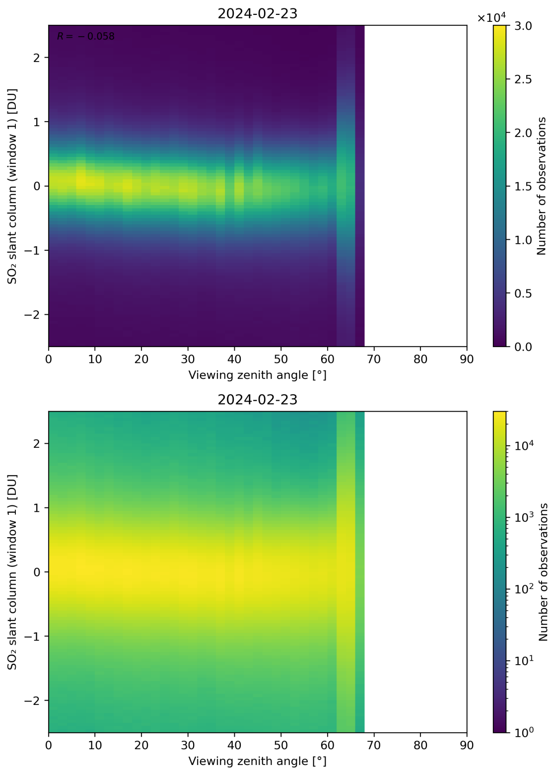
Figure 320: Scatter density plot of “Viewing zenith angle” against “SO 2 slant column (window 1)” for 2024-02-22 to 2024-02-24.
