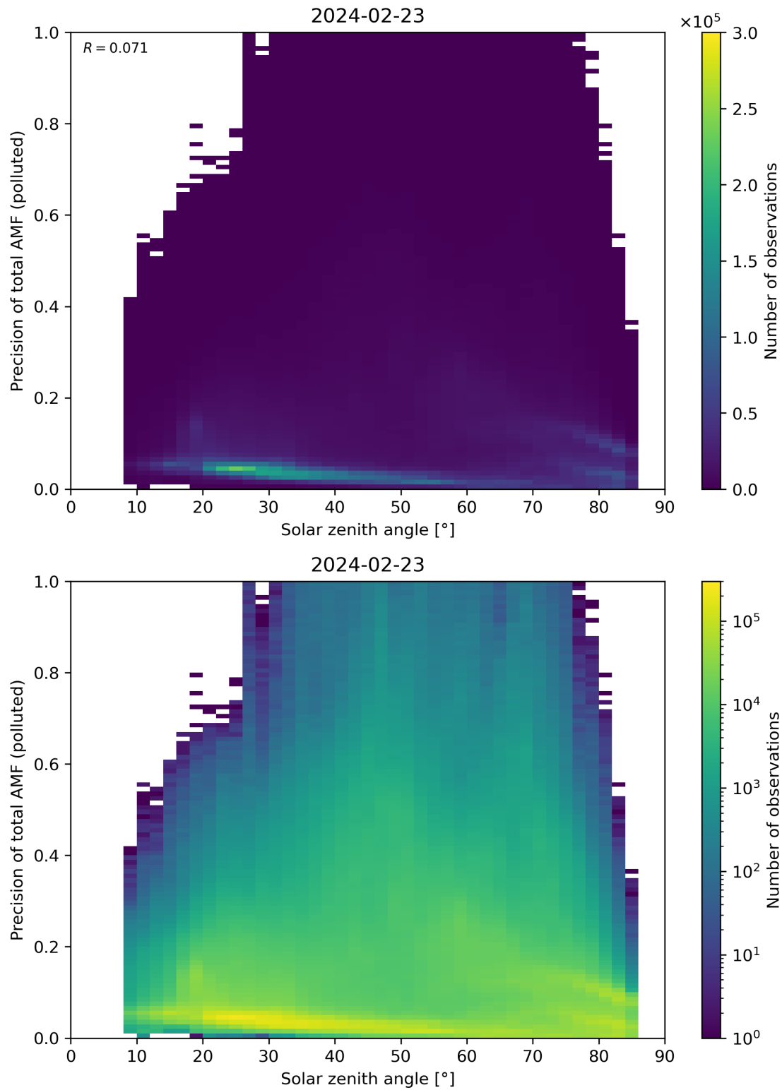
Figure 175: Scatter density plot of “Solar zenith angle” against “Precision of total AMF (polluted)” for 2024-02-22 to 2024-02-24.
