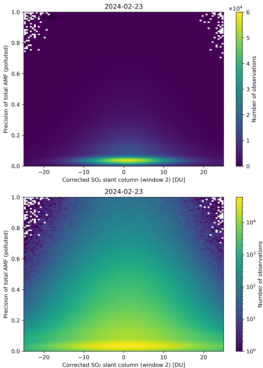
Figure 204: Scatter density plot of “Corrected SO 2 slant column (window 2)” against “Precision of total AMF (polluted)” for 2024-02-22 to 2024-02-24.
