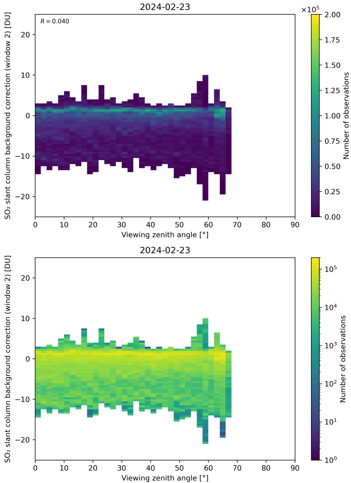
Figure 309: Scatter density plot of “Viewing zenith angle” against “SO 2 slant column background correction (window 2)” for 2024-02-22 to 2024-02-24.
