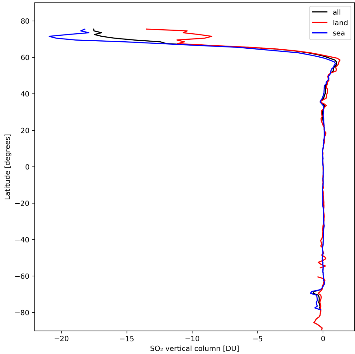
Figure 30: Zonal average of “SO 2 vertical column” for 2024-02-22 to 2024-02-24.
