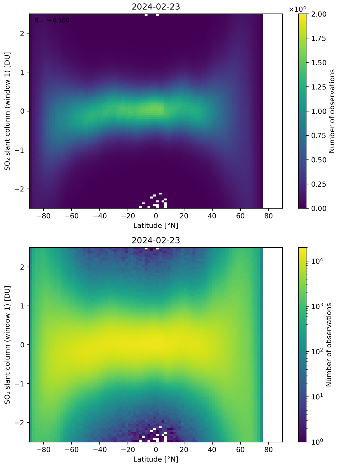
Figure 149: Scatter density plot of “Latitude” against “SO 2 slant column (window 1)” for 2024-02-22 to 2024-02-24.
