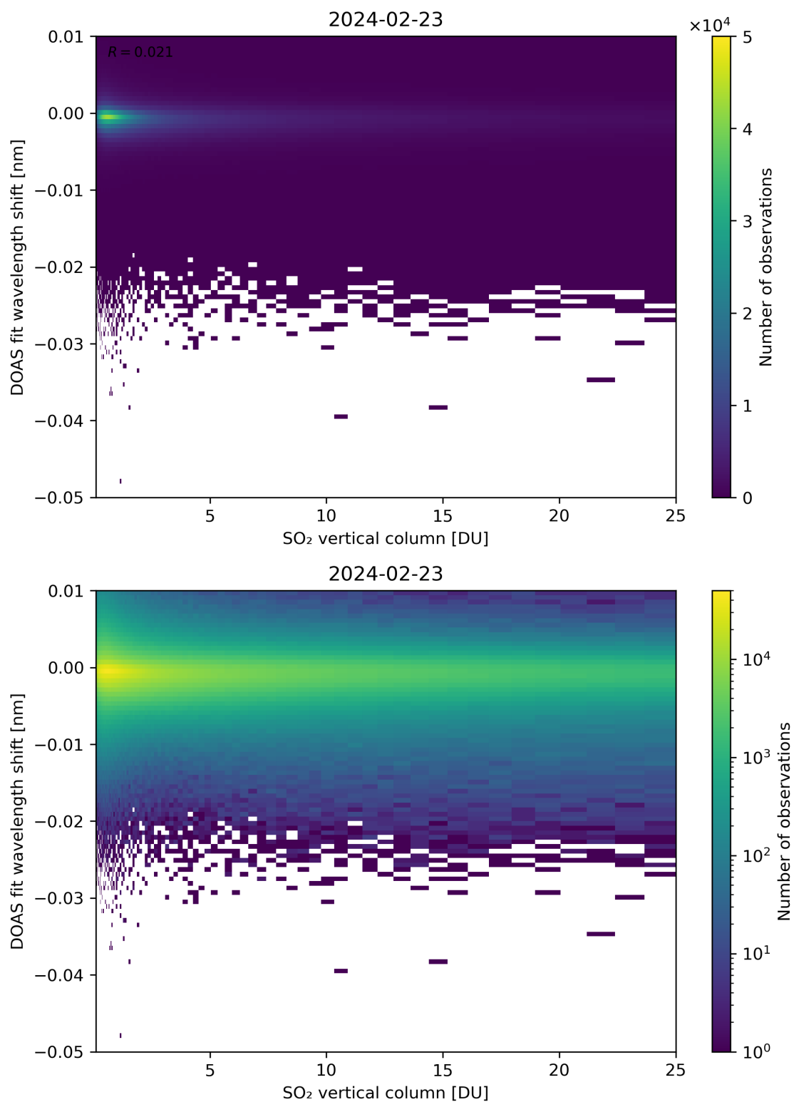
Figure 276: Scatter density plot of “SO 2 vertical column” against “DOAS fit wavelength shift” for 2024-02-22 to 2024-02-24.
