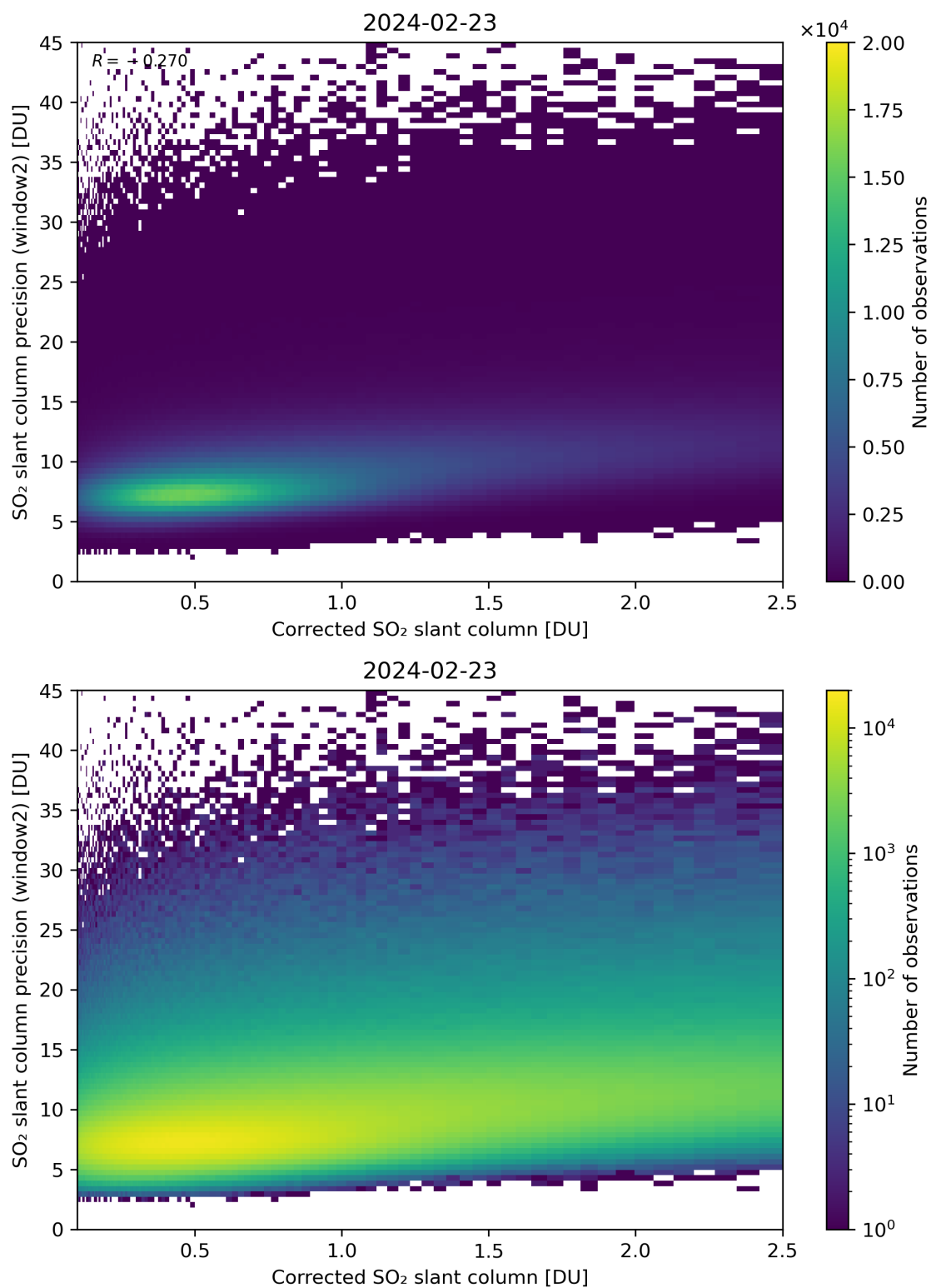
Figure 189: Scatter density plot of “Corrected SO 2 slant column” against “SO 2 slant column precision (window2)” for 2024-02-22 to 2024-02-24.
