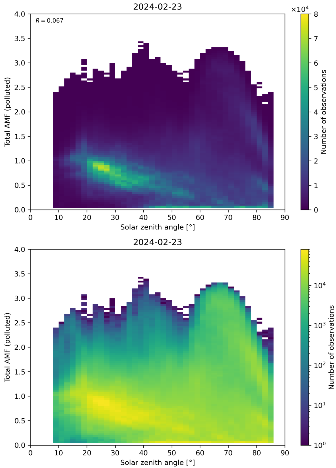
Figure 174: Scatter density plot of “Solar zenith angle” against “Total AMF (polluted)” for 2024-02-22 to 2024-02-24.
