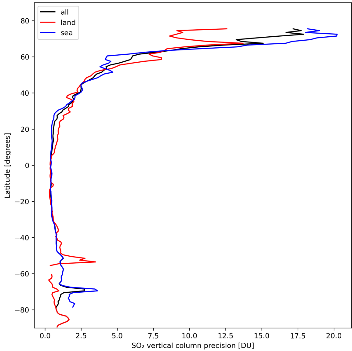
Figure 31: Zonal average of “SO 2 vertical column precision” for 2024-02-22 to 2024-02-24.
