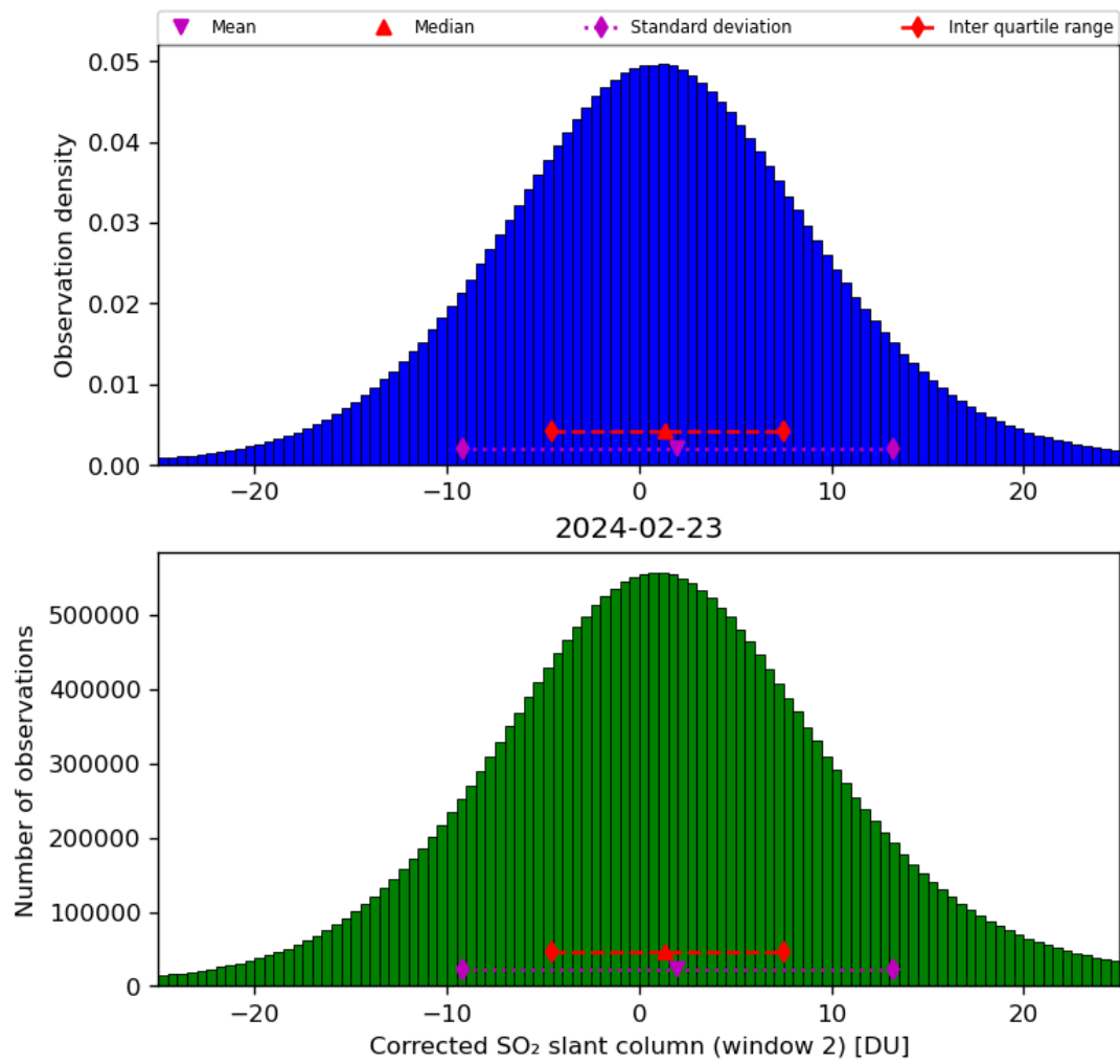
Figure 62: Histogram of “Corrected SO 2 slant column (window 2)” for 2024-02-22 to 2024-02-24
