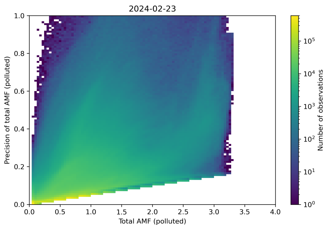
Figure 272: Scatter density plot of “Total AMF (polluted)” against “Precision of total AMF (polluted)” for 2024-02-22 to 2024-02-24.
