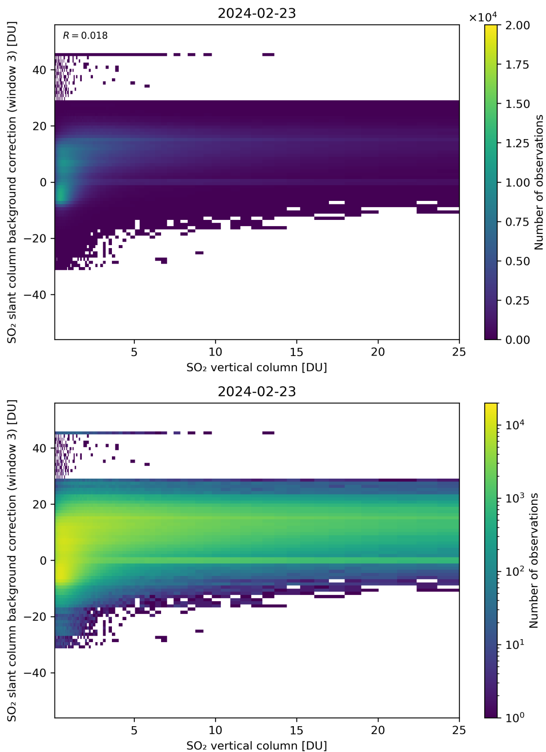
Figure 275: Scatter density plot of “SO 2 vertical column” against “SO 2 slant column background correction (window 3)” for 2024-02-22 to 2024-02-24.
