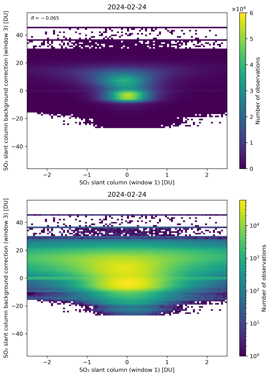
Figure 214: Scatter density plot of “SO 2 slant column (window 1)” against “SO 2 slant column background correction (window 3)” for 2024-02-23 to 2024-02-25.
