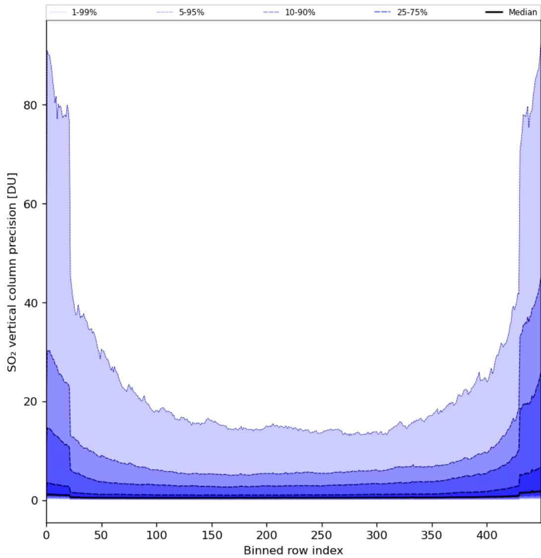
Figure 77: Along track statistics of “SO 2 vertical column precision” for 2024-02-23 to 2024-02-25
