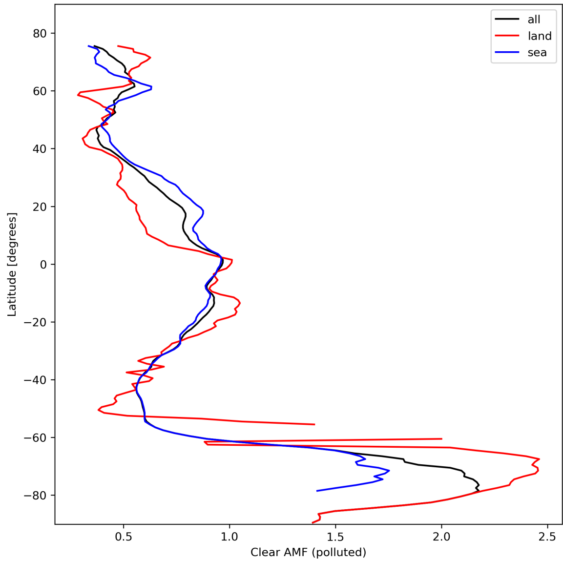
Figure 50: Zonal average of “Clear AMF (polluted)” for 2024-02-23 to 2024-02-25.
