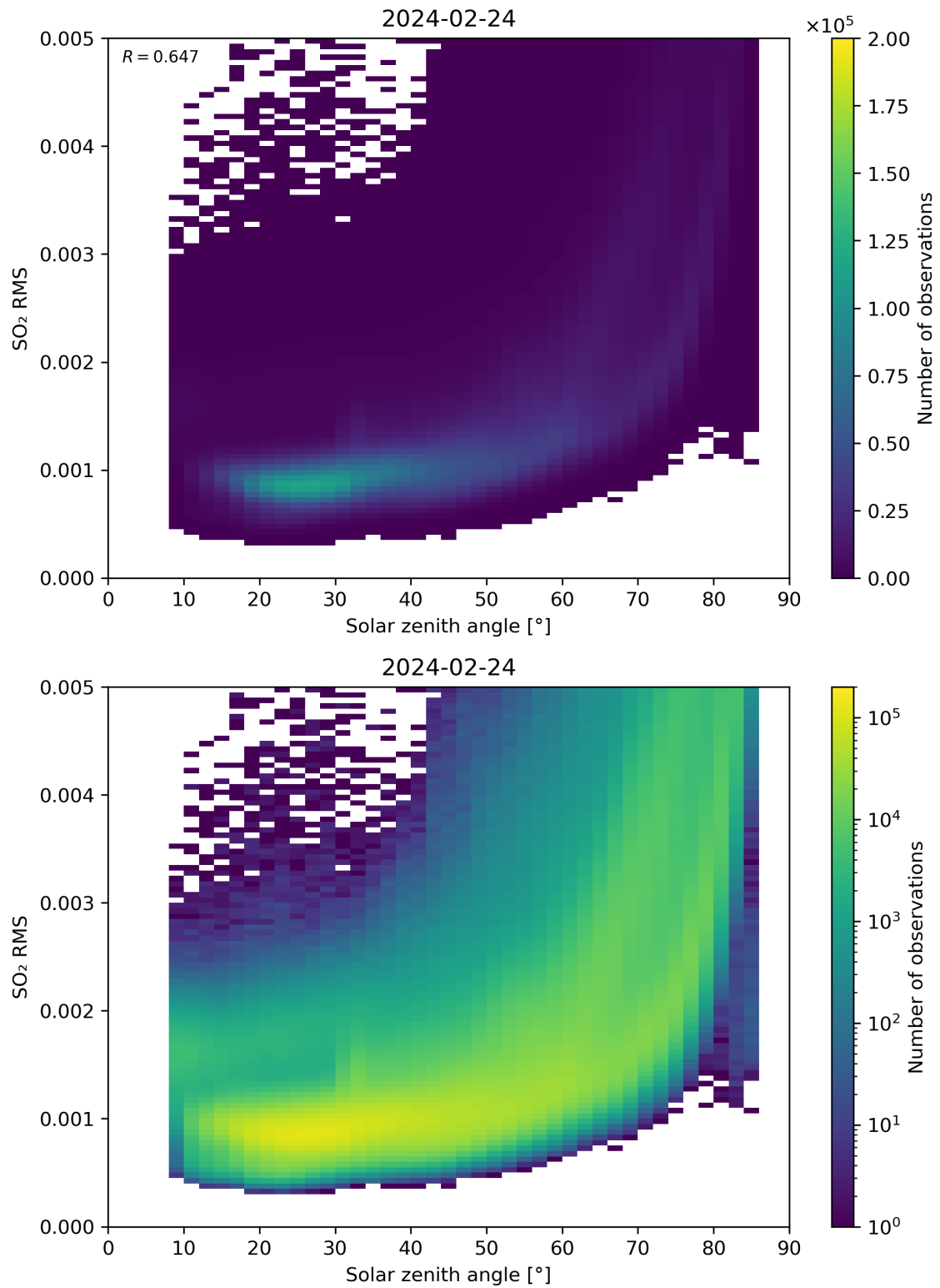
Figure 163: Scatter density plot of “Solar zenith angle” against “SO 2 RMS” for 2024-02-23 to 2024-02-25.
