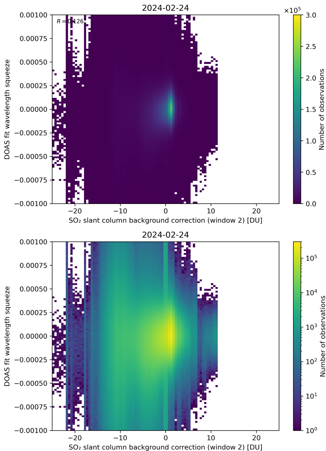
Figure 113: Scatter density plot of “SO 2 slant column background correction (window 2)” against “DOAS fit wavelength squeeze” for 2024-02-23 to 2024-02-25.
