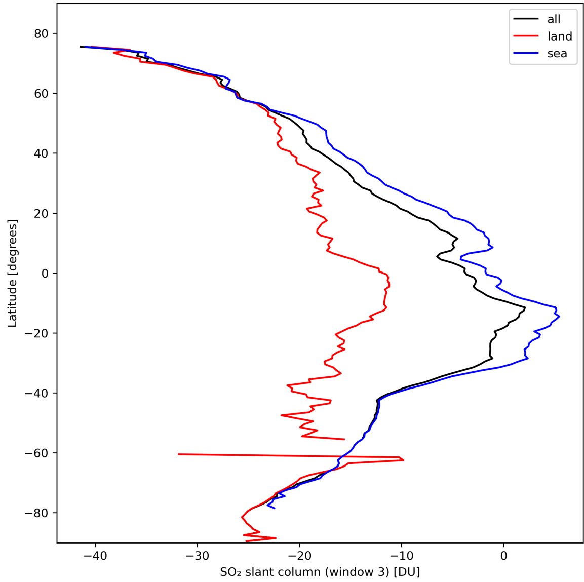
Figure 41: Zonal average of “SO 2 slant column (window 3)” for 2024-02-23 to 2024-02-25.
