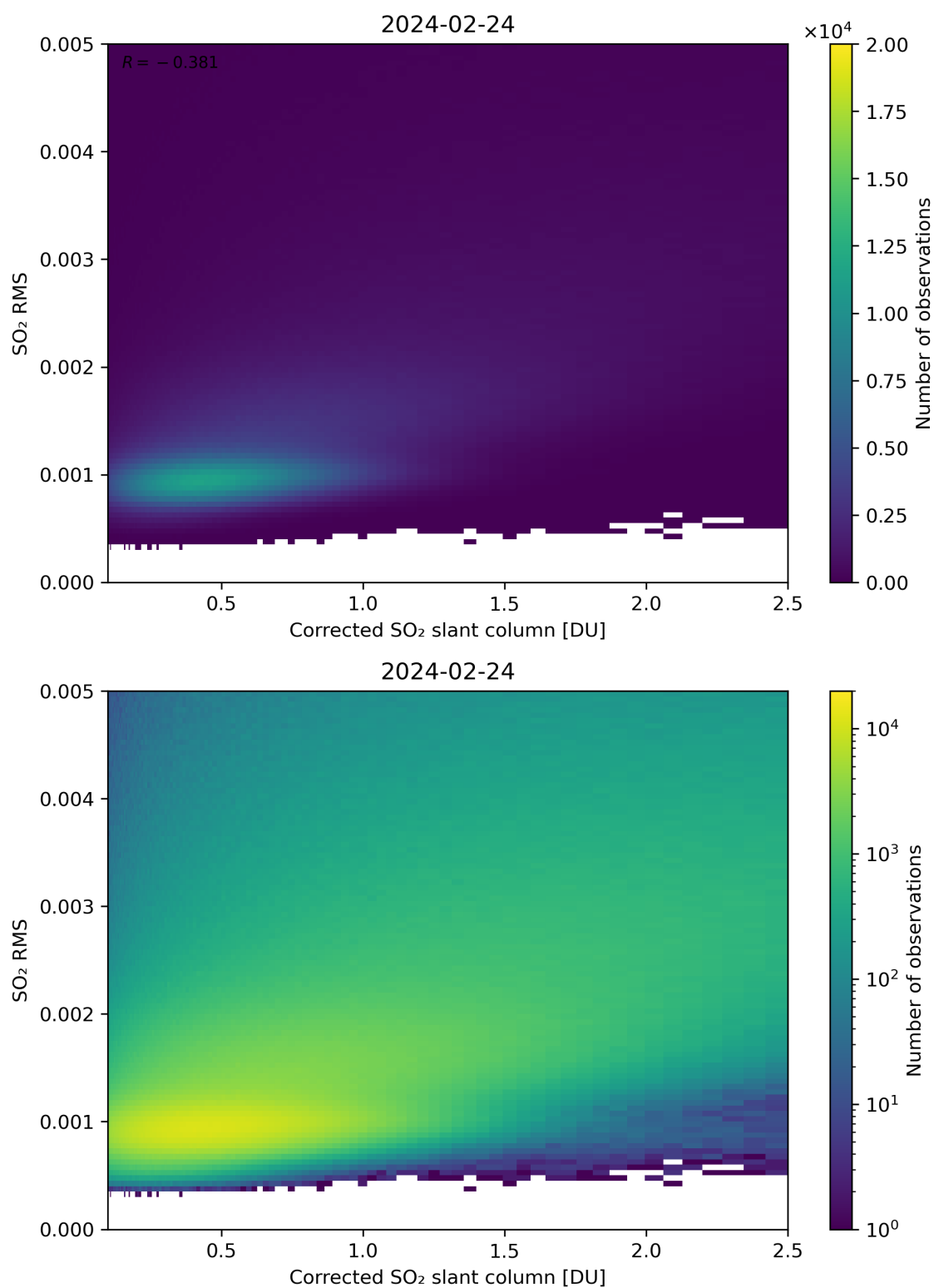
Figure 183: Scatter density plot of “Corrected SO 2 slant column” against “SO 2 RMS” for 2024-02-23 to 2024-02-25.
