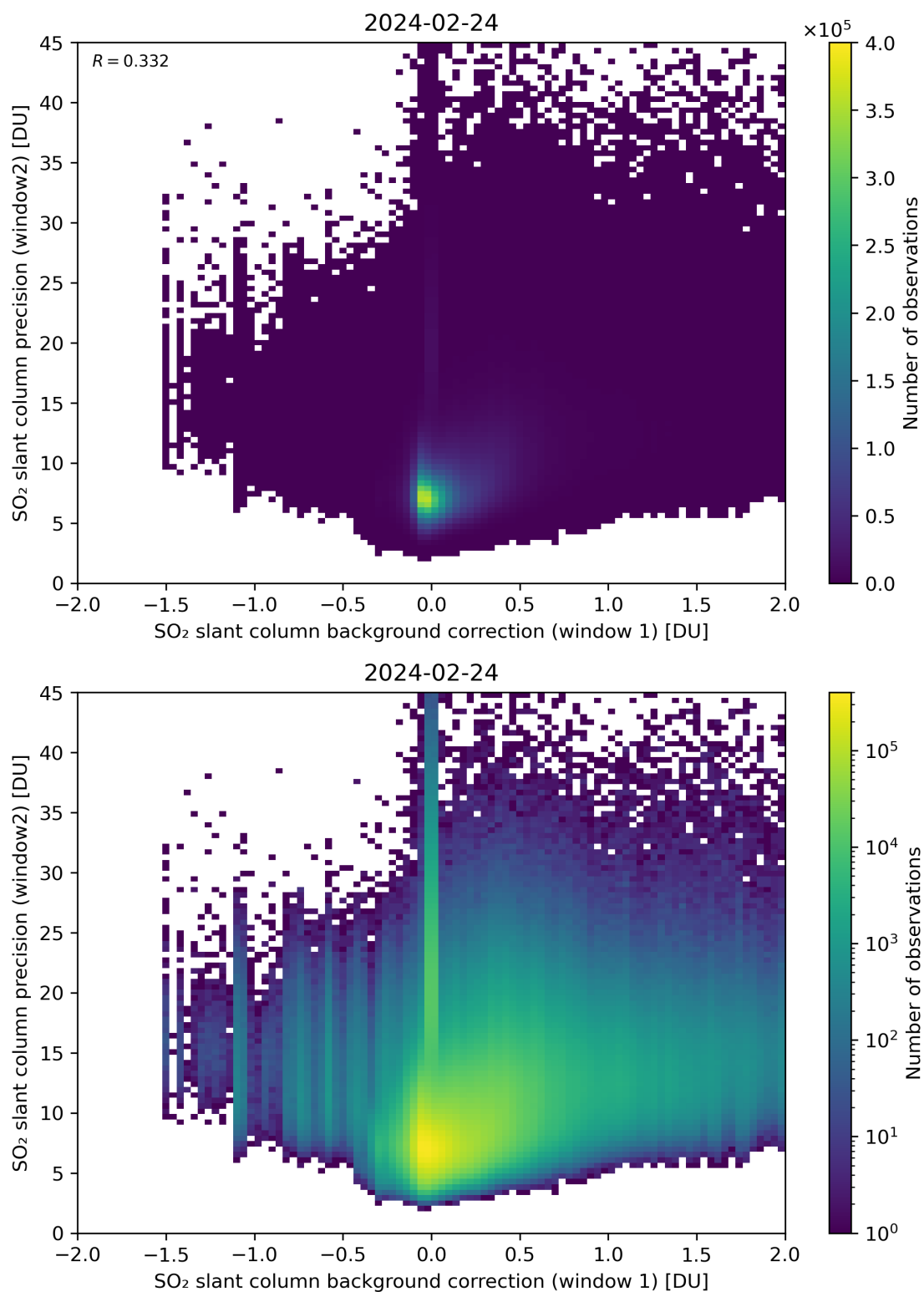
Figure 106: Scatter density plot of “SO 2 slant column background correction (window 1)” against “SO 2 slant column precision (window2)” for 2024-02-23 to 2024-02-25.
