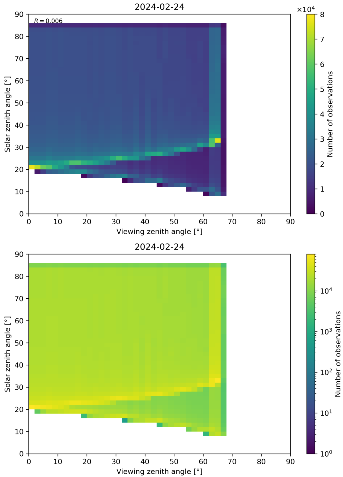
Figure 315: Scatter density plot of “Viewing zenith angle” against “Solar zenith angle” for 2024-02-23 to 2024-02-25.
