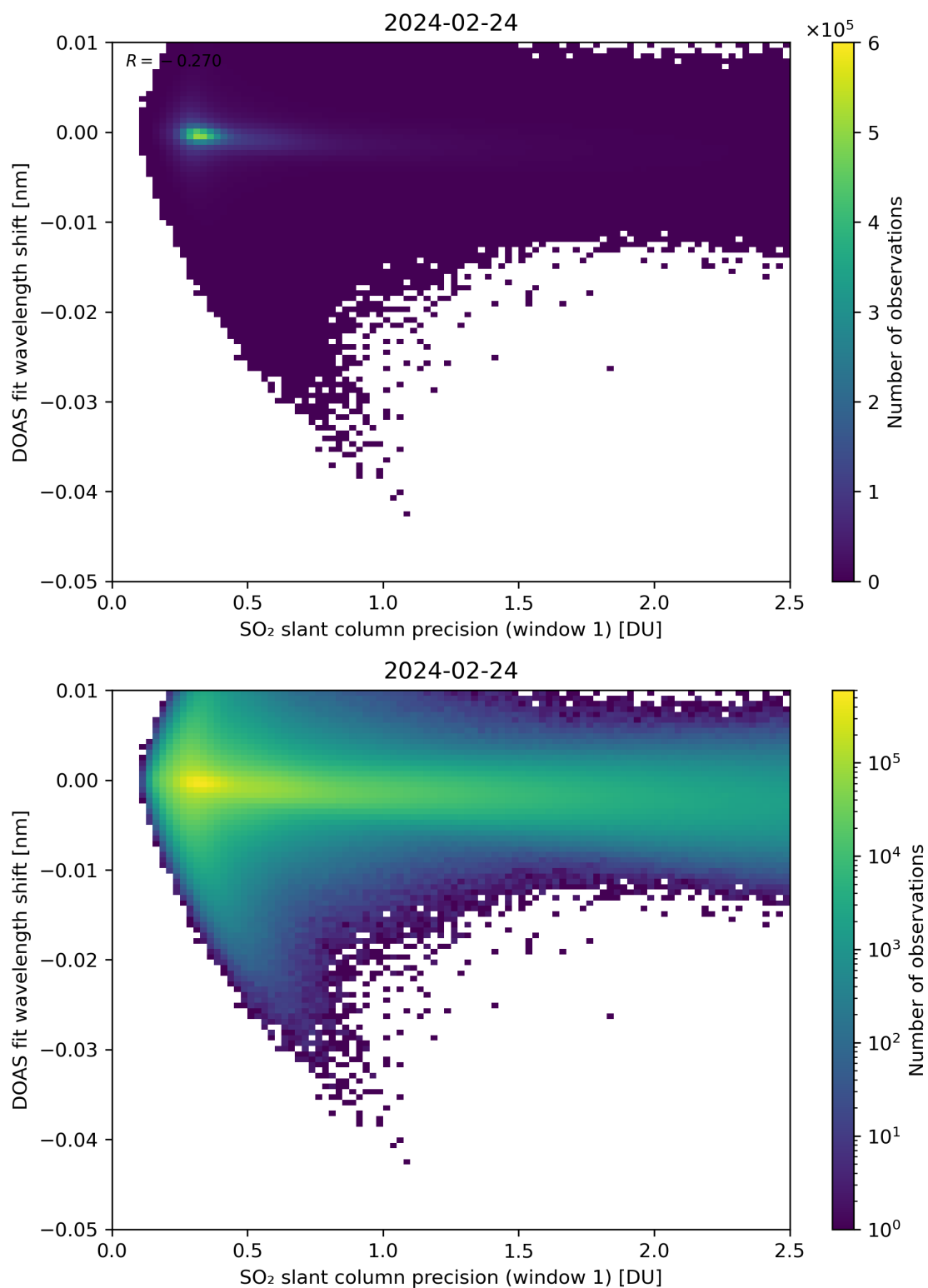
Figure 221: Scatter density plot of “SO 2 slant column precision (window 1)” against “DOAS fit wavelength shift” for 2024-02-23 to 2024-02-25.
