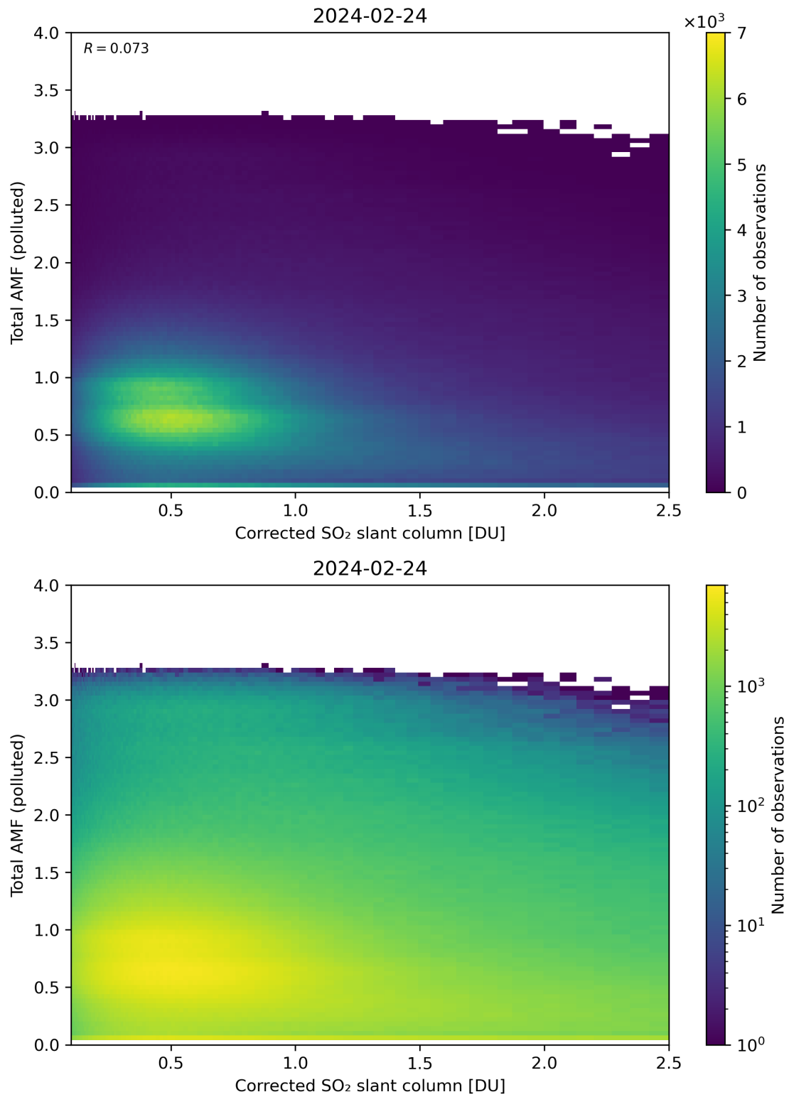
Figure 192: Scatter density plot of “Corrected SO 2 slant column” against “Total AMF (polluted)” for 2024-02-23 to 2024-02-25.
