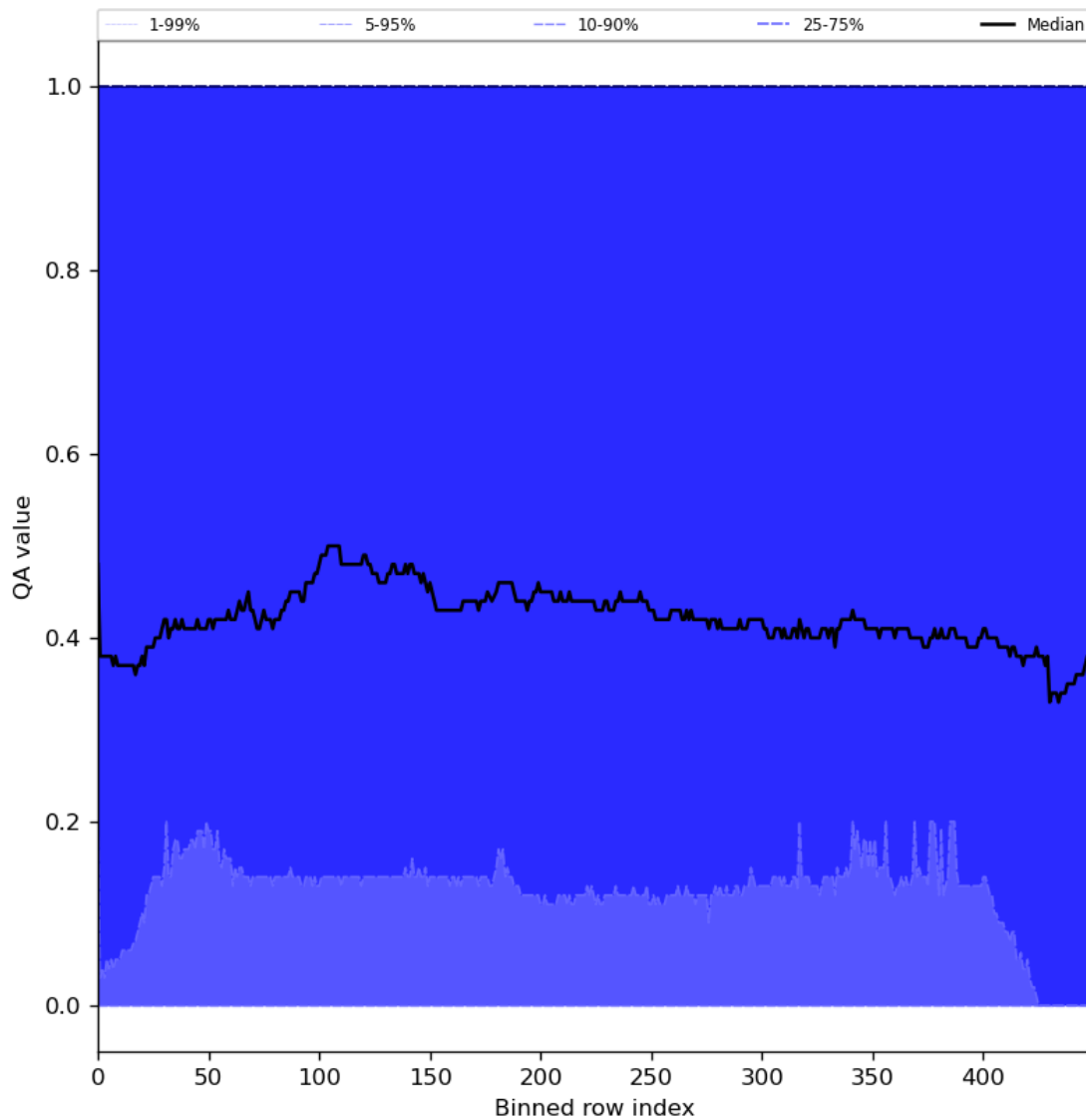
Figure 75: Along track statistics of “QA value” for 2024-02-23 to 2024-02-25
