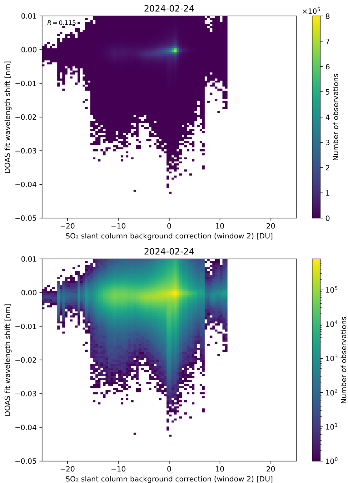
Figure 112: Scatter density plot of “SO 2 slant column background correction (window 2)” against “DOAS fit wavelength shift” for 2024-02-23 to 2024-02-25.
