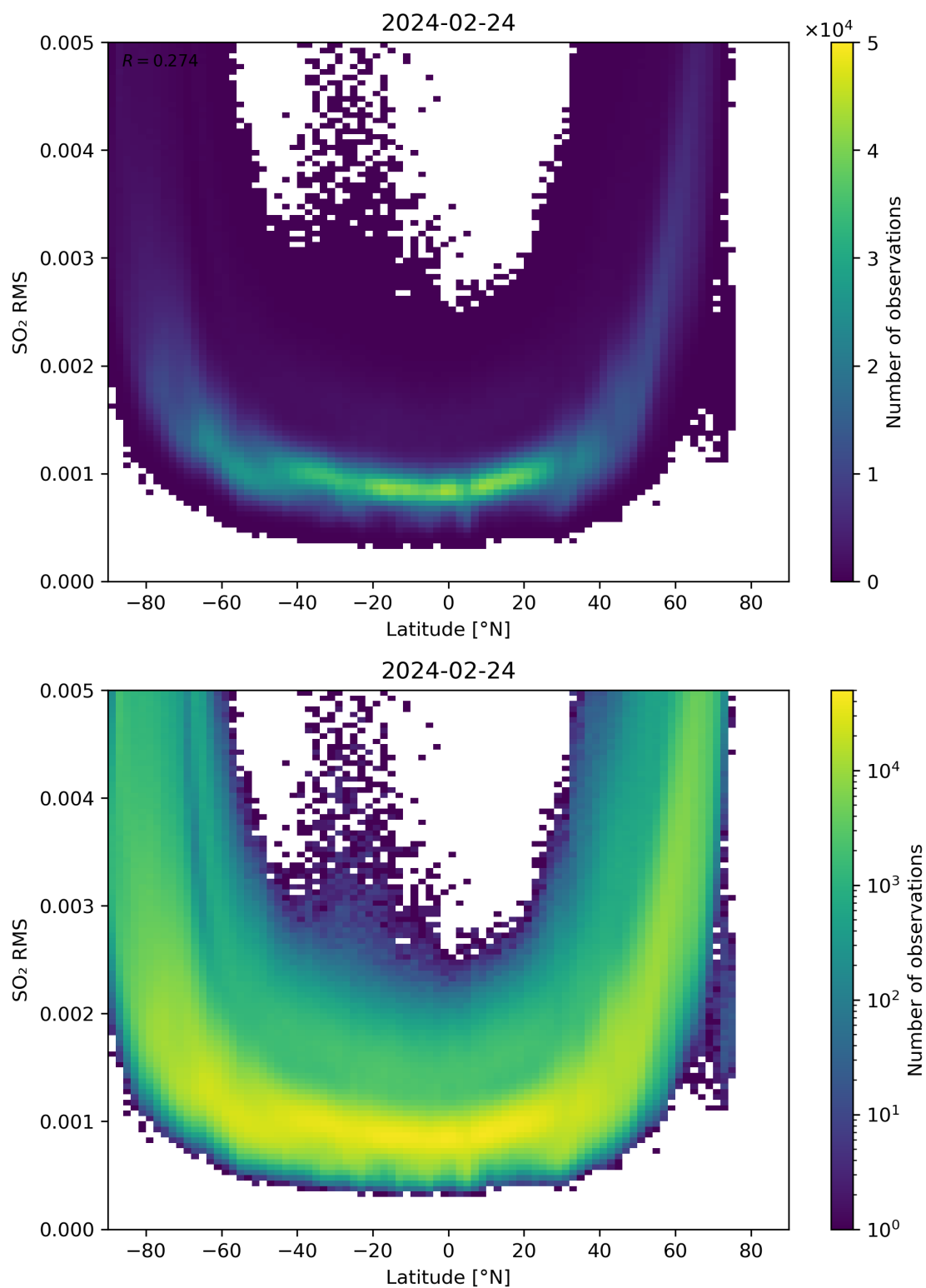
Figure 144: Scatter density plot of “Latitude” against “SO 2 RMS” for 2024-02-23 to 2024-02-25.
