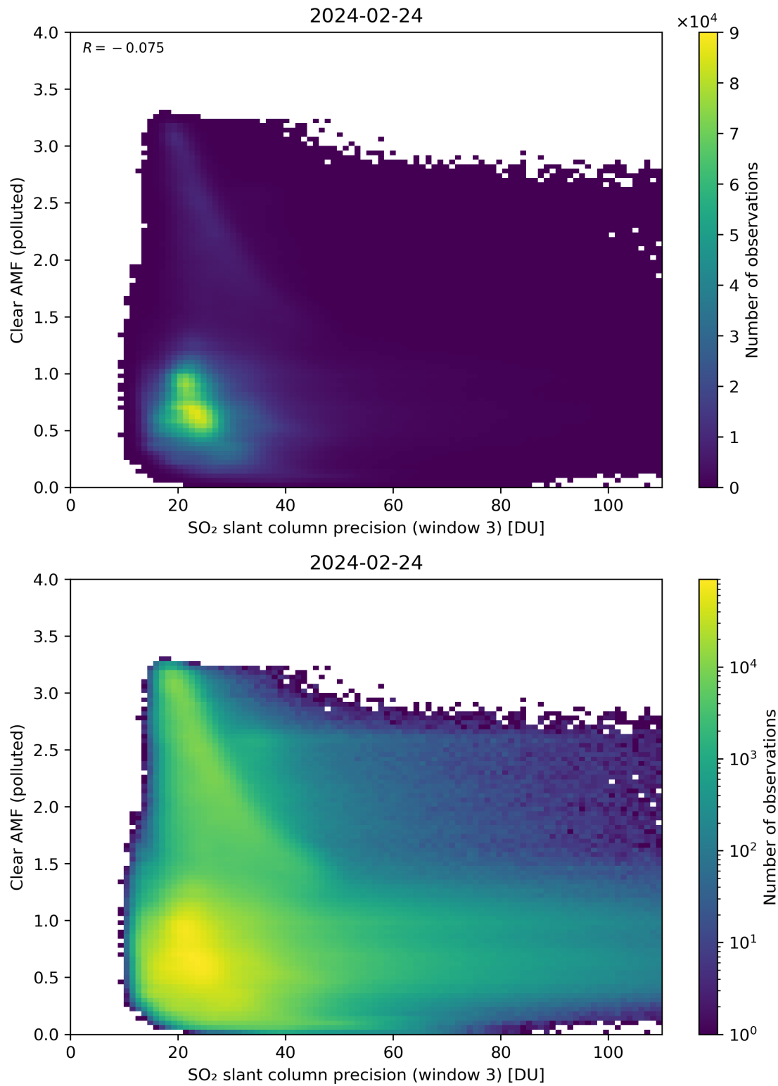
Figure 261: Scatter density plot of “SO 2 slant column precision (window 3)” against “Clear AMF (polluted)” for 2024-02-23 to 2024-02-25.
