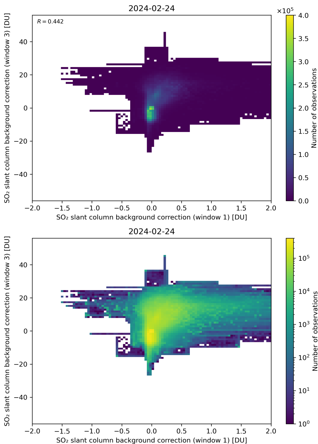
Figure 99: Scatter density plot of “SO 2 slant column background correction (window 1)” against “SO 2 slant column background correction (window 3)” for 2024-02-23 to 2024-02-25.
