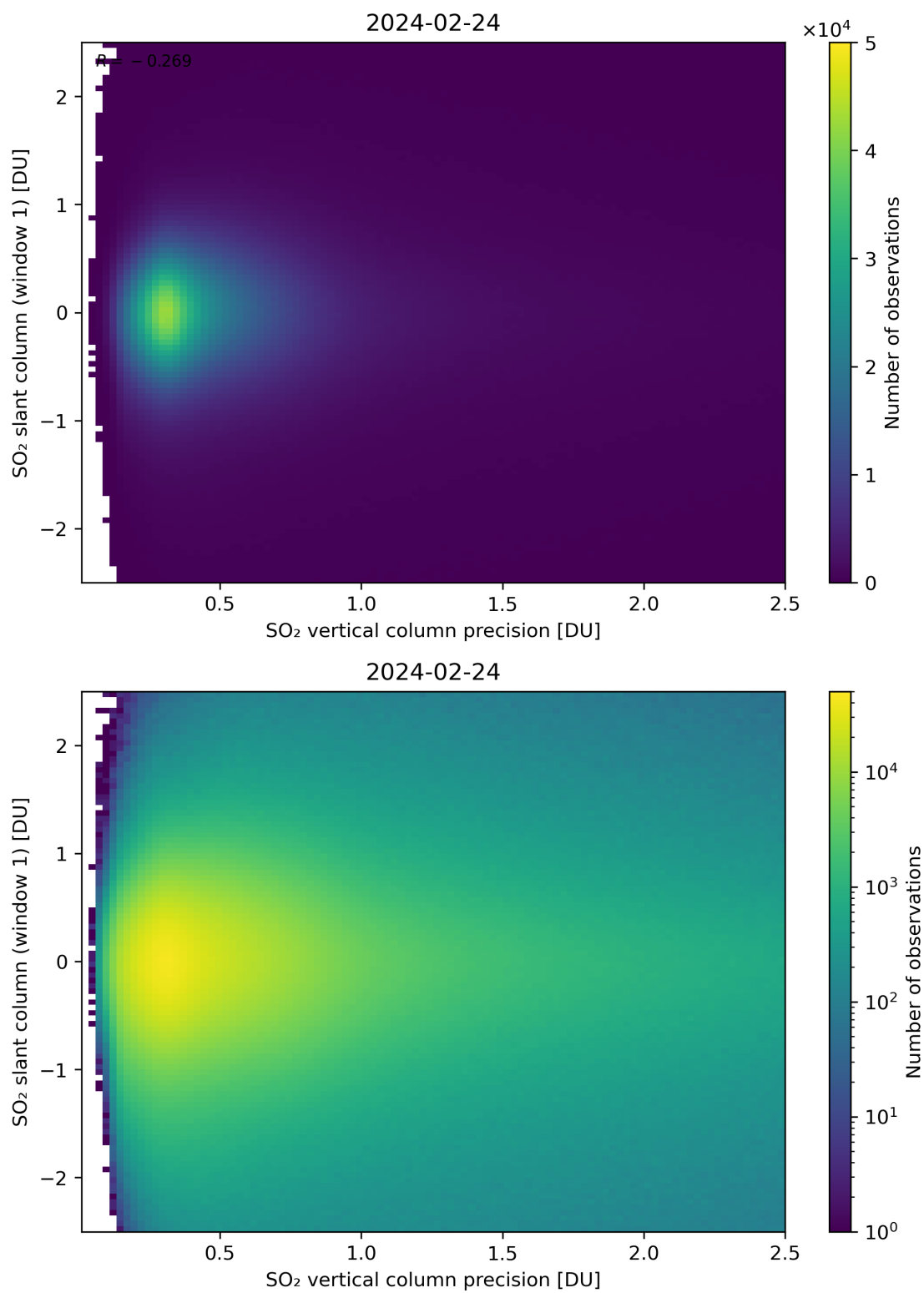
Figure 289: Scatter density plot of “SO 2 vertical column precision” against “SO 2 slant column (window 1)” for 2024-02-23 to 2024-02-25.
