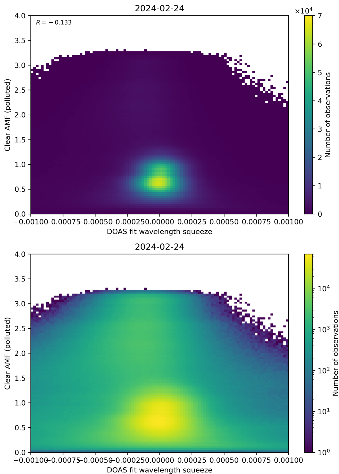
Figure 133: Scatter density plot of “DOAS fit wavelength squeeze” against “Clear AMF (polluted)” for 2024-02-23 to 2024-02-25.
