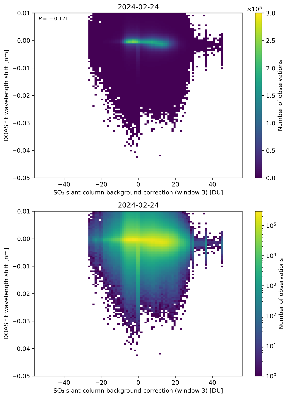
Figure 121: Scatter density plot of “SO 2 slant column background correction (window 3)” against “DOAS fit wavelength shift” for 2024-02-23 to 2024-02-25.
