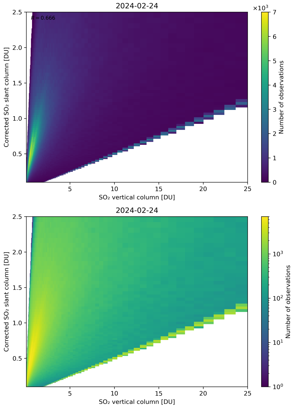
Figure 297: Scatter density plot of “SO 2 vertical column” against “Corrected SO 2 slant column” for 2024-02-23 to 2024-02-25.
