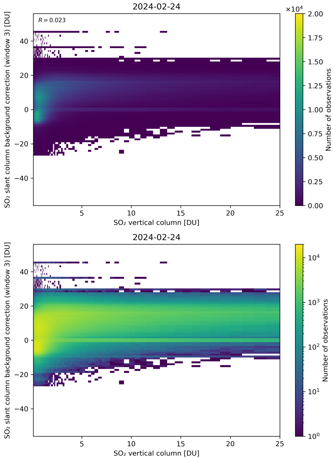
Figure 275: Scatter density plot of “SO 2 vertical column” against “SO 2 slant column background correction (window 3)” for 2024-02-23 to 2024-02-25.
