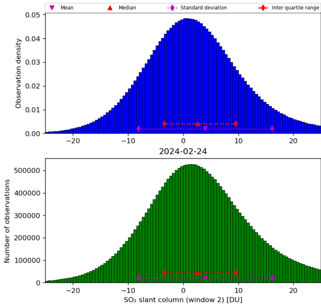
Figure 60: Histogram of “SO 2 slant column (window 2)” for 2024-02-23 to 2024-02-25
