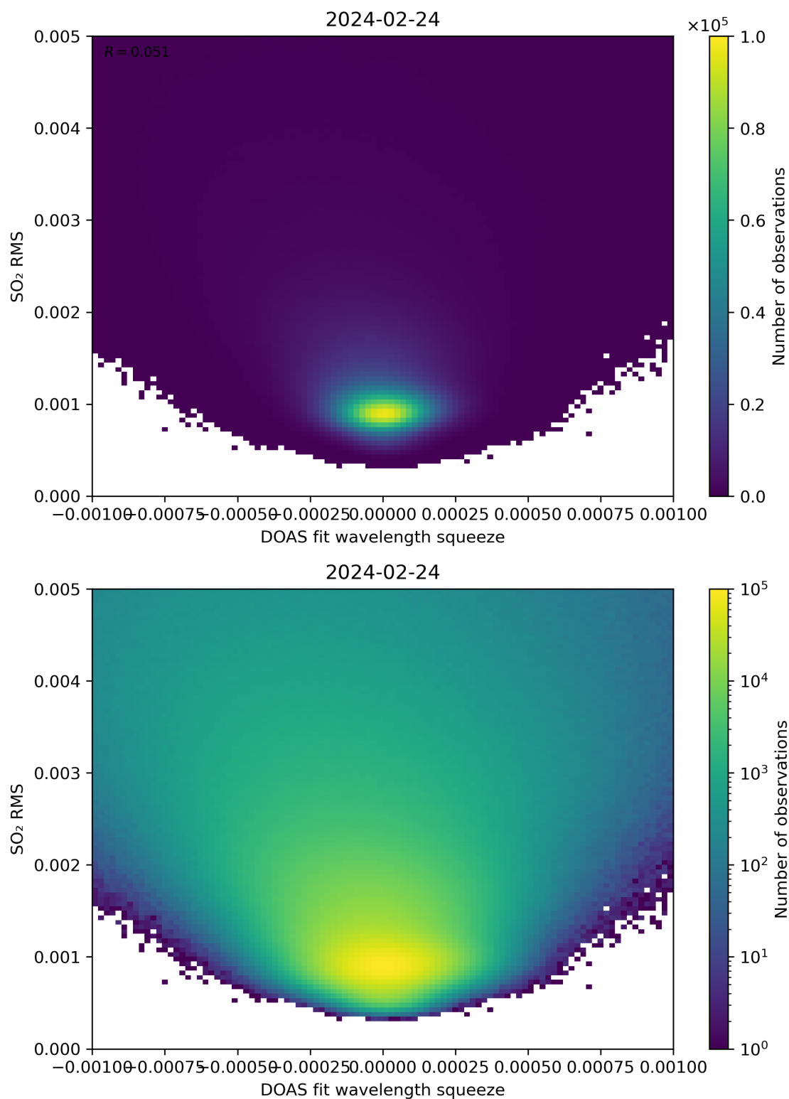
Figure 132: Scatter density plot of “DOAS fit wavelength squeeze” against “SO 2 RMS” for 2024-02-23 to 2024-02-25.
