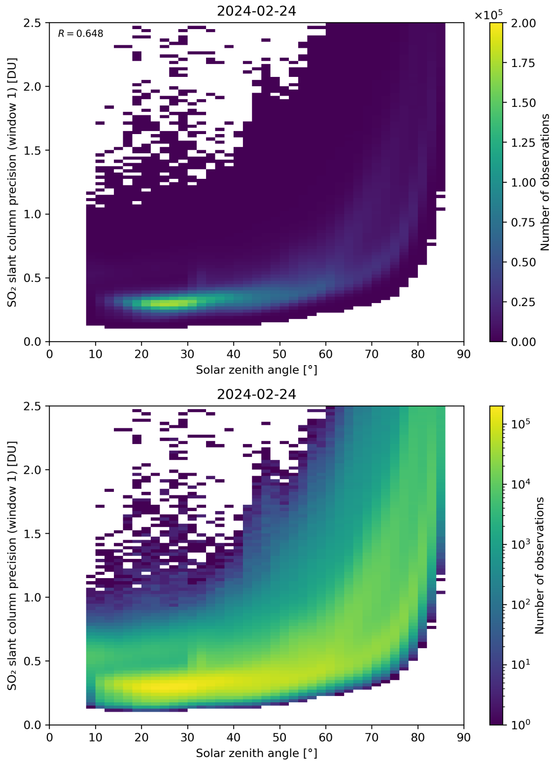
Figure 170: Scatter density plot of “Solar zenith angle” against “SO 2 slant column precision (window 1)” for 2024-02-23 to 2024-02-25.
