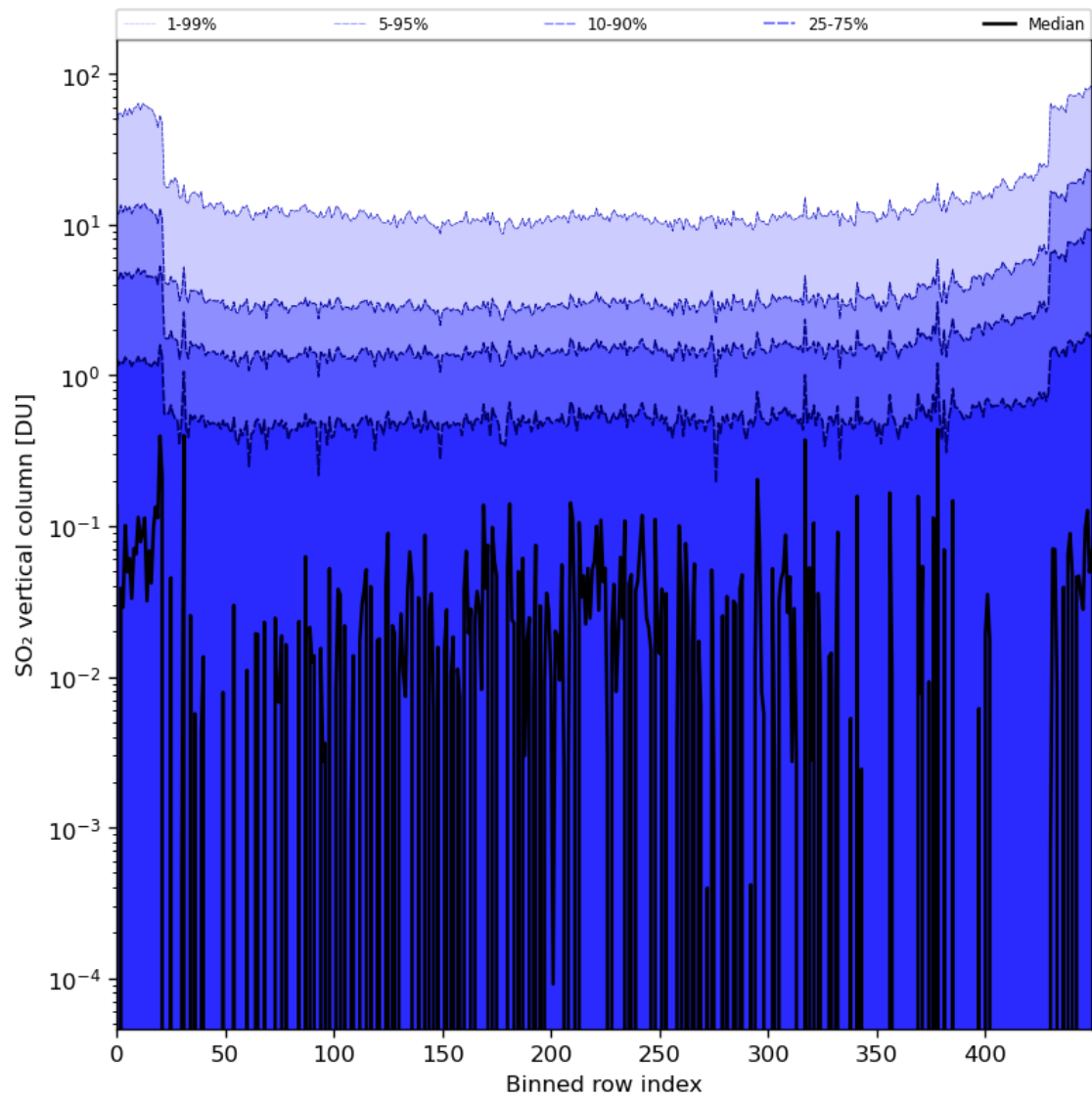
Figure 76: Along track statistics of “SO 2 vertical column” for 2024-02-23 to 2024-02-25
