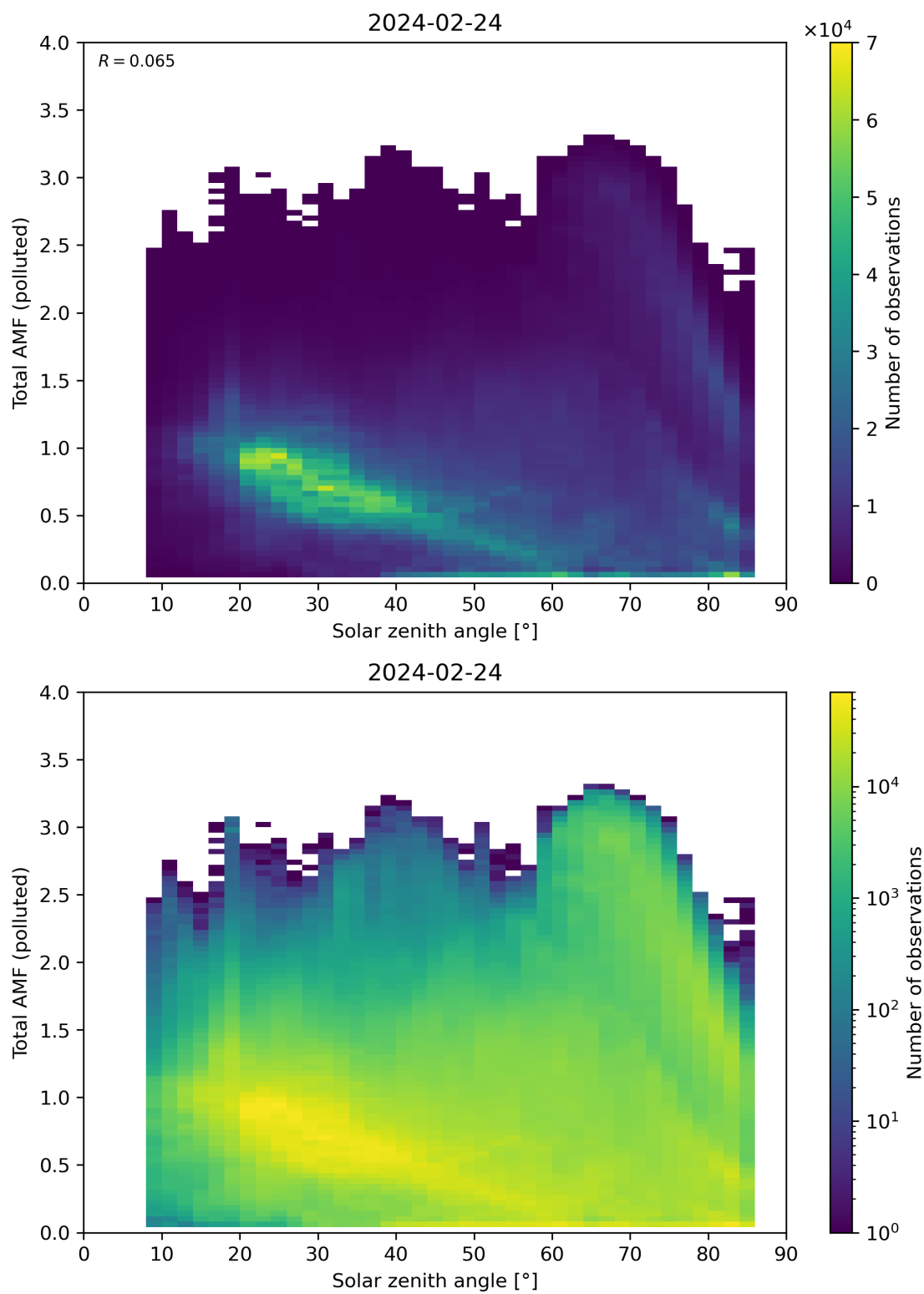
Figure 174: Scatter density plot of “Solar zenith angle” against “Total AMF (polluted)” for 2024-02-23 to 2024-02-25.
