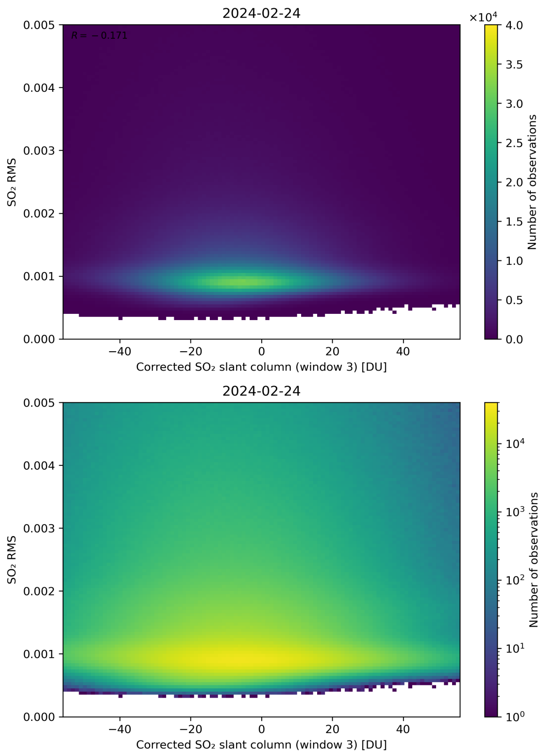
Figure 208: Scatter density plot of “Corrected SO 2 slant column (window 3)” against “SO 2 RMS” for 2024-02-23 to 2024-02-25.
