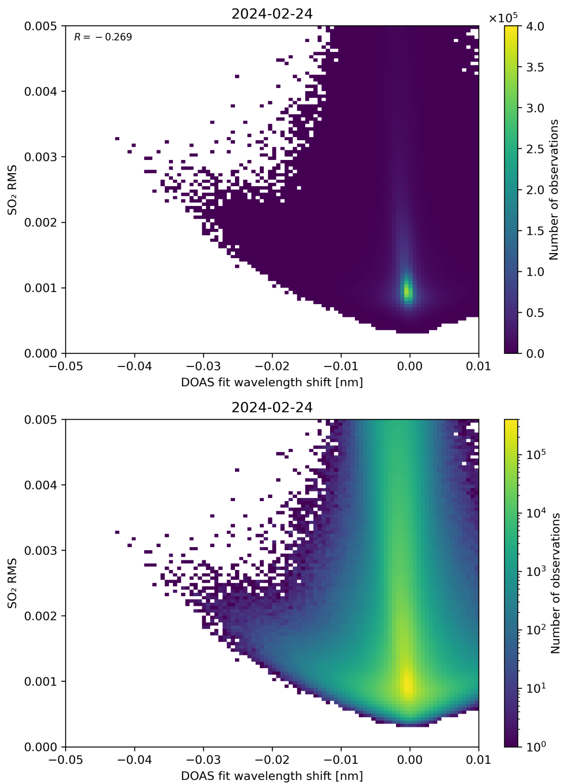
Figure 128: Scatter density plot of “DOAS fit wavelength shift” against “SO 2 RMS” for 2024-02-23 to 2024-02-25.
