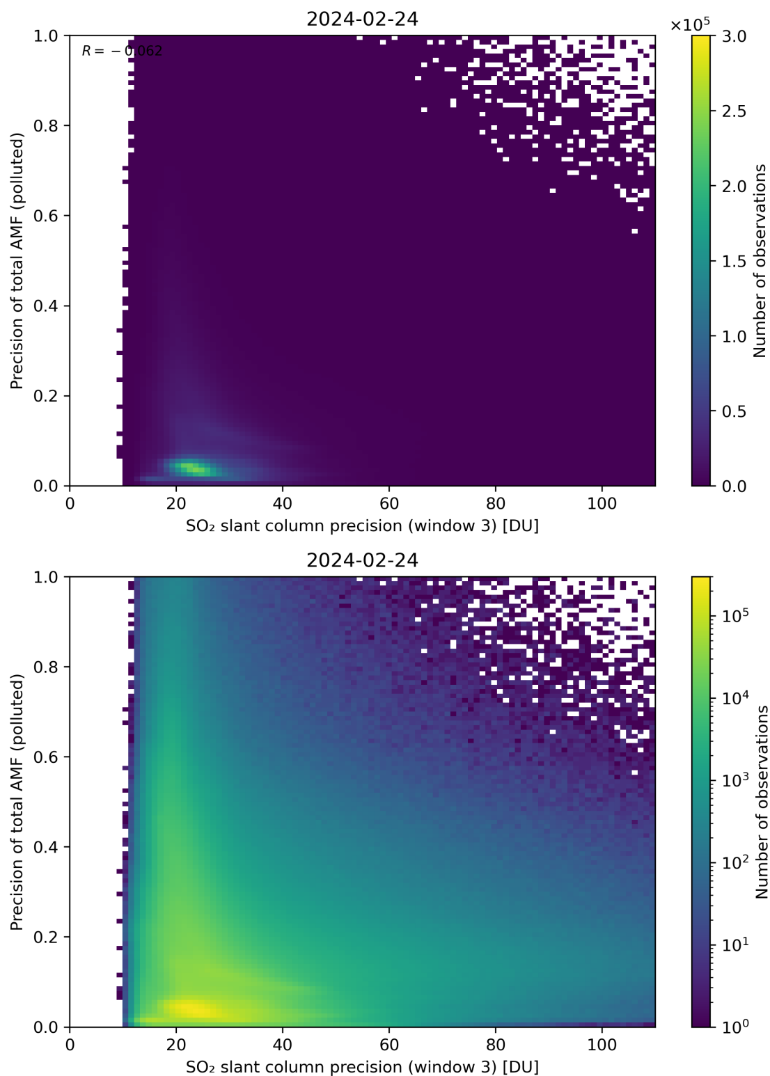
Figure 264: Scatter density plot of “SO 2 slant column precision (window 3)” against “Precision of total AMF (polluted)” for 2024-02-23 to 2024-02-25.
