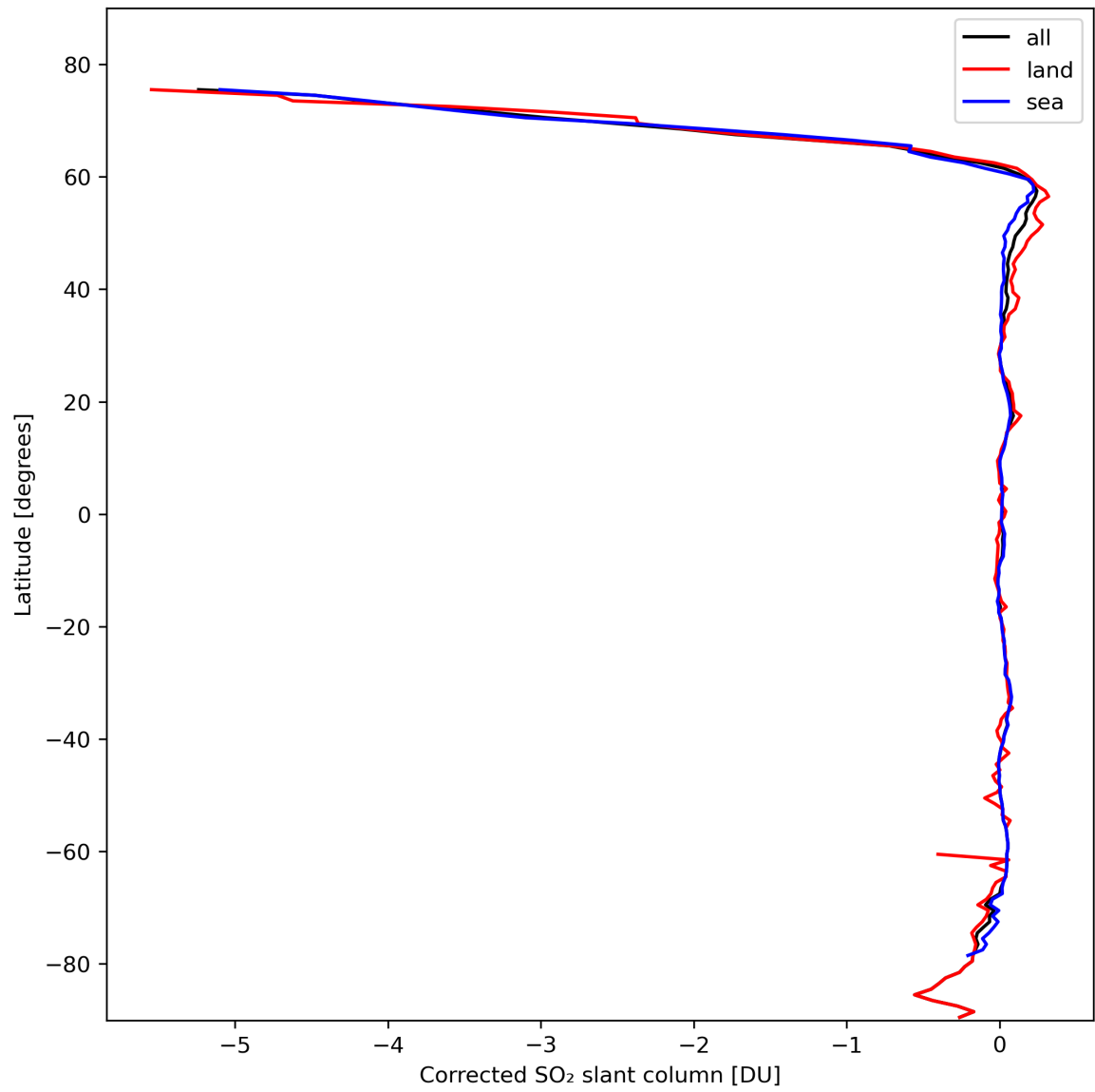
Figure 32: Zonal average of “Corrected SO 2 slant column” for 2024-02-23 to 2024-02-25.
