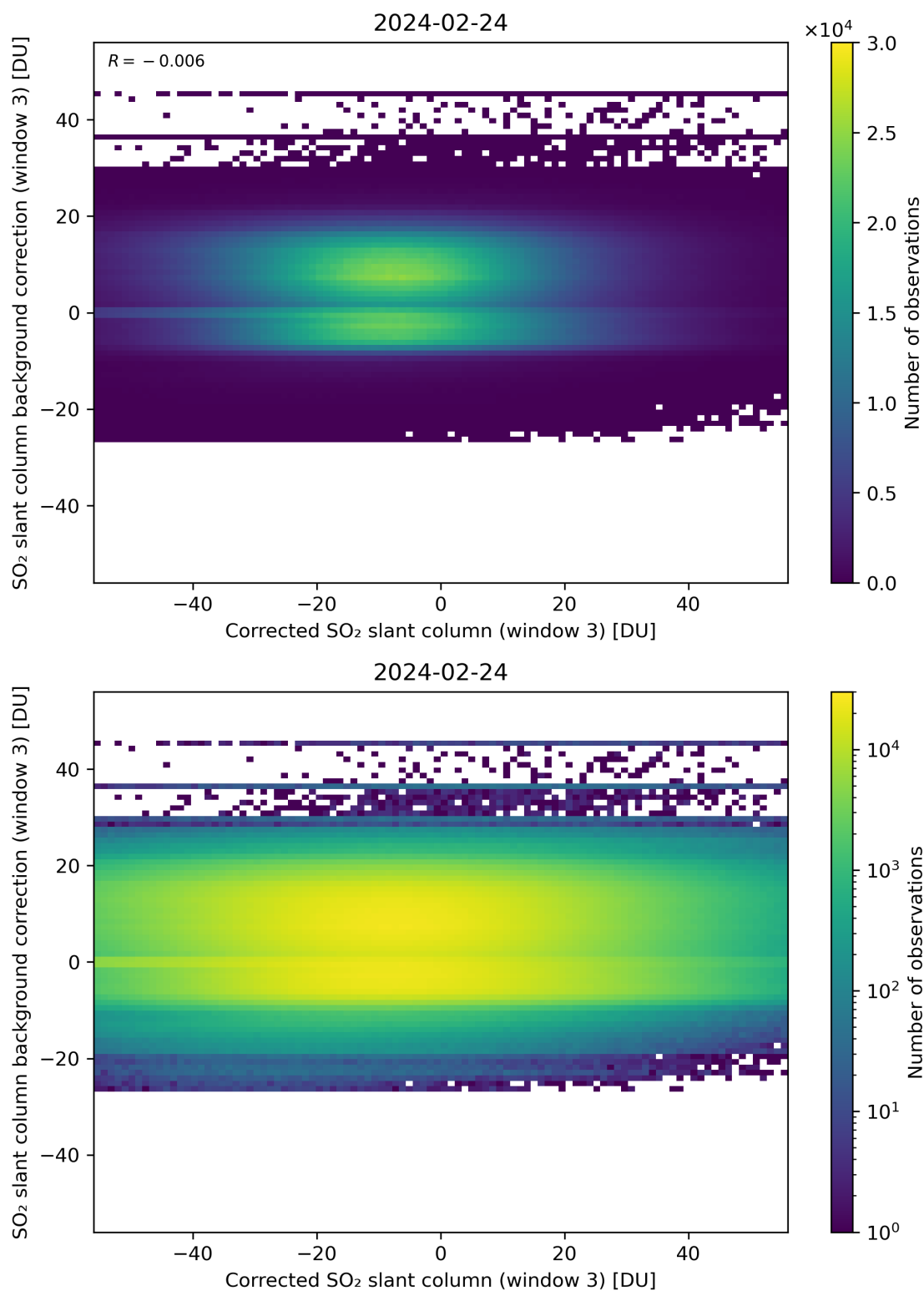
Figure 205: Scatter density plot of “Corrected SO 2 slant column (window 3)” against “SO 2 slant column background correction (window 3)” for 2024-02-23 to 2024-02-25.
