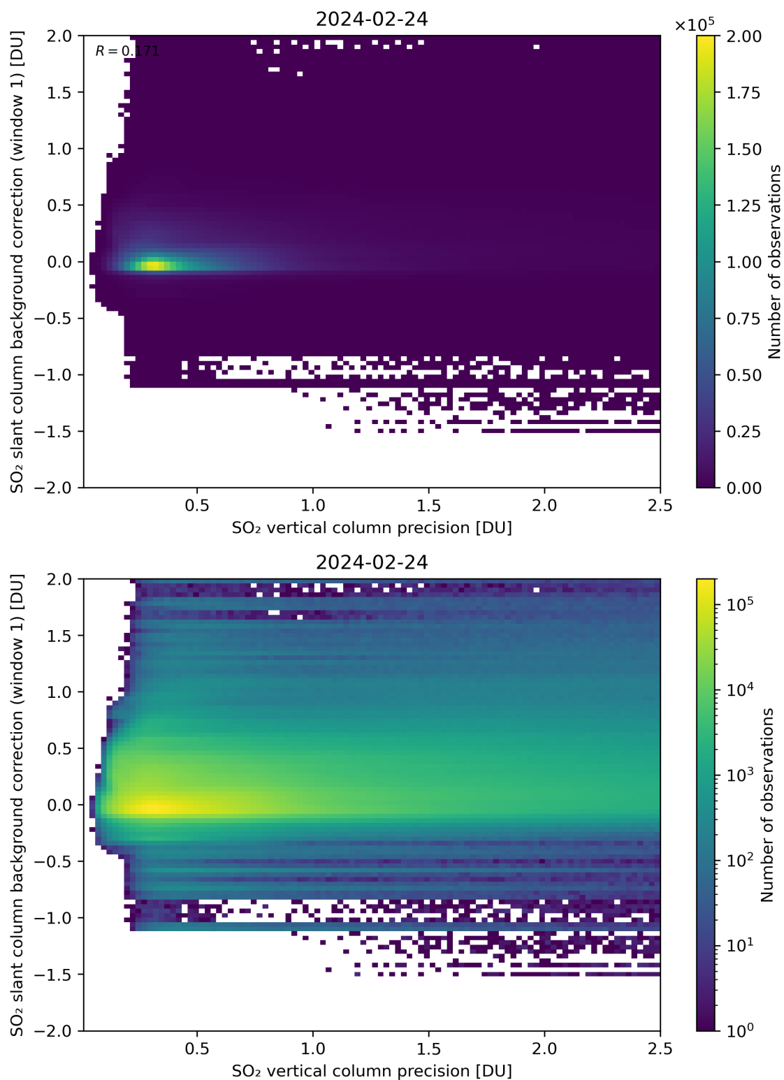
Figure 279: Scatter density plot of “SO 2 vertical column precision” against “SO 2 slant column background correction (window 1)” for 2024-02-23 to 2024-02-25.
