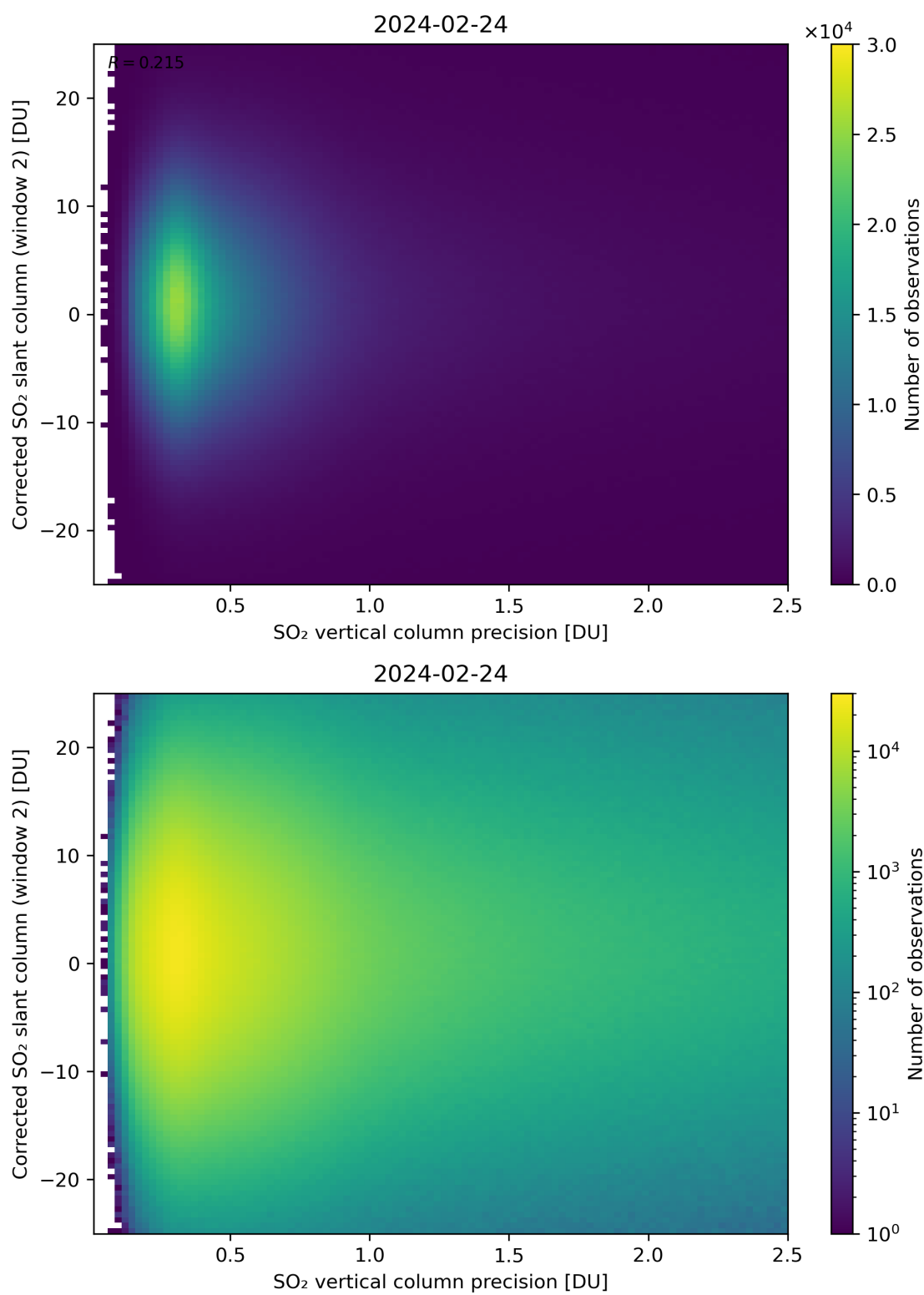
Figure 287: Scatter density plot of “SO 2 vertical column precision” against “Corrected SO 2 slant column (window 2)” for 2024-02-23 to 2024-02-25.
