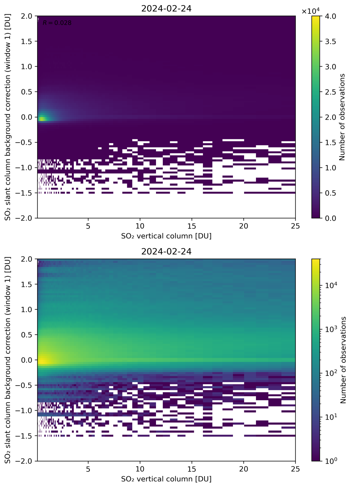
Figure 273: Scatter density plot of “SO 2 vertical column” against “SO 2 slant column background correction (window 1)” for 2024-02-23 to 2024-02-25.
