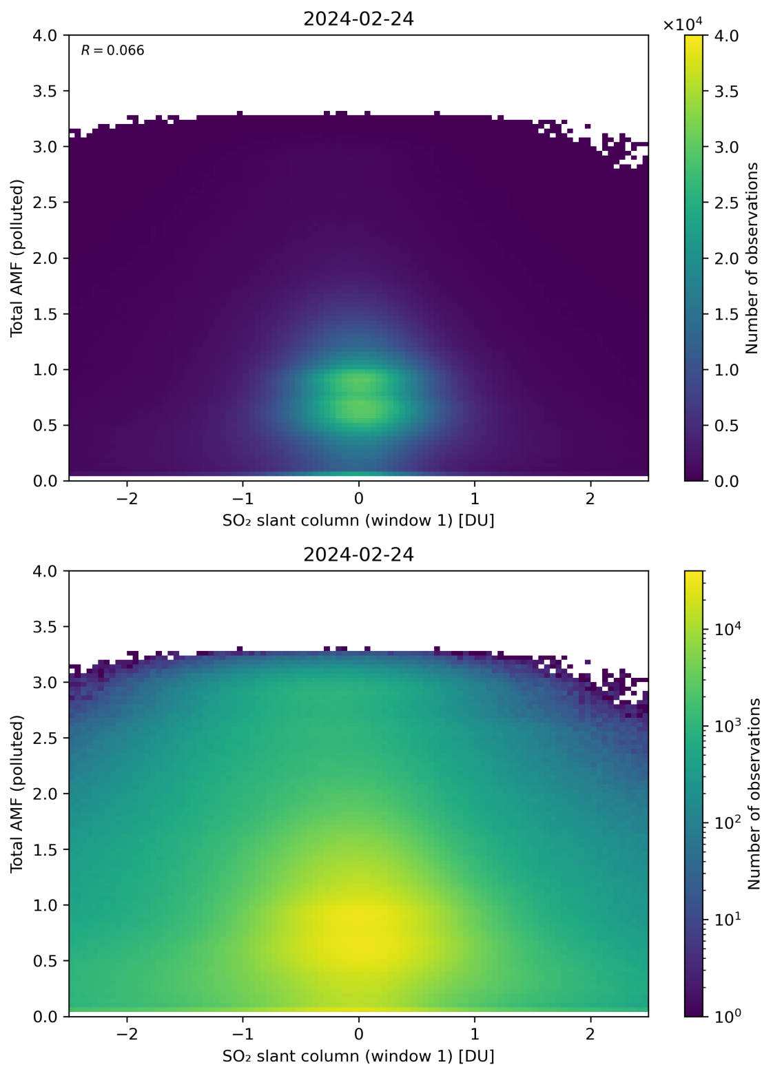
Figure 239: Scatter density plot of “SO 2 slant column (window 1)” against “Total AMF (polluted)” for 2024-02-23 to 2024-02-25.
