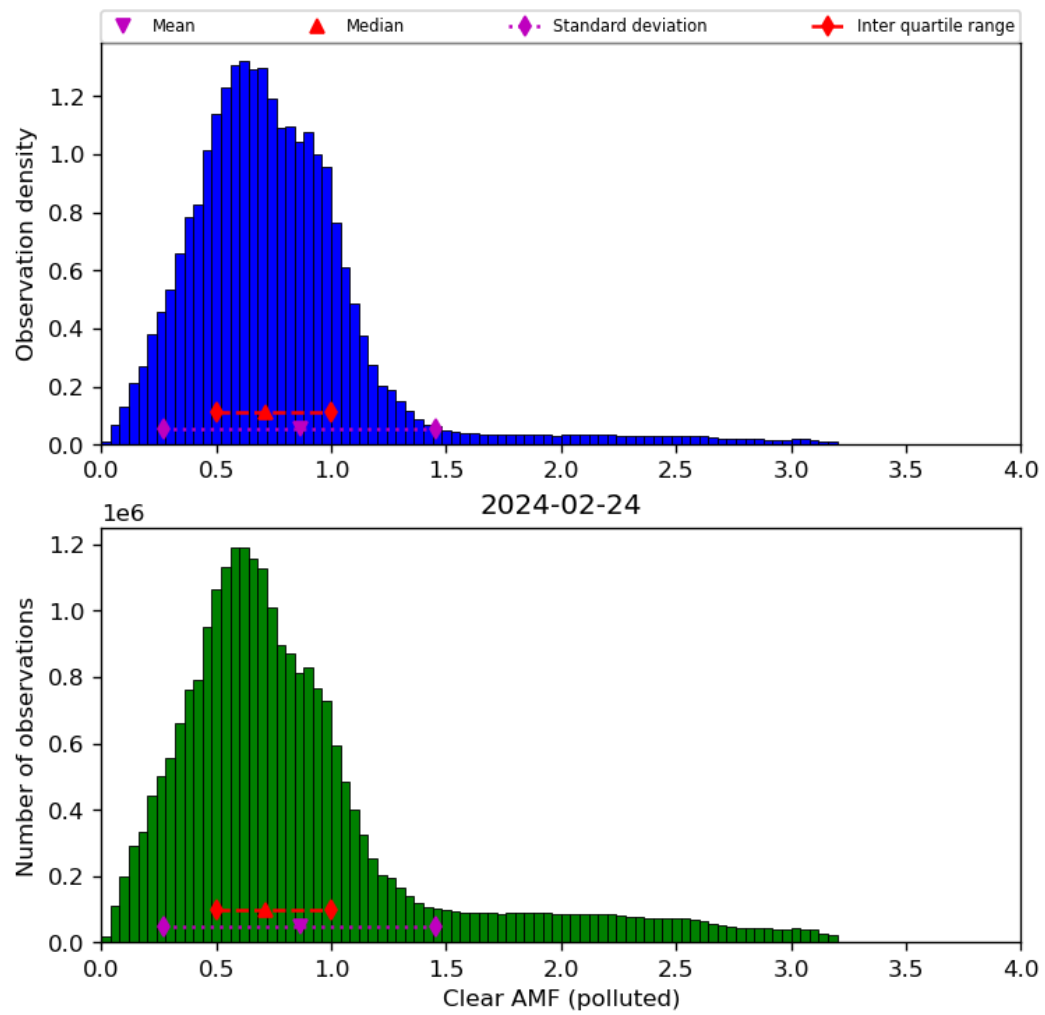
Figure 73: Histogram of “Clear AMF (polluted)” for 2024-02-23 to 2024-02-25
