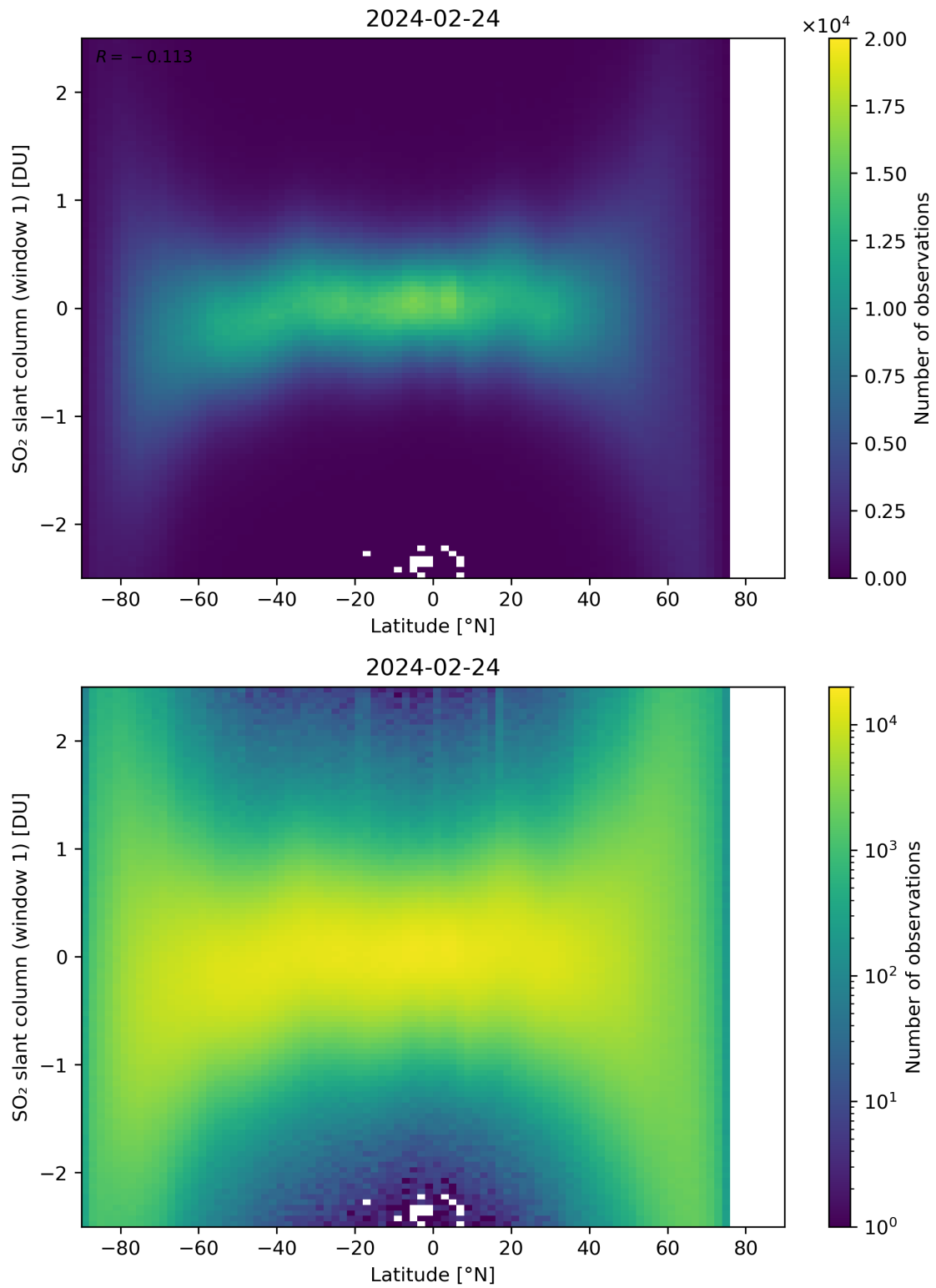
Figure 149: Scatter density plot of “Latitude” against “SO 2 slant column (window 1)” for 2024-02-23 to 2024-02-25.
