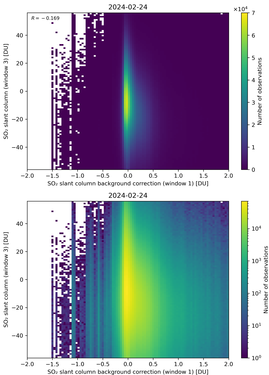
Figure 107: Scatter density plot of “SO 2 slant column background correction (window 1)” against “SO 2 slant column (window 3)” for 2024-02-23 to 2024-02-25.
