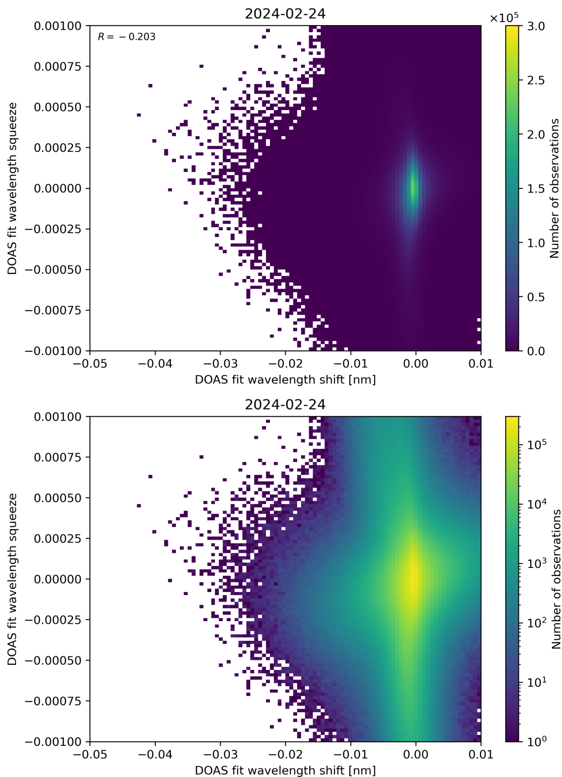
Figure 127: Scatter density plot of “DOAS fit wavelength shift” against “DOAS fit wavelength squeeze” for 2024-02-23 to 2024-02-25.
