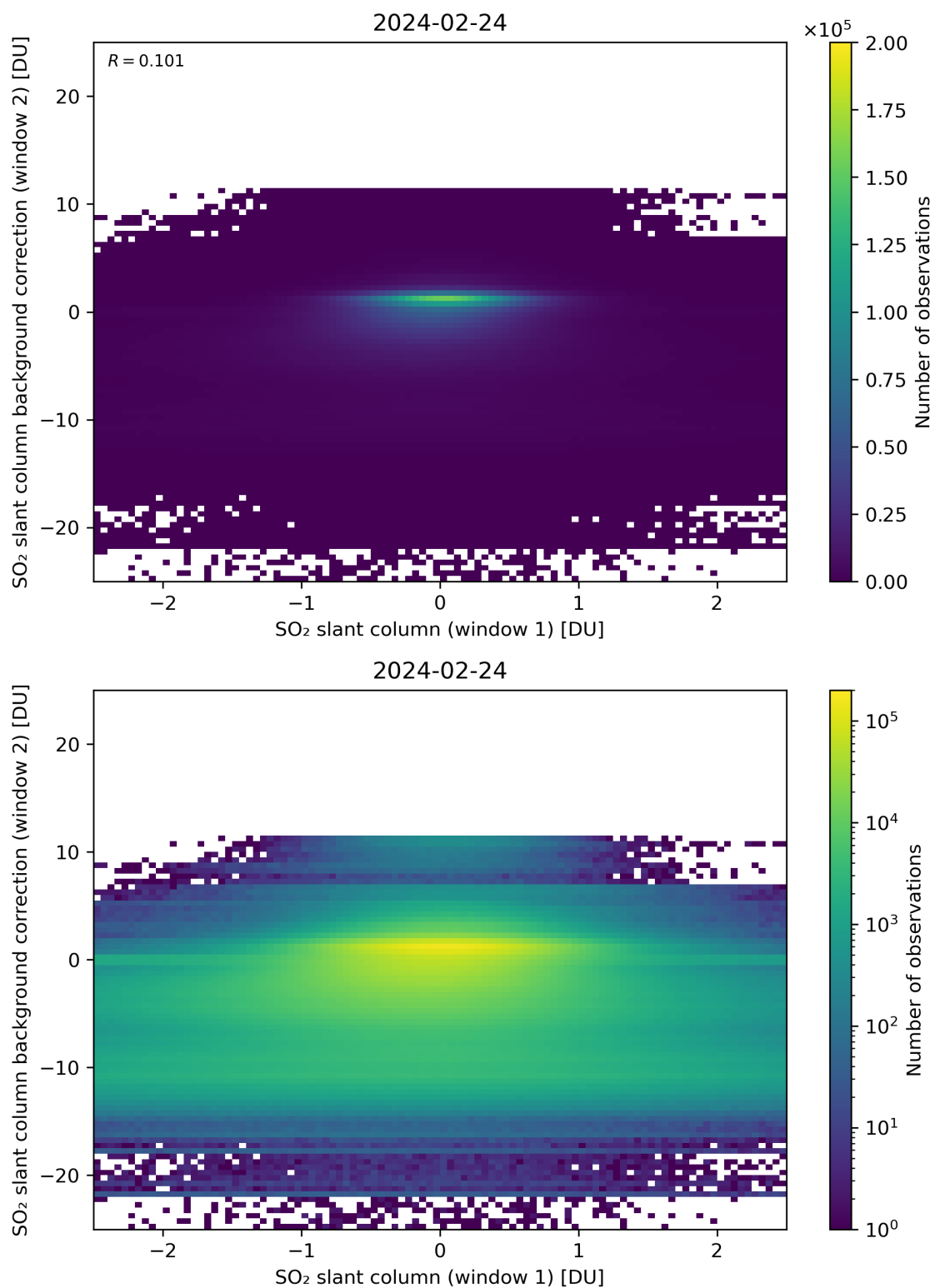
Figure 213: Scatter density plot of “SO 2 slant column (window 1)” against “SO 2 slant column background correction (window 2)” for 2024-02-23 to 2024-02-25.
