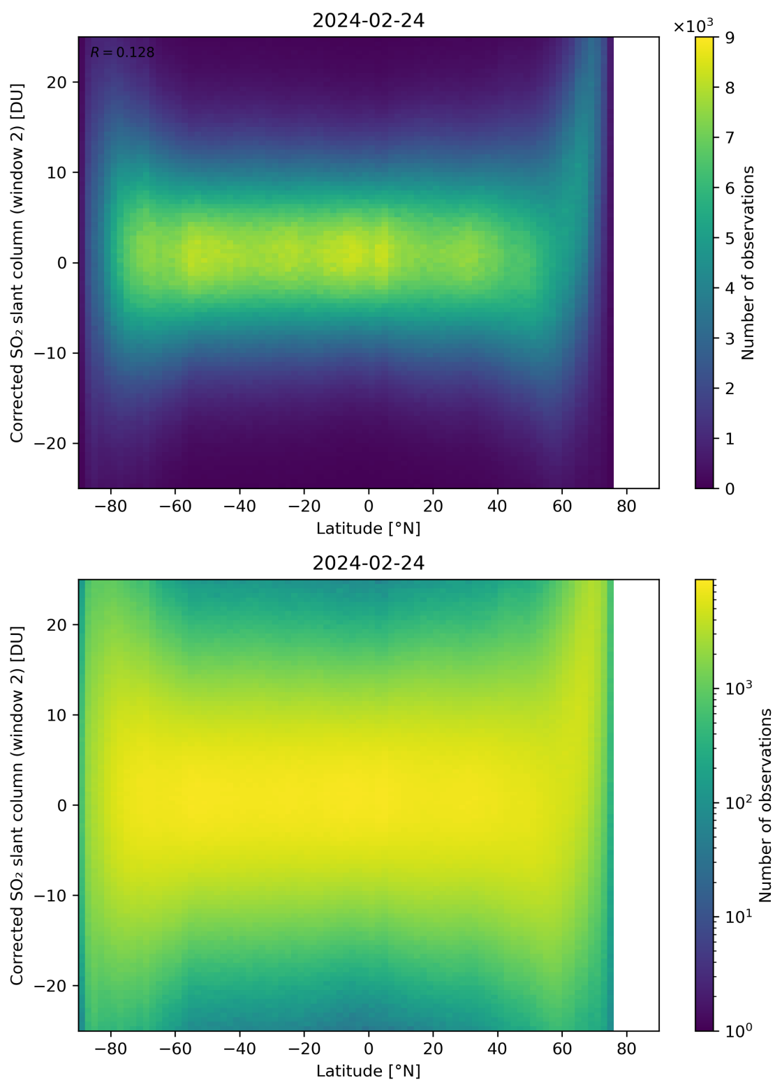
Figure 147: Scatter density plot of “Latitude” against “Corrected SO 2 slant column (window 2)” for 2024-02-23 to 2024-02-25.
