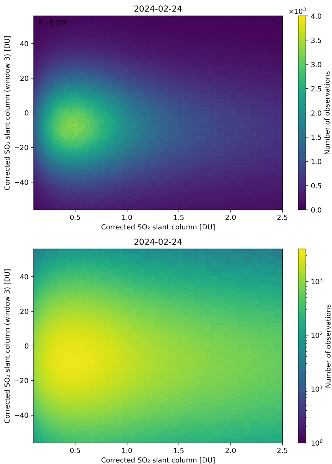
Figure 186: Scatter density plot of “Corrected SO 2 slant column” against “Corrected SO 2 slant column (window 3)” for 2024-02-23 to 2024-02-25.
