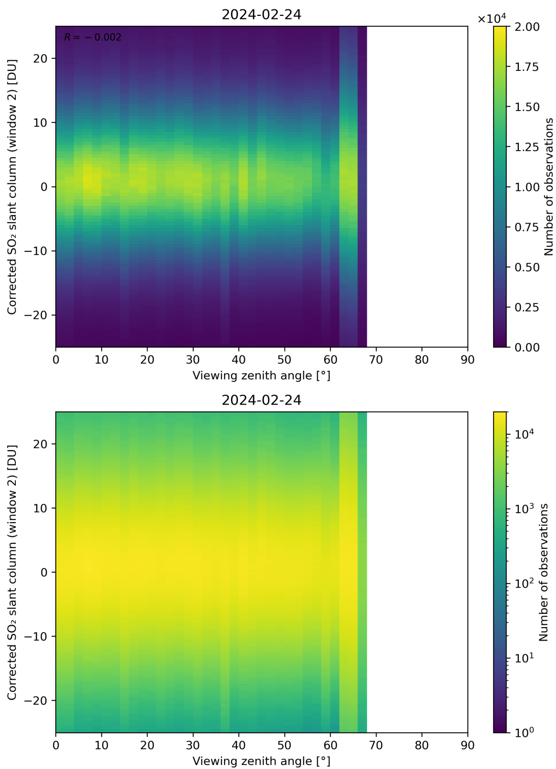
Figure 318: Scatter density plot of “Viewing zenith angle” against “Corrected SO 2 slant column (window 2)” for 2024-02-23 to 2024-02-25.
