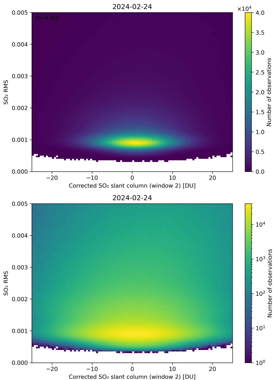
Figure 198: Scatter density plot of “Corrected SO 2 slant column (window 2)” against “SO 2 RMS” for 2024-02-23 to 2024-02-25.
