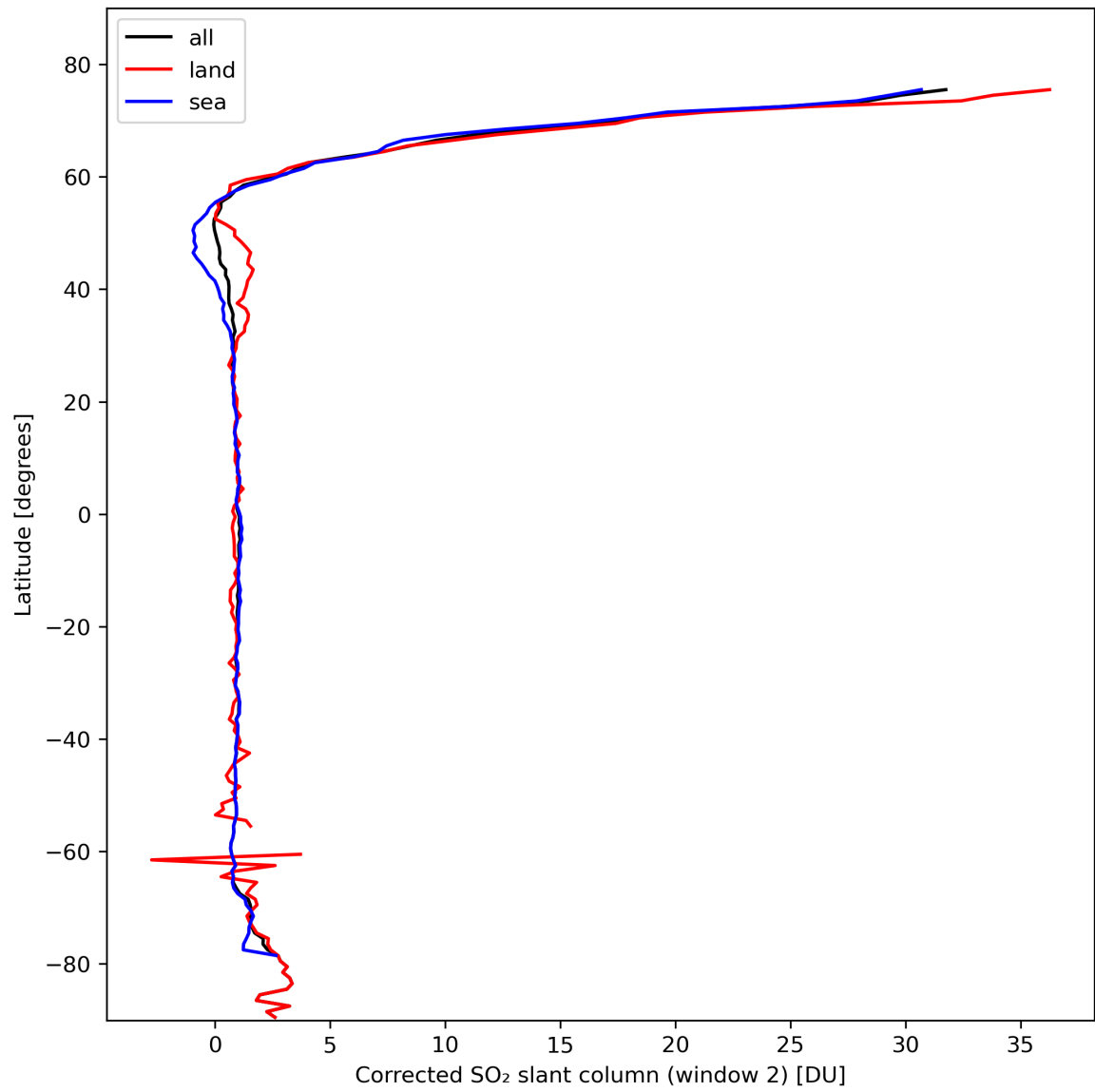
Figure 39: Zonal average of “Corrected SO 2 slant column (window 2)” for 2024-02-23 to 2024-02-25.
