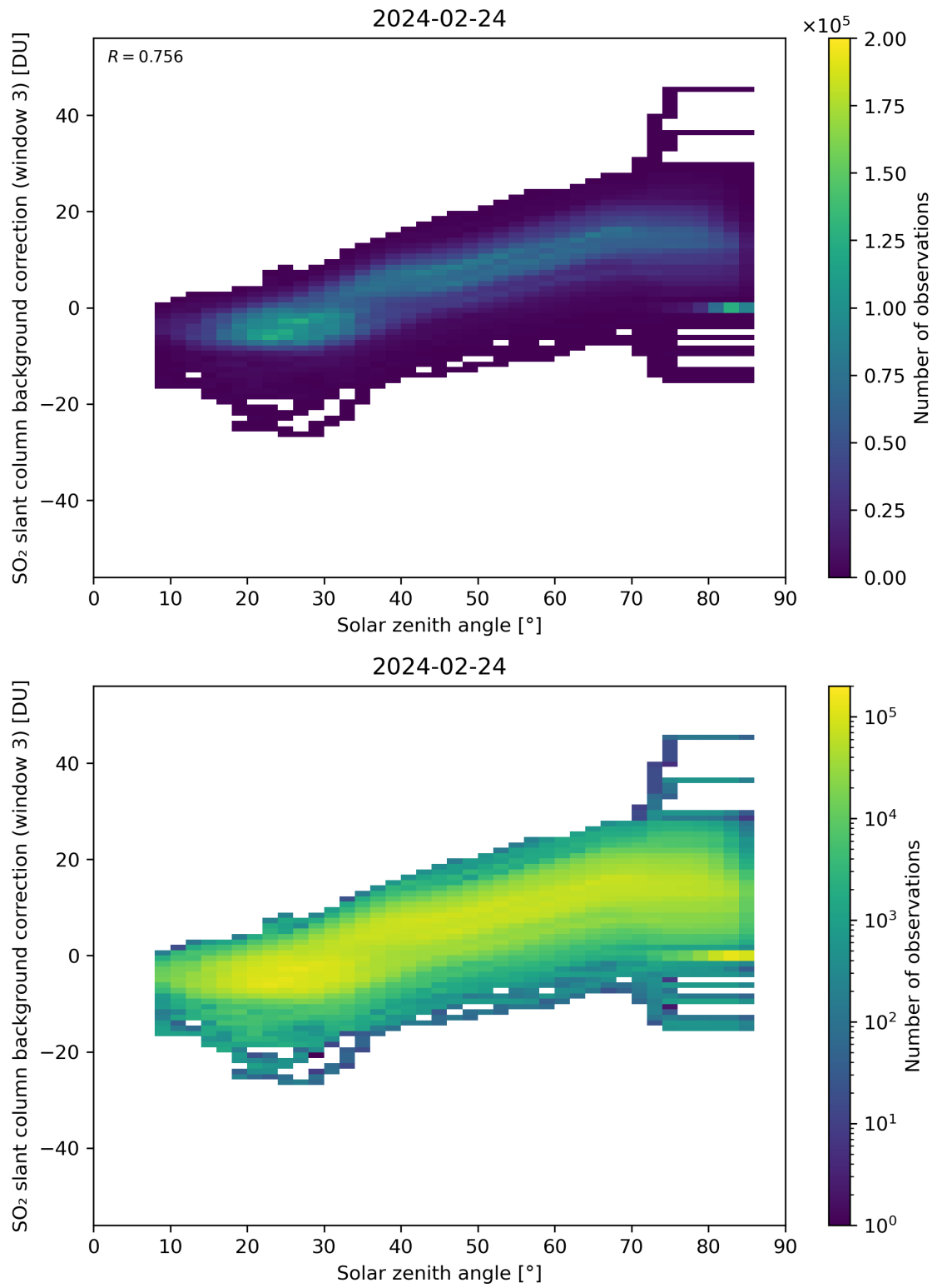
Figure 160: Scatter density plot of “Solar zenith angle” against “SO 2 slant column background correction (window 3)” for 2024-02-23 to 2024-02-25.
