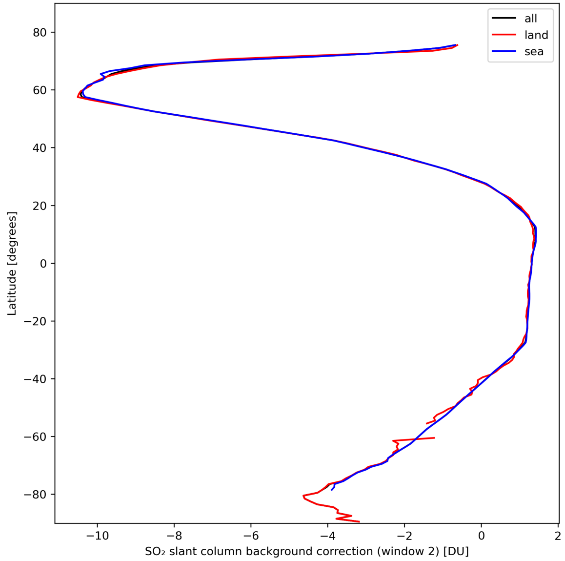
Figure 40: Zonal average of “SO 2 slant column background correction (window 2)” for 2024-02-23 to 2024-02-25.
