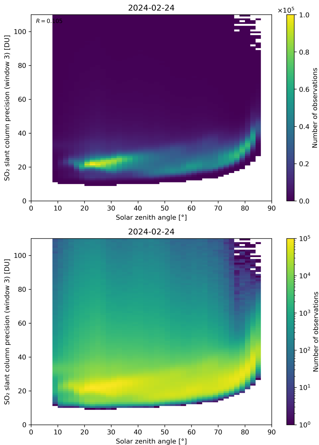
Figure 173: Scatter density plot of “Solar zenith angle” against “SO 2 slant column precision (window 3)” for 2024-02-23 to 2024-02-25.
