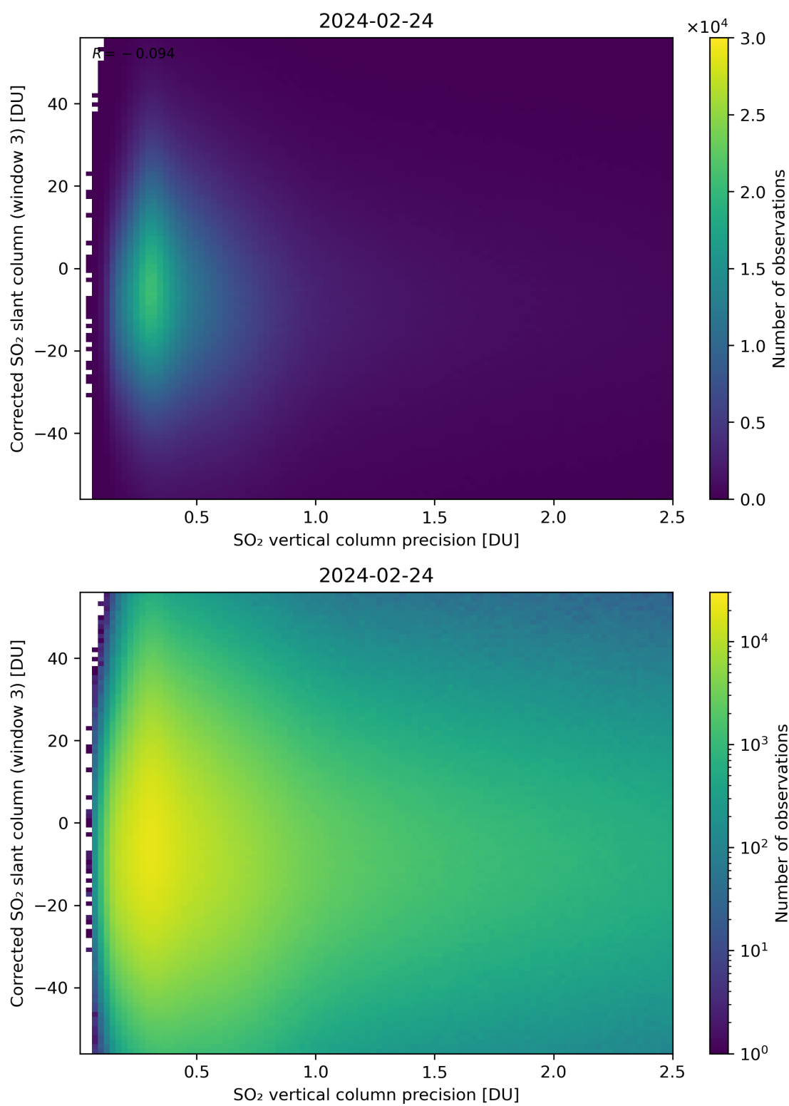
Figure 288: Scatter density plot of “SO 2 vertical column precision” against “Corrected SO 2 slant column (window 3)” for 2024-02-23 to 2024-02-25.
