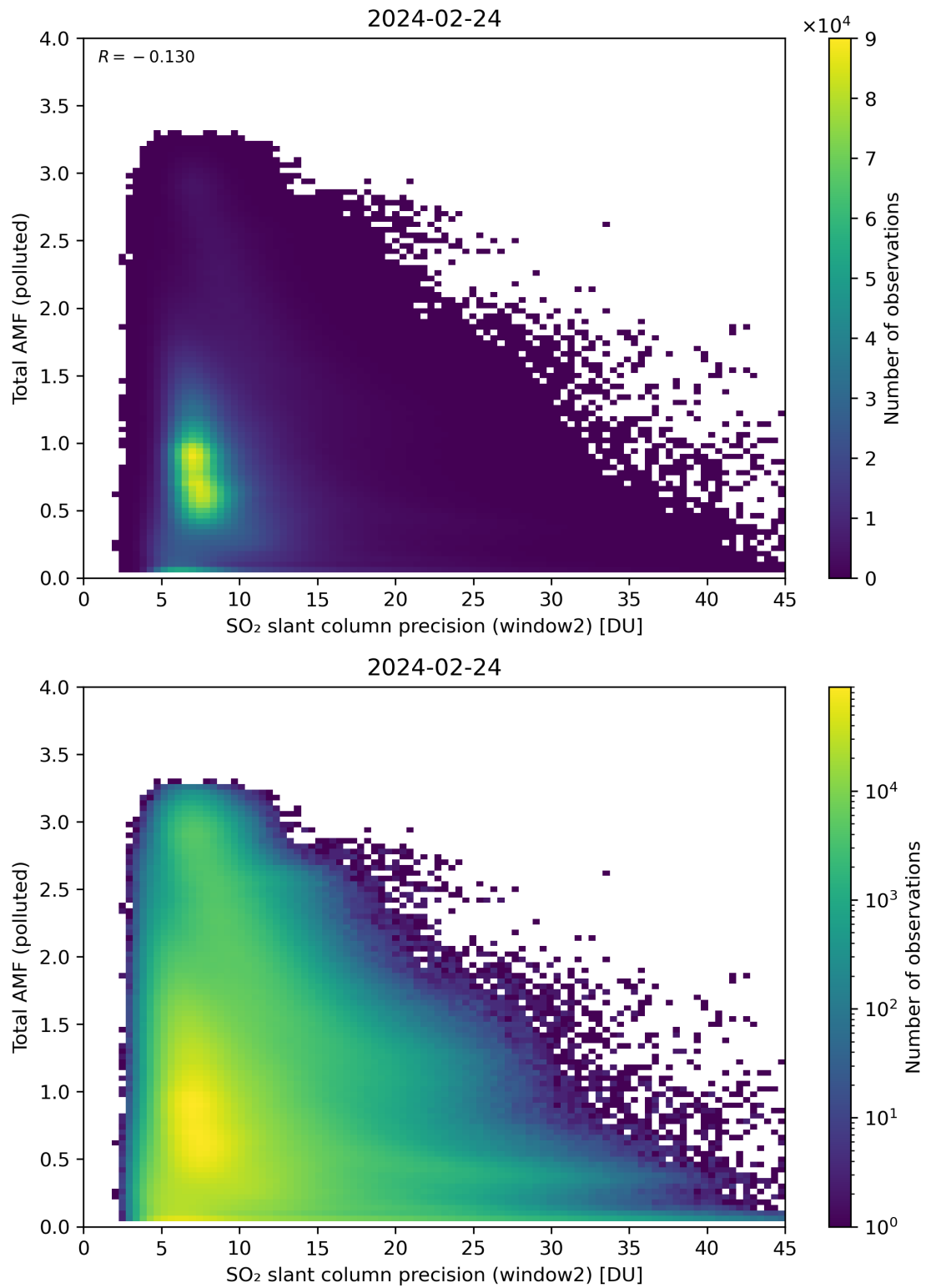
Figure 251: Scatter density plot of “SO 2 slant column precision (window2)” against “Total AMF (polluted)” for 2024-02-23 to 2024-02-25.
