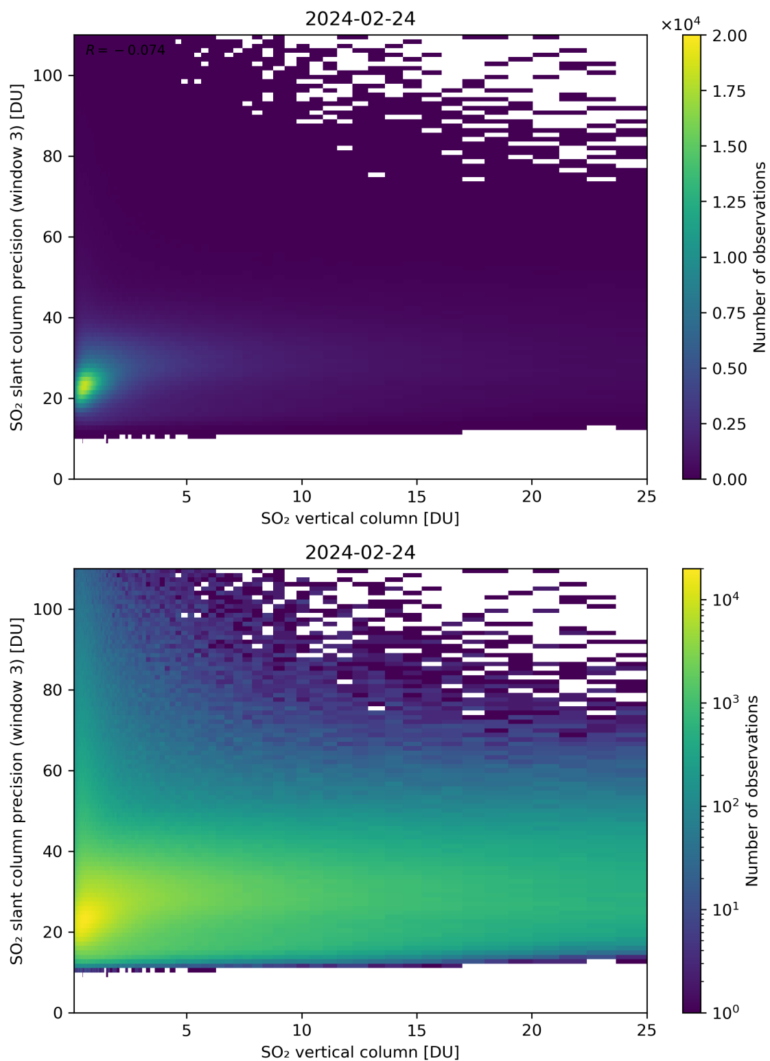
Figure 304: Scatter density plot of “SO 2 vertical column” against “SO 2 slant column precision (window 3)” for 2024-02-23 to 2024-02-25.
