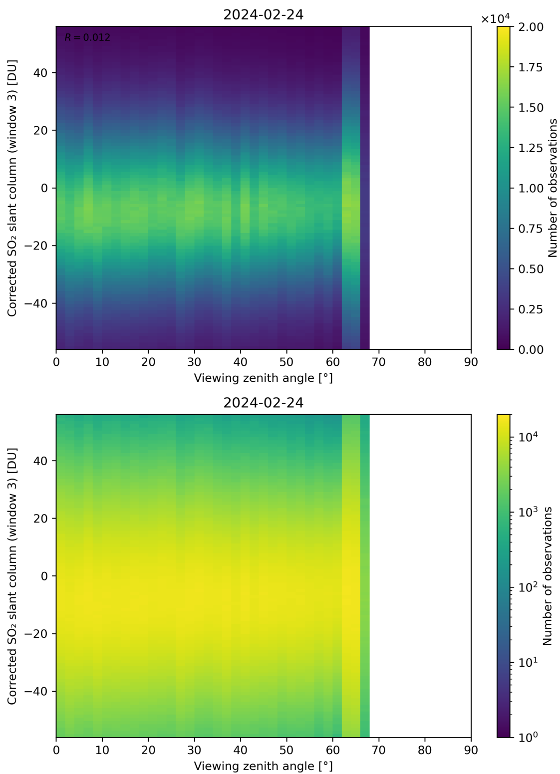
Figure 319: Scatter density plot of “Viewing zenith angle” against “Corrected SO 2 slant column (window 3)” for 2024-02-23 to 2024-02-25.
