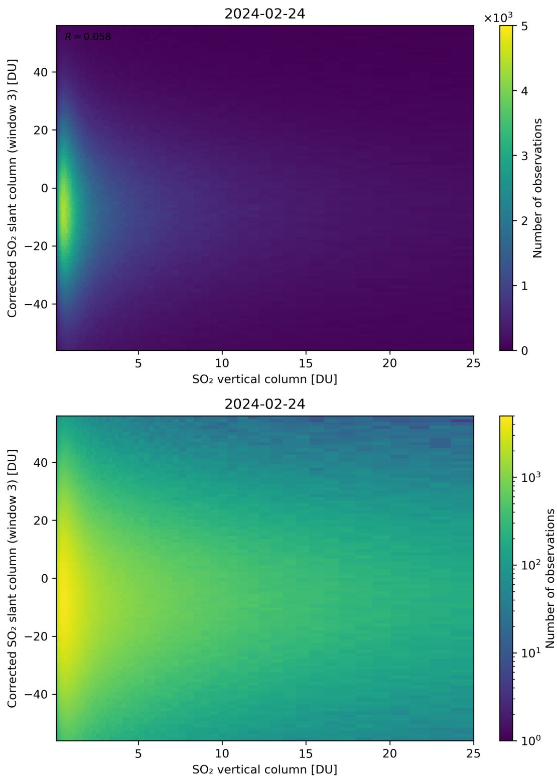
Figure 299: Scatter density plot of “SO 2 vertical column” against “Corrected SO 2 slant column (window 3)” for 2024-02-23 to 2024-02-25.
