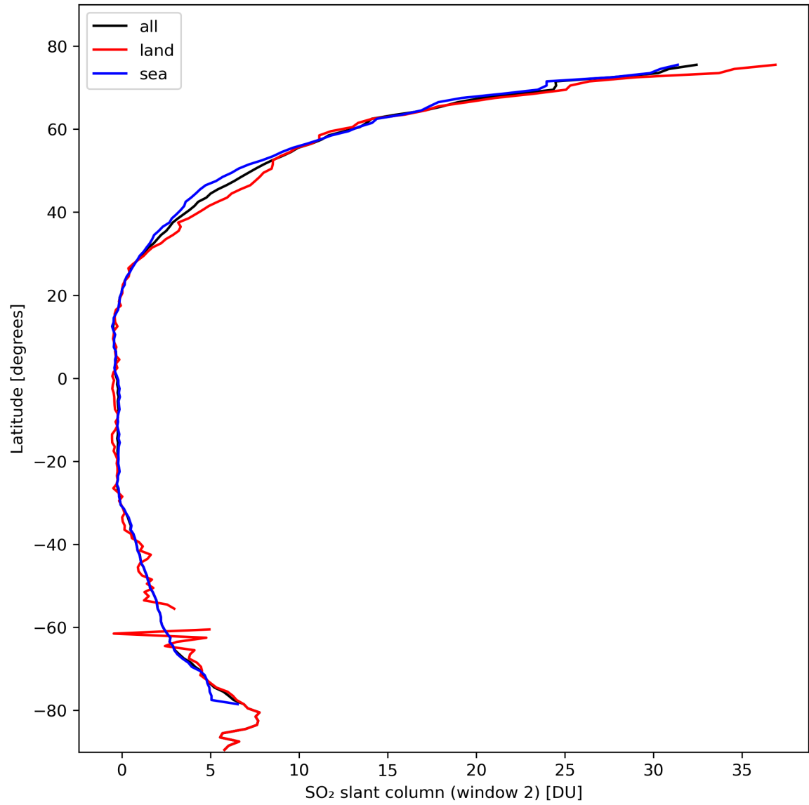
Figure 37: Zonal average of “SO 2 slant column (window 2)” for 2024-02-23 to 2024-02-25.
