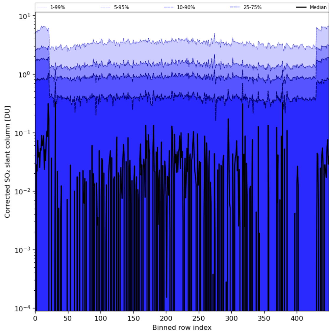
Figure 78: Along track statistics of “Corrected SO 2 slant column” for 2024-02-23 to 2024-02-25
