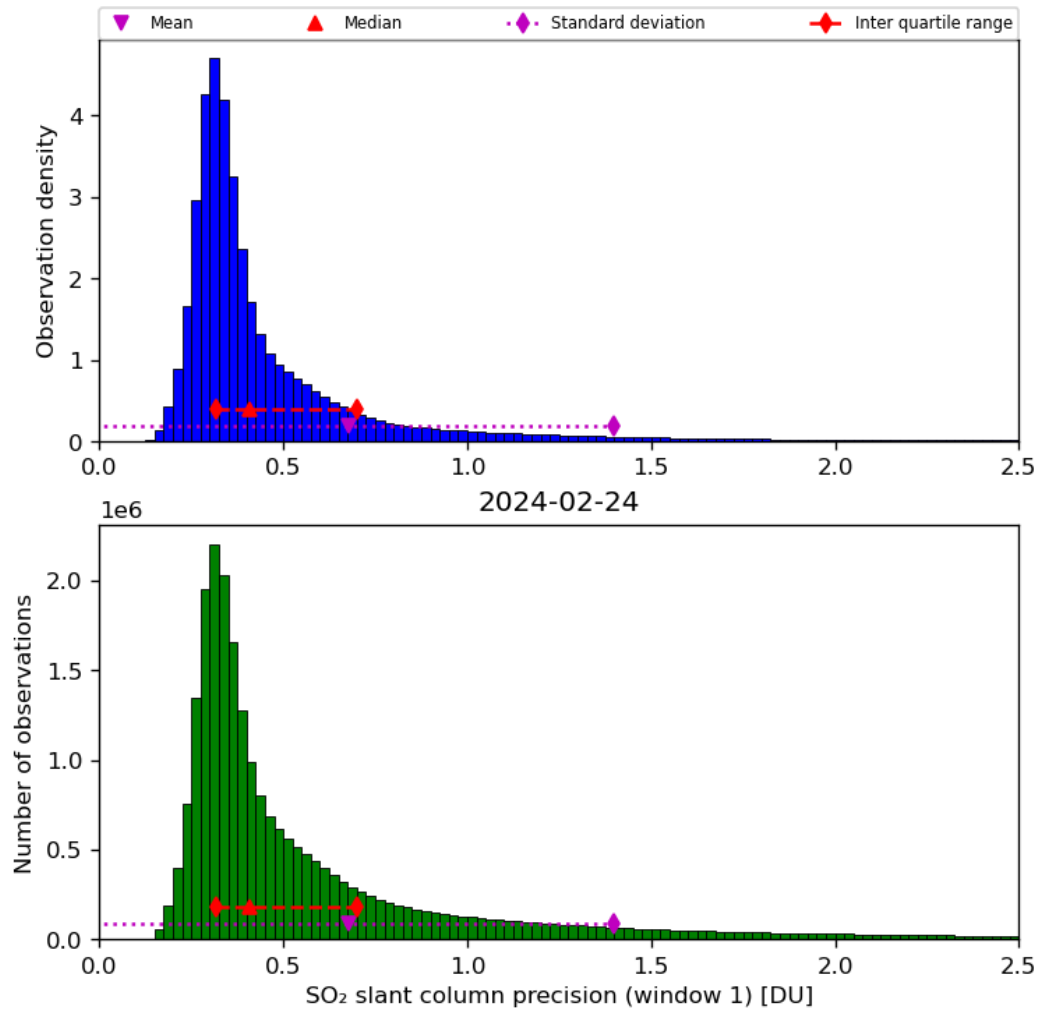
Figure 57: Histogram of “SO 2 slant column precision (window 1)” for 2024-02-23 to 2024-02-25
