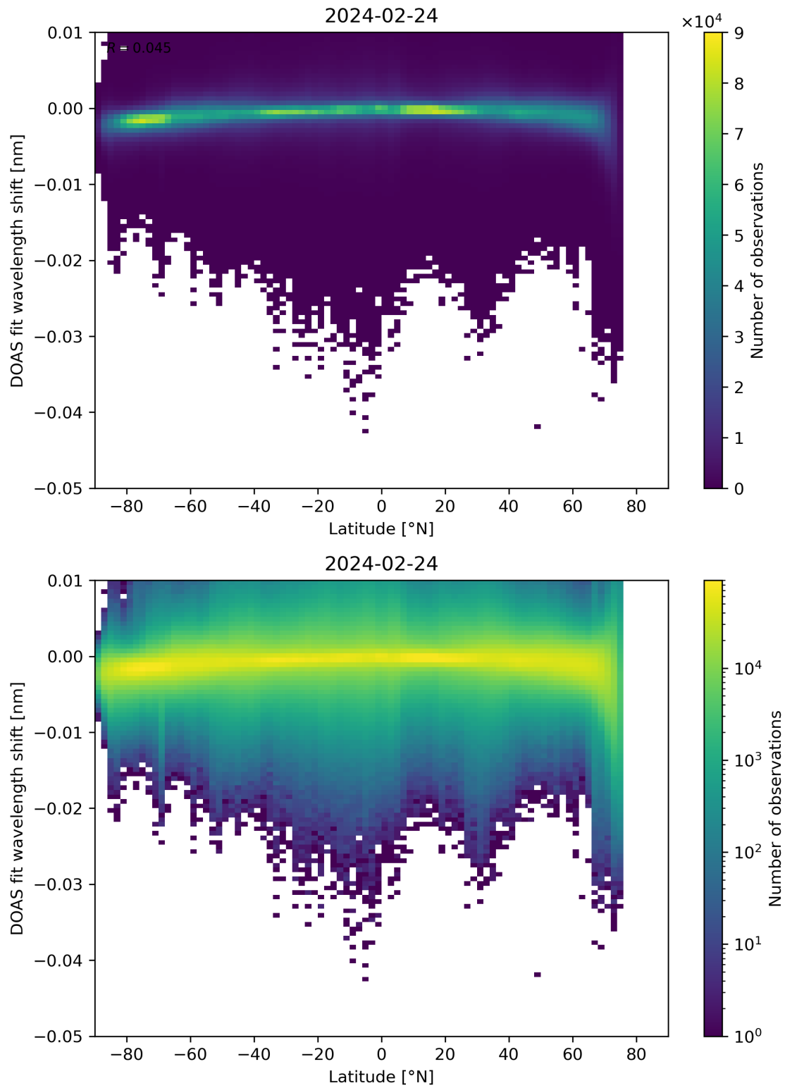
Figure 142: Scatter density plot of “Latitude” against “DOAS fit wavelength shift” for 2024-02-23 to 2024-02-25.
