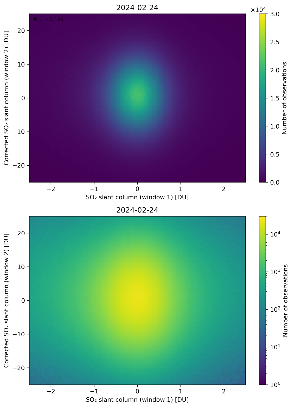
Figure 233: Scatter density plot of “SO 2 slant column (window 1)” against “Corrected SO 2 slant column (window 2)” for 2024-02-23 to 2024-02-25.
