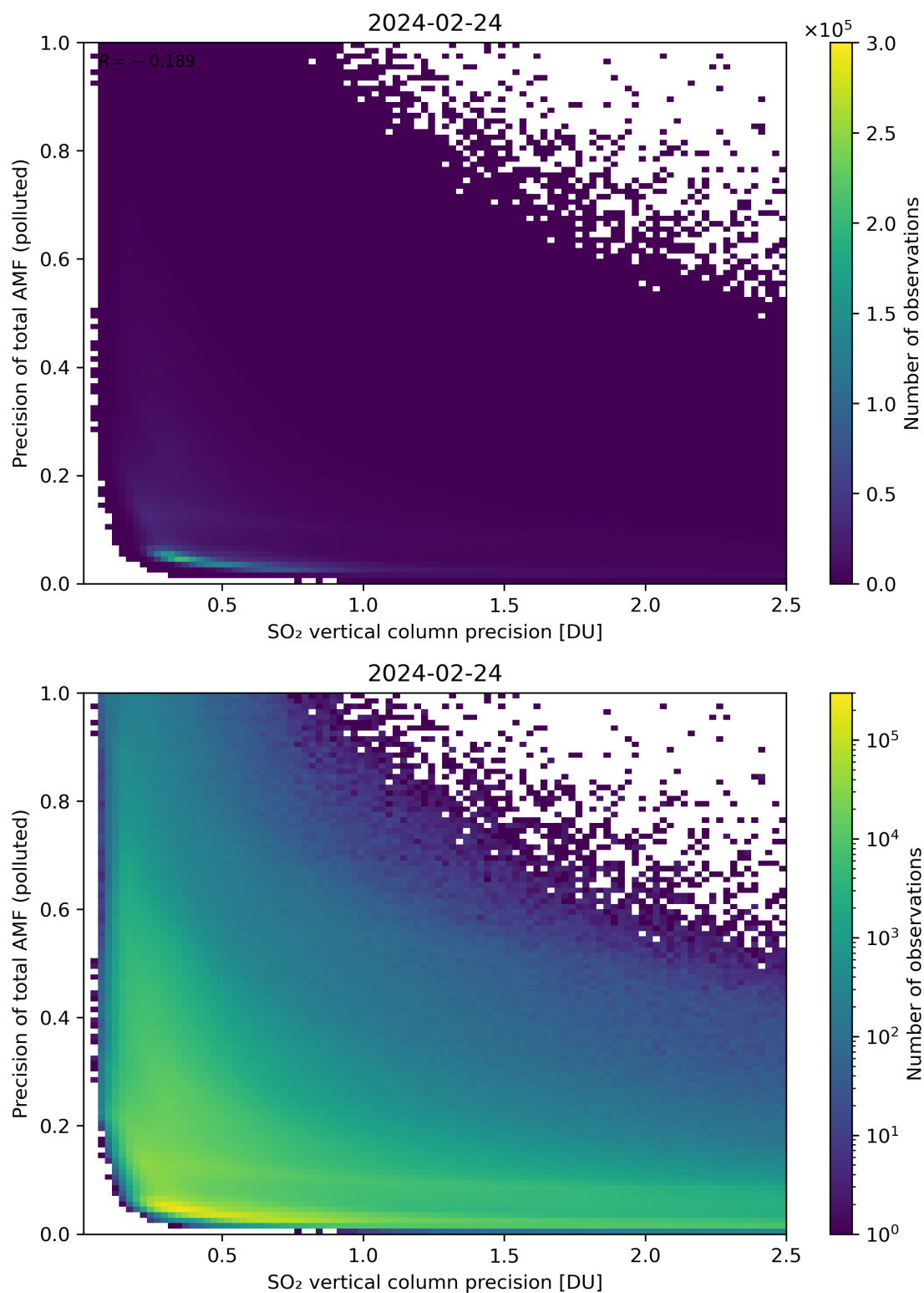
Figure 295: Scatter density plot of “SO 2 vertical column precision” against “Precision of total AMF (polluted)” for 2024-02-23 to 2024-02-25.
