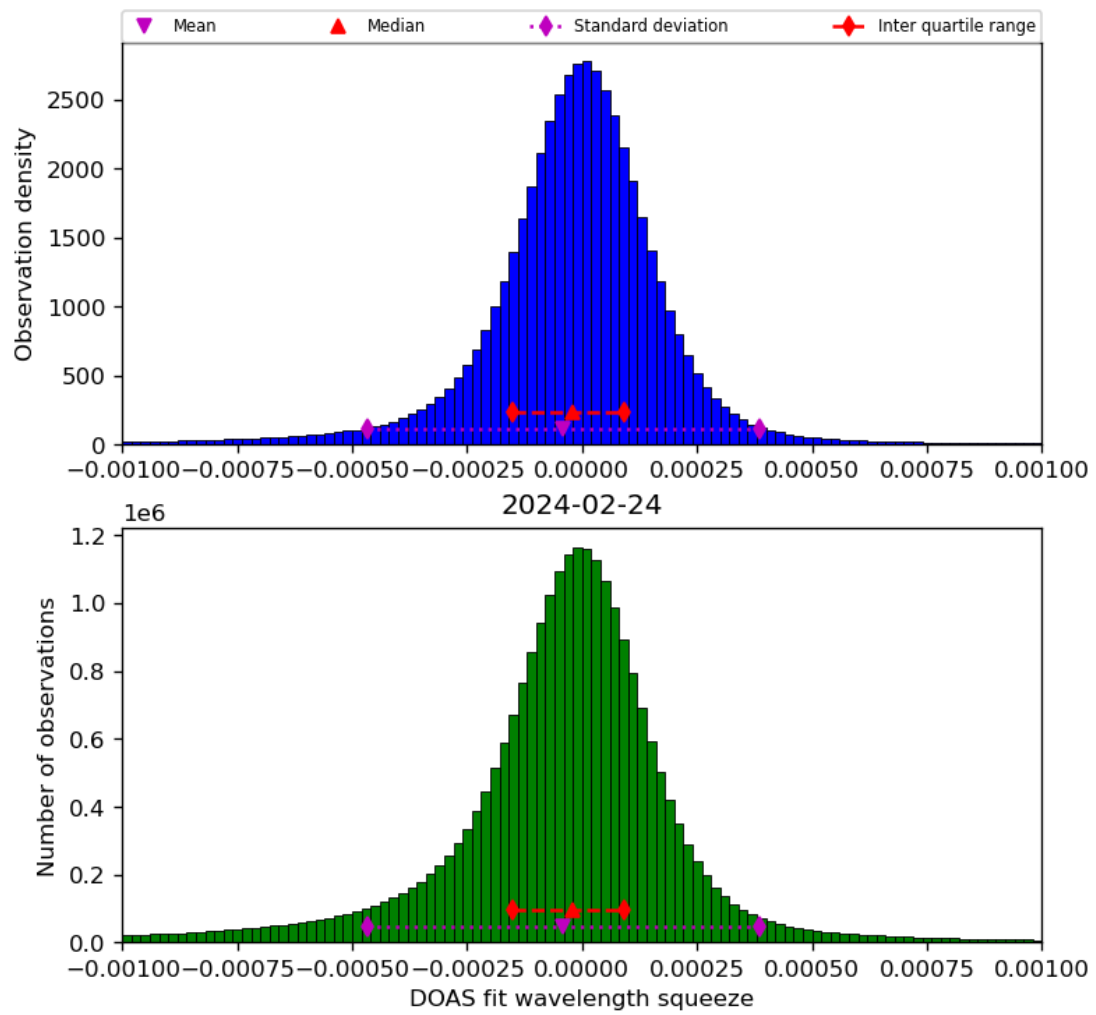
Figure 69: Histogram of “DOAS fit wavelength squeeze” for 2024-02-23 to 2024-02-25
