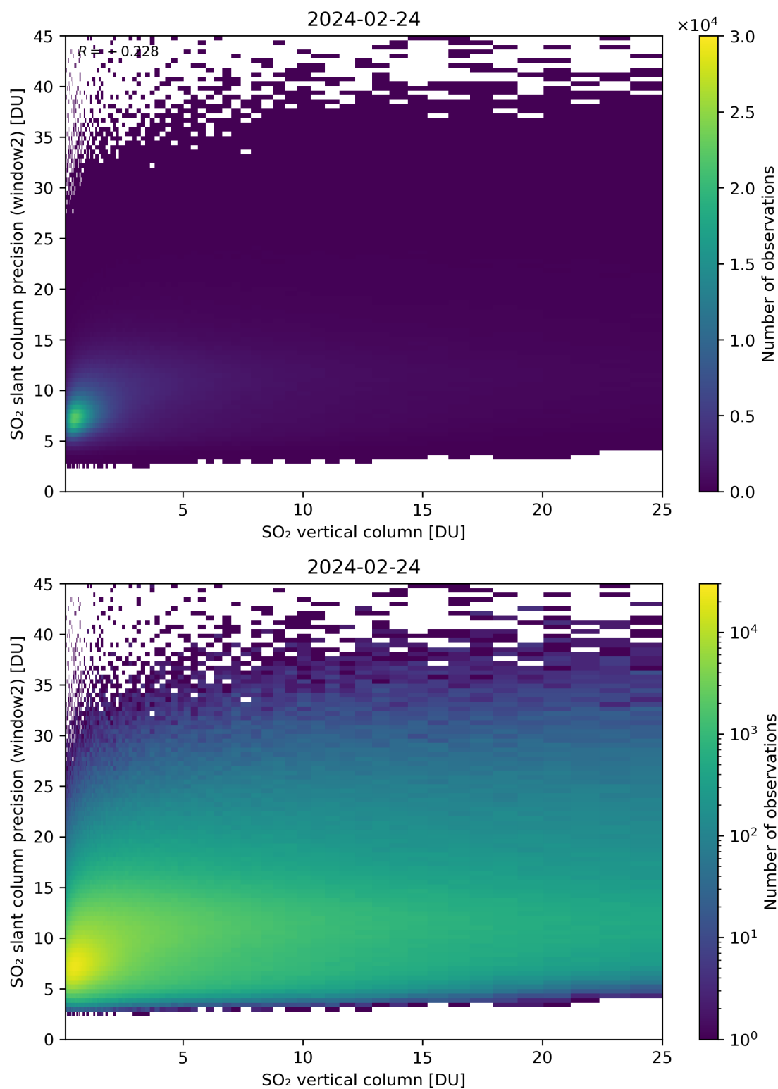
Figure 302: Scatter density plot of “SO 2 vertical column” against “SO 2 slant column precision (window2)” for 2024-02-23 to 2024-02-25.
