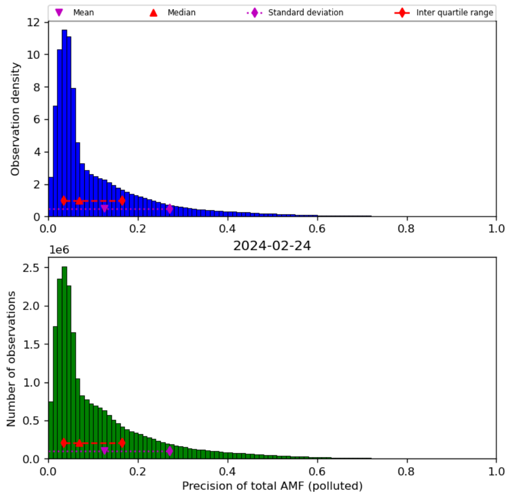
Figure 72: Histogram of “Precision of total AMF (polluted)” for 2024-02-23 to 2024-02-25
