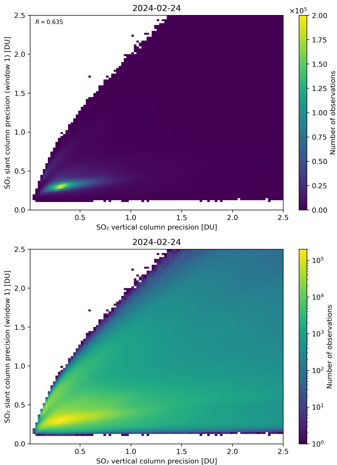
Figure 290: Scatter density plot of “SO 2 vertical column precision” against “SO 2 slant column precision (window 1)” for 2024-02-23 to 2024-02-25.
