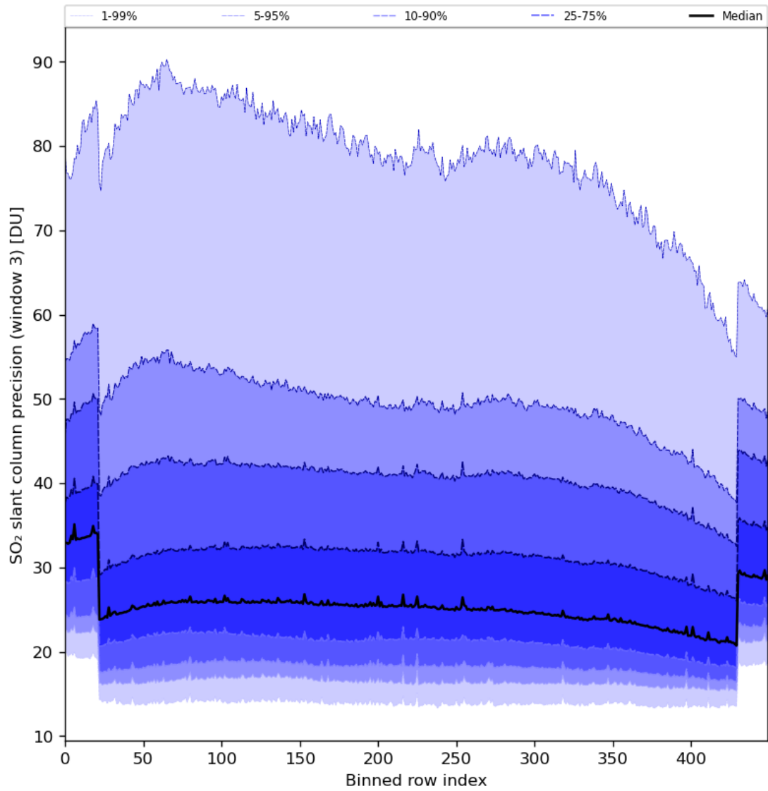
Figure 88: Along track statistics of “SO 2 slant column precision (window 3)” for 2024-02-23 to 2024-02-25
