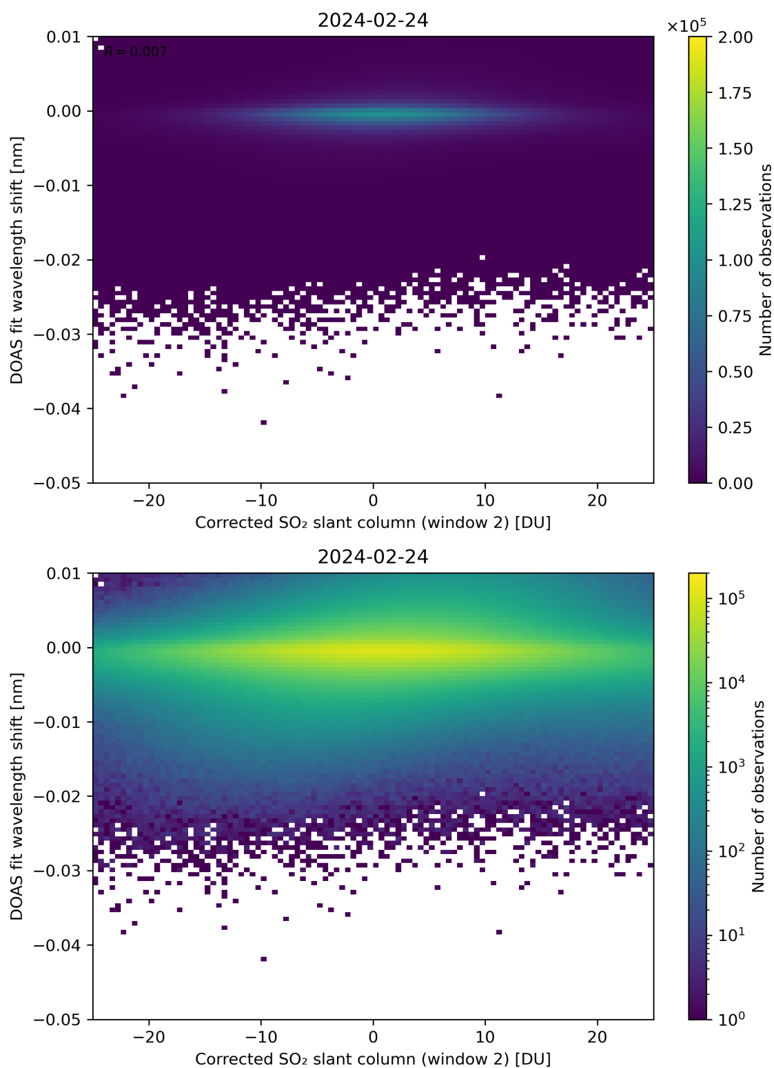
Figure 196: Scatter density plot of “Corrected SO 2 slant column (window 2)” against “DOAS fit wavelength shift” for 2024-02-23 to 2024-02-25.
