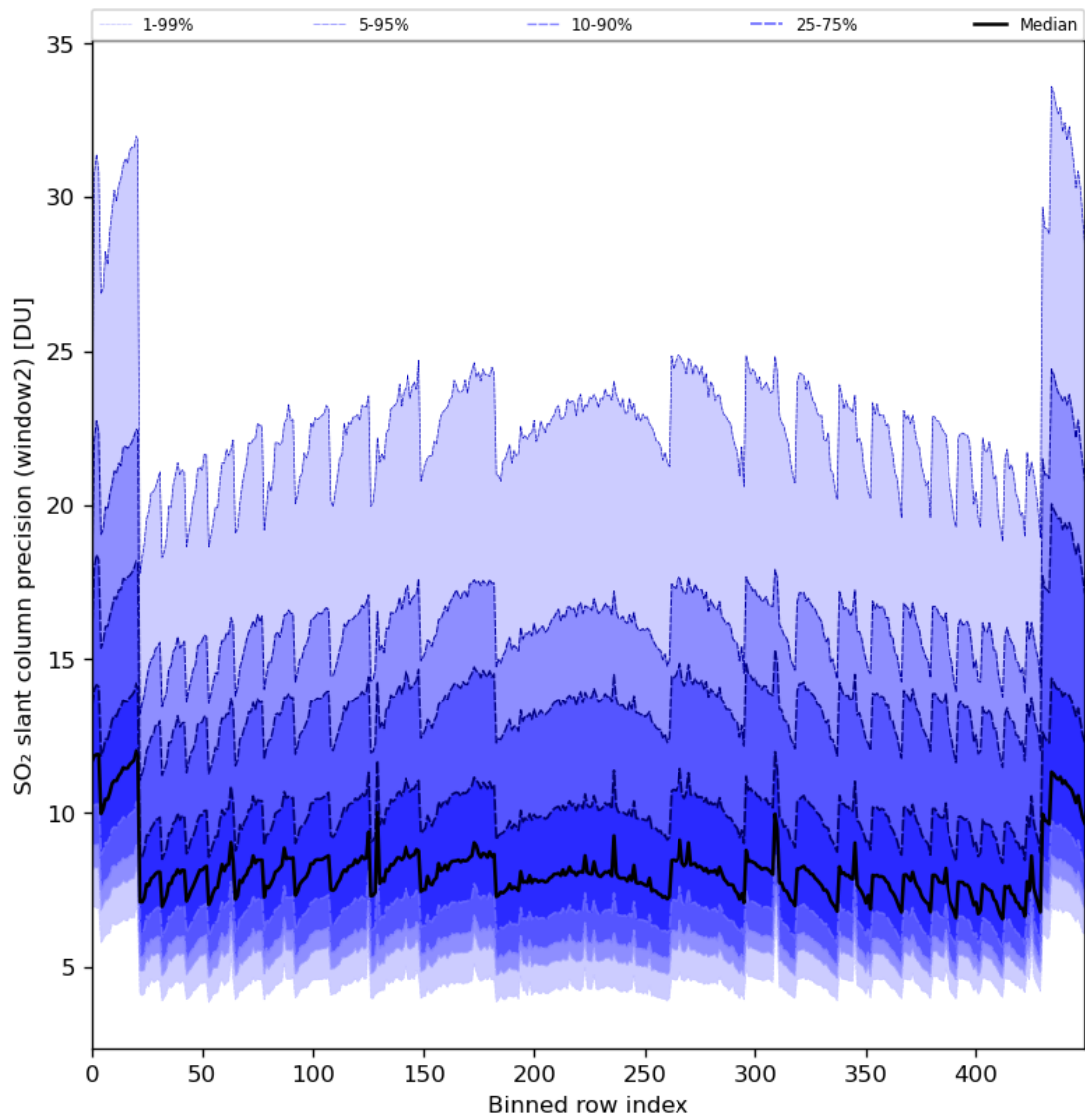
Figure 84: Along track statistics of “SO 2 slant column precision (window2)” for 2024-02-23 to 2024-02-25
