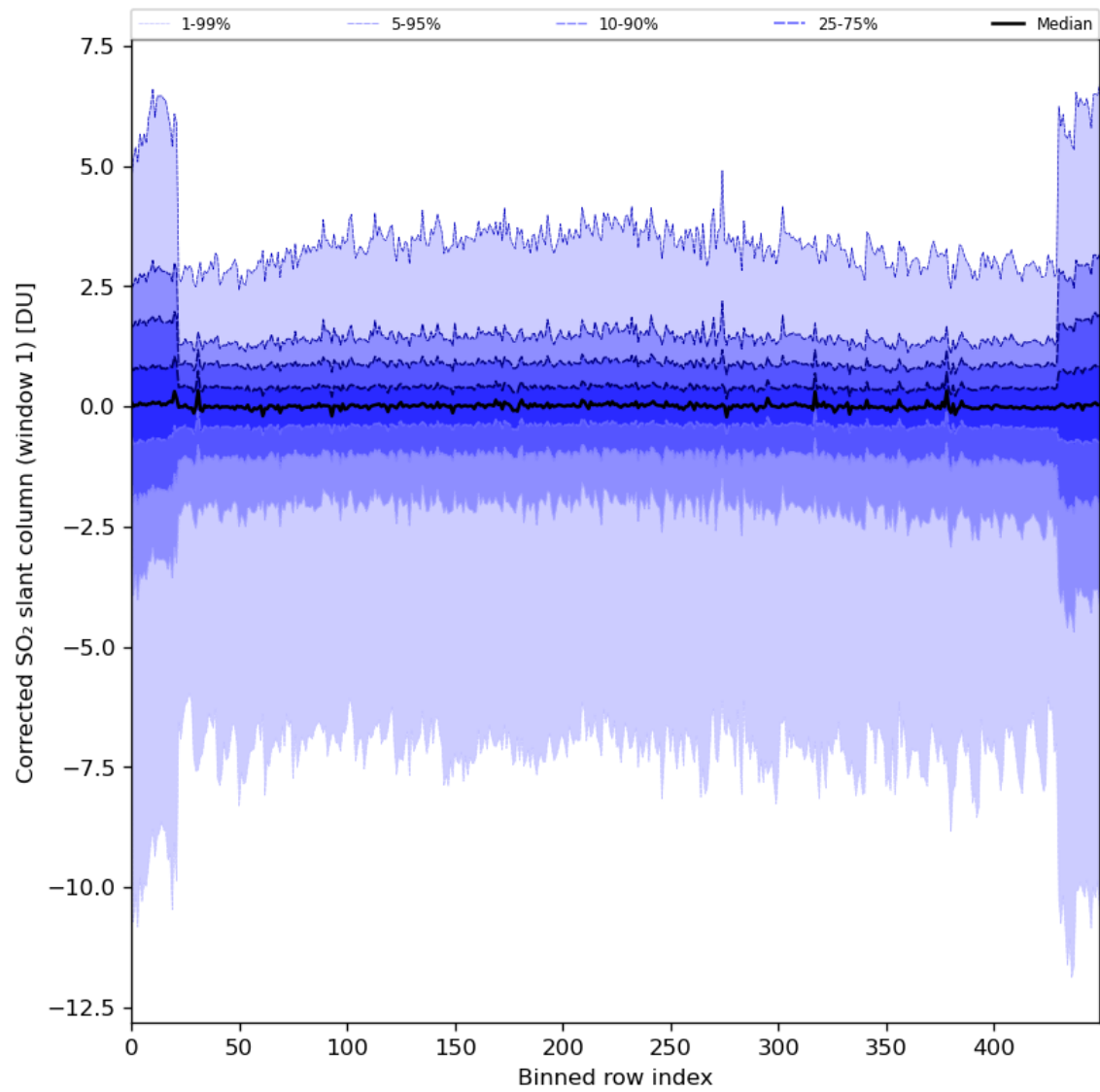
Figure 81: Along track statistics of “Corrected SO 2 slant column (window 1)” for 2024-02-23 to 2024-02-25
