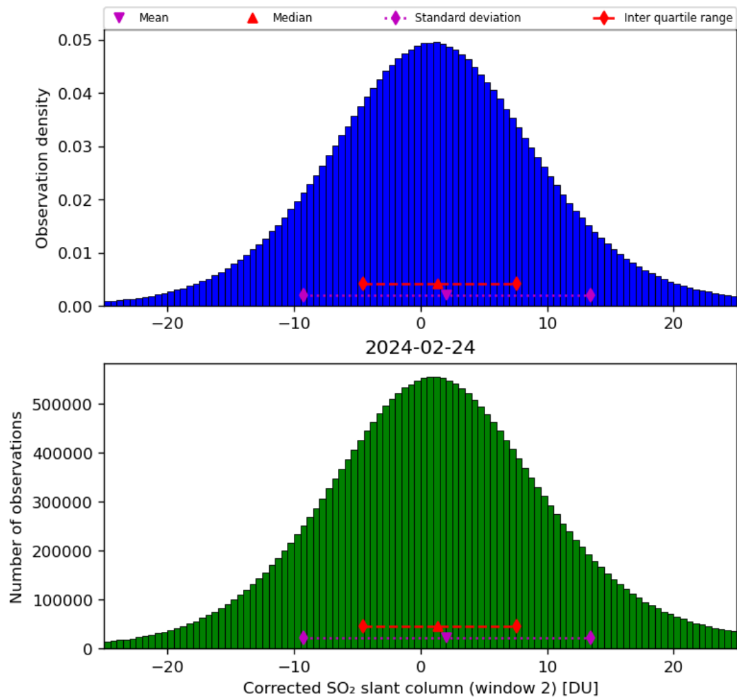
Figure 62: Histogram of “Corrected SO 2 slant column (window 2)” for 2024-02-23 to 2024-02-25
