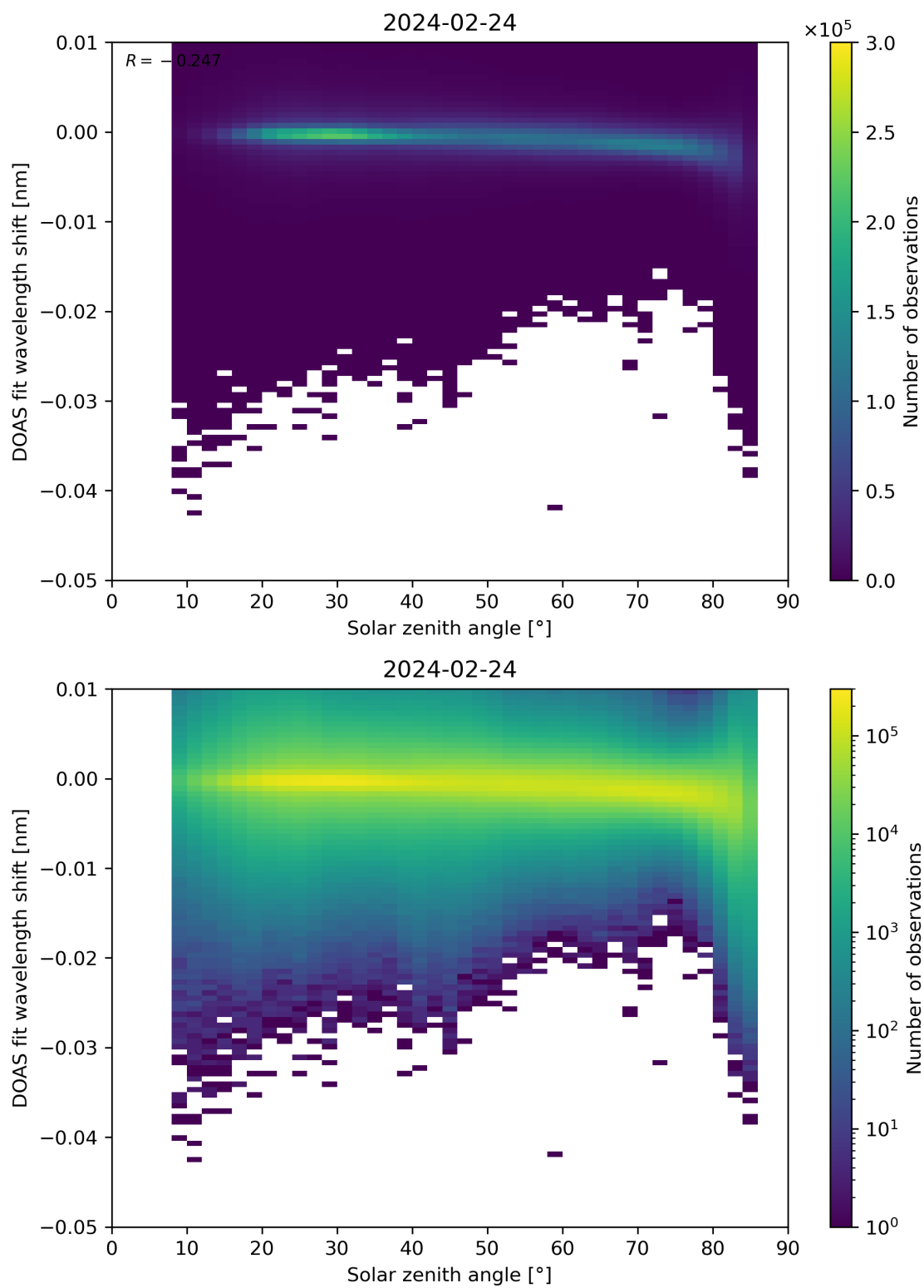
Figure 161: Scatter density plot of “Solar zenith angle” against “DOAS fit wavelength shift” for 2024-02-23 to 2024-02-25.
