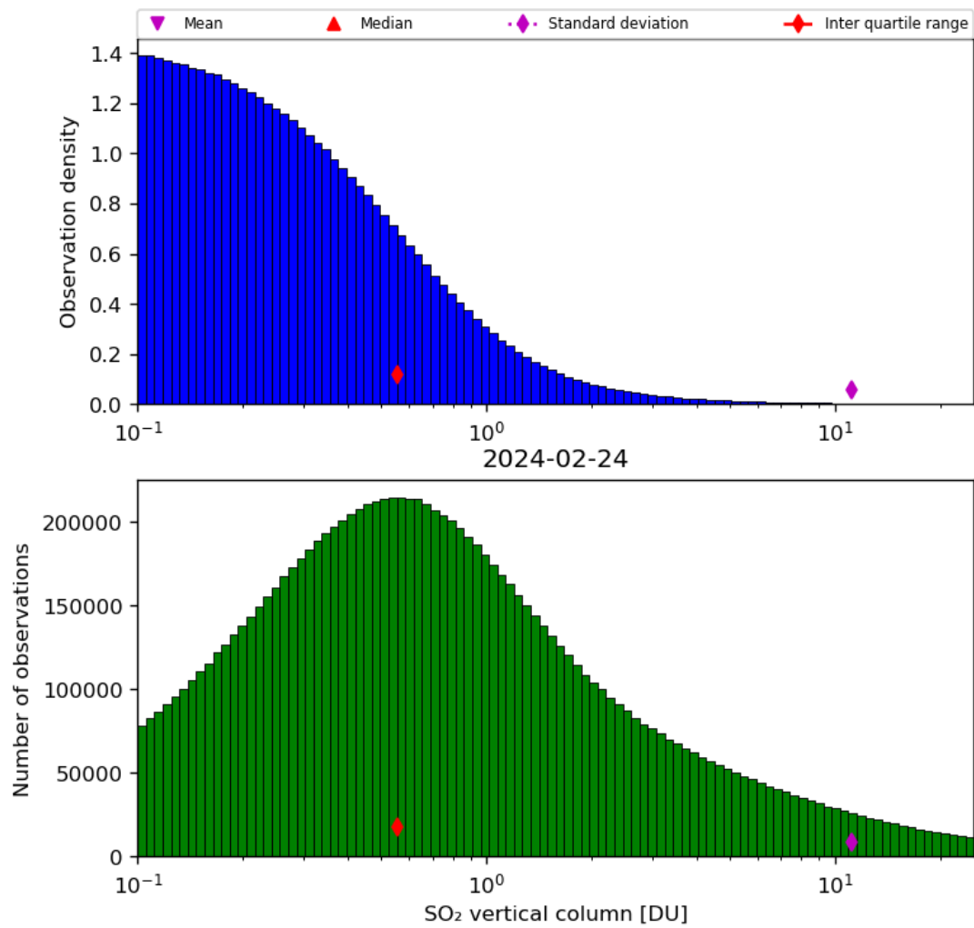
Figure 53: Histogram of “SO 2 vertical column” for 2024-02-23 to 2024-02-25
