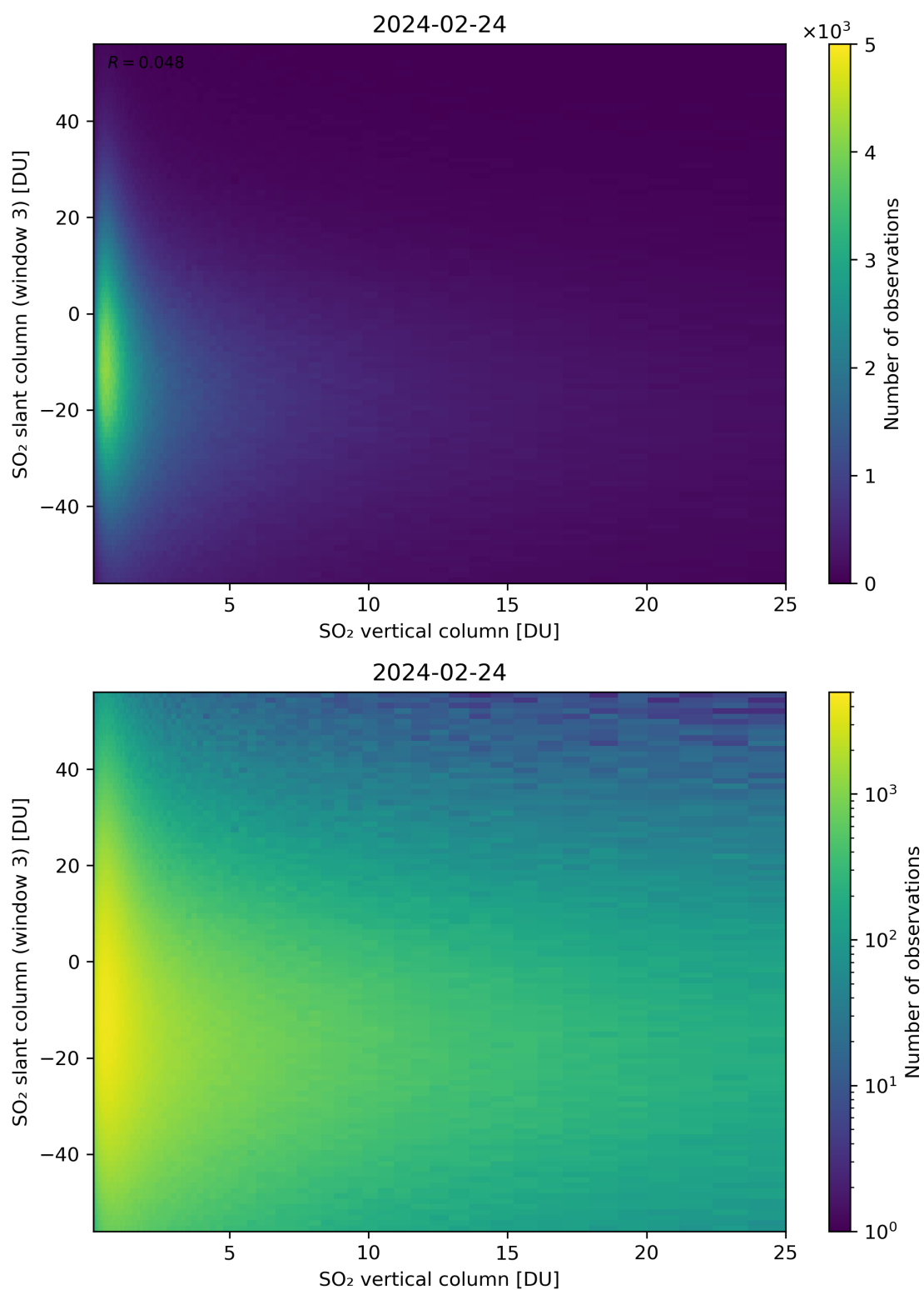
Figure 303: Scatter density plot of “SO 2 vertical column” against “SO 2 slant column (window 3)” for 2024-02-23 to 2024-02-25.
