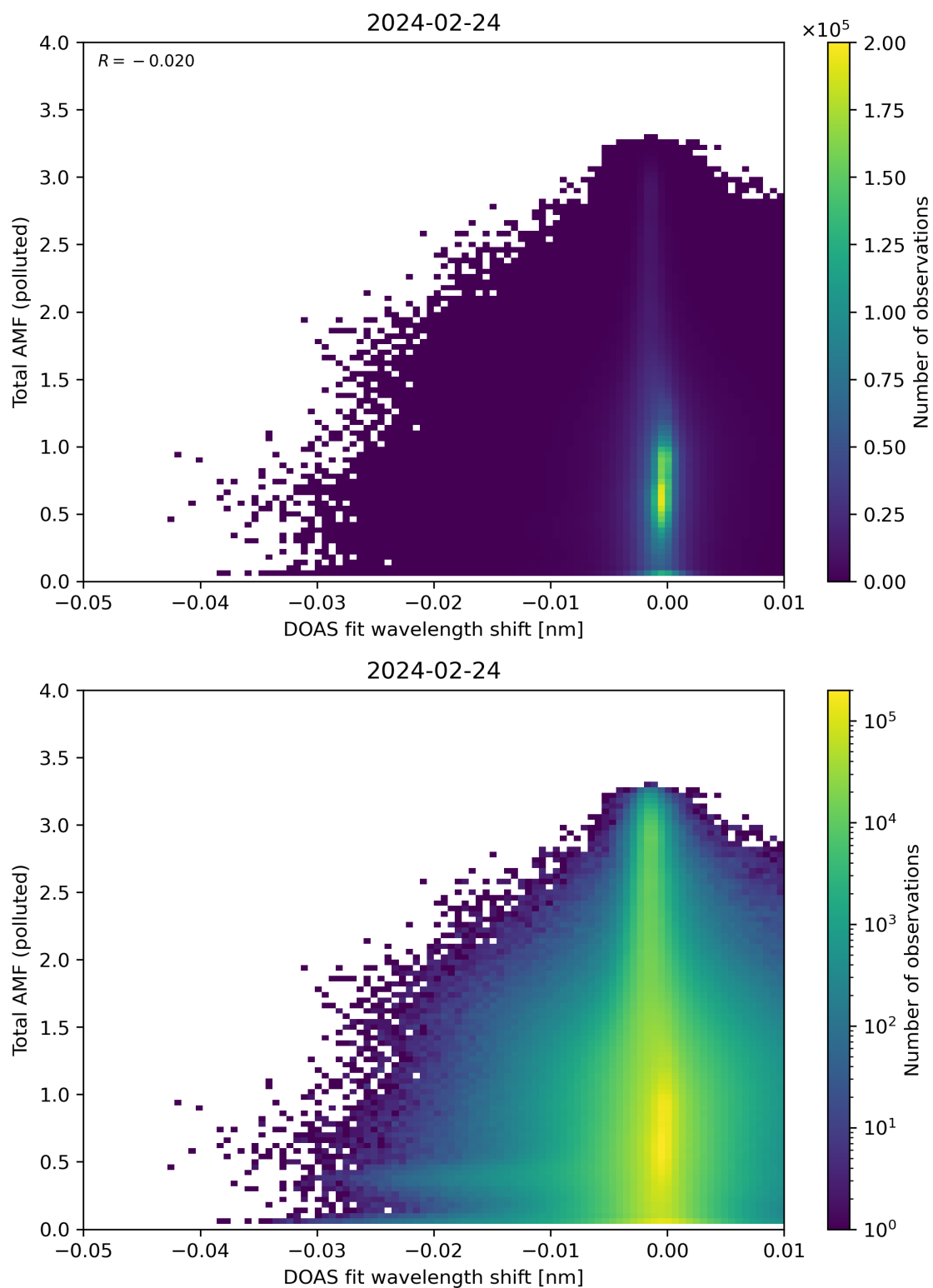
Figure 130: Scatter density plot of “DOAS fit wavelength shift” against “Total AMF (polluted)” for 2024-02-23 to 2024-02-25.
