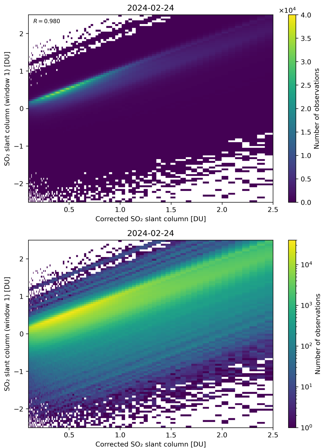
Figure 187: Scatter density plot of “Corrected SO 2 slant column” against “SO 2 slant column (window 1)” for 2024-02-23 to 2024-02-25.
