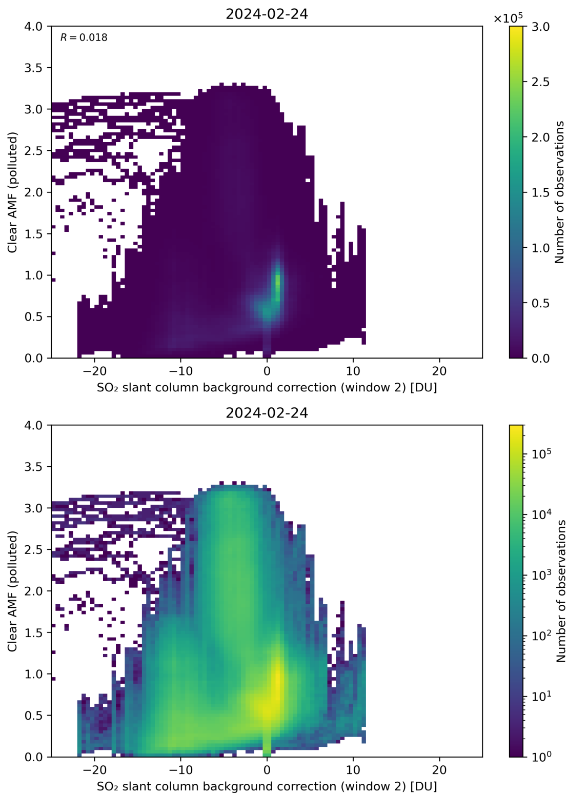
Figure 115: Scatter density plot of “SO 2 slant column background correction (window 2)” against “Clear AMF (polluted)” for 2024-02-23 to 2024-02-25.
