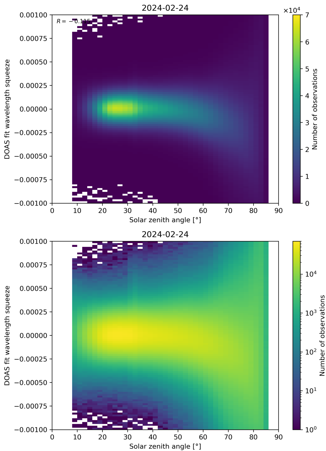
Figure 162: Scatter density plot of “Solar zenith angle” against “DOAS fit wavelength squeeze” for 2024-02-23 to 2024-02-25.
