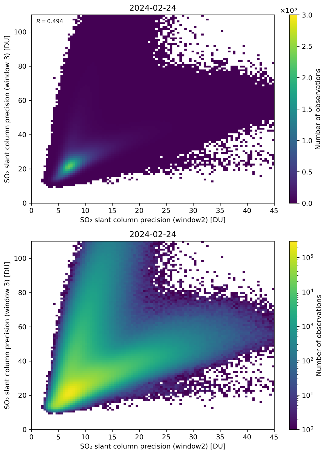
Figure 250: Scatter density plot of “SO 2 slant column precision (window2)” against “SO 2 slant column precision (window 3)” for 2024-02-23 to 2024-02-25.
