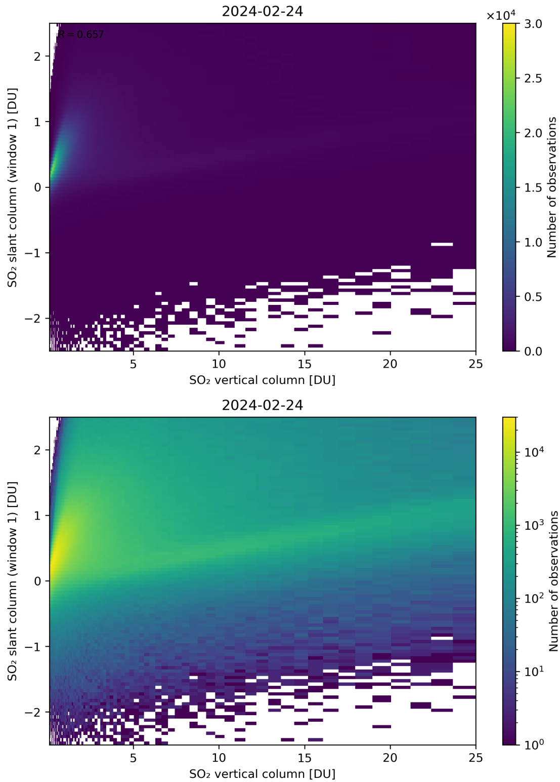
Figure 300: Scatter density plot of “SO 2 vertical column” against “SO 2 slant column (window 1)” for 2024-02-23 to 2024-02-25.
