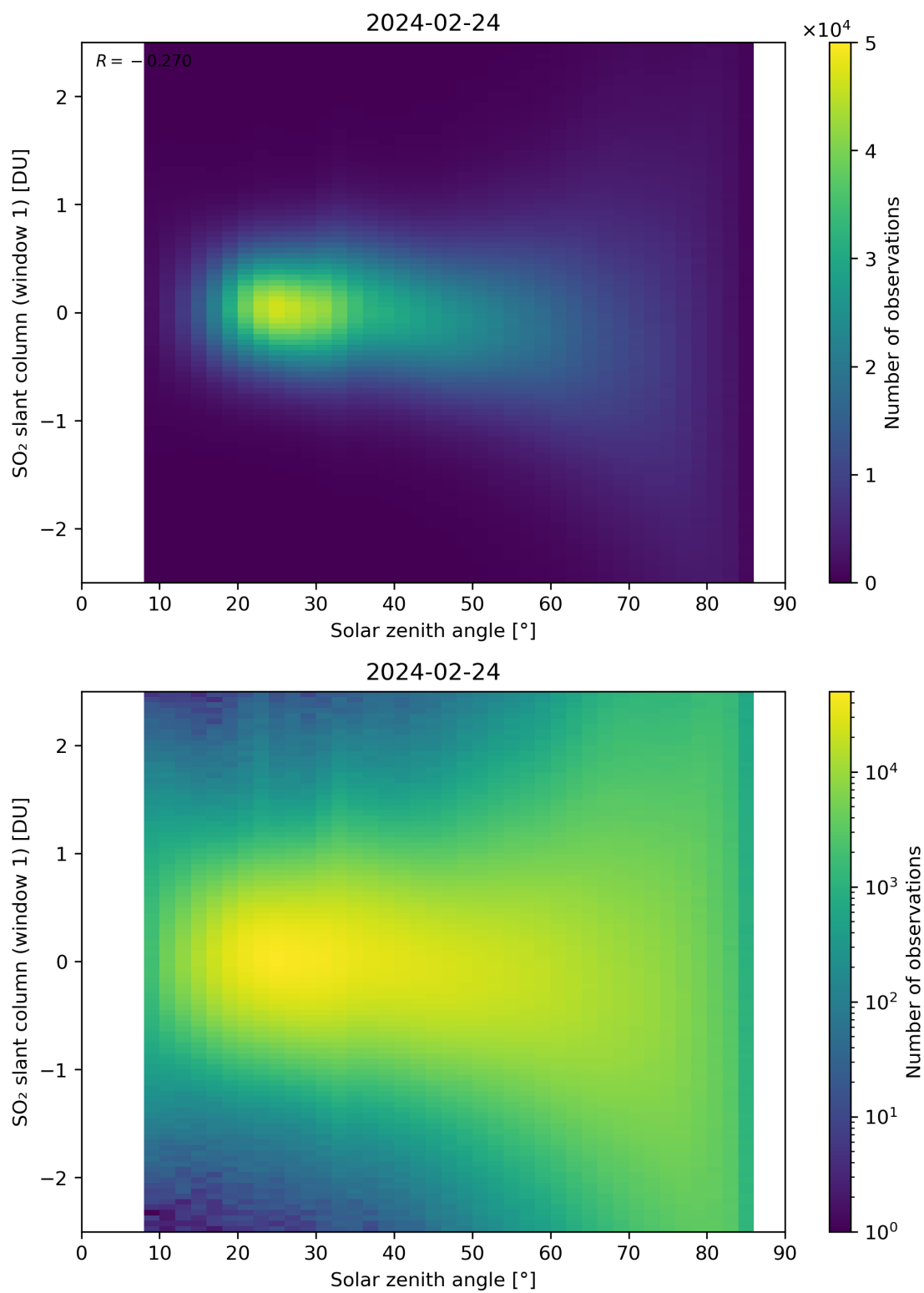
Figure 169: Scatter density plot of “Solar zenith angle” against “SO 2 slant column (window 1)” for 2024-02-23 to 2024-02-25.
