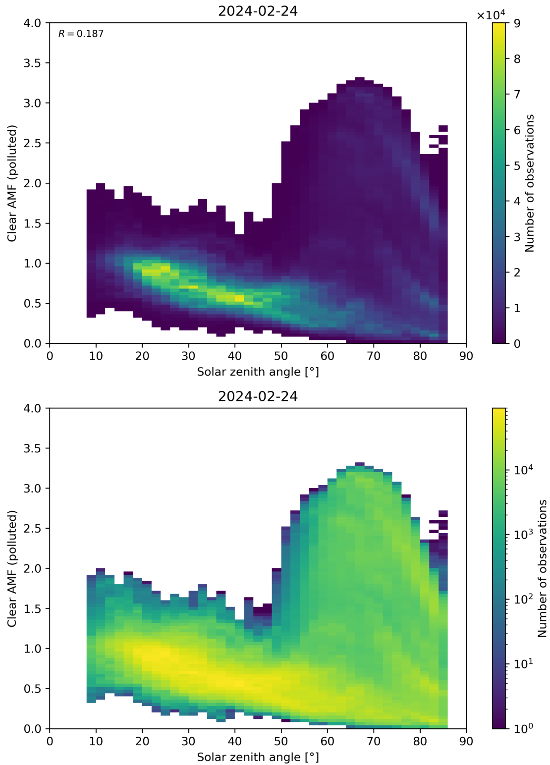
Figure 165: Scatter density plot of “Solar zenith angle” against “Clear AMF (polluted)” for 2024-02-23 to 2024-02-25.
