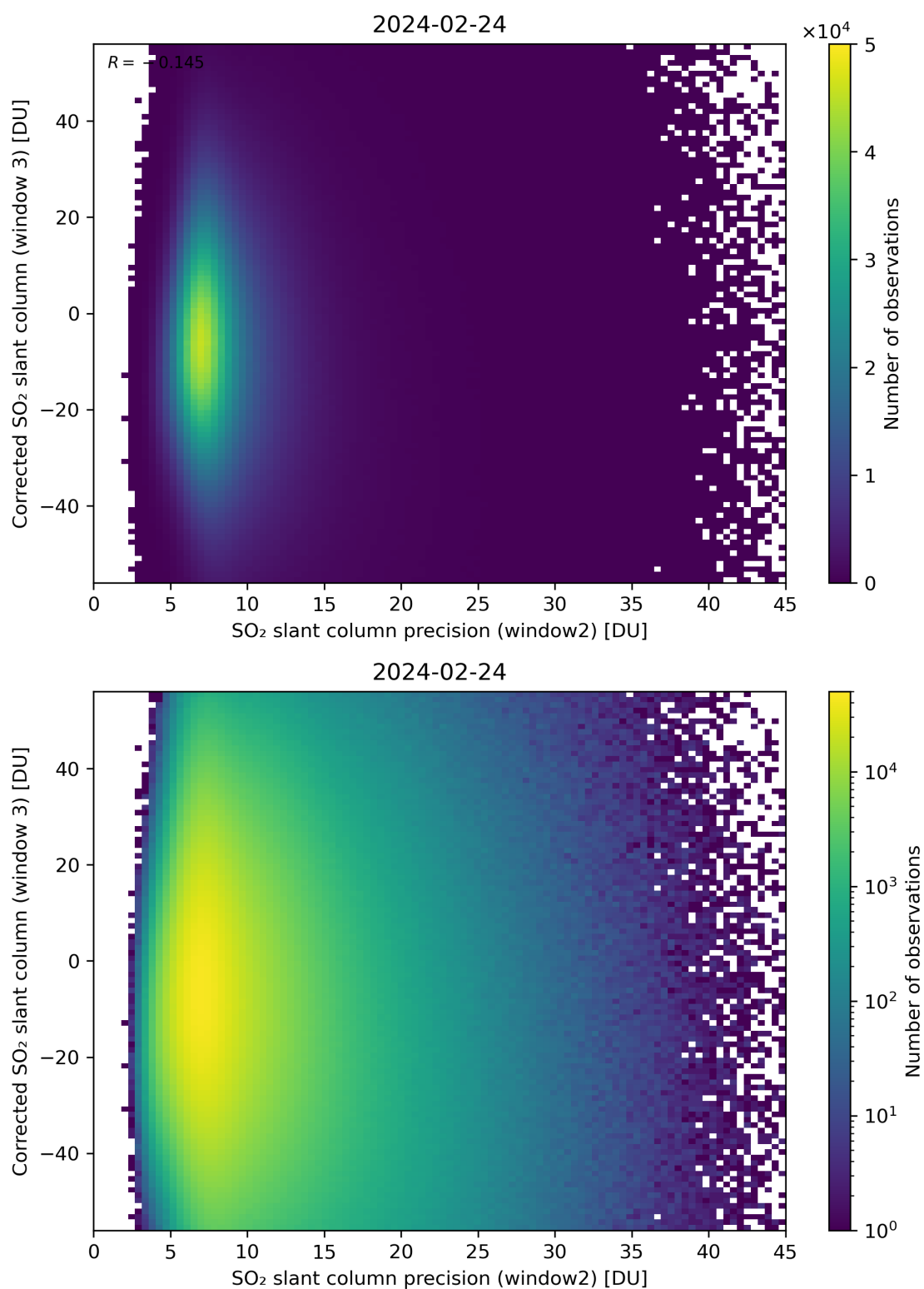
Figure 248: Scatter density plot of “SO 2 slant column precision (window2)” against “Corrected SO 2 slant column (window 3)” for 2024-02-23 to 2024-02-25.
