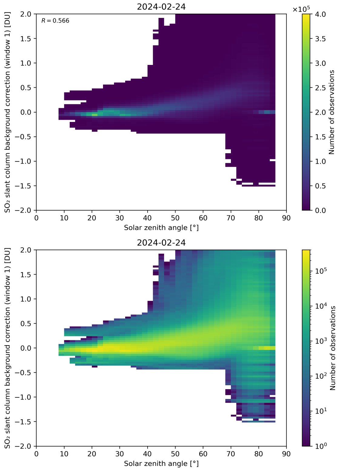
Figure 158: Scatter density plot of “Solar zenith angle” against “SO 2 slant column background correction (window 1)” for 2024-02-23 to 2024-02-25.
