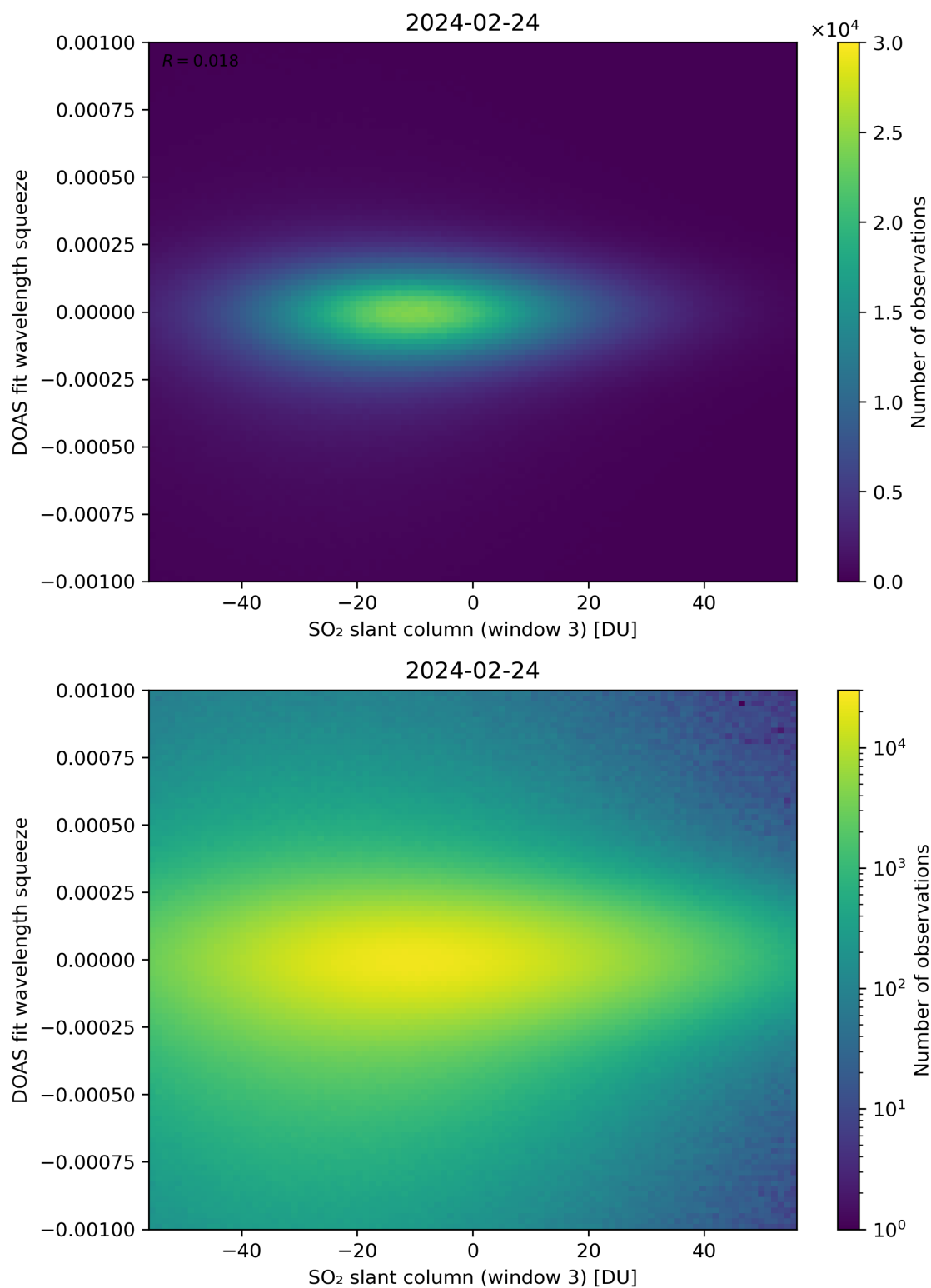
Figure 255: Scatter density plot of “SO 2 slant column (window 3)” against “DOAS fit wavelength squeeze” for 2024-02-23 to 2024-02-25.
