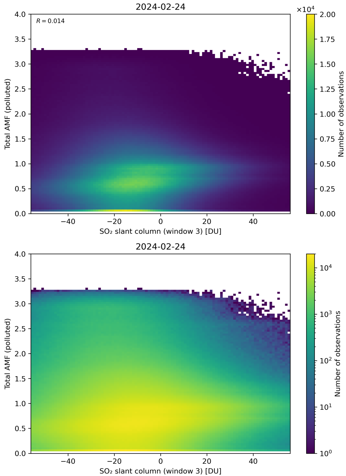
Figure 268: Scatter density plot of “SO 2 slant column (window 3)” against “Total AMF (polluted)” for 2024-02-23 to 2024-02-25.
