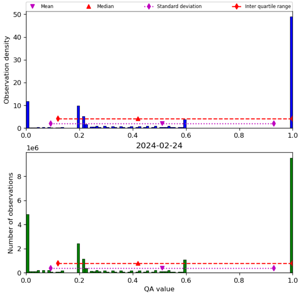
Figure 52: Histogram of “QA value” for 2024-02-23 to 2024-02-25
