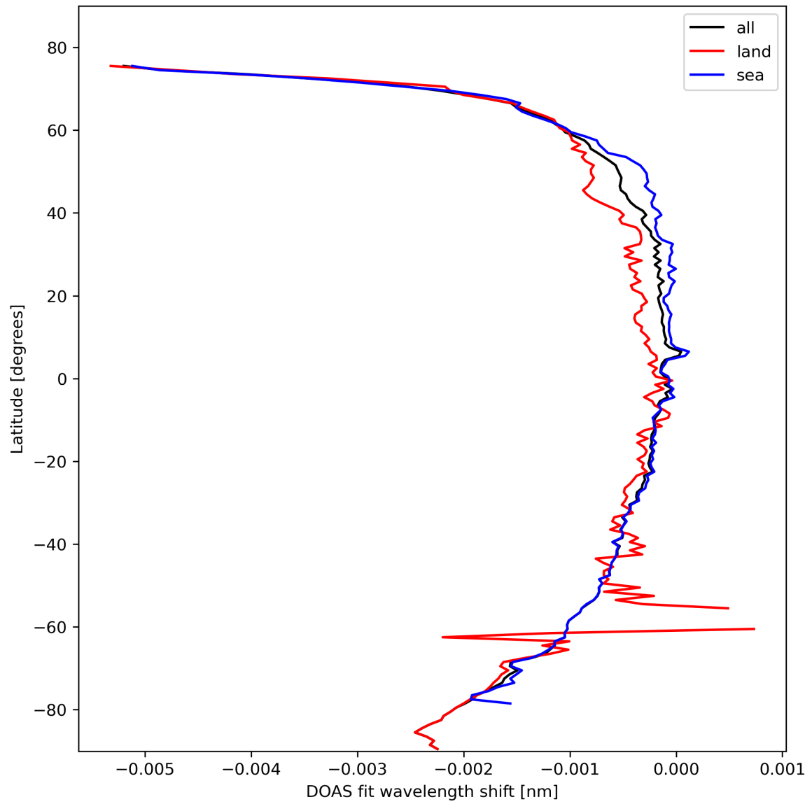
Figure 45: Zonal average of “DOAS fit wavelength shift” for 2024-02-23 to 2024-02-25.
