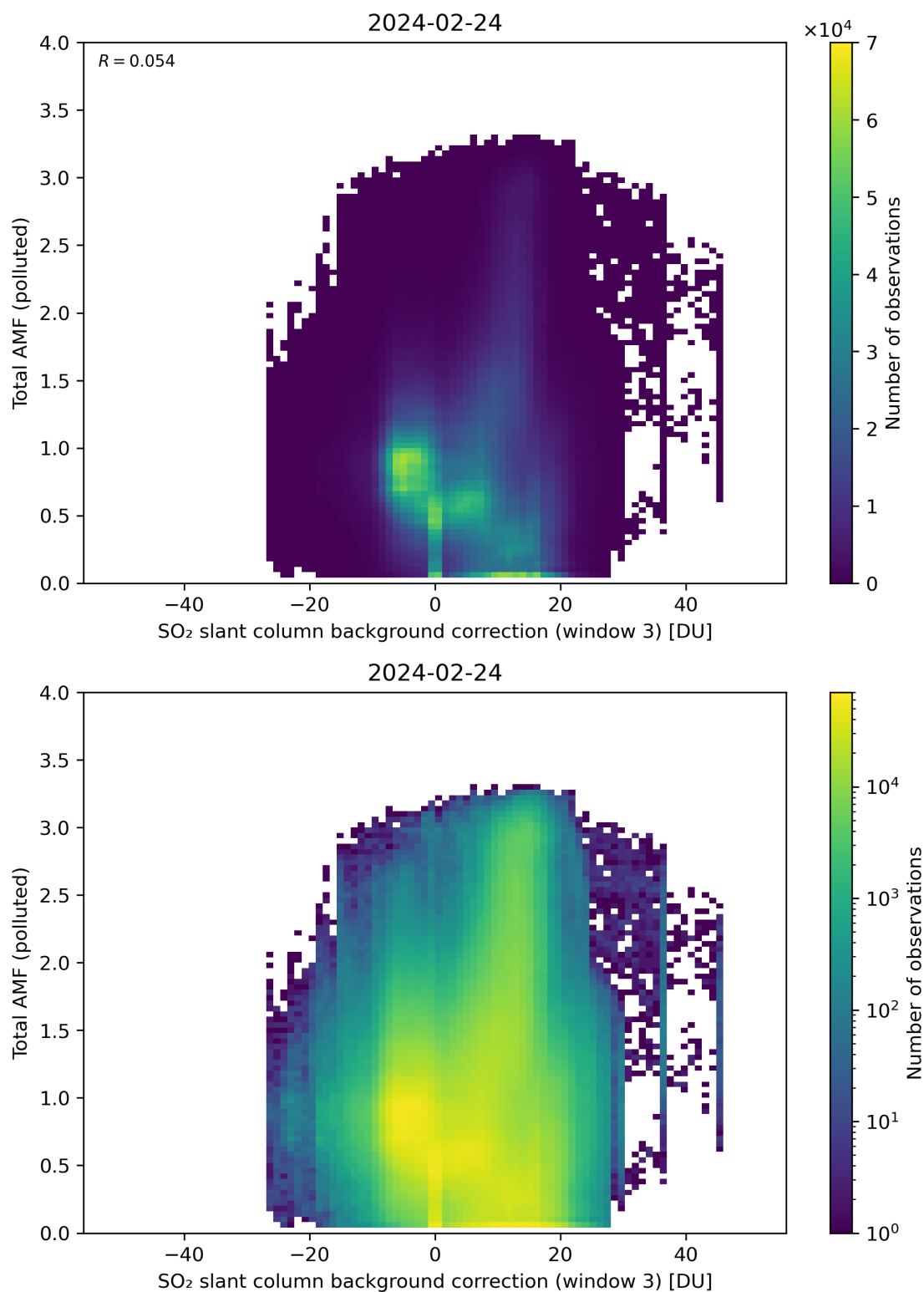
Figure 125: Scatter density plot of “SO 2 slant column background correction (window 3)” against “Total AMF (polluted)” for 2024-02-23 to 2024-02-25.
