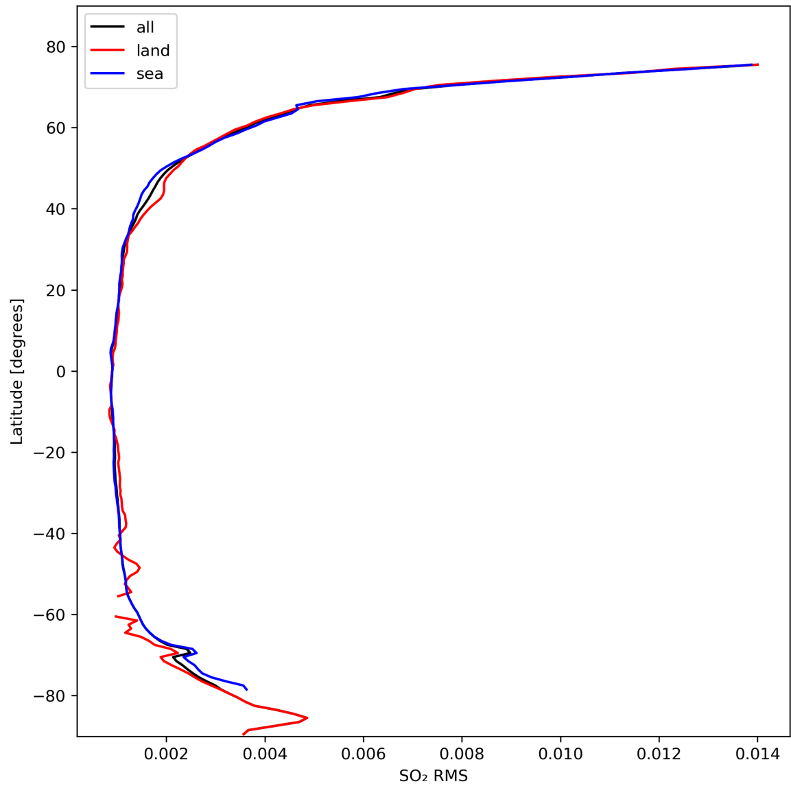
Figure 47: Zonal average of “SO 2 RMS” for 2024-02-23 to 2024-02-25.
