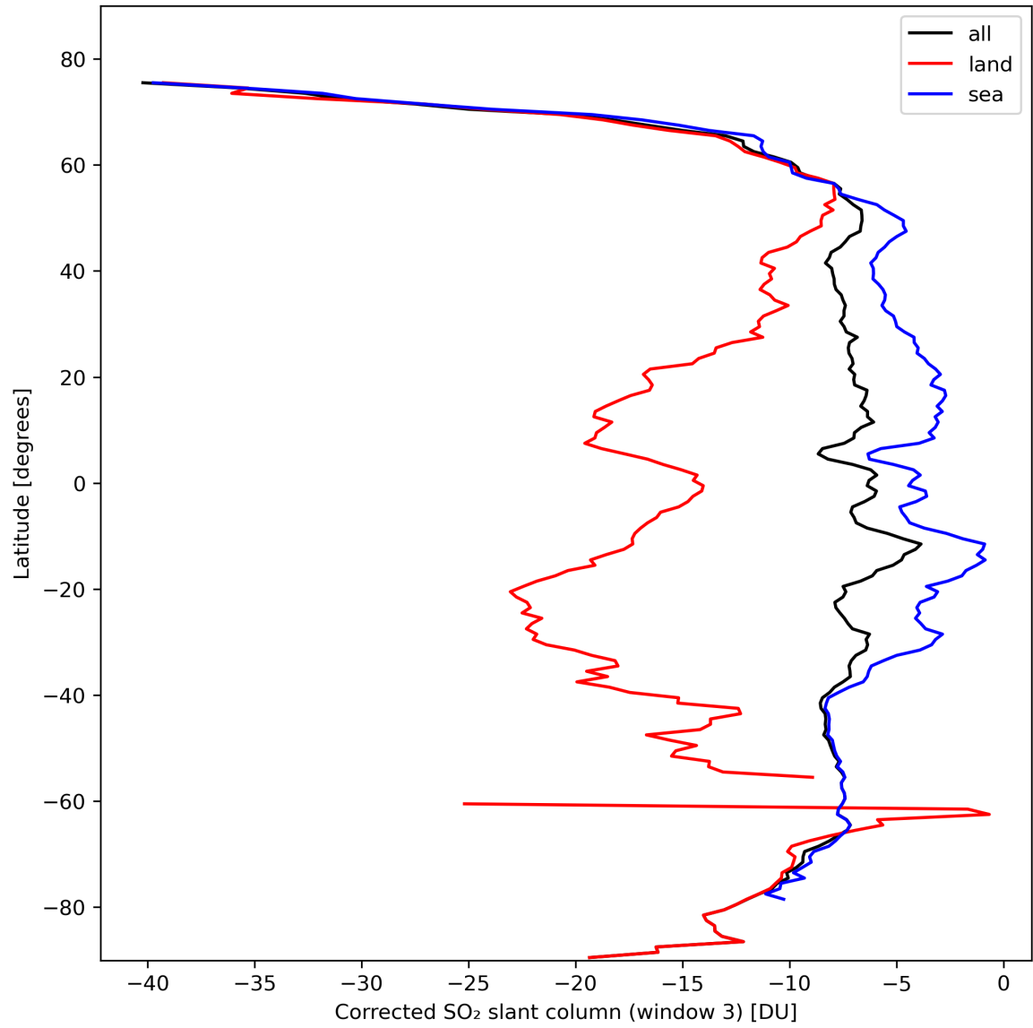
Figure 43: Zonal average of “Corrected SO 2 slant column (window 3)” for 2024-02-23 to 2024-02-25.
