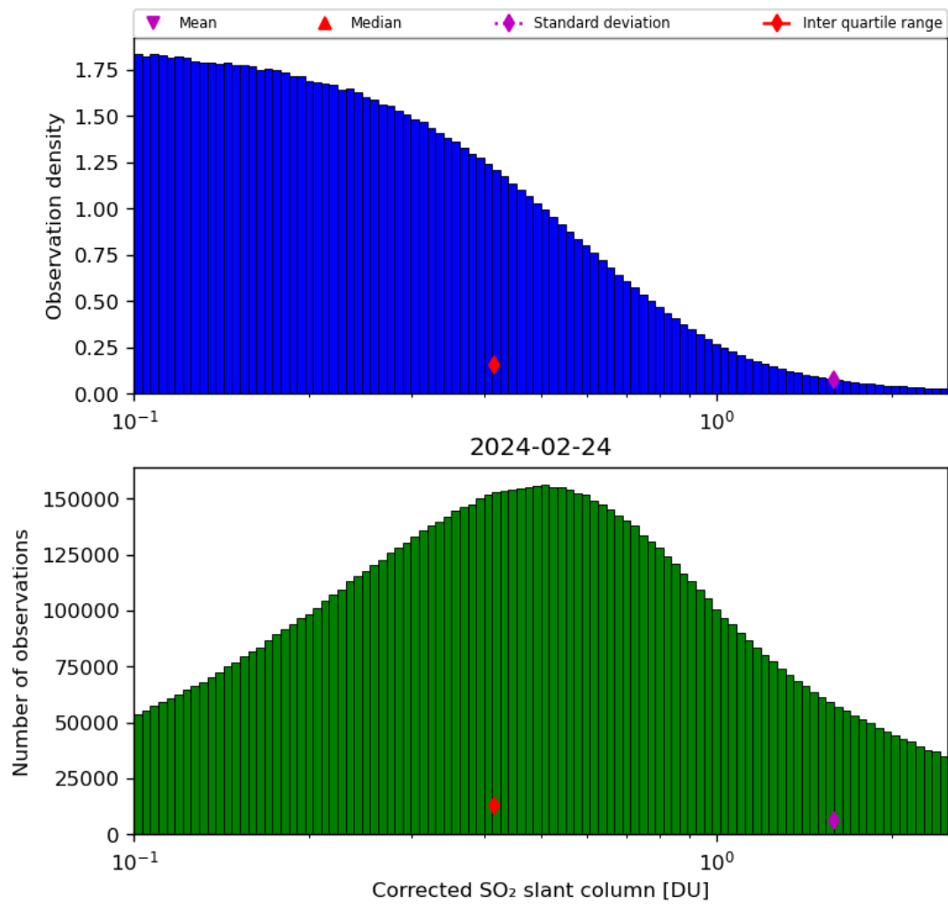
Figure 55: Histogram of “Corrected SO 2 slant column” for 2024-02-23 to 2024-02-25
