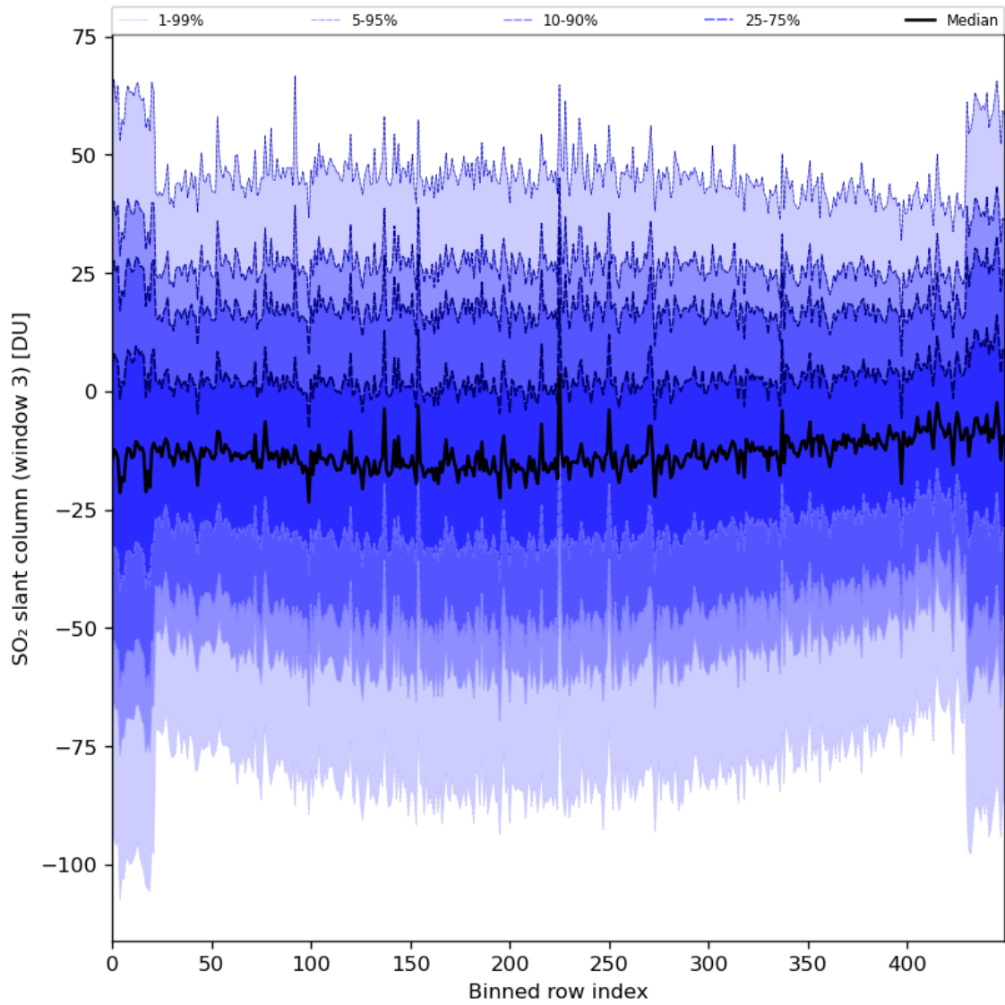
Figure 87: Along track statistics of “SO 2 slant column (window 3)” for 2024-02-23 to 2024-02-25
