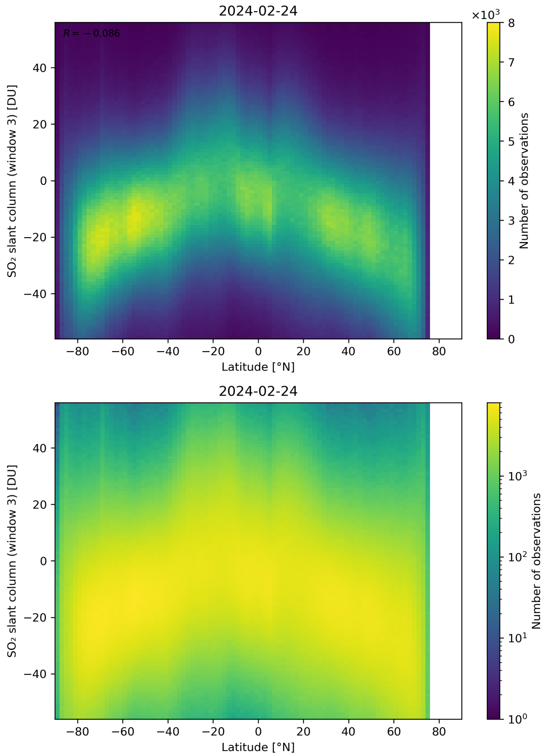
Figure 152: Scatter density plot of “Latitude” against “SO 2 slant column (window 3)” for 2024-02-23 to 2024-02-25.
