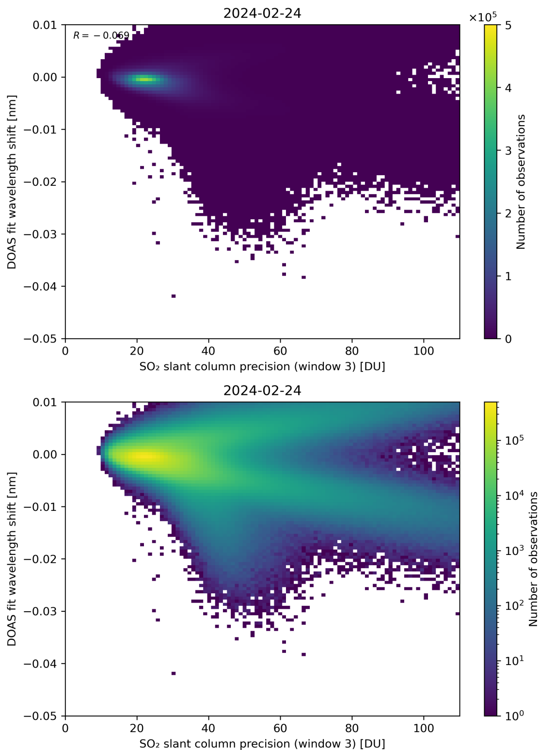
Figure 258: Scatter density plot of “SO 2 slant column precision (window 3)” against “DOAS fit wavelength shift” for 2024-02-23 to 2024-02-25.
