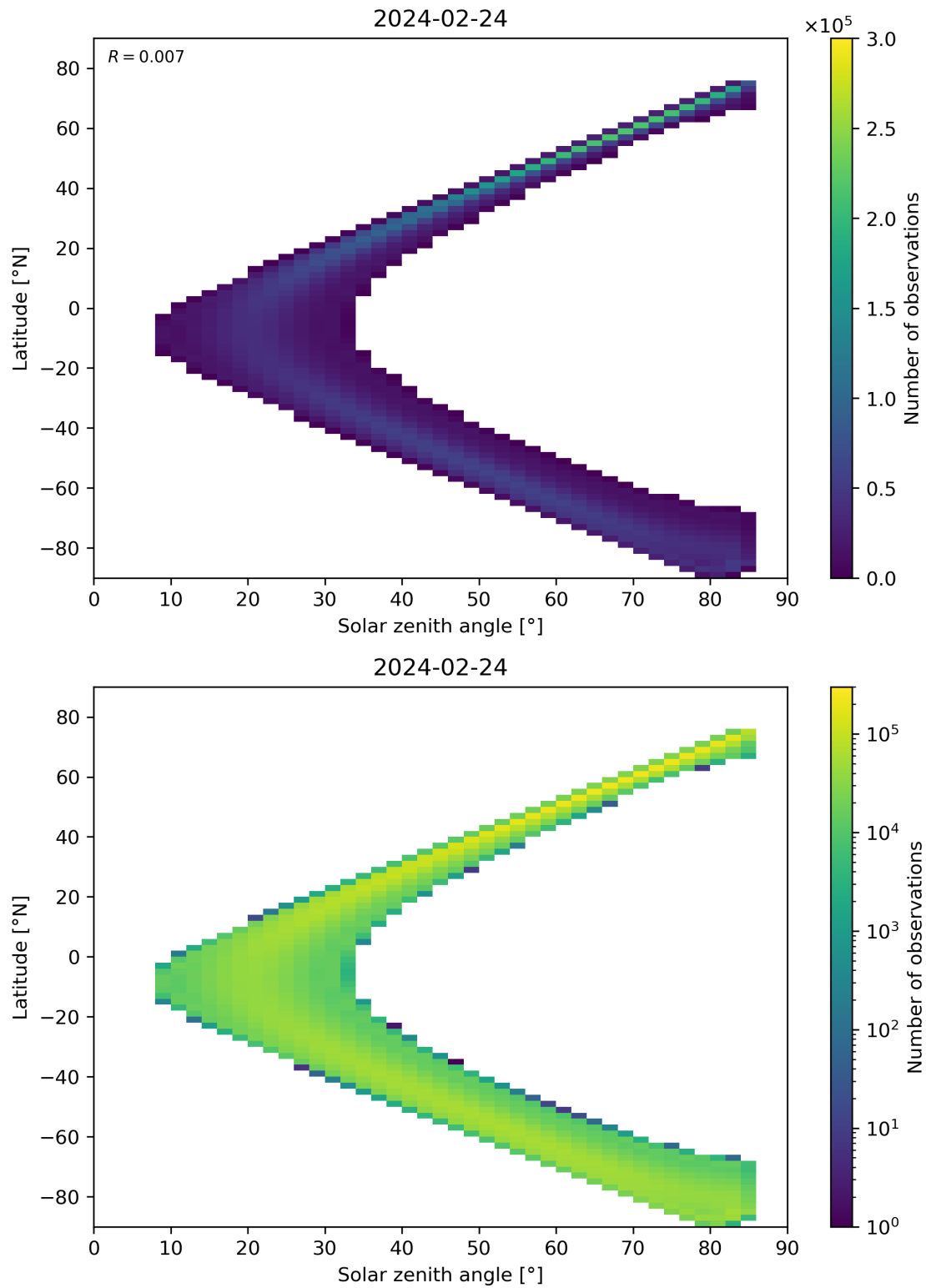
Figure 164: Scatter density plot of “Solar zenith angle” against “Latitude” for 2024-02-23 to 2024-02-25.
