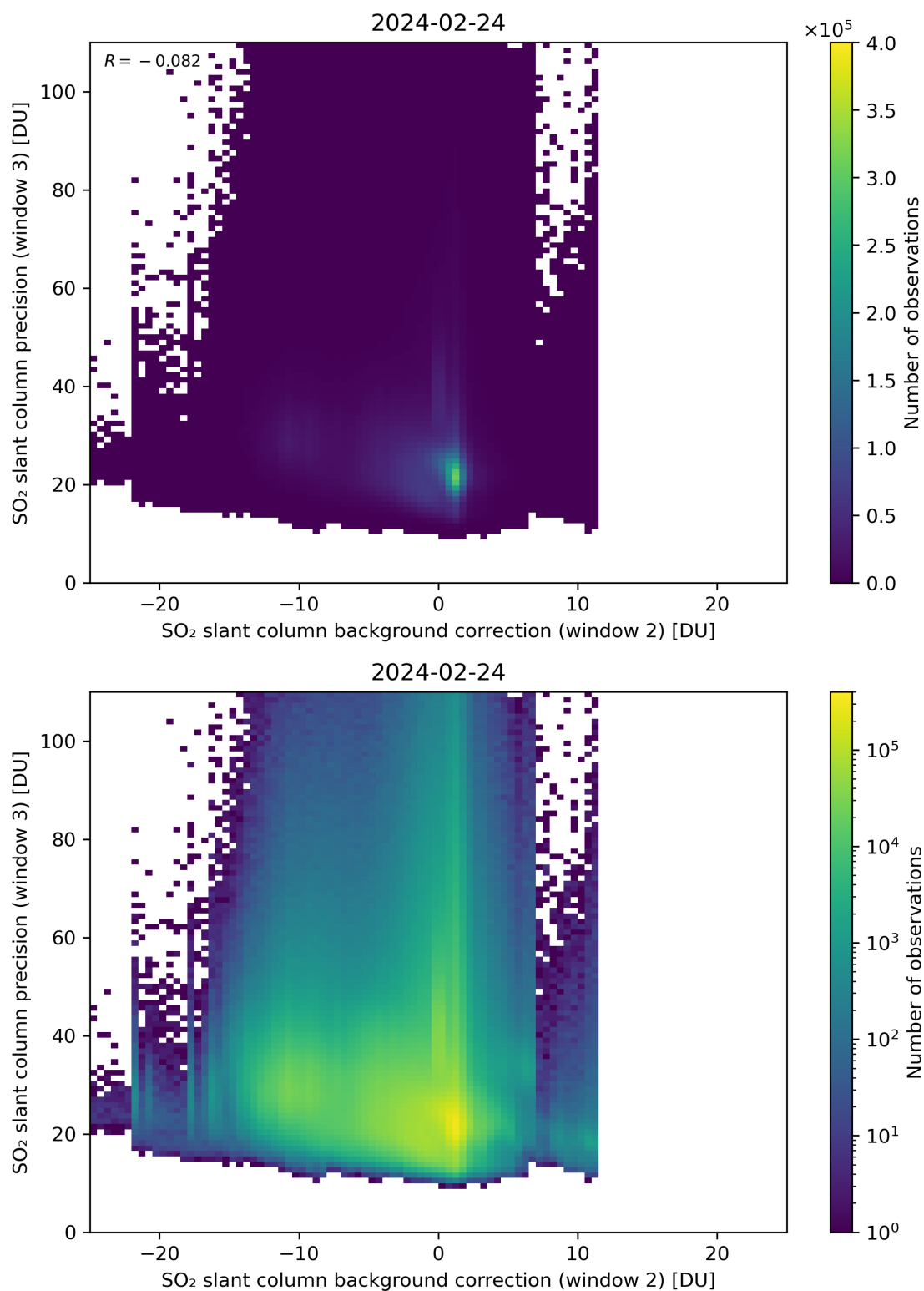
Figure 118: Scatter density plot of “SO 2 slant column background correction (window 2)” against “SO 2 slant column precision (window 3)” for 2024-02-23 to 2024-02-25.
