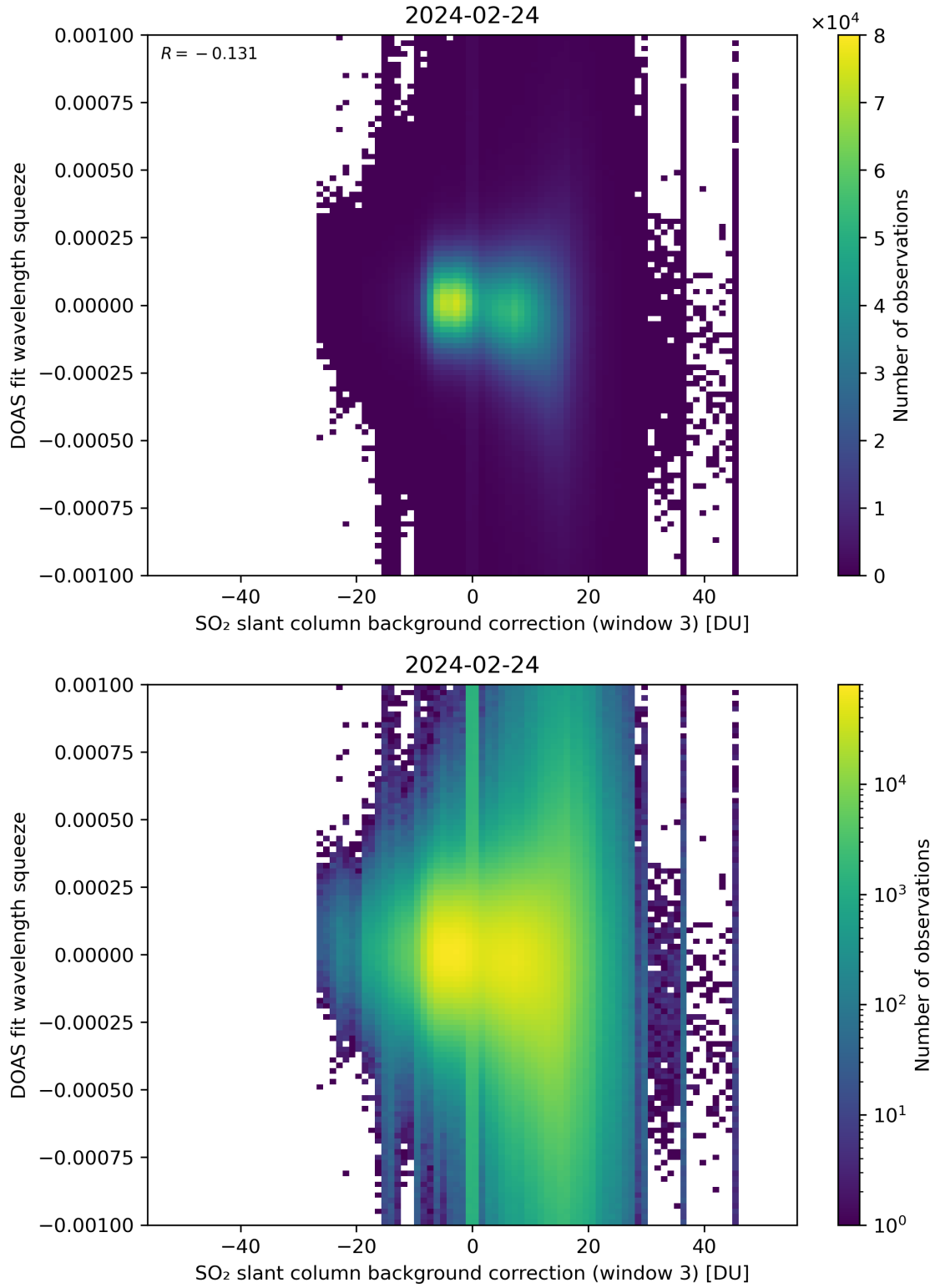
Figure 122: Scatter density plot of “SO 2 slant column background correction (window 3)” against “DOAS fit wavelength squeeze” for 2024-02-23 to 2024-02-25.
