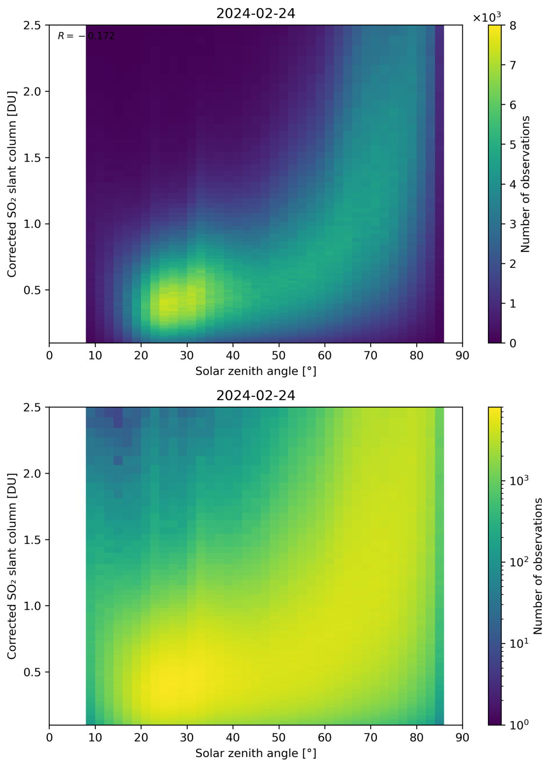
Figure 166: Scatter density plot of “Solar zenith angle” against “Corrected SO 2 slant column” for 2024-02-23 to 2024-02-25.
