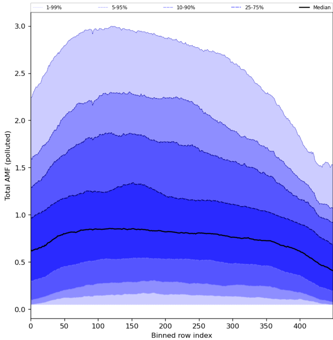
Figure 94: Along track statistics of “Total AMF (polluted)” for 2024-02-23 to 2024-02-25
