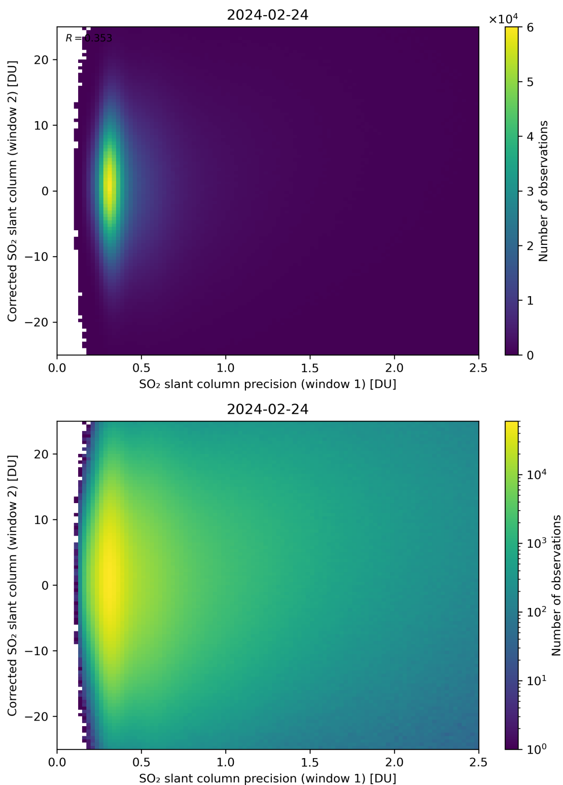
Figure 225: Scatter density plot of “SO 2 slant column precision (window 1)” against “Corrected SO 2 slant column (window 2)” for 2024-02-23 to 2024-02-25.
