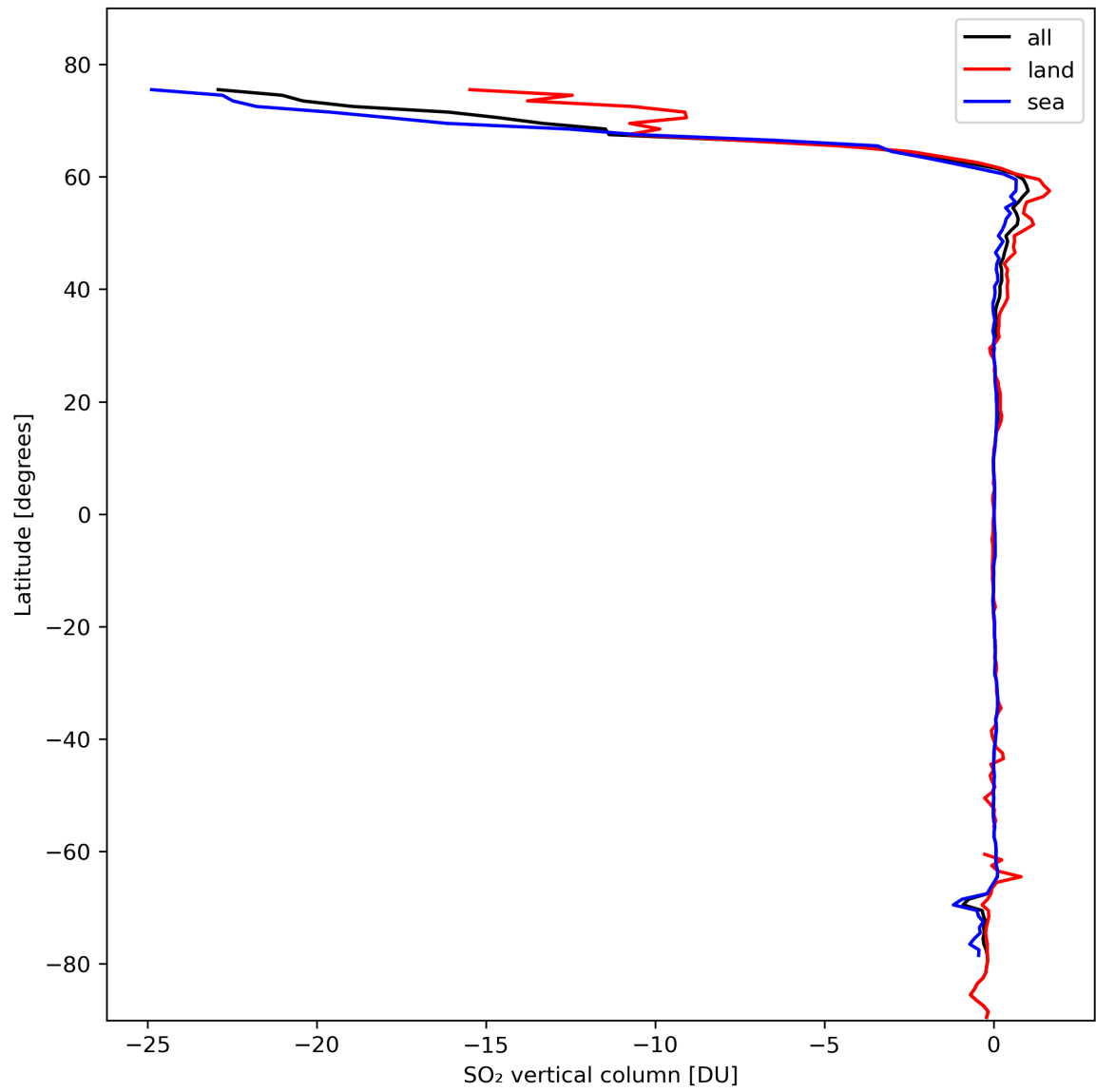
Figure 30: Zonal average of “SO 2 vertical column” for 2024-02-23 to 2024-02-25.
