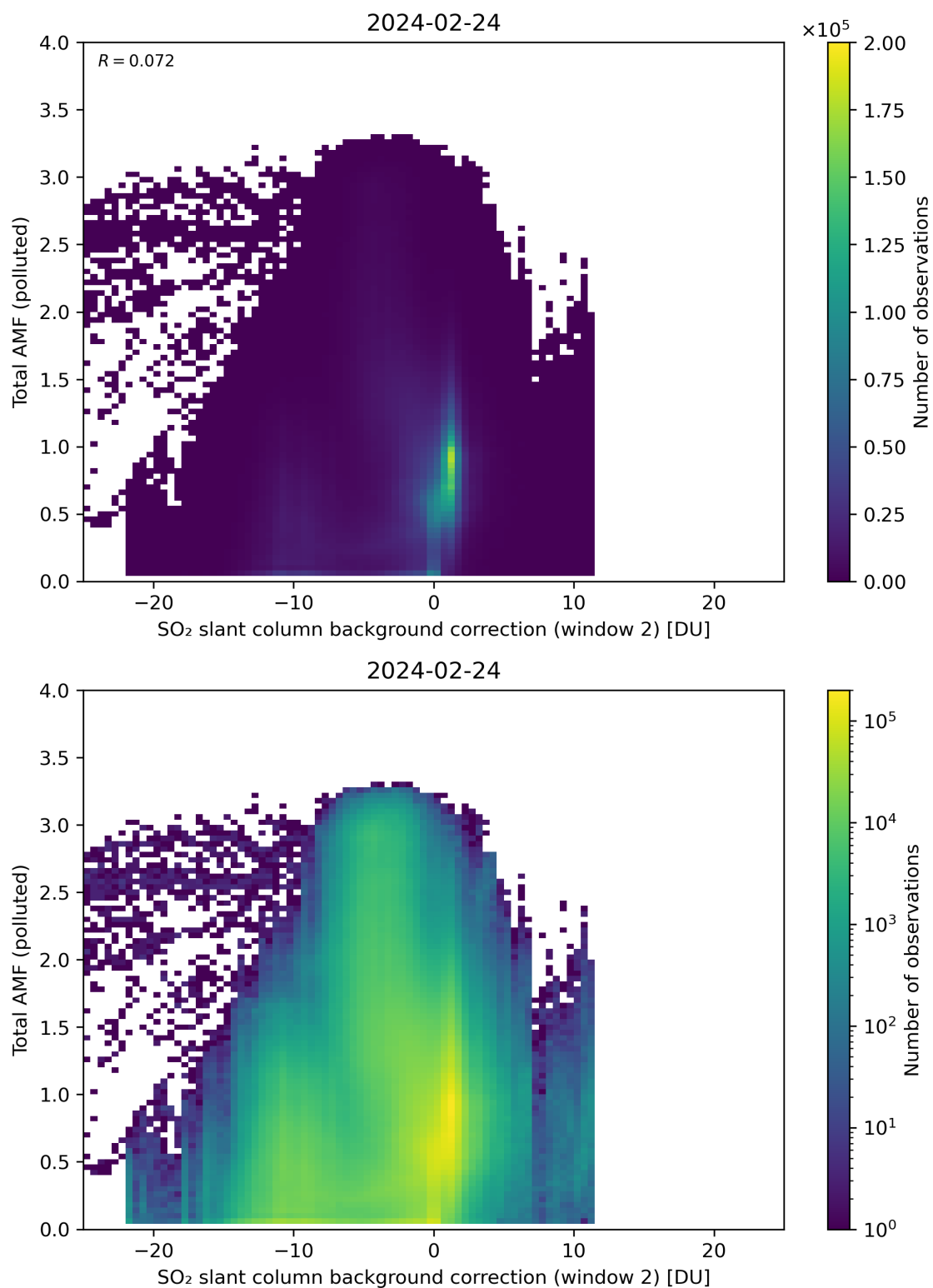
Figure 119: Scatter density plot of “SO 2 slant column background correction (window 2)” against “Total AMF (polluted)” for 2024-02-23 to 2024-02-25.
