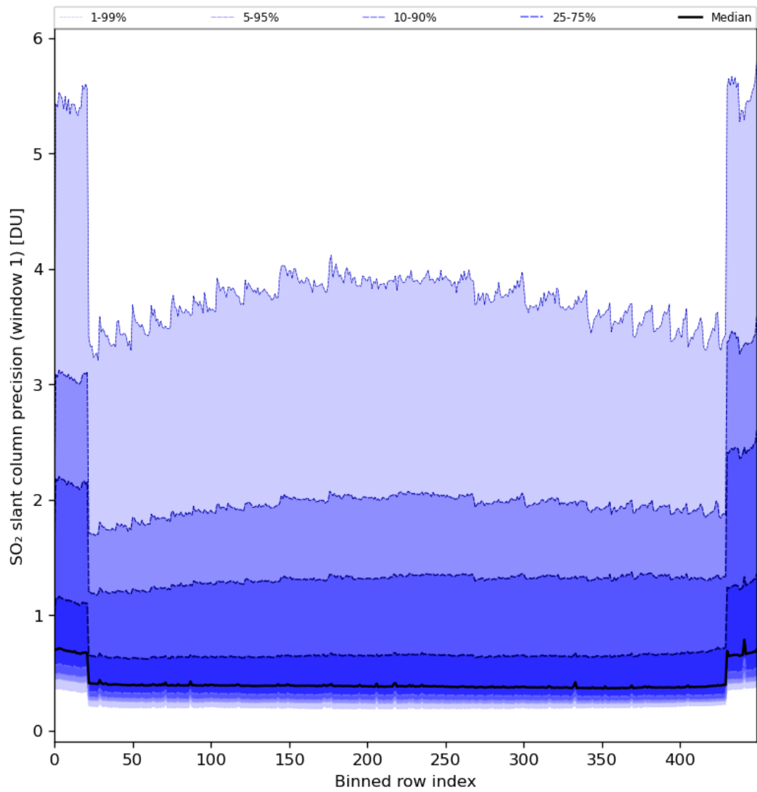
Figure 80: Along track statistics of “SO 2 slant column precision (window 1)” for 2024-02-23 to 2024-02-25
