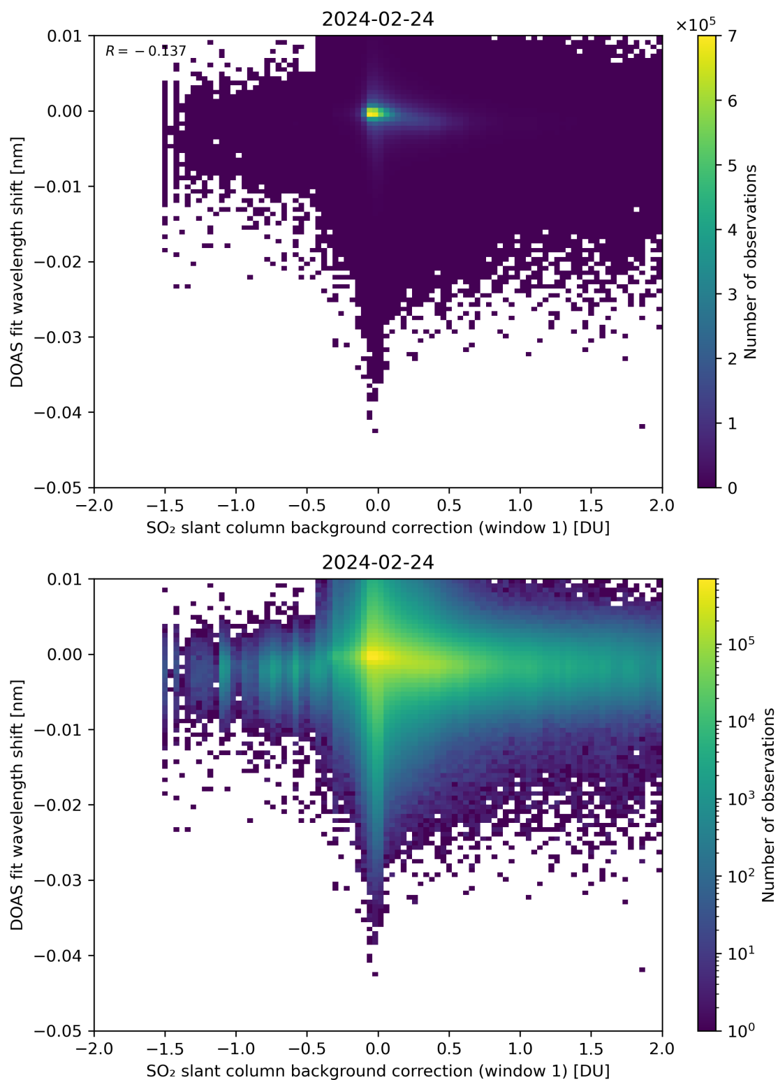
Figure 100: Scatter density plot of “SO 2 slant column background correction (window 1)” against “DOAS fit wavelength shift” for 2024-02-23 to 2024-02-25.
