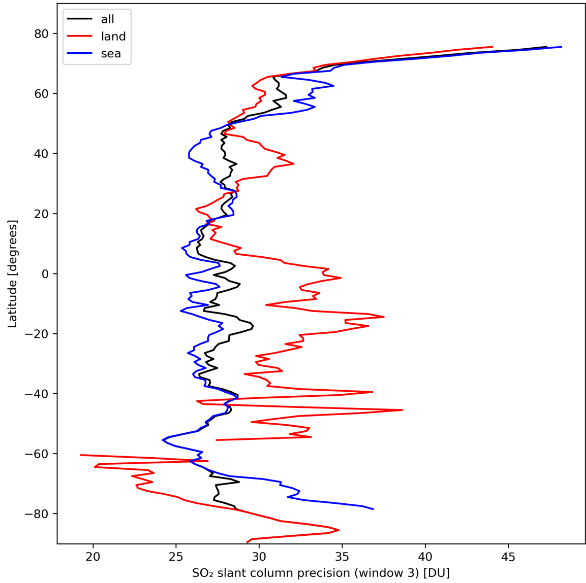
Figure 42: Zonal average of “SO 2 slant column precision (window 3)” for 2024-02-23 to 2024-02-25.
