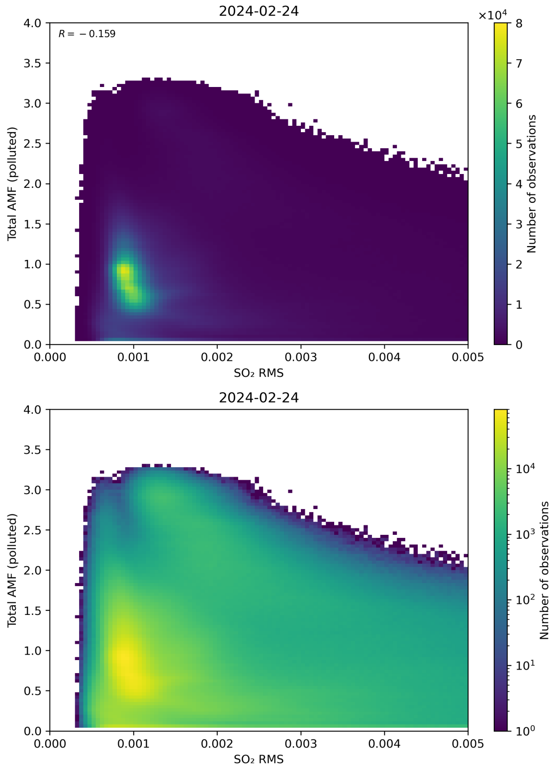
Figure 137: Scatter density plot of “SO 2 RMS” against “Total AMF (polluted)” for 2024-02-23 to 2024-02-25.
