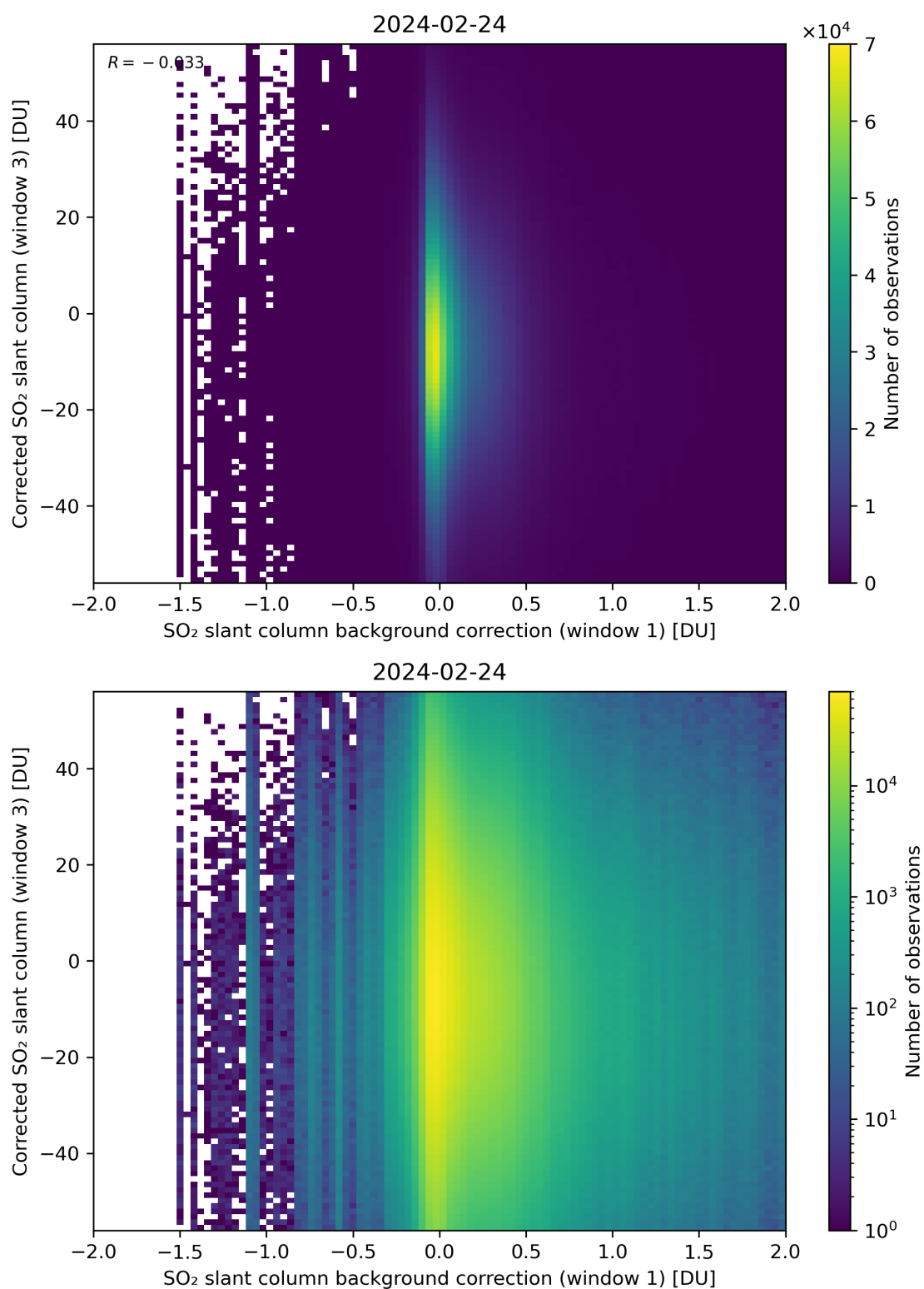
Figure 105: Scatter density plot of “SO 2 slant column background correction (window 1)” against “Corrected SO 2 slant column (window 3)” for 2024-02-23 to 2024-02-25.
