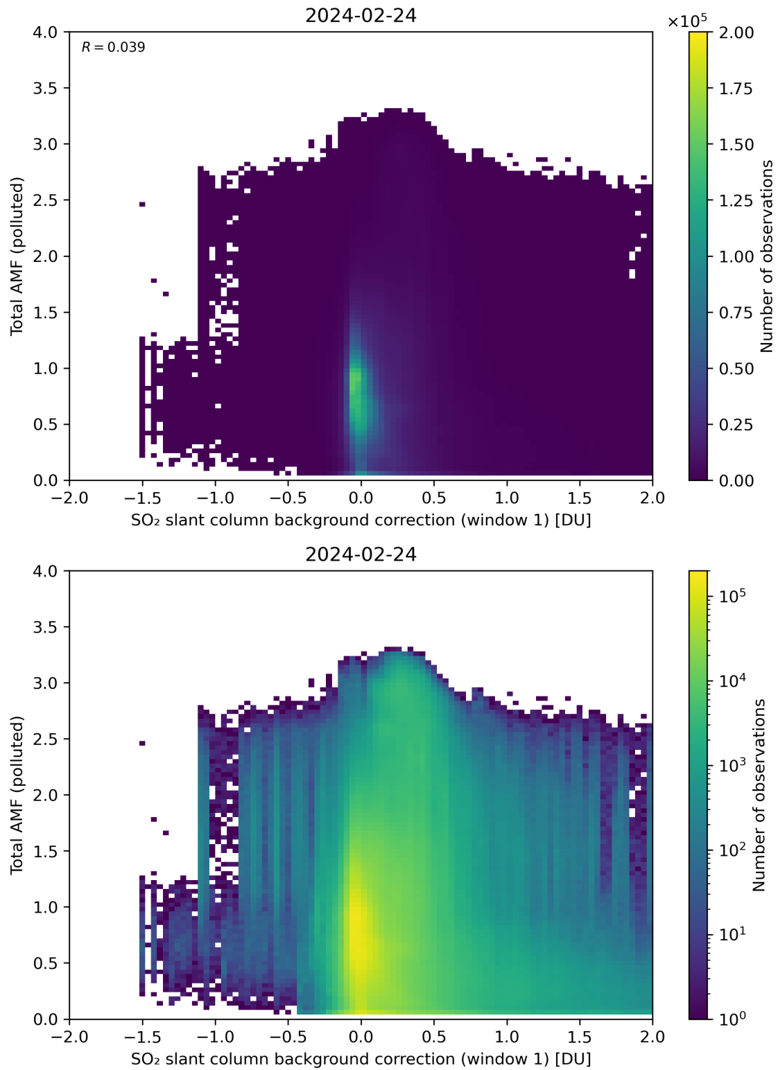
Figure 109: Scatter density plot of “SO 2 slant column background correction (window 1)” against “Total AMF (polluted)” for 2024-02-23 to 2024-02-25.
