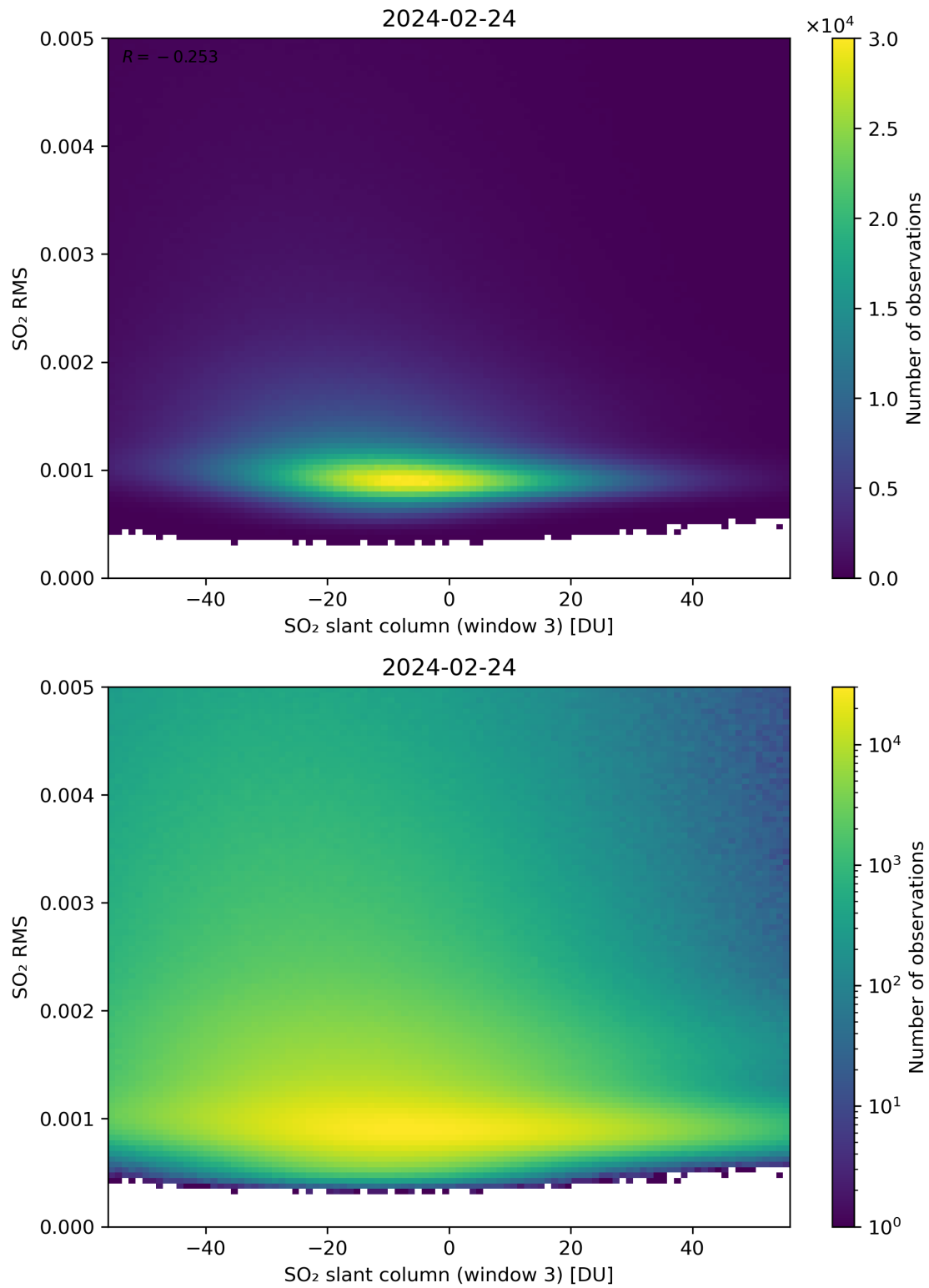
Figure 256: Scatter density plot of “SO 2 slant column (window 3)” against “SO 2 RMS” for 2024-02-23 to 2024-02-25.
