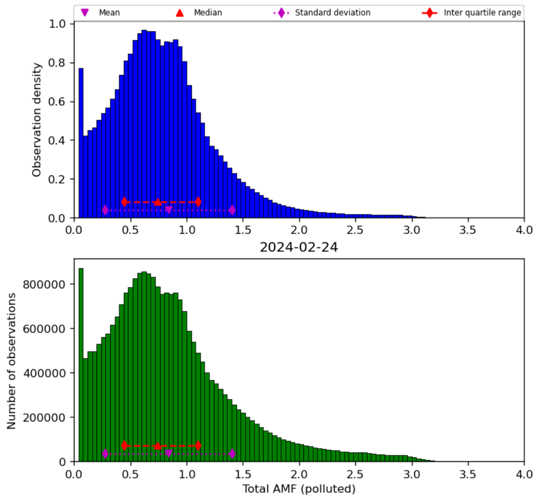
Figure 71: Histogram of “Total AMF (polluted)” for 2024-02-23 to 2024-02-25
