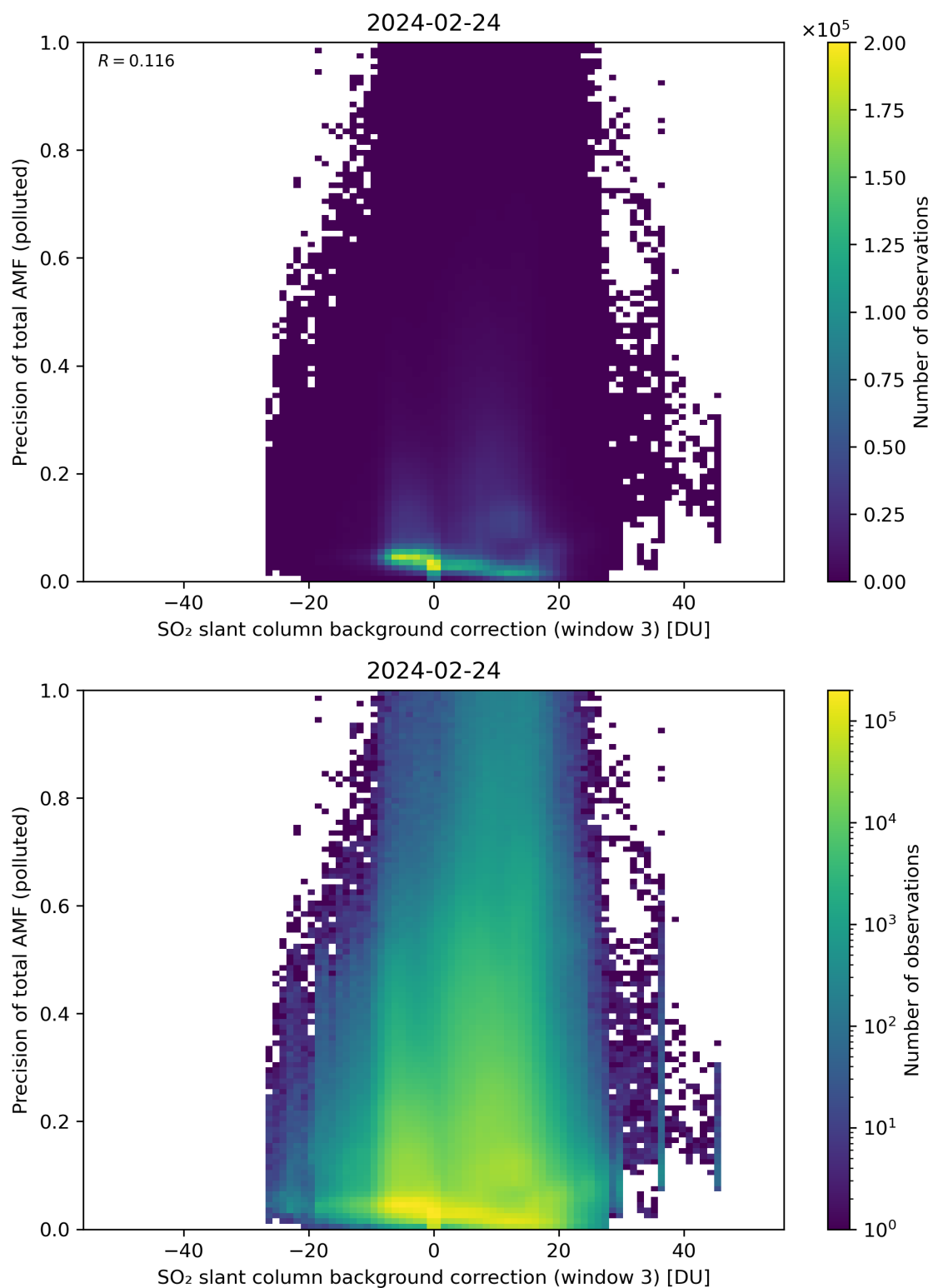
Figure 126: Scatter density plot of “SO 2 slant column background correction (window 3)” against “Precision of total AMF (polluted)” for 2024-02-23 to 2024-02-25.
