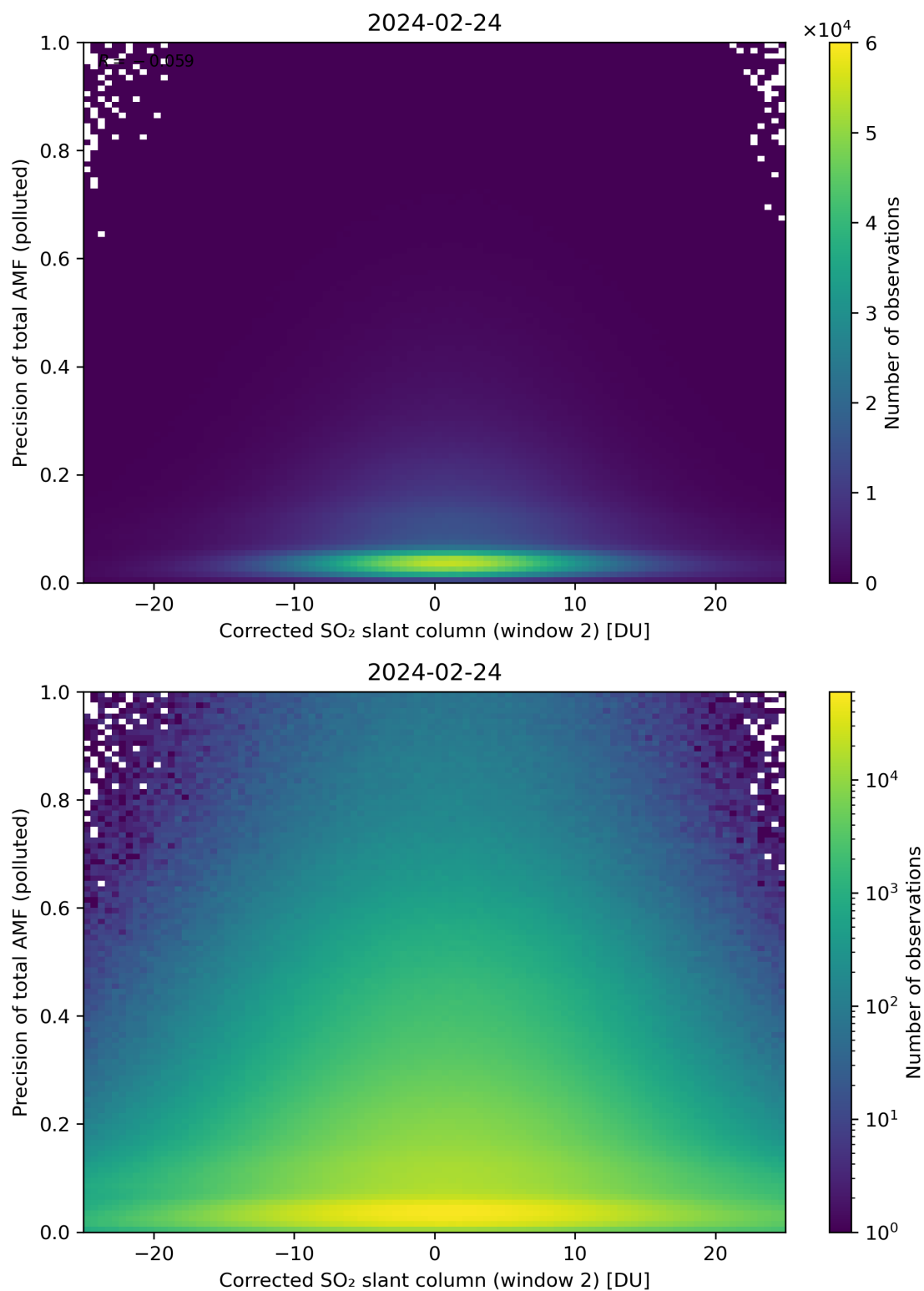
Figure 204: Scatter density plot of “Corrected SO 2 slant column (window 2)” against “Precision of total AMF (polluted)” for 2024-02-23 to 2024-02-25.
