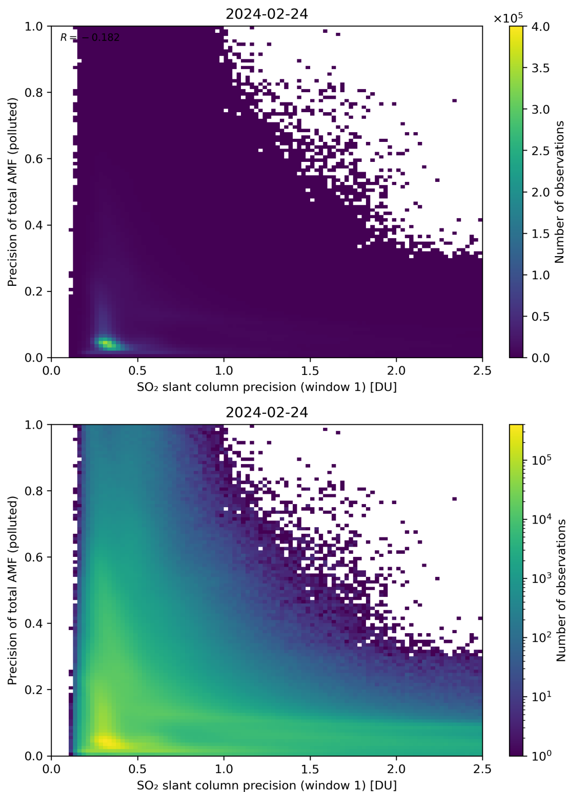
Figure 231: Scatter density plot of “SO 2 slant column precision (window 1)” against “Precision of total AMF (polluted)” for 2024-02-23 to 2024-02-25.
