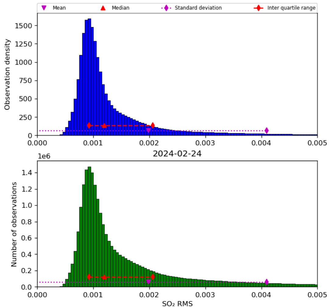
Figure 70: Histogram of “SO 2 RMS” for 2024-02-23 to 2024-02-25
