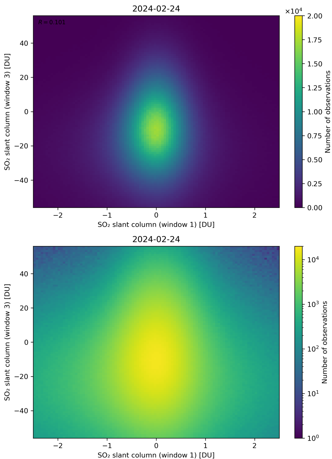
Figure 237: Scatter density plot of “SO 2 slant column (window 1)” against “SO 2 slant column (window 3)” for 2024-02-23 to 2024-02-25.
