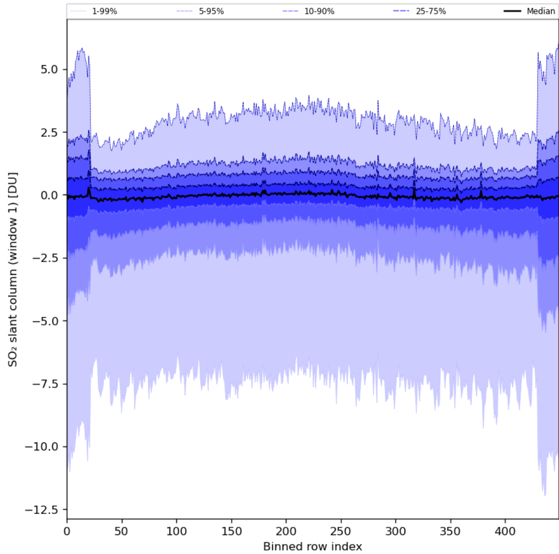
Figure 79: Along track statistics of “SO 2 slant column (window 1)” for 2024-02-23 to 2024-02-25
