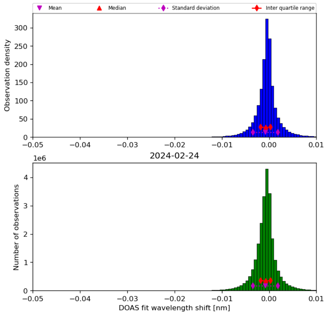
Figure 68: Histogram of “DOAS fit wavelength shift” for 2024-02-23 to 2024-02-25
