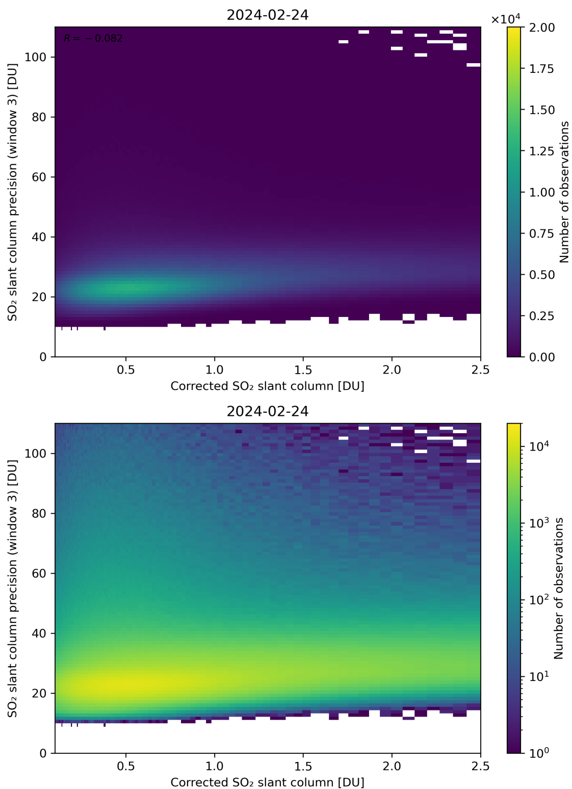
Figure 191: Scatter density plot of “Corrected SO 2 slant column” against “SO 2 slant column precision (window 3)” for 2024-02-23 to 2024-02-25.
