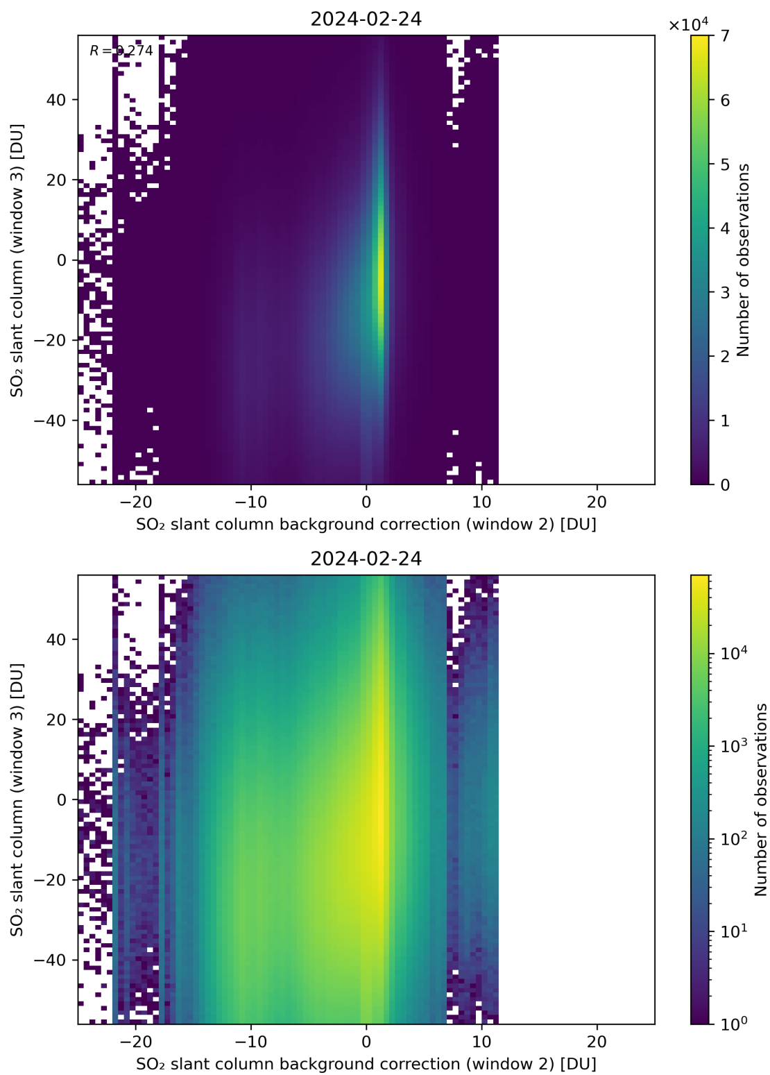
Figure 117: Scatter density plot of “SO 2 slant column background correction (window 2)” against “SO 2 slant column (window 3)” for 2024-02-23 to 2024-02-25.
