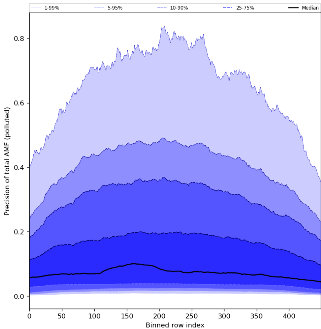
Figure 95: Along track statistics of “Precision of total AMF (polluted)” for 2024-02-23 to 2024-02-25
