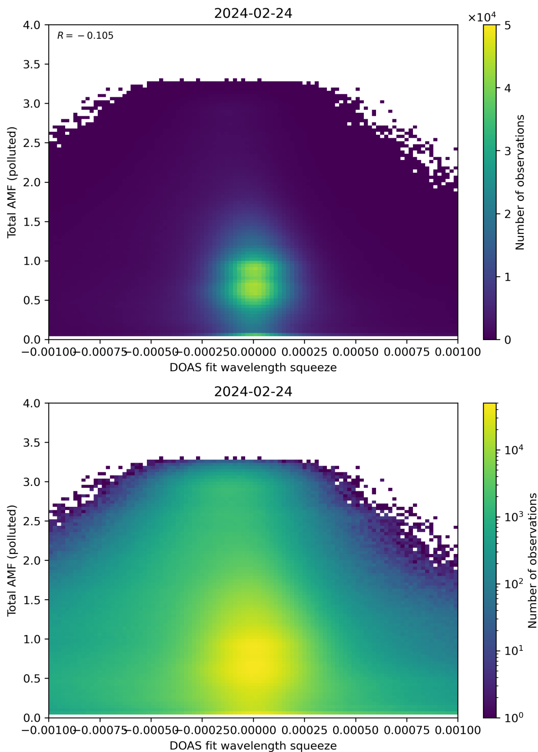
Figure 134: Scatter density plot of “DOAS fit wavelength squeeze” against “Total AMF (polluted)” for 2024-02-23 to 2024-02-25.
