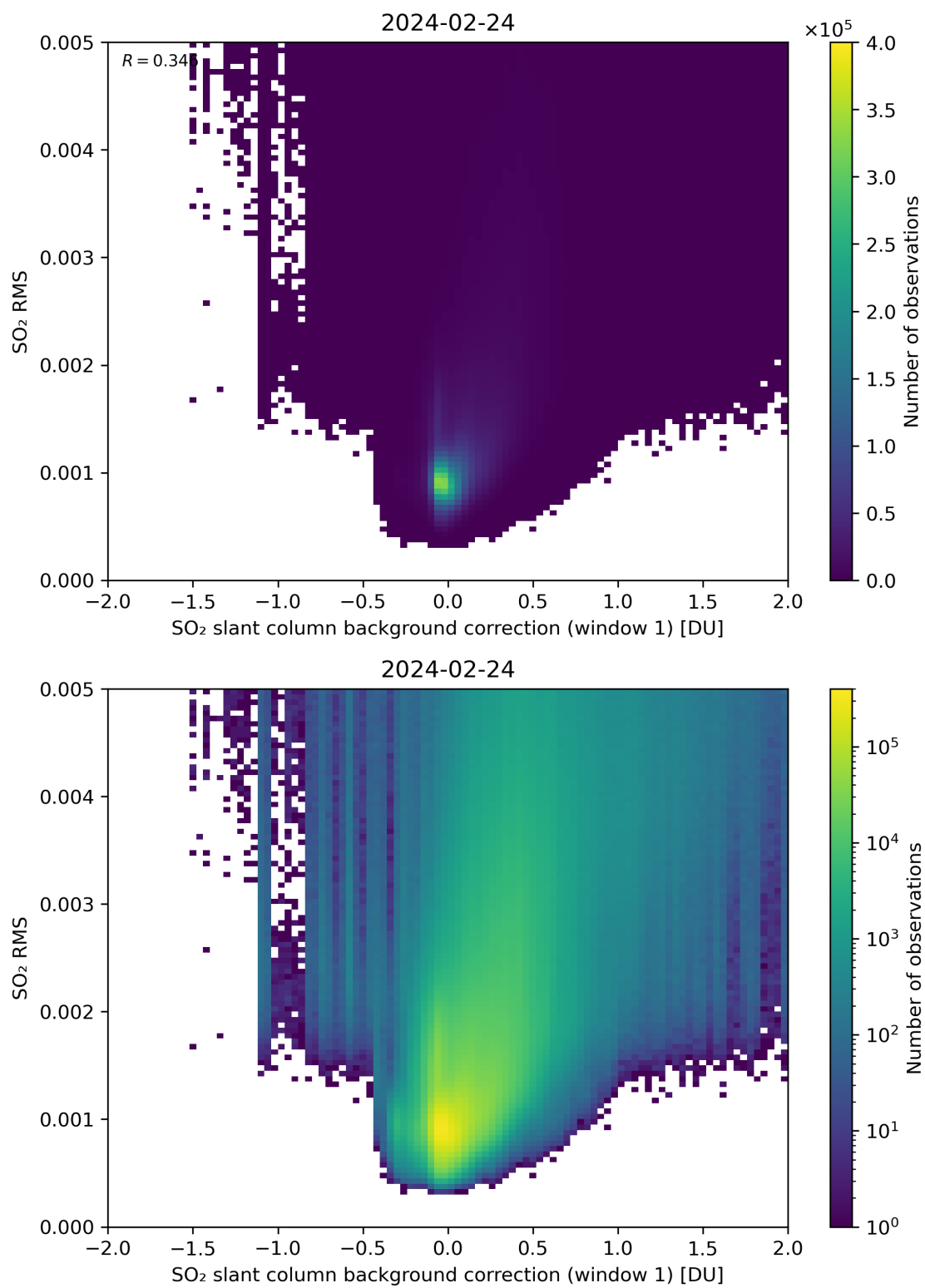
Figure 102: Scatter density plot of “SO 2 slant column background correction (window 1)” against “SO 2 RMS” for 2024-02-23 to 2024-02-25.
