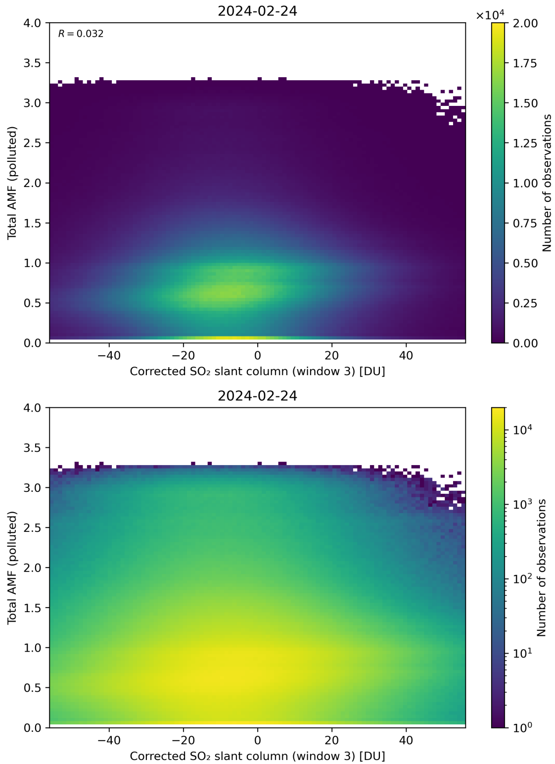
Figure 210: Scatter density plot of “Corrected SO 2 slant column (window 3)” against “Total AMF (polluted)” for 2024-02-23 to 2024-02-25.
