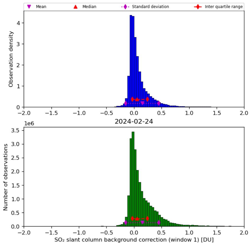
Figure 59: Histogram of “SO 2 slant column background correction (window 1)” for 2024-02-23 to 2024-02-25
