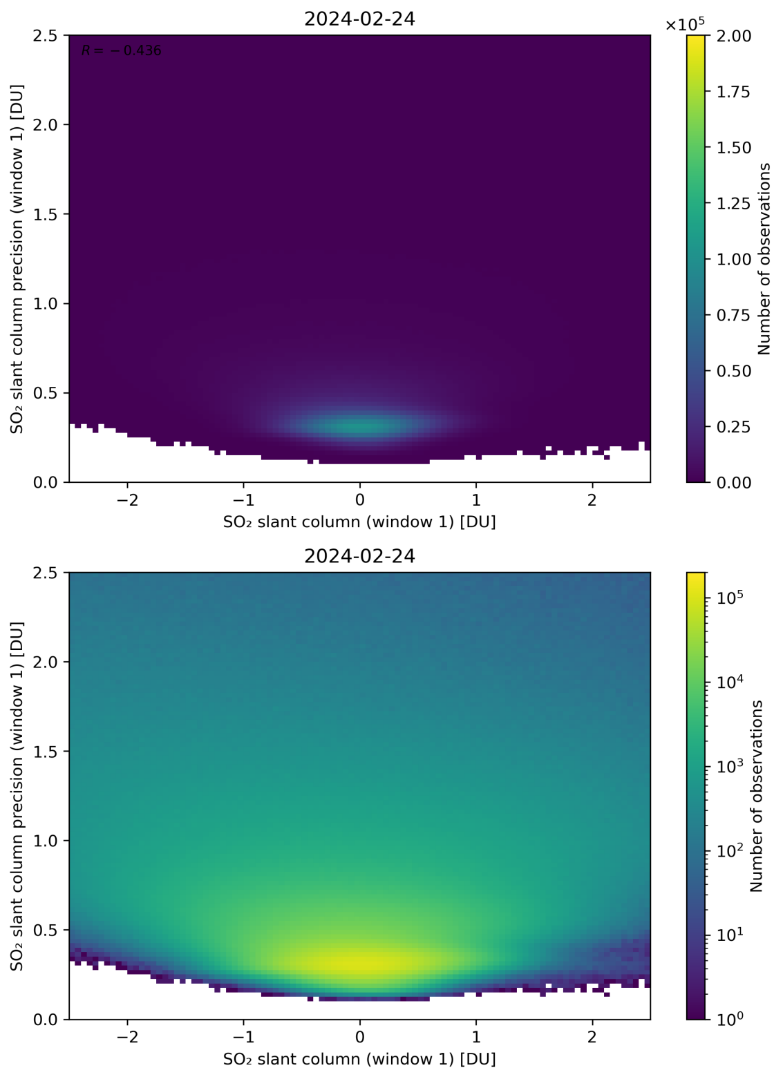
Figure 235: Scatter density plot of “SO 2 slant column (window 1)” against “SO 2 slant column precision (window 1)” for 2024-02-23 to 2024-02-25.
