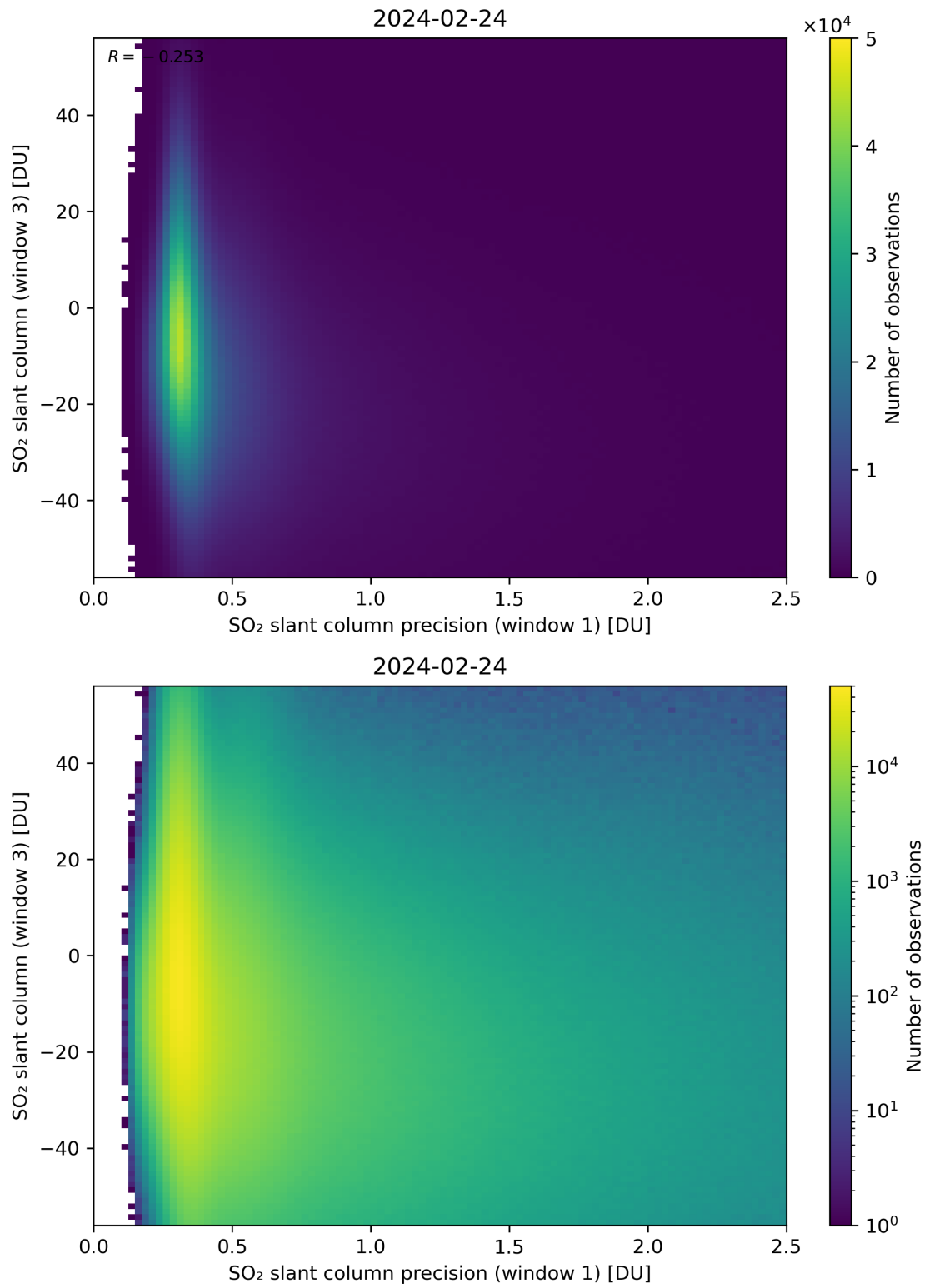
Figure 228: Scatter density plot of “SO 2 slant column precision (window 1)” against “SO 2 slant column (window 3)” for 2024-02-23 to 2024-02-25.
