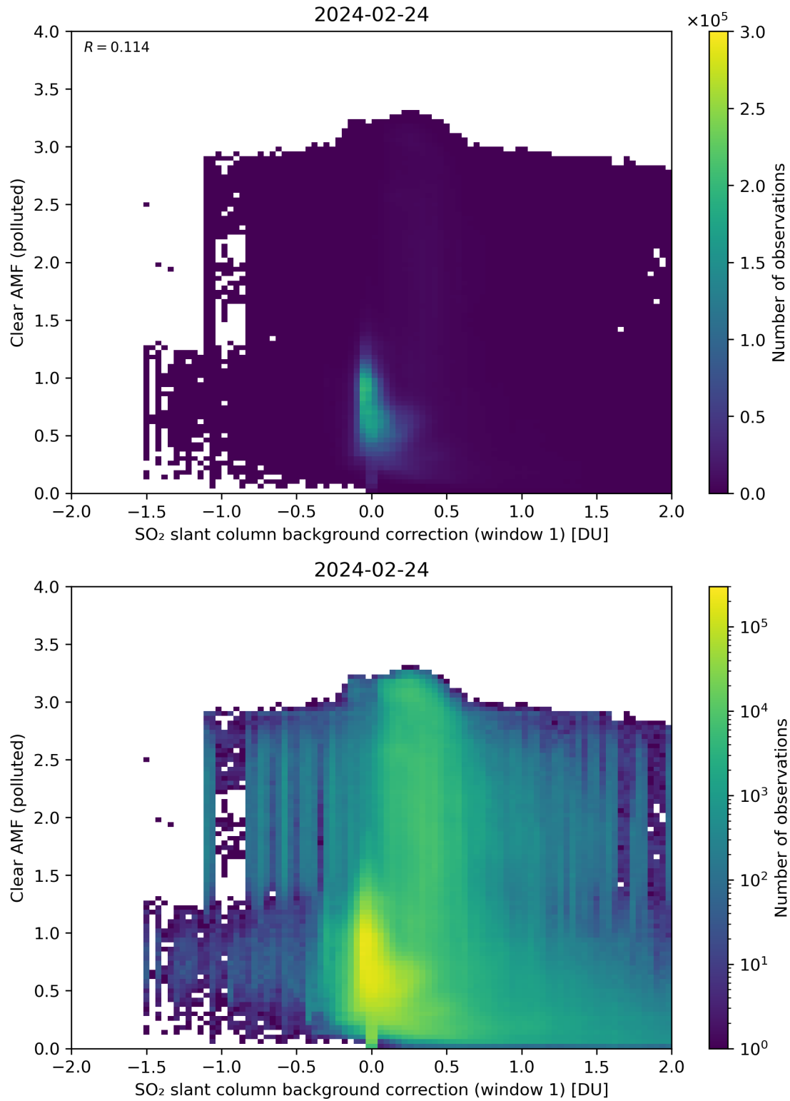
Figure 103: Scatter density plot of “SO 2 slant column background correction (window 1)” against “Clear AMF (polluted)” for 2024-02-23 to 2024-02-25.
