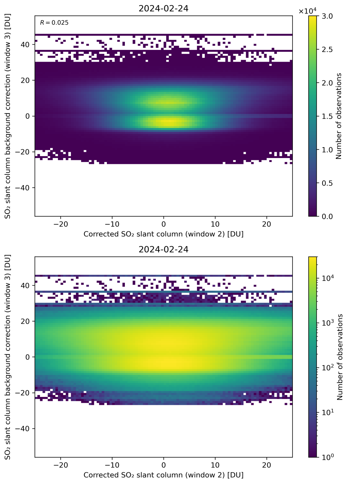
Figure 195: Scatter density plot of “Corrected SO 2 slant column (window 2)” against “SO 2 slant column background correction (window 3)” for 2024-02-23 to 2024-02-25.
