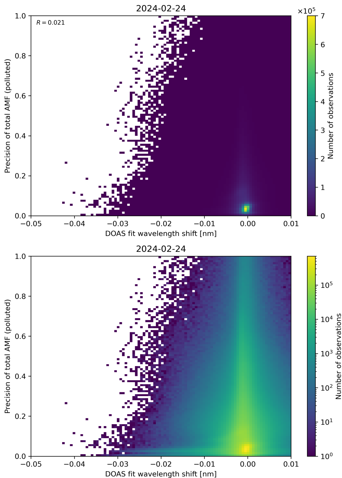
Figure 131: Scatter density plot of “DOAS fit wavelength shift” against “Precision of total AMF (polluted)” for 2024-02-23 to 2024-02-25.
