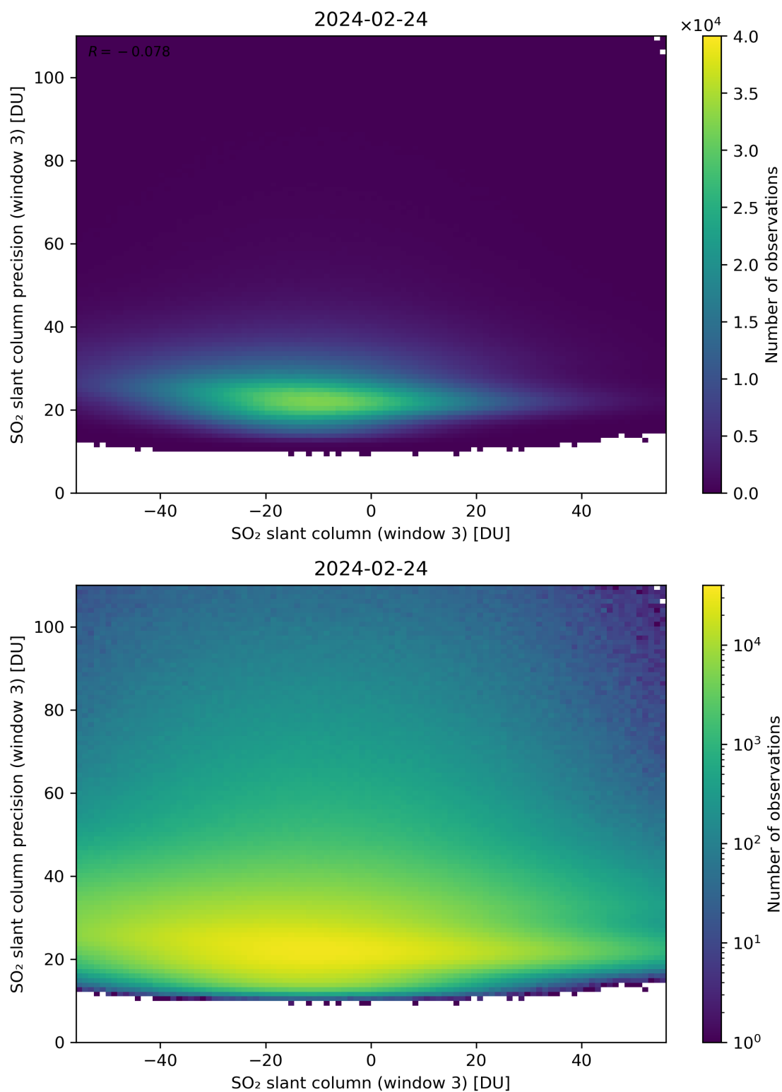
Figure 267: Scatter density plot of “SO 2 slant column (window 3)” against “SO 2 slant column precision (window 3)” for 2024-02-23 to 2024-02-25.
