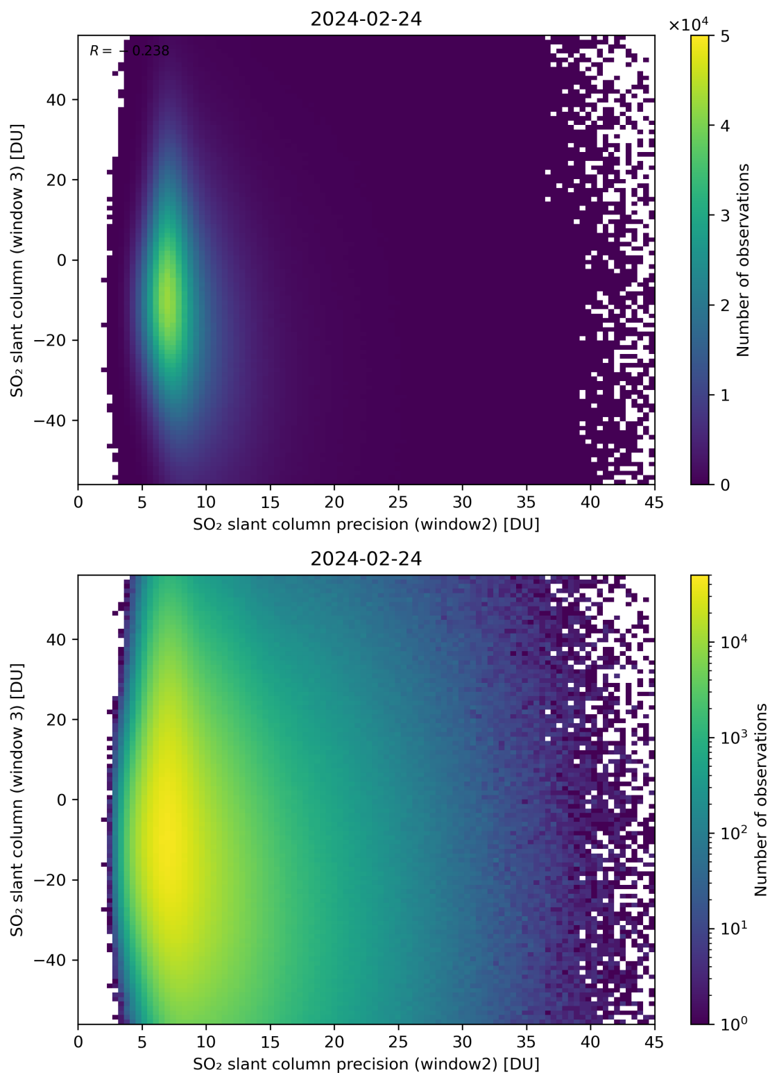
Figure 249: Scatter density plot of “SO 2 slant column precision (window2)” against “SO 2 slant column (window 3)” for 2024-02-23 to 2024-02-25.
