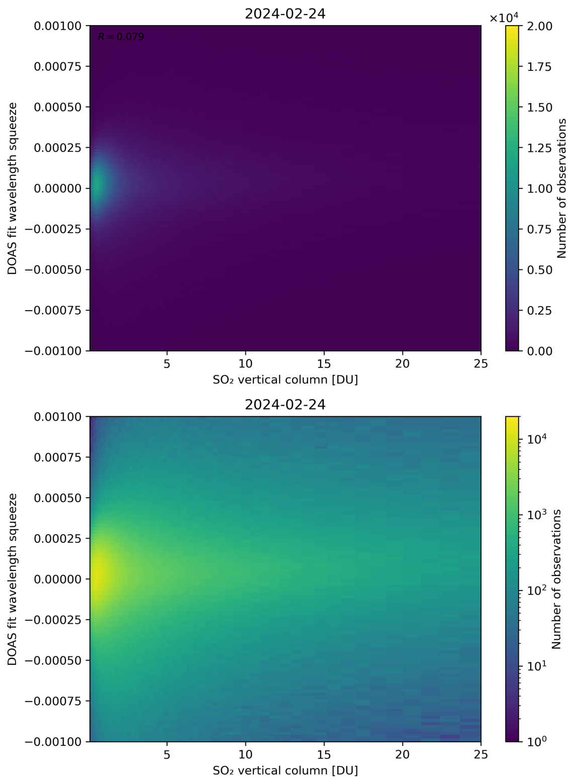
Figure 277: Scatter density plot of “SO 2 vertical column” against “DOAS fit wavelength squeeze” for 2024-02-23 to 2024-02-25.
