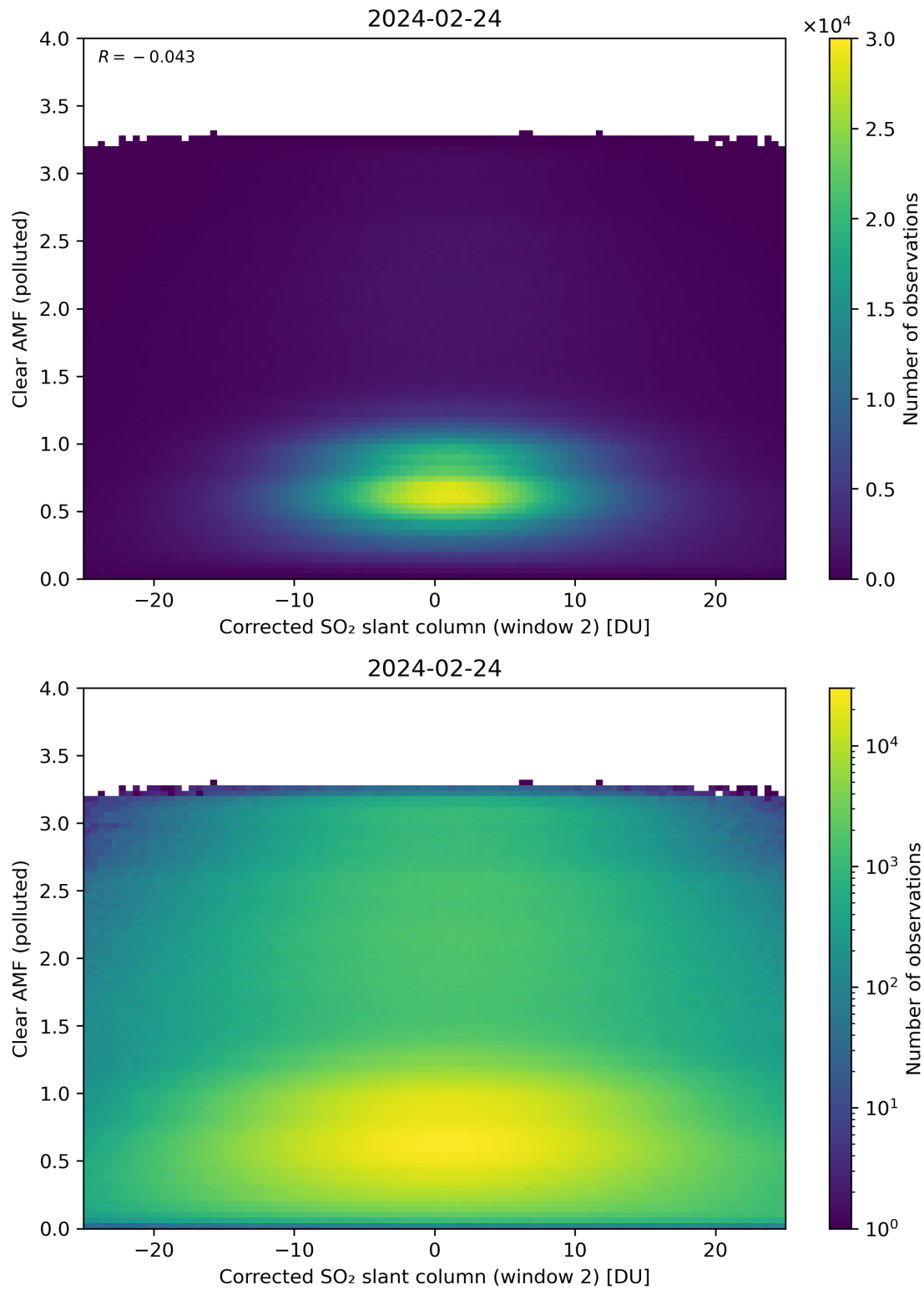
Figure 199: Scatter density plot of “Corrected SO 2 slant column (window 2)” against “Clear AMF (polluted)” for 2024-02-23 to 2024-02-25.
