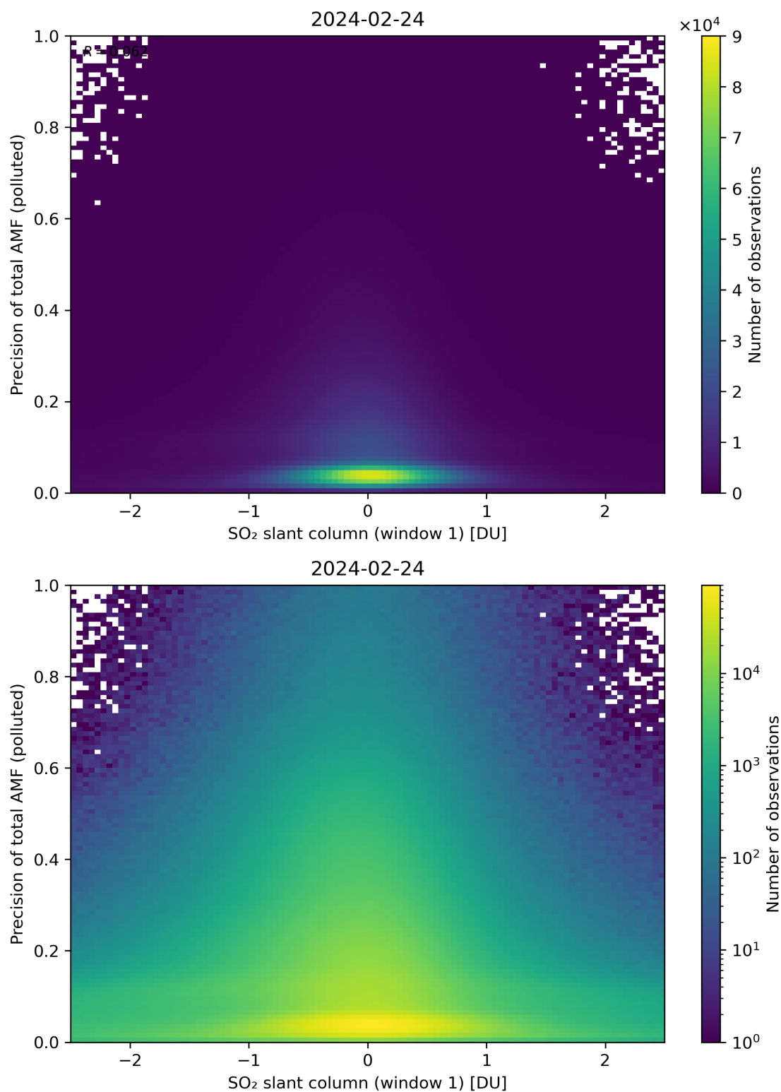
Figure 240: Scatter density plot of “SO 2 slant column (window 1)” against “Precision of total AMF (polluted)” for 2024-02-23 to 2024-02-25.
