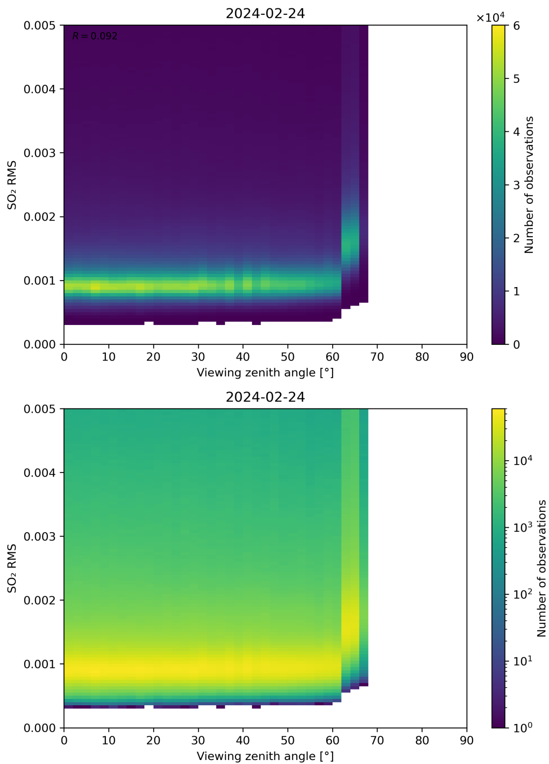
Figure 313: Scatter density plot of “Viewing zenith angle” against “SO 2 RMS” for 2024-02-23 to 2024-02-25.
