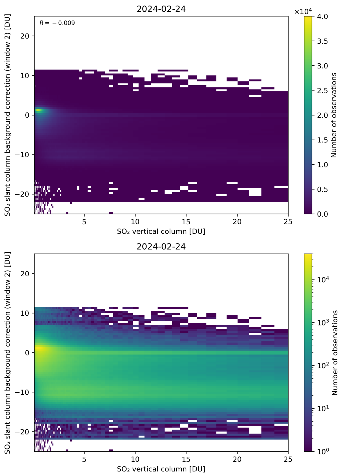
Figure 274: Scatter density plot of “SO 2 vertical column” against “SO 2 slant column background correction (window 2)” for 2024-02-23 to 2024-02-25.
