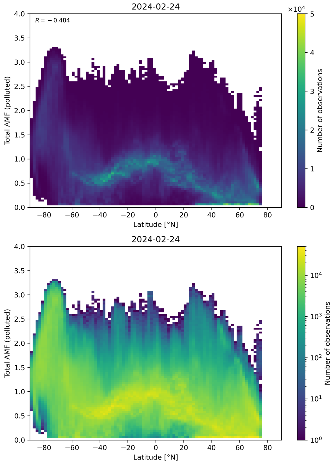
Figure 154: Scatter density plot of “Latitude” against “Total AMF (polluted)” for 2024-02-23 to 2024-02-25.
