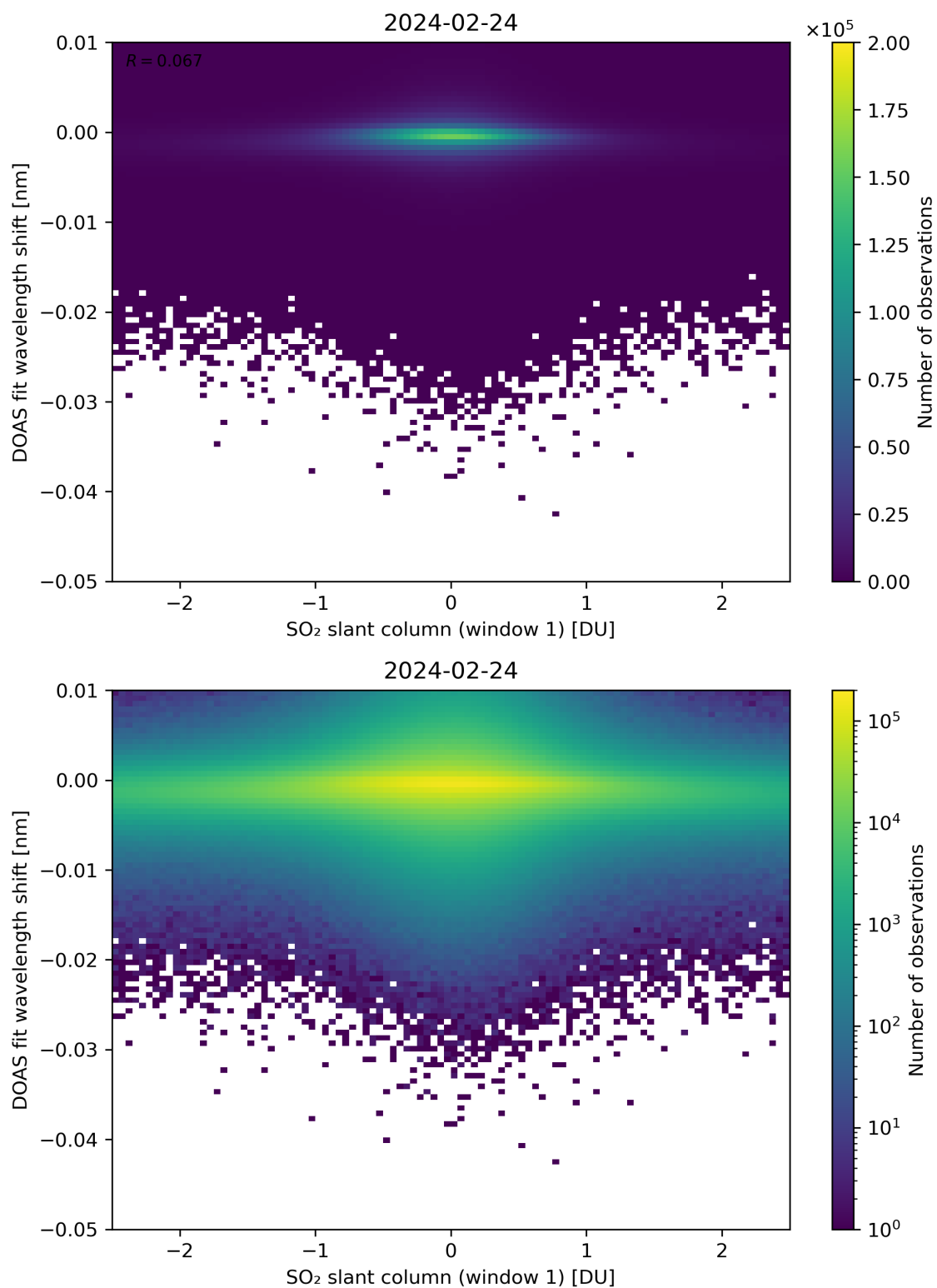
Figure 215: Scatter density plot of “SO 2 slant column (window 1)” against “DOAS fit wavelength shift” for 2024-02-23 to 2024-02-25.
