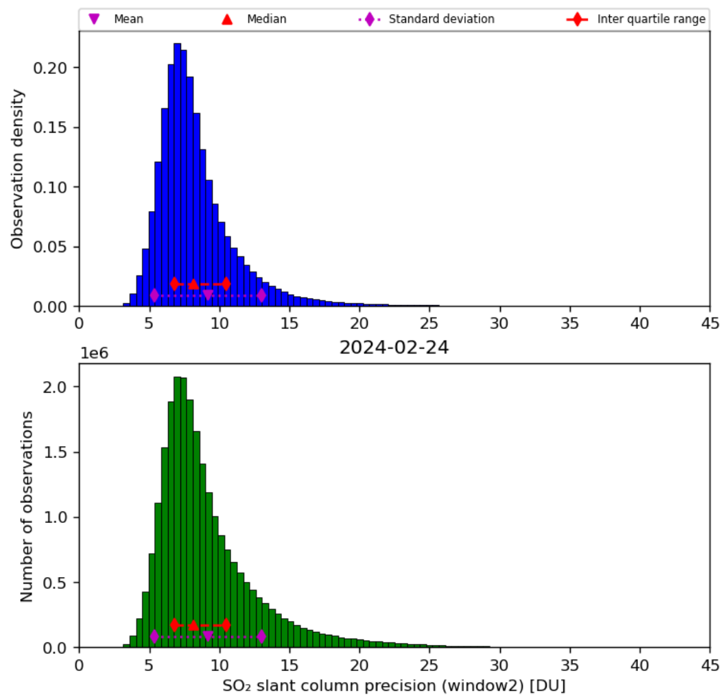
Figure 61: Histogram of “SO 2 slant column precision (window2)” for 2024-02-23 to 2024-02-25
