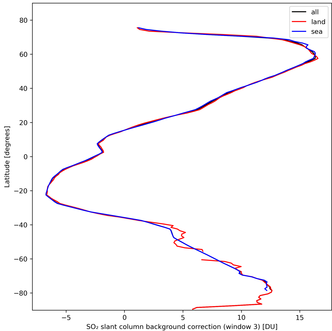
Figure 44: Zonal average of “SO 2 slant column background correction (window 3)” for 2024-02-23 to 2024-02-25.
