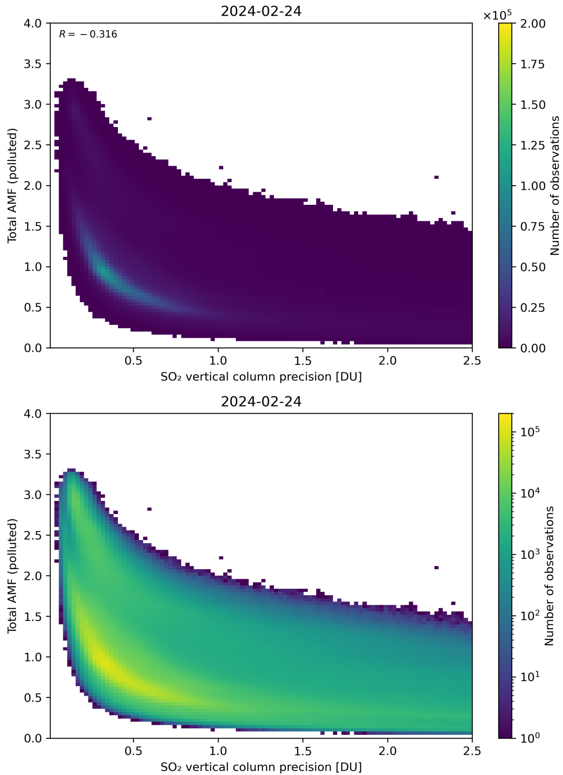
Figure 294: Scatter density plot of “SO 2 vertical column precision” against “Total AMF (polluted)” for 2024-02-23 to 2024-02-25.
