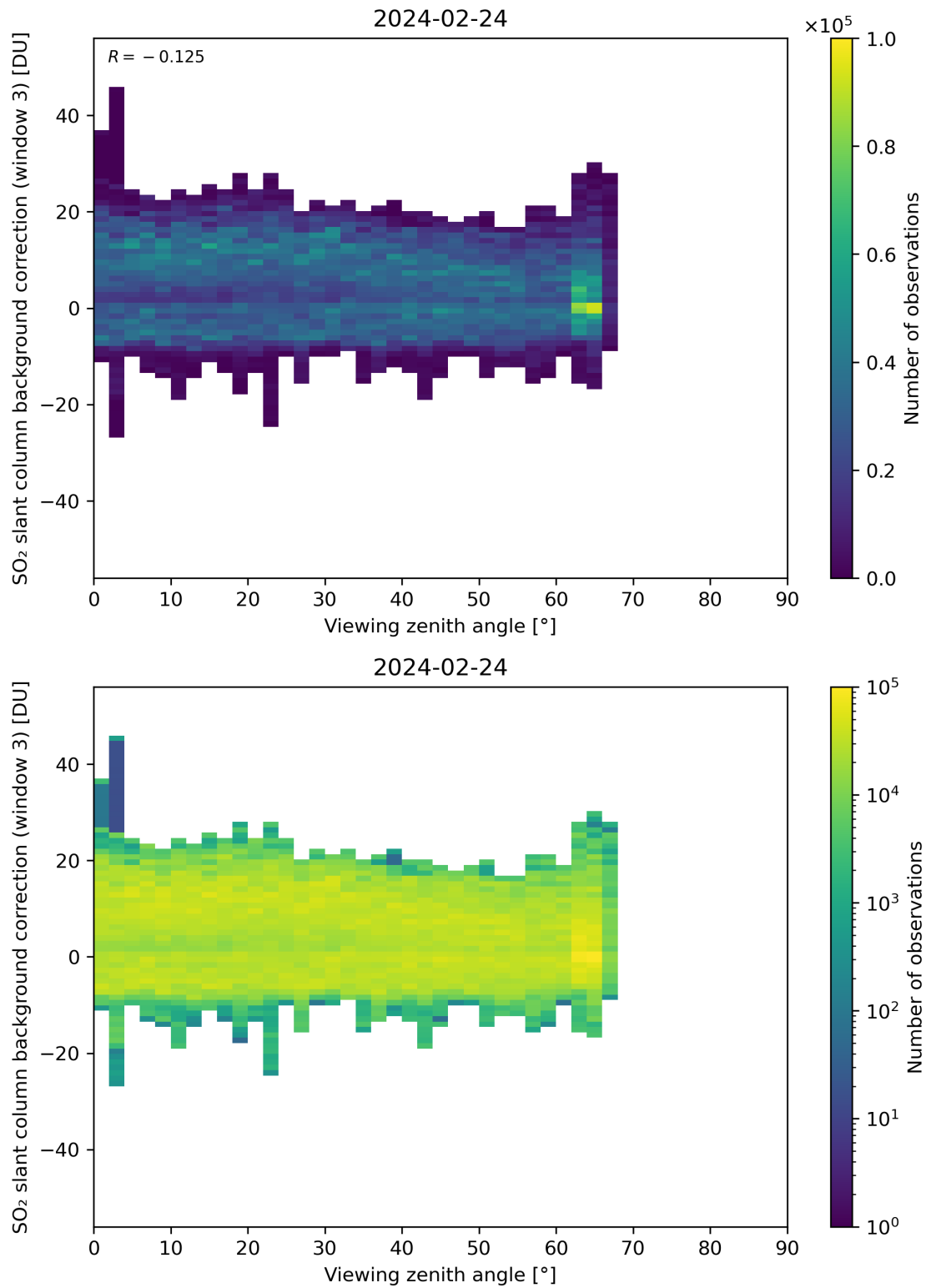
Figure 310: Scatter density plot of “Viewing zenith angle” against “SO 2 slant column background correction (window 3)” for 2024-02-23 to 2024-02-25.
