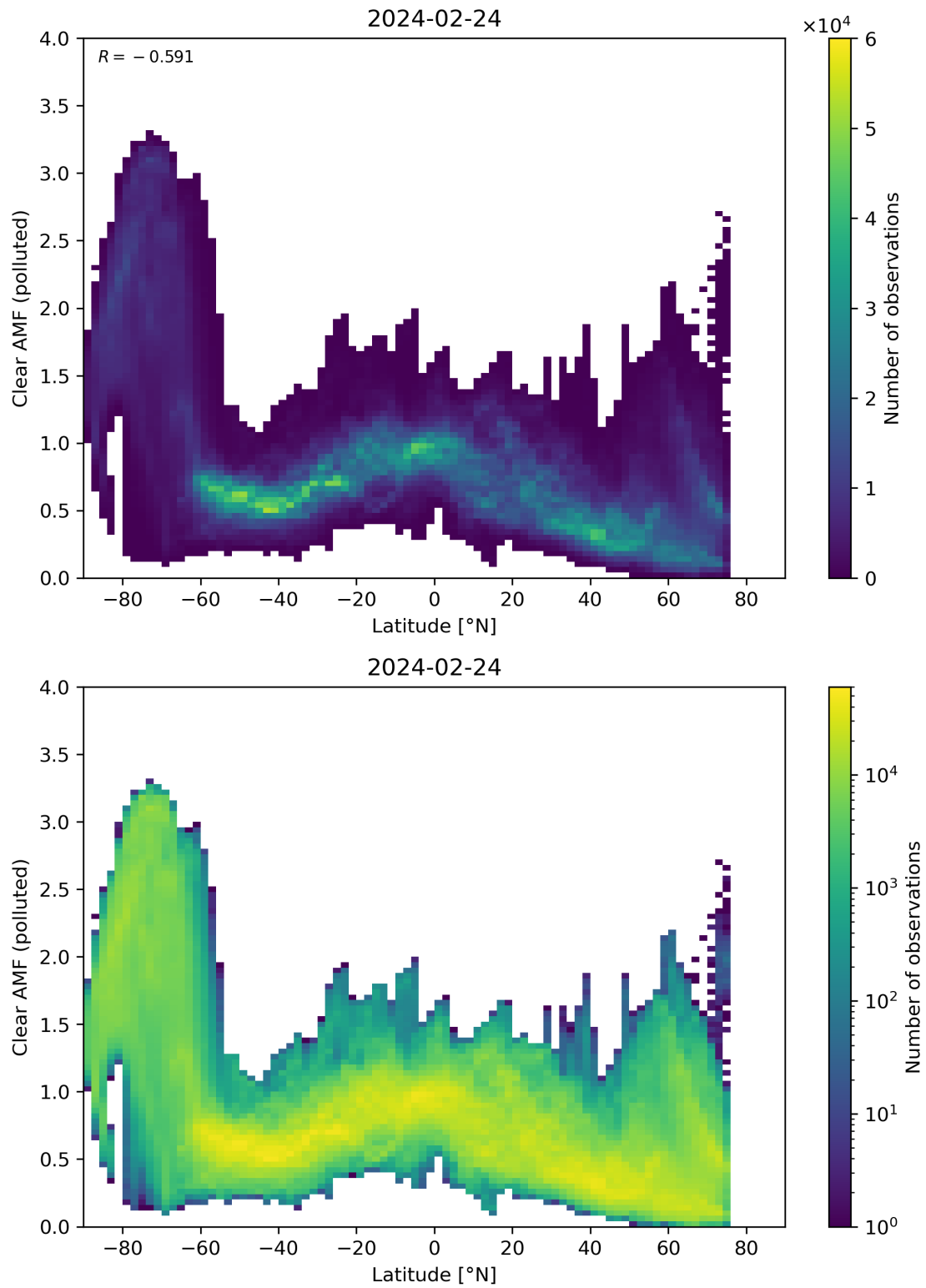
Figure 145: Scatter density plot of “Latitude” against “Clear AMF (polluted)” for 2024-02-23 to 2024-02-25.
