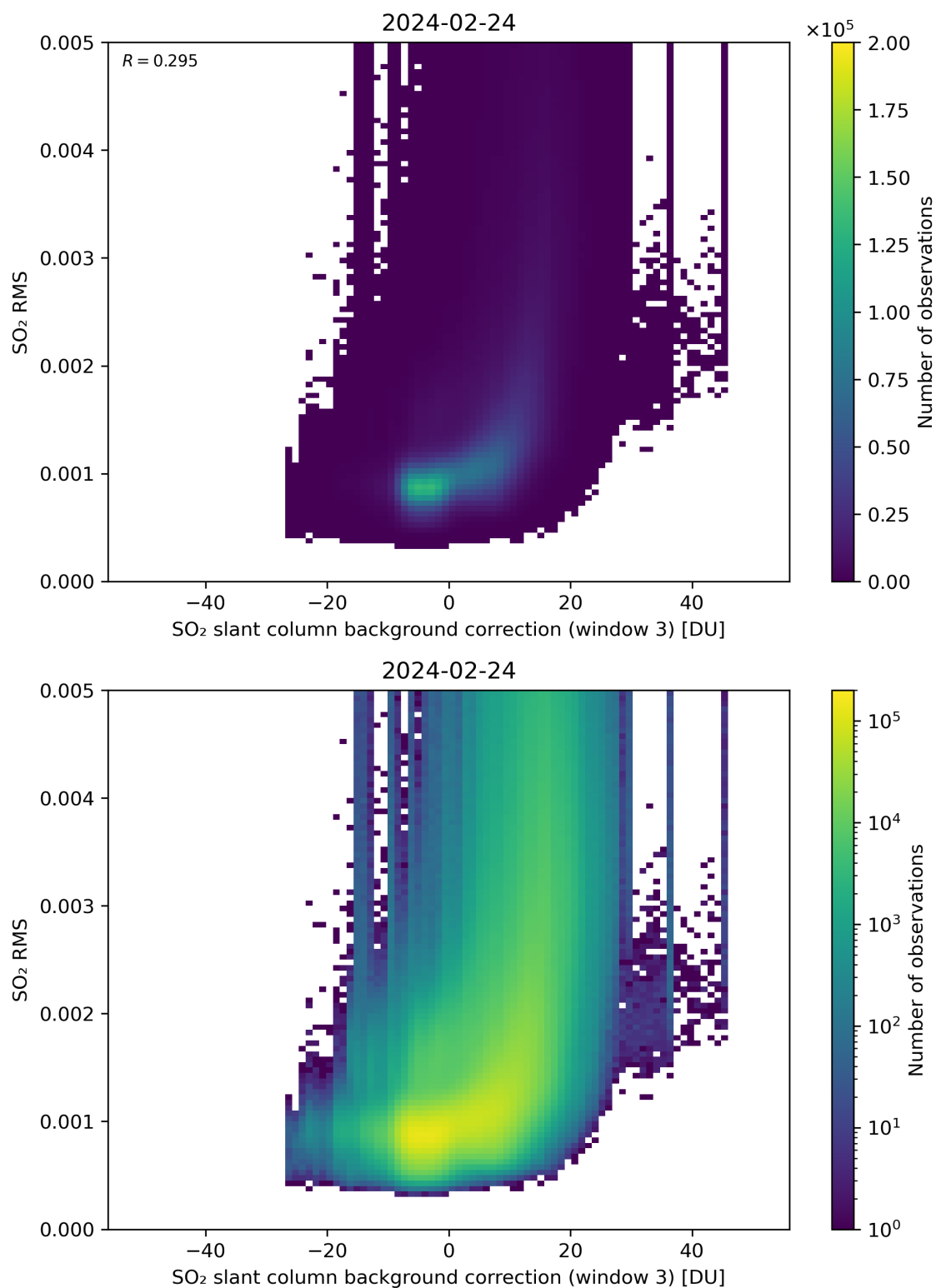
Figure 123: Scatter density plot of “SO 2 slant column background correction (window 3)” against “SO 2 RMS” for 2024-02-23 to 2024-02-25.
