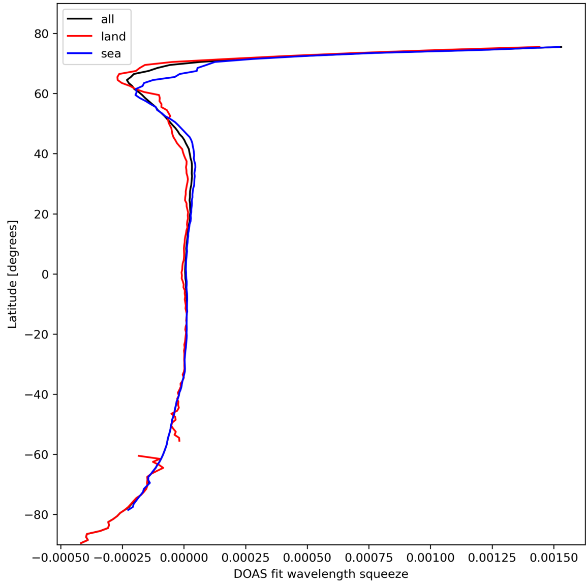
Figure 46: Zonal average of “DOAS fit wavelength squeeze” for 2024-02-23 to 2024-02-25.
