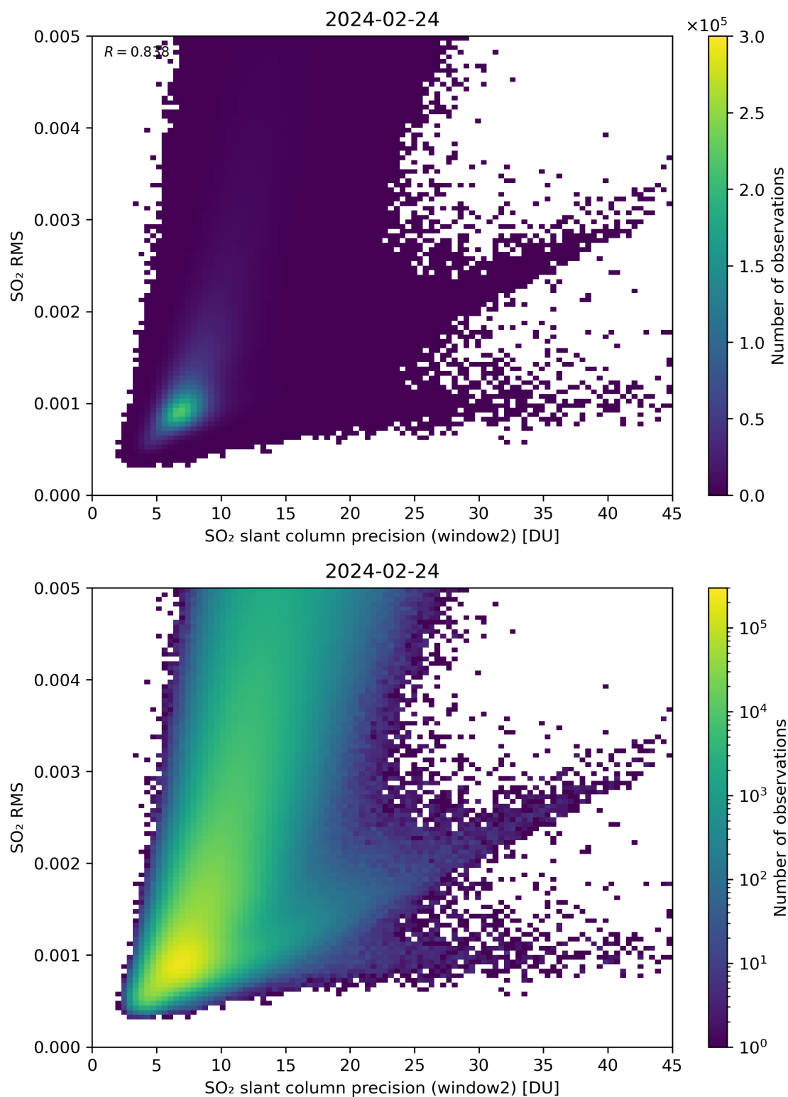
Figure 245: Scatter density plot of “SO 2 slant column precision (window2)” against “SO 2 RMS” for 2024-02-23 to 2024-02-25.
