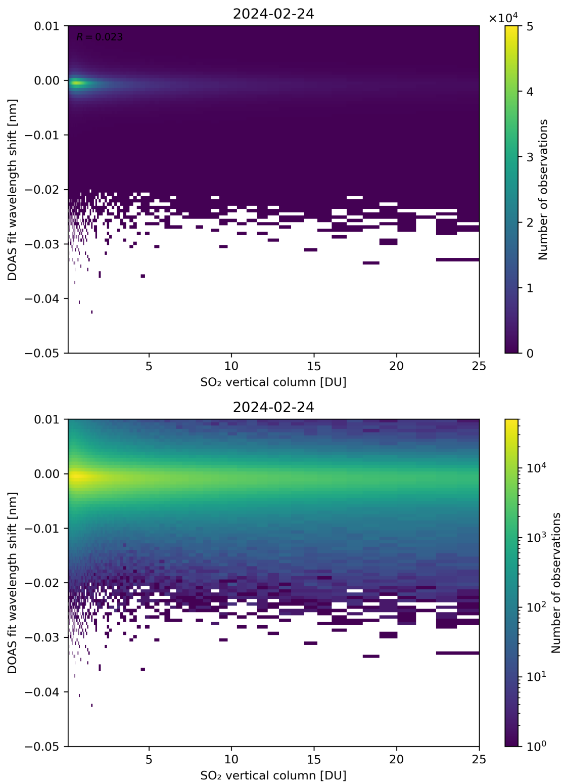
Figure 276: Scatter density plot of “SO 2 vertical column” against “DOAS fit wavelength shift” for 2024-02-23 to 2024-02-25.
