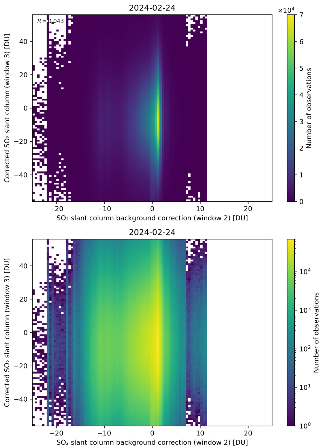
Figure 116: Scatter density plot of “SO 2 slant column background correction (window 2)” against “Corrected SO 2 slant column (window 3)” for 2024-02-23 to 2024-02-25.
