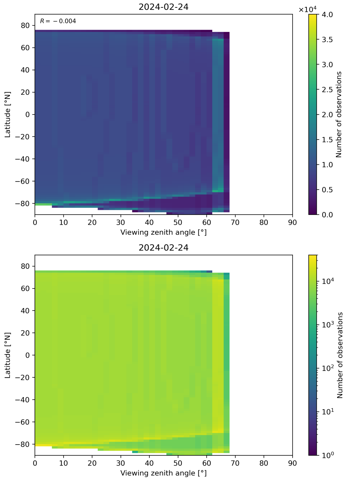
Figure 314: Scatter density plot of “Viewing zenith angle” against “Latitude” for 2024-02-23 to 2024-02-25.
