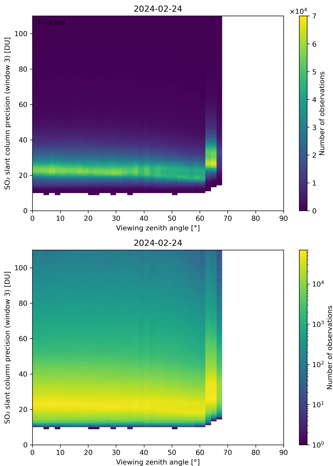
Figure 324: Scatter density plot of “Viewing zenith angle” against “SO 2 slant column precision (window 3)” for 2024-02-23 to 2024-02-25.
