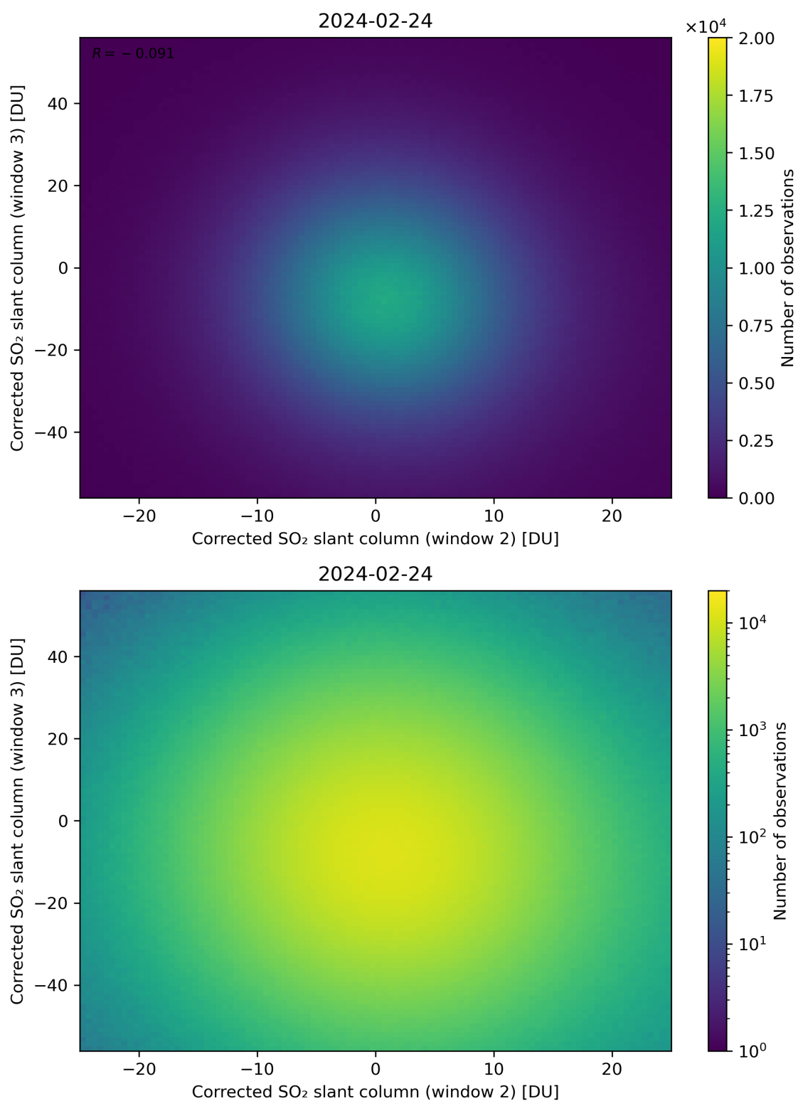
Figure 200: Scatter density plot of “Corrected SO 2 slant column (window 2)” against “Corrected SO 2 slant column (window 3)” for 2024-02-23 to 2024-02-25.
