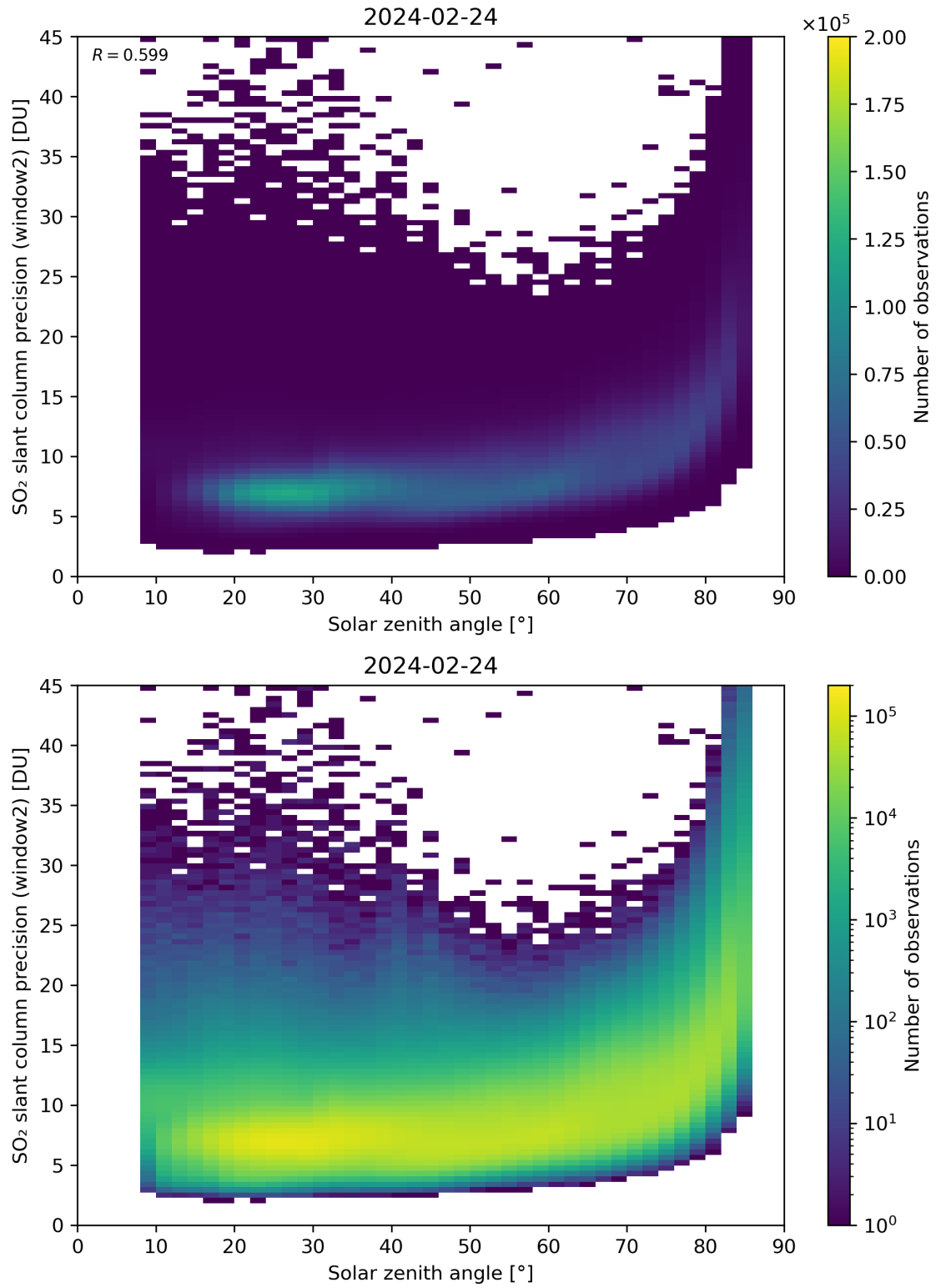
Figure 171: Scatter density plot of “Solar zenith angle” against “SO 2 slant column precision (window2)” for 2024-02-23 to 2024-02-25.
