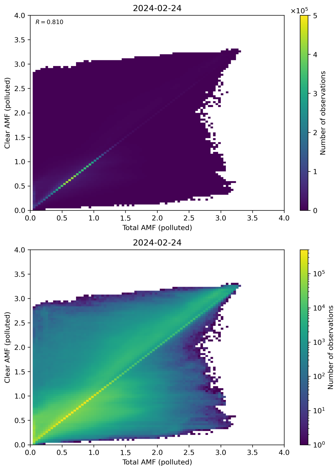
Figure 271: Scatter density plot of “Total AMF (polluted)” against “Clear AMF (polluted)” for 2024-02-23 to 2024-02-25.
