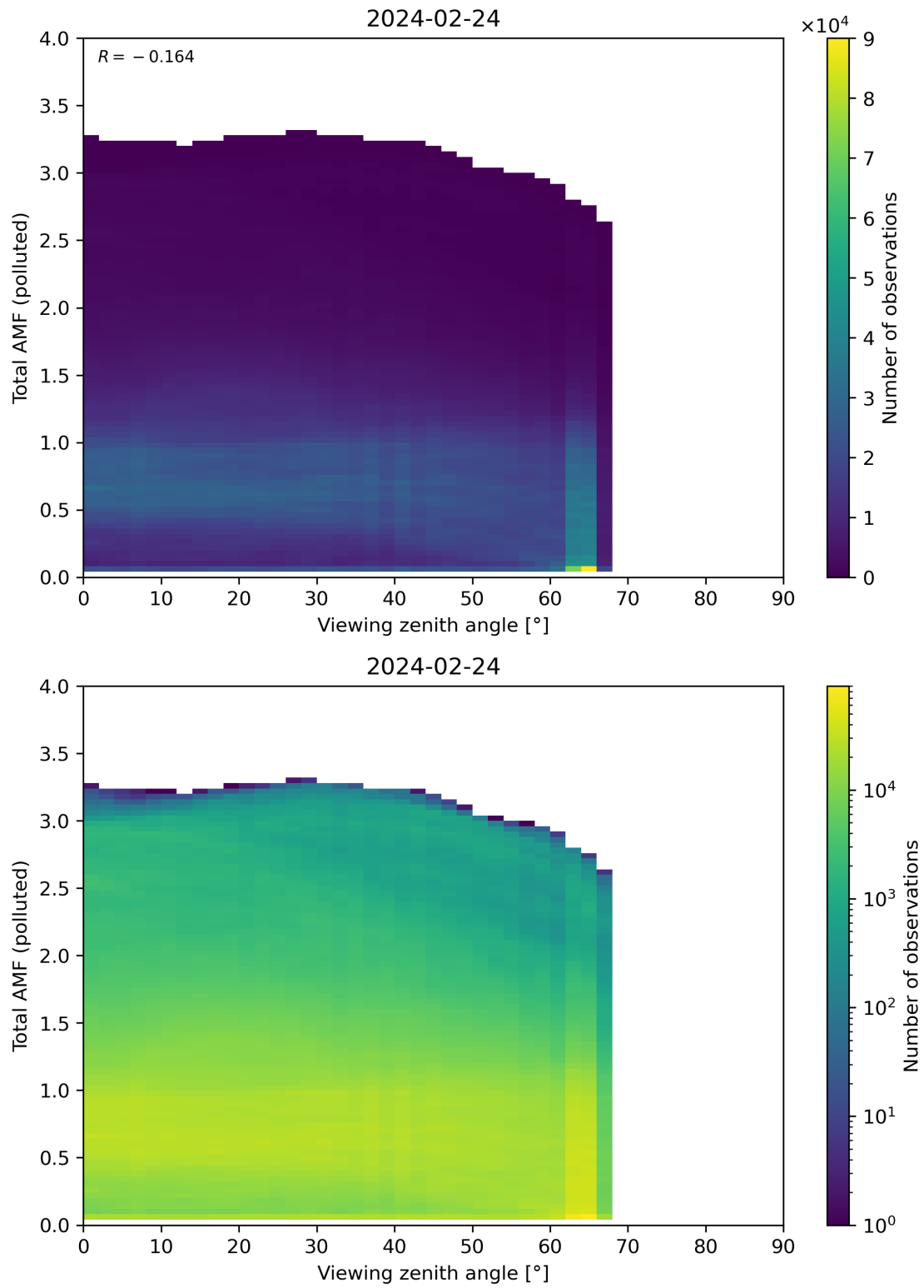
Figure 325: Scatter density plot of “Viewing zenith angle” against “Total AMF (polluted)” for 2024-02-23 to 2024-02-25.
