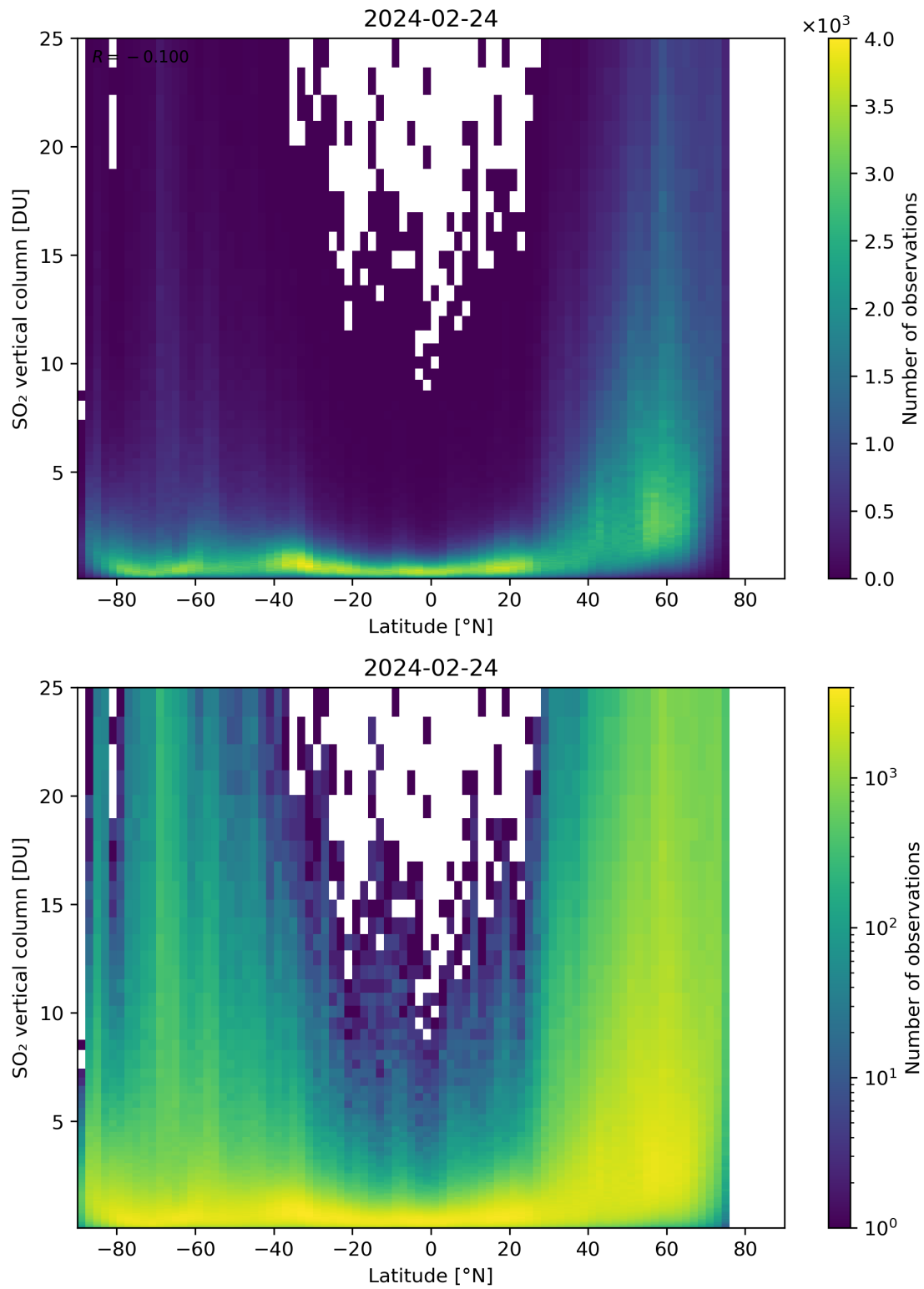
Figure 156: Scatter density plot of “Latitude” against “SO 2 vertical column” for 2024-02-23 to 2024-02-25.
