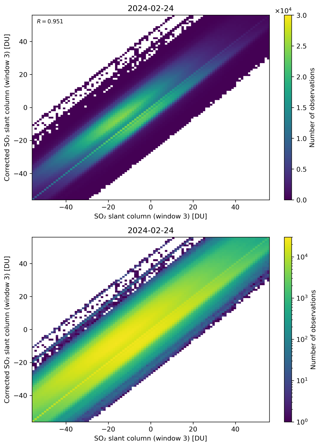
Figure 266: Scatter density plot of “SO 2 slant column (window 3)” against “Corrected SO 2 slant column (window 3)” for 2024-02-23 to 2024-02-25.
