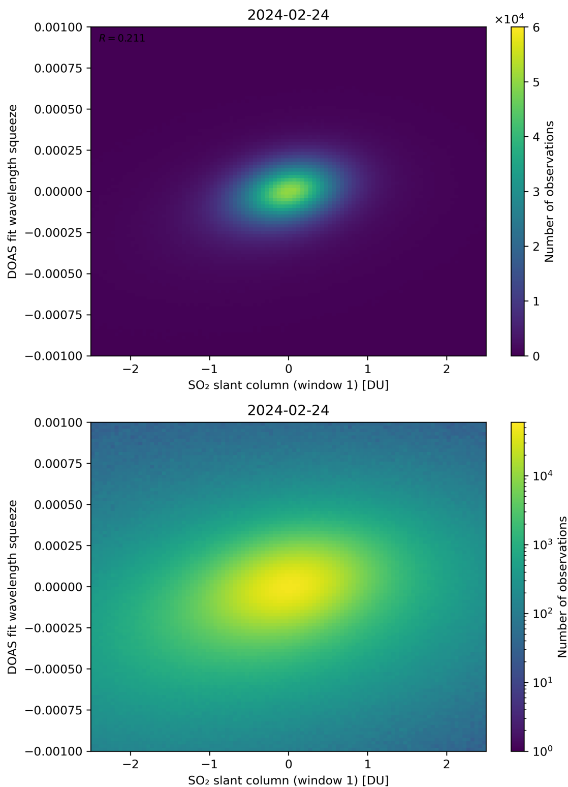
Figure 216: Scatter density plot of “SO 2 slant column (window 1)” against “DOAS fit wavelength squeeze” for 2024-02-23 to 2024-02-25.
