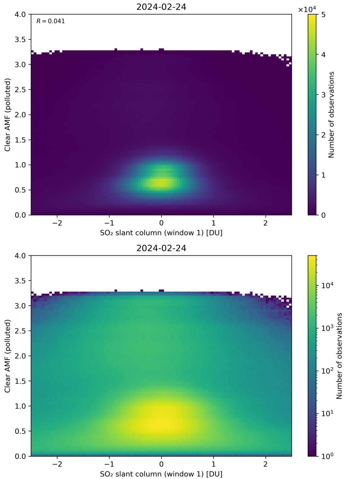
Figure 232: Scatter density plot of “SO 2 slant column (window 1)” against “Clear AMF (polluted)” for 2024-02-23 to 2024-02-25.
