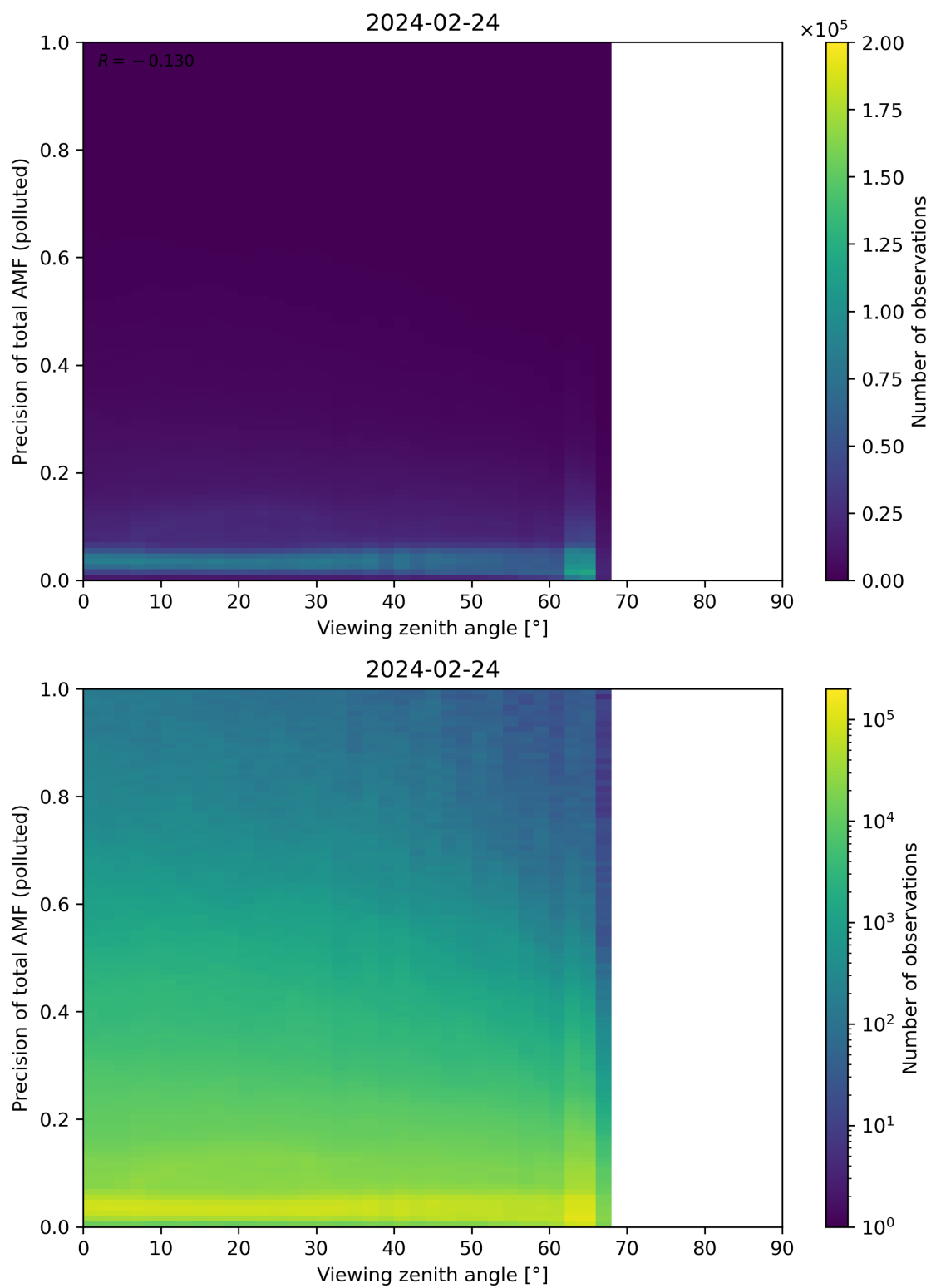
Figure 326: Scatter density plot of “Viewing zenith angle” against “Precision of total AMF (polluted)” for 2024-02-23 to 2024-02-25.
