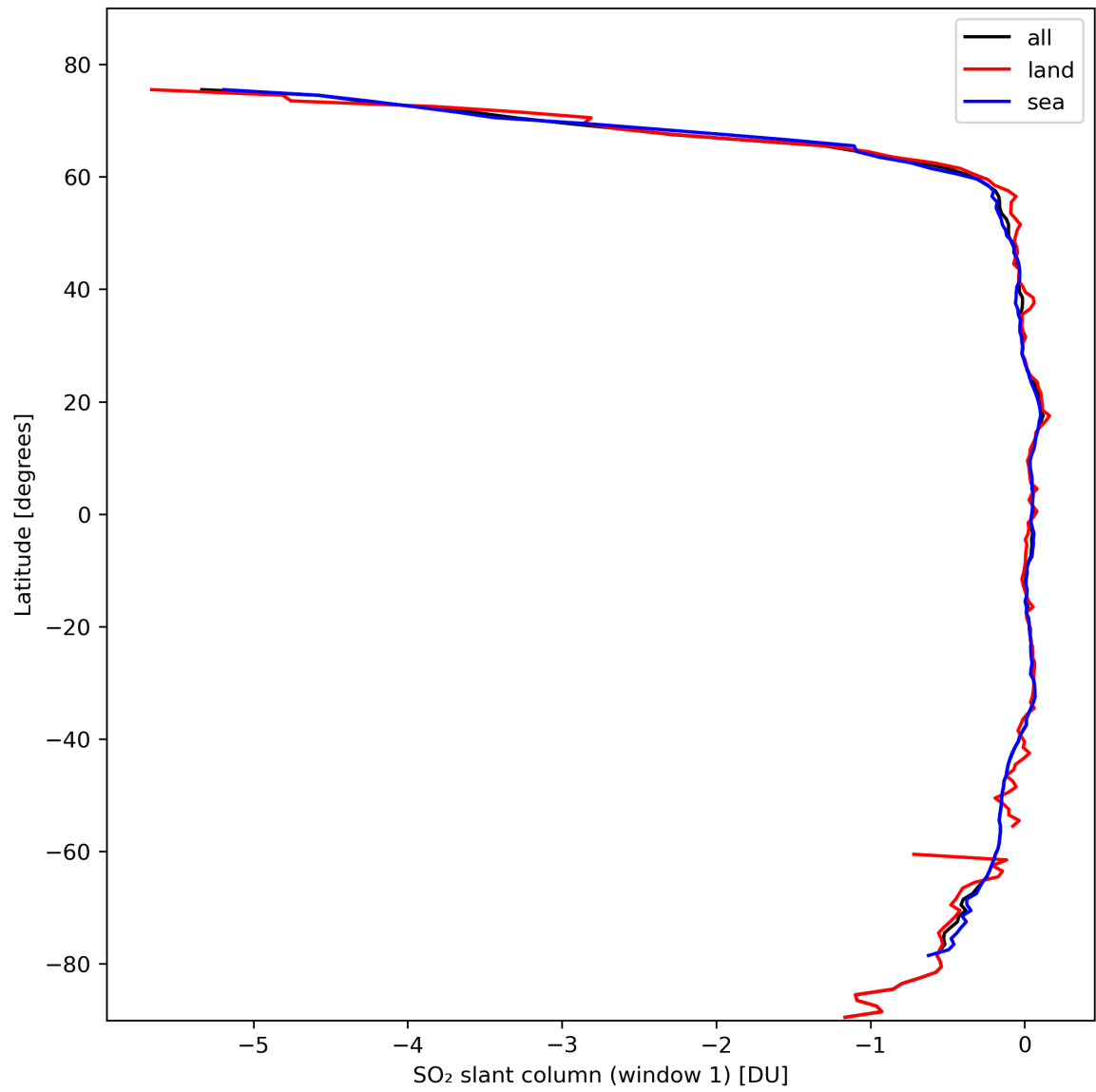
Figure 33: Zonal average of “SO 2 slant column (window 1)” for 2024-02-23 to 2024-02-25.
