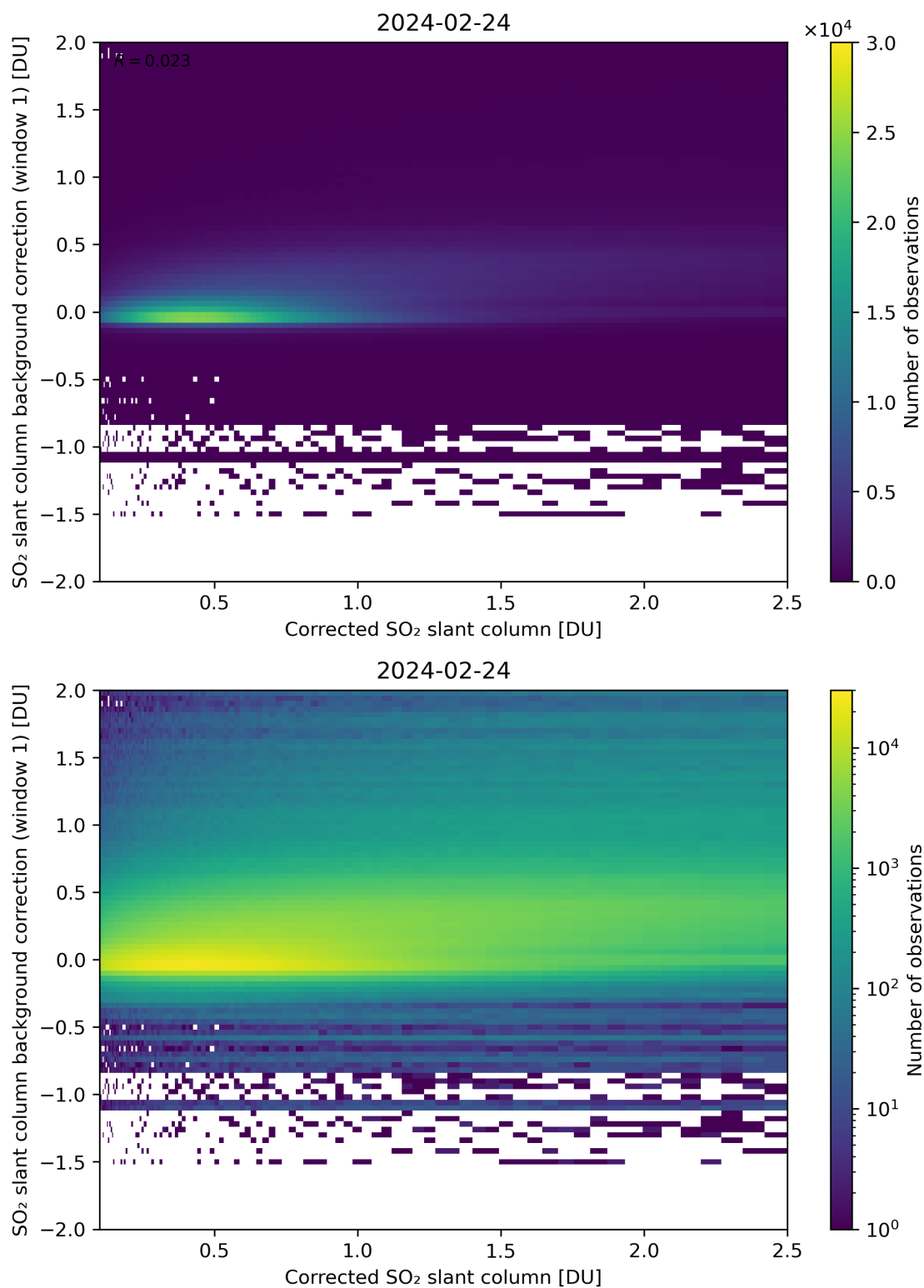
Figure 178: Scatter density plot of “Corrected SO 2 slant column” against “SO 2 slant column background correction (window 1)” for 2024-02-23 to 2024-02-25.
