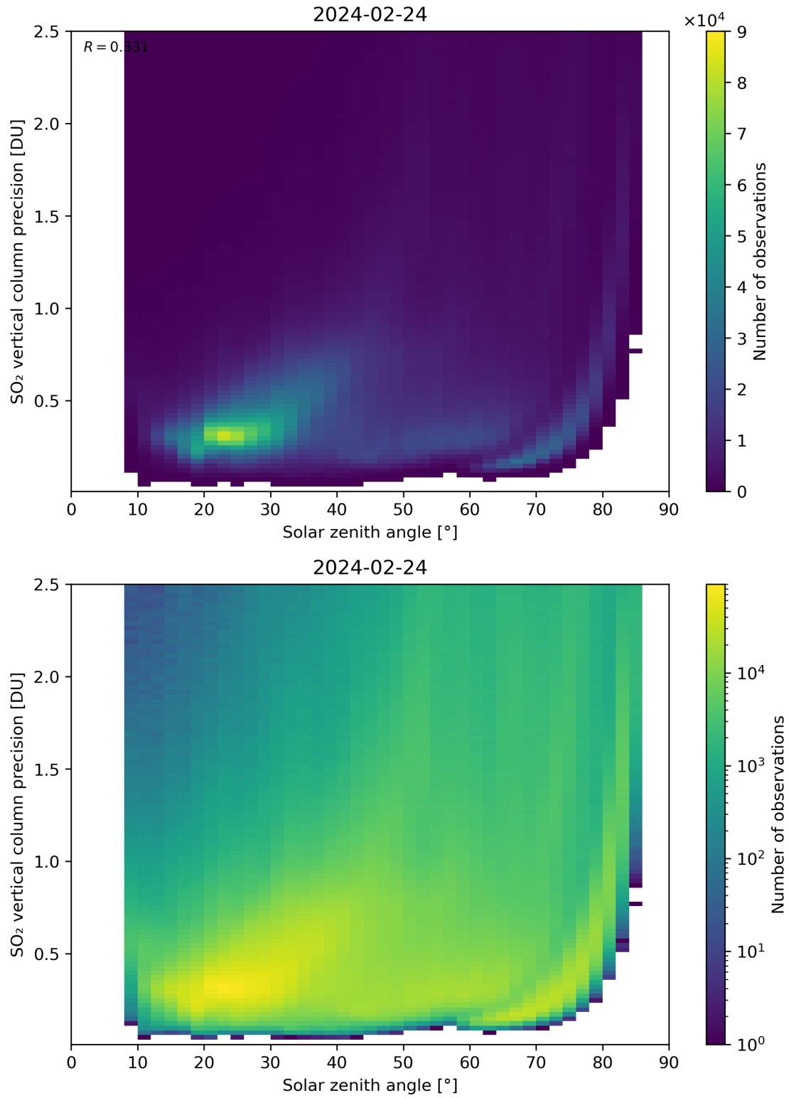
Figure 177: Scatter density plot of “Solar zenith angle” against “SO 2 vertical column precision” for 2024-02-23 to 2024-02-25.
