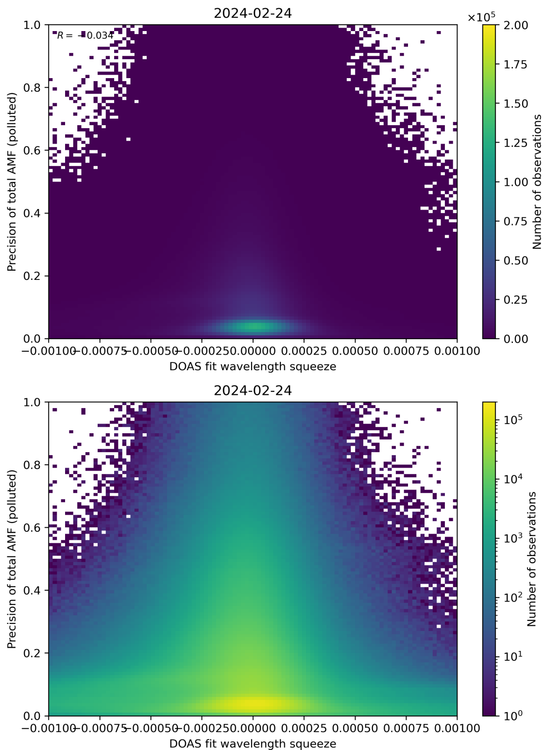
Figure 135: Scatter density plot of “DOAS fit wavelength squeeze” against “Precision of total AMF (polluted)” for 2024-02-23 to 2024-02-25.
