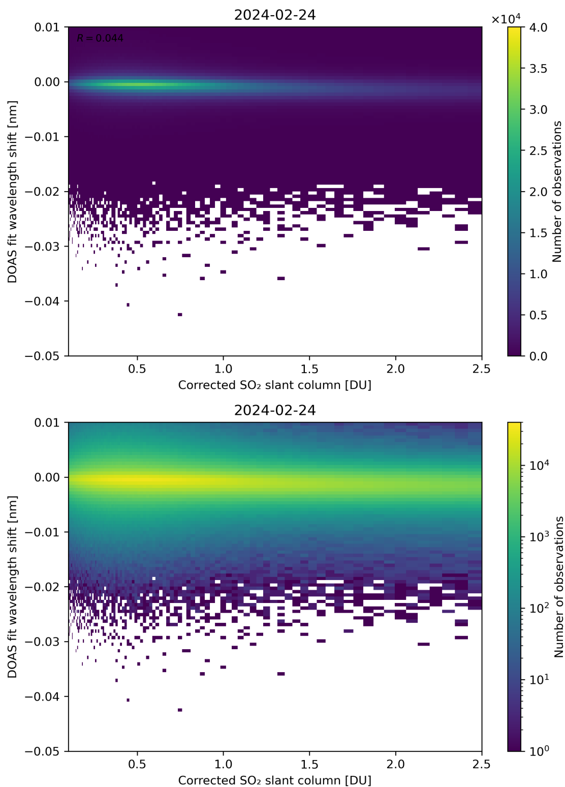
Figure 181: Scatter density plot of “Corrected SO 2 slant column” against “DOAS fit wavelength shift” for 2024-02-23 to 2024-02-25.
