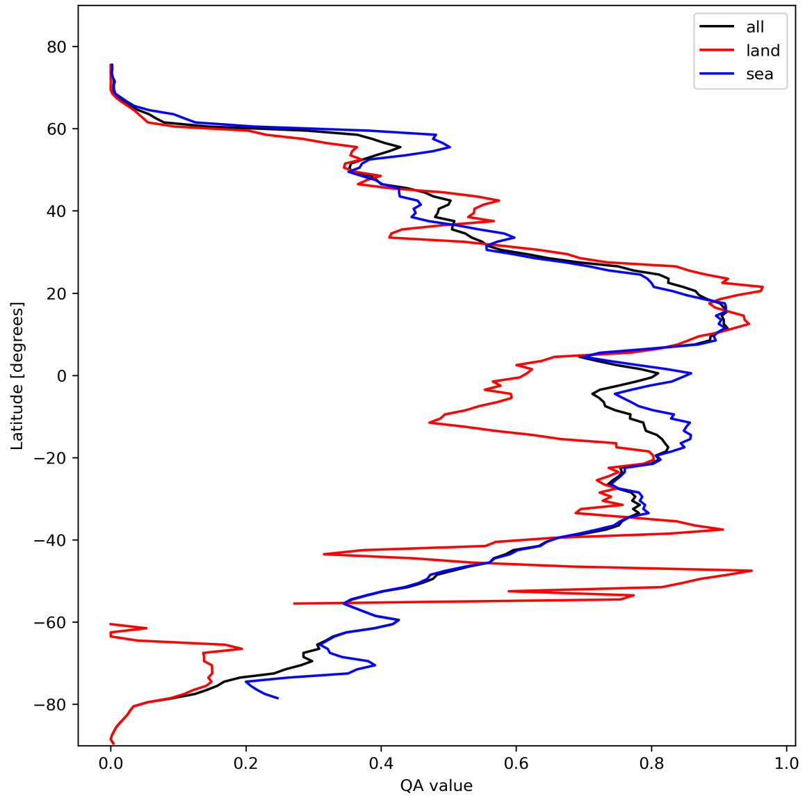
Figure 29: Zonal average of “QA value” for 2024-02-23 to 2024-02-25.
