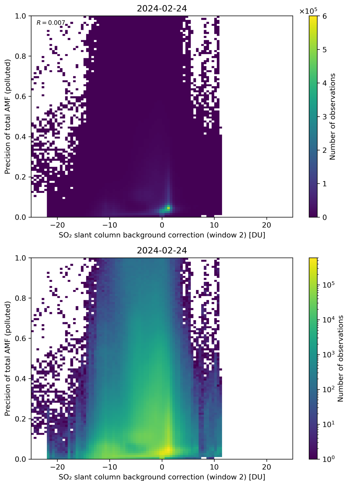
Figure 120: Scatter density plot of “SO 2 slant column background correction (window 2)” against “Precision of total AMF (polluted)” for 2024-02-23 to 2024-02-25.
