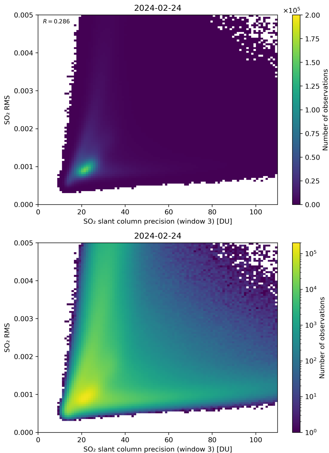
Figure 260: Scatter density plot of “SO 2 slant column precision (window 3)” against “SO 2 RMS” for 2024-02-23 to 2024-02-25.
