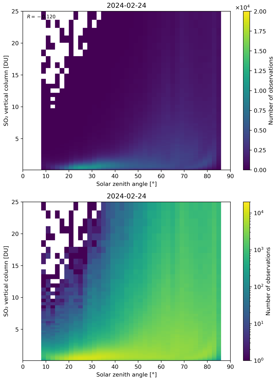
Figure 176: Scatter density plot of “Solar zenith angle” against “SO 2 vertical column” for 2024-02-23 to 2024-02-25.
