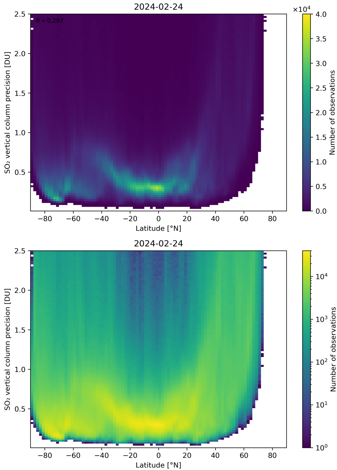
Figure 157: Scatter density plot of “Latitude” against “SO 2 vertical column precision” for 2024-02-23 to 2024-02-25.
