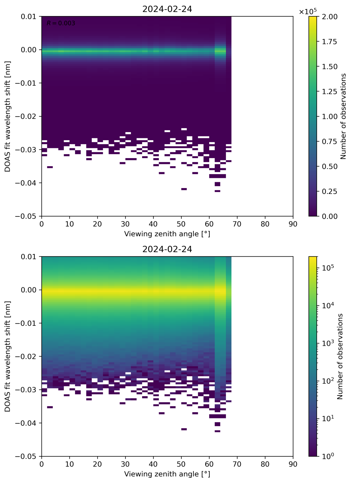
Figure 311: Scatter density plot of “Viewing zenith angle” against “DOAS fit wavelength shift” for 2024-02-23 to 2024-02-25.
