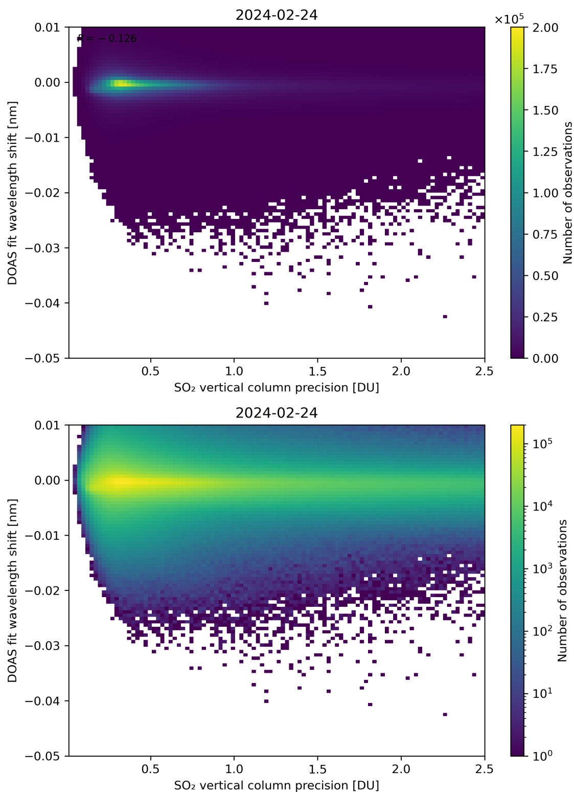
Figure 282: Scatter density plot of “SO 2 vertical column precision” against “DOAS fit wavelength shift” for 2024-02-23 to 2024-02-25.
