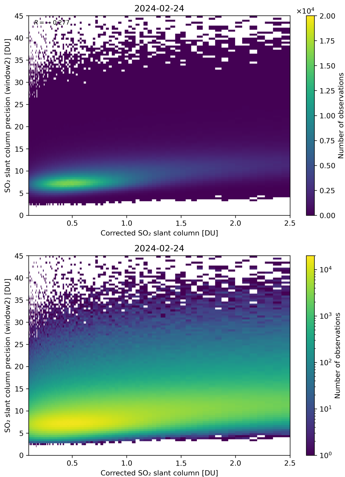
Figure 189: Scatter density plot of “Corrected SO 2 slant column” against “SO 2 slant column precision (window2)” for 2024-02-23 to 2024-02-25.
