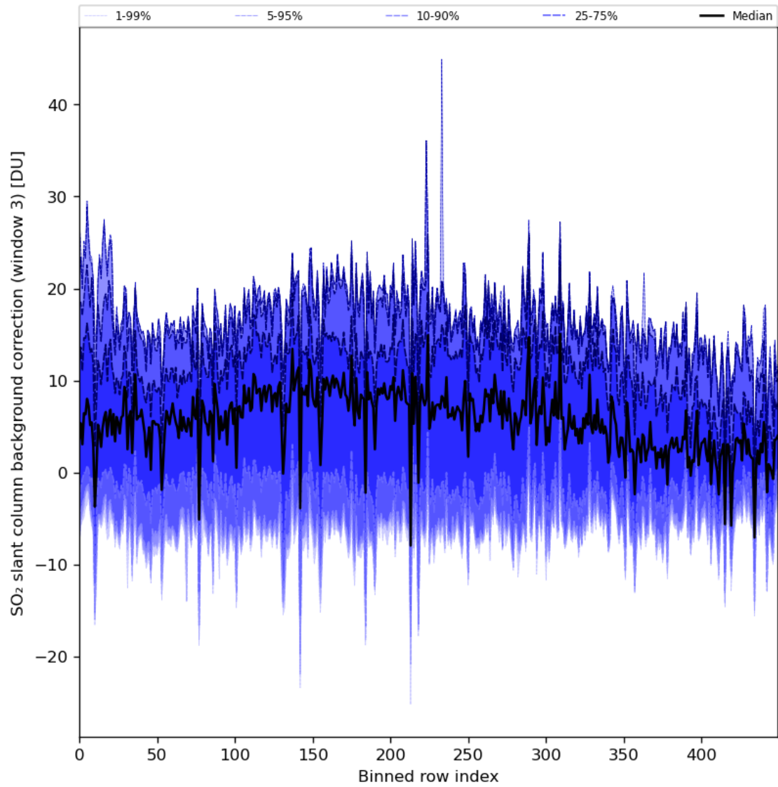
Figure 90: Along track statistics of “SO 2 slant column background correction (window 3)” for 2024-02-23 to 2024-02-25
