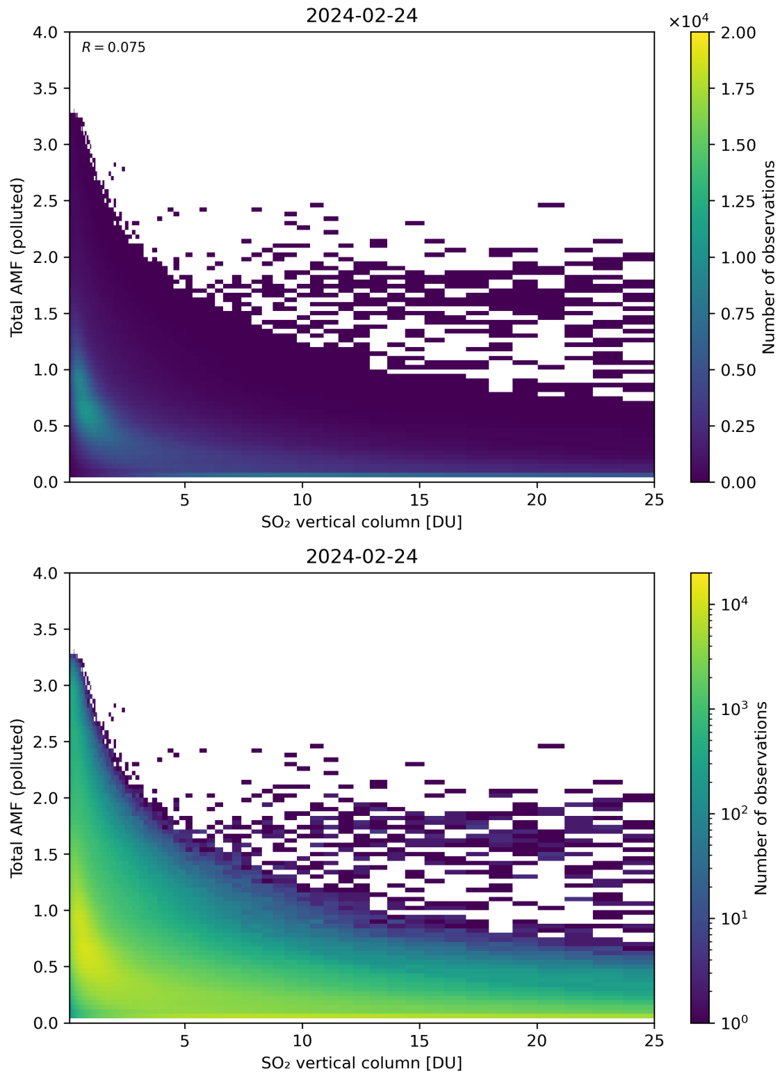
Figure 305: Scatter density plot of “SO 2 vertical column” against “Total AMF (polluted)” for 2024-02-23 to 2024-02-25.
