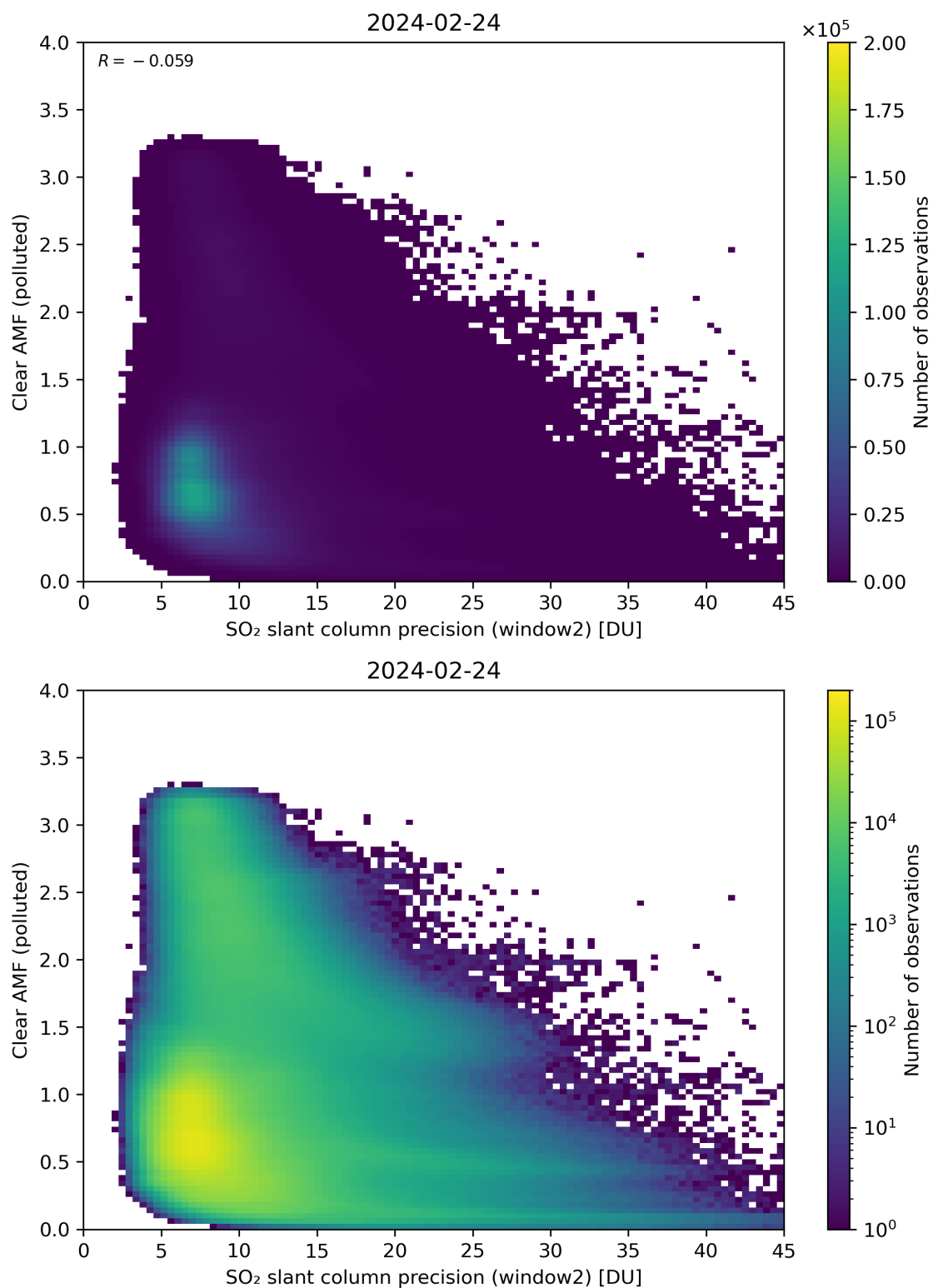
Figure 246: Scatter density plot of “SO 2 slant column precision (window2)” against “Clear AMF (polluted)” for 2024-02-23 to 2024-02-25.
