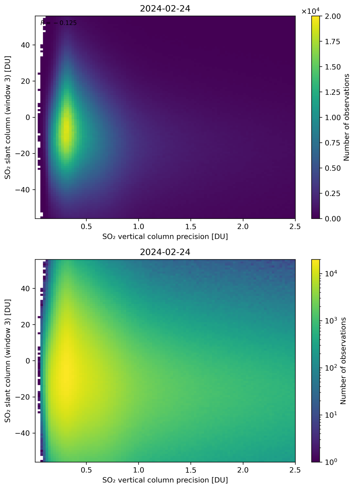
Figure 292: Scatter density plot of “SO 2 vertical column precision” against “SO 2 slant column (window 3)” for 2024-02-23 to 2024-02-25.
