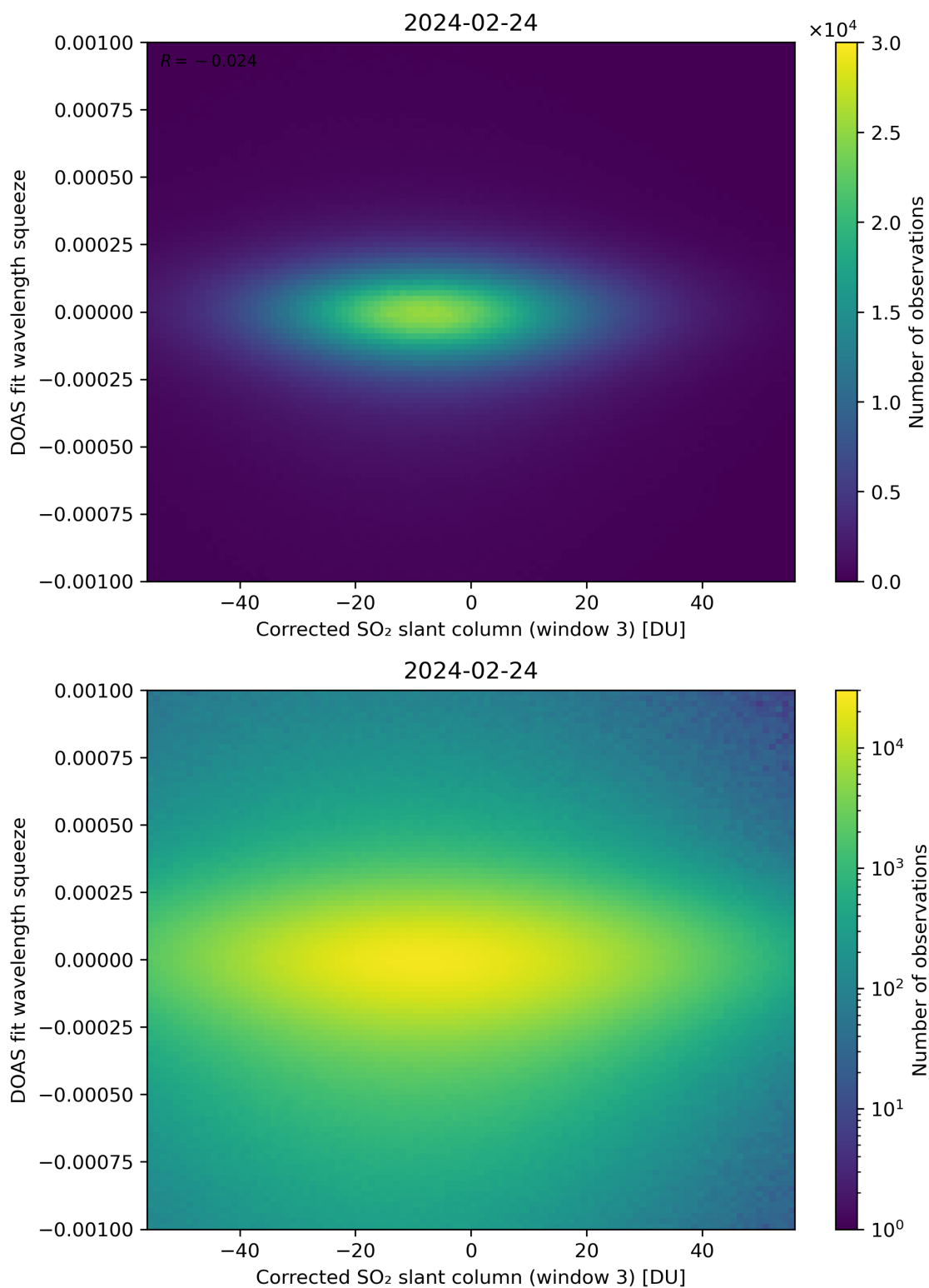
Figure 207: Scatter density plot of “Corrected SO 2 slant column (window 3)” against “DOAS fit wavelength squeeze” for 2024-02-23 to 2024-02-25.
