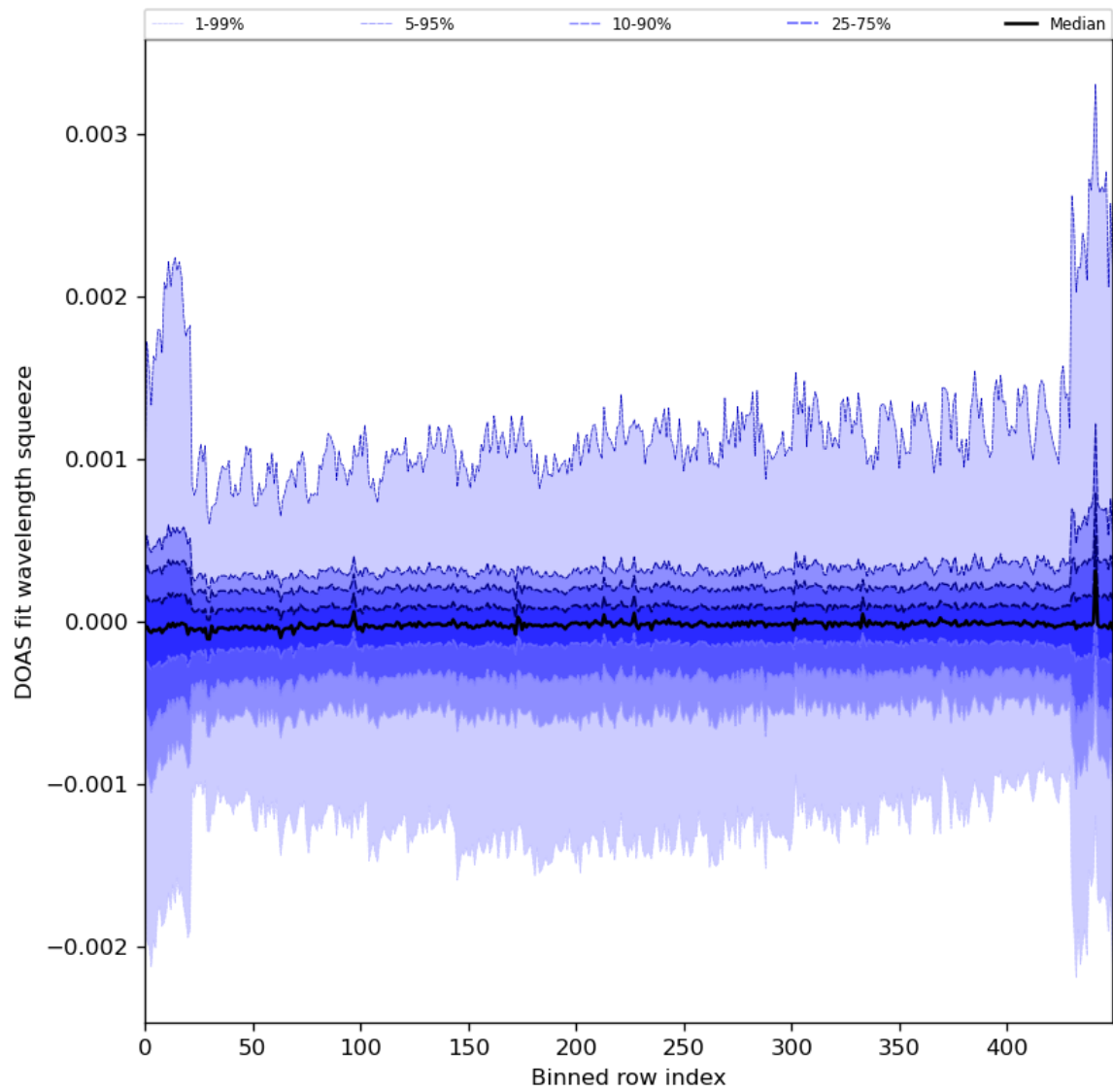
Figure 92: Along track statistics of “DOAS fit wavelength squeeze” for 2024-02-23 to 2024-02-25
