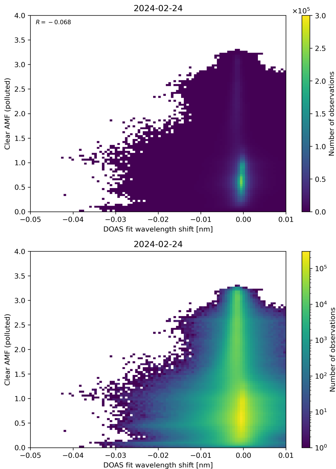
Figure 129: Scatter density plot of “DOAS fit wavelength shift” against “Clear AMF (polluted)” for 2024-02-23 to 2024-02-25.
