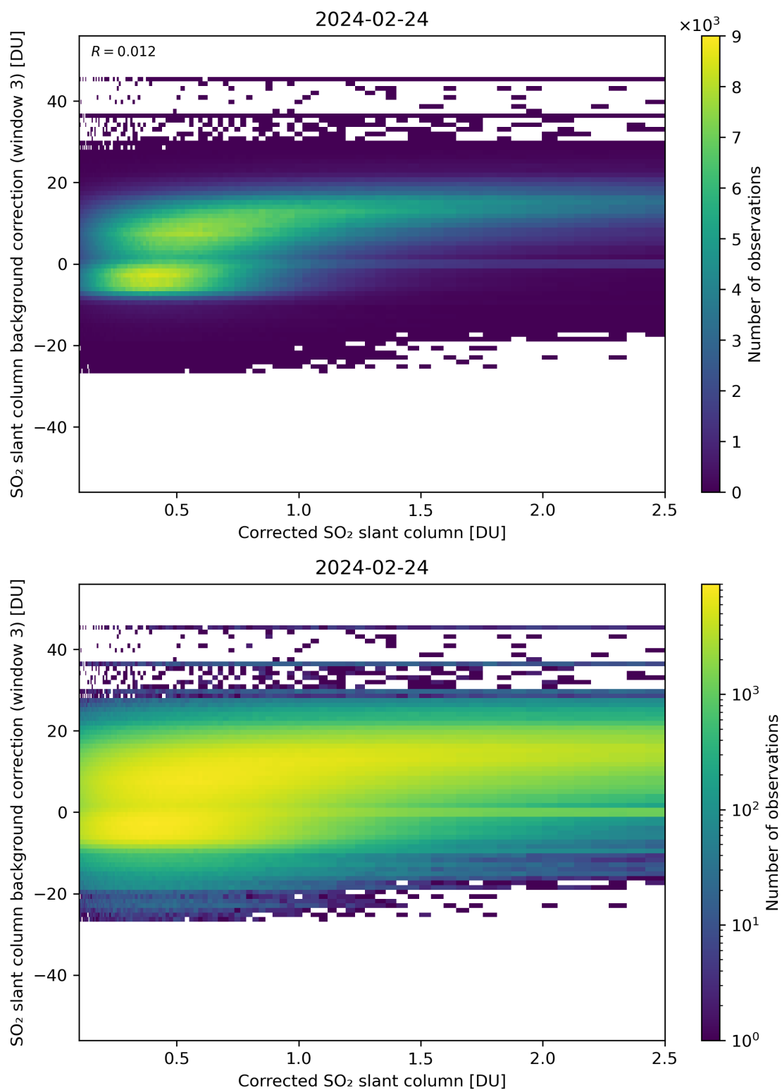
Figure 180: Scatter density plot of “Corrected SO 2 slant column” against “SO 2 slant column background correction (window 3)” for 2024-02-23 to 2024-02-25.
