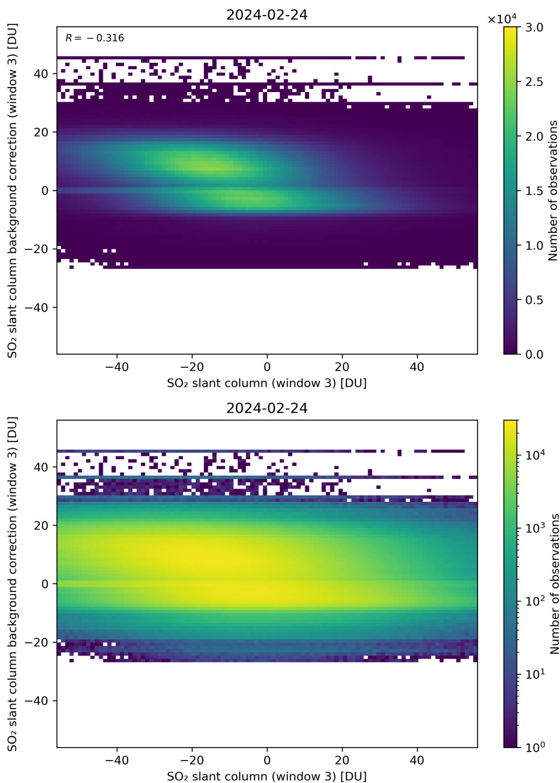
Figure 253: Scatter density plot of “SO 2 slant column (window 3)” against “SO 2 slant column background correction (window 3)” for 2024-02-23 to 2024-02-25.
