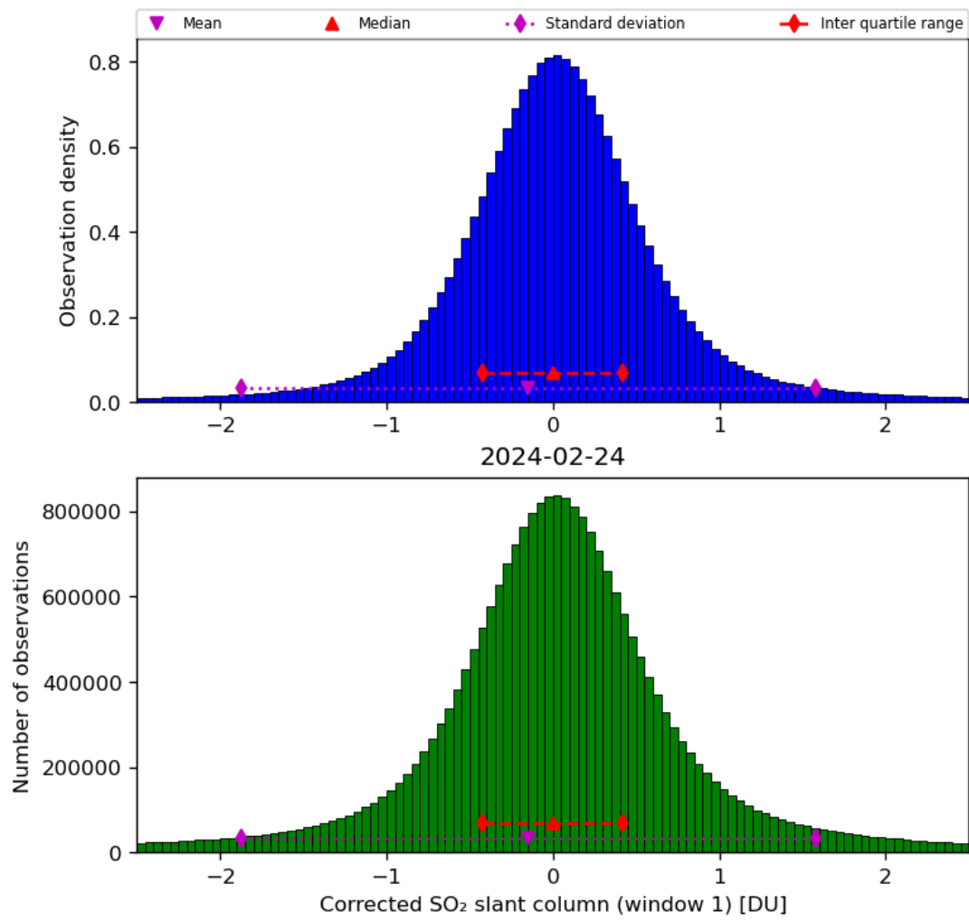
Figure 58: Histogram of “Corrected SO 2 slant column (window 1)” for 2024-02-23 to 2024-02-25
