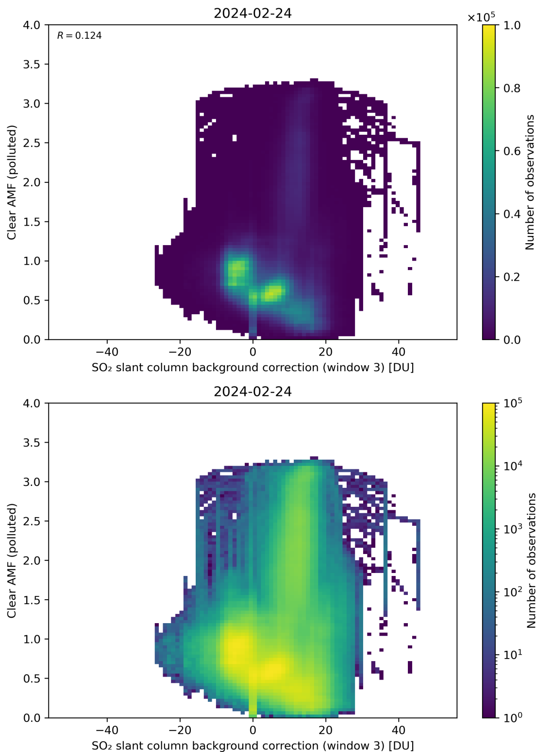
Figure 124: Scatter density plot of “SO 2 slant column background correction (window 3)” against “Clear AMF (polluted)” for 2024-02-23 to 2024-02-25.
