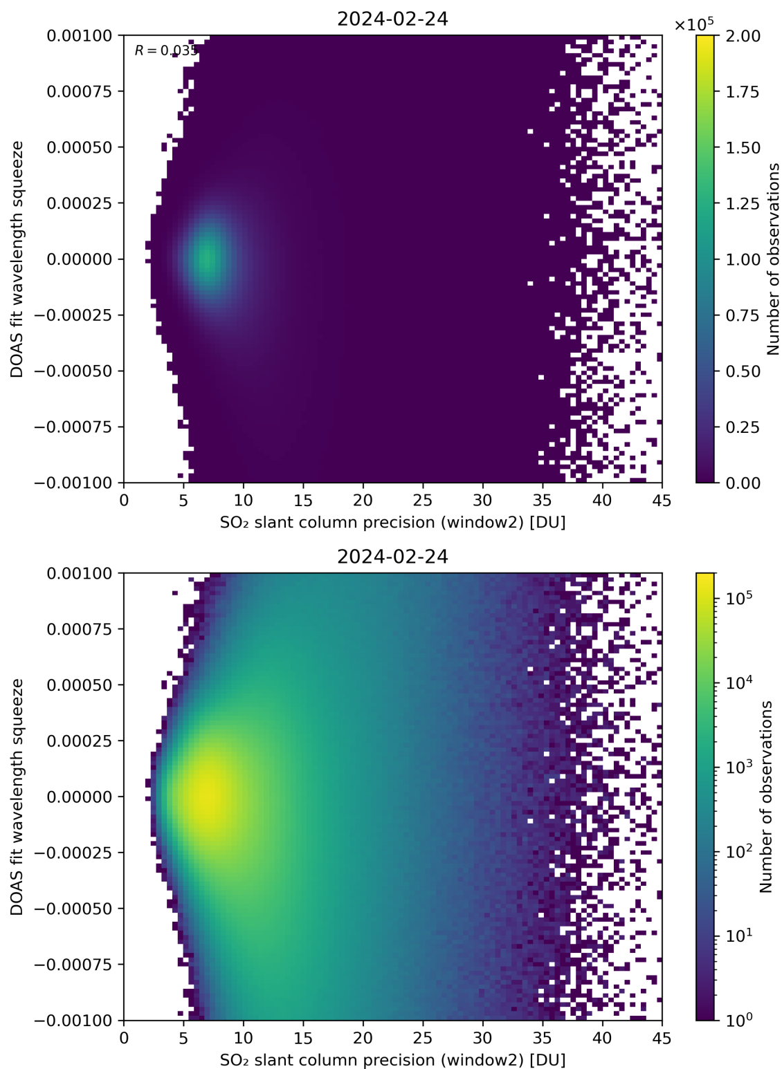
Figure 244: Scatter density plot of “SO 2 slant column precision (window2)” against “DOAS fit wavelength squeeze” for 2024-02-23 to 2024-02-25.
