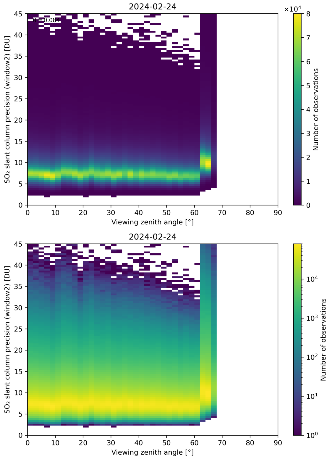
Figure 322: Scatter density plot of “Viewing zenith angle” against “SO 2 slant column precision (window2)” for 2024-02-23 to 2024-02-25.
