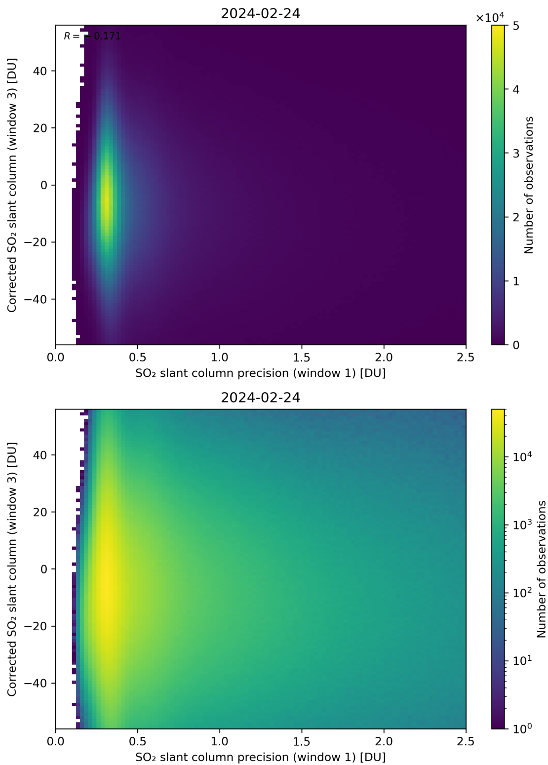
Figure 226: Scatter density plot of “SO 2 slant column precision (window 1)” against “Corrected SO 2 slant column (window 3)” for 2024-02-23 to 2024-02-25.
