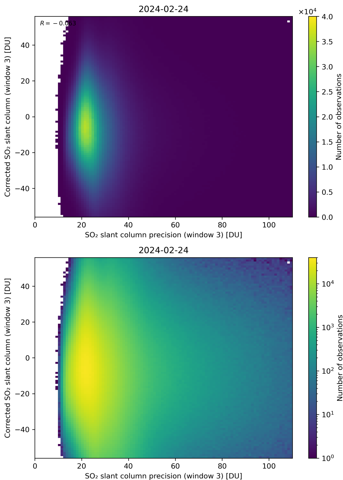
Figure 262: Scatter density plot of “SO 2 slant column precision (window 3)” against “Corrected SO 2 slant column (window 3)” for 2024-02-23 to 2024-02-25.
