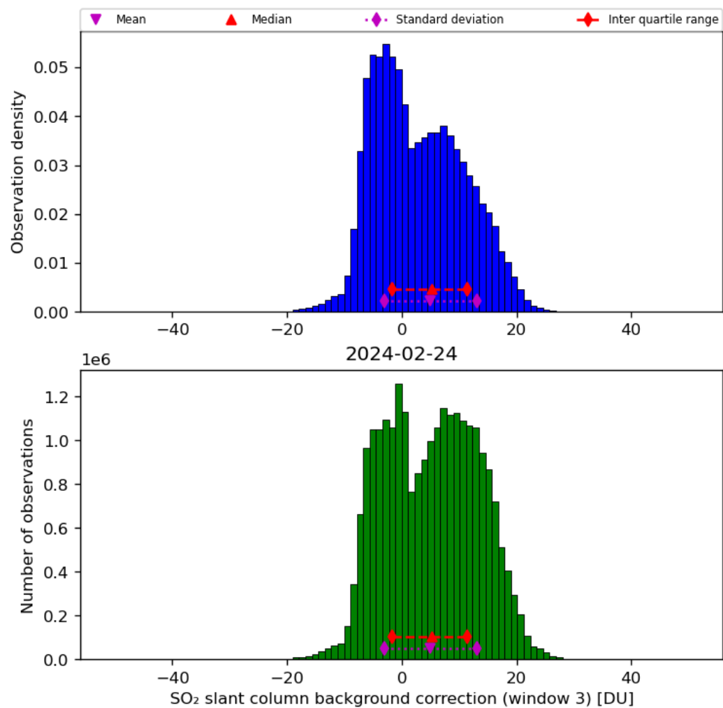
Figure 67: Histogram of “SO 2 slant column background correction (window 3)” for 2024-02-23 to 2024-02-25
