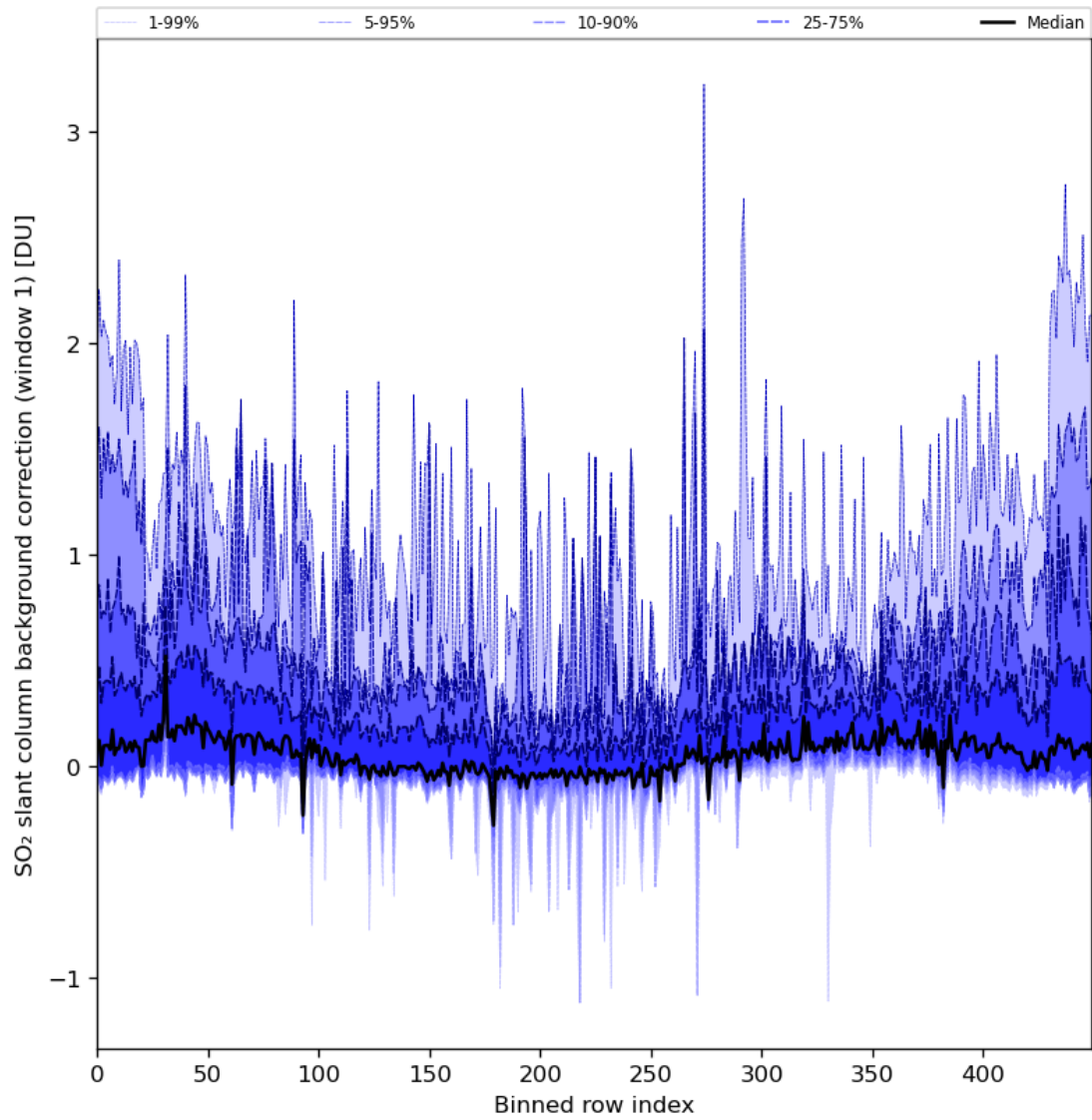
Figure 82: Along track statistics of “SO 2 slant column background correction (window 1)” for 2024-02-23 to 2024-02-25
