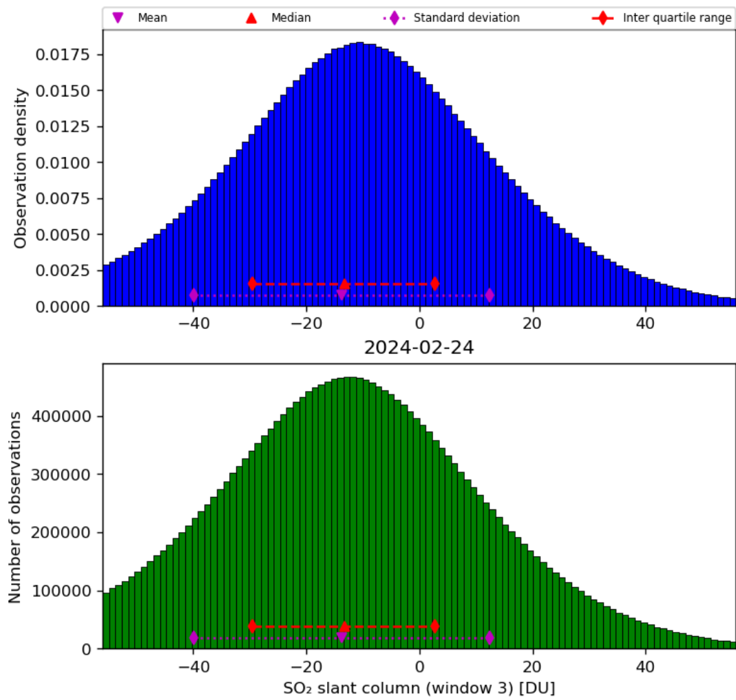
Figure 64: Histogram of “SO 2 slant column (window 3)” for 2024-02-23 to 2024-02-25
