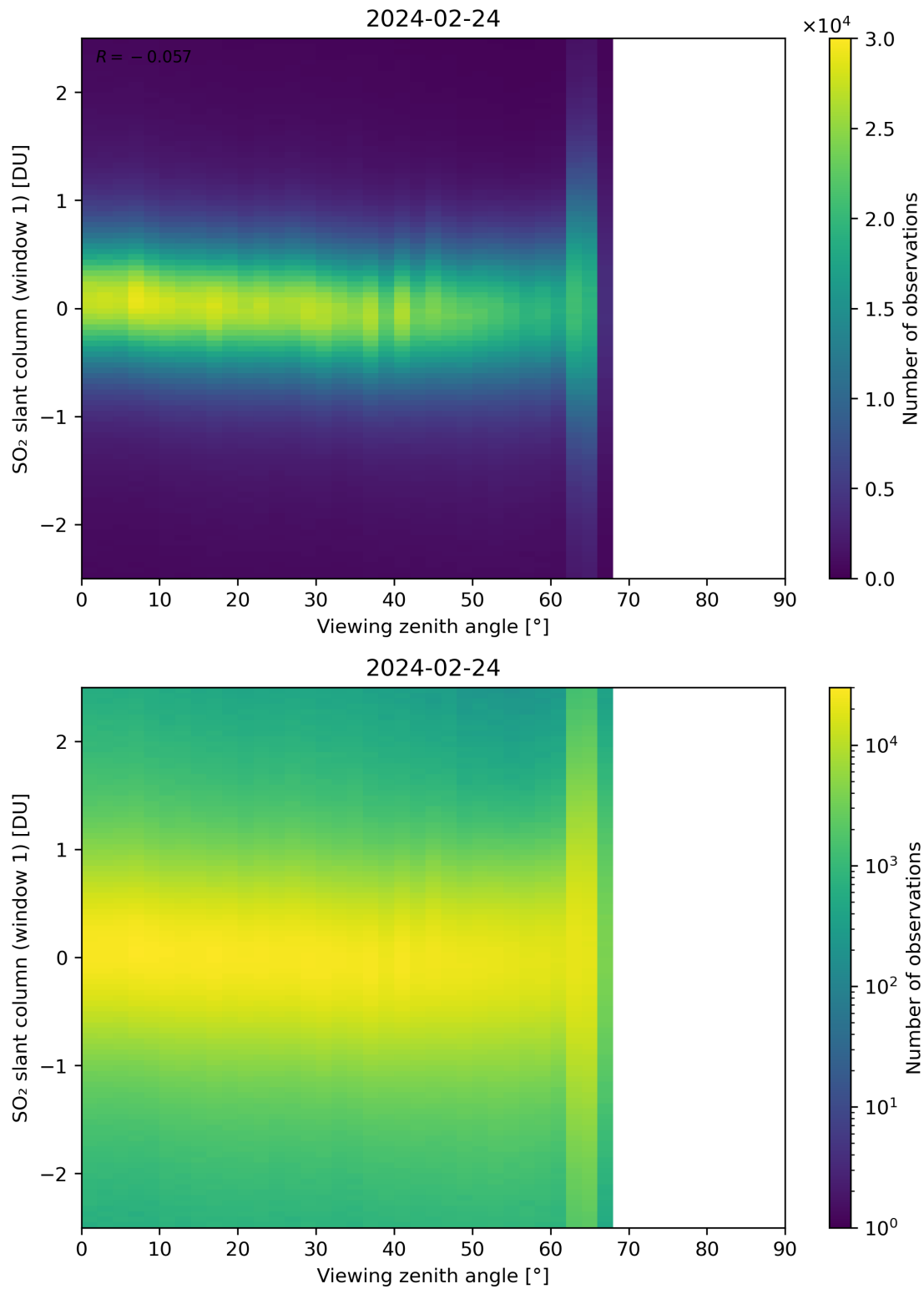
Figure 320: Scatter density plot of “Viewing zenith angle” against “SO 2 slant column (window 1)” for 2024-02-23 to 2024-02-25.
