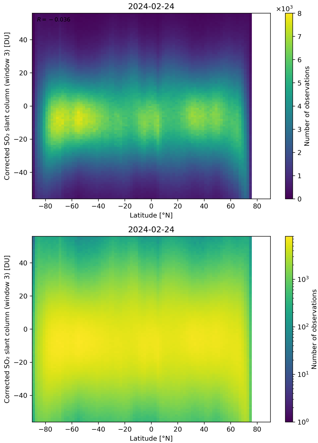
Figure 148: Scatter density plot of “Latitude” against “Corrected SO 2 slant column (window 3)” for 2024-02-23 to 2024-02-25.
