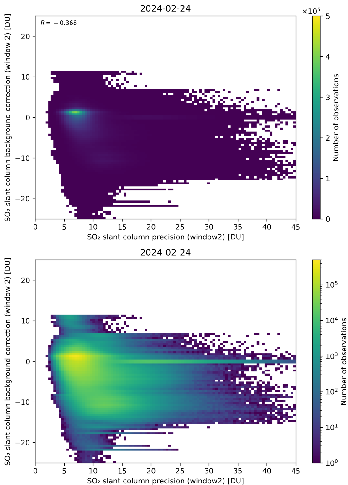
Figure 241: Scatter density plot of “SO 2 slant column precision (window2)” against “SO 2 slant column background correction (window 2)” for 2024-02-23 to 2024-02-25.
