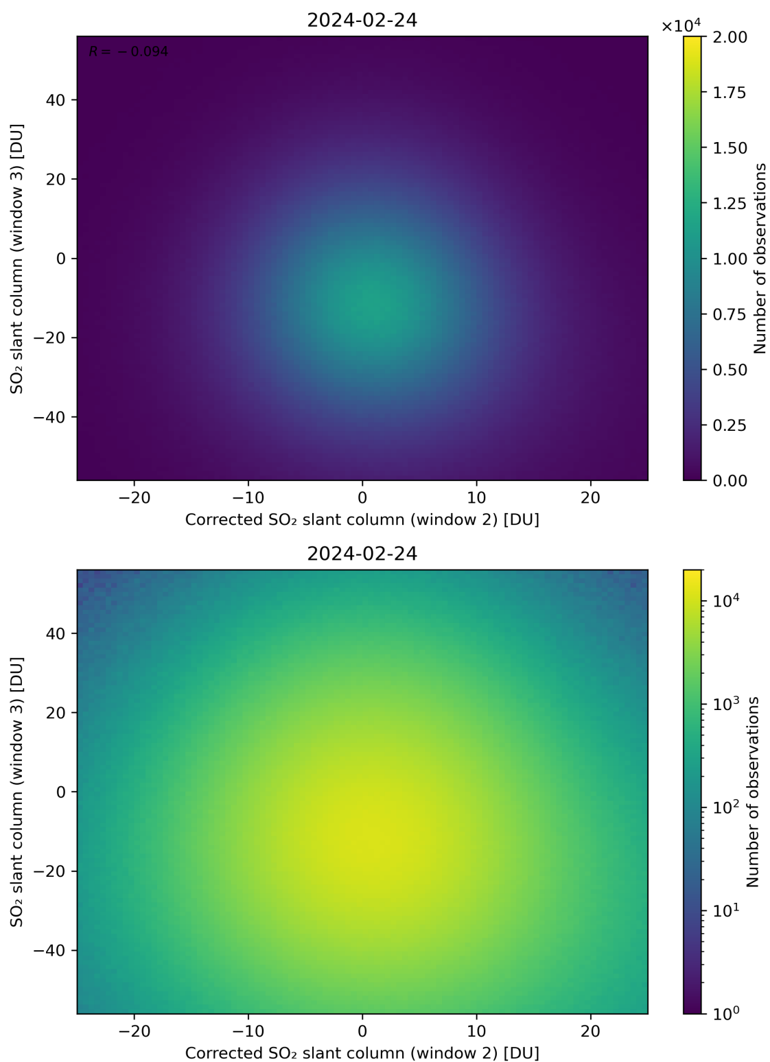
Figure 201: Scatter density plot of “Corrected SO 2 slant column (window 2)” against “SO 2 slant column (window 3)” for 2024-02-23 to 2024-02-25.
