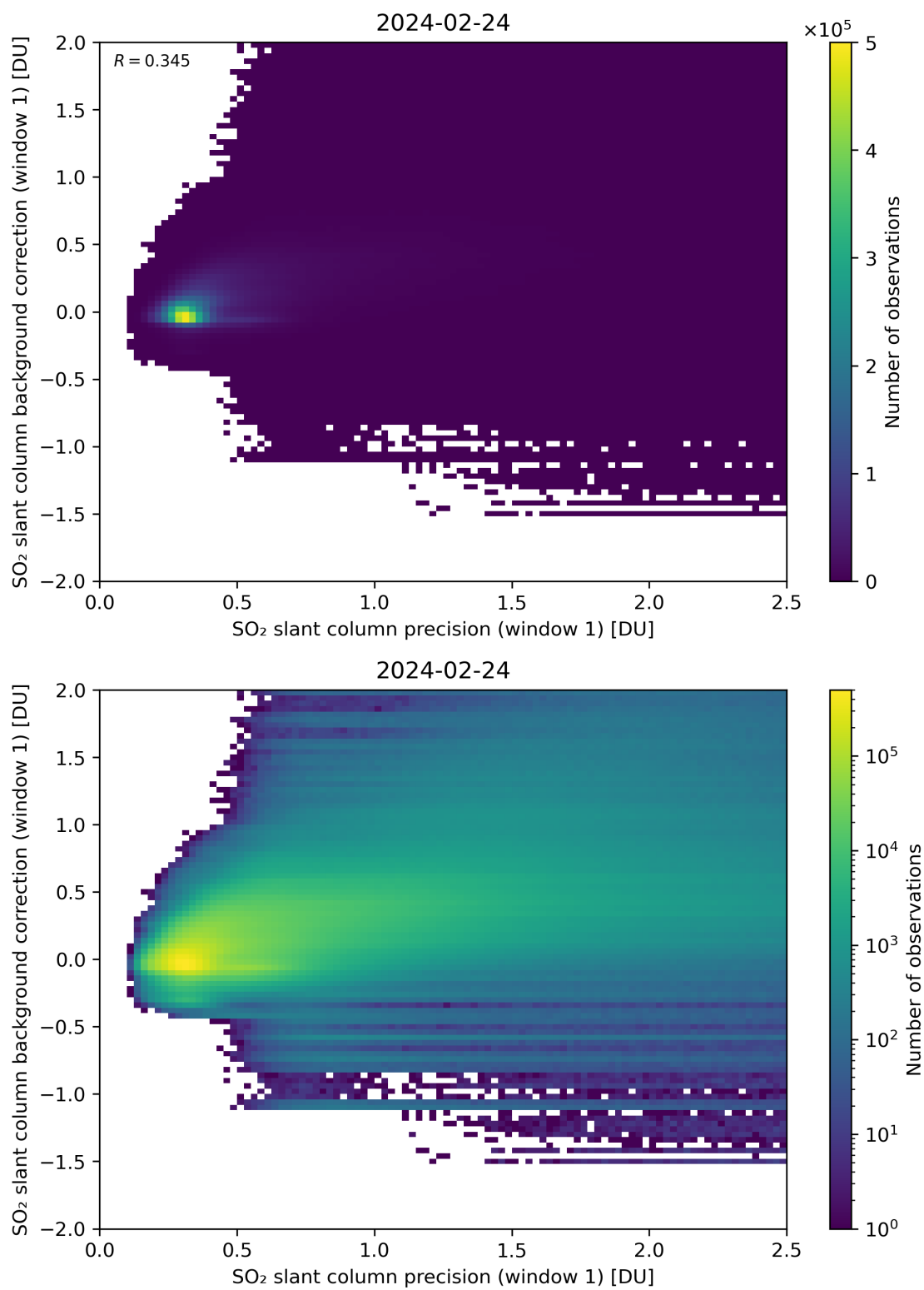
Figure 218: Scatter density plot of “SO 2 slant column precision (window 1)” against “SO 2 slant column background correction (window 1)” for 2024-02-23 to 2024-02-25.
