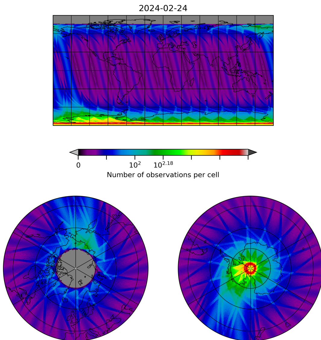
Figure 28: Map of the number of observations for 2024-02-23 to 2024-02-25
