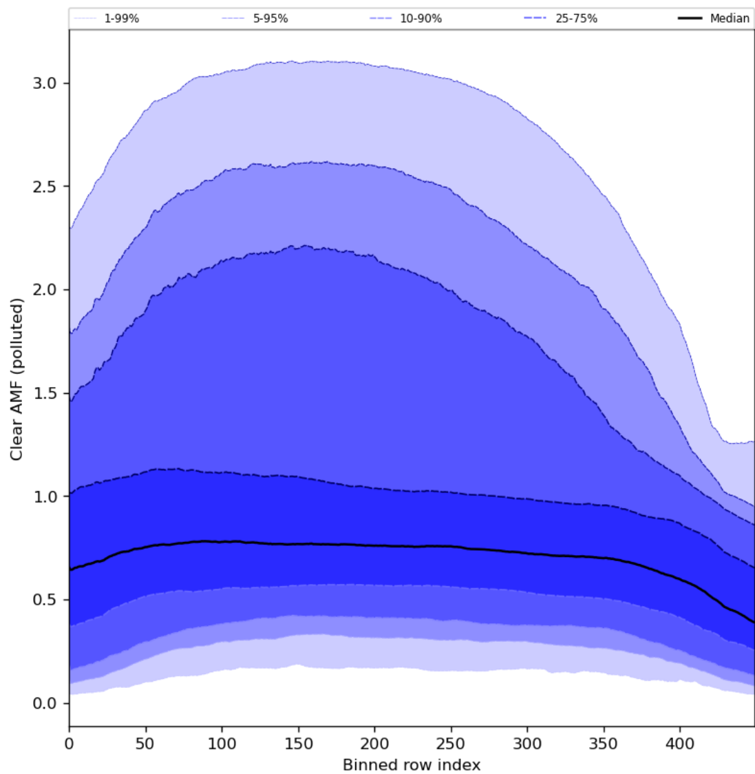
Figure 96: Along track statistics of “Clear AMF (polluted)” for 2024-02-23 to 2024-02-25
