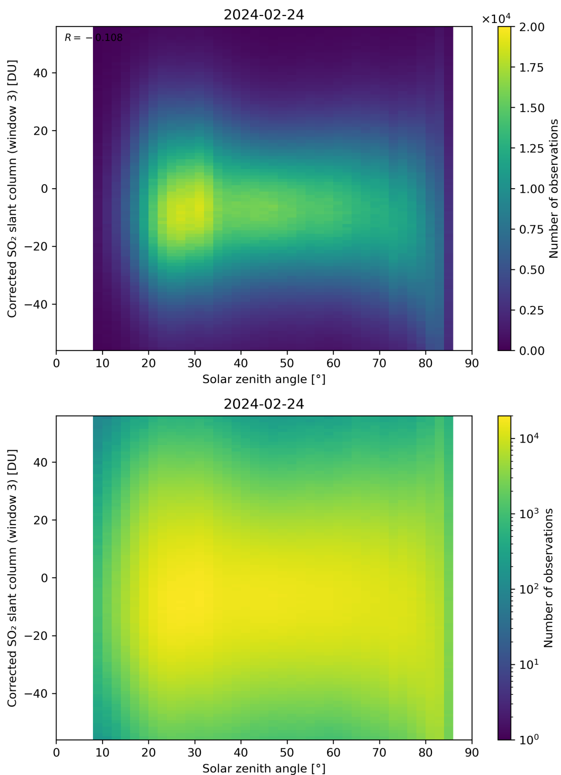
Figure 168: Scatter density plot of “Solar zenith angle” against “Corrected SO 2 slant column (window 3)” for 2024-02-23 to 2024-02-25.
