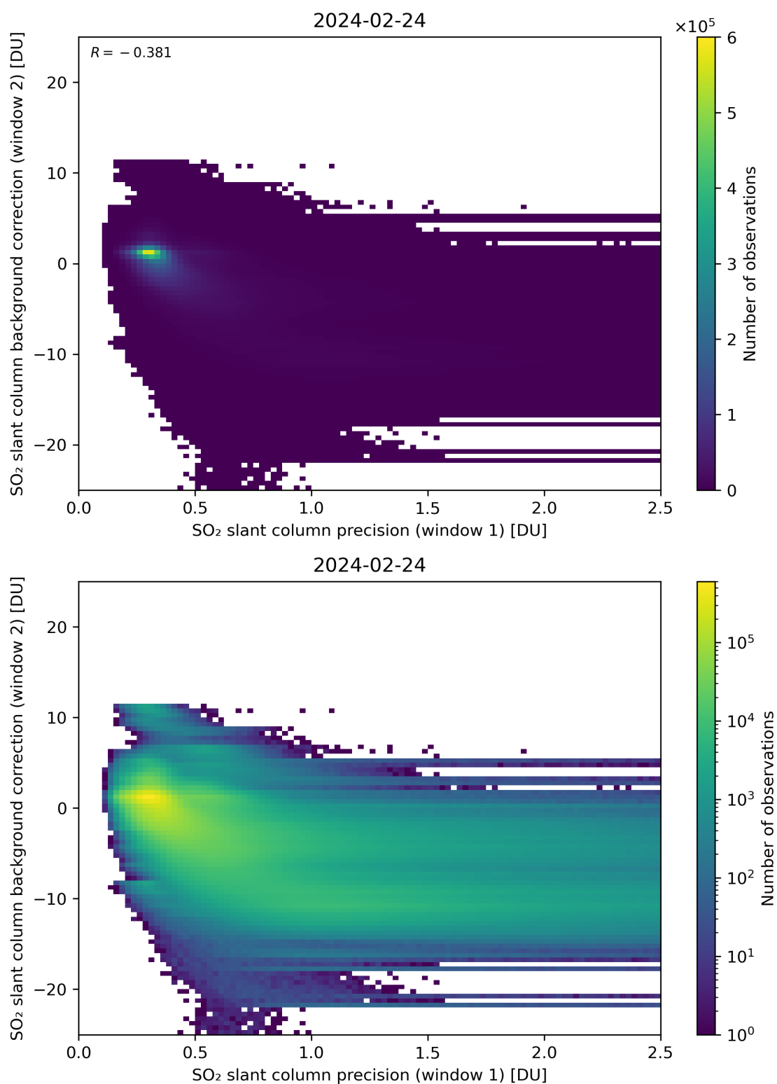
Figure 219: Scatter density plot of “SO 2 slant column precision (window 1)” against “SO 2 slant column background correction (window 2)” for 2024-02-23 to 2024-02-25.
