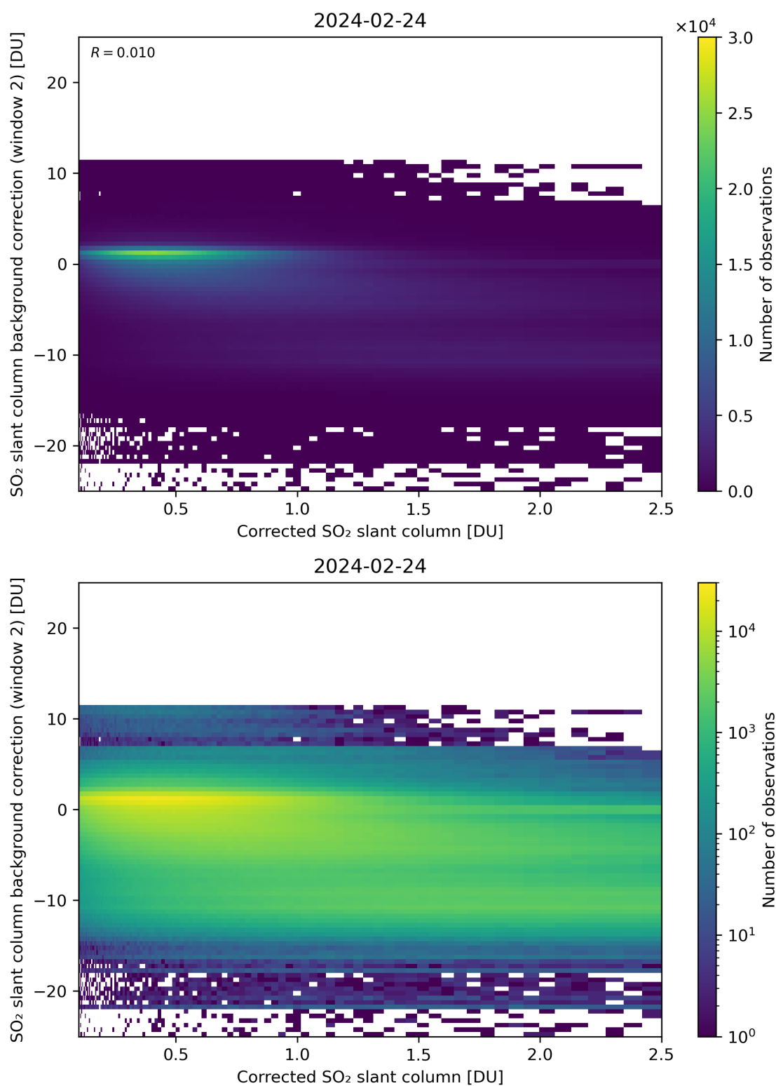
Figure 179: Scatter density plot of “Corrected SO 2 slant column” against “SO 2 slant column background correction (window 2)” for 2024-02-23 to 2024-02-25.
