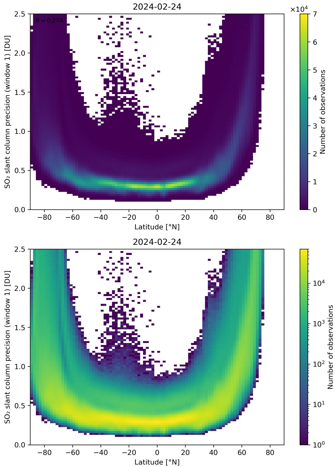
Figure 150: Scatter density plot of “Latitude” against “SO 2 slant column precision (window 1)” for 2024-02-23 to 2024-02-25.
