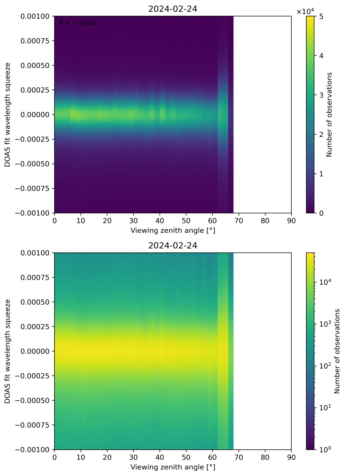
Figure 312: Scatter density plot of “Viewing zenith angle” against “DOAS fit wavelength squeeze” for 2024-02-23 to 2024-02-25.
