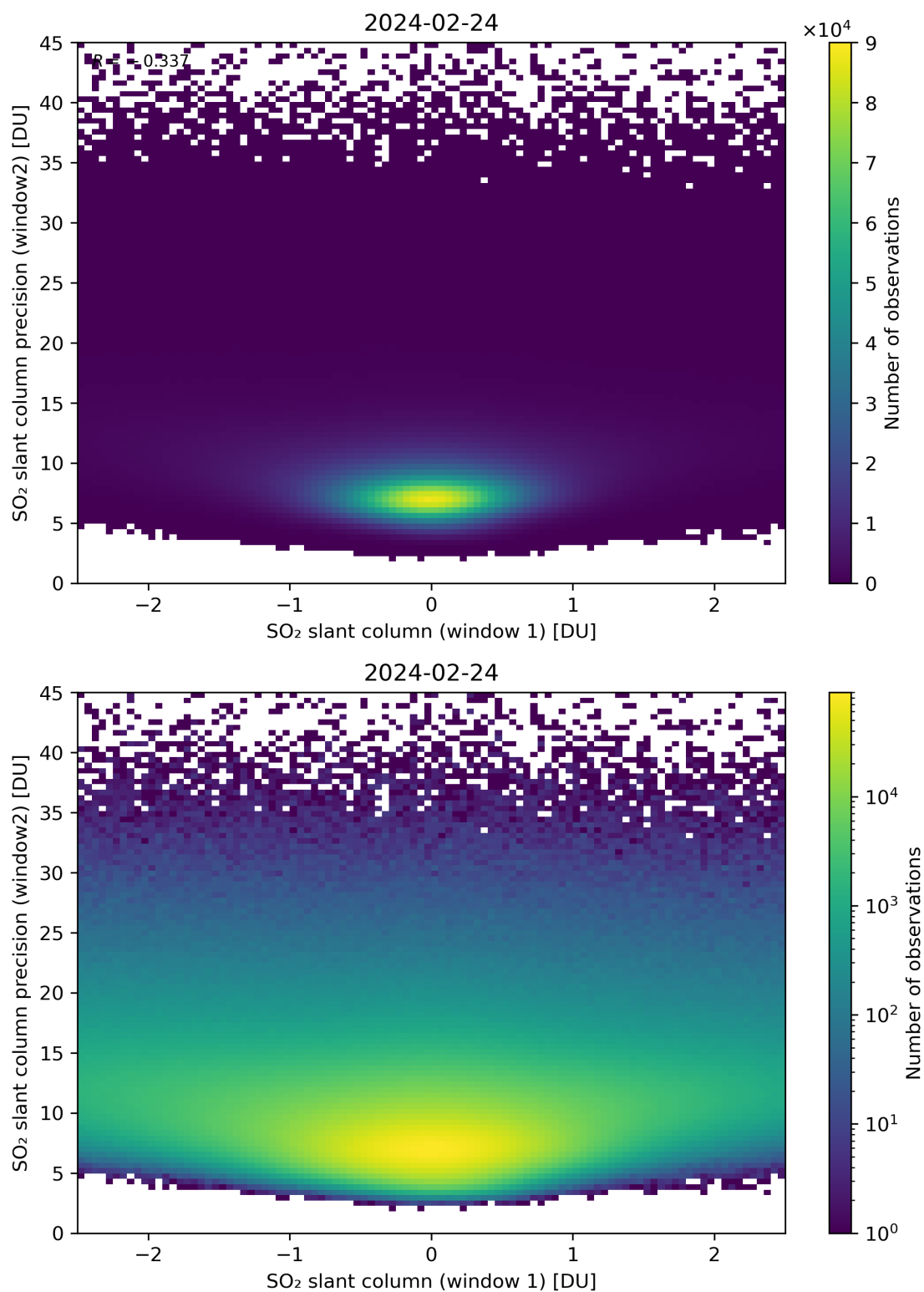
Figure 236: Scatter density plot of “SO 2 slant column (window 1)” against “SO 2 slant column precision (window2)” for 2024-02-23 to 2024-02-25.
