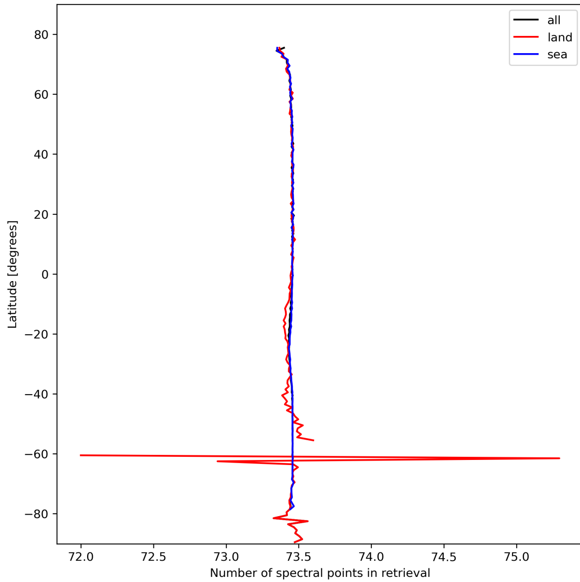
Figure 51: Zonal average of “Number of spectral points in retrieval” for 2024-02-23 to 2024-02-25.
