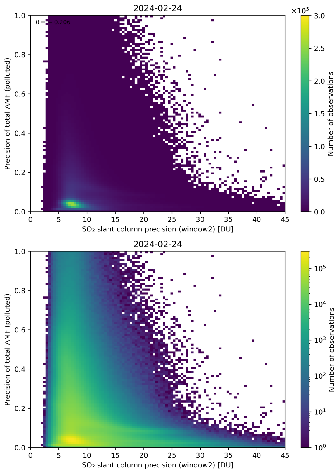
Figure 252: Scatter density plot of “SO 2 slant column precision (window2)” against “Precision of total AMF (polluted)” for 2024-02-23 to 2024-02-25.
