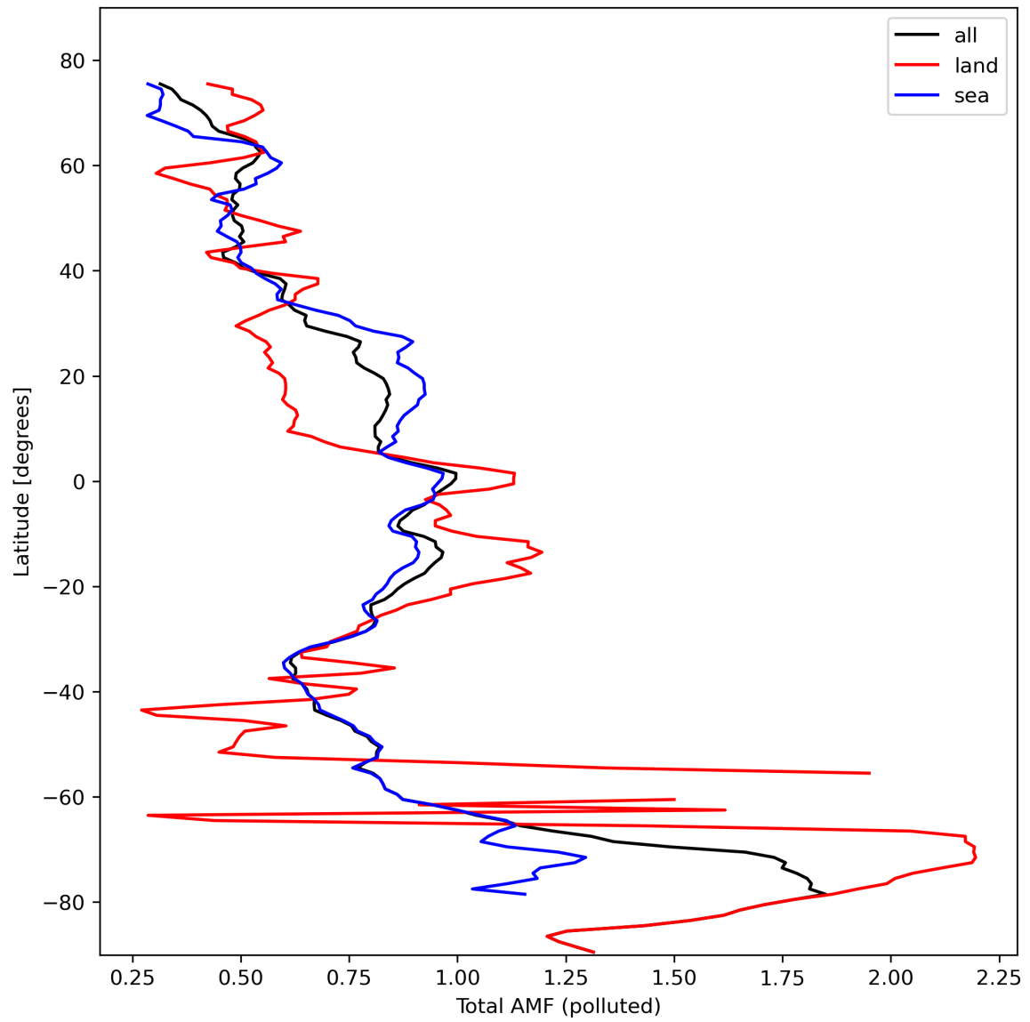
Figure 48: Zonal average of “Total AMF (polluted)” for 2024-02-23 to 2024-02-25.
