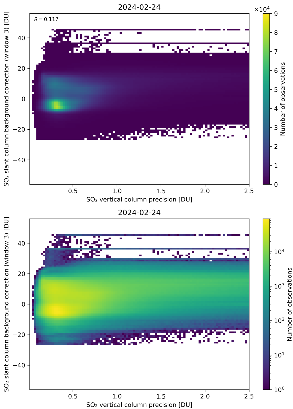
Figure 281: Scatter density plot of “SO 2 vertical column precision” against “SO 2 slant column background correction (window 3)” for 2024-02-23 to 2024-02-25.
