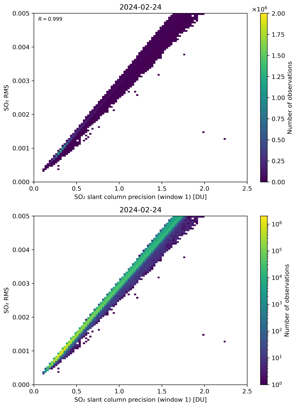
Figure 223: Scatter density plot of “SO 2 slant column precision (window 1)” against “SO 2 RMS” for 2024-02-23 to 2024-02-25.
