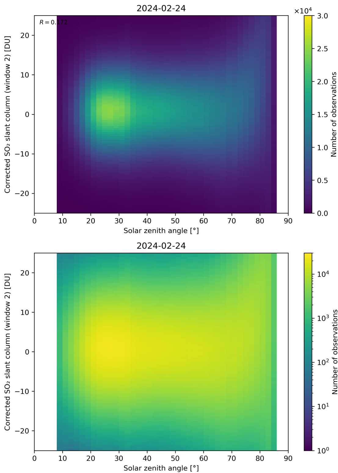
Figure 167: Scatter density plot of “Solar zenith angle” against “Corrected SO 2 slant column (window 2)” for 2024-02-23 to 2024-02-25.
