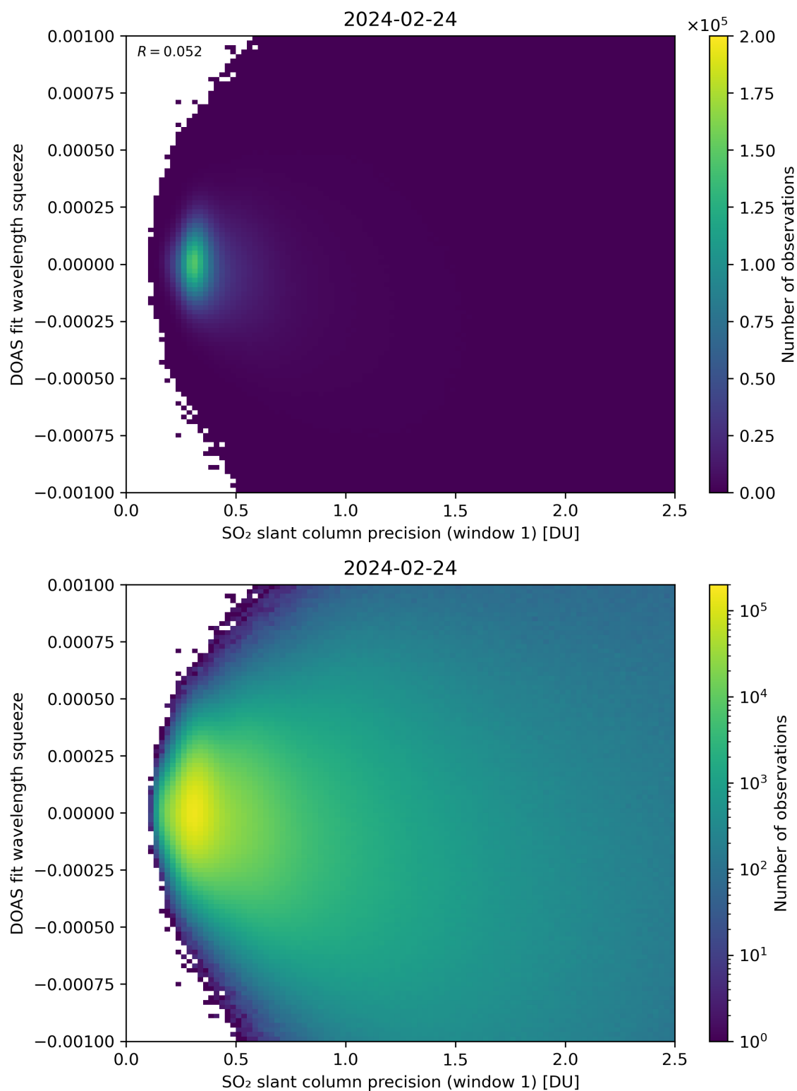
Figure 222: Scatter density plot of “SO 2 slant column precision (window 1)” against “DOAS fit wavelength squeeze” for 2024-02-23 to 2024-02-25.
