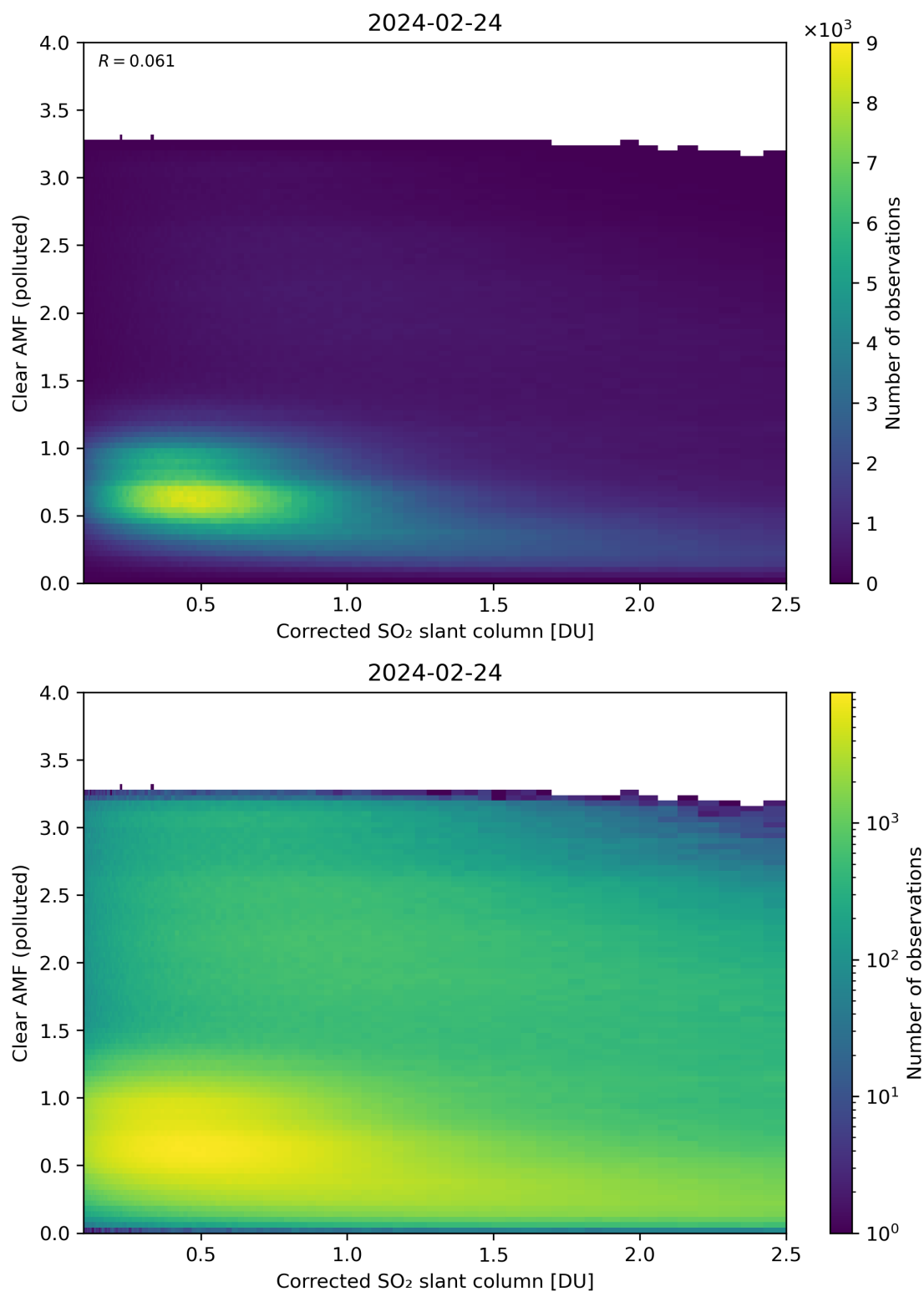
Figure 184: Scatter density plot of “Corrected SO 2 slant column” against “Clear AMF (polluted)” for 2024-02-23 to 2024-02-25.
