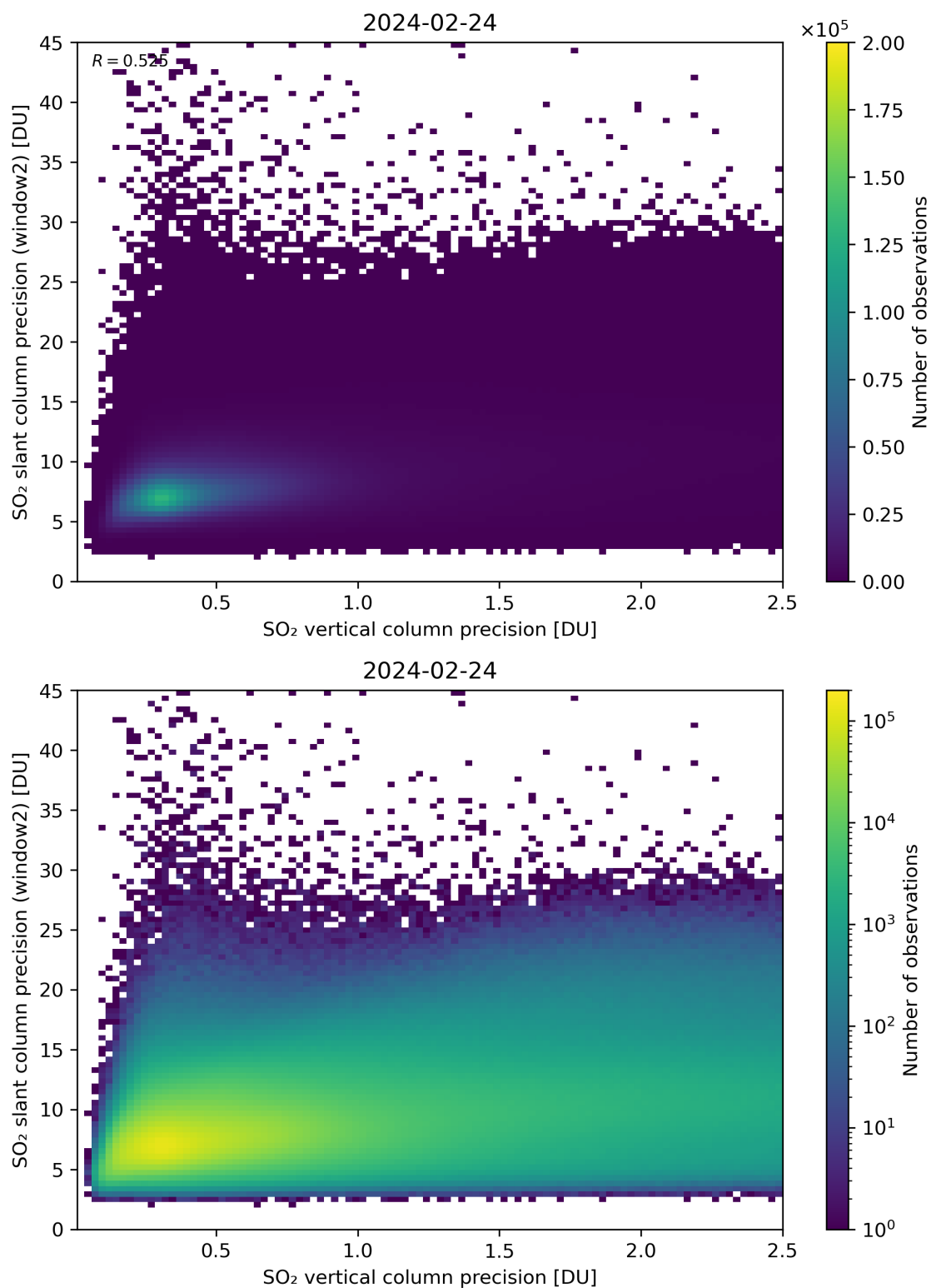
Figure 291: Scatter density plot of “SO 2 vertical column precision” against “SO 2 slant column precision (window2)” for 2024-02-23 to 2024-02-25.
