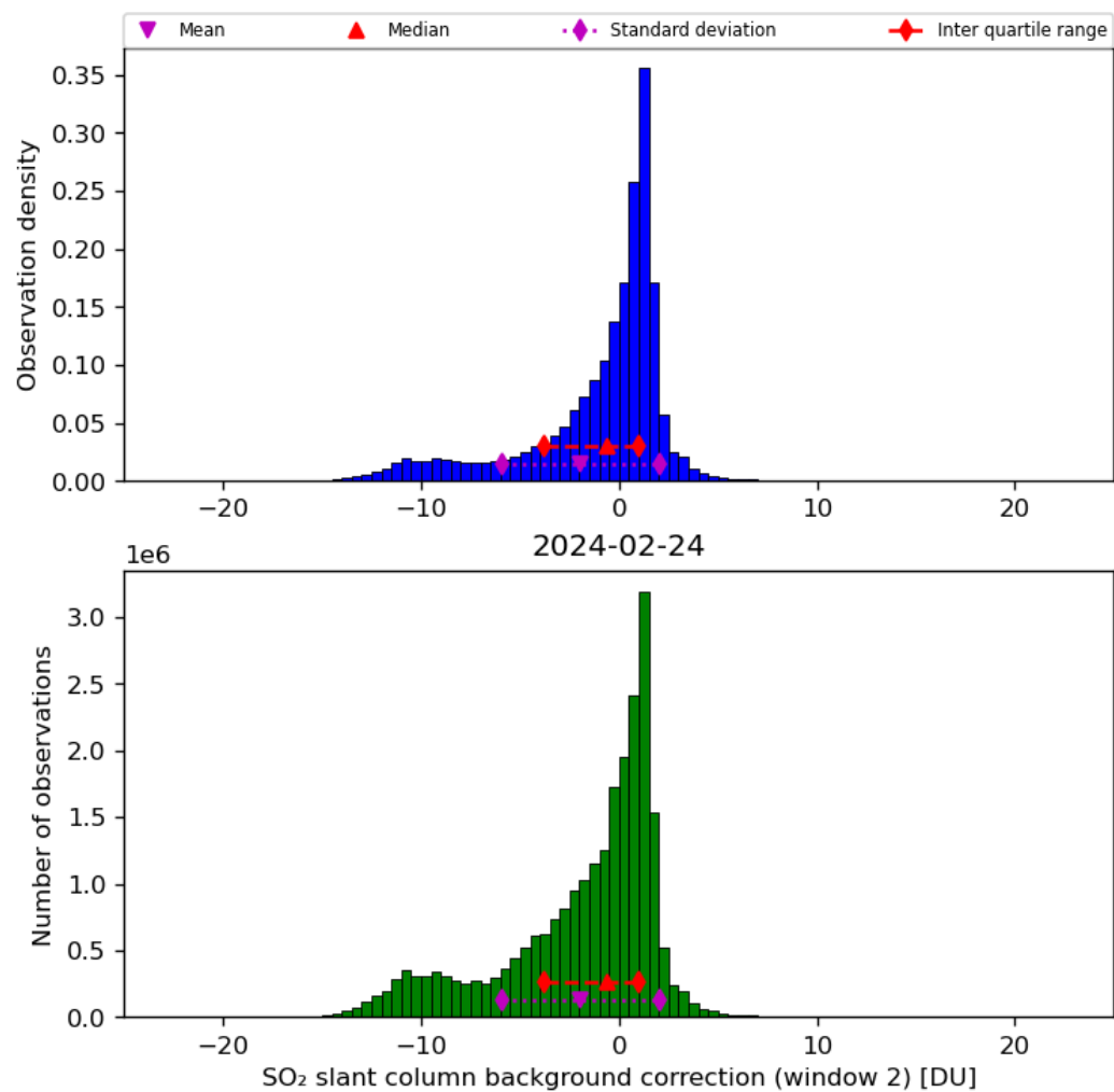
Figure 63: Histogram of “SO 2 slant column background correction (window 2)” for 2024-02-23 to 2024-02-25
