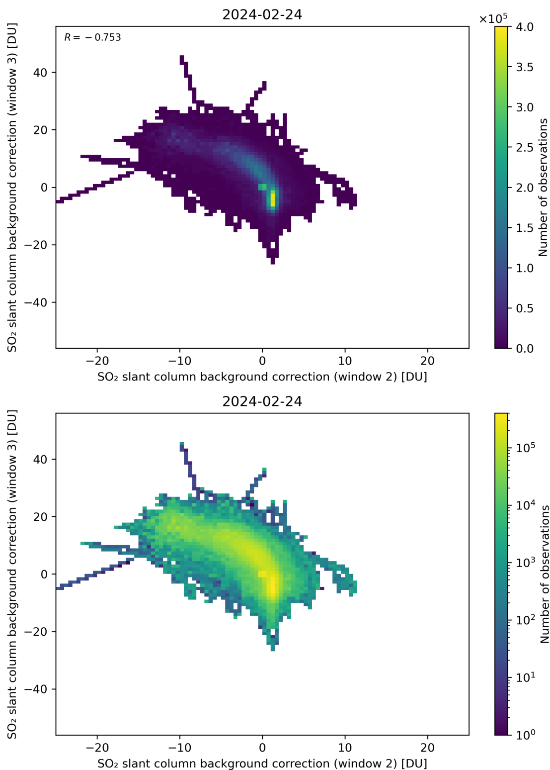
Figure 111: Scatter density plot of “SO 2 slant column background correction (window 2)” against “SO 2 slant column background correction (window 3)” for 2024-02-23 to 2024-02-25.
