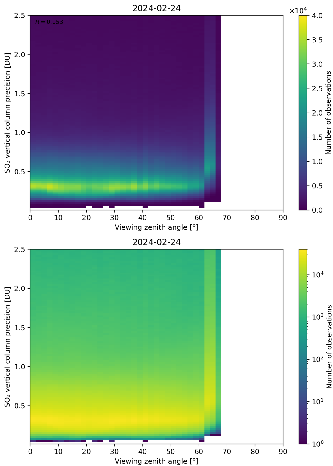
Figure 328: Scatter density plot of “Viewing zenith angle” against “SO 2 vertical column precision” for 2024-02-23 to 2024-02-25.
