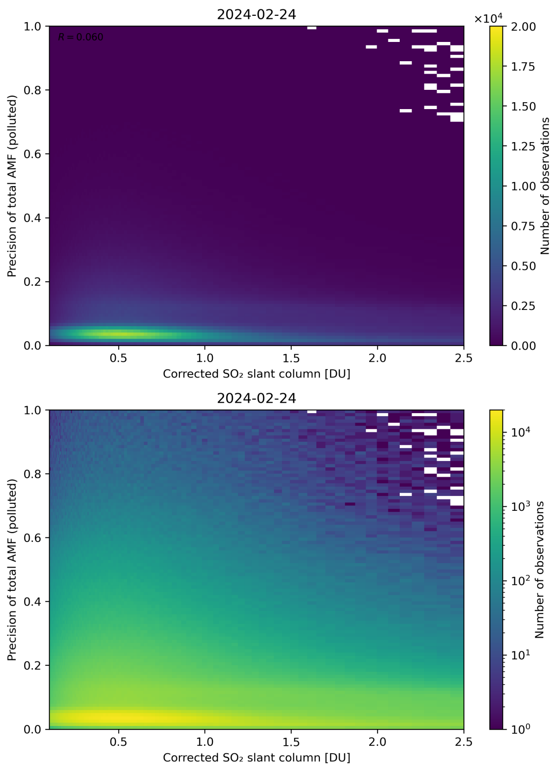
Figure 193: Scatter density plot of “Corrected SO 2 slant column” against “Precision of total AMF (polluted)” for 2024-02-23 to 2024-02-25.
