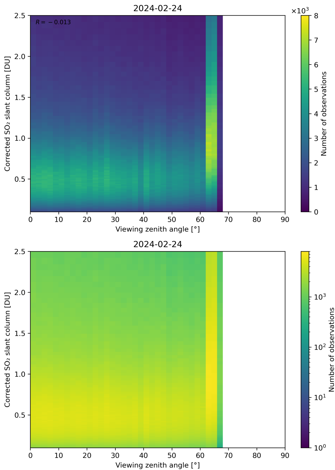
Figure 317: Scatter density plot of “Viewing zenith angle” against “Corrected SO 2 slant column” for 2024-02-23 to 2024-02-25.
