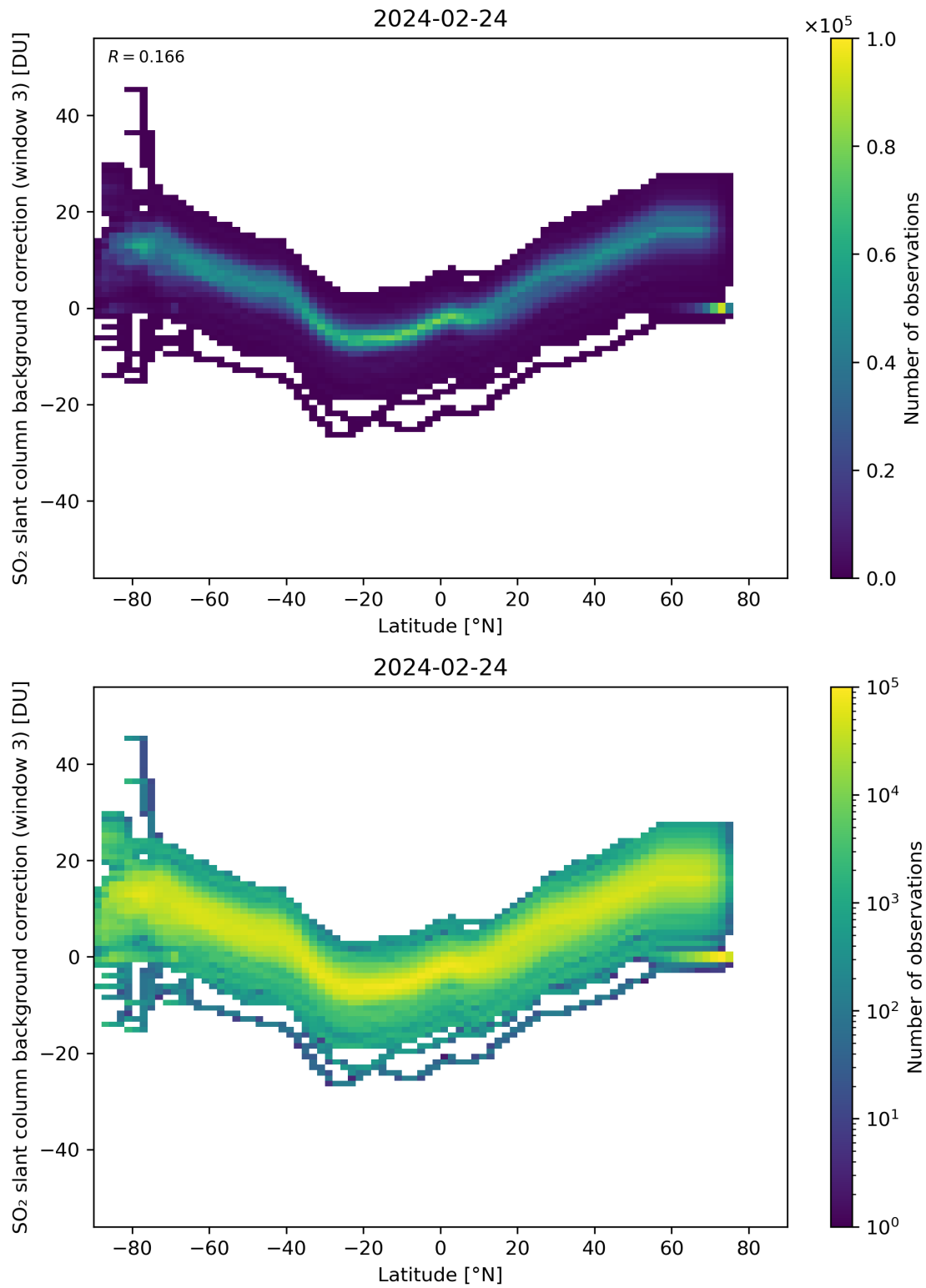
Figure 141: Scatter density plot of “Latitude” against “SO 2 slant column background correction (window 3)” for 2024-02-23 to 2024-02-25.
