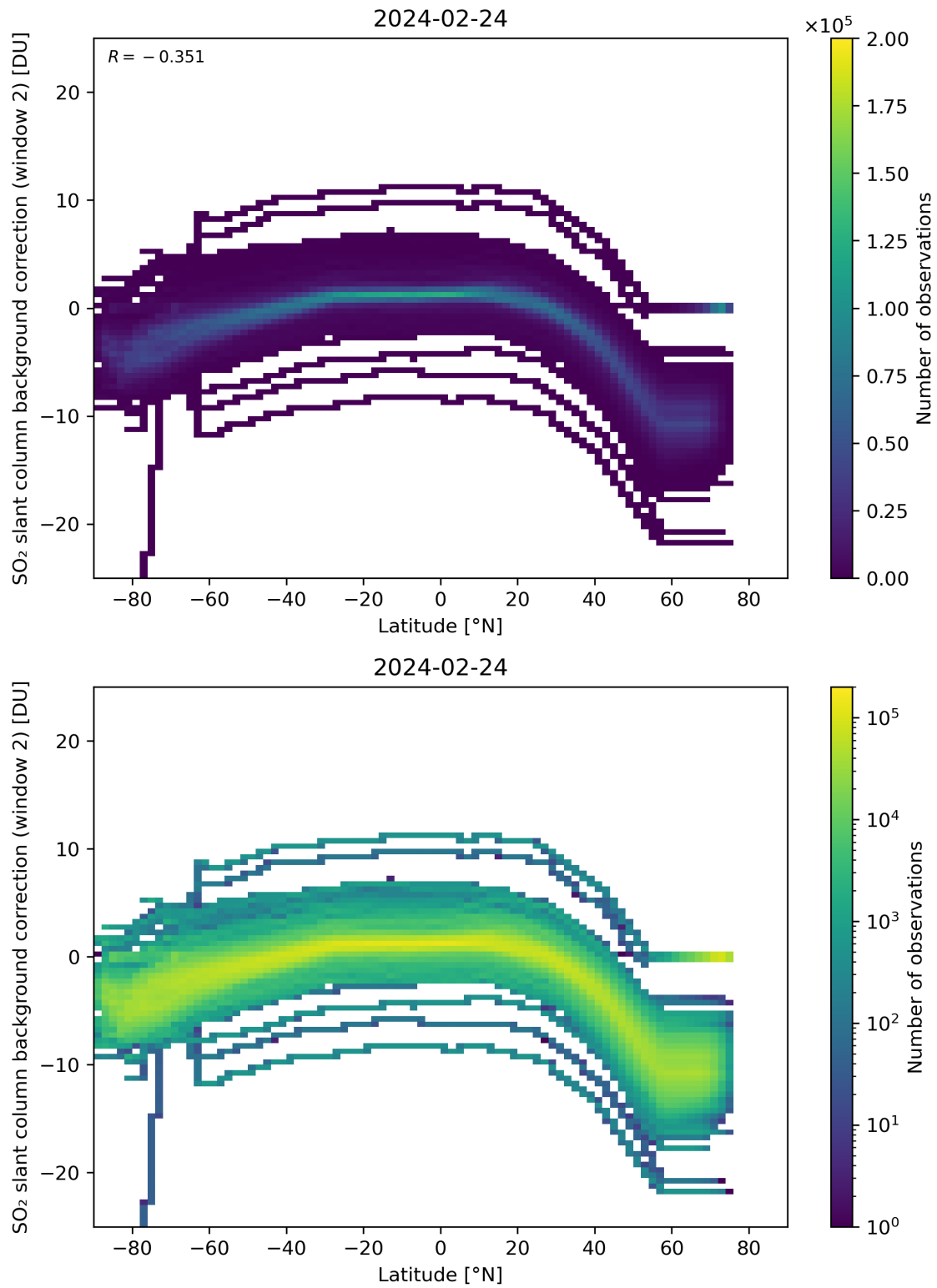
Figure 140: Scatter density plot of “Latitude” against “SO 2 slant column background correction (window 2)” for 2024-02-23 to 2024-02-25.
