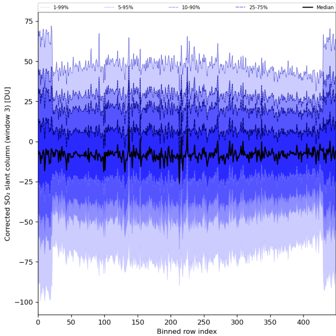
Figure 89: Along track statistics of “Corrected SO 2 slant column (window 3)” for 2024-02-23 to 2024-02-25
