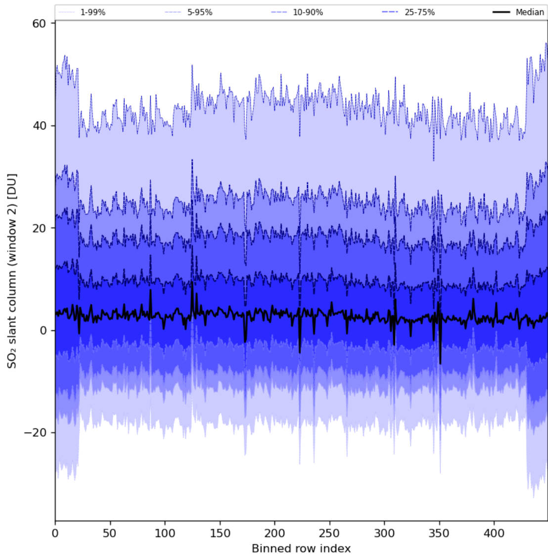
Figure 83: Along track statistics of “SO 2 slant column (window 2)” for 2024-02-23 to 2024-02-25
