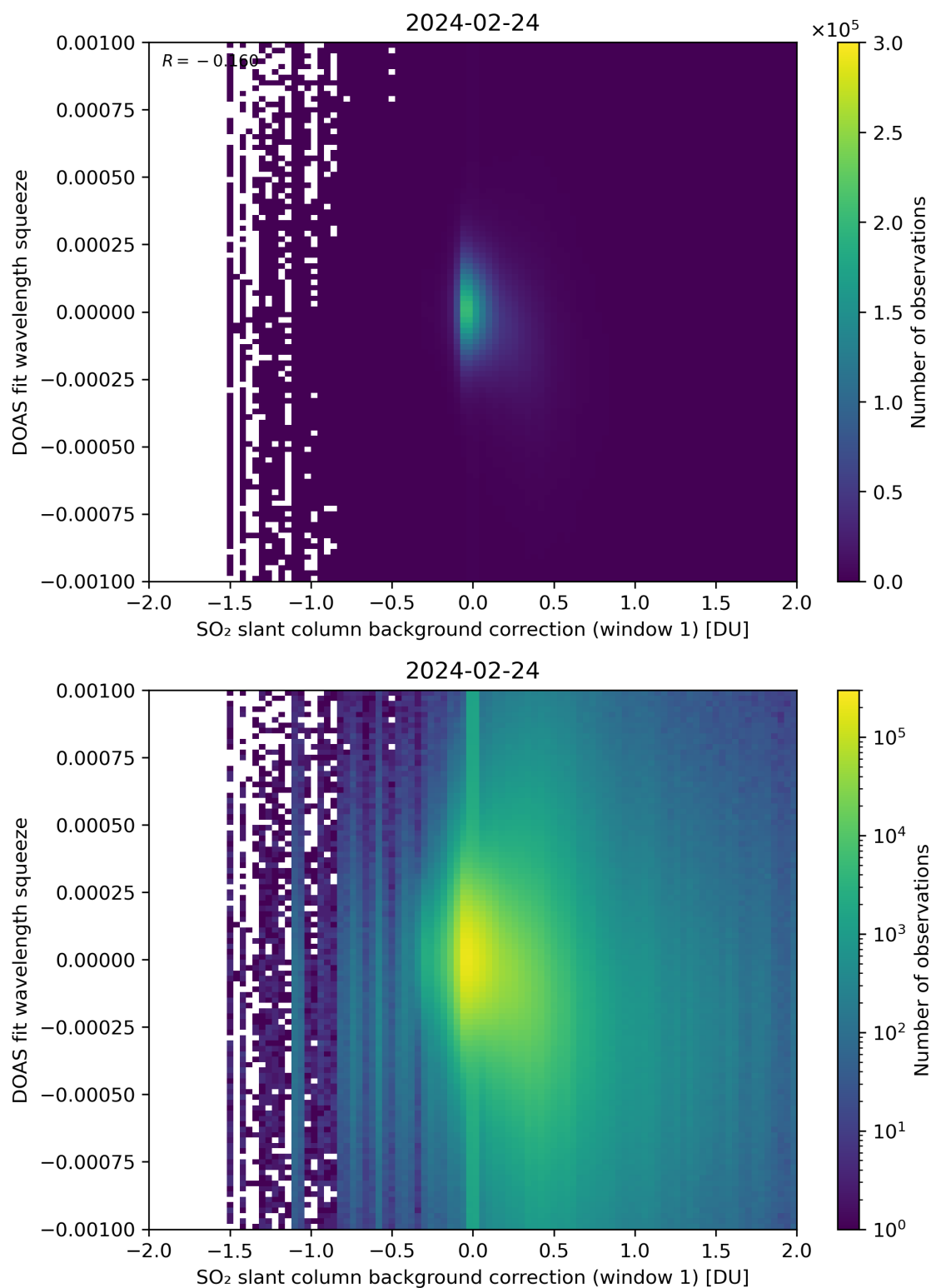
Figure 101: Scatter density plot of “SO 2 slant column background correction (window 1)” against “DOAS fit wavelength squeeze” for 2024-02-23 to 2024-02-25.
