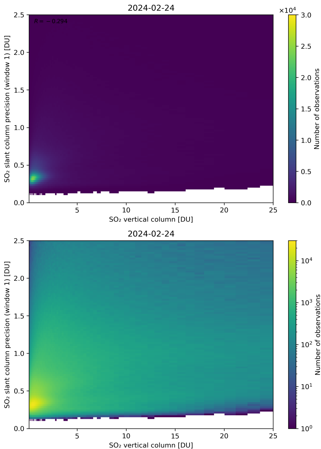
Figure 301: Scatter density plot of “SO 2 vertical column” against “SO 2 slant column precision (window 1)” for 2024-02-23 to 2024-02-25.
