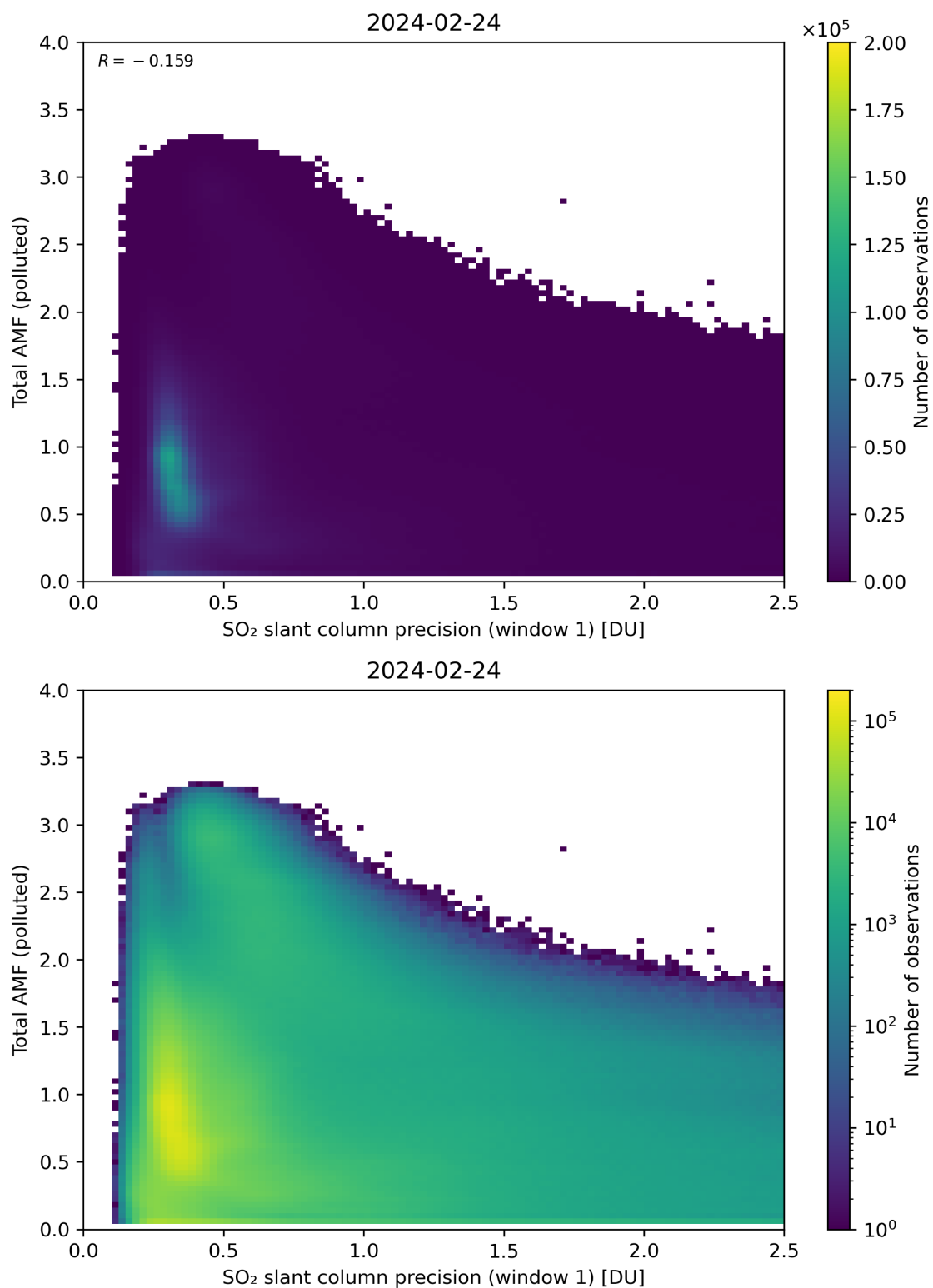
Figure 230: Scatter density plot of “SO 2 slant column precision (window 1)” against “Total AMF (polluted)” for 2024-02-23 to 2024-02-25.
