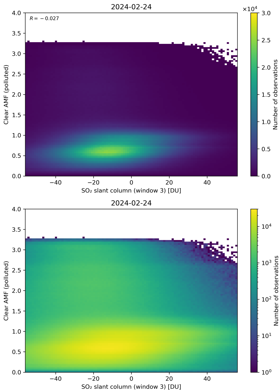
Figure 265: Scatter density plot of “SO 2 slant column (window 3)” against “Clear AMF (polluted)” for 2024-02-23 to 2024-02-25.
