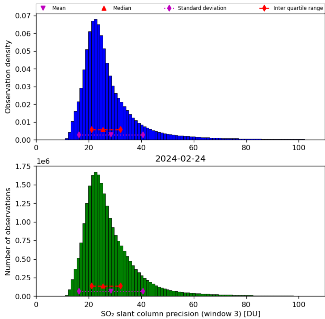
Figure 65: Histogram of “SO 2 slant column precision (window 3)” for 2024-02-23 to 2024-02-25
