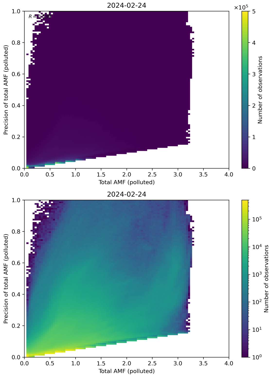
Figure 272: Scatter density plot of “Total AMF (polluted)” against “Precision of total AMF (polluted)” for 2024-02-23 to 2024-02-25.
