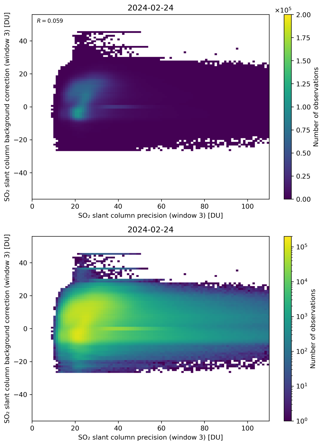
Figure 257: Scatter density plot of “SO 2 slant column precision (window 3)” against “SO 2 slant column background correction (window 3)” for 2024-02-23 to 2024-02-25.
