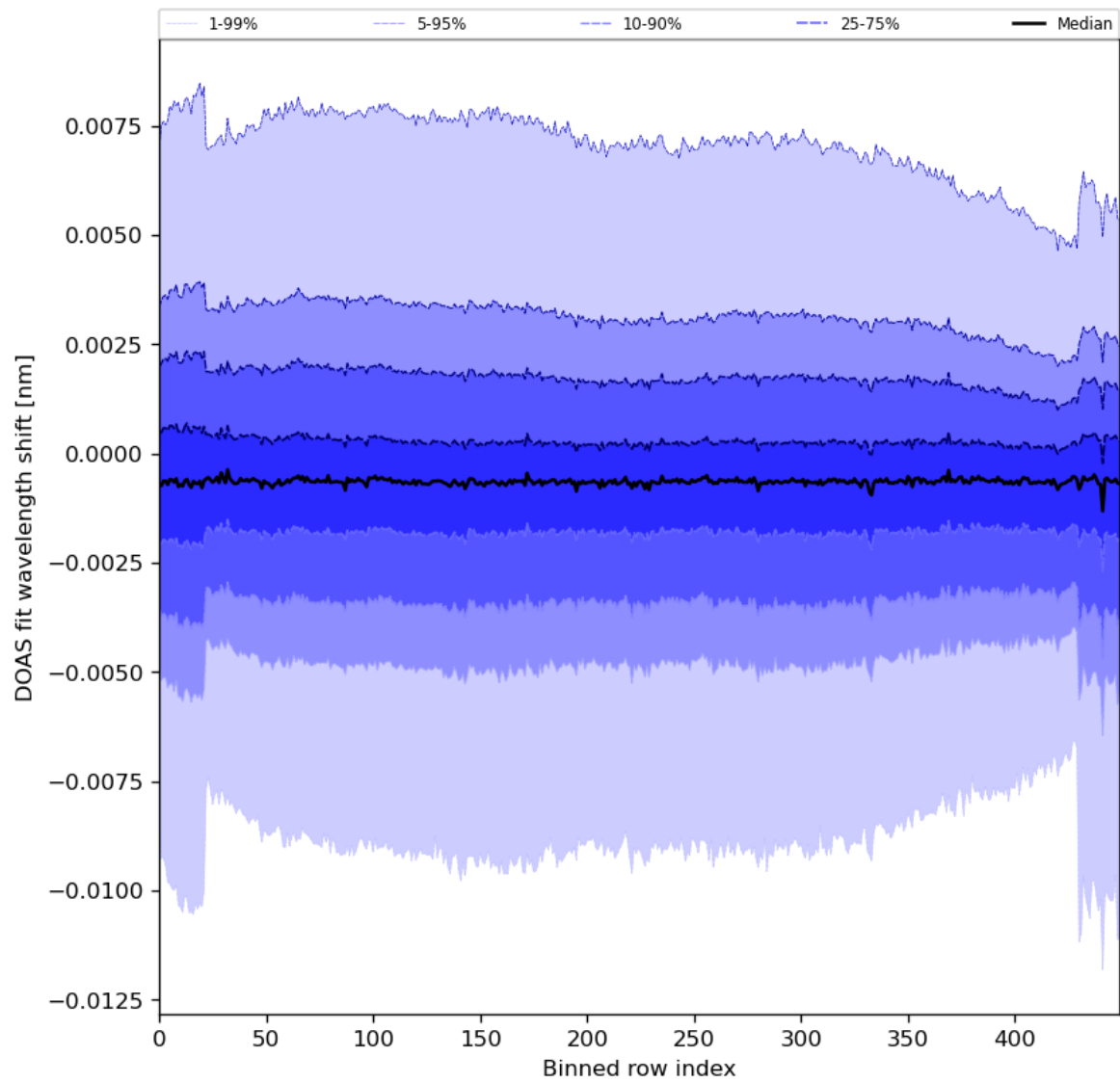
Figure 91: Along track statistics of “DOAS fit wavelength shift” for 2024-02-23 to 2024-02-25
