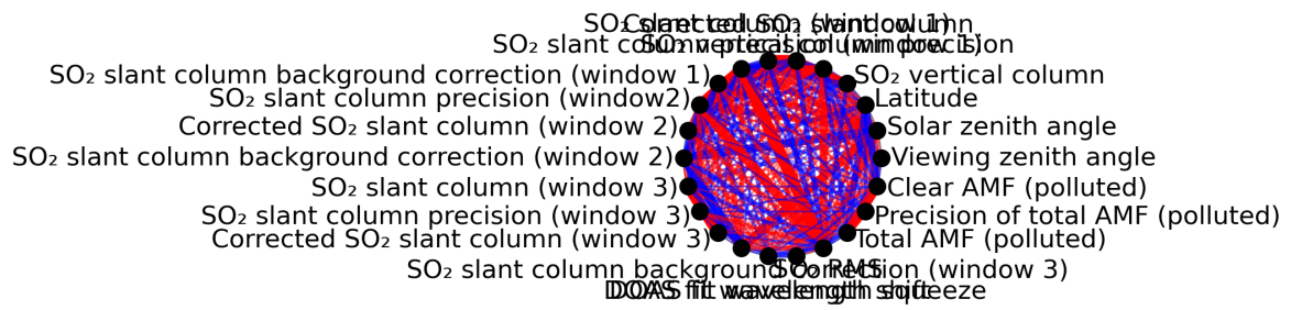
Figure 1: Map of correlation graph for 2024-02-23 to 2024-02-25.
