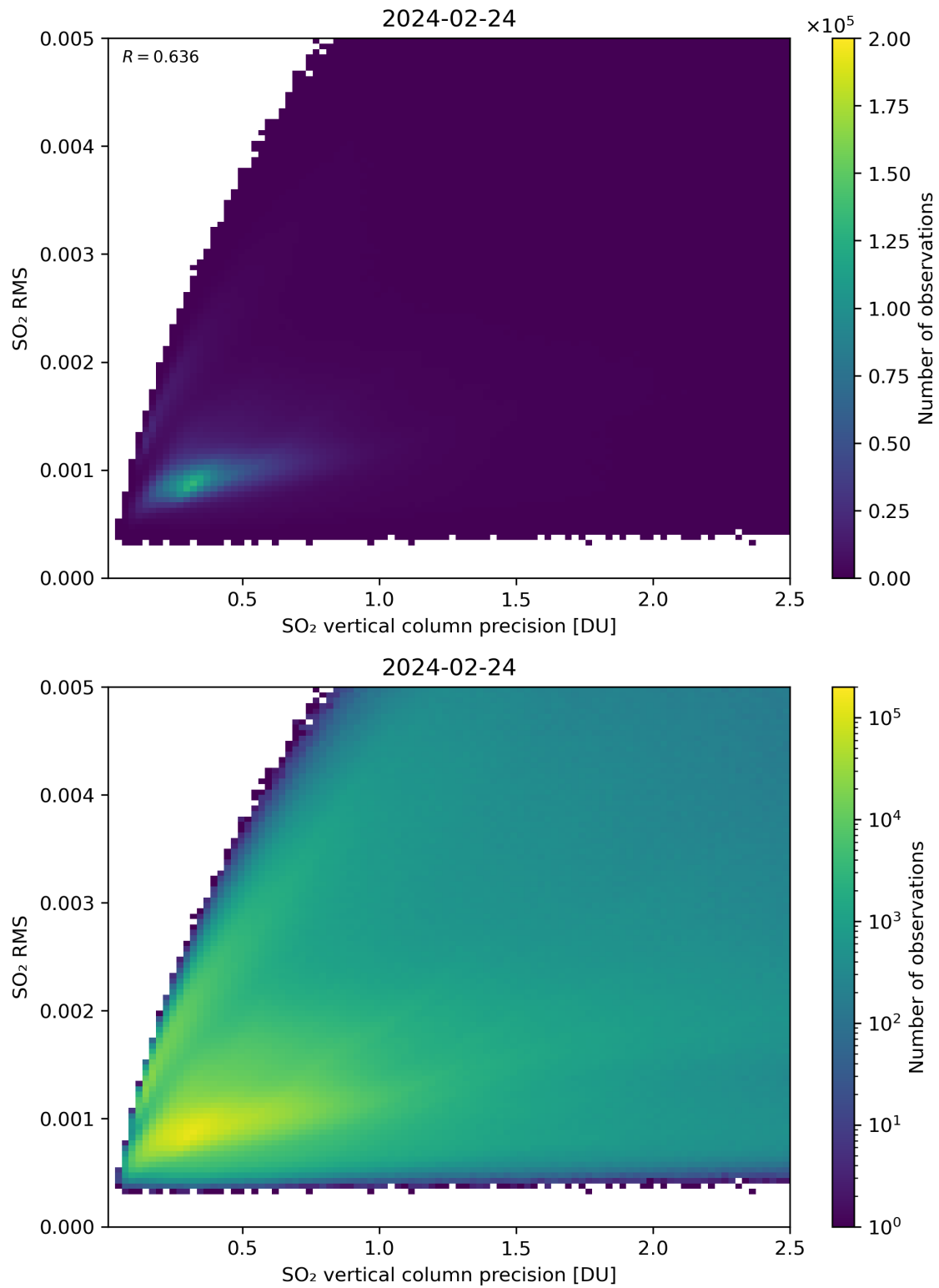
Figure 284: Scatter density plot of “SO 2 vertical column precision” against “SO 2 RMS” for 2024-02-23 to 2024-02-25.
