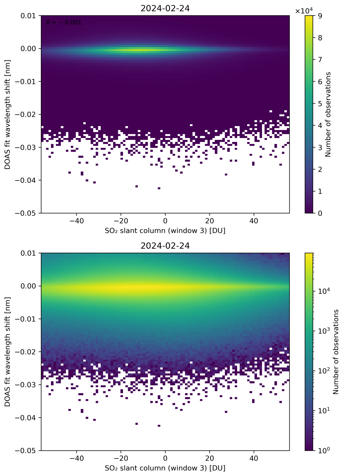
Figure 254: Scatter density plot of “SO 2 slant column (window 3)” against “DOAS fit wavelength shift” for 2024-02-23 to 2024-02-25.
