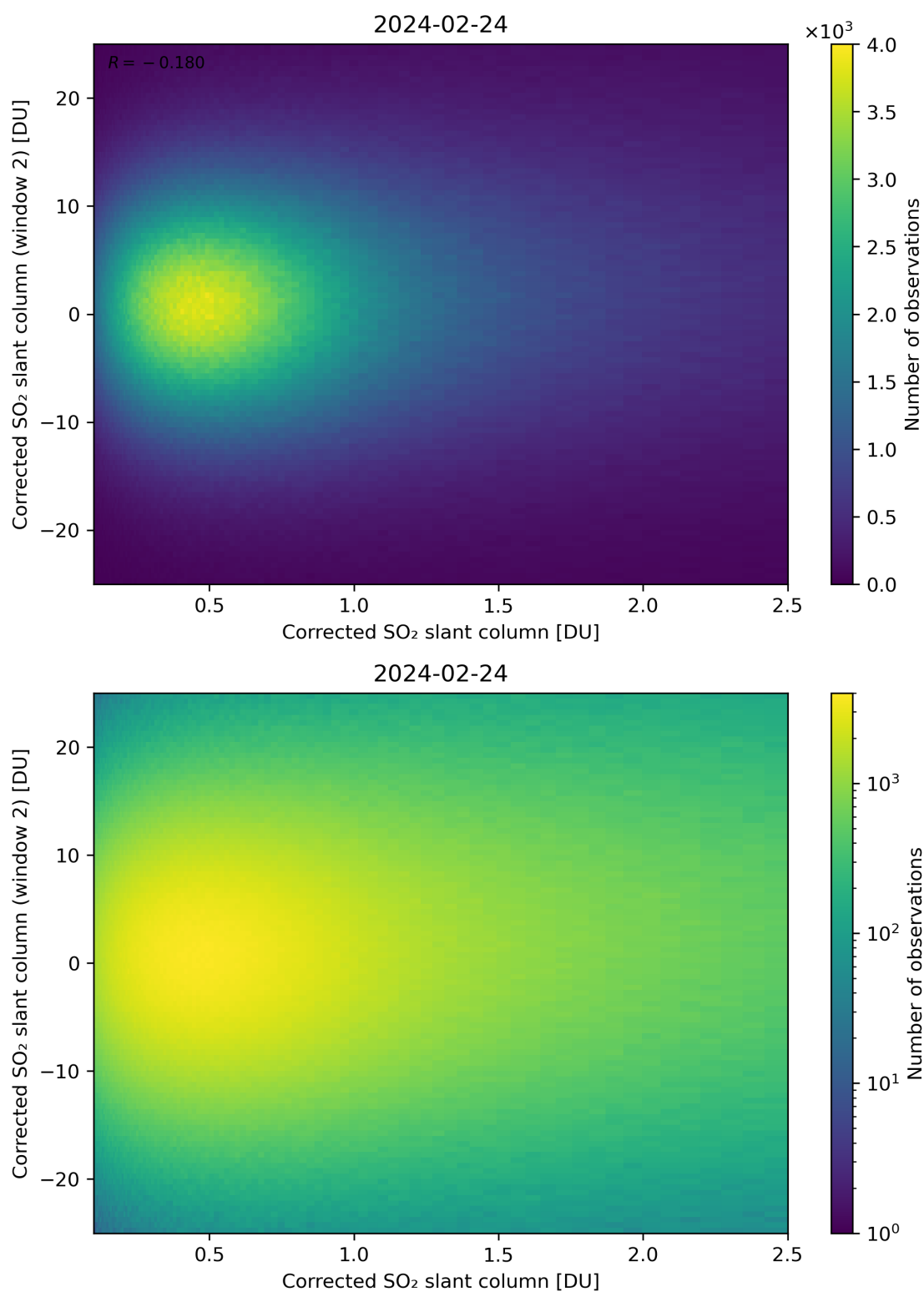
Figure 185: Scatter density plot of “Corrected SO 2 slant column” against “Corrected SO 2 slant column (window 2)” for 2024-02-23 to 2024-02-25.
