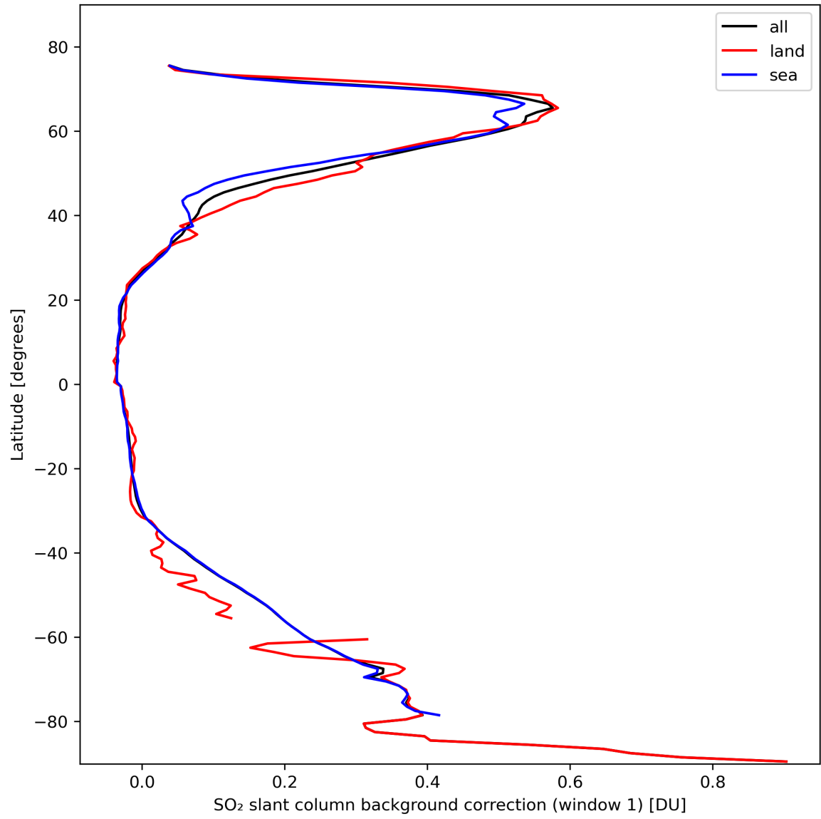
Figure 36: Zonal average of “SO 2 slant column background correction (window 1)” for 2024-02-23 to 2024-02-25.
