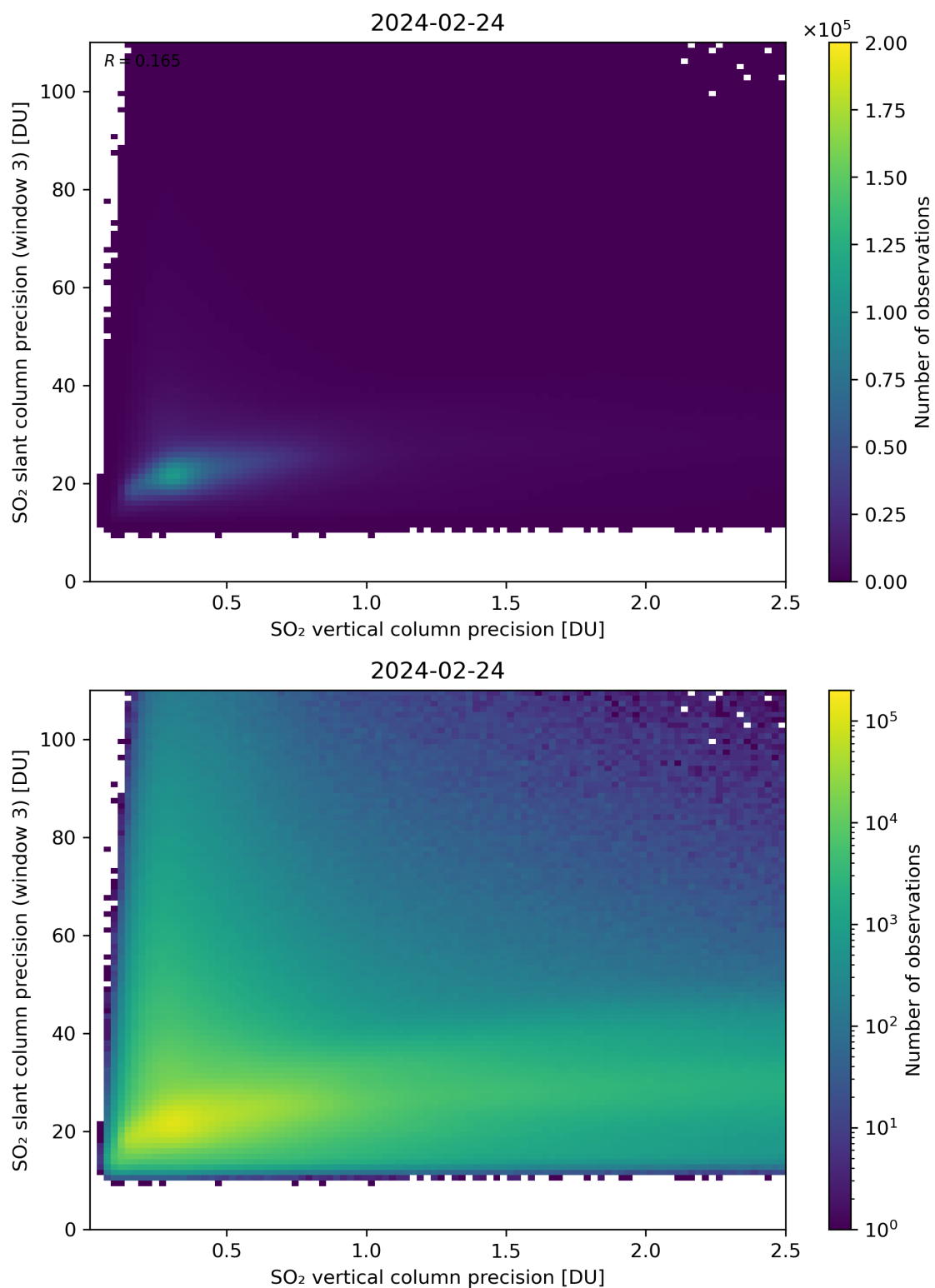
Figure 293: Scatter density plot of “SO 2 vertical column precision” against “SO 2 slant column precision (window 3)” for 2024-02-23 to 2024-02-25.
