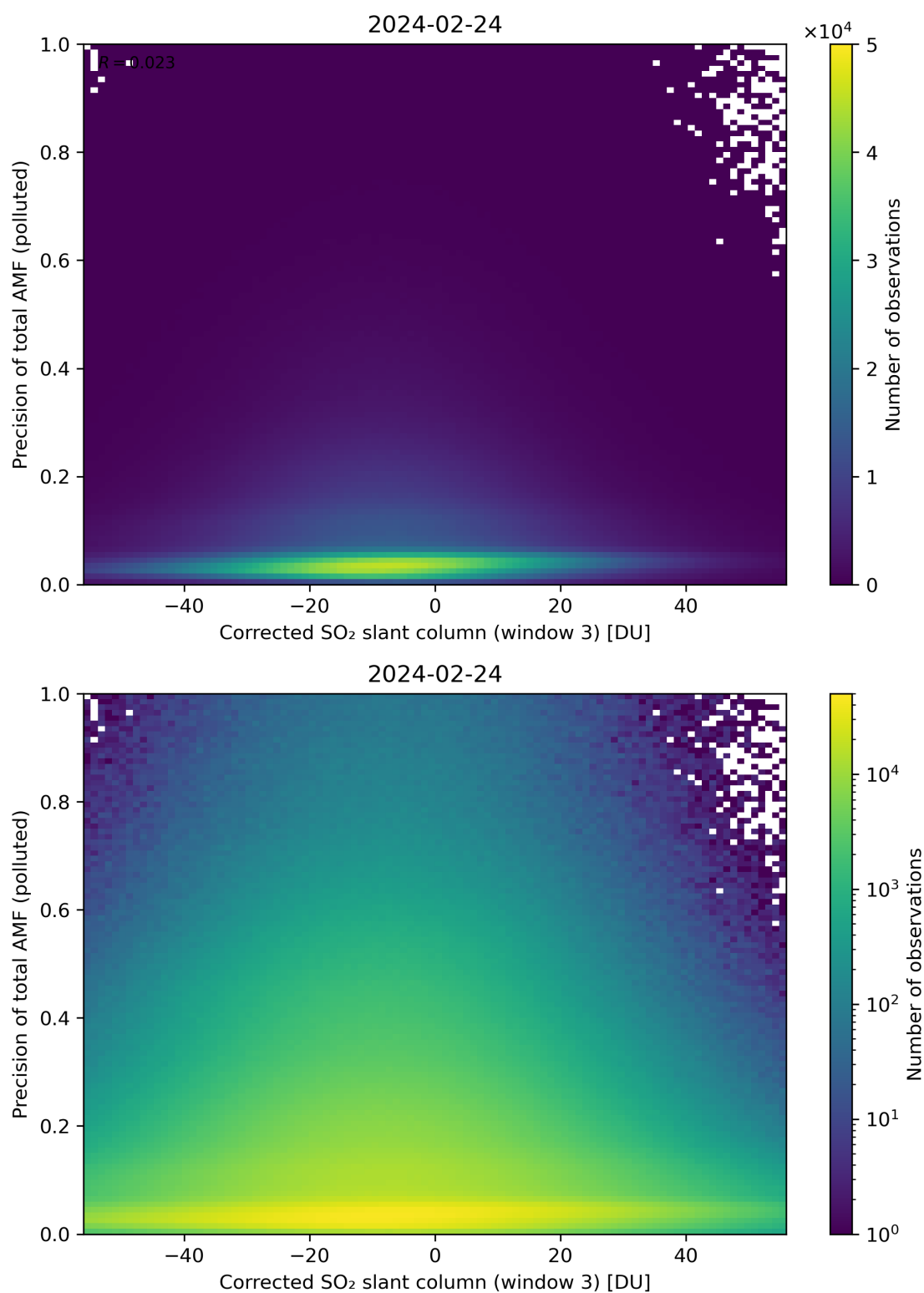
Figure 211: Scatter density plot of “Corrected SO 2 slant column (window 3)” against “Precision of total AMF (polluted)” for 2024-02-23 to 2024-02-25.
