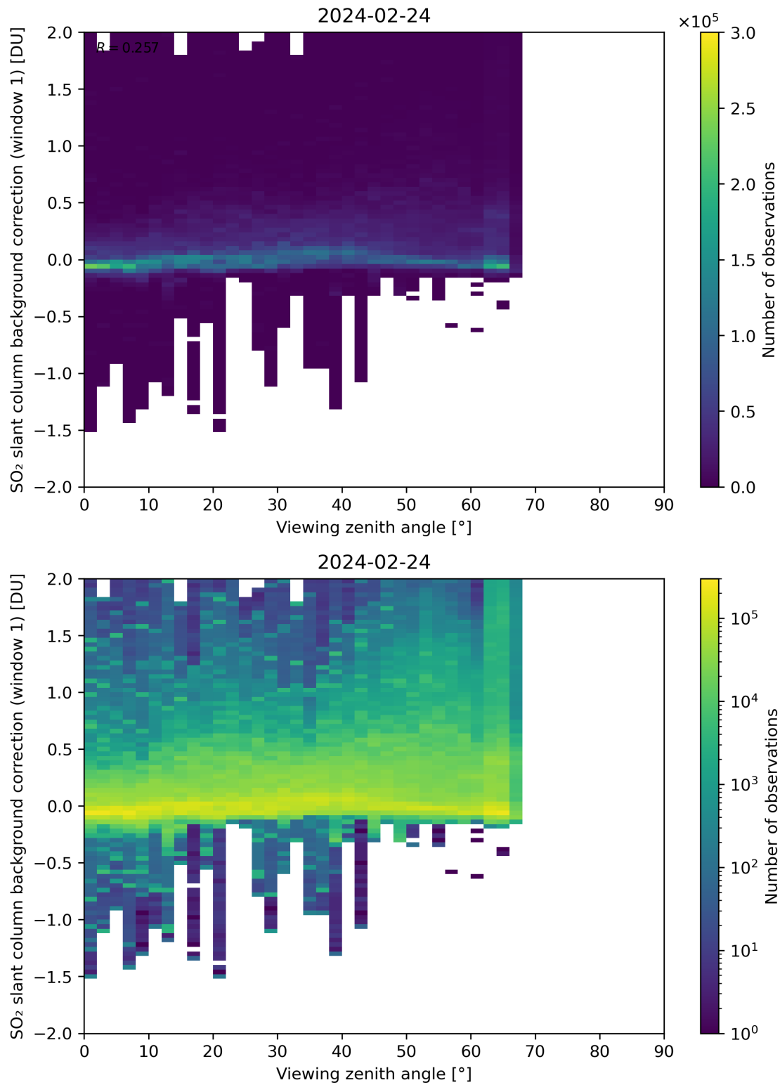
Figure 308: Scatter density plot of “Viewing zenith angle” against “SO 2 slant column background correction (window 1)” for 2024-02-23 to 2024-02-25.
