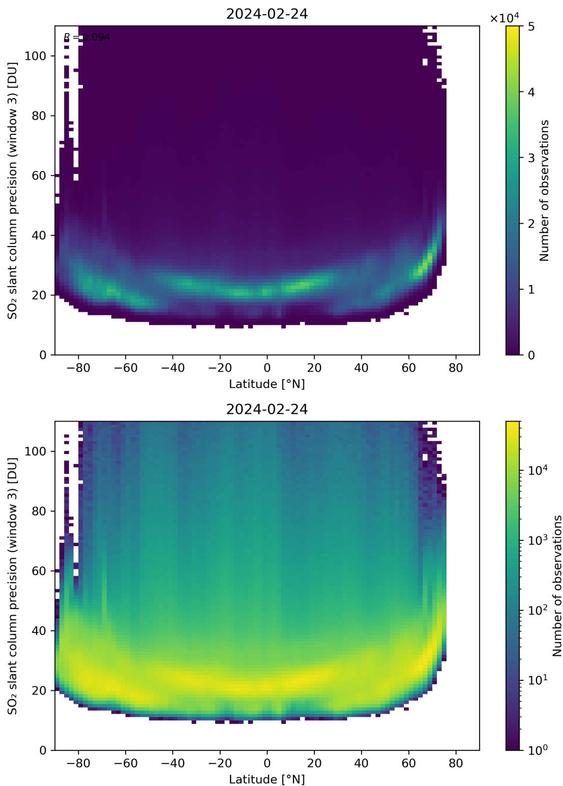
Figure 153: Scatter density plot of “Latitude” against “SO 2 slant column precision (window 3)” for 2024-02-23 to 2024-02-25.
