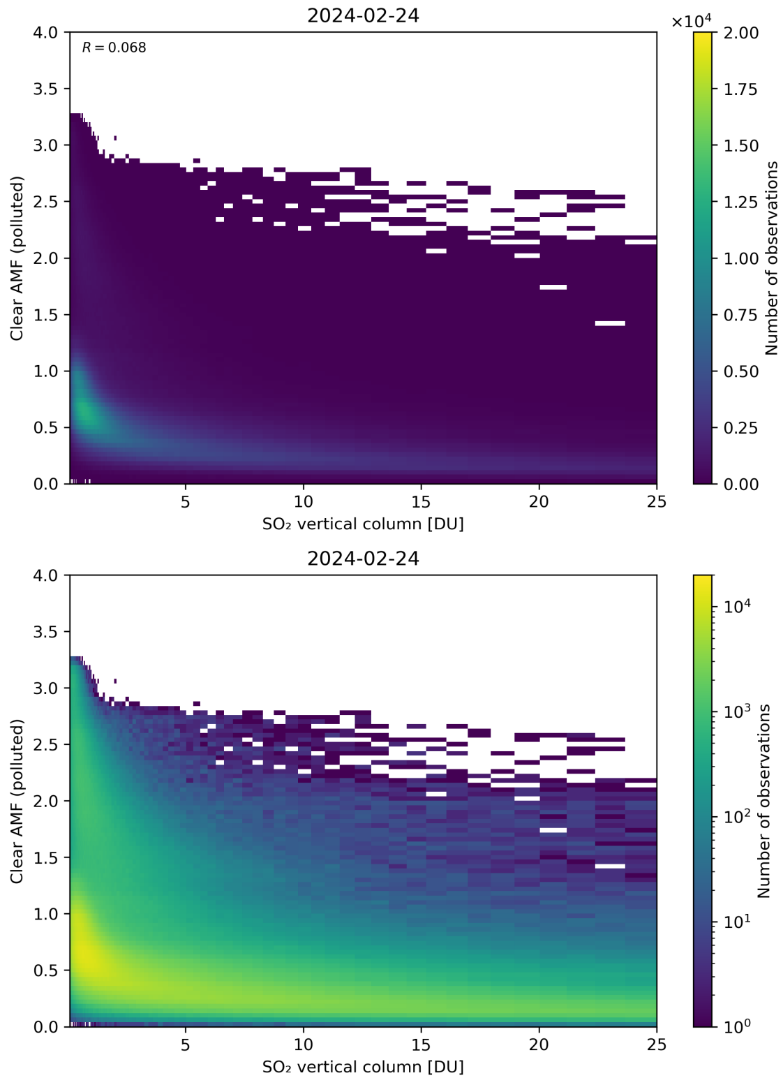
Figure 296: Scatter density plot of “SO 2 vertical column” against “Clear AMF (polluted)” for 2024-02-23 to 2024-02-25.
