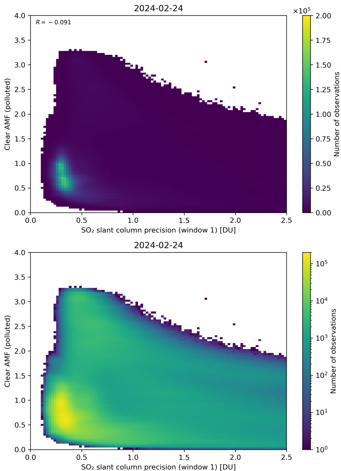
Figure 224: Scatter density plot of “SO 2 slant column precision (window 1)” against “Clear AMF (polluted)” for 2024-02-23 to 2024-02-25.
