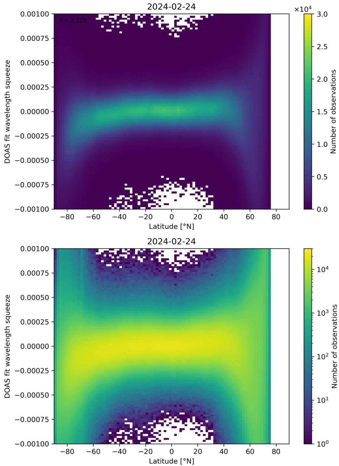
Figure 143: Scatter density plot of “Latitude” against “DOAS fit wavelength squeeze” for 2024-02-23 to 2024-02-25.
