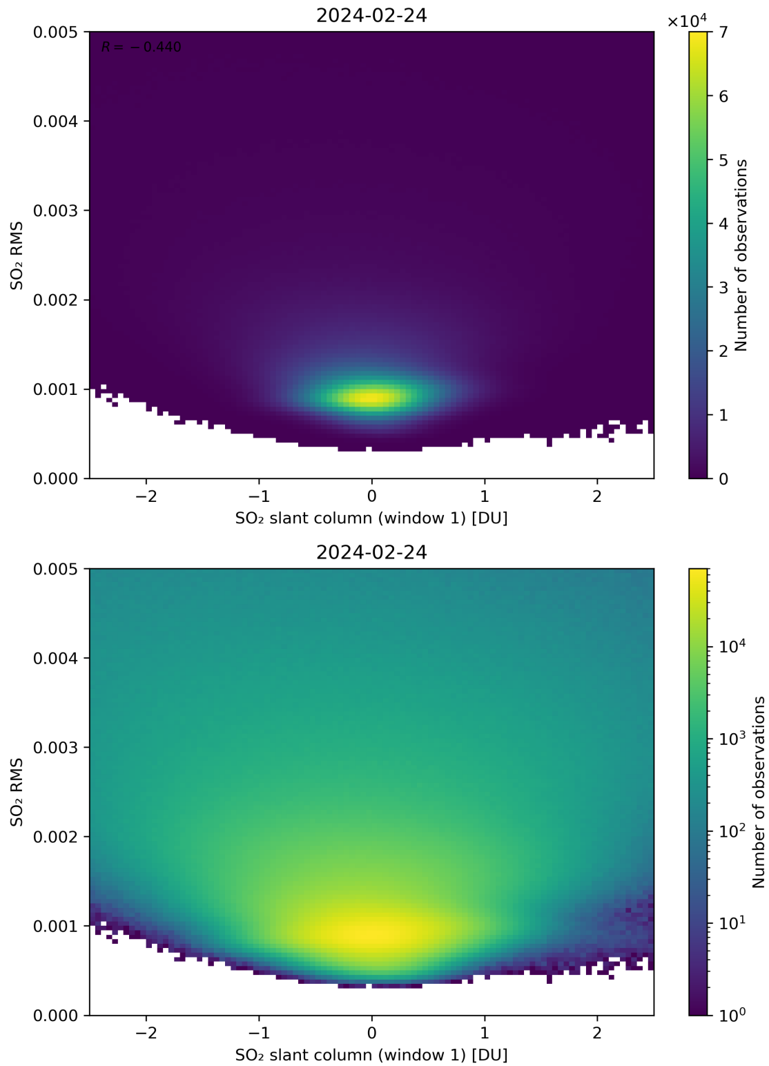
Figure 217: Scatter density plot of “SO 2 slant column (window 1)” against “SO 2 RMS” for 2024-02-23 to 2024-02-25.
