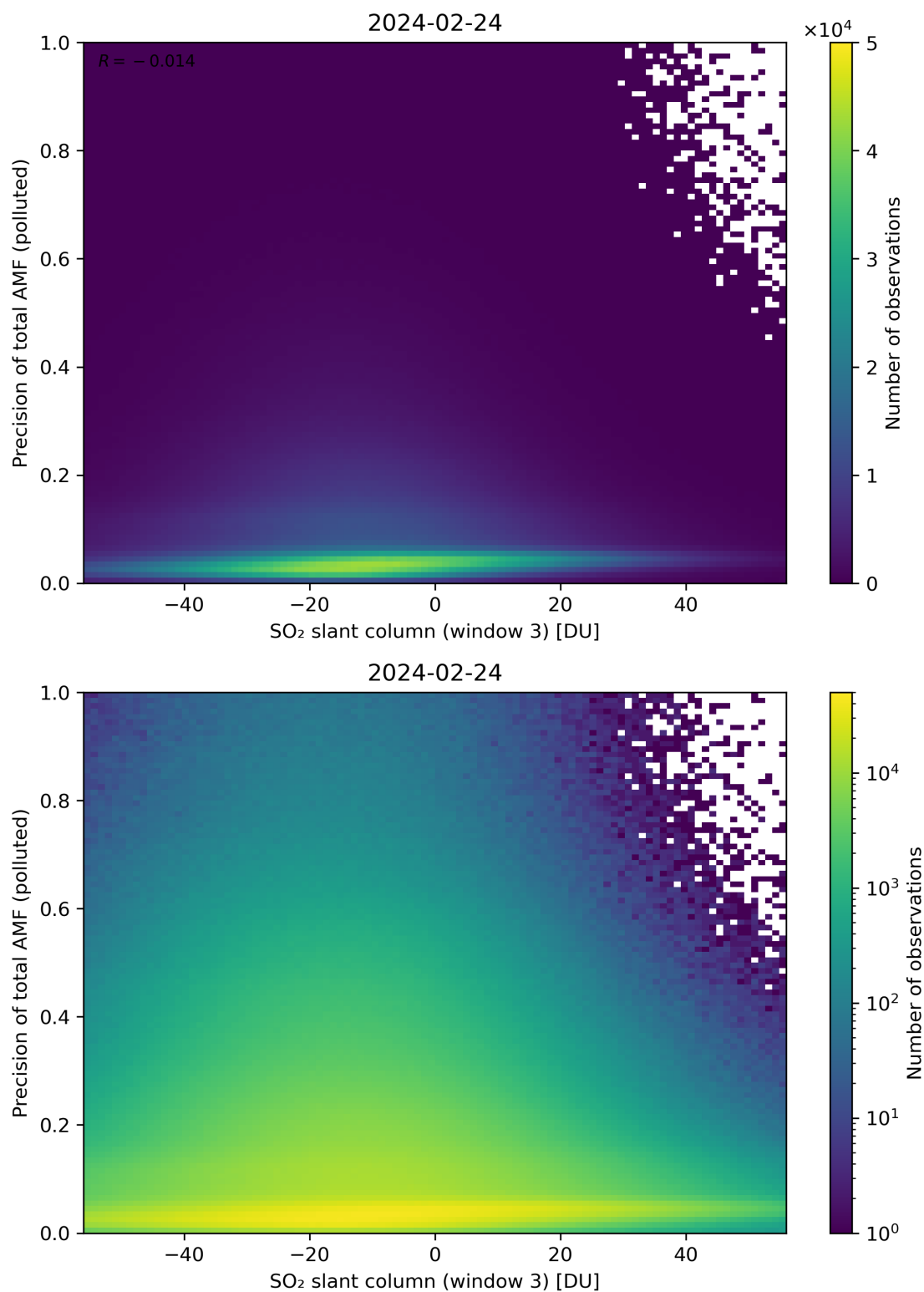
Figure 269: Scatter density plot of “SO 2 slant column (window 3)” against “Precision of total AMF (polluted)” for 2024-02-23 to 2024-02-25.
