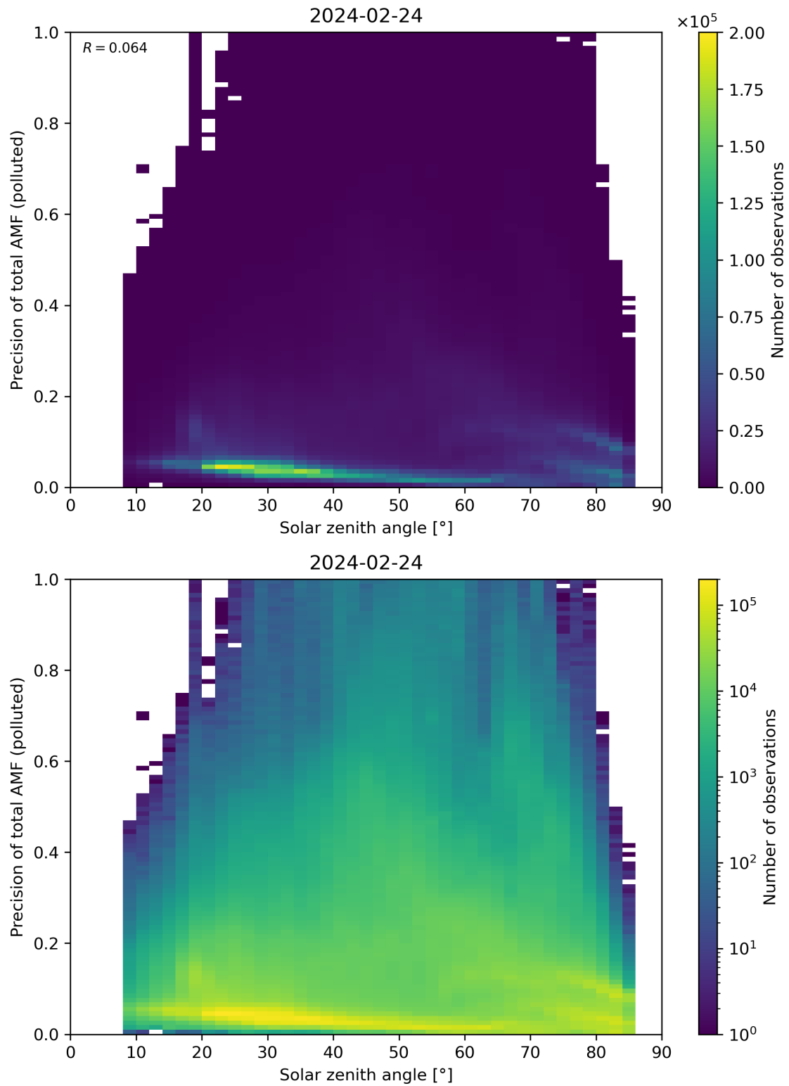
Figure 175: Scatter density plot of “Solar zenith angle” against “Precision of total AMF (polluted)” for 2024-02-23 to 2024-02-25.
