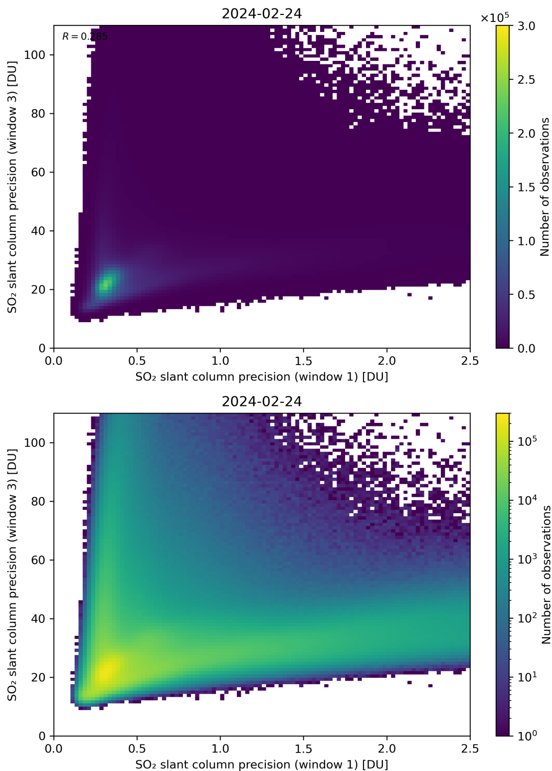
Figure 229: Scatter density plot of “SO 2 slant column precision (window 1)” against “SO 2 slant column precision (window 3)” for 2024-02-23 to 2024-02-25.
