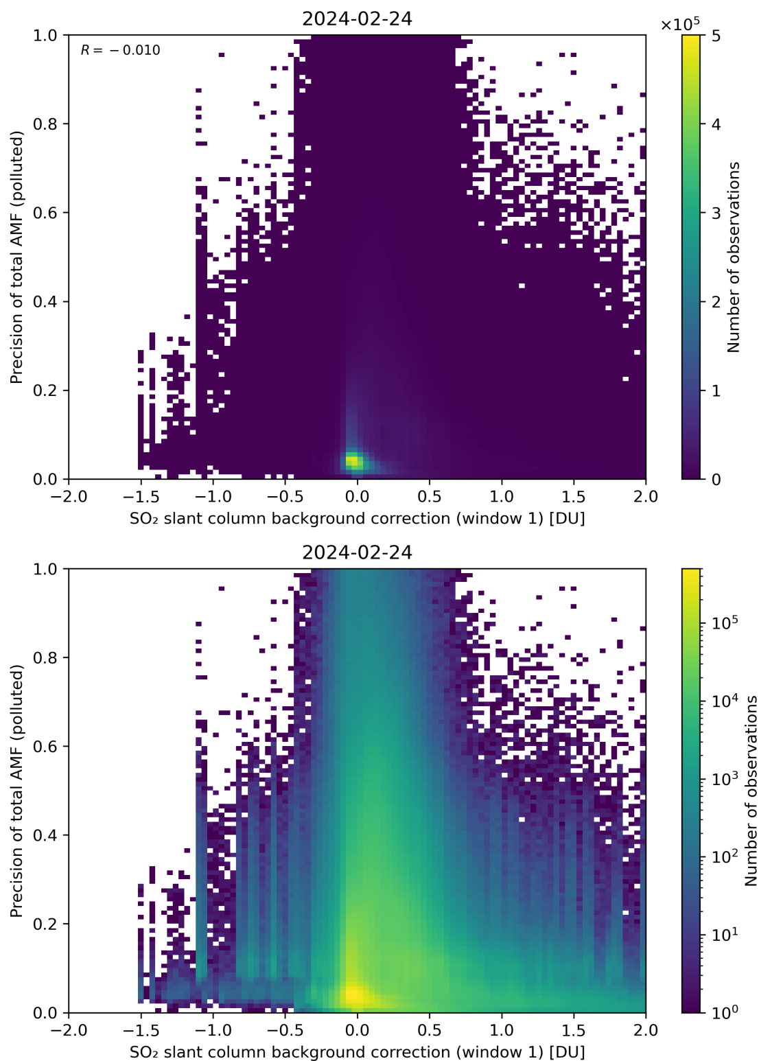
Figure 110: Scatter density plot of “SO 2 slant column background correction (window 1)” against “Precision of total AMF (polluted)” for 2024-02-23 to 2024-02-25.
