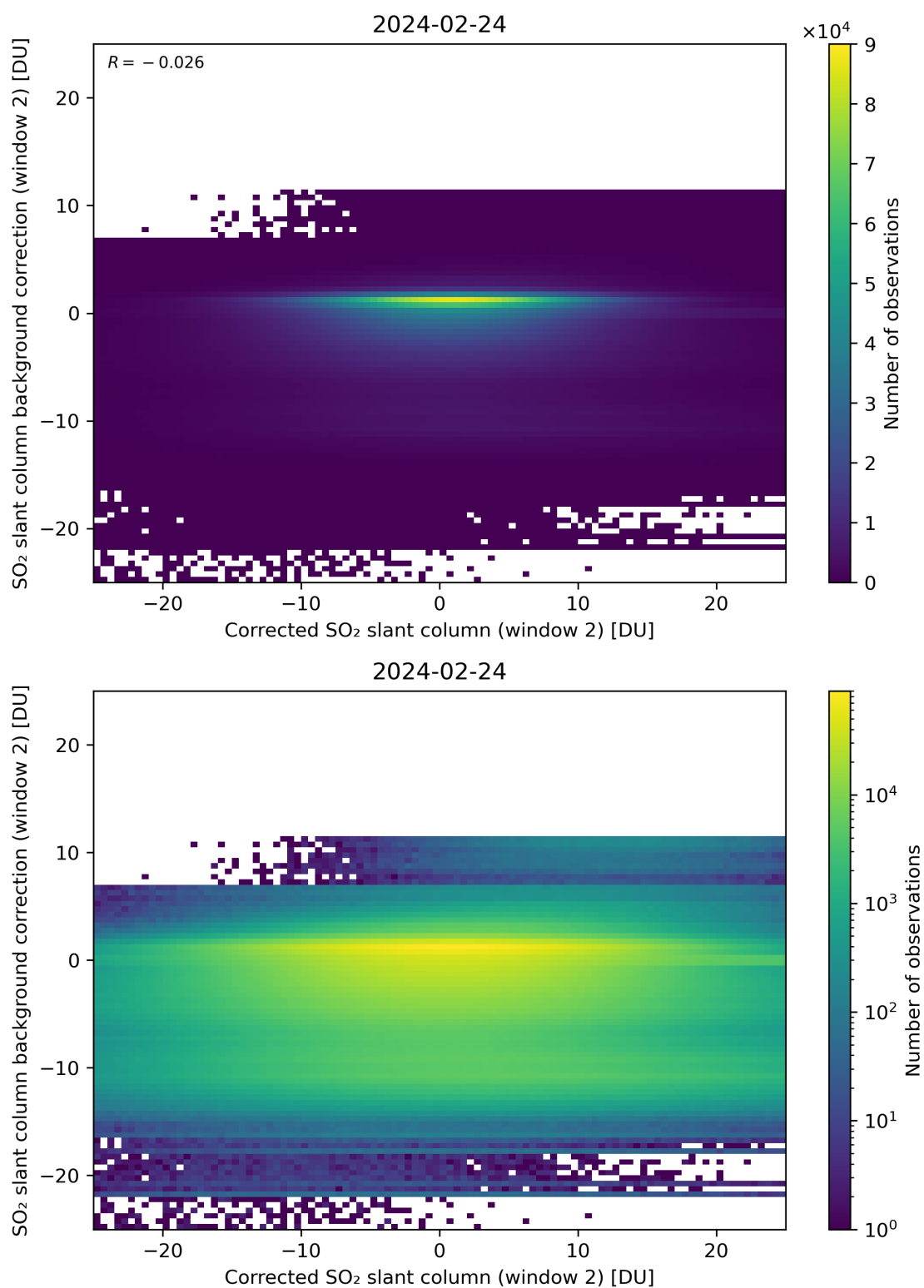
Figure 194: Scatter density plot of “Corrected SO 2 slant column (window 2)” against “SO 2 slant column background correction (window 2)” for 2024-02-23 to 2024-02-25.
