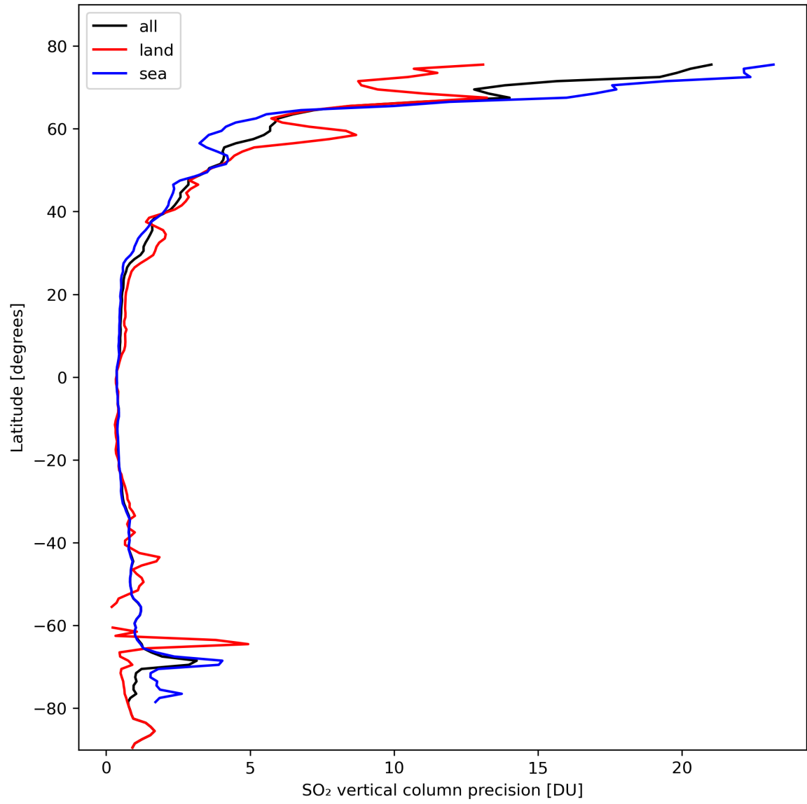
Figure 31: Zonal average of “SO 2 vertical column precision” for 2024-02-23 to 2024-02-25.
