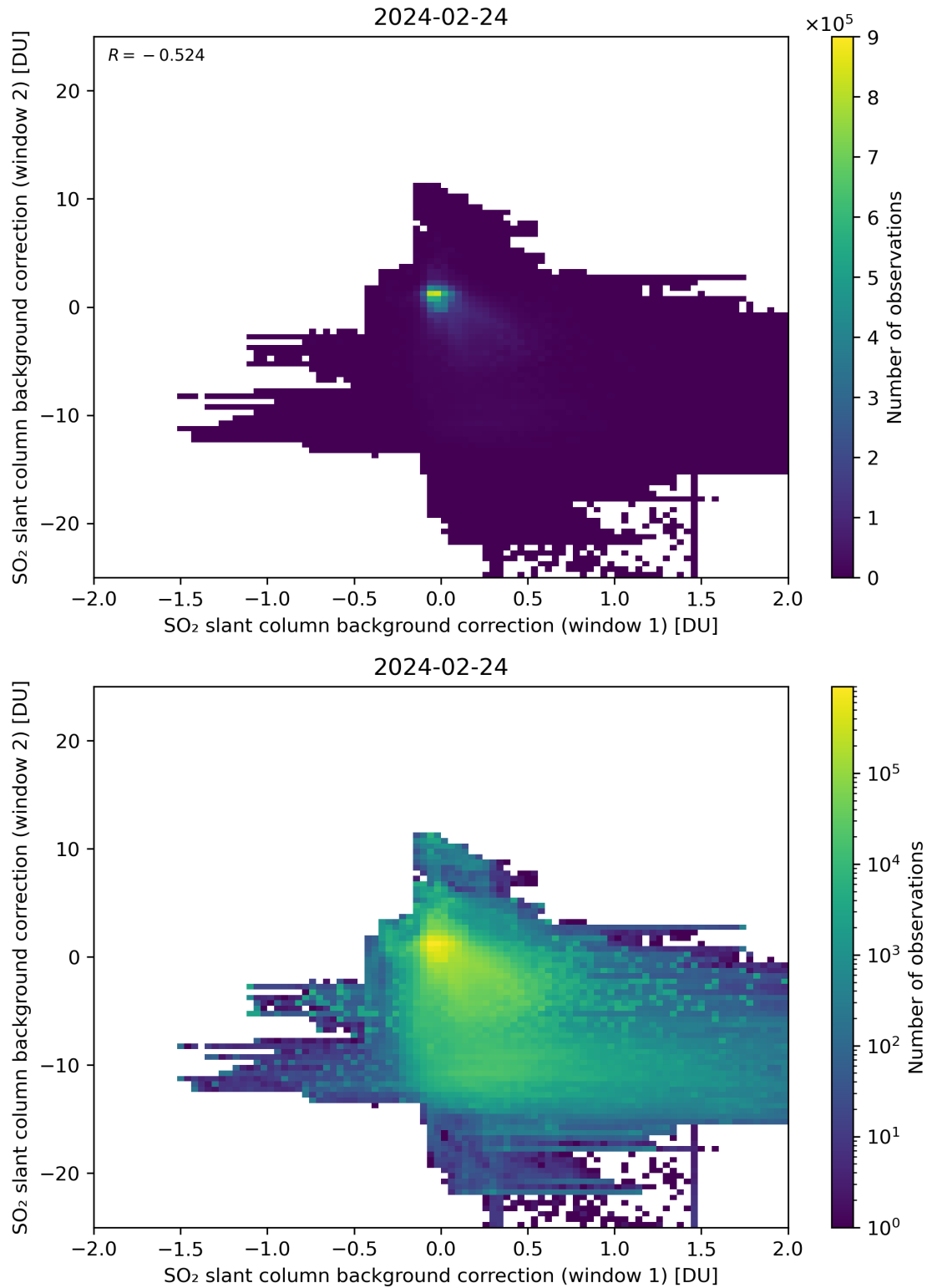
Figure 98: Scatter density plot of “SO 2 slant column background correction (window 1)” against “SO 2 slant column background correction (window 2)” for 2024-02-23 to 2024-02-25.
