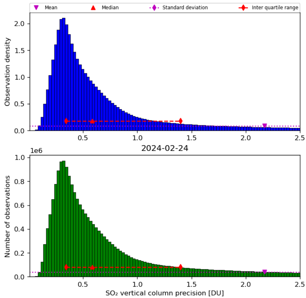
Figure 54: Histogram of “SO 2 vertical column precision” for 2024-02-23 to 2024-02-25
