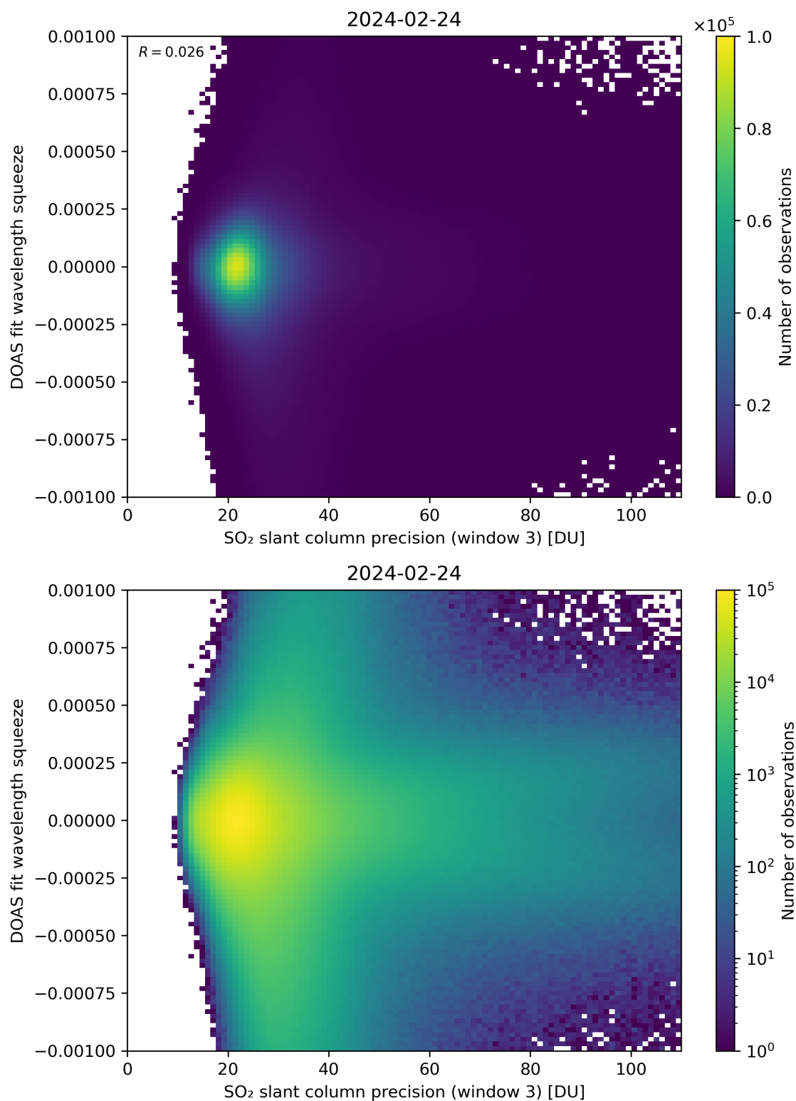
Figure 259: Scatter density plot of “SO 2 slant column precision (window 3)” against “DOAS fit wavelength squeeze” for 2024-02-23 to 2024-02-25.
