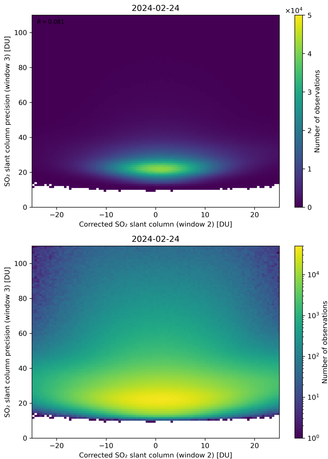
Figure 202: Scatter density plot of “Corrected SO 2 slant column (window 2)” against “SO 2 slant column precision (window 3)” for 2024-02-23 to 2024-02-25.
