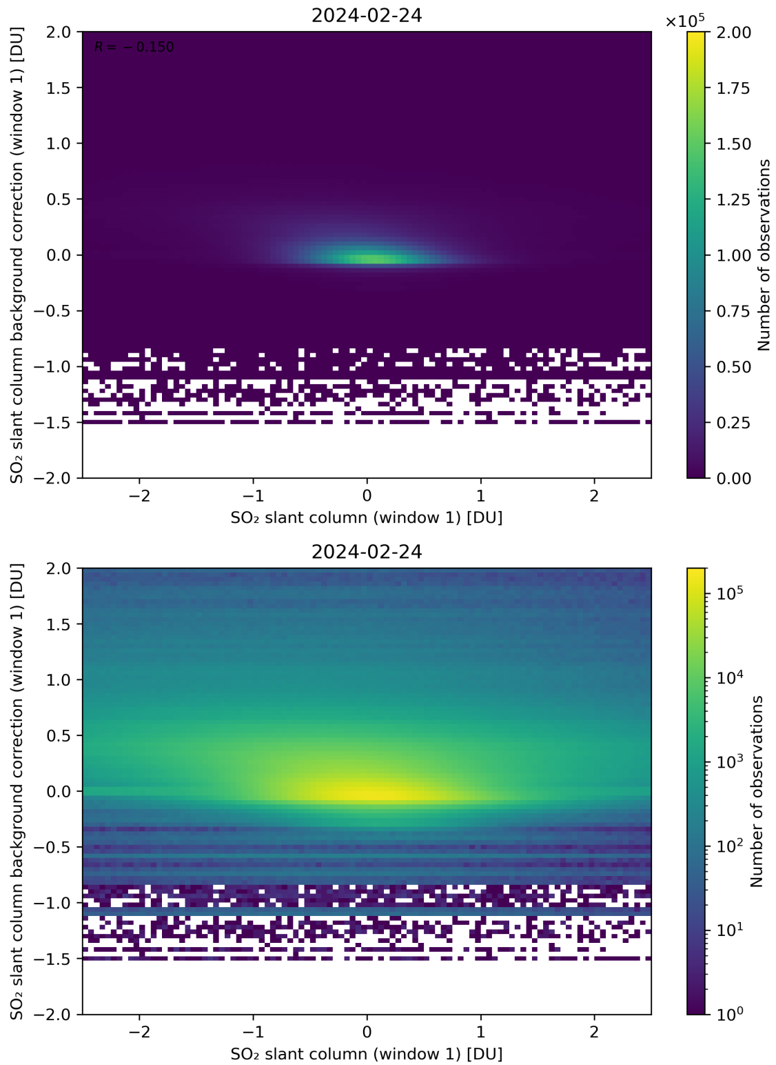
Figure 212: Scatter density plot of “SO 2 slant column (window 1)” against “SO 2 slant column background correction (window 1)” for 2024-02-23 to 2024-02-25.
