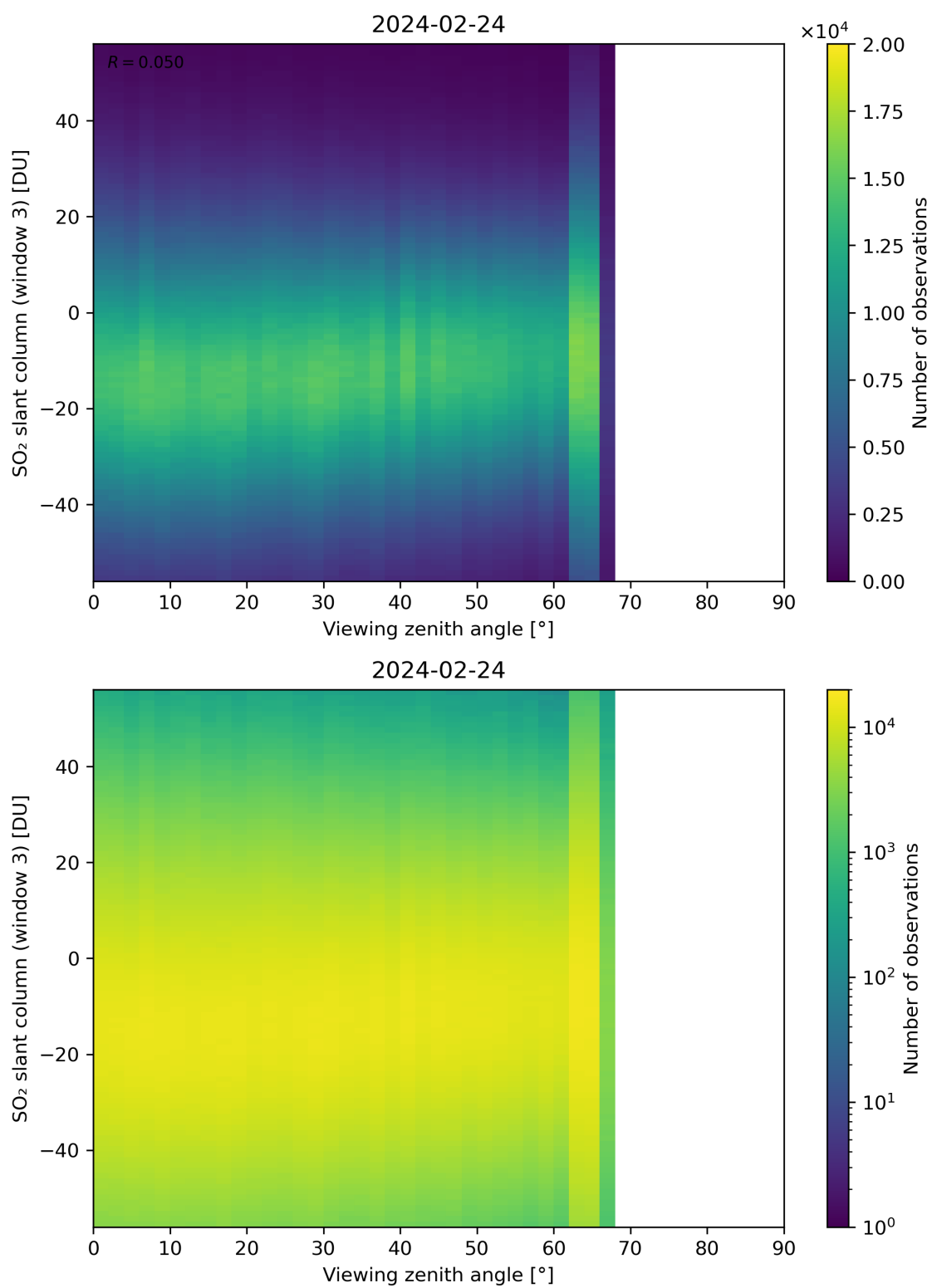
Figure 323: Scatter density plot of “Viewing zenith angle” against “SO 2 slant column (window 3)” for 2024-02-23 to 2024-02-25.
