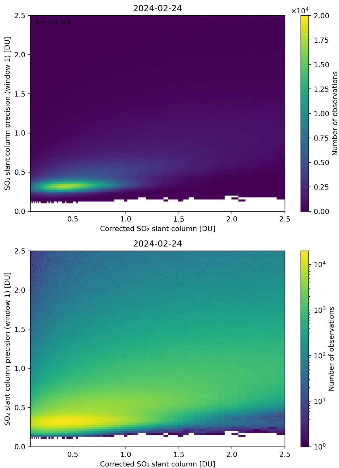
Figure 188: Scatter density plot of “Corrected SO 2 slant column” against “SO 2 slant column precision (window 1)” for 2024-02-23 to 2024-02-25.
