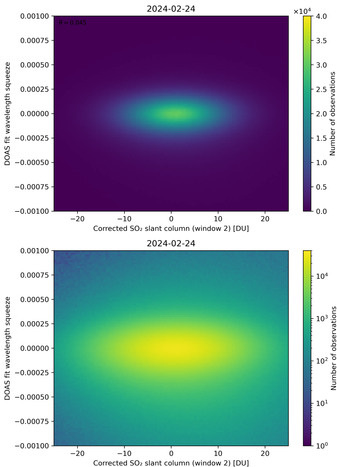
Figure 197: Scatter density plot of “Corrected SO 2 slant column (window 2)” against “DOAS fit wavelength squeeze” for 2024-02-23 to 2024-02-25.
