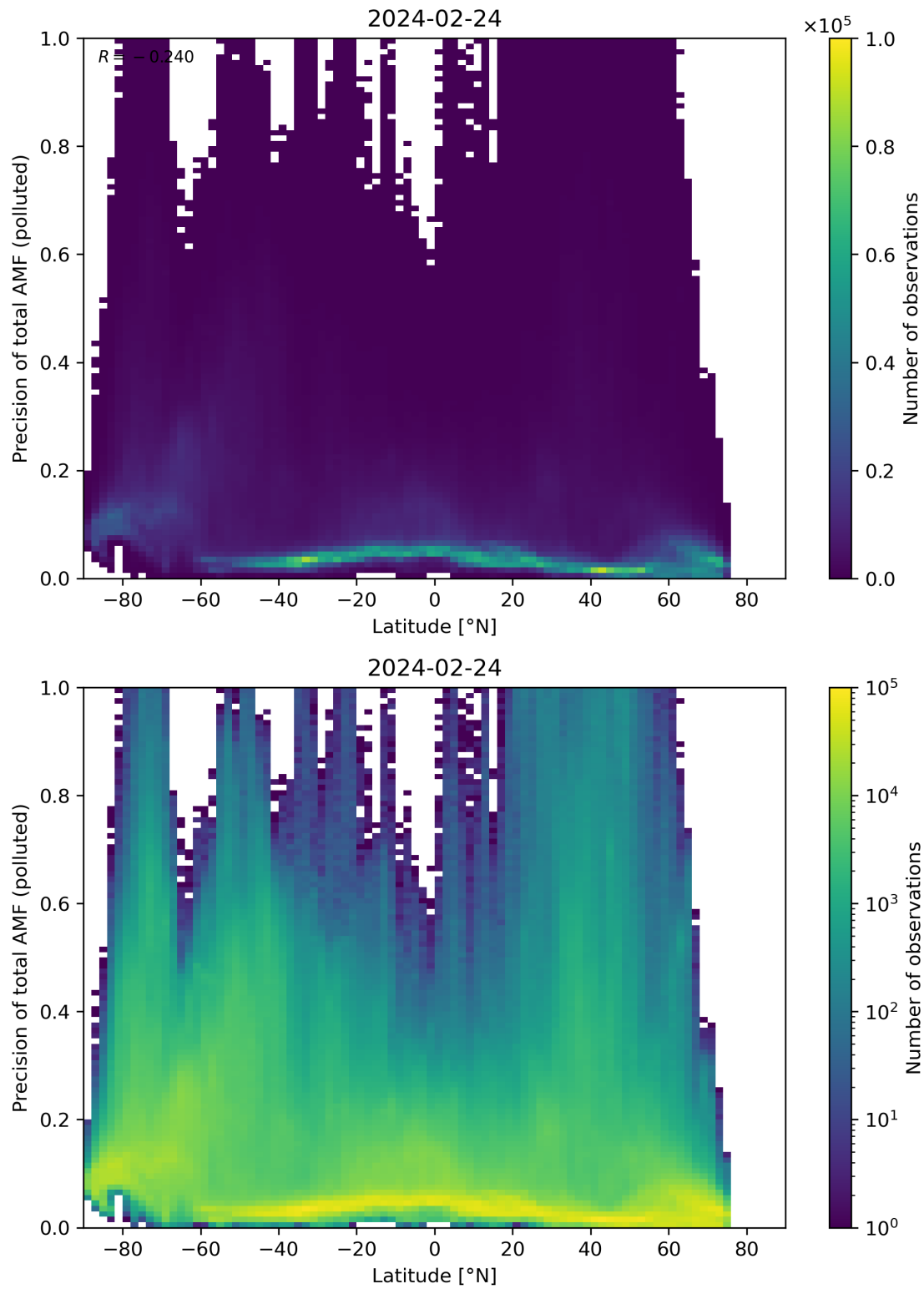
Figure 155: Scatter density plot of “Latitude” against “Precision of total AMF (polluted)” for 2024-02-23 to 2024-02-25.
