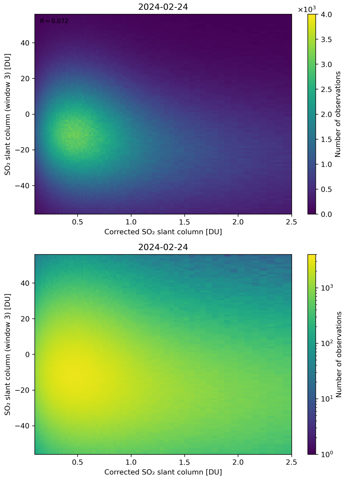
Figure 190: Scatter density plot of “Corrected SO 2 slant column” against “SO 2 slant column (window 3)” for 2024-02-23 to 2024-02-25.
