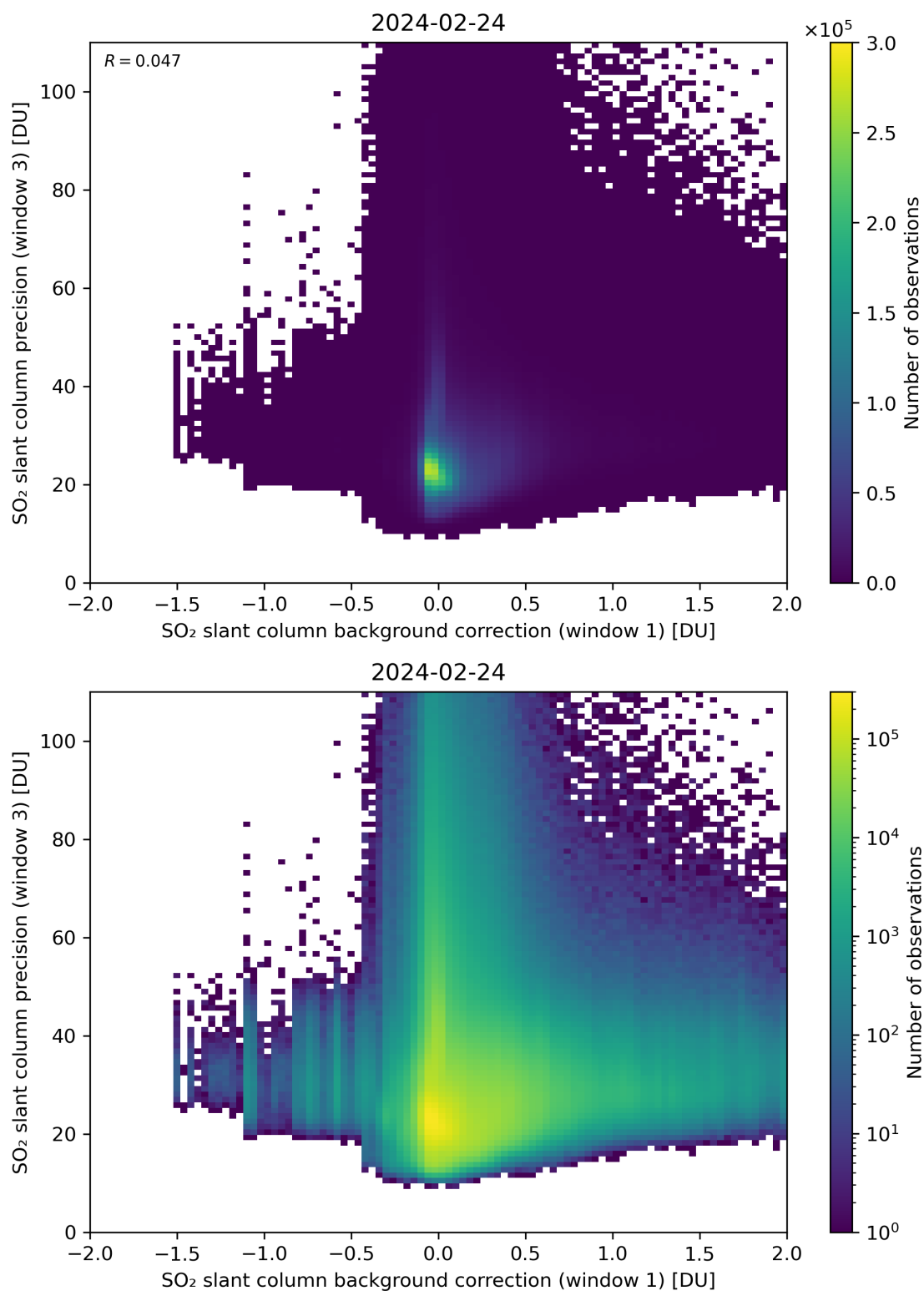
Figure 108: Scatter density plot of “SO 2 slant column background correction (window 1)” against “SO 2 slant column precision (window 3)” for 2024-02-23 to 2024-02-25.
