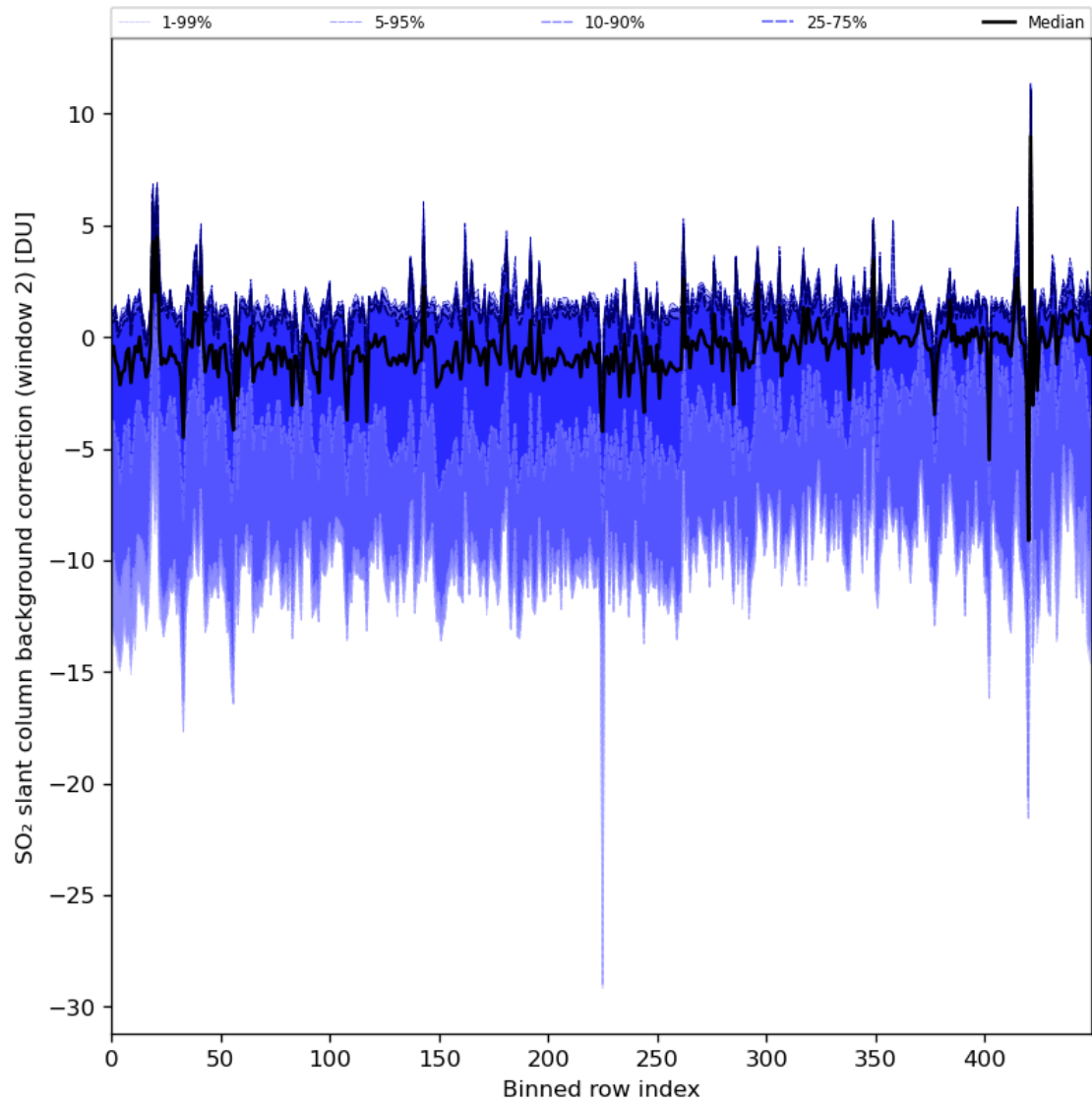
Figure 86: Along track statistics of “SO 2 slant column background correction (window 2)” for 2024-02-23 to 2024-02-25
