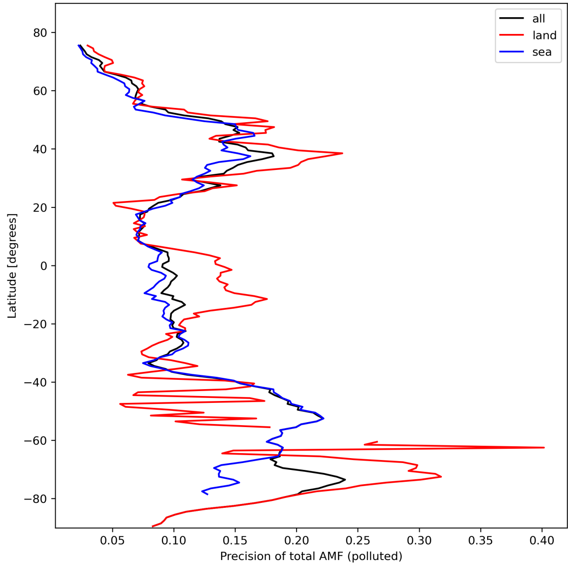
Figure 49: Zonal average of “Precision of total AMF (polluted)” for 2024-02-23 to 2024-02-25.
