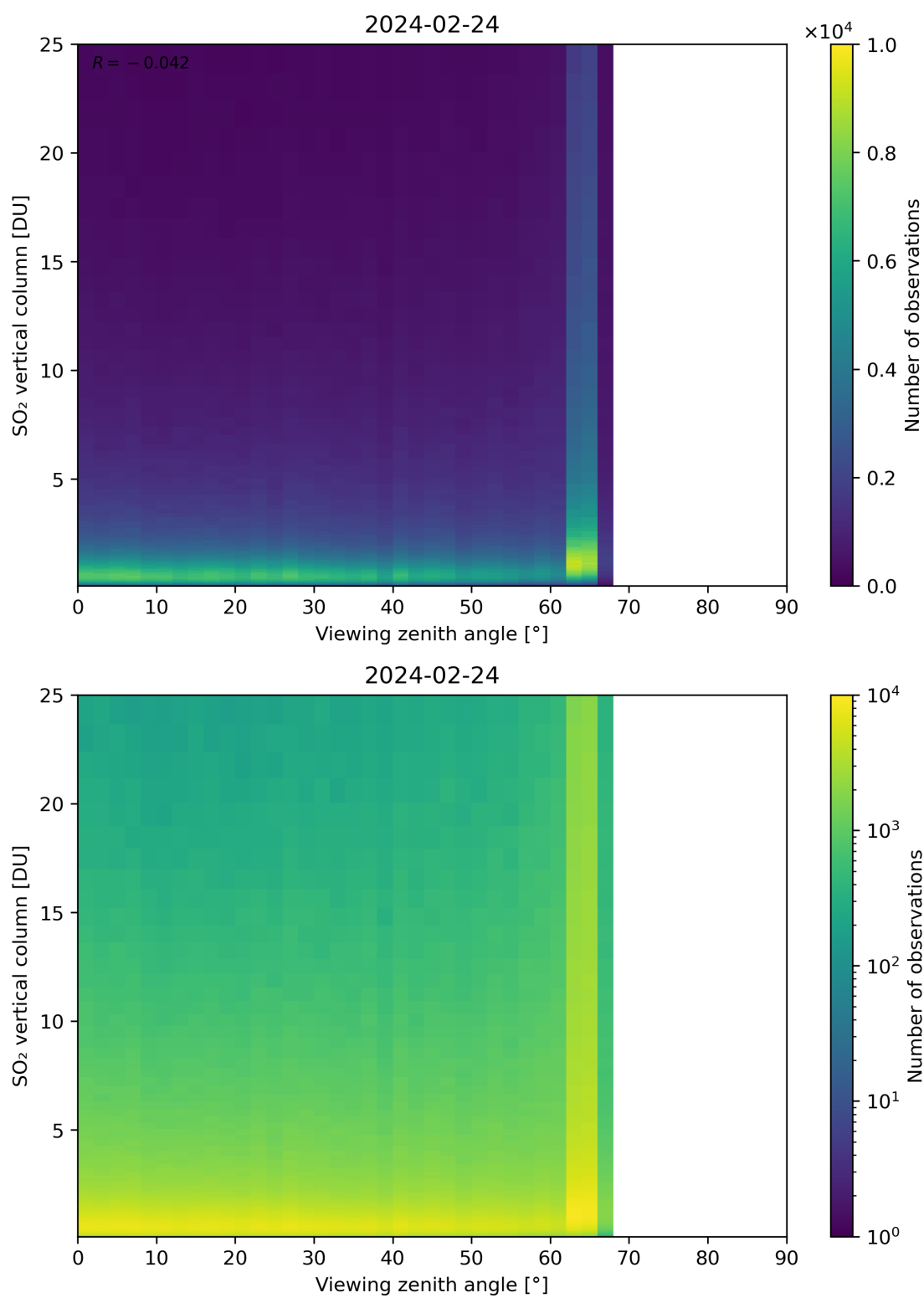
Figure 327: Scatter density plot of “Viewing zenith angle” against “SO 2 vertical column” for 2024-02-23 to 2024-02-25.
