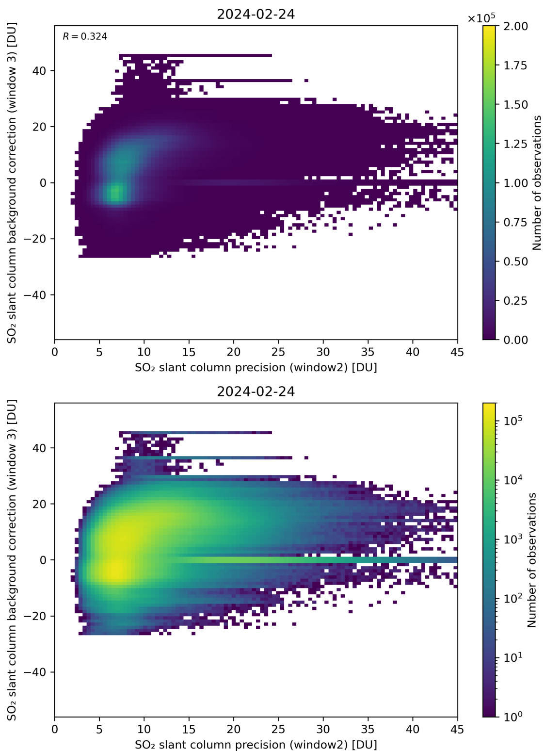
Figure 242: Scatter density plot of “SO 2 slant column precision (window2)” against “SO 2 slant column background correction (window 3)” for 2024-02-23 to 2024-02-25.
