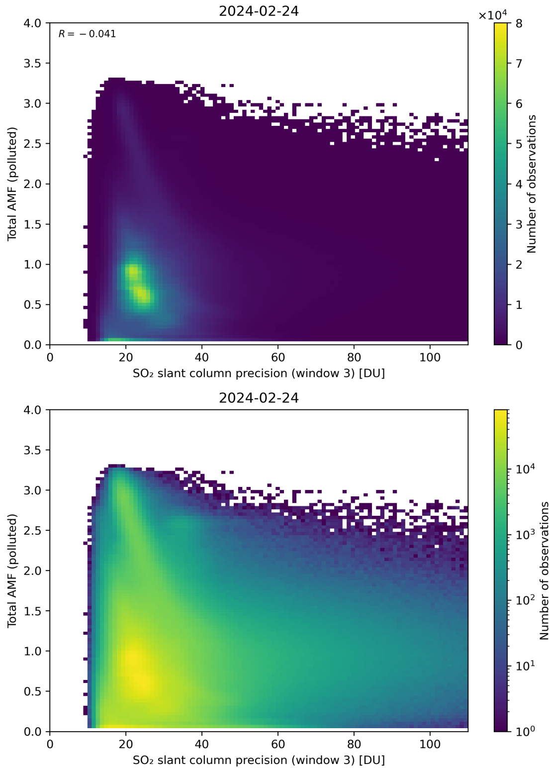
Figure 263: Scatter density plot of “SO 2 slant column precision (window 3)” against “Total AMF (polluted)” for 2024-02-23 to 2024-02-25.
