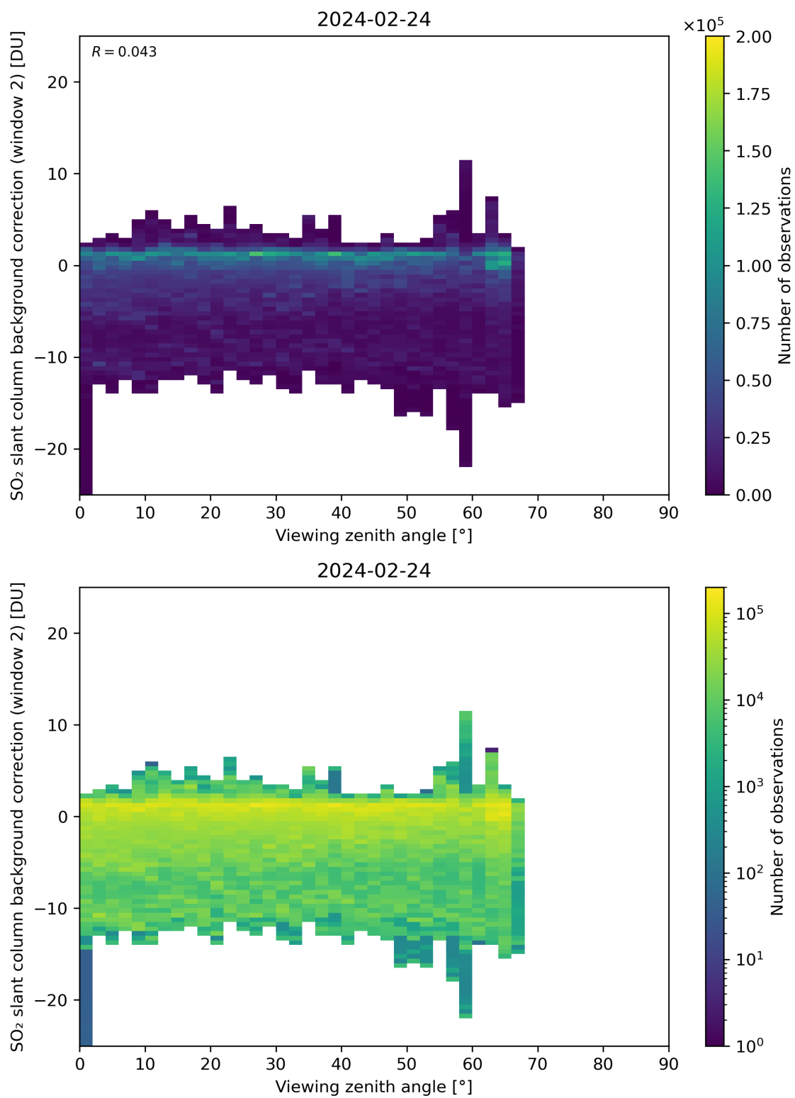
Figure 309: Scatter density plot of “Viewing zenith angle” against “SO 2 slant column background correction (window 2)” for 2024-02-23 to 2024-02-25.
