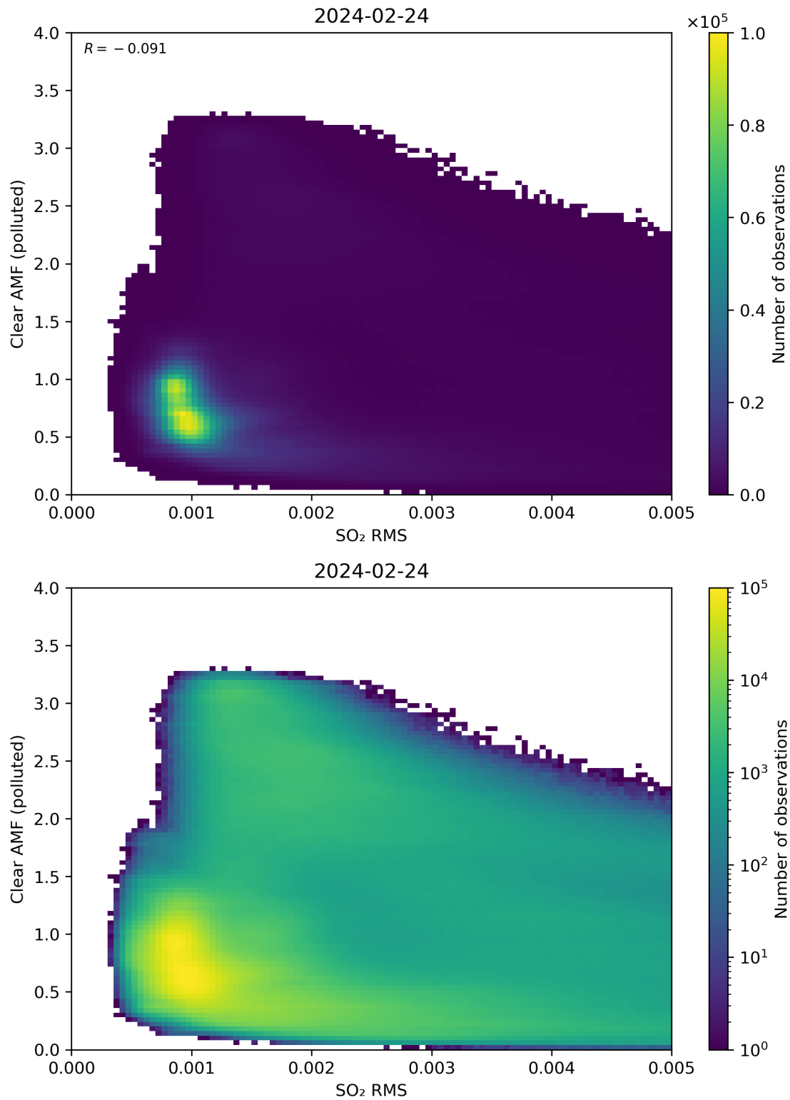
Figure 136: Scatter density plot of “SO 2 RMS” against “Clear AMF (polluted)” for 2024-02-23 to 2024-02-25.
