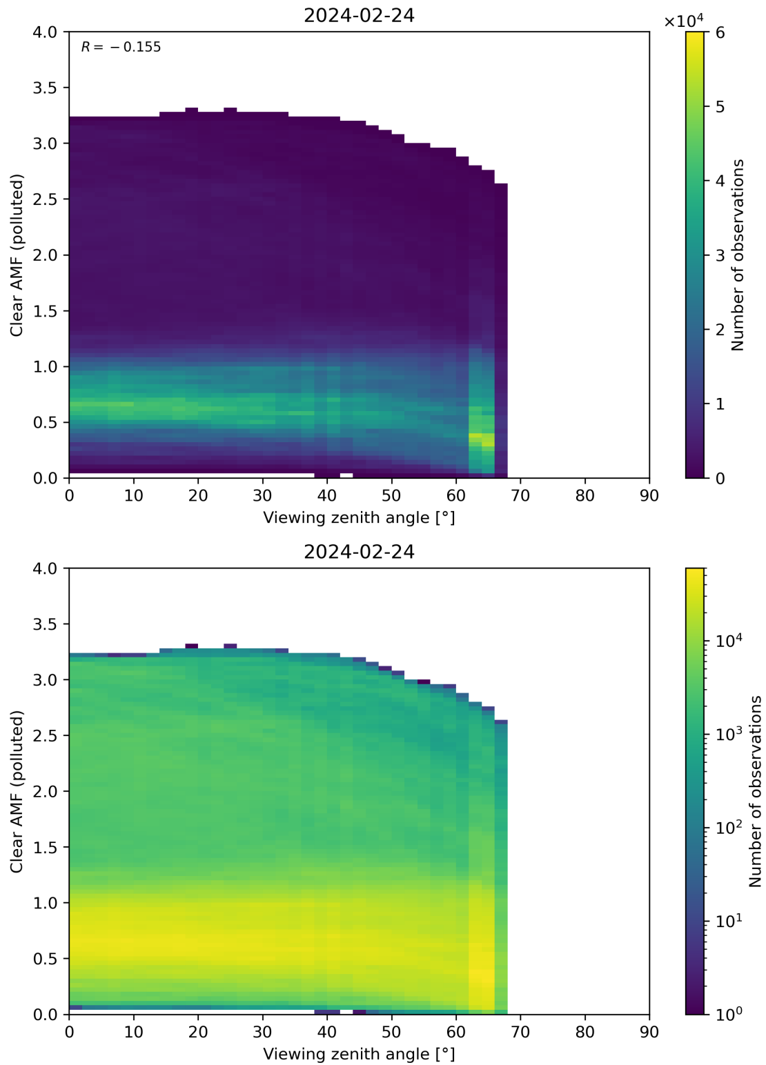
Figure 316: Scatter density plot of “Viewing zenith angle” against “Clear AMF (polluted)” for 2024-02-23 to 2024-02-25.
