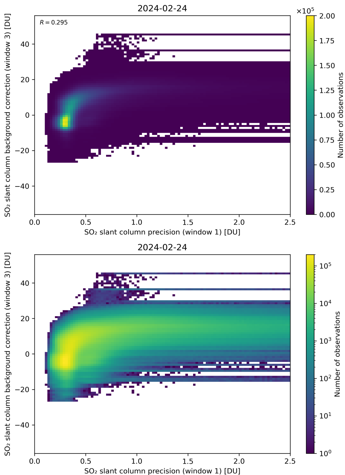
Figure 220: Scatter density plot of “SO 2 slant column precision (window 1)” against “SO 2 slant column background correction (window 3)” for 2024-02-23 to 2024-02-25.
