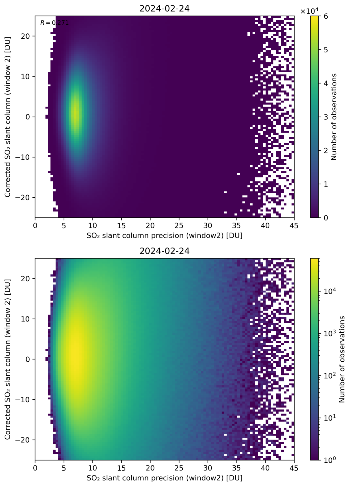
Figure 247: Scatter density plot of “SO 2 slant column precision (window2)” against “Corrected SO 2 slant column (window 2)” for 2024-02-23 to 2024-02-25.
