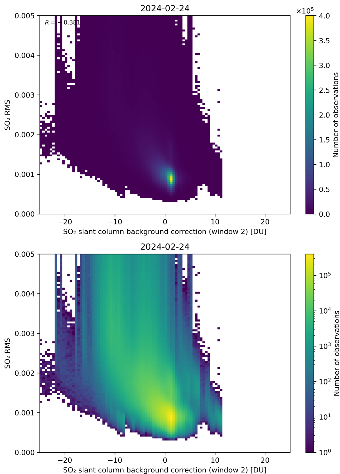
Figure 114: Scatter density plot of “SO 2 slant column background correction (window 2)” against “SO 2 RMS” for 2024-02-23 to 2024-02-25.
