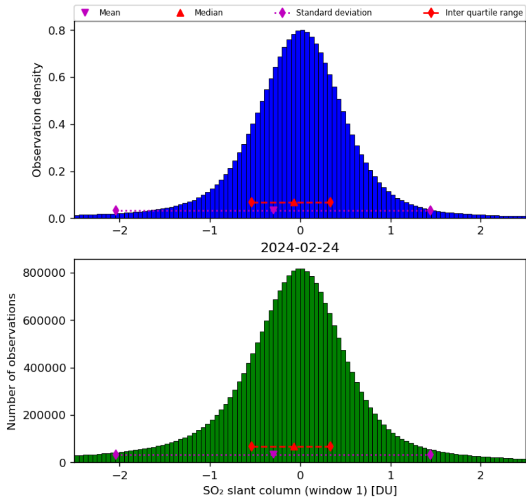
Figure 56: Histogram of “SO 2 slant column (window 1)” for 2024-02-23 to 2024-02-25
