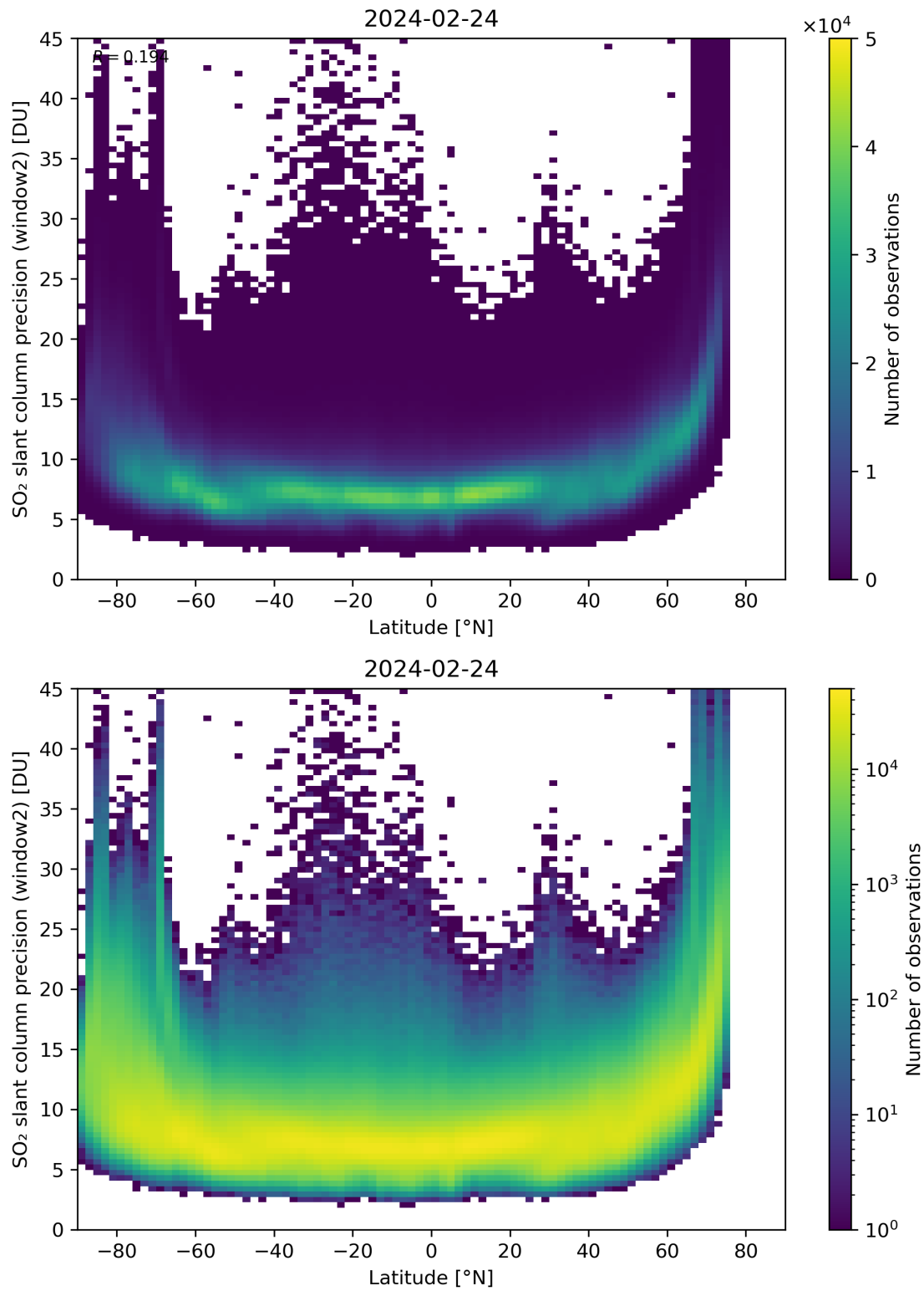
Figure 151: Scatter density plot of “Latitude” against “SO 2 slant column precision (window2)” for 2024-02-23 to 2024-02-25.
