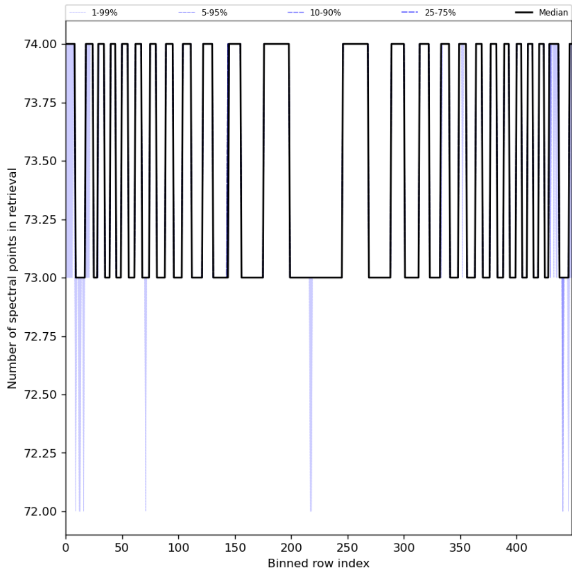
Figure 97: Along track statistics of “Number of spectral points in retrieval” for 2024-02-23 to 2024-02-25
