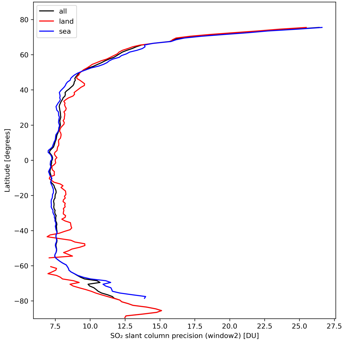
Figure 38: Zonal average of “SO 2 slant column precision (window2)” for 2024-02-23 to 2024-02-25.
