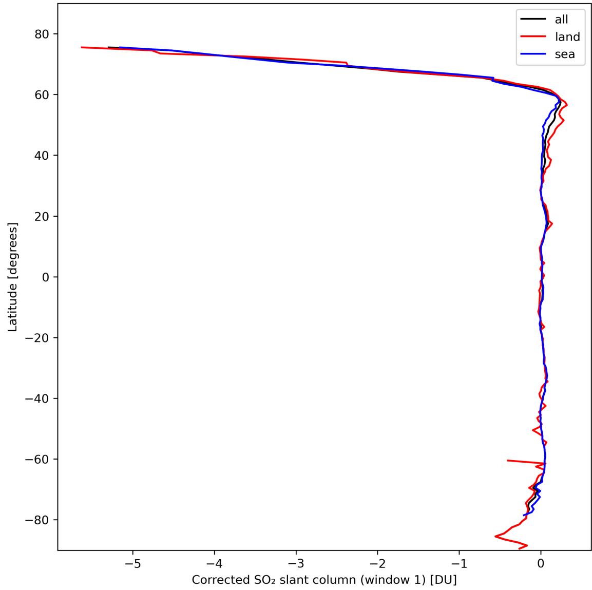
Figure 35: Zonal average of “Corrected SO 2 slant column (window 1)” for 2024-02-23 to 2024-02-25.
