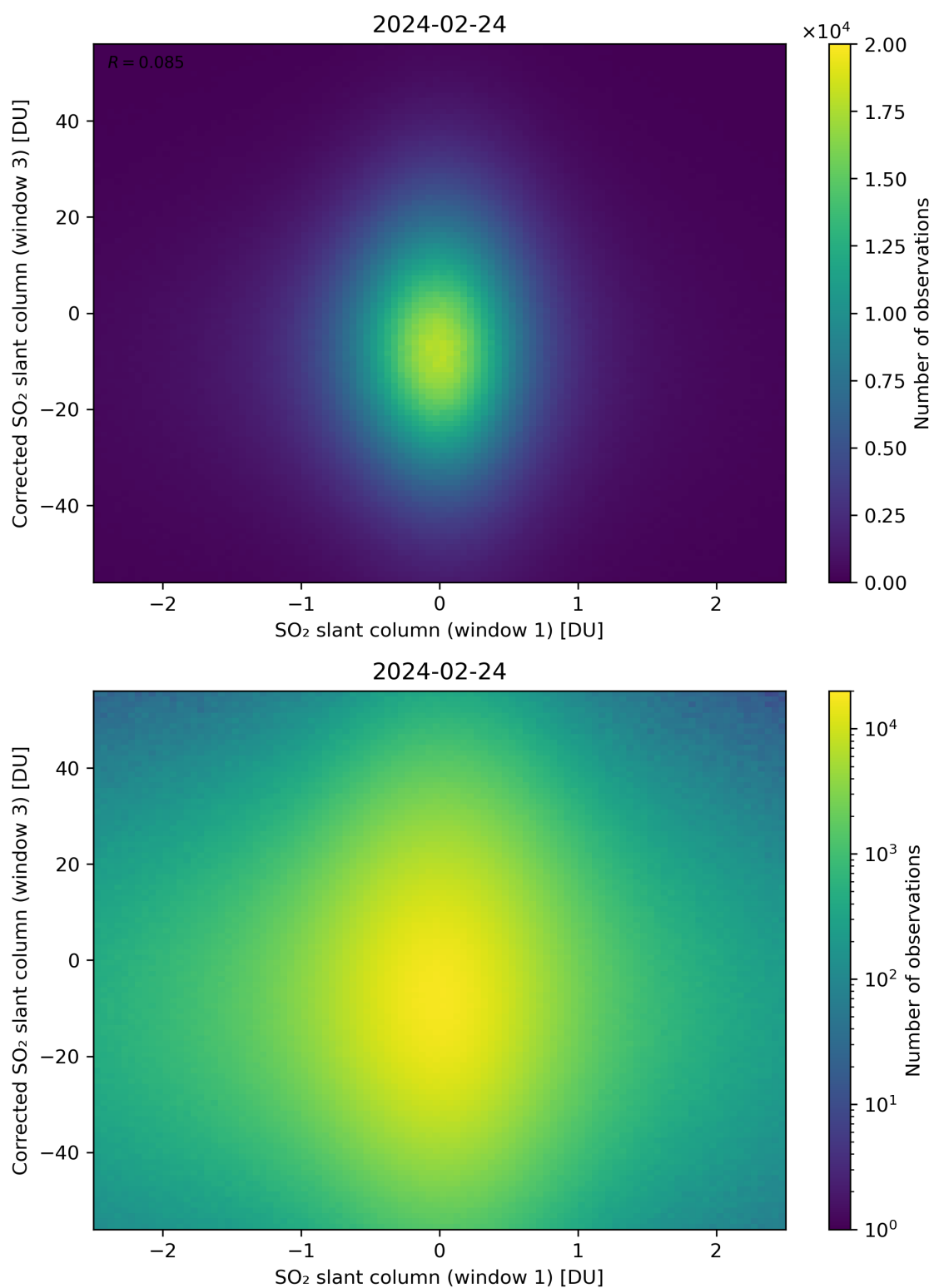
Figure 234: Scatter density plot of “SO 2 slant column (window 1)” against “Corrected SO 2 slant column (window 3)” for 2024-02-23 to 2024-02-25.
