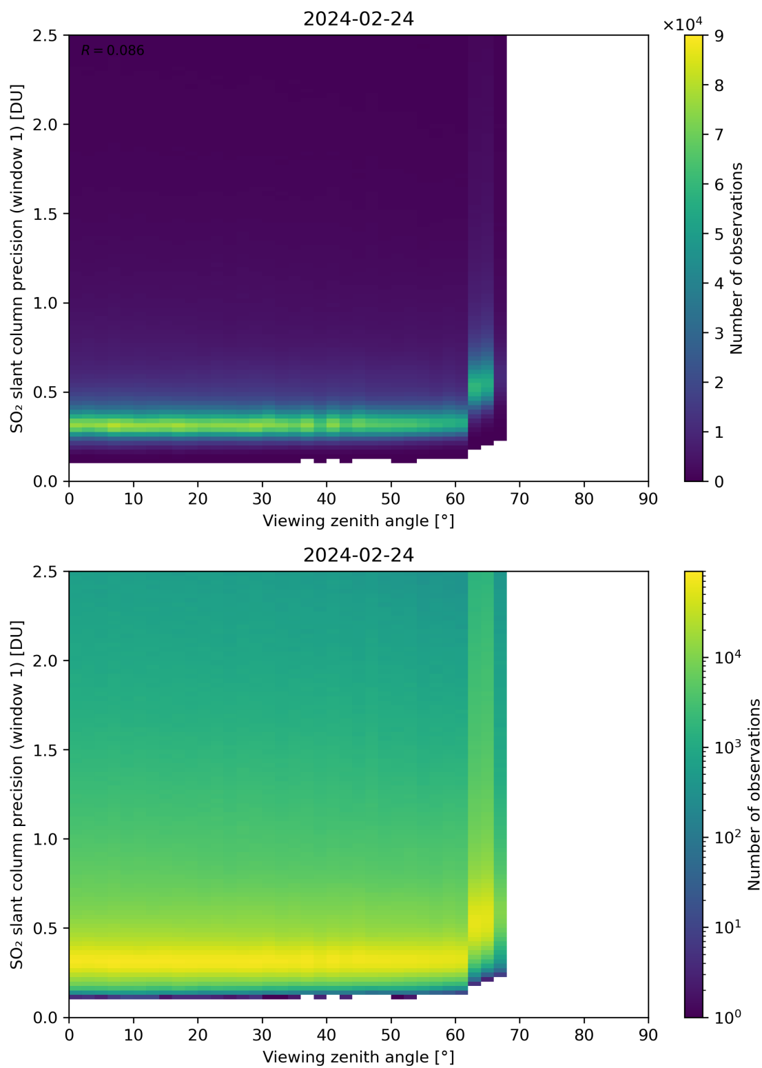
Figure 321: Scatter density plot of “Viewing zenith angle” against “SO 2 slant column precision (window 1)” for 2024-02-23 to 2024-02-25.
