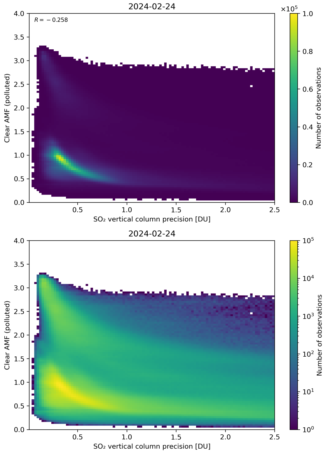
Figure 285: Scatter density plot of “SO 2 vertical column precision” against “Clear AMF (polluted)” for 2024-02-23 to 2024-02-25.
