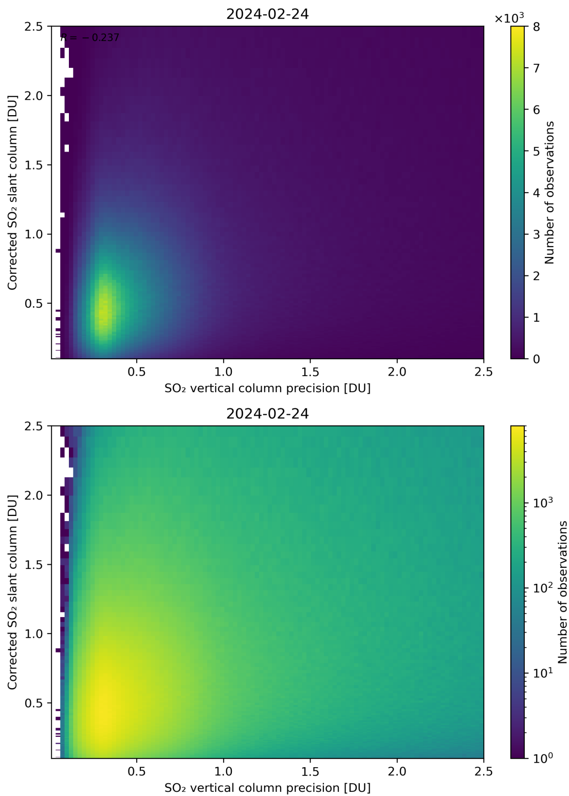
Figure 286: Scatter density plot of “SO 2 vertical column precision” against “Corrected SO 2 slant column” for 2024-02-23 to 2024-02-25.
