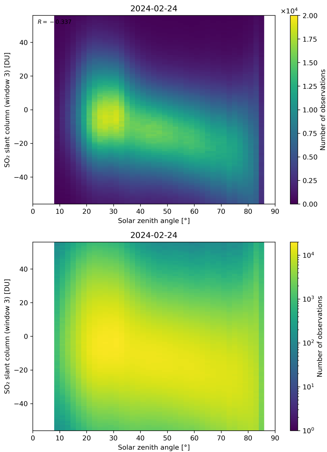
Figure 172: Scatter density plot of “Solar zenith angle” against “SO 2 slant column (window 3)” for 2024-02-23 to 2024-02-25.
