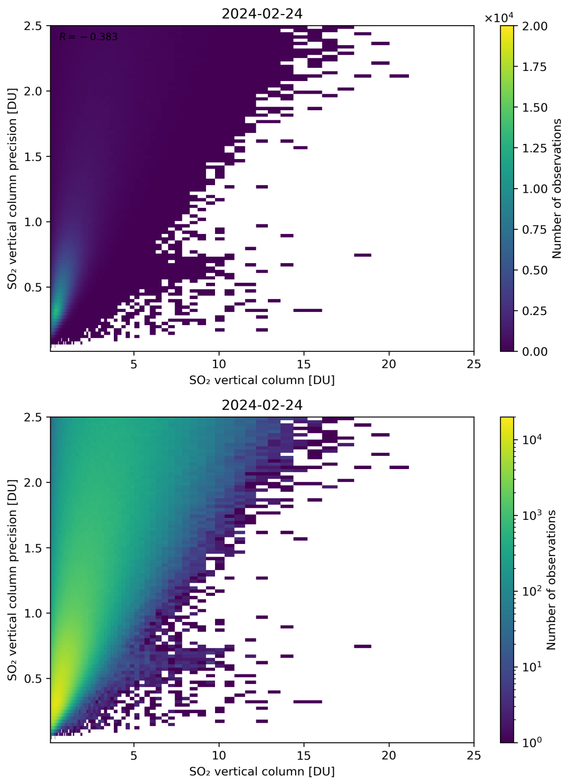
Figure 307: Scatter density plot of “SO 2 vertical column” against “SO 2 vertical column precision” for 2024-02-23 to 2024-02-25.
