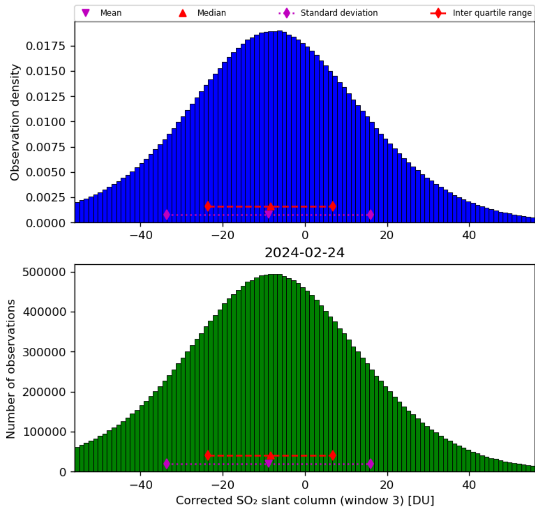
Figure 66: Histogram of “Corrected SO 2 slant column (window 3)” for 2024-02-23 to 2024-02-25
