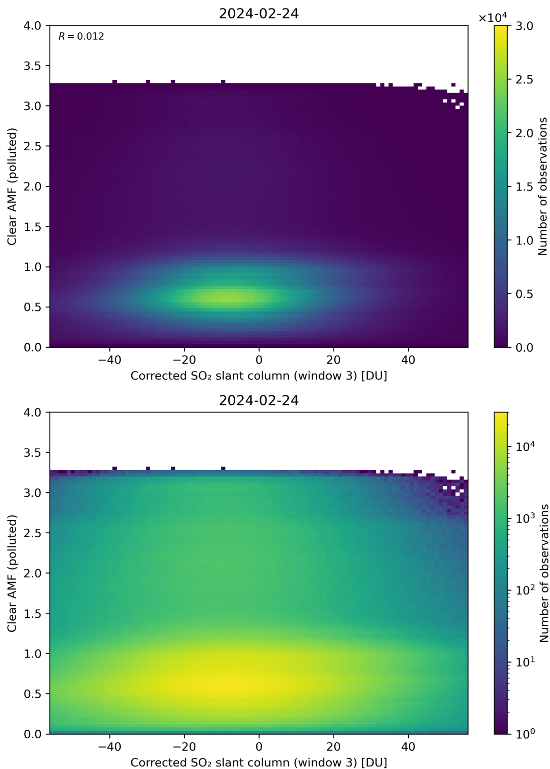
Figure 209: Scatter density plot of “Corrected SO 2 slant column (window 3)” against “Clear AMF (polluted)” for 2024-02-23 to 2024-02-25.
