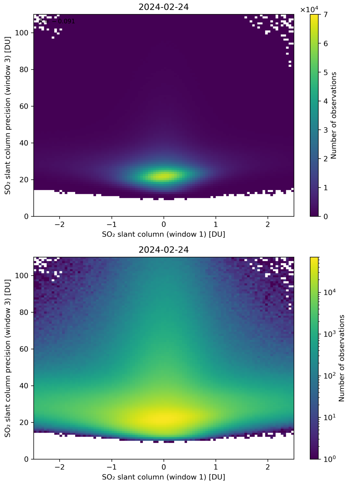
Figure 238: Scatter density plot of “SO 2 slant column (window 1)” against “SO 2 slant column precision (window 3)” for 2024-02-23 to 2024-02-25.
