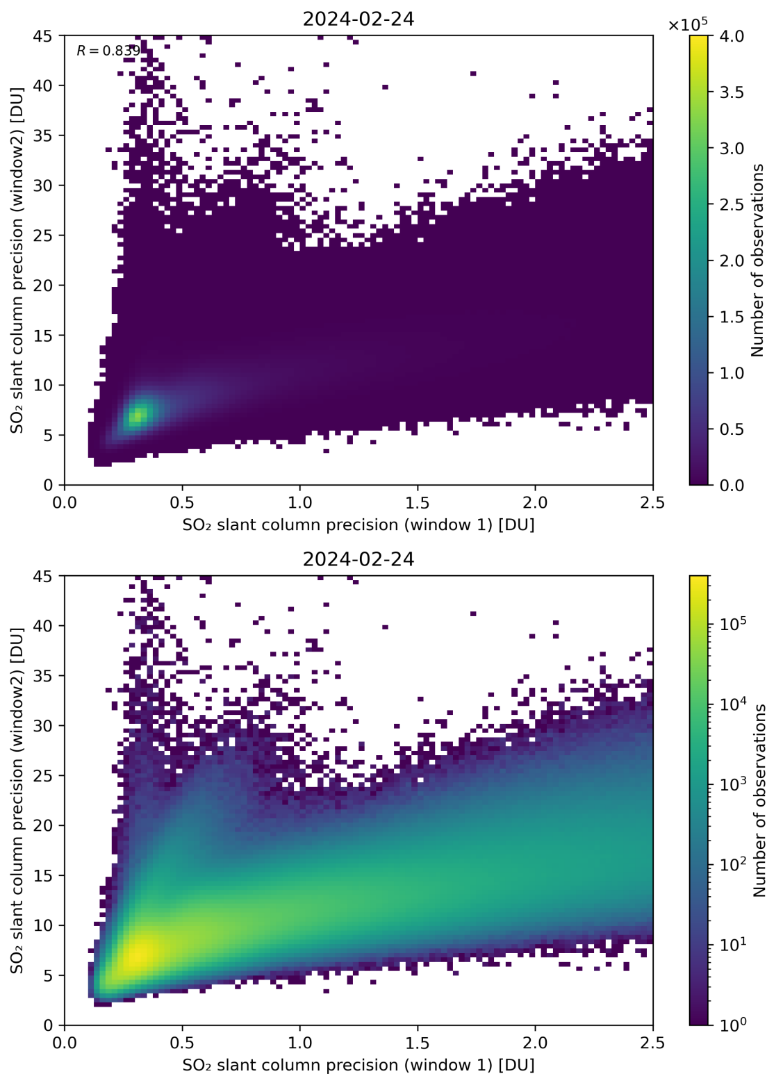
Figure 227: Scatter density plot of “SO 2 slant column precision (window 1)” against “SO 2 slant column precision (window2)” for 2024-02-23 to 2024-02-25.
