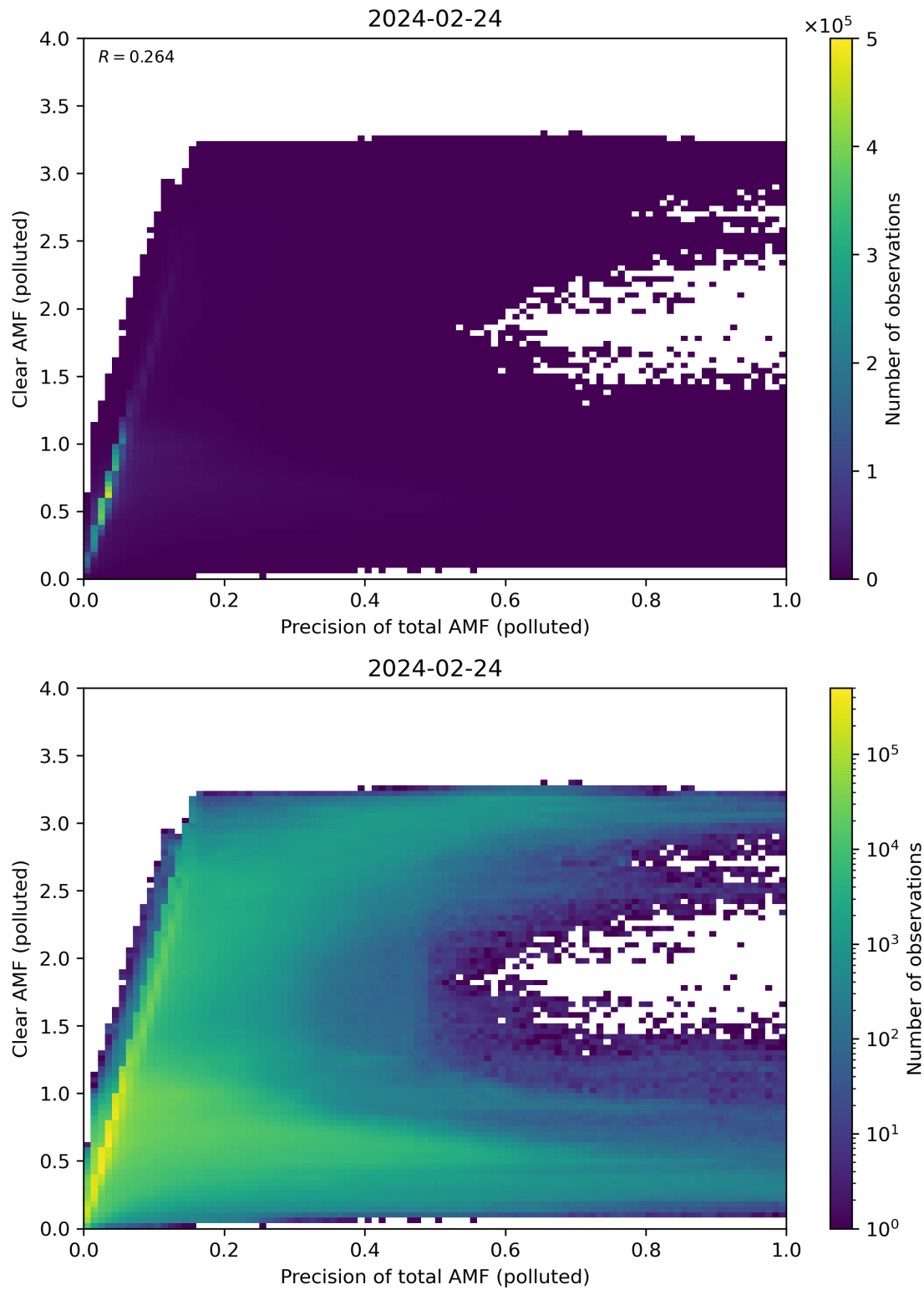
Figure 270: Scatter density plot of “Precision of total AMF (polluted)” against “Clear AMF (polluted)” for 2024-02-23 to 2024-02-25.
