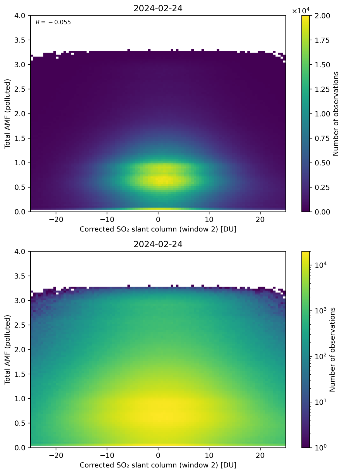
Figure 203: Scatter density plot of “Corrected SO 2 slant column (window 2)” against “Total AMF (polluted)” for 2024-02-23 to 2024-02-25.
