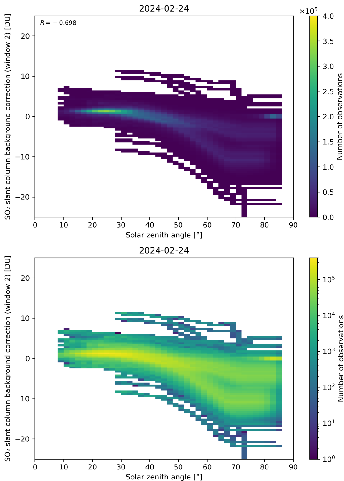
Figure 159: Scatter density plot of “Solar zenith angle” against “SO 2 slant column background correction (window 2)” for 2024-02-23 to 2024-02-25.
