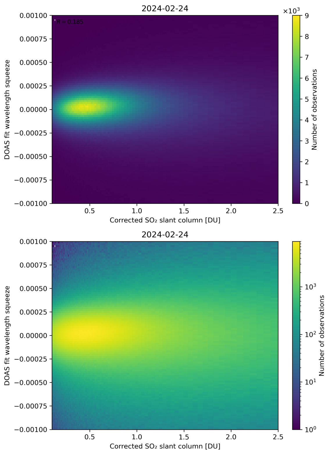
Figure 182: Scatter density plot of “Corrected SO 2 slant column” against “DOAS fit wavelength squeeze” for 2024-02-23 to 2024-02-25.
