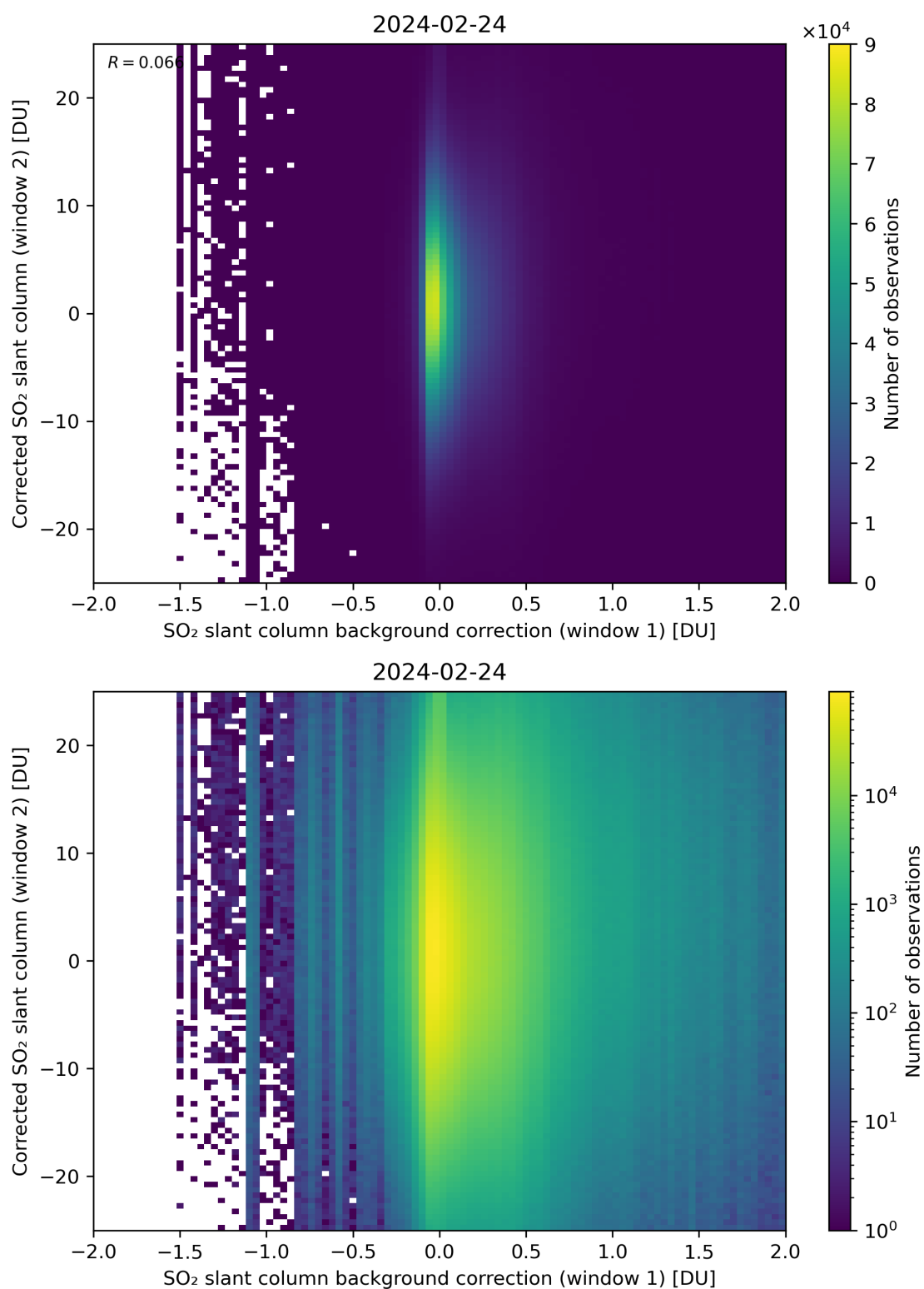
Figure 104: Scatter density plot of “SO 2 slant column background correction (window 1)” against “Corrected SO 2 slant column (window 2)” for 2024-02-23 to 2024-02-25.
