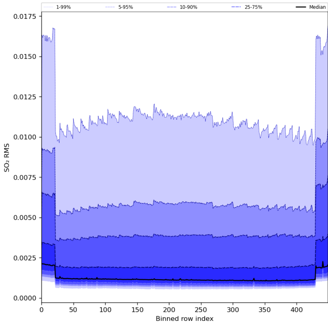
Figure 93: Along track statistics of “SO 2 RMS” for 2024-02-23 to 2024-02-25
