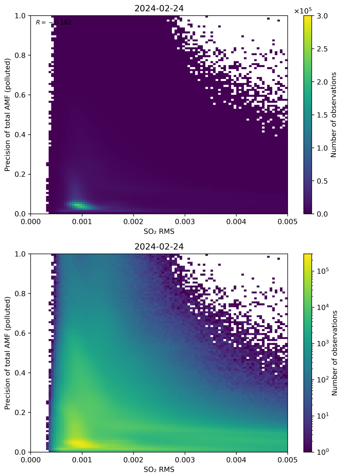
Figure 138: Scatter density plot of “SO 2 RMS” against “Precision of total AMF (polluted)” for 2024-02-23 to 2024-02-25.
