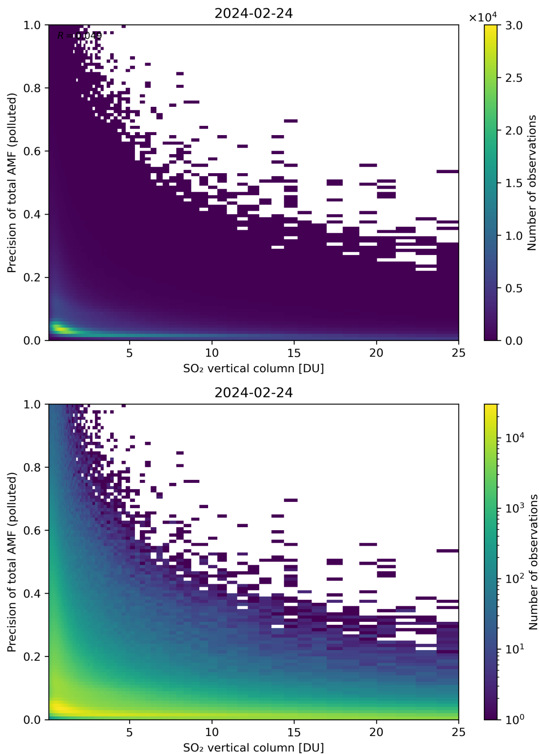
Figure 306: Scatter density plot of “SO 2 vertical column” against “Precision of total AMF (polluted)” for 2024-02-23 to 2024-02-25.
