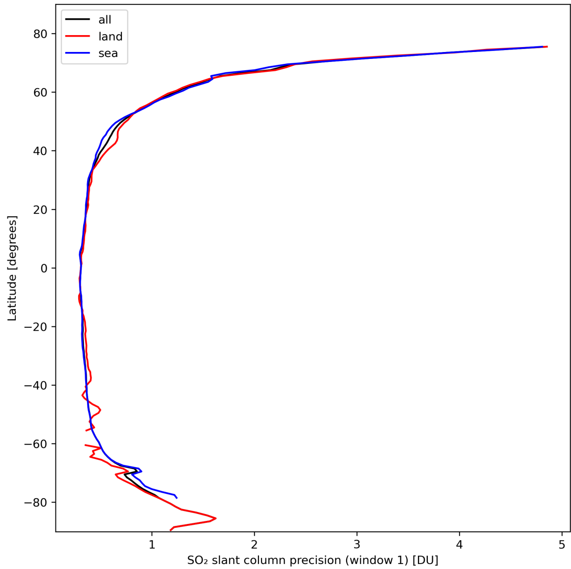
Figure 34: Zonal average of “SO 2 slant column precision (window 1)” for 2024-02-23 to 2024-02-25.
