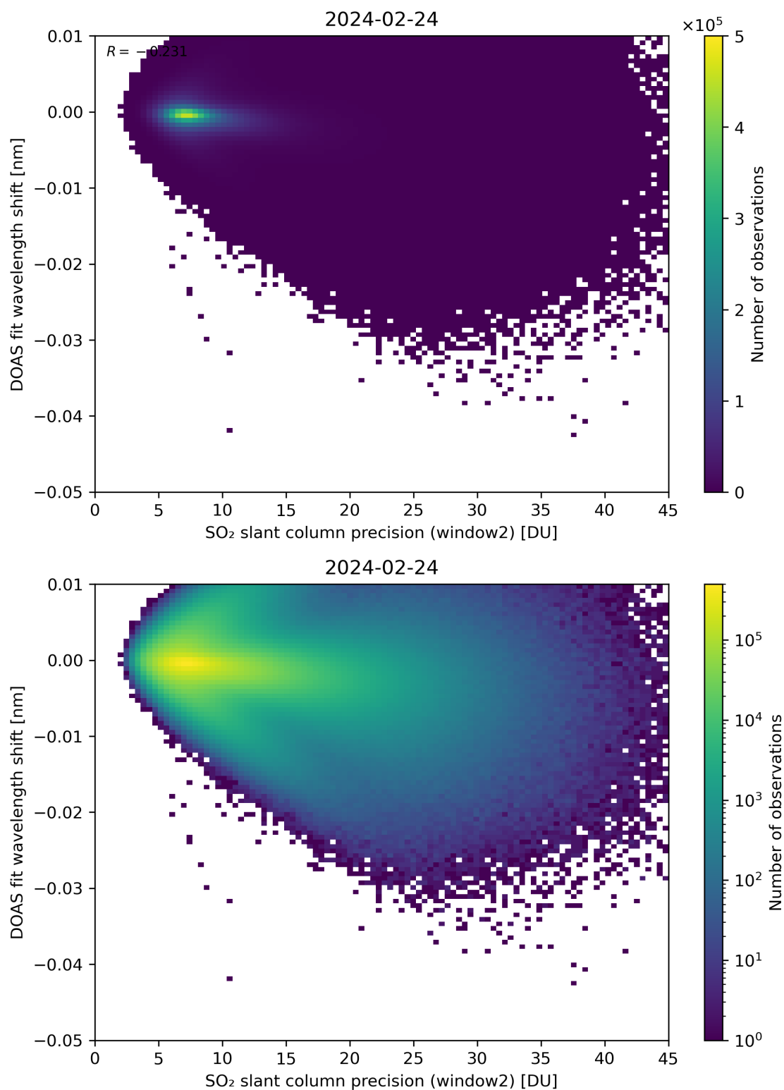
Figure 243: Scatter density plot of “SO 2 slant column precision (window2)” against “DOAS fit wavelength shift” for 2024-02-23 to 2024-02-25.
