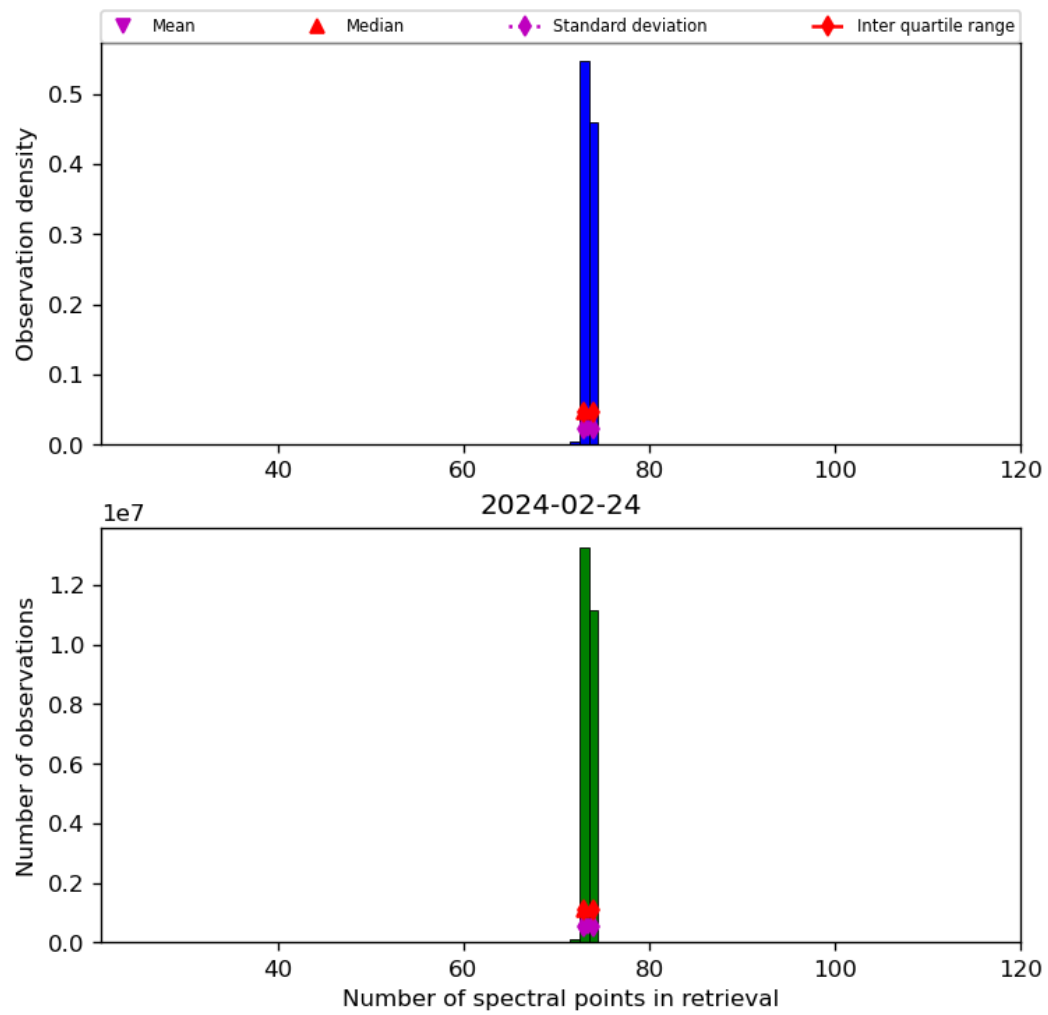
Figure 74: Histogram of “Number of spectral points in retrieval” for 2024-02-23 to 2024-02-25
