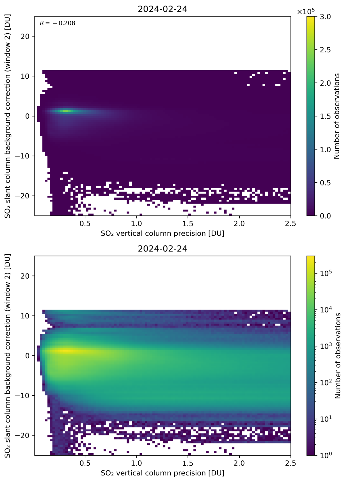
Figure 280: Scatter density plot of “SO 2 vertical column precision” against “SO 2 slant column background correction (window 2)” for 2024-02-23 to 2024-02-25.
