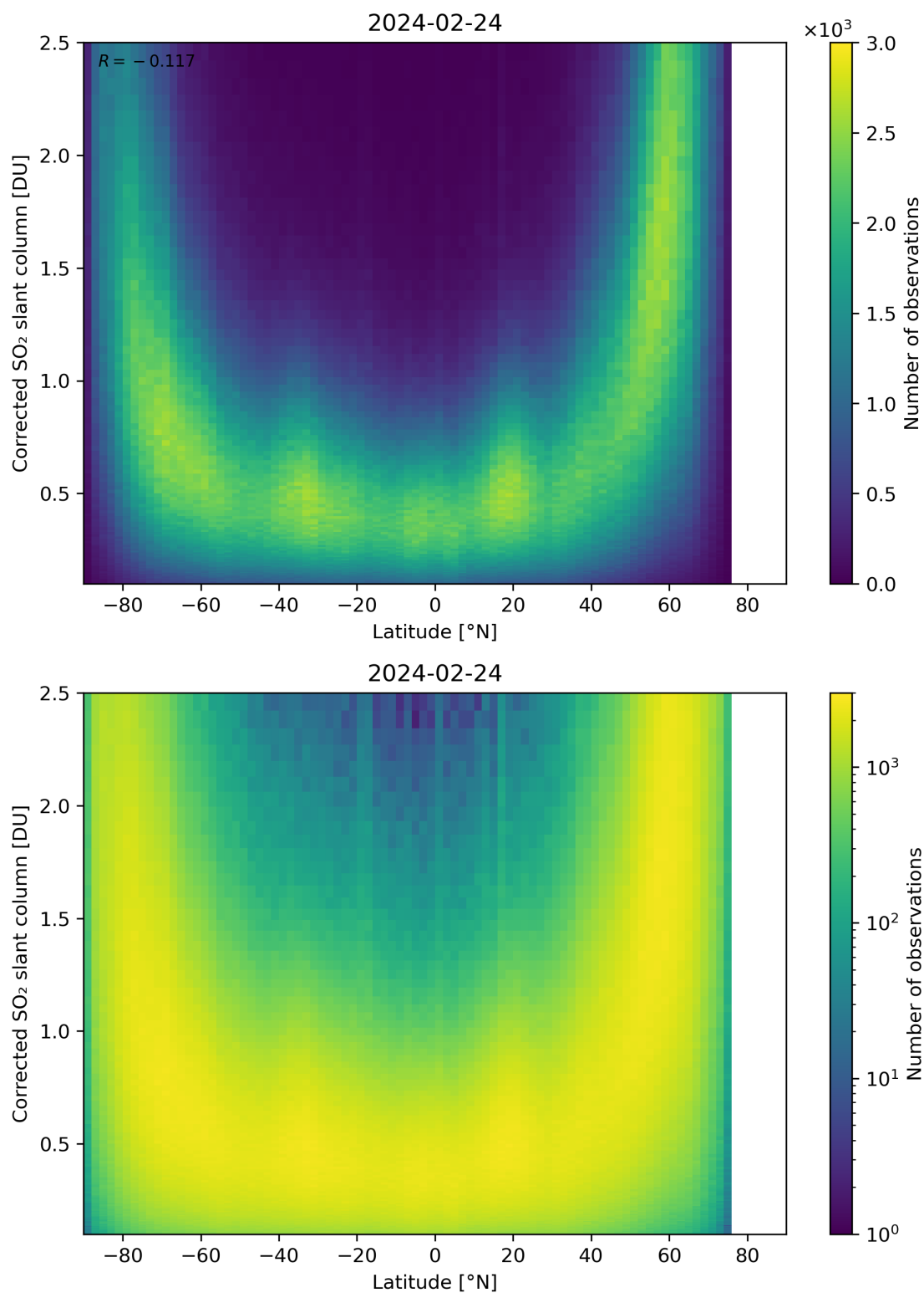
Figure 146: Scatter density plot of “Latitude” against “Corrected SO 2 slant column” for 2024-02-23 to 2024-02-25.
