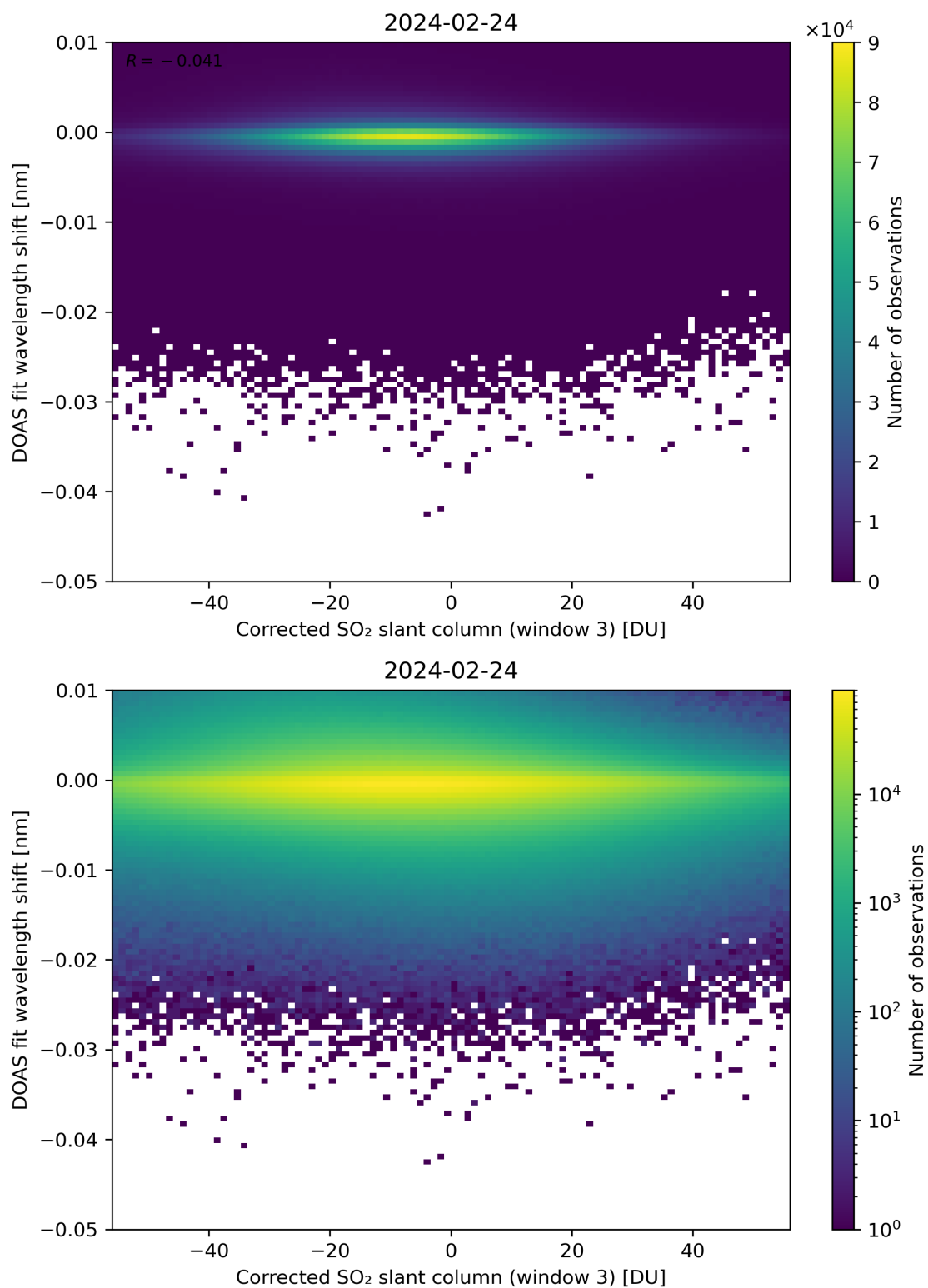
Figure 206: Scatter density plot of “Corrected SO 2 slant column (window 3)” against “DOAS fit wavelength shift” for 2024-02-23 to 2024-02-25.
