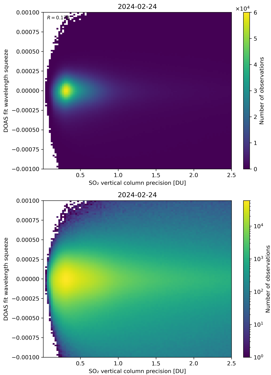
Figure 283: Scatter density plot of “SO 2 vertical column precision” against “DOAS fit wavelength squeeze” for 2024-02-23 to 2024-02-25.
