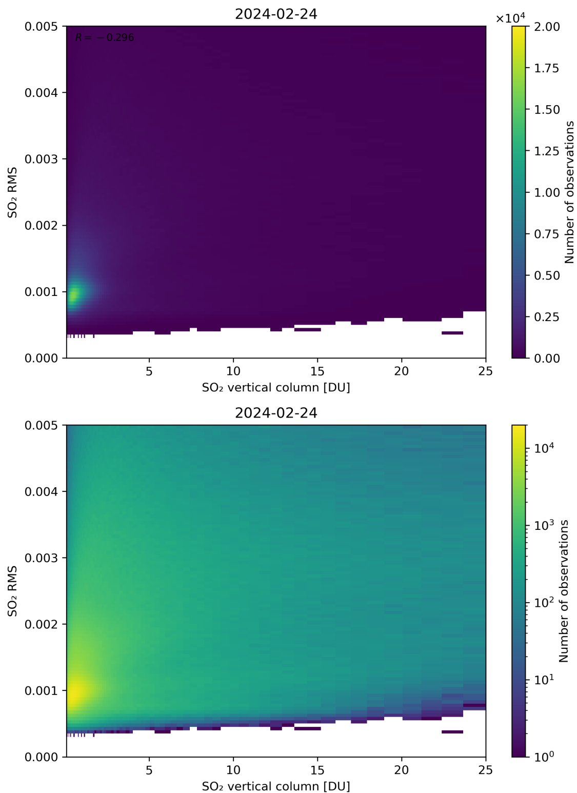
Figure 278: Scatter density plot of “SO 2 vertical column” against “SO 2 RMS” for 2024-02-23 to 2024-02-25.
