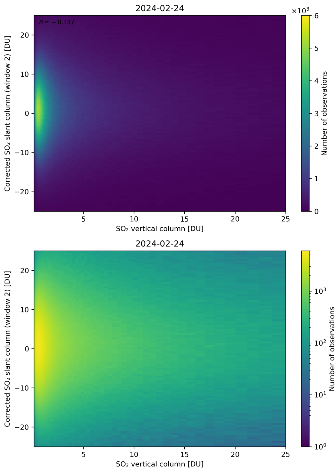
Figure 298: Scatter density plot of “SO 2 vertical column” against “Corrected SO 2 slant column (window 2)” for 2024-02-23 to 2024-02-25.
