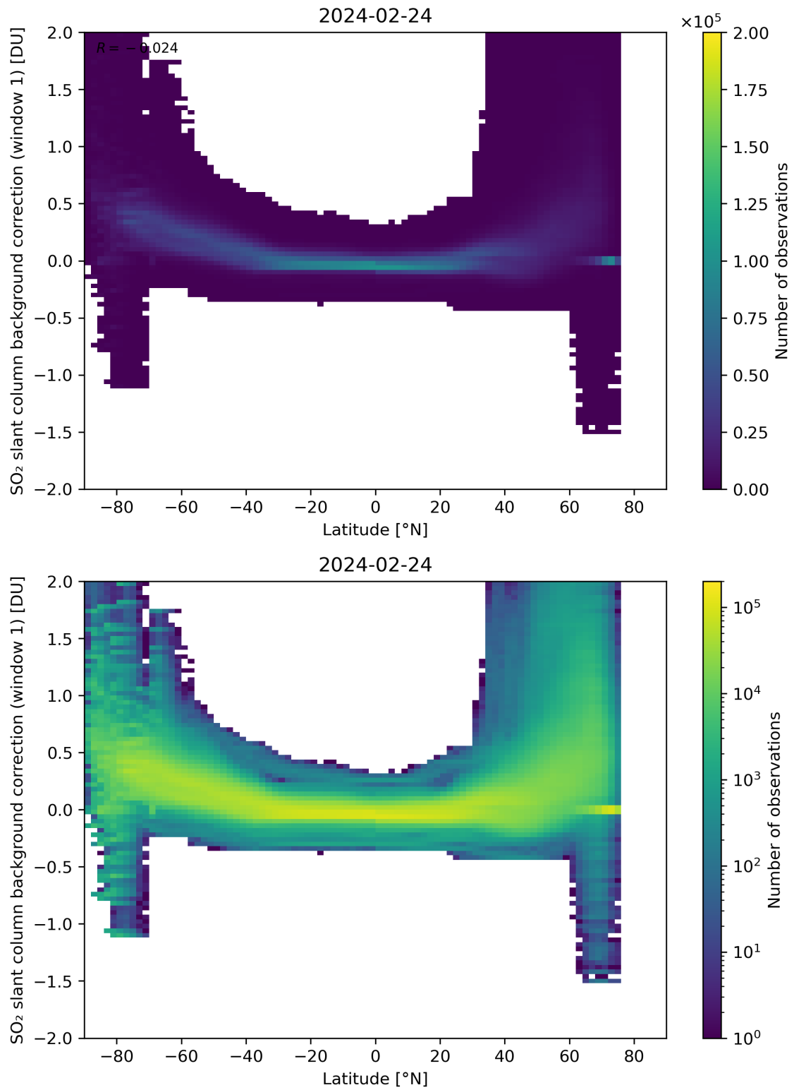
Figure 139: Scatter density plot of “Latitude” against “SO 2 slant column background correction (window 1)” for 2024-02-23 to 2024-02-25.
