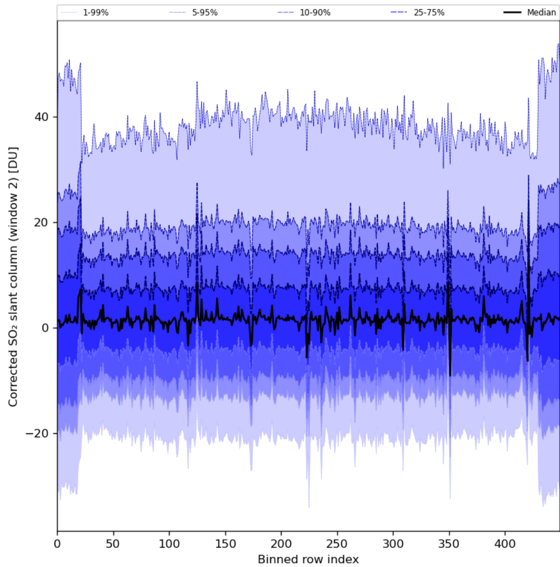
Figure 85: Along track statistics of “Corrected SO 2 slant column (window 2)” for 2024-02-23 to 2024-02-25
