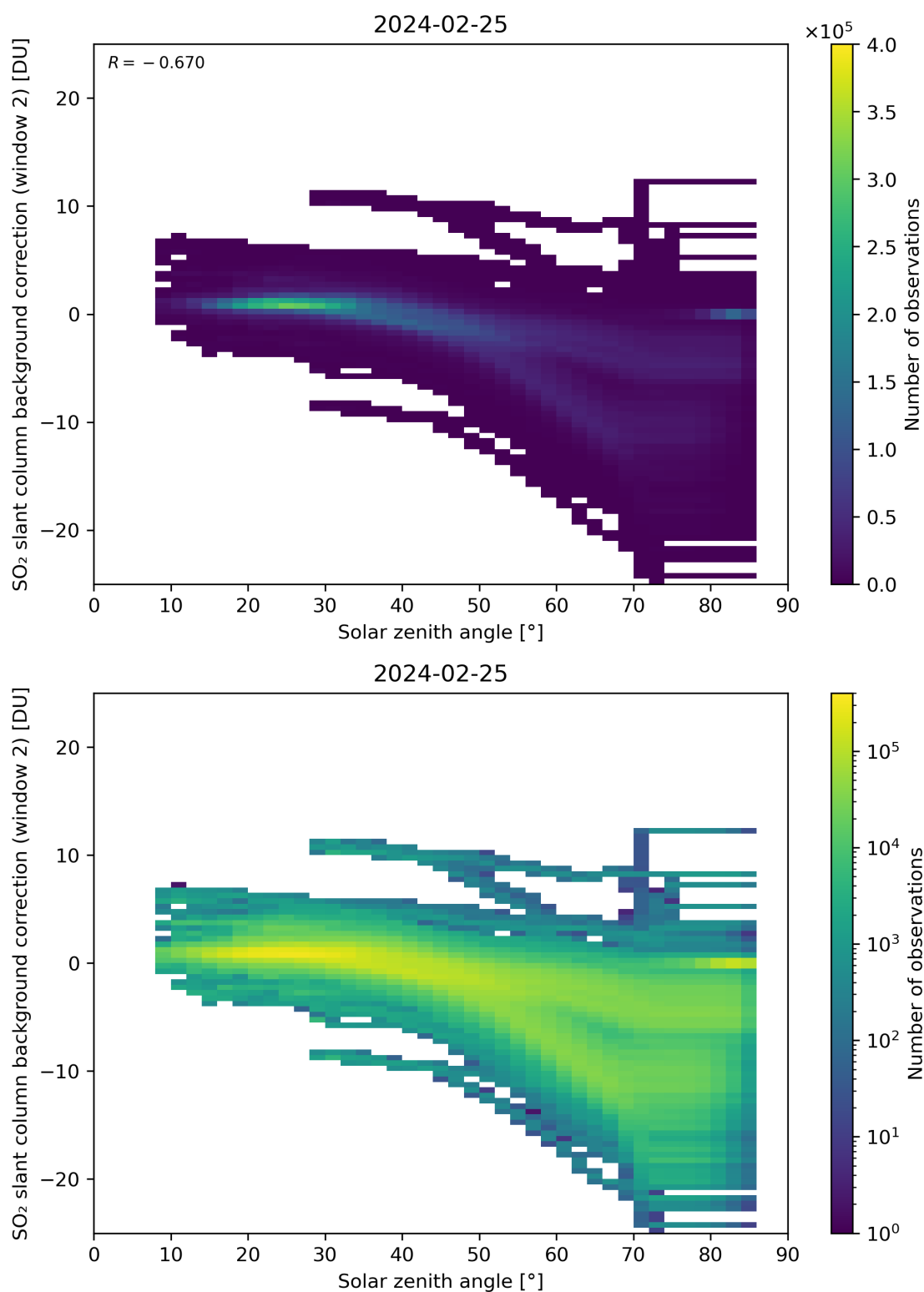
Figure 159: Scatter density plot of “Solar zenith angle” against “SO 2 slant column background correction (window 2)” for 2024-02-24 to 2024-02-26.
