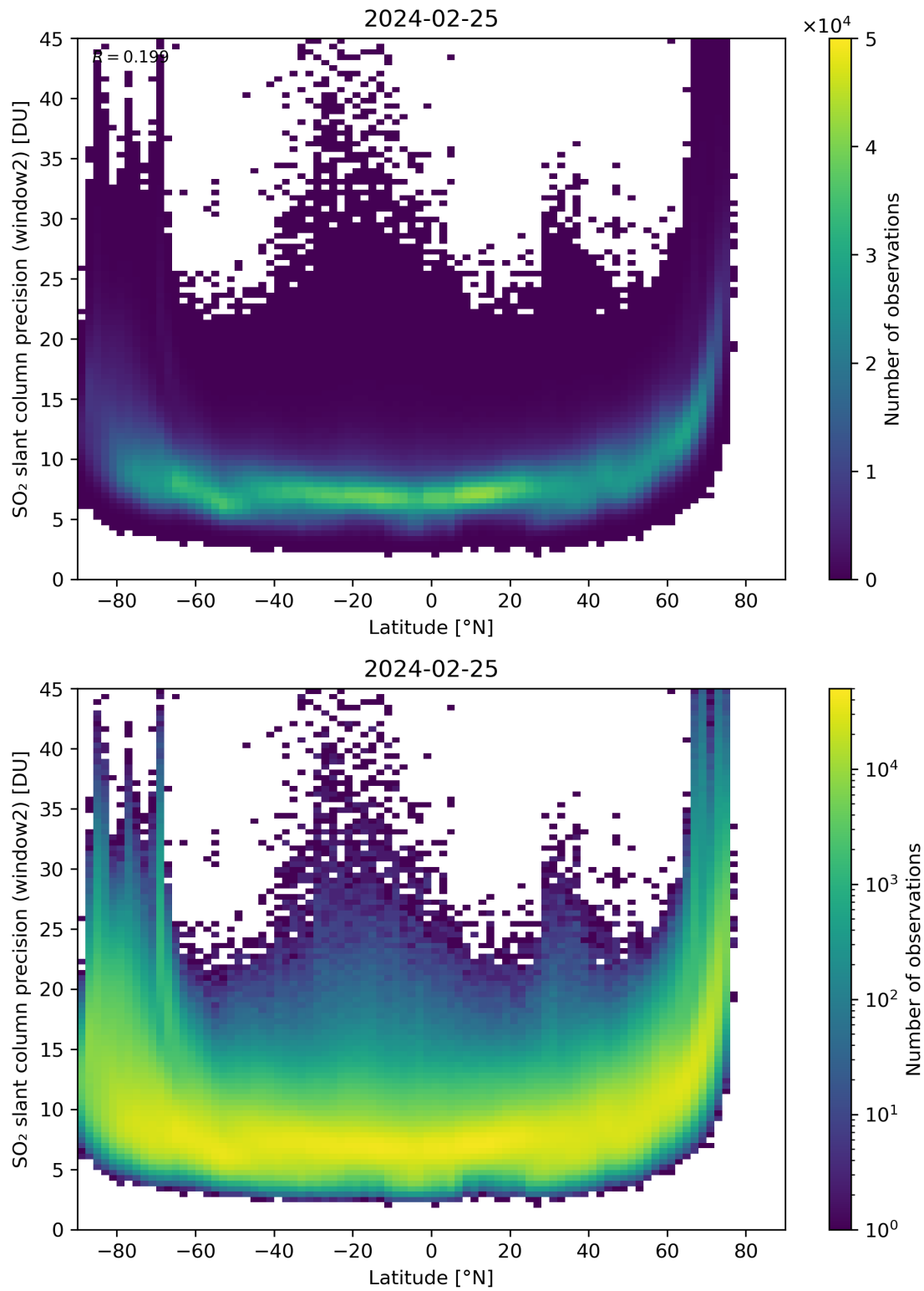
Figure 151: Scatter density plot of “Latitude” against “SO 2 slant column precision (window2)” for 2024-02-24 to 2024-02-26.
