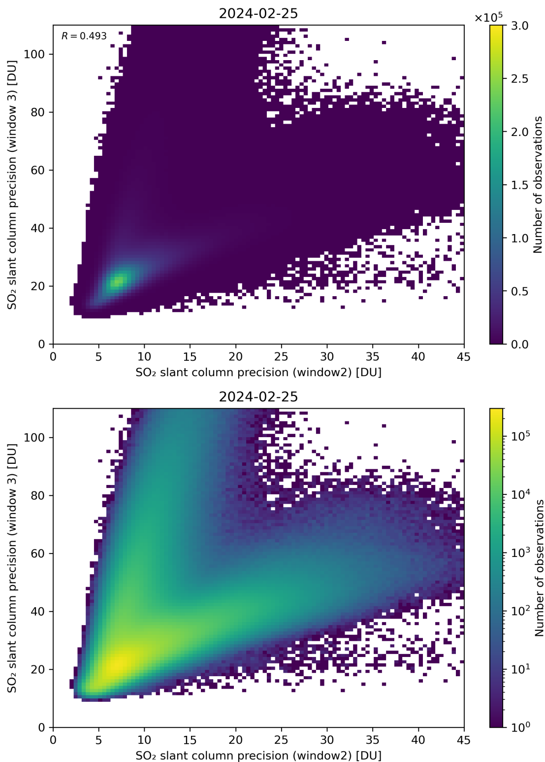
Figure 250: Scatter density plot of “SO 2 slant column precision (window2)” against “SO 2 slant column precision (window 3)” for 2024-02-24 to 2024-02-26.
