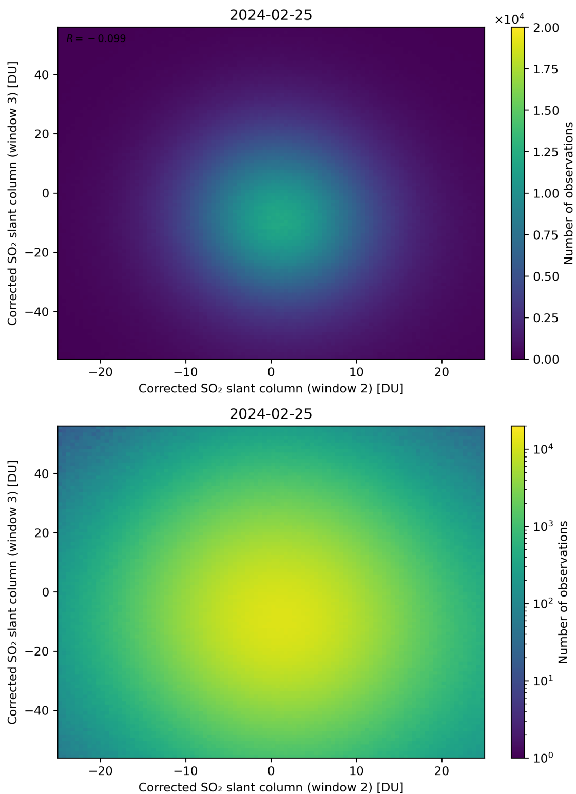
Figure 200: Scatter density plot of “Corrected SO 2 slant column (window 2)” against “Corrected SO 2 slant column (window 3)” for 2024-02-24 to 2024-02-26.
