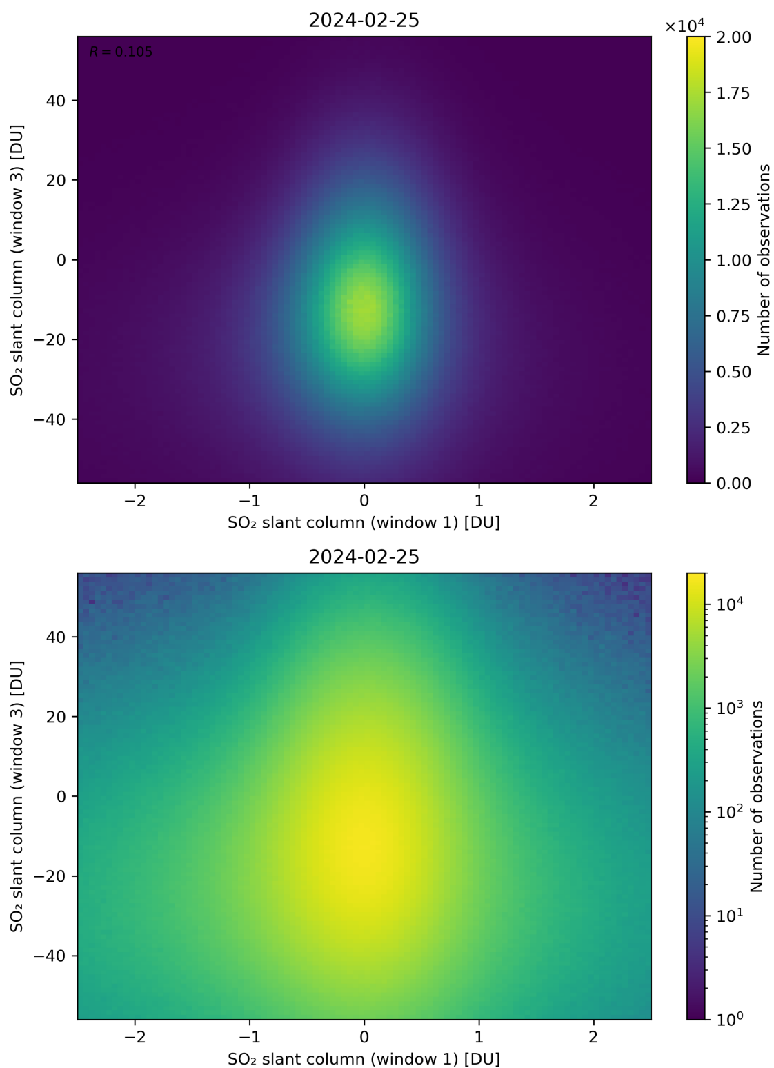
Figure 237: Scatter density plot of “SO 2 slant column (window 1)” against “SO 2 slant column (window 3)” for 2024-02-24 to 2024-02-26.
