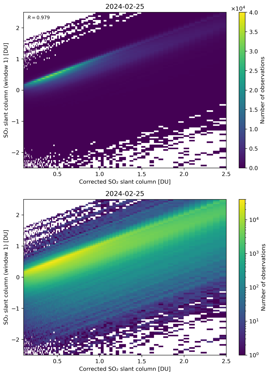
Figure 187: Scatter density plot of “Corrected SO 2 slant column” against “SO 2 slant column (window 1)” for 2024-02-24 to 2024-02-26.
