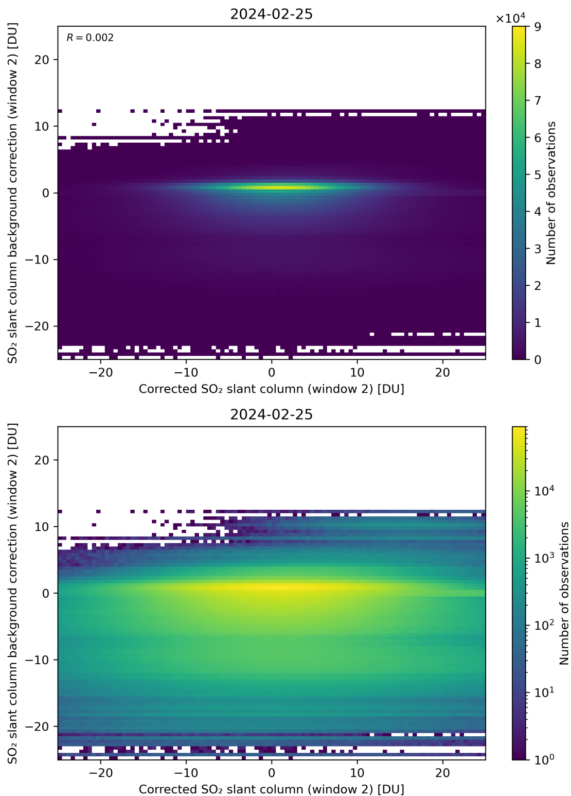
Figure 194: Scatter density plot of “Corrected SO 2 slant column (window 2)” against “SO 2 slant column background correction (window 2)” for 2024-02-24 to 2024-02-26.
