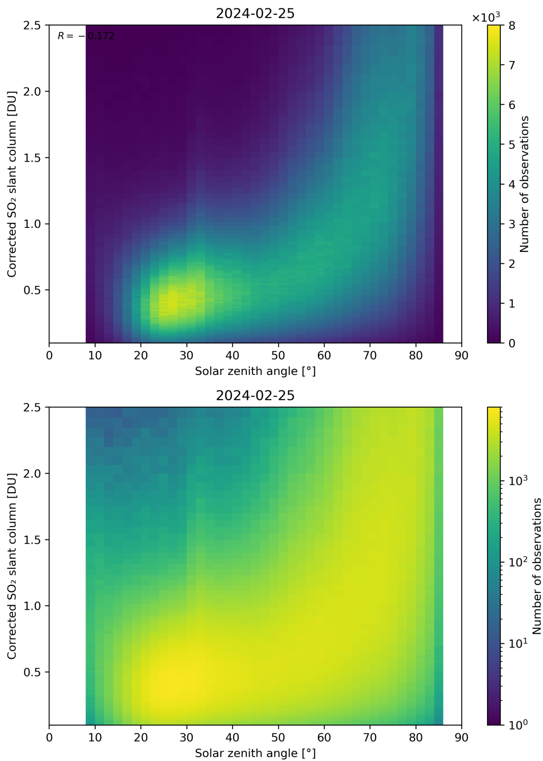
Figure 166: Scatter density plot of “Solar zenith angle” against “Corrected SO 2 slant column” for 2024-02-24 to 2024-02-26.
