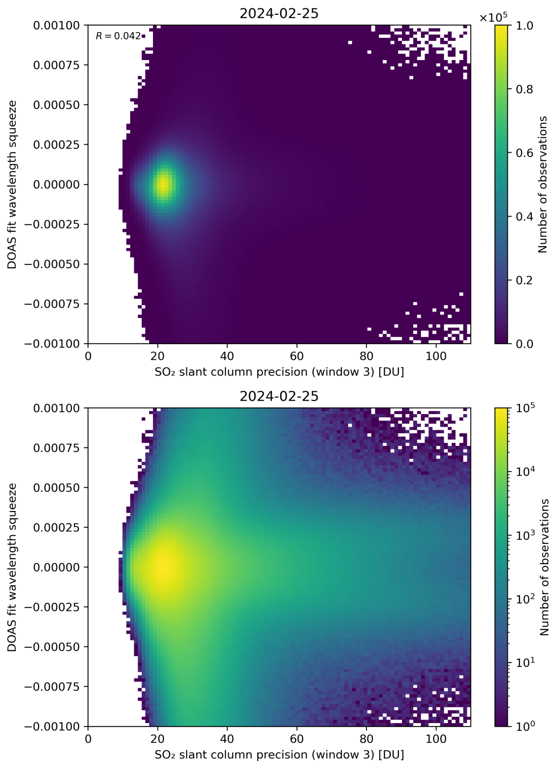
Figure 259: Scatter density plot of “SO 2 slant column precision (window 3)” against “DOAS fit wavelength squeeze” for 2024-02-24 to 2024-02-26.
