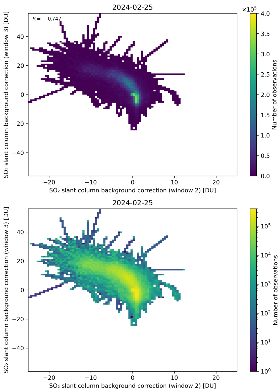
Figure 111: Scatter density plot of “SO 2 slant column background correction (window 2)” against “SO 2 slant column background correction (window 3)” for 2024-02-24 to 2024-02-26.
