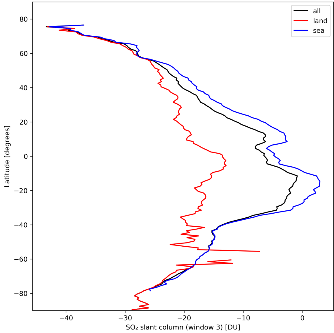
Figure 41: Zonal average of “SO 2 slant column (window 3)” for 2024-02-24 to 2024-02-26.
