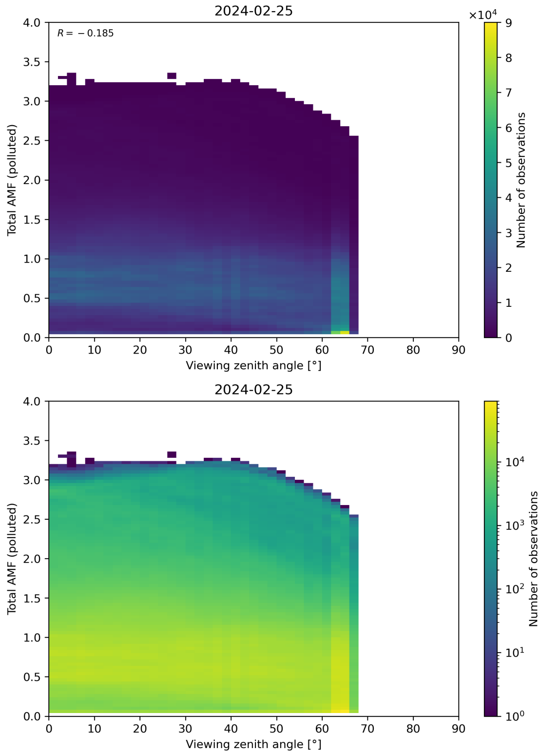
Figure 325: Scatter density plot of “Viewing zenith angle” against “Total AMF (polluted)” for 2024-02-24 to 2024-02-26.
