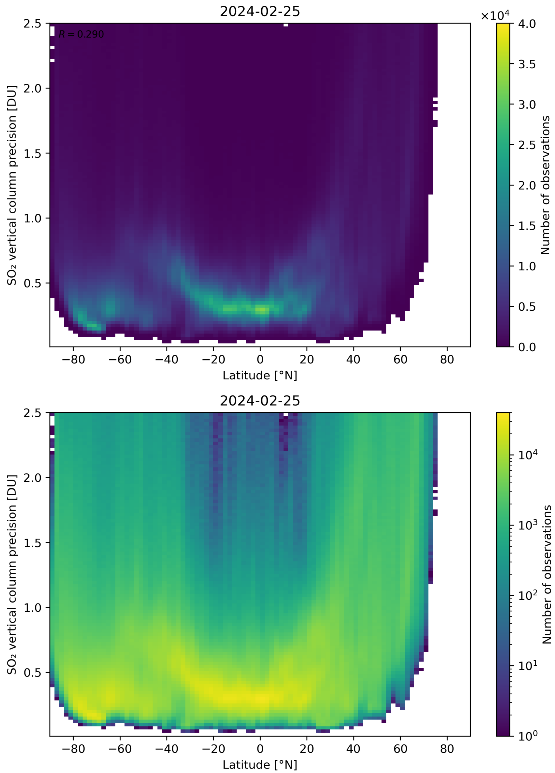
Figure 157: Scatter density plot of “Latitude” against “SO 2 vertical column precision” for 2024-02-24 to 2024-02-26.
