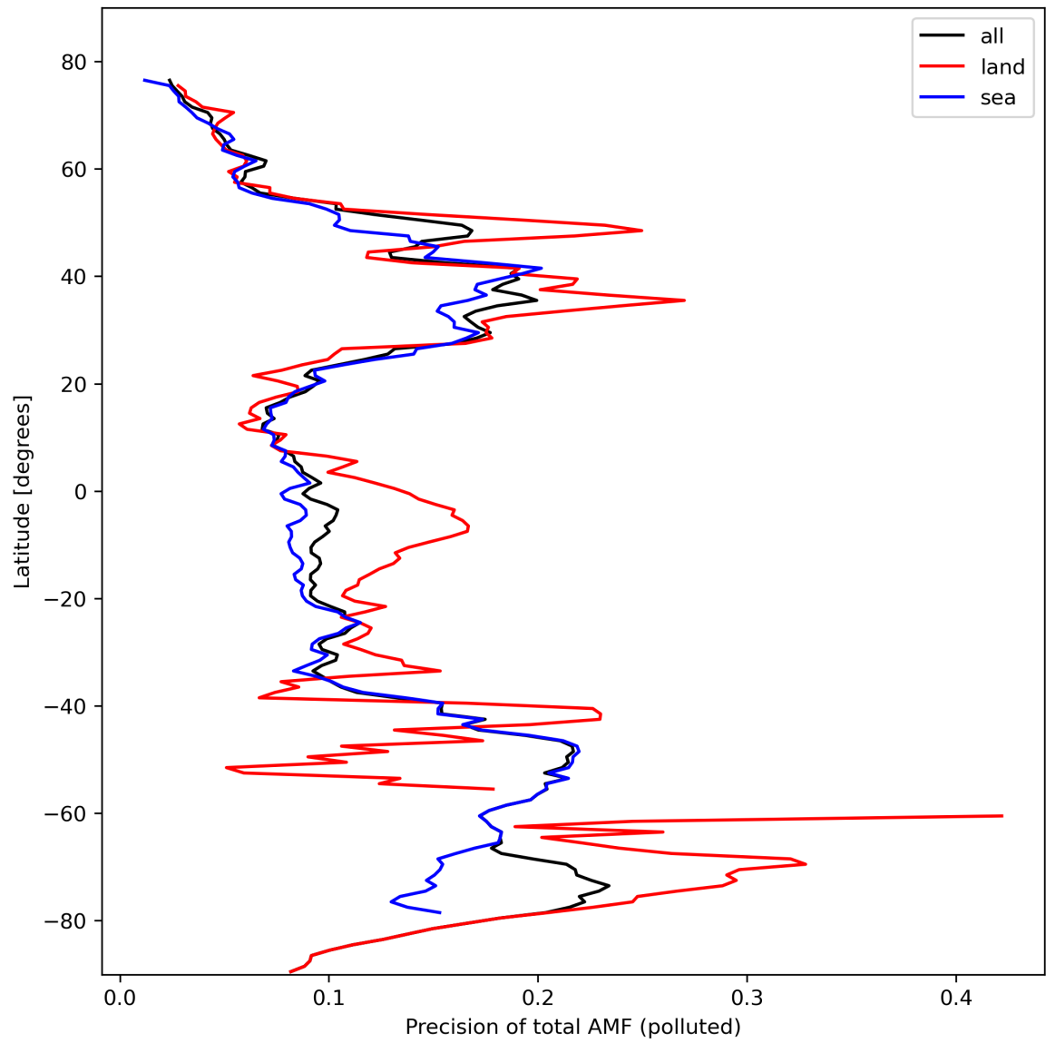
Figure 49: Zonal average of “Precision of total AMF (polluted)” for 2024-02-24 to 2024-02-26.
