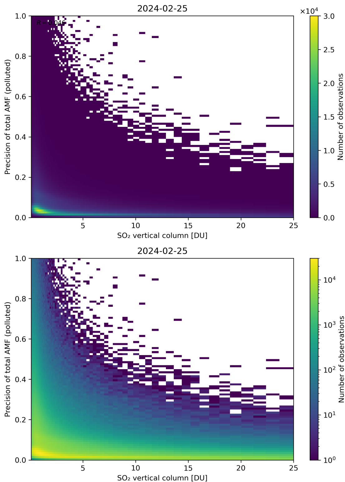
Figure 306: Scatter density plot of “SO 2 vertical column” against “Precision of total AMF (polluted)” for 2024-02-24 to 2024-02-26.
