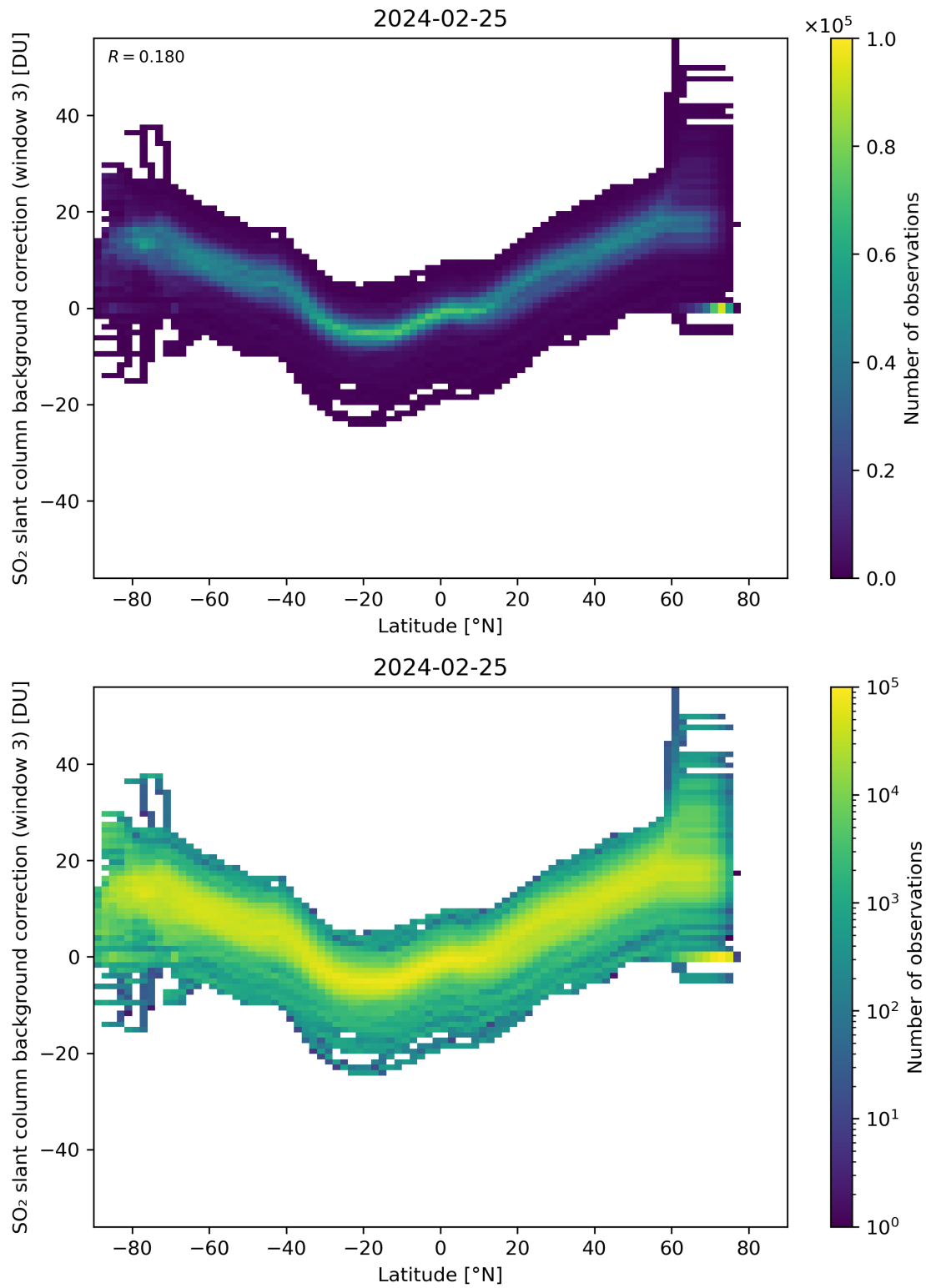
Figure 141: Scatter density plot of “Latitude” against “SO 2 slant column background correction (window 3)” for 2024-02-24 to 2024-02-26.
