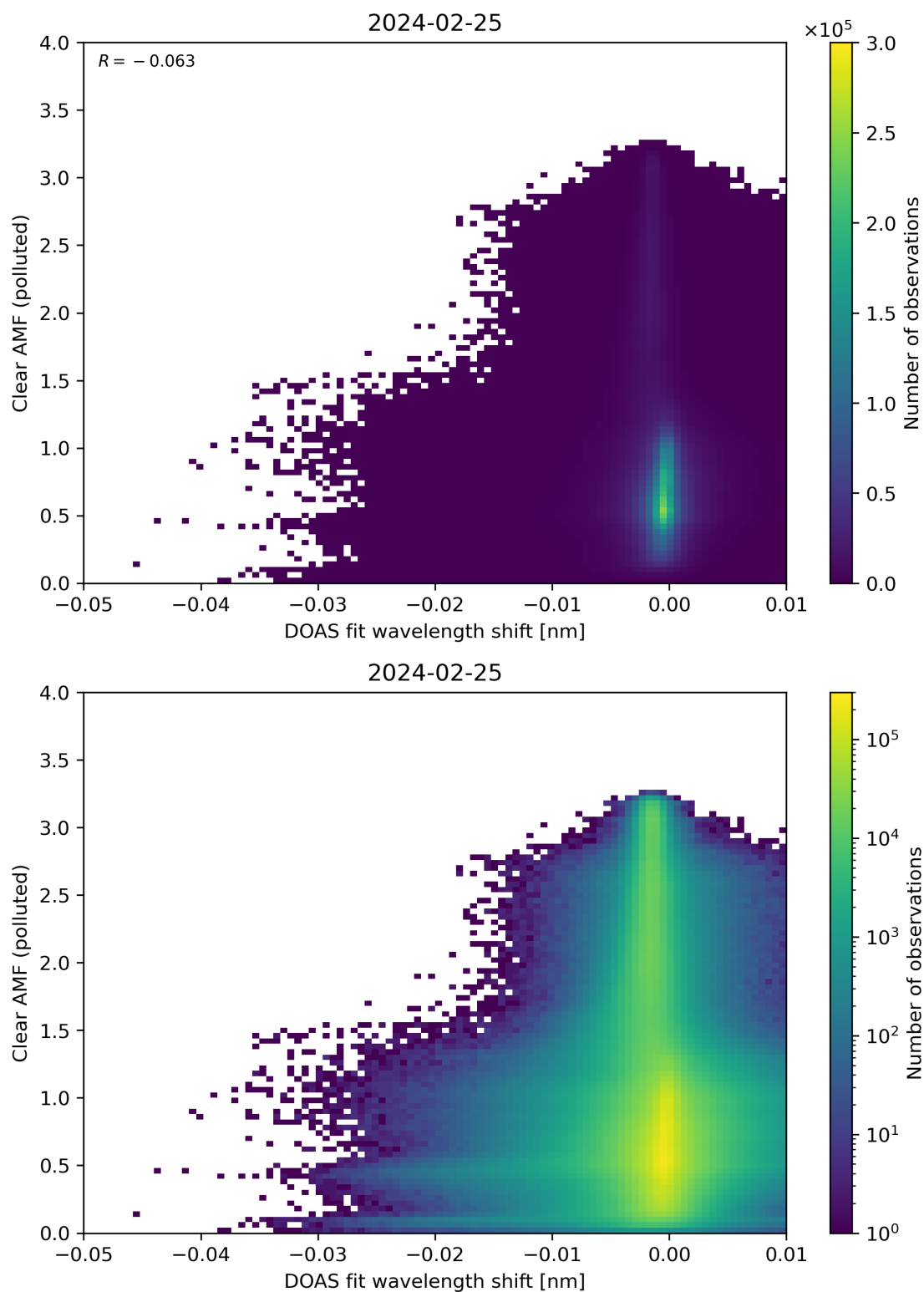
Figure 129: Scatter density plot of “DOAS fit wavelength shift” against “Clear AMF (polluted)” for 2024-02-24 to 2024-02-26.
