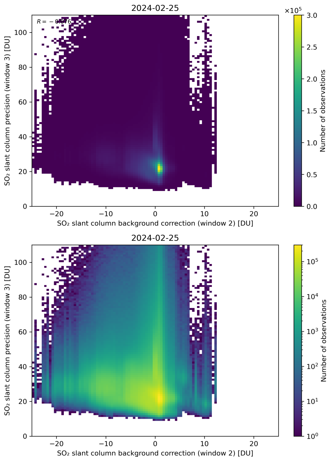
Figure 118: Scatter density plot of “SO 2 slant column background correction (window 2)” against “SO 2 slant column precision (window 3)” for 2024-02-24 to 2024-02-26.
