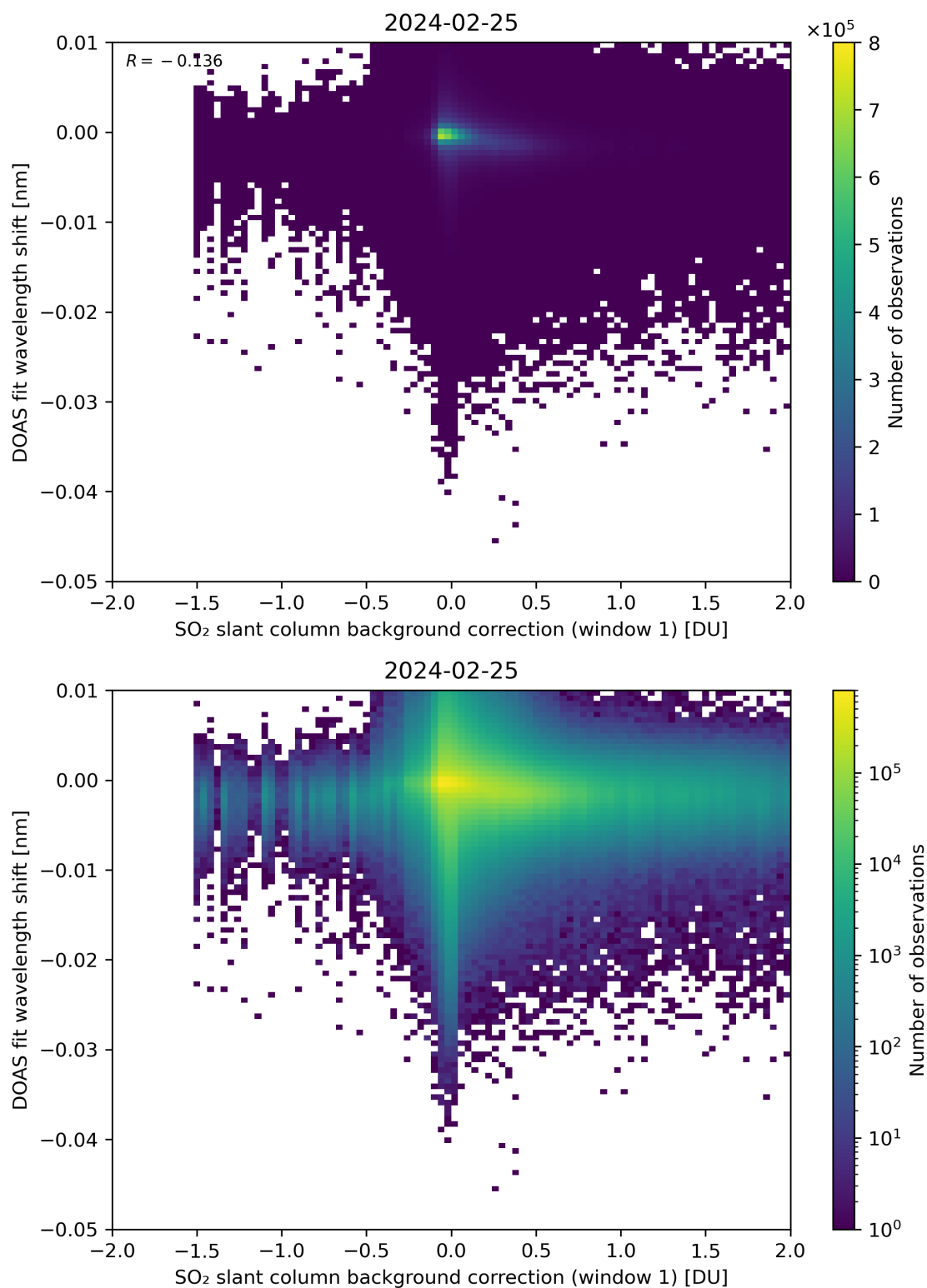
Figure 100: Scatter density plot of “SO 2 slant column background correction (window 1)” against “DOAS fit wavelength shift” for 2024-02-24 to 2024-02-26.
