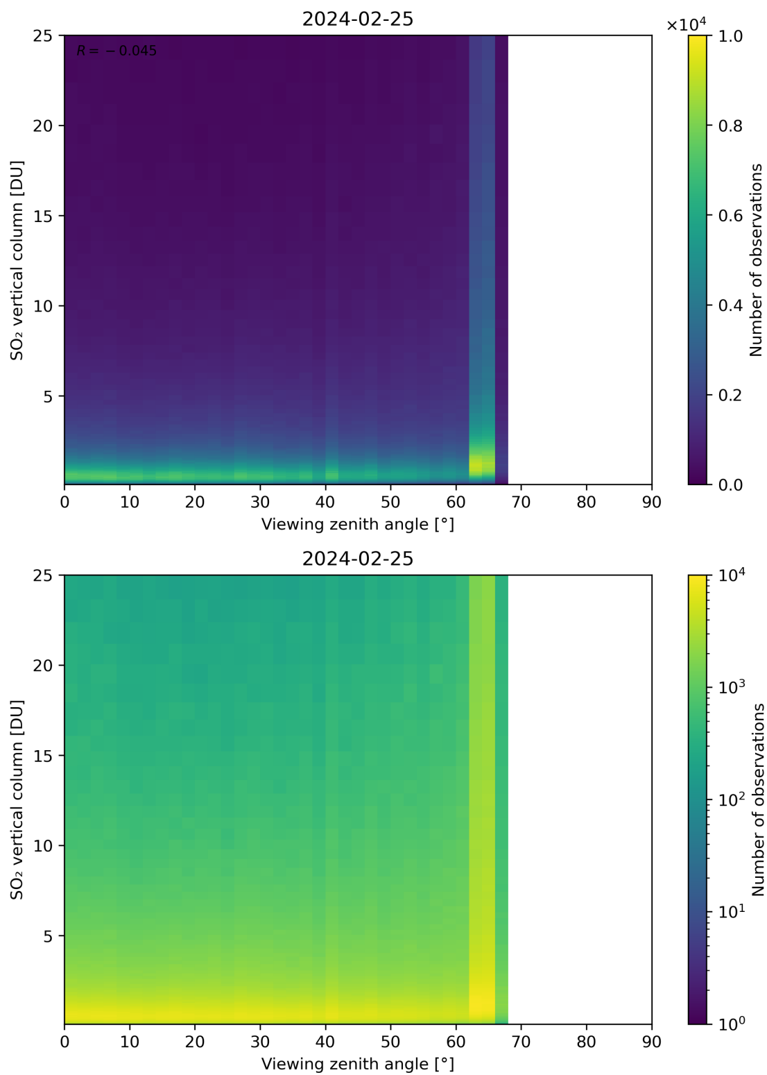
Figure 327: Scatter density plot of “Viewing zenith angle” against “SO 2 vertical column” for 2024-02-24 to 2024-02-26.
