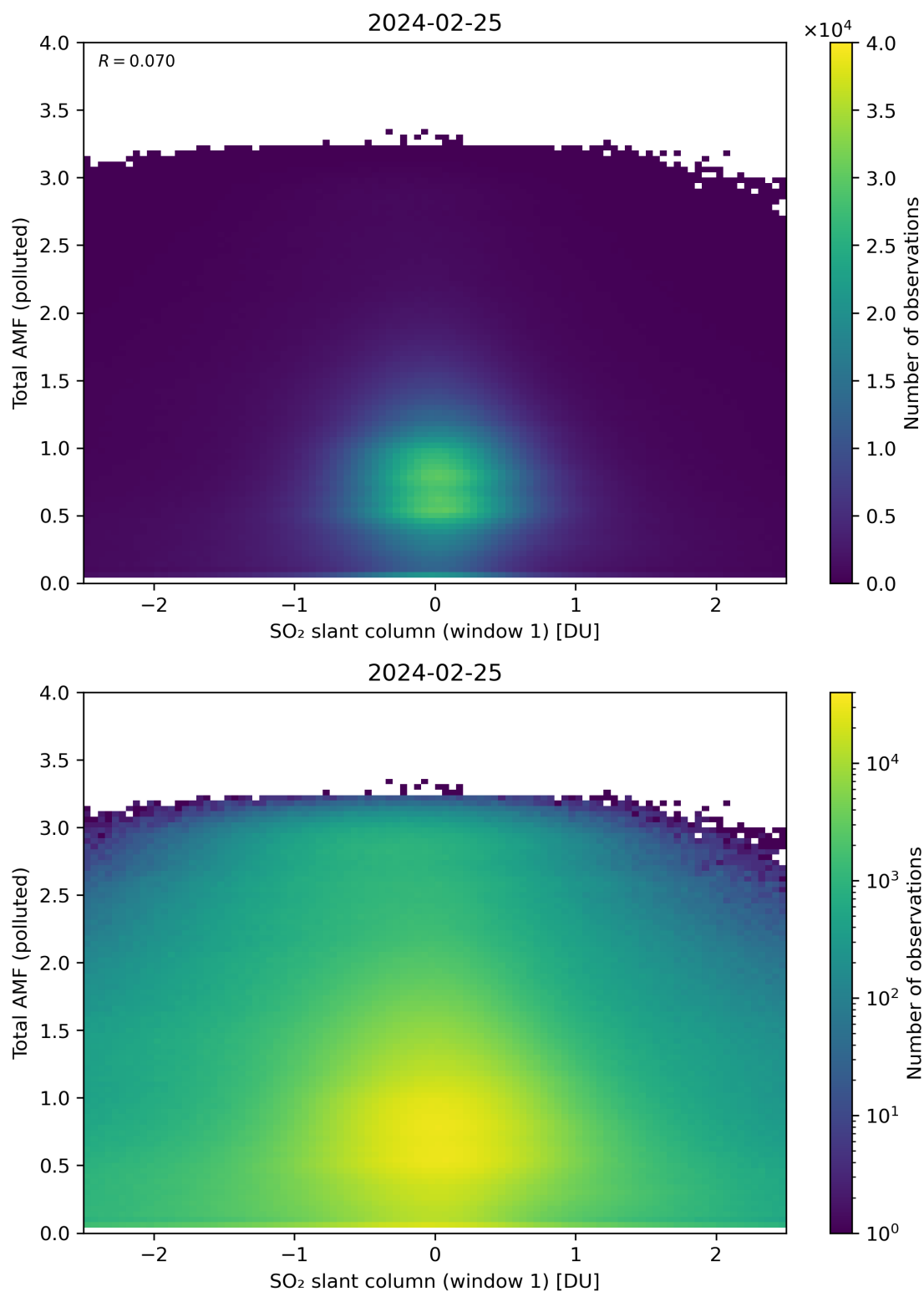
Figure 239: Scatter density plot of “SO 2 slant column (window 1)” against “Total AMF (polluted)” for 2024-02-24 to 2024-02-26.
