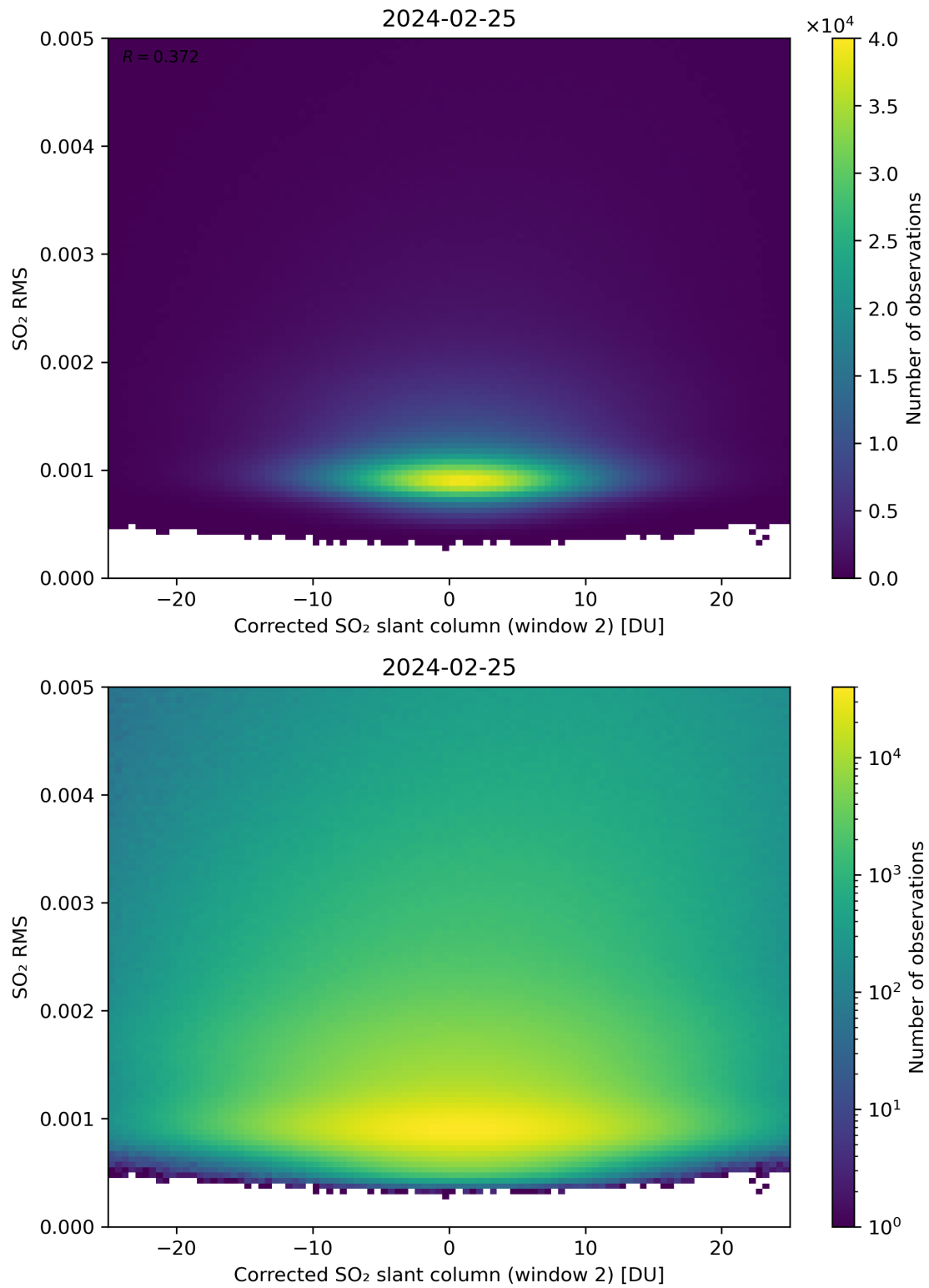
Figure 198: Scatter density plot of “Corrected SO 2 slant column (window 2)” against “SO 2 RMS” for 2024-02-24 to 2024-02-26.
