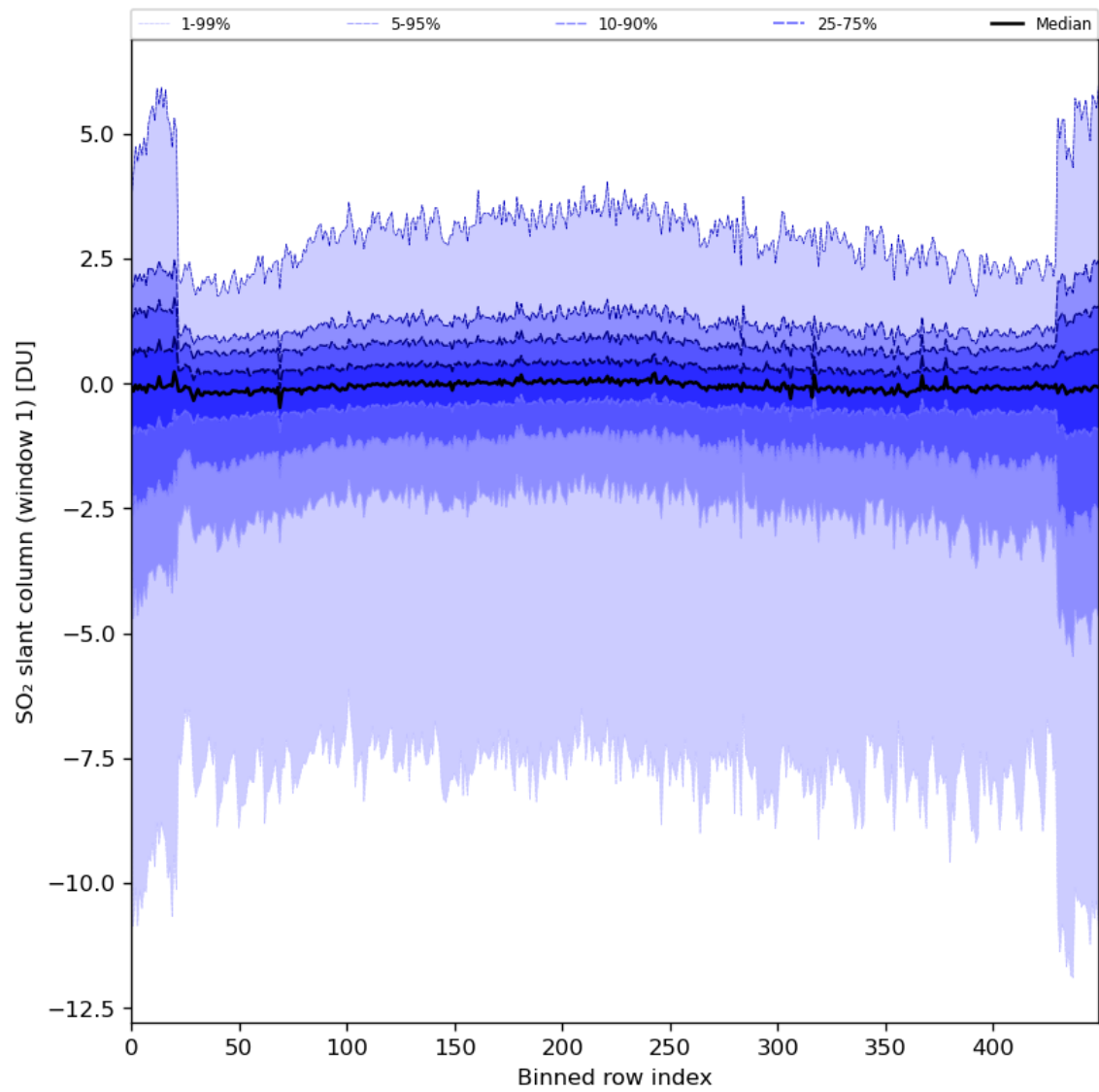
Figure 79: Along track statistics of “SO 2 slant column (window 1)” for 2024-02-24 to 2024-02-26
