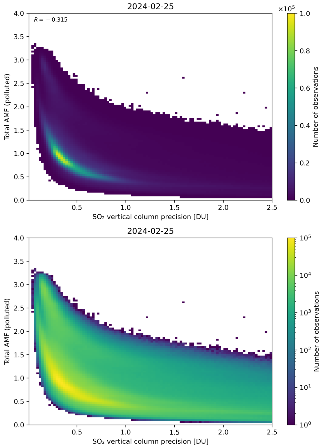
Figure 294: Scatter density plot of “SO 2 vertical column precision” against “Total AMF (polluted)” for 2024-02-24 to 2024-02-26.
