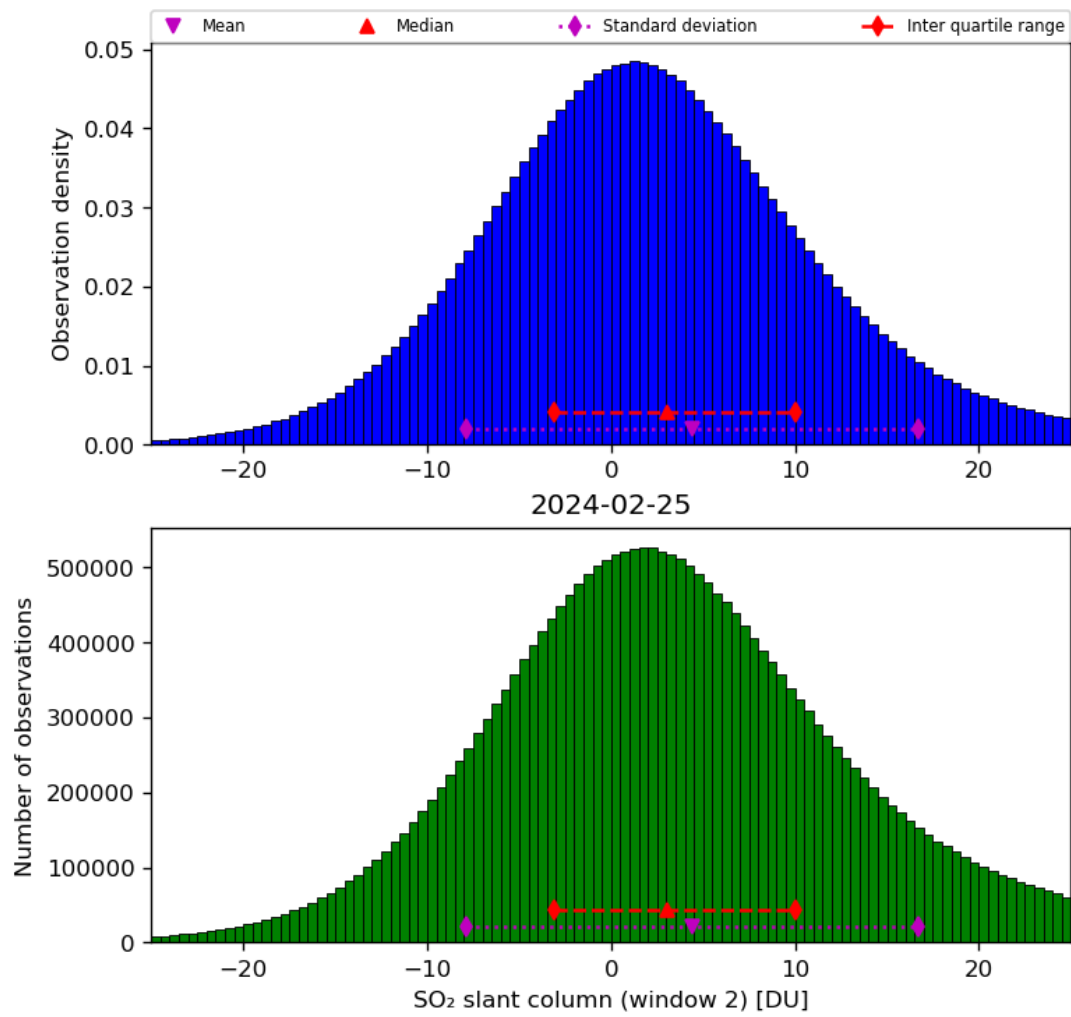
Figure 60: Histogram of “SO 2 slant column (window 2)” for 2024-02-24 to 2024-02-26
