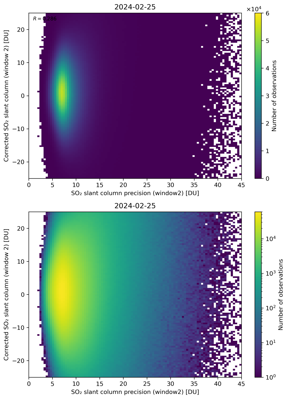
Figure 247: Scatter density plot of “SO 2 slant column precision (window2)” against “Corrected SO 2 slant column (window 2)” for 2024-02-24 to 2024-02-26.
