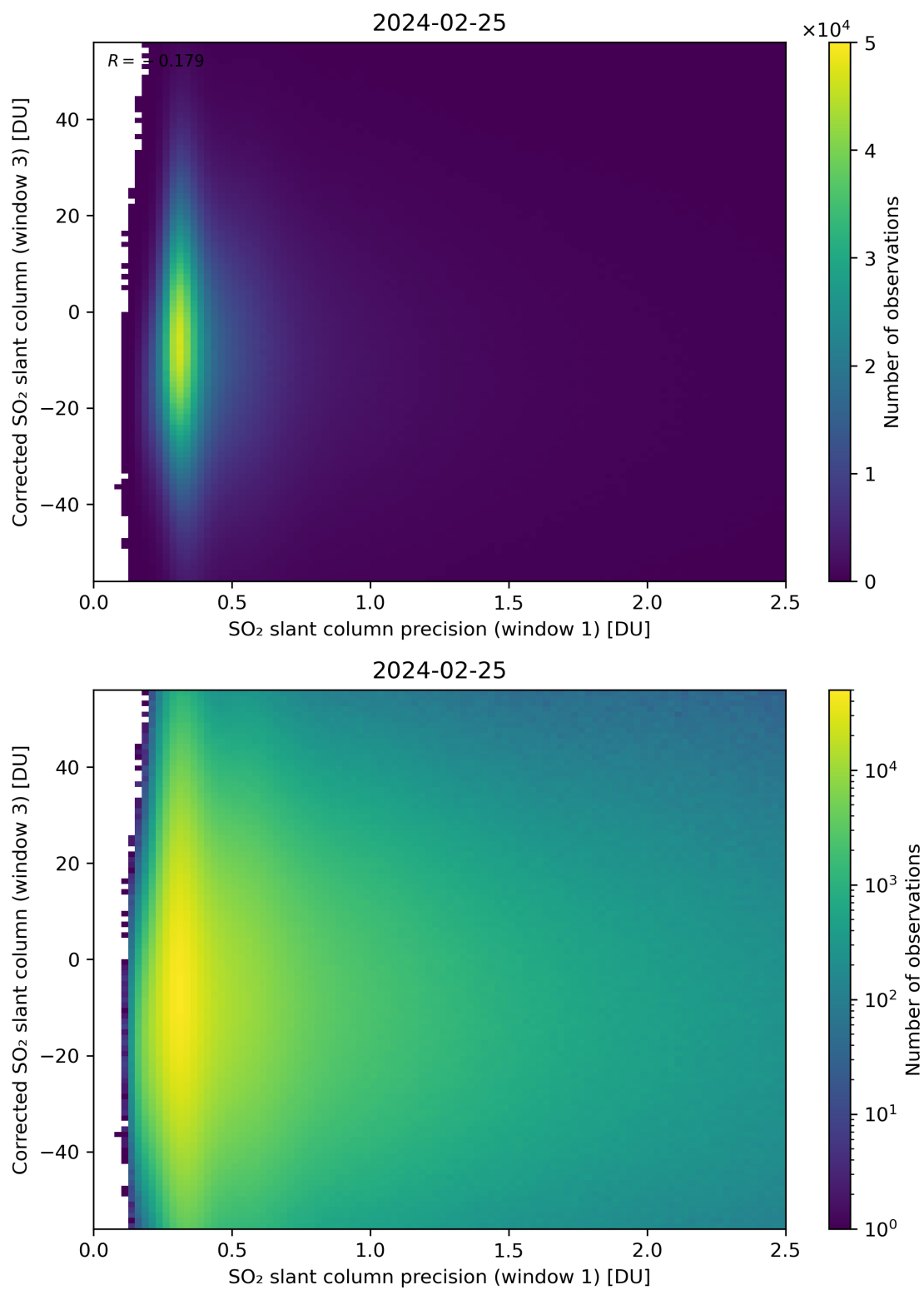
Figure 226: Scatter density plot of “SO 2 slant column precision (window 1)” against “Corrected SO 2 slant column (window 3)” for 2024-02-24 to 2024-02-26.
