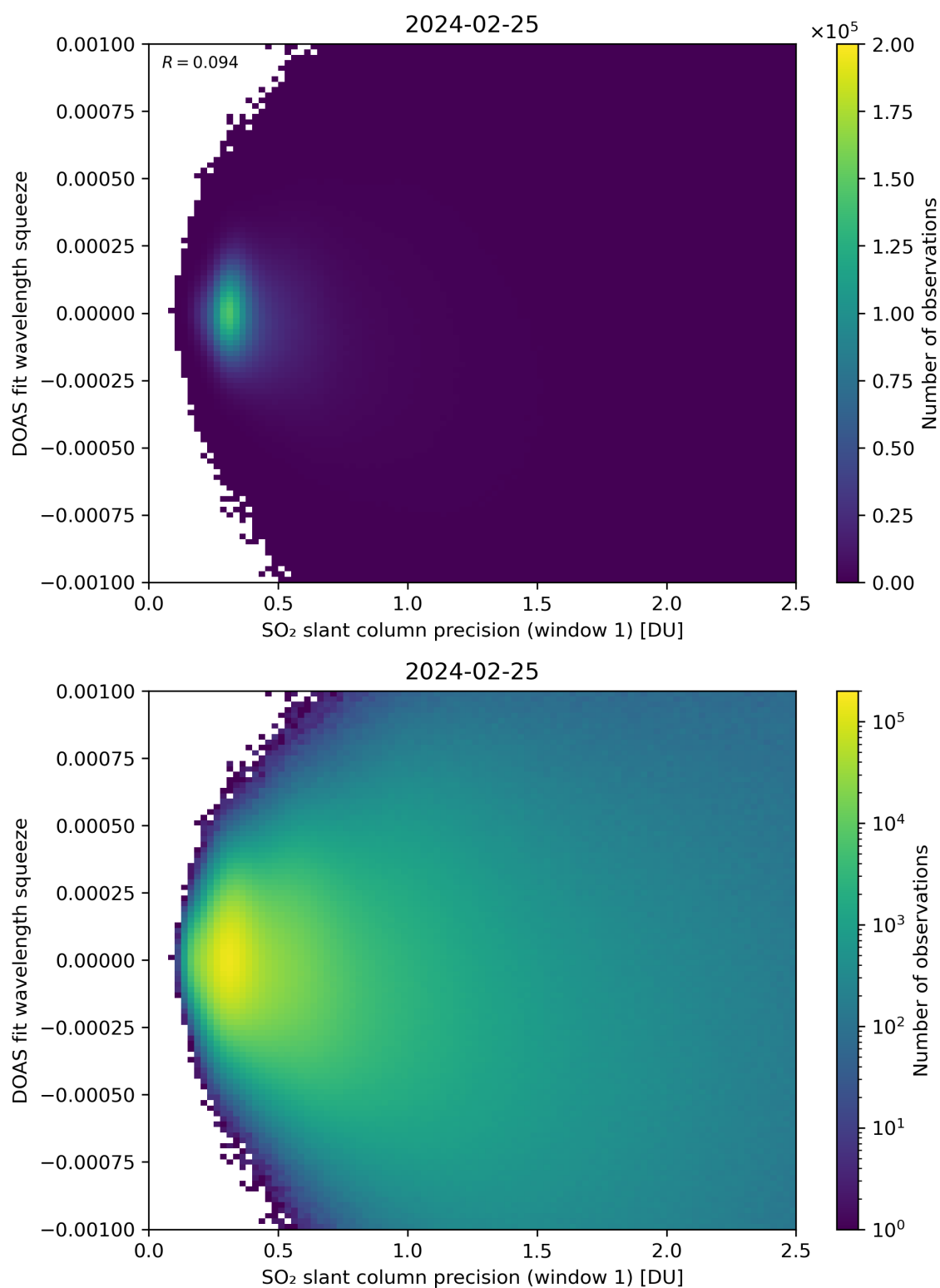
Figure 222: Scatter density plot of “SO 2 slant column precision (window 1)” against “DOAS fit wavelength squeeze” for 2024-02-24 to 2024-02-26.
