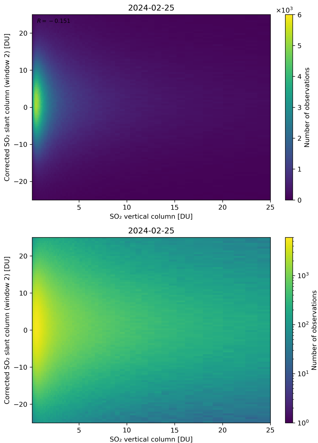
Figure 298: Scatter density plot of “SO 2 vertical column” against “Corrected SO 2 slant column (window 2)” for 2024-02-24 to 2024-02-26.
