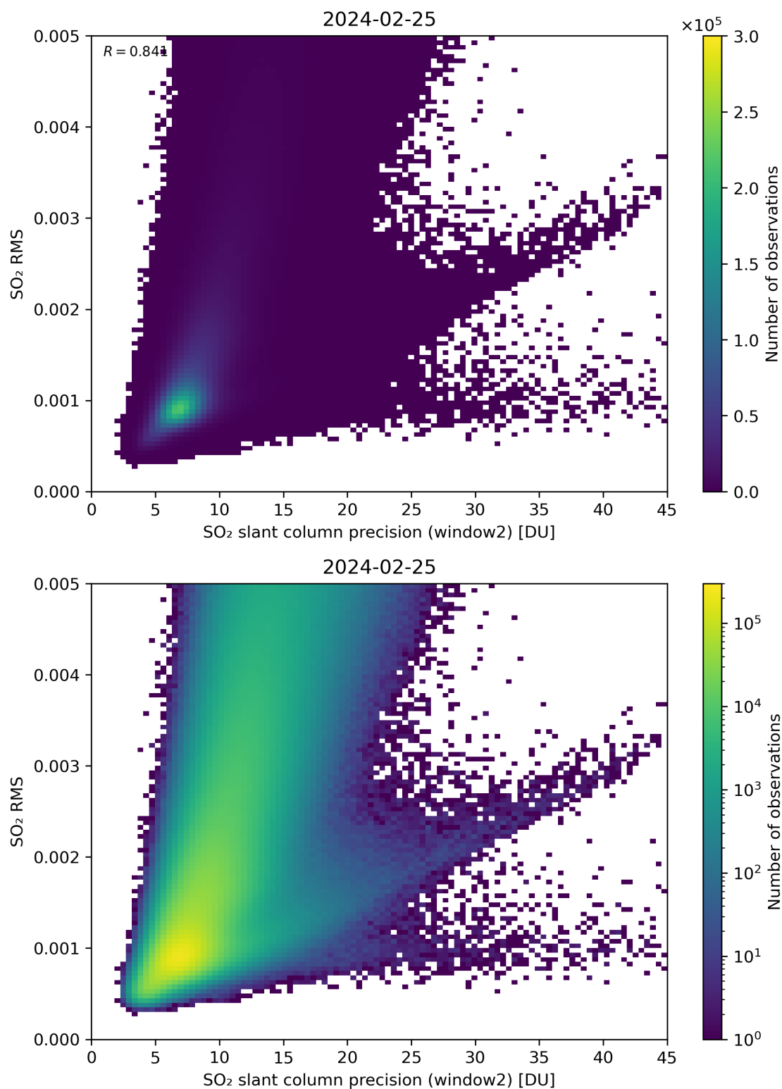
Figure 245: Scatter density plot of “SO 2 slant column precision (window2)” against “SO 2 RMS” for 2024-02-24 to 2024-02-26.
