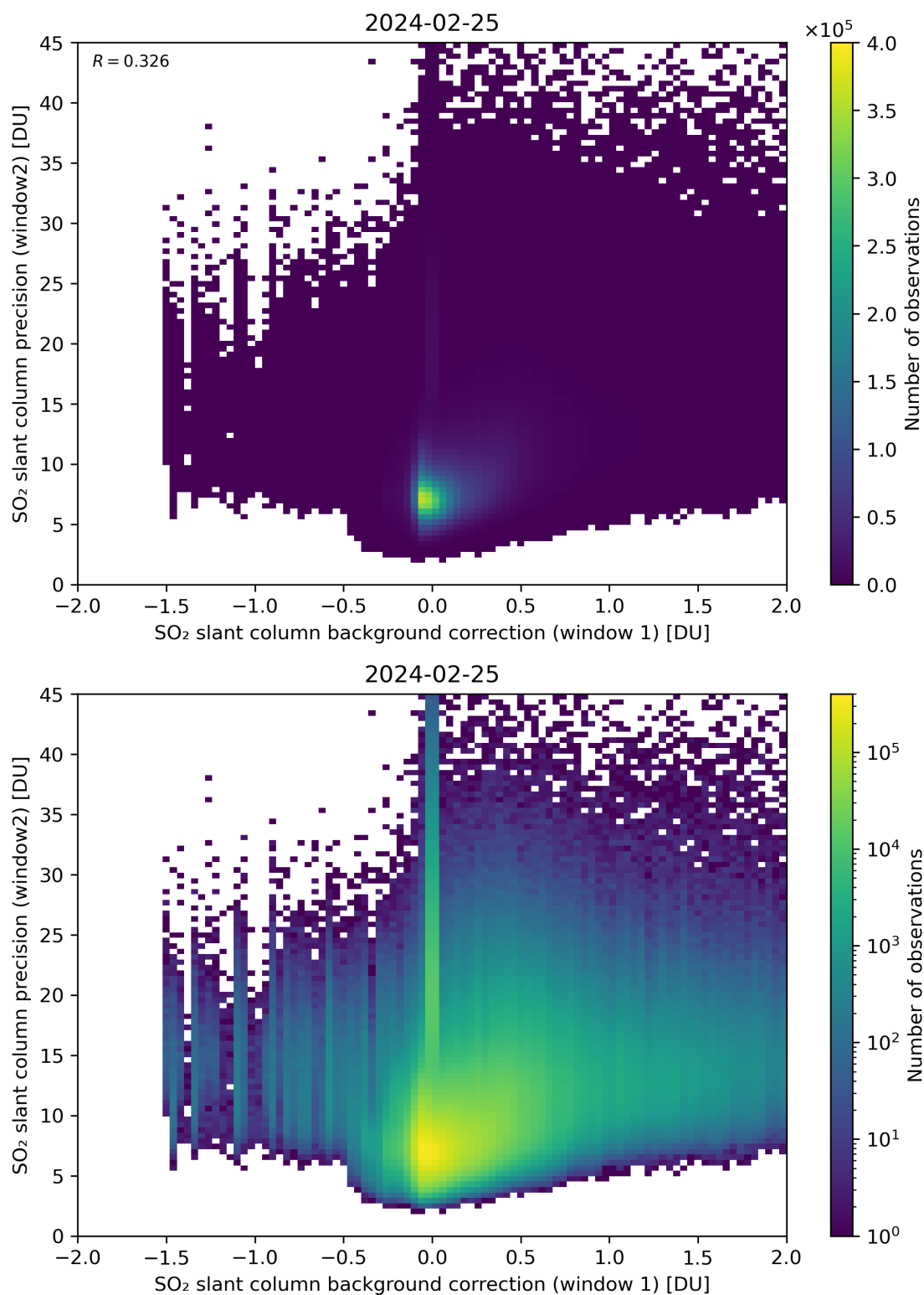
Figure 106: Scatter density plot of “SO 2 slant column background correction (window 1)” against “SO 2 slant column precision (window2)” for 2024-02-24 to 2024-02-26.
