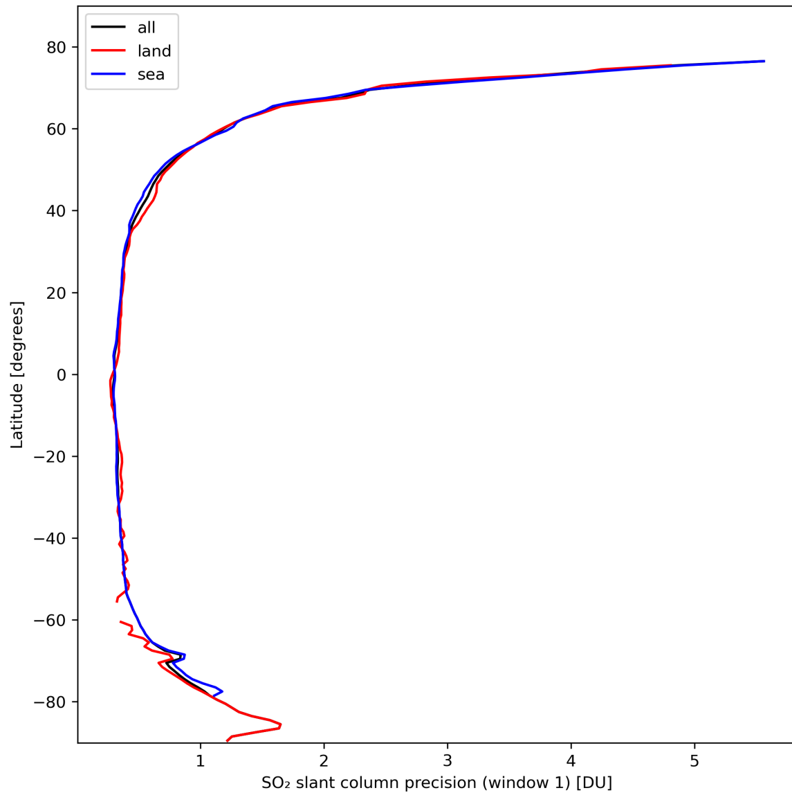
Figure 34: Zonal average of “SO 2 slant column precision (window 1)” for 2024-02-24 to 2024-02-26.
