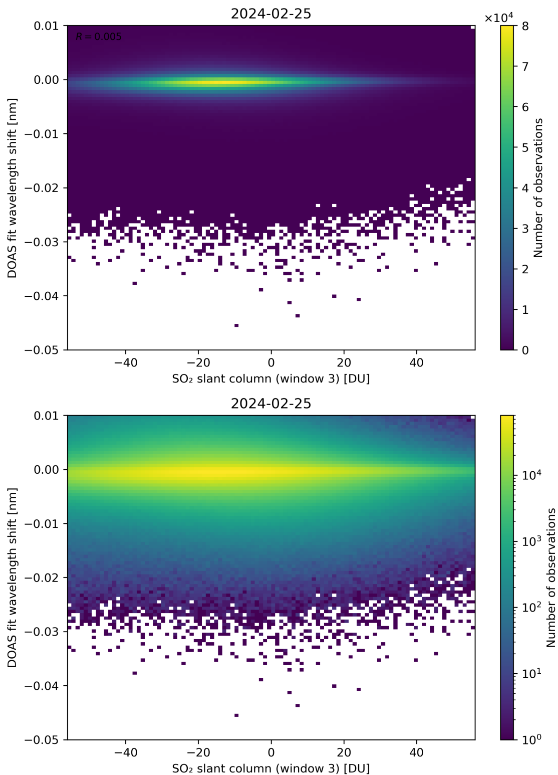
Figure 254: Scatter density plot of “SO 2 slant column (window 3)” against “DOAS fit wavelength shift” for 2024-02-24 to 2024-02-26.
