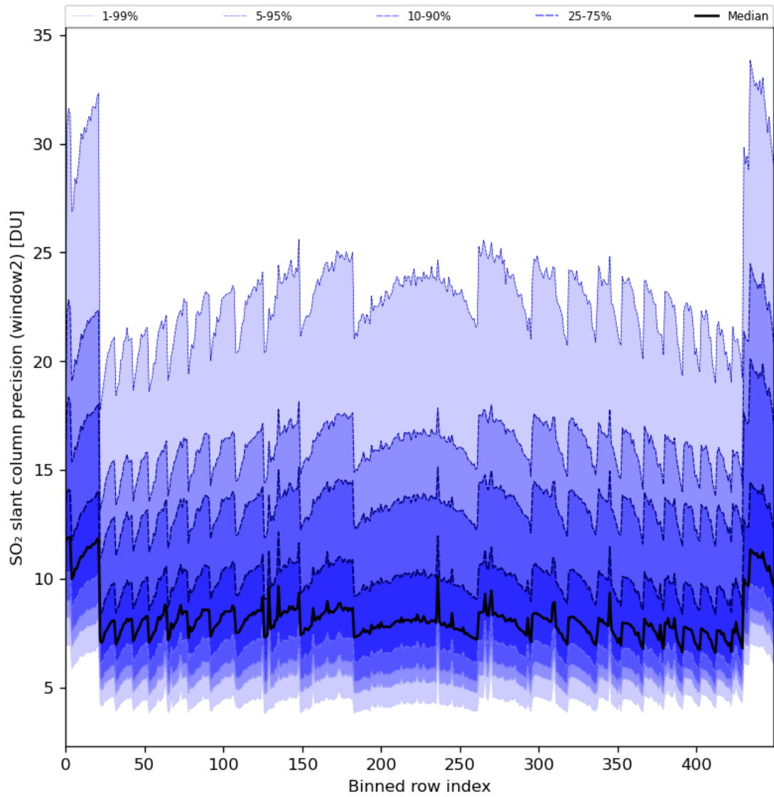
Figure 84: Along track statistics of “SO 2 slant column precision (window2)” for 2024-02-24 to 2024-02-26
