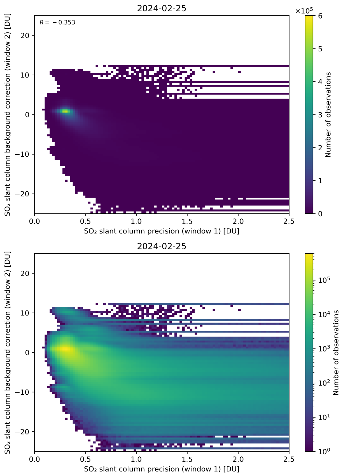
Figure 219: Scatter density plot of “SO 2 slant column precision (window 1)” against “SO 2 slant column background correction (window 2)” for 2024-02-24 to 2024-02-26.
