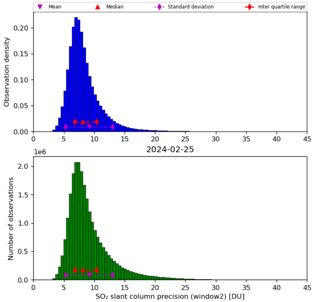
Figure 61: Histogram of “SO 2 slant column precision (window2)” for 2024-02-24 to 2024-02-26
