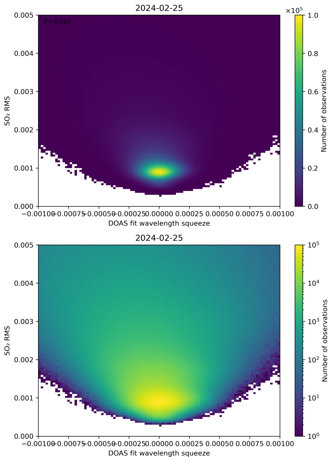
Figure 132: Scatter density plot of “DOAS fit wavelength squeeze” against “SO 2 RMS” for 2024-02-24 to 2024-02-26.
