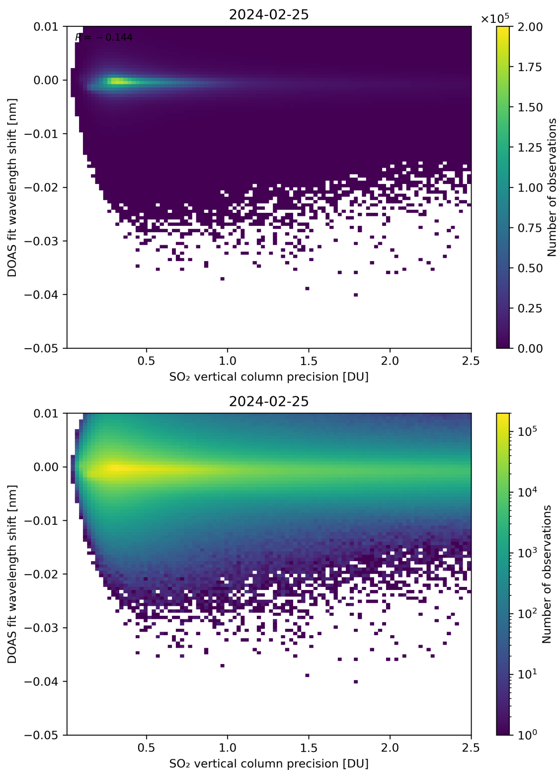
Figure 282: Scatter density plot of “SO 2 vertical column precision” against “DOAS fit wavelength shift” for 2024-02-24 to 2024-02-26.
