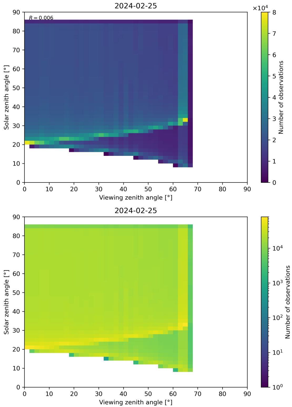
Figure 315: Scatter density plot of “Viewing zenith angle” against “Solar zenith angle” for 2024-02-24 to 2024-02-26.
