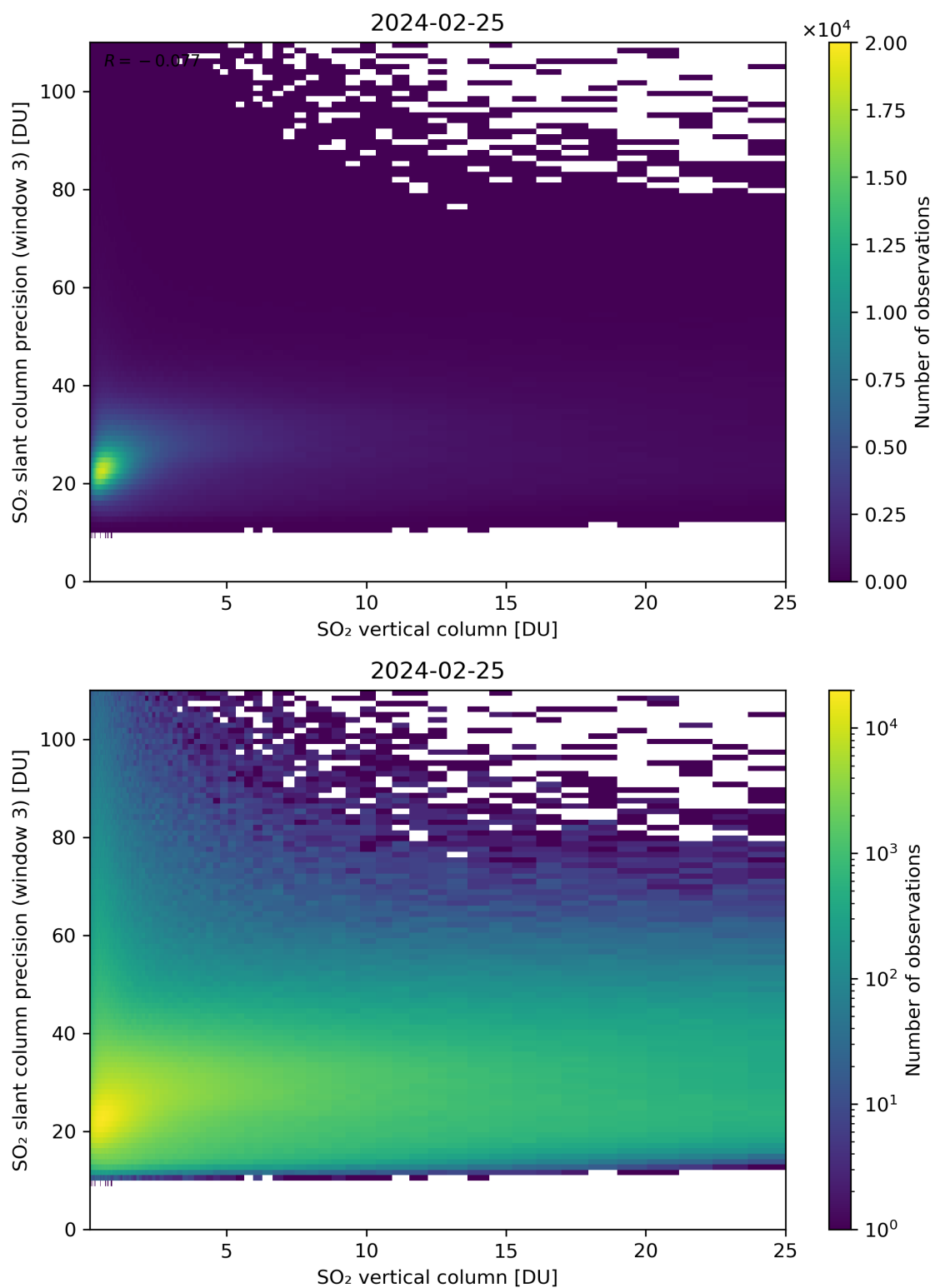
Figure 304: Scatter density plot of “SO 2 vertical column” against “SO 2 slant column precision (window 3)” for 2024-02-24 to 2024-02-26.
