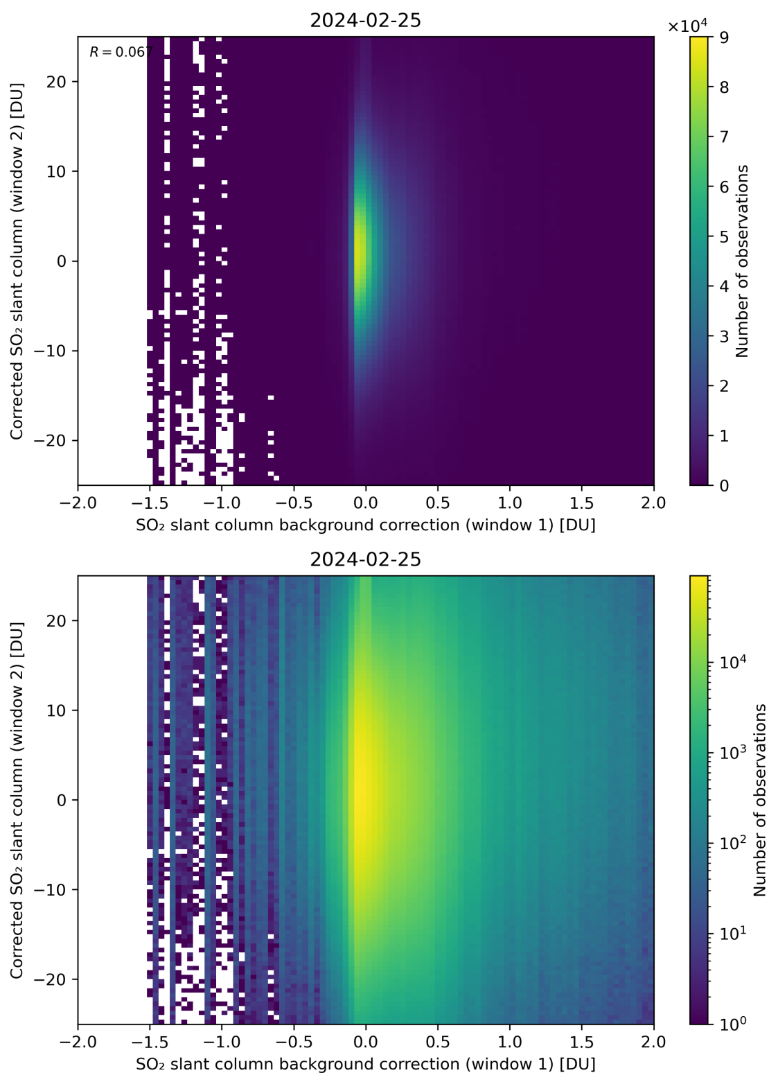
Figure 104: Scatter density plot of “SO 2 slant column background correction (window 1)” against “Corrected SO 2 slant column (window 2)” for 2024-02-24 to 2024-02-26.
