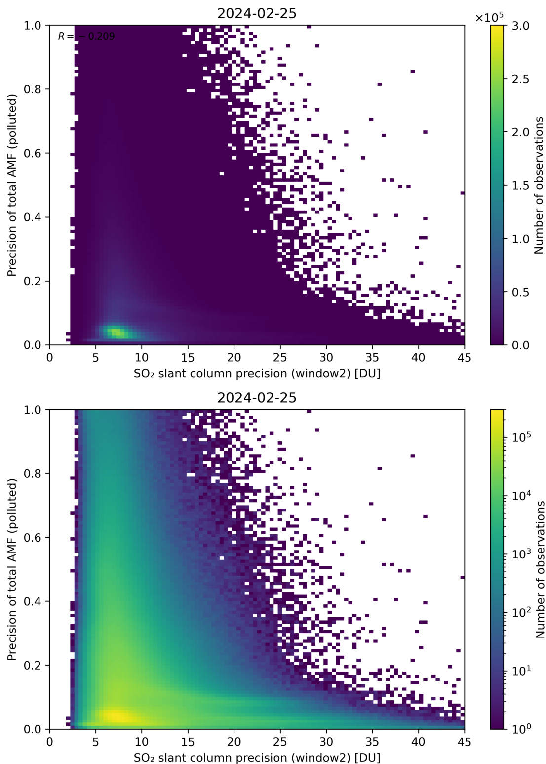
Figure 252: Scatter density plot of “SO 2 slant column precision (window2)” against “Precision of total AMF (polluted)” for 2024-02-24 to 2024-02-26.
