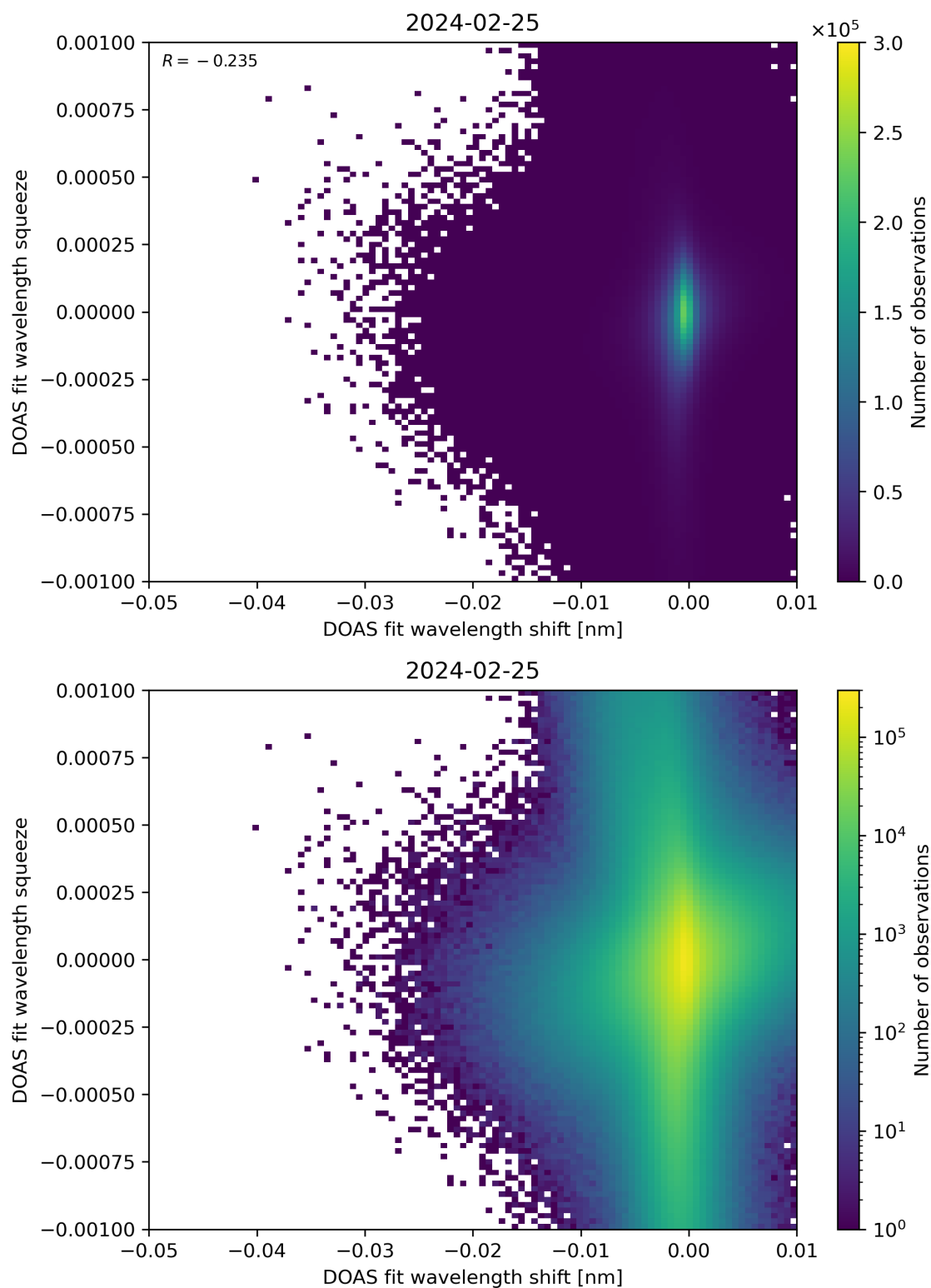
Figure 127: Scatter density plot of “DOAS fit wavelength shift” against “DOAS fit wavelength squeeze” for 2024-02-24 to 2024-02-26.
