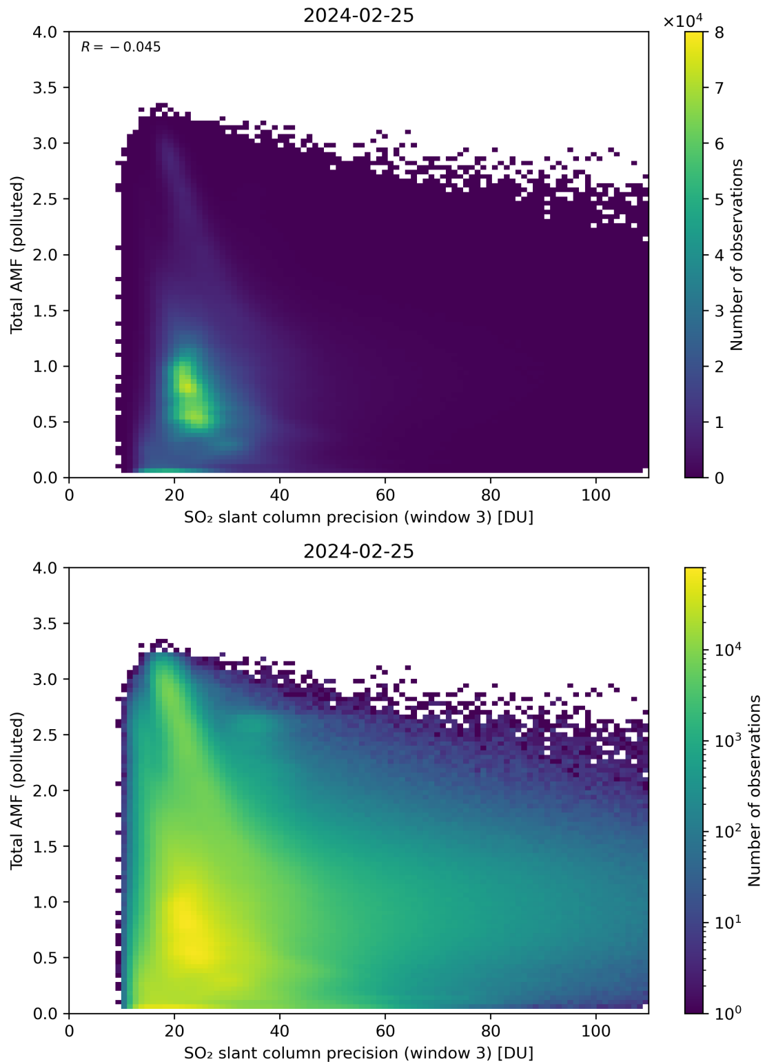
Figure 263: Scatter density plot of “SO 2 slant column precision (window 3)” against “Total AMF (polluted)” for 2024-02-24 to 2024-02-26.
