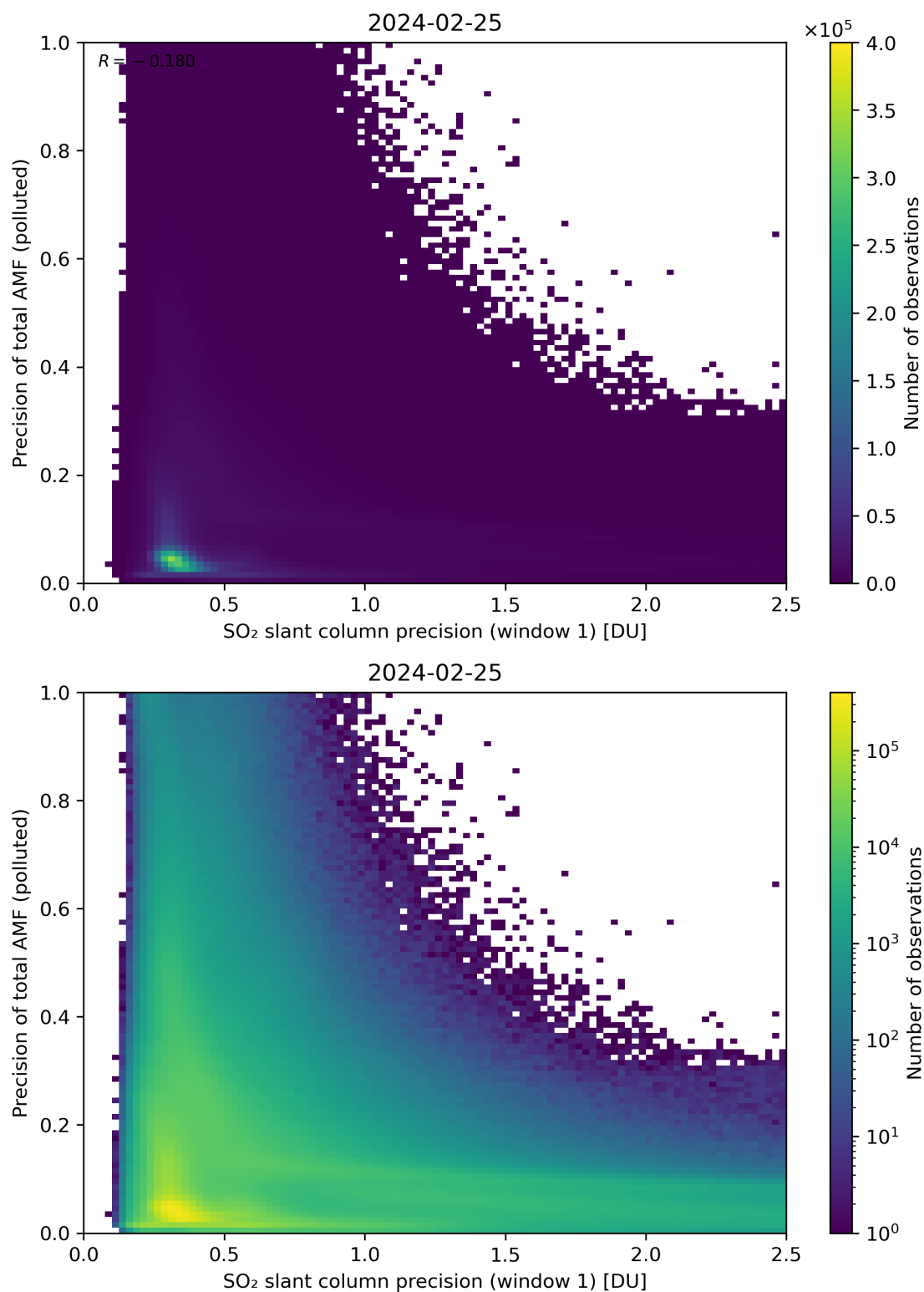
Figure 231: Scatter density plot of “SO 2 slant column precision (window 1)” against “Precision of total AMF (polluted)” for 2024-02-24 to 2024-02-26.
