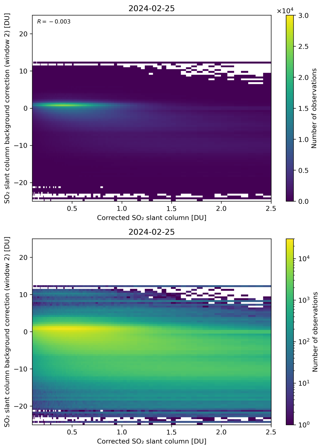
Figure 179: Scatter density plot of “Corrected SO 2 slant column” against “SO 2 slant column background correction (window 2)” for 2024-02-24 to 2024-02-26.
