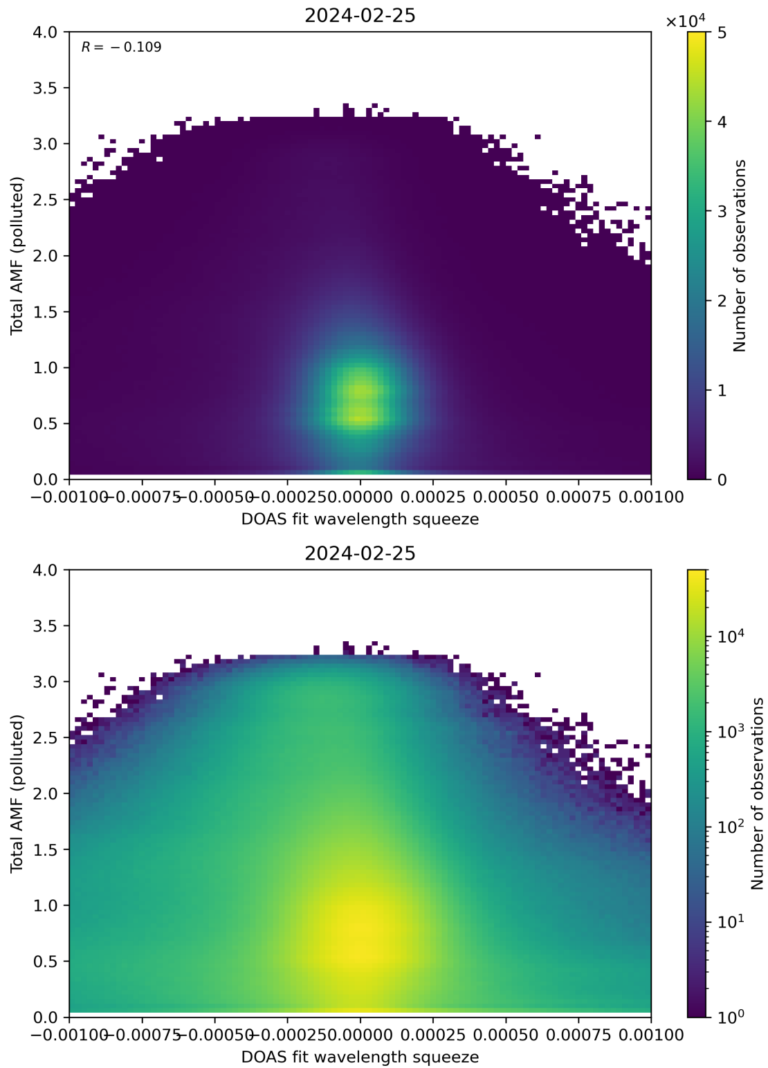
Figure 134: Scatter density plot of “DOAS fit wavelength squeeze” against “Total AMF (polluted)” for 2024-02-24 to 2024-02-26.
