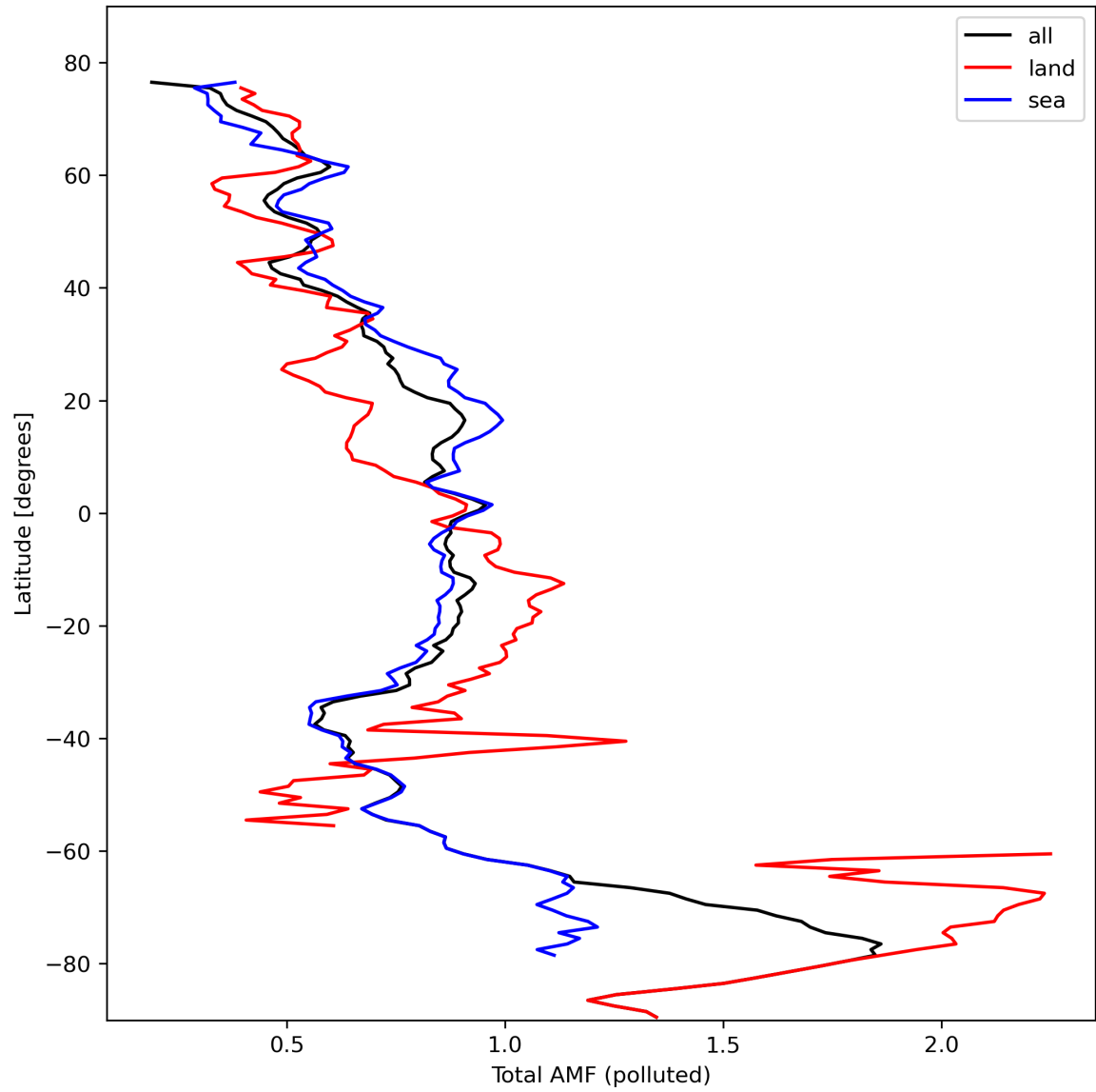
Figure 48: Zonal average of “Total AMF (polluted)” for 2024-02-24 to 2024-02-26.
