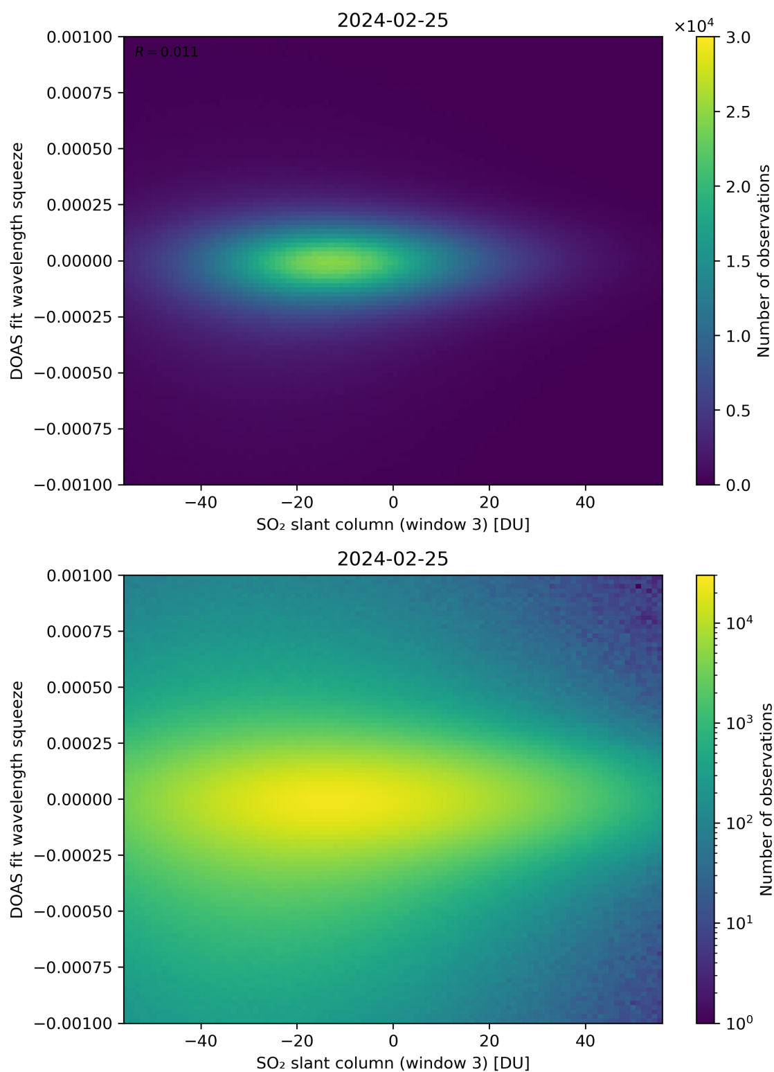
Figure 255: Scatter density plot of “SO 2 slant column (window 3)” against “DOAS fit wavelength squeeze” for 2024-02-24 to 2024-02-26.
