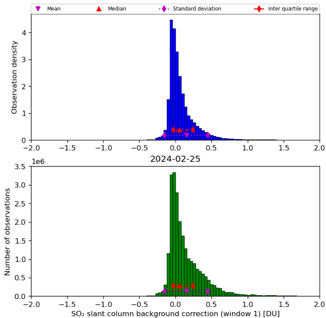
Figure 59: Histogram of “SO 2 slant column background correction (window 1)” for 2024-02-24 to 2024-02-26
