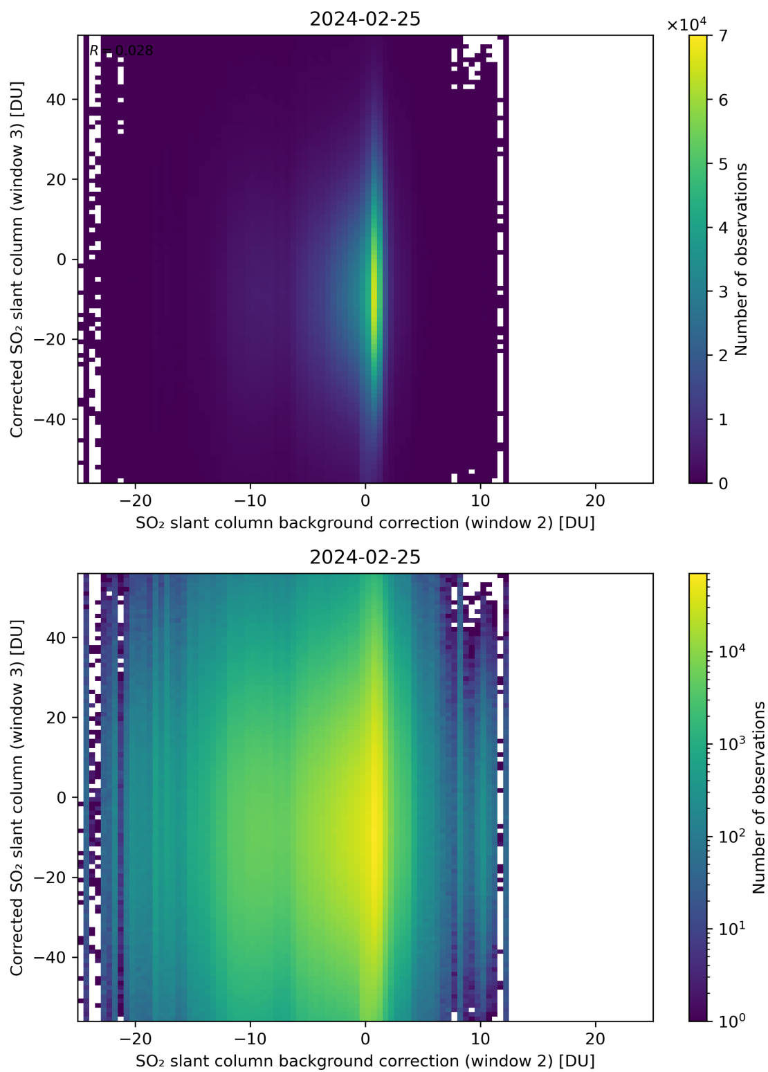
Figure 116: Scatter density plot of “SO 2 slant column background correction (window 2)” against “Corrected SO 2 slant column (window 3)” for 2024-02-24 to 2024-02-26.
