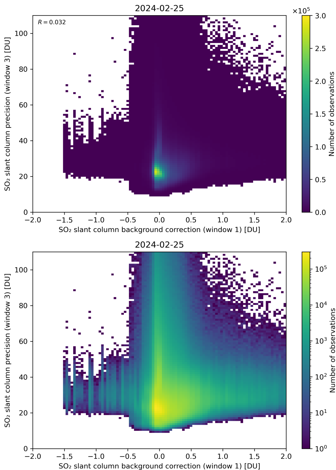
Figure 108: Scatter density plot of “SO 2 slant column background correction (window 1)” against “SO 2 slant column precision (window 3)” for 2024-02-24 to 2024-02-26.
