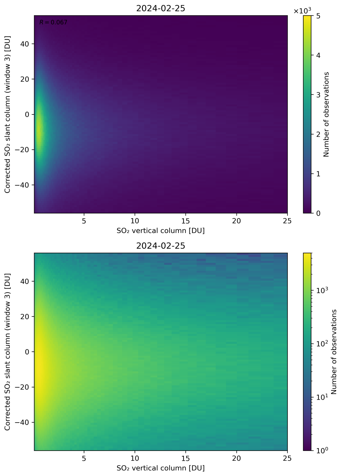
Figure 299: Scatter density plot of “SO 2 vertical column” against “Corrected SO 2 slant column (window 3)” for 2024-02-24 to 2024-02-26.
