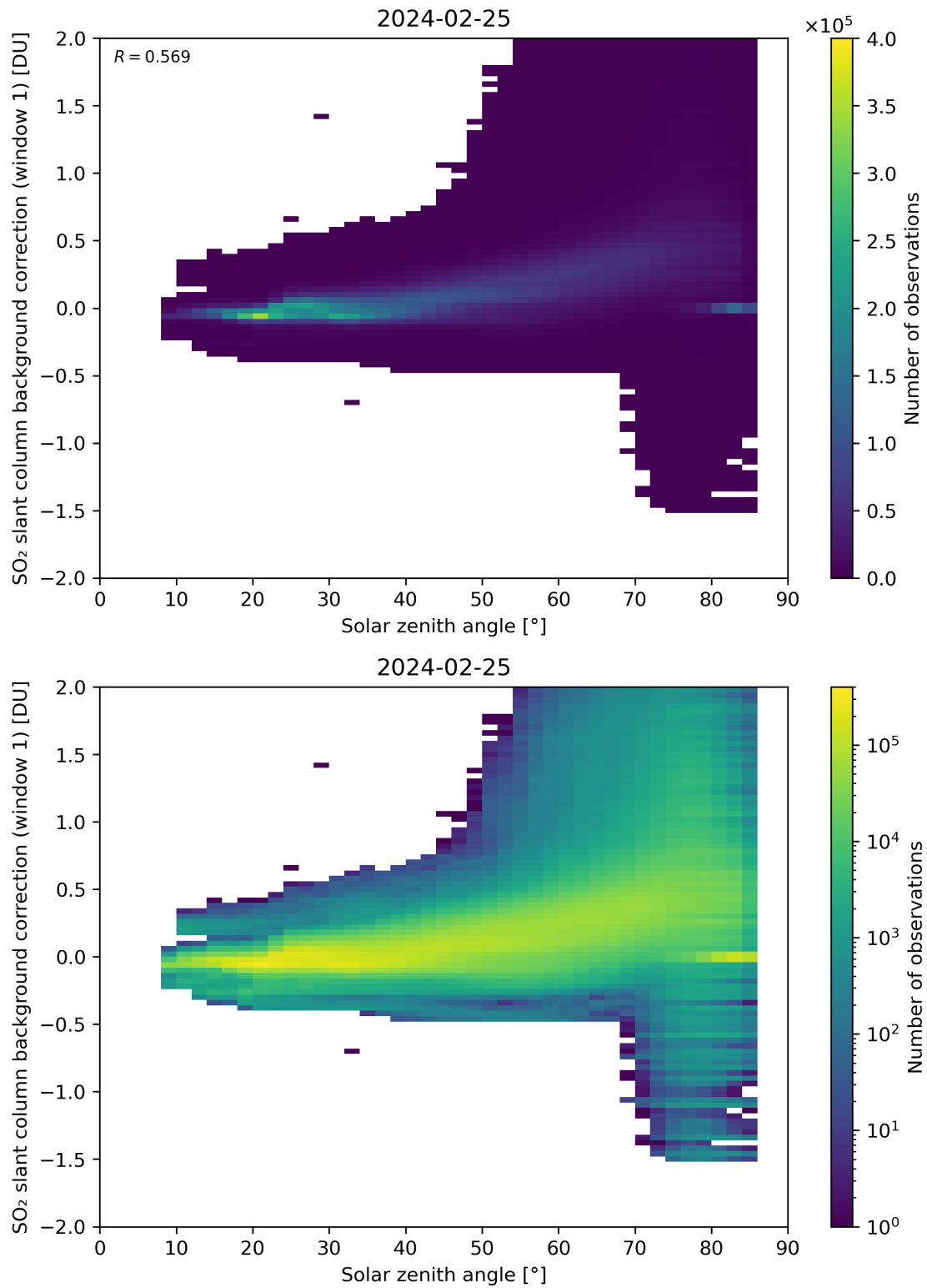
Figure 158: Scatter density plot of “Solar zenith angle” against “SO 2 slant column background correction (window 1)” for 2024-02-24 to 2024-02-26.
