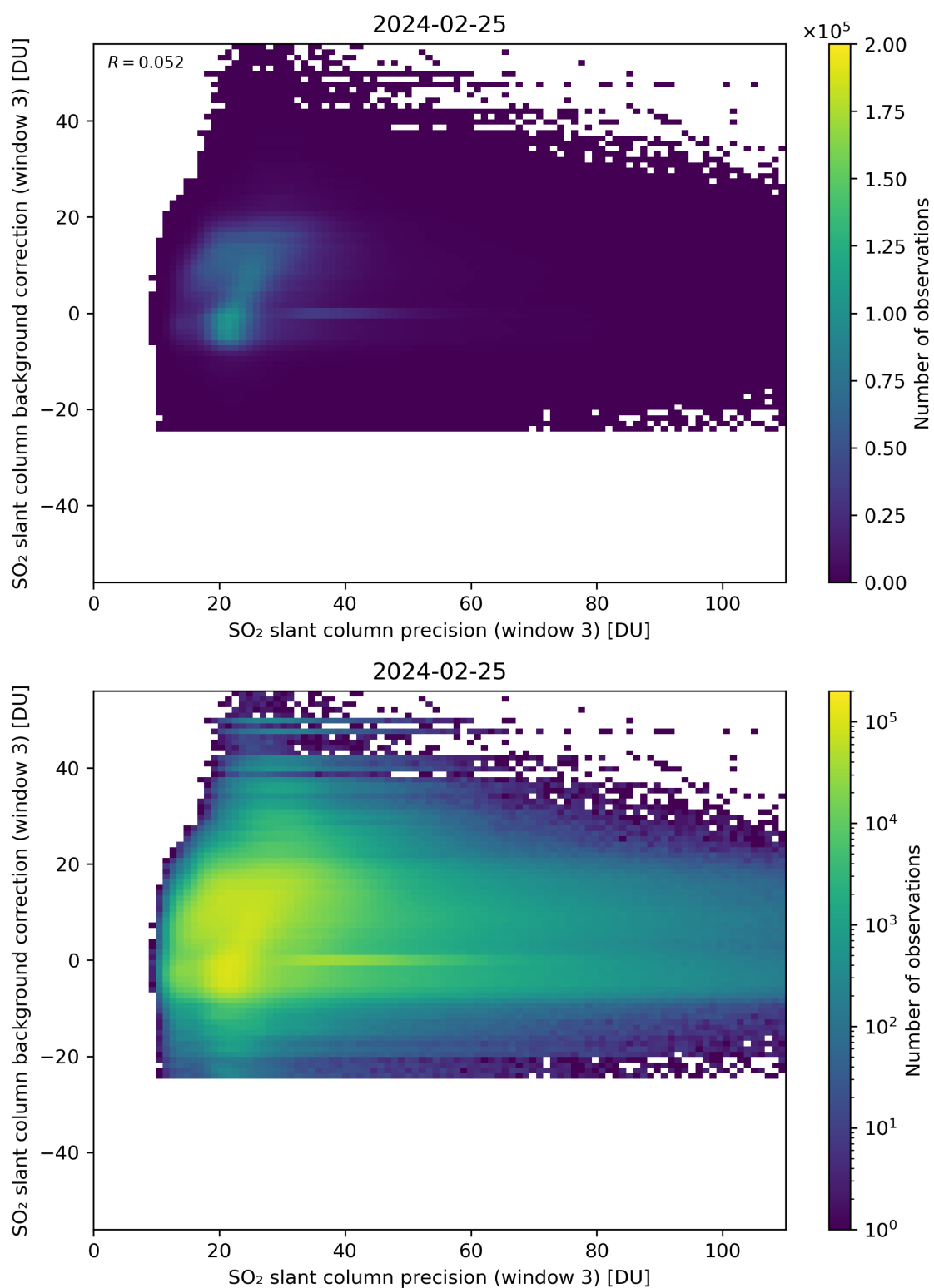
Figure 257: Scatter density plot of “SO 2 slant column precision (window 3)” against “SO 2 slant column background correction (window 3)” for 2024-02-24 to 2024-02-26.
