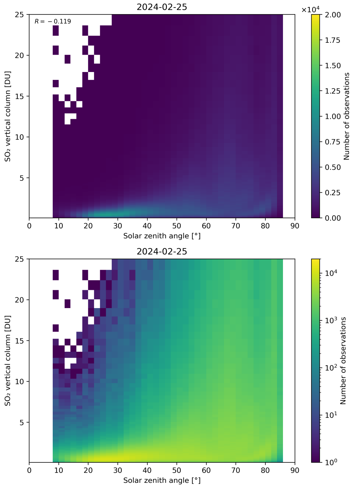
Figure 176: Scatter density plot of “Solar zenith angle” against “SO 2 vertical column” for 2024-02-24 to 2024-02-26.
