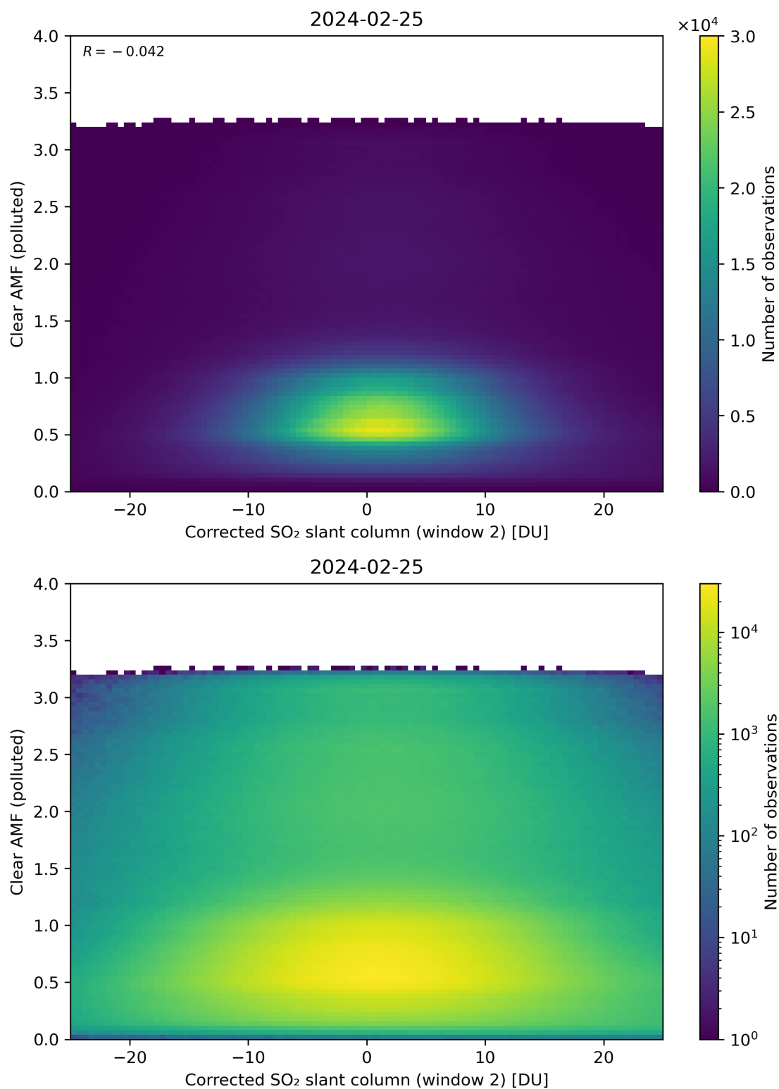
Figure 199: Scatter density plot of “Corrected SO 2 slant column (window 2)” against “Clear AMF (polluted)” for 2024-02-24 to 2024-02-26.
