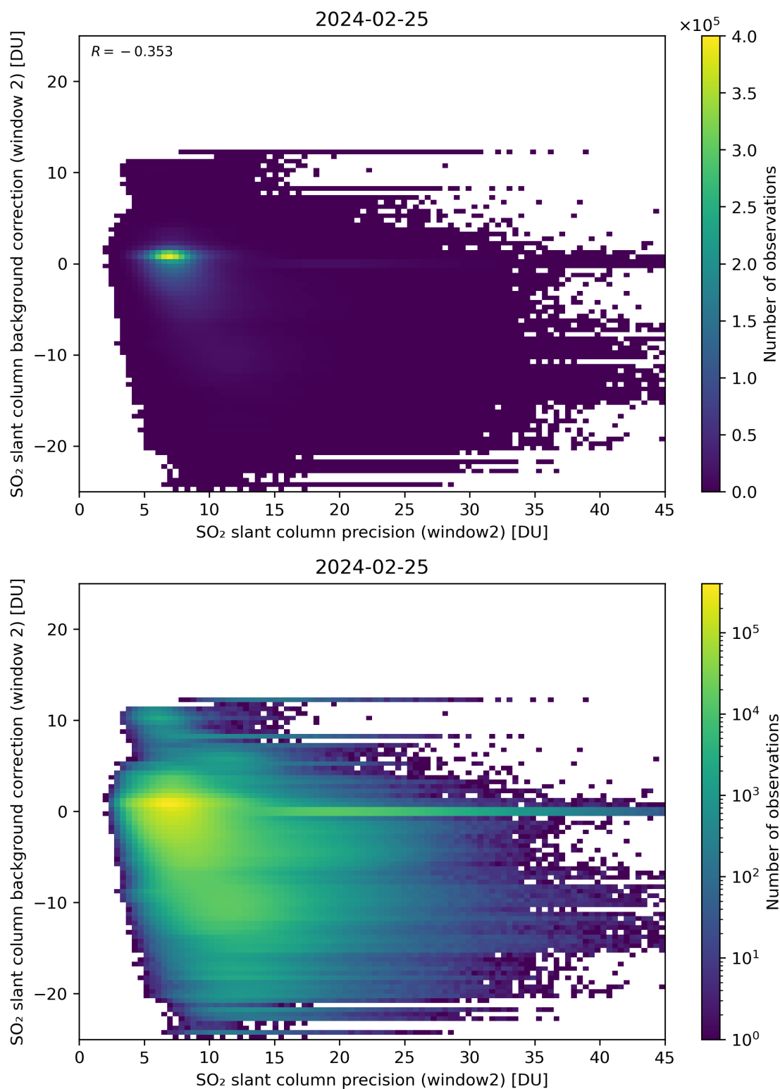
Figure 241: Scatter density plot of “SO 2 slant column precision (window2)” against “SO 2 slant column background correction (window 2)” for 2024-02-24 to 2024-02-26.
