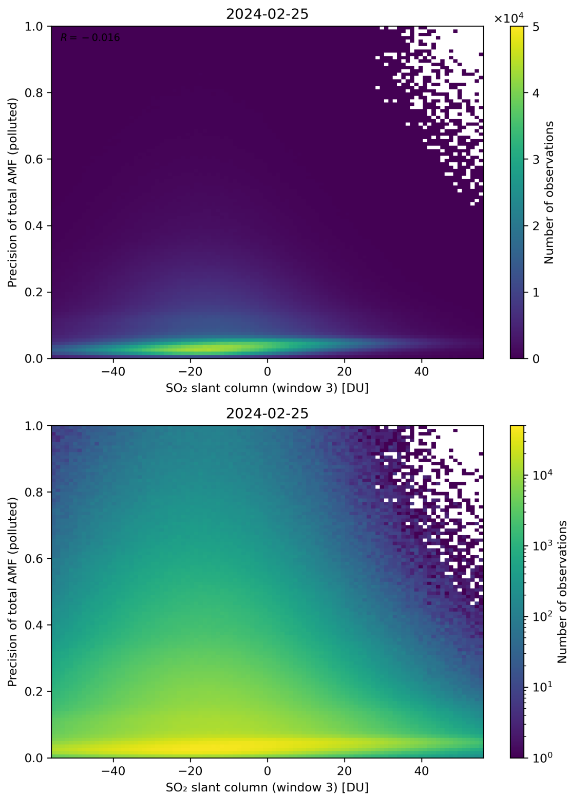
Figure 269: Scatter density plot of “SO 2 slant column (window 3)” against “Precision of total AMF (polluted)” for 2024-02-24 to 2024-02-26.
