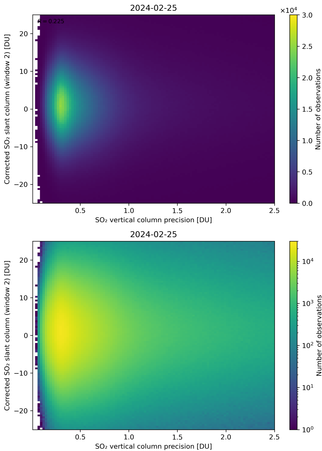
Figure 287: Scatter density plot of “SO 2 vertical column precision” against “Corrected SO 2 slant column (window 2)” for 2024-02-24 to 2024-02-26.
