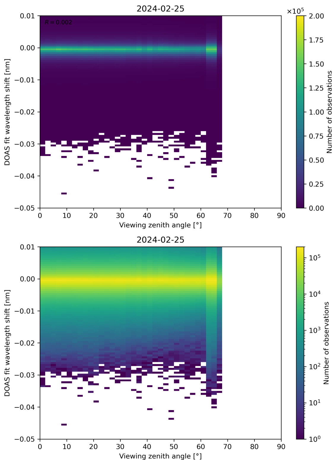
Figure 311: Scatter density plot of “Viewing zenith angle” against “DOAS fit wavelength shift” for 2024-02-24 to 2024-02-26.
