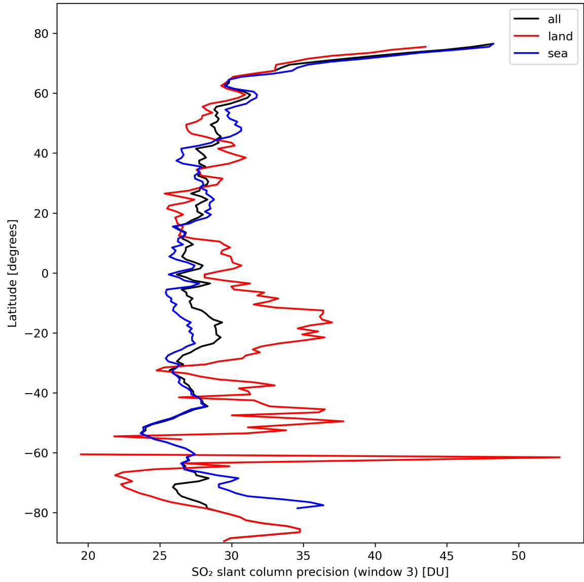
Figure 42: Zonal average of “SO 2 slant column precision (window 3)” for 2024-02-24 to 2024-02-26.
