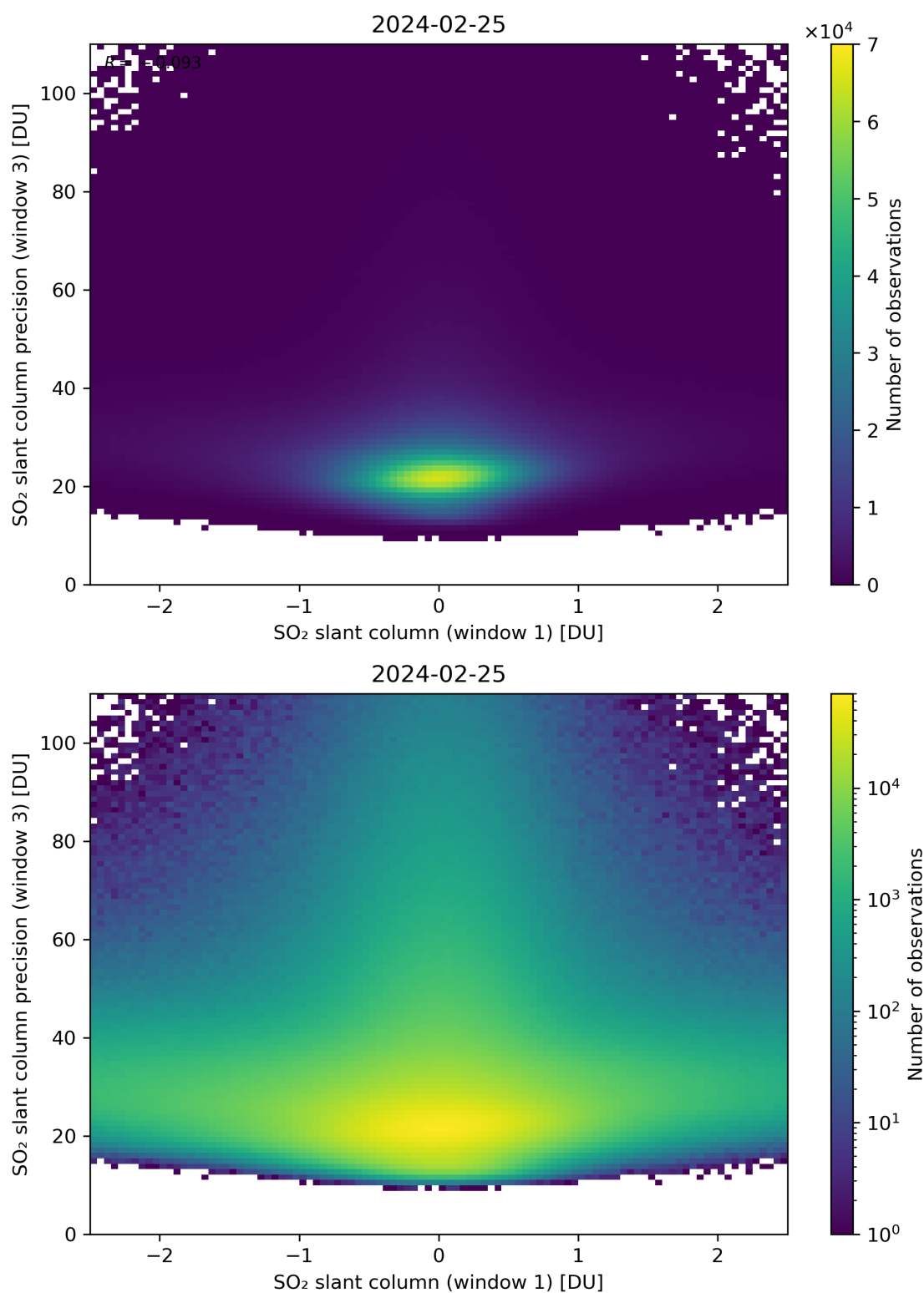
Figure 238: Scatter density plot of “SO 2 slant column (window 1)” against “SO 2 slant column precision (window 3)” for 2024-02-24 to 2024-02-26.
