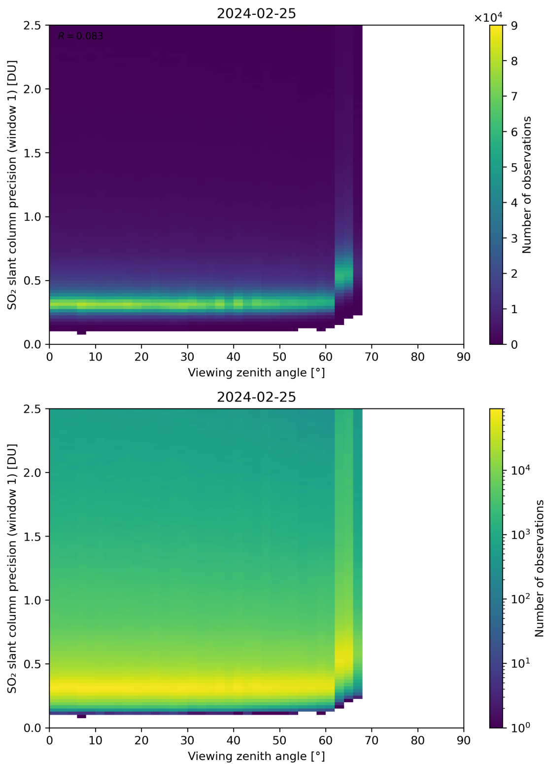
Figure 321: Scatter density plot of “Viewing zenith angle” against “SO 2 slant column precision (window 1)” for 2024-02-24 to 2024-02-26.
