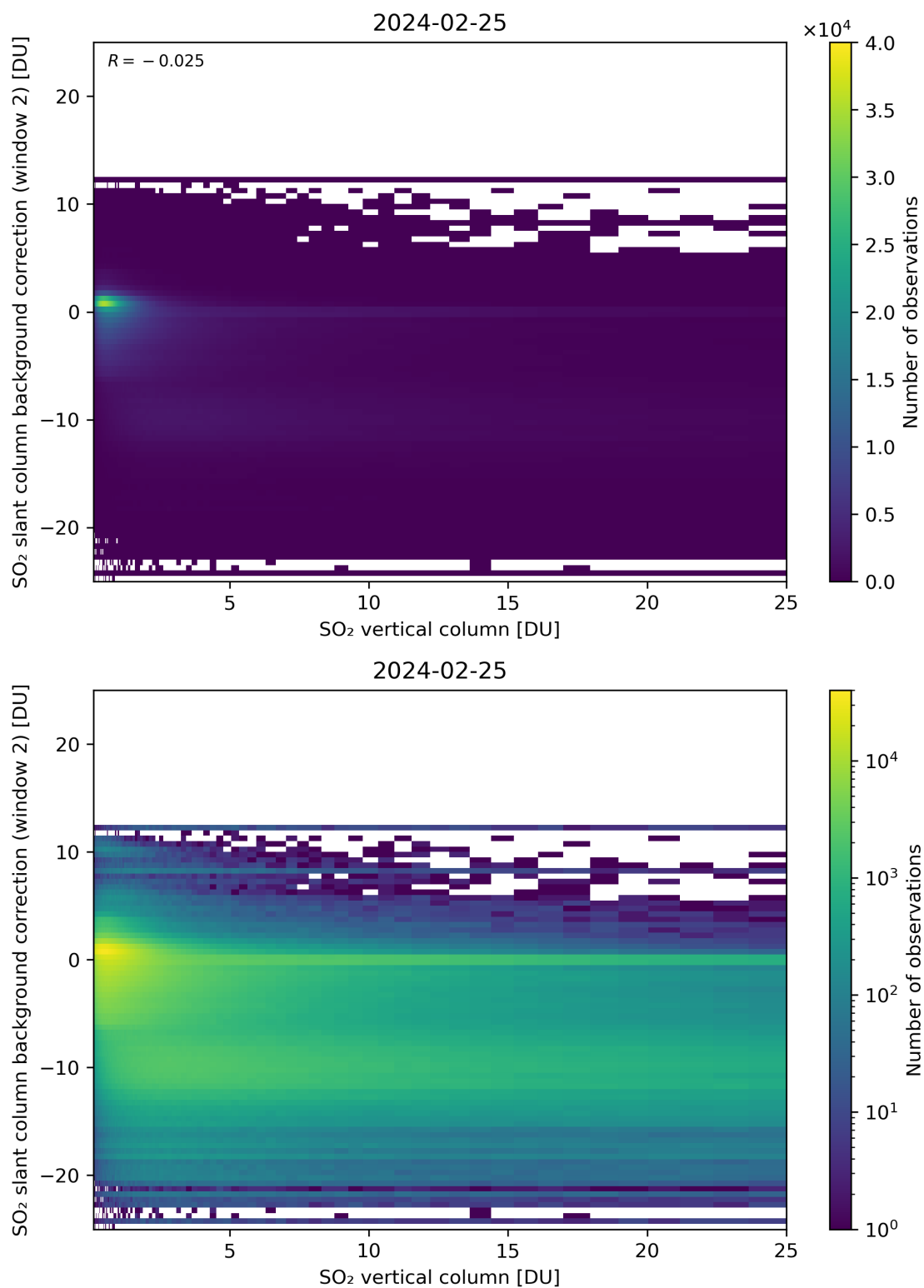
Figure 274: Scatter density plot of “SO 2 vertical column” against “SO 2 slant column background correction (window 2)” for 2024-02-24 to 2024-02-26.
