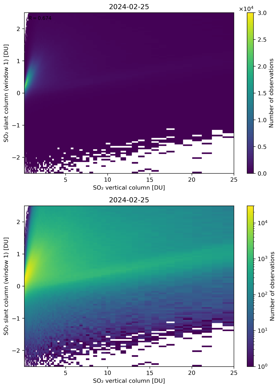
Figure 300: Scatter density plot of “SO 2 vertical column” against “SO 2 slant column (window 1)” for 2024-02-24 to 2024-02-26.
