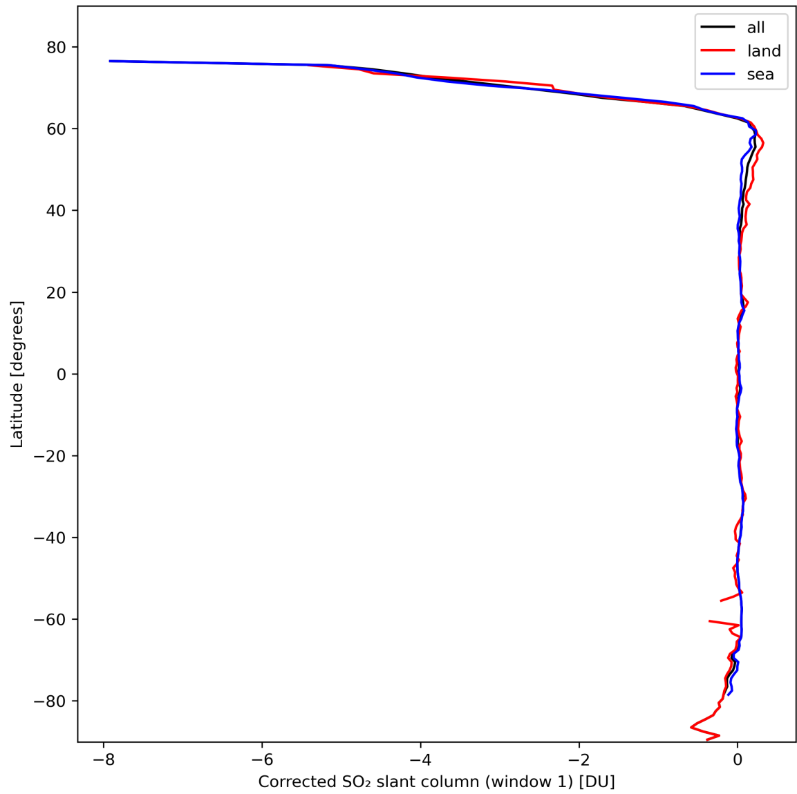
Figure 35: Zonal average of “Corrected SO 2 slant column (window 1)” for 2024-02-24 to 2024-02-26.
