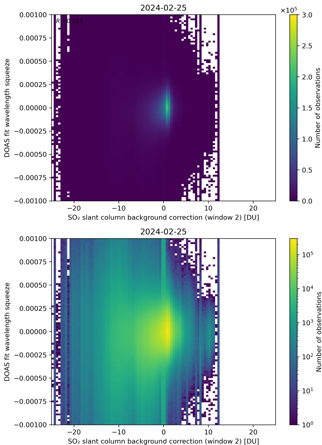
Figure 113: Scatter density plot of “SO 2 slant column background correction (window 2)” against “DOAS fit wavelength squeeze” for 2024-02-24 to 2024-02-26.
