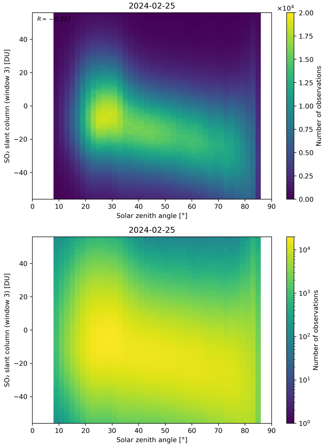
Figure 172: Scatter density plot of “Solar zenith angle” against “SO 2 slant column (window 3)” for 2024-02-24 to 2024-02-26.
