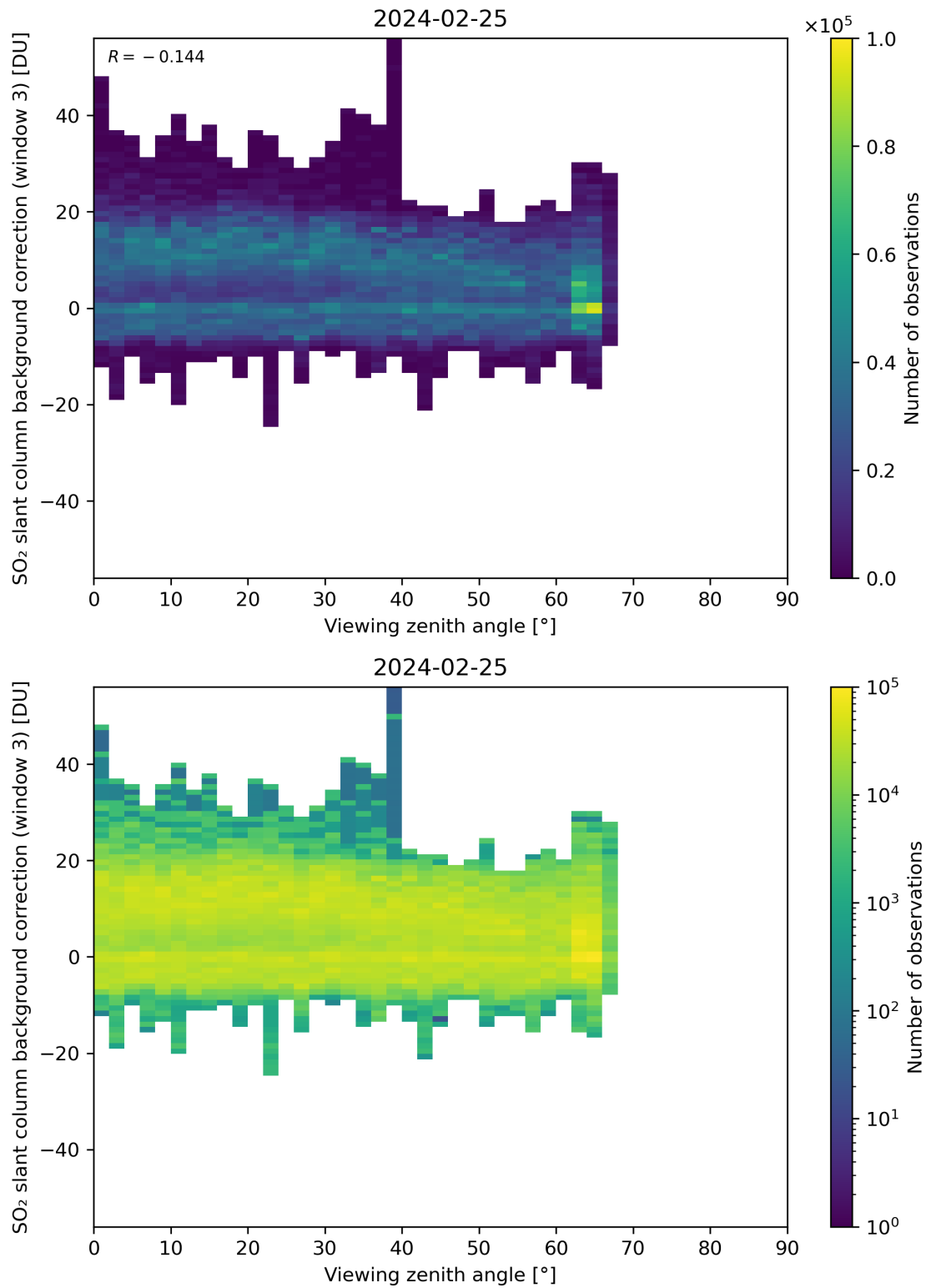
Figure 310: Scatter density plot of “Viewing zenith angle” against “SO 2 slant column background correction (window 3)” for 2024-02-24 to 2024-02-26.
