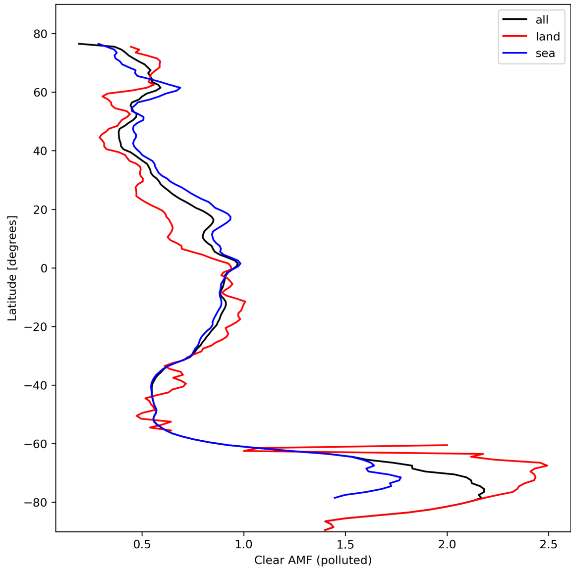
Figure 50: Zonal average of “Clear AMF (polluted)” for 2024-02-24 to 2024-02-26.
