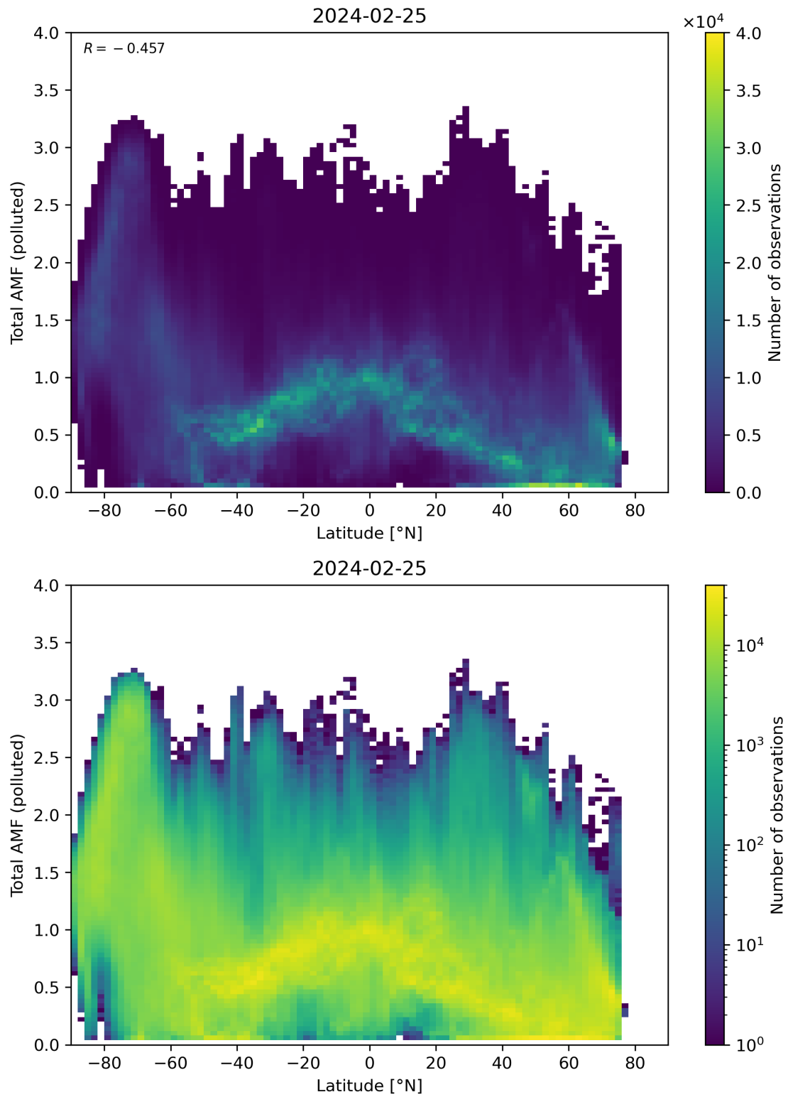
Figure 154: Scatter density plot of “Latitude” against “Total AMF (polluted)” for 2024-02-24 to 2024-02-26.
