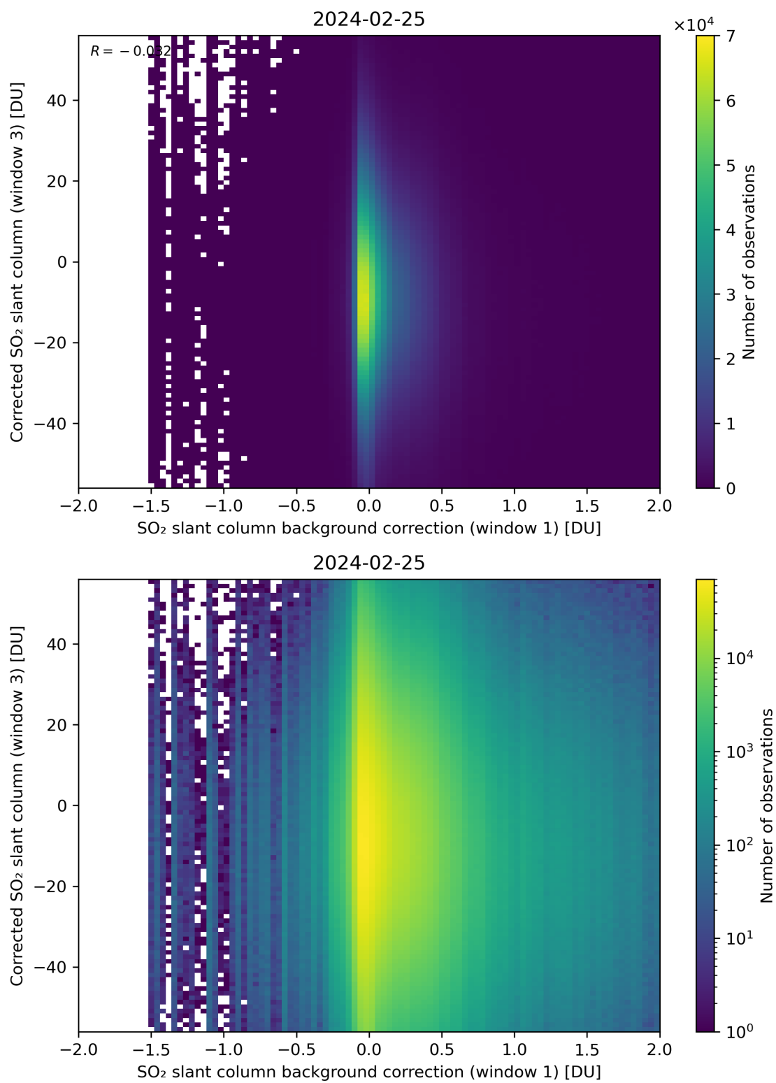
Figure 105: Scatter density plot of “SO 2 slant column background correction (window 1)” against “Corrected SO 2 slant column (window 3)” for 2024-02-24 to 2024-02-26.
