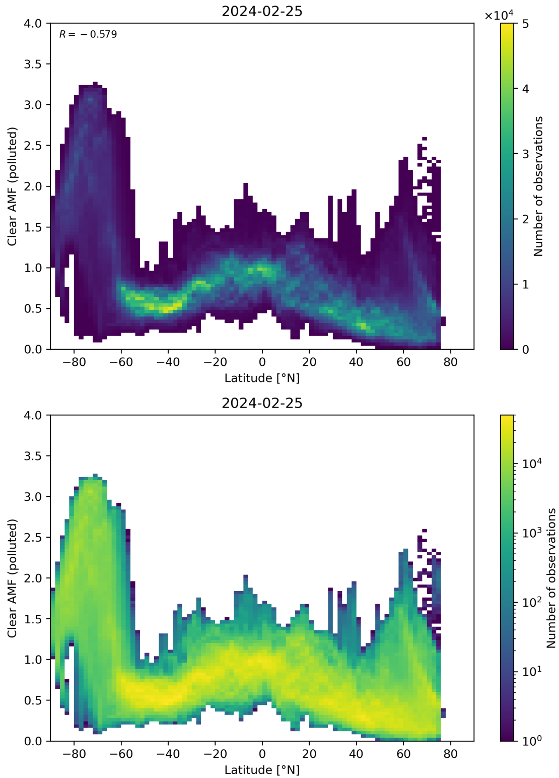
Figure 145: Scatter density plot of “Latitude” against “Clear AMF (polluted)” for 2024-02-24 to 2024-02-26.
