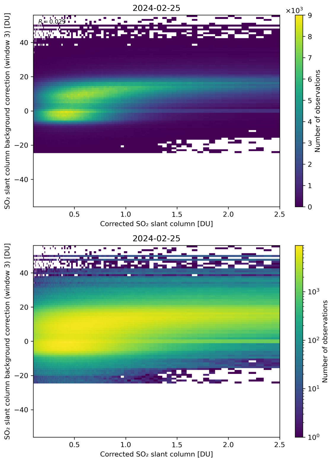
Figure 180: Scatter density plot of “Corrected SO 2 slant column” against “SO 2 slant column background correction (window 3)” for 2024-02-24 to 2024-02-26.
