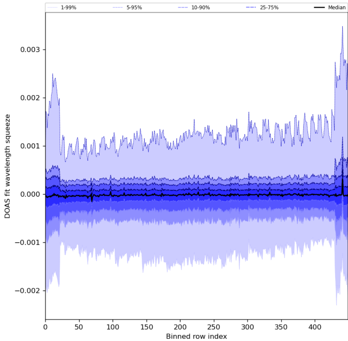
Figure 92: Along track statistics of “DOAS fit wavelength squeeze” for 2024-02-24 to 2024-02-26
