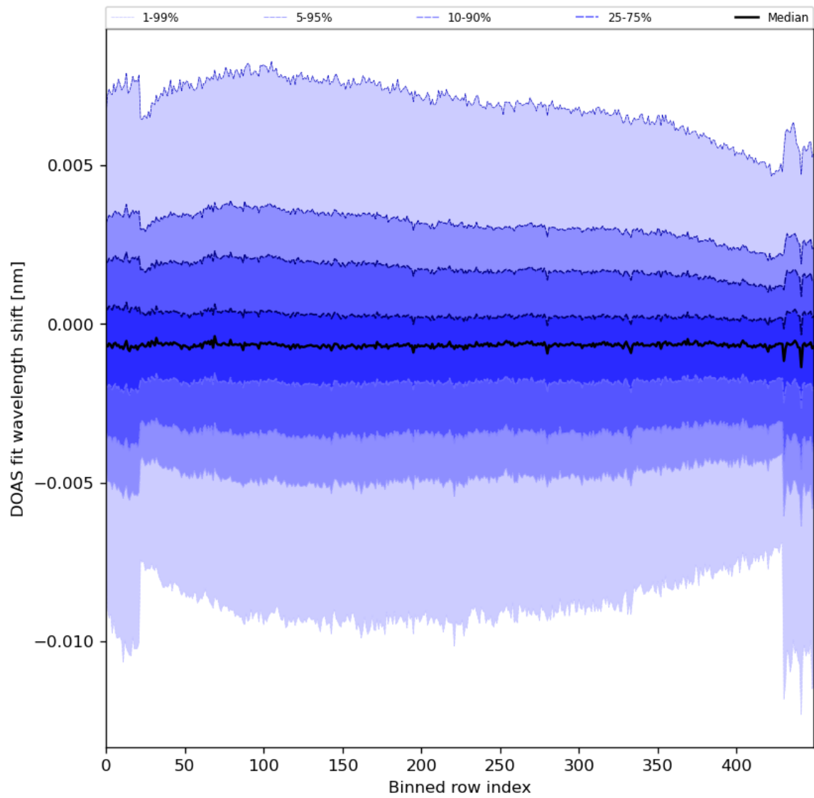
Figure 91: Along track statistics of “DOAS fit wavelength shift” for 2024-02-24 to 2024-02-26
