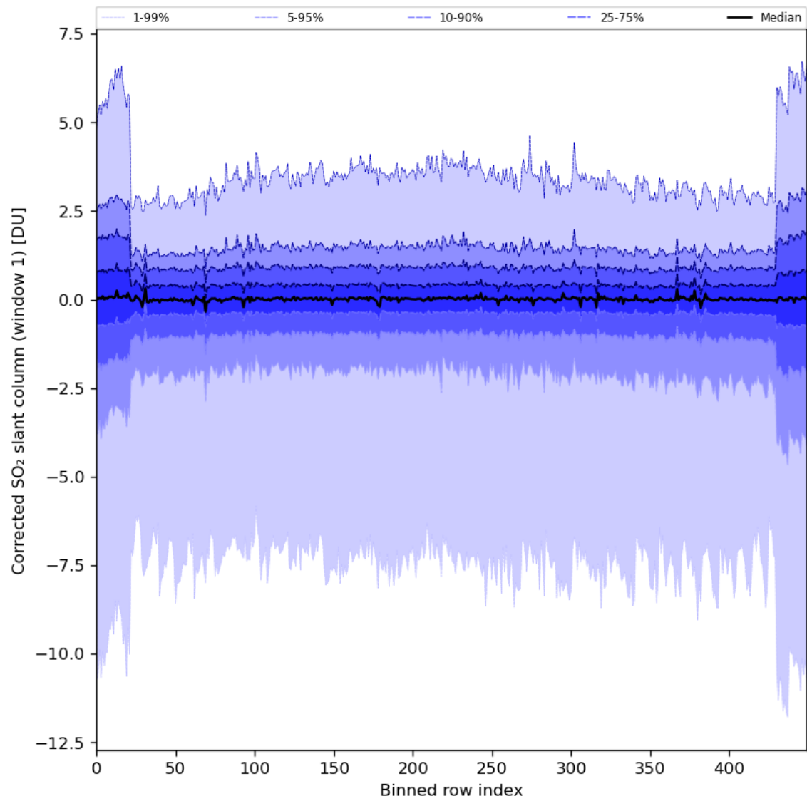
Figure 81: Along track statistics of “Corrected SO 2 slant column (window 1)” for 2024-02-24 to 2024-02-26
