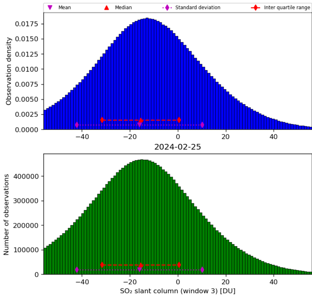
Figure 64: Histogram of “SO 2 slant column (window 3)” for 2024-02-24 to 2024-02-26
