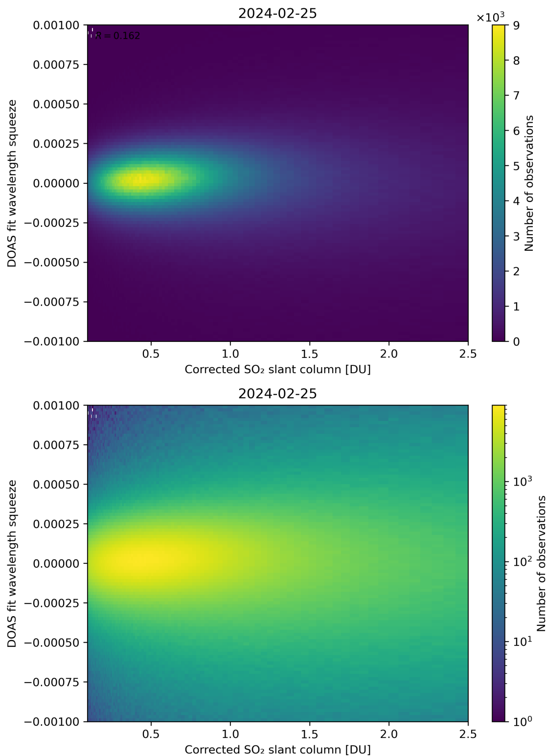
Figure 182: Scatter density plot of “Corrected SO 2 slant column” against “DOAS fit wavelength squeeze” for 2024-02-24 to 2024-02-26.
