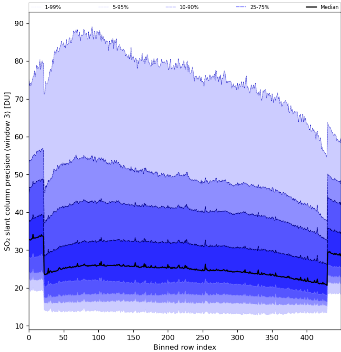
Figure 88: Along track statistics of “SO 2 slant column precision (window 3)” for 2024-02-24 to 2024-02-26
