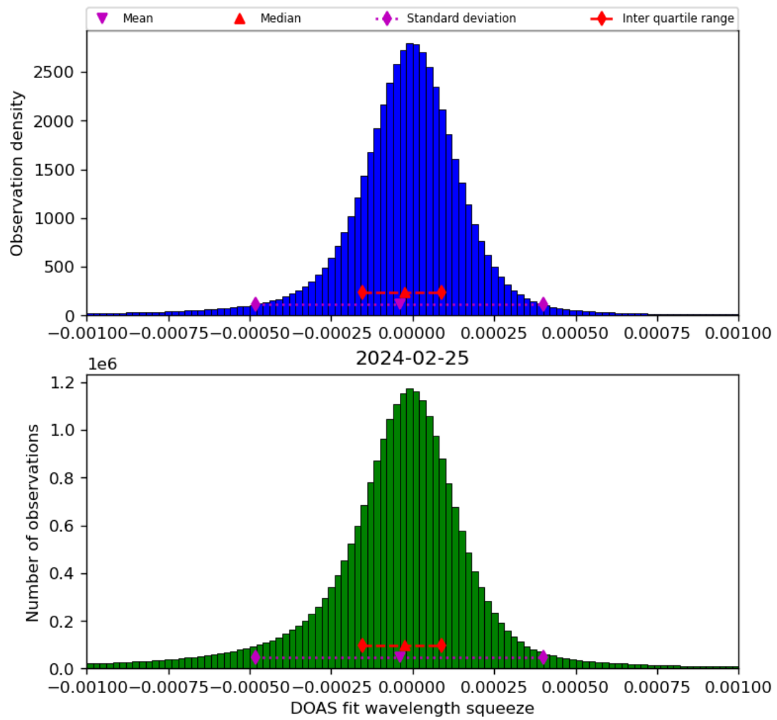
Figure 69: Histogram of “DOAS fit wavelength squeeze” for 2024-02-24 to 2024-02-26
