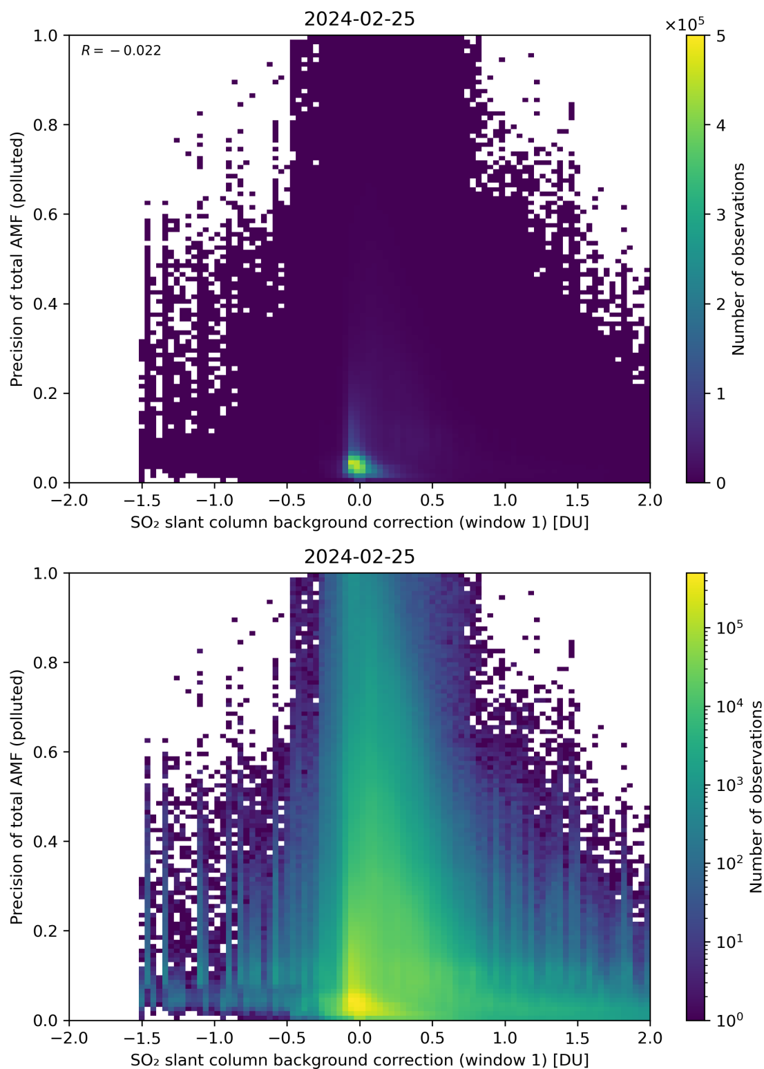
Figure 110: Scatter density plot of “SO 2 slant column background correction (window 1)” against “Precision of total AMF (polluted)” for 2024-02-24 to 2024-02-26.
