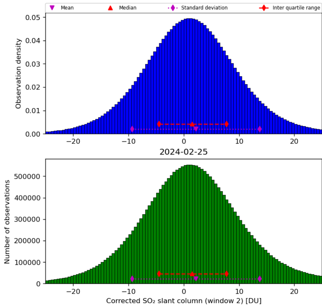
Figure 62: Histogram of “Corrected SO 2 slant column (window 2)” for 2024-02-24 to 2024-02-26
