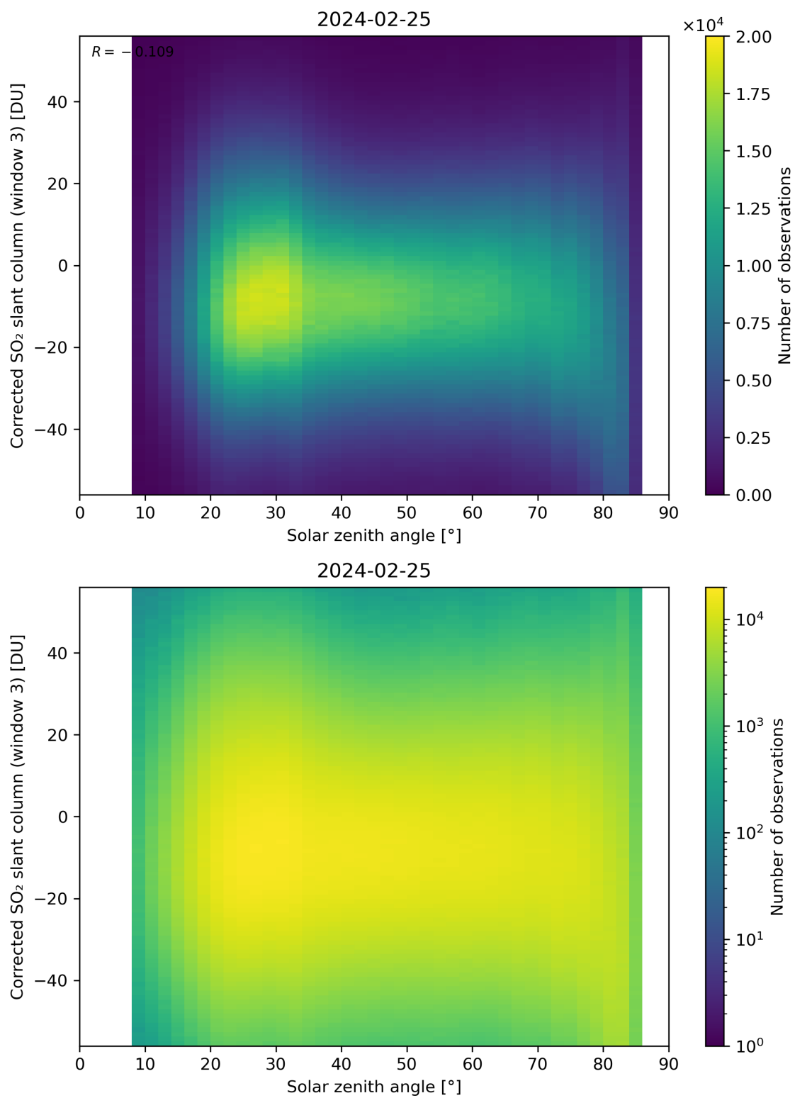
Figure 168: Scatter density plot of “Solar zenith angle” against “Corrected SO 2 slant column (window 3)” for 2024-02-24 to 2024-02-26.
