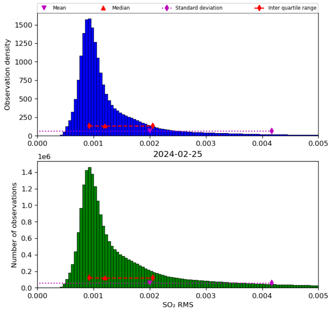
Figure 70: Histogram of “SO 2 RMS” for 2024-02-24 to 2024-02-26
