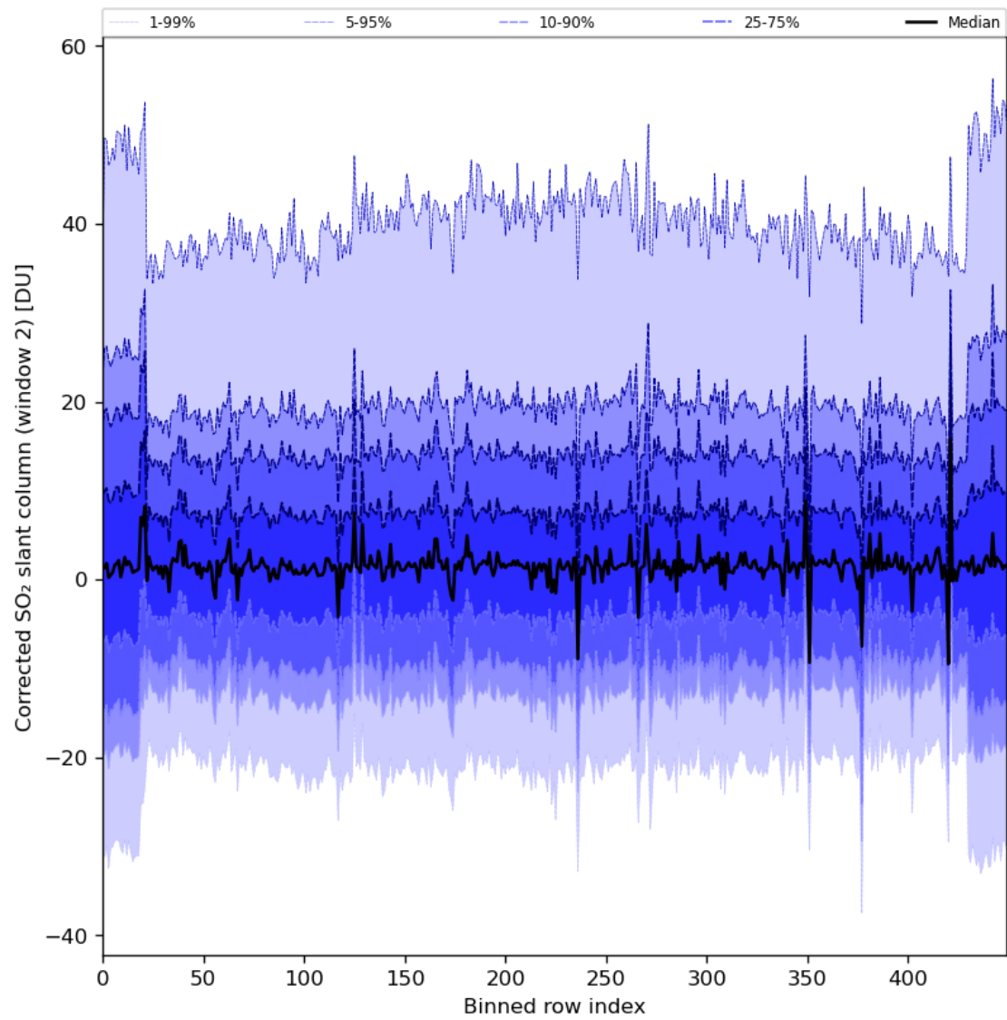
Figure 85: Along track statistics of “Corrected SO 2 slant column (window 2)” for 2024-02-24 to 2024-02-26
