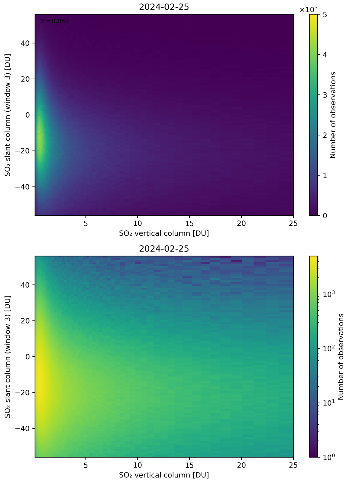
Figure 303: Scatter density plot of “SO 2 vertical column” against “SO 2 slant column (window 3)” for 2024-02-24 to 2024-02-26.
