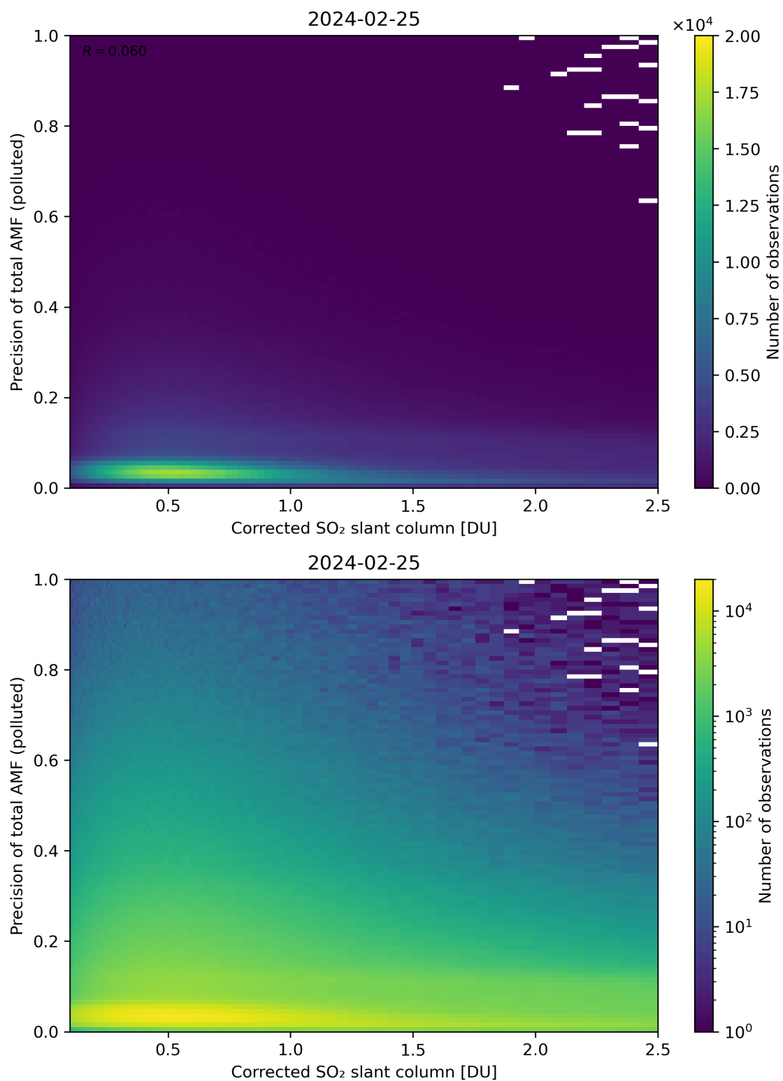
Figure 193: Scatter density plot of “Corrected SO 2 slant column” against “Precision of total AMF (polluted)” for 2024-02-24 to 2024-02-26.
