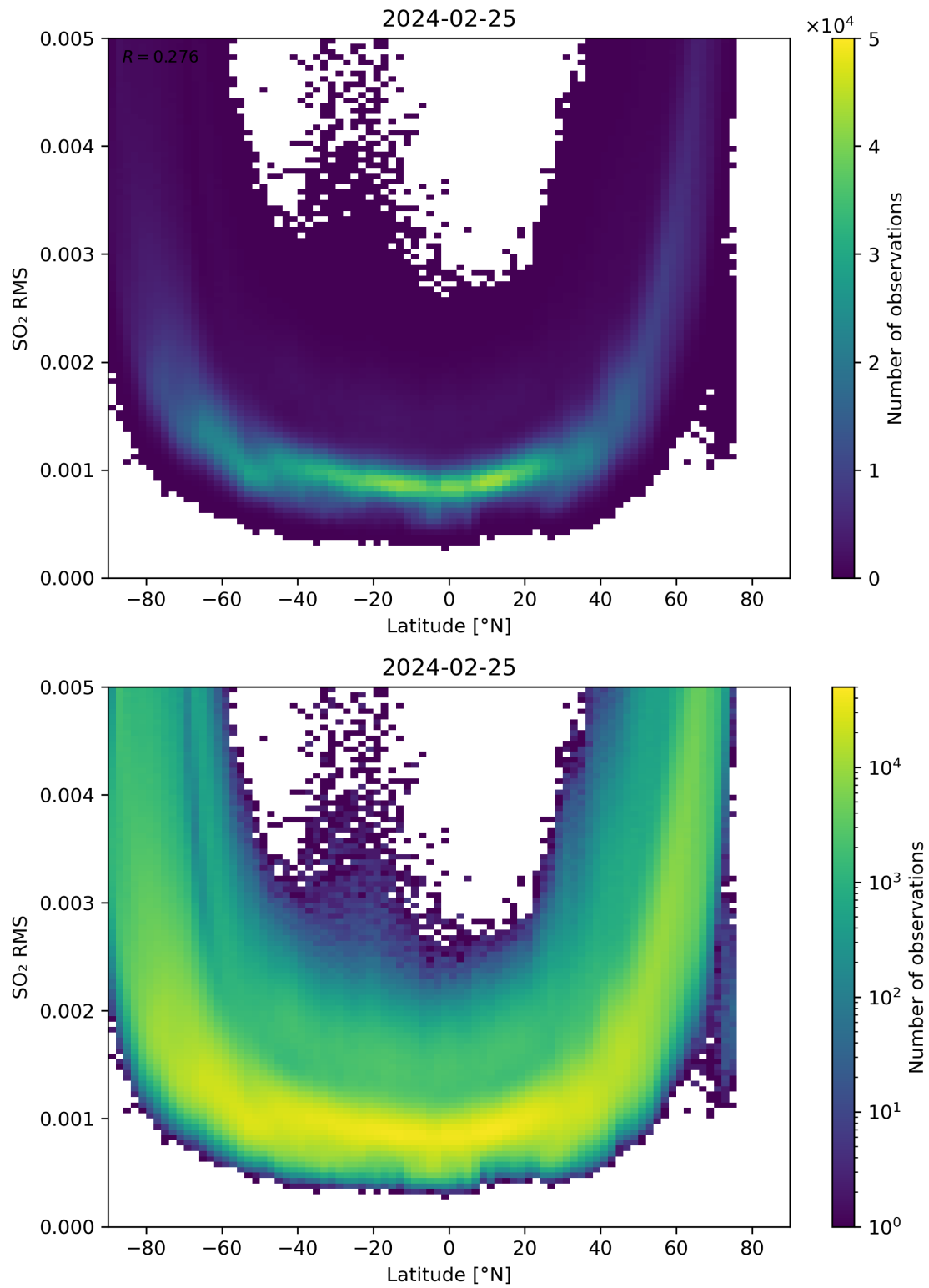
Figure 144: Scatter density plot of “Latitude” against “SO 2 RMS” for 2024-02-24 to 2024-02-26.
