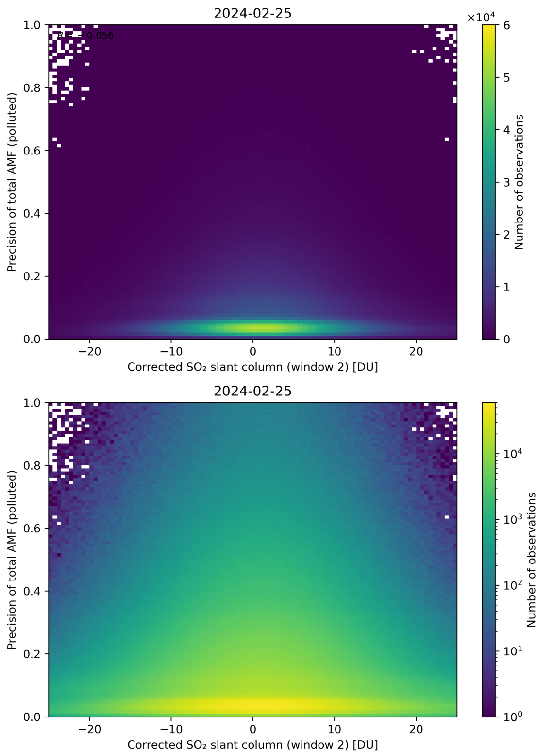
Figure 204: Scatter density plot of “Corrected SO 2 slant column (window 2)” against “Precision of total AMF (polluted)” for 2024-02-24 to 2024-02-26.
