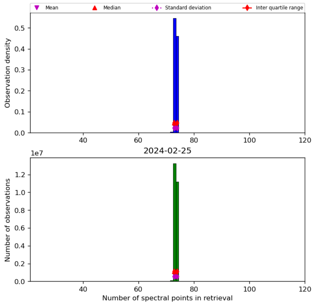
Figure 74: Histogram of “Number of spectral points in retrieval” for 2024-02-24 to 2024-02-26
