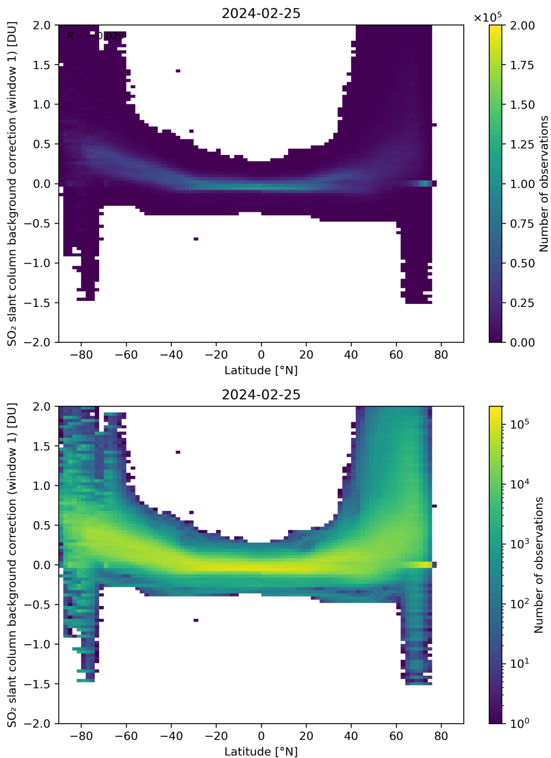
Figure 139: Scatter density plot of “Latitude” against “SO 2 slant column background correction (window 1)” for 2024-02-24 to 2024-02-26.
