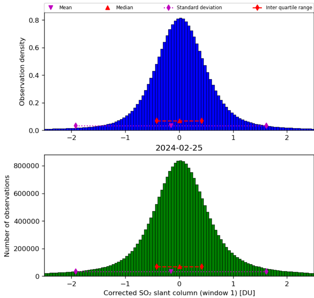
Figure 58: Histogram of “Corrected SO 2 slant column (window 1)” for 2024-02-24 to 2024-02-26
