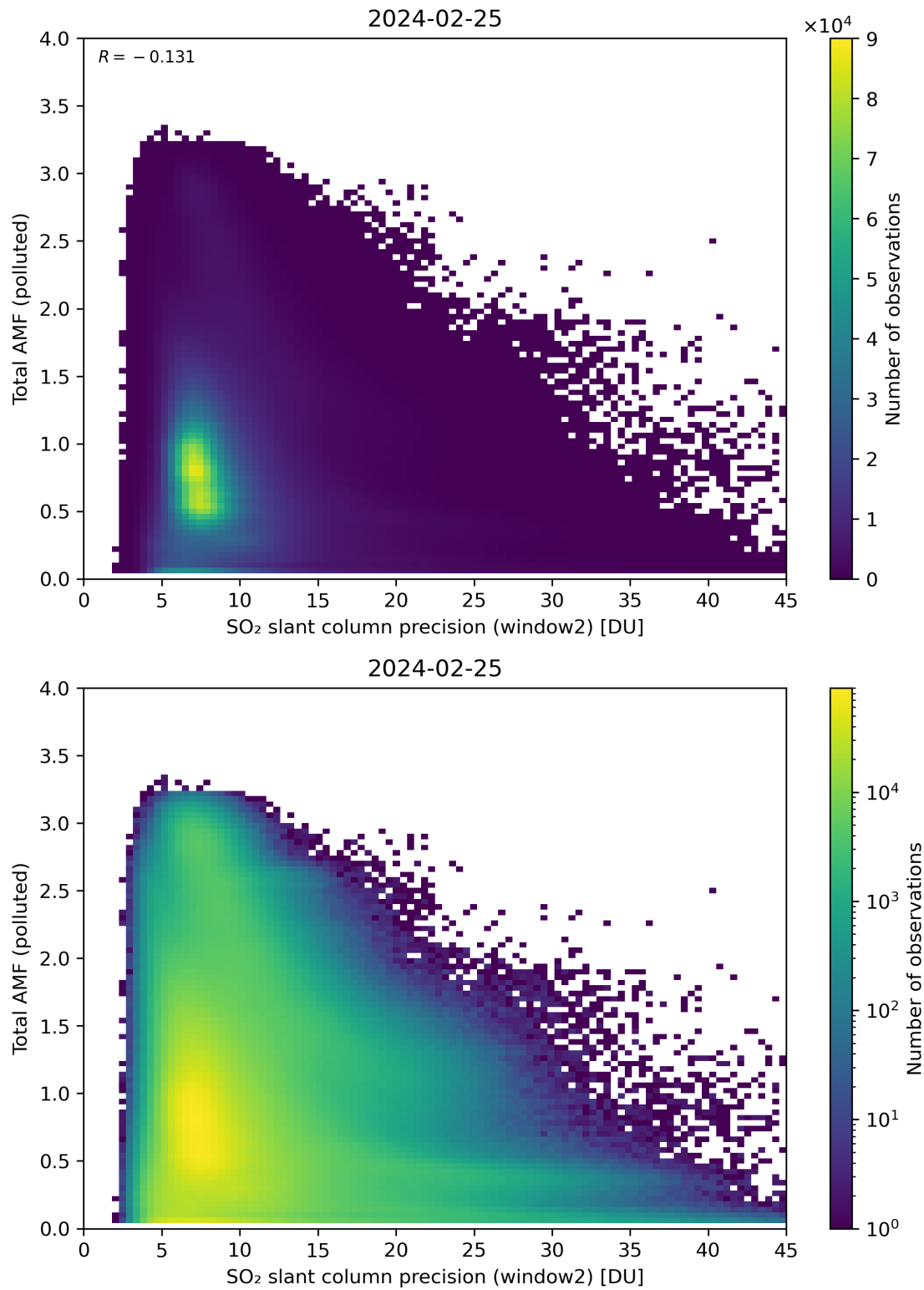
Figure 251: Scatter density plot of “SO 2 slant column precision (window2)” against “Total AMF (polluted)” for 2024-02-24 to 2024-02-26.
