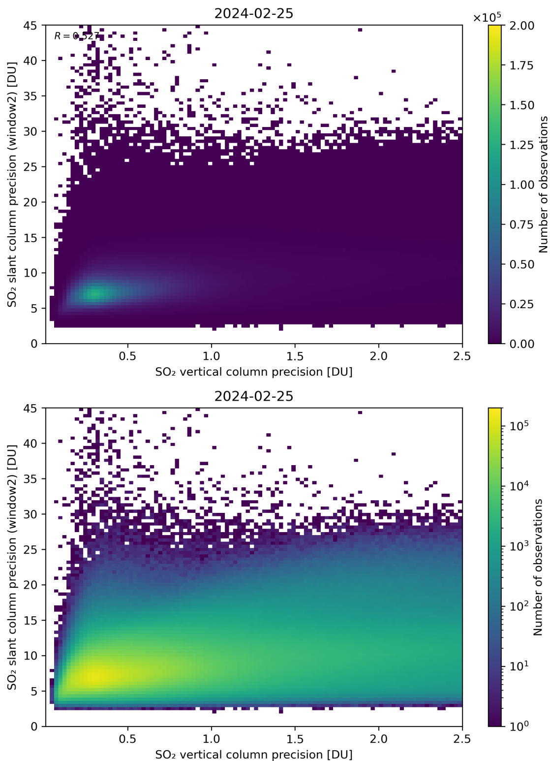
Figure 291: Scatter density plot of “SO 2 vertical column precision” against “SO 2 slant column precision (window2)” for 2024-02-24 to 2024-02-26.
