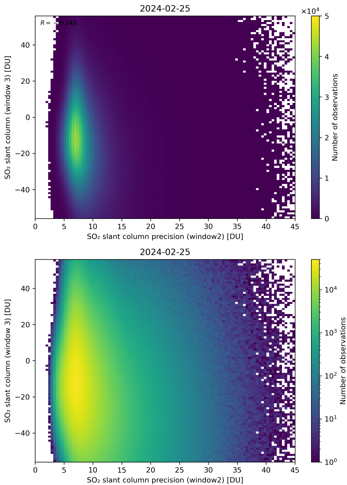
Figure 249: Scatter density plot of “SO 2 slant column precision (window2)” against “SO 2 slant column (window 3)” for 2024-02-24 to 2024-02-26.
