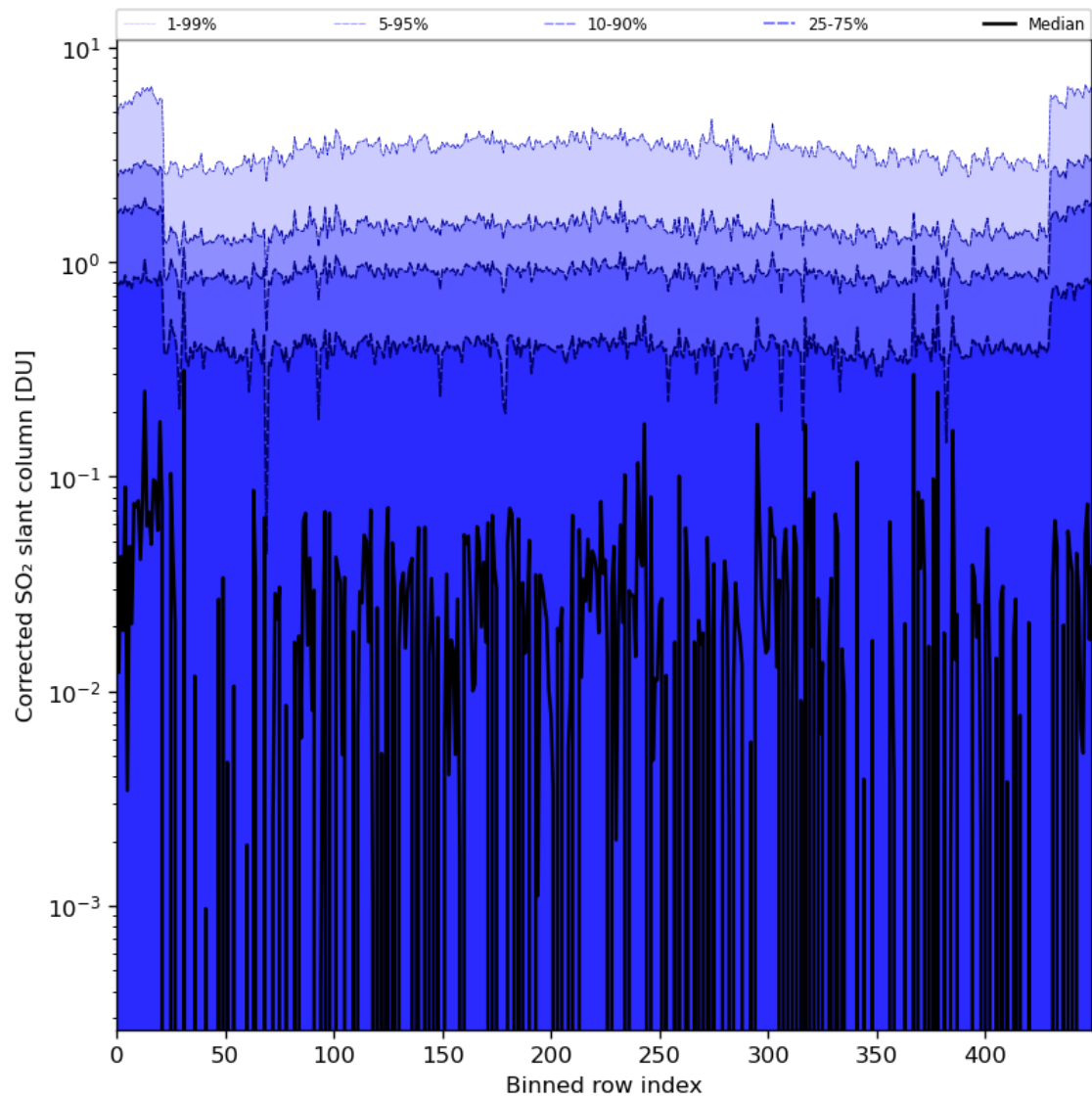
Figure 78: Along track statistics of “Corrected SO 2 slant column” for 2024-02-24 to 2024-02-26
