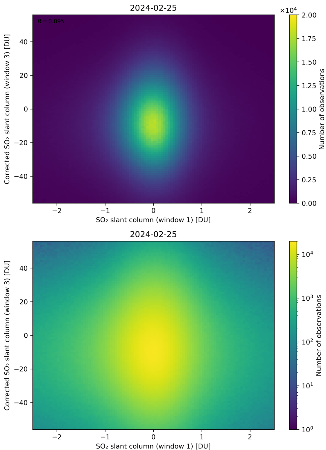
Figure 234: Scatter density plot of “SO 2 slant column (window 1)” against “Corrected SO 2 slant column (window 3)” for 2024-02-24 to 2024-02-26.
