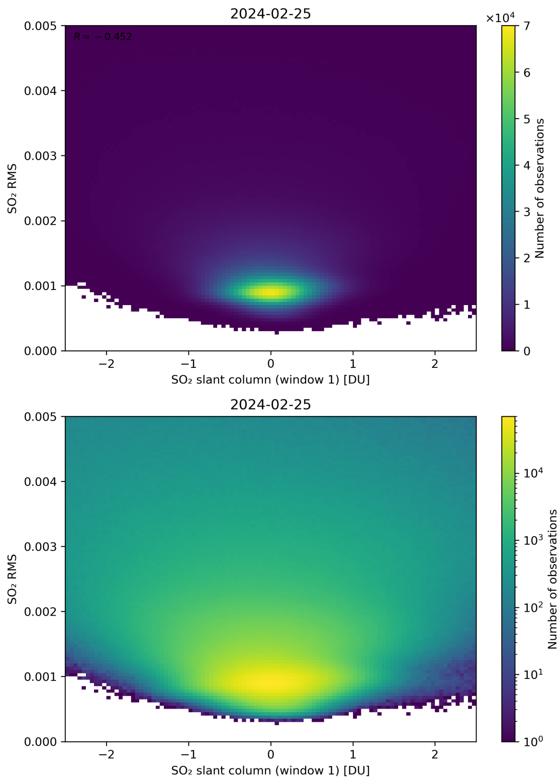
Figure 217: Scatter density plot of “SO 2 slant column (window 1)” against “SO 2 RMS” for 2024-02-24 to 2024-02-26.
