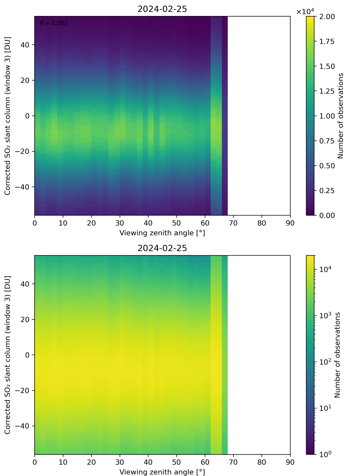
Figure 319: Scatter density plot of “Viewing zenith angle” against “Corrected SO 2 slant column (window 3)” for 2024-02-24 to 2024-02-26.
