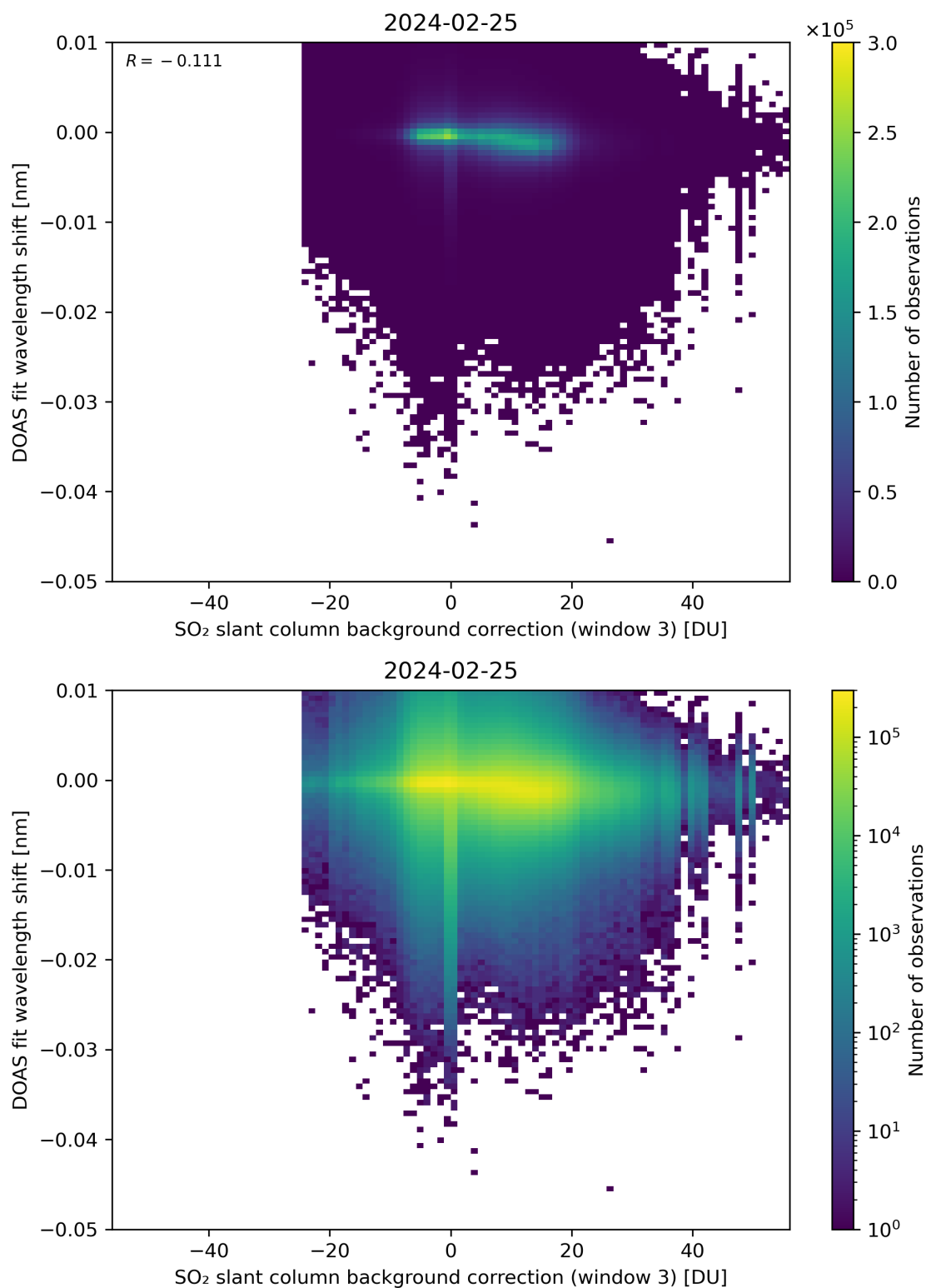
Figure 121: Scatter density plot of “SO 2 slant column background correction (window 3)” against “DOAS fit wavelength shift” for 2024-02-24 to 2024-02-26.
