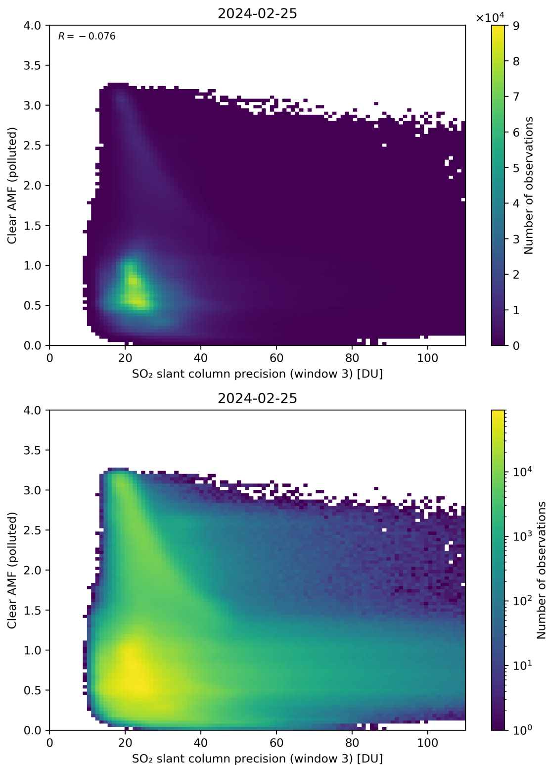
Figure 261: Scatter density plot of “SO 2 slant column precision (window 3)” against “Clear AMF (polluted)” for 2024-02-24 to 2024-02-26.
