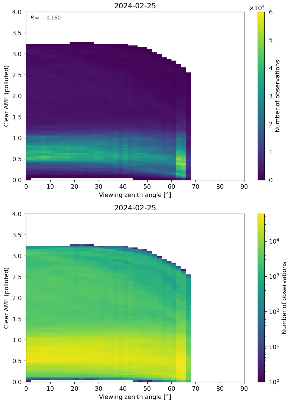
Figure 316: Scatter density plot of “Viewing zenith angle” against “Clear AMF (polluted)” for 2024-02-24 to 2024-02-26.
