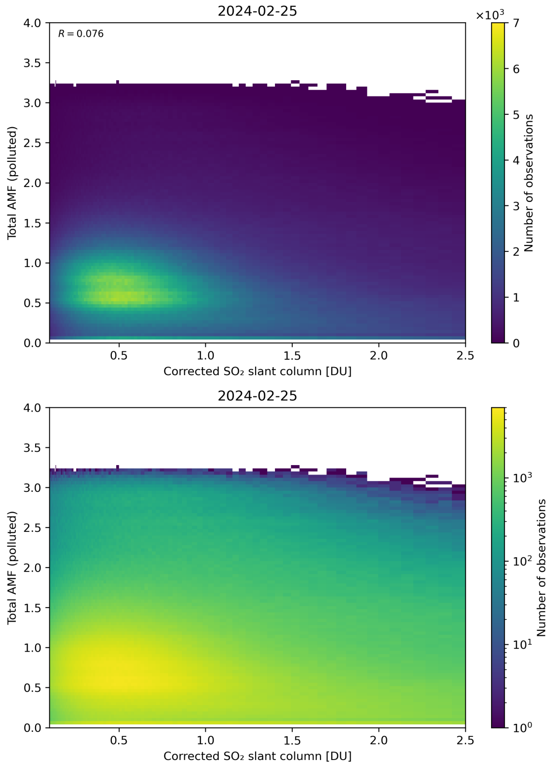
Figure 192: Scatter density plot of “Corrected SO 2 slant column” against “Total AMF (polluted)” for 2024-02-24 to 2024-02-26.
