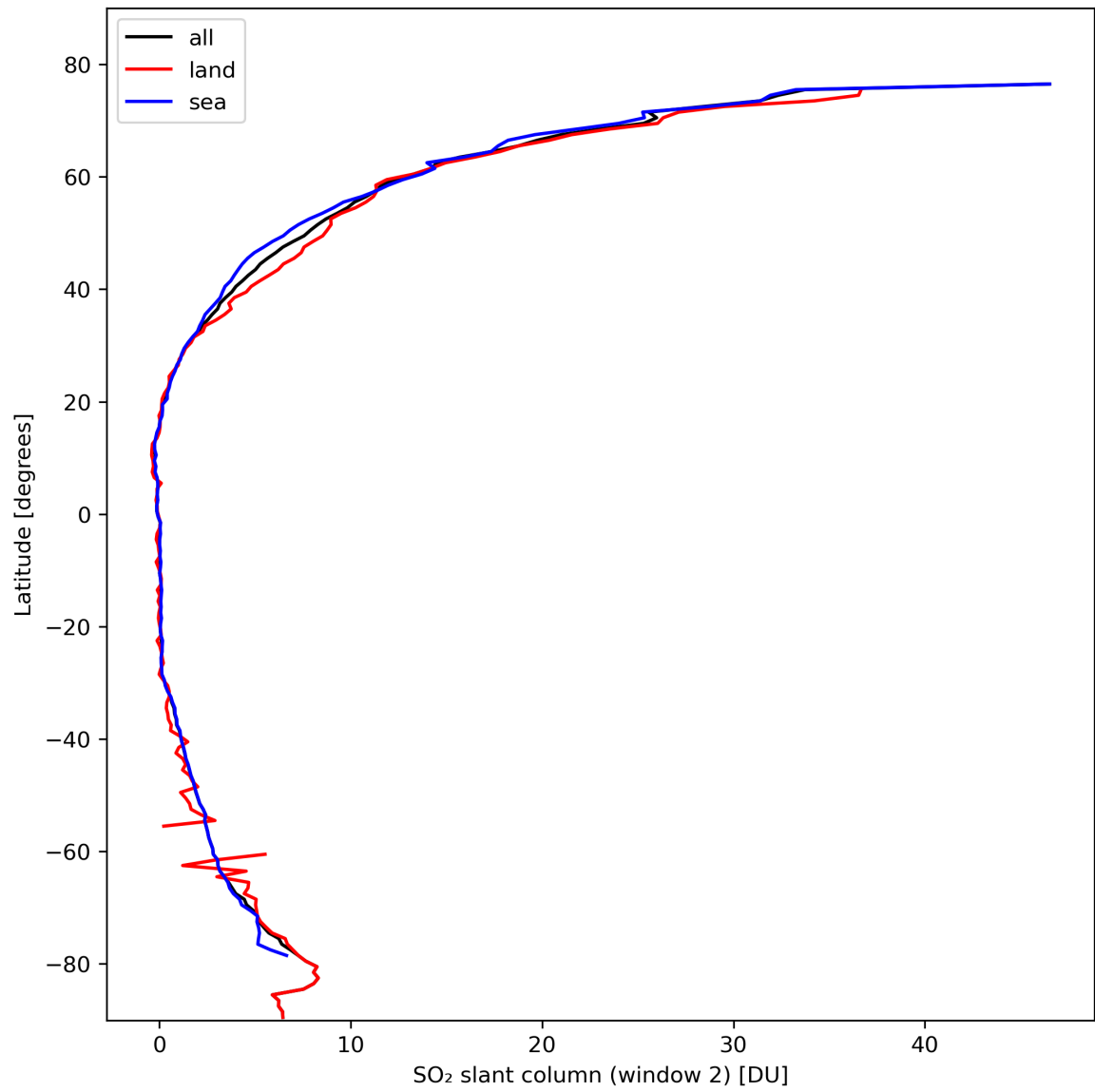
Figure 37: Zonal average of “SO 2 slant column (window 2)” for 2024-02-24 to 2024-02-26.
