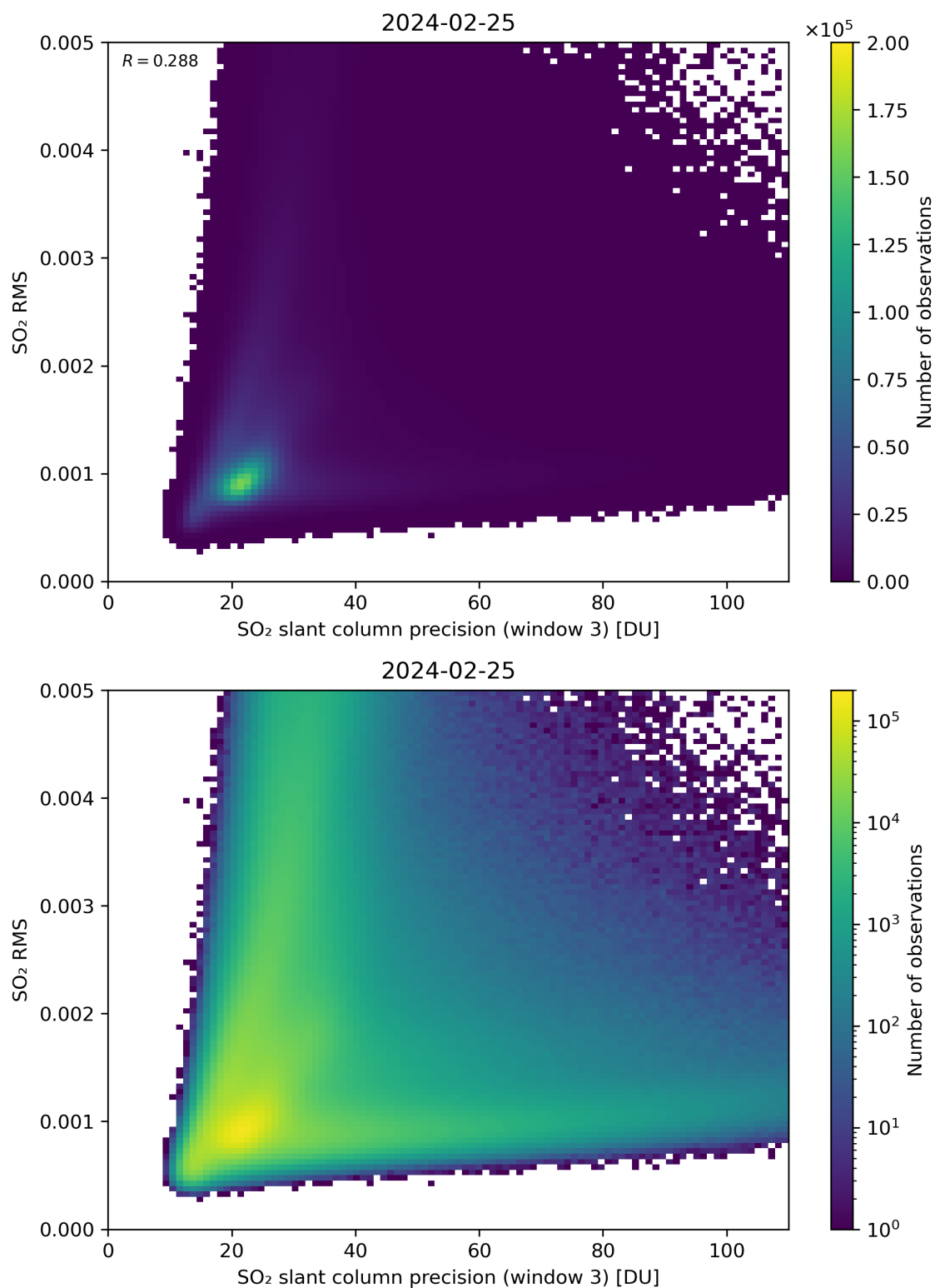
Figure 260: Scatter density plot of “SO 2 slant column precision (window 3)” against “SO 2 RMS” for 2024-02-24 to 2024-02-26.
