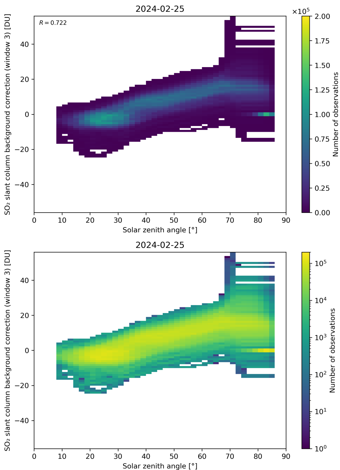
Figure 160: Scatter density plot of “Solar zenith angle” against “SO 2 slant column background correction (window 3)” for 2024-02-24 to 2024-02-26.
