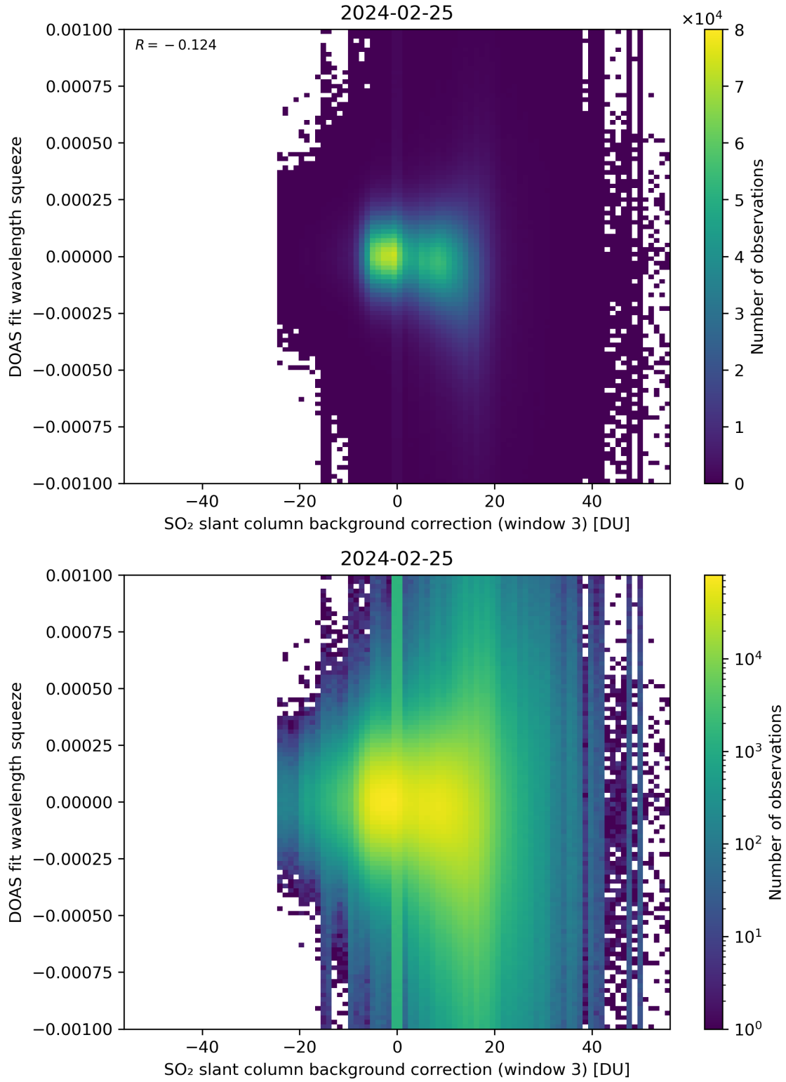
Figure 122: Scatter density plot of “SO 2 slant column background correction (window 3)” against “DOAS fit wavelength squeeze” for 2024-02-24 to 2024-02-26.
