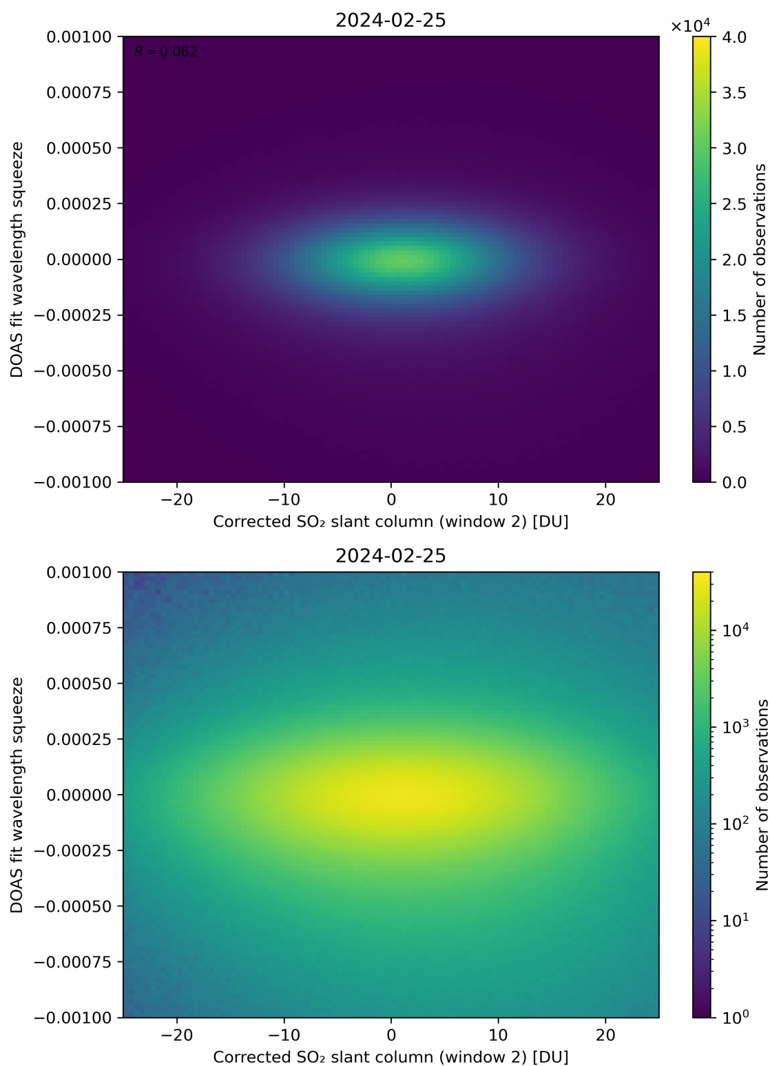
Figure 197: Scatter density plot of “Corrected SO 2 slant column (window 2)” against “DOAS fit wavelength squeeze” for 2024-02-24 to 2024-02-26.
