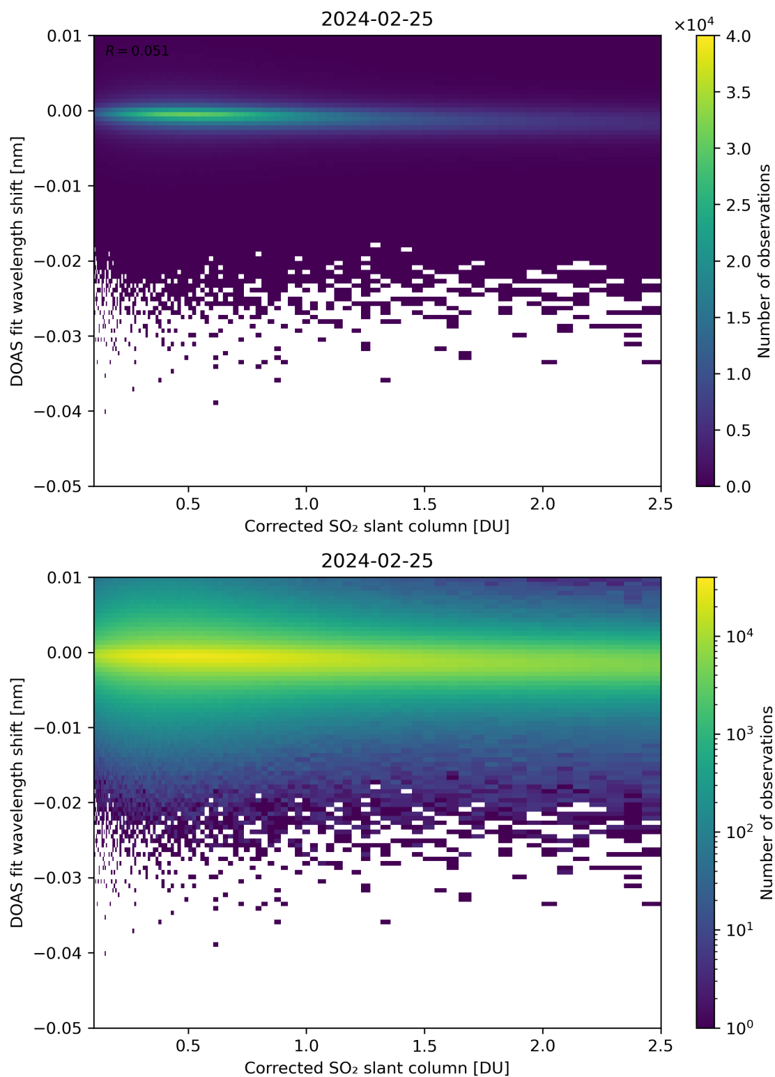
Figure 181: Scatter density plot of “Corrected SO 2 slant column” against “DOAS fit wavelength shift” for 2024-02-24 to 2024-02-26.
