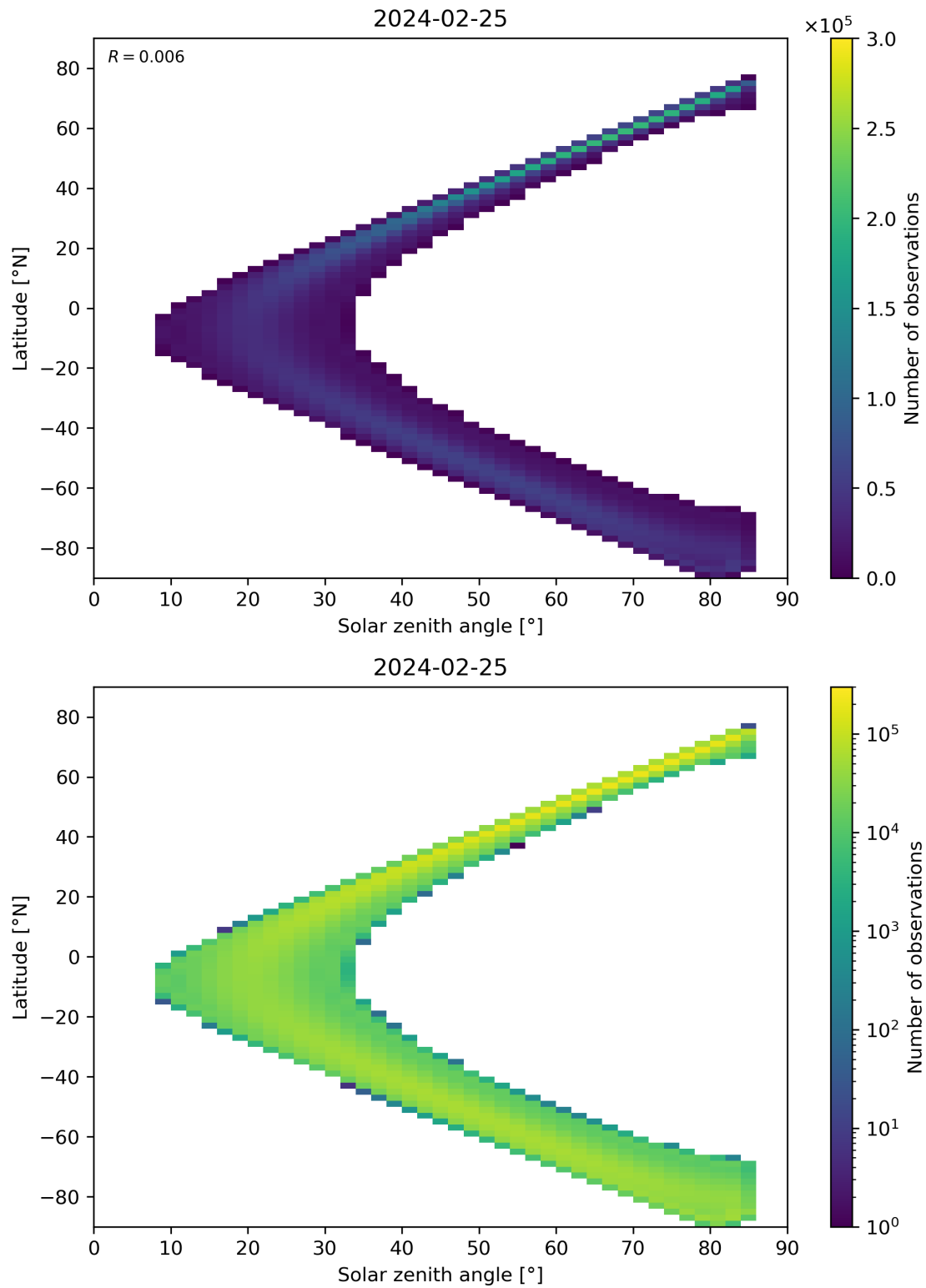
Figure 164: Scatter density plot of “Solar zenith angle” against “Latitude” for 2024-02-24 to 2024-02-26.
