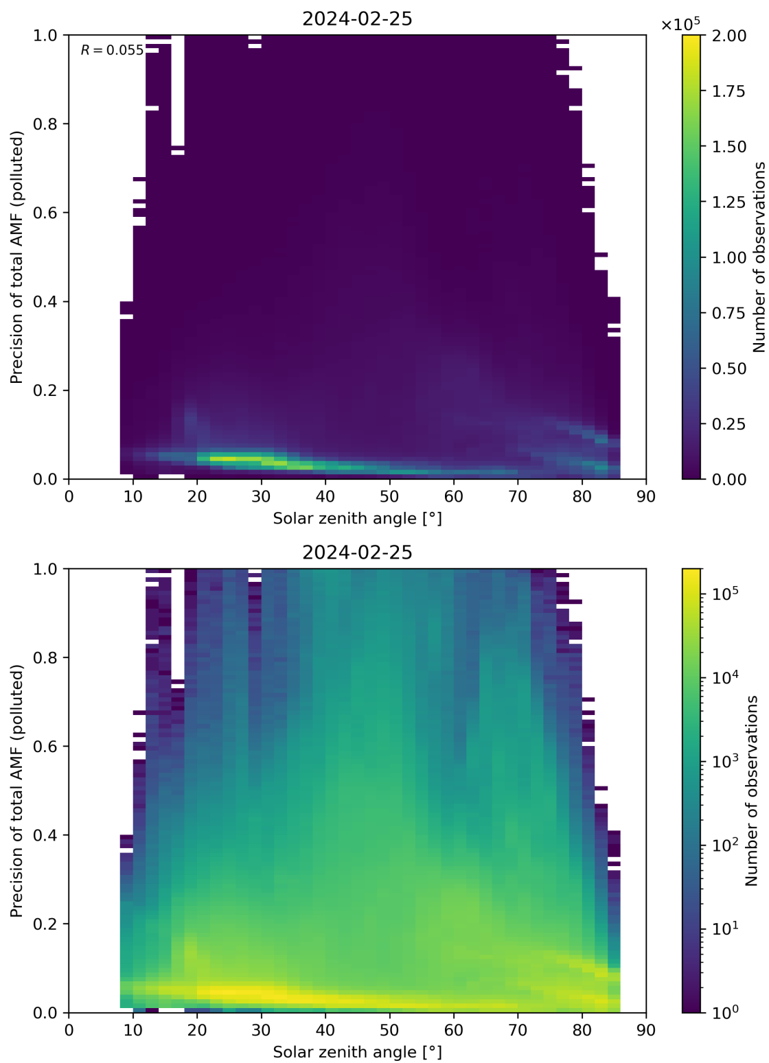
Figure 175: Scatter density plot of “Solar zenith angle” against “Precision of total AMF (polluted)” for 2024-02-24 to 2024-02-26.
