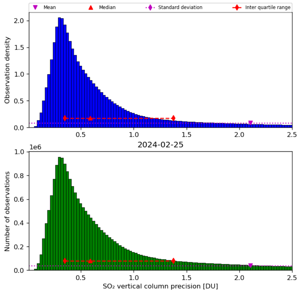
Figure 54: Histogram of “SO 2 vertical column precision” for 2024-02-24 to 2024-02-26
