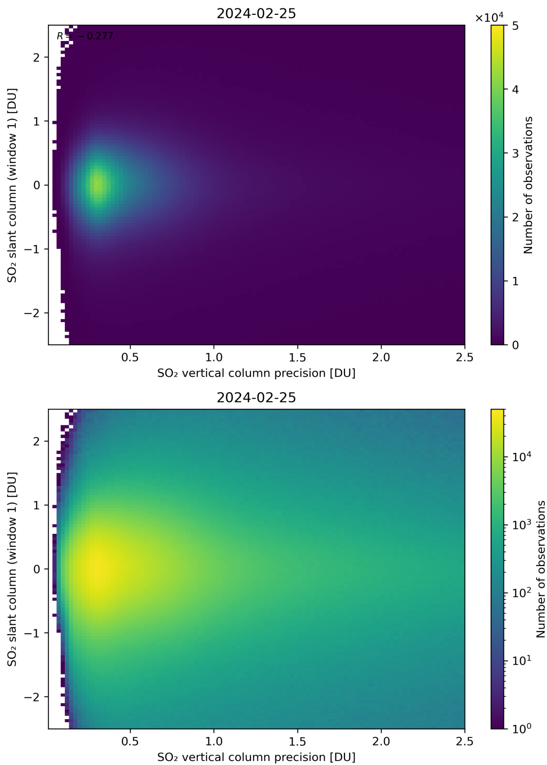
Figure 289: Scatter density plot of “SO 2 vertical column precision” against “SO 2 slant column (window 1)” for 2024-02-24 to 2024-02-26.
