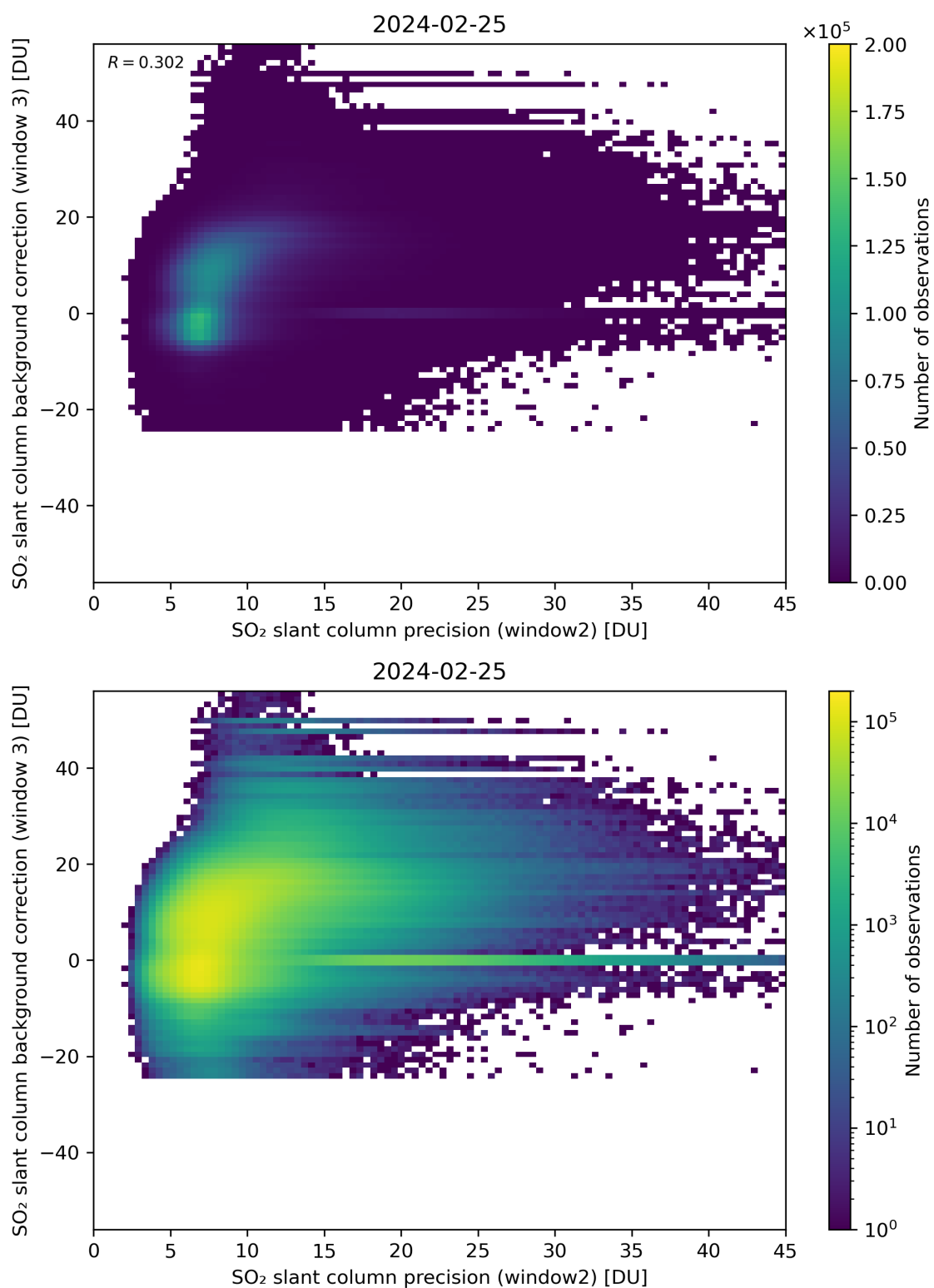
Figure 242: Scatter density plot of “SO 2 slant column precision (window2)” against “SO 2 slant column background correction (window 3)” for 2024-02-24 to 2024-02-26.
