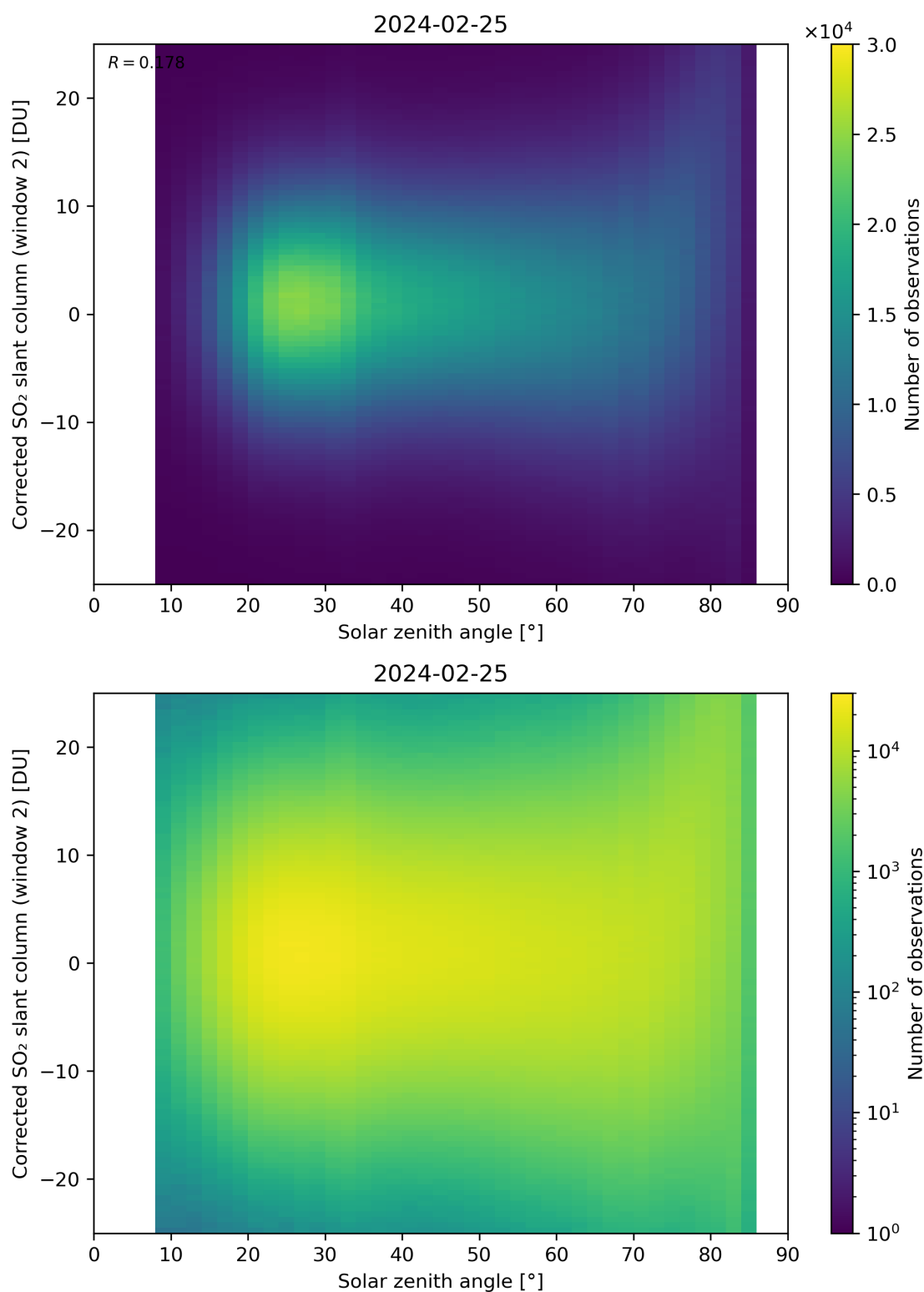
Figure 167: Scatter density plot of “Solar zenith angle” against “Corrected SO 2 slant column (window 2)” for 2024-02-24 to 2024-02-26.
