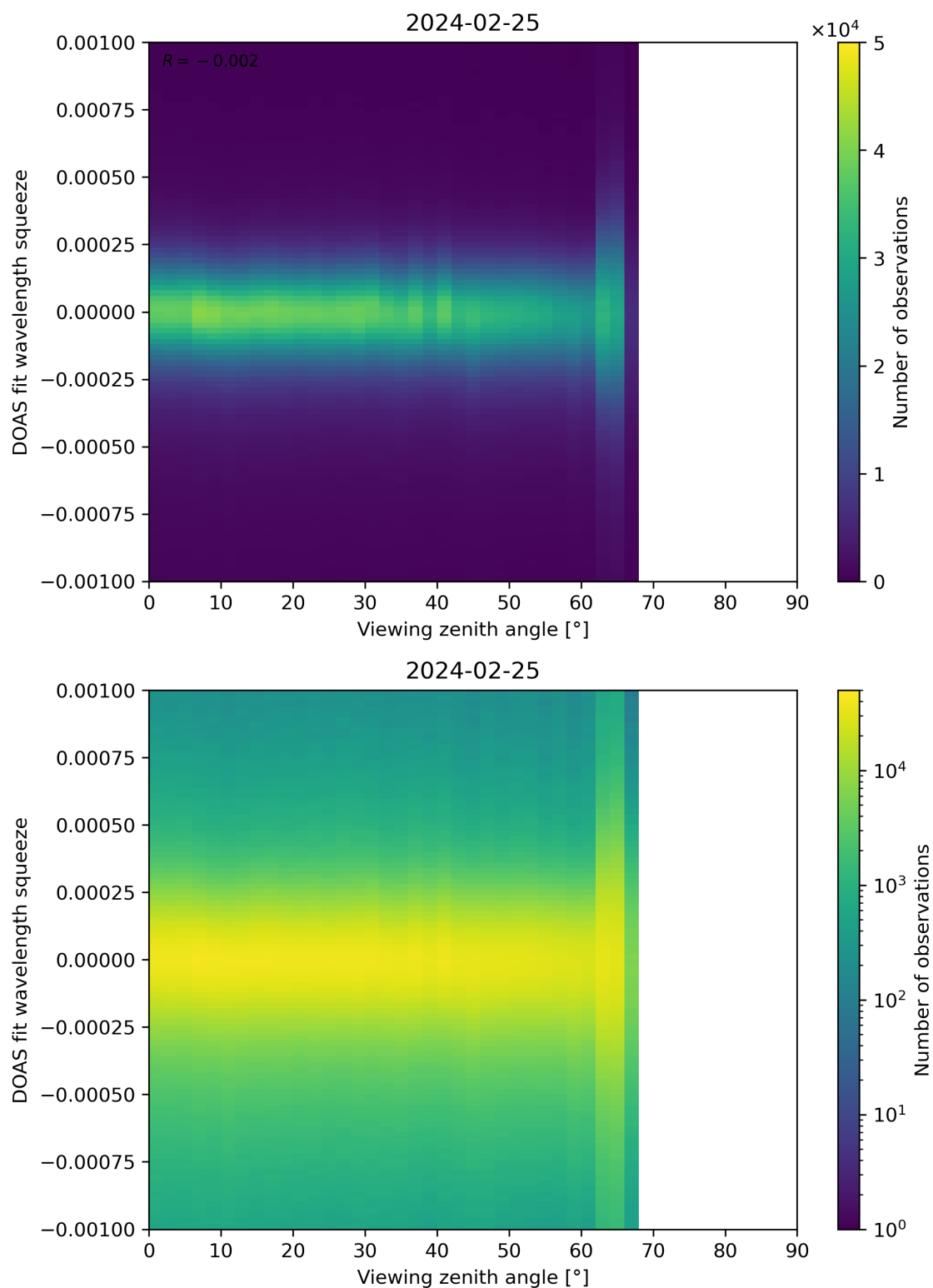
Figure 312: Scatter density plot of “Viewing zenith angle” against “DOAS fit wavelength squeeze” for 2024-02-24 to 2024-02-26.
