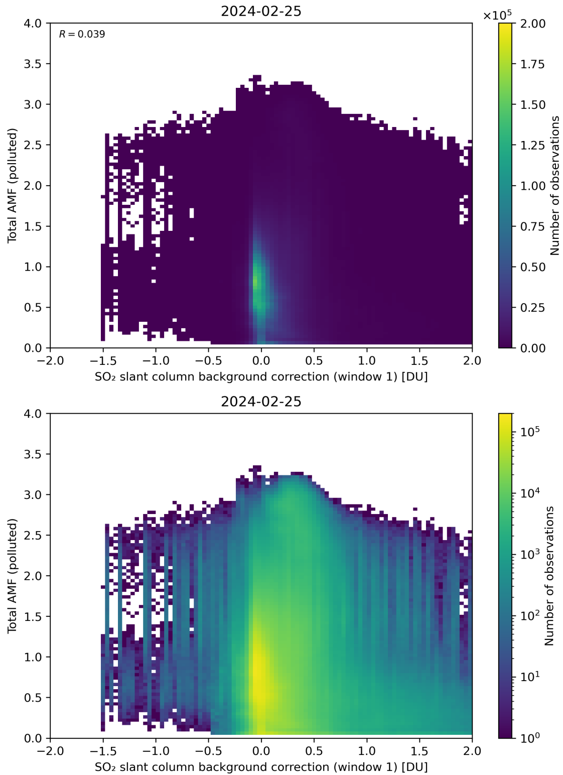
Figure 109: Scatter density plot of “SO 2 slant column background correction (window 1)” against “Total AMF (polluted)” for 2024-02-24 to 2024-02-26.
