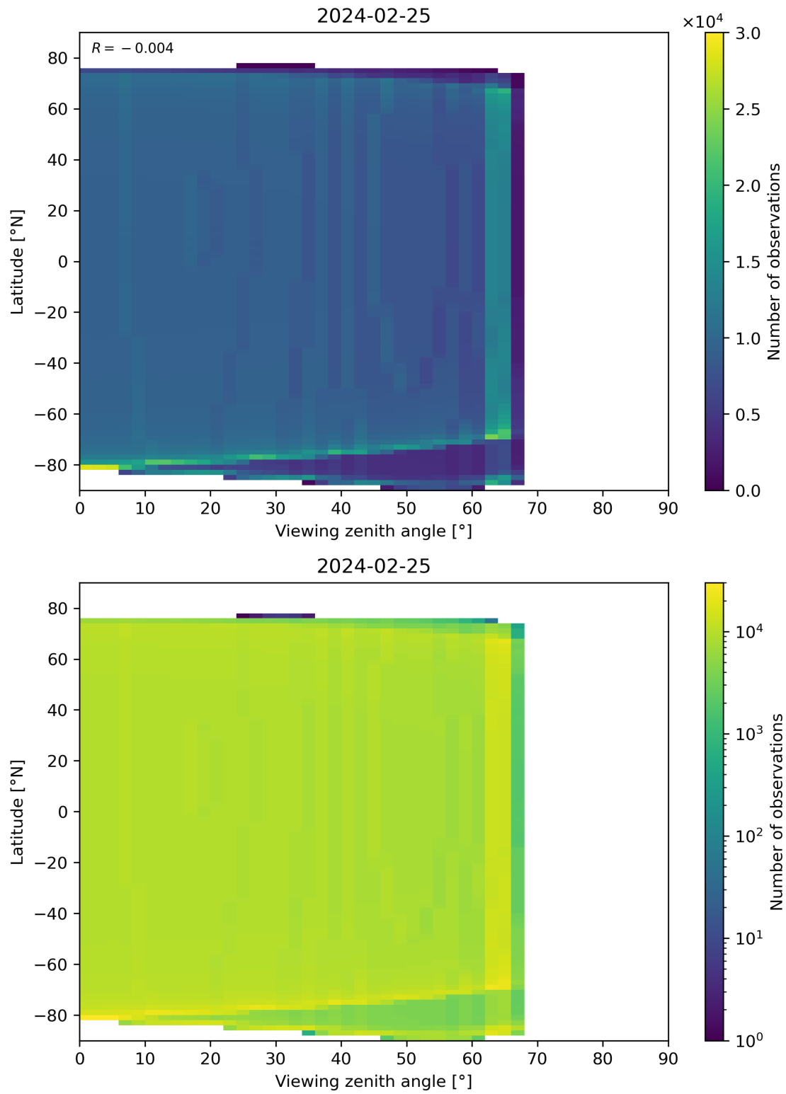
Figure 314: Scatter density plot of “Viewing zenith angle” against “Latitude” for 2024-02-24 to 2024-02-26.
