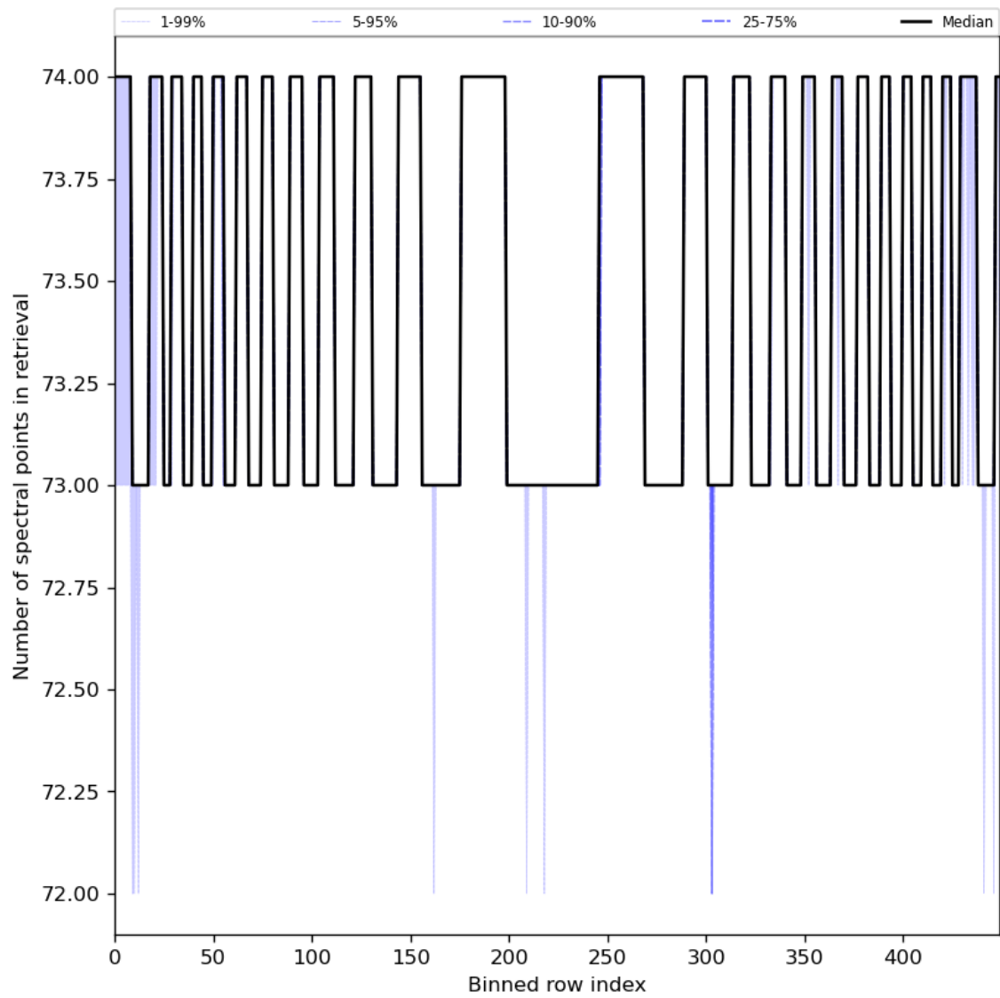
Figure 97: Along track statistics of “Number of spectral points in retrieval” for 2024-02-24 to 2024-02-26
