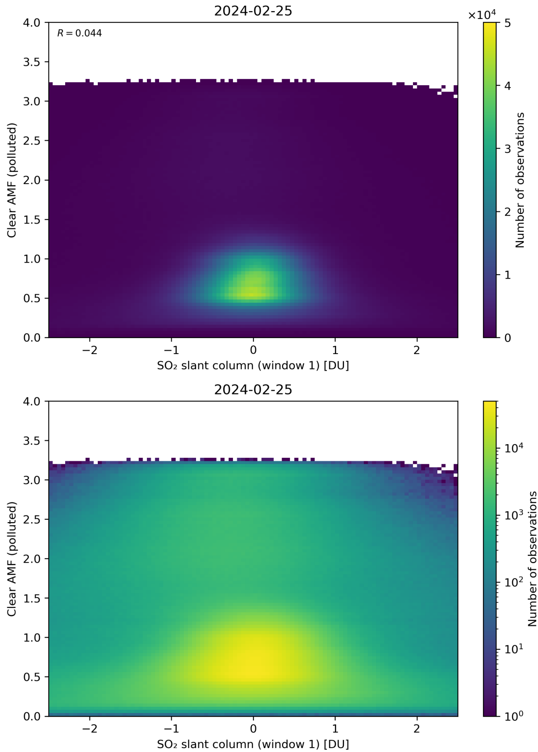
Figure 232: Scatter density plot of “SO 2 slant column (window 1)” against “Clear AMF (polluted)” for 2024-02-24 to 2024-02-26.
