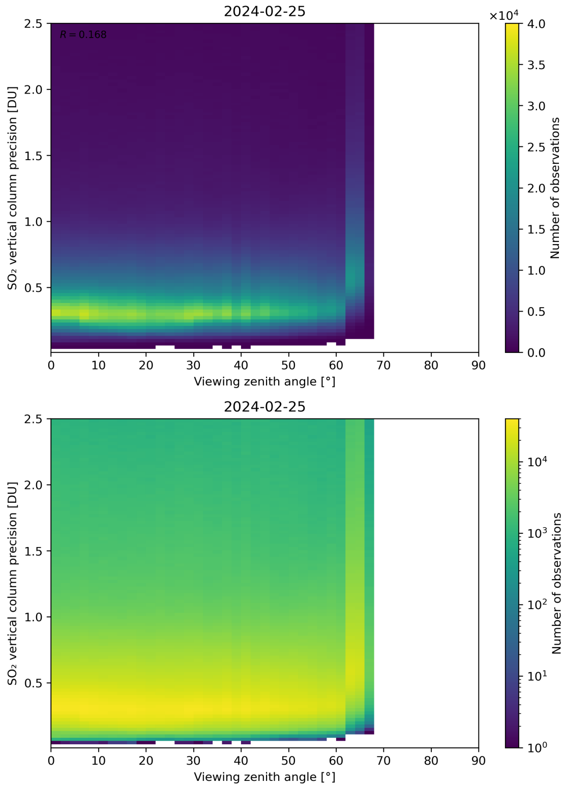
Figure 328: Scatter density plot of “Viewing zenith angle” against “SO 2 vertical column precision” for 2024-02-24 to 2024-02-26.
