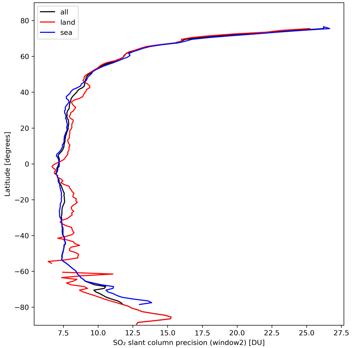
Figure 38: Zonal average of “SO 2 slant column precision (window2)” for 2024-02-24 to 2024-02-26.
