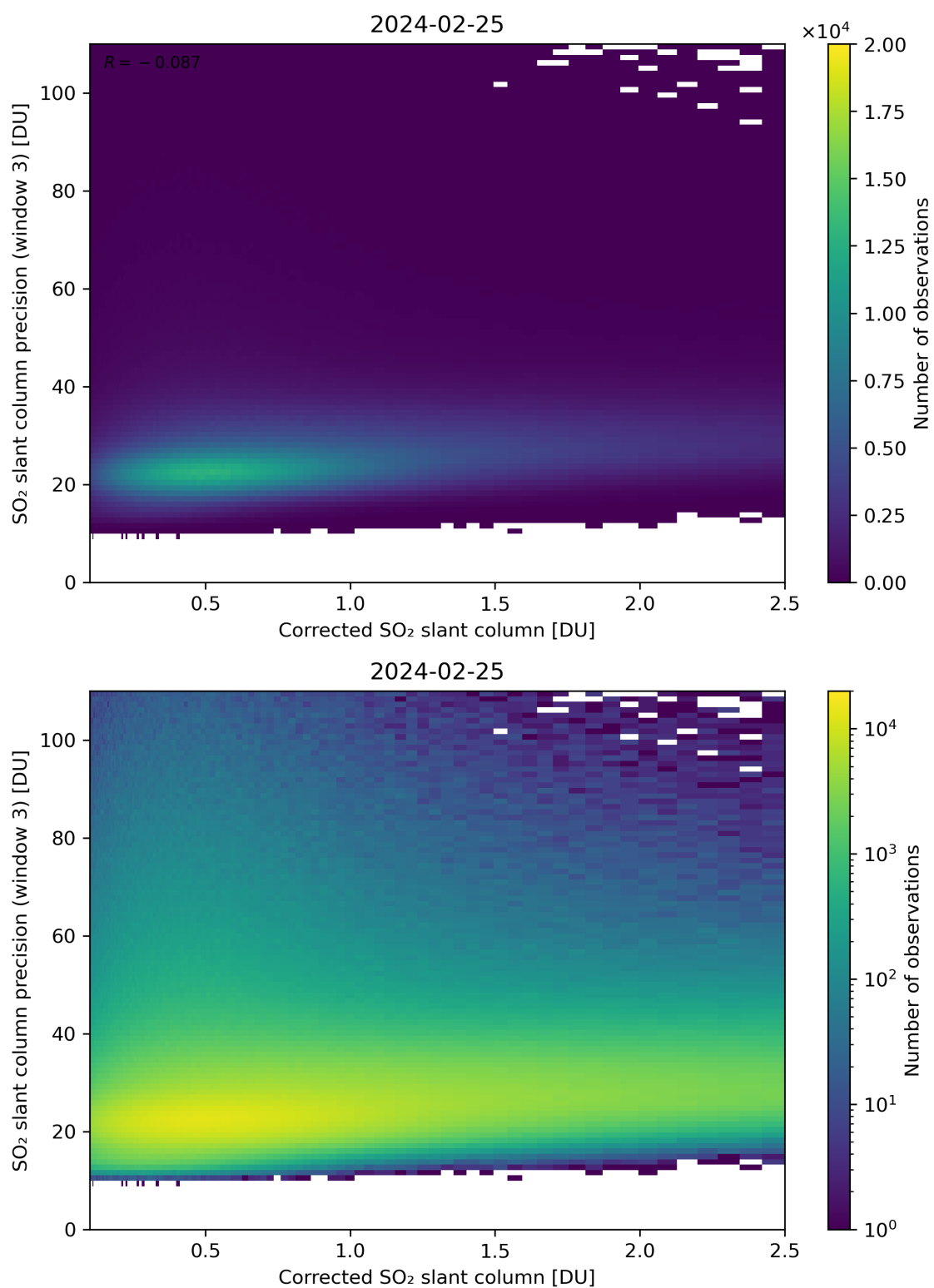
Figure 191: Scatter density plot of “Corrected SO 2 slant column” against “SO 2 slant column precision (window 3)” for 2024-02-24 to 2024-02-26.
