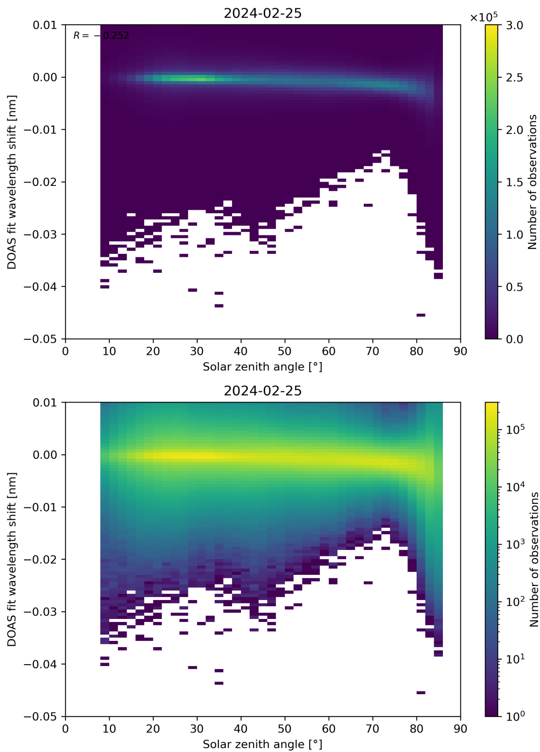
Figure 161: Scatter density plot of “Solar zenith angle” against “DOAS fit wavelength shift” for 2024-02-24 to 2024-02-26.
