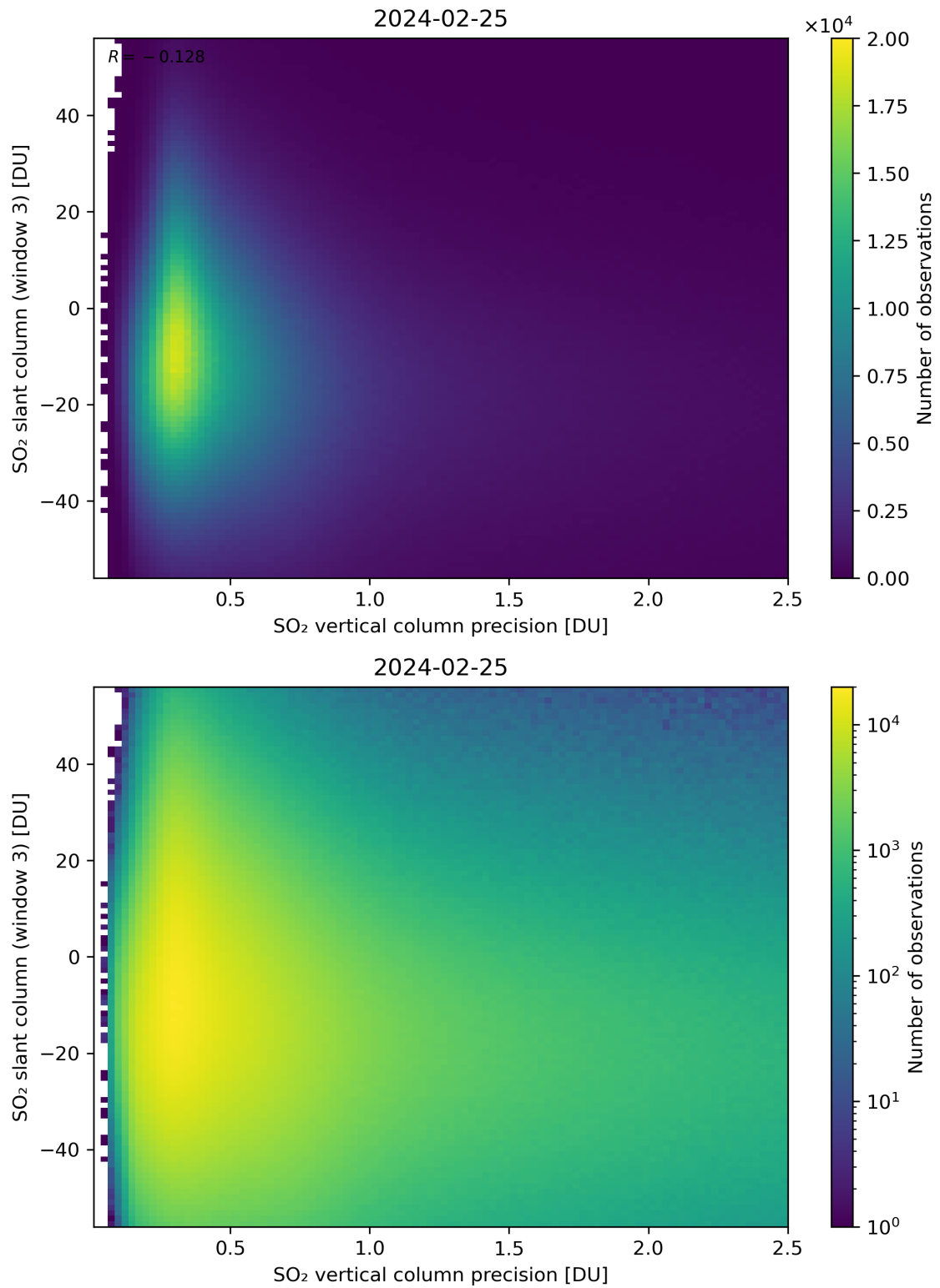
Figure 292: Scatter density plot of “SO 2 vertical column precision” against “SO 2 slant column (window 3)” for 2024-02-24 to 2024-02-26.
