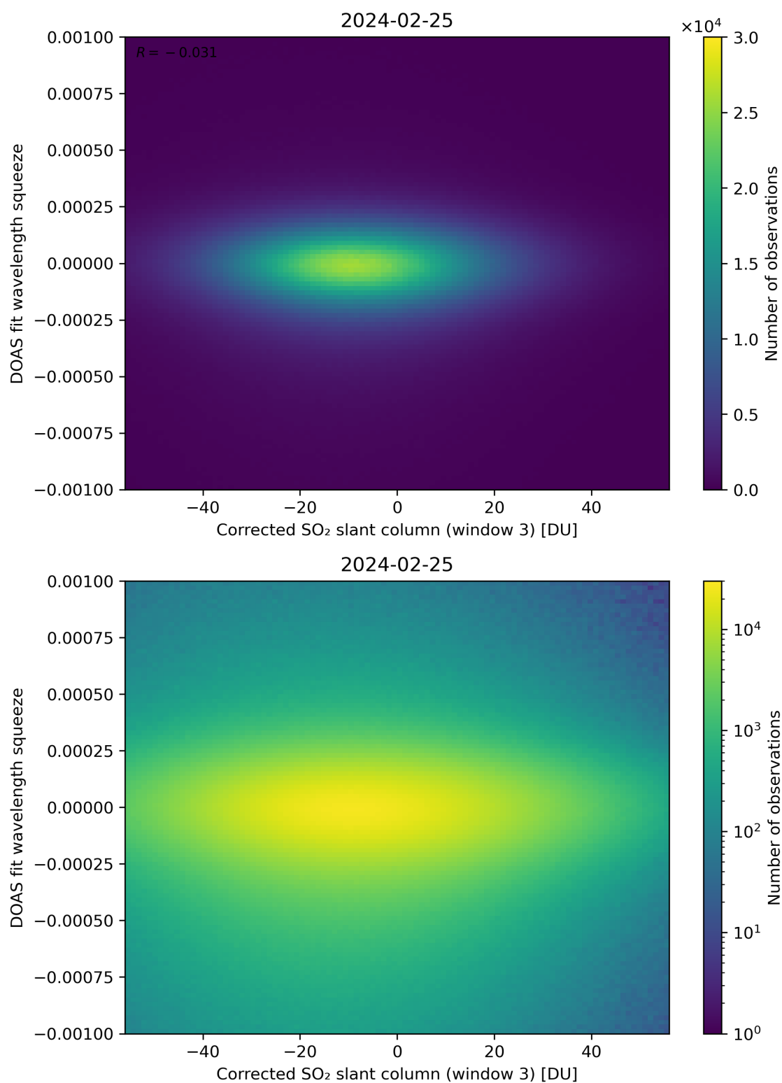
Figure 207: Scatter density plot of “Corrected SO 2 slant column (window 3)” against “DOAS fit wavelength squeeze” for 2024-02-24 to 2024-02-26.
