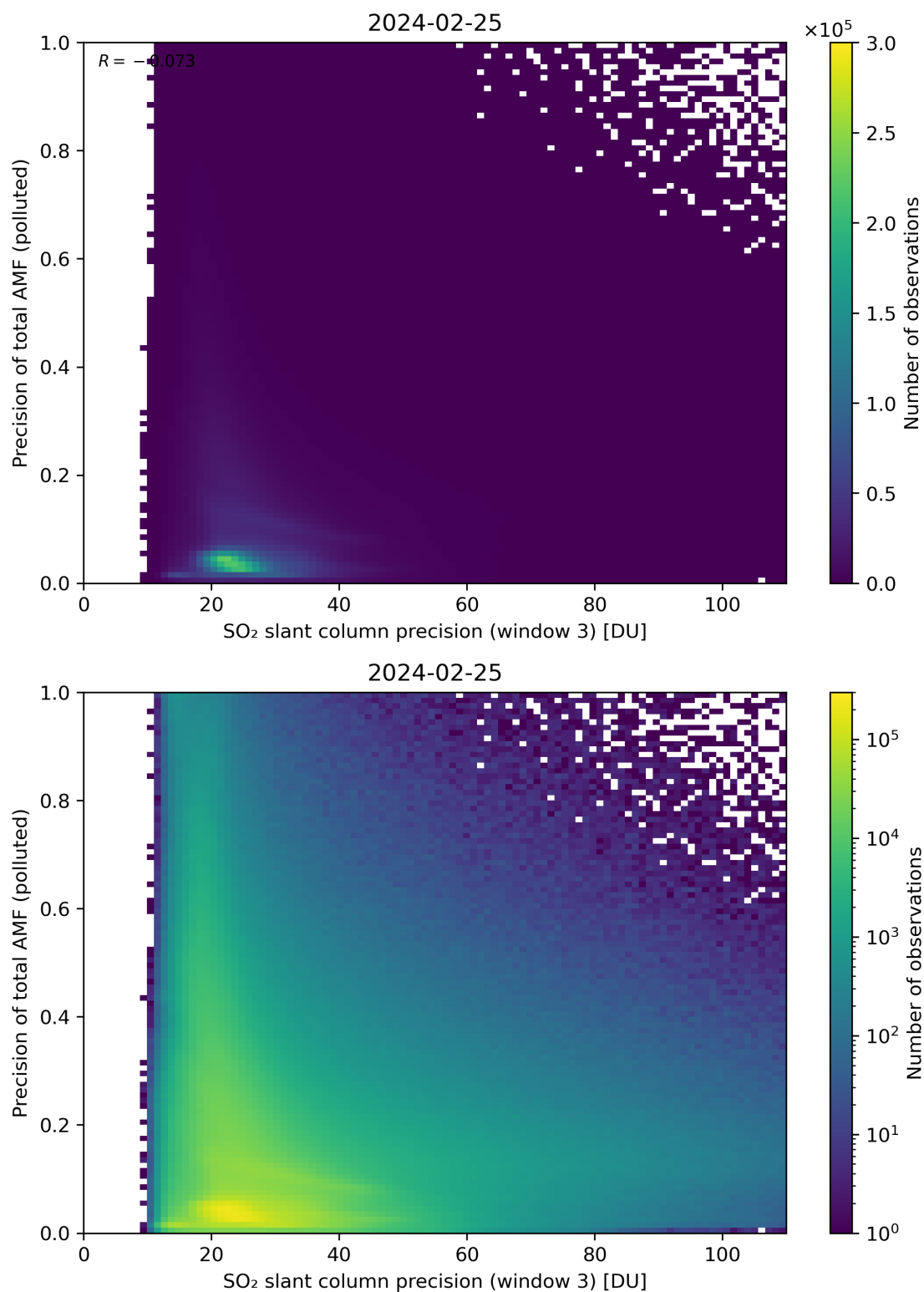
Figure 264: Scatter density plot of “SO 2 slant column precision (window 3)” against “Precision of total AMF (polluted)” for 2024-02-24 to 2024-02-26.
