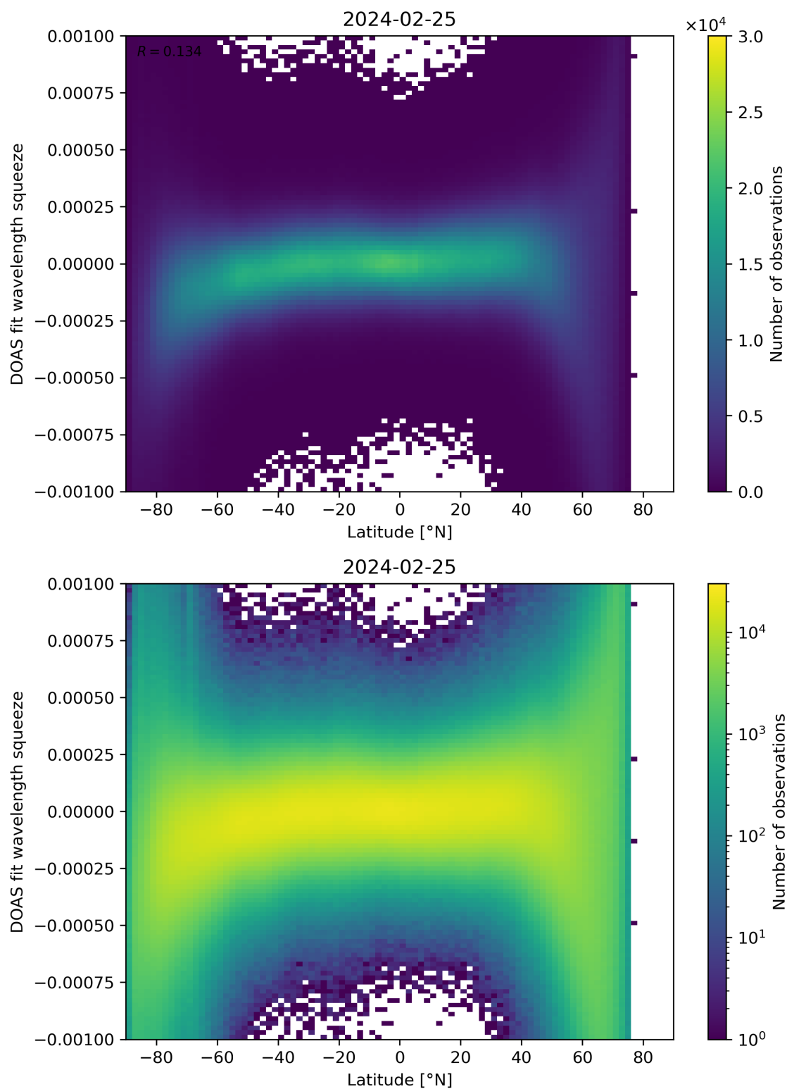
Figure 143: Scatter density plot of “Latitude” against “DOAS fit wavelength squeeze” for 2024-02-24 to 2024-02-26.
