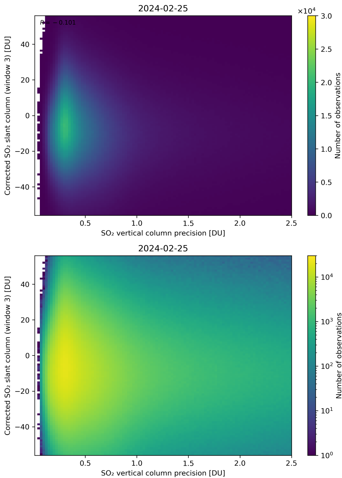
Figure 288: Scatter density plot of “SO 2 vertical column precision” against “Corrected SO 2 slant column (window 3)” for 2024-02-24 to 2024-02-26.
