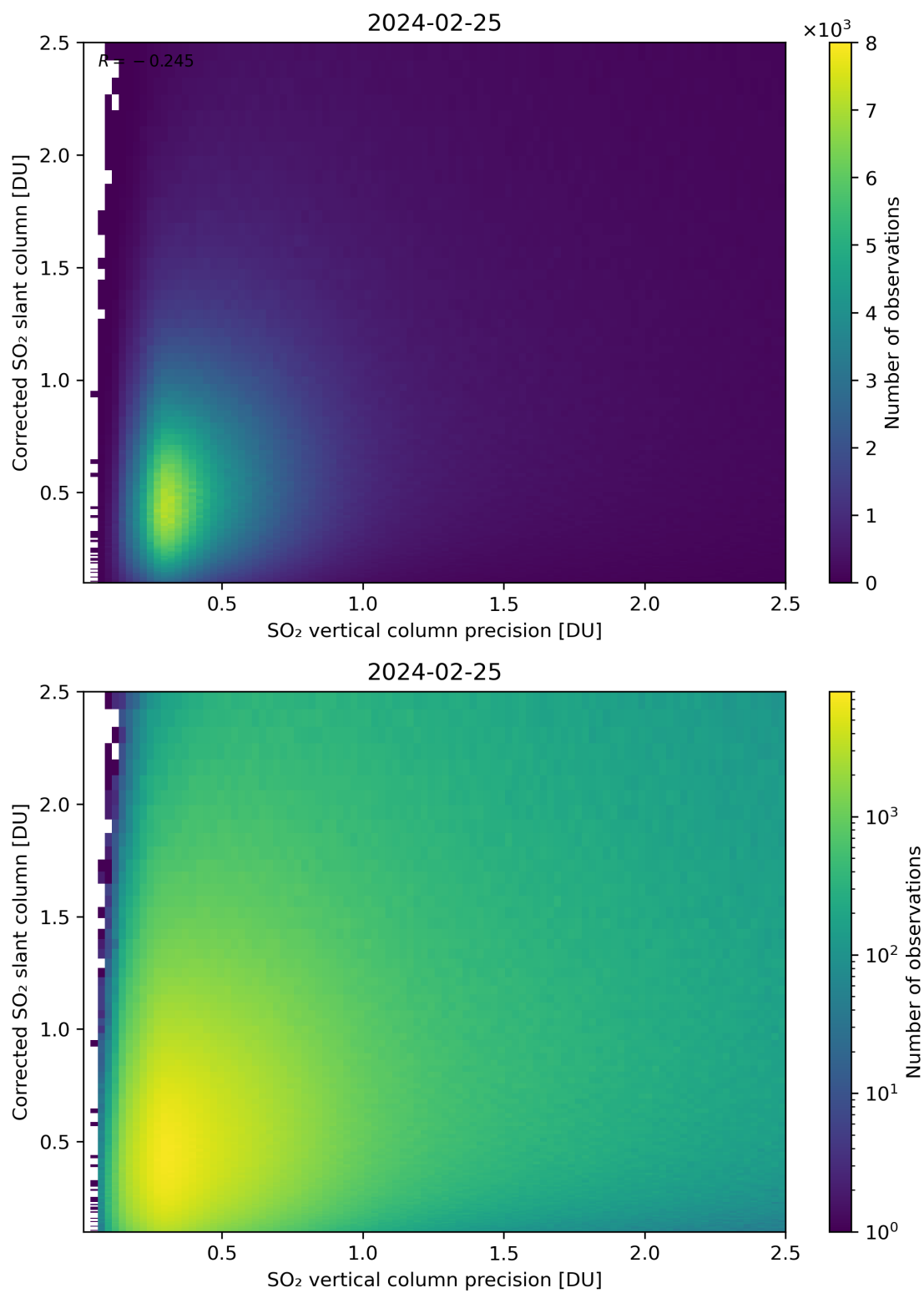
Figure 286: Scatter density plot of “SO 2 vertical column precision” against “Corrected SO 2 slant column” for 2024-02-24 to 2024-02-26.
