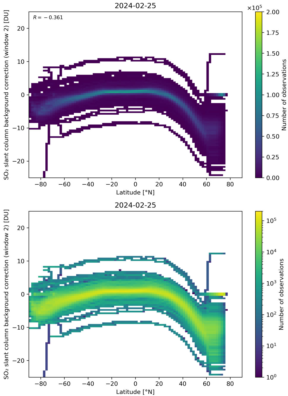
Figure 140: Scatter density plot of “Latitude” against “SO 2 slant column background correction (window 2)” for 2024-02-24 to 2024-02-26.
