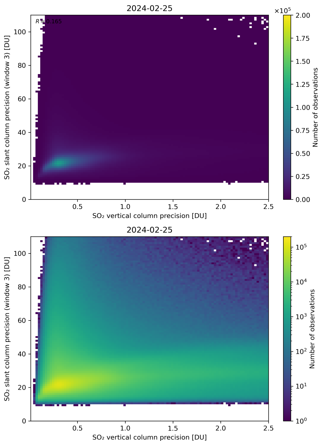
Figure 293: Scatter density plot of “SO 2 vertical column precision” against “SO 2 slant column precision (window 3)” for 2024-02-24 to 2024-02-26.
