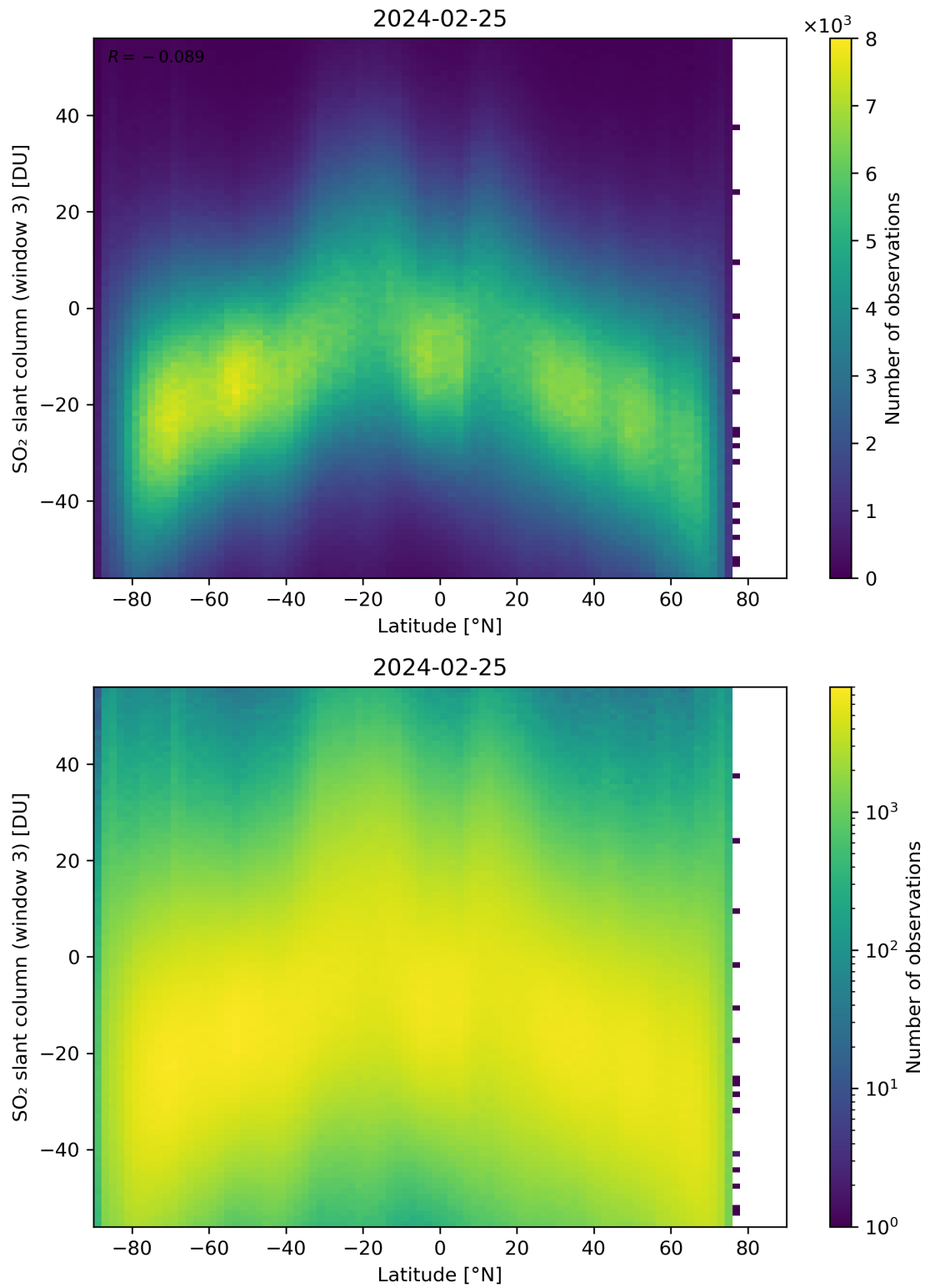
Figure 152: Scatter density plot of “Latitude” against “SO 2 slant column (window 3)” for 2024-02-24 to 2024-02-26.
