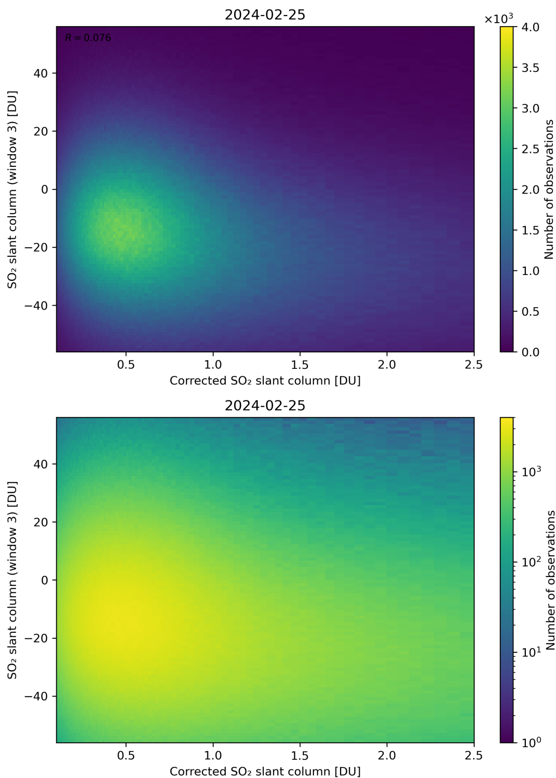
Figure 190: Scatter density plot of “Corrected SO 2 slant column” against “SO 2 slant column (window 3)” for 2024-02-24 to 2024-02-26.
