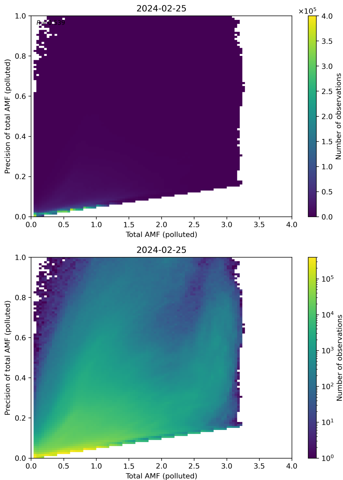
Figure 272: Scatter density plot of “Total AMF (polluted)” against “Precision of total AMF (polluted)” for 2024-02-24 to 2024-02-26.
