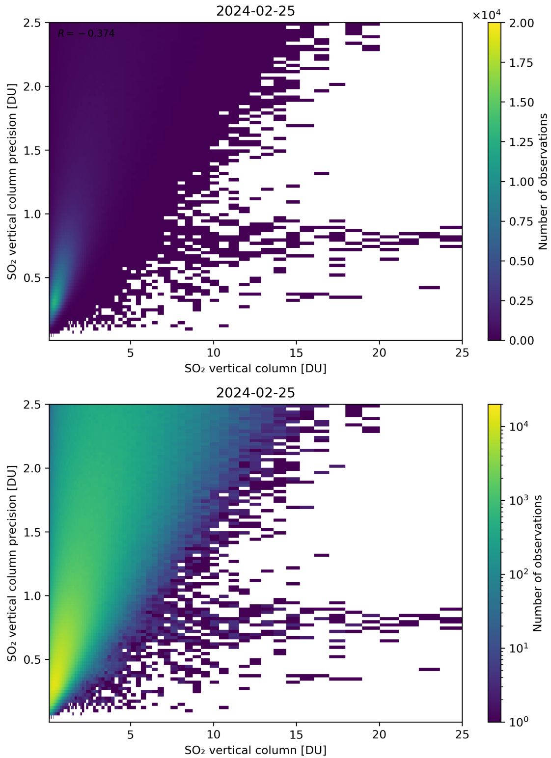
Figure 307: Scatter density plot of “SO 2 vertical column” against “SO 2 vertical column precision” for 2024-02-24 to 2024-02-26.
