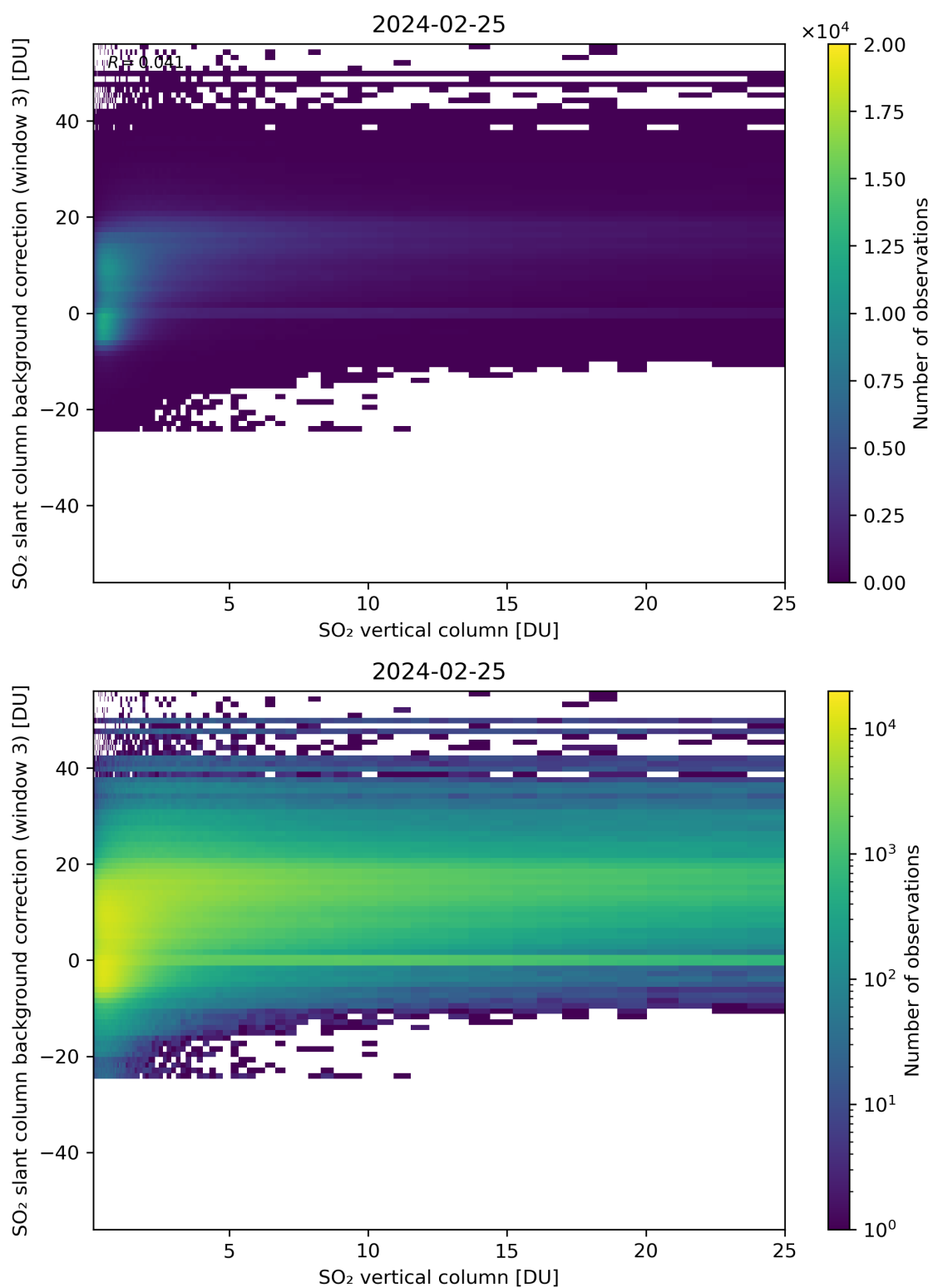
Figure 275: Scatter density plot of “SO 2 vertical column” against “SO 2 slant column background correction (window 3)” for 2024-02-24 to 2024-02-26.
