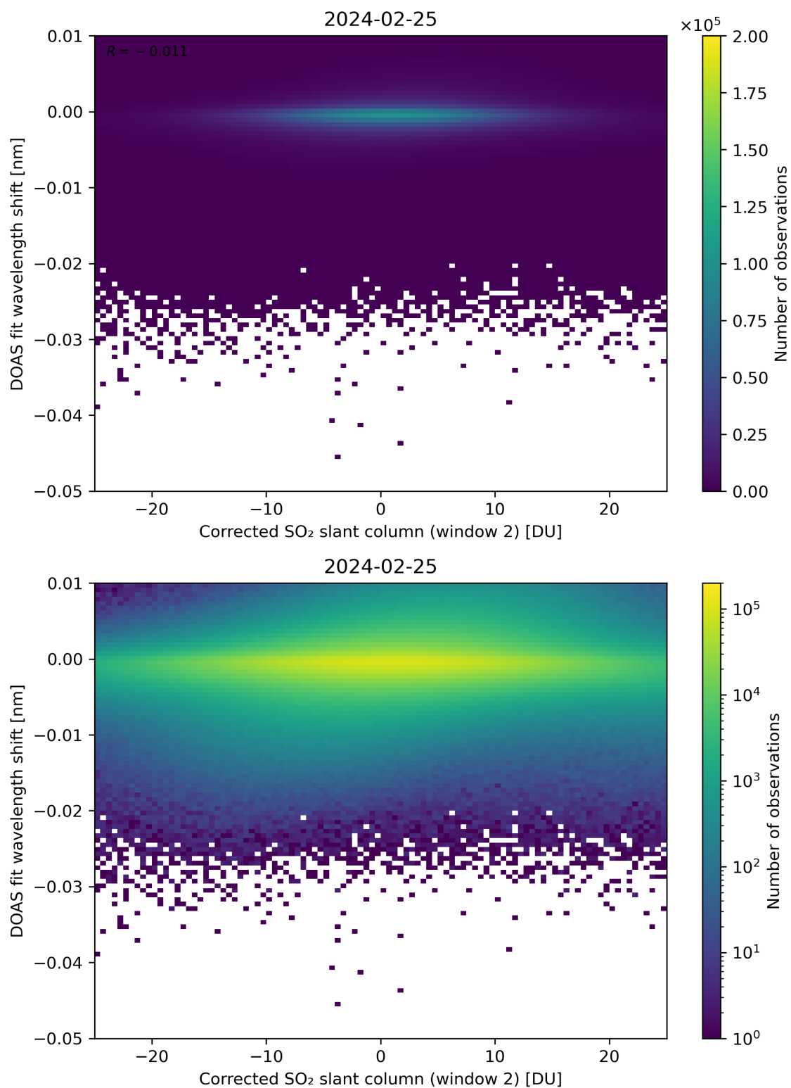
Figure 196: Scatter density plot of “Corrected SO 2 slant column (window 2)” against “DOAS fit wavelength shift” for 2024-02-24 to 2024-02-26.
