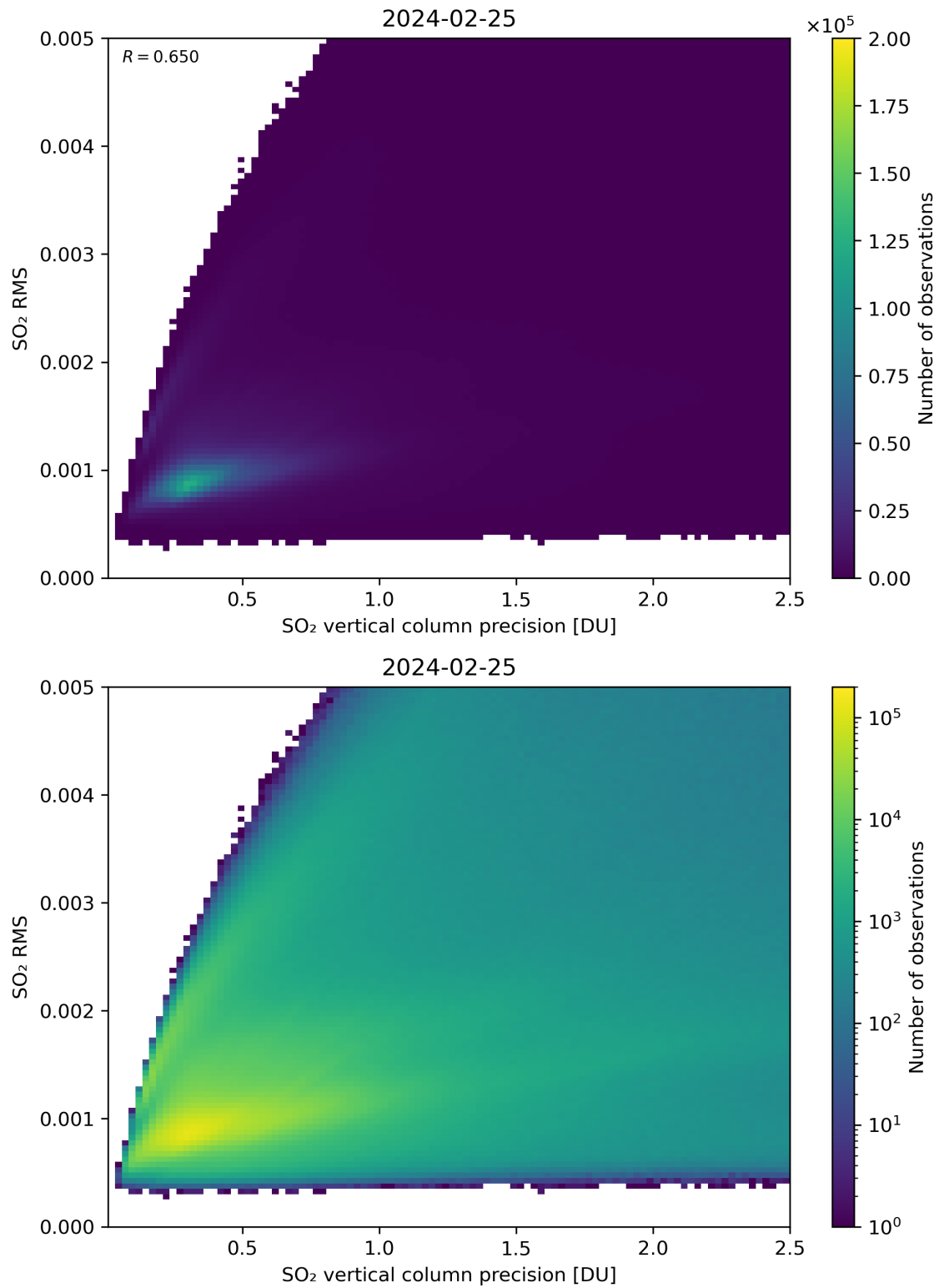
Figure 284: Scatter density plot of “SO 2 vertical column precision” against “SO 2 RMS” for 2024-02-24 to 2024-02-26.
