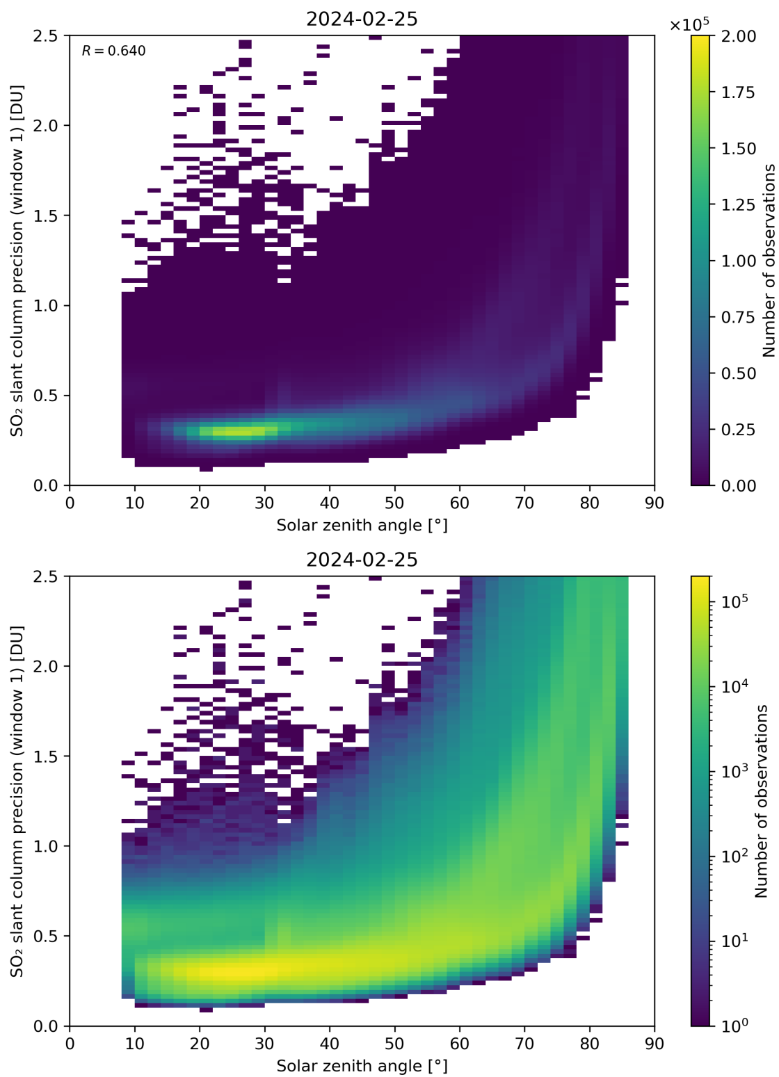
Figure 170: Scatter density plot of “Solar zenith angle” against “SO 2 slant column precision (window 1)” for 2024-02-24 to 2024-02-26.
