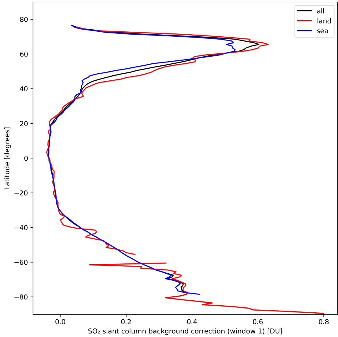
Figure 36: Zonal average of "SO 2 slant column background correction (window 1)" for 2024-02-24 to 2024-02-26.
