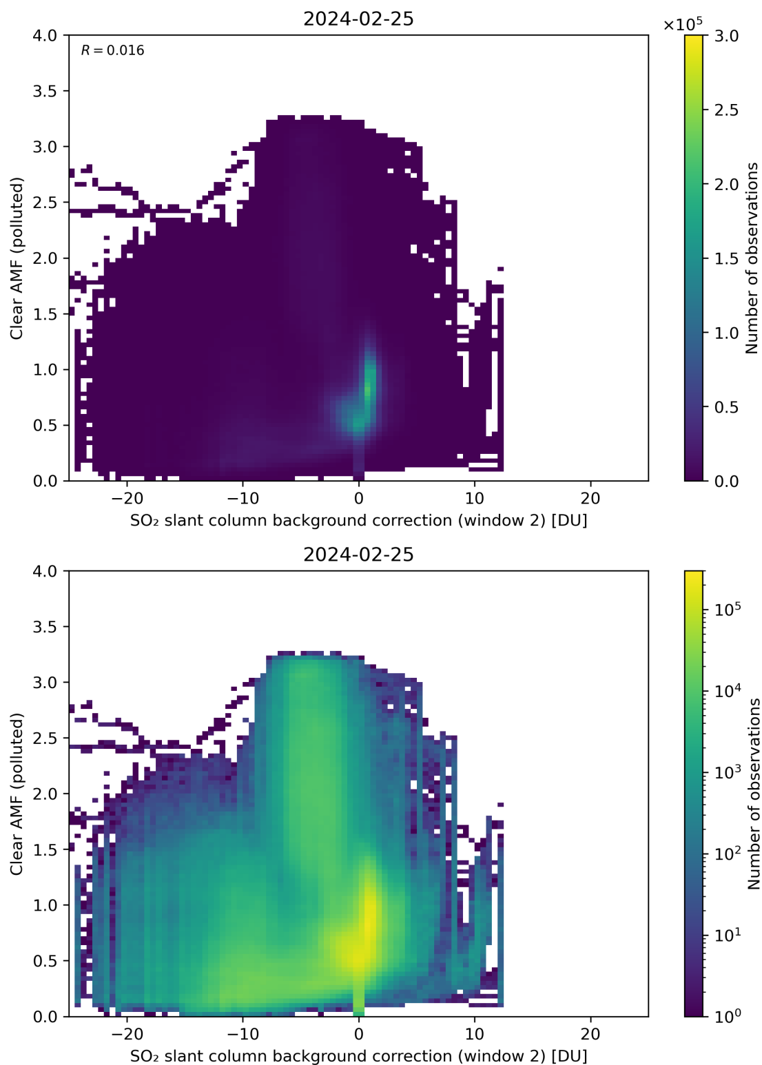
Figure 115: Scatter density plot of “SO 2 slant column background correction (window 2)” against “Clear AMF (polluted)” for 2024-02-24 to 2024-02-26.
