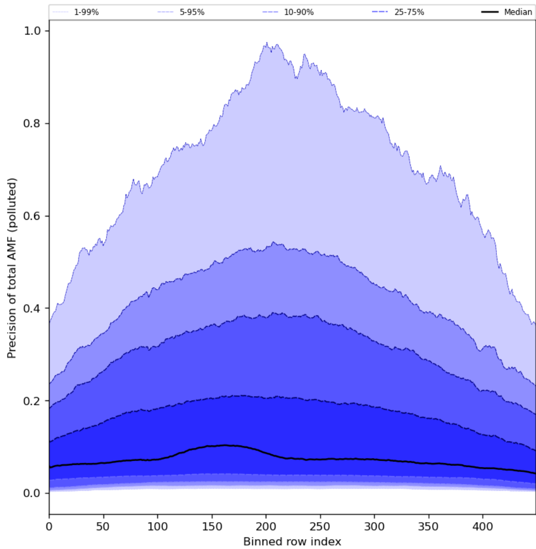
Figure 95: Along track statistics of “Precision of total AMF (polluted)” for 2024-02-24 to 2024-02-26
