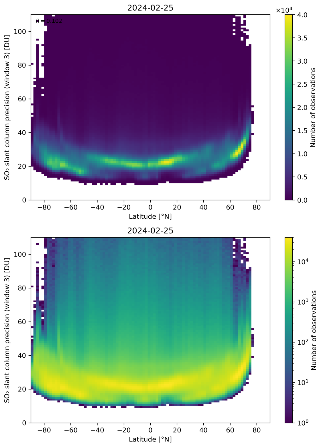
Figure 153: Scatter density plot of “Latitude” against “SO 2 slant column precision (window 3)” for 2024-02-24 to 2024-02-26.
