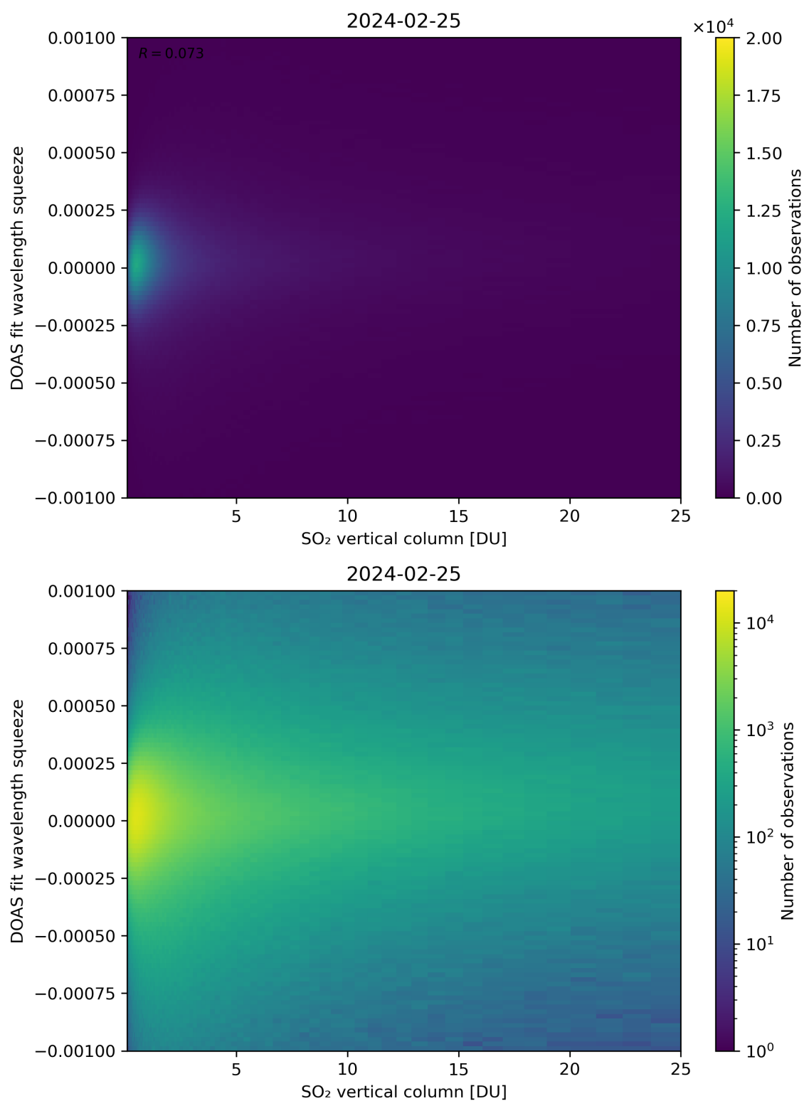
Figure 277: Scatter density plot of “SO 2 vertical column” against “DOAS fit wavelength squeeze” for 2024-02-24 to 2024-02-26.
