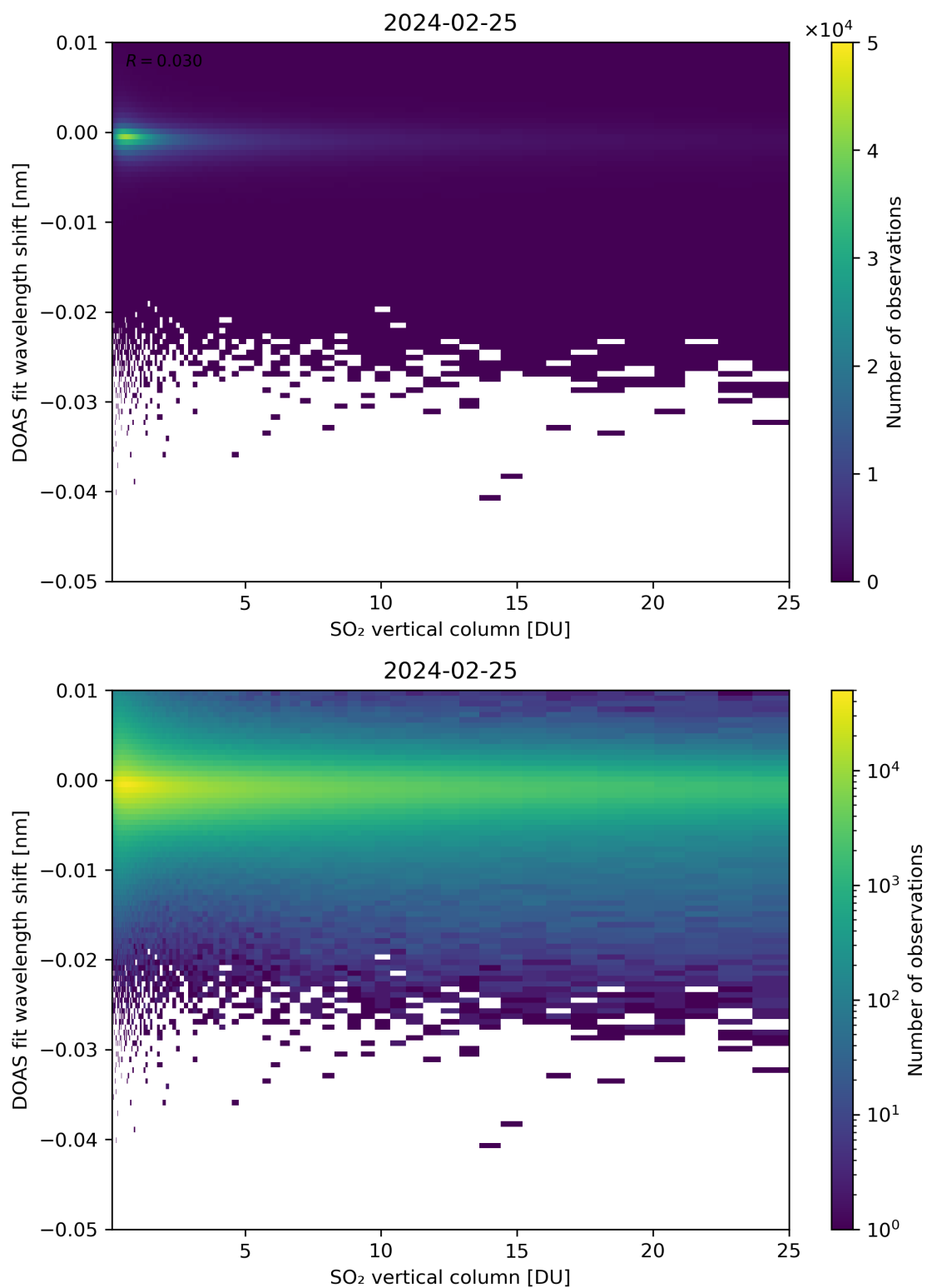
Figure 276: Scatter density plot of “SO 2 vertical column” against “DOAS fit wavelength shift” for 2024-02-24 to 2024-02-26.
