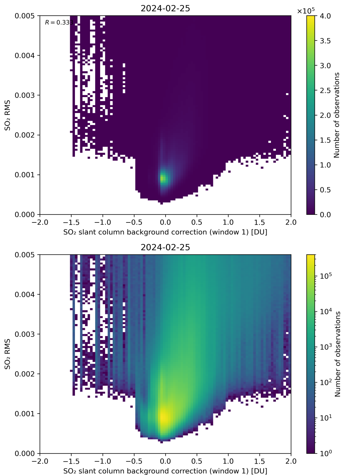
Figure 102: Scatter density plot of “SO 2 slant column background correction (window 1)” against “SO 2 RMS” for 2024-02-24 to 2024-02-26.
