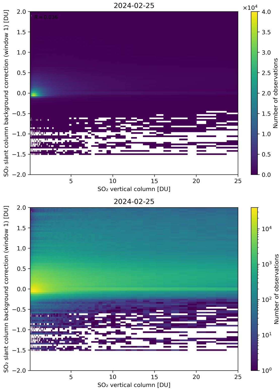
Figure 273: Scatter density plot of “SO 2 vertical column” against “SO 2 slant column background correction (window 1)” for 2024-02-24 to 2024-02-26.
