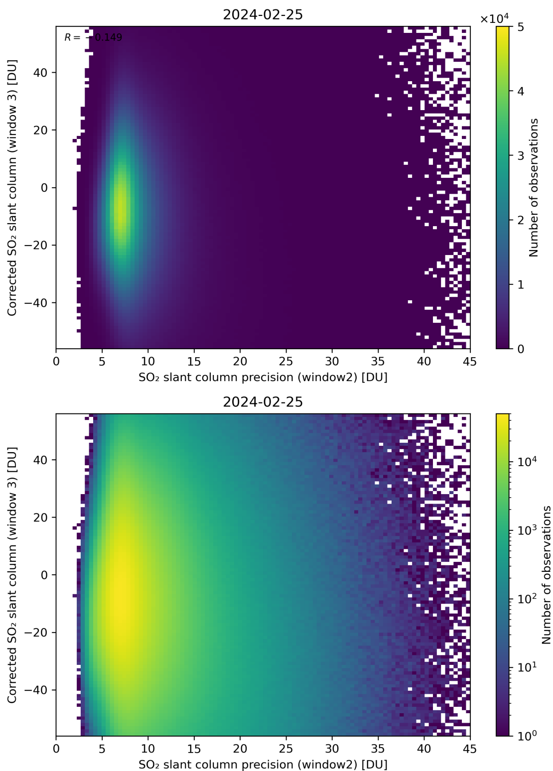
Figure 248: Scatter density plot of “SO 2 slant column precision (window2)” against “Corrected SO 2 slant column (window 3)” for 2024-02-24 to 2024-02-26.
