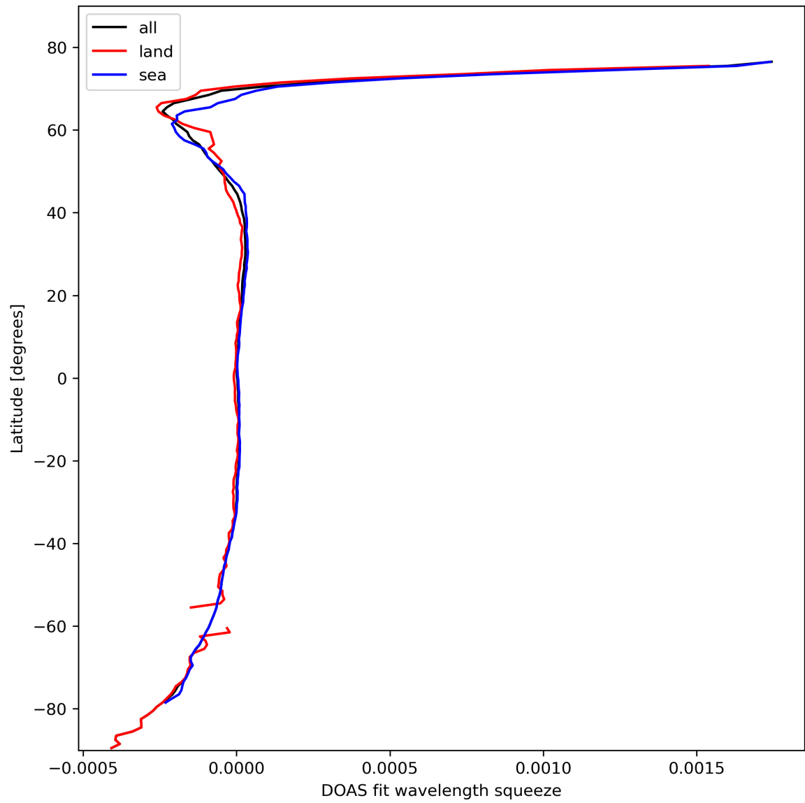
Figure 46: Zonal average of “DOAS fit wavelength squeeze” for 2024-02-24 to 2024-02-26.
