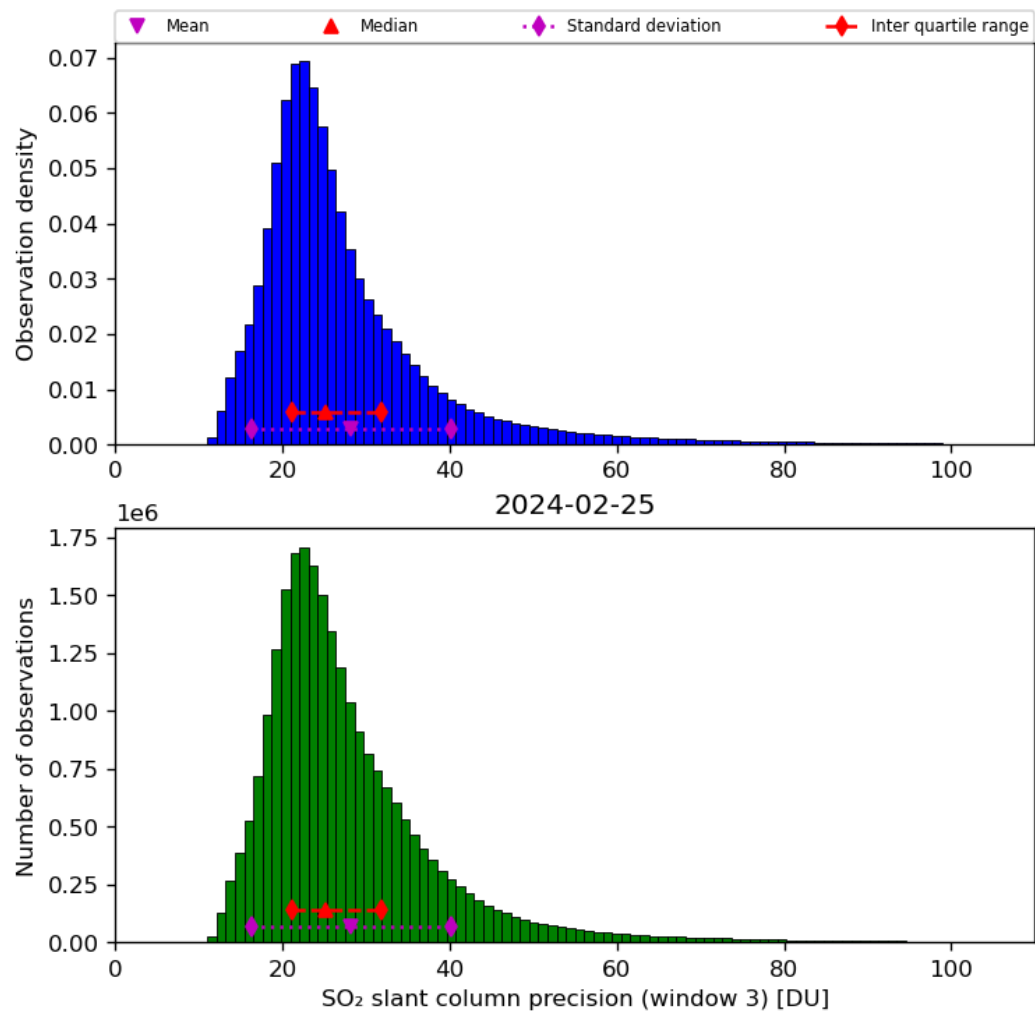
Figure 65: Histogram of “SO 2 slant column precision (window 3)” for 2024-02-24 to 2024-02-26
