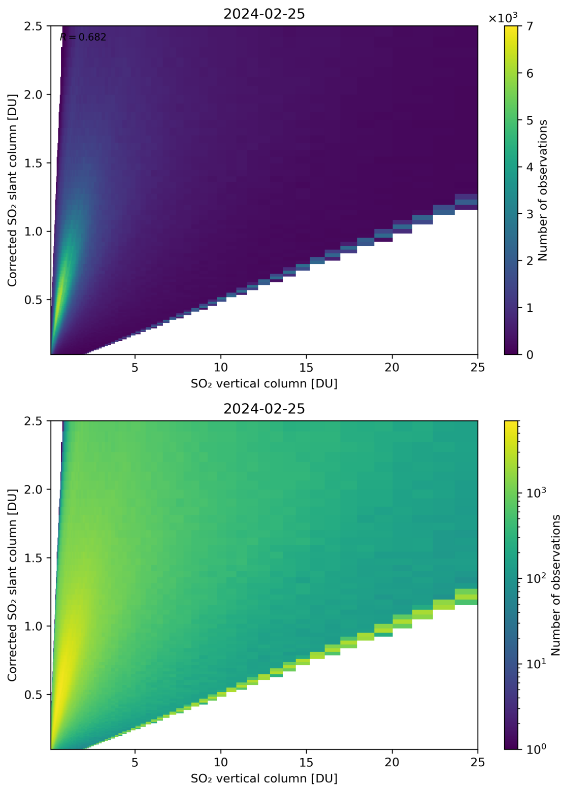
Figure 297: Scatter density plot of “SO 2 vertical column” against “Corrected SO 2 slant column” for 2024-02-24 to 2024-02-26.
