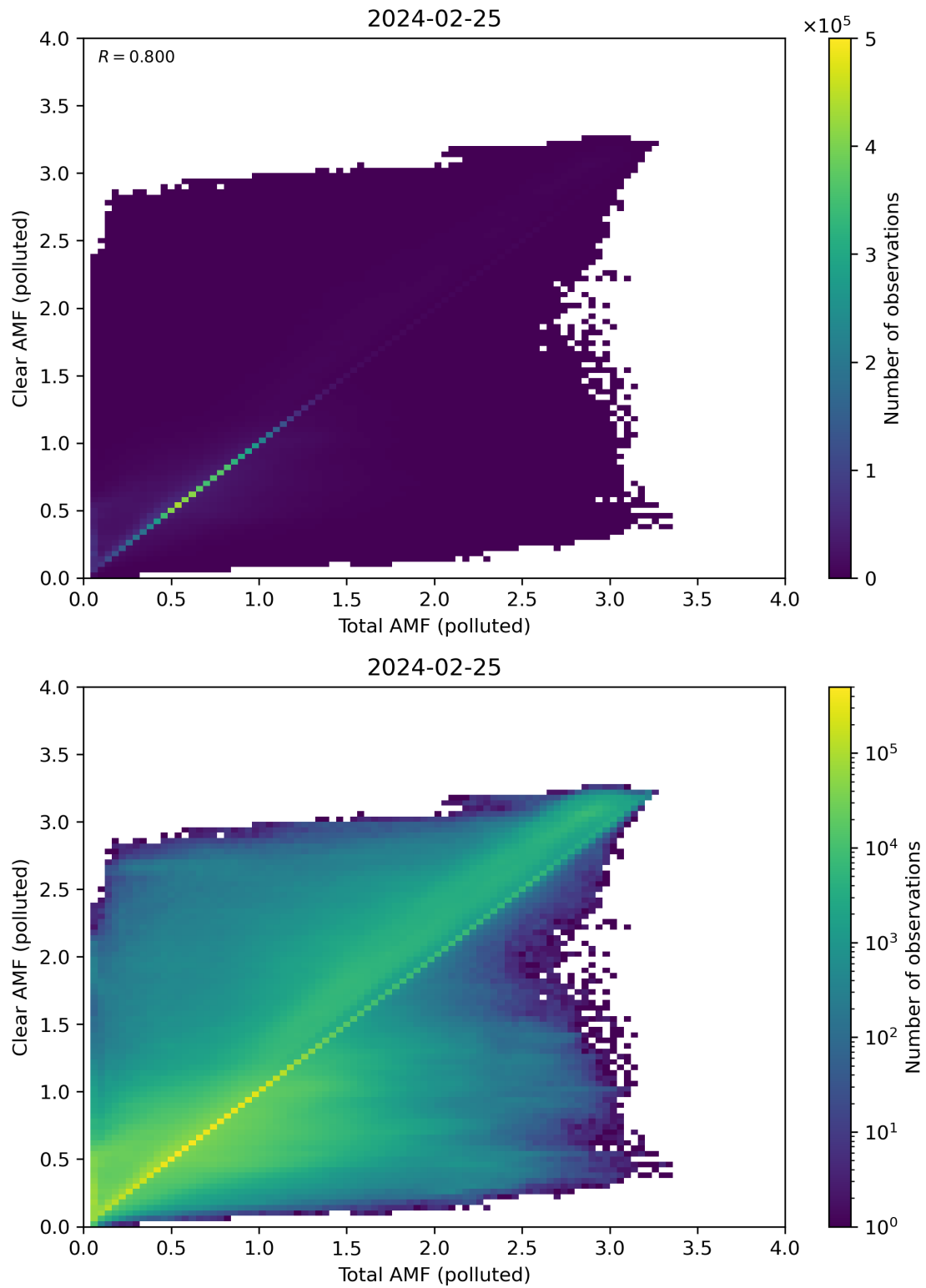
Figure 271: Scatter density plot of “Total AMF (polluted)” against “Clear AMF (polluted)” for 2024-02-24 to 2024-02-26.
