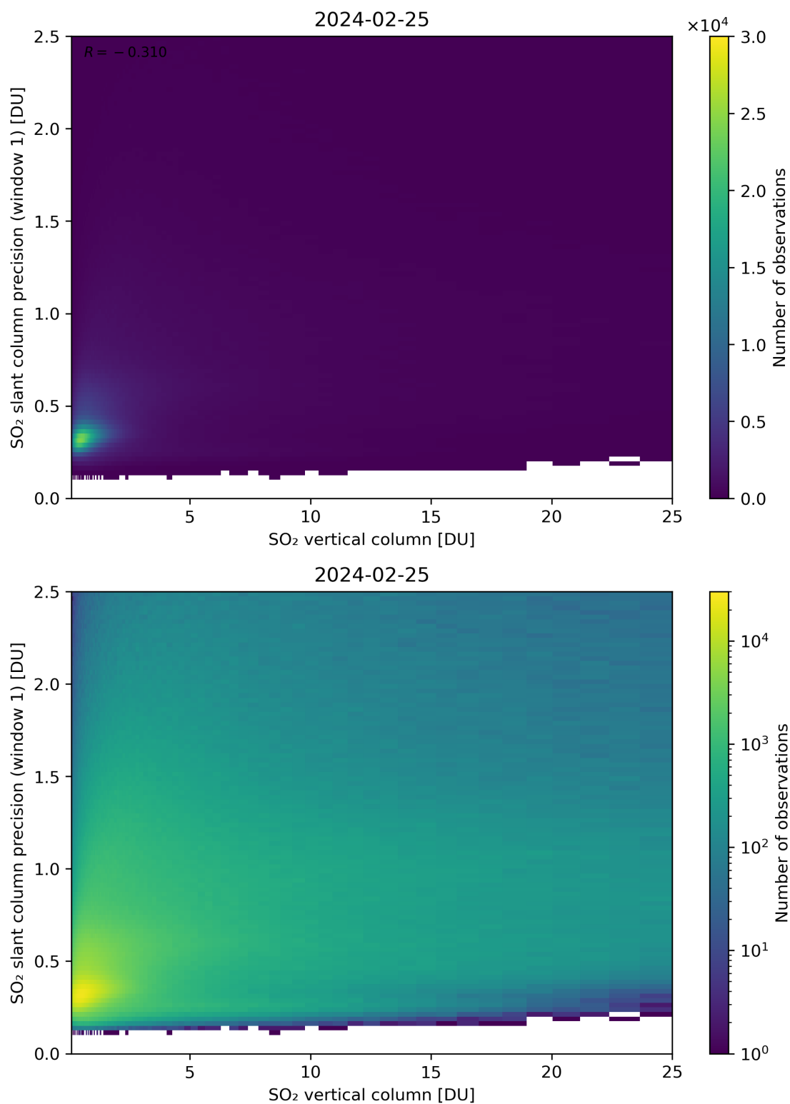
Figure 301: Scatter density plot of “SO 2 vertical column” against “SO 2 slant column precision (window 1)” for 2024-02-24 to 2024-02-26.
