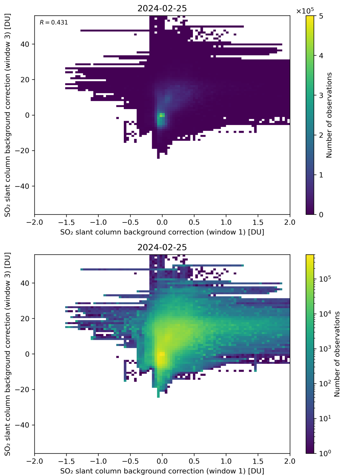
Figure 99: Scatter density plot of “SO 2 slant column background correction (window 1)” against “SO 2 slant column background correction (window 3)” for 2024-02-24 to 2024-02-26.
