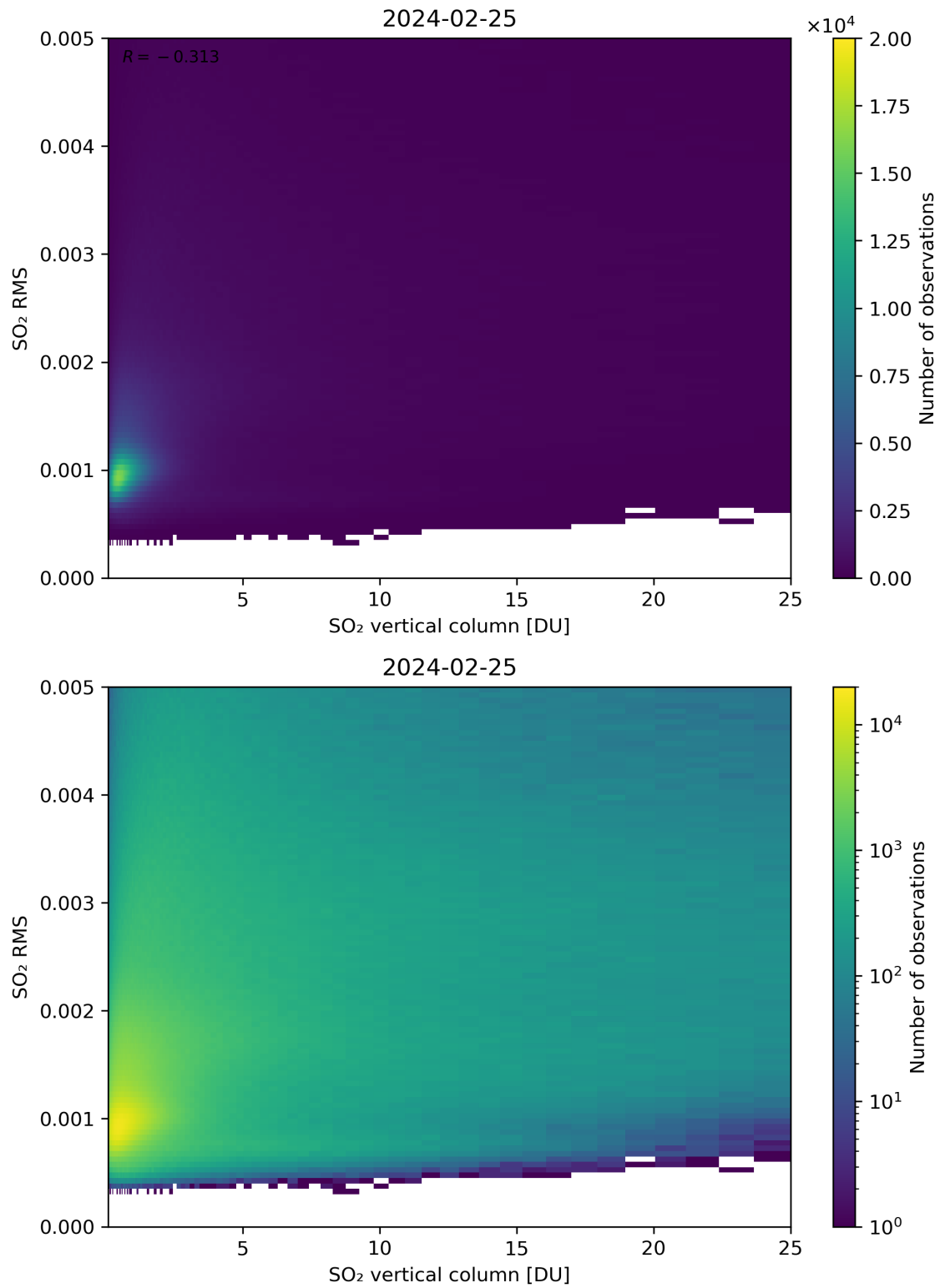
Figure 278: Scatter density plot of “SO 2 vertical column” against “SO 2 RMS” for 2024-02-24 to 2024-02-26.
