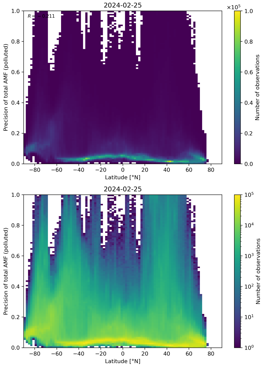
Figure 155: Scatter density plot of “Latitude” against “Precision of total AMF (polluted)” for 2024-02-24 to 2024-02-26.
