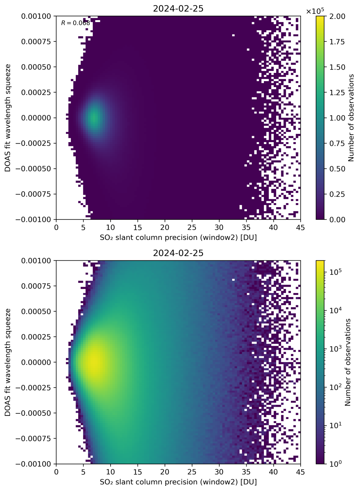
Figure 244: Scatter density plot of “SO 2 slant column precision (window2)” against “DOAS fit wavelength squeeze” for 2024-02-24 to 2024-02-26.
