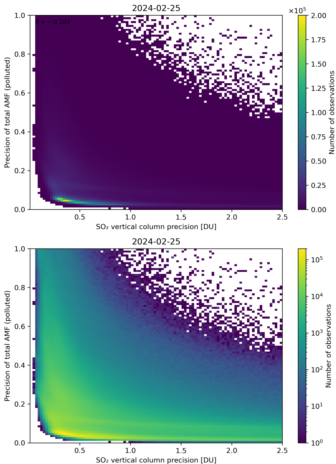
Figure 295: Scatter density plot of “SO 2 vertical column precision” against “Precision of total AMF (polluted)” for 2024-02-24 to 2024-02-26.
