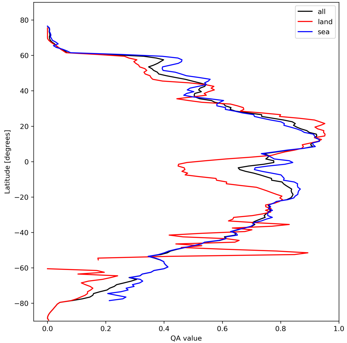
Figure 29: Zonal average of “QA value” for 2024-02-24 to 2024-02-26.
