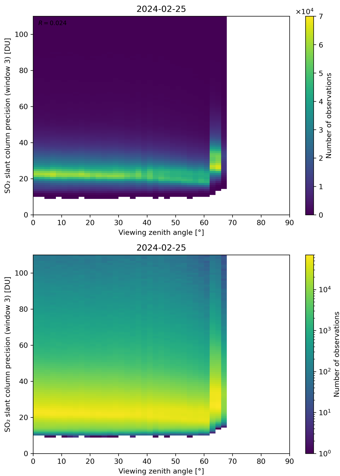
Figure 324: Scatter density plot of “Viewing zenith angle” against “SO 2 slant column precision (window 3)” for 2024-02-24 to 2024-02-26.
