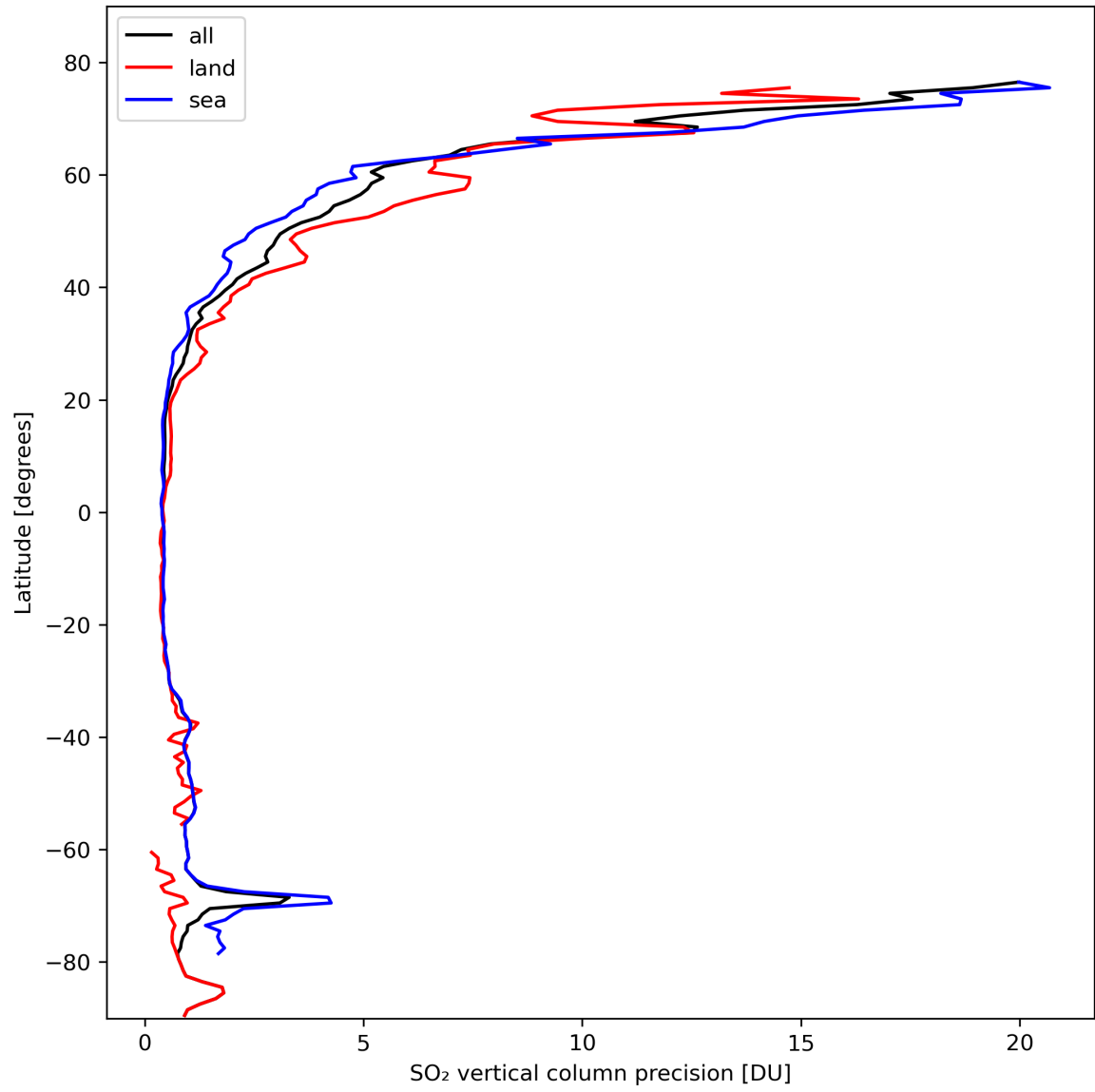
Figure 31: Zonal average of “SO 2 vertical column precision” for 2024-02-24 to 2024-02-26.
