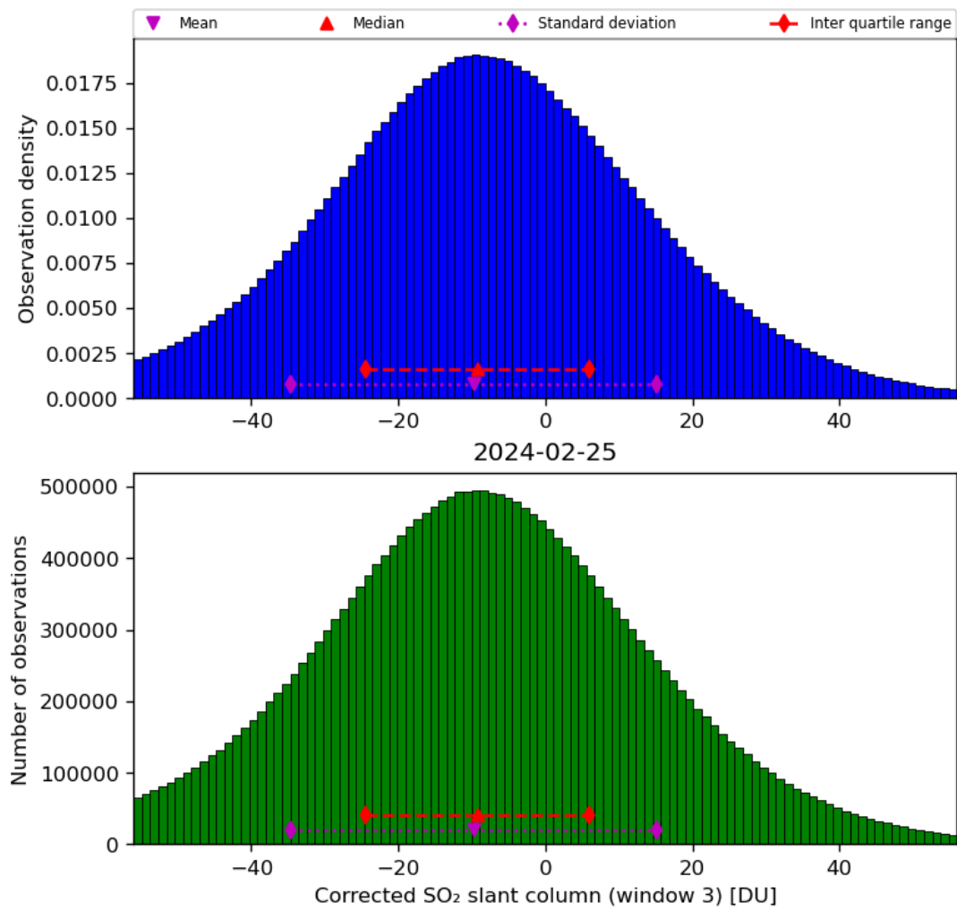
Figure 66: Histogram of “Corrected SO 2 slant column (window 3)” for 2024-02-24 to 2024-02-26
