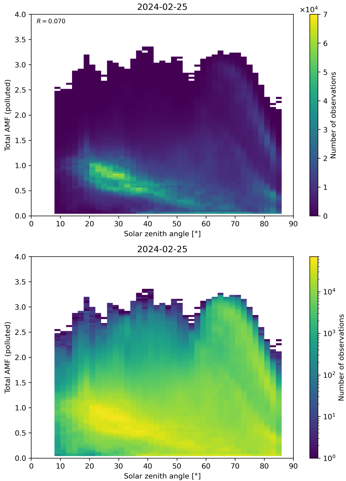
Figure 174: Scatter density plot of “Solar zenith angle” against “Total AMF (polluted)” for 2024-02-24 to 2024-02-26.
