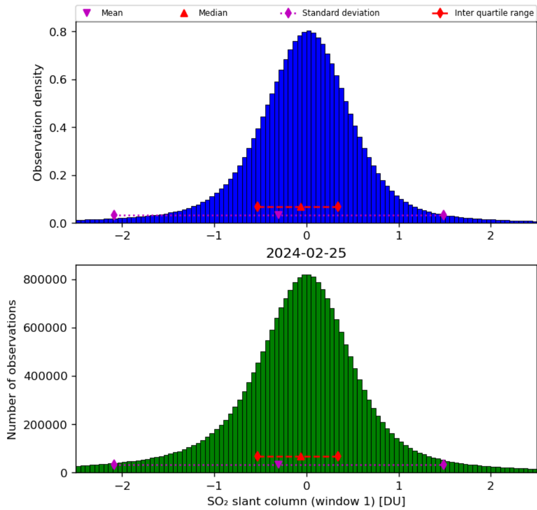
Figure 56: Histogram of “SO 2 slant column (window 1)” for 2024-02-24 to 2024-02-26
