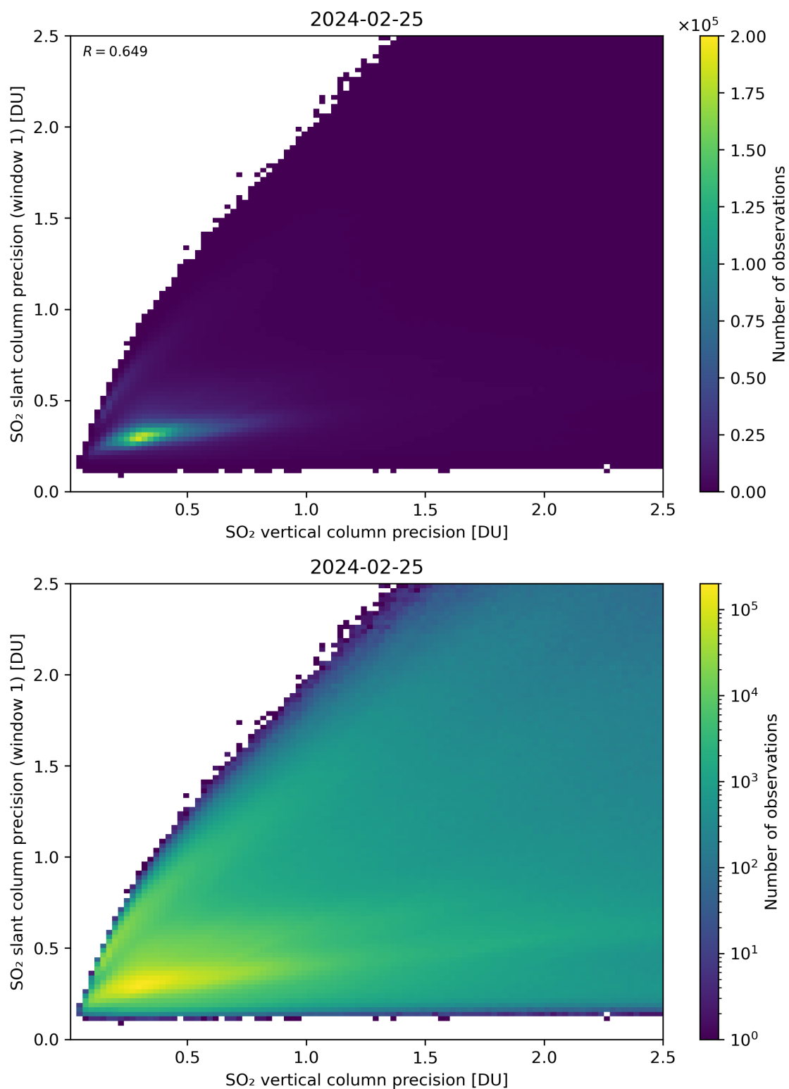
Figure 290: Scatter density plot of “SO 2 vertical column precision” against “SO 2 slant column precision (window 1)” for 2024-02-24 to 2024-02-26.
