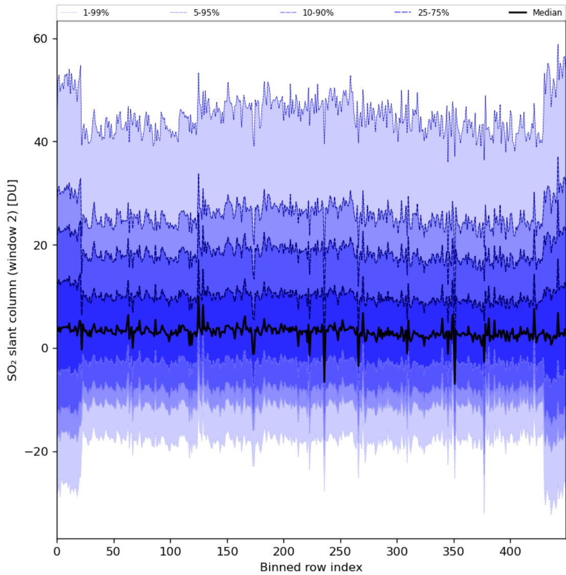
Figure 83: Along track statistics of “SO 2 slant column (window 2)” for 2024-02-24 to 2024-02-26
