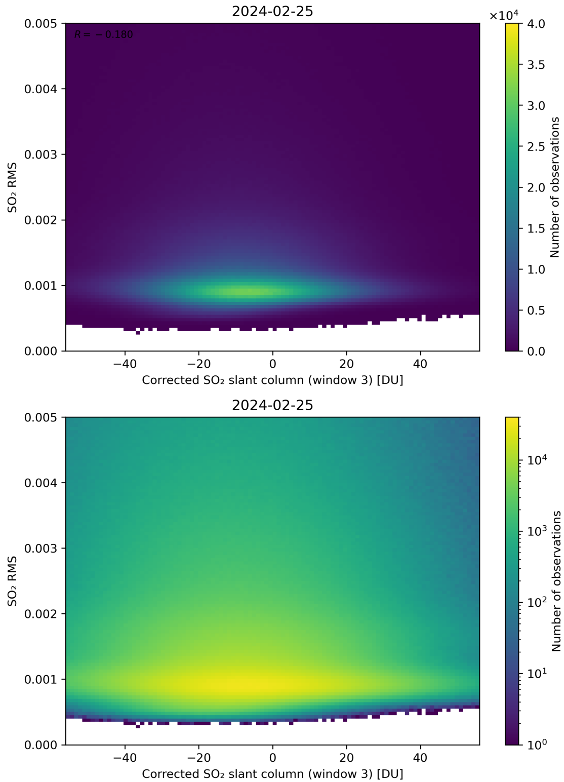
Figure 208: Scatter density plot of “Corrected SO 2 slant column (window 3)” against “SO 2 RMS” for 2024-02-24 to 2024-02-26.
