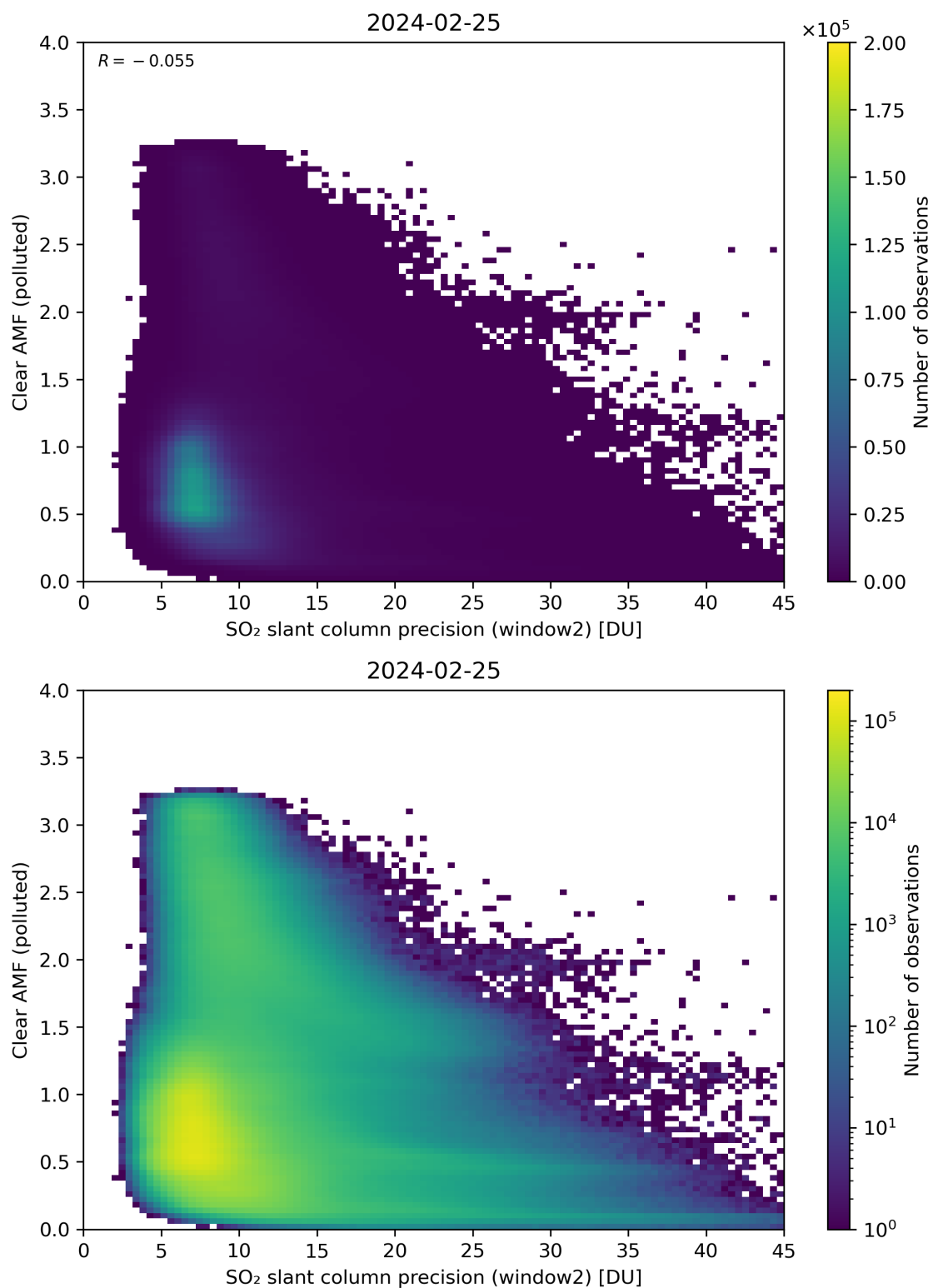
Figure 246: Scatter density plot of “SO 2 slant column precision (window2)” against “Clear AMF (polluted)” for 2024-02-24 to 2024-02-26.
