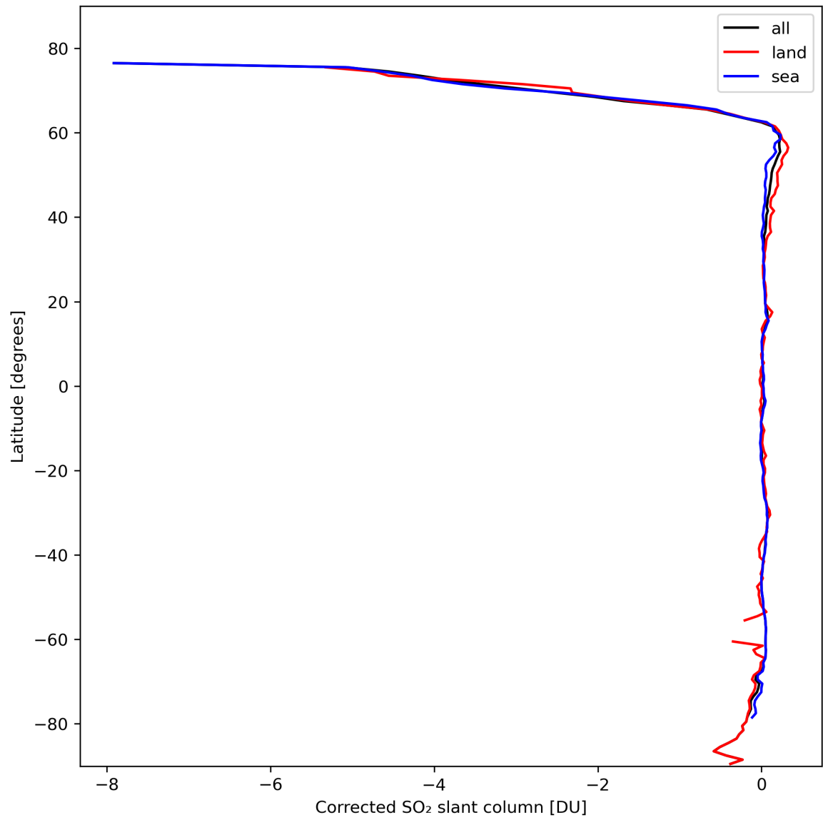
Figure 32: Zonal average of “Corrected SO 2 slant column” for 2024-02-24 to 2024-02-26.
