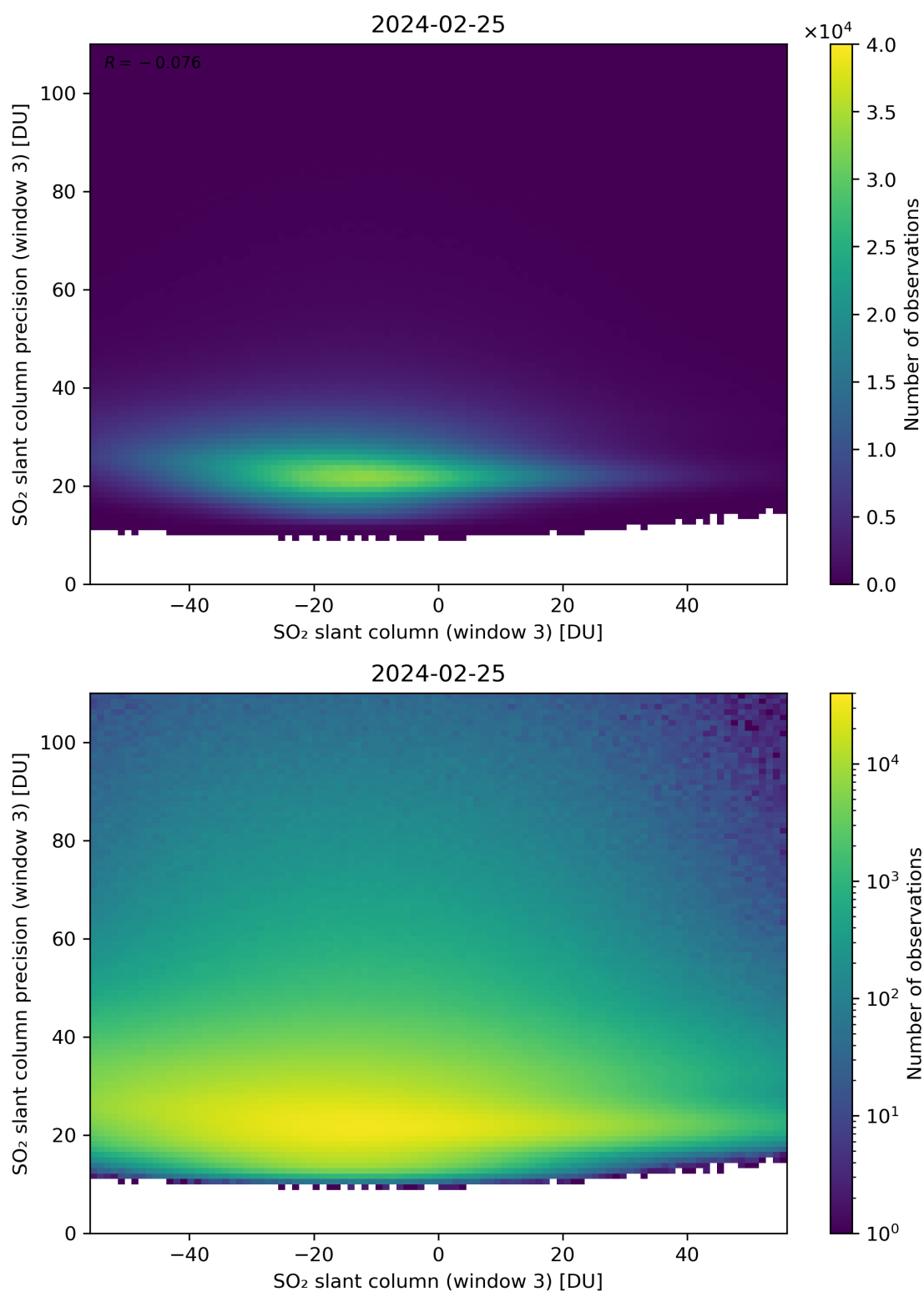
Figure 267: Scatter density plot of “SO 2 slant column (window 3)” against “SO 2 slant column precision (window 3)” for 2024-02-24 to 2024-02-26.
