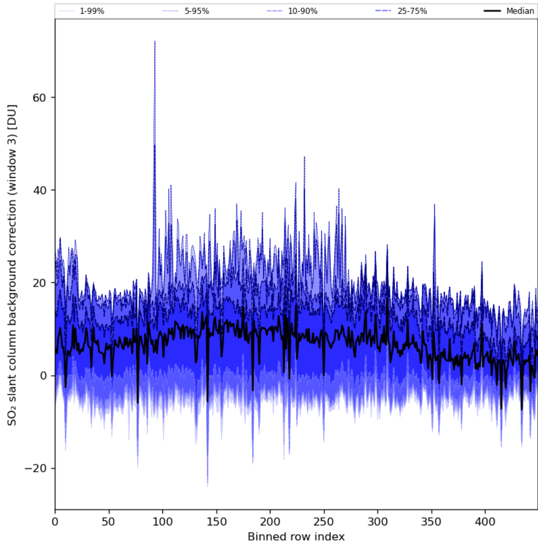
Figure 90: Along track statistics of “SO 2 slant column background correction (window 3)” for 2024-02-24 to 2024-02-26
