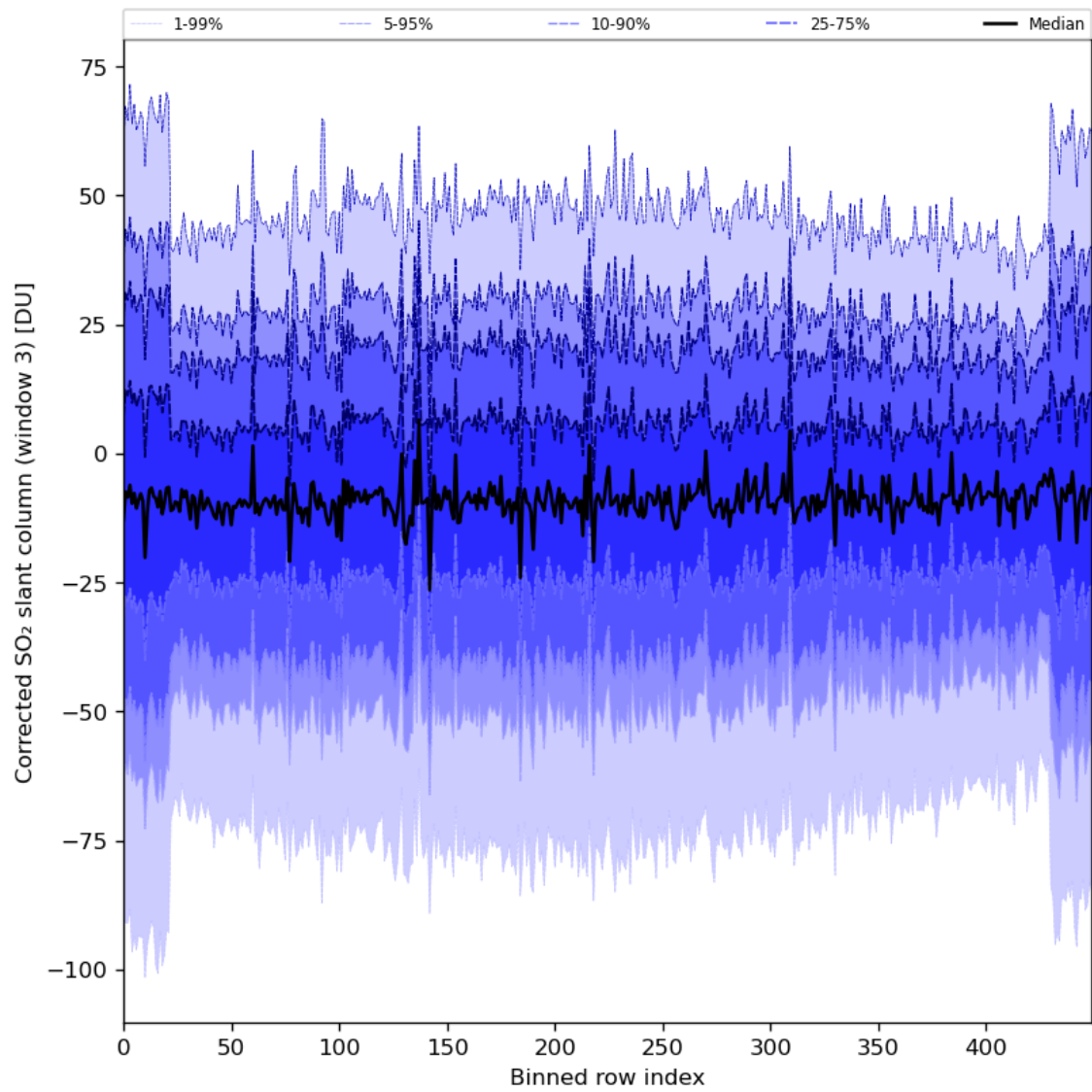
Figure 89: Along track statistics of “Corrected SO 2 slant column (window 3)” for 2024-02-24 to 2024-02-26
