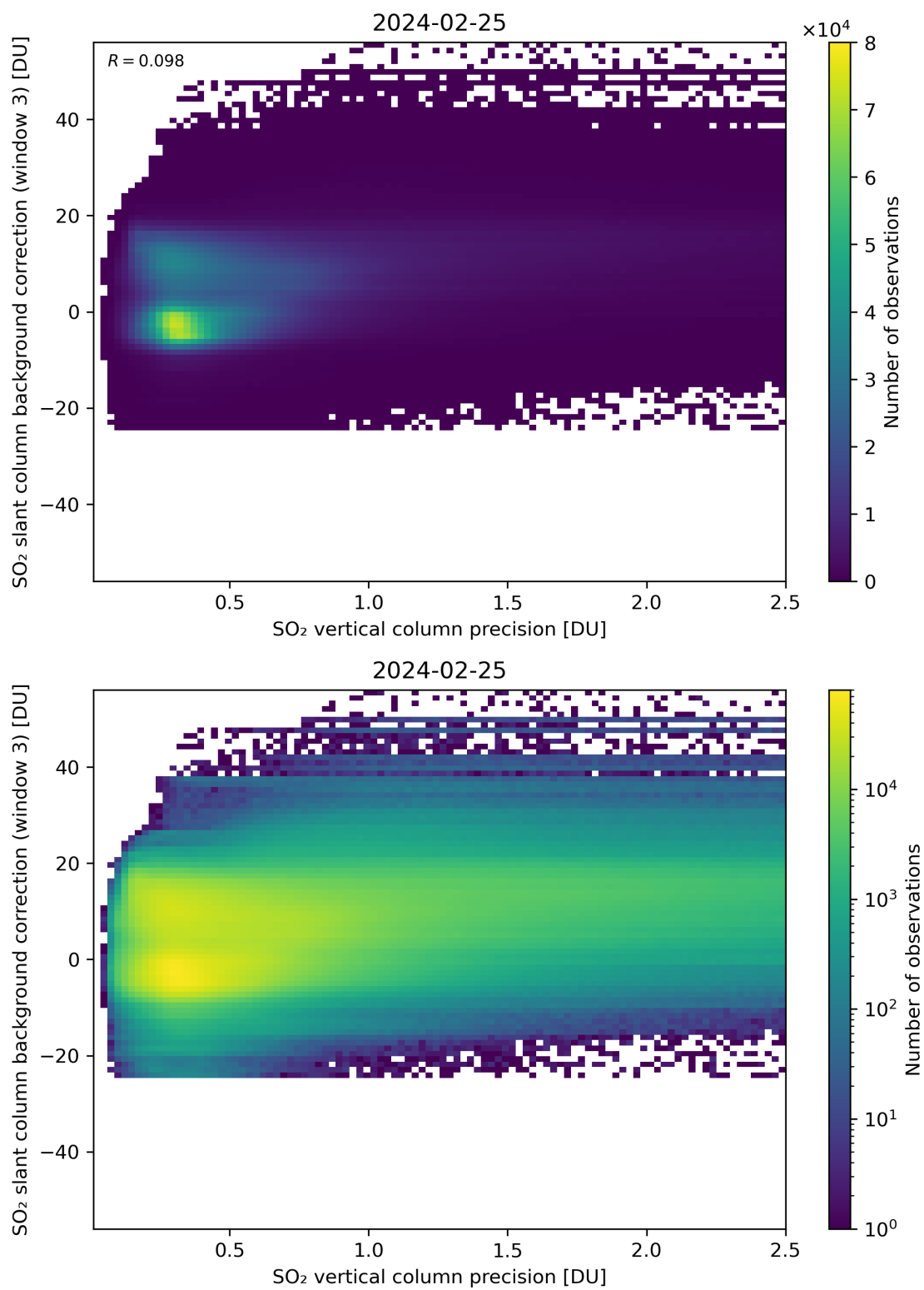
Figure 281: Scatter density plot of “SO 2 vertical column precision” against “SO 2 slant column background correction (window 3)” for 2024-02-24 to 2024-02-26.
