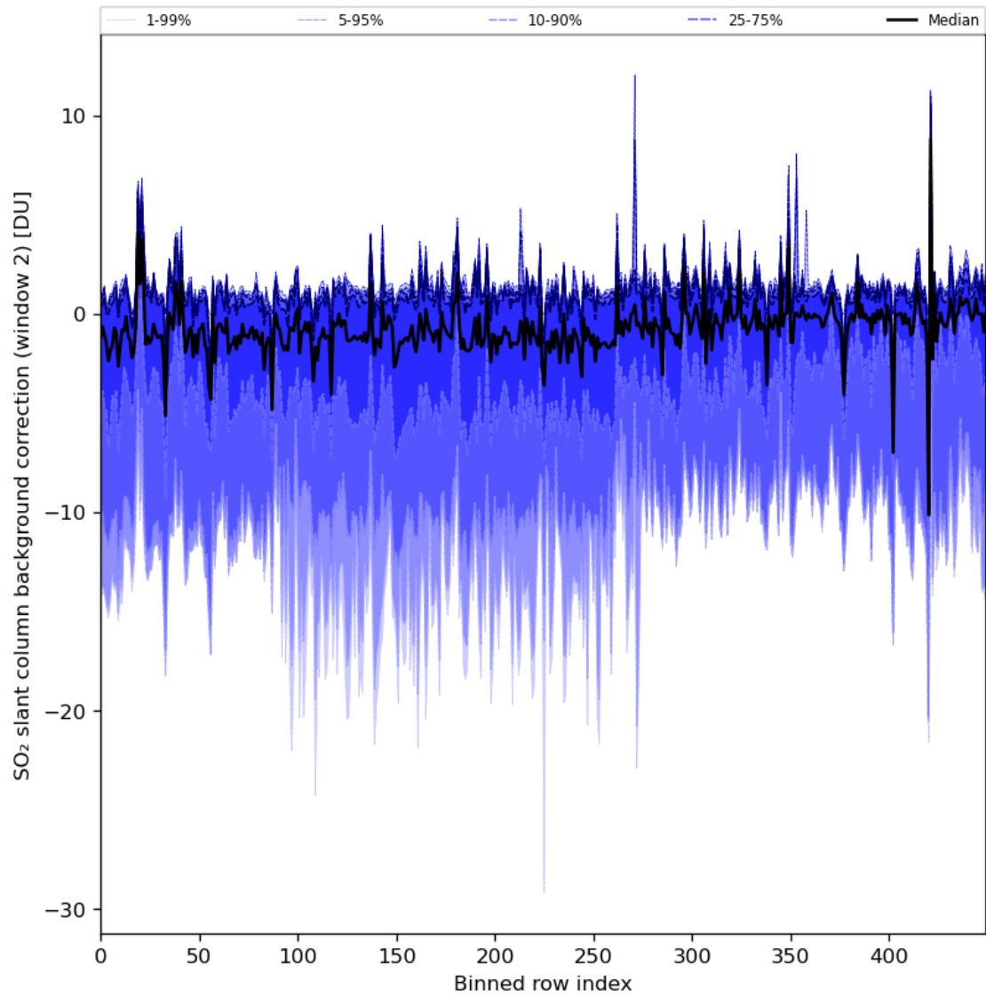
Figure 86: Along track statistics of “SO 2 slant column background correction (window 2)” for 2024-02-24 to 2024-02-26
