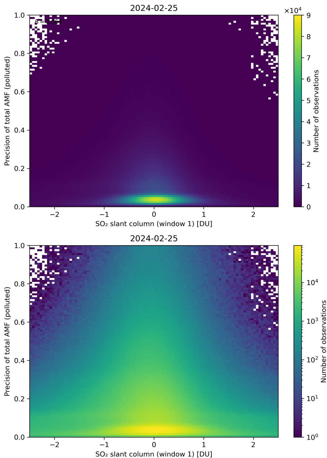
Figure 240: Scatter density plot of “SO 2 slant column (window 1)” against “Precision of total AMF (polluted)” for 2024-02-24 to 2024-02-26.
