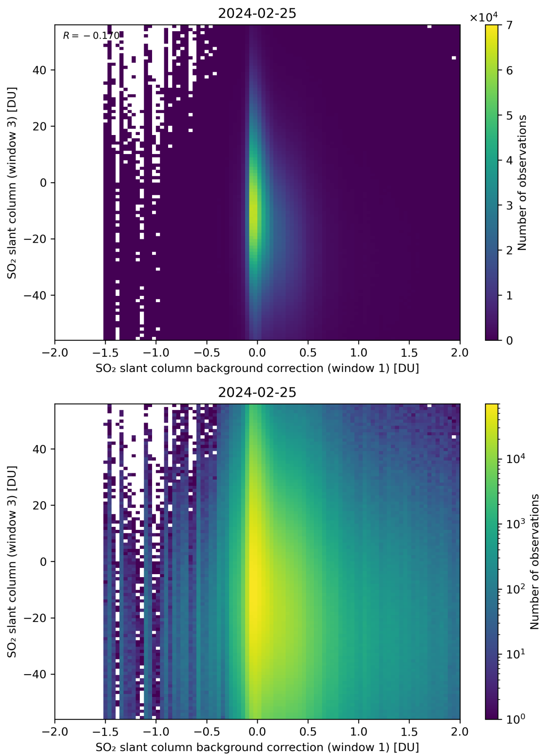
Figure 107: Scatter density plot of “SO 2 slant column background correction (window 1)” against “SO 2 slant column (window 3)” for 2024-02-24 to 2024-02-26.
