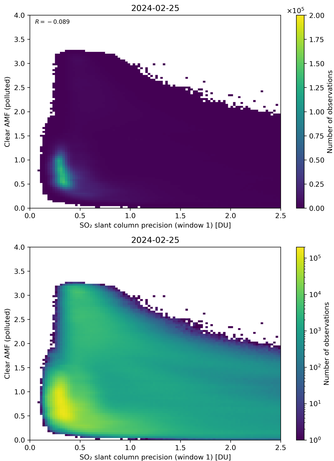
Figure 224: Scatter density plot of “SO 2 slant column precision (window 1)” against “Clear AMF (polluted)” for 2024-02-24 to 2024-02-26.
