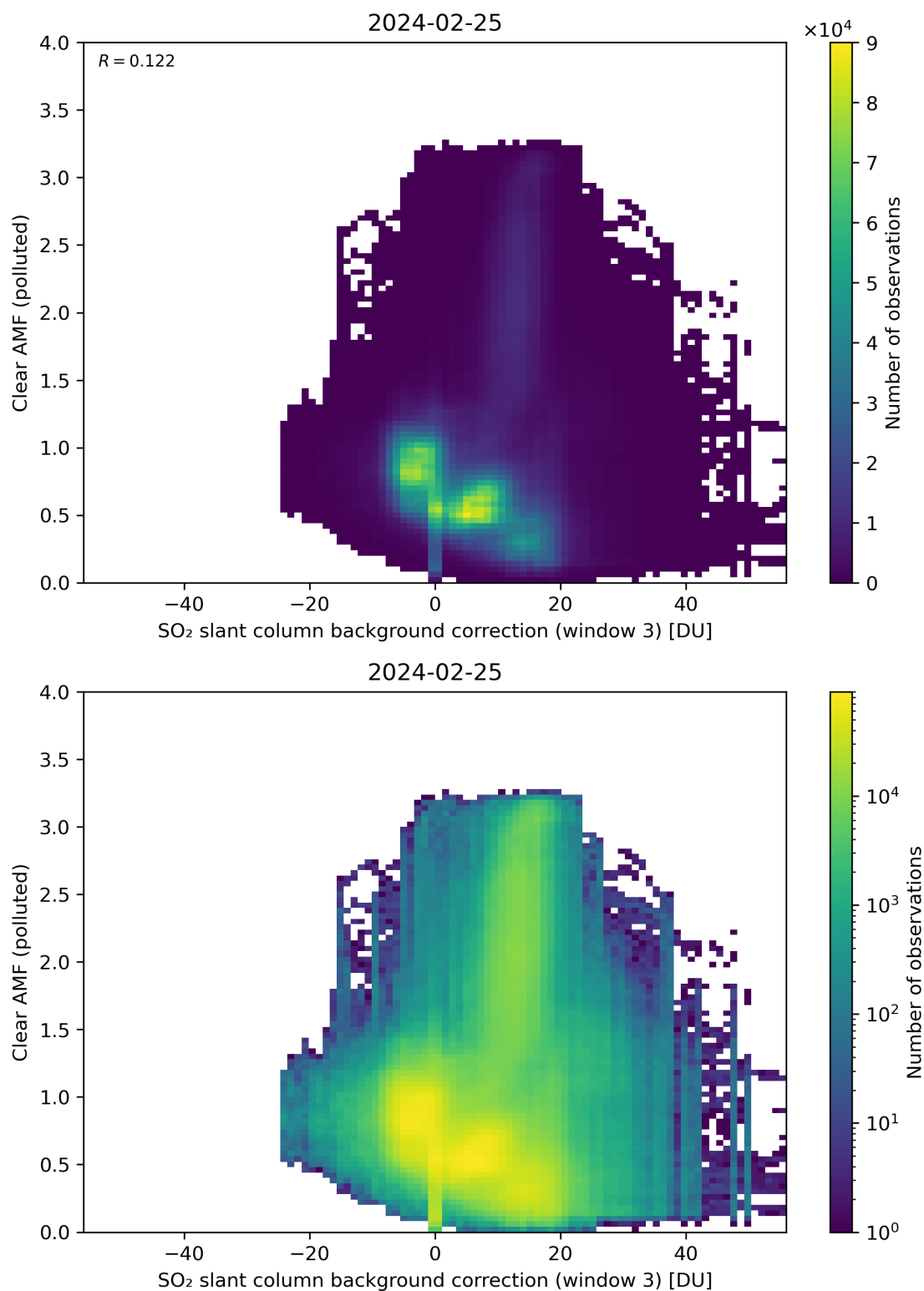
Figure 124: Scatter density plot of “SO 2 slant column background correction (window 3)” against “Clear AMF (polluted)” for 2024-02-24 to 2024-02-26.
