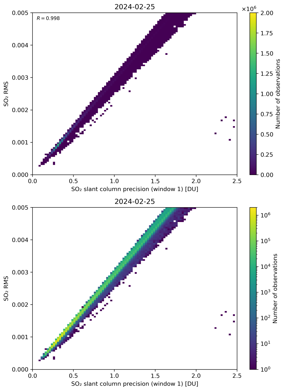
Figure 223: Scatter density plot of “SO 2 slant column precision (window 1)” against “SO 2 RMS” for 2024-02-24 to 2024-02-26.
