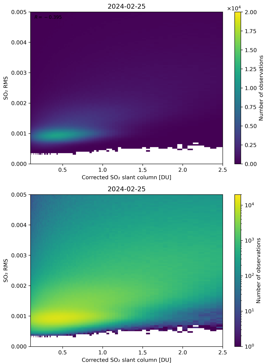
Figure 183: Scatter density plot of “Corrected SO 2 slant column” against “SO 2 RMS” for 2024-02-24 to 2024-02-26.
