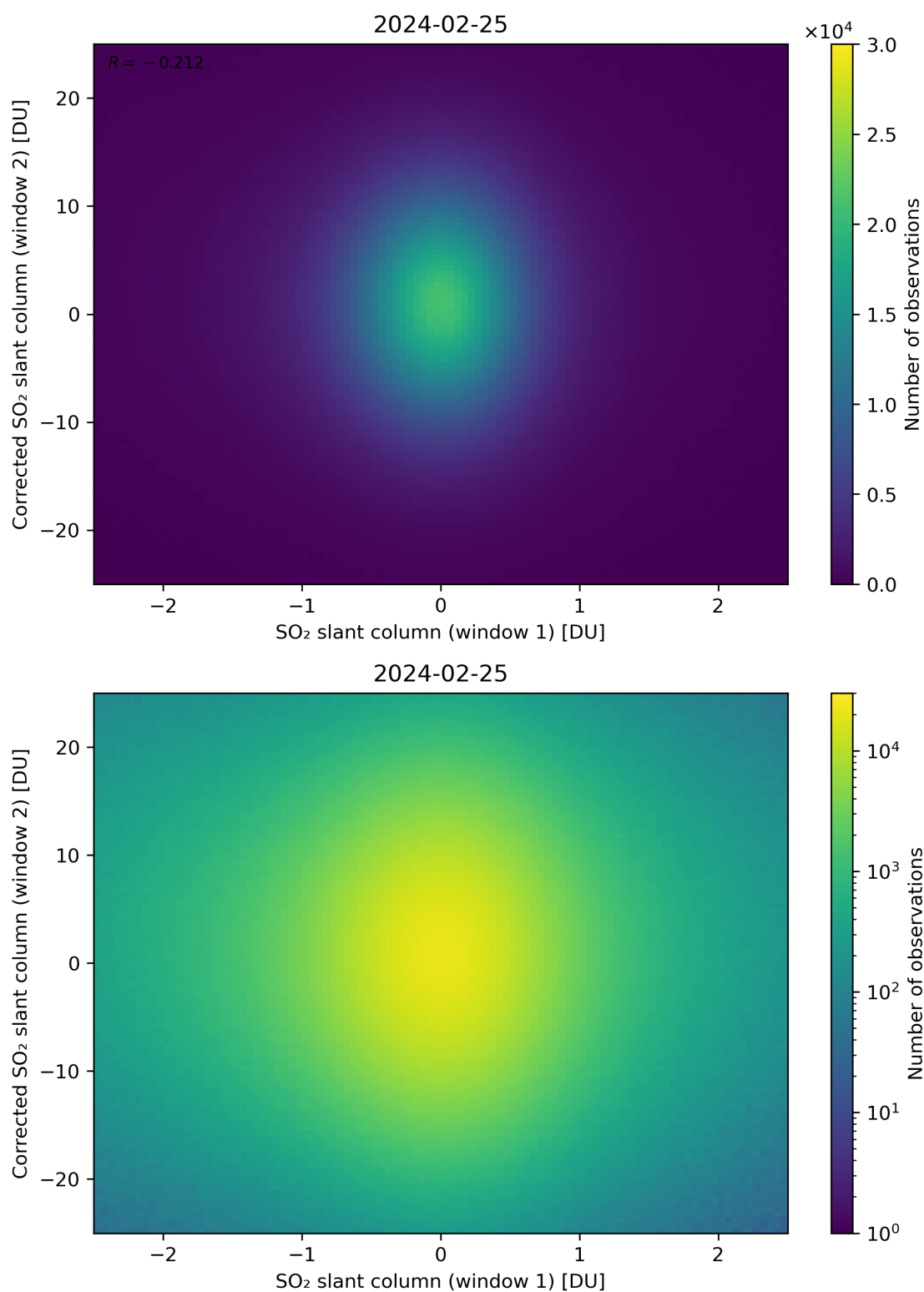
Figure 233: Scatter density plot of “SO 2 slant column (window 1)” against “Corrected SO 2 slant column (window 2)” for 2024-02-24 to 2024-02-26.
