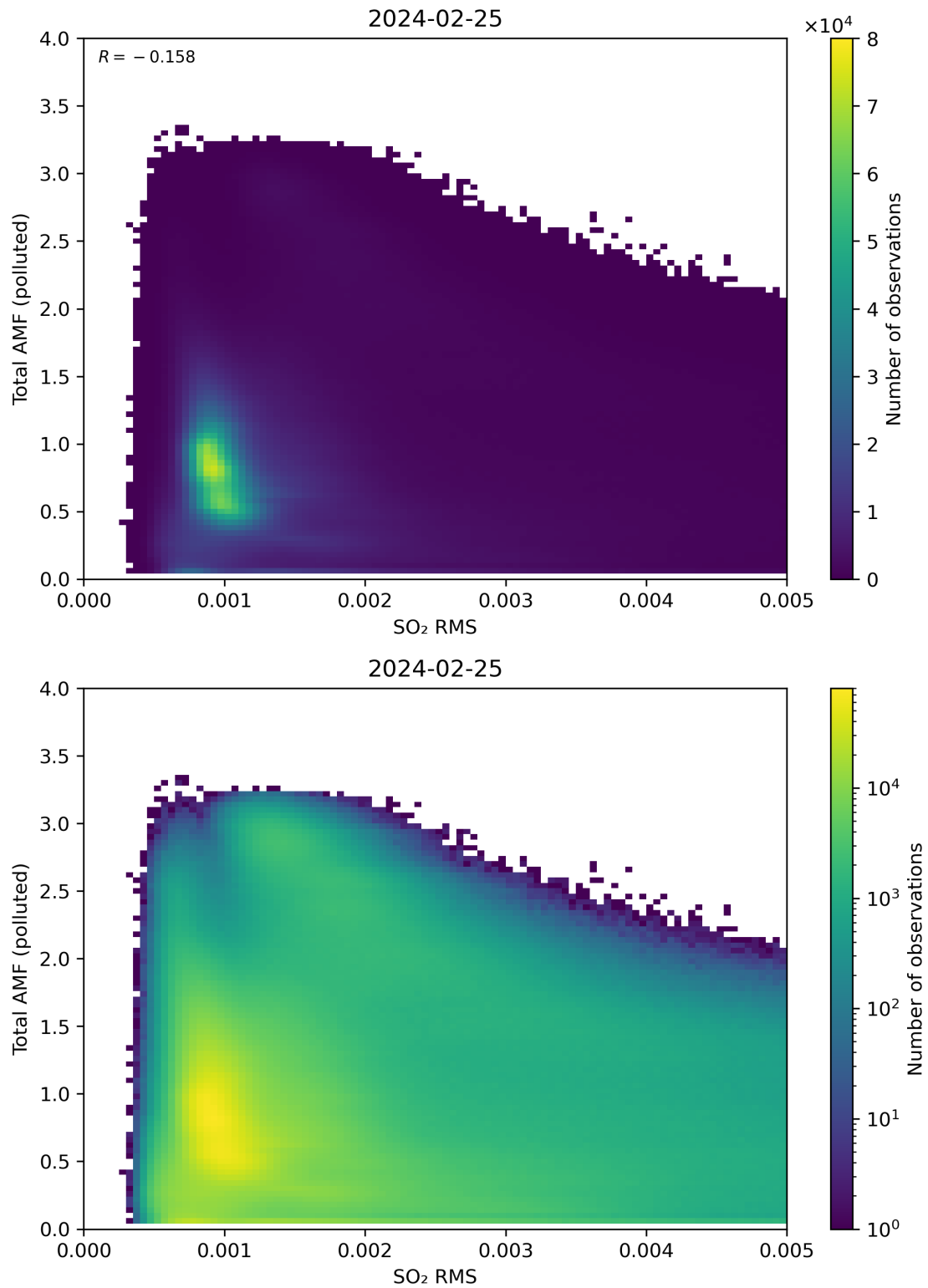
Figure 137: Scatter density plot of “SO 2 RMS” against “Total AMF (polluted)” for 2024-02-24 to 2024-02-26.
