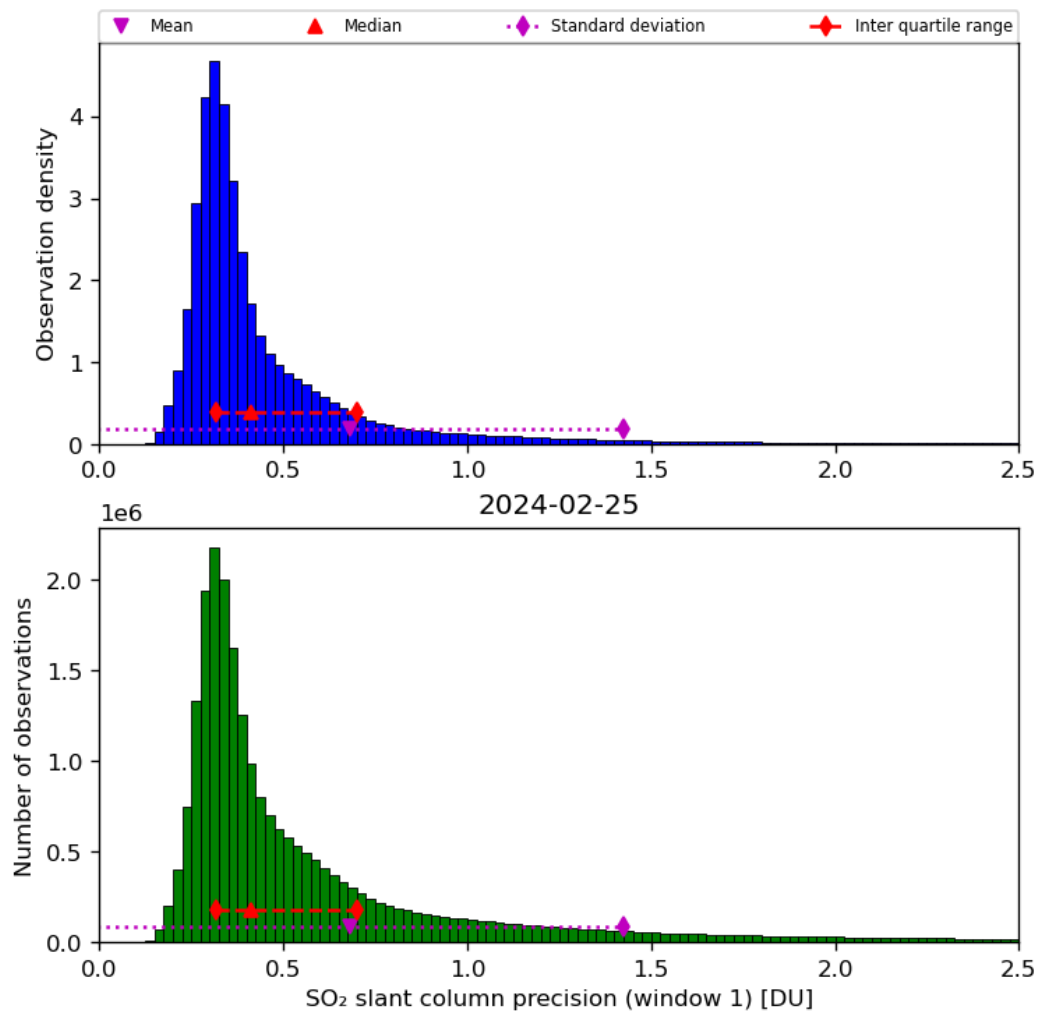
Figure 57: Histogram of “SO 2 slant column precision (window 1)” for 2024-02-24 to 2024-02-26
