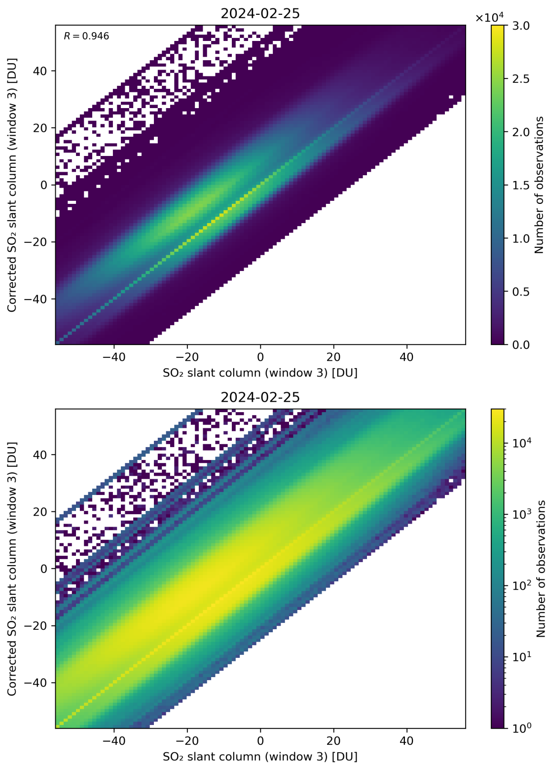
Figure 266: Scatter density plot of “SO 2 slant column (window 3)” against “Corrected SO 2 slant column (window 3)” for 2024-02-24 to 2024-02-26.
