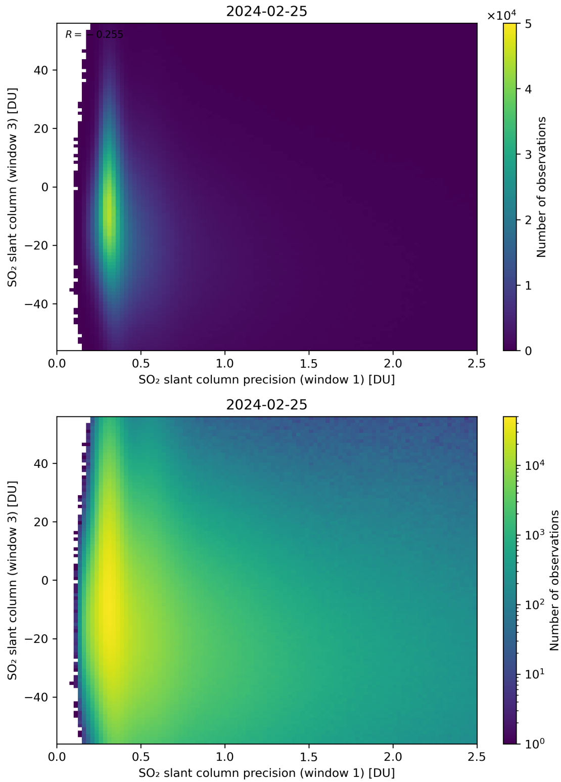
Figure 228: Scatter density plot of “SO 2 slant column precision (window 1)” against “SO 2 slant column (window 3)” for 2024-02-24 to 2024-02-26.
