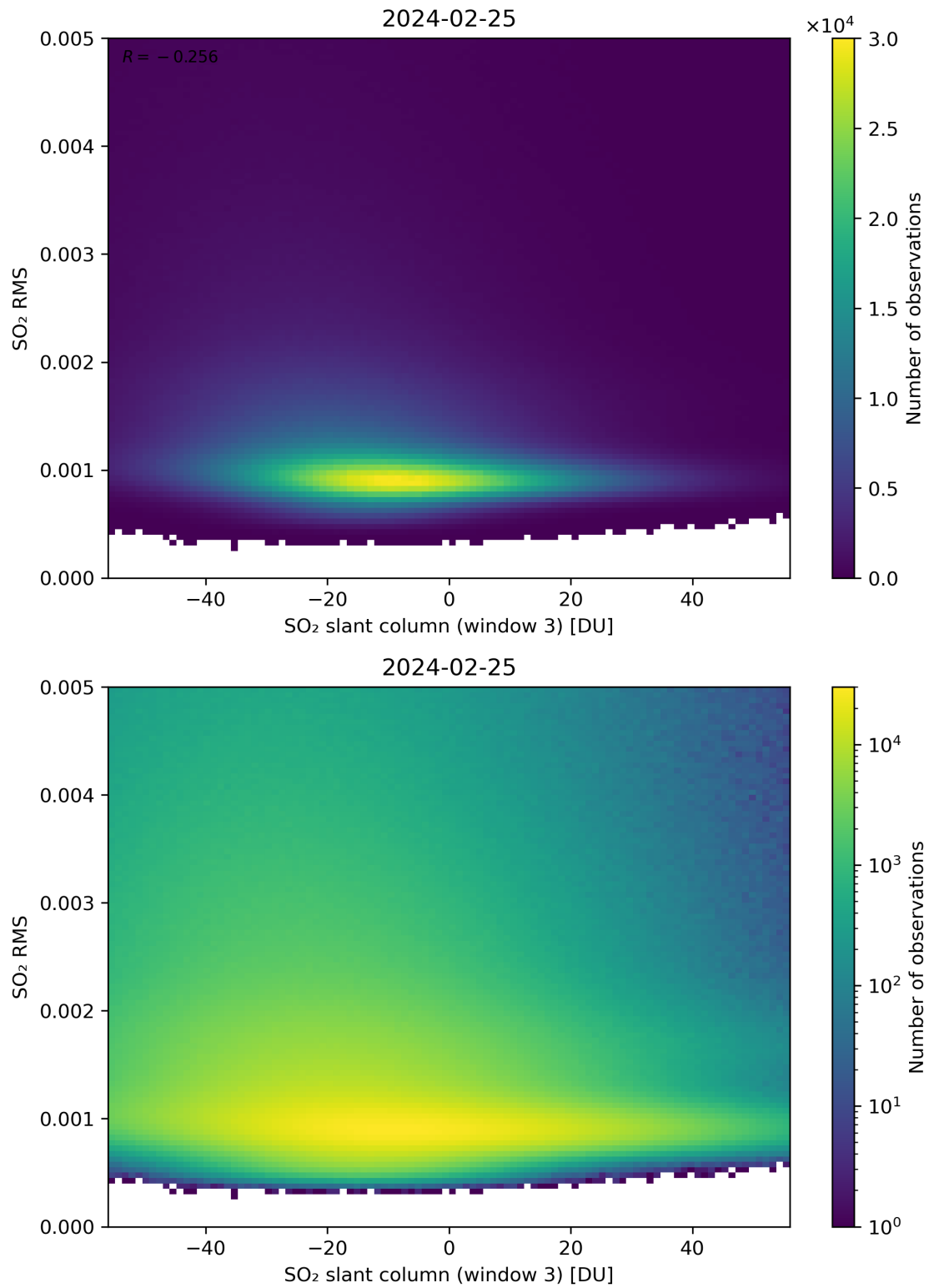
Figure 256: Scatter density plot of “SO 2 slant column (window 3)” against “SO 2 RMS” for 2024-02-24 to 2024-02-26.
