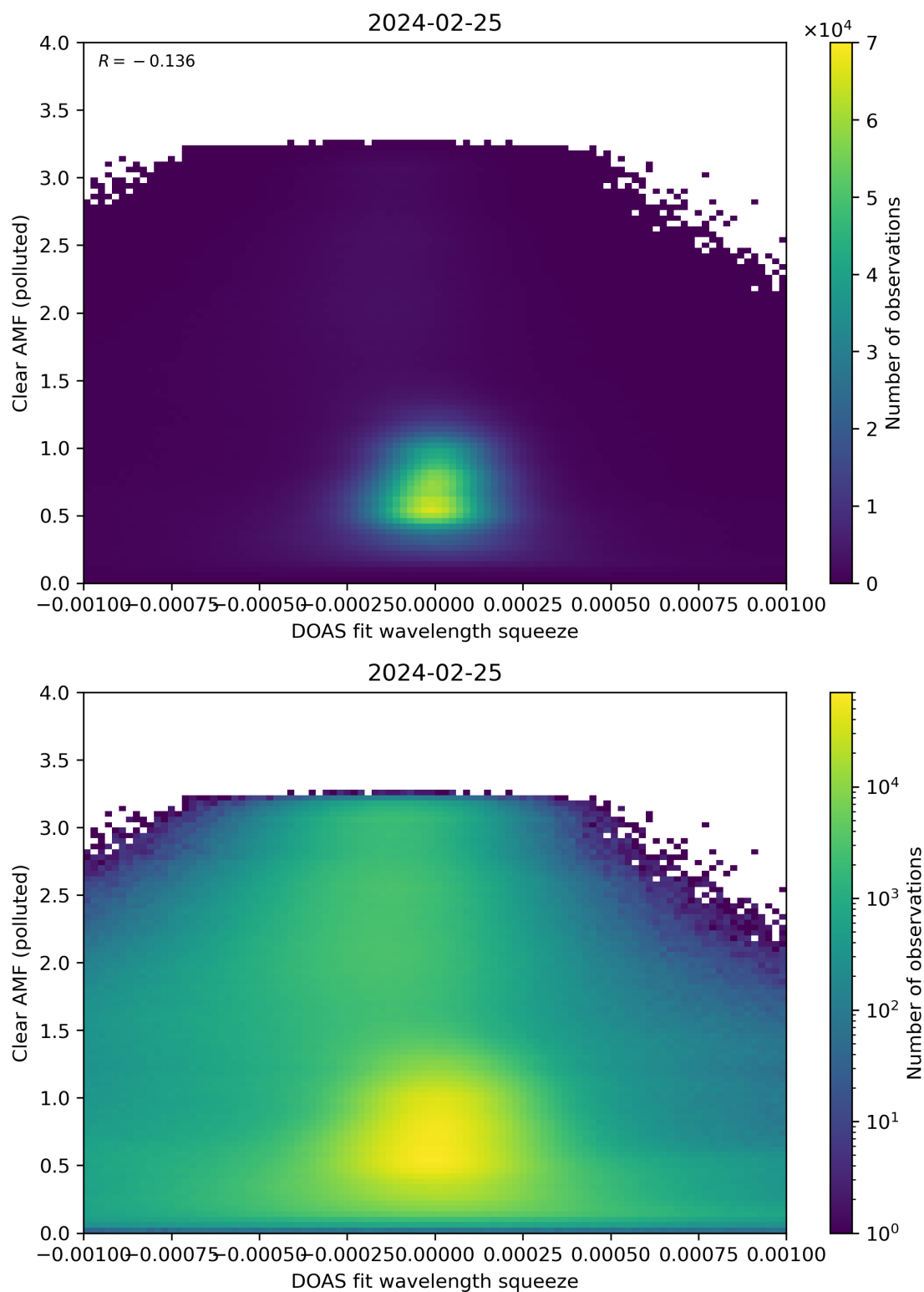
Figure 133: Scatter density plot of “DOAS fit wavelength squeeze” against “Clear AMF (polluted)” for 2024-02-24 to 2024-02-26.
