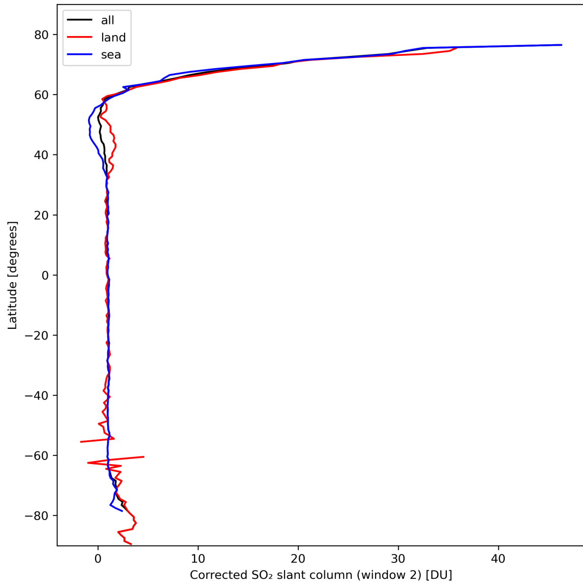
Figure 39: Zonal average of “Corrected SO 2 slant column (window 2)” for 2024-02-24 to 2024-02-26.
