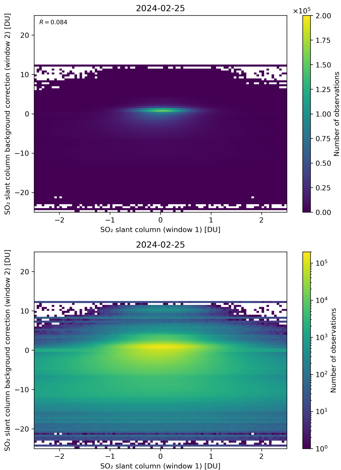
Figure 213: Scatter density plot of “SO 2 slant column (window 1)” against “SO 2 slant column background correction (window 2)” for 2024-02-24 to 2024-02-26.
