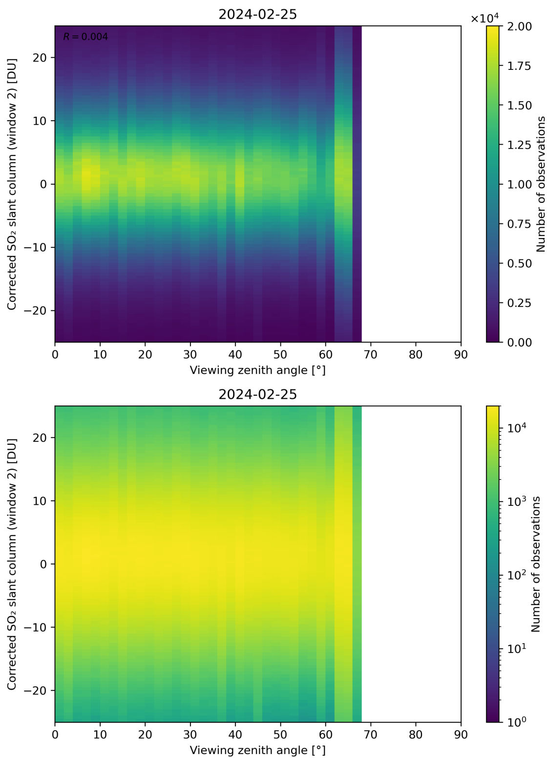
Figure 318: Scatter density plot of “Viewing zenith angle” against “Corrected SO 2 slant column (window 2)” for 2024-02-24 to 2024-02-26.
