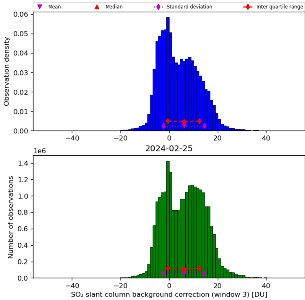
Figure 67: Histogram of “SO 2 slant column background correction (window 3)” for 2024-02-24 to 2024-02-26
