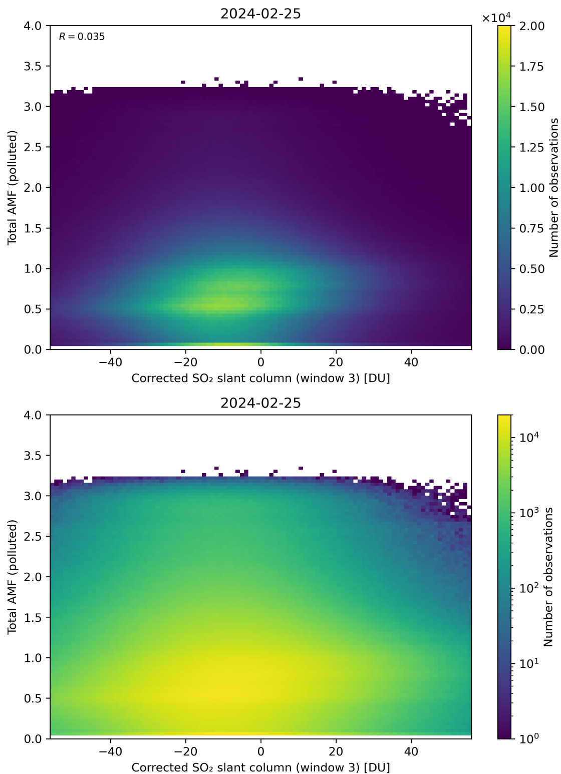
Figure 210: Scatter density plot of “Corrected SO 2 slant column (window 3)” against “Total AMF (polluted)” for 2024-02-24 to 2024-02-26.
