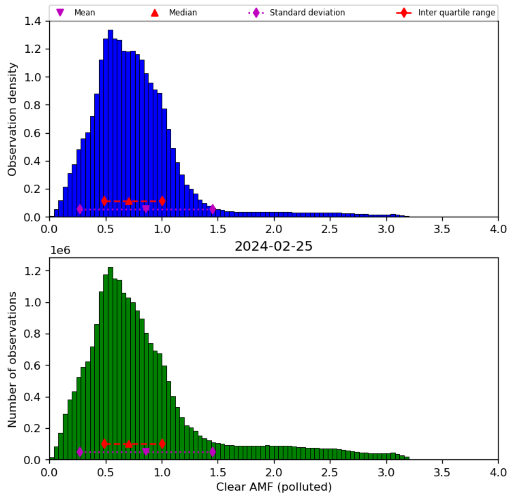
Figure 73: Histogram of “Clear AMF (polluted)” for 2024-02-24 to 2024-02-26
