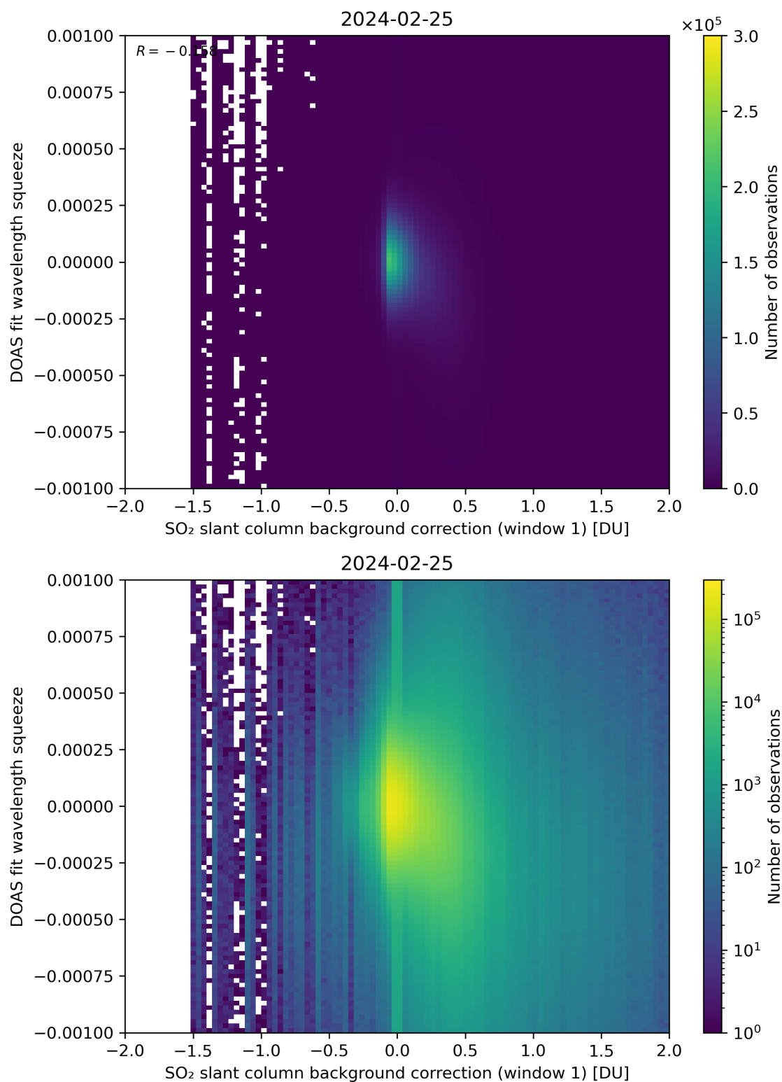
Figure 101: Scatter density plot of “SO 2 slant column background correction (window 1)” against “DOAS fit wavelength squeeze” for 2024-02-24 to 2024-02-26.
