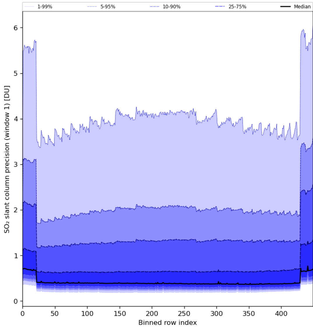
Figure 80: Along track statistics of “SO 2 slant column precision (window 1)” for 2024-02-24 to 2024-02-26
