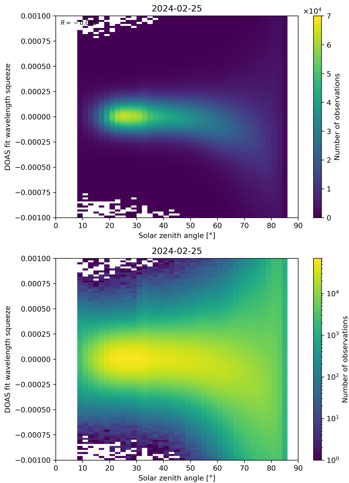
Figure 162: Scatter density plot of “Solar zenith angle” against “DOAS fit wavelength squeeze” for 2024-02-24 to 2024-02-26.
