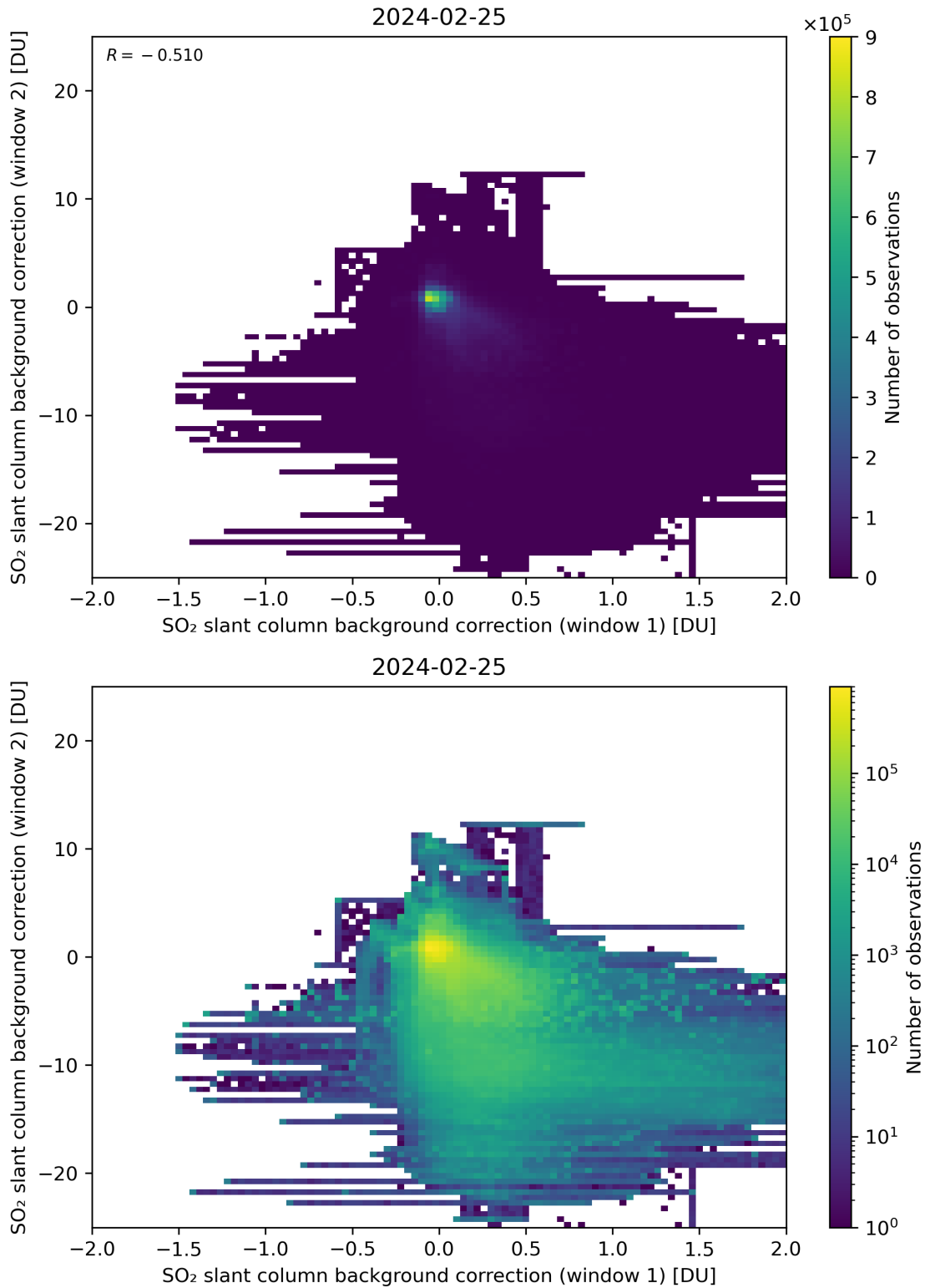
Figure 98: Scatter density plot of “SO 2 slant column background correction (window 1)” against “SO 2 slant column background correction (window 2)” for 2024-02-24 to 2024-02-26.
