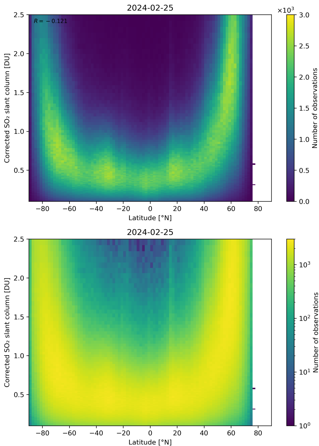
Figure 146: Scatter density plot of “Latitude” against “Corrected SO 2 slant column” for 2024-02-24 to 2024-02-26.
