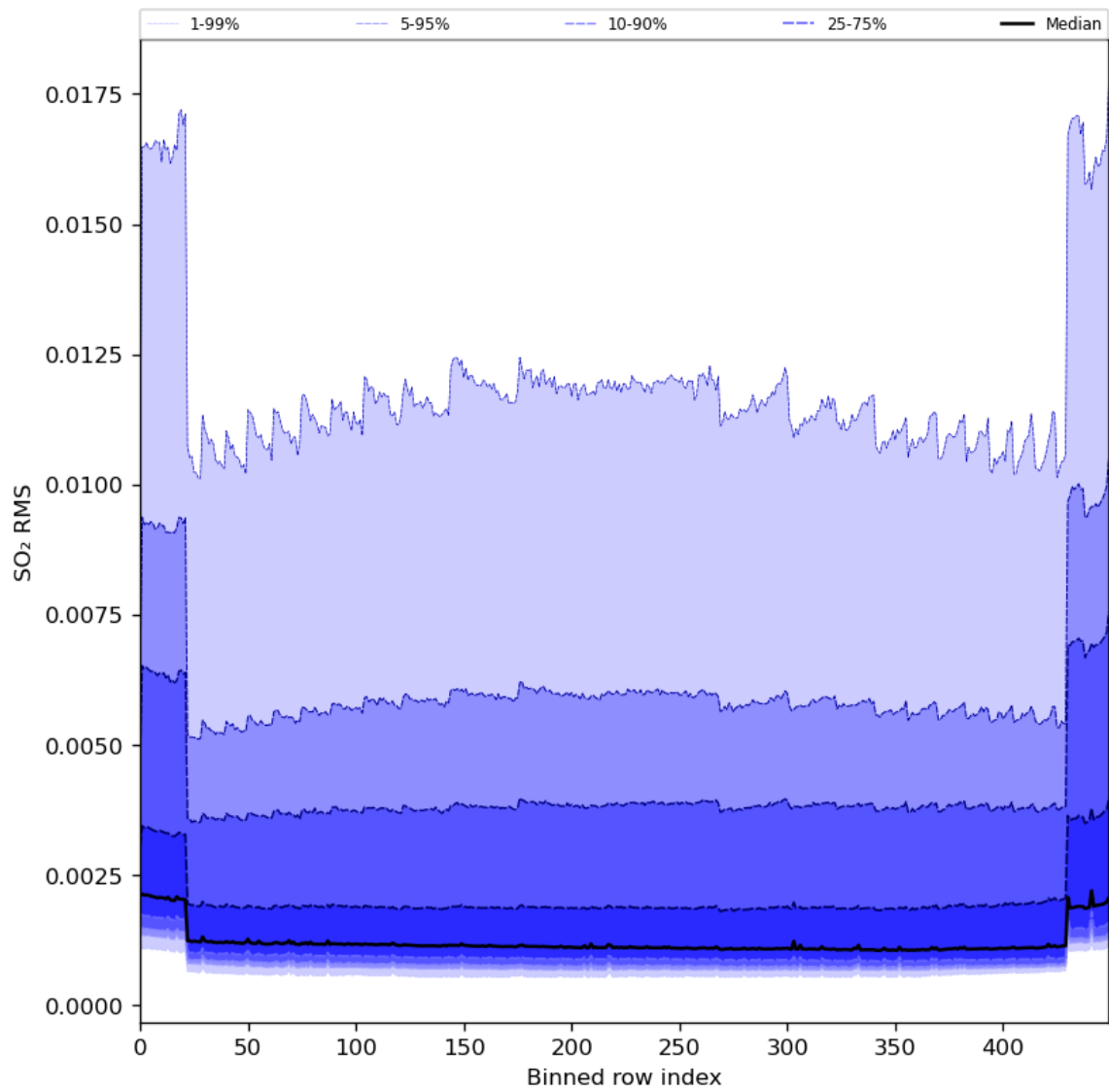
Figure 93: Along track statistics of “SO 2 RMS” for 2024-02-24 to 2024-02-26
