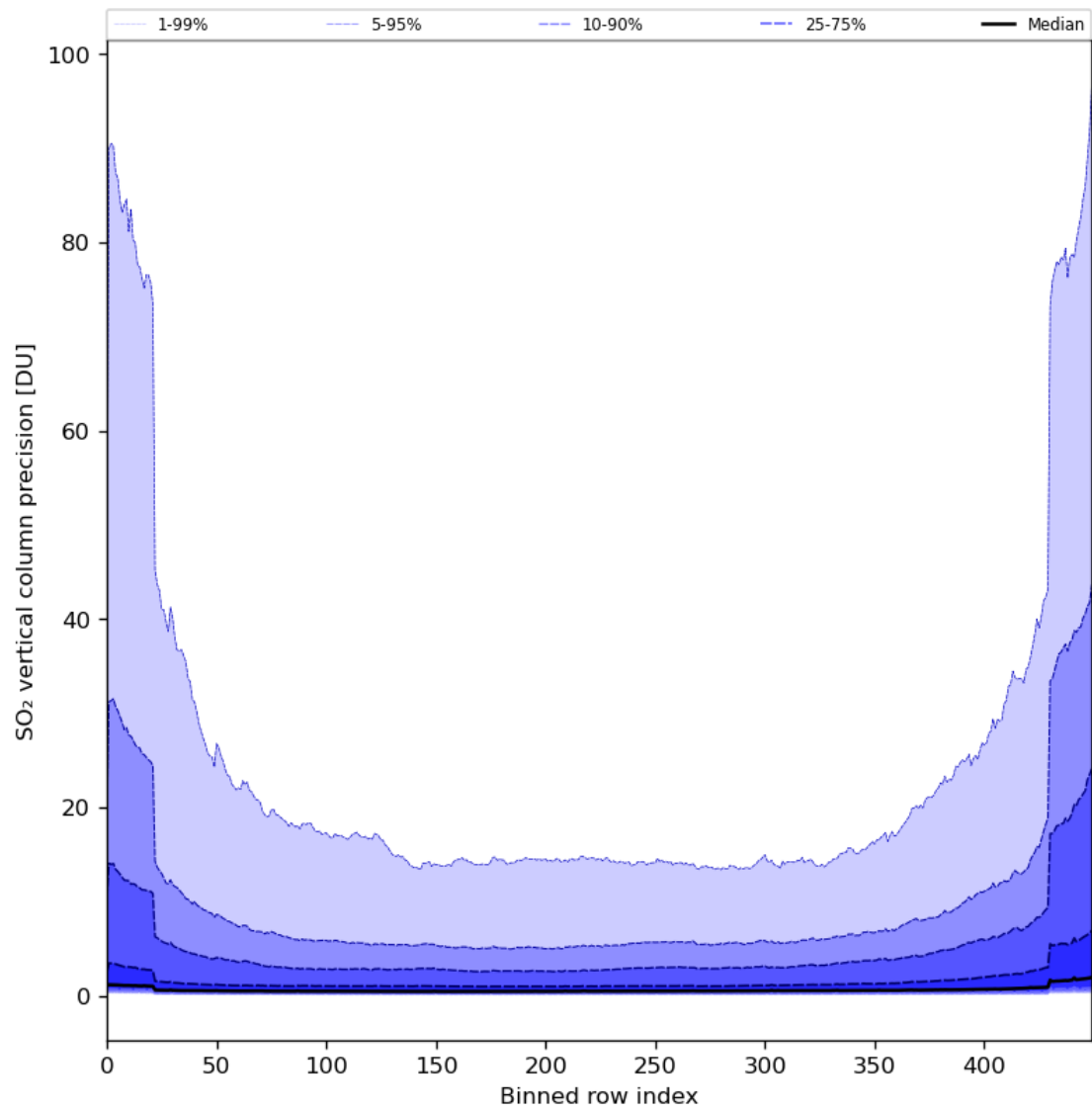
Figure 77: Along track statistics of “SO 2 vertical column precision” for 2024-02-24 to 2024-02-26
