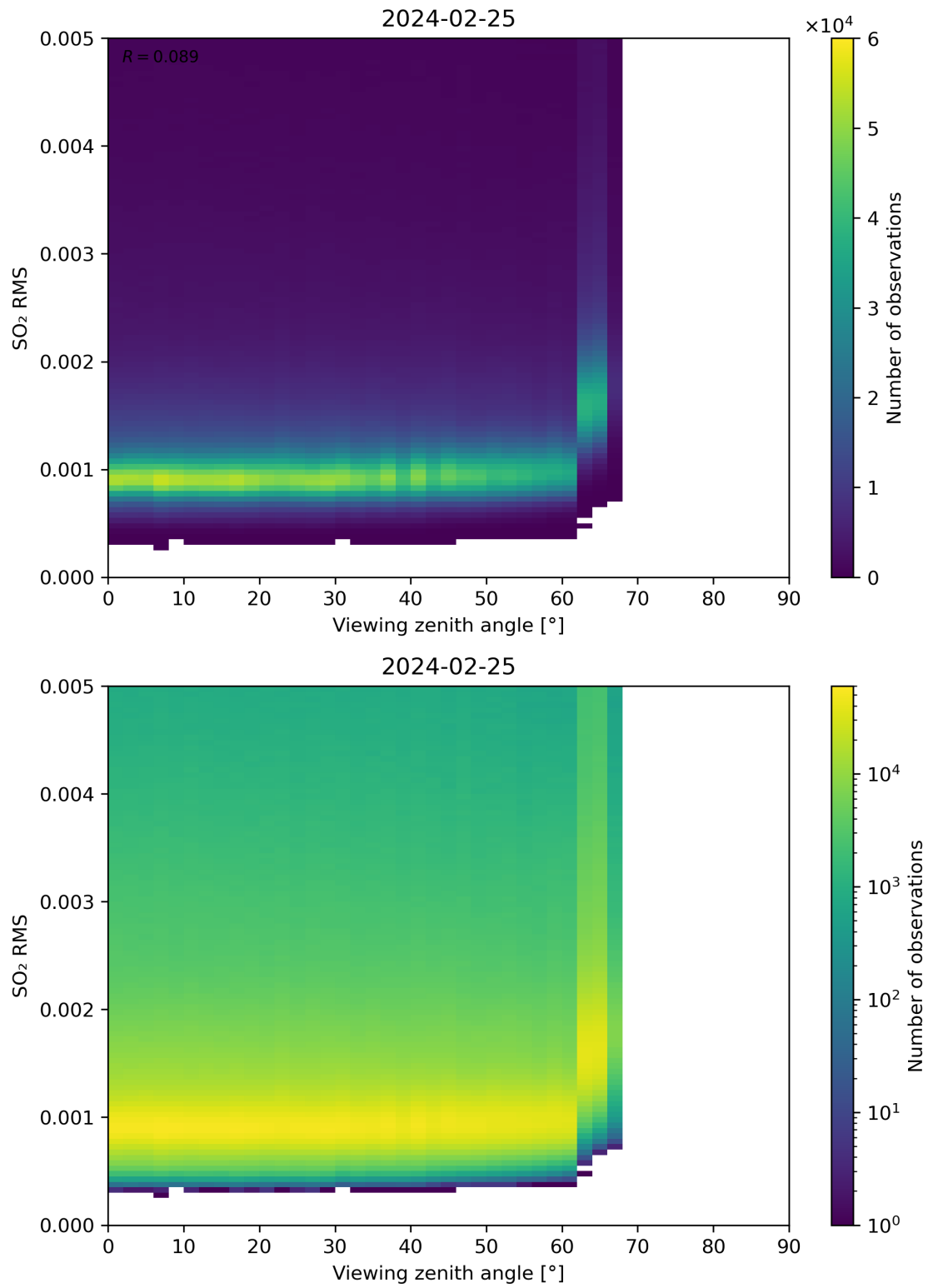
Figure 313: Scatter density plot of “Viewing zenith angle” against “SO 2 RMS” for 2024-02-24 to 2024-02-26.
