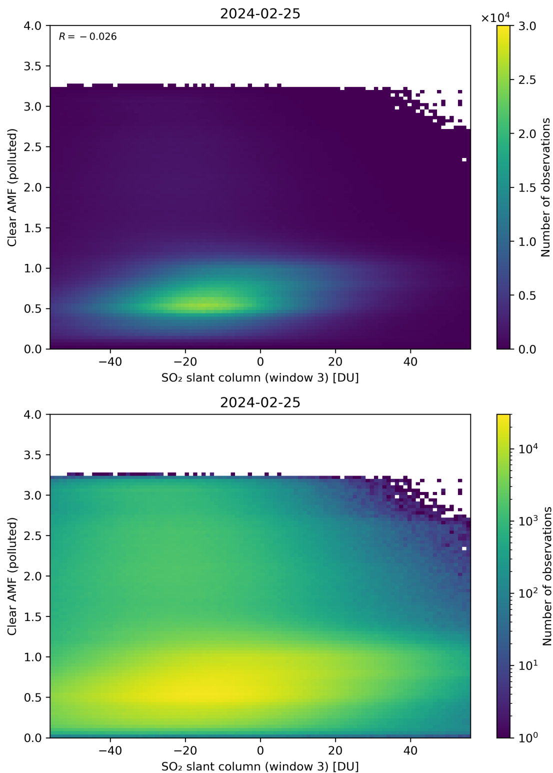
Figure 265: Scatter density plot of “SO 2 slant column (window 3)” against “Clear AMF (polluted)” for 2024-02-24 to 2024-02-26.
