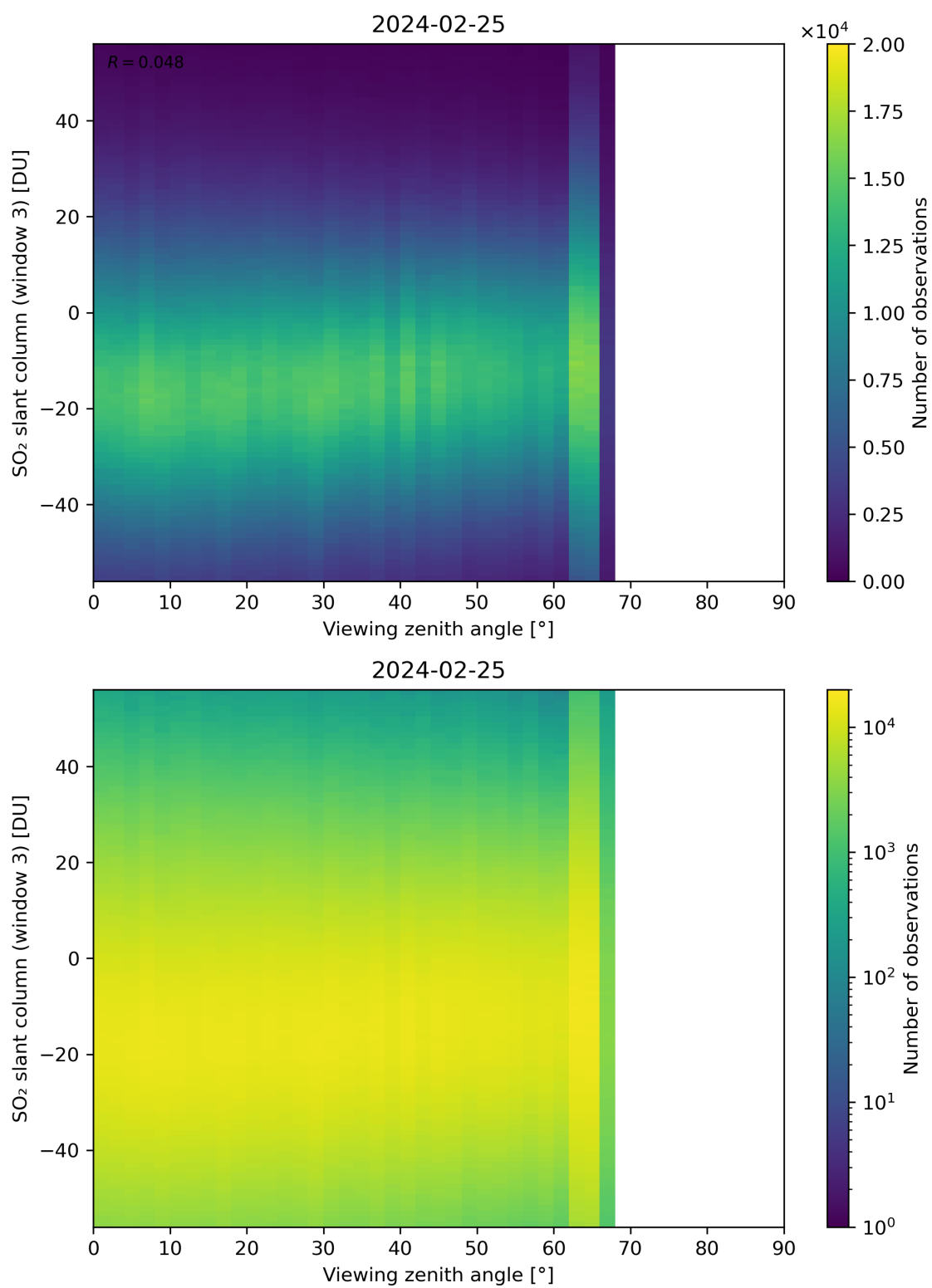
Figure 323: Scatter density plot of “Viewing zenith angle” against “SO 2 slant column (window 3)” for 2024-02-24 to 2024-02-26.
