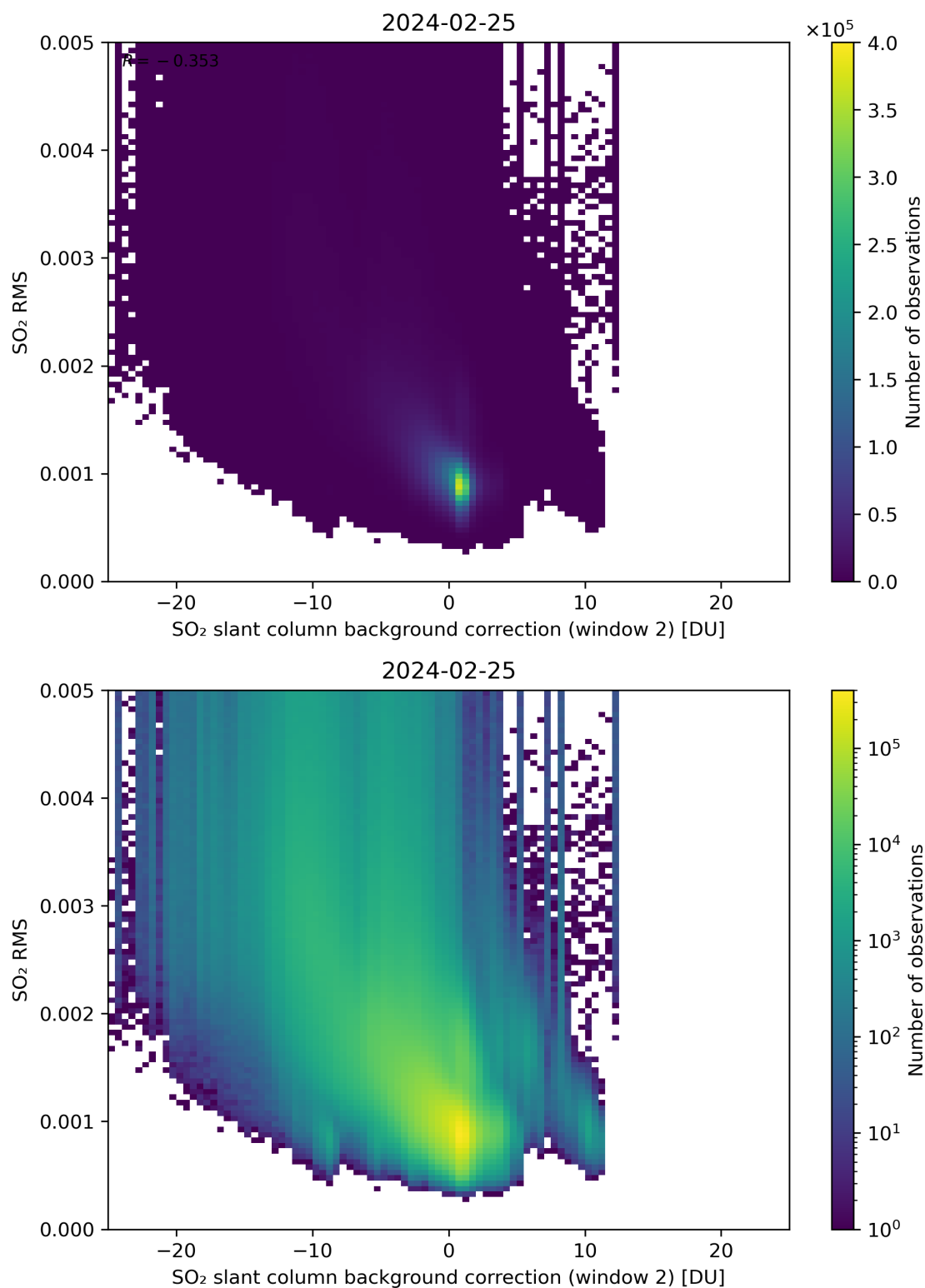
Figure 114: Scatter density plot of “SO 2 slant column background correction (window 2)” against “SO 2 RMS” for 2024-02-24 to 2024-02-26.
