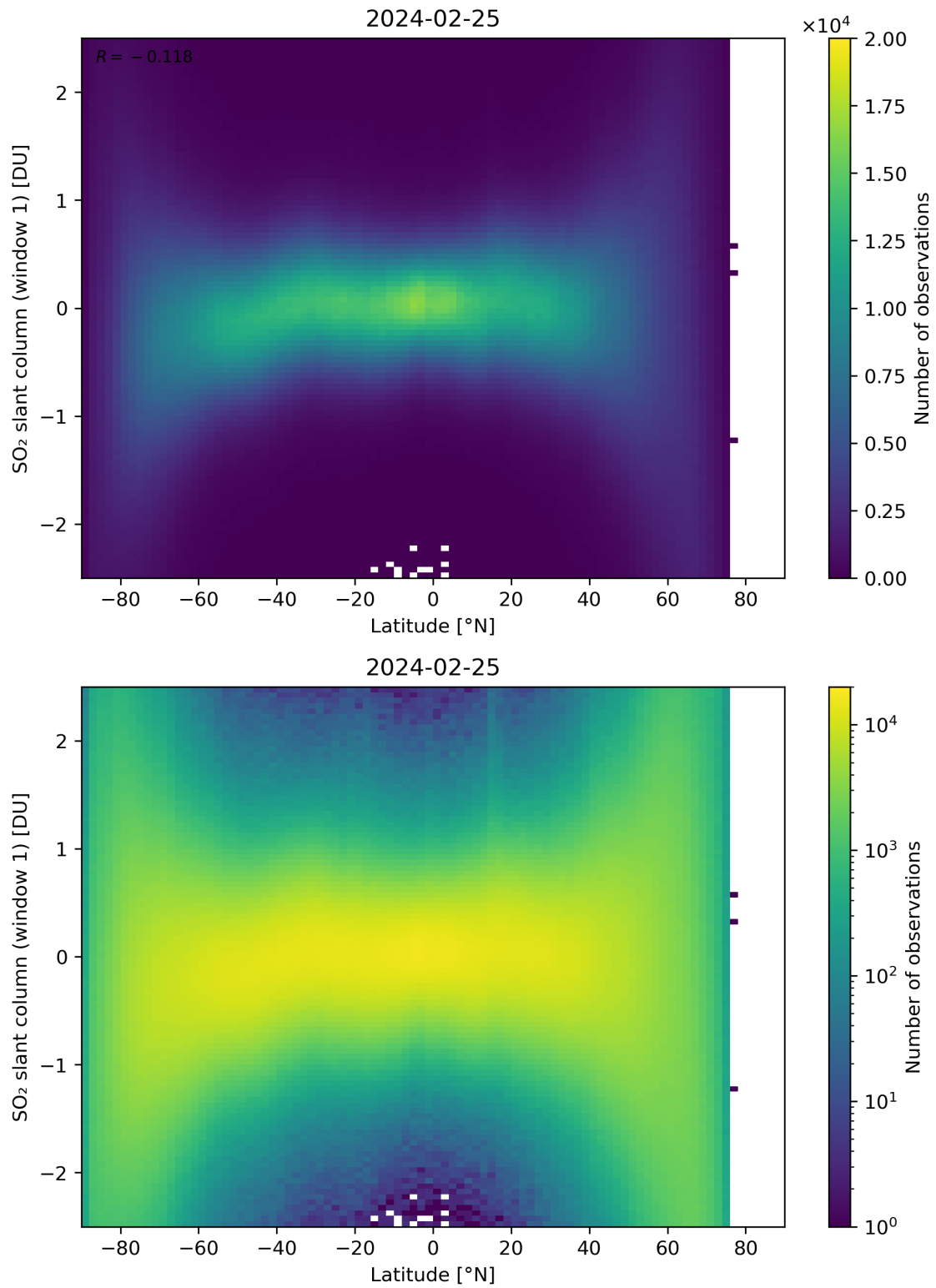
Figure 149: Scatter density plot of “Latitude” against “SO 2 slant column (window 1)” for 2024-02-24 to 2024-02-26.
