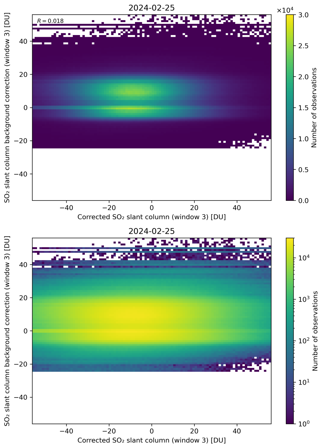
Figure 205: Scatter density plot of “Corrected SO 2 slant column (window 3)” against “SO 2 slant column background correction (window 3)” for 2024-02-24 to 2024-02-26.
