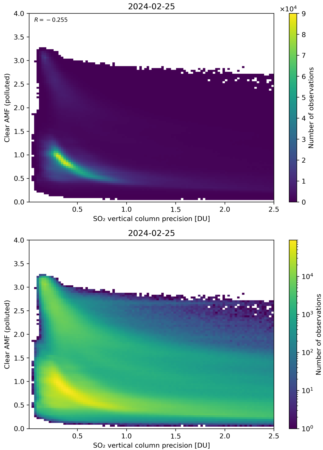
Figure 285: Scatter density plot of “SO 2 vertical column precision” against “Clear AMF (polluted)” for 2024-02-24 to 2024-02-26.
