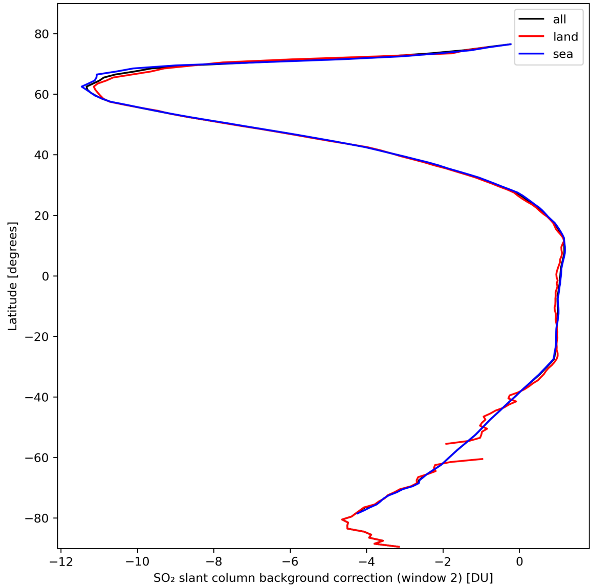
Figure 40: Zonal average of “SO 2 slant column background correction (window 2)” for 2024-02-24 to 2024-02-26.
