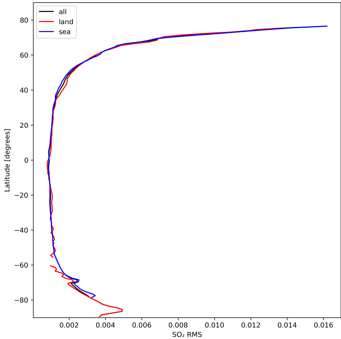
Figure 47: Zonal average of “SO 2 RMS” for 2024-02-24 to 2024-02-26.
