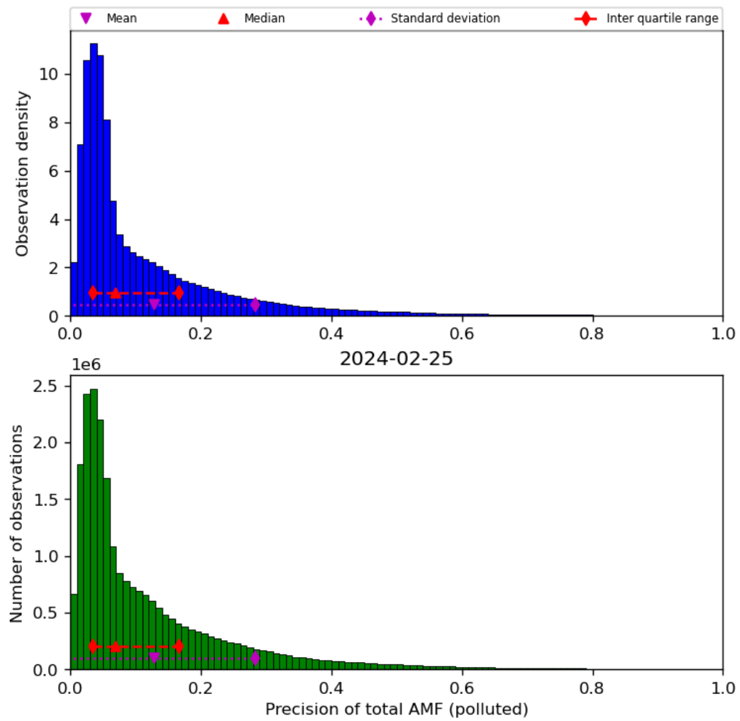
Figure 72: Histogram of “Precision of total AMF (polluted)” for 2024-02-24 to 2024-02-26
