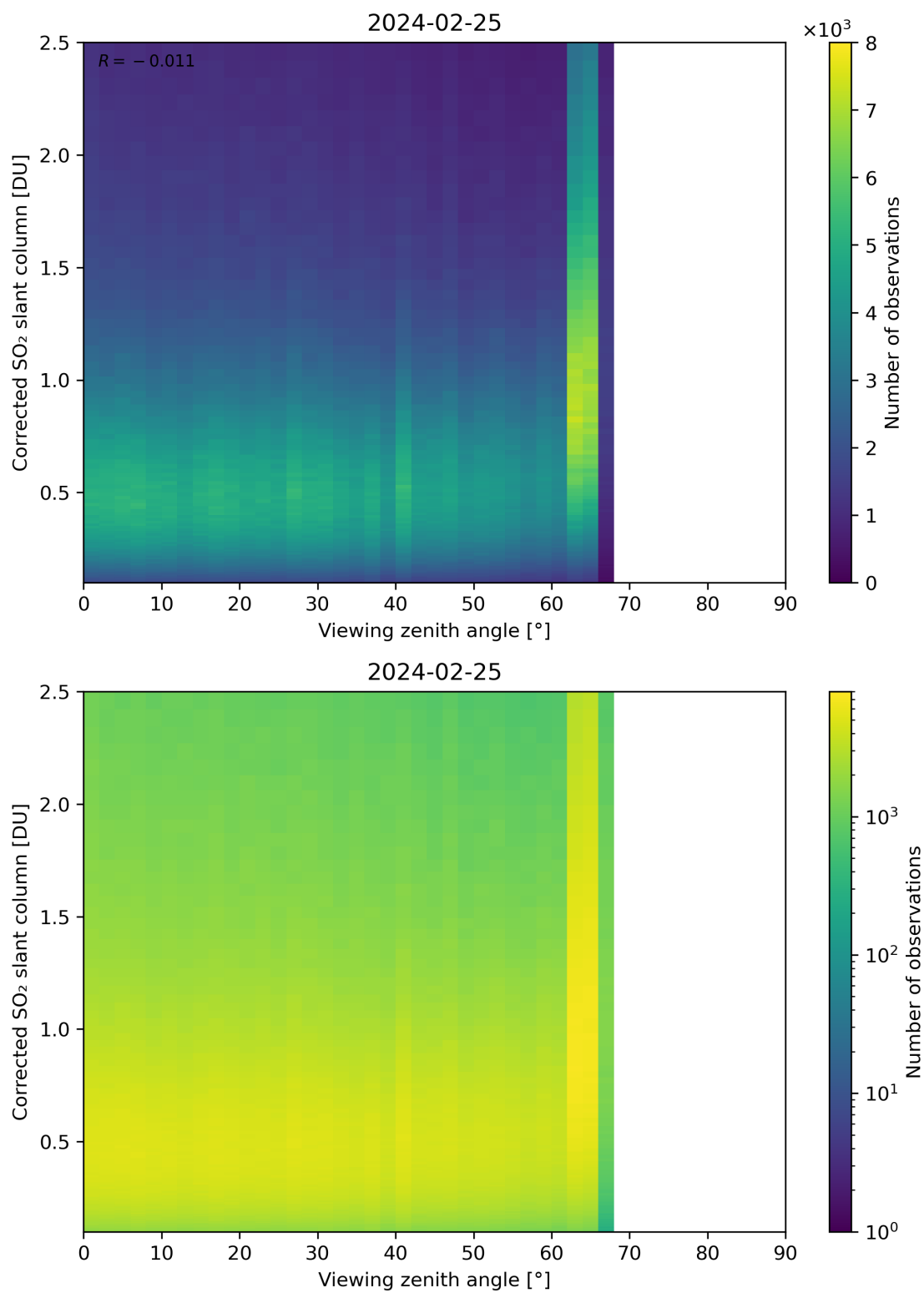
Figure 317: Scatter density plot of “Viewing zenith angle” against “Corrected SO 2 slant column” for 2024-02-24 to 2024-02-26.
