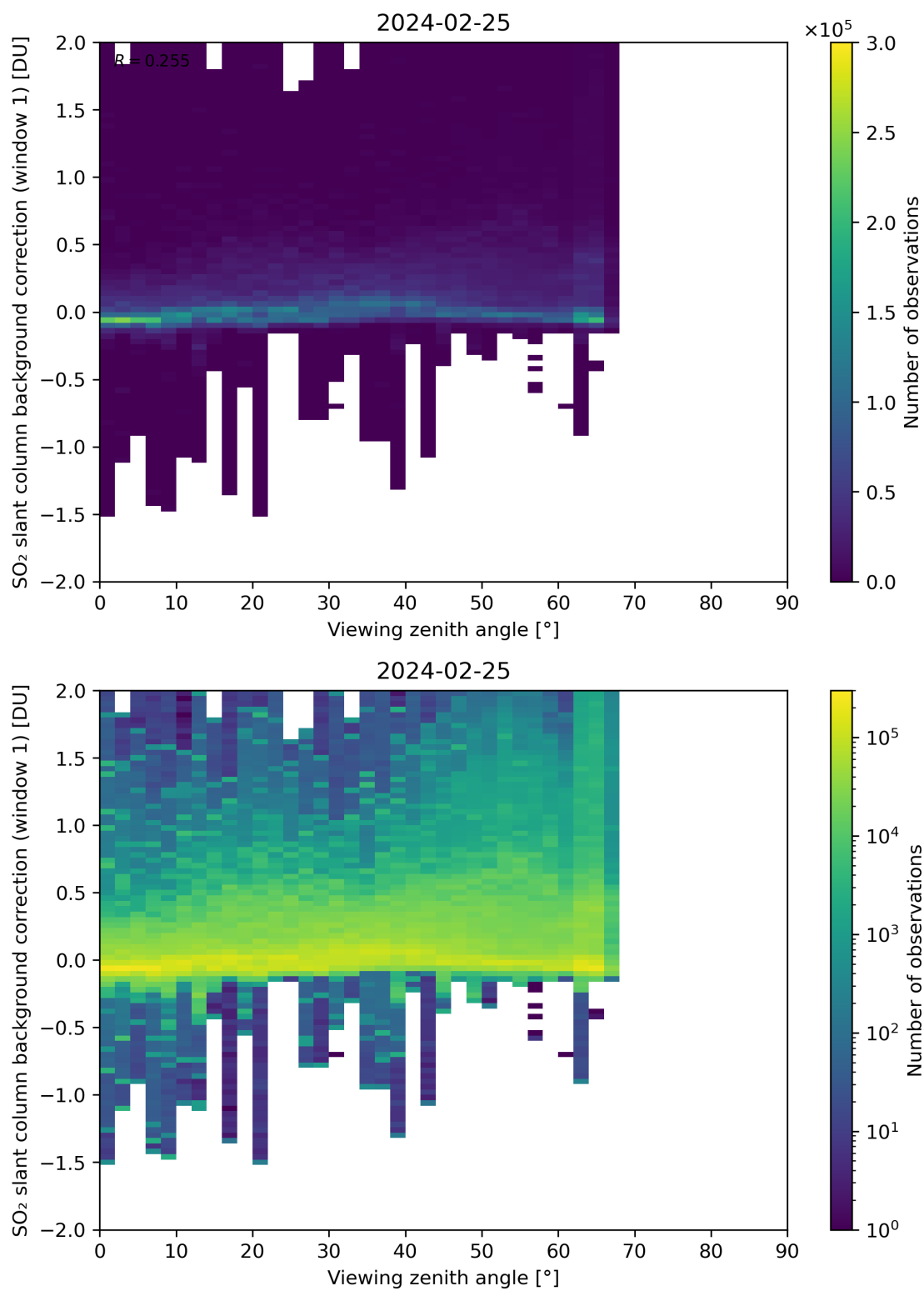
Figure 308: Scatter density plot of “Viewing zenith angle” against “SO 2 slant column background correction (window 1)” for 2024-02-24 to 2024-02-26.
