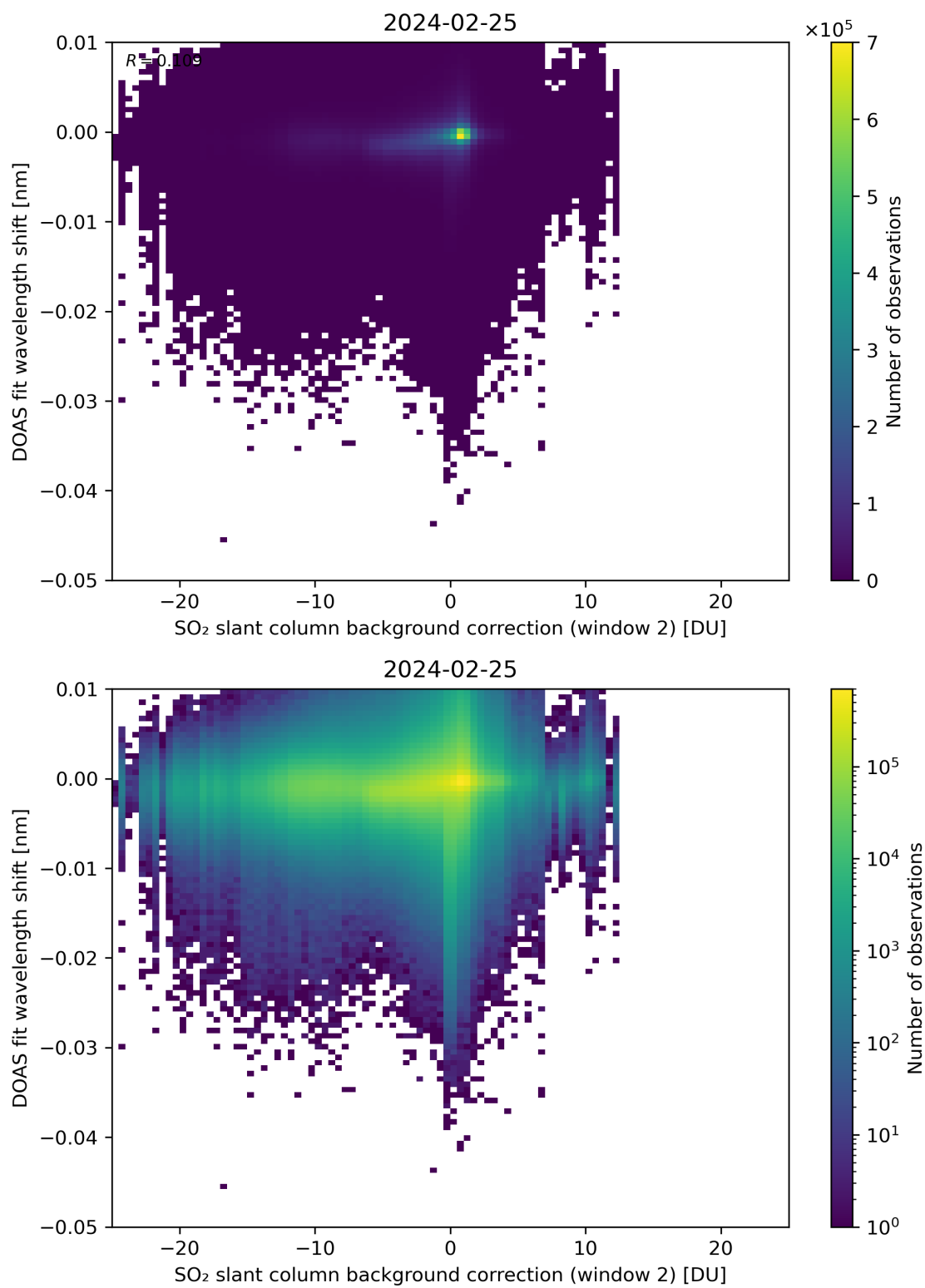
Figure 112: Scatter density plot of “SO 2 slant column background correction (window 2)” against “DOAS fit wavelength shift” for 2024-02-24 to 2024-02-26.
