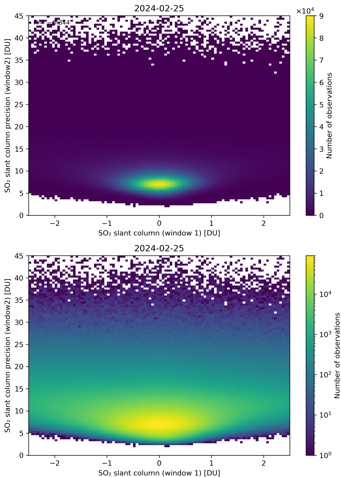
Figure 236: Scatter density plot of “SO 2 slant column (window 1)” against “SO 2 slant column precision (window2)” for 2024-02-24 to 2024-02-26.
