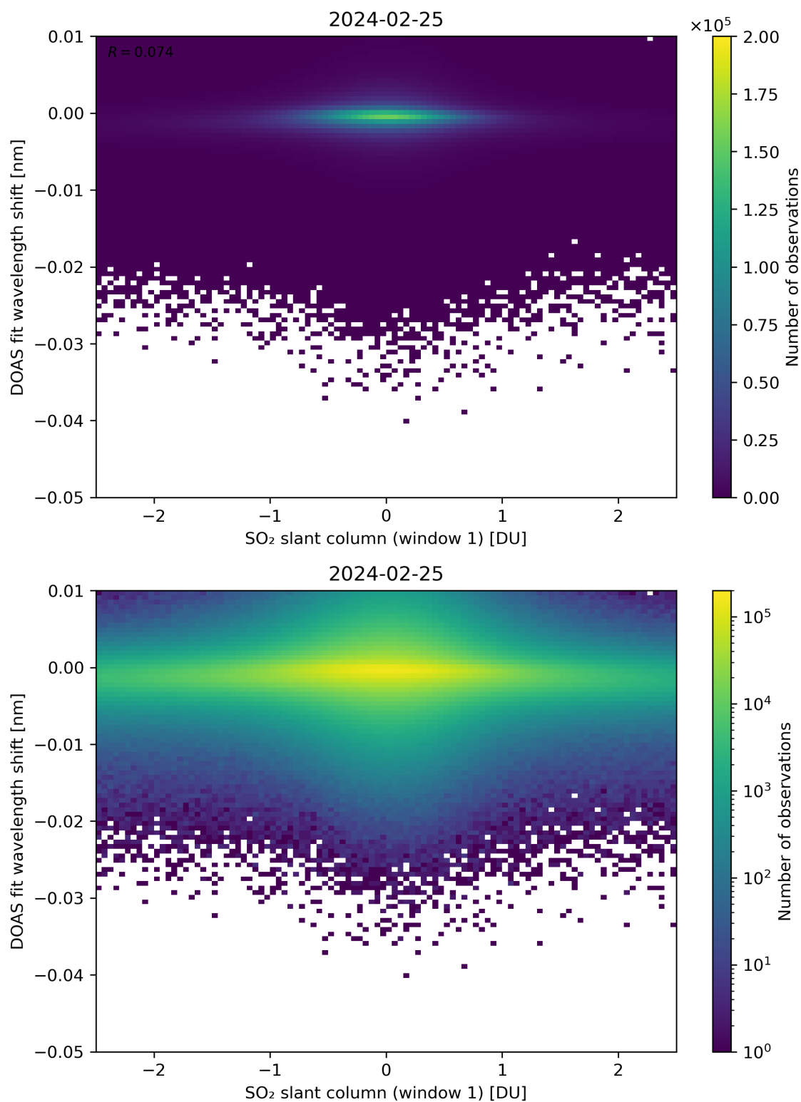
Figure 215: Scatter density plot of “SO 2 slant column (window 1)” against “DOAS fit wavelength shift” for 2024-02-24 to 2024-02-26.
