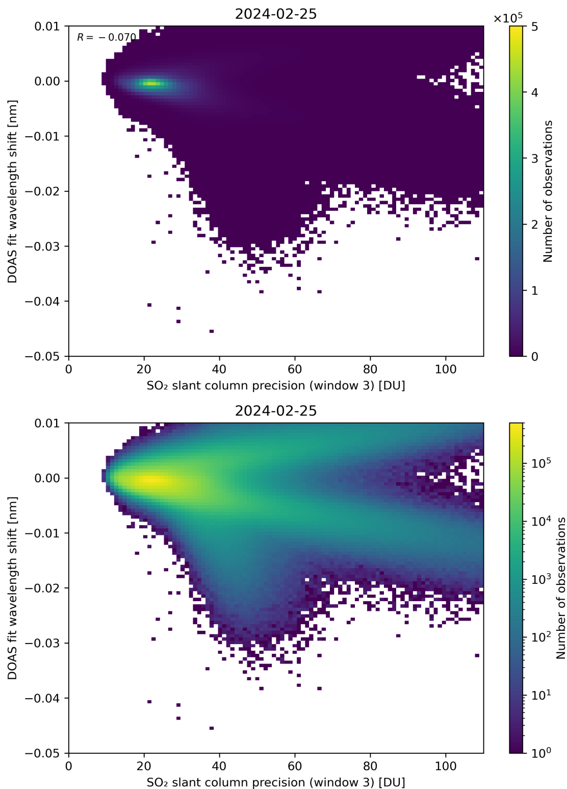
Figure 258: Scatter density plot of “SO 2 slant column precision (window 3)” against “DOAS fit wavelength shift” for 2024-02-24 to 2024-02-26.
