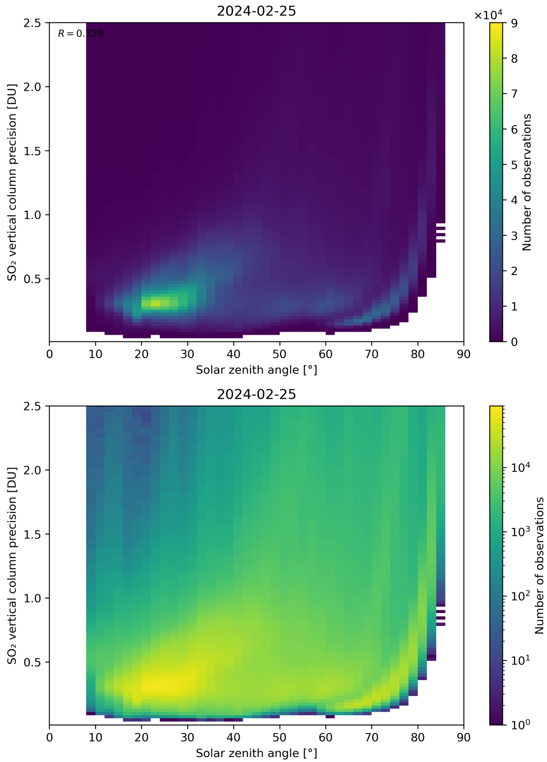
Figure 177: Scatter density plot of “Solar zenith angle” against “SO 2 vertical column precision” for 2024-02-24 to 2024-02-26.
