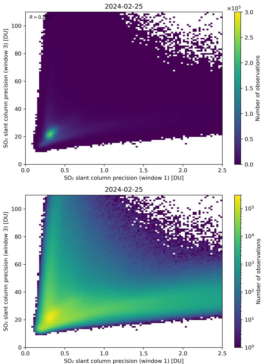
Figure 229: Scatter density plot of “SO 2 slant column precision (window 1)” against “SO 2 slant column precision (window 3)” for 2024-02-24 to 2024-02-26.
