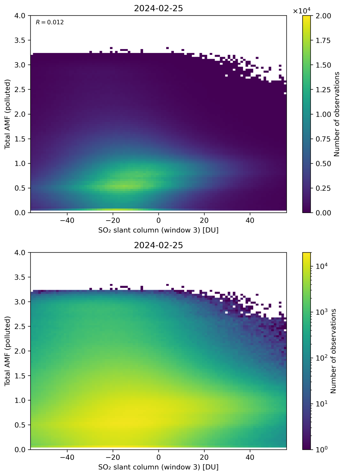
Figure 268: Scatter density plot of “SO 2 slant column (window 3)” against “Total AMF (polluted)” for 2024-02-24 to 2024-02-26.
