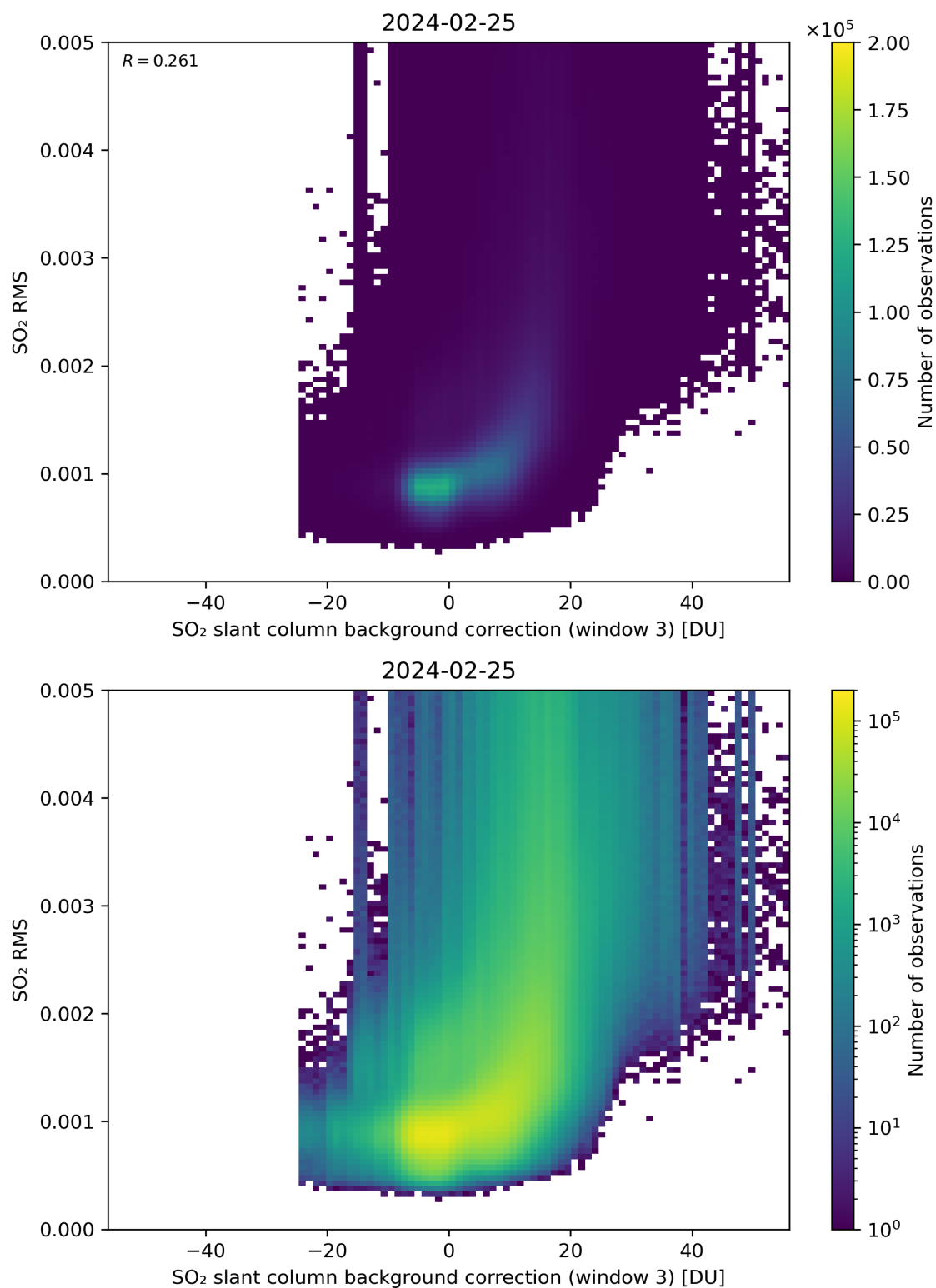
Figure 123: Scatter density plot of “SO 2 slant column background correction (window 3)” against “SO 2 RMS” for 2024-02-24 to 2024-02-26.
