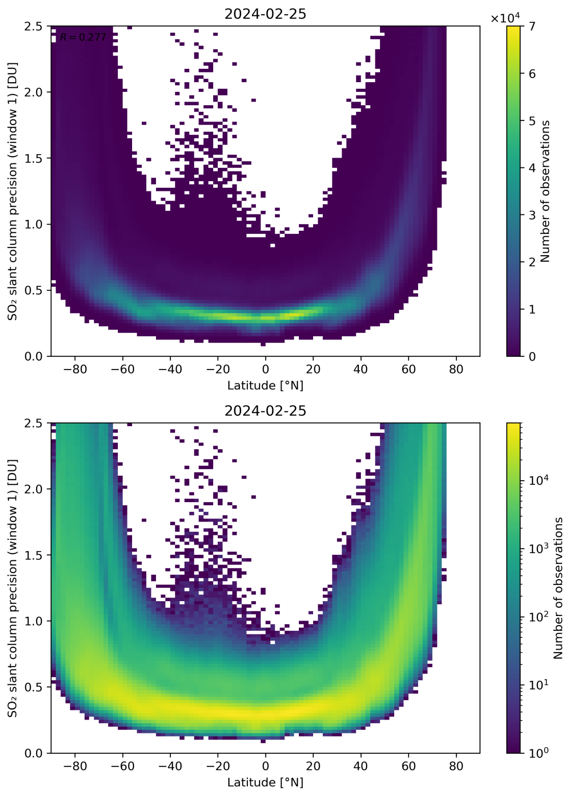
Figure 150: Scatter density plot of “Latitude” against “SO 2 slant column precision (window 1)” for 2024-02-24 to 2024-02-26.
