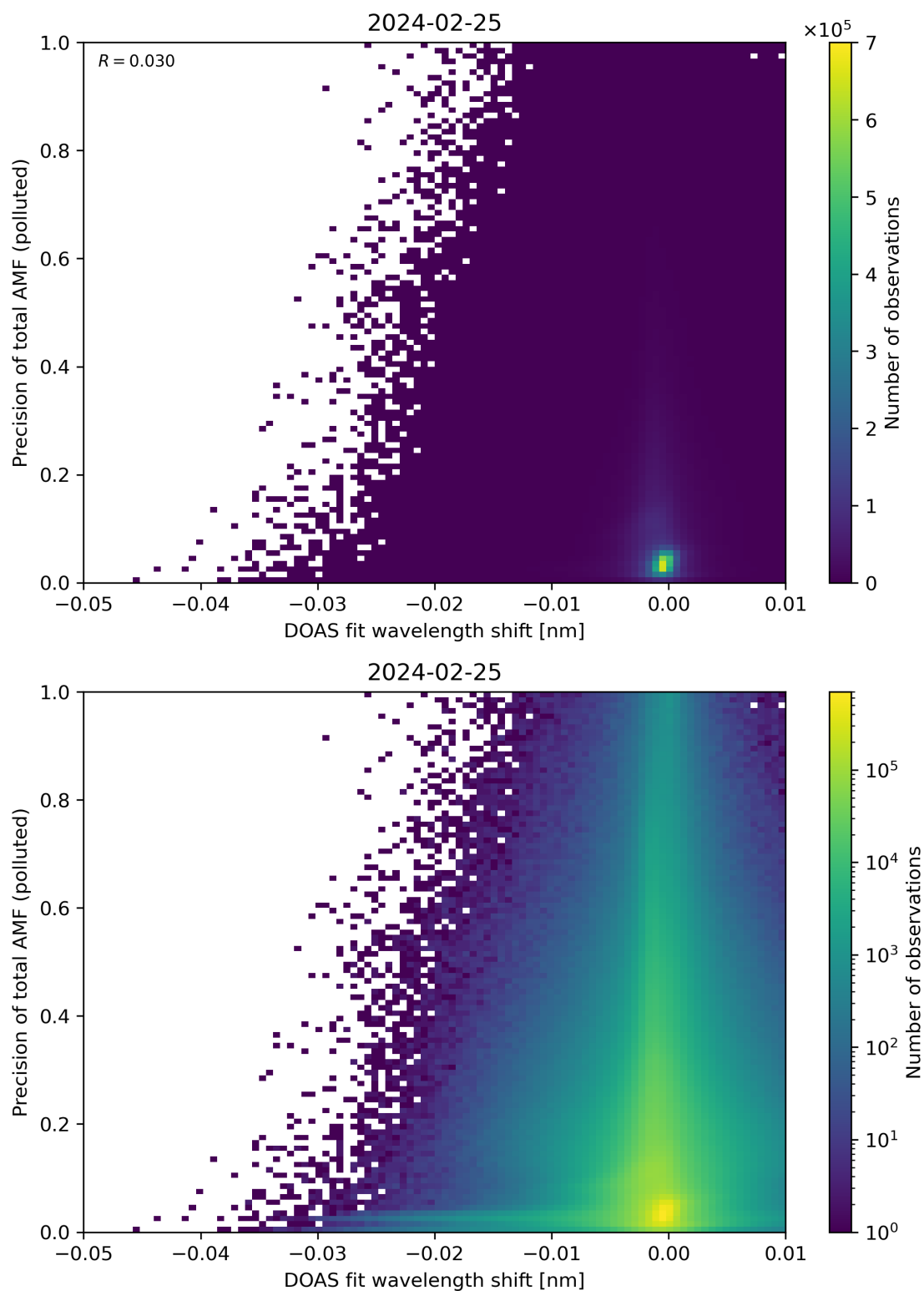
Figure 131: Scatter density plot of “DOAS fit wavelength shift” against “Precision of total AMF (polluted)” for 2024-02-24 to 2024-02-26.
