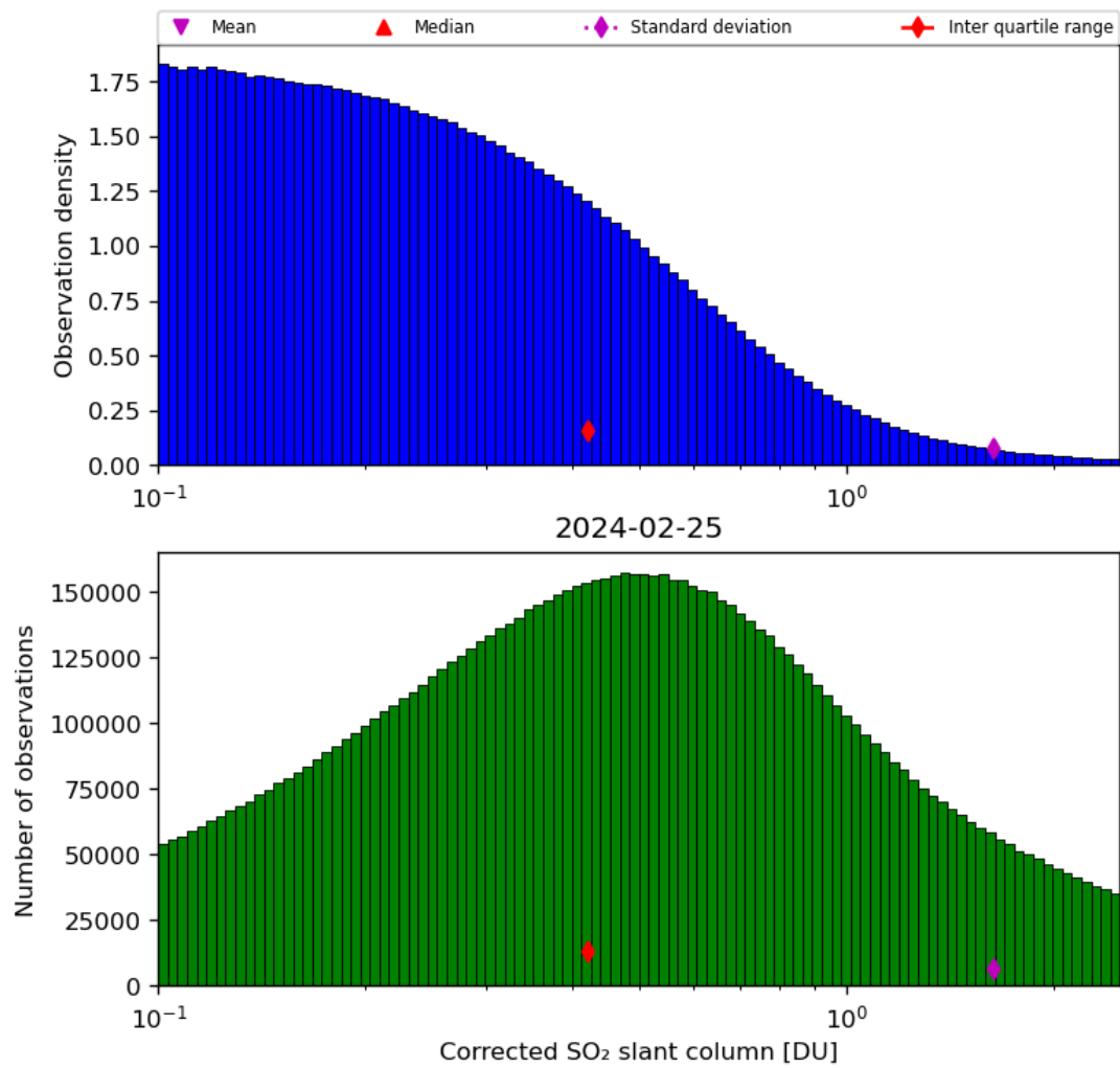
Figure 55: Histogram of “Corrected SO 2 slant column” for 2024-02-24 to 2024-02-26
