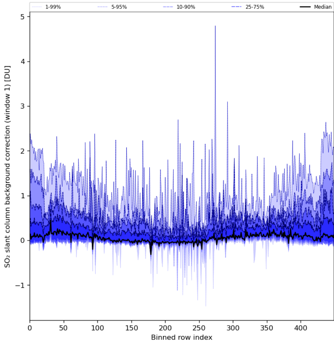
Figure 82: Along track statistics of “SO 2 slant column background correction (window 1)” for 2024-02-24 to 2024-02-26
