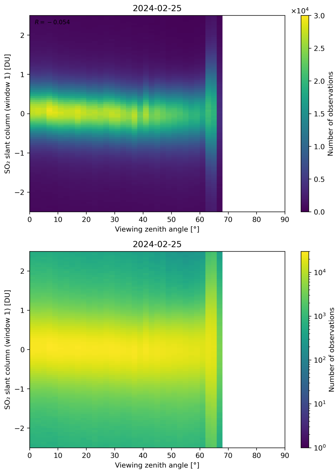
Figure 320: Scatter density plot of “Viewing zenith angle” against “SO 2 slant column (window 1)” for 2024-02-24 to 2024-02-26.
