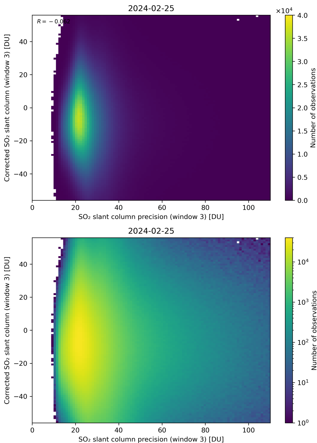
Figure 262: Scatter density plot of “SO 2 slant column precision (window 3)” against “Corrected SO 2 slant column (window 3)” for 2024-02-24 to 2024-02-26.
