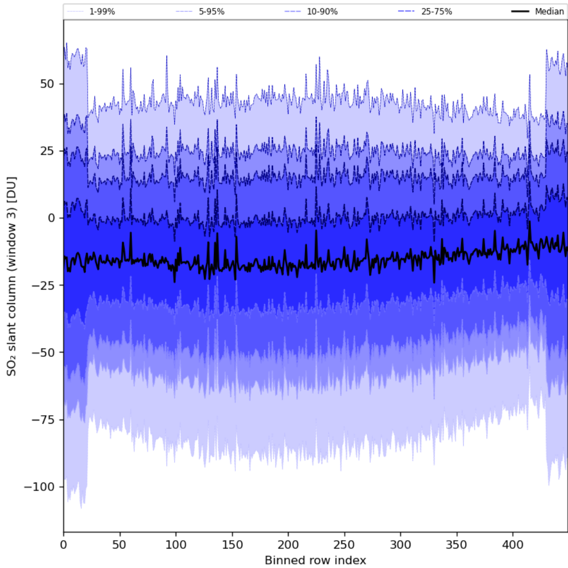
Figure 87: Along track statistics of “SO 2 slant column (window 3)” for 2024-02-24 to 2024-02-26
