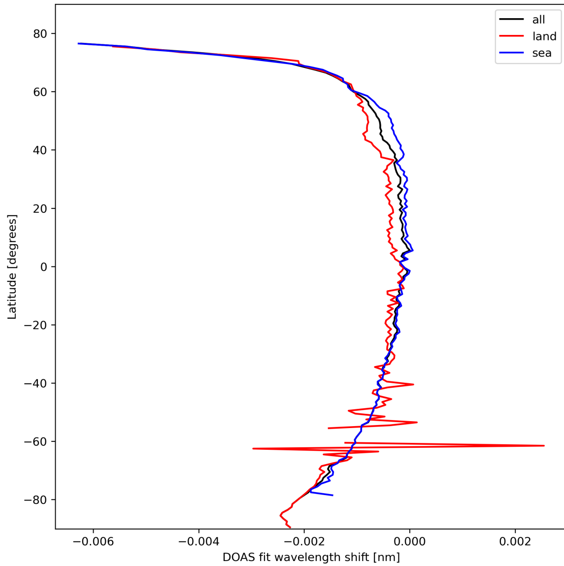
Figure 45: Zonal average of “DOAS fit wavelength shift” for 2024-02-24 to 2024-02-26.
