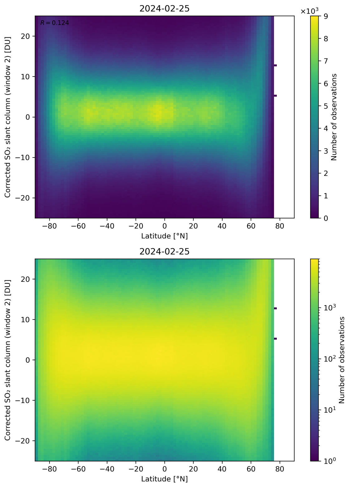
Figure 147: Scatter density plot of “Latitude” against “Corrected SO 2 slant column (window 2)” for 2024-02-24 to 2024-02-26.
