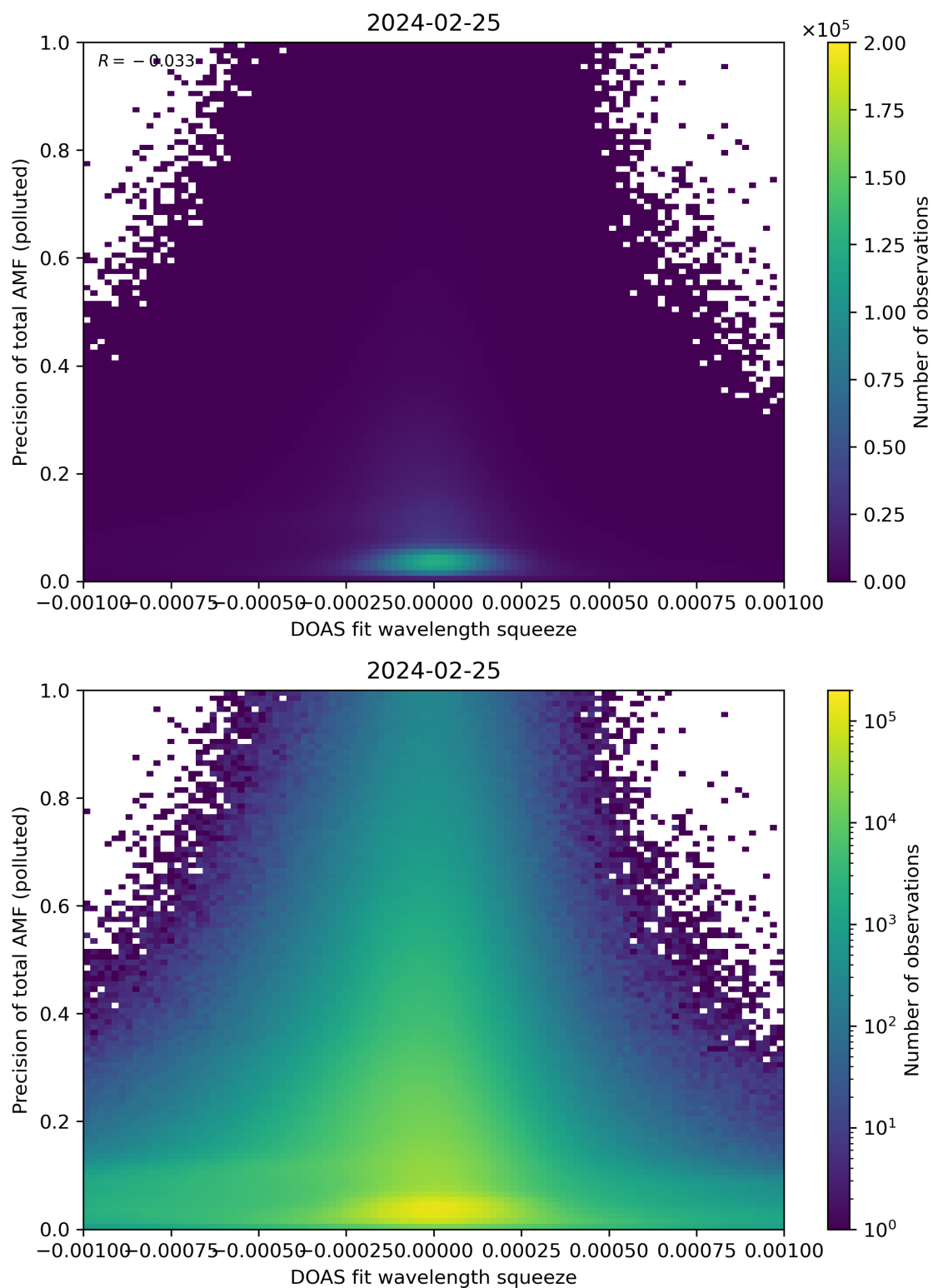
Figure 135: Scatter density plot of “DOAS fit wavelength squeeze” against “Precision of total AMF (polluted)” for 2024-02-24 to 2024-02-26.
