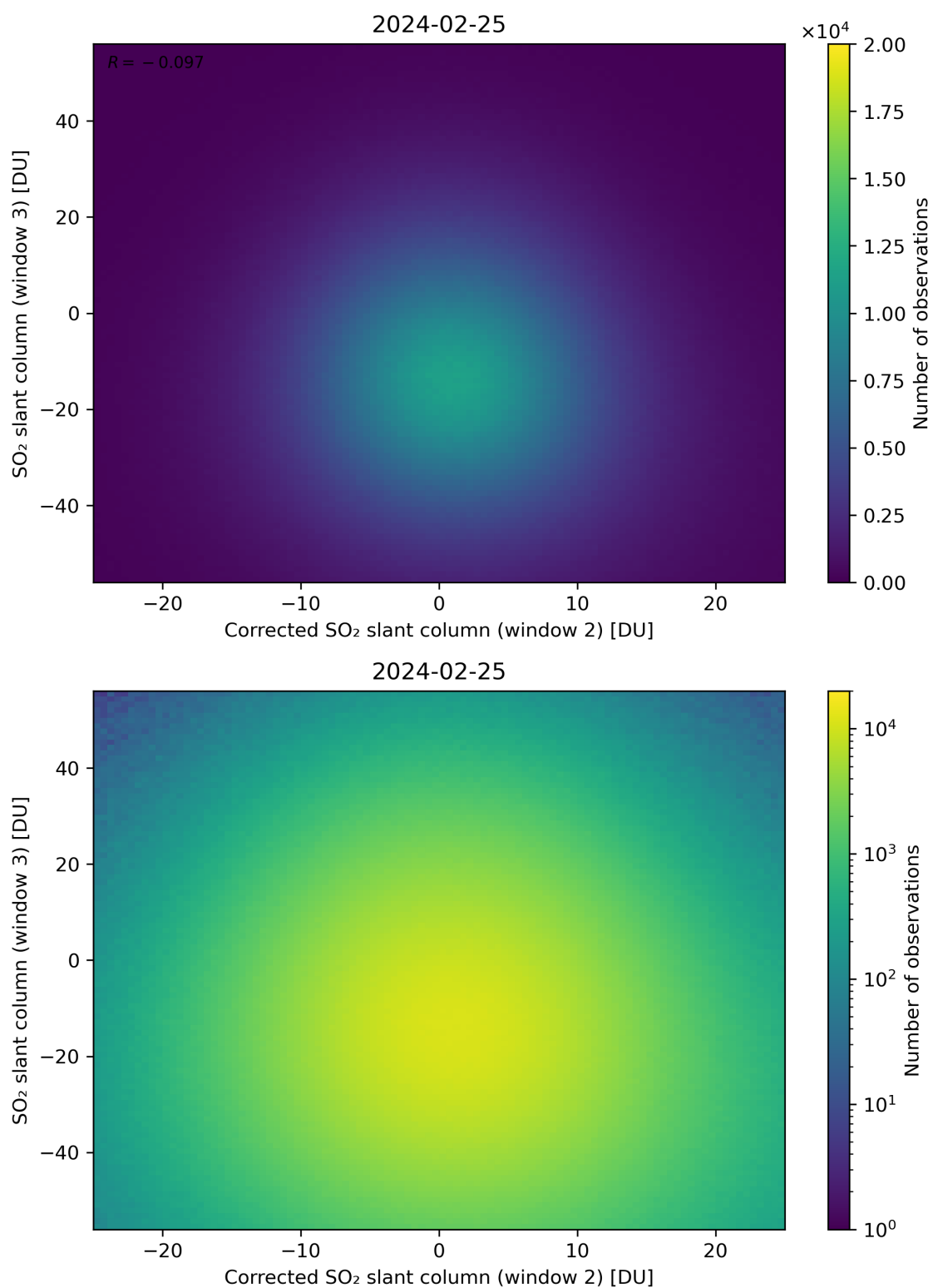
Figure 201: Scatter density plot of “Corrected SO 2 slant column (window 2)” against “SO 2 slant column (window 3)” for 2024-02-24 to 2024-02-26.
