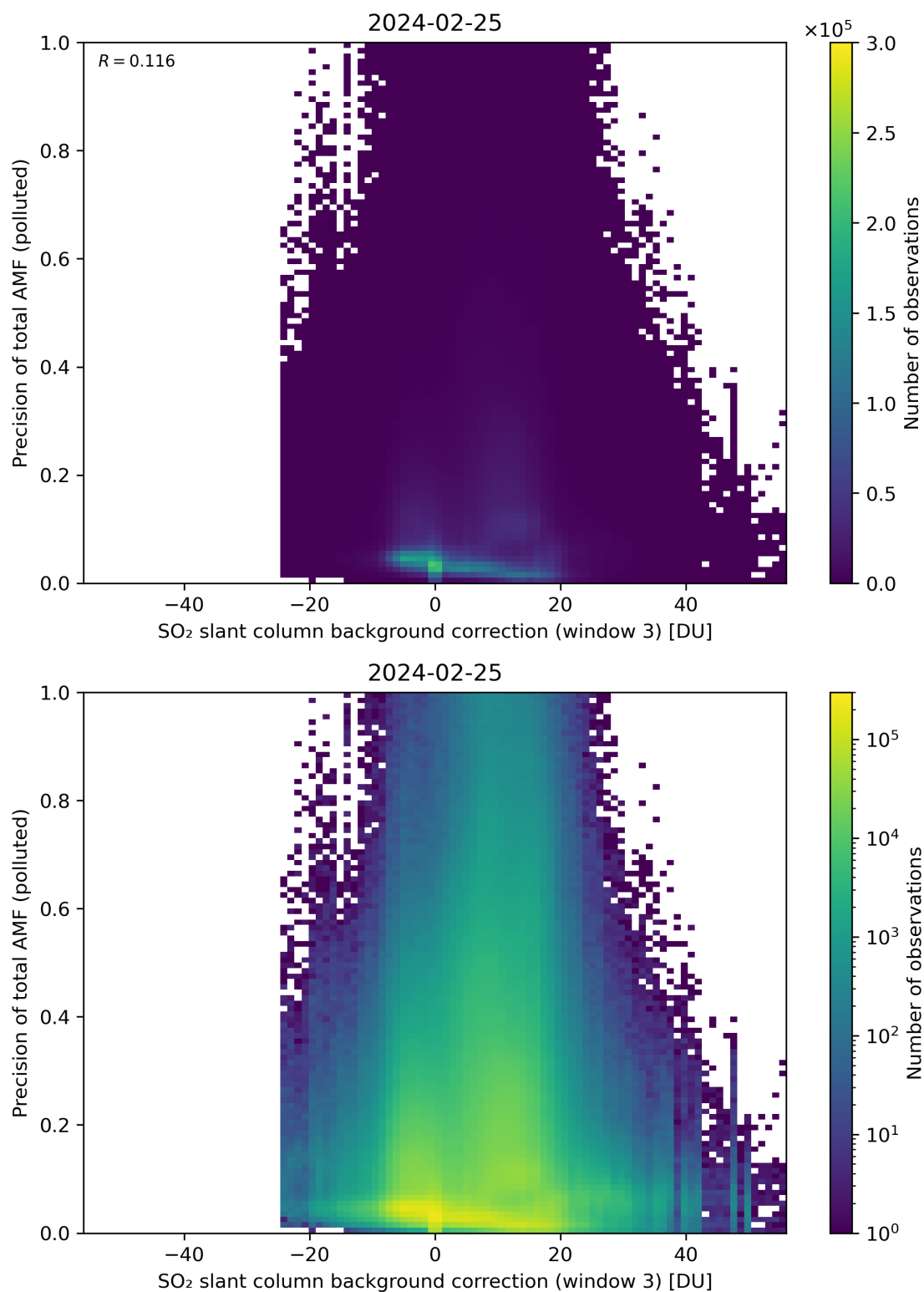
Figure 126: Scatter density plot of “SO 2 slant column background correction (window 3)” against “Precision of total AMF (polluted)” for 2024-02-24 to 2024-02-26.
