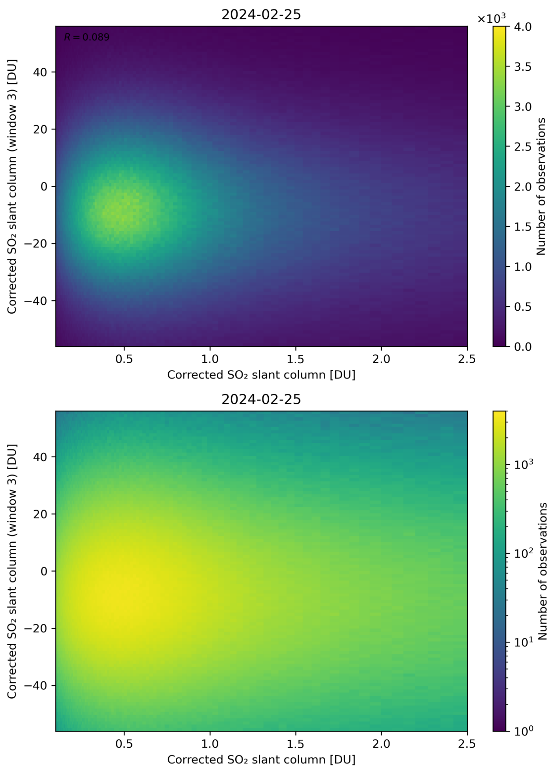
Figure 186: Scatter density plot of “Corrected SO 2 slant column” against “Corrected SO 2 slant column (window 3)” for 2024-02-24 to 2024-02-26.
