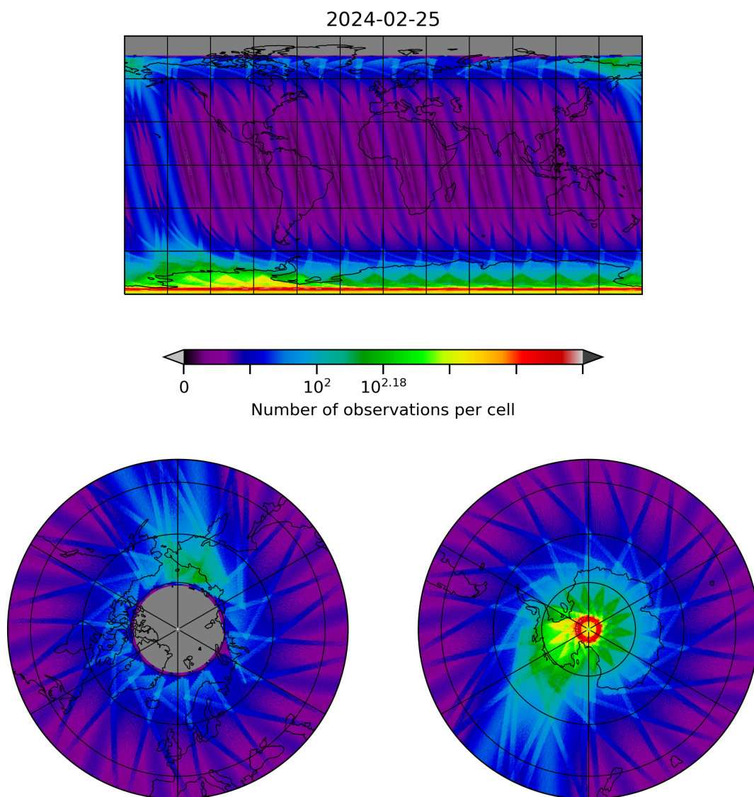
Figure 28: Map of the number of observations for 2024-02-24 to 2024-02-26
