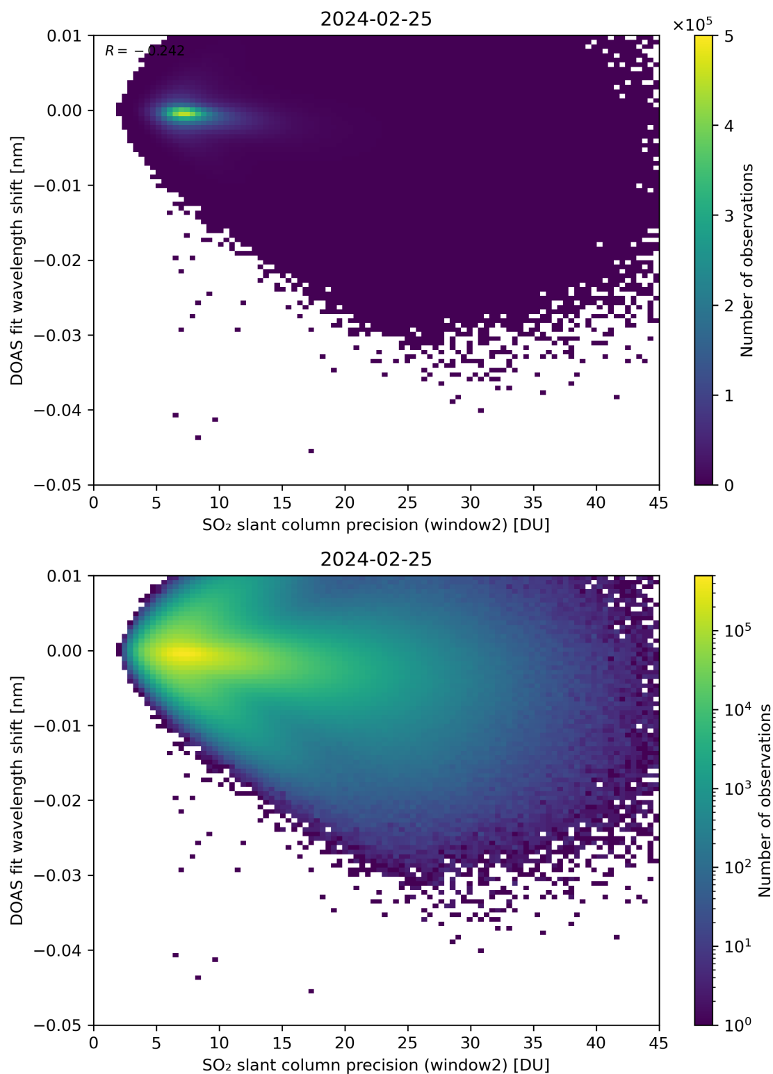
Figure 243: Scatter density plot of “SO 2 slant column precision (window2)” against “DOAS fit wavelength shift” for 2024-02-24 to 2024-02-26.
