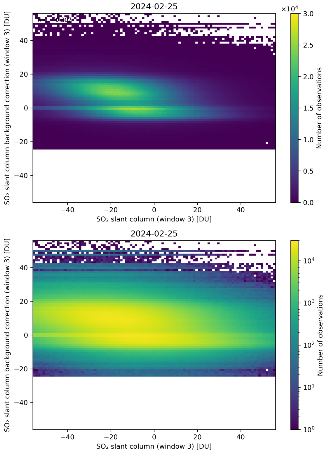
Figure 253: Scatter density plot of “SO 2 slant column (window 3)” against “SO 2 slant column background correction (window 3)” for 2024-02-24 to 2024-02-26.
