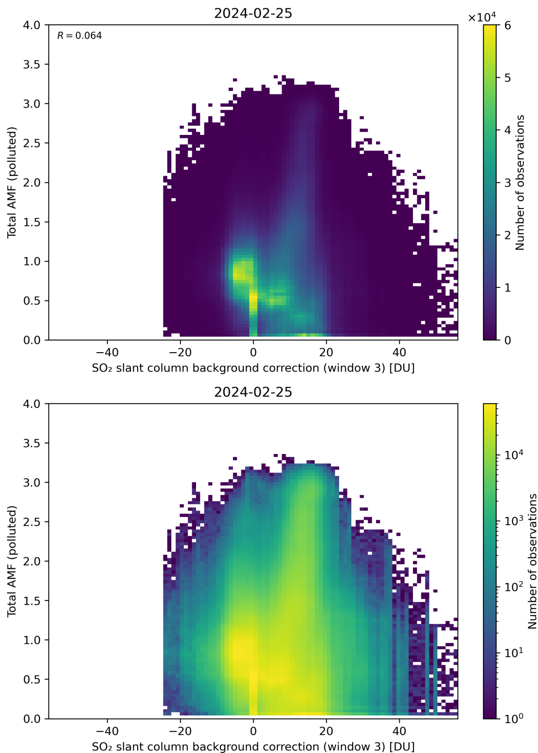
Figure 125: Scatter density plot of “SO 2 slant column background correction (window 3)” against “Total AMF (polluted)” for 2024-02-24 to 2024-02-26.
