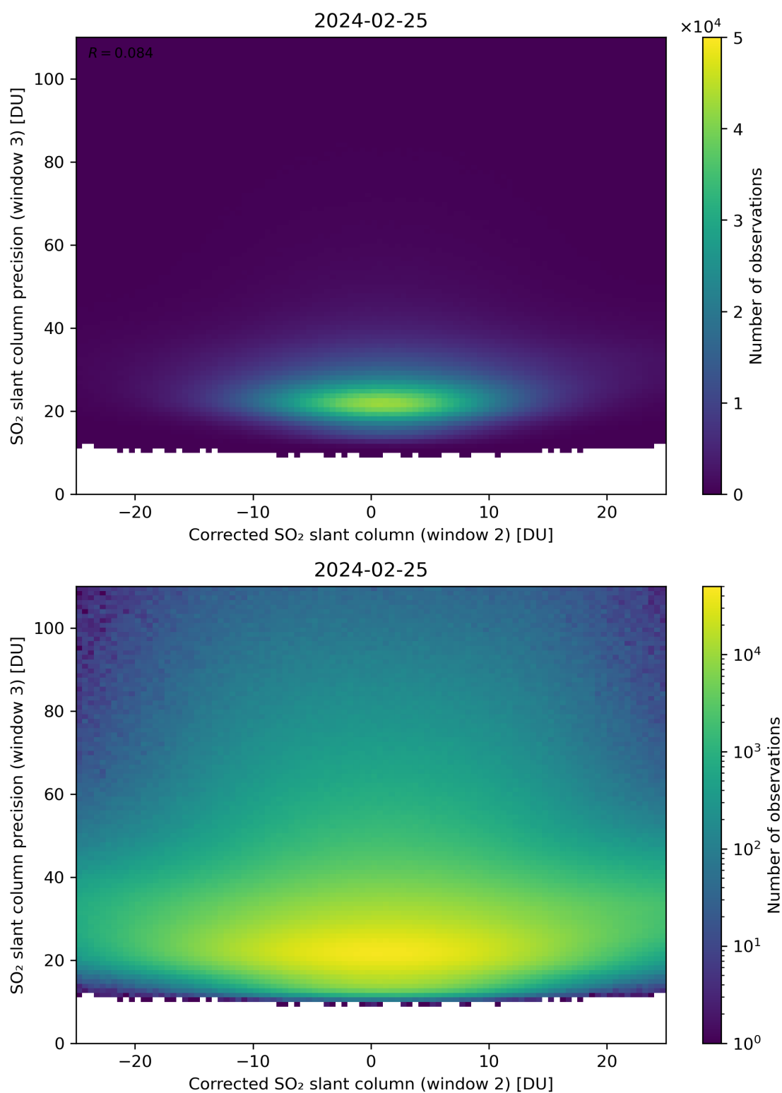
Figure 202: Scatter density plot of “Corrected SO 2 slant column (window 2)” against “SO 2 slant column precision (window 3)” for 2024-02-24 to 2024-02-26.
