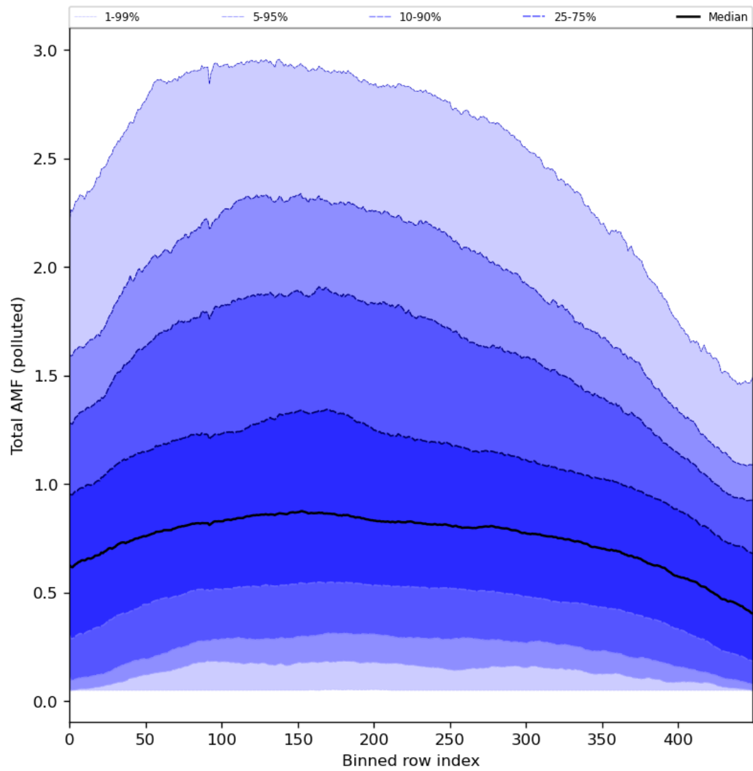
Figure 94: Along track statistics of “Total AMF (polluted)” for 2024-02-24 to 2024-02-26
