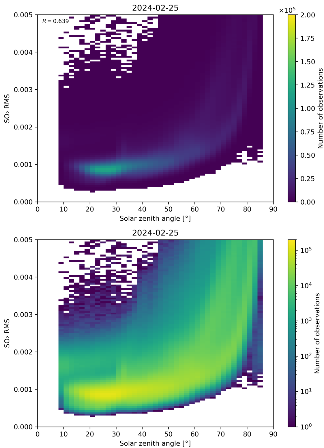
Figure 163: Scatter density plot of “Solar zenith angle” against “SO 2 RMS” for 2024-02-24 to 2024-02-26.
