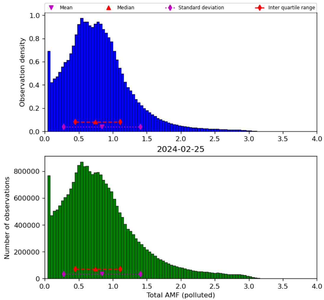
Figure 71: Histogram of “Total AMF (polluted)” for 2024-02-24 to 2024-02-26
