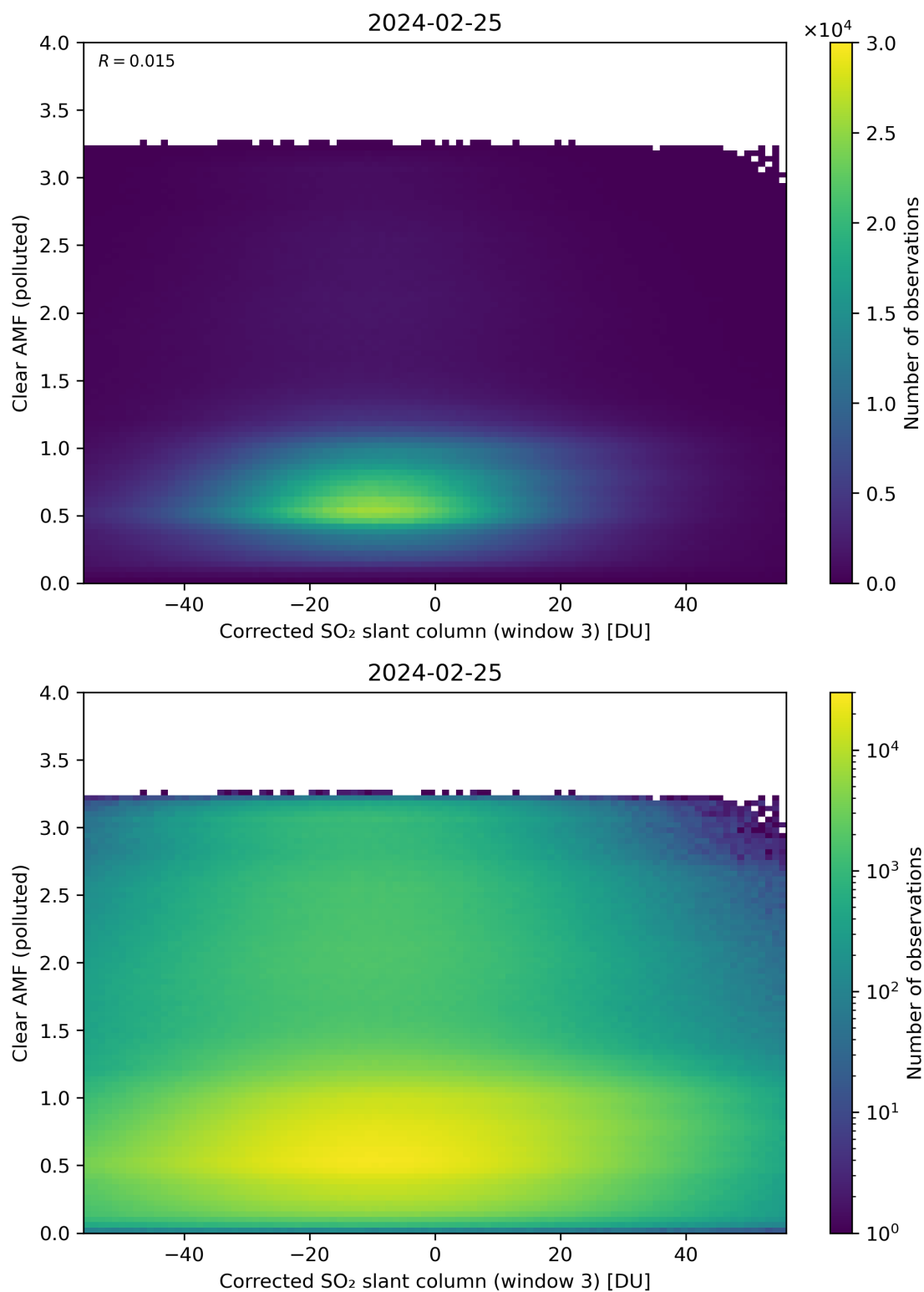
Figure 209: Scatter density plot of “Corrected SO 2 slant column (window 3)” against “Clear AMF (polluted)” for 2024-02-24 to 2024-02-26.
