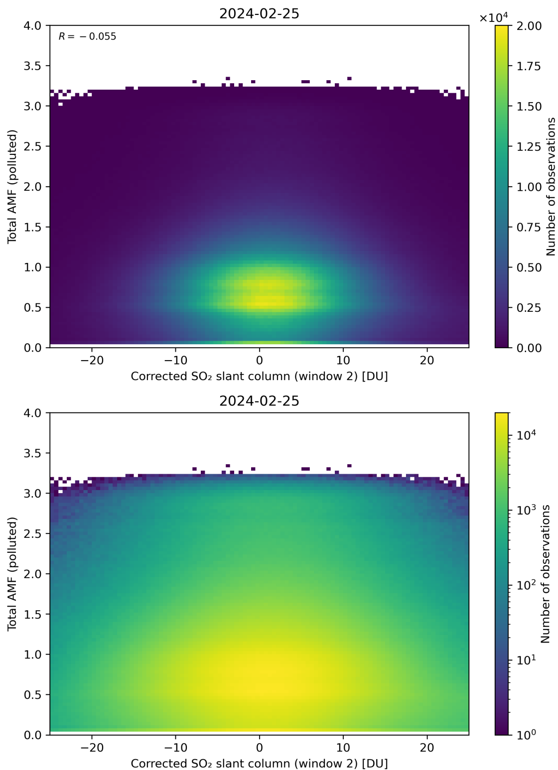
Figure 203: Scatter density plot of “Corrected SO 2 slant column (window 2)” against “Total AMF (polluted)” for 2024-02-24 to 2024-02-26.
