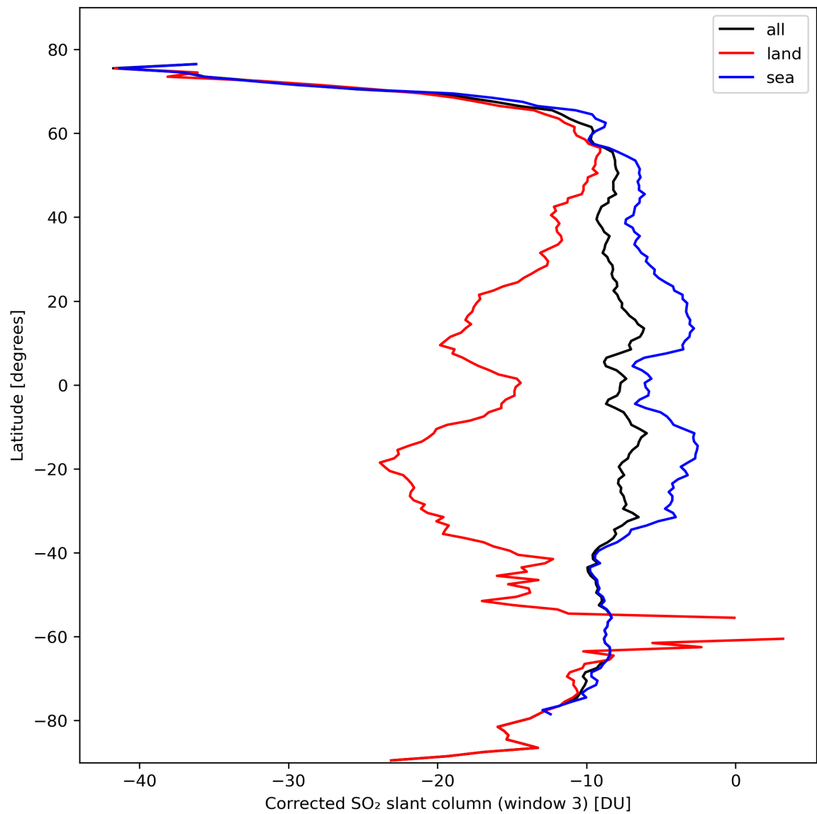
Figure 43: Zonal average of “Corrected SO 2 slant column (window 3)” for 2024-02-24 to 2024-02-26.
