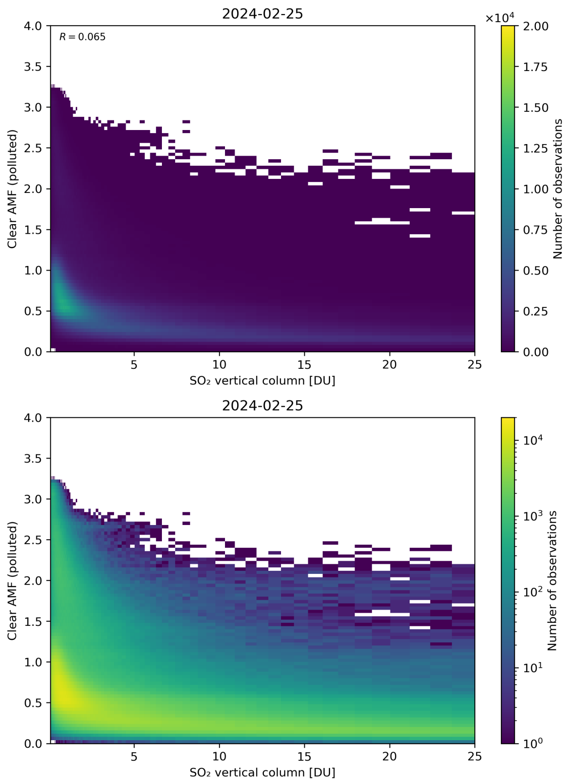
Figure 296: Scatter density plot of “SO 2 vertical column” against “Clear AMF (polluted)” for 2024-02-24 to 2024-02-26.
