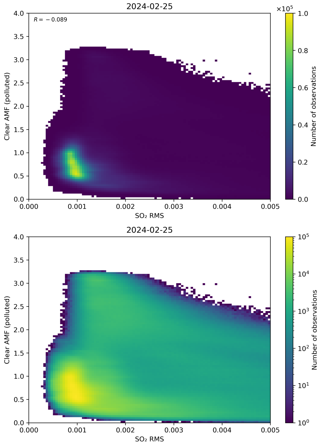
Figure 136: Scatter density plot of “SO 2 RMS” against “Clear AMF (polluted)” for 2024-02-24 to 2024-02-26.
