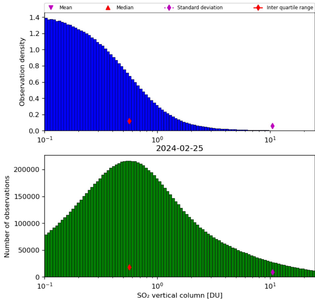
Figure 53: Histogram of “SO 2 vertical column” for 2024-02-24 to 2024-02-26
