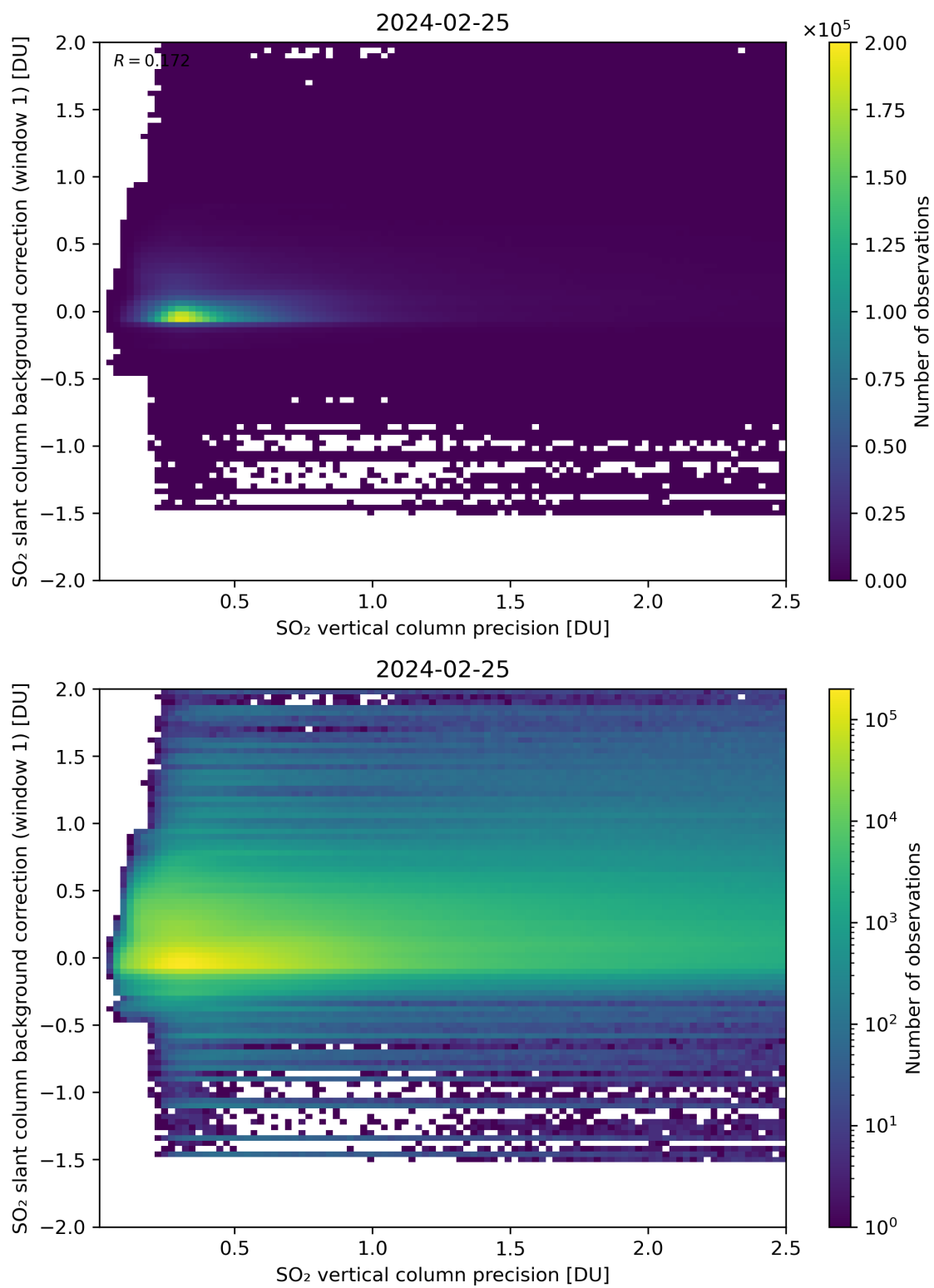
Figure 279: Scatter density plot of “SO 2 vertical column precision” against “SO 2 slant column background correction (window 1)” for 2024-02-24 to 2024-02-26.
