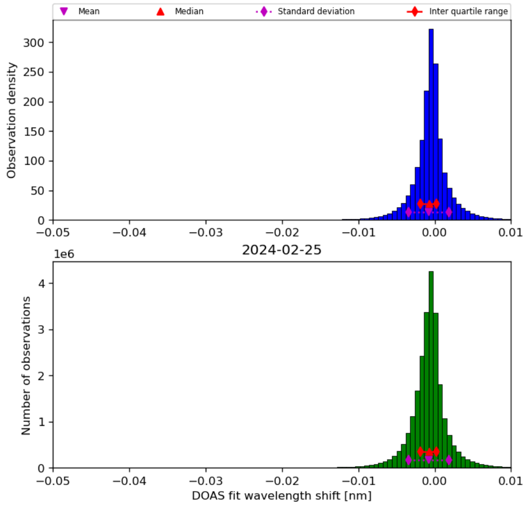
Figure 68: Histogram of “DOAS fit wavelength shift” for 2024-02-24 to 2024-02-26
