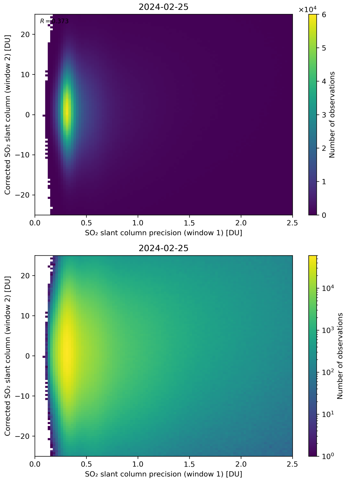
Figure 225: Scatter density plot of “SO 2 slant column precision (window 1)” against “Corrected SO 2 slant column (window 2)” for 2024-02-24 to 2024-02-26.
