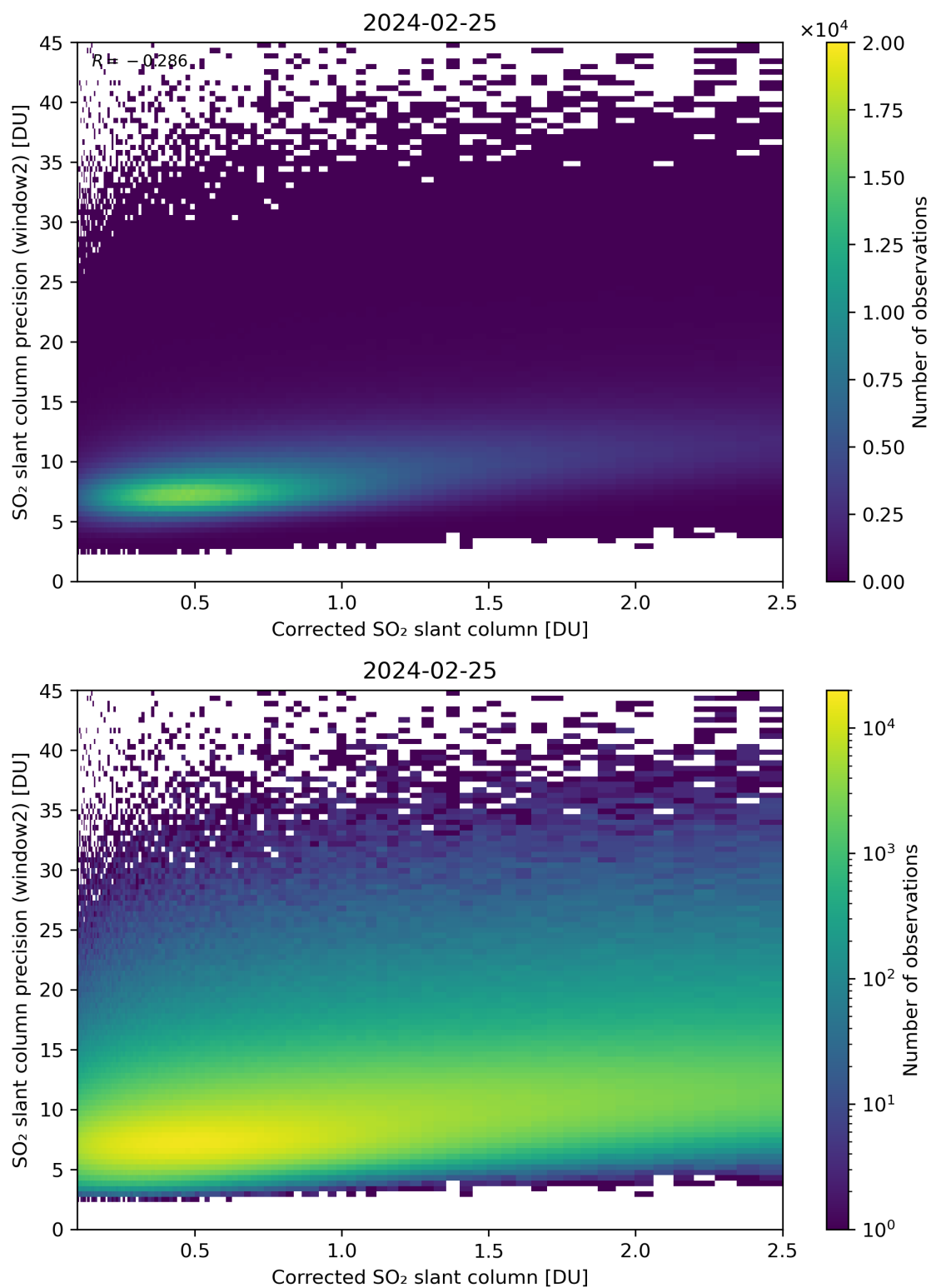
Figure 189: Scatter density plot of “Corrected SO 2 slant column” against “SO 2 slant column precision (window2)” for 2024-02-24 to 2024-02-26.
