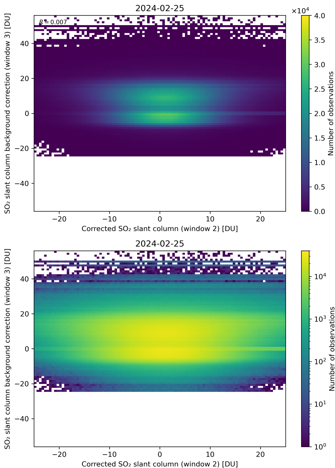
Figure 195: Scatter density plot of “Corrected SO 2 slant column (window 2)” against “SO 2 slant column background correction (window 3)” for 2024-02-24 to 2024-02-26.
