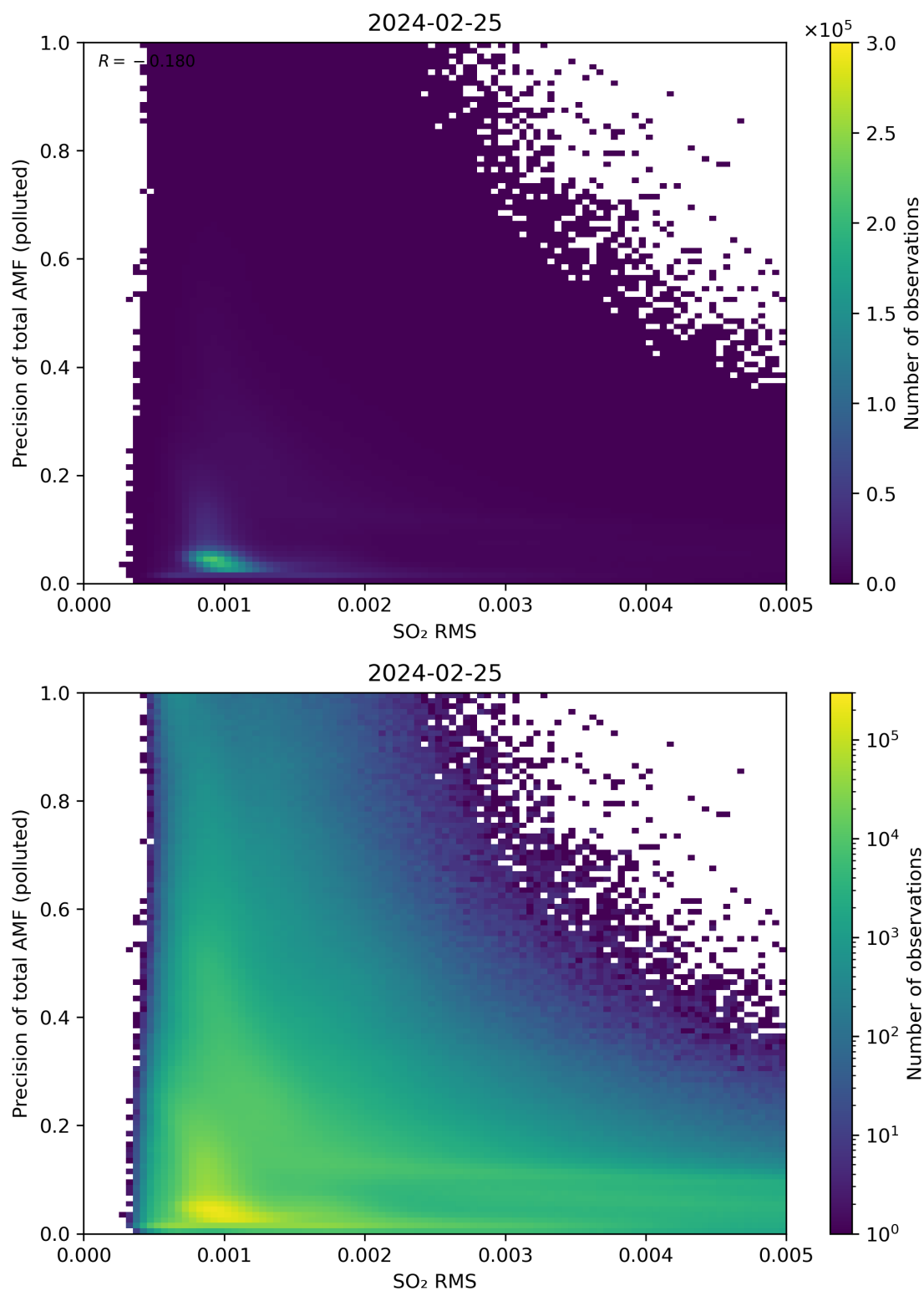
Figure 138: Scatter density plot of “SO 2 RMS” against “Precision of total AMF (polluted)” for 2024-02-24 to 2024-02-26.
