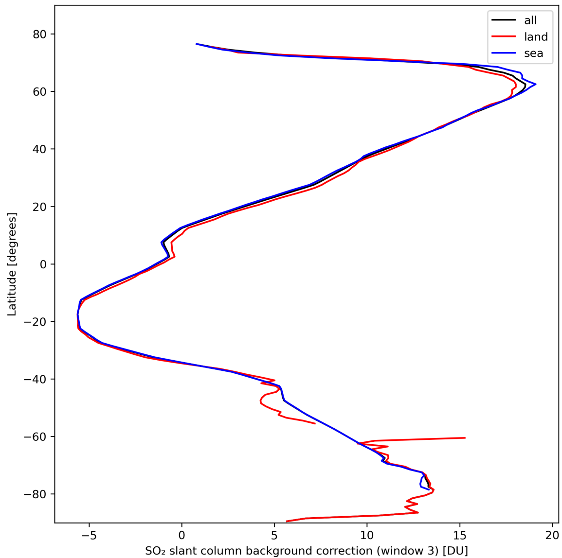
Figure 44: Zonal average of “SO 2 slant column background correction (window 3)” for 2024-02-24 to 2024-02-26.
