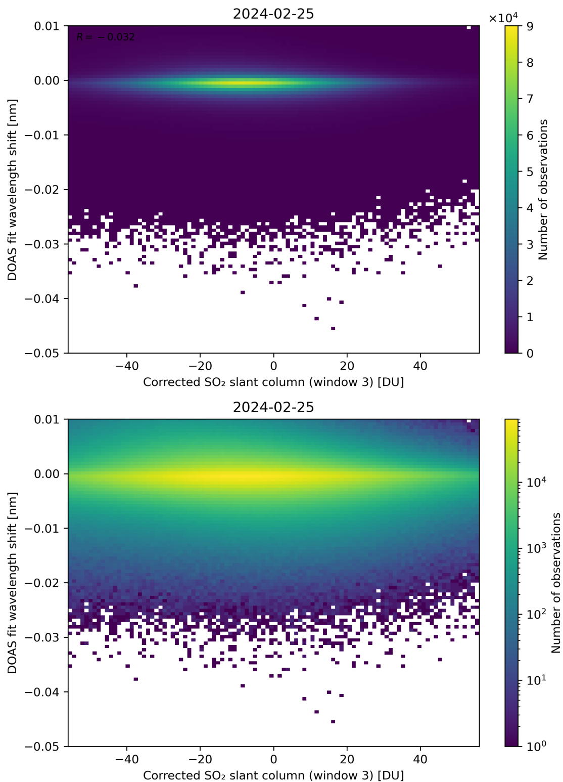
Figure 206: Scatter density plot of “Corrected SO 2 slant column (window 3)” against “DOAS fit wavelength shift” for 2024-02-24 to 2024-02-26.
