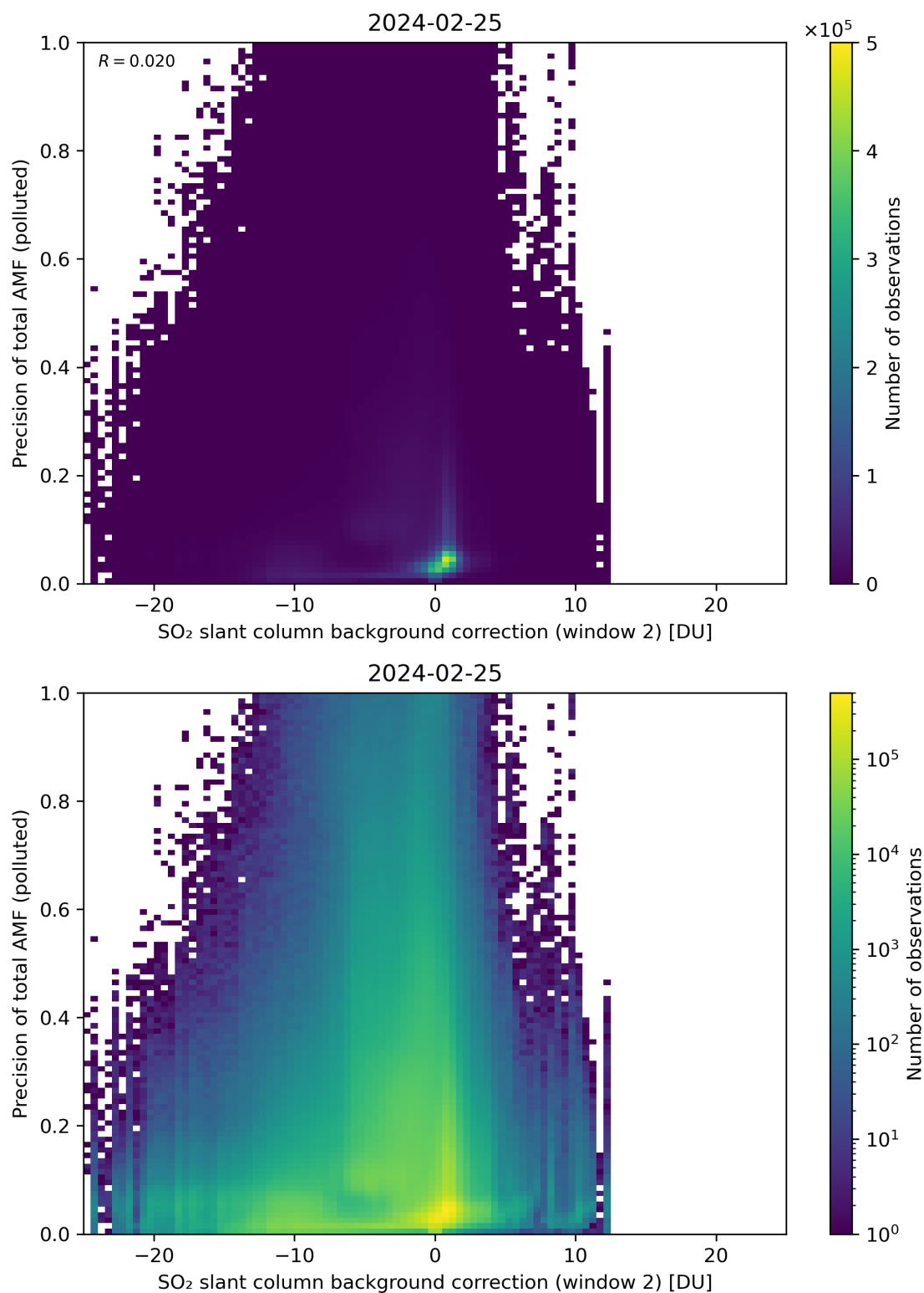
Figure 120: Scatter density plot of “SO 2 slant column background correction (window 2)” against “Precision of total AMF (polluted)” for 2024-02-24 to 2024-02-26.
