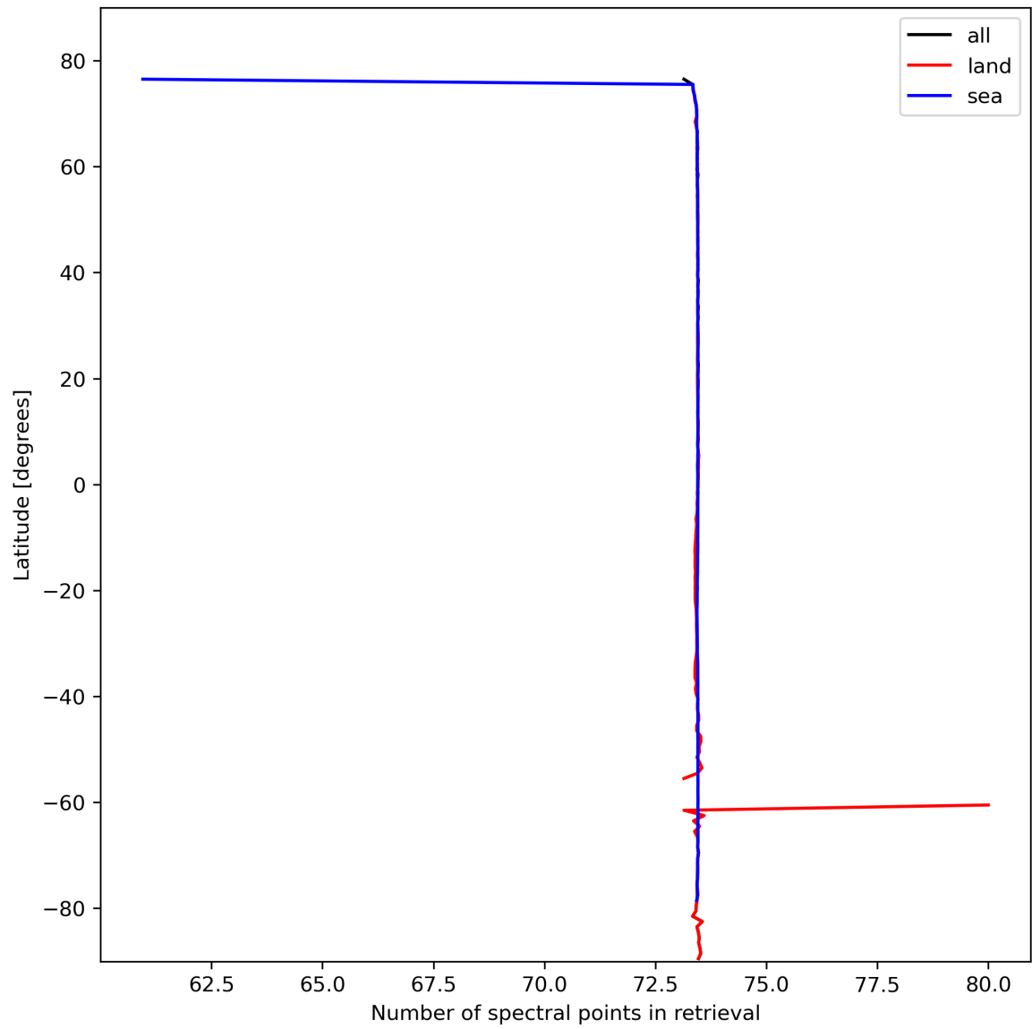
Figure 51: Zonal average of “Number of spectral points in retrieval” for 2024-02-24 to 2024-02-26.
