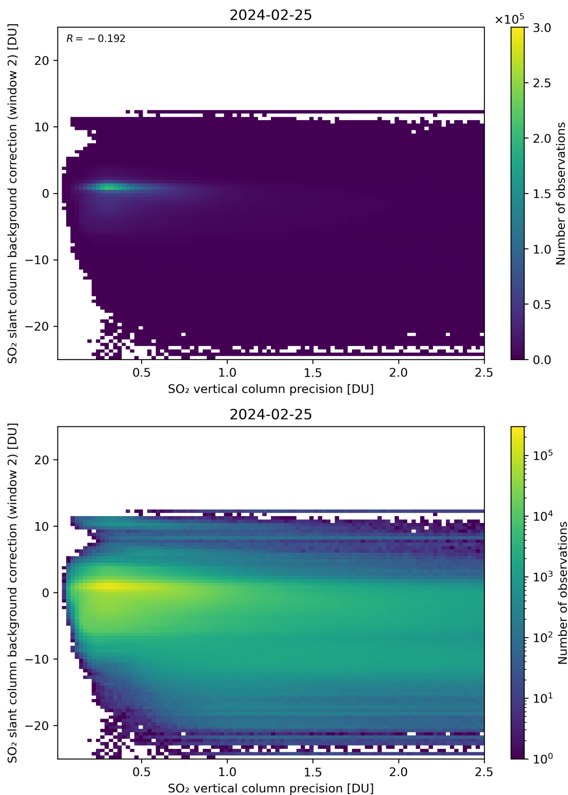
Figure 280: Scatter density plot of “SO 2 vertical column precision” against “SO 2 slant column background correction (window 2)” for 2024-02-24 to 2024-02-26.
