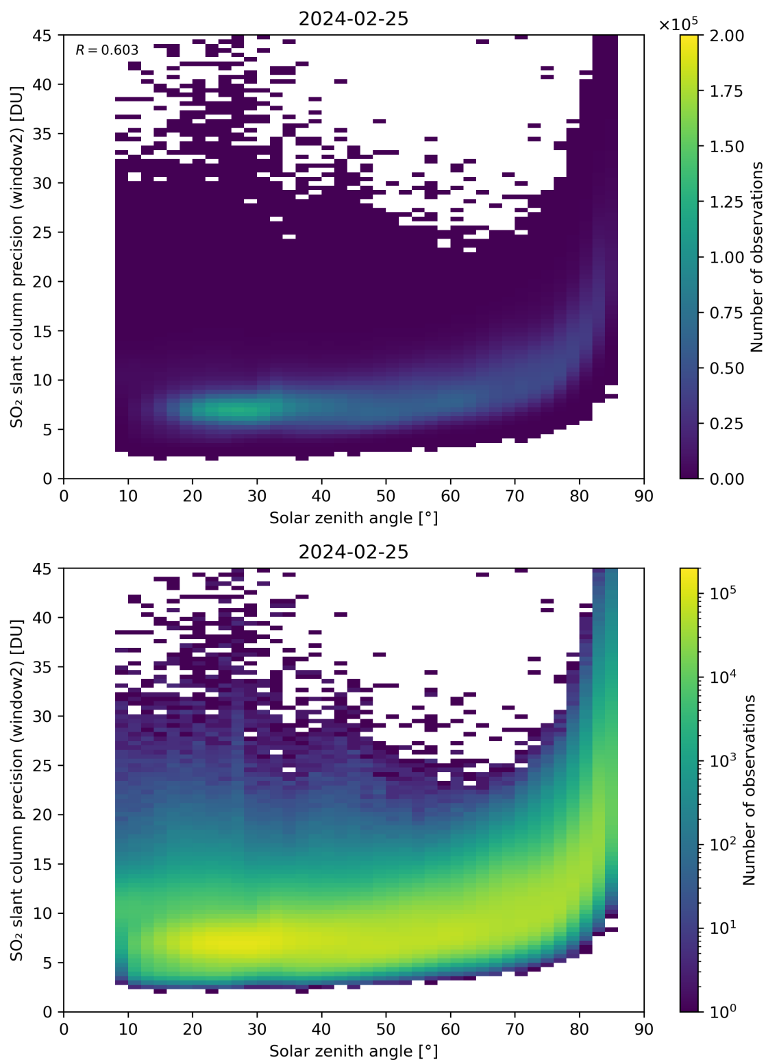
Figure 171: Scatter density plot of “Solar zenith angle” against “SO 2 slant column precision (window2)” for 2024-02-24 to 2024-02-26.
