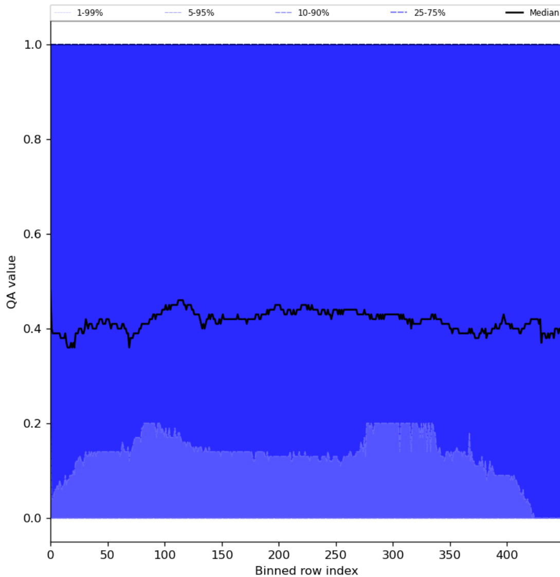
Figure 75: Along track statistics of “QA value” for 2024-02-24 to 2024-02-26
