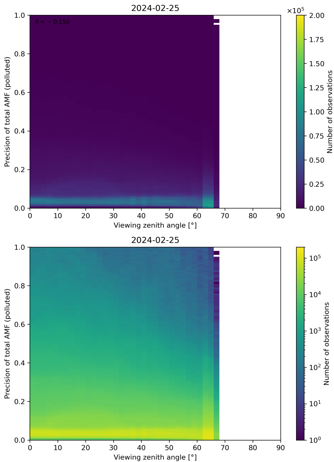
Figure 326: Scatter density plot of “Viewing zenith angle” against “Precision of total AMF (polluted)” for 2024-02-24 to 2024-02-26.
