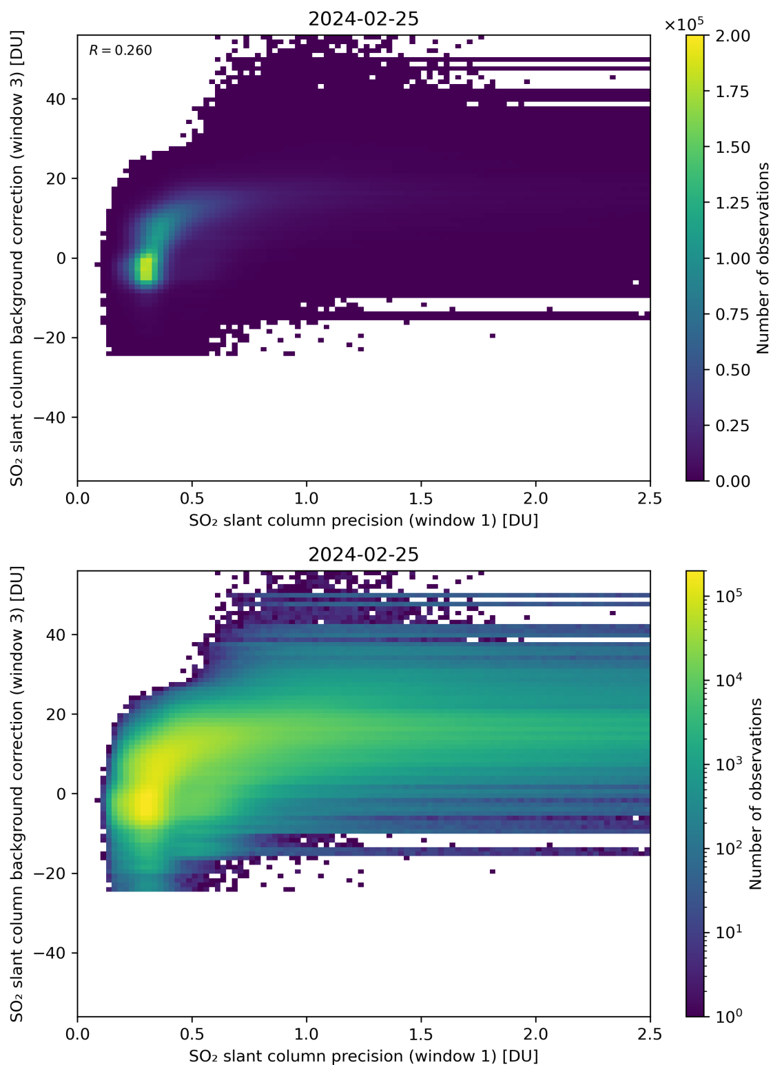
Figure 220: Scatter density plot of “SO 2 slant column precision (window 1)” against “SO 2 slant column background correction (window 3)” for 2024-02-24 to 2024-02-26.
