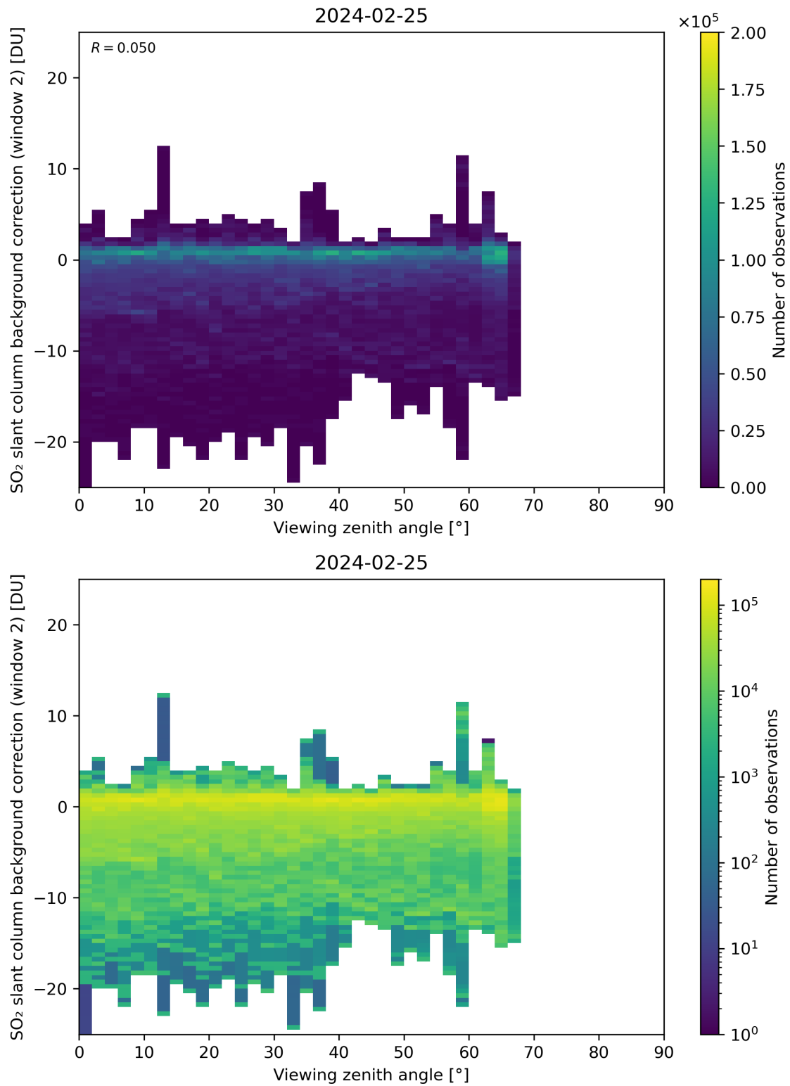
Figure 309: Scatter density plot of “Viewing zenith angle” against “SO 2 slant column background correction (window 2)” for 2024-02-24 to 2024-02-26.
