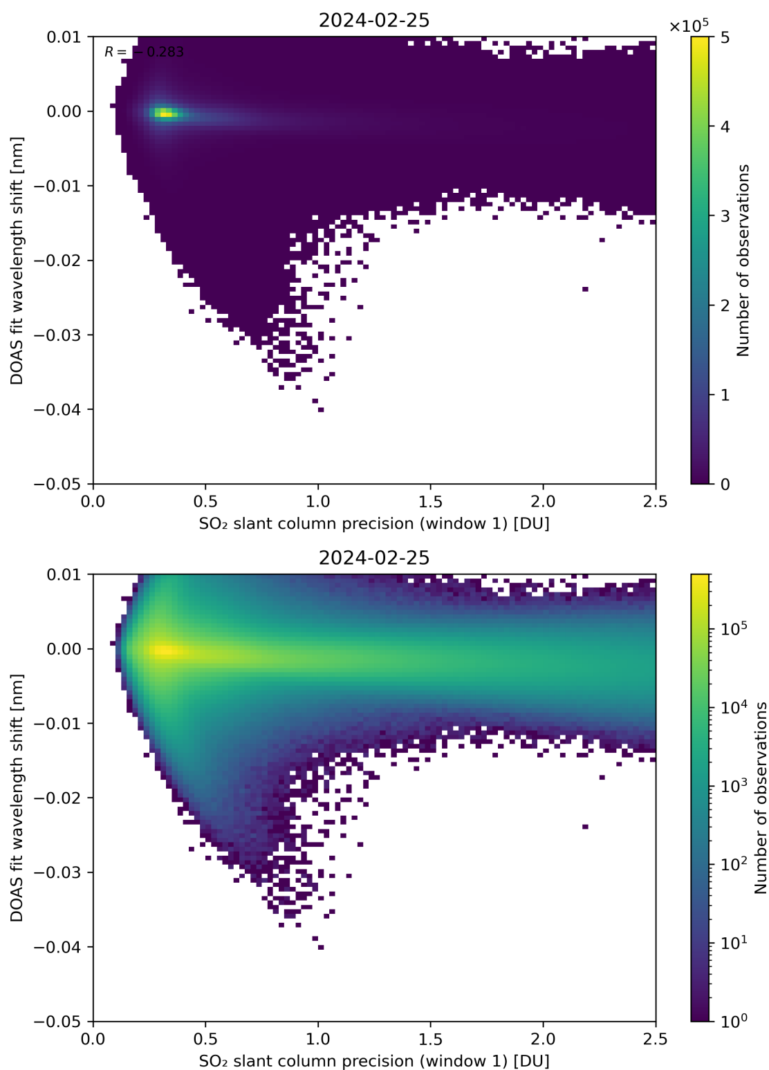
Figure 221: Scatter density plot of “SO 2 slant column precision (window 1)” against “DOAS fit wavelength shift” for 2024-02-24 to 2024-02-26.
