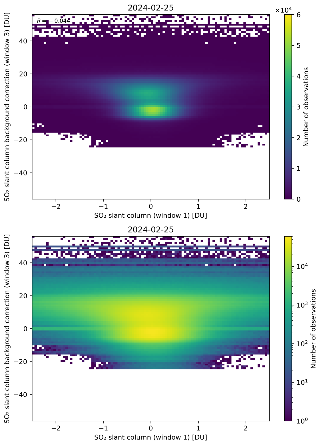
Figure 214: Scatter density plot of “SO 2 slant column (window 1)” against “SO 2 slant column background correction (window 3)” for 2024-02-24 to 2024-02-26.
