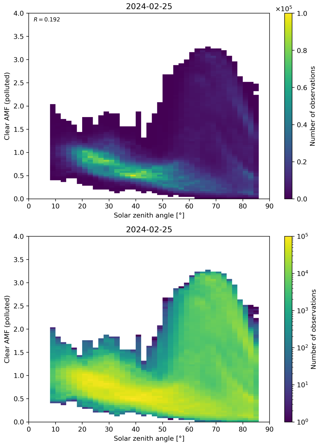
Figure 165: Scatter density plot of “Solar zenith angle” against “Clear AMF (polluted)” for 2024-02-24 to 2024-02-26.
