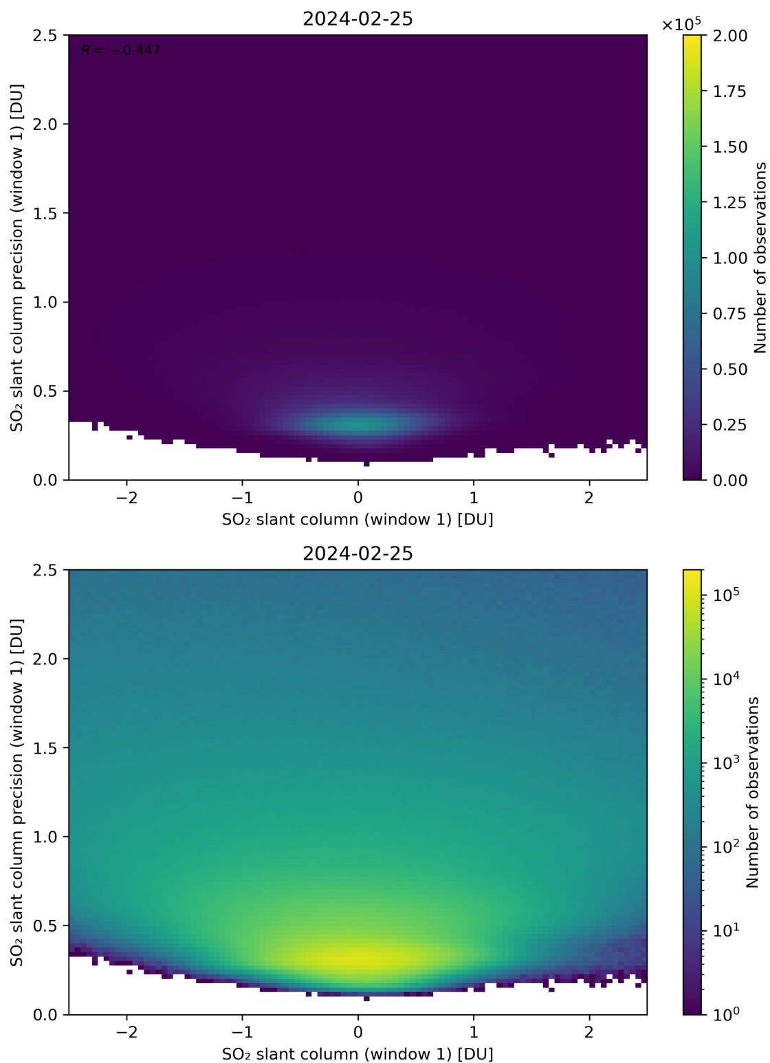
Figure 235: Scatter density plot of “SO 2 slant column (window 1)” against “SO 2 slant column precision (window 1)” for 2024-02-24 to 2024-02-26.
