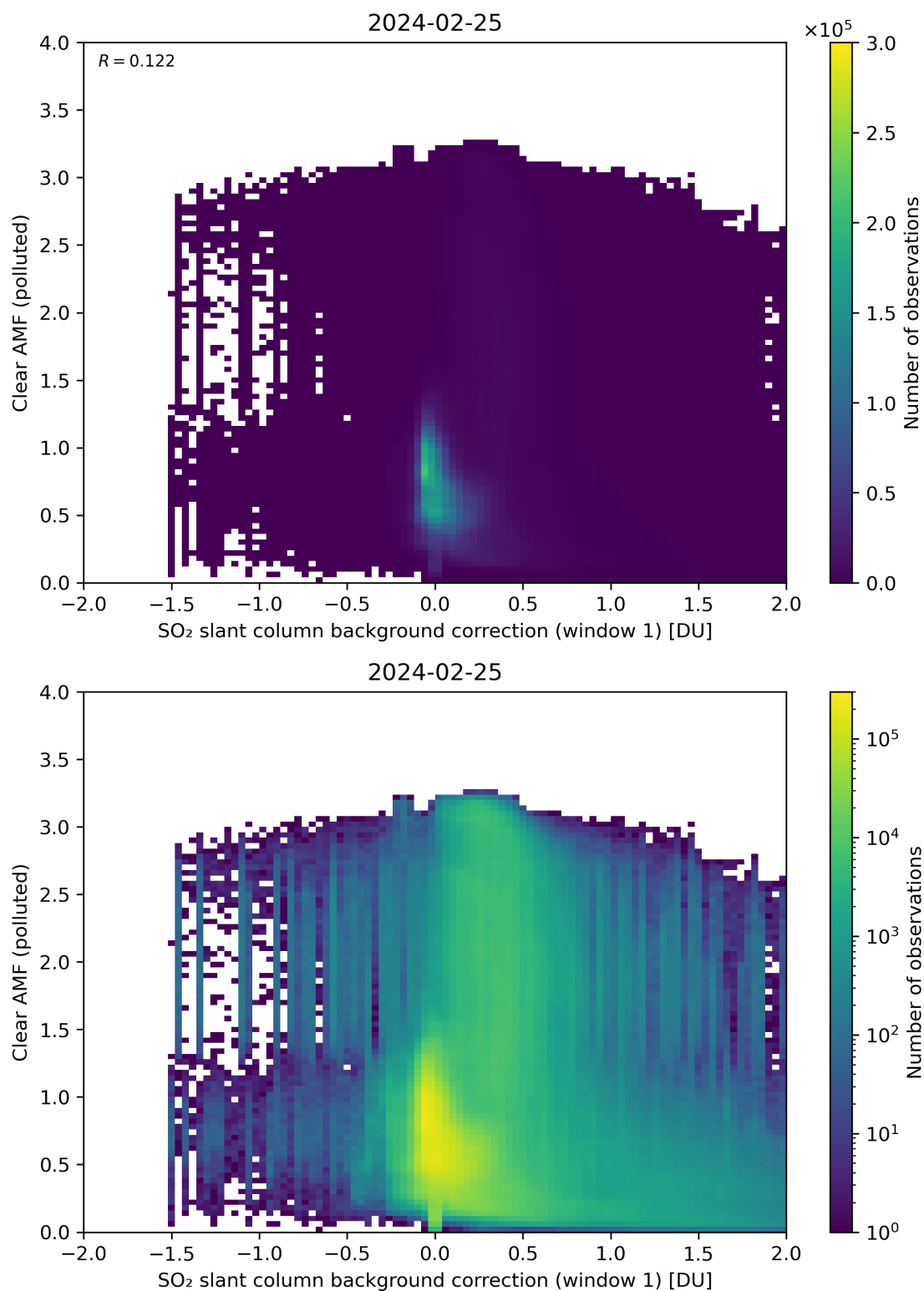
Figure 103: Scatter density plot of “SO 2 slant column background correction (window 1)” against “Clear AMF (polluted)” for 2024-02-24 to 2024-02-26.
