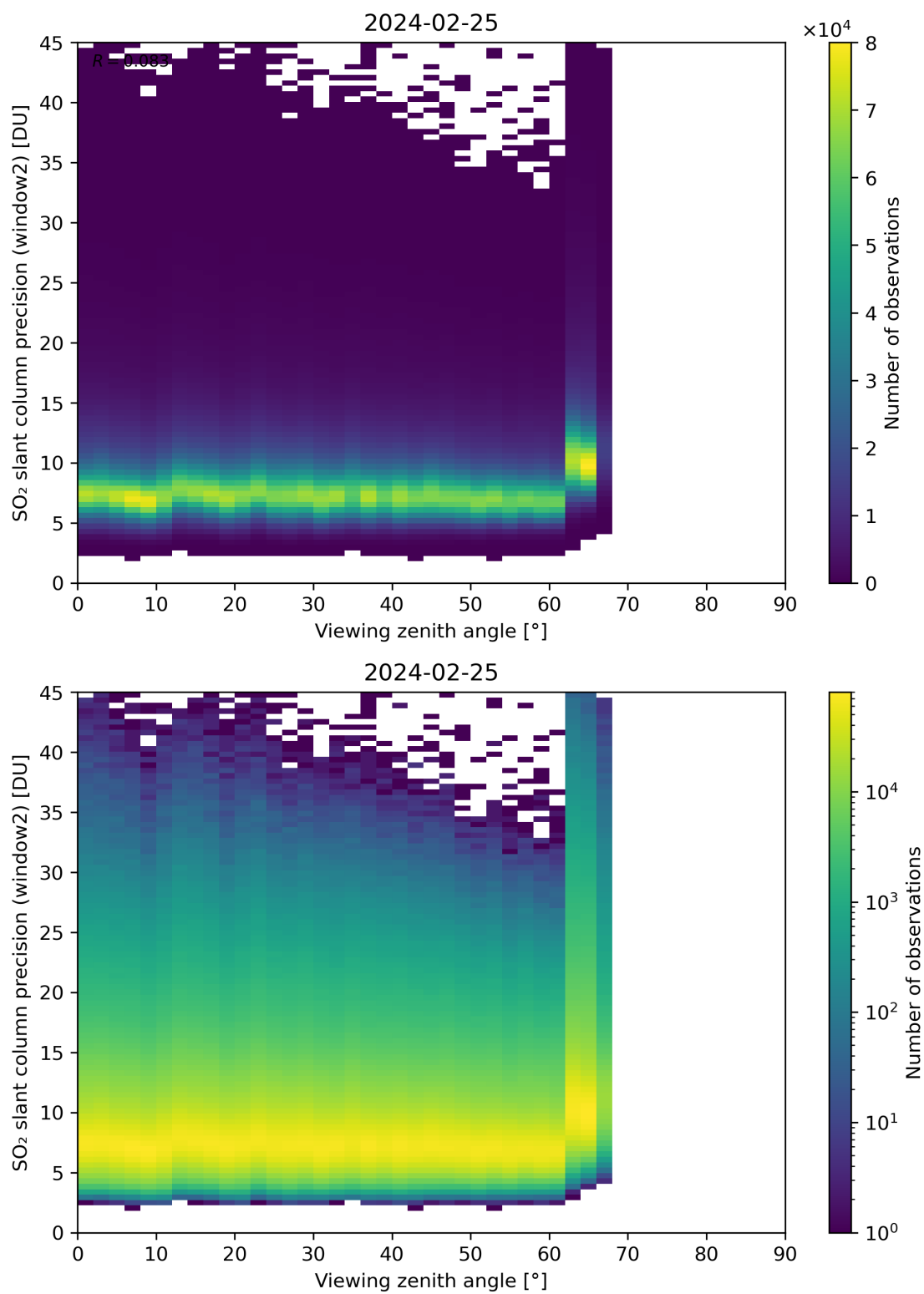
Figure 322: Scatter density plot of “Viewing zenith angle” against “SO 2 slant column precision (window2)” for 2024-02-24 to 2024-02-26.
