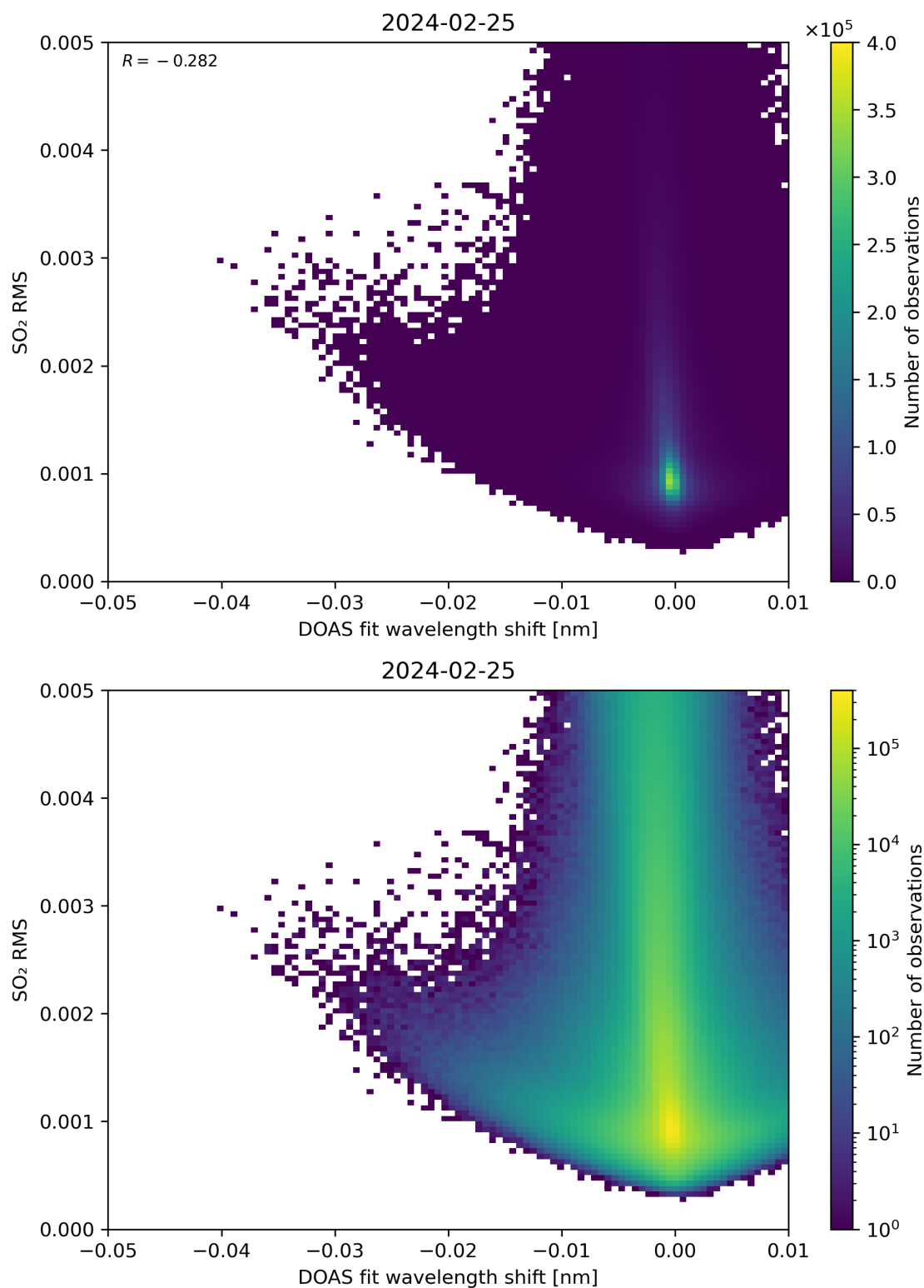
Figure 128: Scatter density plot of “DOAS fit wavelength shift” against “SO 2 RMS” for 2024-02-24 to 2024-02-26.
