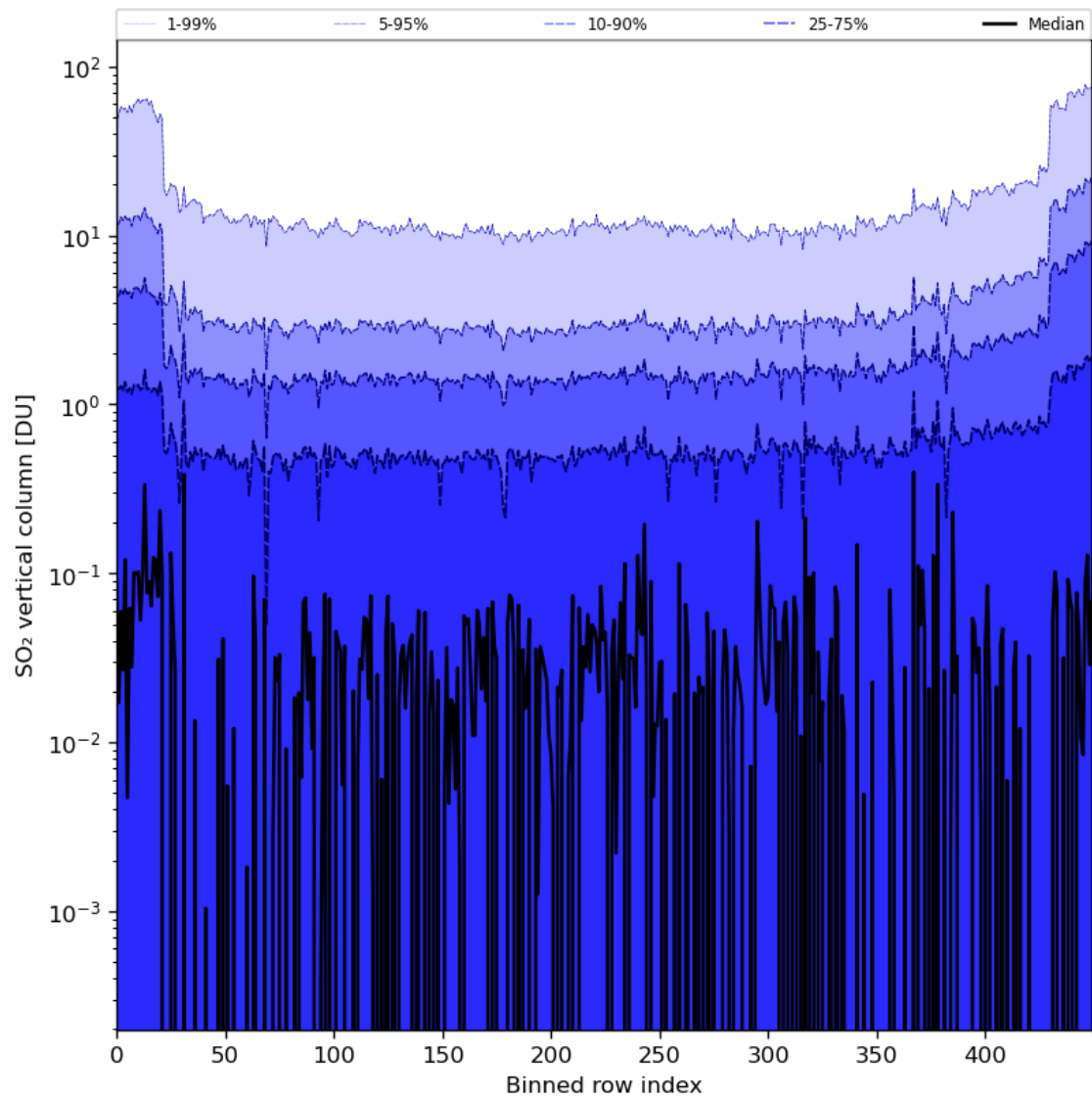
Figure 76: Along track statistics of “SO 2 vertical column” for 2024-02-24 to 2024-02-26
