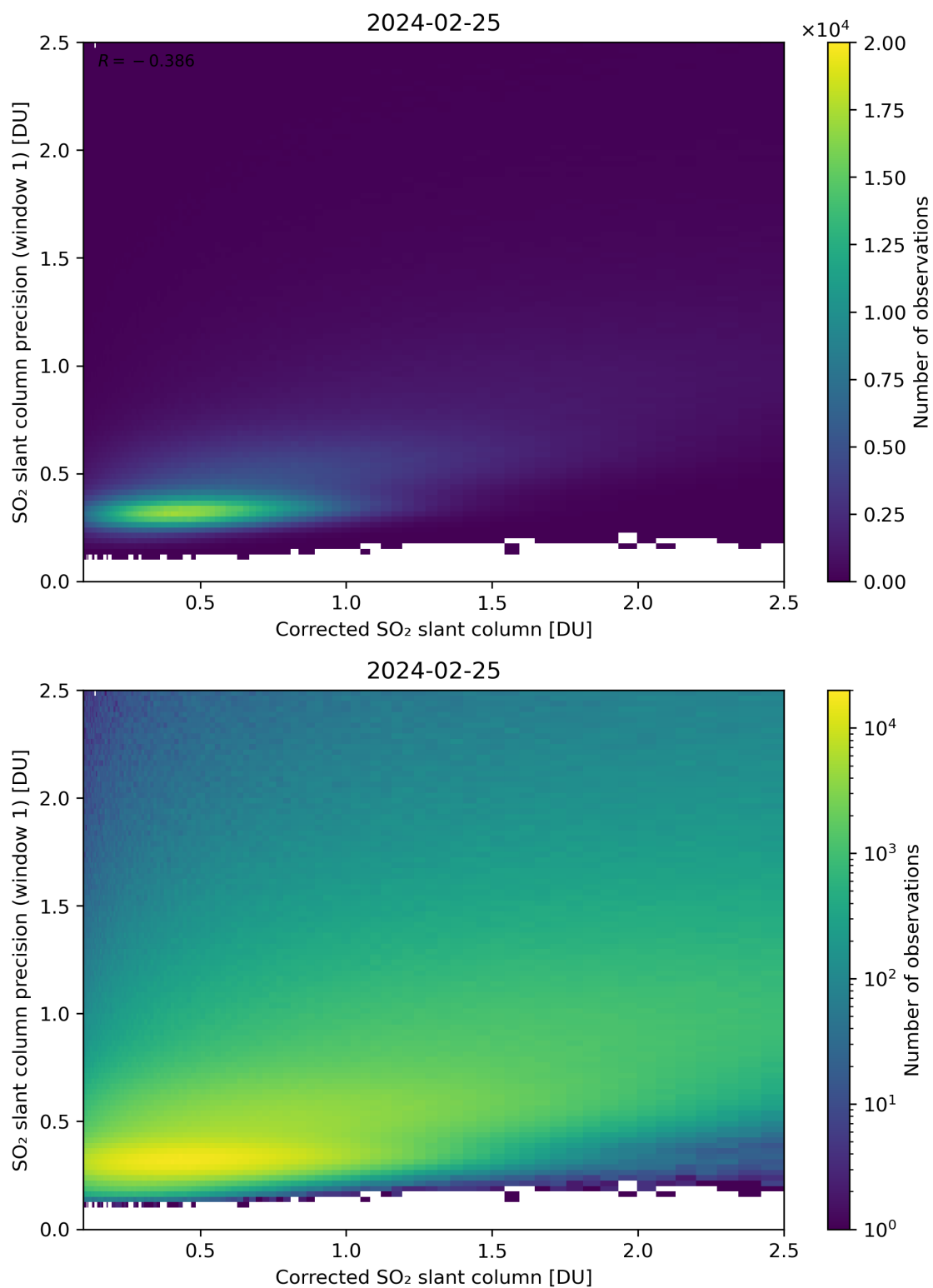
Figure 188: Scatter density plot of “Corrected SO 2 slant column” against “SO 2 slant column precision (window 1)” for 2024-02-24 to 2024-02-26.
