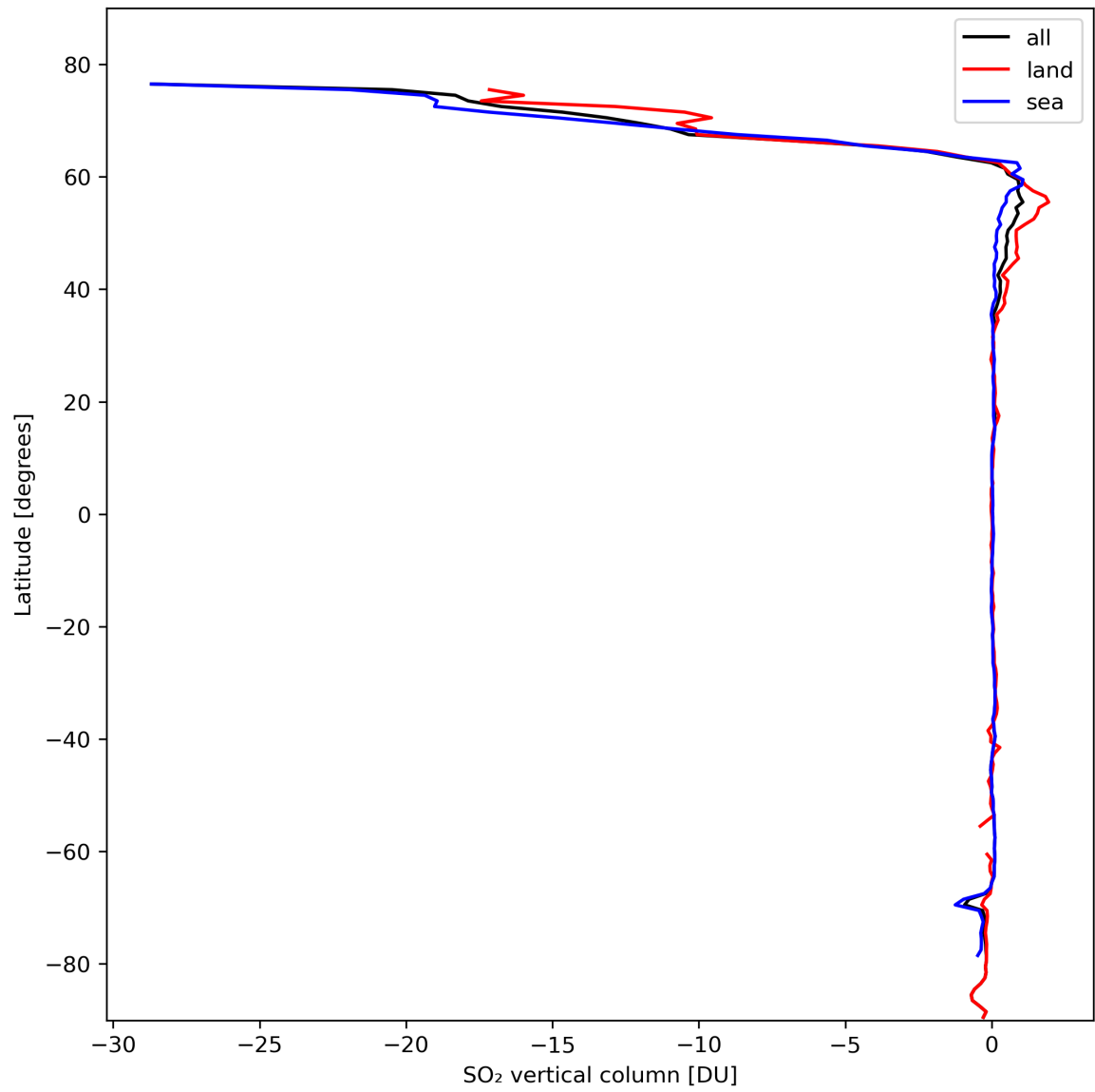
Figure 30: Zonal average of “SO 2 vertical column” for 2024-02-24 to 2024-02-26.
