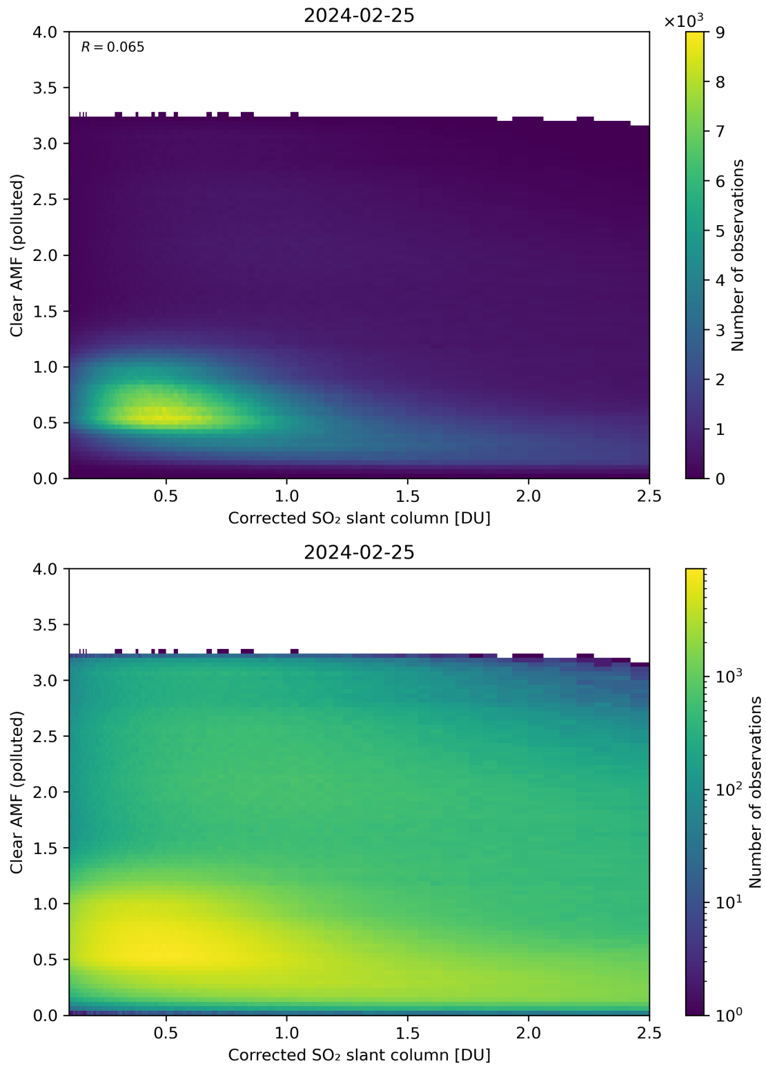
Figure 184: Scatter density plot of “Corrected SO 2 slant column” against “Clear AMF (polluted)” for 2024-02-24 to 2024-02-26.
