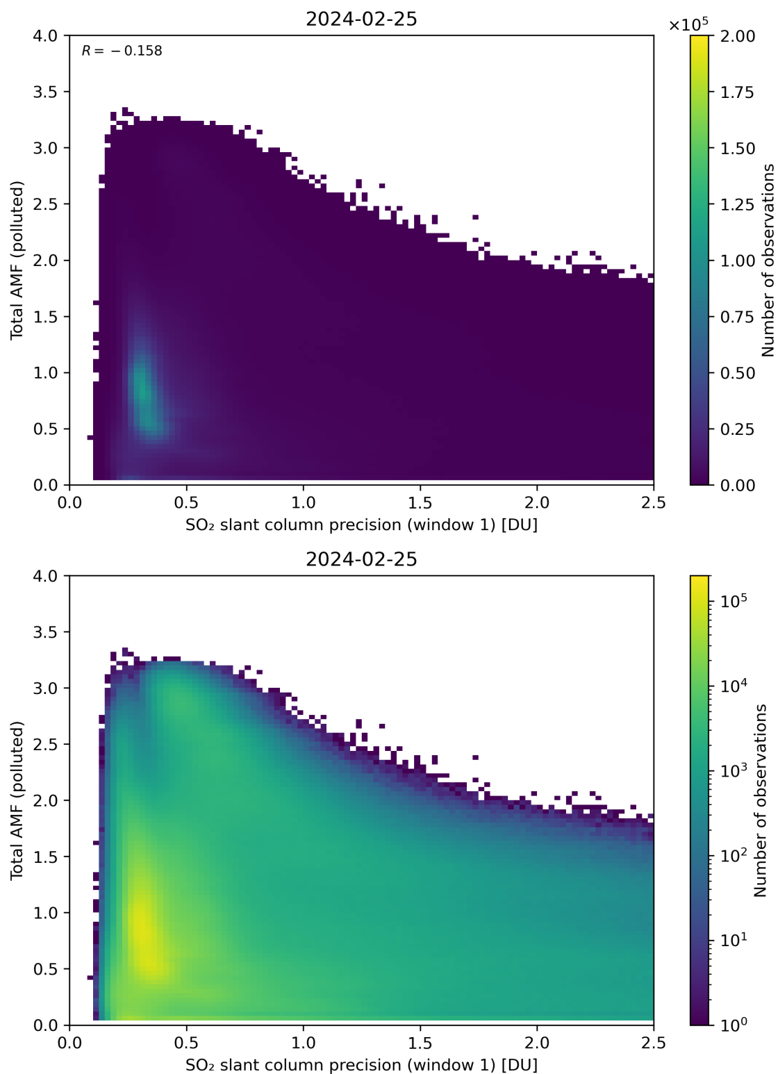
Figure 230: Scatter density plot of “SO 2 slant column precision (window 1)” against “Total AMF (polluted)” for 2024-02-24 to 2024-02-26.
