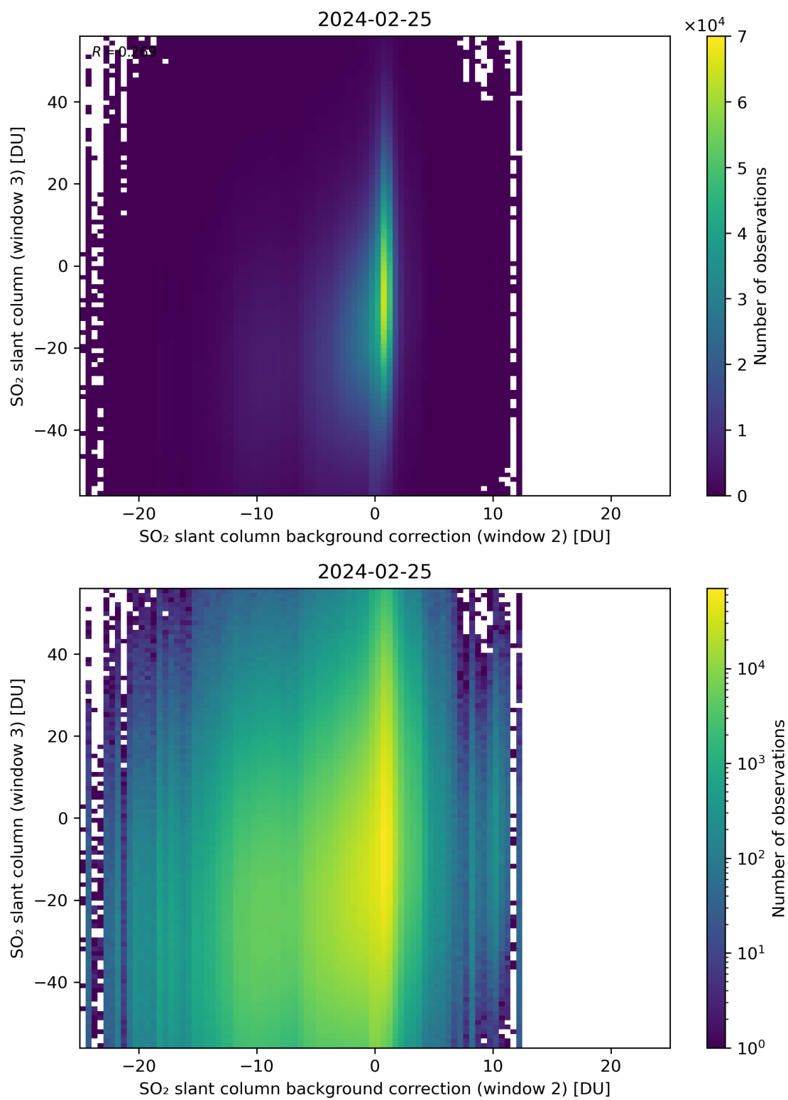
Figure 117: Scatter density plot of “SO 2 slant column background correction (window 2)” against “SO 2 slant column (window 3)” for 2024-02-24 to 2024-02-26.
