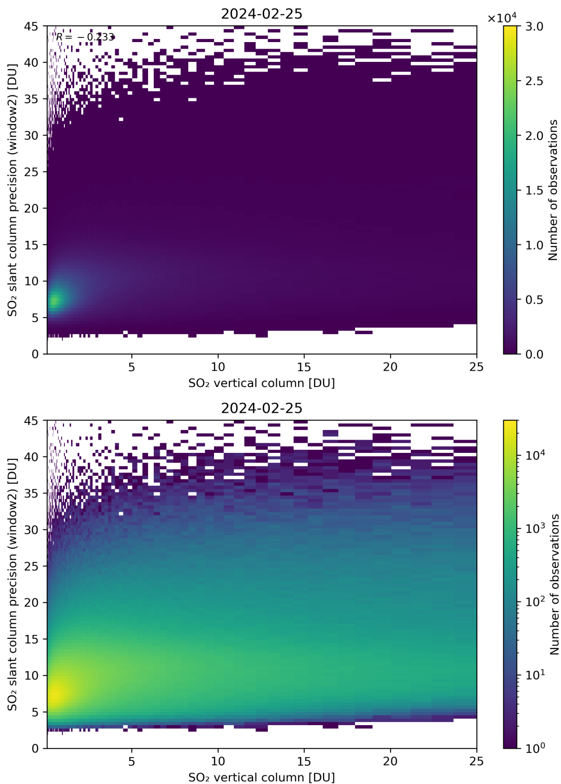
Figure 302: Scatter density plot of “SO 2 vertical column” against “SO 2 slant column precision (window2)” for 2024-02-24 to 2024-02-26.
