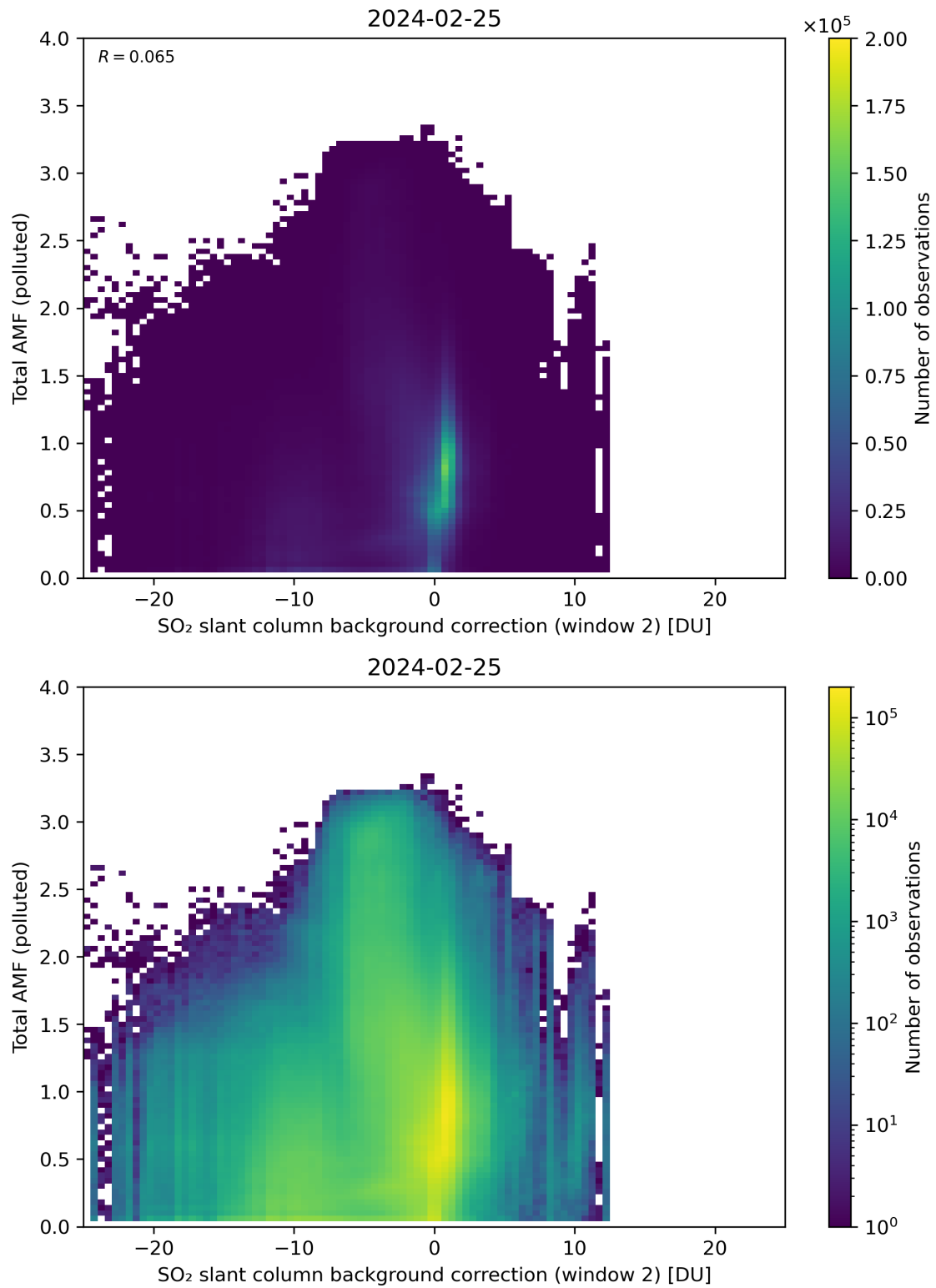
Figure 119: Scatter density plot of “SO 2 slant column background correction (window 2)” against “Total AMF (polluted)” for 2024-02-24 to 2024-02-26.
