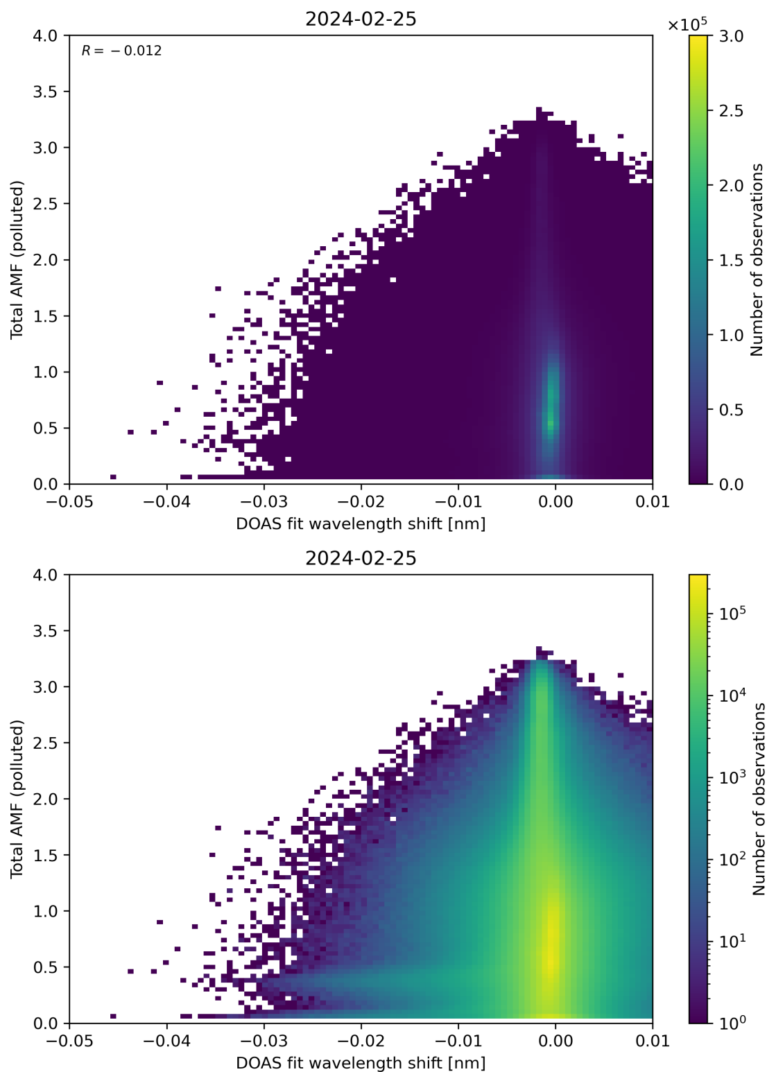
Figure 130: Scatter density plot of “DOAS fit wavelength shift” against “Total AMF (polluted)” for 2024-02-24 to 2024-02-26.
