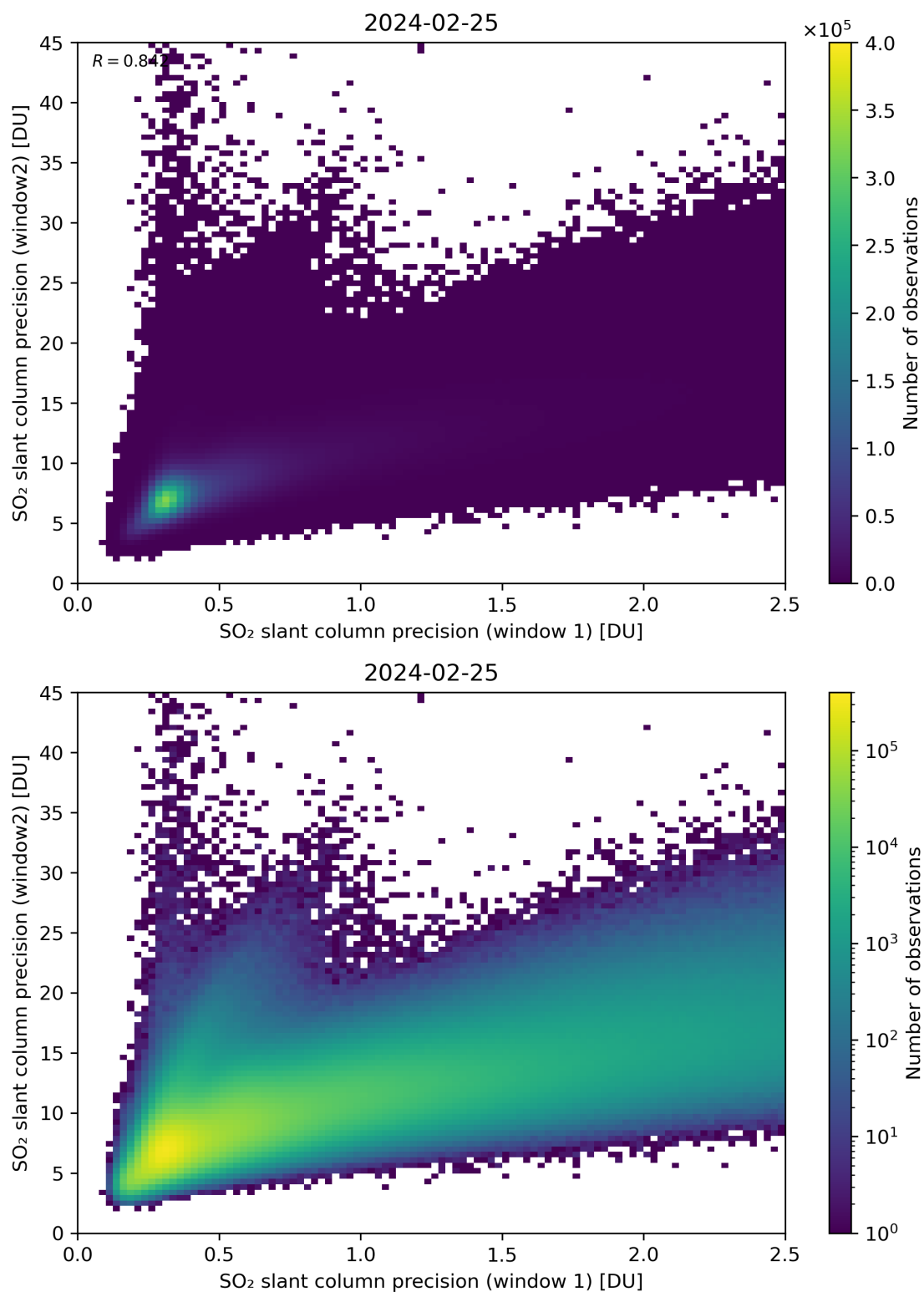
Figure 227: Scatter density plot of “SO 2 slant column precision (window 1)” against “SO 2 slant column precision (window2)” for 2024-02-24 to 2024-02-26.
