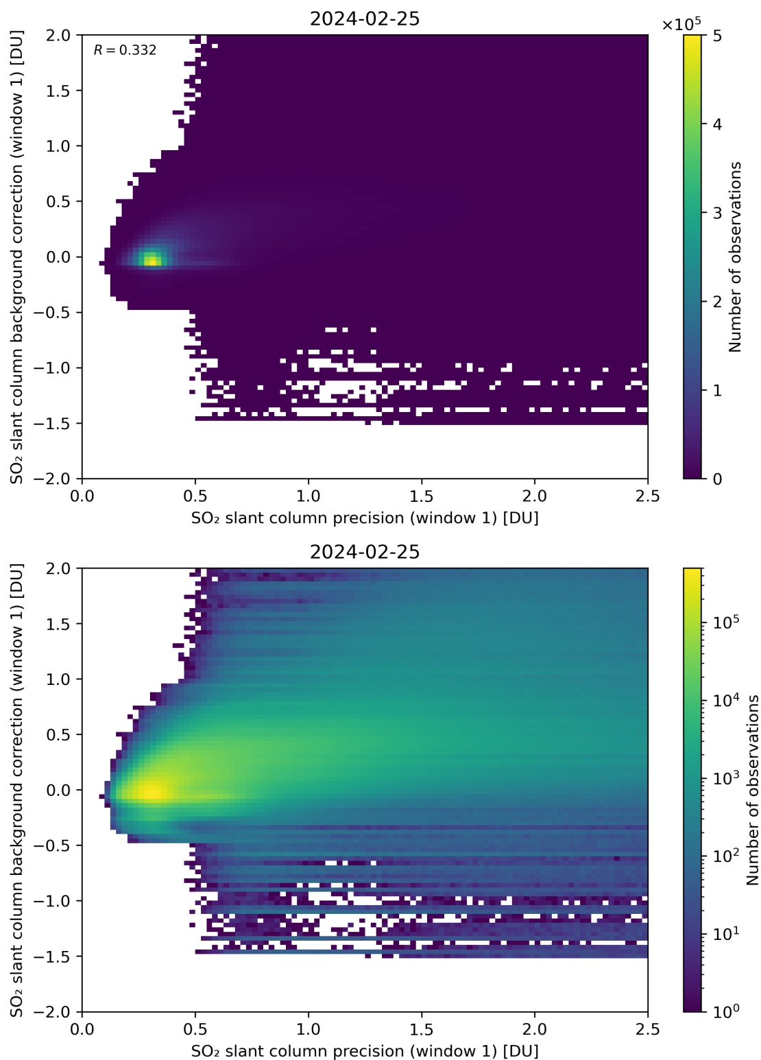
Figure 218: Scatter density plot of “SO 2 slant column precision (window 1)” against “SO 2 slant column background correction (window 1)” for 2024-02-24 to 2024-02-26.
