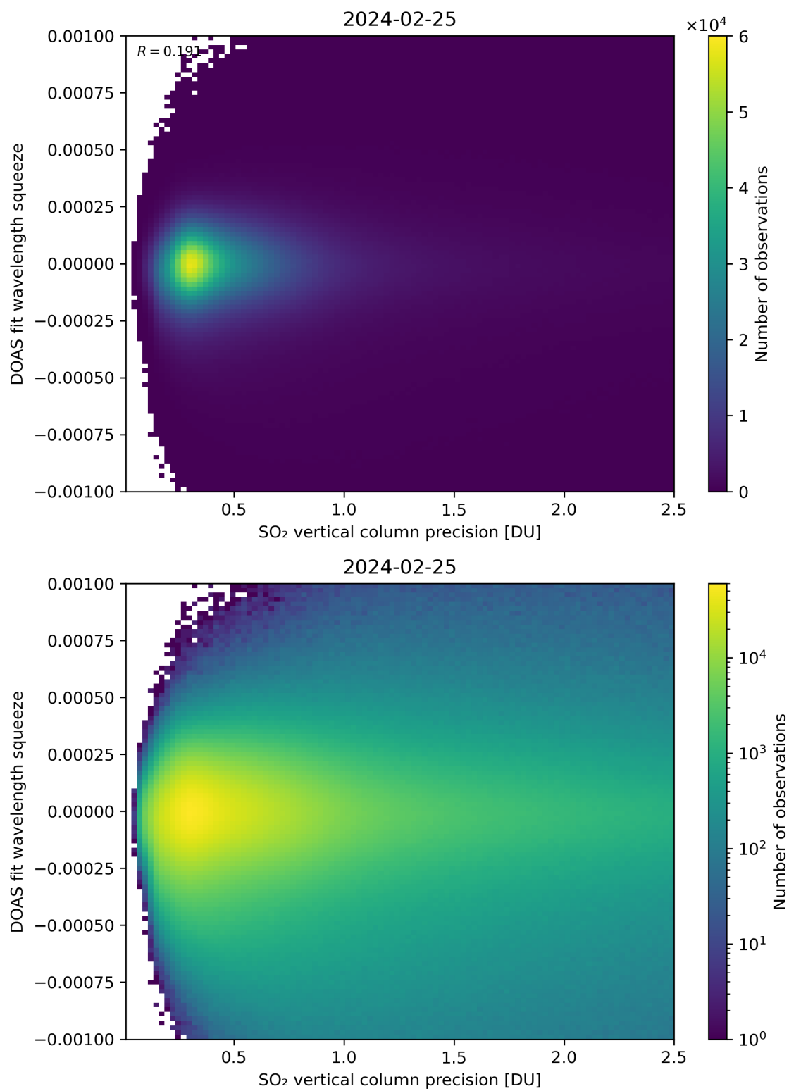
Figure 283: Scatter density plot of “SO 2 vertical column precision” against “DOAS fit wavelength squeeze” for 2024-02-24 to 2024-02-26.
