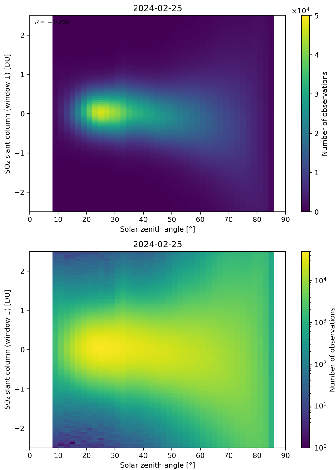
Figure 169: Scatter density plot of “Solar zenith angle” against “SO 2 slant column (window 1)” for 2024-02-24 to 2024-02-26.
