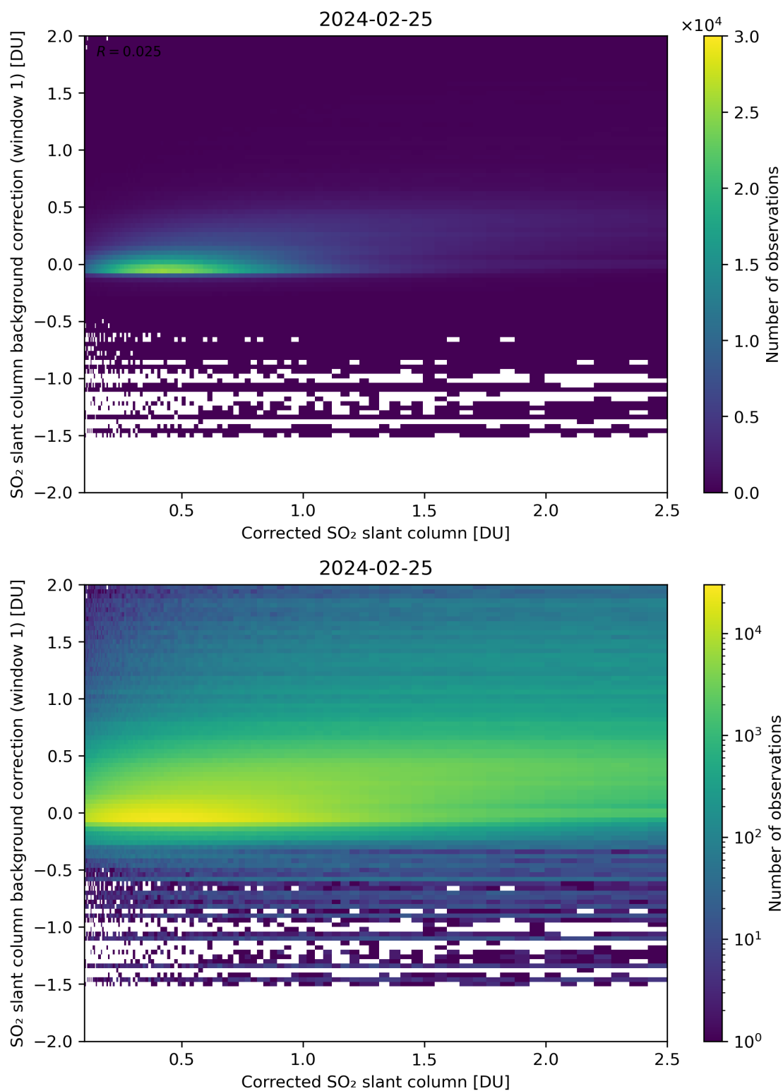
Figure 178: Scatter density plot of “Corrected SO 2 slant column” against “SO 2 slant column background correction (window 1)” for 2024-02-24 to 2024-02-26.
