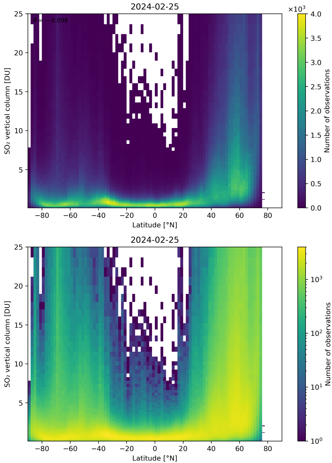
Figure 156: Scatter density plot of “Latitude” against “SO 2 vertical column” for 2024-02-24 to 2024-02-26.
