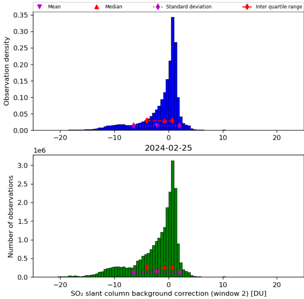
Figure 63: Histogram of “SO 2 slant column background correction (window 2)” for 2024-02-24 to 2024-02-26
