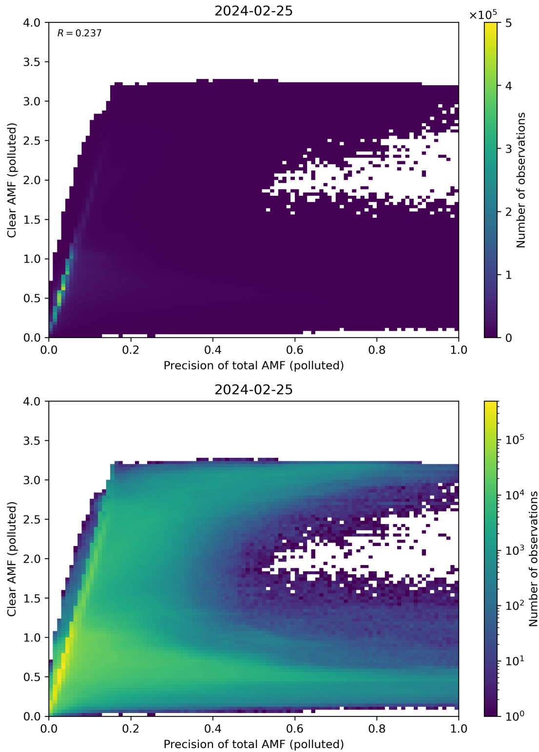
Figure 270: Scatter density plot of “Precision of total AMF (polluted)” against “Clear AMF (polluted)” for 2024-02-24 to 2024-02-26.
