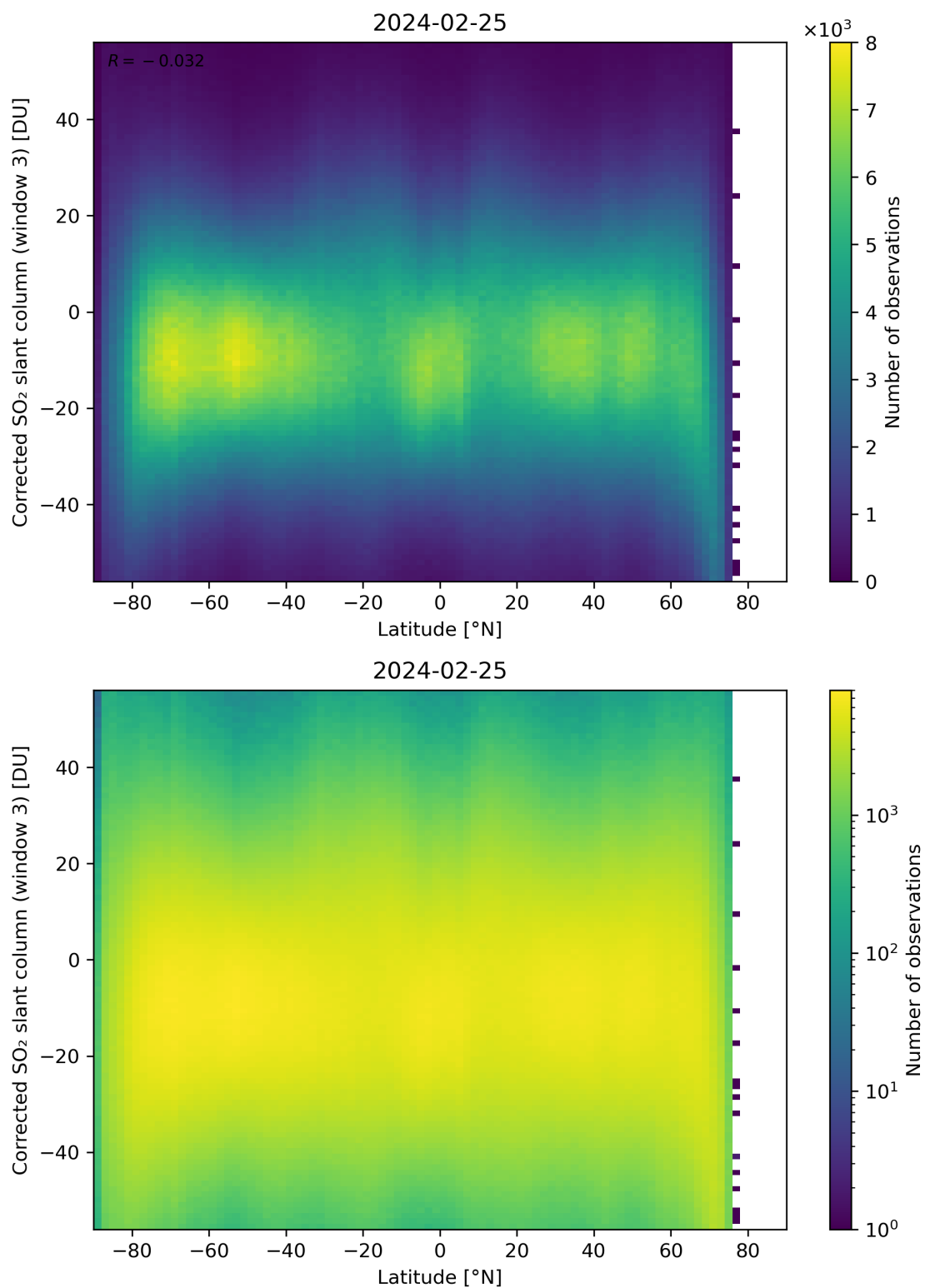
Figure 148: Scatter density plot of “Latitude” against “Corrected SO 2 slant column (window 3)” for 2024-02-24 to 2024-02-26.
