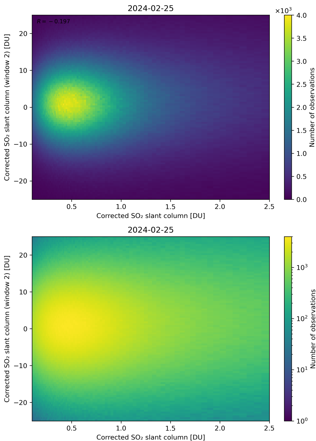
Figure 185: Scatter density plot of “Corrected SO 2 slant column” against “Corrected SO 2 slant column (window 2)” for 2024-02-24 to 2024-02-26.
