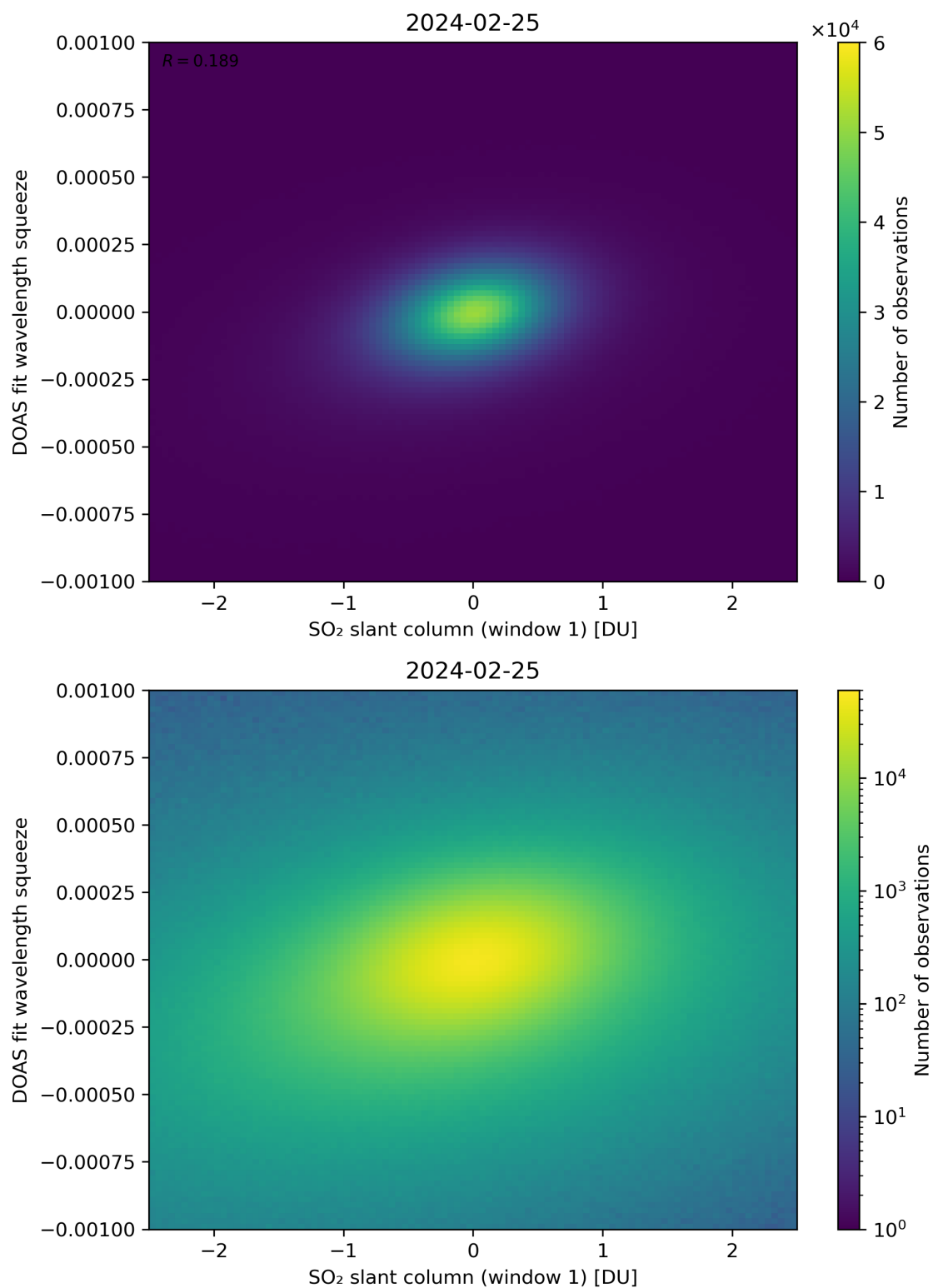
Figure 216: Scatter density plot of “SO 2 slant column (window 1)” against “DOAS fit wavelength squeeze” for 2024-02-24 to 2024-02-26.
