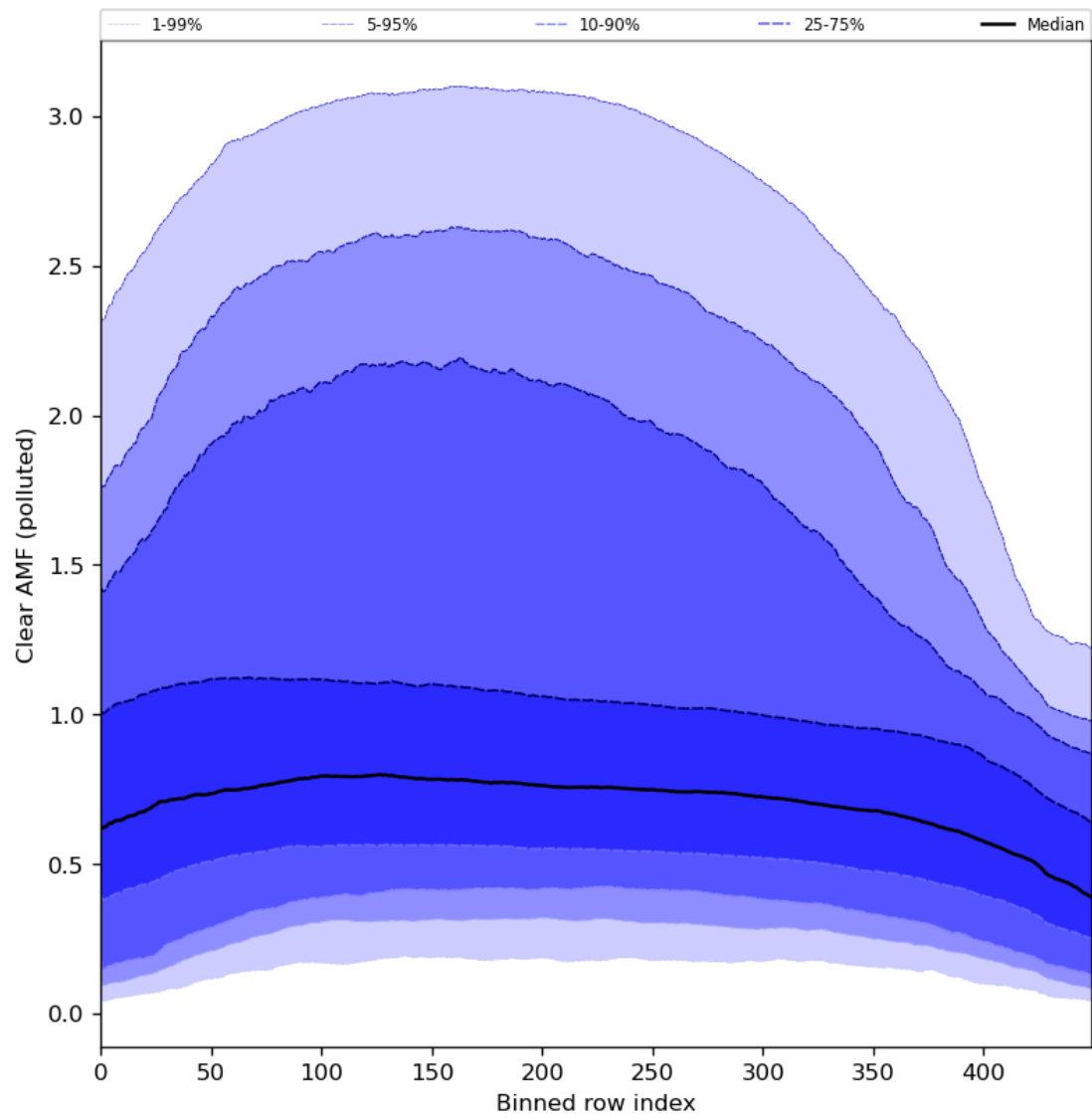
Figure 96: Along track statistics of “Clear AMF (polluted)” for 2024-02-24 to 2024-02-26
