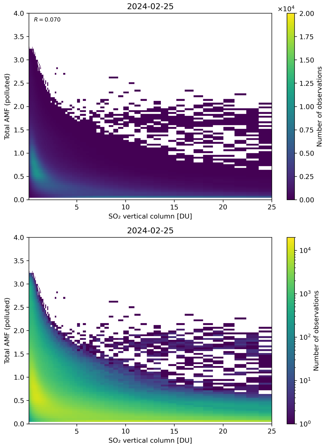
Figure 305: Scatter density plot of “SO 2 vertical column” against “Total AMF (polluted)” for 2024-02-24 to 2024-02-26.
