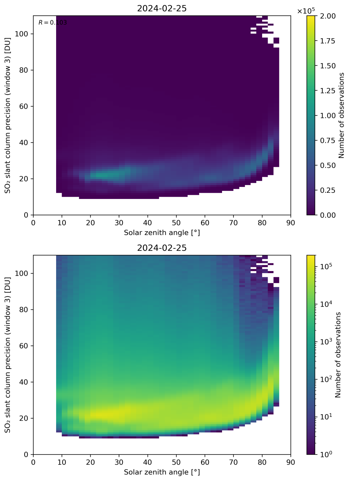
Figure 173: Scatter density plot of “Solar zenith angle” against “SO 2 slant column precision (window 3)” for 2024-02-24 to 2024-02-26.
