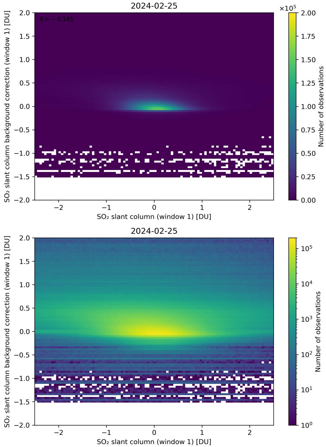
Figure 212: Scatter density plot of “SO 2 slant column (window 1)” against “SO 2 slant column background correction (window 1)” for 2024-02-24 to 2024-02-26.
