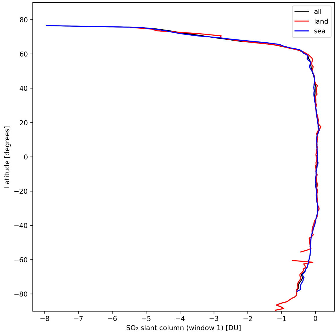
Figure 33: Zonal average of “SO 2 slant column (window 1)” for 2024-02-24 to 2024-02-26.
