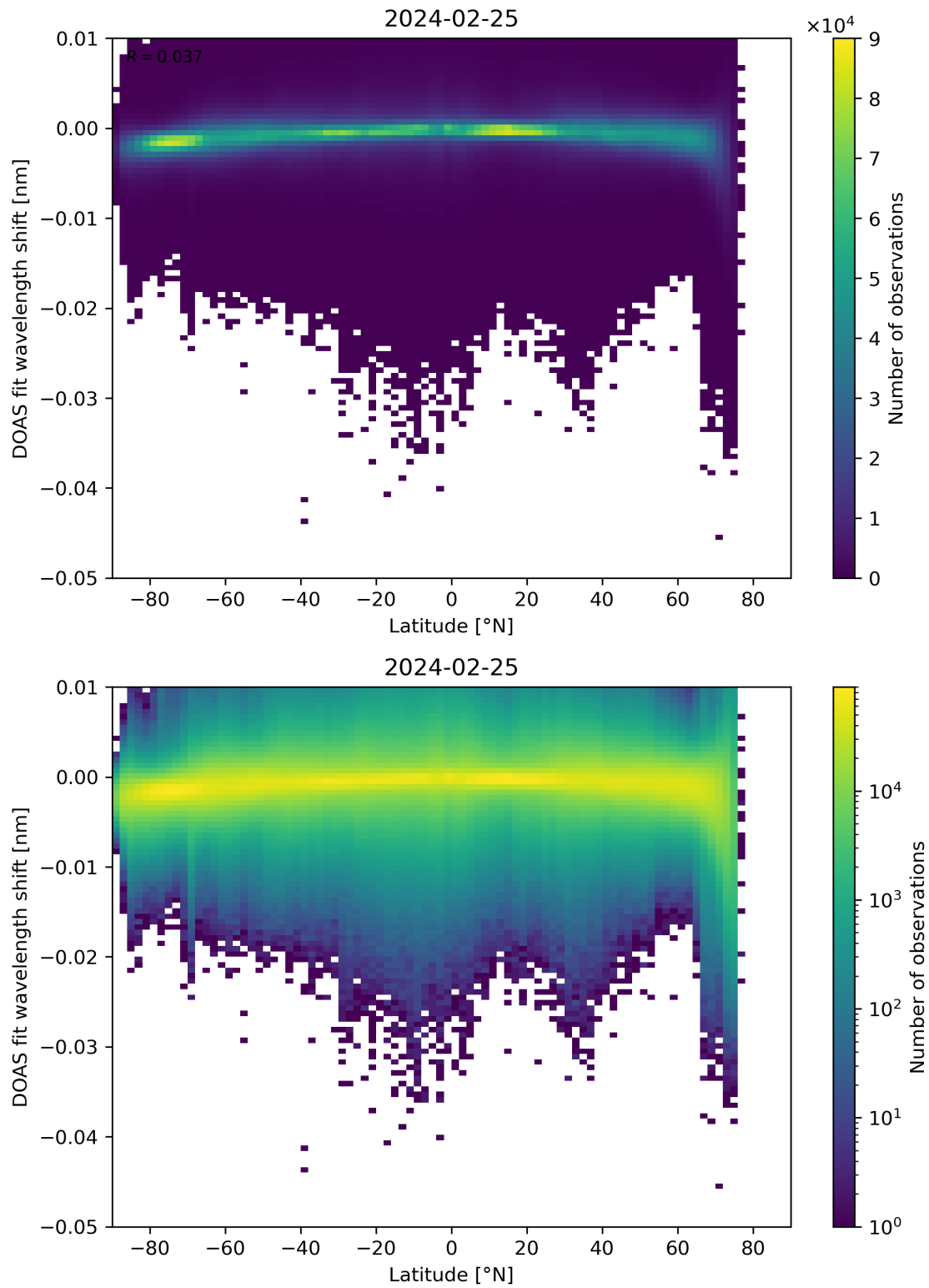
Figure 142: Scatter density plot of “Latitude” against “DOAS fit wavelength shift” for 2024-02-24 to 2024-02-26.
