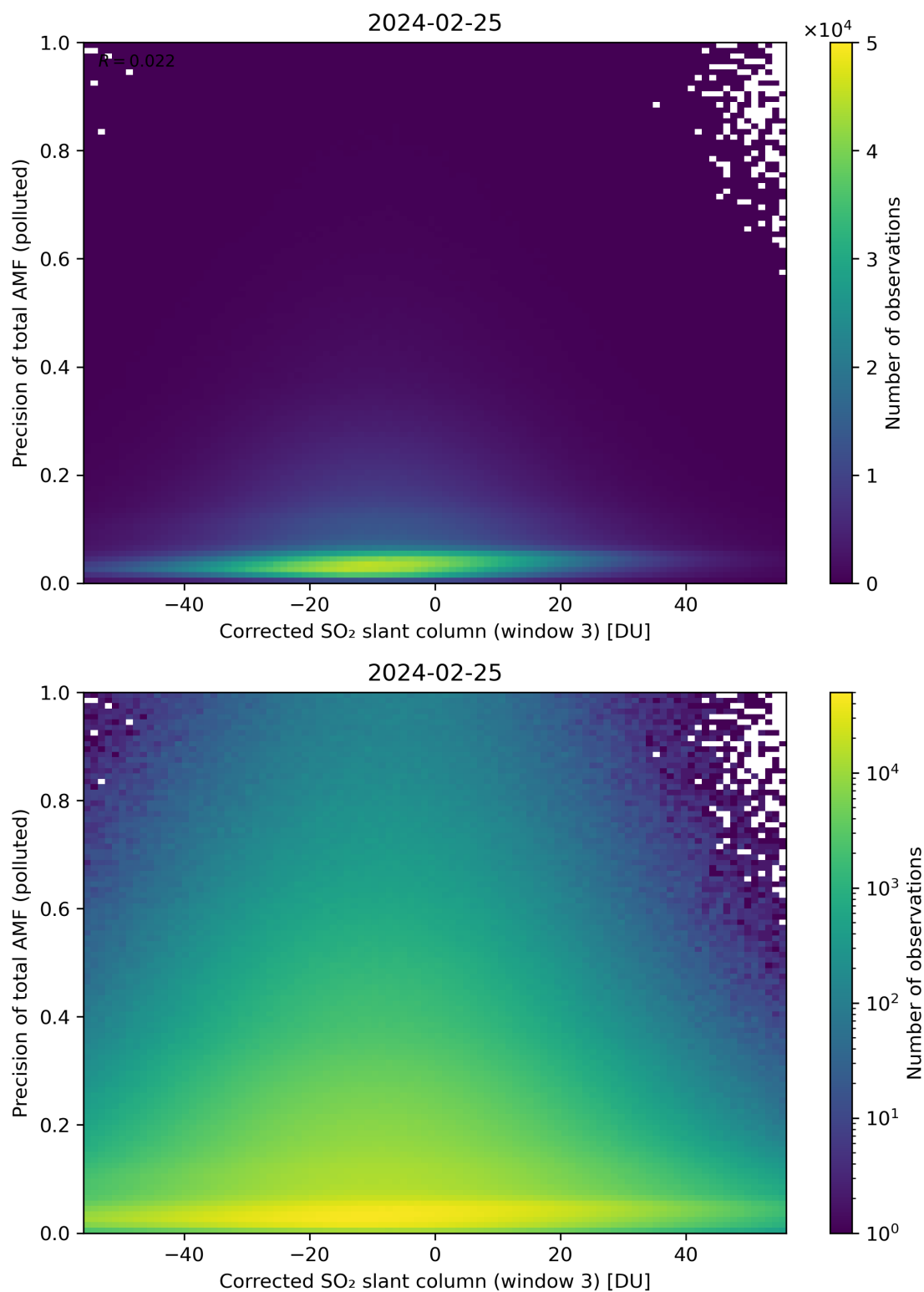
Figure 211: Scatter density plot of “Corrected SO 2 slant column (window 3)” against “Precision of total AMF (polluted)” for 2024-02-24 to 2024-02-26.
