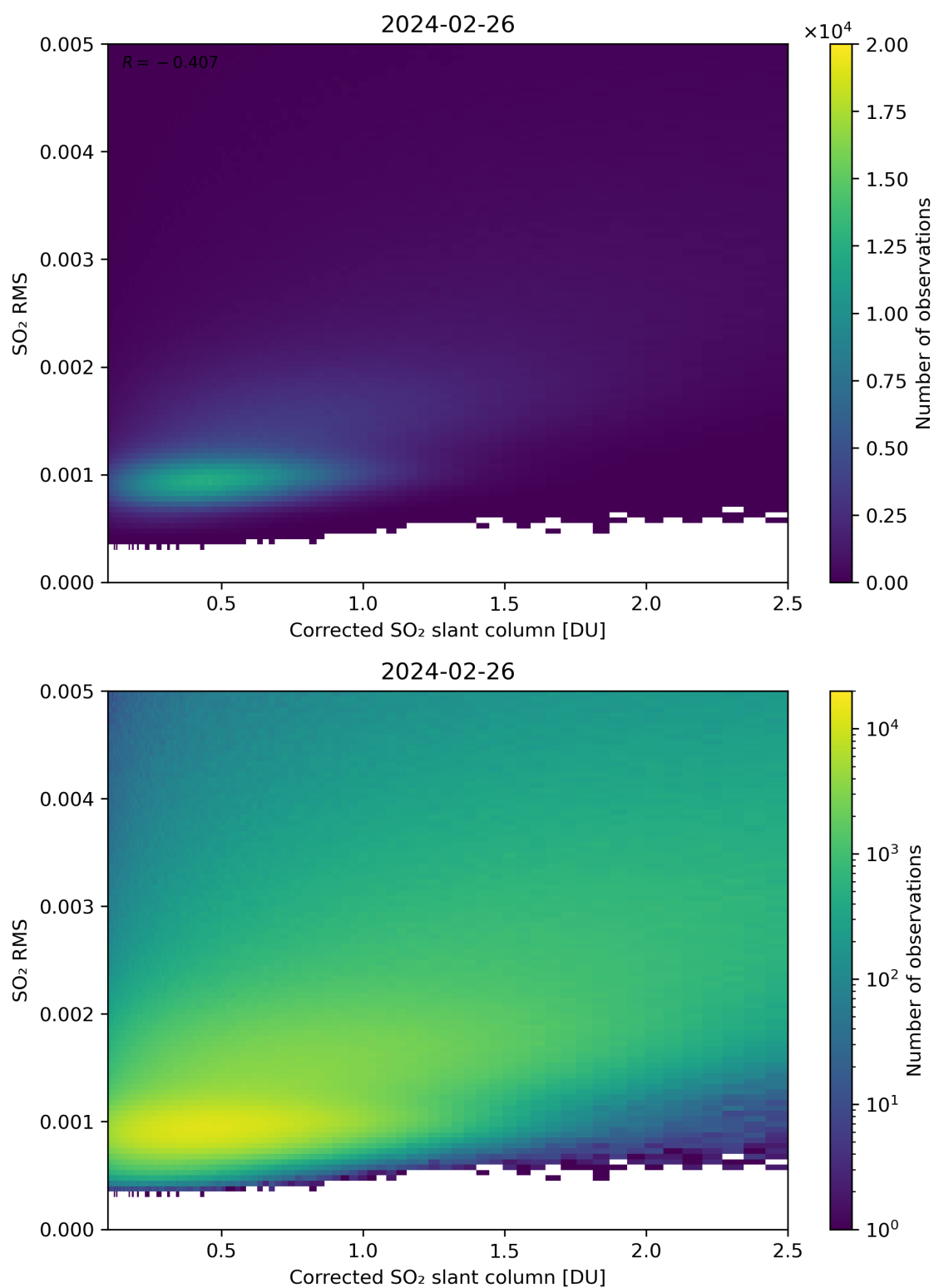
Figure 183: Scatter density plot of “Corrected SO 2 slant column” against “SO 2 RMS” for 2024-02-25 to 2024-02-27.
