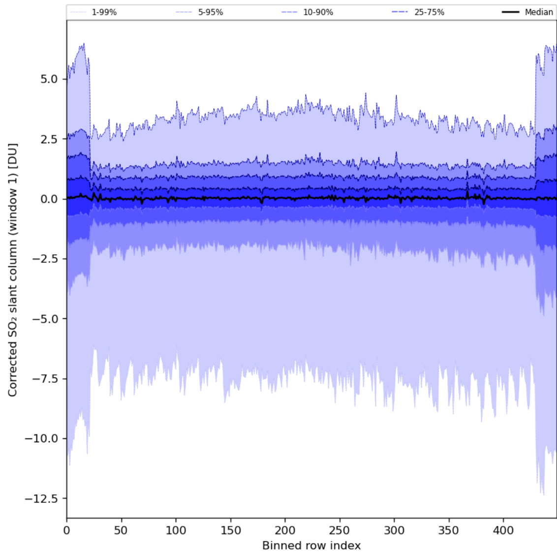
Figure 81: Along track statistics of “Corrected SO 2 slant column (window 1)” for 2024-02-25 to 2024-02-27
