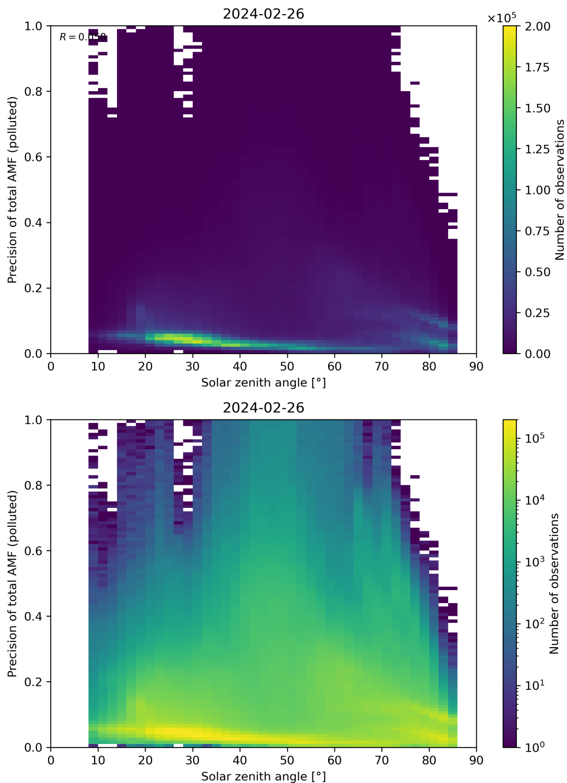
Figure 175: Scatter density plot of “Solar zenith angle” against “Precision of total AMF (polluted)” for 2024-02-25 to 2024-02-27.
