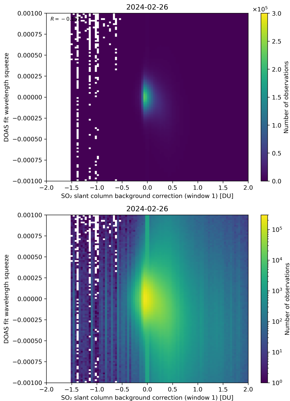
Figure 101: Scatter density plot of “SO 2 slant column background correction (window 1)” against “DOAS fit wavelength squeeze” for 2024-02-25 to 2024-02-27.
