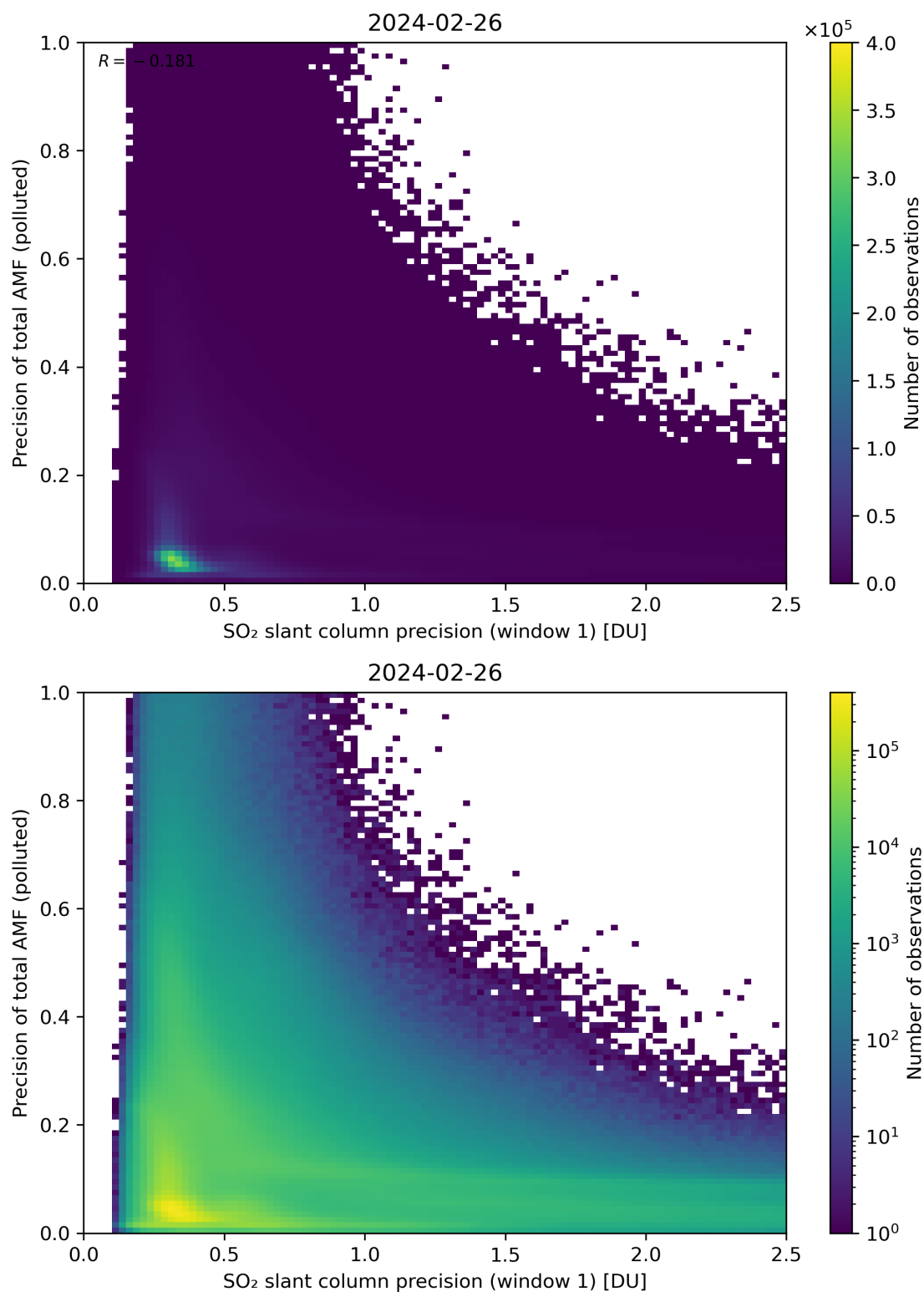
Figure 231: Scatter density plot of “SO 2 slant column precision (window 1)” against “Precision of total AMF (polluted)” for 2024-02-25 to 2024-02-27.
