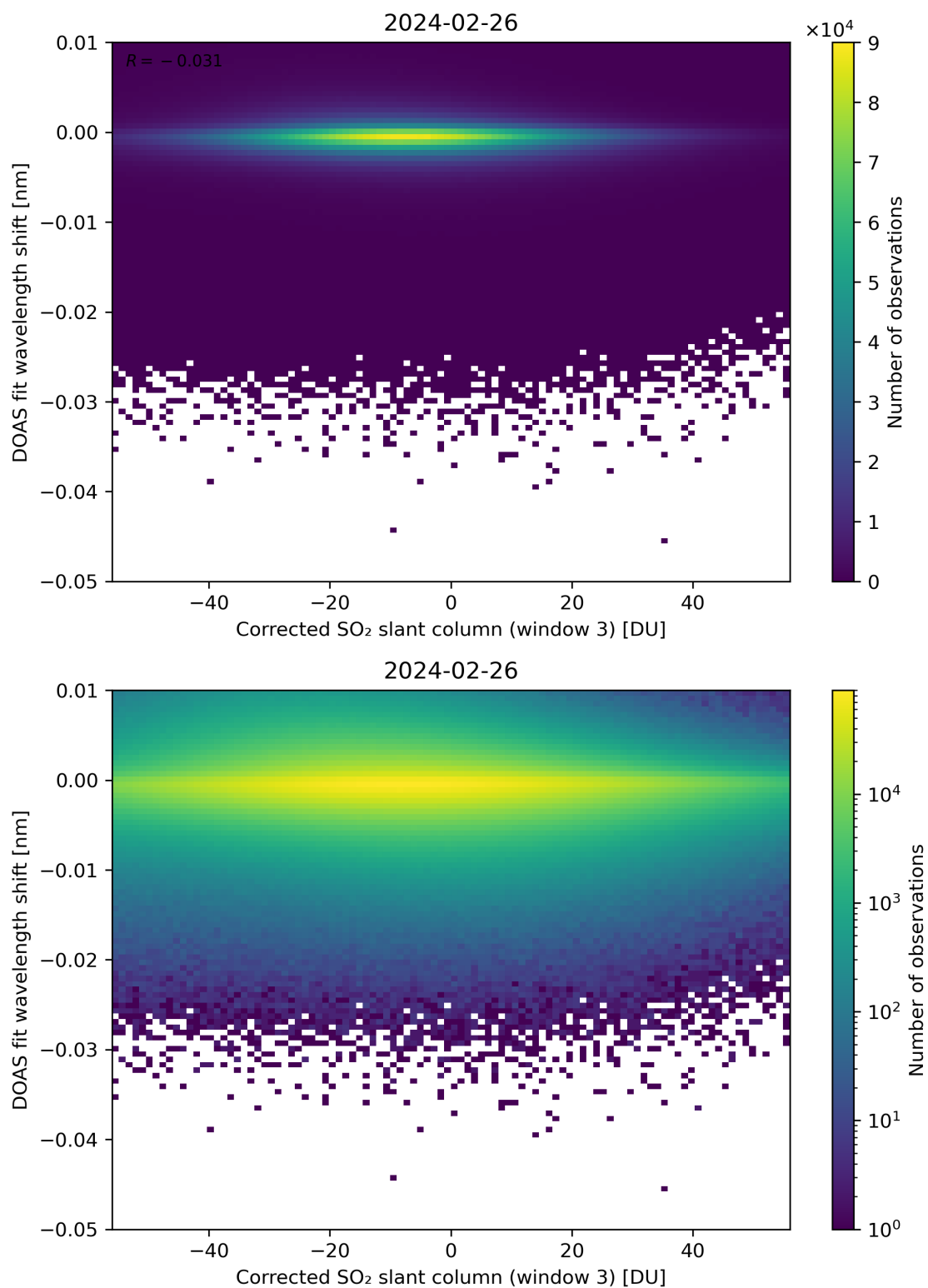
Figure 206: Scatter density plot of “Corrected SO 2 slant column (window 3)” against “DOAS fit wavelength shift” for 2024-02-25 to 2024-02-27.
