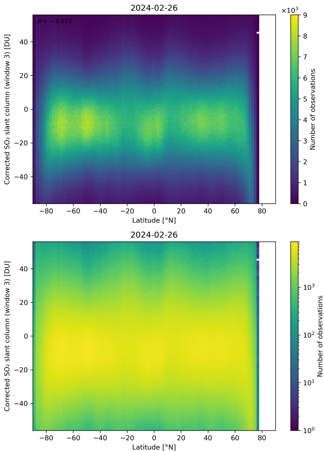
Figure 148: Scatter density plot of “Latitude” against “Corrected SO 2 slant column (window 3)” for 2024-02-25 to 2024-02-27.
