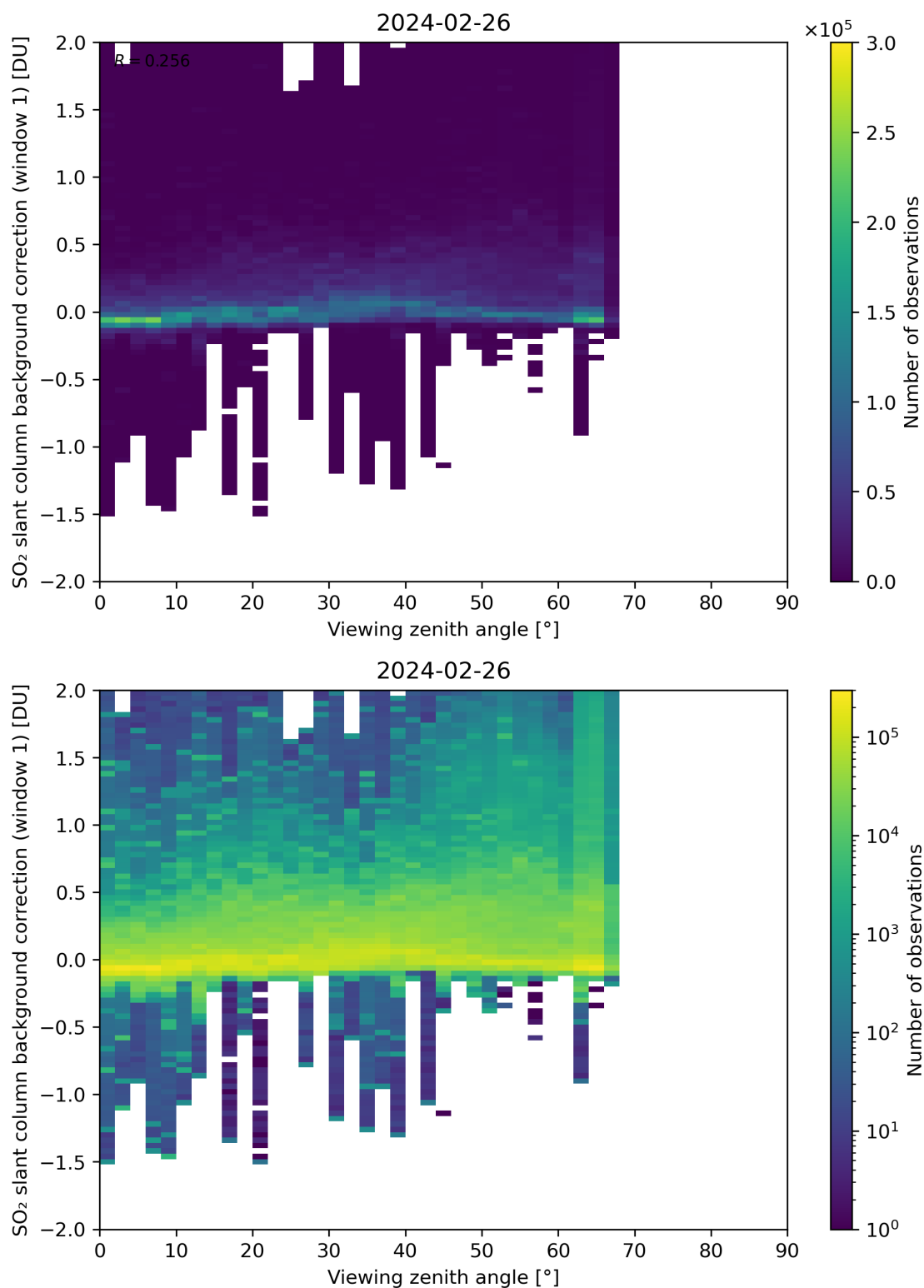
Figure 308: Scatter density plot of “Viewing zenith angle” against “SO 2 slant column background correction (window 1)” for 2024-02-25 to 2024-02-27.
