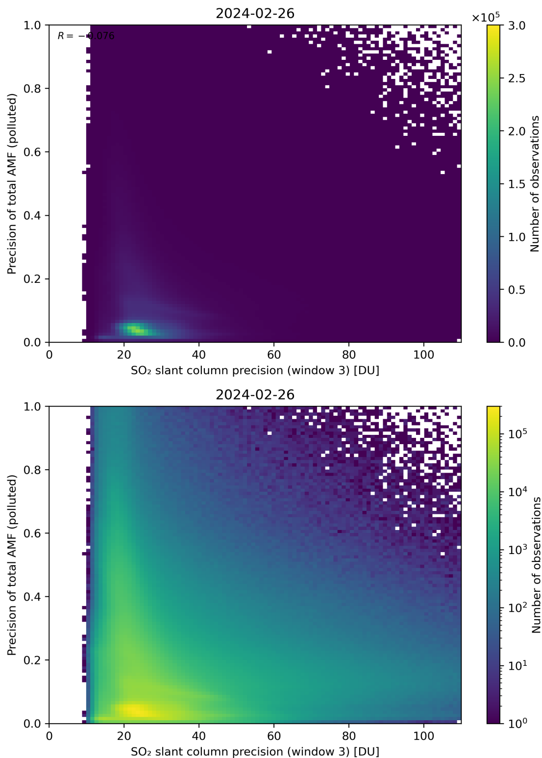
Figure 264: Scatter density plot of “SO 2 slant column precision (window 3)” against “Precision of total AMF (polluted)” for 2024-02-25 to 2024-02-27.
