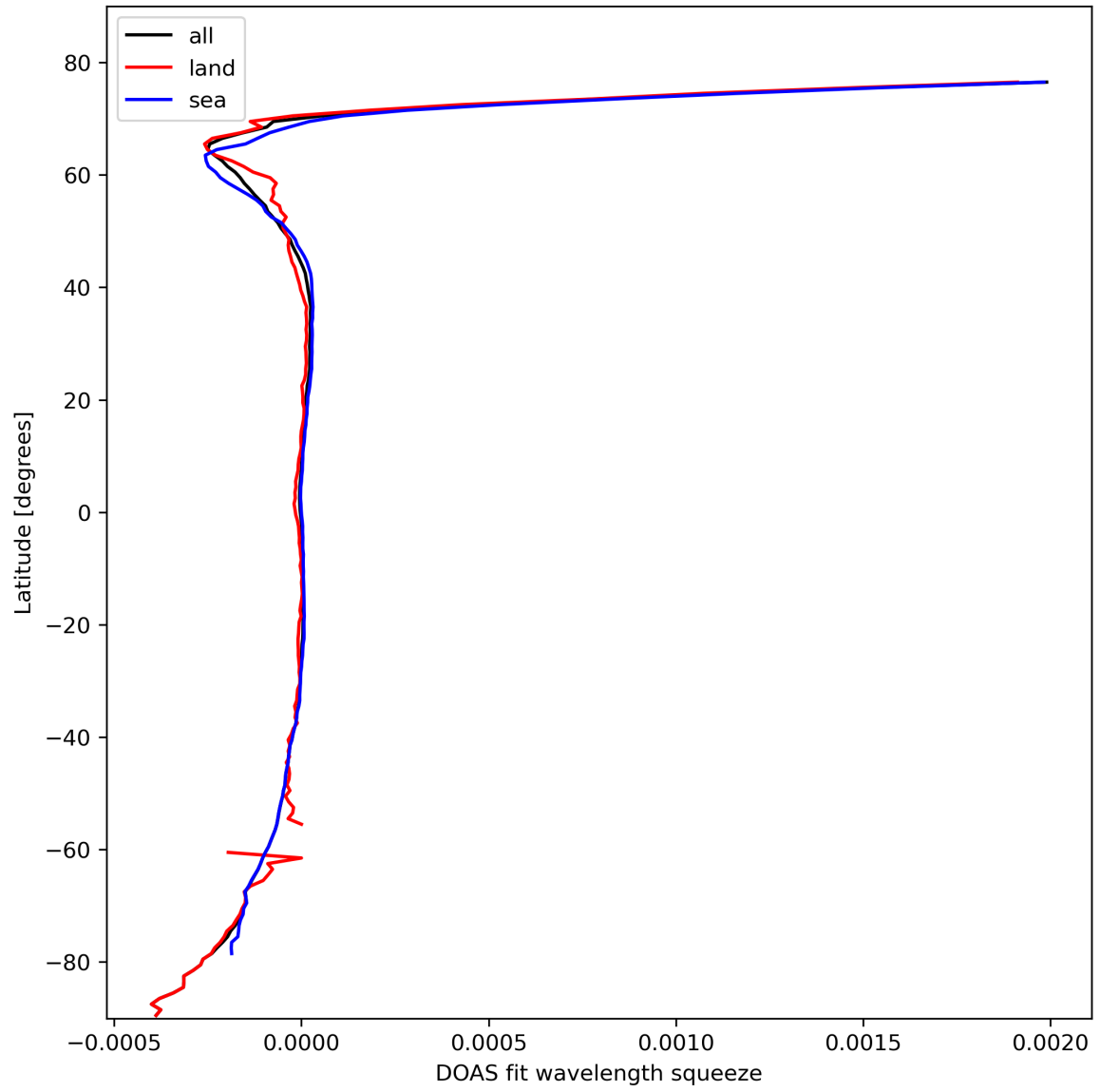
Figure 46: Zonal average of “DOAS fit wavelength squeeze” for 2024-02-25 to 2024-02-27.
