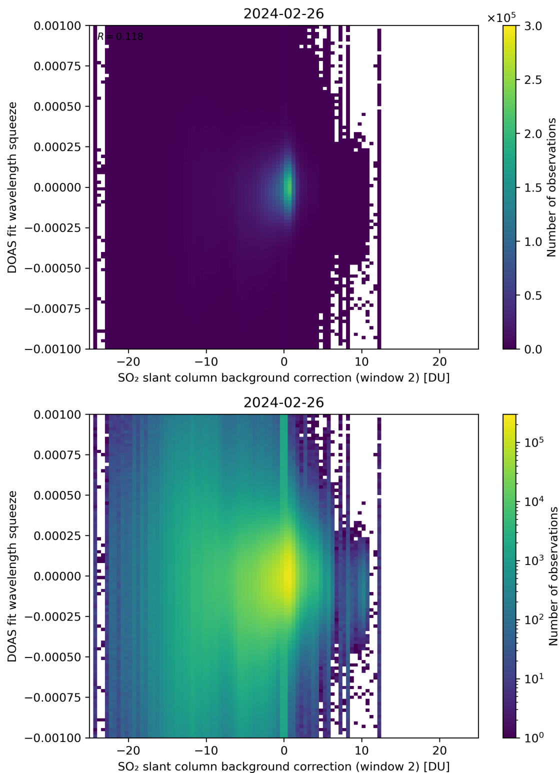
Figure 113: Scatter density plot of “SO 2 slant column background correction (window 2)” against “DOAS fit wavelength squeeze” for 2024-02-25 to 2024-02-27.
