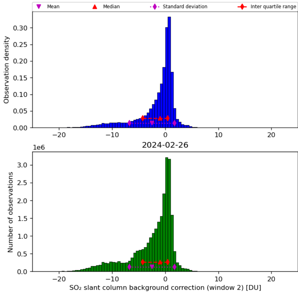
Figure 63: Histogram of “SO 2 slant column background correction (window 2)” for 2024-02-25 to 2024-02-27
