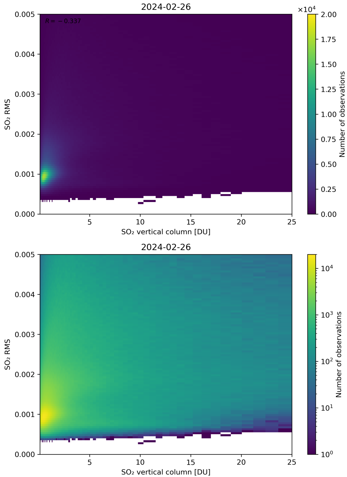
Figure 278: Scatter density plot of “SO 2 vertical column” against “SO 2 RMS” for 2024-02-25 to 2024-02-27.
