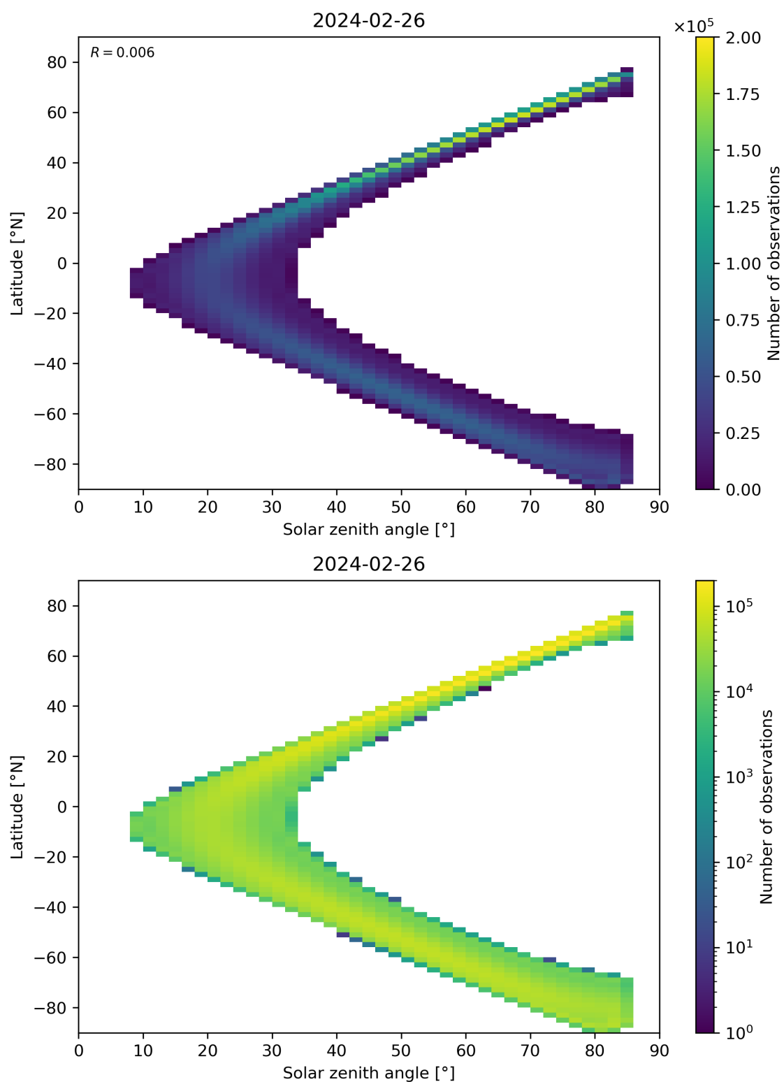
Figure 164: Scatter density plot of “Solar zenith angle” against “Latitude” for 2024-02-25 to 2024-02-27.
