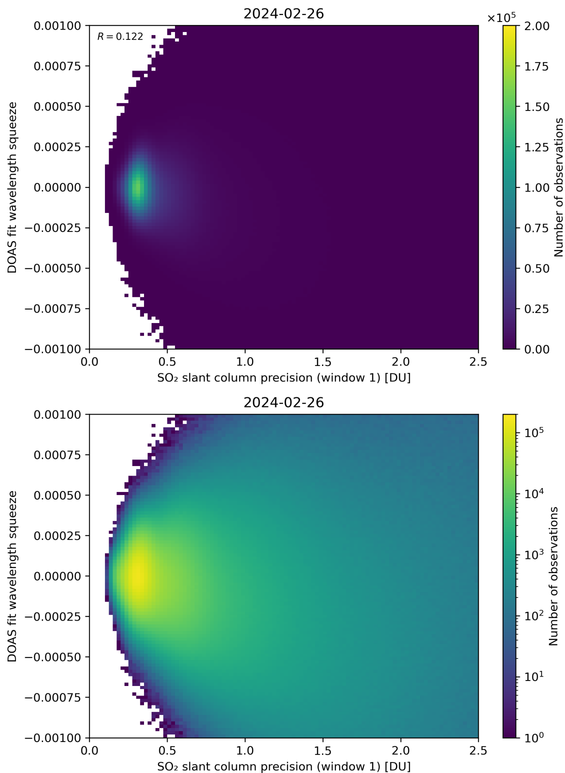
Figure 222: Scatter density plot of “SO 2 slant column precision (window 1)” against “DOAS fit wavelength squeeze” for 2024-02-25 to 2024-02-27.
