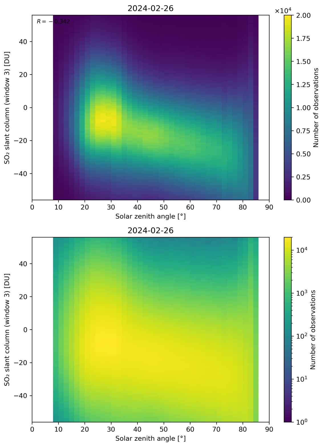
Figure 172: Scatter density plot of “Solar zenith angle” against “SO 2 slant column (window 3)” for 2024-02-25 to 2024-02-27.
