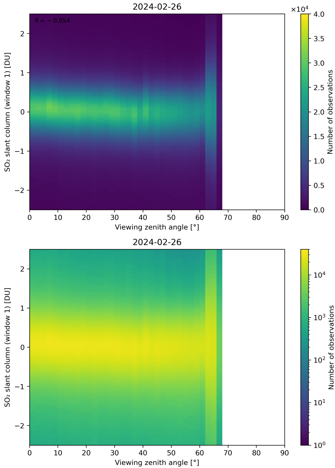
Figure 320: Scatter density plot of “Viewing zenith angle” against “SO 2 slant column (window 1)” for 2024-02-25 to 2024-02-27.
