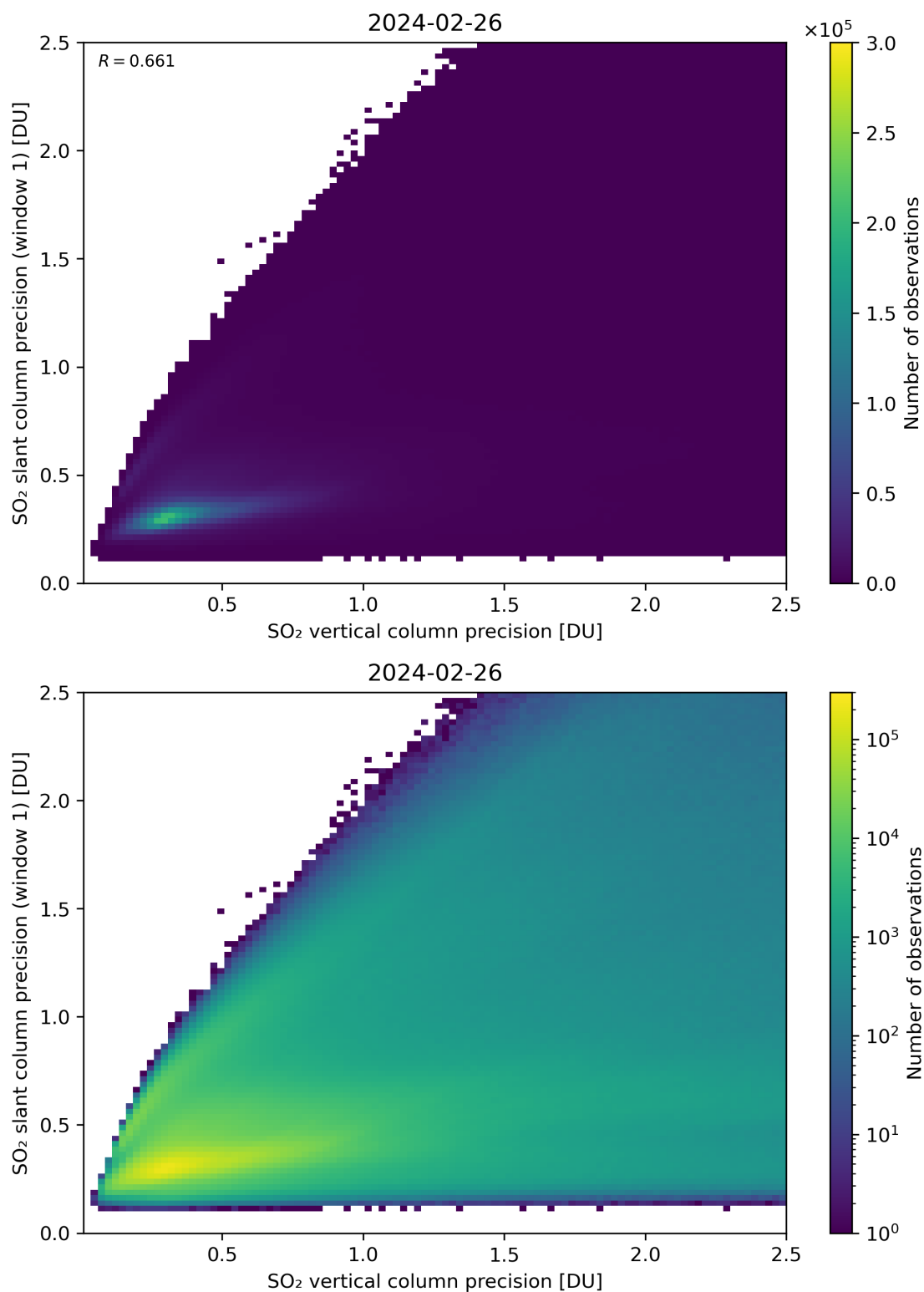
Figure 290: Scatter density plot of “SO 2 vertical column precision” against “SO 2 slant column precision (window 1)” for 2024-02-25 to 2024-02-27.
