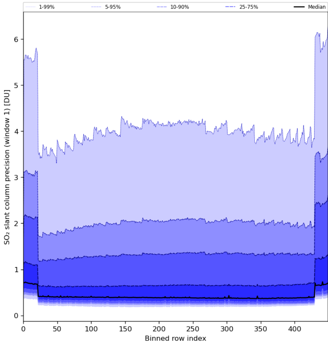
Figure 80: Along track statistics of “SO 2 slant column precision (window 1)” for 2024-02-25 to 2024-02-27
