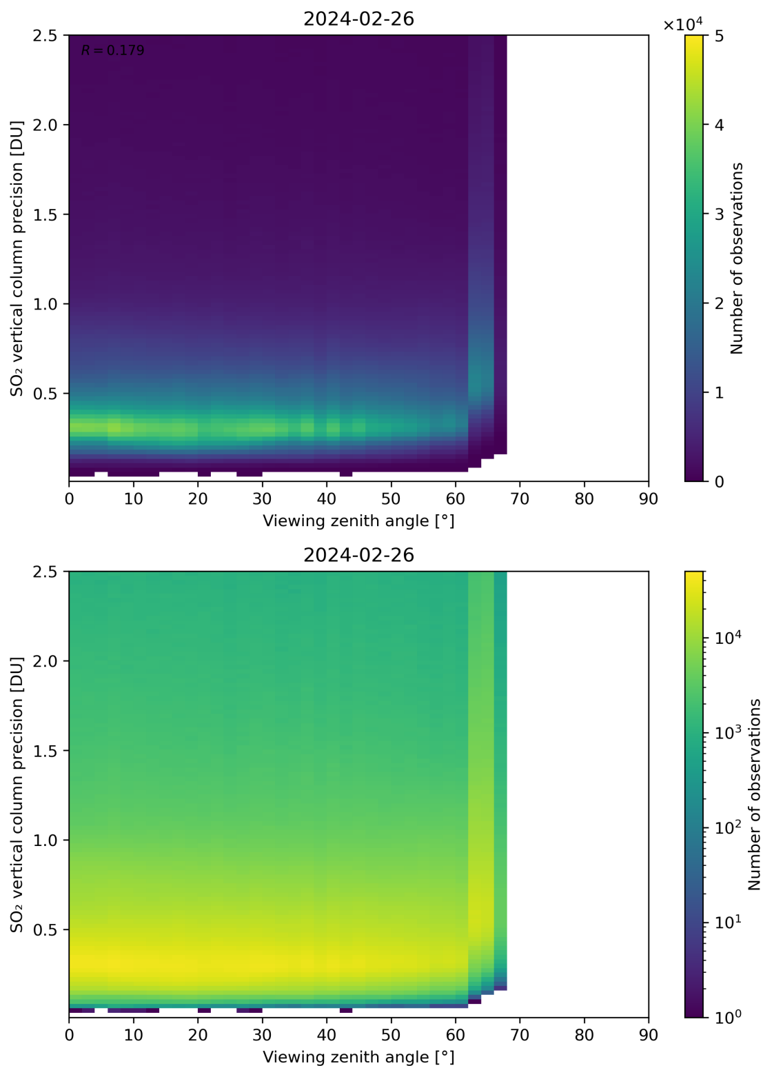
Figure 328: Scatter density plot of “Viewing zenith angle” against “SO 2 vertical column precision” for 2024-02-25 to 2024-02-27.
