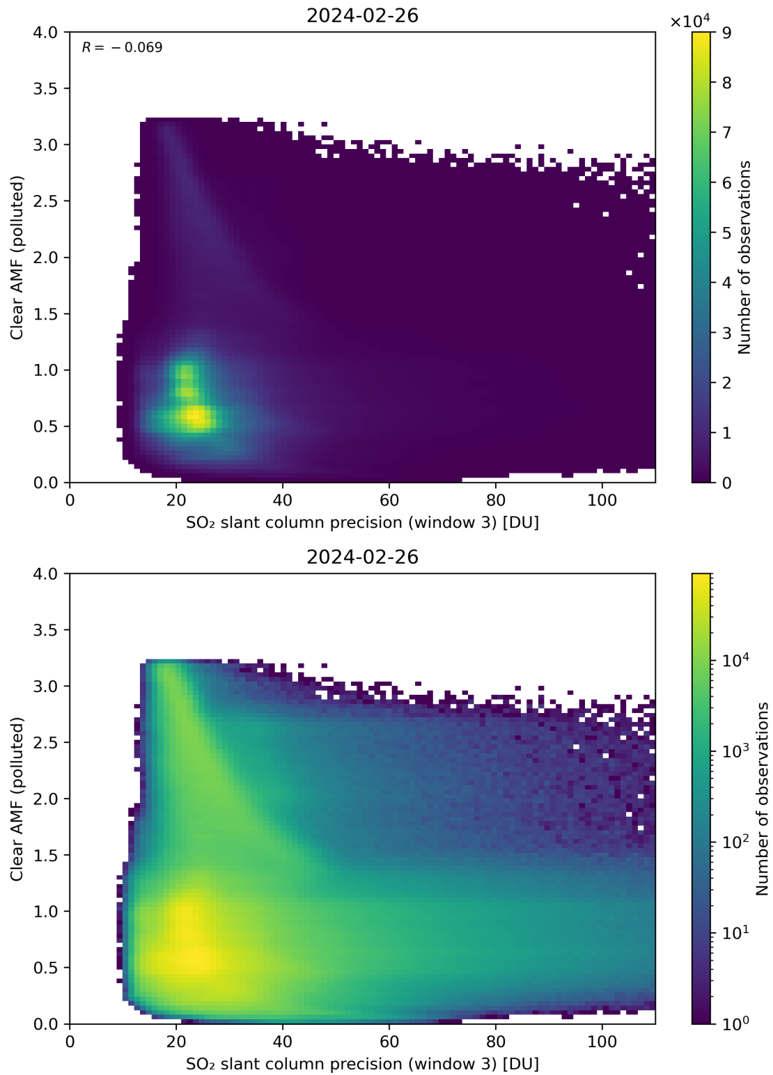
Figure 261: Scatter density plot of “SO 2 slant column precision (window 3)” against “Clear AMF (polluted)” for 2024-02-25 to 2024-02-27.
