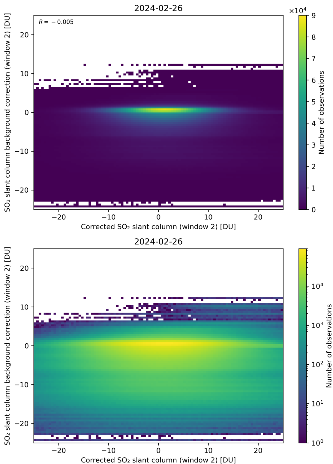
Figure 194: Scatter density plot of “Corrected SO 2 slant column (window 2)” against “SO 2 slant column background correction (window 2)” for 2024-02-25 to 2024-02-27.
