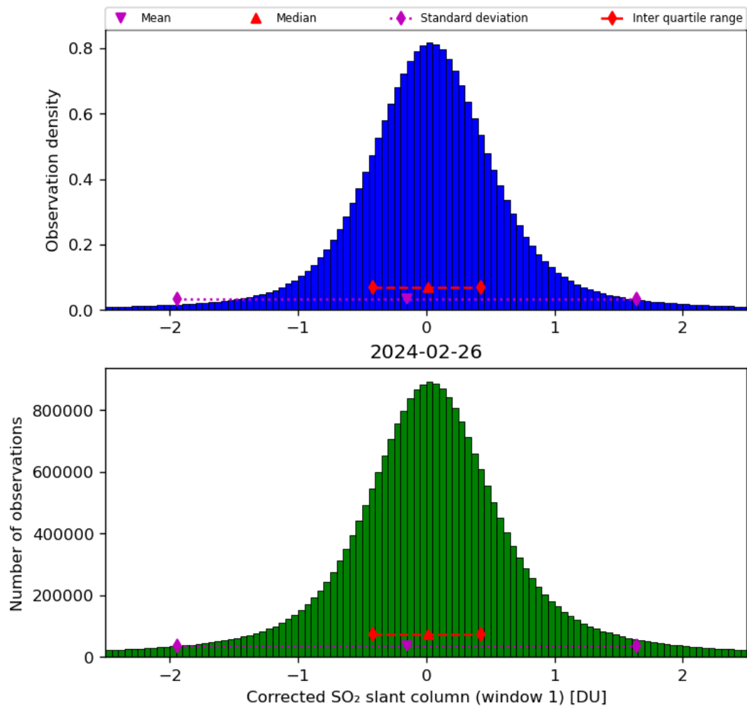
Figure 58: Histogram of “Corrected SO 2 slant column (window 1)” for 2024-02-25 to 2024-02-27
