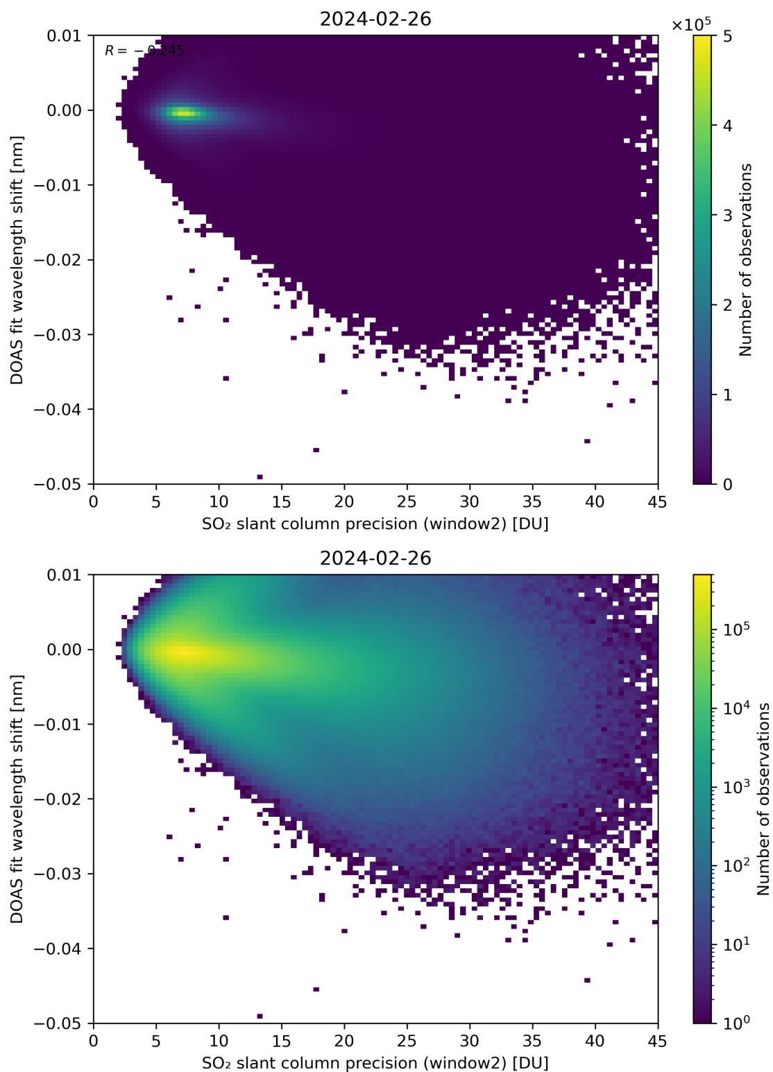
Figure 243: Scatter density plot of “SO 2 slant column precision (window2)” against “DOAS fit wavelength shift” for 2024-02-25 to 2024-02-27.
