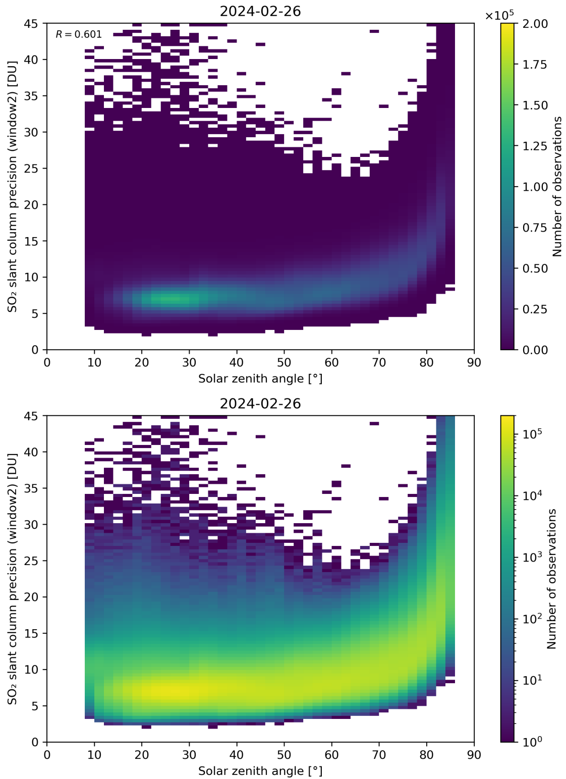
Figure 171: Scatter density plot of “Solar zenith angle” against “SO 2 slant column precision (window2)” for 2024-02-25 to 2024-02-27.
