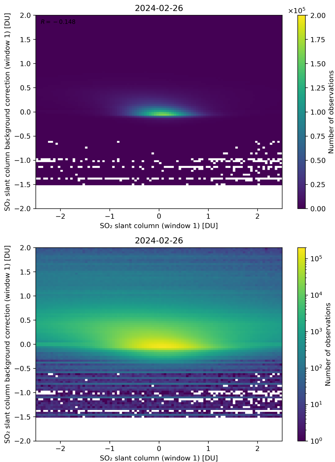
Figure 212: Scatter density plot of “SO 2 slant column (window 1)” against “SO 2 slant column background correction (window 1)” for 2024-02-25 to 2024-02-27.
