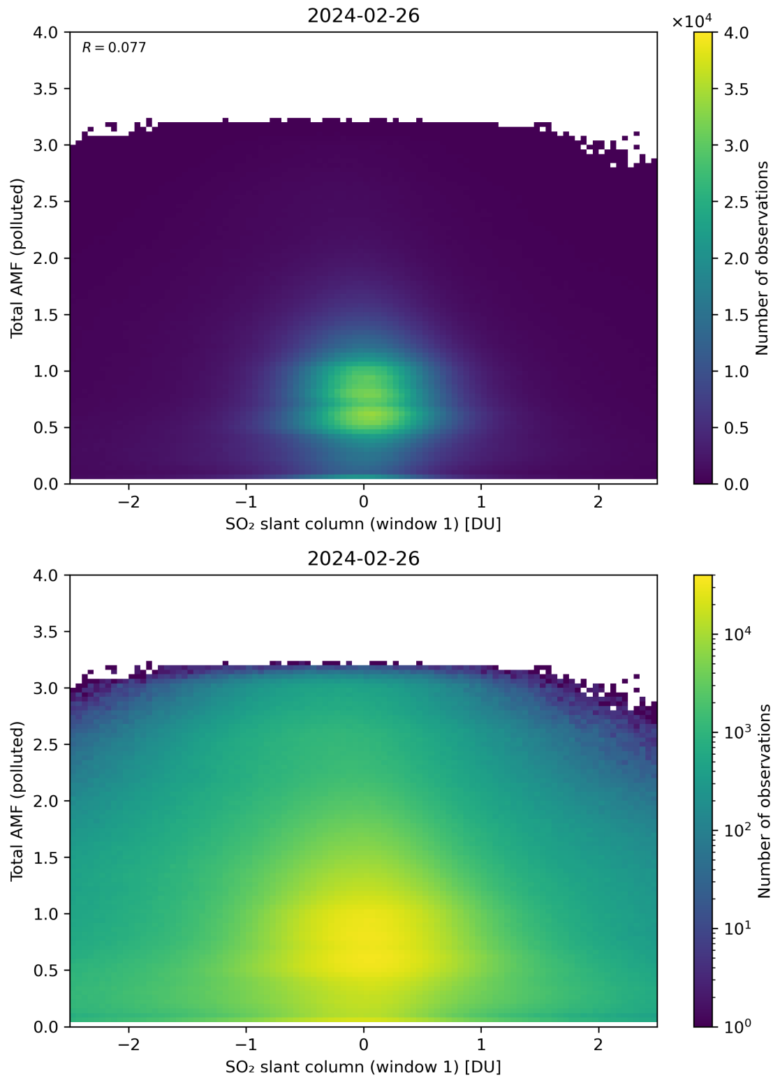
Figure 239: Scatter density plot of “SO 2 slant column (window 1)” against “Total AMF (polluted)” for 2024-02-25 to 2024-02-27.
