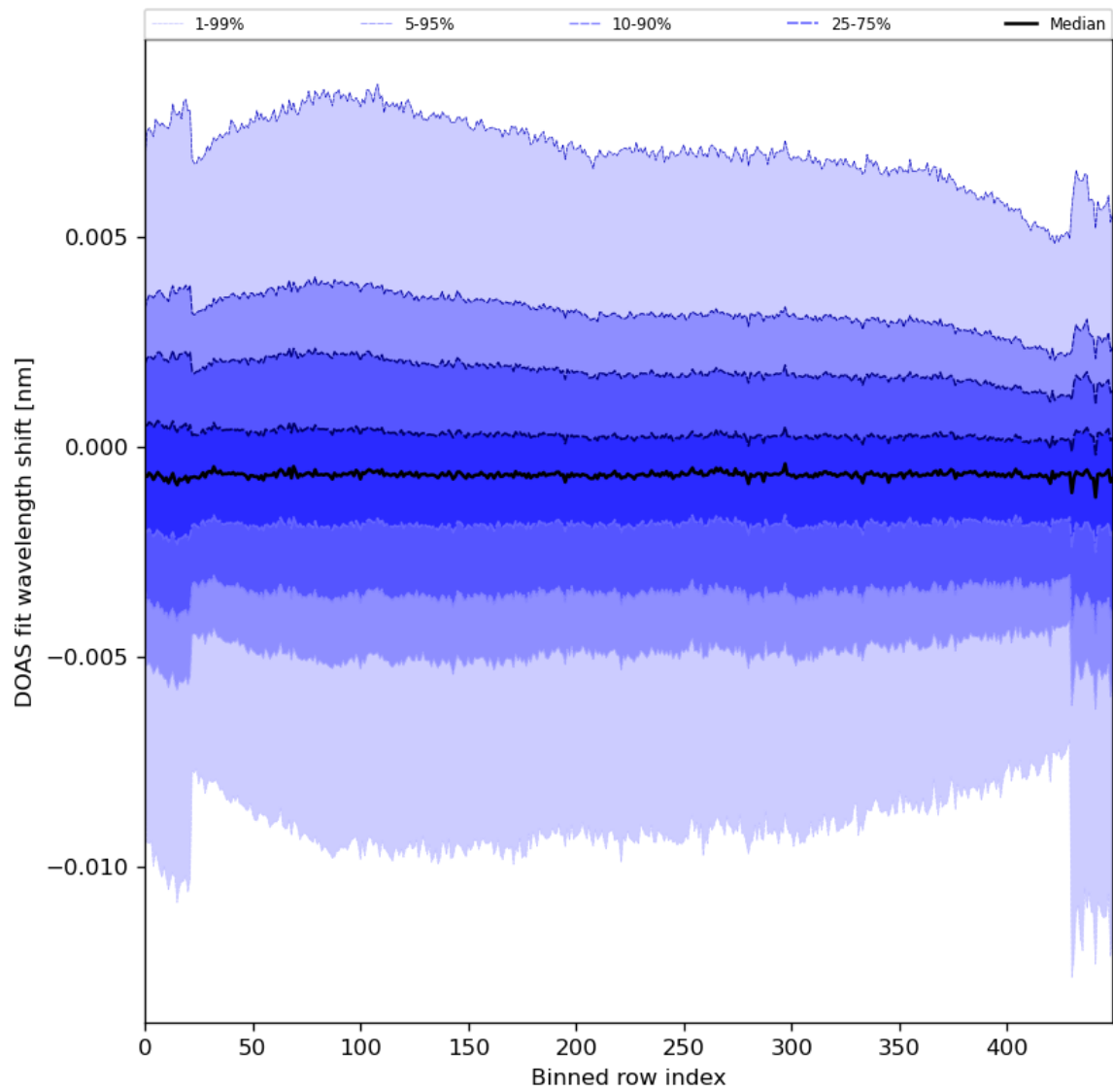
Figure 91: Along track statistics of “DOAS fit wavelength shift” for 2024-02-25 to 2024-02-27
