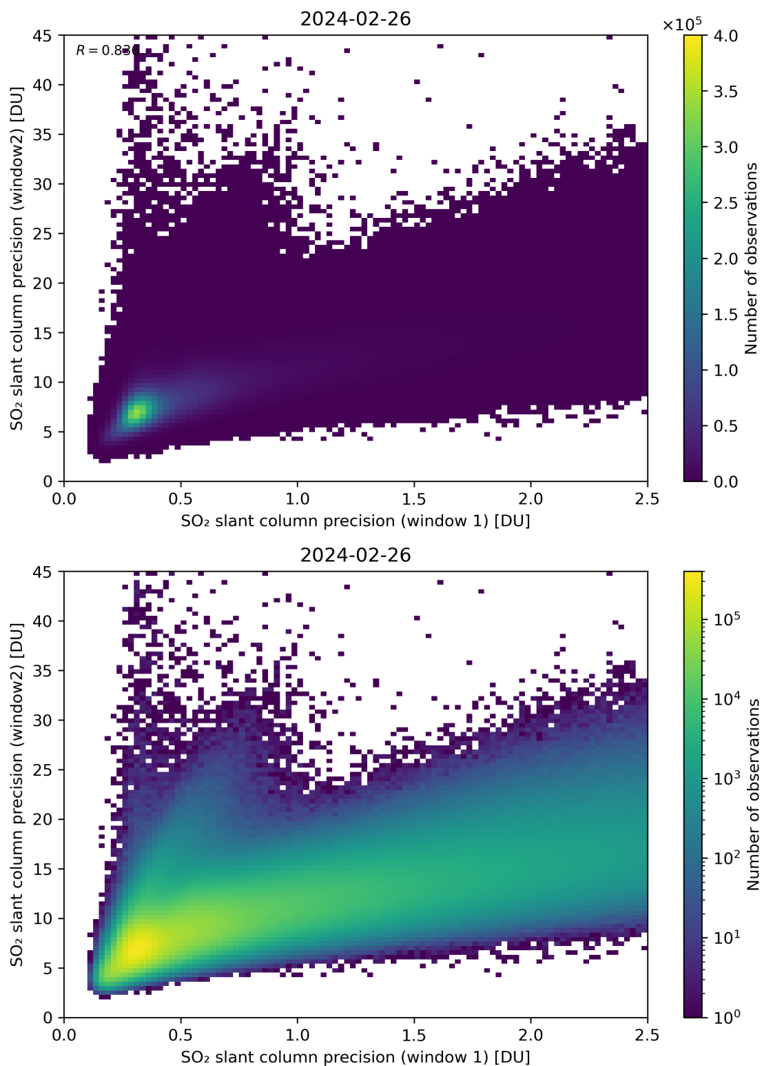
Figure 227: Scatter density plot of “SO 2 slant column precision (window 1)” against “SO 2 slant column precision (window 2)” for 2024-02-25 to 2024-02-27.
