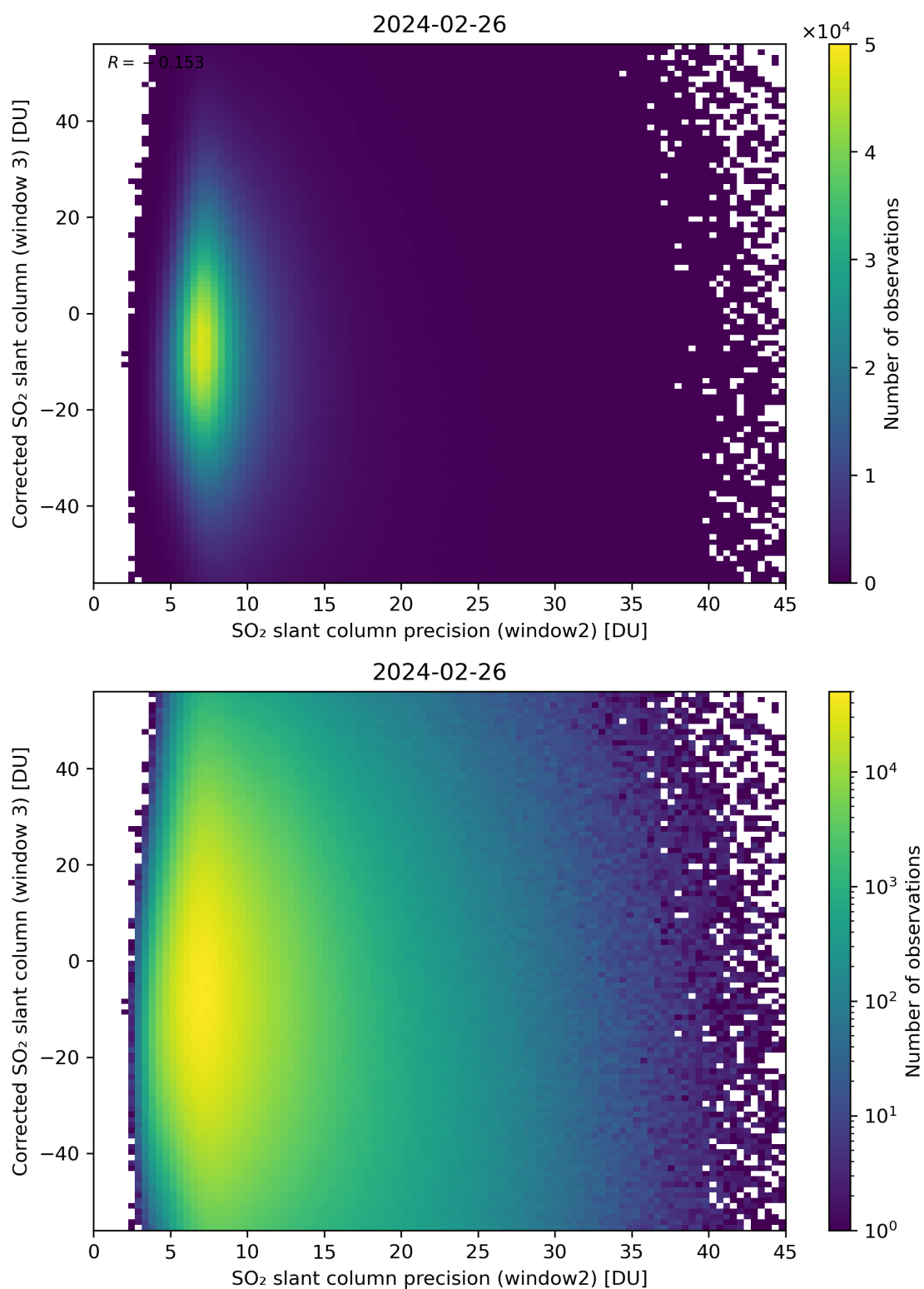
Figure 248: Scatter density plot of “SO 2 slant column precision (window2)” against “Corrected SO 2 slant column (window 3)” for 2024-02-25 to 2024-02-27.
