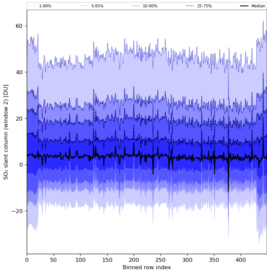
Figure 83: Along track statistics of “SO 2 slant column (window 2)” for 2024-02-25 to 2024-02-27
