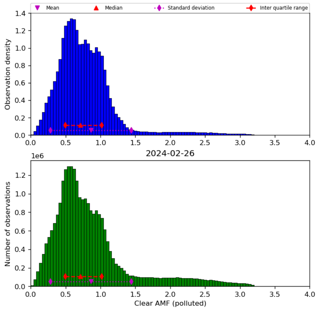
Figure 73: Histogram of “Clear AMF (polluted)” for 2024-02-25 to 2024-02-27
