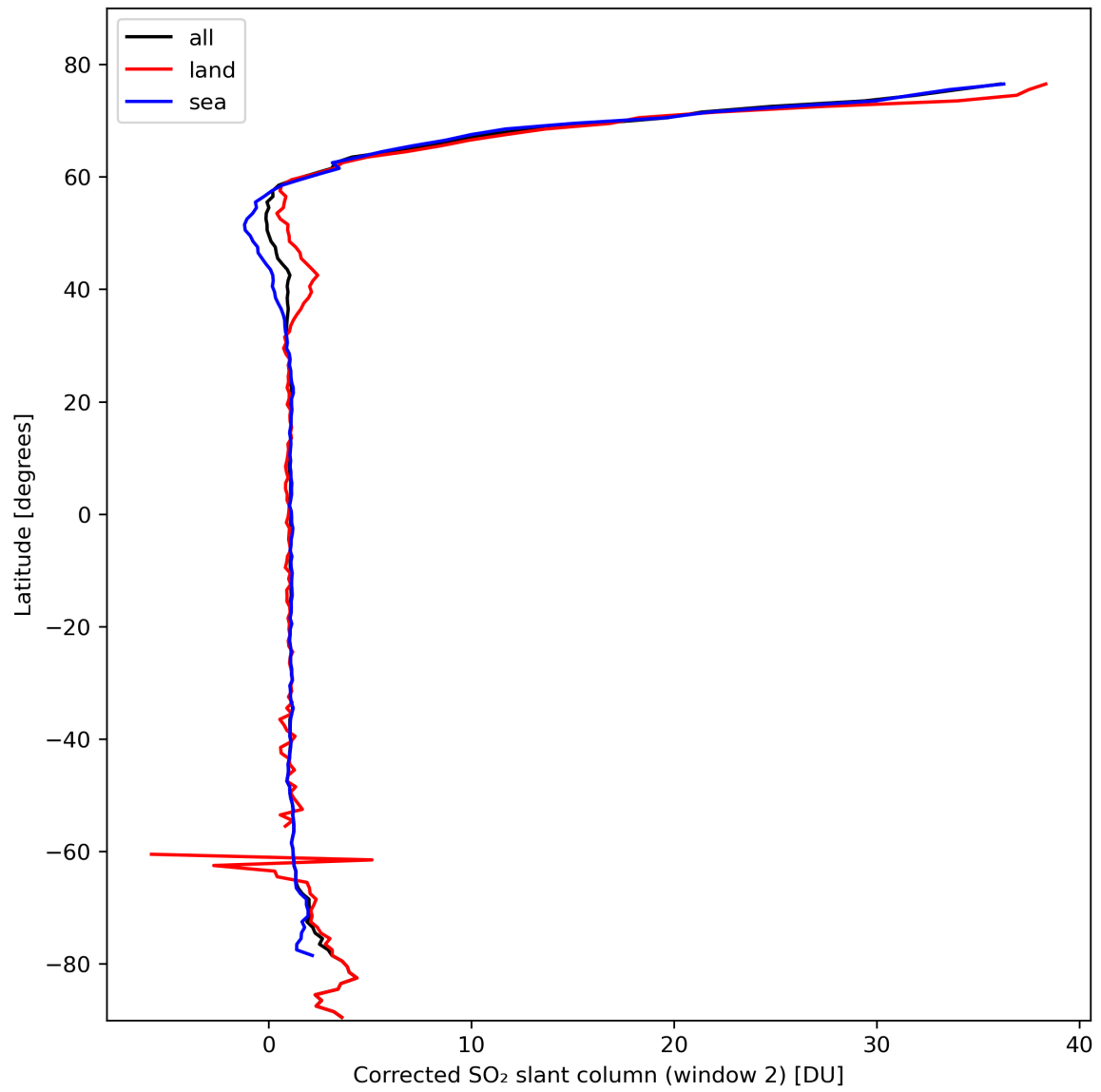
Figure 39: Zonal average of “Corrected SO 2 slant column (window 2)” for 2024-02-25 to 2024-02-27.
