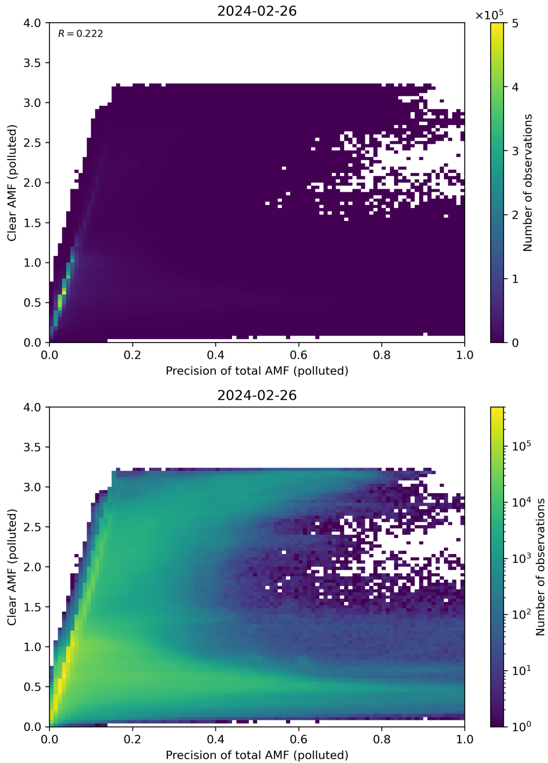
Figure 270: Scatter density plot of “Precision of total AMF (polluted)” against “Clear AMF (polluted)” for 2024-02-25 to 2024-02-27.
