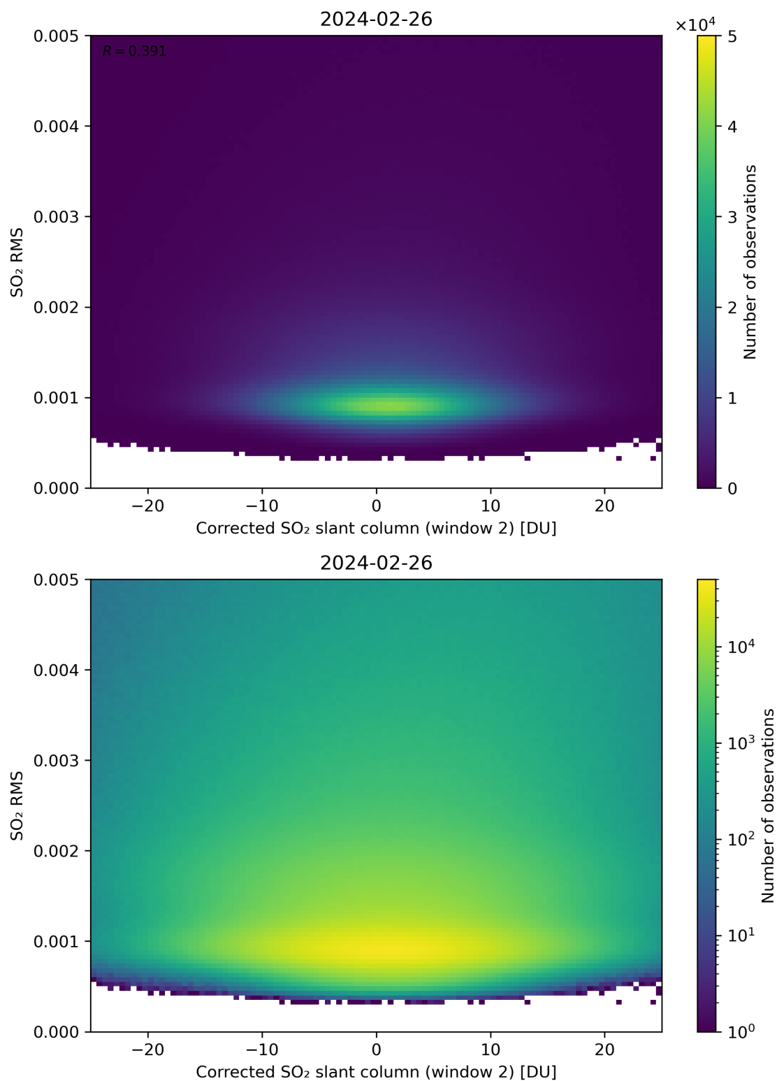
Figure 198: Scatter density plot of “Corrected SO 2 slant column (window 2)” against “SO 2 RMS” for 2024-02-25 to 2024-02-27.
