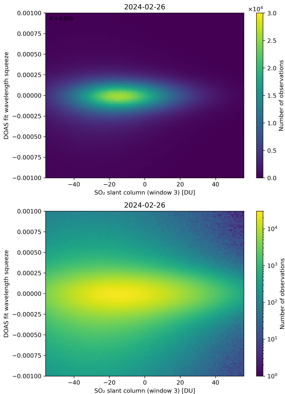
Figure 255: Scatter density plot of “SO 2 slant column (window 3)” against “DOAS fit wavelength squeeze” for 2024-02-25 to 2024-02-27.
