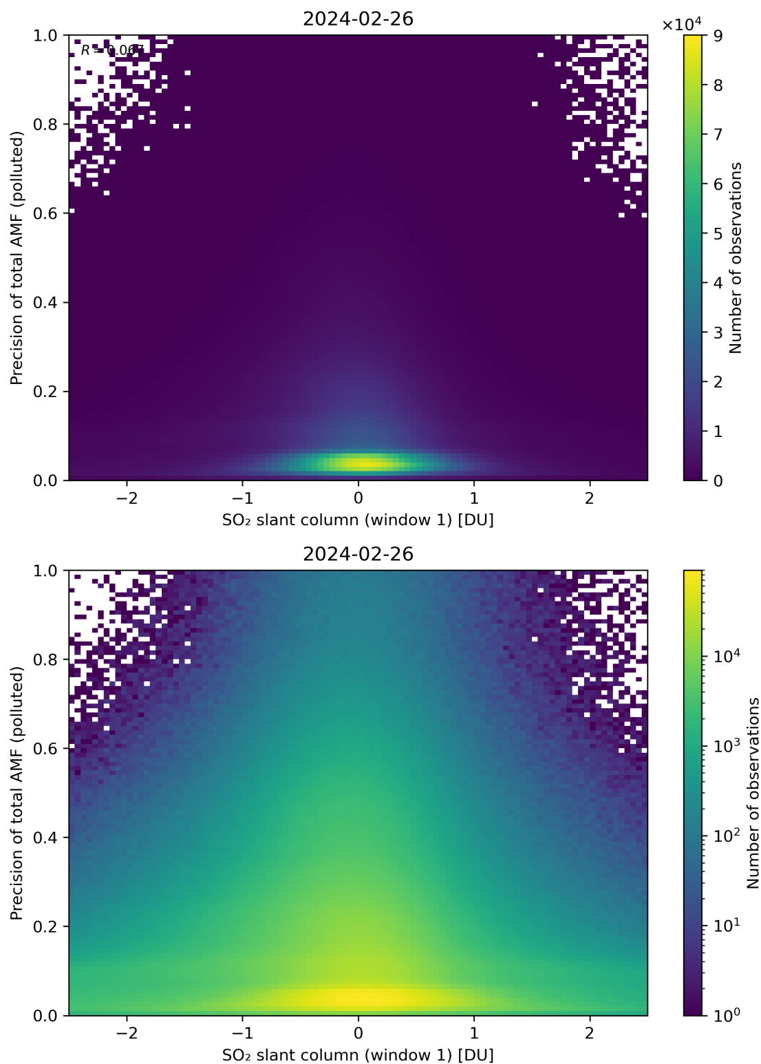
Figure 240: Scatter density plot of “SO 2 slant column (window 1)” against “Precision of total AMF (polluted)” for 2024-02-25 to 2024-02-27.
