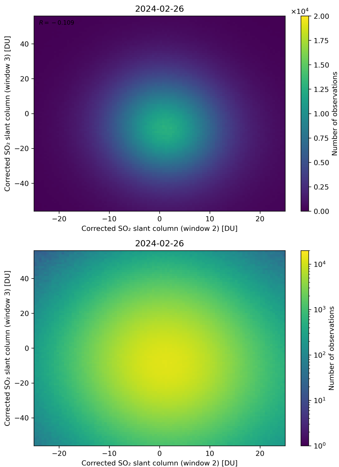
Figure 200: Scatter density plot of “Corrected SO 2 slant column (window 2)” against “Corrected SO 2 slant column (window 3)” for 2024-02-25 to 2024-02-27.
