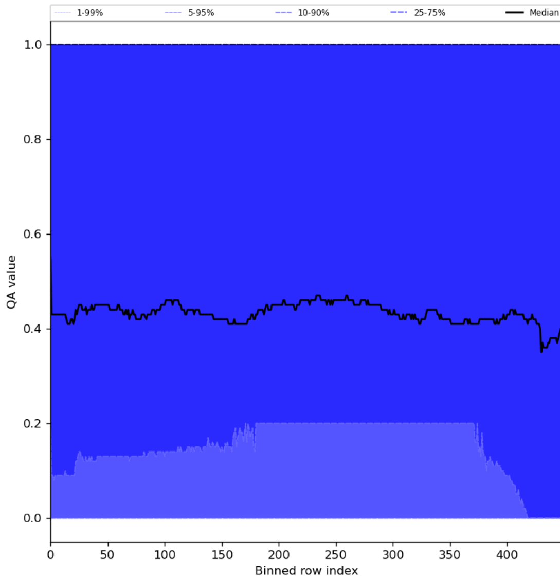
Figure 75: Along track statistics of “QA value” for 2024-02-25 to 2024-02-27
