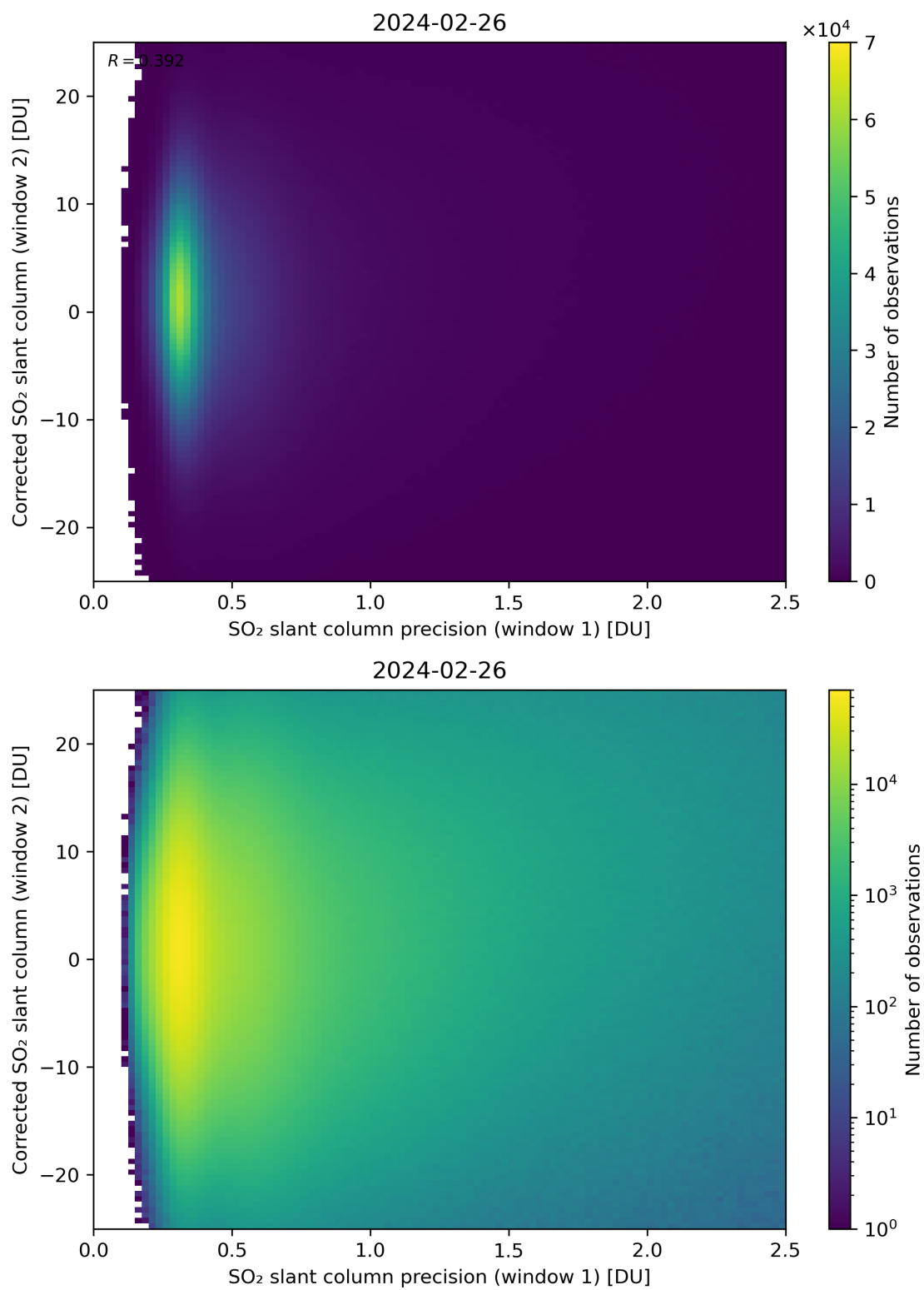
Figure 225: Scatter density plot of “SO 2 slant column precision (window 1)” against “Corrected SO 2 slant column (window 2)” for 2024-02-25 to 2024-02-27.
