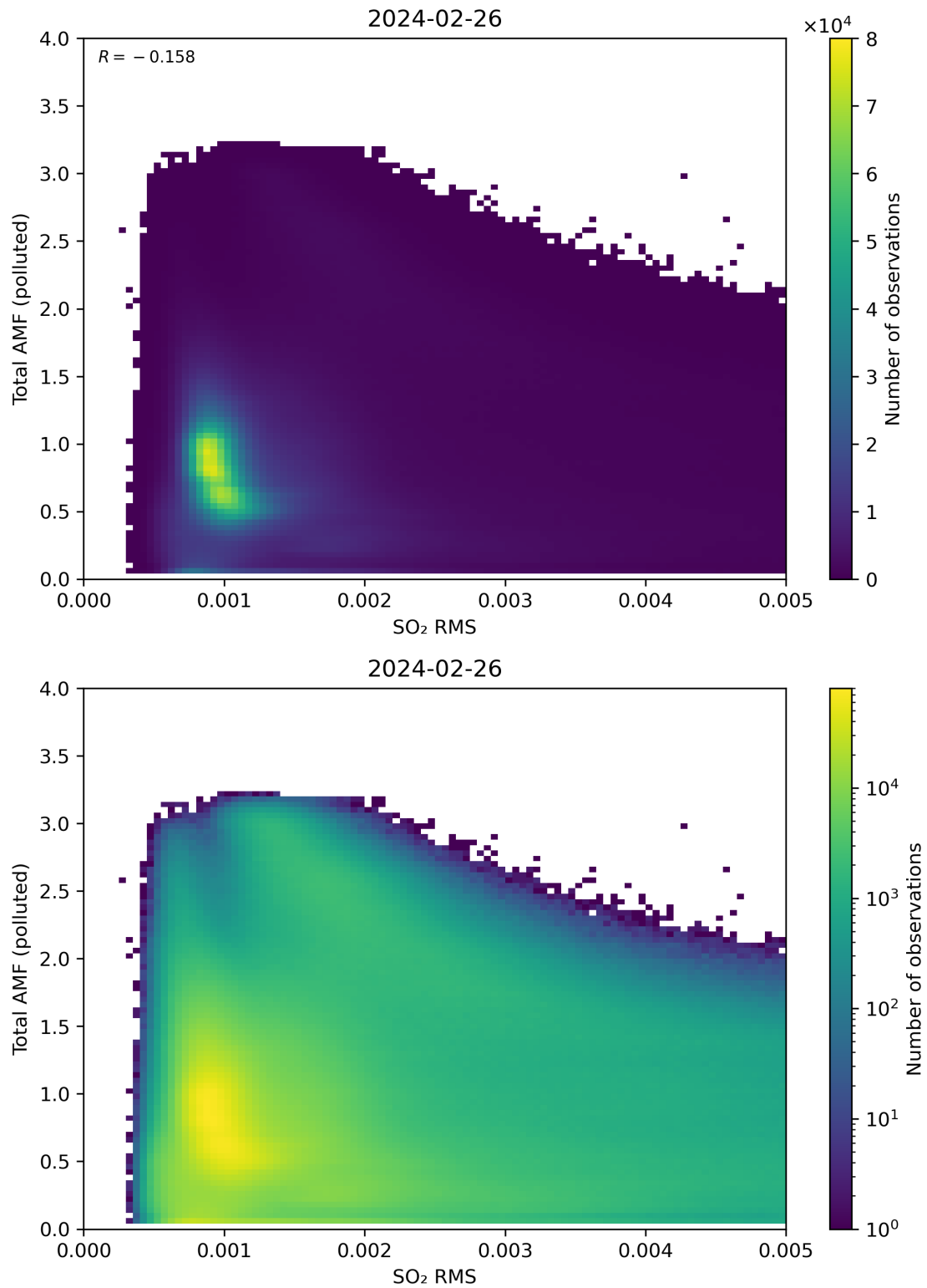
Figure 137: Scatter density plot of “SO 2 RMS” against “Total AMF (polluted)” for 2024-02-25 to 2024-02-27.
