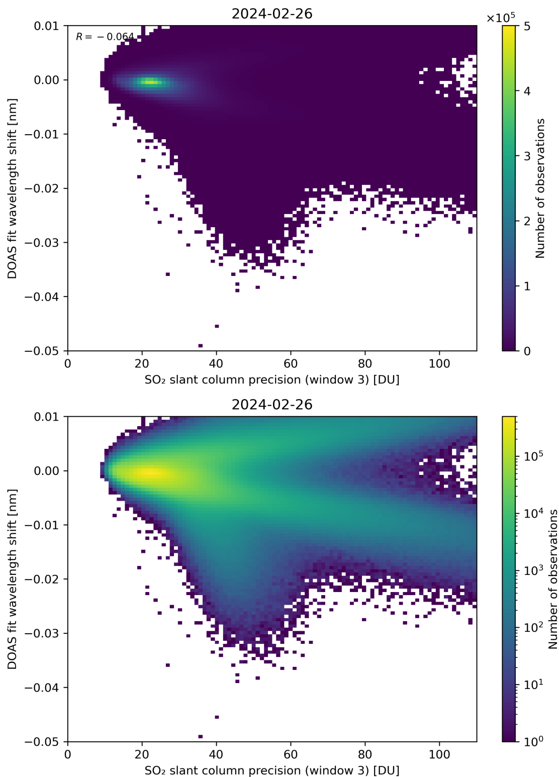
Figure 258: Scatter density plot of “SO 2 slant column precision (window 3)” against “DOAS fit wavelength shift” for 2024-02-25 to 2024-02-27.
