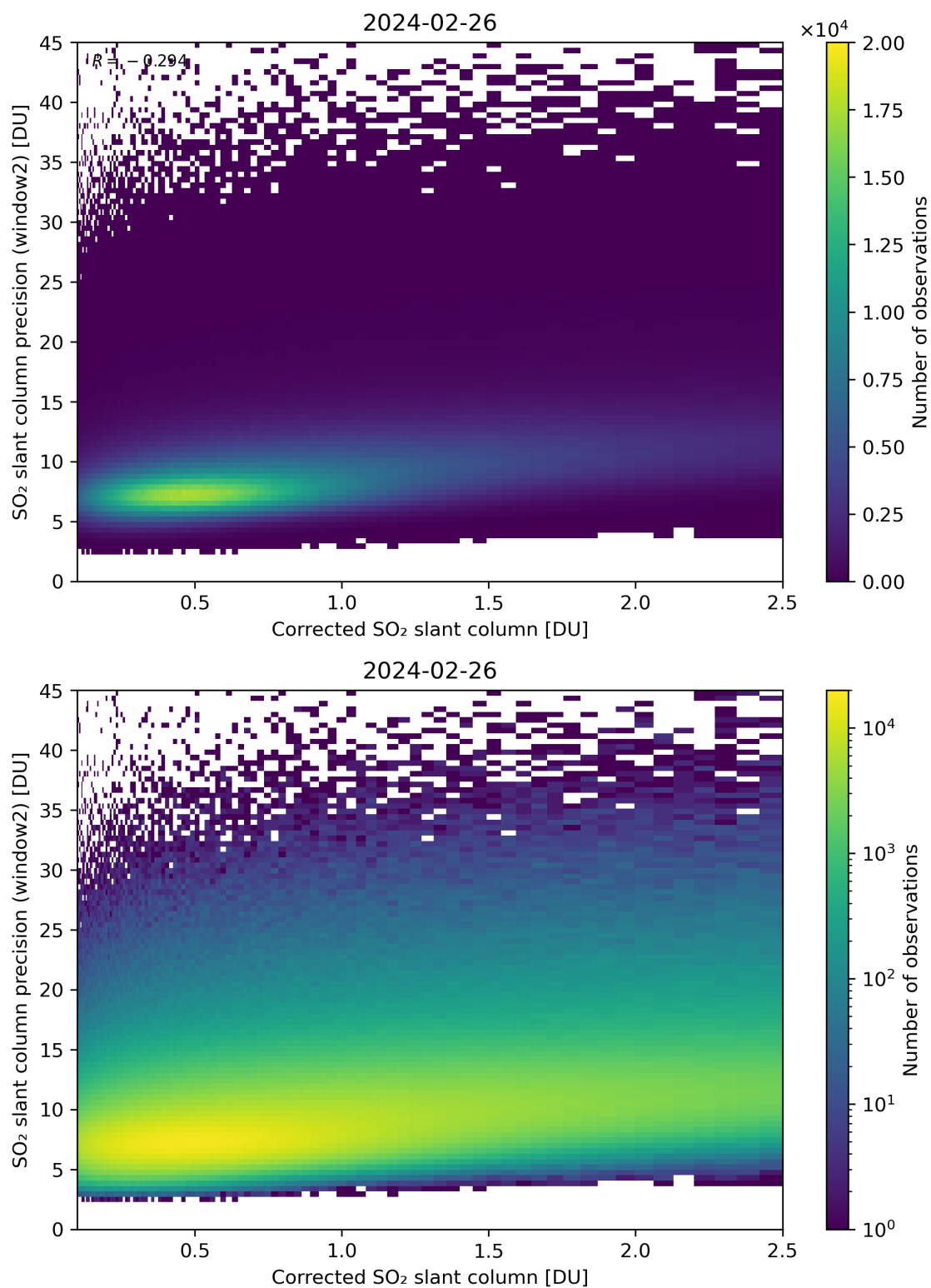
Figure 189: Scatter density plot of “Corrected SO 2 slant column” against “SO 2 slant column precision (window2)” for 2024-02-25 to 2024-02-27.
