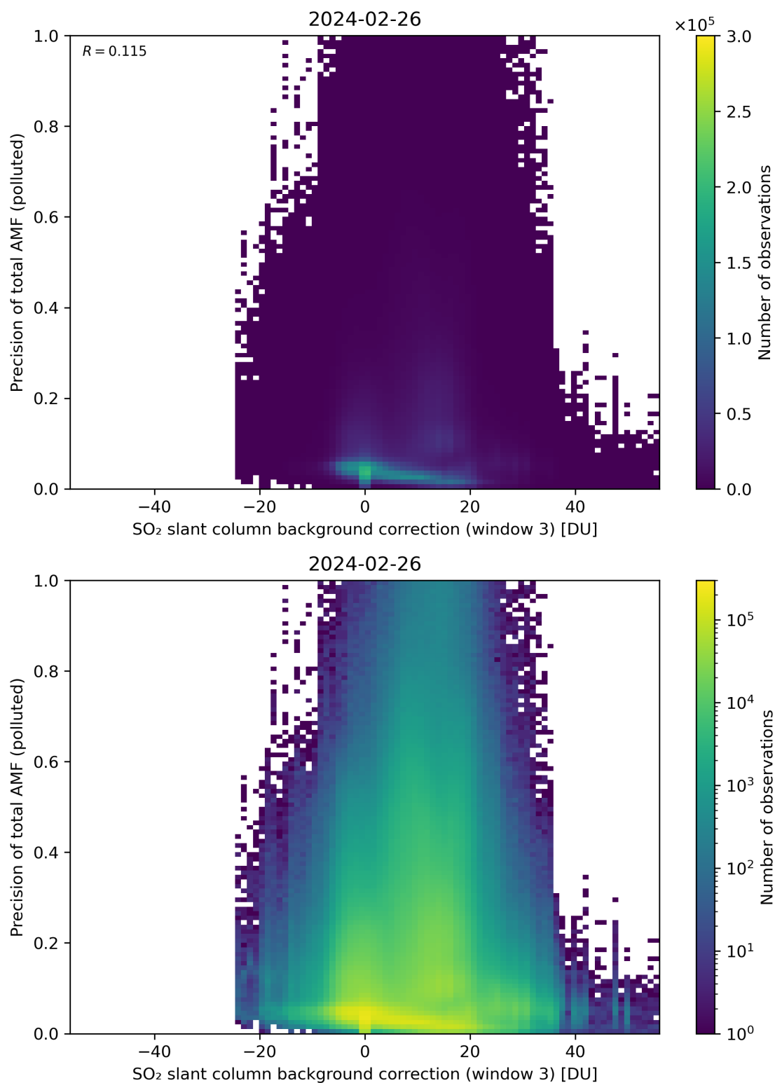
Figure 126: Scatter density plot of “SO 2 slant column background correction (window 3)” against “Precision of total AMF (polluted)” for 2024-02-25 to 2024-02-27.
