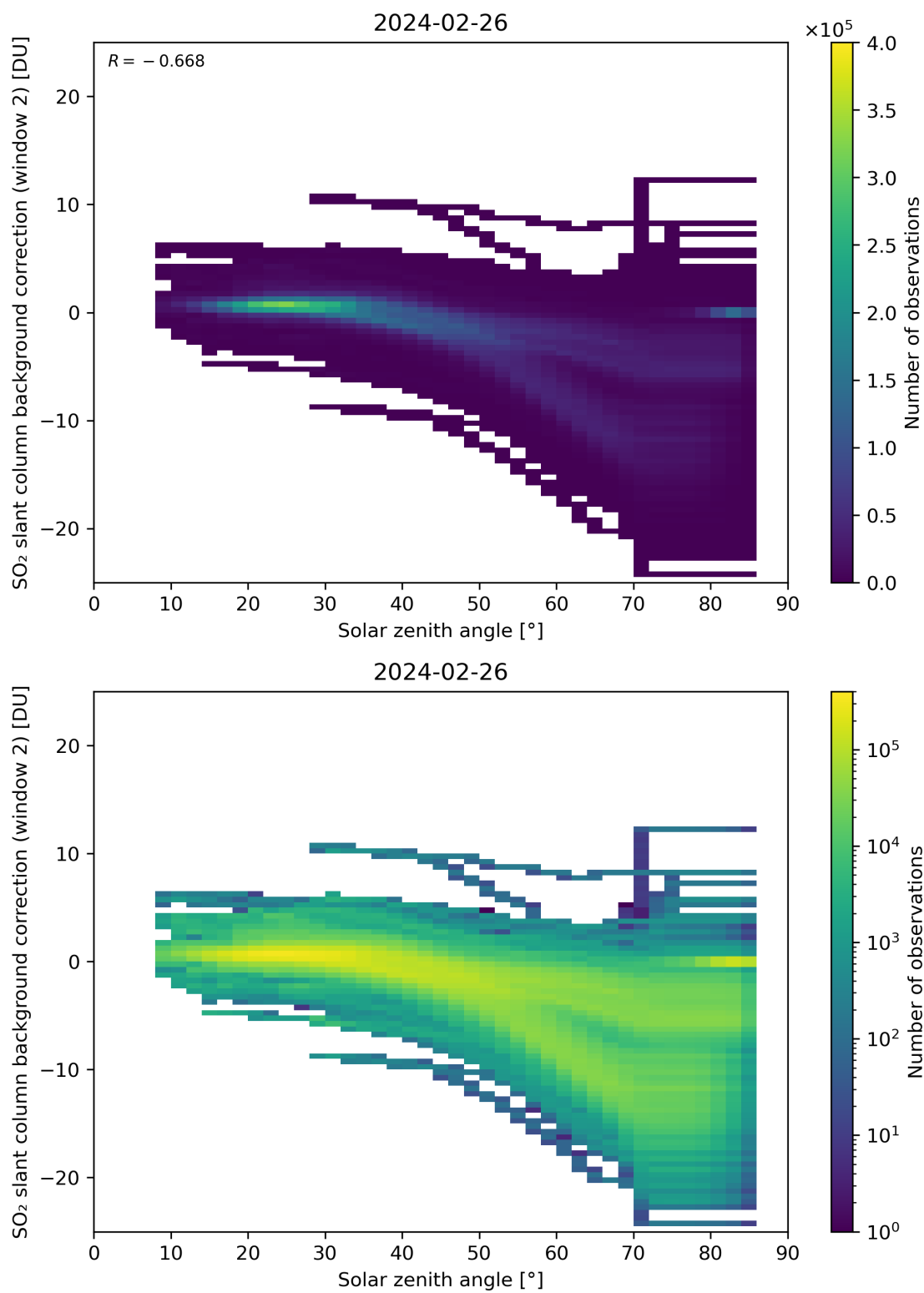
Figure 159: Scatter density plot of “Solar zenith angle” against “SO 2 slant column background correction (window 2)” for 2024-02-25 to 2024-02-27.
