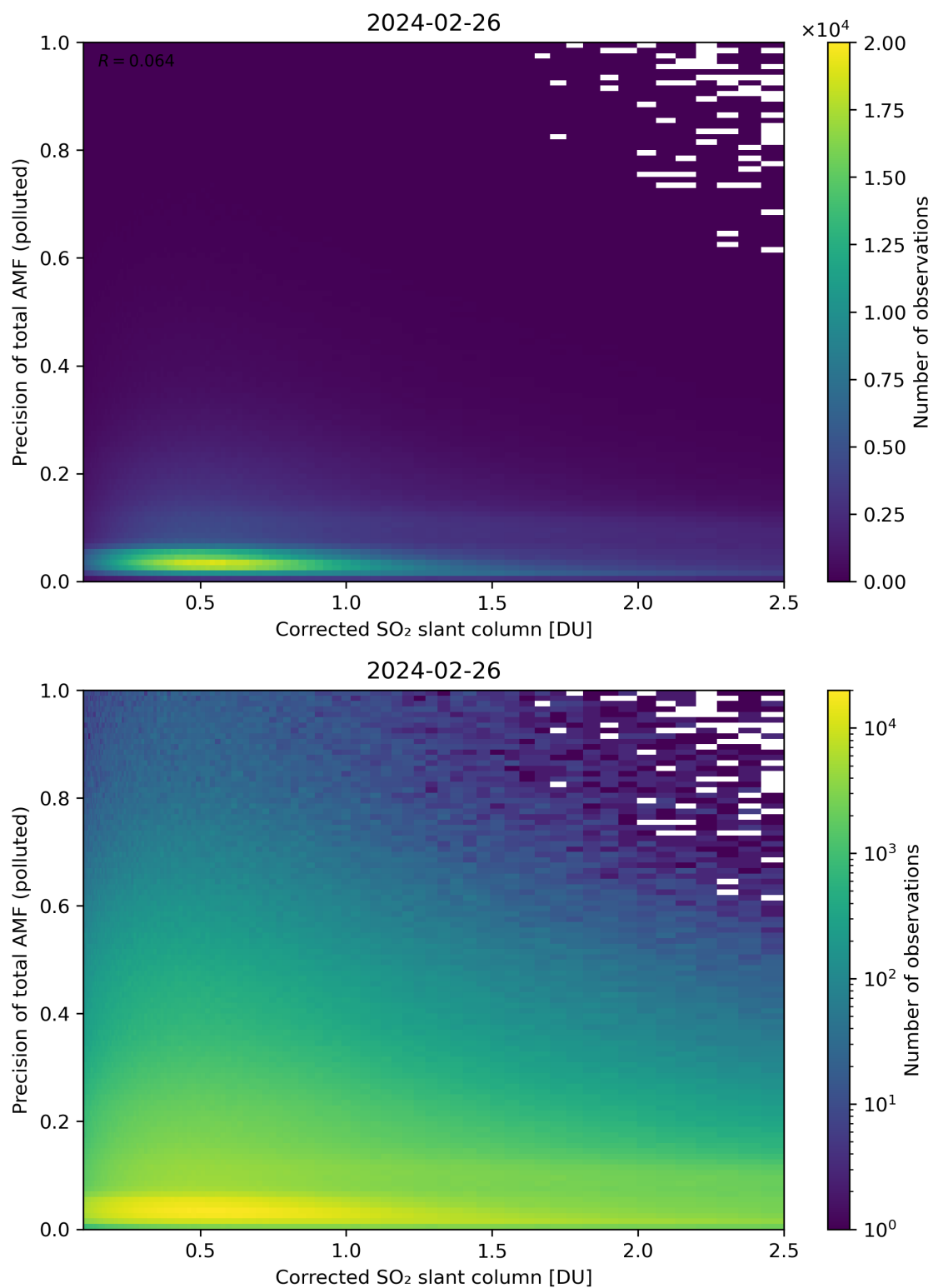
Figure 193: Scatter density plot of “Corrected SO 2 slant column” against “Precision of total AMF (polluted)” for 2024-02-25 to 2024-02-27.
