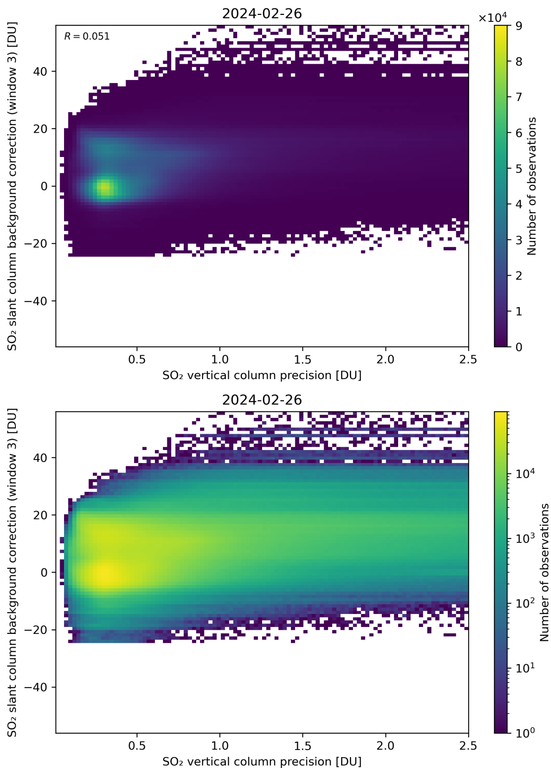
Figure 281: Scatter density plot of “SO 2 vertical column precision” against “SO 2 slant column background correction (window 3)” for 2024-02-25 to 2024-02-27.
