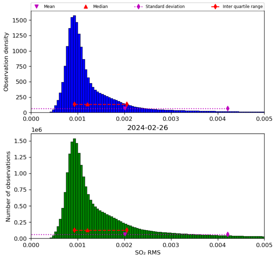
Figure 70: Histogram of “SO 2 RMS” for 2024-02-25 to 2024-02-27
