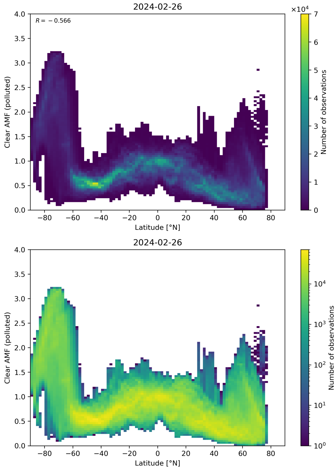
Figure 145: Scatter density plot of “Latitude” against “Clear AMF (polluted)” for 2024-02-25 to 2024-02-27.
