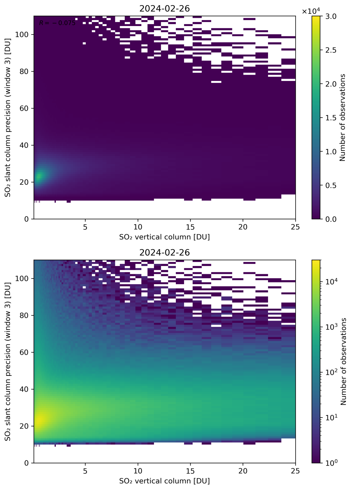
Figure 304: Scatter density plot of “SO 2 vertical column” against “SO 2 slant column precision (window 3)” for 2024-02-25 to 2024-02-27.
