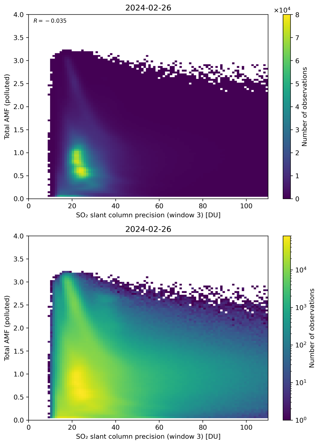
Figure 263: Scatter density plot of “SO 2 slant column precision (window 3)” against “Total AMF (polluted)” for 2024-02-25 to 2024-02-27.
