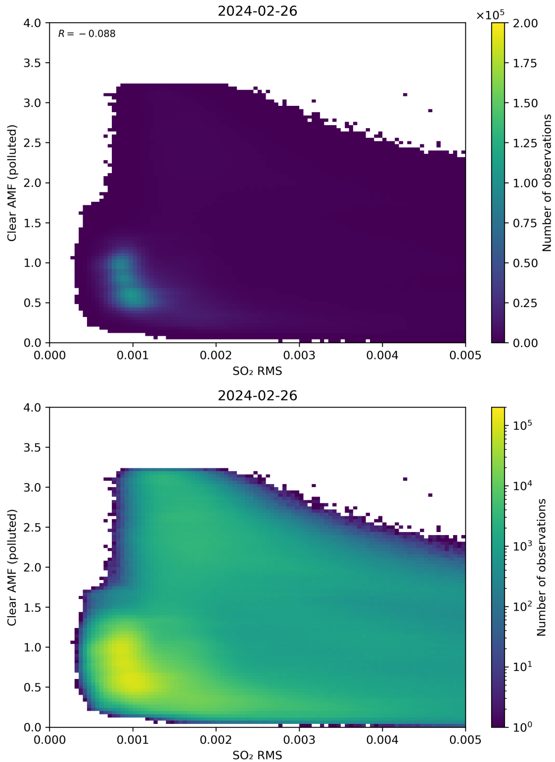
Figure 136: Scatter density plot of “SO 2 RMS” against “Clear AMF (polluted)” for 2024-02-25 to 2024-02-27.
