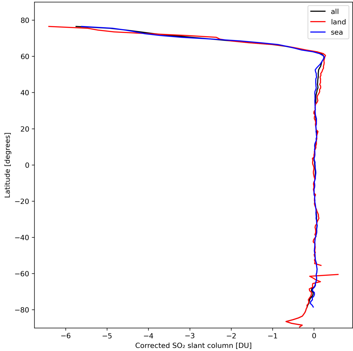
Figure 32: Zonal average of “Corrected SO 2 slant column” for 2024-02-25 to 2024-02-27.
