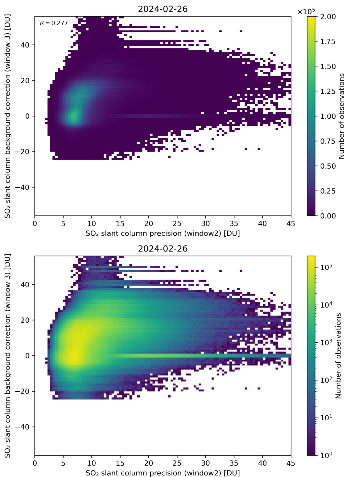
Figure 242: Scatter density plot of “SO 2 slant column precision (window2)” against “SO 2 slant column background correction (window 3)” for 2024-02-25 to 2024-02-27.
