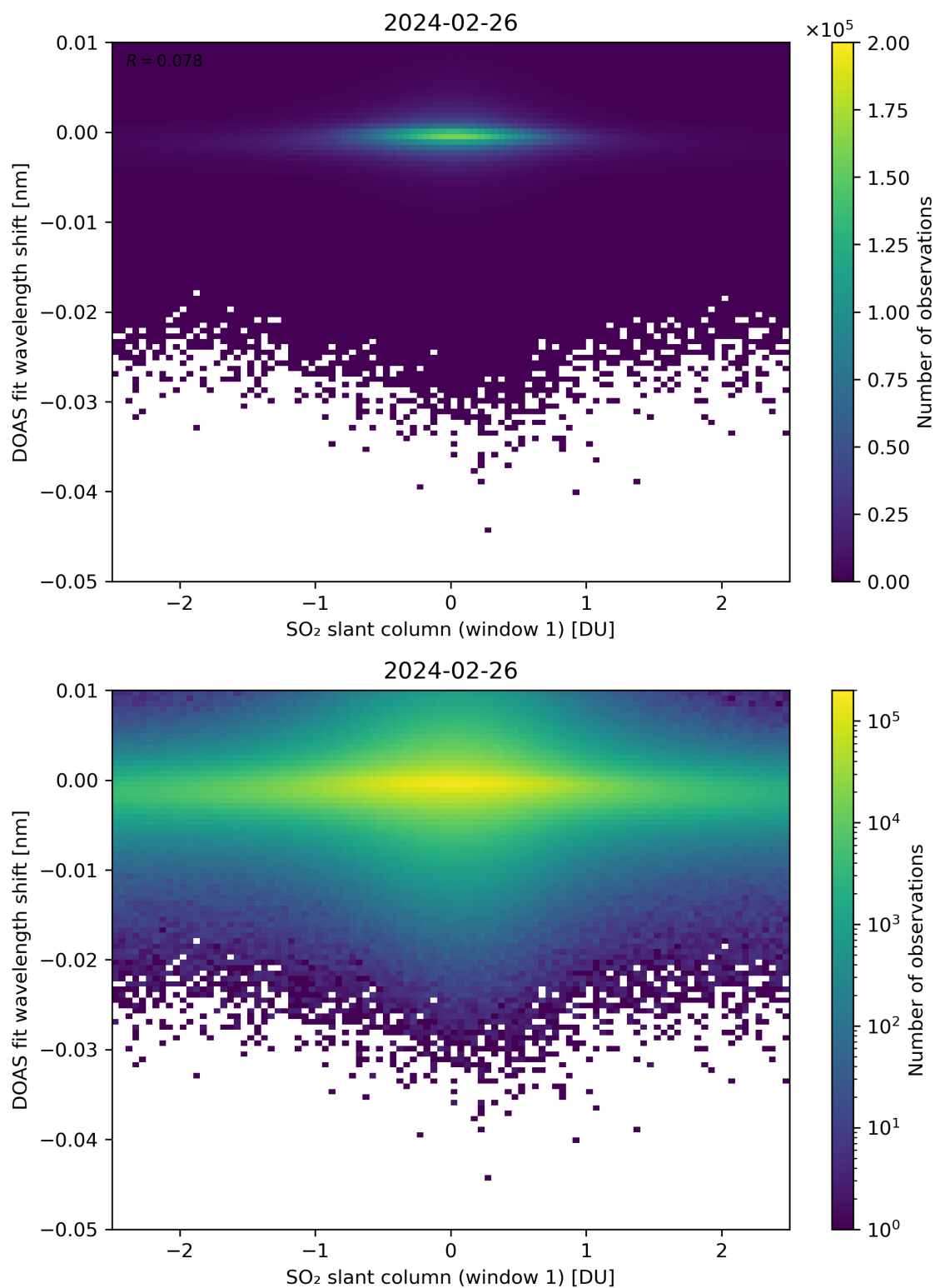
Figure 215: Scatter density plot of “SO 2 slant column (window 1)” against “DOAS fit wavelength shift” for 2024-02-25 to 2024-02-27.
