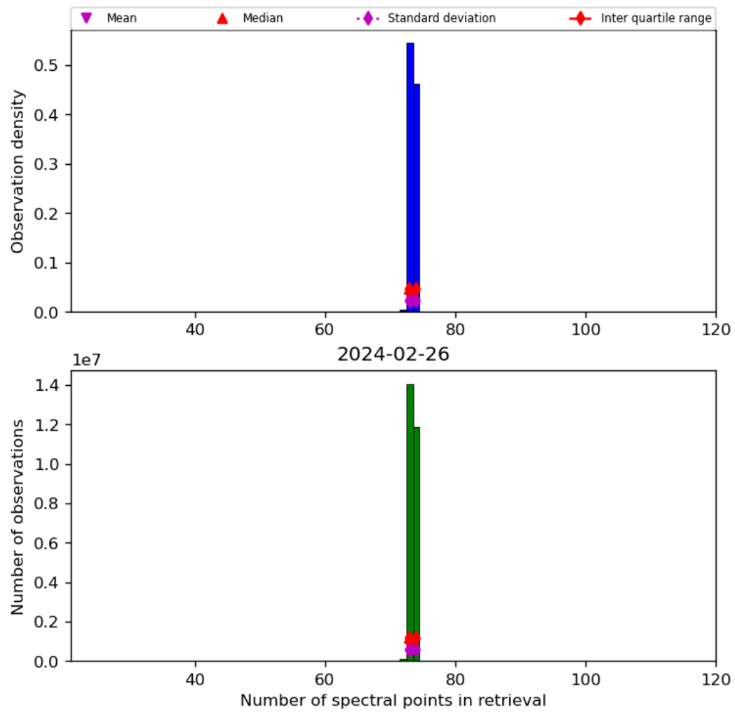
Figure 74: Histogram of “Number of spectral points in retrieval” for 2024-02-25 to 2024-02-27
