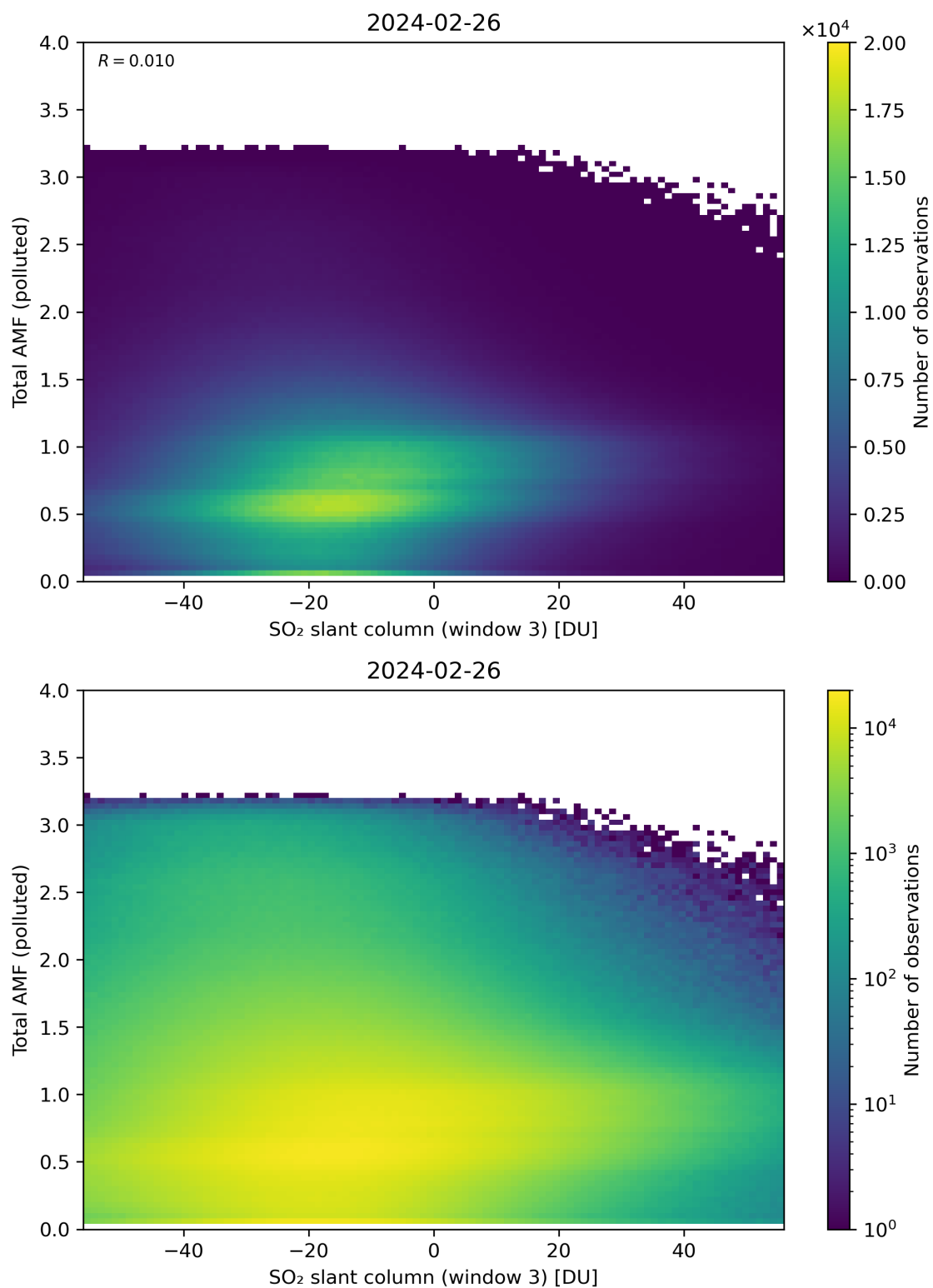
Figure 268: Scatter density plot of “SO 2 slant column (window 3)” against “Total AMF (polluted)” for 2024-02-25 to 2024-02-27.
