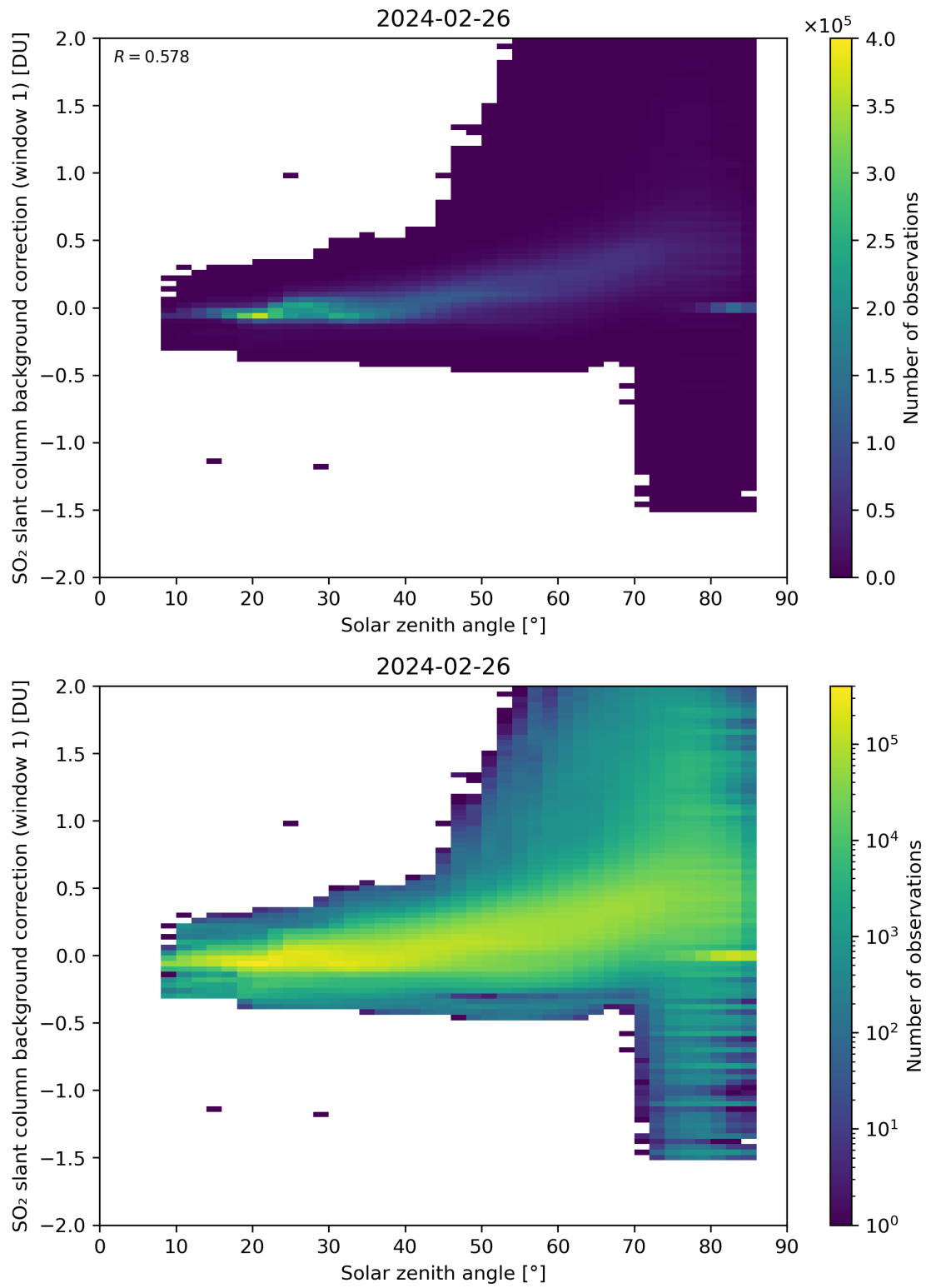
Figure 158: Scatter density plot of “Solar zenith angle” against “SO 2 slant column background correction (window 1)” for 2024-02-25 to 2024-02-27.
