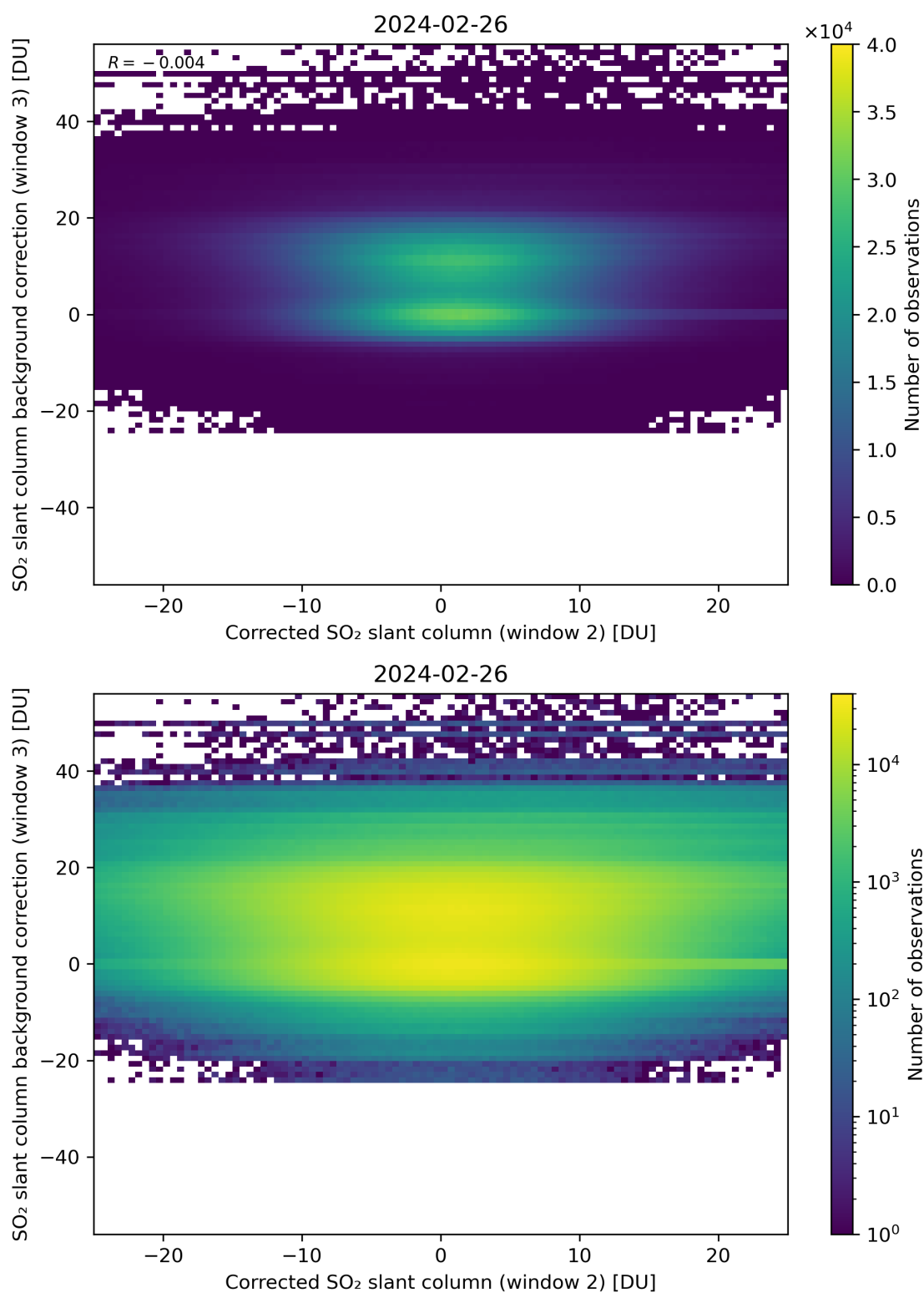
Figure 195: Scatter density plot of “Corrected SO 2 slant column (window 2)” against “SO 2 slant column background correction (window 3)” for 2024-02-25 to 2024-02-27.
