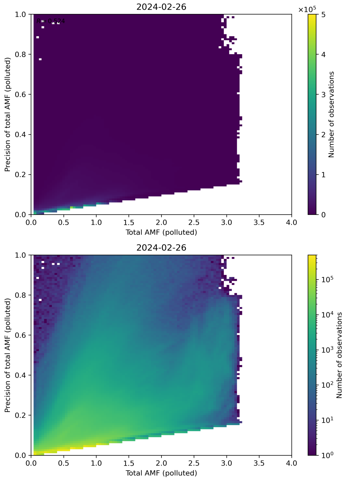
Figure 272: Scatter density plot of “Total AMF (polluted)” against “Precision of total AMF (polluted)” for 2024-02-25 to 2024-02-27.
