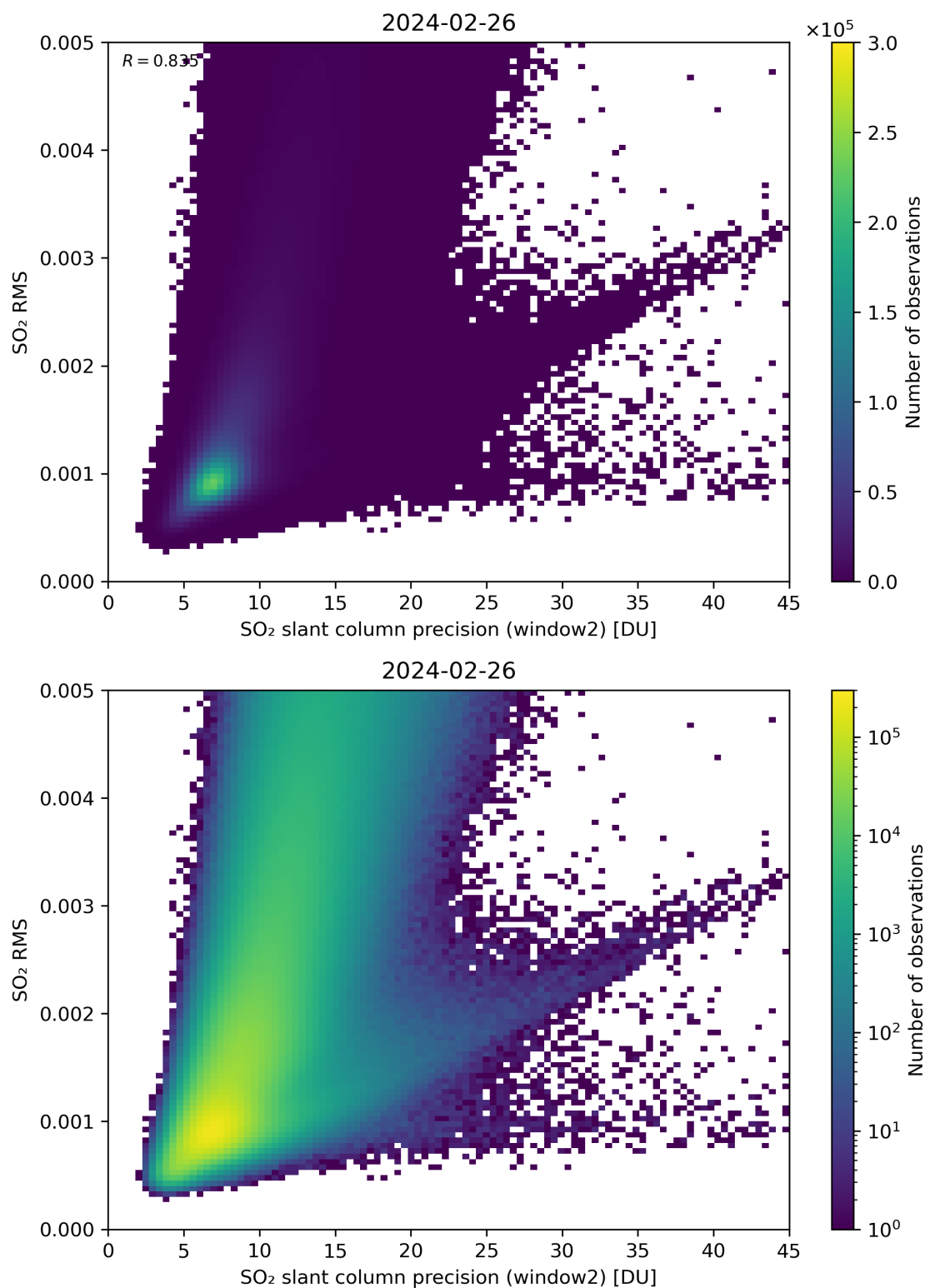
Figure 245: Scatter density plot of “SO 2 slant column precision (window2)” against “SO 2 RMS” for 2024-02-25 to 2024-02-27.
