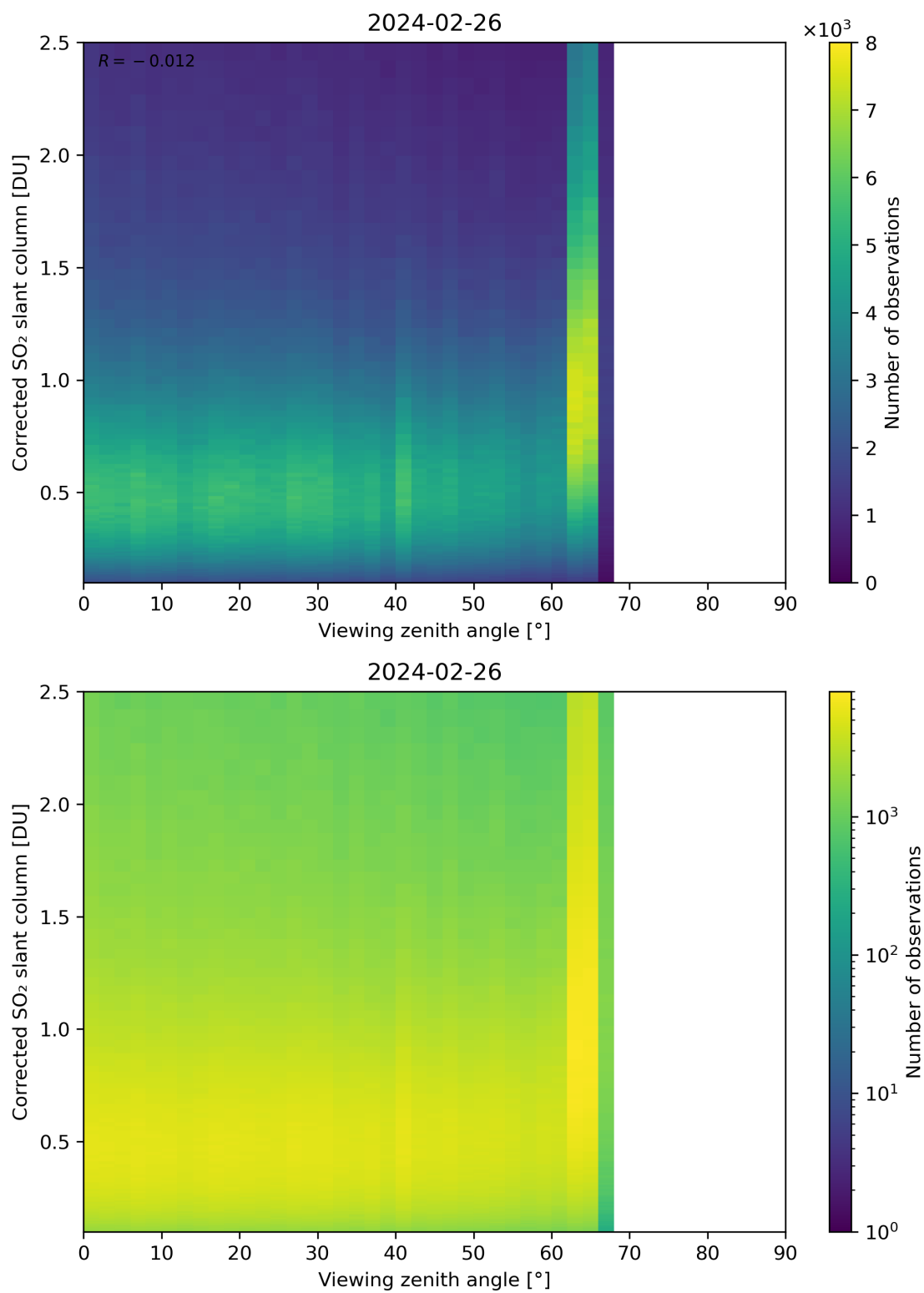
Figure 317: Scatter density plot of “Viewing zenith angle” against “Corrected SO 2 slant column” for 2024-02-25 to 2024-02-27.
