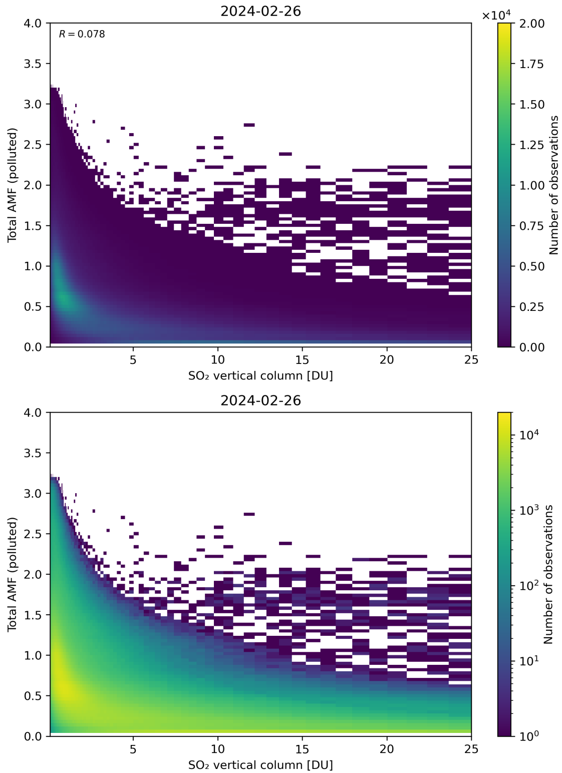
Figure 305: Scatter density plot of “SO 2 vertical column” against “Total AMF (polluted)” for 2024-02-25 to 2024-02-27.
