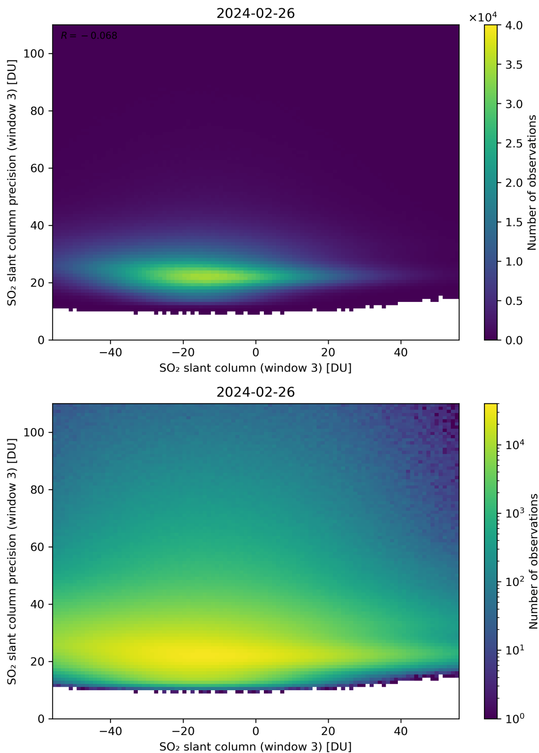
Figure 267: Scatter density plot of “SO 2 slant column (window 3)” against “SO 2 slant column precision (window 3)” for 2024-02-25 to 2024-02-27.
