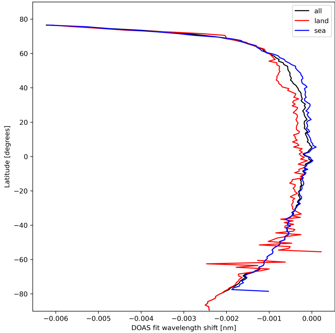
Figure 45: Zonal average of “DOAS fit wavelength shift” for 2024-02-25 to 2024-02-27.
