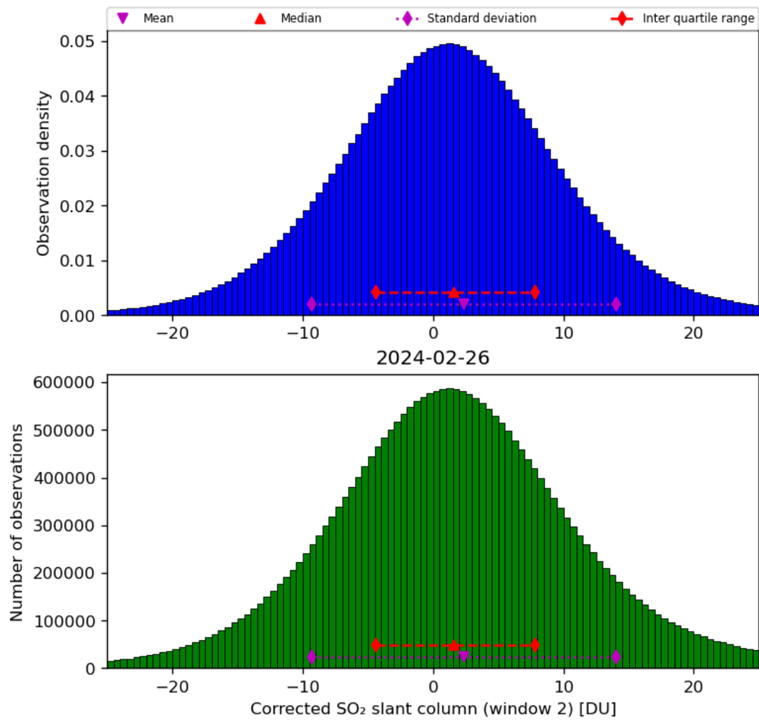
Figure 62: Histogram of “Corrected SO 2 slant column (window 2)” for 2024-02-25 to 2024-02-27
