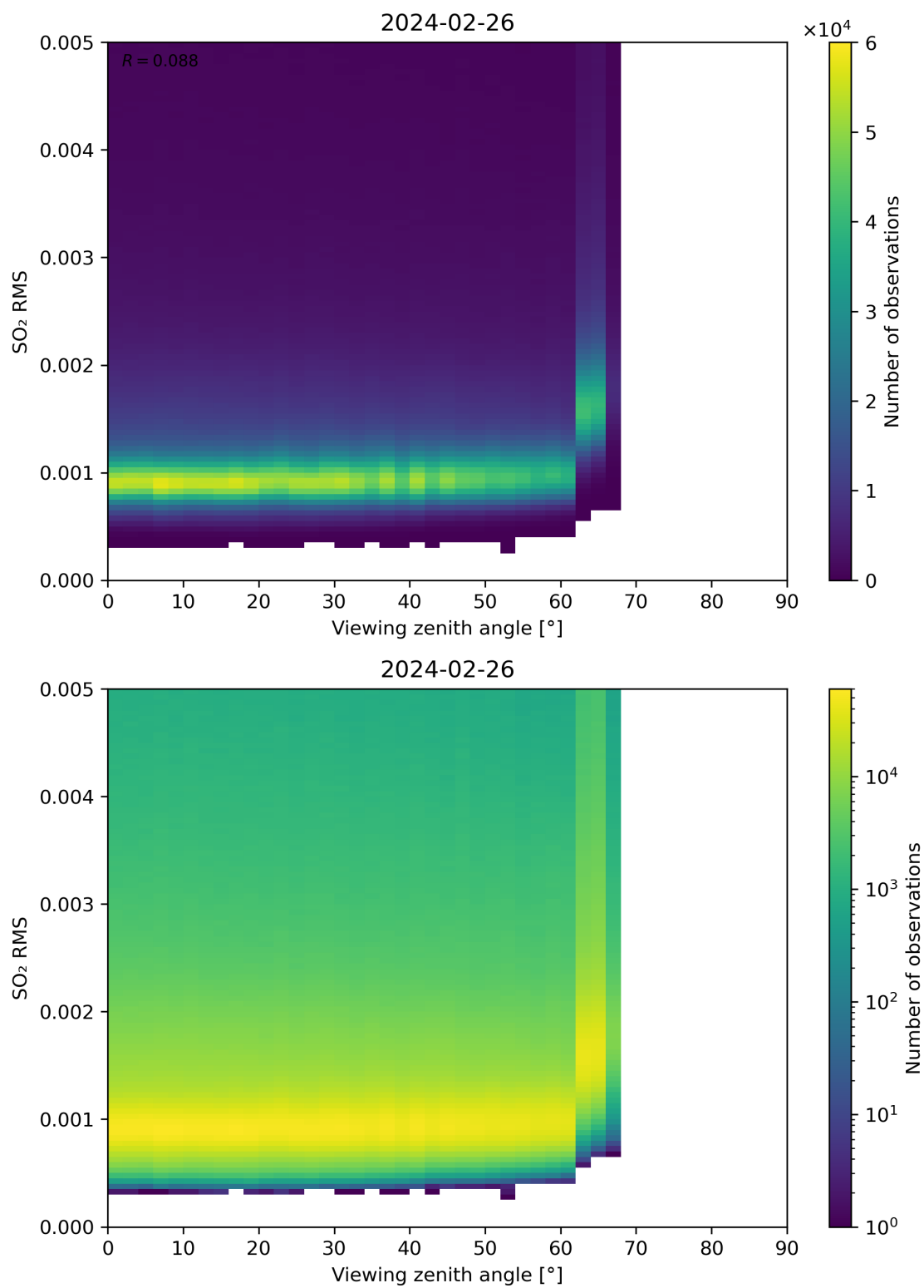
Figure 313: Scatter density plot of “Viewing zenith angle” against “SO 2 RMS” for 2024-02-25 to 2024-02-27.
