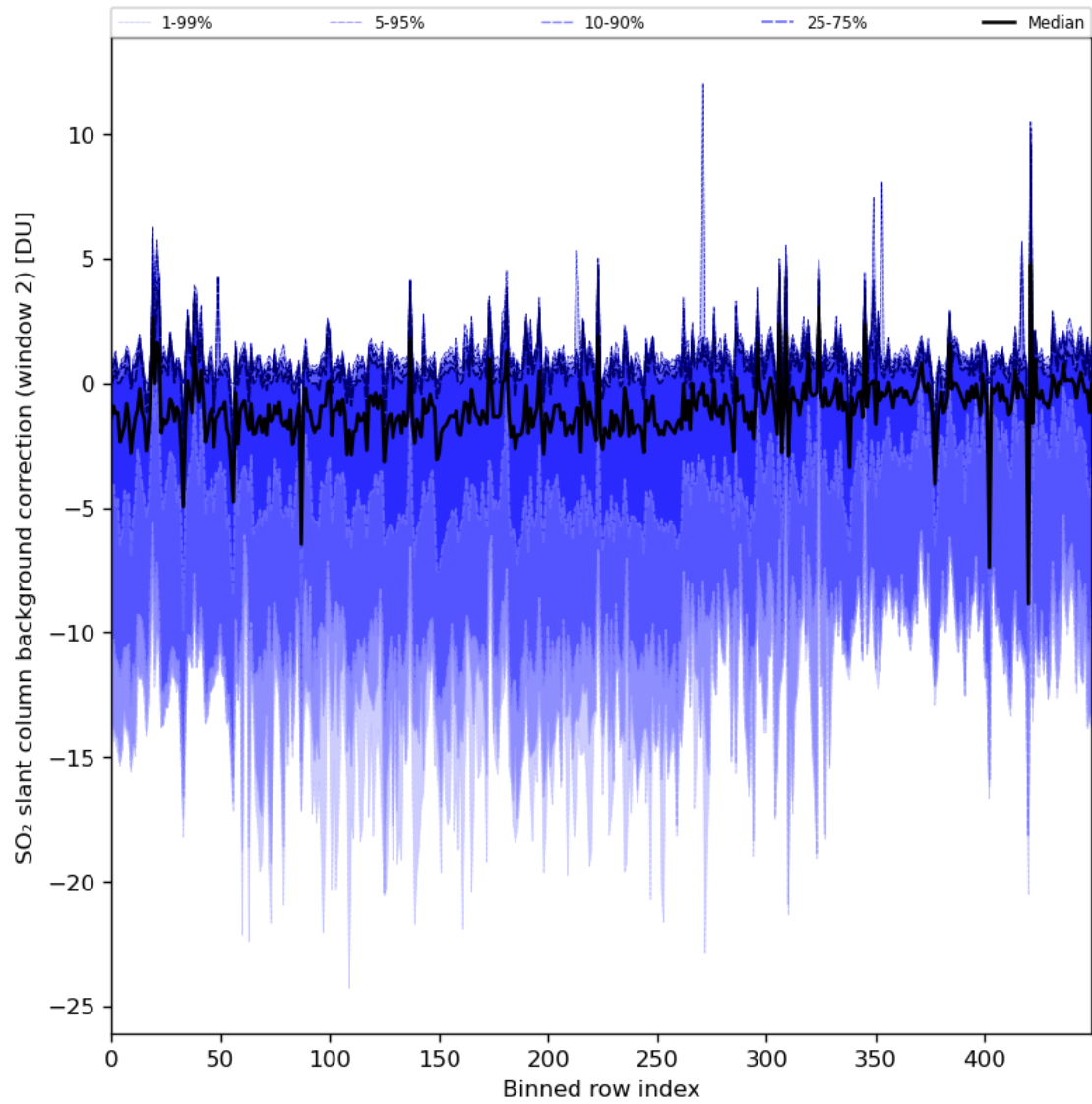
Figure 86: Along track statistics of “SO 2 slant column background correction (window 2)” for 2024-02-25 to 2024-02-27
