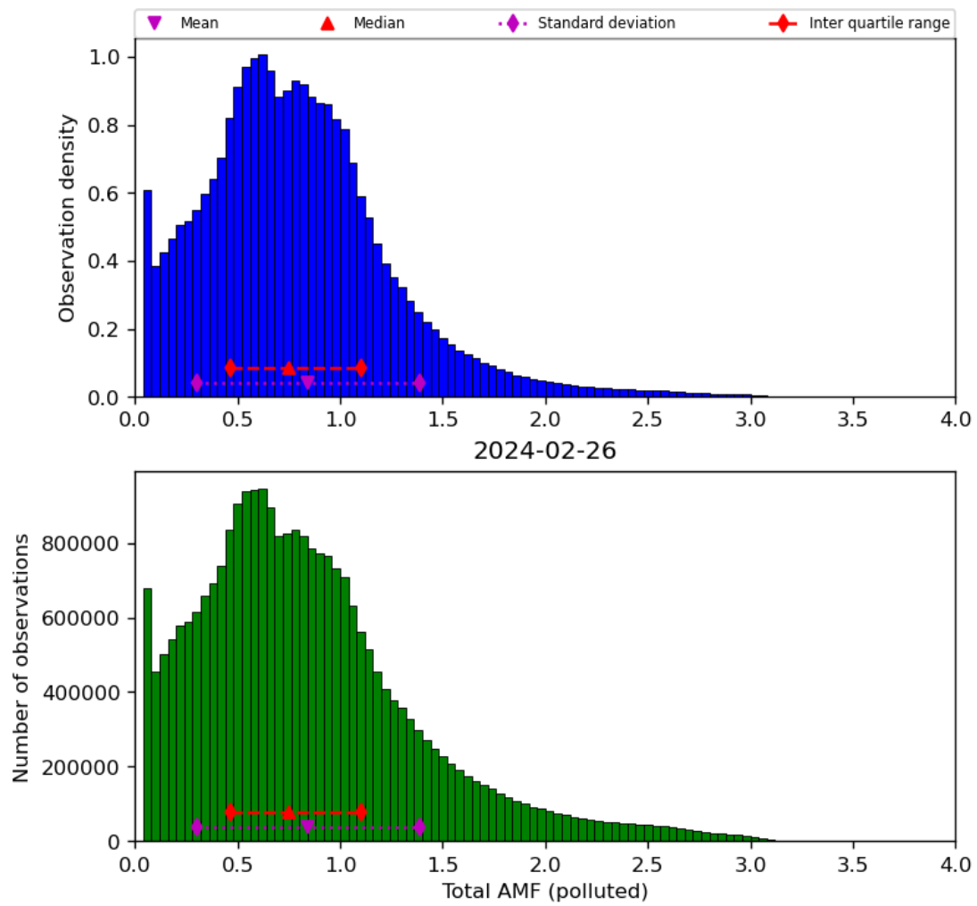
Figure 71: Histogram of “Total AMF (polluted)” for 2024-02-25 to 2024-02-27
