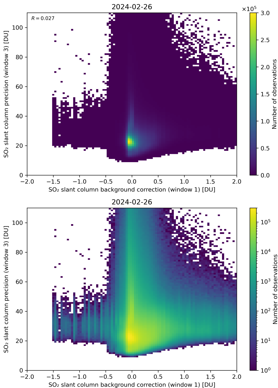
Figure 108: Scatter density plot of “SO 2 slant column background correction (window 1)” against “SO 2 slant column precision (window 3)” for 2024-02-25 to 2024-02-27.
