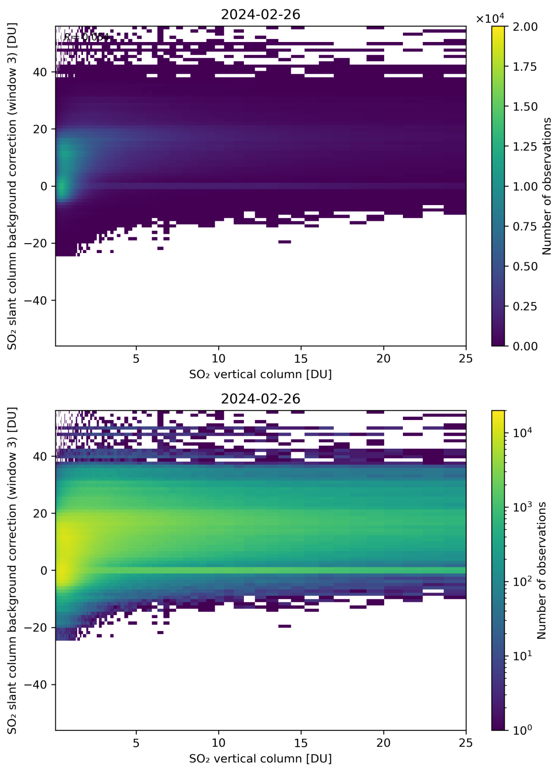
Figure 275: Scatter density plot of “SO 2 vertical column” against “SO 2 slant column background correction (window 3)” for 2024-02-25 to 2024-02-27.
