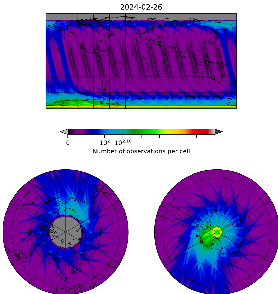
Figure 28: Map of the number of observations for 2024-02-25 to 2024-02-27
