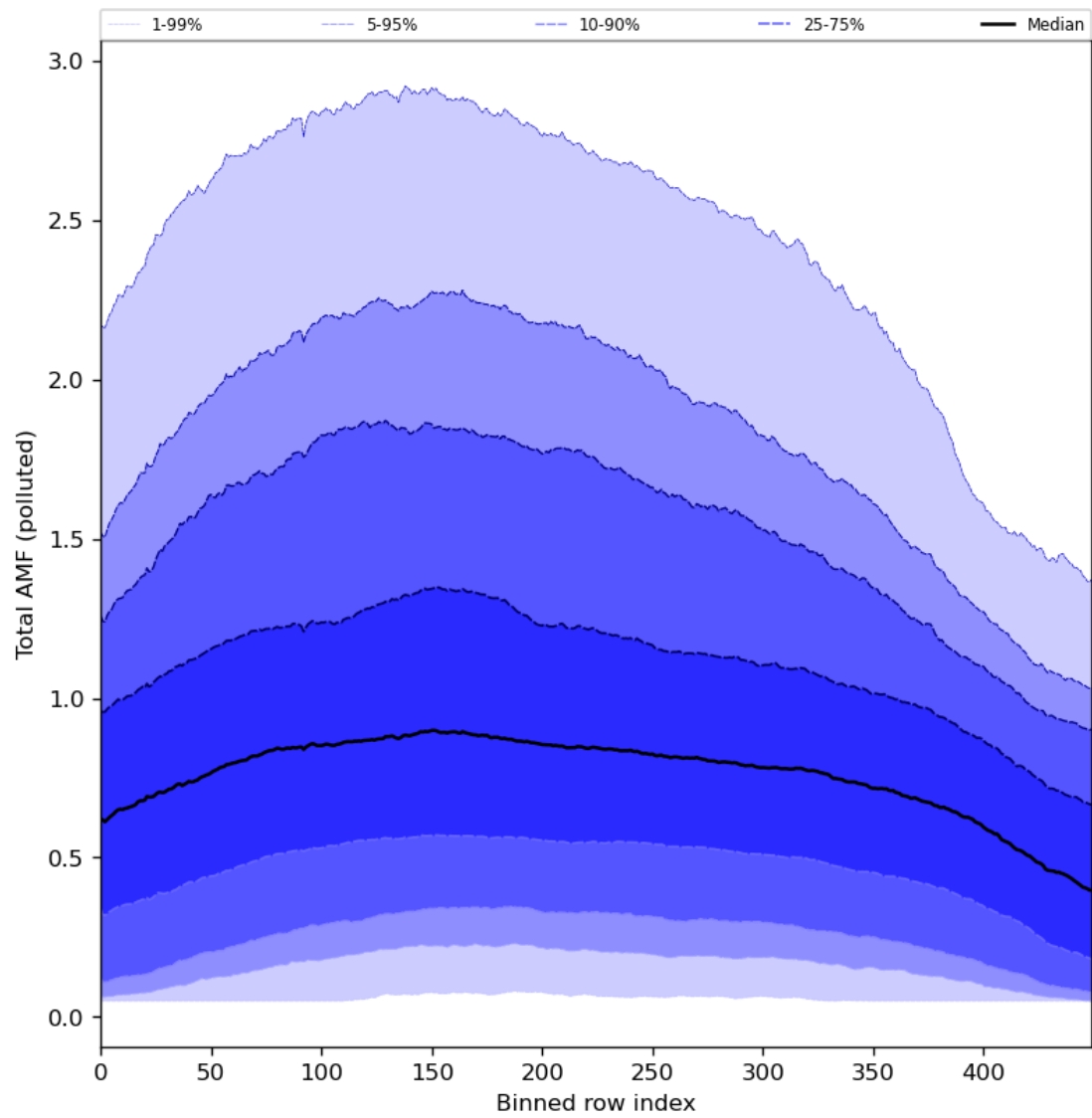
Figure 94: Along track statistics of “Total AMF (polluted)” for 2024-02-25 to 2024-02-27
