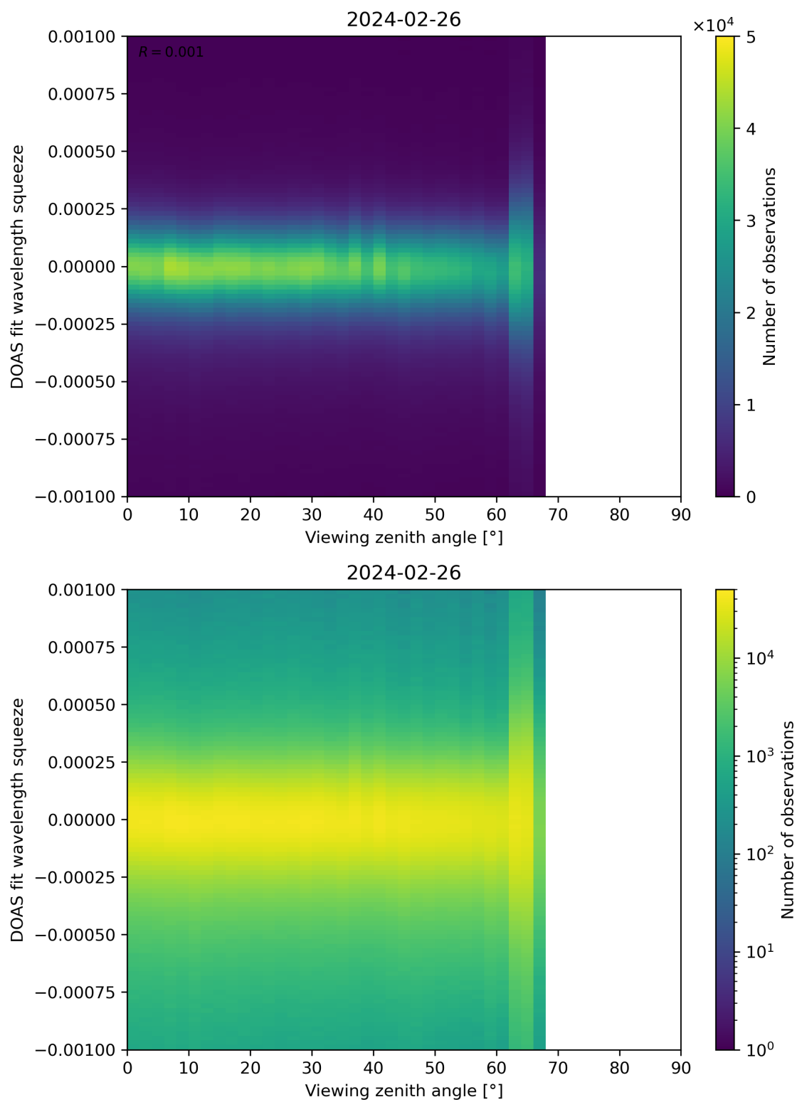
Figure 312: Scatter density plot of “Viewing zenith angle” against “DOAS fit wavelength squeeze” for 2024-02-25 to 2024-02-27.
