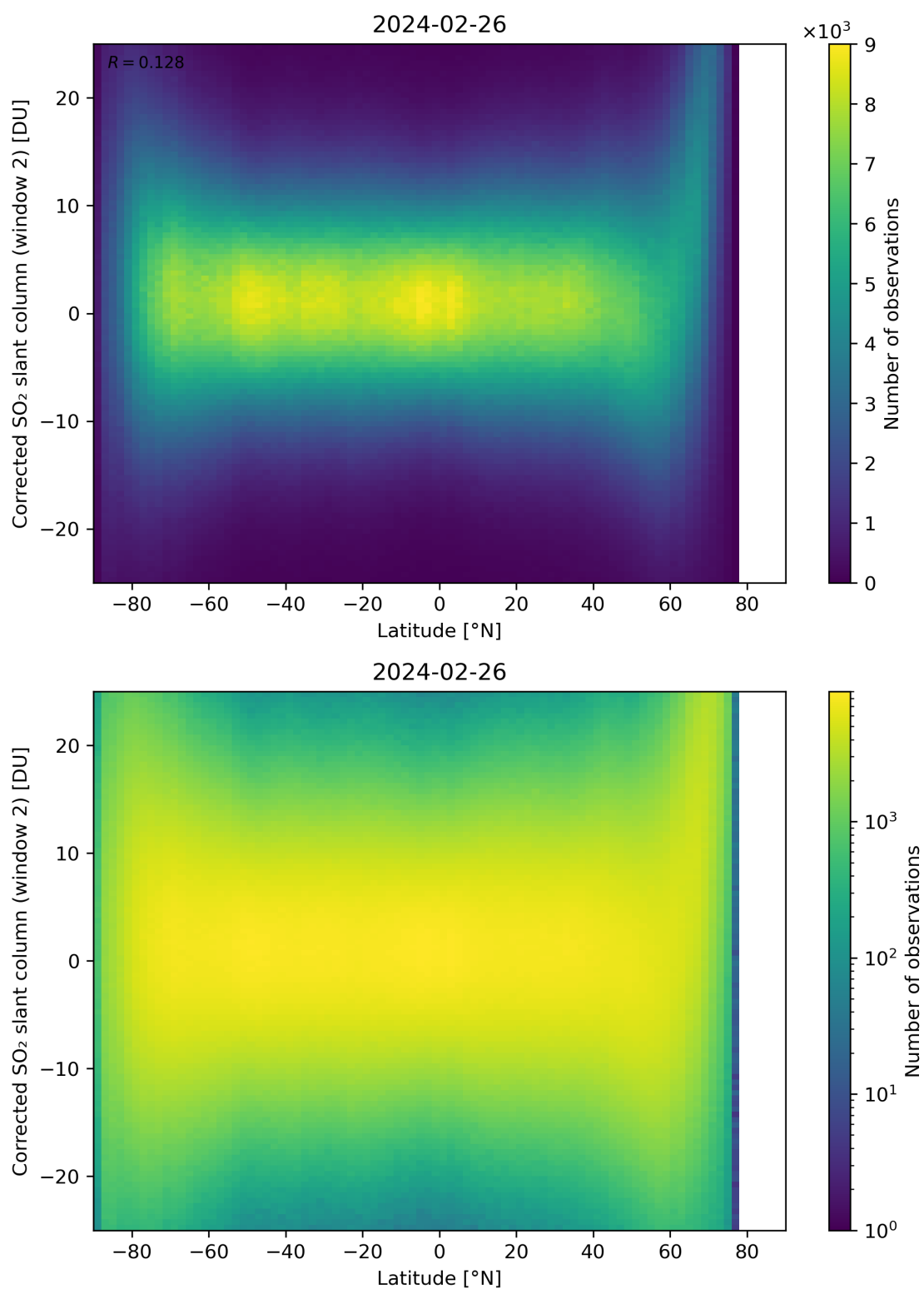
Figure 147: Scatter density plot of “Latitude” against “Corrected SO 2 slant column (window 2)” for 2024-02-25 to 2024-02-27.
