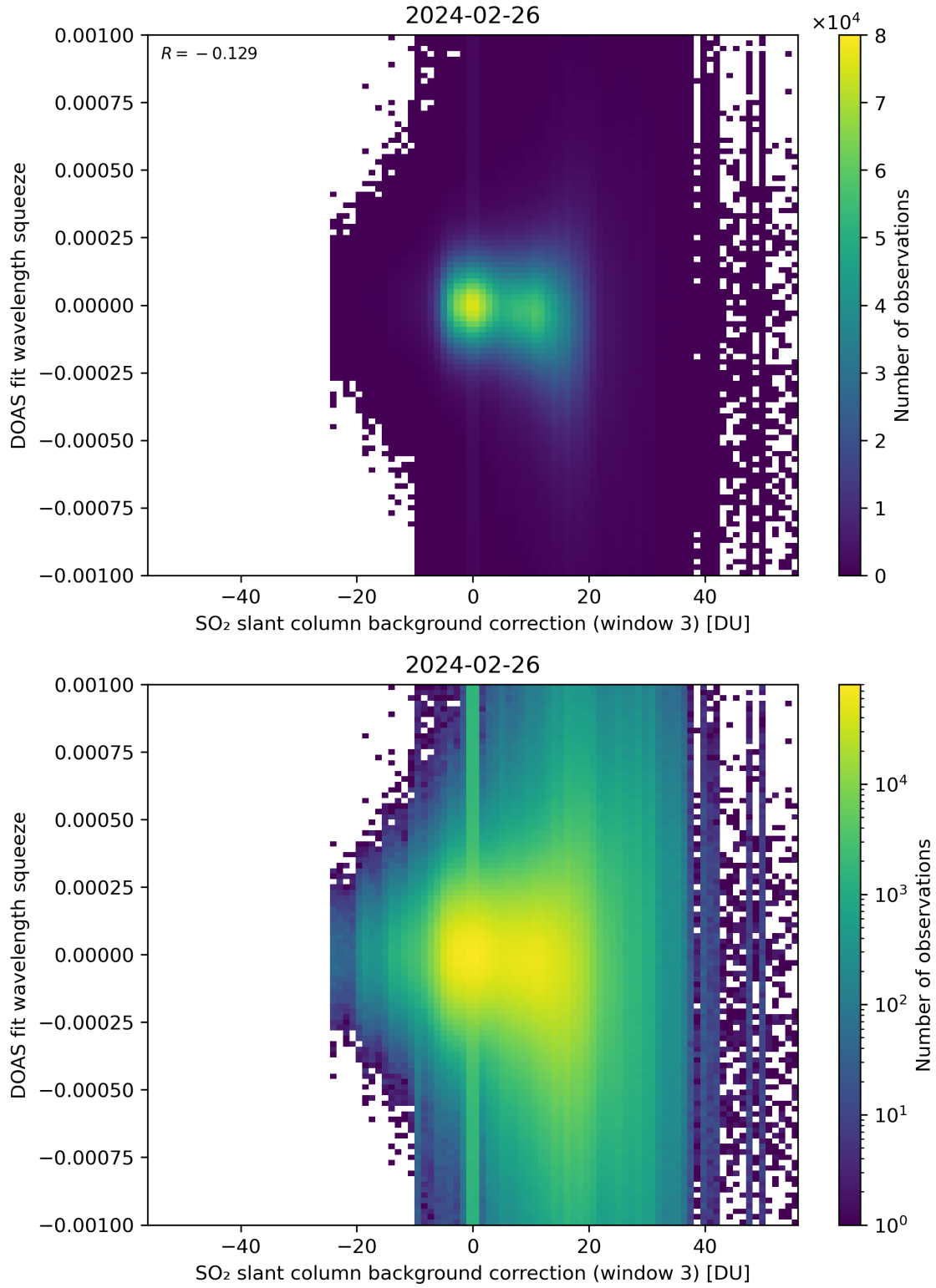
Figure 122: Scatter density plot of “SO 2 slant column background correction (window 3)” against “DOAS fit wavelength squeeze” for 2024-02-25 to 2024-02-27.
