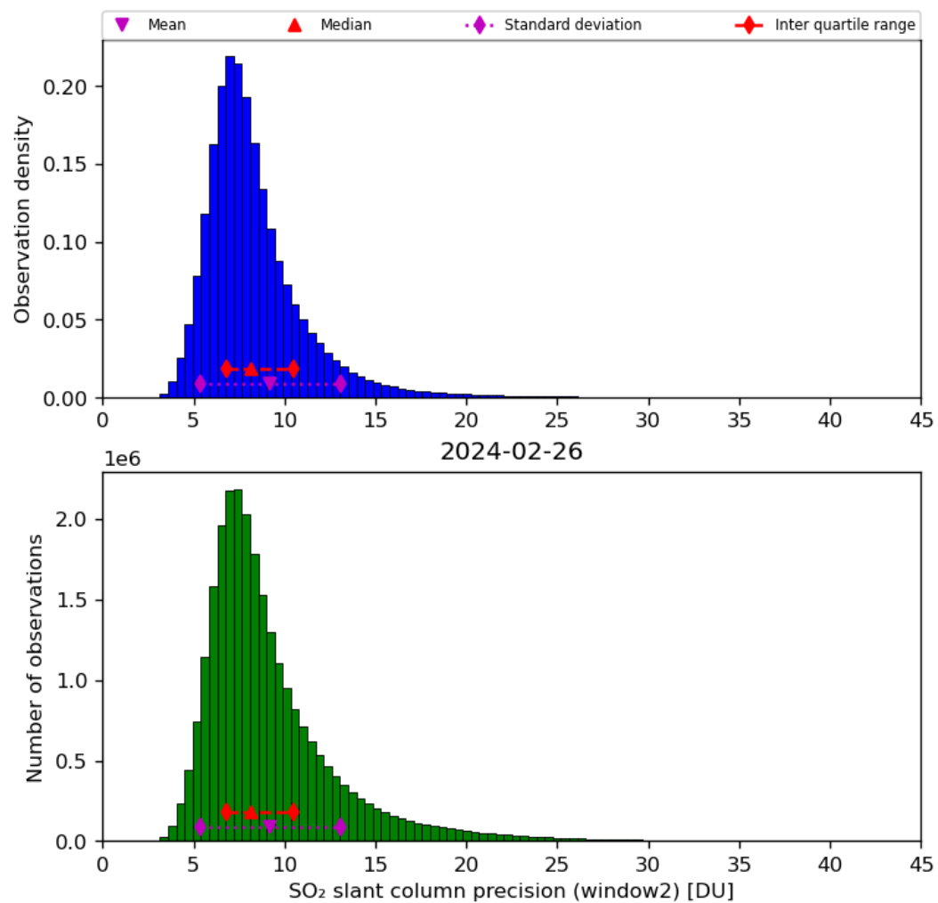
Figure 61: Histogram of “SO 2 slant column precision (window2)” for 2024-02-25 to 2024-02-27
