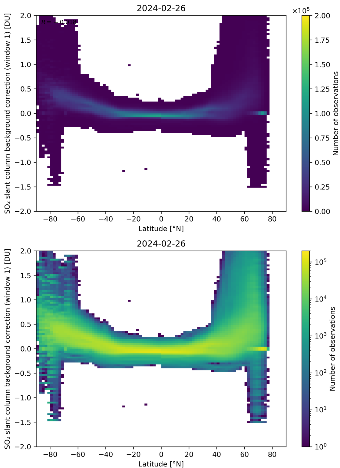
Figure 139: Scatter density plot of “Latitude” against “SO 2 slant column background correction (window 1)” for 2024-02-25 to 2024-02-27.
