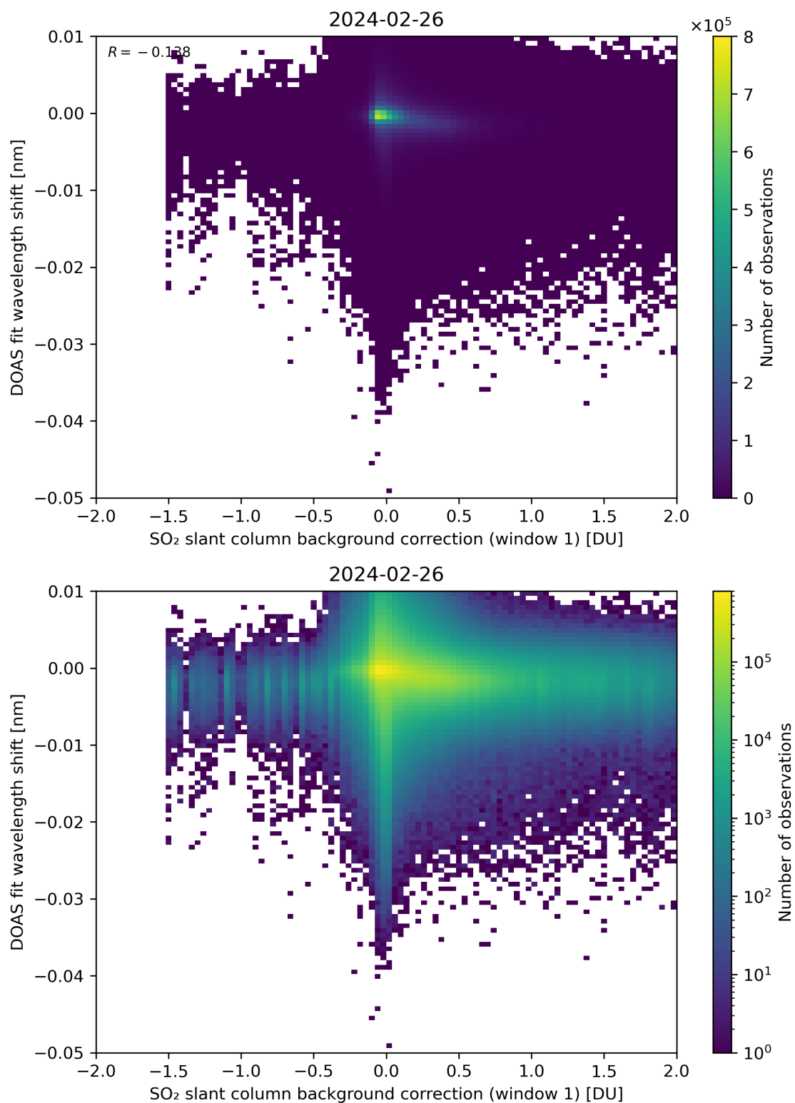
Figure 100: Scatter density plot of “SO 2 slant column background correction (window 1)” against “DOAS fit wavelength shift” for 2024-02-25 to 2024-02-27.
