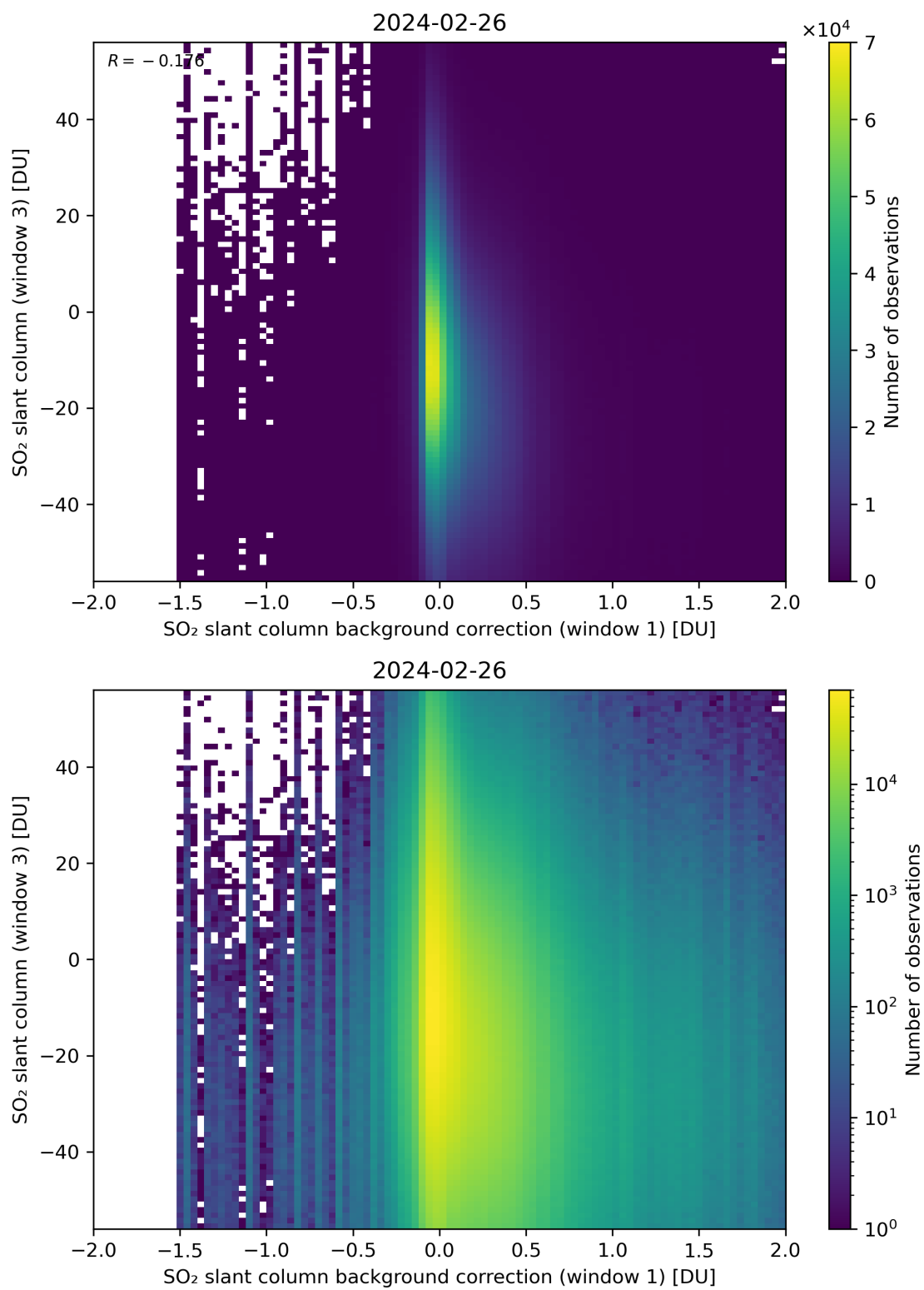
Figure 107: Scatter density plot of “SO 2 slant column background correction (window 1)” against “SO 2 slant column (window 3)” for 2024-02-25 to 2024-02-27.
