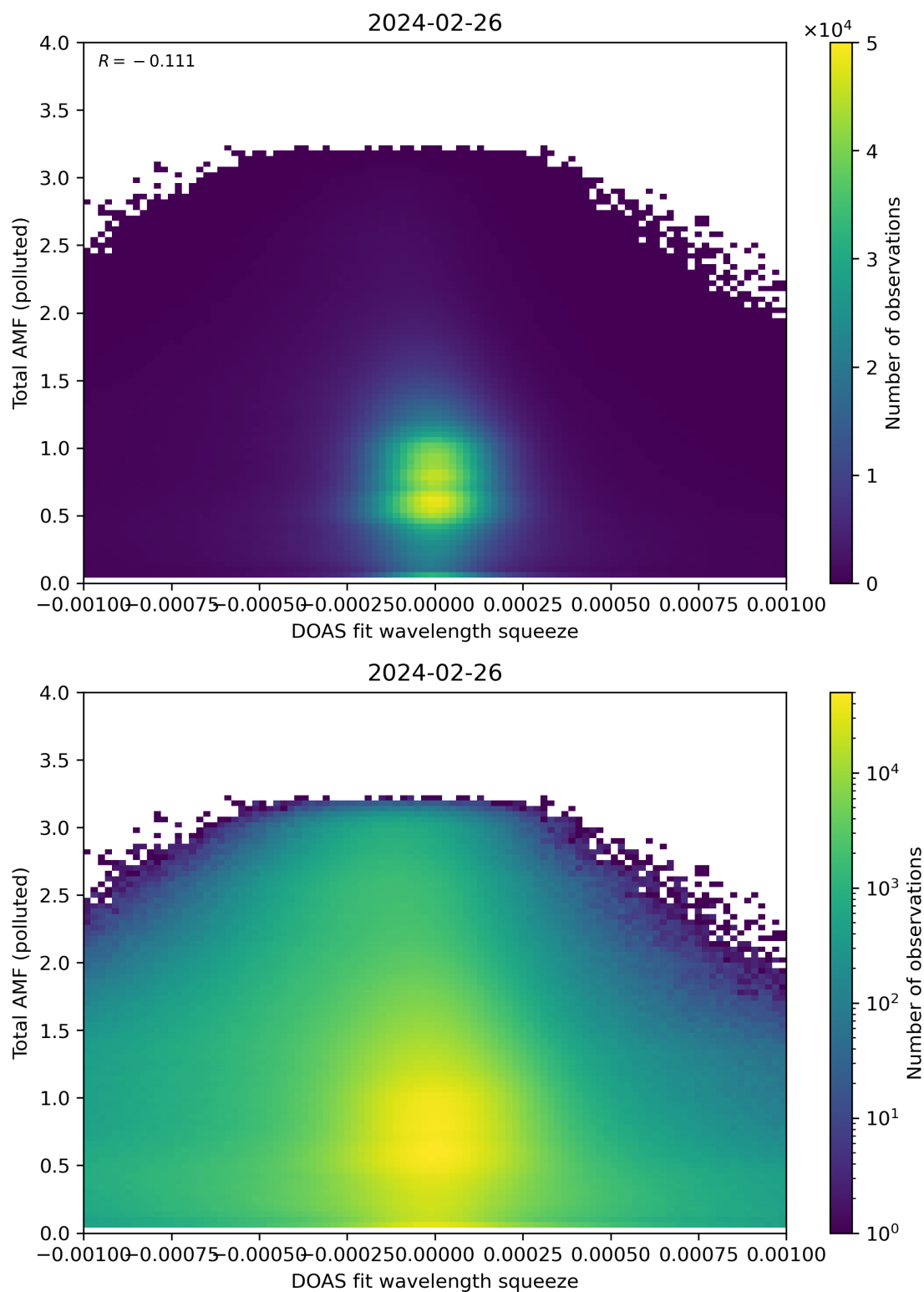
Figure 134: Scatter density plot of “DOAS fit wavelength squeeze” against “Total AMF (polluted)” for 2024-02-25 to 2024-02-27.
