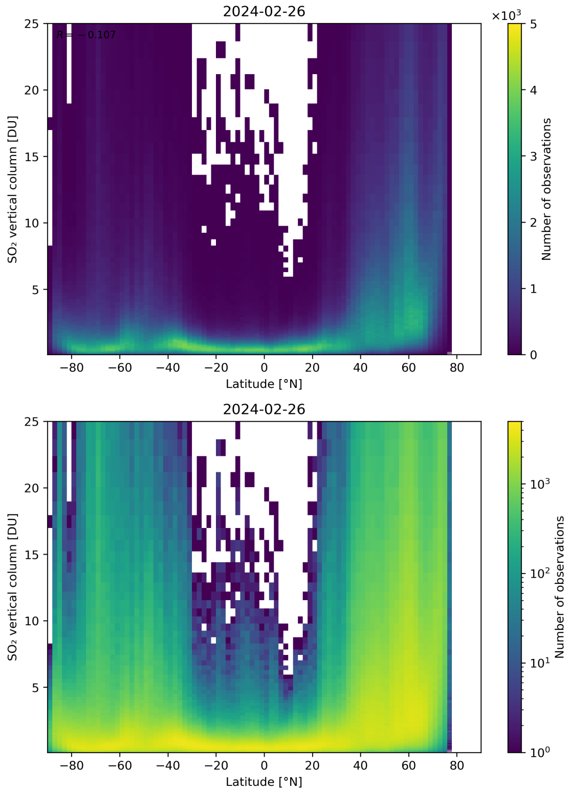
Figure 156: Scatter density plot of “Latitude” against “SO 2 vertical column” for 2024-02-25 to 2024-02-27.
