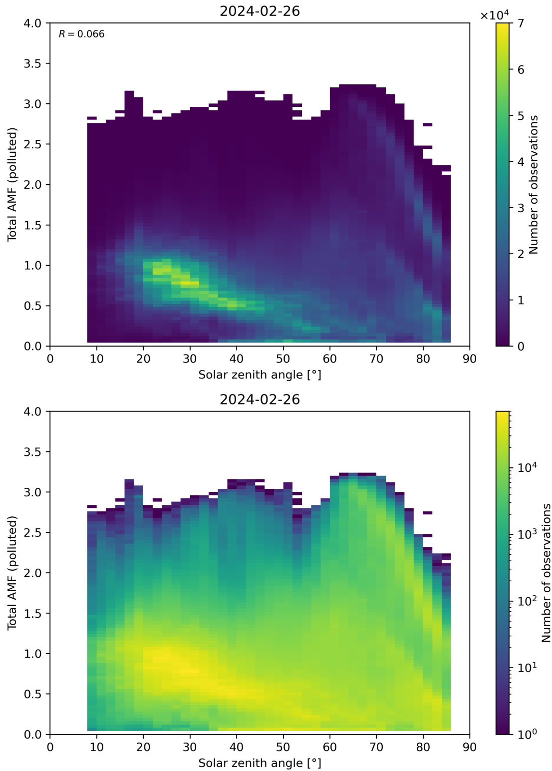
Figure 174: Scatter density plot of “Solar zenith angle” against “Total AMF (polluted)” for 2024-02-25 to 2024-02-27.
