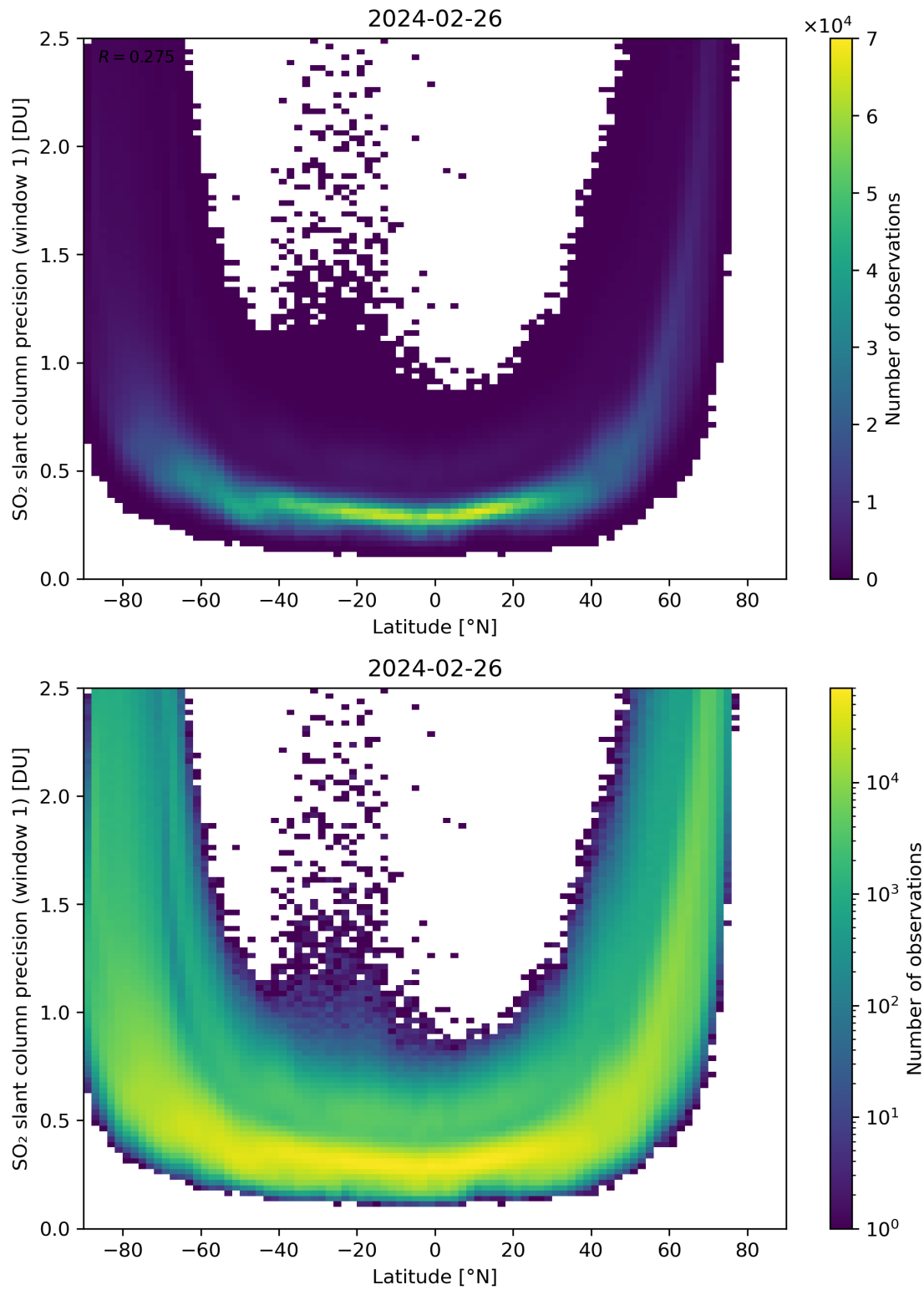
Figure 150: Scatter density plot of “Latitude” against “SO 2 slant column precision (window 1)” for 2024-02-25 to 2024-02-27.
