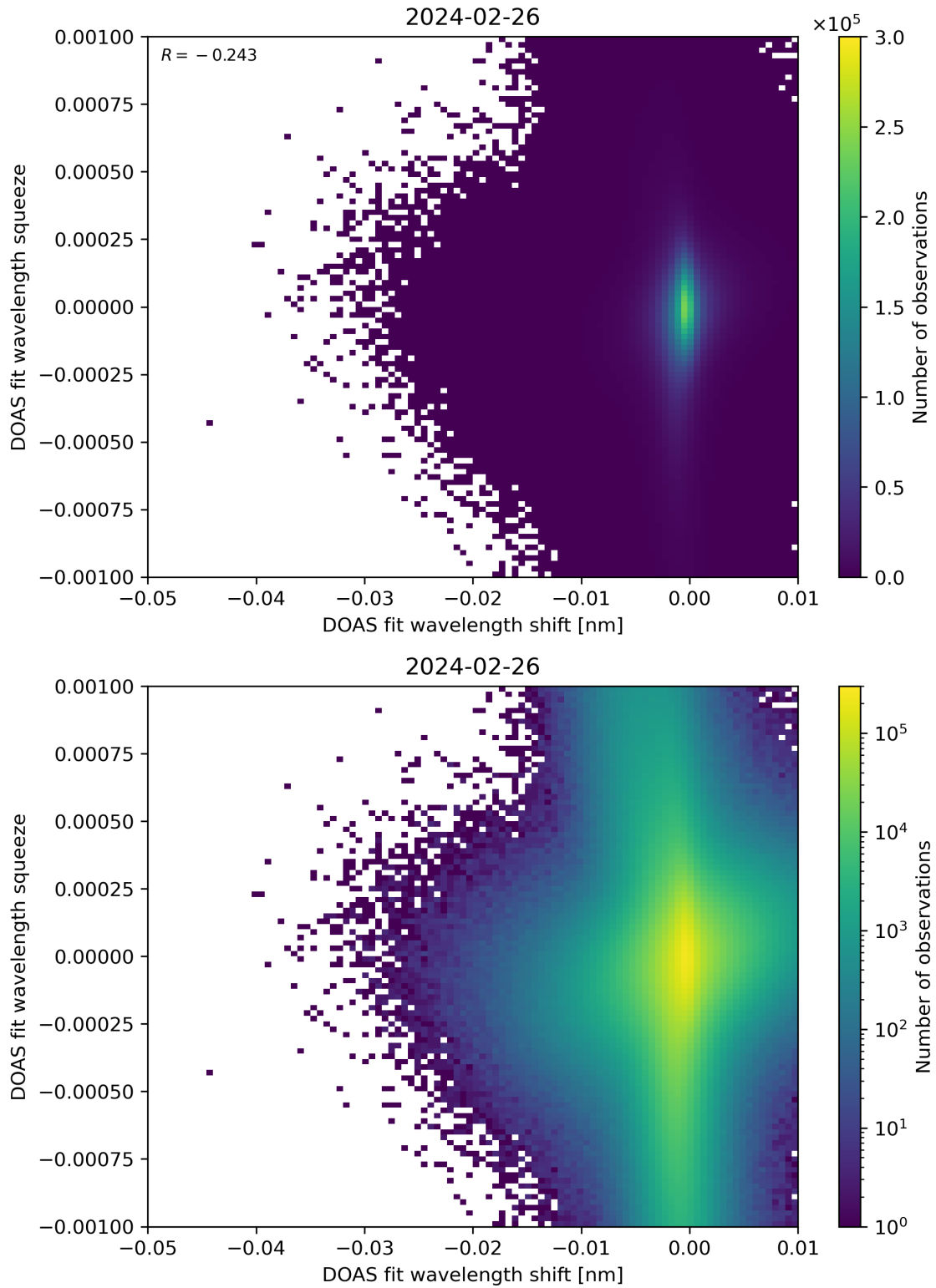
Figure 127: Scatter density plot of “DOAS fit wavelength shift” against “DOAS fit wavelength squeeze” for 2024-02-25 to 2024-02-27.
