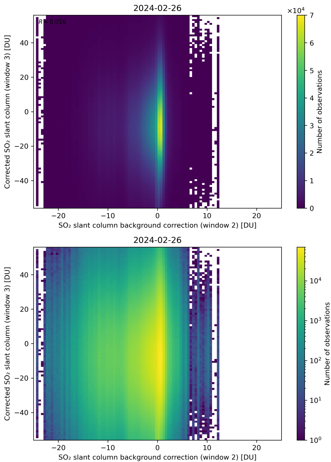
Figure 116: Scatter density plot of “SO 2 slant column background correction (window 2)” against “Corrected SO 2 slant column (window 3)” for 2024-02-25 to 2024-02-27.
