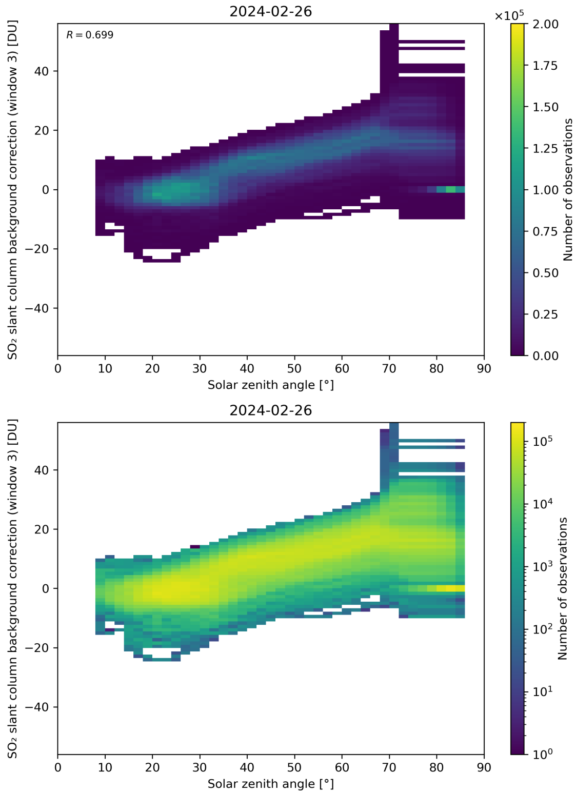
Figure 160: Scatter density plot of “Solar zenith angle” against “SO 2 slant column background correction (window 3)” for 2024-02-25 to 2024-02-27.
