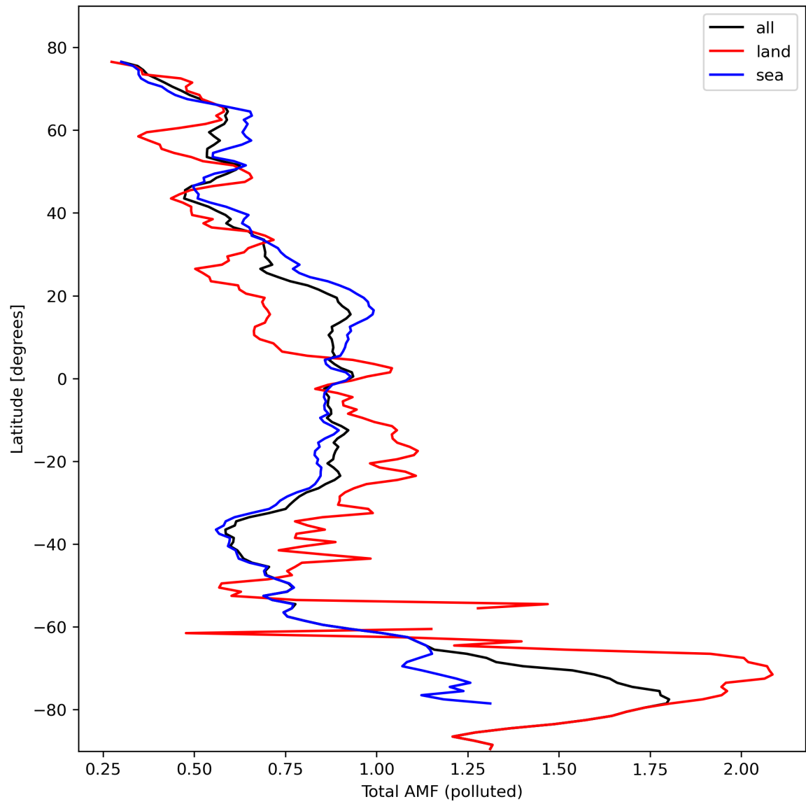
Figure 48: Zonal average of “Total AMF (polluted)” for 2024-02-25 to 2024-02-27.
