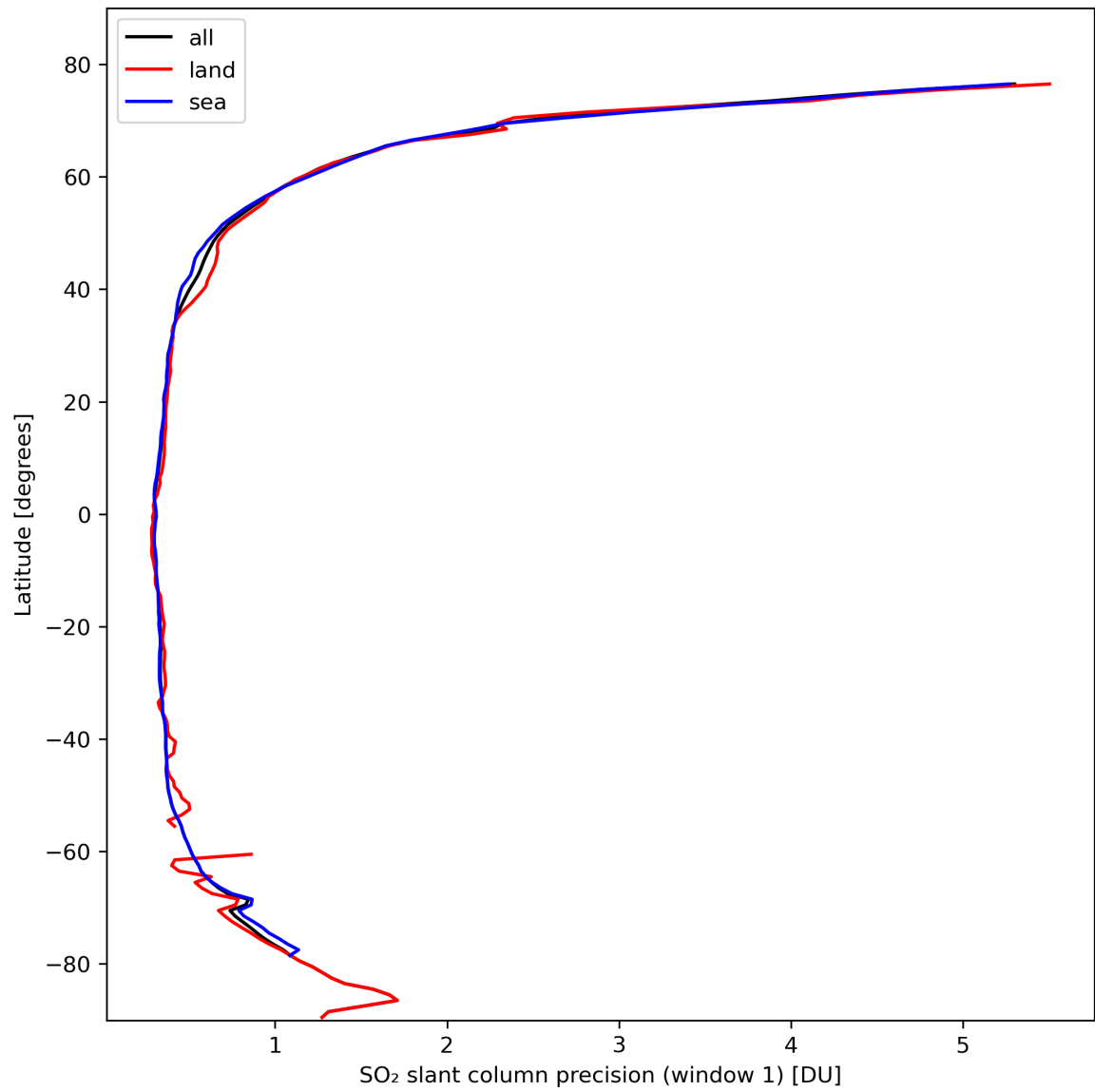
Figure 34: Zonal average of “SO 2 slant column precision (window 1)” for 2024-02-25 to 2024-02-27.
