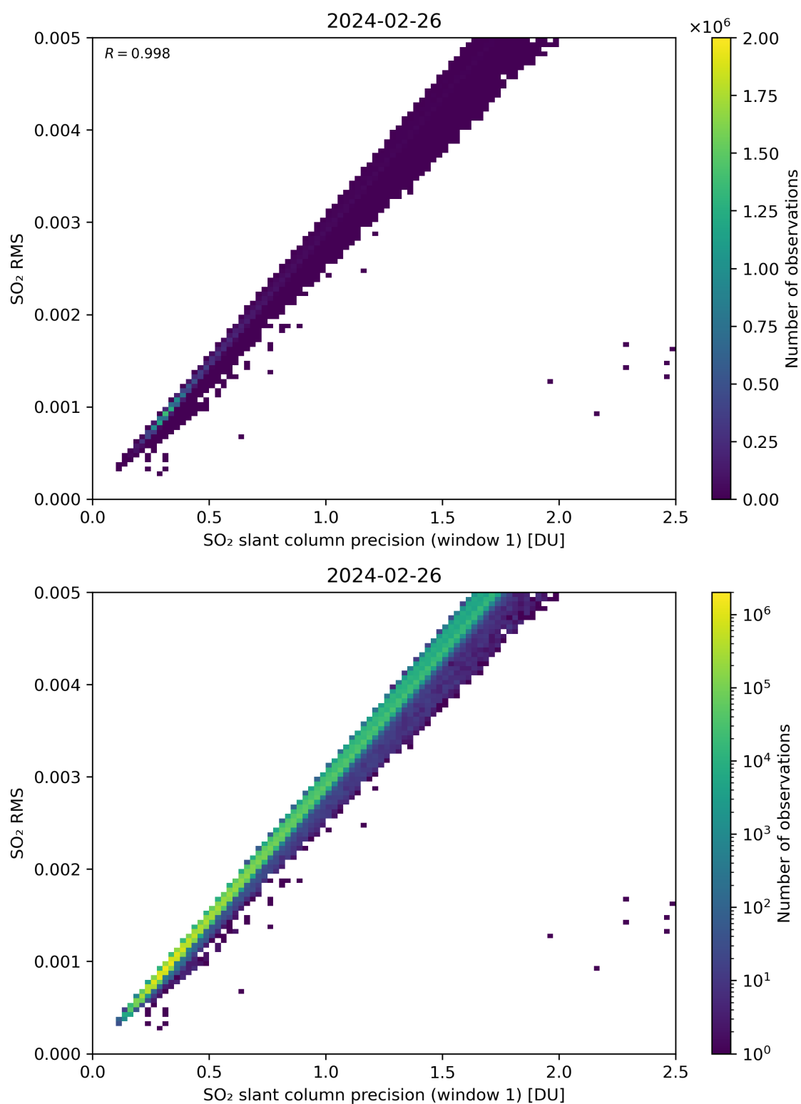
Figure 223: Scatter density plot of “SO 2 slant column precision (window 1)” against “SO 2 RMS” for 2024-02-25 to 2024-02-27.
