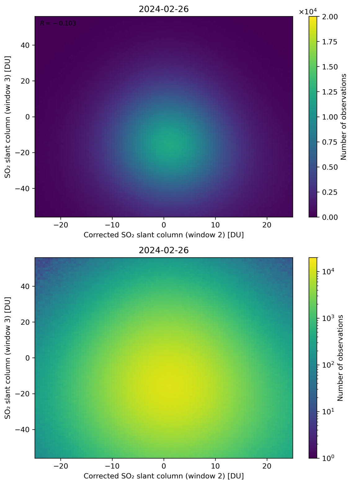
Figure 201: Scatter density plot of “Corrected SO 2 slant column (window 2)” against “SO 2 slant column (window 3)” for 2024-02-25 to 2024-02-27.
