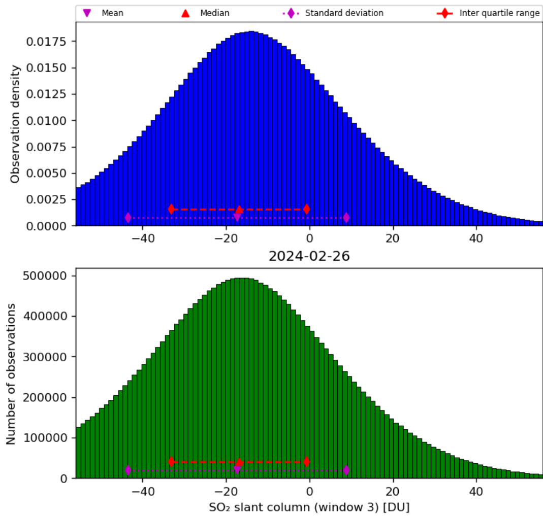
Figure 64: Histogram of “SO 2 slant column (window 3)” for 2024-02-25 to 2024-02-27
