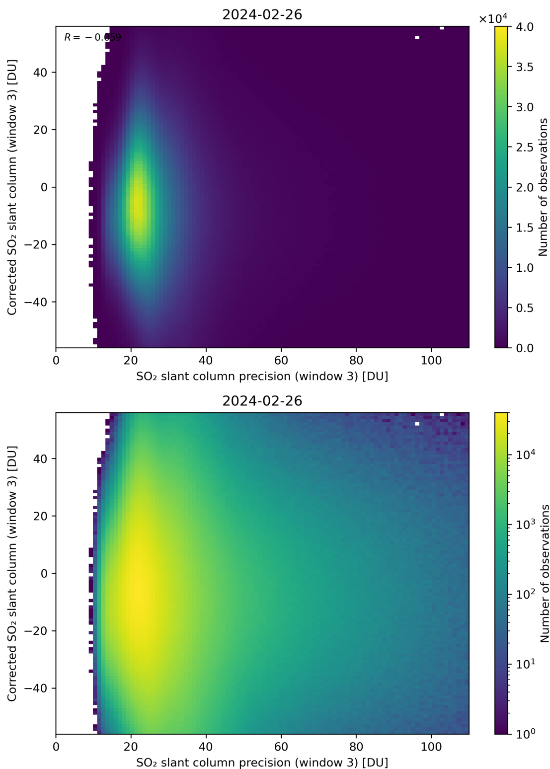
Figure 262: Scatter density plot of “SO 2 slant column precision (window 3)” against “Corrected SO 2 slant column (window 3)” for 2024-02-25 to 2024-02-27.
