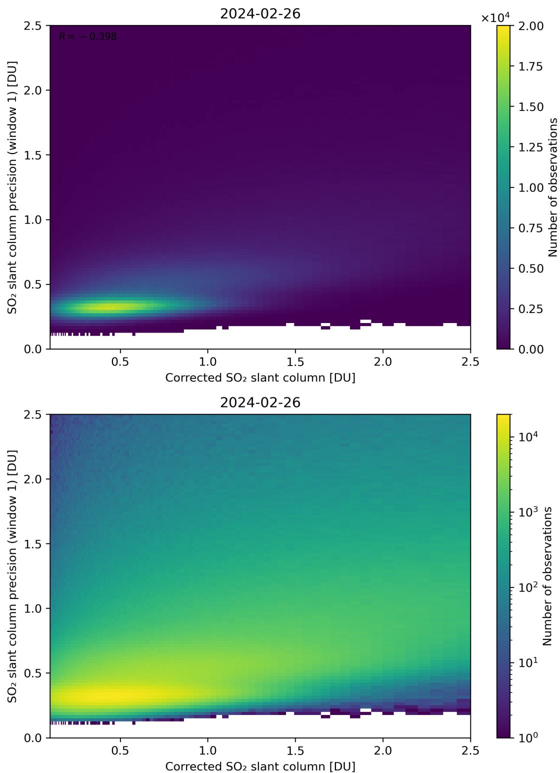
Figure 188: Scatter density plot of “Corrected SO 2 slant column” against “SO 2 slant column precision (window 1)” for 2024-02-25 to 2024-02-27.
