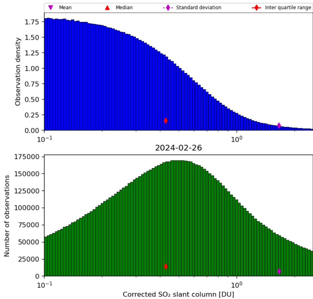
Figure 55: Histogram of “Corrected SO 2 slant column” for 2024-02-25 to 2024-02-27
