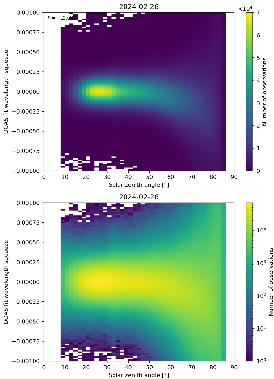
Figure 162: Scatter density plot of “Solar zenith angle” against “DOAS fit wavelength squeeze” for 2024-02-25 to 2024-02-27.
