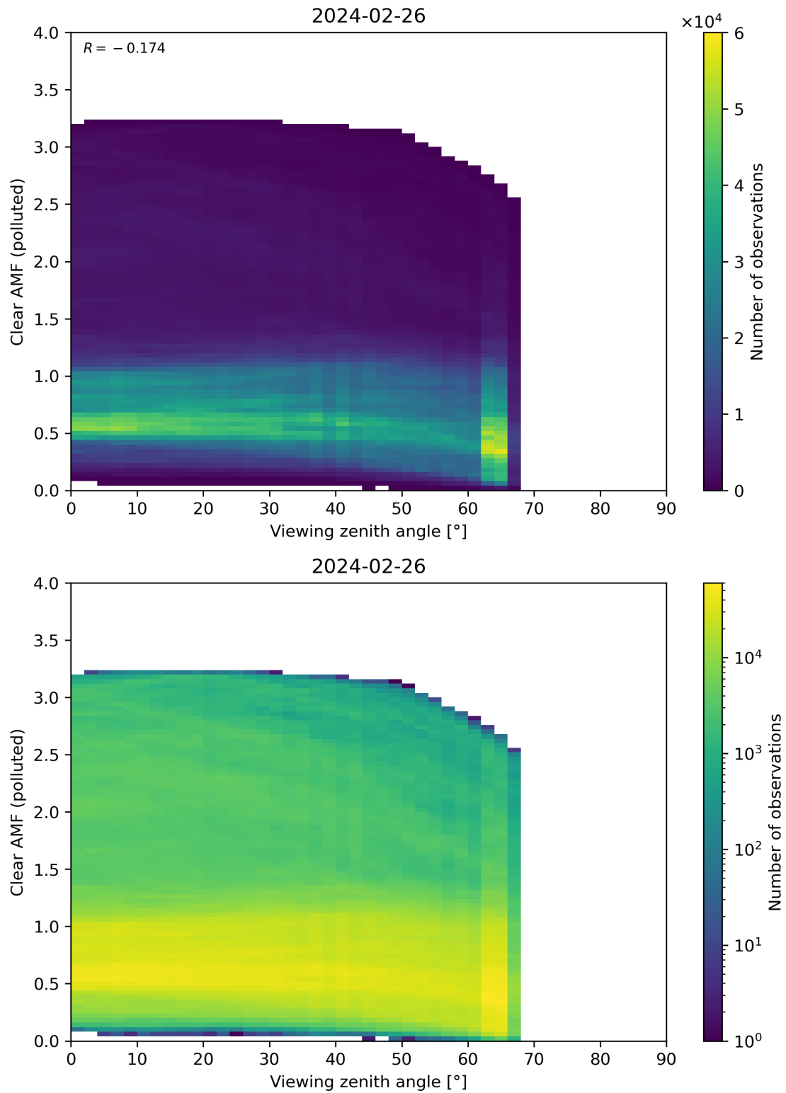
Figure 316: Scatter density plot of “Viewing zenith angle” against “Clear AMF (polluted)” for 2024-02-25 to 2024-02-27.
