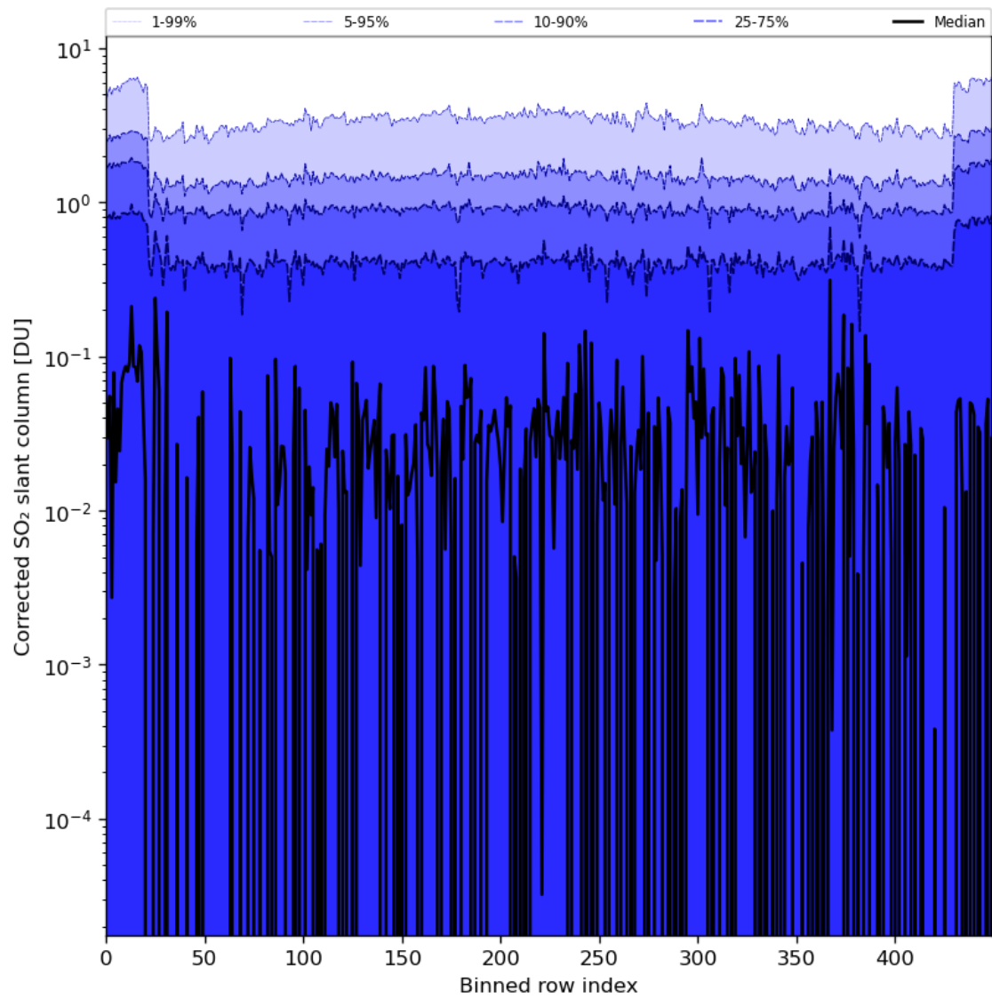
Figure 78: Along track statistics of “Corrected SO 2 slant column” for 2024-02-25 to 2024-02-27
