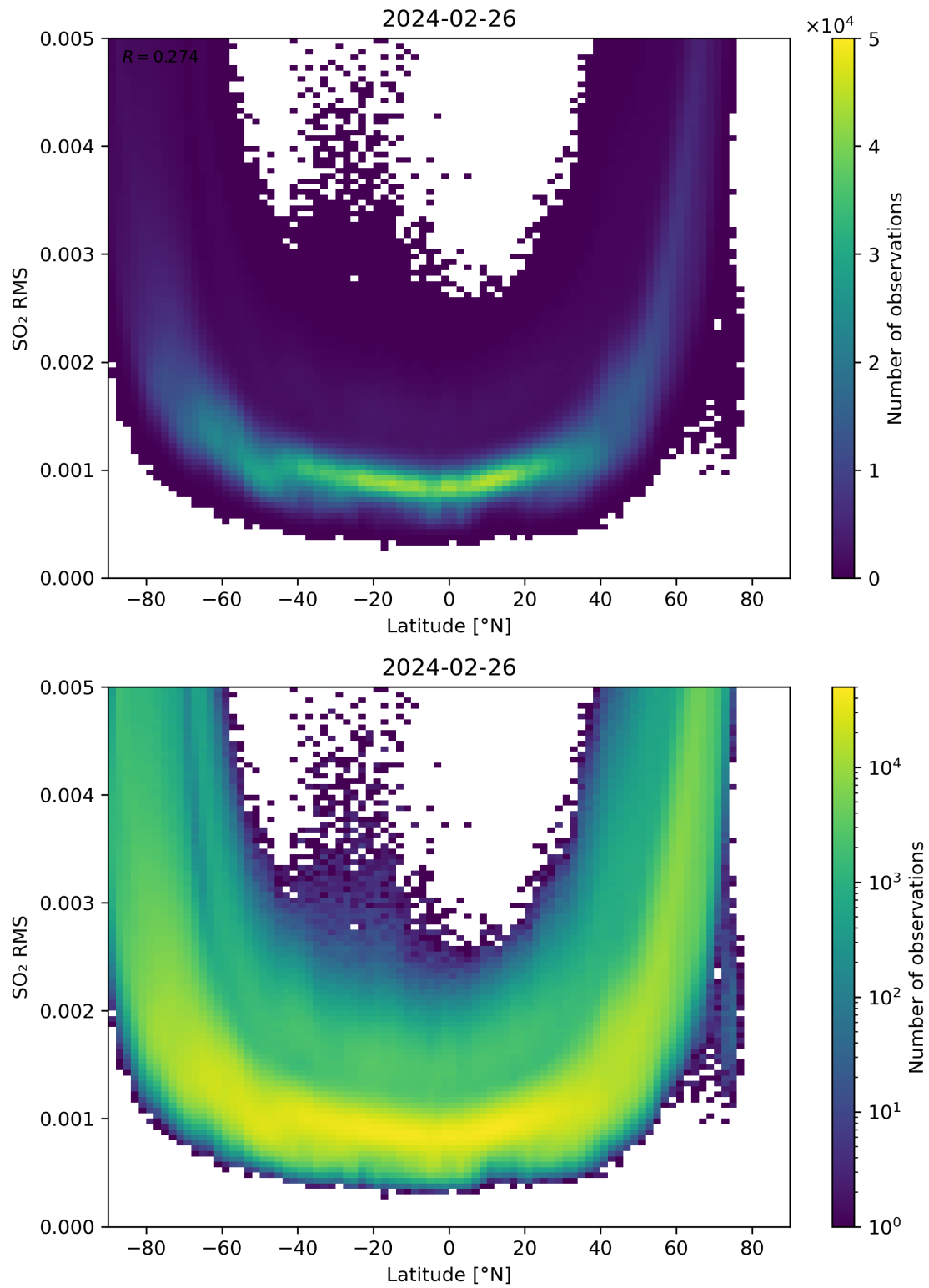
Figure 144: Scatter density plot of “Latitude” against “SO 2 RMS” for 2024-02-25 to 2024-02-27.
