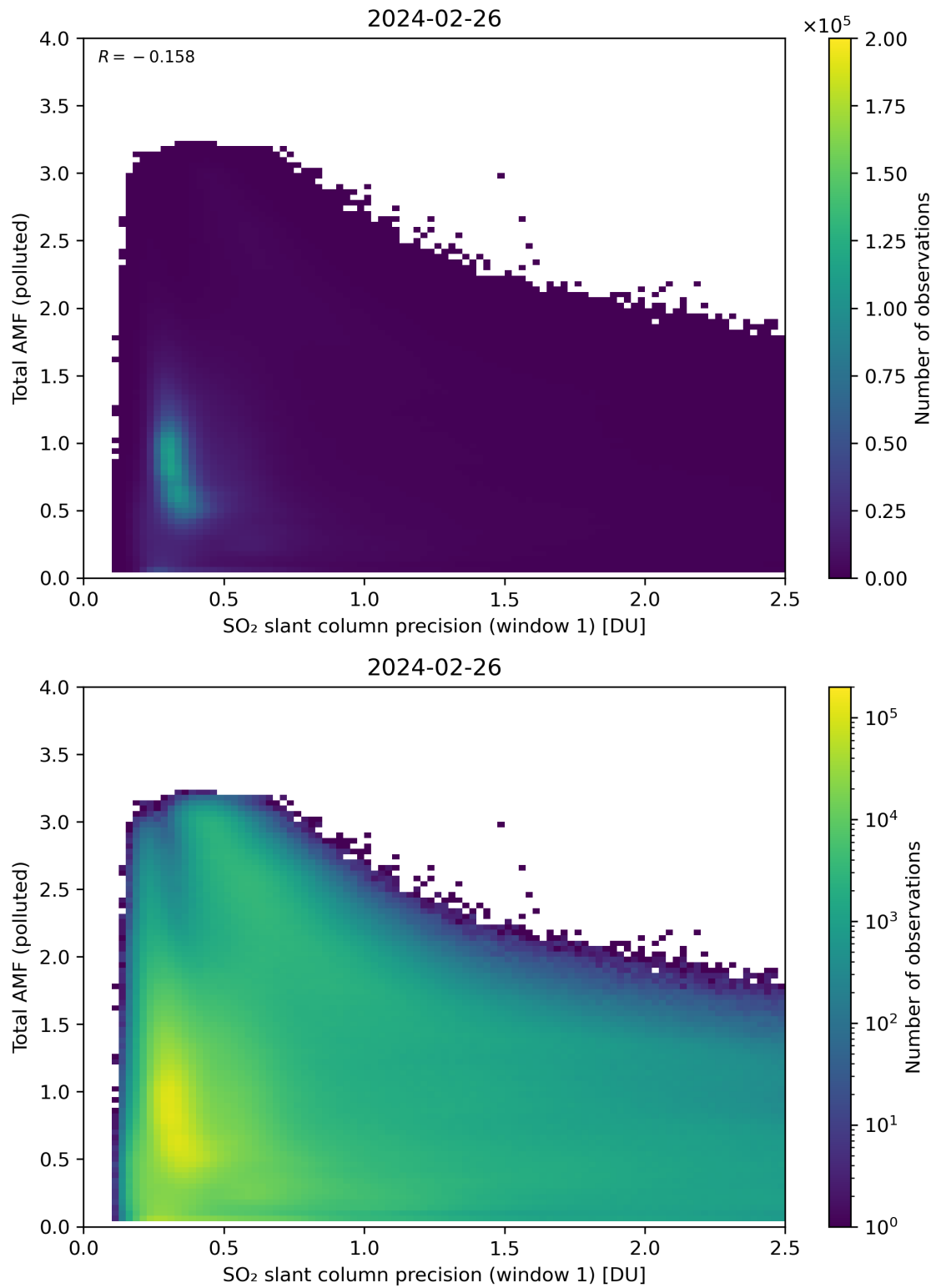
Figure 230: Scatter density plot of “SO 2 slant column precision (window 1)” against “Total AMF (polluted)” for 2024-02-25 to 2024-02-27.
