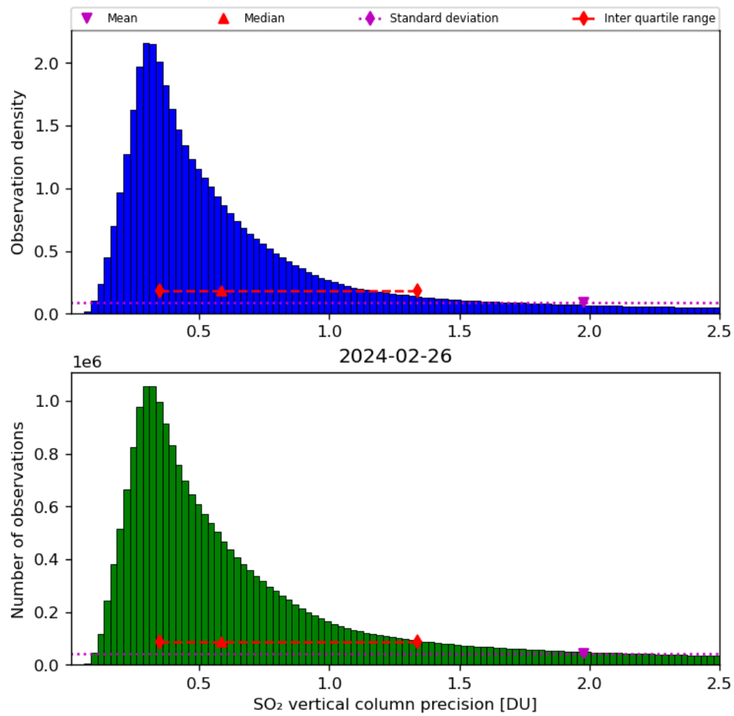
Figure 54: Histogram of “SO 2 vertical column precision” for 2024-02-25 to 2024-02-27
