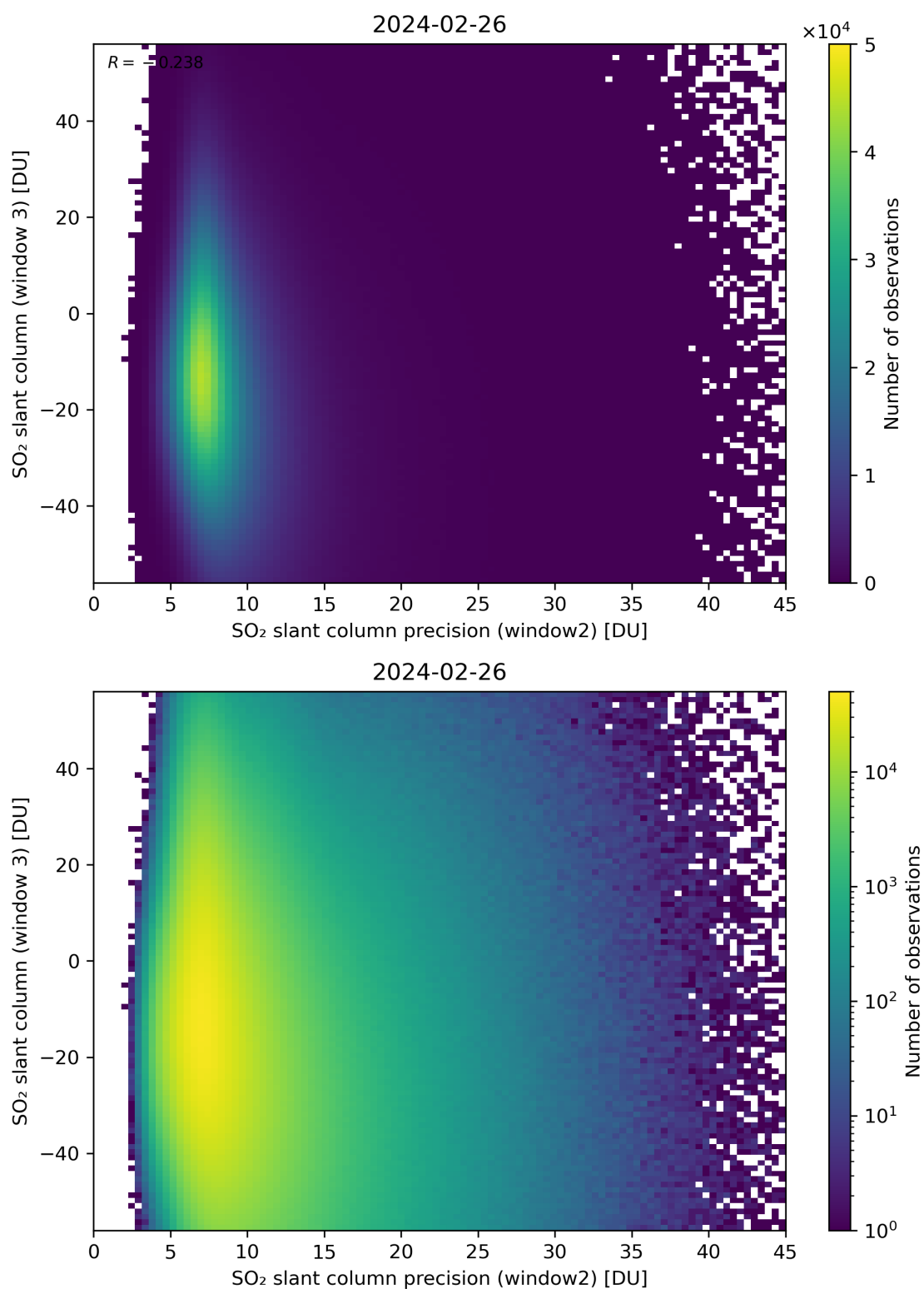
Figure 249: Scatter density plot of “SO 2 slant column precision (window2)” against “SO 2 slant column (window 3)” for 2024-02-25 to 2024-02-27.
