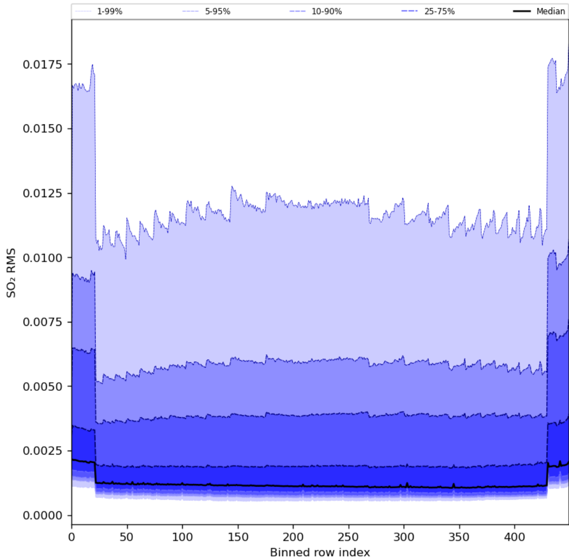
Figure 93: Along track statistics of “SO 2 RMS” for 2024-02-25 to 2024-02-27
