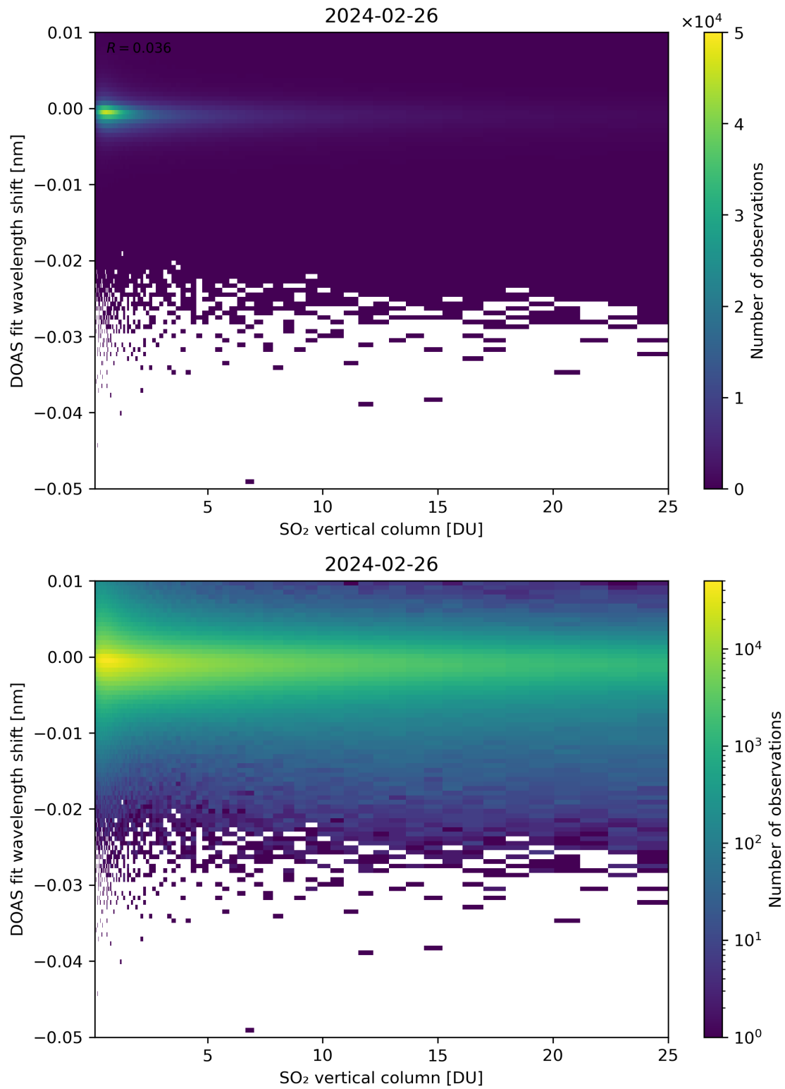
Figure 276: Scatter density plot of “SO 2 vertical column” against “DOAS fit wavelength shift” for 2024-02-25 to 2024-02-27.
