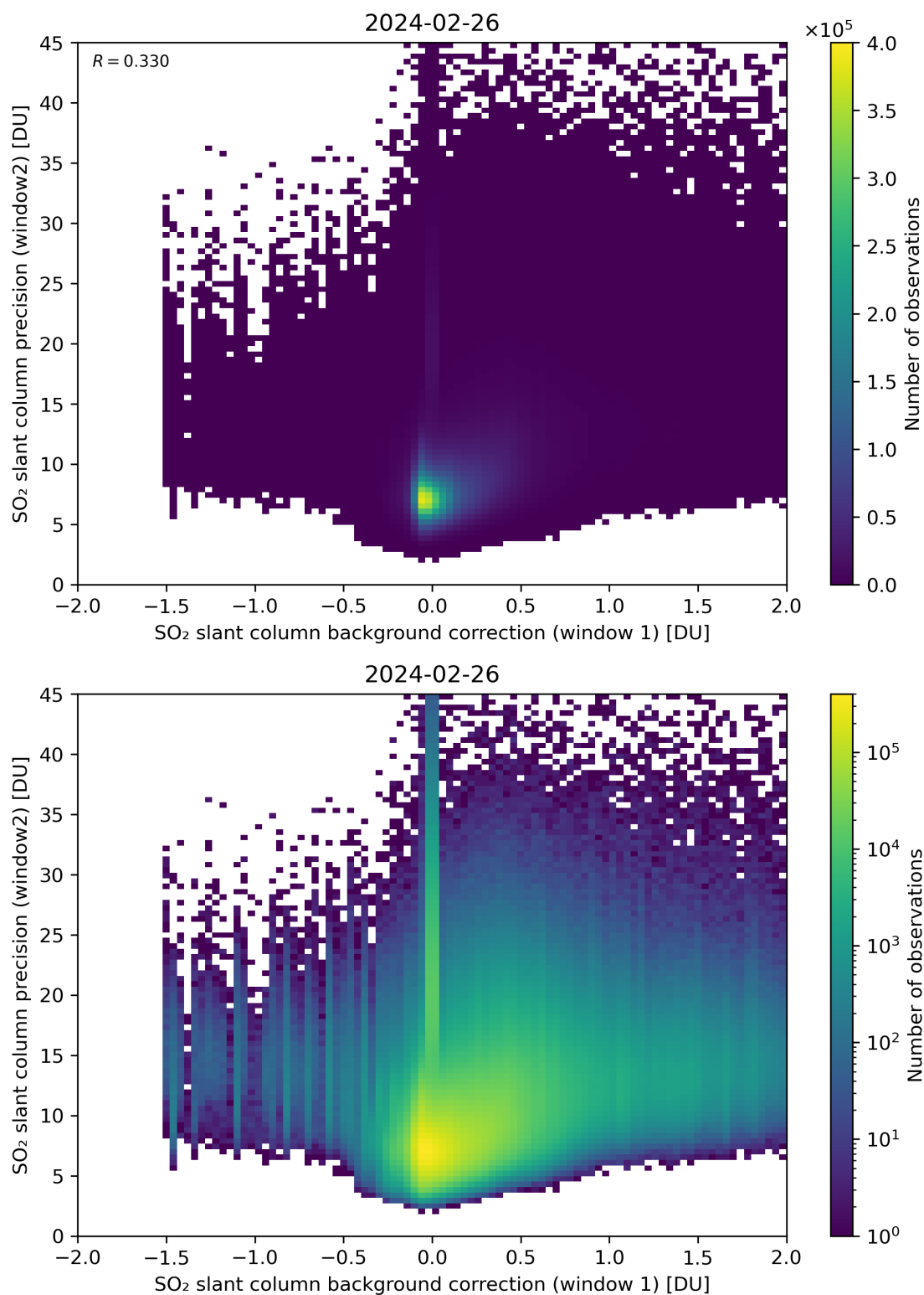
Figure 106: Scatter density plot of “SO 2 slant column background correction (window 1)” against “SO 2 slant column precision (window2)” for 2024-02-25 to 2024-02-27.
