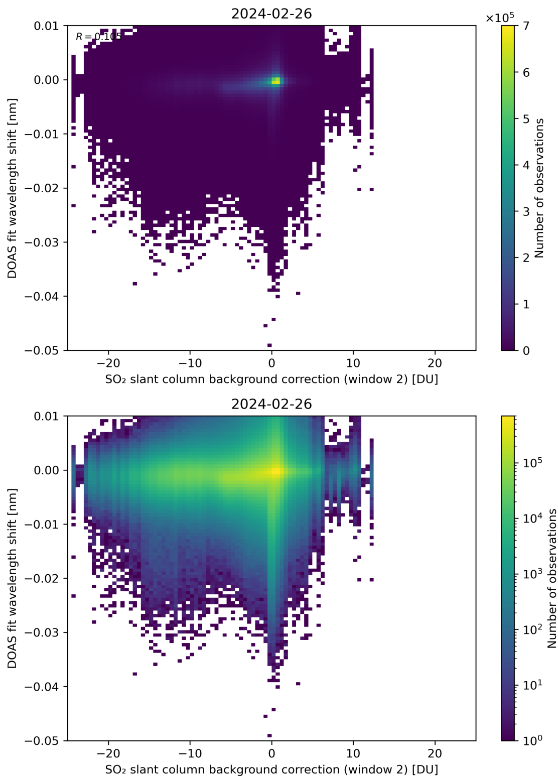
Figure 112: Scatter density plot of “SO 2 slant column background correction (window 2)” against “DOAS fit wavelength shift” for 2024-02-25 to 2024-02-27.
