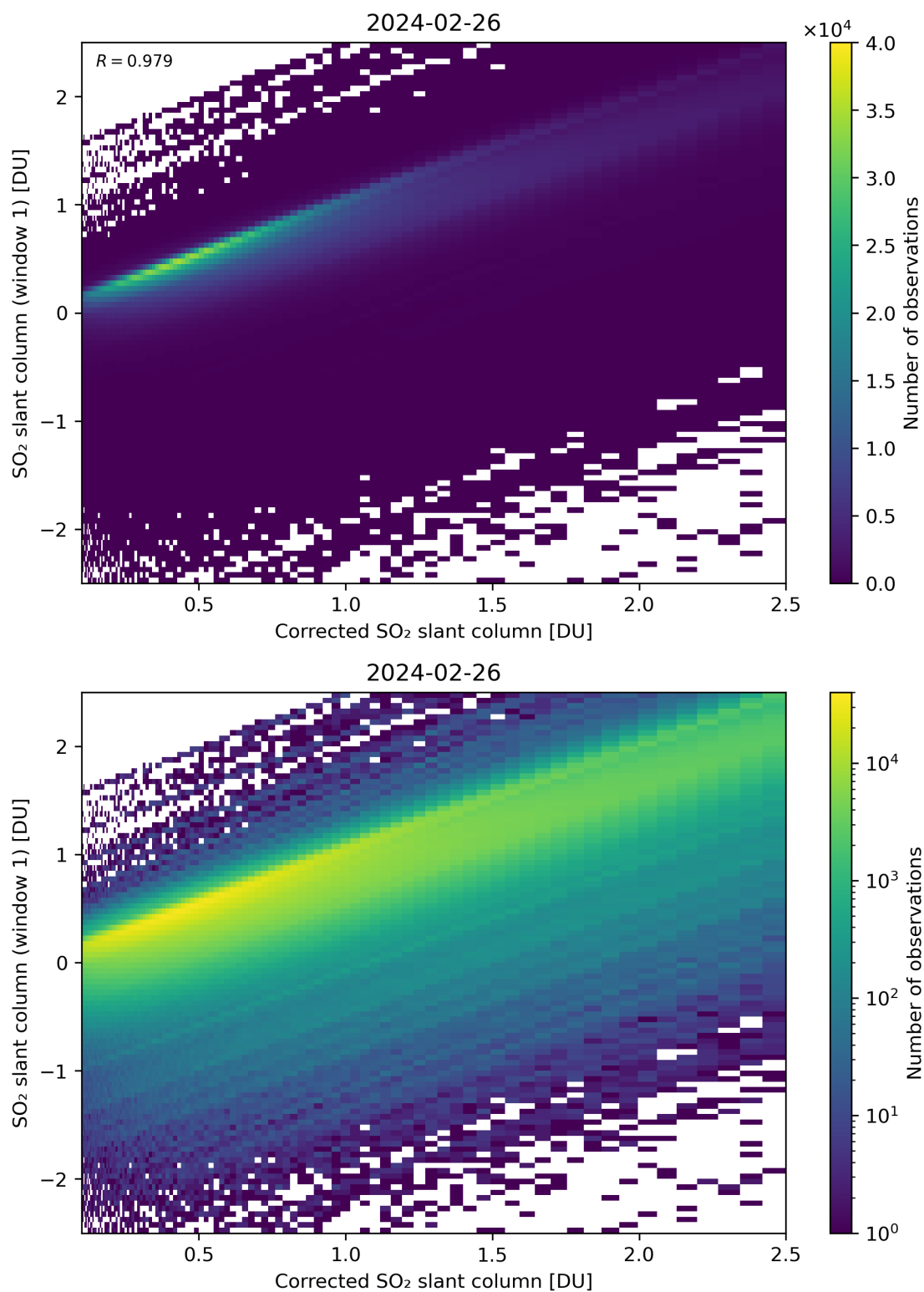
Figure 187: Scatter density plot of “Corrected SO 2 slant column” against “SO 2 slant column (window 1)” for 2024-02-25 to 2024-02-27.
