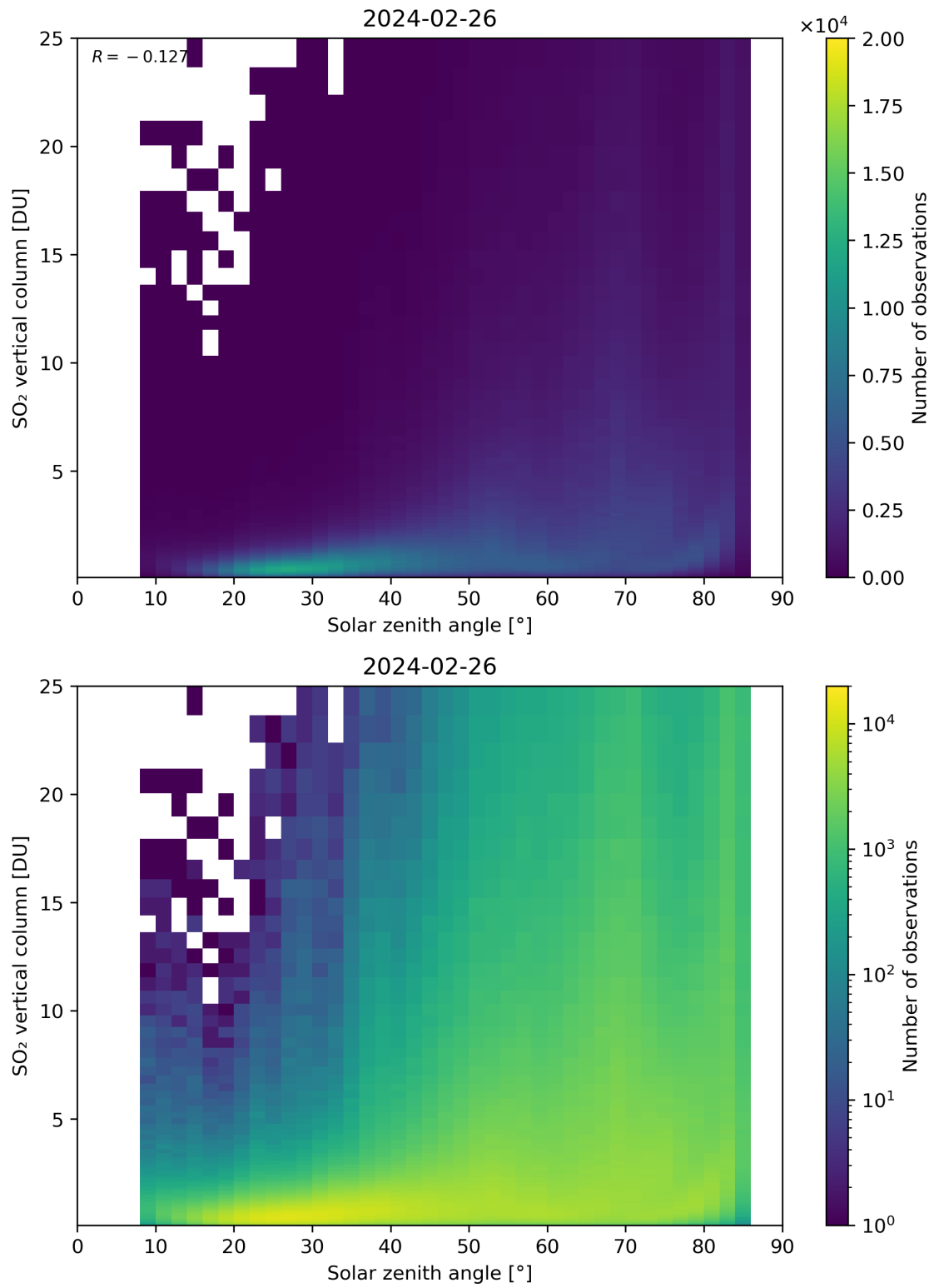
Figure 176: Scatter density plot of “Solar zenith angle” against “SO 2 vertical column” for 2024-02-25 to 2024-02-27.
