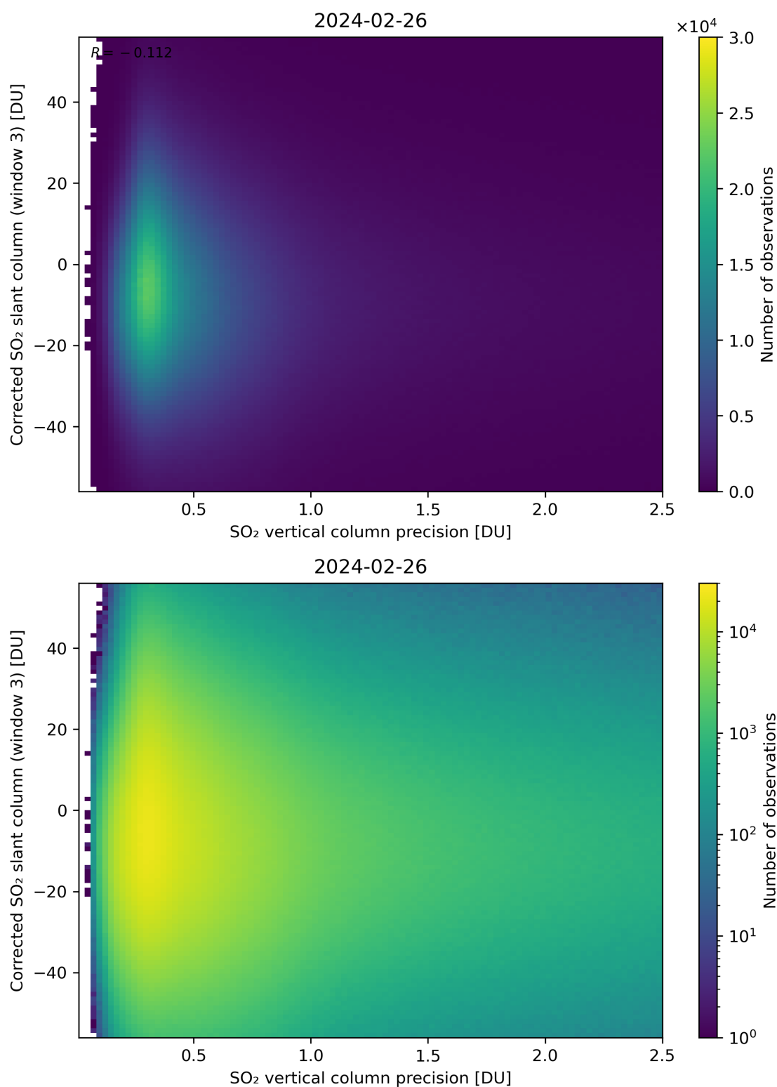
Figure 288: Scatter density plot of “SO 2 vertical column precision” against “Corrected SO 2 slant column (window 3)” for 2024-02-25 to 2024-02-27.
