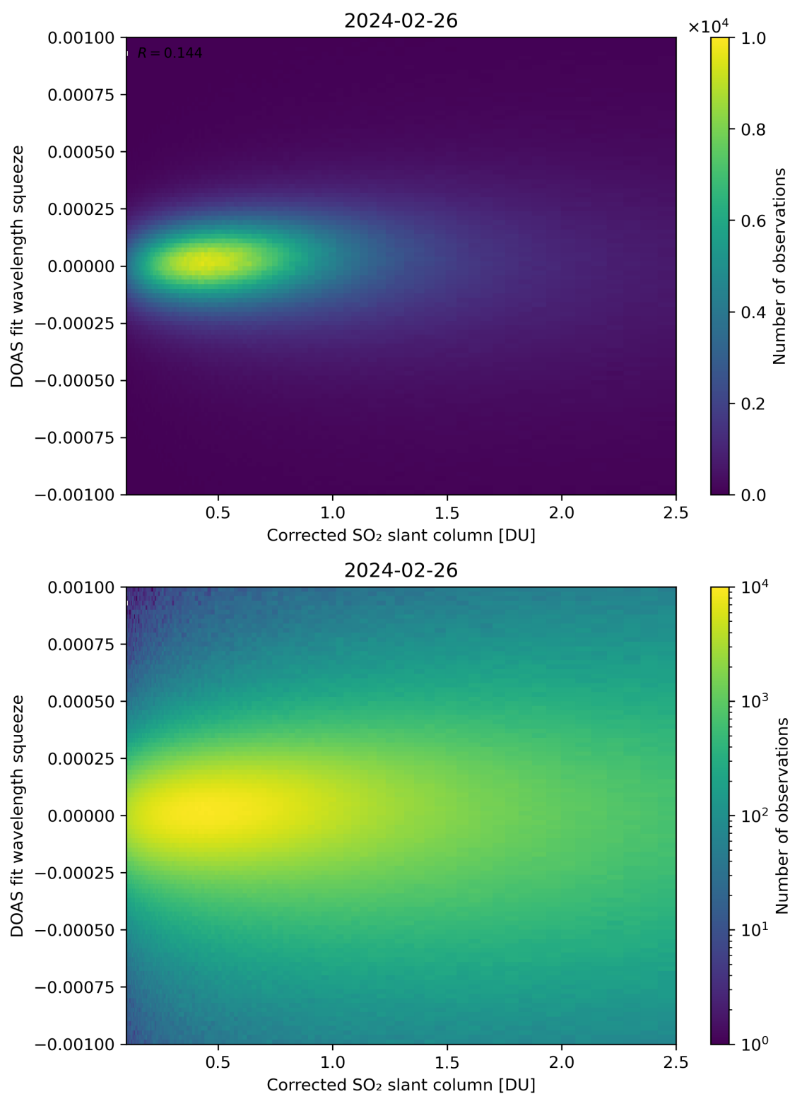
Figure 182: Scatter density plot of “Corrected SO 2 slant column” against “DOAS fit wavelength squeeze” for 2024-02-25 to 2024-02-27.
