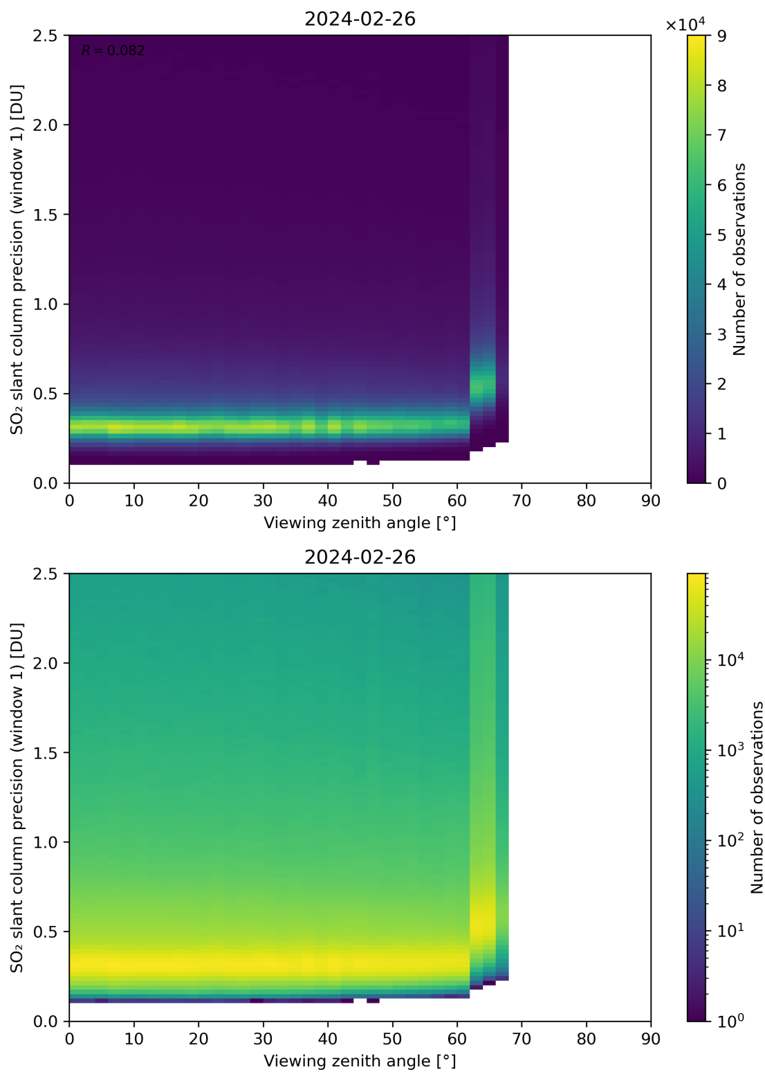
Figure 321: Scatter density plot of “Viewing zenith angle” against “SO 2 slant column precision (window 1)” for 2024-02-25 to 2024-02-27.
