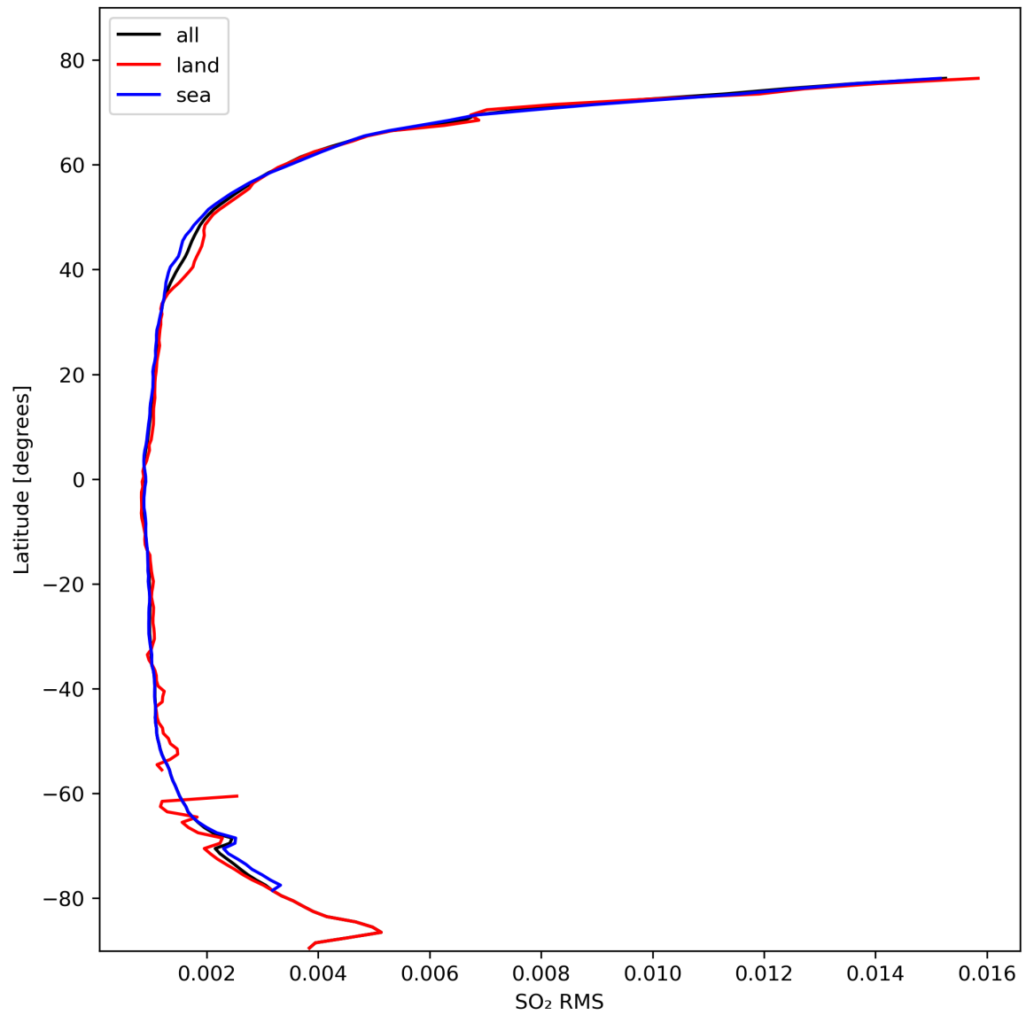
Figure 47: Zonal average of “SO 2 RMS” for 2024-02-25 to 2024-02-27.
