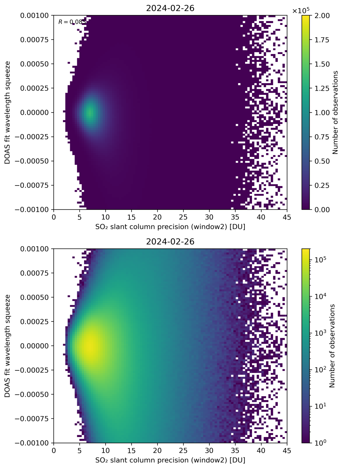
Figure 244: Scatter density plot of “SO 2 slant column precision (window2)” against “DOAS fit wavelength squeeze” for 2024-02-25 to 2024-02-27.
