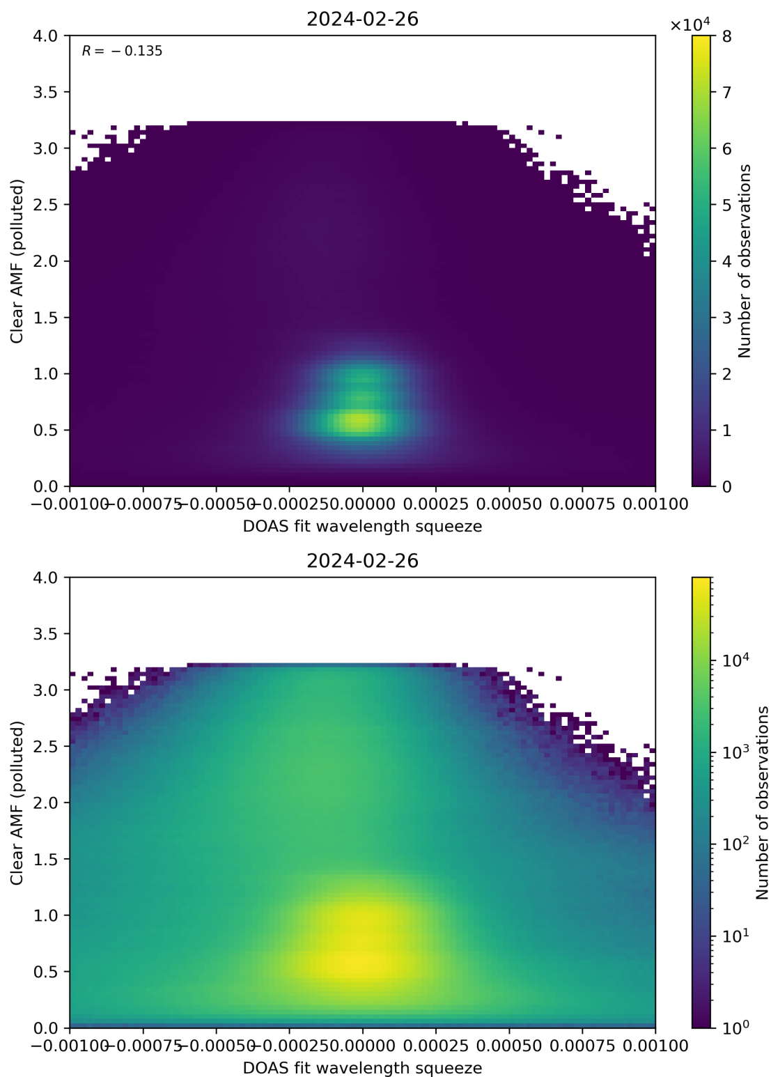
Figure 133: Scatter density plot of “DOAS fit wavelength squeeze” against “Clear AMF (polluted)” for 2024-02-25 to 2024-02-27.
