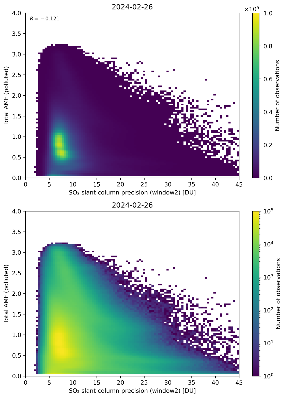
Figure 251: Scatter density plot of “SO 2 slant column precision (window2)” against “Total AMF (polluted)” for 2024-02-25 to 2024-02-27.
