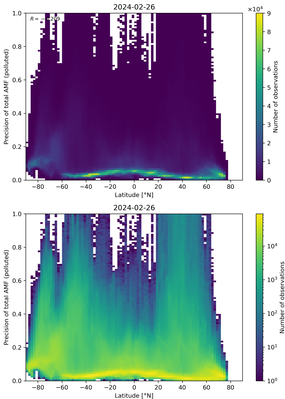
Figure 155: Scatter density plot of “Latitude” against “Precision of total AMF (polluted)” for 2024-02-25 to 2024-02-27.
