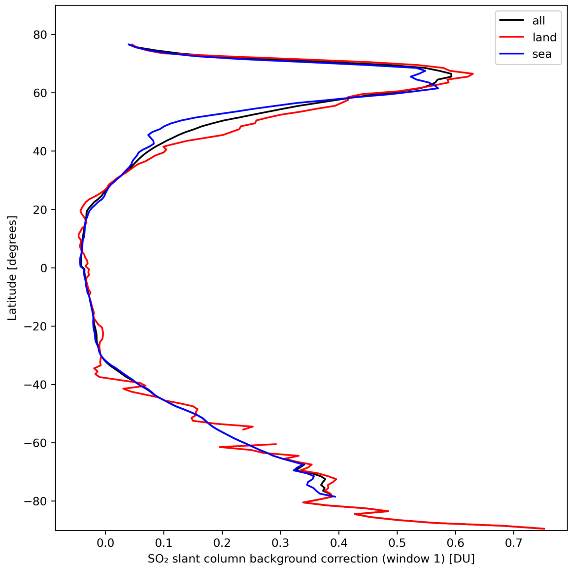
Figure 36: Zonal average of “SO 2 slant column background correction (window 1)” for 2024-02-25 to 2024-02-27.
