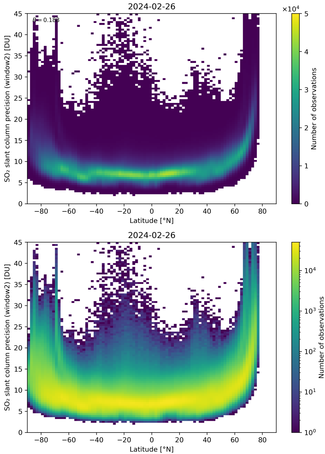
Figure 151: Scatter density plot of “Latitude” against “SO 2 slant column precision (window2)” for 2024-02-25 to 2024-02-27.
