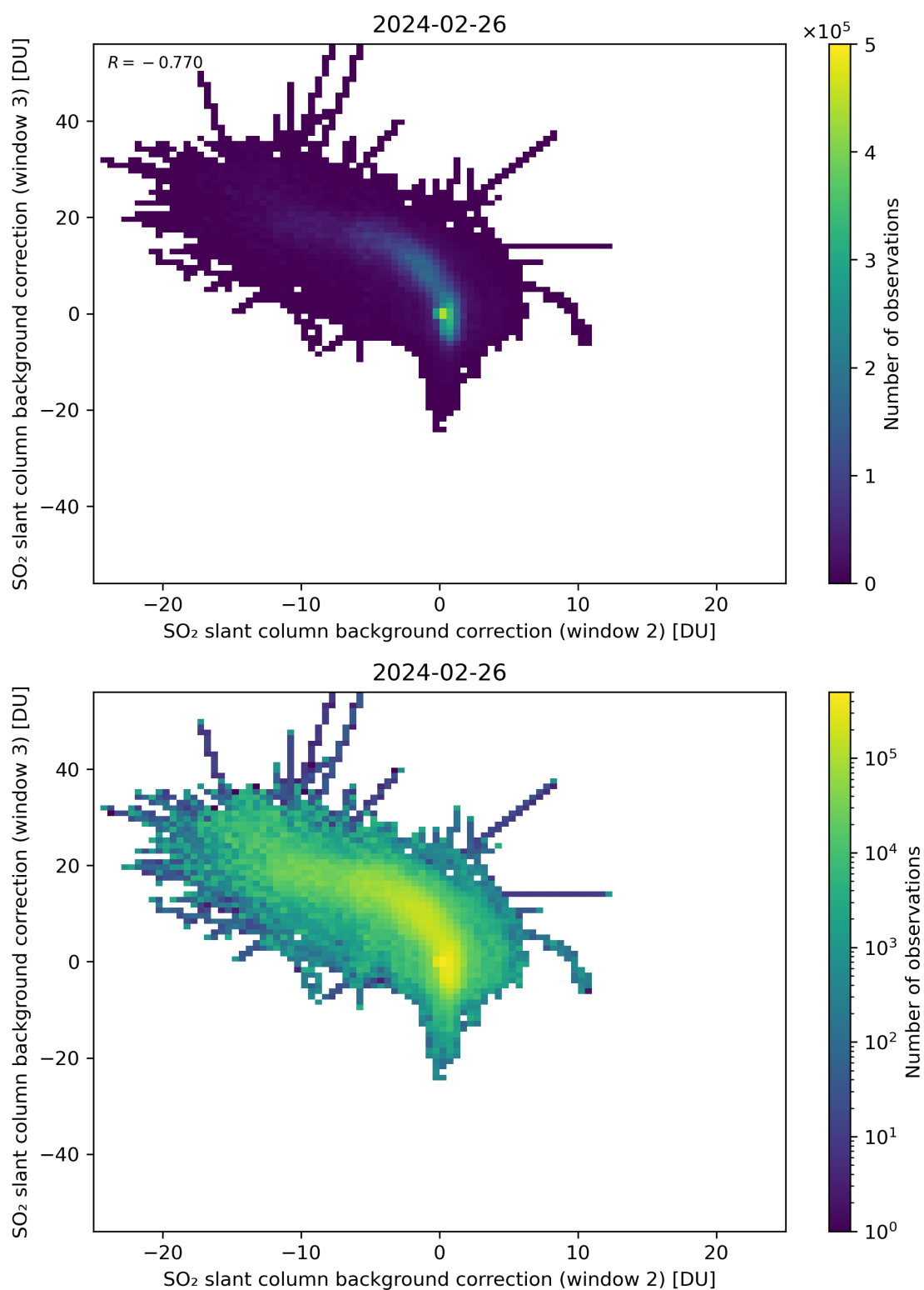
Figure 111: Scatter density plot of “SO 2 slant column background correction (window 2)” against “SO 2 slant column background correction (window 3)” for 2024-02-25 to 2024-02-27.
