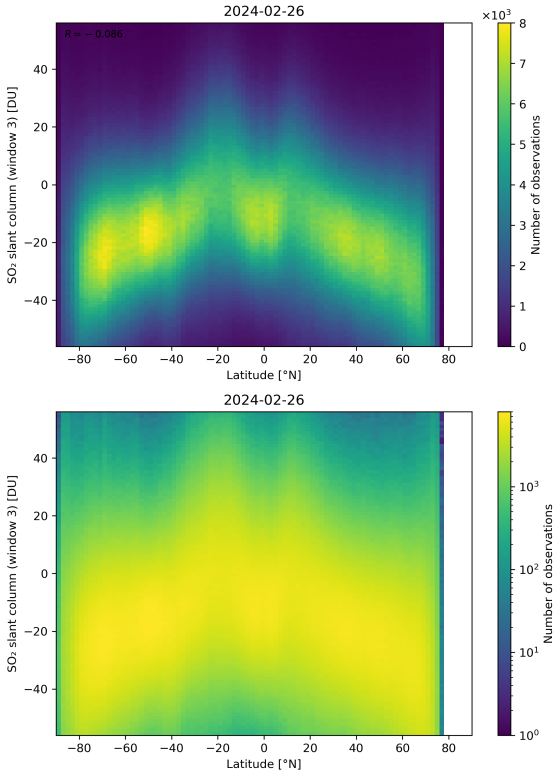
Figure 152: Scatter density plot of “Latitude” against “SO 2 slant column (window 3)” for 2024-02-25 to 2024-02-27.
