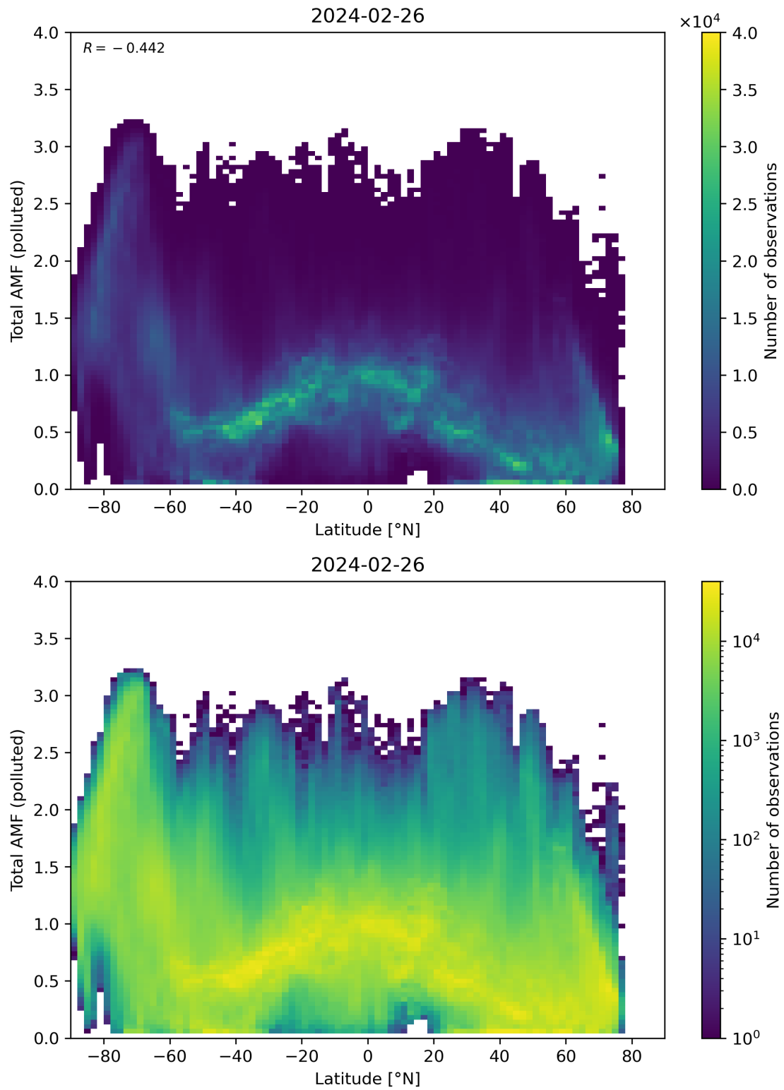
Figure 154: Scatter density plot of “Latitude” against “Total AMF (polluted)” for 2024-02-25 to 2024-02-27.
