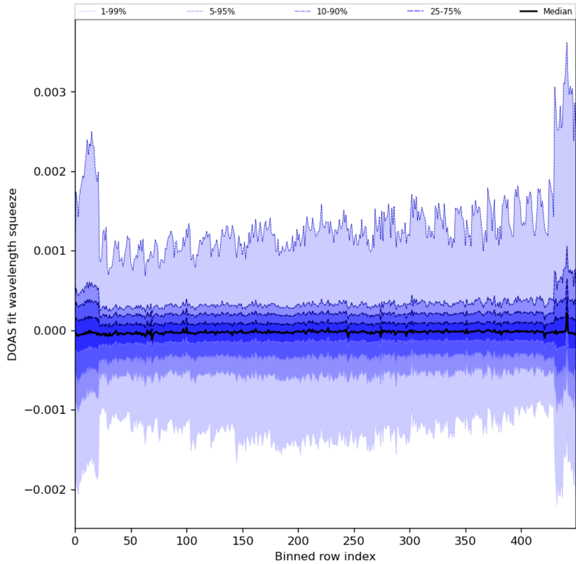
Figure 92: Along track statistics of “DOAS fit wavelength squeeze” for 2024-02-25 to 2024-02-27
