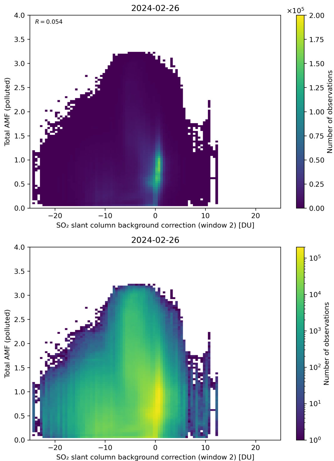
Figure 119: Scatter density plot of “SO 2 slant column background correction (window 2)” against “Total AMF (polluted)” for 2024-02-25 to 2024-02-27.
