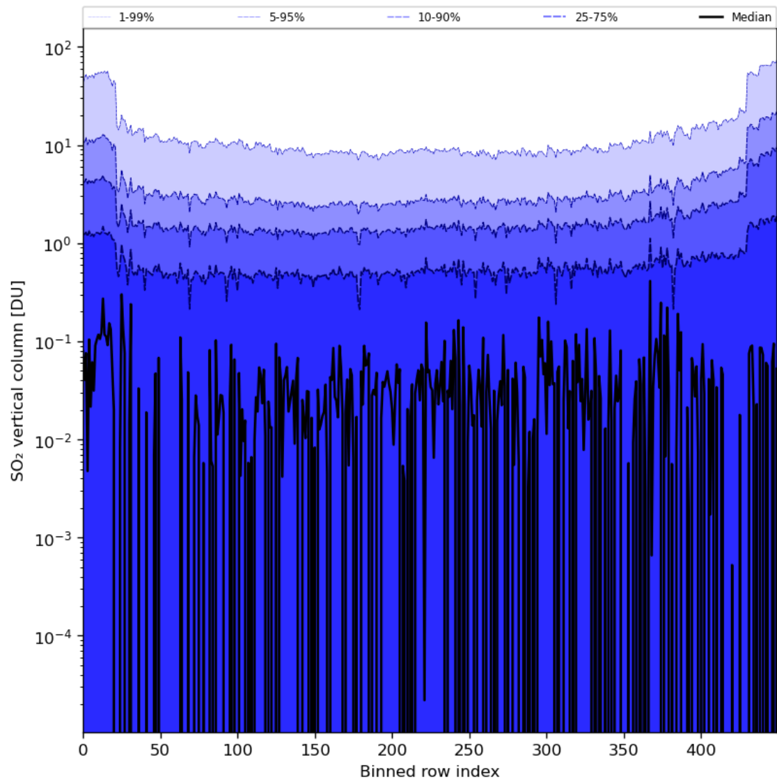
Figure 76: Along track statistics of “SO 2 vertical column” for 2024-02-25 to 2024-02-27
