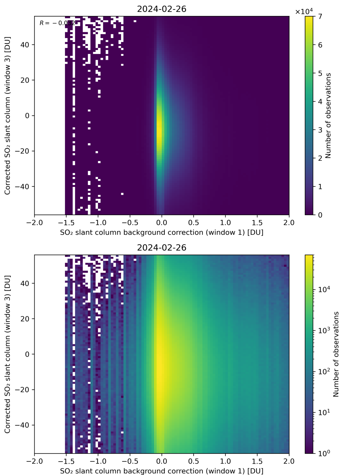
Figure 105: Scatter density plot of “SO 2 slant column background correction (window 1)” against “Corrected SO 2 slant column (window 3)” for 2024-02-25 to 2024-02-27.
