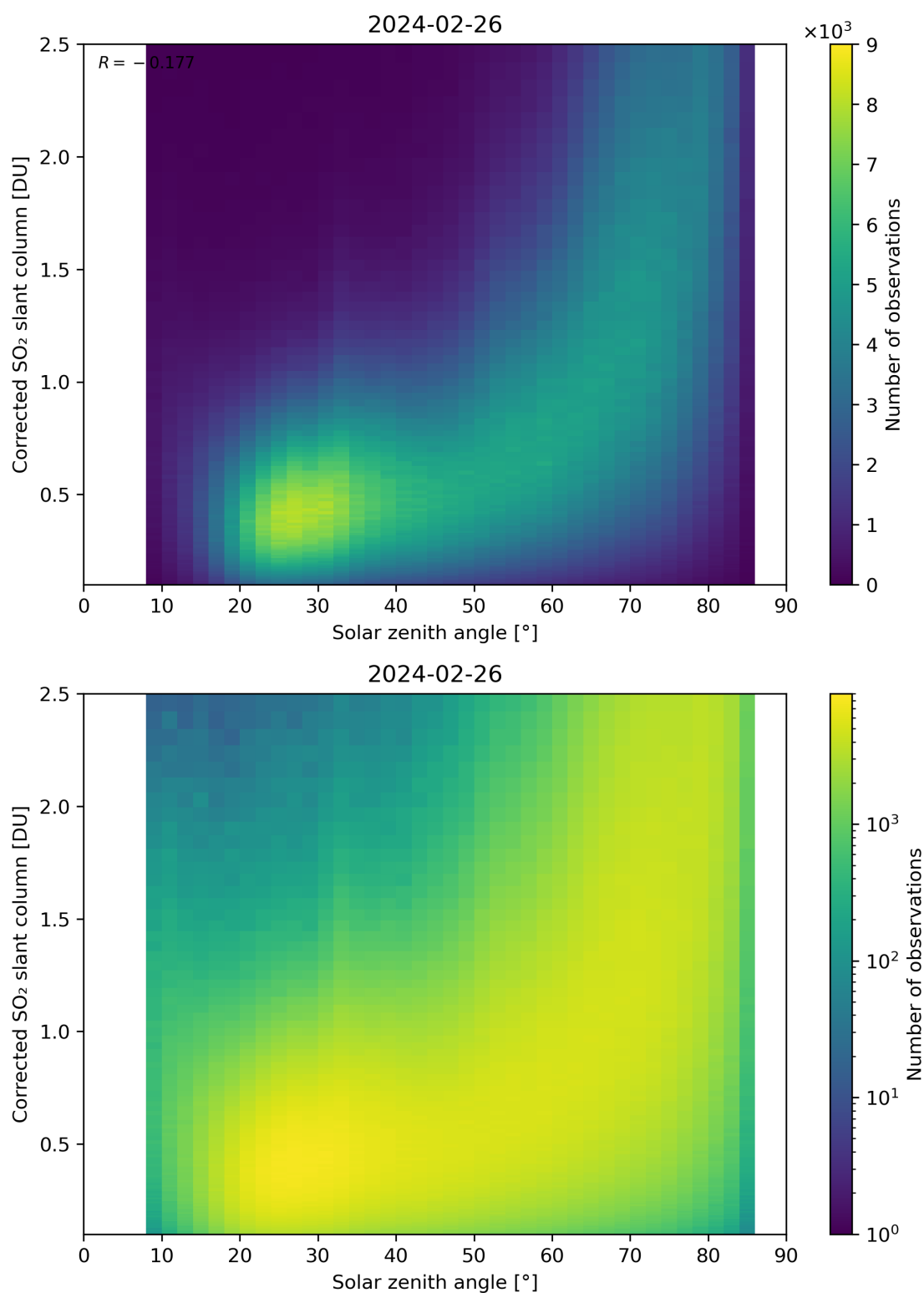
Figure 166: Scatter density plot of “Solar zenith angle” against “Corrected SO 2 slant column” for 2024-02-25 to 2024-02-27.
