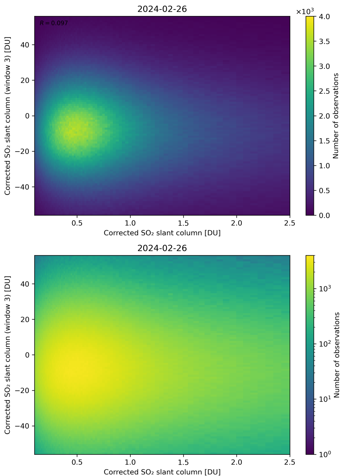
Figure 186: Scatter density plot of “Corrected SO 2 slant column” against “Corrected SO 2 slant column (window 3)” for 2024-02-25 to 2024-02-27.
