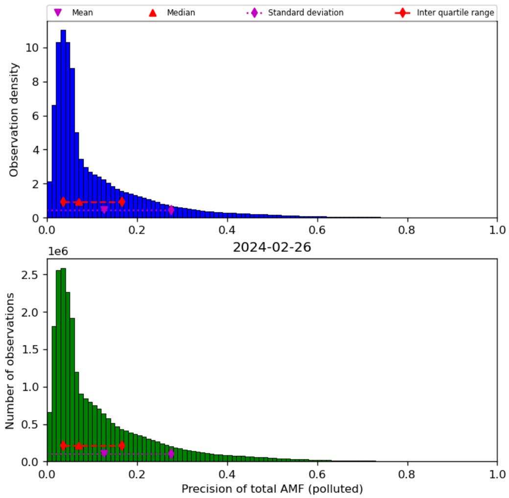
Figure 72: Histogram of “Precision of total AMF (polluted)” for 2024-02-25 to 2024-02-27
