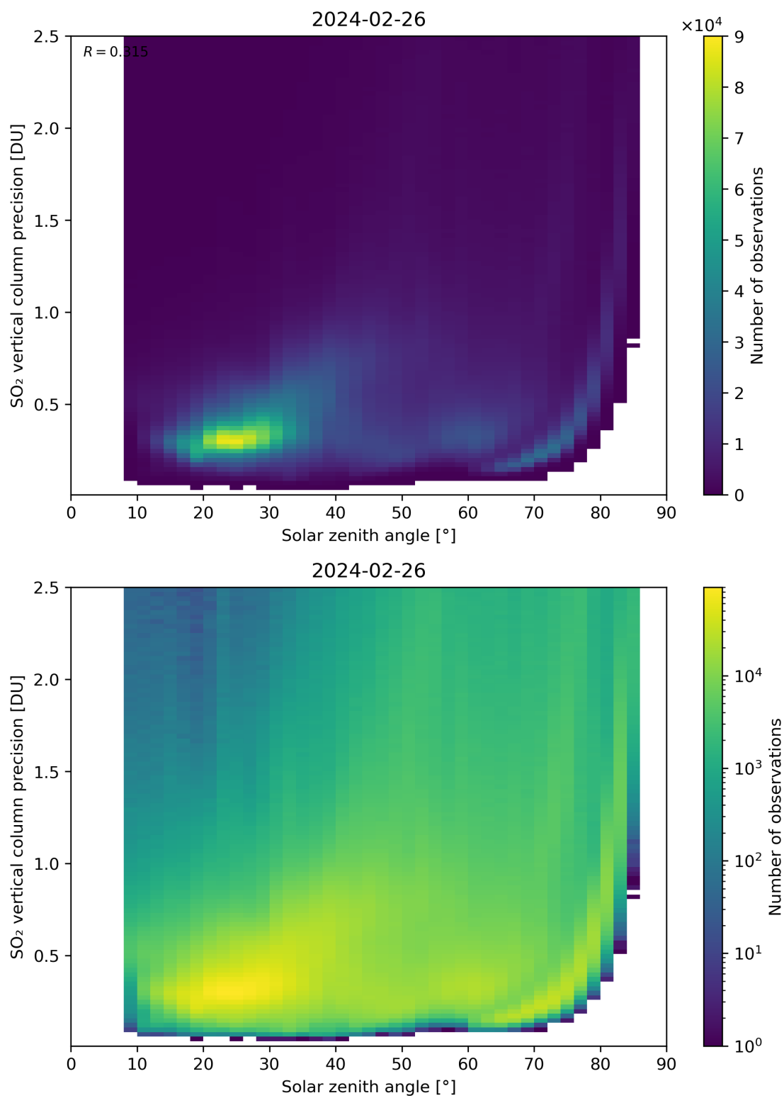
Figure 177: Scatter density plot of “Solar zenith angle” against “SO 2 vertical column precision” for 2024-02-25 to 2024-02-27.
