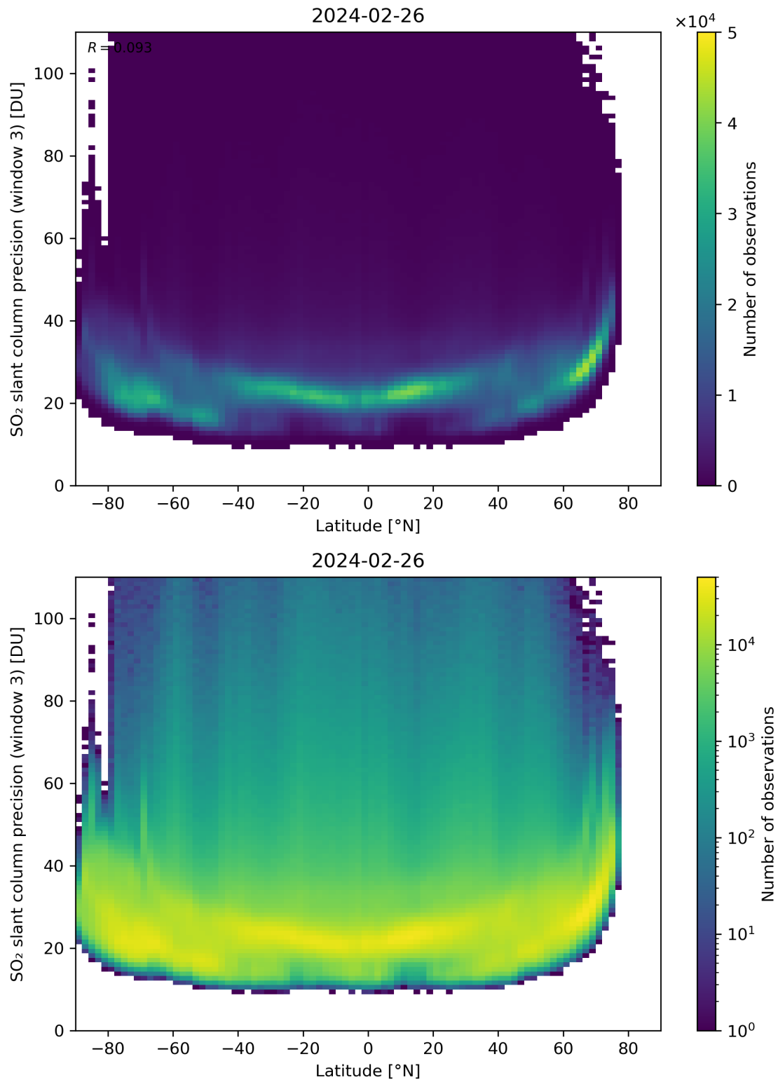
Figure 153: Scatter density plot of “Latitude” against “SO 2 slant column precision (window 3)” for 2024-02-25 to 2024-02-27.
