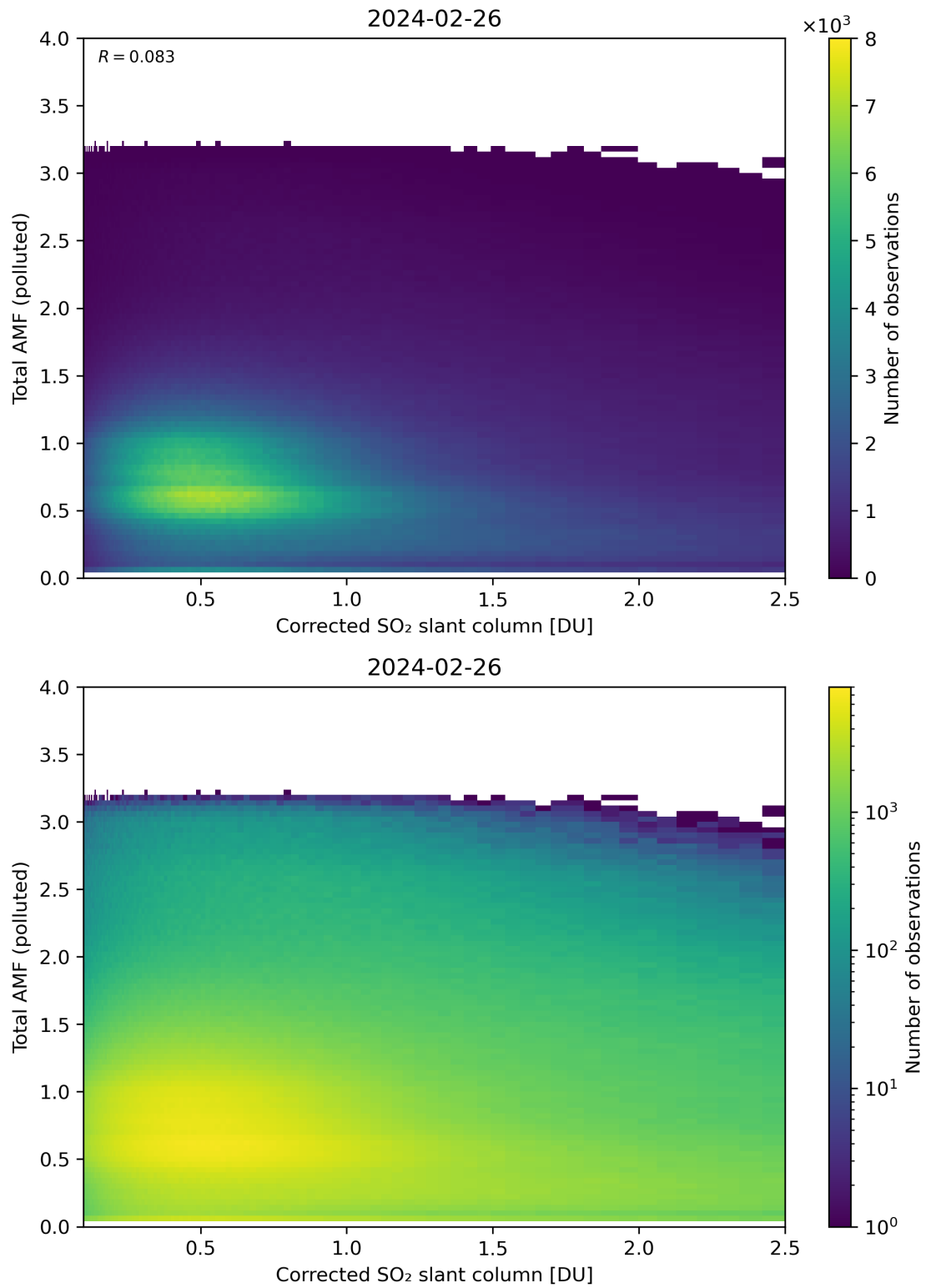
Figure 192: Scatter density plot of “Corrected SO 2 slant column” against “Total AMF (polluted)” for 2024-02-25 to 2024-02-27.
