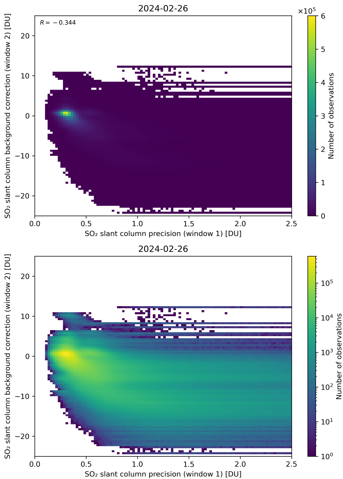
Figure 219: Scatter density plot of “SO 2 slant column precision (window 1)” against “SO 2 slant column background correction (window 2)” for 2024-02-25 to 2024-02-27.
