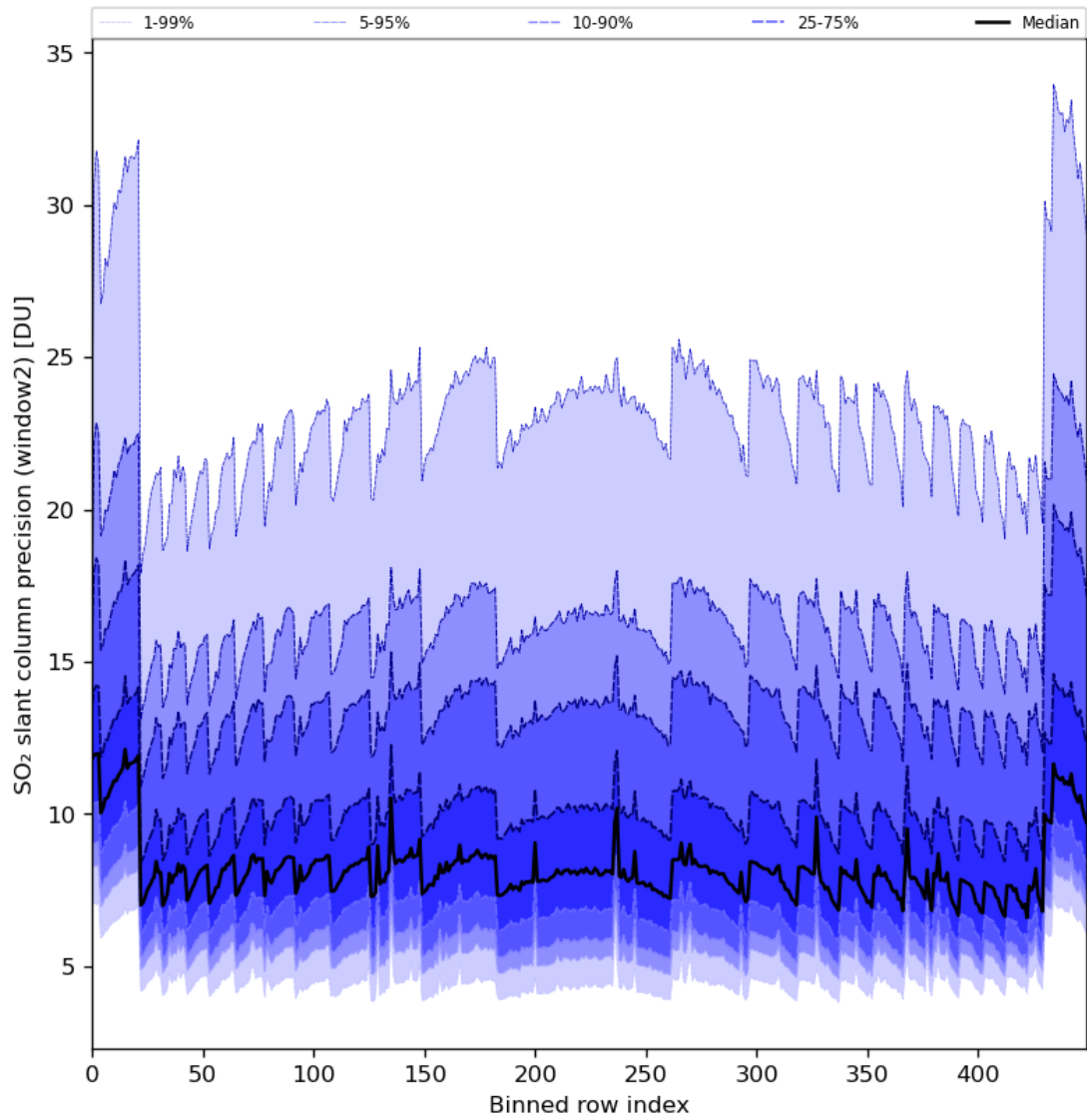
Figure 84: Along track statistics of “SO 2 slant column precision (window2)” for 2024-02-25 to 2024-02-27
