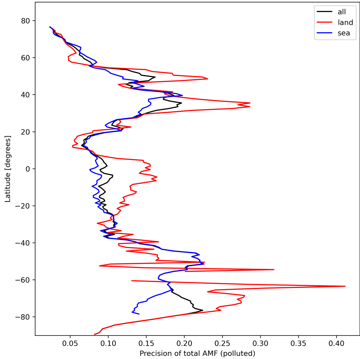
Figure 49: Zonal average of “Precision of total AMF (polluted)” for 2024-02-25 to 2024-02-27.
