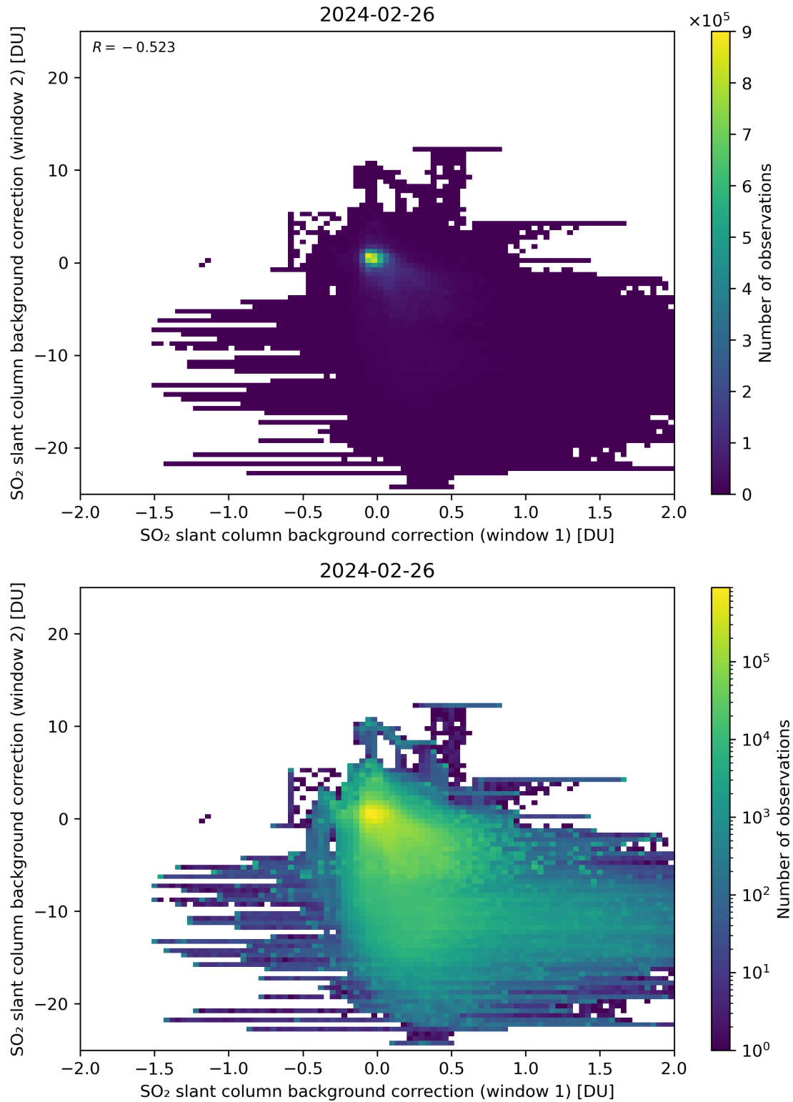
Figure 98: Scatter density plot of “SO 2 slant column background correction (window 1)” against “SO 2 slant column background correction (window 2)” for 2024-02-25 to 2024-02-27.
