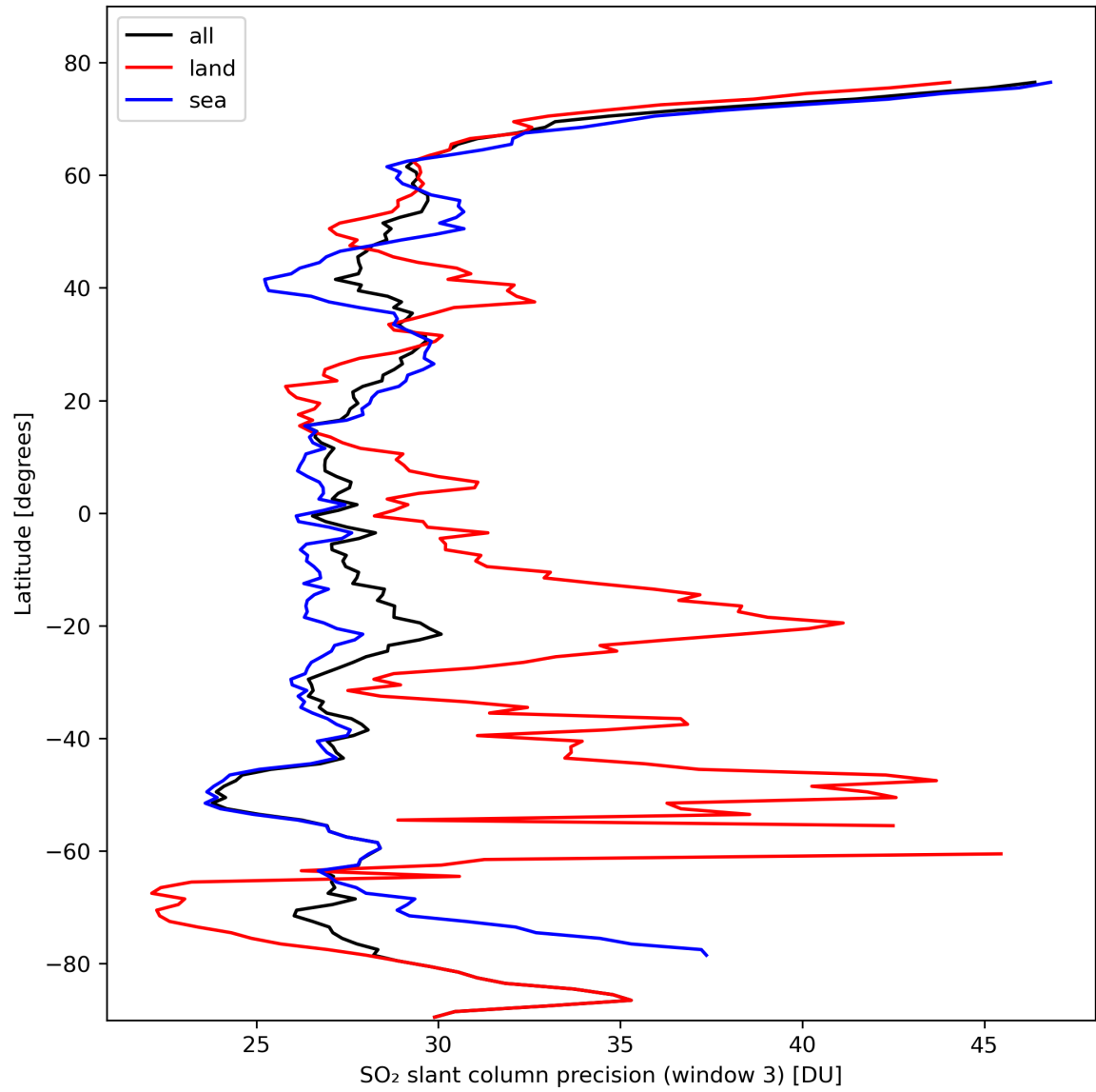
Figure 42: Zonal average of “SO 2 slant column precision (window 3)” for 2024-02-25 to 2024-02-27.
