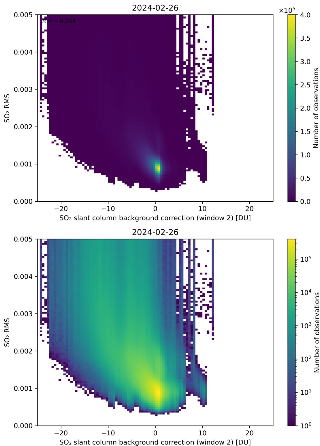
Figure 114: Scatter density plot of “SO 2 slant column background correction (window 2)” against “SO 2 RMS” for 2024-02-25 to 2024-02-27.
