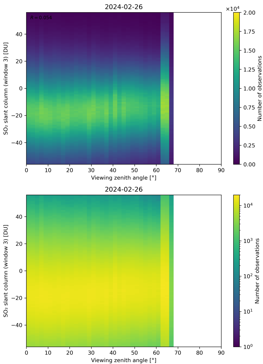
Figure 323: Scatter density plot of “Viewing zenith angle” against “SO 2 slant column (window 3)” for 2024-02-25 to 2024-02-27.
