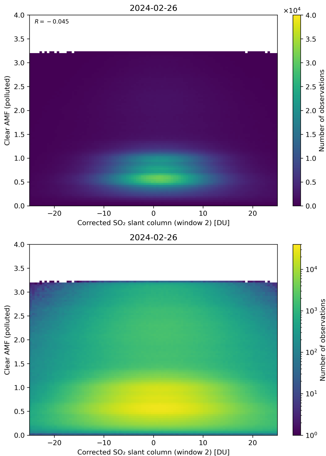
Figure 199: Scatter density plot of “Corrected SO 2 slant column (window 2)” against “Clear AMF (polluted)” for 2024-02-25 to 2024-02-27.
