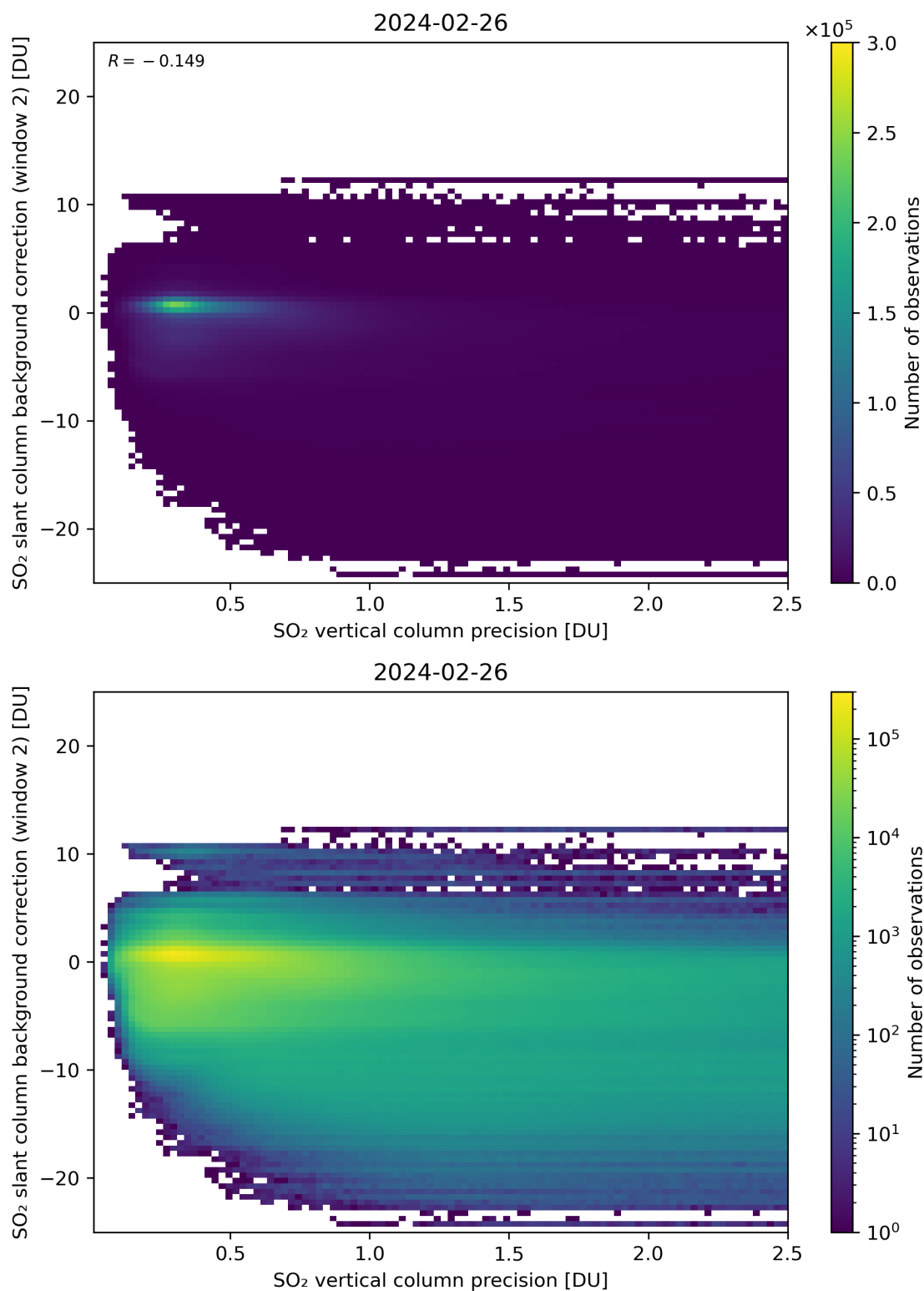
Figure 280: Scatter density plot of “SO 2 vertical column precision” against “SO 2 slant column background correction (window 2)” for 2024-02-25 to 2024-02-27.
