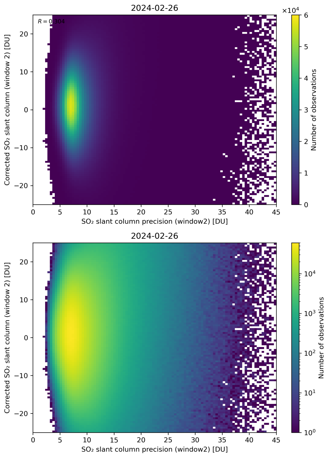
Figure 247: Scatter density plot of “SO 2 slant column precision (window2)” against “Corrected SO 2 slant column (window 2)” for 2024-02-25 to 2024-02-27.
