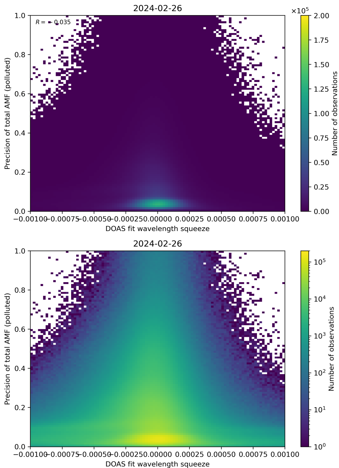
Figure 135: Scatter density plot of “DOAS fit wavelength squeeze” against “Precision of total AMF (polluted)” for 2024-02-25 to 2024-02-27.
