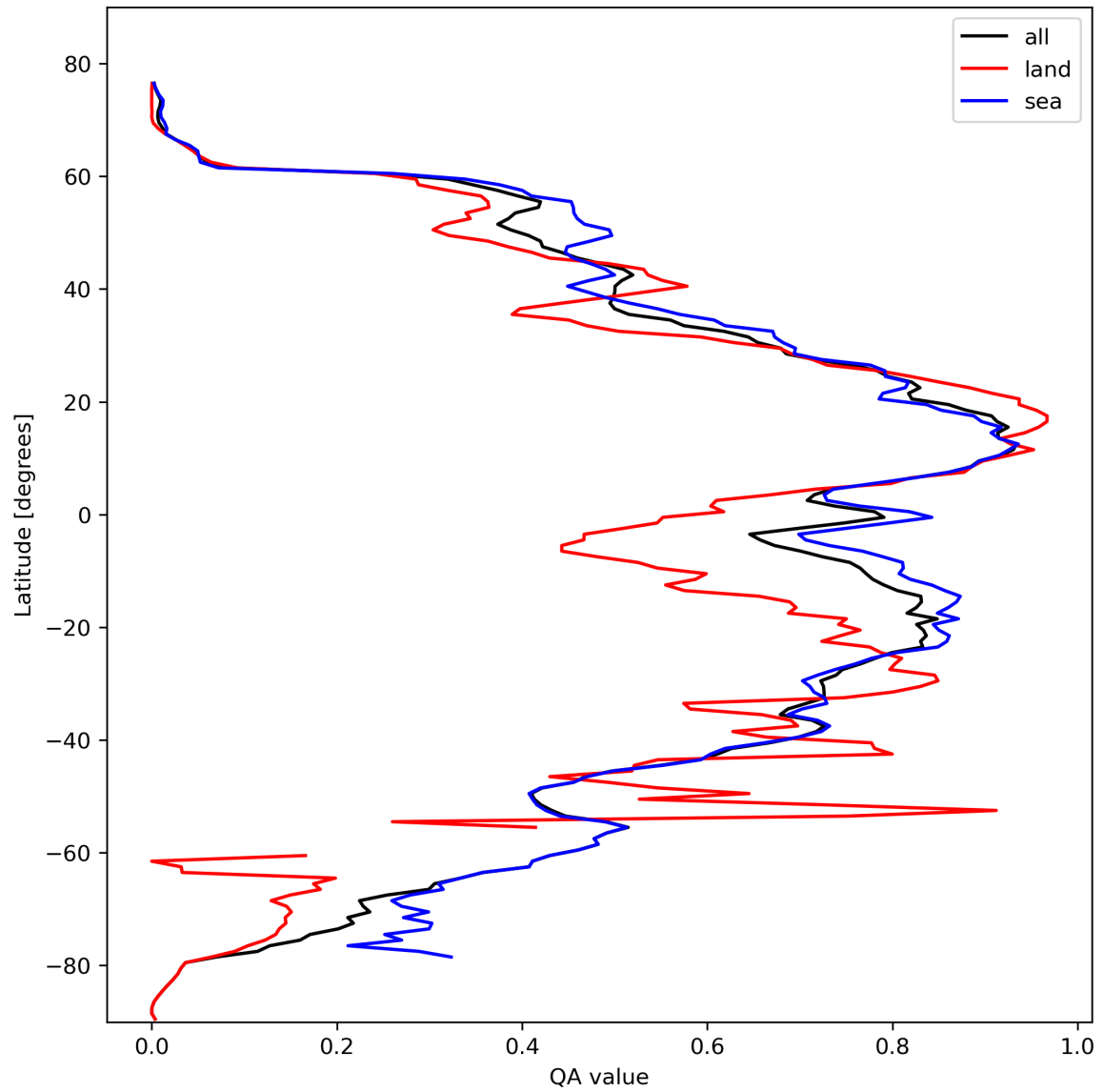
Figure 29: Zonal average of “QA value” for 2024-02-25 to 2024-02-27.
