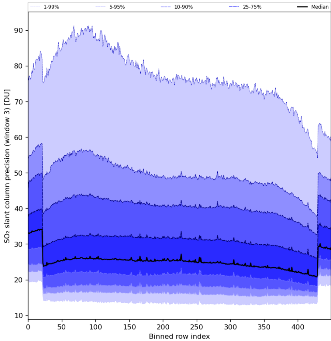
Figure 88: Along track statistics of “SO 2 slant column precision (window 3)” for 2024-02-25 to 2024-02-27
