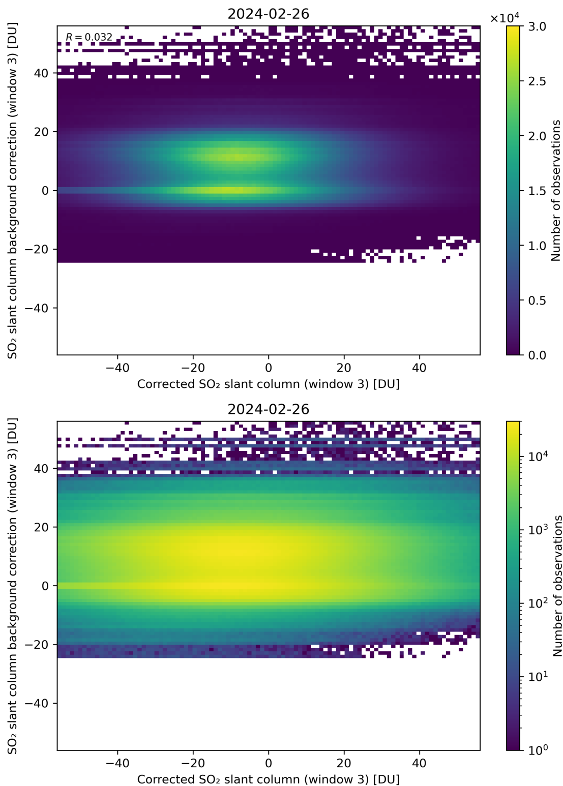
Figure 205: Scatter density plot of “Corrected SO 2 slant column (window 3)” against “SO 2 slant column background correction (window 3)” for 2024-02-25 to 2024-02-27.
