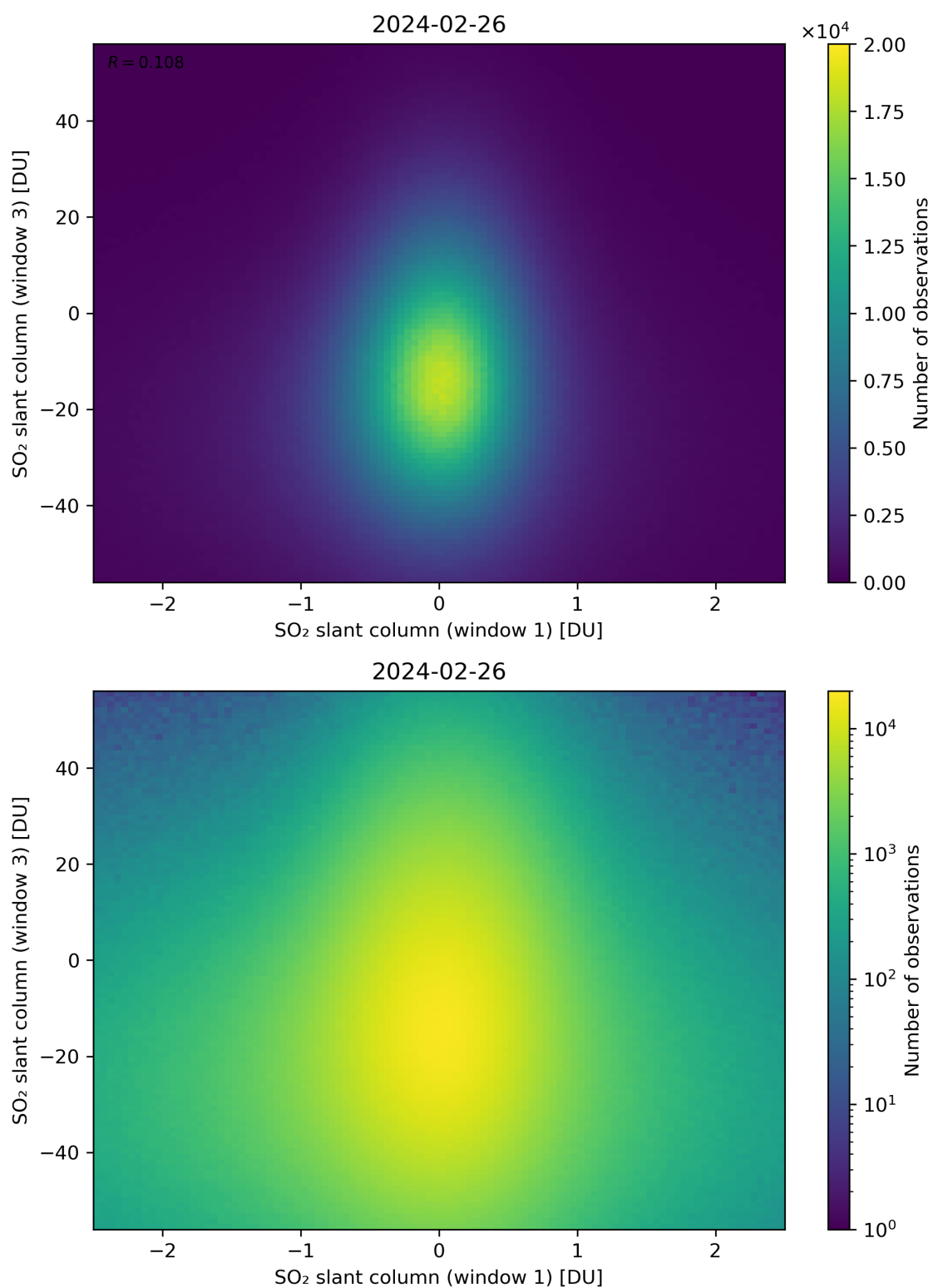
Figure 237: Scatter density plot of “SO 2 slant column (window 1)” against “SO 2 slant column (window 3)” for 2024-02-25 to 2024-02-27.
