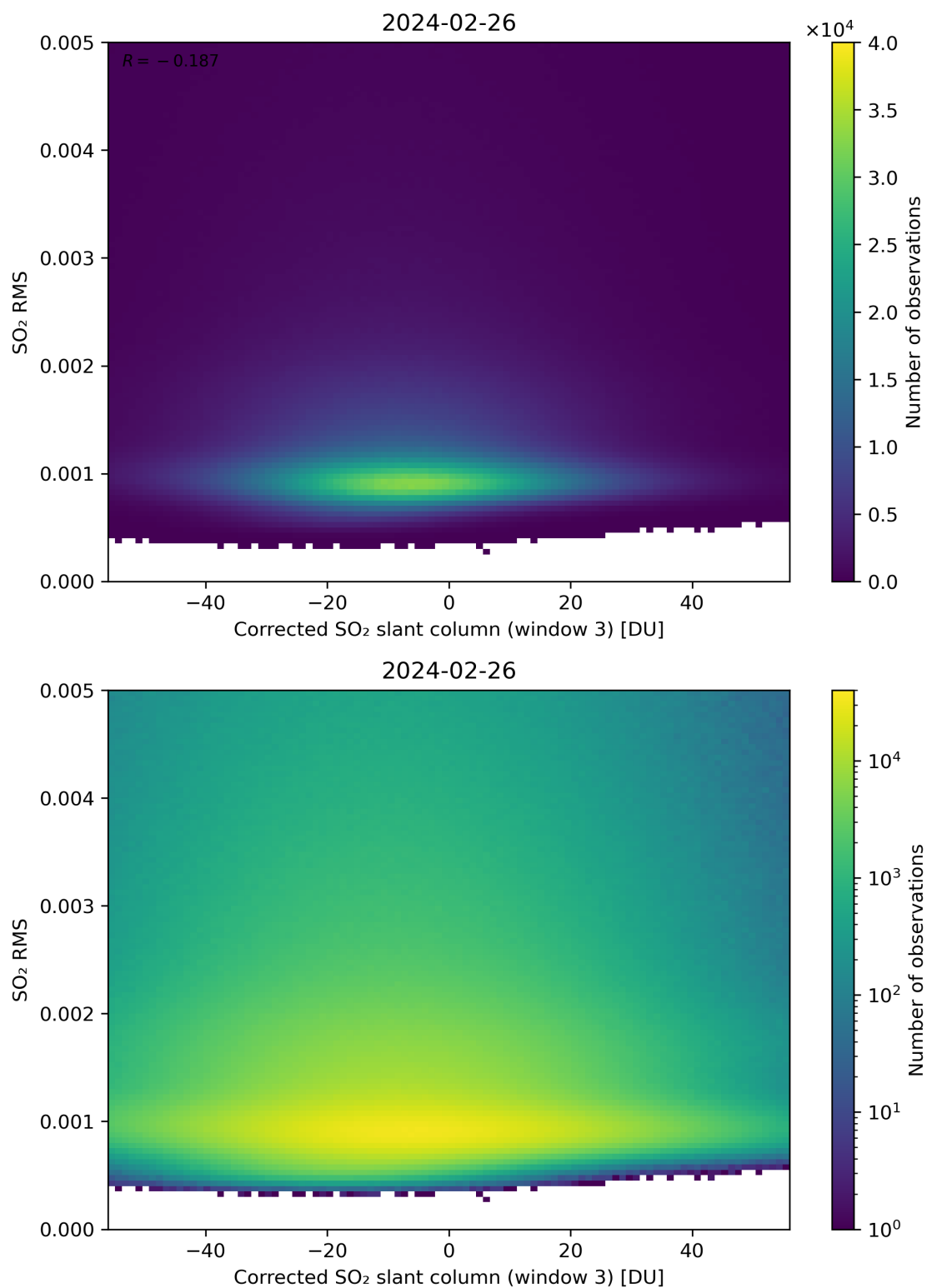
Figure 208: Scatter density plot of “Corrected SO 2 slant column (window 3)” against “SO 2 RMS” for 2024-02-25 to 2024-02-27.
