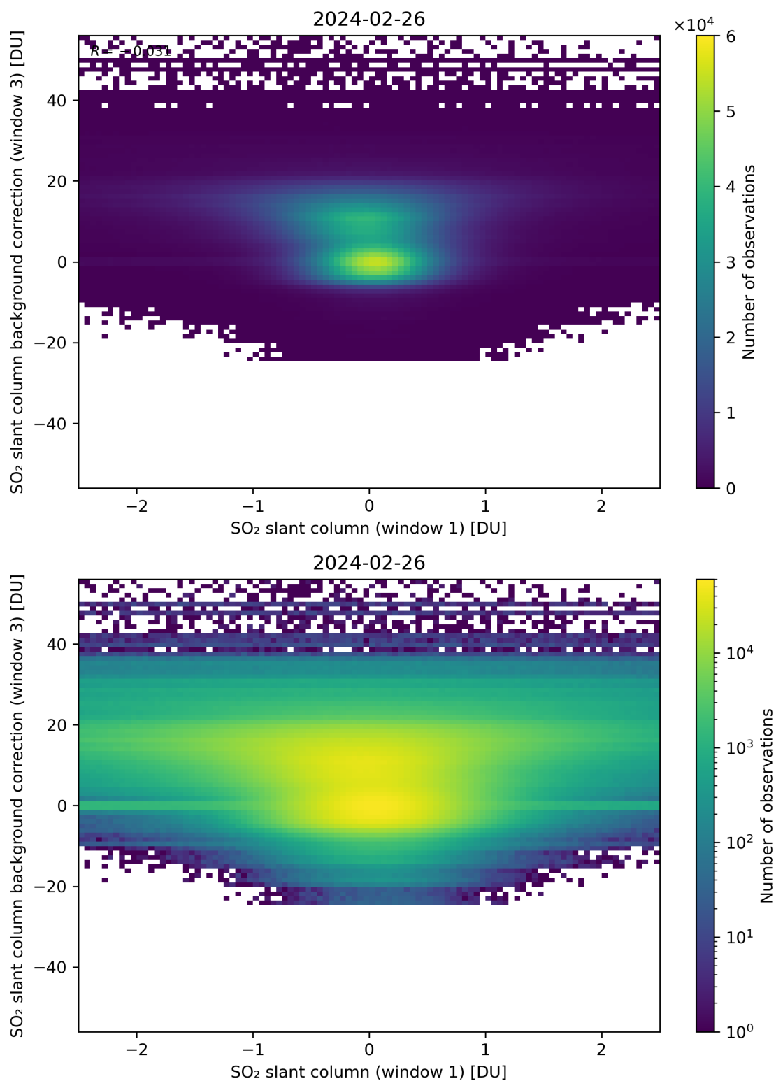
Figure 214: Scatter density plot of “SO 2 slant column (window 1)” against “SO 2 slant column background correction (window 3)” for 2024-02-25 to 2024-02-27.
