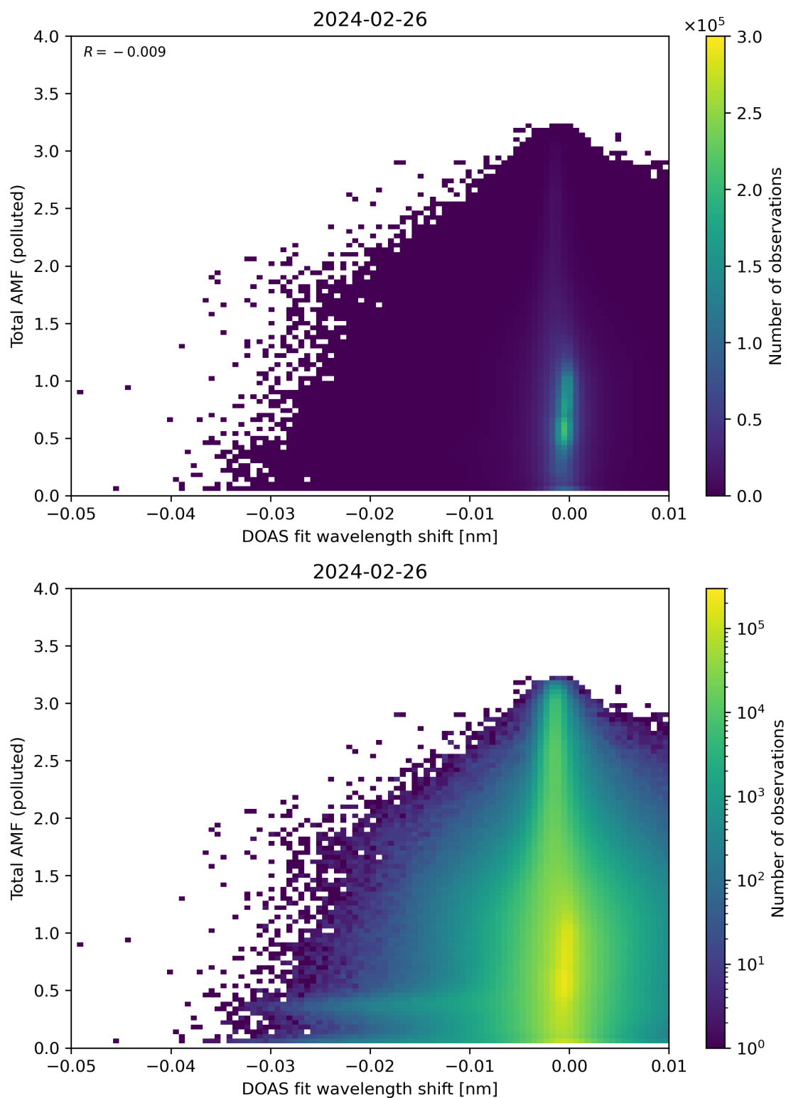
Figure 130: Scatter density plot of “DOAS fit wavelength shift” against “Total AMF (polluted)” for 2024-02-25 to 2024-02-27.
