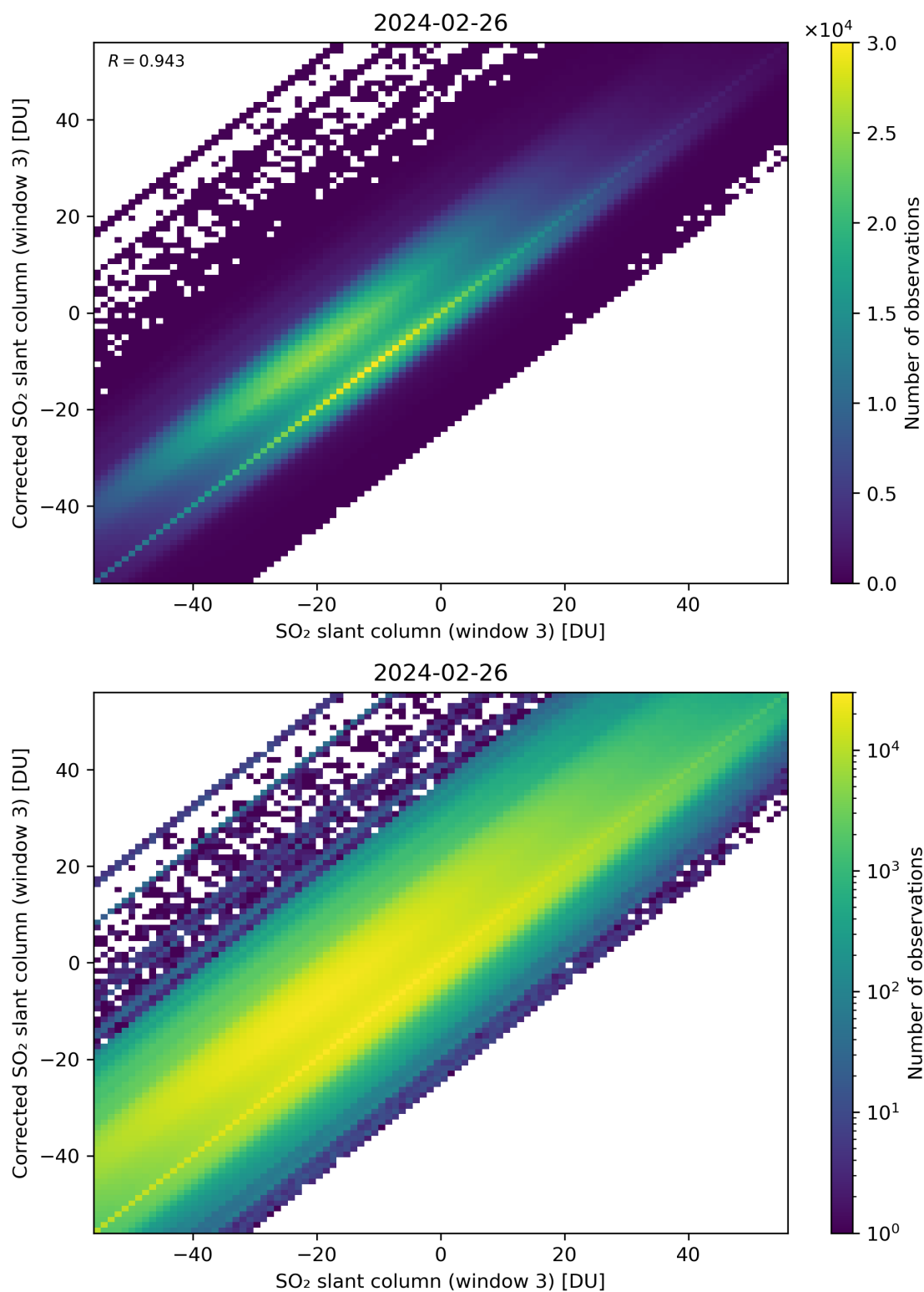
Figure 266: Scatter density plot of “SO 2 slant column (window 3)” against “Corrected SO 2 slant column (window 3)” for 2024-02-25 to 2024-02-27.
