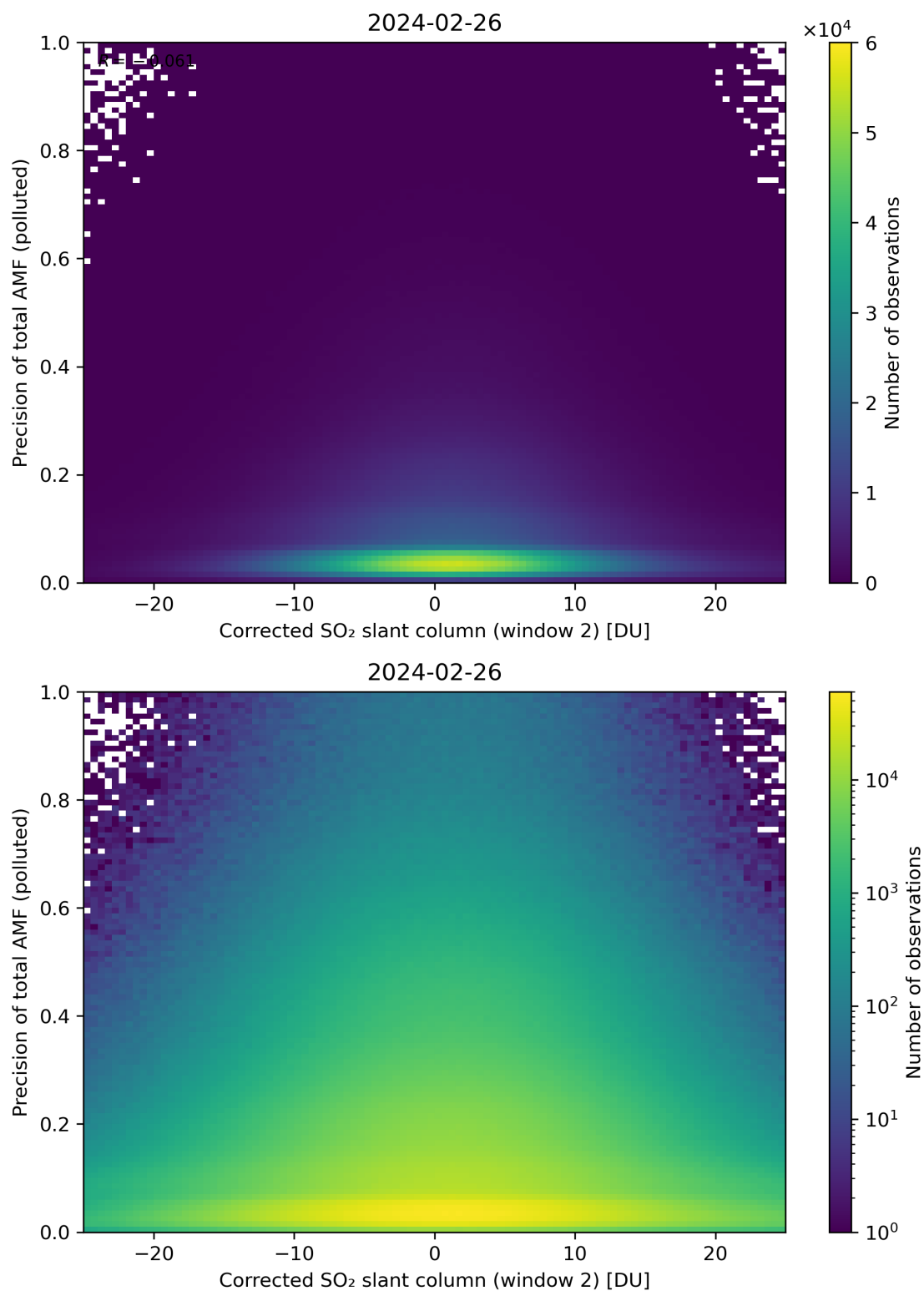
Figure 204: Scatter density plot of “Corrected SO 2 slant column (window 2)” against “Precision of total AMF (polluted)” for 2024-02-25 to 2024-02-27.
