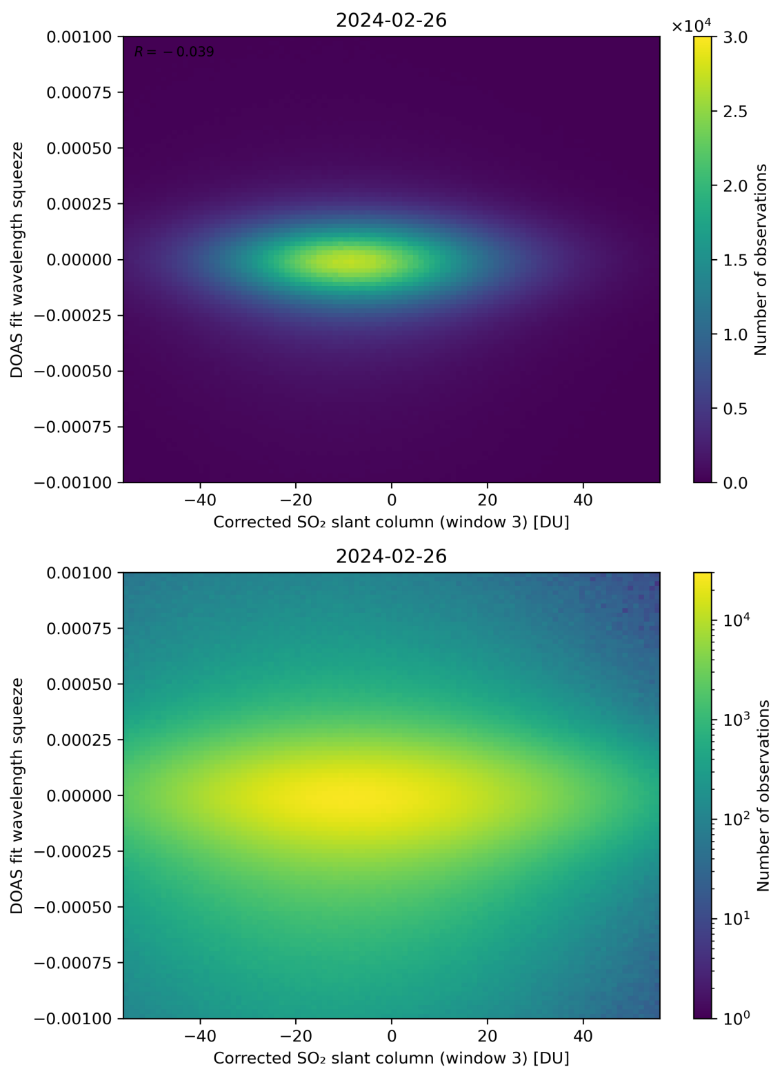
Figure 207: Scatter density plot of “Corrected SO 2 slant column (window 3)” against “DOAS fit wavelength squeeze” for 2024-02-25 to 2024-02-27.
