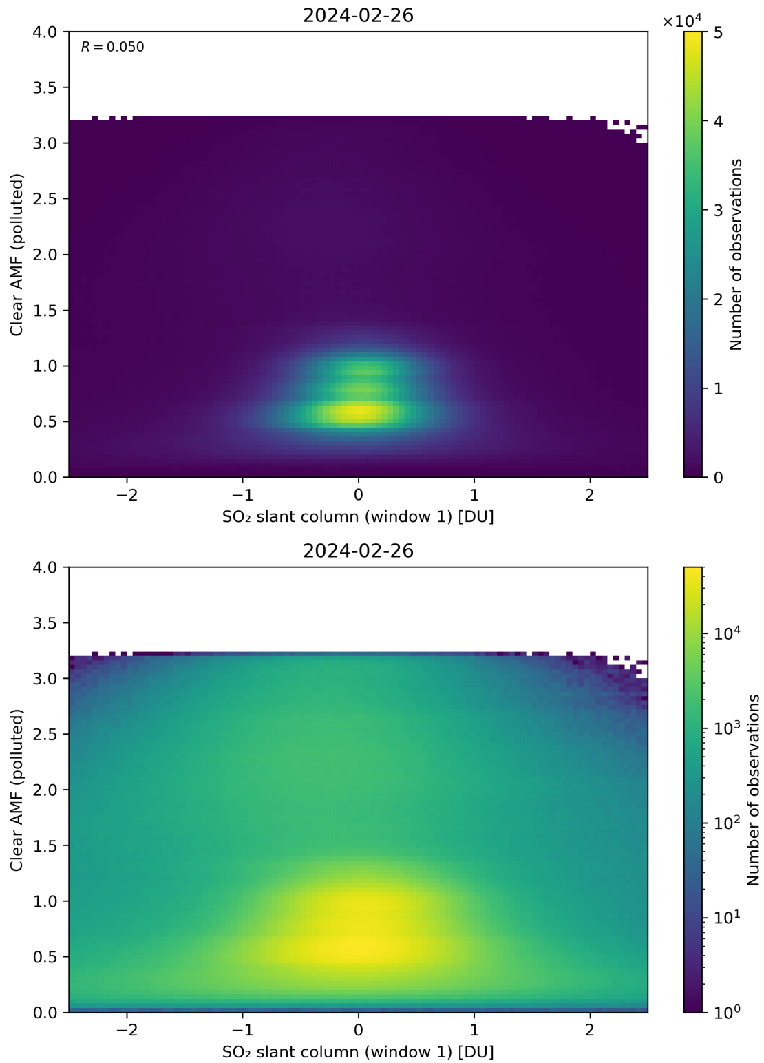
Figure 232: Scatter density plot of “SO 2 slant column (window 1)” against “Clear AMF (polluted)” for 2024-02-25 to 2024-02-27.
