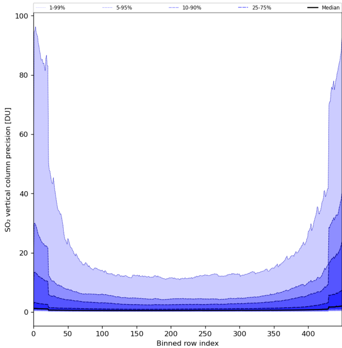
Figure 77: Along track statistics of “SO 2 vertical column precision” for 2024-02-25 to 2024-02-27
