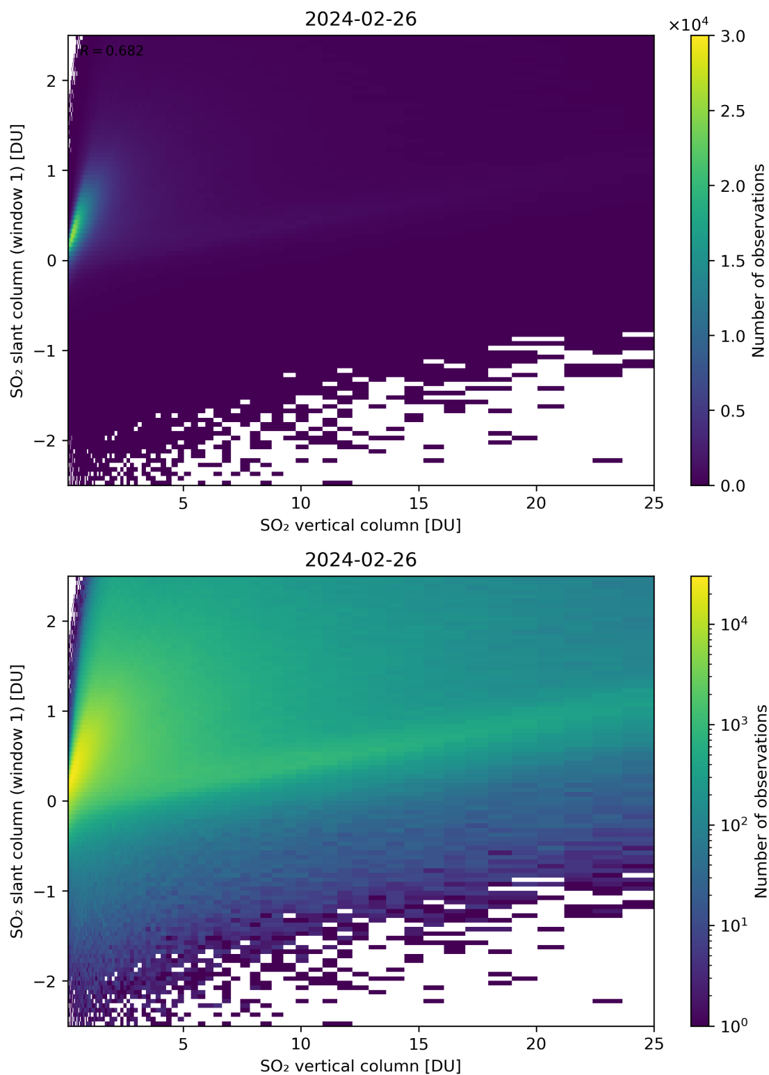
Figure 300: Scatter density plot of “SO 2 vertical column” against “SO 2 slant column (window 1)” for 2024-02-25 to 2024-02-27.
