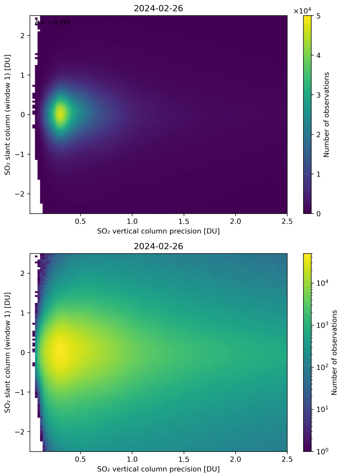
Figure 289: Scatter density plot of “SO 2 vertical column precision” against “SO 2 slant column (window 1)” for 2024-02-25 to 2024-02-27.
