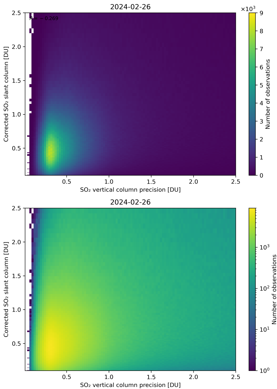
Figure 286: Scatter density plot of “SO 2 vertical column precision” against “Corrected SO 2 slant column” for 2024-02-25 to 2024-02-27.
