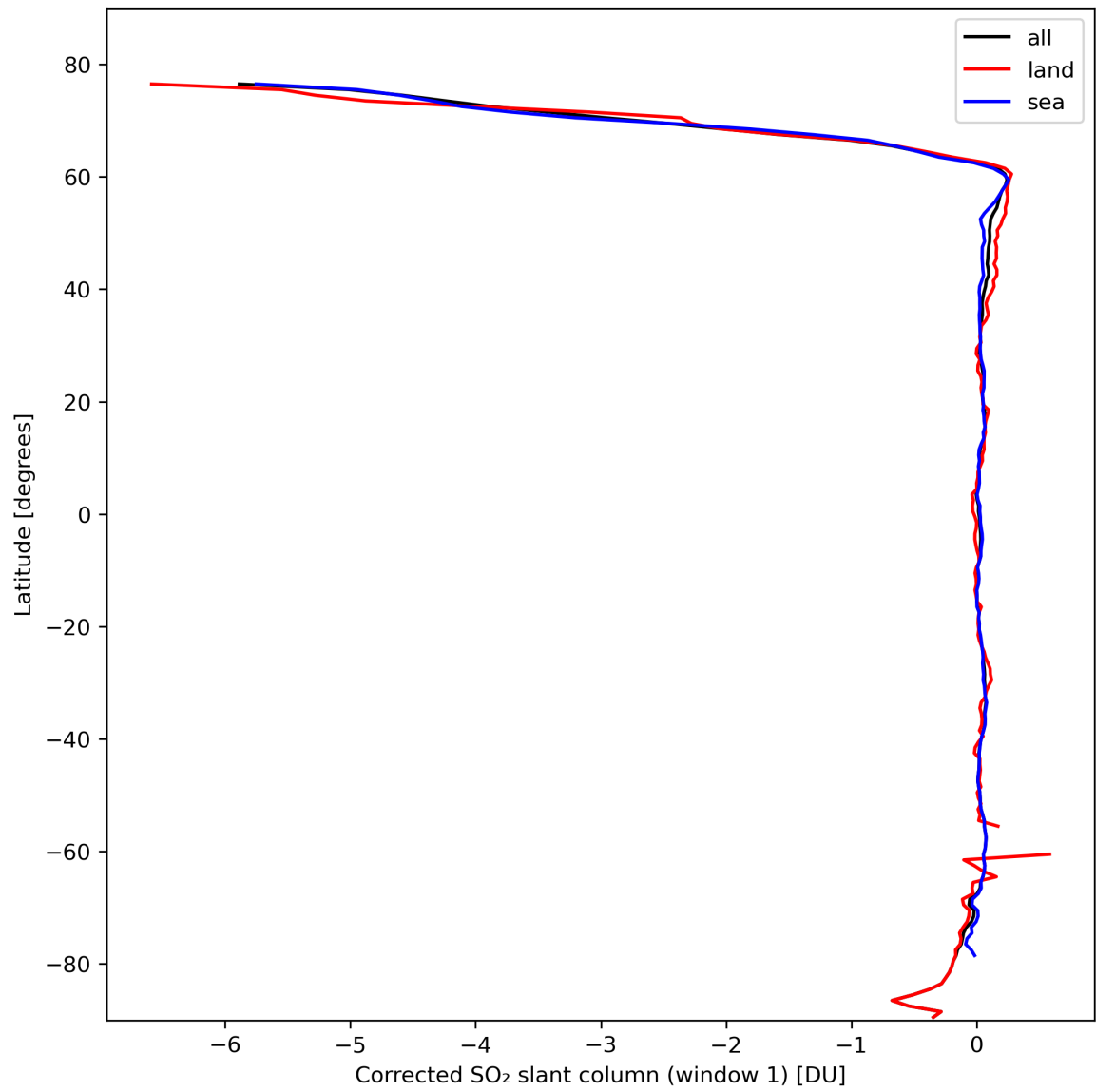
Figure 35: Zonal average of “Corrected SO 2 slant column (window 1)” for 2024-02-25 to 2024-02-27.
