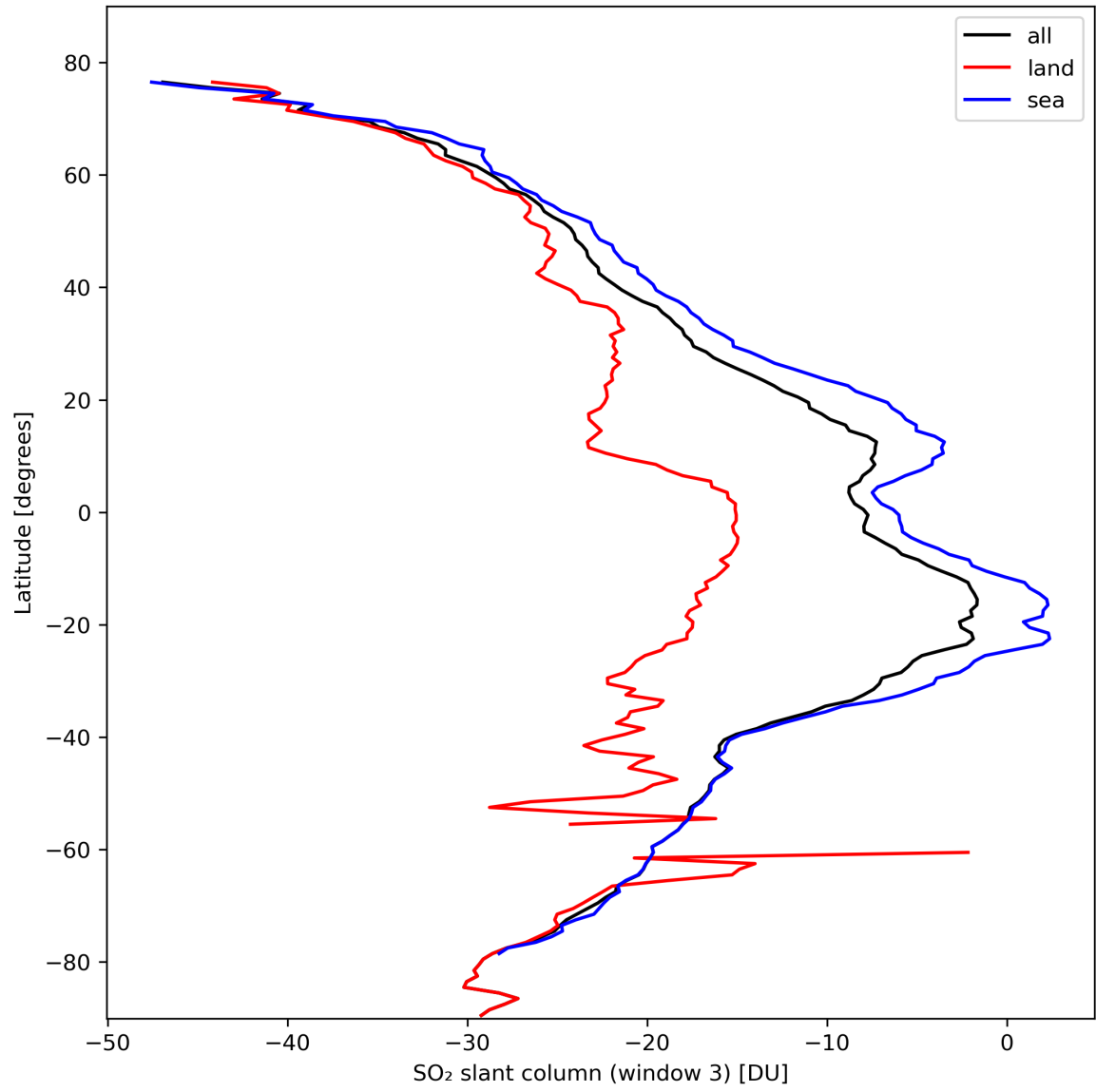
Figure 41: Zonal average of “SO 2 slant column (window 3)” for 2024-02-25 to 2024-02-27.
