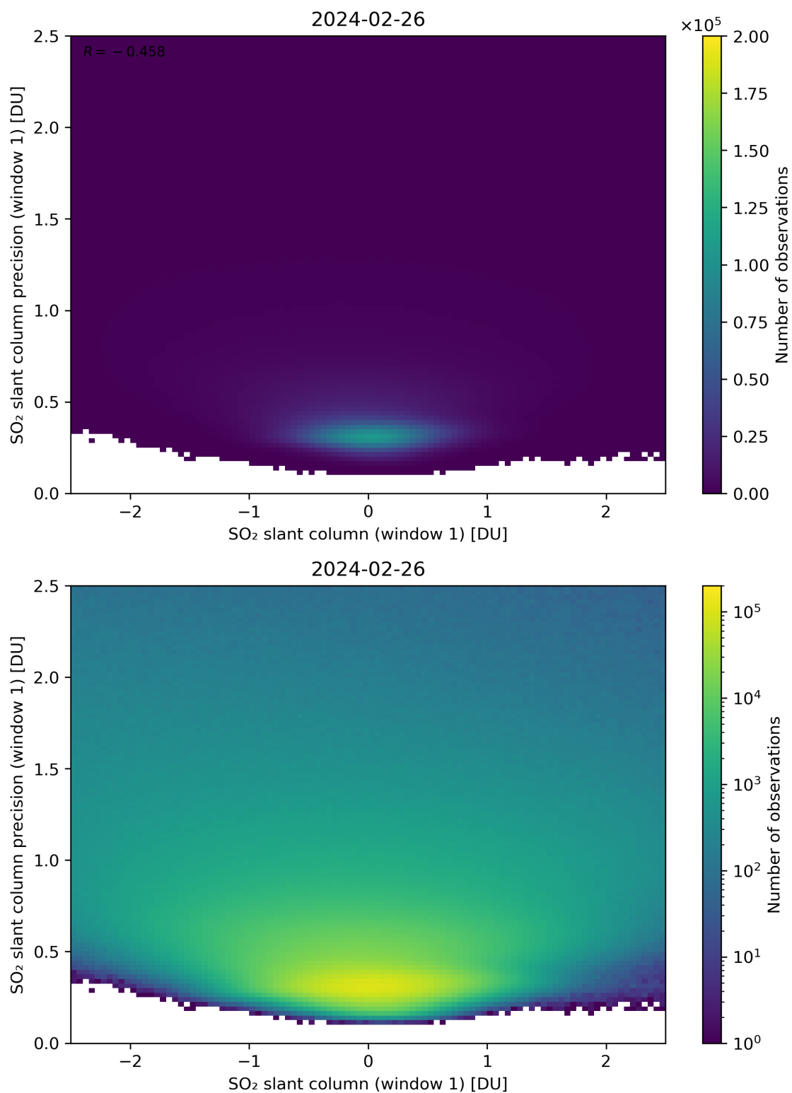
Figure 235: Scatter density plot of “SO 2 slant column (window 1)” against “SO 2 slant column precision (window 1)” for 2024-02-25 to 2024-02-27.
