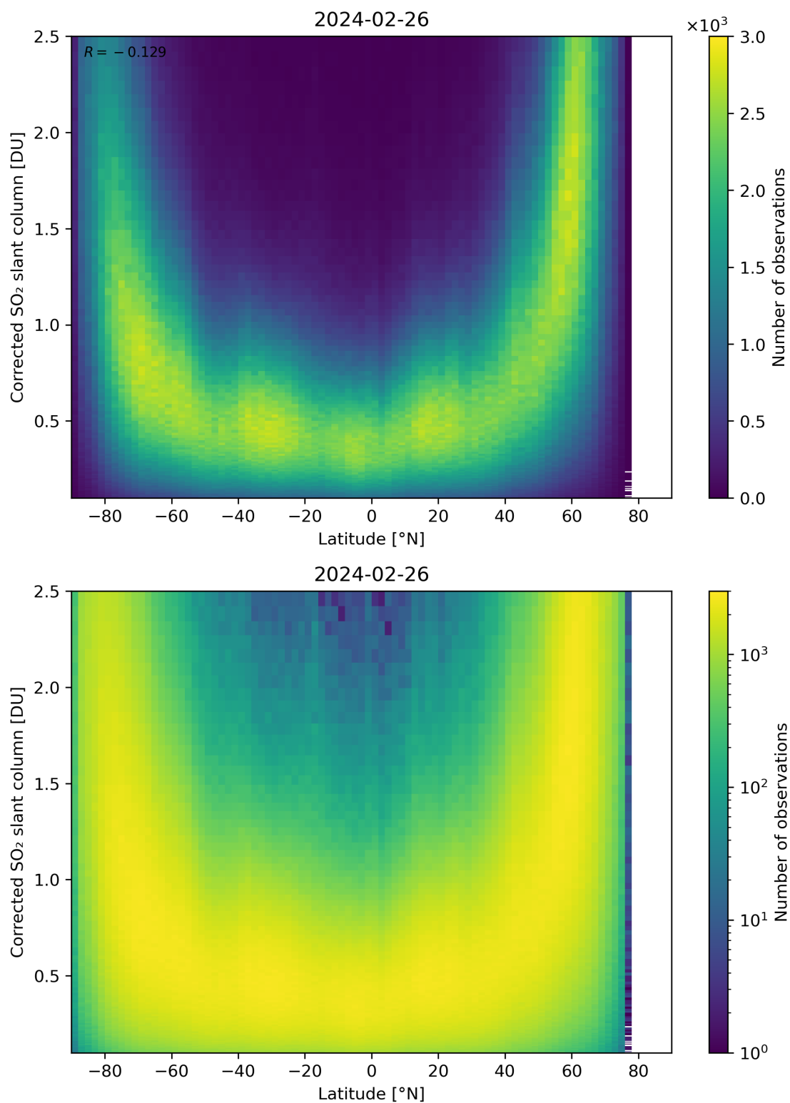
Figure 146: Scatter density plot of “Latitude” against “Corrected SO 2 slant column” for 2024-02-25 to 2024-02-27.
