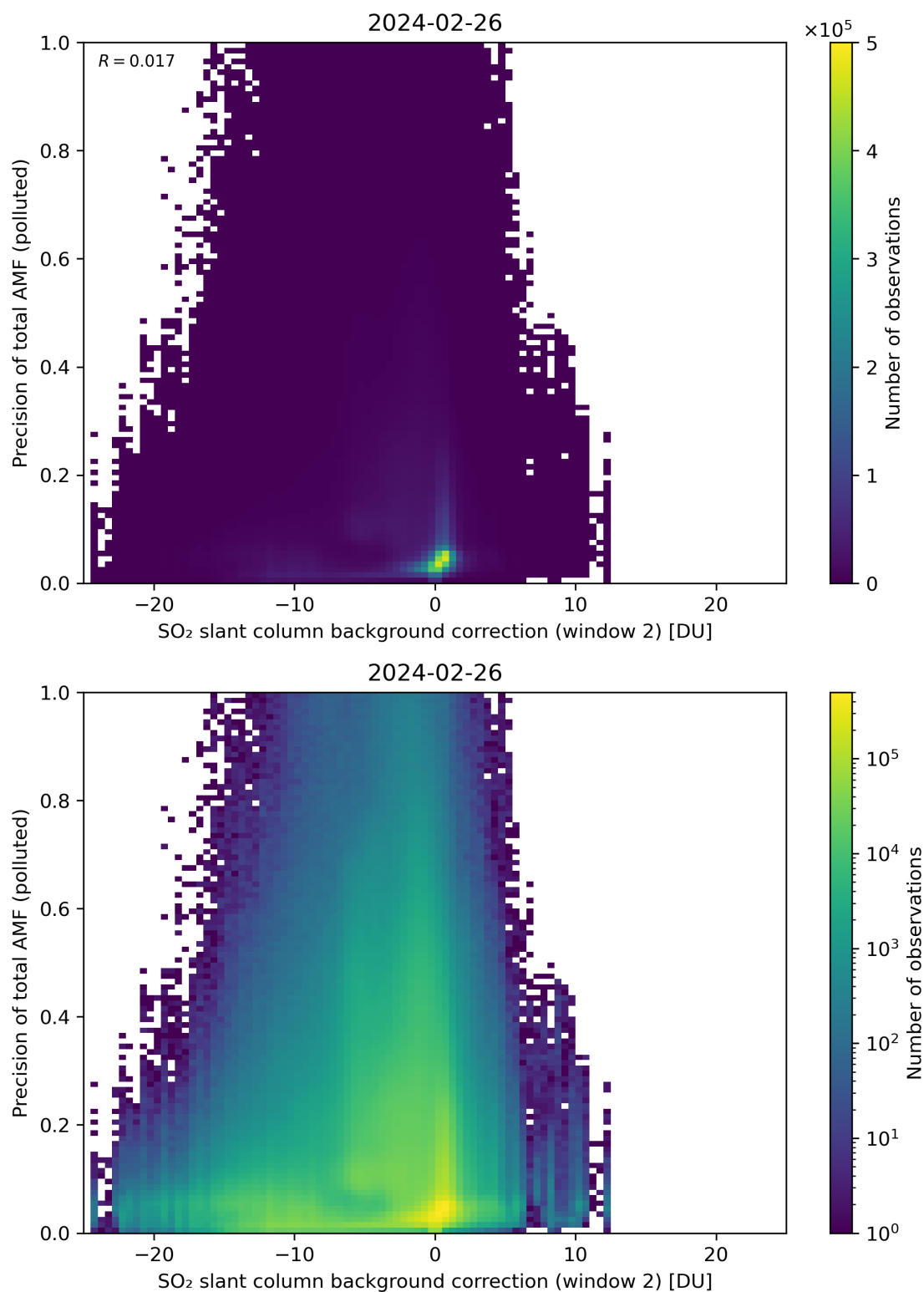
Figure 120: Scatter density plot of “SO 2 slant column background correction (window 2)” against “Precision of total AMF (polluted)” for 2024-02-25 to 2024-02-27.
