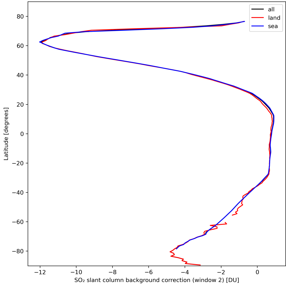
Figure 40: Zonal average of “SO 2 slant column background correction (window 2)” for 2024-02-25 to 2024-02-27.
