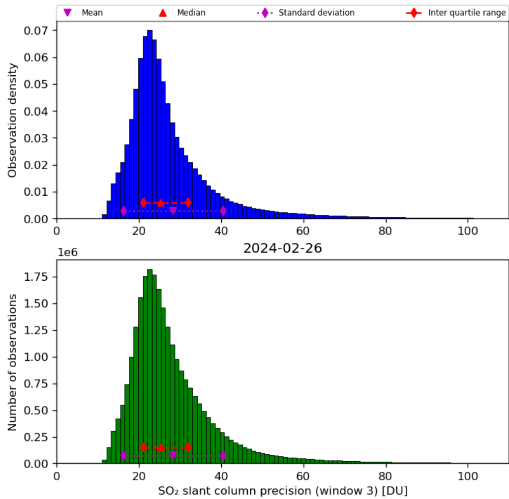
Figure 65: Histogram of “SO 2 slant column precision (window 3)” for 2024-02-25 to 2024-02-27
