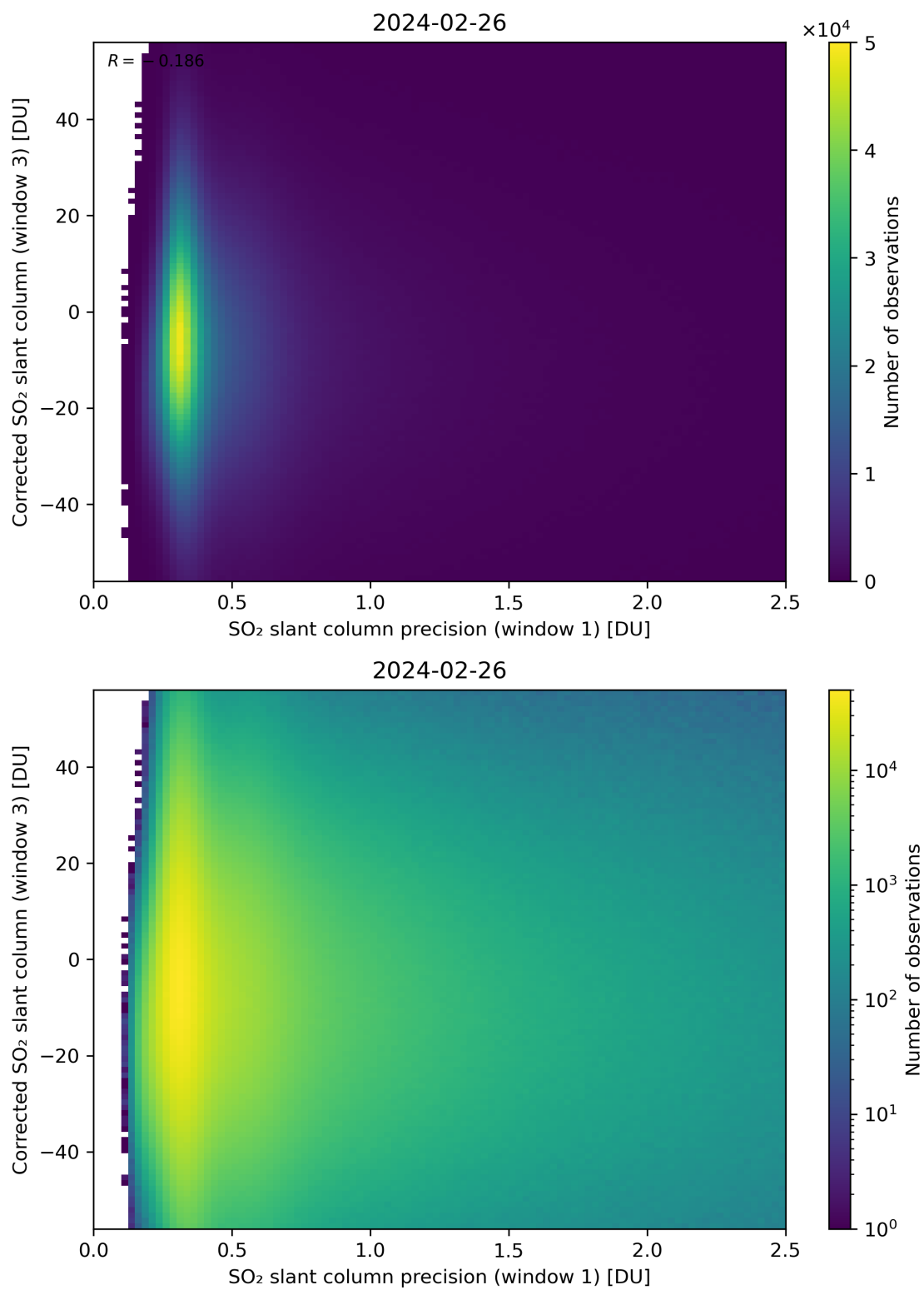
Figure 226: Scatter density plot of “SO 2 slant column precision (window 1)” against “Corrected SO 2 slant column (window 3)” for 2024-02-25 to 2024-02-27.
