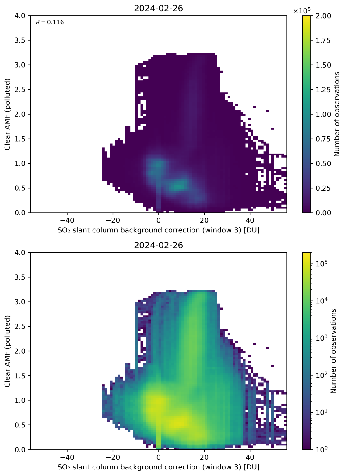
Figure 124: Scatter density plot of “SO 2 slant column background correction (window 3)” against “Clear AMF (polluted)” for 2024-02-25 to 2024-02-27.
