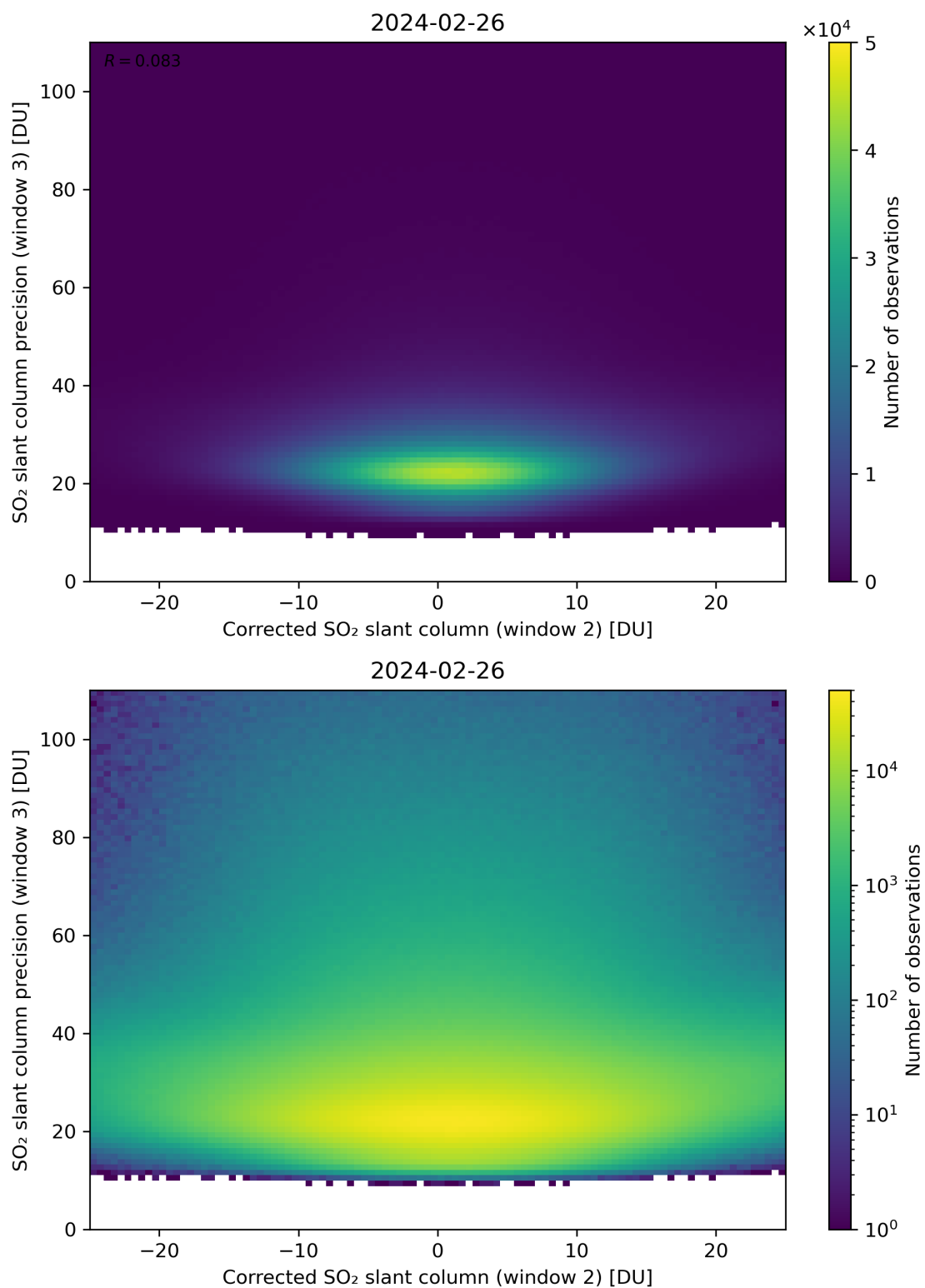
Figure 202: Scatter density plot of “Corrected SO 2 slant column (window 2)” against “SO 2 slant column precision (window 3)” for 2024-02-25 to 2024-02-27.
