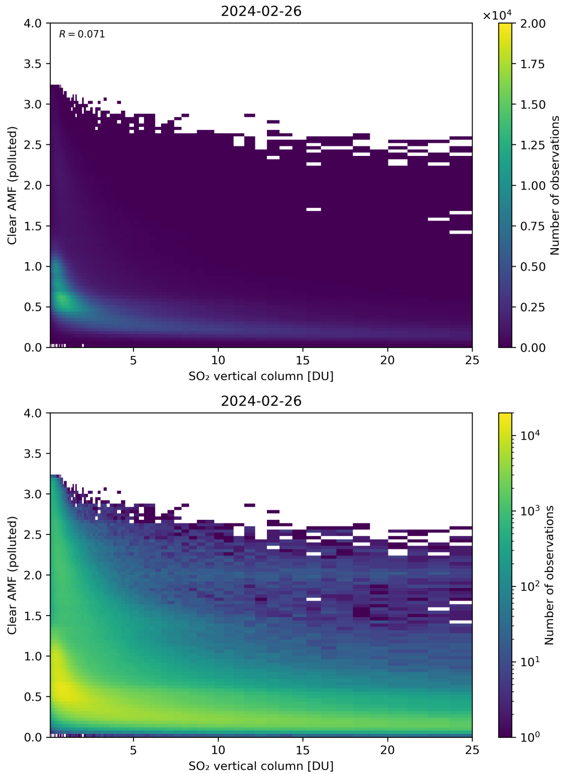
Figure 296: Scatter density plot of “SO 2 vertical column” against “Clear AMF (polluted)” for 2024-02-25 to 2024-02-27.
