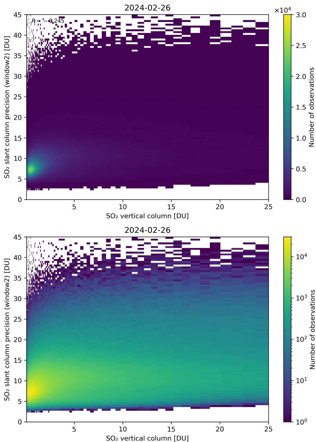
Figure 302: Scatter density plot of “SO 2 vertical column” against “SO 2 slant column precision (window2)” for 2024-02-25 to 2024-02-27.
