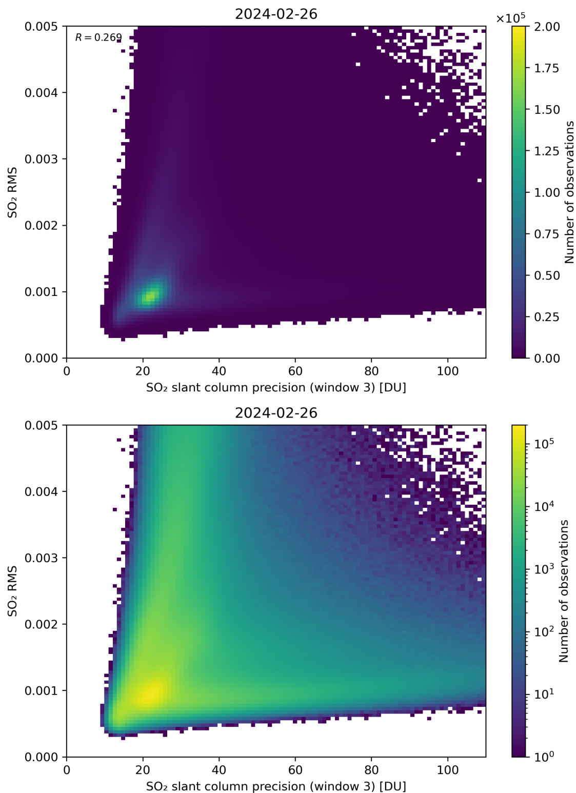
Figure 260: Scatter density plot of “SO 2 slant column precision (window 3)” against “SO 2 RMS” for 2024-02-25 to 2024-02-27.
