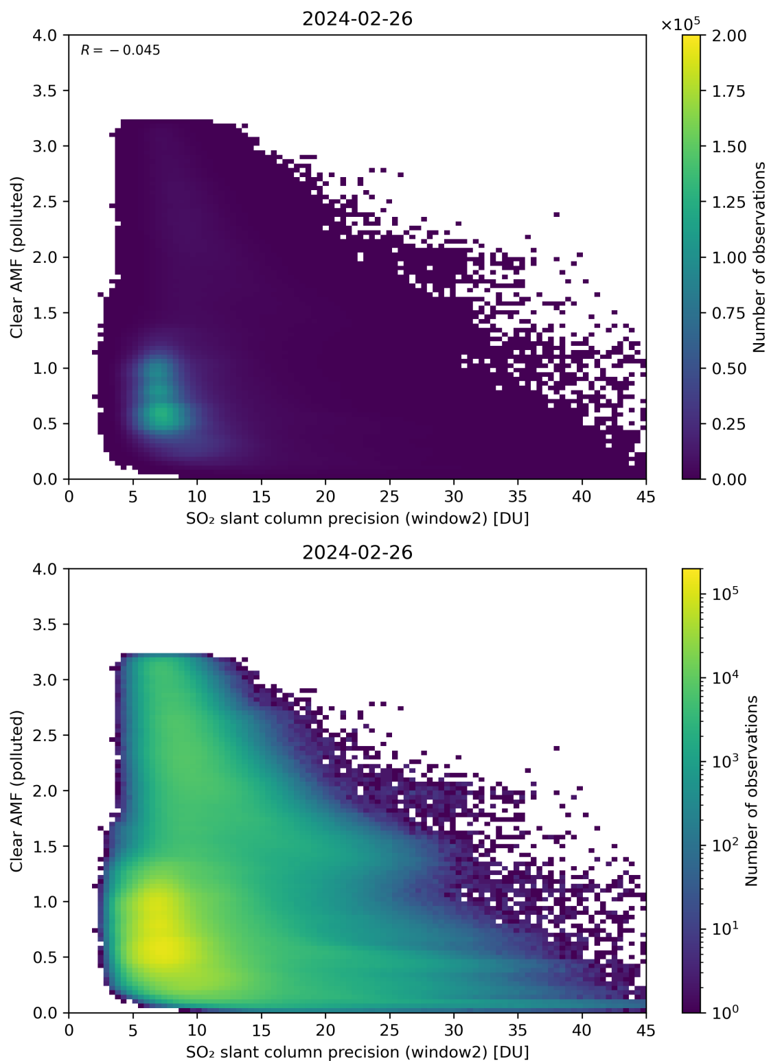
Figure 246: Scatter density plot of “SO 2 slant column precision (window2)” against “Clear AMF (polluted)” for 2024-02-25 to 2024-02-27.
