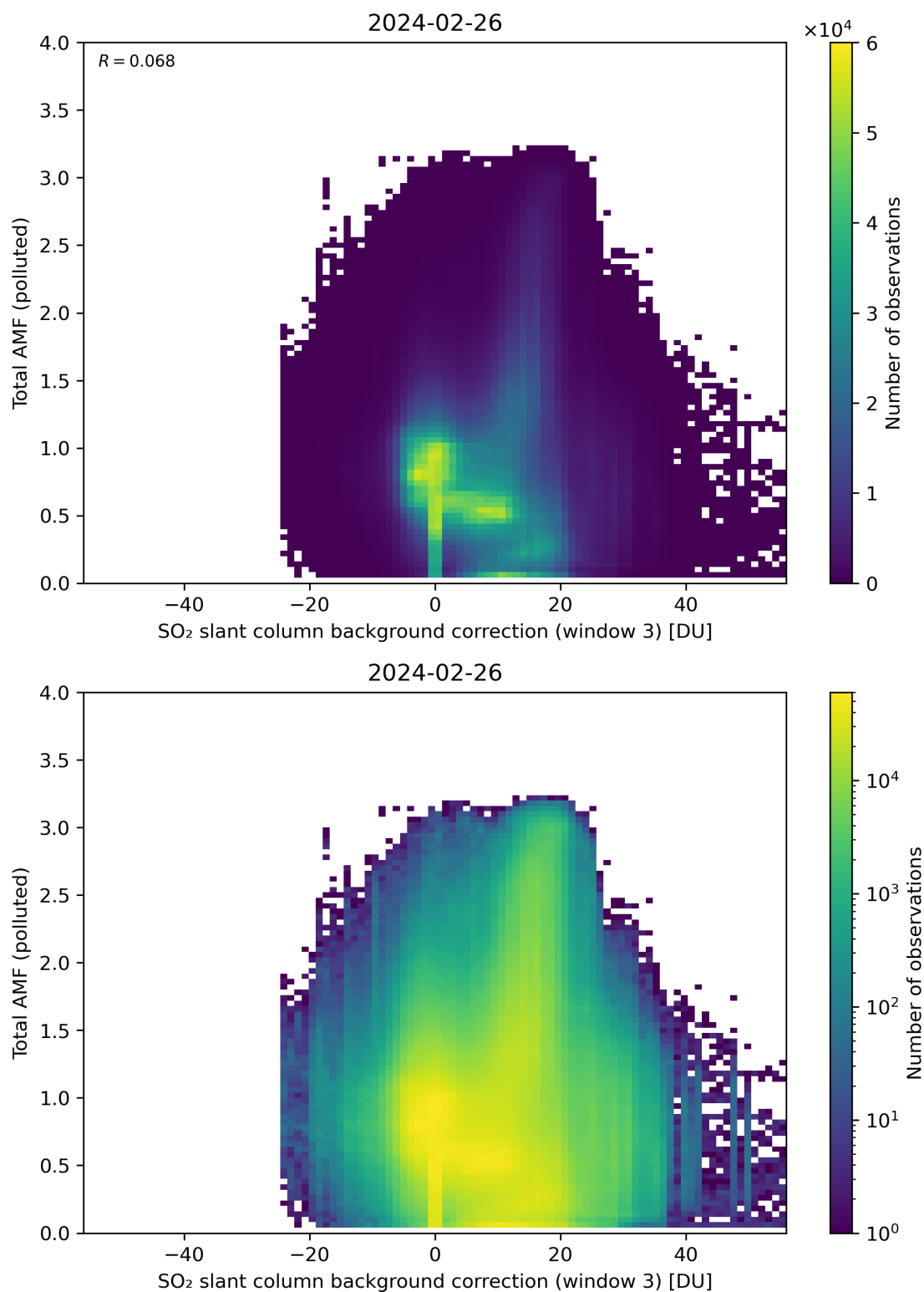
Figure 125: Scatter density plot of “SO 2 slant column background correction (window 3)” against “Total AMF (polluted)” for 2024-02-25 to 2024-02-27.
