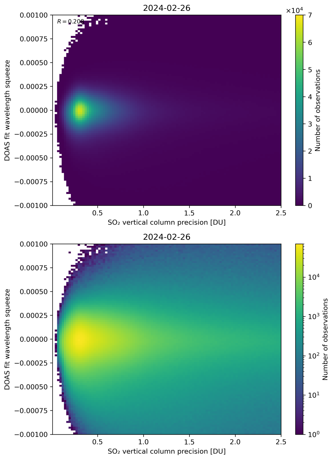
Figure 283: Scatter density plot of “SO 2 vertical column precision” against “DOAS fit wavelength squeeze” for 2024-02-25 to 2024-02-27.
