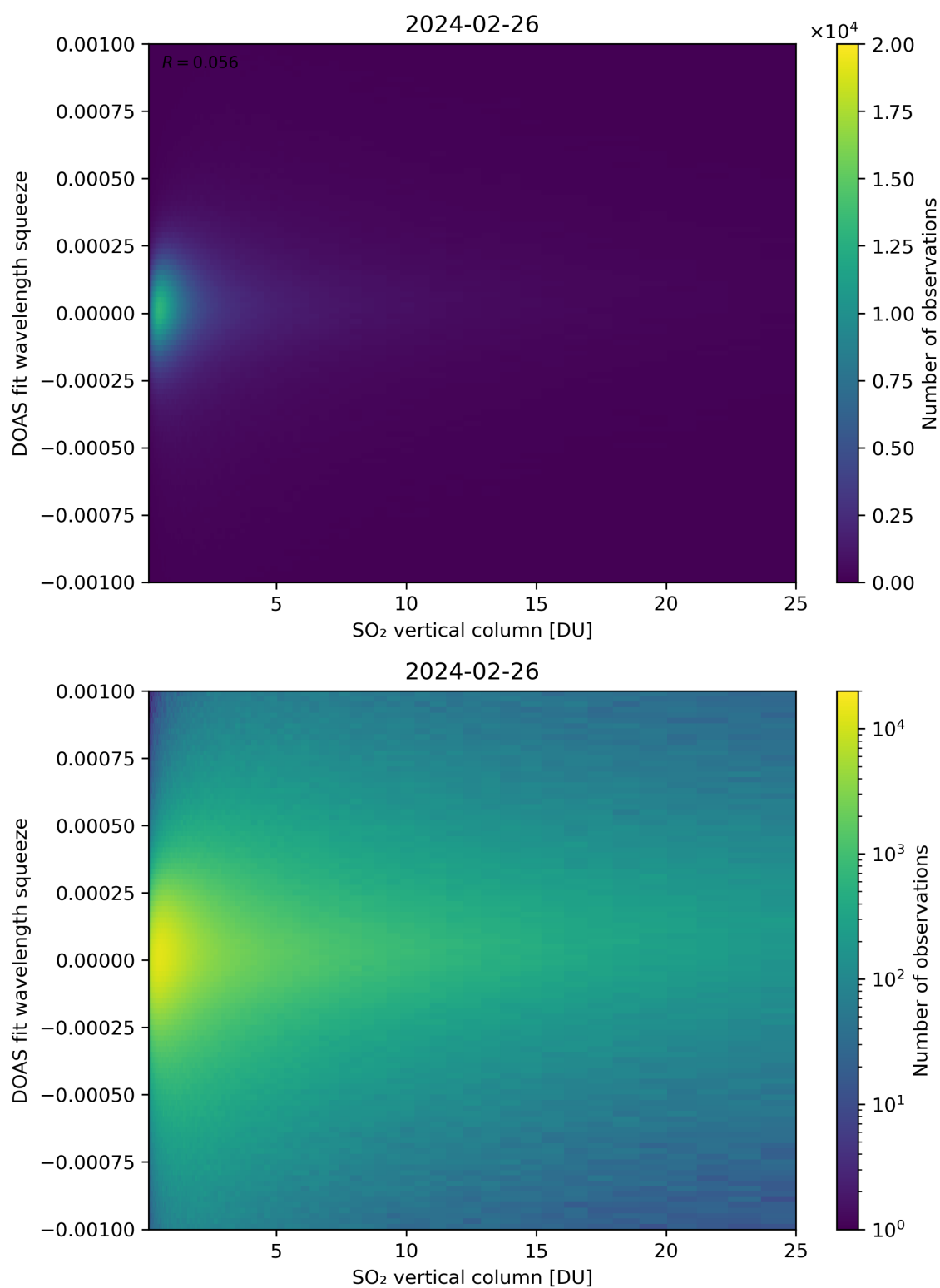
Figure 277: Scatter density plot of “SO 2 vertical column” against “DOAS fit wavelength squeeze” for 2024-02-25 to 2024-02-27.
