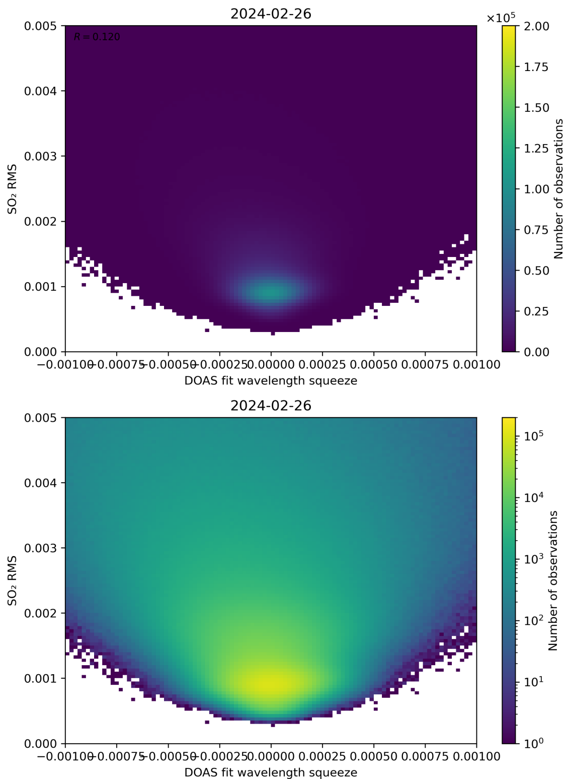
Figure 132: Scatter density plot of “DOAS fit wavelength squeeze” against “SO 2 RMS” for 2024-02-25 to 2024-02-27.
