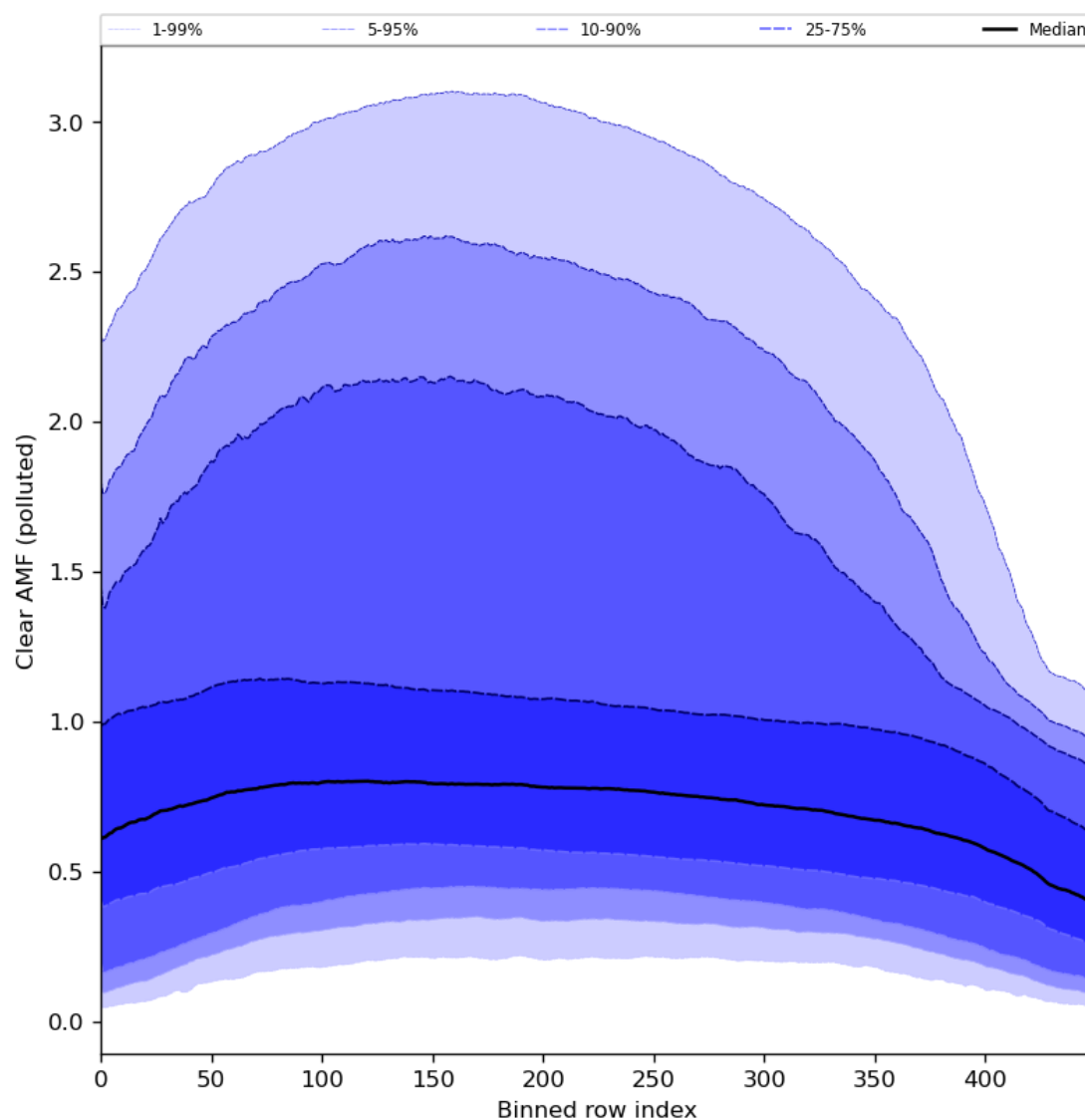
Figure 96: Along track statistics of “Clear AMF (polluted)” for 2024-02-25 to 2024-02-27
