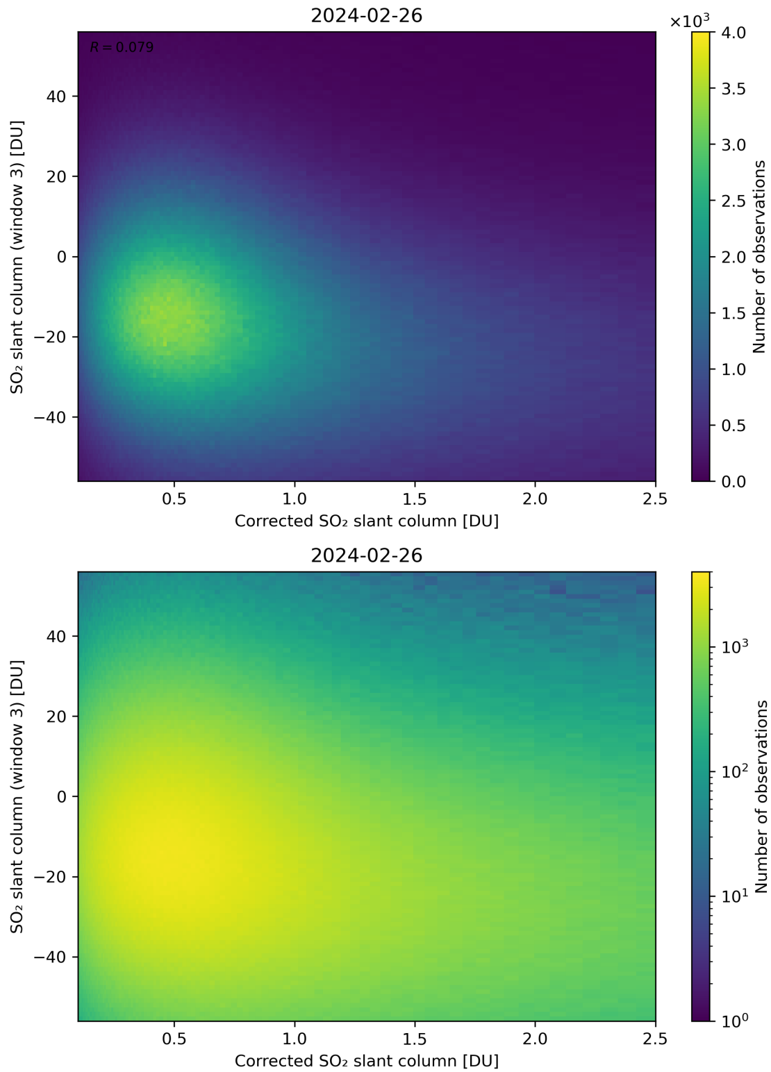
Figure 190: Scatter density plot of “Corrected SO 2 slant column” against “SO 2 slant column (window 3)” for 2024-02-25 to 2024-02-27.
