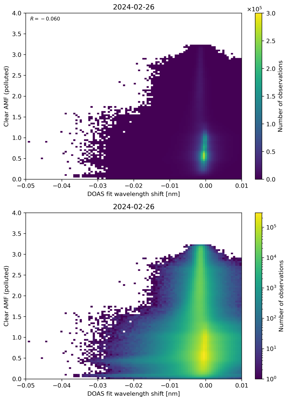
Figure 129: Scatter density plot of “DOAS fit wavelength shift” against “Clear AMF (polluted)” for 2024-02-25 to 2024-02-27.
