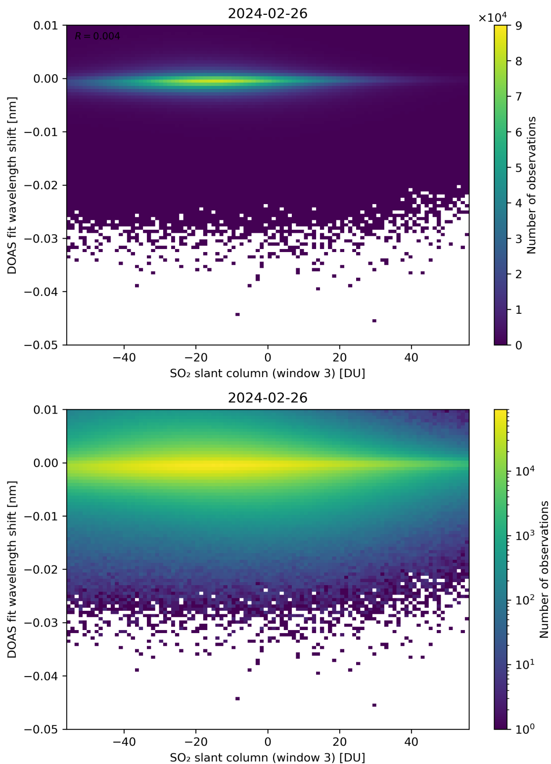
Figure 254: Scatter density plot of “SO 2 slant column (window 3)” against “DOAS fit wavelength shift” for 2024-02-25 to 2024-02-27.
