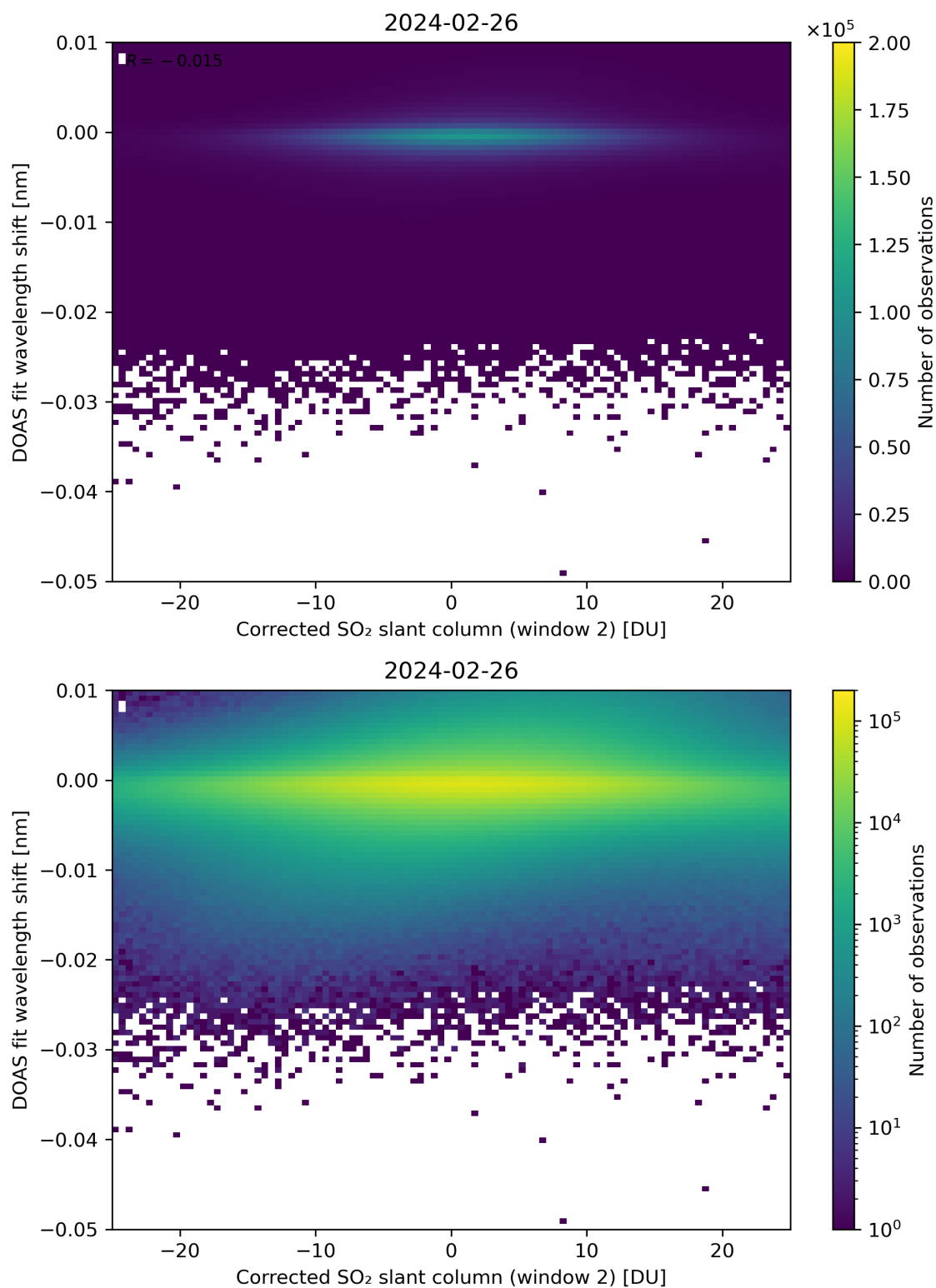
Figure 196: Scatter density plot of “Corrected SO 2 slant column (window 2)” against “DOAS fit wavelength shift” for 2024-02-25 to 2024-02-27.
