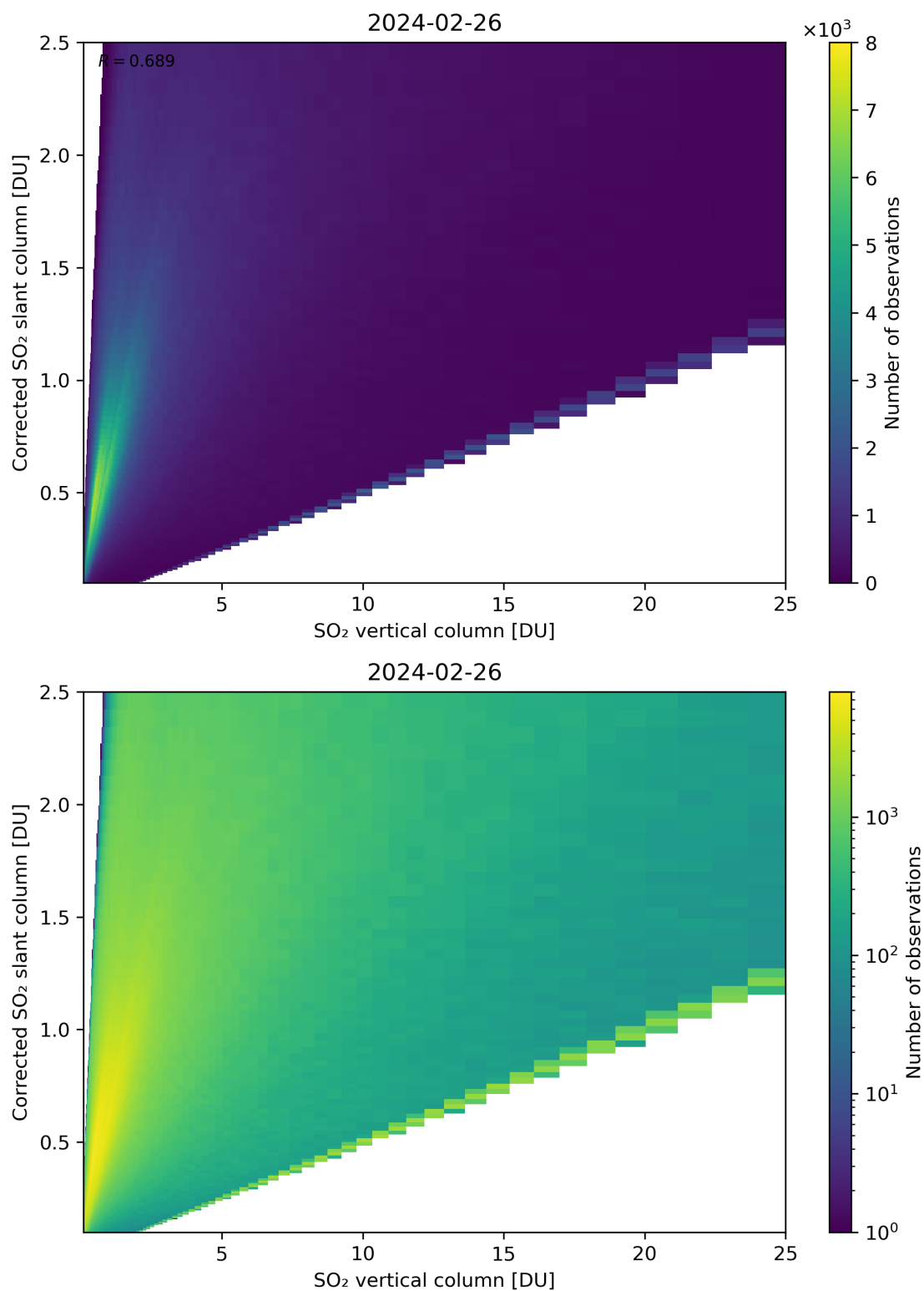
Figure 297: Scatter density plot of “SO 2 vertical column” against “Corrected SO 2 slant column” for 2024-02-25 to 2024-02-27.
