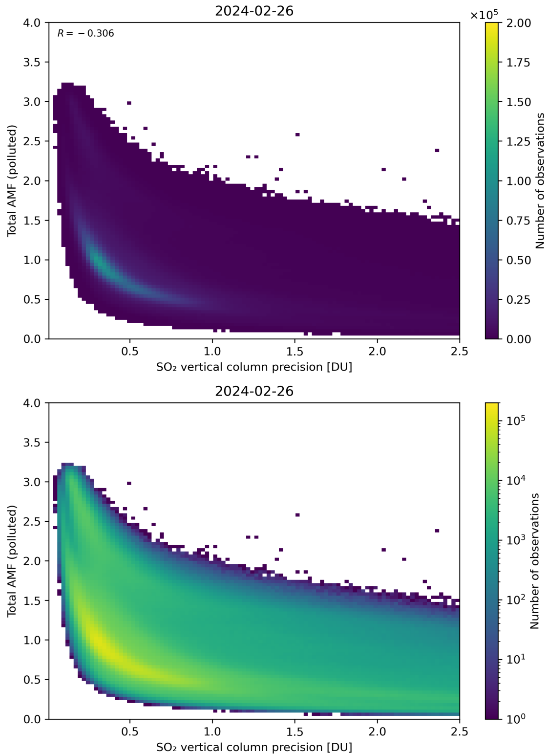
Figure 294: Scatter density plot of “SO 2 vertical column precision” against “Total AMF (polluted)” for 2024-02-25 to 2024-02-27.
