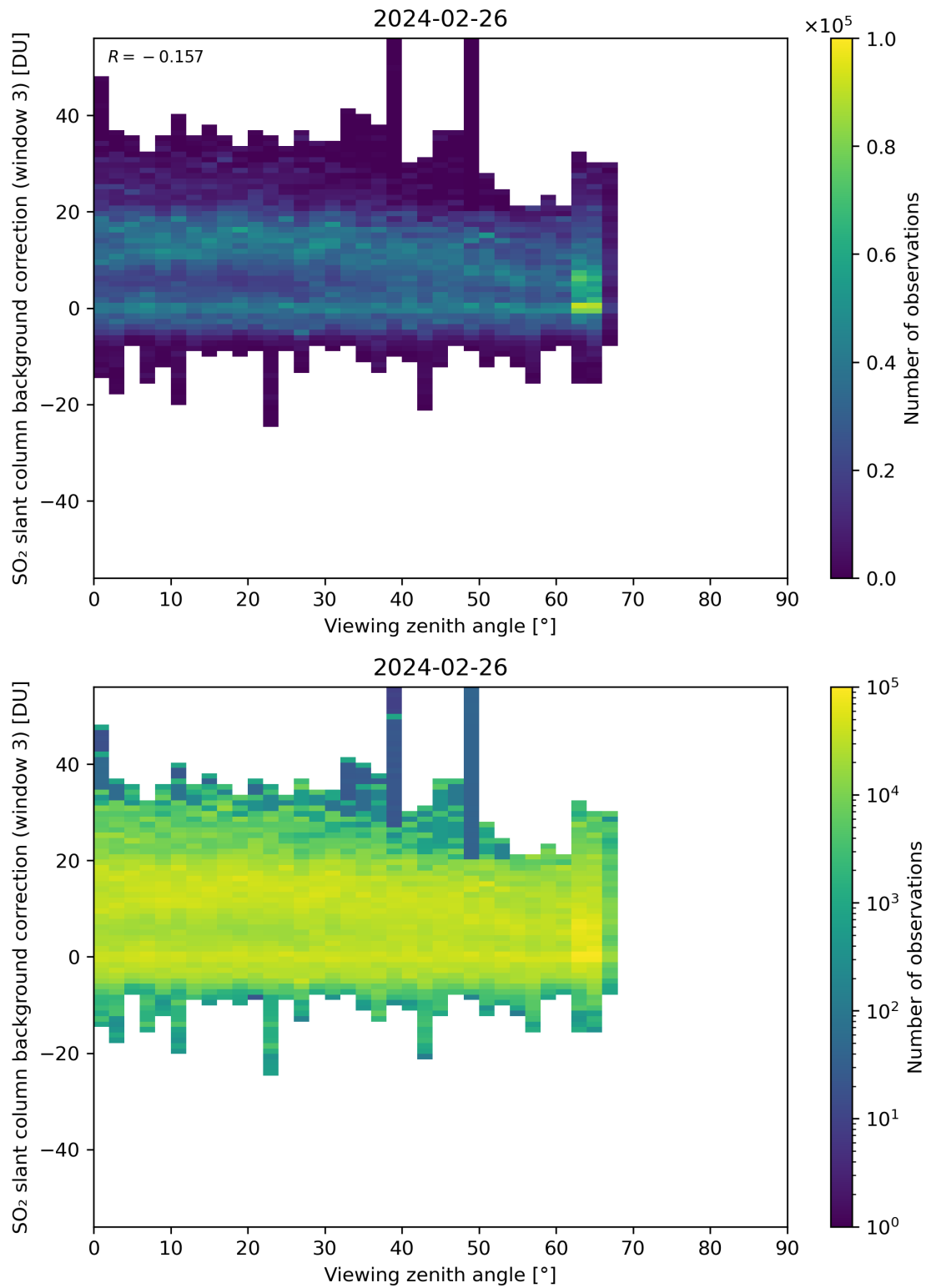
Figure 310: Scatter density plot of “Viewing zenith angle” against “SO 2 slant column background correction (window 3)” for 2024-02-25 to 2024-02-27.
