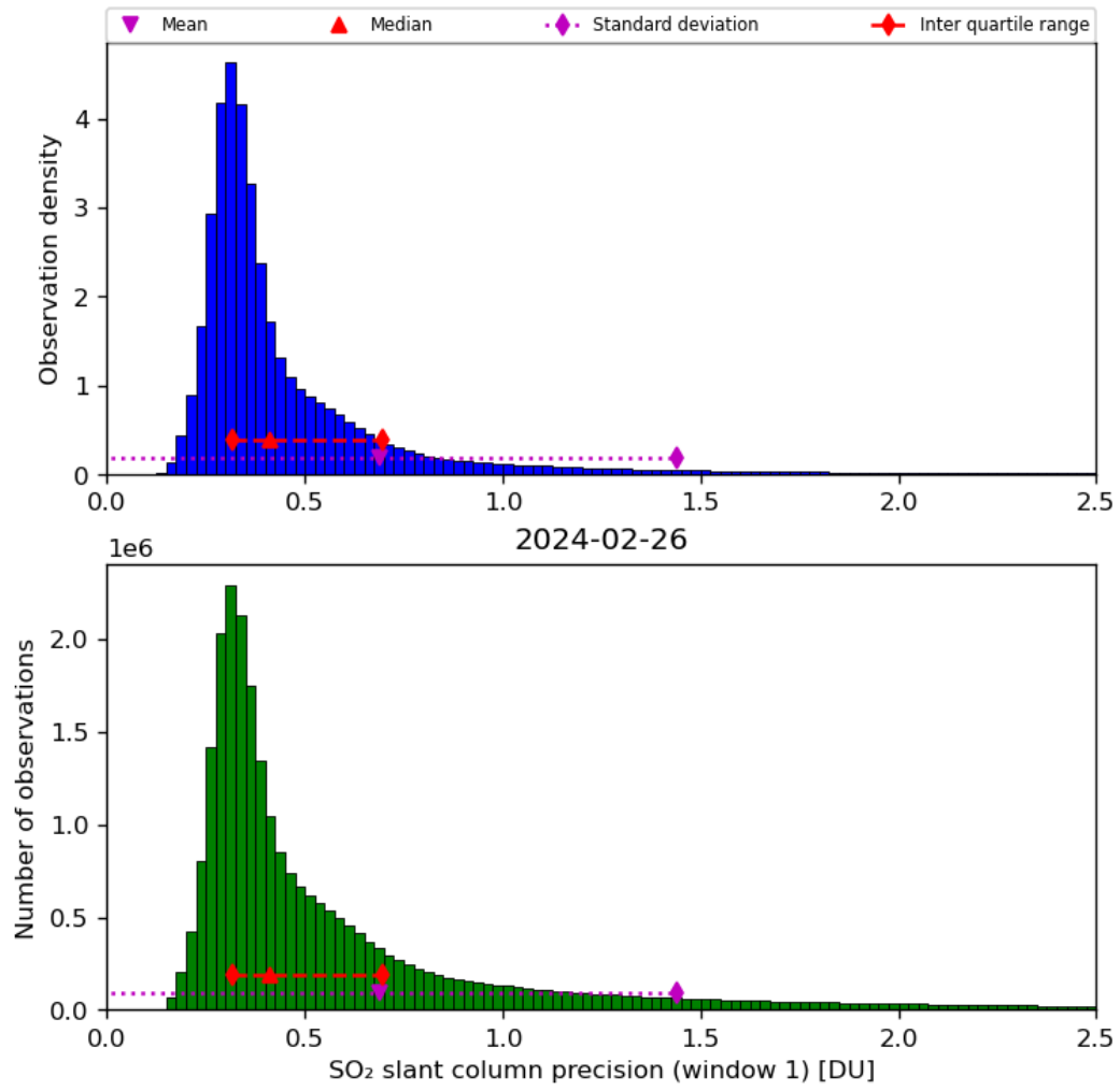
Figure 57: Histogram of “SO 2 slant column precision (window 1)” for 2024-02-25 to 2024-02-27
