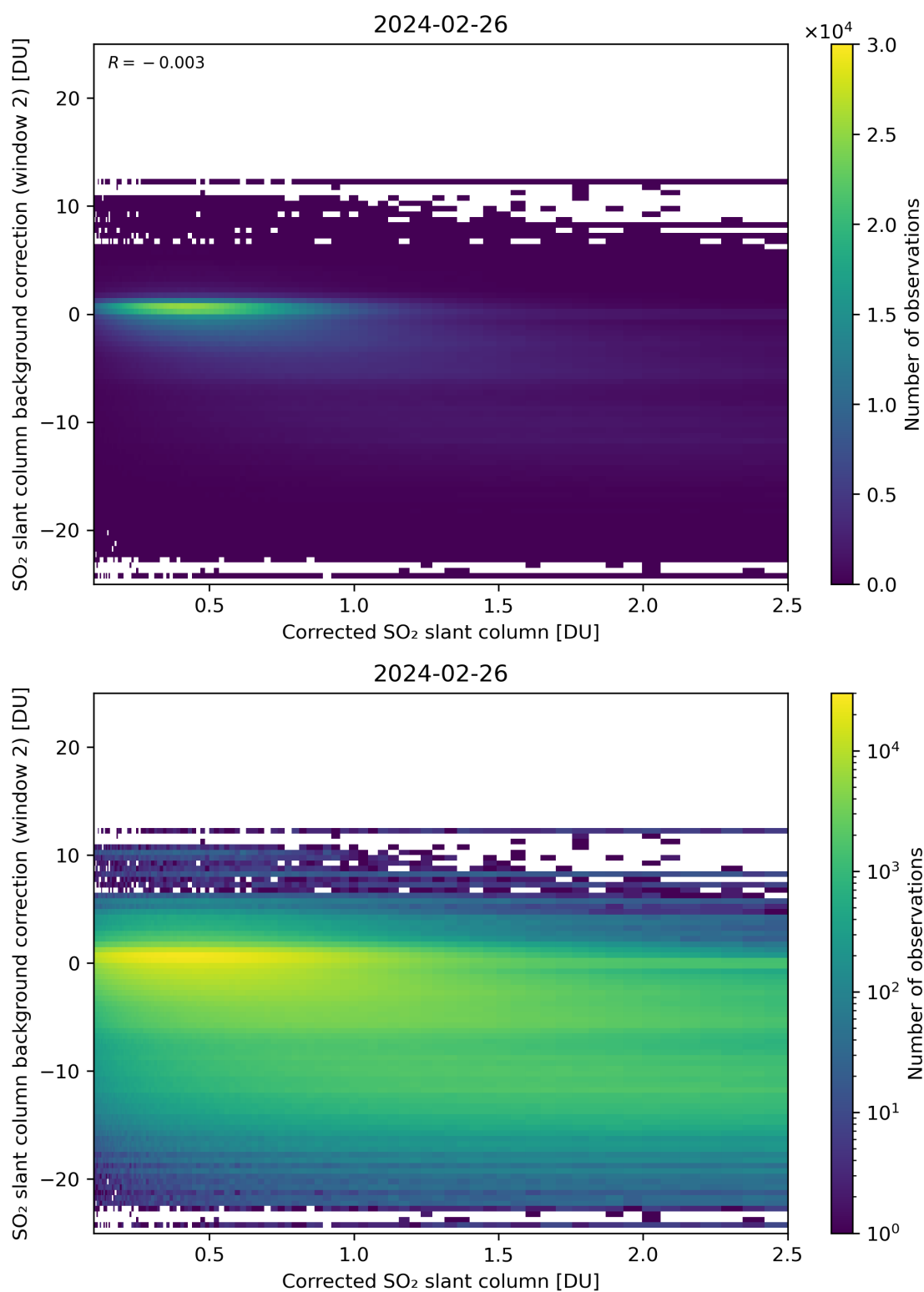
Figure 179: Scatter density plot of “Corrected SO 2 slant column” against “SO 2 slant column background correction (window 2)” for 2024-02-25 to 2024-02-27.
