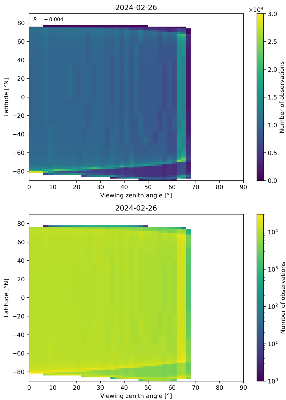
Figure 314: Scatter density plot of “Viewing zenith angle” against “Latitude” for 2024-02-25 to 2024-02-27.
