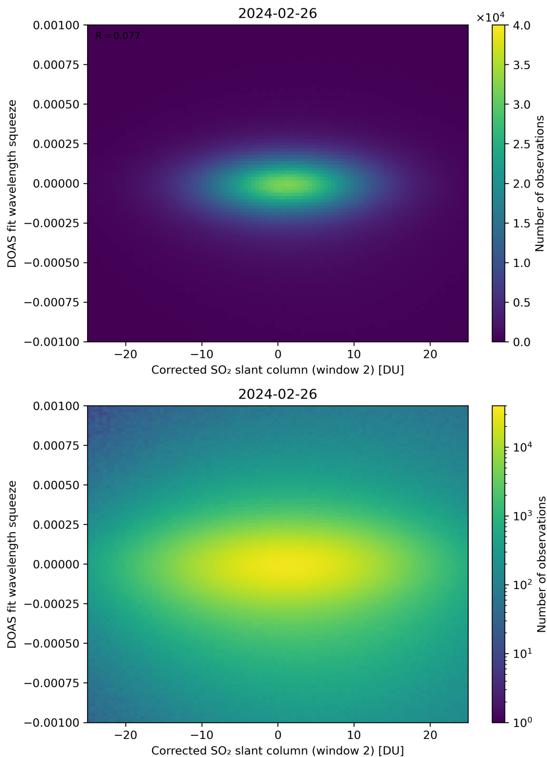
Figure 197: Scatter density plot of “Corrected SO 2 slant column (window 2)” against “DOAS fit wavelength squeeze” for 2024-02-25 to 2024-02-27.
