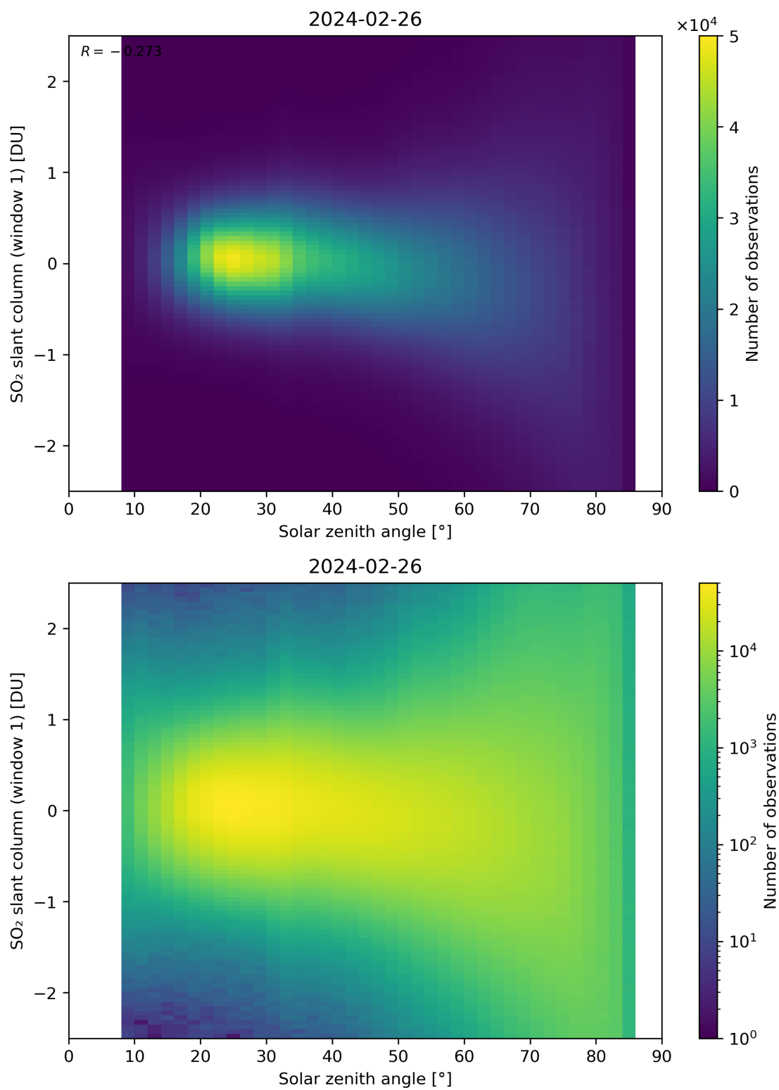
Figure 169: Scatter density plot of “Solar zenith angle” against “SO 2 slant column (window 1)” for 2024-02-25 to 2024-02-27.
