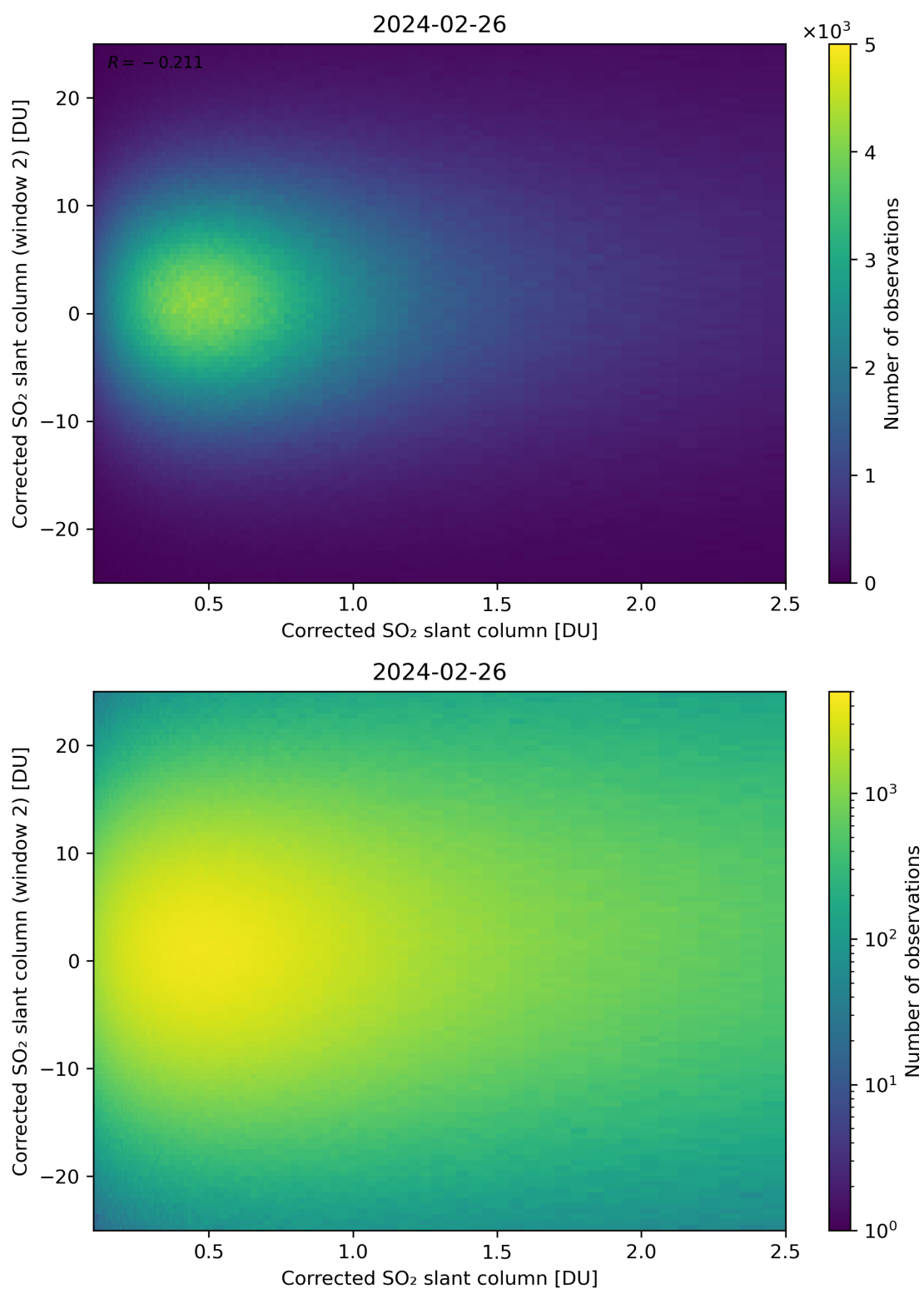
Figure 185: Scatter density plot of “Corrected SO 2 slant column” against “Corrected SO 2 slant column (window 2)” for 2024-02-25 to 2024-02-27.
