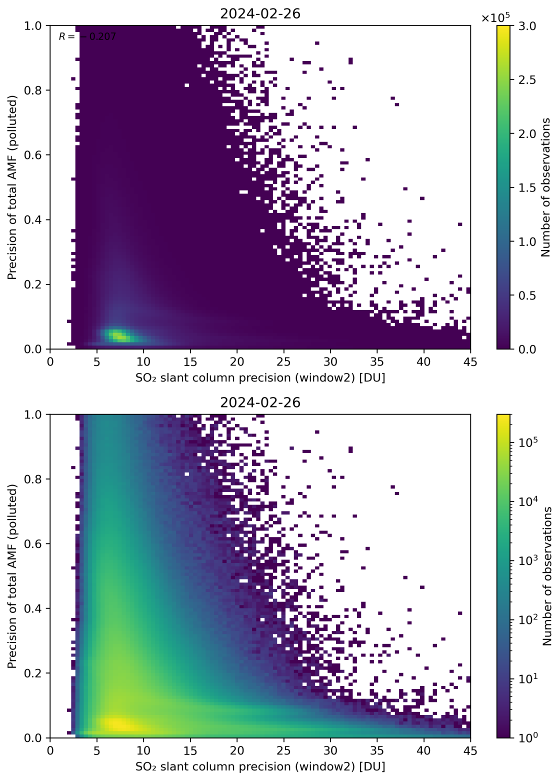
Figure 252: Scatter density plot of “SO 2 slant column precision (window2)” against “Precision of total AMF (polluted)” for 2024-02-25 to 2024-02-27.
