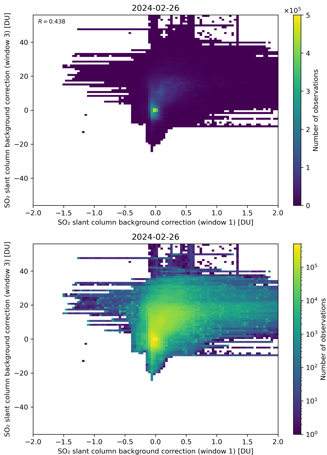
Figure 99: Scatter density plot of “SO 2 slant column background correction (window 1)” against “SO 2 slant column background correction (window 3)” for 2024-02-25 to 2024-02-27.
