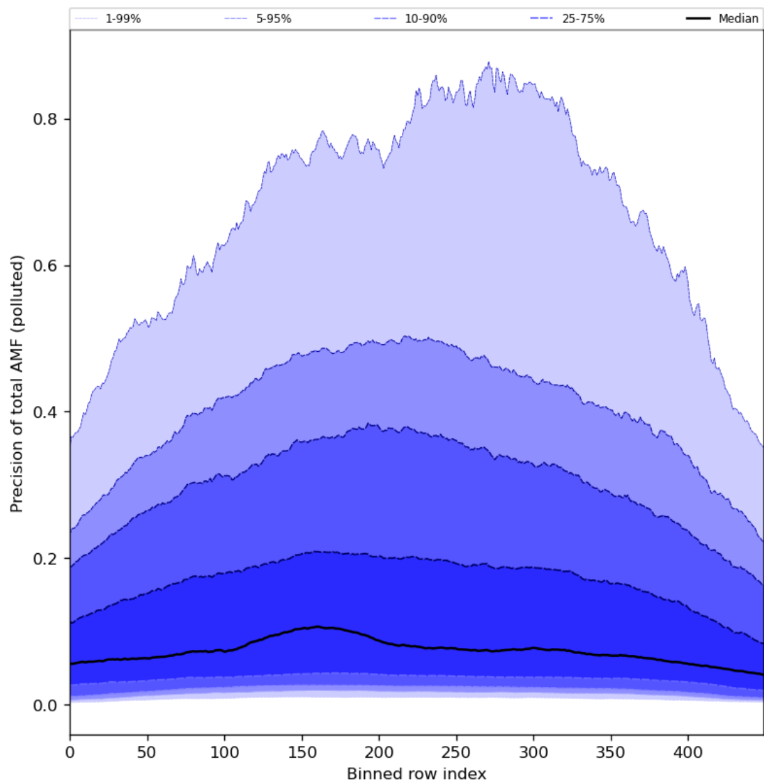
Figure 95: Along track statistics of “Precision of total AMF (polluted)” for 2024-02-25 to 2024-02-27
