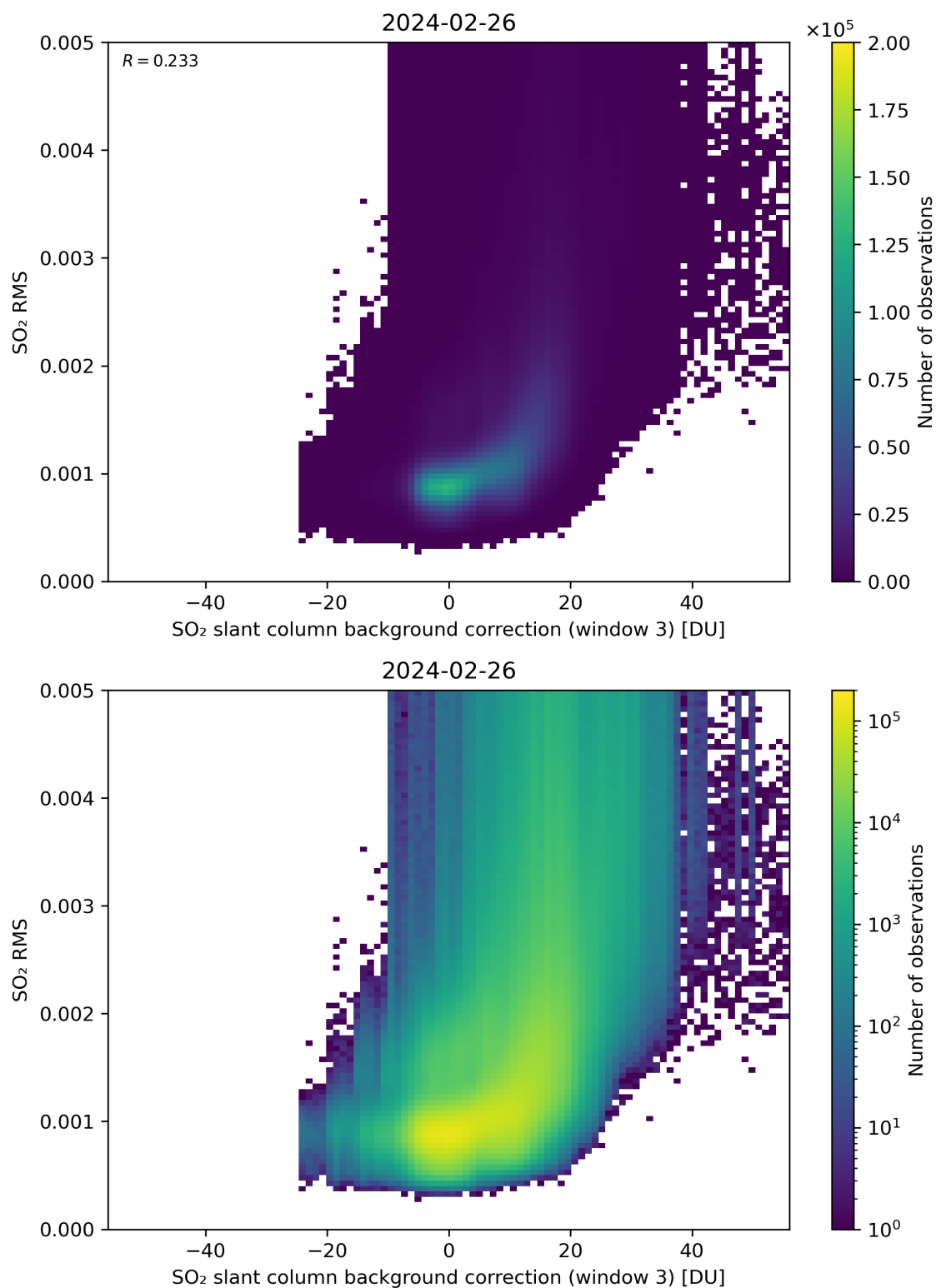
Figure 123: Scatter density plot of “SO 2 slant column background correction (window 3)” against “SO 2 RMS” for 2024-02-25 to 2024-02-27.
