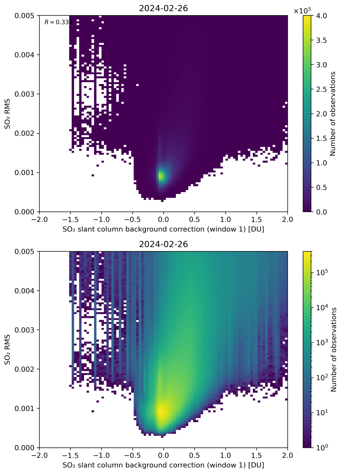
Figure 102: Scatter density plot of “SO 2 slant column background correction (window 1)” against “SO 2 RMS” for 2024-02-25 to 2024-02-27.
