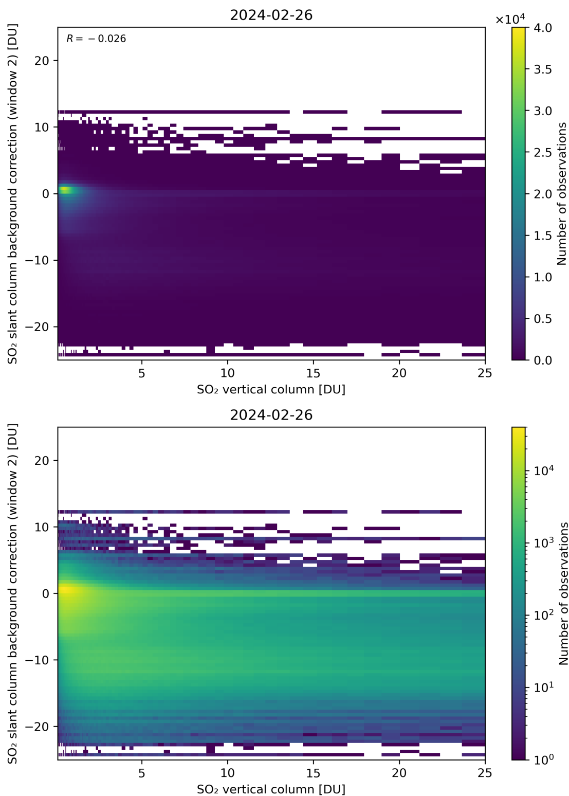
Figure 274: Scatter density plot of “SO 2 vertical column” against “SO 2 slant column background correction (window 2)” for 2024-02-25 to 2024-02-27.
