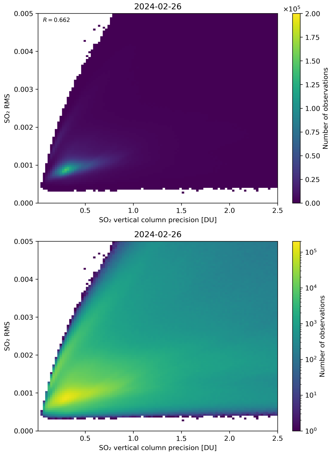
Figure 284: Scatter density plot of “SO 2 vertical column precision” against “SO 2 RMS” for 2024-02-25 to 2024-02-27.
