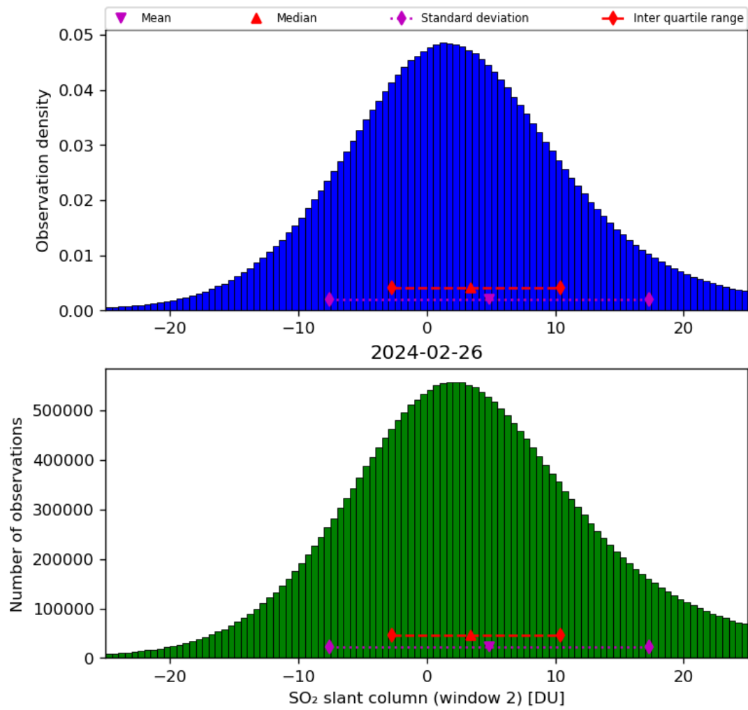
Figure 60: Histogram of “SO 2 slant column (window 2)” for 2024-02-25 to 2024-02-27
