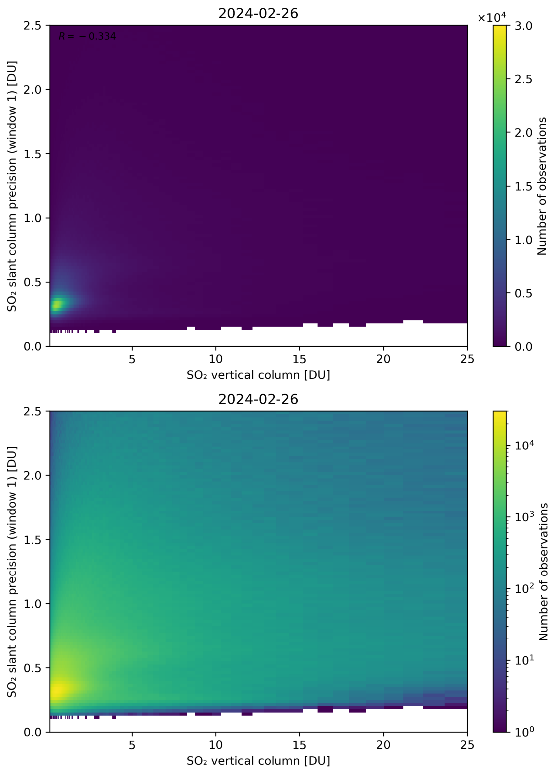
Figure 301: Scatter density plot of “SO 2 vertical column” against “SO 2 slant column precision (window 1)” for 2024-02-25 to 2024-02-27.
