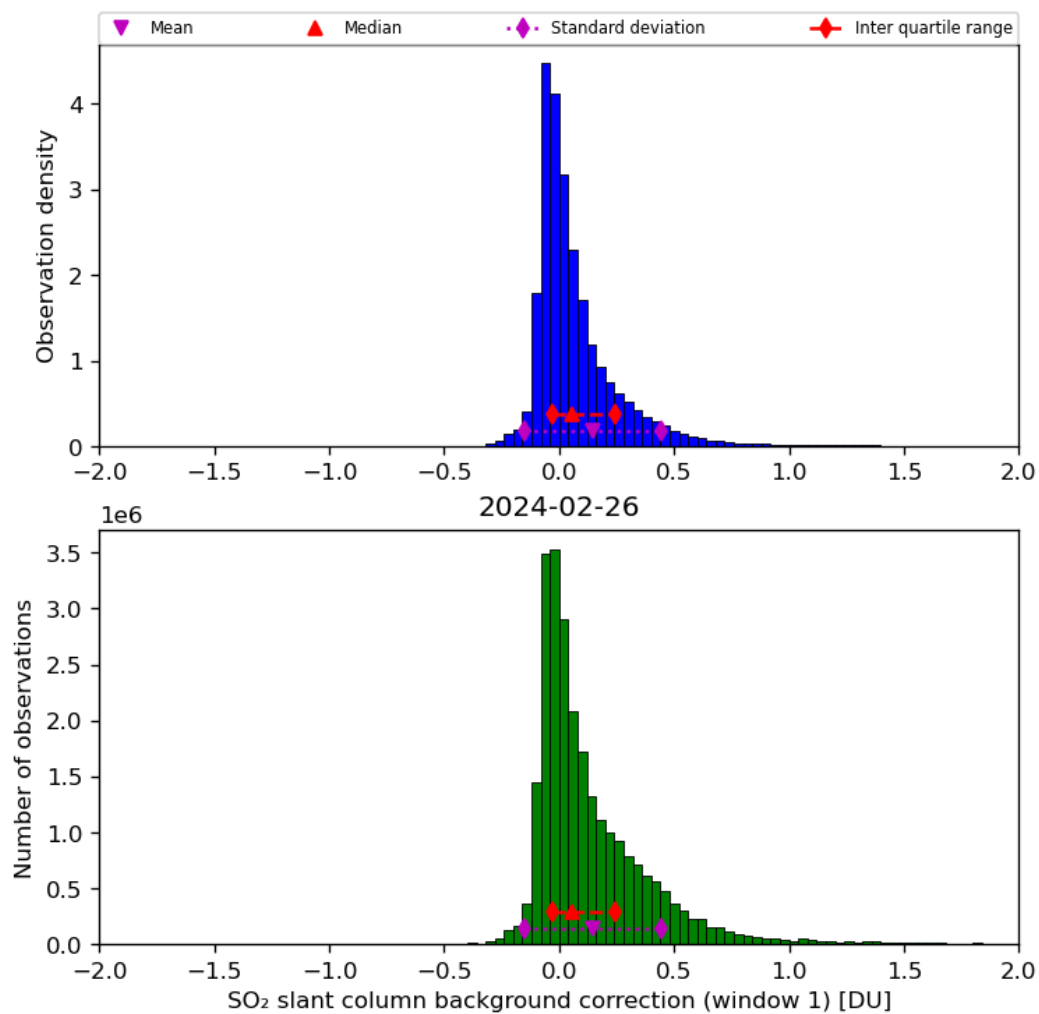
Figure 59: Histogram of “SO 2 slant column background correction (window 1)” for 2024-02-25 to 2024-02-27
