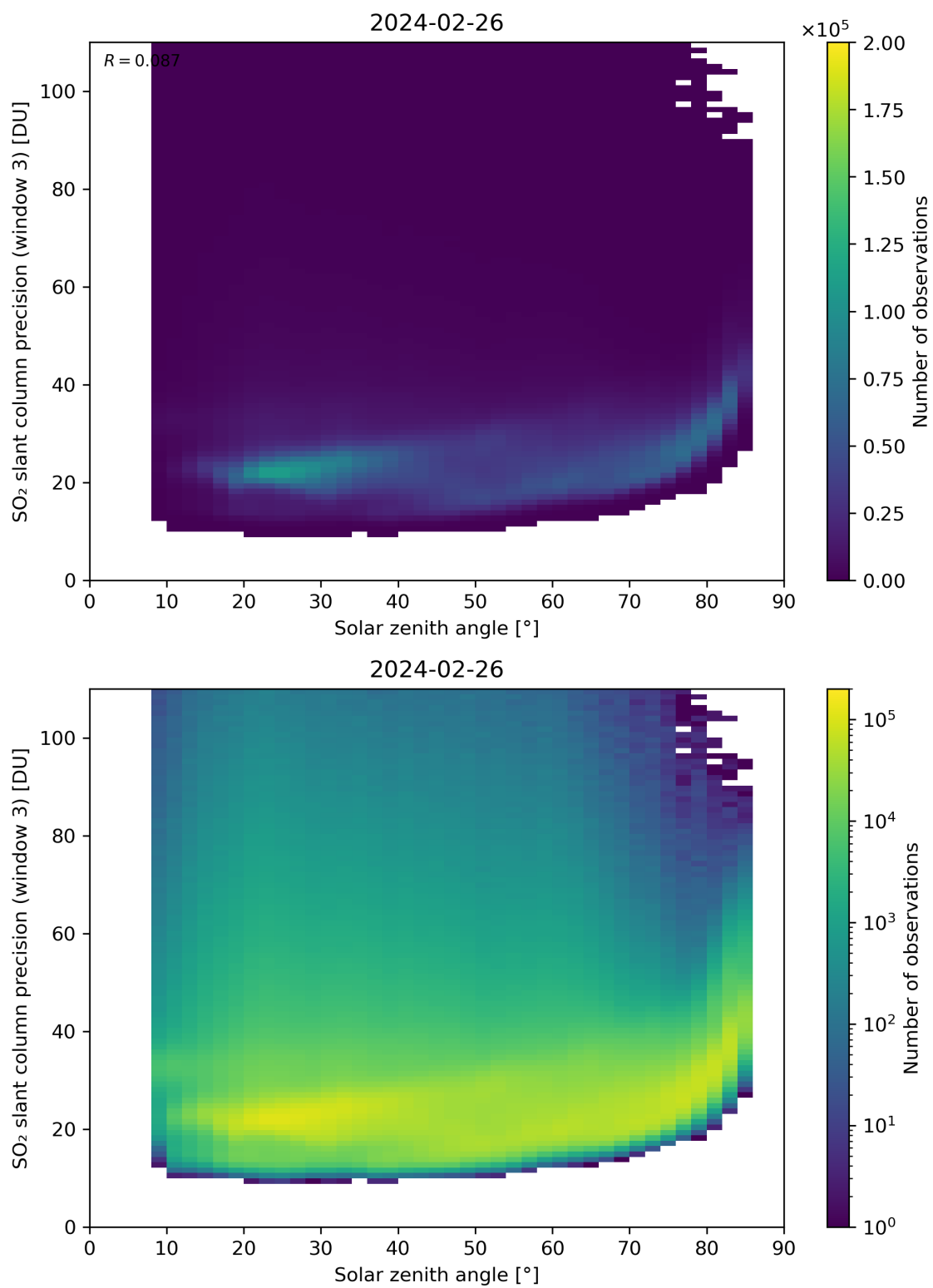
Figure 173: Scatter density plot of “Solar zenith angle” against “SO 2 slant column precision (window 3)” for 2024-02-25 to 2024-02-27.
