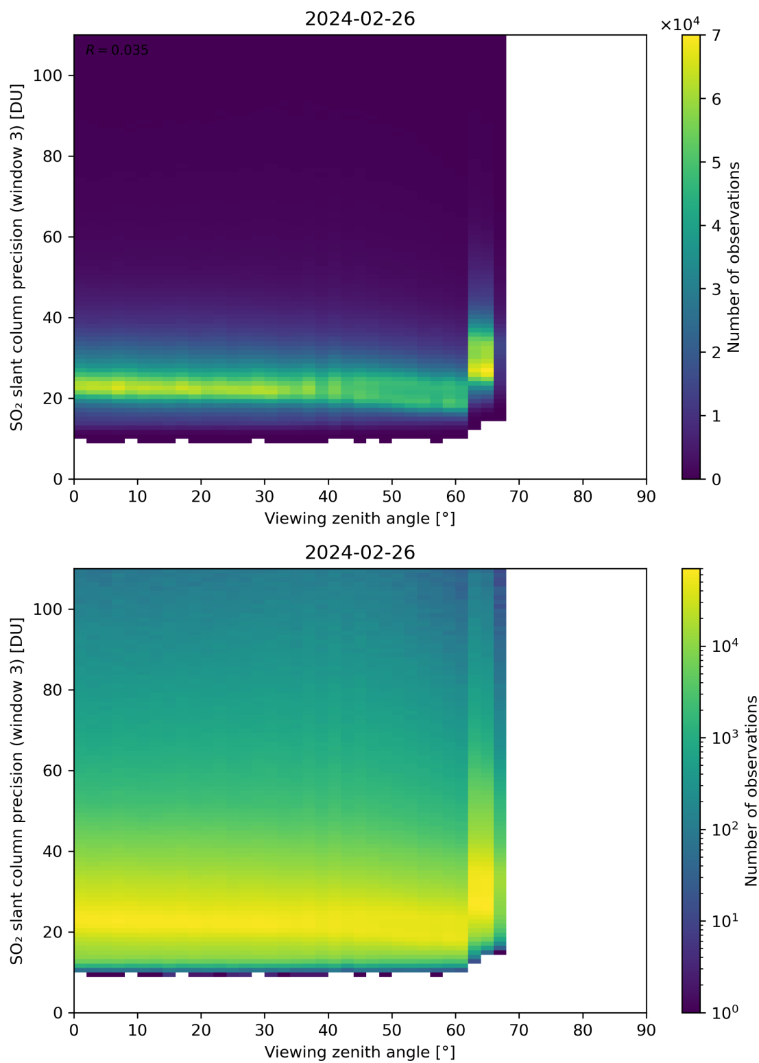
Figure 324: Scatter density plot of “Viewing zenith angle” against “SO 2 slant column precision (window 3)” for 2024-02-25 to 2024-02-27.
