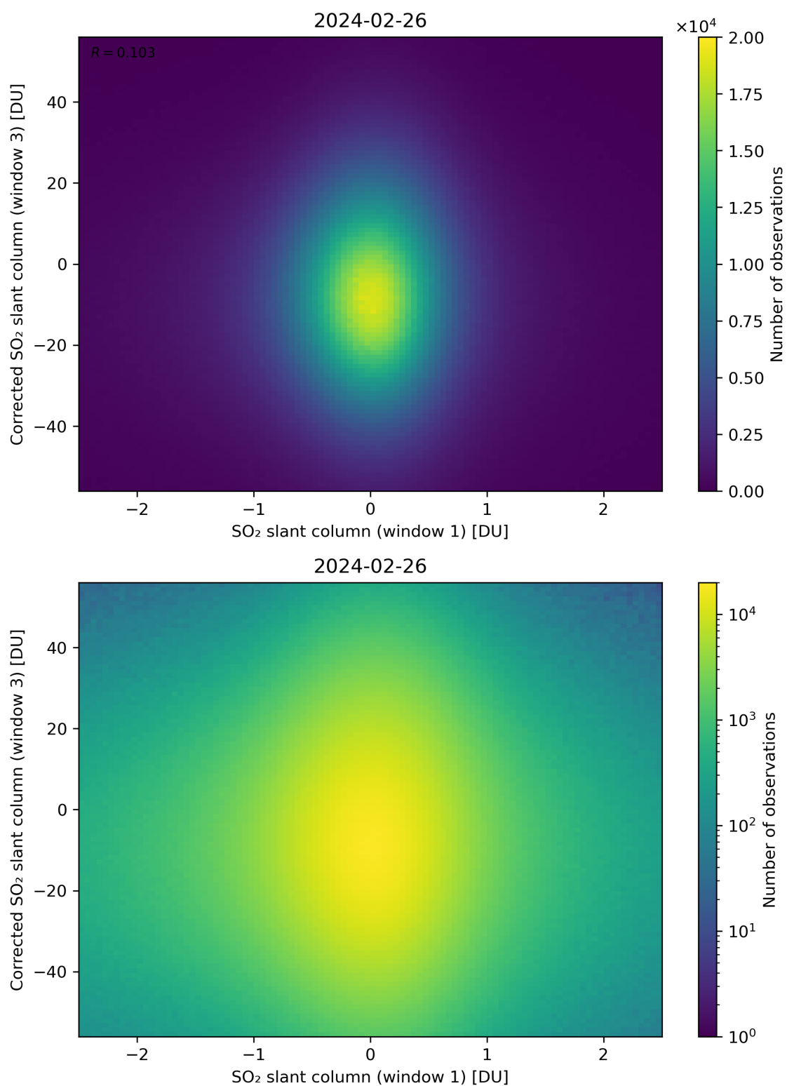
Figure 234: Scatter density plot of “SO 2 slant column (window 1)” against “Corrected SO 2 slant column (window 3)” for 2024-02-25 to 2024-02-27.
