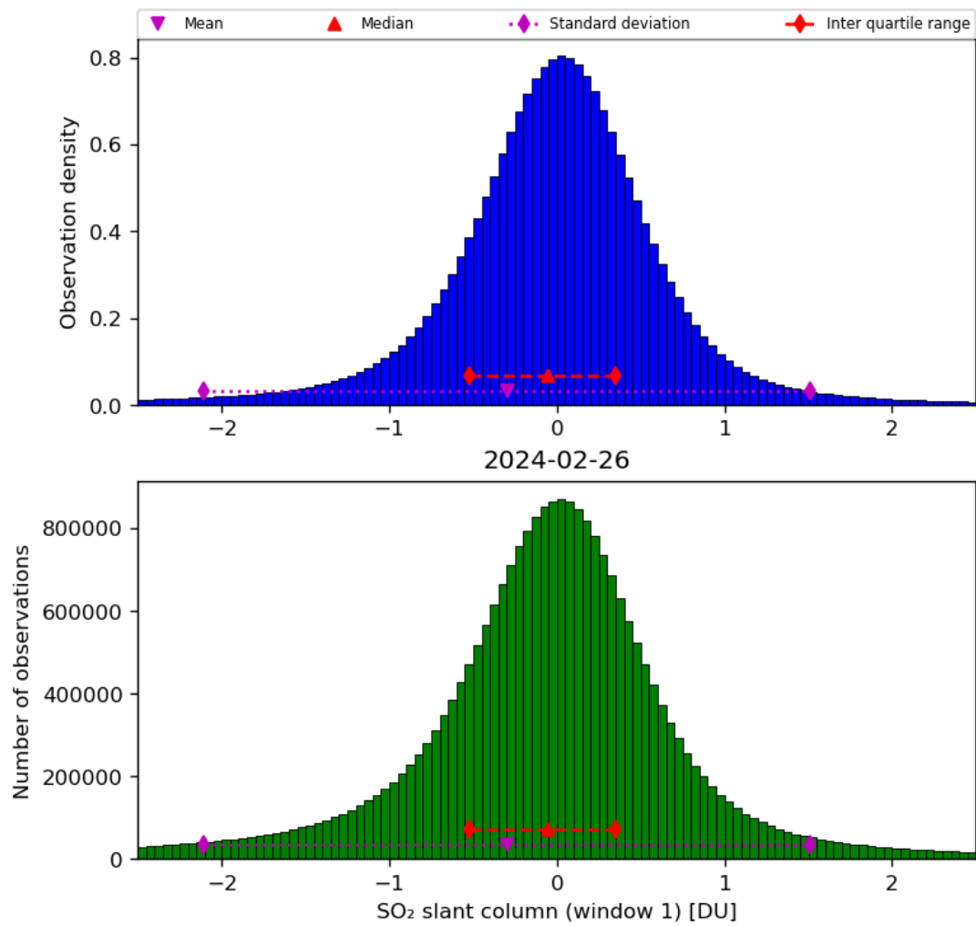
Figure 56: Histogram of “SO 2 slant column (window 1)” for 2024-02-25 to 2024-02-27
