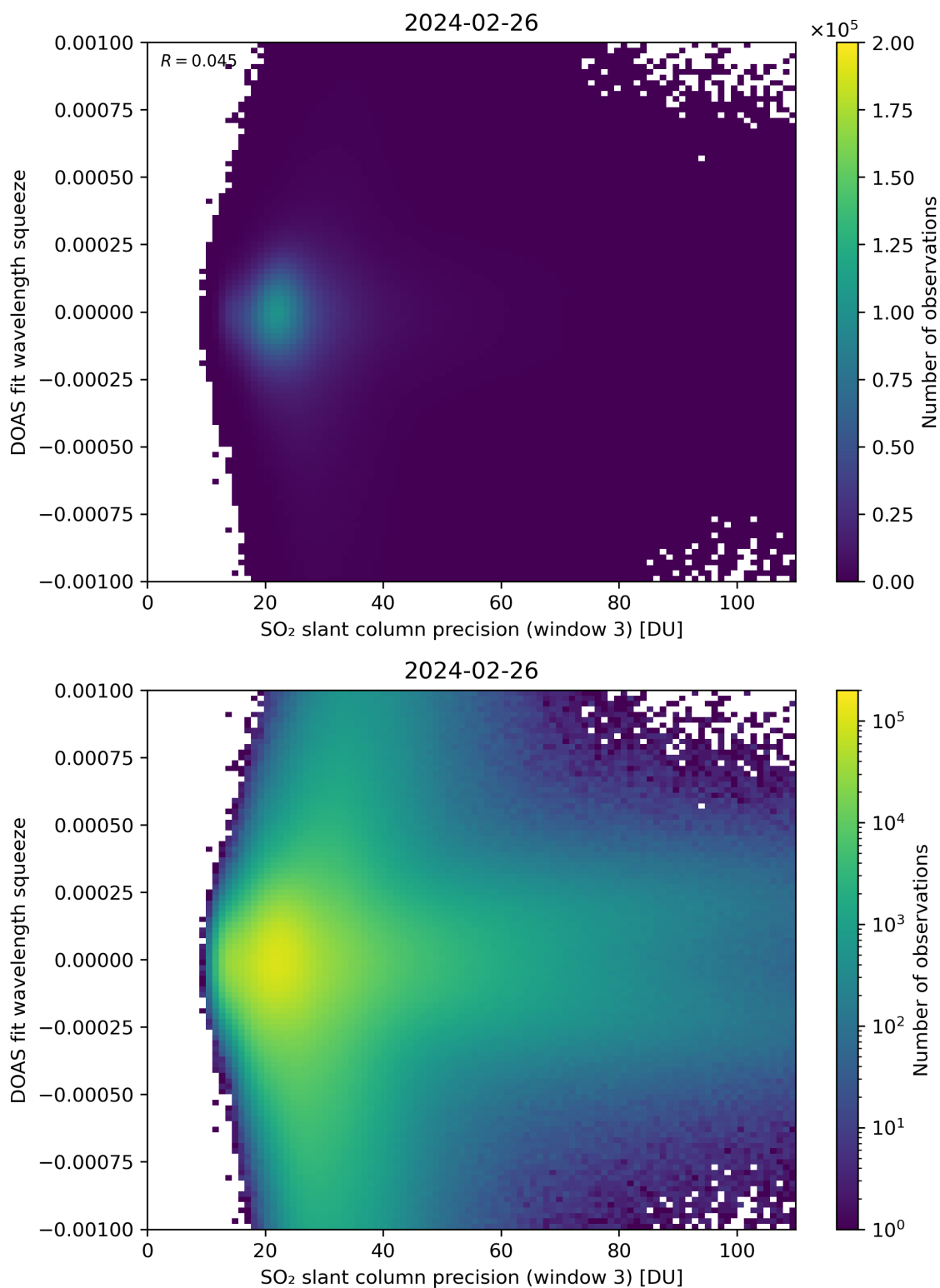
Figure 259: Scatter density plot of “SO 2 slant column precision (window 3)” against “DOAS fit wavelength squeeze” for 2024-02-25 to 2024-02-27.
