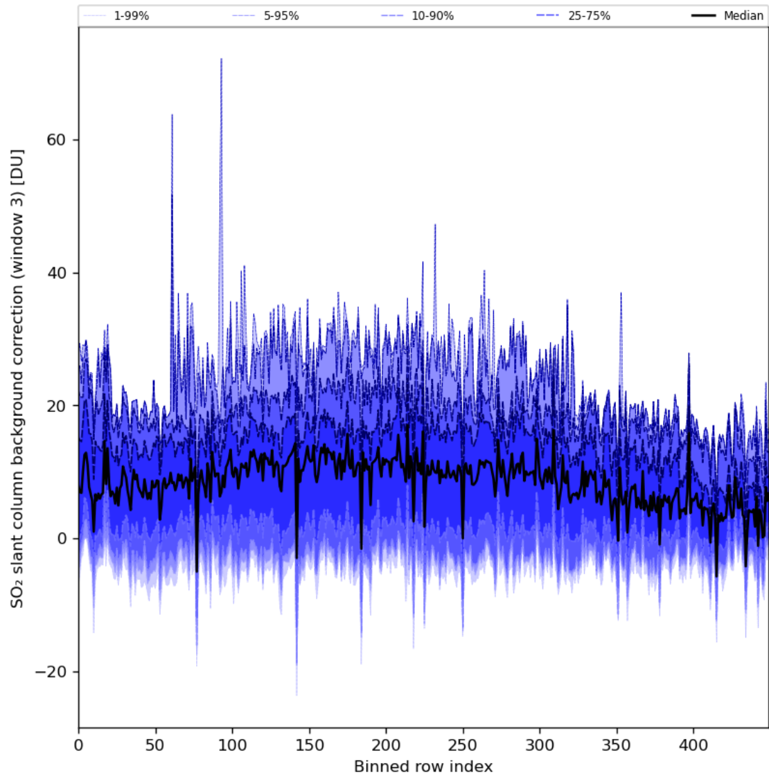
Figure 90: Along track statistics of “SO 2 slant column background correction (window 3)” for 2024-02-25 to 2024-02-27
