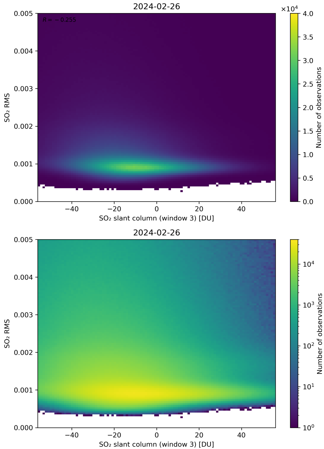
Figure 256: Scatter density plot of “SO 2 slant column (window 3)” against “SO 2 RMS” for 2024-02-25 to 2024-02-27.
