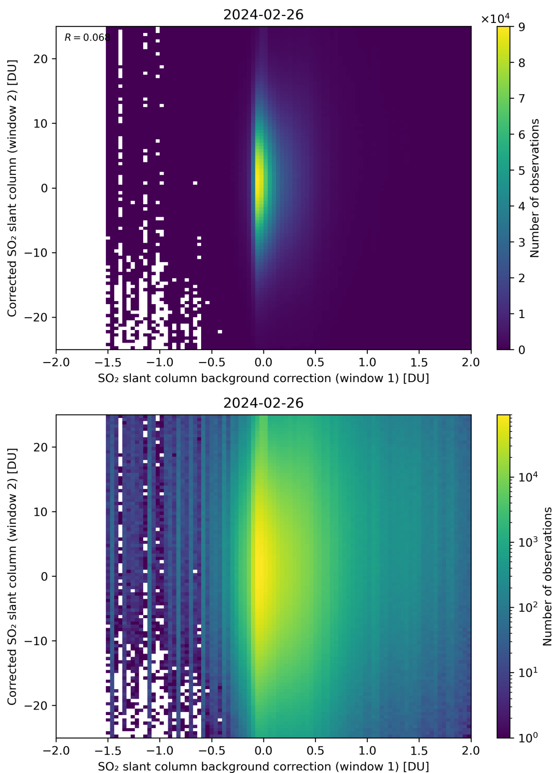
Figure 104: Scatter density plot of “SO 2 slant column background correction (window 1)” against “Corrected SO 2 slant column (window 2)” for 2024-02-25 to 2024-02-27.
