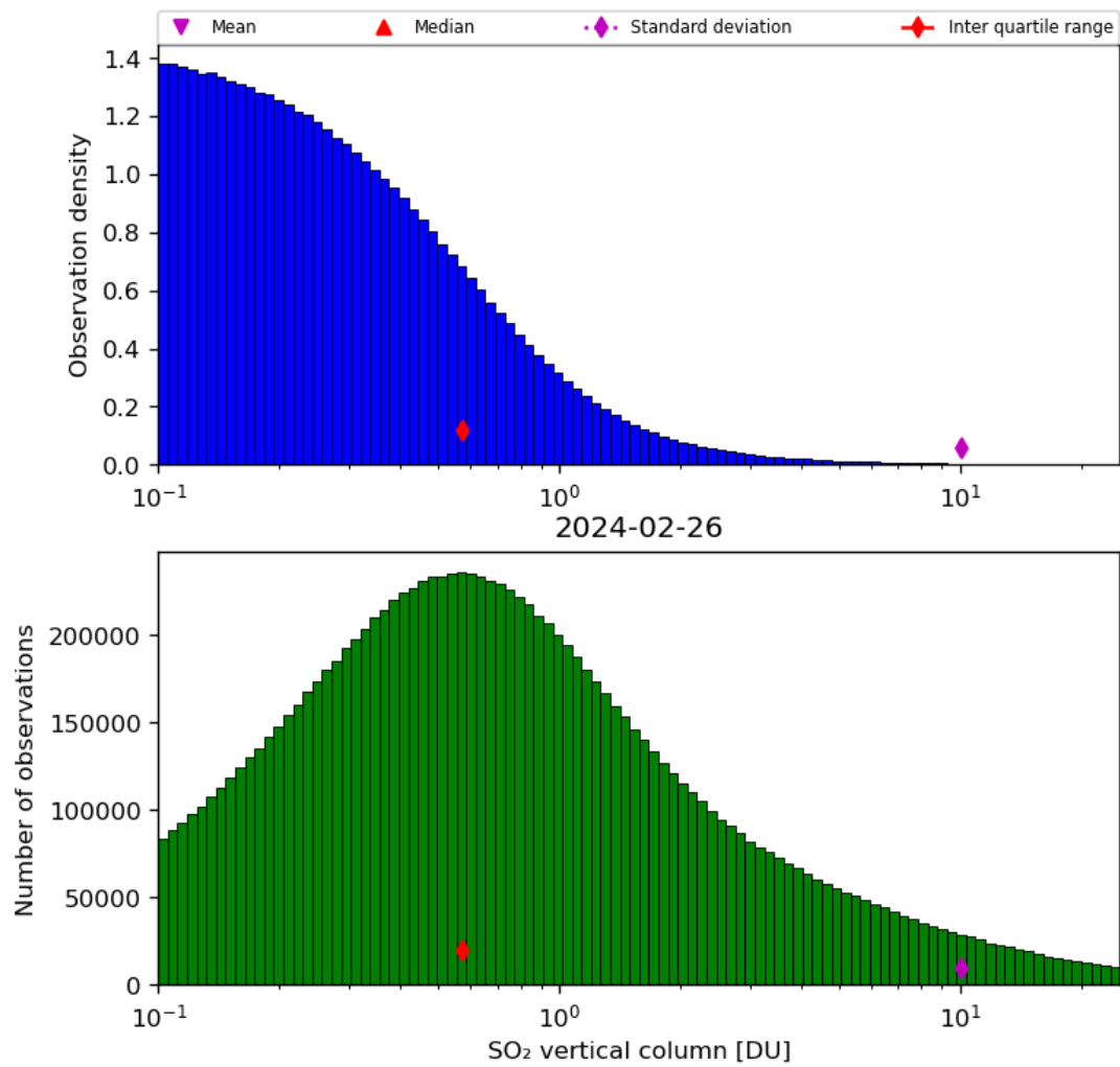
Figure 53: Histogram of “SO 2 vertical column” for 2024-02-25 to 2024-02-27
