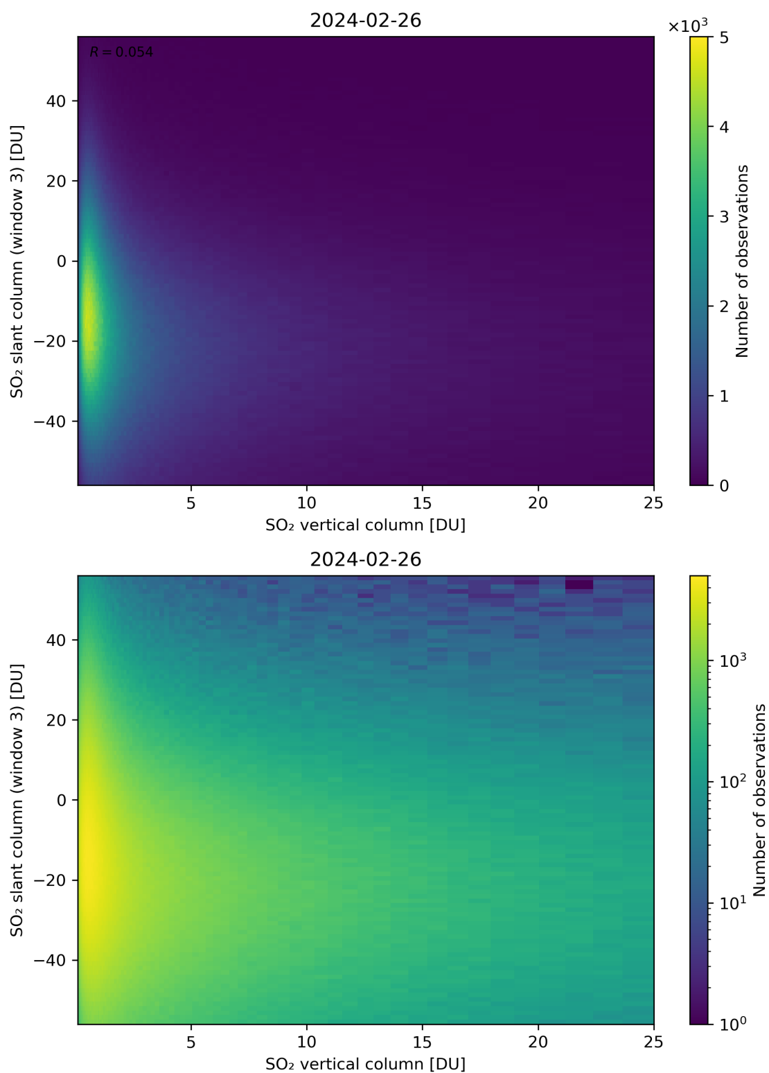
Figure 303: Scatter density plot of “SO 2 vertical column” against “SO 2 slant column (window 3)” for 2024-02-25 to 2024-02-27.
