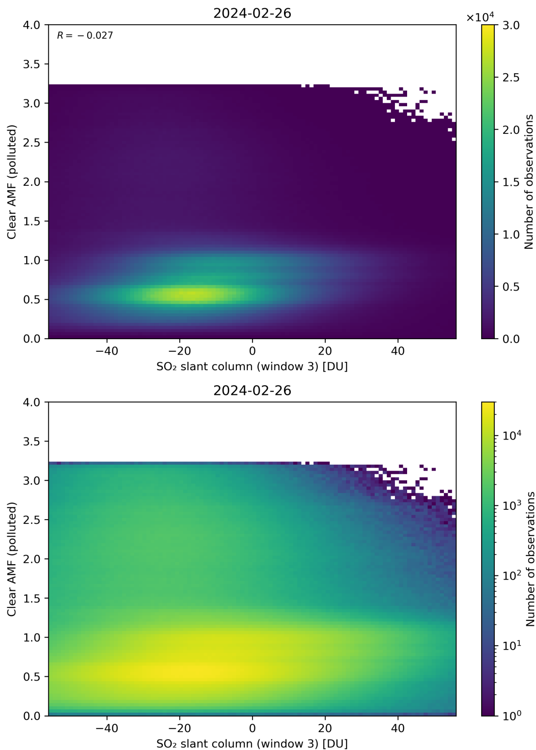
Figure 265: Scatter density plot of “SO 2 slant column (window 3)” against “Clear AMF (polluted)” for 2024-02-25 to 2024-02-27.
