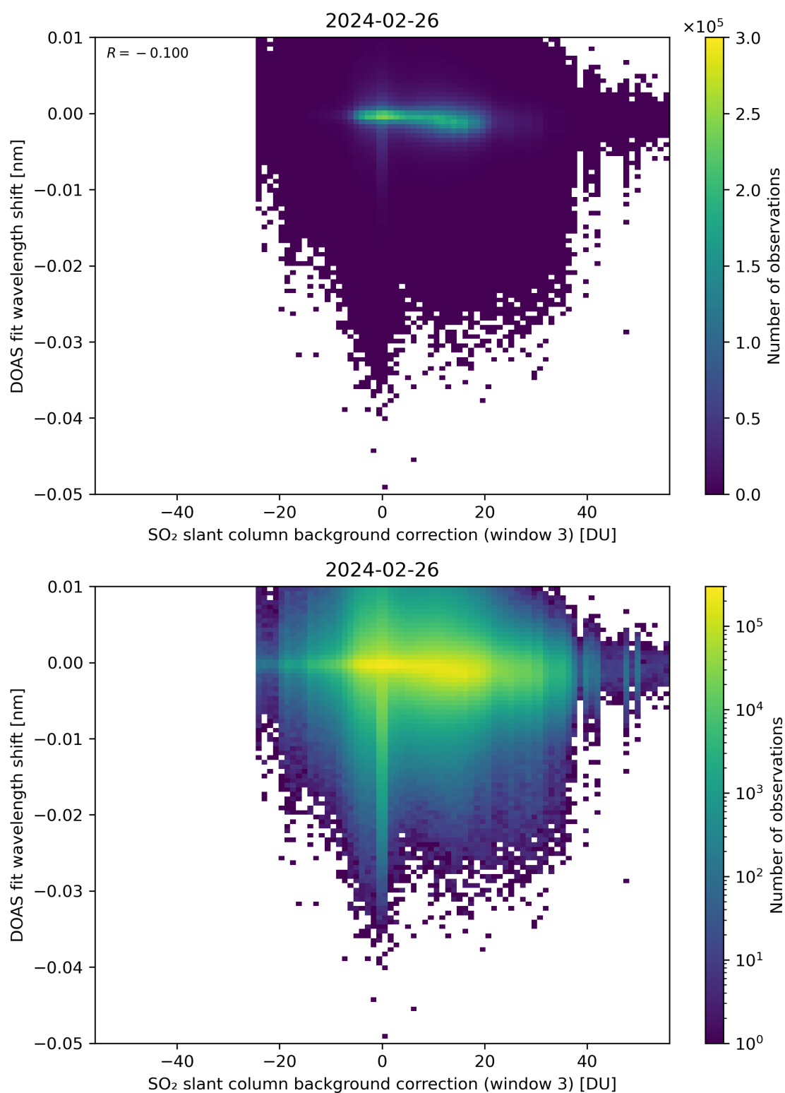
Figure 121: Scatter density plot of “SO 2 slant column background correction (window 3)” against “DOAS fit wavelength shift” for 2024-02-25 to 2024-02-27.
