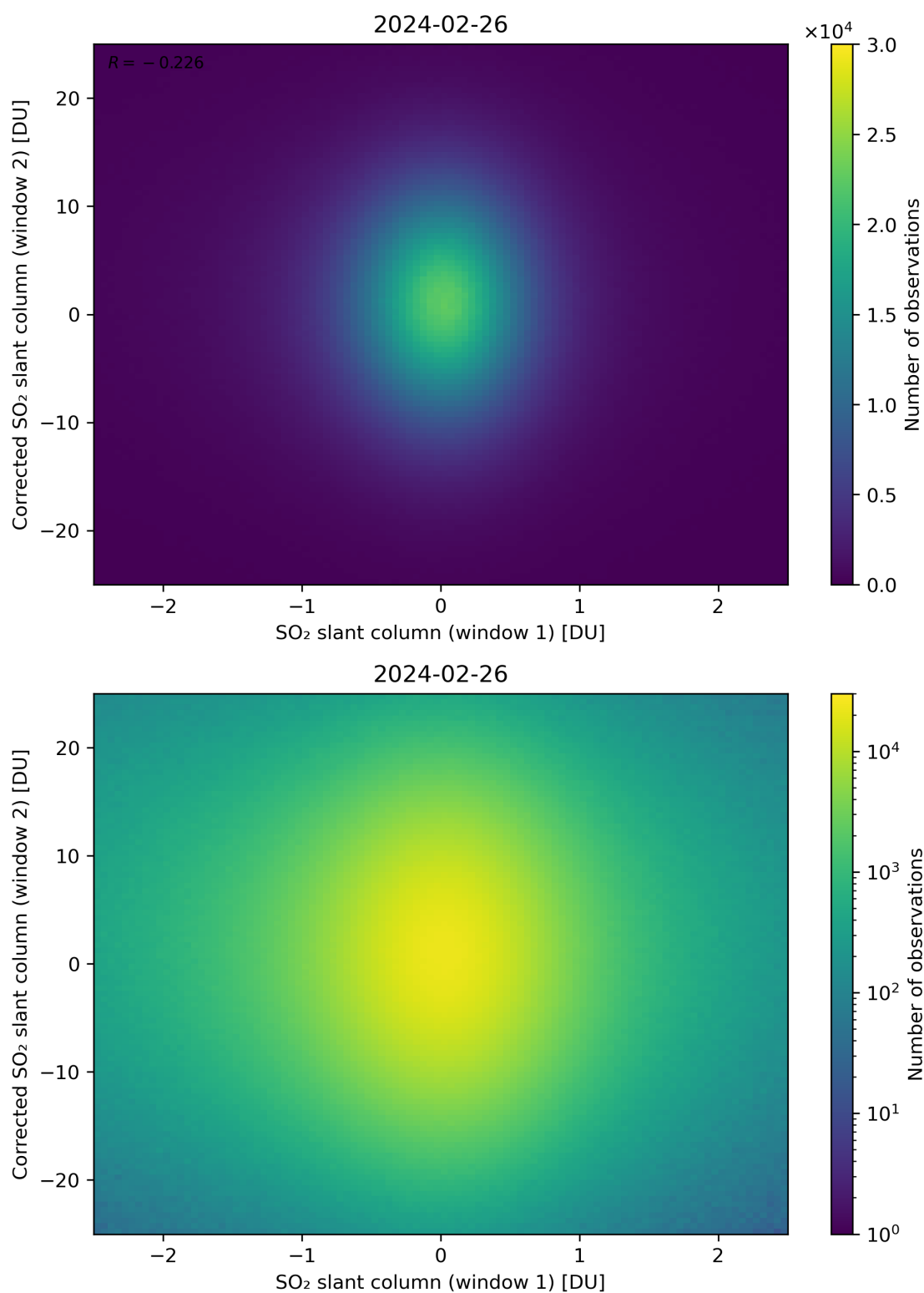
Figure 233: Scatter density plot of “SO 2 slant column (window 1)” against “Corrected SO 2 slant column (window 2)” for 2024-02-25 to 2024-02-27.
