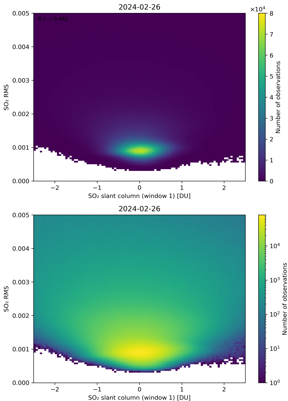
Figure 217: Scatter density plot of “SO 2 slant column (window 1)” against “SO 2 RMS” for 2024-02-25 to 2024-02-27.
