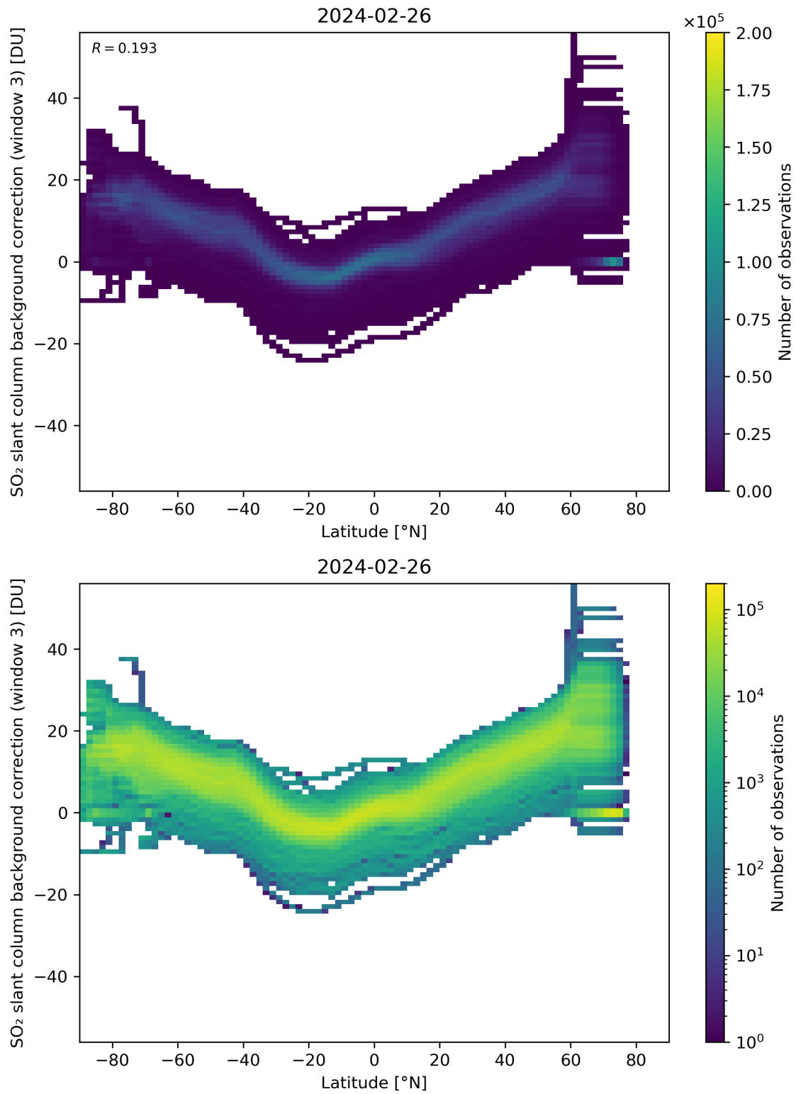
Figure 141: Scatter density plot of “Latitude” against “SO 2 slant column background correction (window 3)” for 2024-02-25 to 2024-02-27.
