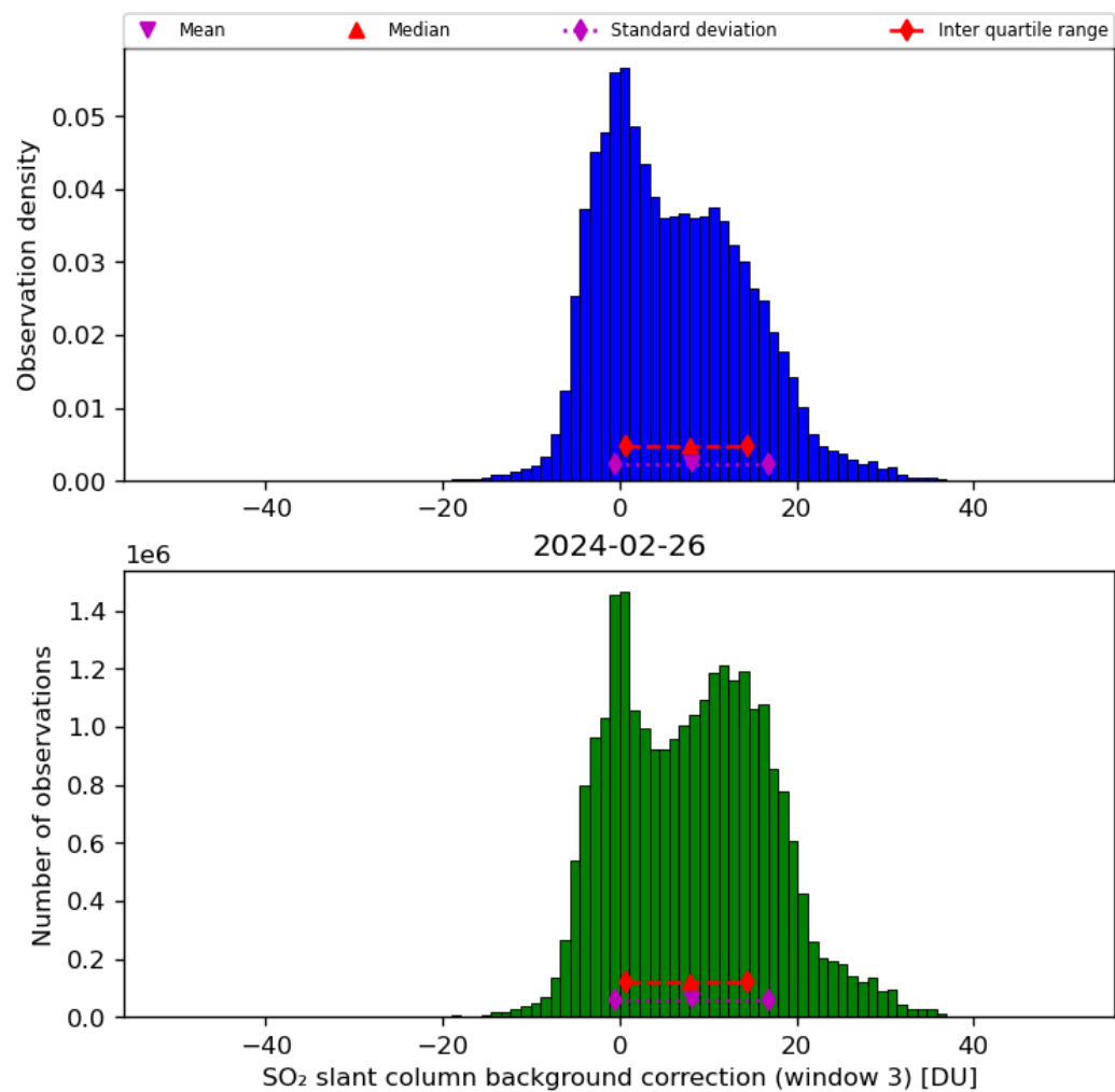
Figure 67: Histogram of “SO 2 slant column background correction (window 3)” for 2024-02-25 to 2024-02-27
