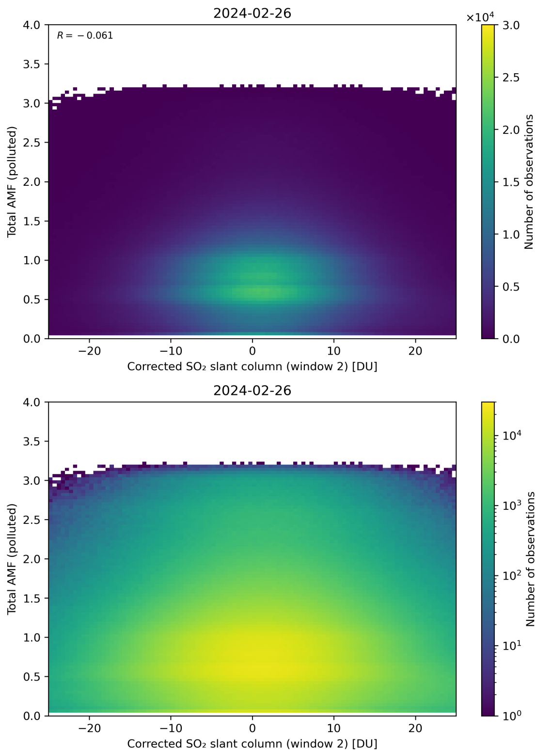
Figure 203: Scatter density plot of “Corrected SO 2 slant column (window 2)” against “Total AMF (polluted)” for 2024-02-25 to 2024-02-27.
