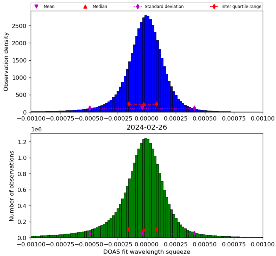
Figure 69: Histogram of “DOAS fit wavelength squeeze” for 2024-02-25 to 2024-02-27
