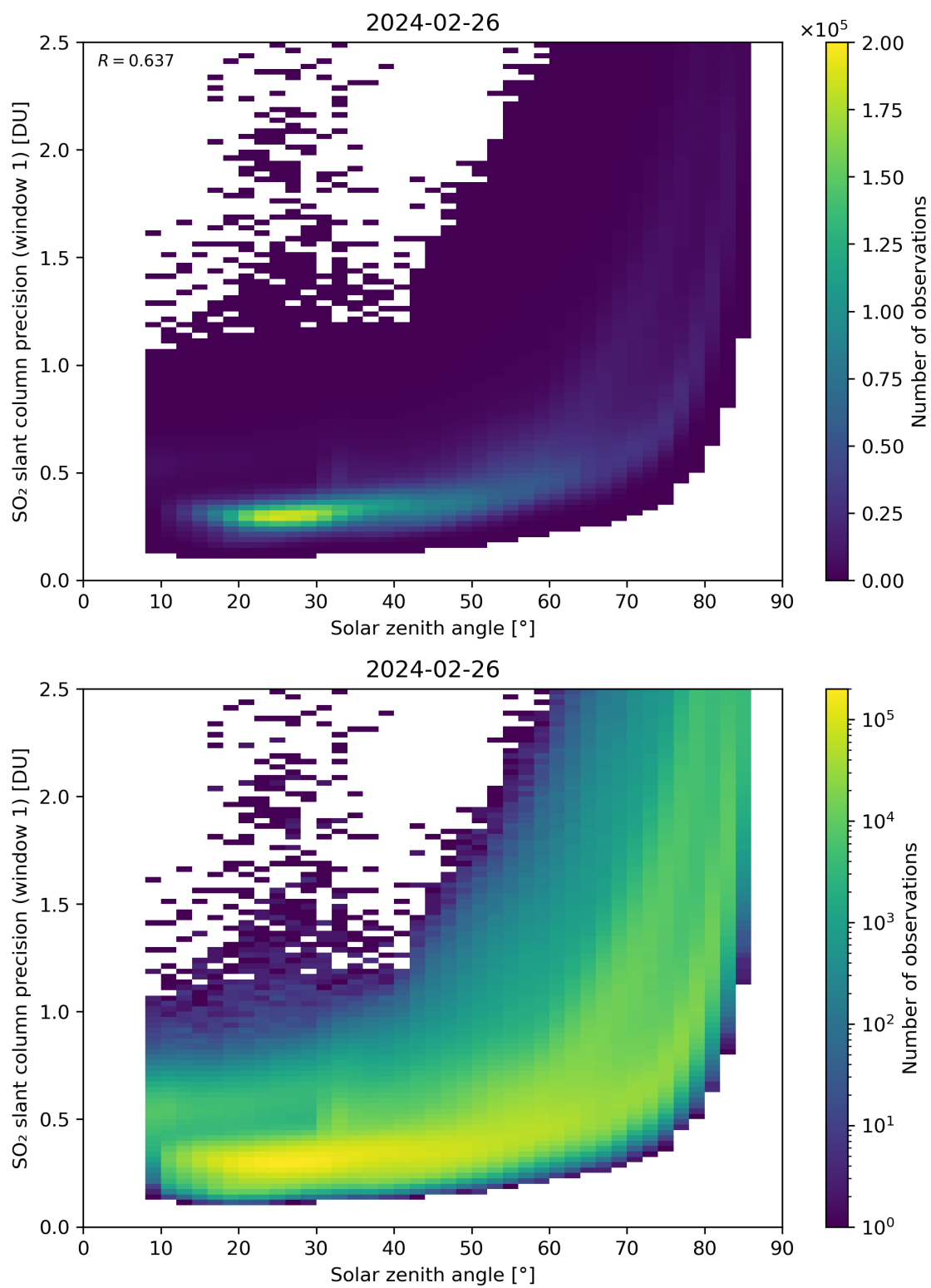
Figure 170: Scatter density plot of “Solar zenith angle” against “SO 2 slant column precision (window 1)” for 2024-02-25 to 2024-02-27.
