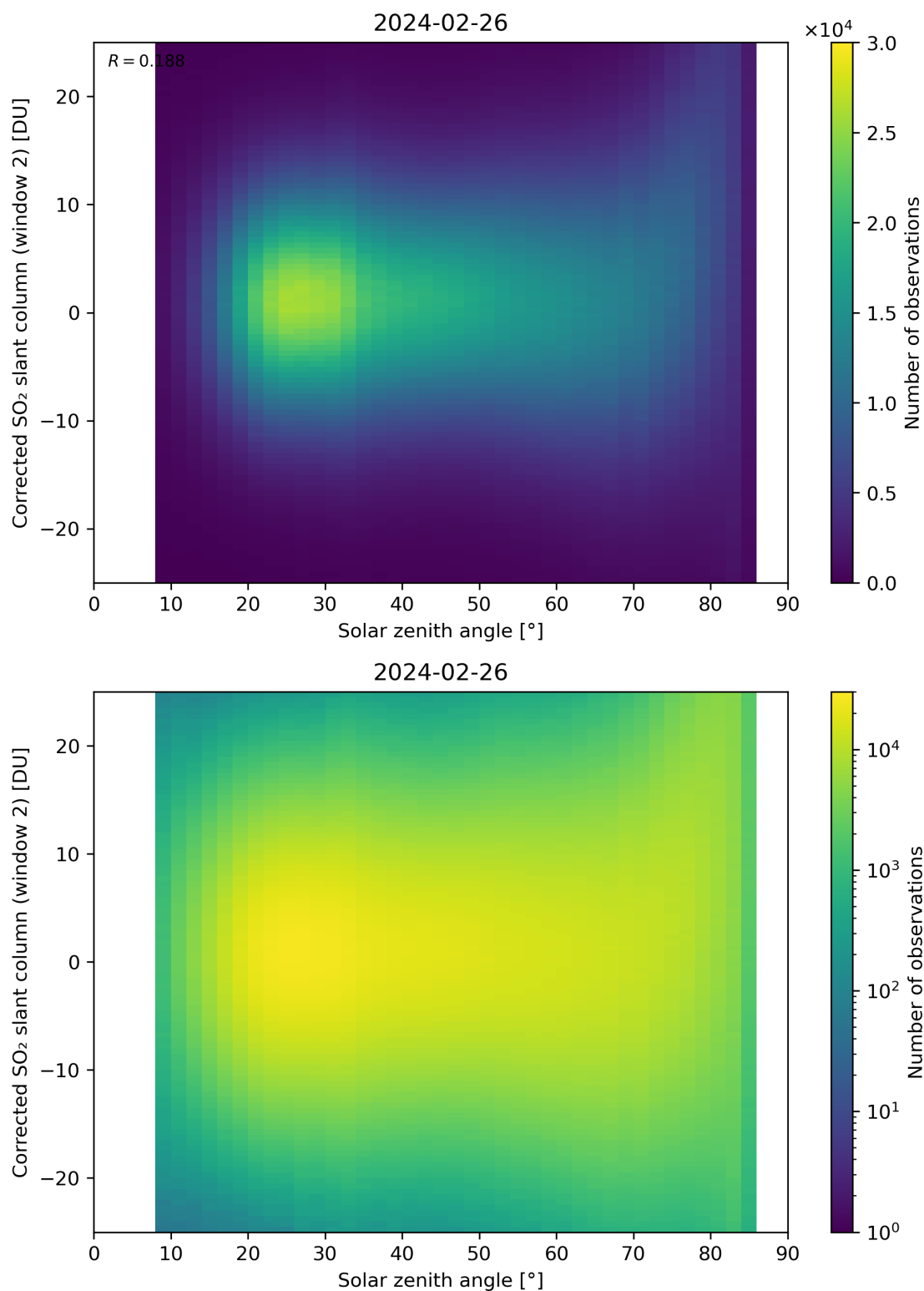
Figure 167: Scatter density plot of “Solar zenith angle” against “Corrected SO 2 slant column (window 2)” for 2024-02-25 to 2024-02-27.
