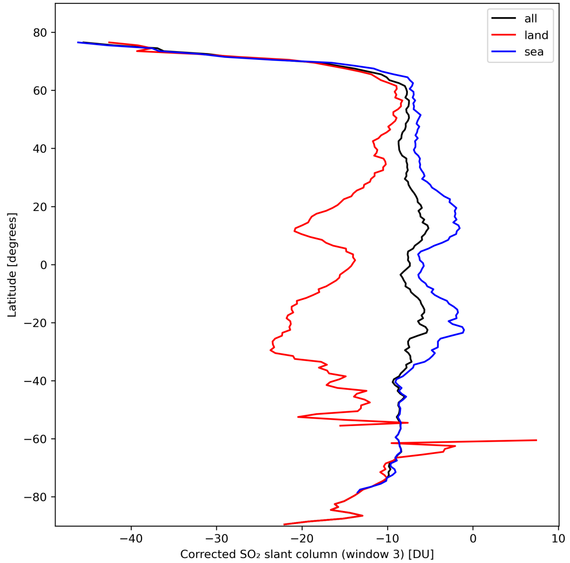
Figure 43: Zonal average of “Corrected SO 2 slant column (window 3)” for 2024-02-25 to 2024-02-27.
