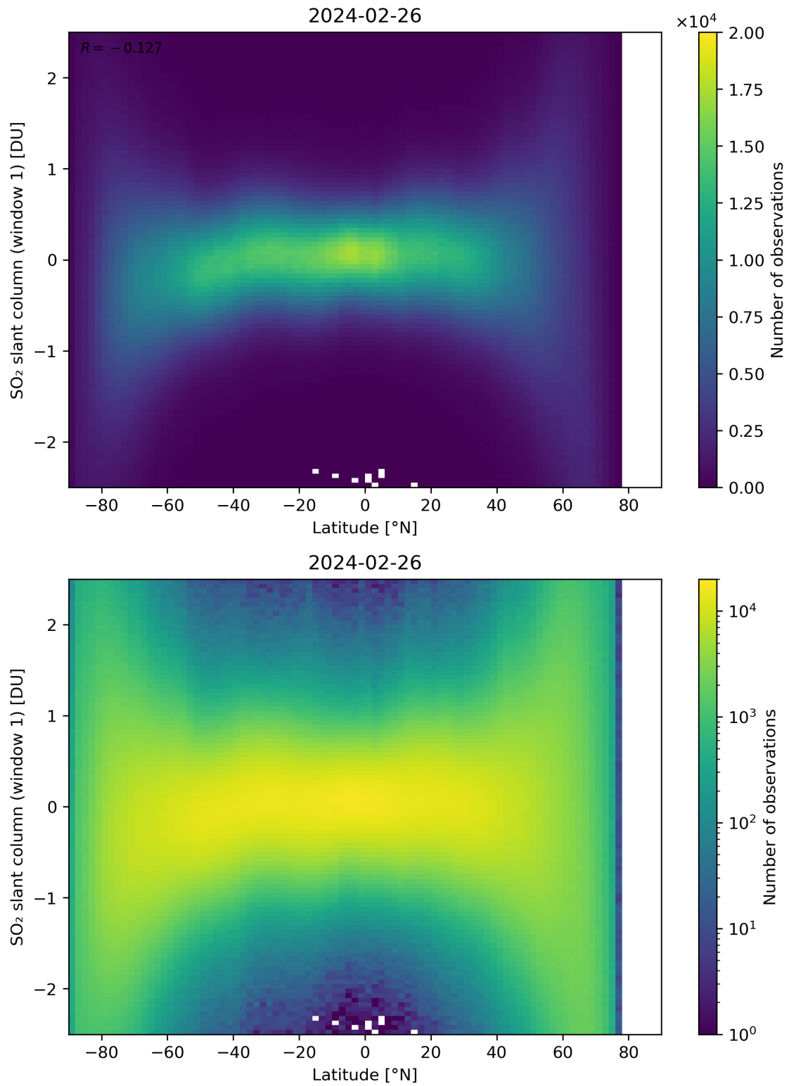
Figure 149: Scatter density plot of “Latitude” against “SO 2 slant column (window 1)” for 2024-02-25 to 2024-02-27.
