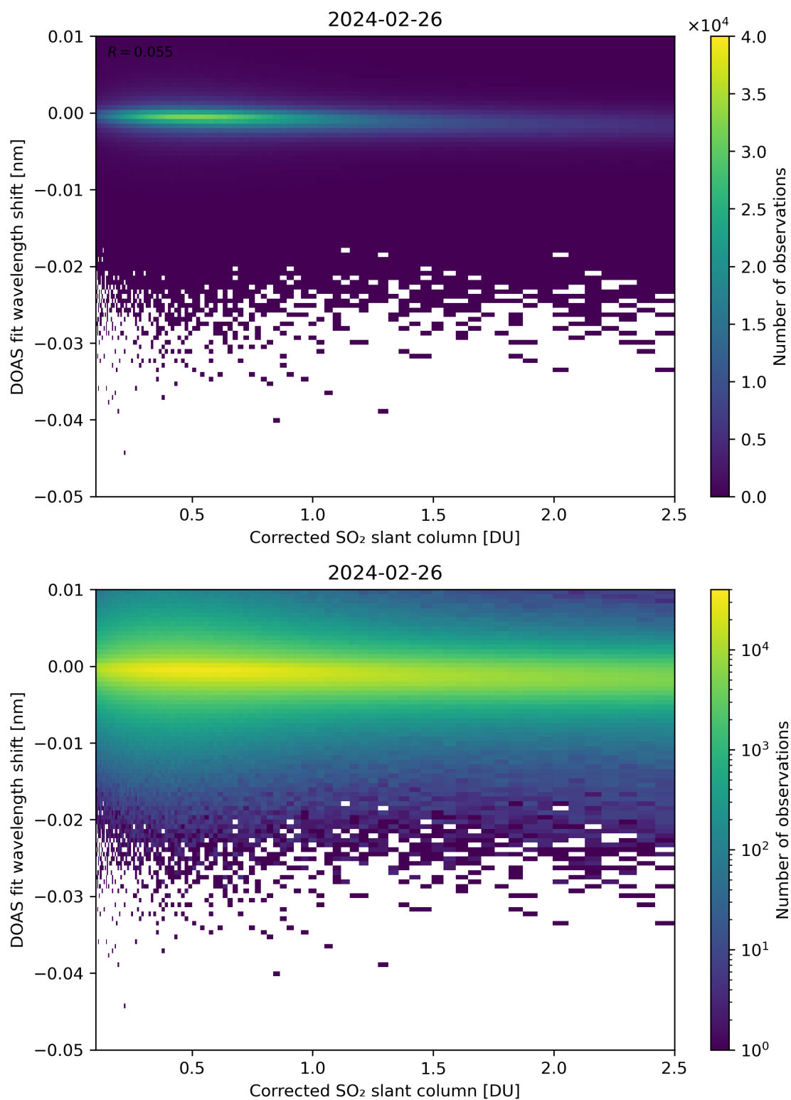
Figure 181: Scatter density plot of “Corrected SO 2 slant column” against “DOAS fit wavelength shift” for 2024-02-25 to 2024-02-27.
