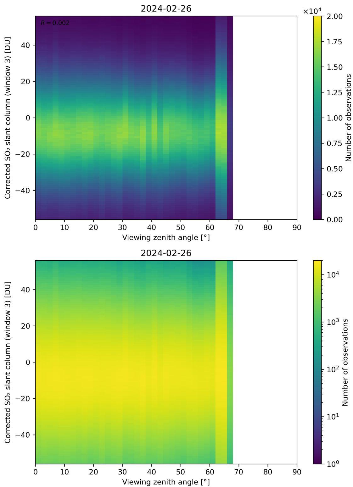
Figure 319: Scatter density plot of “Viewing zenith angle” against “Corrected SO 2 slant column (window 3)” for 2024-02-25 to 2024-02-27.
