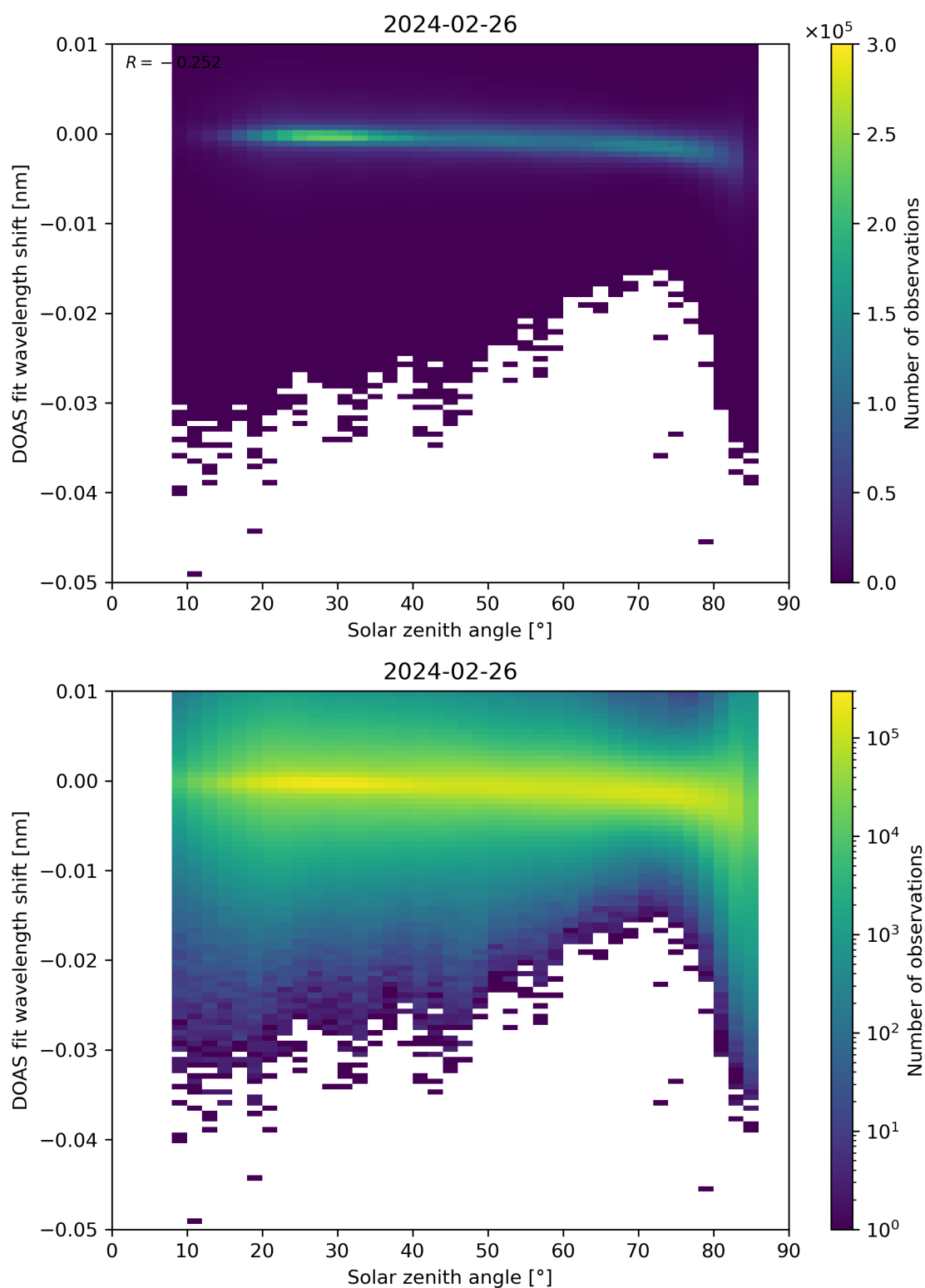
Figure 161: Scatter density plot of “Solar zenith angle” against “DOAS fit wavelength shift” for 2024-02-25 to 2024-02-27.
