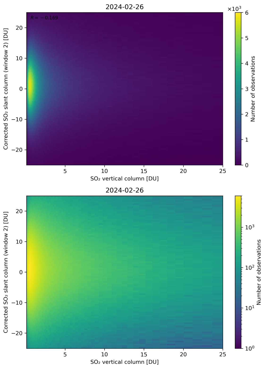
Figure 298: Scatter density plot of “SO 2 vertical column” against “Corrected SO 2 slant column (window 2)” for 2024-02-25 to 2024-02-27.
