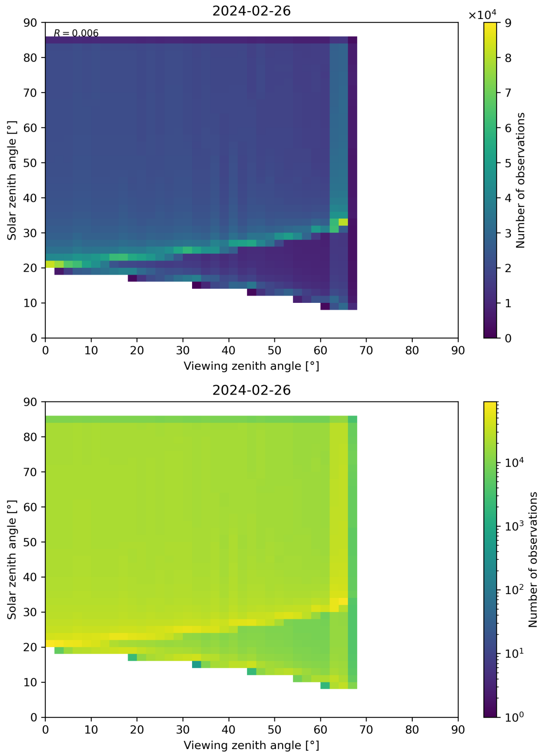
Figure 315: Scatter density plot of “Viewing zenith angle” against “Solar zenith angle” for 2024-02-25 to 2024-02-27.
