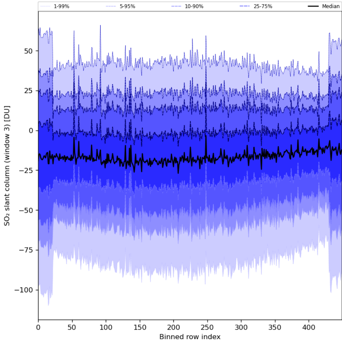
Figure 87: Along track statistics of “SO 2 slant column (window 3)” for 2024-02-25 to 2024-02-27
