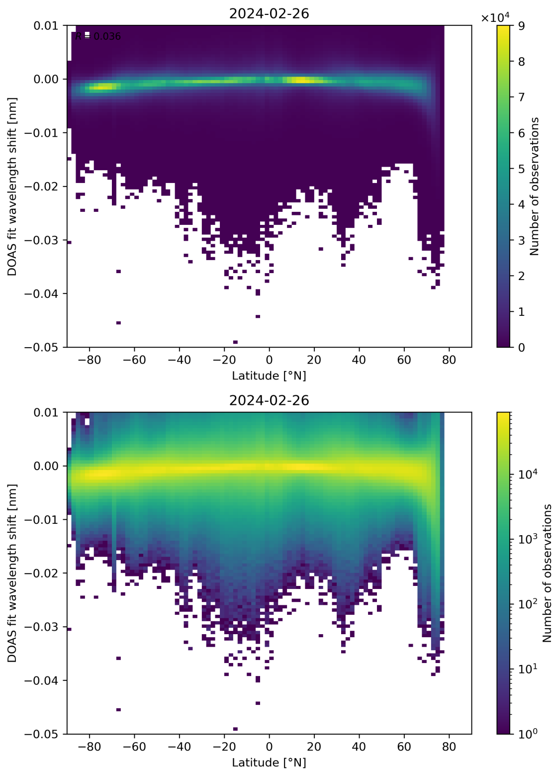
Figure 142: Scatter density plot of “Latitude” against “DOAS fit wavelength shift” for 2024-02-25 to 2024-02-27.
