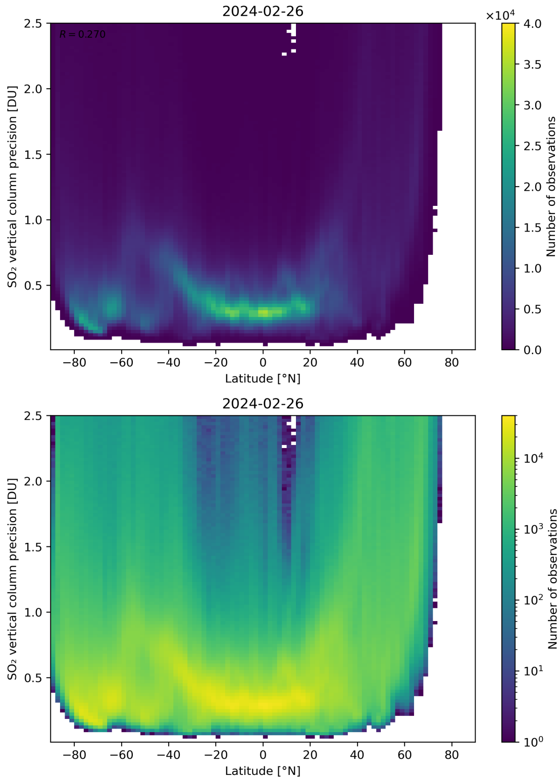
Figure 157: Scatter density plot of “Latitude” against “SO 2 vertical column precision” for 2024-02-25 to 2024-02-27.
