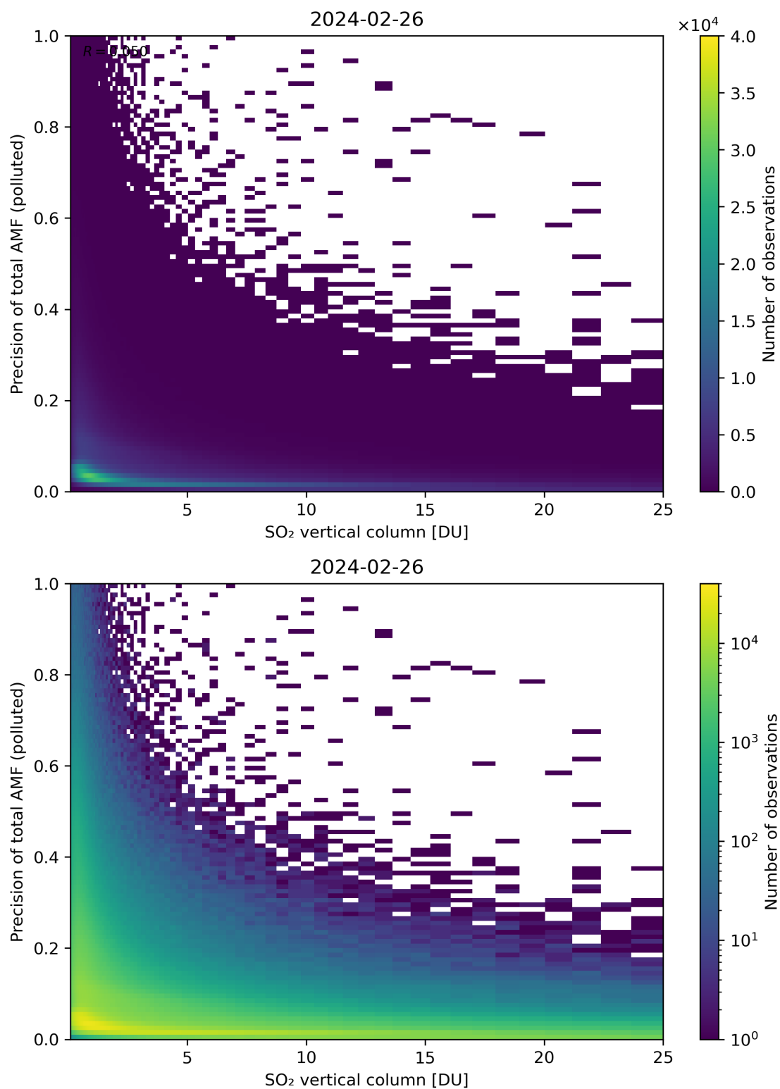
Figure 306: Scatter density plot of “SO 2 vertical column” against “Precision of total AMF (polluted)” for 2024-02-25 to 2024-02-27.
