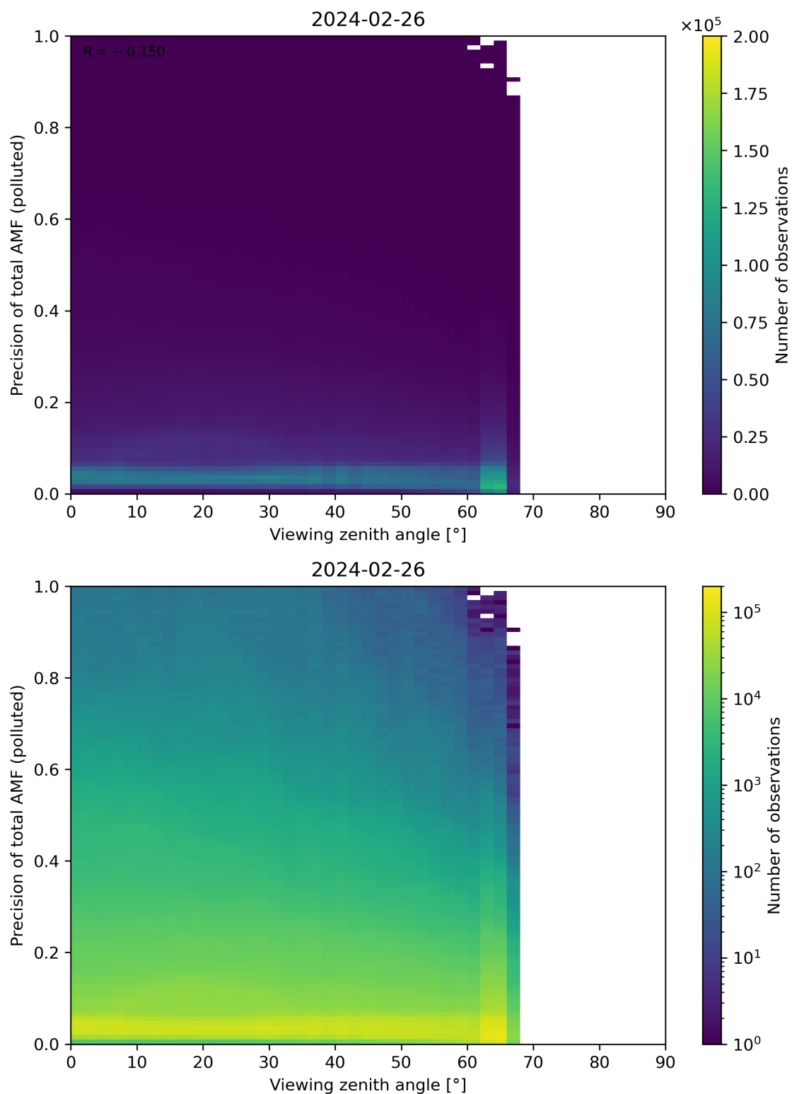
Figure 326: Scatter density plot of “Viewing zenith angle” against “Precision of total AMF (polluted)” for 2024-02-25 to 2024-02-27.
