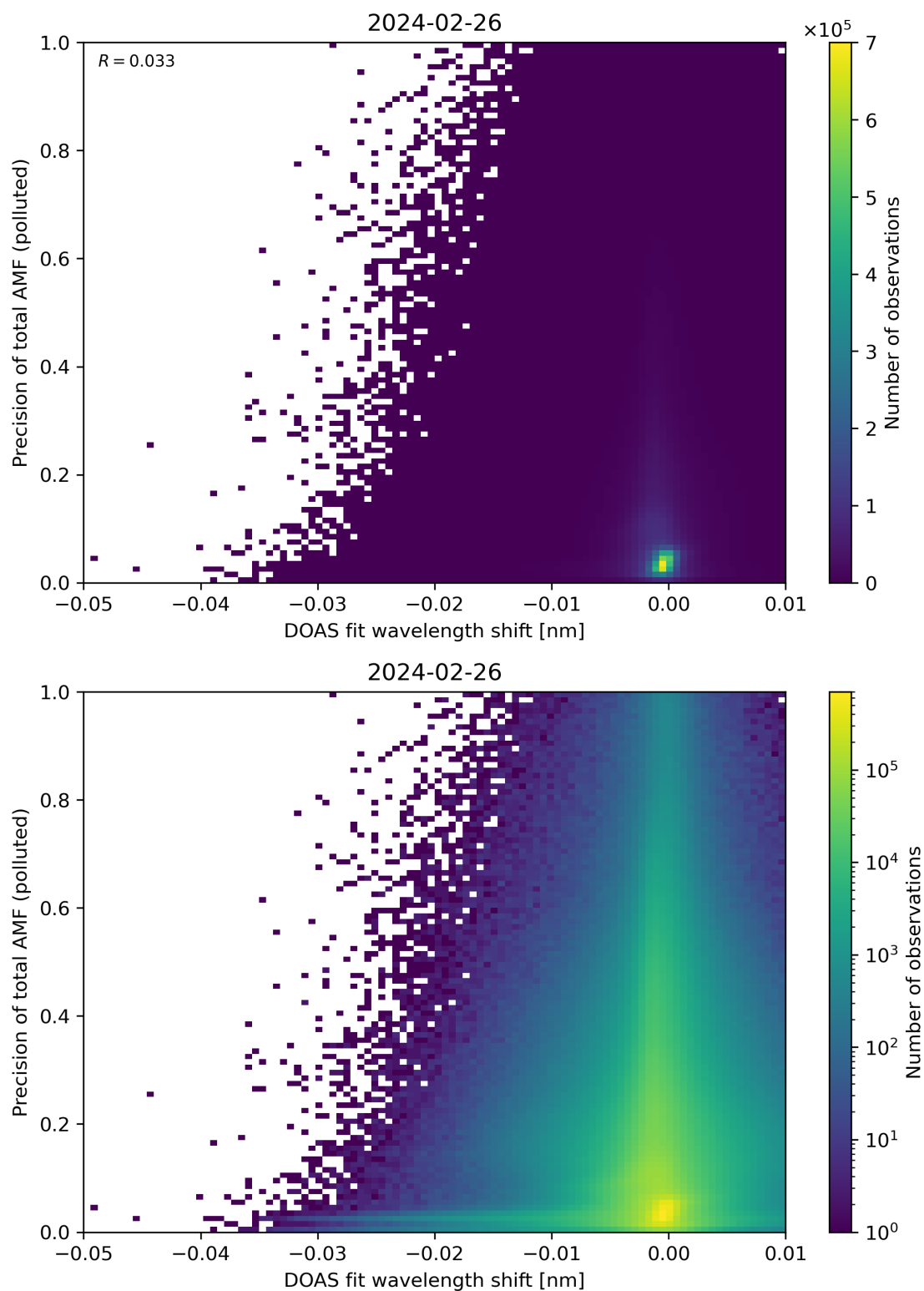
Figure 131: Scatter density plot of “DOAS fit wavelength shift” against “Precision of total AMF (polluted)” for 2024-02-25 to 2024-02-27.
