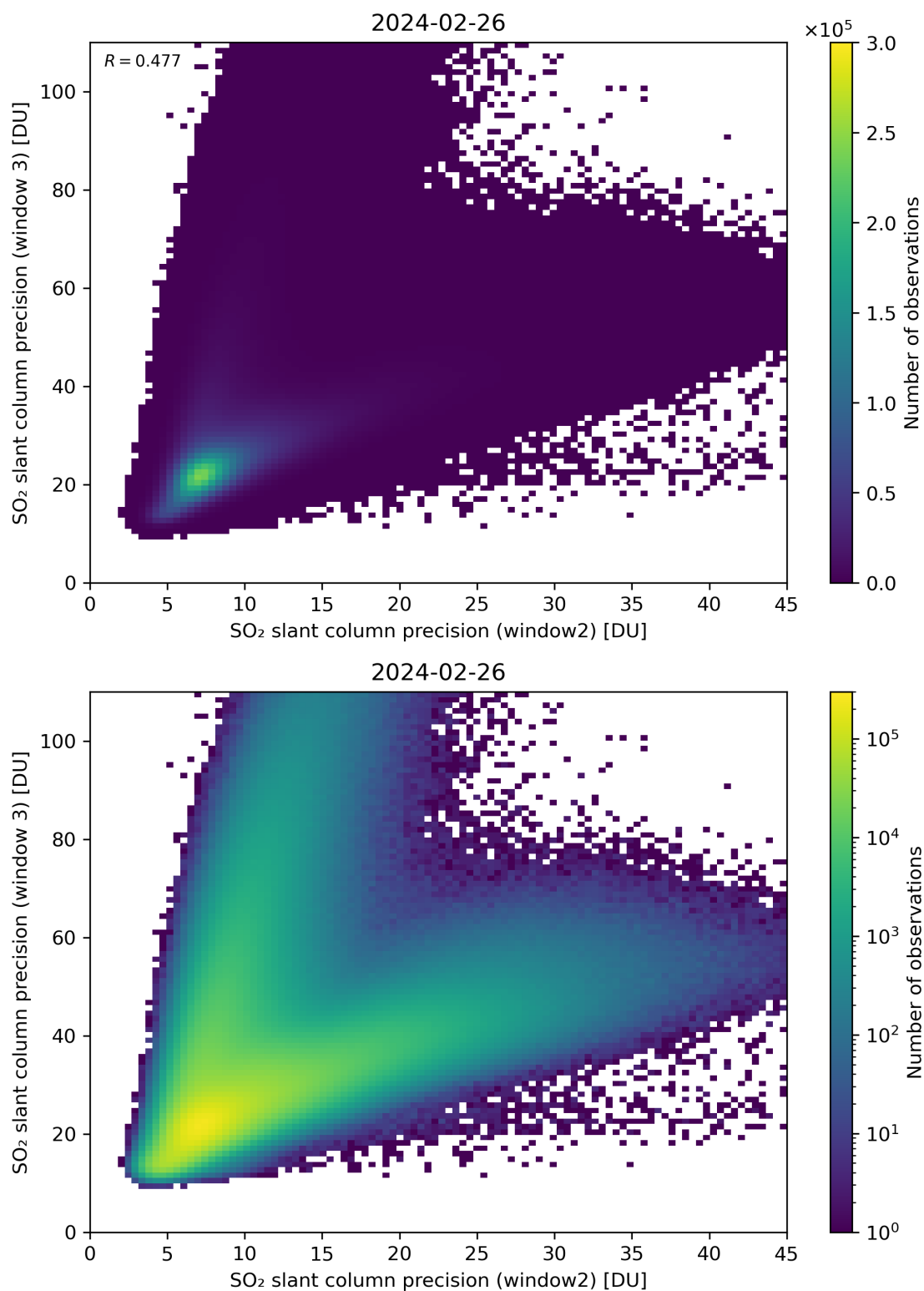
Figure 250: Scatter density plot of “SO 2 slant column precision (window2)” against “SO 2 slant column precision (window 3)” for 2024-02-25 to 2024-02-27.
