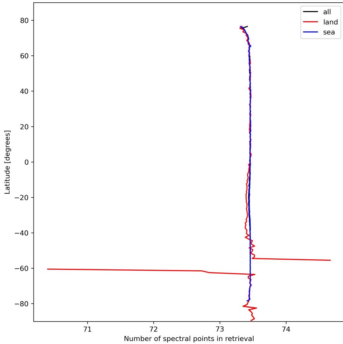
Figure 51: Zonal average of “Number of spectral points in retrieval” for 2024-02-25 to 2024-02-27.
