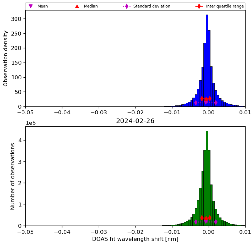
Figure 68: Histogram of “DOAS fit wavelength shift” for 2024-02-25 to 2024-02-27
