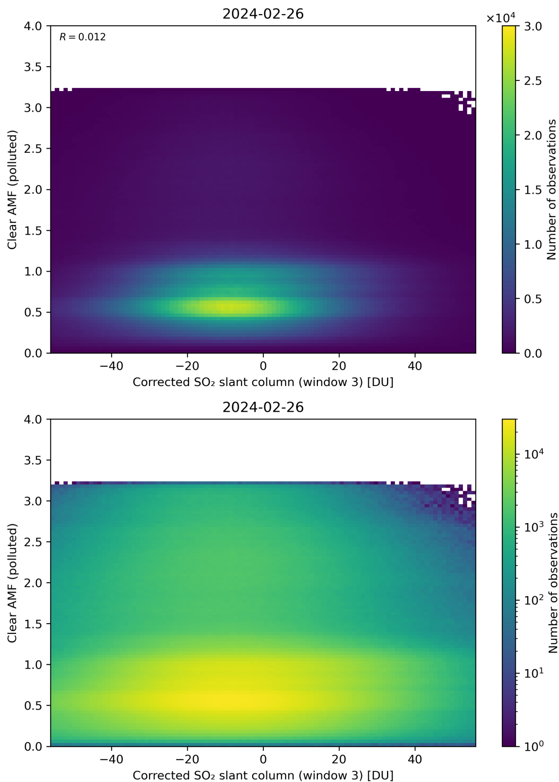
Figure 209: Scatter density plot of “Corrected SO 2 slant column (window 3)” against “Clear AMF (polluted)” for 2024-02-25 to 2024-02-27.
