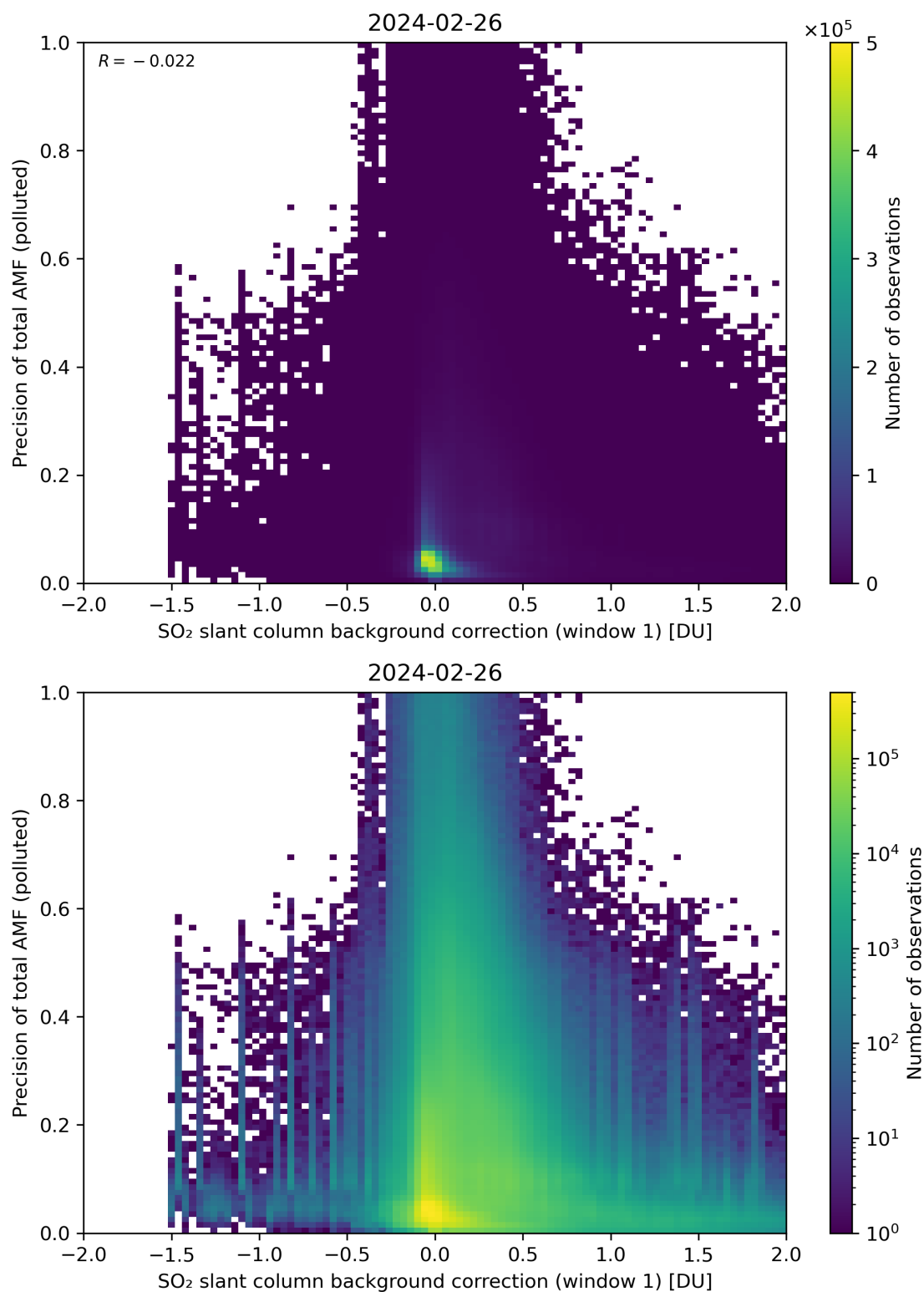
Figure 110: Scatter density plot of “SO 2 slant column background correction (window 1)” against “Precision of total AMF (polluted)” for 2024-02-25 to 2024-02-27.
