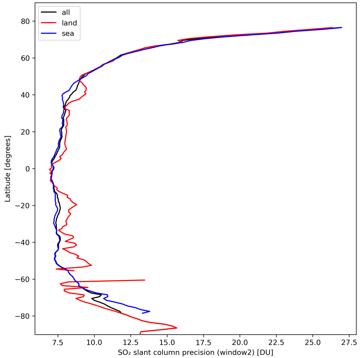
Figure 38: Zonal average of “SO 2 slant column precision (window2)” for 2024-02-25 to 2024-02-27.
