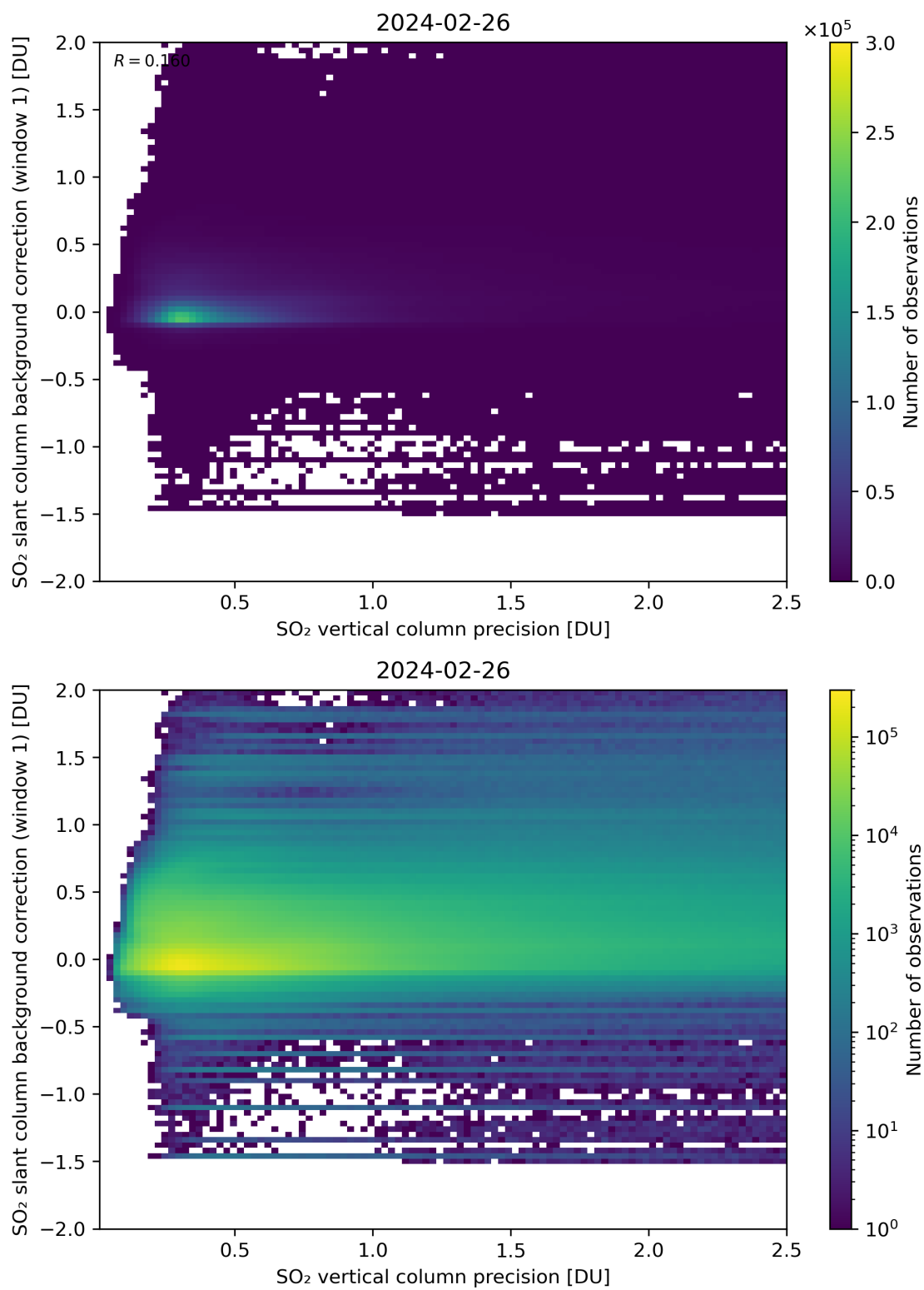
Figure 279: Scatter density plot of “SO 2 vertical column precision” against “SO 2 slant column background correction (window 1)” for 2024-02-25 to 2024-02-27.
