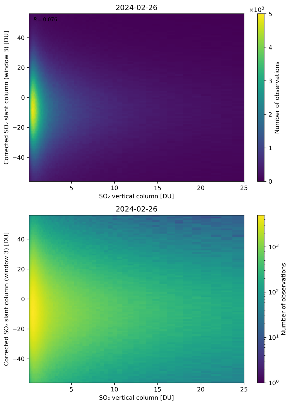
Figure 299: Scatter density plot of “SO 2 vertical column” against “Corrected SO 2 slant column (window 3)” for 2024-02-25 to 2024-02-27.
