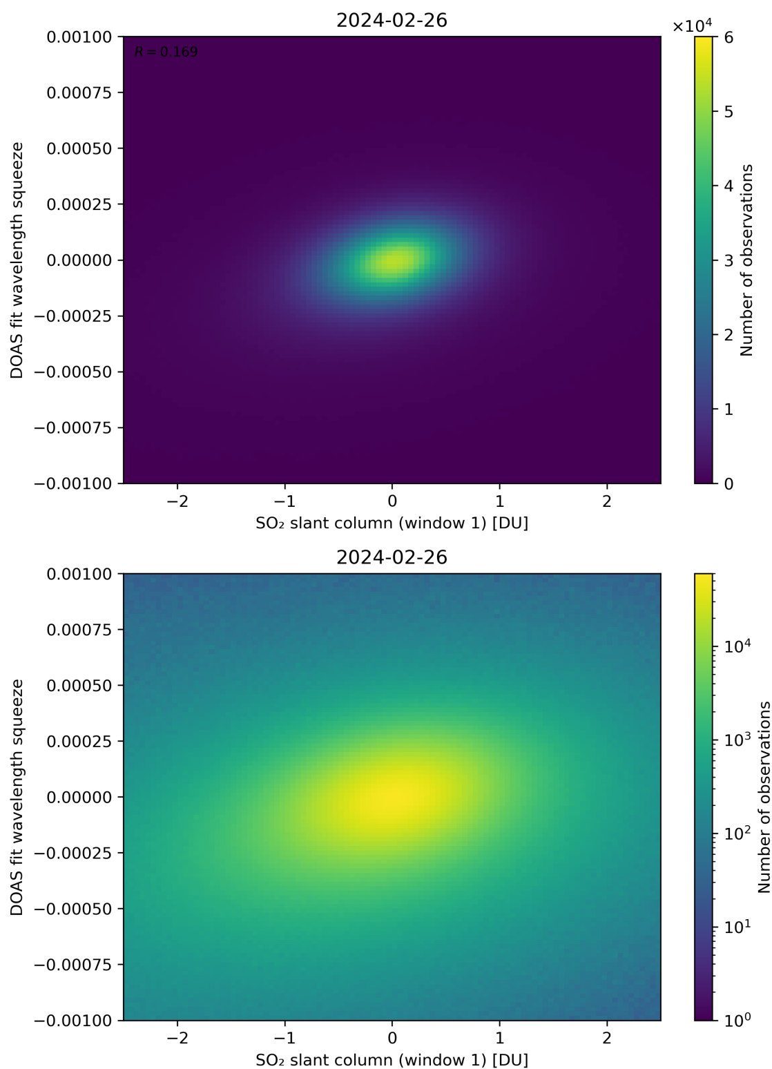
Figure 216: Scatter density plot of “SO 2 slant column (window 1)” against “DOAS fit wavelength squeeze” for 2024-02-25 to 2024-02-27.
