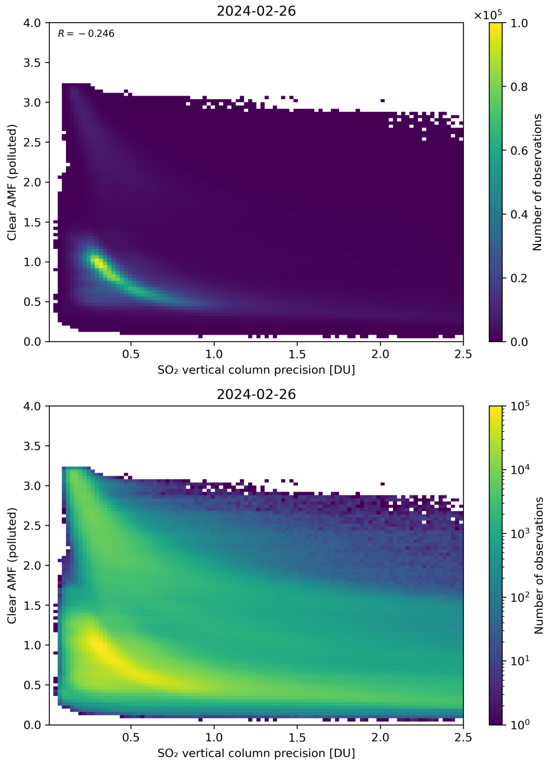
Figure 285: Scatter density plot of “SO 2 vertical column precision” against “Clear AMF (polluted)” for 2024-02-25 to 2024-02-27.
