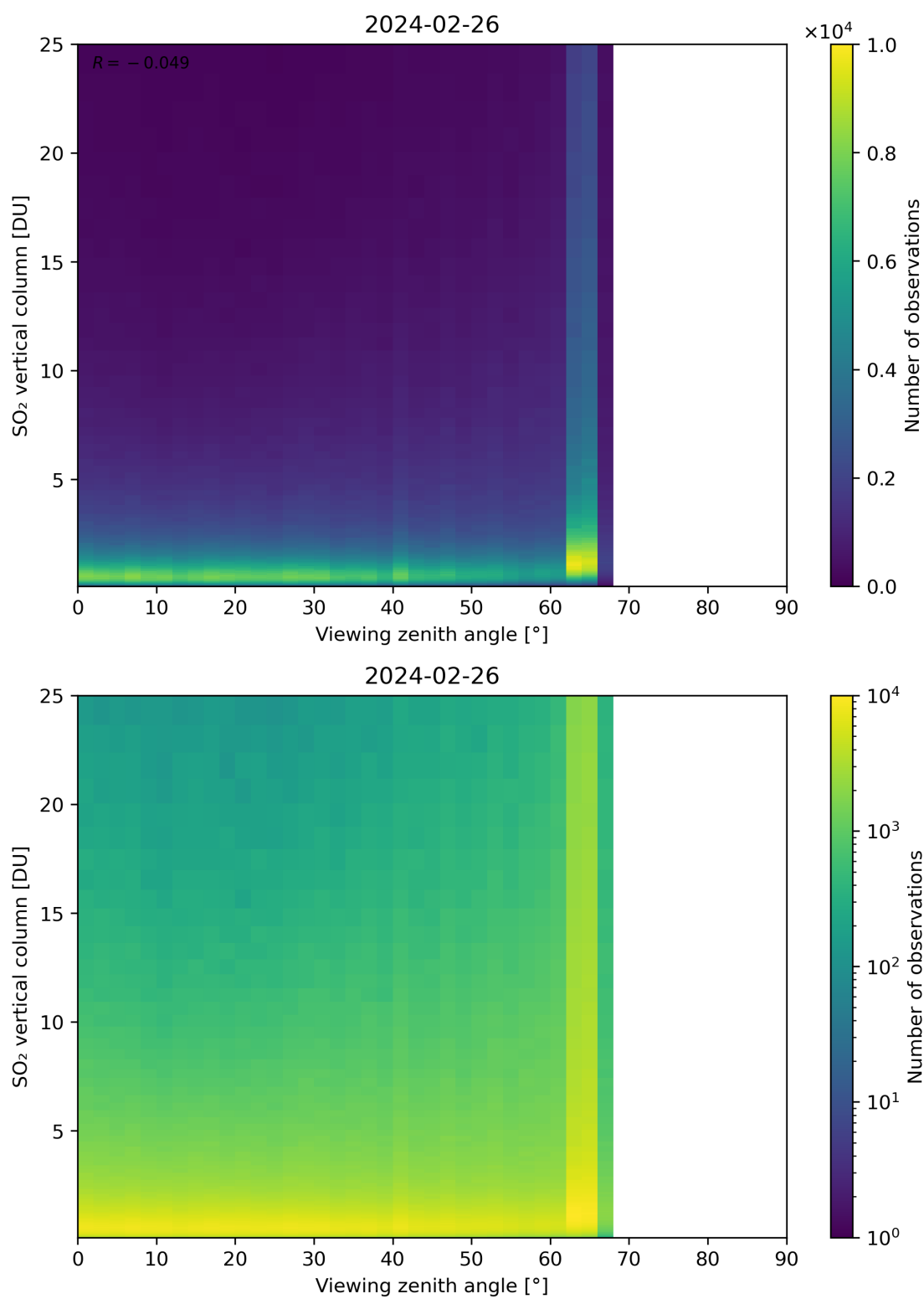
Figure 327: Scatter density plot of “Viewing zenith angle” against “SO 2 vertical column” for 2024-02-25 to 2024-02-27.
