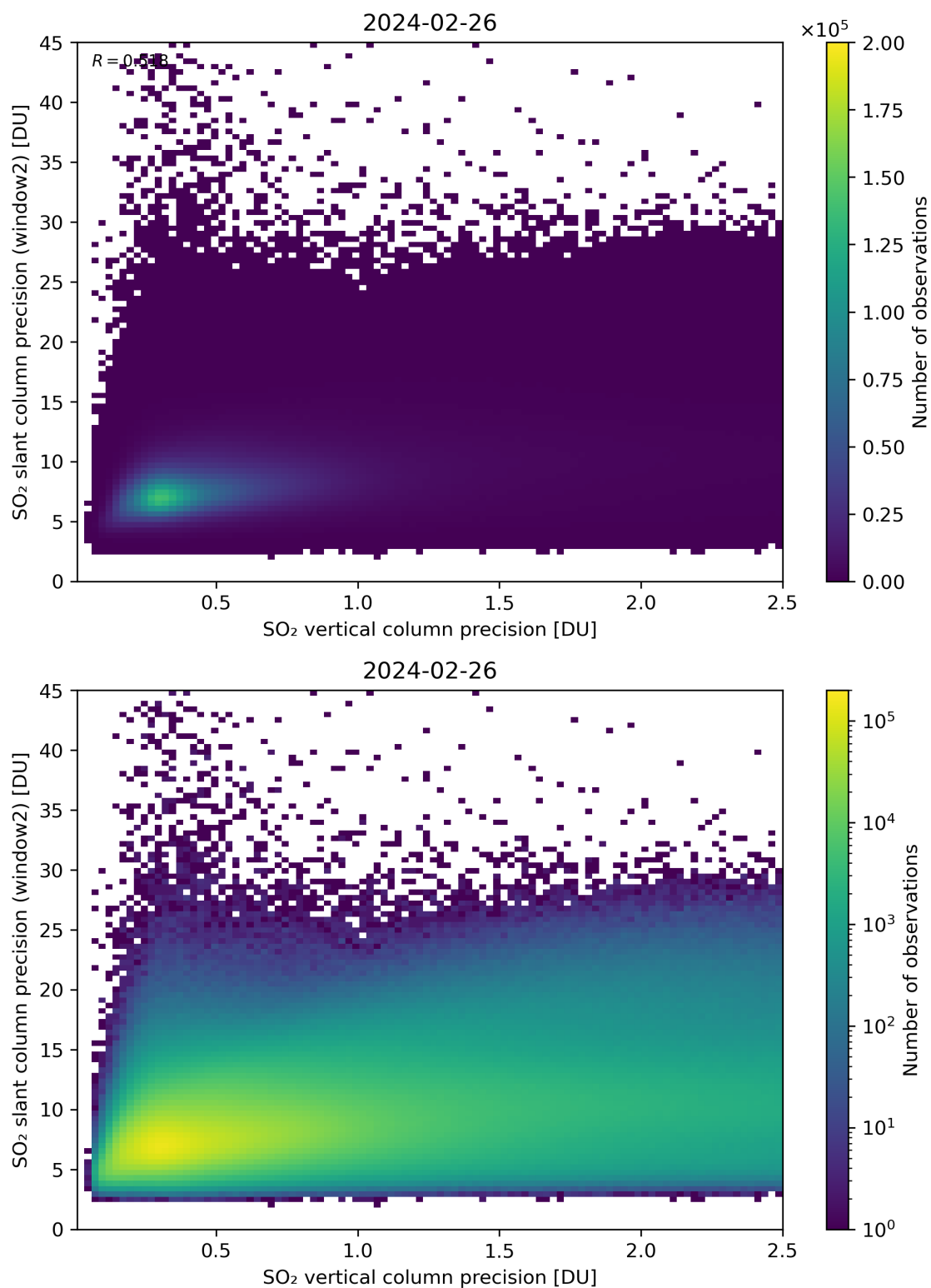
Figure 291: Scatter density plot of “SO 2 vertical column precision” against “SO 2 slant column precision (window2)” for 2024-02-25 to 2024-02-27.
