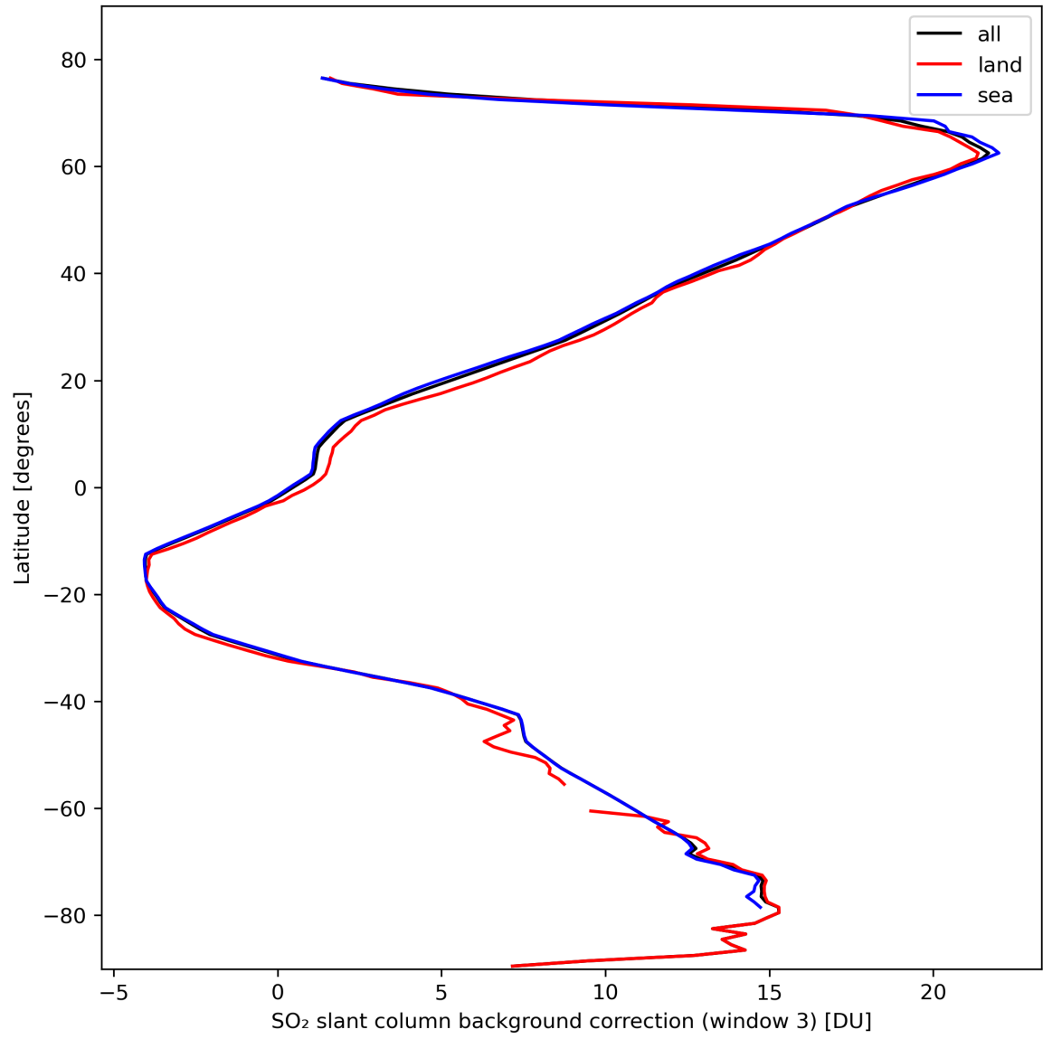
Figure 44: Zonal average of “SO 2 slant column background correction (window 3)” for 2024-02-25 to 2024-02-27.
