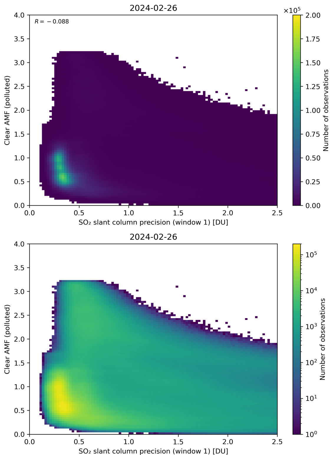
Figure 224: Scatter density plot of “SO 2 slant column precision (window 1)” against “Clear AMF (polluted)” for 2024-02-25 to 2024-02-27.
