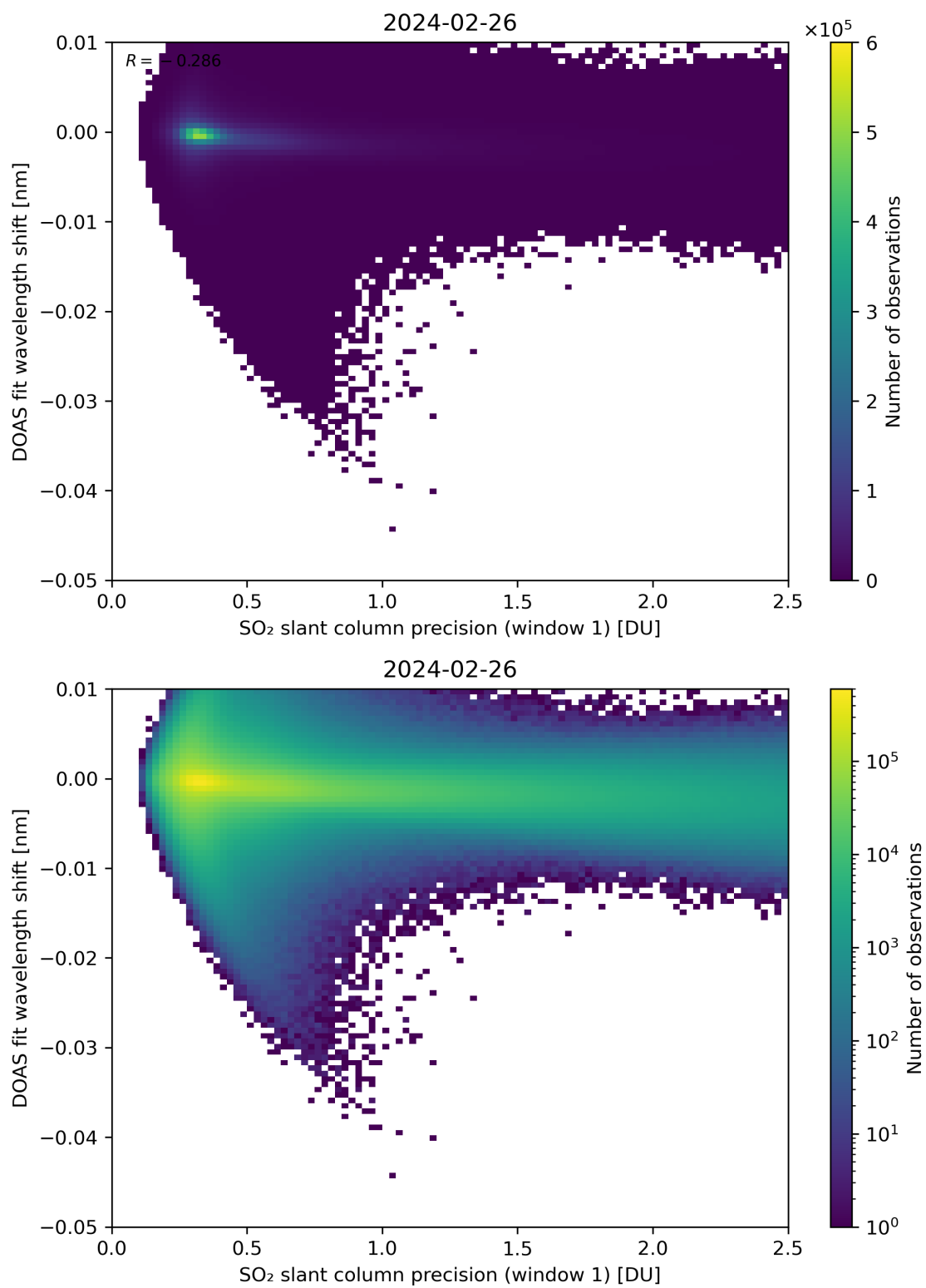
Figure 221: Scatter density plot of “SO 2 slant column precision (window 1)” against “DOAS fit wavelength shift” for 2024-02-25 to 2024-02-27.
