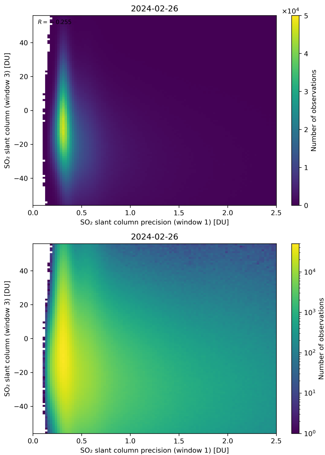
Figure 228: Scatter density plot of “SO 2 slant column precision (window 1)” against “SO 2 slant column (window 3)” for 2024-02-25 to 2024-02-27.
