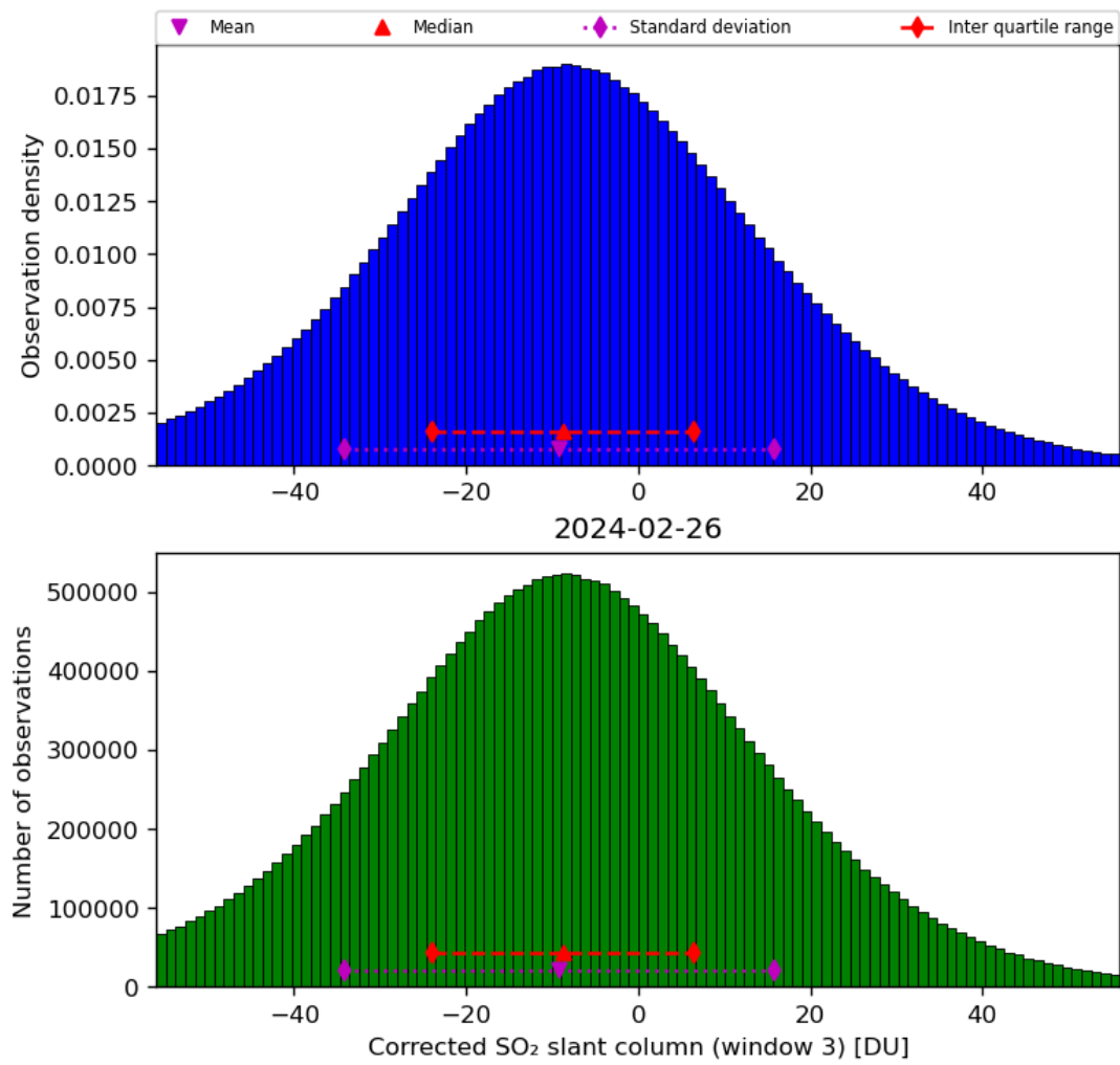
Figure 66: Histogram of “Corrected SO 2 slant column (window 3)” for 2024-02-25 to 2024-02-27
