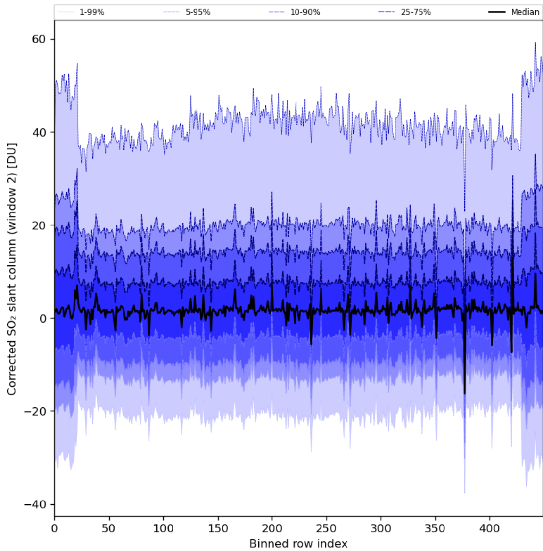
Figure 85: Along track statistics of “Corrected SO 2 slant column (window 2)” for 2024-02-25 to 2024-02-27
