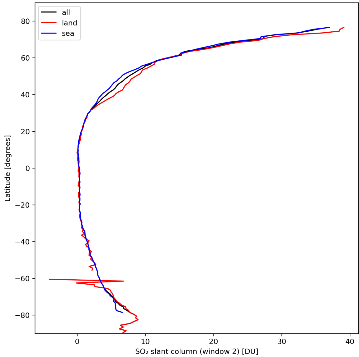
Figure 37: Zonal average of “SO 2 slant column (window 2)” for 2024-02-25 to 2024-02-27.
