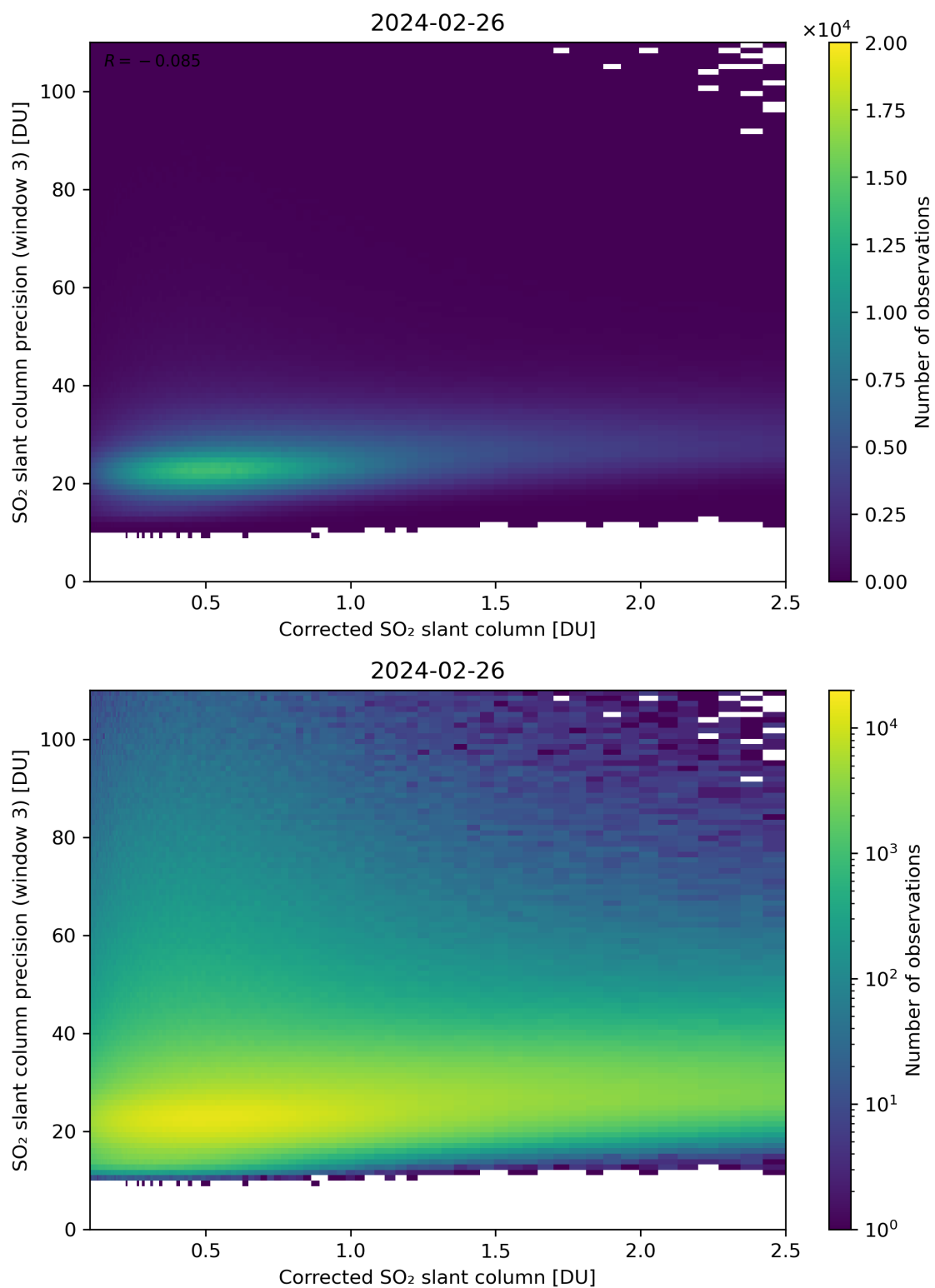
Figure 191: Scatter density plot of “Corrected SO 2 slant column” against “SO 2 slant column precision (window 3)” for 2024-02-25 to 2024-02-27.
