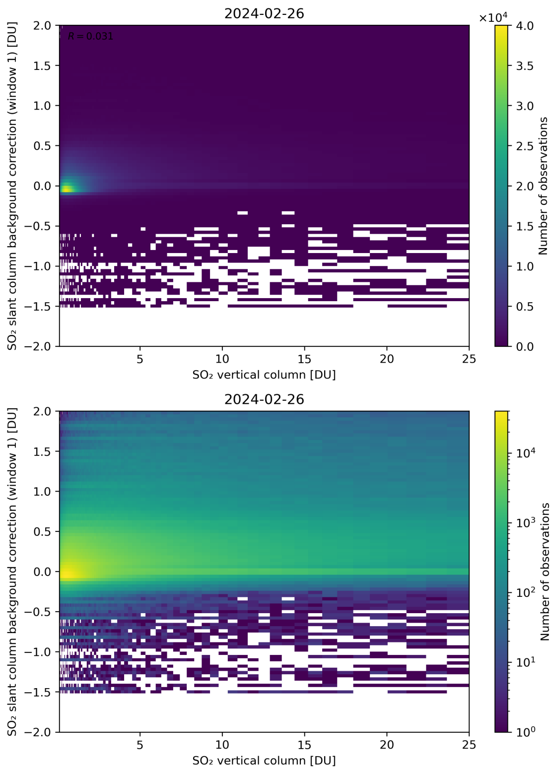
Figure 273: Scatter density plot of “SO 2 vertical column” against “SO 2 slant column background correction (window 1)” for 2024-02-25 to 2024-02-27.
