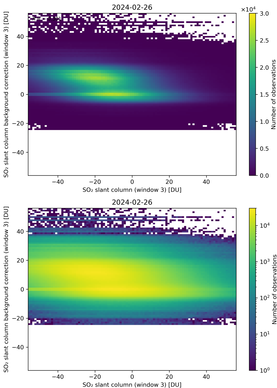
Figure 253: Scatter density plot of “SO 2 slant column (window 3)” against “SO 2 slant column background correction (window 3)” for 2024-02-25 to 2024-02-27.
