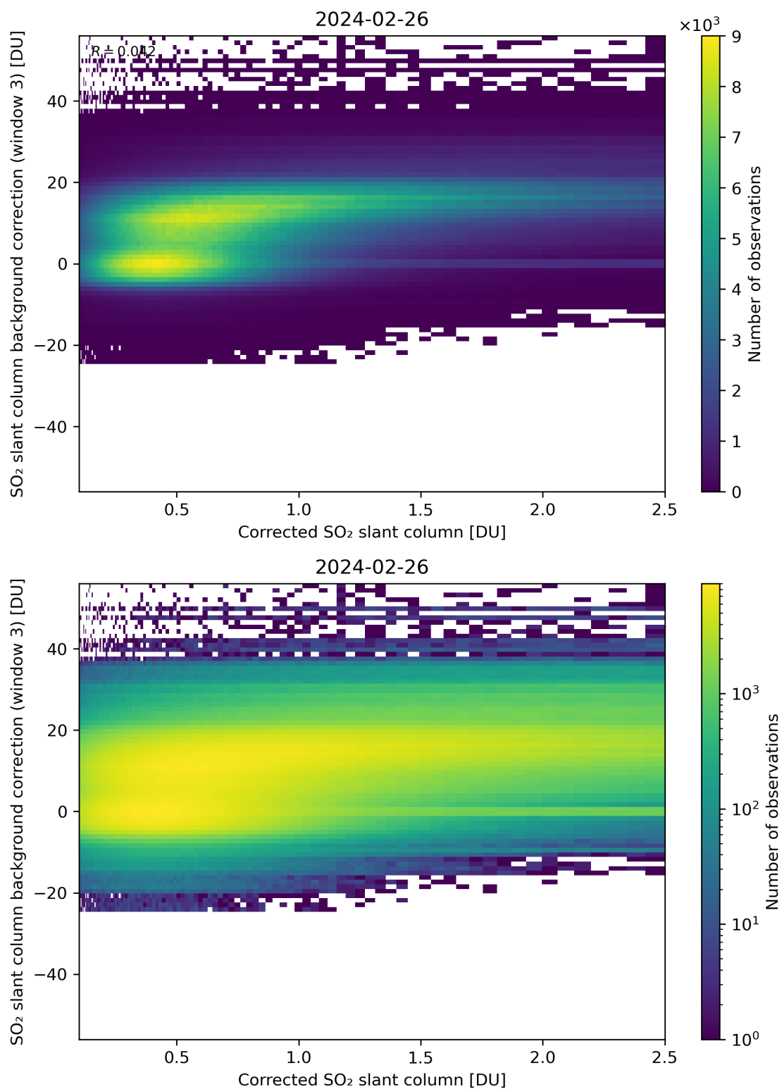
Figure 180: Scatter density plot of “Corrected SO 2 slant column” against “SO 2 slant column background correction (window 3)” for 2024-02-25 to 2024-02-27.
