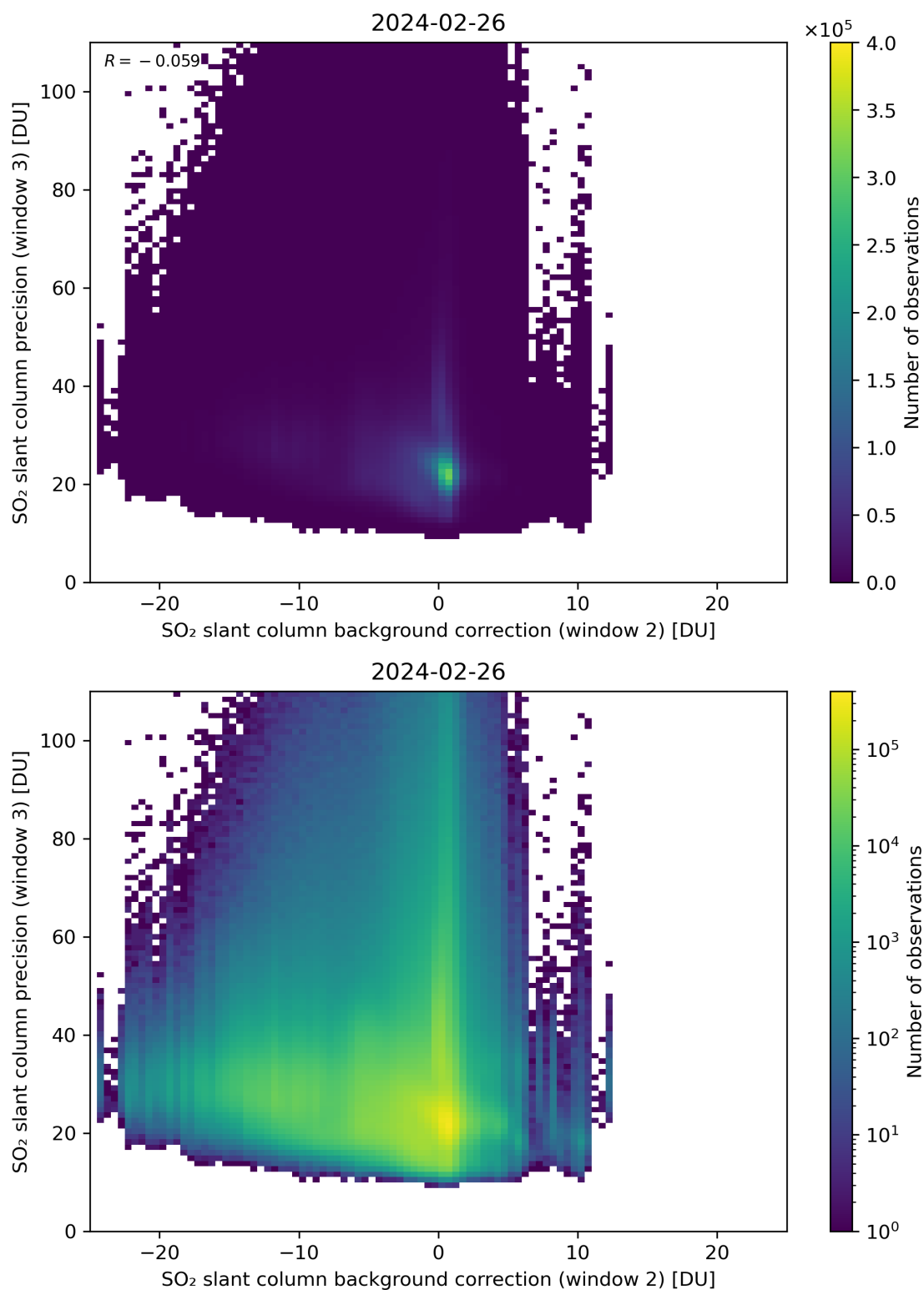
Figure 118: Scatter density plot of “SO 2 slant column background correction (window 2)” against “SO 2 slant column precision (window 3)” for 2024-02-25 to 2024-02-27.
