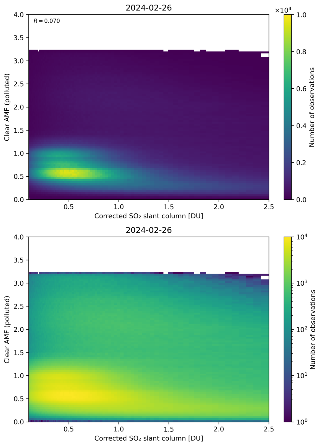
Figure 184: Scatter density plot of “Corrected SO 2 slant column” against “Clear AMF (polluted)” for 2024-02-25 to 2024-02-27.
