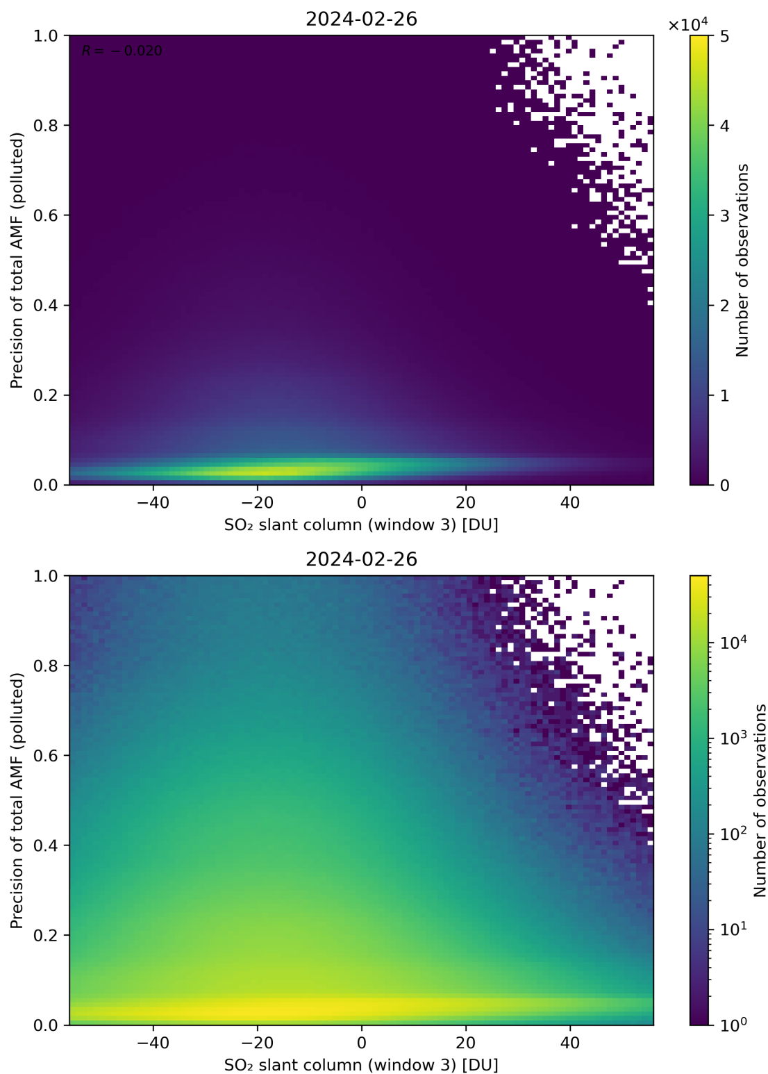
Figure 269: Scatter density plot of “SO 2 slant column (window 3)” against “Precision of total AMF (polluted)” for 2024-02-25 to 2024-02-27.
