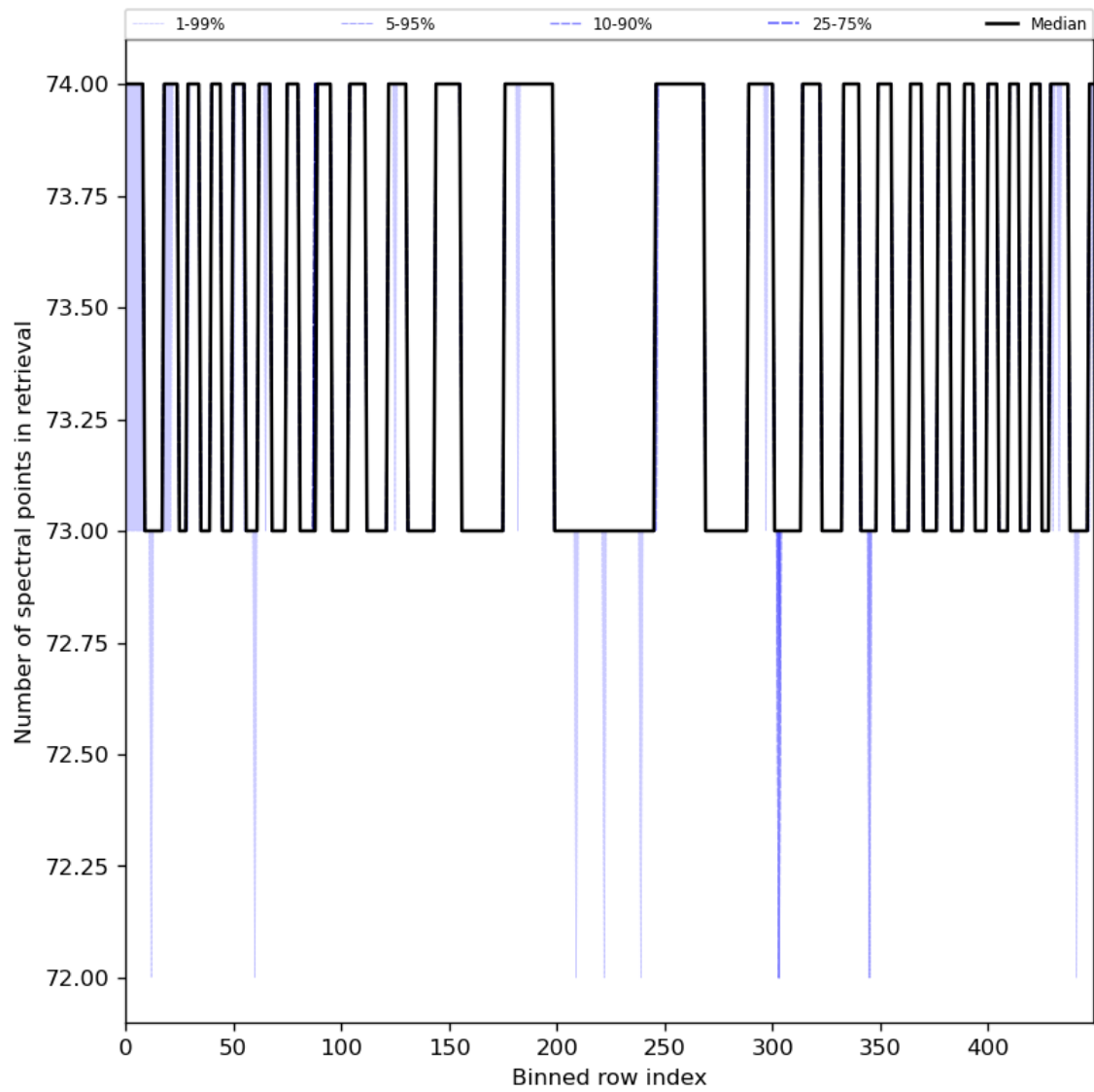
Figure 97: Along track statistics of “Number of spectral points in retrieval” for 2024-02-25 to 2024-02-27
