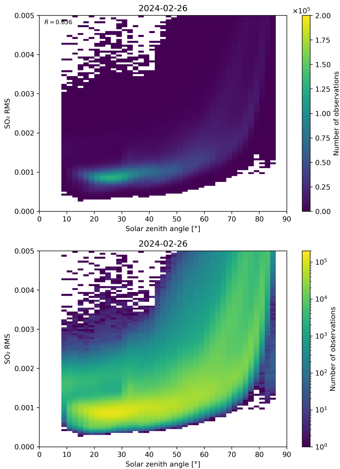
Figure 163: Scatter density plot of “Solar zenith angle” against “SO 2 RMS” for 2024-02-25 to 2024-02-27.
