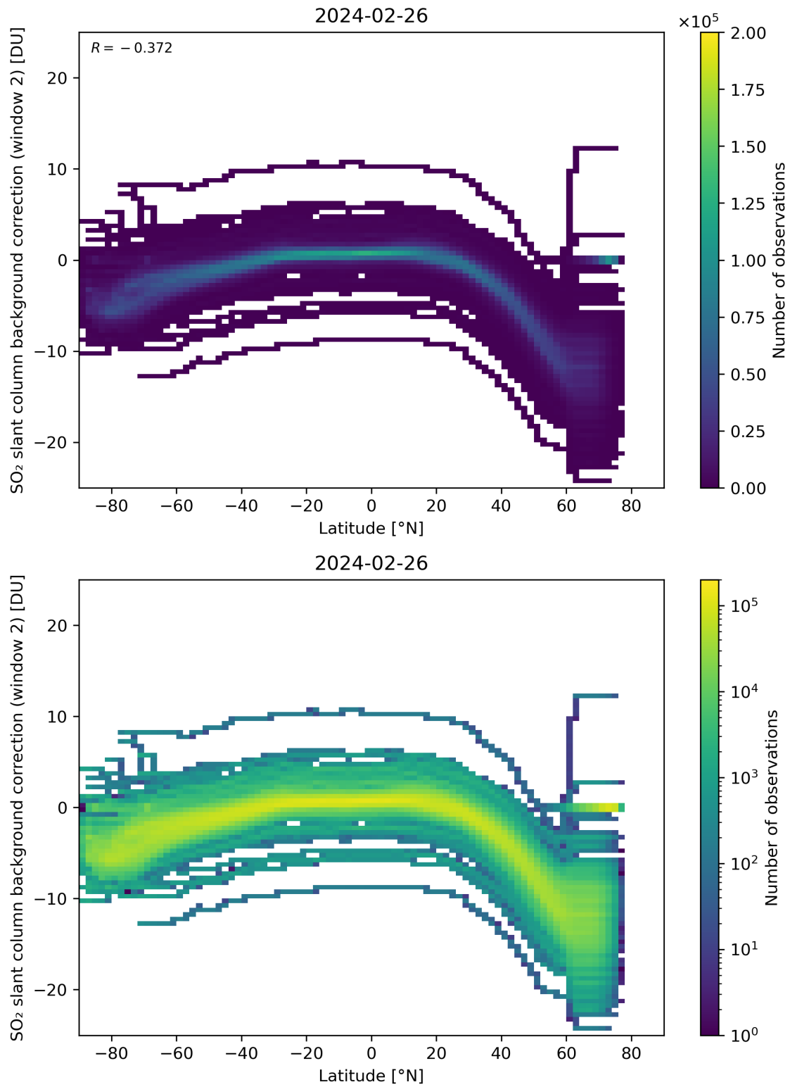
Figure 140: Scatter density plot of “Latitude” against “SO 2 slant column background correction (window 2)” for 2024-02-25 to 2024-02-27.
