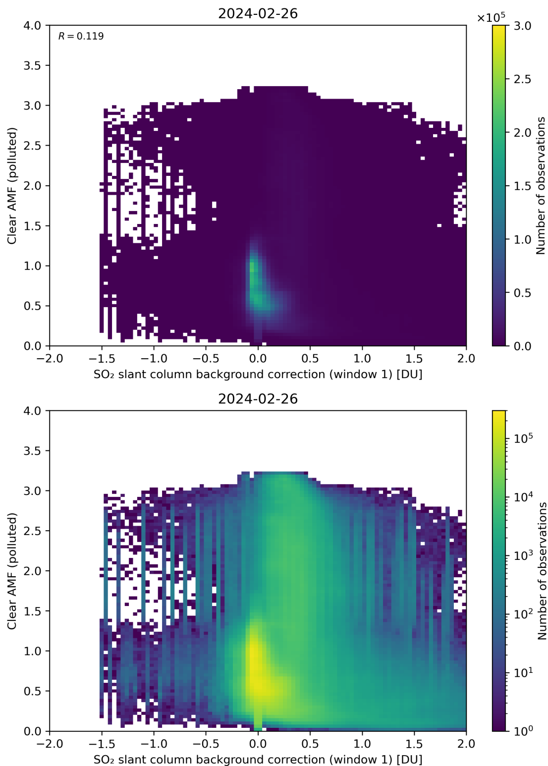
Figure 103: Scatter density plot of “SO 2 slant column background correction (window 1)” against “Clear AMF (polluted)” for 2024-02-25 to 2024-02-27.
