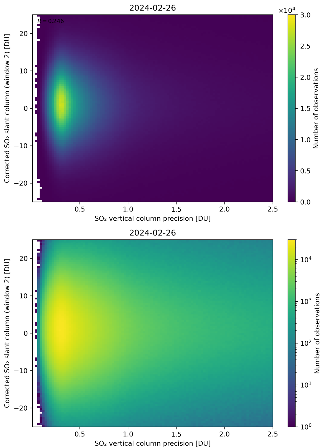
Figure 287: Scatter density plot of “SO 2 vertical column precision” against “Corrected SO 2 slant column (window 2)” for 2024-02-25 to 2024-02-27.
