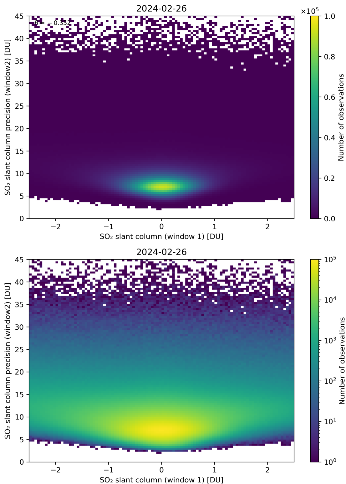
Figure 236: Scatter density plot of “SO 2 slant column (window 1)” against “SO 2 slant column precision (window2)” for 2024-02-25 to 2024-02-27.
