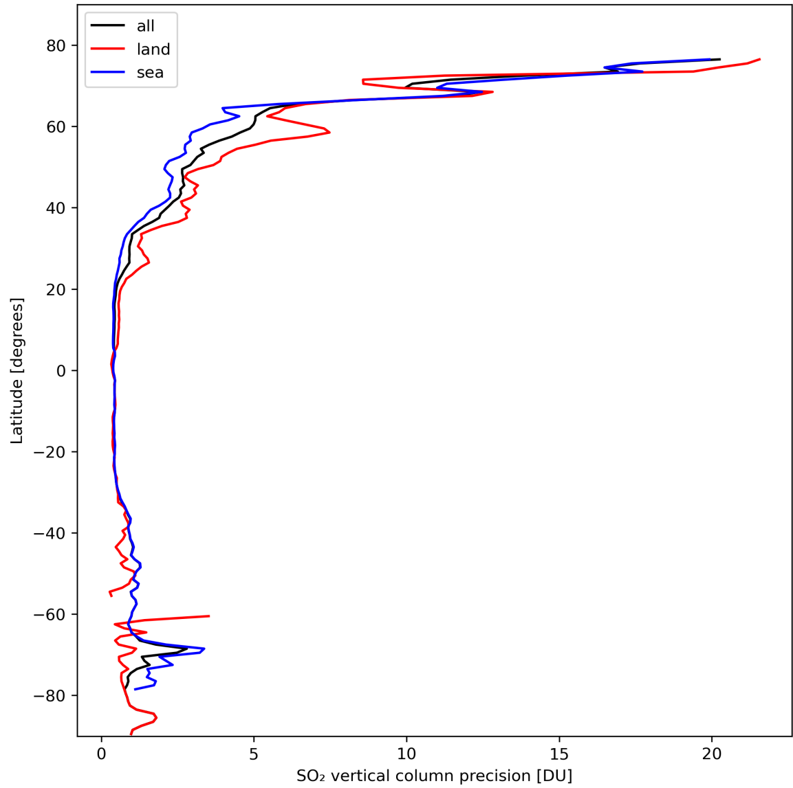
Figure 31: Zonal average of “SO 2 vertical column precision” for 2024-02-25 to 2024-02-27.
