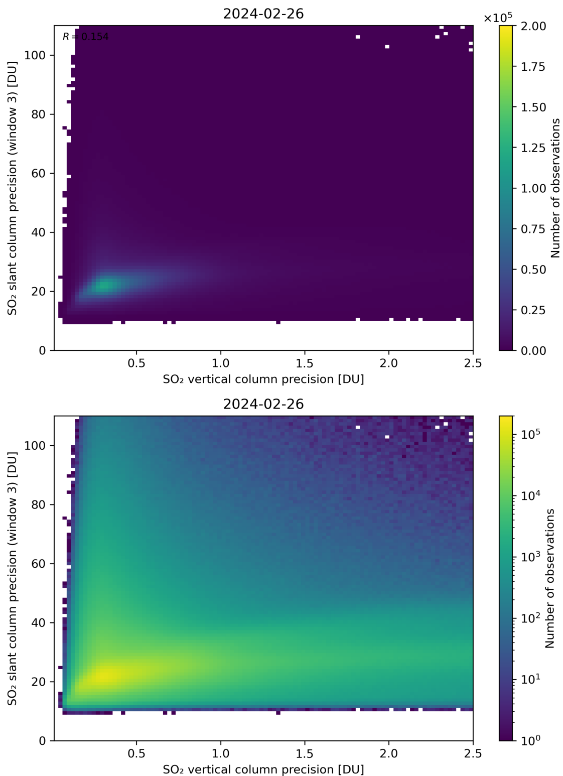
Figure 293: Scatter density plot of “SO 2 vertical column precision” against “SO 2 slant column precision (window 3)” for 2024-02-25 to 2024-02-27.
