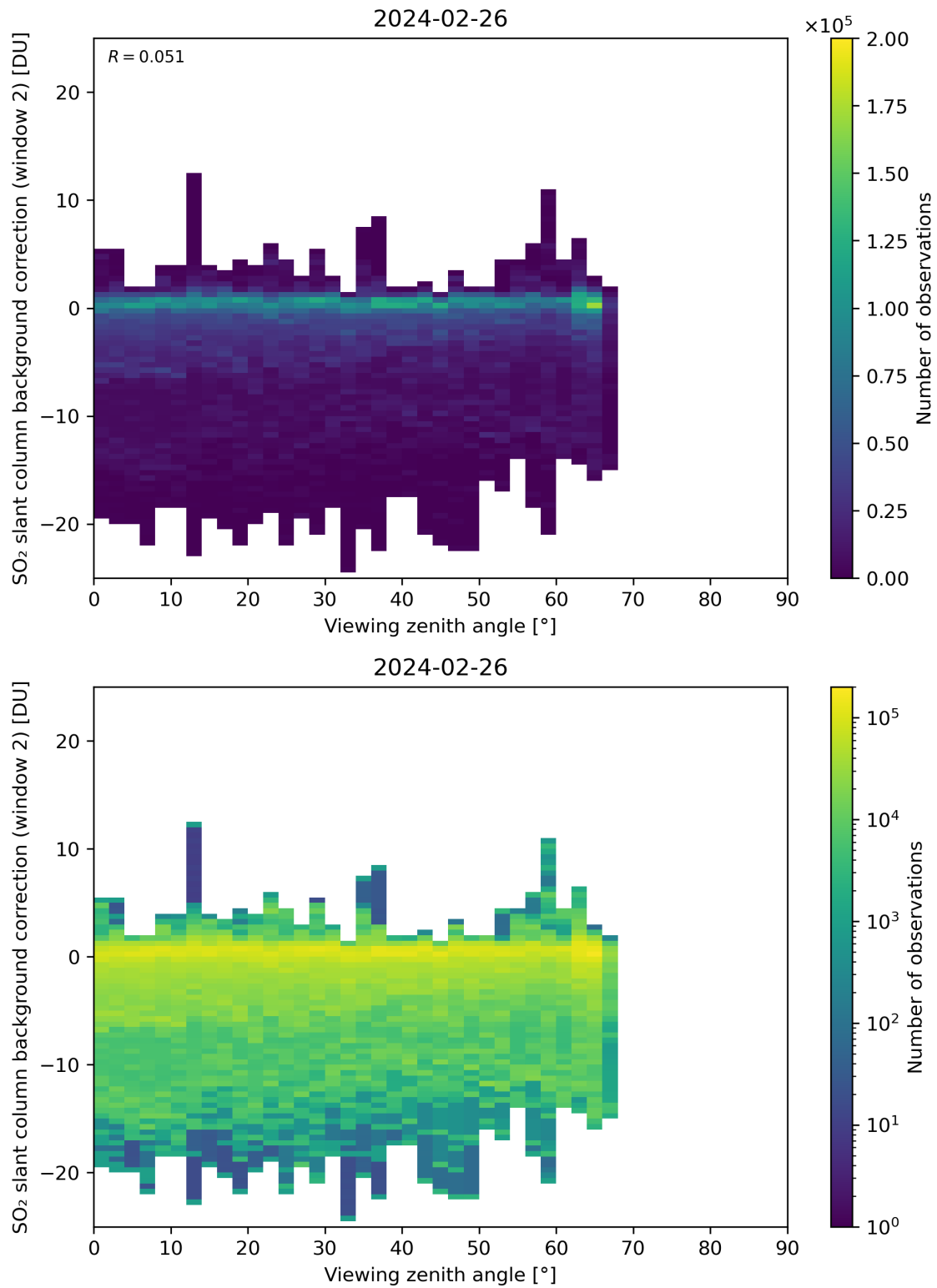
Figure 309: Scatter density plot of “Viewing zenith angle” against “SO 2 slant column background correction (window 2)” for 2024-02-25 to 2024-02-27.
