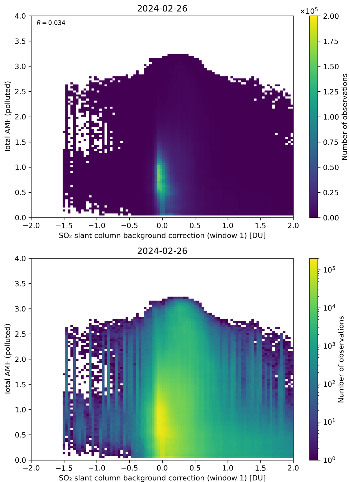
Figure 109: Scatter density plot of “SO 2 slant column background correction (window 1)” against “Total AMF (polluted)” for 2024-02-25 to 2024-02-27.
