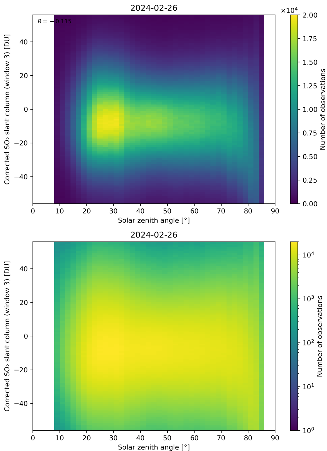
Figure 168: Scatter density plot of “Solar zenith angle” against “Corrected SO 2 slant column (window 3)” for 2024-02-25 to 2024-02-27.
