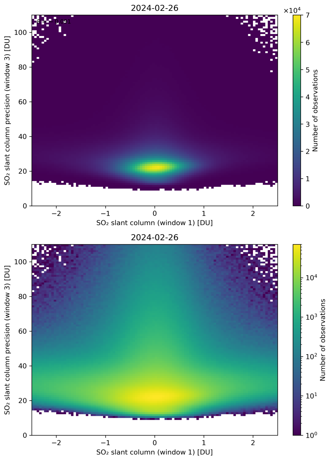
Figure 238: Scatter density plot of “SO 2 slant column (window 1)” against “SO 2 slant column precision (window 3)” for 2024-02-25 to 2024-02-27.
