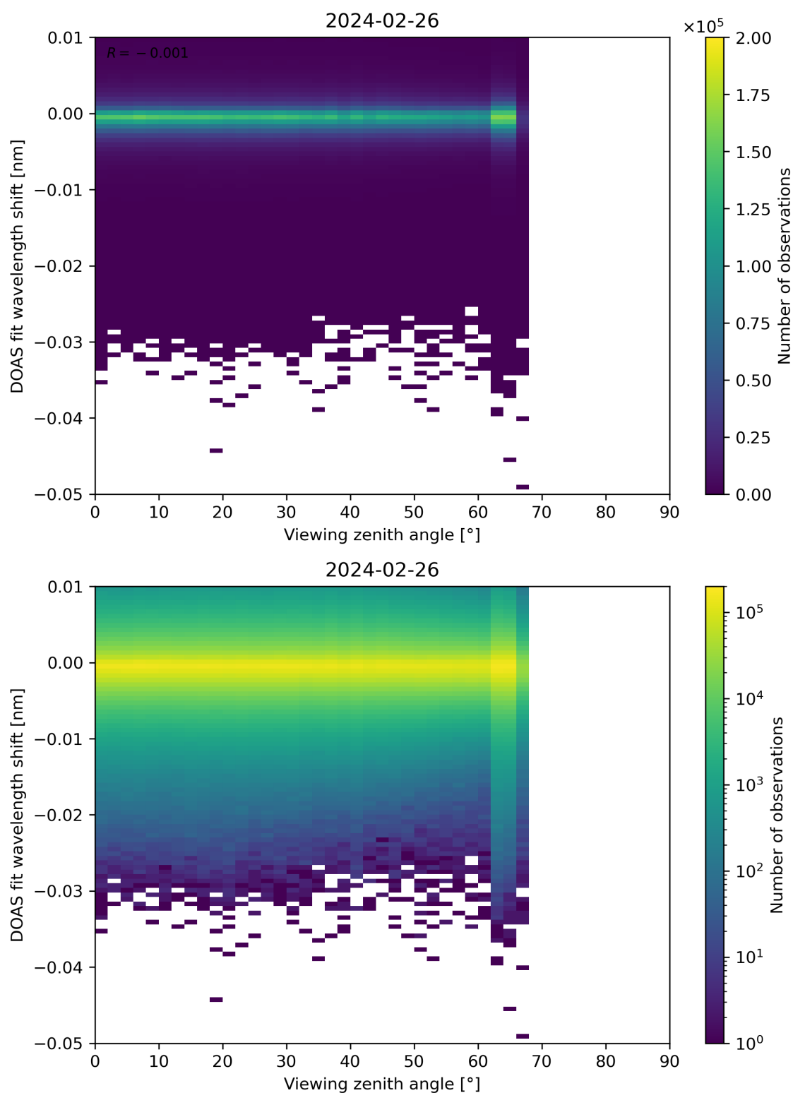
Figure 311: Scatter density plot of “Viewing zenith angle” against “DOAS fit wavelength shift” for 2024-02-25 to 2024-02-27.
