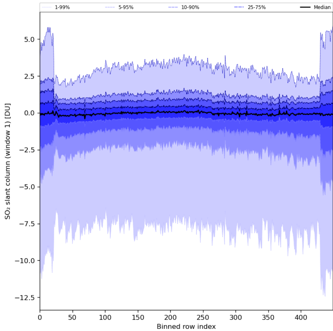
Figure 79: Along track statistics of “SO 2 slant column (window 1)” for 2024-02-25 to 2024-02-27
