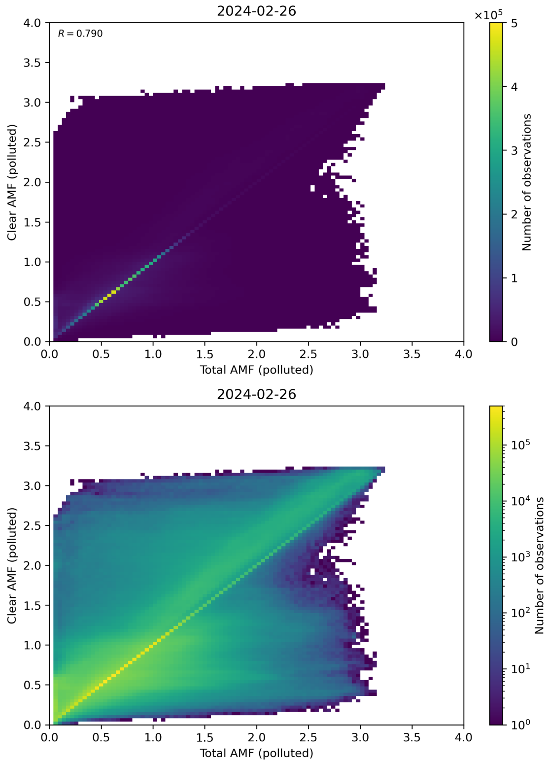
Figure 271: Scatter density plot of “Total AMF (polluted)” against “Clear AMF (polluted)” for 2024-02-25 to 2024-02-27.
