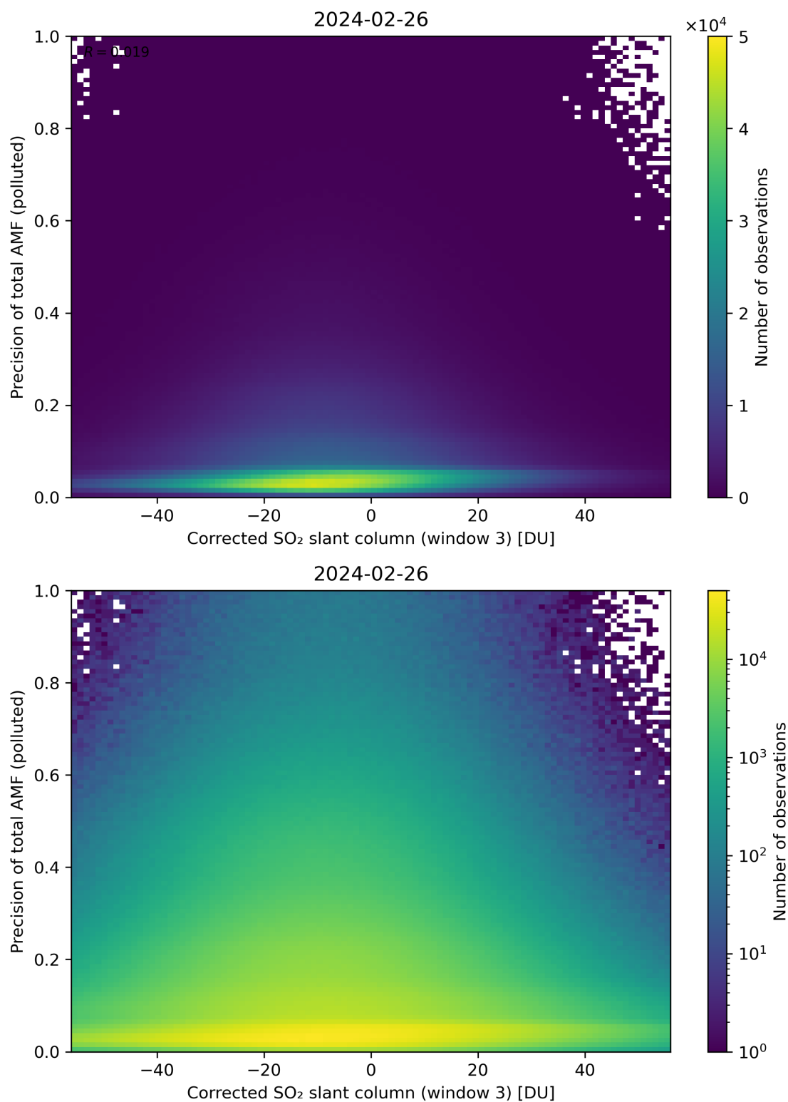
Figure 211: Scatter density plot of “Corrected SO 2 slant column (window 3)” against “Precision of total AMF (polluted)” for 2024-02-25 to 2024-02-27.
