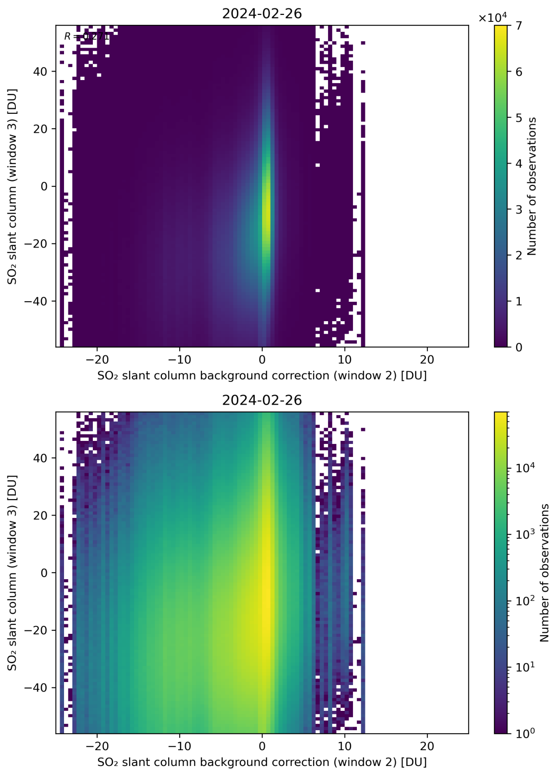
Figure 117: Scatter density plot of “SO 2 slant column background correction (window 2)” against “SO 2 slant column (window 3)” for 2024-02-25 to 2024-02-27.
