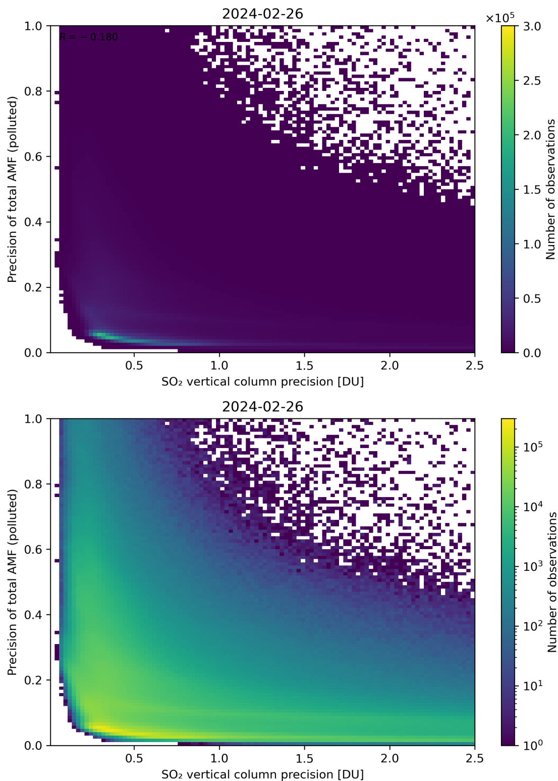
Figure 295: Scatter density plot of “SO 2 vertical column precision” against “Precision of total AMF (polluted)” for 2024-02-25 to 2024-02-27.
