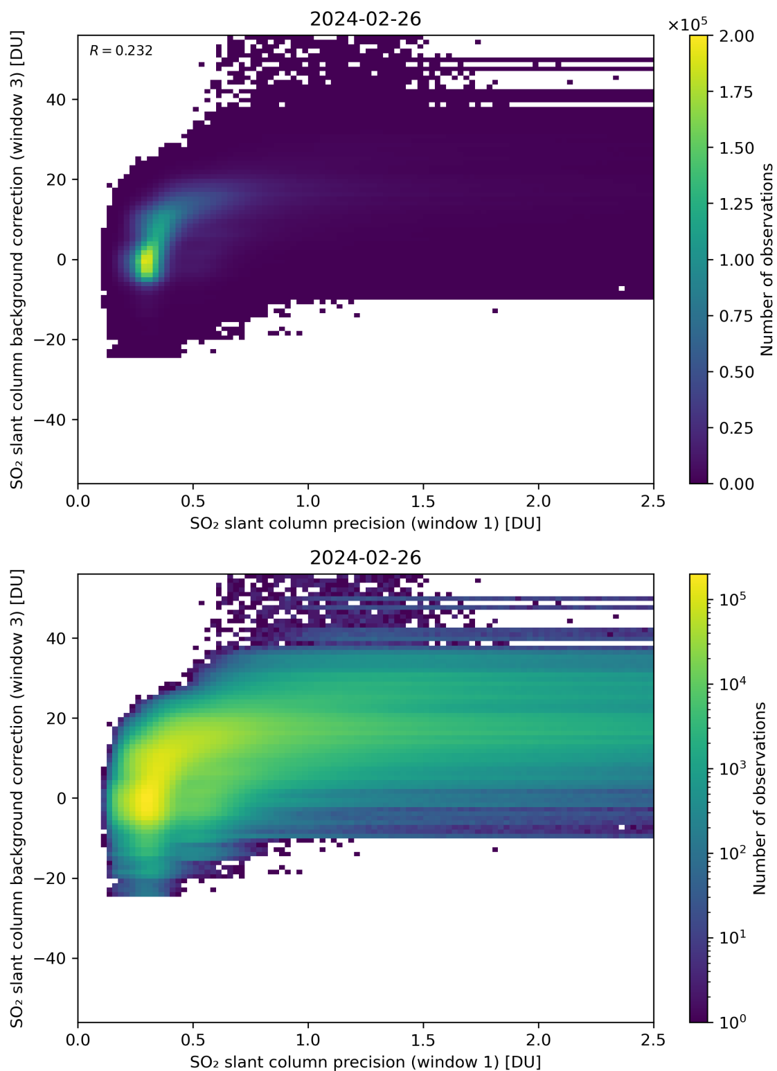
Figure 220: Scatter density plot of “SO 2 slant column precision (window 1)” against “SO 2 slant column background correction (window 3)” for 2024-02-25 to 2024-02-27.
