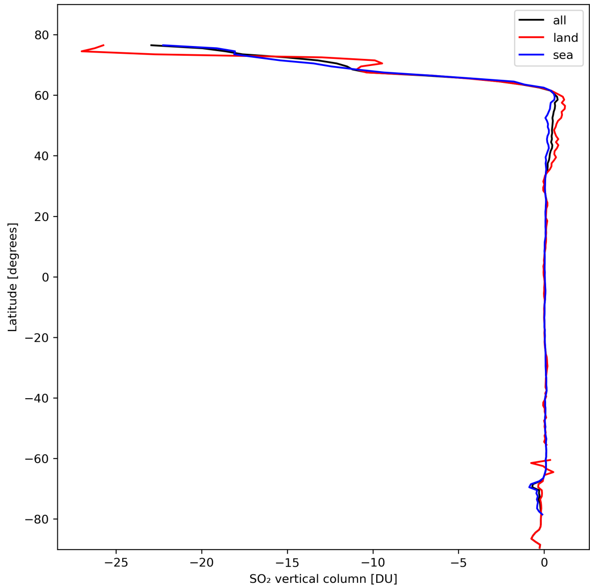
Figure 30: Zonal average of “SO 2 vertical column” for 2024-02-25 to 2024-02-27.
