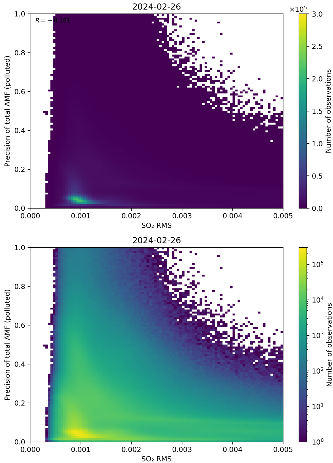
Figure 138: Scatter density plot of “SO 2 RMS” against “Precision of total AMF (polluted)” for 2024-02-25 to 2024-02-27.
