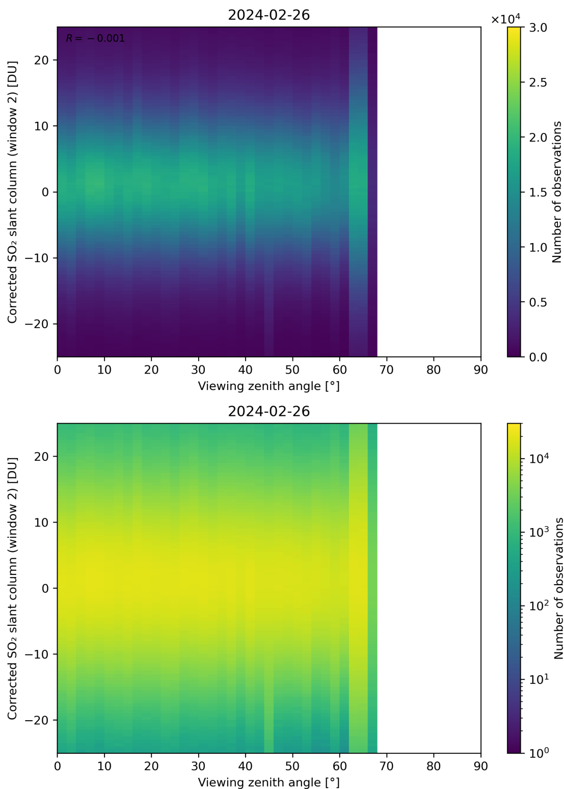
Figure 318: Scatter density plot of “Viewing zenith angle” against “Corrected SO 2 slant column (window 2)” for 2024-02-25 to 2024-02-27.
