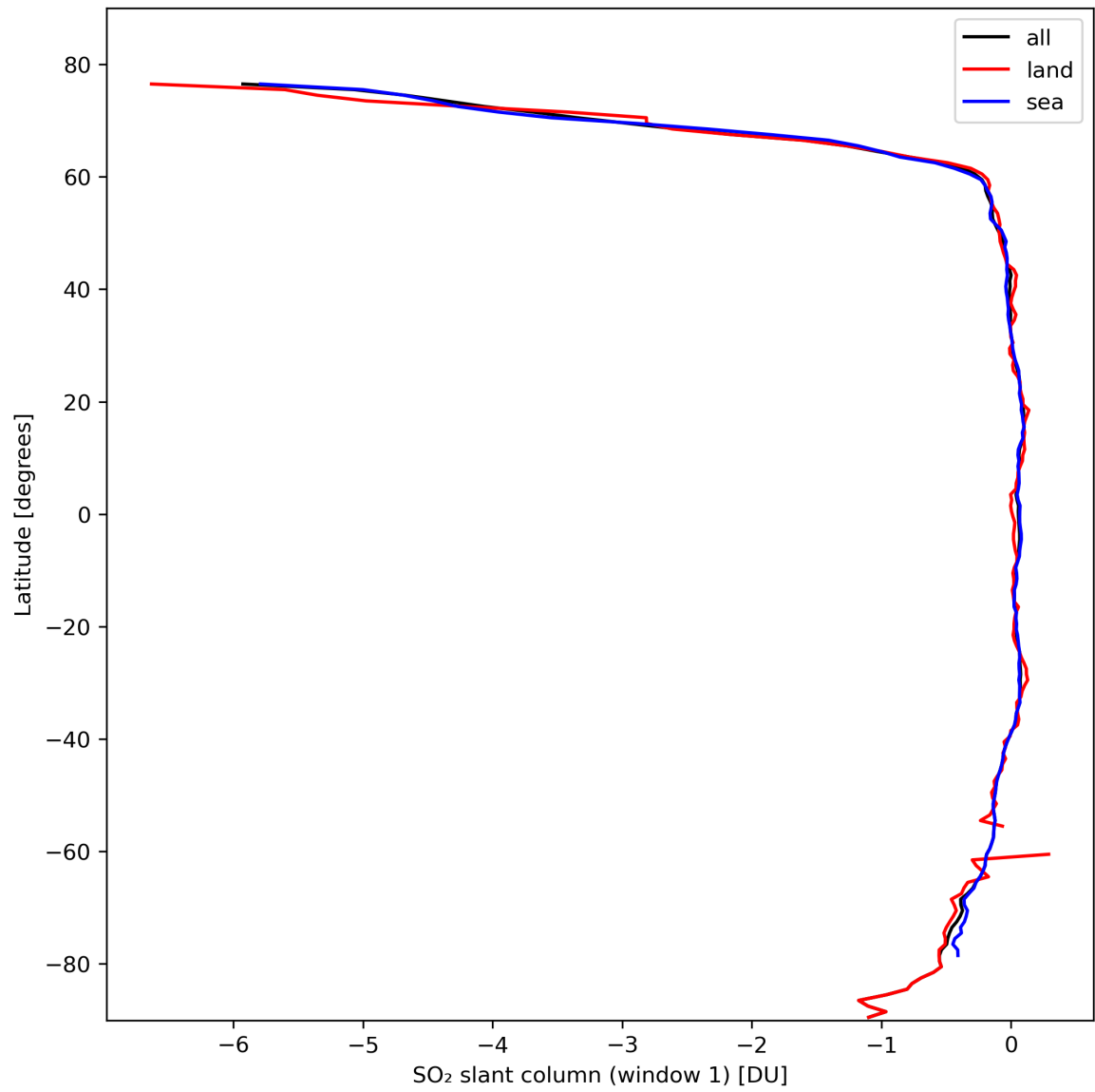
Figure 33: Zonal average of “SO 2 slant column (window 1)” for 2024-02-25 to 2024-02-27.
