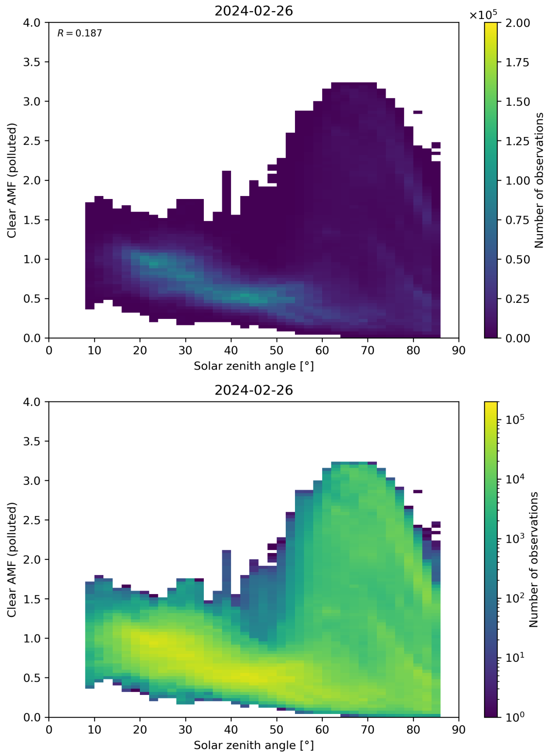
Figure 165: Scatter density plot of “Solar zenith angle” against “Clear AMF (polluted)” for 2024-02-25 to 2024-02-27.
