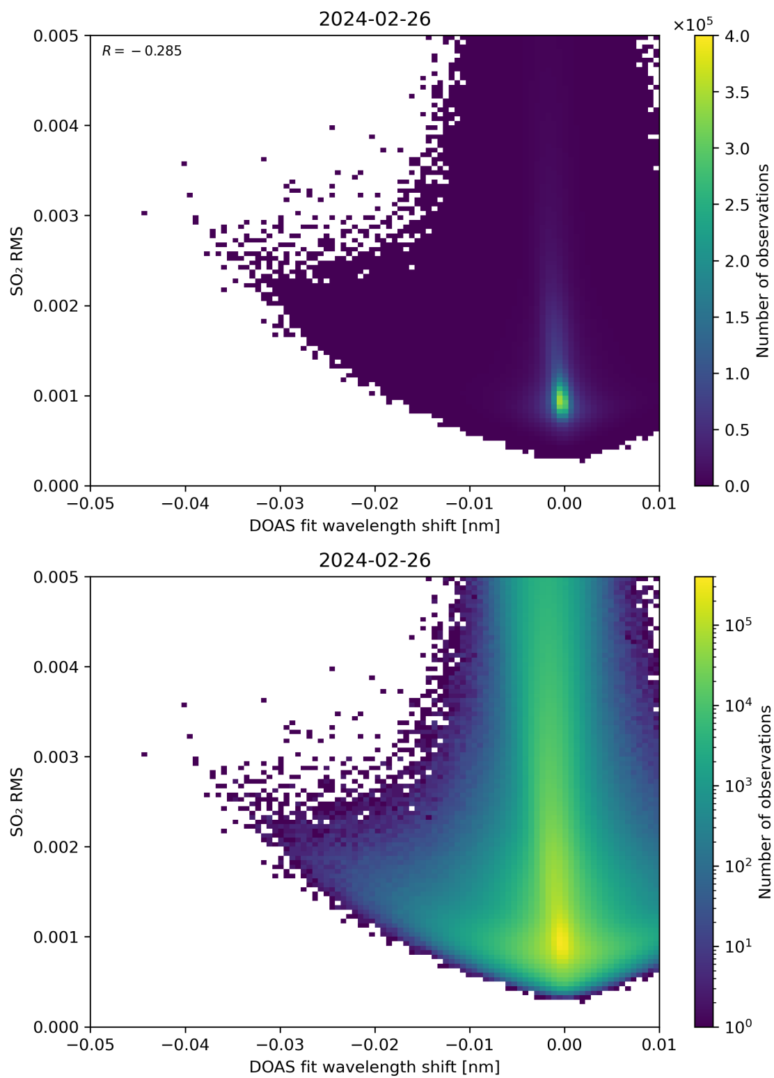
Figure 128: Scatter density plot of “DOAS fit wavelength shift” against “SO 2 RMS” for 2024-02-25 to 2024-02-27.
