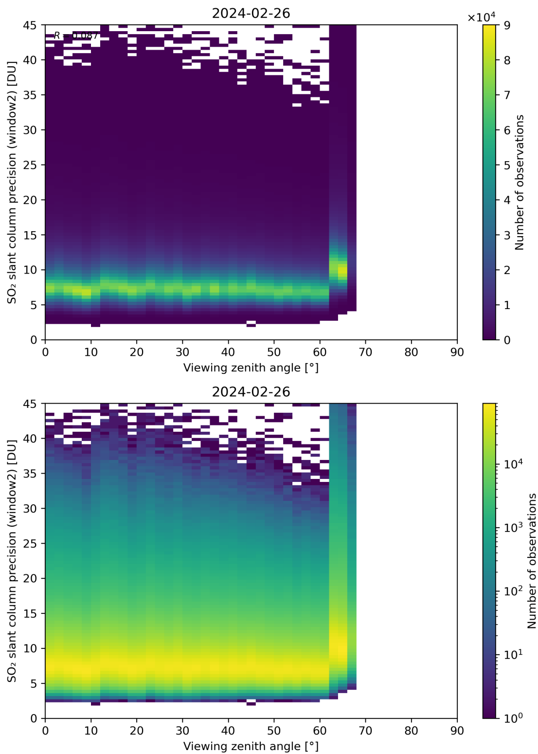
Figure 322: Scatter density plot of “Viewing zenith angle” against “SO 2 slant column precision (window2)” for 2024-02-25 to 2024-02-27.
