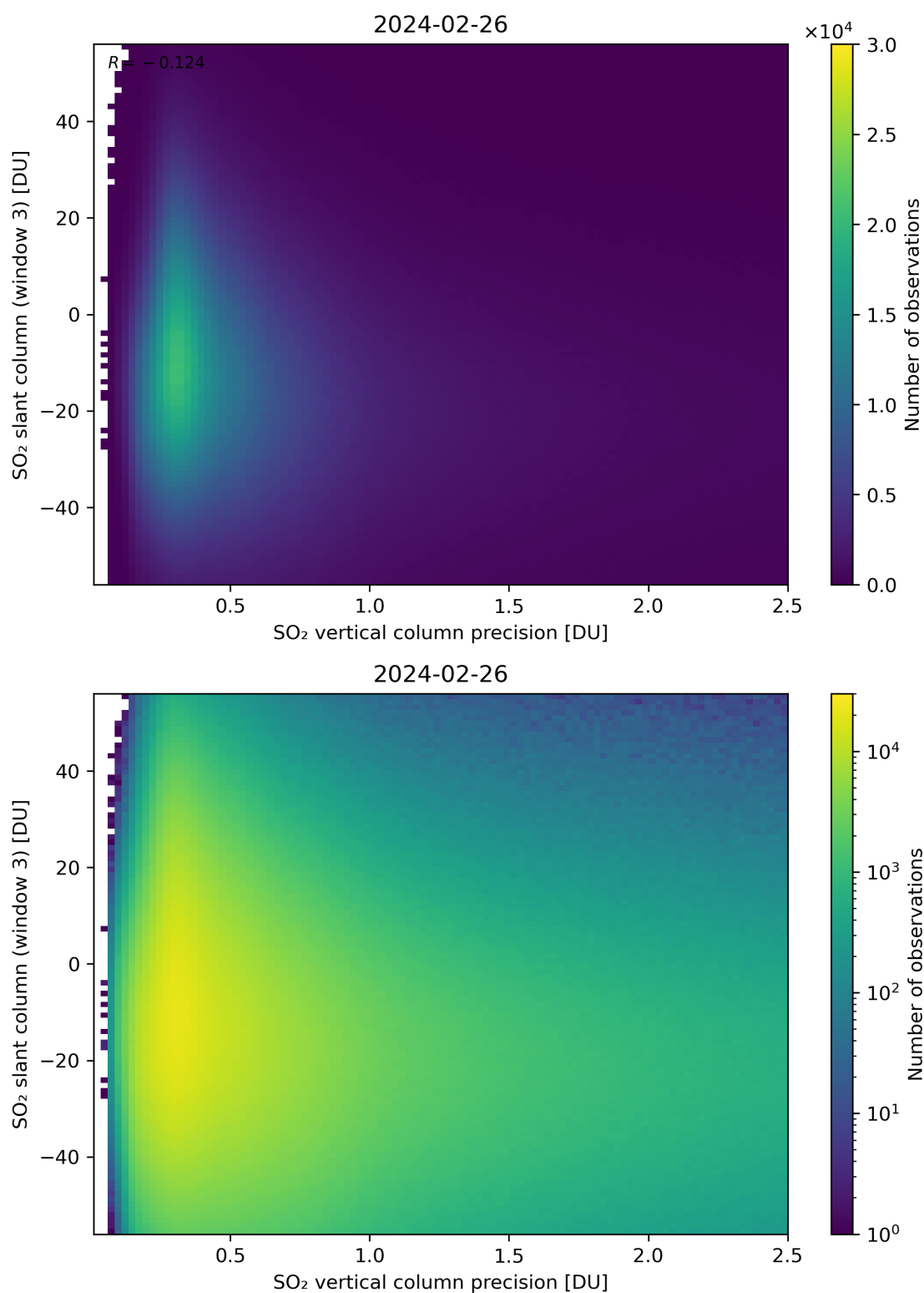
Figure 292: Scatter density plot of “SO 2 vertical column precision” against “SO 2 slant column (window 3)” for 2024-02-25 to 2024-02-27.
