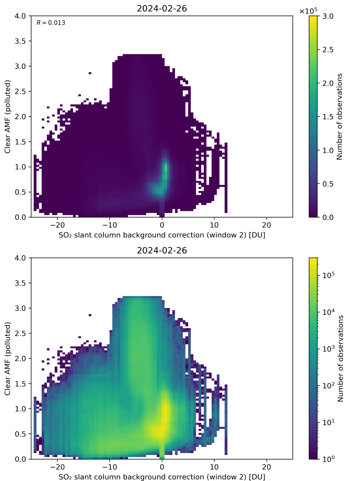
Figure 115: Scatter density plot of “SO 2 slant column background correction (window 2)” against “Clear AMF (polluted)” for 2024-02-25 to 2024-02-27.
