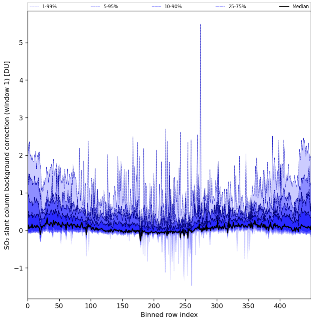
Figure 82: Along track statistics of “SO 2 slant column background correction (window 1)” for 2024-02-25 to 2024-02-27
