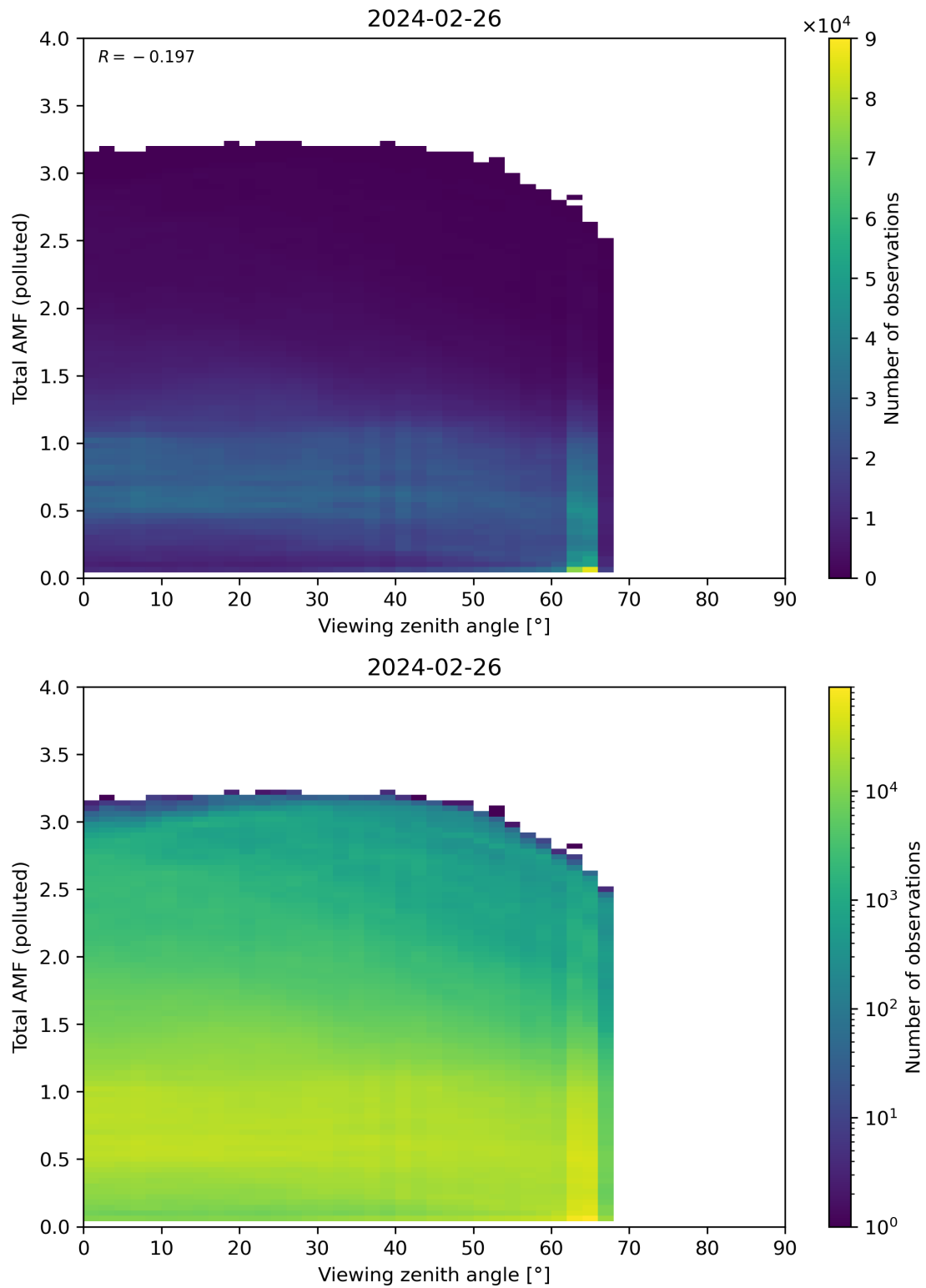
Figure 325: Scatter density plot of “Viewing zenith angle” against “Total AMF (polluted)” for 2024-02-25 to 2024-02-27.
