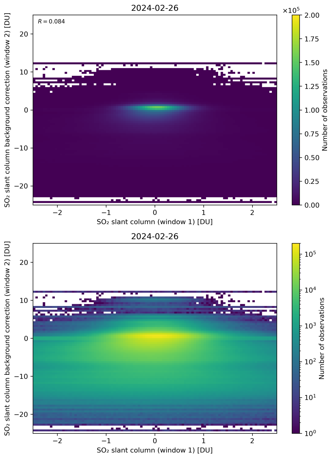
Figure 213: Scatter density plot of “SO 2 slant column (window 1)” against “SO 2 slant column background correction (window 2)” for 2024-02-25 to 2024-02-27.
