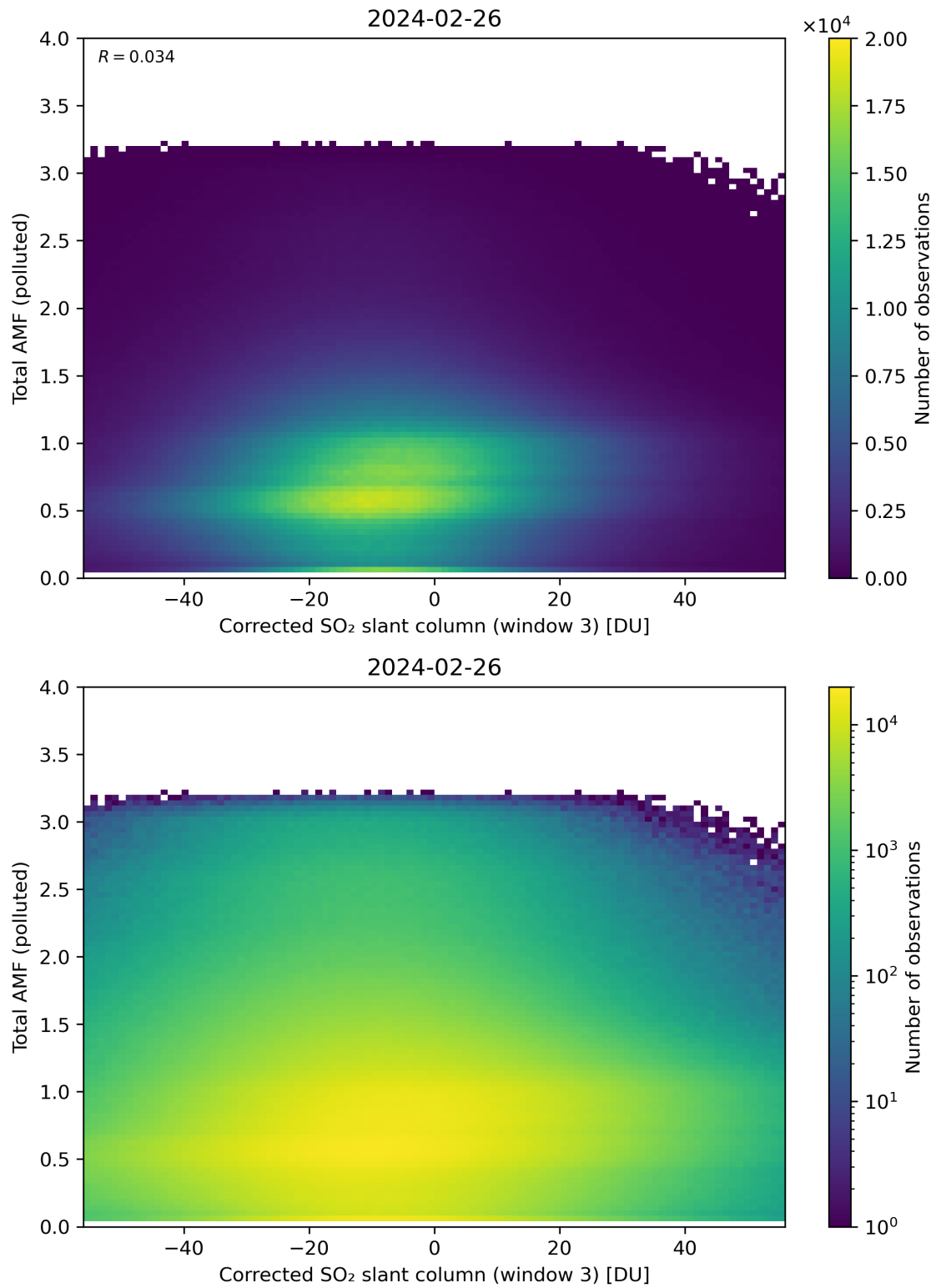
Figure 210: Scatter density plot of “Corrected SO 2 slant column (window 3)” against “Total AMF (polluted)” for 2024-02-25 to 2024-02-27.
