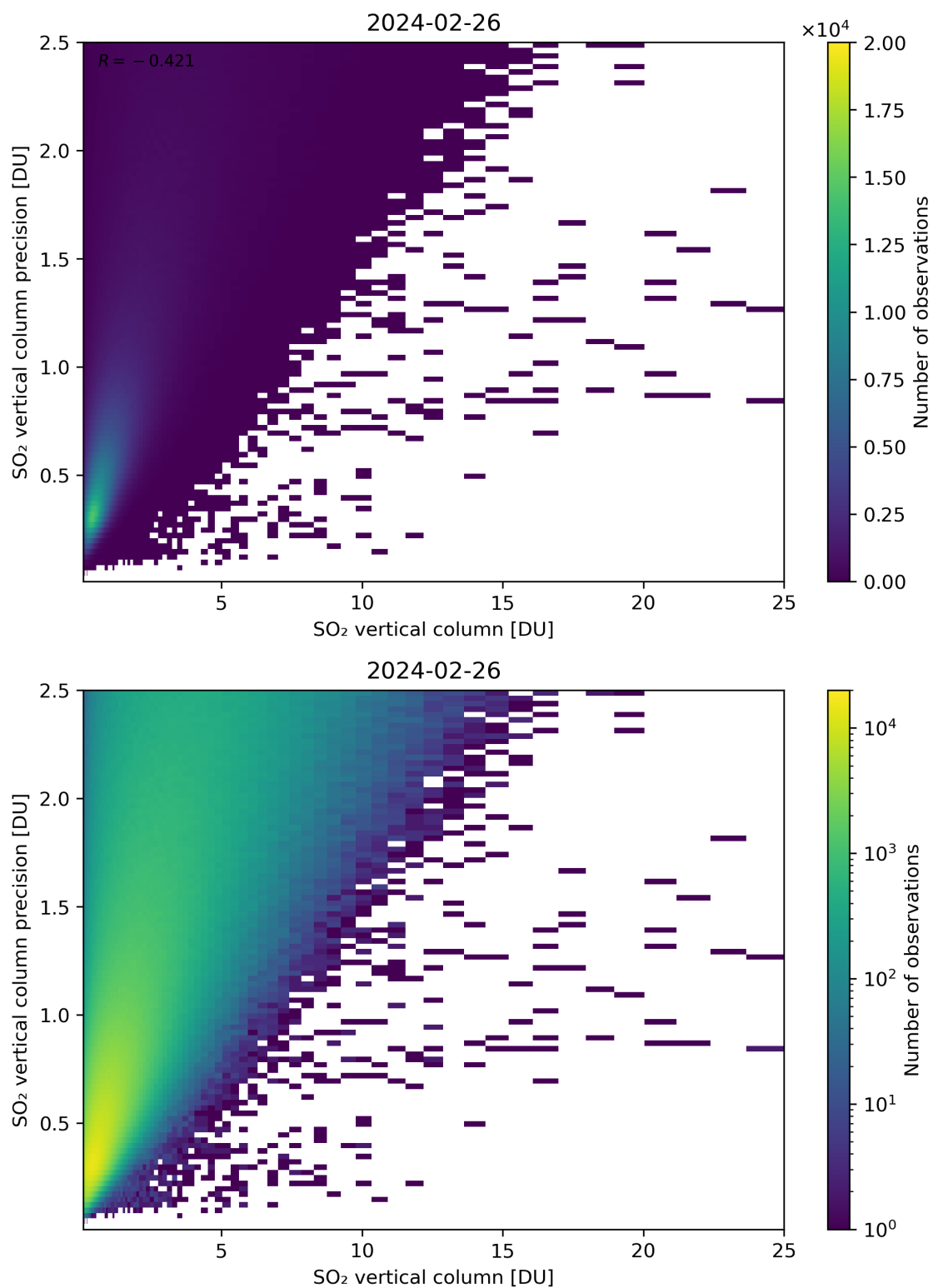
Figure 307: Scatter density plot of “SO 2 vertical column” against “SO 2 vertical column precision” for 2024-02-25 to 2024-02-27.
