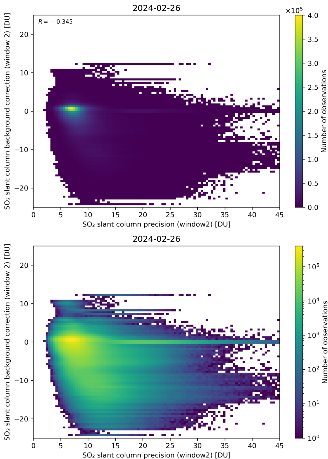
Figure 241: Scatter density plot of “SO 2 slant column precision (window2)” against “SO 2 slant column background correction (window 2)” for 2024-02-25 to 2024-02-27.
