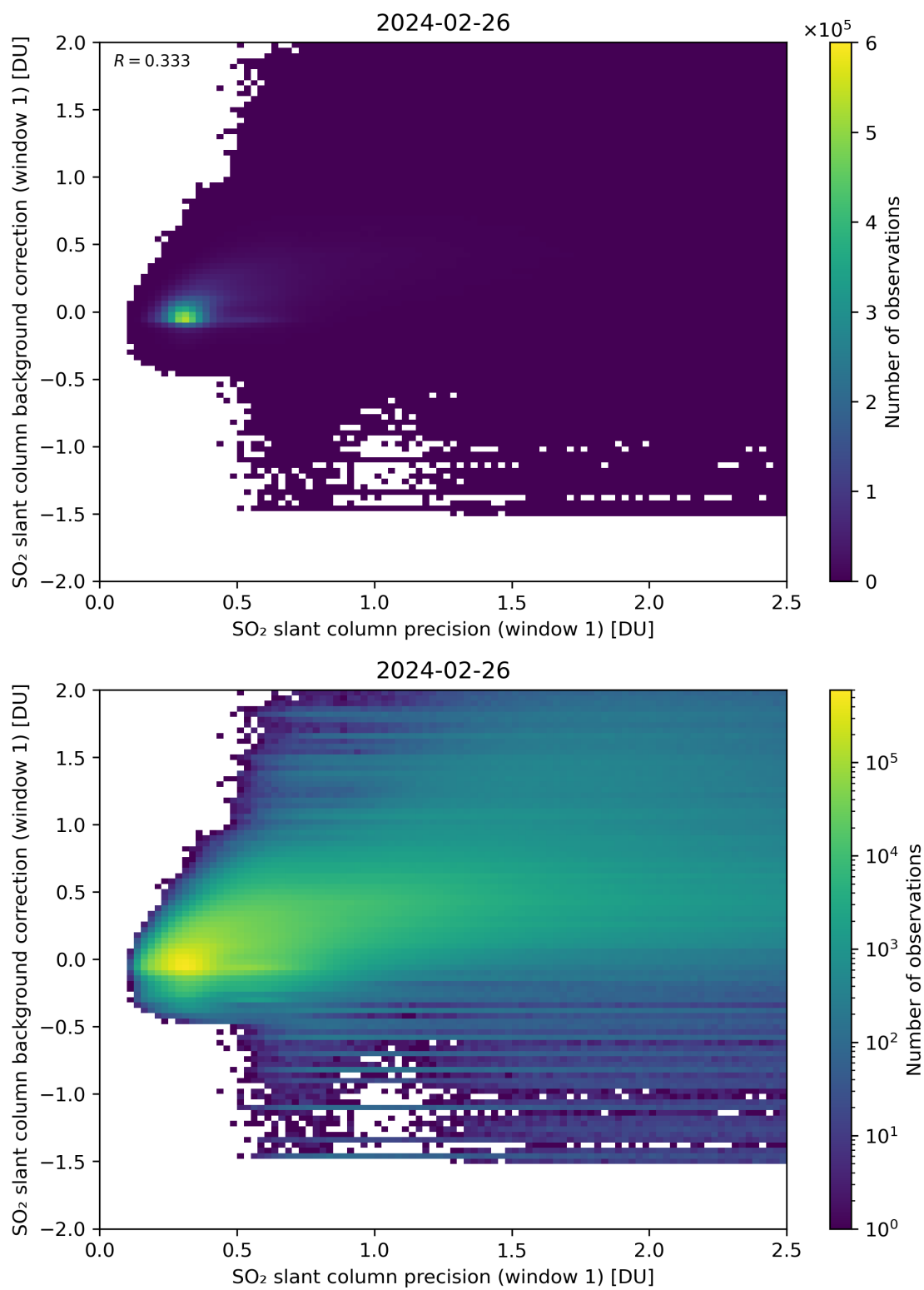
Figure 218: Scatter density plot of “SO 2 slant column precision (window 1)” against “SO 2 slant column background correction (window 1)” for 2024-02-25 to 2024-02-27.
