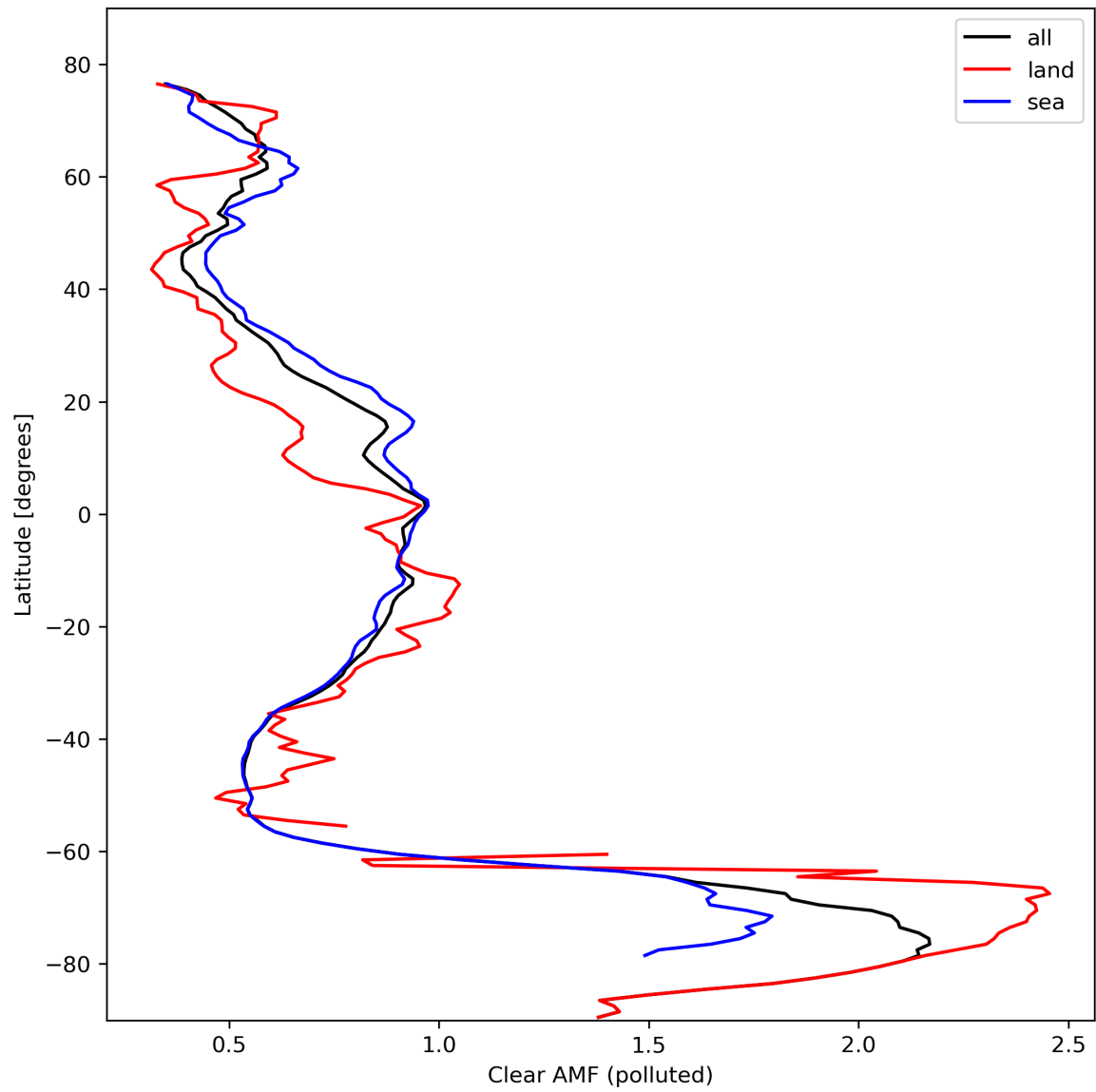
Figure 50: Zonal average of “Clear AMF (polluted)” for 2024-02-25 to 2024-02-27.
