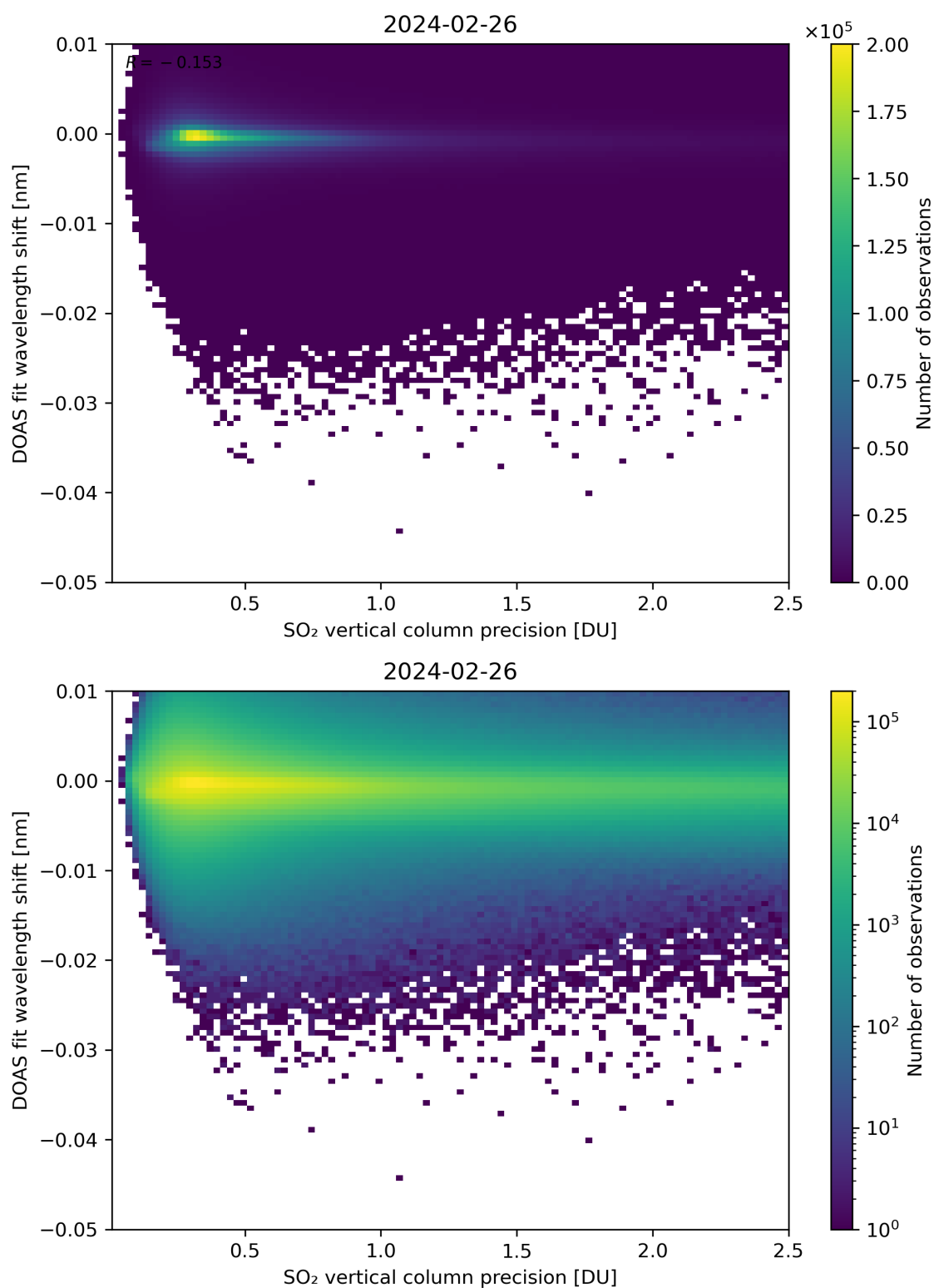
Figure 282: Scatter density plot of “SO 2 vertical column precision” against “DOAS fit wavelength shift” for 2024-02-25 to 2024-02-27.
