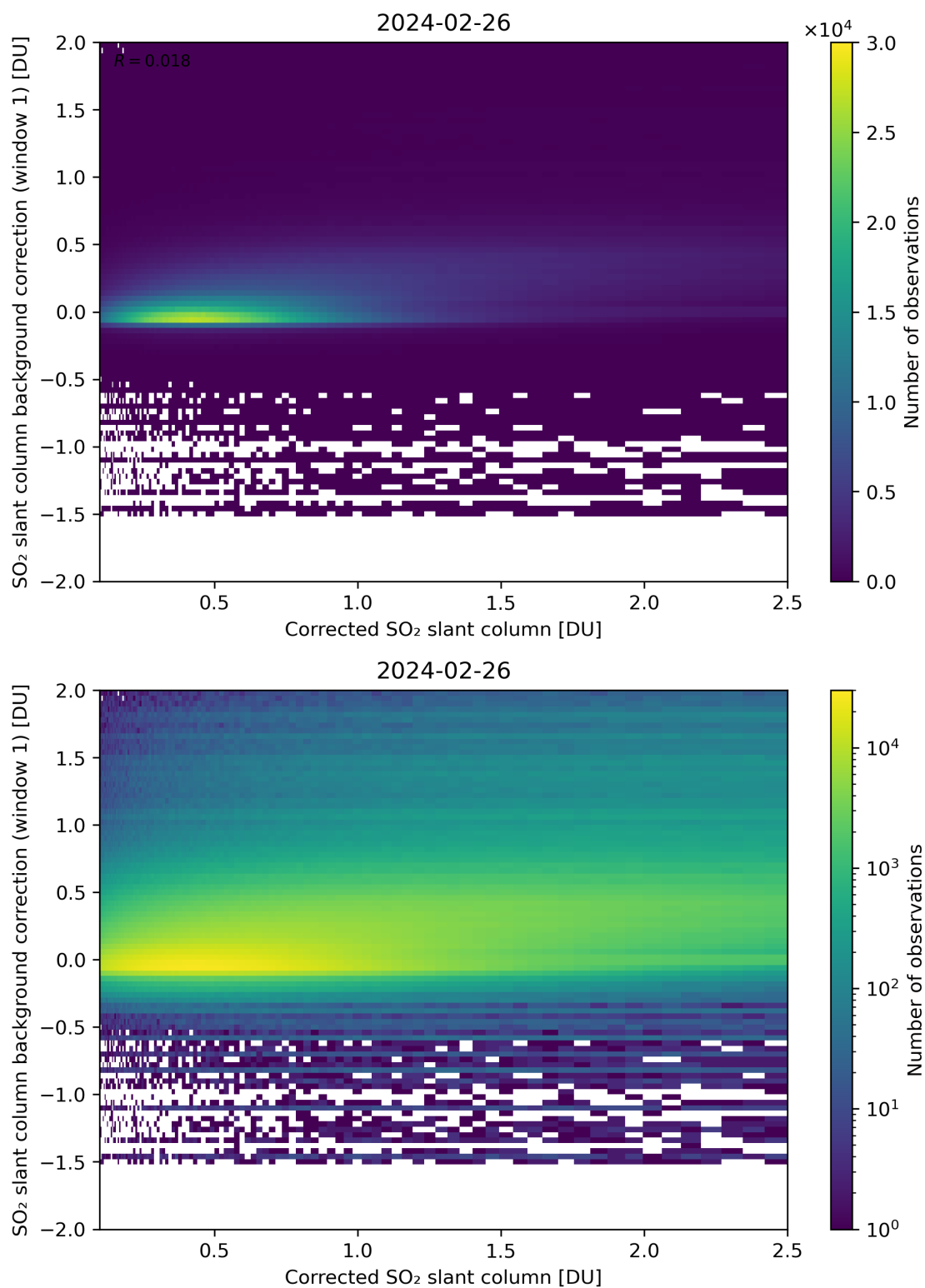
Figure 178: Scatter density plot of “Corrected SO 2 slant column” against “SO 2 slant column background correction (window 1)” for 2024-02-25 to 2024-02-27.
