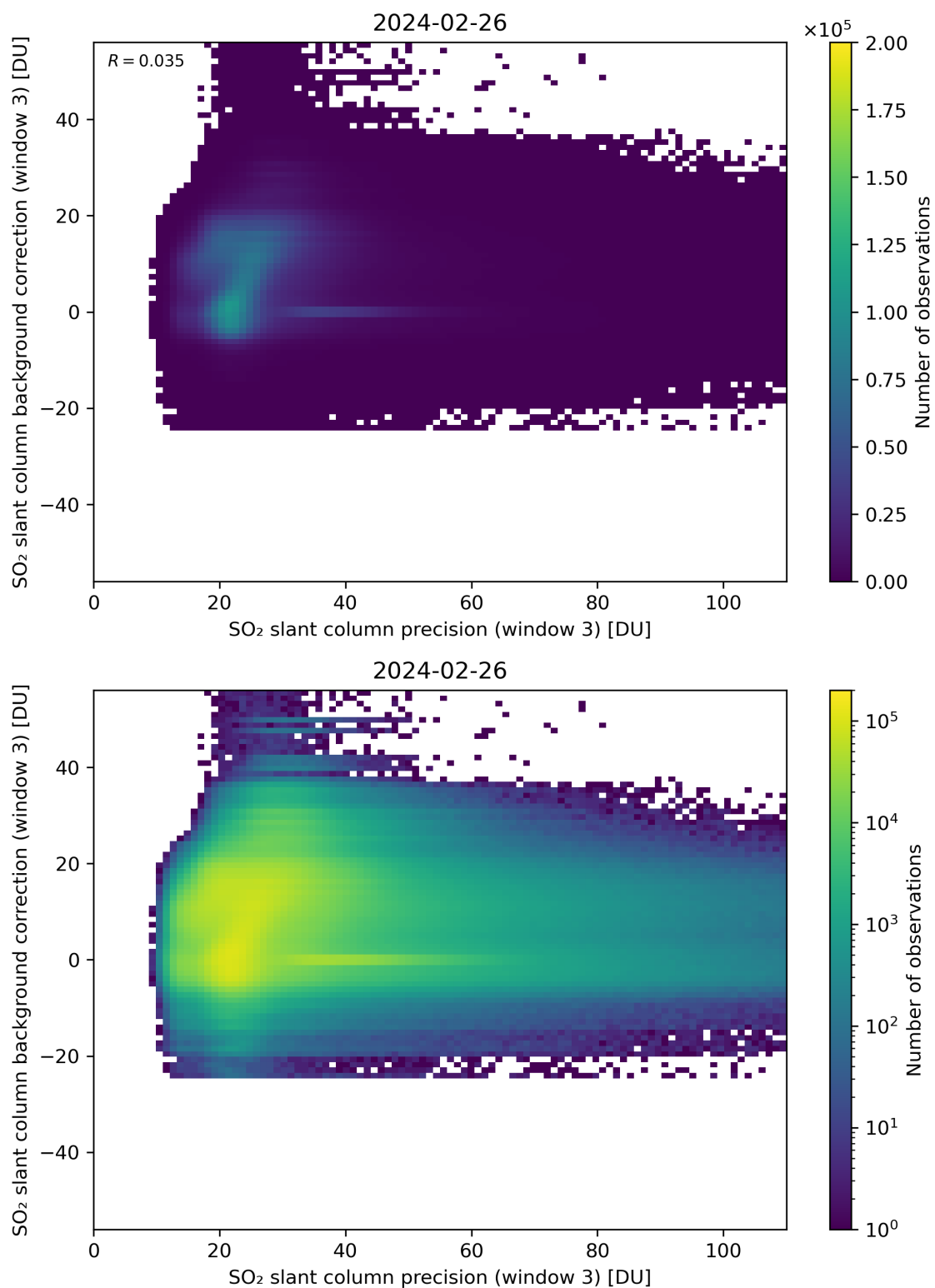
Figure 257: Scatter density plot of “SO 2 slant column precision (window 3)” against “SO 2 slant column background correction (window 3)” for 2024-02-25 to 2024-02-27.
