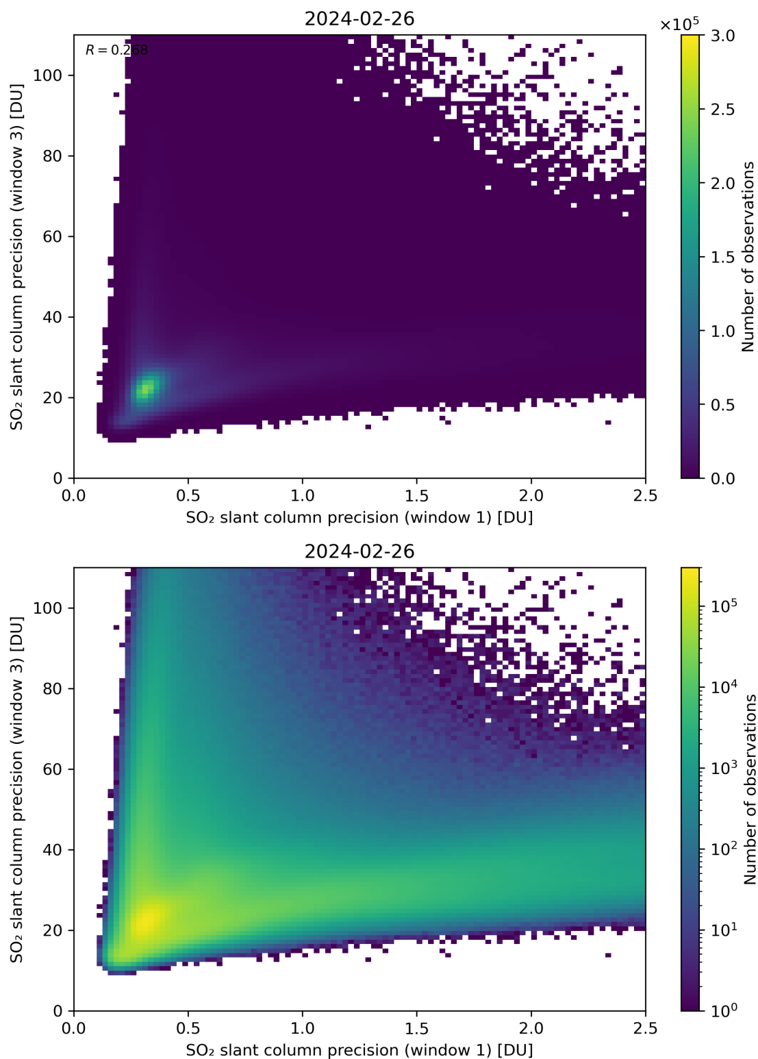
Figure 229: Scatter density plot of “SO 2 slant column precision (window 1)” against “SO 2 slant column precision (window 3)” for 2024-02-25 to 2024-02-27.
