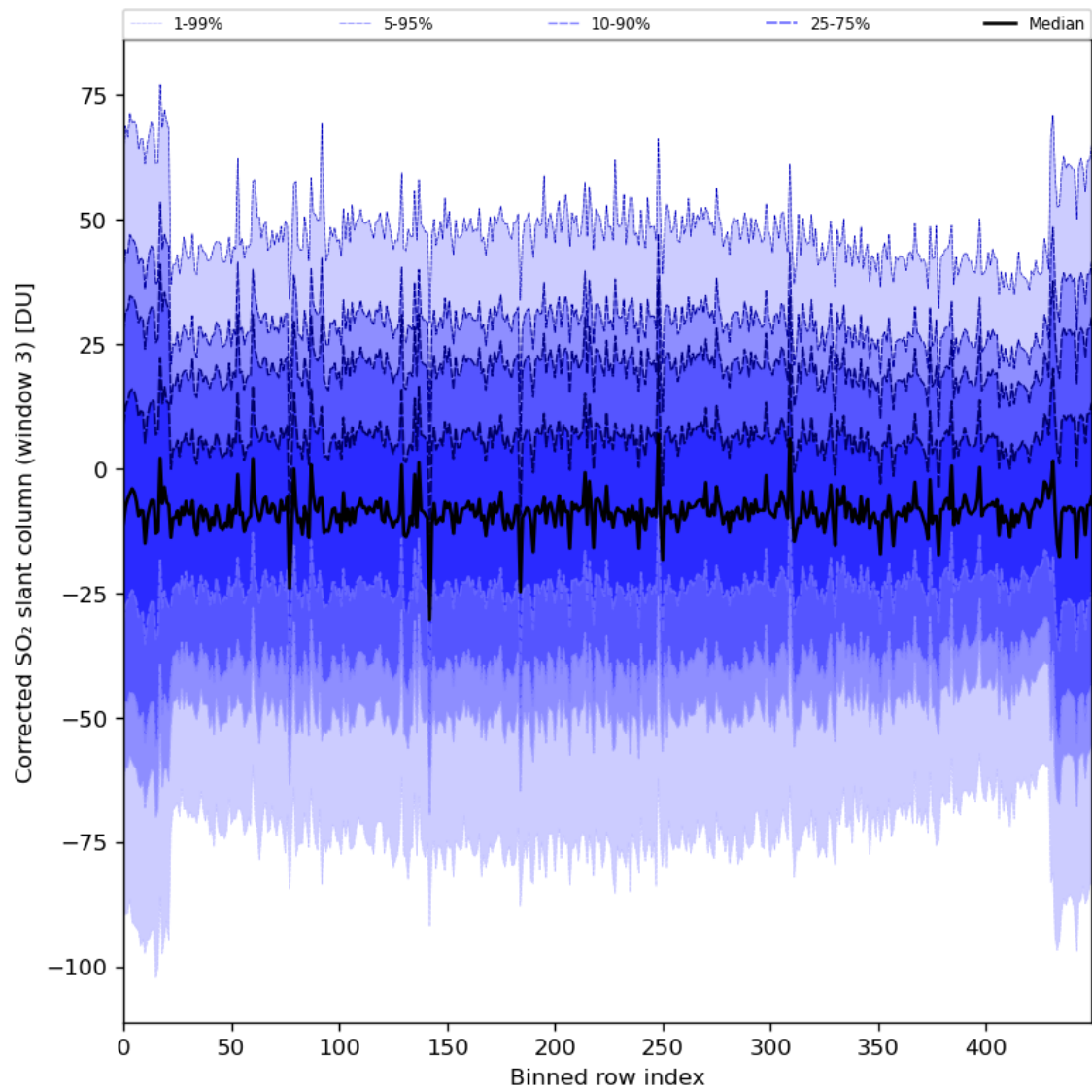
Figure 89: Along track statistics of “Corrected SO 2 slant column (window 3)” for 2024-02-25 to 2024-02-27
