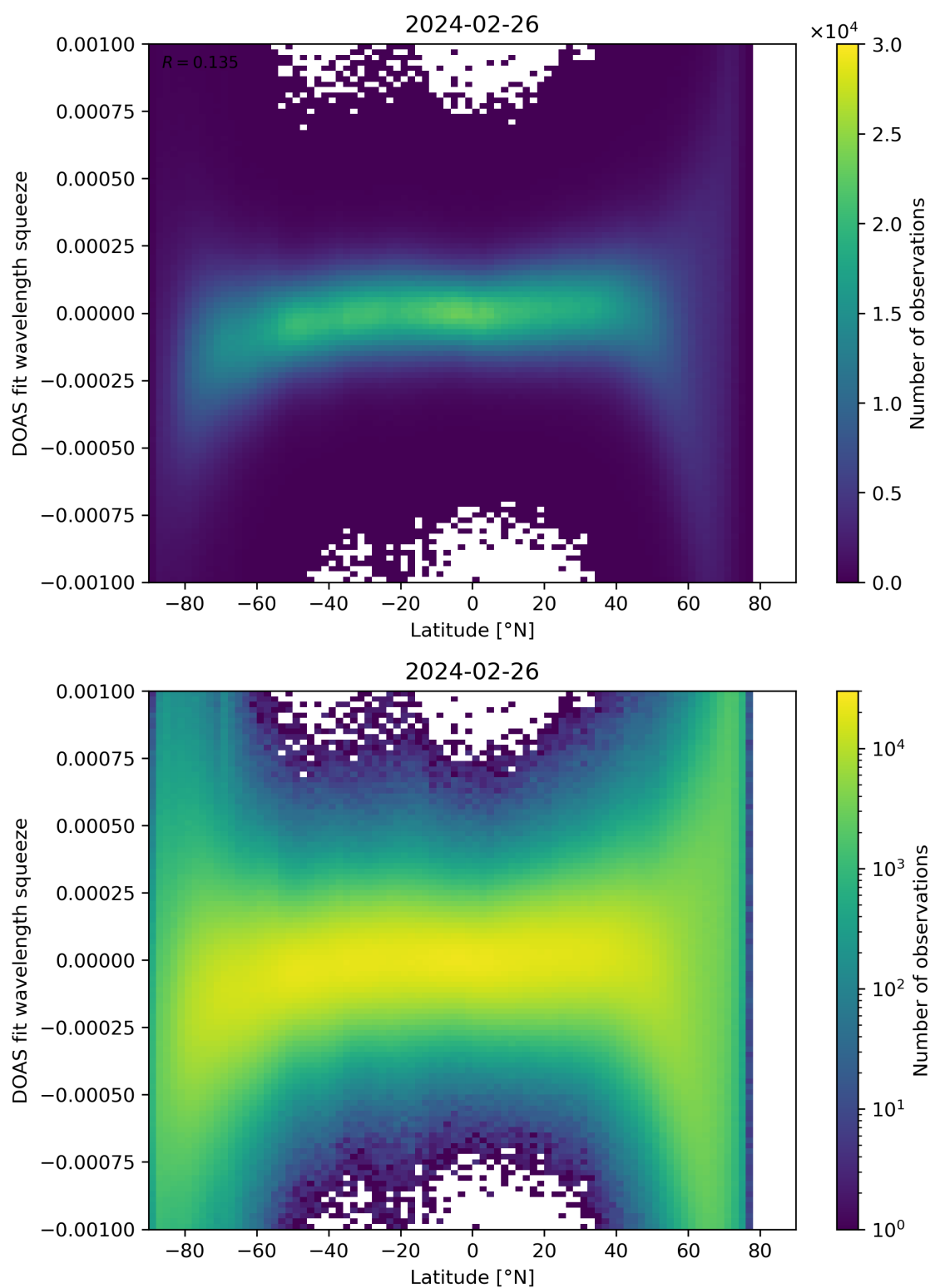
Figure 143: Scatter density plot of “Latitude” against “DOAS fit wavelength squeeze” for 2024-02-25 to 2024-02-27.
