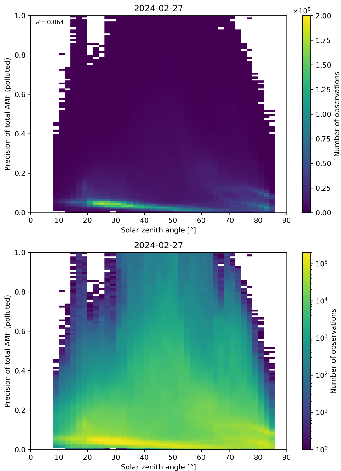
Figure 175: Scatter density plot of “Solar zenith angle” against “Precision of total AMF (polluted)” for 2024-02-27 to 2024-02-28.
