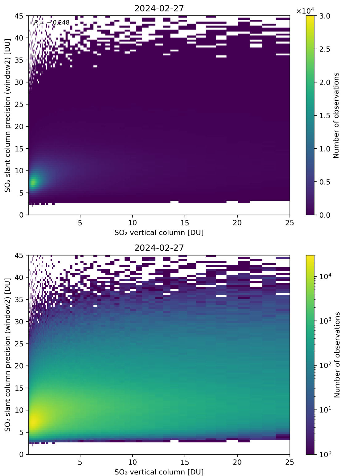
Figure 302: Scatter density plot of “SO 2 vertical column” against “SO 2 slant column precision (window2)” for 2024-02-27 to 2024-02-28.
