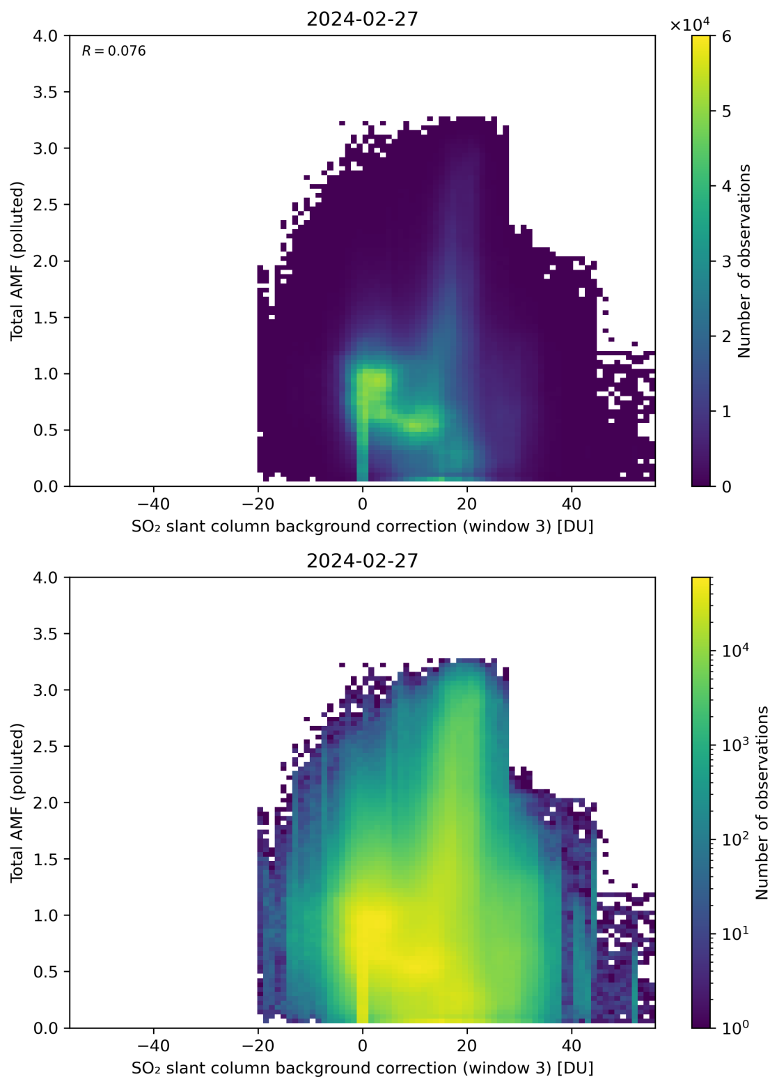
Figure 125: Scatter density plot of “SO 2 slant column background correction (window 3)” against “Total AMF (polluted)” for 2024-02-27 to 2024-02-28.
