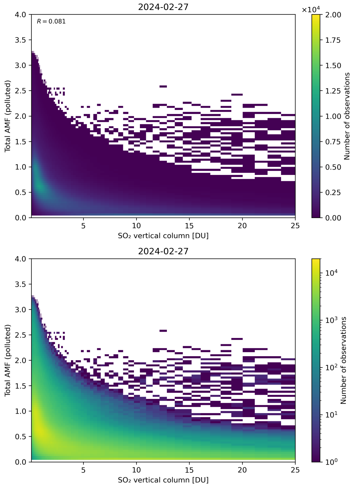
Figure 305: Scatter density plot of “SO 2 vertical column” against “Total AMF (polluted)” for 2024-02-27 to 2024-02-28.
