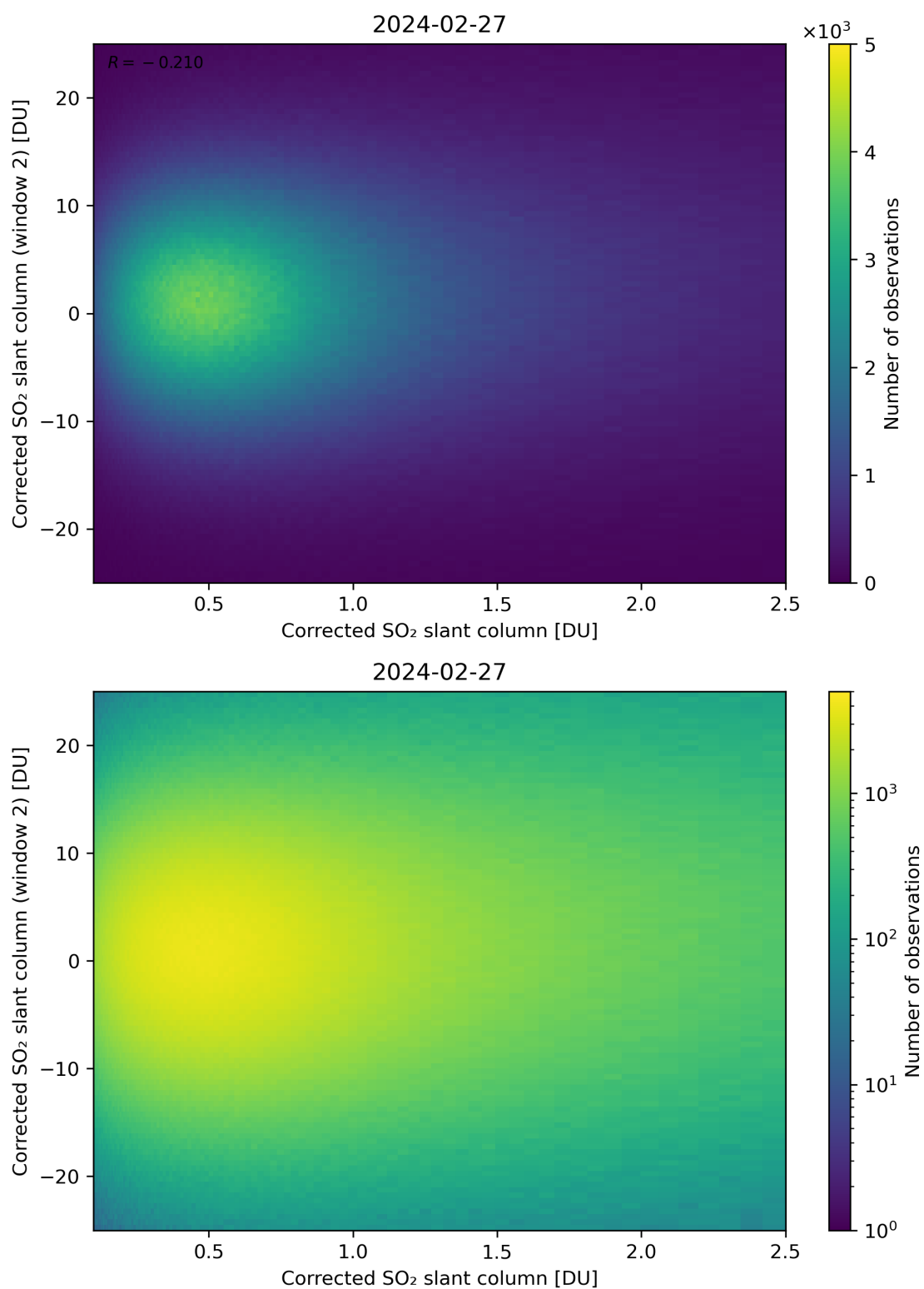
Figure 185: Scatter density plot of “Corrected SO 2 slant column” against “Corrected SO 2 slant column (window 2)” for 2024-02-27 to 2024-02-28.
