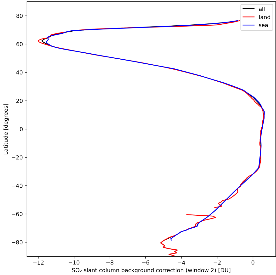
Figure 40: Zonal average of “SO 2 slant column background correction (window 2)” for 2024-02-27 to 2024-02-28.
