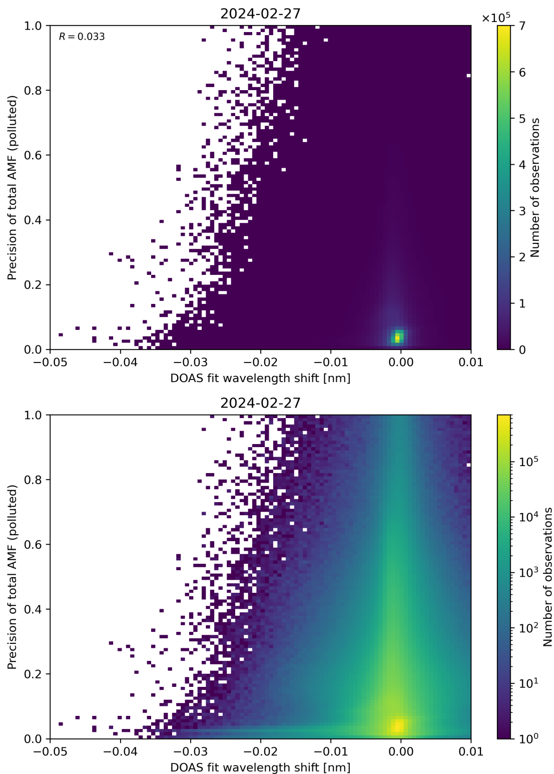
Figure 131: Scatter density plot of “DOAS fit wavelength shift” against “Precision of total AMF (polluted)” for 2024-02-27 to 2024-02-28.
