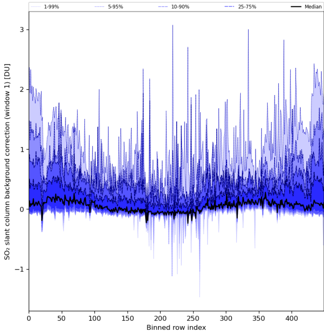
Figure 82: Along track statistics of “SO 2 slant column background correction (window 1)” for 2024-02-27 to 2024-02-28
