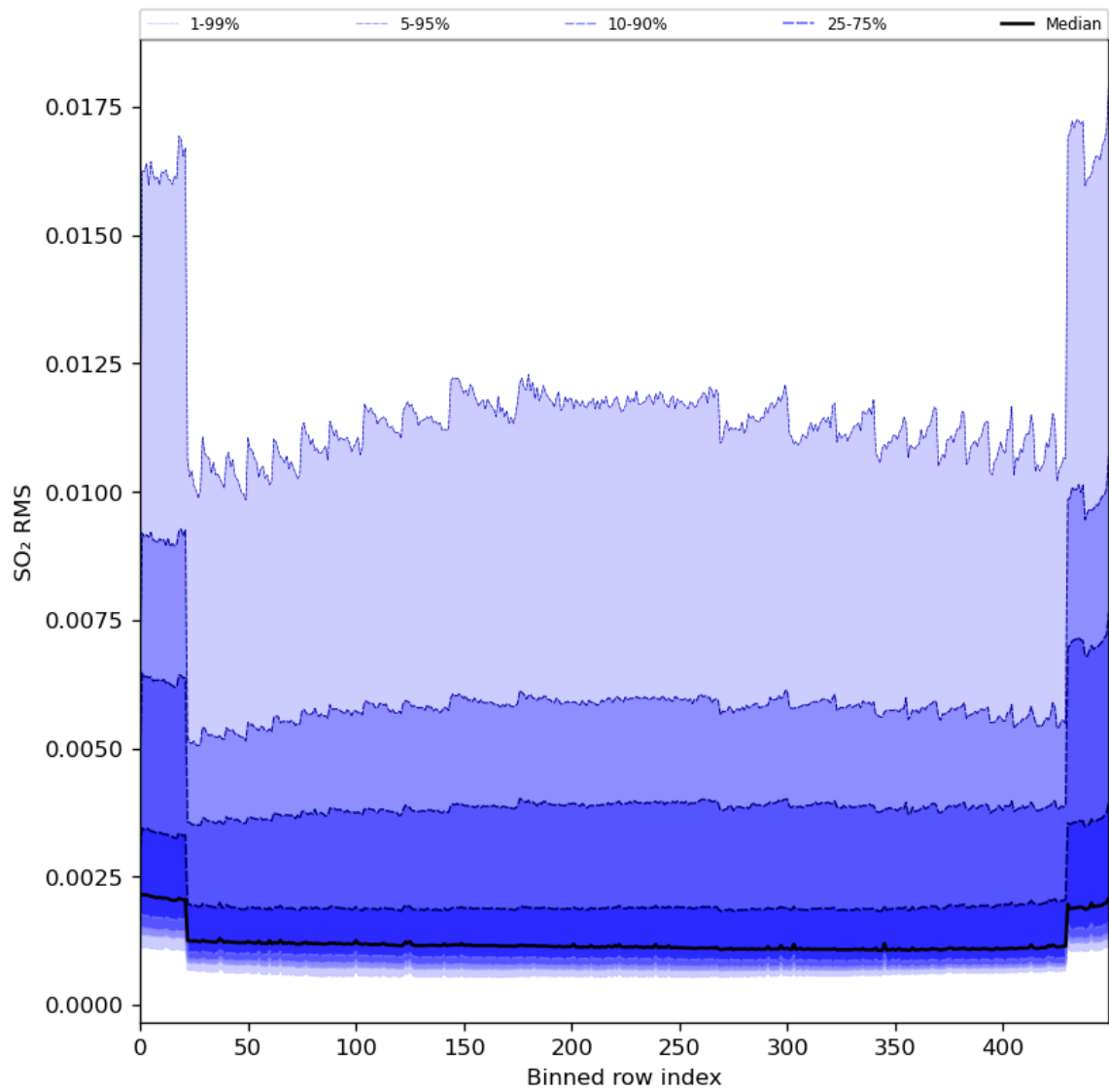
Figure 93: Along track statistics of “SO 2 RMS” for 2024-02-27 to 2024-02-28
