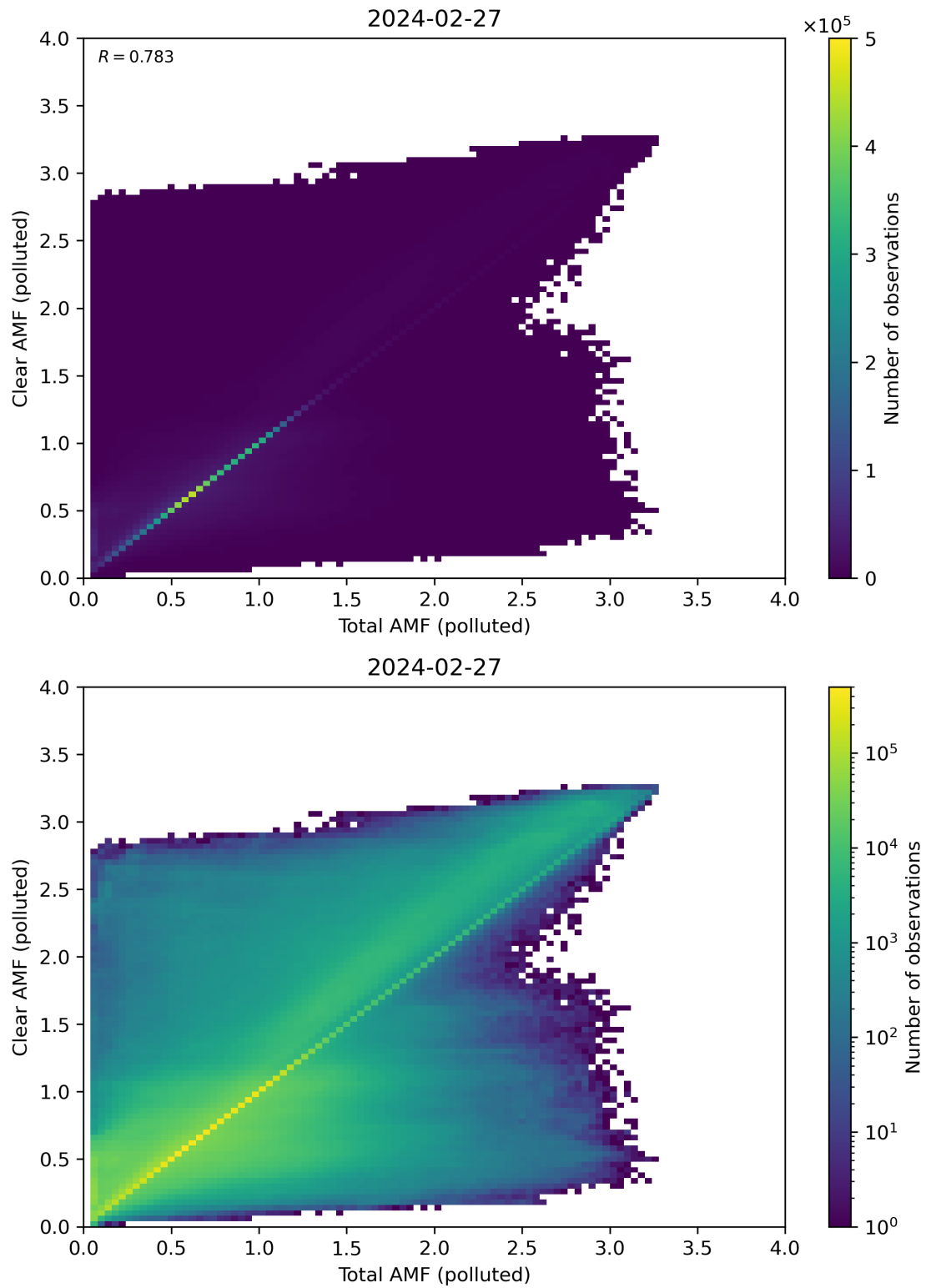
Figure 271: Scatter density plot of “Total AMF (polluted)” against “Clear AMF (polluted)” for 2024-02-27 to 2024-02-28.
