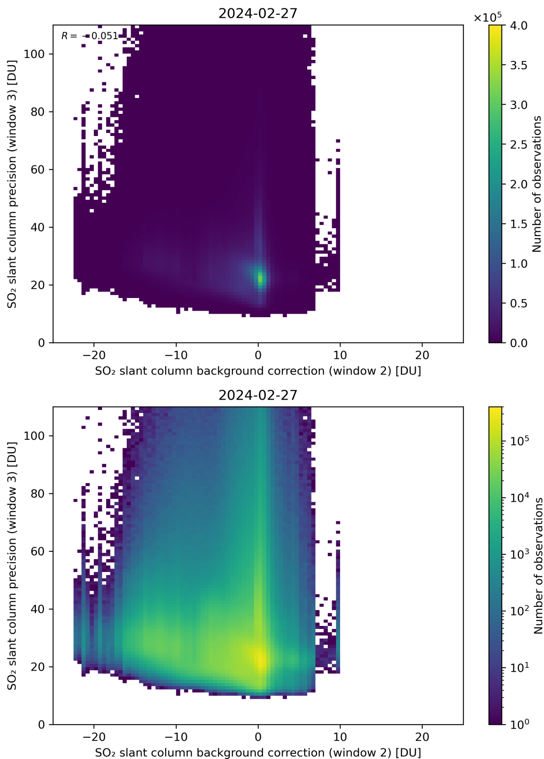
Figure 118: Scatter density plot of “SO 2 slant column background correction (window 2)” against “SO 2 slant column precision (window 3)” for 2024-02-27 to 2024-02-28.
