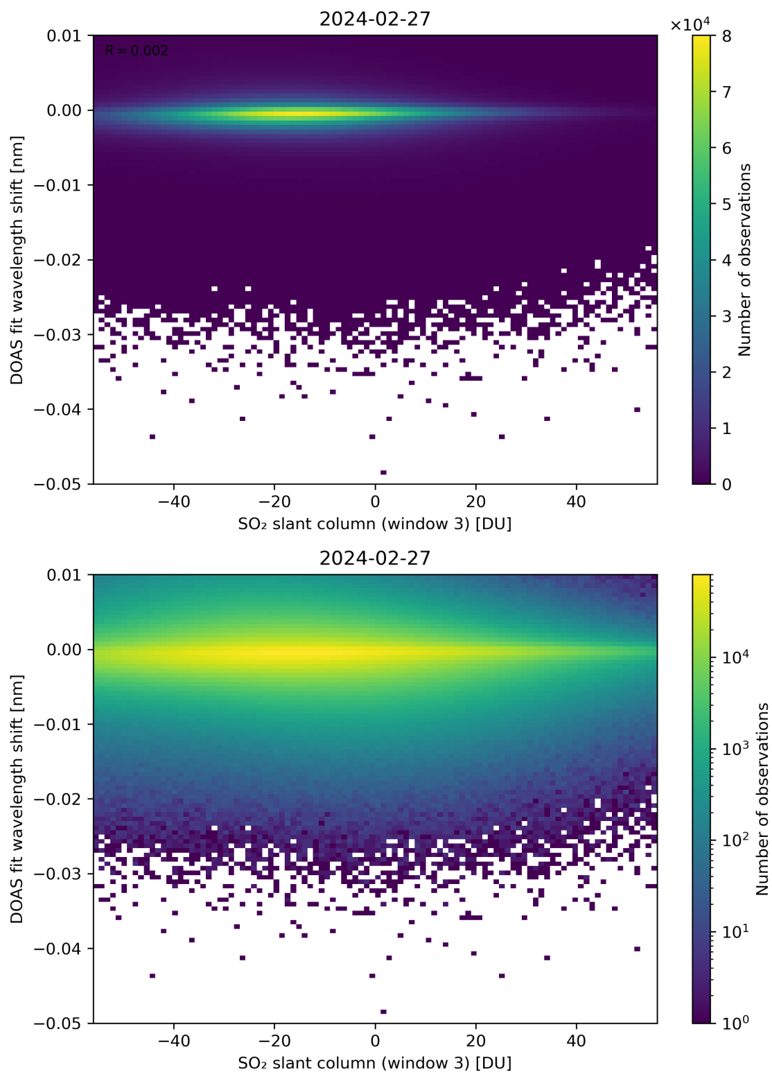
Figure 254: Scatter density plot of “SO 2 slant column (window 3)” against “DOAS fit wavelength shift” for 2024-02-27 to 2024-02-28.
