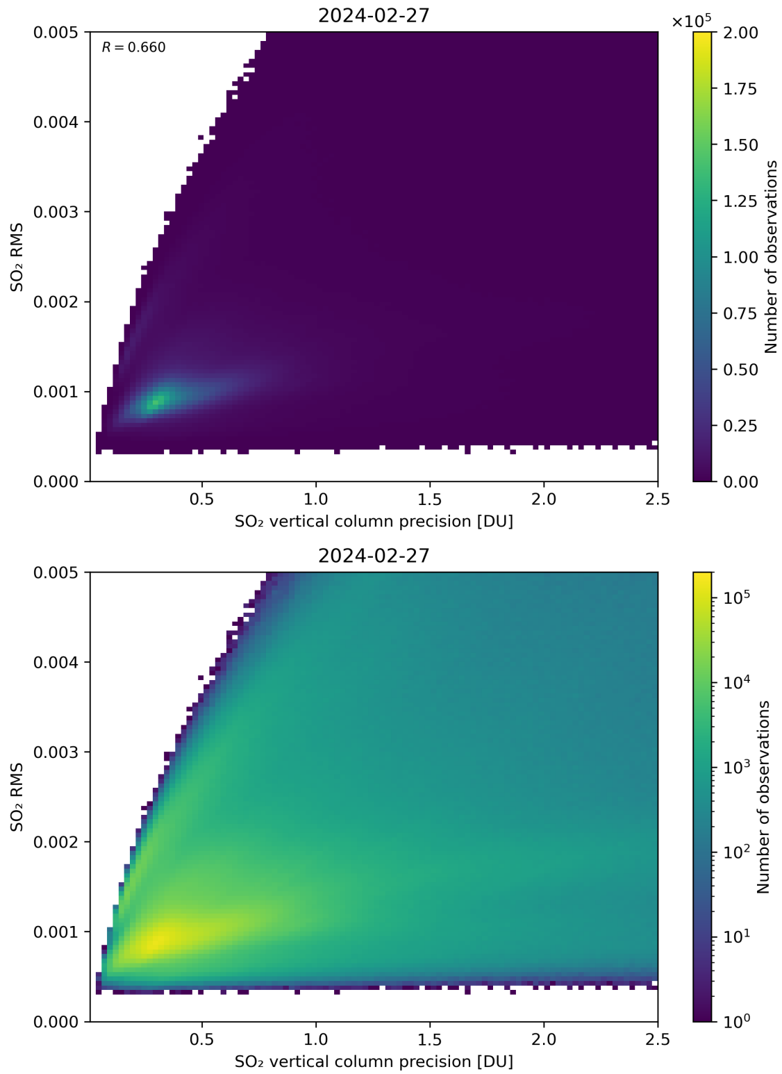
Figure 284: Scatter density plot of “SO 2 vertical column precision” against “SO 2 RMS” for 2024-02-27 to 2024-02-28.
