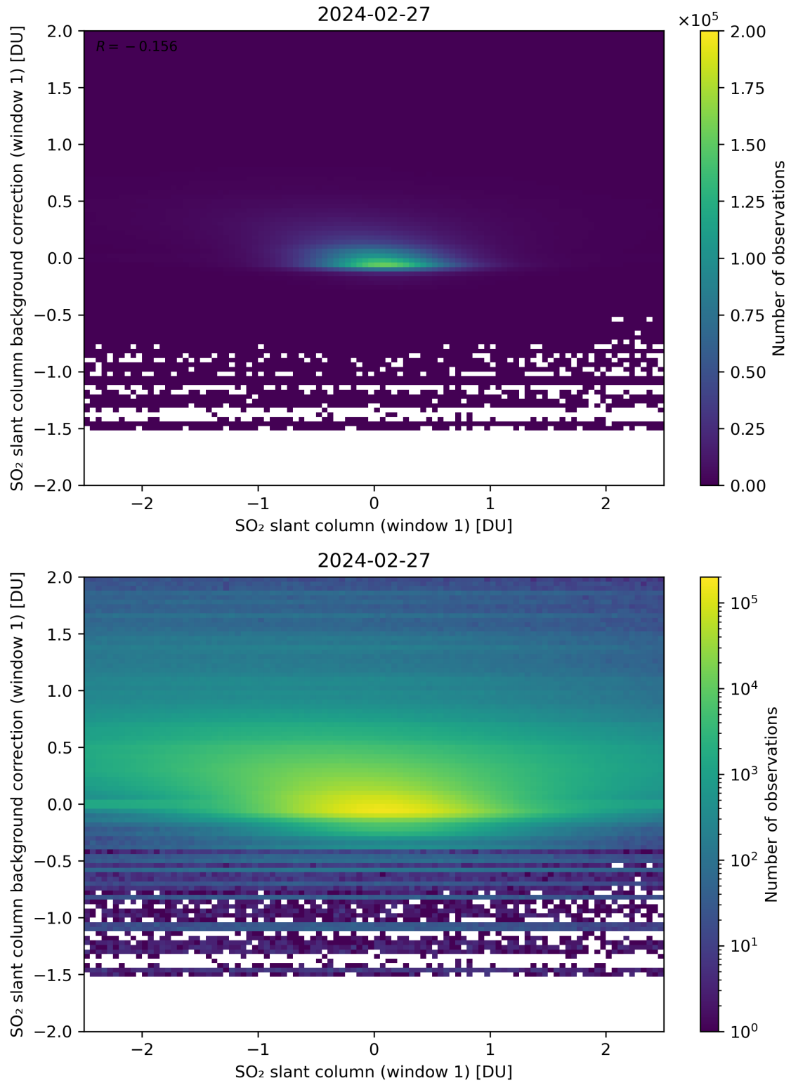
Figure 212: Scatter density plot of “SO 2 slant column (window 1)” against “SO 2 slant column background correction (window 1)” for 2024-02-27 to 2024-02-28.
