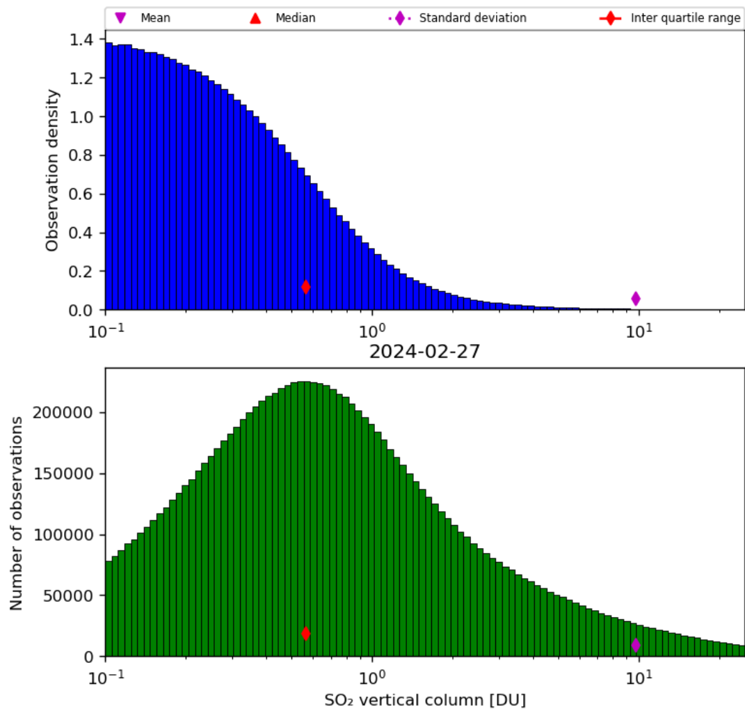
Figure 53: Histogram of “SO 2 vertical column” for 2024-02-27 to 2024-02-28
