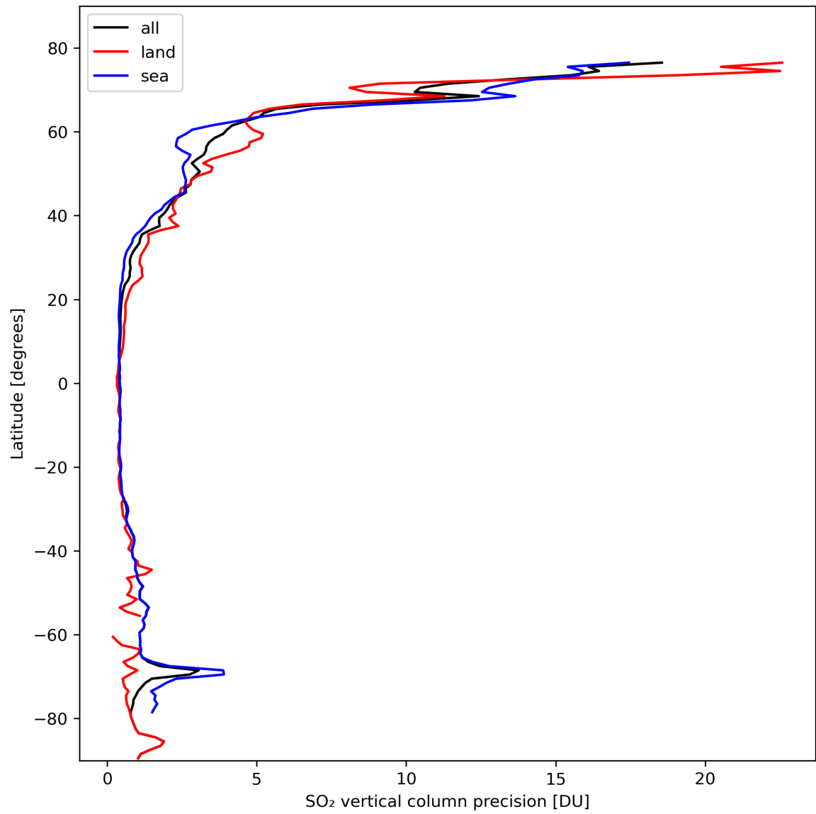
Figure 31: Zonal average of “SO 2 vertical column precision” for 2024-02-27 to 2024-02-28.
