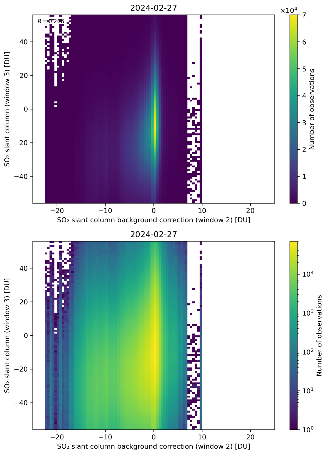
Figure 117: Scatter density plot of “SO 2 slant column background correction (window 2)” against “SO 2 slant column (window 3)” for 2024-02-27 to 2024-02-28.
