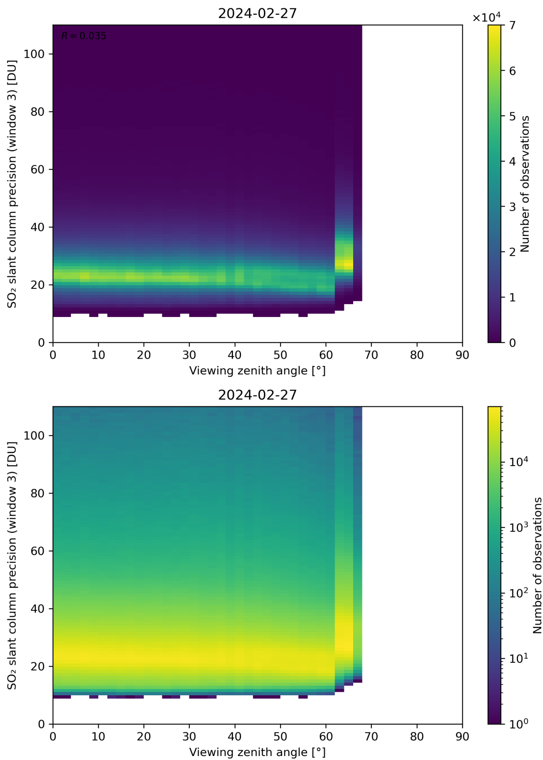
Figure 324: Scatter density plot of “Viewing zenith angle” against “SO 2 slant column precision (window 3)” for 2024-02-27 to 2024-02-28.
