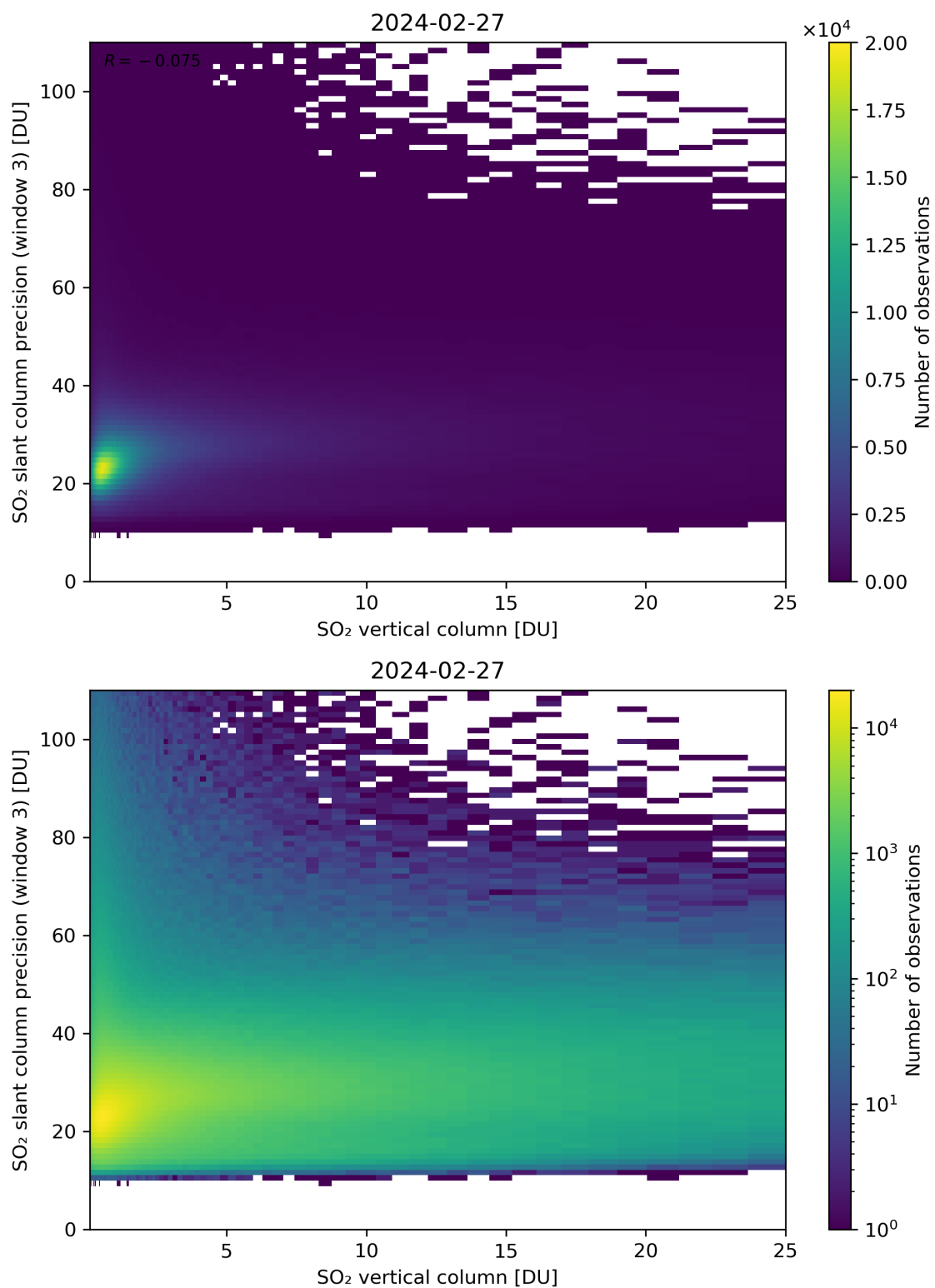
Figure 304: Scatter density plot of “SO 2 vertical column” against “SO 2 slant column precision (window 3)” for 2024-02-27 to 2024-02-28.
