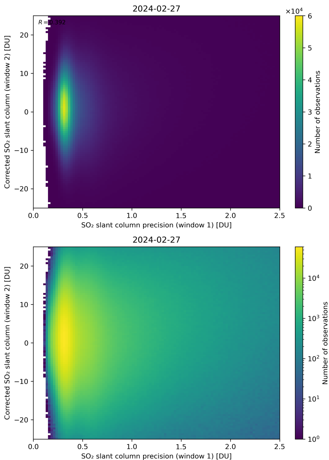
Figure 225: Scatter density plot of “SO 2 slant column precision (window 1)” against “Corrected SO 2 slant column (window 2)” for 2024-02-27 to 2024-02-28.
