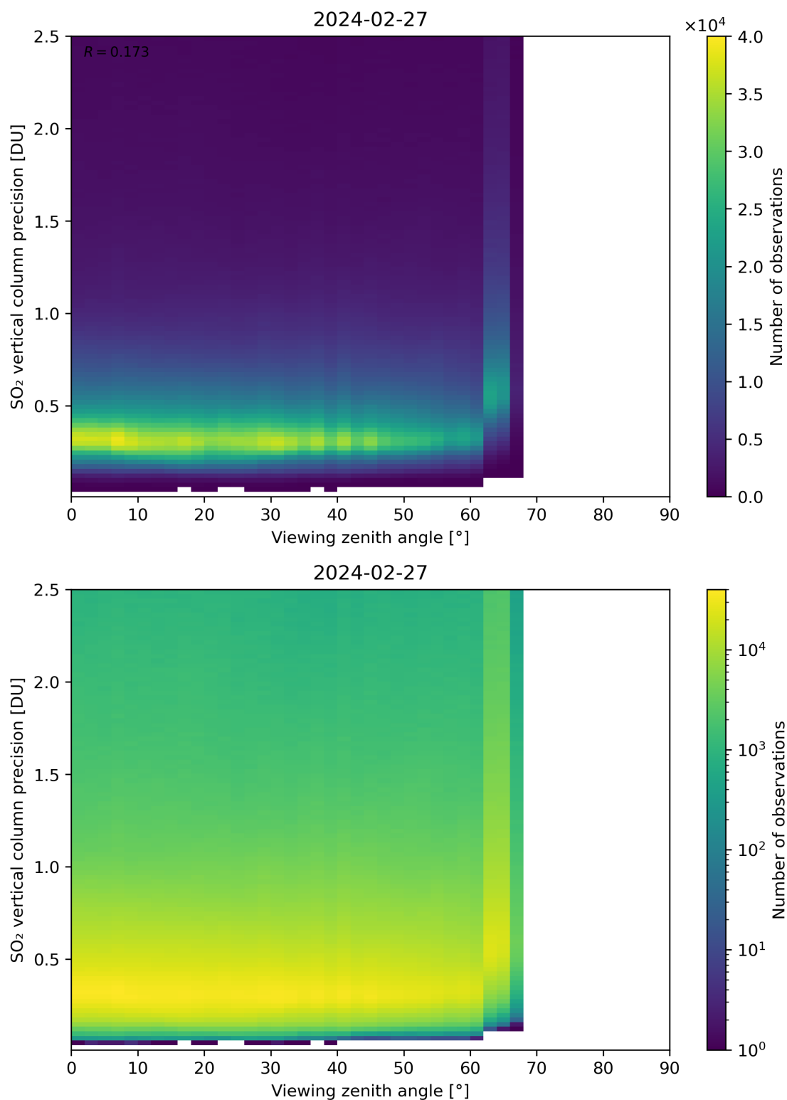
Figure 328: Scatter density plot of “Viewing zenith angle” against “SO 2 vertical column precision” for 2024-02-27 to 2024-02-28.
