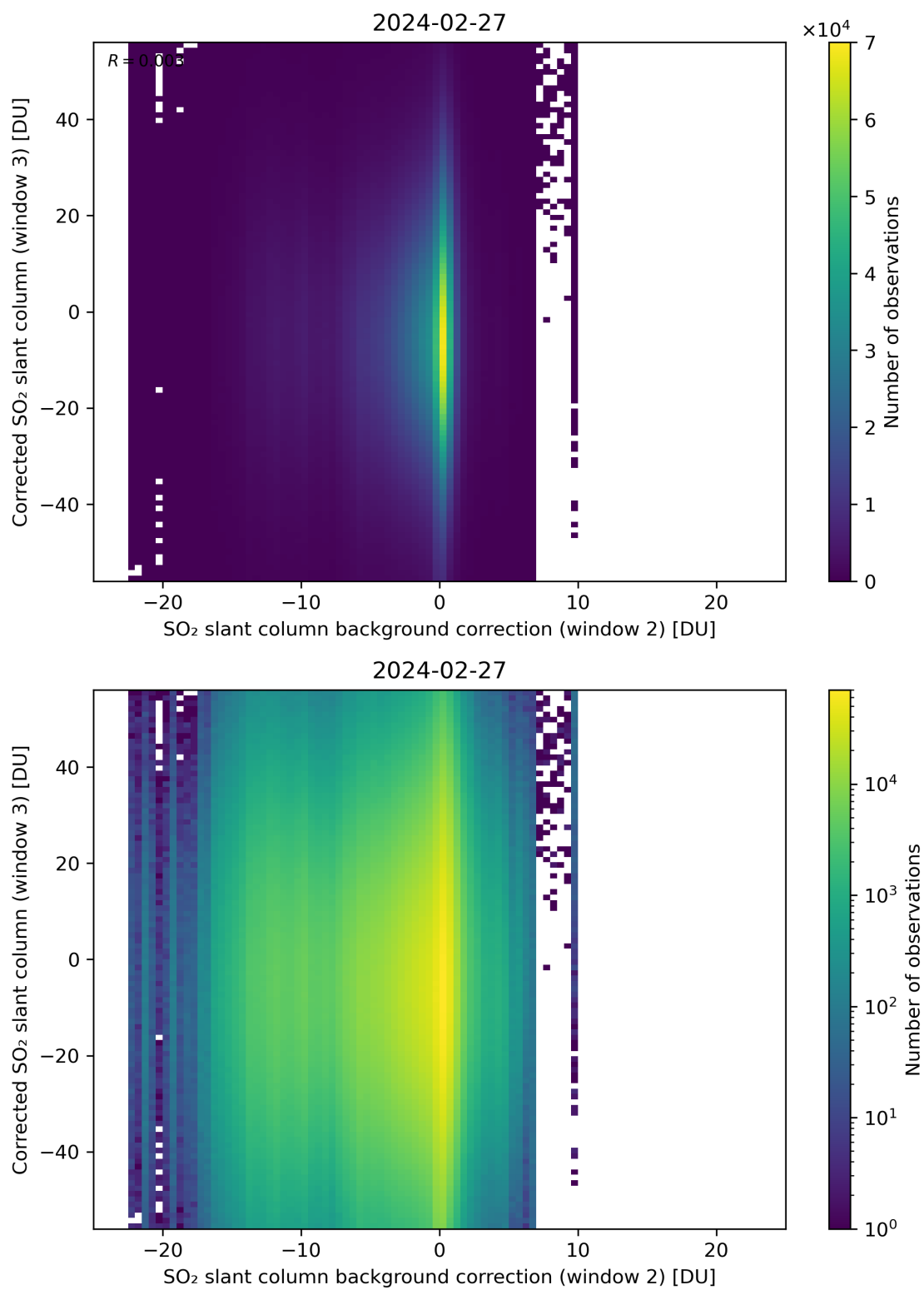
Figure 116: Scatter density plot of “SO 2 slant column background correction (window 2)” against “Corrected SO 2 slant column (window 3)” for 2024-02-27 to 2024-02-28.
