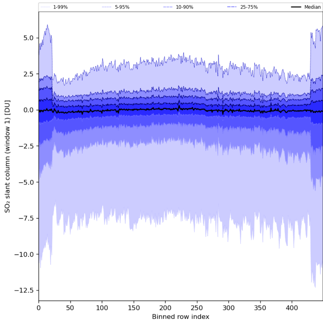
Figure 79: Along track statistics of “SO 2 slant column (window 1)” for 2024-02-27 to 2024-02-28
