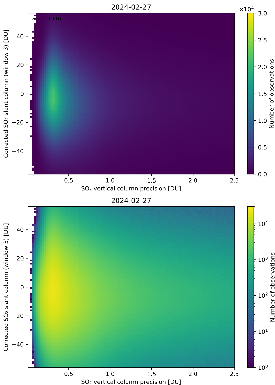
Figure 288: Scatter density plot of “SO 2 vertical column precision” against “Corrected SO 2 slant column (window 3)” for 2024-02-27 to 2024-02-28.
