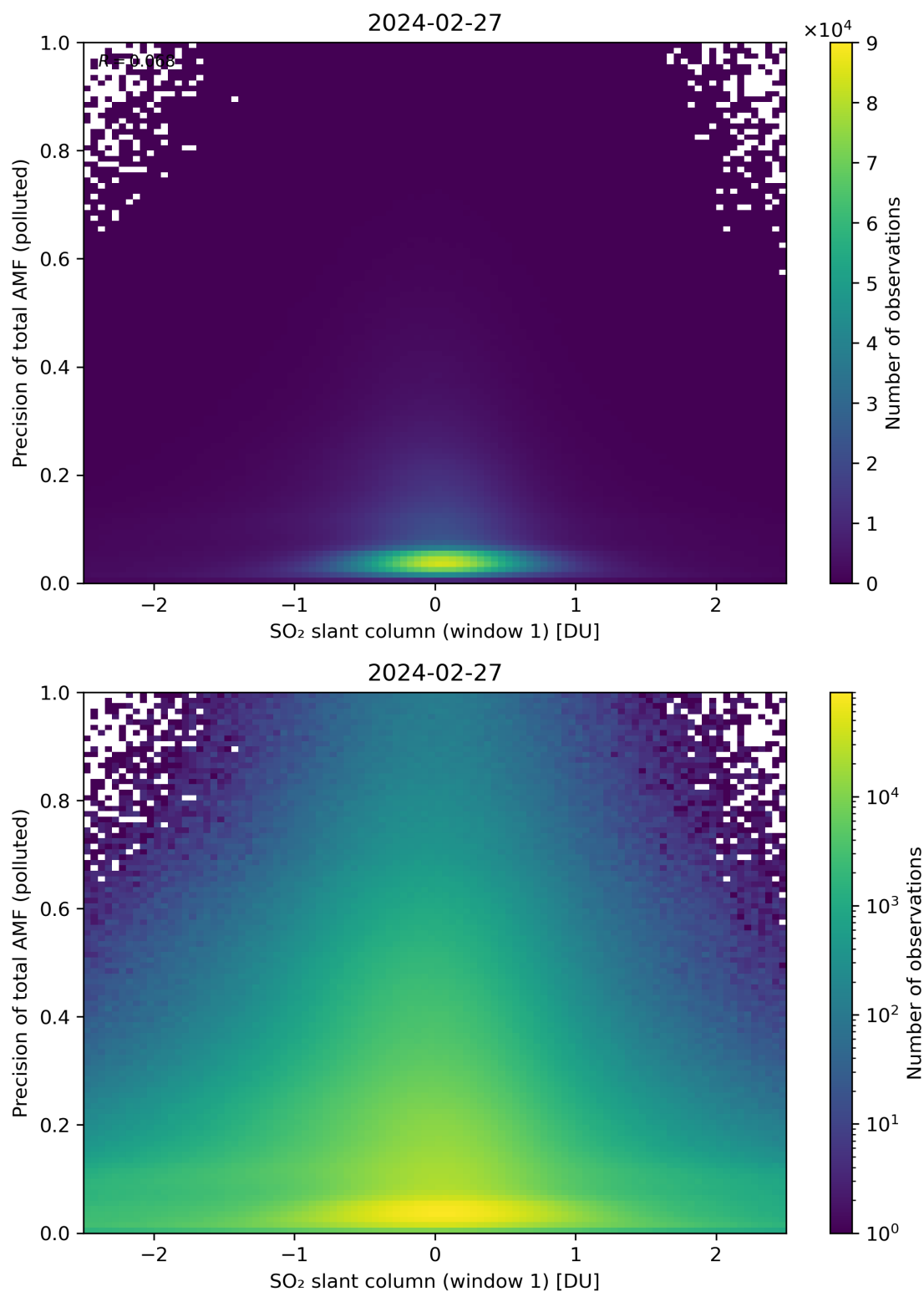
Figure 240: Scatter density plot of “SO 2 slant column (window 1)” against “Precision of total AMF (polluted)” for 2024-02-27 to 2024-02-28.
