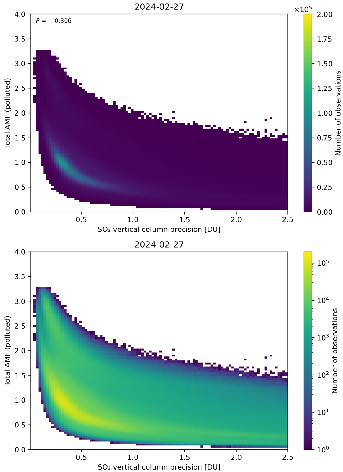
Figure 294: Scatter density plot of “SO 2 vertical column precision” against “Total AMF (polluted)” for 2024-02-27 to 2024-02-28.
