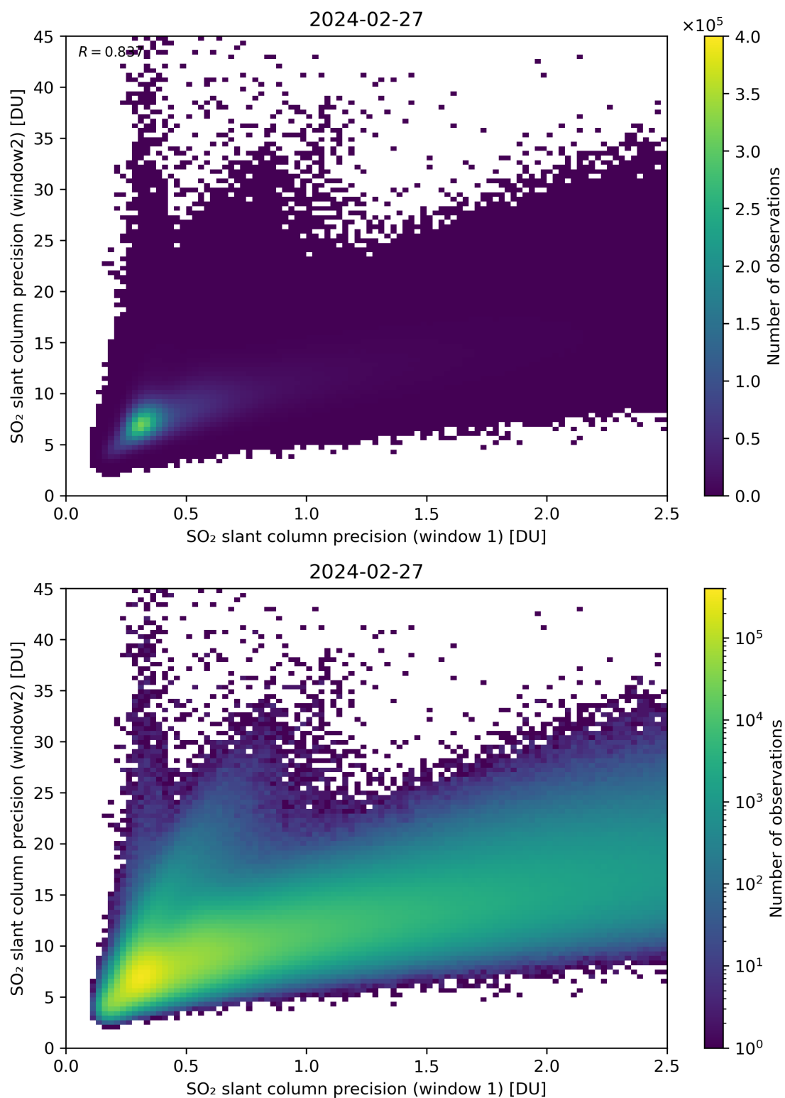
Figure 227: Scatter density plot of “SO 2 slant column precision (window 1)” against “SO 2 slant column precision (window2)” for 2024-02-27 to 2024-02-28.
