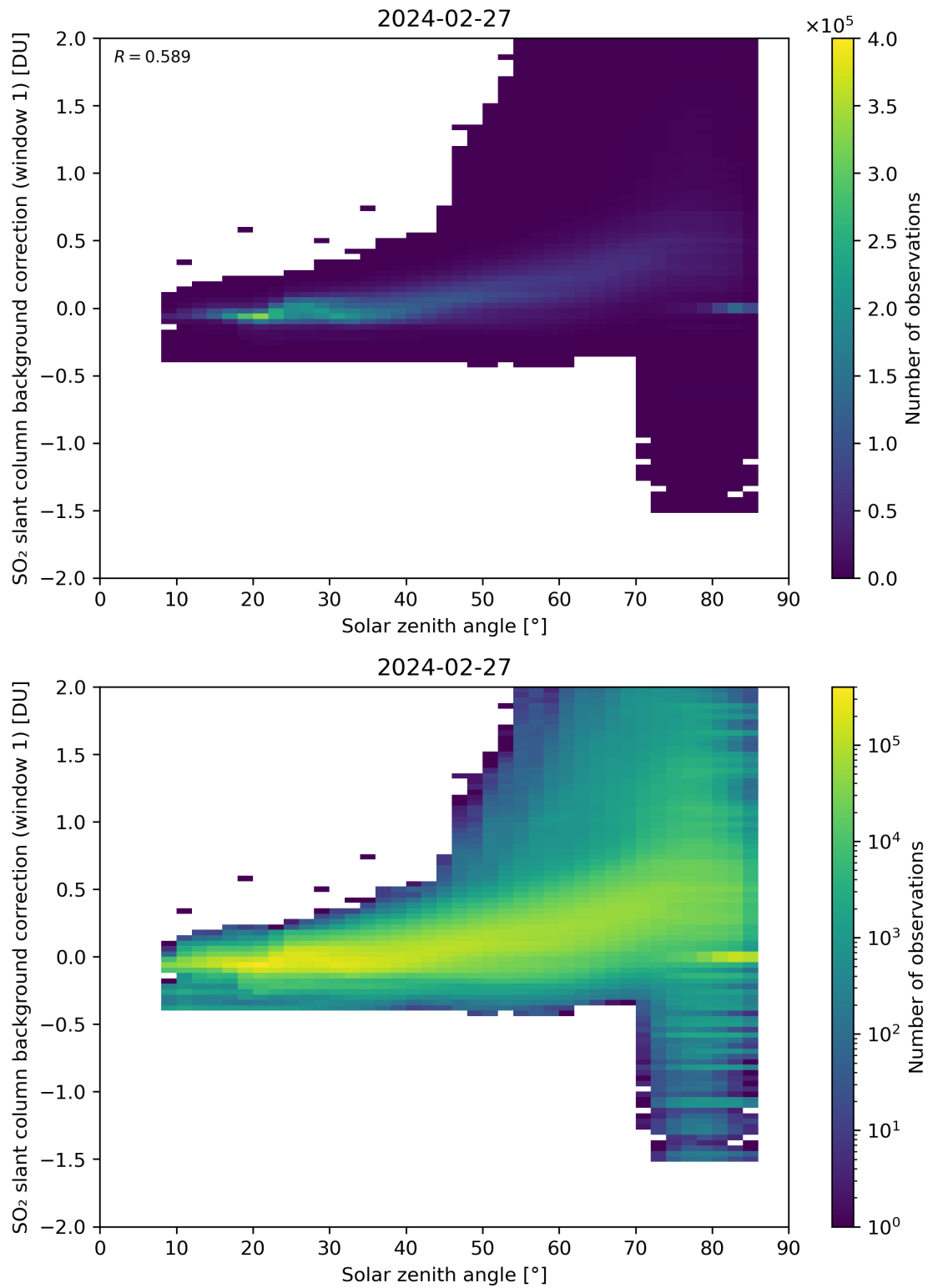
Figure 158: Scatter density plot of “Solar zenith angle” against “SO 2 slant column background correction (window 1)” for 2024-02-27 to 2024-02-28.
