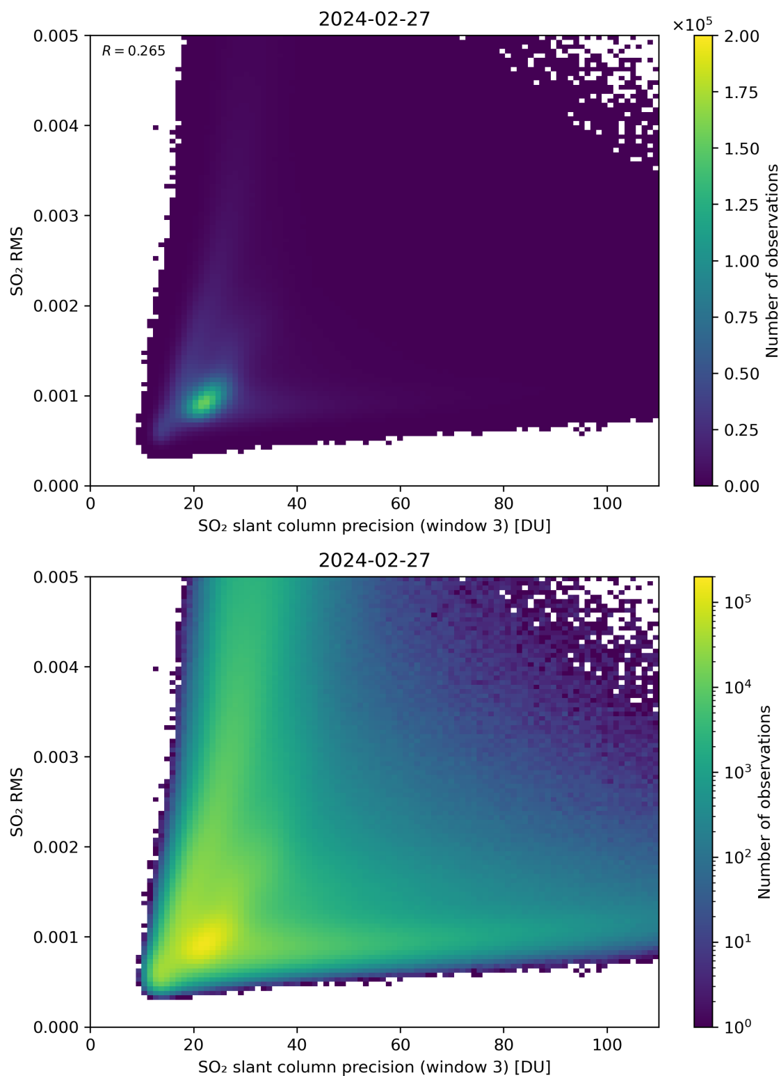
Figure 260: Scatter density plot of “SO 2 slant column precision (window 3)” against “SO 2 RMS” for 2024-02-27 to 2024-02-28.
