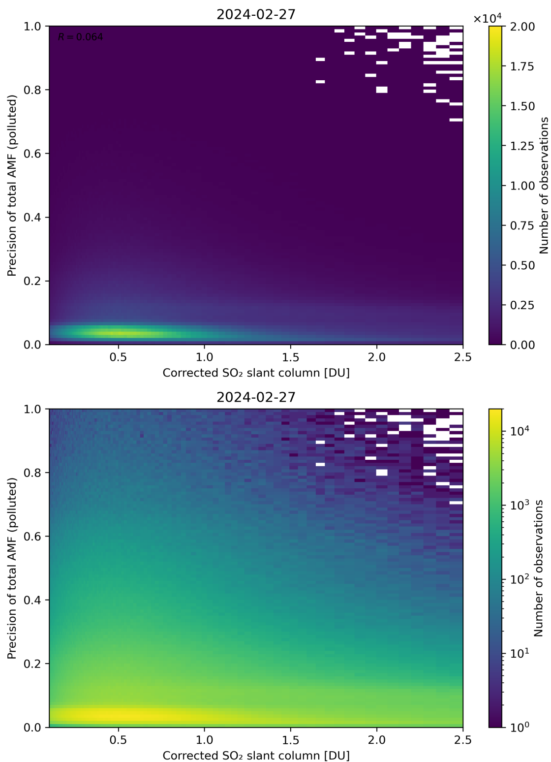
Figure 193: Scatter density plot of “Corrected SO 2 slant column” against “Precision of total AMF (polluted)” for 2024-02-27 to 2024-02-28.
