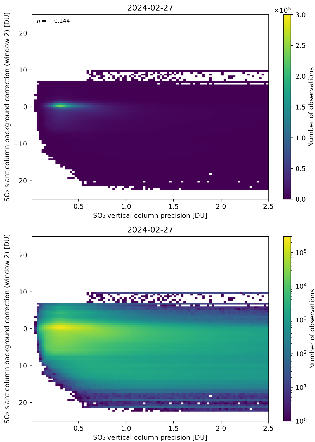
Figure 280: Scatter density plot of “SO 2 vertical column precision” against “SO 2 slant column background correction (window 2)” for 2024-02-27 to 2024-02-28.
