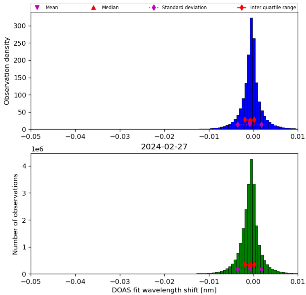
Figure 68: Histogram of “DOAS fit wavelength shift” for 2024-02-27 to 2024-02-28
