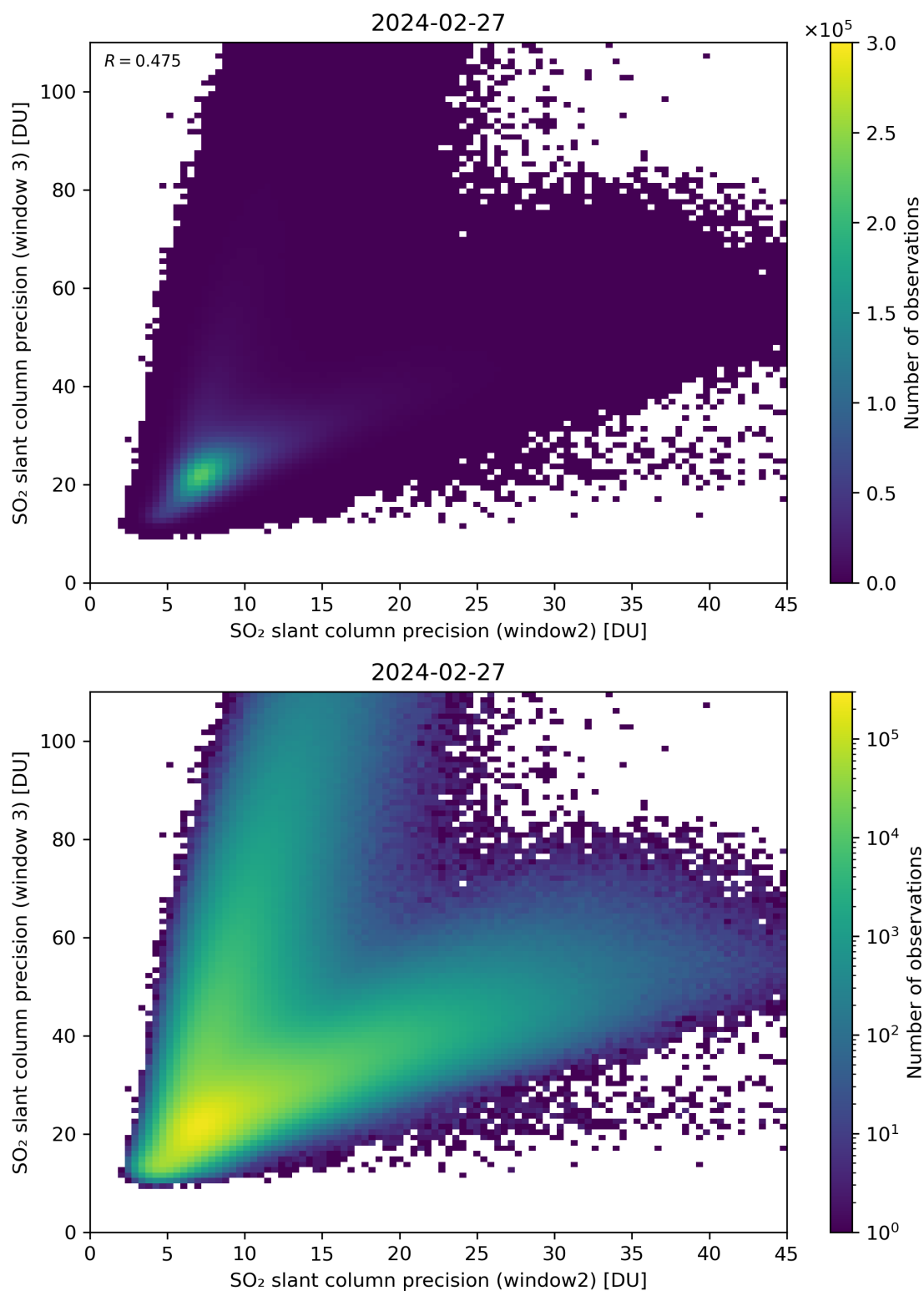
Figure 250: Scatter density plot of “SO 2 slant column precision (window2)” against “SO 2 slant column precision (window 3)” for 2024-02-27 to 2024-02-28.
