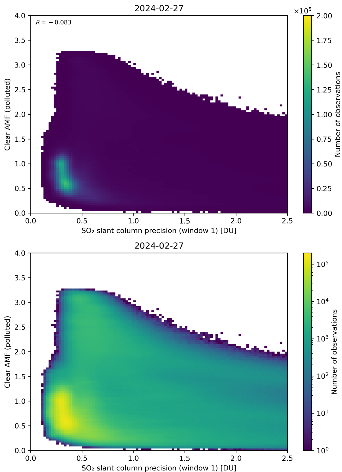
Figure 224: Scatter density plot of “SO 2 slant column precision (window 1)” against “Clear AMF (polluted)” for 2024-02-27 to 2024-02-28.
