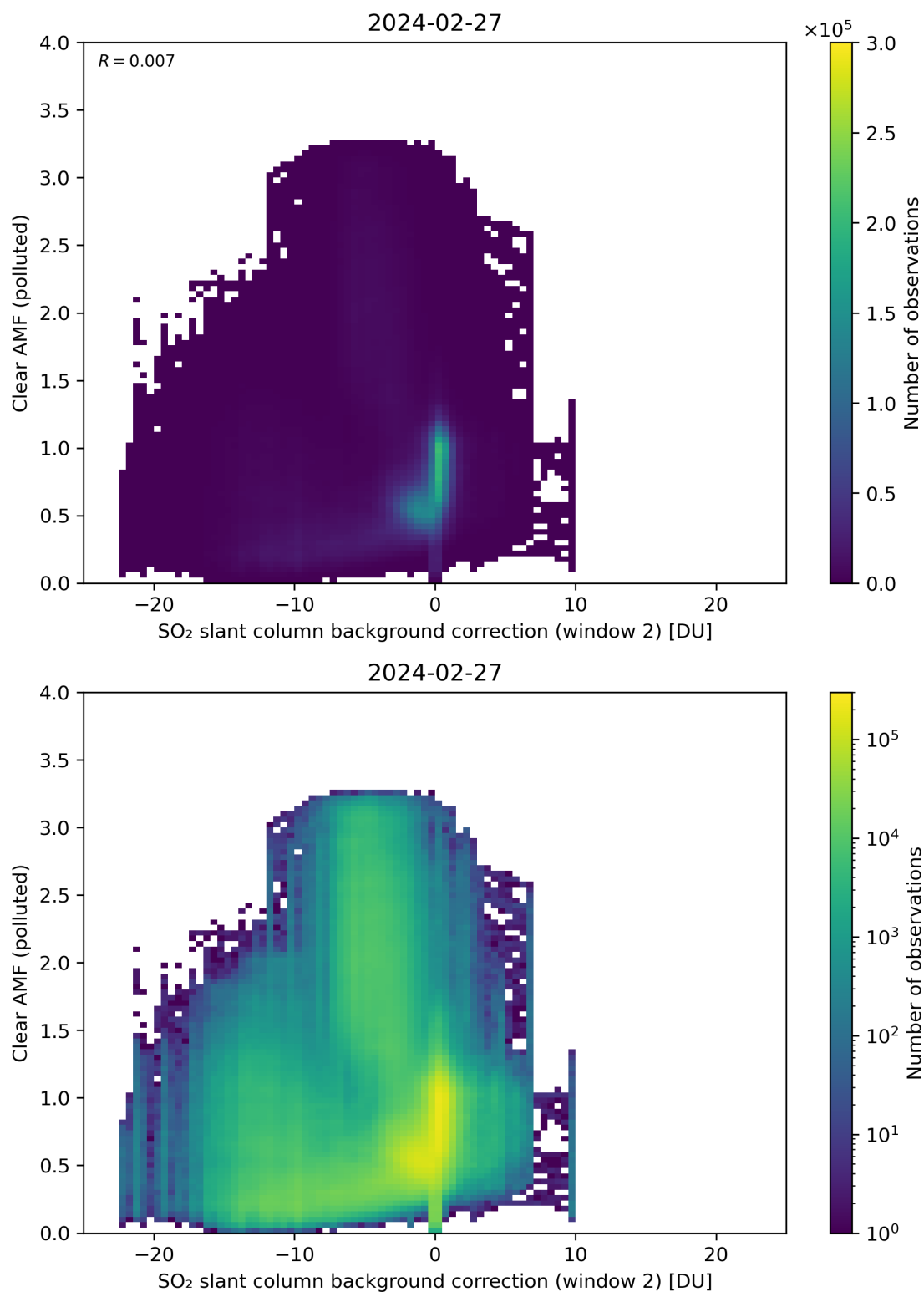
Figure 115: Scatter density plot of “SO 2 slant column background correction (window 2)” against “Clear AMF (polluted)” for 2024-02-27 to 2024-02-28.
