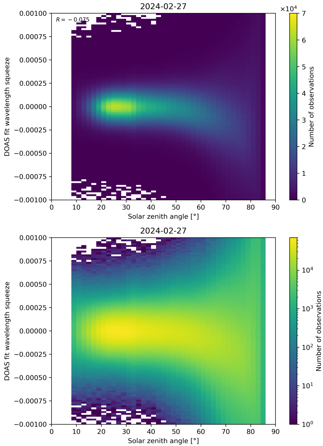
Figure 162: Scatter density plot of “Solar zenith angle” against “DOAS fit wavelength squeeze” for 2024-02-27 to 2024-02-28.
