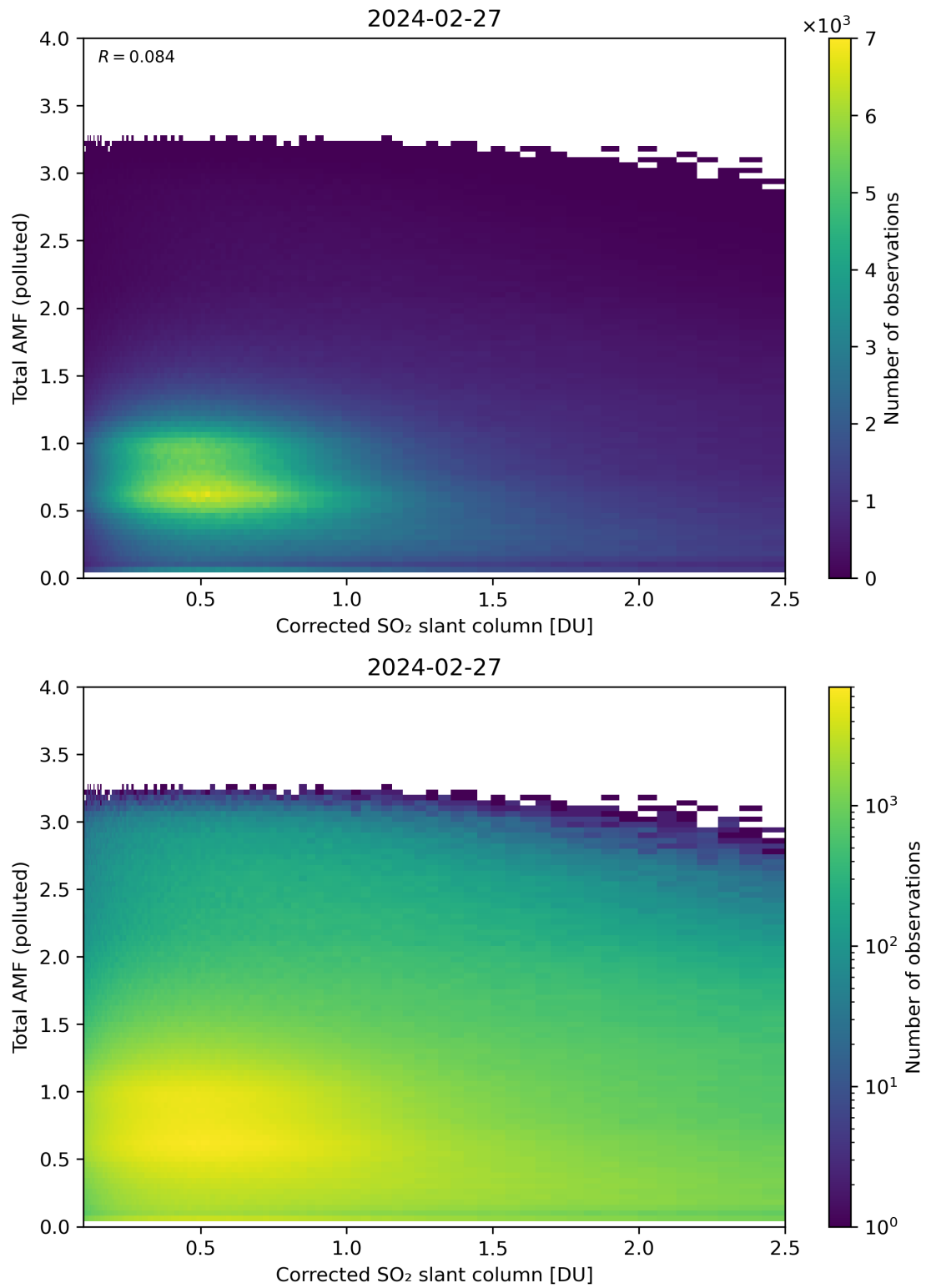
Figure 192: Scatter density plot of “Corrected SO 2 slant column” against “Total AMF (polluted)” for 2024-02-27 to 2024-02-28.
