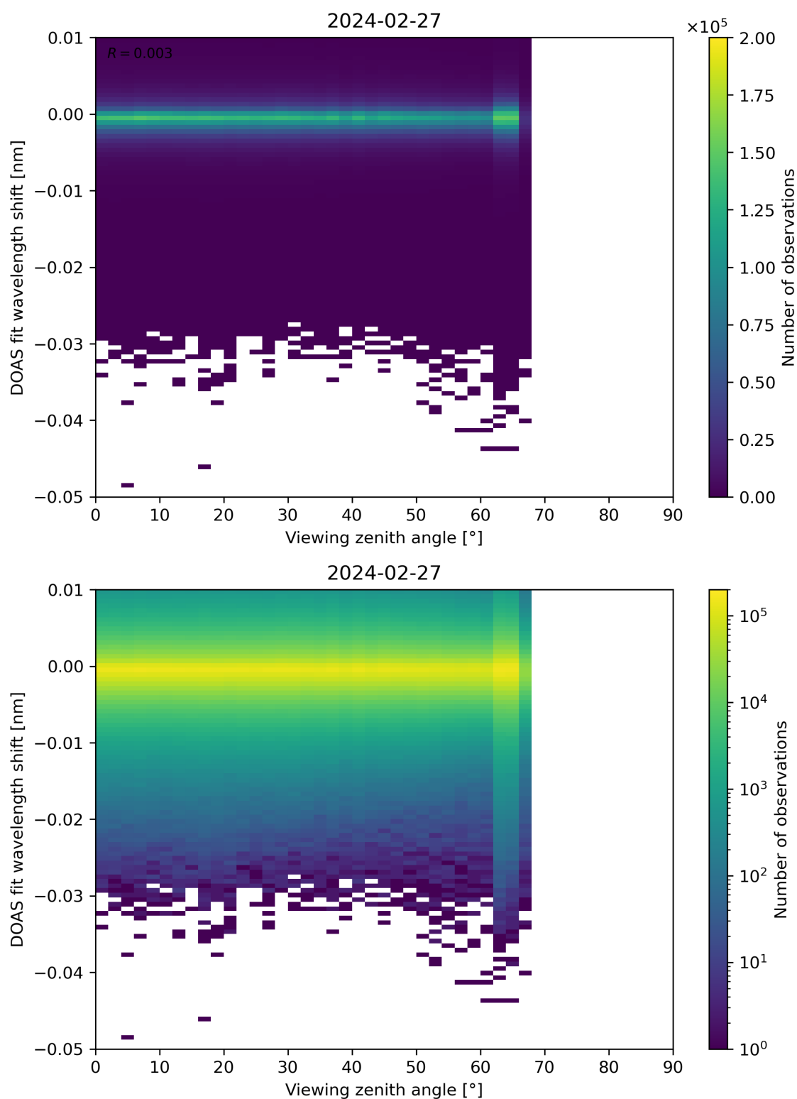
Figure 311: Scatter density plot of “Viewing zenith angle” against “DOAS fit wavelength shift” for 2024-02-27 to 2024-02-28.
