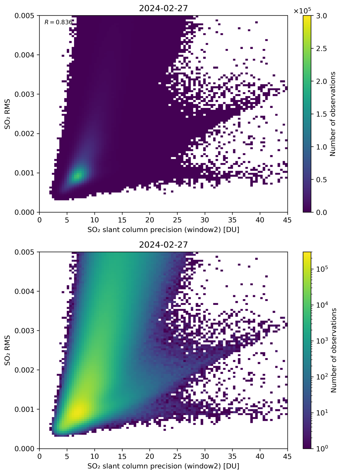
Figure 245: Scatter density plot of “SO 2 slant column precision (window2)” against “SO 2 RMS” for 2024-02-27 to 2024-02-28.
