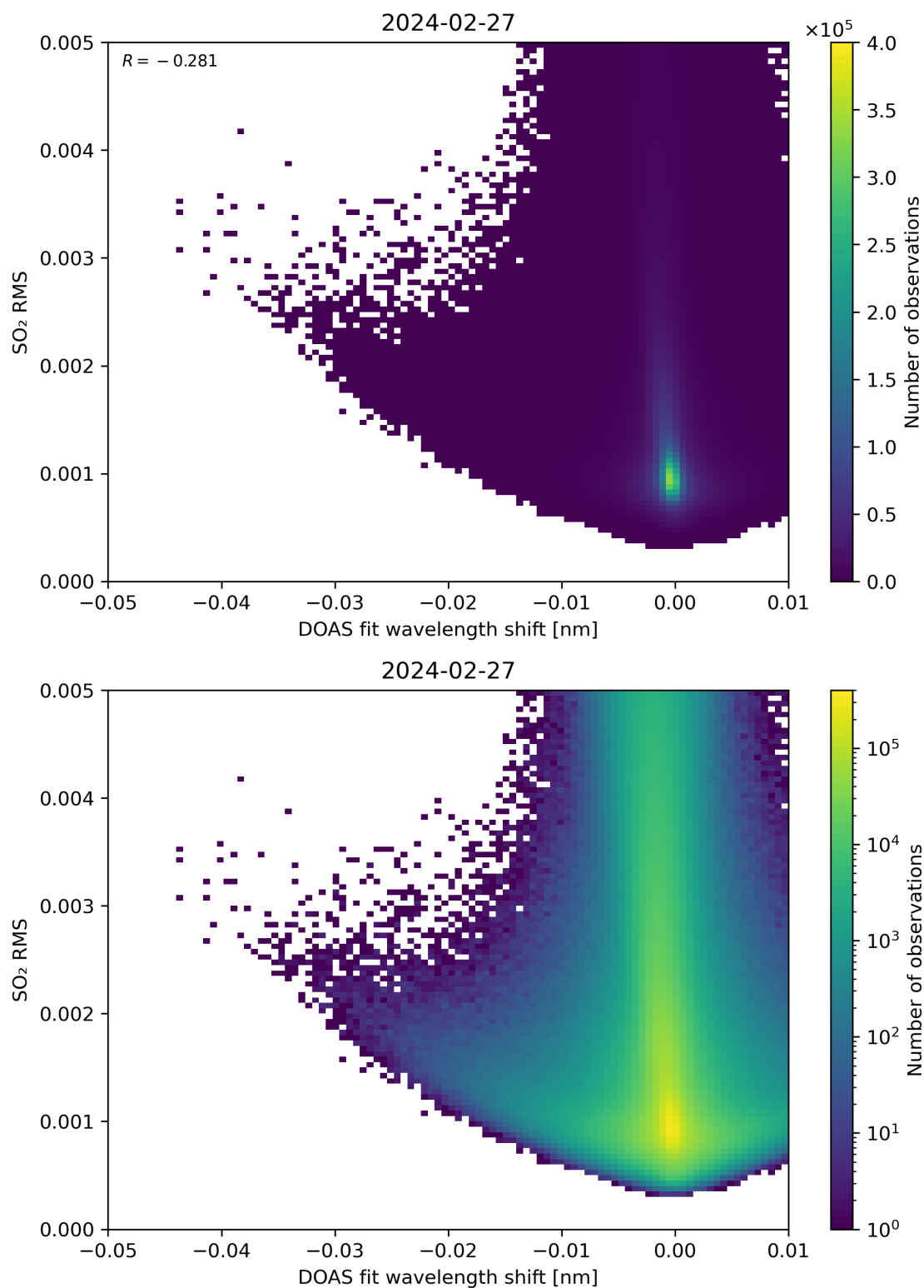
Figure 128: Scatter density plot of “DOAS fit wavelength shift” against “SO 2 RMS” for 2024-02-27 to 2024-02-28.
