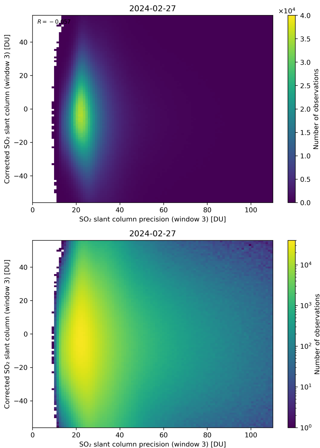
Figure 262: Scatter density plot of “SO 2 slant column precision (window 3)” against “Corrected SO 2 slant column (window 3)” for 2024-02-27 to 2024-02-28.
