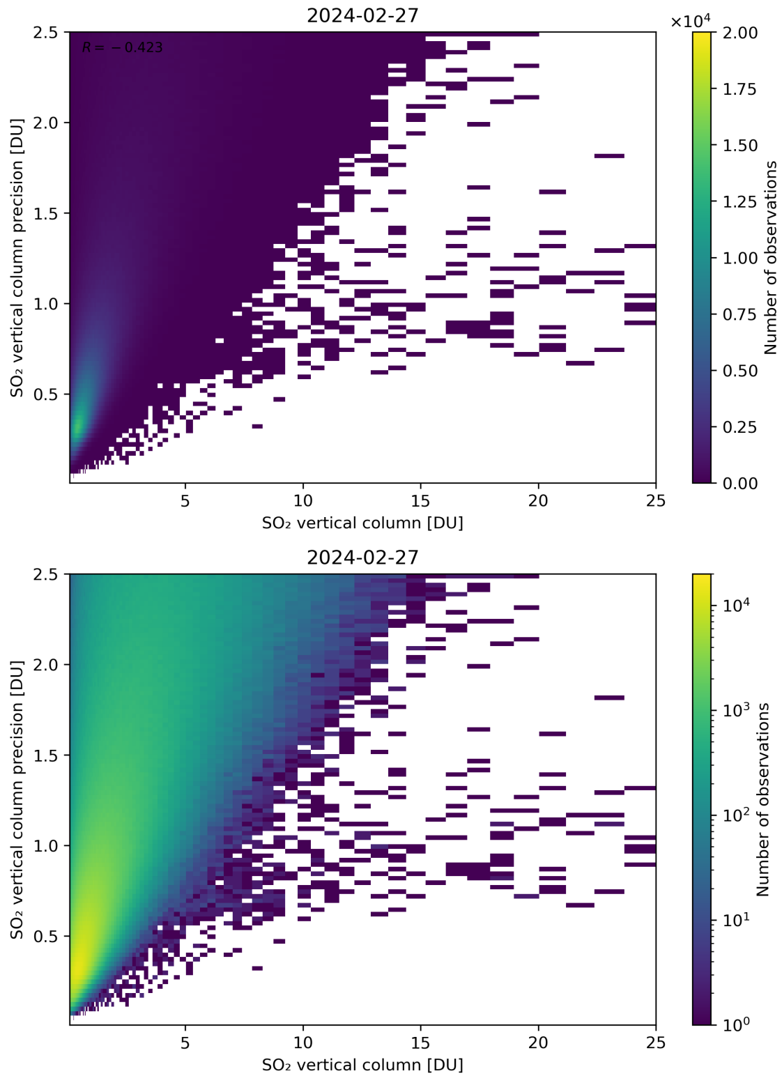
Figure 307: Scatter density plot of “SO 2 vertical column” against “SO 2 vertical column precision” for 2024-02-27 to 2024-02-28.
