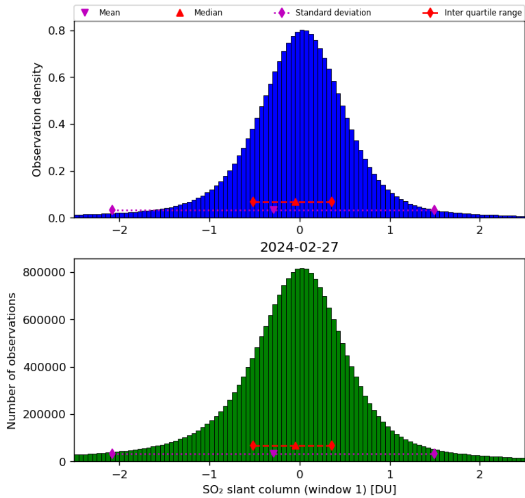
Figure 56: Histogram of “SO 2 slant column (window 1)” for 2024-02-27 to 2024-02-28
