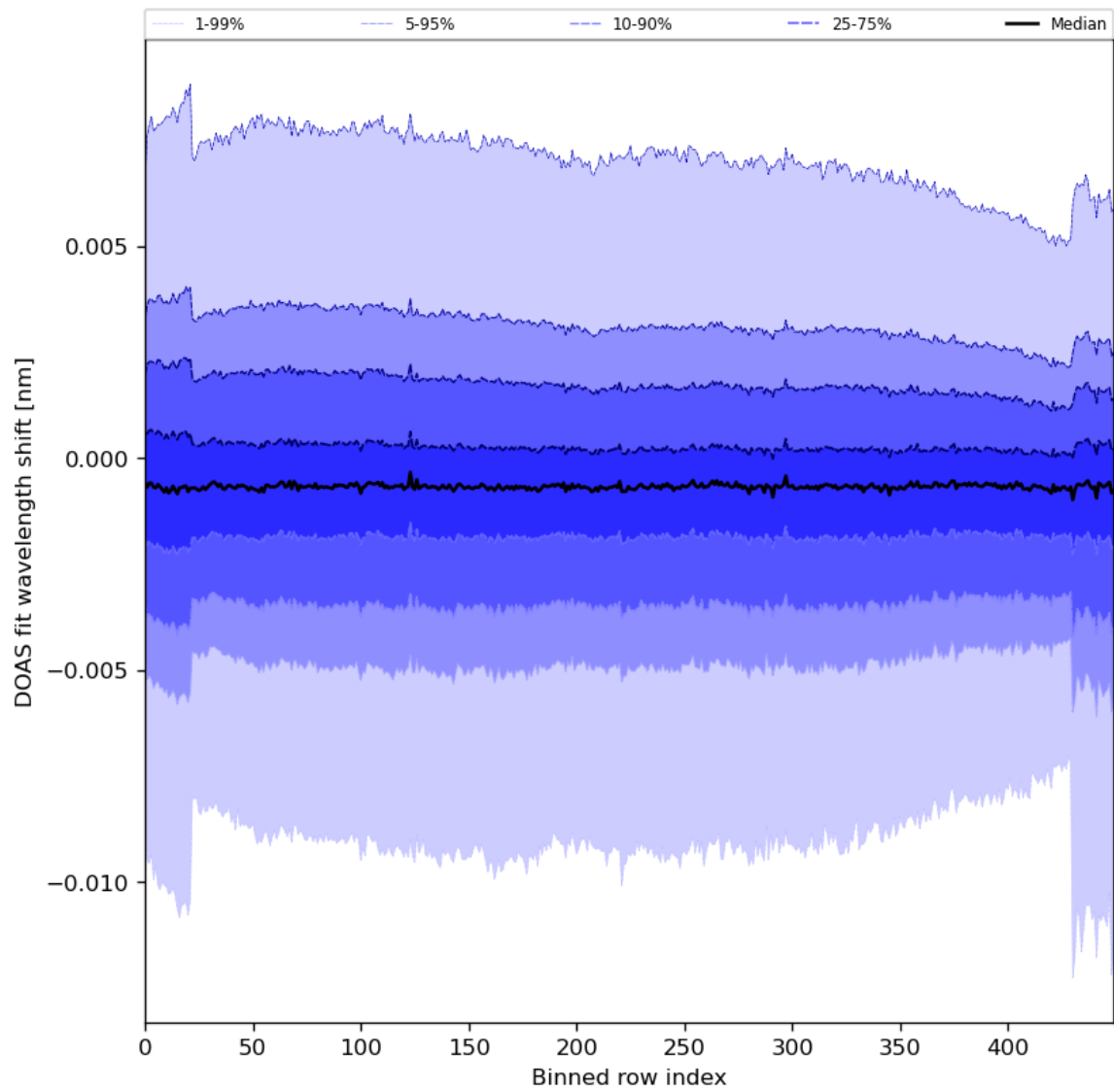
Figure 91: Along track statistics of “DOAS fit wavelength shift” for 2024-02-27 to 2024-02-28
