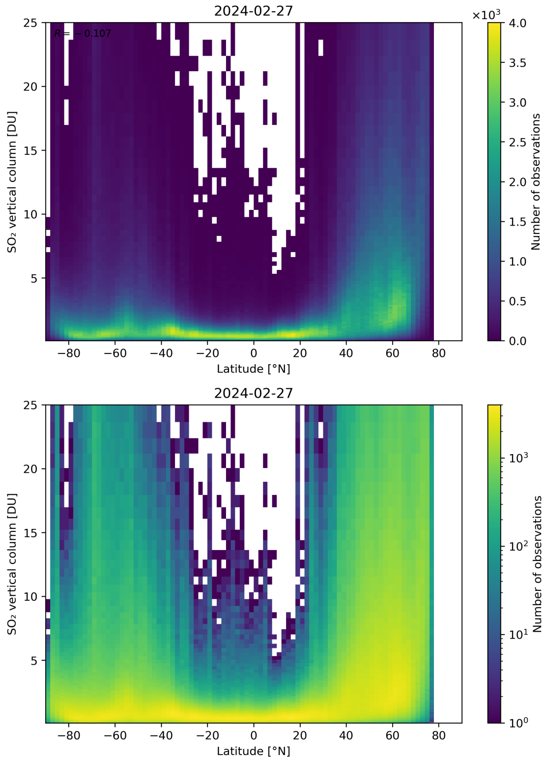
Figure 156: Scatter density plot of “Latitude” against “SO 2 vertical column” for 2024-02-27 to 2024-02-28.
