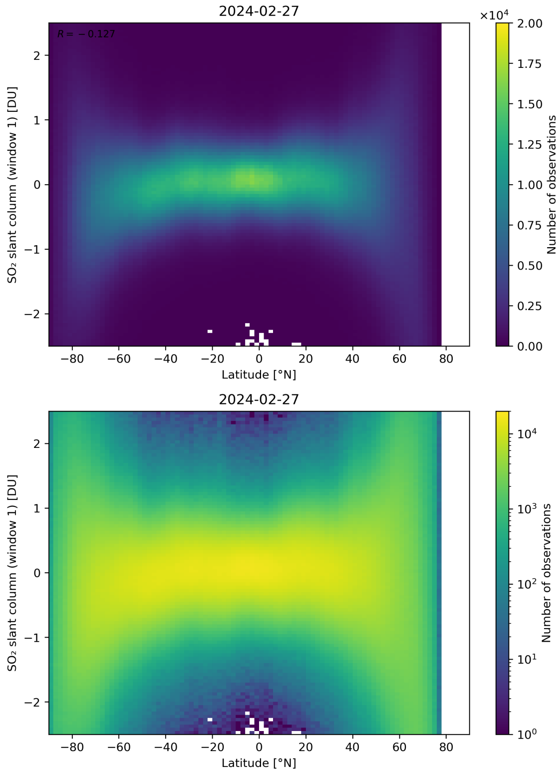
Figure 149: Scatter density plot of “Latitude” against “SO 2 slant column (window 1)” for 2024-02-27 to 2024-02-28.
