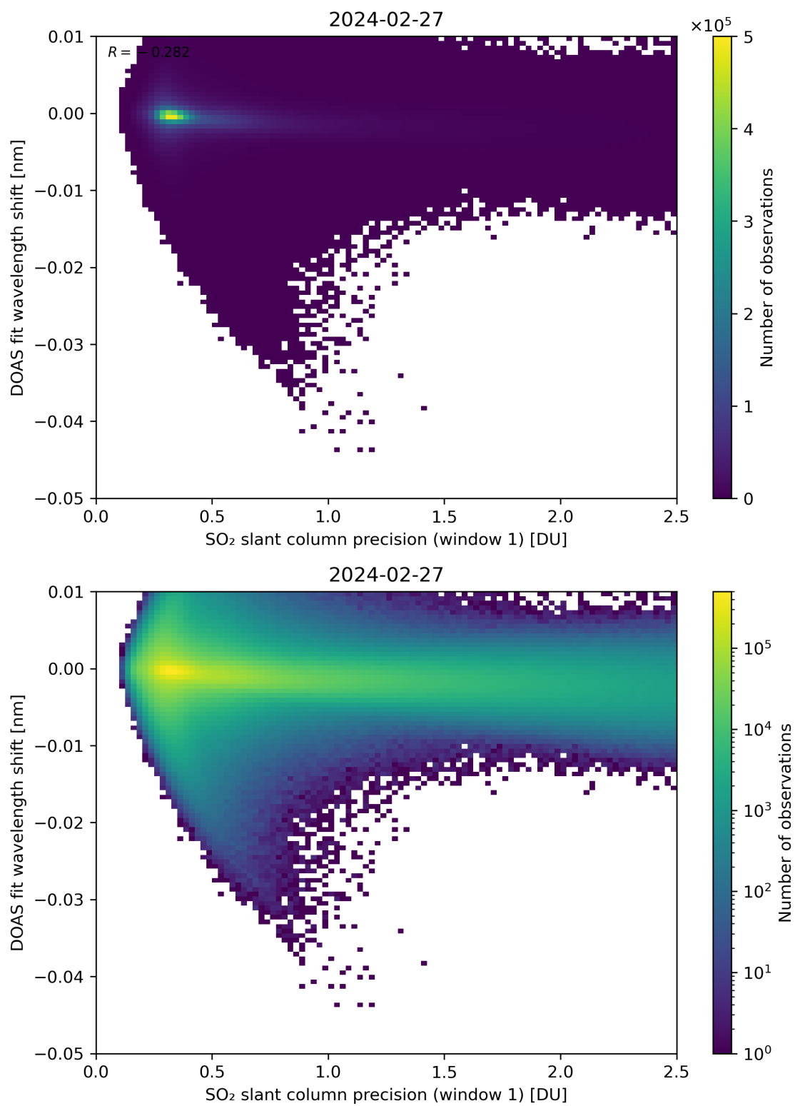
Figure 221: Scatter density plot of “SO 2 slant column precision (window 1)” against “DOAS fit wavelength shift” for 2024-02-27 to 2024-02-28.
