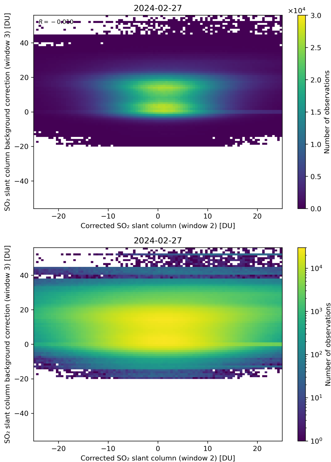
Figure 195: Scatter density plot of “Corrected SO 2 slant column (window 2)” against “SO 2 slant column background correction (window 3)” for 2024-02-27 to 2024-02-28.
