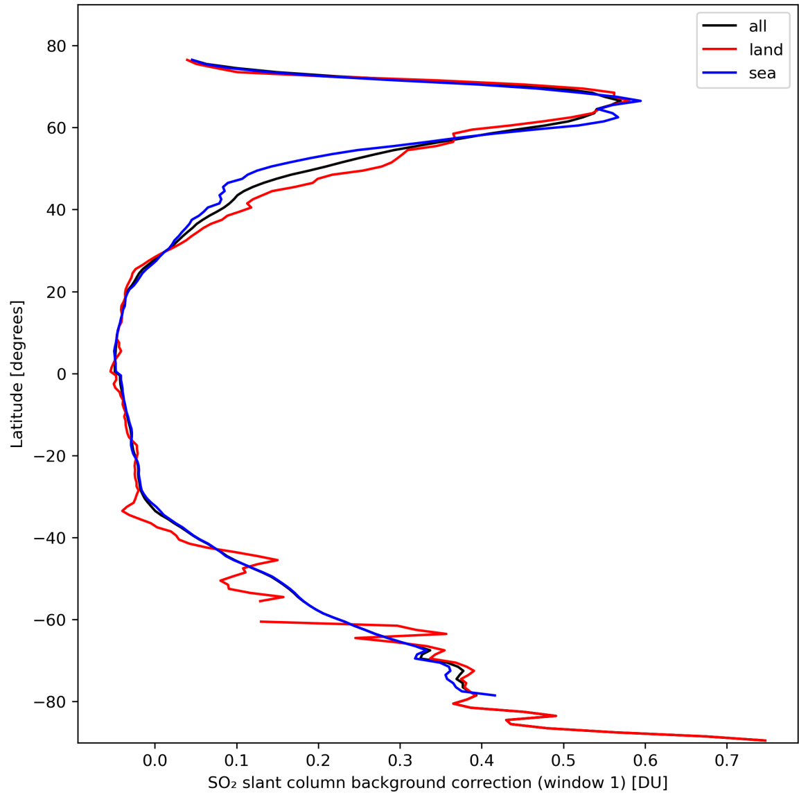
Figure 36: Zonal average of “SO 2 slant column background correction (window 1)” for 2024-02-27 to 2024-02-28.
