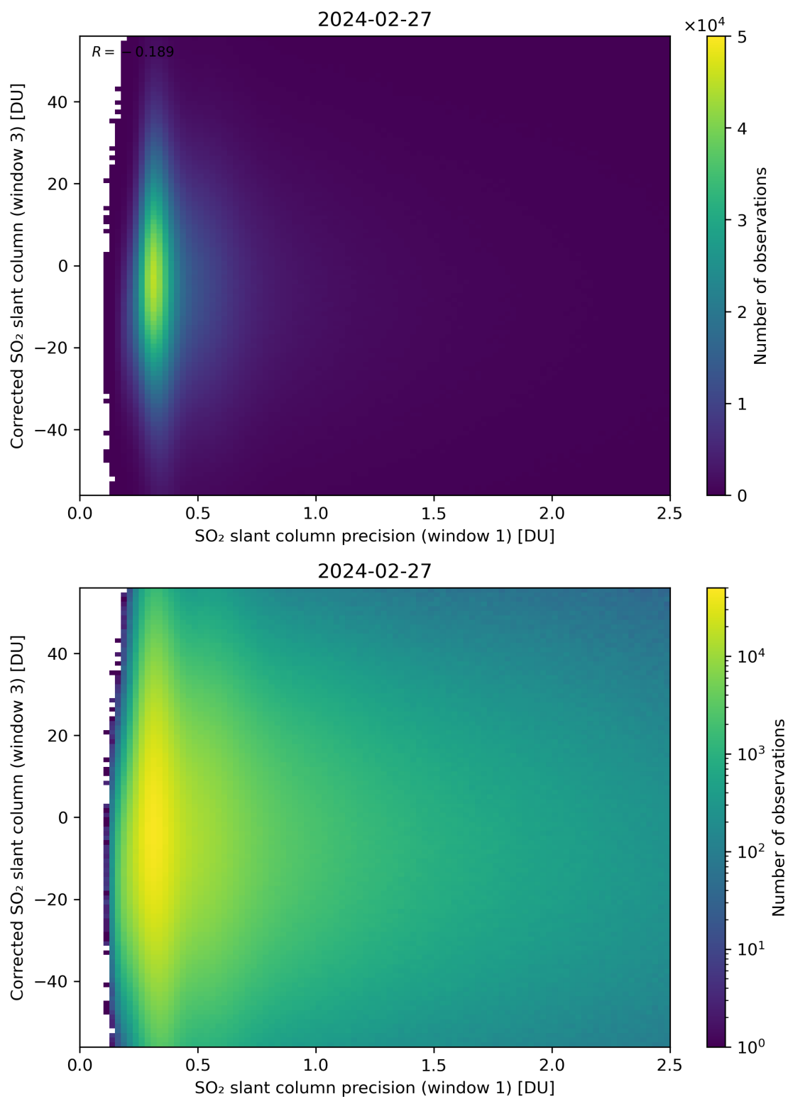
Figure 226: Scatter density plot of “SO 2 slant column precision (window 1)” against “Corrected SO 2 slant column (window 3)” for 2024-02-27 to 2024-02-28.
