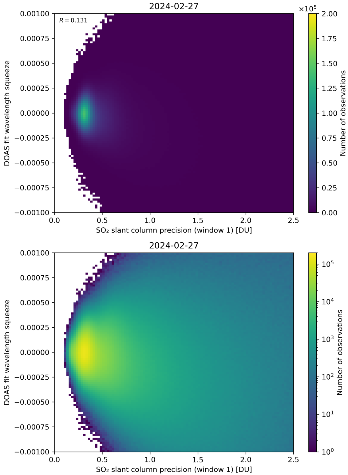
Figure 222: Scatter density plot of “SO 2 slant column precision (window 1)” against “DOAS fit wavelength squeeze” for 2024-02-27 to 2024-02-28.
