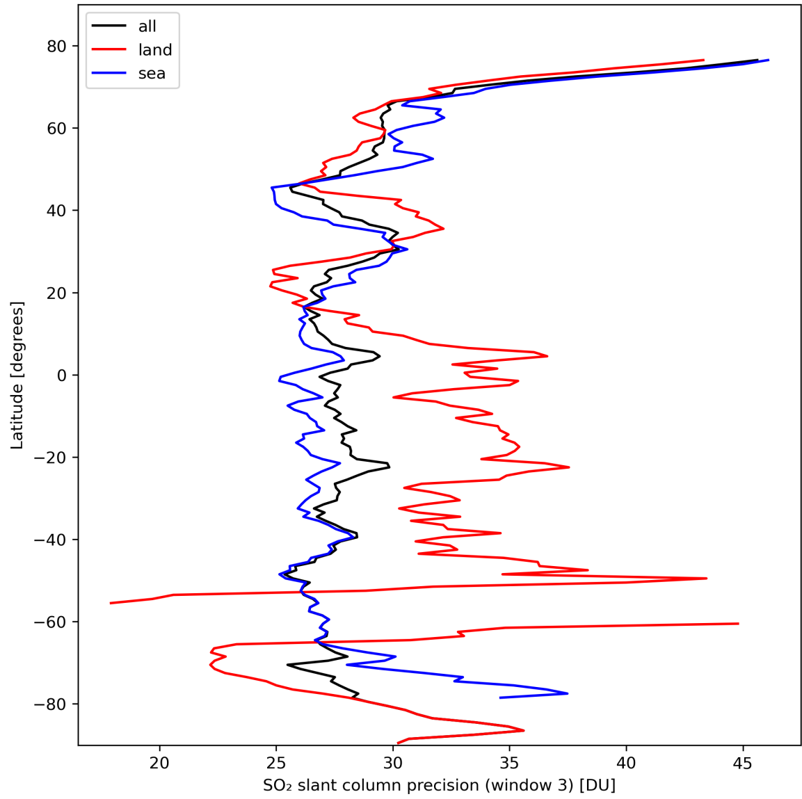
Figure 42: Zonal average of “SO 2 slant column precision (window 3)” for 2024-02-27 to 2024-02-28.
