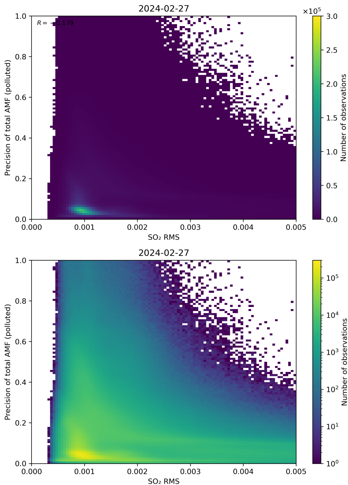
Figure 138: Scatter density plot of “SO 2 RMS” against “Precision of total AMF (polluted)” for 2024-02-27 to 2024-02-28.
