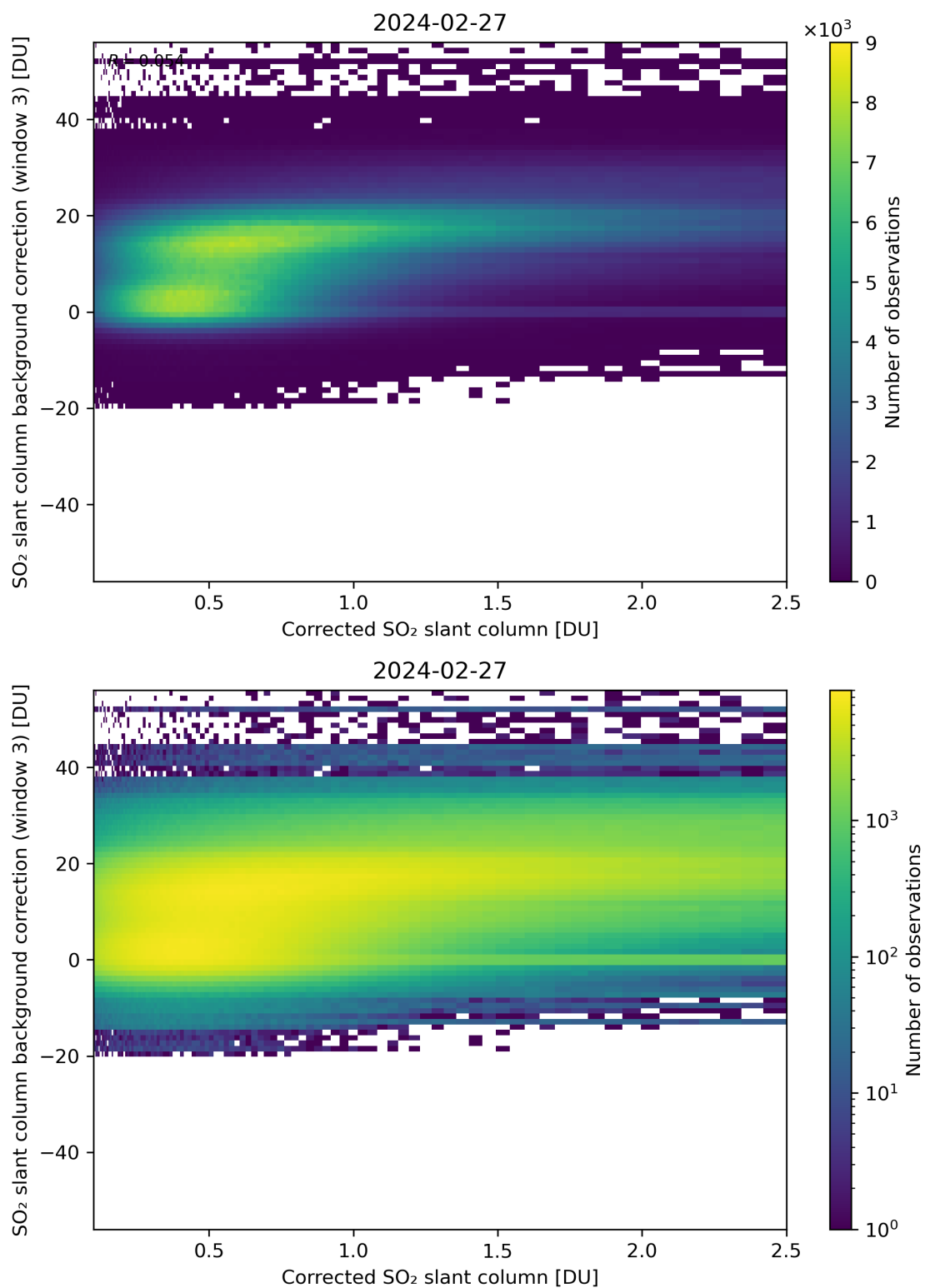
Figure 180: Scatter density plot of “Corrected SO 2 slant column” against “SO 2 slant column background correction (window 3)” for 2024-02-27 to 2024-02-28.
