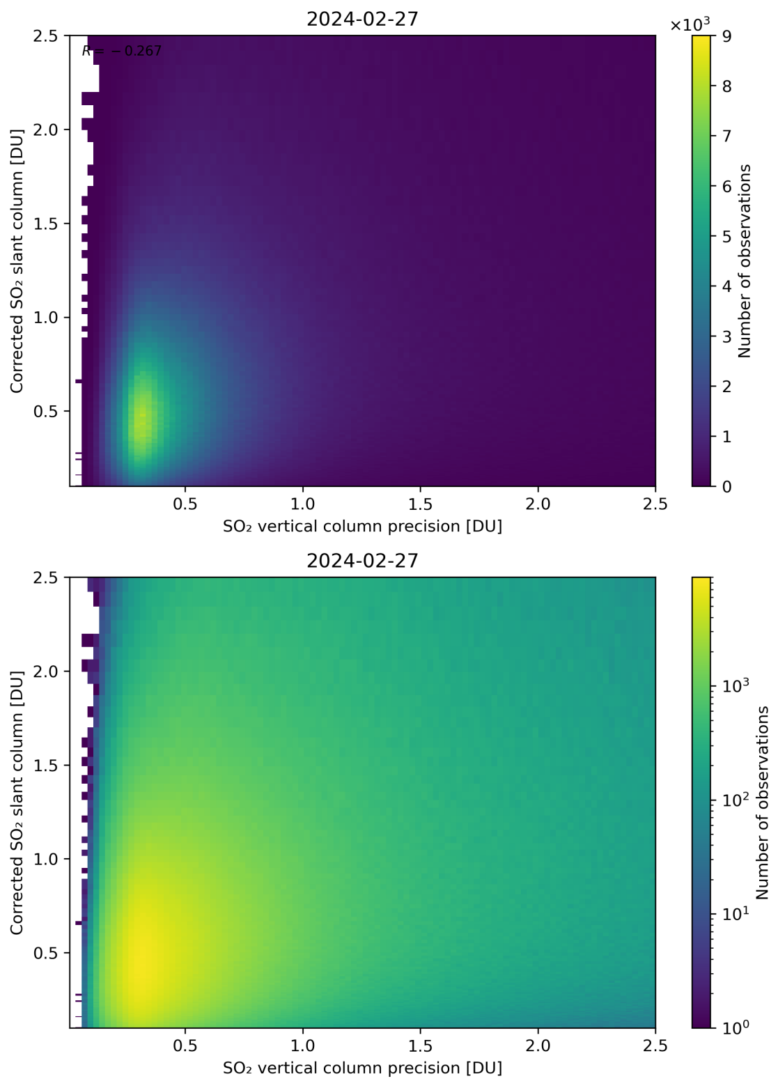
Figure 286: Scatter density plot of “SO 2 vertical column precision” against “Corrected SO 2 slant column” for 2024-02-27 to 2024-02-28.
