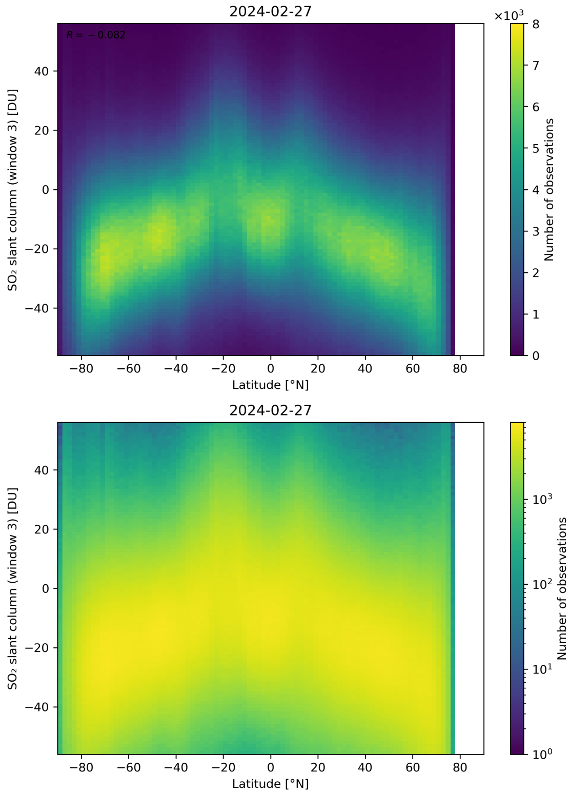
Figure 152: Scatter density plot of “Latitude” against “SO 2 slant column (window 3)” for 2024-02-27 to 2024-02-28.
