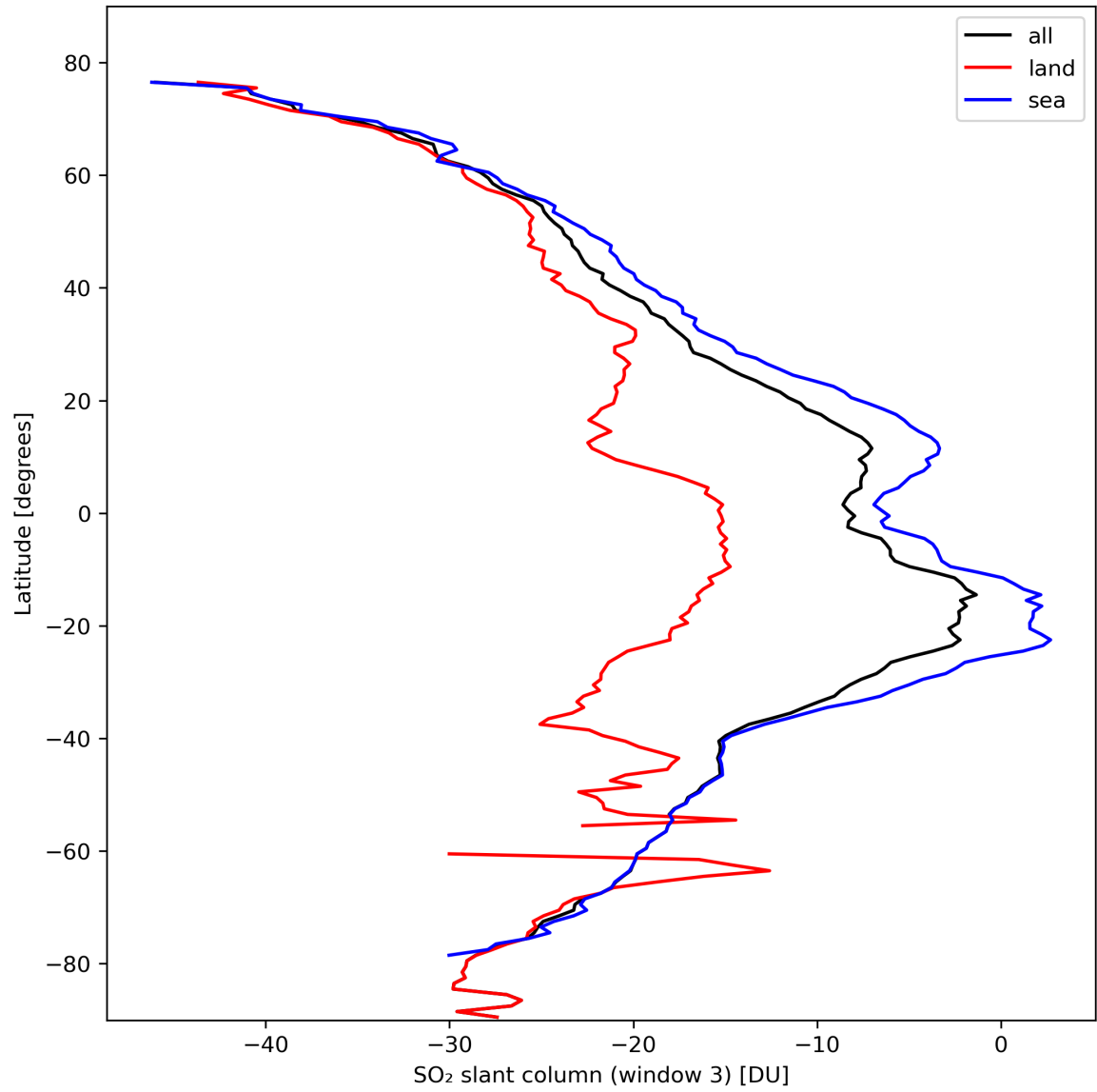
Figure 41: Zonal average of “SO 2 slant column (window 3)” for 2024-02-27 to 2024-02-28.
