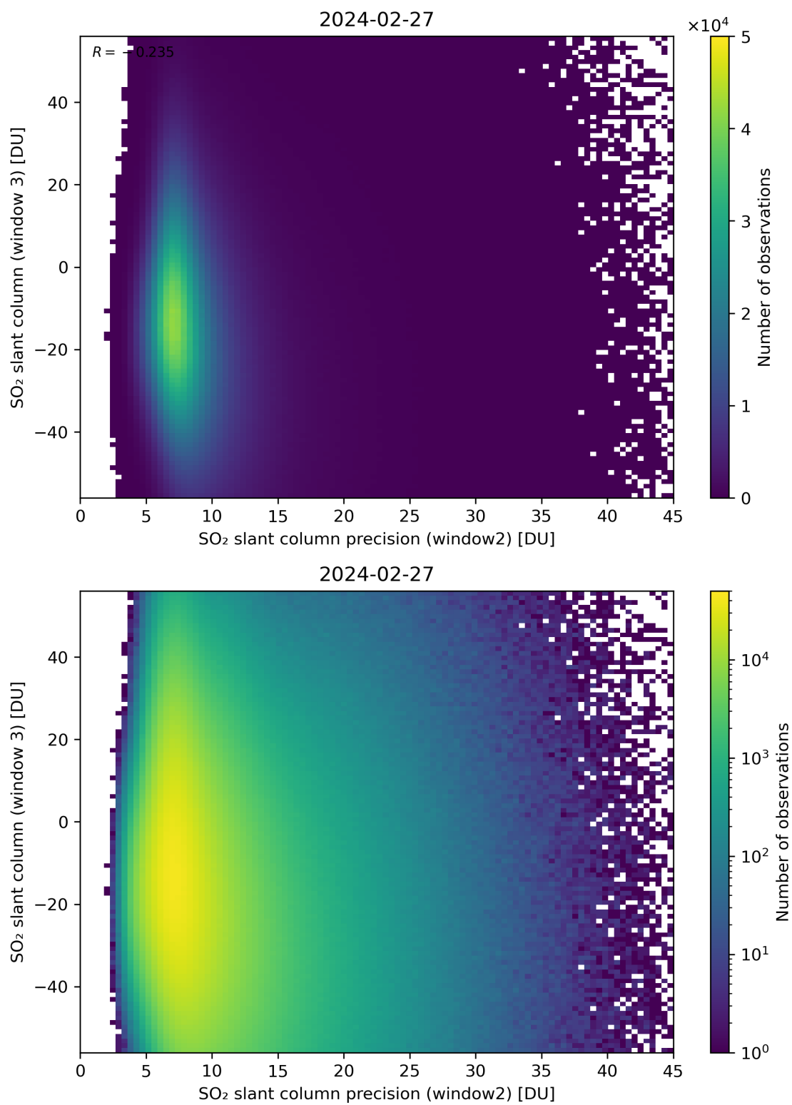
Figure 249: Scatter density plot of “SO 2 slant column precision (window2)” against “SO 2 slant column (window 3)” for 2024-02-27 to 2024-02-28.
