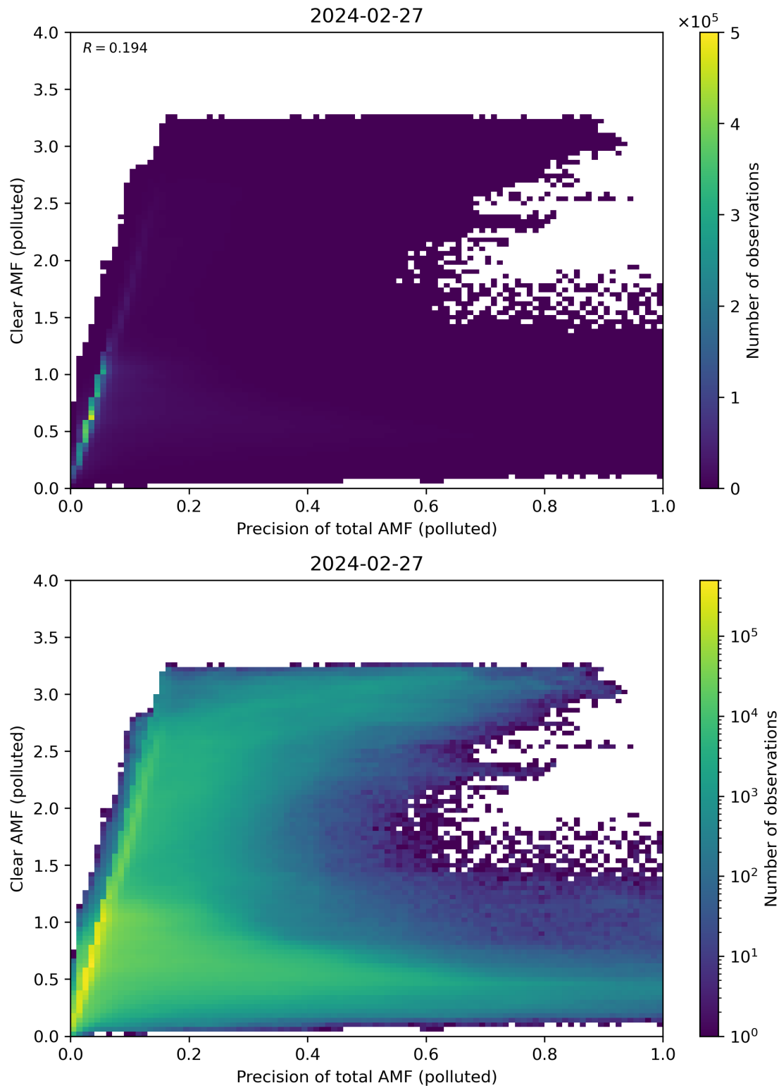
Figure 270: Scatter density plot of “Precision of total AMF (polluted)” against “Clear AMF (polluted)” for 2024-02-27 to 2024-02-28.
