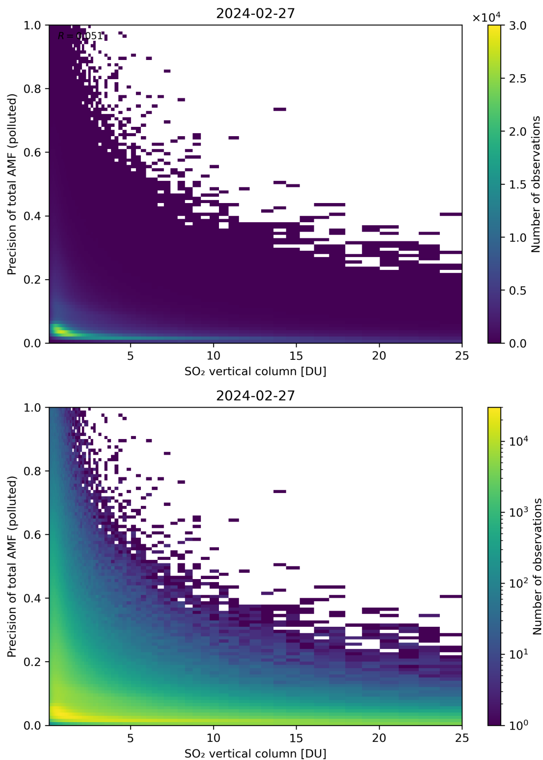
Figure 306: Scatter density plot of “SO 2 vertical column” against “Precision of total AMF (polluted)” for 2024-02-27 to 2024-02-28.
