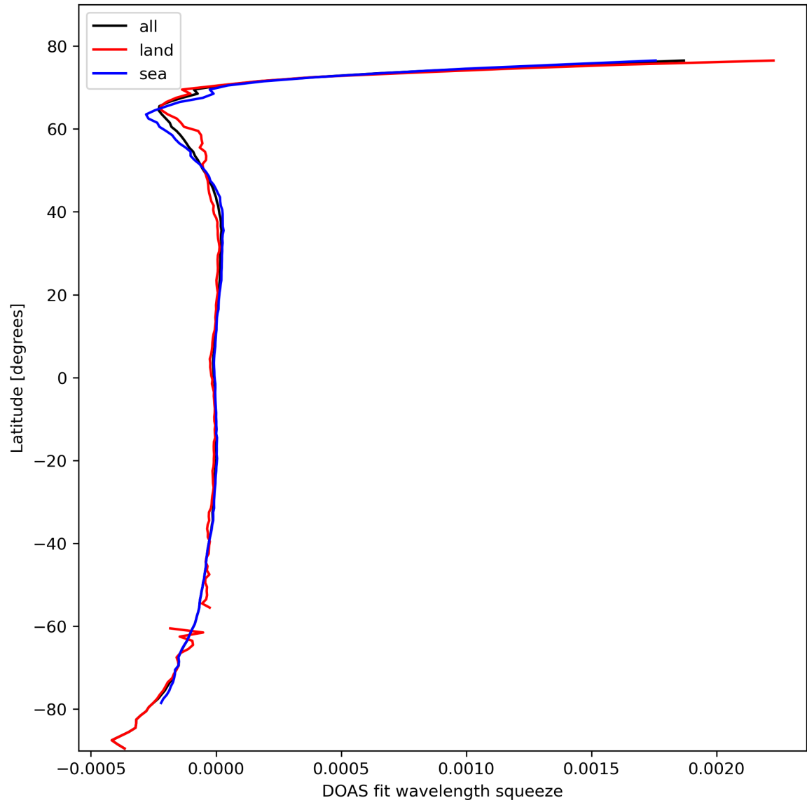
Figure 46: Zonal average of “DOAS fit wavelength squeeze” for 2024-02-27 to 2024-02-28.
