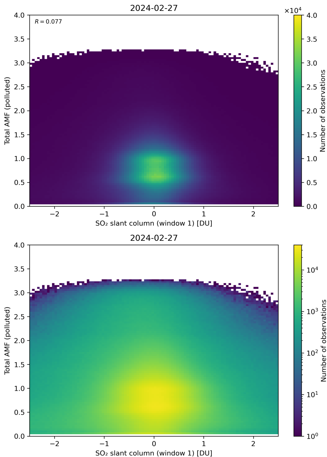
Figure 239: Scatter density plot of “SO 2 slant column (window 1)” against “Total AMF (polluted)” for 2024-02-27 to 2024-02-28.
