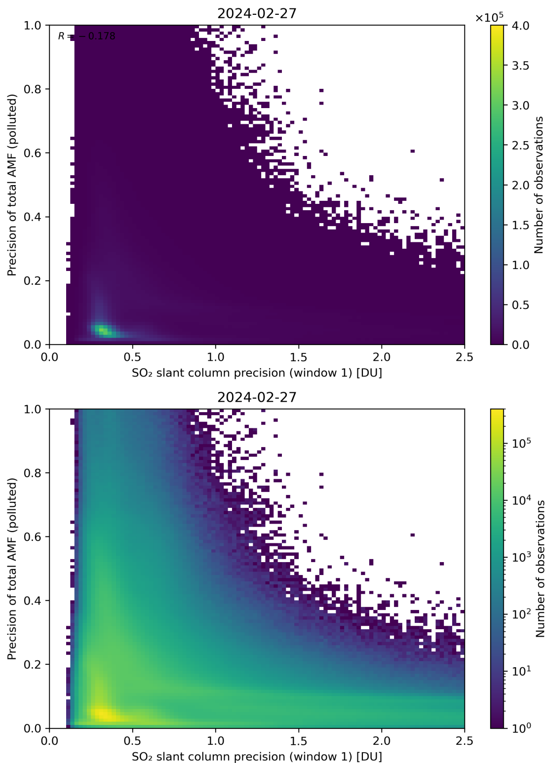
Figure 231: Scatter density plot of “SO 2 slant column precision (window 1)” against “Precision of total AMF (polluted)” for 2024-02-27 to 2024-02-28.
