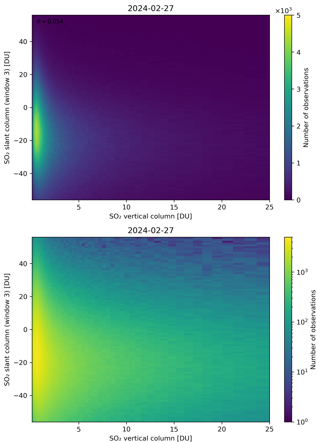
Figure 303: Scatter density plot of “SO 2 vertical column” against “SO 2 slant column (window 3)” for 2024-02-27 to 2024-02-28.
