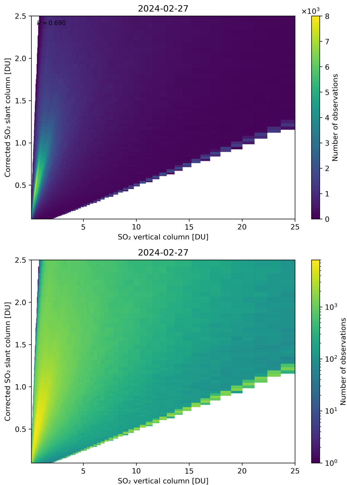
Figure 297: Scatter density plot of “SO 2 vertical column” against “Corrected SO 2 slant column” for 2024-02-27 to 2024-02-28.
