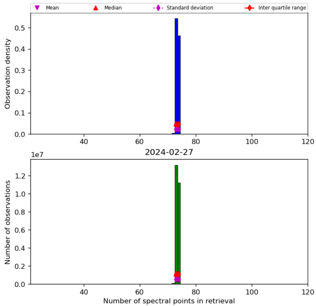
Figure 74: Histogram of “Number of spectral points in retrieval” for 2024-02-27 to 2024-02-28
