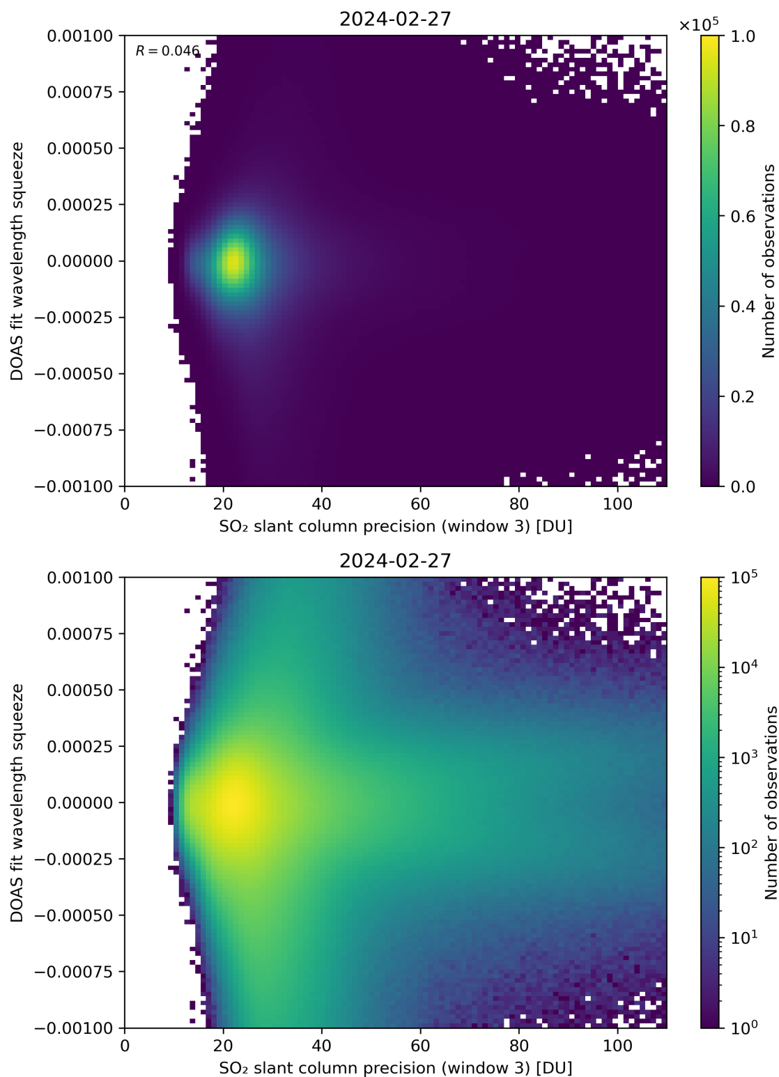
Figure 259: Scatter density plot of “SO 2 slant column precision (window 3)” against “DOAS fit wavelength squeeze” for 2024-02-27 to 2024-02-28.
