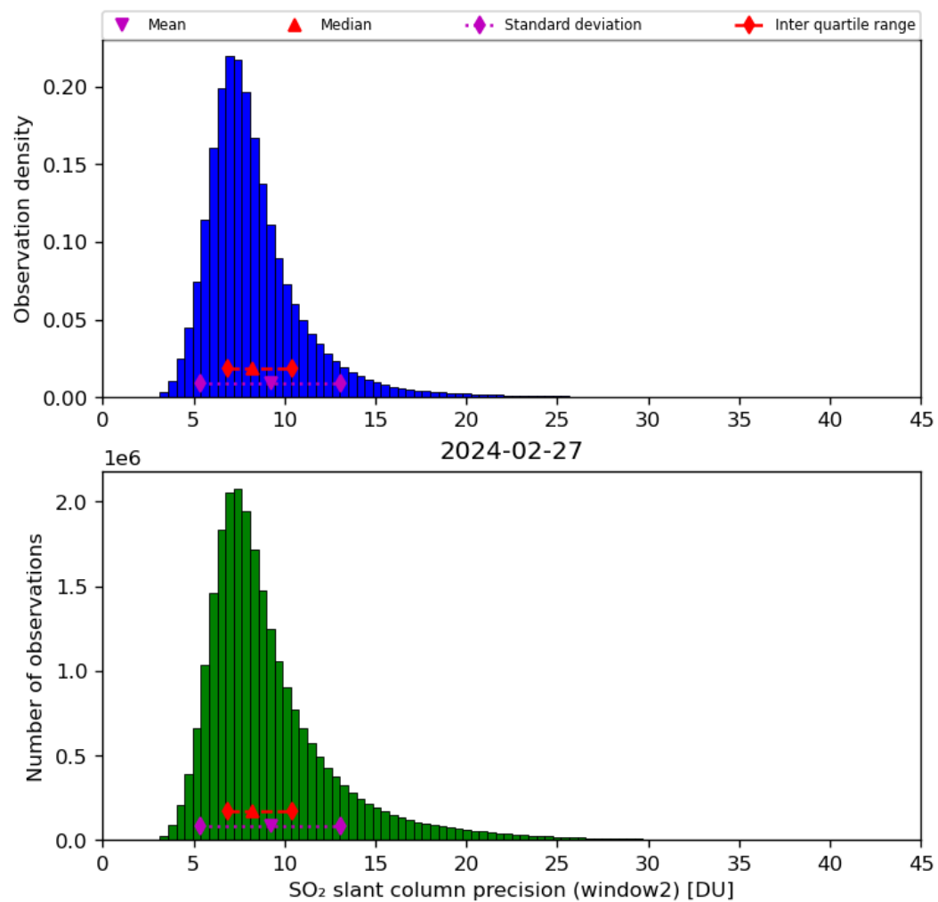
Figure 61: Histogram of “SO 2 slant column precision (window2)” for 2024-02-27 to 2024-02-28
