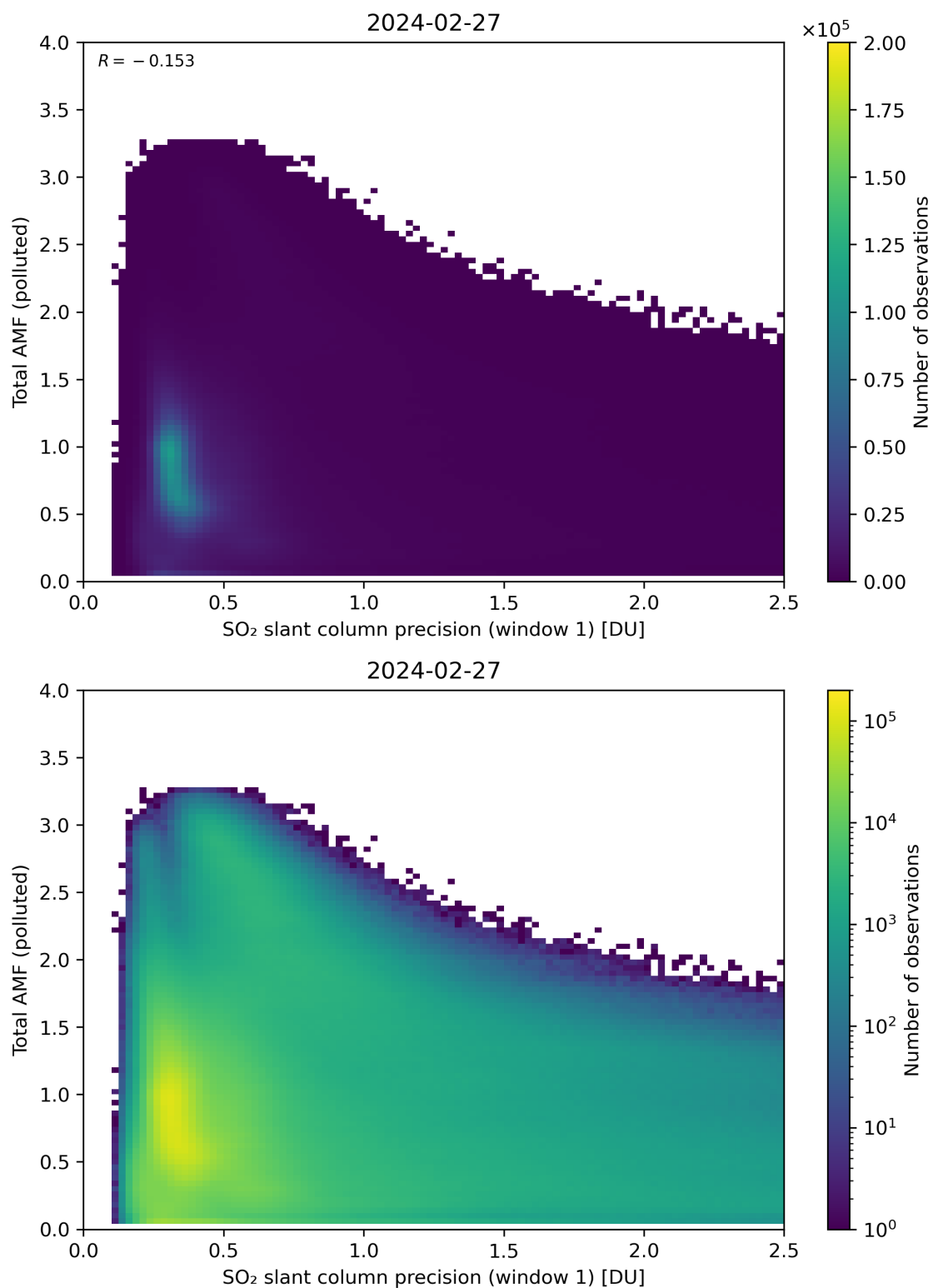
Figure 230: Scatter density plot of “SO 2 slant column precision (window 1)” against “Total AMF (polluted)” for 2024-02-27 to 2024-02-28.
