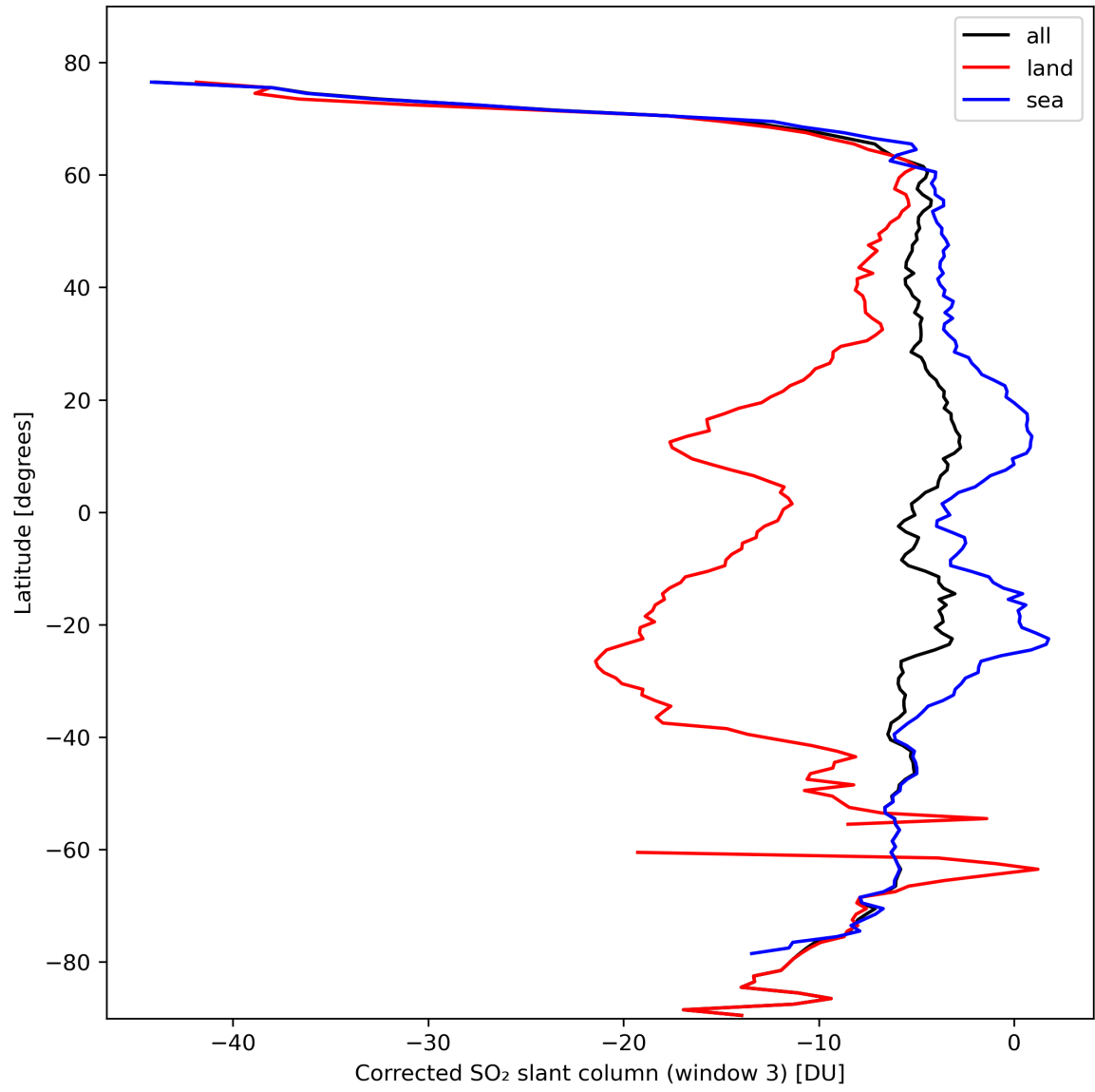
Figure 43: Zonal average of “Corrected SO 2 slant column (window 3)” for 2024-02-27 to 2024-02-28.
