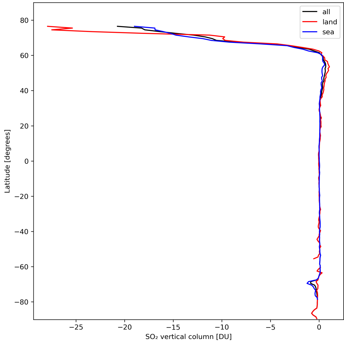
Figure 30: Zonal average of “SO 2 vertical column” for 2024-02-27 to 2024-02-28.
