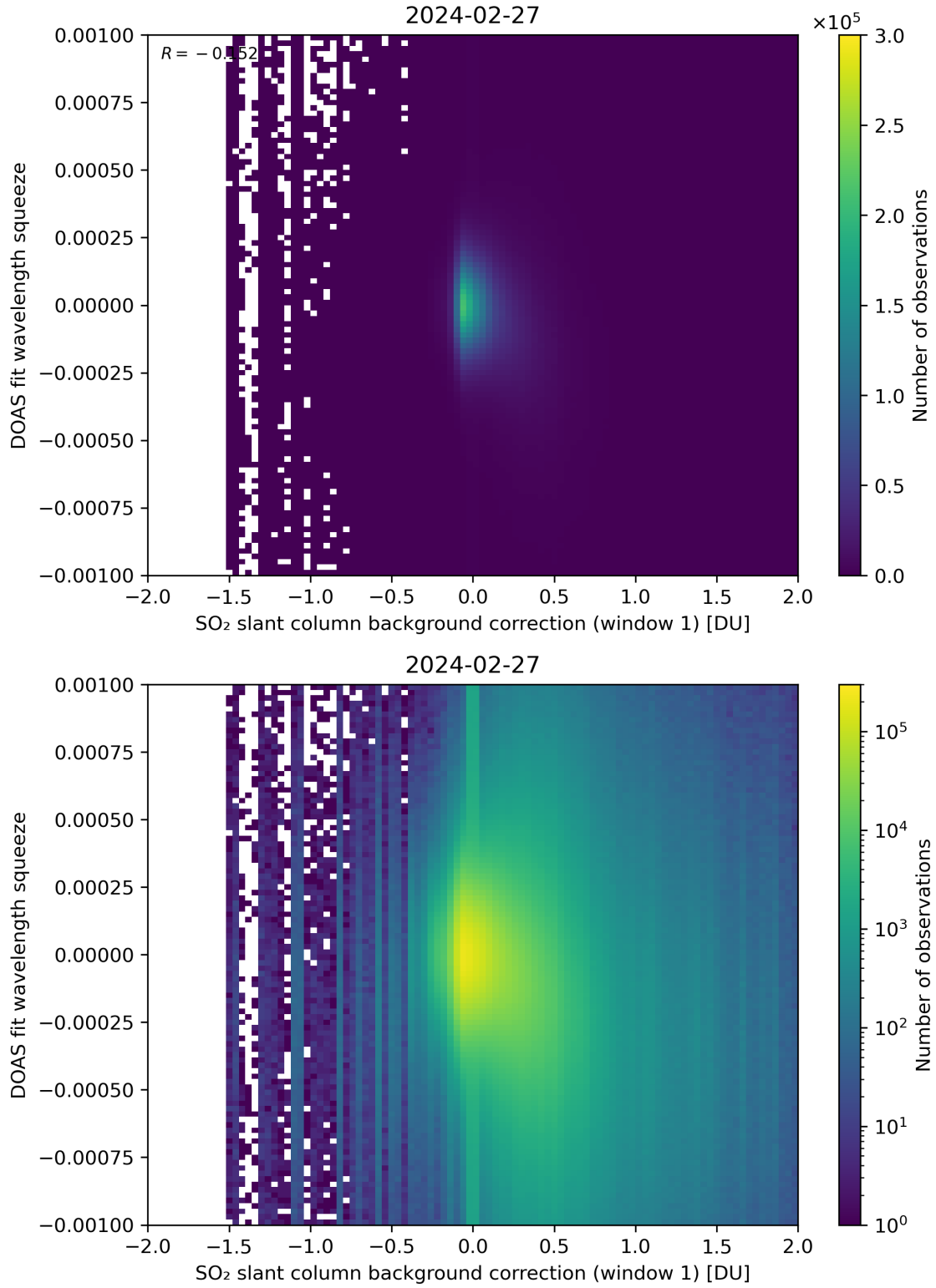
Figure 101: Scatter density plot of “SO 2 slant column background correction (window 1)” against “DOAS fit wavelength squeeze” for 2024-02-27 to 2024-02-28.
