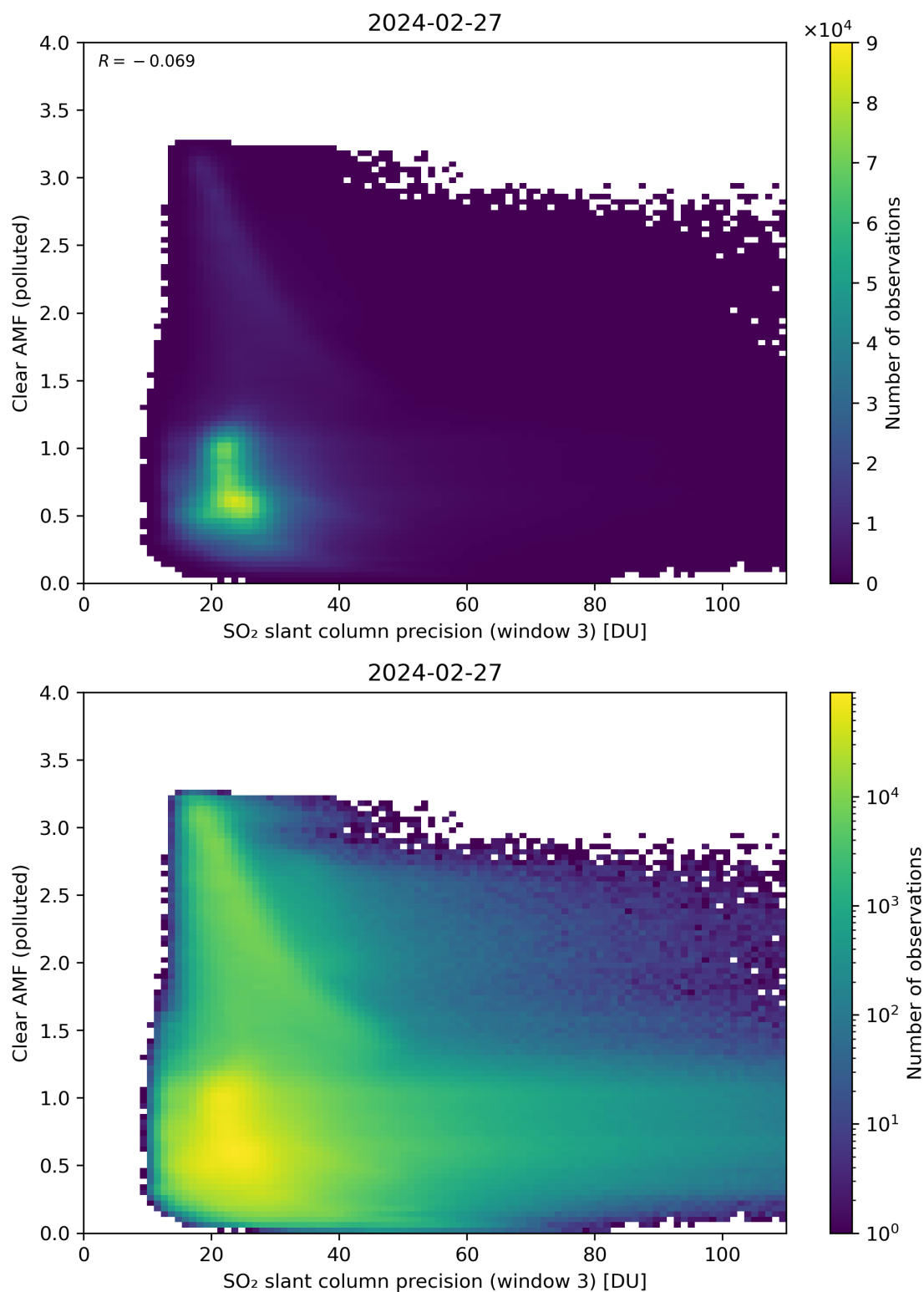
Figure 261: Scatter density plot of “SO 2 slant column precision (window 3)” against “Clear AMF (polluted)” for 2024-02-27 to 2024-02-28.
