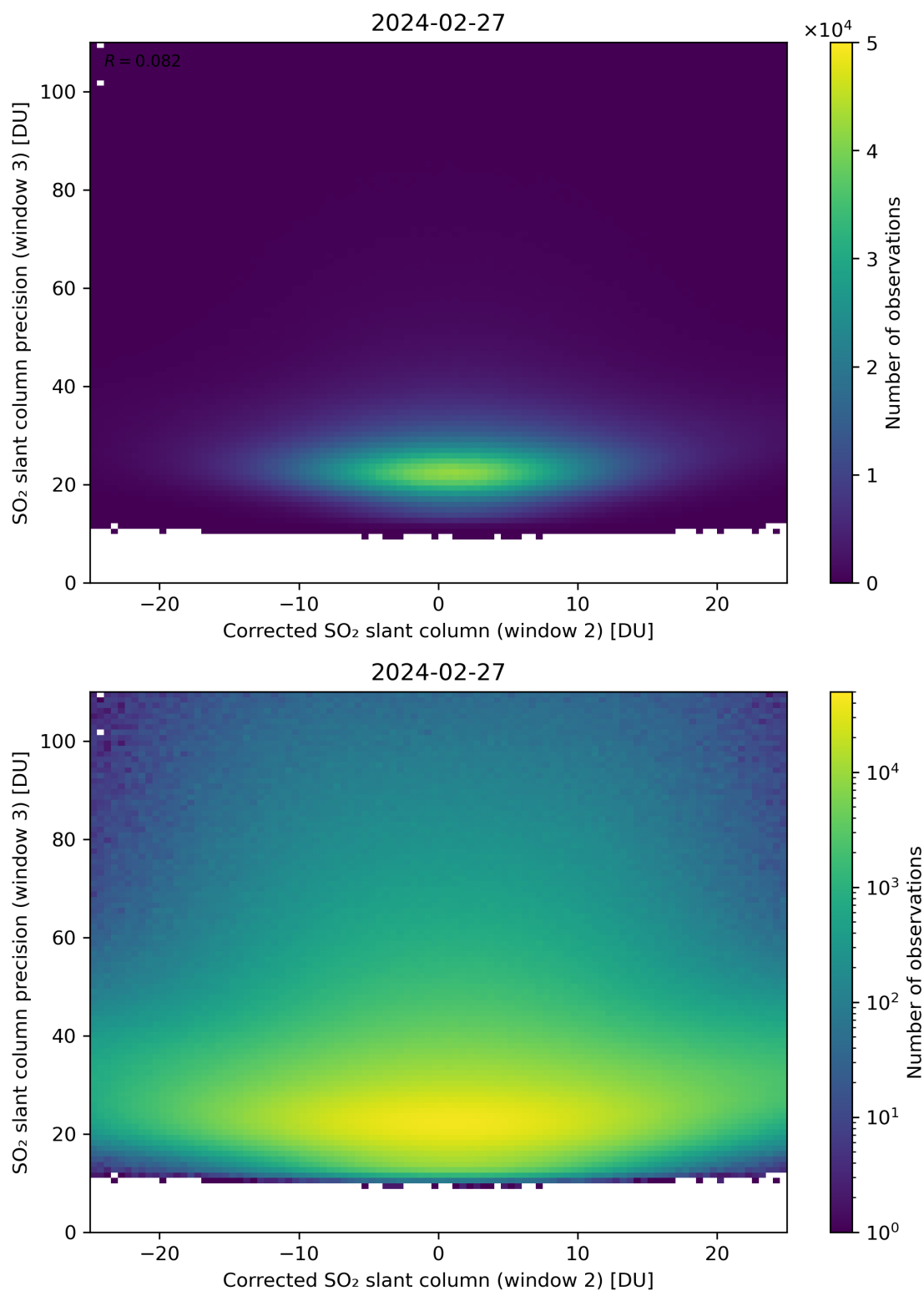
Figure 202: Scatter density plot of “Corrected SO 2 slant column (window 2)” against “SO 2 slant column precision (window 3)” for 2024-02-27 to 2024-02-28.
