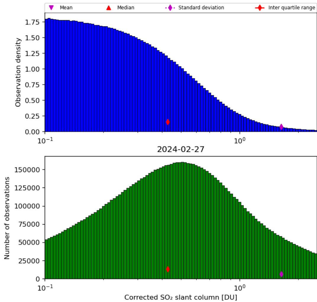
Figure 55: Histogram of “Corrected SO 2 slant column” for 2024-02-27 to 2024-02-28
