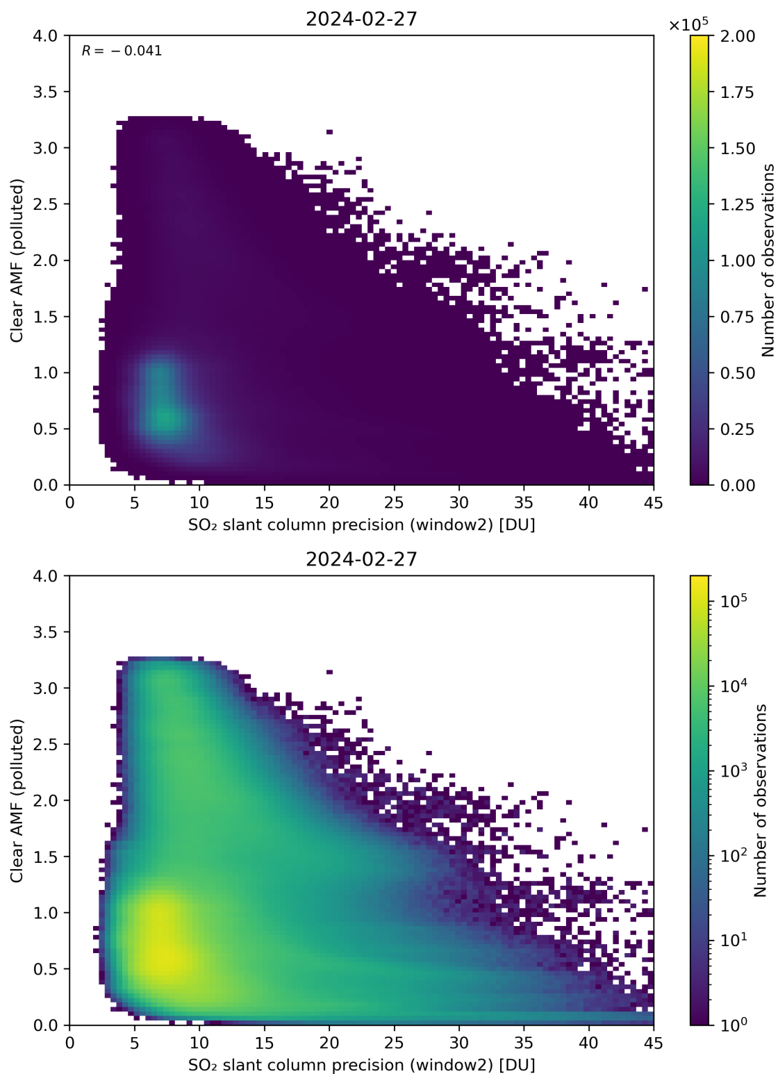
Figure 246: Scatter density plot of “SO 2 slant column precision (window2)” against “Clear AMF (polluted)” for 2024-02-27 to 2024-02-28.
