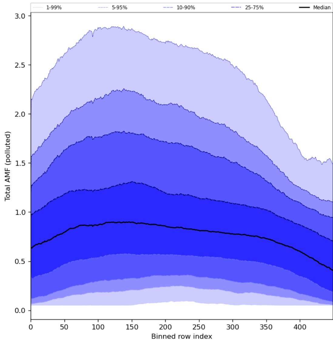
Figure 94: Along track statistics of “Total AMF (polluted)” for 2024-02-27 to 2024-02-28
