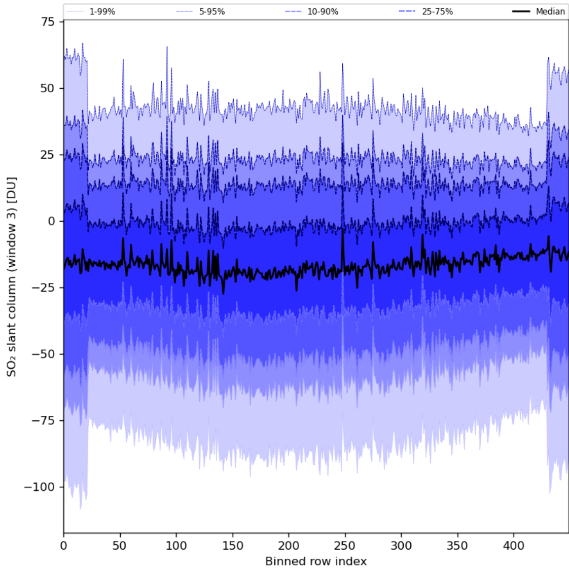
Figure 87: Along track statistics of “SO 2 slant column (window 3)” for 2024-02-27 to 2024-02-28
