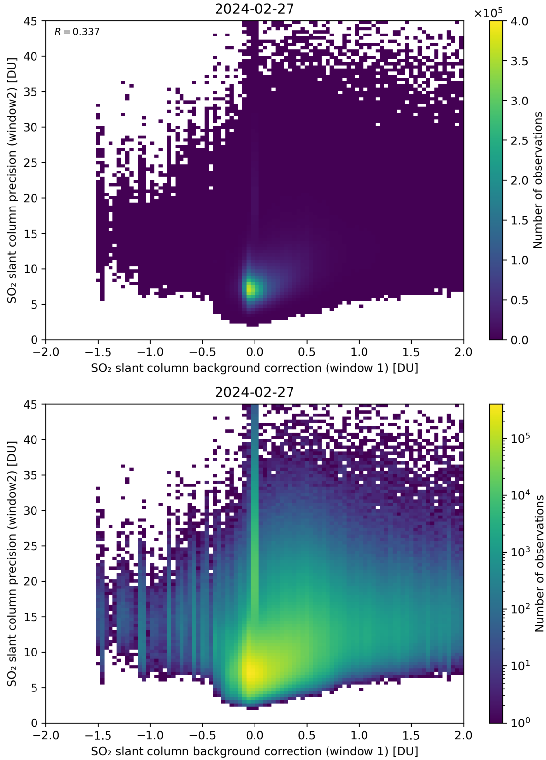
Figure 106: Scatter density plot of “SO 2 slant column background correction (window 1)” against “SO 2 slant column precision (window2)” for 2024-02-27 to 2024-02-28.
