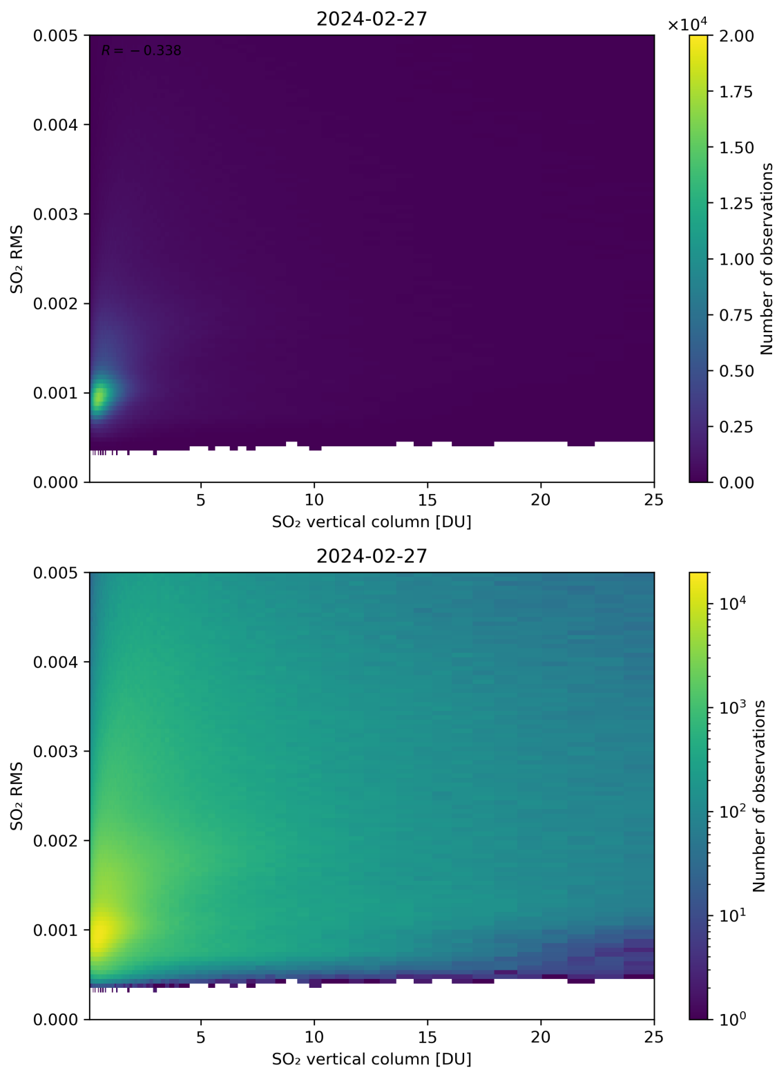
Figure 278: Scatter density plot of “SO 2 vertical column” against “SO 2 RMS” for 2024-02-27 to 2024-02-28.
