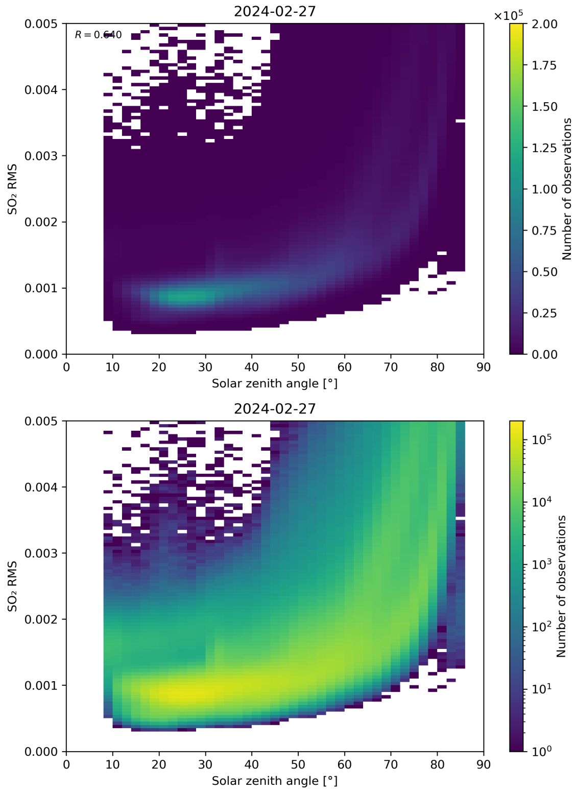
Figure 163: Scatter density plot of “Solar zenith angle” against “SO 2 RMS” for 2024-02-27 to 2024-02-28.
