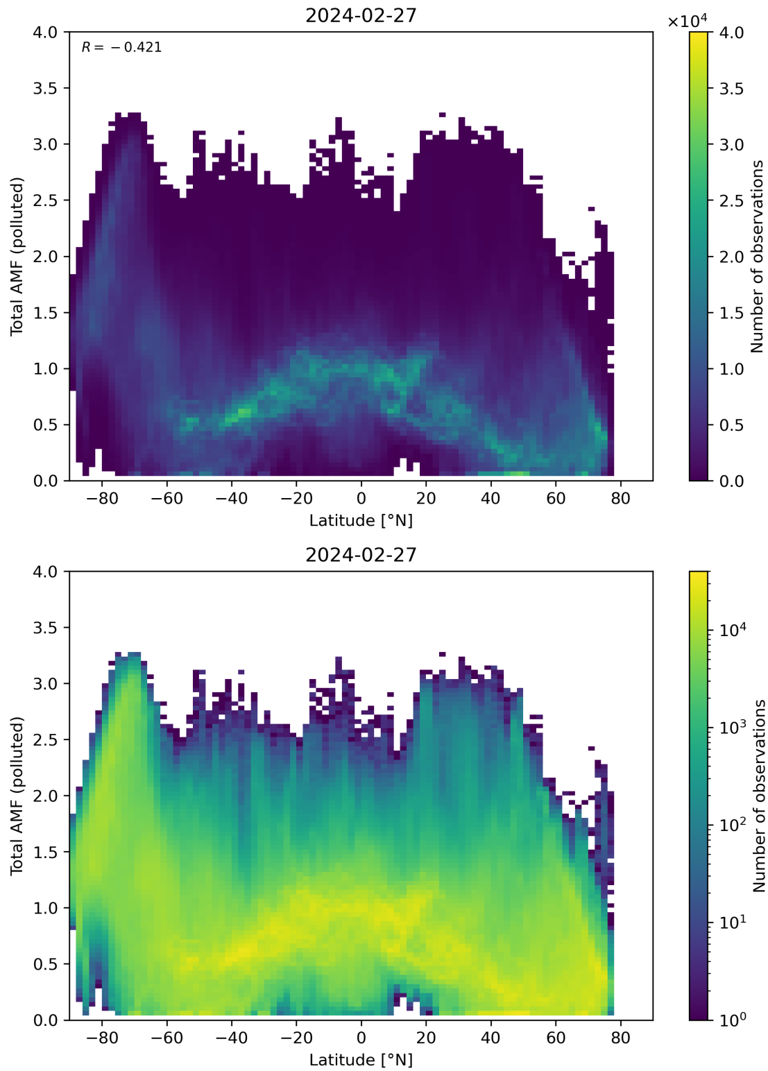
Figure 154: Scatter density plot of “Latitude” against “Total AMF (polluted)” for 2024-02-27 to 2024-02-28.
