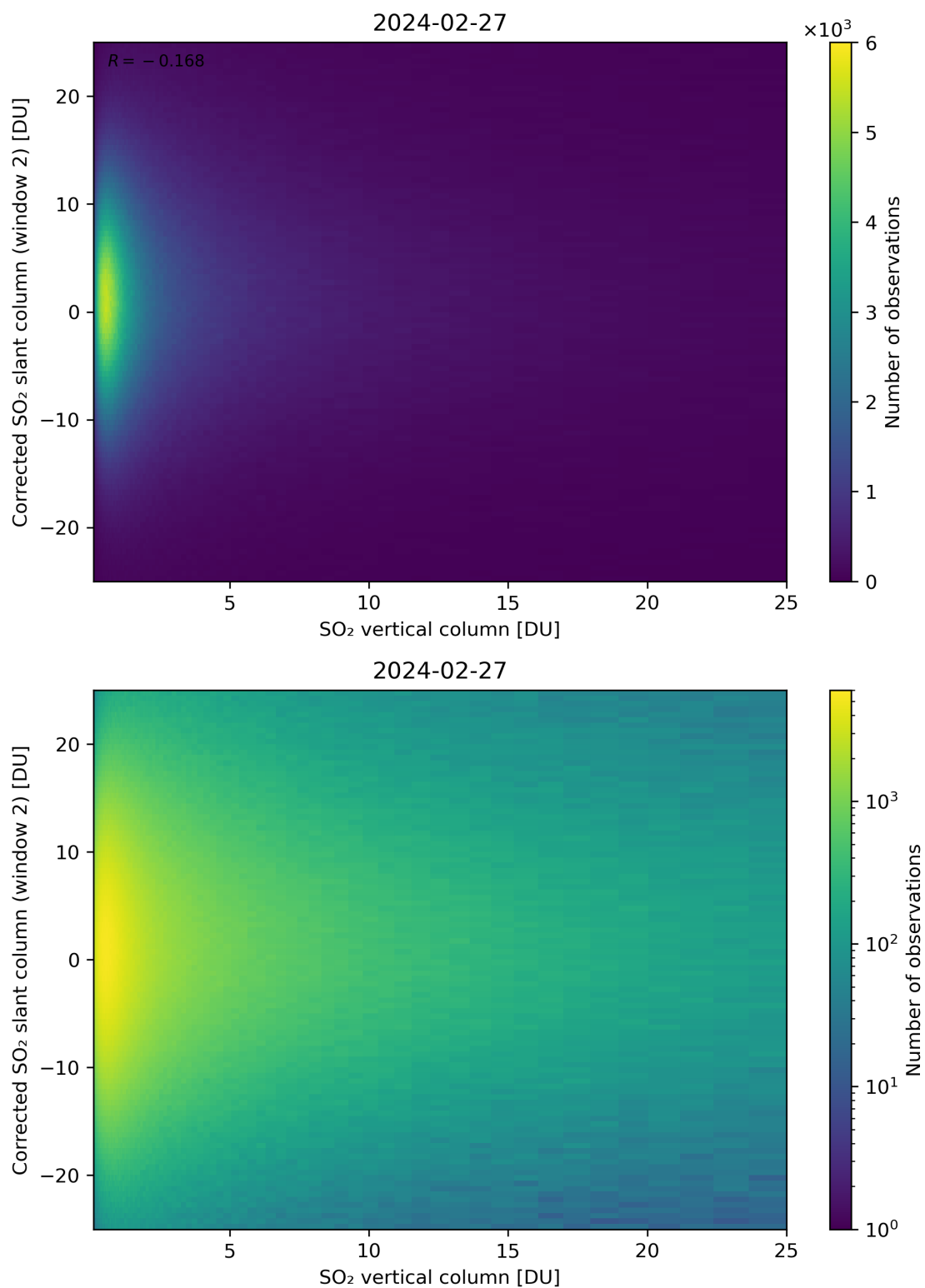
Figure 298: Scatter density plot of “SO 2 vertical column” against “Corrected SO 2 slant column (window 2)” for 2024-02-27 to 2024-02-28.
