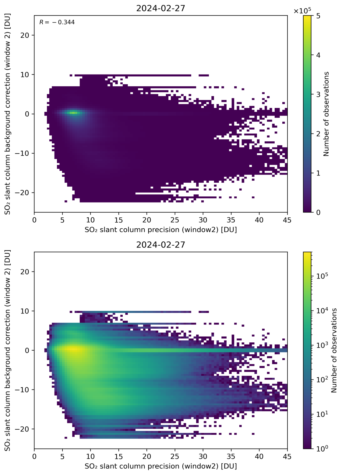
Figure 241: Scatter density plot of “SO 2 slant column precision (window2)” against “SO 2 slant column background correction (window 2)” for 2024-02-27 to 2024-02-28.
