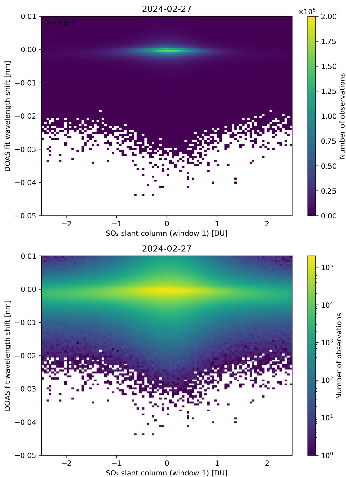
Figure 215: Scatter density plot of “SO 2 slant column (window 1)” against “DOAS fit wavelength shift” for 2024-02-27 to 2024-02-28.
