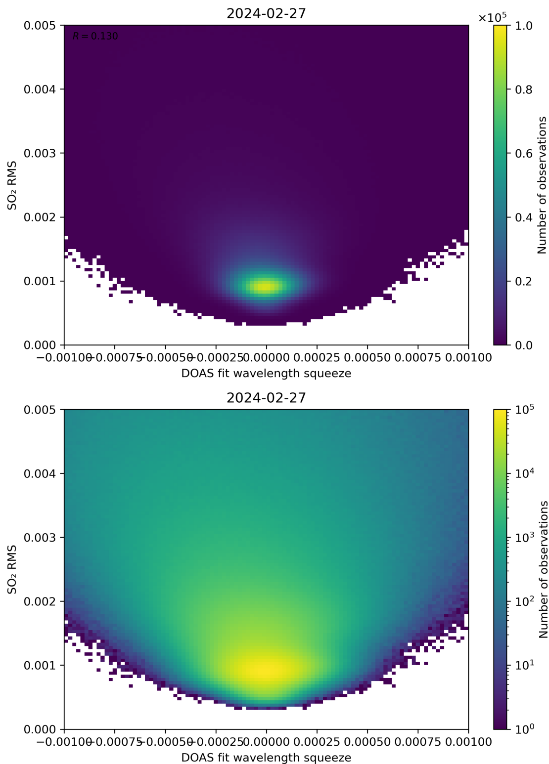
Figure 132: Scatter density plot of “DOAS fit wavelength squeeze” against “SO 2 RMS” for 2024-02-27 to 2024-02-28.
