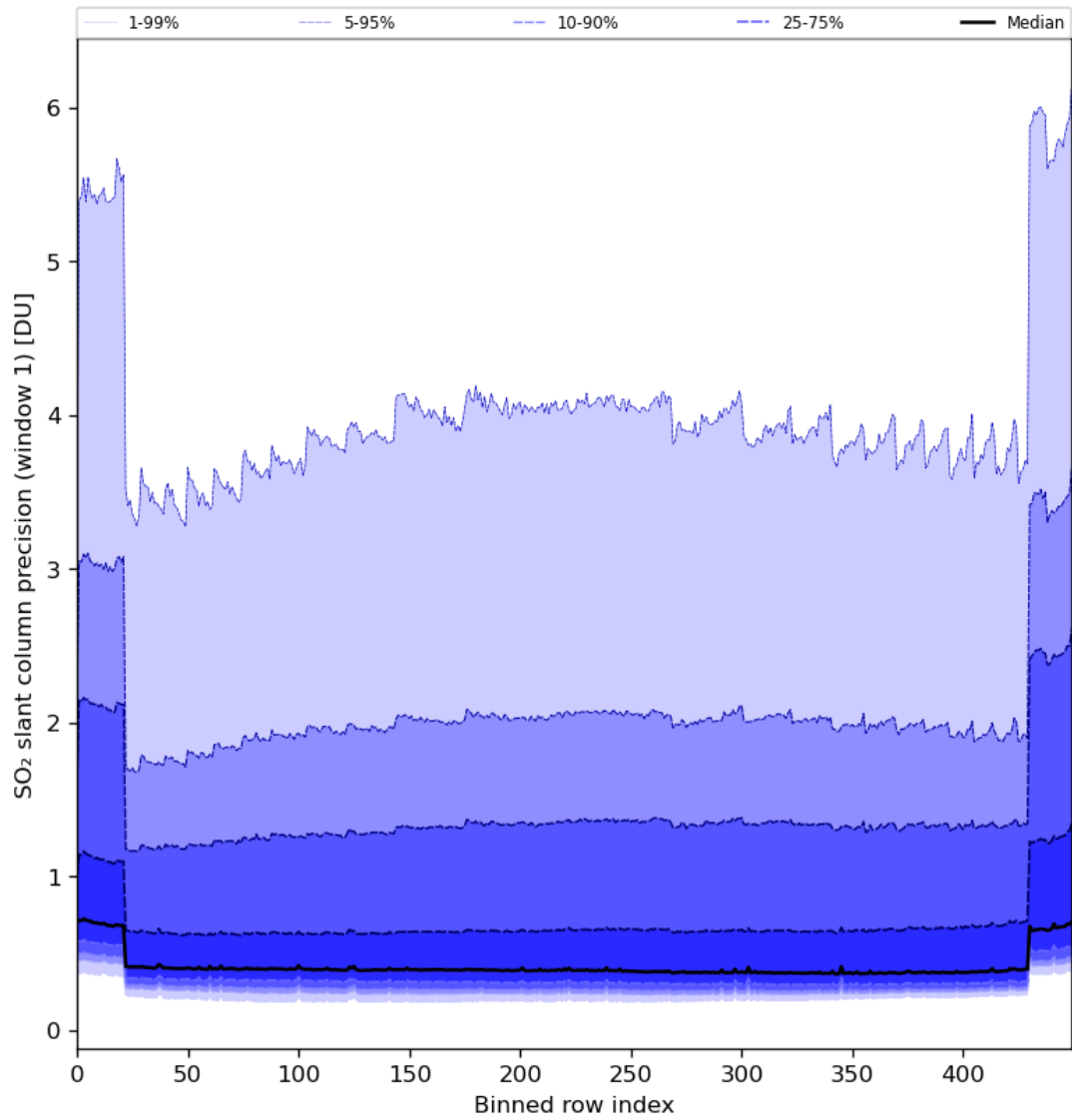
Figure 80: Along track statistics of “SO 2 slant column precision (window 1)” for 2024-02-27 to 2024-02-28
