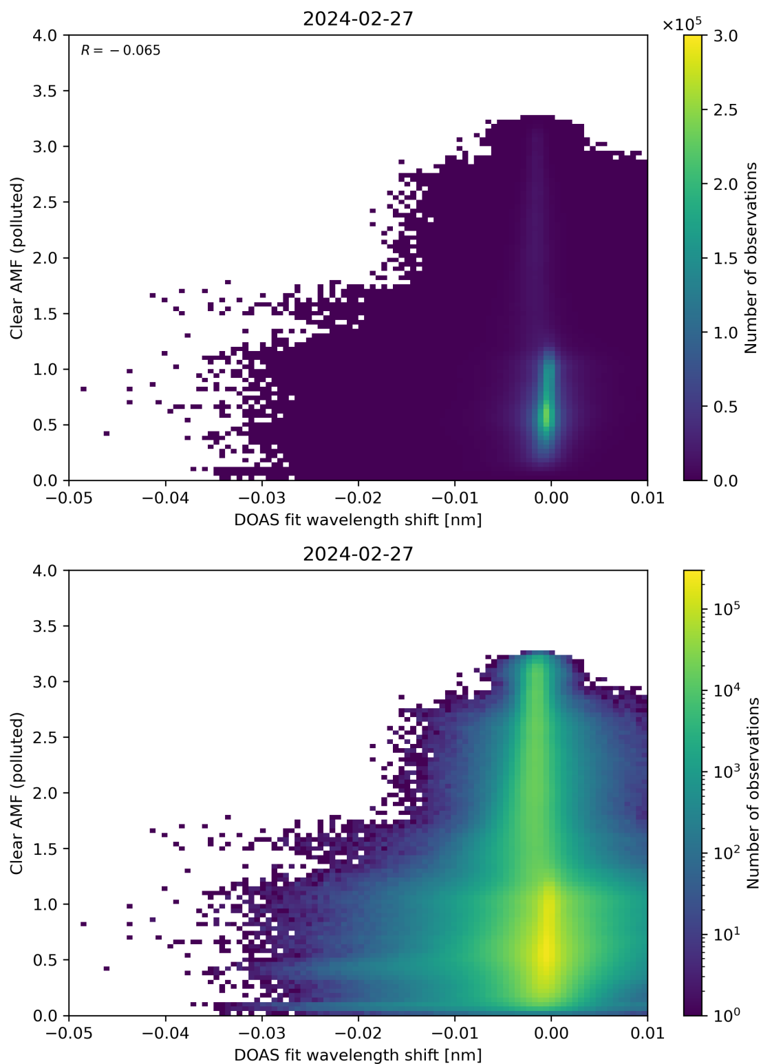
Figure 129: Scatter density plot of “DOAS fit wavelength shift” against “Clear AMF (polluted)” for 2024-02-27 to 2024-02-28.
