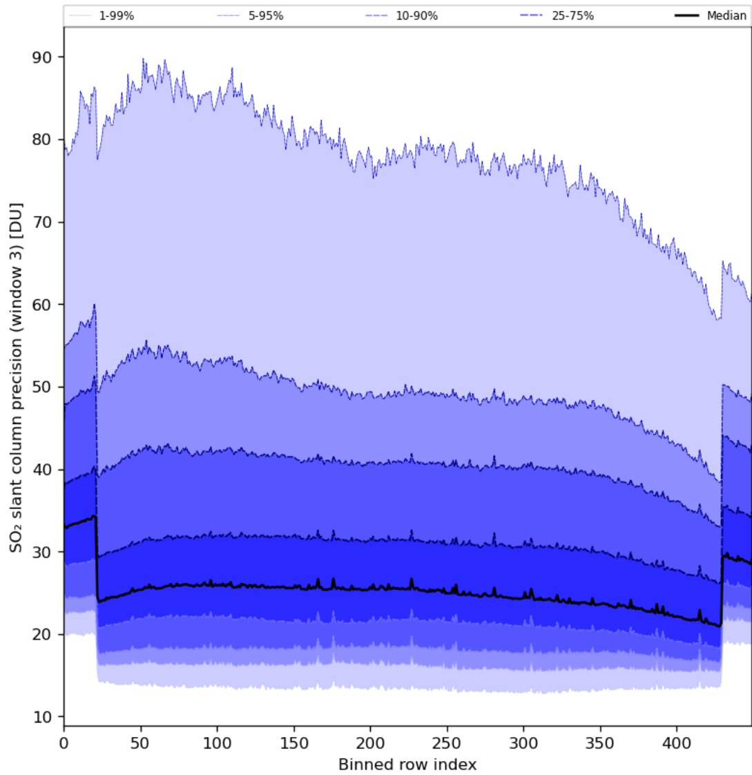
Figure 88: Along track statistics of “SO 2 slant column precision (window 3)” for 2024-02-27 to 2024-02-28
