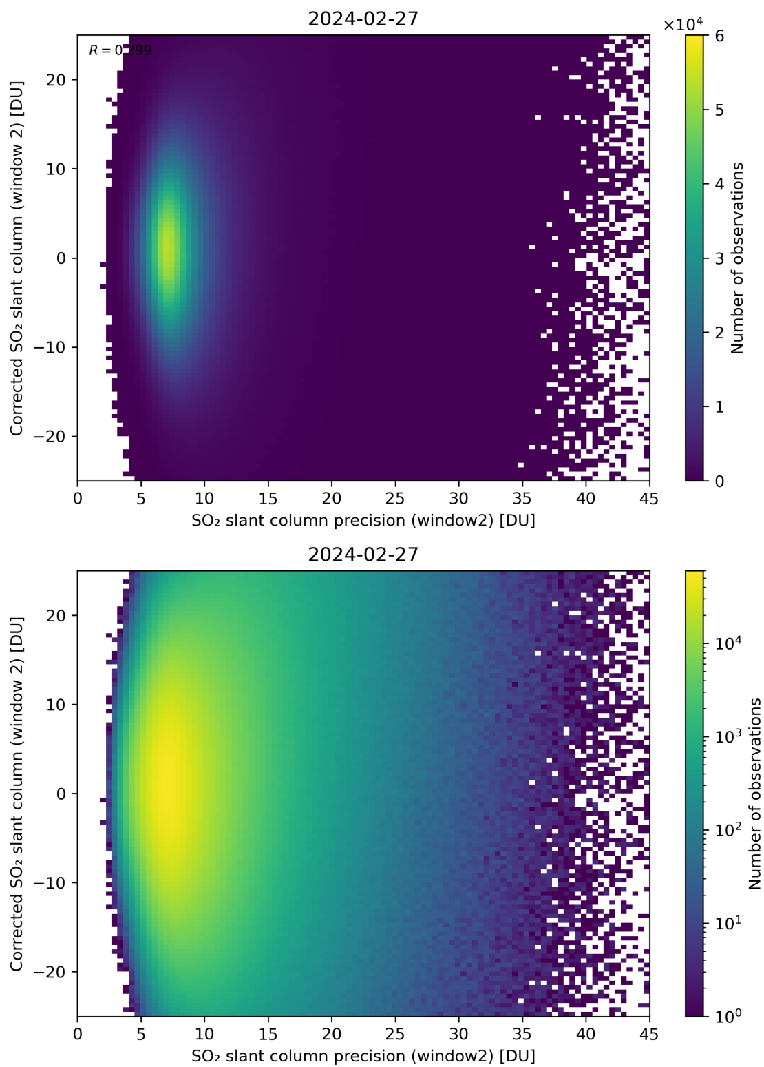
Figure 247: Scatter density plot of “SO 2 slant column precision (window2)” against “Corrected SO 2 slant column (window 2)” for 2024-02-27 to 2024-02-28.
