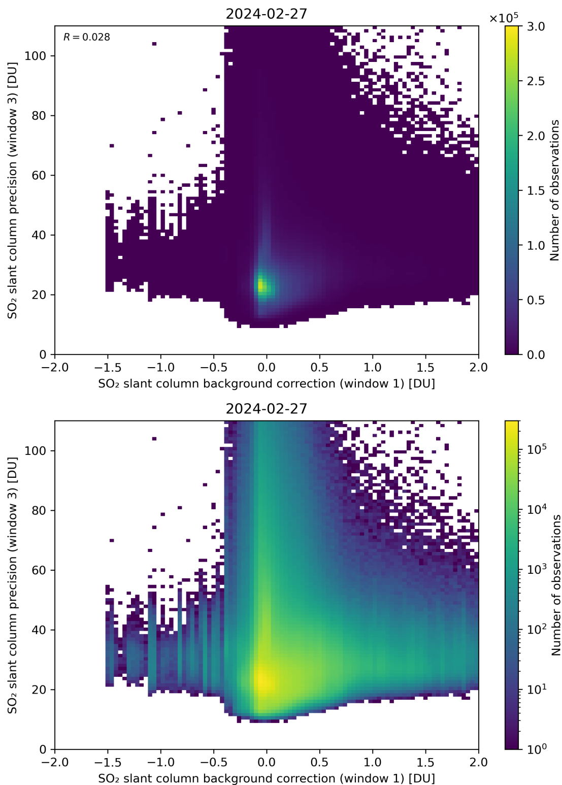
Figure 108: Scatter density plot of “SO 2 slant column background correction (window 1)” against “SO 2 slant column precision (window 3)” for 2024-02-27 to 2024-02-28.
