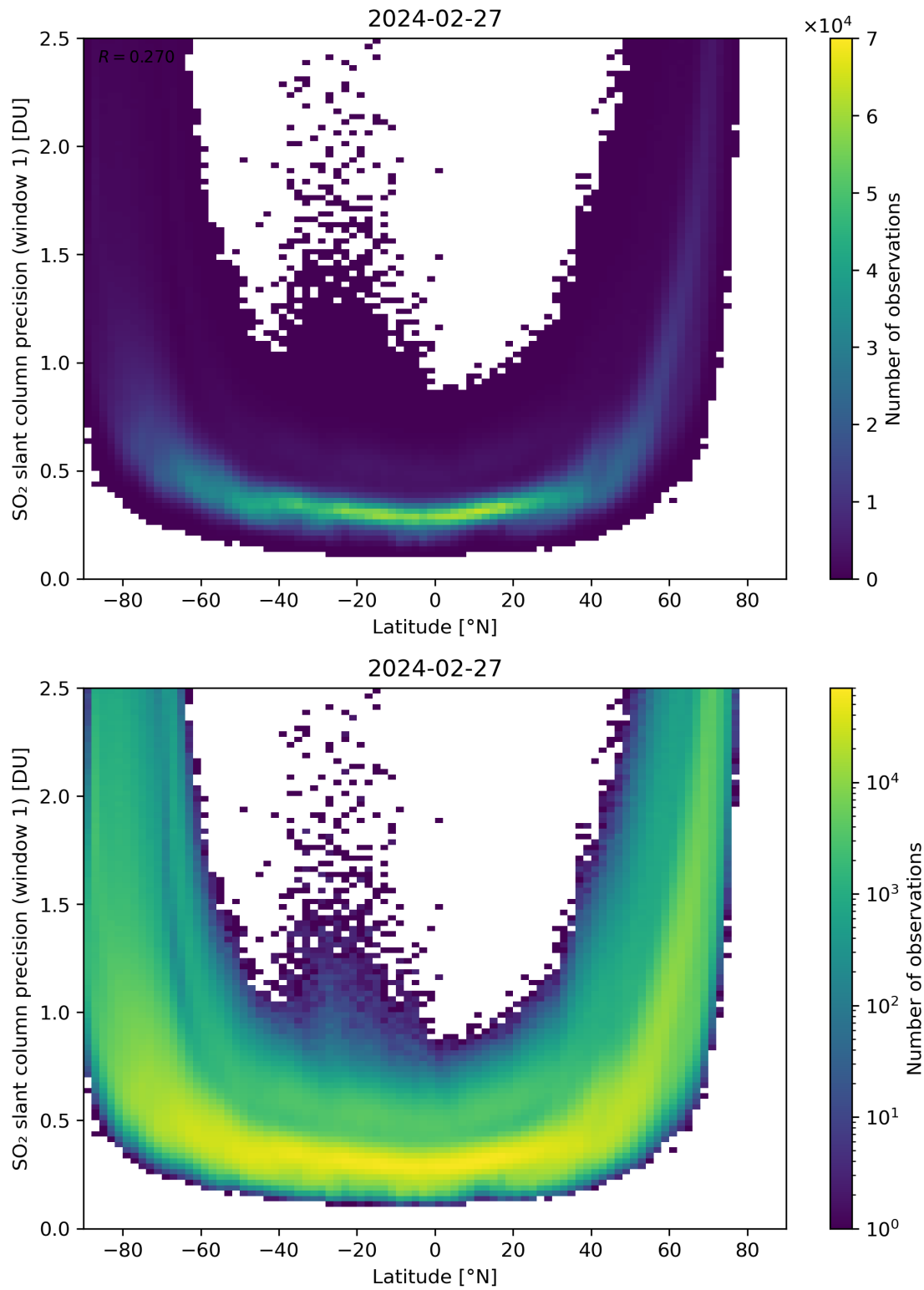
Figure 150: Scatter density plot of “Latitude” against “SO 2 slant column precision (window 1)” for 2024-02-27 to 2024-02-28.
