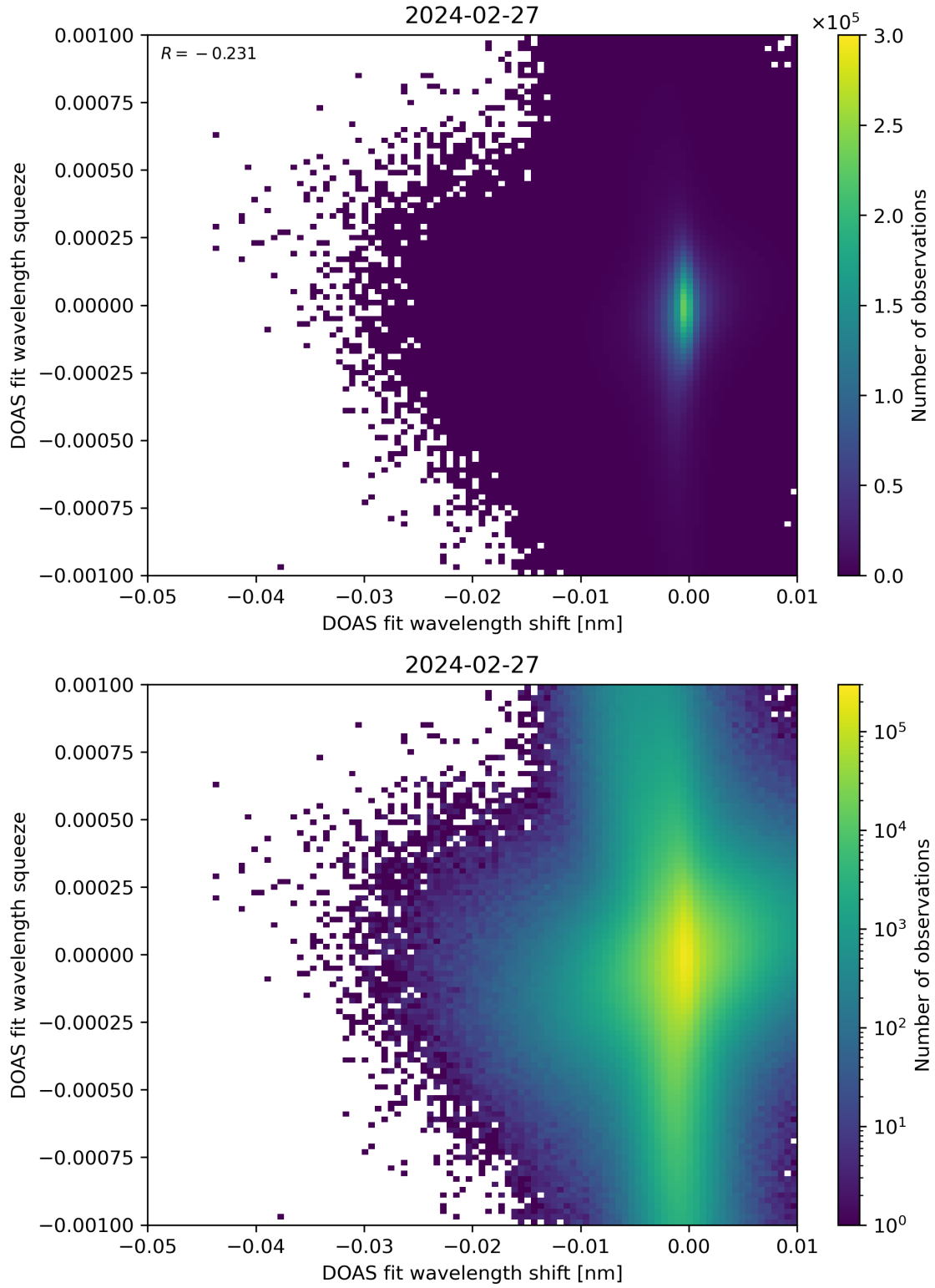
Figure 127: Scatter density plot of “DOAS fit wavelength shift” against “DOAS fit wavelength squeeze” for 2024-02-27 to 2024-02-28.
