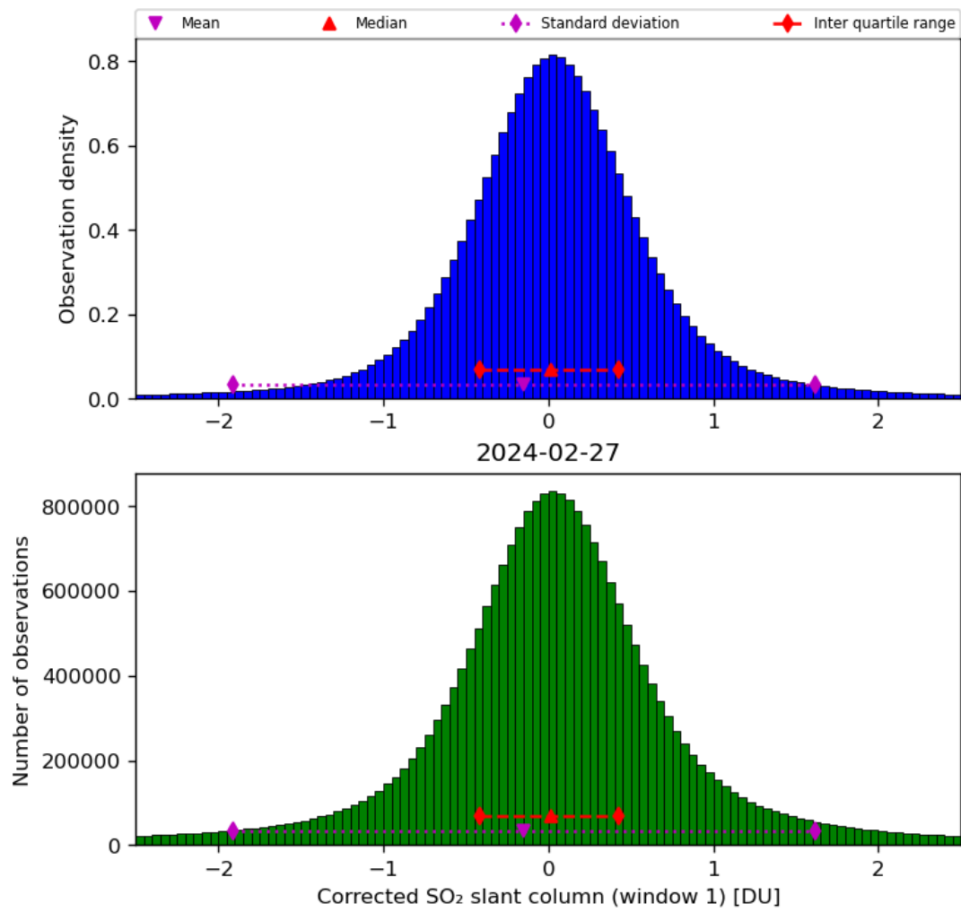
Figure 58: Histogram of “Corrected SO 2 slant column (window 1)” for 2024-02-27 to 2024-02-28
