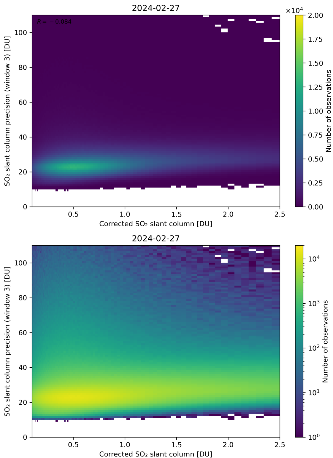
Figure 191: Scatter density plot of “Corrected SO 2 slant column” against “SO 2 slant column precision (window 3)” for 2024-02-27 to 2024-02-28.
