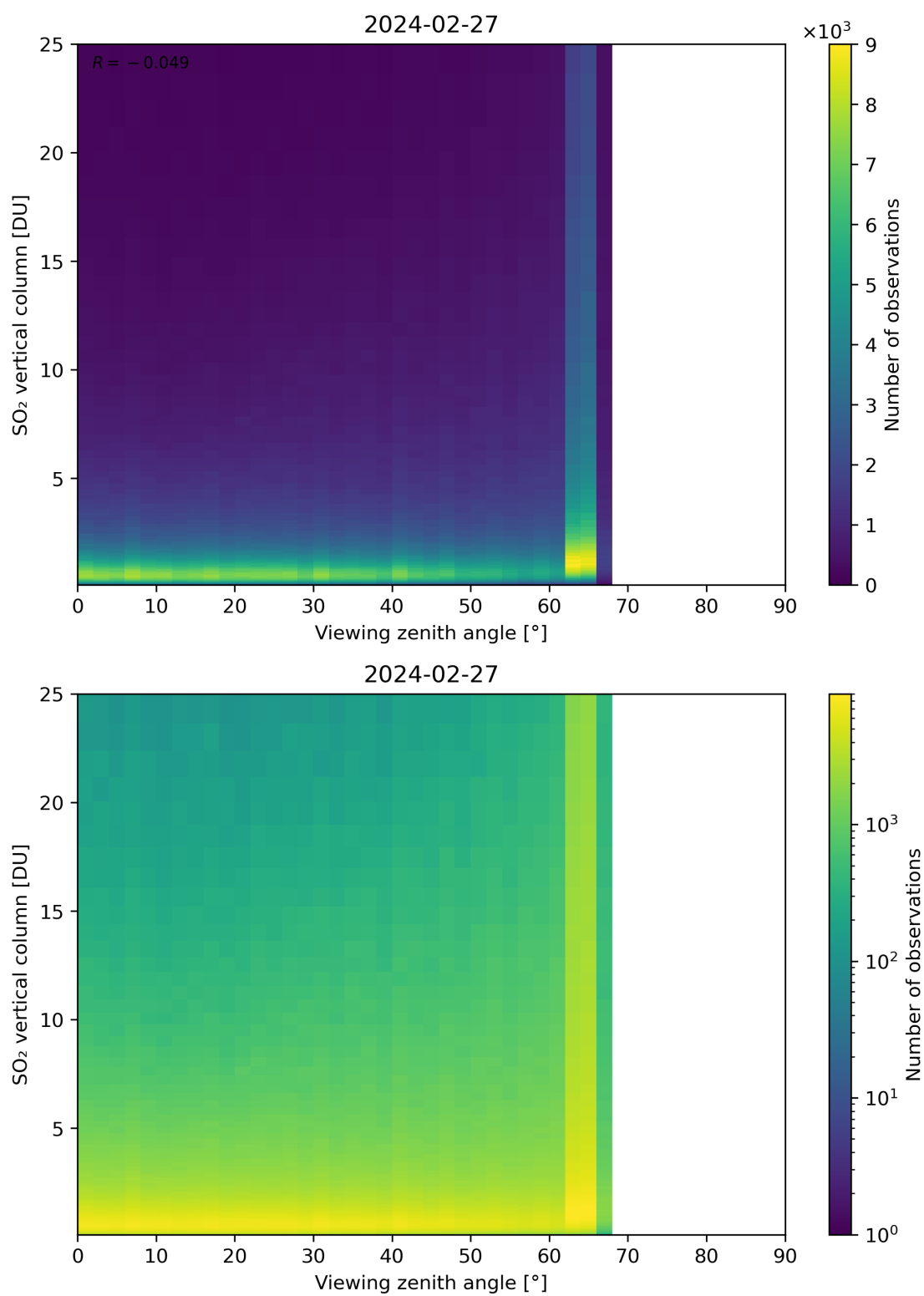
Figure 327: Scatter density plot of “Viewing zenith angle” against “SO 2 vertical column” for 2024-02-27 to 2024-02-28.
