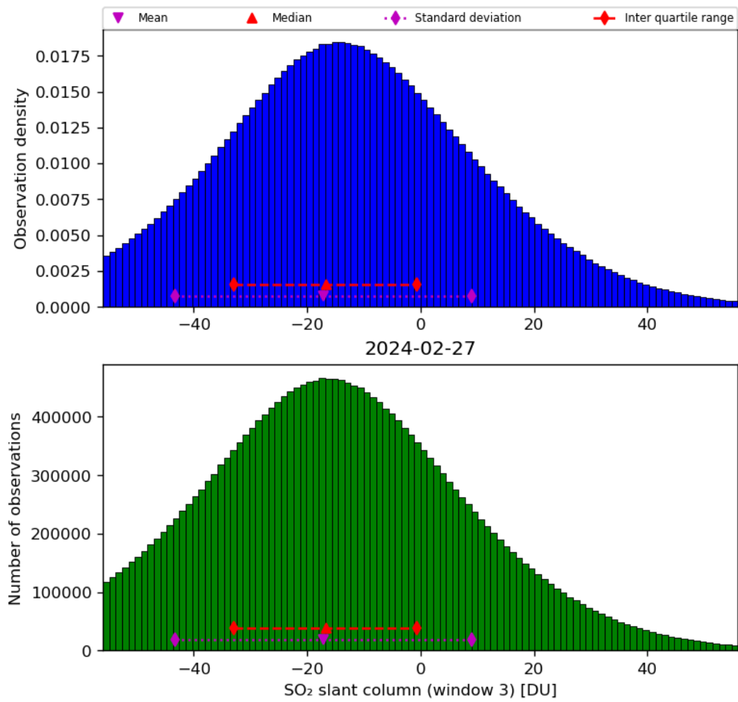
Figure 64: Histogram of “SO 2 slant column (window 3)” for 2024-02-27 to 2024-02-28
