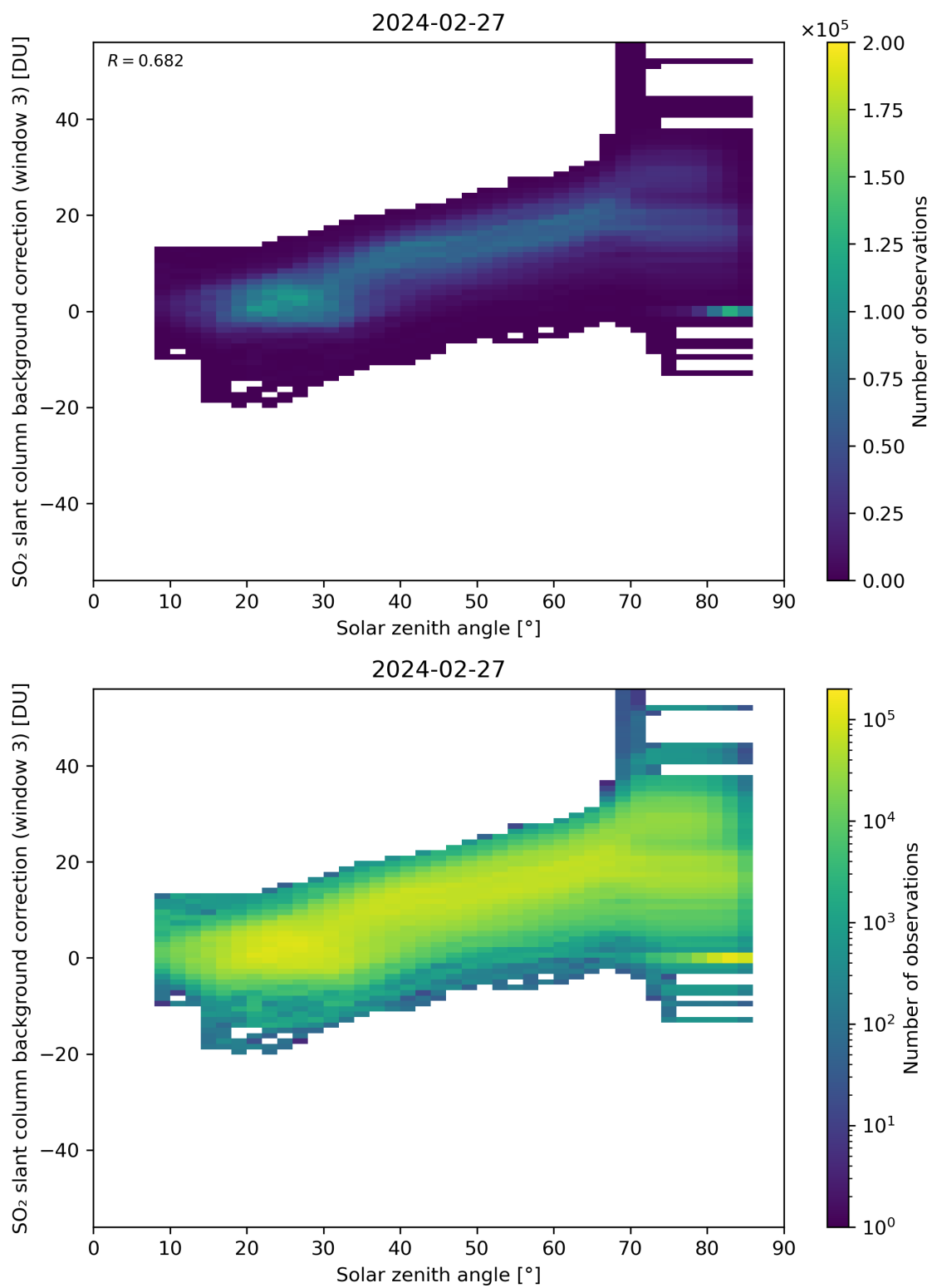
Figure 160: Scatter density plot of “Solar zenith angle” against “SO 2 slant column background correction (window 3)” for 2024-02-27 to 2024-02-28.
