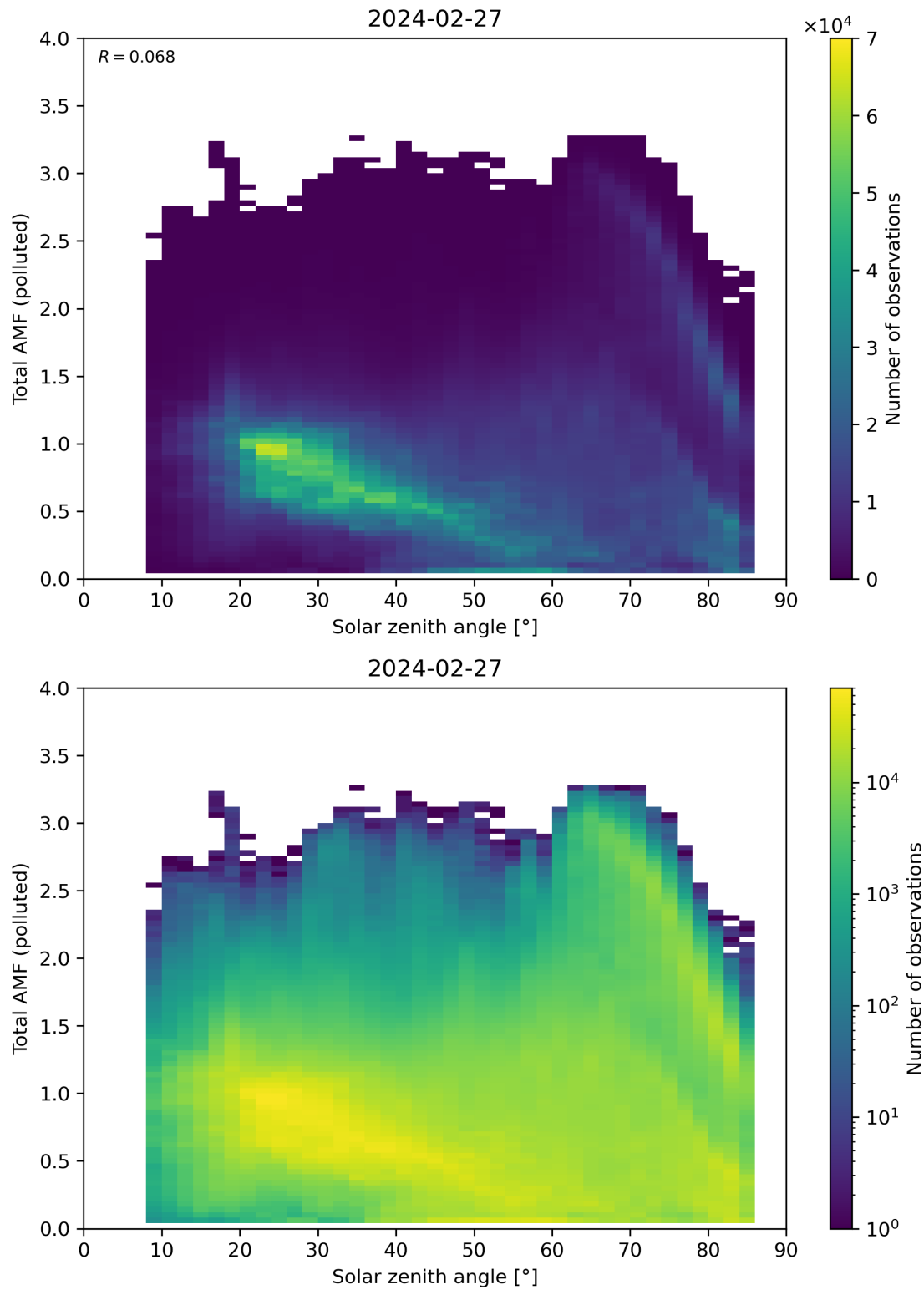
Figure 174: Scatter density plot of “Solar zenith angle” against “Total AMF (polluted)” for 2024-02-27 to 2024-02-28.
