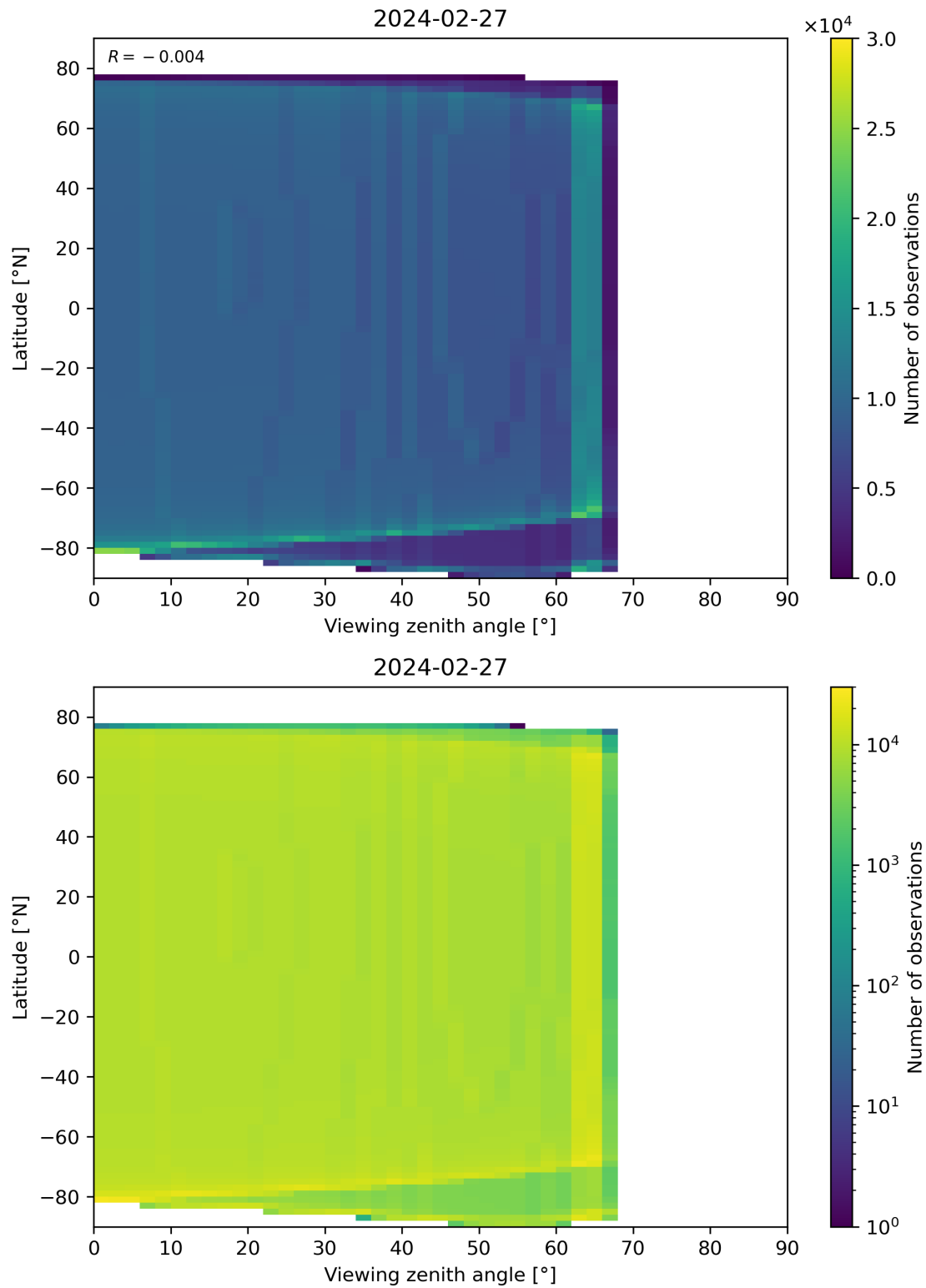
Figure 314: Scatter density plot of “Viewing zenith angle” against “Latitude” for 2024-02-27 to 2024-02-28.
