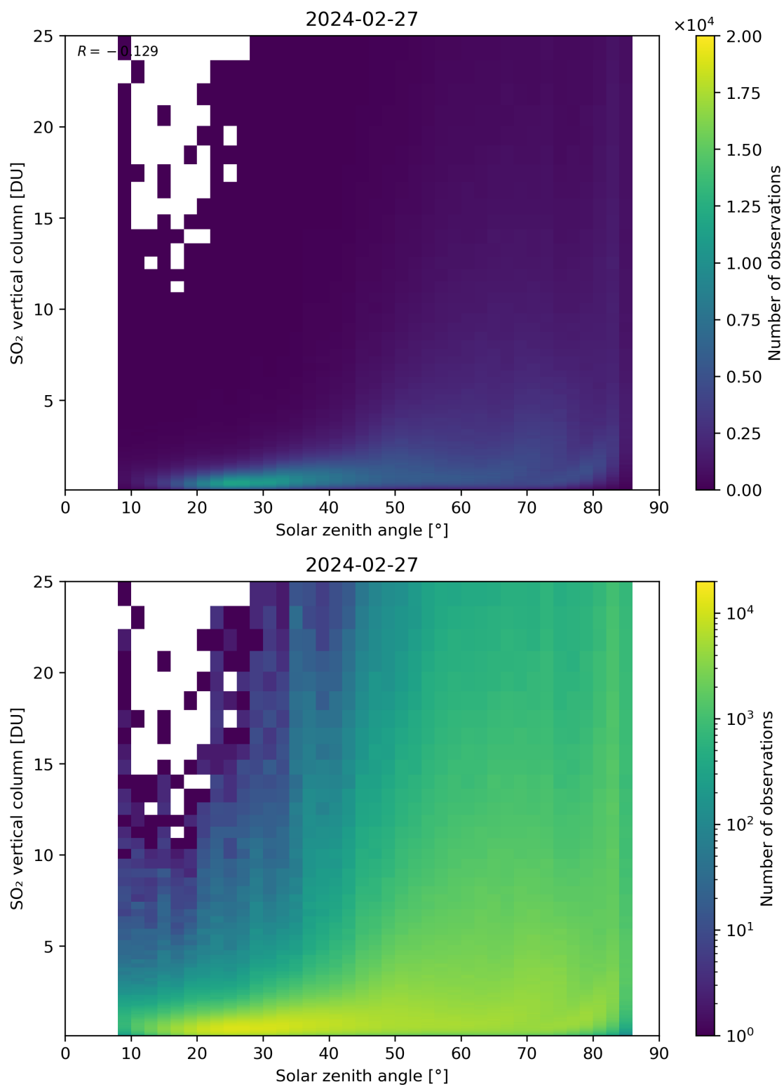
Figure 176: Scatter density plot of “Solar zenith angle” against “SO 2 vertical column” for 2024-02-27 to 2024-02-28.
