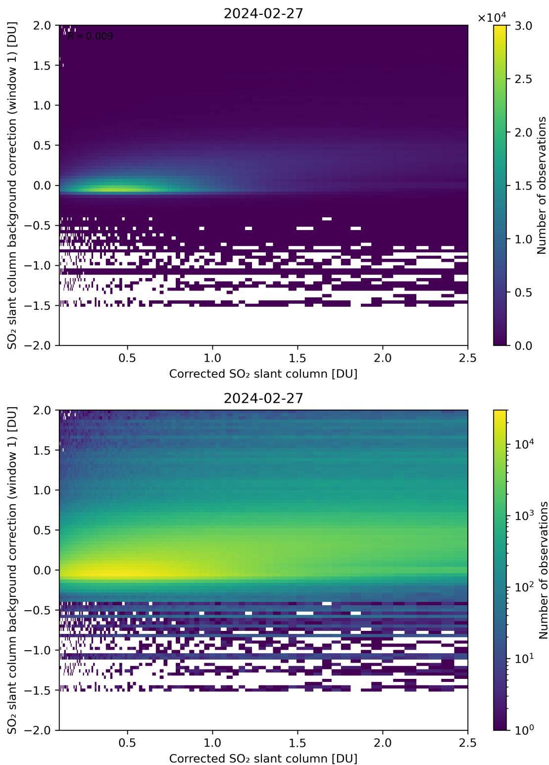
Figure 178: Scatter density plot of “Corrected SO 2 slant column” against “SO 2 slant column background correction (window 1)” for 2024-02-27 to 2024-02-28.
