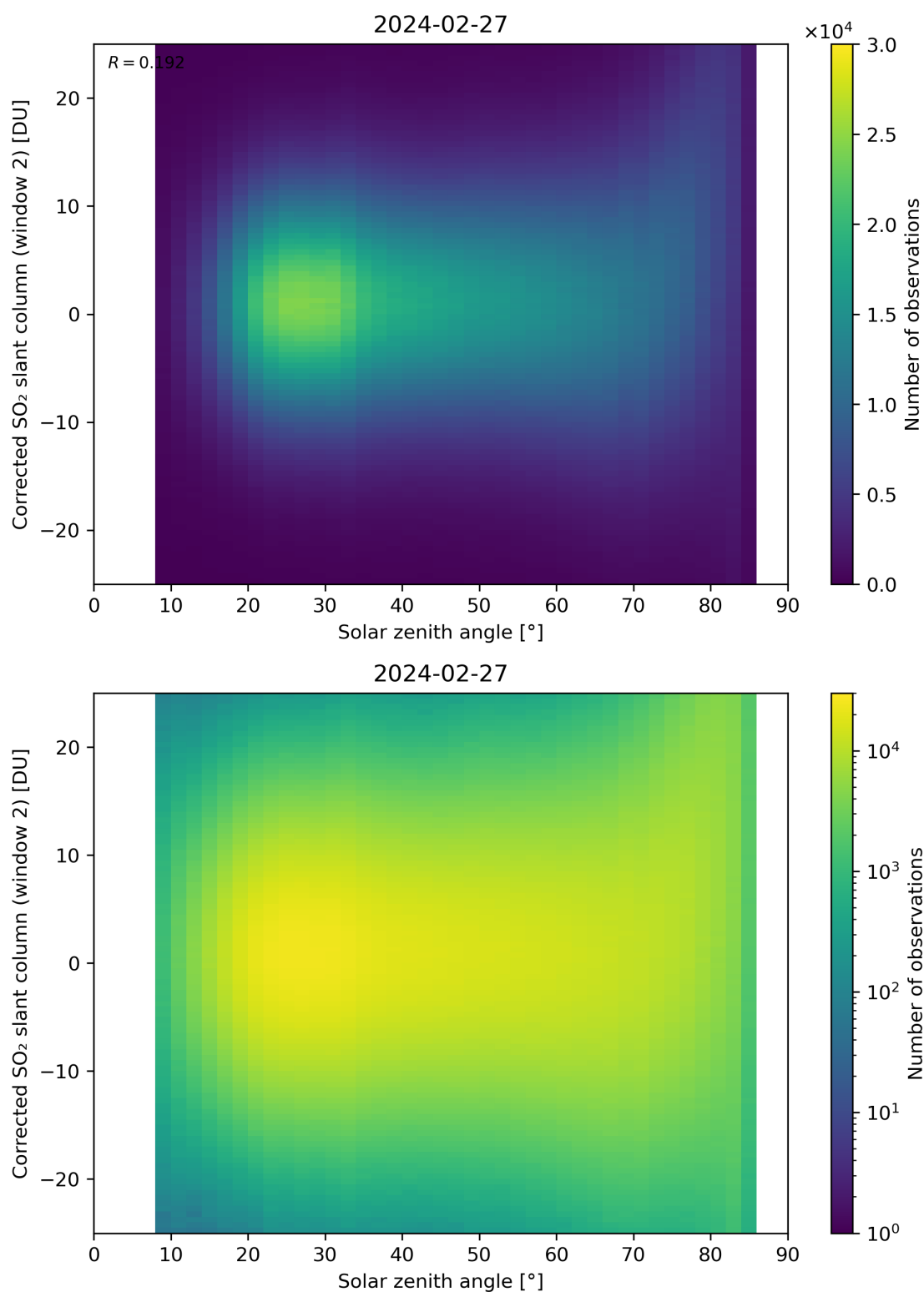
Figure 167: Scatter density plot of “Solar zenith angle” against “Corrected SO 2 slant column (window 2)” for 2024-02-27 to 2024-02-28.
