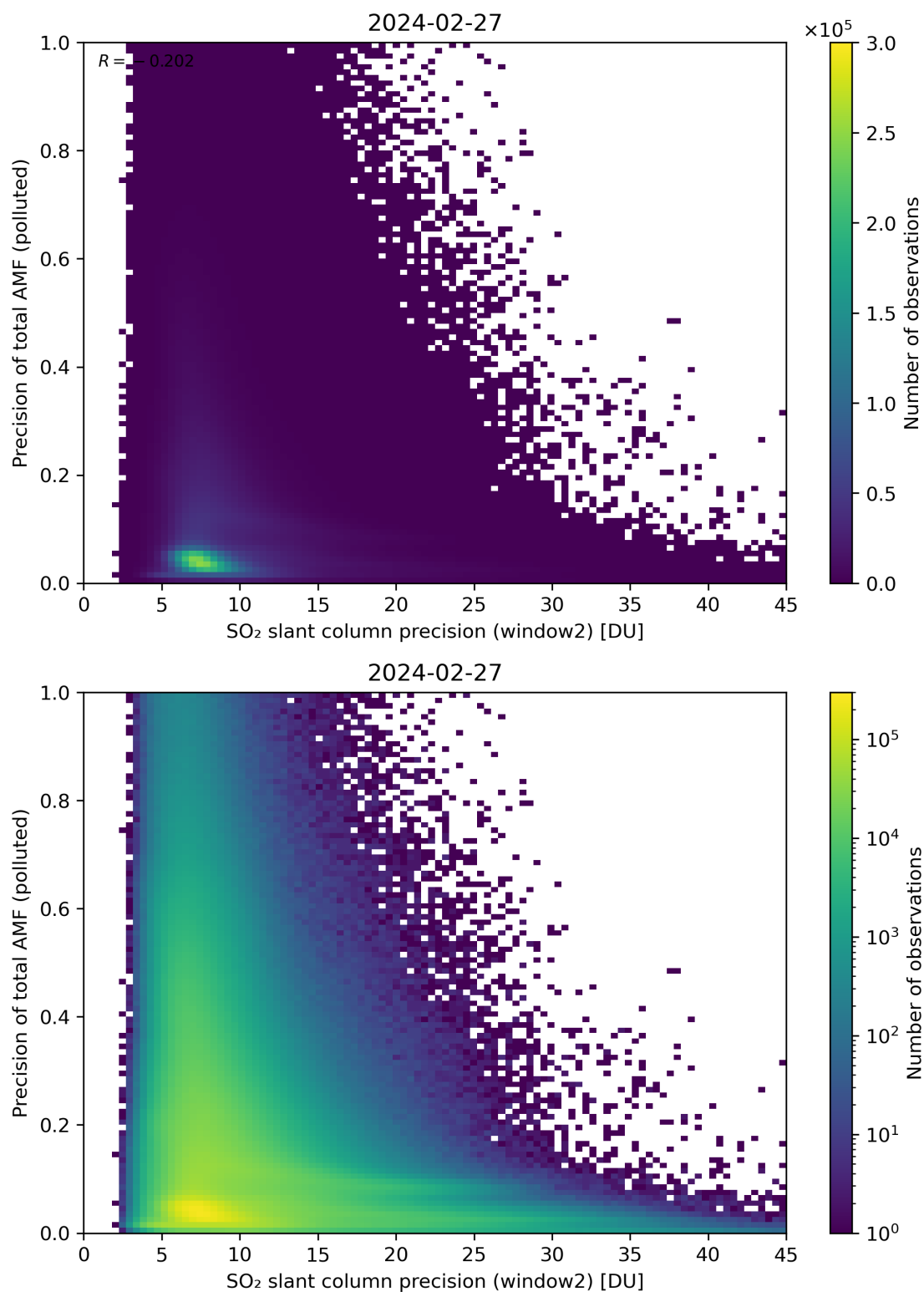
Figure 252: Scatter density plot of “SO 2 slant column precision (window2)” against “Precision of total AMF (polluted)” for 2024-02-27 to 2024-02-28.
