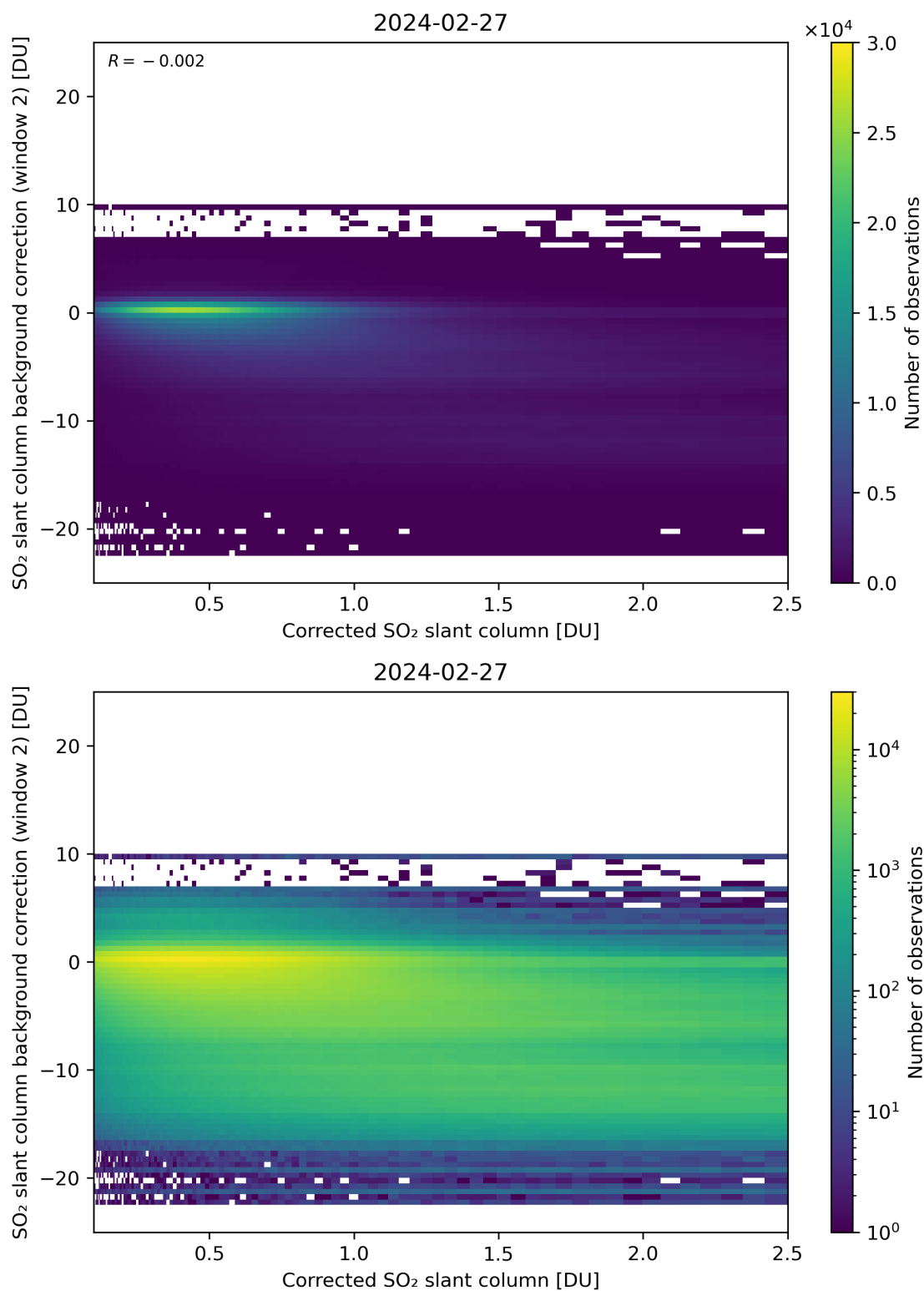
Figure 179: Scatter density plot of “Corrected SO 2 slant column” against “SO 2 slant column background correction (window 2)” for 2024-02-27 to 2024-02-28.
