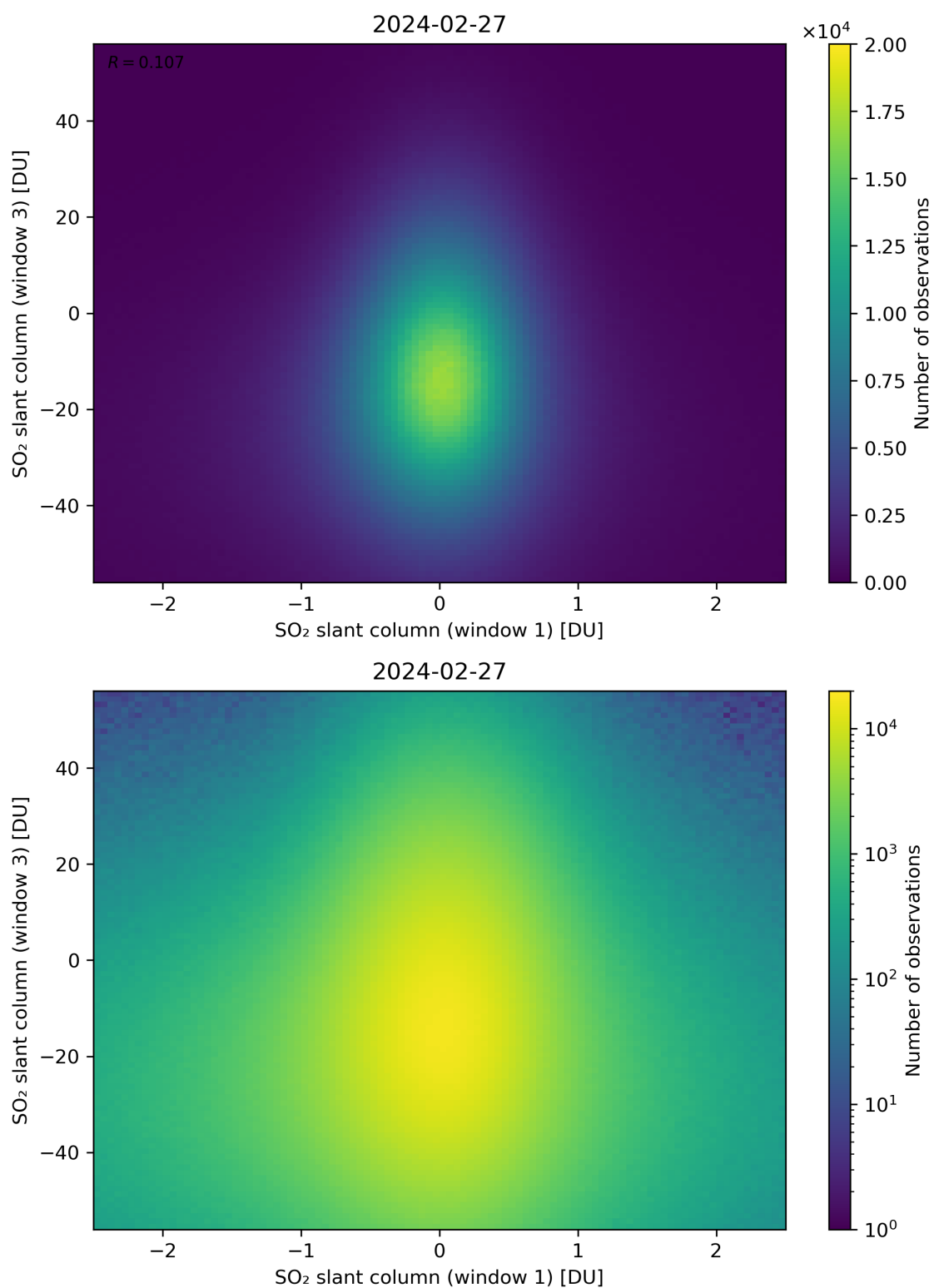
Figure 237: Scatter density plot of “SO 2 slant column (window 1)” against “SO 2 slant column (window 3)” for 2024-02-27 to 2024-02-28.
