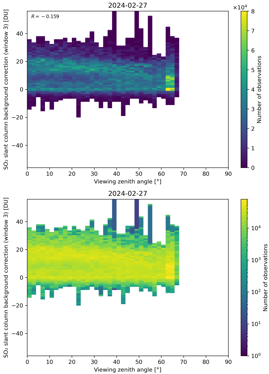
Figure 310: Scatter density plot of “Viewing zenith angle” against “SO 2 slant column background correction (window 3)” for 2024-02-27 to 2024-02-28.
