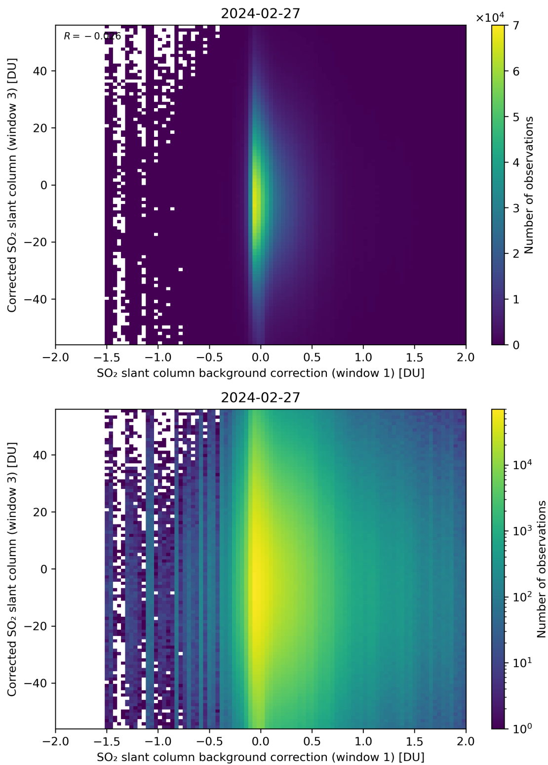
Figure 105: Scatter density plot of “SO 2 slant column background correction (window 1)” against “Corrected SO 2 slant column (window 3)” for 2024-02-27 to 2024-02-28.
