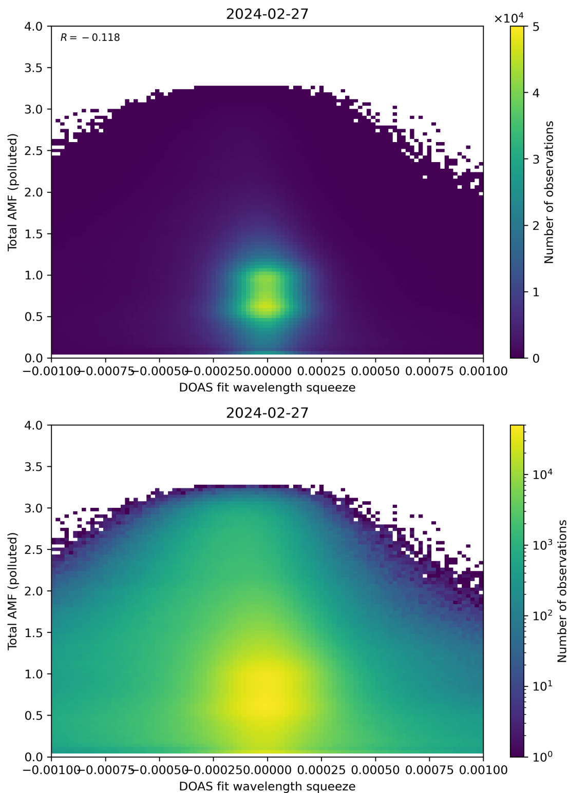
Figure 134: Scatter density plot of “DOAS fit wavelength squeeze” against “Total AMF (polluted)” for 2024-02-27 to 2024-02-28.
