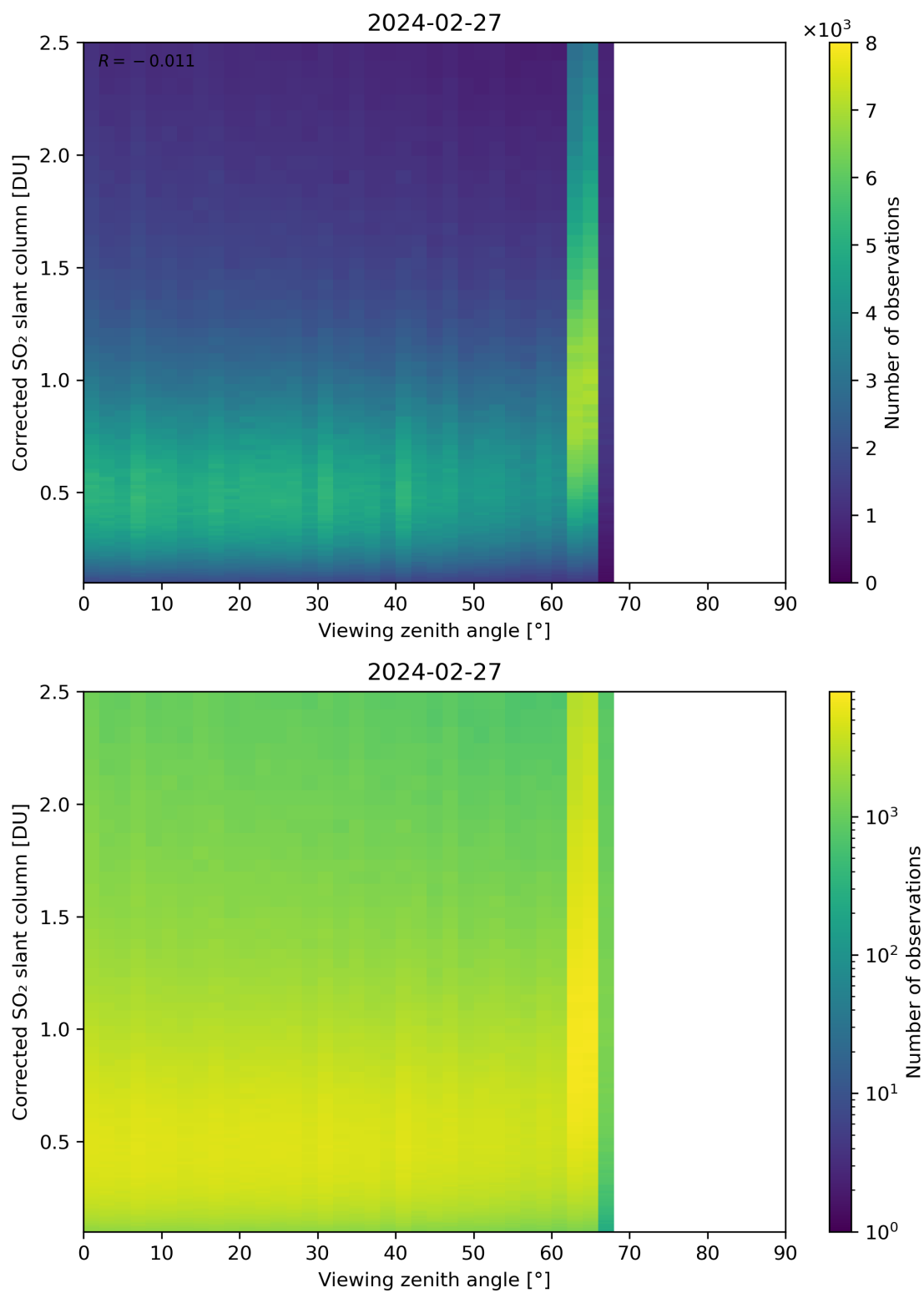
Figure 317: Scatter density plot of “Viewing zenith angle” against “Corrected SO 2 slant column” for 2024-02-27 to 2024-02-28.
