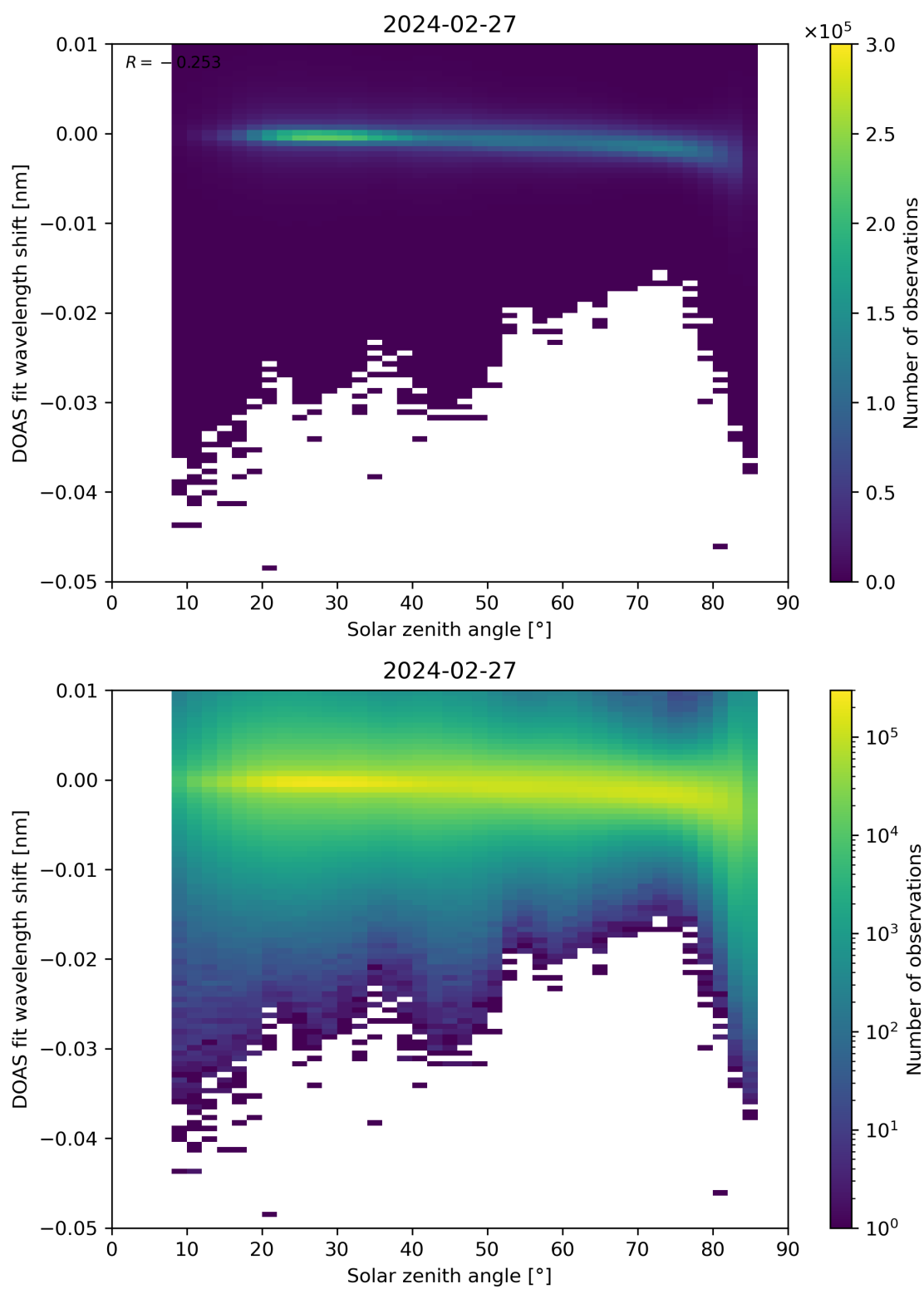
Figure 161: Scatter density plot of “Solar zenith angle” against “DOAS fit wavelength shift” for 2024-02-27 to 2024-02-28.
