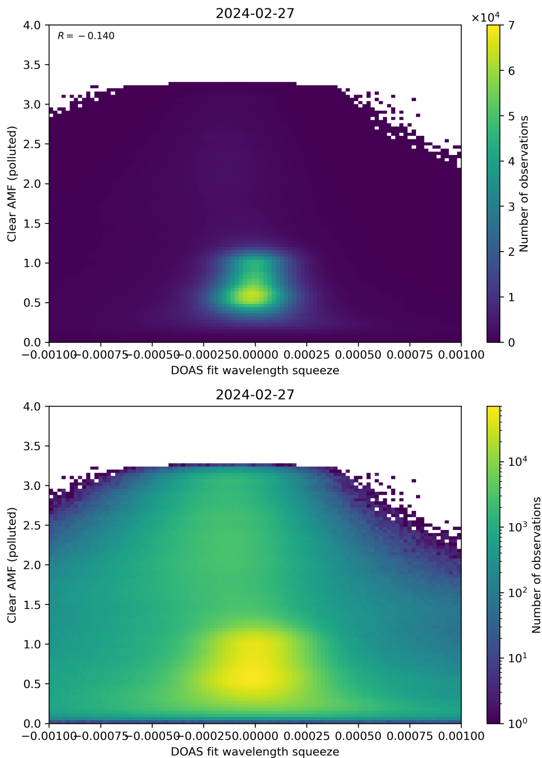
Figure 133: Scatter density plot of “DOAS fit wavelength squeeze” against “Clear AMF (polluted)” for 2024-02-27 to 2024-02-28.
