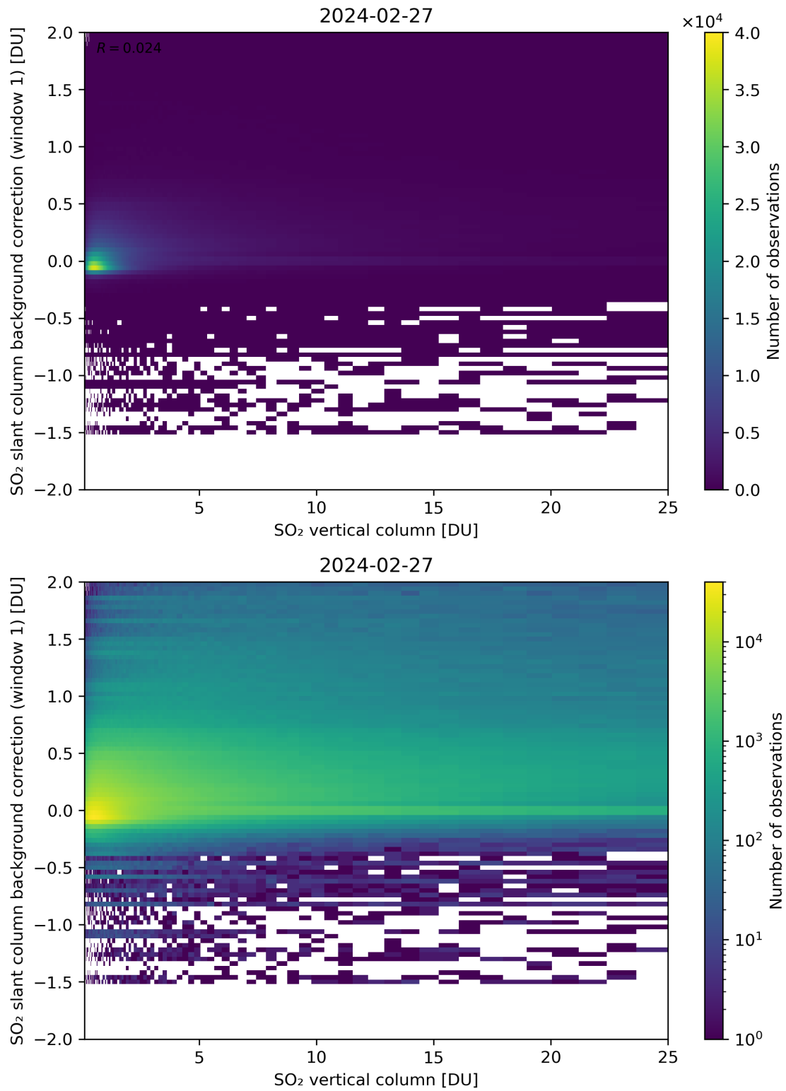
Figure 273: Scatter density plot of “SO 2 vertical column” against “SO 2 slant column background correction (window 1)” for 2024-02-27 to 2024-02-28.
