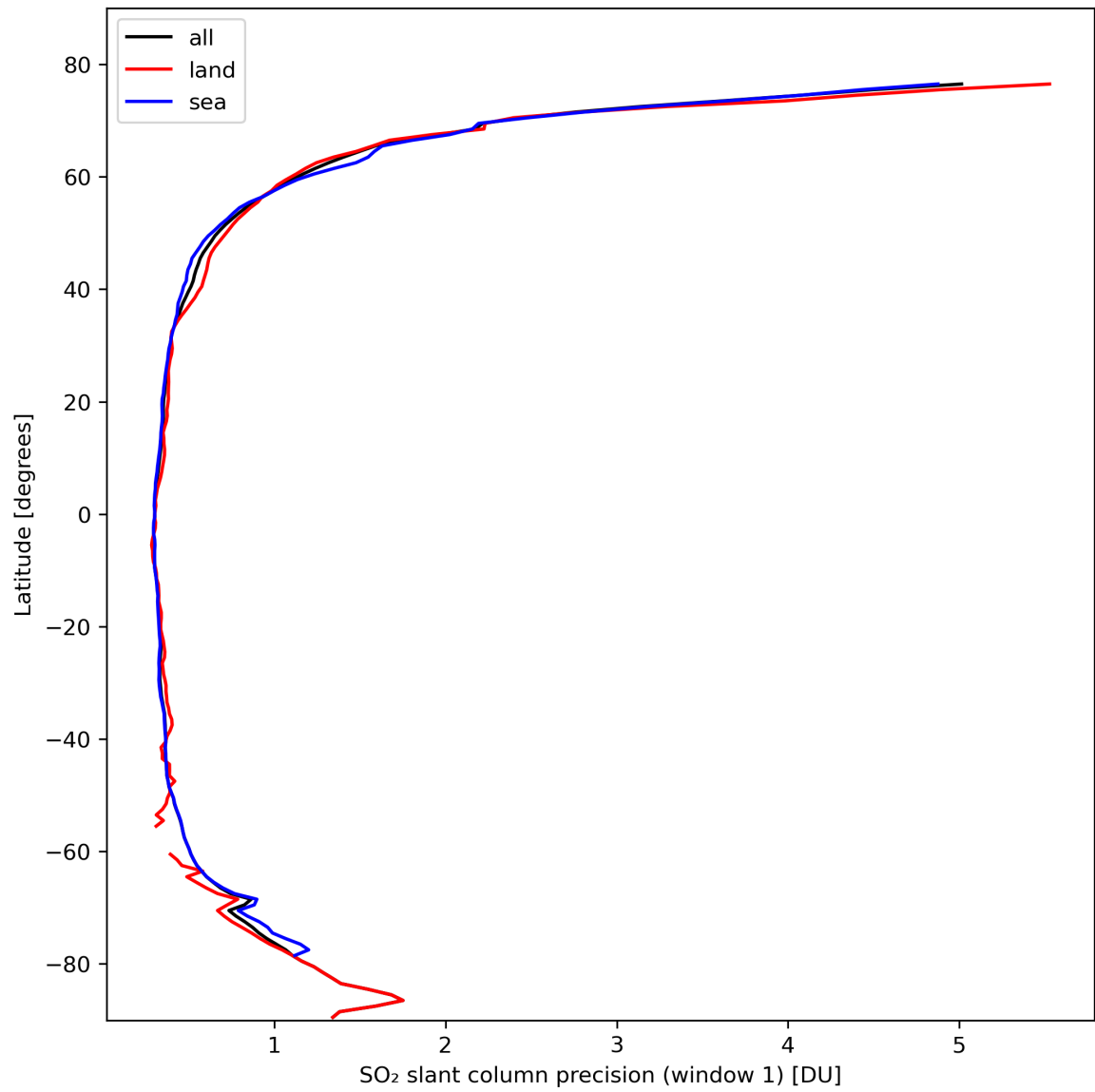
Figure 34: Zonal average of “SO 2 slant column precision (window 1)” for 2024-02-27 to 2024-02-28.
