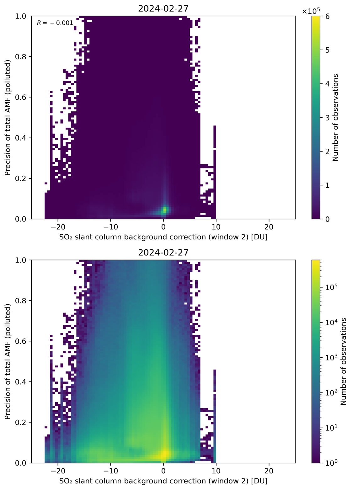
Figure 120: Scatter density plot of “SO 2 slant column background correction (window 2)” against “Precision of total AMF (polluted)” for 2024-02-27 to 2024-02-28.
