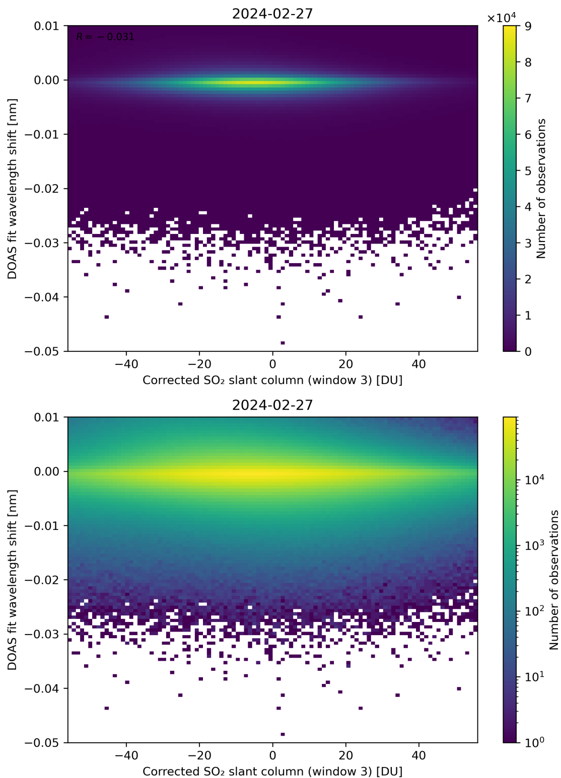
Figure 206: Scatter density plot of “Corrected SO 2 slant column (window 3)” against “DOAS fit wavelength shift” for 2024-02-27 to 2024-02-28.
