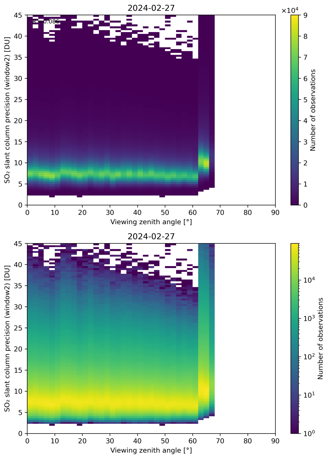
Figure 322: Scatter density plot of “Viewing zenith angle” against “SO 2 slant column precision (window2)” for 2024-02-27 to 2024-02-28.
