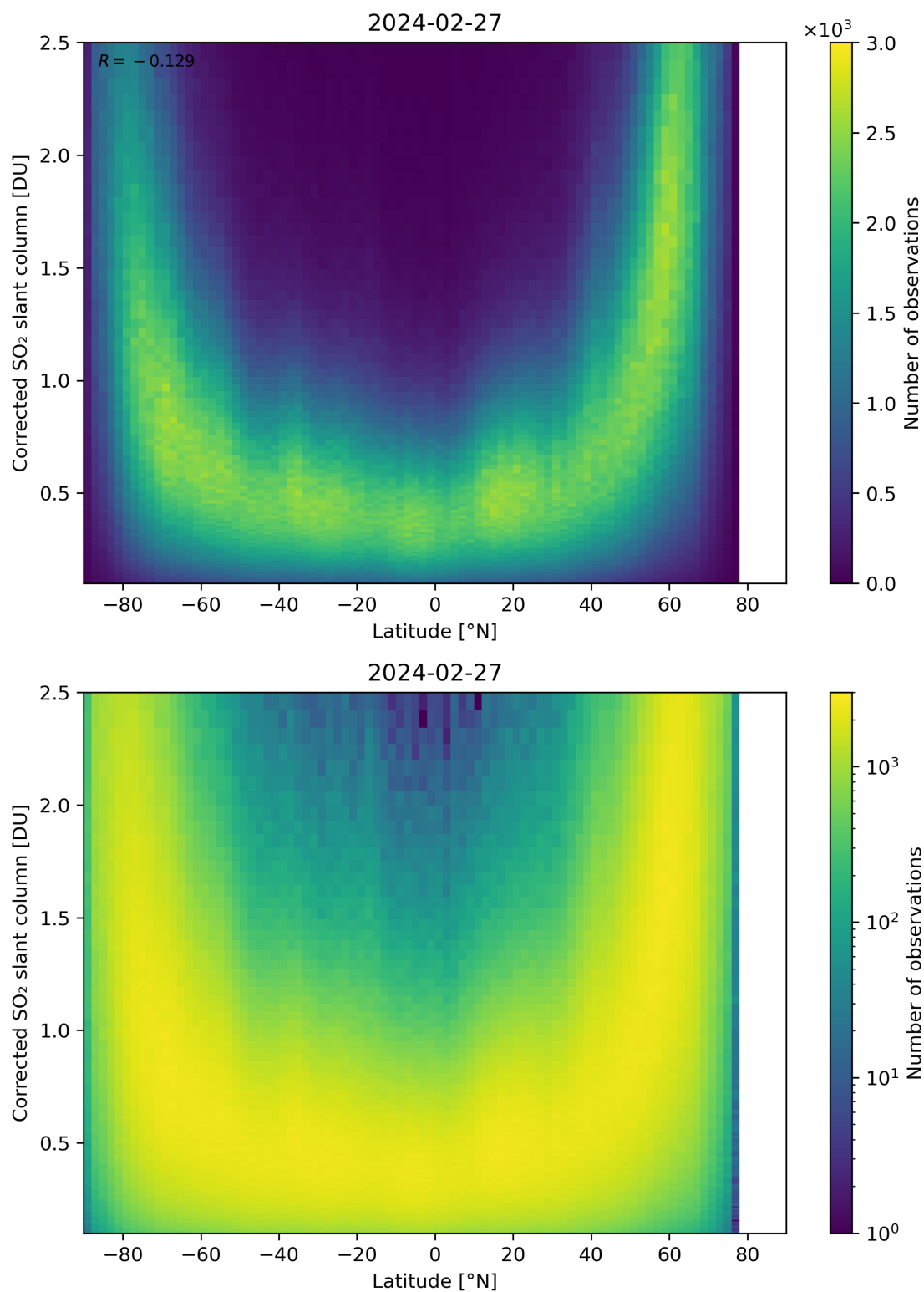
Figure 146: Scatter density plot of “Latitude” against “Corrected SO 2 slant column” for 2024-02-27 to 2024-02-28.
