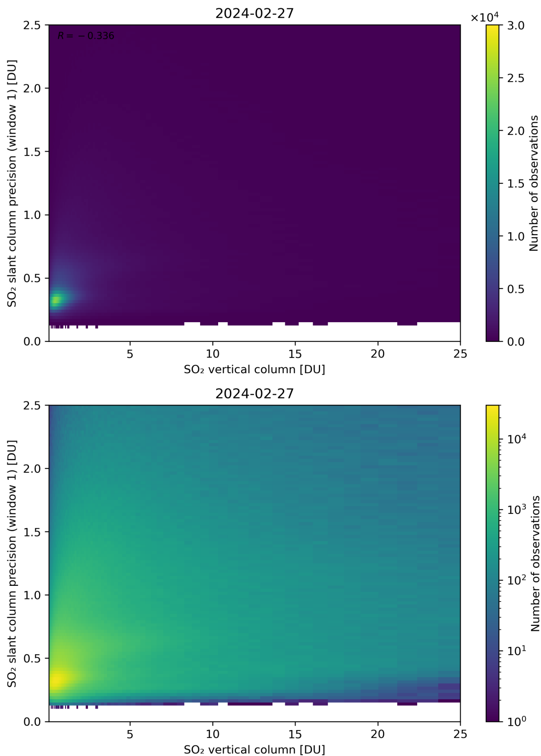
Figure 301: Scatter density plot of “SO 2 vertical column” against “SO 2 slant column precision (window 1)” for 2024-02-27 to 2024-02-28.
