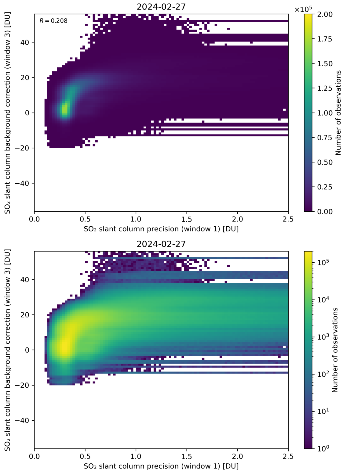
Figure 220: Scatter density plot of “SO 2 slant column precision (window 1)” against “SO 2 slant column background correction (window 3)” for 2024-02-27 to 2024-02-28.
