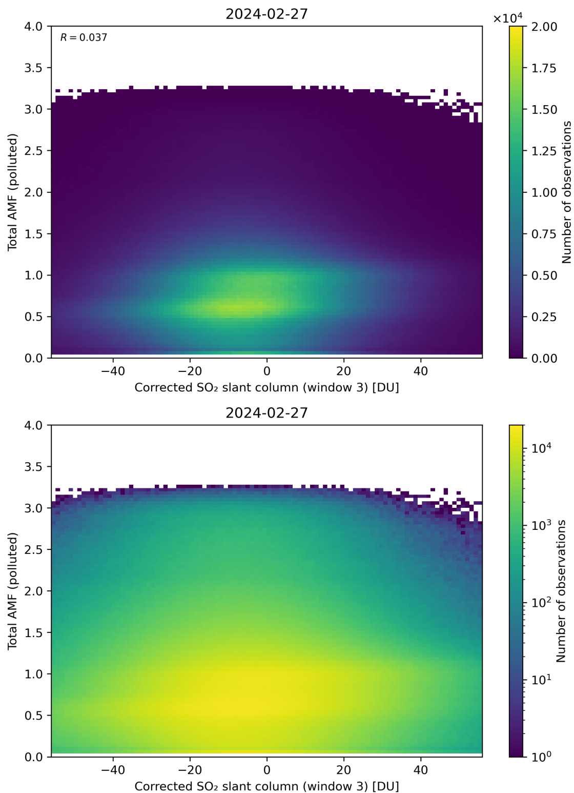
Figure 210: Scatter density plot of “Corrected SO 2 slant column (window 3)” against “Total AMF (polluted)” for 2024-02-27 to 2024-02-28.
