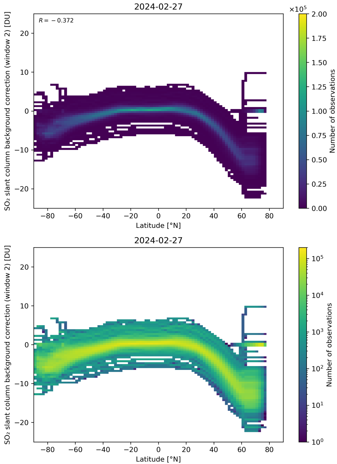
Figure 140: Scatter density plot of “Latitude” against “SO 2 slant column background correction (window 2)” for 2024-02-27 to 2024-02-28.
