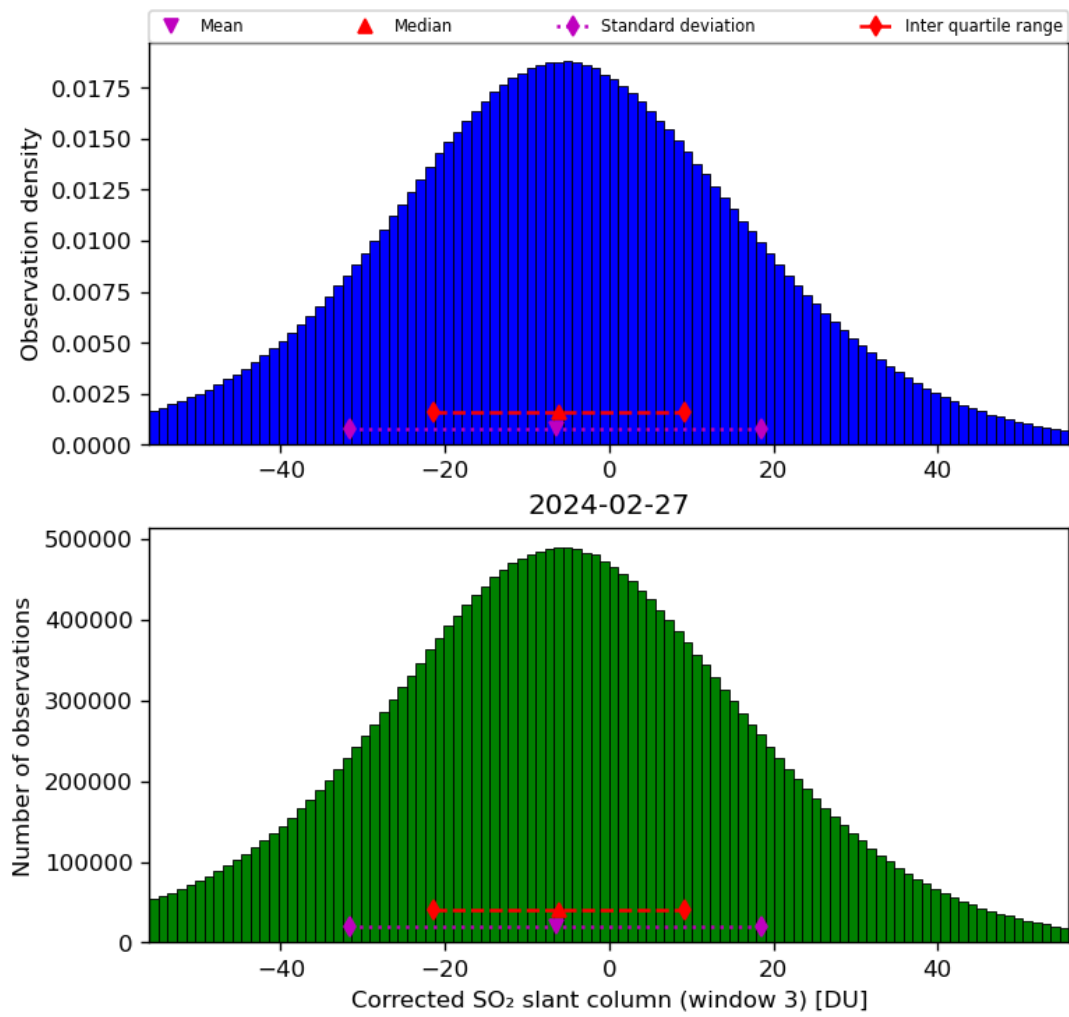
Figure 66: Histogram of “Corrected SO 2 slant column (window 3)” for 2024-02-27 to 2024-02-28
