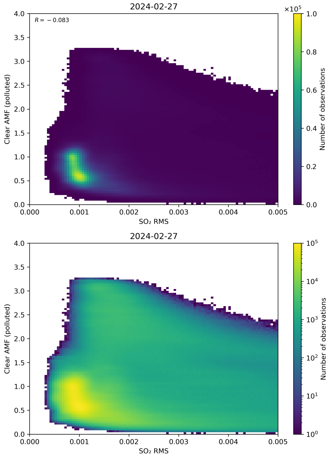
Figure 136: Scatter density plot of “SO 2 RMS” against “Clear AMF (polluted)” for 2024-02-27 to 2024-02-28.
