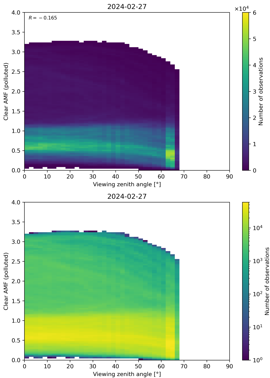
Figure 316: Scatter density plot of “Viewing zenith angle” against “Clear AMF (polluted)” for 2024-02-27 to 2024-02-28.
