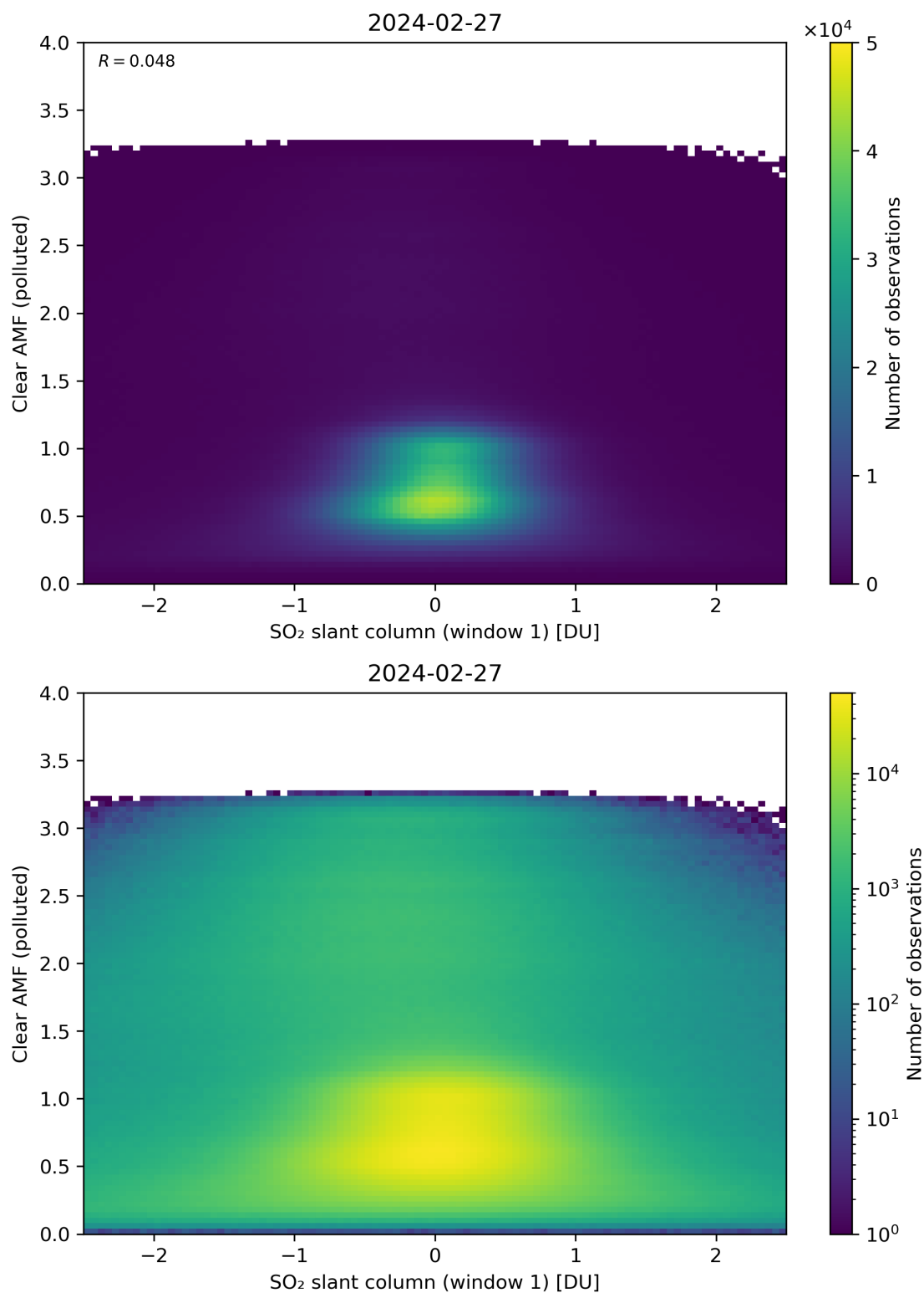
Figure 232: Scatter density plot of “SO 2 slant column (window 1)” against “Clear AMF (polluted)” for 2024-02-27 to 2024-02-28.
