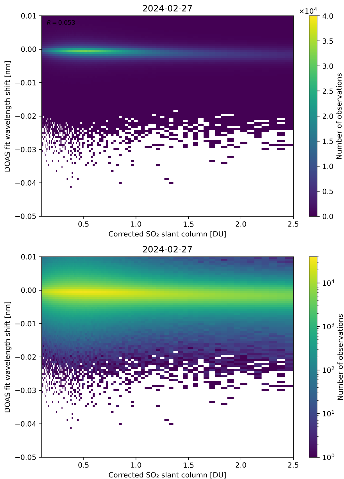
Figure 181: Scatter density plot of “Corrected SO 2 slant column” against “DOAS fit wavelength shift” for 2024-02-27 to 2024-02-28.
