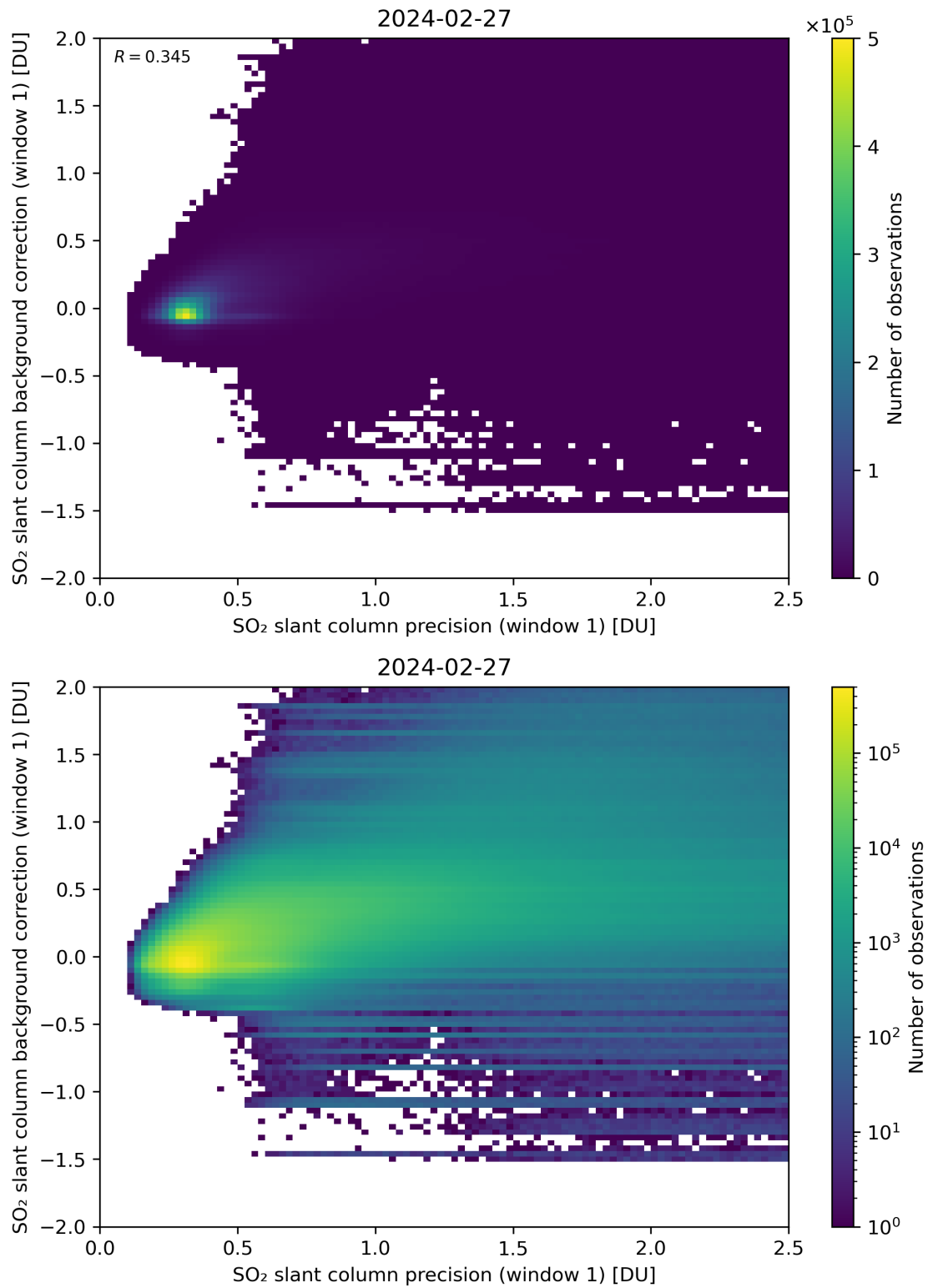
Figure 218: Scatter density plot of “SO 2 slant column precision (window 1)” against “SO 2 slant column background correction (window 1)” for 2024-02-27 to 2024-02-28.
