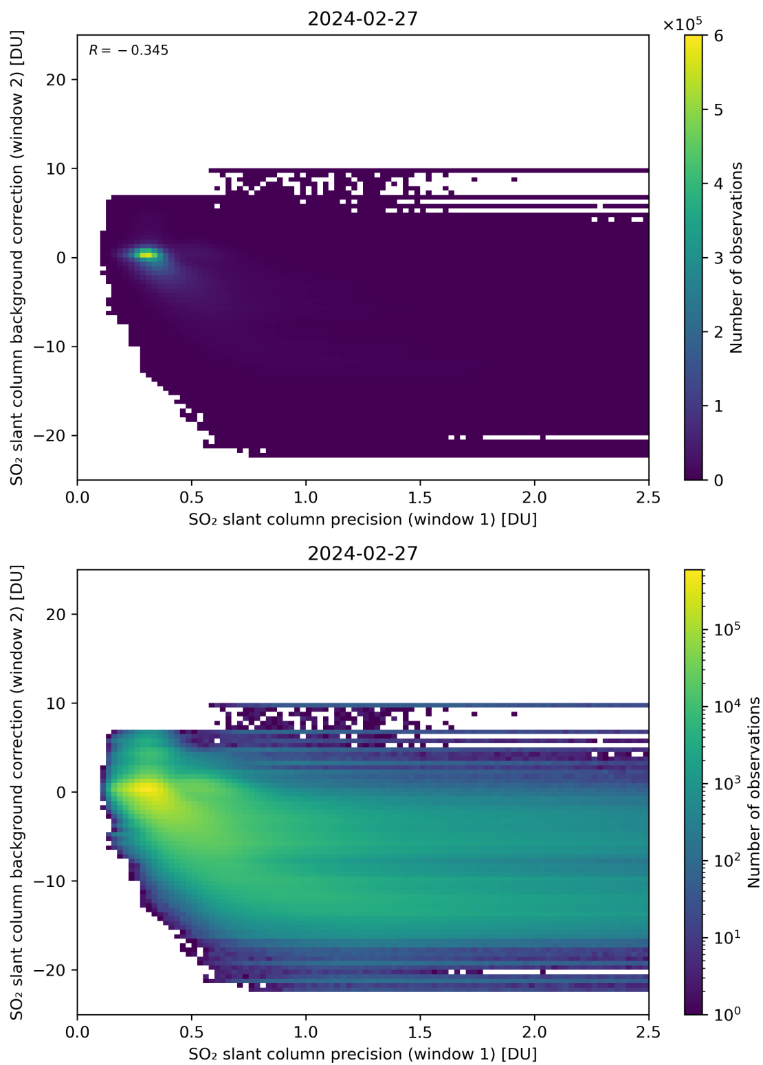
Figure 219: Scatter density plot of “SO 2 slant column precision (window 1)” against “SO 2 slant column background correction (window 2)” for 2024-02-27 to 2024-02-28.
