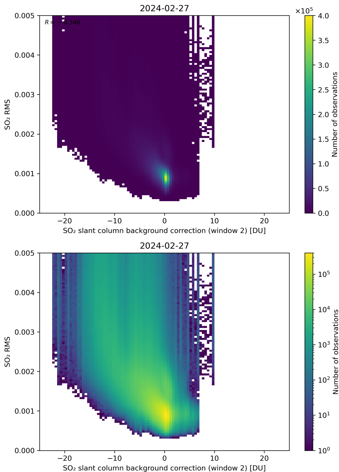
Figure 114: Scatter density plot of “SO 2 slant column background correction (window 2)” against “SO 2 RMS” for 2024-02-27 to 2024-02-28.
