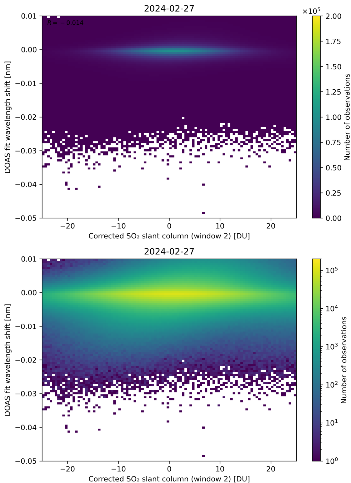
Figure 196: Scatter density plot of “Corrected SO 2 slant column (window 2)” against “DOAS fit wavelength shift” for 2024-02-27 to 2024-02-28.
