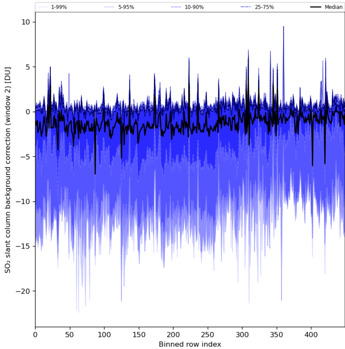
Figure 86: Along track statistics of “SO 2 slant column background correction (window 2)” for 2024-02-27 to 2024-02-28
