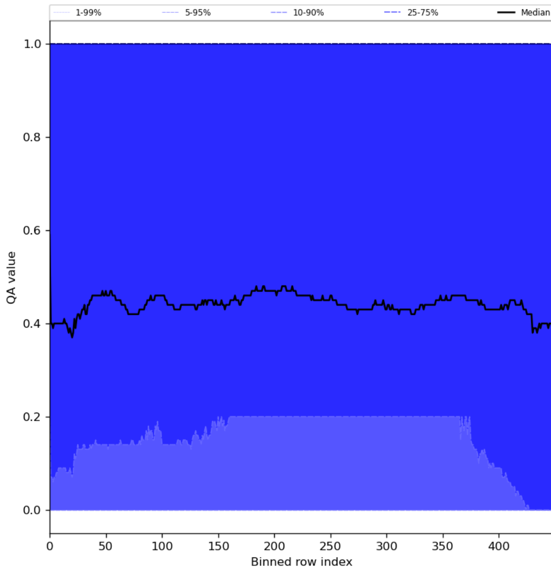
Figure 75: Along track statistics of “QA value” for 2024-02-27 to 2024-02-28
