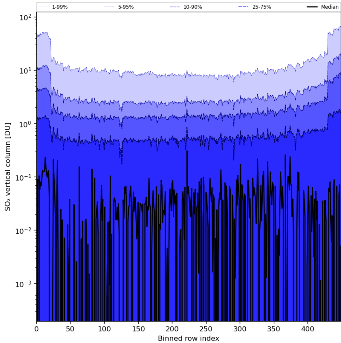
Figure 76: Along track statistics of “SO 2 vertical column” for 2024-02-27 to 2024-02-28
