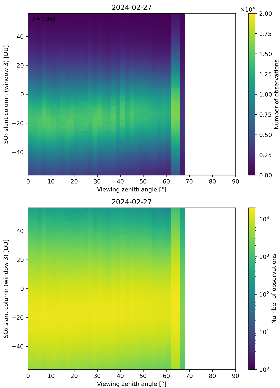
Figure 323: Scatter density plot of “Viewing zenith angle” against “SO 2 slant column (window 3)” for 2024-02-27 to 2024-02-28.
