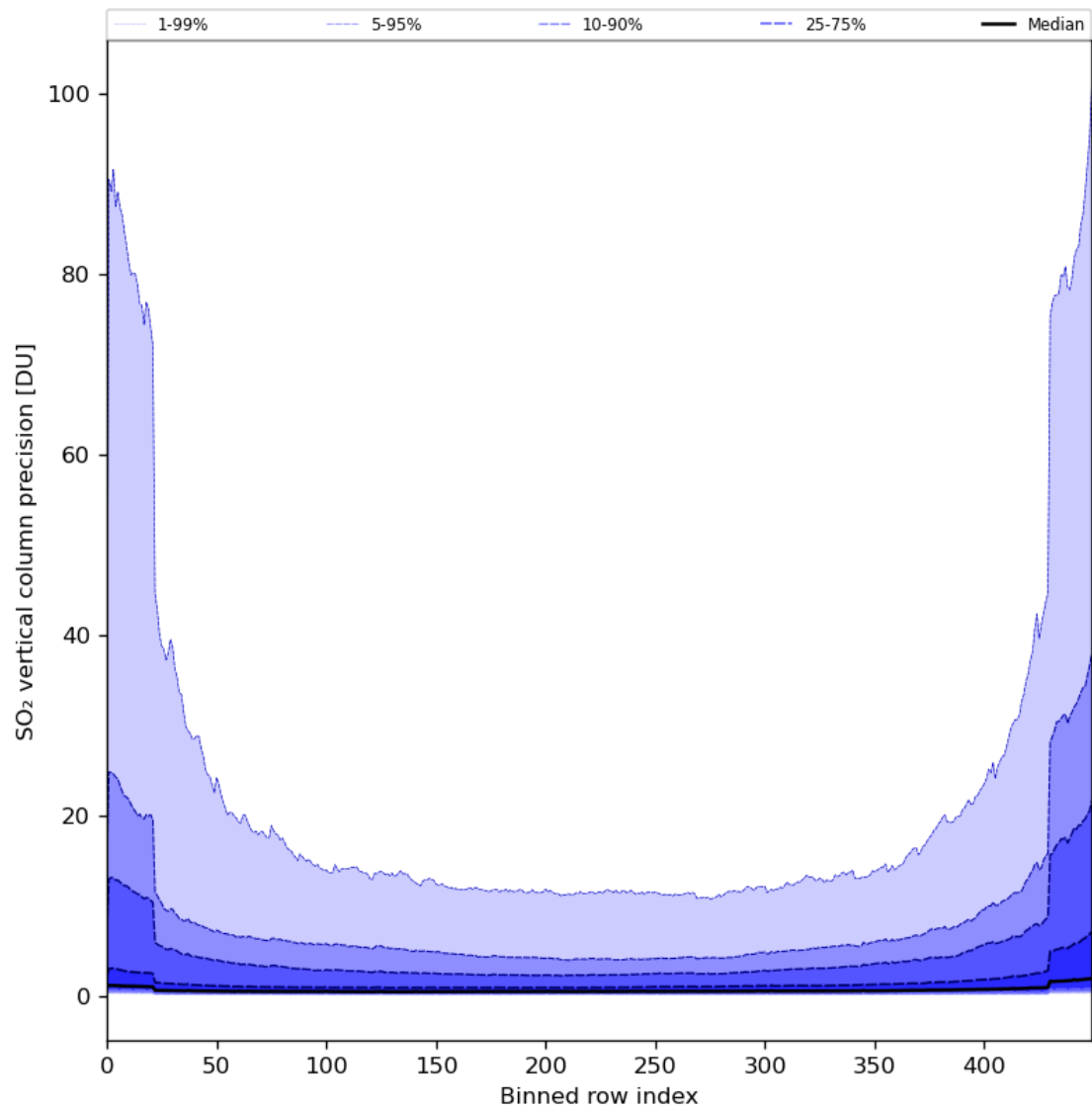
Figure 77: Along track statistics of “SO 2 vertical column precision” for 2024-02-27 to 2024-02-28
