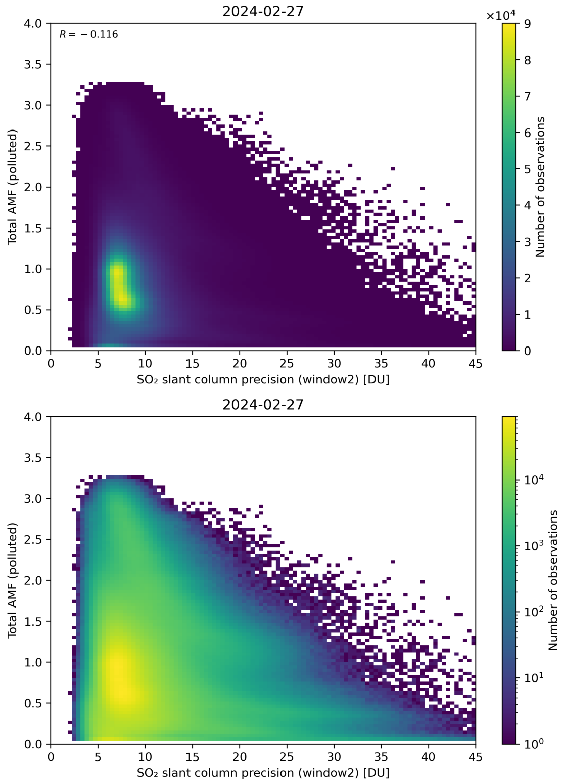
Figure 251: Scatter density plot of “SO 2 slant column precision (window2)” against “Total AMF (polluted)” for 2024-02-27 to 2024-02-28.
