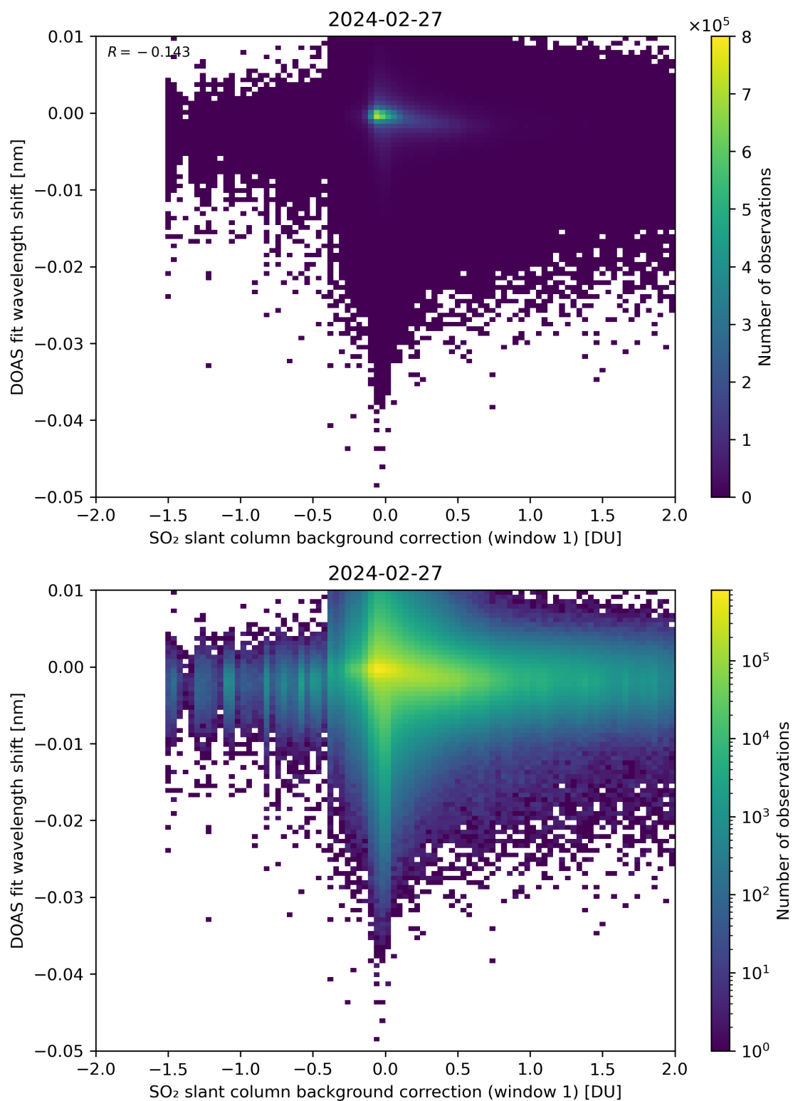
Figure 100: Scatter density plot of “SO 2 slant column background correction (window 1)” against “DOAS fit wavelength shift” for 2024-02-27 to 2024-02-28.
