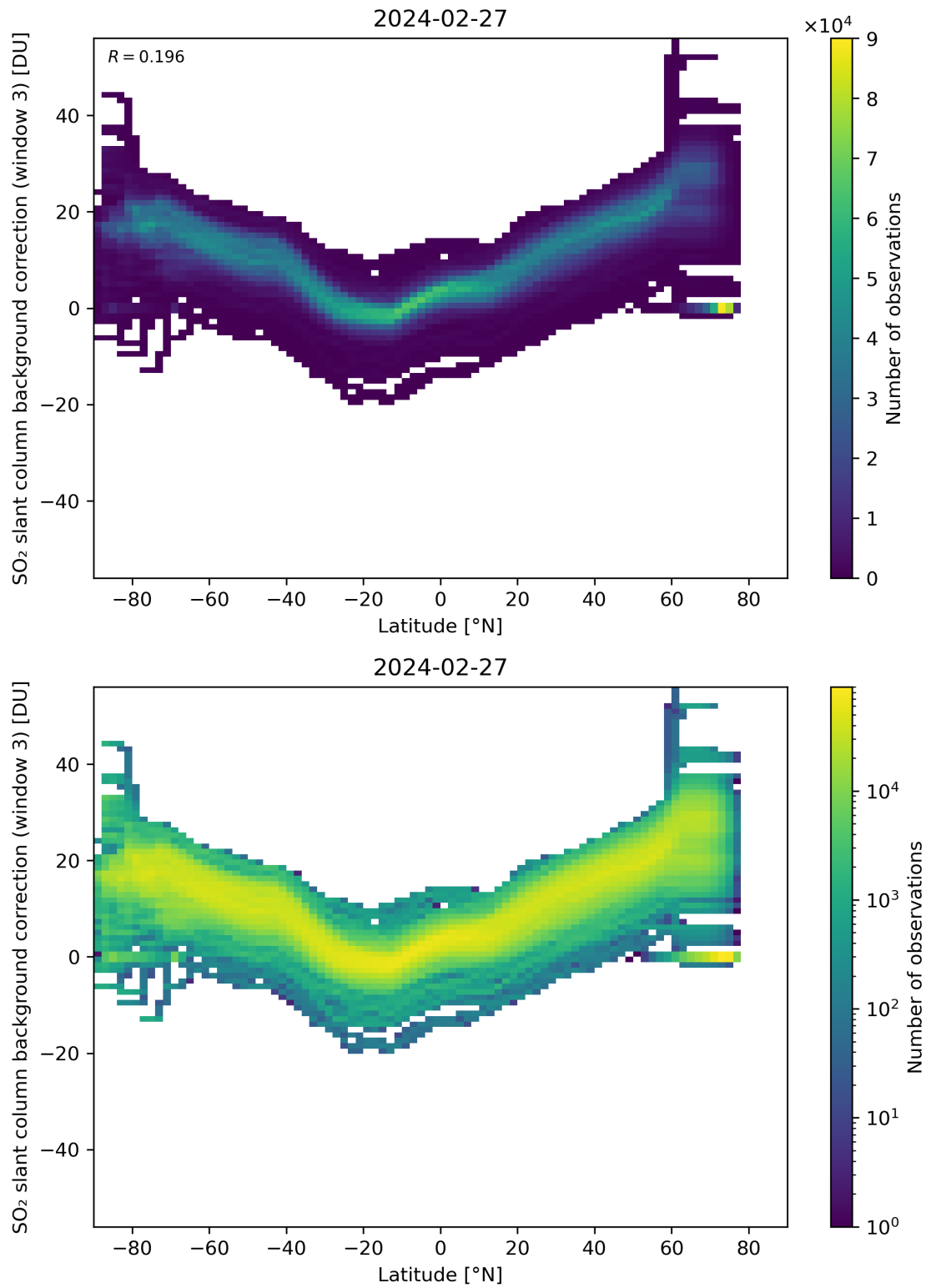
Figure 141: Scatter density plot of “Latitude” against “SO 2 slant column background correction (window 3)” for 2024-02-27 to 2024-02-28.
