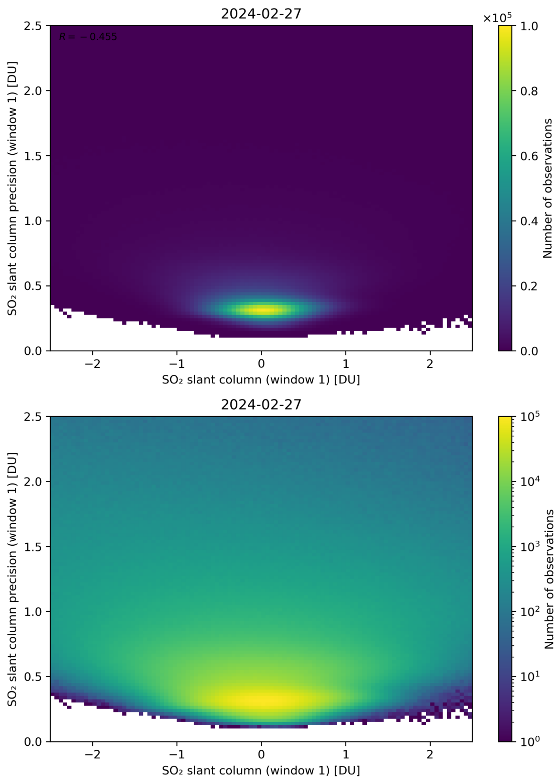
Figure 235: Scatter density plot of “SO 2 slant column (window 1)” against “SO 2 slant column precision (window 1)” for 2024-02-27 to 2024-02-28.
