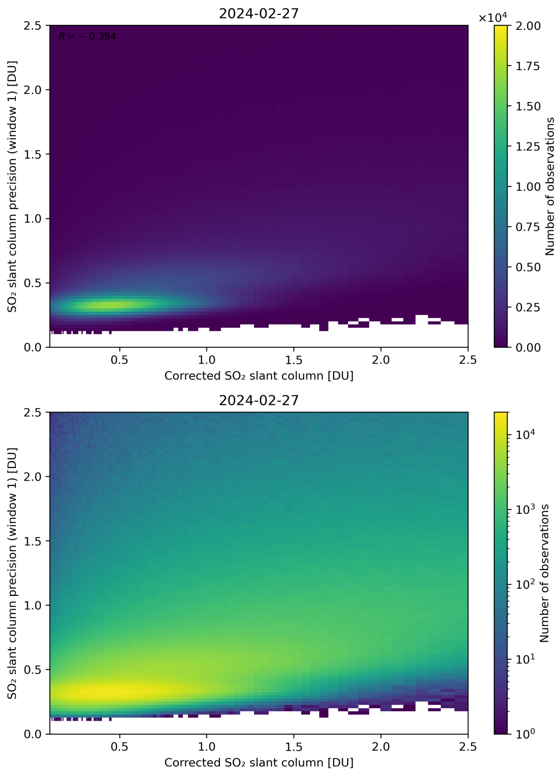
Figure 188: Scatter density plot of “Corrected SO 2 slant column” against “SO 2 slant column precision (window 1)” for 2024-02-27 to 2024-02-28.
