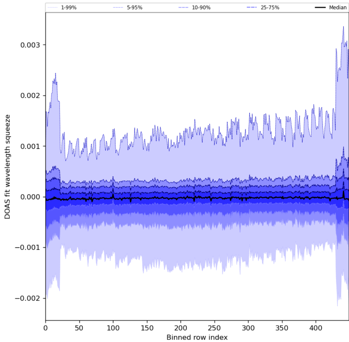
Figure 92: Along track statistics of “DOAS fit wavelength squeeze” for 2024-02-27 to 2024-02-28
