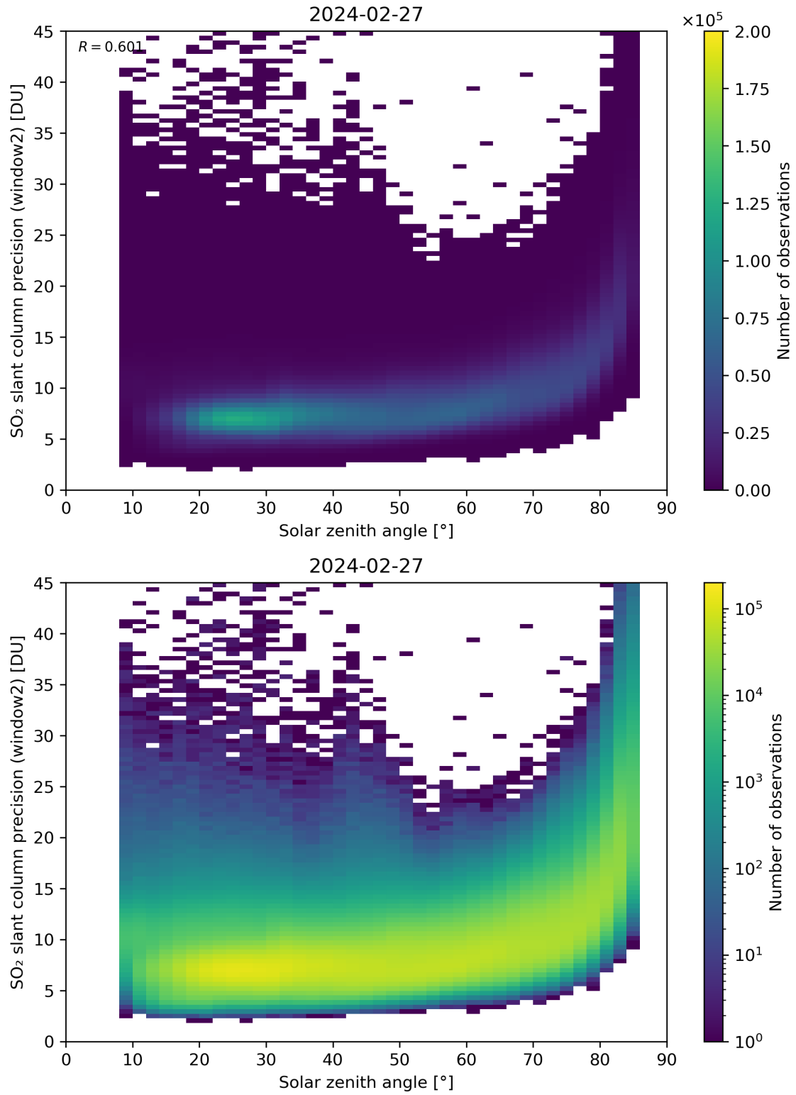
Figure 171: Scatter density plot of “Solar zenith angle” against “SO 2 slant column precision (window2)” for 2024-02-27 to 2024-02-28.
