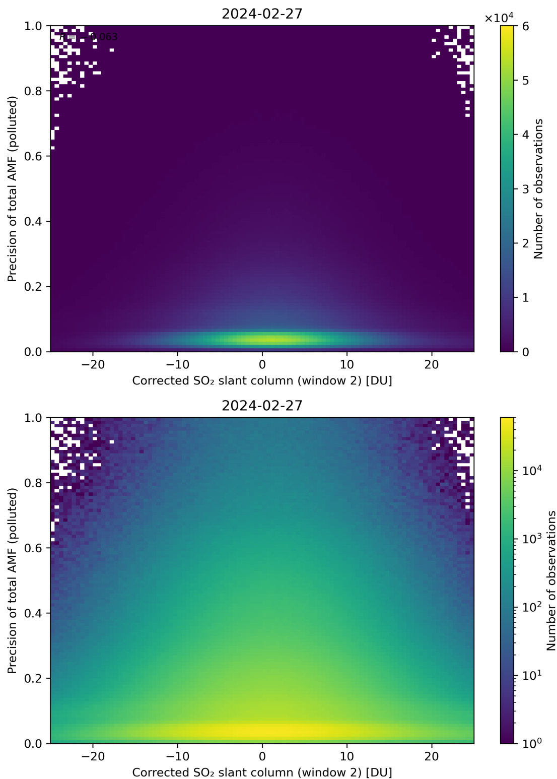
Figure 204: Scatter density plot of “Corrected SO 2 slant column (window 2)” against “Precision of total AMF (polluted)” for 2024-02-27 to 2024-02-28.
