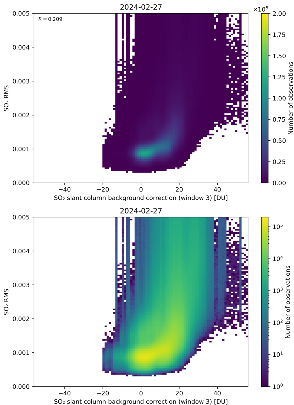
Figure 123: Scatter density plot of “SO 2 slant column background correction (window 3)” against “SO 2 RMS” for 2024-02-27 to 2024-02-28.
