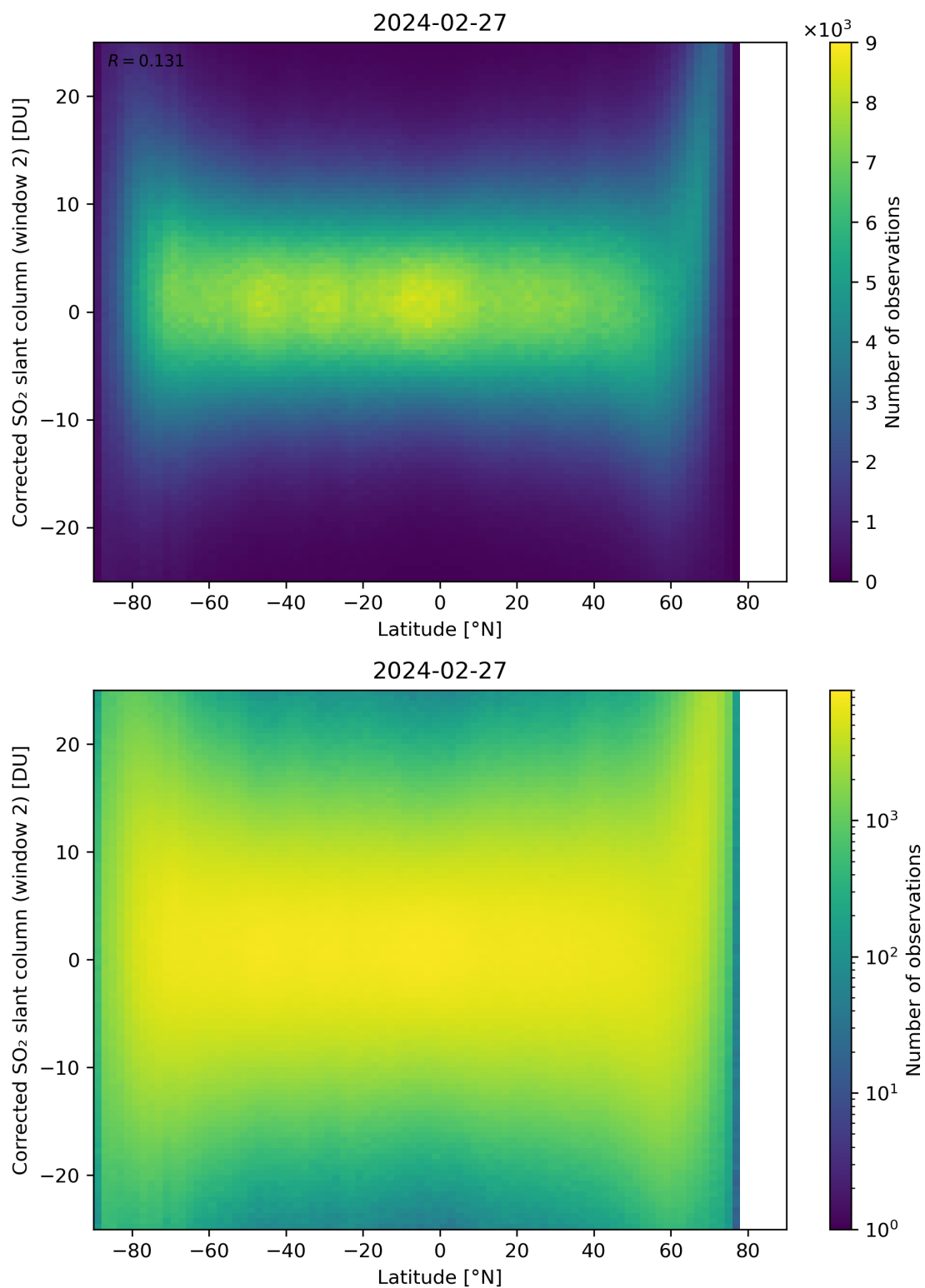
Figure 147: Scatter density plot of “Latitude” against “Corrected SO 2 slant column (window 2)” for 2024-02-27 to 2024-02-28.
