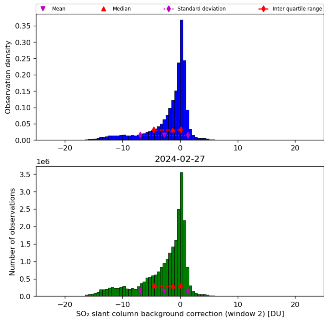
Figure 63: Histogram of “SO 2 slant column background correction (window 2)” for 2024-02-27 to 2024-02-28
