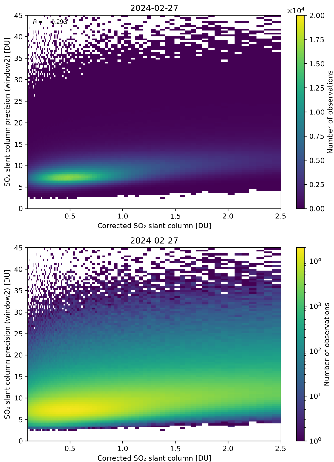
Figure 189: Scatter density plot of “Corrected SO 2 slant column” against “SO 2 slant column precision (window2)” for 2024-02-27 to 2024-02-28.
