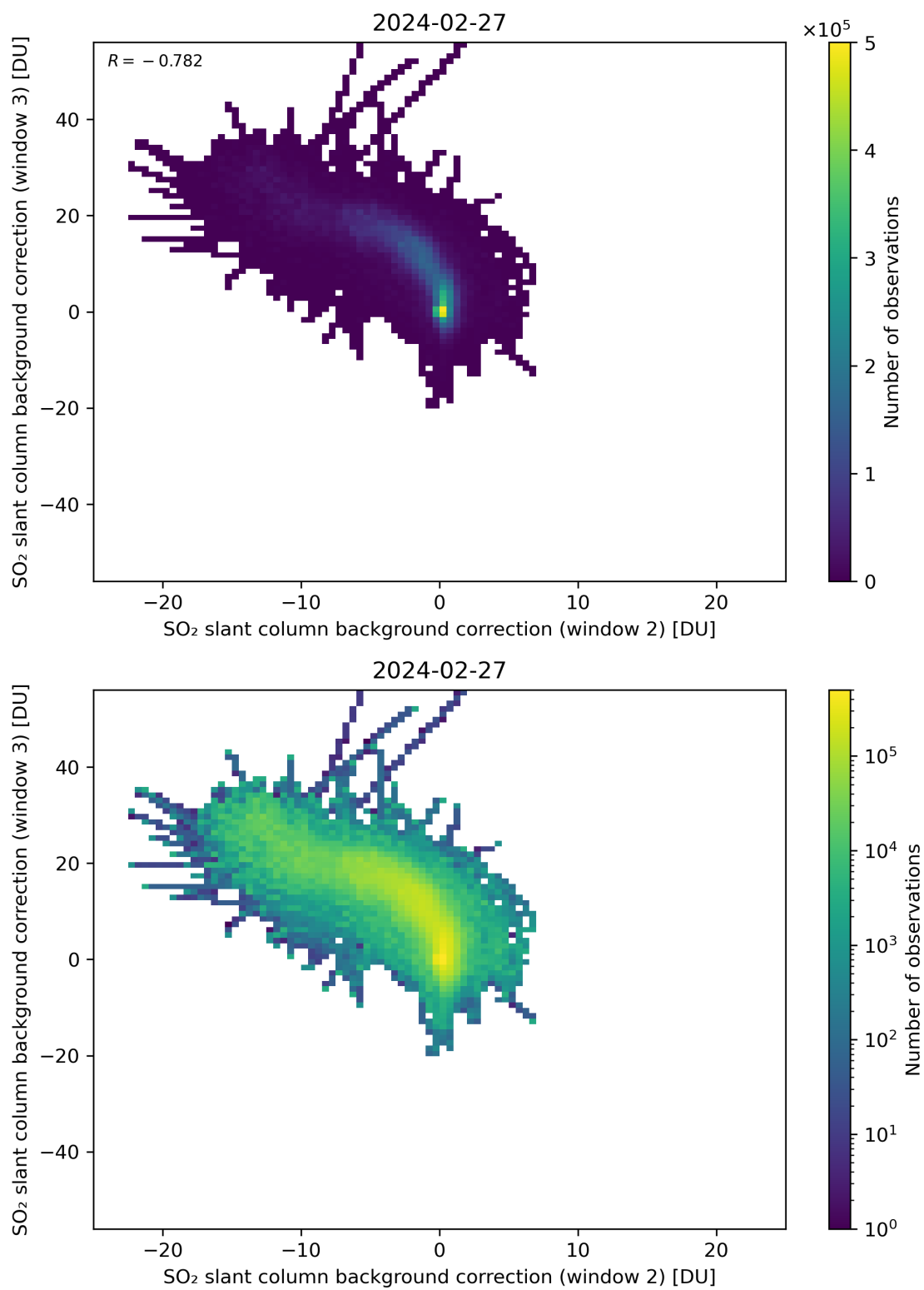
Figure 111: Scatter density plot of “SO 2 slant column background correction (window 2)” against “SO 2 slant column background correction (window 3)” for 2024-02-27 to 2024-02-28.
