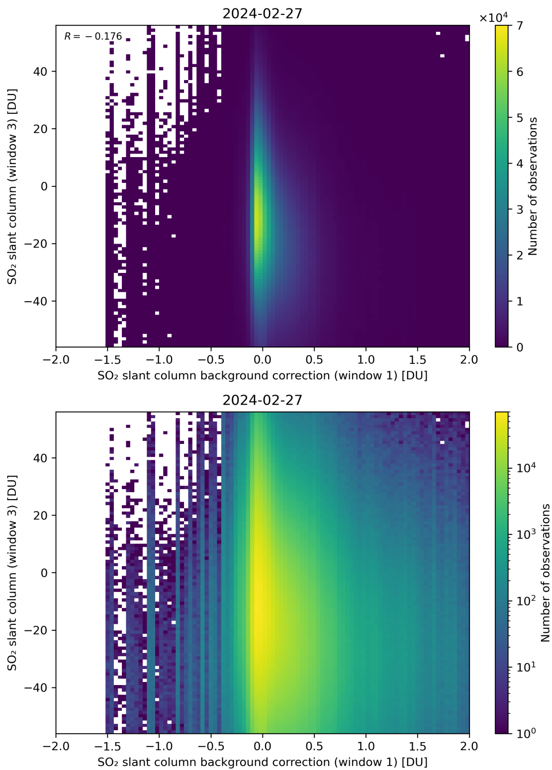
Figure 107: Scatter density plot of “SO 2 slant column background correction (window 1)” against “SO 2 slant column (window 3)” for 2024-02-27 to 2024-02-28.
