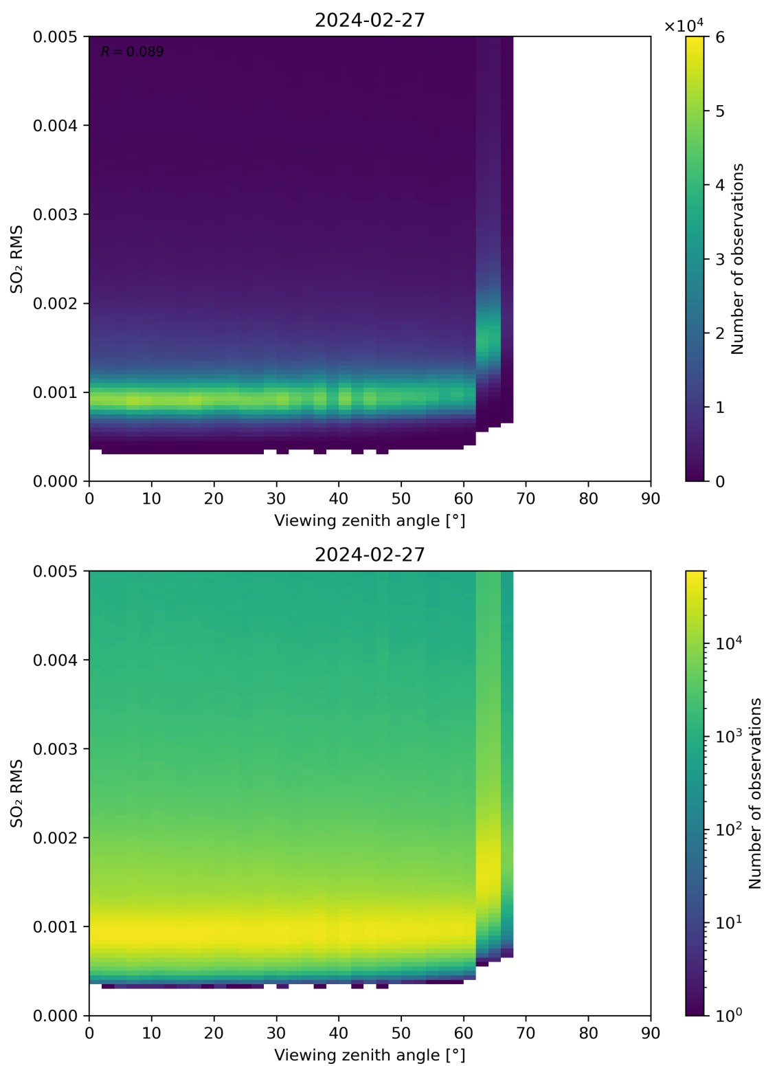
Figure 313: Scatter density plot of “Viewing zenith angle” against “SO 2 RMS” for 2024-02-27 to 2024-02-28.
