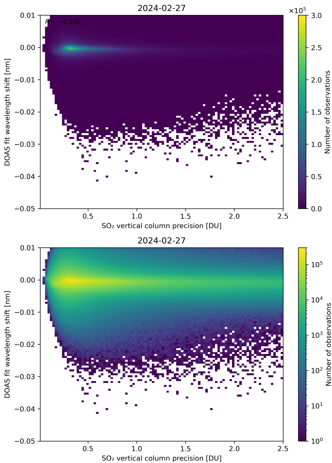
Figure 282: Scatter density plot of “SO 2 vertical column precision” against “DOAS fit wavelength shift” for 2024-02-27 to 2024-02-28.
