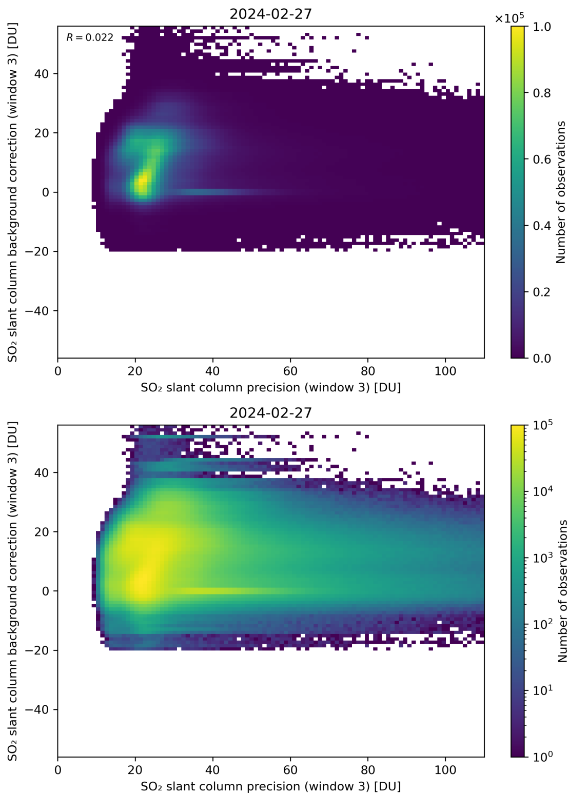
Figure 257: Scatter density plot of “SO 2 slant column precision (window 3)” against “SO 2 slant column background correction (window 3)” for 2024-02-27 to 2024-02-28.
