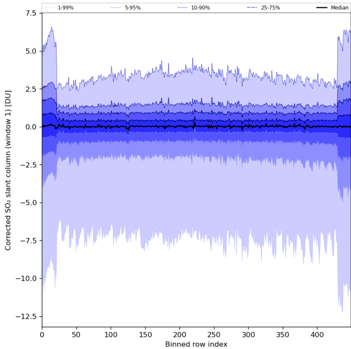
Figure 81: Along track statistics of “Corrected SO 2 slant column (window 1)” for 2024-02-27 to 2024-02-28
