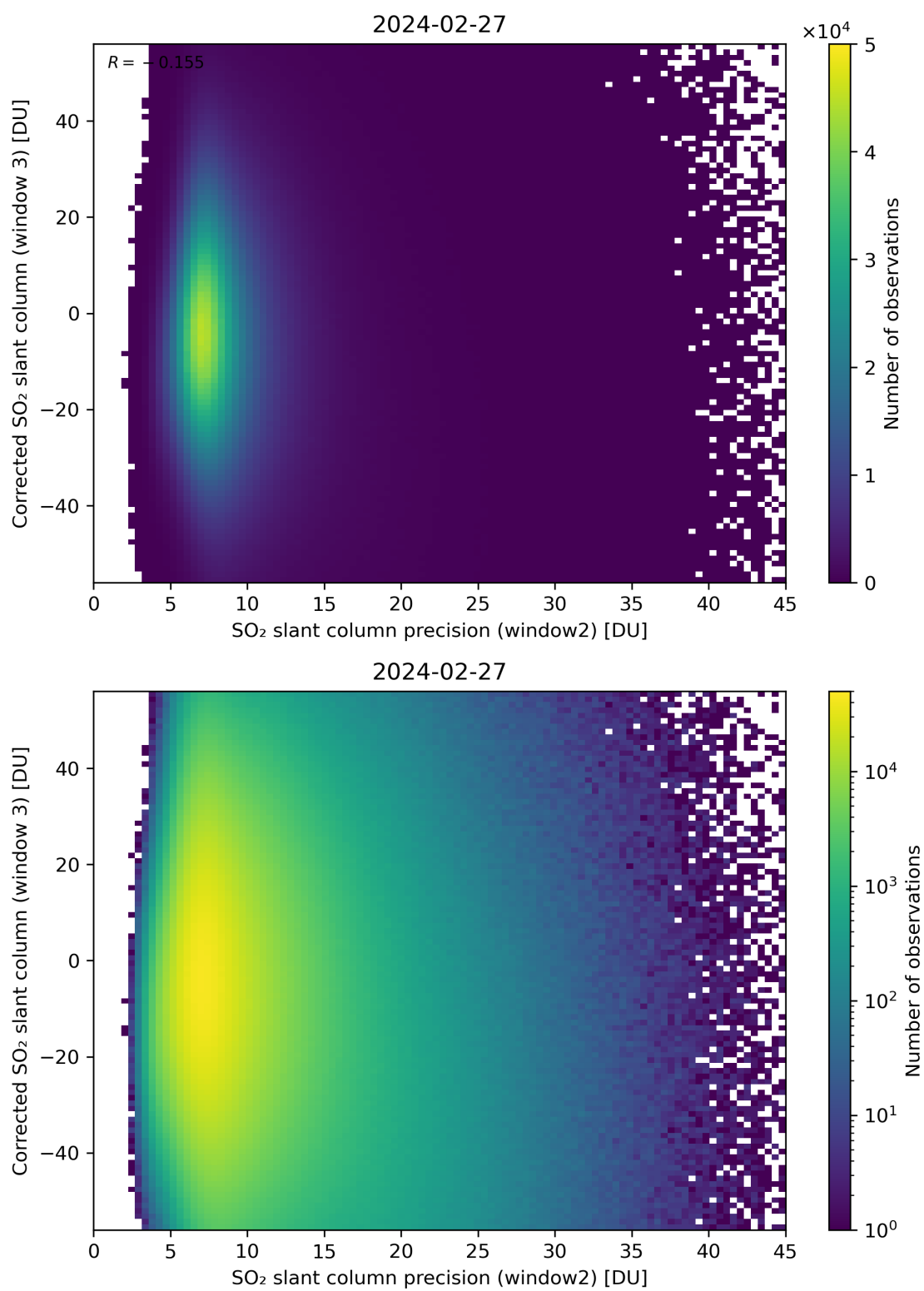
Figure 248: Scatter density plot of “SO 2 slant column precision (window2)” against “Corrected SO 2 slant column (window 3)” for 2024-02-27 to 2024-02-28.
