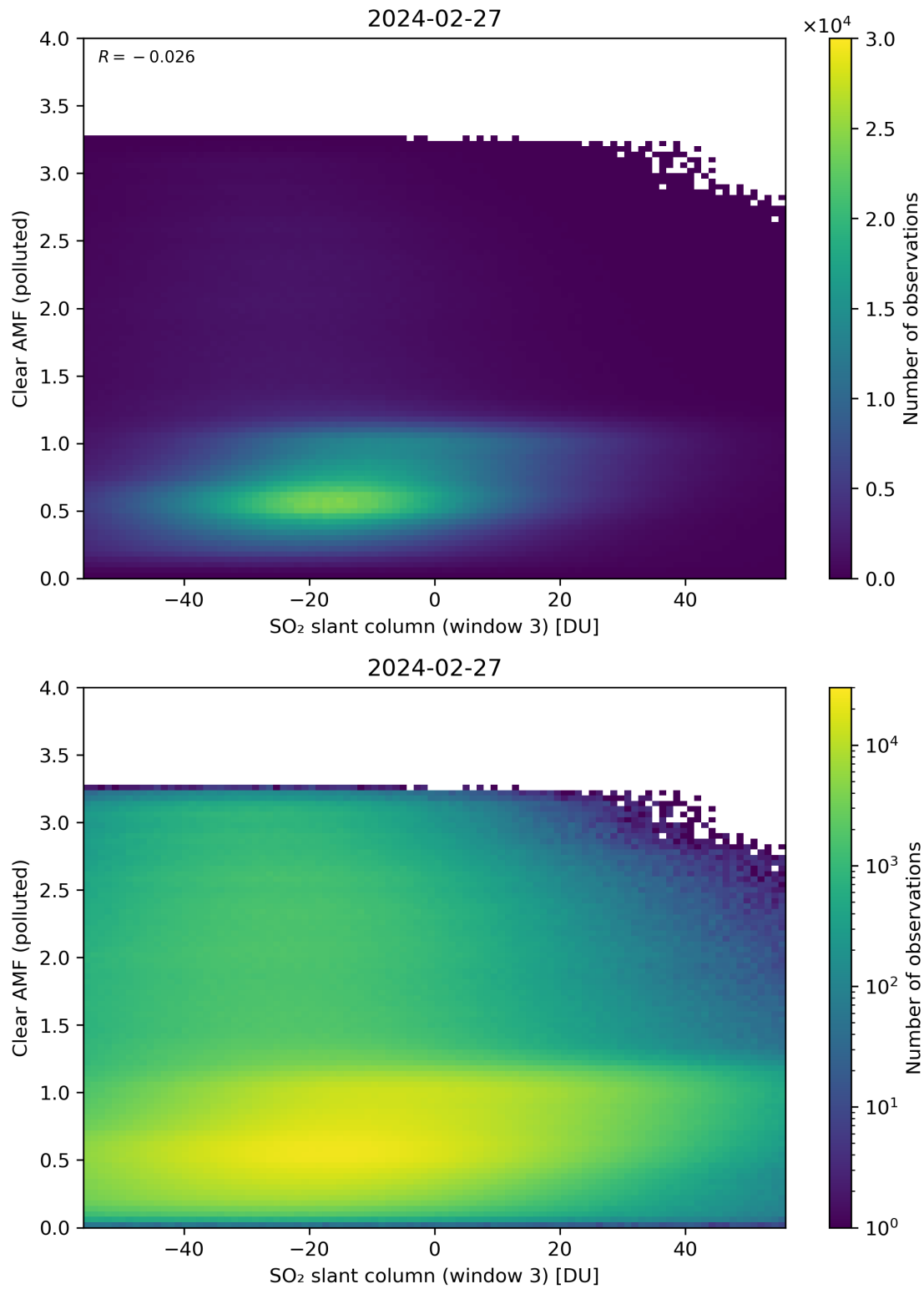
Figure 265: Scatter density plot of “SO 2 slant column (window 3)” against “Clear AMF (polluted)” for 2024-02-27 to 2024-02-28.
