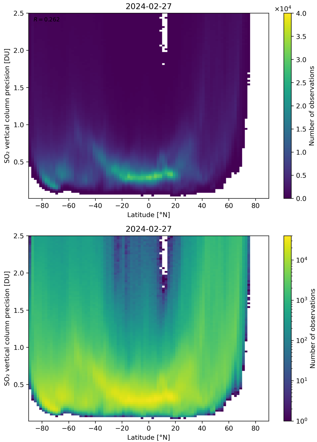
Figure 157: Scatter density plot of “Latitude” against “SO 2 vertical column precision” for 2024-02-27 to 2024-02-28.
