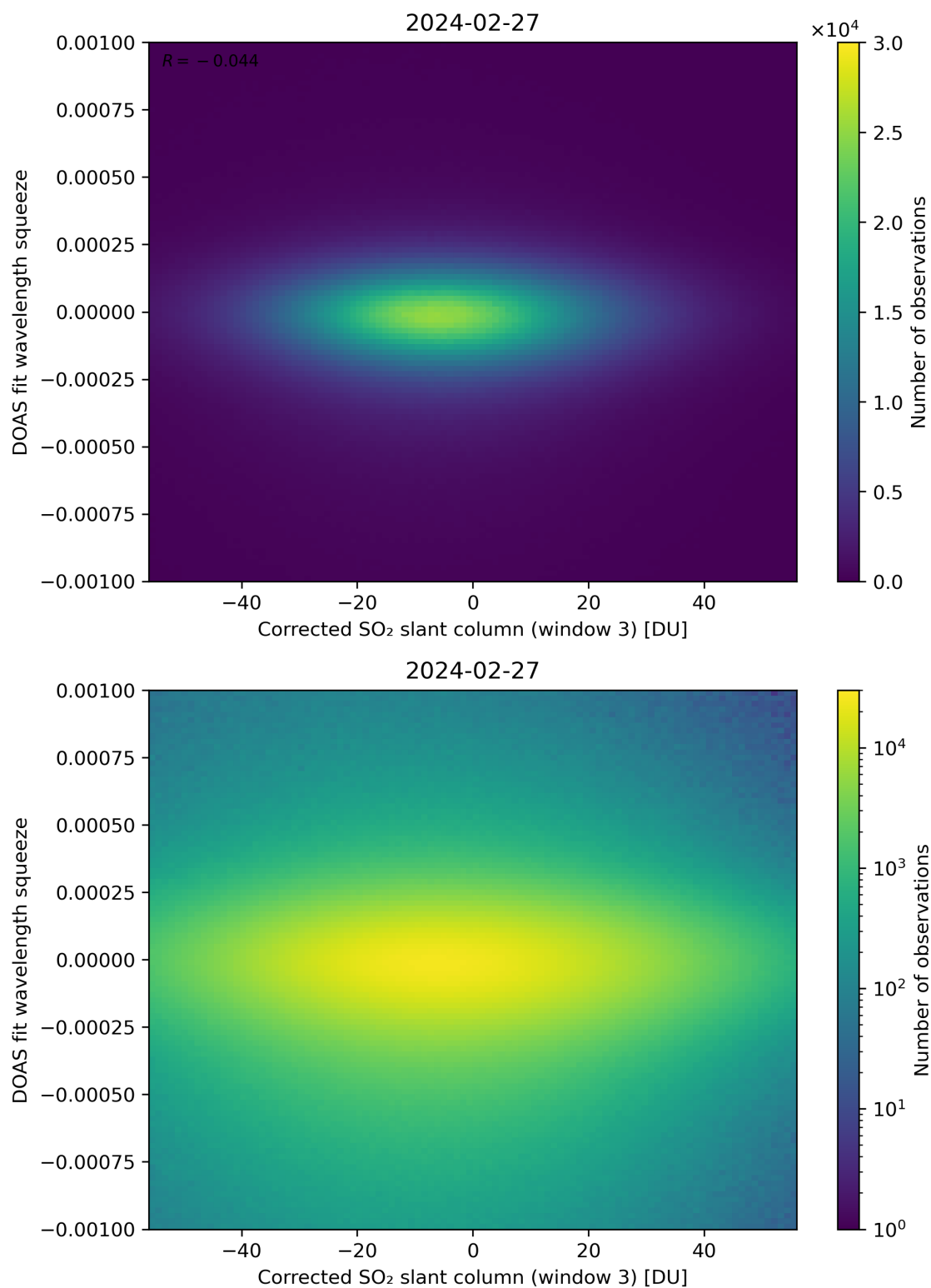
Figure 207: Scatter density plot of “Corrected SO 2 slant column (window 3)” against “DOAS fit wavelength squeeze” for 2024-02-27 to 2024-02-28.
