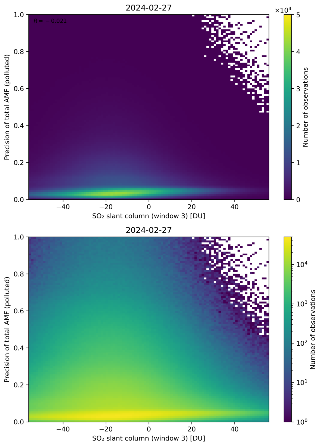
Figure 269: Scatter density plot of “SO 2 slant column (window 3)” against “Precision of total AMF (polluted)” for 2024-02-27 to 2024-02-28.
