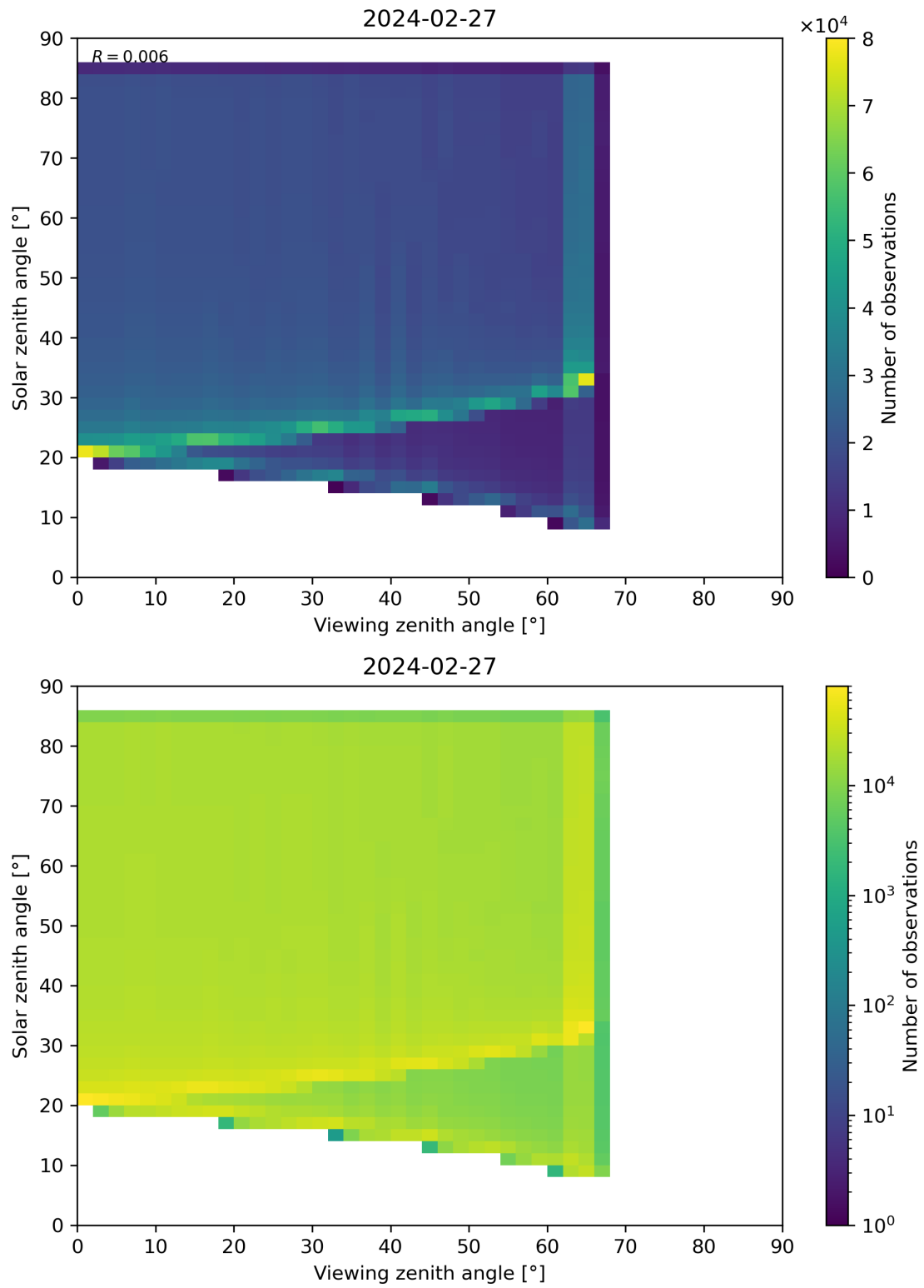
Figure 315: Scatter density plot of “Viewing zenith angle” against “Solar zenith angle” for 2024-02-27 to 2024-02-28.
