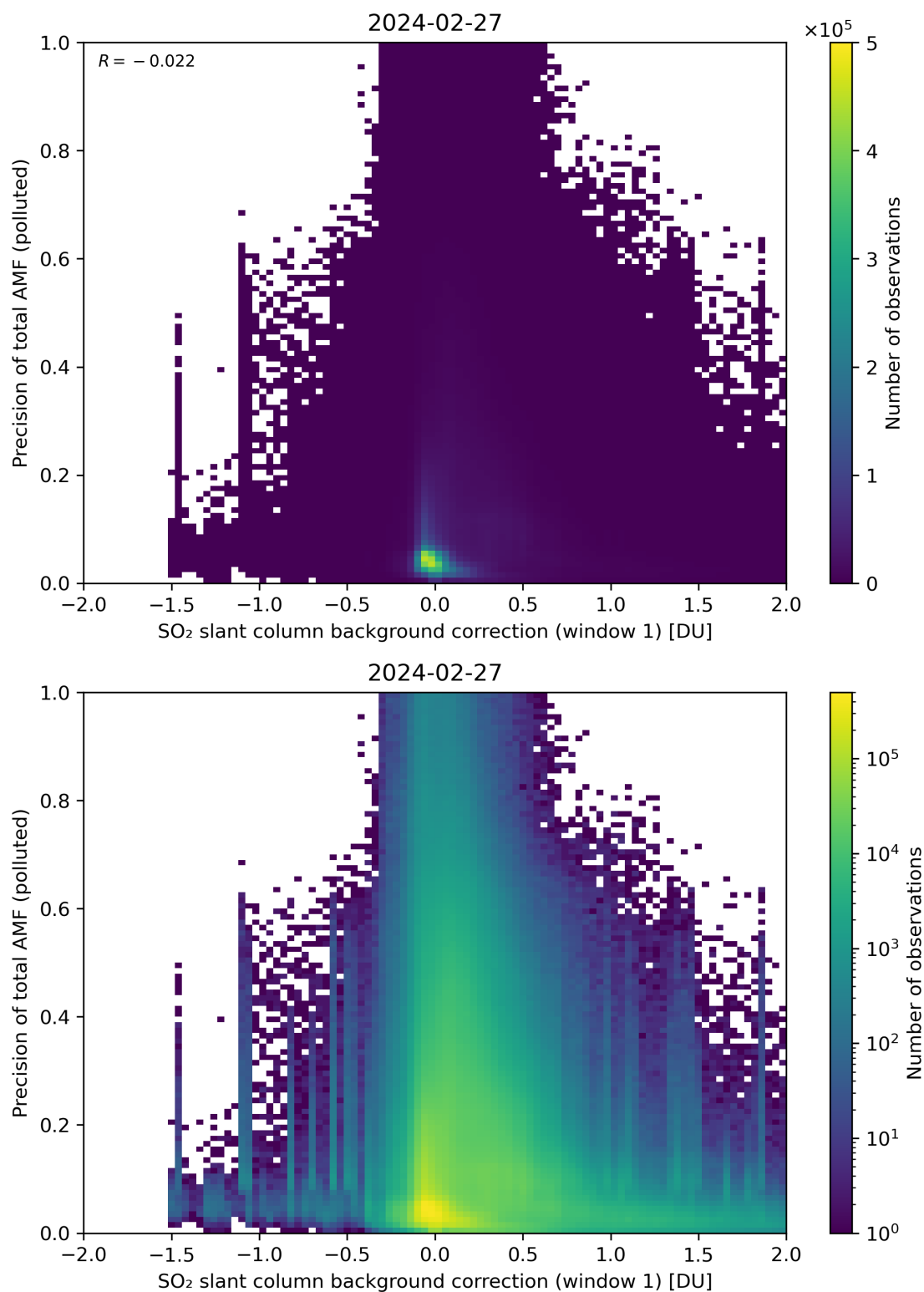
Figure 110: Scatter density plot of “SO 2 slant column background correction (window 1)” against “Precision of total AMF (polluted)” for 2024-02-27 to 2024-02-28.
