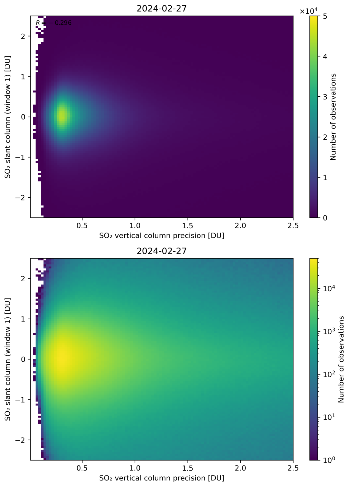
Figure 289: Scatter density plot of “SO 2 vertical column precision” against “SO 2 slant column (window 1)” for 2024-02-27 to 2024-02-28.
