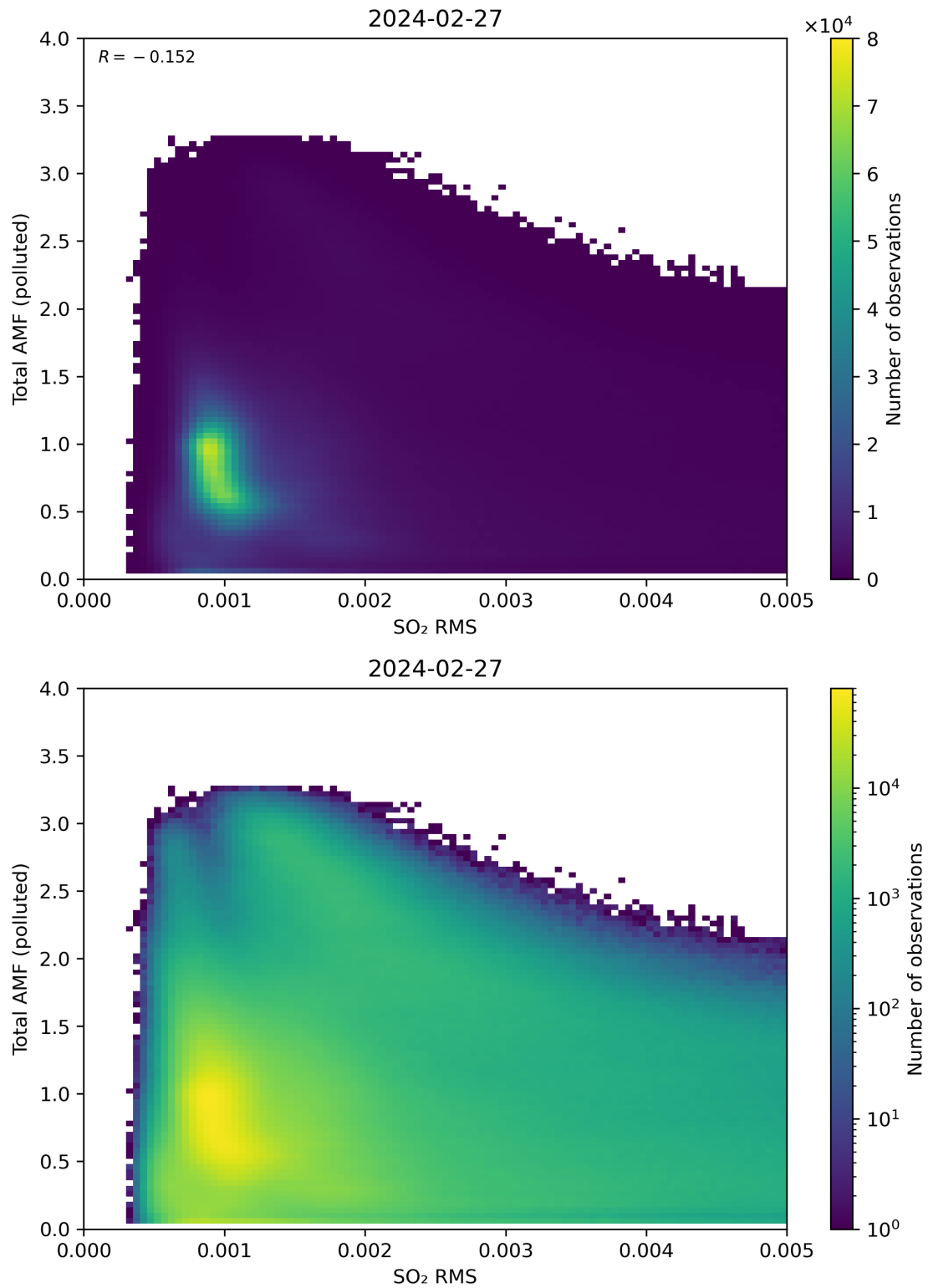
Figure 137: Scatter density plot of “SO 2 RMS” against “Total AMF (polluted)” for 2024-02-27 to 2024-02-28.
