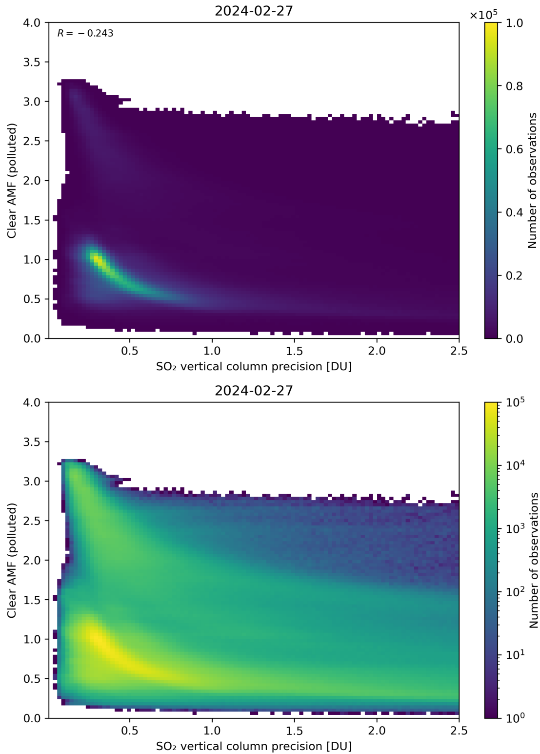
Figure 285: Scatter density plot of “SO 2 vertical column precision” against “Clear AMF (polluted)” for 2024-02-27 to 2024-02-28.
