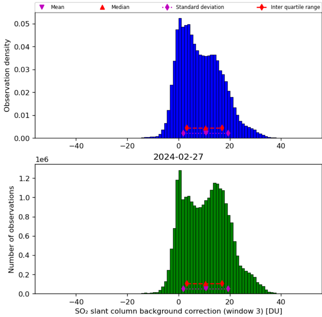
Figure 67: Histogram of “SO 2 slant column background correction (window 3)” for 2024-02-27 to 2024-02-28
