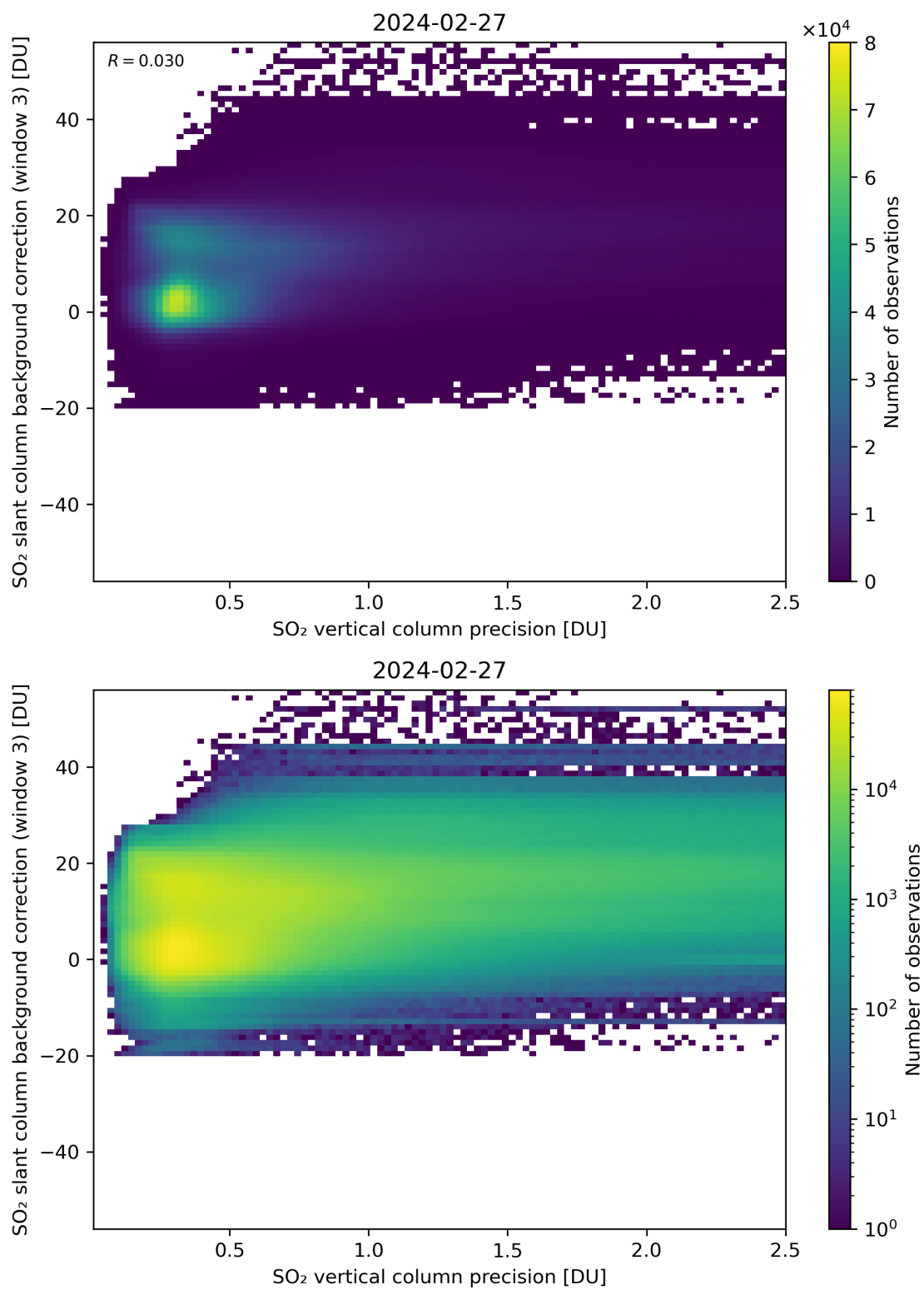
Figure 281: Scatter density plot of “SO 2 vertical column precision” against “SO 2 slant column background correction (window 3)” for 2024-02-27 to 2024-02-28.
