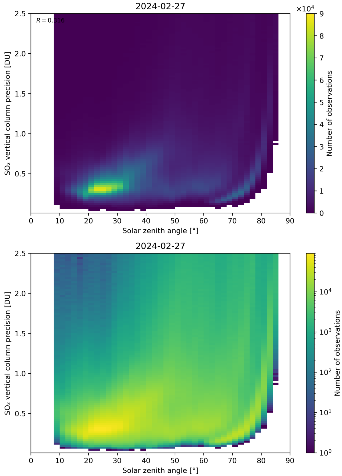
Figure 177: Scatter density plot of “Solar zenith angle” against “SO 2 vertical column precision” for 2024-02-27 to 2024-02-28.
