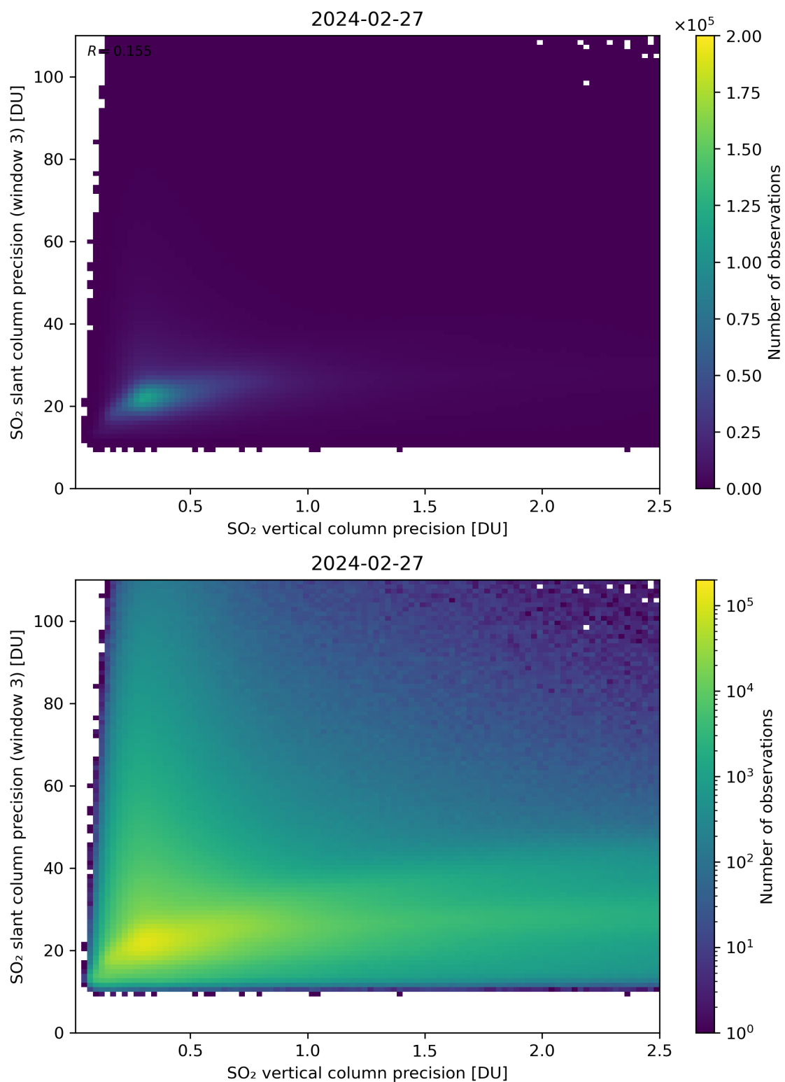
Figure 293: Scatter density plot of “SO 2 vertical column precision” against “SO 2 slant column precision (window 3)” for 2024-02-27 to 2024-02-28.
