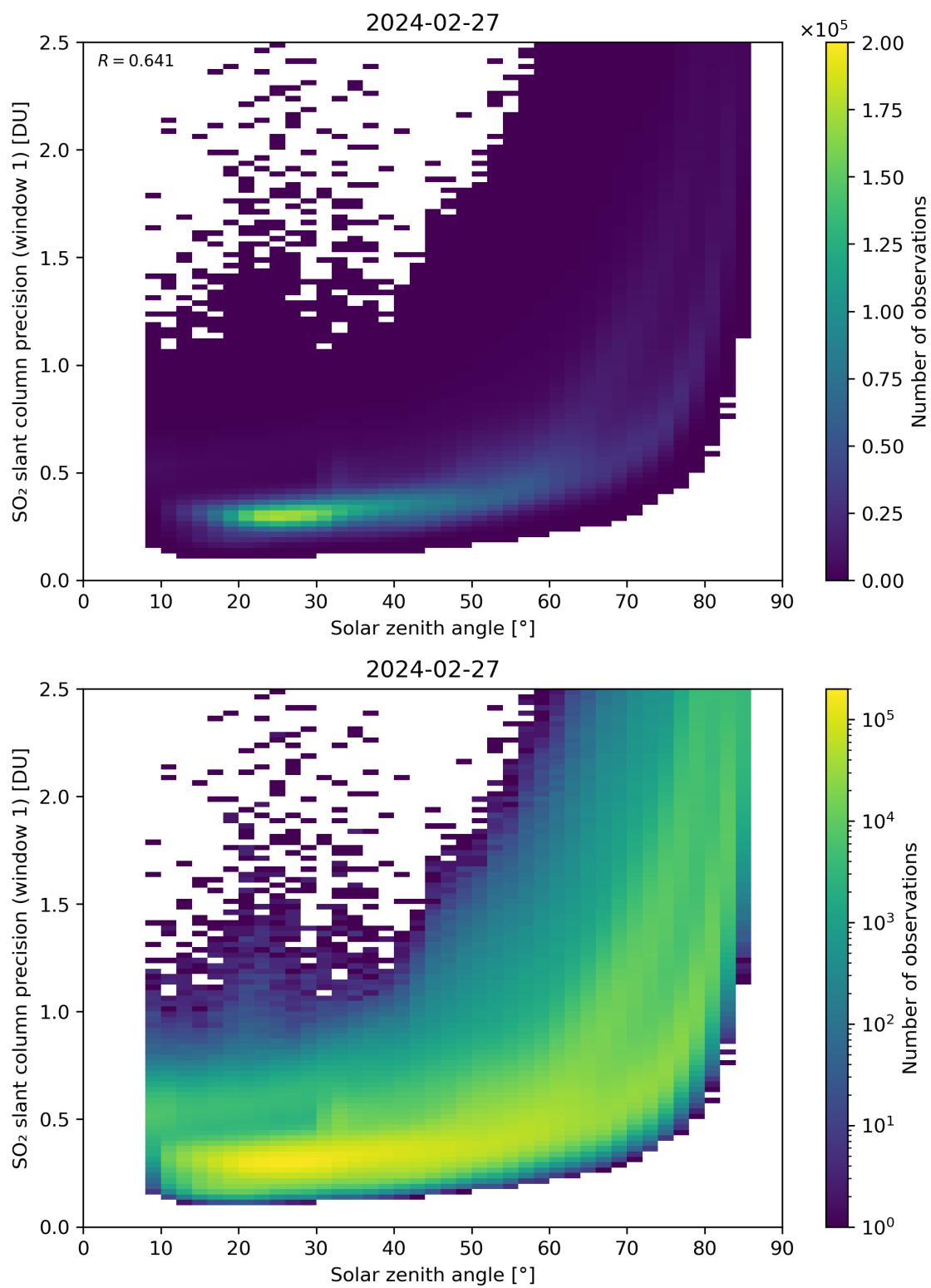
Figure 170: Scatter density plot of “Solar zenith angle” against “SO 2 slant column precision (window 1)” for 2024-02-27 to 2024-02-28.
