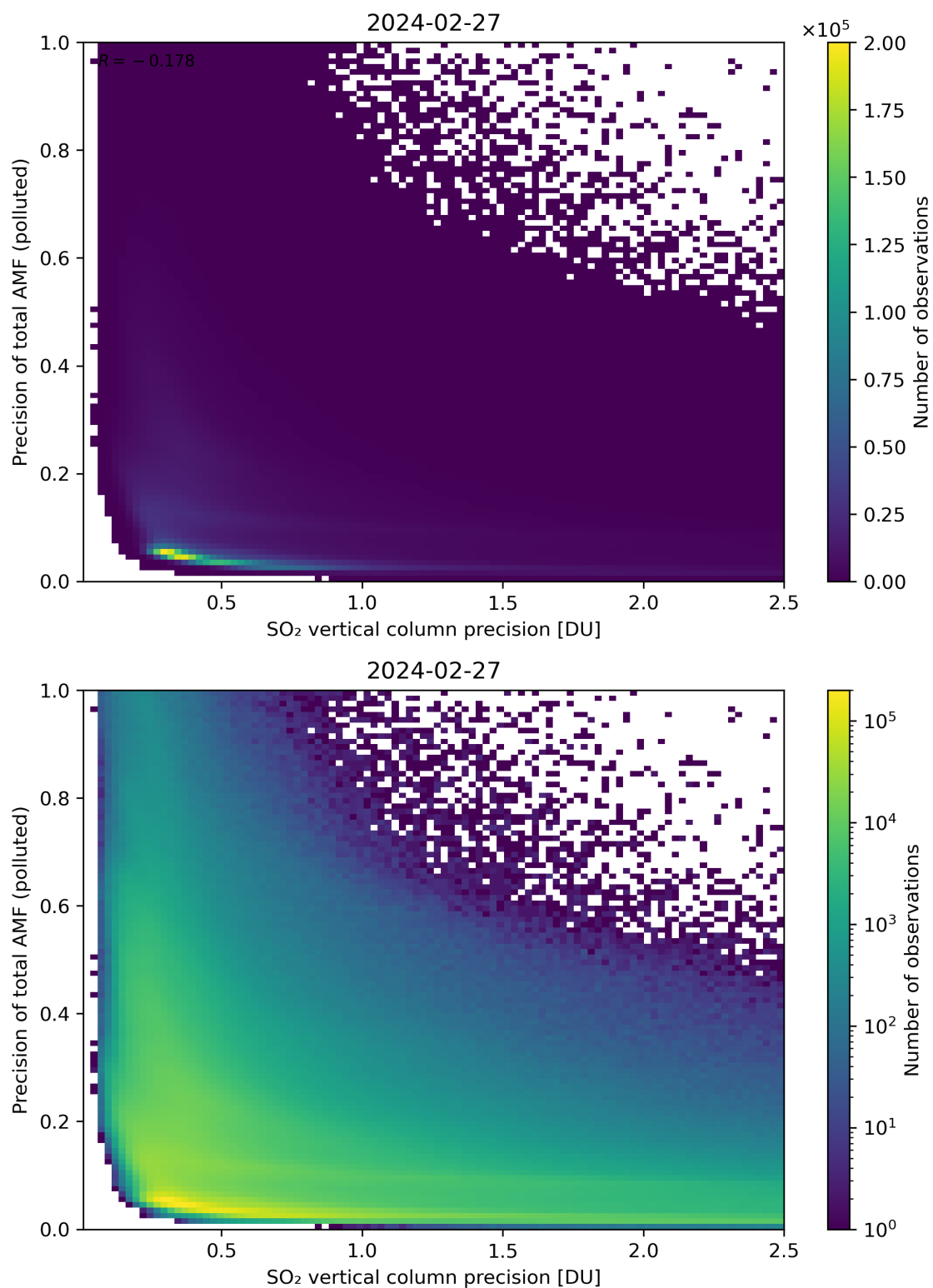
Figure 295: Scatter density plot of “SO 2 vertical column precision” against “Precision of total AMF (polluted)” for 2024-02-27 to 2024-02-28.
