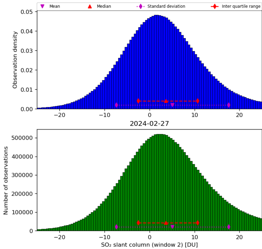
Figure 60: Histogram of “SO 2 slant column (window 2)” for 2024-02-27 to 2024-02-28
