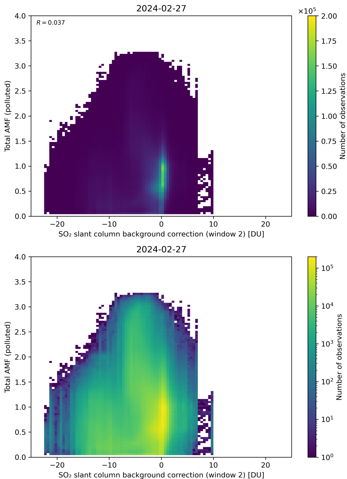
Figure 119: Scatter density plot of “SO 2 slant column background correction (window 2)” against “Total AMF (polluted)” for 2024-02-27 to 2024-02-28.
