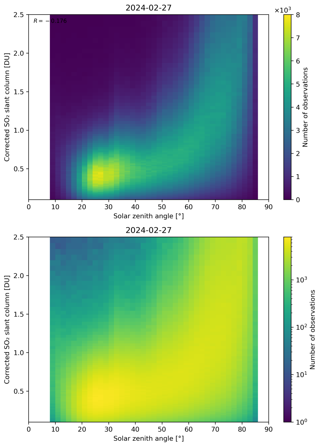
Figure 166: Scatter density plot of “Solar zenith angle” against “Corrected SO 2 slant column” for 2024-02-27 to 2024-02-28.
