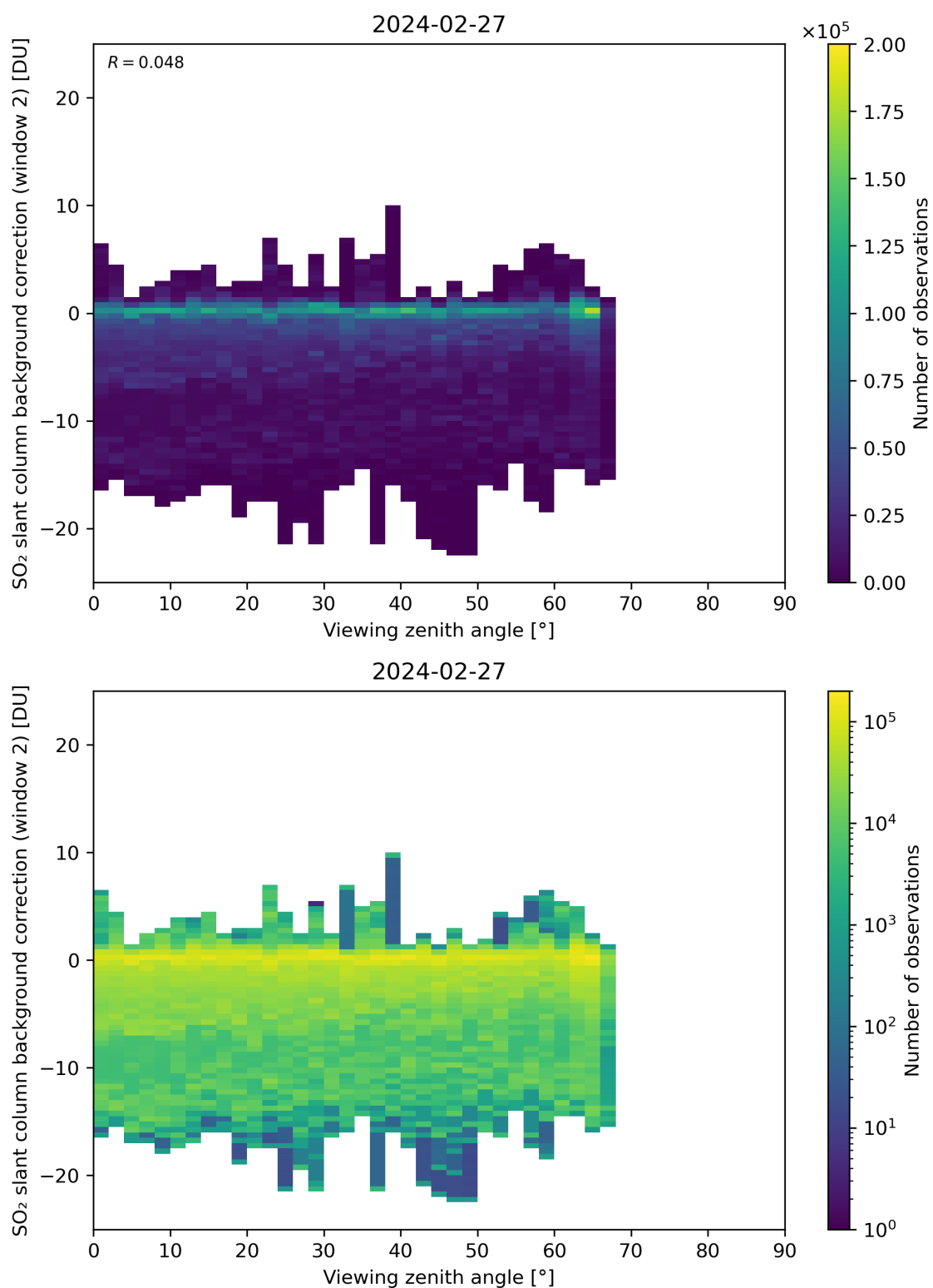
Figure 309: Scatter density plot of “Viewing zenith angle” against “SO 2 slant column background correction (window 2)” for 2024-02-27 to 2024-02-28.
