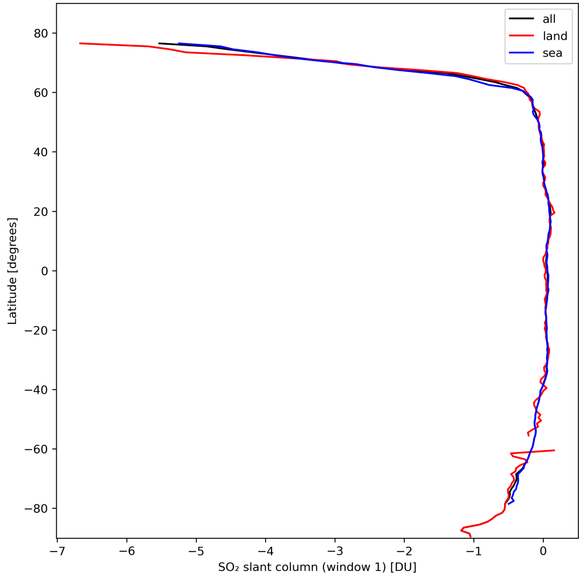
Figure 33: Zonal average of “SO 2 slant column (window 1)” for 2024-02-27 to 2024-02-28.
