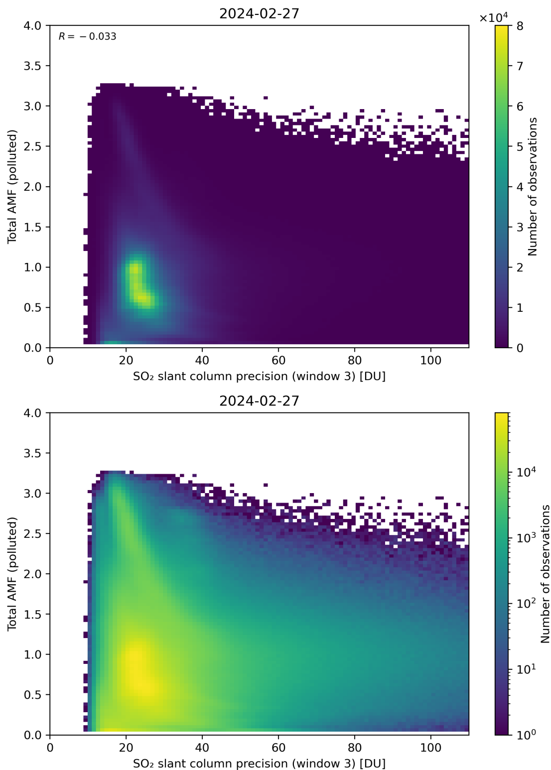
Figure 263: Scatter density plot of “SO 2 slant column precision (window 3)” against “Total AMF (polluted)” for 2024-02-27 to 2024-02-28.
