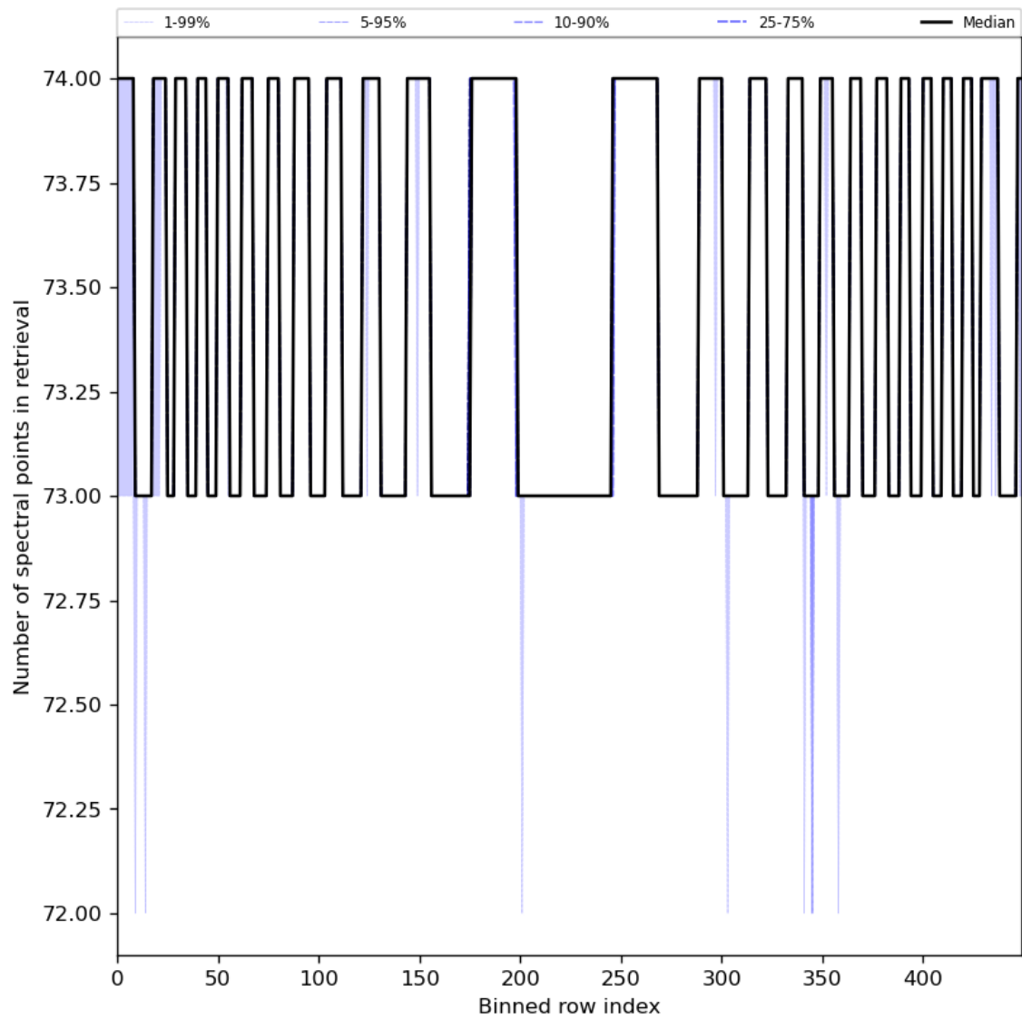
Figure 97: Along track statistics of “Number of spectral points in retrieval” for 2024-02-27 to 2024-02-28
