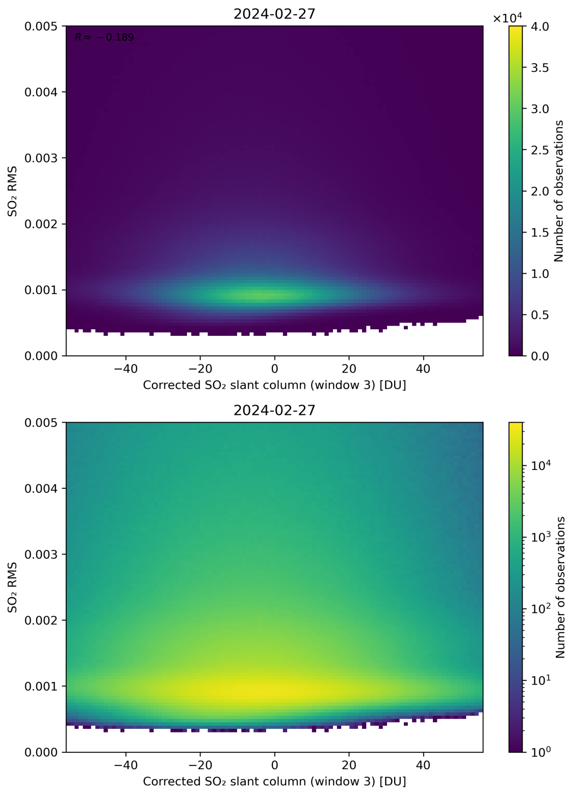
Figure 208: Scatter density plot of “Corrected SO 2 slant column (window 3)” against “SO 2 RMS” for 2024-02-27 to 2024-02-28.
