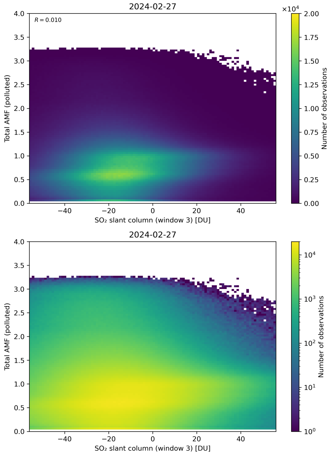
Figure 268: Scatter density plot of “SO 2 slant column (window 3)” against “Total AMF (polluted)” for 2024-02-27 to 2024-02-28.
