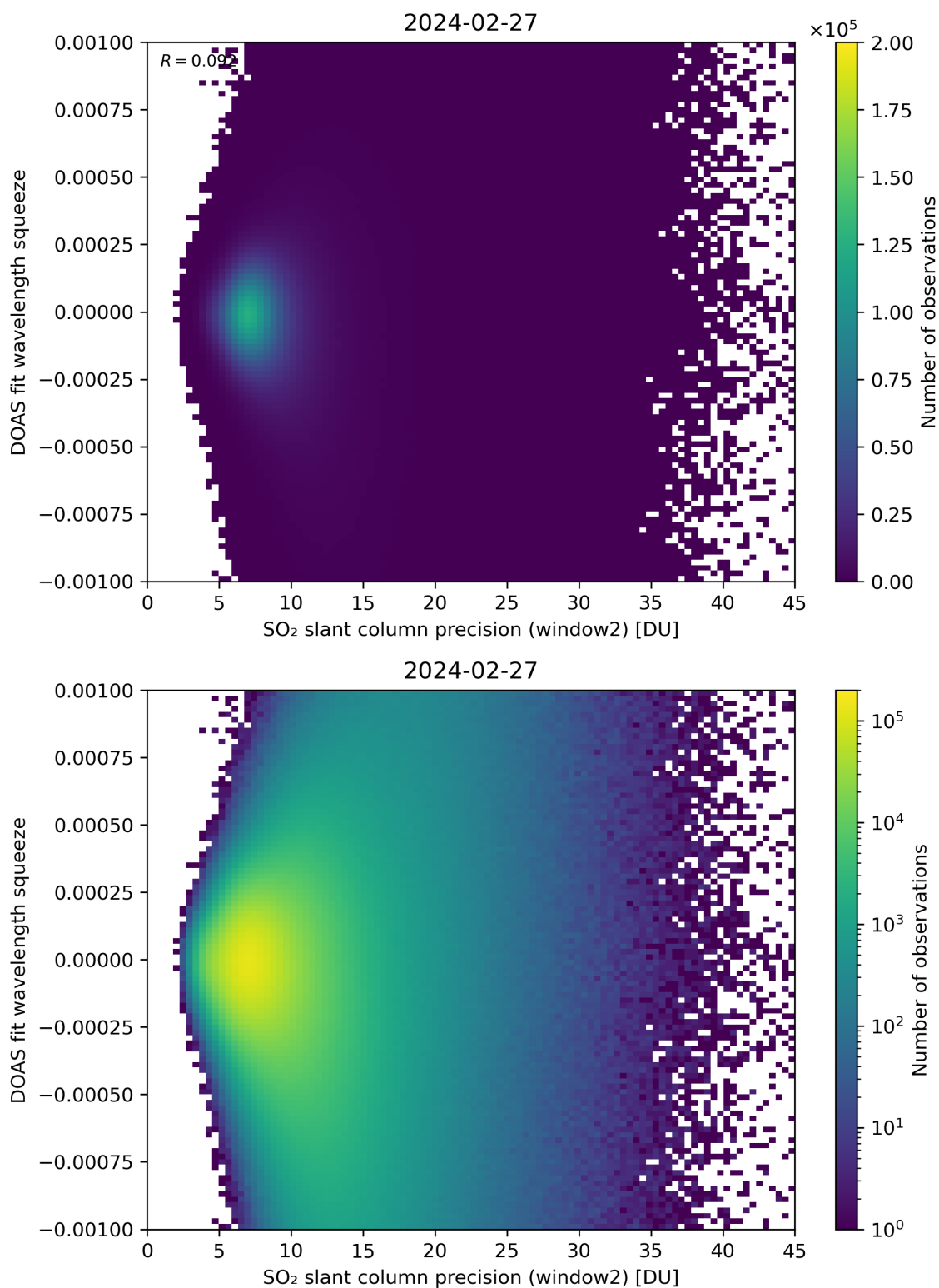
Figure 244: Scatter density plot of “SO 2 slant column precision (window2)” against “DOAS fit wavelength squeeze” for 2024-02-27 to 2024-02-28.
