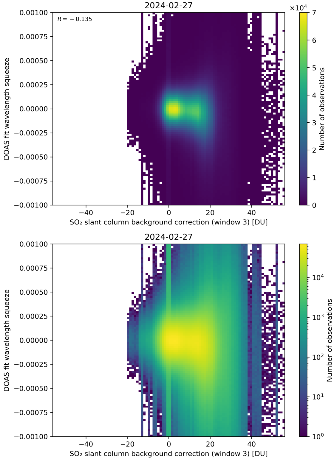
Figure 122: Scatter density plot of “SO 2 slant column background correction (window 3)” against “DOAS fit wavelength squeeze” for 2024-02-27 to 2024-02-28.
