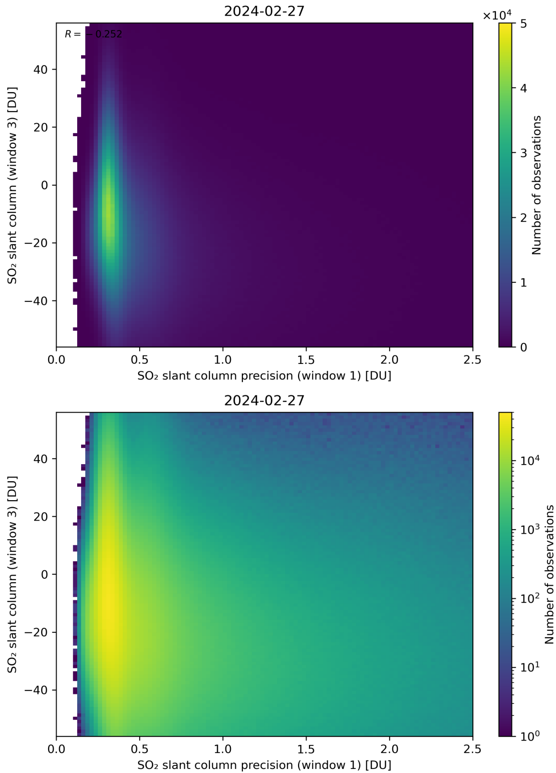
Figure 228: Scatter density plot of “SO 2 slant column precision (window 1)” against “SO 2 slant column (window 3)” for 2024-02-27 to 2024-02-28.
