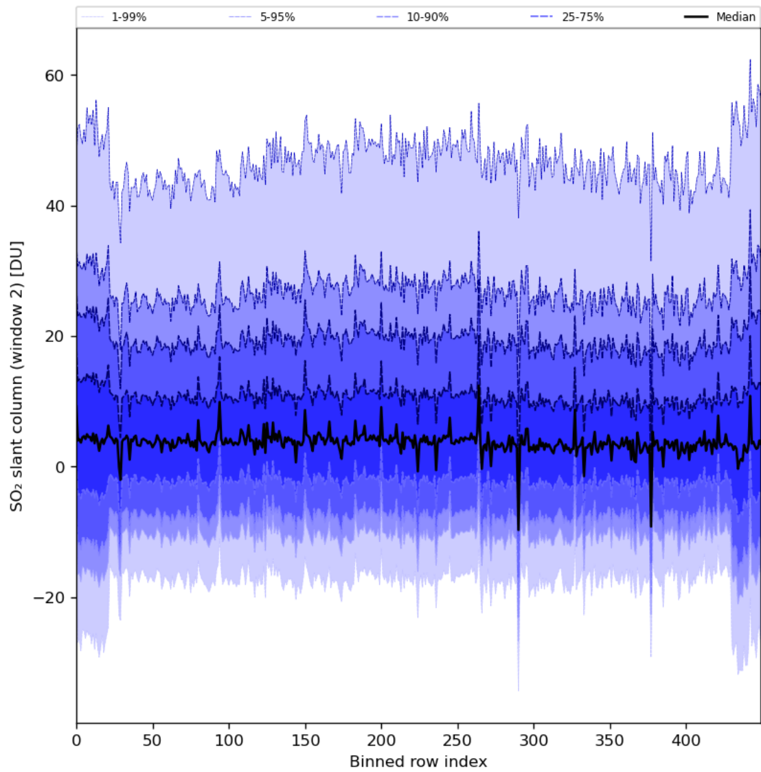
Figure 83: Along track statistics of “SO 2 slant column (window 2)” for 2024-02-27 to 2024-02-28
