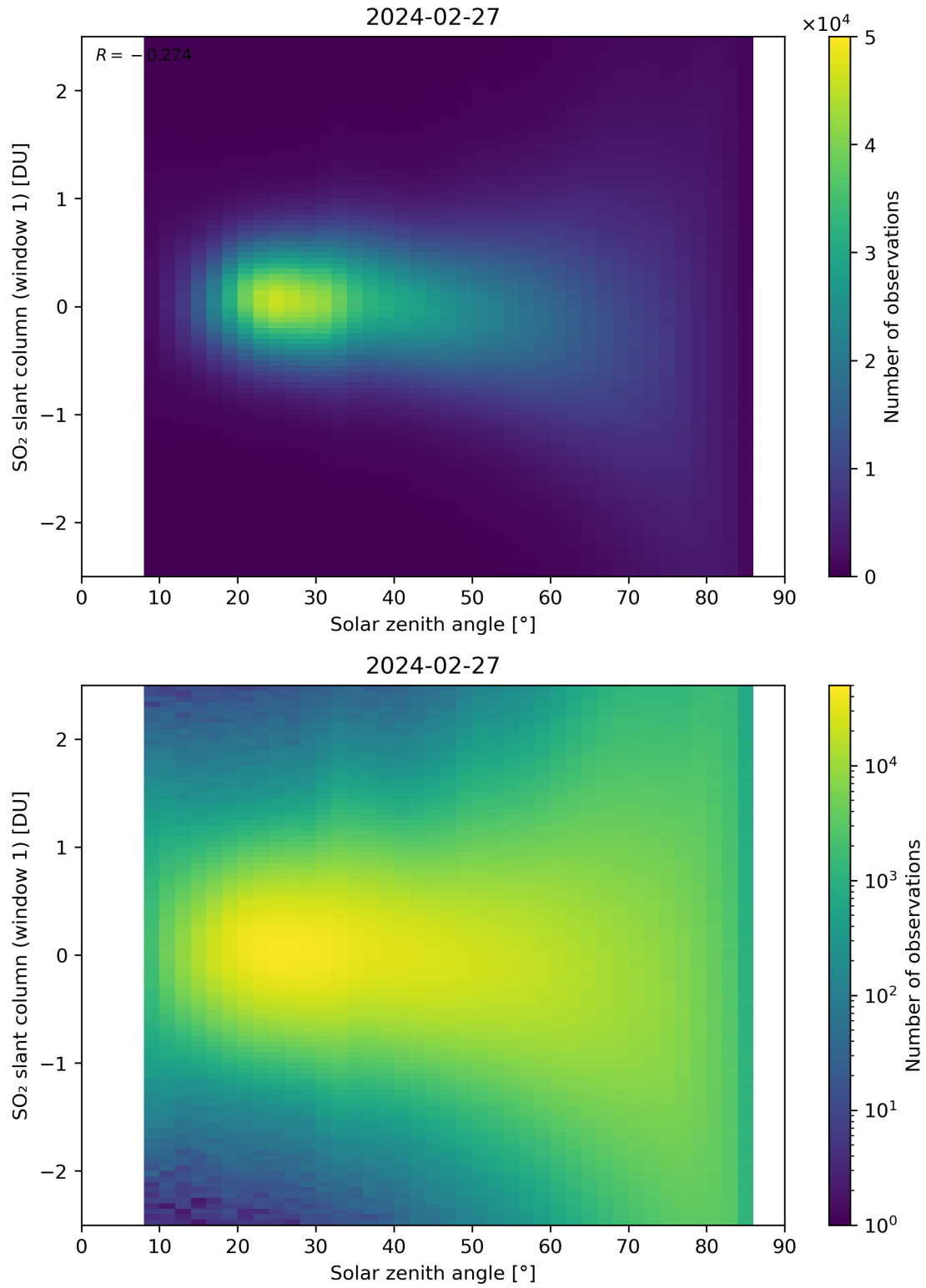
Figure 169: Scatter density plot of “Solar zenith angle” against “SO 2 slant column (window 1)” for 2024-02-27 to 2024-02-28.
