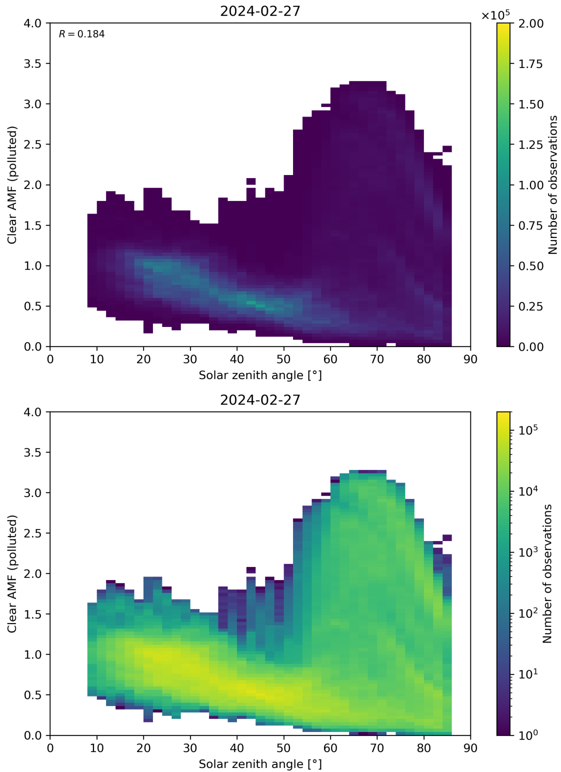
Figure 165: Scatter density plot of “Solar zenith angle” against “Clear AMF (polluted)” for 2024-02-27 to 2024-02-28.
