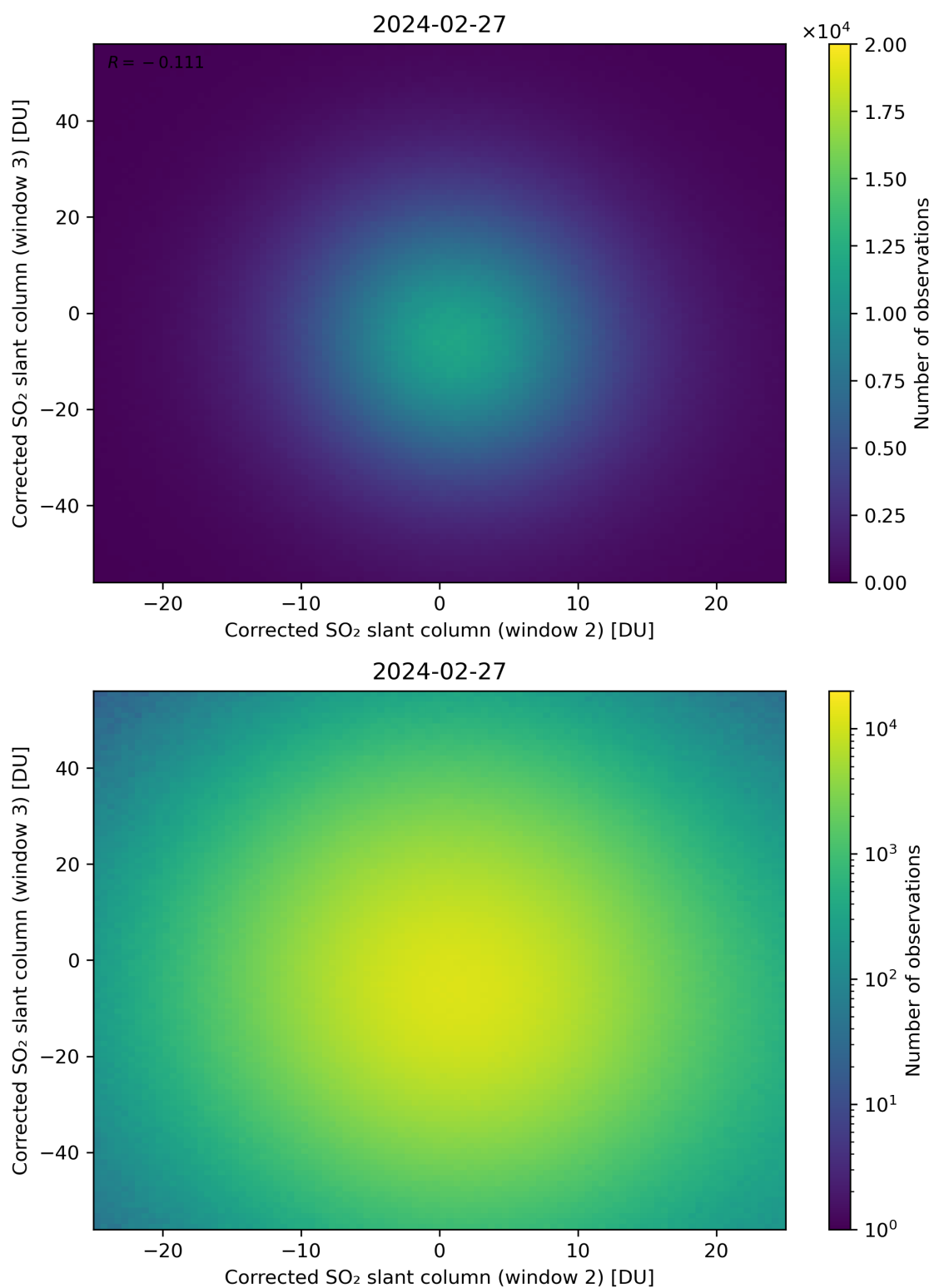
Figure 200: Scatter density plot of “Corrected SO 2 slant column (window 2)” against “Corrected SO 2 slant column (window 3)” for 2024-02-27 to 2024-02-28.
