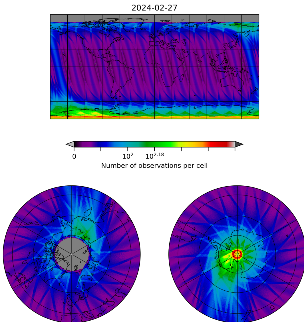
Figure 28: Map of the number of observations for 2024-02-27 to 2024-02-28
