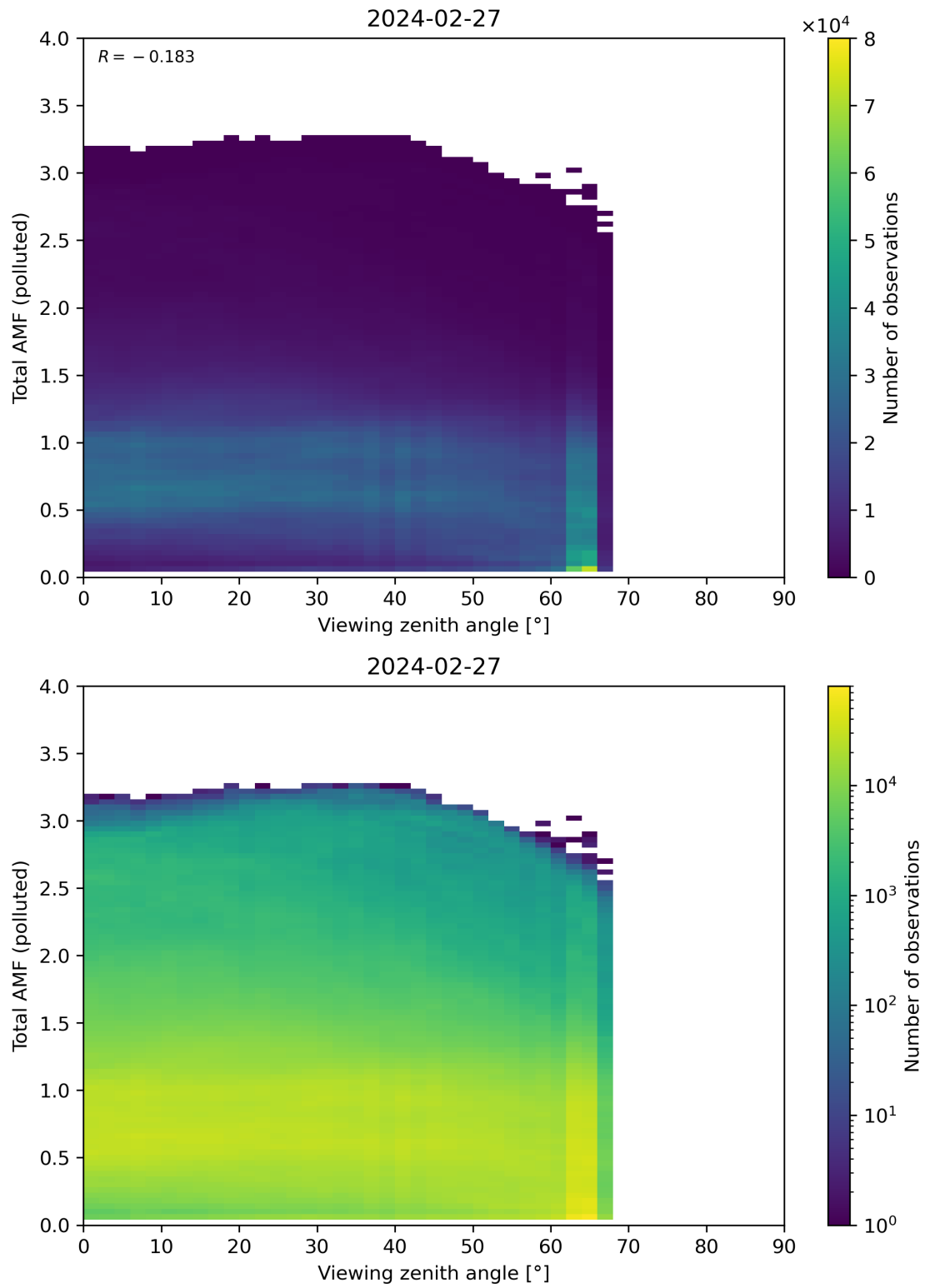
Figure 325: Scatter density plot of “Viewing zenith angle” against “Total AMF (polluted)” for 2024-02-27 to 2024-02-28.
