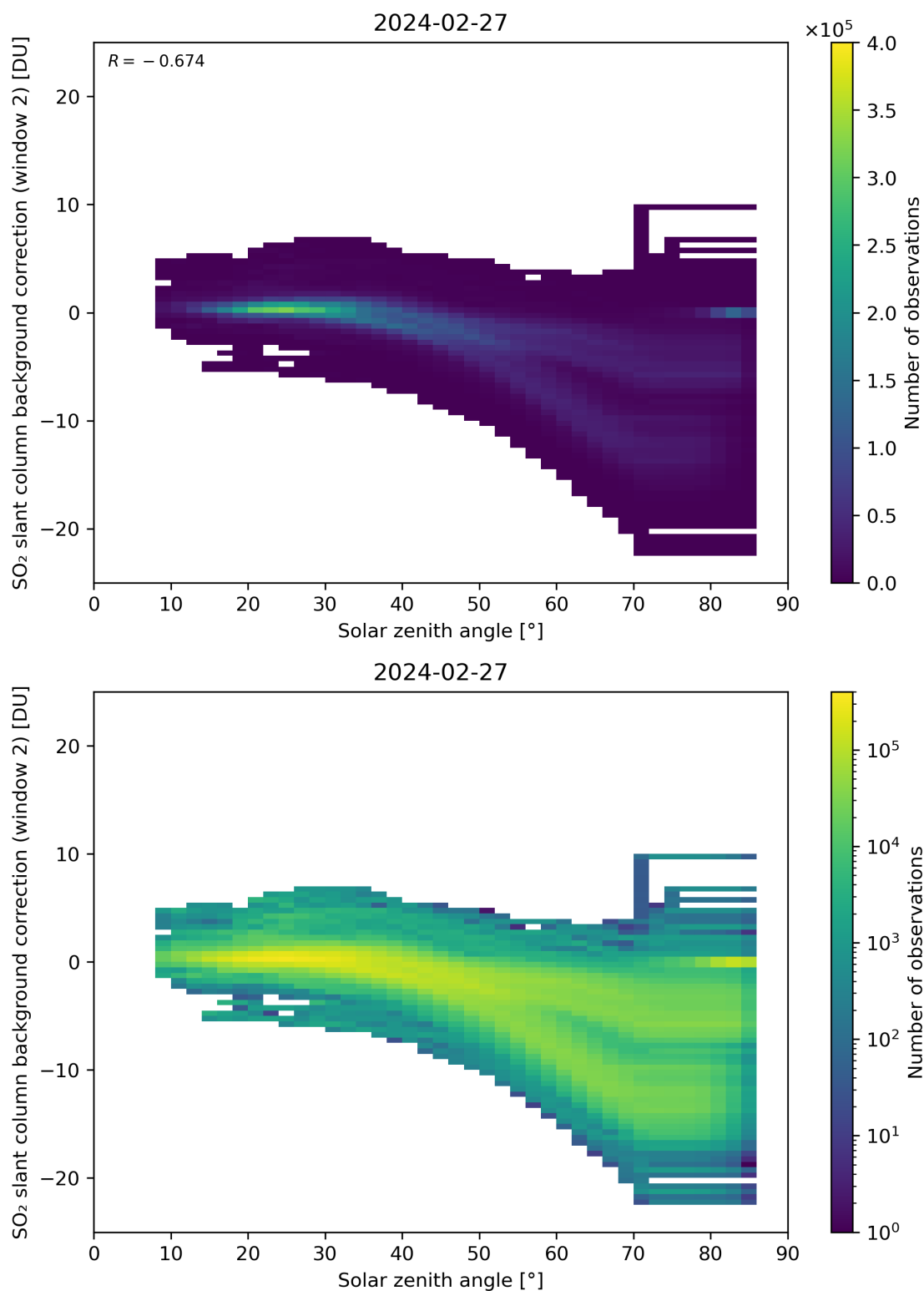
Figure 159: Scatter density plot of “Solar zenith angle” against “SO 2 slant column background correction (window 2)” for 2024-02-27 to 2024-02-28.
