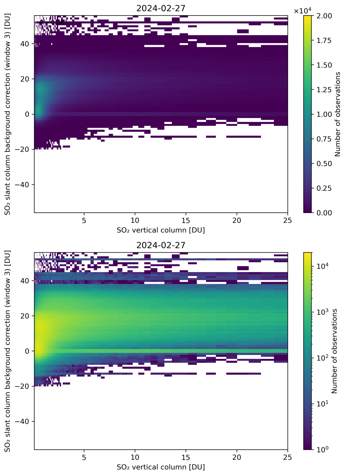
Figure 275: Scatter density plot of “SO 2 vertical column” against “SO 2 slant column background correction (window 3)” for 2024-02-27 to 2024-02-28.
