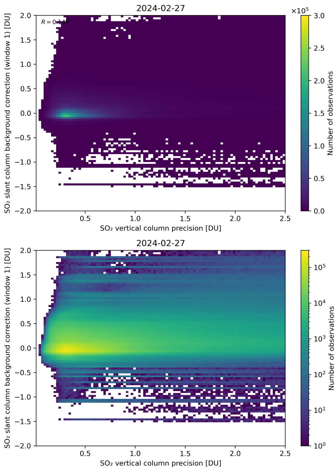
Figure 279: Scatter density plot of “SO 2 vertical column precision” against “SO 2 slant column background correction (window 1)” for 2024-02-27 to 2024-02-28.
