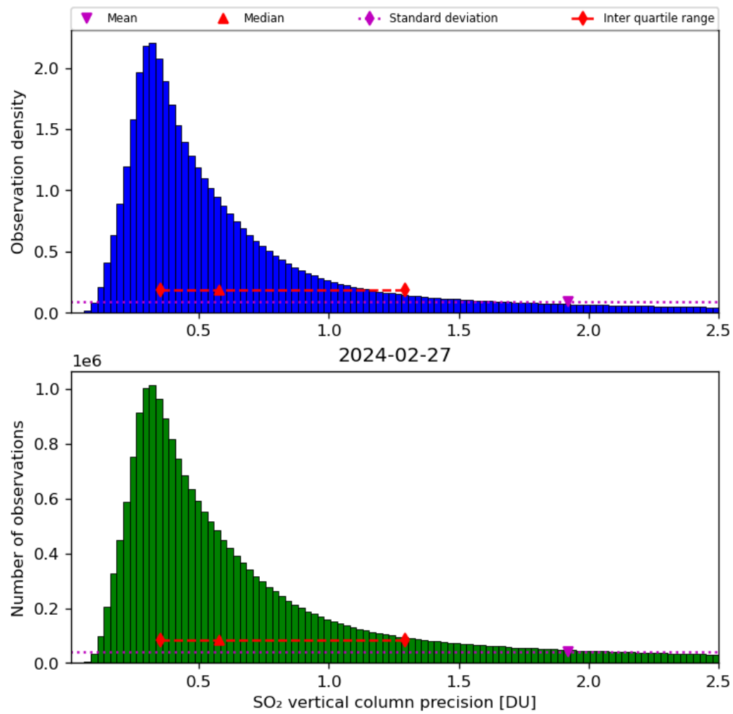
Figure 54: Histogram of “SO 2 vertical column precision” for 2024-02-27 to 2024-02-28
