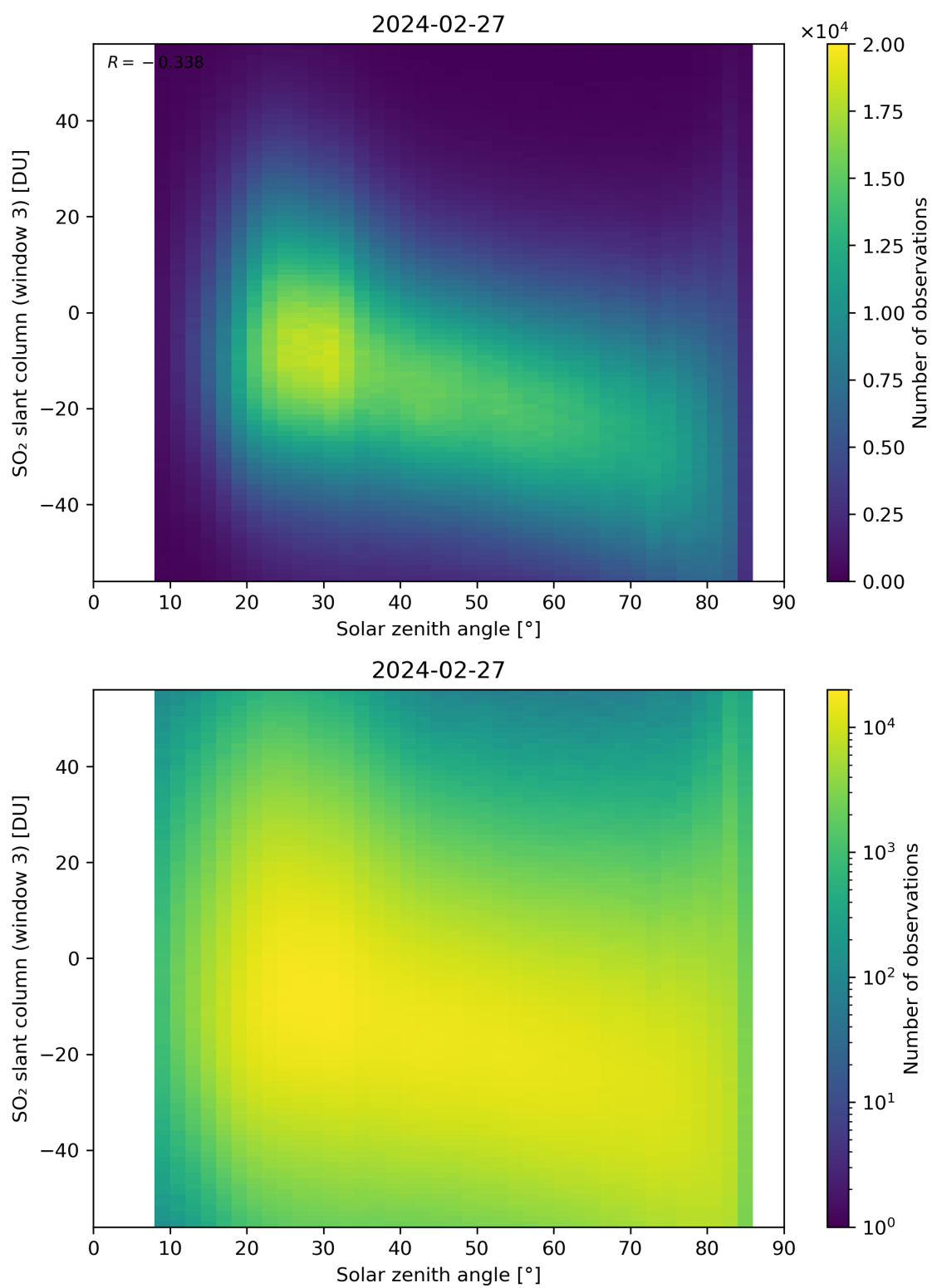
Figure 172: Scatter density plot of “Solar zenith angle” against “SO 2 slant column (window 3)” for 2024-02-27 to 2024-02-28.
