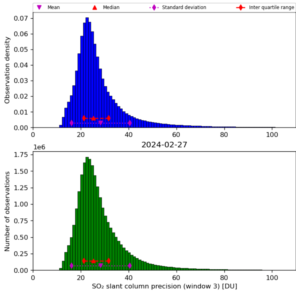
Figure 65: Histogram of “SO 2 slant column precision (window 3)” for 2024-02-27 to 2024-02-28
