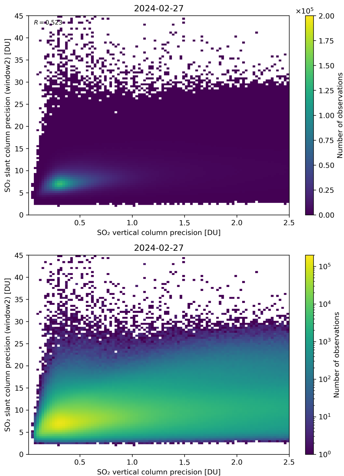
Figure 291: Scatter density plot of “SO 2 vertical column precision” against “SO 2 slant column precision (window2)” for 2024-02-27 to 2024-02-28.
