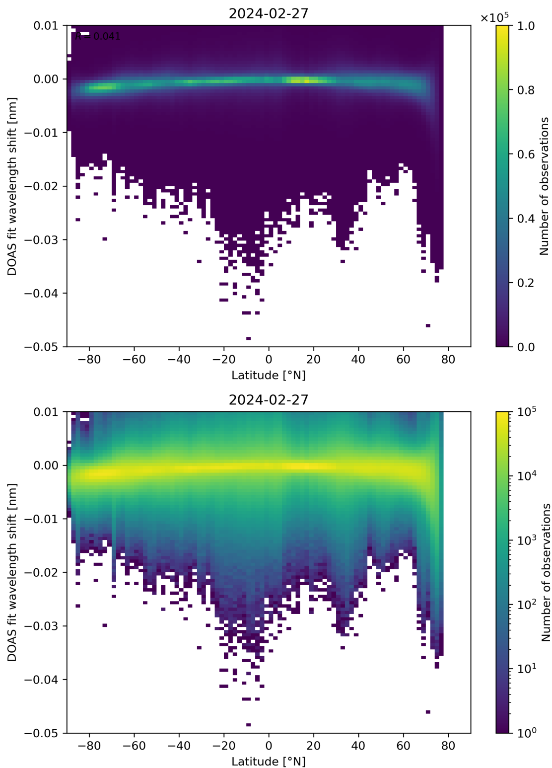
Figure 142: Scatter density plot of “Latitude” against “DOAS fit wavelength shift” for 2024-02-27 to 2024-02-28.
