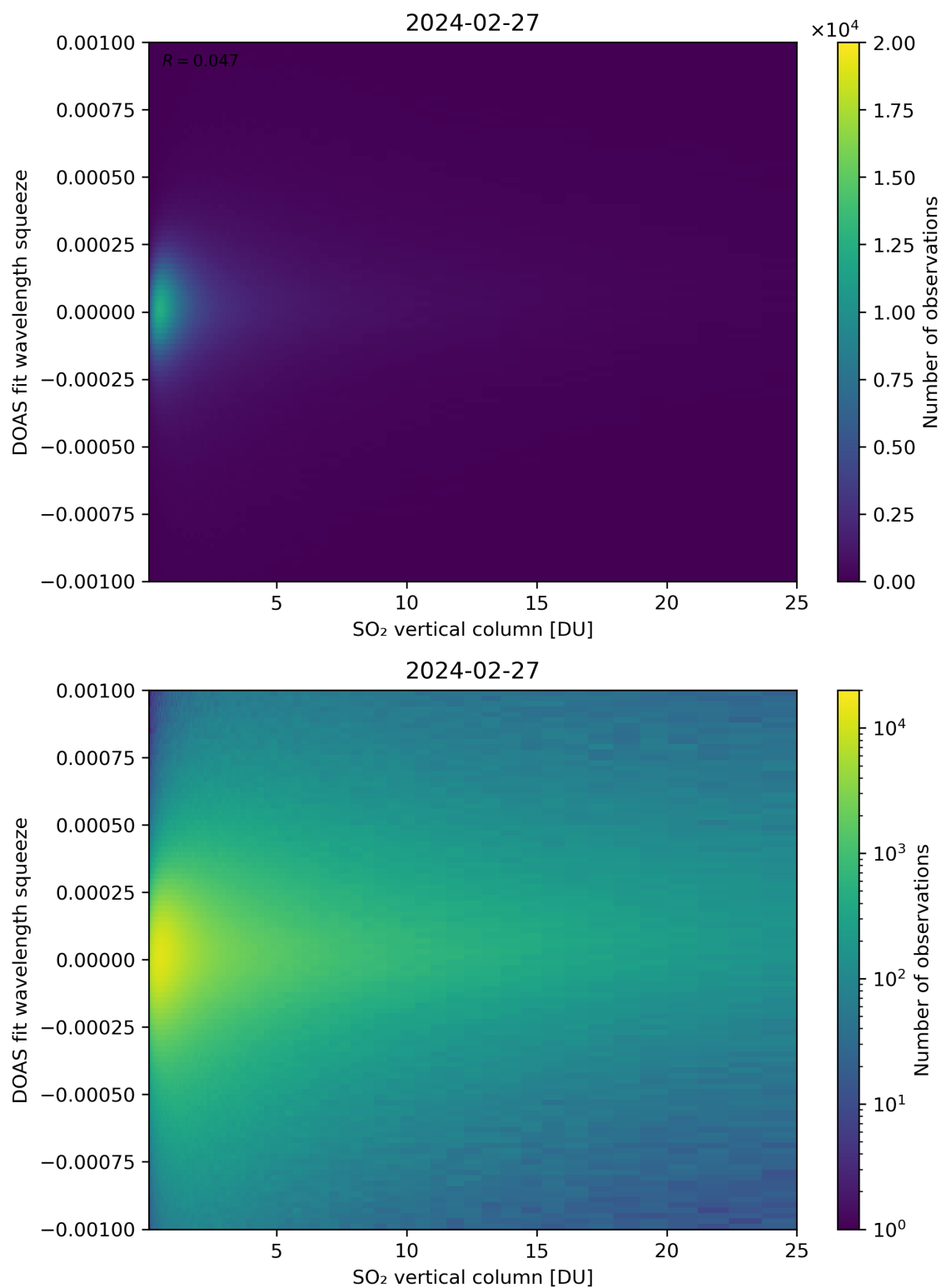
Figure 277: Scatter density plot of “SO 2 vertical column” against “DOAS fit wavelength squeeze” for 2024-02-27 to 2024-02-28.
