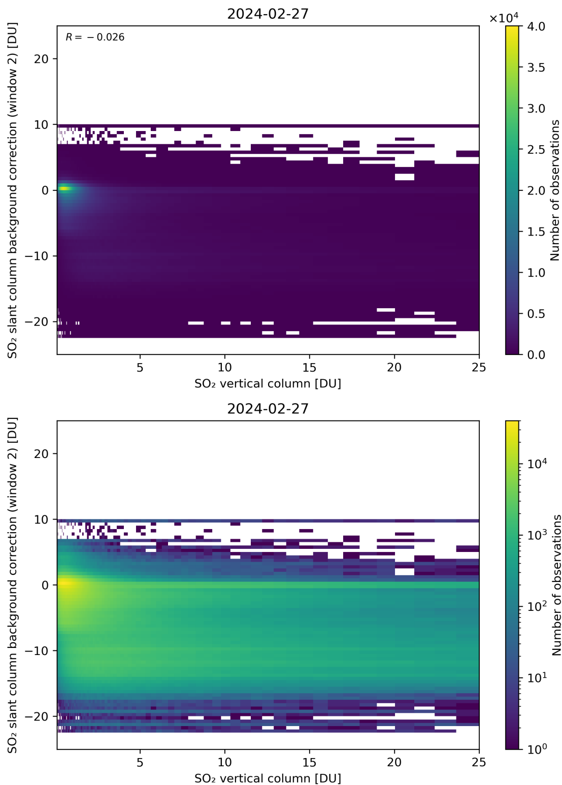
Figure 274: Scatter density plot of “SO 2 vertical column” against “SO 2 slant column background correction (window 2)” for 2024-02-27 to 2024-02-28.
