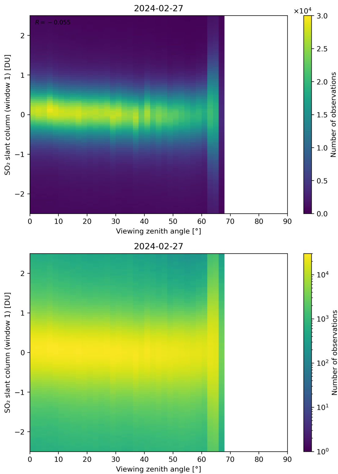
Figure 320: Scatter density plot of “Viewing zenith angle” against “SO 2 slant column (window 1)” for 2024-02-27 to 2024-02-28.
