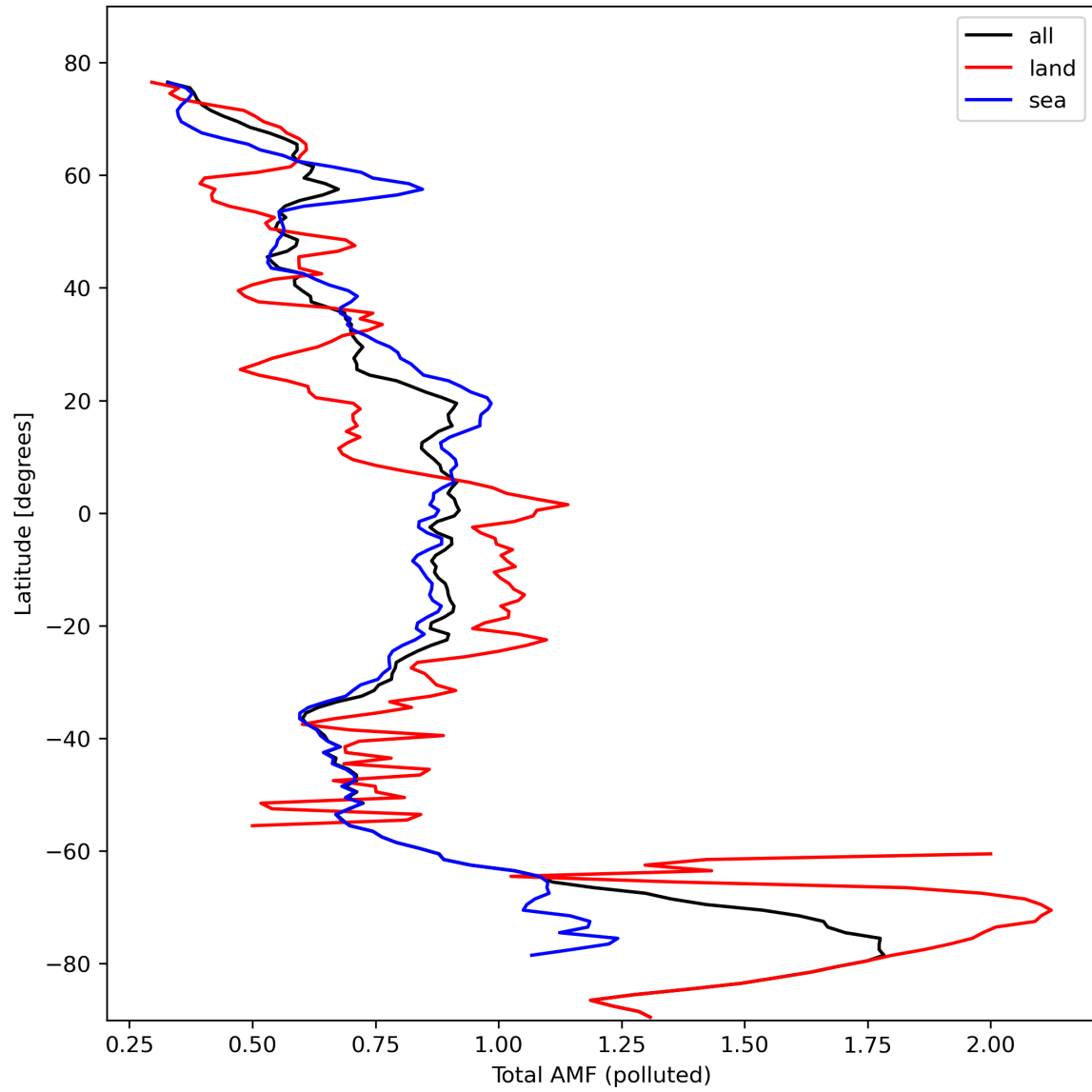
Figure 48: Zonal average of “Total AMF (polluted)” for 2024-02-27 to 2024-02-28.
