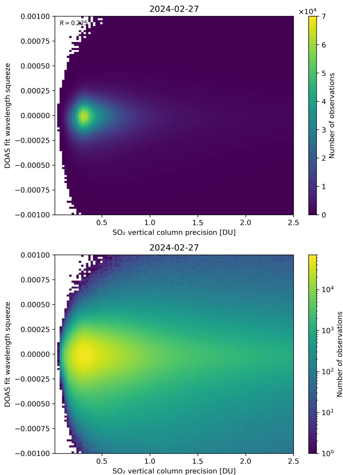
Figure 283: Scatter density plot of “SO 2 vertical column precision” against “DOAS fit wavelength squeeze” for 2024-02-27 to 2024-02-28.
