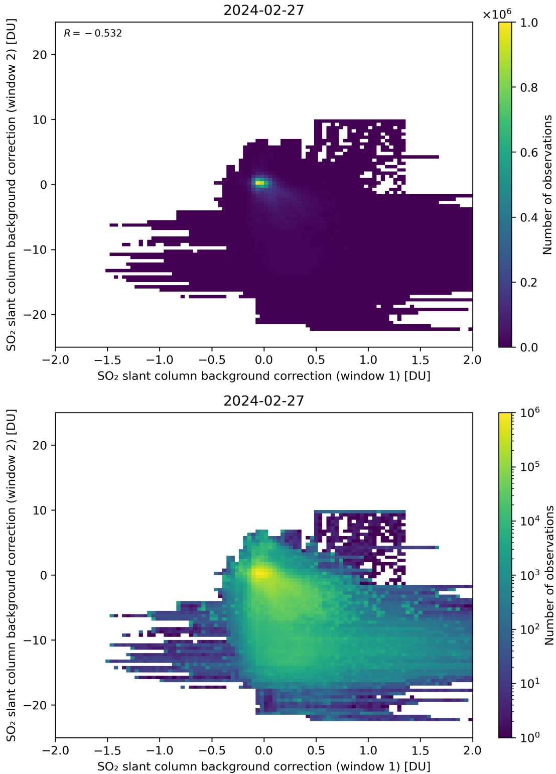
Figure 98: Scatter density plot of “SO 2 slant column background correction (window 1)” against “SO 2 slant column background correction (window 2)” for 2024-02-27 to 2024-02-28.
