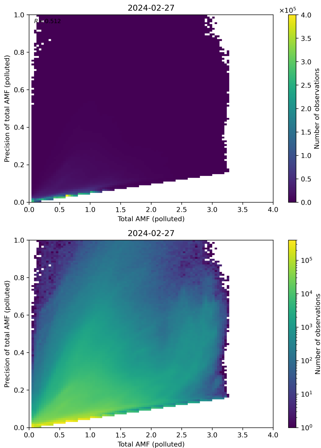
Figure 272: Scatter density plot of “Total AMF (polluted)” against “Precision of total AMF (polluted)” for 2024-02-27 to 2024-02-28.
