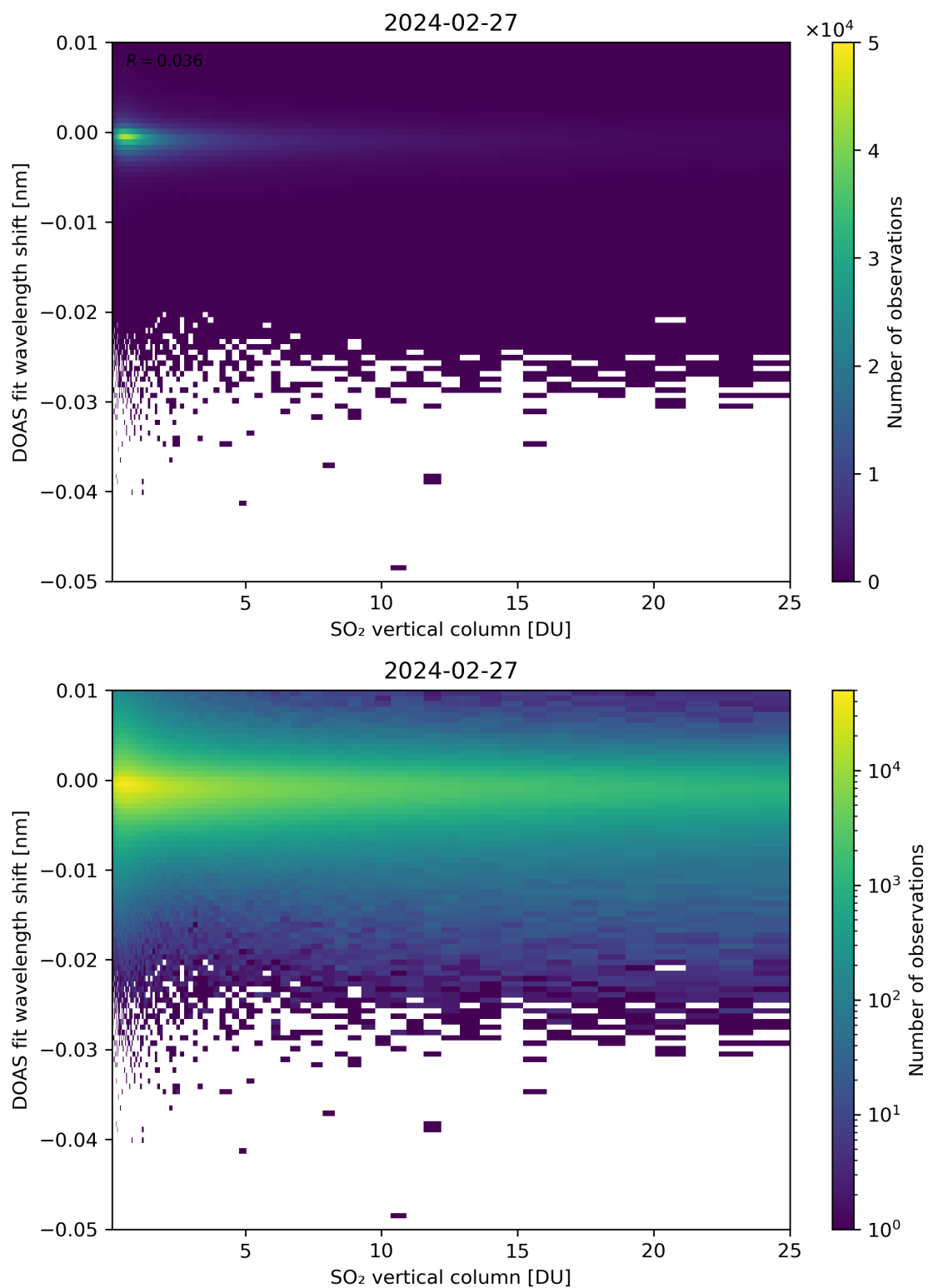
Figure 276: Scatter density plot of “SO 2 vertical column” against “DOAS fit wavelength shift” for 2024-02-27 to 2024-02-28.
