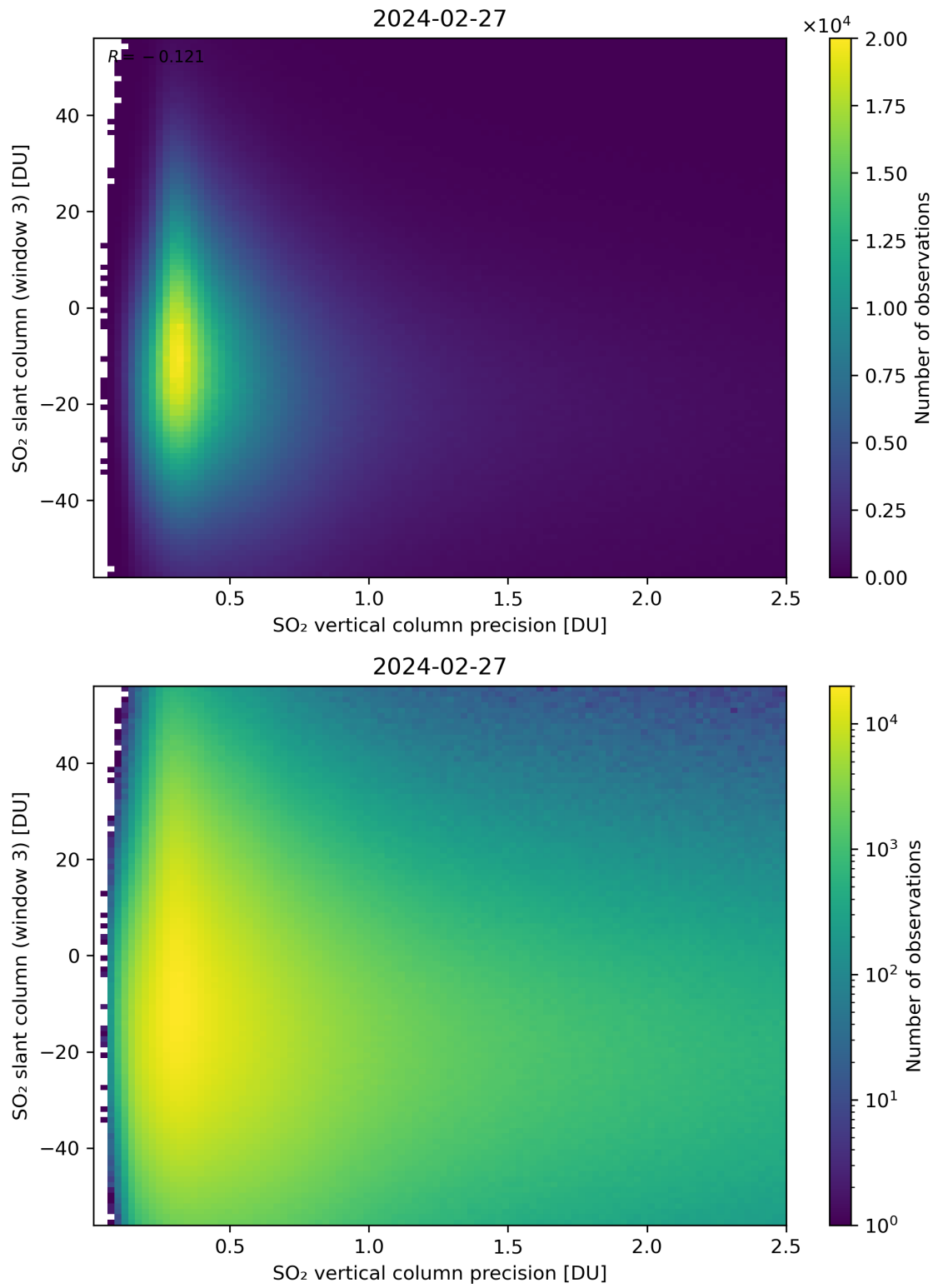
Figure 292: Scatter density plot of “SO 2 vertical column precision” against “SO 2 slant column (window 3)” for 2024-02-27 to 2024-02-28.
