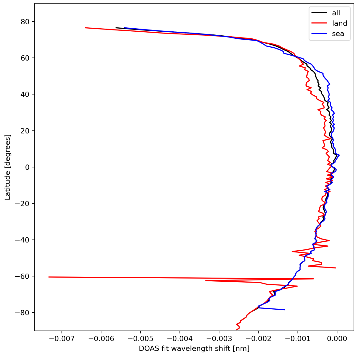
Figure 45: Zonal average of “DOAS fit wavelength shift” for 2024-02-27 to 2024-02-28.
