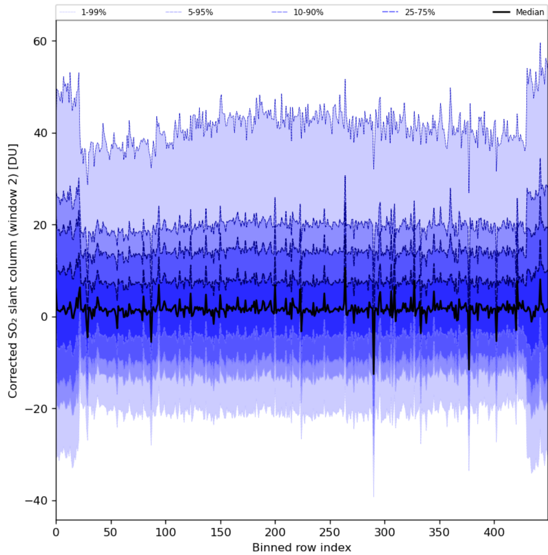
Figure 85: Along track statistics of “Corrected SO 2 slant column (window 2)” for 2024-02-27 to 2024-02-28
