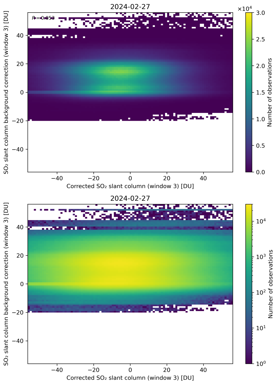
Figure 205: Scatter density plot of “Corrected SO 2 slant column (window 3)” against “SO 2 slant column background correction (window 3)” for 2024-02-27 to 2024-02-28.
