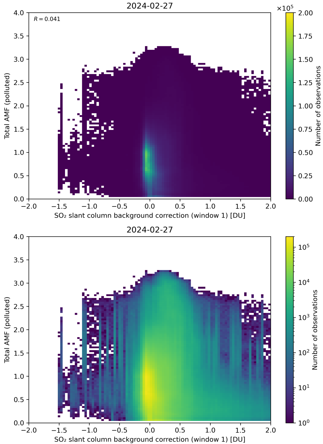
Figure 109: Scatter density plot of “SO 2 slant column background correction (window 1)” against “Total AMF (polluted)” for 2024-02-27 to 2024-02-28.
