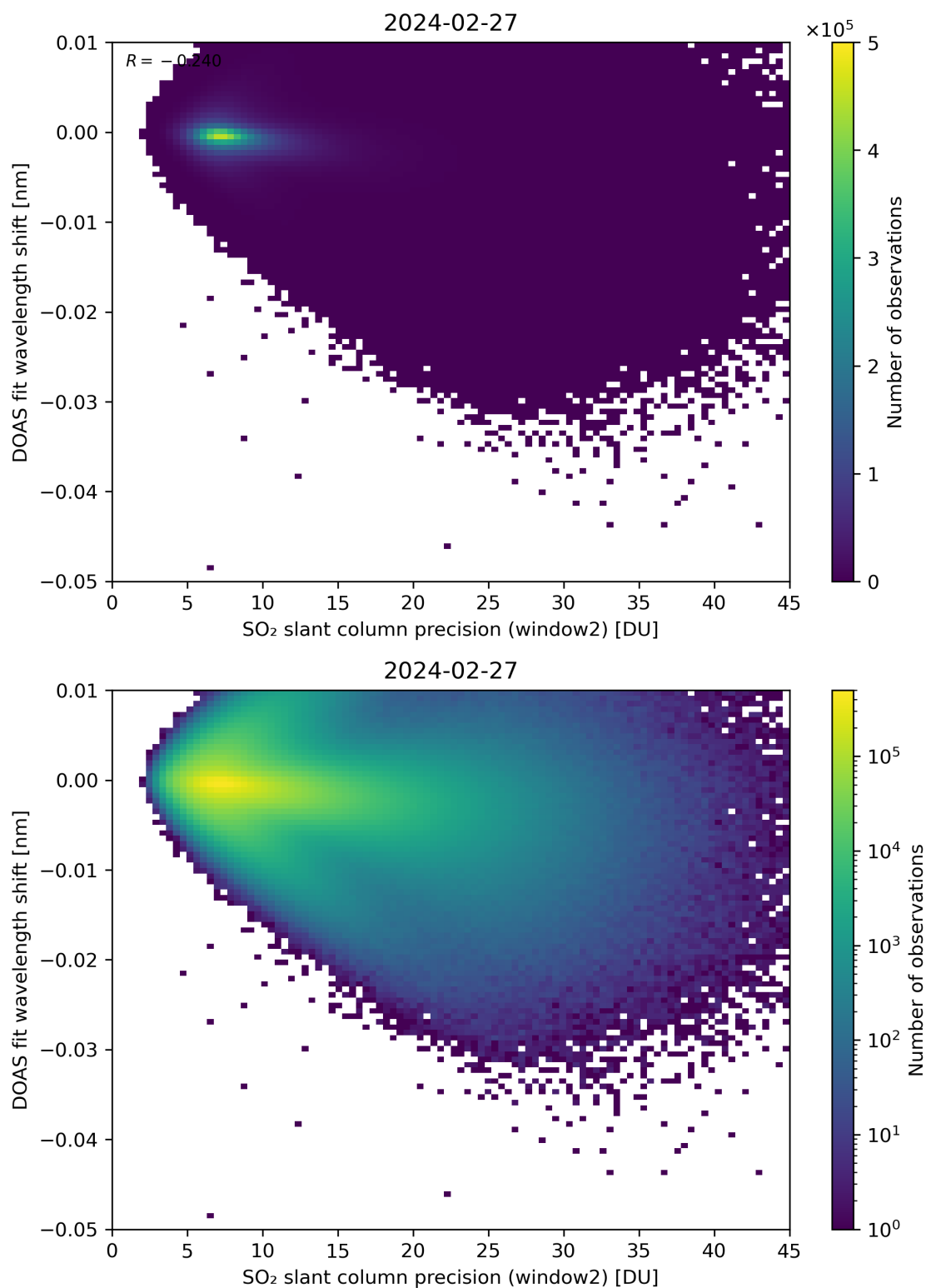
Figure 243: Scatter density plot of “SO 2 slant column precision (window2)” against “DOAS fit wavelength shift” for 2024-02-27 to 2024-02-28.
