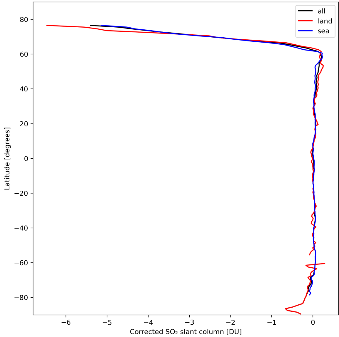
Figure 32: Zonal average of “Corrected SO 2 slant column” for 2024-02-27 to 2024-02-28.
