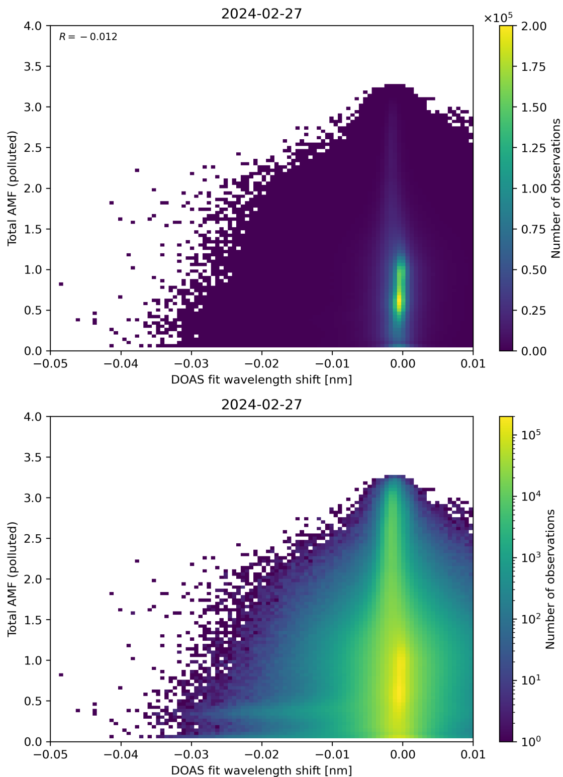
Figure 130: Scatter density plot of “DOAS fit wavelength shift” against “Total AMF (polluted)” for 2024-02-27 to 2024-02-28.
