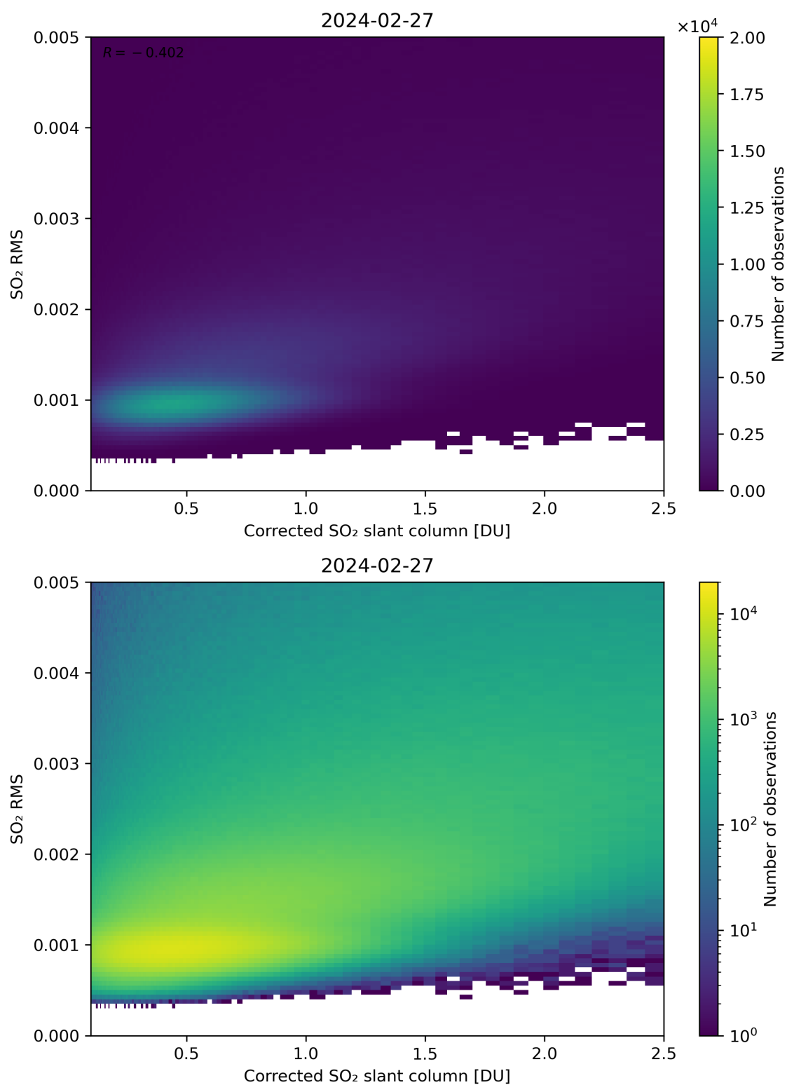
Figure 183: Scatter density plot of “Corrected SO 2 slant column” against “SO 2 RMS” for 2024-02-27 to 2024-02-28.
