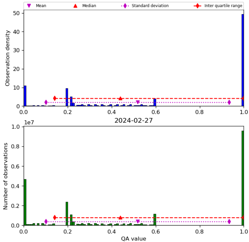
Figure 52: Histogram of “QA value” for 2024-02-27 to 2024-02-28
