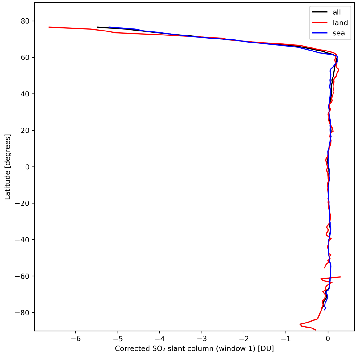
Figure 35: Zonal average of “Corrected SO 2 slant column (window 1)” for 2024-02-27 to 2024-02-28.
