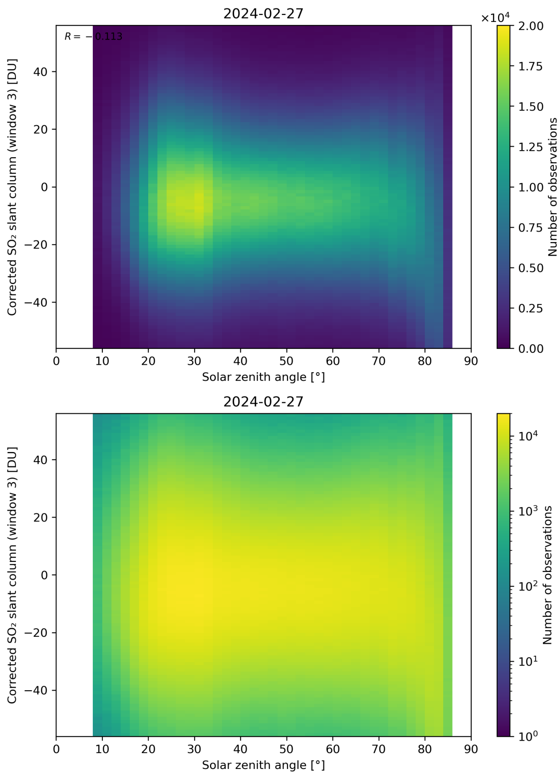
Figure 168: Scatter density plot of “Solar zenith angle” against “Corrected SO 2 slant column (window 3)” for 2024-02-27 to 2024-02-28.
