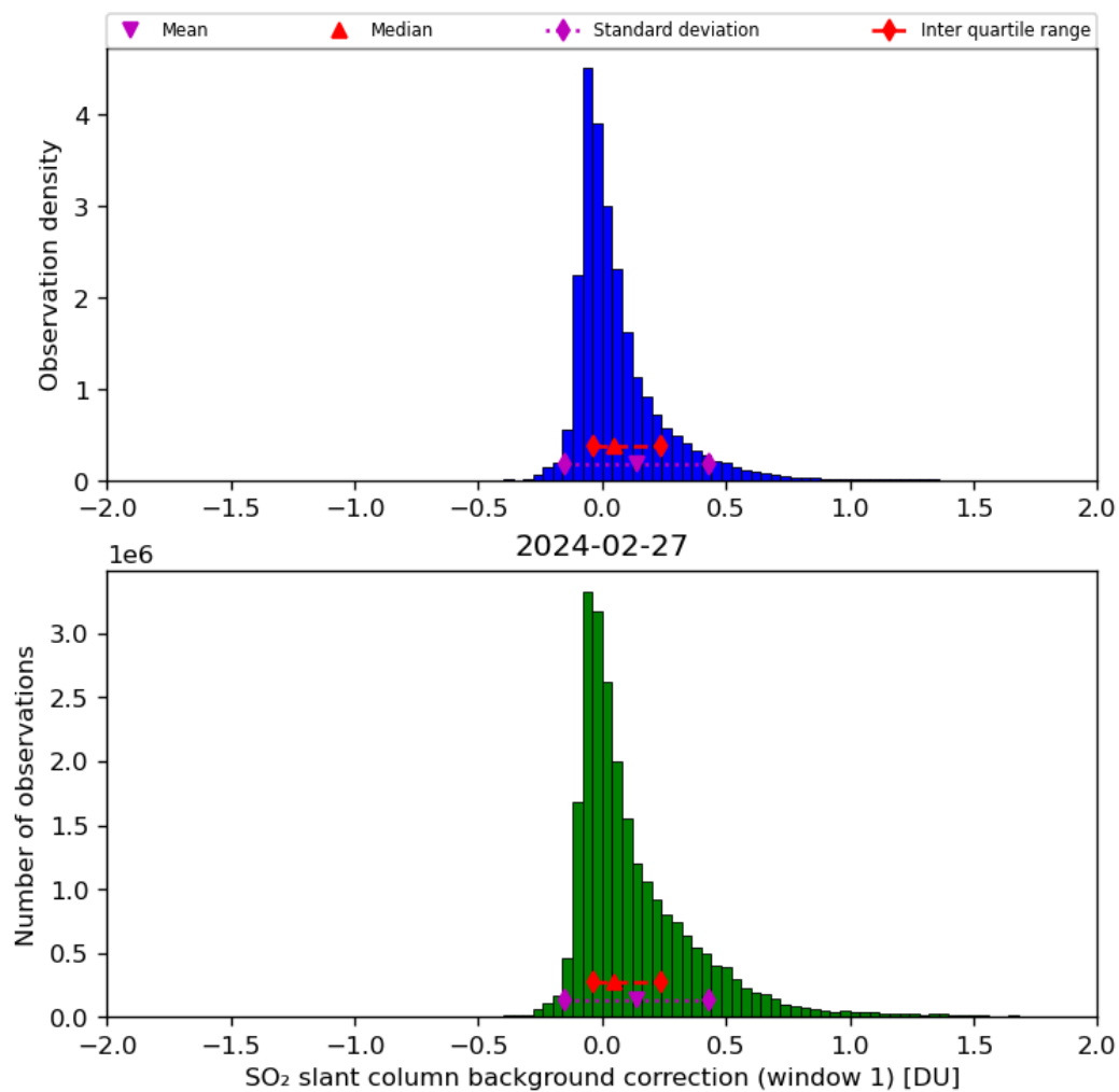
Figure 59: Histogram of “SO 2 slant column background correction (window 1)” for 2024-02-27 to 2024-02-28
