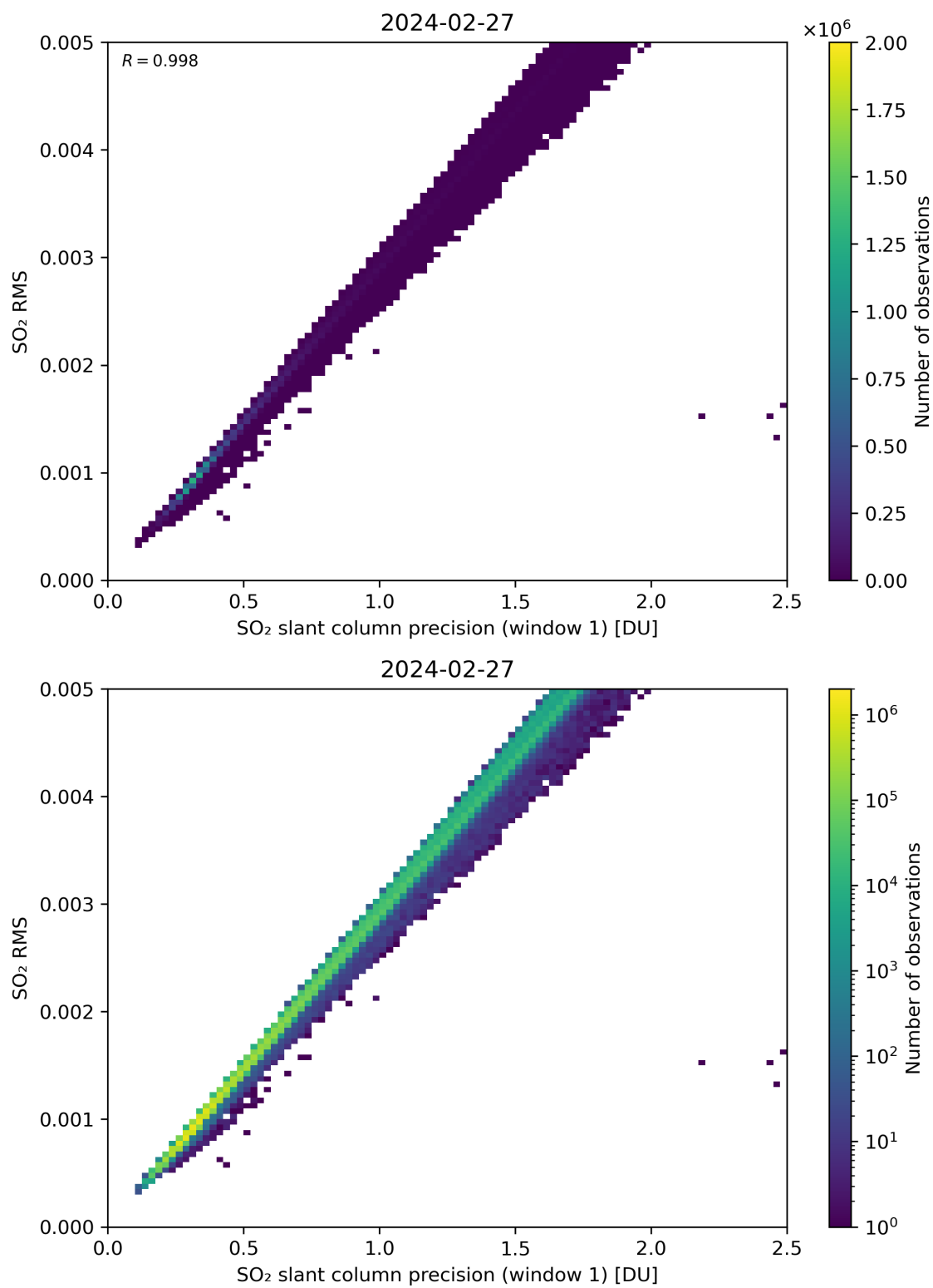
Figure 223: Scatter density plot of “SO 2 slant column precision (window 1)” against “SO 2 RMS” for 2024-02-27 to 2024-02-28.
