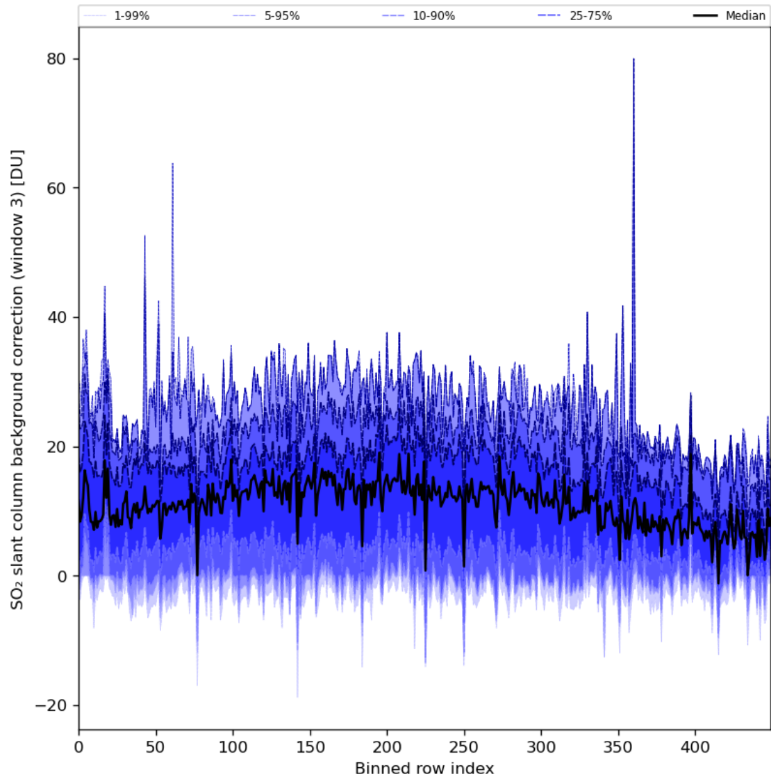
Figure 90: Along track statistics of “SO 2 slant column background correction (window 3)” for 2024-02-27 to 2024-02-28
