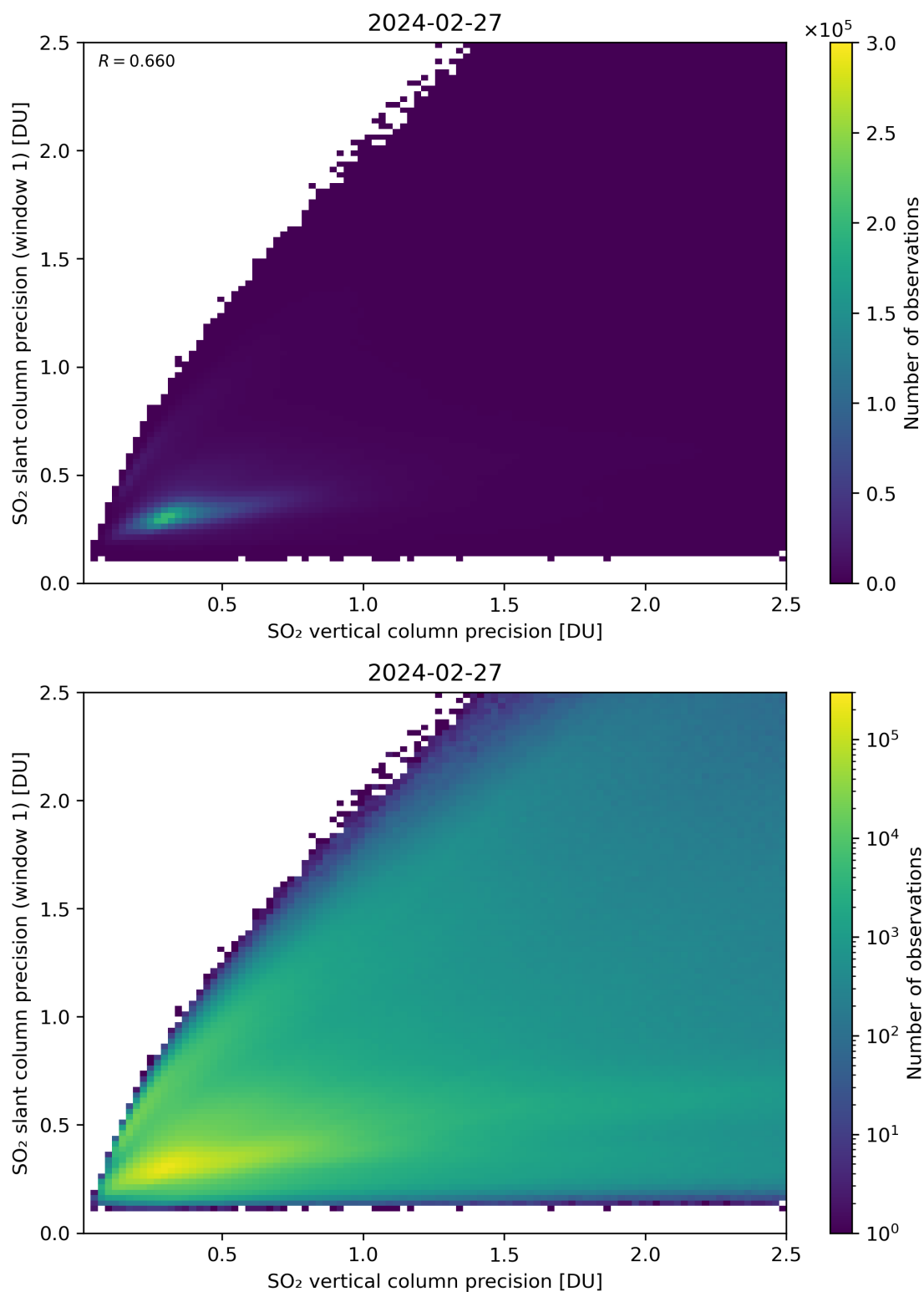
Figure 290: Scatter density plot of “SO 2 vertical column precision” against “SO 2 slant column precision (window 1)” for 2024-02-27 to 2024-02-28.
