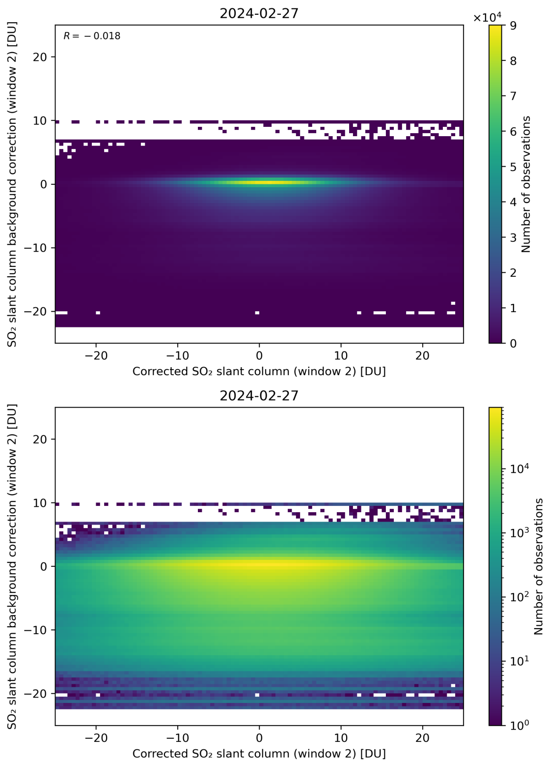
Figure 194: Scatter density plot of “Corrected SO 2 slant column (window 2)” against “SO 2 slant column background correction (window 2)” for 2024-02-27 to 2024-02-28.
