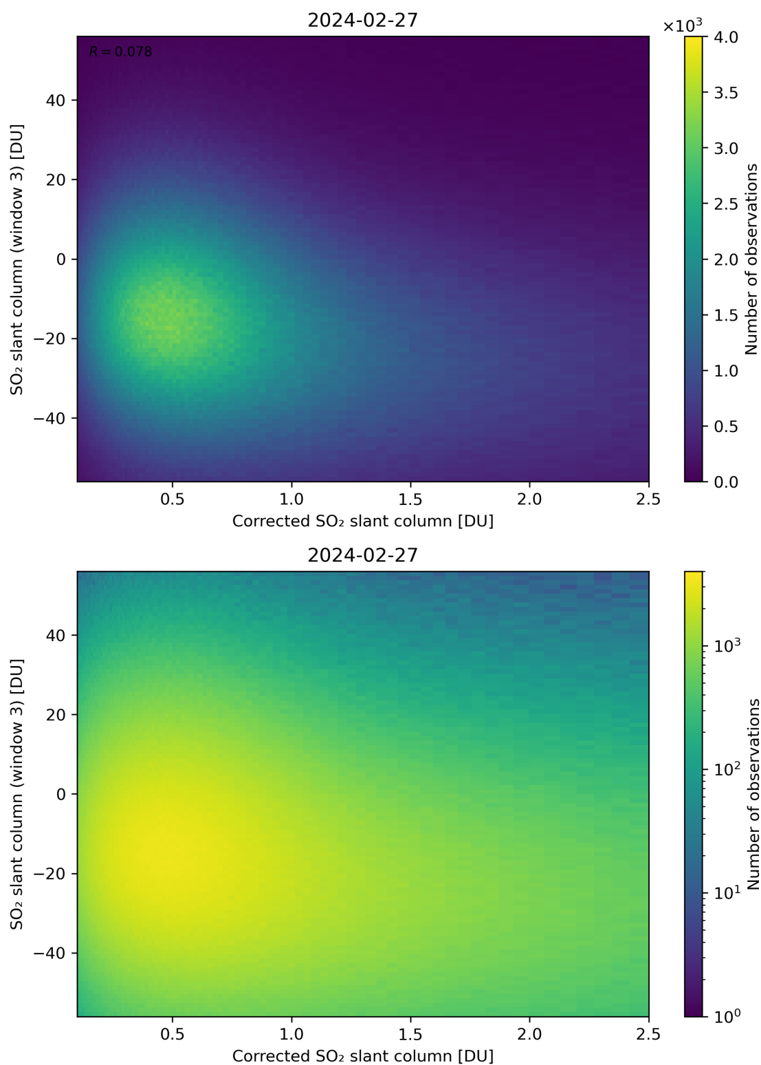
Figure 190: Scatter density plot of “Corrected SO 2 slant column” against “SO 2 slant column (window 3)” for 2024-02-27 to 2024-02-28.
