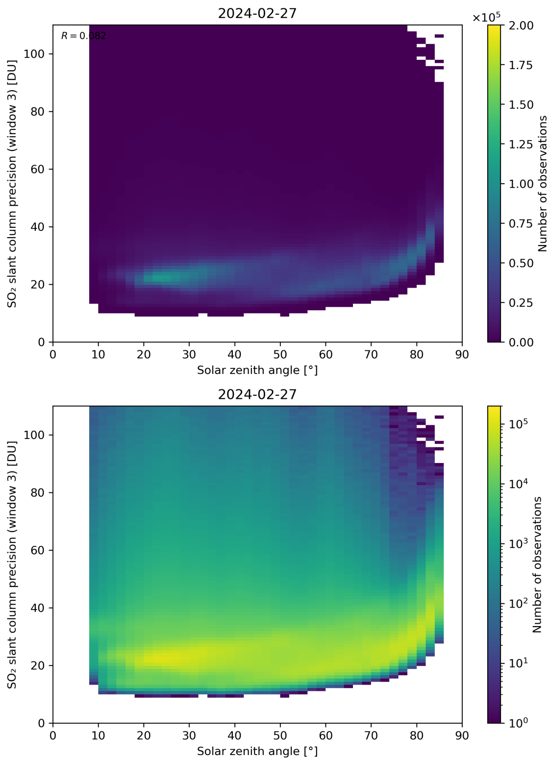
Figure 173: Scatter density plot of “Solar zenith angle” against “SO 2 slant column precision (window 3)” for 2024-02-27 to 2024-02-28.
