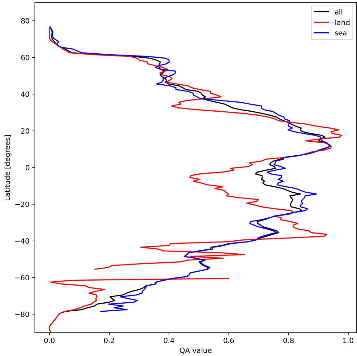
Figure 29: Zonal average of “QA value” for 2024-02-27 to 2024-02-28.
