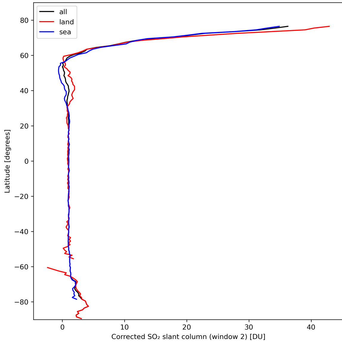
Figure 39: Zonal average of “Corrected SO 2 slant column (window 2)” for 2024-02-27 to 2024-02-28.
