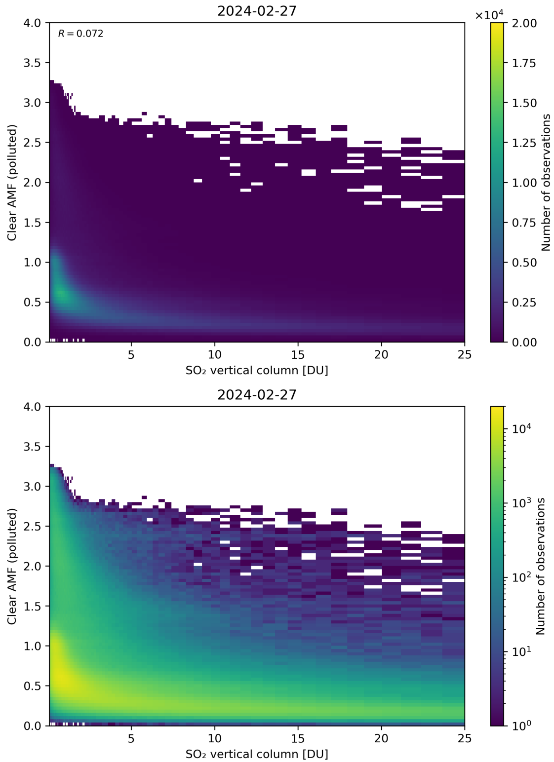
Figure 296: Scatter density plot of “SO 2 vertical column” against “Clear AMF (polluted)” for 2024-02-27 to 2024-02-28.
