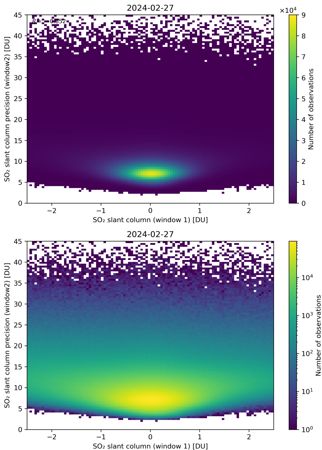
Figure 236: Scatter density plot of “SO 2 slant column (window 1)” against “SO 2 slant column precision (window2)” for 2024-02-27 to 2024-02-28.
