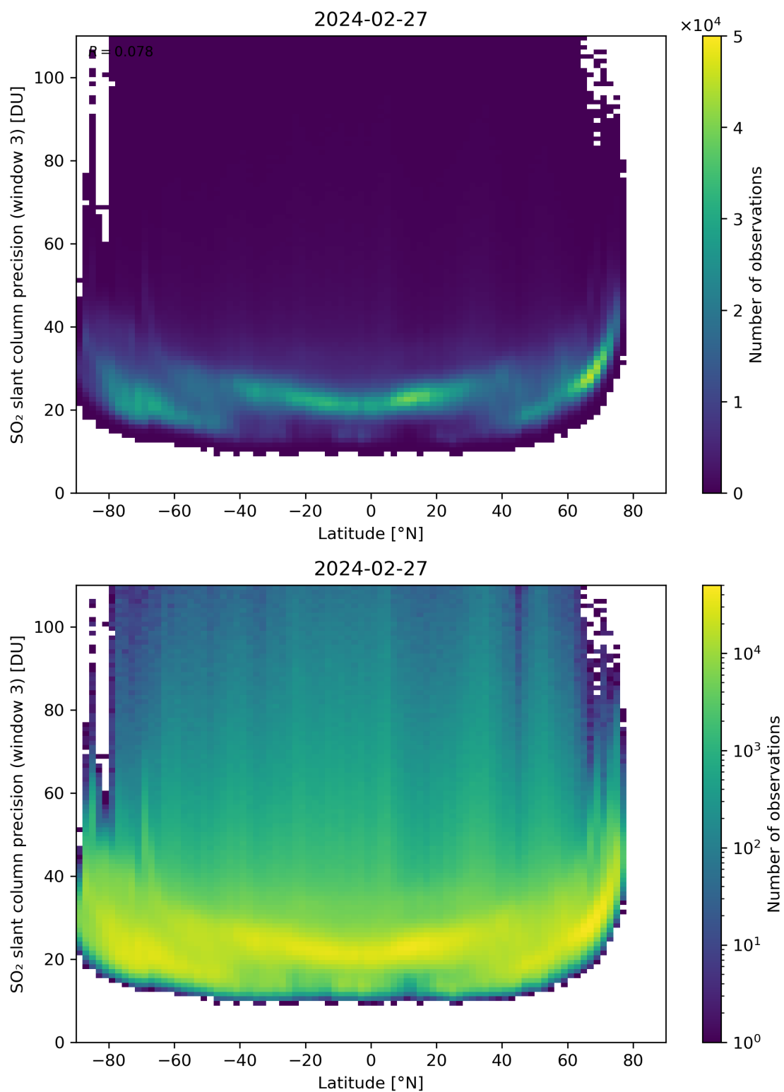
Figure 153: Scatter density plot of “Latitude” against “SO 2 slant column precision (window 3)” for 2024-02-27 to 2024-02-28.
