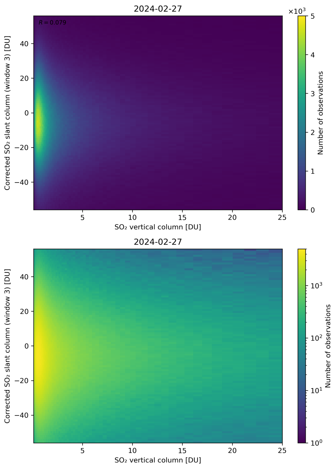
Figure 299: Scatter density plot of “SO 2 vertical column” against “Corrected SO 2 slant column (window 3)” for 2024-02-27 to 2024-02-28.
