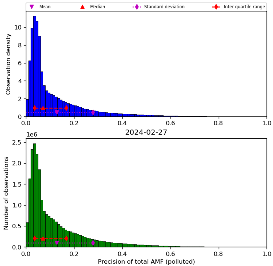
Figure 72: Histogram of “Precision of total AMF (polluted)” for 2024-02-27 to 2024-02-28
