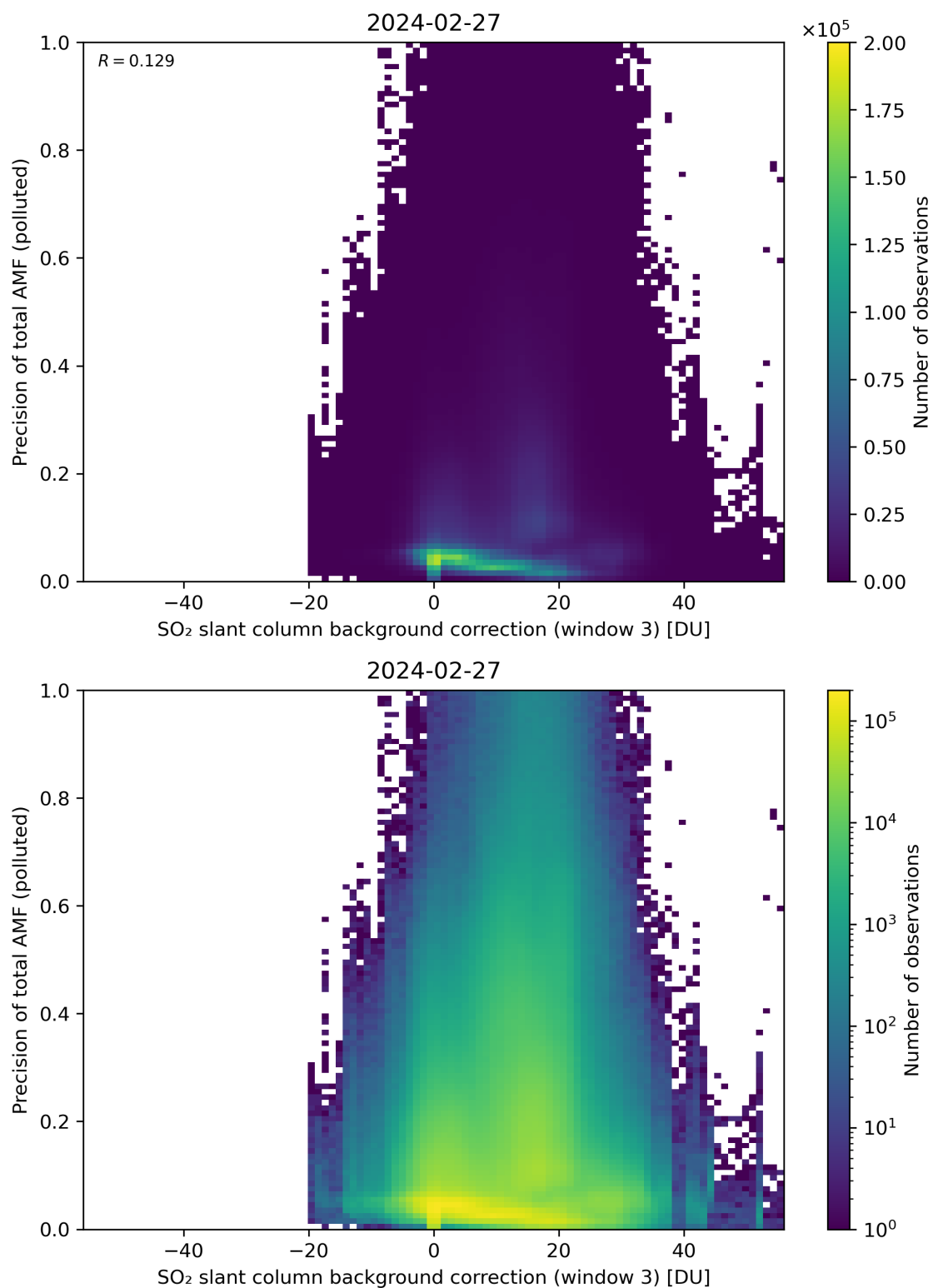
Figure 126: Scatter density plot of “SO 2 slant column background correction (window 3)” against “Precision of total AMF (polluted)” for 2024-02-27 to 2024-02-28.
