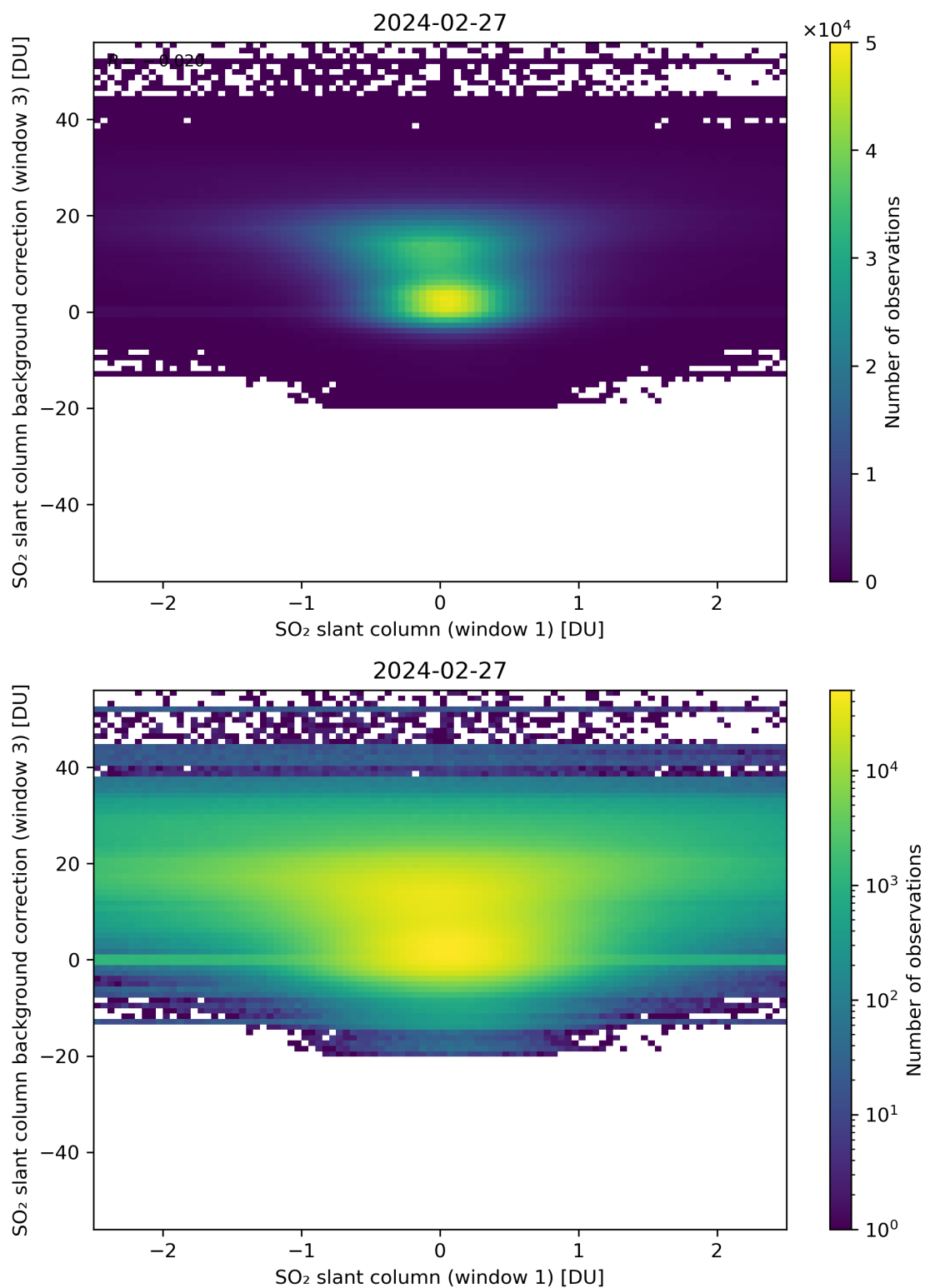
Figure 214: Scatter density plot of “SO 2 slant column (window 1)” against “SO 2 slant column background correction (window 3)” for 2024-02-27 to 2024-02-28.
