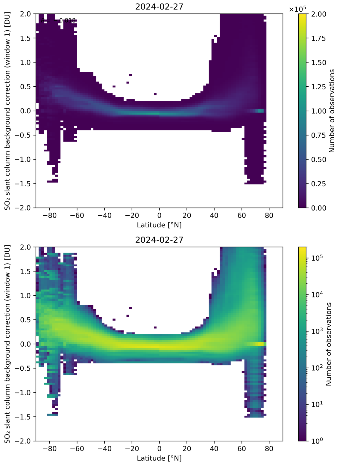
Figure 139: Scatter density plot of “Latitude” against “SO 2 slant column background correction (window 1)” for 2024-02-27 to 2024-02-28.
