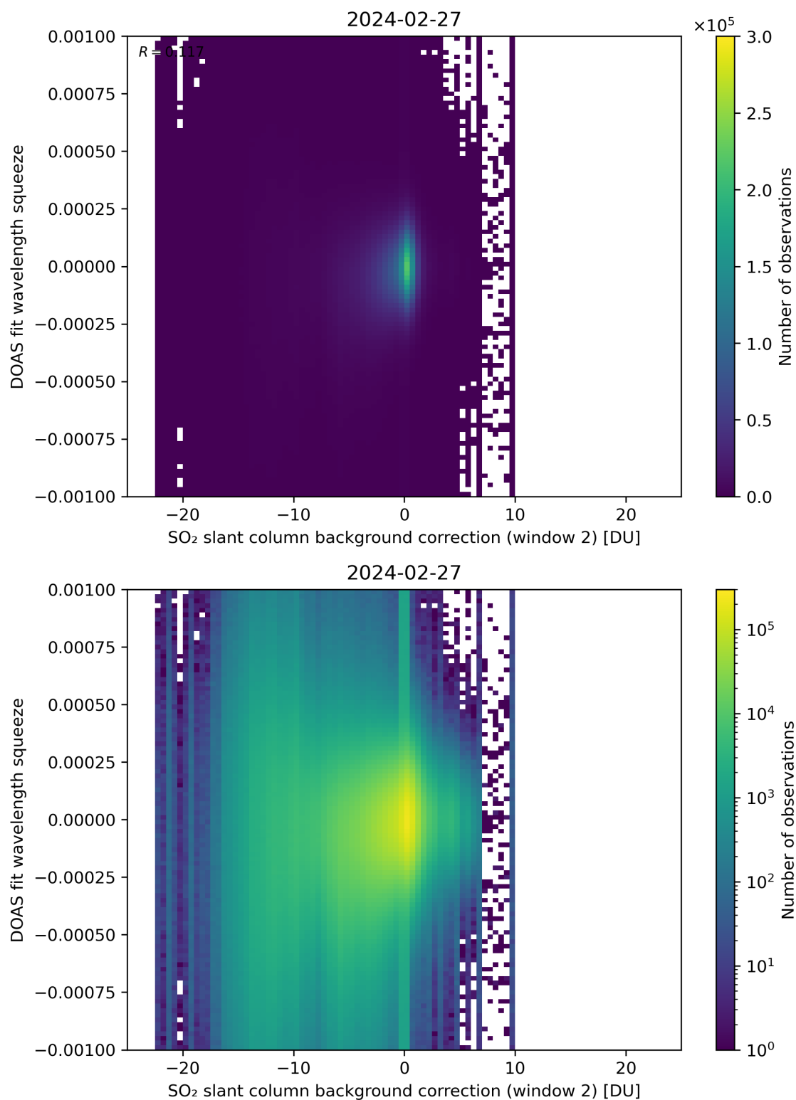
Figure 113: Scatter density plot of “SO 2 slant column background correction (window 2)” against “DOAS fit wavelength squeeze” for 2024-02-27 to 2024-02-28.
