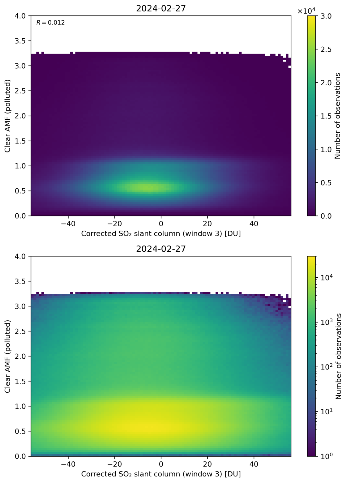
Figure 209: Scatter density plot of “Corrected SO 2 slant column (window 3)” against “Clear AMF (polluted)” for 2024-02-27 to 2024-02-28.
