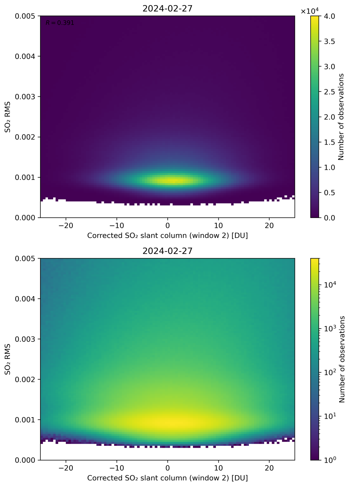
Figure 198: Scatter density plot of “Corrected SO 2 slant column (window 2)” against “SO 2 RMS” for 2024-02-27 to 2024-02-28.
