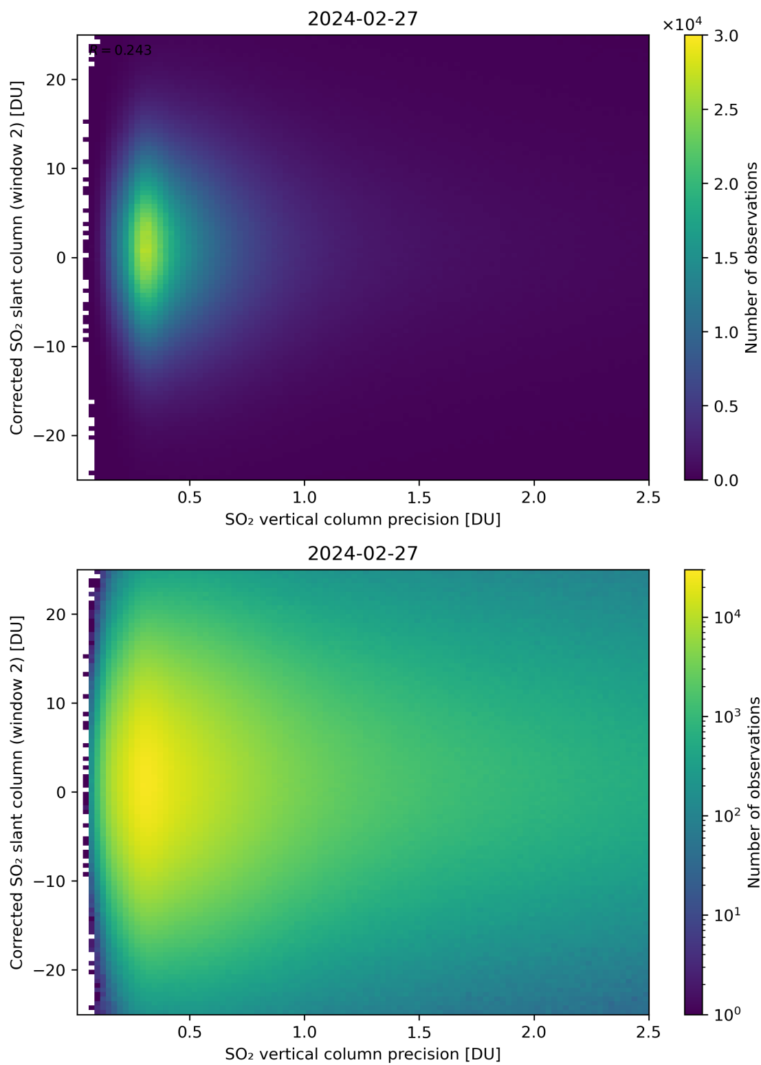
Figure 287: Scatter density plot of “SO 2 vertical column precision” against “Corrected SO 2 slant column (window 2)” for 2024-02-27 to 2024-02-28.
