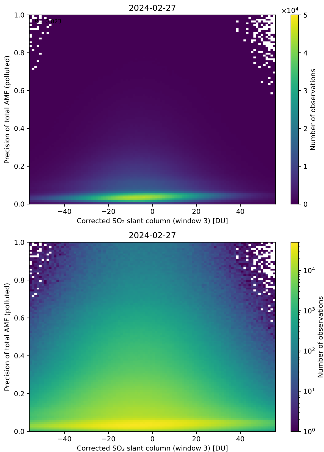
Figure 211: Scatter density plot of “Corrected SO 2 slant column (window 3)” against “Precision of total AMF (polluted)” for 2024-02-27 to 2024-02-28.
