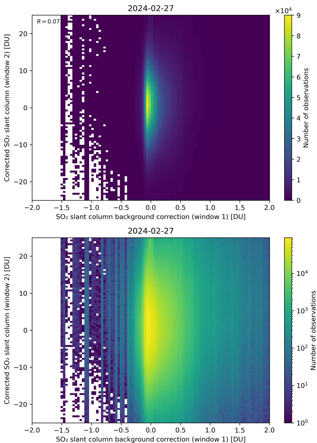
Figure 104: Scatter density plot of “SO 2 slant column background correction (window 1)” against “Corrected SO 2 slant column (window 2)” for 2024-02-27 to 2024-02-28.
