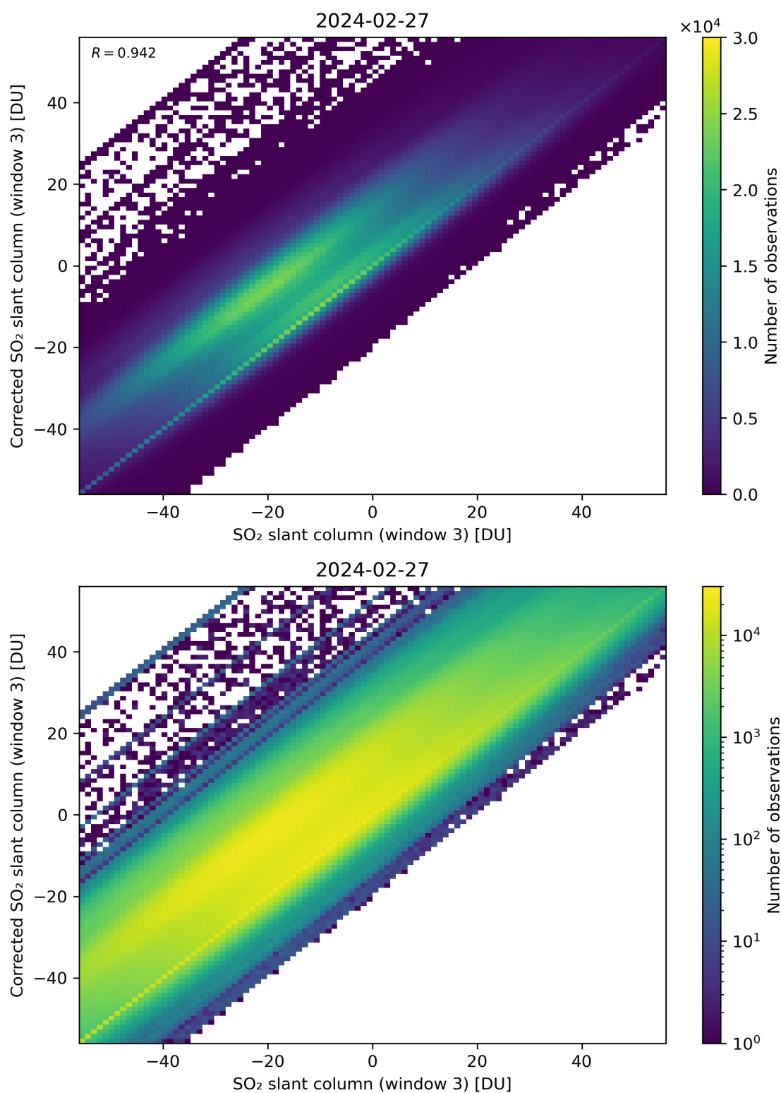
Figure 266: Scatter density plot of “SO 2 slant column (window 3)” against “Corrected SO 2 slant column (window 3)” for 2024-02-27 to 2024-02-28.
