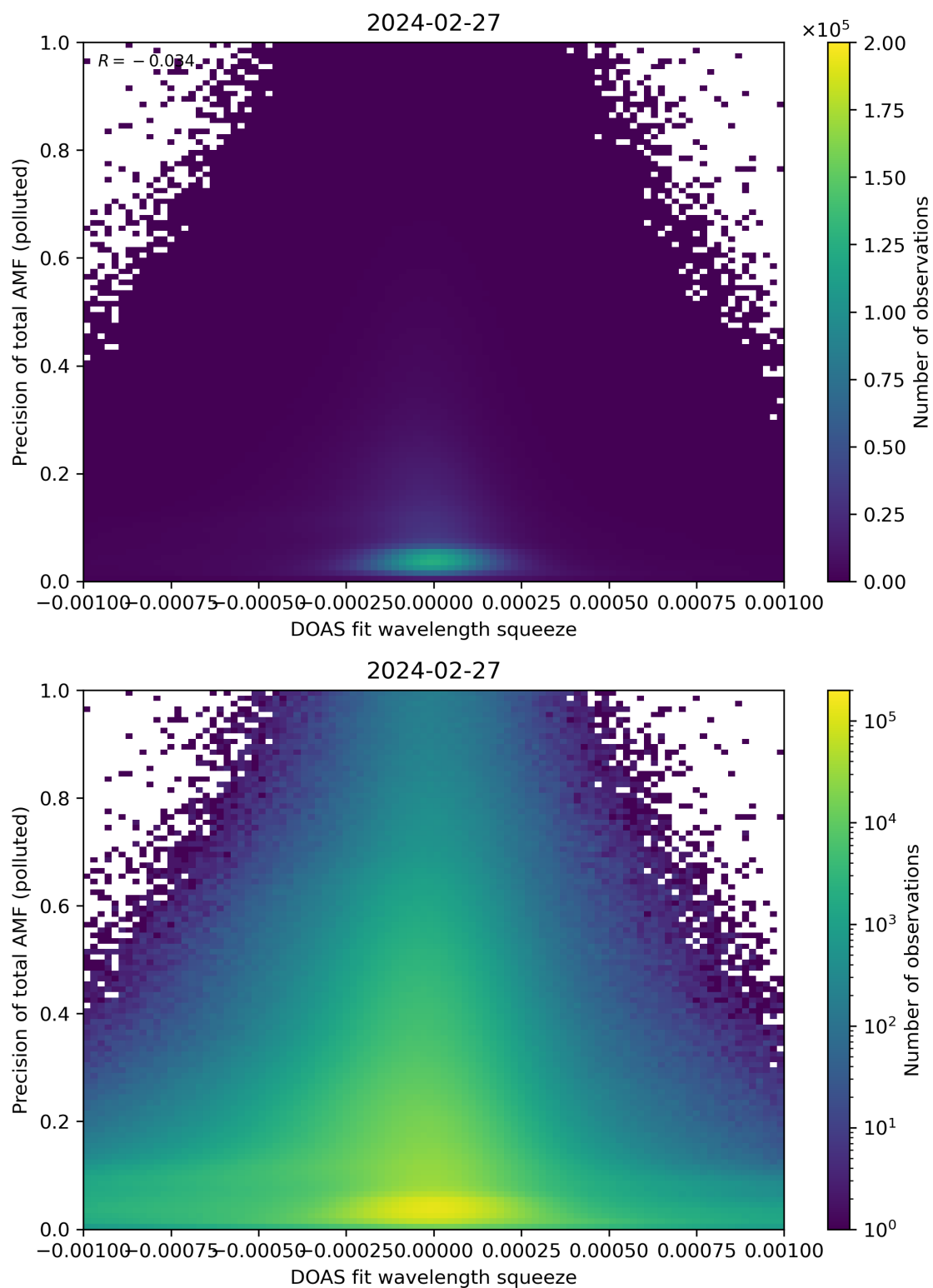
Figure 135: Scatter density plot of “DOAS fit wavelength squeeze” against “Precision of total AMF (polluted)” for 2024-02-27 to 2024-02-28.
