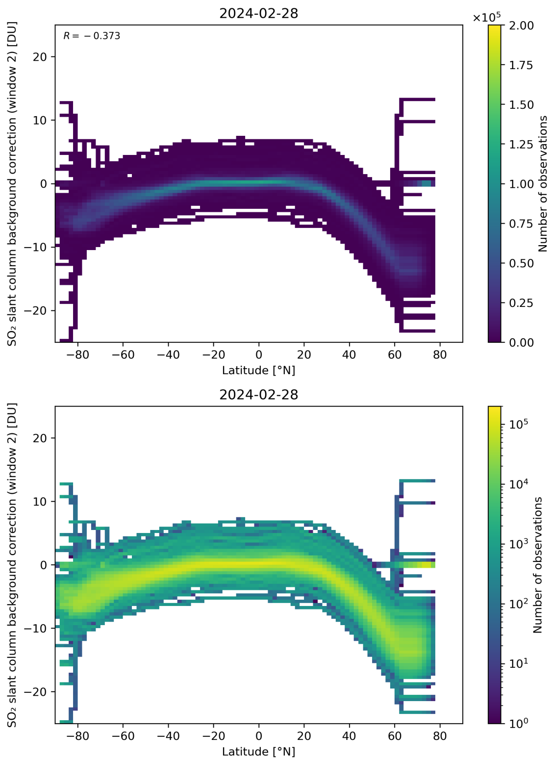
Figure 140: Scatter density plot of “Latitude” against “SO 2 slant column background correction (window 2)” for 2024-02-27 to 2024-02-29.
