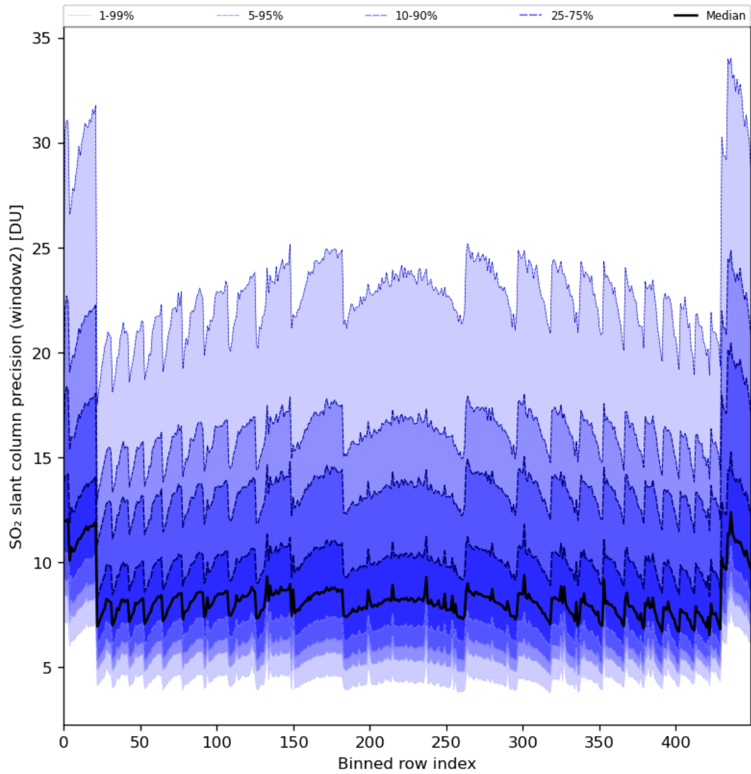
Figure 84: Along track statistics of “SO 2 slant column precision (window2)” for 2024-02-27 to 2024-02-29
