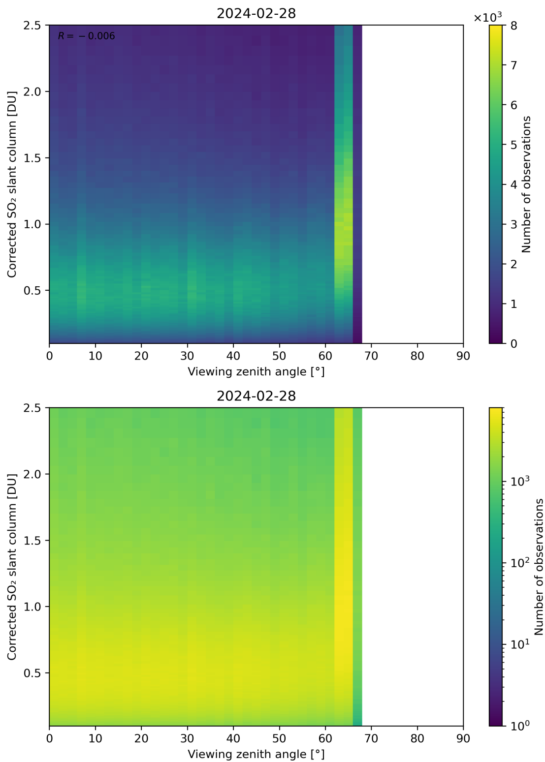
Figure 317: Scatter density plot of “Viewing zenith angle” against “Corrected SO 2 slant column” for 2024-02-27 to 2024-02-29.
