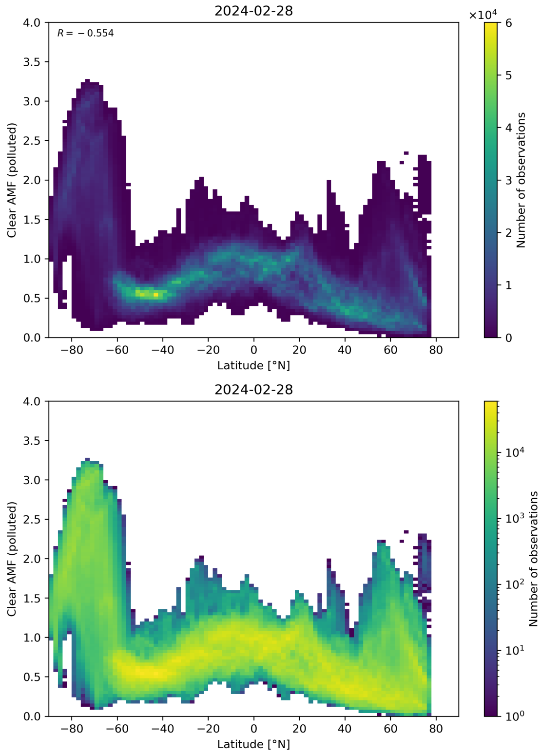
Figure 145: Scatter density plot of “Latitude” against “Clear AMF (polluted)” for 2024-02-27 to 2024-02-29.
