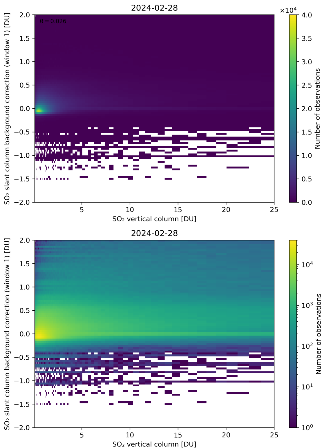
Figure 273: Scatter density plot of “SO 2 vertical column” against “SO 2 slant column background correction (window 1)” for 2024-02-27 to 2024-02-29.
