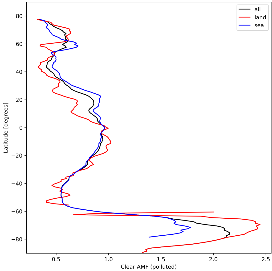
Figure 50: Zonal average of “Clear AMF (polluted)” for 2024-02-27 to 2024-02-29.
