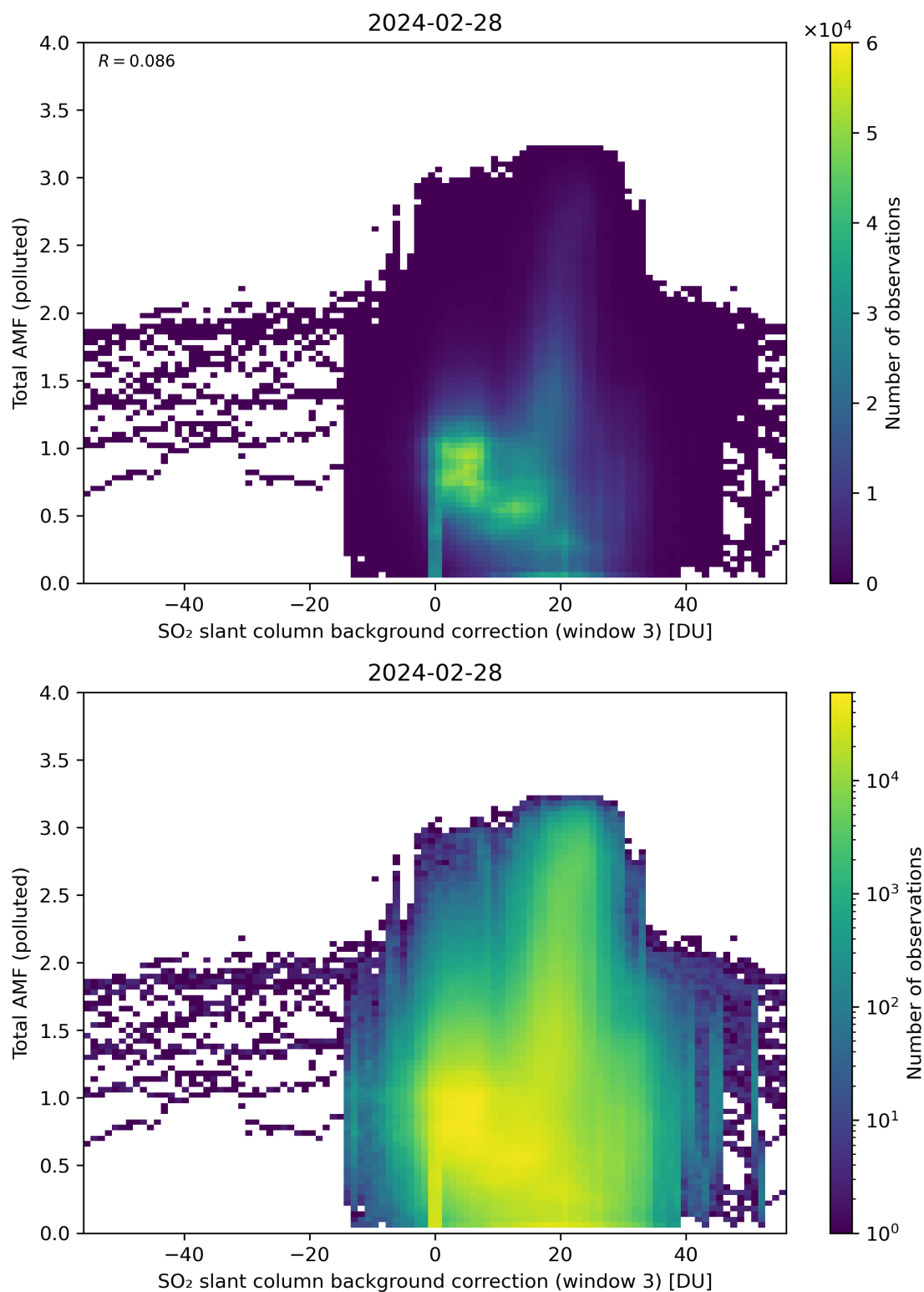
Figure 125: Scatter density plot of “SO 2 slant column background correction (window 3)” against “Total AMF (polluted)” for 2024-02-27 to 2024-02-29.
