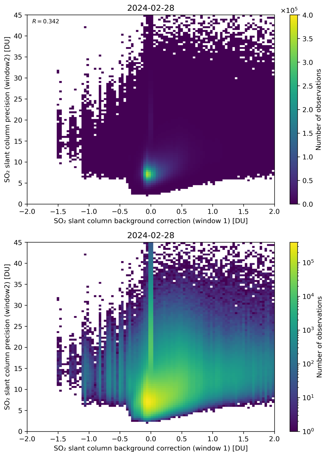
Figure 106: Scatter density plot of “SO 2 slant column background correction (window 1)” against “SO 2 slant column precision (window2)” for 2024-02-27 to 2024-02-29.
