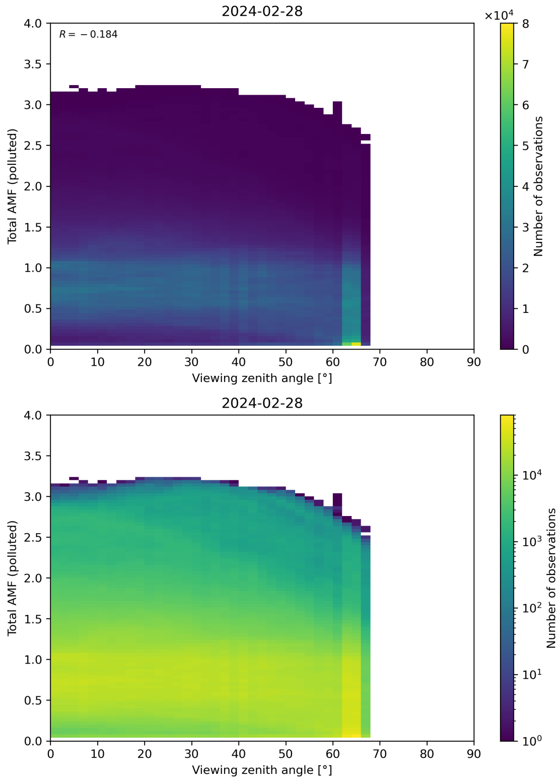
Figure 325: Scatter density plot of “Viewing zenith angle” against “Total AMF (polluted)” for 2024-02-27 to 2024-02-29.
