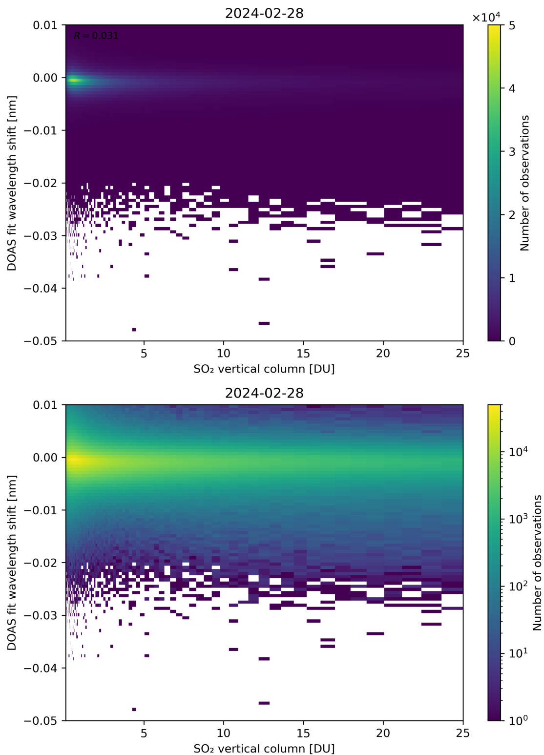
Figure 276: Scatter density plot of “SO 2 vertical column” against “DOAS fit wavelength shift” for 2024-02-27 to 2024-02-29.
