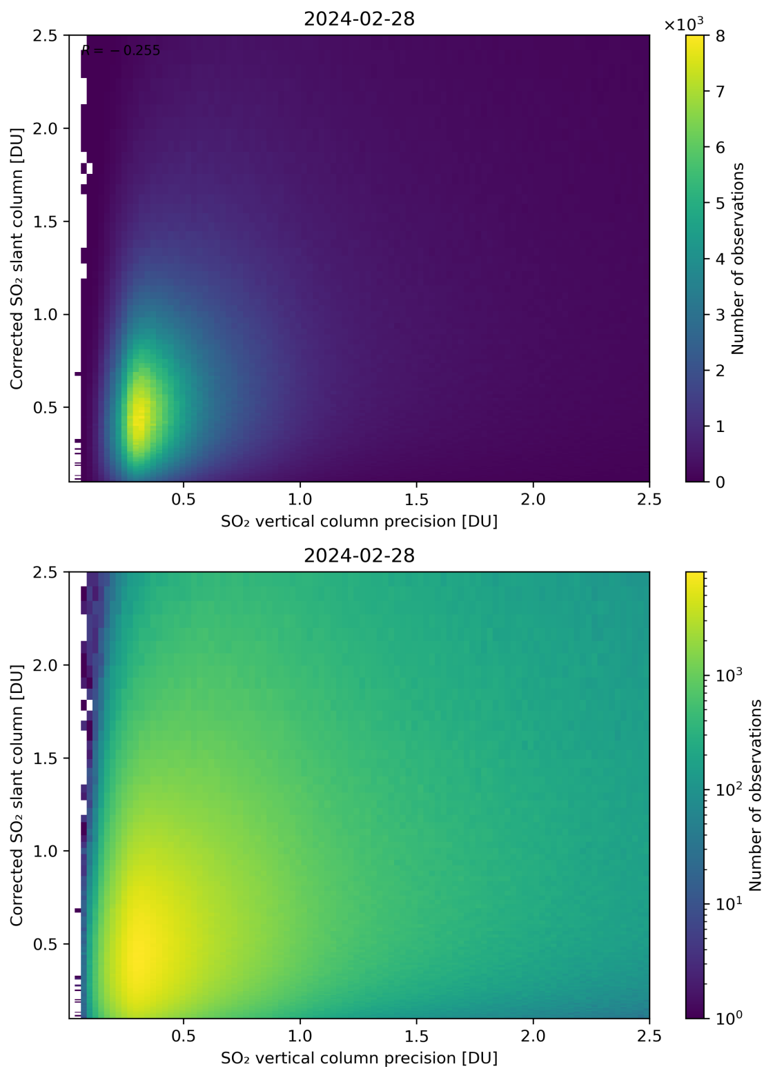
Figure 286: Scatter density plot of “SO 2 vertical column precision” against “Corrected SO 2 slant column” for 2024-02-27 to 2024-02-29.
