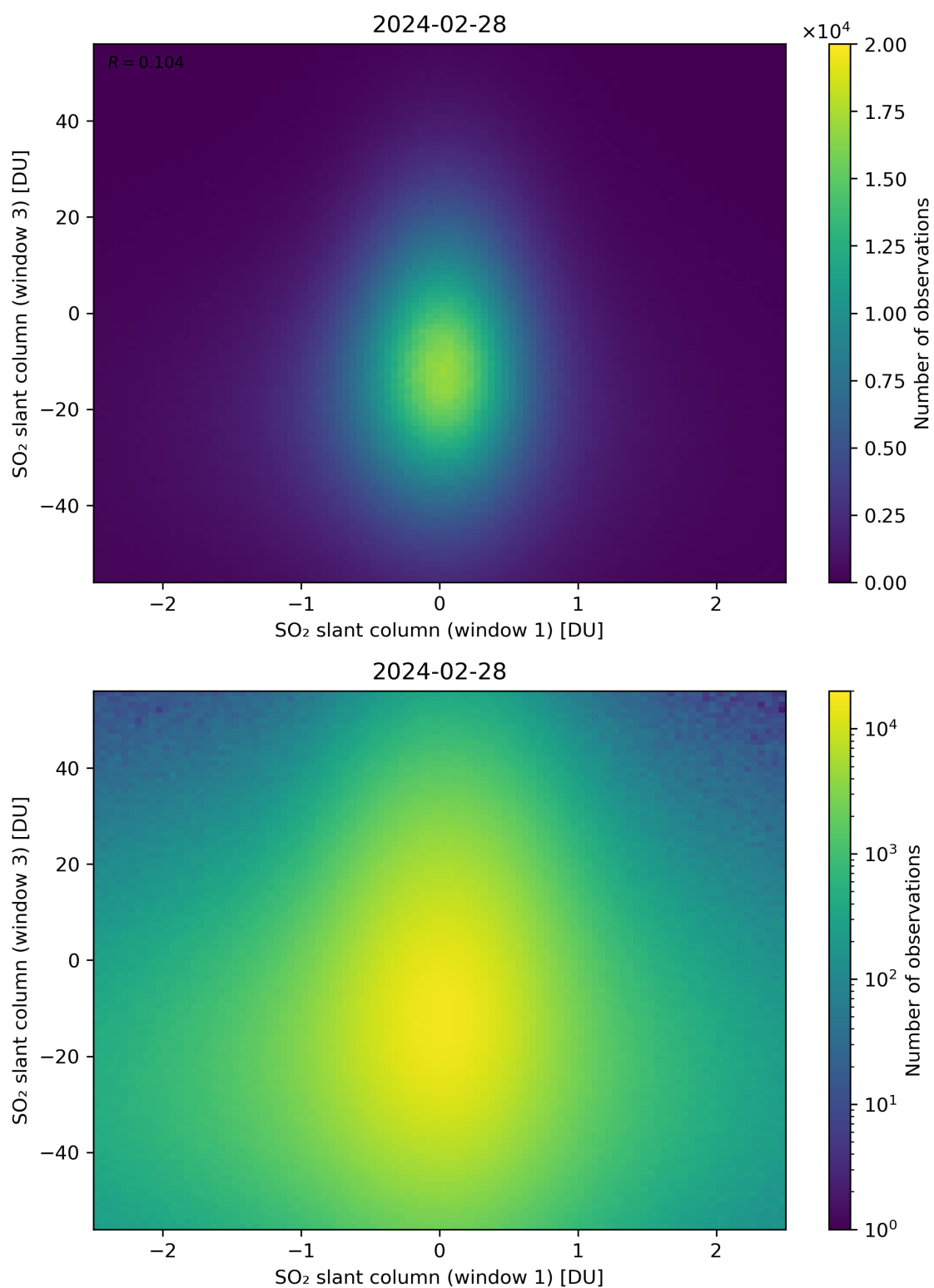
Figure 237: Scatter density plot of “SO 2 slant column (window 1)” against “SO 2 slant column (window 3)” for 2024-02-27 to 2024-02-29.
