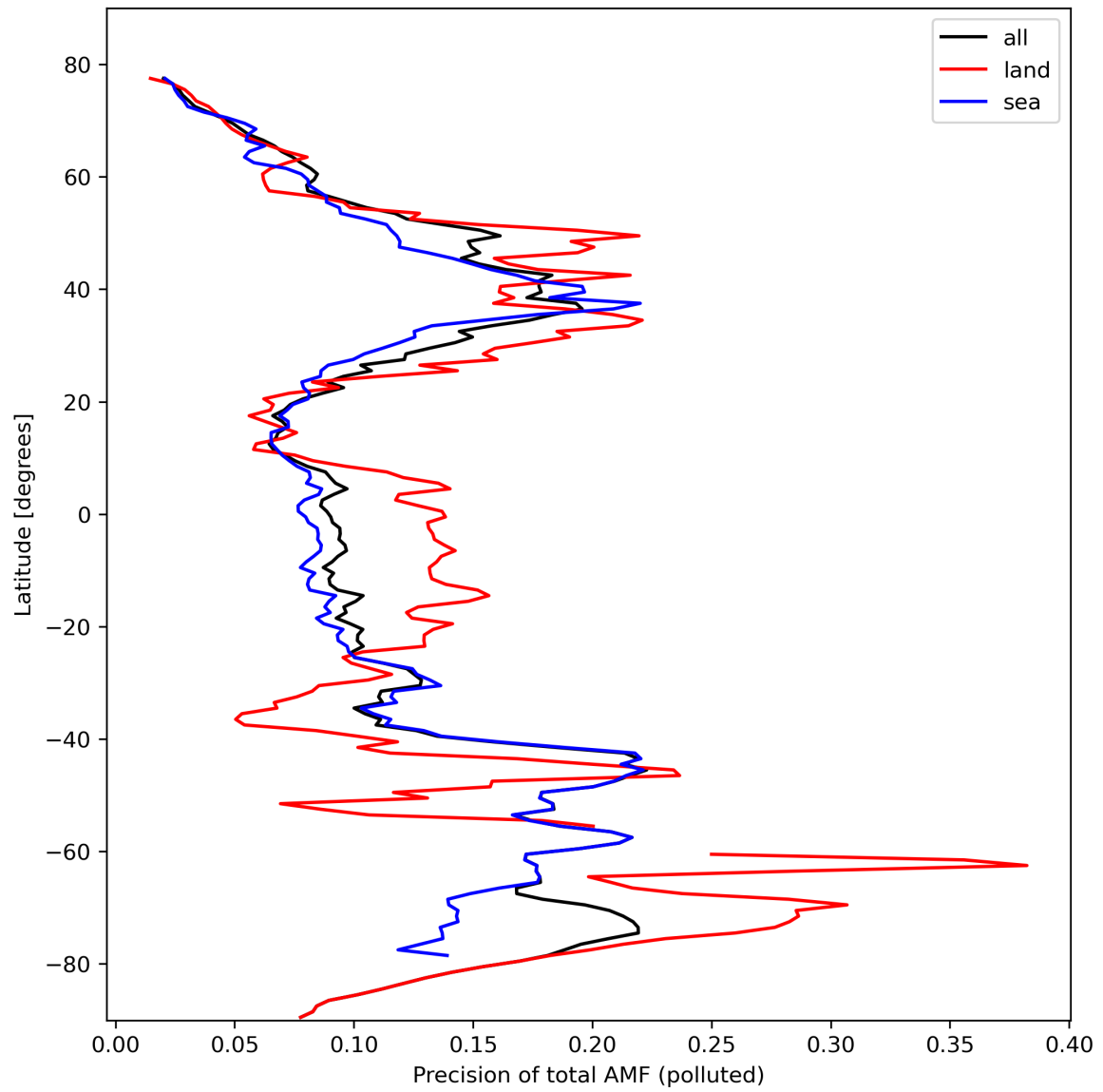
Figure 49: Zonal average of “Precision of total AMF (polluted)” for 2024-02-27 to 2024-02-29.
