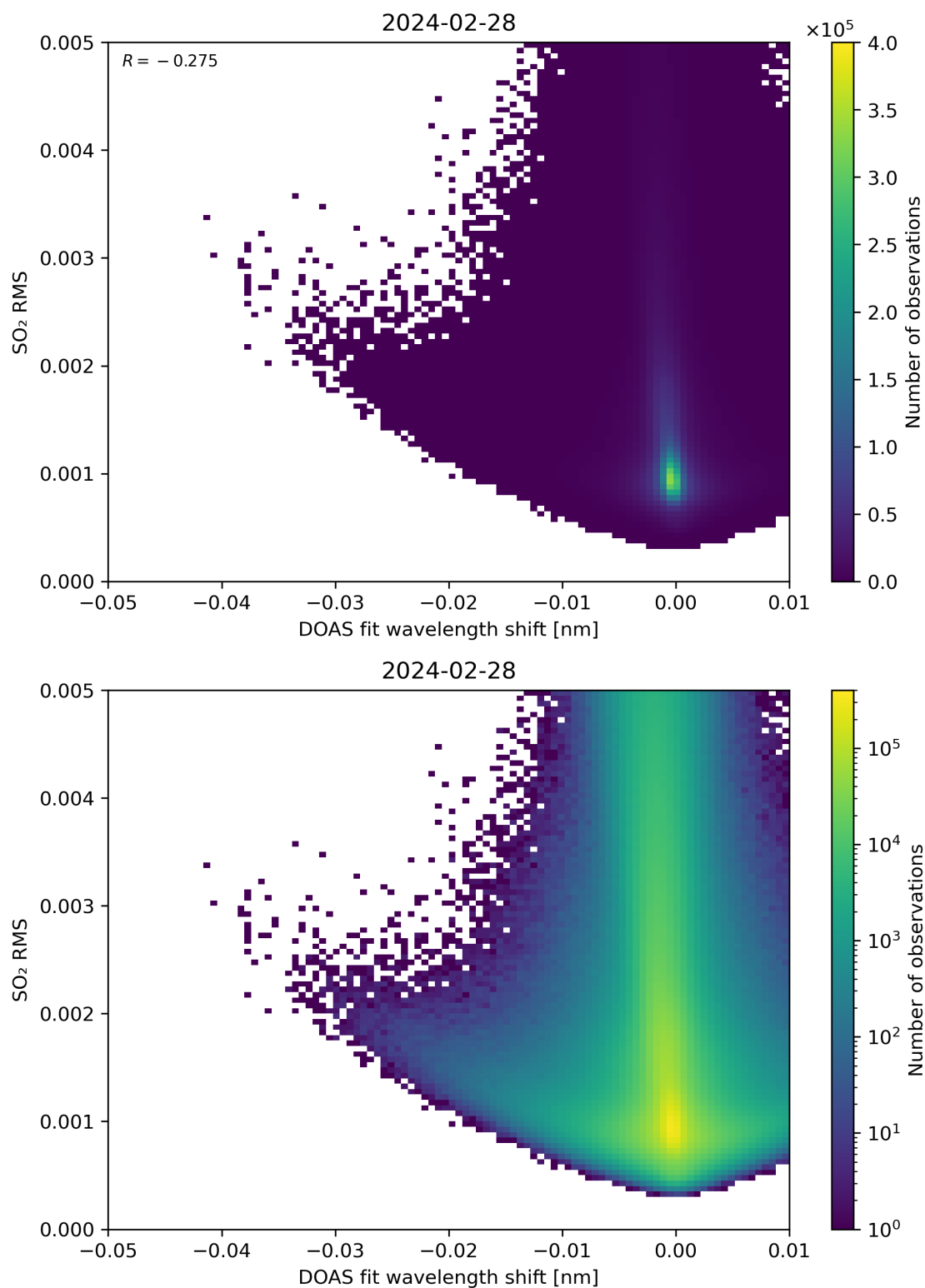
Figure 128: Scatter density plot of “DOAS fit wavelength shift” against “SO 2 RMS” for 2024-02-27 to 2024-02-29.
