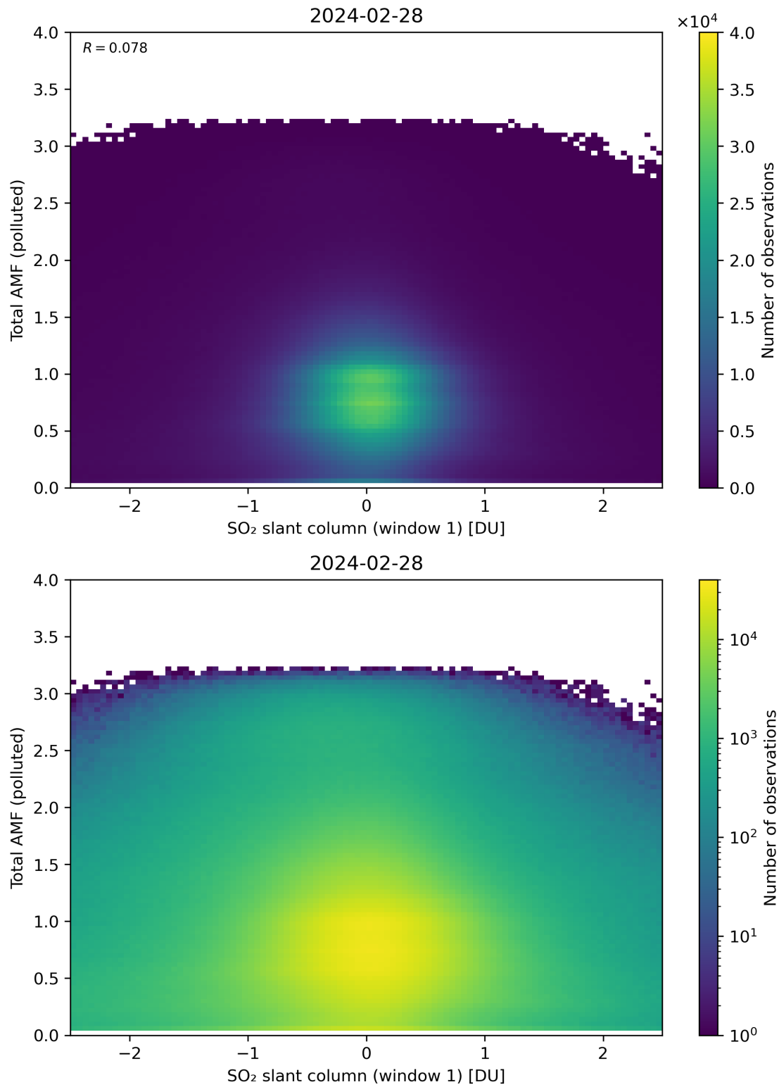
Figure 239: Scatter density plot of “SO 2 slant column (window 1)” against “Total AMF (polluted)” for 2024-02-27 to 2024-02-29.
