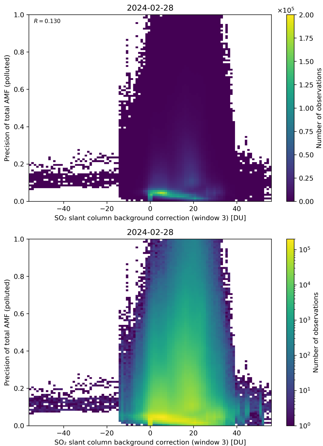
Figure 126: Scatter density plot of “SO 2 slant column background correction (window 3)” against “Precision of total AMF (polluted)” for 2024-02-27 to 2024-02-29.
