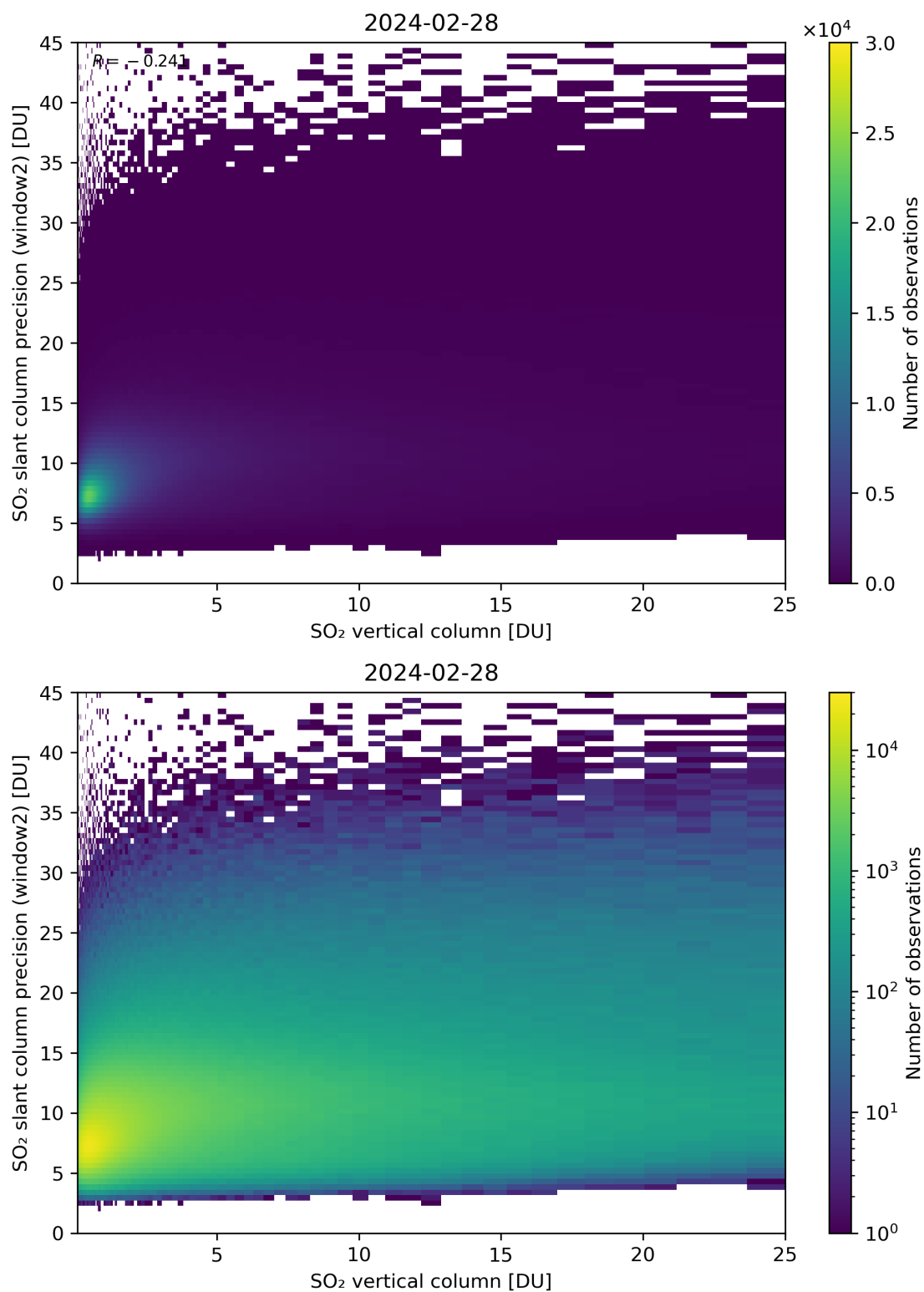
Figure 302: Scatter density plot of “SO 2 vertical column” against “SO 2 slant column precision (window2)” for 2024-02-27 to 2024-02-29.
