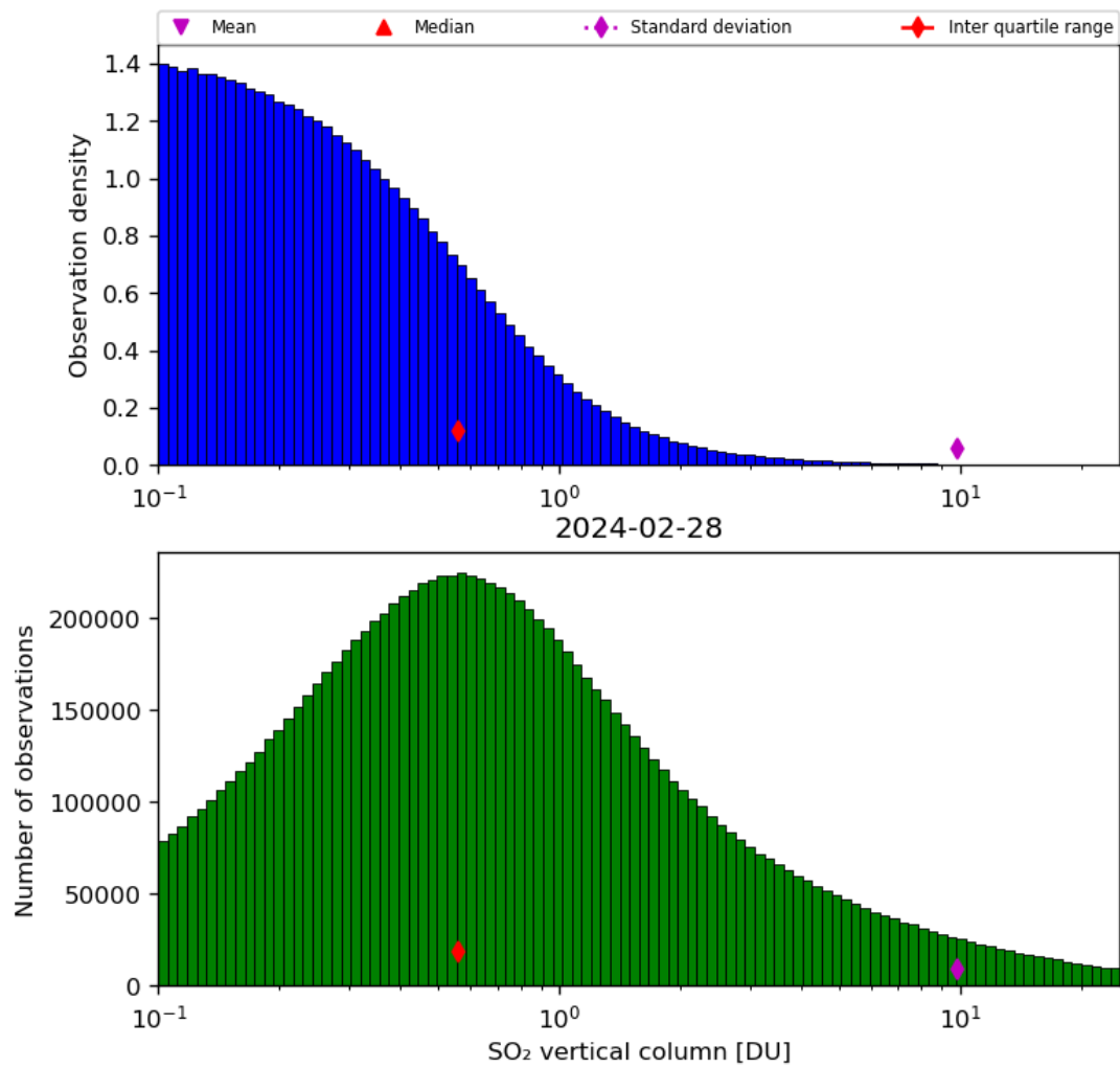
Figure 53: Histogram of “SO 2 vertical column” for 2024-02-27 to 2024-02-29
