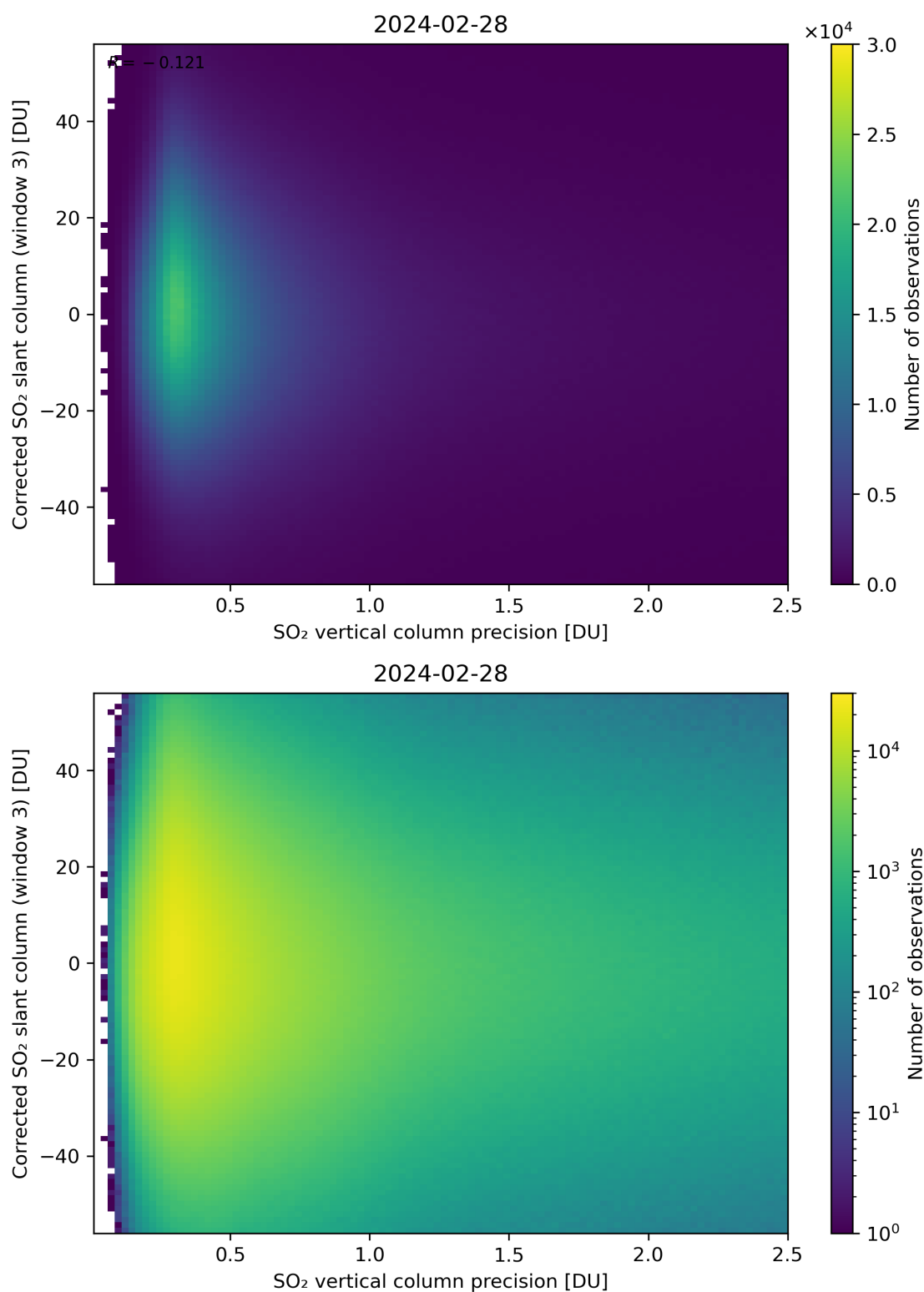
Figure 288: Scatter density plot of “SO 2 vertical column precision” against “Corrected SO 2 slant column (window 3)” for 2024-02-27 to 2024-02-29.
