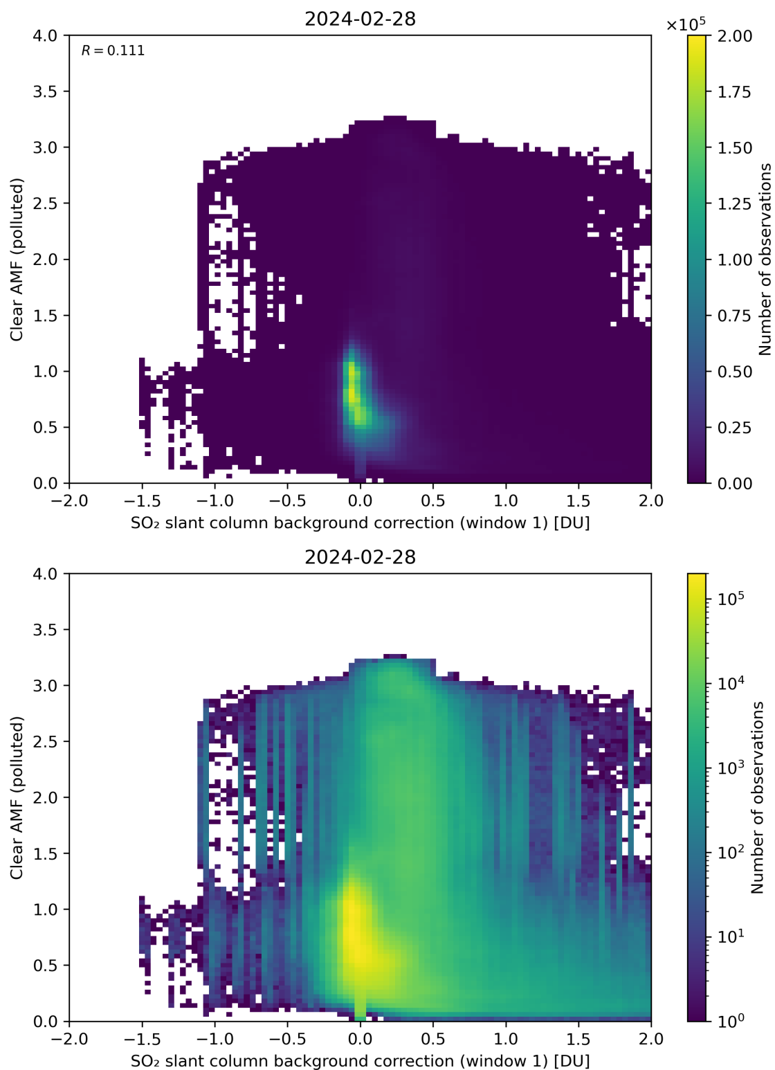
Figure 103: Scatter density plot of “SO 2 slant column background correction (window 1)” against “Clear AMF (polluted)” for 2024-02-27 to 2024-02-29.
