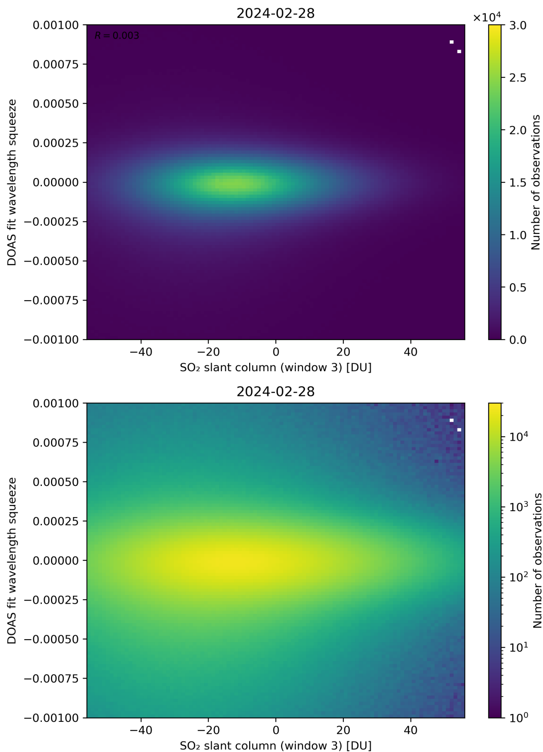
Figure 255: Scatter density plot of “SO 2 slant column (window 3)” against “DOAS fit wavelength squeeze” for 2024-02-27 to 2024-02-29.
