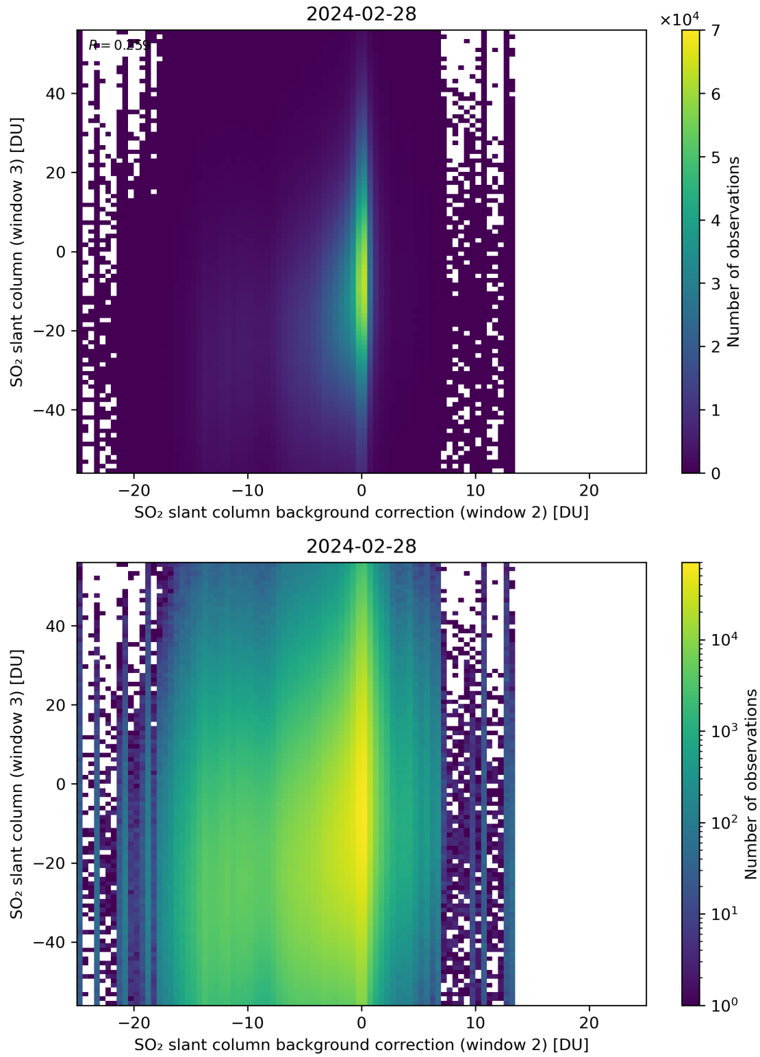
Figure 117: Scatter density plot of “SO 2 slant column background correction (window 2)” against “SO 2 slant column (window 3)” for 2024-02-27 to 2024-02-29.
