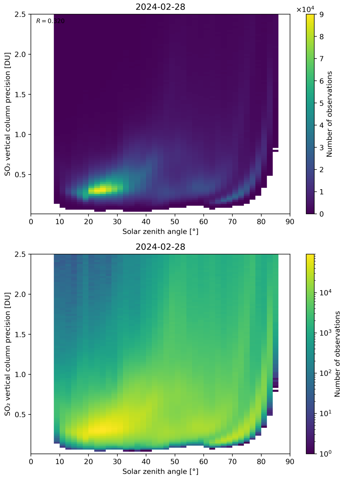
Figure 177: Scatter density plot of “Solar zenith angle” against “SO 2 vertical column precision” for 2024-02-27 to 2024-02-29.
