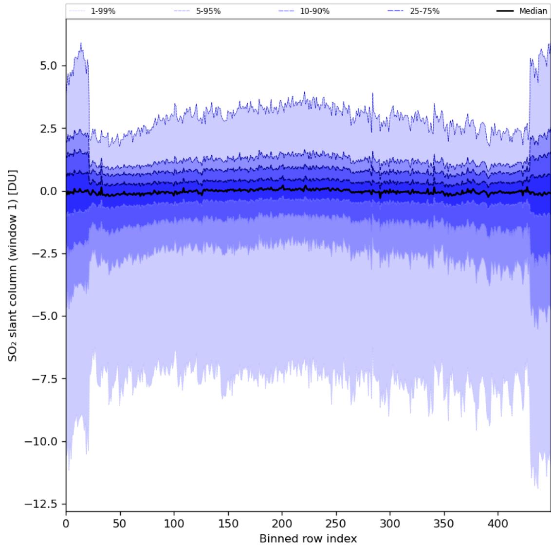
Figure 79: Along track statistics of “SO 2 slant column (window 1)” for 2024-02-27 to 2024-02-29
