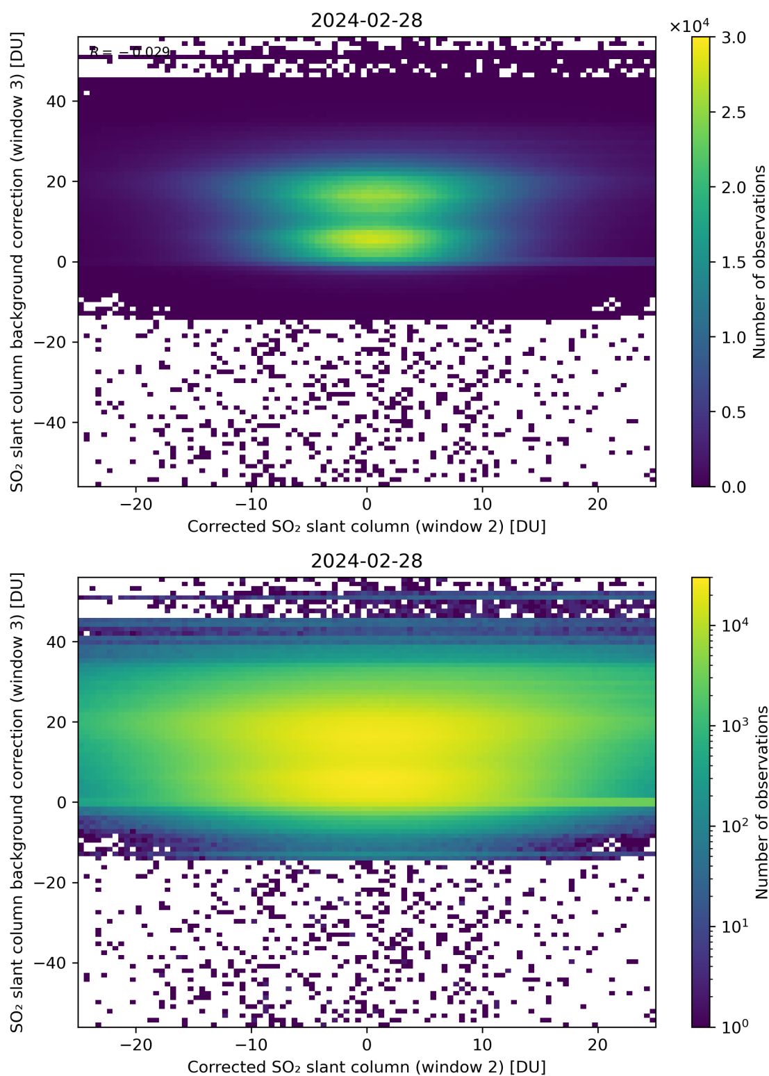
Figure 195: Scatter density plot of “Corrected SO 2 slant column (window 2)” against “SO 2 slant column background correction (window 3)” for 2024-02-27 to 2024-02-29.
