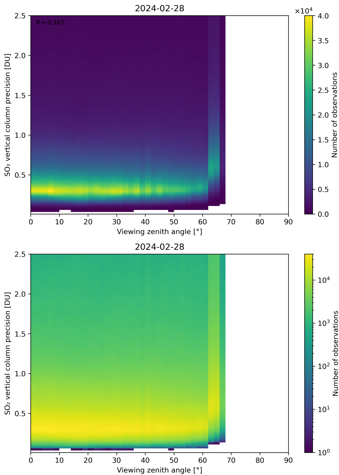
Figure 328: Scatter density plot of “Viewing zenith angle” against “SO 2 vertical column precision” for 2024-02-27 to 2024-02-29.
