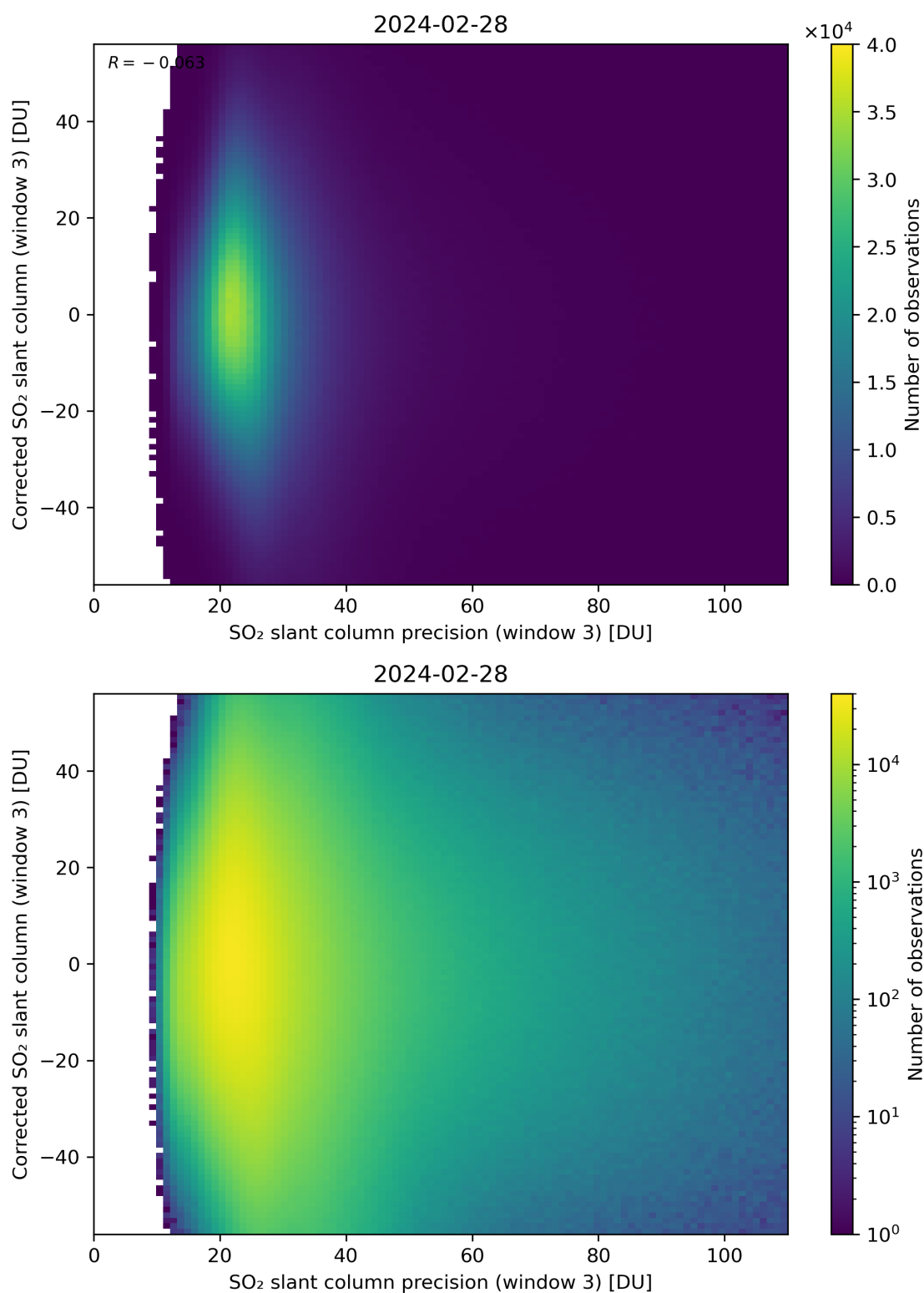
Figure 262: Scatter density plot of “SO 2 slant column precision (window 3)” against “Corrected SO 2 slant column (window 3)” for 2024-02-27 to 2024-02-29.
