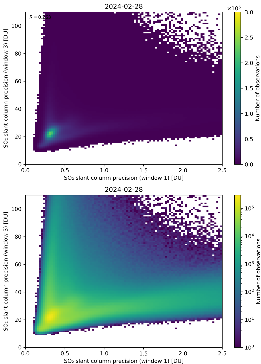
Figure 229: Scatter density plot of “SO 2 slant column precision (window 1)” against “SO 2 slant column precision (window 3)” for 2024-02-27 to 2024-02-29.
