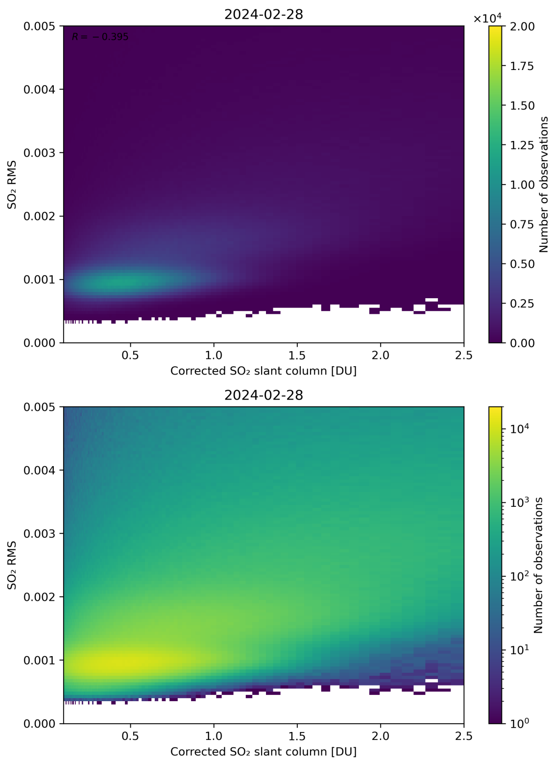
Figure 183: Scatter density plot of “Corrected SO 2 slant column” against “SO 2 RMS” for 2024-02-27 to 2024-02-29.
