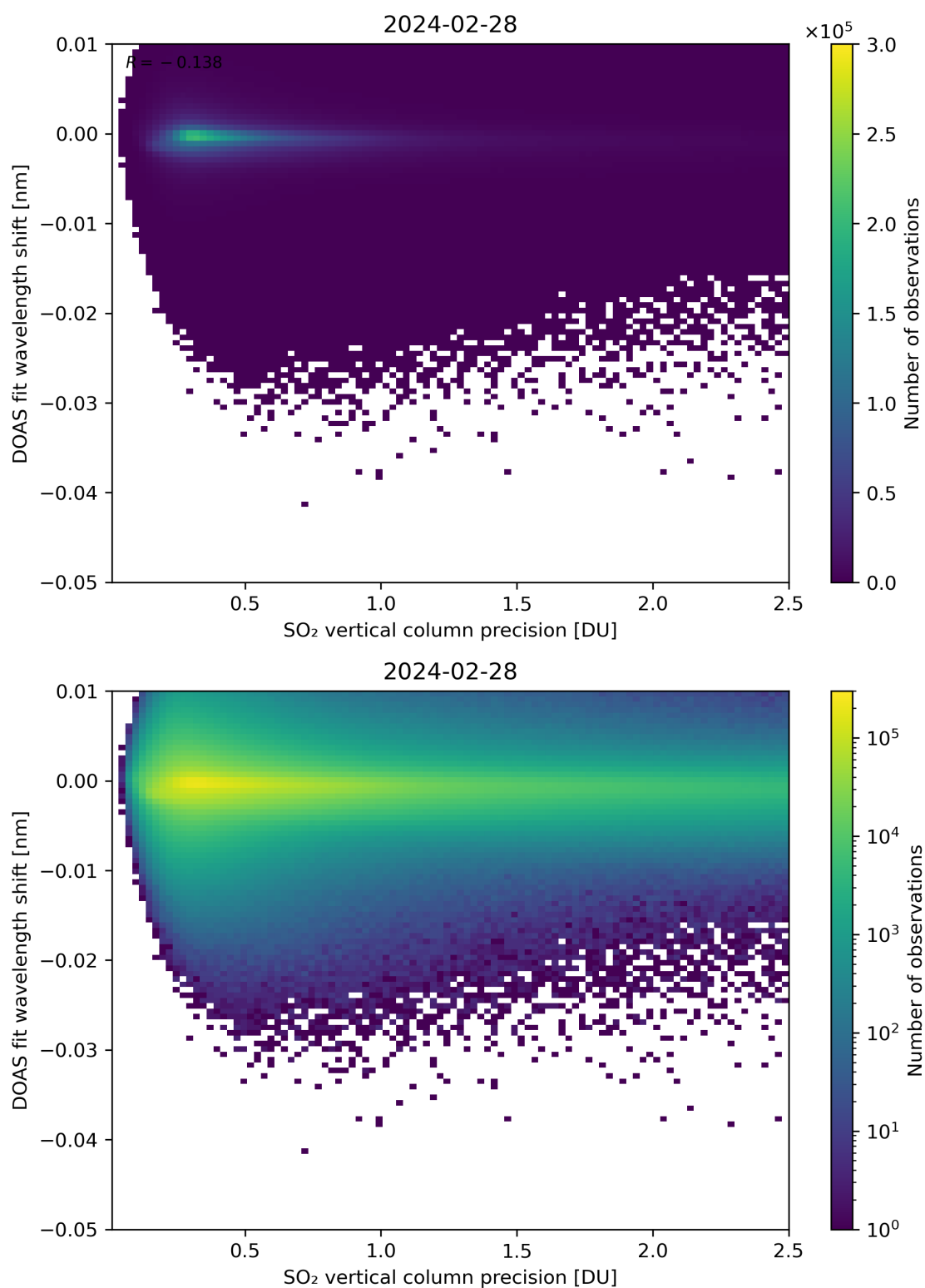
Figure 282: Scatter density plot of “SO 2 vertical column precision” against “DOAS fit wavelength shift” for 2024-02-27 to 2024-02-29.
