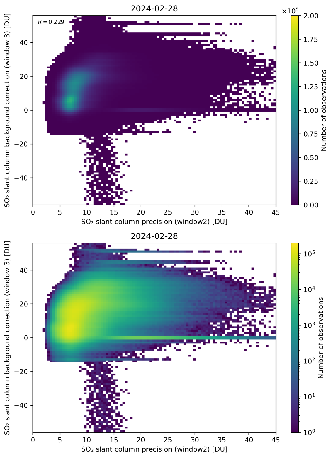
Figure 242: Scatter density plot of “SO 2 slant column precision (window2)” against “SO 2 slant column background correction (window 3)” for 2024-02-27 to 2024-02-29.
