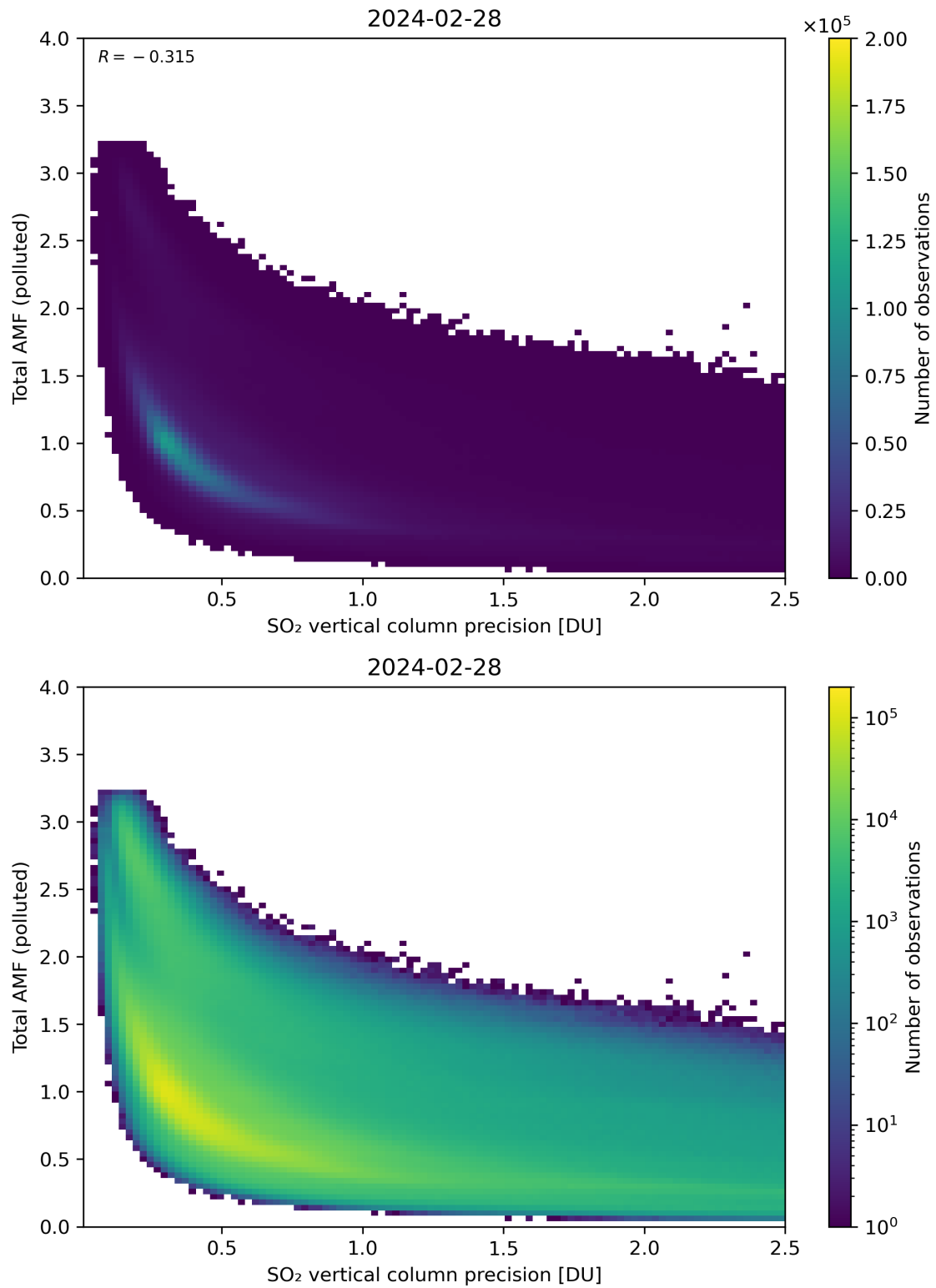
Figure 294: Scatter density plot of “SO 2 vertical column precision” against “Total AMF (polluted)” for 2024-02-27 to 2024-02-29.
