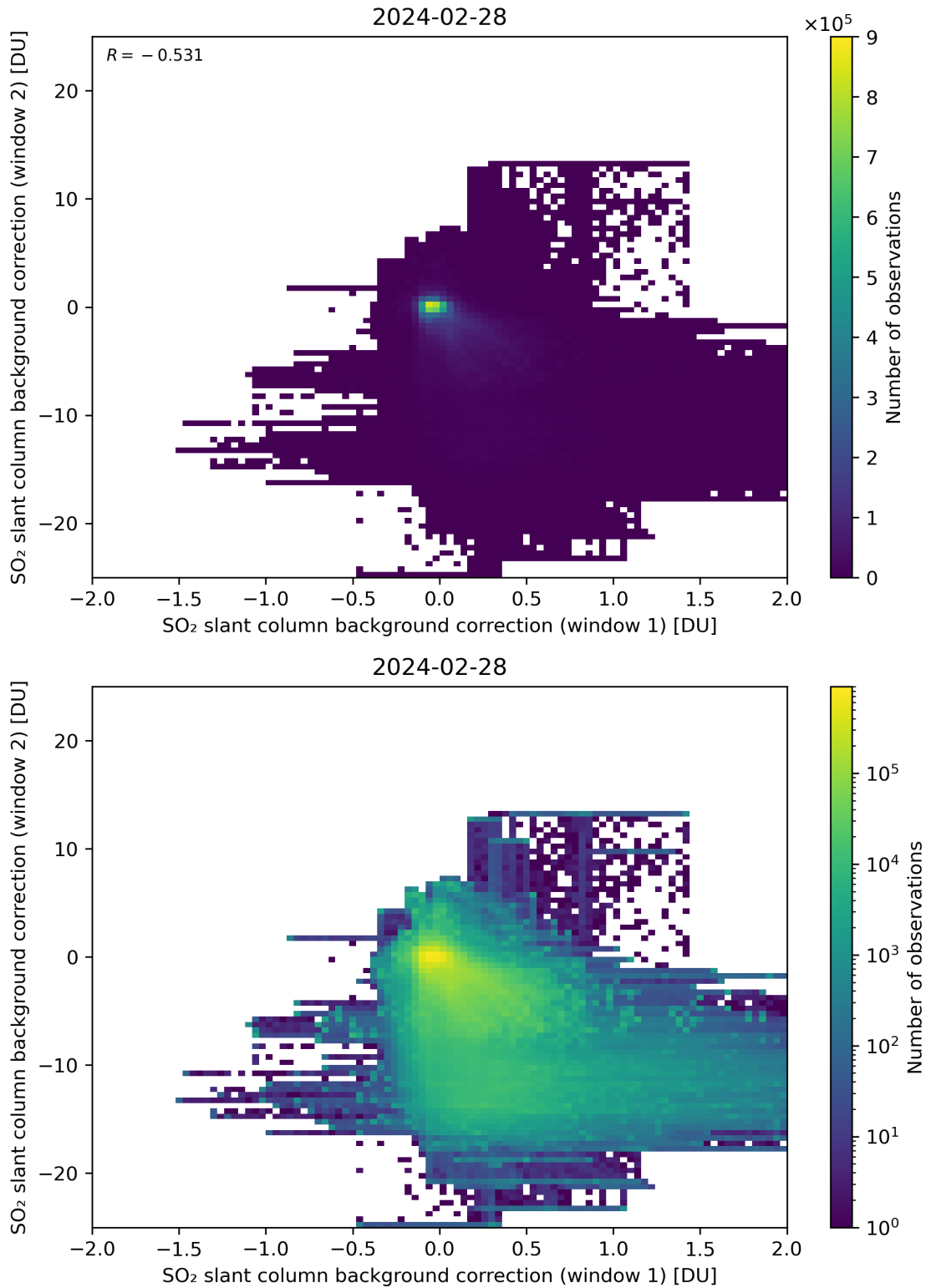
Figure 98: Scatter density plot of “SO 2 slant column background correction (window 1)” against “SO 2 slant column background correction (window 2)” for 2024-02-27 to 2024-02-29.
