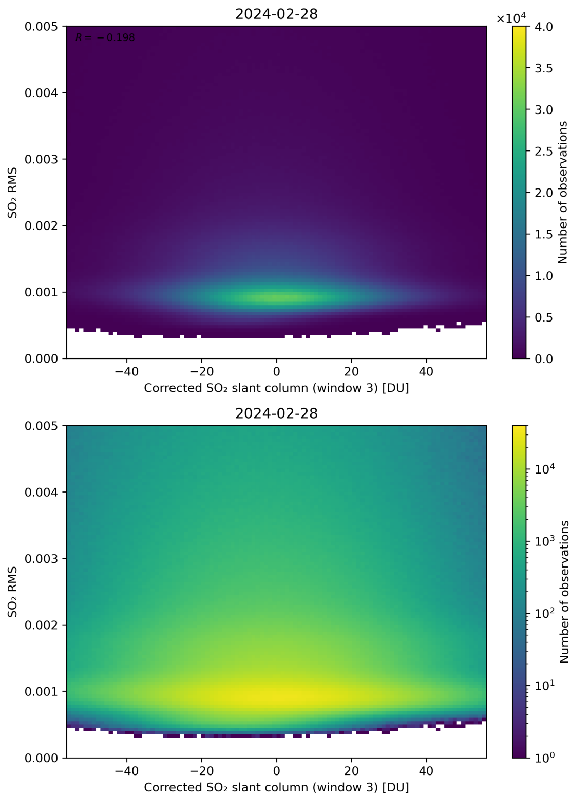
Figure 208: Scatter density plot of “Corrected SO 2 slant column (window 3)” against “SO 2 RMS” for 2024-02-27 to 2024-02-29.
