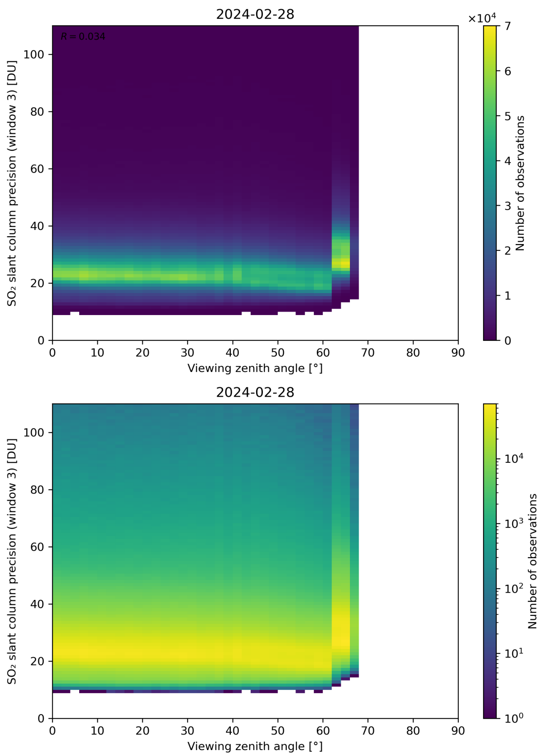
Figure 324: Scatter density plot of “Viewing zenith angle” against “SO 2 slant column precision (window 3)” for 2024-02-27 to 2024-02-29.
