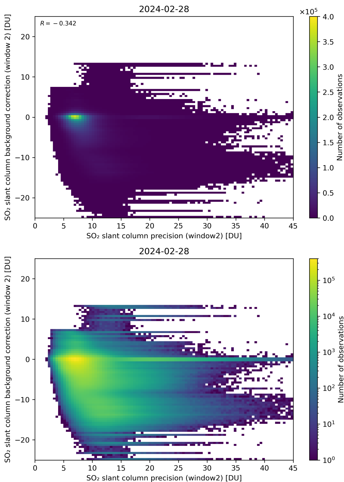
Figure 241: Scatter density plot of “SO 2 slant column precision (window2)” against “SO 2 slant column background correction (window 2)” for 2024-02-27 to 2024-02-29.
