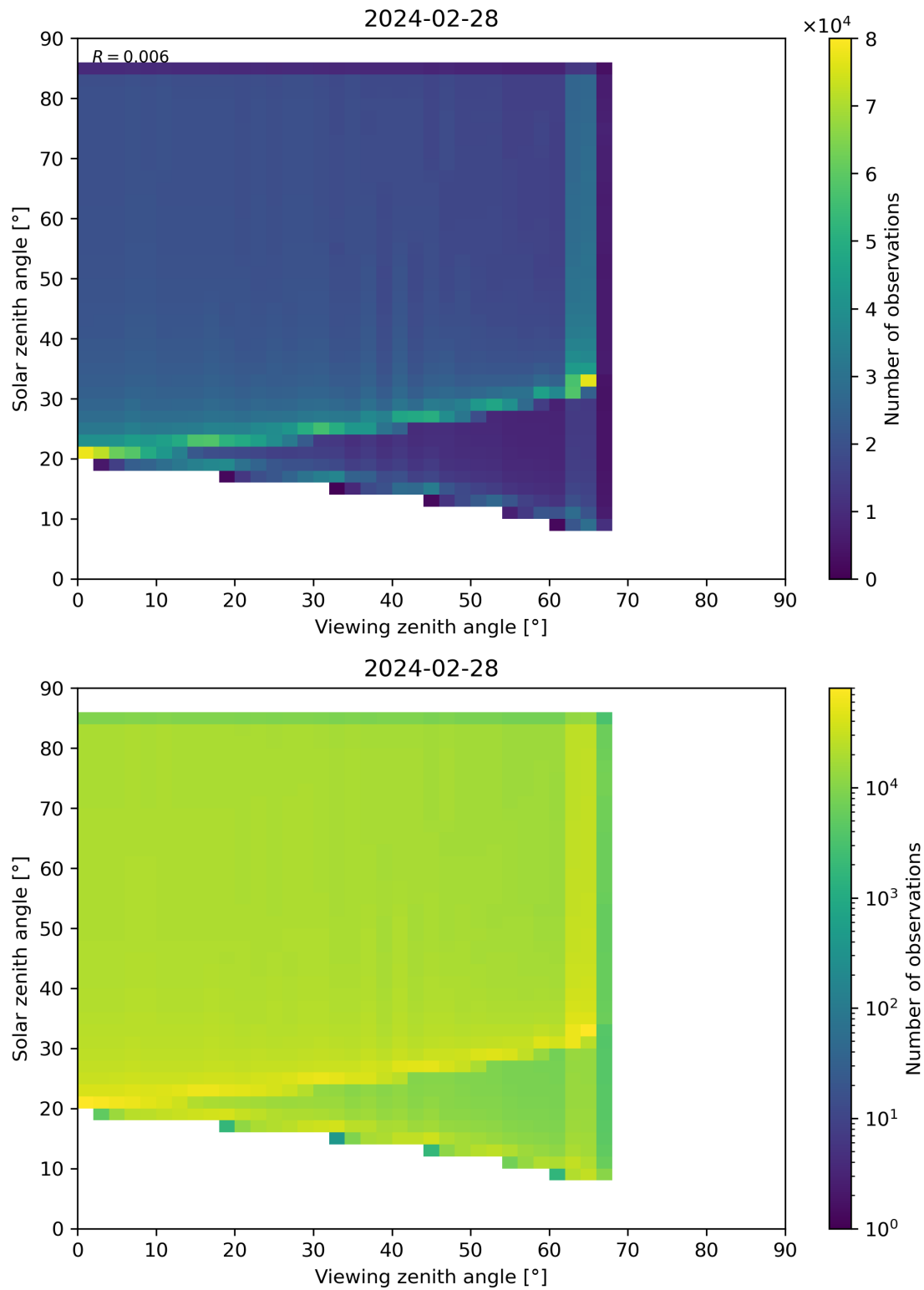
Figure 315: Scatter density plot of “Viewing zenith angle” against “Solar zenith angle” for 2024-02-27 to 2024-02-29.
