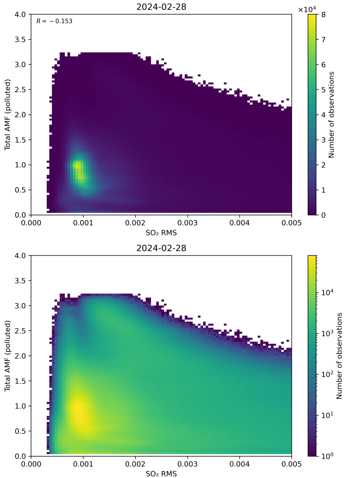
Figure 137: Scatter density plot of “SO 2 RMS” against “Total AMF (polluted)” for 2024-02-27 to 2024-02-29.
