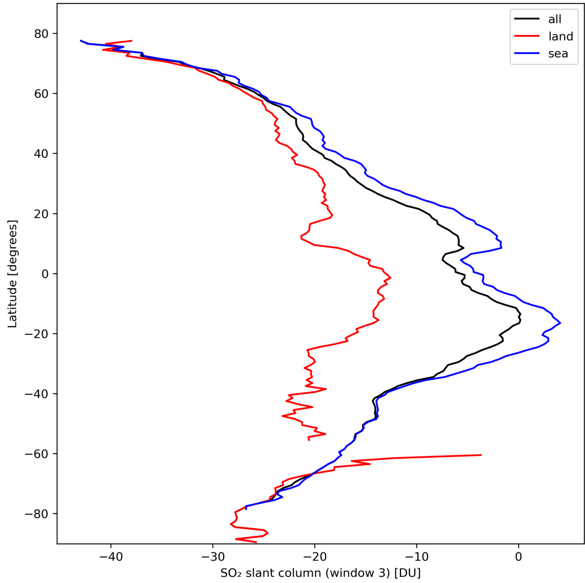
Figure 41: Zonal average of “SO 2 slant column (window 3)” for 2024-02-27 to 2024-02-29.
