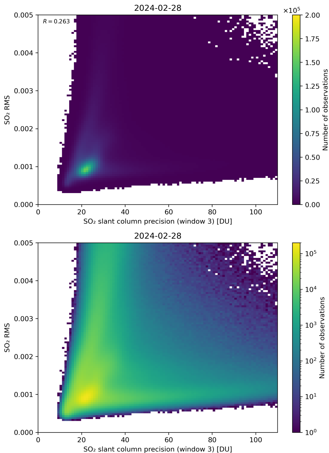
Figure 260: Scatter density plot of “SO 2 slant column precision (window 3)” against “SO 2 RMS” for 2024-02-27 to 2024-02-29.
