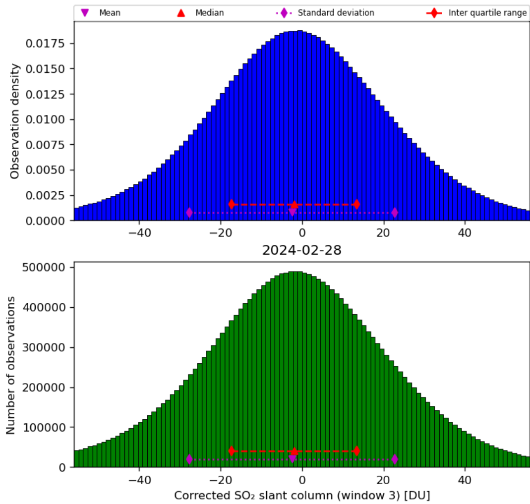
Figure 66: Histogram of “Corrected SO 2 slant column (window 3)” for 2024-02-27 to 2024-02-29
