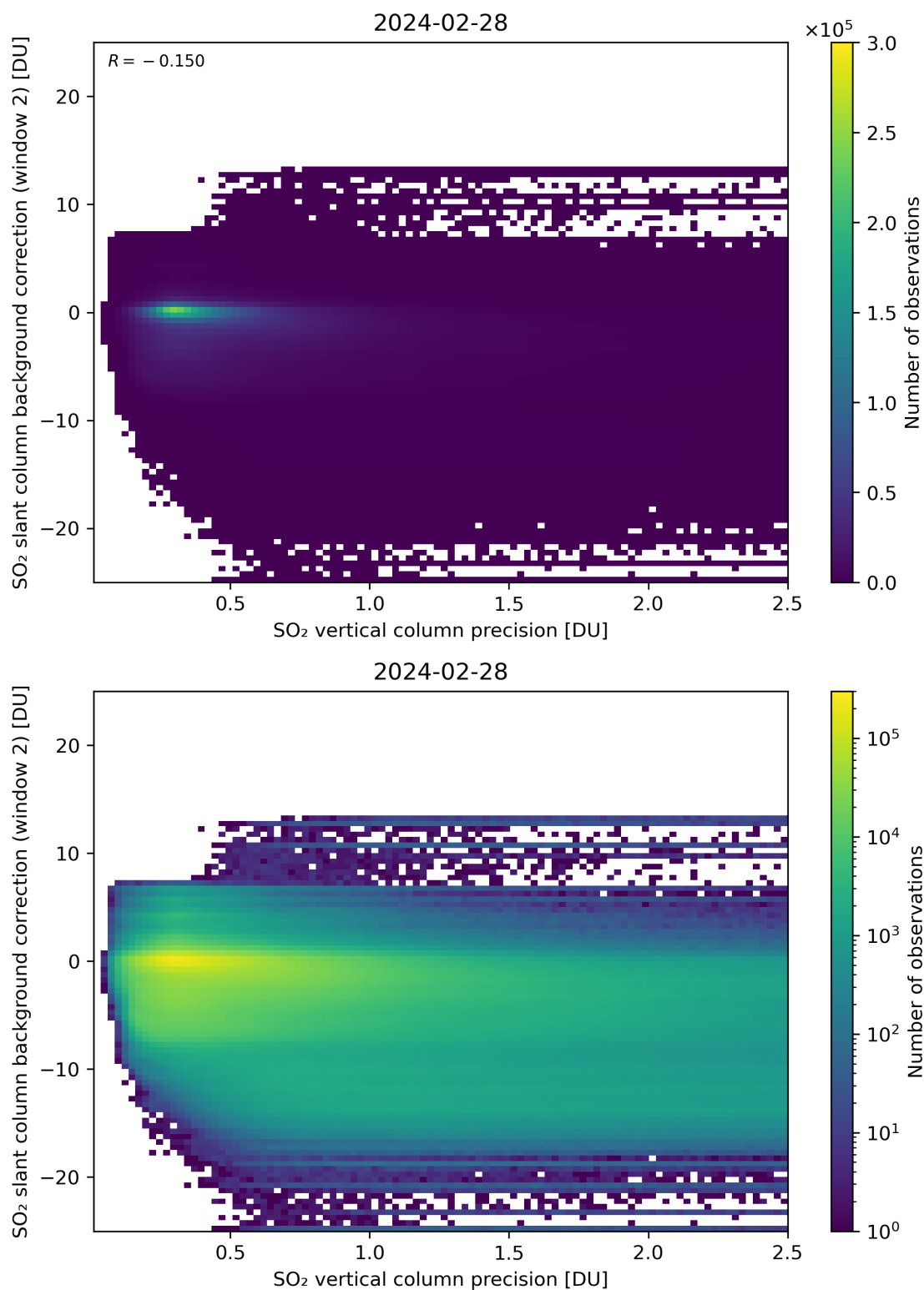
Figure 280: Scatter density plot of “SO 2 vertical column precision” against “SO 2 slant column background correction (window 2)” for 2024-02-27 to 2024-02-29.
