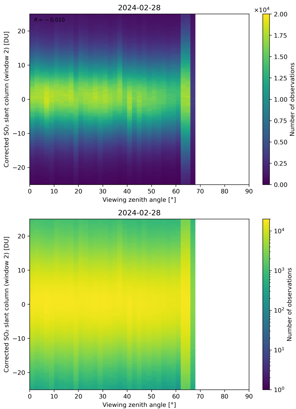
Figure 318: Scatter density plot of “Viewing zenith angle” against “Corrected SO 2 slant column (window 2)” for 2024-02-27 to 2024-02-29.
