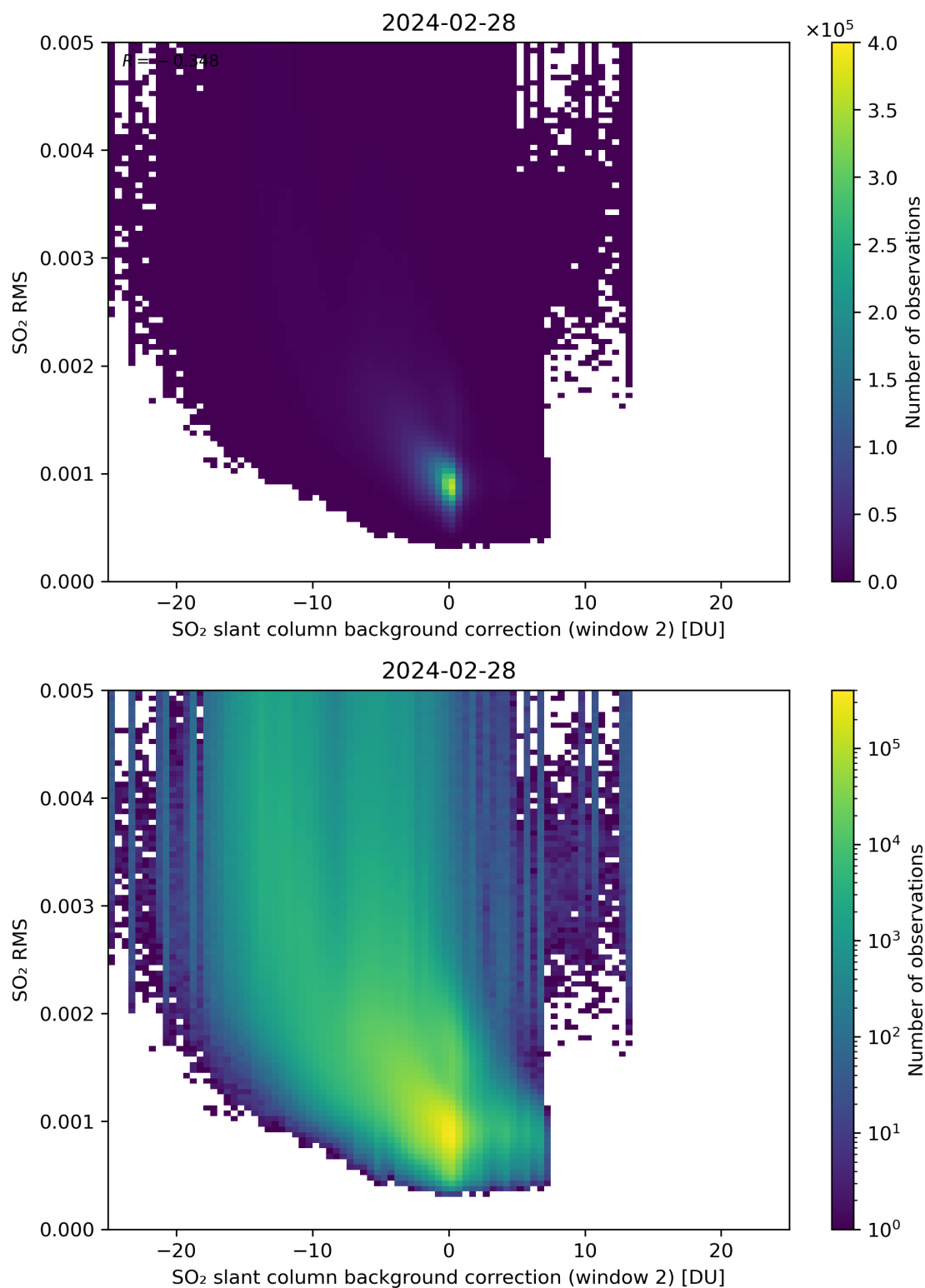
Figure 114: Scatter density plot of “SO 2 slant column background correction (window 2)” against “SO 2 RMS” for 2024-02-27 to 2024-02-29.
