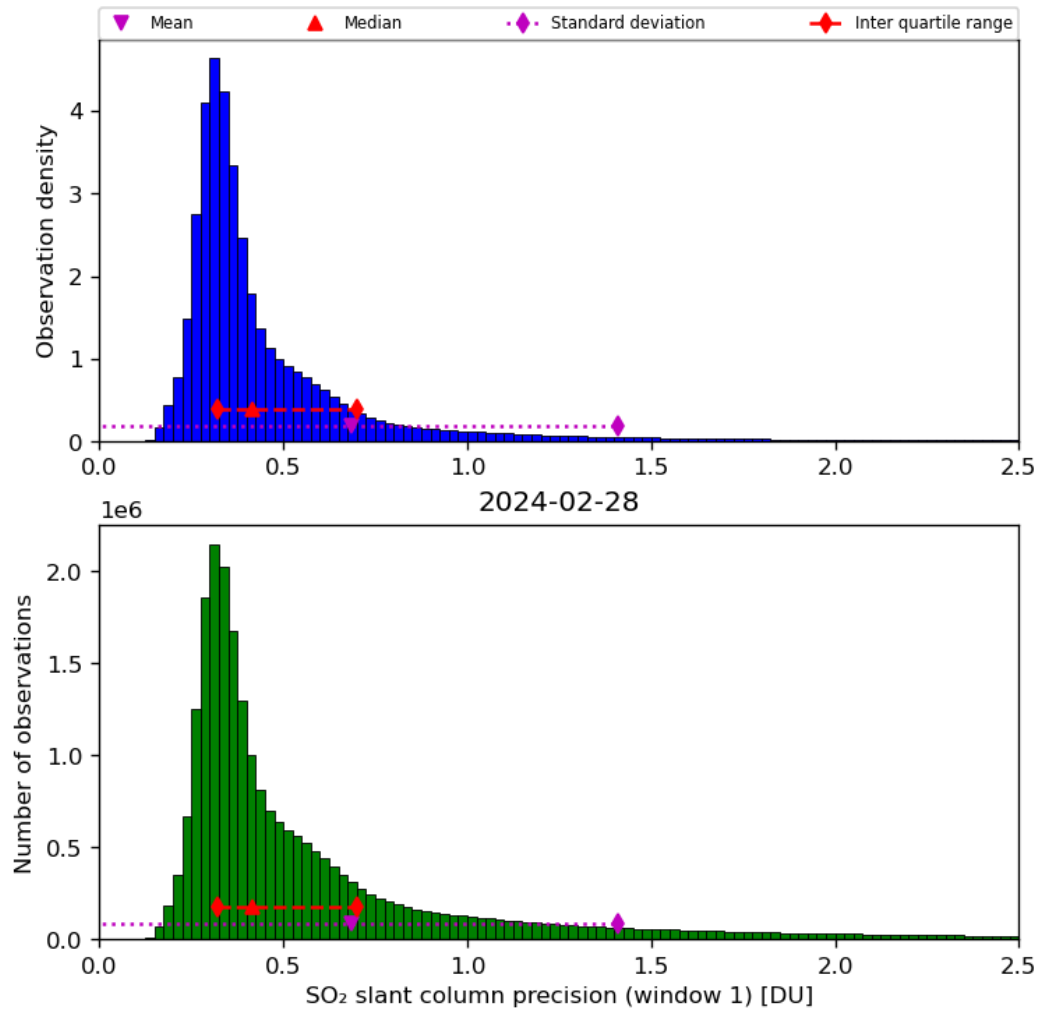
Figure 57: Histogram of “SO 2 slant column precision (window 1)” for 2024-02-27 to 2024-02-29
