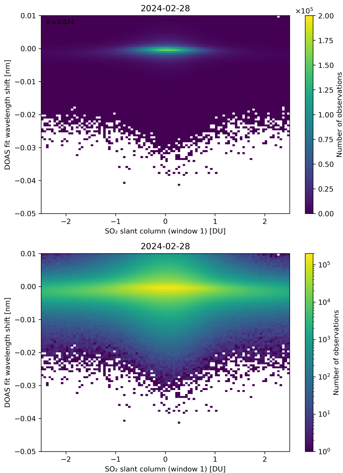
Figure 215: Scatter density plot of “SO 2 slant column (window 1)” against “DOAS fit wavelength shift” for 2024-02-27 to 2024-02-29.
