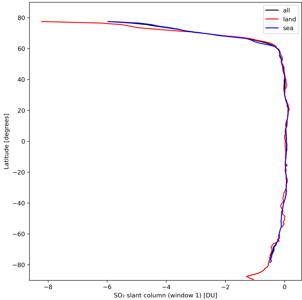
Figure 33: Zonal average of “SO 2 slant column (window 1)” for 2024-02-27 to 2024-02-29.
