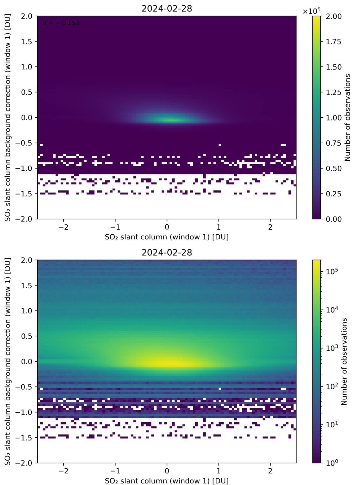
Figure 212: Scatter density plot of “SO 2 slant column (window 1)” against “SO 2 slant column background correction (window 1)” for 2024-02-27 to 2024-02-29.
