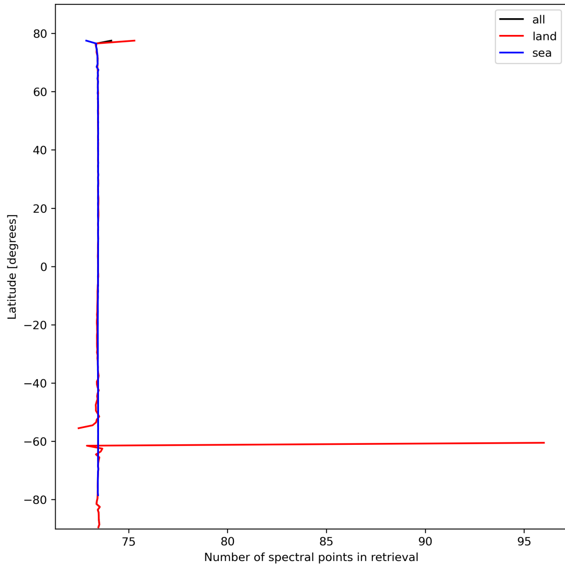
Figure 51: Zonal average of “Number of spectral points in retrieval” for 2024-02-27 to 2024-02-29.
