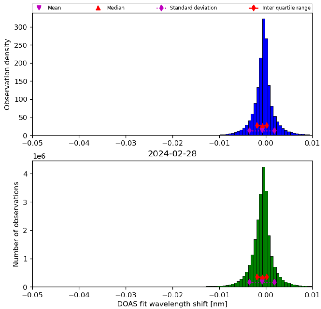
Figure 68: Histogram of “DOAS fit wavelength shift” for 2024-02-27 to 2024-02-29
