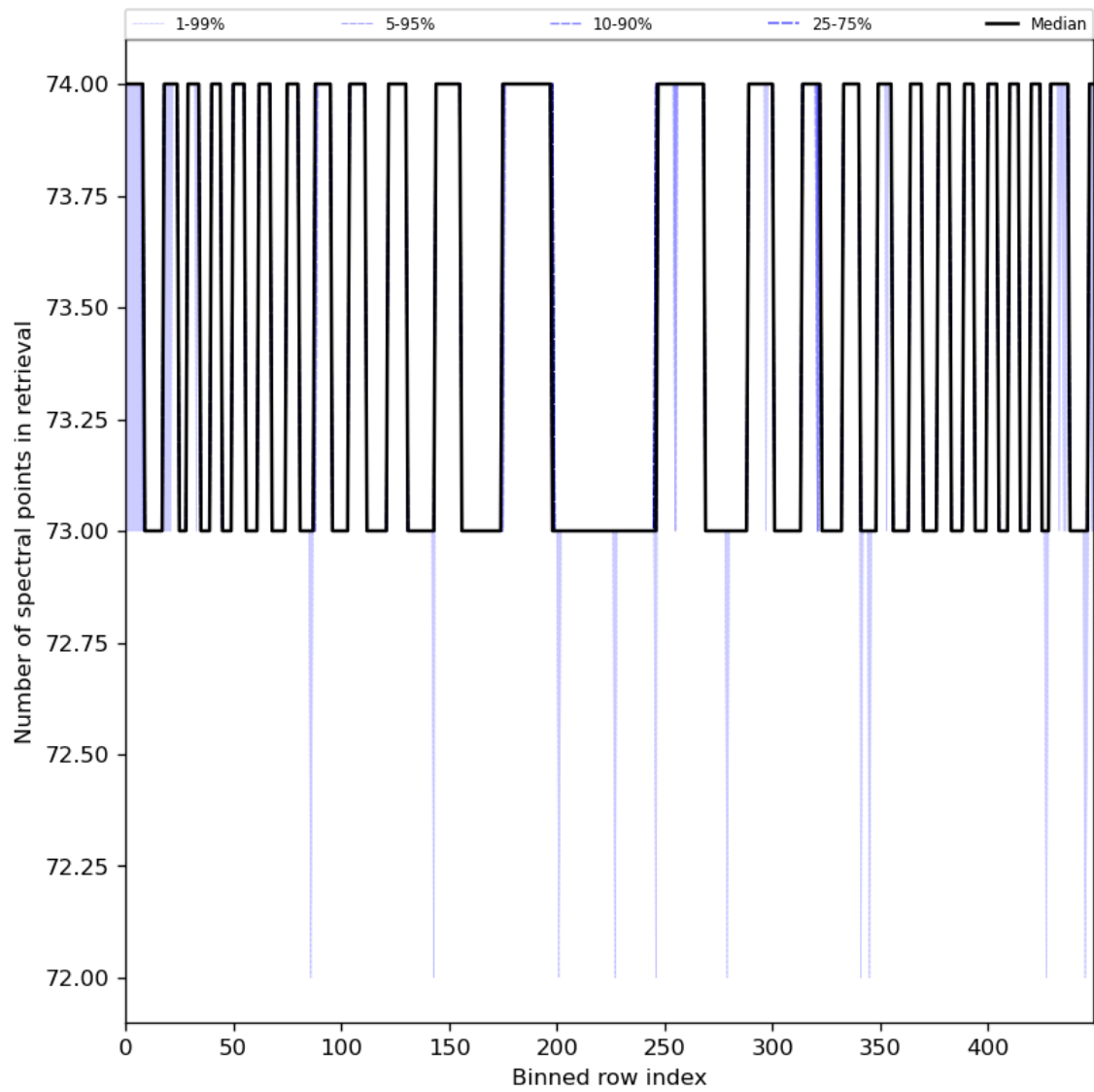
Figure 97: Along track statistics of “Number of spectral points in retrieval” for 2024-02-27 to 2024-02-29
