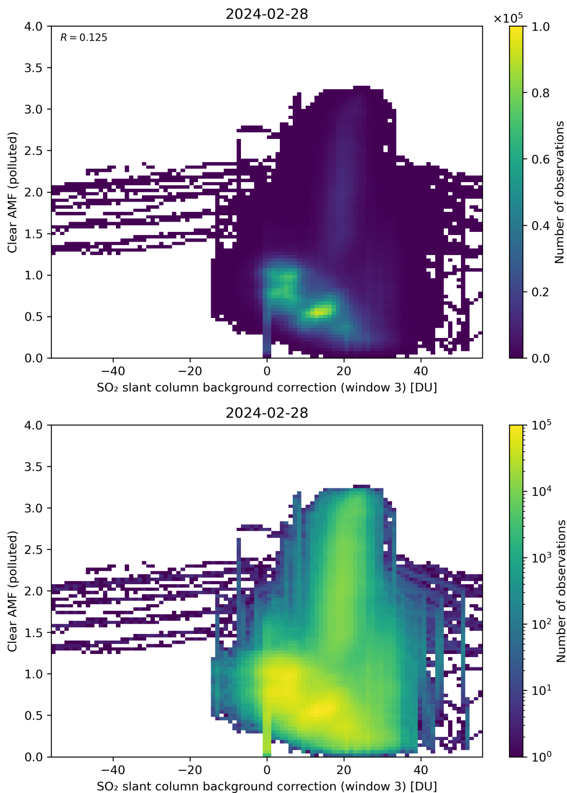
Figure 124: Scatter density plot of “SO 2 slant column background correction (window 3)” against “Clear AMF (polluted)” for 2024-02-27 to 2024-02-29.
