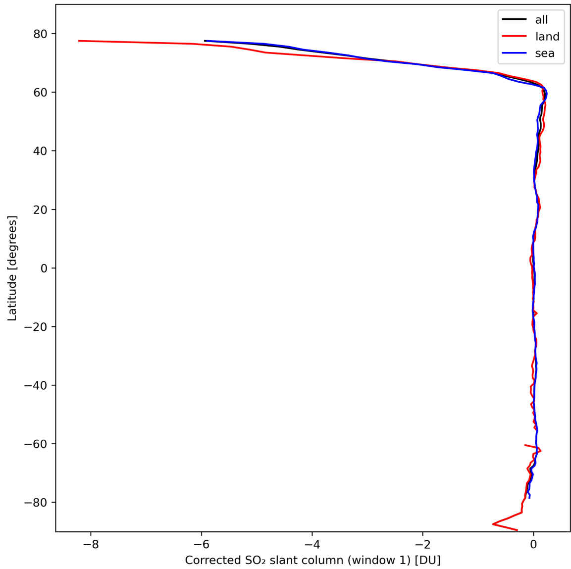
Figure 35: Zonal average of “Corrected SO 2 slant column (window 1)” for 2024-02-27 to 2024-02-29.
