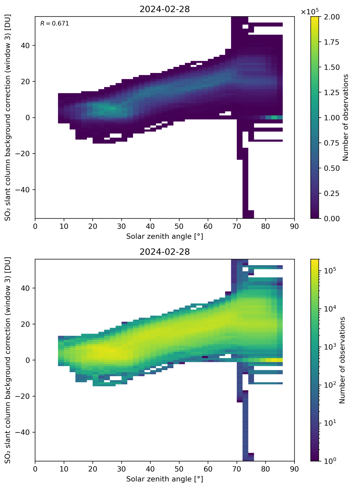
Figure 160: Scatter density plot of “Solar zenith angle” against “SO 2 slant column background correction (window 3)” for 2024-02-27 to 2024-02-29.
