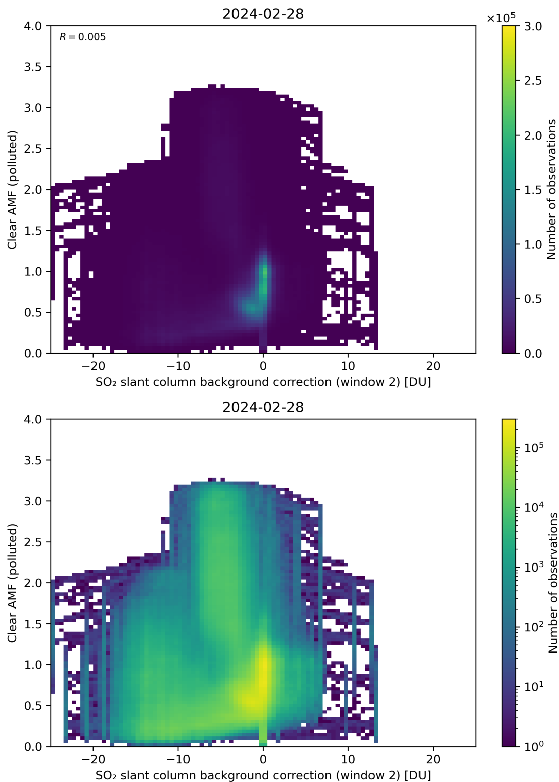
Figure 115: Scatter density plot of “SO 2 slant column background correction (window 2)” against “Clear AMF (polluted)” for 2024-02-27 to 2024-02-29.
