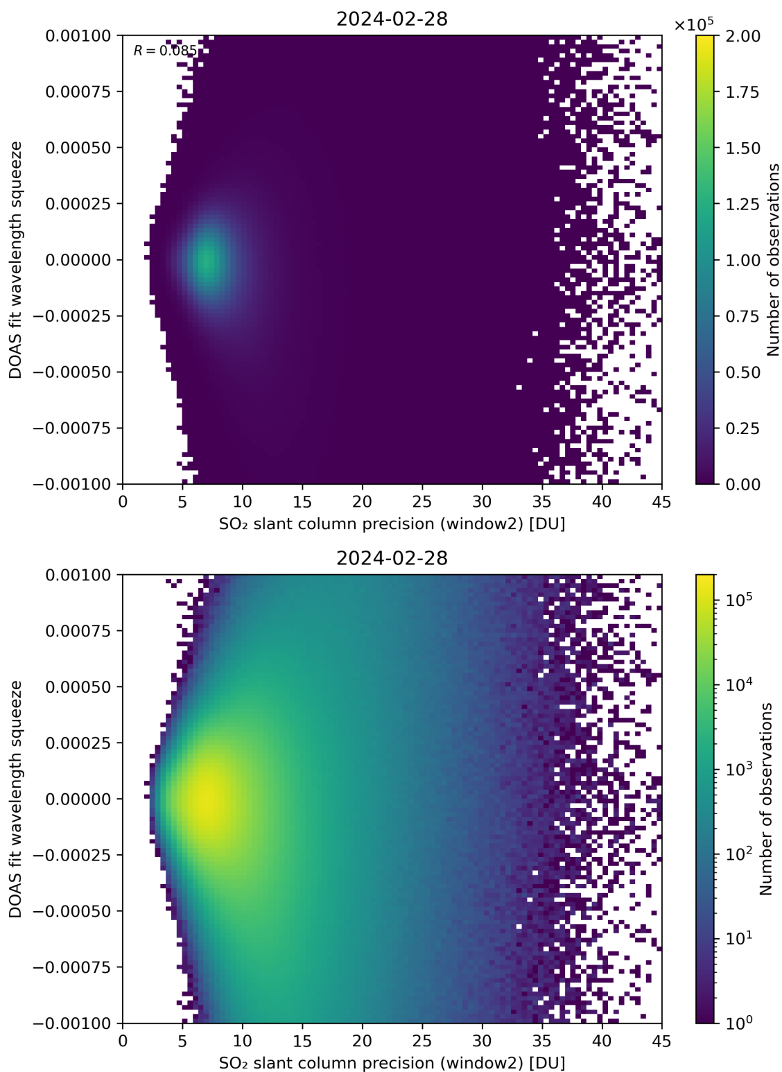
Figure 244: Scatter density plot of “SO 2 slant column precision (window2)” against “DOAS fit wavelength squeeze” for 2024-02-27 to 2024-02-29.
