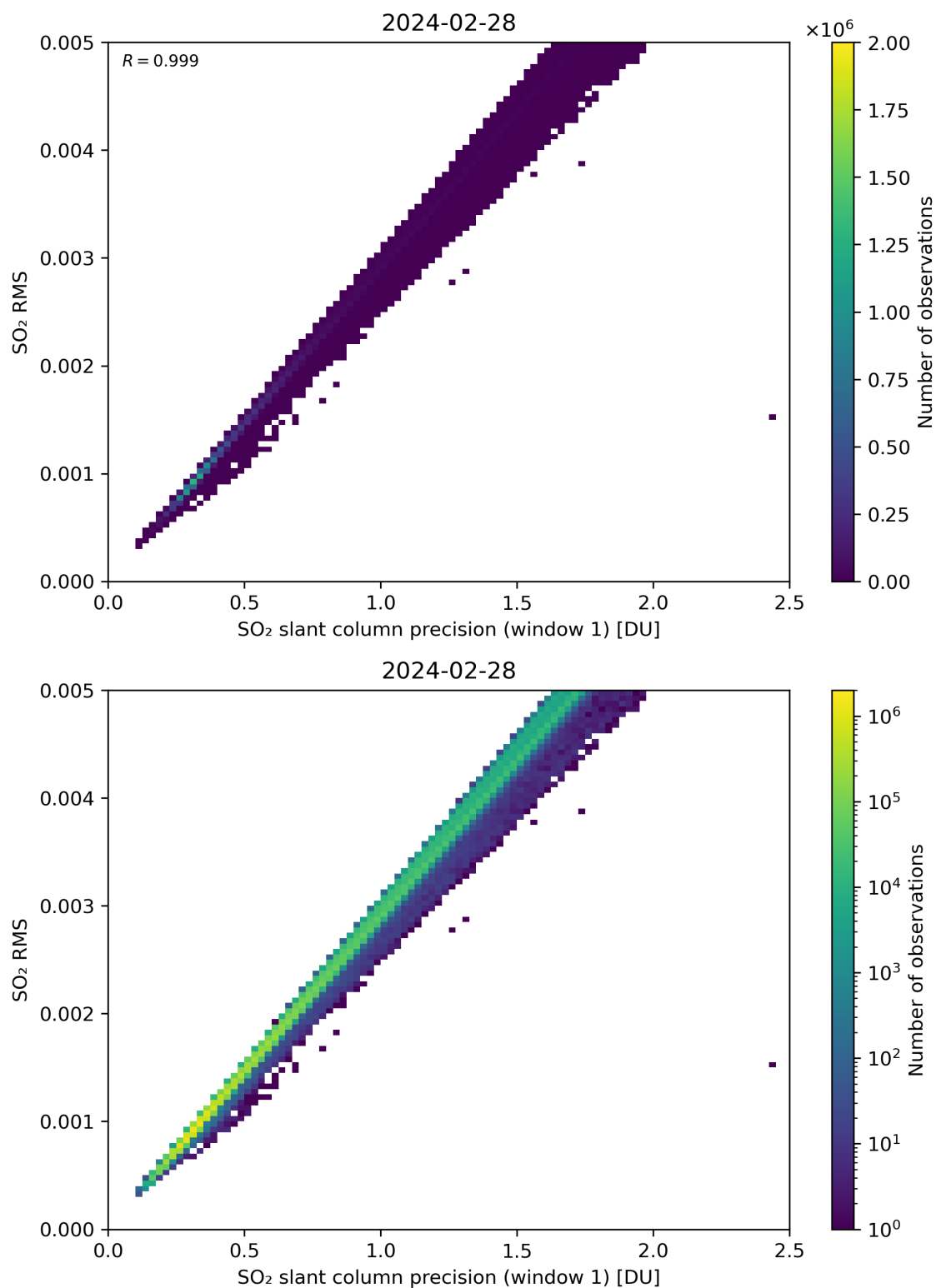
Figure 223: Scatter density plot of “SO 2 slant column precision (window 1)” against “SO 2 RMS” for 2024-02-27 to 2024-02-29.
