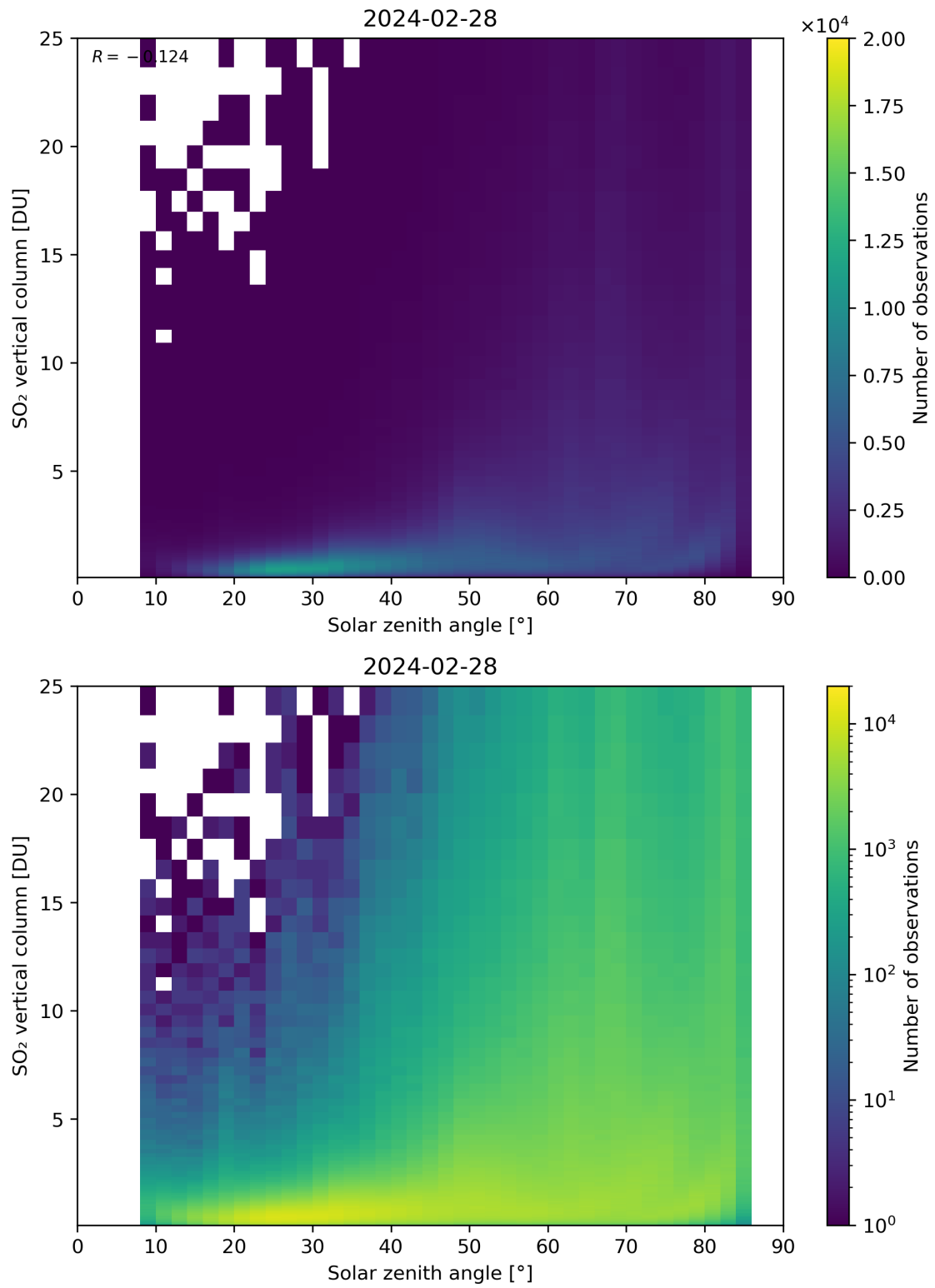
Figure 176: Scatter density plot of “Solar zenith angle” against “SO 2 vertical column” for 2024-02-27 to 2024-02-29.
