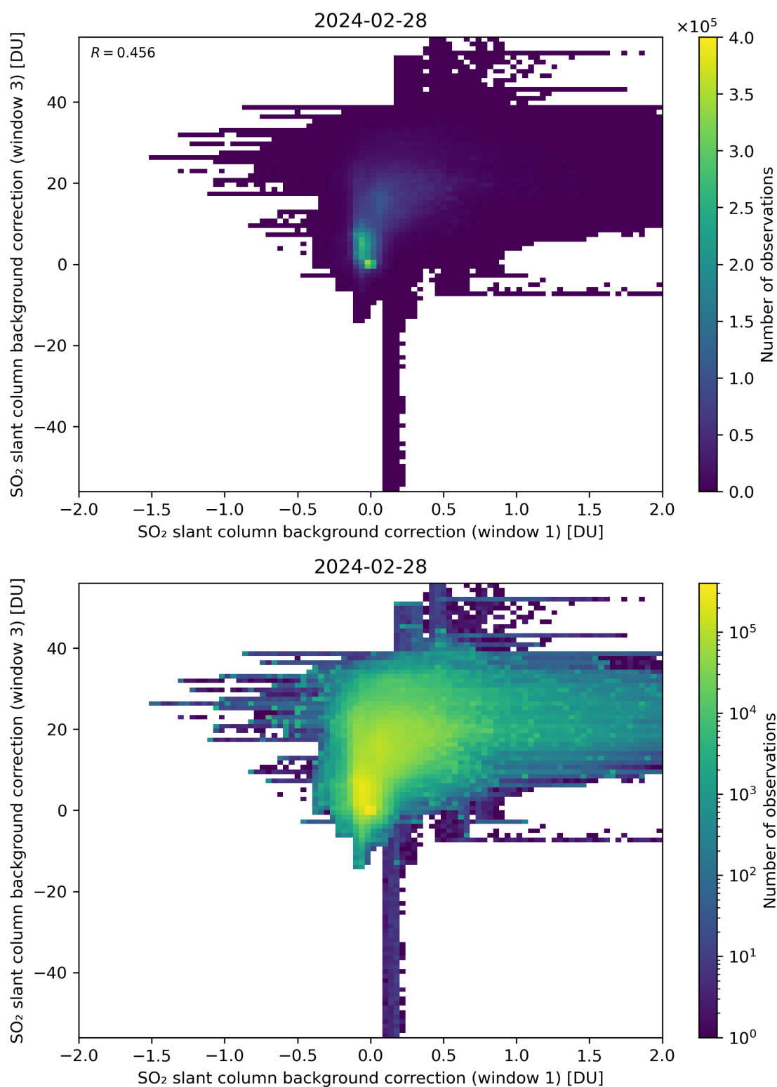
Figure 99: Scatter density plot of “SO 2 slant column background correction (window 1)” against “SO 2 slant column background correction (window 3)” for 2024-02-27 to 2024-02-29.
