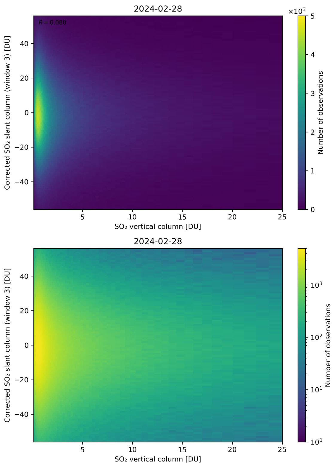
Figure 299: Scatter density plot of “SO 2 vertical column” against “Corrected SO 2 slant column (window 3)” for 2024-02-27 to 2024-02-29.
