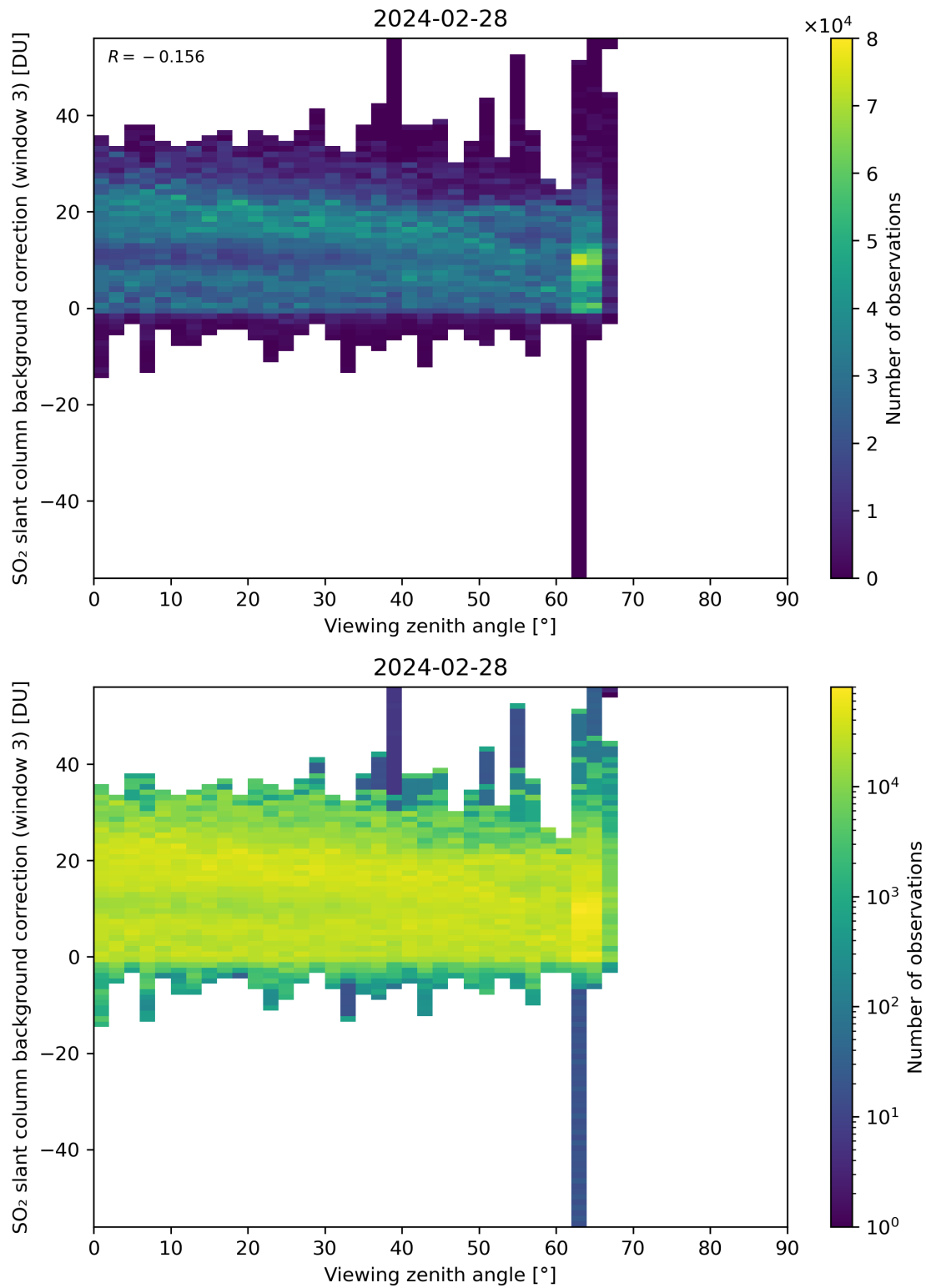
Figure 310: Scatter density plot of “Viewing zenith angle” against “SO 2 slant column background correction (window 3)” for 2024-02-27 to 2024-02-29.
