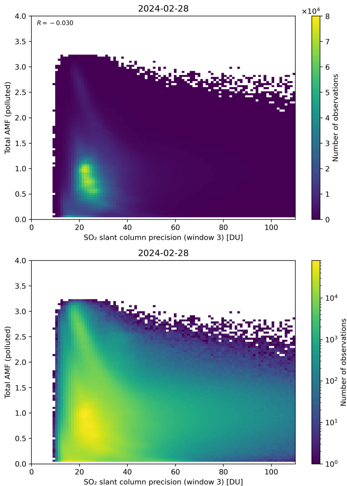
Figure 263: Scatter density plot of “SO 2 slant column precision (window 3)” against “Total AMF (polluted)” for 2024-02-27 to 2024-02-29.
