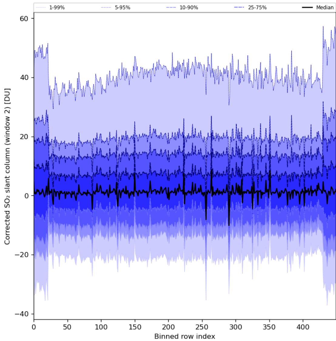
Figure 85: Along track statistics of “Corrected SO 2 slant column (window 2)” for 2024-02-27 to 2024-02-29
