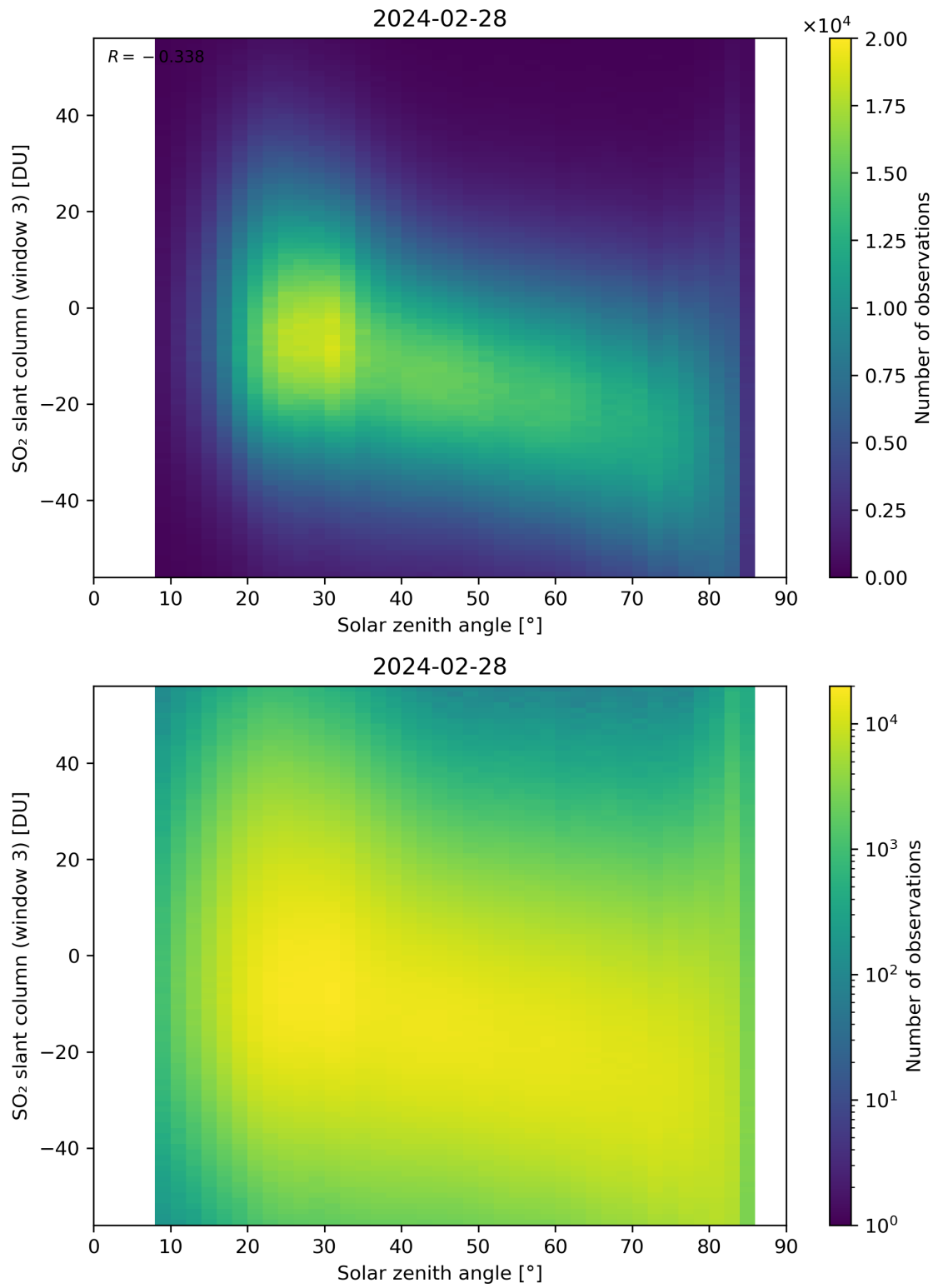
Figure 172: Scatter density plot of “Solar zenith angle” against “SO 2 slant column (window 3)” for 2024-02-27 to 2024-02-29.
