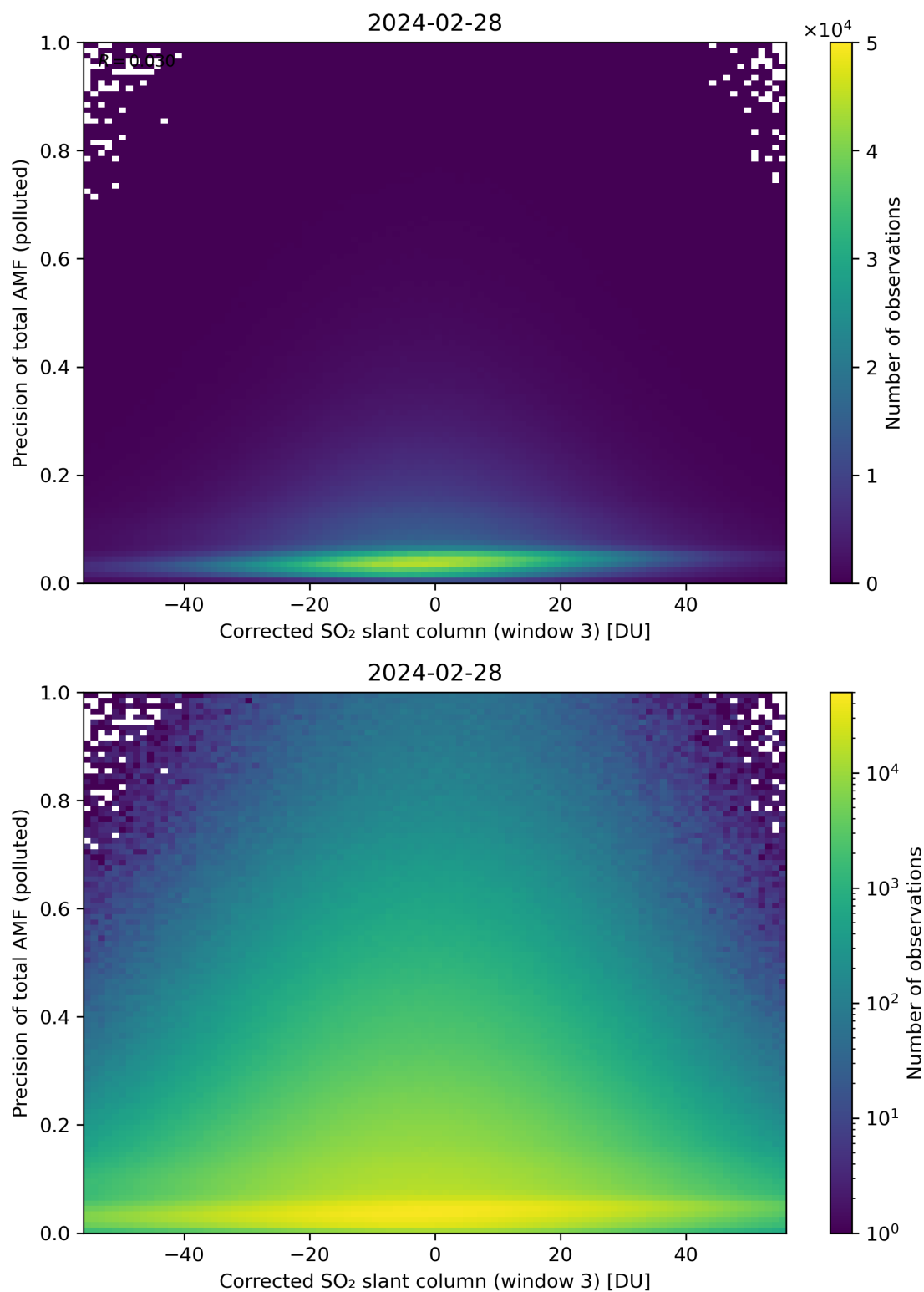
Figure 211: Scatter density plot of “Corrected SO 2 slant column (window 3)” against “Precision of total AMF (polluted)” for 2024-02-27 to 2024-02-29.
