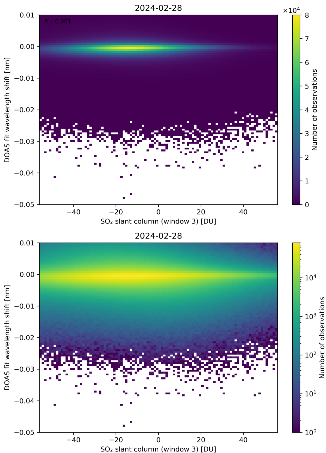
Figure 254: Scatter density plot of “SO 2 slant column (window 3)” against “DOAS fit wavelength shift” for 2024-02-27 to 2024-02-29.
