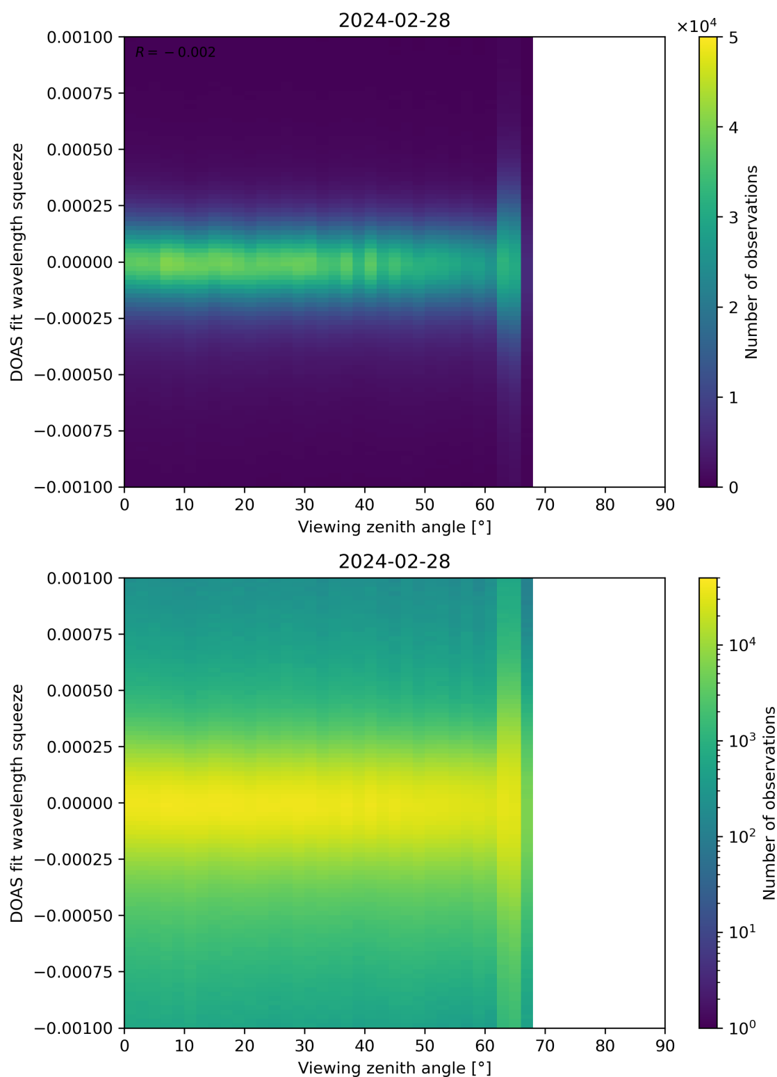
Figure 312: Scatter density plot of “Viewing zenith angle” against “DOAS fit wavelength squeeze” for 2024-02-27 to 2024-02-29.
