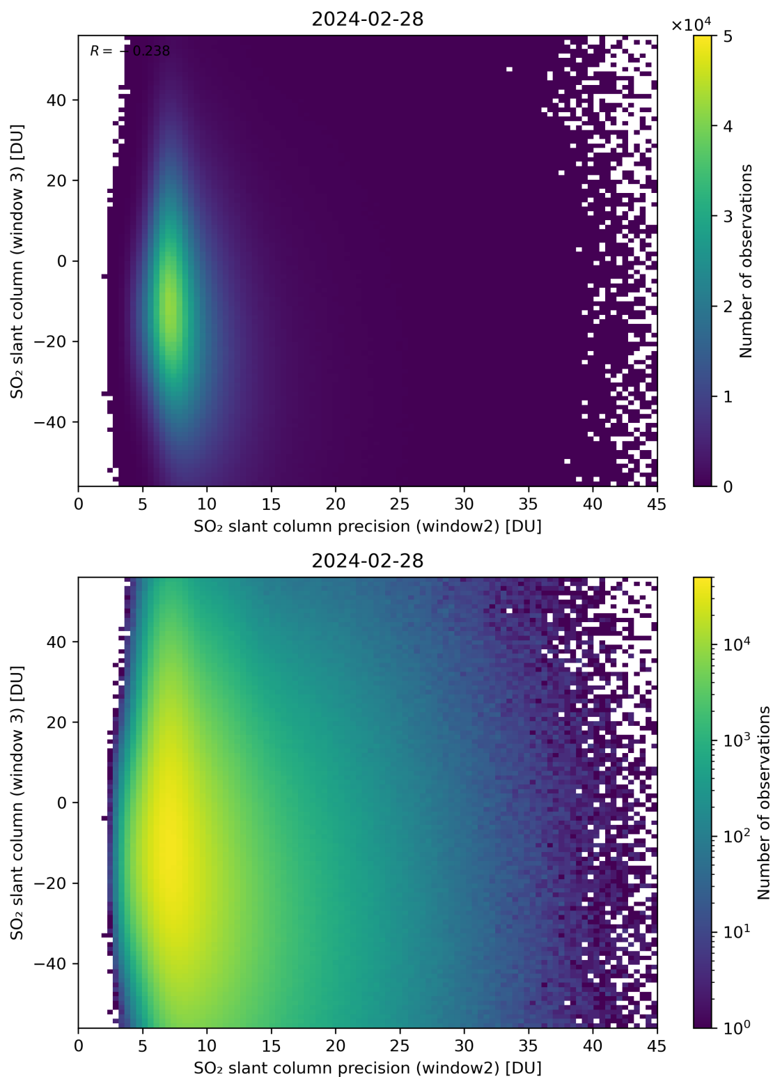
Figure 249: Scatter density plot of “SO 2 slant column precision (window2)” against “SO 2 slant column (window 3)” for 2024-02-27 to 2024-02-29.
