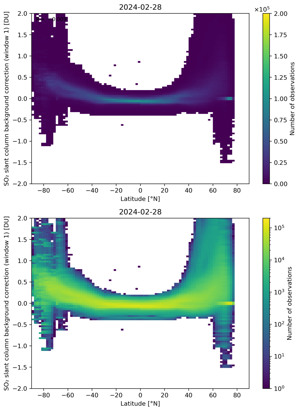
Figure 139: Scatter density plot of “Latitude” against “SO 2 slant column background correction (window 1)” for 2024-02-27 to 2024-02-29.
