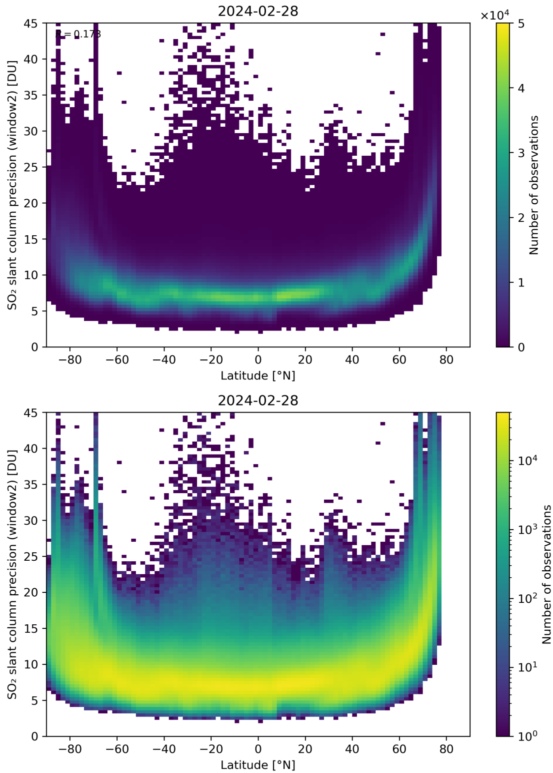
Figure 151: Scatter density plot of “Latitude” against “SO 2 slant column precision (window2)” for 2024-02-27 to 2024-02-29.
