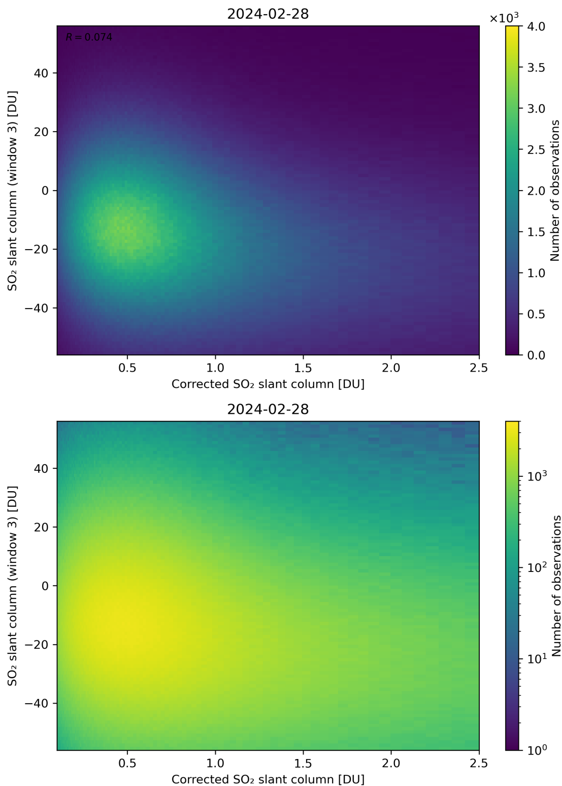
Figure 190: Scatter density plot of “Corrected SO 2 slant column” against “SO 2 slant column (window 3)” for 2024-02-27 to 2024-02-29.
