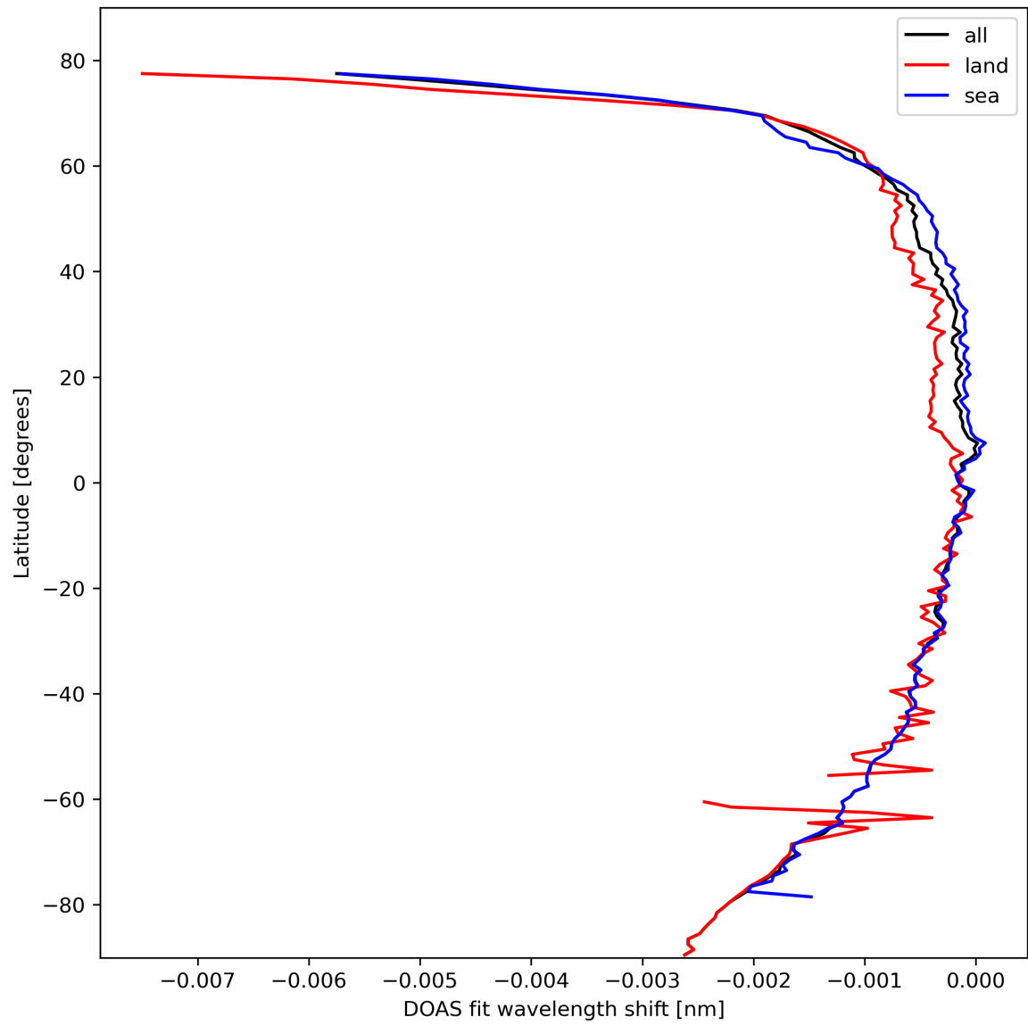
Figure 45: Zonal average of “DOAS fit wavelength shift” for 2024-02-27 to 2024-02-29.
