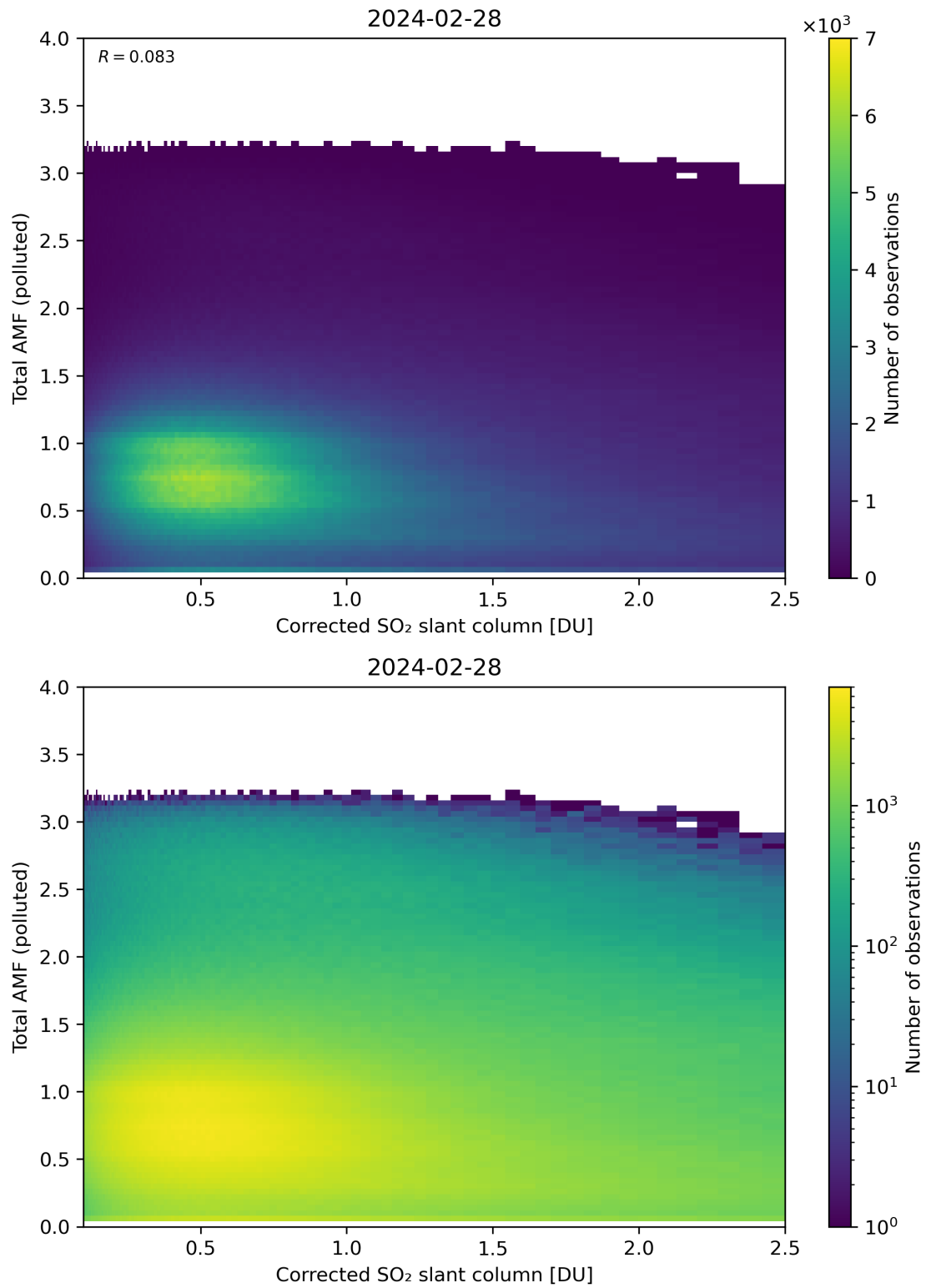
Figure 192: Scatter density plot of “Corrected SO 2 slant column” against “Total AMF (polluted)” for 2024-02-27 to 2024-02-29.
