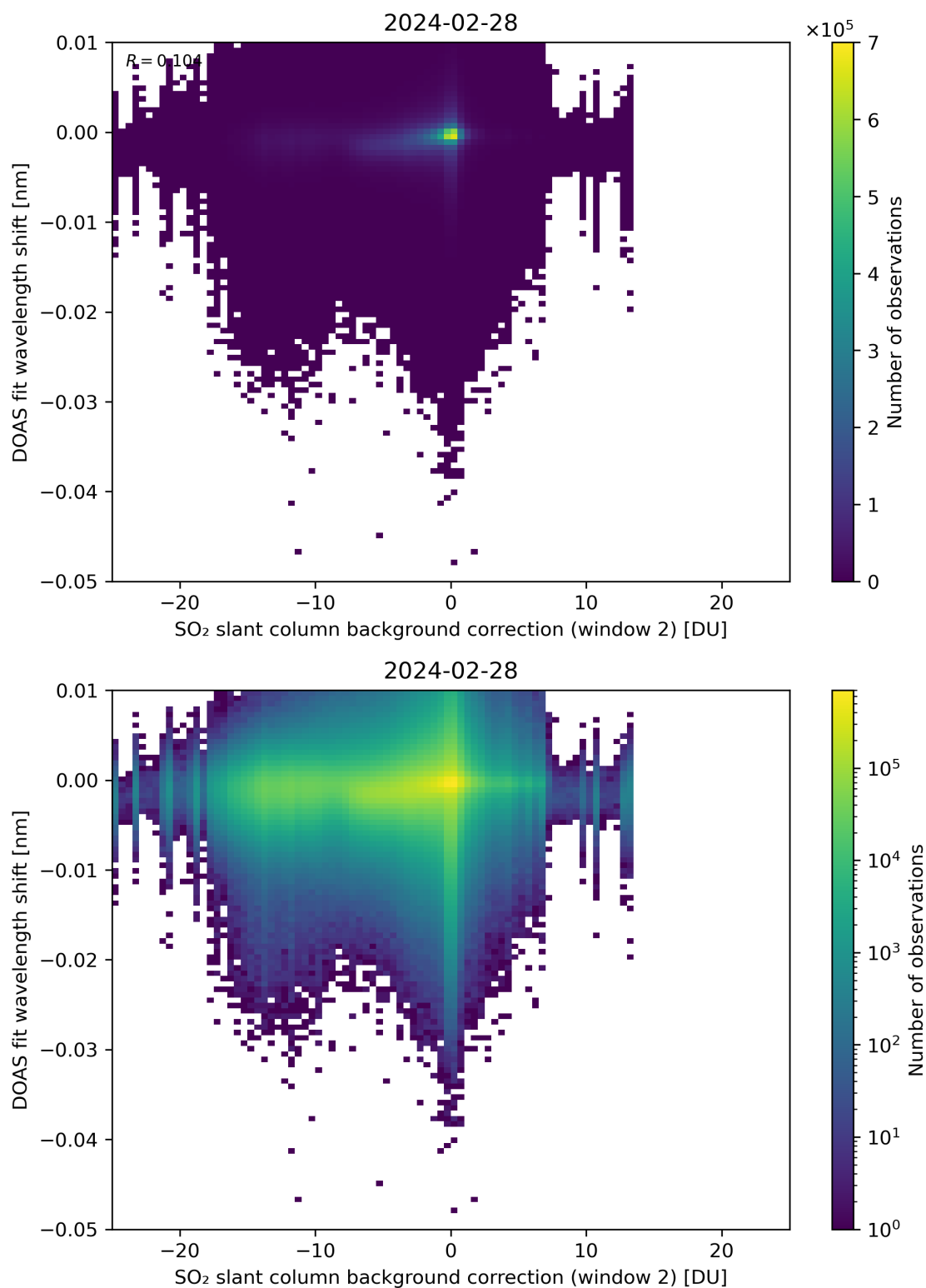
Figure 112: Scatter density plot of “SO 2 slant column background correction (window 2)” against “DOAS fit wavelength shift” for 2024-02-27 to 2024-02-29.
