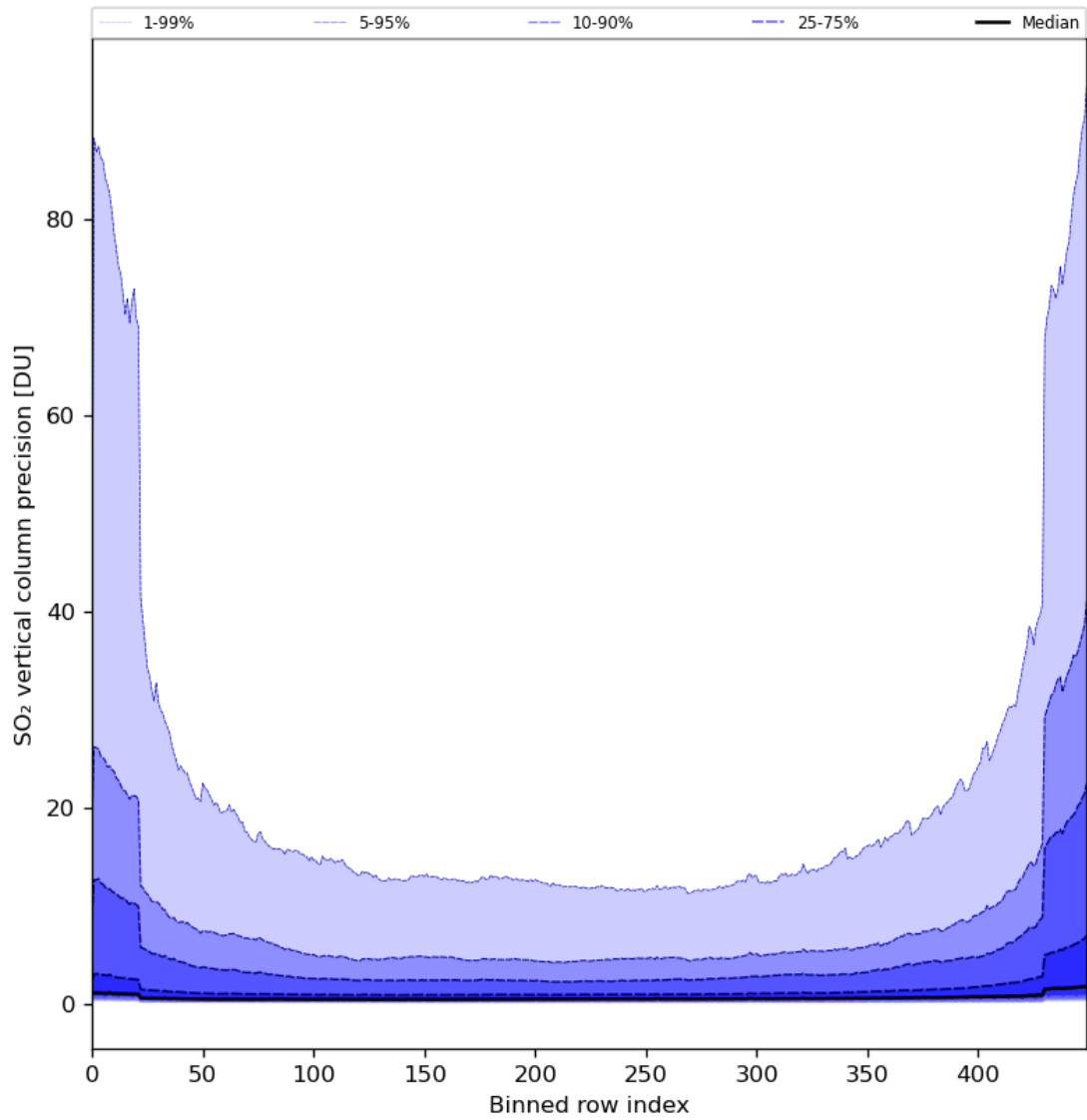
Figure 77: Along track statistics of “SO 2 vertical column precision” for 2024-02-27 to 2024-02-29
