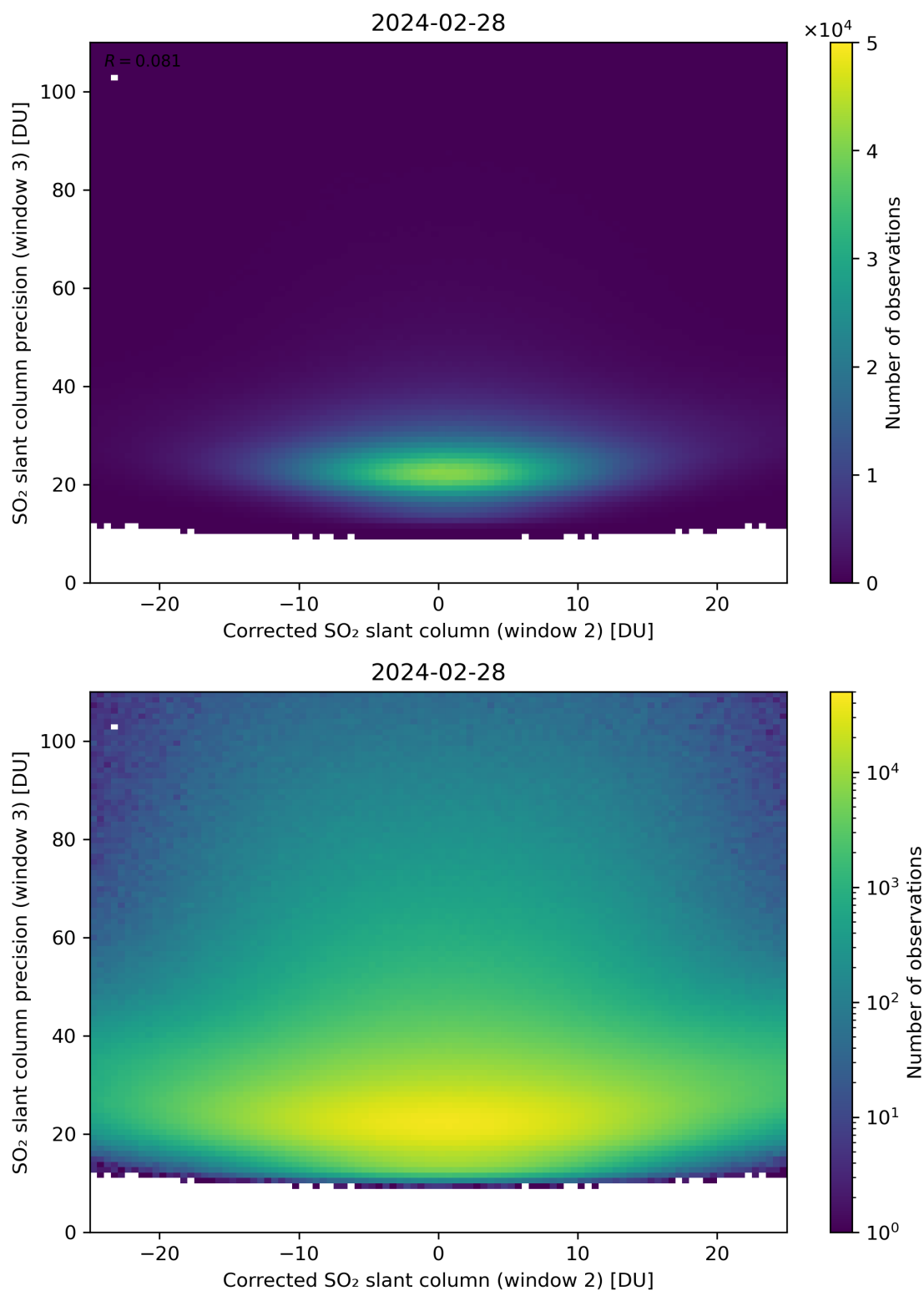
Figure 202: Scatter density plot of “Corrected SO 2 slant column (window 2)” against “SO 2 slant column precision (window 3)” for 2024-02-27 to 2024-02-29.
