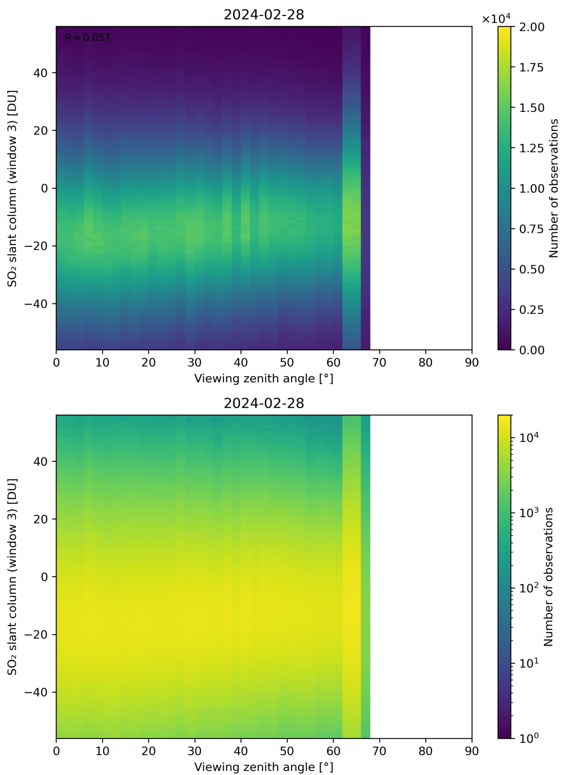
Figure 323: Scatter density plot of “Viewing zenith angle” against “SO 2 slant column (window 3)” for 2024-02-27 to 2024-02-29.
