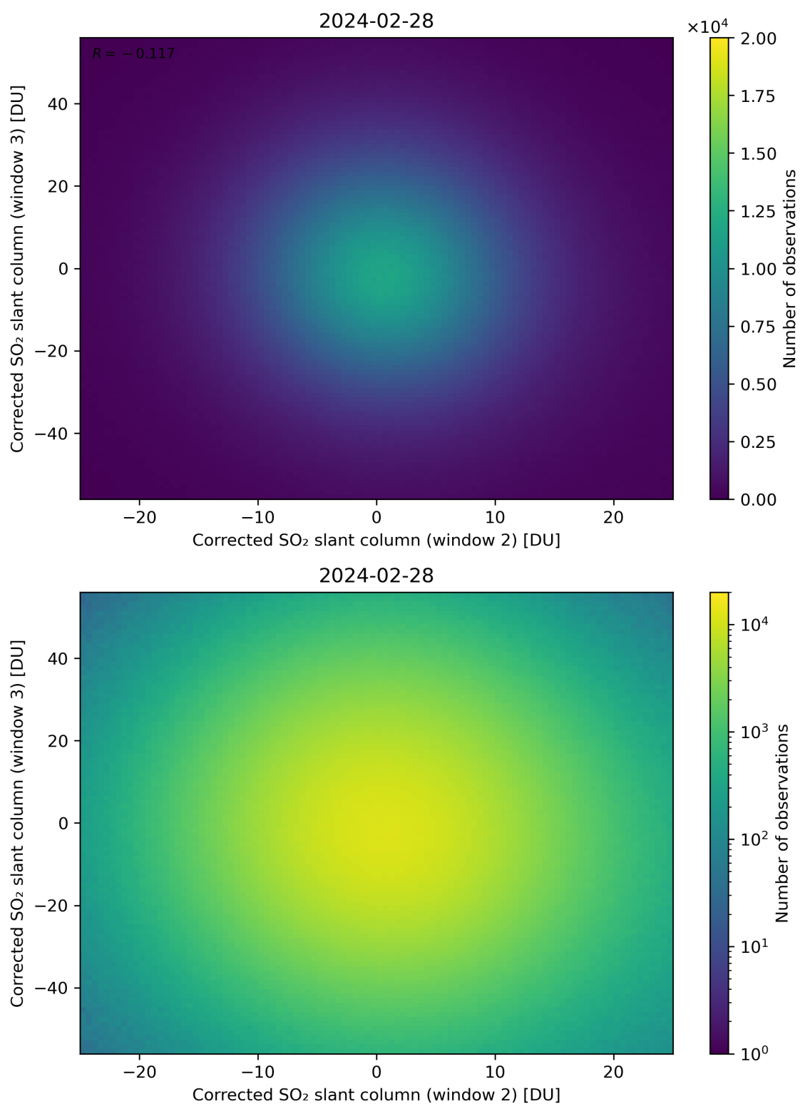
Figure 200: Scatter density plot of “Corrected SO 2 slant column (window 2)” against “Corrected SO 2 slant column (window 3)” for 2024-02-27 to 2024-02-29.
