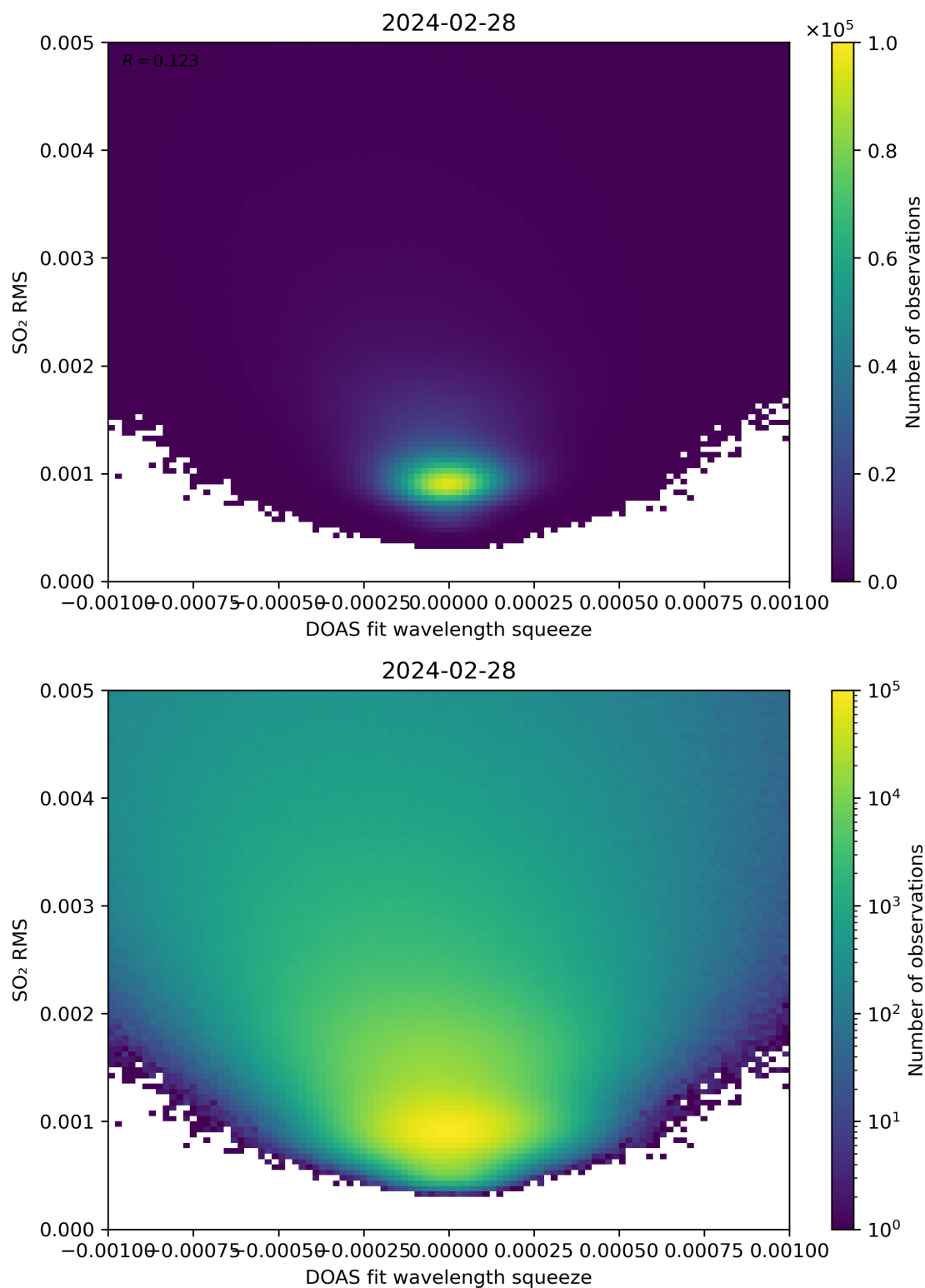
Figure 132: Scatter density plot of “DOAS fit wavelength squeeze” against “SO 2 RMS” for 2024-02-27 to 2024-02-29.
