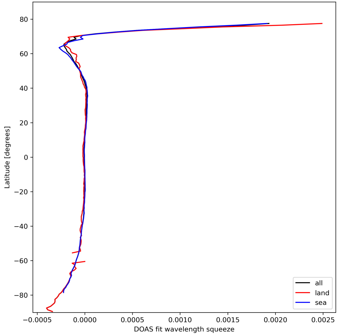
Figure 46: Zonal average of “DOAS fit wavelength squeeze” for 2024-02-27 to 2024-02-29.
