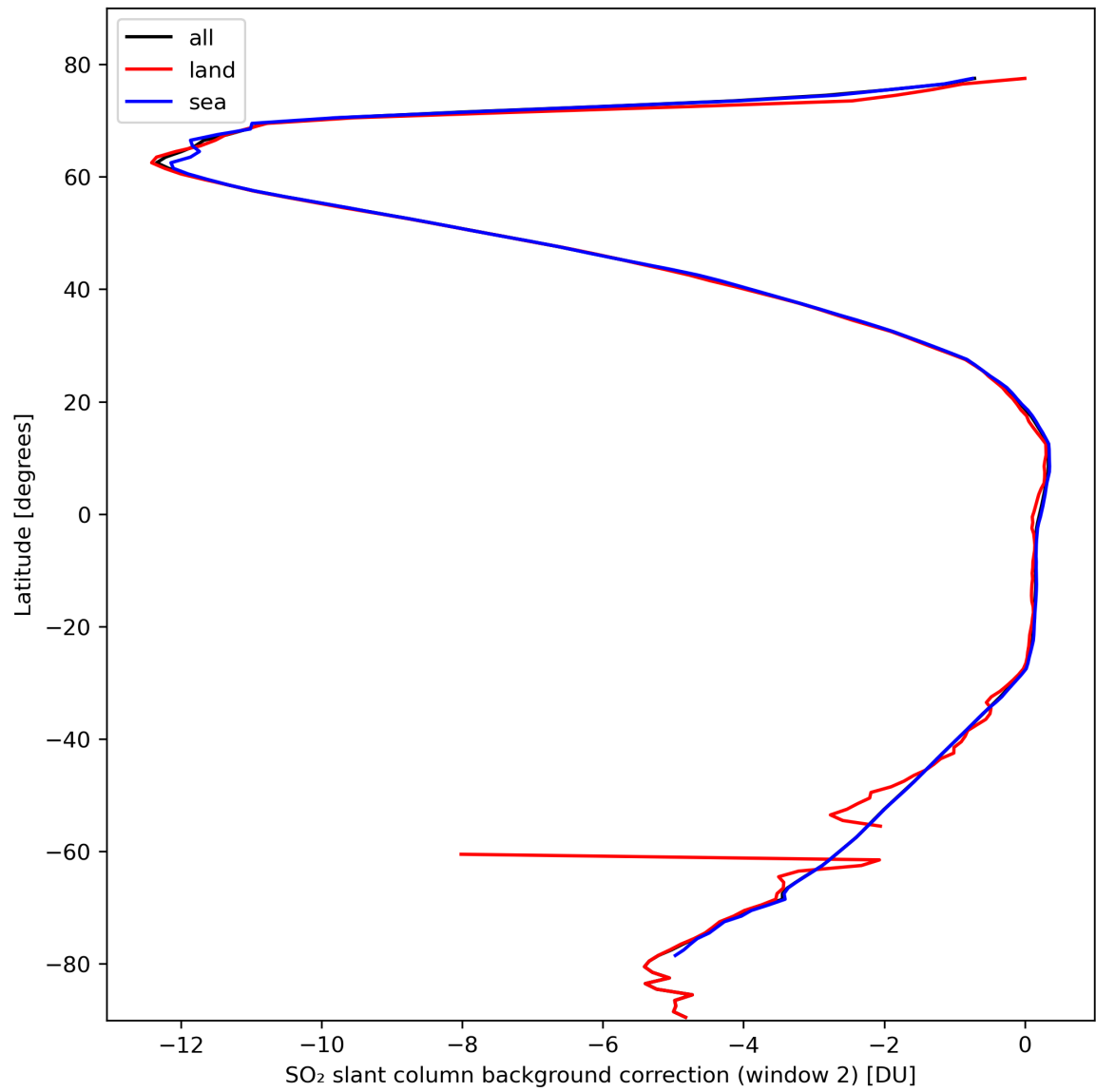
Figure 40: Zonal average of “SO 2 slant column background correction (window 2)” for 2024-02-27 to 2024-02-29.
