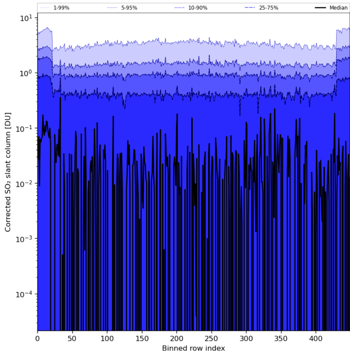
Figure 78: Along track statistics of “Corrected SO 2 slant column” for 2024-02-27 to 2024-02-29
