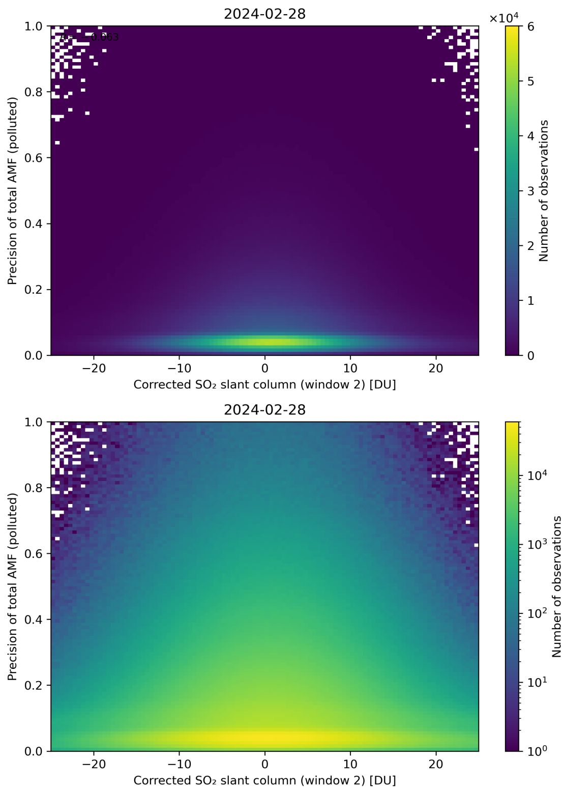
Figure 204: Scatter density plot of “Corrected SO 2 slant column (window 2)” against “Precision of total AMF (polluted)” for 2024-02-27 to 2024-02-29.
