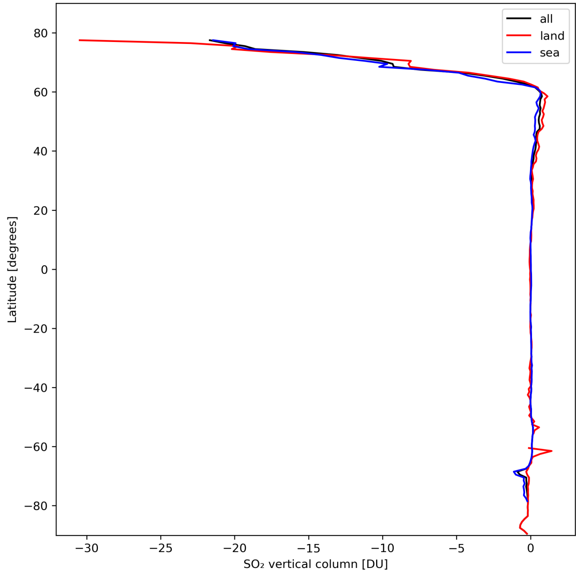
Figure 30: Zonal average of “SO 2 vertical column” for 2024-02-27 to 2024-02-29.
