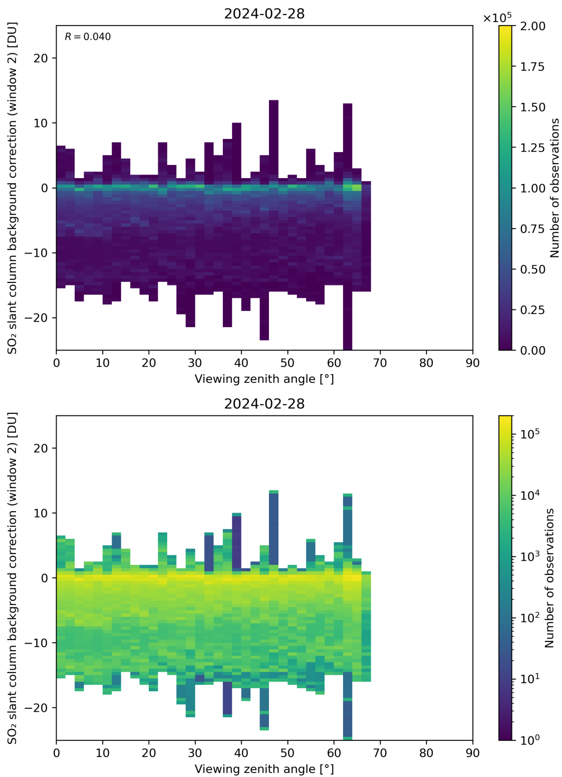
Figure 309: Scatter density plot of “Viewing zenith angle” against “SO 2 slant column background correction (window 2)” for 2024-02-27 to 2024-02-29.
