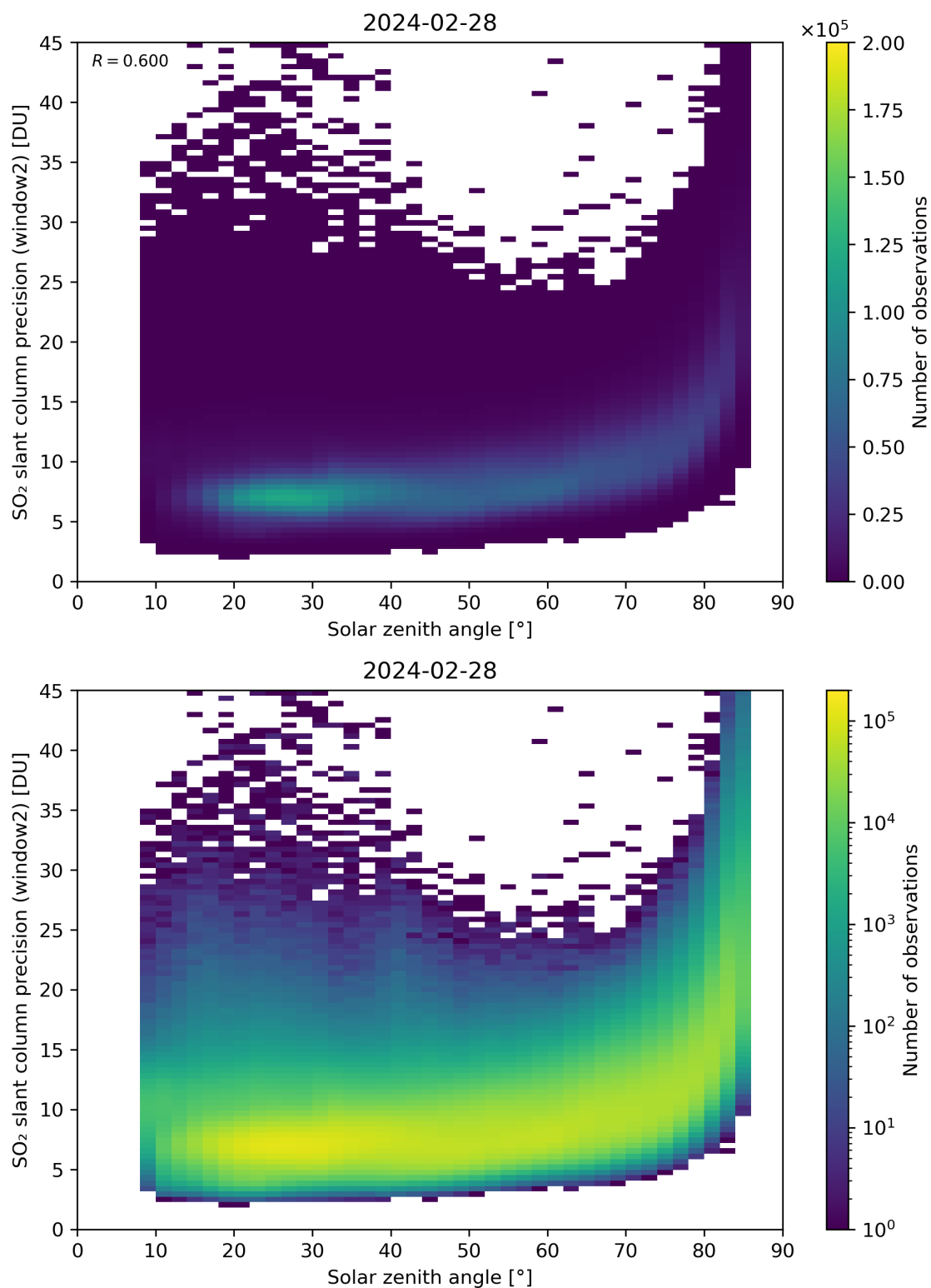
Figure 171: Scatter density plot of “Solar zenith angle” against “SO 2 slant column precision (window2)” for 2024-02-27 to 2024-02-29.
