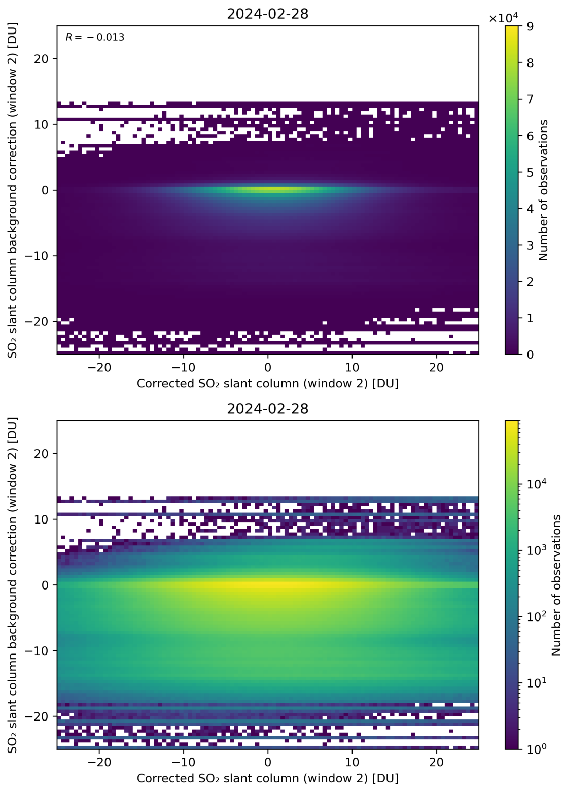
Figure 194: Scatter density plot of “Corrected SO 2 slant column (window 2)” against “SO 2 slant column background correction (window 2)” for 2024-02-27 to 2024-02-29.
