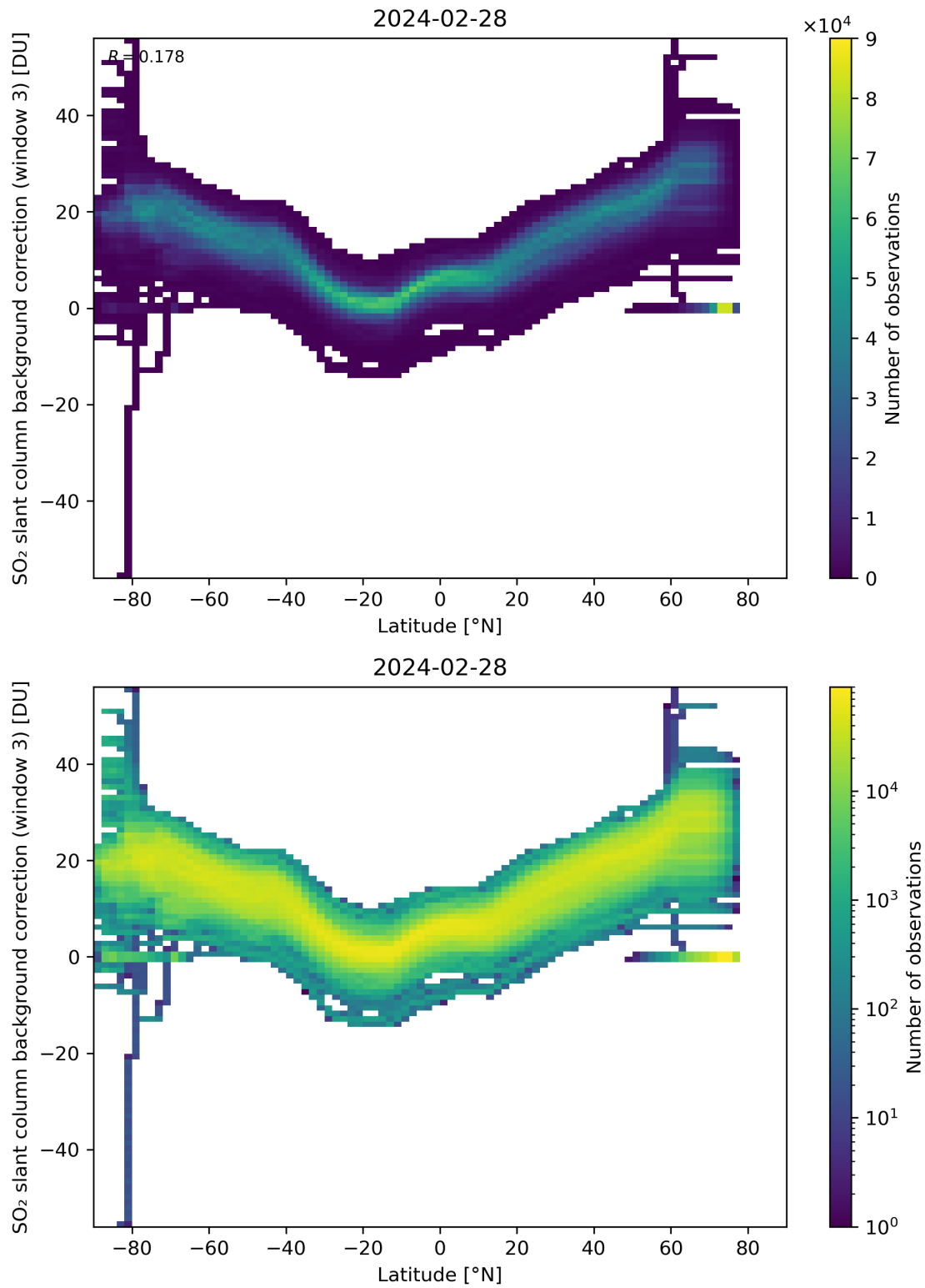
Figure 141: Scatter density plot of “Latitude” against “SO 2 slant column background correction (window 3)” for 2024-02-27 to 2024-02-29.
