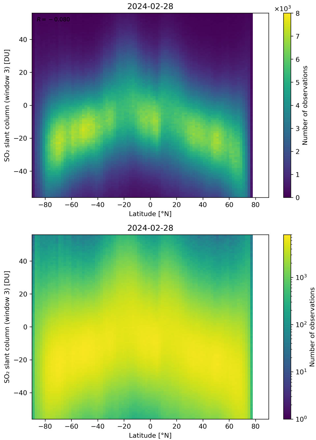
Figure 152: Scatter density plot of “Latitude” against “SO 2 slant column (window 3)” for 2024-02-27 to 2024-02-29.
