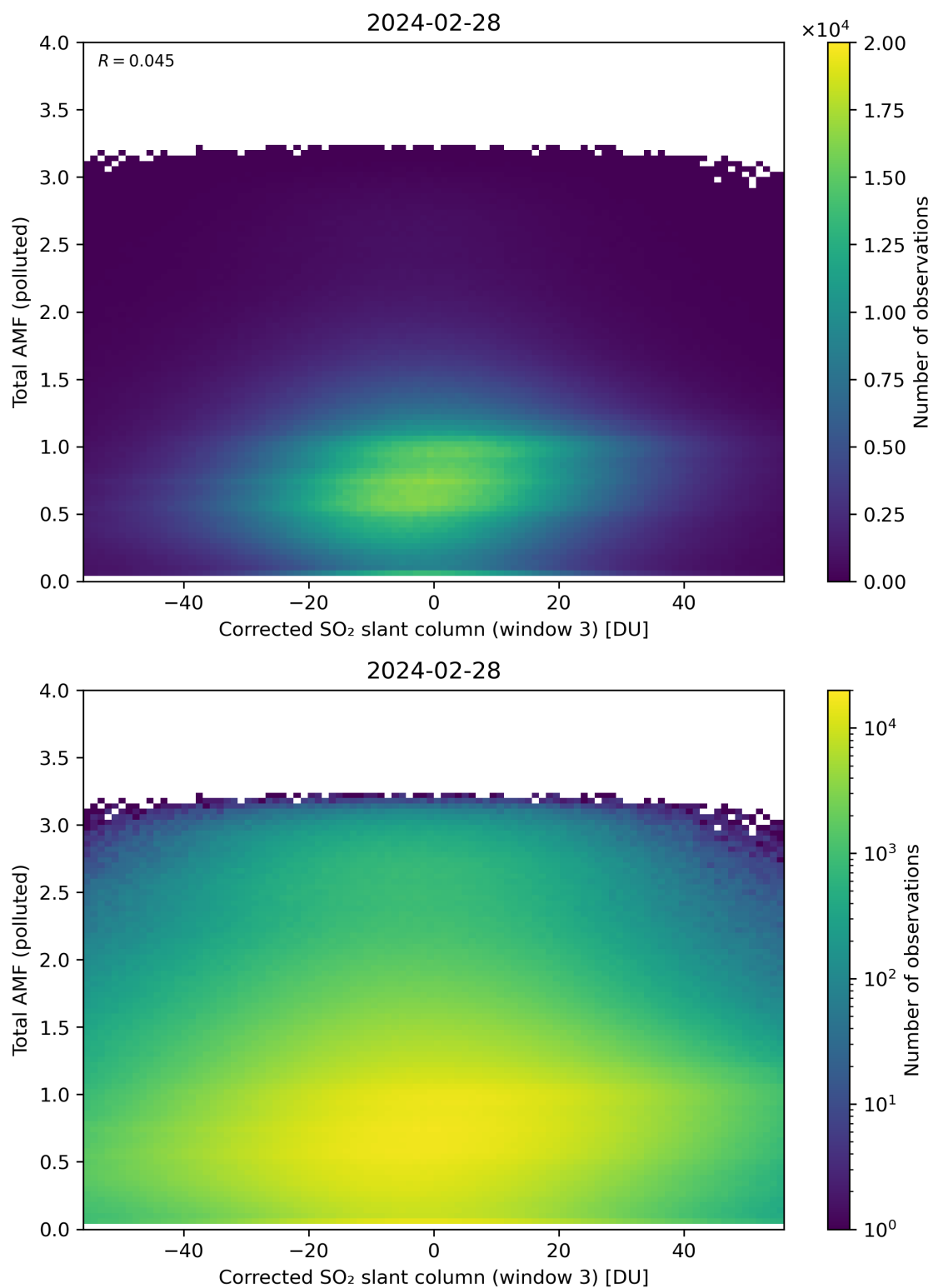
Figure 210: Scatter density plot of “Corrected SO 2 slant column (window 3)” against “Total AMF (polluted)” for 2024-02-27 to 2024-02-29.
