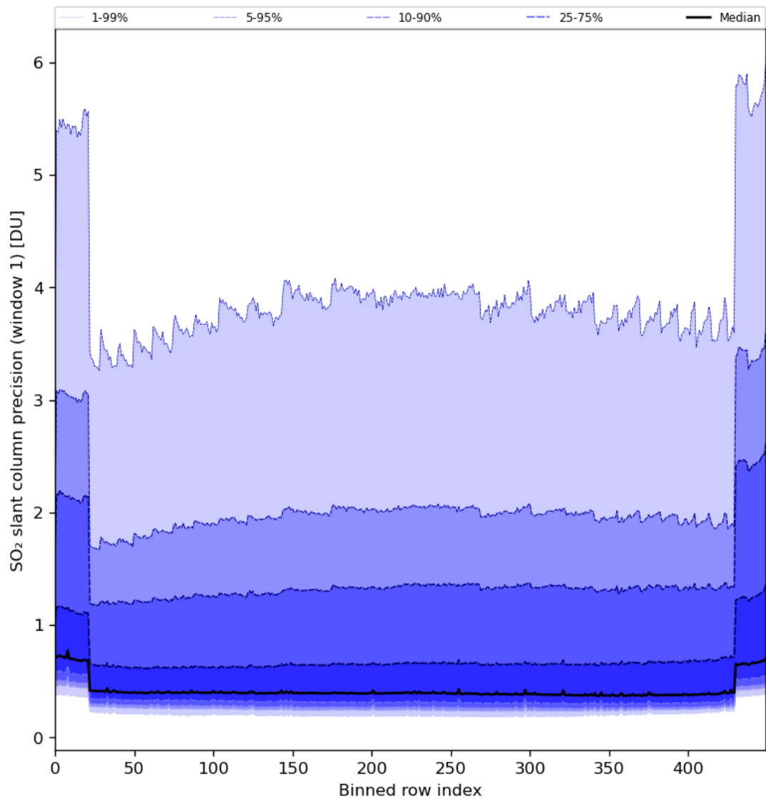
Figure 80: Along track statistics of “SO 2 slant column precision (window 1)” for 2024-02-27 to 2024-02-29
