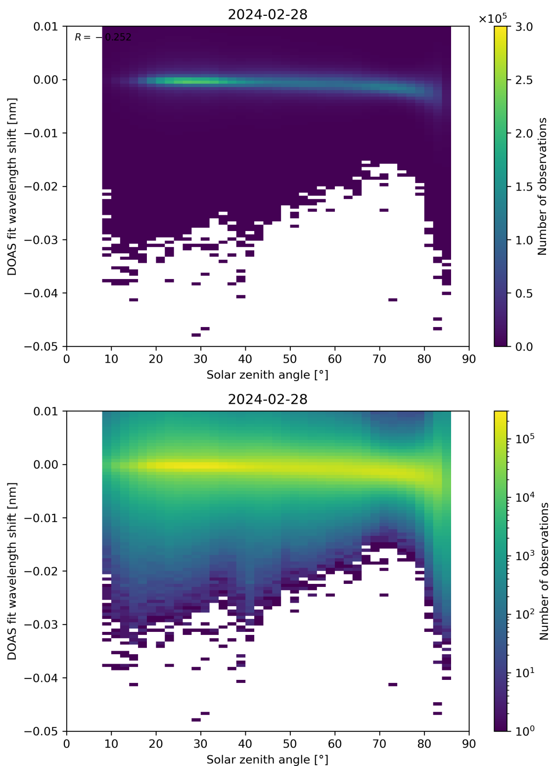
Figure 161: Scatter density plot of “Solar zenith angle” against “DOAS fit wavelength shift” for 2024-02-27 to 2024-02-29.
