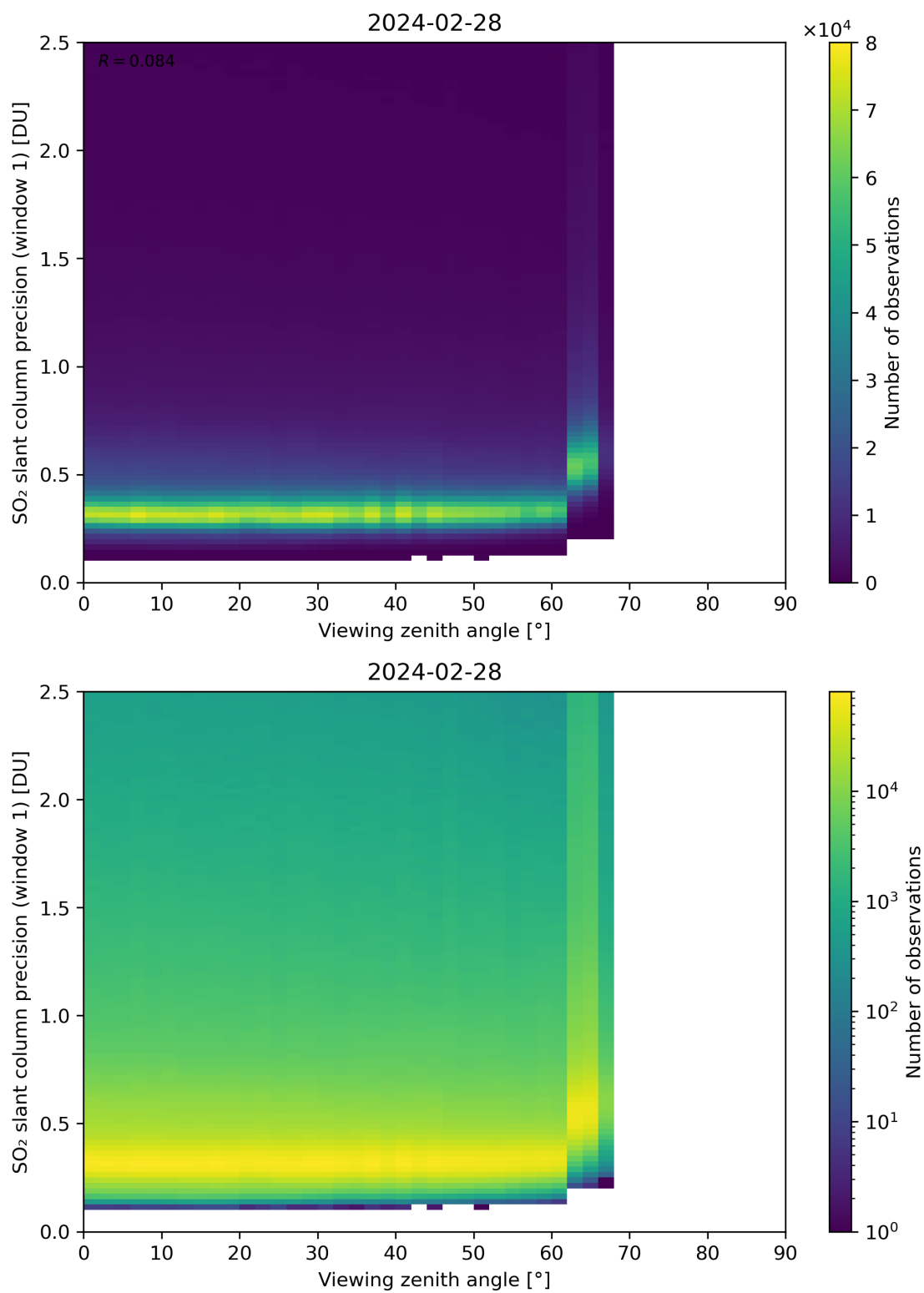
Figure 321: Scatter density plot of “Viewing zenith angle” against “SO 2 slant column precision (window 1)” for 2024-02-27 to 2024-02-29.
