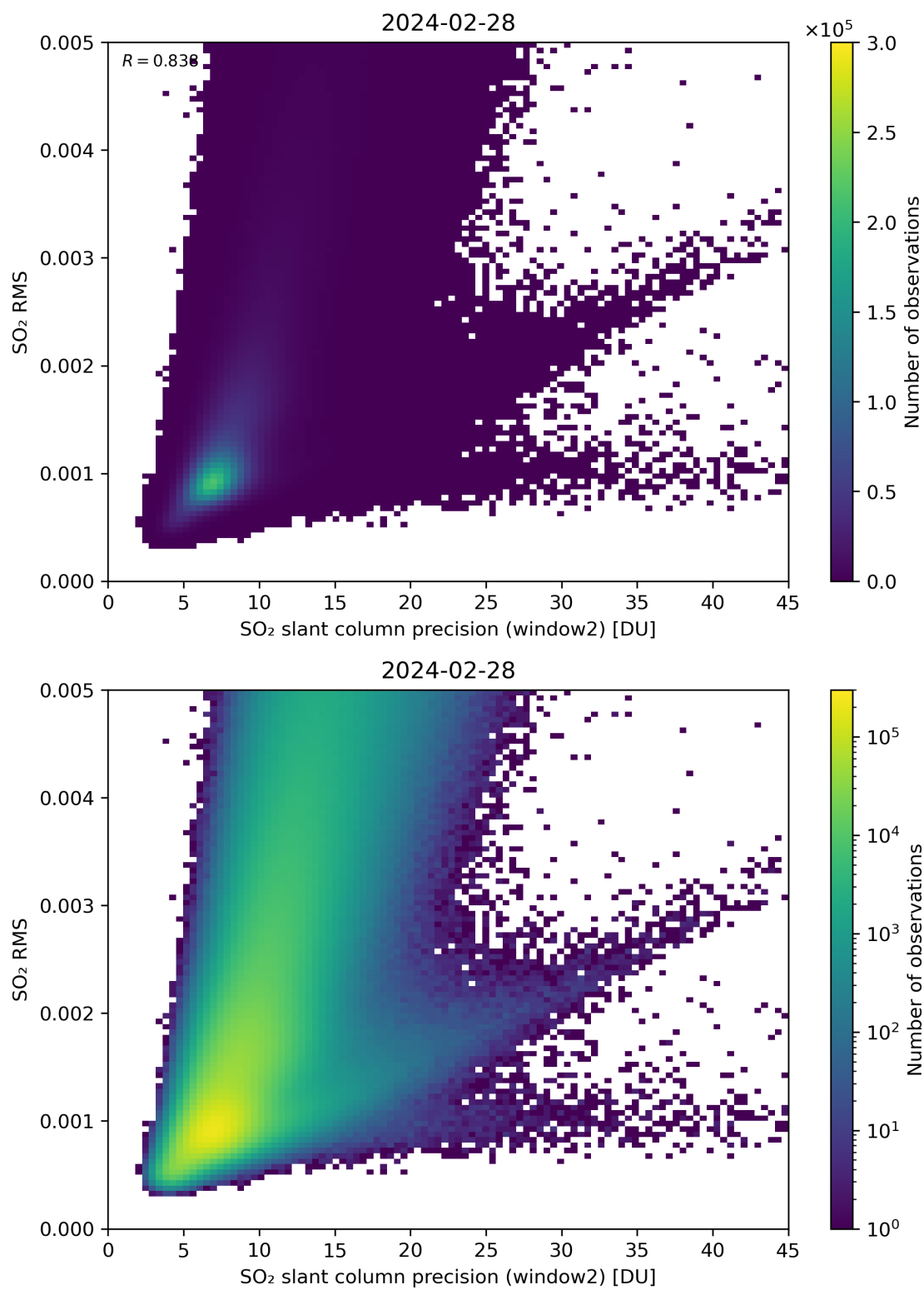
Figure 245: Scatter density plot of “SO 2 slant column precision (window2)” against “SO 2 RMS” for 2024-02-27 to 2024-02-29.
