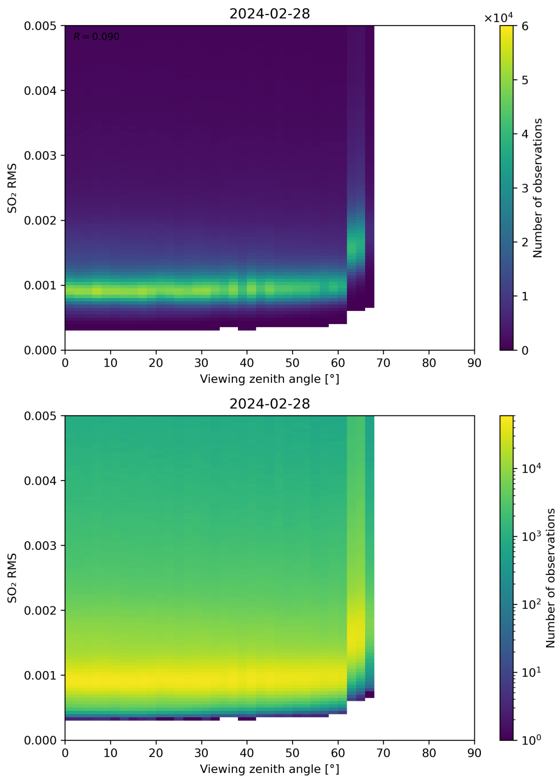
Figure 313: Scatter density plot of “Viewing zenith angle” against “SO 2 RMS” for 2024-02-27 to 2024-02-29.
