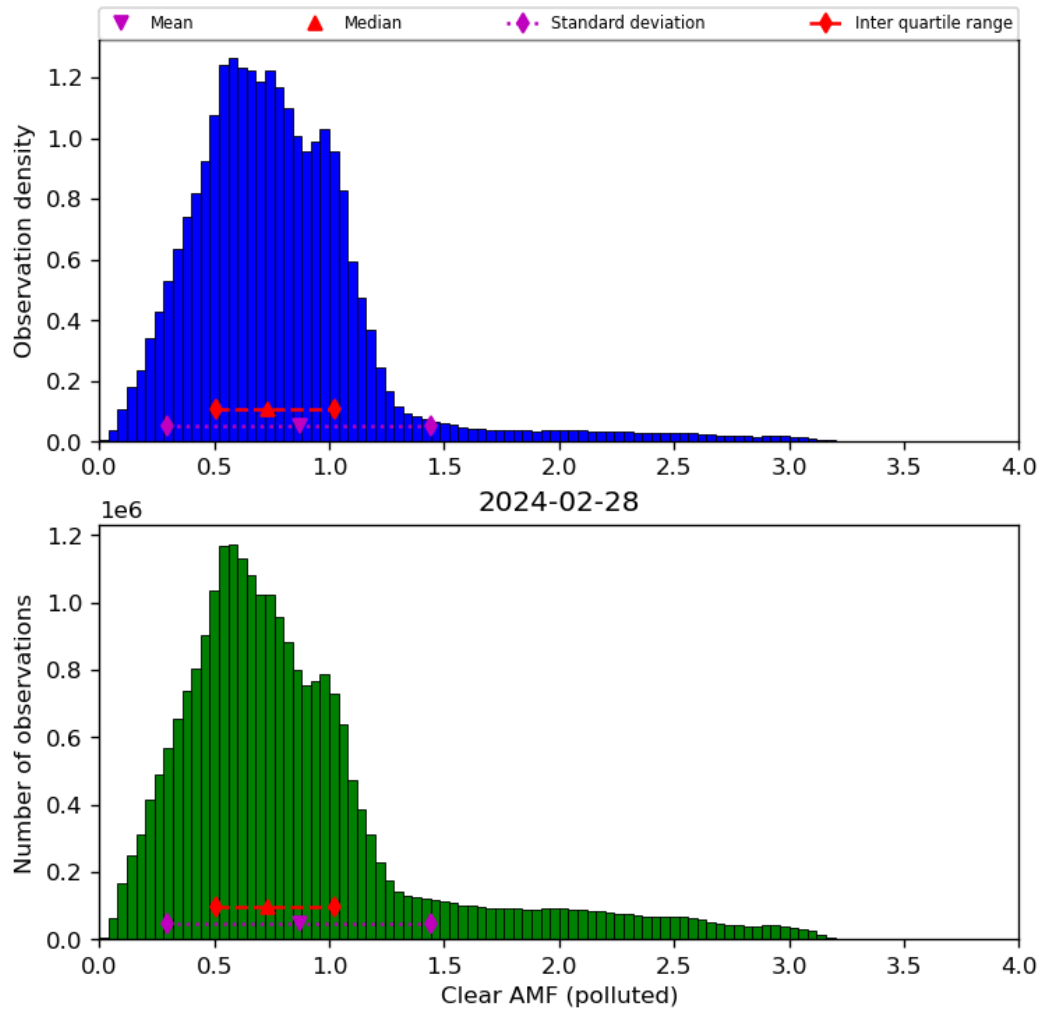
Figure 73: Histogram of “Clear AMF (polluted)” for 2024-02-27 to 2024-02-29
