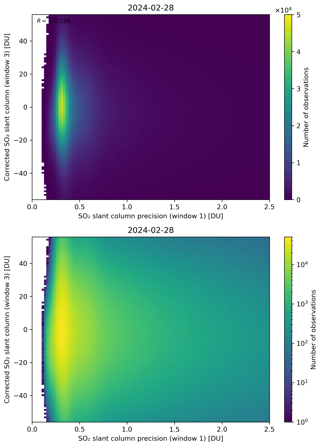
Figure 226: Scatter density plot of “SO 2 slant column precision (window 1)” against “Corrected SO 2 slant column (window 3)” for 2024-02-27 to 2024-02-29.
