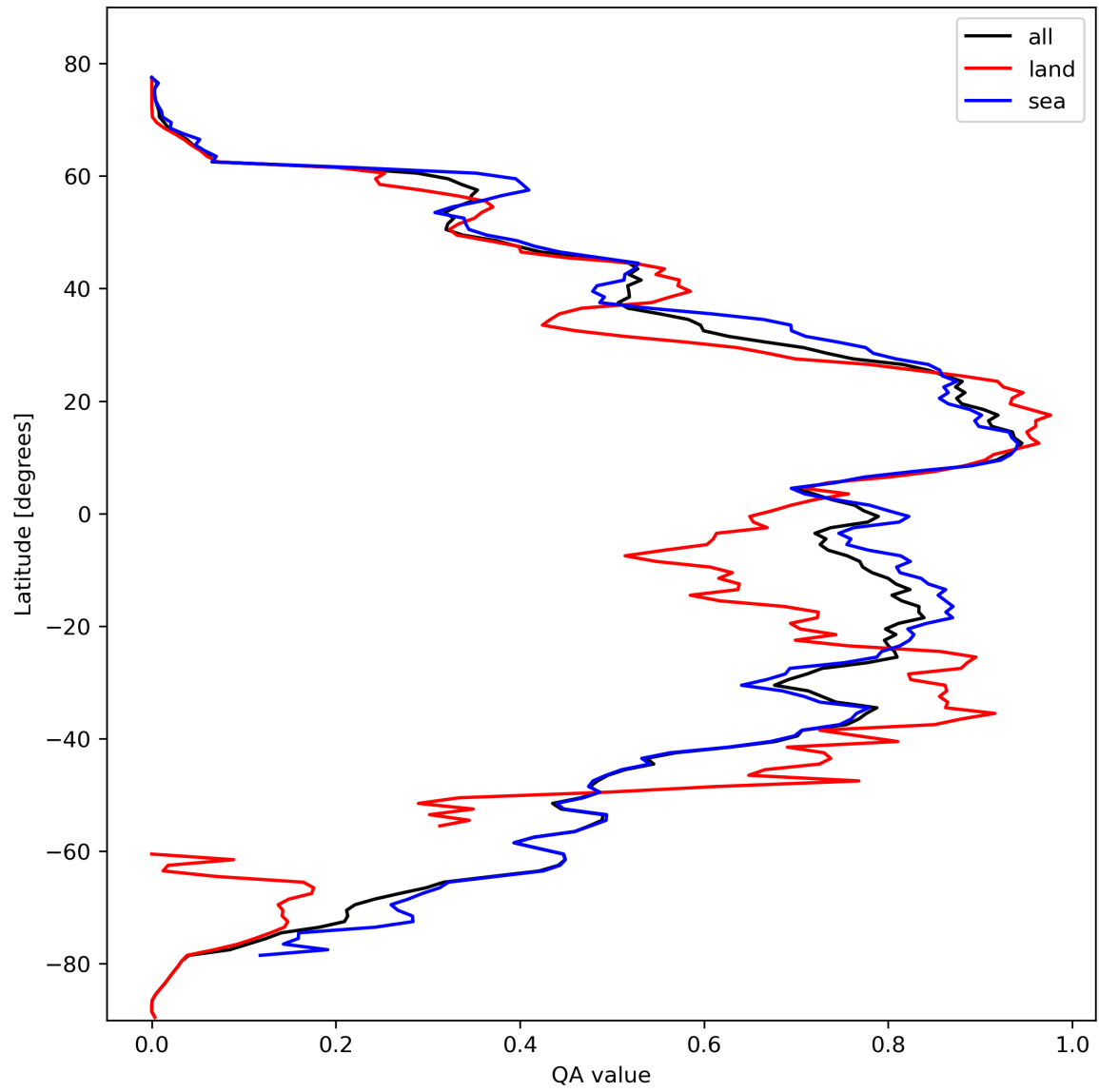
Figure 29: Zonal average of “QA value” for 2024-02-27 to 2024-02-29.
