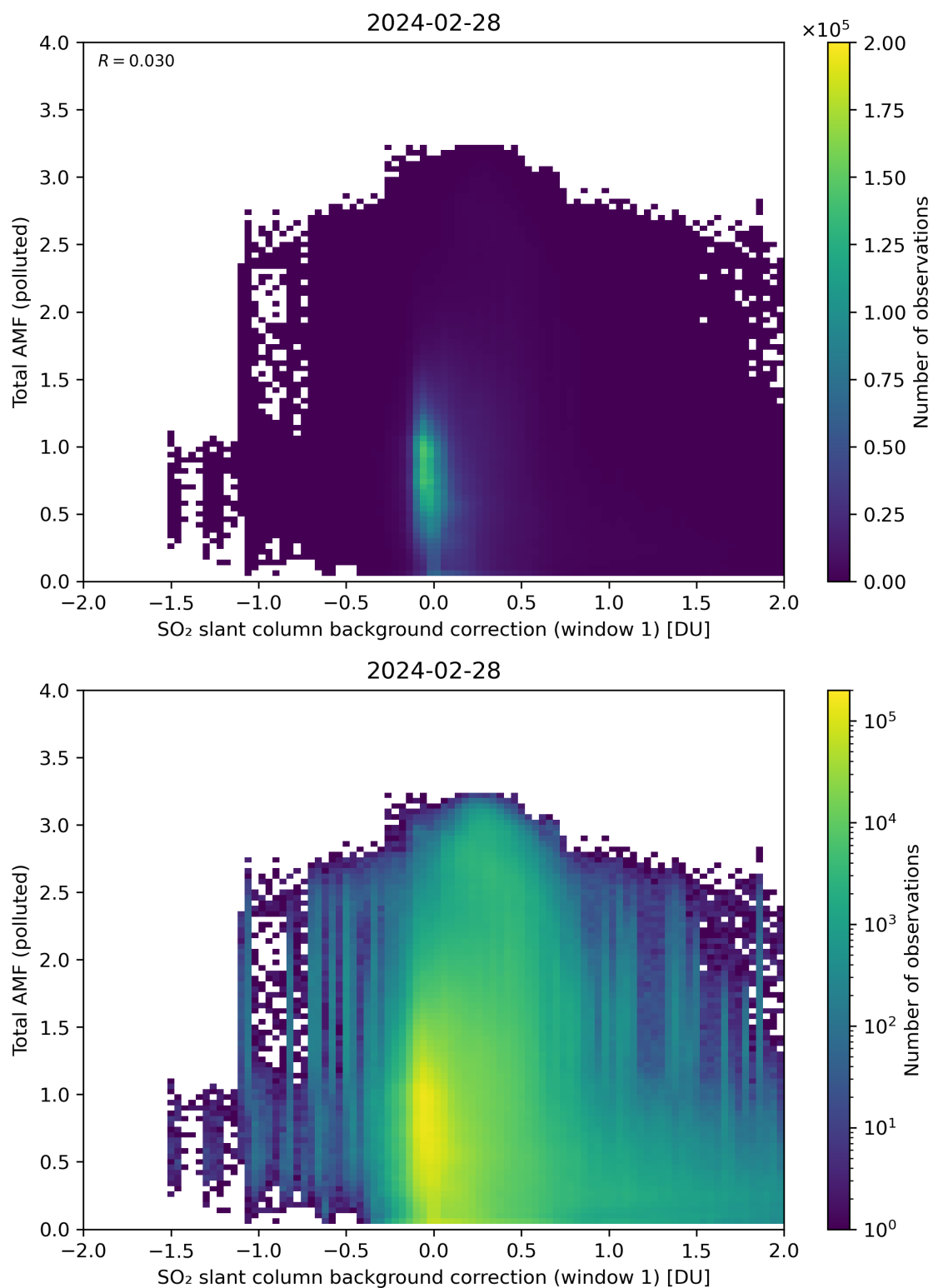
Figure 109: Scatter density plot of “SO 2 slant column background correction (window 1)” against “Total AMF (polluted)” for 2024-02-27 to 2024-02-29.
