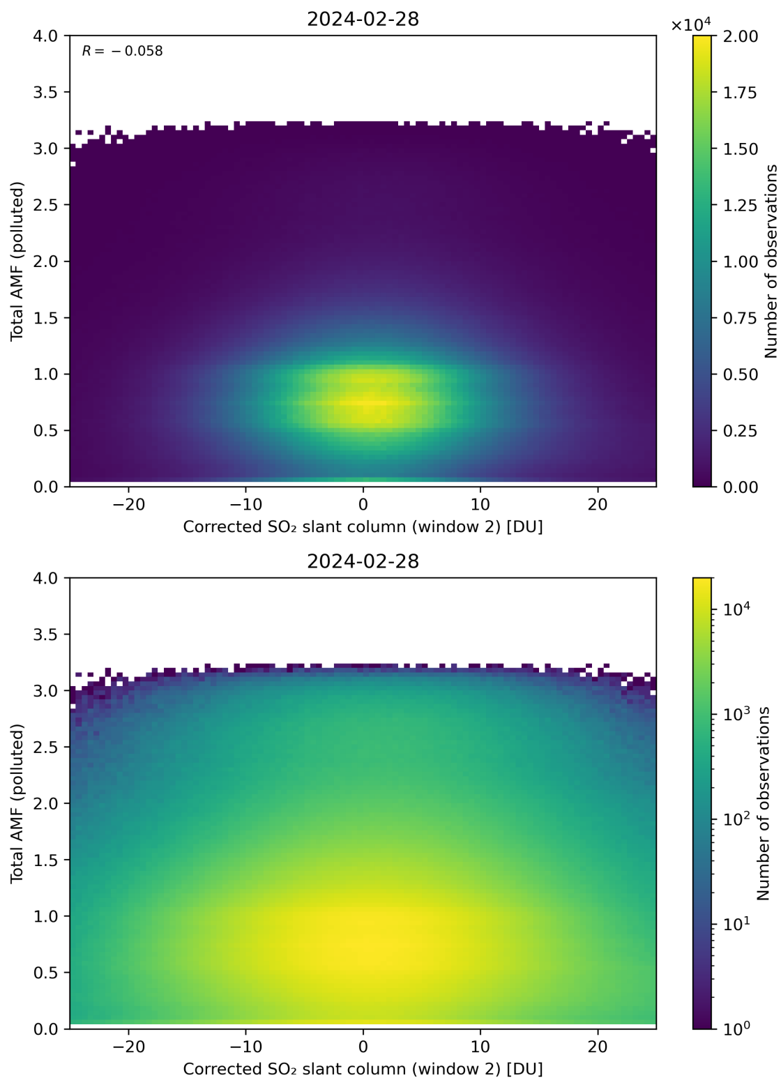
Figure 203: Scatter density plot of “Corrected SO 2 slant column (window 2)” against “Total AMF (polluted)” for 2024-02-27 to 2024-02-29.
