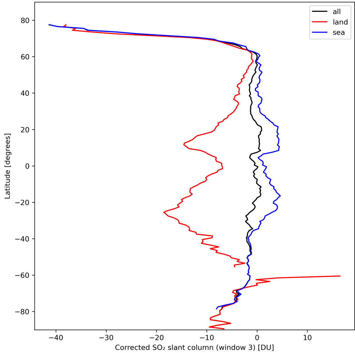
Figure 43: Zonal average of “Corrected SO 2 slant column (window 3)” for 2024-02-27 to 2024-02-29.
