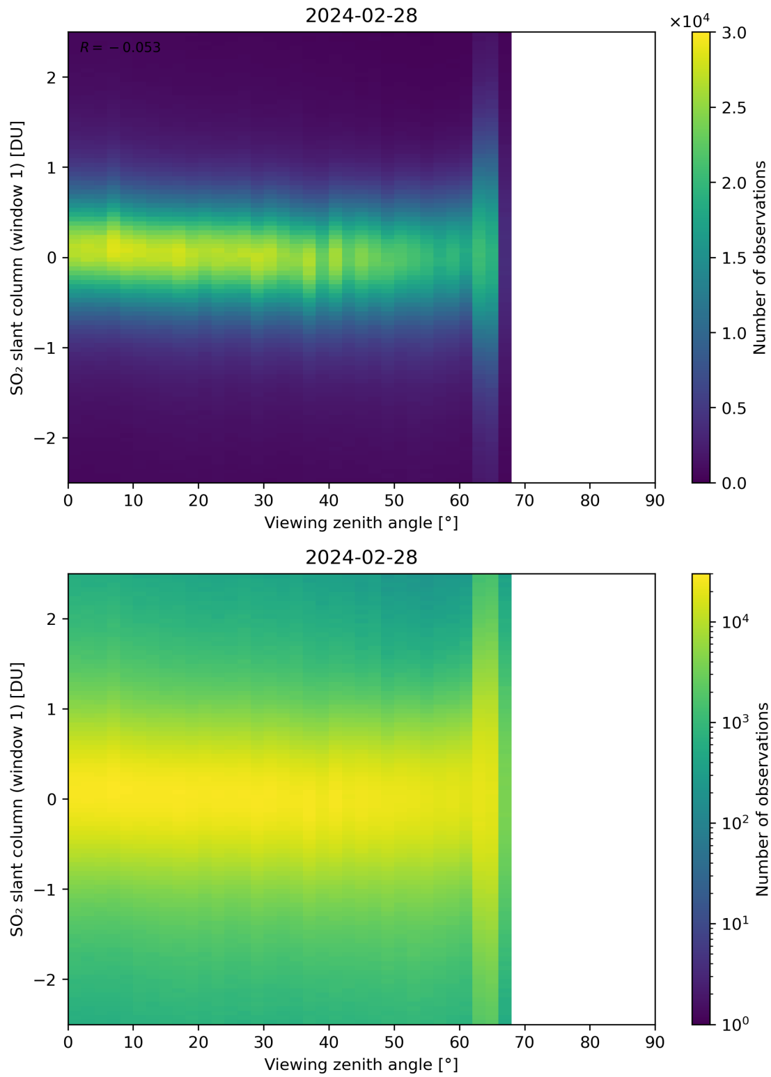
Figure 320: Scatter density plot of “Viewing zenith angle” against “SO 2 slant column (window 1)” for 2024-02-27 to 2024-02-29.
