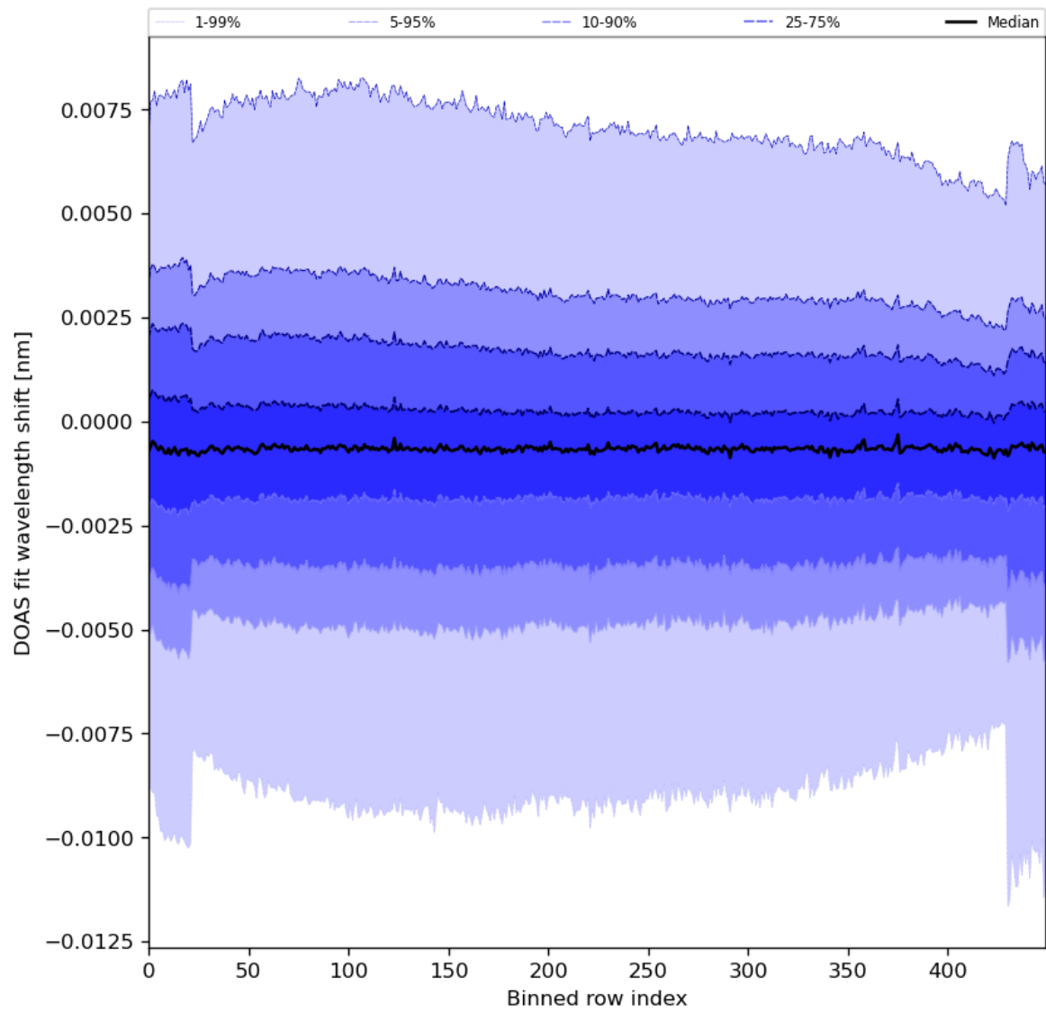
Figure 91: Along track statistics of “DOAS fit wavelength shift” for 2024-02-27 to 2024-02-29
