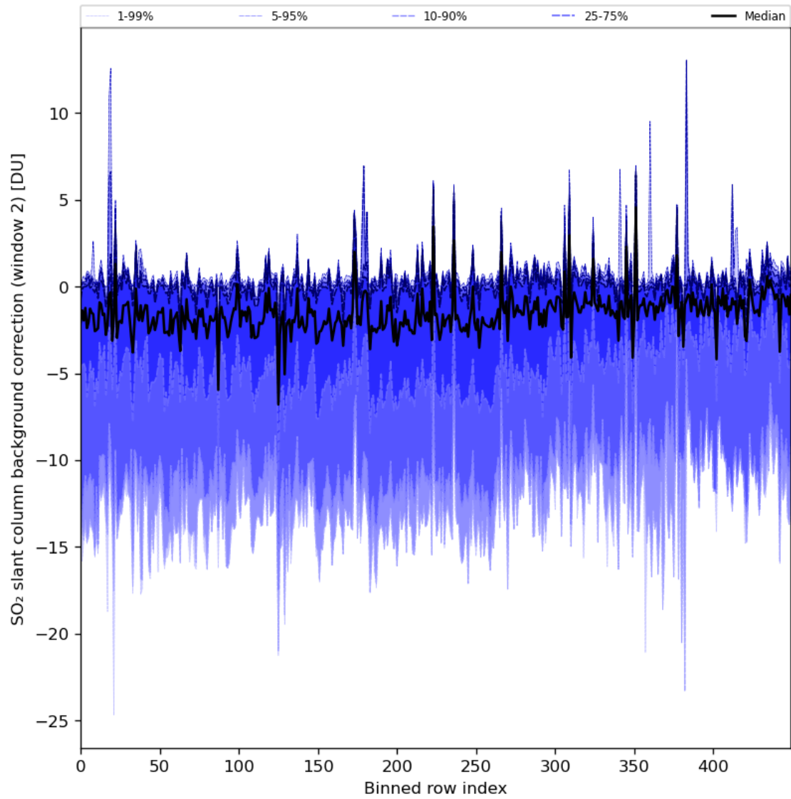
Figure 86: Along track statistics of “SO 2 slant column background correction (window 2)” for 2024-02-27 to 2024-02-29
