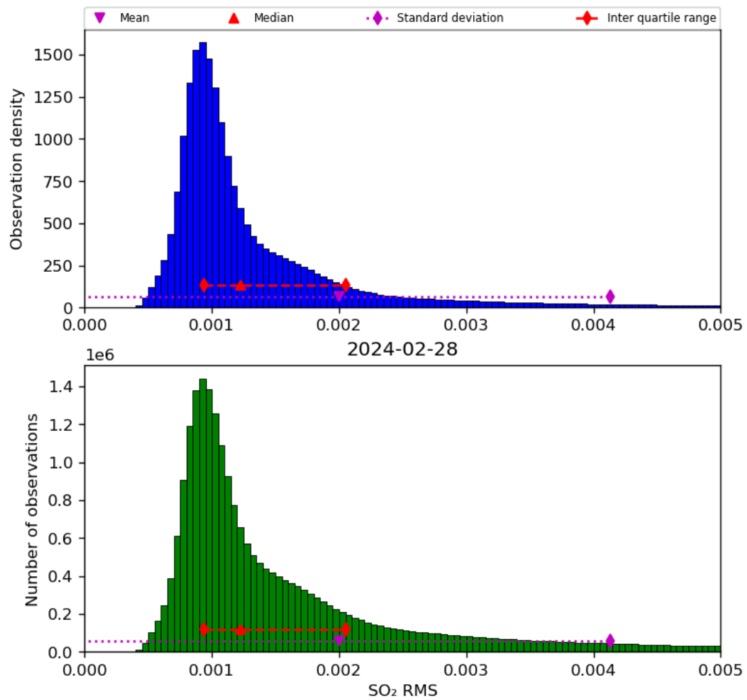
Figure 70: Histogram of “SO 2 RMS” for 2024-02-27 to 2024-02-29
