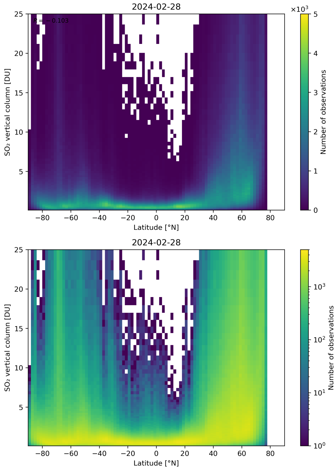
Figure 156: Scatter density plot of “Latitude” against “SO 2 vertical column” for 2024-02-27 to 2024-02-29.
