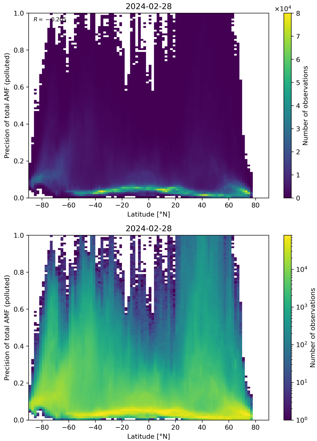
Figure 155: Scatter density plot of “Latitude” against “Precision of total AMF (polluted)” for 2024-02-27 to 2024-02-29.
