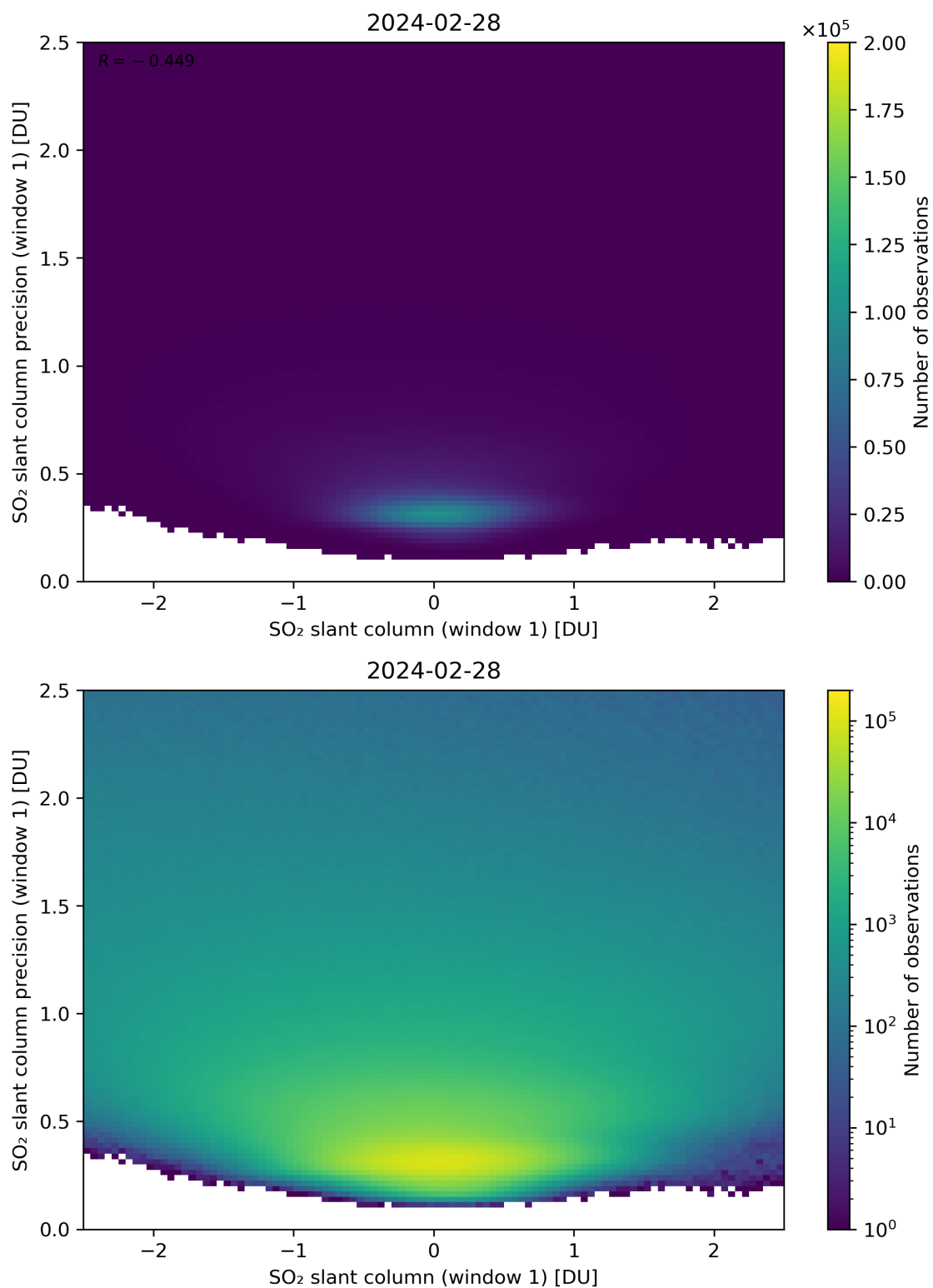
Figure 235: Scatter density plot of “SO 2 slant column (window 1)” against “SO 2 slant column precision (window 1)” for 2024-02-27 to 2024-02-29.
