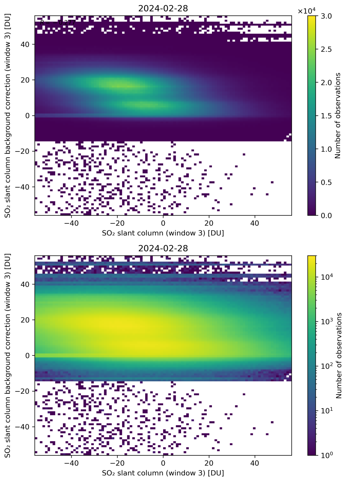
Figure 253: Scatter density plot of “SO 2 slant column (window 3)” against “SO 2 slant column background correction (window 3)” for 2024-02-27 to 2024-02-29.
