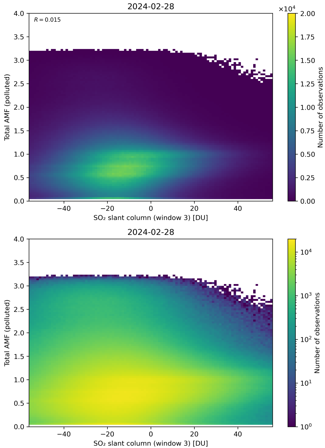
Figure 268: Scatter density plot of “SO 2 slant column (window 3)” against “Total AMF (polluted)” for 2024-02-27 to 2024-02-29.
