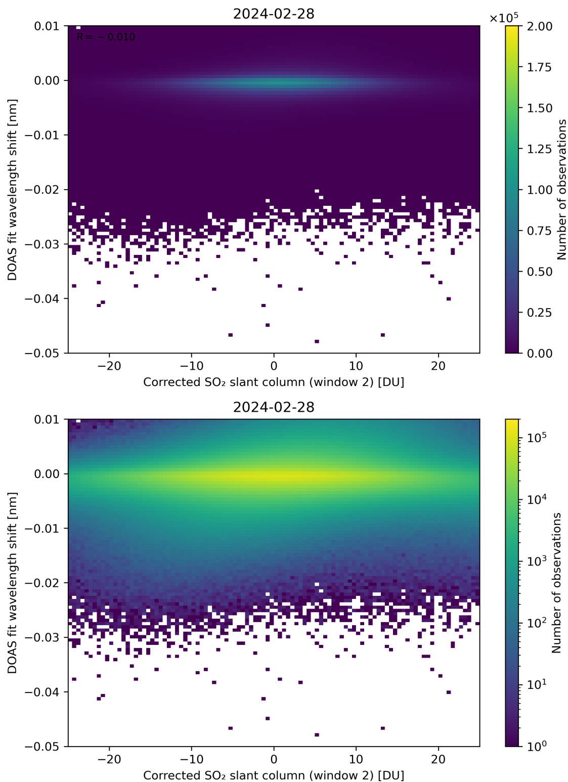
Figure 196: Scatter density plot of “Corrected SO 2 slant column (window 2)” against “DOAS fit wavelength shift” for 2024-02-27 to 2024-02-29.
