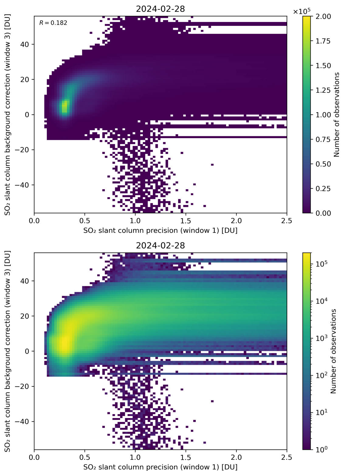
Figure 220: Scatter density plot of “SO 2 slant column precision (window 1)” against “SO 2 slant column background correction (window 3)” for 2024-02-27 to 2024-02-29.
