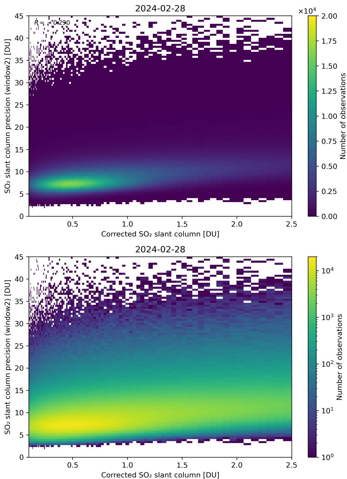
Figure 189: Scatter density plot of “Corrected SO 2 slant column” against “SO 2 slant column precision (window2)” for 2024-02-27 to 2024-02-29.
