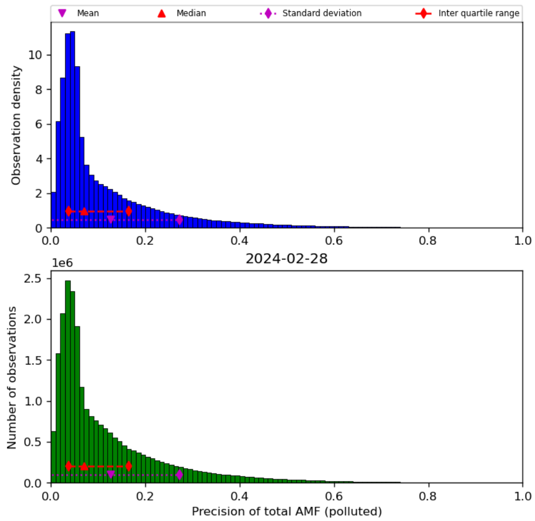
Figure 72: Histogram of “Precision of total AMF (polluted)” for 2024-02-27 to 2024-02-29
