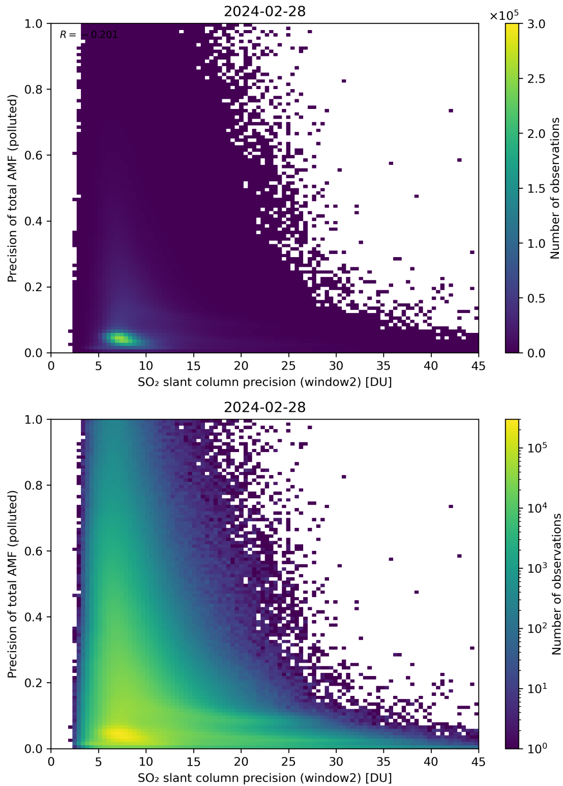
Figure 252: Scatter density plot of “SO 2 slant column precision (window2)” against “Precision of total AMF (polluted)” for 2024-02-27 to 2024-02-29.
