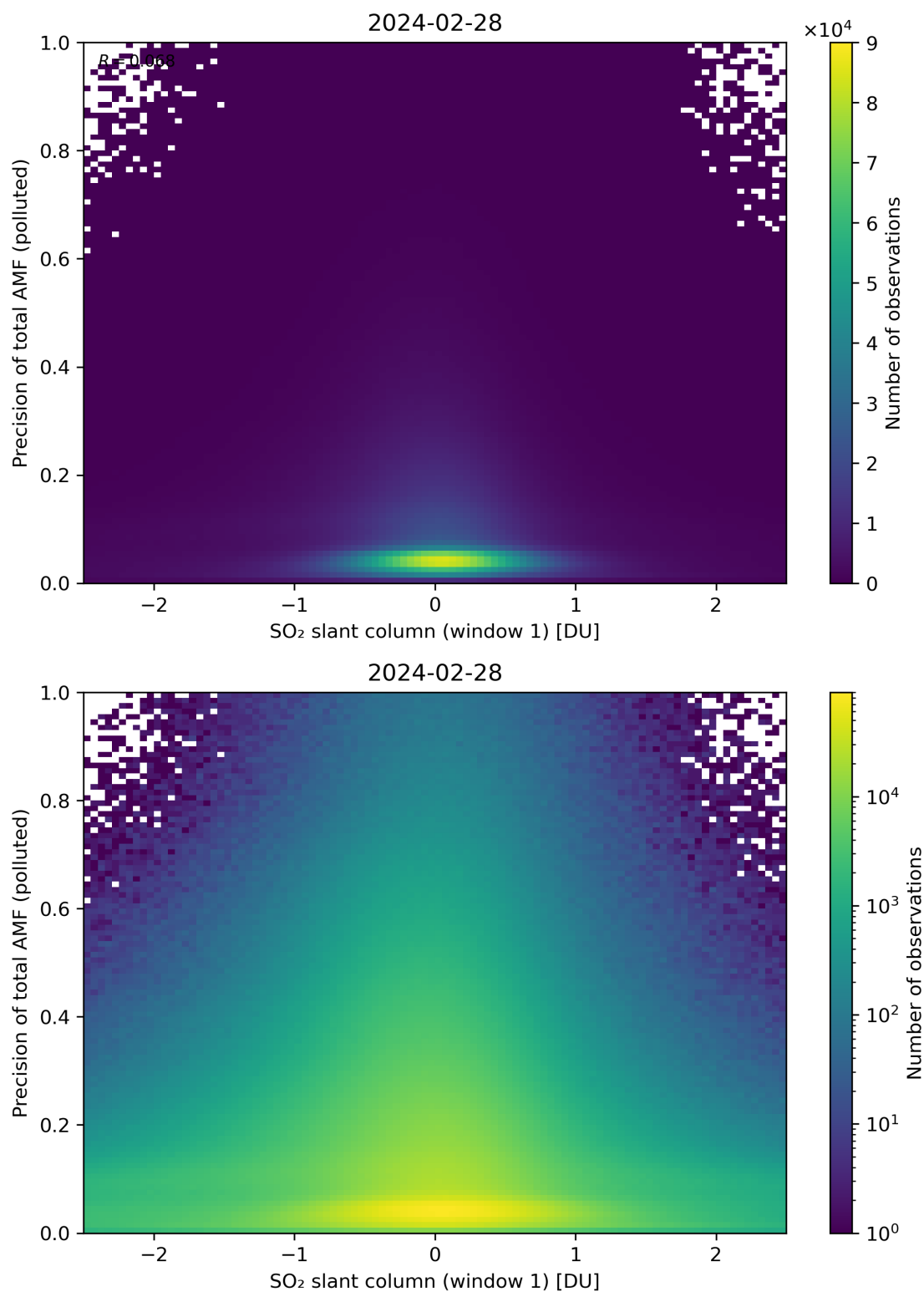
Figure 240: Scatter density plot of “SO 2 slant column (window 1)” against “Precision of total AMF (polluted)” for 2024-02-27 to 2024-02-29.
