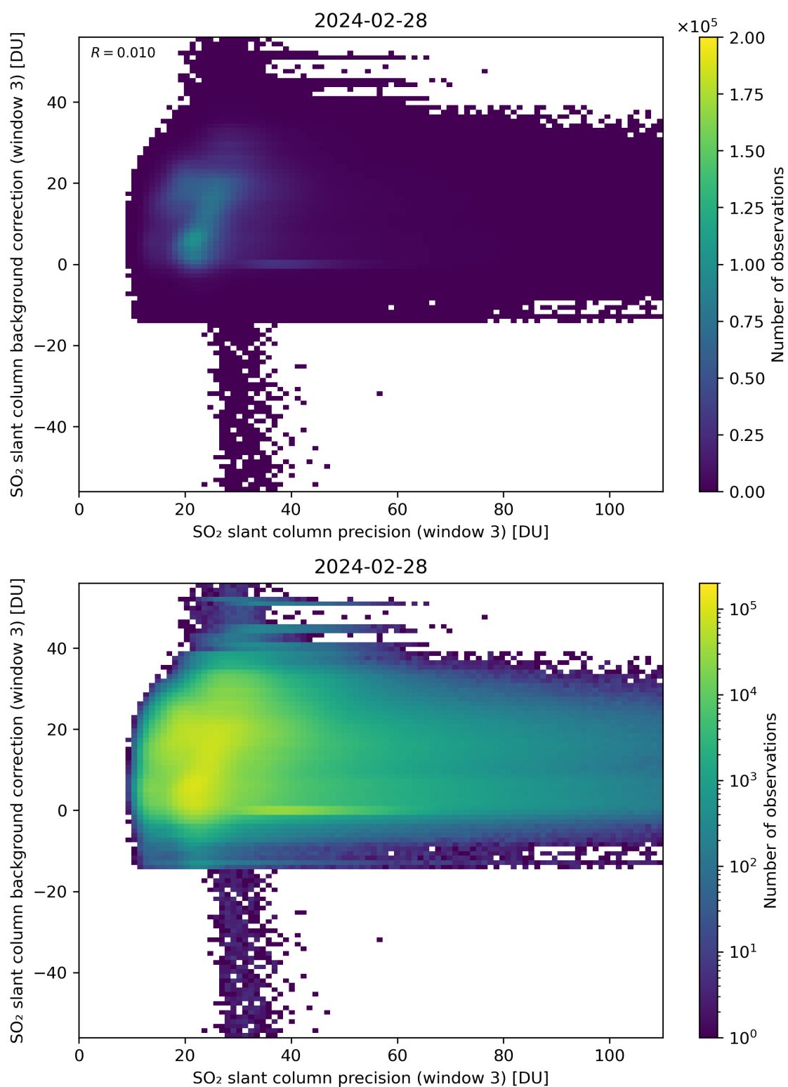
Figure 257: Scatter density plot of “SO 2 slant column precision (window 3)” against “SO 2 slant column background correction (window 3)” for 2024-02-27 to 2024-02-29.
