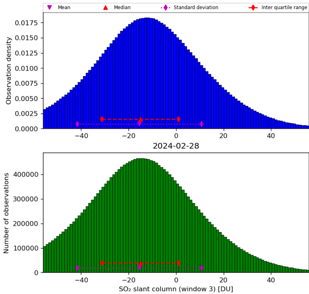
Figure 64: Histogram of “SO 2 slant column (window 3)” for 2024-02-27 to 2024-02-29
