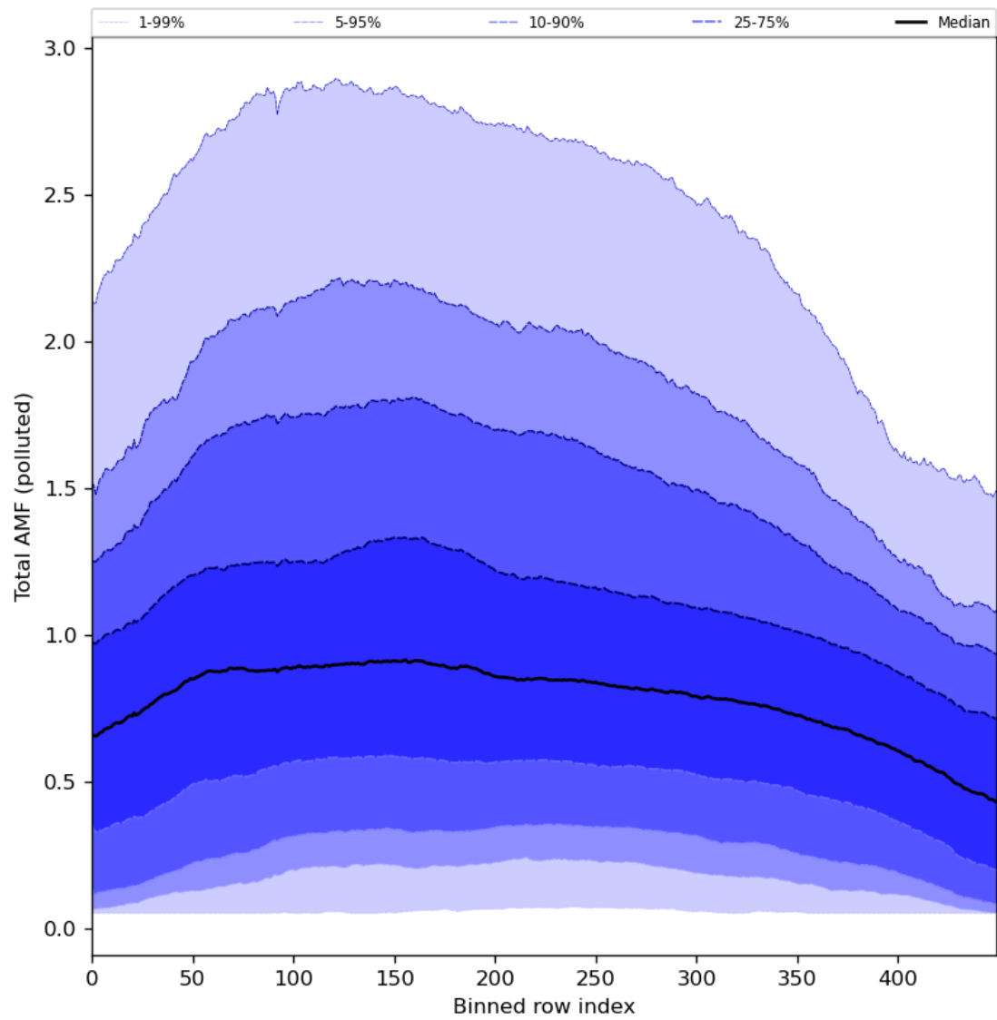
Figure 94: Along track statistics of “Total AMF (polluted)” for 2024-02-27 to 2024-02-29
