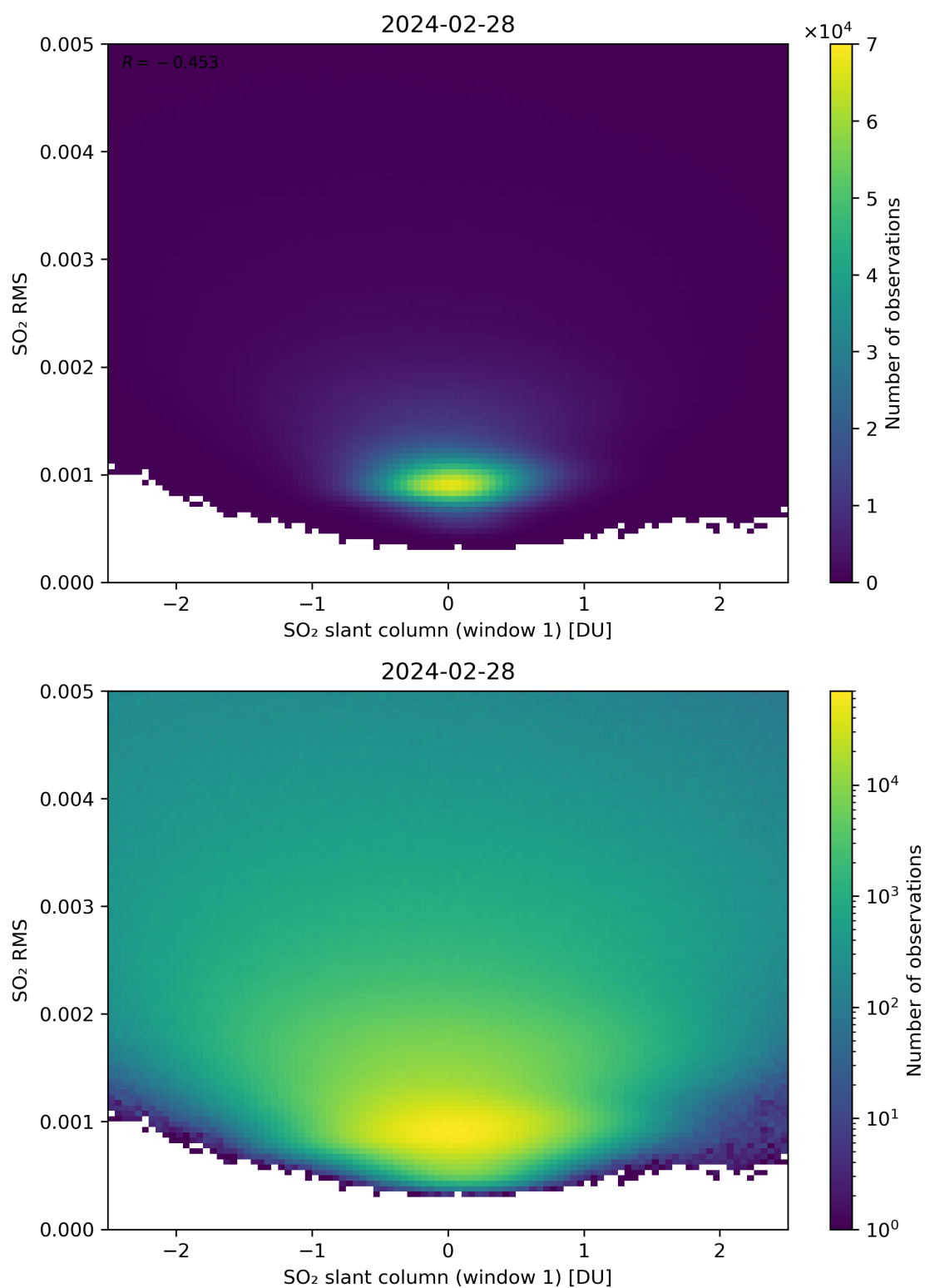
Figure 217: Scatter density plot of “SO 2 slant column (window 1)” against “SO 2 RMS” for 2024-02-27 to 2024-02-29.
