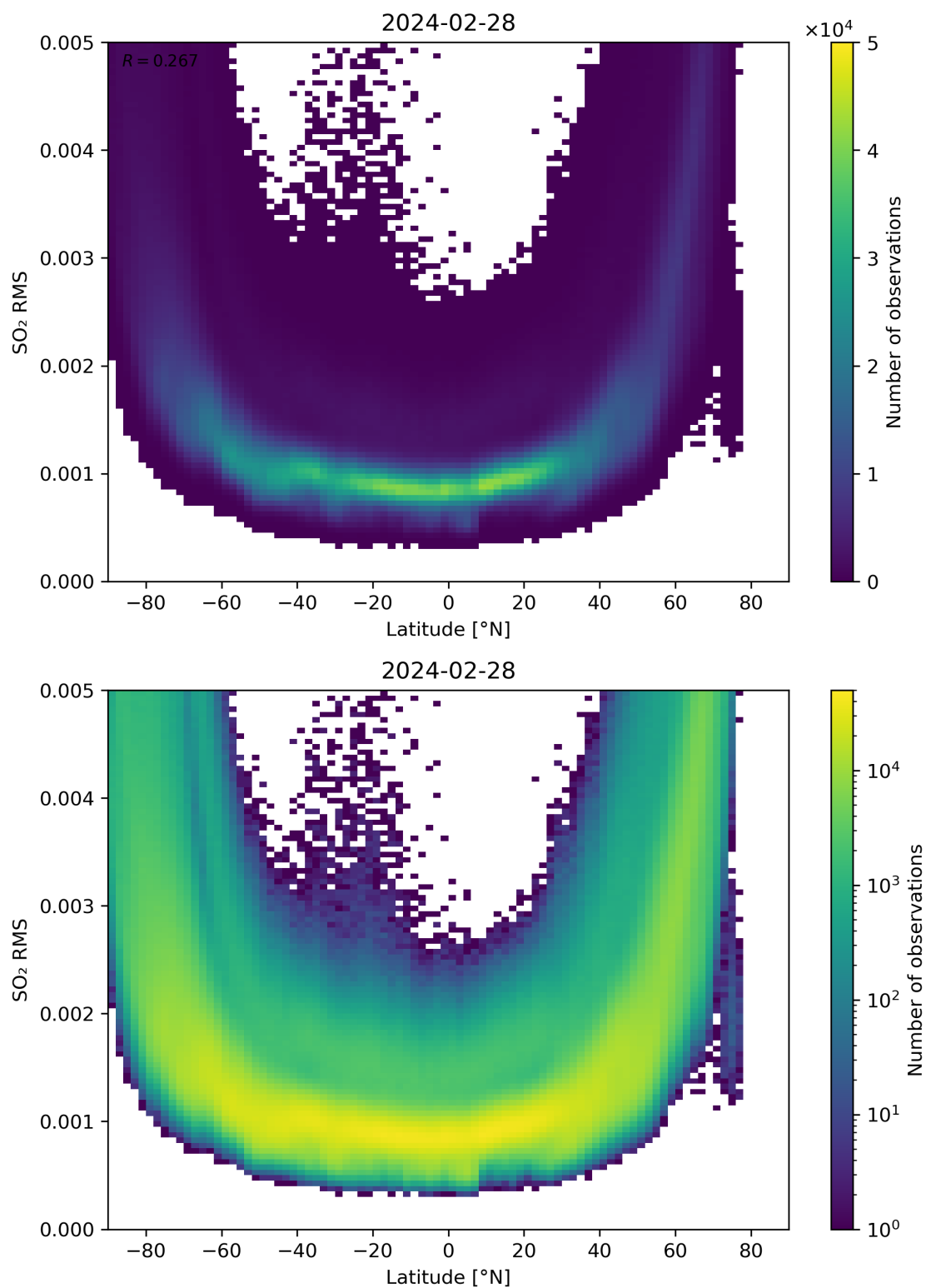
Figure 144: Scatter density plot of “Latitude” against “SO 2 RMS” for 2024-02-27 to 2024-02-29.
