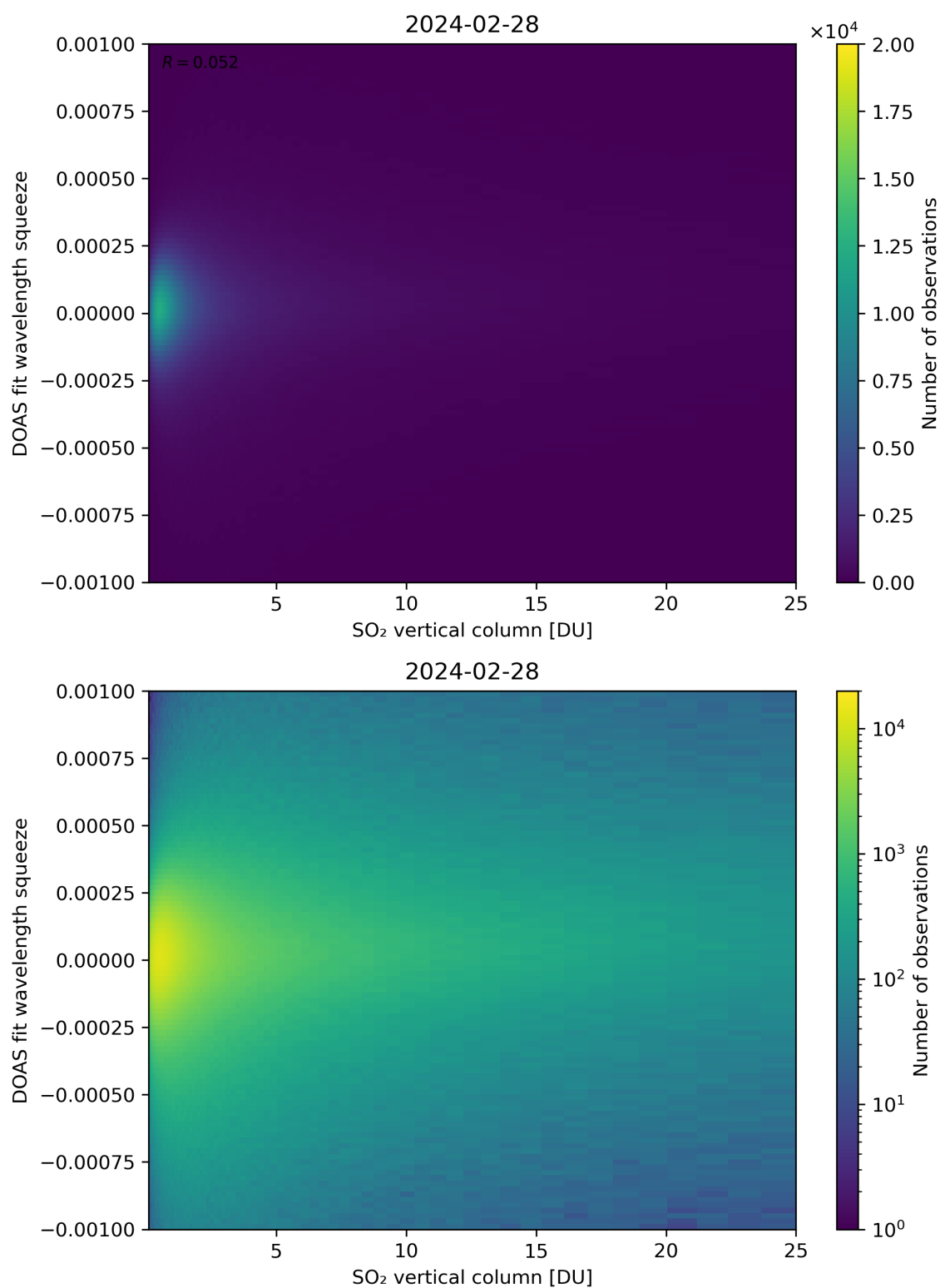
Figure 277: Scatter density plot of “SO 2 vertical column” against “DOAS fit wavelength squeeze” for 2024-02-27 to 2024-02-29.
