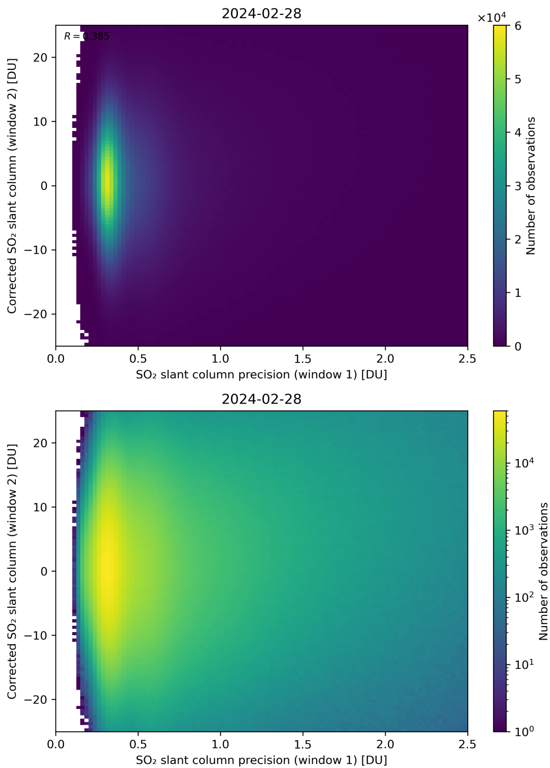
Figure 225: Scatter density plot of “SO 2 slant column precision (window 1)” against “Corrected SO 2 slant column (window 2)” for 2024-02-27 to 2024-02-29.
