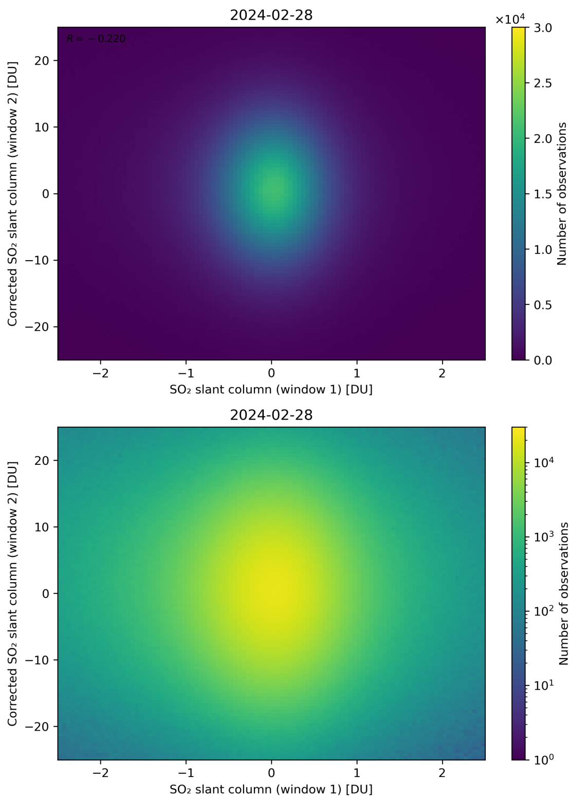
Figure 233: Scatter density plot of “SO 2 slant column (window 1)” against “Corrected SO 2 slant column (window 2)” for 2024-02-27 to 2024-02-29.
