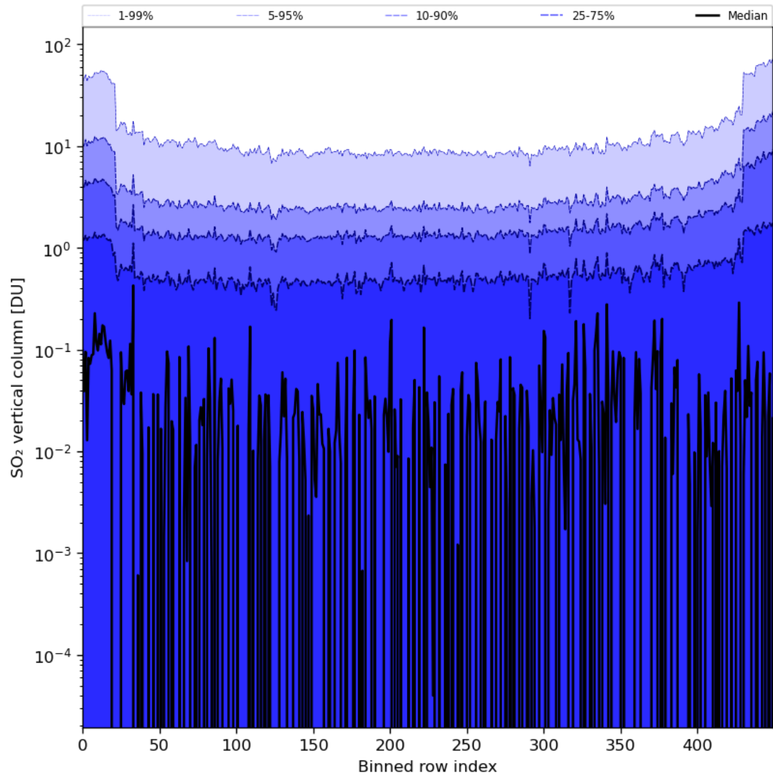
Figure 76: Along track statistics of “SO 2 vertical column” for 2024-02-27 to 2024-02-29
