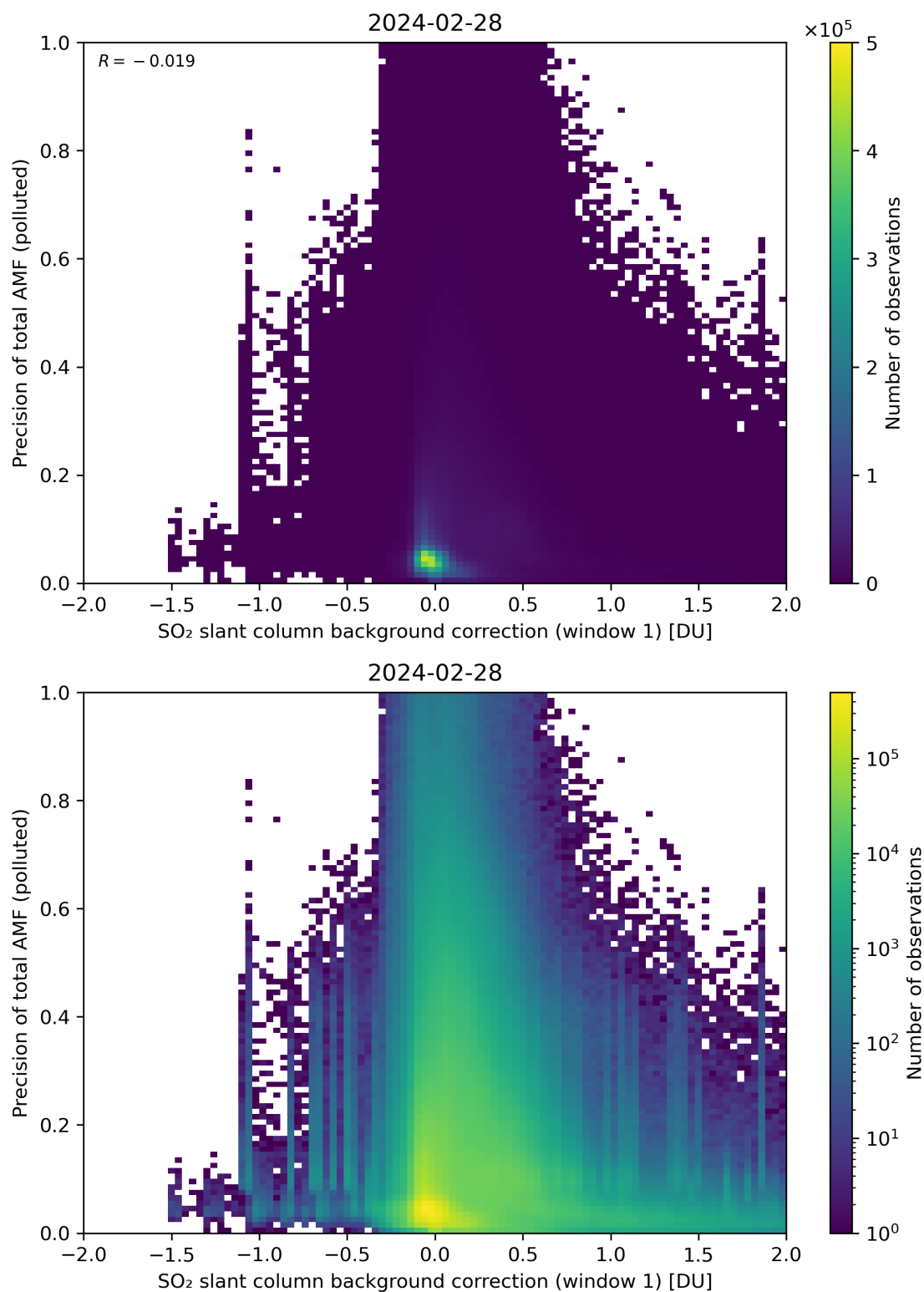
Figure 110: Scatter density plot of “SO 2 slant column background correction (window 1)” against “Precision of total AMF (polluted)” for 2024-02-27 to 2024-02-29.
