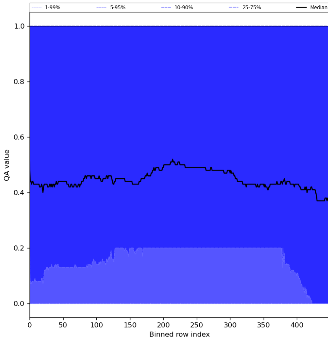
Figure 75: Along track statistics of “QA value” for 2024-02-27 to 2024-02-29
