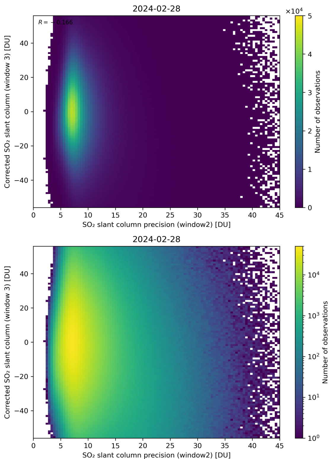
Figure 248: Scatter density plot of “SO 2 slant column precision (window2)” against “Corrected SO 2 slant column (window 3)” for 2024-02-27 to 2024-02-29.
