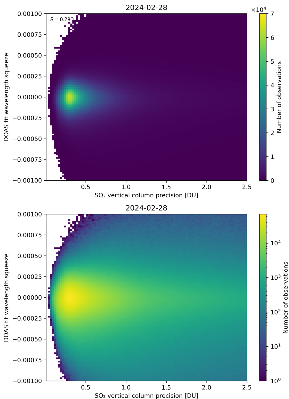
Figure 283: Scatter density plot of “SO 2 vertical column precision” against “DOAS fit wavelength squeeze” for 2024-02-27 to 2024-02-29.
