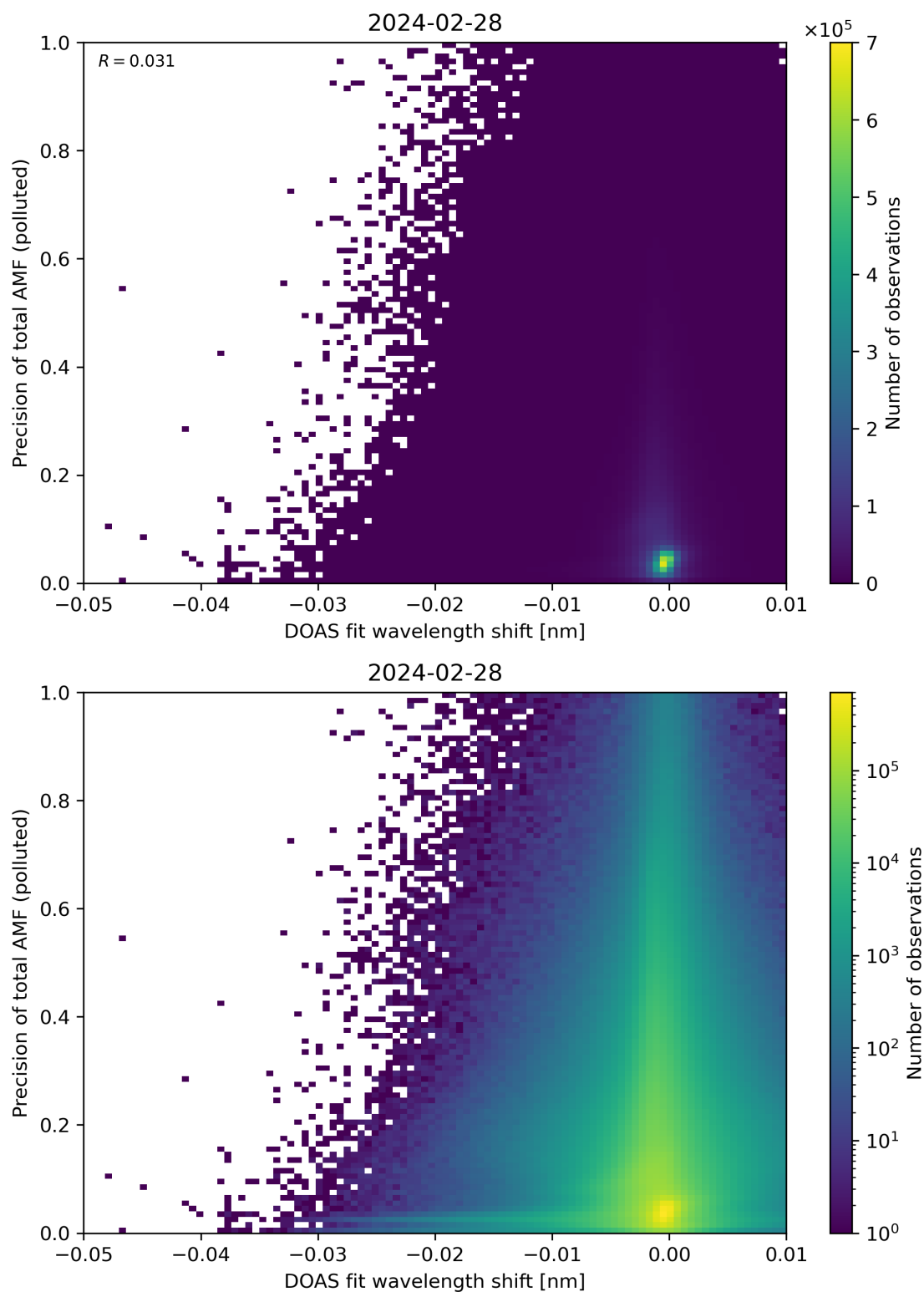
Figure 131: Scatter density plot of “DOAS fit wavelength shift” against “Precision of total AMF (polluted)” for 2024-02-27 to 2024-02-29.
