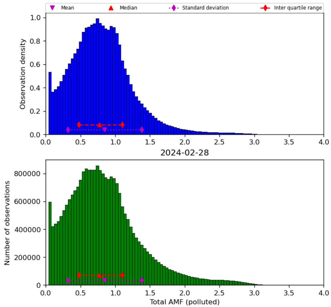
Figure 71: Histogram of “Total AMF (polluted)” for 2024-02-27 to 2024-02-29
