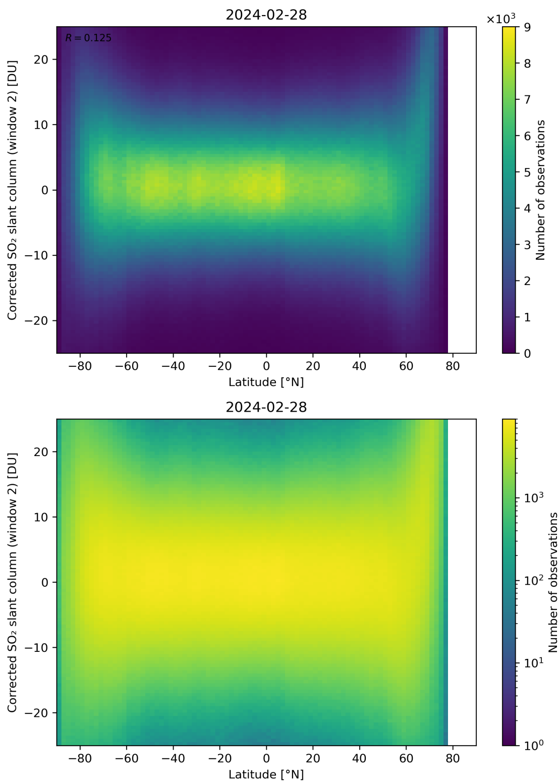
Figure 147: Scatter density plot of “Latitude” against “Corrected SO 2 slant column (window 2)” for 2024-02-27 to 2024-02-29.
