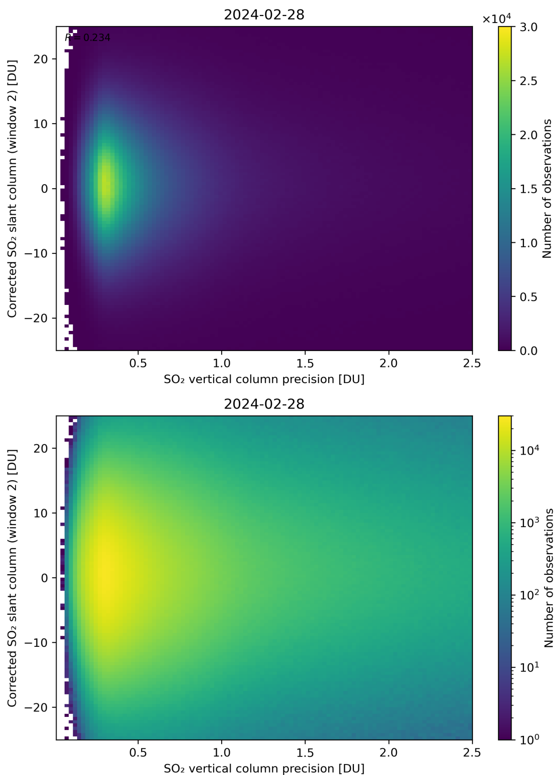
Figure 287: Scatter density plot of “SO 2 vertical column precision” against “Corrected SO 2 slant column (window 2)” for 2024-02-27 to 2024-02-29.
