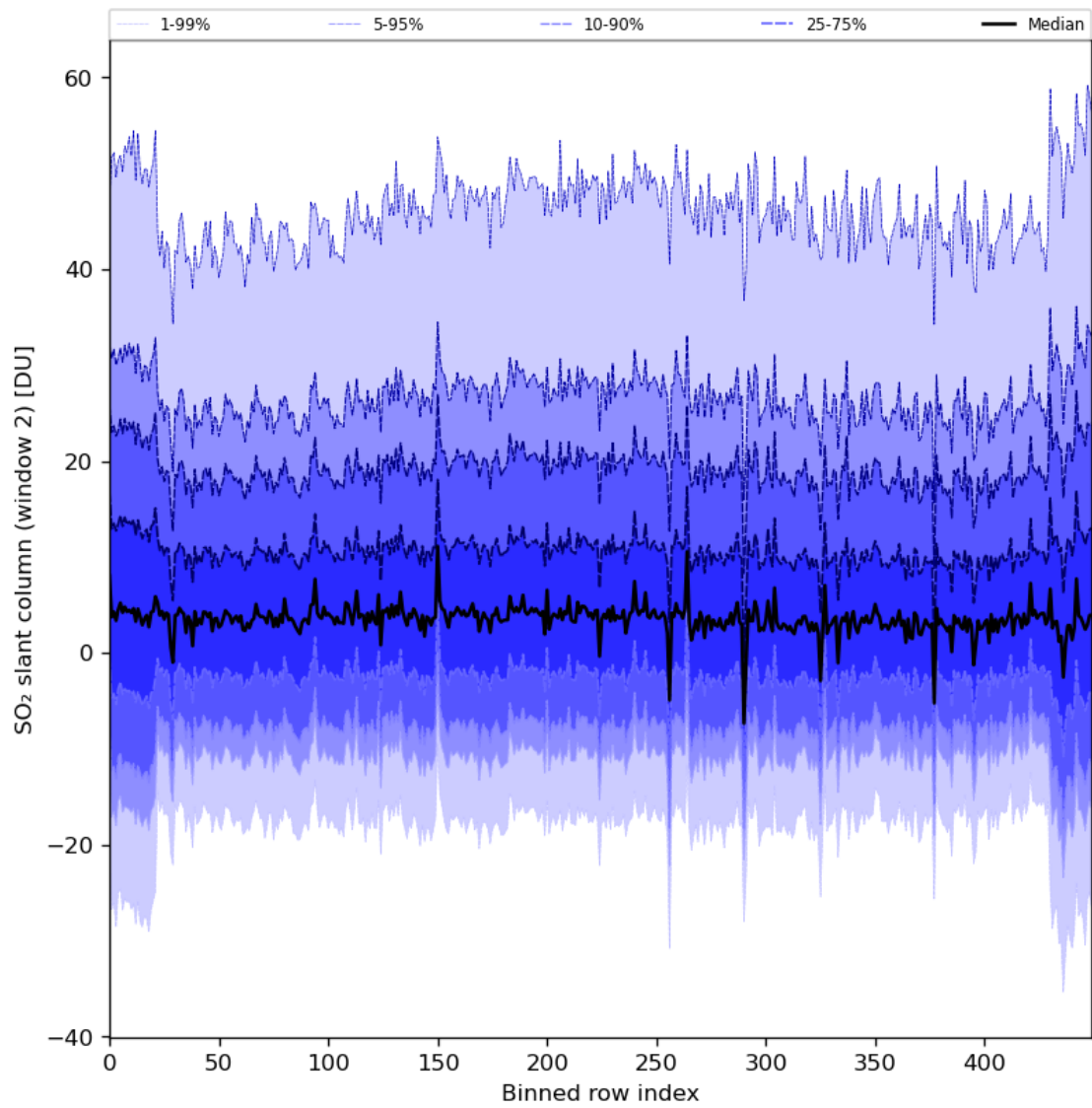
Figure 83: Along track statistics of “SO 2 slant column (window 2)” for 2024-02-27 to 2024-02-29
