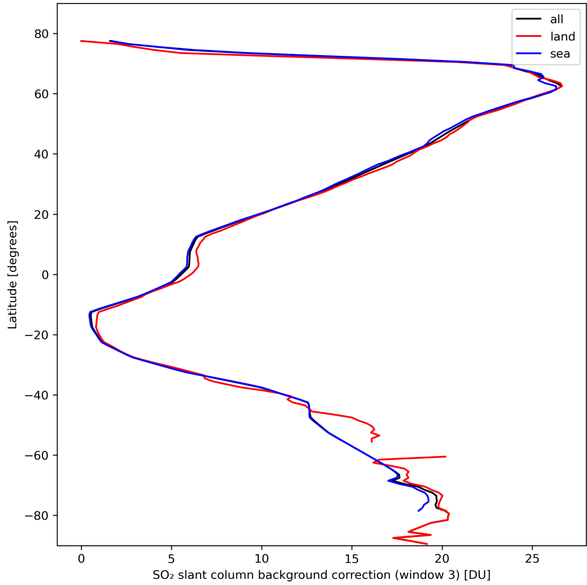
Figure 44: Zonal average of “SO 2 slant column background correction (window 3)” for 2024-02-27 to 2024-02-29.
