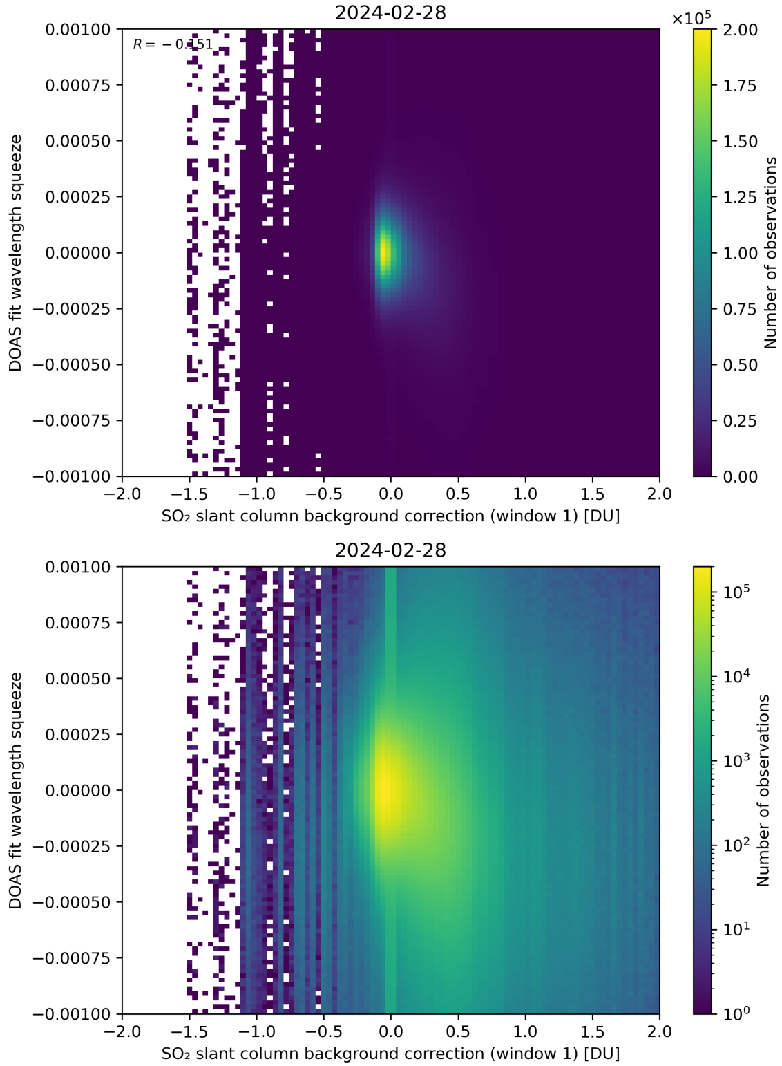
Figure 101: Scatter density plot of “SO 2 slant column background correction (window 1)” against “DOAS fit wavelength squeeze” for 2024-02-27 to 2024-02-29.
