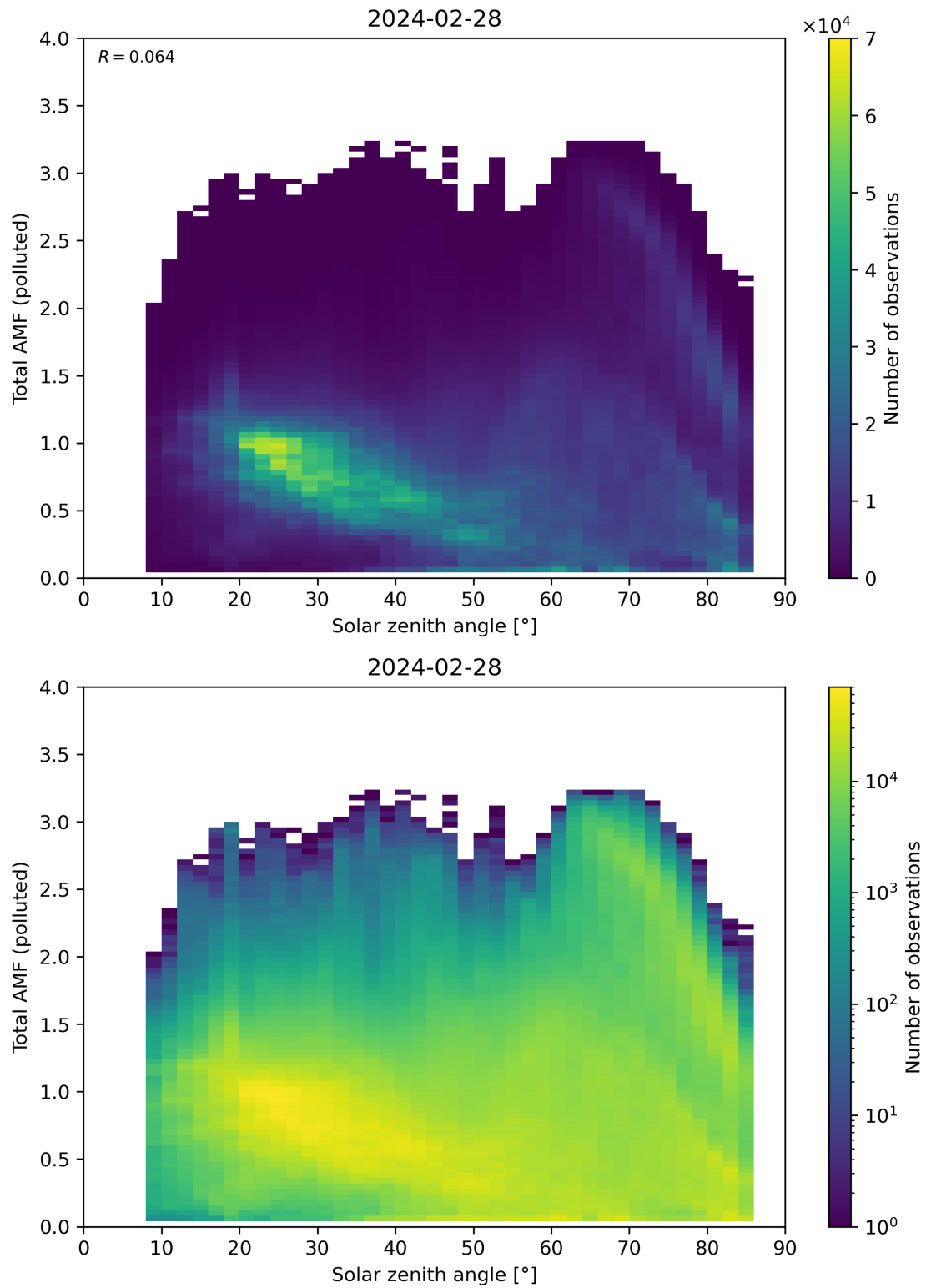
Figure 174: Scatter density plot of “Solar zenith angle” against “Total AMF (polluted)” for 2024-02-27 to 2024-02-29.
