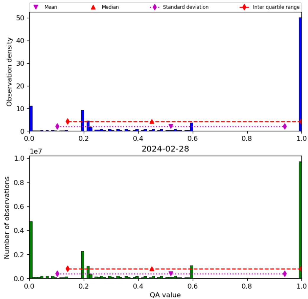
Figure 52: Histogram of “QA value” for 2024-02-27 to 2024-02-29
