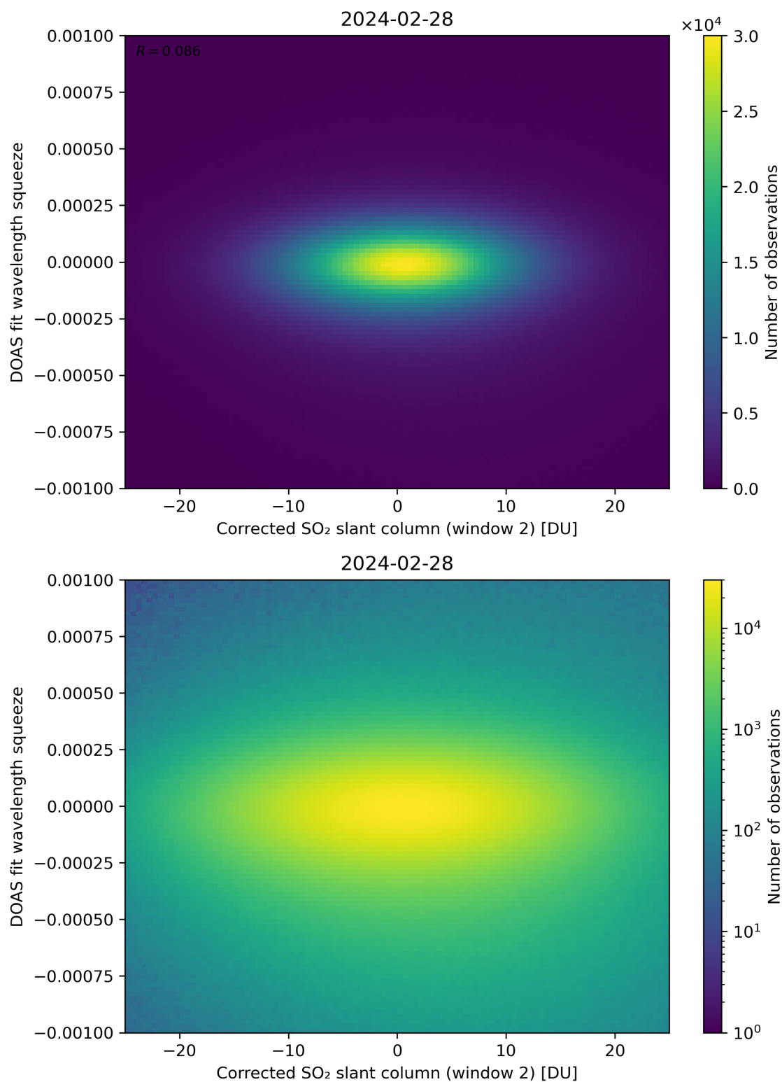
Figure 197: Scatter density plot of “Corrected SO 2 slant column (window 2)” against “DOAS fit wavelength squeeze” for 2024-02-27 to 2024-02-29.
