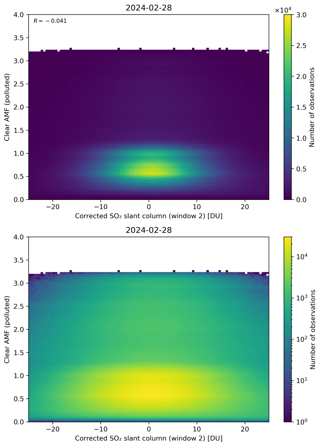
Figure 199: Scatter density plot of “Corrected SO 2 slant column (window 2)” against “Clear AMF (polluted)” for 2024-02-27 to 2024-02-29.
