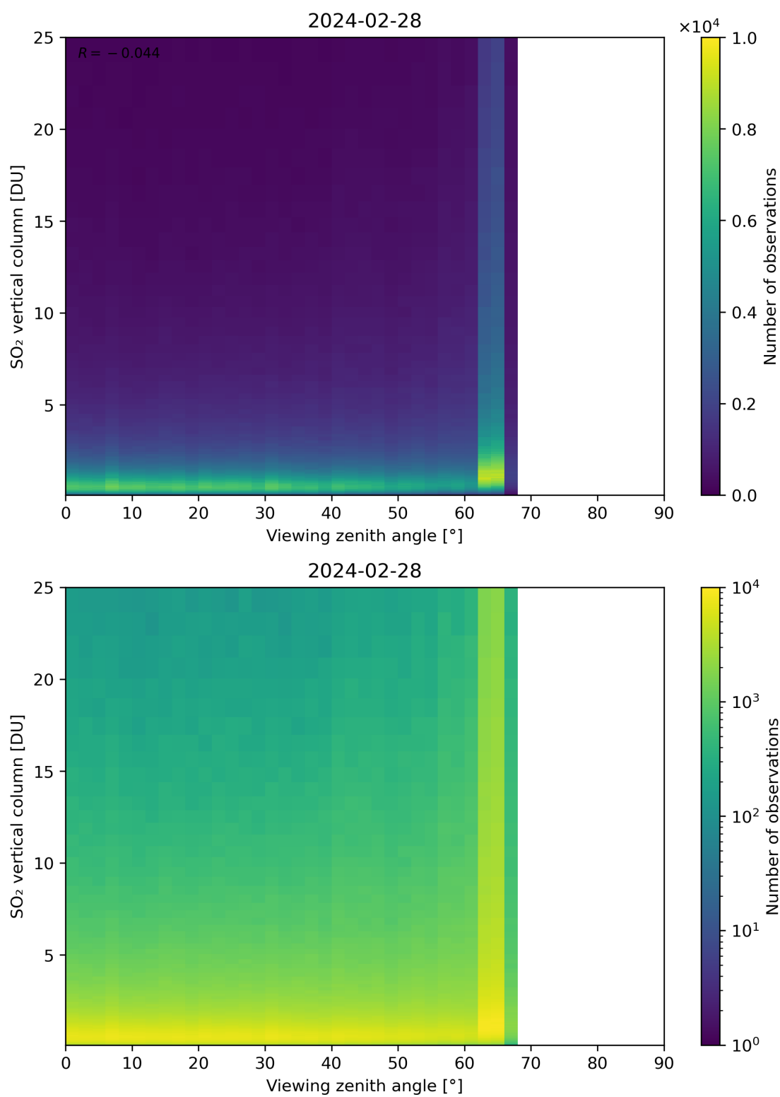
Figure 327: Scatter density plot of “Viewing zenith angle” against “SO 2 vertical column” for 2024-02-27 to 2024-02-29.
