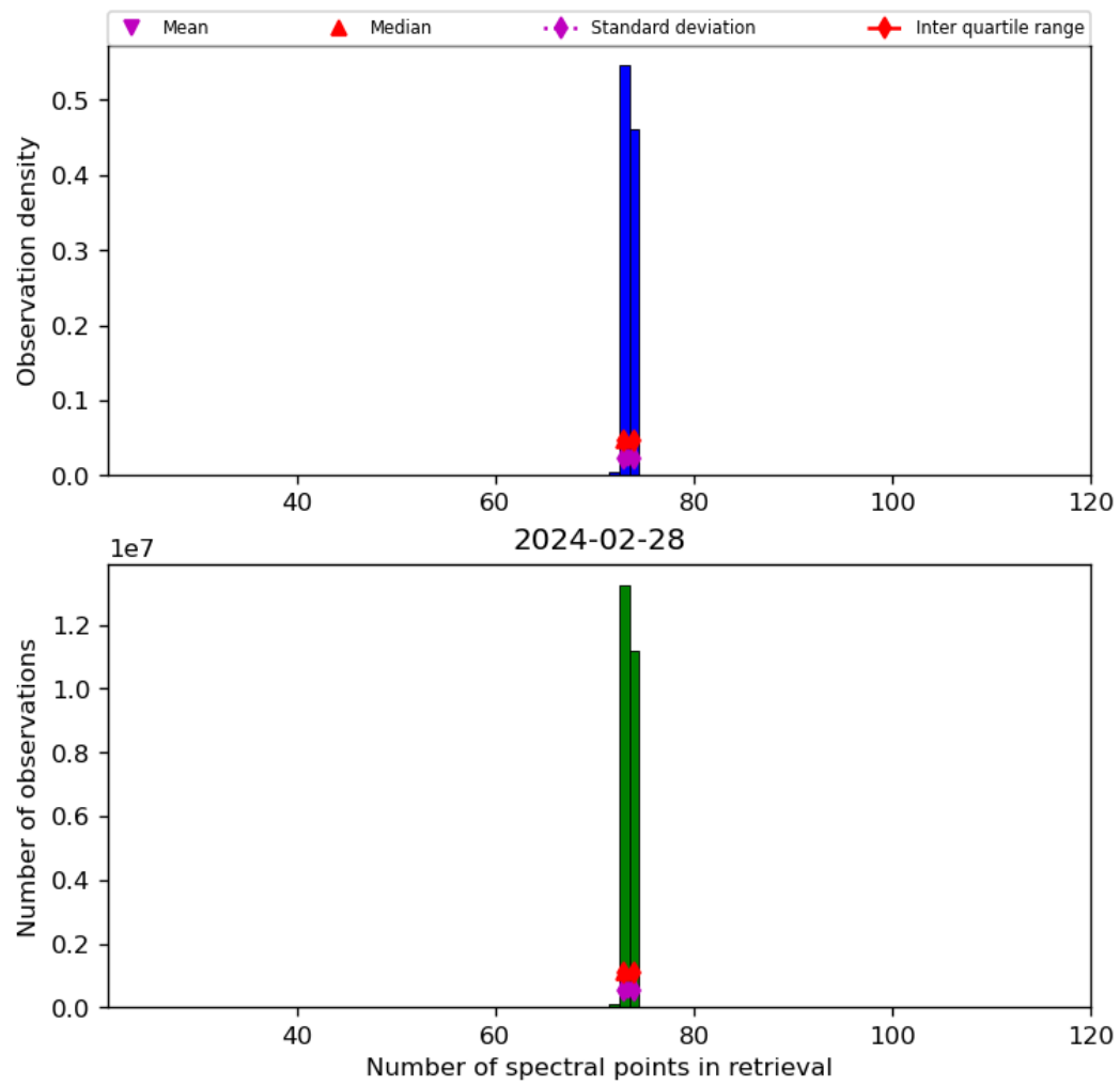
Figure 74: Histogram of “Number of spectral points in retrieval” for 2024-02-27 to 2024-02-29
