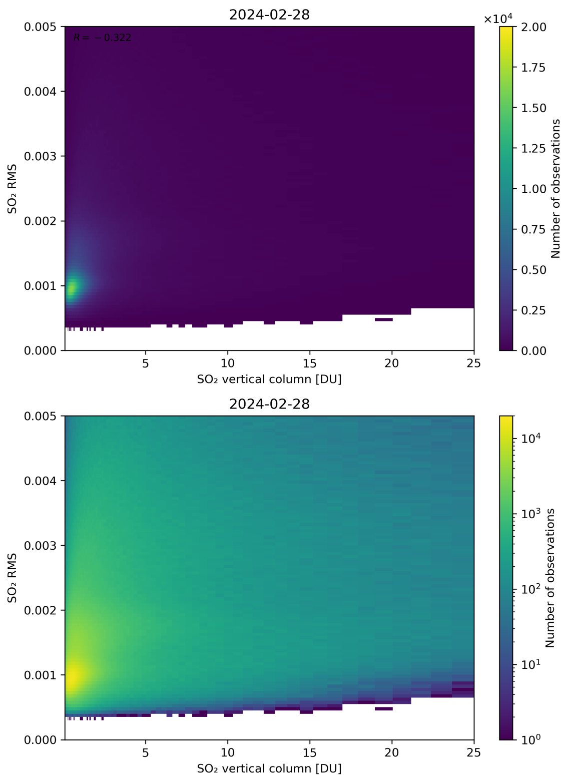
Figure 278: Scatter density plot of “SO 2 vertical column” against “SO 2 RMS” for 2024-02-27 to 2024-02-29.
