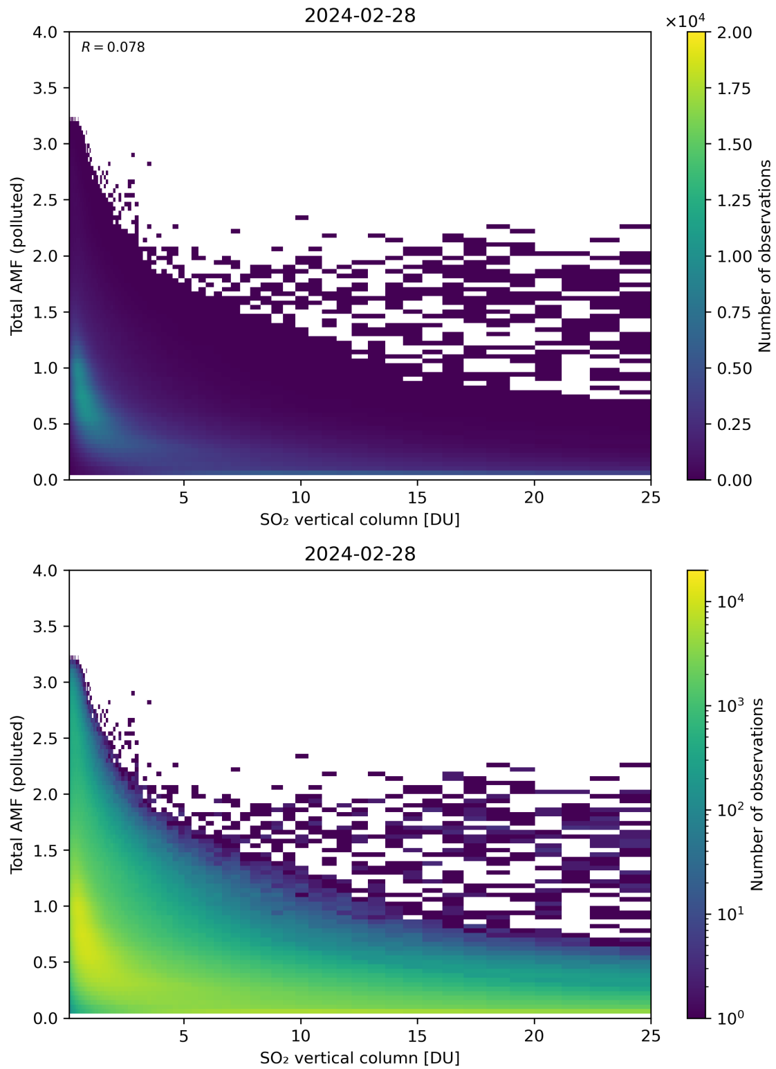
Figure 305: Scatter density plot of “SO 2 vertical column” against “Total AMF (polluted)” for 2024-02-27 to 2024-02-29.
