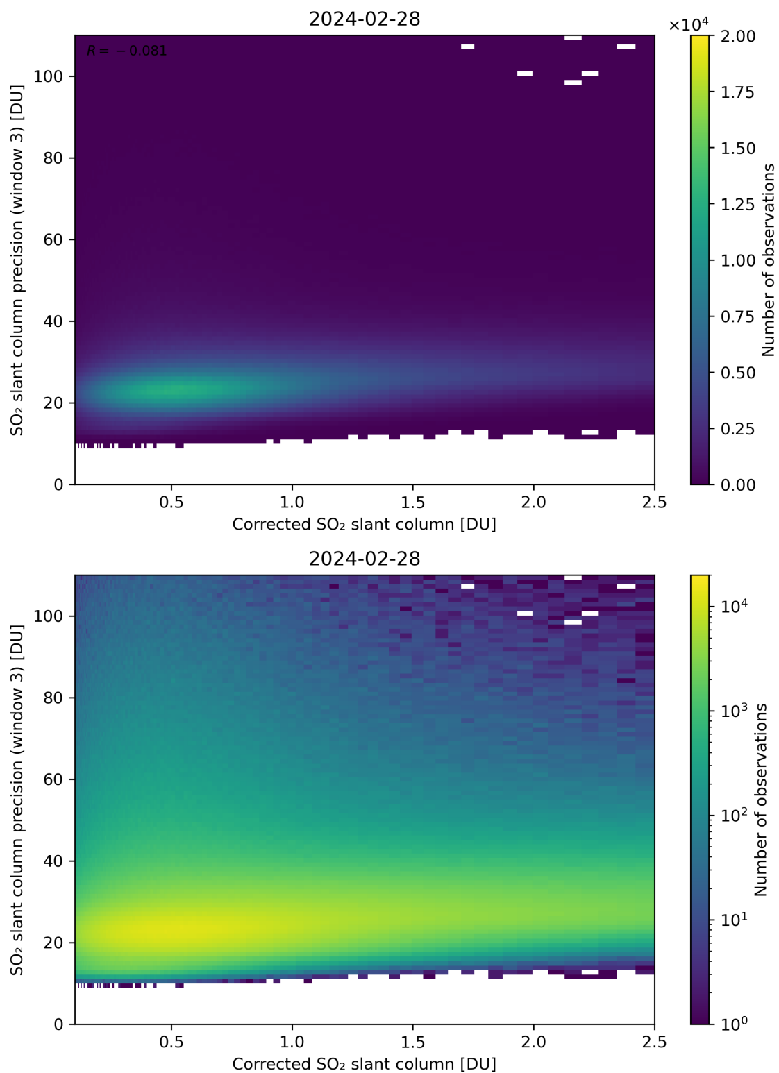
Figure 191: Scatter density plot of “Corrected SO 2 slant column” against “SO 2 slant column precision (window 3)” for 2024-02-27 to 2024-02-29.
