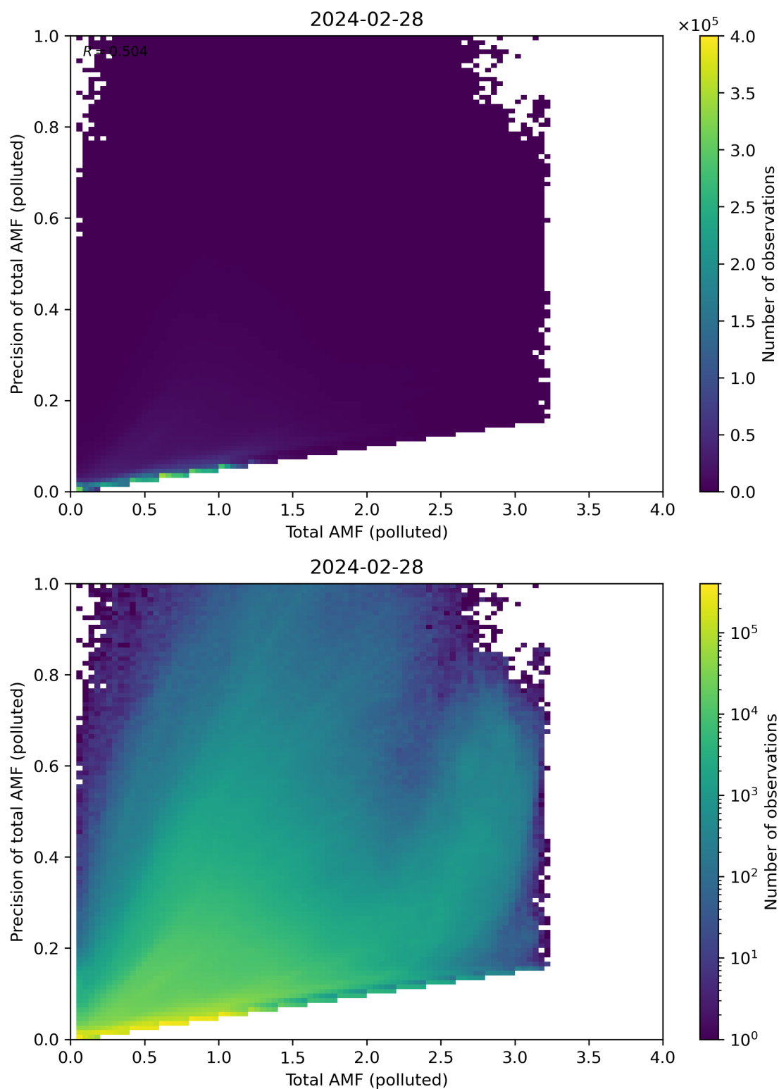
Figure 272: Scatter density plot of “Total AMF (polluted)” against “Precision of total AMF (polluted)” for 2024-02-27 to 2024-02-29.
