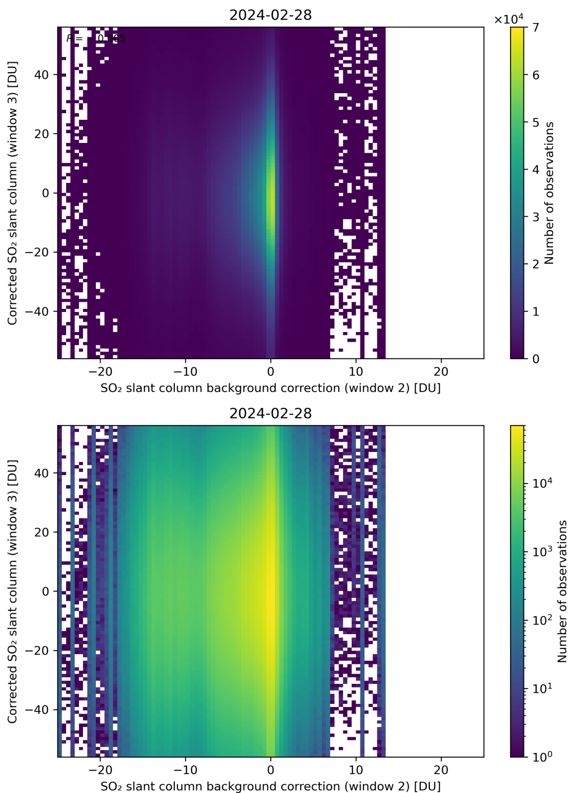
Figure 116: Scatter density plot of “SO 2 slant column background correction (window 2)” against “Corrected SO 2 slant column (window 3)” for 2024-02-27 to 2024-02-29.
