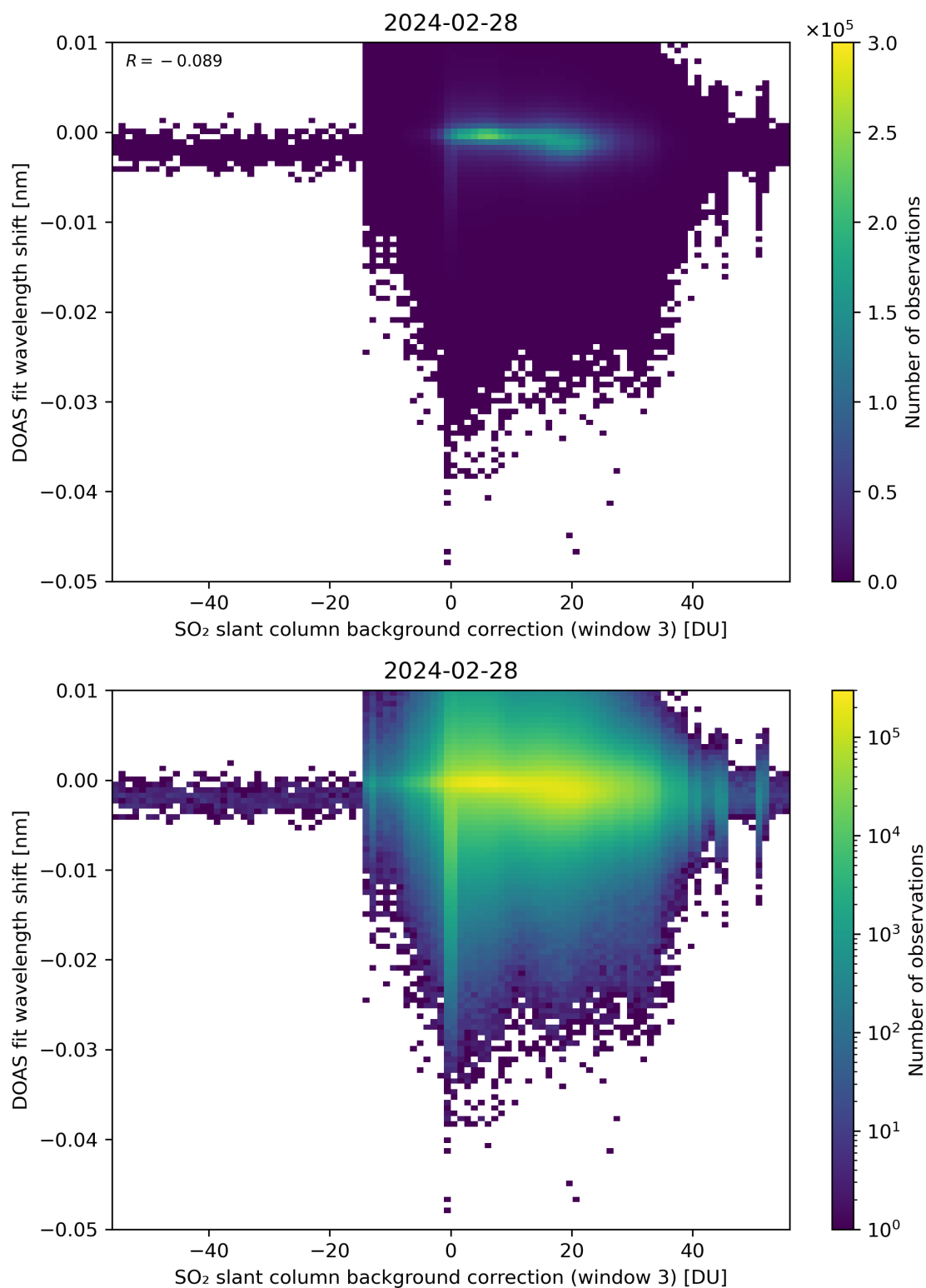
Figure 121: Scatter density plot of “SO 2 slant column background correction (window 3)” against “DOAS fit wavelength shift” for 2024-02-27 to 2024-02-29.
