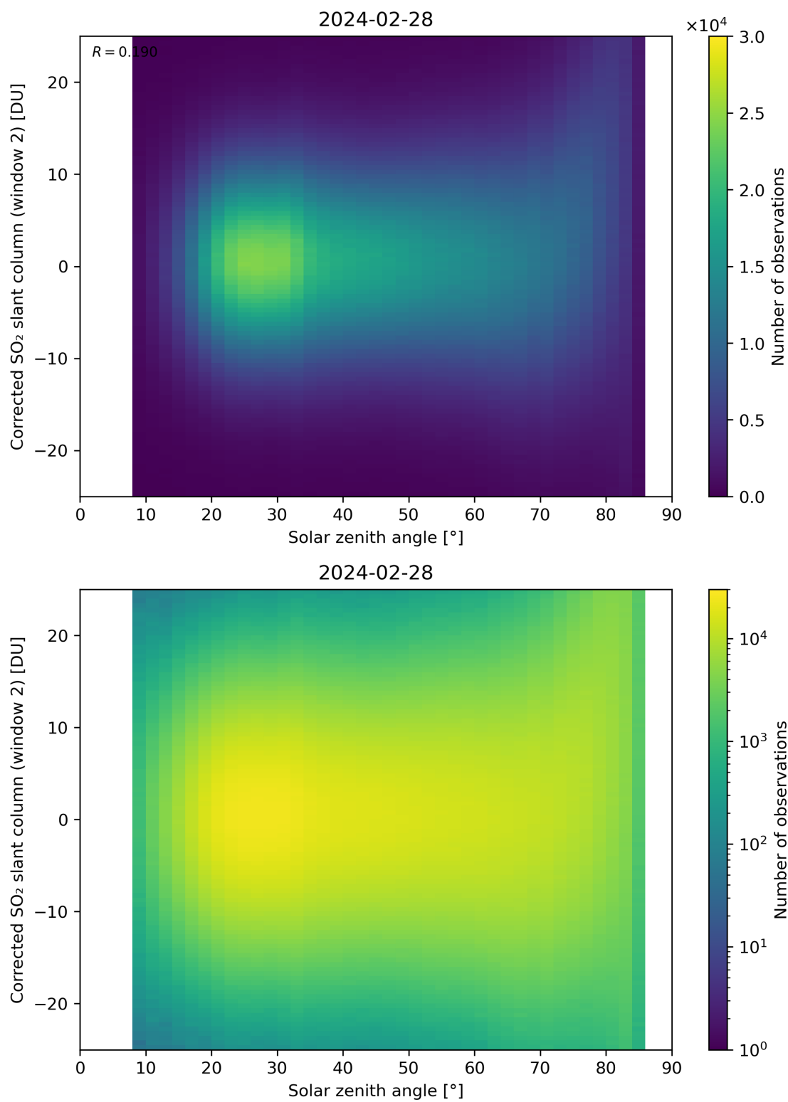
Figure 167: Scatter density plot of “Solar zenith angle” against “Corrected SO 2 slant column (window 2)” for 2024-02-27 to 2024-02-29.
