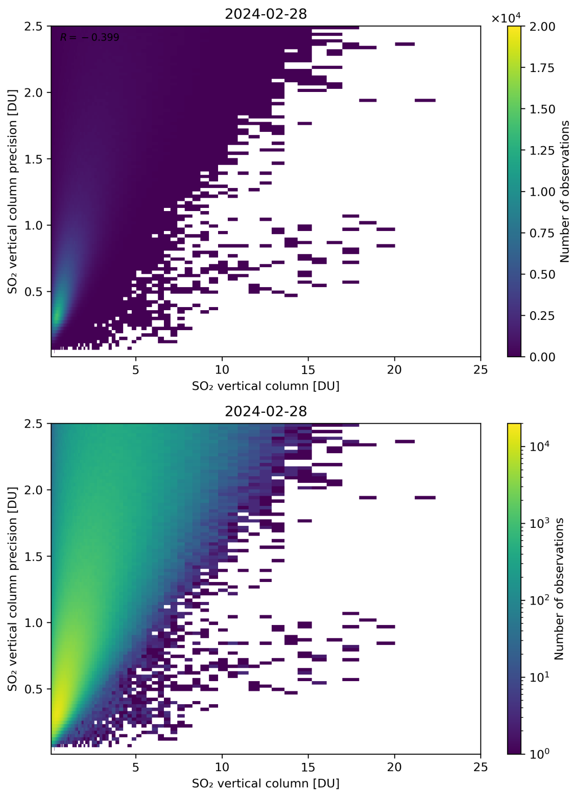
Figure 307: Scatter density plot of “SO 2 vertical column” against “SO 2 vertical column precision” for 2024-02-27 to 2024-02-29.
