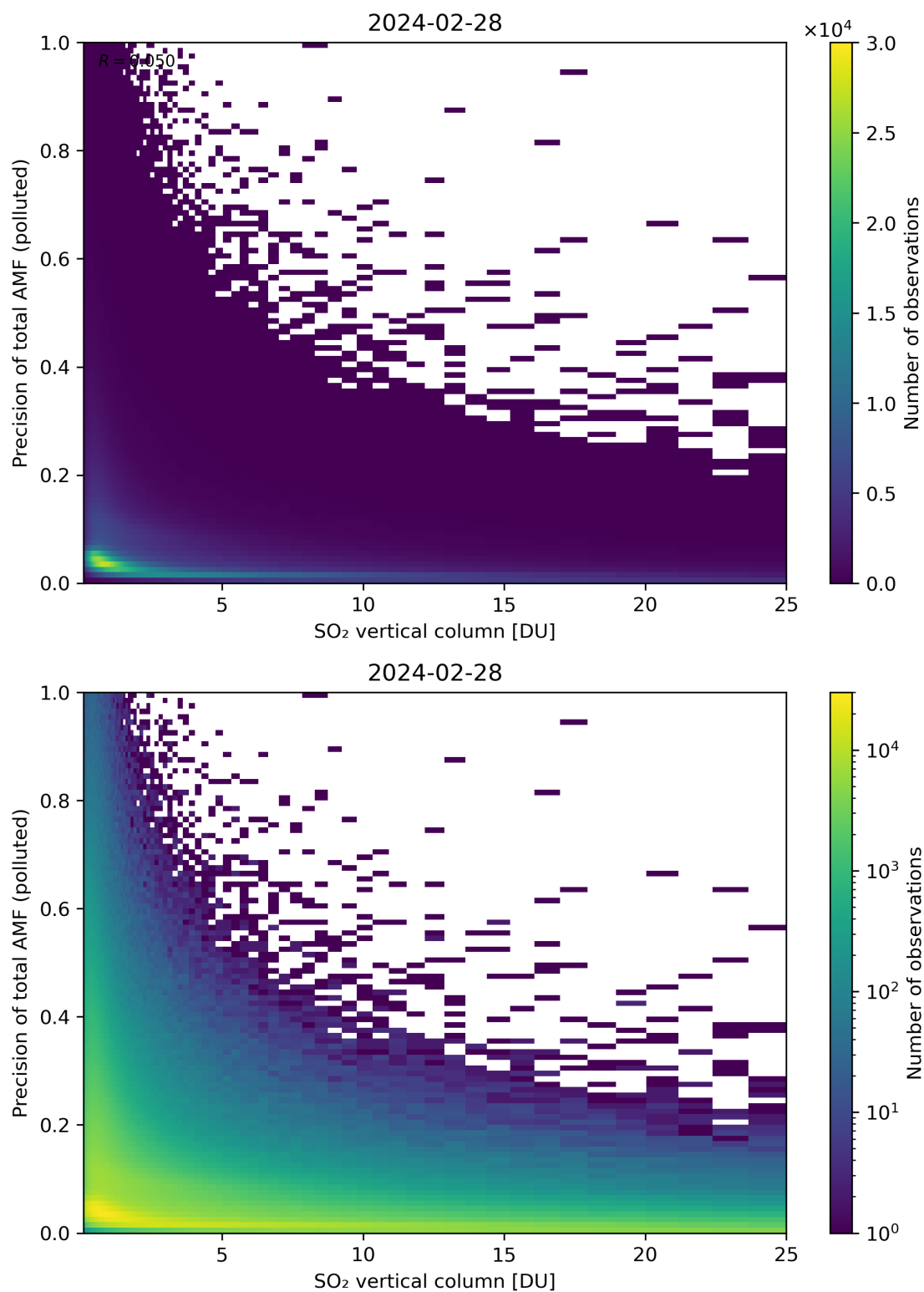
Figure 306: Scatter density plot of “SO 2 vertical column” against “Precision of total AMF (polluted)” for 2024-02-27 to 2024-02-29.
