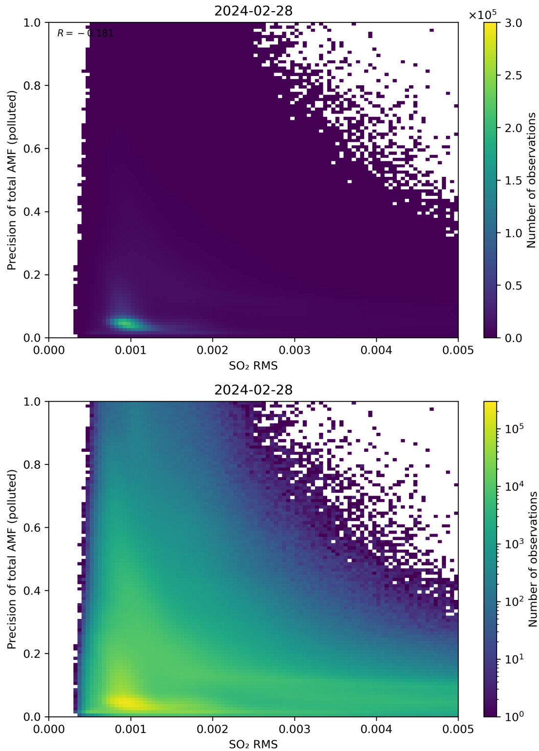
Figure 138: Scatter density plot of “SO 2 RMS” against “Precision of total AMF (polluted)” for 2024-02-27 to 2024-02-29.
