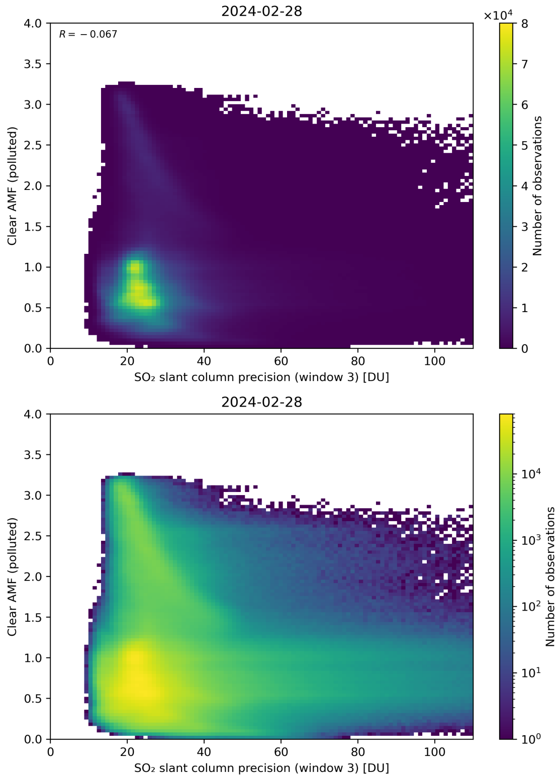
Figure 261: Scatter density plot of “SO 2 slant column precision (window 3)” against “Clear AMF (polluted)” for 2024-02-27 to 2024-02-29.
