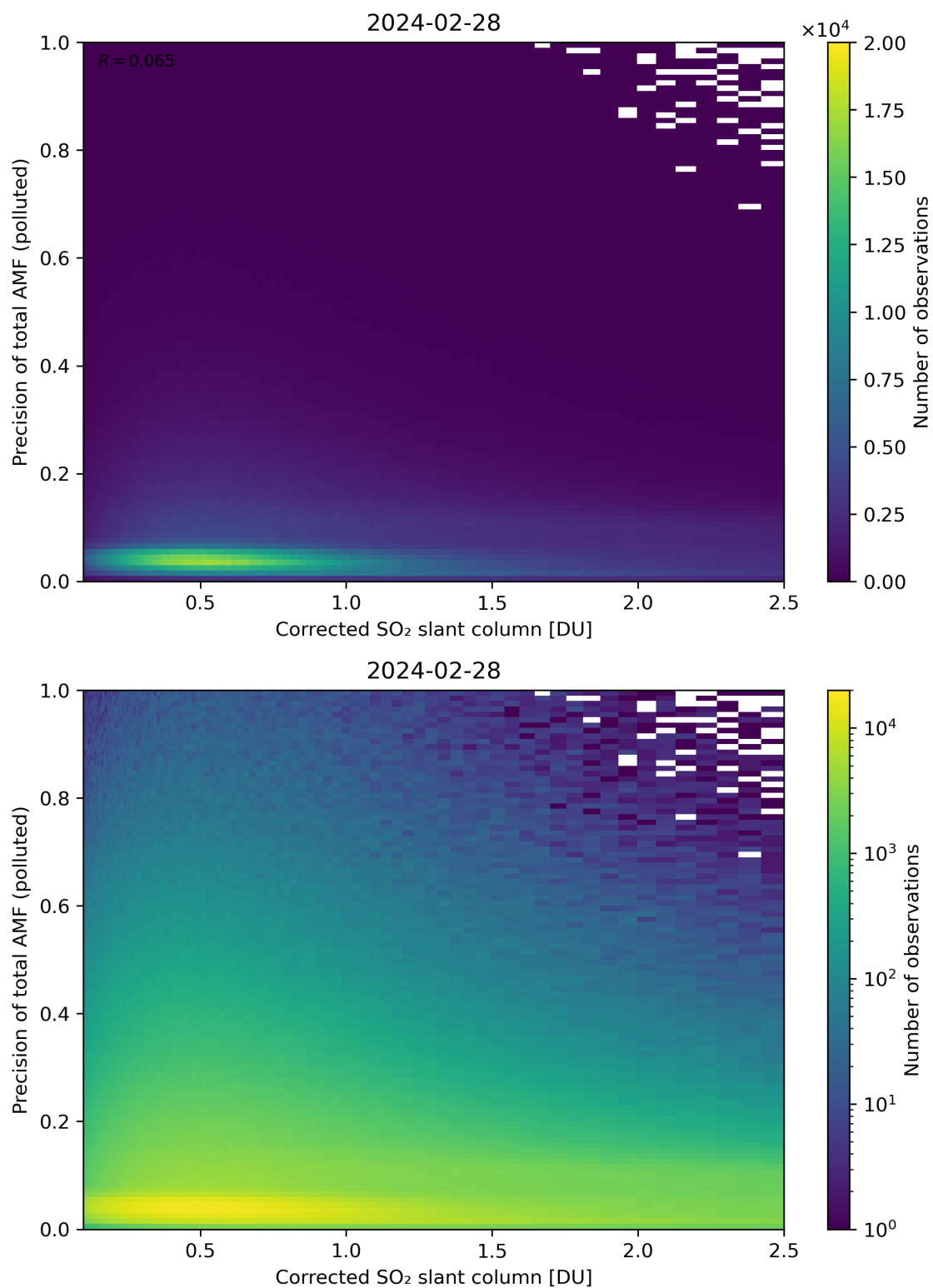
Figure 193: Scatter density plot of “Corrected SO 2 slant column” against “Precision of total AMF (polluted)” for 2024-02-27 to 2024-02-29.
