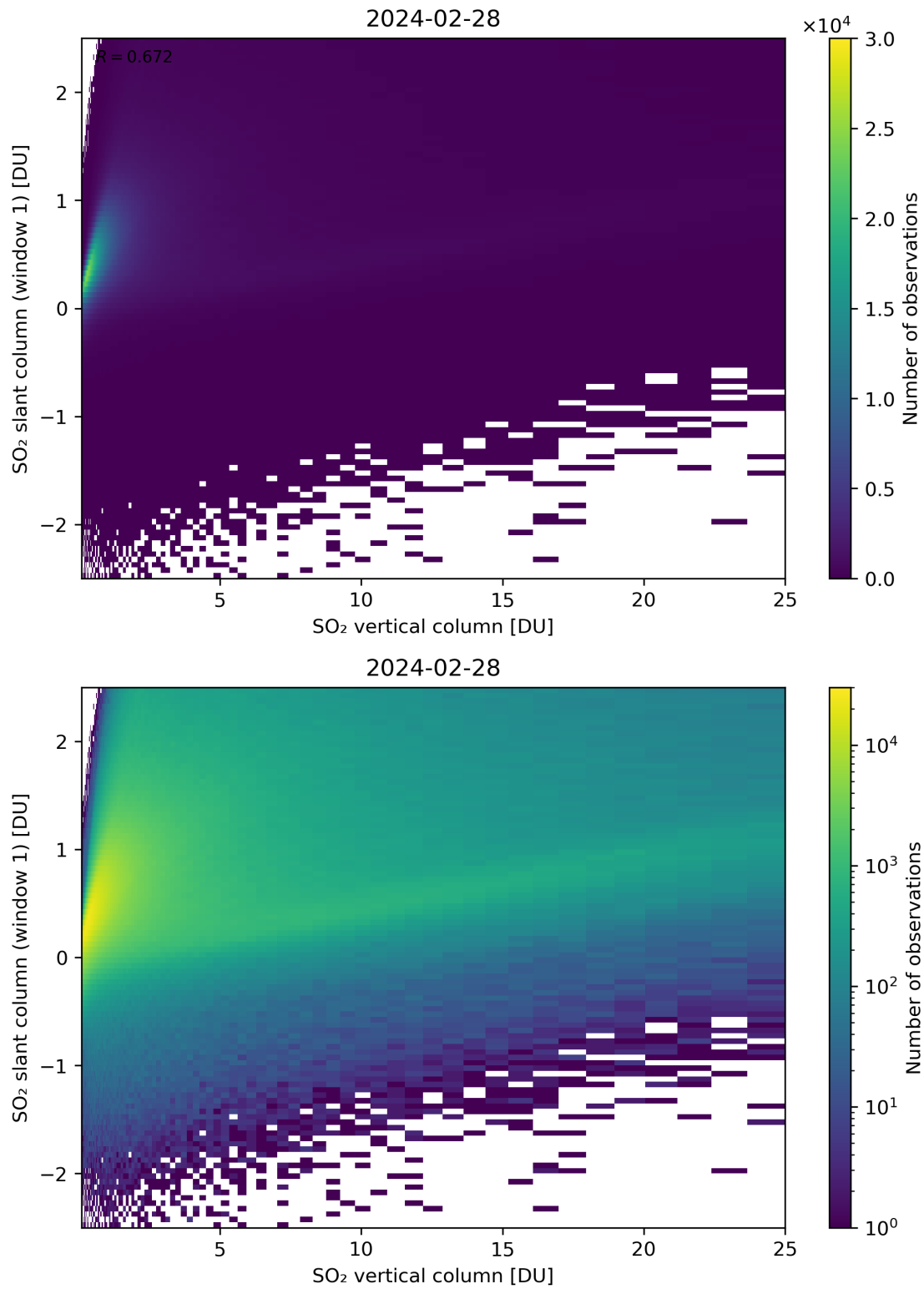
Figure 300: Scatter density plot of “SO 2 vertical column” against “SO 2 slant column (window 1)” for 2024-02-27 to 2024-02-29.
