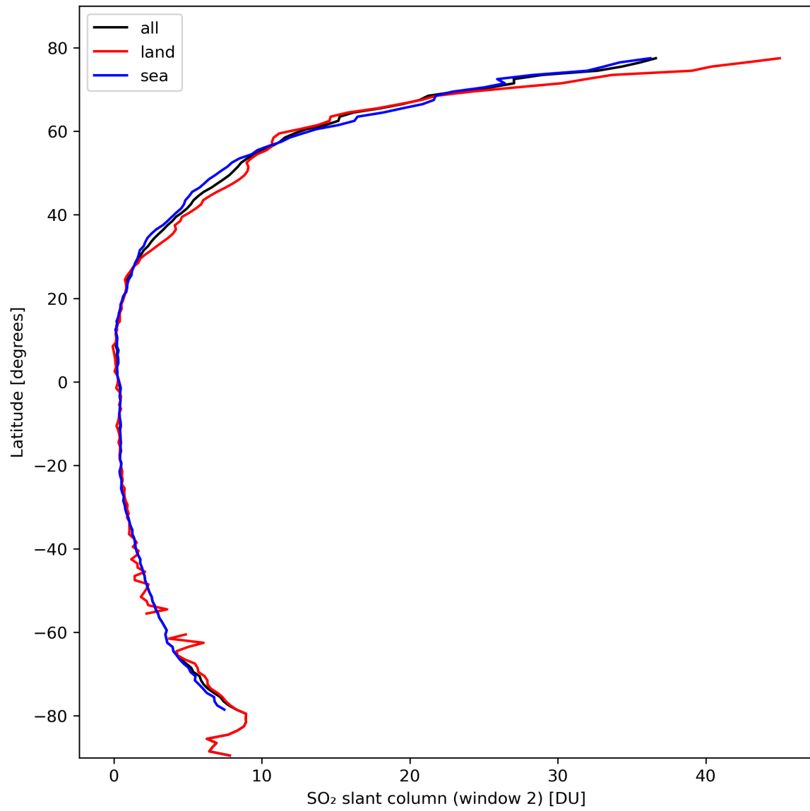
Figure 37: Zonal average of “SO 2 slant column (window 2)” for 2024-02-27 to 2024-02-29.
