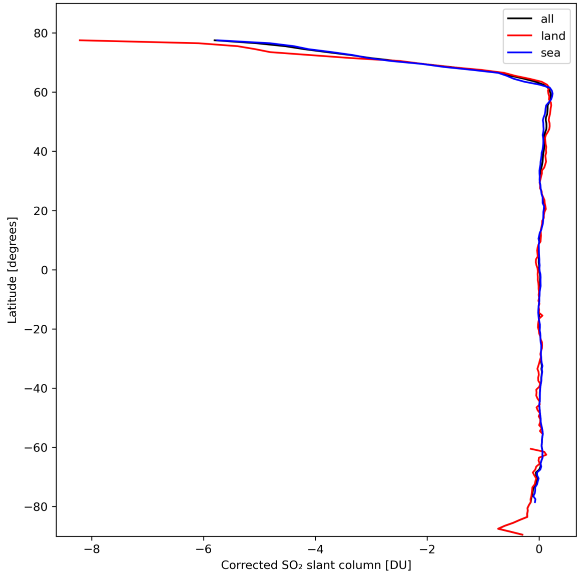
Figure 32: Zonal average of “Corrected SO 2 slant column” for 2024-02-27 to 2024-02-29.
