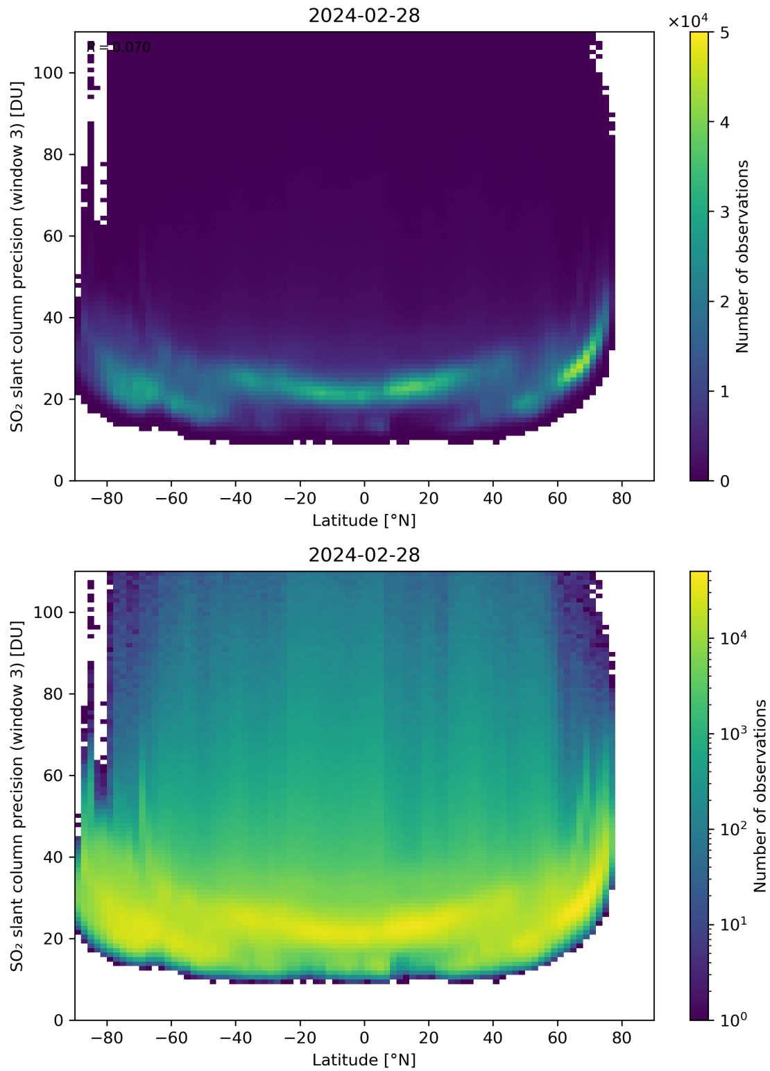
Figure 153: Scatter density plot of “Latitude” against “SO 2 slant column precision (window 3)” for 2024-02-27 to 2024-02-29.
