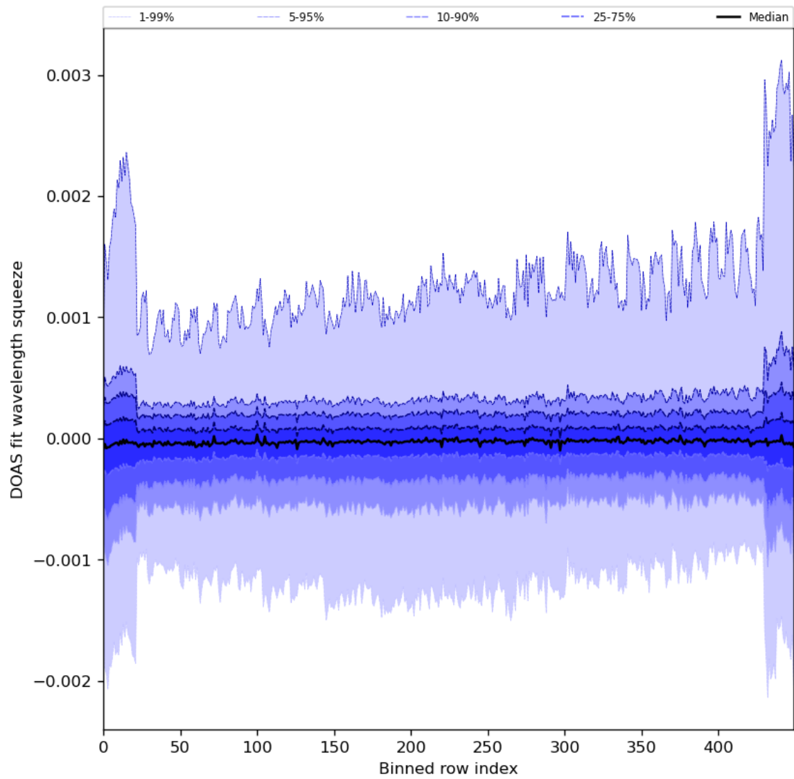
Figure 92: Along track statistics of “DOAS fit wavelength squeeze” for 2024-02-27 to 2024-02-29
