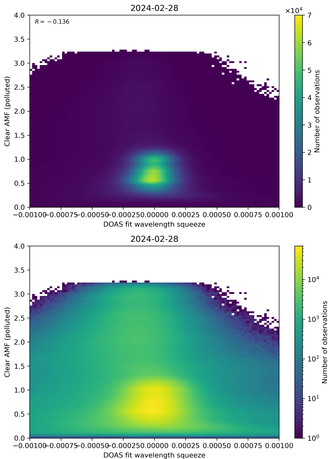
Figure 133: Scatter density plot of “DOAS fit wavelength squeeze” against “Clear AMF (polluted)” for 2024-02-27 to 2024-02-29.
