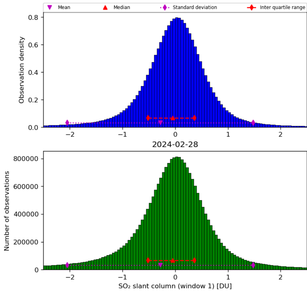
Figure 56: Histogram of “SO 2 slant column (window 1)” for 2024-02-27 to 2024-02-29
