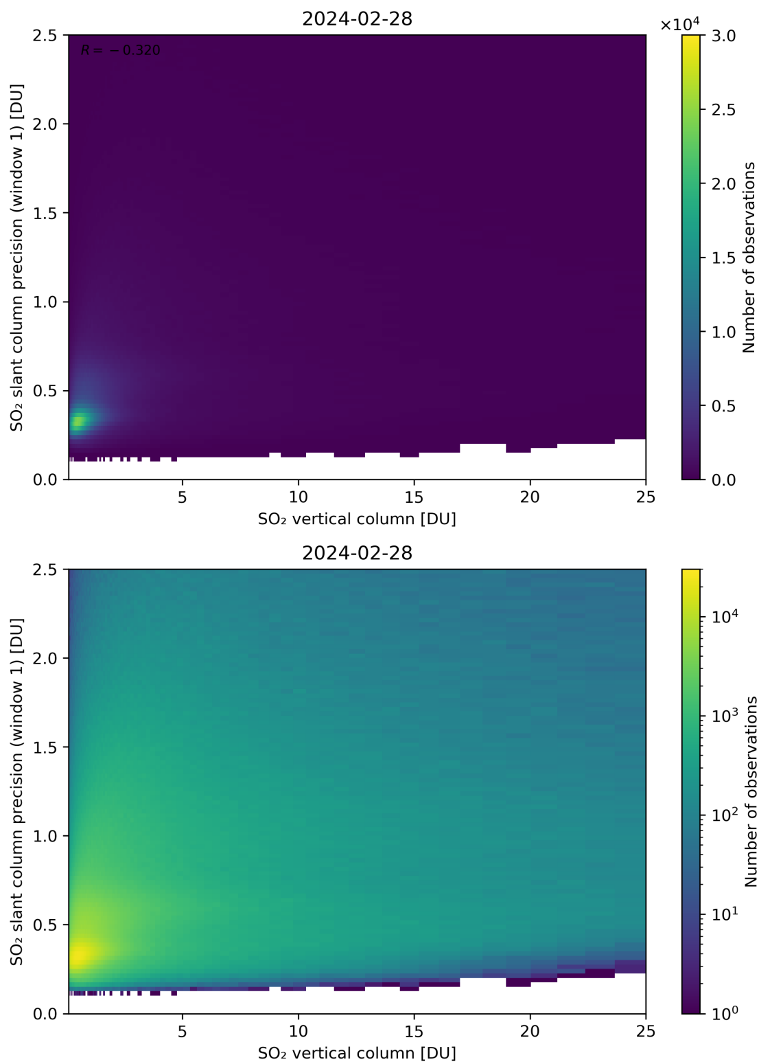
Figure 301: Scatter density plot of “SO 2 vertical column” against “SO 2 slant column precision (window 1)” for 2024-02-27 to 2024-02-29.
