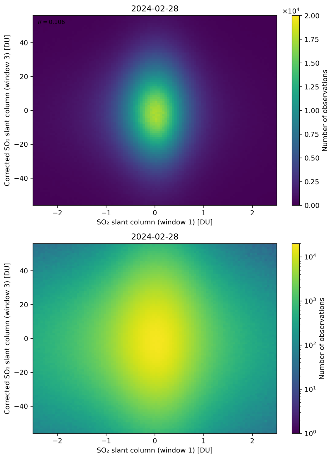
Figure 234: Scatter density plot of “SO 2 slant column (window 1)” against “Corrected SO 2 slant column (window 3)” for 2024-02-27 to 2024-02-29.
