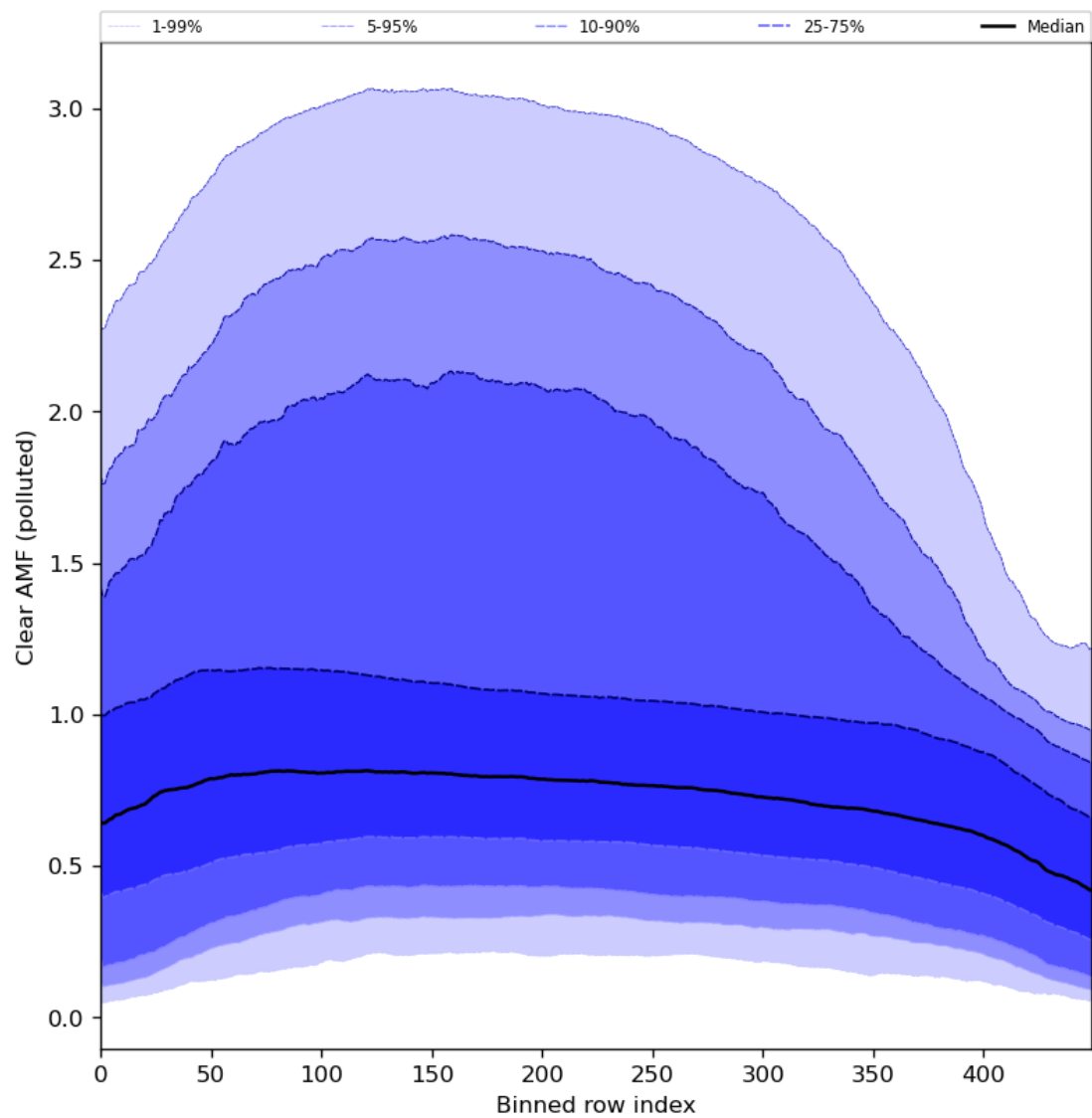
Figure 96: Along track statistics of “Clear AMF (polluted)” for 2024-02-27 to 2024-02-29
