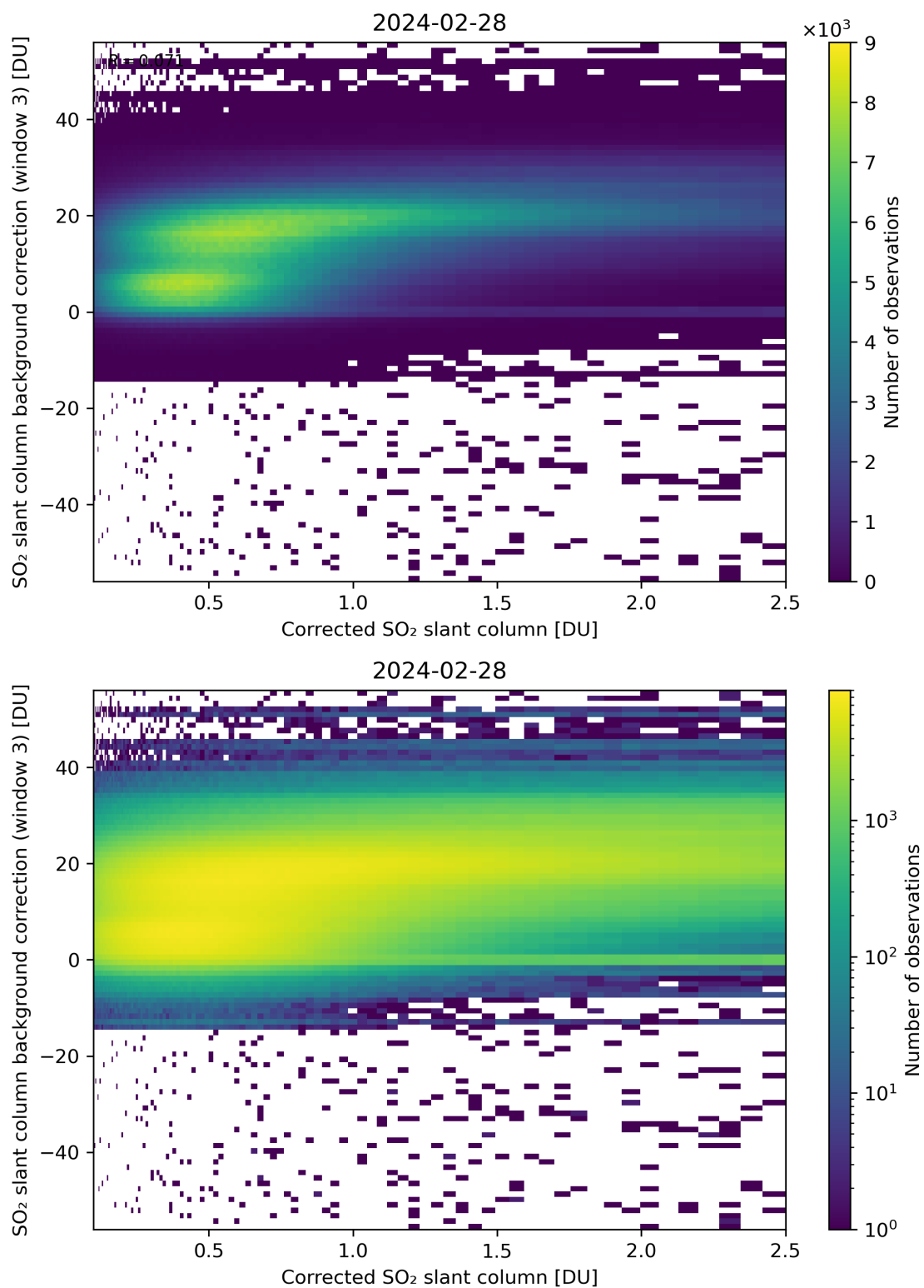
Figure 180: Scatter density plot of “Corrected SO 2 slant column” against “SO 2 slant column background correction (window 3)” for 2024-02-27 to 2024-02-29.
