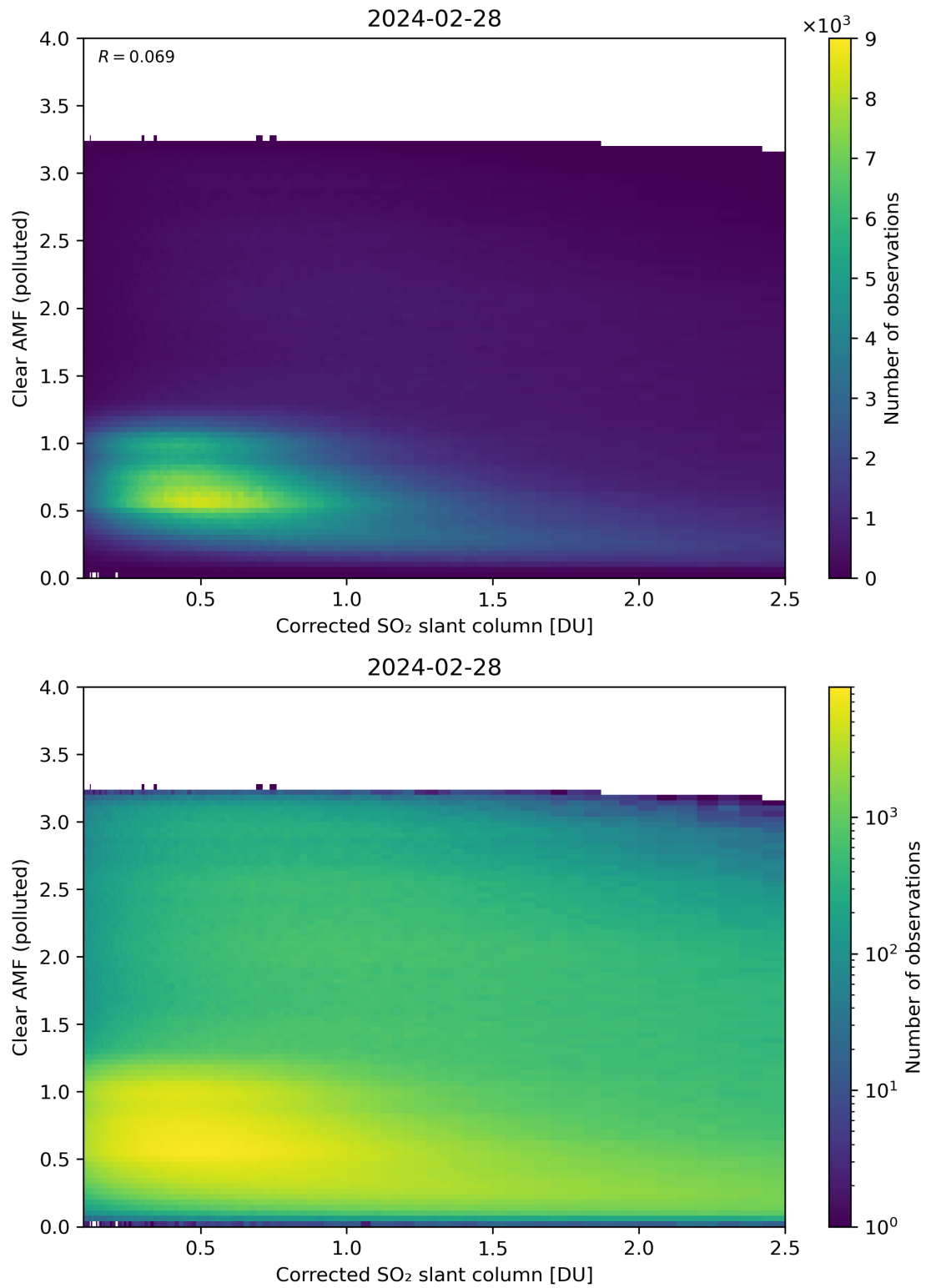
Figure 184: Scatter density plot of “Corrected SO 2 slant column” against “Clear AMF (polluted)” for 2024-02-27 to 2024-02-29.
