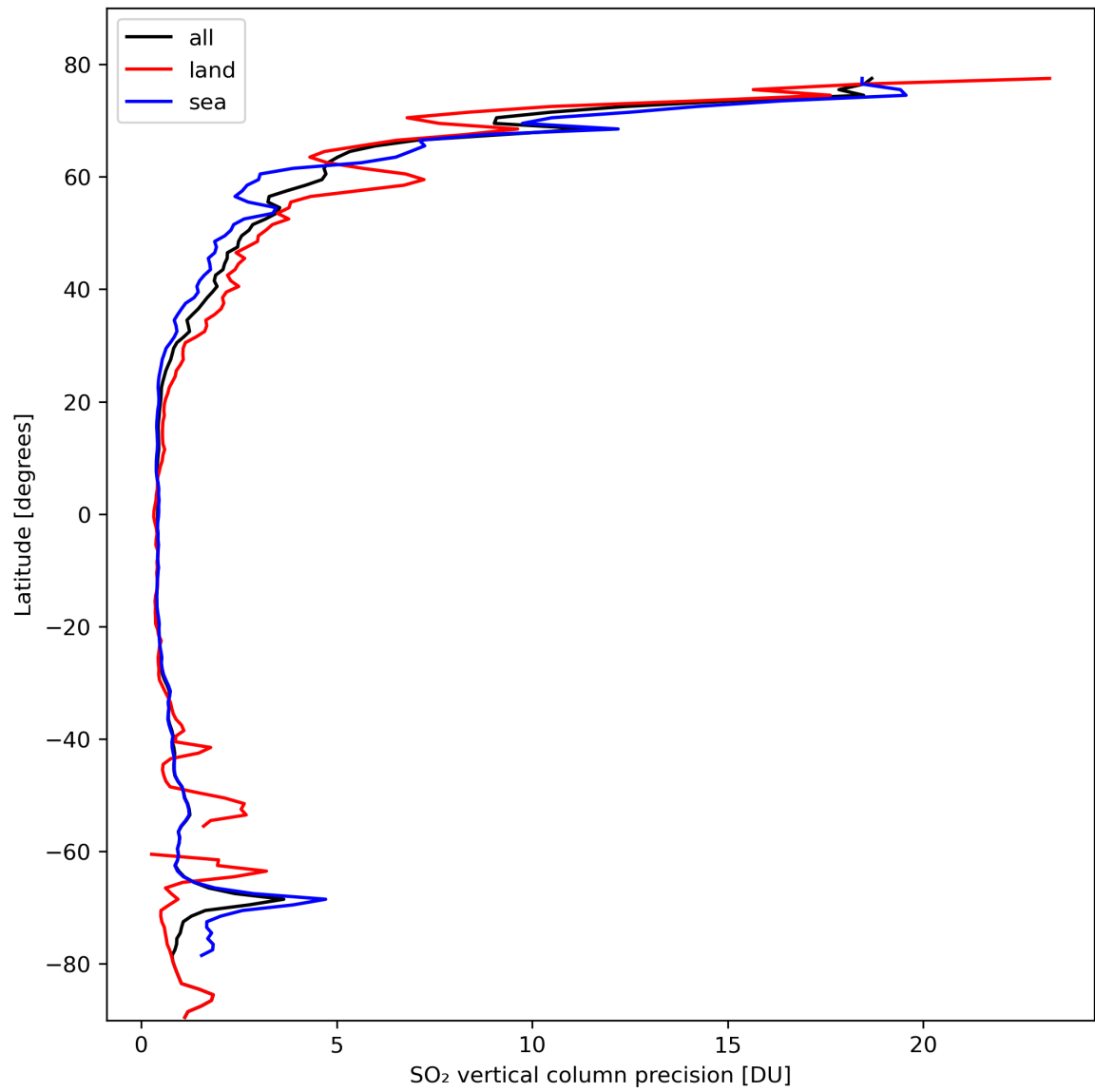
Figure 31: Zonal average of “SO 2 vertical column precision” for 2024-02-27 to 2024-02-29.
