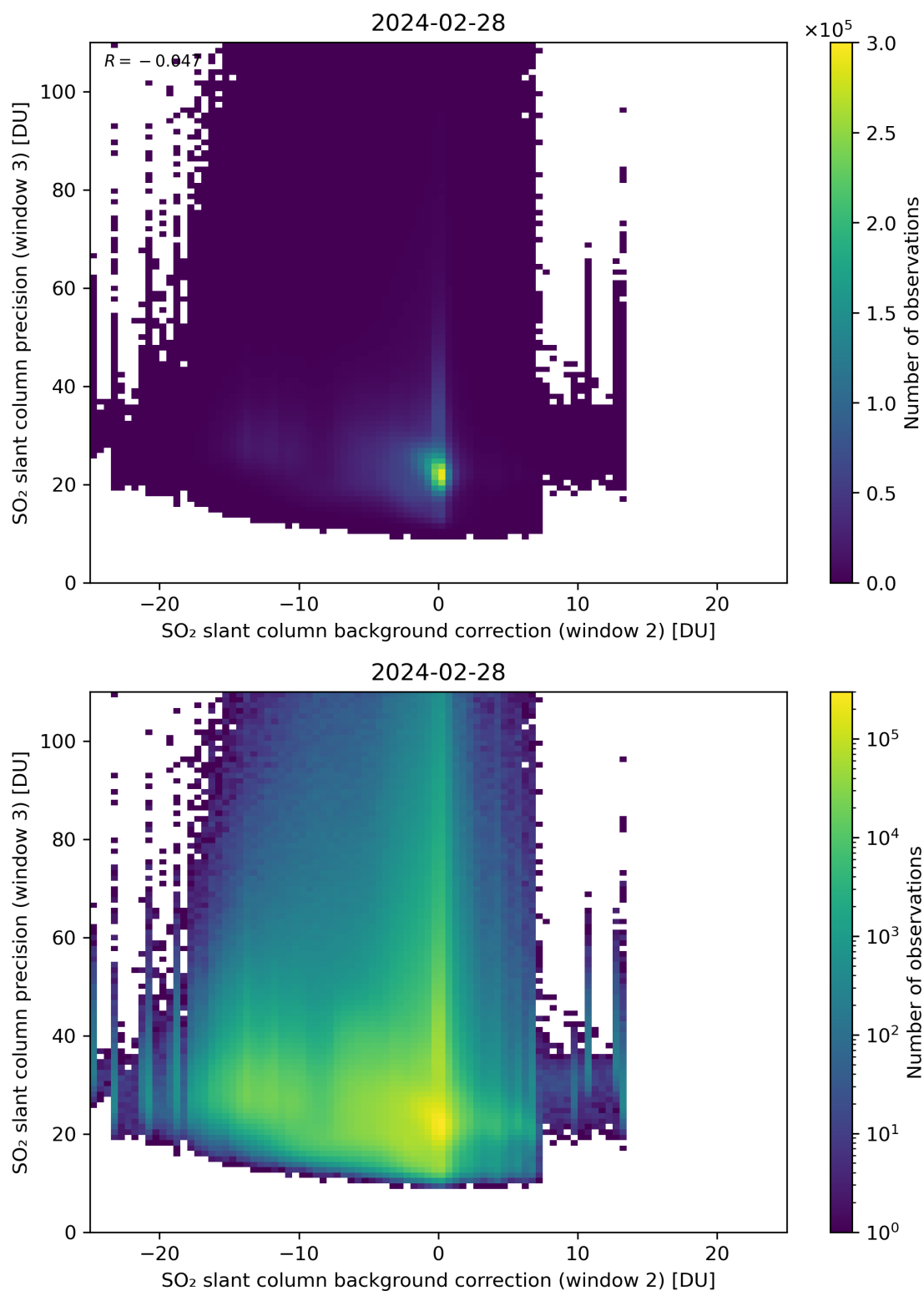
Figure 118: Scatter density plot of “SO 2 slant column background correction (window 2)” against “SO 2 slant column precision (window 3)” for 2024-02-27 to 2024-02-29.
