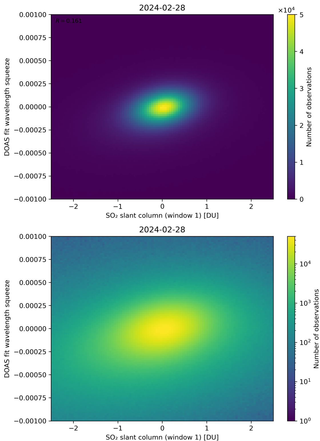
Figure 216: Scatter density plot of “SO 2 slant column (window 1)” against “DOAS fit wavelength squeeze” for 2024-02-27 to 2024-02-29.
