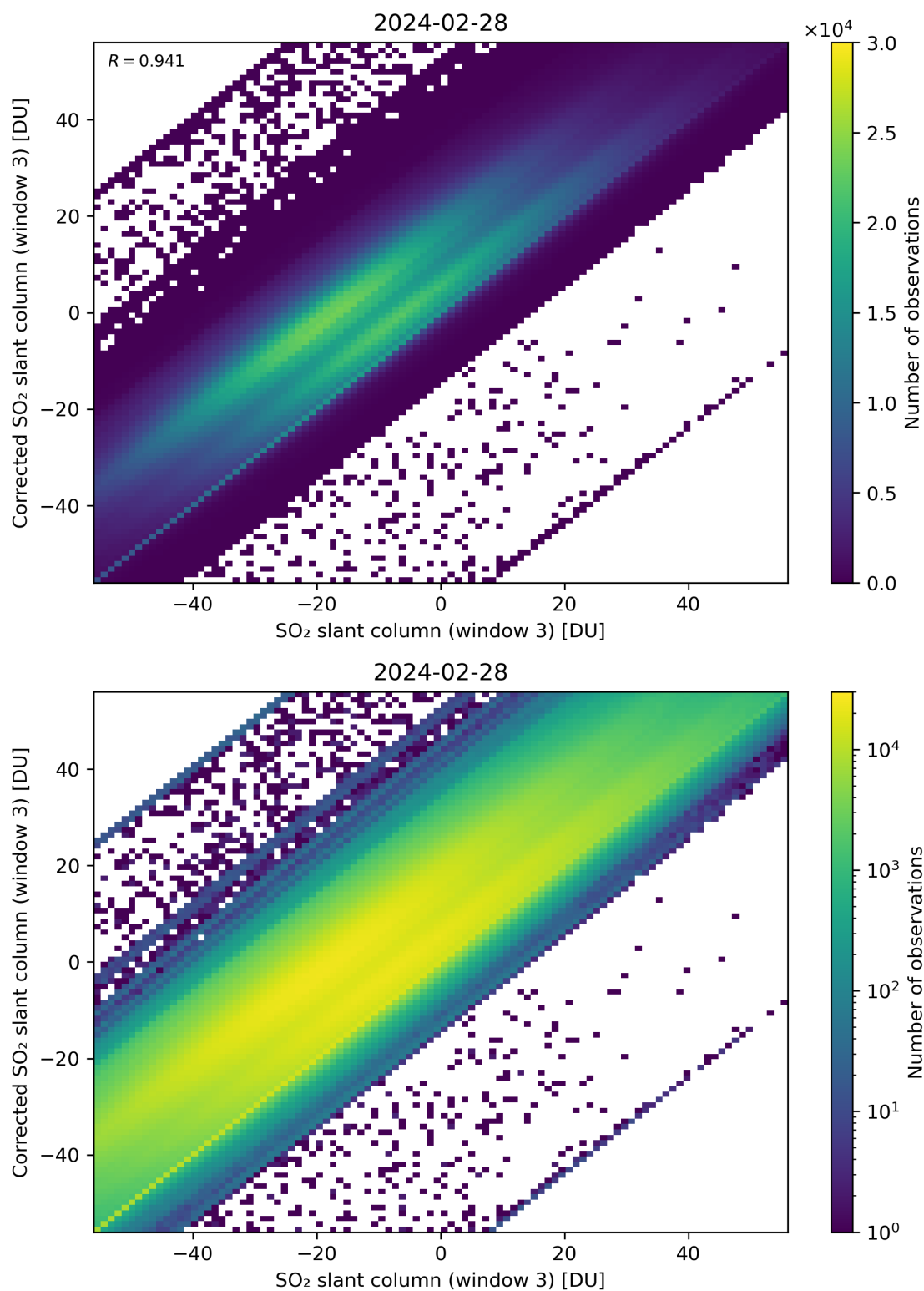
Figure 266: Scatter density plot of “SO 2 slant column (window 3)” against “Corrected SO 2 slant column (window 3)” for 2024-02-27 to 2024-02-29.
