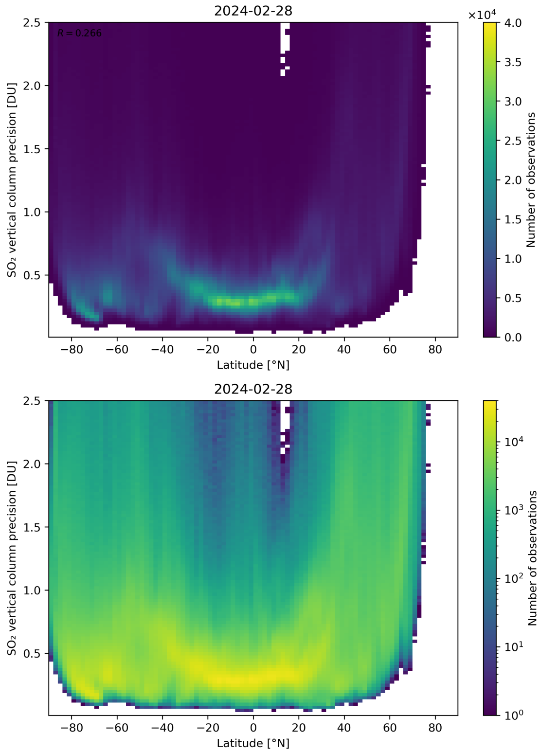
Figure 157: Scatter density plot of “Latitude” against “SO 2 vertical column precision” for 2024-02-27 to 2024-02-29.
