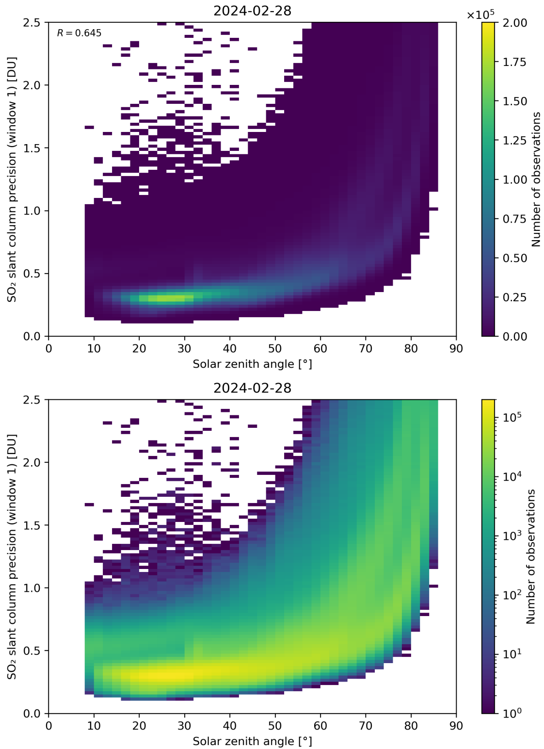
Figure 170: Scatter density plot of “Solar zenith angle” against “SO 2 slant column precision (window 1)” for 2024-02-27 to 2024-02-29.
