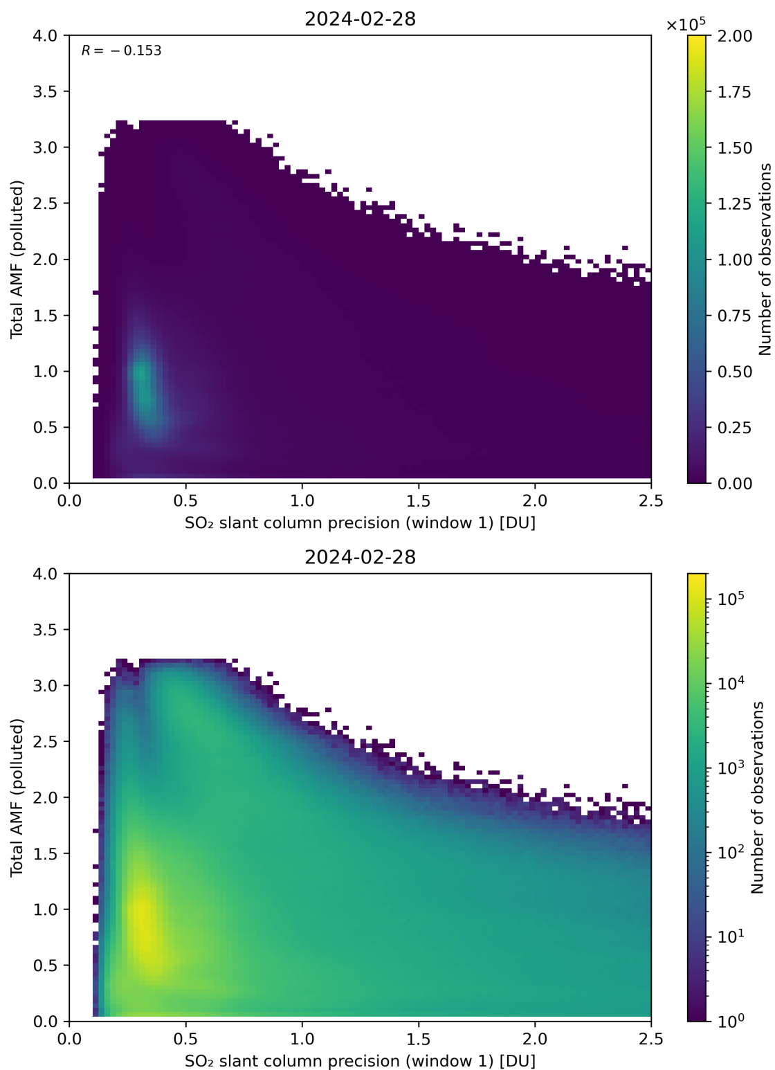
Figure 230: Scatter density plot of “SO 2 slant column precision (window 1)” against “Total AMF (polluted)” for 2024-02-27 to 2024-02-29.
