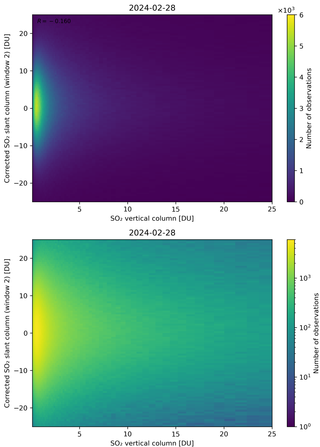
Figure 298: Scatter density plot of “SO 2 vertical column” against “Corrected SO 2 slant column (window 2)” for 2024-02-27 to 2024-02-29.
