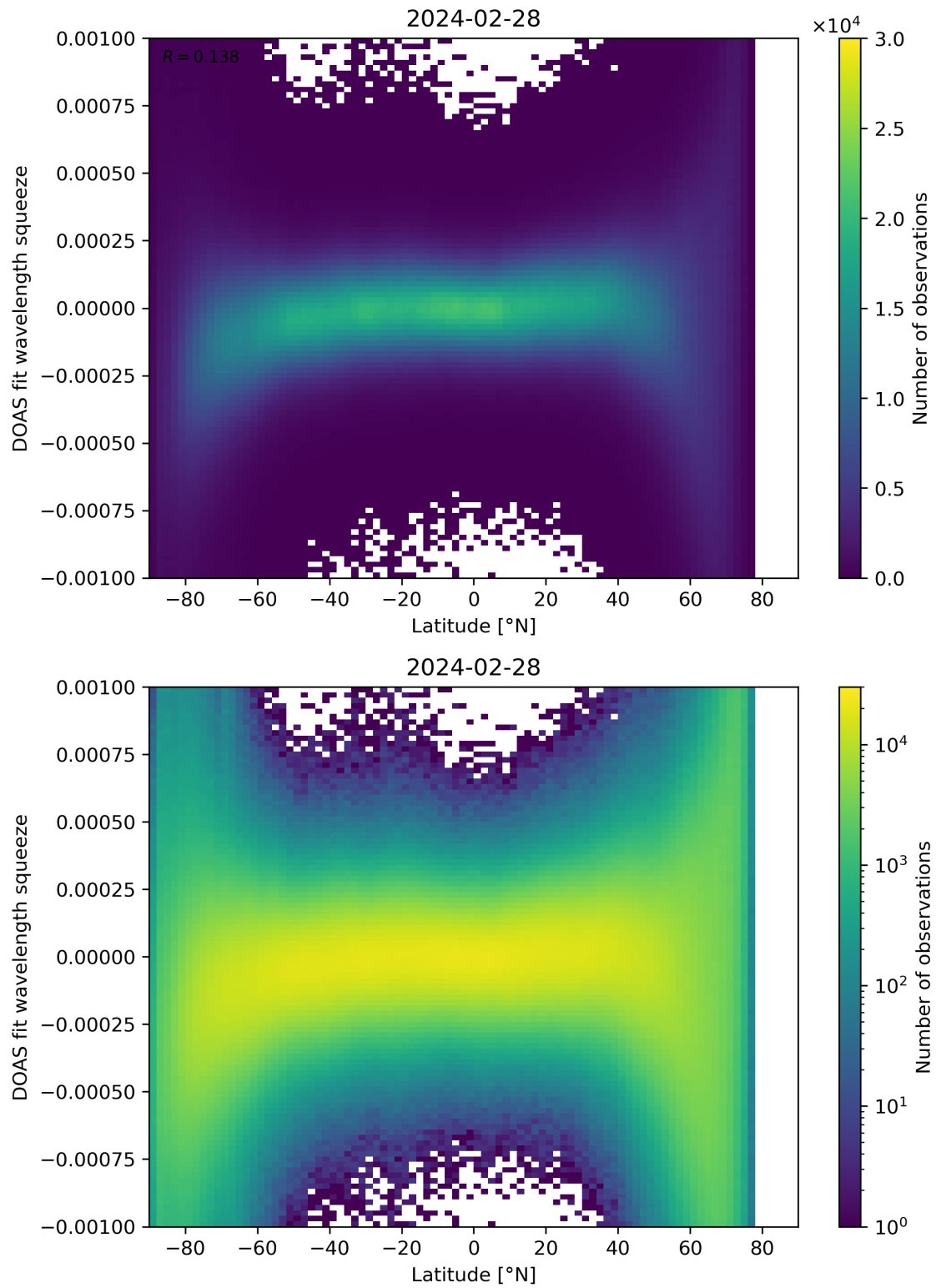
Figure 143: Scatter density plot of “Latitude” against “DOAS fit wavelength squeeze” for 2024-02-27 to 2024-02-29.
