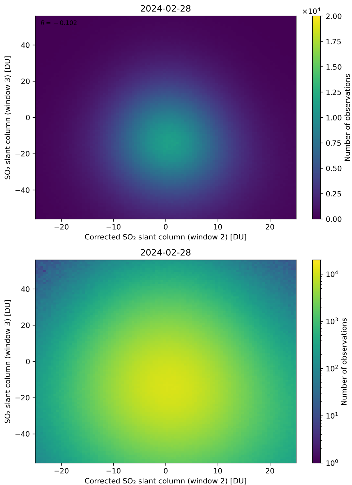
Figure 201: Scatter density plot of “Corrected SO 2 slant column (window 2)” against “SO 2 slant column (window 3)” for 2024-02-27 to 2024-02-29.
