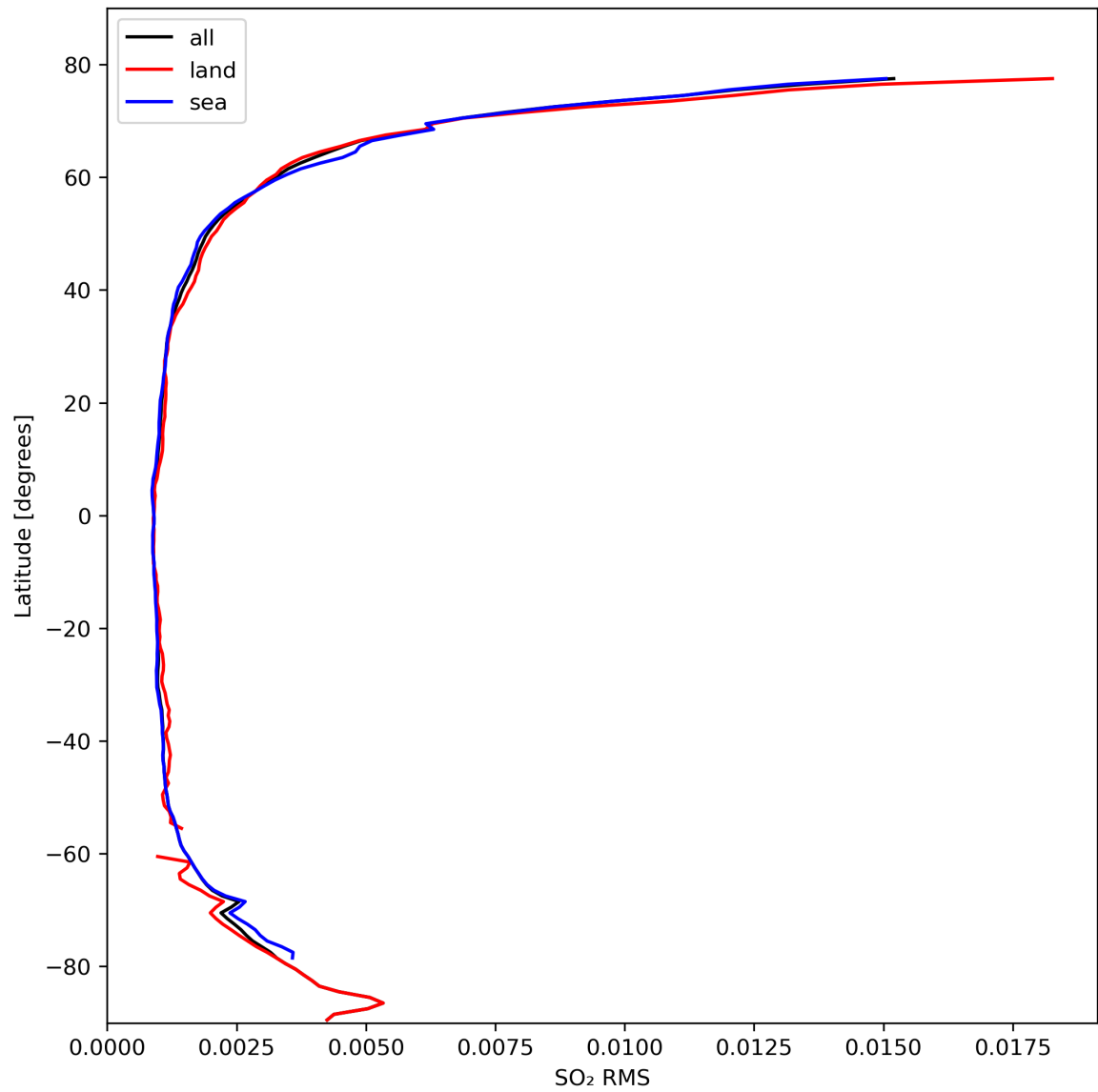
Figure 47: Zonal average of “SO 2 RMS” for 2024-02-27 to 2024-02-29.
