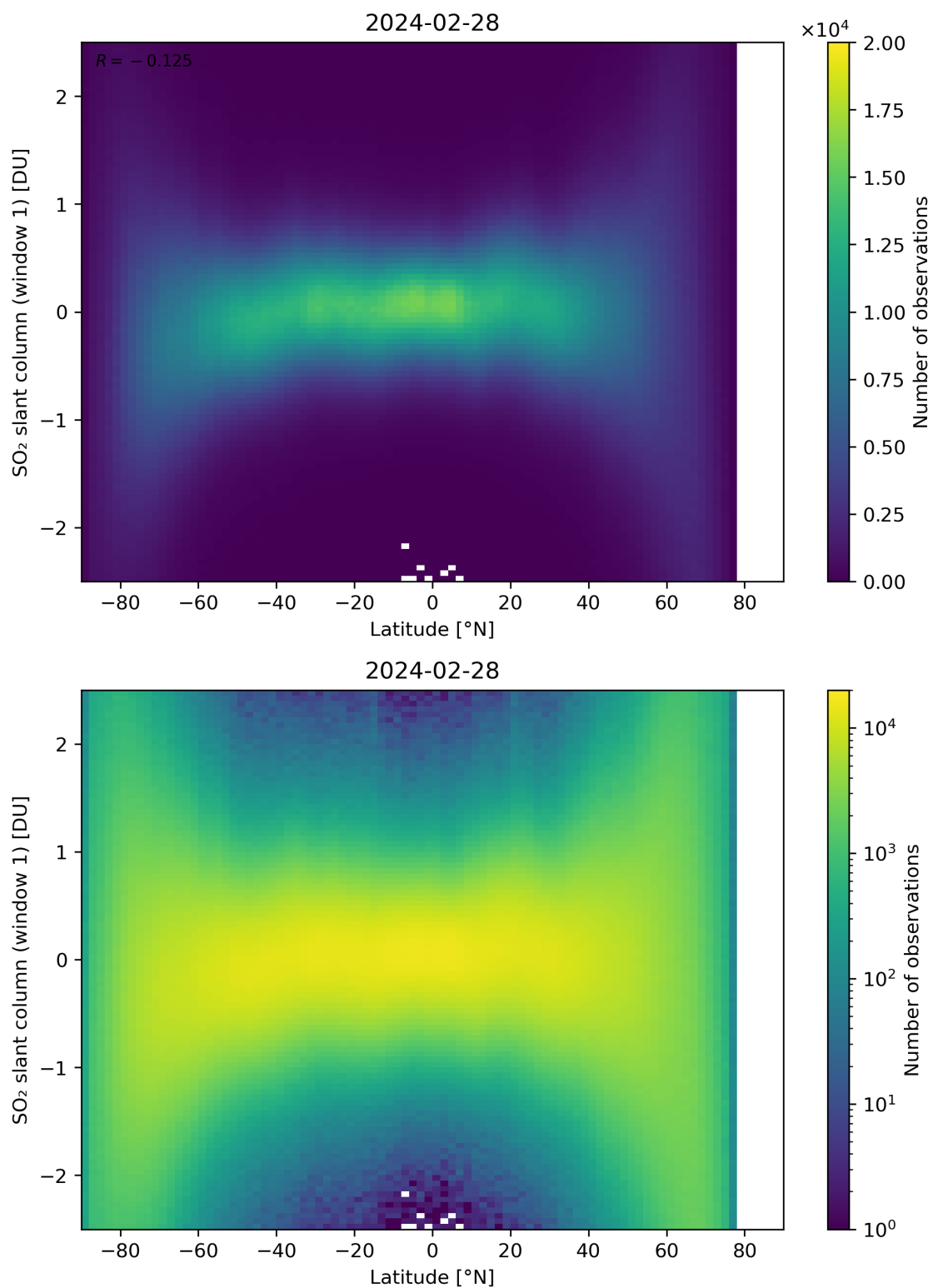
Figure 149: Scatter density plot of “Latitude” against “SO 2 slant column (window 1)” for 2024-02-27 to 2024-02-29.
