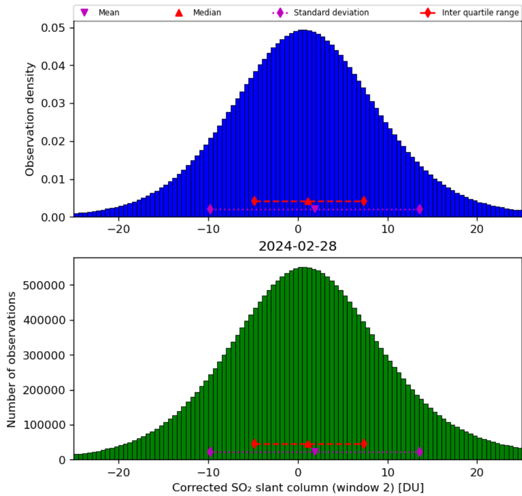
Figure 62: Histogram of “Corrected SO 2 slant column (window 2)” for 2024-02-27 to 2024-02-29
