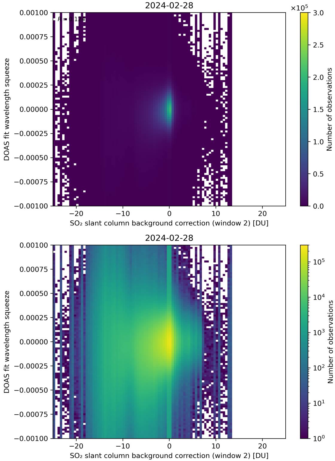
Figure 113: Scatter density plot of “SO 2 slant column background correction (window 2)” against “DOAS fit wavelength squeeze” for 2024-02-27 to 2024-02-29.
