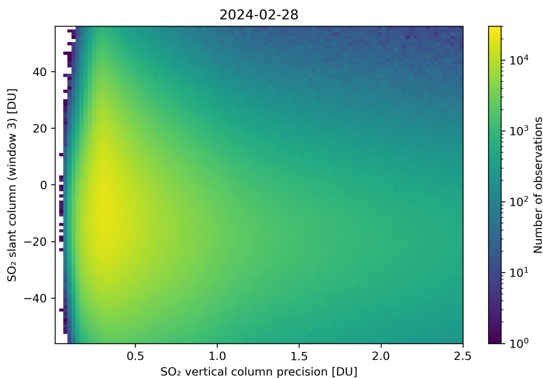
Figure 292: Scatter density plot of “SO 2 vertical column precision” against “SO 2 slant column (window 3)” for 2024-02-27 to 2024-02-29.
