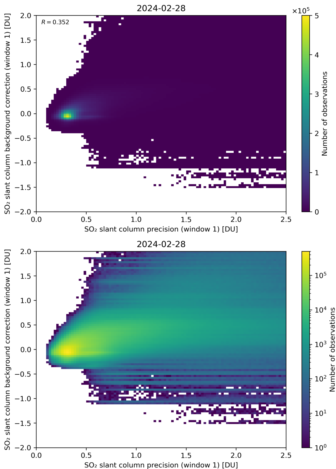
Figure 218: Scatter density plot of “SO 2 slant column precision (window 1)” against “SO 2 slant column background correction (window 1)” for 2024-02-27 to 2024-02-29.
