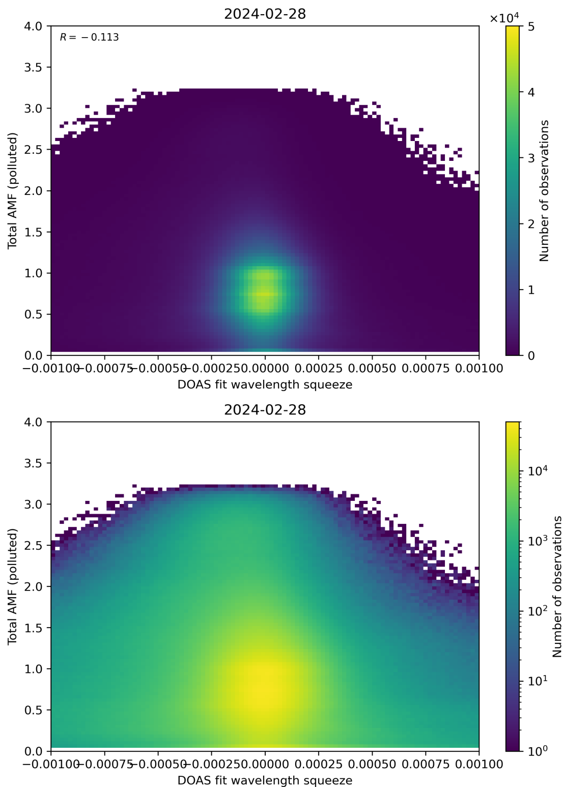
Figure 134: Scatter density plot of “DOAS fit wavelength squeeze” against “Total AMF (polluted)” for 2024-02-27 to 2024-02-29.
