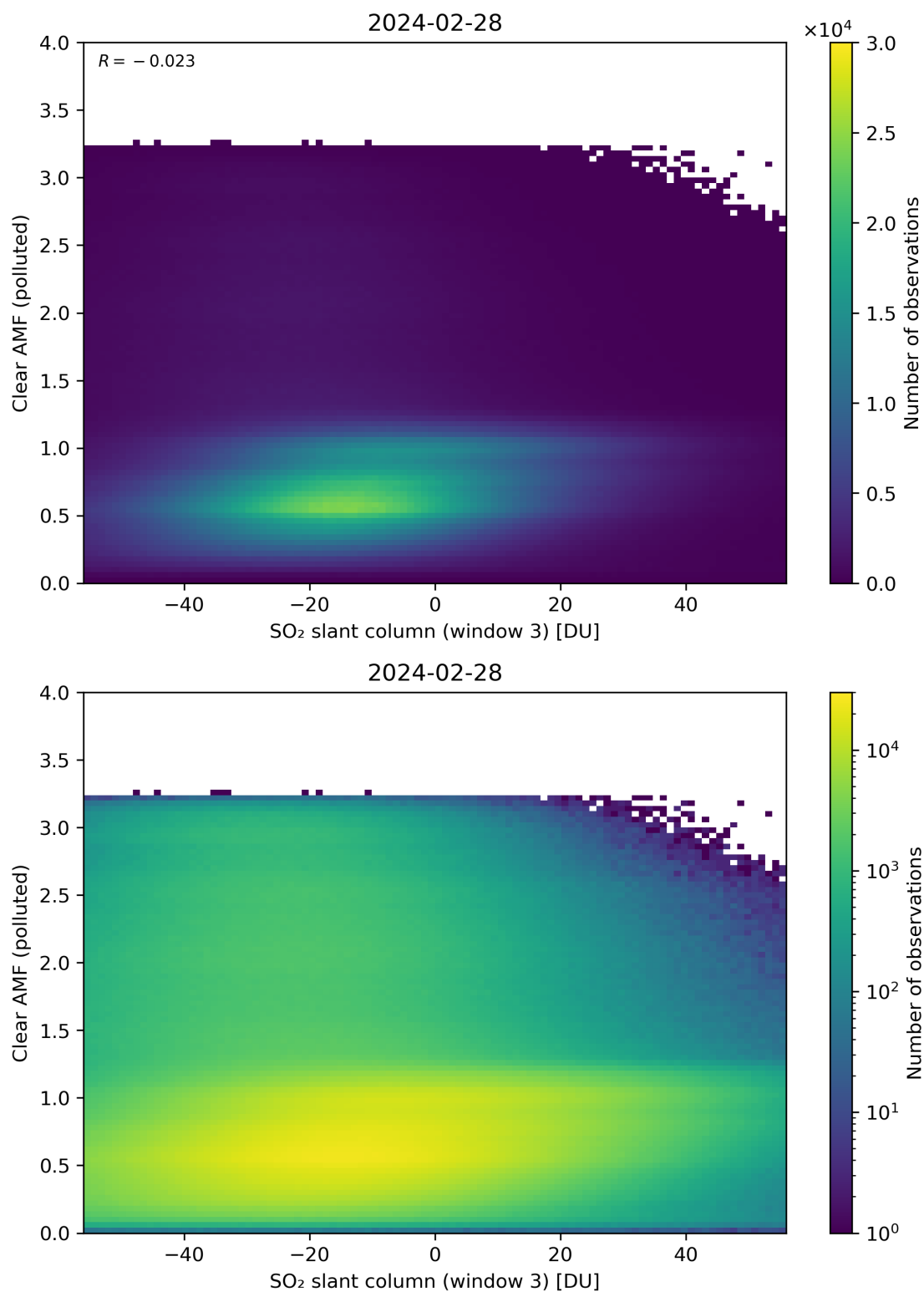
Figure 265: Scatter density plot of “SO 2 slant column (window 3)” against “Clear AMF (polluted)” for 2024-02-27 to 2024-02-29.
