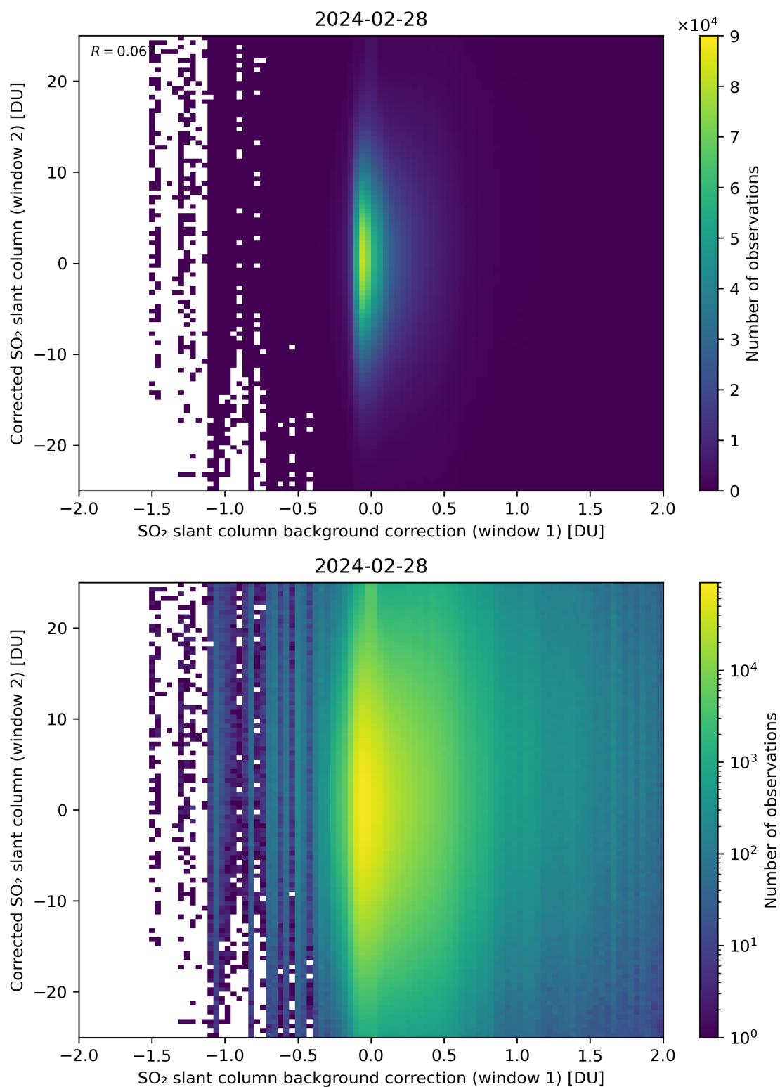
Figure 104: Scatter density plot of “SO 2 slant column background correction (window 1)” against “Corrected SO 2 slant column (window 2)” for 2024-02-27 to 2024-02-29.
