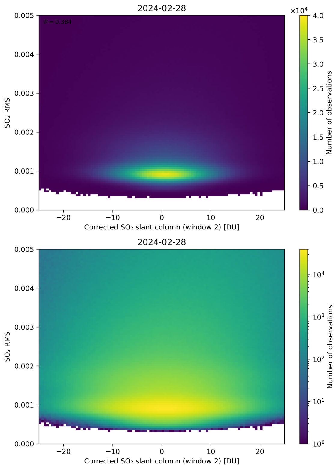
Figure 198: Scatter density plot of “Corrected SO 2 slant column (window 2)” against “SO 2 RMS” for 2024-02-27 to 2024-02-29.
