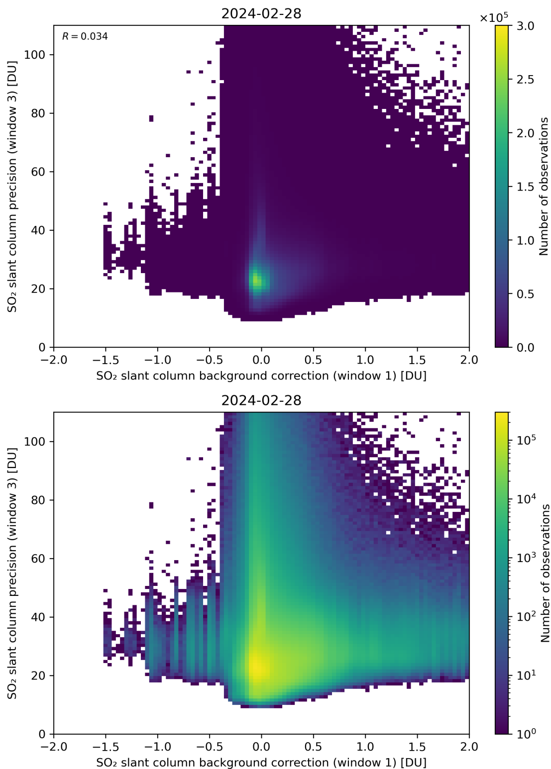
Figure 108: Scatter density plot of “SO 2 slant column background correction (window 1)” against “SO 2 slant column precision (window 3)” for 2024-02-27 to 2024-02-29.
