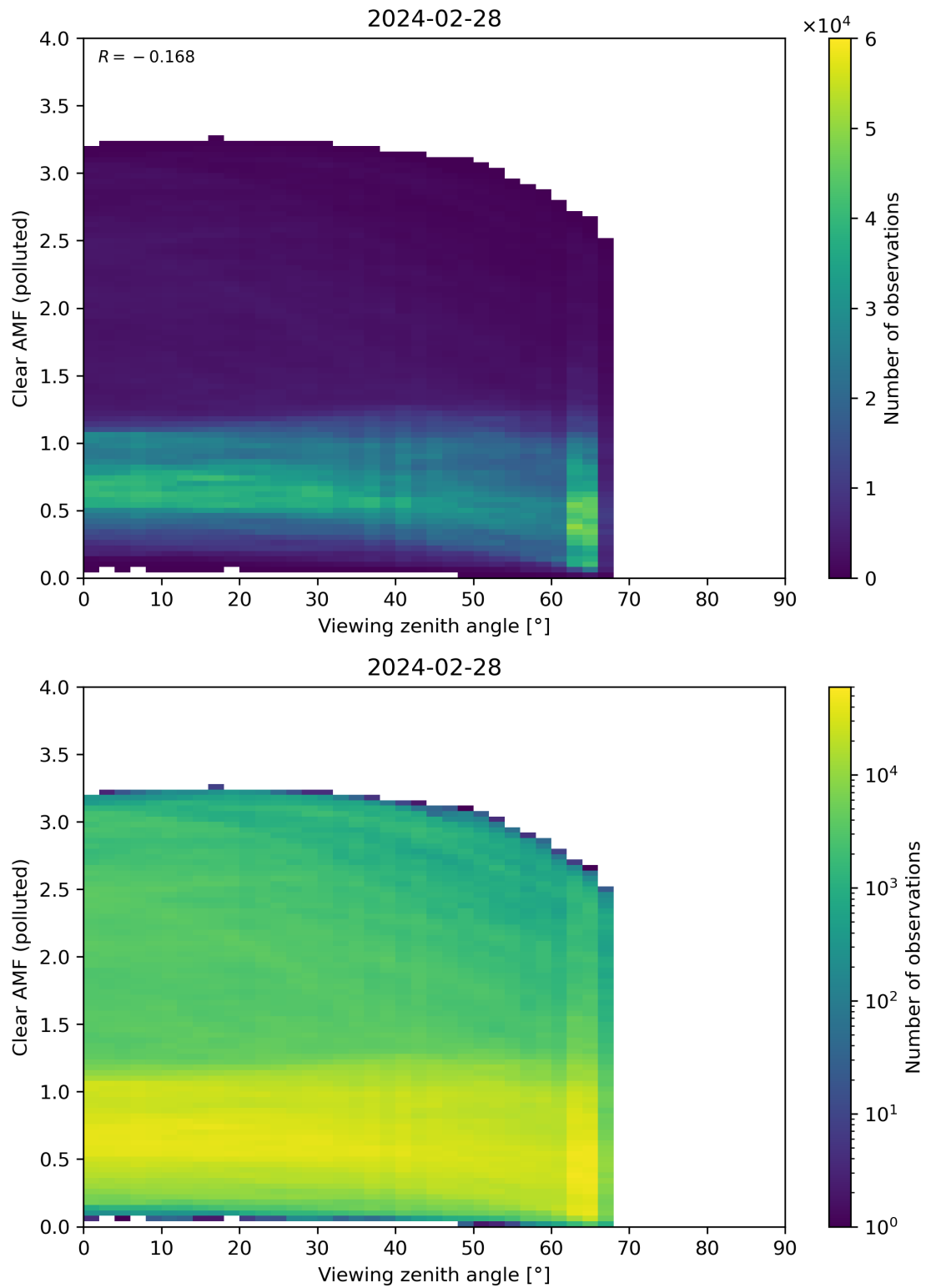
Figure 316: Scatter density plot of “Viewing zenith angle” against “Clear AMF (polluted)” for 2024-02-27 to 2024-02-29.
