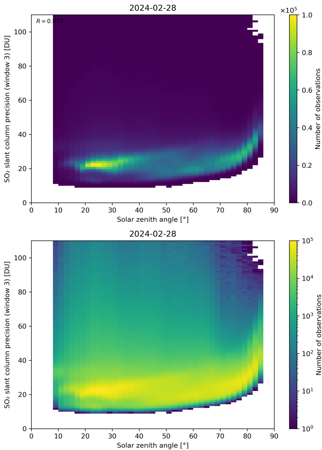
Figure 173: Scatter density plot of “Solar zenith angle” against “SO 2 slant column precision (window 3)” for 2024-02-27 to 2024-02-29.
