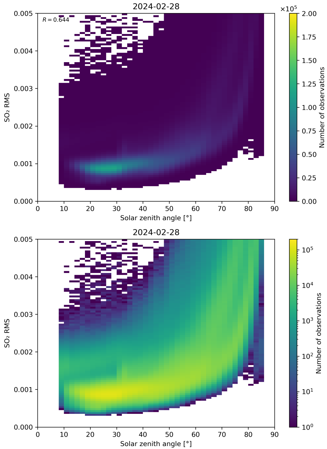
Figure 163: Scatter density plot of “Solar zenith angle” against “SO 2 RMS” for 2024-02-27 to 2024-02-29.
