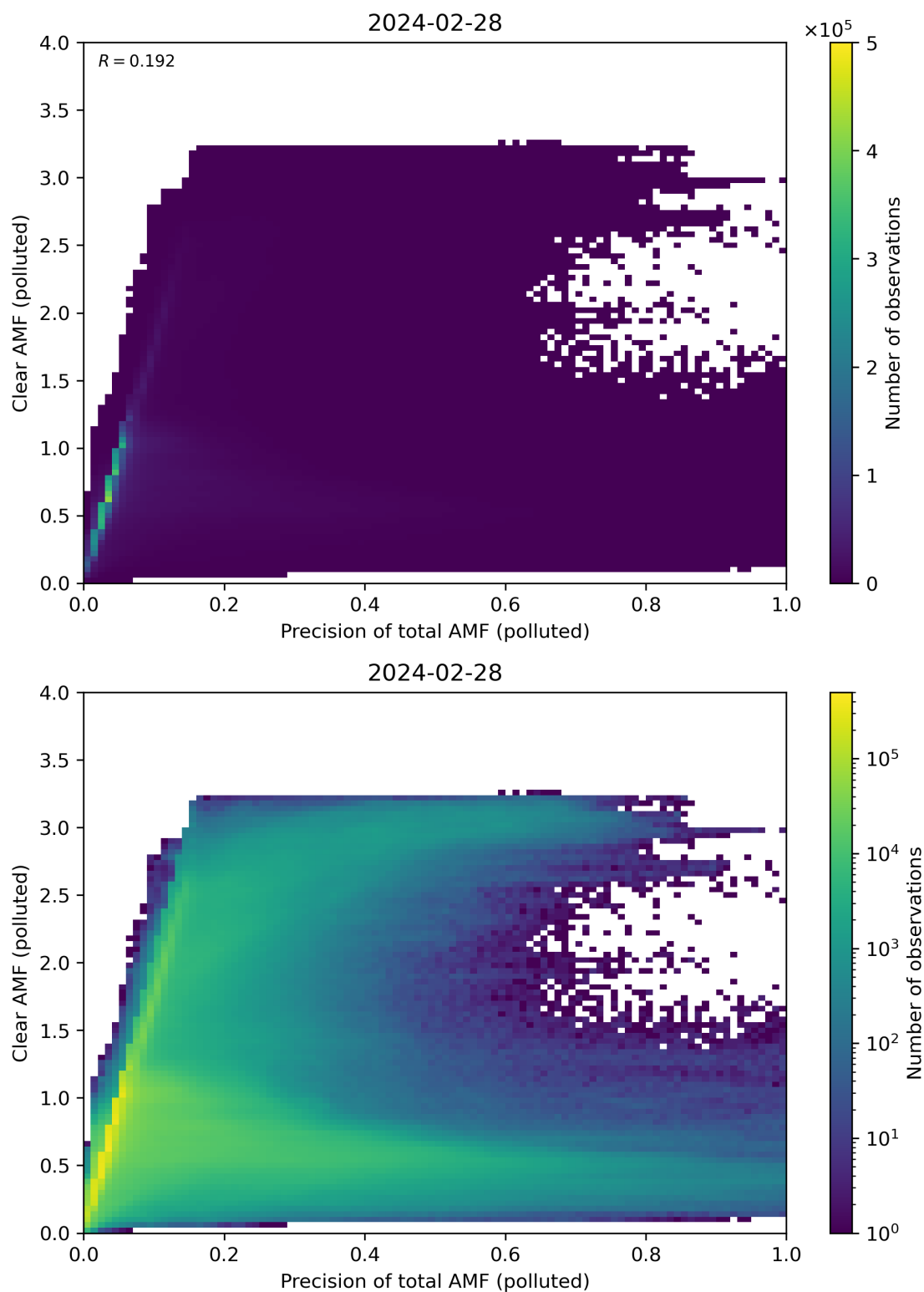
Figure 270: Scatter density plot of “Precision of total AMF (polluted)” against “Clear AMF (polluted)” for 2024-02-27 to 2024-02-29.
