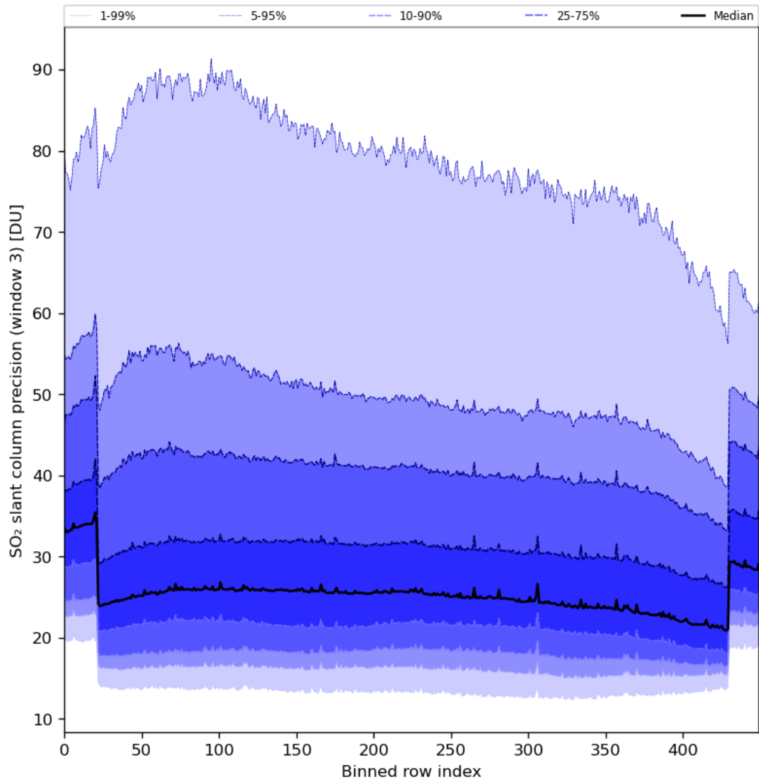
Figure 88: Along track statistics of “SO 2 slant column precision (window 3)” for 2024-02-27 to 2024-02-29
