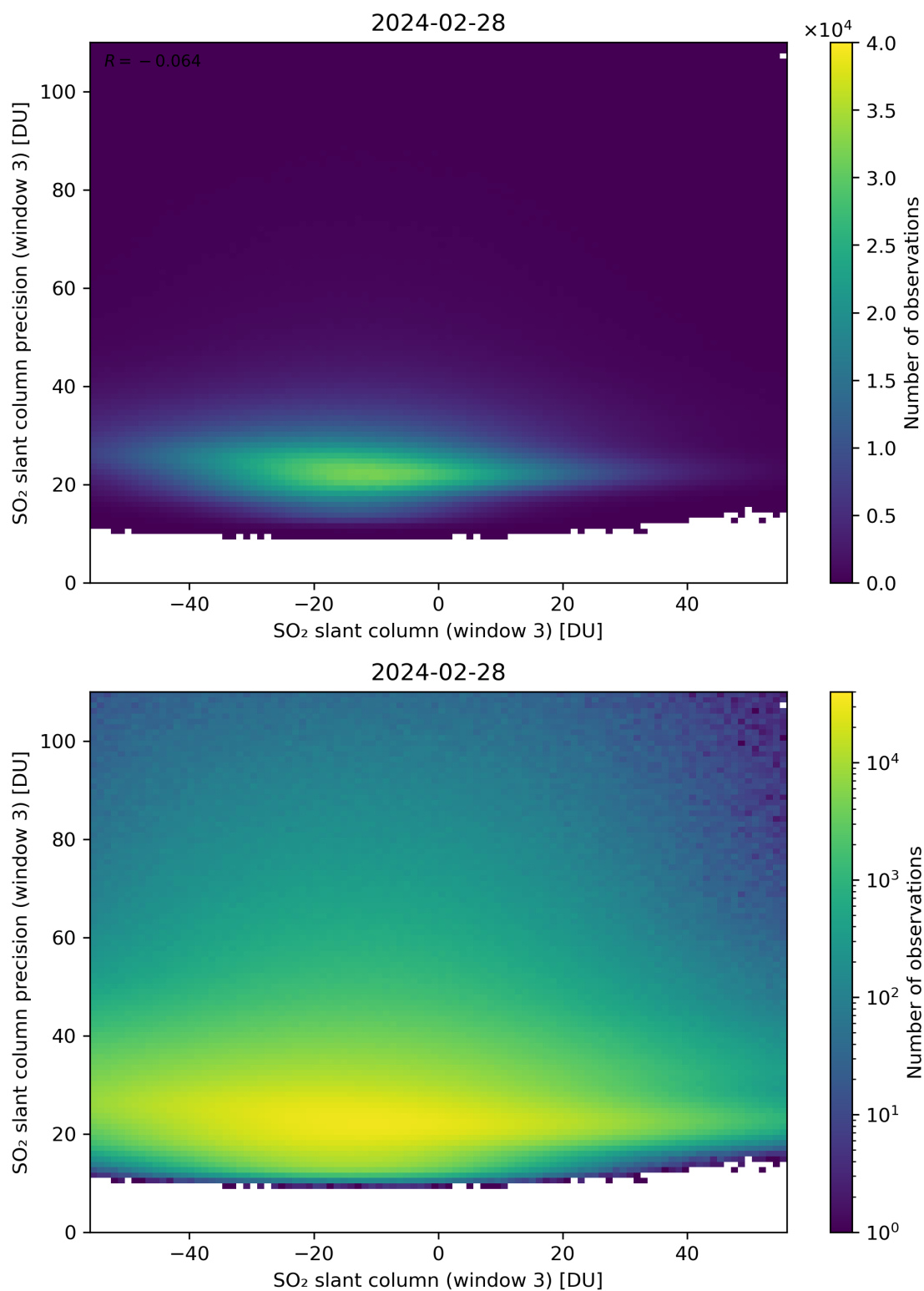
Figure 267: Scatter density plot of “SO 2 slant column (window 3)” against “SO 2 slant column precision (window 3)” for 2024-02-27 to 2024-02-29.
