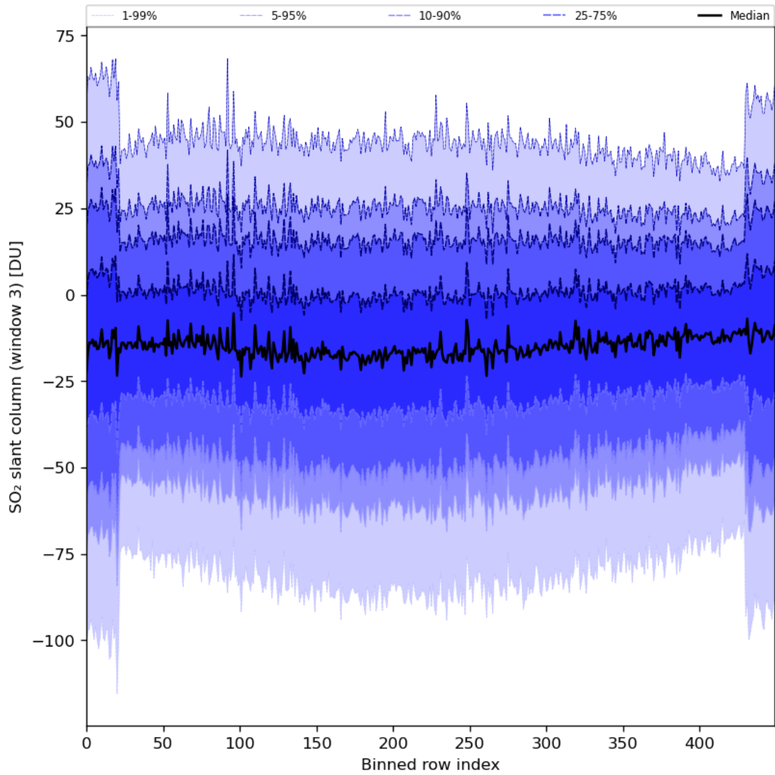
Figure 87: Along track statistics of “SO 2 slant column (window 3)” for 2024-02-27 to 2024-02-29
