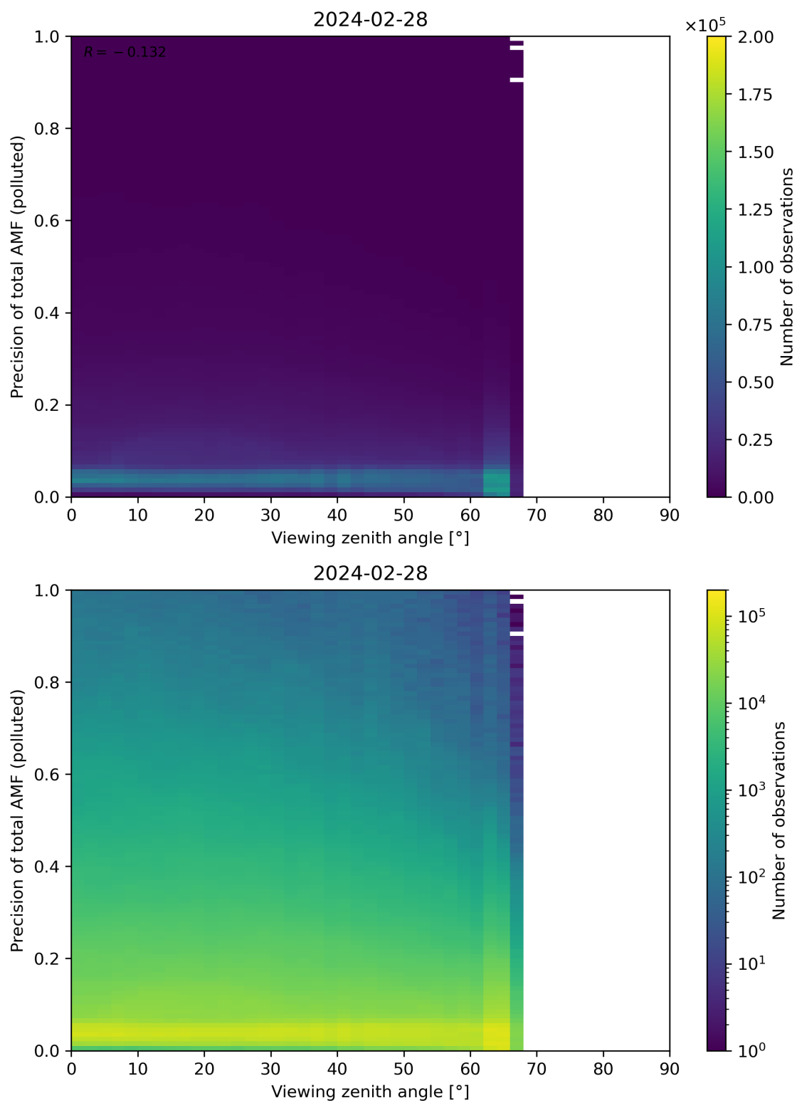
Figure 326: Scatter density plot of “Viewing zenith angle” against “Precision of total AMF (polluted)” for 2024-02-27 to 2024-02-29.
