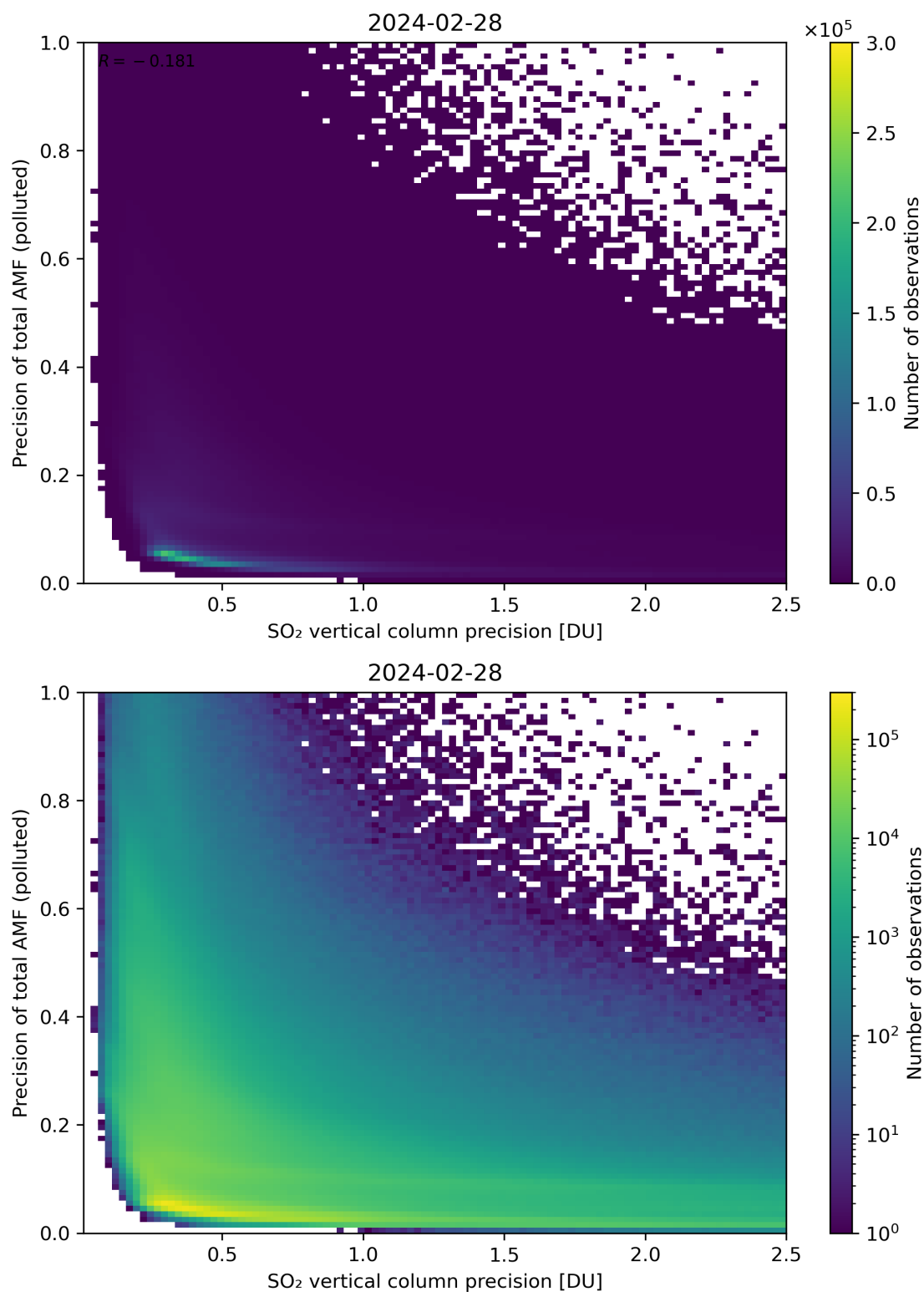
Figure 295: Scatter density plot of “SO 2 vertical column precision” against “Precision of total AMF (polluted)” for 2024-02-27 to 2024-02-29.
