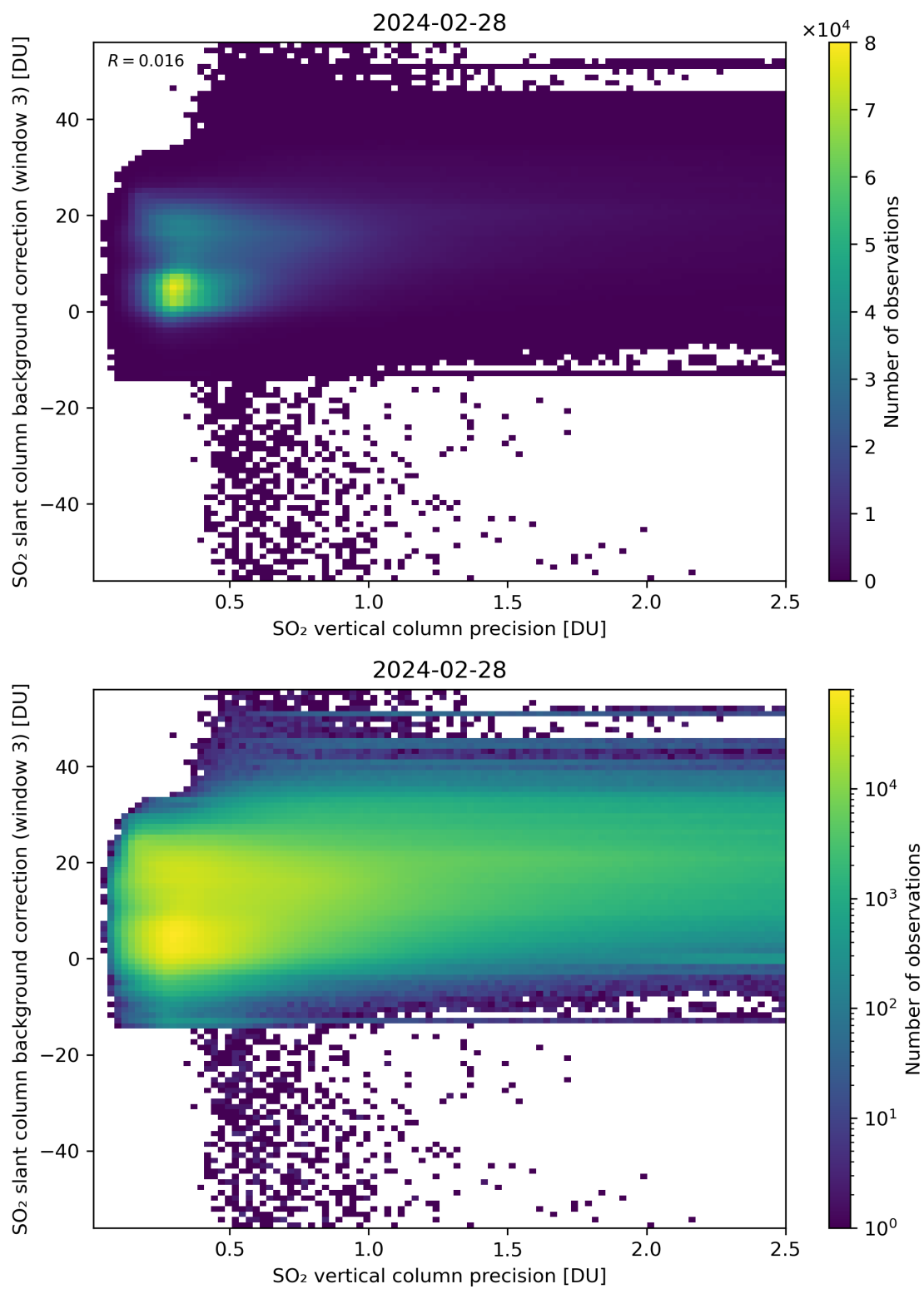
Figure 281: Scatter density plot of “SO 2 vertical column precision” against “SO 2 slant column background correction (window 3)” for 2024-02-27 to 2024-02-29.
