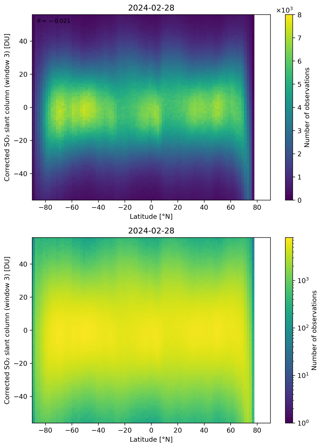
Figure 148: Scatter density plot of “Latitude” against “Corrected SO 2 slant column (window 3)” for 2024-02-27 to 2024-02-29.
