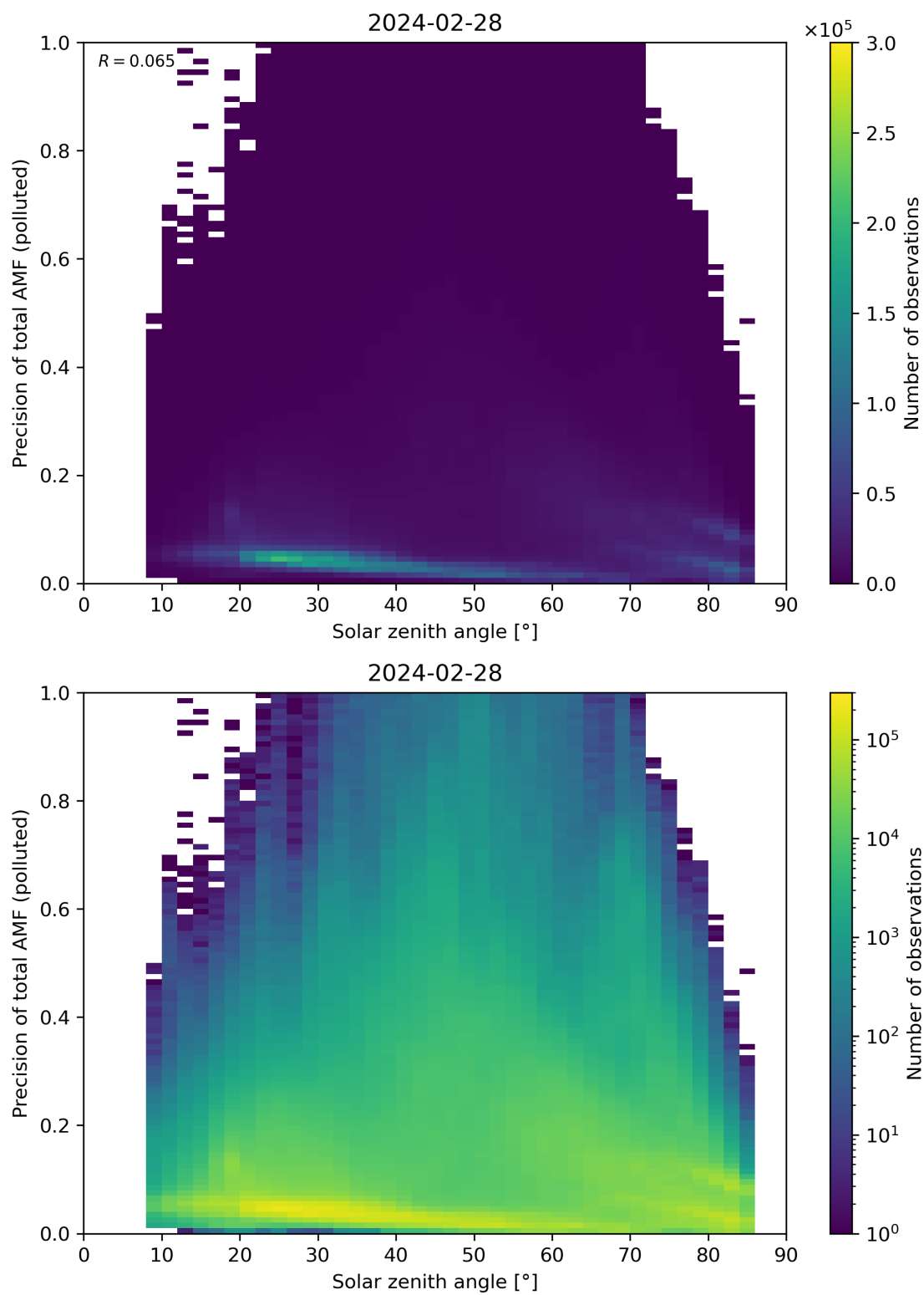
Figure 175: Scatter density plot of “Solar zenith angle” against “Precision of total AMF (polluted)” for 2024-02-27 to 2024-02-29.
