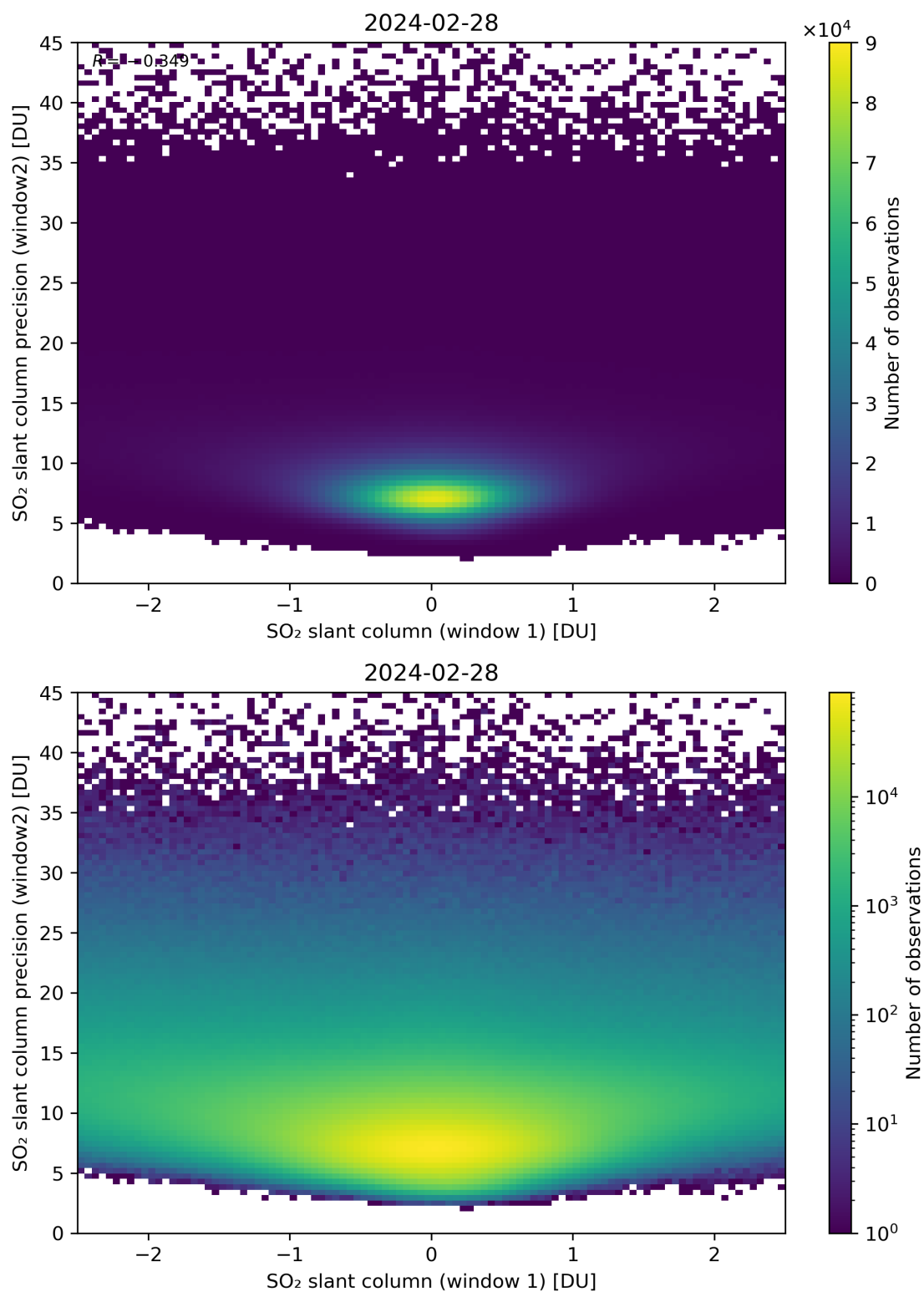
Figure 236: Scatter density plot of “SO 2 slant column (window 1)” against “SO 2 slant column precision (window2)” for 2024-02-27 to 2024-02-29.
