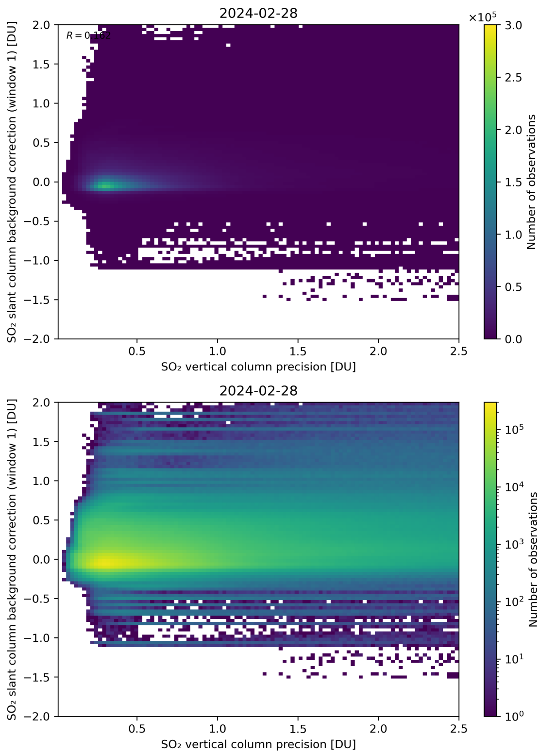
Figure 279: Scatter density plot of “SO 2 vertical column precision” against “SO 2 slant column background correction (window 1)” for 2024-02-27 to 2024-02-29.
