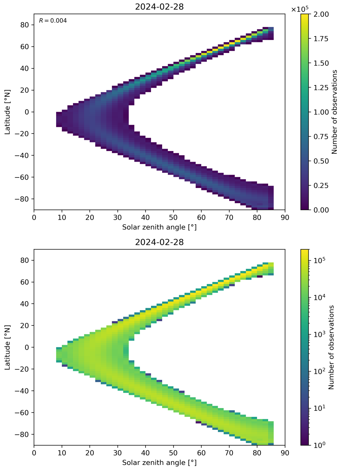
Figure 164: Scatter density plot of “Solar zenith angle” against “Latitude” for 2024-02-27 to 2024-02-29.
