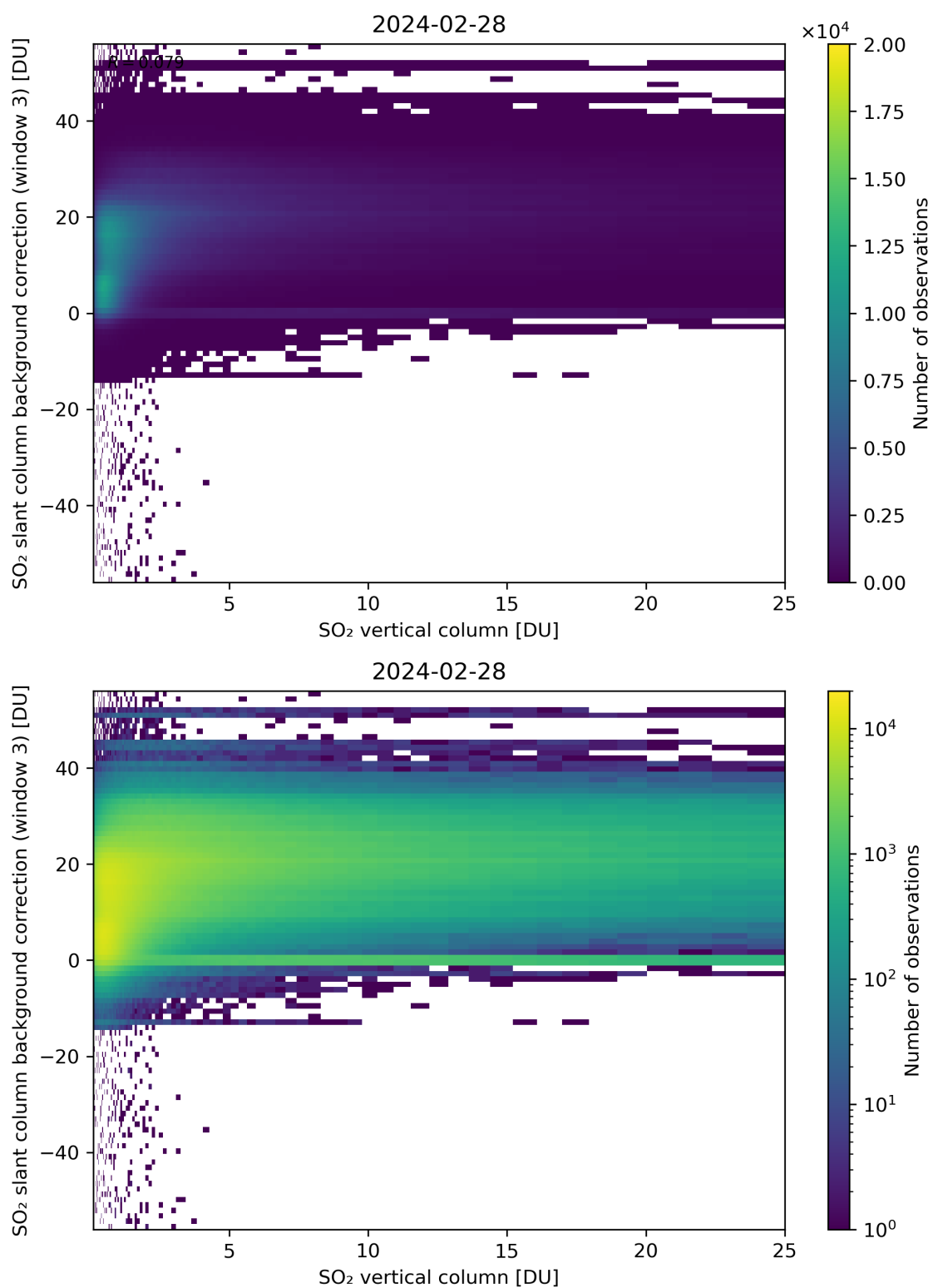
Figure 275: Scatter density plot of “SO 2 vertical column” against “SO 2 slant column background correction (window 3)” for 2024-02-27 to 2024-02-29.
