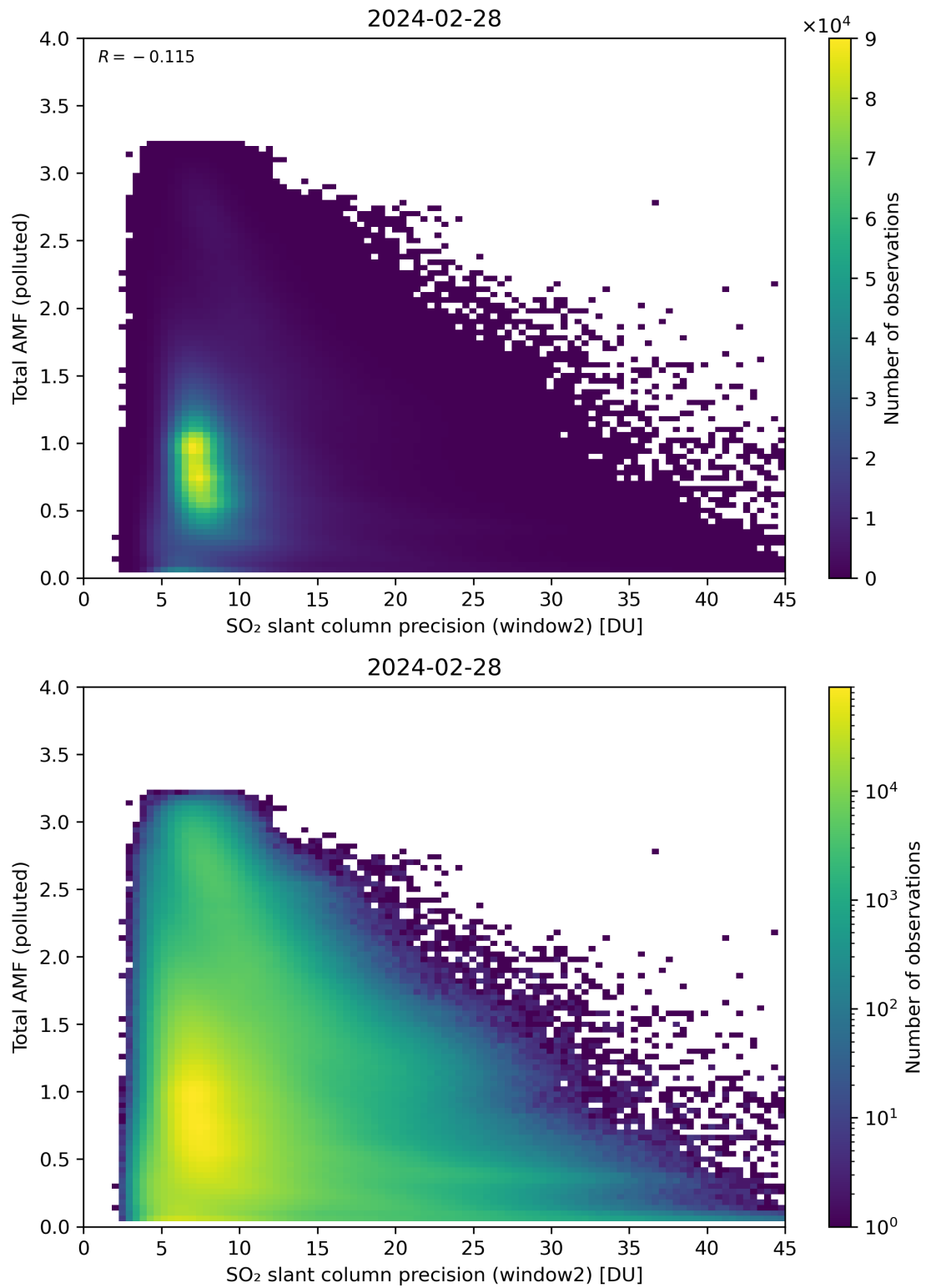
Figure 251: Scatter density plot of “SO 2 slant column precision (window2)” against “Total AMF (polluted)” for 2024-02-27 to 2024-02-29.
