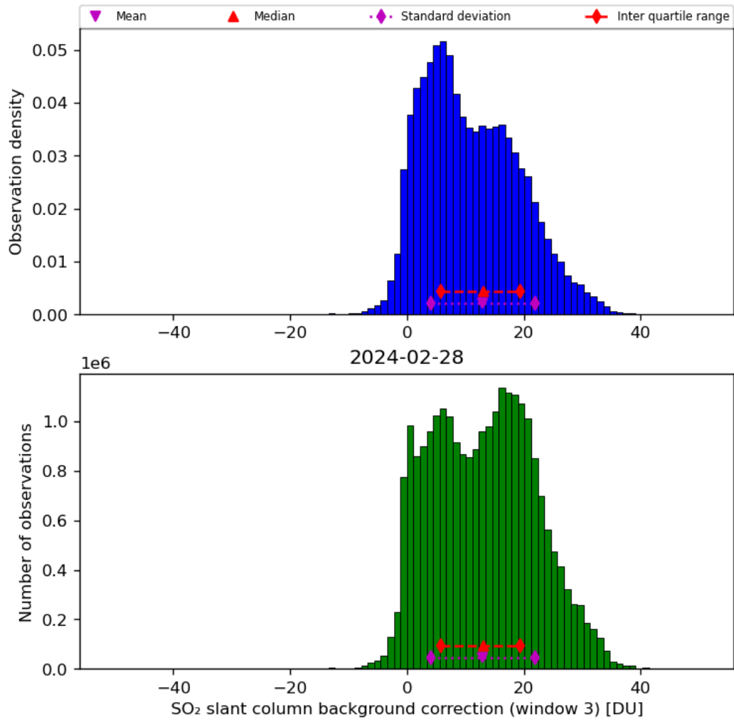
Figure 67: Histogram of “SO 2 slant column background correction (window 3)” for 2024-02-27 to 2024-02-29
