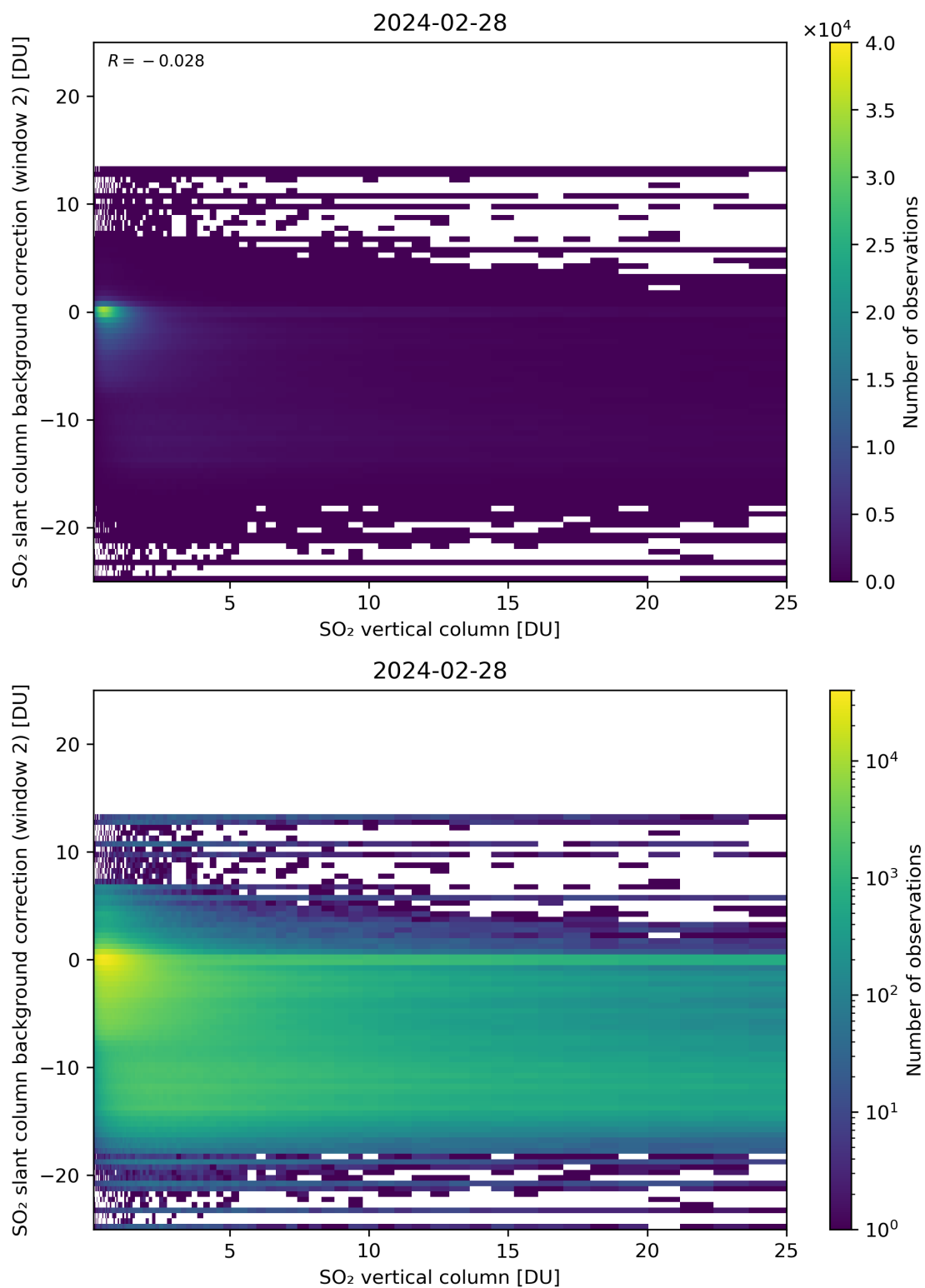
Figure 274: Scatter density plot of “SO 2 vertical column” against “SO 2 slant column background correction (window 2)” for 2024-02-27 to 2024-02-29.
