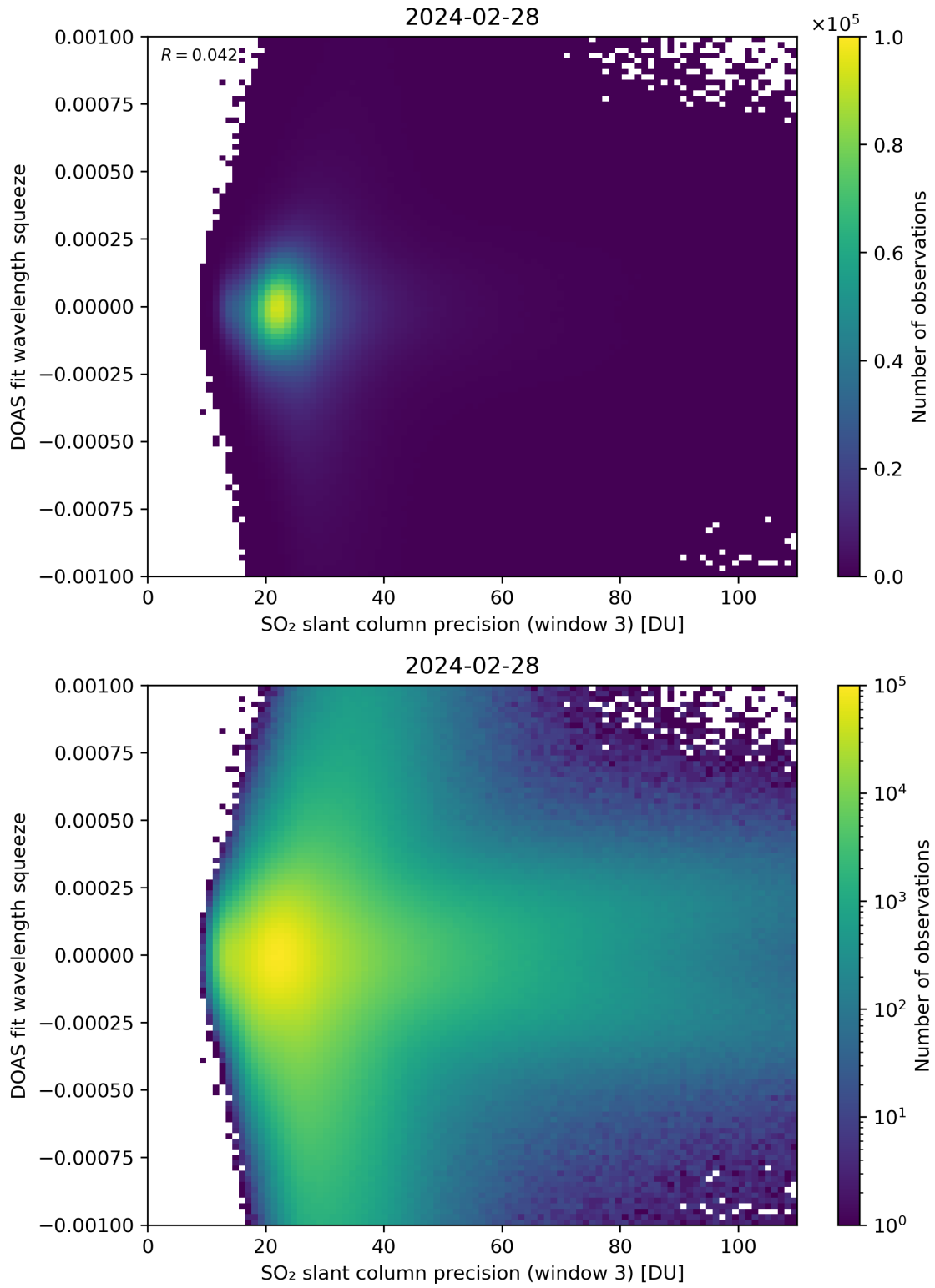
Figure 259: Scatter density plot of “SO 2 slant column precision (window 3)” against “DOAS fit wavelength squeeze” for 2024-02-27 to 2024-02-29.
