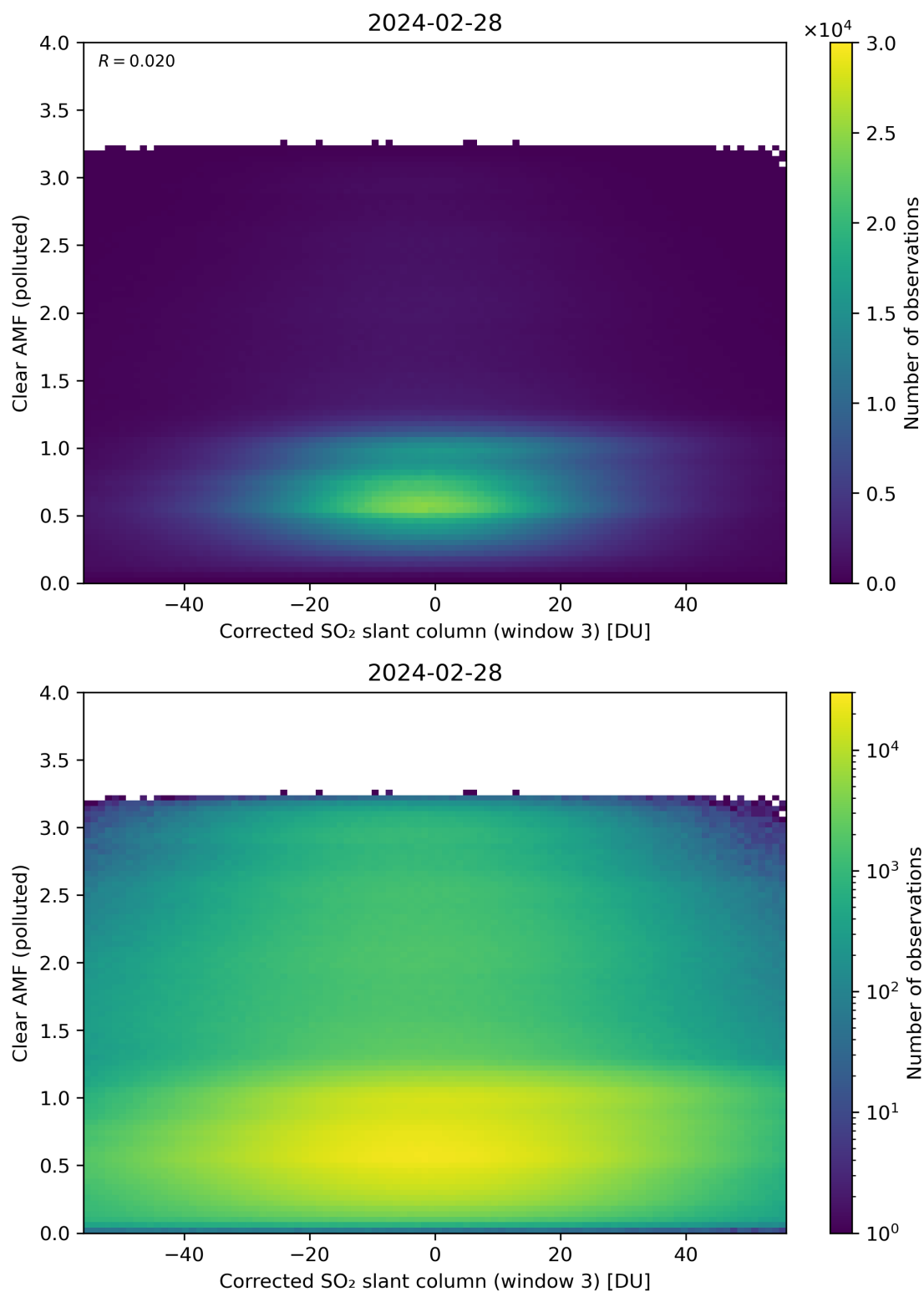
Figure 209: Scatter density plot of “Corrected SO 2 slant column (window 3)” against “Clear AMF (polluted)” for 2024-02-27 to 2024-02-29.
