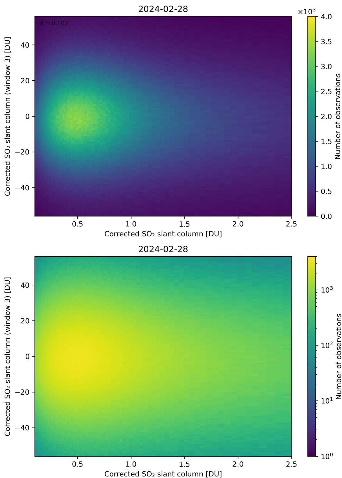
Figure 186: Scatter density plot of “Corrected SO 2 slant column” against “Corrected SO 2 slant column (window 3)” for 2024-02-27 to 2024-02-29.
