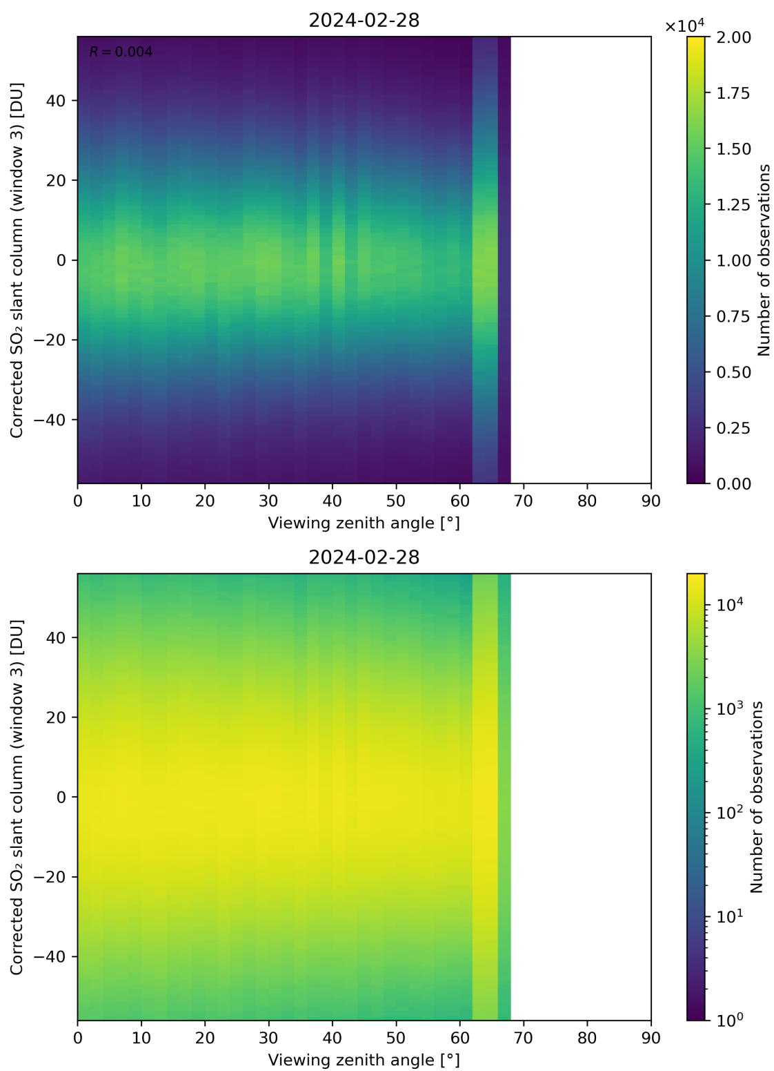
Figure 319: Scatter density plot of “Viewing zenith angle” against “Corrected SO 2 slant column (window 3)” for 2024-02-27 to 2024-02-29.
