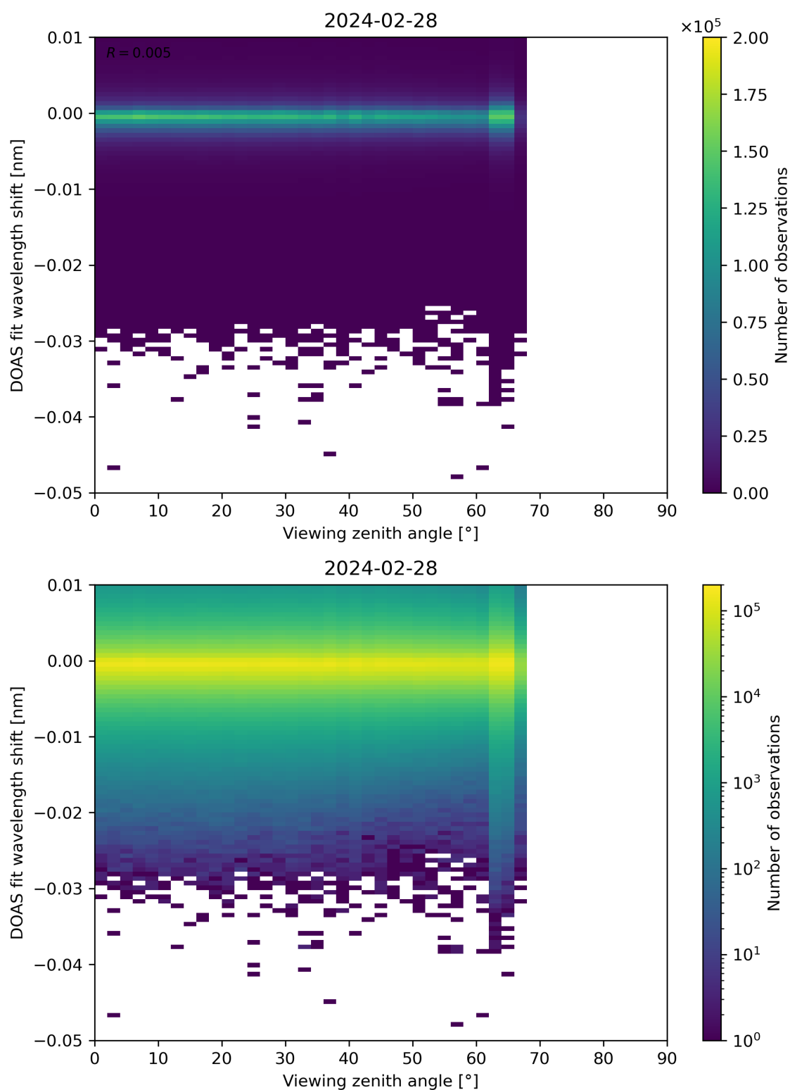
Figure 311: Scatter density plot of “Viewing zenith angle” against “DOAS fit wavelength shift” for 2024-02-27 to 2024-02-29.
