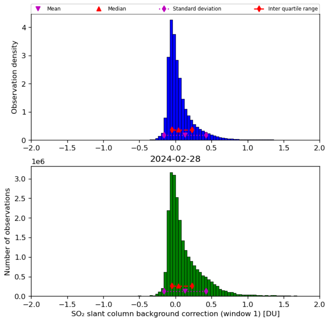
Figure 59: Histogram of “SO 2 slant column background correction (window 1)” for 2024-02-27 to 2024-02-29
