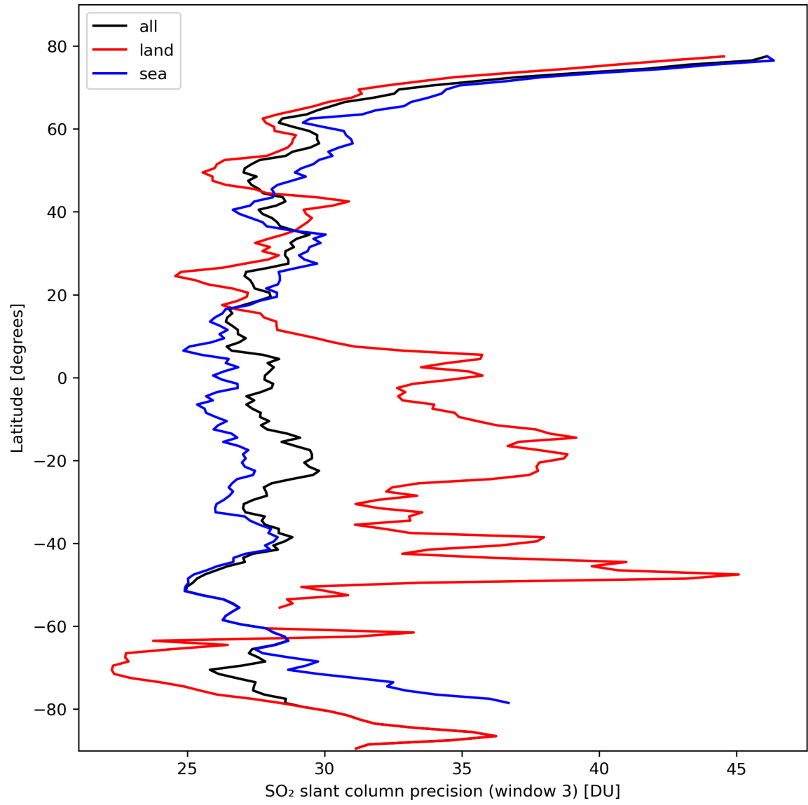
Figure 42: Zonal average of “SO 2 slant column precision (window 3)” for 2024-02-27 to 2024-02-29.
