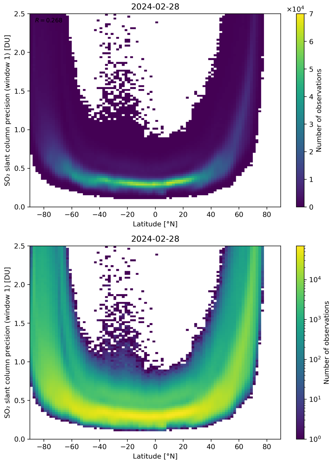
Figure 150: Scatter density plot of “Latitude” against “SO 2 slant column precision (window 1)” for 2024-02-27 to 2024-02-29.
