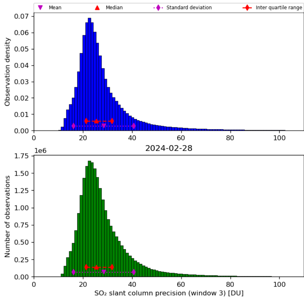
Figure 65: Histogram of “SO 2 slant column precision (window 3)” for 2024-02-27 to 2024-02-29
