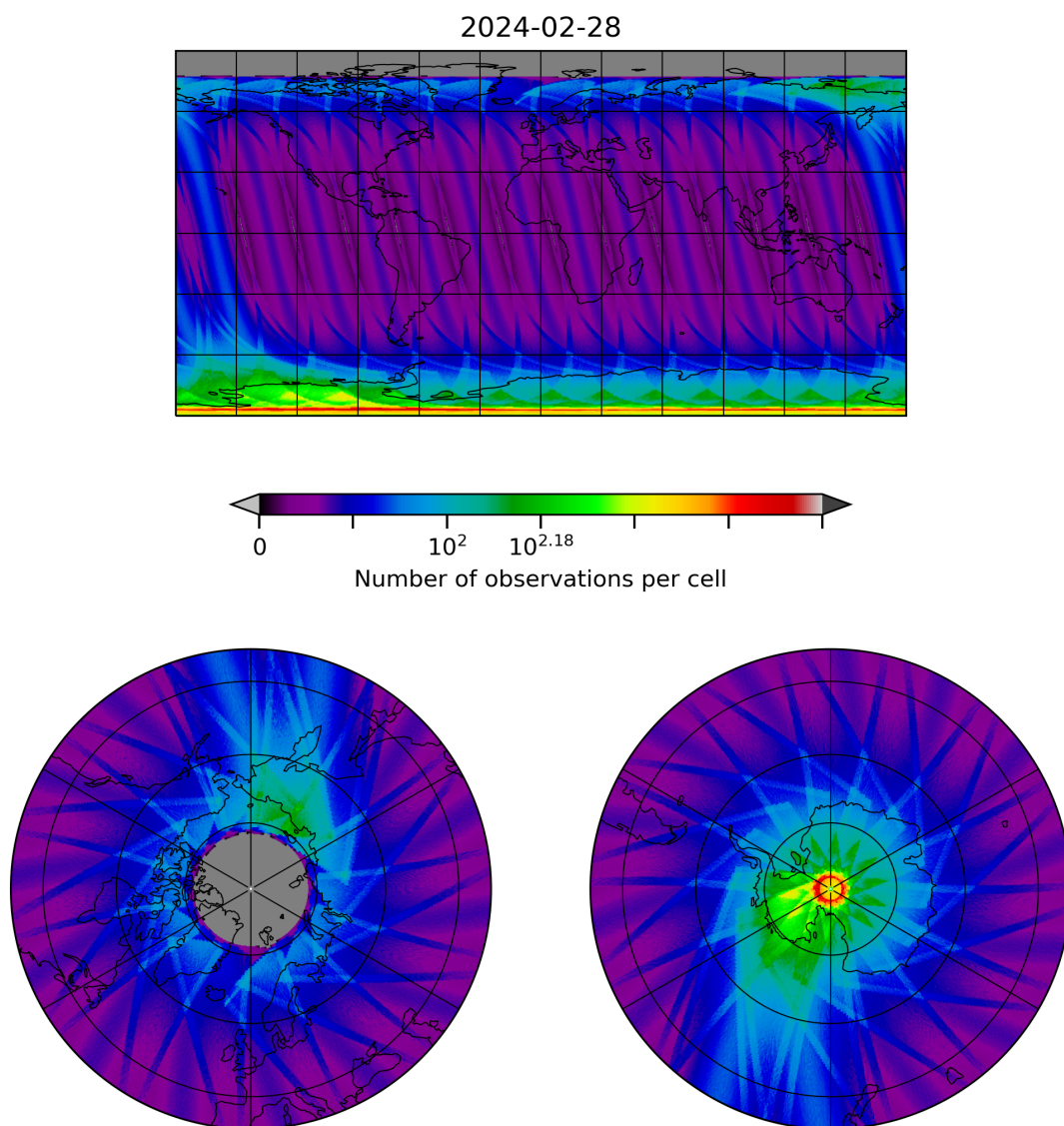
Figure 28: Map of the number of observations for 2024-02-27 to 2024-02-29
