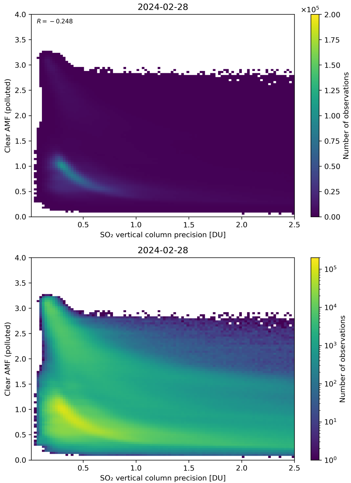
Figure 285: Scatter density plot of “SO 2 vertical column precision” against “Clear AMF (polluted)” for 2024-02-27 to 2024-02-29.
