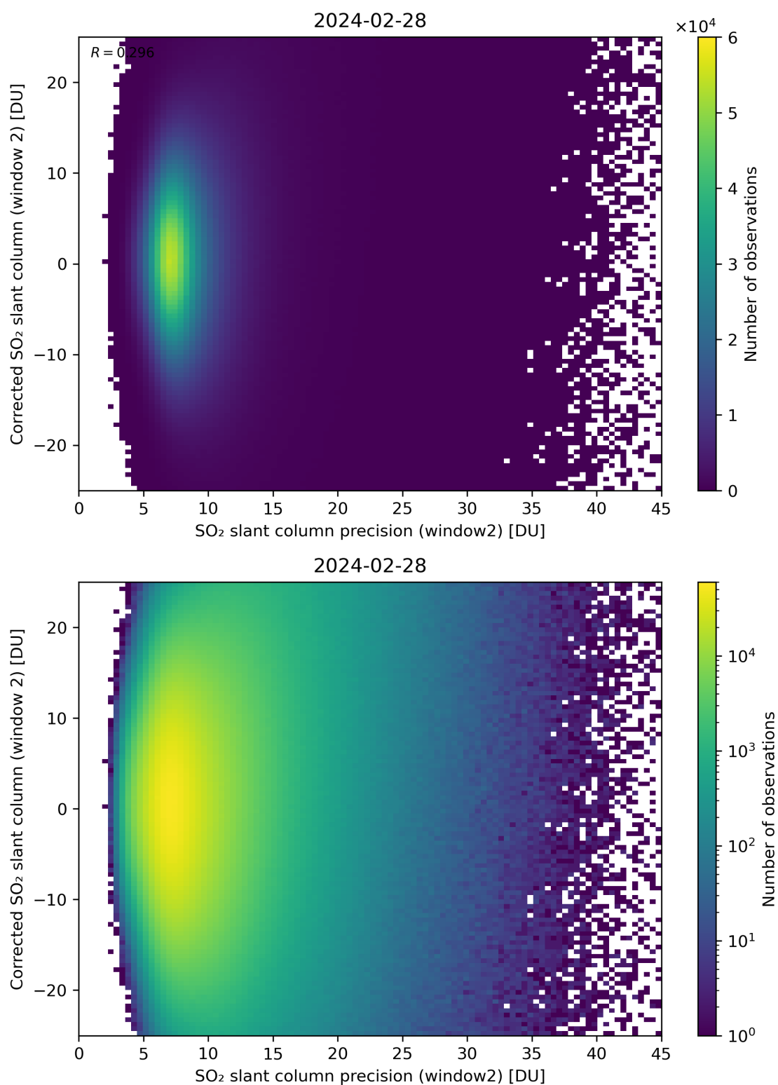
Figure 247: Scatter density plot of “SO 2 slant column precision (window2)” against “Corrected SO 2 slant column (window 2)” for 2024-02-27 to 2024-02-29.
