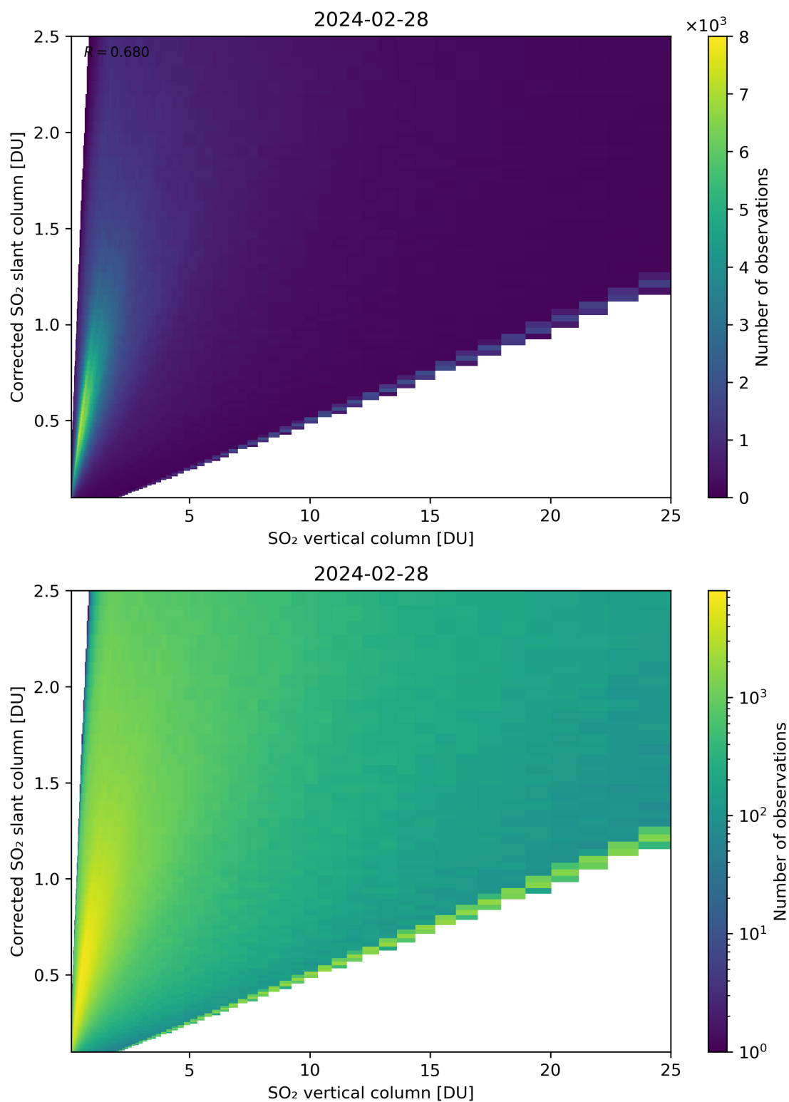
Figure 297: Scatter density plot of “SO 2 vertical column” against “Corrected SO 2 slant column” for 2024-02-27 to 2024-02-29.
