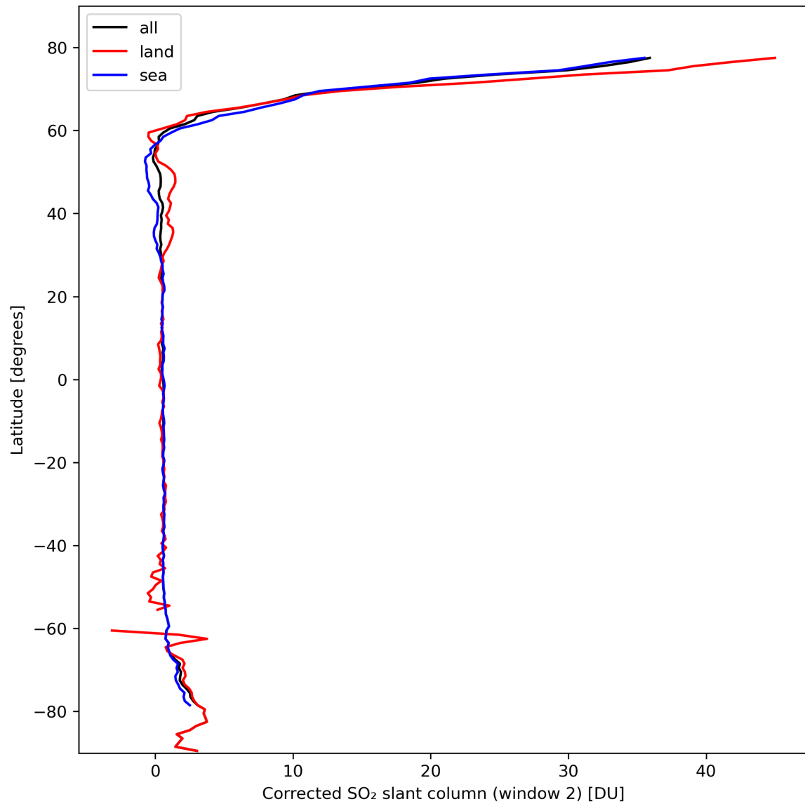
Figure 39: Zonal average of “Corrected SO 2 slant column (window 2)” for 2024-02-27 to 2024-02-29.
