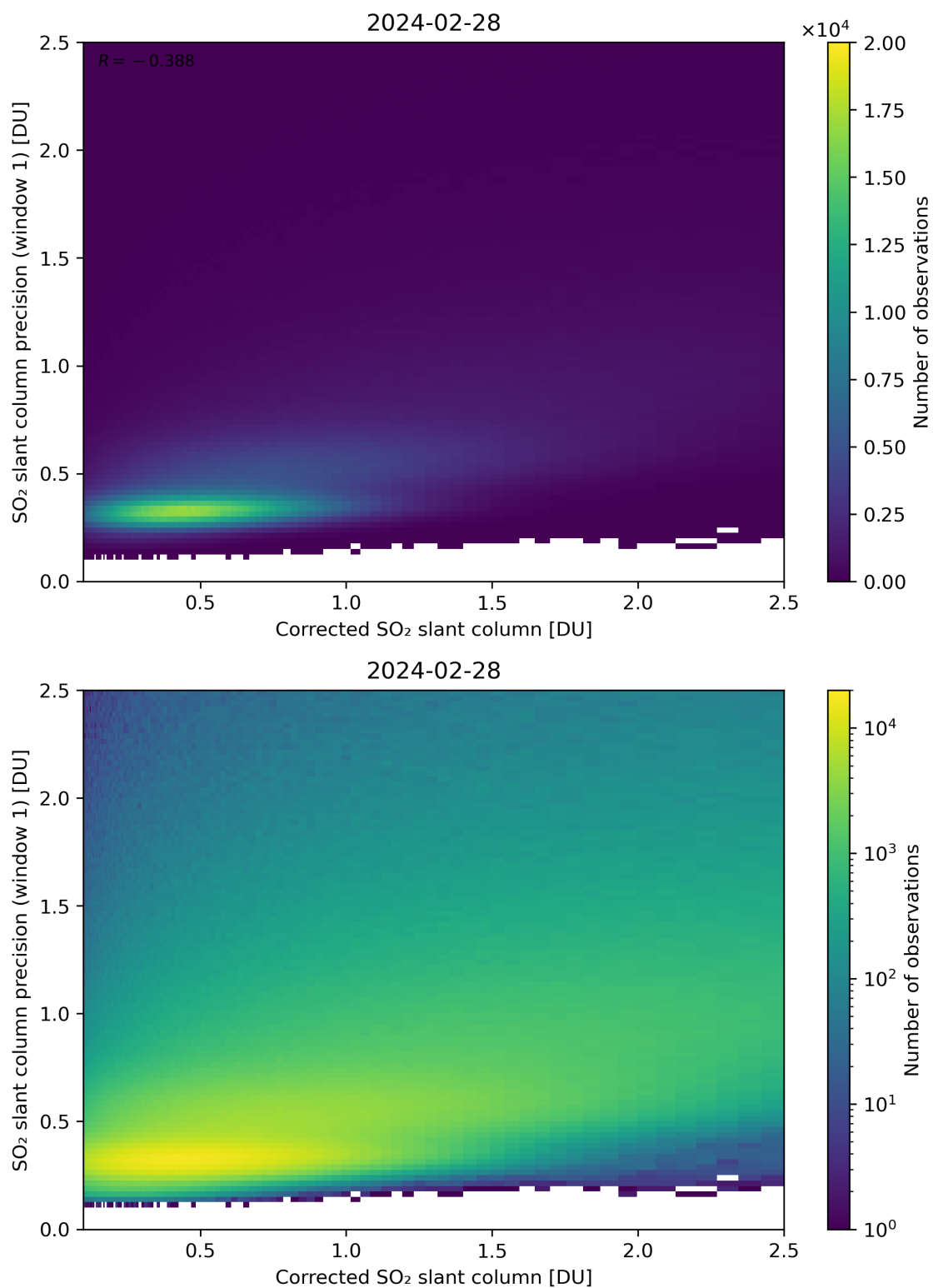
Figure 188: Scatter density plot of “Corrected SO 2 slant column” against “SO 2 slant column precision (window 1)” for 2024-02-27 to 2024-02-29.
