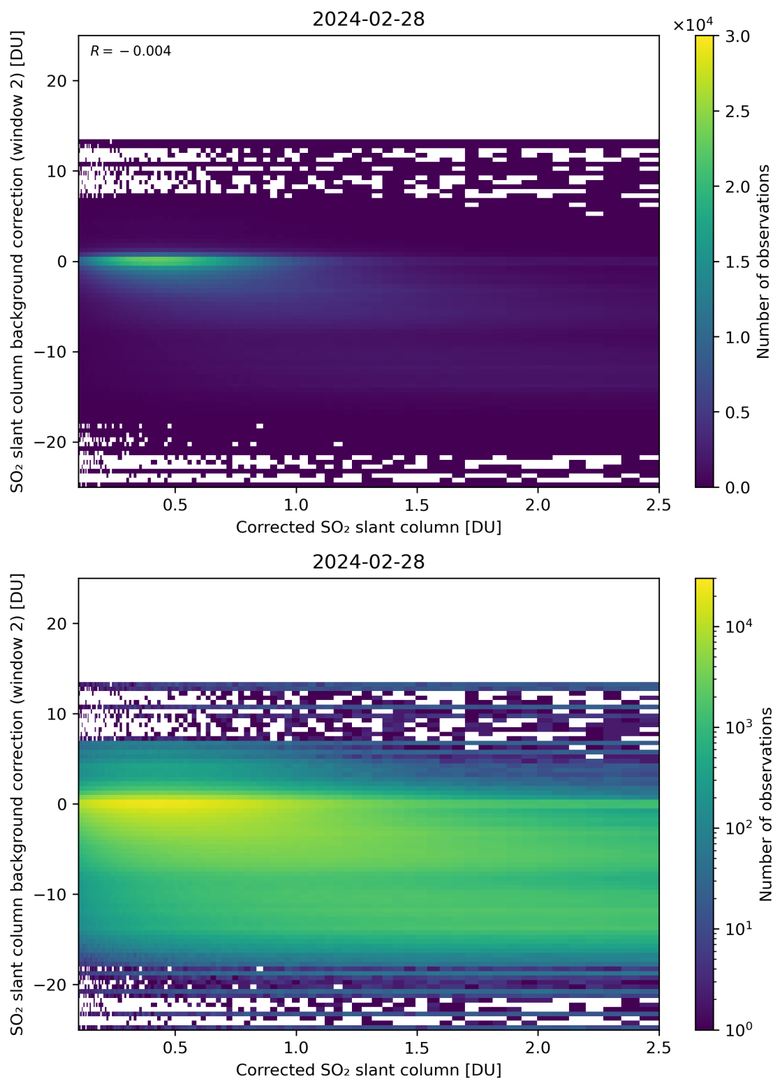
Figure 179: Scatter density plot of “Corrected SO 2 slant column” against “SO 2 slant column background correction (window 2)” for 2024-02-27 to 2024-02-29.
