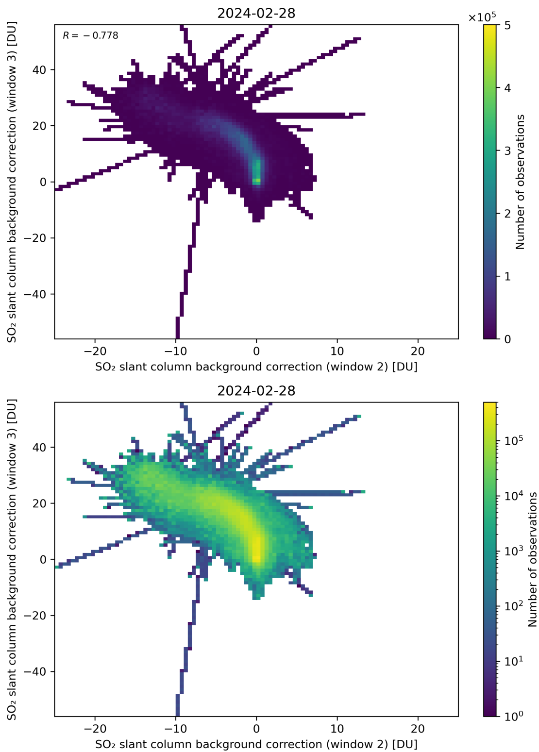
Figure 111: Scatter density plot of “SO 2 slant column background correction (window 2)” against “SO 2 slant column background correction (window 3)” for 2024-02-27 to 2024-02-29.
