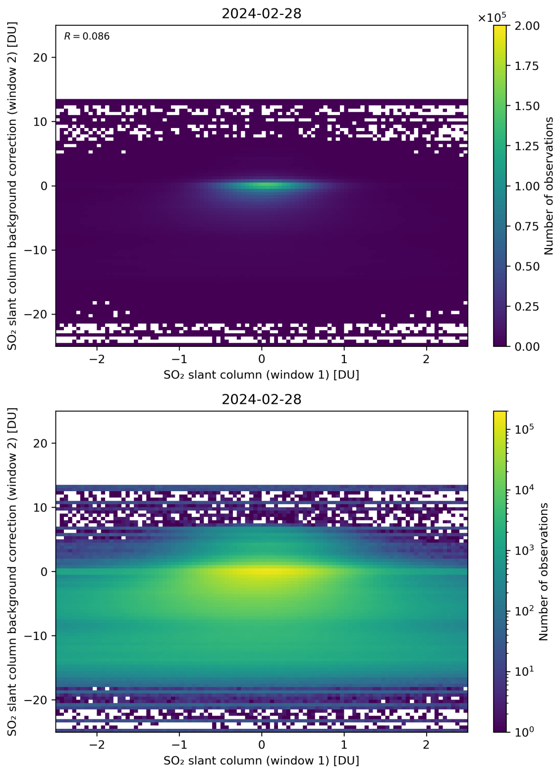
Figure 213: Scatter density plot of “SO 2 slant column (window 1)” against “SO 2 slant column background correction (window 2)” for 2024-02-27 to 2024-02-29.
