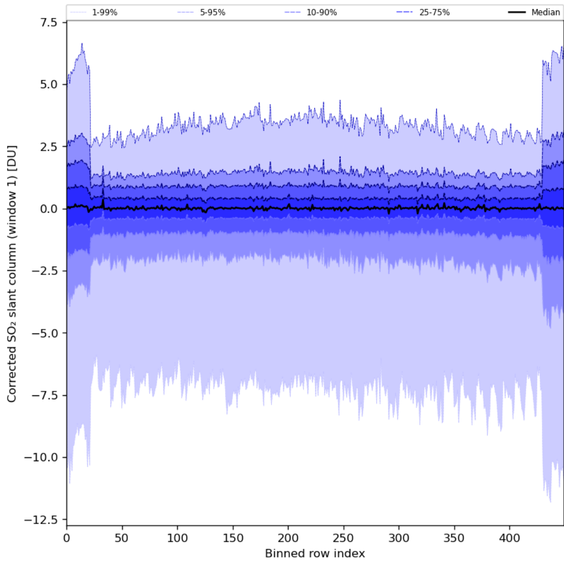
Figure 81: Along track statistics of “Corrected SO 2 slant column (window 1)” for 2024-02-27 to 2024-02-29
