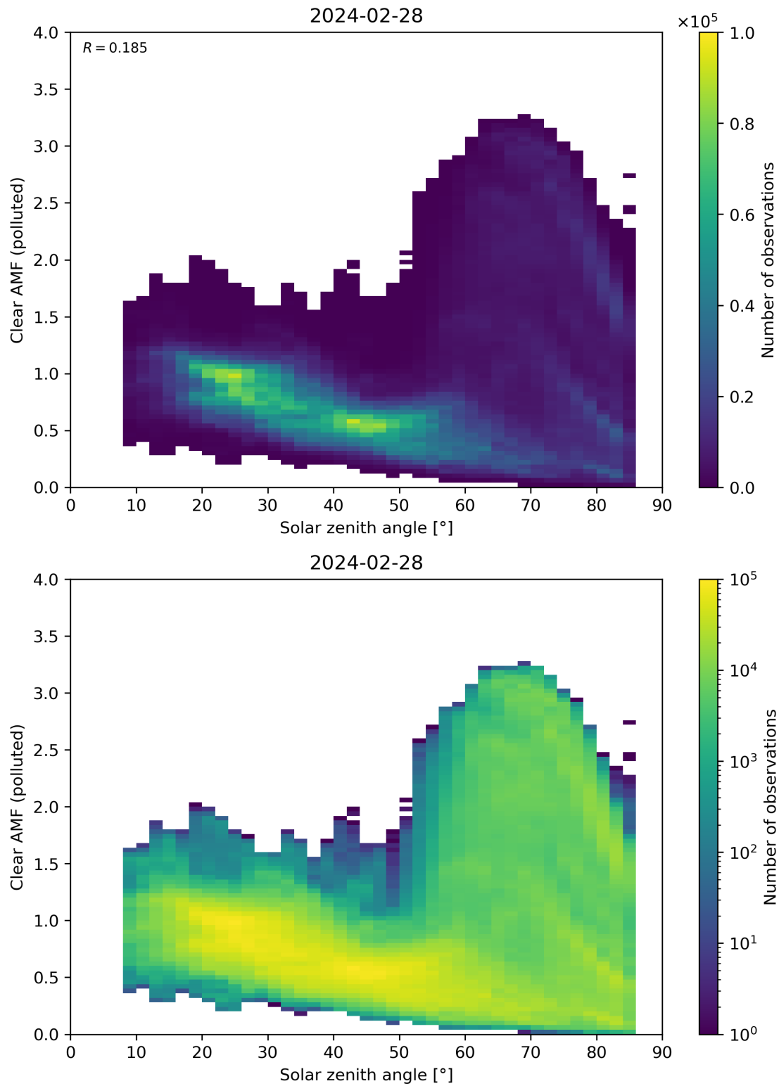
Figure 165: Scatter density plot of “Solar zenith angle” against “Clear AMF (polluted)” for 2024-02-27 to 2024-02-29.
