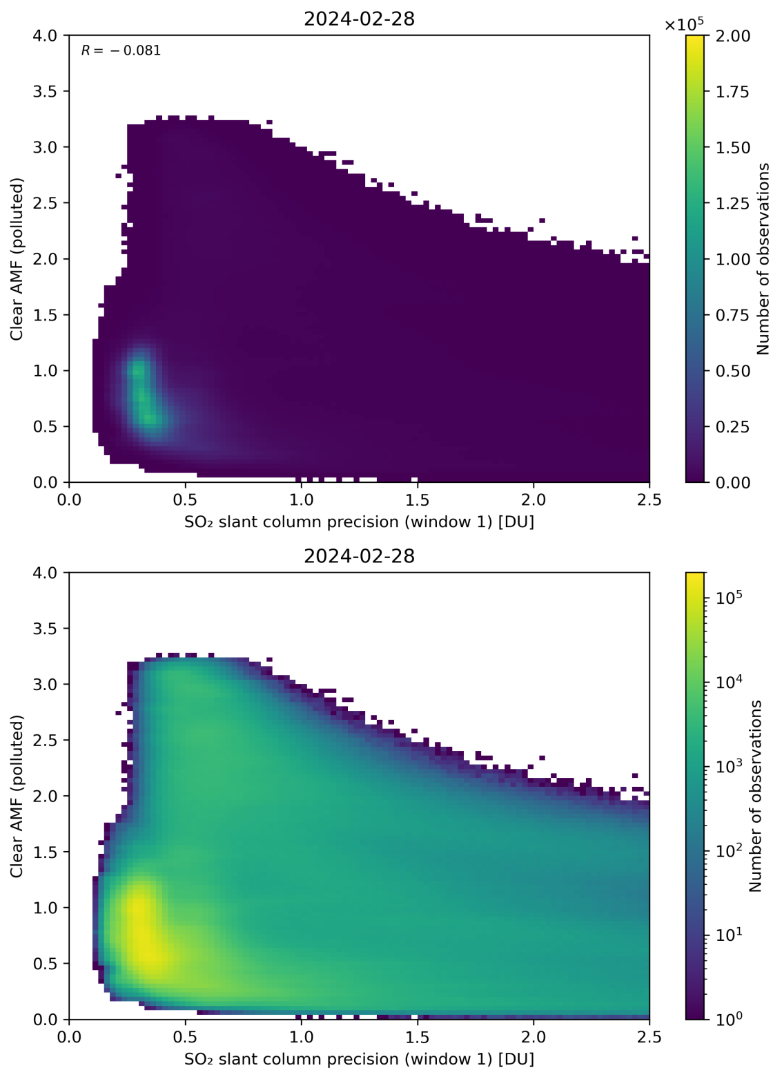
Figure 224: Scatter density plot of “SO 2 slant column precision (window 1)” against “Clear AMF (polluted)” for 2024-02-27 to 2024-02-29.
