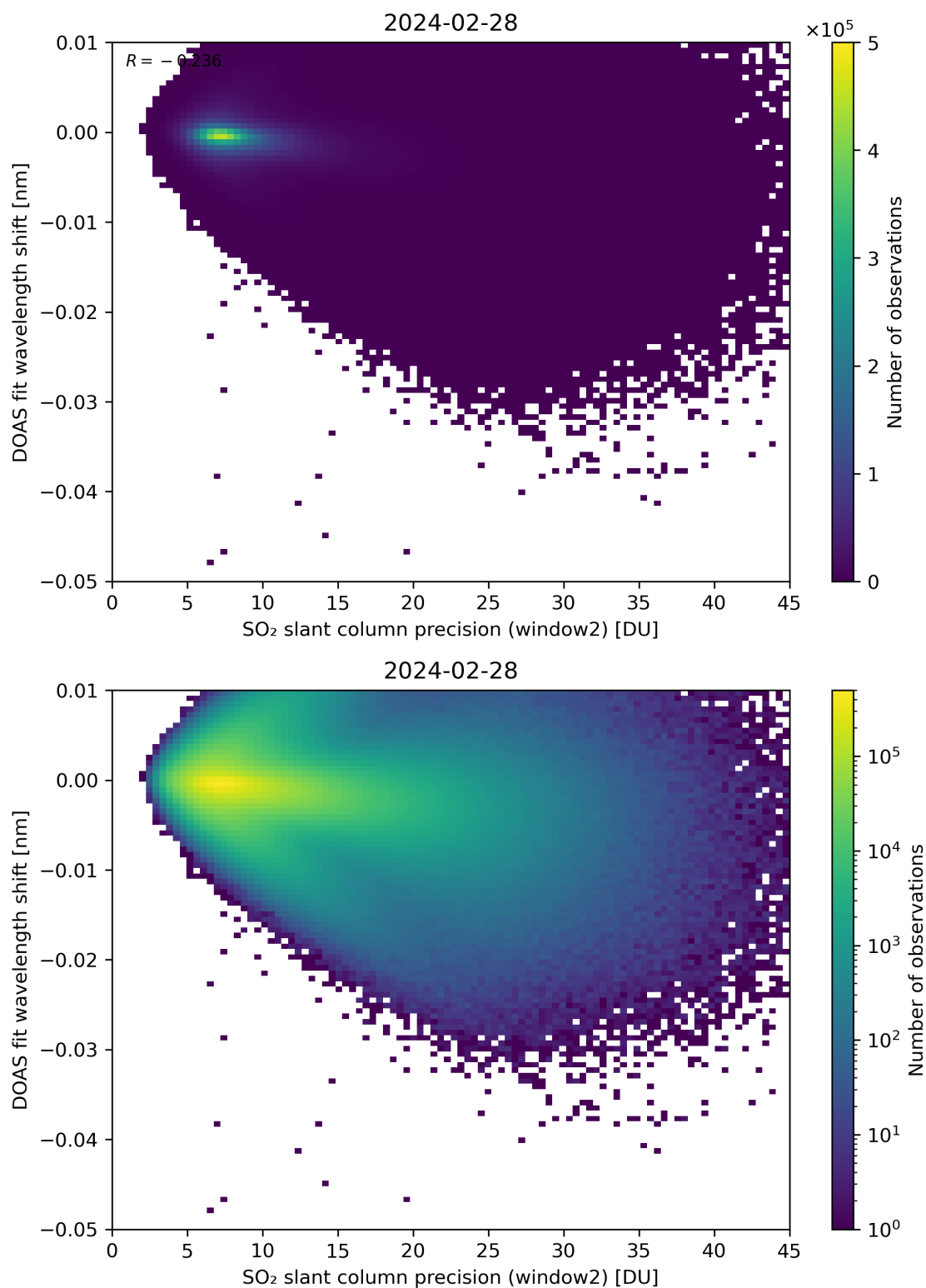
Figure 243: Scatter density plot of “SO 2 slant column precision (window2)” against “DOAS fit wavelength shift” for 2024-02-27 to 2024-02-29.
