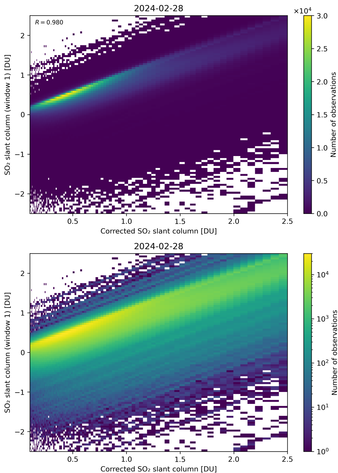
Figure 187: Scatter density plot of “Corrected SO 2 slant column” against “SO 2 slant column (window 1)” for 2024-02-27 to 2024-02-29.
