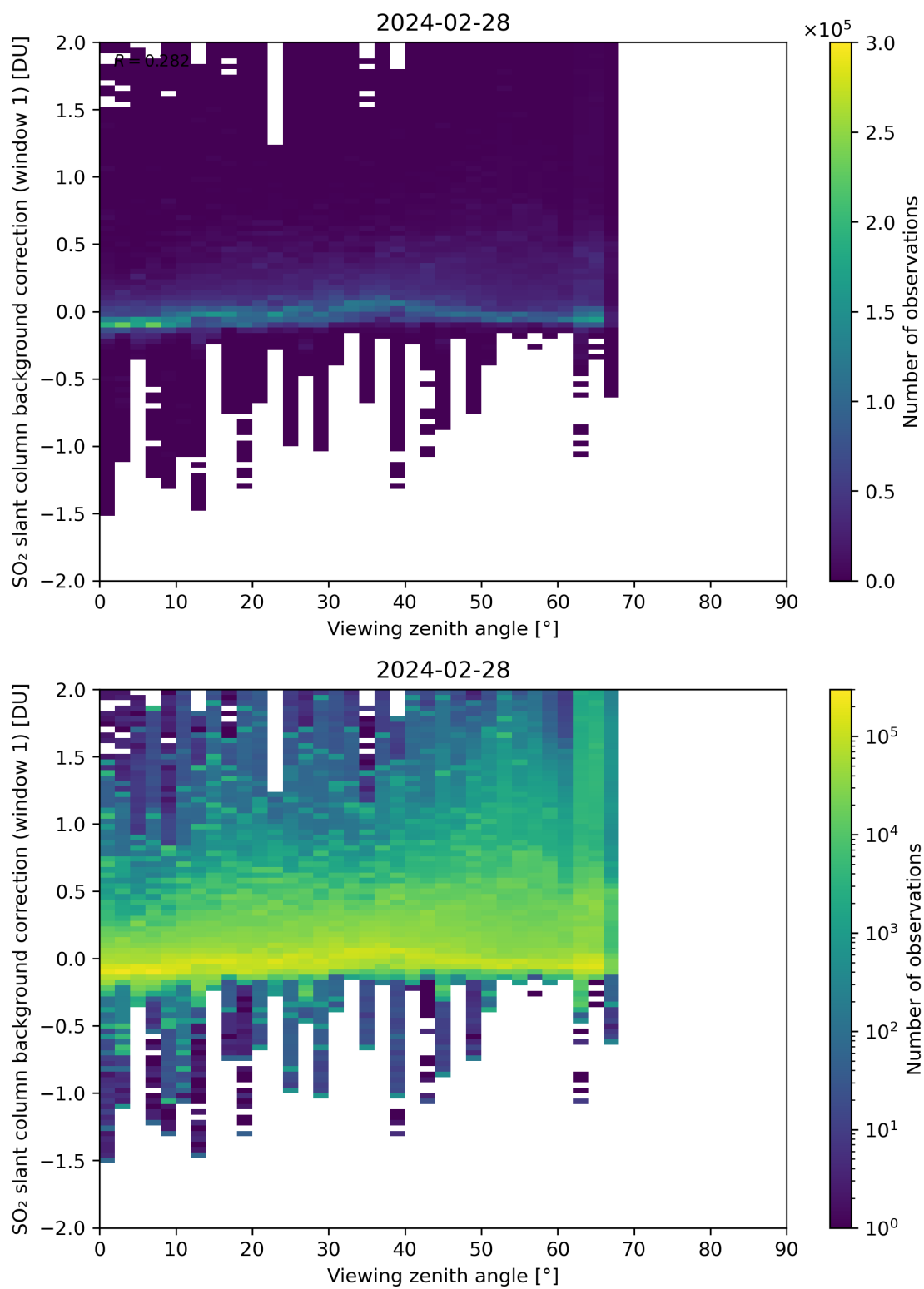
Figure 308: Scatter density plot of “Viewing zenith angle” against “SO 2 slant column background correction (window 1)” for 2024-02-27 to 2024-02-29.
