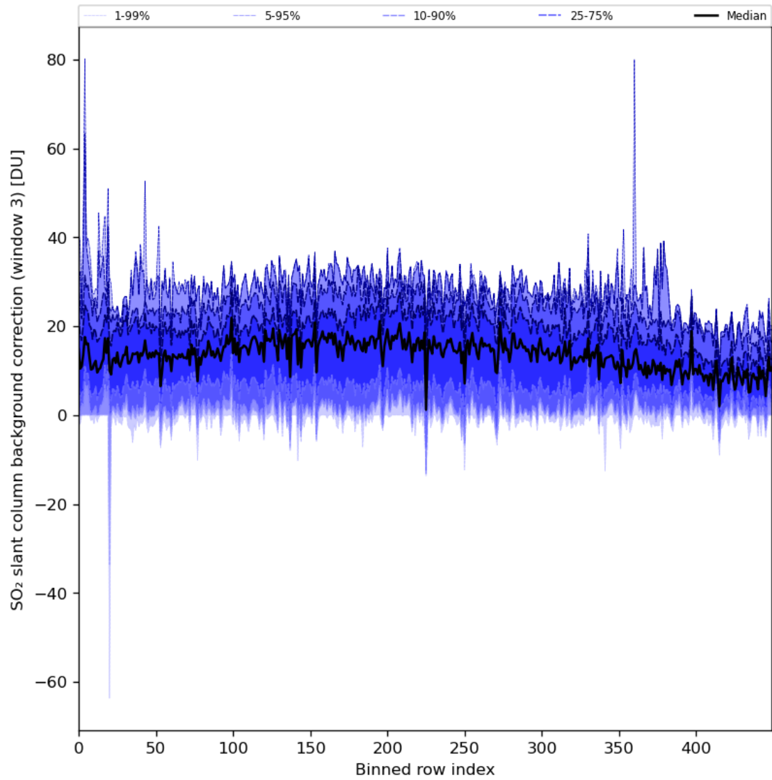
Figure 90: Along track statistics of “SO 2 slant column background correction (window 3)” for 2024-02-27 to 2024-02-29
