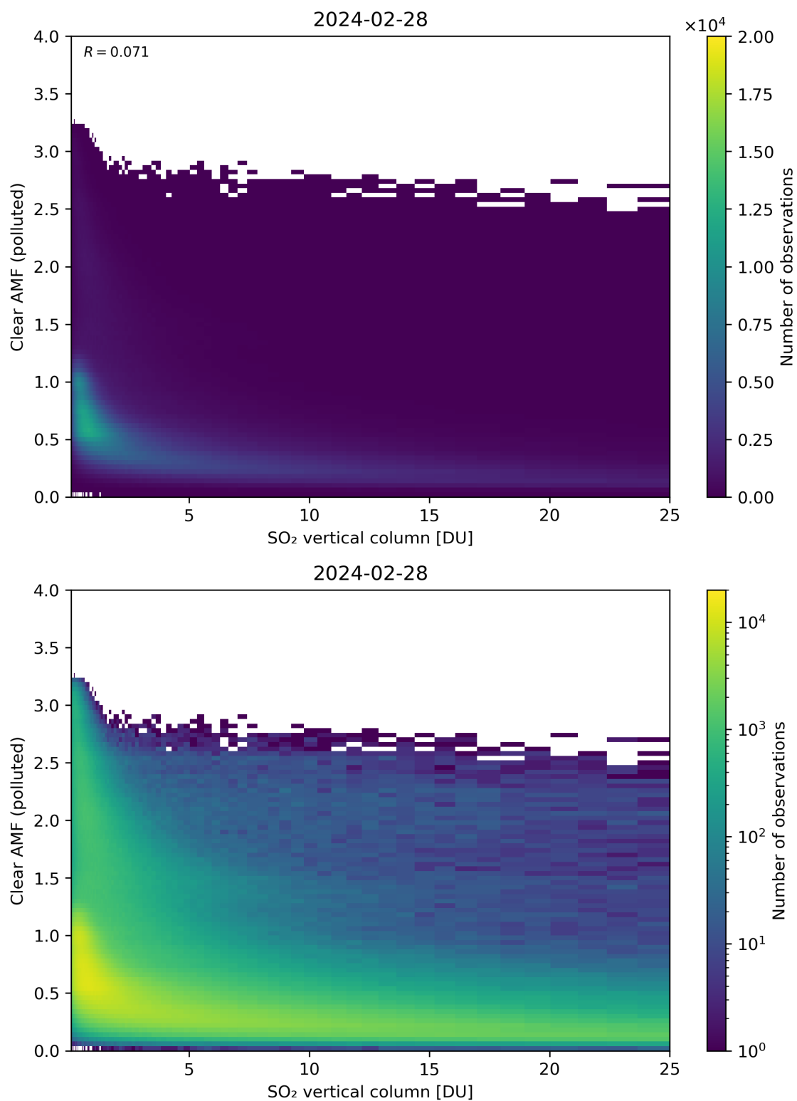
Figure 296: Scatter density plot of “SO 2 vertical column” against “Clear AMF (polluted)” for 2024-02-27 to 2024-02-29.
