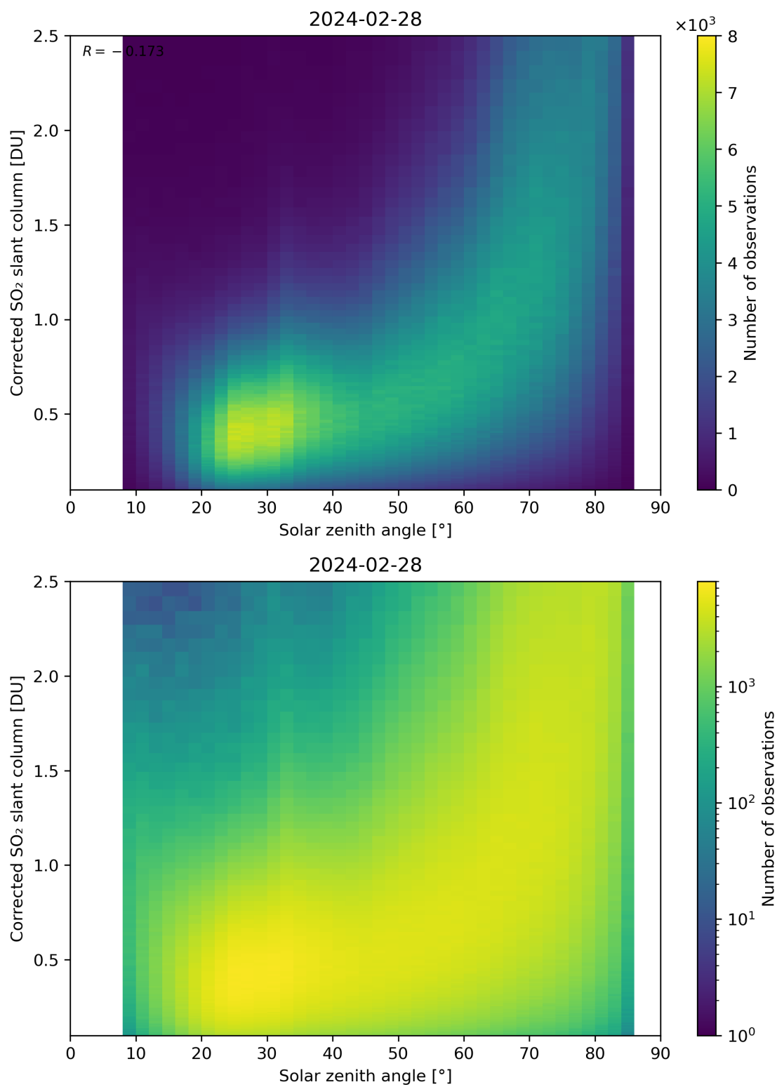
Figure 166: Scatter density plot of “Solar zenith angle” against “Corrected SO 2 slant column” for 2024-02-27 to 2024-02-29.
