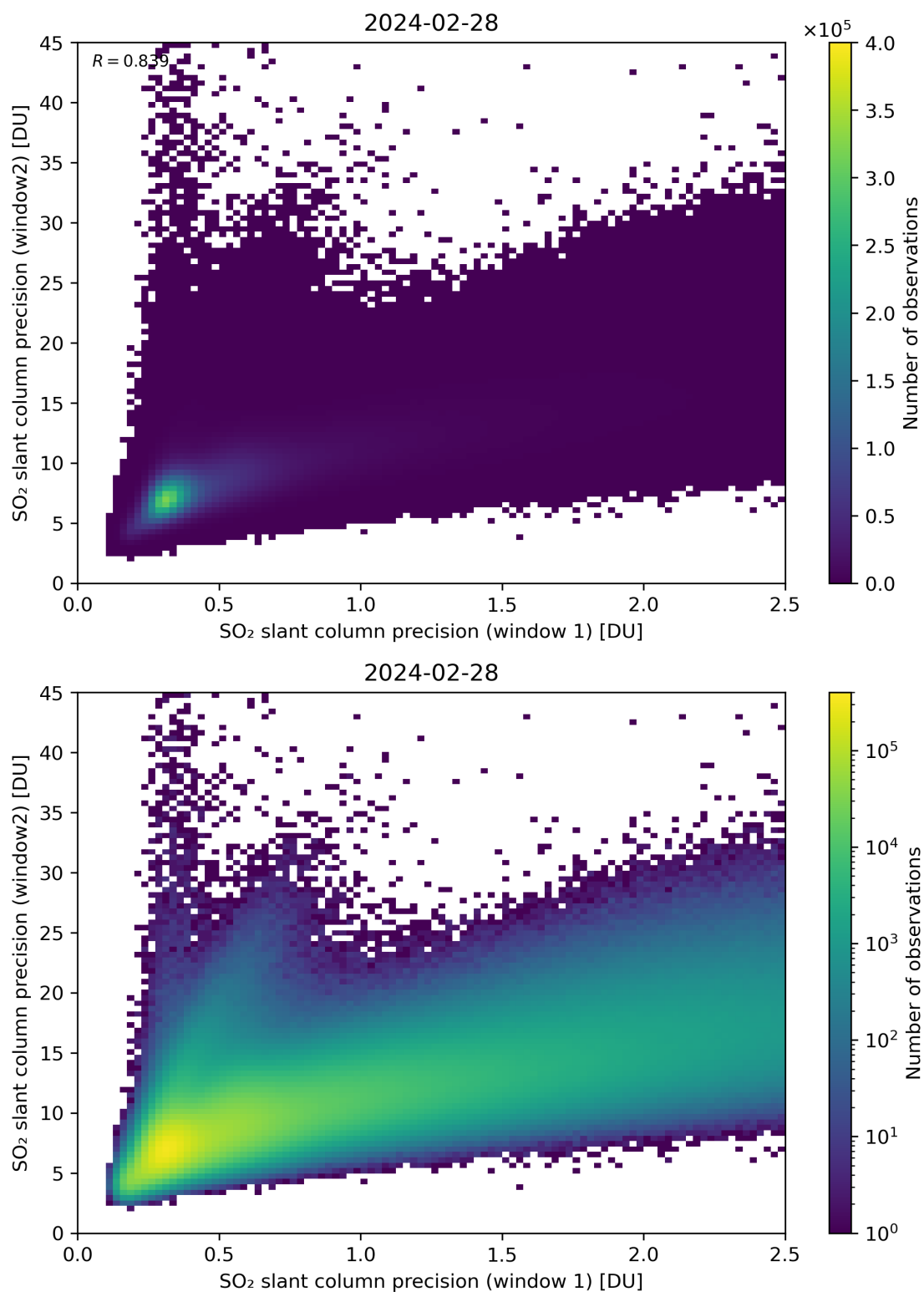
Figure 227: Scatter density plot of “SO 2 slant column precision (window 1)” against “SO 2 slant column precision (window2)” for 2024-02-27 to 2024-02-29.
