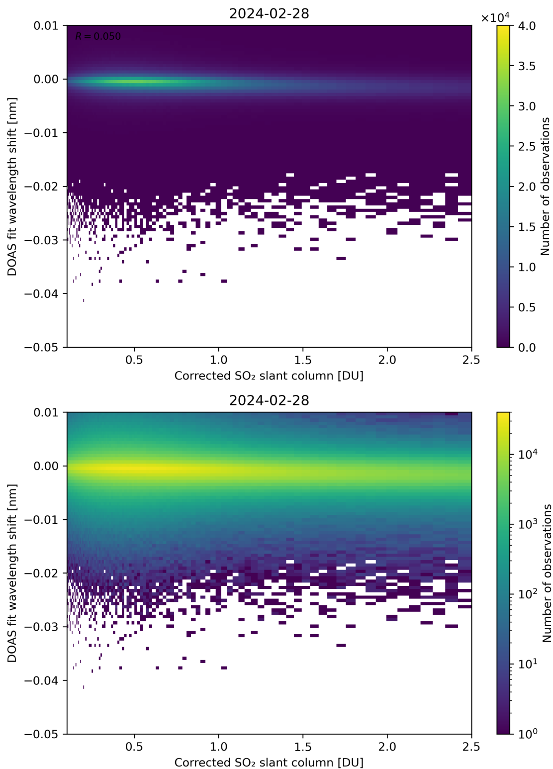
Figure 181: Scatter density plot of “Corrected SO 2 slant column” against “DOAS fit wavelength shift” for 2024-02-27 to 2024-02-29.
