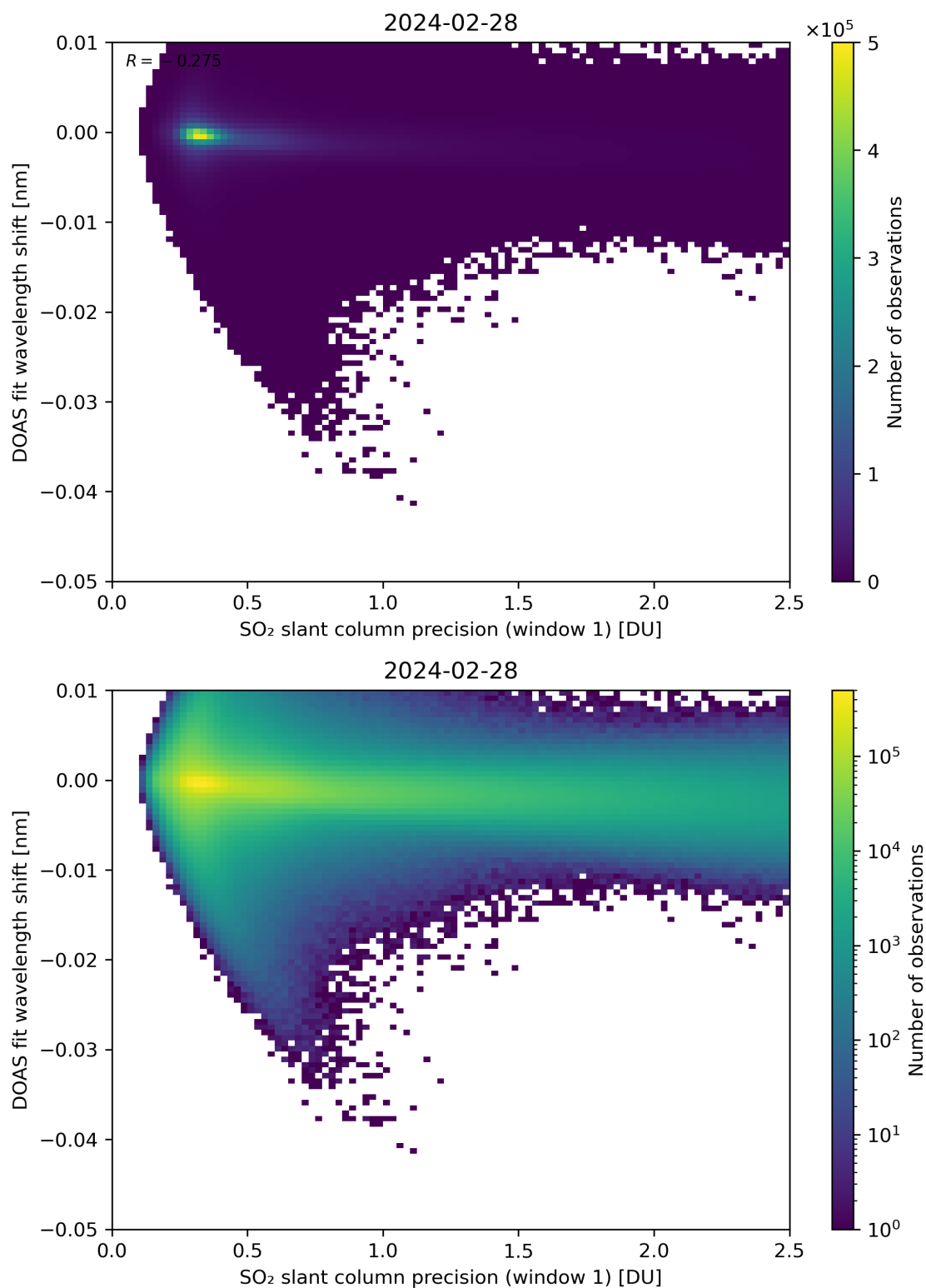
Figure 221: Scatter density plot of “SO 2 slant column precision (window 1)” against “DOAS fit wavelength shift” for 2024-02-27 to 2024-02-29.
