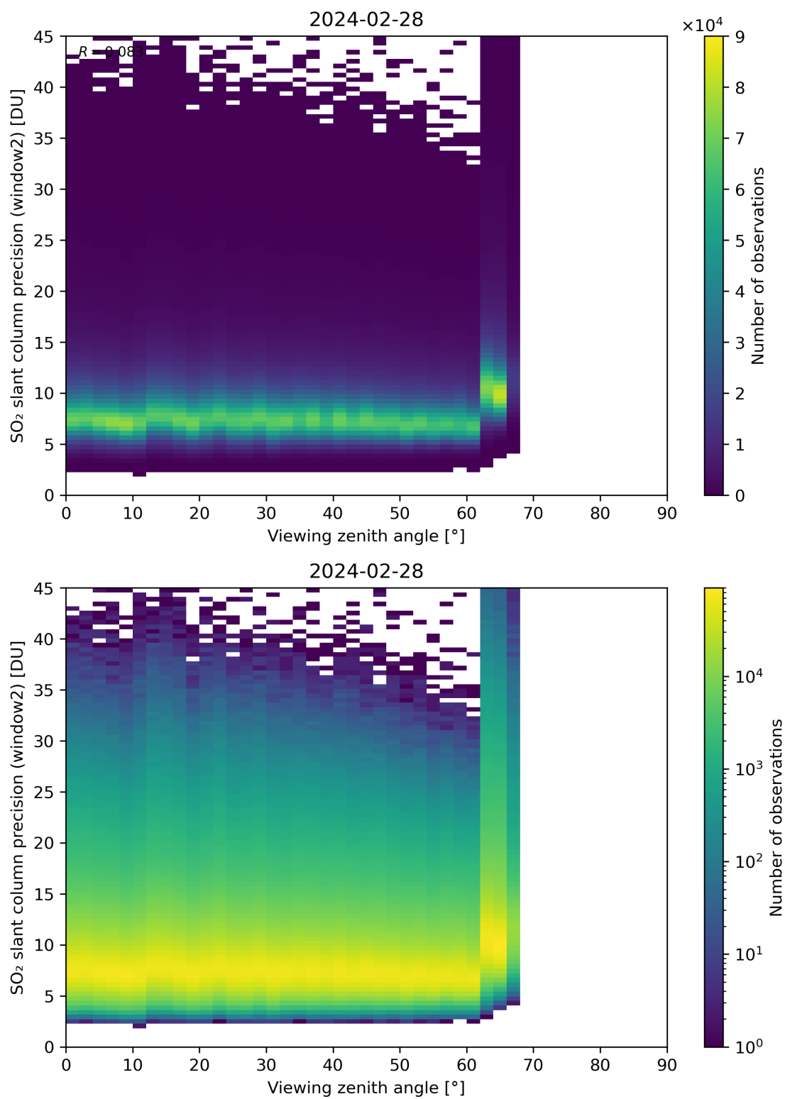
Figure 322: Scatter density plot of “Viewing zenith angle” against “SO 2 slant column precision (window2)” for 2024-02-27 to 2024-02-29.
