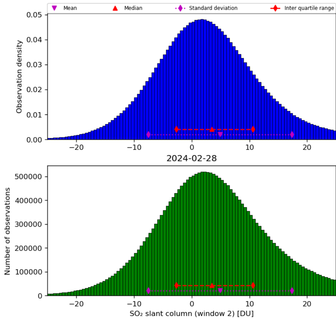
Figure 60: Histogram of “SO 2 slant column (window 2)” for 2024-02-27 to 2024-02-29
