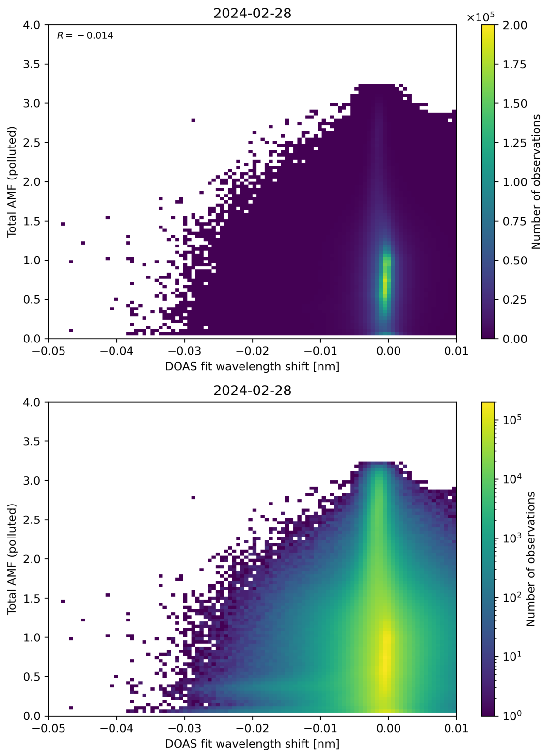
Figure 130: Scatter density plot of “DOAS fit wavelength shift” against “Total AMF (polluted)” for 2024-02-27 to 2024-02-29.
