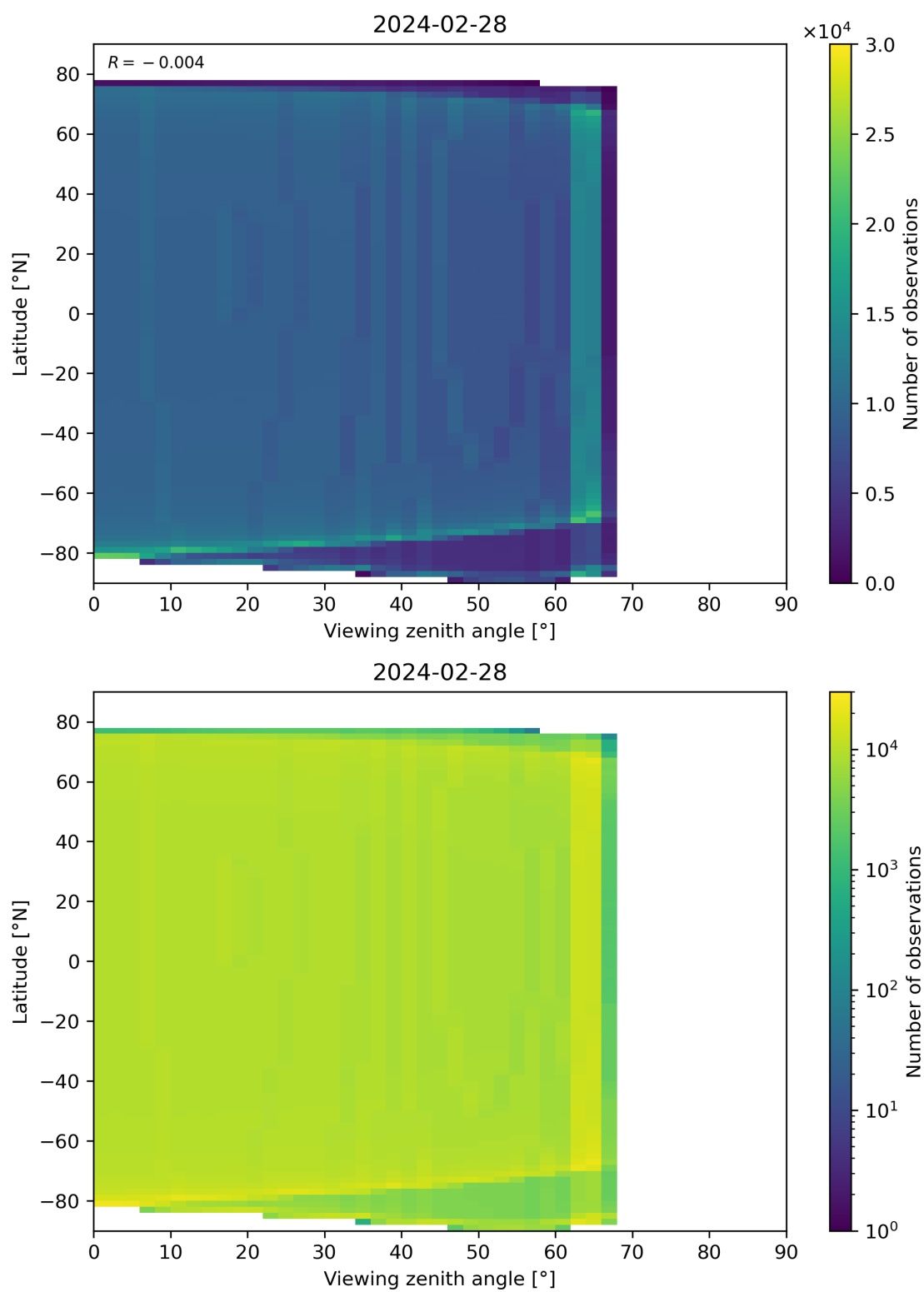
Figure 314: Scatter density plot of “Viewing zenith angle” against “Latitude” for 2024-02-27 to 2024-02-29.
