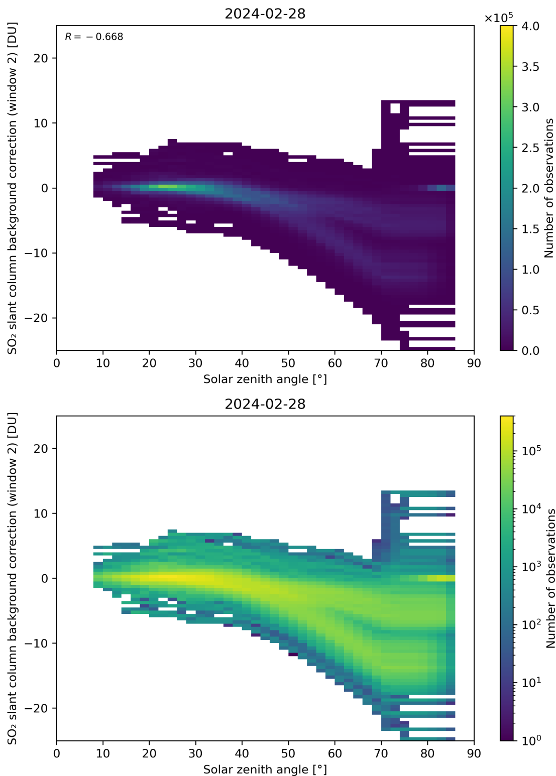
Figure 159: Scatter density plot of “Solar zenith angle” against “SO 2 slant column background correction (window 2)” for 2024-02-27 to 2024-02-29.
