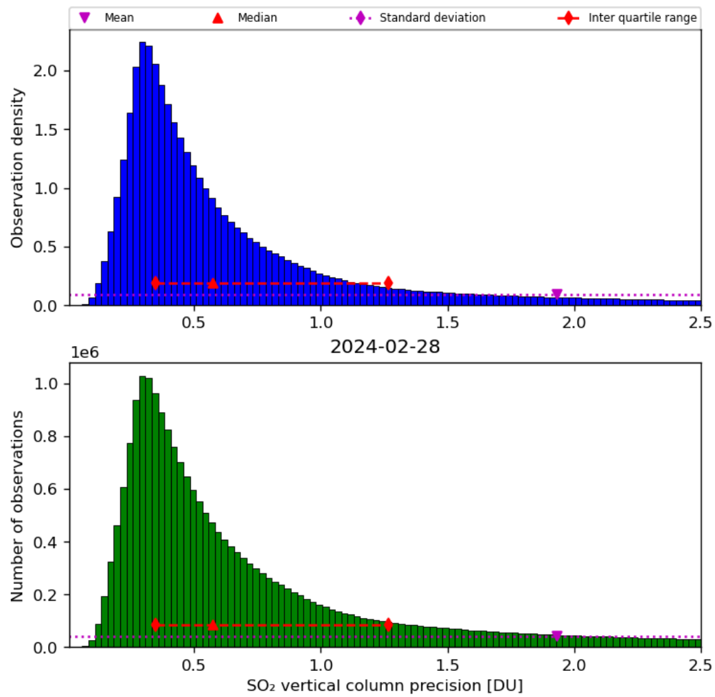
Figure 54: Histogram of “SO 2 vertical column precision” for 2024-02-27 to 2024-02-29
