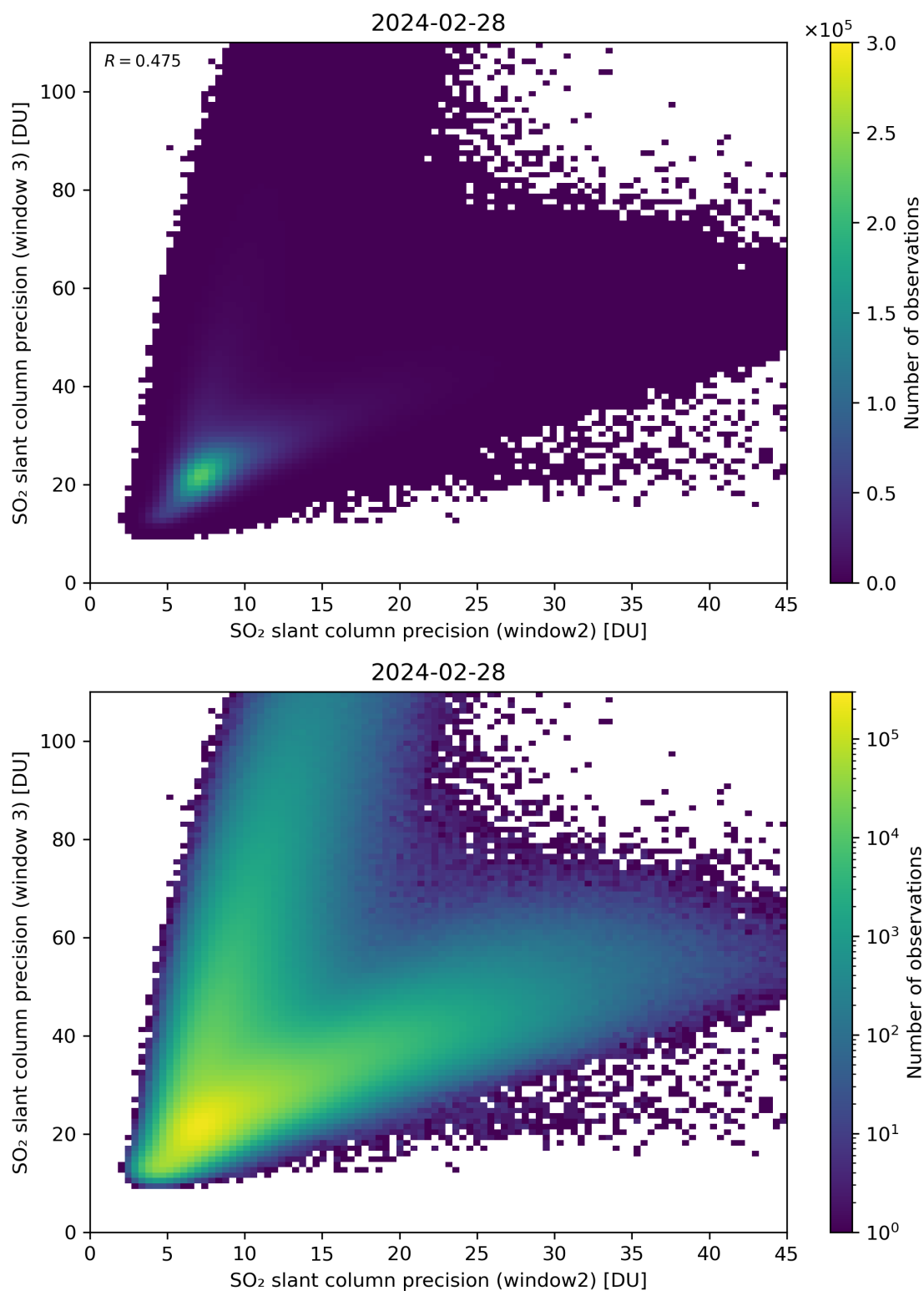
Figure 250: Scatter density plot of “SO 2 slant column precision (window2)” against “SO 2 slant column precision (window 3)” for 2024-02-27 to 2024-02-29.
