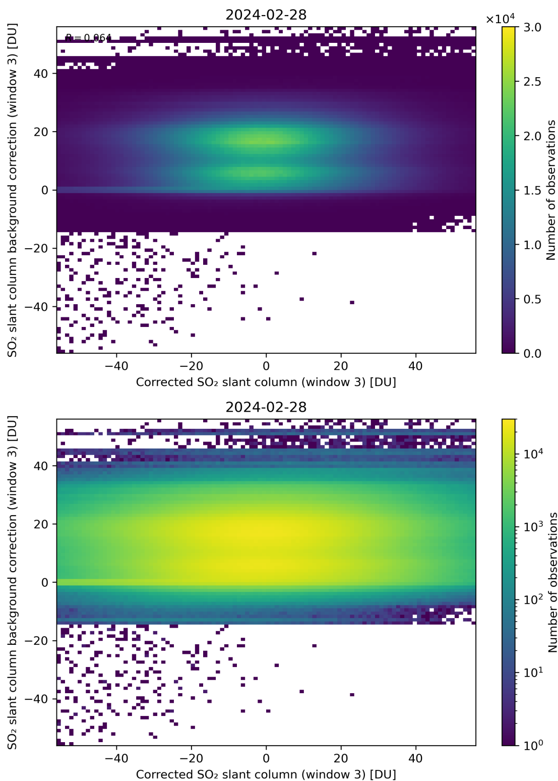
Figure 205: Scatter density plot of “Corrected SO 2 slant column (window 3)” against “SO 2 slant column background correction (window 3)” for 2024-02-27 to 2024-02-29.
