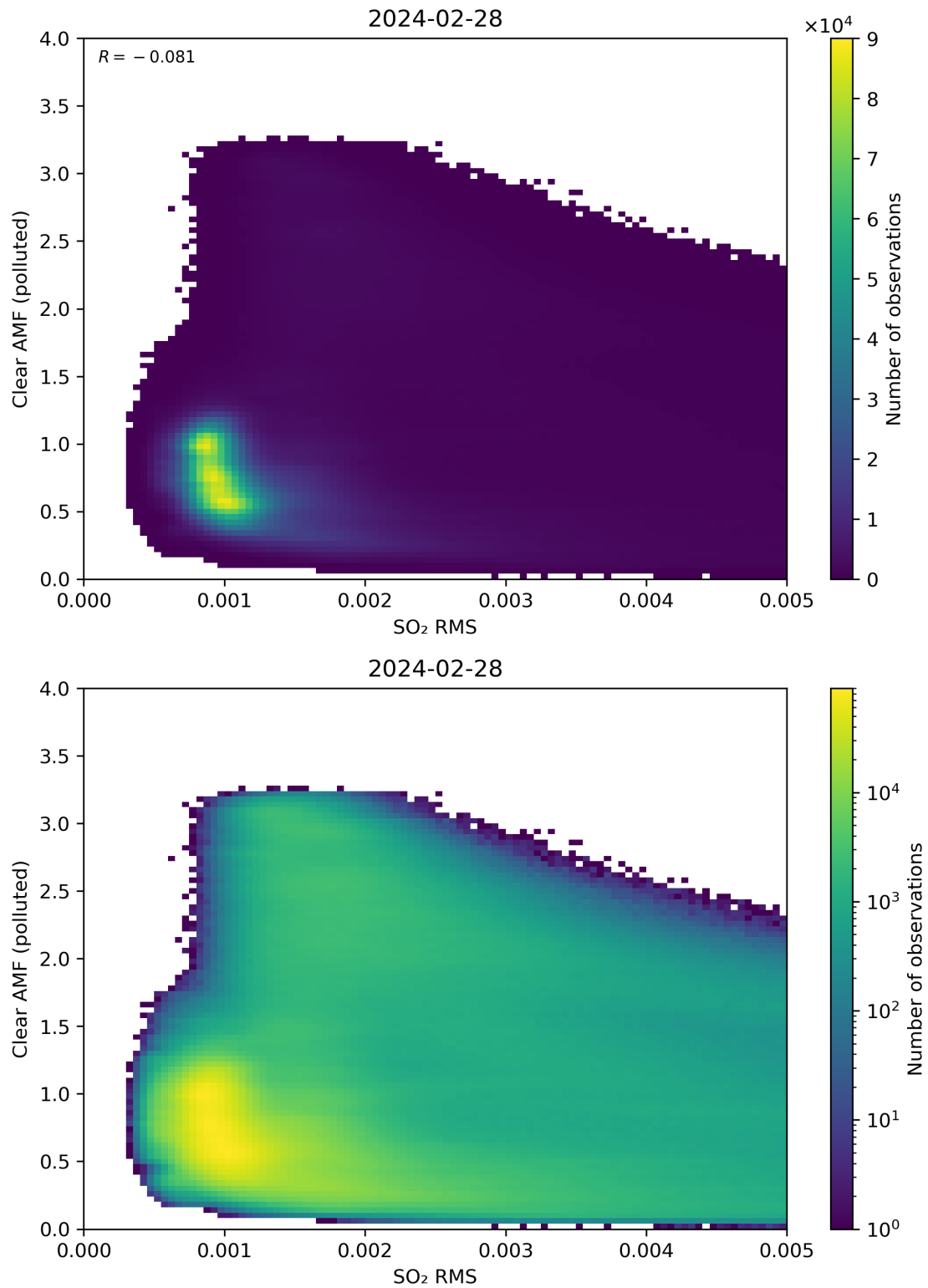
Figure 136: Scatter density plot of “SO 2 RMS” against “Clear AMF (polluted)” for 2024-02-27 to 2024-02-29.
