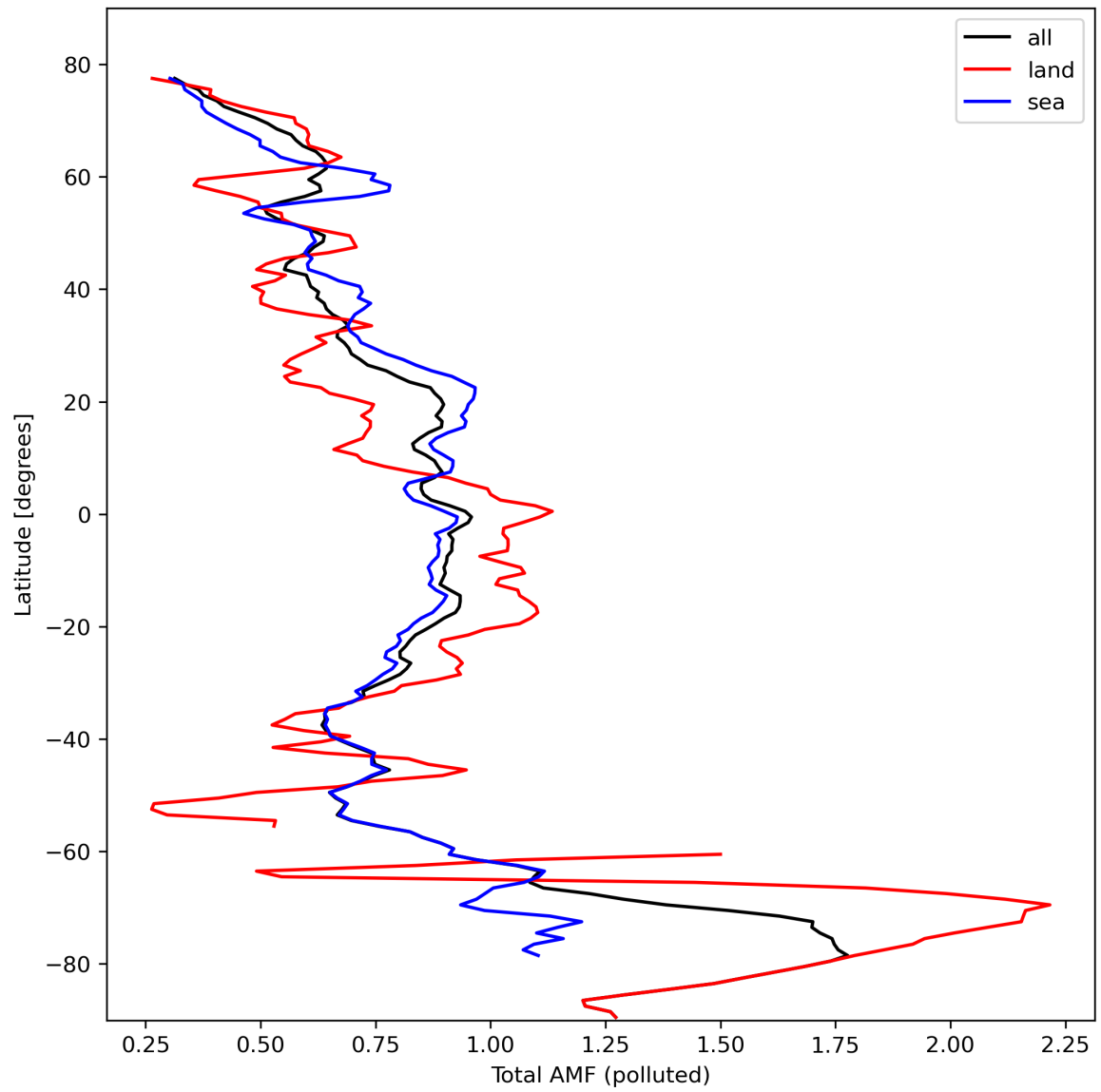
Figure 48: Zonal average of “Total AMF (polluted)” for 2024-02-27 to 2024-02-29.
