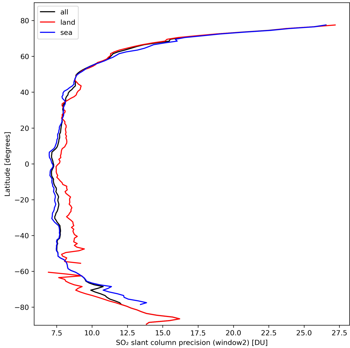
Figure 38: Zonal average of “SO 2 slant column precision (window2)” for 2024-02-27 to 2024-02-29.
