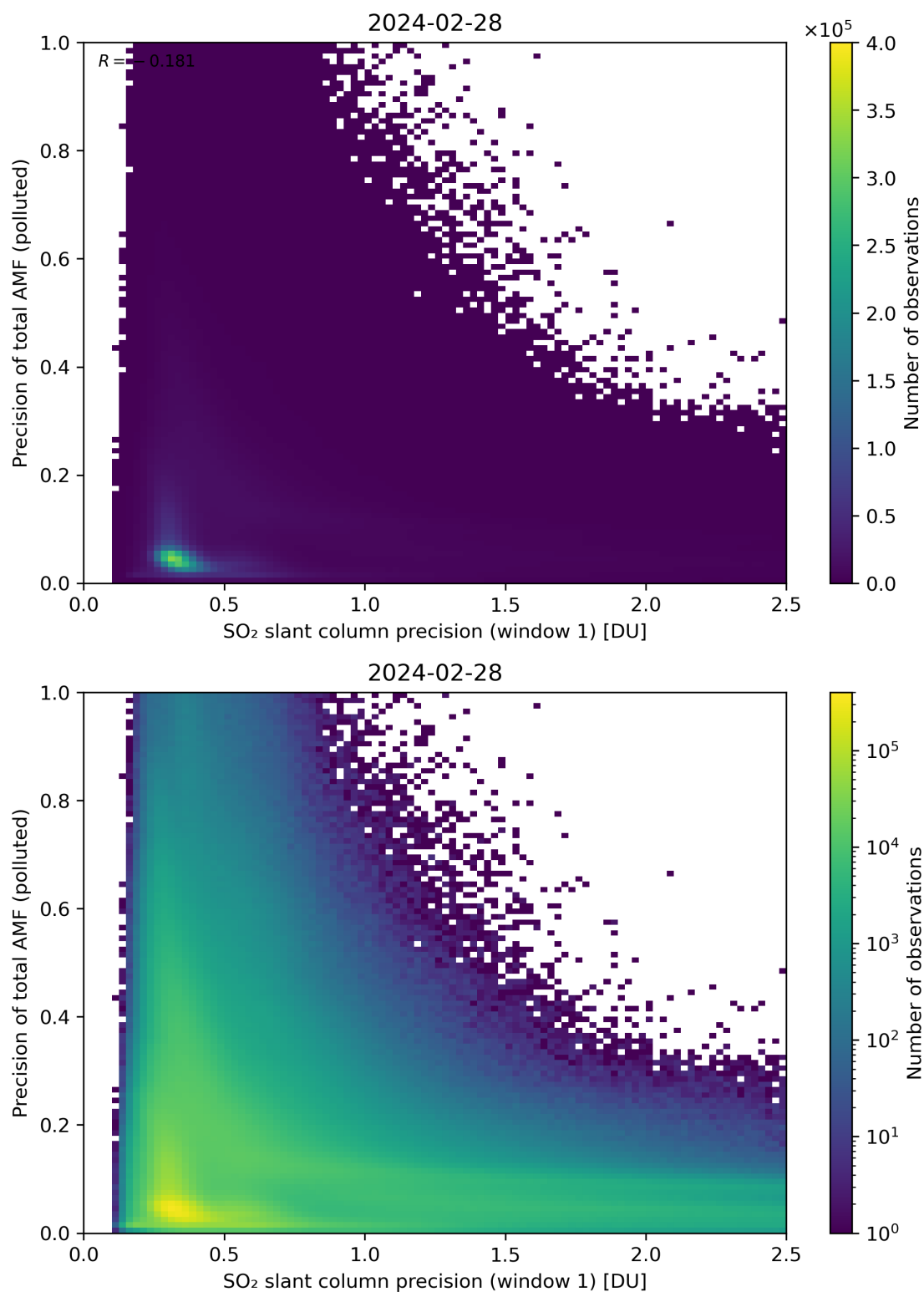
Figure 231: Scatter density plot of “SO 2 slant column precision (window 1)” against “Precision of total AMF (polluted)” for 2024-02-27 to 2024-02-29.
