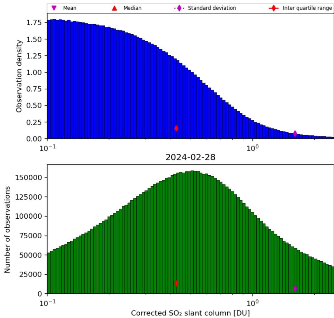
Figure 55: Histogram of “Corrected SO 2 slant column” for 2024-02-27 to 2024-02-29
