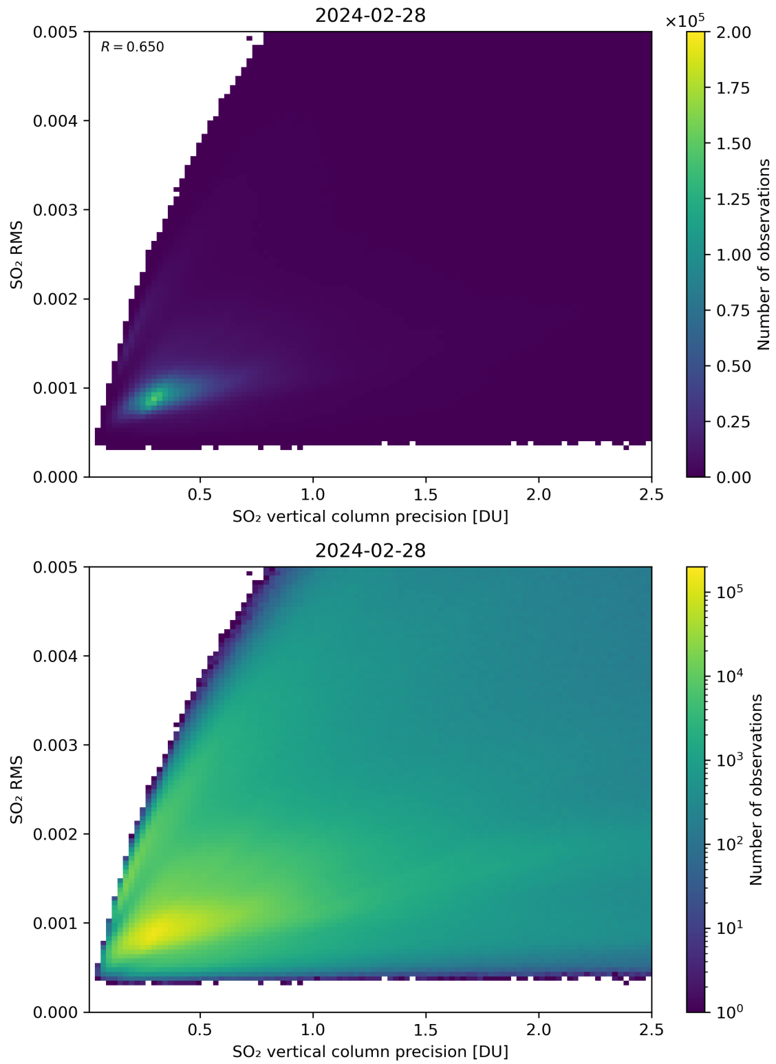
Figure 284: Scatter density plot of “SO 2 vertical column precision” against “SO 2 RMS” for 2024-02-27 to 2024-02-29.
