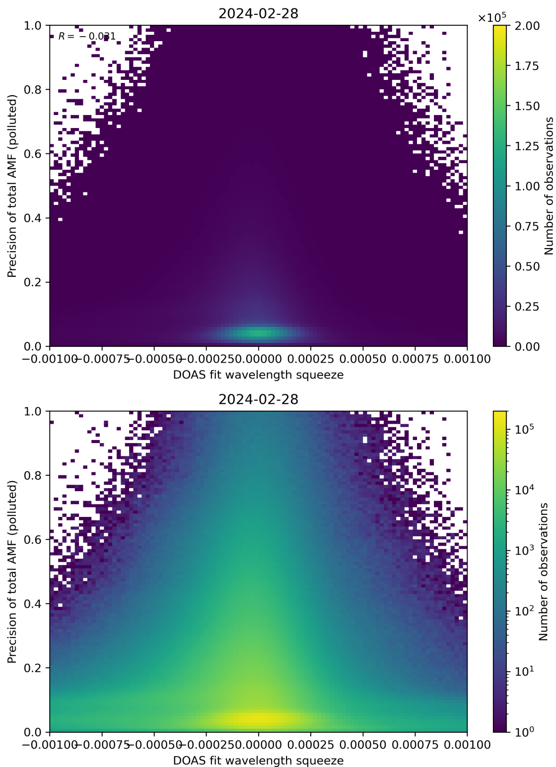
Figure 135: Scatter density plot of “DOAS fit wavelength squeeze” against “Precision of total AMF (polluted)” for 2024-02-27 to 2024-02-29.
