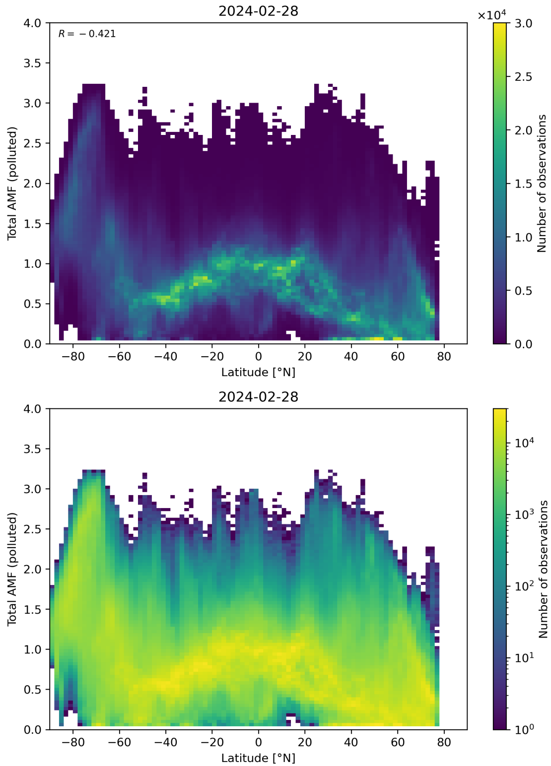
Figure 154: Scatter density plot of “Latitude” against “Total AMF (polluted)” for 2024-02-27 to 2024-02-29.
