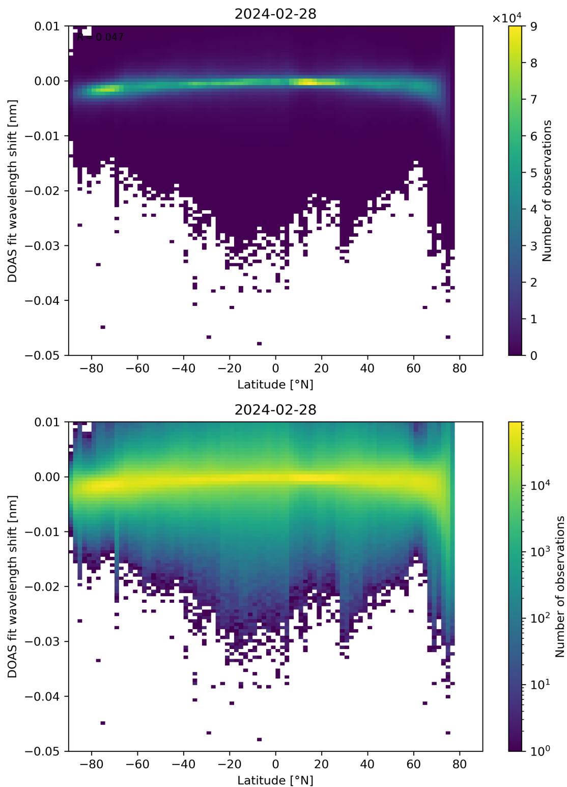
Figure 142: Scatter density plot of “Latitude” against “DOAS fit wavelength shift” for 2024-02-27 to 2024-02-29.
