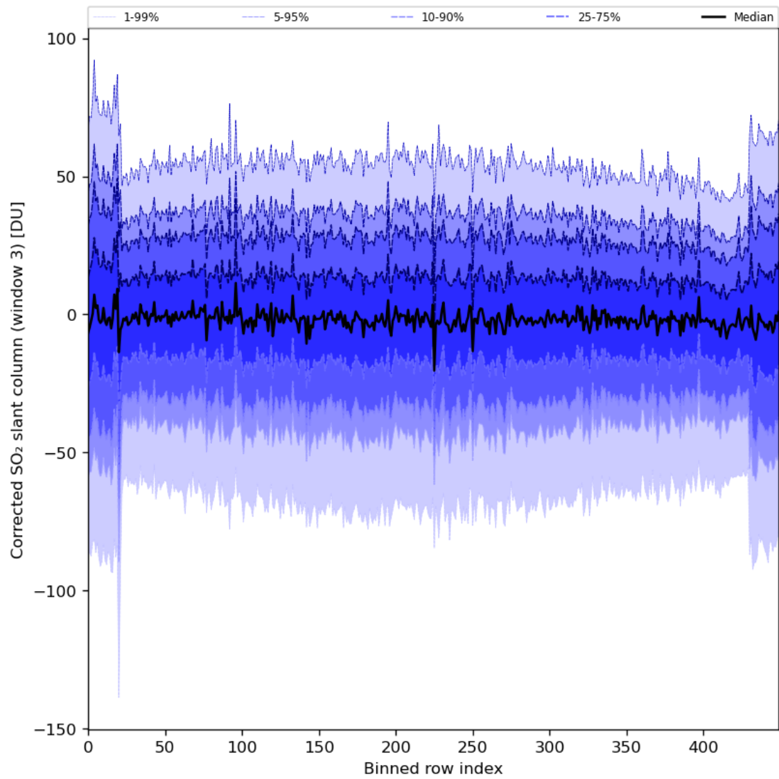
Figure 89: Along track statistics of “Corrected SO 2 slant column (window 3)” for 2024-02-27 to 2024-02-29
