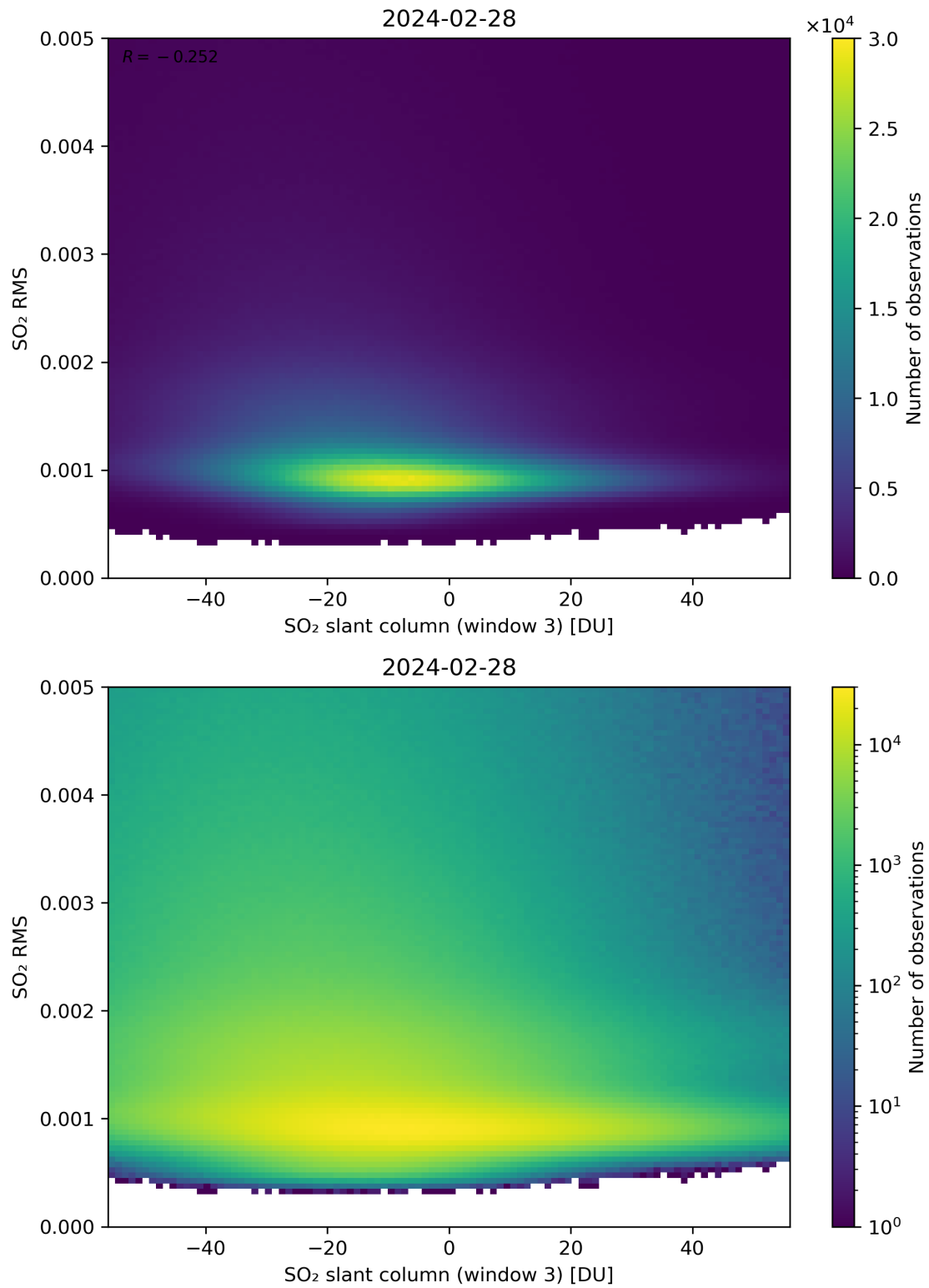
Figure 256: Scatter density plot of “SO 2 slant column (window 3)” against “SO 2 RMS” for 2024-02-27 to 2024-02-29.
