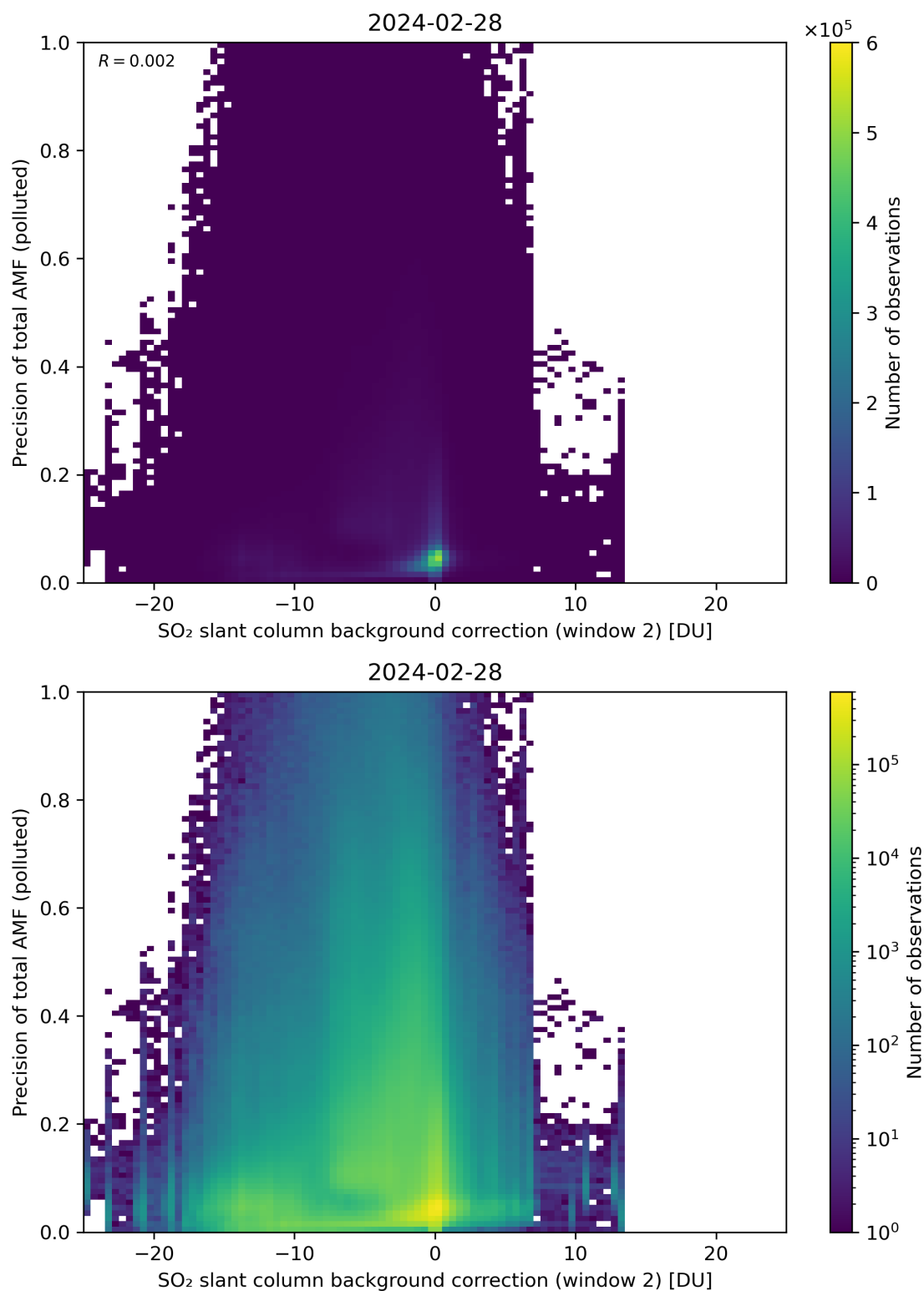
Figure 120: Scatter density plot of “SO 2 slant column background correction (window 2)” against “Precision of total AMF (polluted)” for 2024-02-27 to 2024-02-29.
