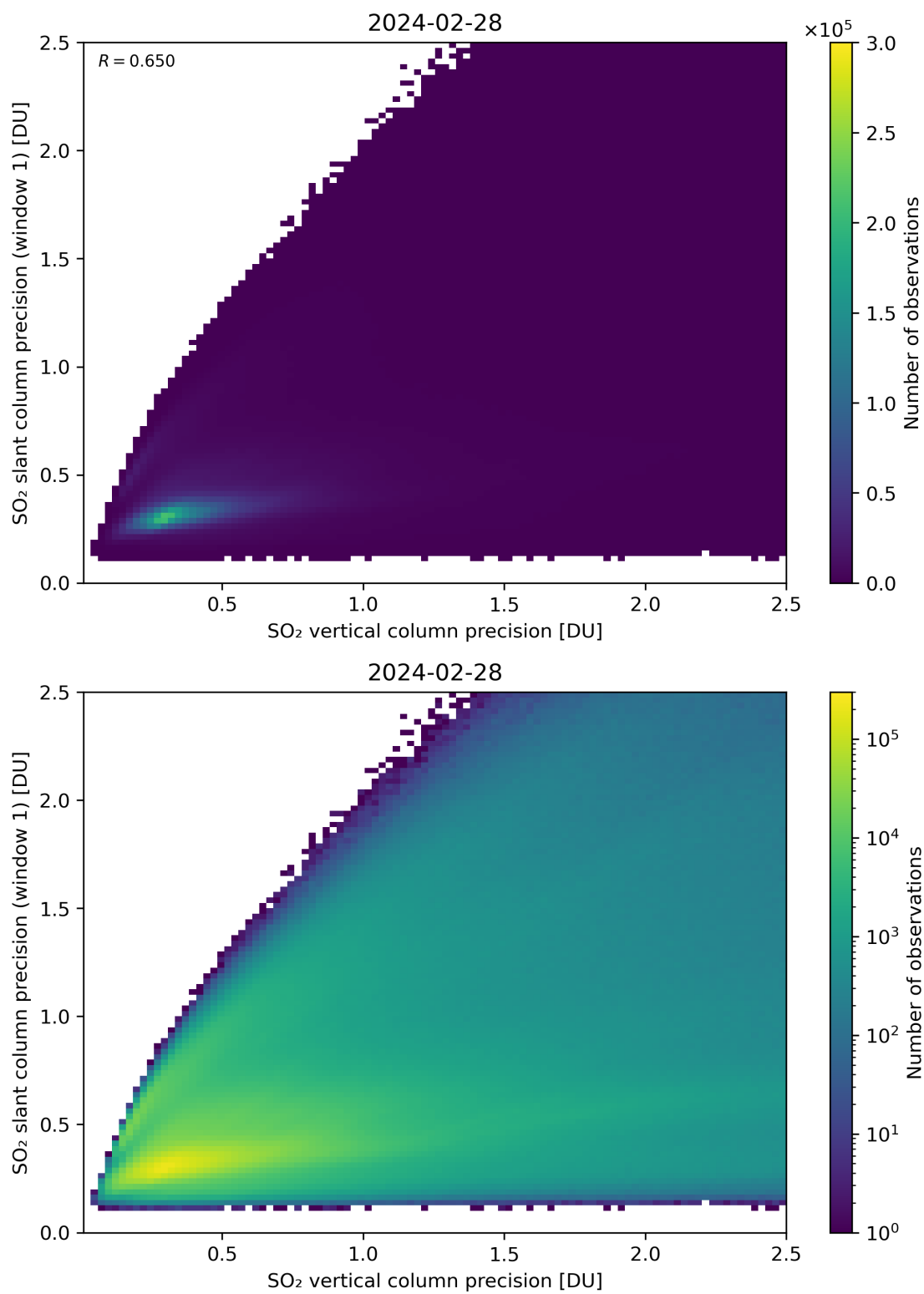
Figure 290: Scatter density plot of “SO 2 vertical column precision” against “SO 2 slant column precision (window 1)” for 2024-02-27 to 2024-02-29.
