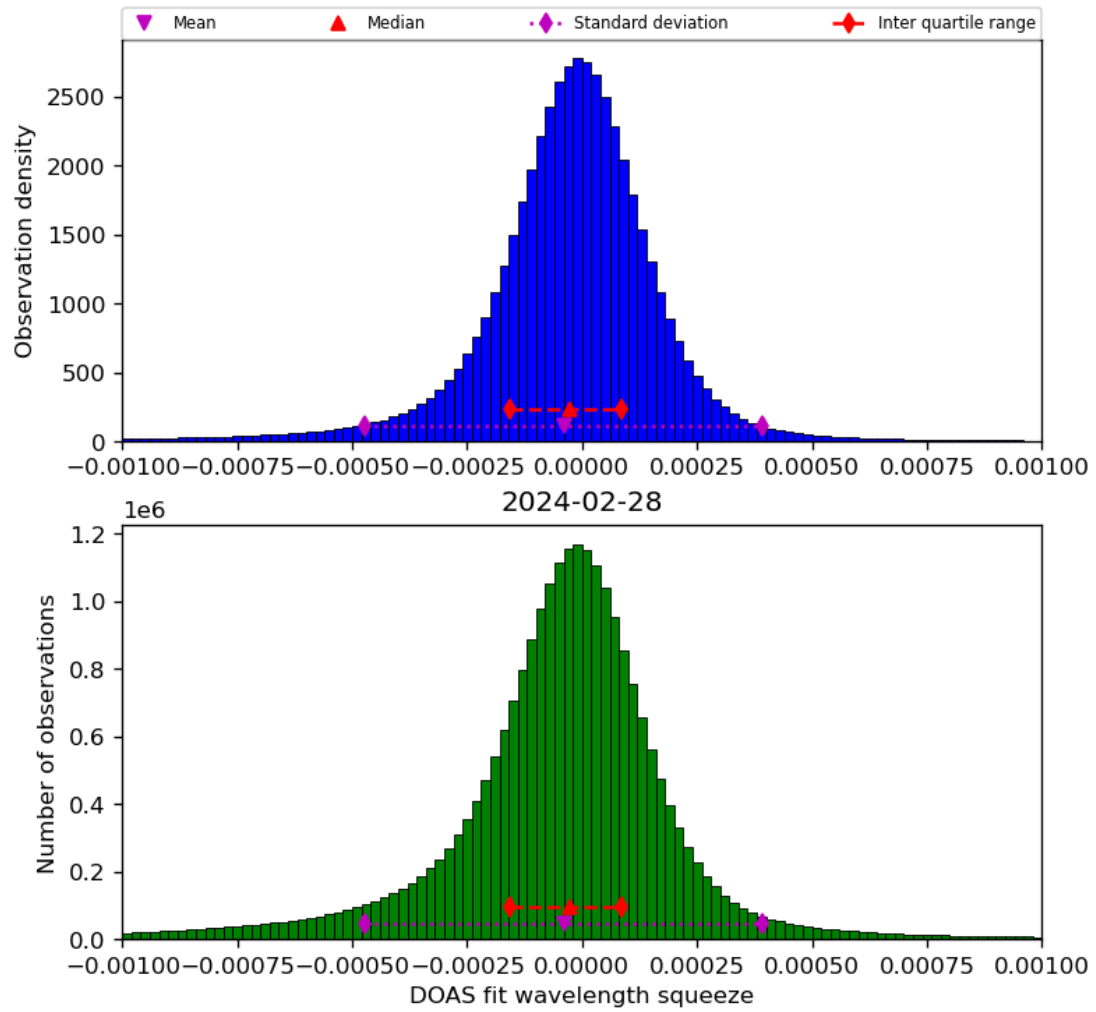
Figure 69: Histogram of “DOAS fit wavelength squeeze” for 2024-02-27 to 2024-02-29
