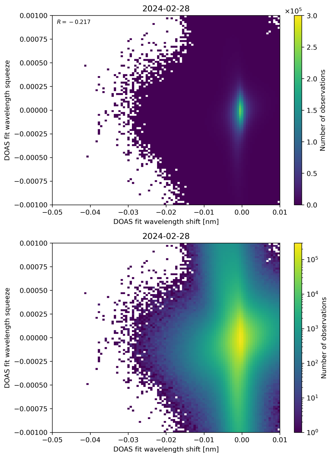
Figure 127: Scatter density plot of “DOAS fit wavelength shift” against “DOAS fit wavelength squeeze” for 2024-02-27 to 2024-02-29.
