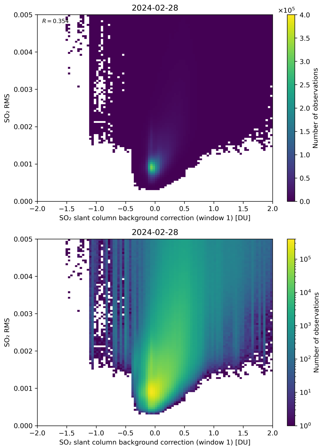
Figure 102: Scatter density plot of “SO 2 slant column background correction (window 1)” against “SO 2 RMS” for 2024-02-27 to 2024-02-29.
