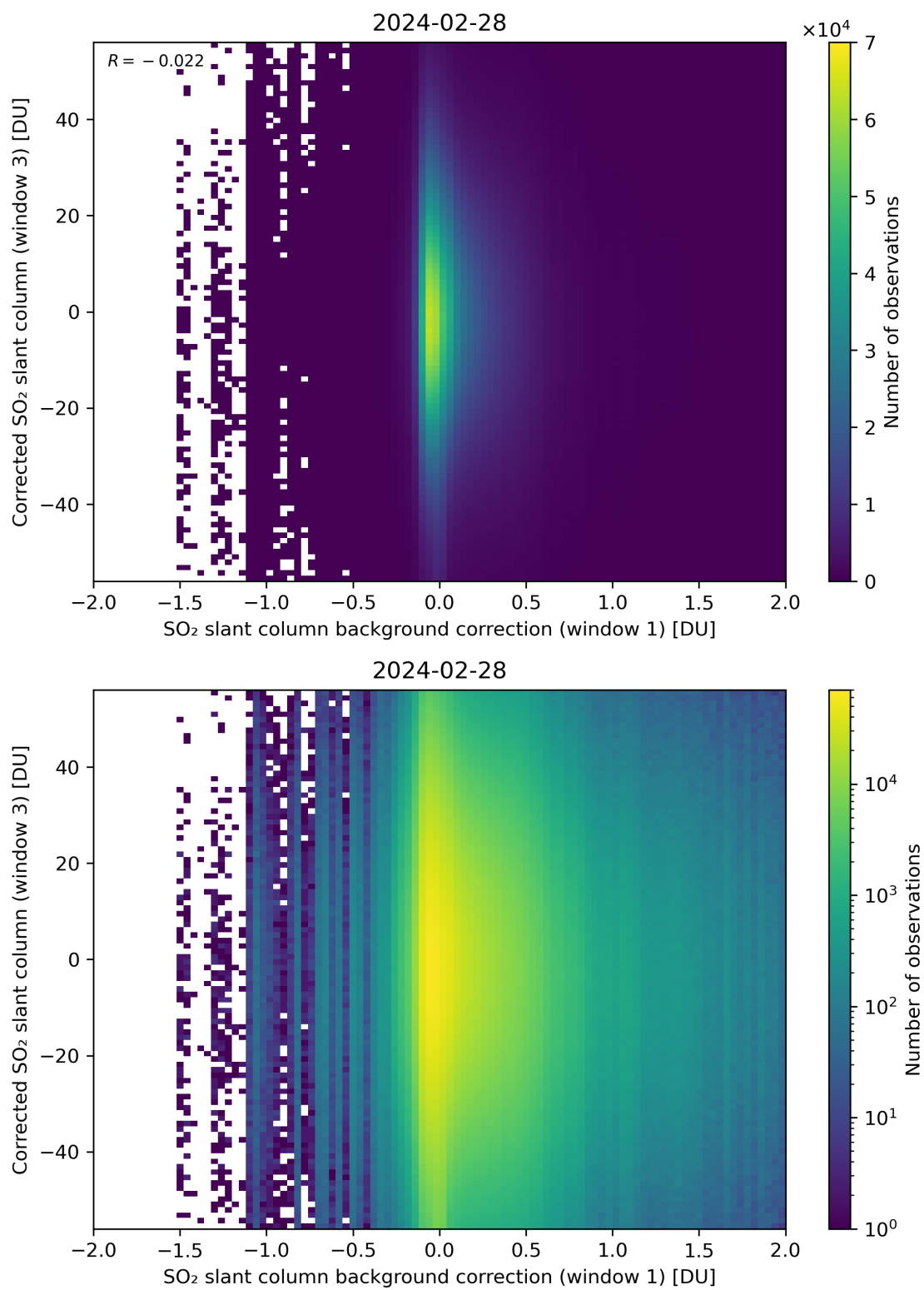
Figure 105: Scatter density plot of “SO 2 slant column background correction (window 1)” against “Corrected SO 2 slant column (window 3)” for 2024-02-27 to 2024-02-29.
