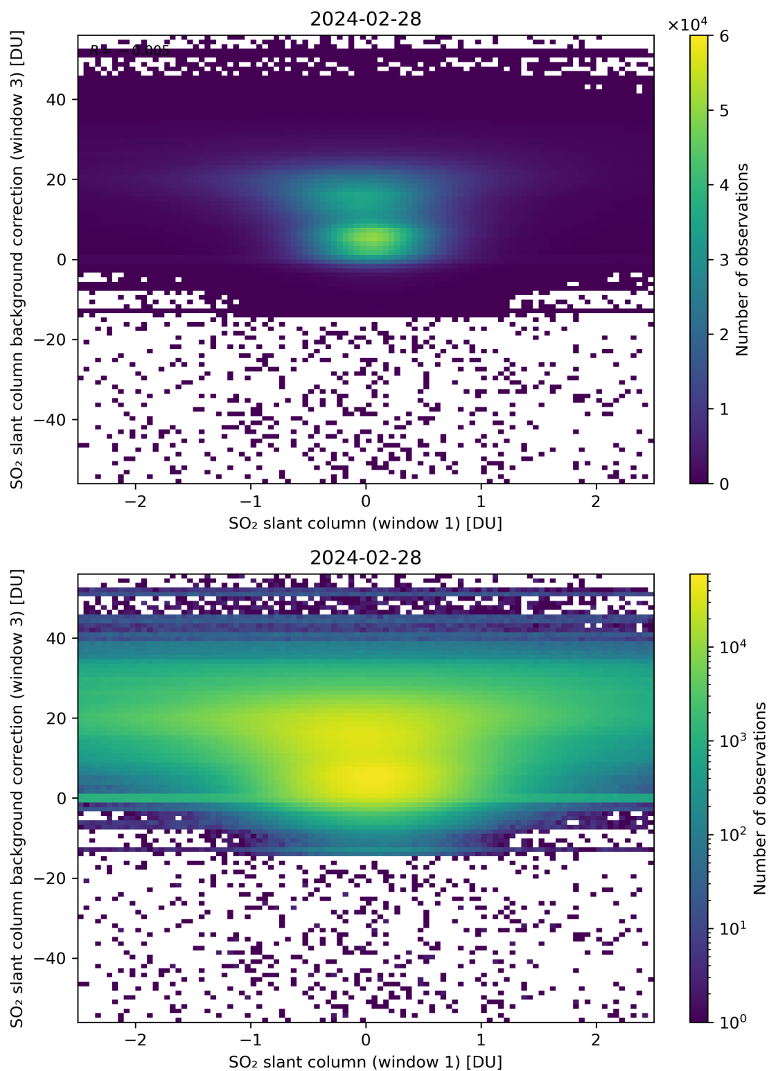
Figure 214: Scatter density plot of “SO 2 slant column (window 1)” against “SO 2 slant column background correction (window 3)” for 2024-02-27 to 2024-02-29.
