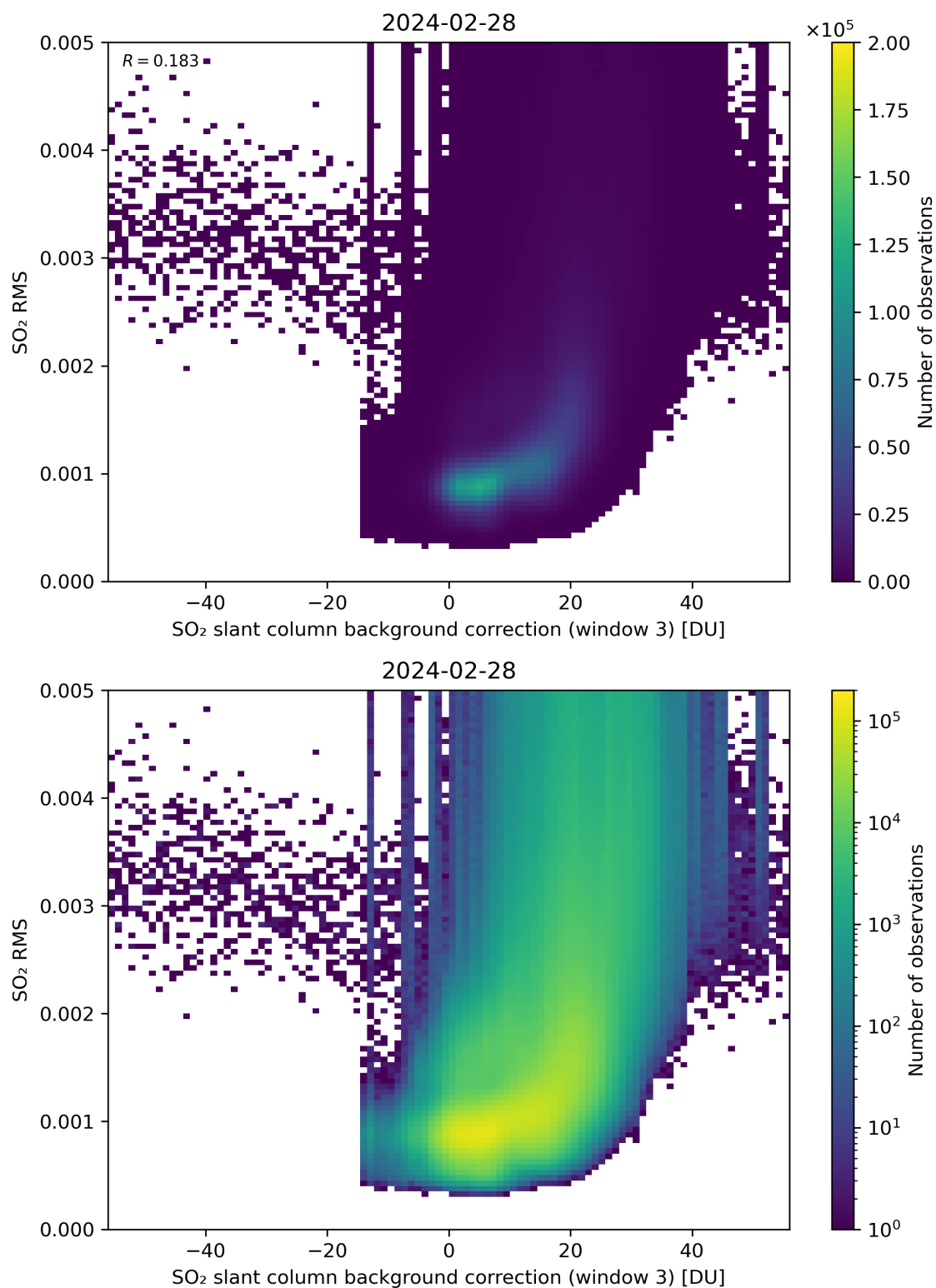
Figure 123: Scatter density plot of “SO 2 slant column background correction (window 3)” against “SO 2 RMS” for 2024-02-27 to 2024-02-29.
