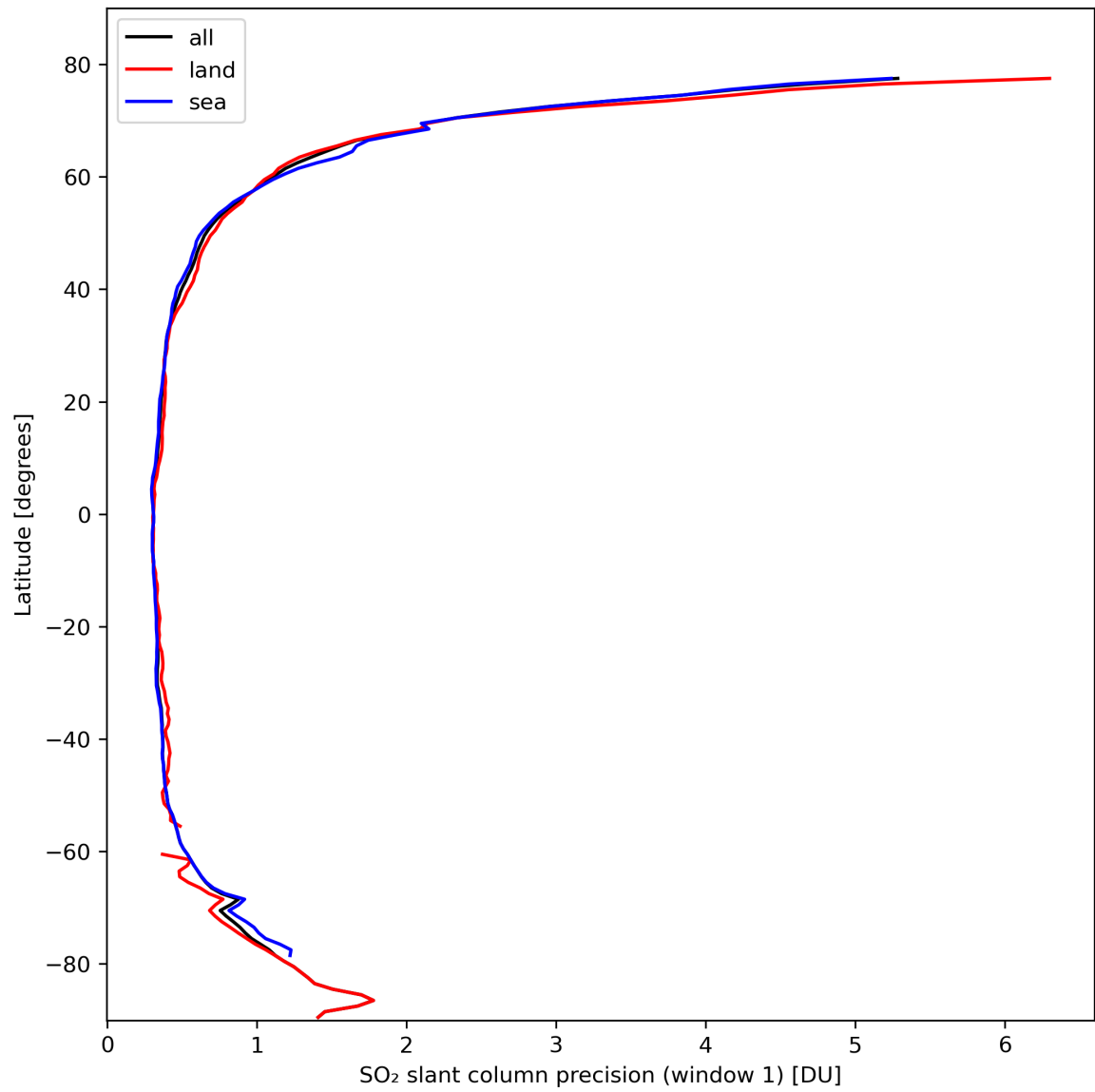
Figure 34: Zonal average of “SO 2 slant column precision (window 1)” for 2024-02-27 to 2024-02-29.
