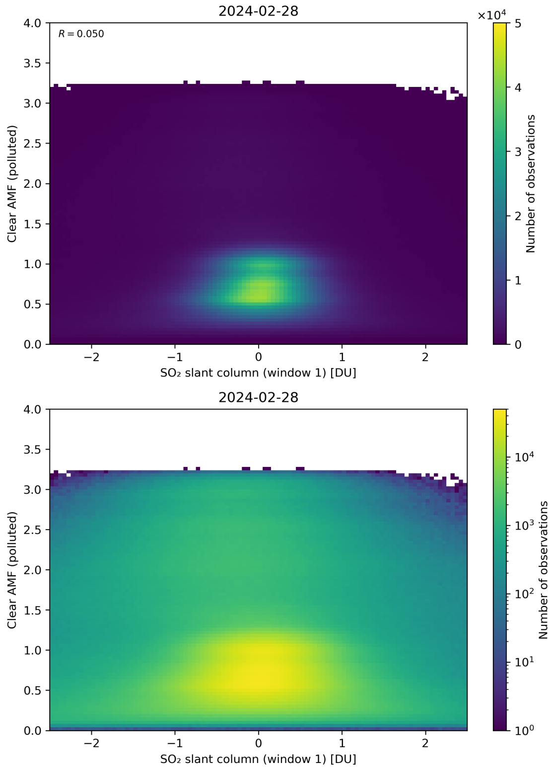
Figure 232: Scatter density plot of “SO 2 slant column (window 1)” against “Clear AMF (polluted)” for 2024-02-27 to 2024-02-29.
