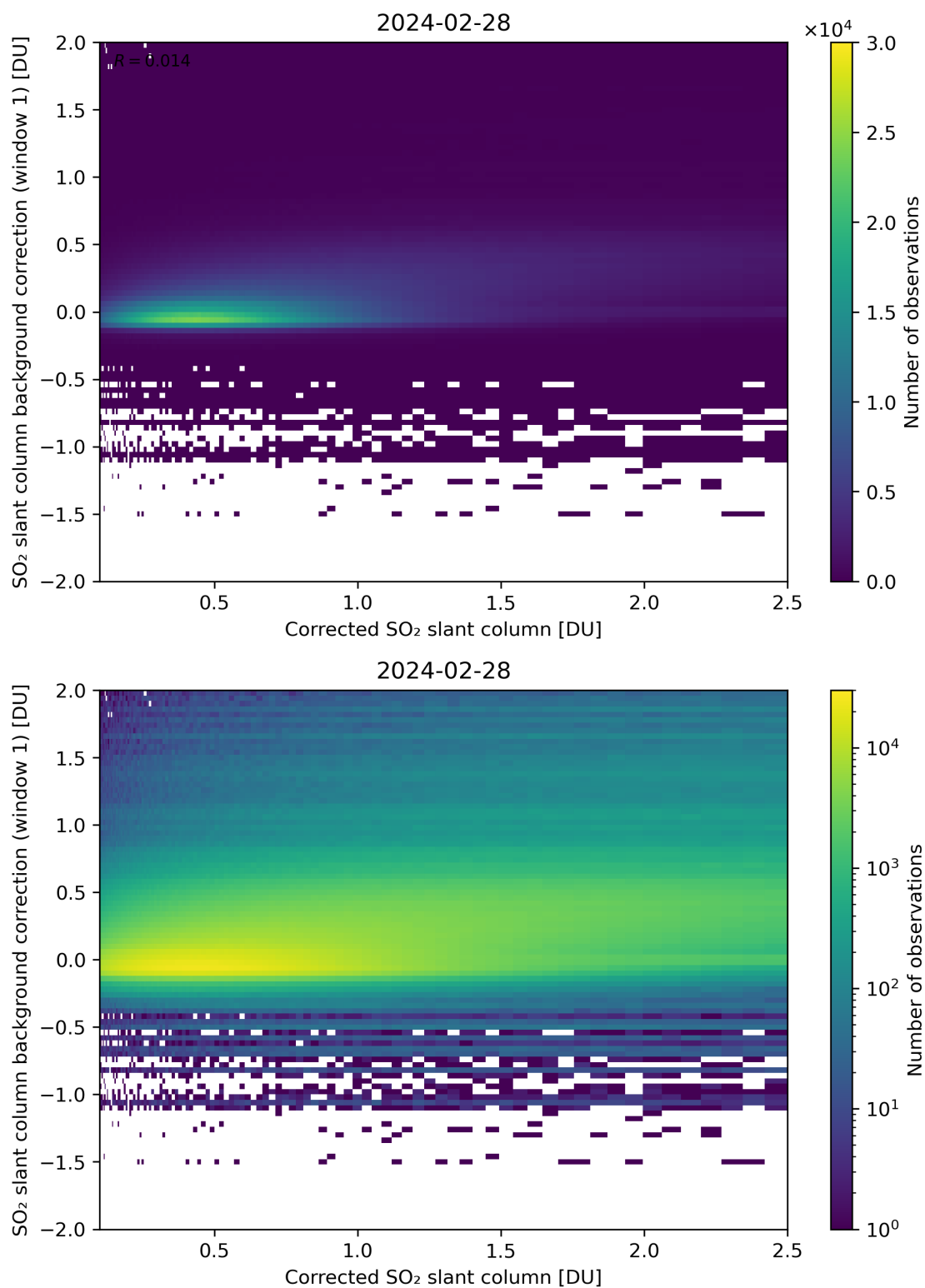
Figure 178: Scatter density plot of “Corrected SO 2 slant column” against “SO 2 slant column background correction (window 1)” for 2024-02-27 to 2024-02-29.
