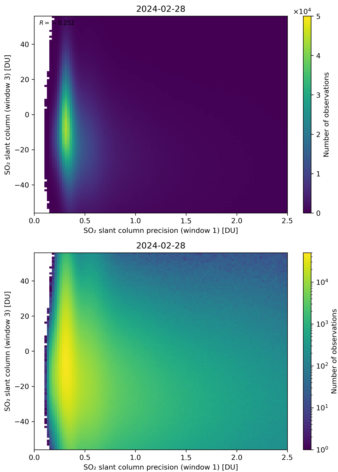
Figure 228: Scatter density plot of “SO 2 slant column precision (window 1)” against “SO 2 slant column (window 3)” for 2024-02-27 to 2024-02-29.
