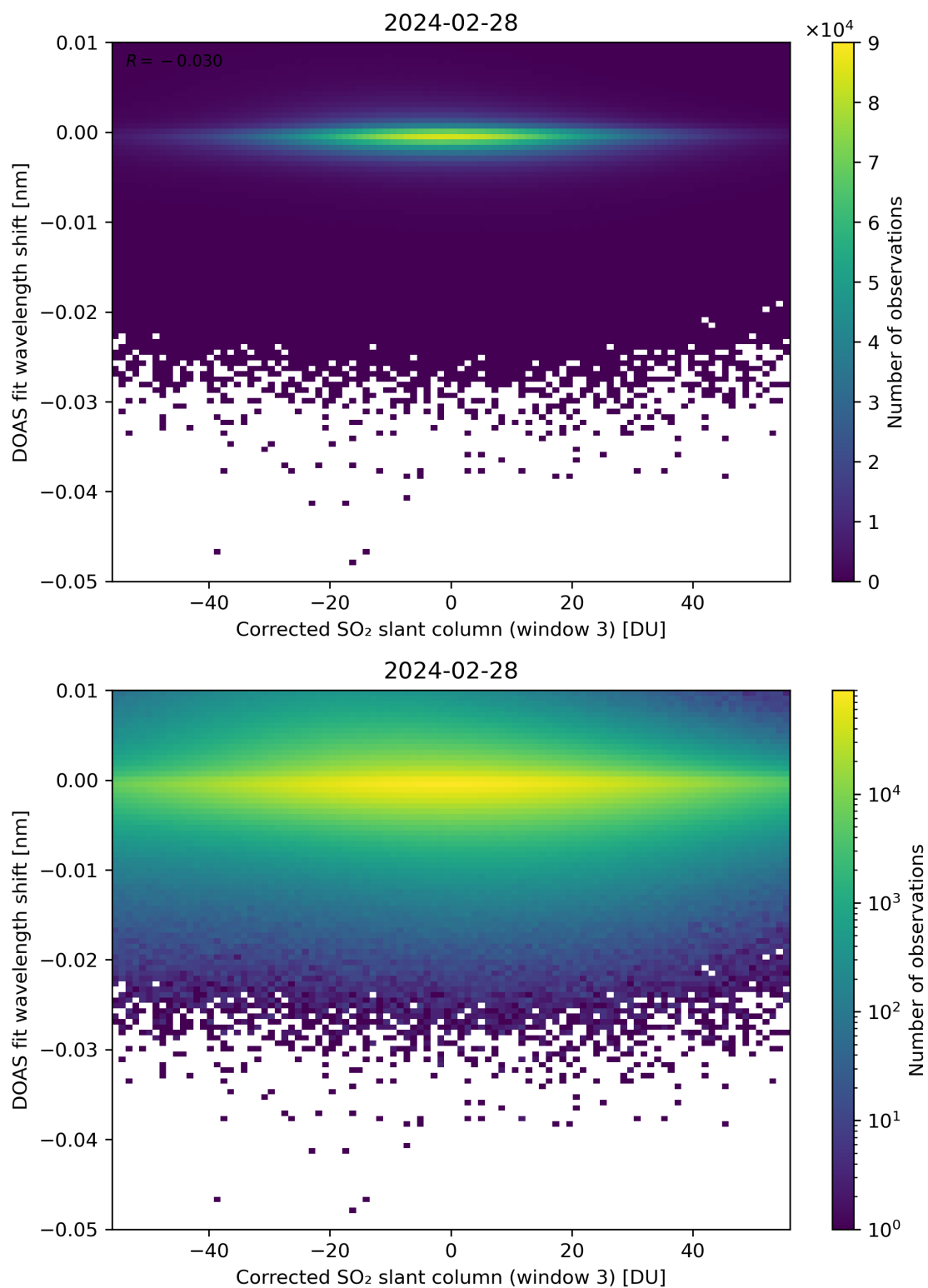
Figure 206: Scatter density plot of “Corrected SO 2 slant column (window 3)” against “DOAS fit wavelength shift” for 2024-02-27 to 2024-02-29.
