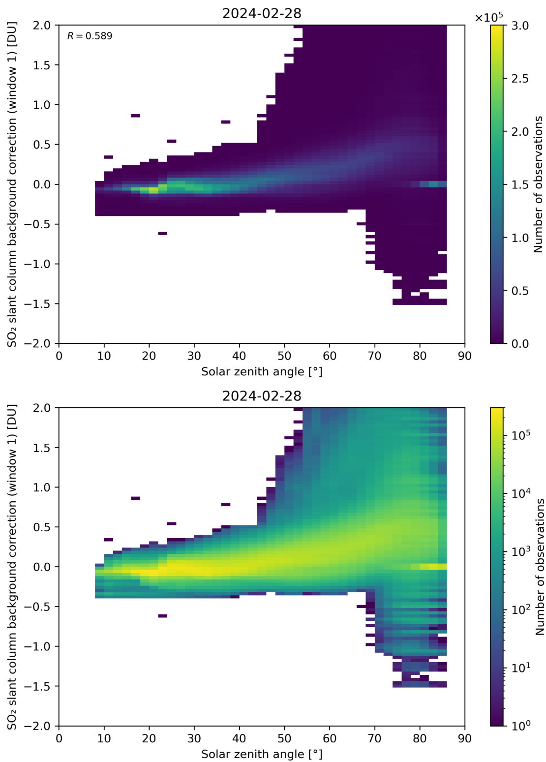
Figure 158: Scatter density plot of “Solar zenith angle” against “SO 2 slant column background correction (window 1)” for 2024-02-27 to 2024-02-29.
