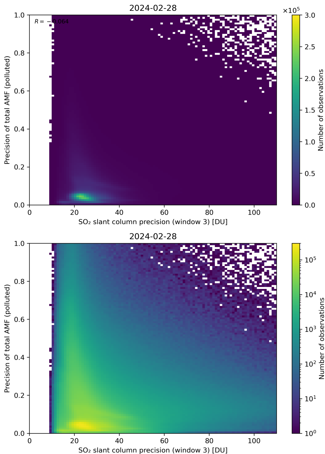
Figure 264: Scatter density plot of “SO 2 slant column precision (window 3)” against “Precision of total AMF (polluted)” for 2024-02-27 to 2024-02-29.
