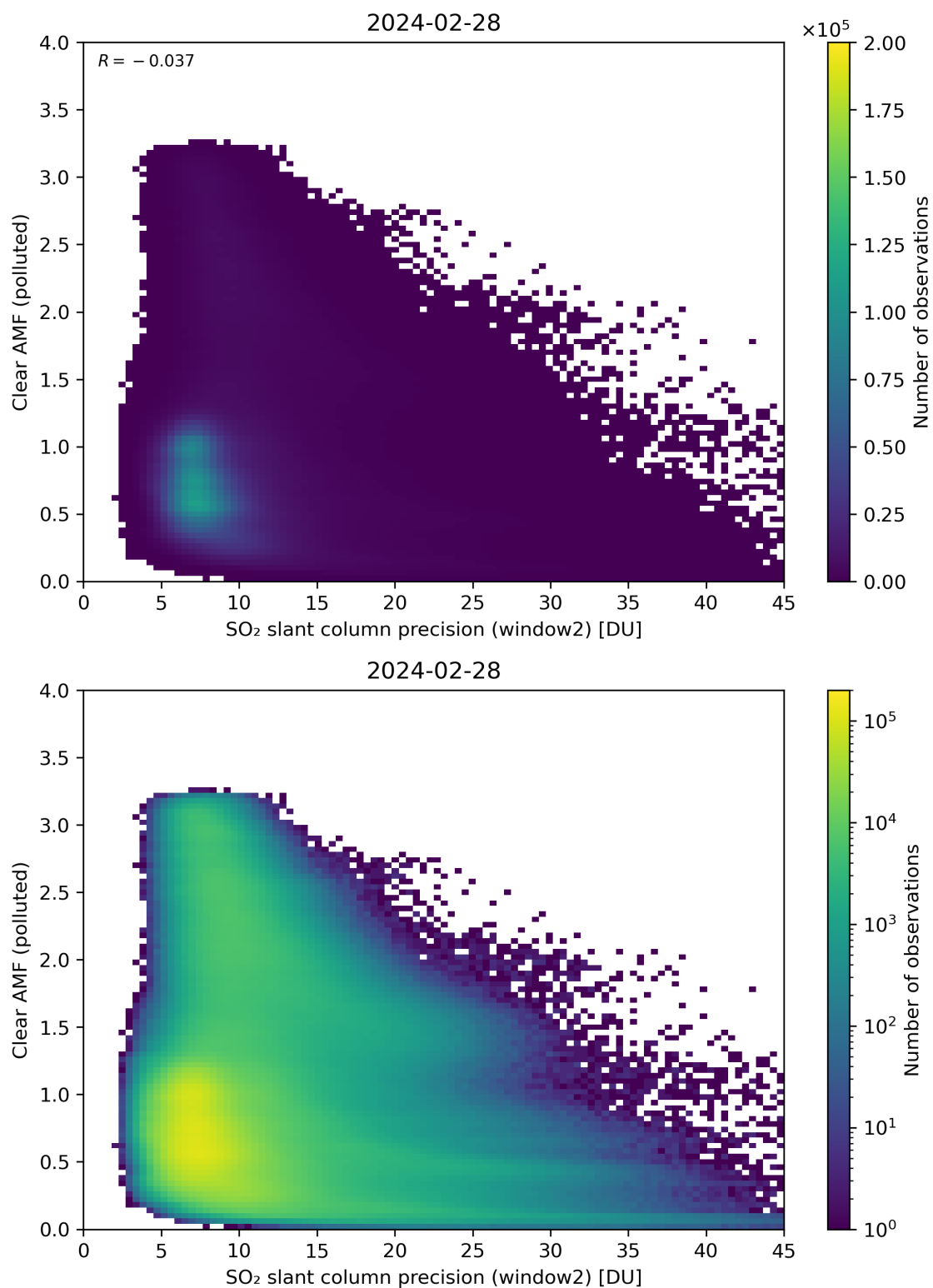
Figure 246: Scatter density plot of “SO 2 slant column precision (window2)” against “Clear AMF (polluted)” for 2024-02-27 to 2024-02-29.
