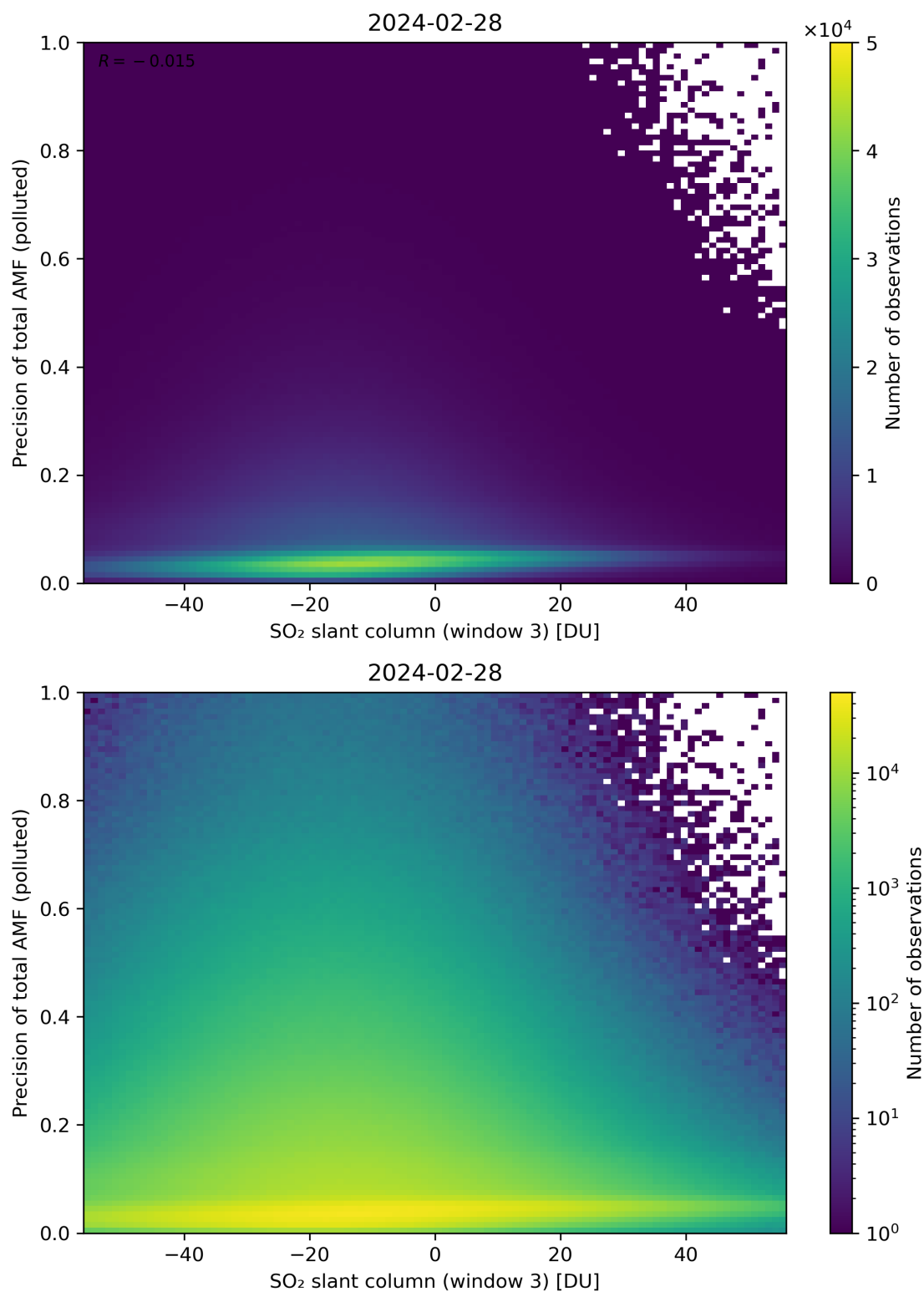
Figure 269: Scatter density plot of “SO 2 slant column (window 3)” against “Precision of total AMF (polluted)” for 2024-02-27 to 2024-02-29.
