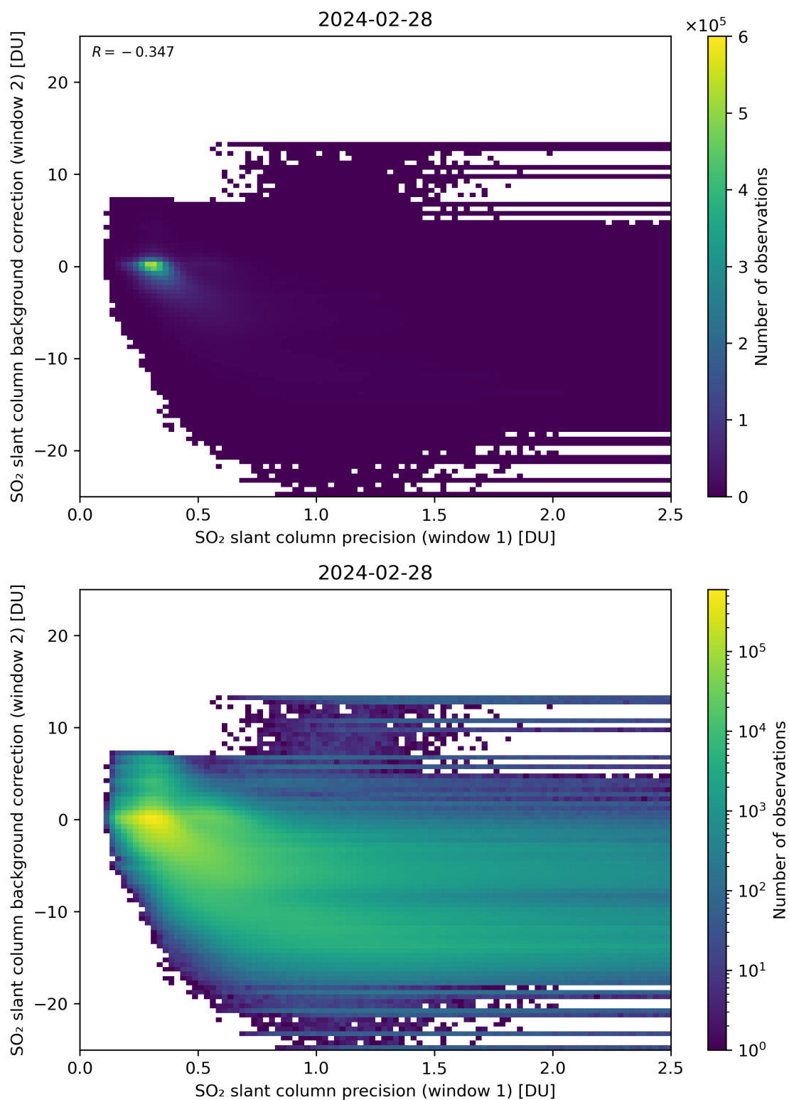
Figure 219: Scatter density plot of “SO 2 slant column precision (window 1)” against “SO 2 slant column background correction (window 2)” for 2024-02-27 to 2024-02-29.
