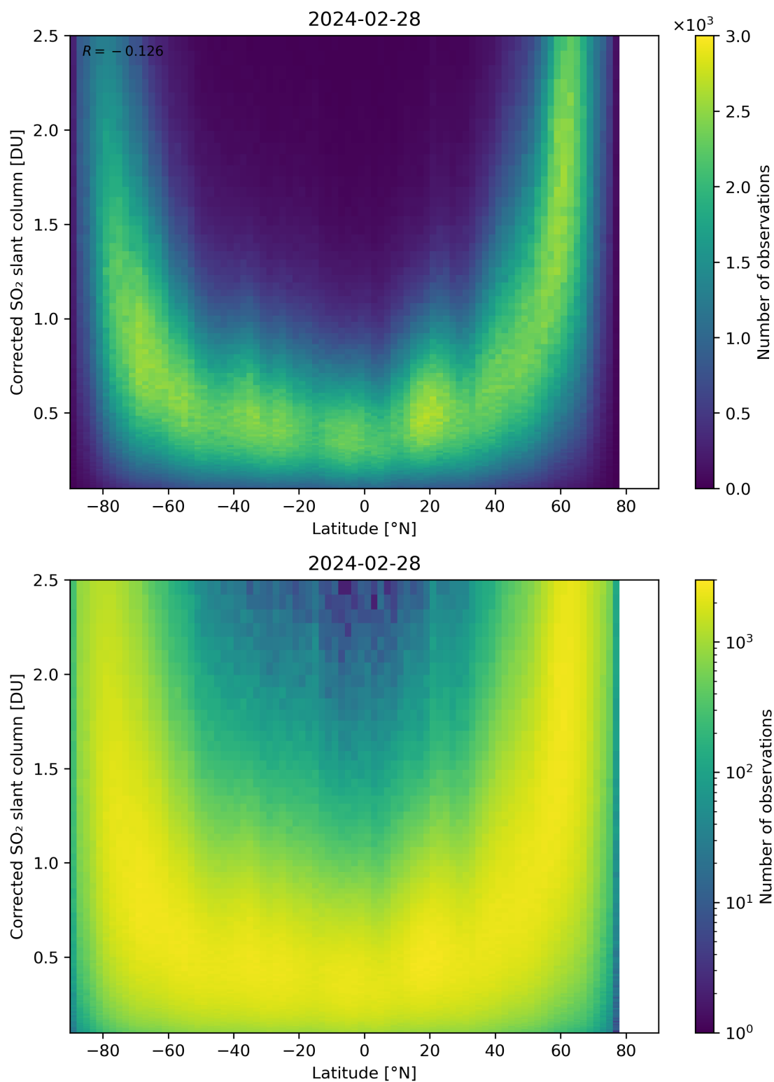
Figure 146: Scatter density plot of “Latitude” against “Corrected SO 2 slant column” for 2024-02-27 to 2024-02-29.
