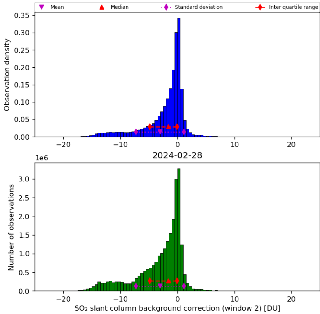
Figure 63: Histogram of “SO 2 slant column background correction (window 2)” for 2024-02-27 to 2024-02-29
