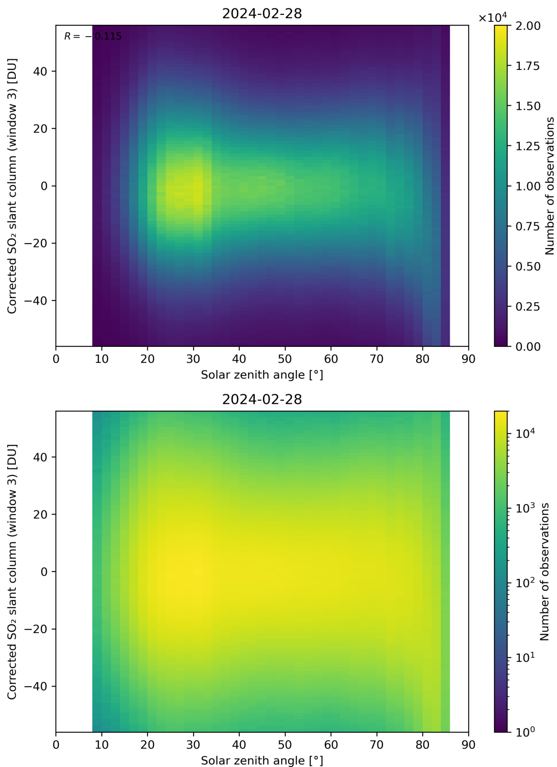
Figure 168: Scatter density plot of “Solar zenith angle” against “Corrected SO 2 slant column (window 3)” for 2024-02-27 to 2024-02-29.
