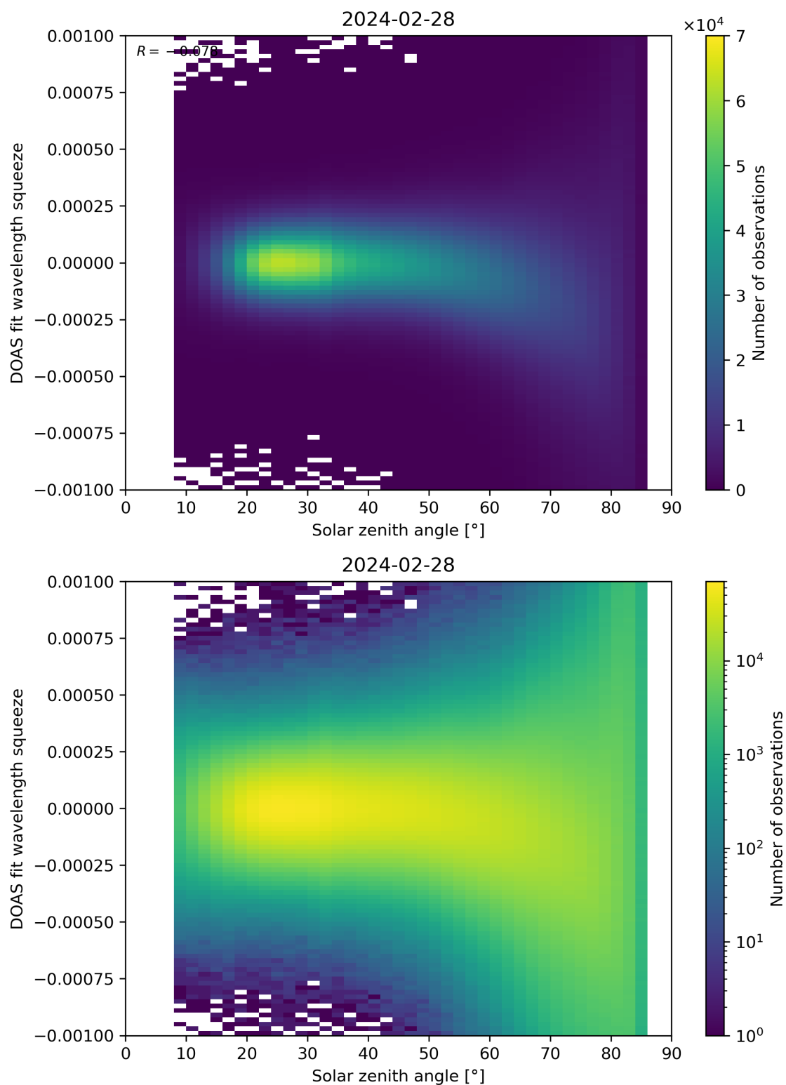
Figure 162: Scatter density plot of “Solar zenith angle” against “DOAS fit wavelength squeeze” for 2024-02-27 to 2024-02-29.
