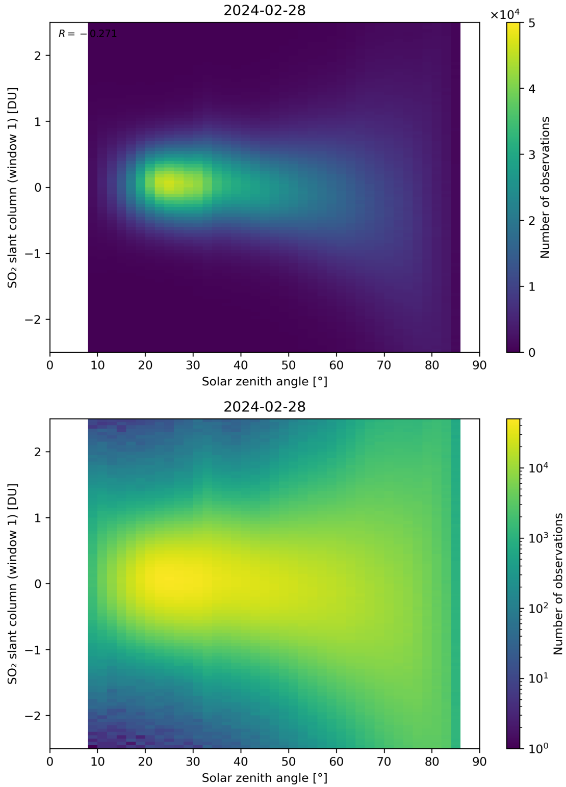
Figure 169: Scatter density plot of “Solar zenith angle” against “SO 2 slant column (window 1)” for 2024-02-27 to 2024-02-29.
