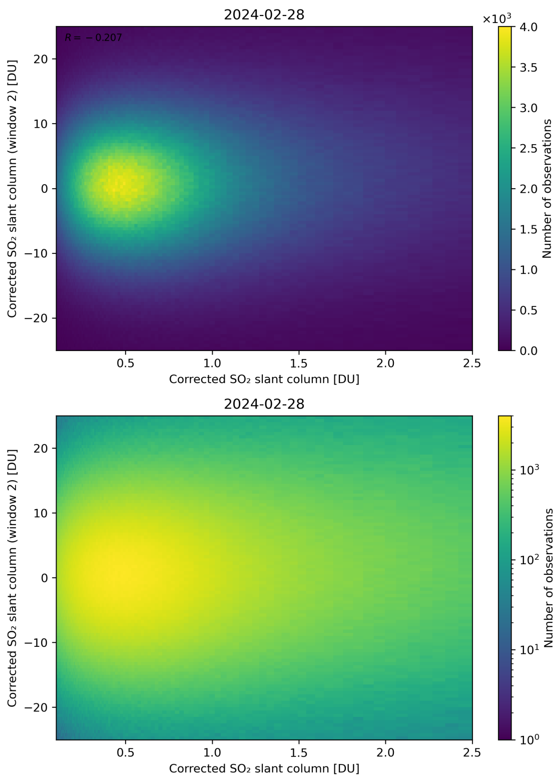
Figure 185: Scatter density plot of “Corrected SO 2 slant column” against “Corrected SO 2 slant column (window 2)” for 2024-02-27 to 2024-02-29.
