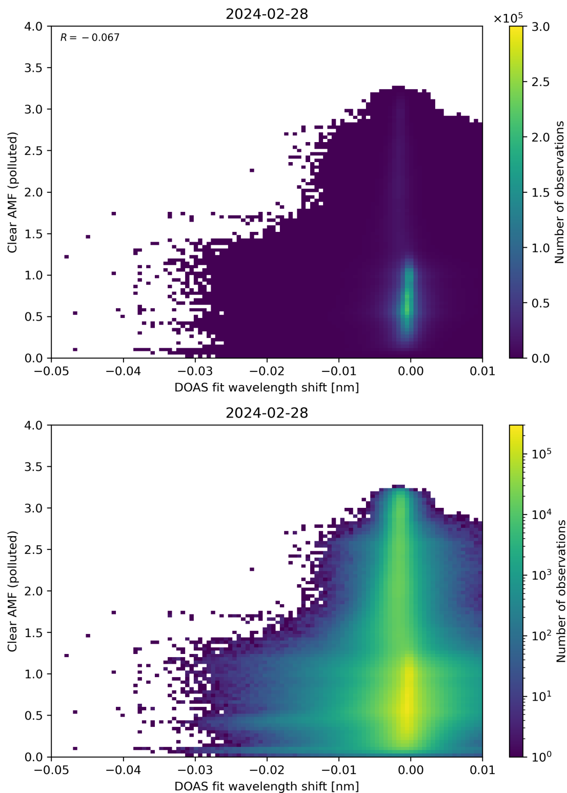
Figure 129: Scatter density plot of “DOAS fit wavelength shift” against “Clear AMF (polluted)” for 2024-02-27 to 2024-02-29.
