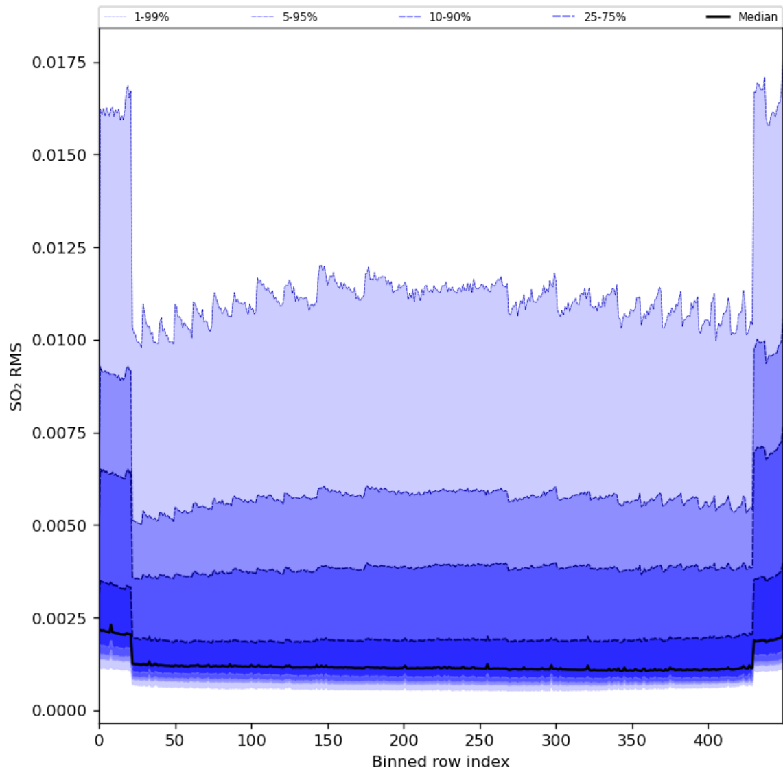
Figure 93: Along track statistics of "SO 2 RMS" for 2024-02-27 to 2024-02-29
