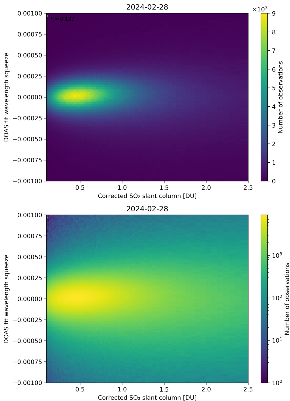
Figure 182: Scatter density plot of “Corrected SO 2 slant column” against “DOAS fit wavelength squeeze” for 2024-02-27 to 2024-02-29.
