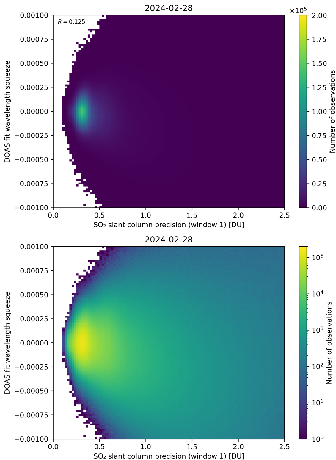
Figure 222: Scatter density plot of “SO 2 slant column precision (window 1)” against “DOAS fit wavelength squeeze” for 2024-02-27 to 2024-02-29.
