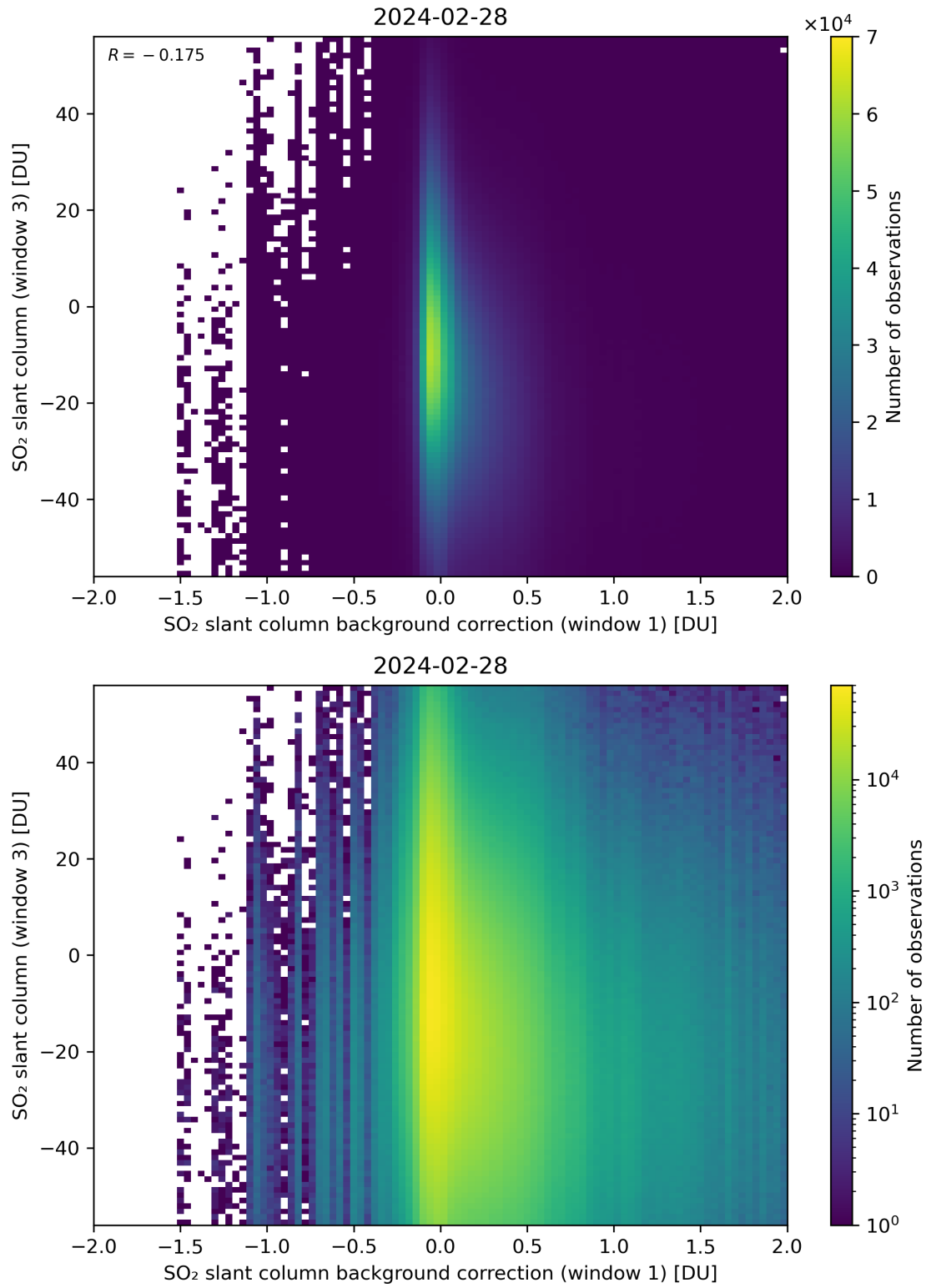
Figure 107: Scatter density plot of “SO 2 slant column background correction (window 1)” against “SO 2 slant column (window 3)” for 2024-02-27 to 2024-02-29.
