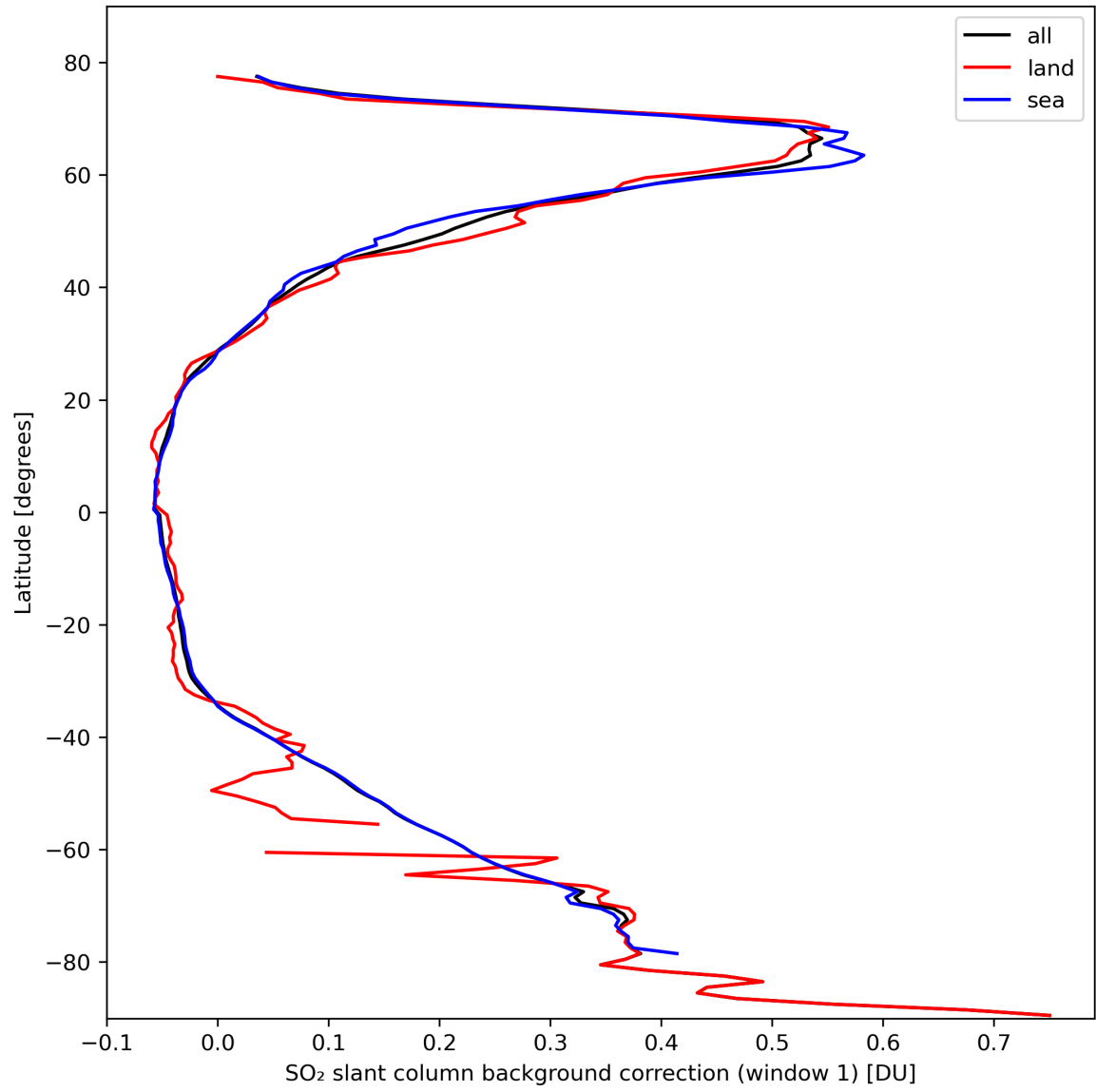
Figure 36: Zonal average of “SO 2 slant column background correction (window 1)” for 2024-02-27 to 2024-02-29.
