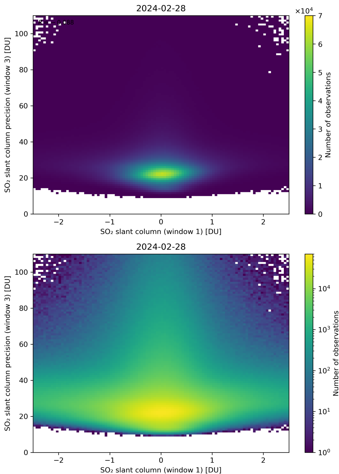
Figure 238: Scatter density plot of “SO 2 slant column (window 1)” against “SO 2 slant column precision (window 3)” for 2024-02-27 to 2024-02-29.
