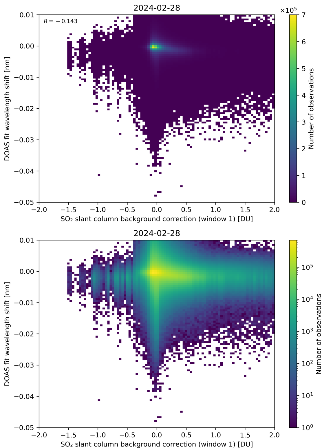
Figure 100: Scatter density plot of “SO 2 slant column background correction (window 1)” against “DOAS fit wavelength shift” for 2024-02-27 to 2024-02-29.
