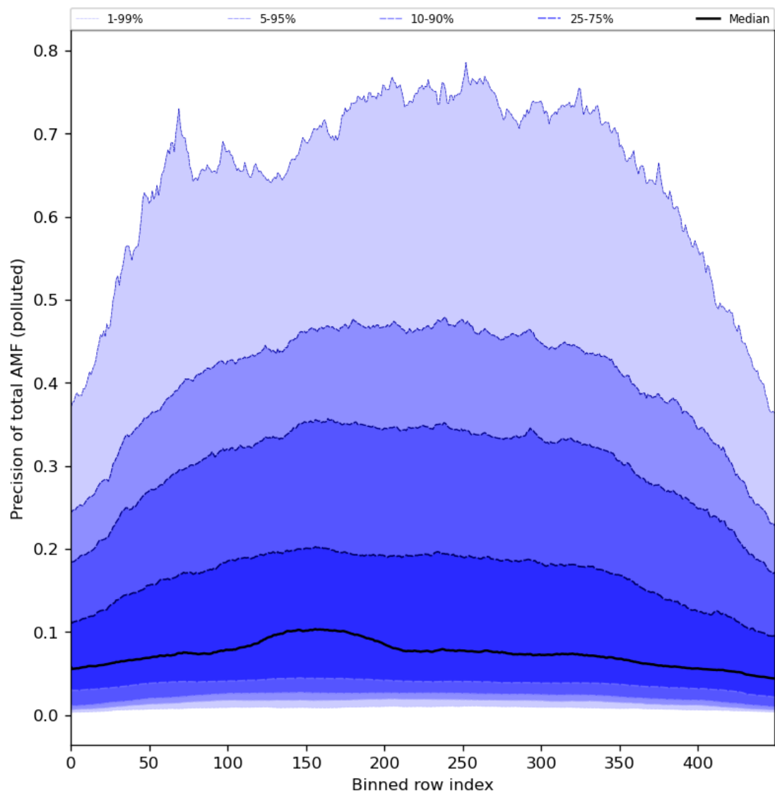
Figure 95: Along track statistics of “Precision of total AMF (polluted)” for 2024-02-27 to 2024-02-29
