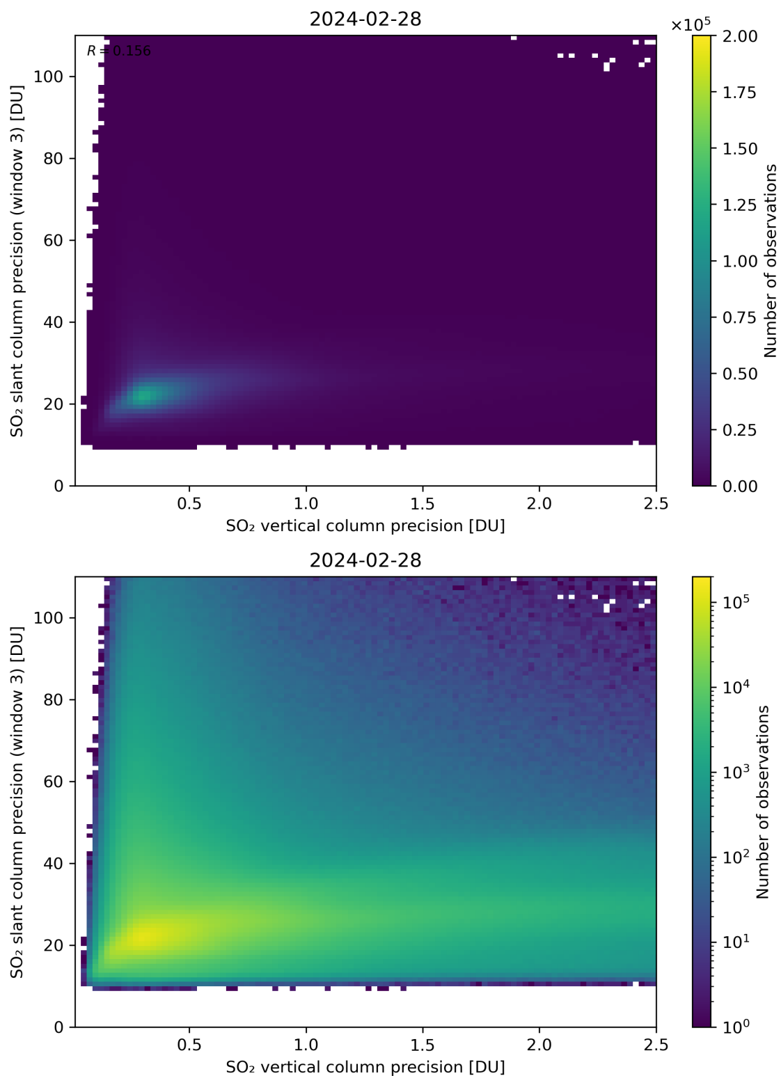
Figure 293: Scatter density plot of “SO 2 vertical column precision” against “SO 2 slant column precision (window 3)” for 2024-02-27 to 2024-02-29.
