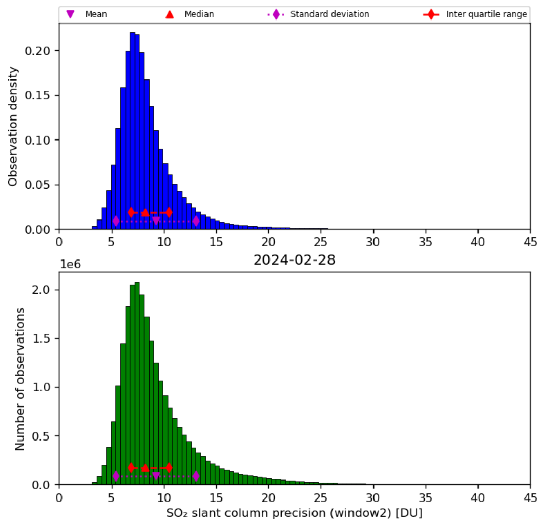
Figure 61: Histogram of “SO 2 slant column precision (window2)” for 2024-02-27 to 2024-02-29
