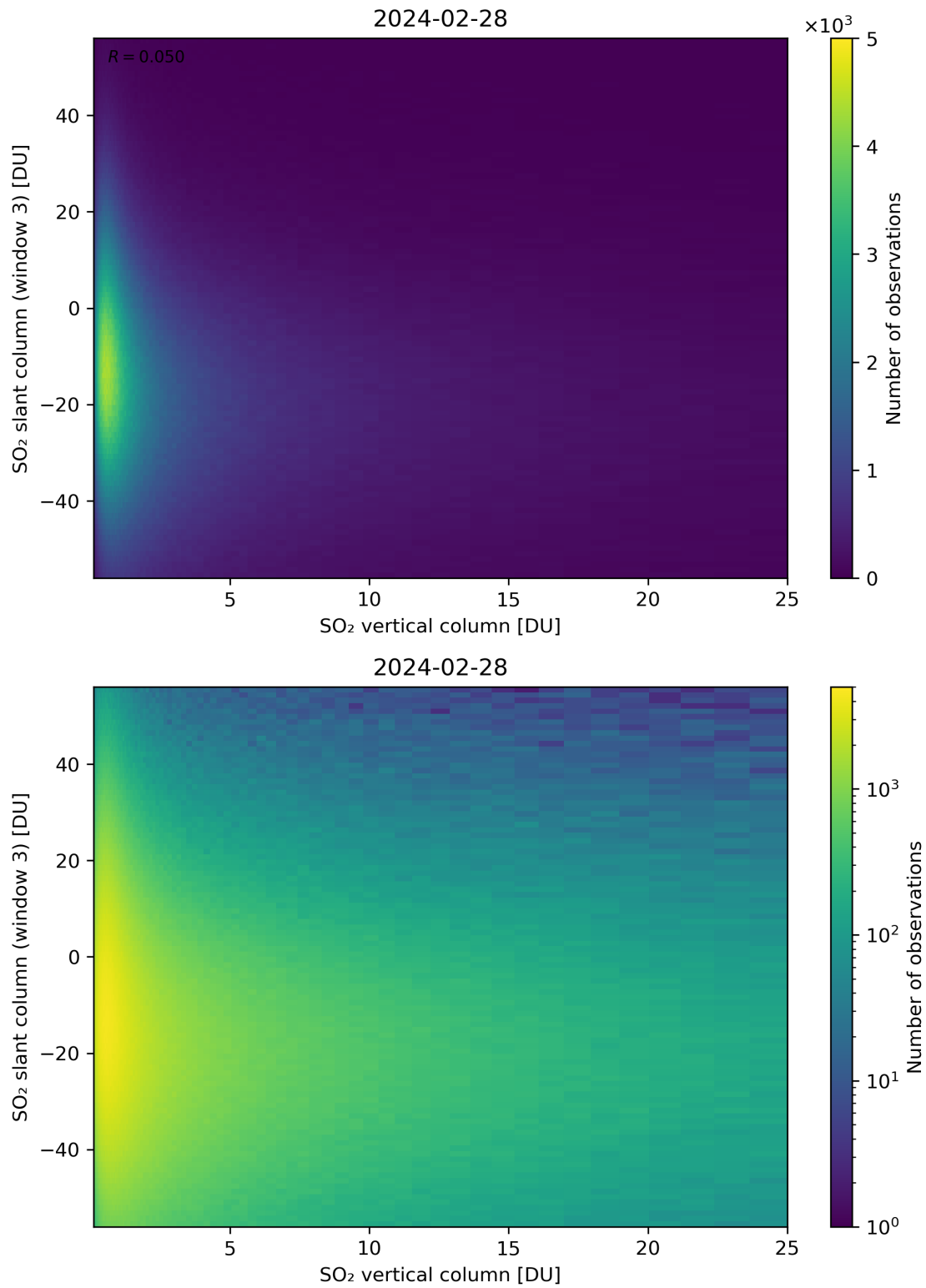
Figure 303: Scatter density plot of “SO 2 vertical column” against “SO 2 slant column (window 3)” for 2024-02-27 to 2024-02-29.
