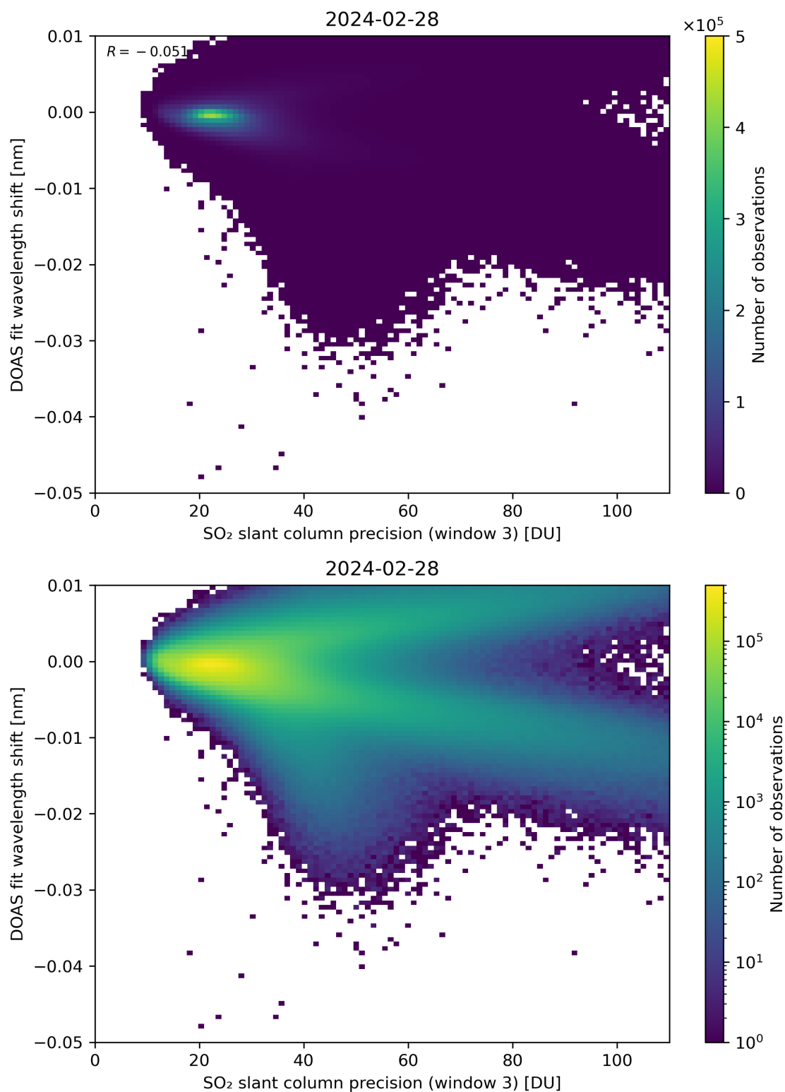
Figure 258: Scatter density plot of “SO 2 slant column precision (window 3)” against “DOAS fit wavelength shift” for 2024-02-27 to 2024-02-29.
