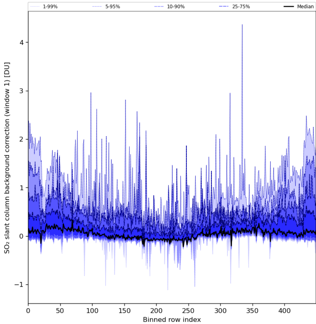
Figure 82: Along track statistics of “SO 2 slant column background correction (window 1)” for 2024-02-27 to 2024-02-29
