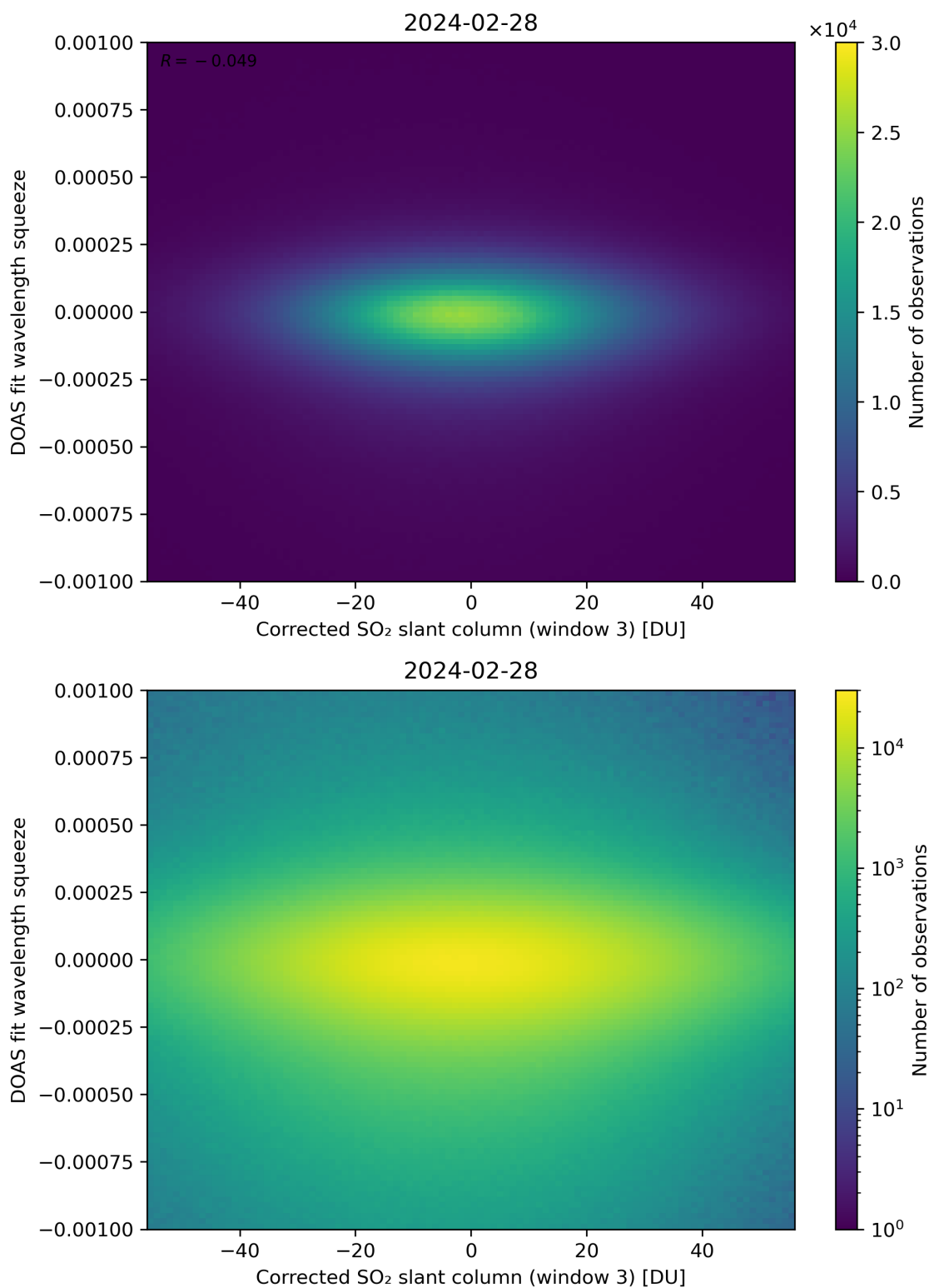
Figure 207: Scatter density plot of “Corrected SO 2 slant column (window 3)” against “DOAS fit wavelength squeeze” for 2024-02-27 to 2024-02-29.
