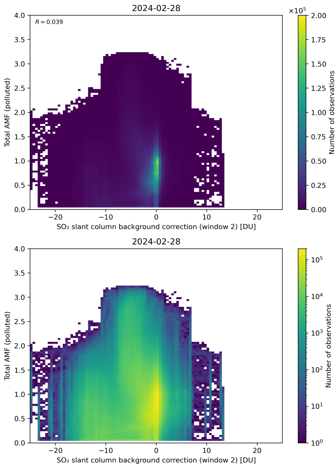
Figure 119: Scatter density plot of “SO 2 slant column background correction (window 2)” against “Total AMF (polluted)” for 2024-02-27 to 2024-02-29.
