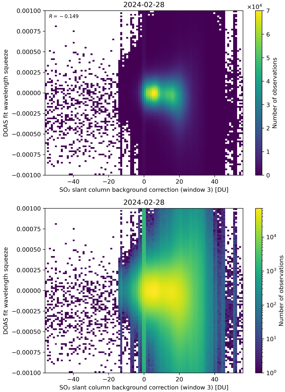
Figure 122: Scatter density plot of “SO 2 slant column background correction (window 3)” against “DOAS fit wavelength squeeze” for 2024-02-27 to 2024-02-29.
