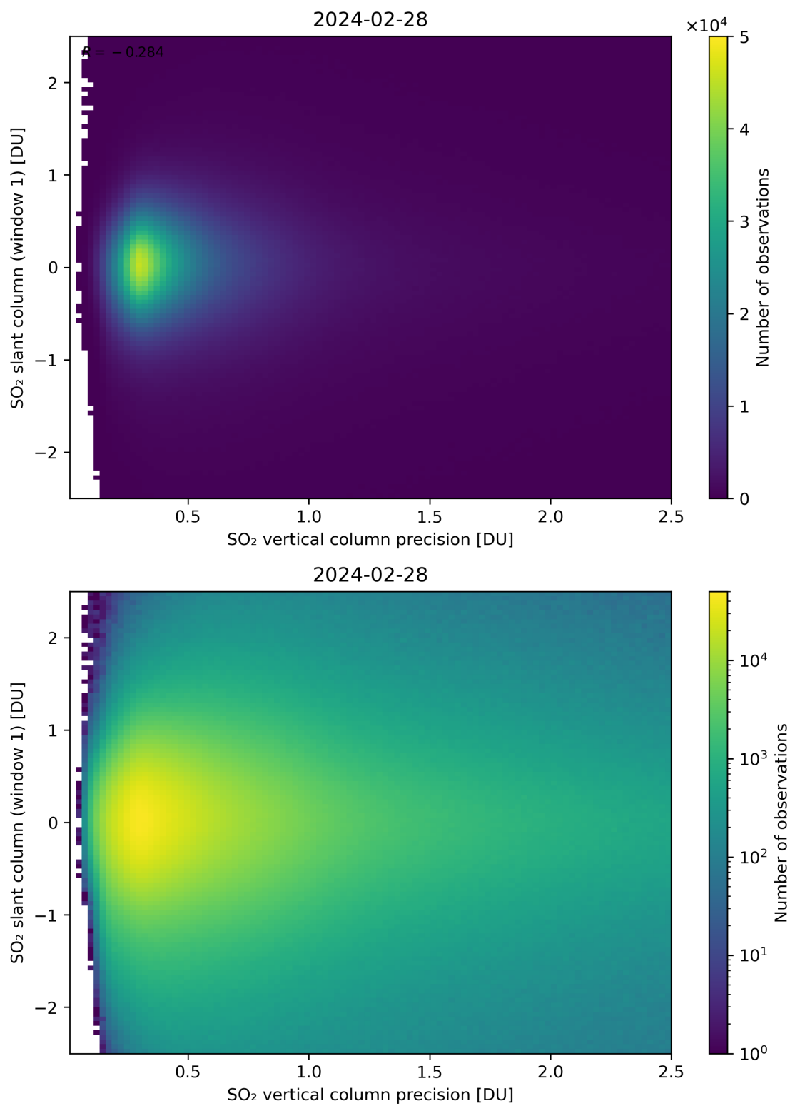
Figure 289: Scatter density plot of “SO 2 vertical column precision” against “SO 2 slant column (window 1)” for 2024-02-27 to 2024-02-29.
