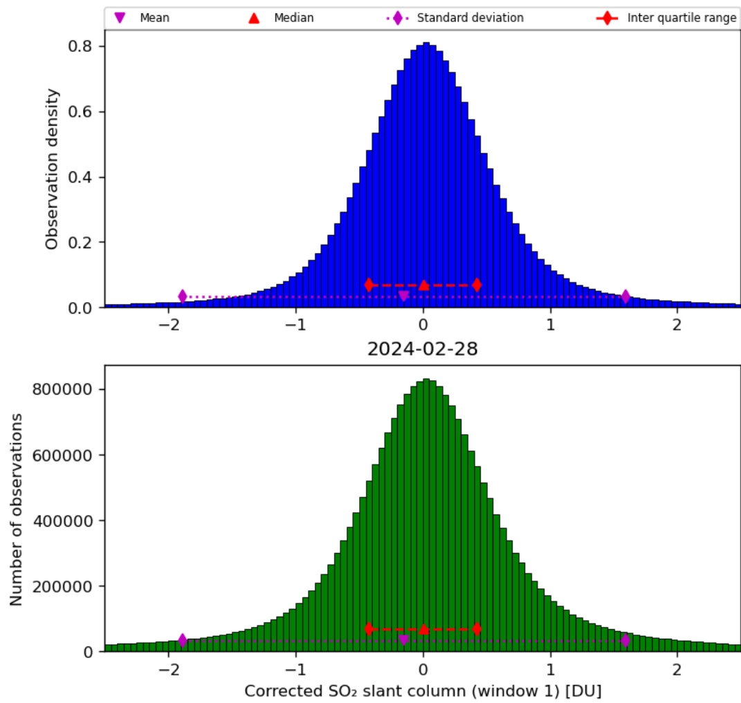
Figure 58: Histogram of “Corrected SO 2 slant column (window 1)” for 2024-02-27 to 2024-02-29
