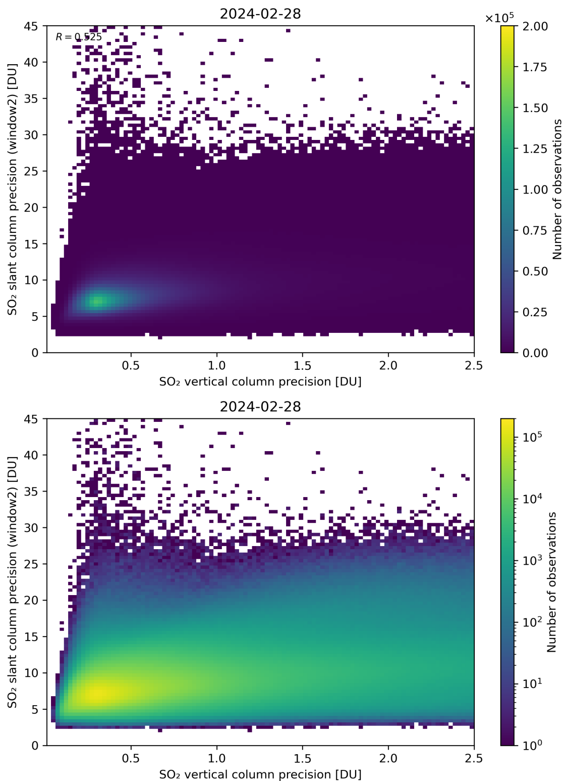
Figure 291: Scatter density plot of “SO 2 vertical column precision” against “SO 2 slant column precision (window2)” for 2024-02-27 to 2024-02-29.
