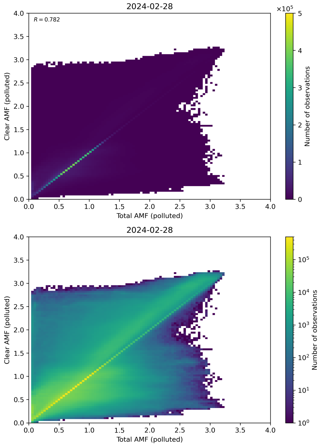
Figure 271: Scatter density plot of “Total AMF (polluted)” against “Clear AMF (polluted)” for 2024-02-27 to 2024-02-29.
