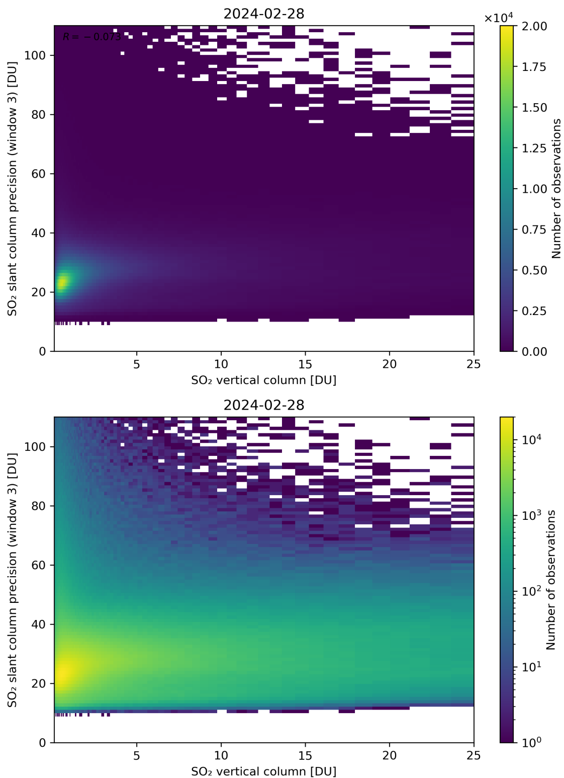
Figure 304: Scatter density plot of “SO 2 vertical column” against “SO 2 slant column precision (window 3)” for 2024-02-27 to 2024-02-29.
