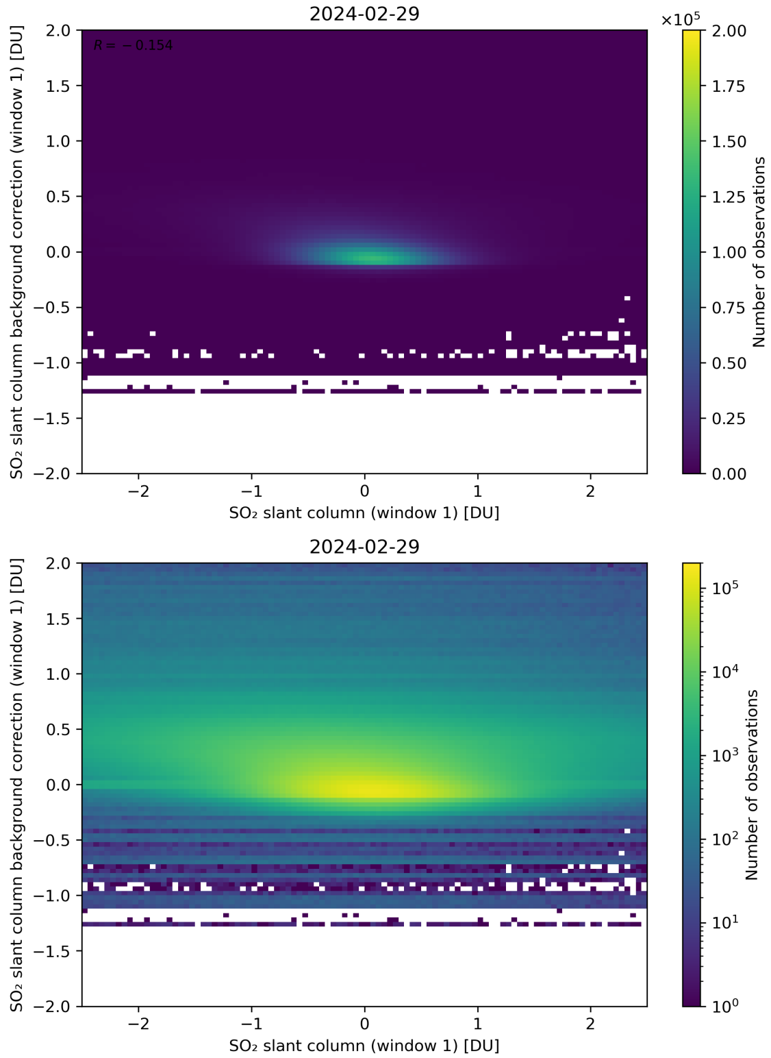
Figure 212: Scatter density plot of “SO 2 slant column (window 1)” against “SO 2 slant column background correction (window 1)” for 2024-02-28 to 2024-03-01.
