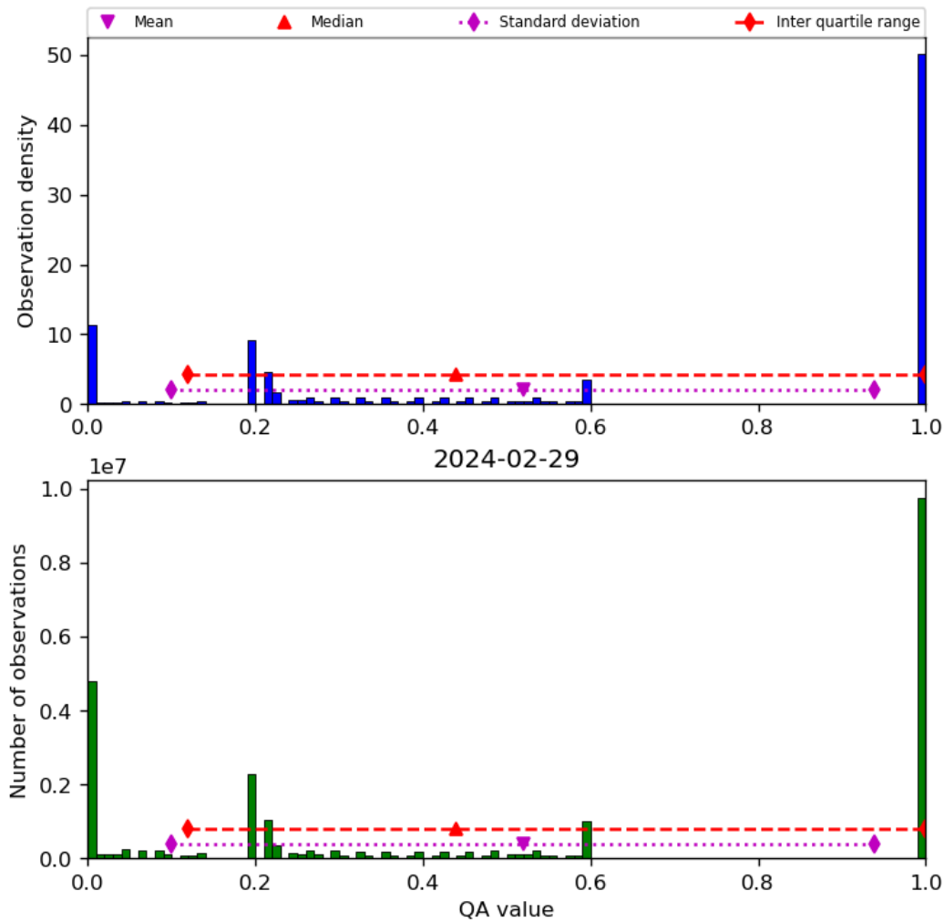
Figure 52: Histogram of “QA value” for 2024-02-28 to 2024-03-01
