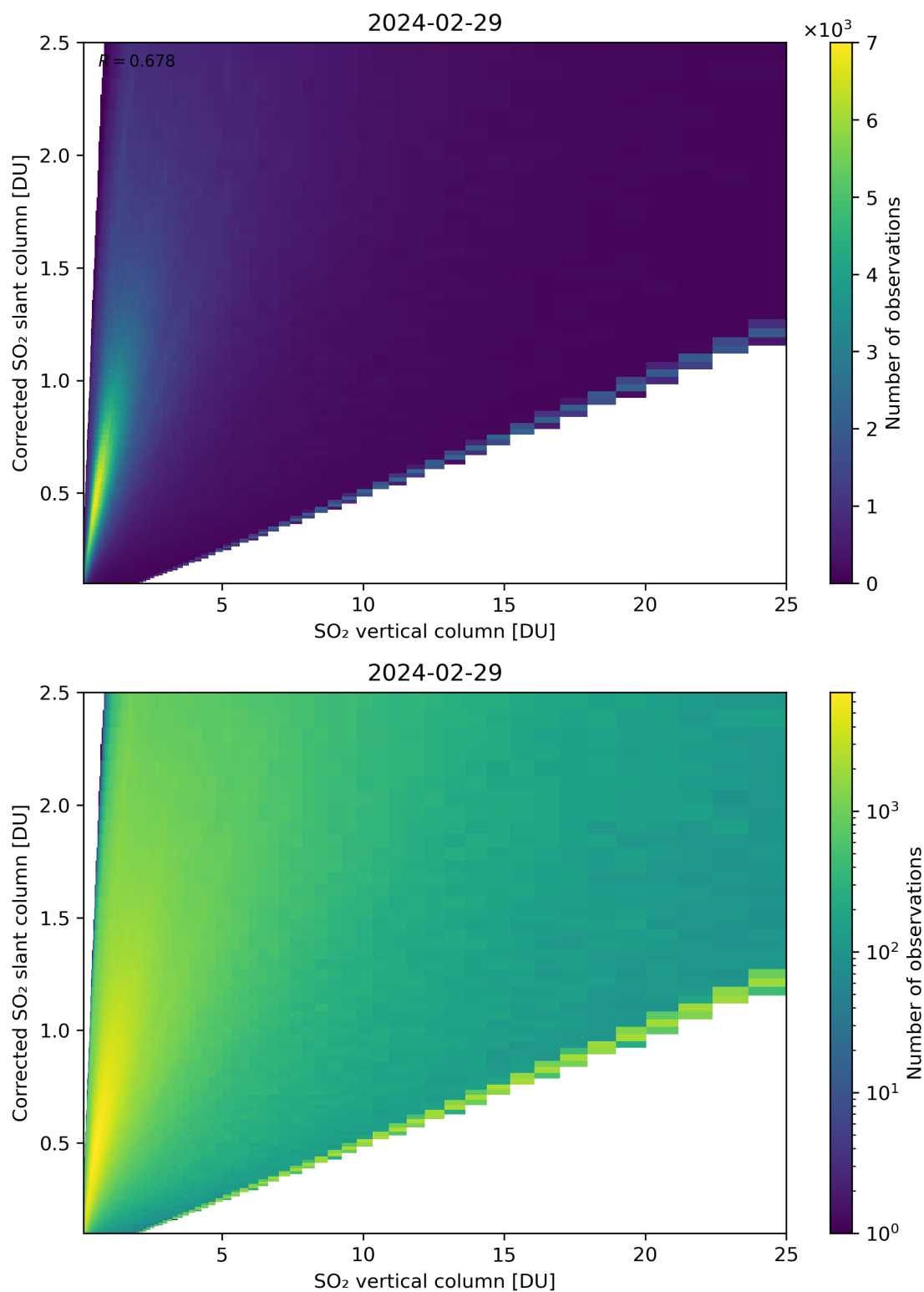
Figure 297: Scatter density plot of “SO 2 vertical column” against “Corrected SO 2 slant column” for 2024-02-28 to 2024-03-01.
