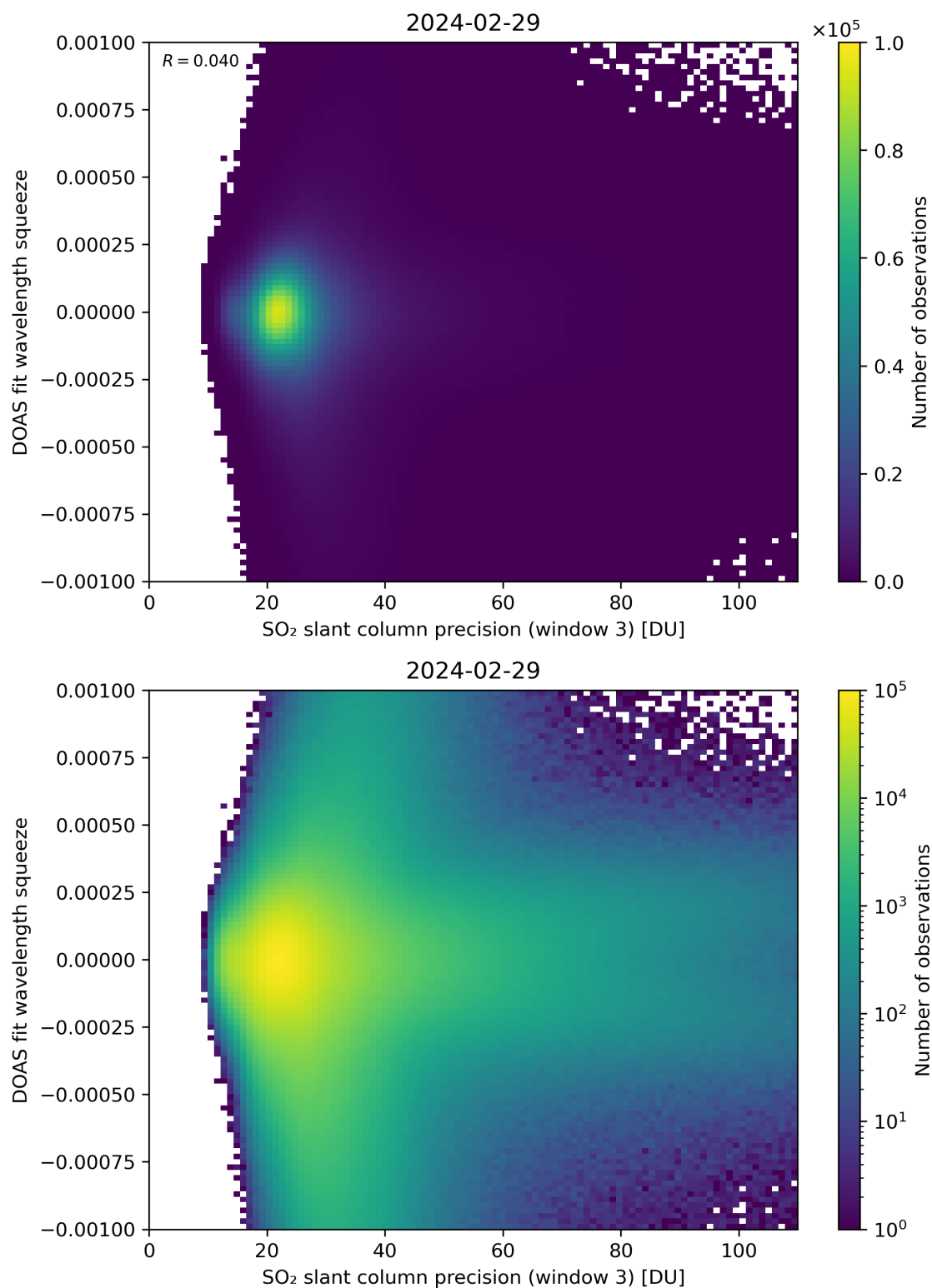
Figure 259: Scatter density plot of “SO 2 slant column precision (window 3)” against “DOAS fit wavelength squeeze” for 2024-02-28 to 2024-03-01.
