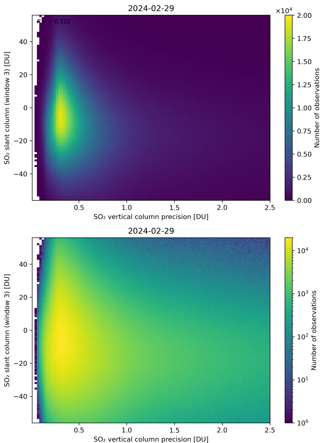
Figure 292: Scatter density plot of “SO 2 vertical column precision” against “SO 2 slant column (window 3)” for 2024-02-28 to 2024-03-01.
