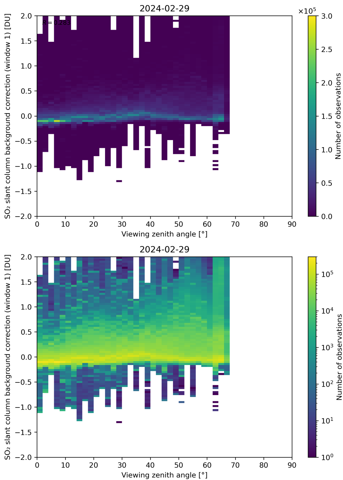
Figure 308: Scatter density plot of “Viewing zenith angle” against “SO 2 slant column background correction (window 1)” for 2024-02-28 to 2024-03-01.
