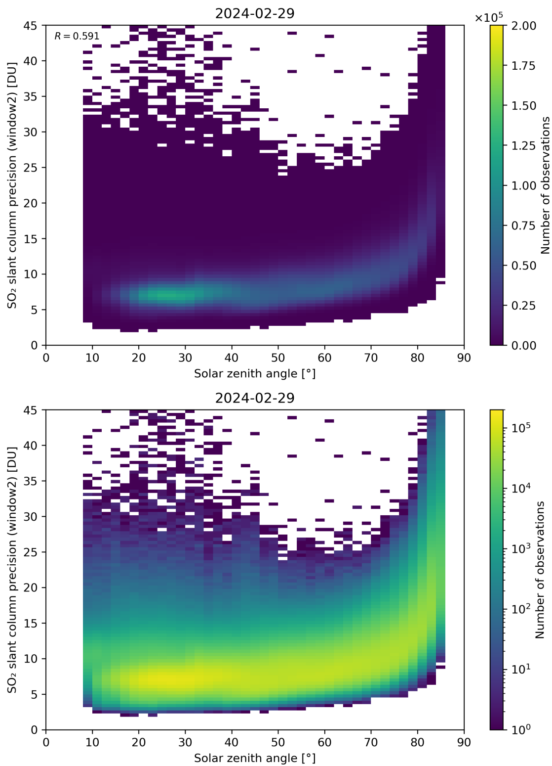
Figure 171: Scatter density plot of “Solar zenith angle” against “SO 2 slant column precision (window2)” for 2024-02-28 to 2024-03-01.
