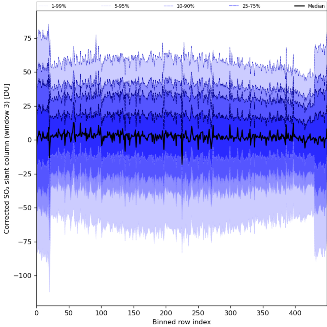
Figure 89: Along track statistics of “Corrected SO 2 slant column (window 3)” for 2024-02-28 to 2024-03-01
