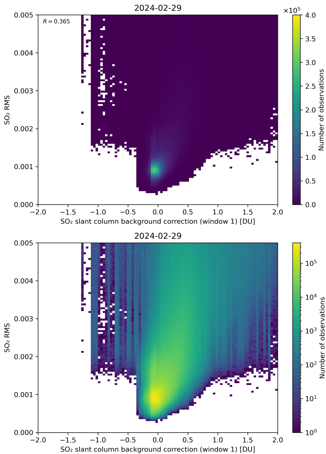
Figure 102: Scatter density plot of “SO 2 slant column background correction (window 1)” against “SO 2 RMS” for 2024-02-28 to 2024-03-01.
