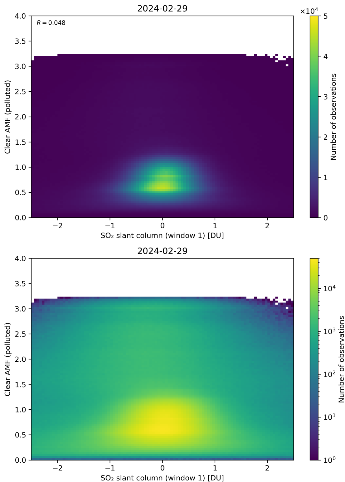
Figure 232: Scatter density plot of “SO 2 slant column (window 1)” against “Clear AMF (polluted)” for 2024-02-28 to 2024-03-01.
