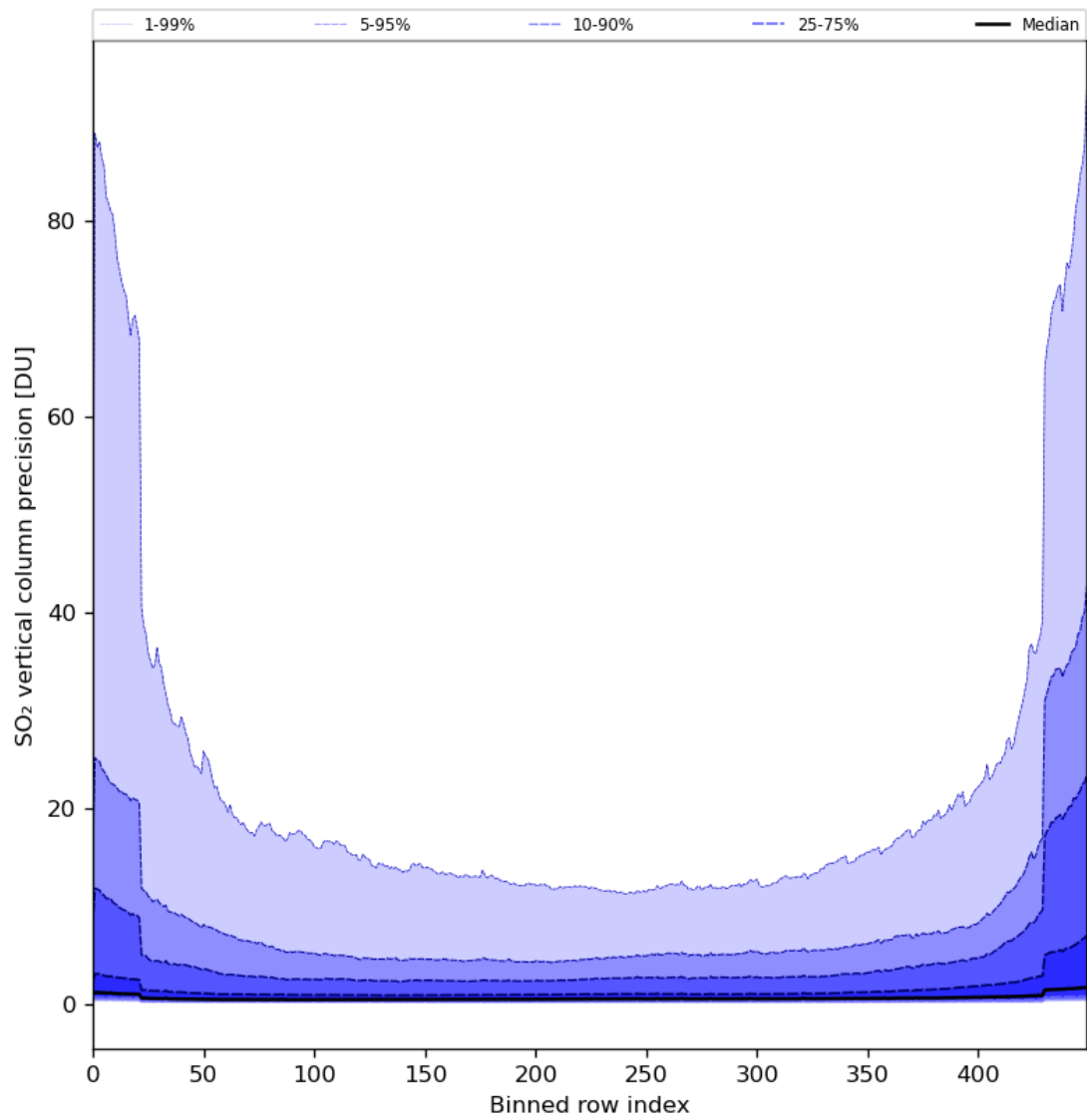
Figure 77: Along track statistics of “SO 2 vertical column precision” for 2024-02-28 to 2024-03-01
