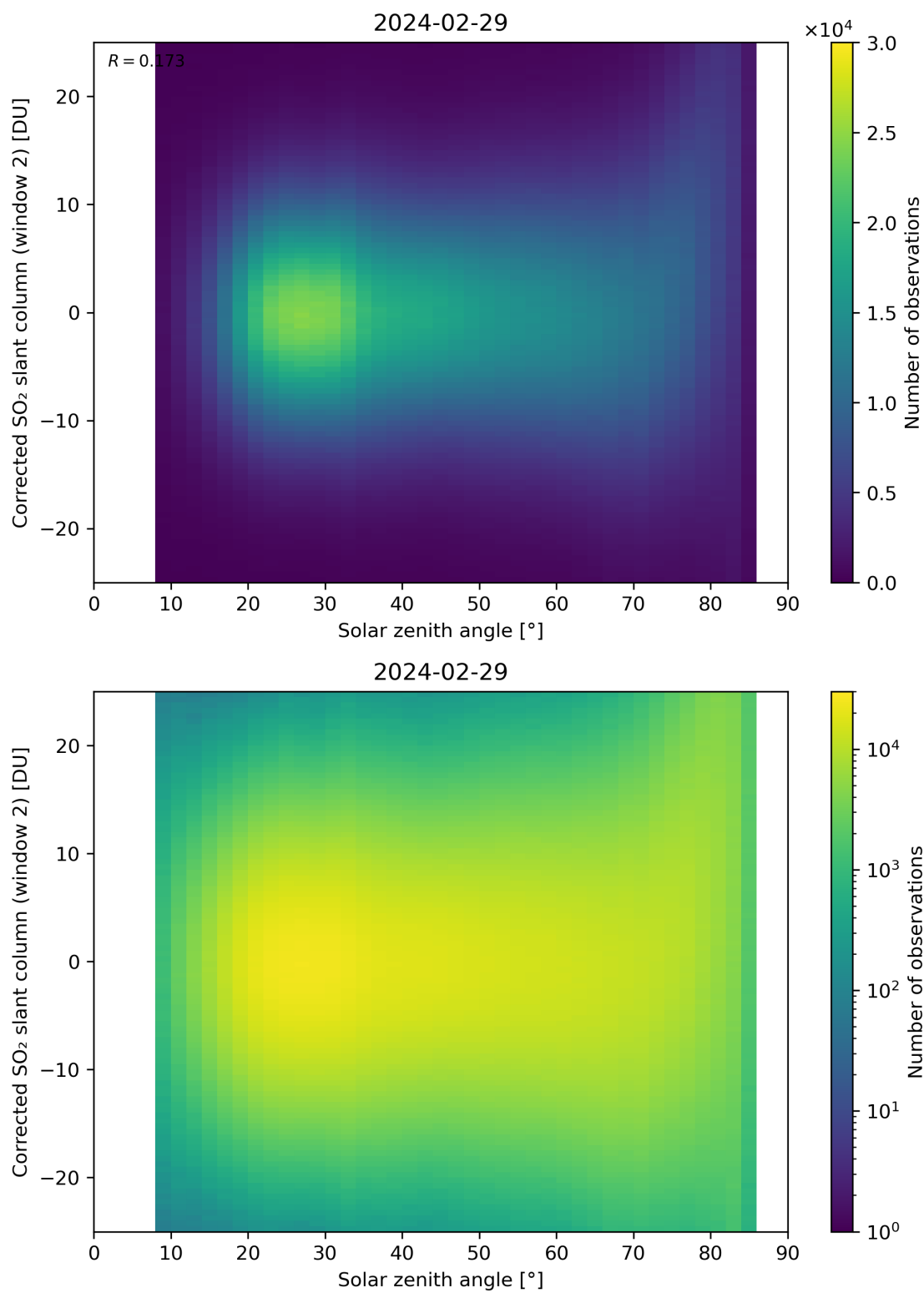
Figure 167: Scatter density plot of “Solar zenith angle” against “Corrected SO 2 slant column (window 2)” for 2024-02-28 to 2024-03-01.
