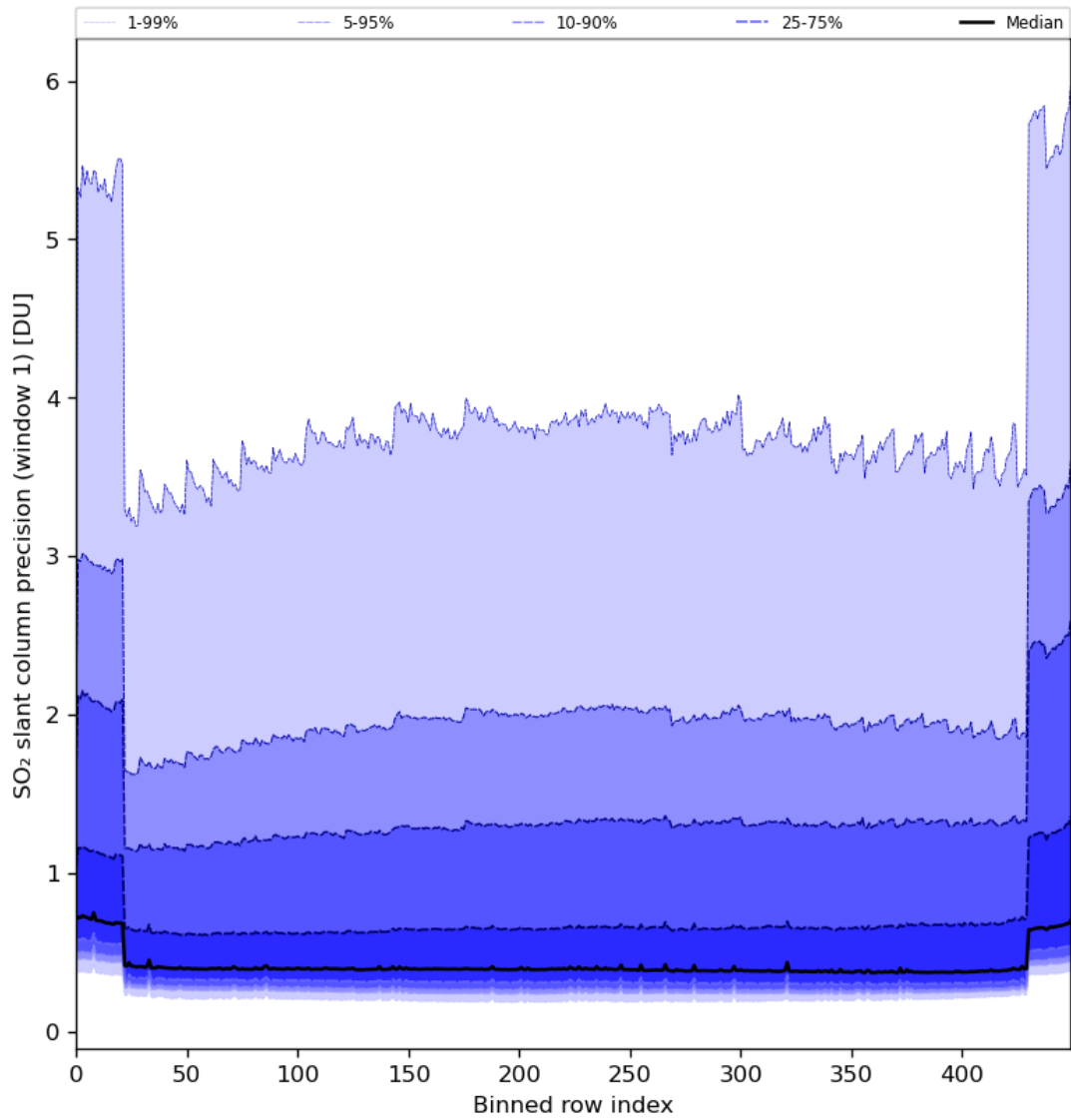
Figure 80: Along track statistics of “SO 2 slant column precision (window 1)” for 2024-02-28 to 2024-03-01
