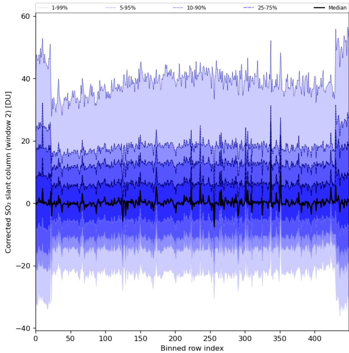
Figure 85: Along track statistics of "Corrected SO 2 slant column (window 2)" for 2024-02-28 to 2024-03-01
