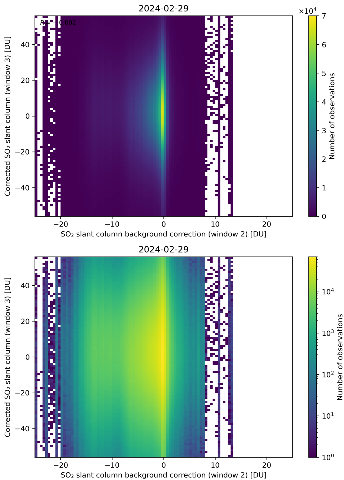
Figure 116: Scatter density plot of “SO 2 slant column background correction (window 2)” against “Corrected SO 2 slant column (window 3)” for 2024-02-28 to 2024-03-01.
