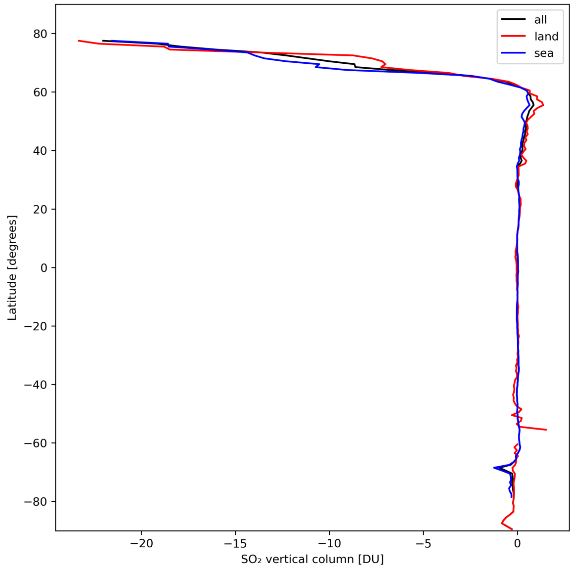
Figure 30: Zonal average of “SO 2 vertical column” for 2024-02-28 to 2024-03-01.
