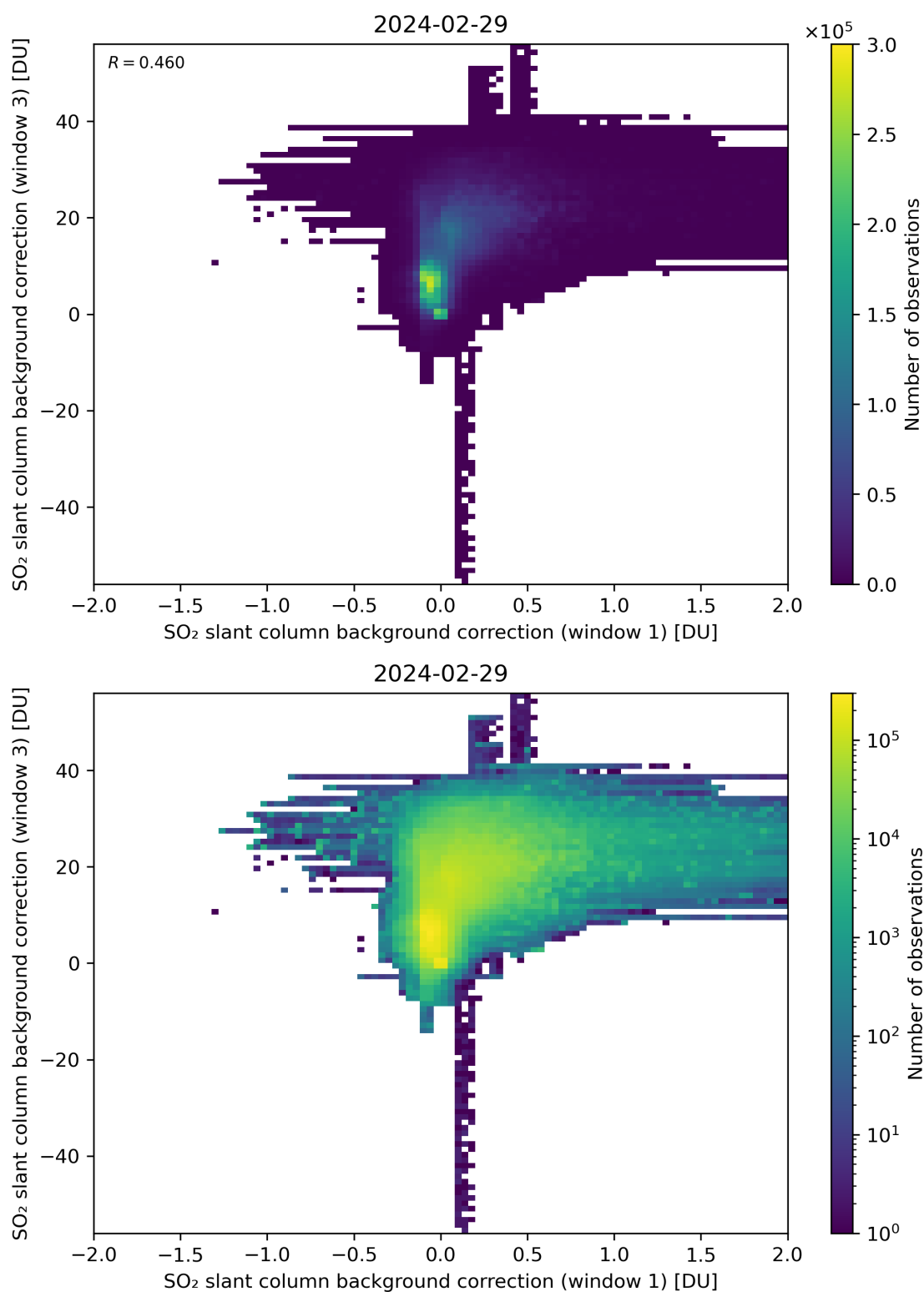
Figure 99: Scatter density plot of “SO 2 slant column background correction (window 1)” against “SO 2 slant column background correction (window 3)” for 2024-02-28 to 2024-03-01.
