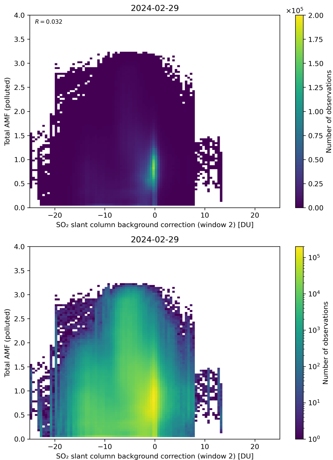
Figure 119: Scatter density plot of “SO 2 slant column background correction (window 2)” against “Total AMF (polluted)” for 2024-02-28 to 2024-03-01.
