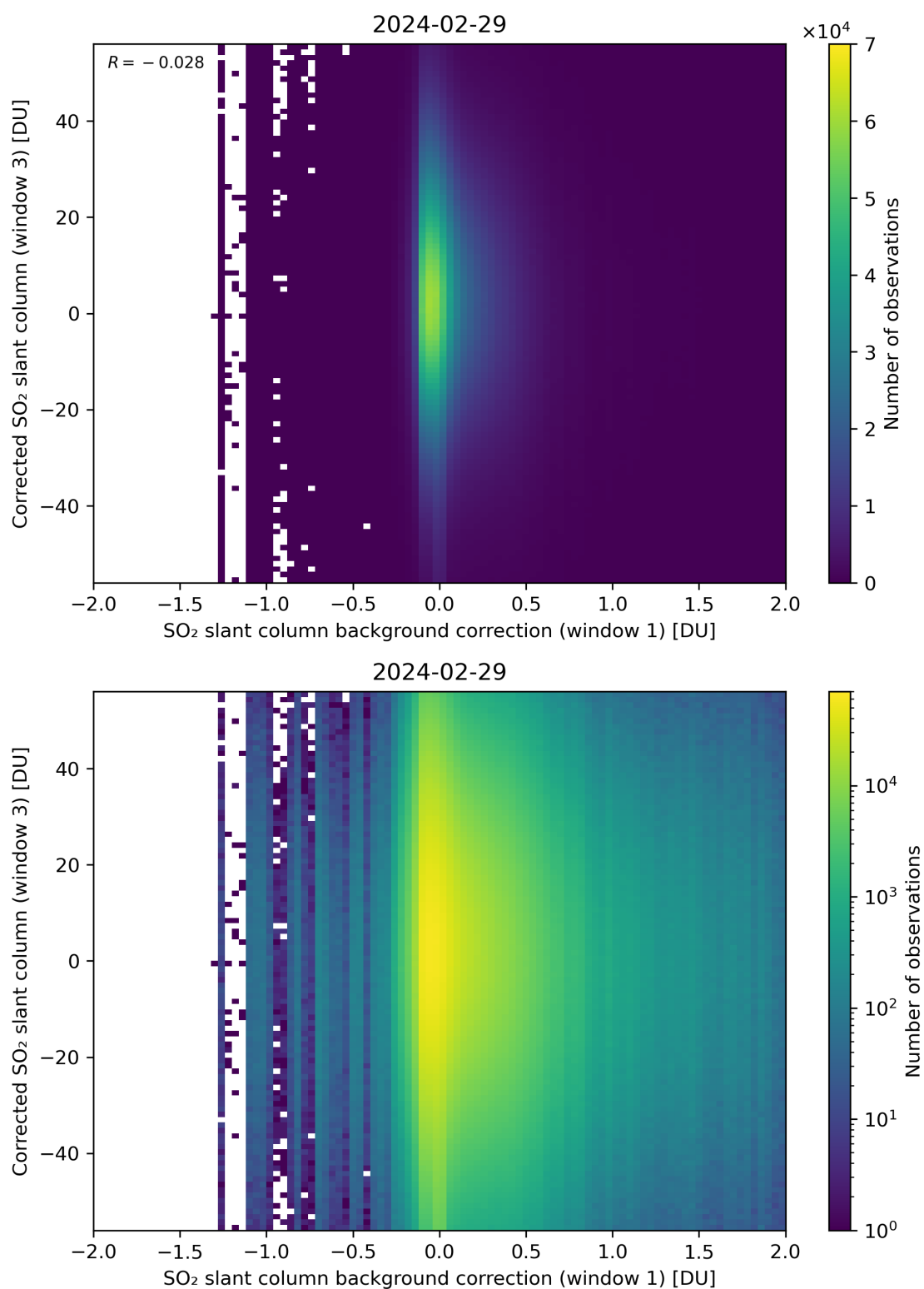
Figure 105: Scatter density plot of “SO 2 slant column background correction (window 1)” against “Corrected SO 2 slant column (window 3)” for 2024-02-28 to 2024-03-01.
