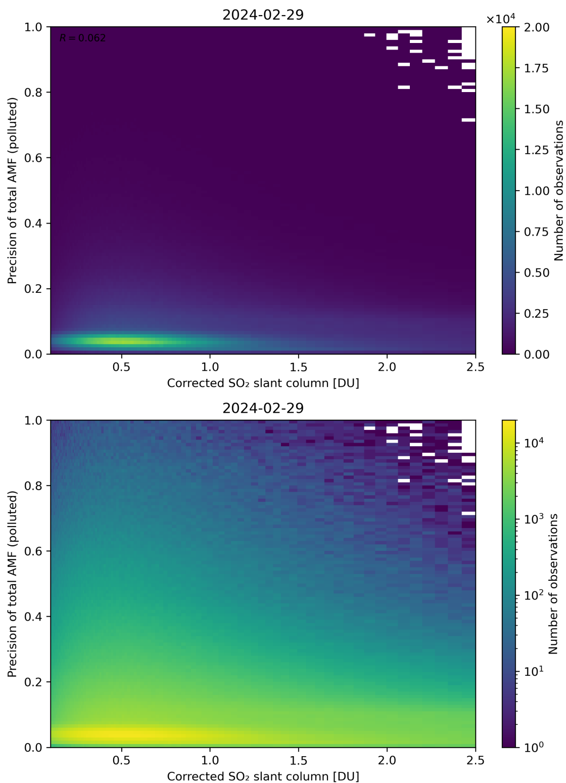
Figure 193: Scatter density plot of “Corrected SO 2 slant column” against “Precision of total AMF (polluted)” for 2024-02-28 to 2024-03-01.
