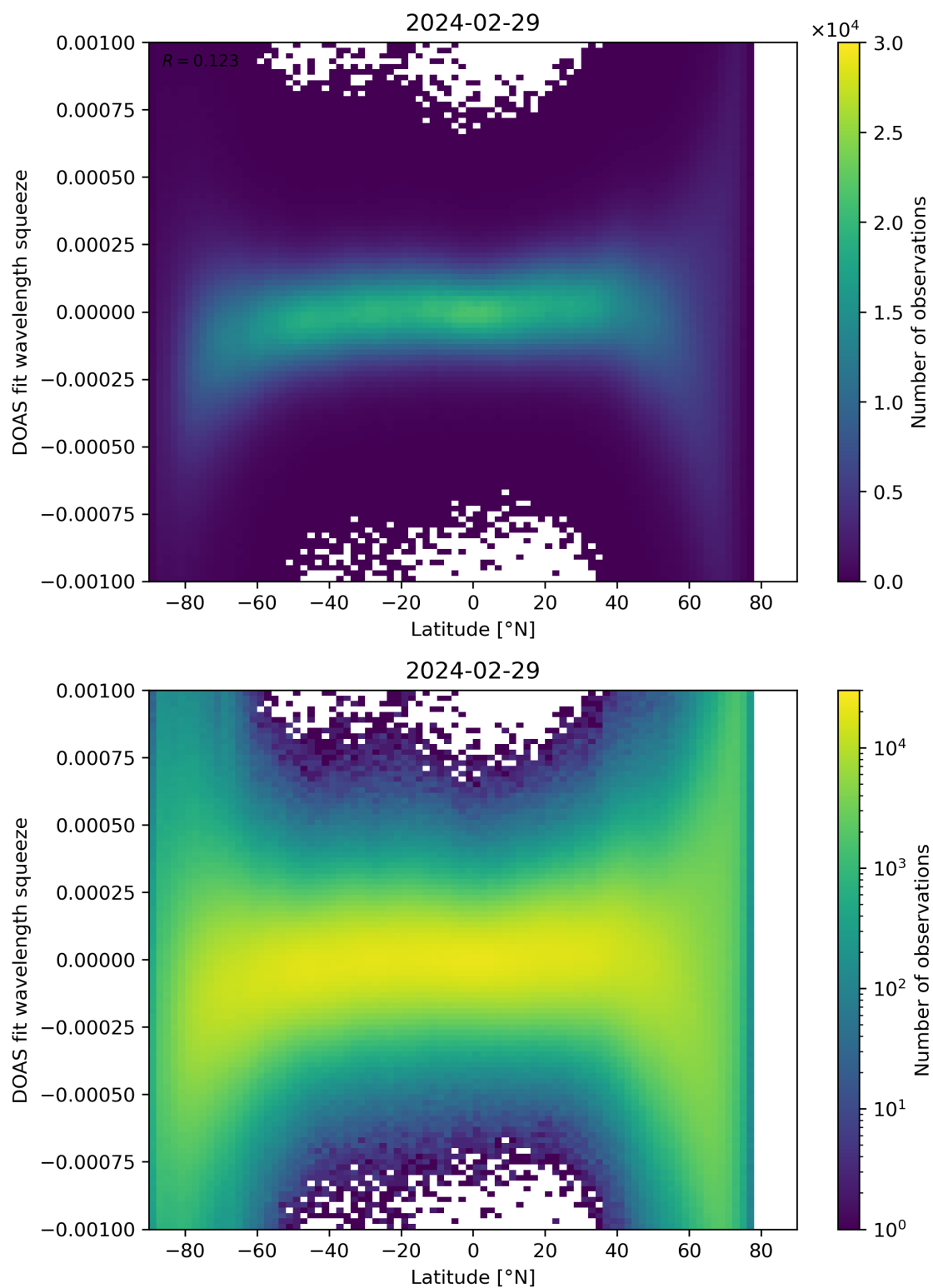
Figure 143: Scatter density plot of “Latitude” against “DOAS fit wavelength squeeze” for 2024-02-28 to 2024-03-01.
