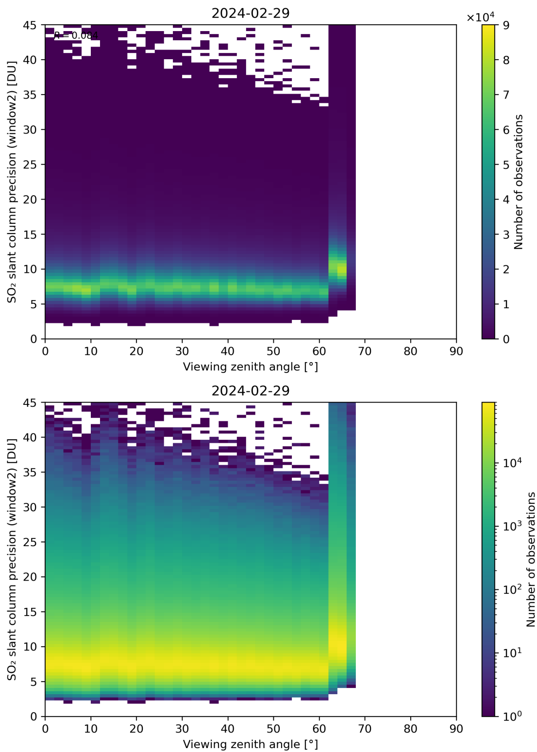
Figure 322: Scatter density plot of “Viewing zenith angle” against “SO 2 slant column precision (window2)” for 2024-02-28 to 2024-03-01.
