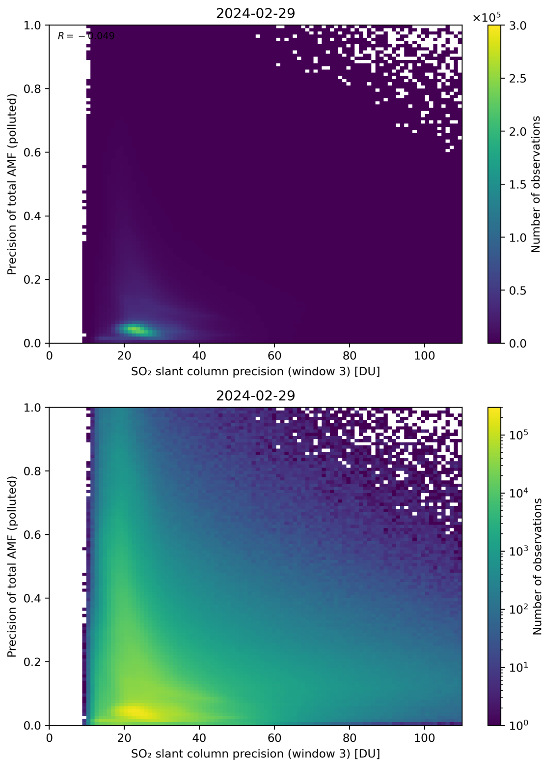
Figure 264: Scatter density plot of “SO 2 slant column precision (window 3)” against “Precision of total AMF (polluted)” for 2024-02-28 to 2024-03-01.
