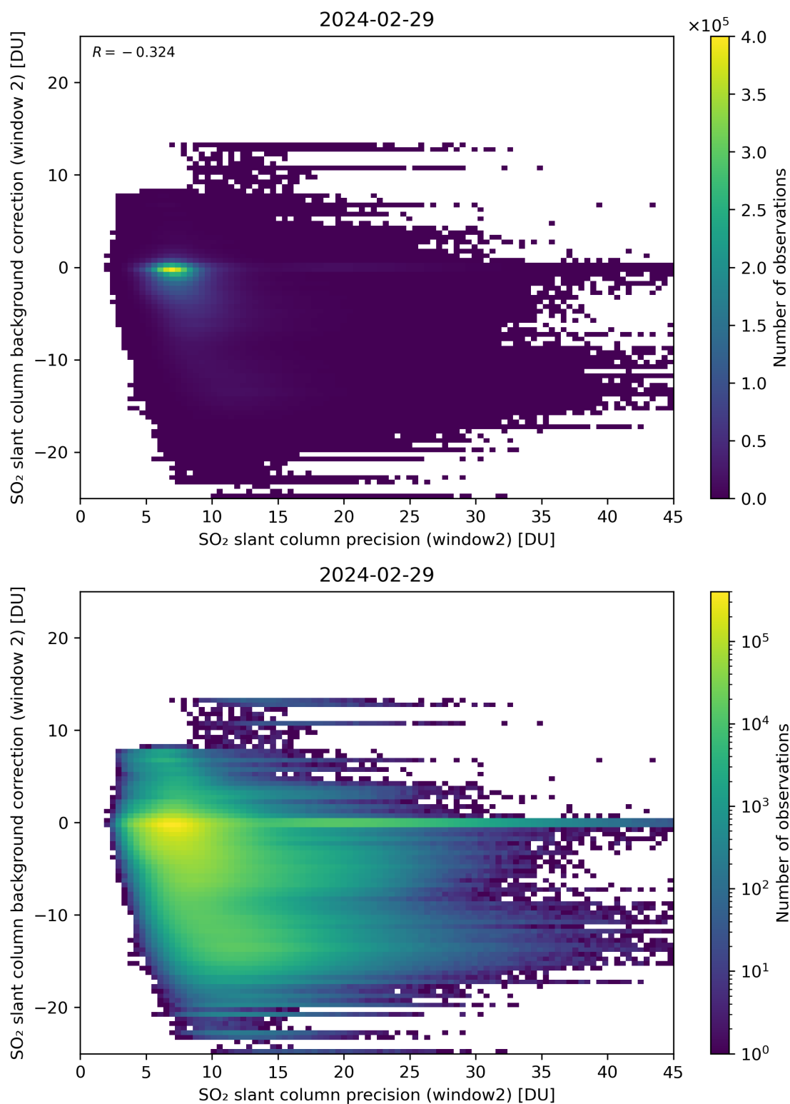
Figure 241: Scatter density plot of “SO 2 slant column precision (window2)” against “SO 2 slant column background correction (window 2)” for 2024-02-28 to 2024-03-01.
