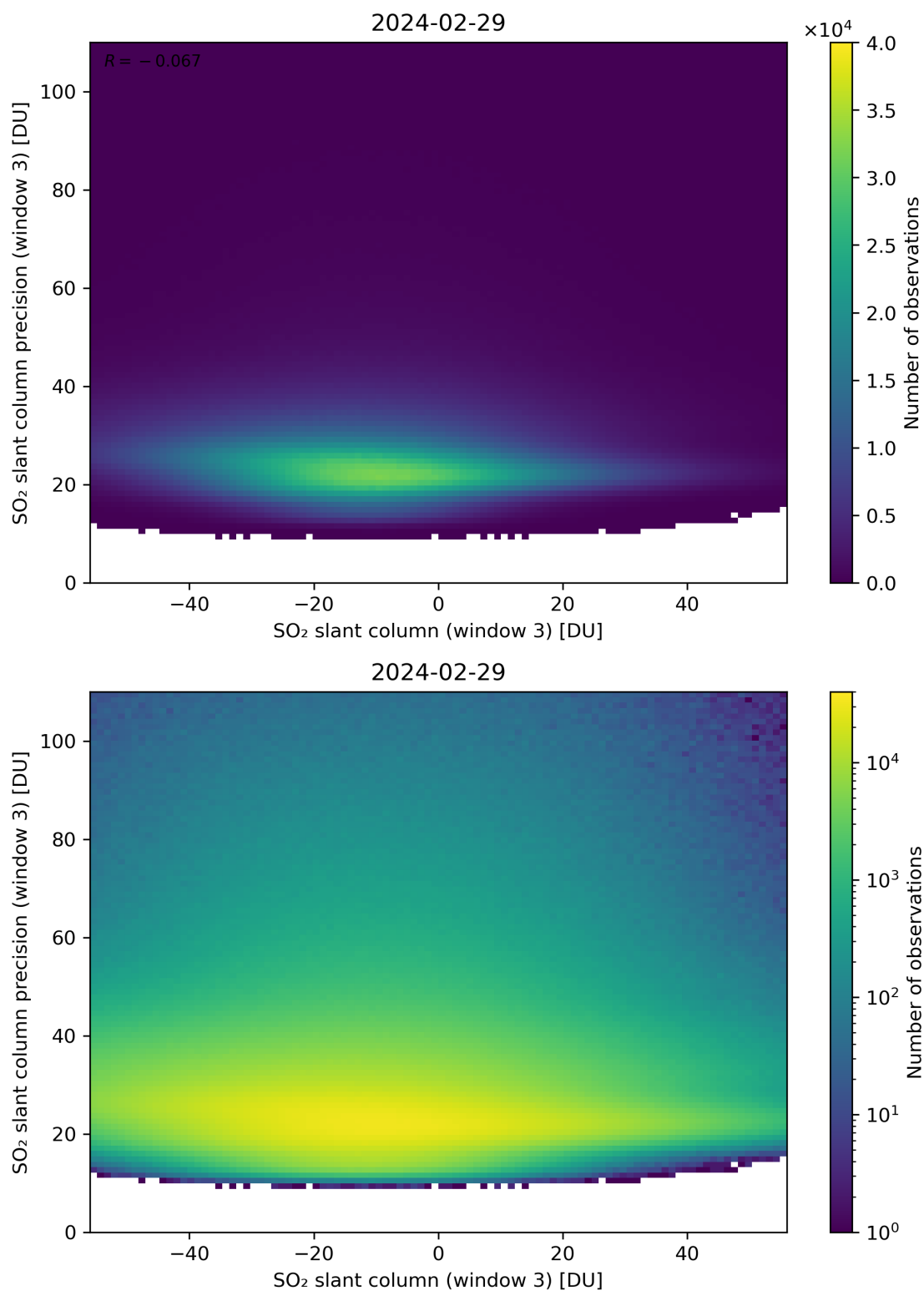
Figure 267: Scatter density plot of “SO 2 slant column (window 3)” against “SO 2 slant column precision (window 3)” for 2024-02-28 to 2024-03-01.
