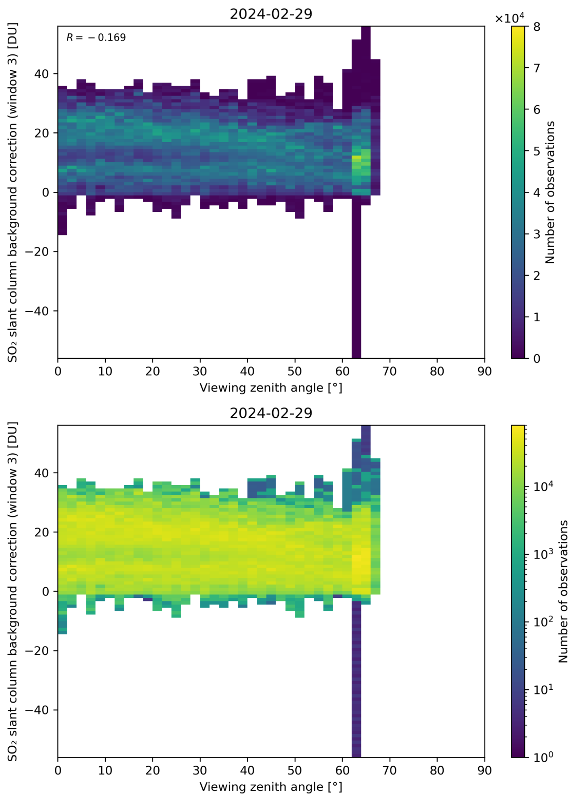
Figure 310: Scatter density plot of “Viewing zenith angle” against “SO 2 slant column background correction (window 3)” for 2024-02-28 to 2024-03-01.
