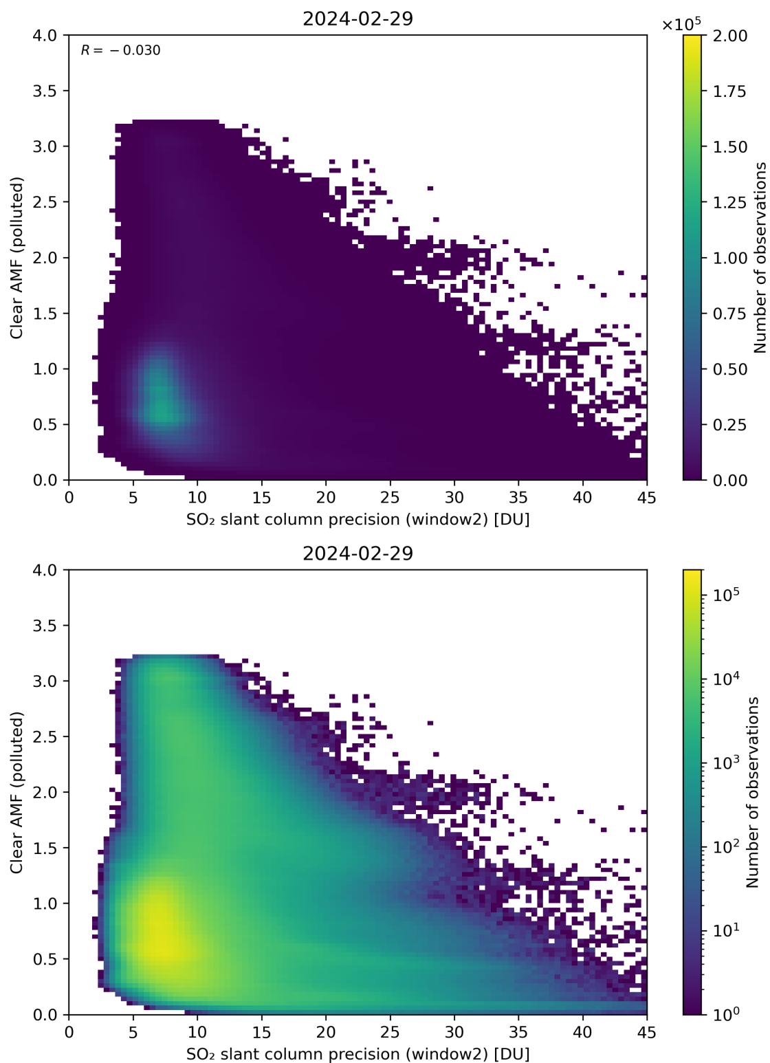
Figure 246: Scatter density plot of “SO 2 slant column precision (window2)” against “Clear AMF (polluted)” for 2024-02-28 to 2024-03-01.
