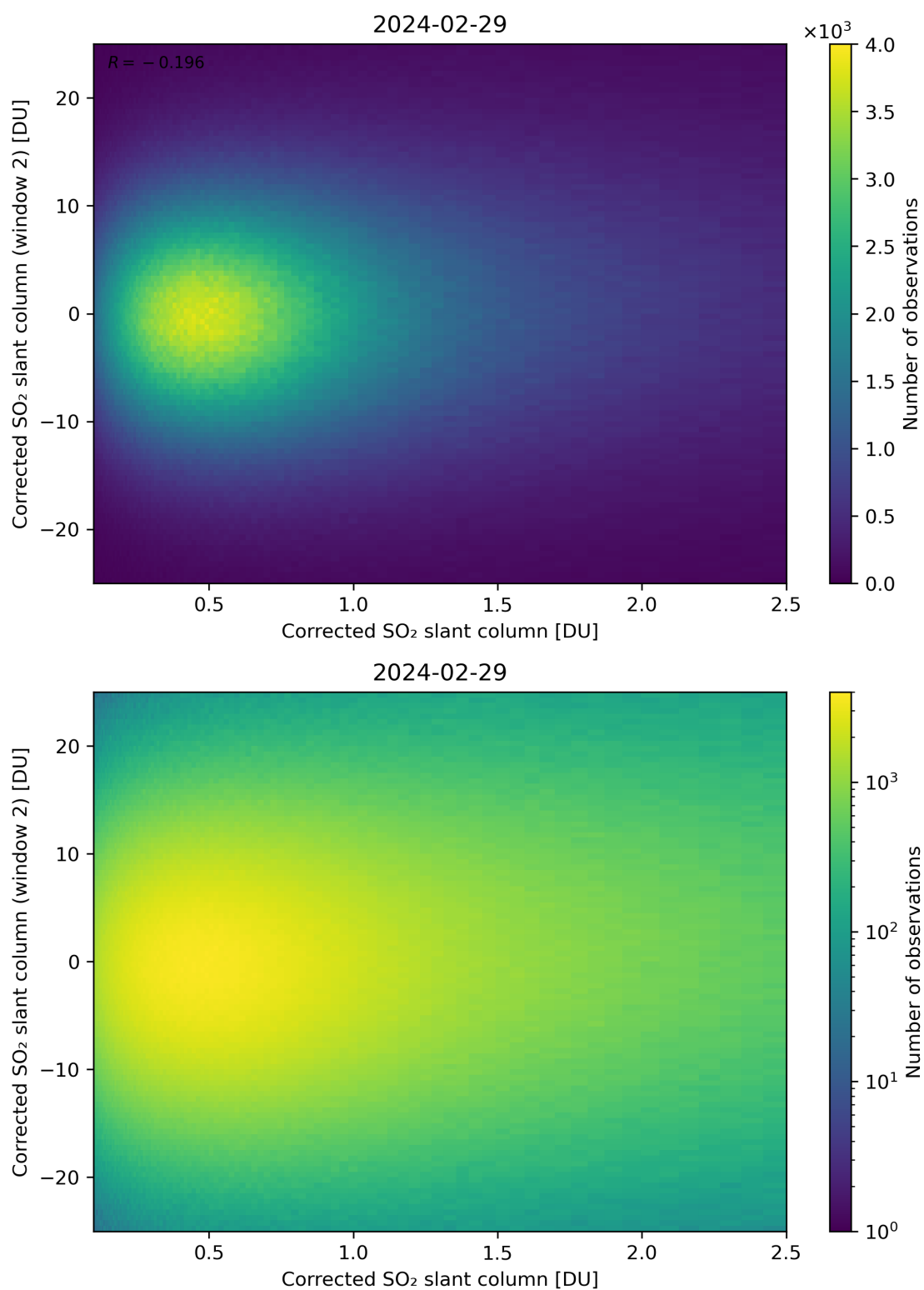
Figure 185: Scatter density plot of “Corrected SO 2 slant column” against “Corrected SO 2 slant column (window 2)” for 2024-02-28 to 2024-03-01.
