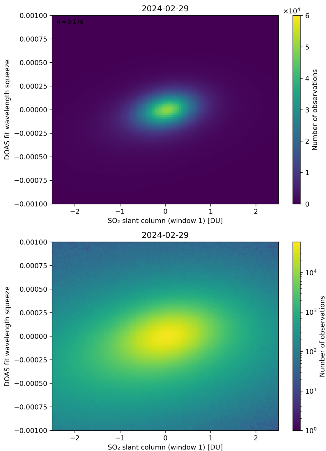
Figure 216: Scatter density plot of “SO 2 slant column (window 1)” against “DOAS fit wavelength squeeze” for 2024-02-28 to 2024-03-01.
