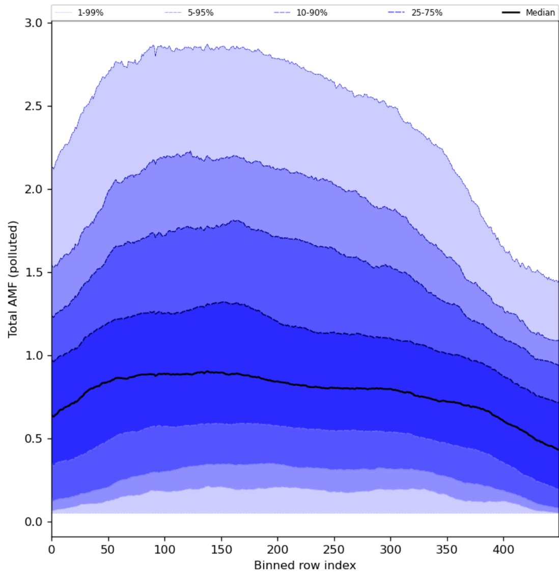
Figure 94: Along track statistics of “Total AMF (polluted)” for 2024-02-28 to 2024-03-01
