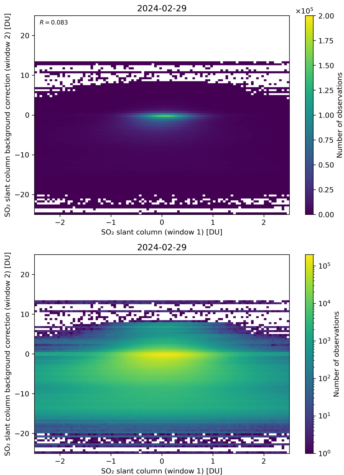
Figure 213: Scatter density plot of “SO 2 slant column (window 1)” against “SO 2 slant column background correction (window 2)” for 2024-02-28 to 2024-03-01.
