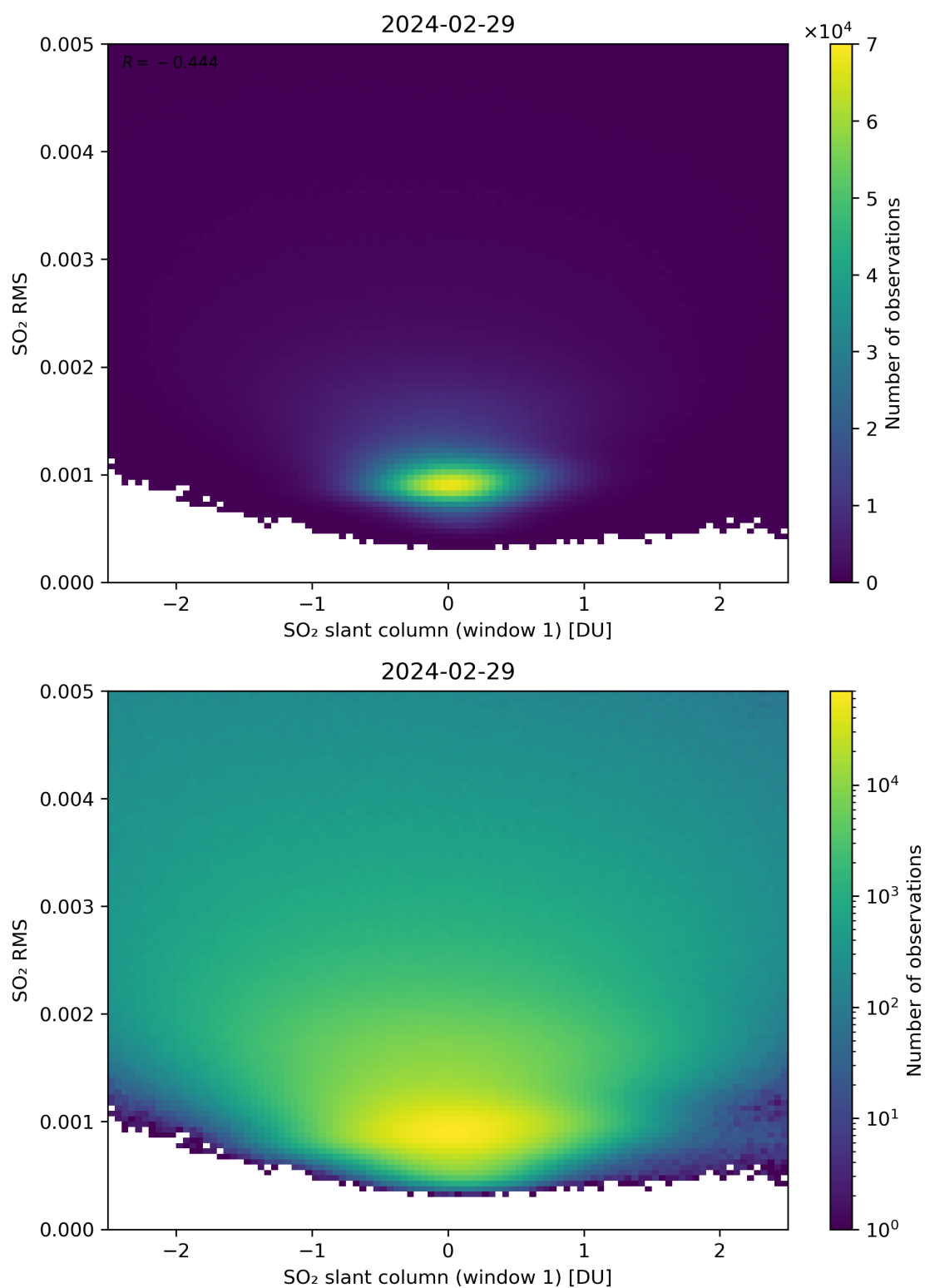
Figure 217: Scatter density plot of “SO 2 slant column (window 1)” against “SO 2 RMS” for 2024-02-28 to 2024-03-01.
