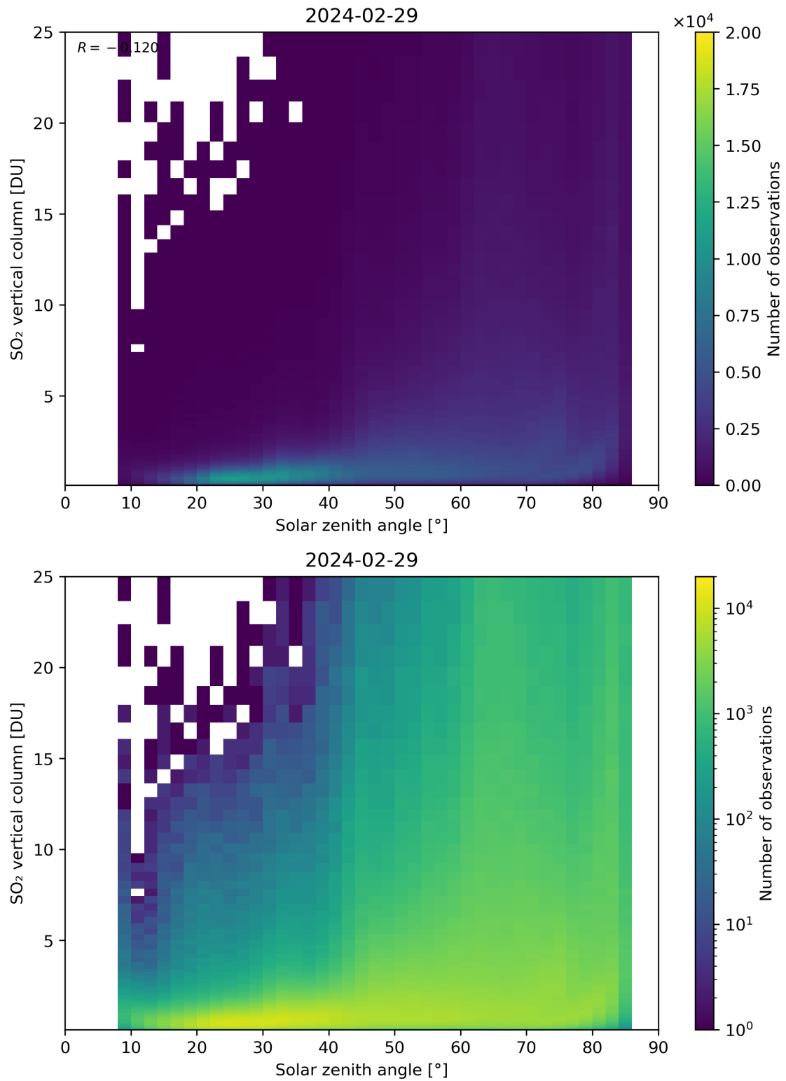
Figure 176: Scatter density plot of “Solar zenith angle” against “SO 2 vertical column” for 2024-02-28 to 2024-03-01.
