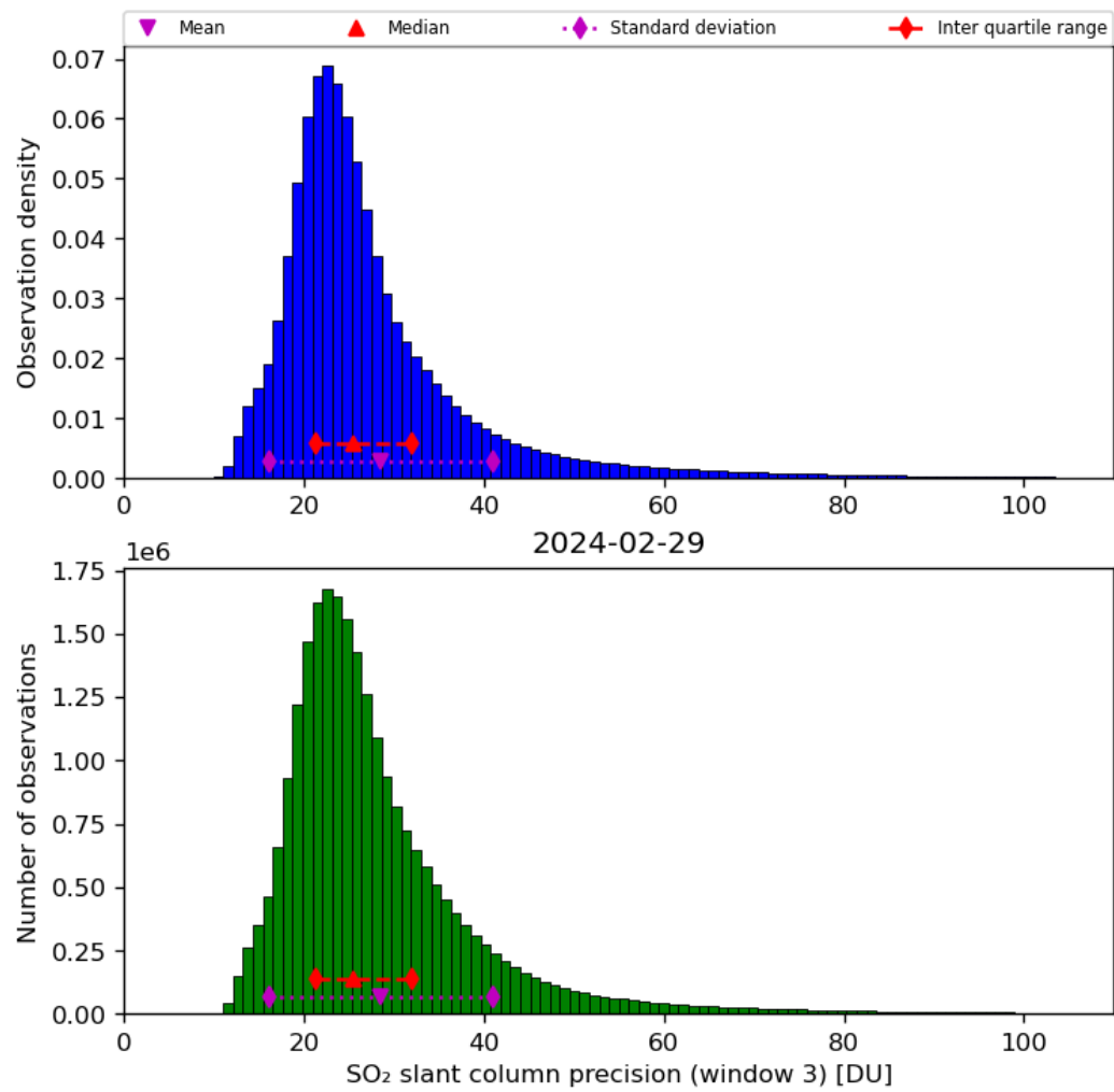
Figure 65: Histogram of “SO 2 slant column precision (window 3)” for 2024-02-28 to 2024-03-01
