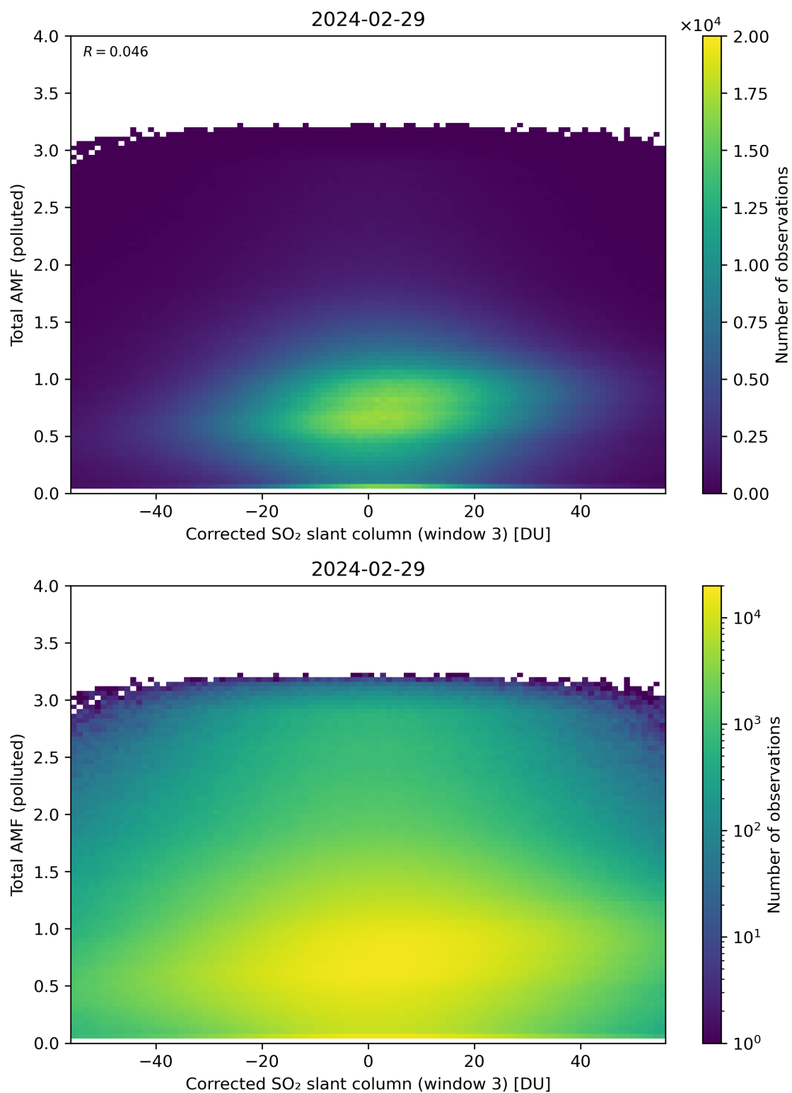
Figure 210: Scatter density plot of “Corrected SO 2 slant column (window 3)” against “Total AMF (polluted)” for 2024-02-28 to 2024-03-01.
