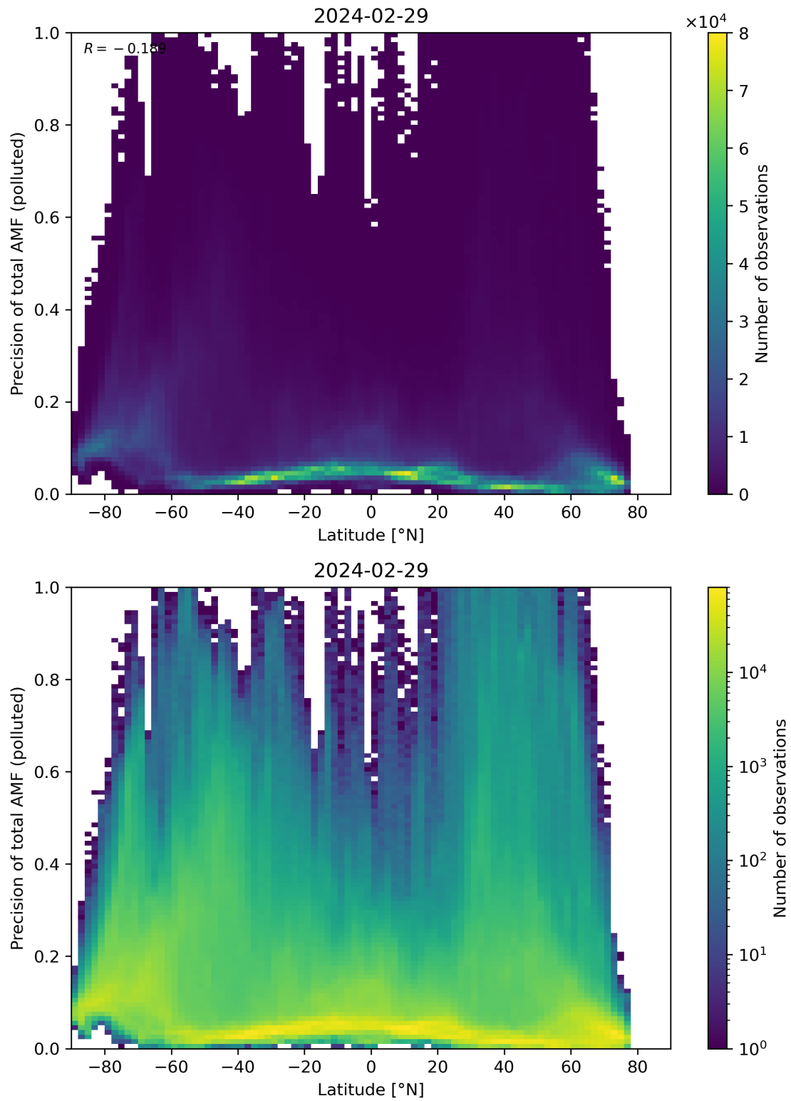
Figure 155: Scatter density plot of “Latitude” against “Precision of total AMF (polluted)” for 2024-02-28 to 2024-03-01.
