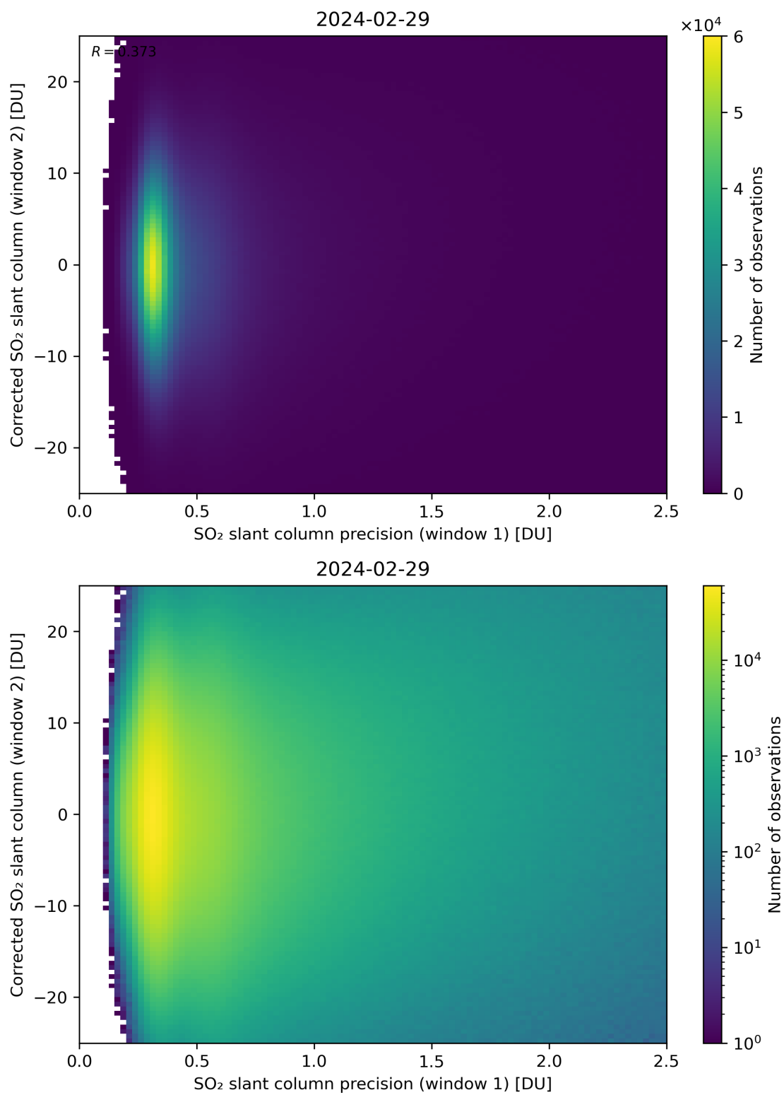
Figure 225: Scatter density plot of “SO 2 slant column precision (window 1)” against “Corrected SO 2 slant column (window 2)” for 2024-02-28 to 2024-03-01.
