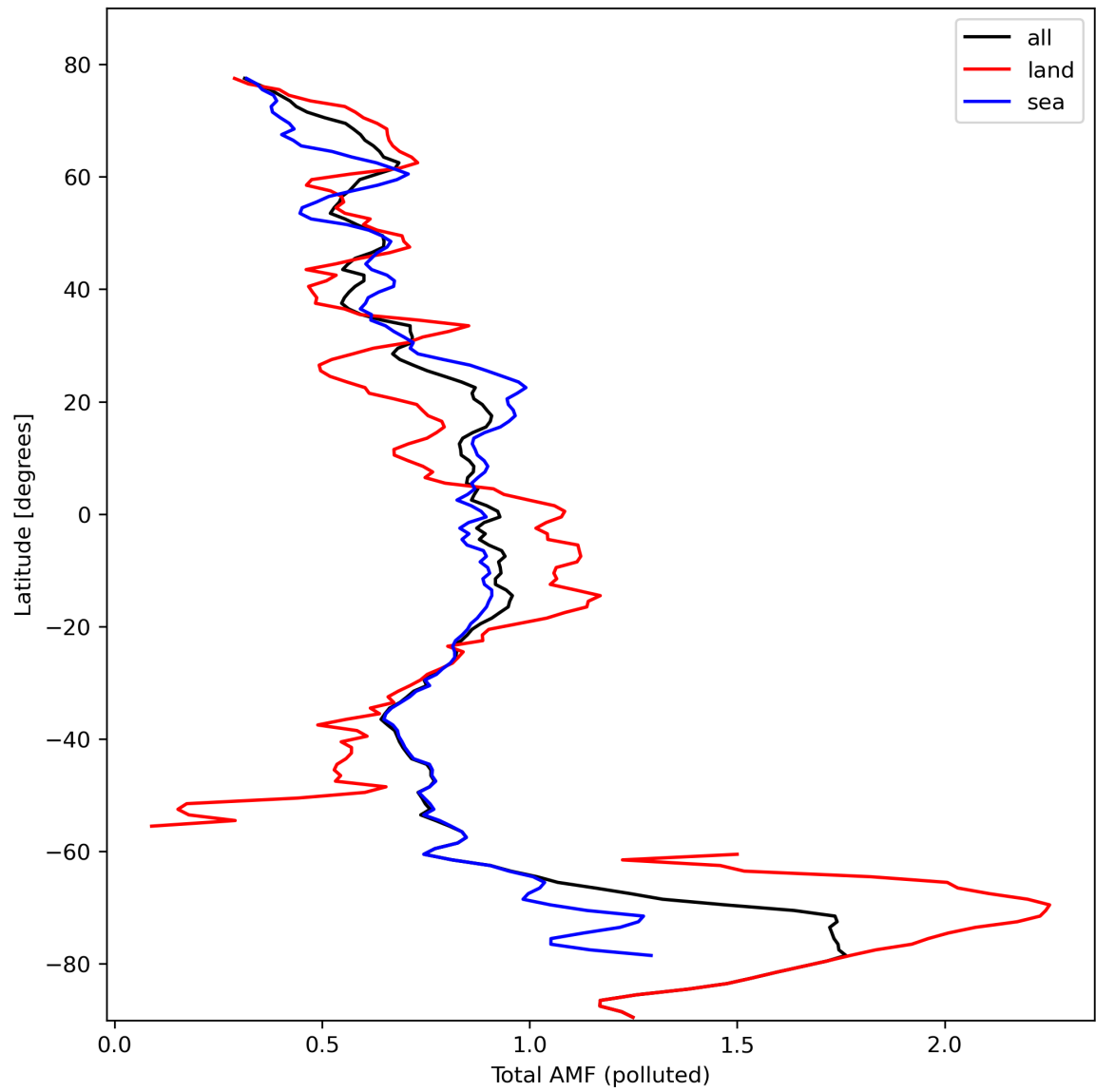
Figure 48: Zonal average of “Total AMF (polluted)” for 2024-02-28 to 2024-03-01.
