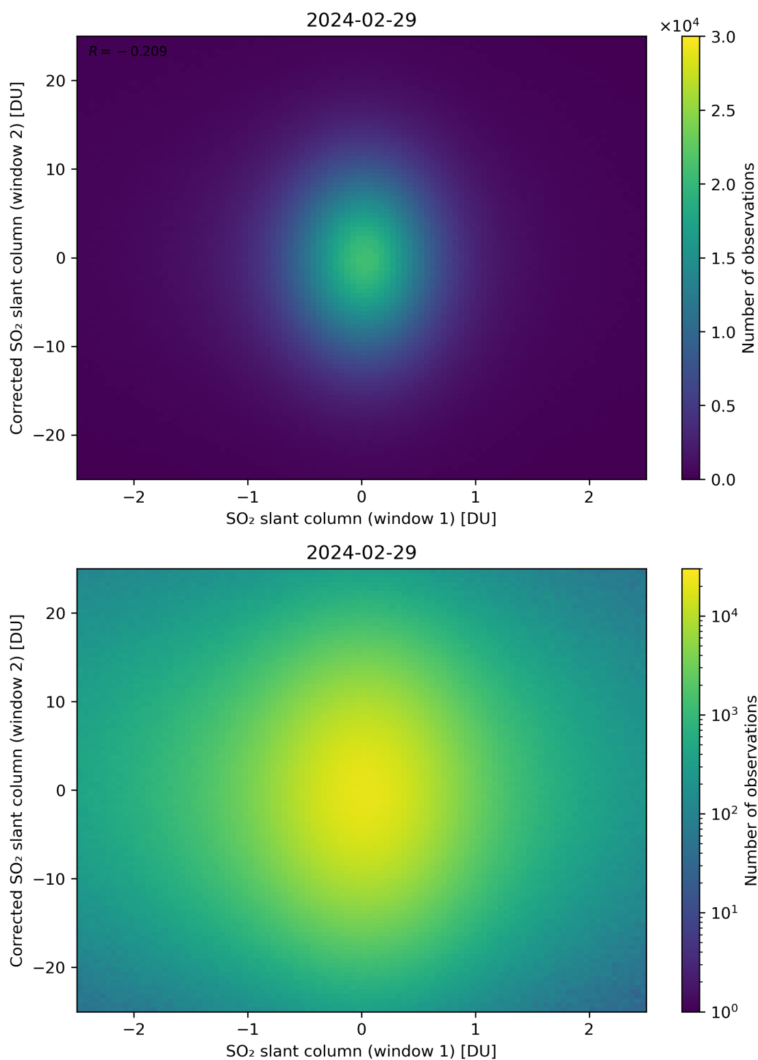
Figure 233: Scatter density plot of “SO 2 slant column (window 1)” against “Corrected SO 2 slant column (window 2)” for 2024-02-28 to 2024-03-01.
