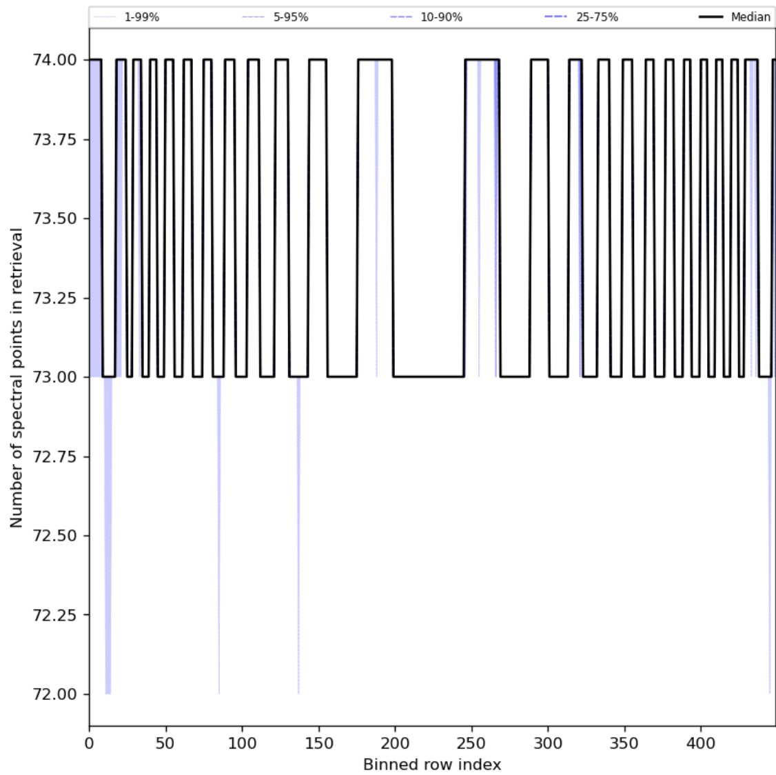
Figure 97: Along track statistics of “Number of spectral points in retrieval” for 2024-02-28 to 2024-03-01
