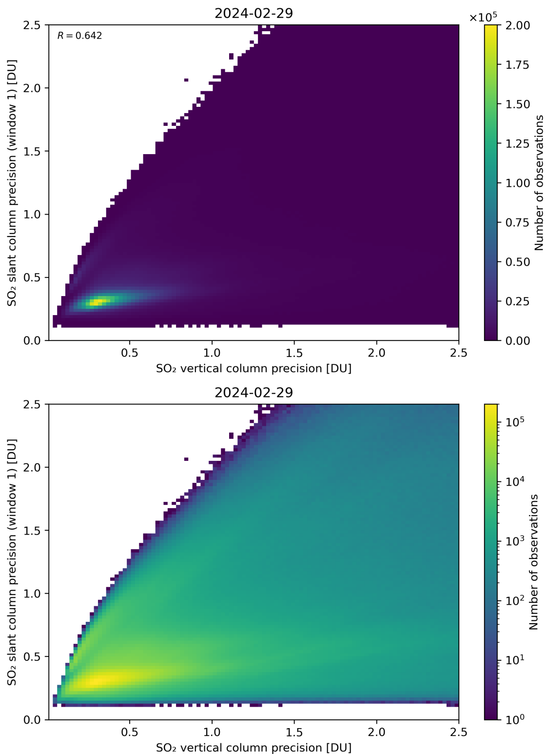
Figure 290: Scatter density plot of “SO 2 vertical column precision” against “SO 2 slant column precision (window 1)” for 2024-02-28 to 2024-03-01.
