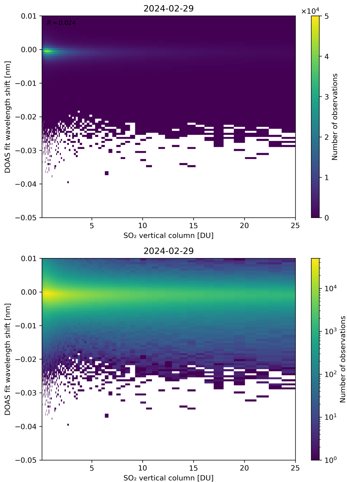
Figure 276: Scatter density plot of “SO 2 vertical column” against “DOAS fit wavelength shift” for 2024-02-28 to 2024-03-01.
