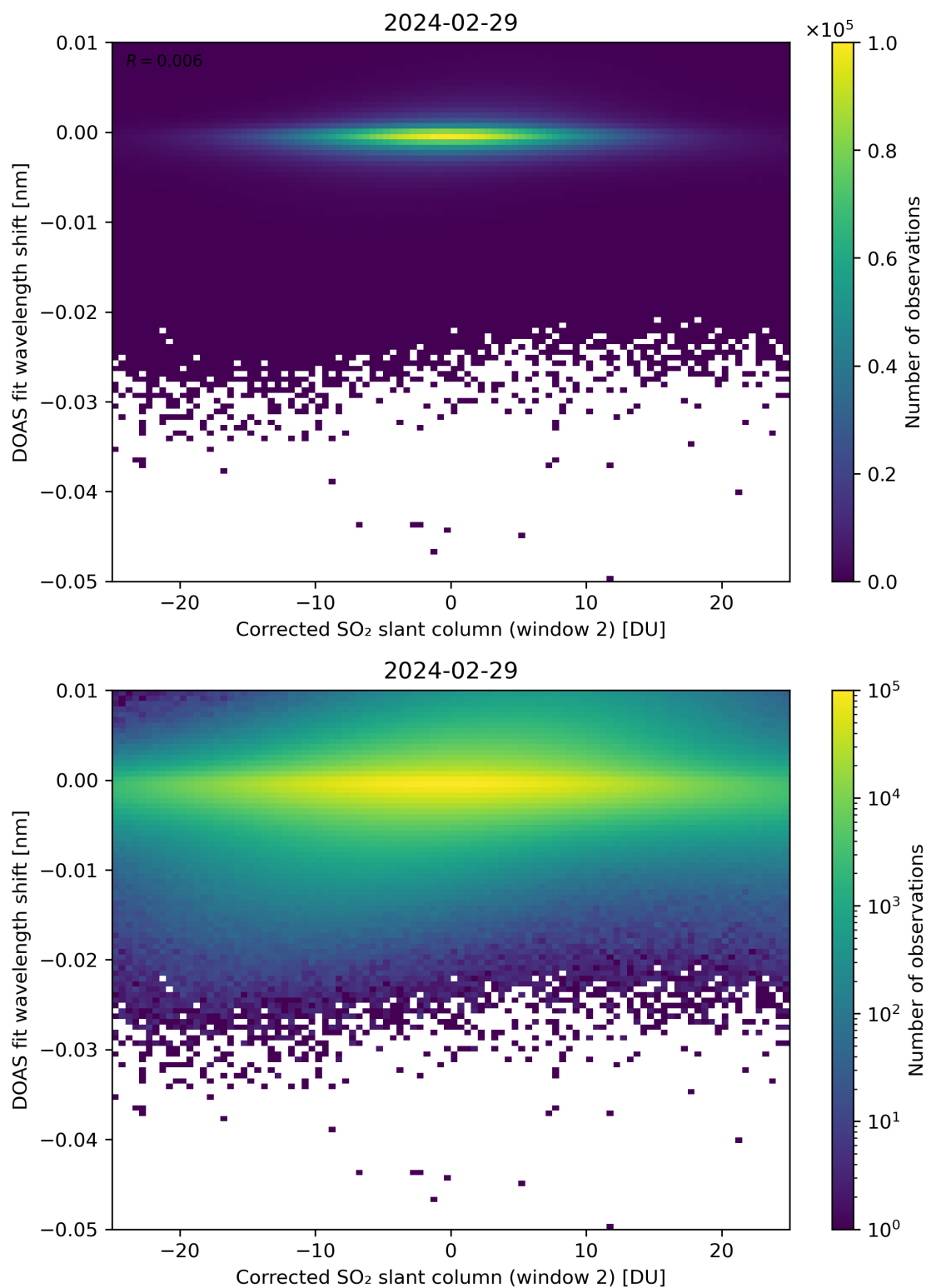
Figure 196: Scatter density plot of “Corrected SO 2 slant column (window 2)” against “DOAS fit wavelength shift” for 2024-02-28 to 2024-03-01.
