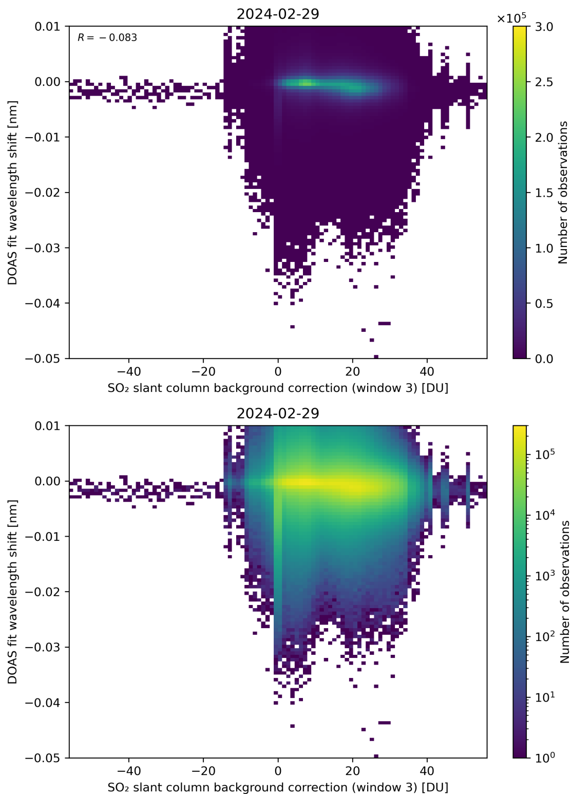
Figure 121: Scatter density plot of “SO 2 slant column background correction (window 3)” against “DOAS fit wavelength shift” for 2024-02-28 to 2024-03-01.
