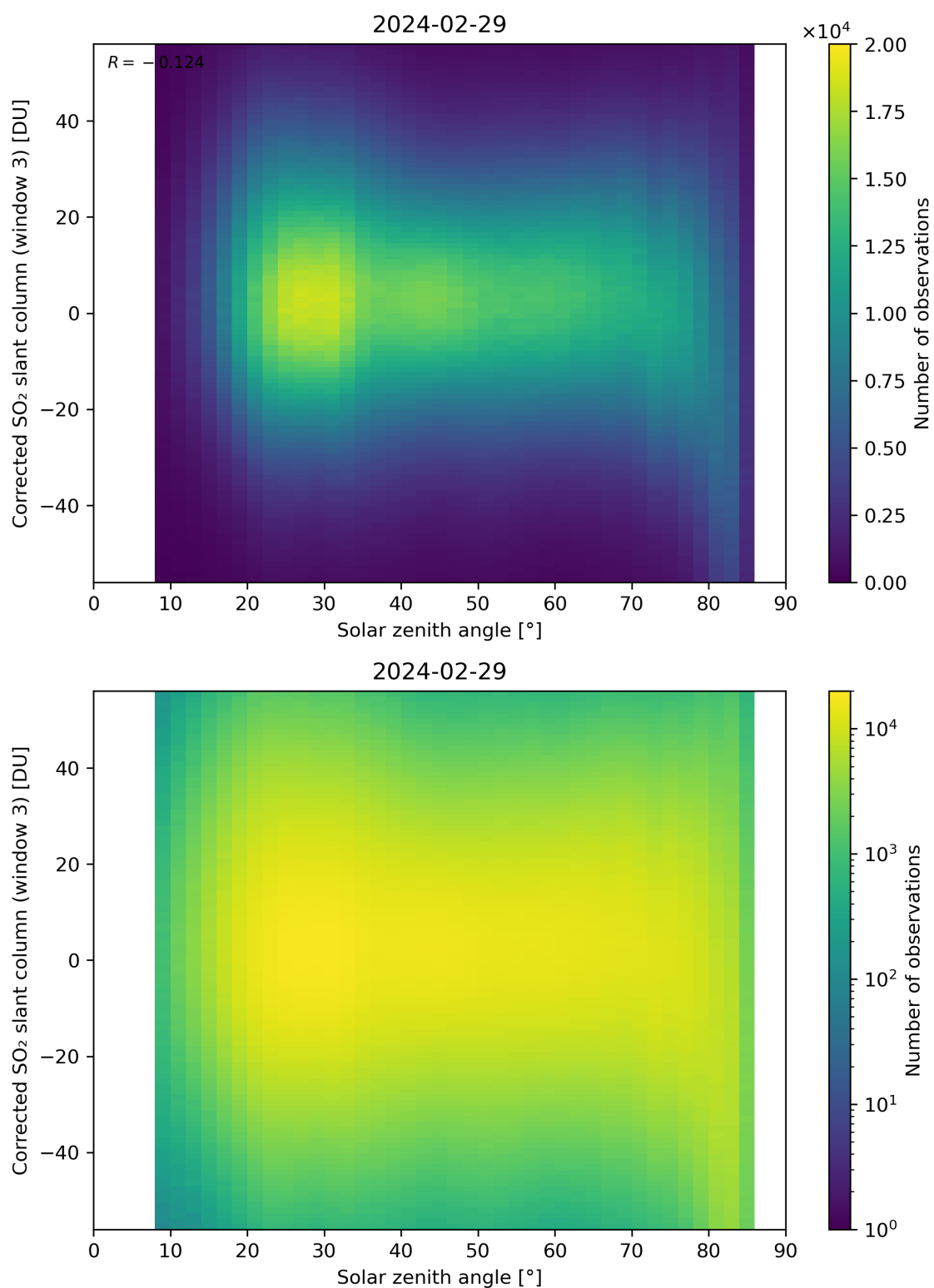
Figure 168: Scatter density plot of “Solar zenith angle” against “Corrected SO 2 slant column (window 3)” for 2024-02-28 to 2024-03-01.
