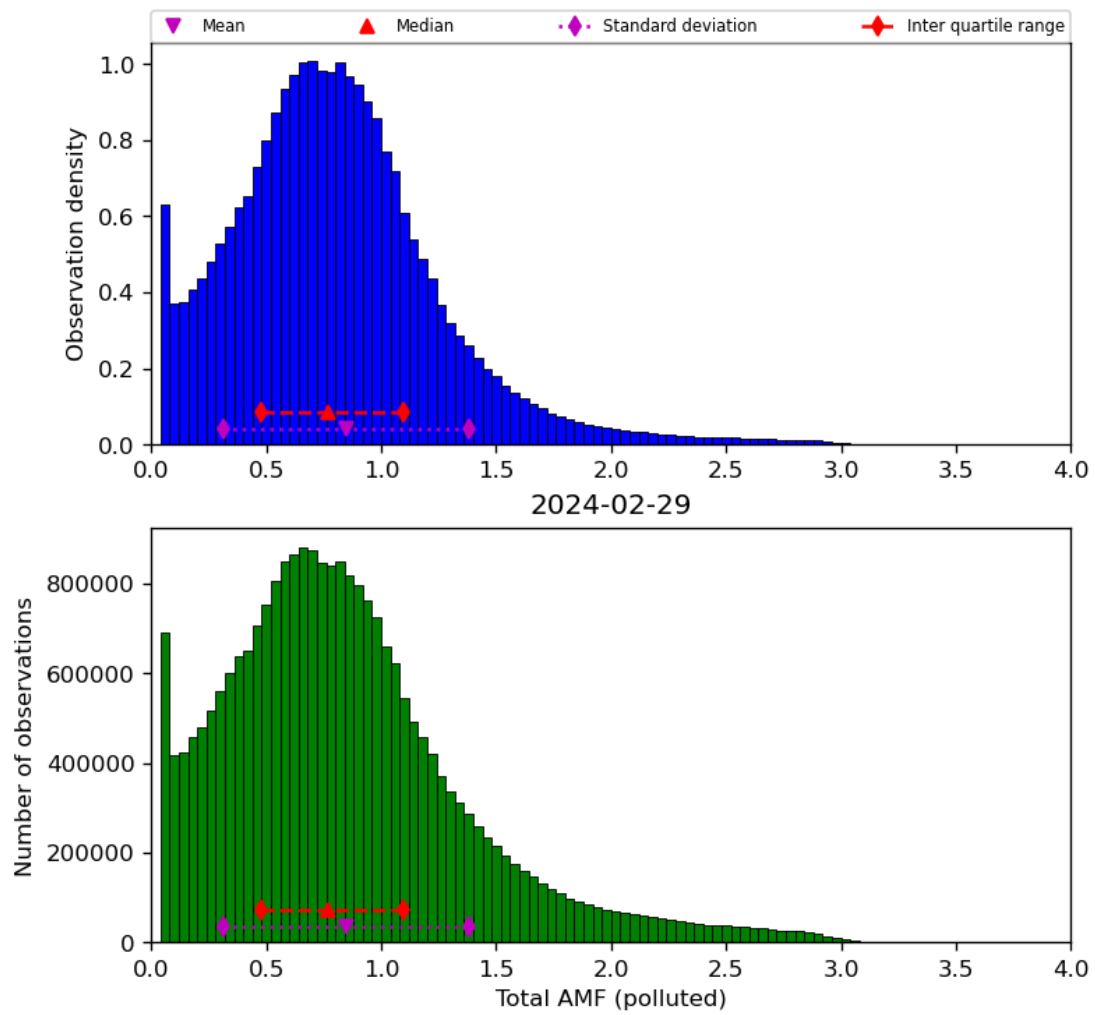
Figure 71: Histogram of “Total AMF (polluted)” for 2024-02-28 to 2024-03-01
