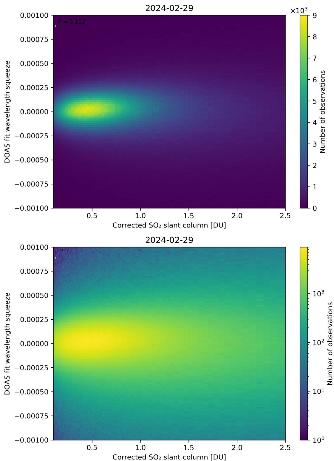
Figure 182: Scatter density plot of “Corrected SO 2 slant column” against “DOAS fit wavelength squeeze” for 2024-02-28 to 2024-03-01.
