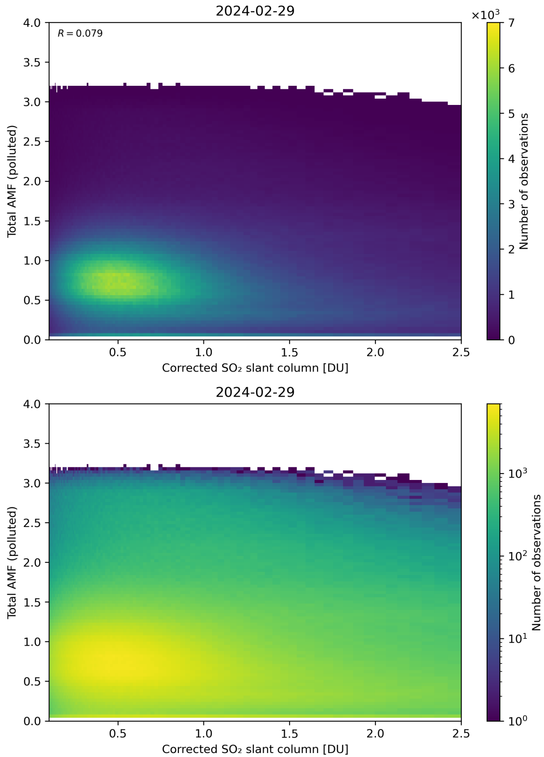
Figure 192: Scatter density plot of “Corrected SO 2 slant column” against “Total AMF (polluted)” for 2024-02-28 to 2024-03-01.
