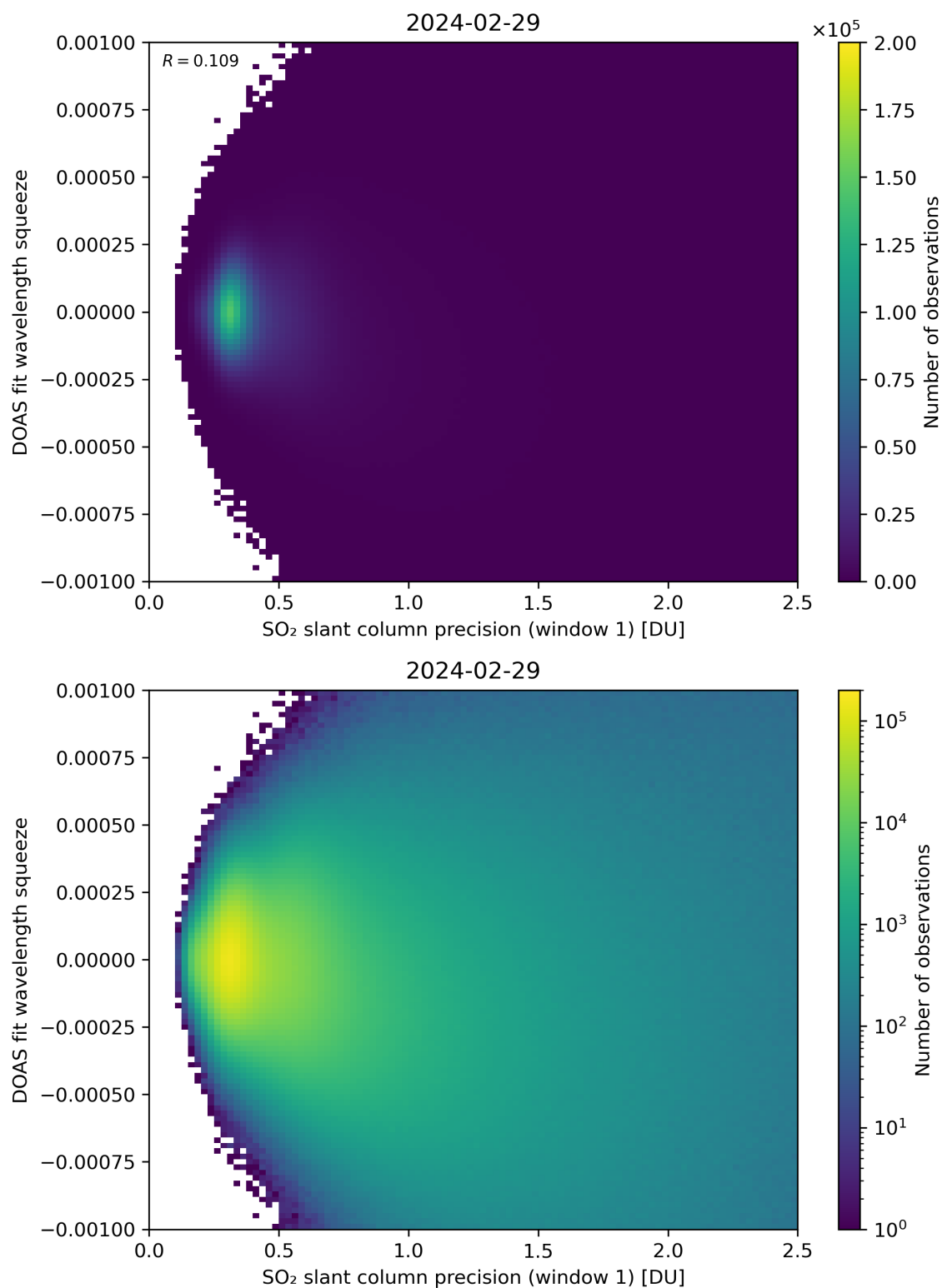
Figure 222: Scatter density plot of “SO 2 slant column precision (window 1)” against “DOAS fit wavelength squeeze” for 2024-02-28 to 2024-03-01.
