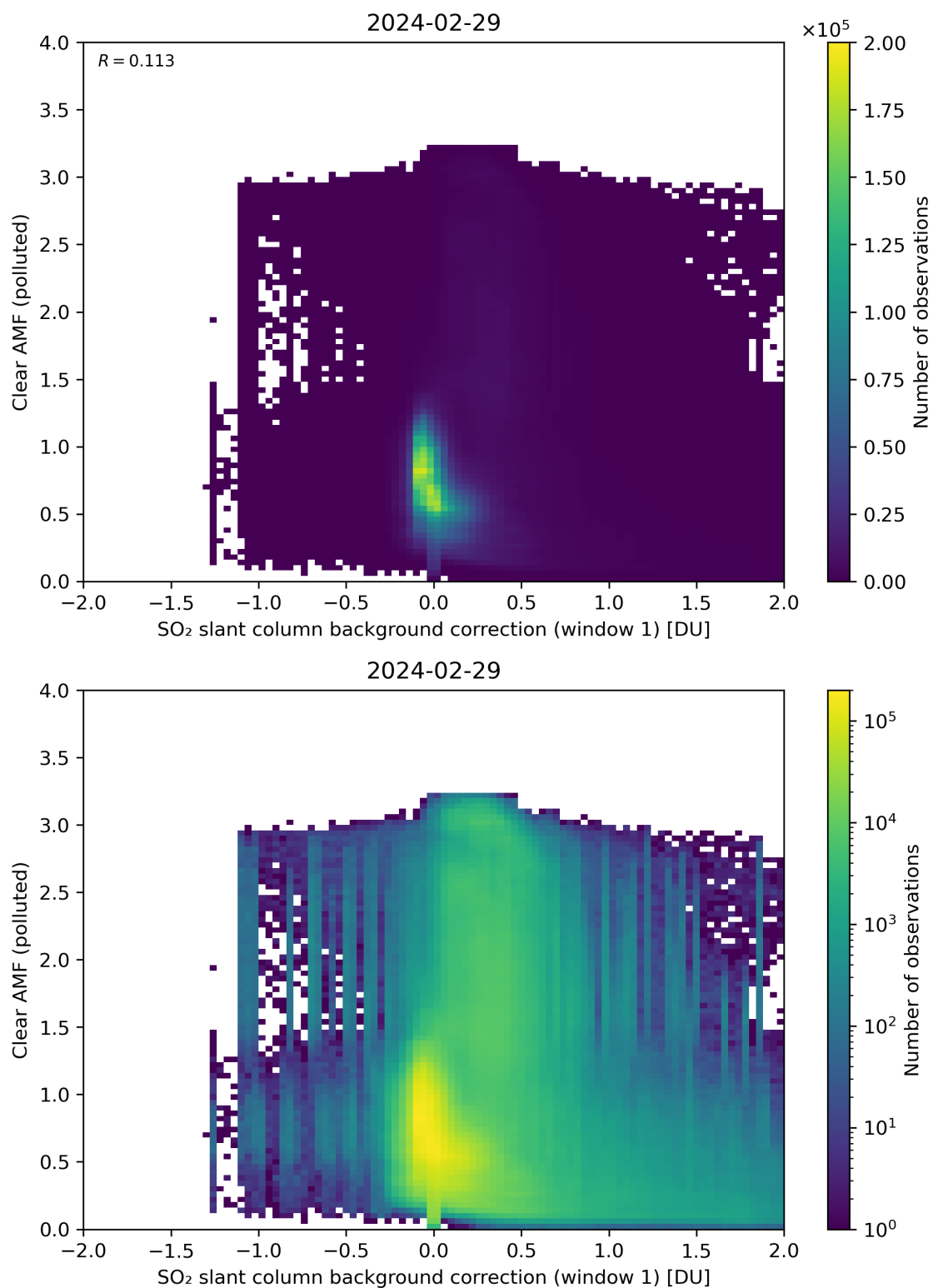
Figure 103: Scatter density plot of “SO 2 slant column background correction (window 1)” against “Clear AMF (polluted)” for 2024-02-28 to 2024-03-01.
