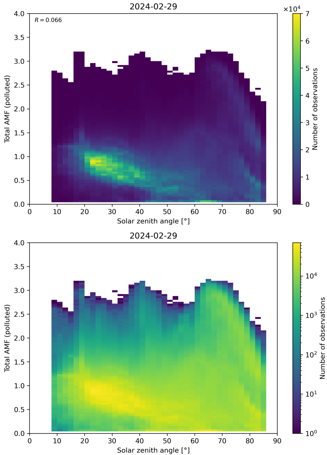
Figure 174: Scatter density plot of “Solar zenith angle” against “Total AMF (polluted)” for 2024-02-28 to 2024-03-01.
