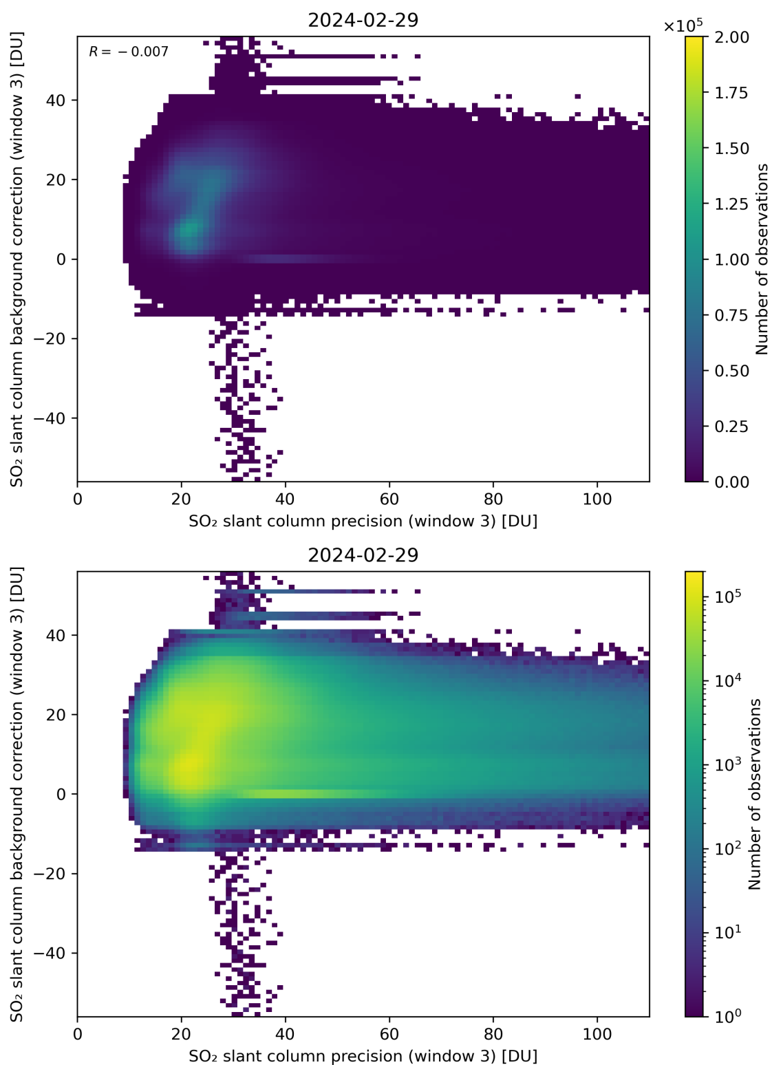
Figure 257: Scatter density plot of “SO 2 slant column precision (window 3)” against “SO 2 slant column background correction (window 3)” for 2024-02-28 to 2024-03-01.
