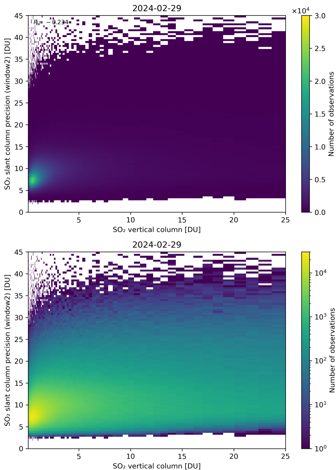
Figure 302: Scatter density plot of “SO 2 vertical column” against “SO 2 slant column precision (window2)” for 2024-02-28 to 2024-03-01.
