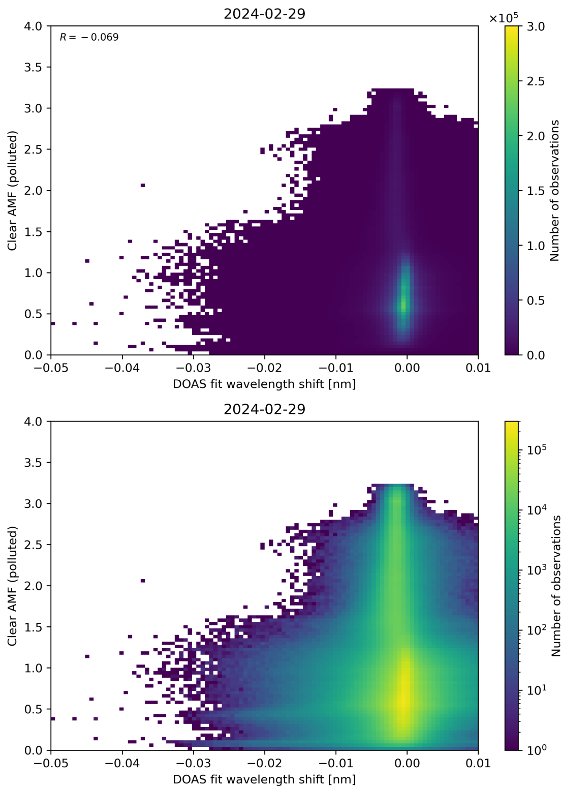
Figure 129: Scatter density plot of “DOAS fit wavelength shift” against “Clear AMF (polluted)” for 2024-02-28 to 2024-03-01.
