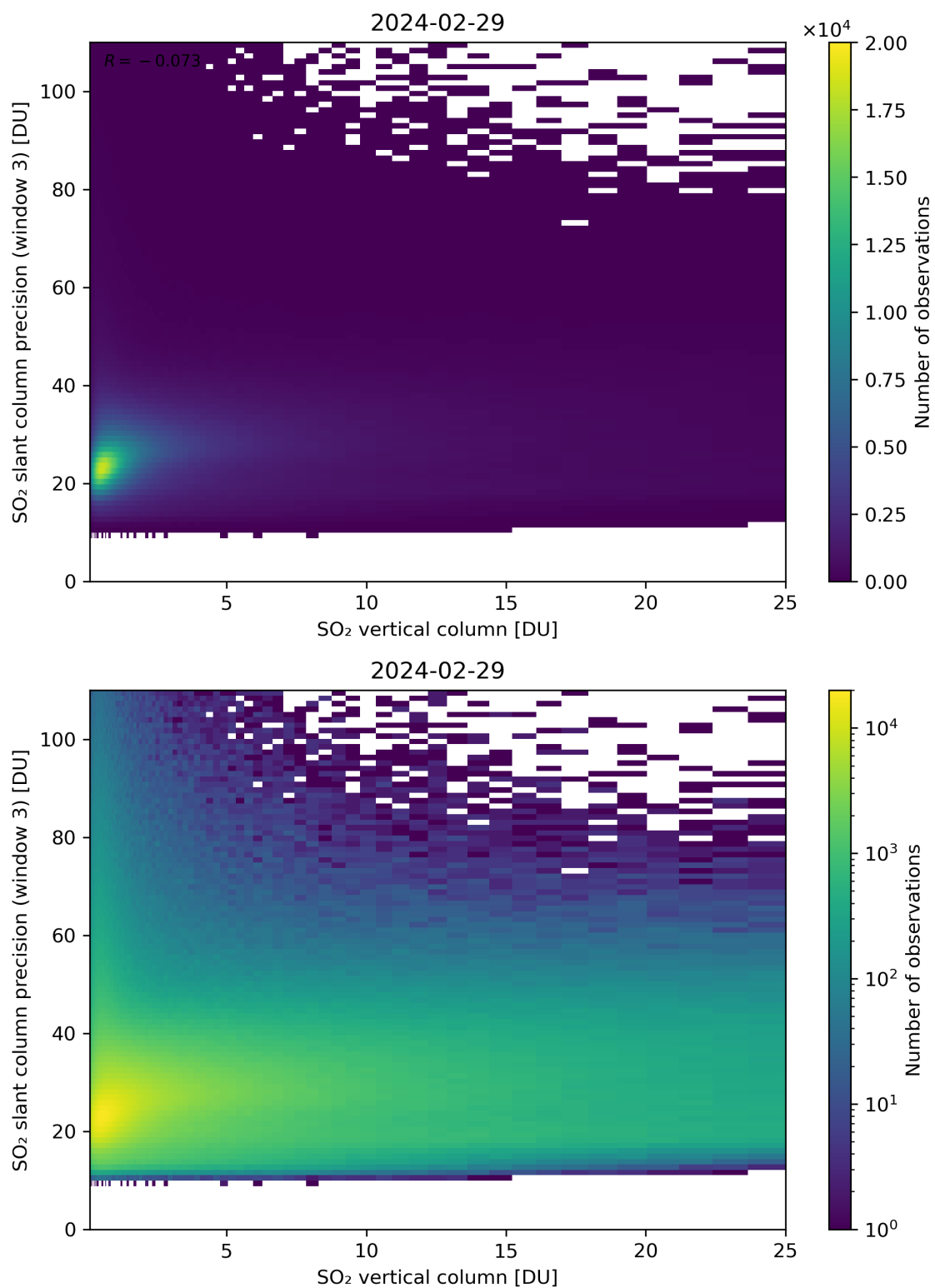
Figure 304: Scatter density plot of “SO 2 vertical column” against “SO 2 slant column precision (window 3)” for 2024-02-28 to 2024-03-01.
