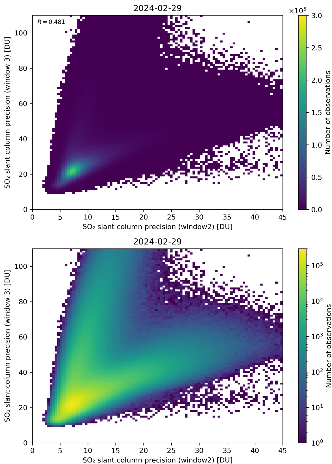
Figure 250: Scatter density plot of “SO 2 slant column precision (window2)” against “SO 2 slant column precision (window 3)” for 2024-02-28 to 2024-03-01.
