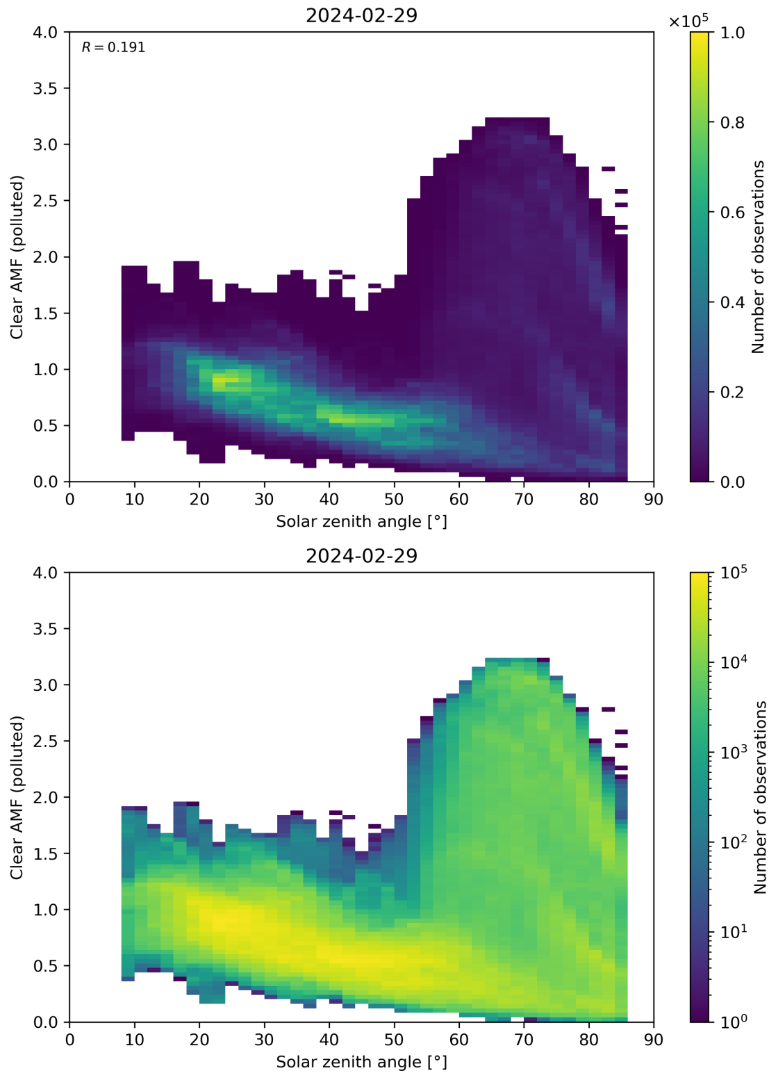
Figure 165: Scatter density plot of “Solar zenith angle” against “Clear AMF (polluted)” for 2024-02-28 to 2024-03-01.
