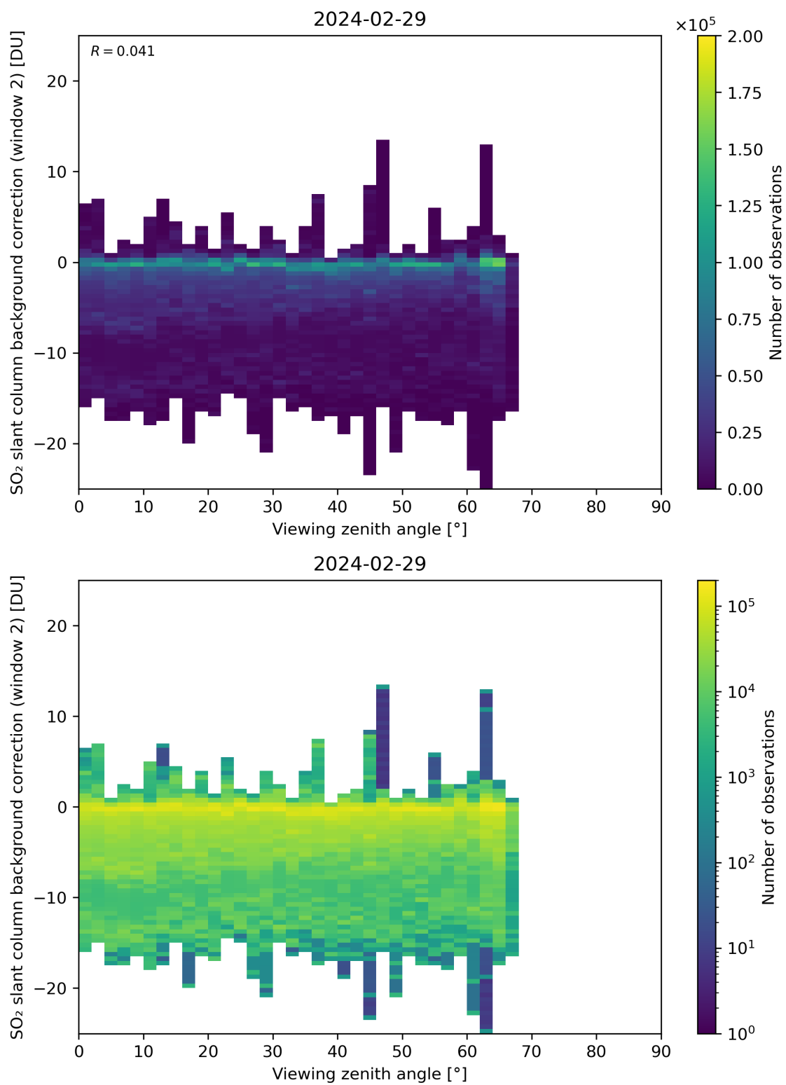
Figure 309: Scatter density plot of “Viewing zenith angle” against “SO 2 slant column background correction (window 2)” for 2024-02-28 to 2024-03-01.
