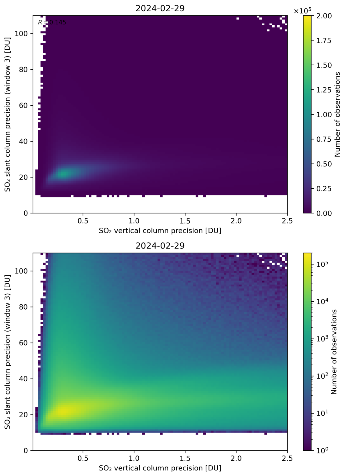
Figure 293: Scatter density plot of “SO 2 vertical column precision” against “SO 2 slant column precision (window 3)” for 2024-02-28 to 2024-03-01.
