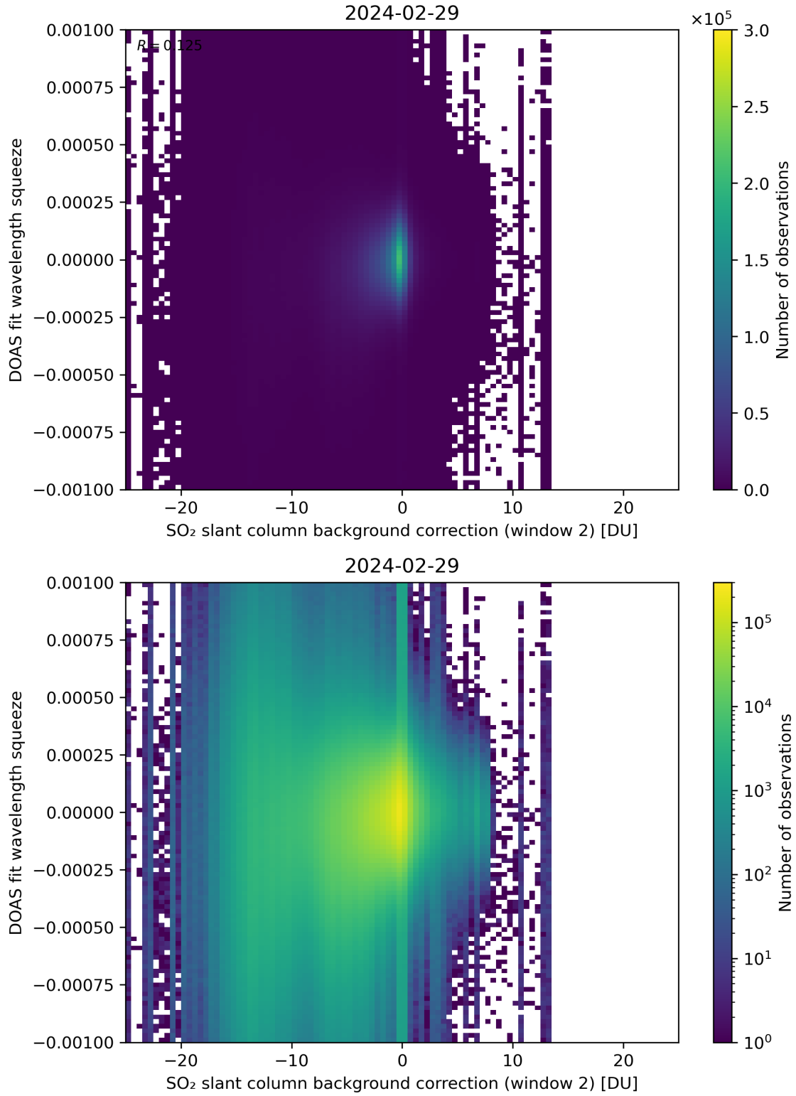
Figure 113: Scatter density plot of “SO 2 slant column background correction (window 2)” against “DOAS fit wavelength squeeze” for 2024-02-28 to 2024-03-01.
