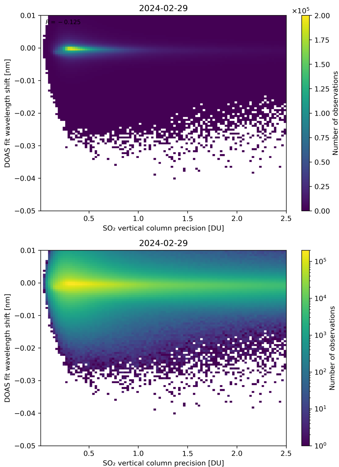
Figure 282: Scatter density plot of “SO 2 vertical column precision” against “DOAS fit wavelength shift” for 2024-02-28 to 2024-03-01.
