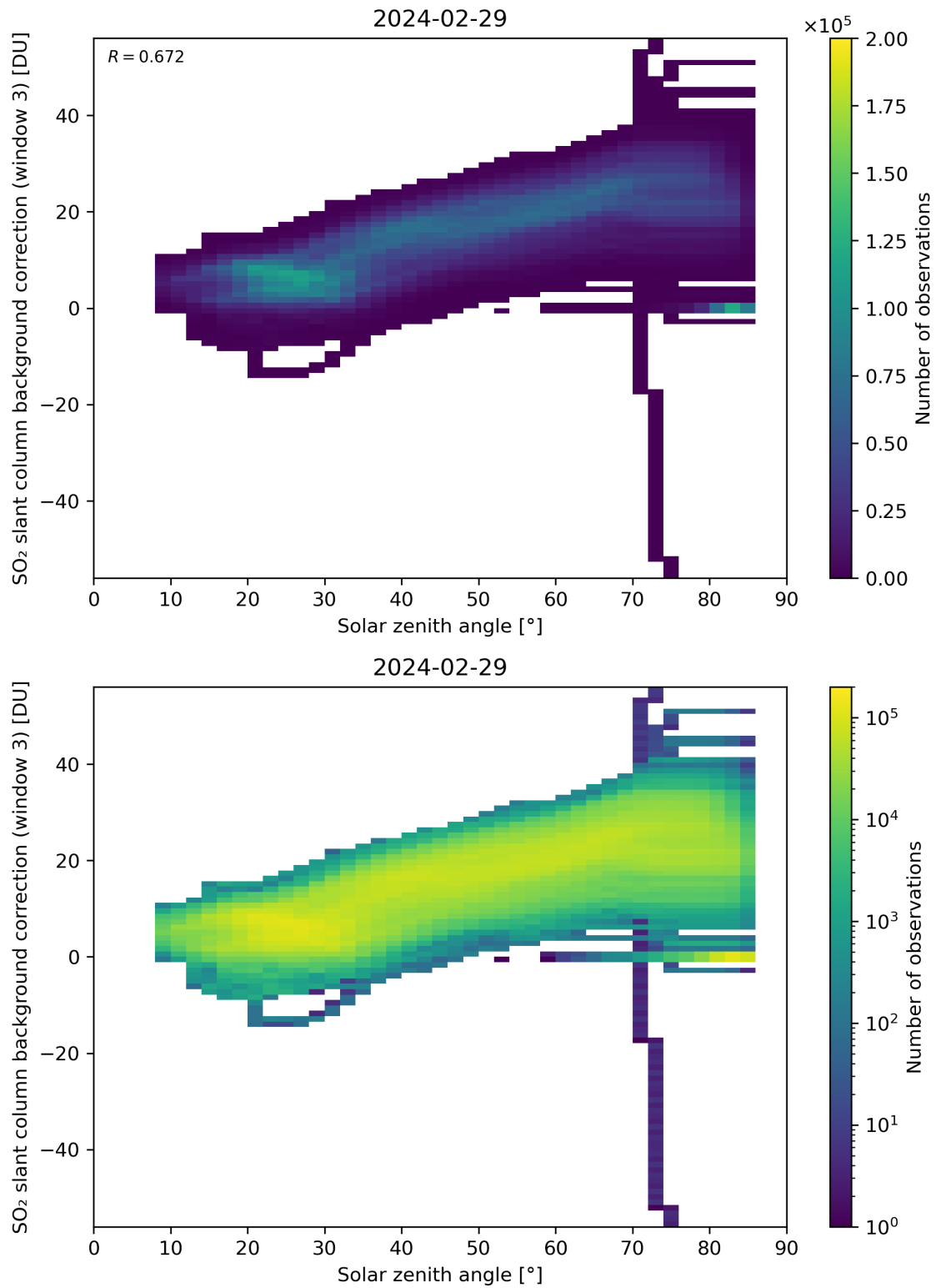
Figure 160: Scatter density plot of “Solar zenith angle” against “SO 2 slant column background correction (window 3)” for 2024-02-28 to 2024-03-01.
