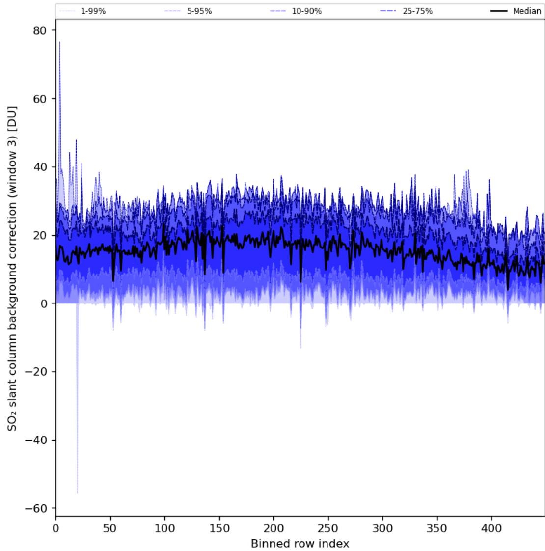
Figure 90: Along track statistics of “SO 2 slant column background correction (window 3)” for 2024-02-28 to 2024-03-01
