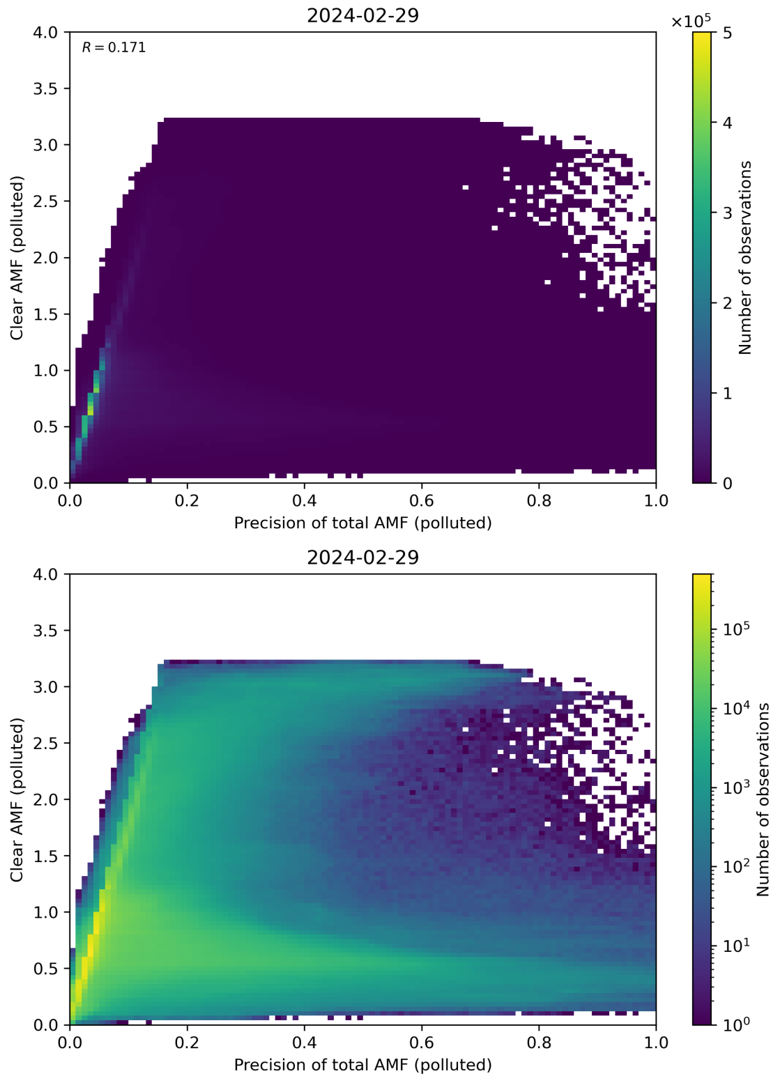
Figure 270: Scatter density plot of “Precision of total AMF (polluted)” against “Clear AMF (polluted)” for 2024-02-28 to 2024-03-01.
