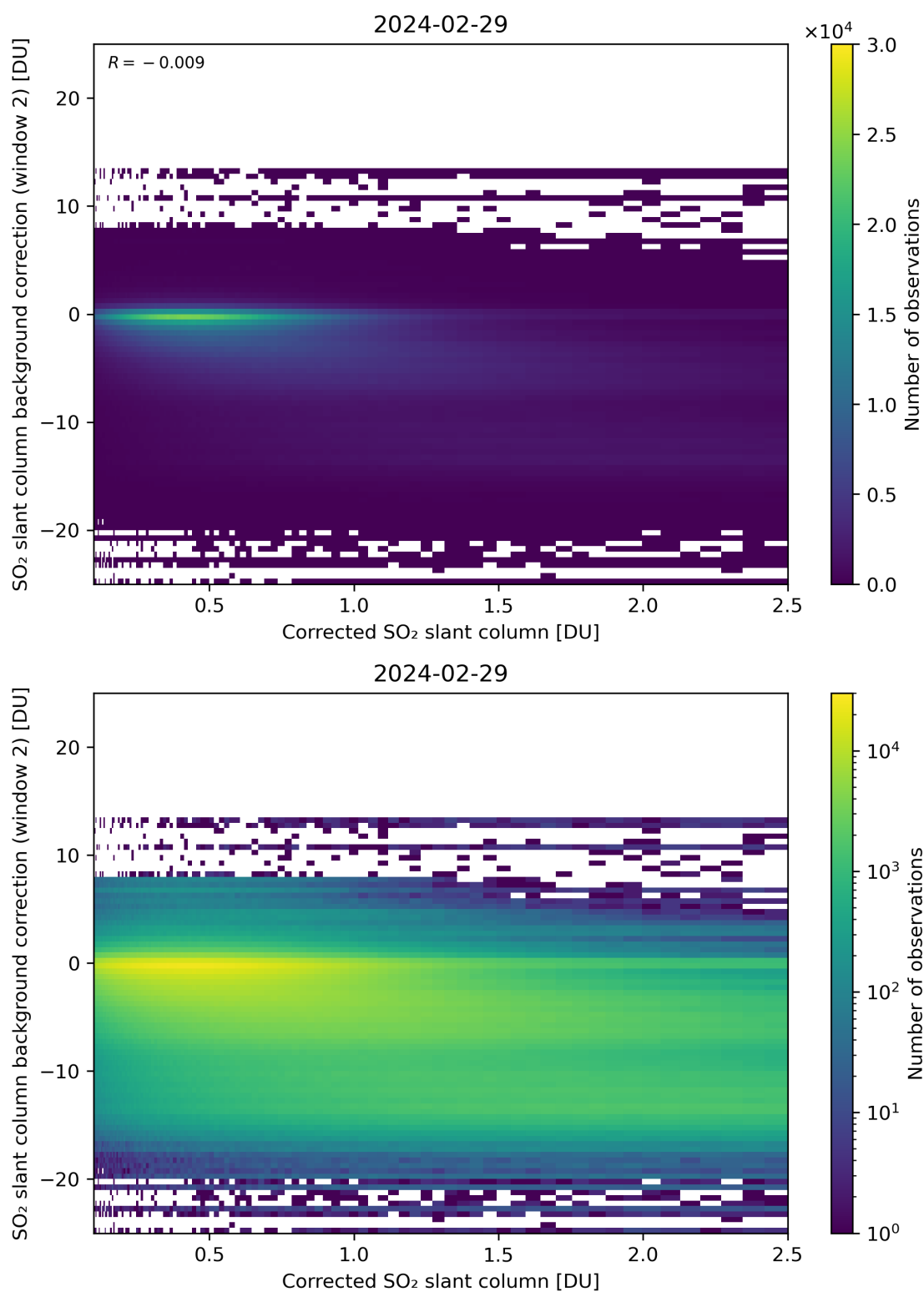
Figure 179: Scatter density plot of “Corrected SO 2 slant column” against “SO 2 slant column background correction (window 2)” for 2024-02-28 to 2024-03-01.
