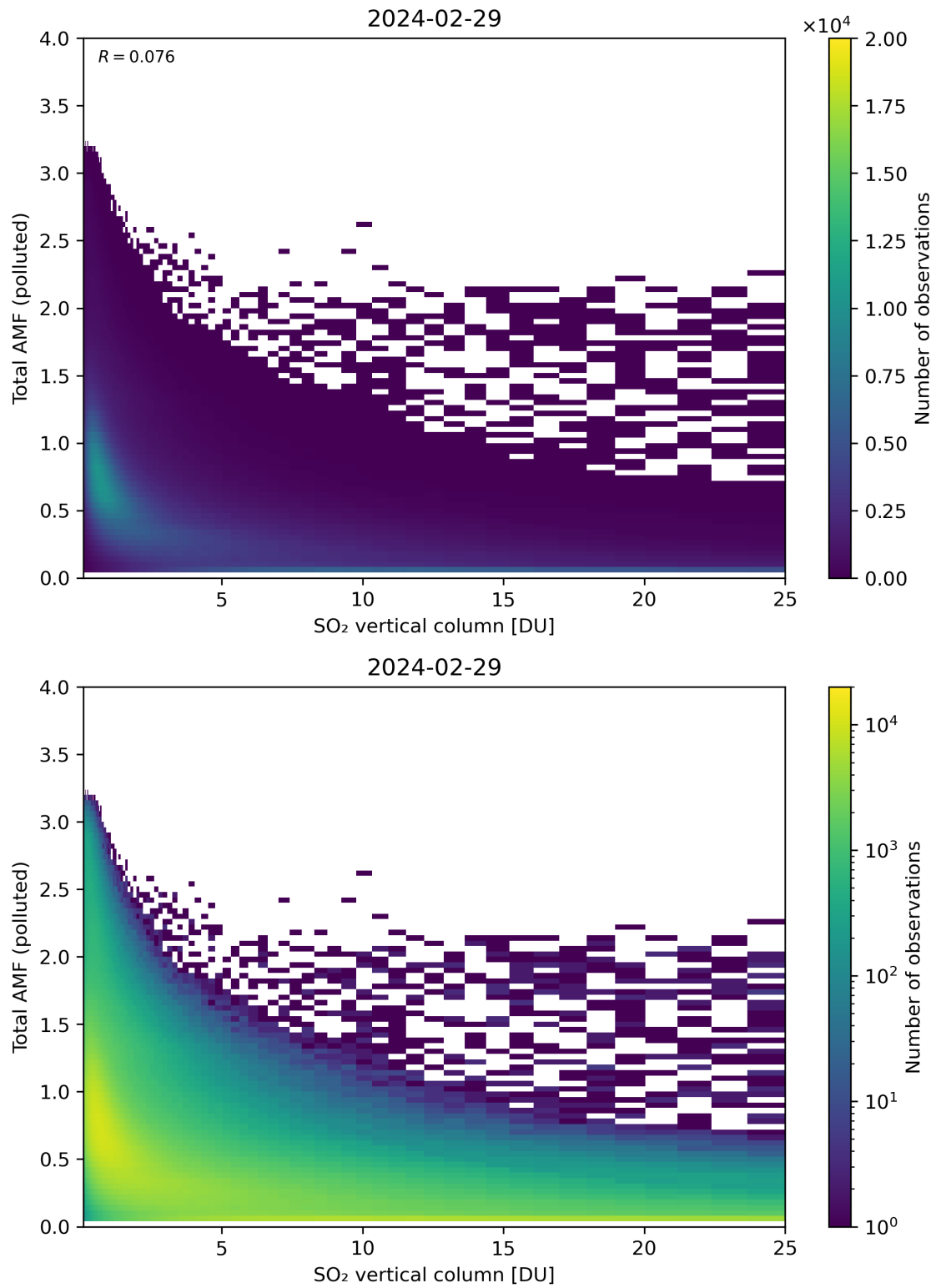
Figure 305: Scatter density plot of “SO 2 vertical column” against “Total AMF (polluted)” for 2024-02-28 to 2024-03-01.
