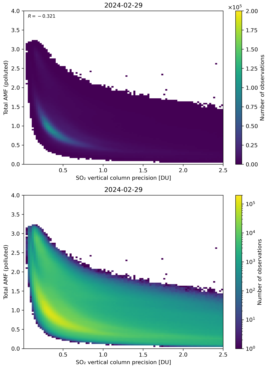
Figure 294: Scatter density plot of “SO 2 vertical column precision” against “Total AMF (polluted)” for 2024-02-28 to 2024-03-01.
