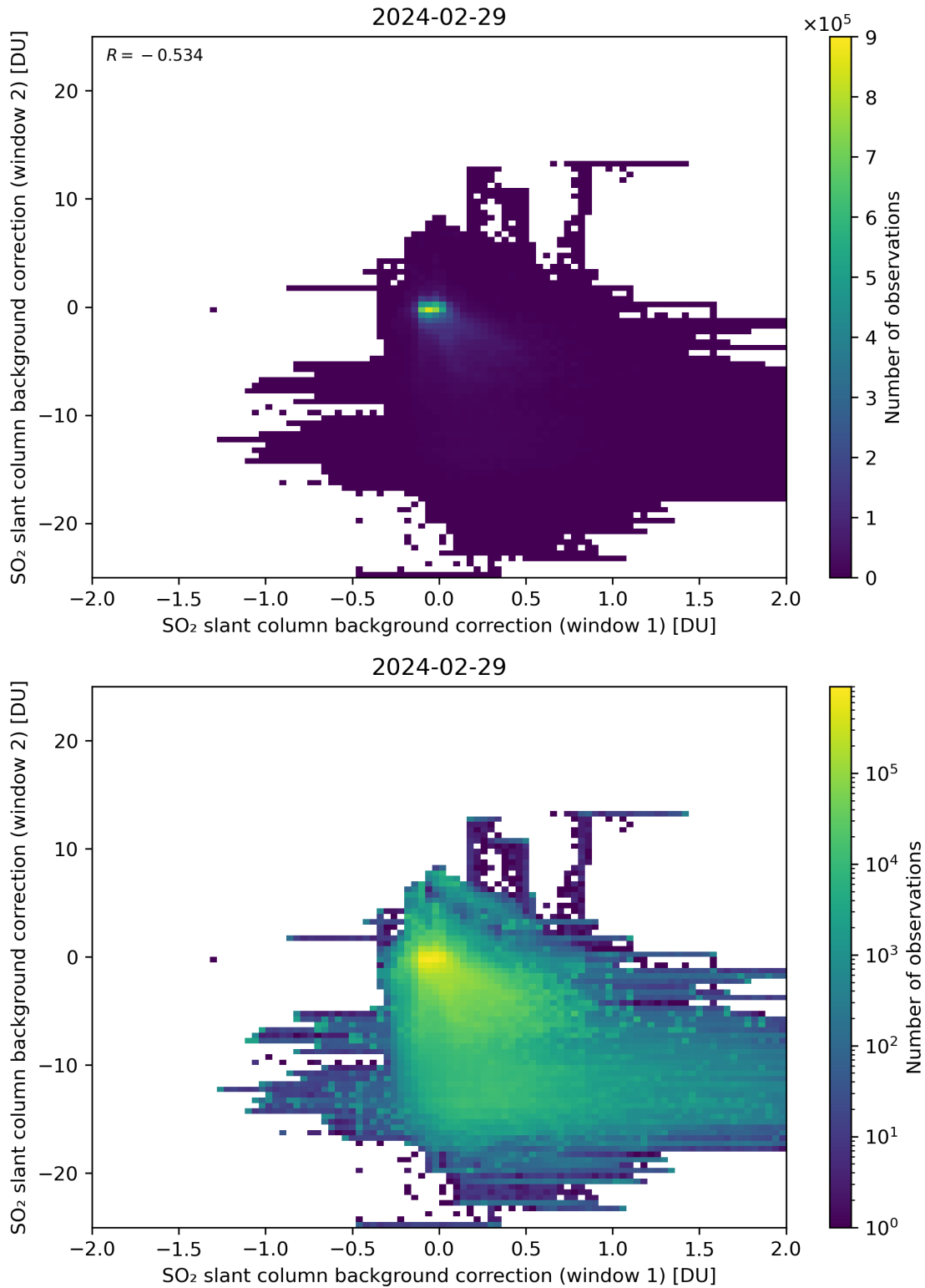
Figure 98: Scatter density plot of “SO 2 slant column background correction (window 1)” against “SO 2 slant column background correction (window 2)” for 2024-02-28 to 2024-03-01.
