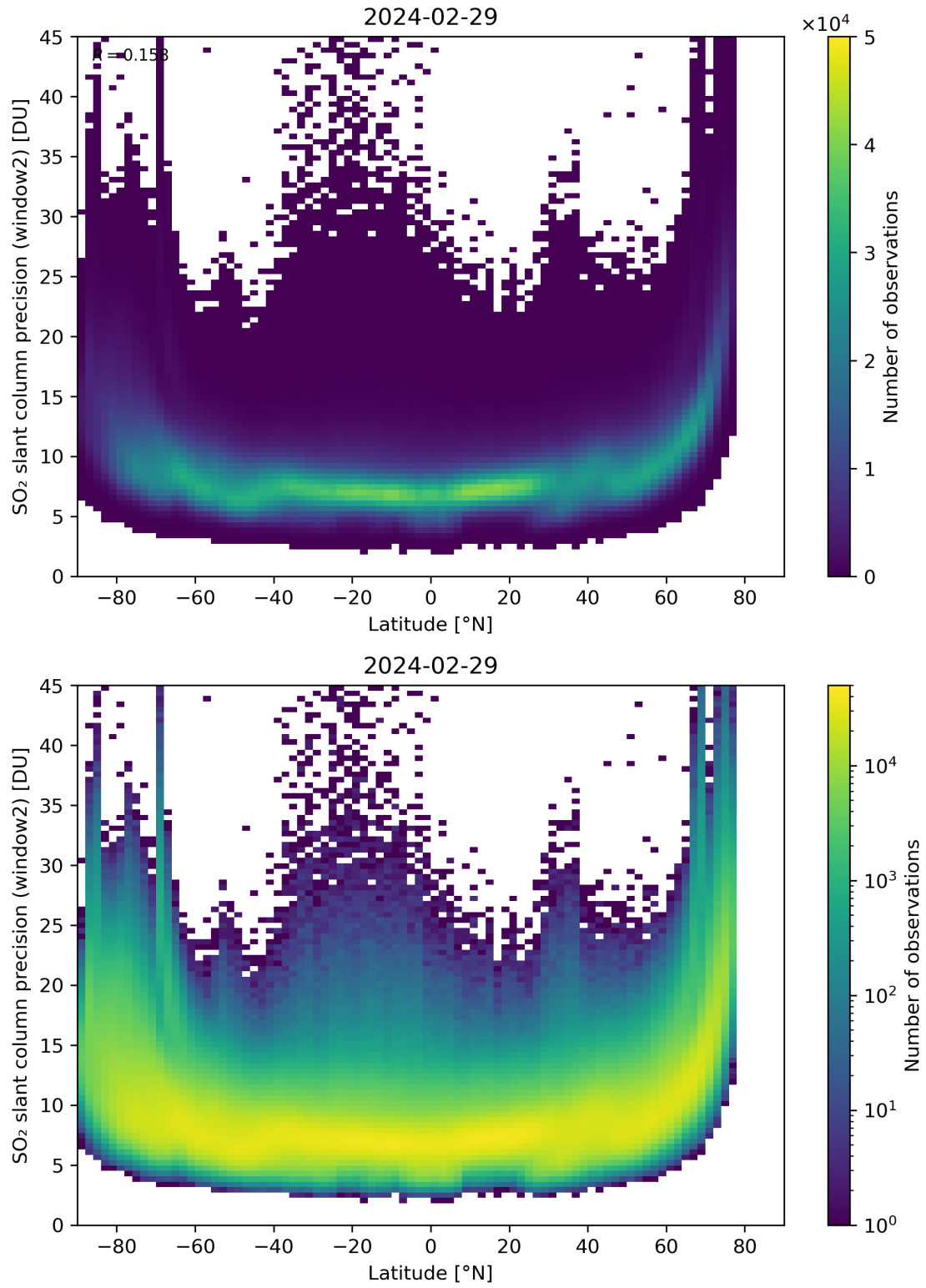
Figure 151: Scatter density plot of “Latitude” against “SO 2 slant column precision (window2)” for 2024-02-28 to 2024-03-01.
