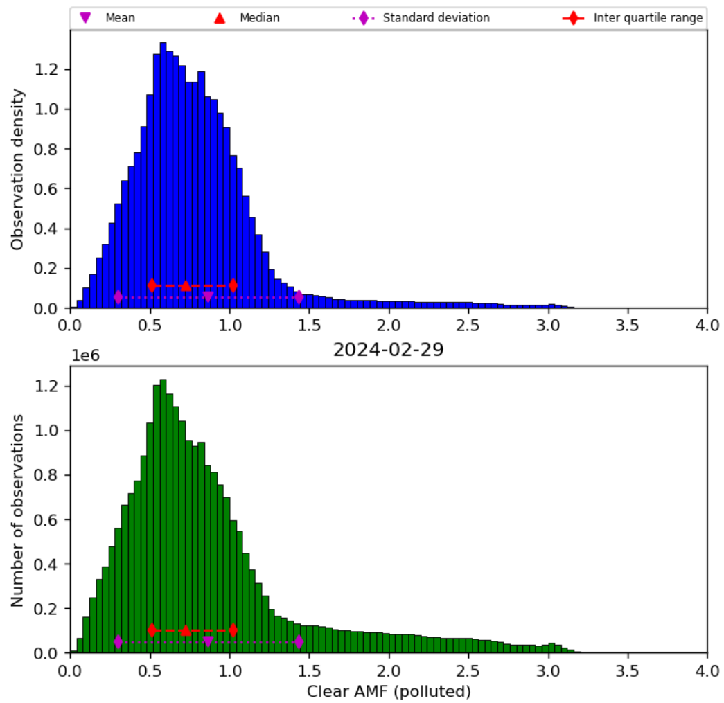
Figure 73: Histogram of “Clear AMF (polluted)” for 2024-02-28 to 2024-03-01
