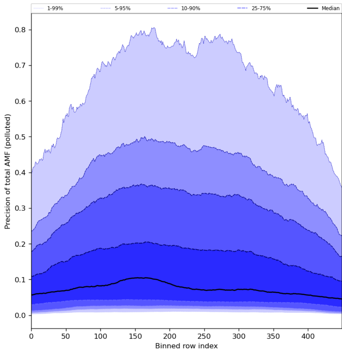
Figure 95: Along track statistics of “Precision of total AMF (polluted)” for 2024-02-28 to 2024-03-01
