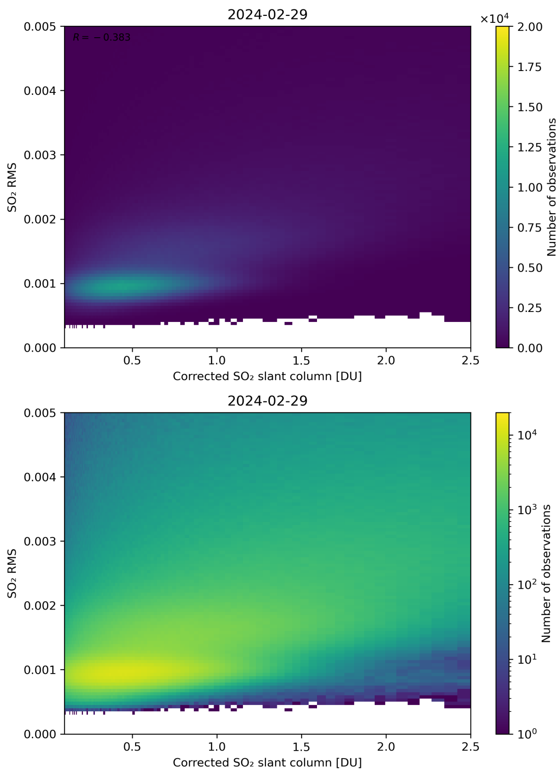
Figure 183: Scatter density plot of “Corrected SO 2 slant column” against “SO 2 RMS” for 2024-02-28 to 2024-03-01.
