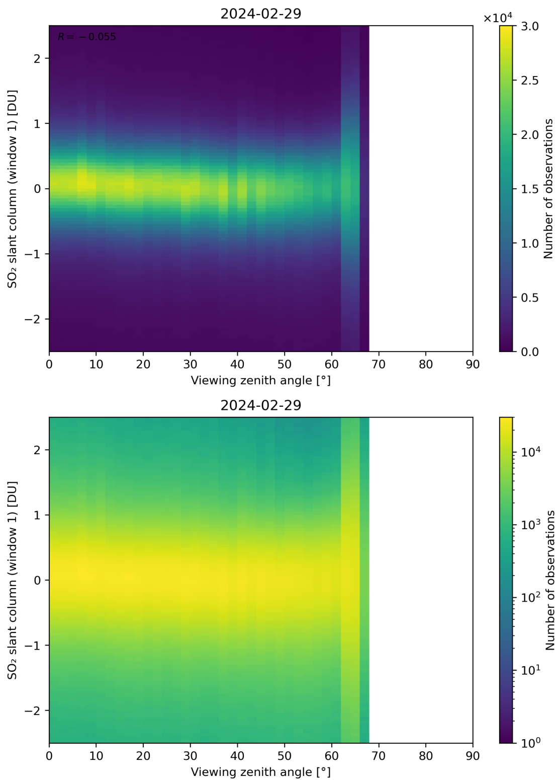
Figure 320: Scatter density plot of “Viewing zenith angle” against “SO 2 slant column (window 1)” for 2024-02-28 to 2024-03-01.
