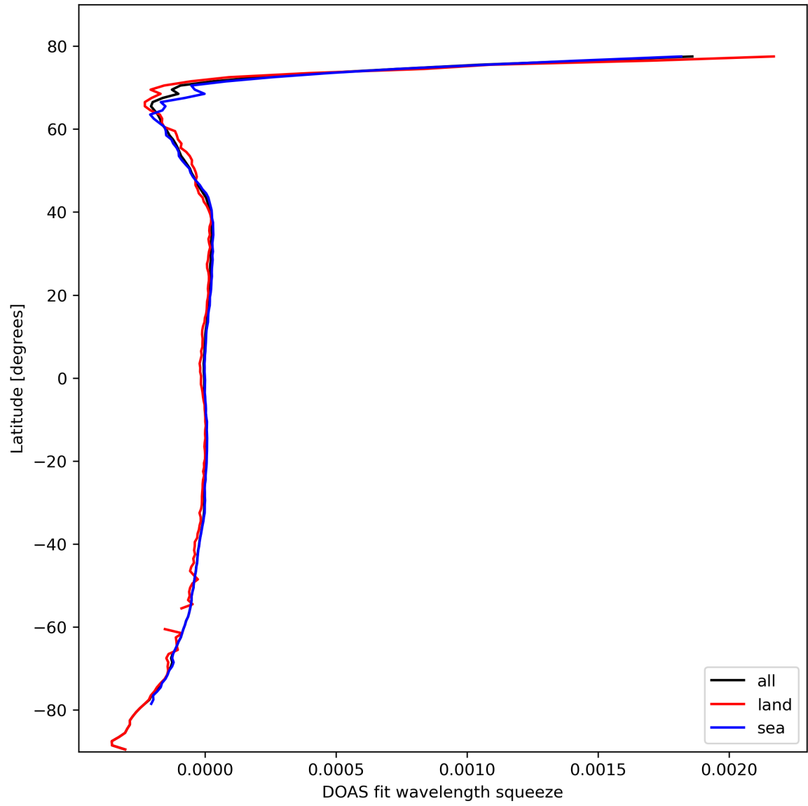
Figure 46: Zonal average of “DOAS fit wavelength squeeze” for 2024-02-28 to 2024-03-01.
