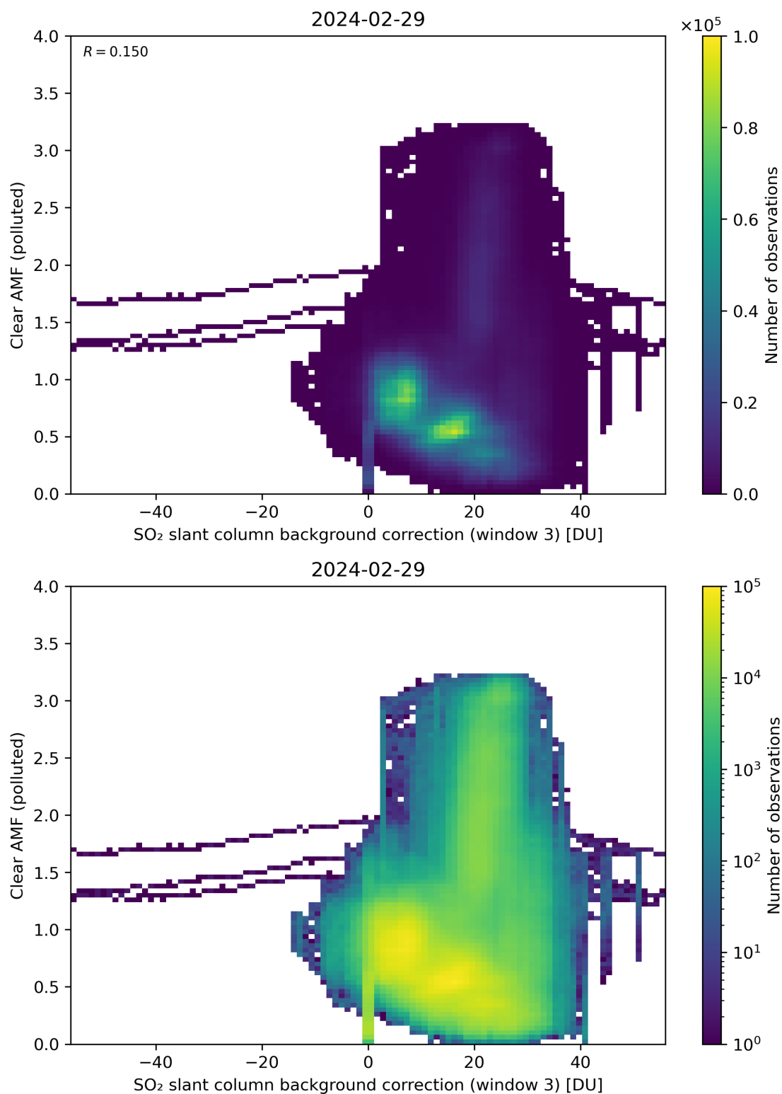
Figure 124: Scatter density plot of “SO 2 slant column background correction (window 3)” against “Clear AMF (polluted)” for 2024-02-28 to 2024-03-01.
