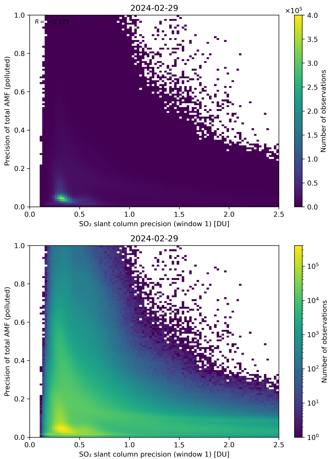
Figure 231: Scatter density plot of “SO 2 slant column precision (window 1)” against “Precision of total AMF (polluted)” for 2024-02-28 to 2024-03-01.
