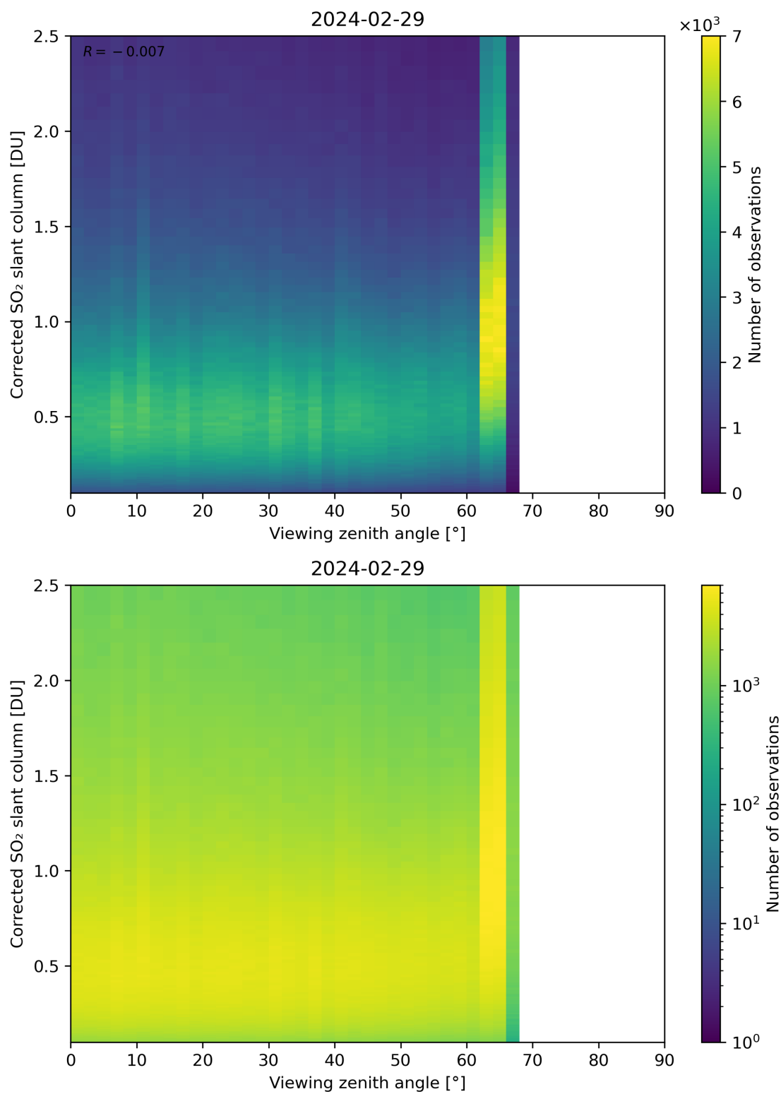
Figure 317: Scatter density plot of “Viewing zenith angle” against “Corrected SO 2 slant column” for 2024-02-28 to 2024-03-01.
