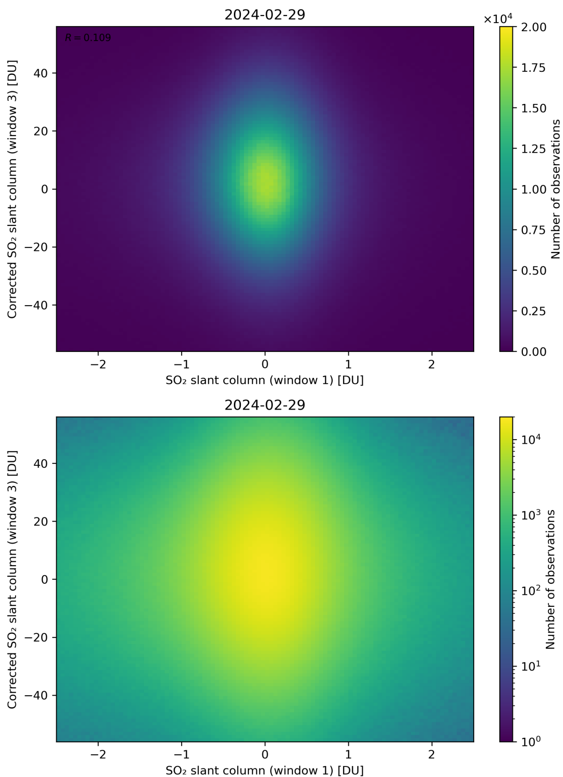
Figure 234: Scatter density plot of “SO 2 slant column (window 1)” against “Corrected SO 2 slant column (window 3)” for 2024-02-28 to 2024-03-01.
