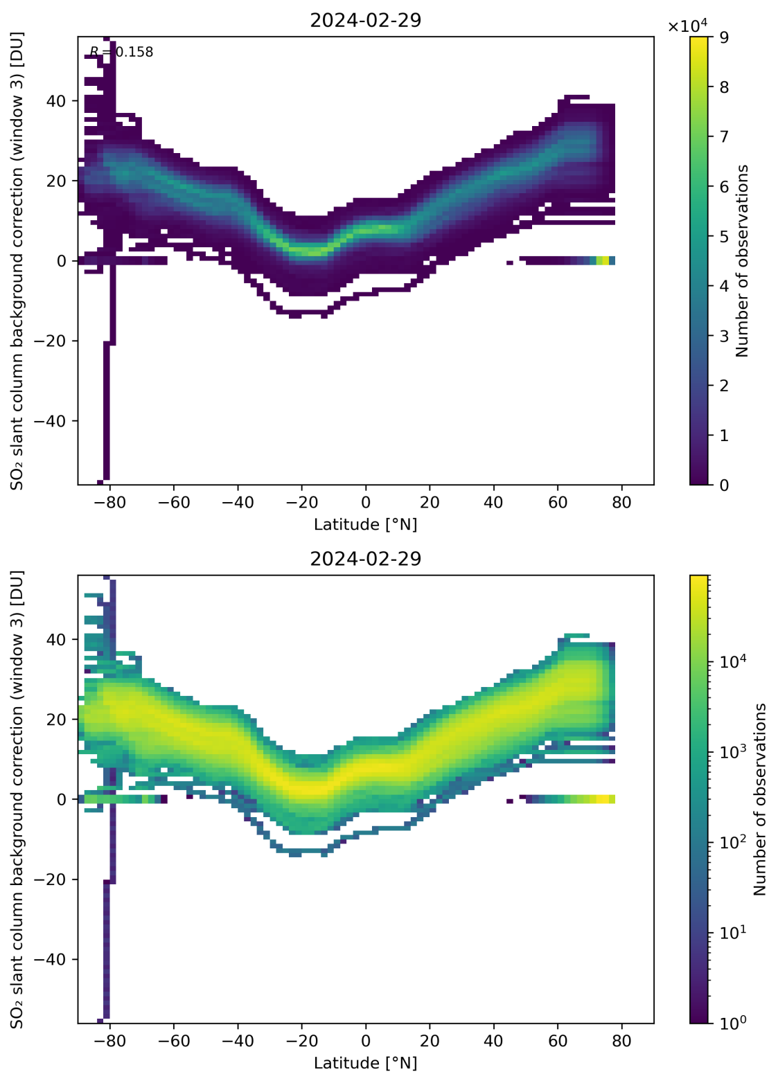
Figure 141: Scatter density plot of “Latitude” against “SO 2 slant column background correction (window 3)” for 2024-02-28 to 2024-03-01.
