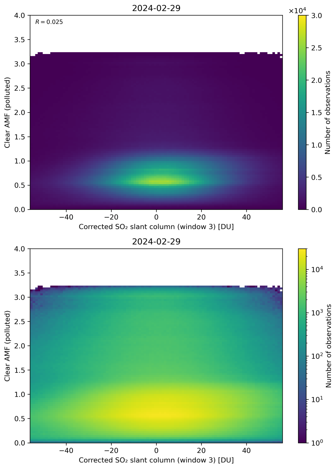
Figure 209: Scatter density plot of “Corrected SO 2 slant column (window 3)” against “Clear AMF (polluted)” for 2024-02-28 to 2024-03-01.
