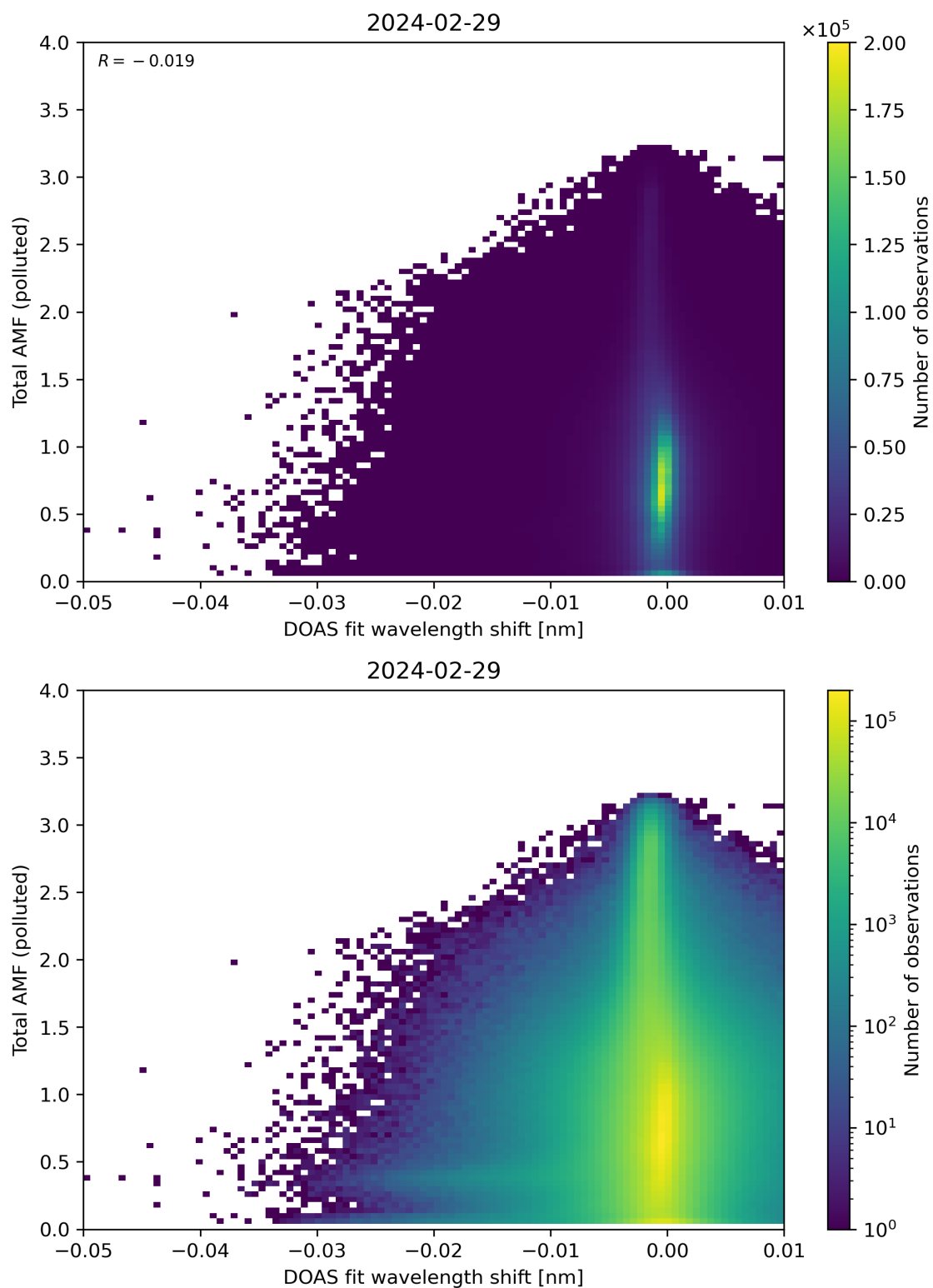
Figure 130: Scatter density plot of “DOAS fit wavelength shift” against “Total AMF (polluted)” for 2024-02-28 to 2024-03-01.
