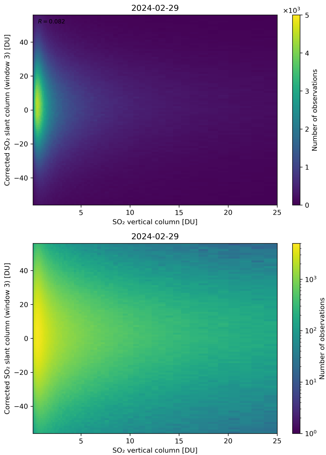
Figure 299: Scatter density plot of “SO 2 vertical column” against “Corrected SO 2 slant column (window 3)” for 2024-02-28 to 2024-03-01.
