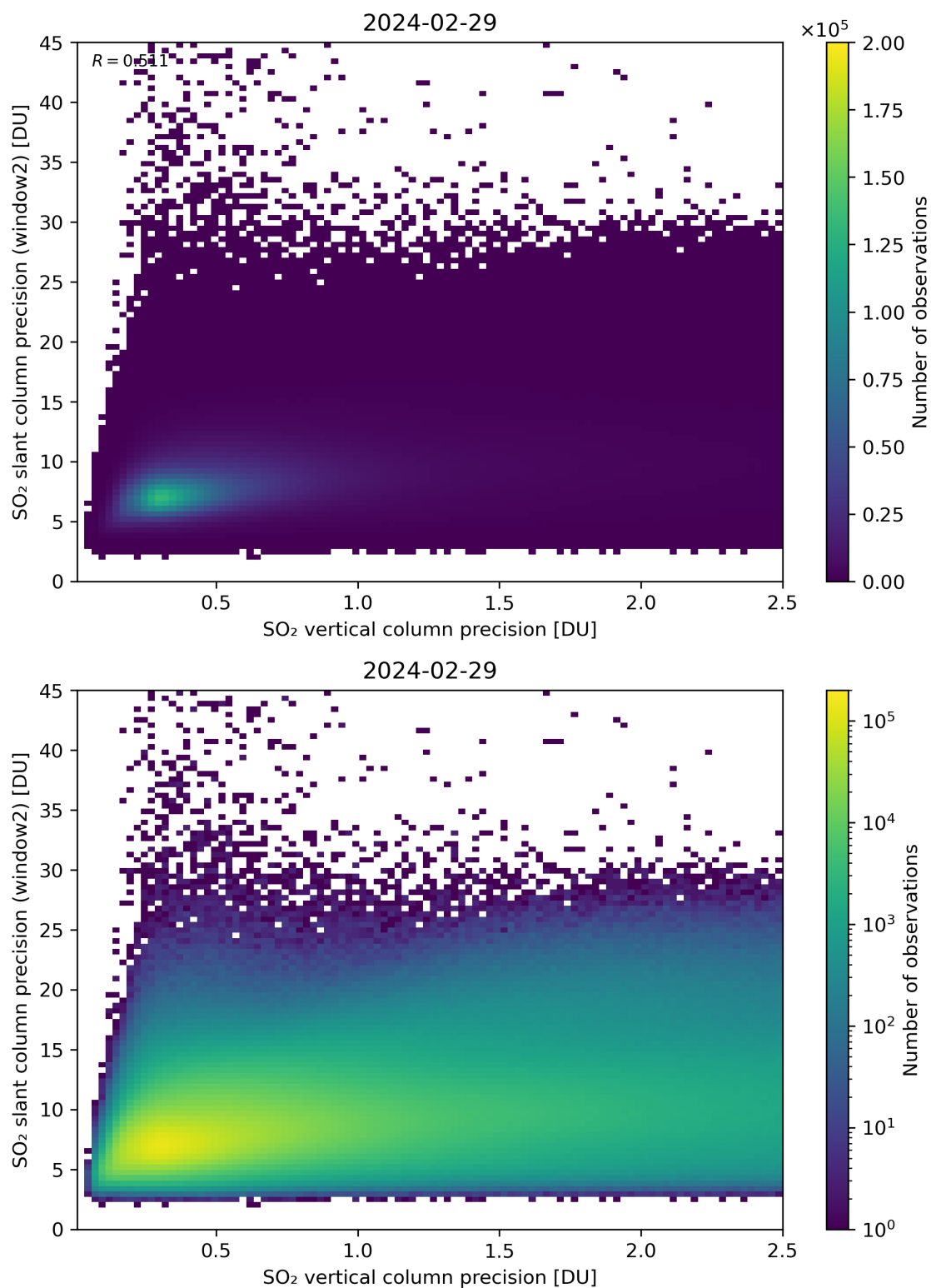
Figure 291: Scatter density plot of “SO 2 vertical column precision” against “SO 2 slant column precision (window2)” for 2024-02-28 to 2024-03-01.
