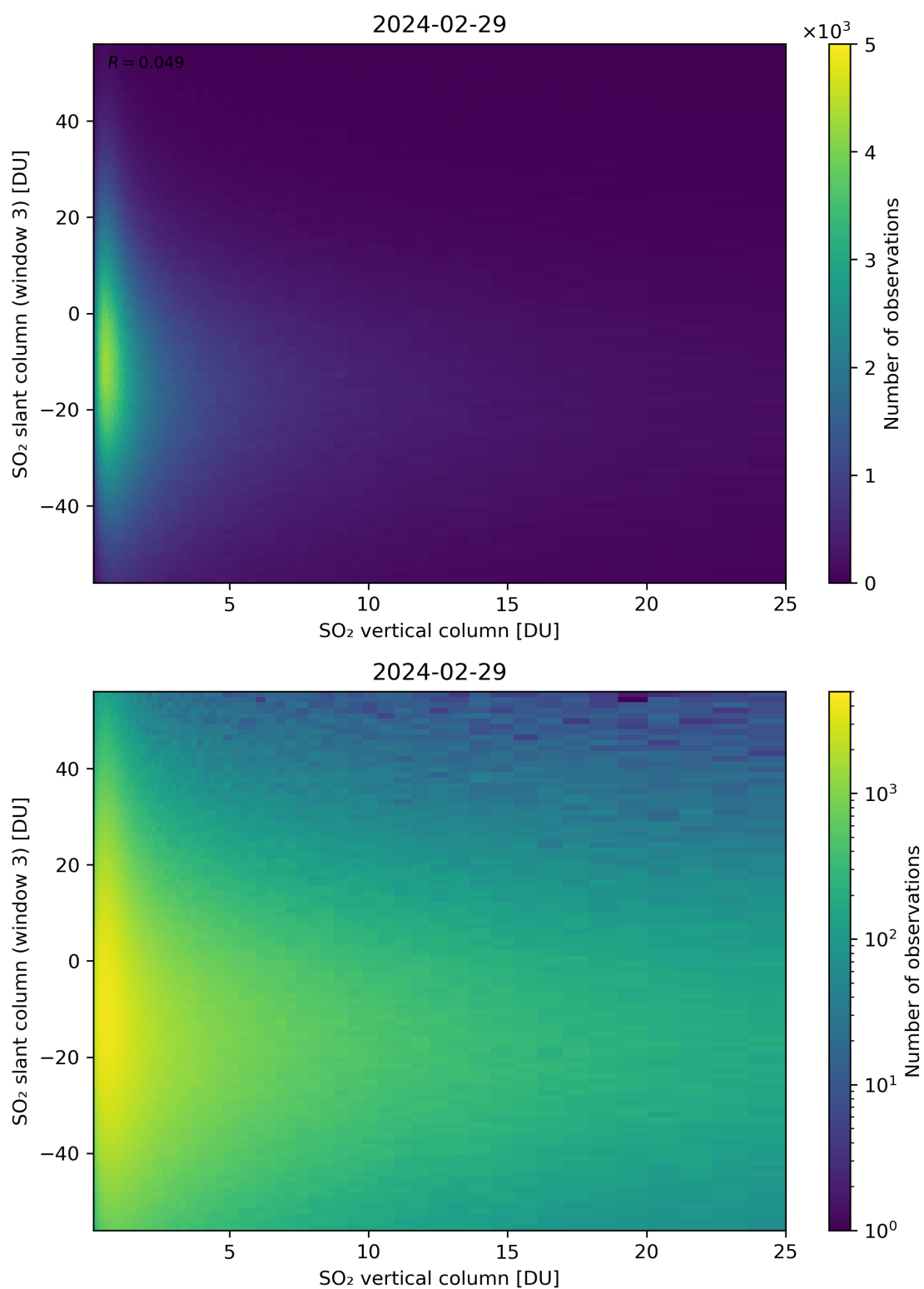
Figure 303: Scatter density plot of “SO 2 vertical column” against “SO 2 slant column (window 3)” for 2024-02-28 to 2024-03-01.
