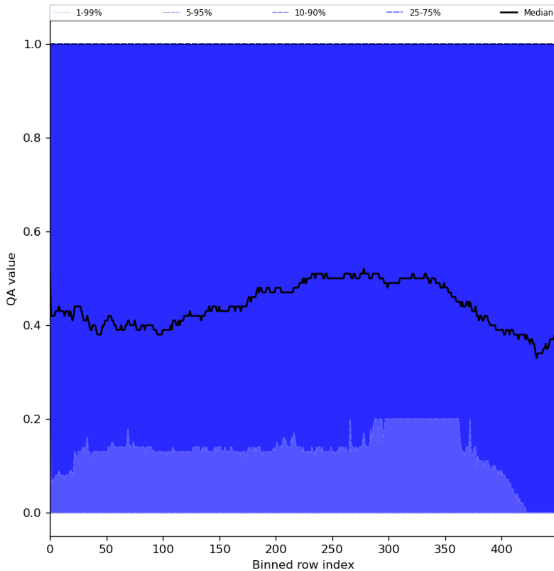
Figure 75: Along track statistics of “QA value” for 2024-02-28 to 2024-03-01
