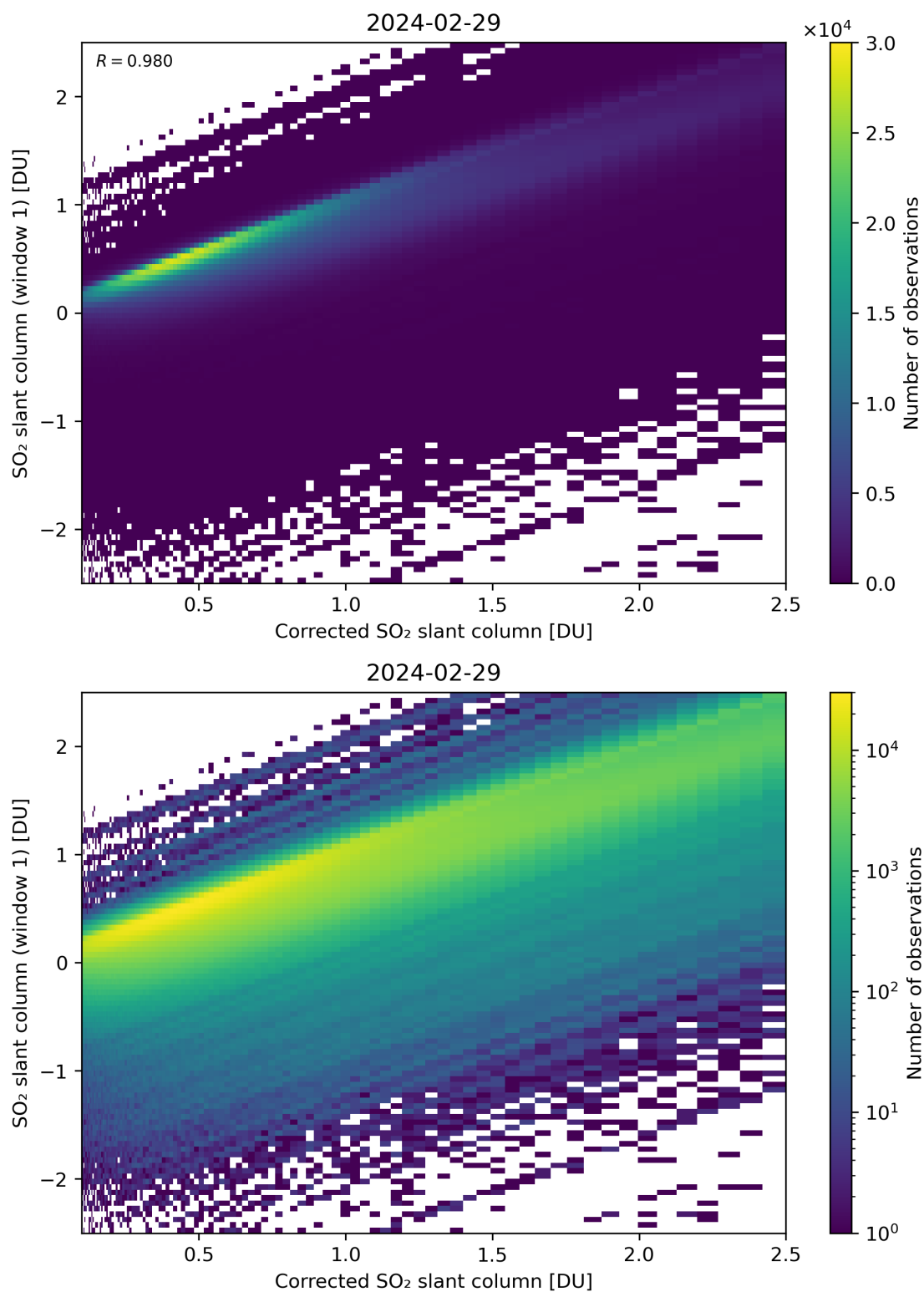
Figure 187: Scatter density plot of “Corrected SO 2 slant column” against “SO 2 slant column (window 1)” for 2024-02-28 to 2024-03-01.
