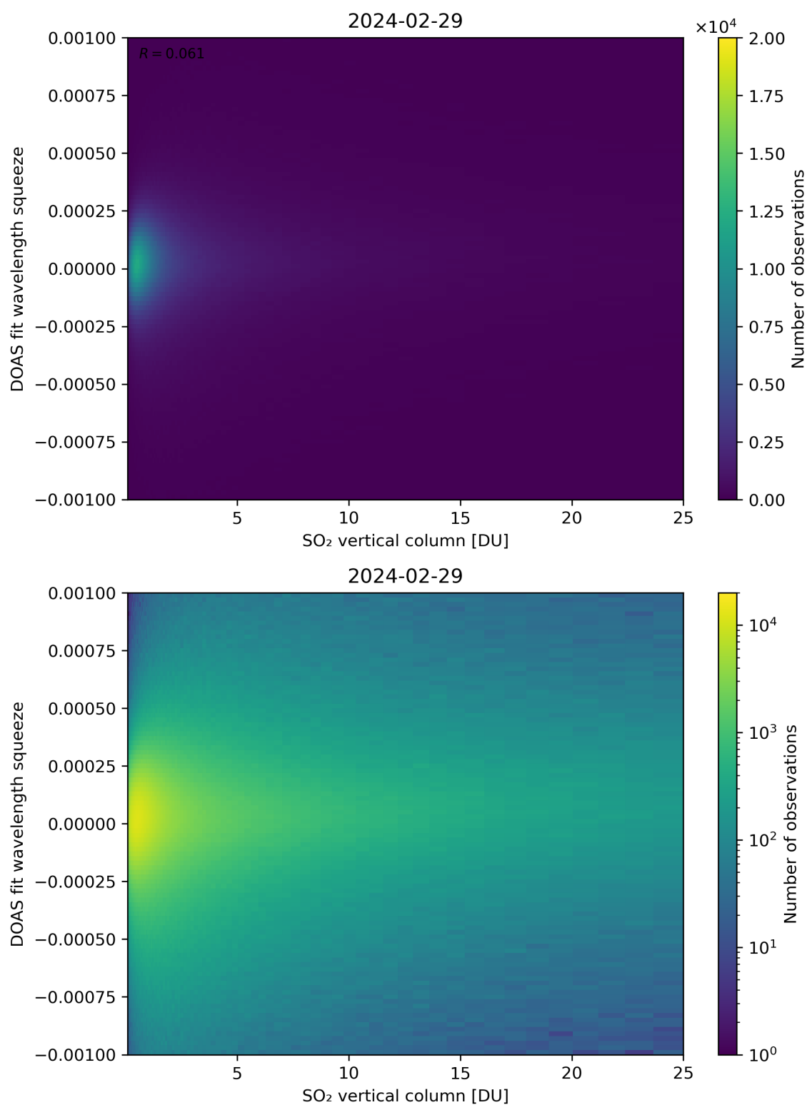
Figure 277: Scatter density plot of “SO 2 vertical column” against “DOAS fit wavelength squeeze” for 2024-02-28 to 2024-03-01.
