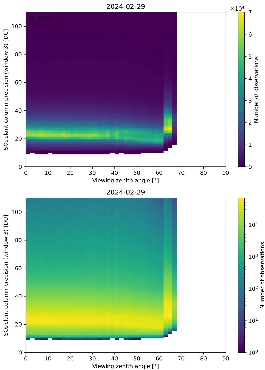
Figure 324: Scatter density plot of “Viewing zenith angle” against “SO 2 slant column precision (window 3)” for 2024-02-28 to 2024-03-01.
