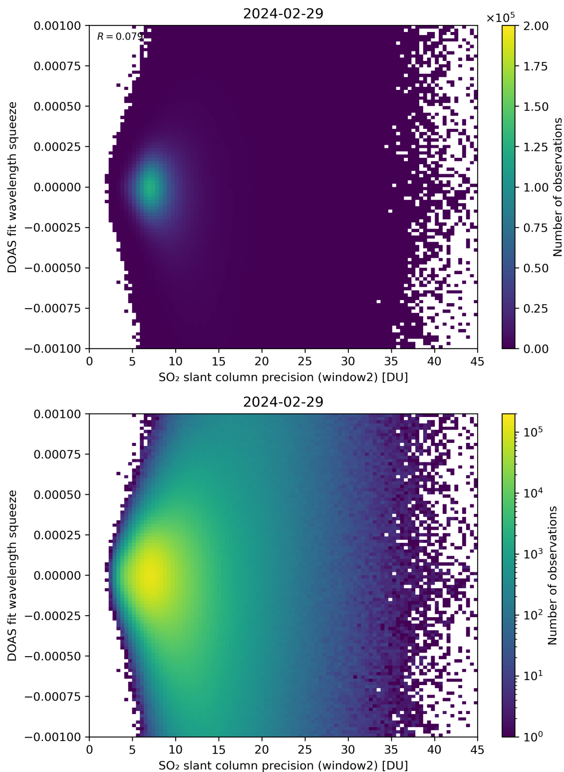
Figure 244: Scatter density plot of “SO 2 slant column precision (window2)” against “DOAS fit wavelength squeeze” for 2024-02-28 to 2024-03-01.
