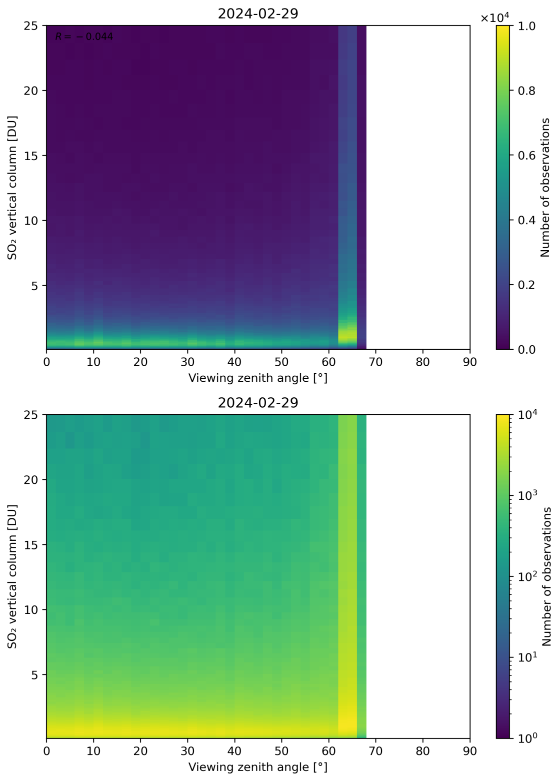
Figure 327: Scatter density plot of “Viewing zenith angle” against “SO 2 vertical column” for 2024-02-28 to 2024-03-01.
