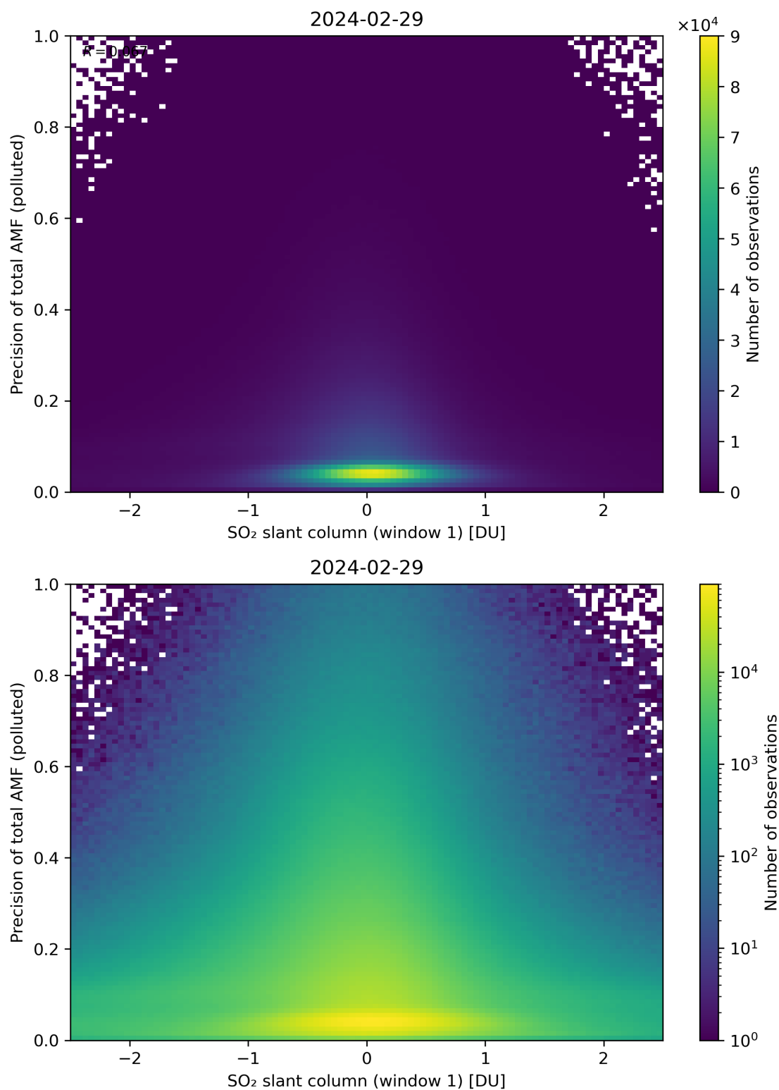
Figure 240: Scatter density plot of “SO 2 slant column (window 1)” against “Precision of total AMF (polluted)” for 2024-02-28 to 2024-03-01.
