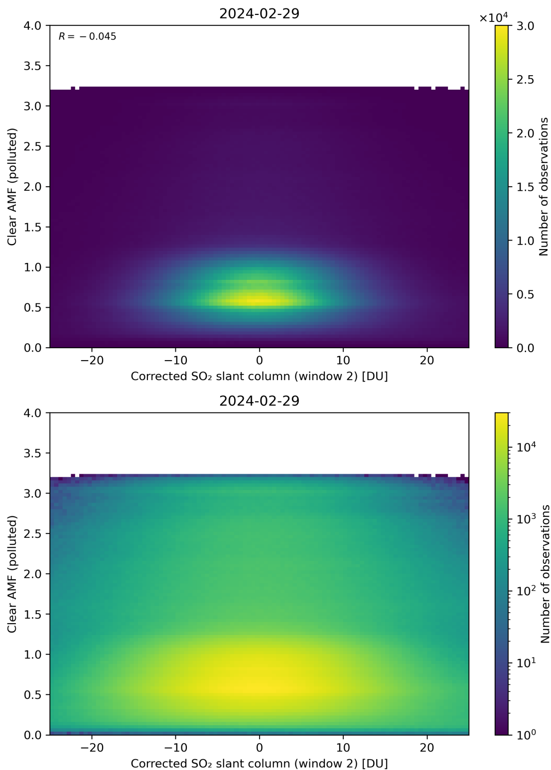
Figure 199: Scatter density plot of “Corrected SO 2 slant column (window 2)” against “Clear AMF (polluted)” for 2024-02-28 to 2024-03-01.
