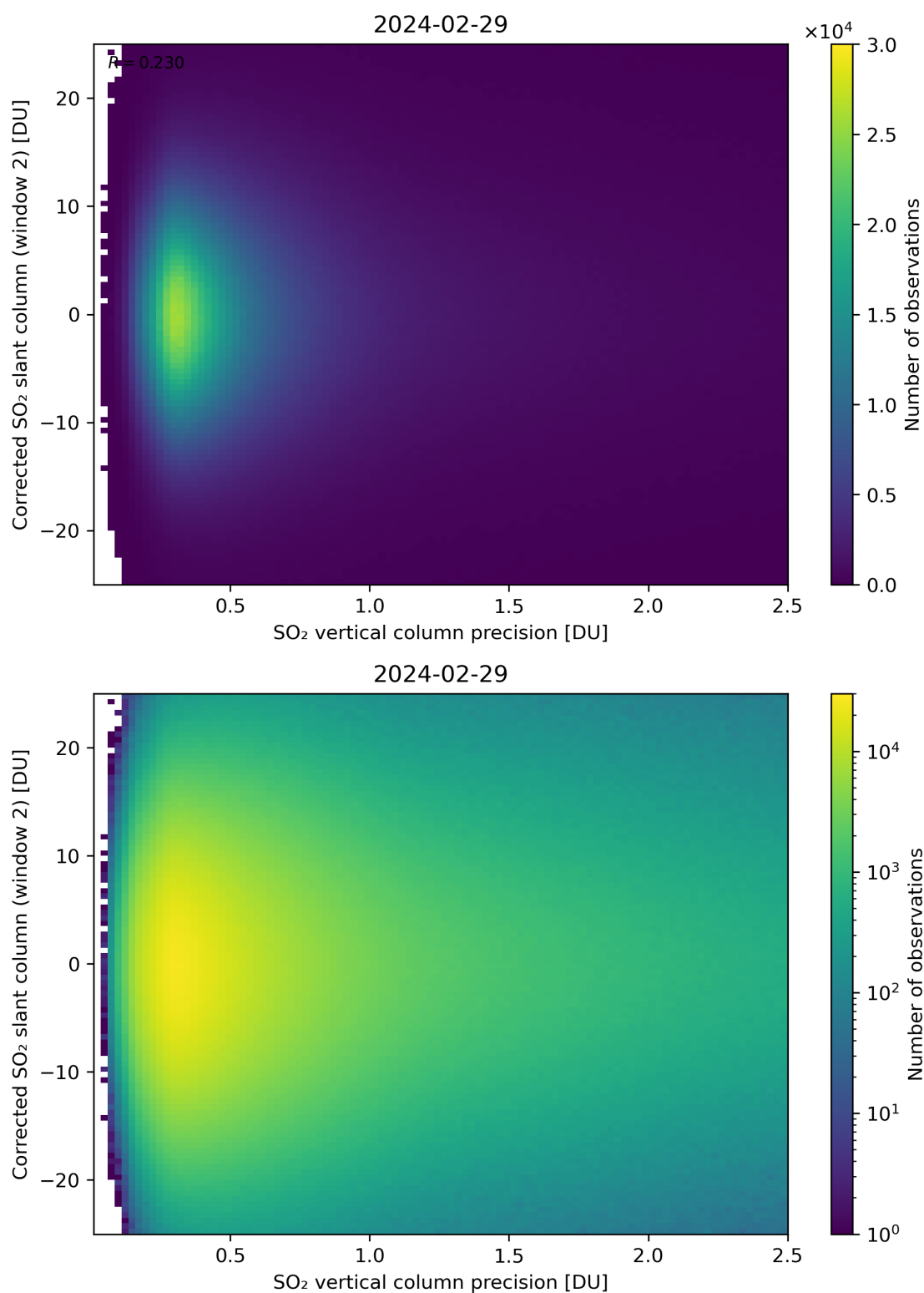
Figure 287: Scatter density plot of “SO 2 vertical column precision” against “Corrected SO 2 slant column (window 2)” for 2024-02-28 to 2024-03-01.
