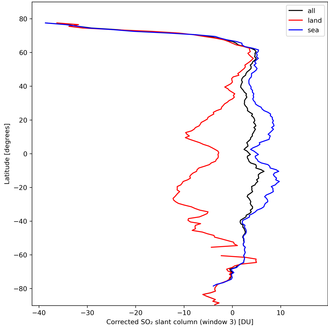
Figure 43: Zonal average of “Corrected SO 2 slant column (window 3)” for 2024-02-28 to 2024-03-01.
