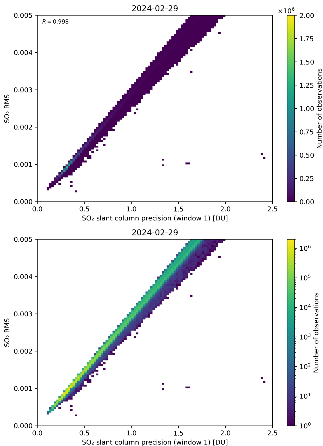
Figure 223: Scatter density plot of “SO 2 slant column precision (window 1)” against “SO 2 RMS” for 2024-02-28 to 2024-03-01.
