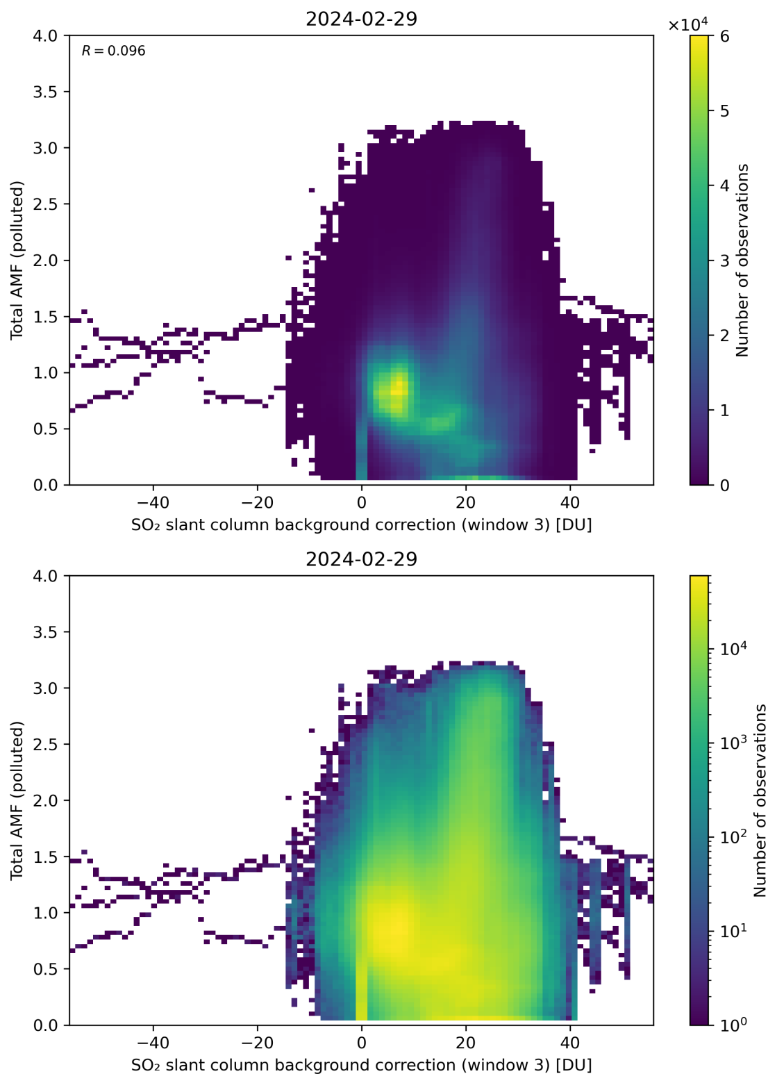
Figure 125: Scatter density plot of “SO 2 slant column background correction (window 3)” against “Total AMF (polluted)” for 2024-02-28 to 2024-03-01.
