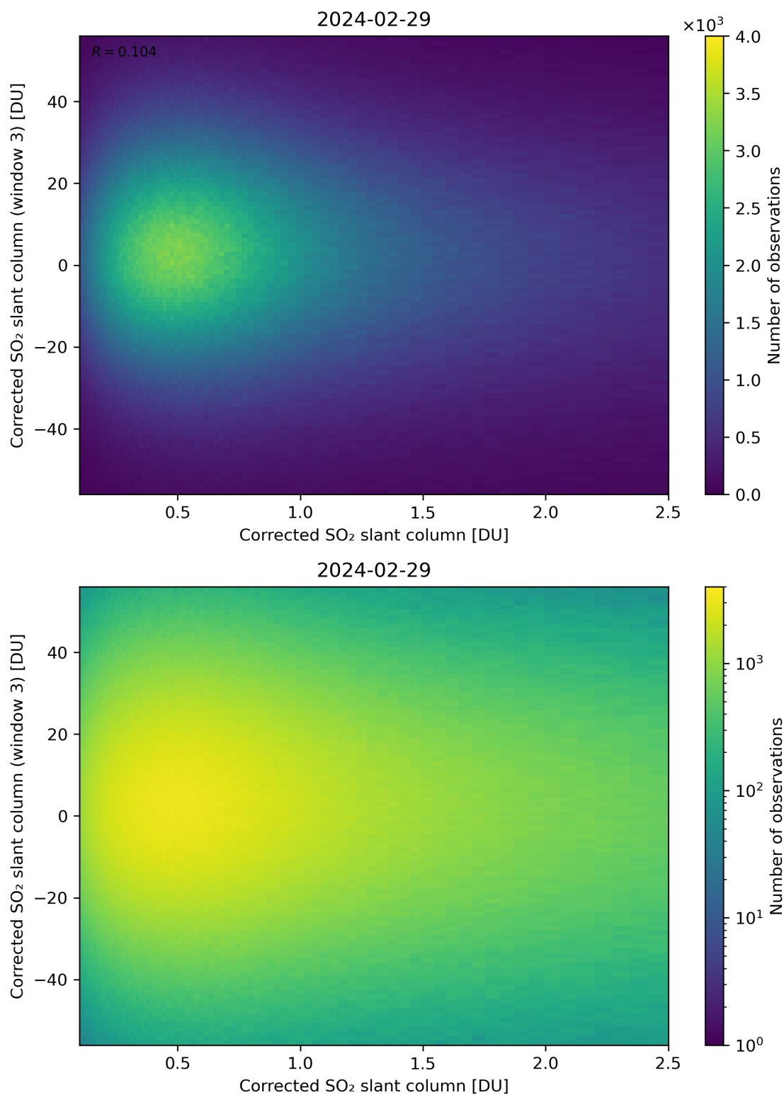
Figure 186: Scatter density plot of “Corrected SO 2 slant column” against “Corrected SO 2 slant column (window 3)” for 2024-02-28 to 2024-03-01.
