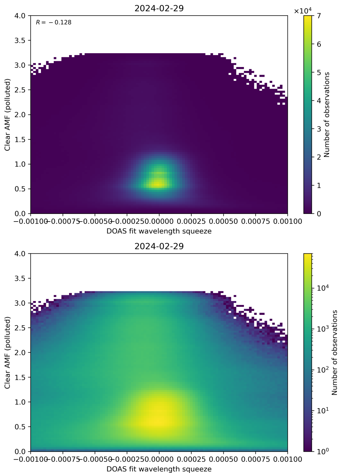
Figure 133: Scatter density plot of “DOAS fit wavelength squeeze” against “Clear AMF (polluted)” for 2024-02-28 to 2024-03-01.
