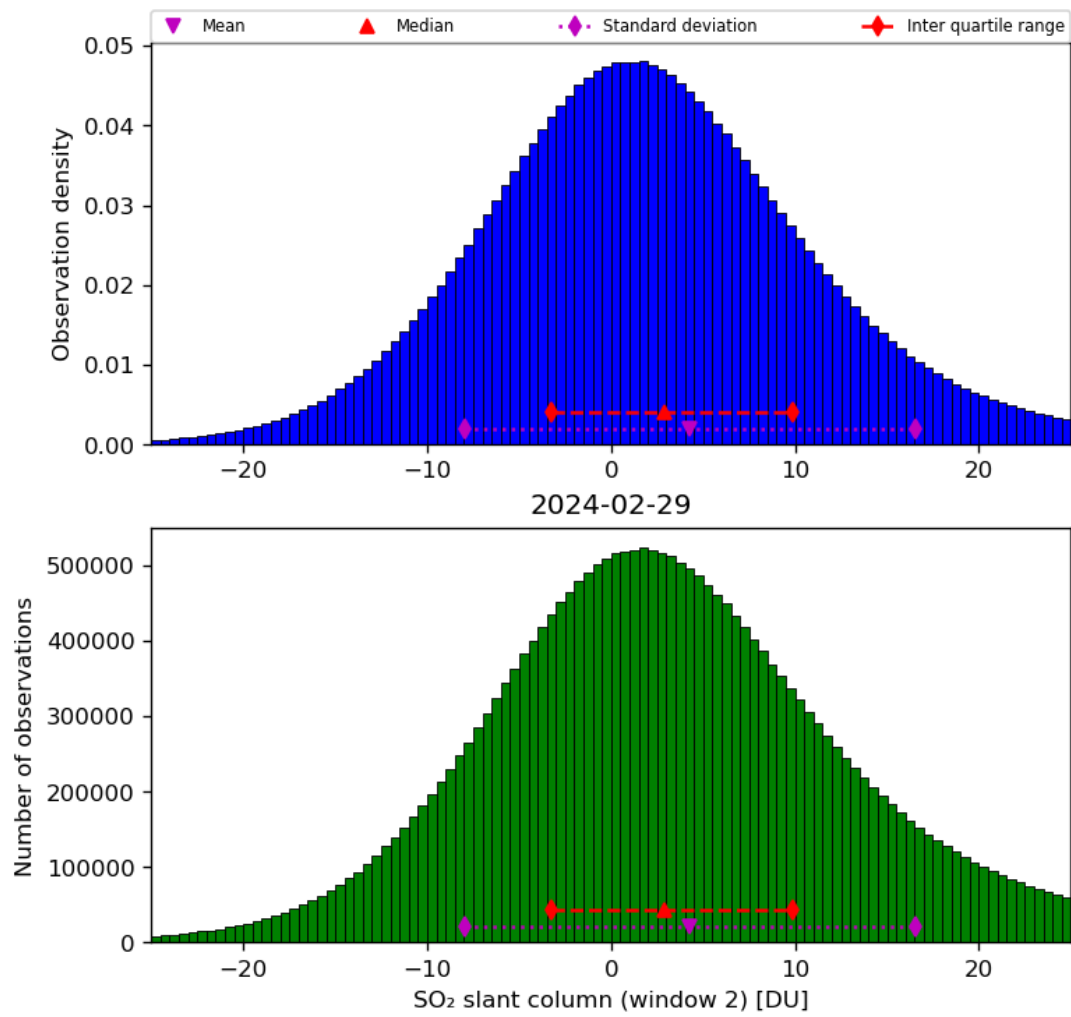
Figure 60: Histogram of “SO 2 slant column (window 2)” for 2024-02-28 to 2024-03-01
