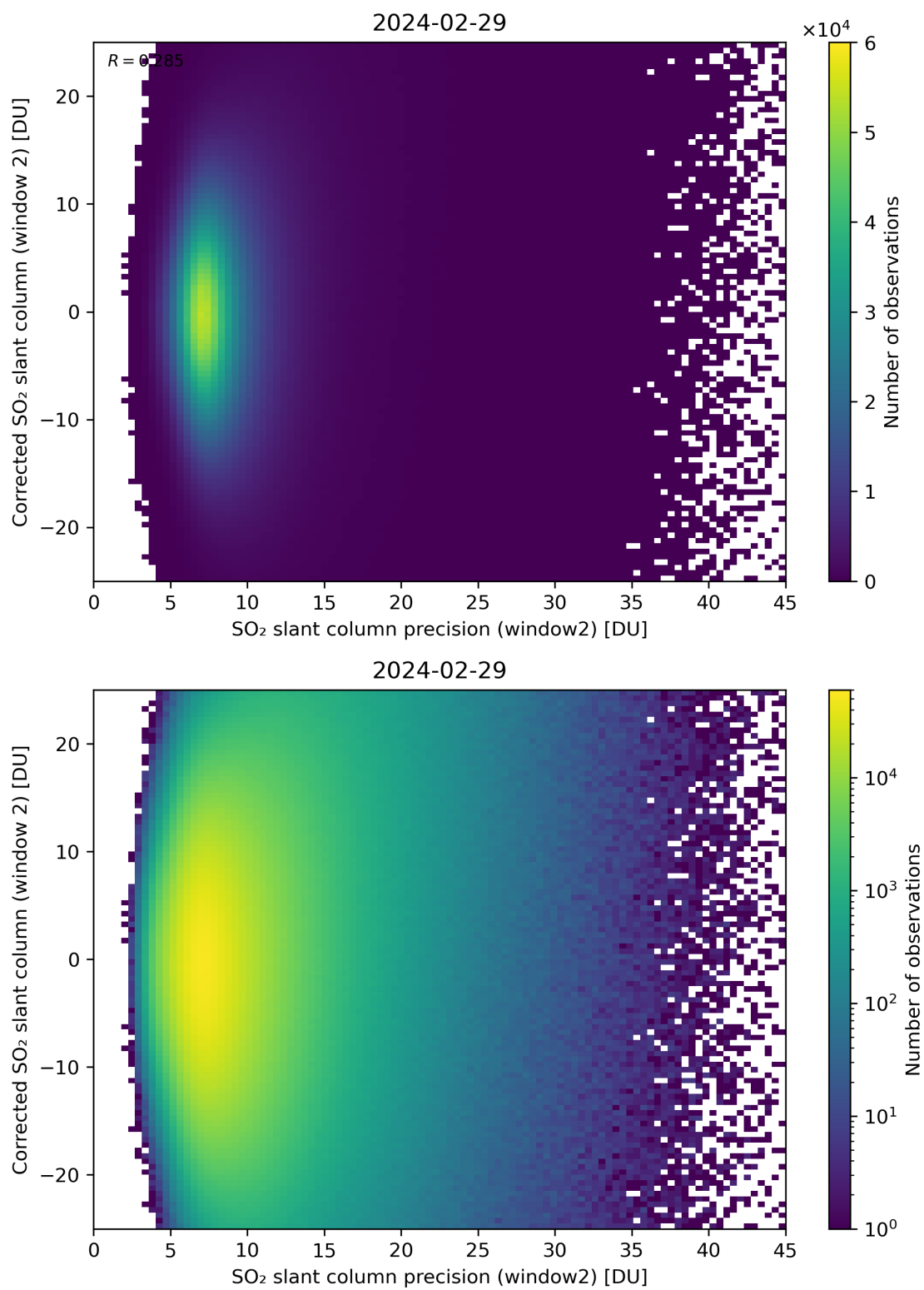
Figure 247: Scatter density plot of “SO 2 slant column precision (window2)” against “Corrected SO 2 slant column (window 2)” for 2024-02-28 to 2024-03-01.
