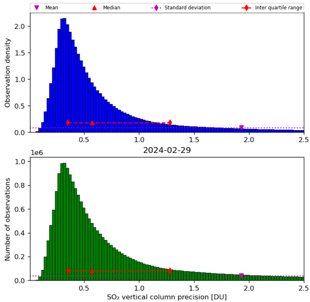
Figure 54: Histogram of “SO 2 vertical column precision” for 2024-02-28 to 2024-03-01
