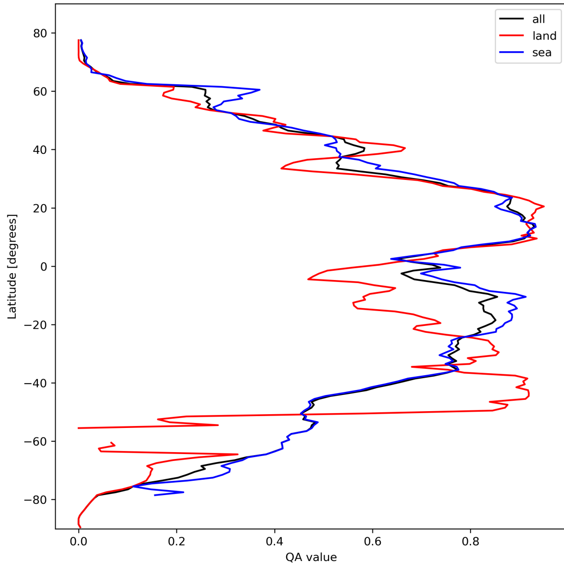
Figure 29: Zonal average of “QA value” for 2024-02-28 to 2024-03-01.
