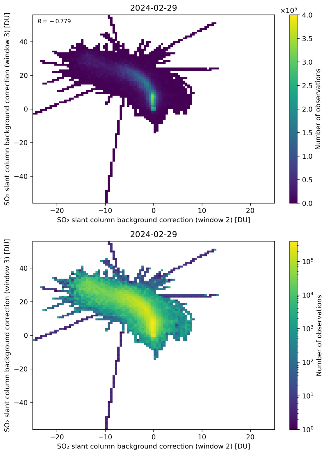
Figure 111: Scatter density plot of “SO 2 slant column background correction (window 2)” against “SO 2 slant column background correction (window 3)” for 2024-02-28 to 2024-03-01.
