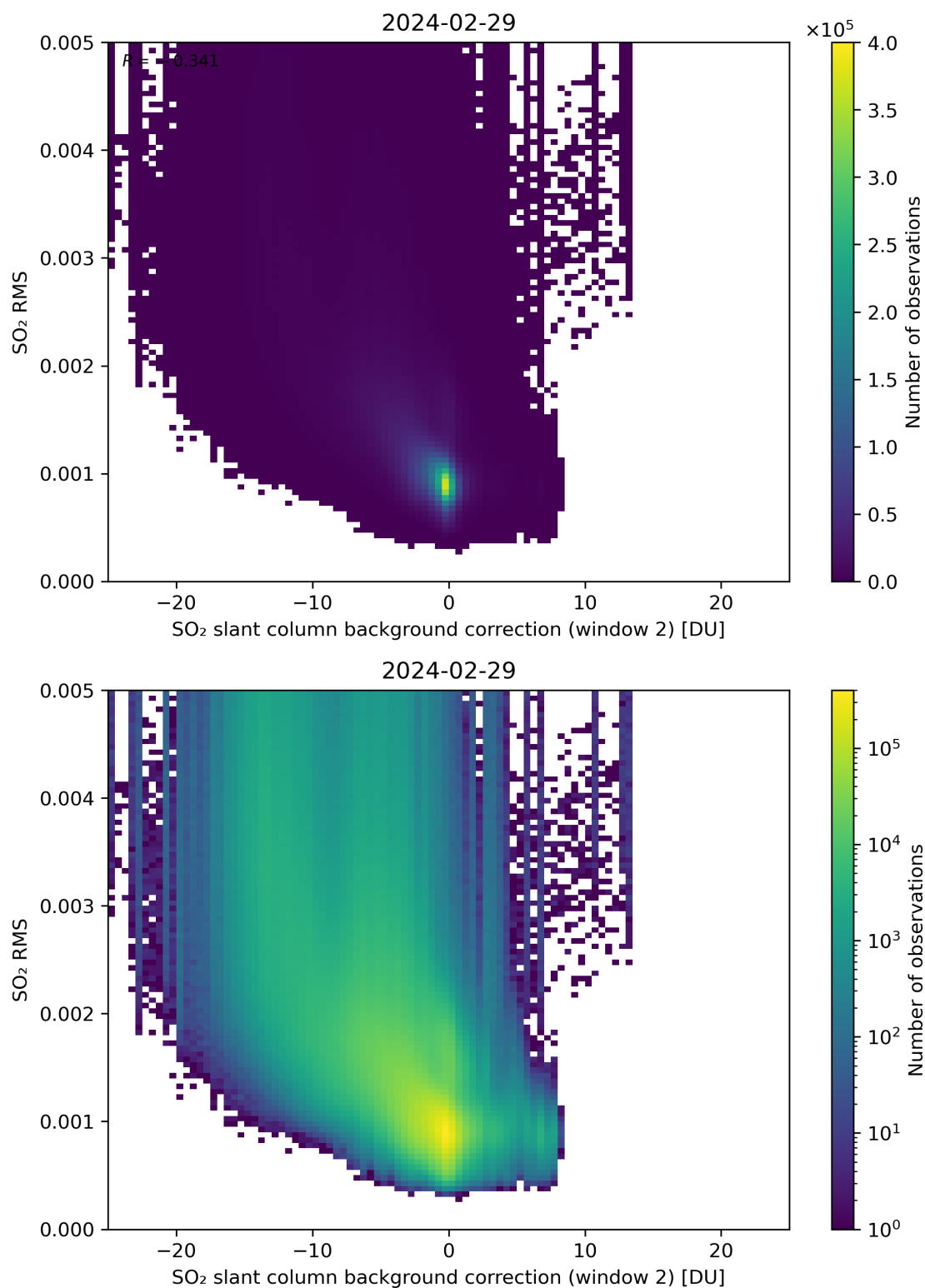
Figure 114: Scatter density plot of “SO 2 slant column background correction (window 2)” against “SO 2 RMS” for 2024-02-28 to 2024-03-01.
