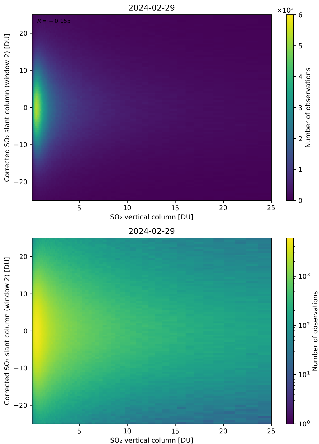
Figure 298: Scatter density plot of “SO 2 vertical column” against “Corrected SO 2 slant column (window 2)” for 2024-02-28 to 2024-03-01.
