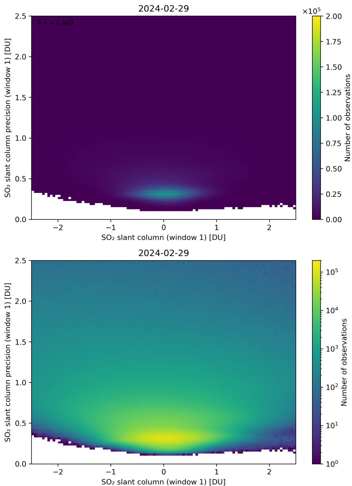
Figure 235: Scatter density plot of “SO 2 slant column (window 1)” against “SO 2 slant column precision (window 1)” for 2024-02-28 to 2024-03-01.
