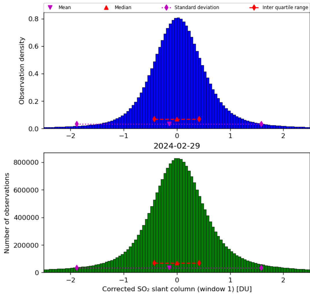
Figure 58: Histogram of “Corrected SO 2 slant column (window 1)” for 2024-02-28 to 2024-03-01
