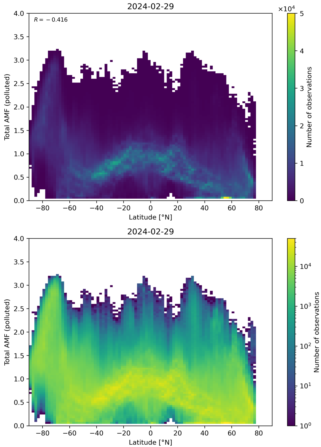
Figure 154: Scatter density plot of “Latitude” against “Total AMF (polluted)” for 2024-02-28 to 2024-03-01.
