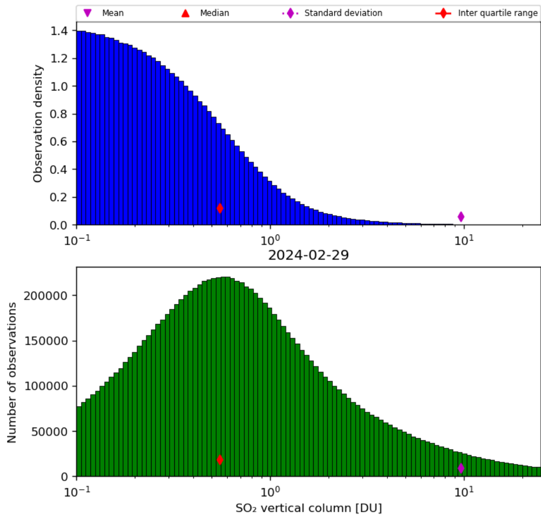
Figure 53: Histogram of “SO 2 vertical column” for 2024-02-28 to 2024-03-01
