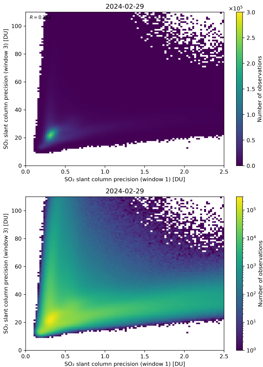
Figure 229: Scatter density plot of “SO 2 slant column precision (window 1)” against “SO 2 slant column precision (window 3)” for 2024-02-28 to 2024-03-01.
