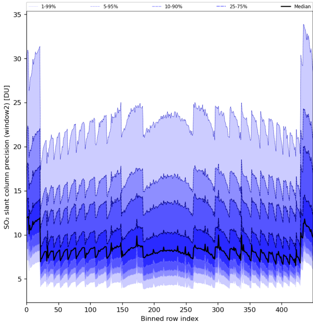
Figure 84: Along track statistics of “SO 2 slant column precision (window2)” for 2024-02-28 to 2024-03-01
