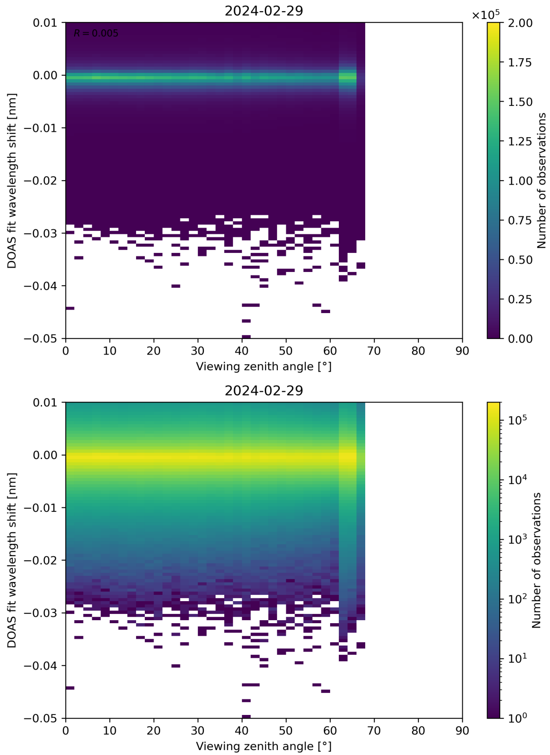
Figure 311: Scatter density plot of “Viewing zenith angle” against “DOAS fit wavelength shift” for 2024-02-28 to 2024-03-01.
