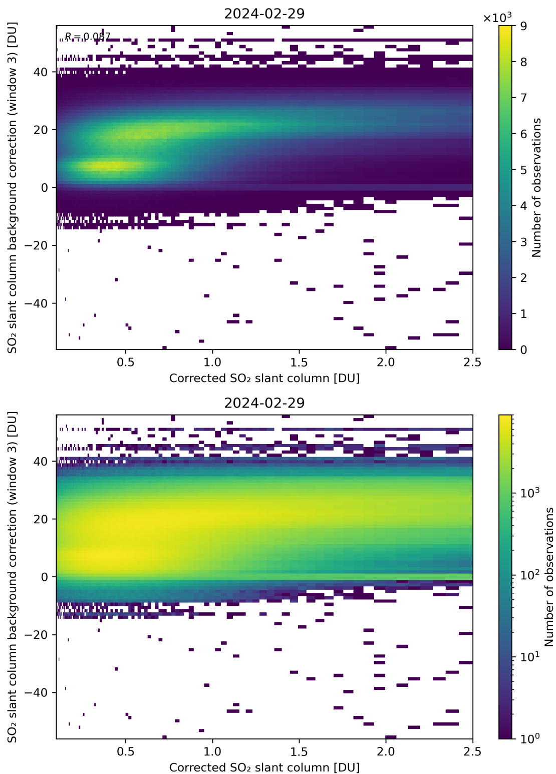
Figure 180: Scatter density plot of “Corrected SO 2 slant column” against “SO 2 slant column background correction (window 3)” for 2024-02-28 to 2024-03-01.
