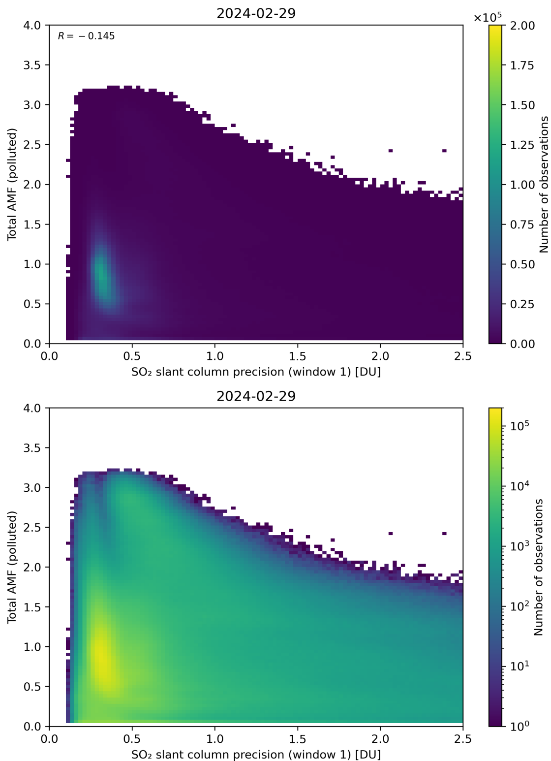
Figure 230: Scatter density plot of “SO 2 slant column precision (window 1)” against “Total AMF (polluted)” for 2024-02-28 to 2024-03-01.
