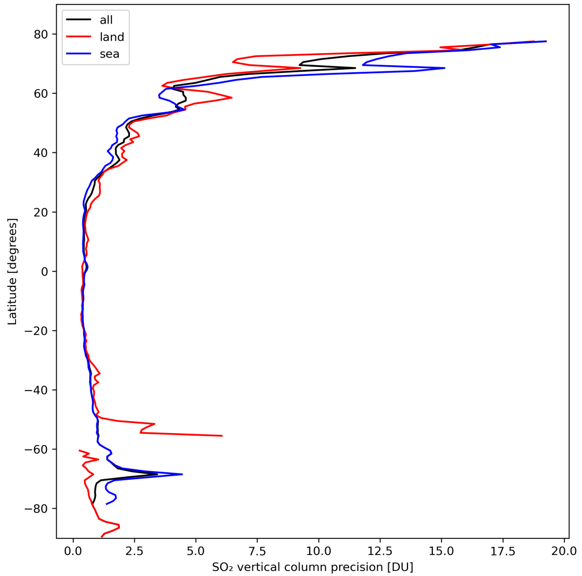
Figure 31: Zonal average of “SO 2 vertical column precision” for 2024-02-28 to 2024-03-01.
