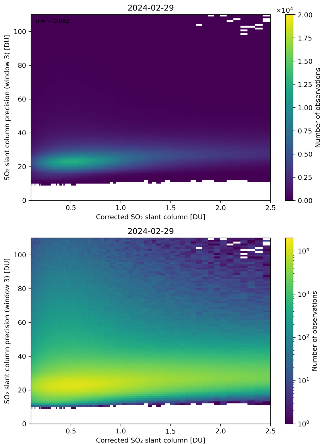
Figure 191: Scatter density plot of “Corrected SO 2 slant column” against “SO 2 slant column precision (window 3)” for 2024-02-28 to 2024-03-01.
