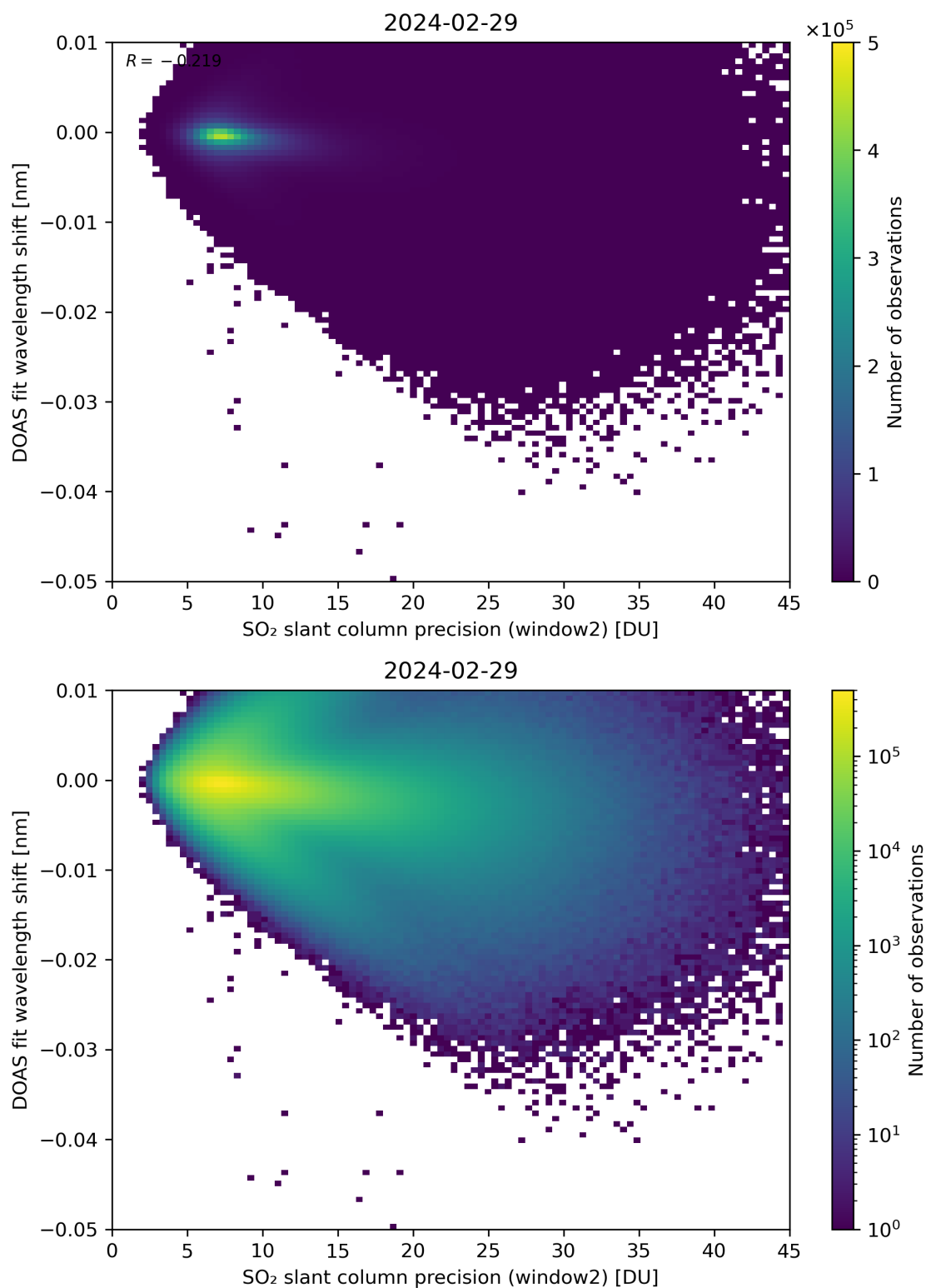
Figure 243: Scatter density plot of “SO 2 slant column precision (window2)” against “DOAS fit wavelength shift” for 2024-02-28 to 2024-03-01.
