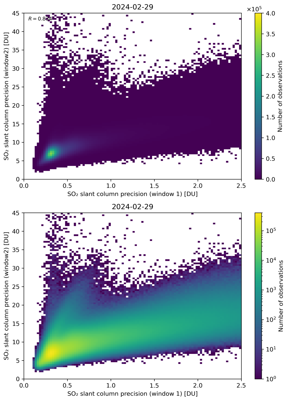
Figure 227: Scatter density plot of “SO 2 slant column precision (window 1)” against “SO 2 slant column precision (window 2)” for 2024-02-28 to 2024-03-01.
