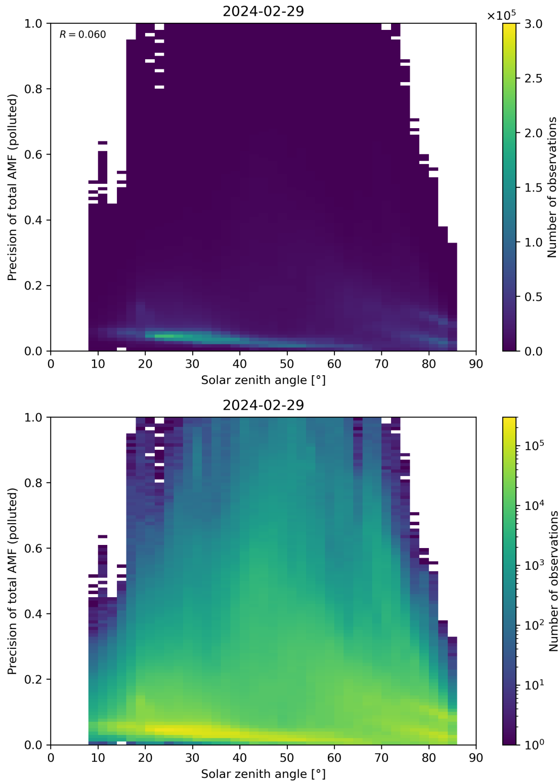
Figure 175: Scatter density plot of “Solar zenith angle” against “Precision of total AMF (polluted)” for 2024-02-28 to 2024-03-01.
