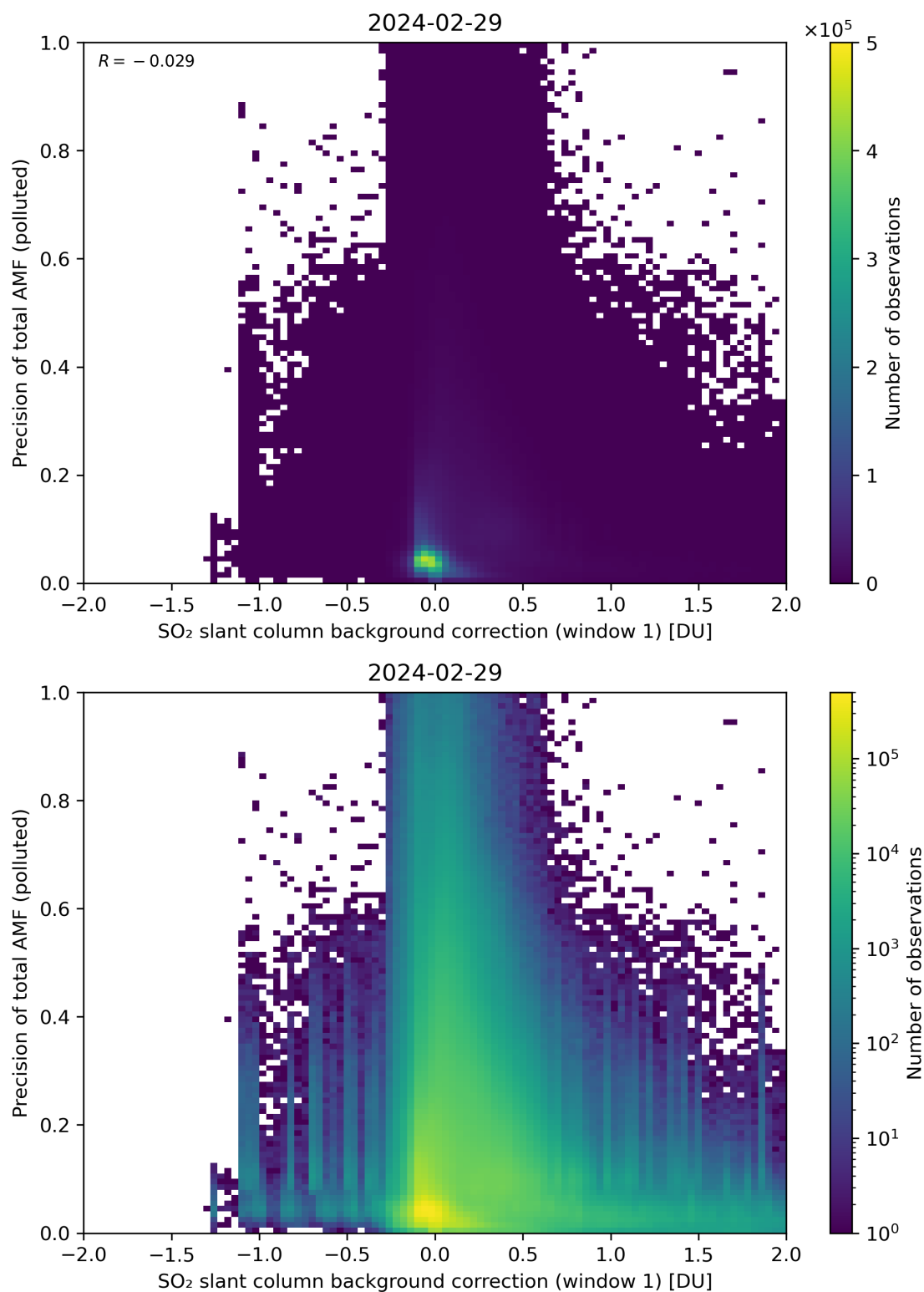
Figure 110: Scatter density plot of “SO 2 slant column background correction (window 1)” against “Precision of total AMF (polluted)” for 2024-02-28 to 2024-03-01.
