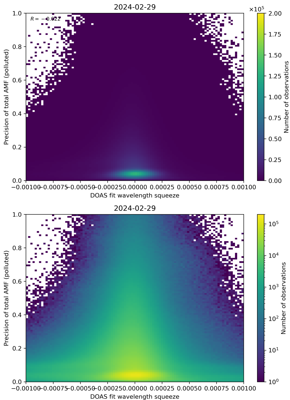
Figure 135: Scatter density plot of “DOAS fit wavelength squeeze” against “Precision of total AMF (polluted)” for 2024-02-28 to 2024-03-01.
