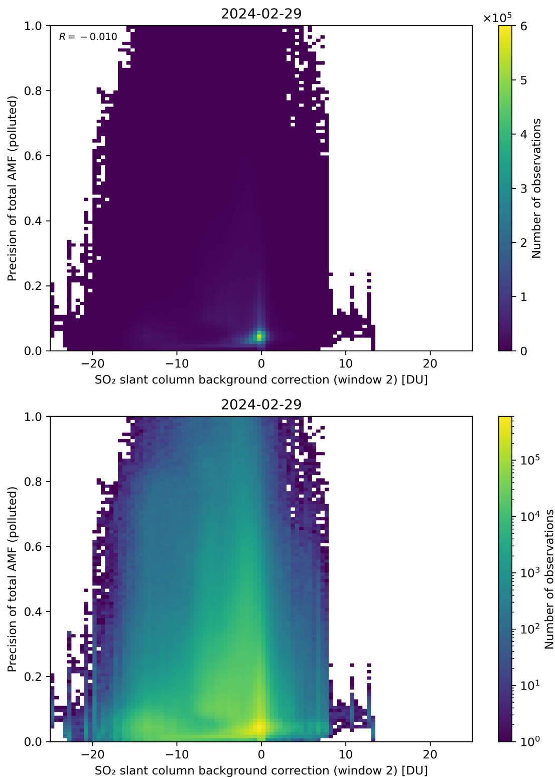
Figure 120: Scatter density plot of “SO 2 slant column background correction (window 2)” against “Precision of total AMF (polluted)” for 2024-02-28 to 2024-03-01.
