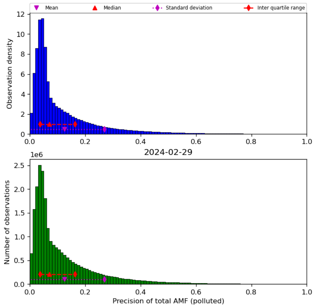
Figure 72: Histogram of “Precision of total AMF (polluted)” for 2024-02-28 to 2024-03-01
