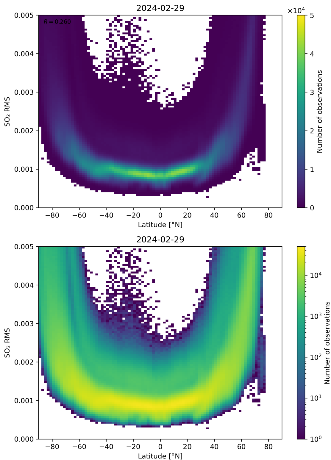
Figure 144: Scatter density plot of “Latitude” against “SO 2 RMS” for 2024-02-28 to 2024-03-01.
