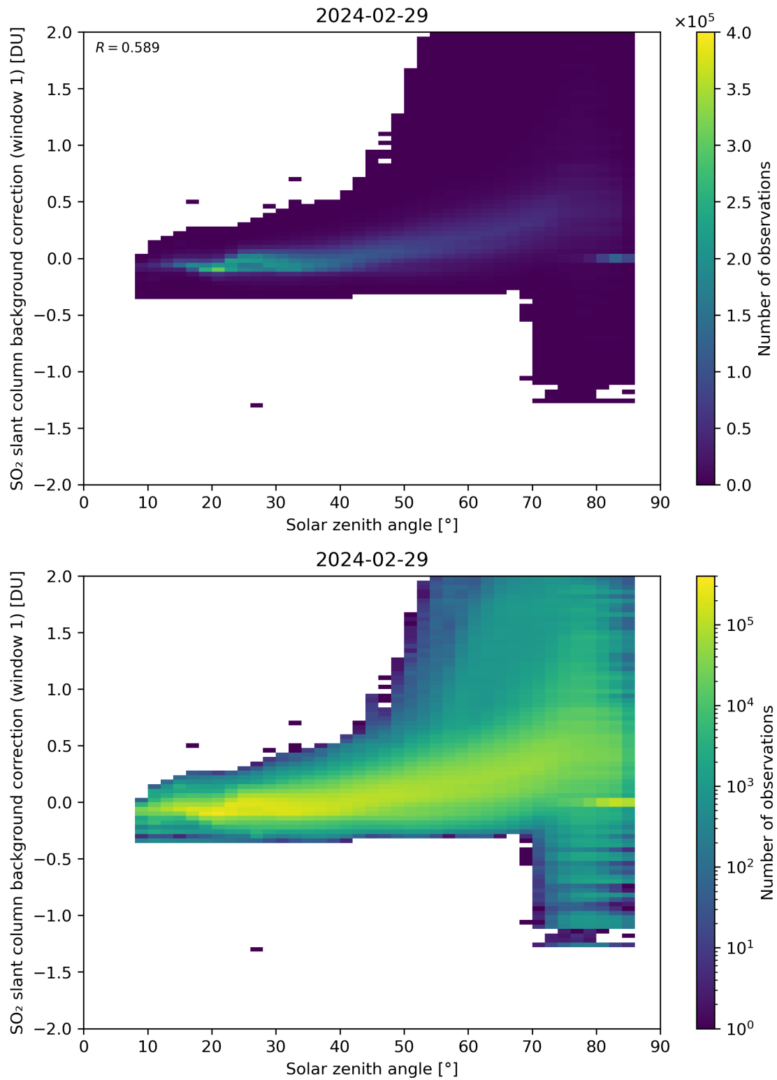
Figure 158: Scatter density plot of “Solar zenith angle” against “SO 2 slant column background correction (window 1)” for 2024-02-28 to 2024-03-01.
