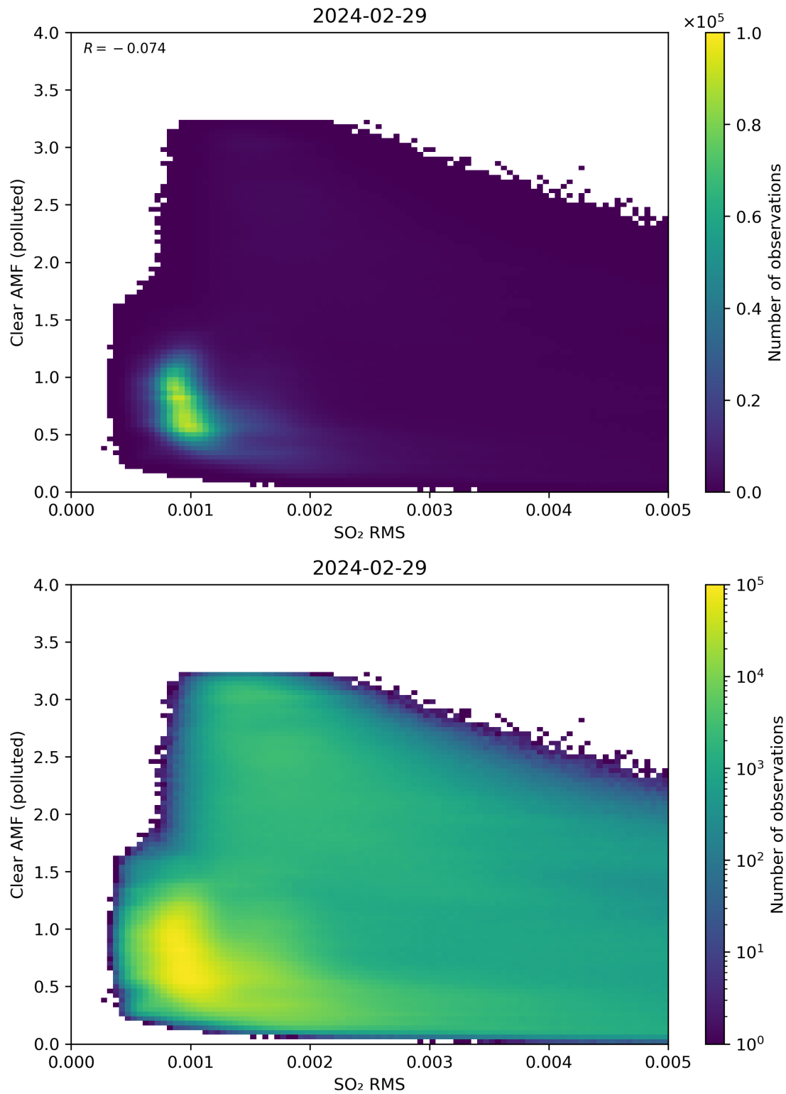
Figure 136: Scatter density plot of “SO 2 RMS” against “Clear AMF (polluted)” for 2024-02-28 to 2024-03-01.
