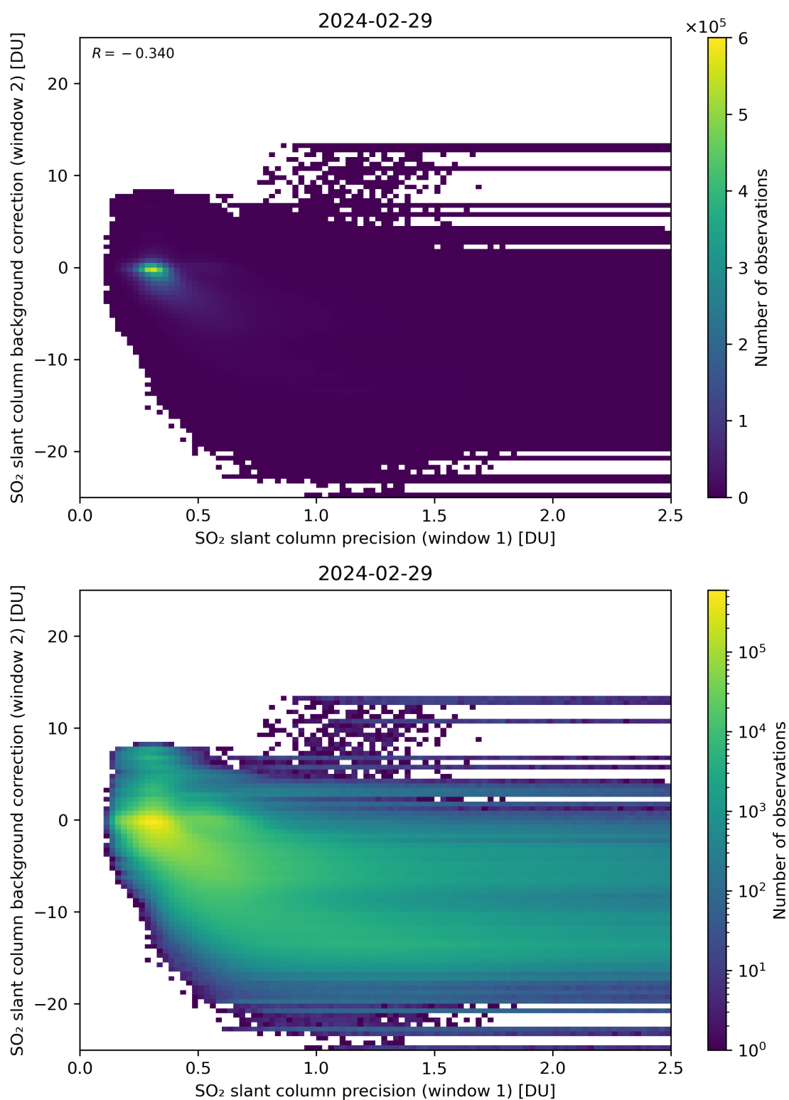
Figure 219: Scatter density plot of “SO 2 slant column precision (window 1)” against “SO 2 slant column background correction (window 2)” for 2024-02-28 to 2024-03-01.
