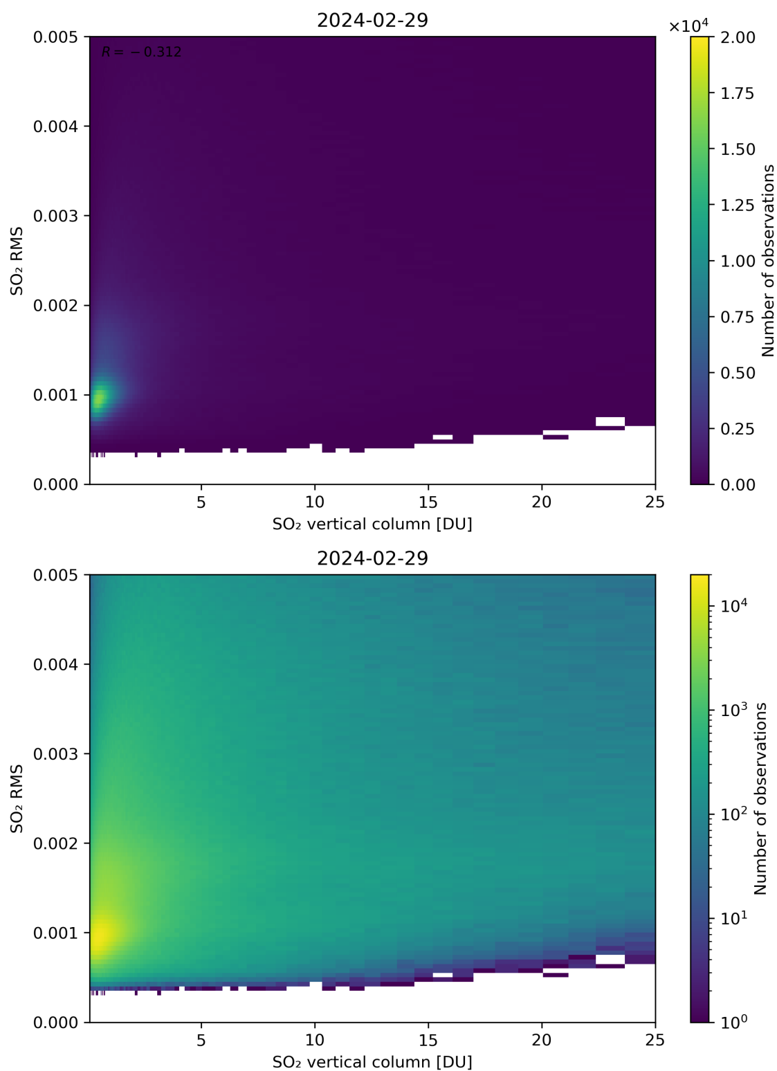
Figure 278: Scatter density plot of “SO 2 vertical column” against “SO 2 RMS” for 2024-02-28 to 2024-03-01.
