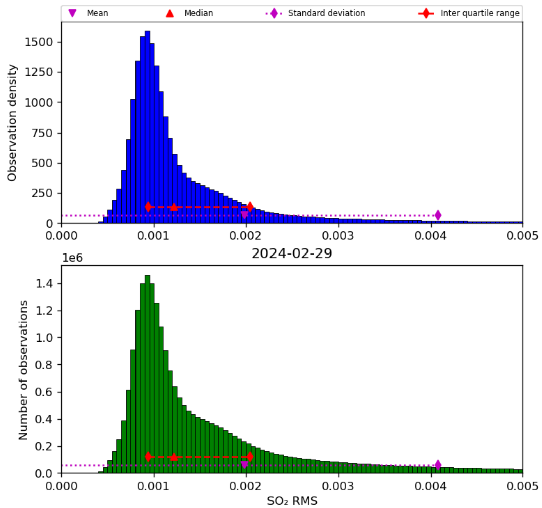
Figure 70: Histogram of “SO 2 RMS” for 2024-02-28 to 2024-03-01
