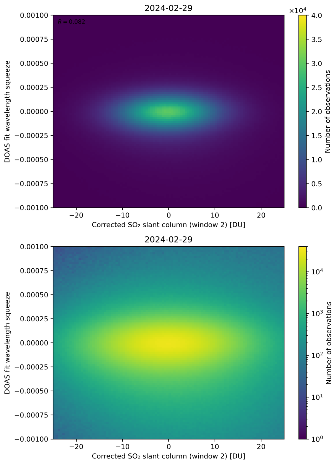
Figure 197: Scatter density plot of “Corrected SO 2 slant column (window 2)” against “DOAS fit wavelength squeeze” for 2024-02-28 to 2024-03-01.
