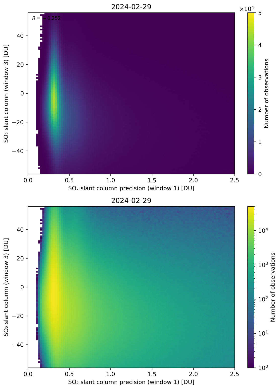
Figure 228: Scatter density plot of “SO 2 slant column precision (window 1)” against “SO 2 slant column (window 3)” for 2024-02-28 to 2024-03-01.
