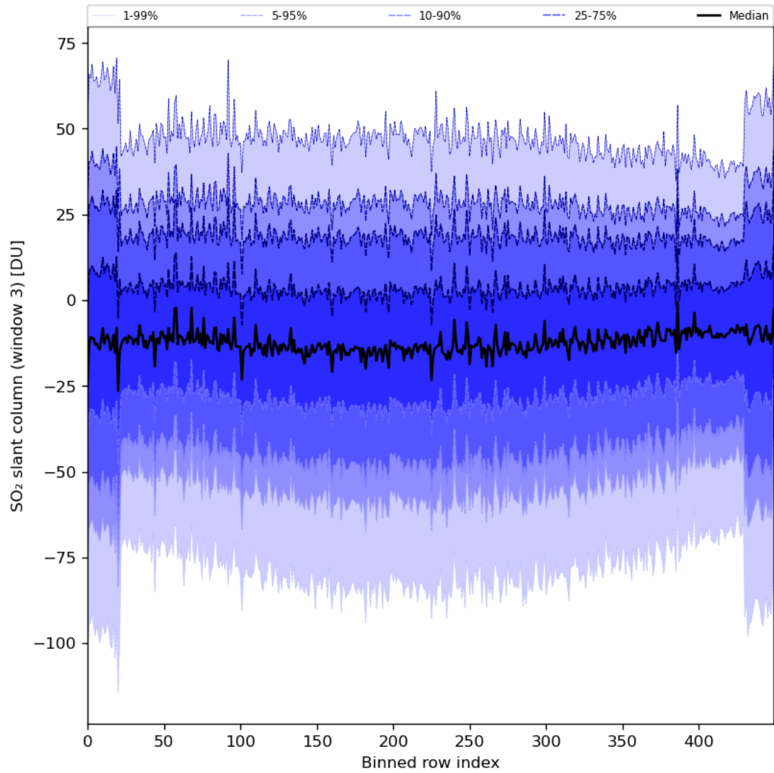
Figure 87: Along track statistics of “SO 2 slant column (window 3)” for 2024-02-28 to 2024-03-01
