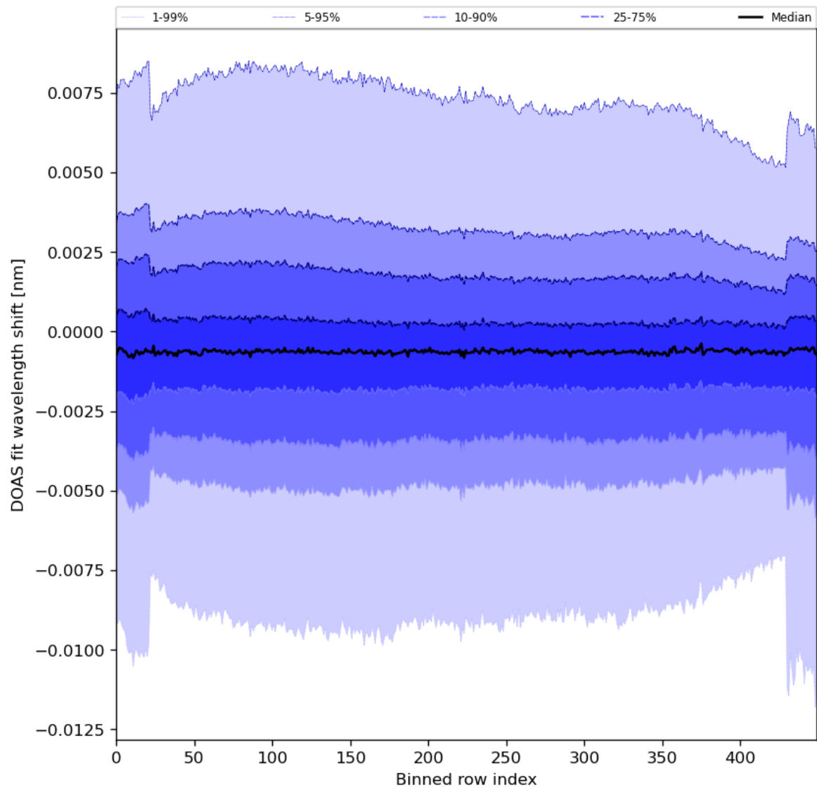
Figure 91: Along track statistics of “DOAS fit wavelength shift” for 2024-02-28 to 2024-03-01
