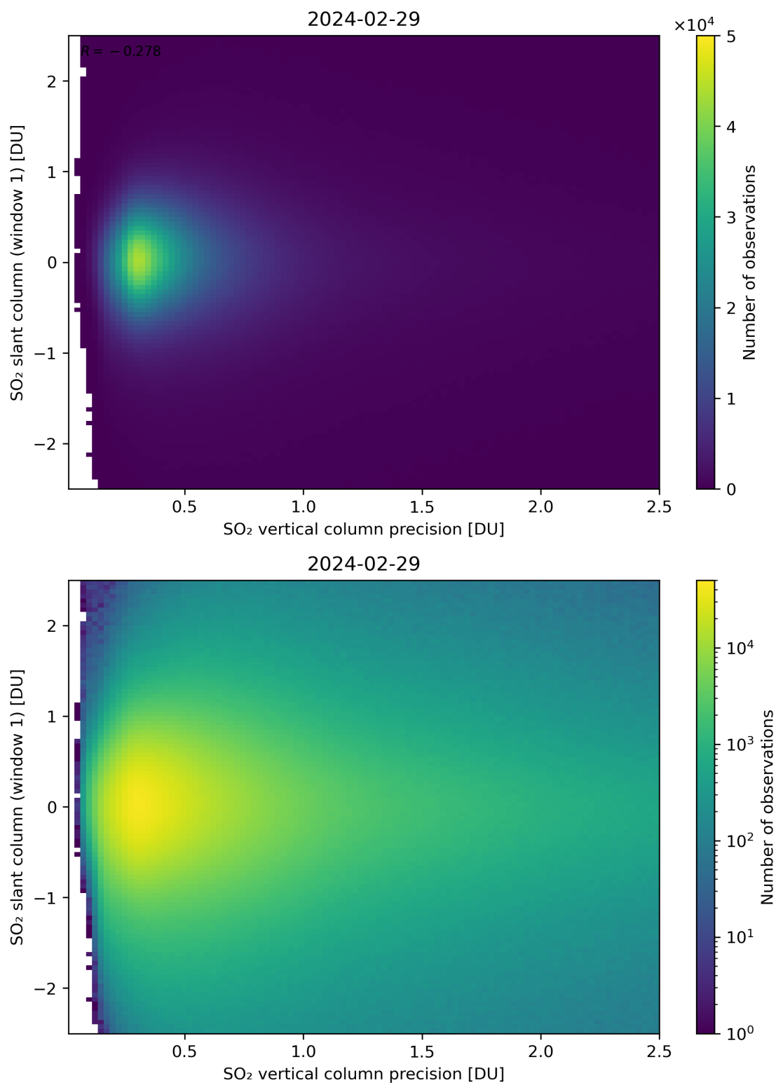
Figure 289: Scatter density plot of “SO 2 vertical column precision” against “SO 2 slant column (window 1)” for 2024-02-28 to 2024-03-01.
