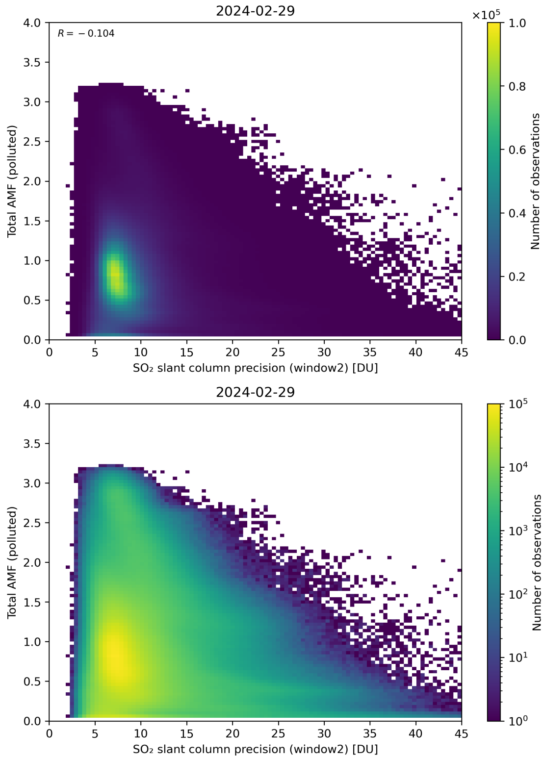
Figure 251: Scatter density plot of “SO 2 slant column precision (window2)” against “Total AMF (polluted)” for 2024-02-28 to 2024-03-01.
