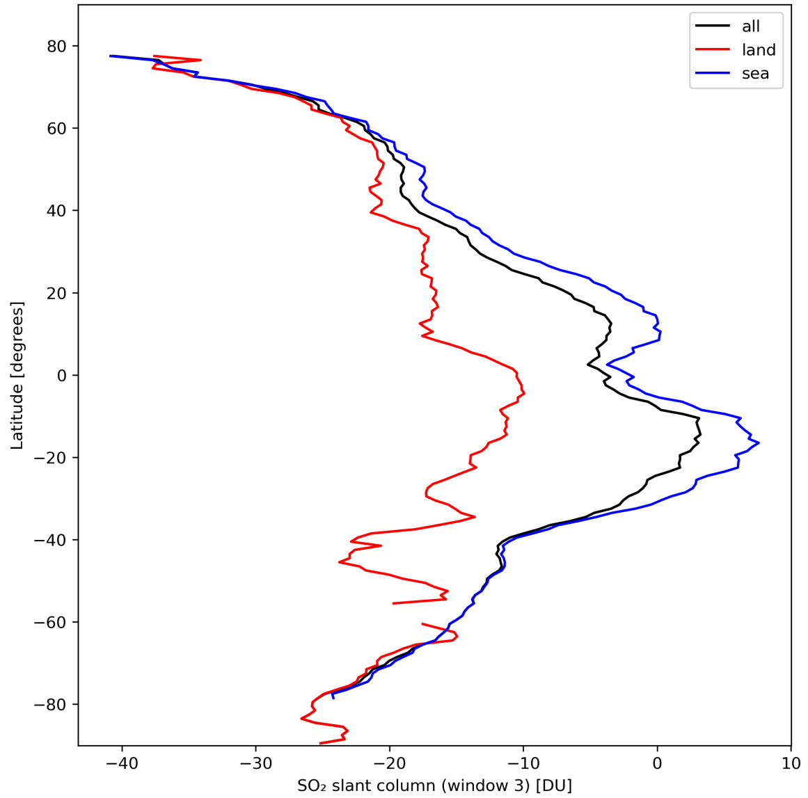
Figure 41: Zonal average of “SO 2 slant column (window 3)” for 2024-02-28 to 2024-03-01.
