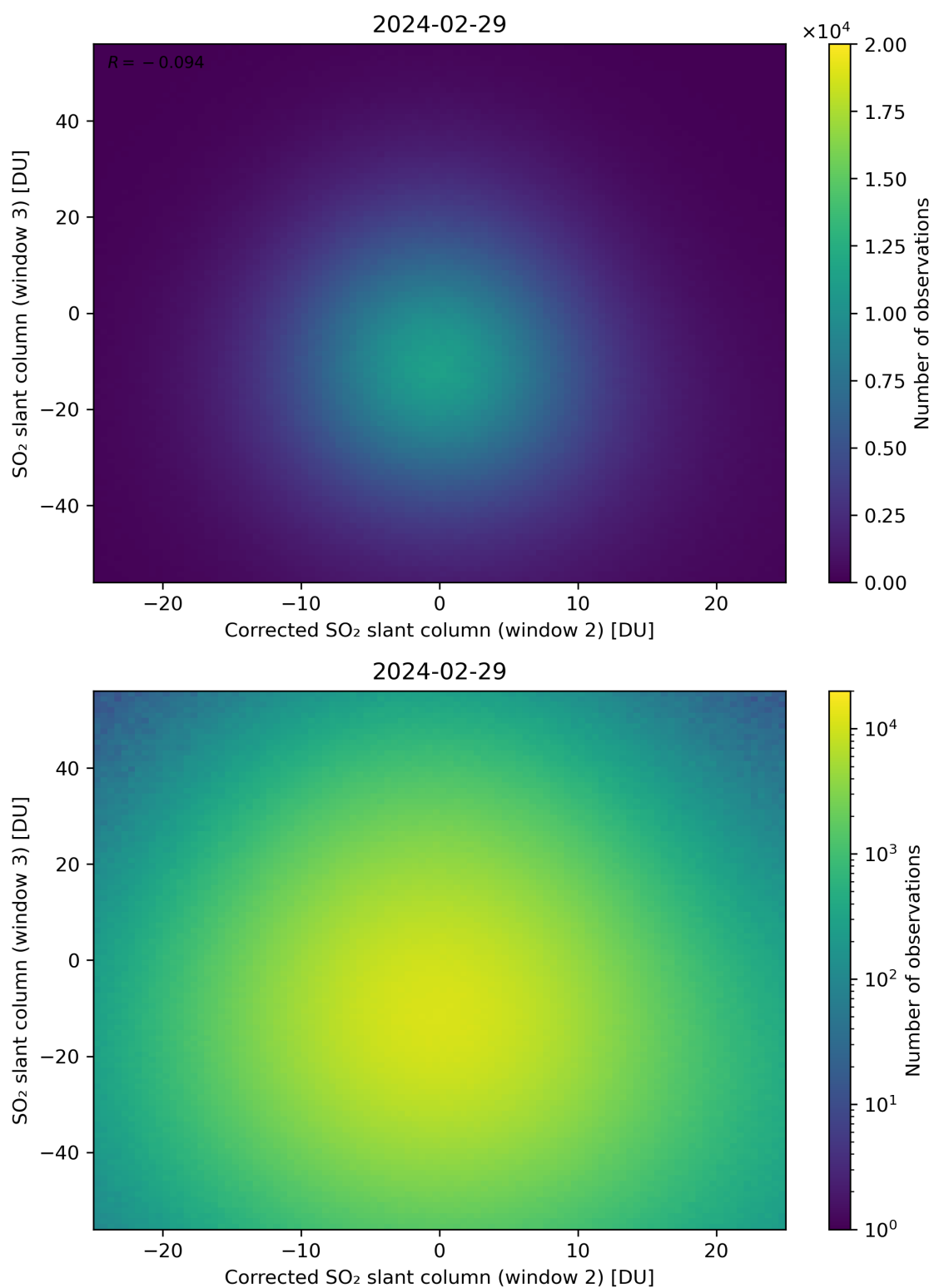
Figure 201: Scatter density plot of “Corrected SO 2 slant column (window 2)” against “SO 2 slant column (window 3)” for 2024-02-28 to 2024-03-01.
