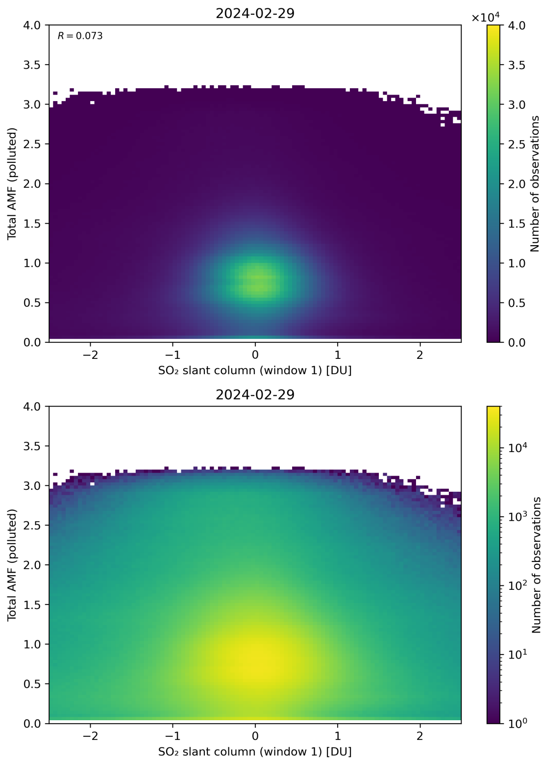
Figure 239: Scatter density plot of “SO 2 slant column (window 1)” against “Total AMF (polluted)” for 2024-02-28 to 2024-03-01.
