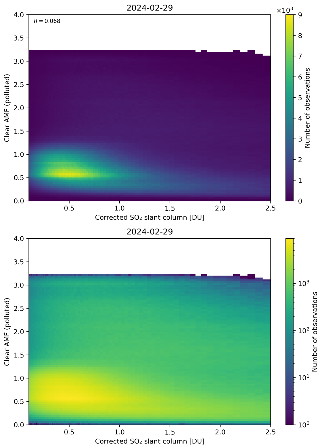
Figure 184: Scatter density plot of “Corrected SO 2 slant column” against “Clear AMF (polluted)” for 2024-02-28 to 2024-03-01.
