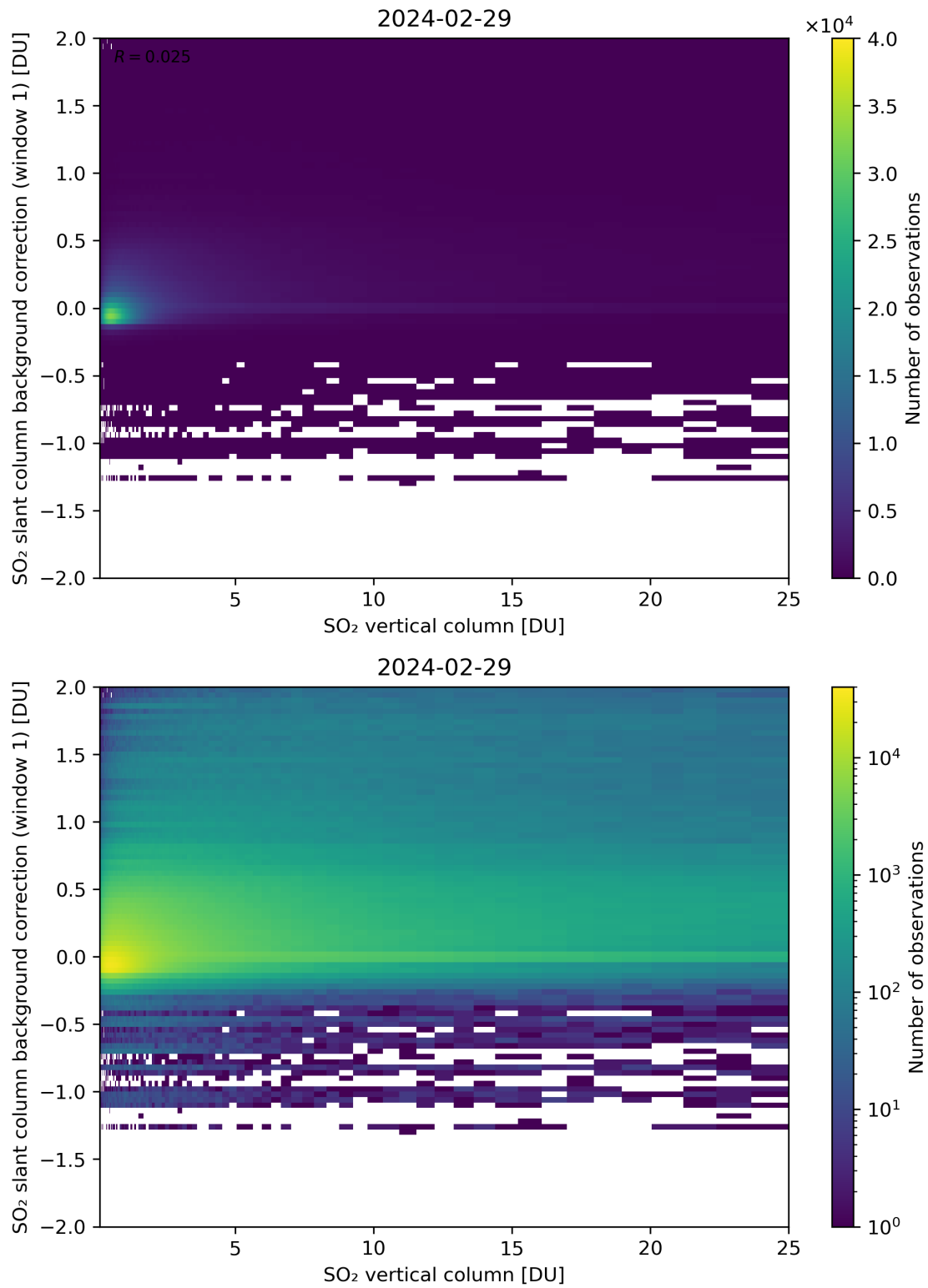
Figure 273: Scatter density plot of “SO 2 vertical column” against “SO 2 slant column background correction (window 1)” for 2024-02-28 to 2024-03-01.
