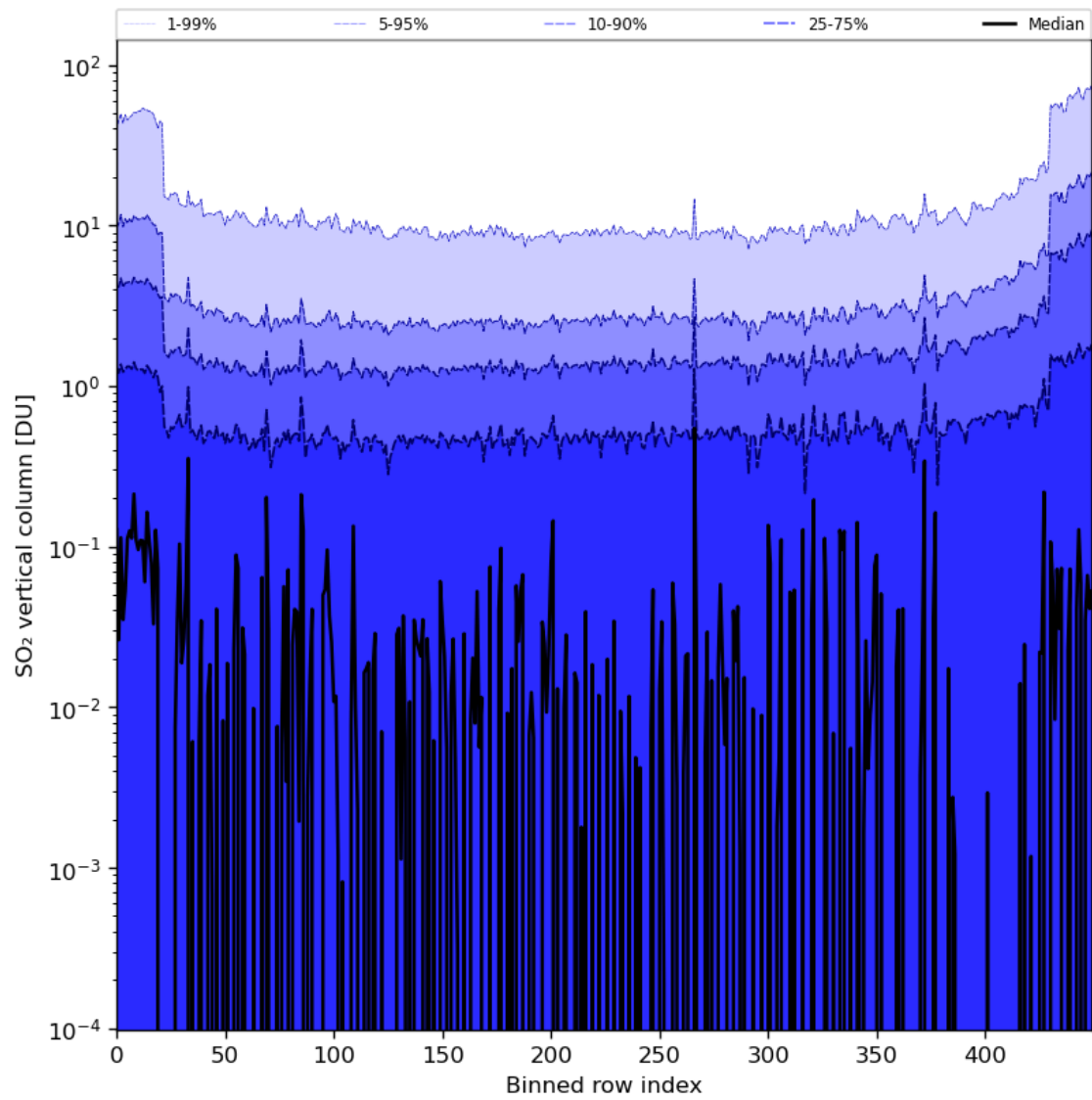
Figure 76: Along track statistics of “SO 2 vertical column” for 2024-02-28 to 2024-03-01
