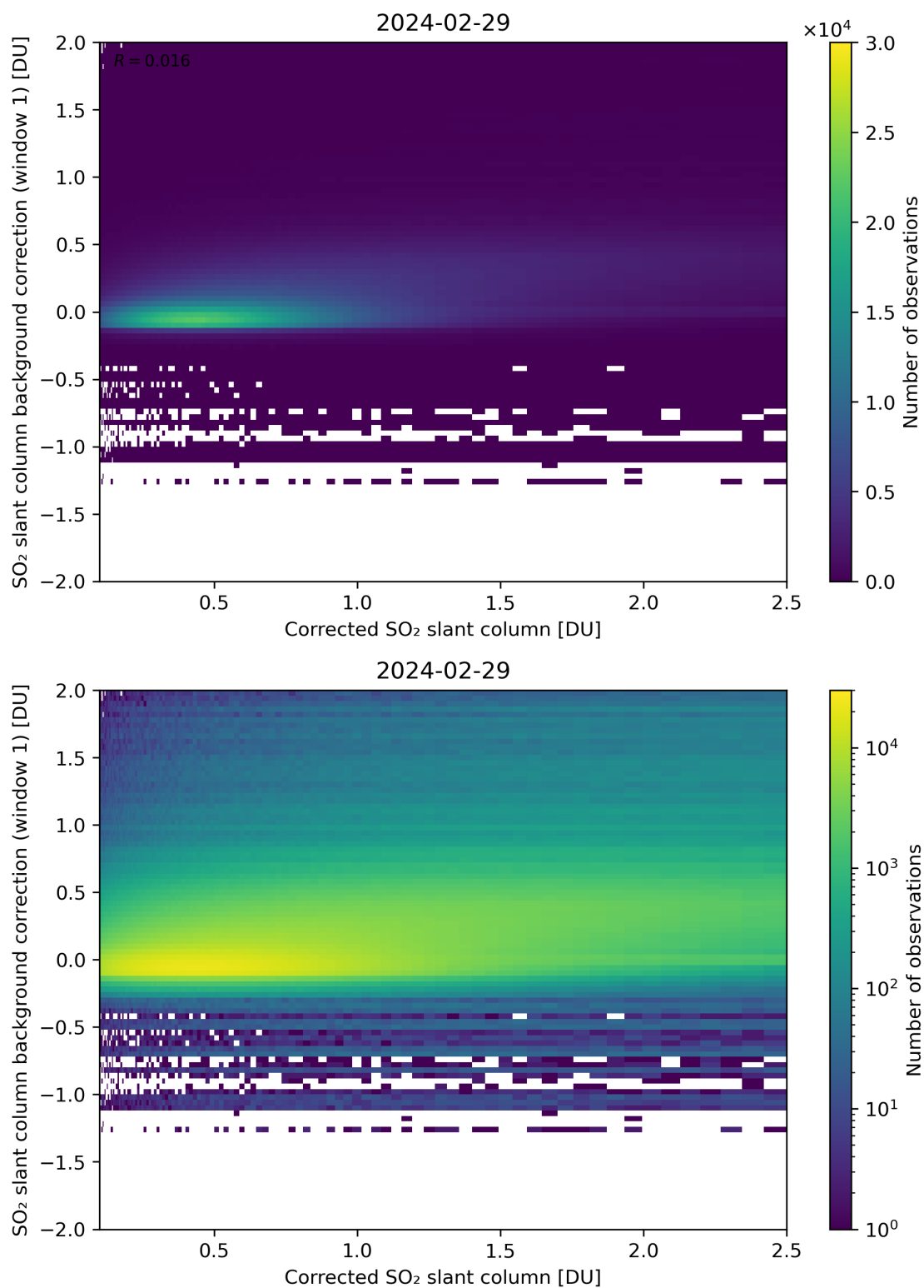
Figure 178: Scatter density plot of “Corrected SO 2 slant column” against “SO 2 slant column background correction (window 1)” for 2024-02-28 to 2024-03-01.
