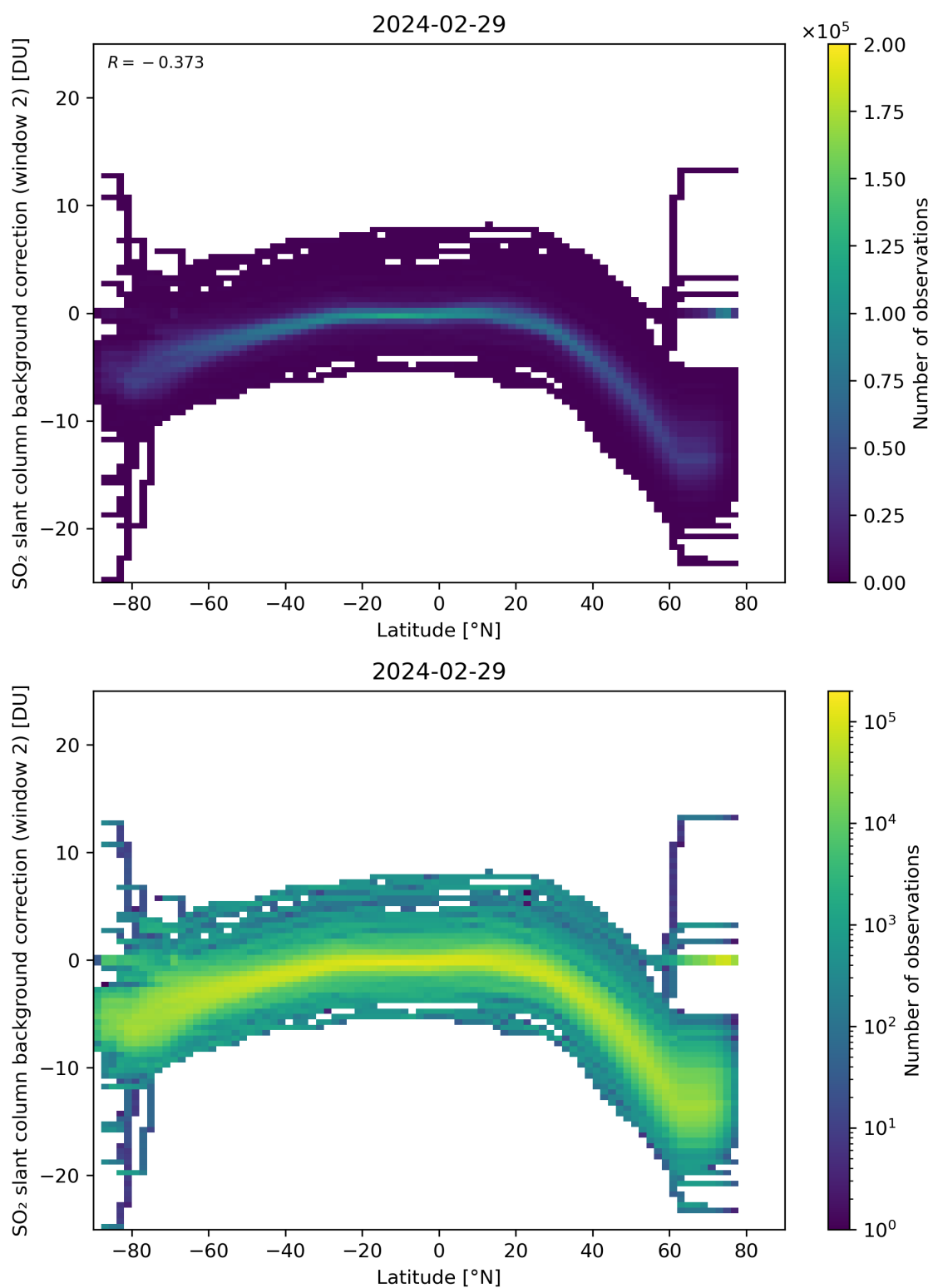
Figure 140: Scatter density plot of “Latitude” against “SO 2 slant column background correction (window 2)” for 2024-02-28 to 2024-03-01.
