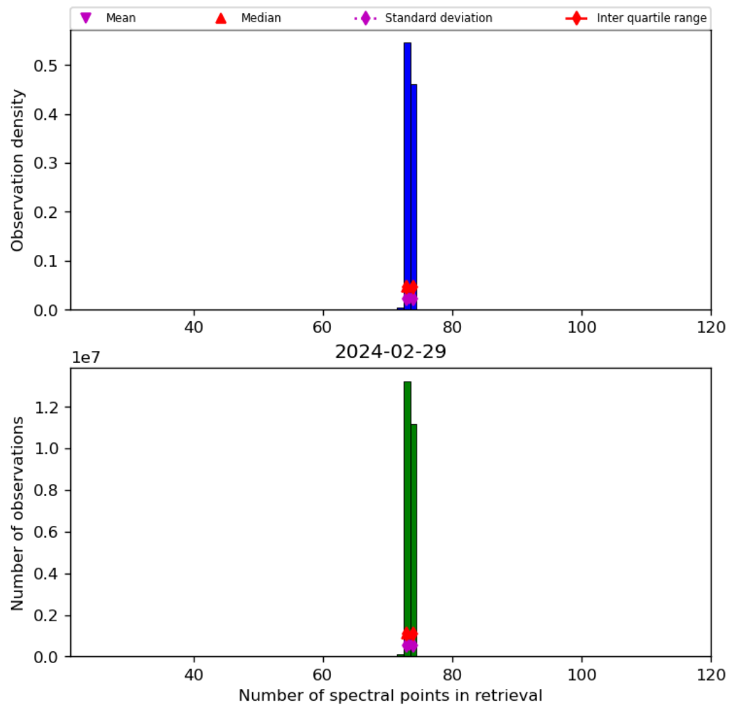
Figure 74: Histogram of “Number of spectral points in retrieval” for 2024-02-28 to 2024-03-01
