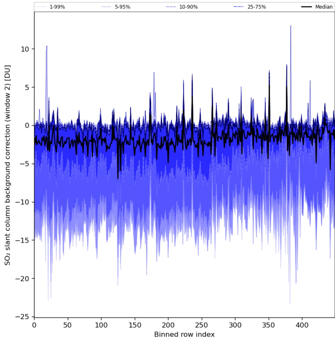
Figure 86: Along track statistics of “SO 2 slant column background correction (window 2)” for 2024-02-28 to 2024-03-01
