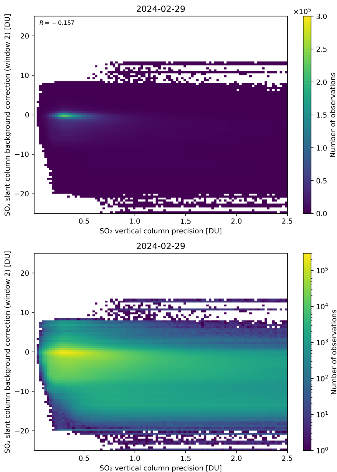
Figure 280: Scatter density plot of “SO 2 vertical column precision” against “SO 2 slant column background correction (window 2)” for 2024-02-28 to 2024-03-01.
