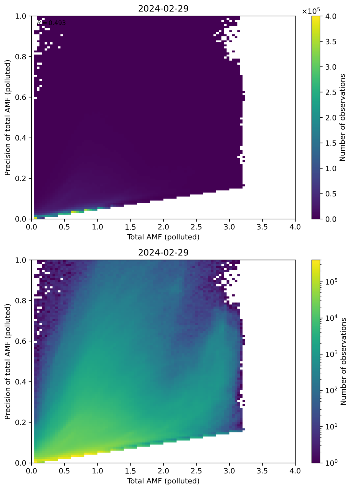
Figure 272: Scatter density plot of “Total AMF (polluted)” against “Precision of total AMF (polluted)” for 2024-02-28 to 2024-03-01.
