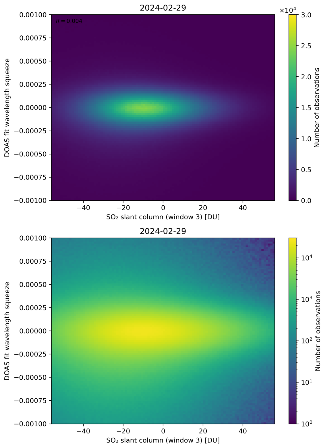
Figure 255: Scatter density plot of “SO 2 slant column (window 3)” against “DOAS fit wavelength squeeze” for 2024-02-28 to 2024-03-01.
