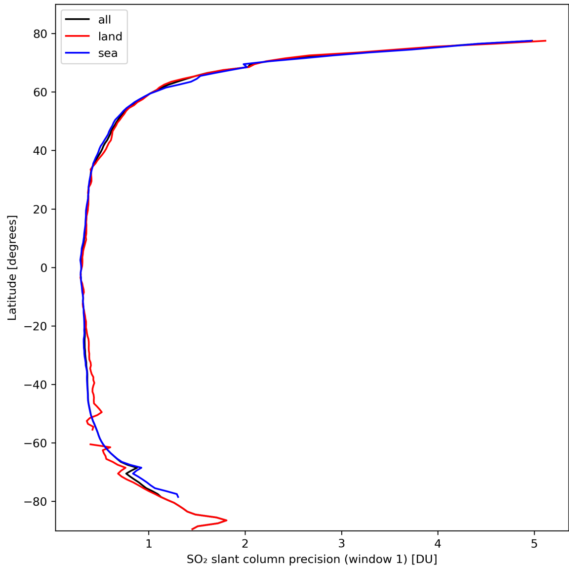
Figure 34: Zonal average of “SO 2 slant column precision (window 1)” for 2024-02-28 to 2024-03-01.
