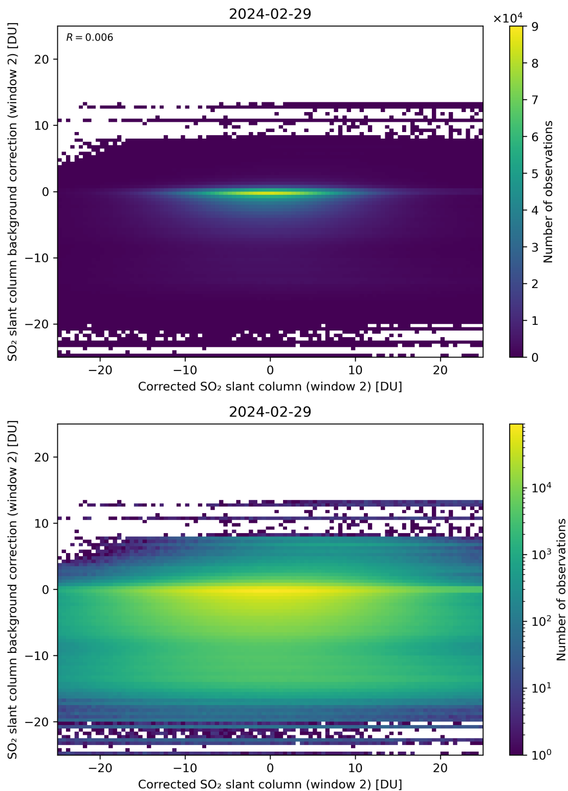
Figure 194: Scatter density plot of “Corrected SO 2 slant column (window 2)” against “SO 2 slant column background correction (window 2)” for 2024-02-28 to 2024-03-01.
