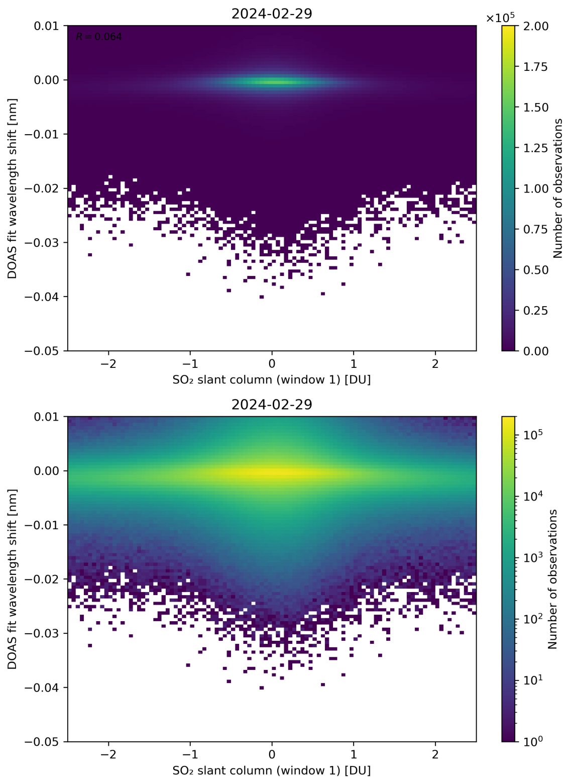
Figure 215: Scatter density plot of “SO 2 slant column (window 1)” against “DOAS fit wavelength shift” for 2024-02-28 to 2024-03-01.
