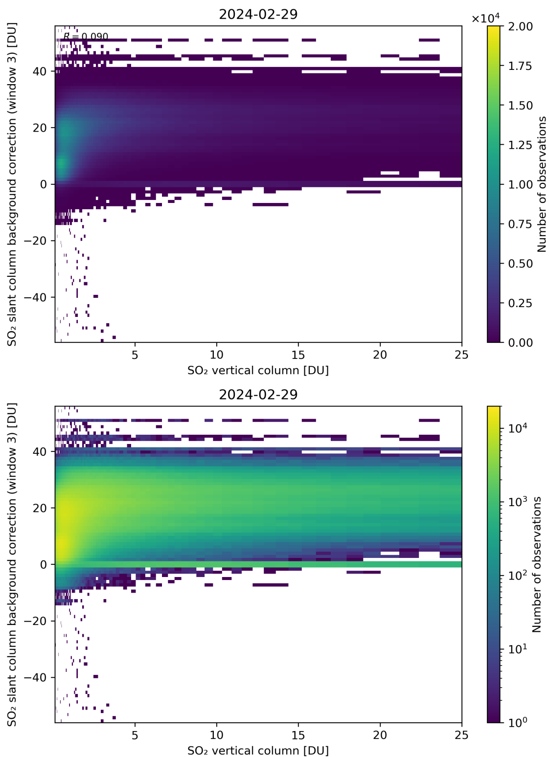
Figure 275: Scatter density plot of “SO 2 vertical column” against “SO 2 slant column background correction (window 3)” for 2024-02-28 to 2024-03-01.
