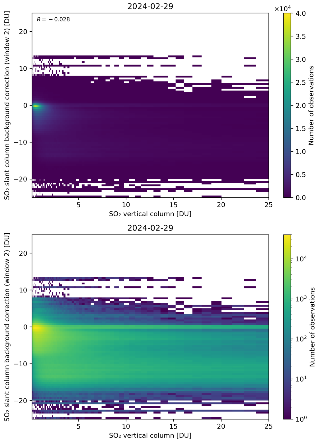
Figure 274: Scatter density plot of “SO 2 vertical column” against “SO 2 slant column background correction (window 2)” for 2024-02-28 to 2024-03-01.
