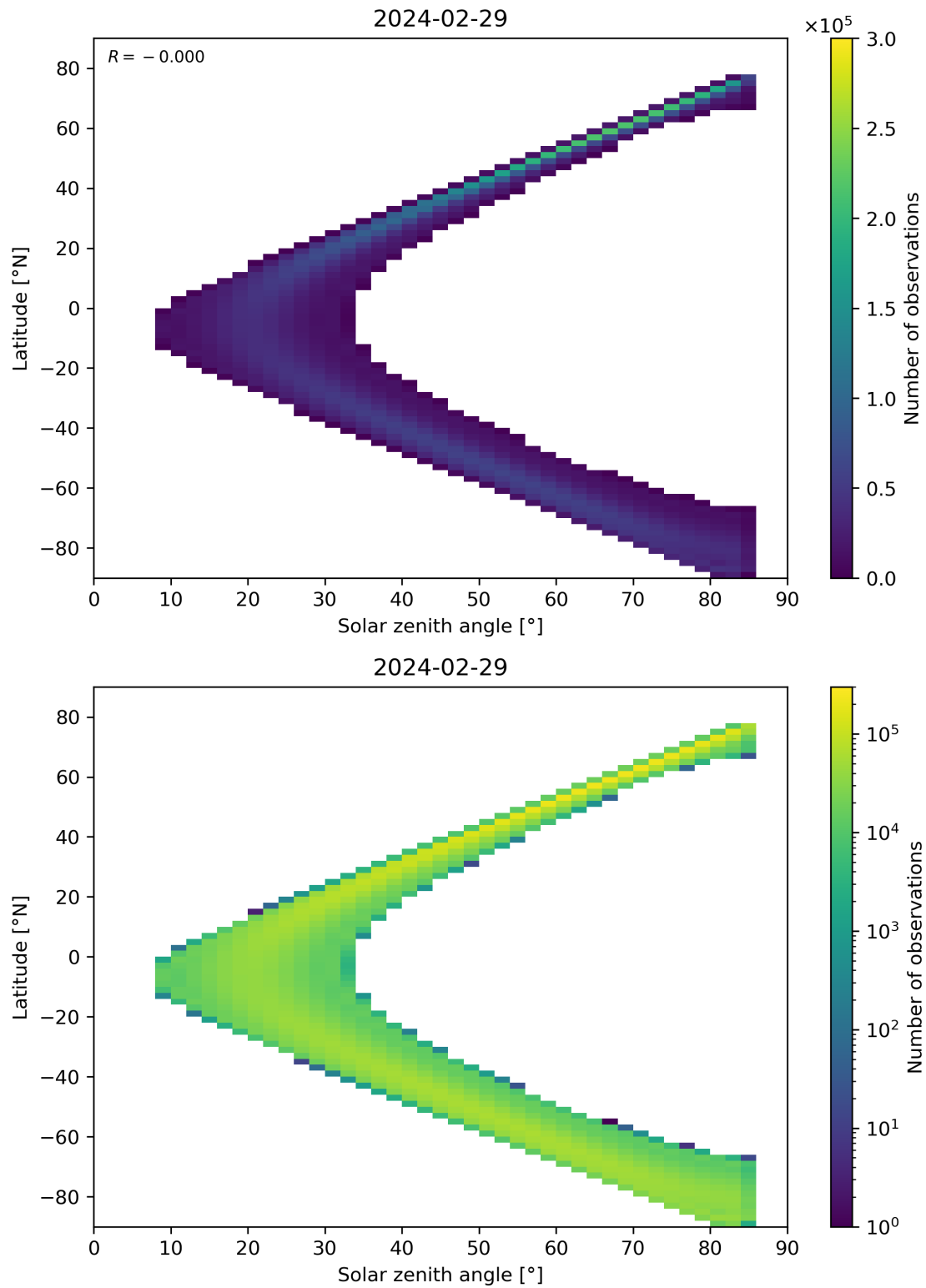
Figure 164: Scatter density plot of “Solar zenith angle” against “Latitude” for 2024-02-28 to 2024-03-01.
