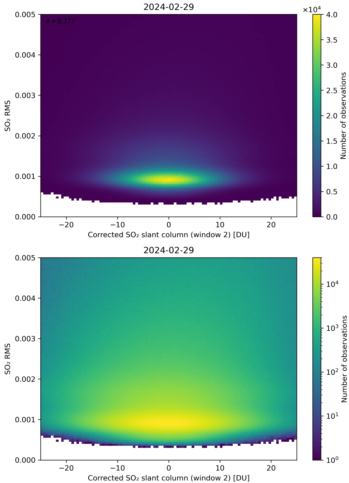
Figure 198: Scatter density plot of “Corrected SO 2 slant column (window 2)” against “SO 2 RMS” for 2024-02-28 to 2024-03-01.
