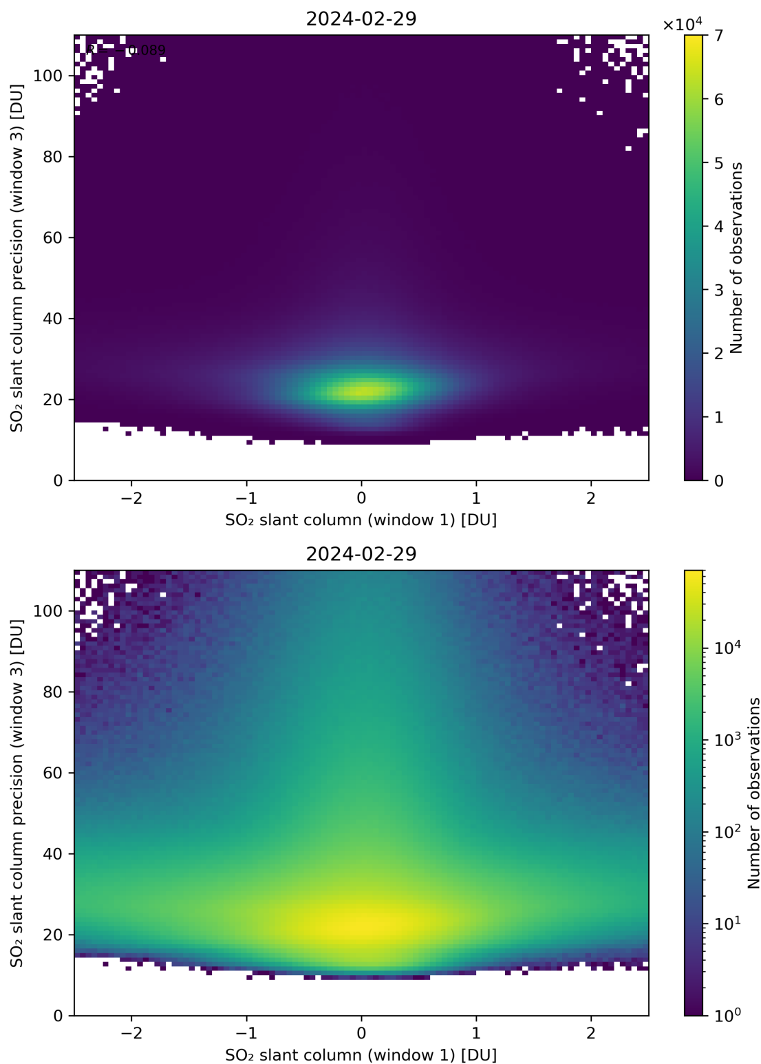
Figure 238: Scatter density plot of “SO 2 slant column (window 1)” against “SO 2 slant column precision (window 3)” for 2024-02-28 to 2024-03-01.
