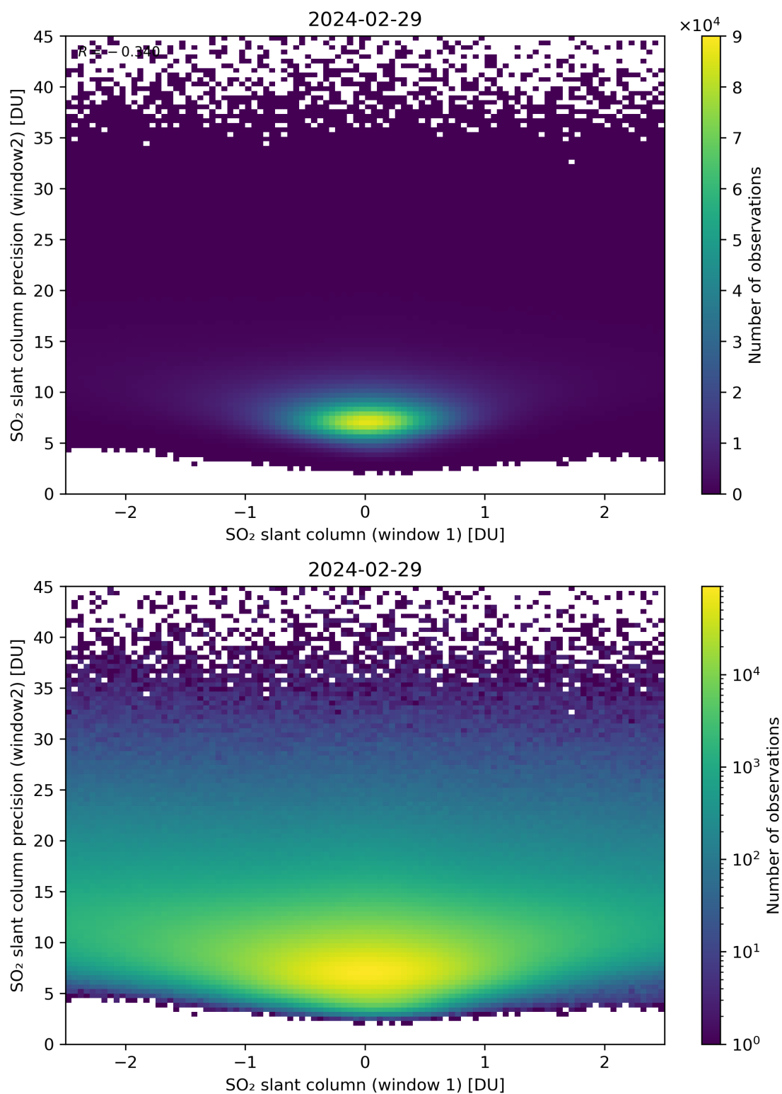
Figure 236: Scatter density plot of “SO 2 slant column (window 1)” against “SO 2 slant column precision (window2)” for 2024-02-28 to 2024-03-01.
