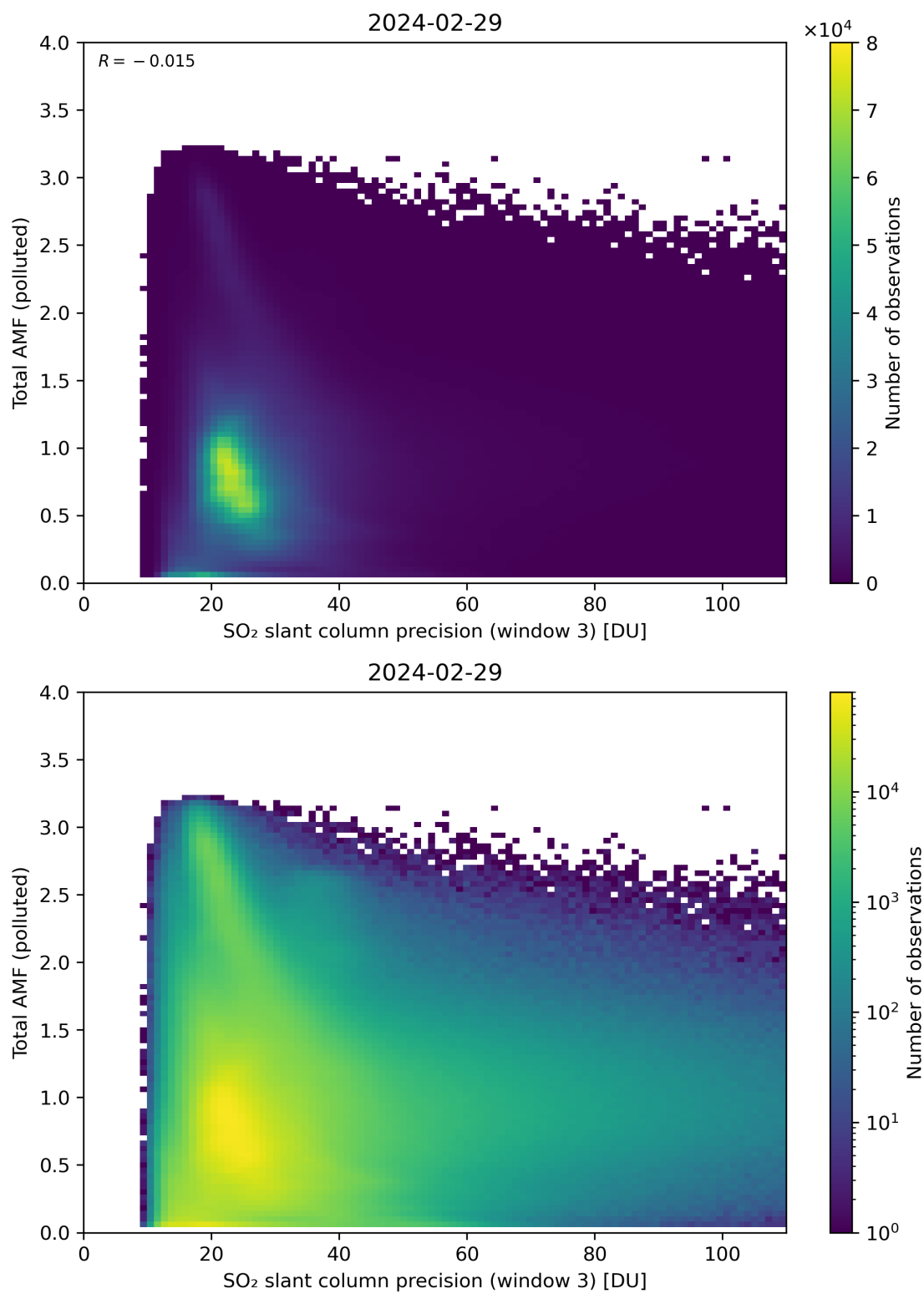
Figure 263: Scatter density plot of “SO 2 slant column precision (window 3)” against “Total AMF (polluted)” for 2024-02-28 to 2024-03-01.
