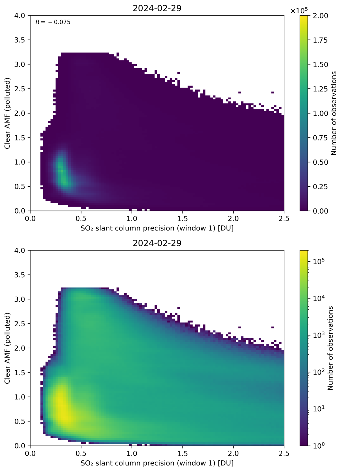
Figure 224: Scatter density plot of “SO 2 slant column precision (window 1)” against “Clear AMF (polluted)” for 2024-02-28 to 2024-03-01.
