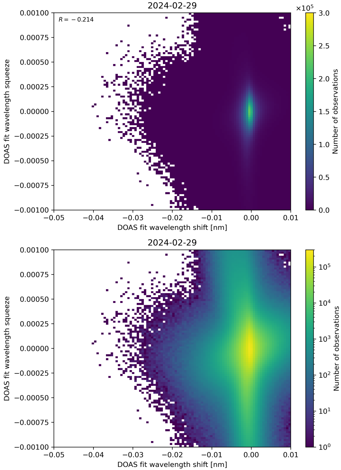
Figure 127: Scatter density plot of “DOAS fit wavelength shift” against “DOAS fit wavelength squeeze” for 2024-02-28 to 2024-03-01.
