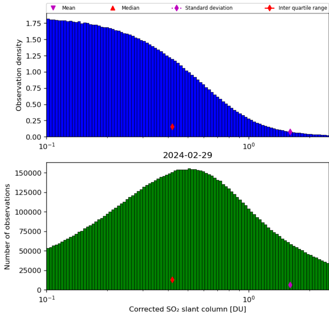
Figure 55: Histogram of “Corrected SO 2 slant column” for 2024-02-28 to 2024-03-01
