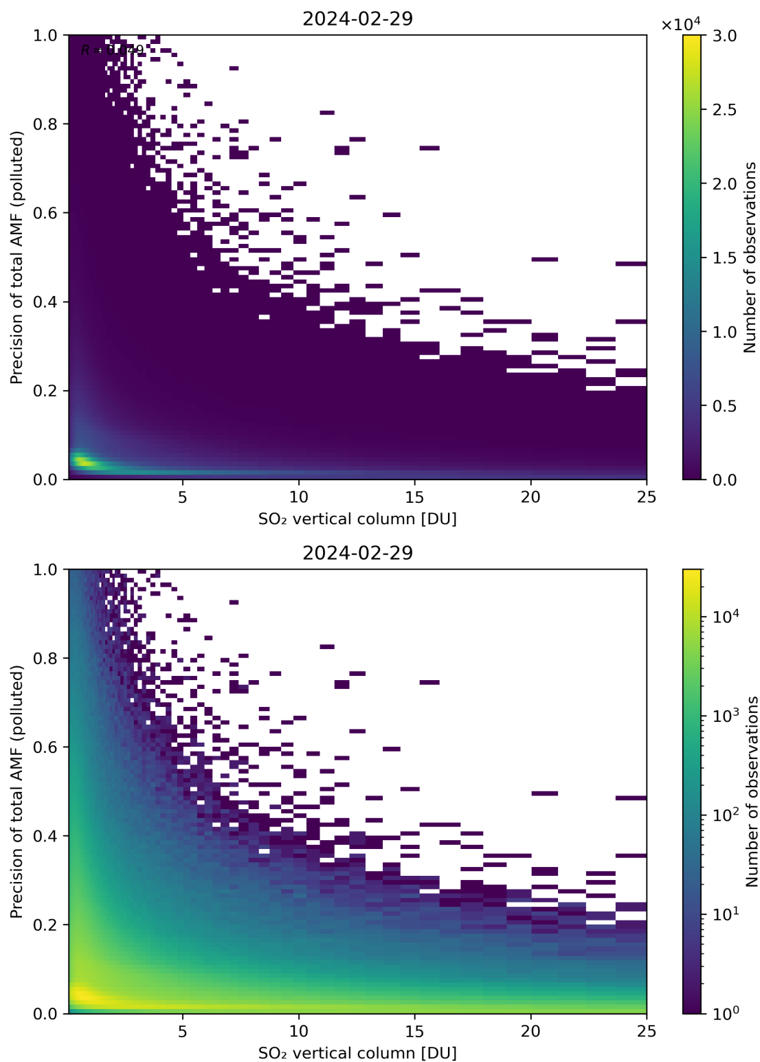
Figure 306: Scatter density plot of “SO 2 vertical column” against “Precision of total AMF (polluted)” for 2024-02-28 to 2024-03-01.
