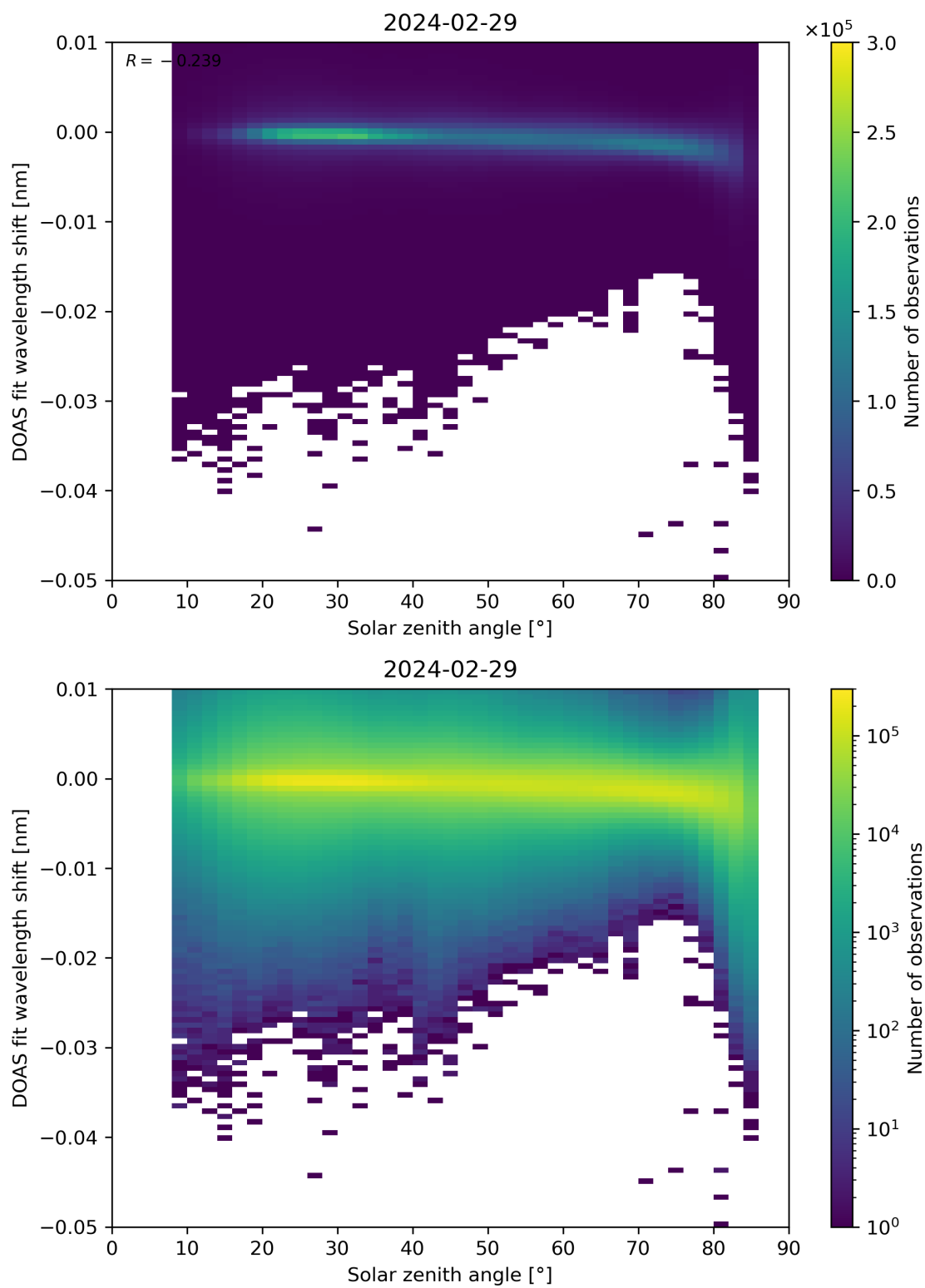
Figure 161: Scatter density plot of “Solar zenith angle” against “DOAS fit wavelength shift” for 2024-02-28 to 2024-03-01.
