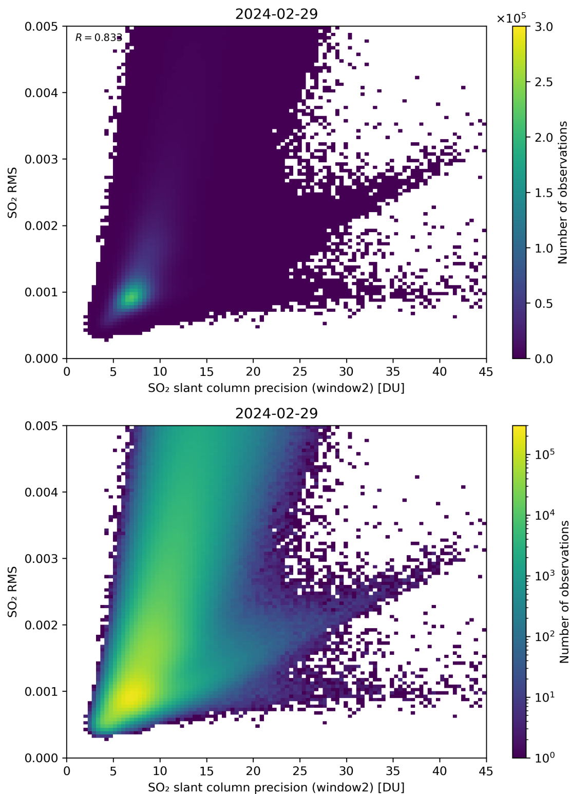
Figure 245: Scatter density plot of “SO 2 slant column precision (window2)” against “SO 2 RMS” for 2024-02-28 to 2024-03-01.
