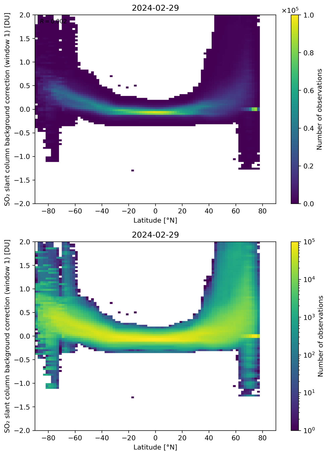
Figure 139: Scatter density plot of “Latitude” against “SO 2 slant column background correction (window 1)” for 2024-02-28 to 2024-03-01.
