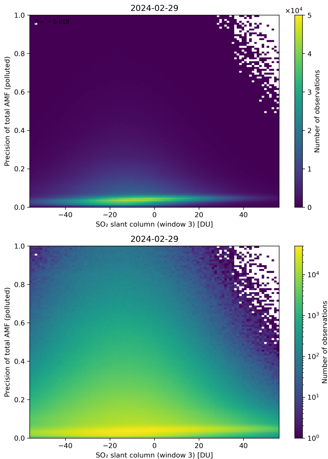
Figure 269: Scatter density plot of “SO 2 slant column (window 3)” against “Precision of total AMF (polluted)” for 2024-02-28 to 2024-03-01.
