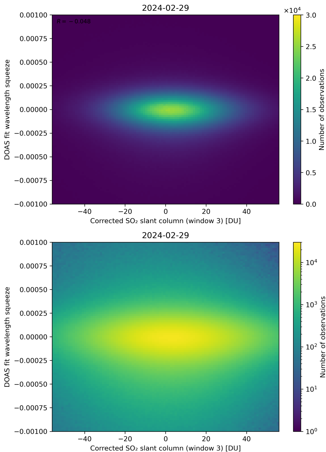
Figure 207: Scatter density plot of “Corrected SO 2 slant column (window 3)” against “DOAS fit wavelength squeeze” for 2024-02-28 to 2024-03-01.
