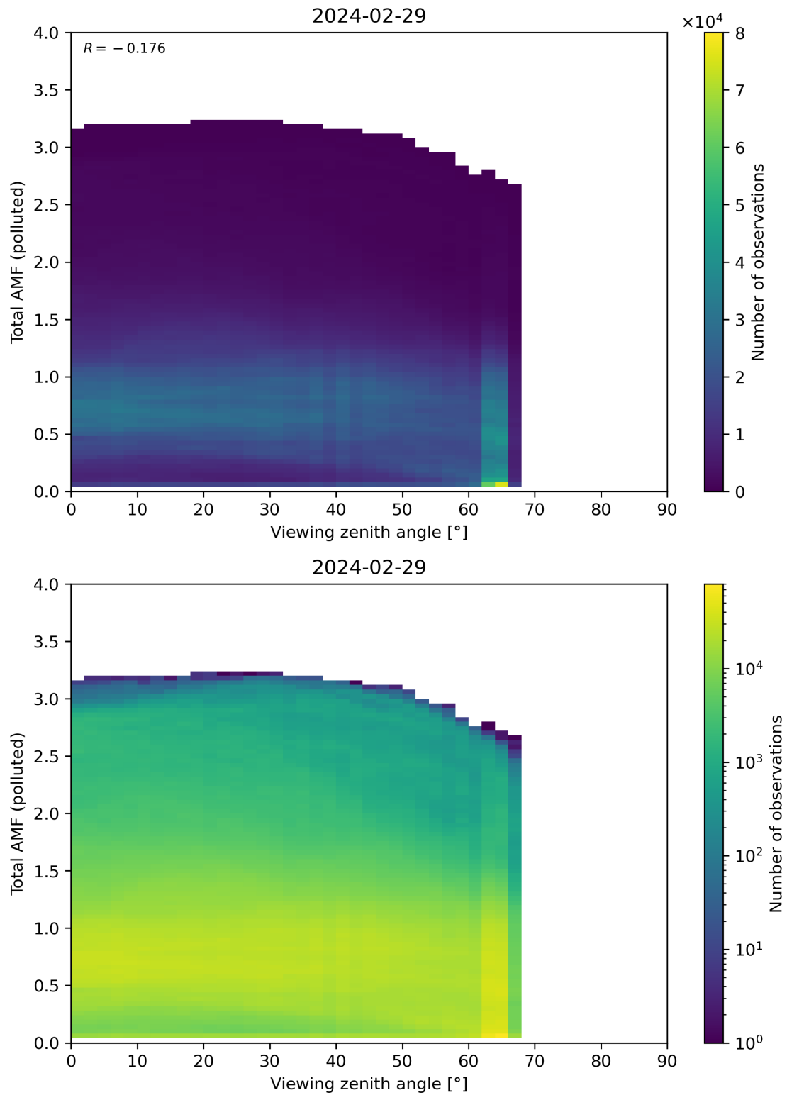
Figure 325: Scatter density plot of “Viewing zenith angle” against “Total AMF (polluted)” for 2024-02-28 to 2024-03-01.
