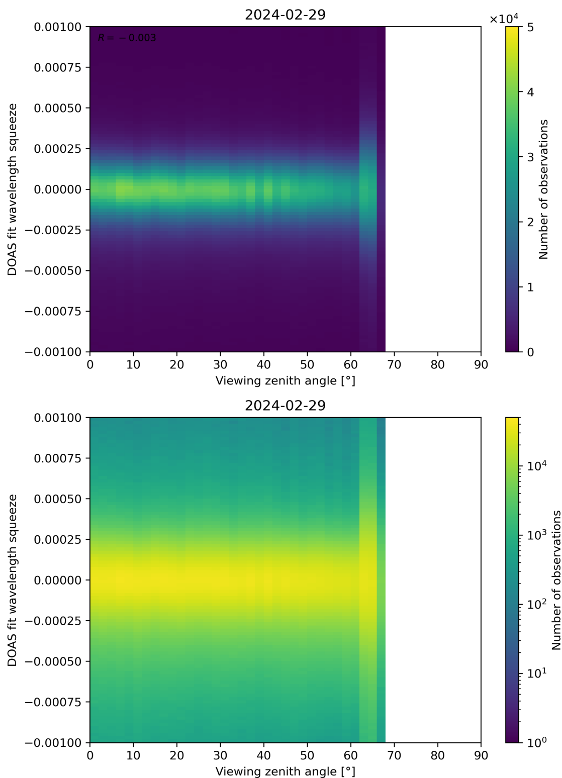
Figure 312: Scatter density plot of “Viewing zenith angle” against “DOAS fit wavelength squeeze” for 2024-02-28 to 2024-03-01.
