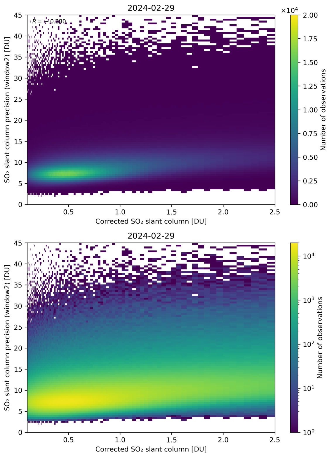
Figure 189: Scatter density plot of “Corrected SO 2 slant column” against “SO 2 slant column precision (window2)” for 2024-02-28 to 2024-03-01.
