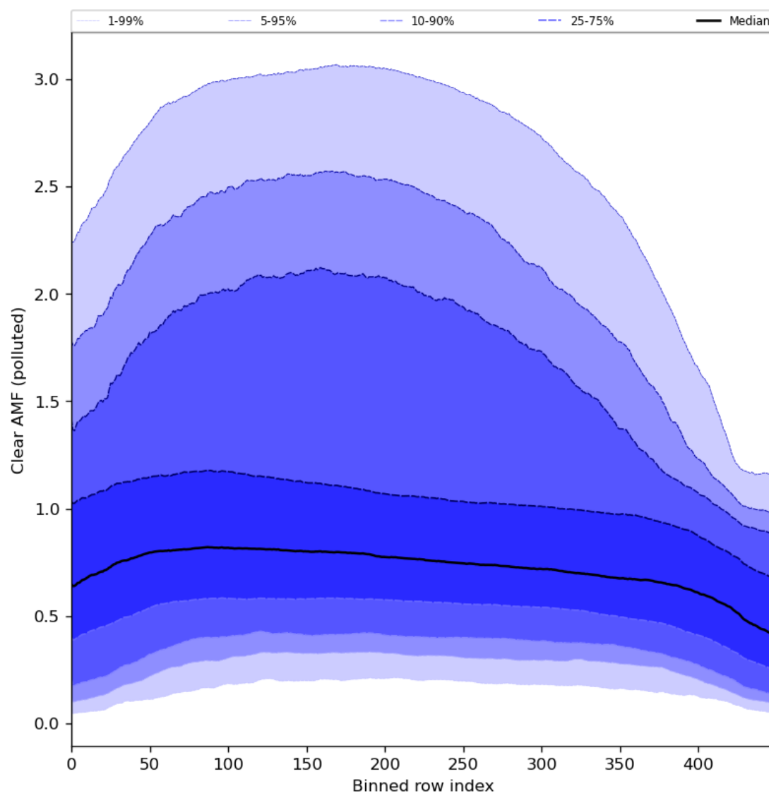
Figure 96: Along track statistics of “Clear AMF (polluted)” for 2024-02-28 to 2024-03-01
