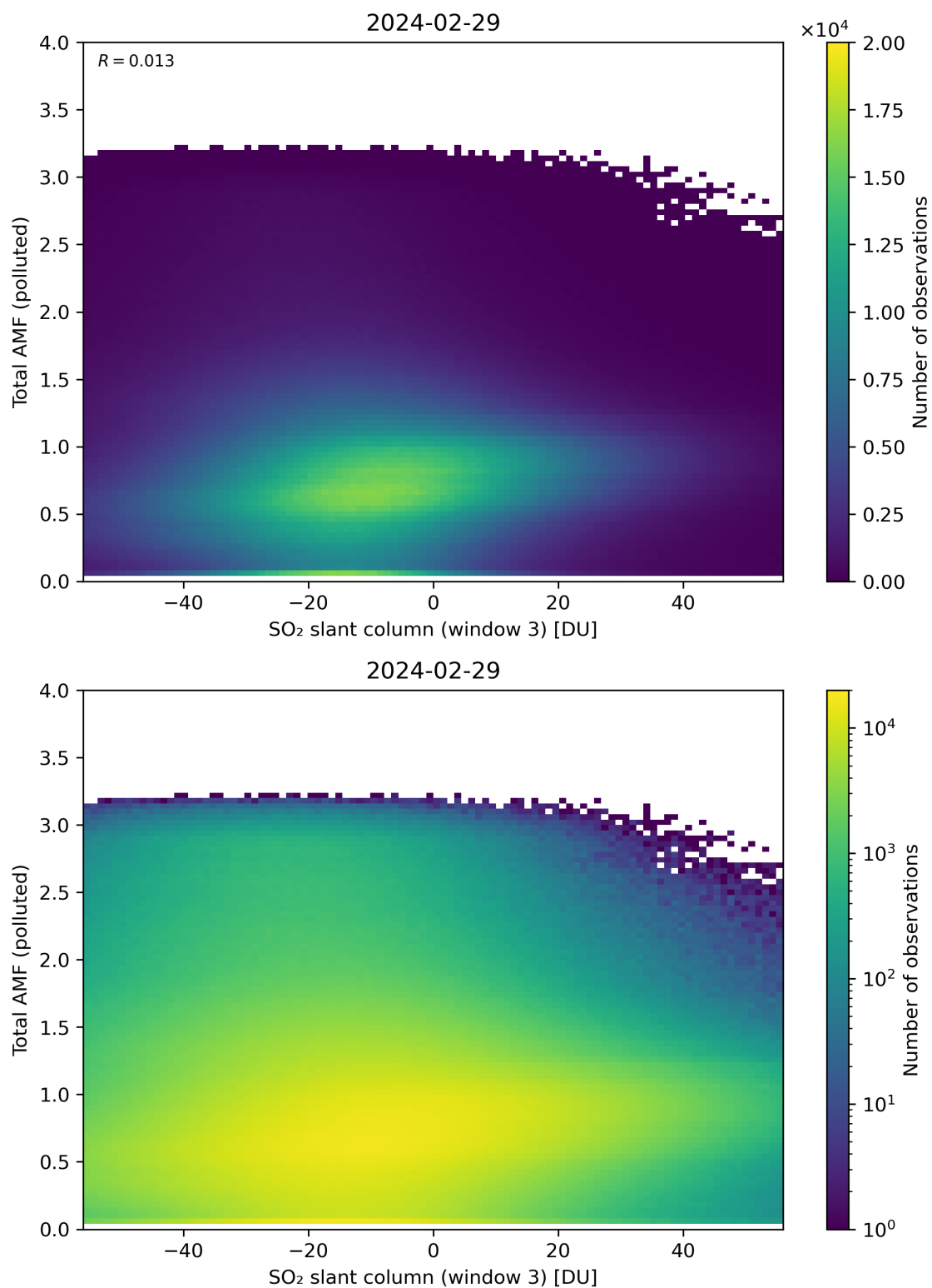
Figure 268: Scatter density plot of “SO 2 slant column (window 3)” against “Total AMF (polluted)” for 2024-02-28 to 2024-03-01.
