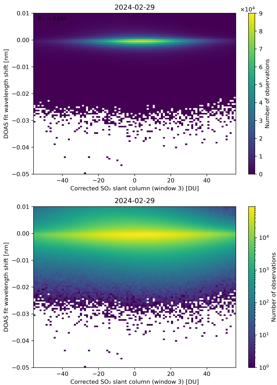
Figure 206: Scatter density plot of “Corrected SO 2 slant column (window 3)” against “DOAS fit wavelength shift” for 2024-02-28 to 2024-03-01.
