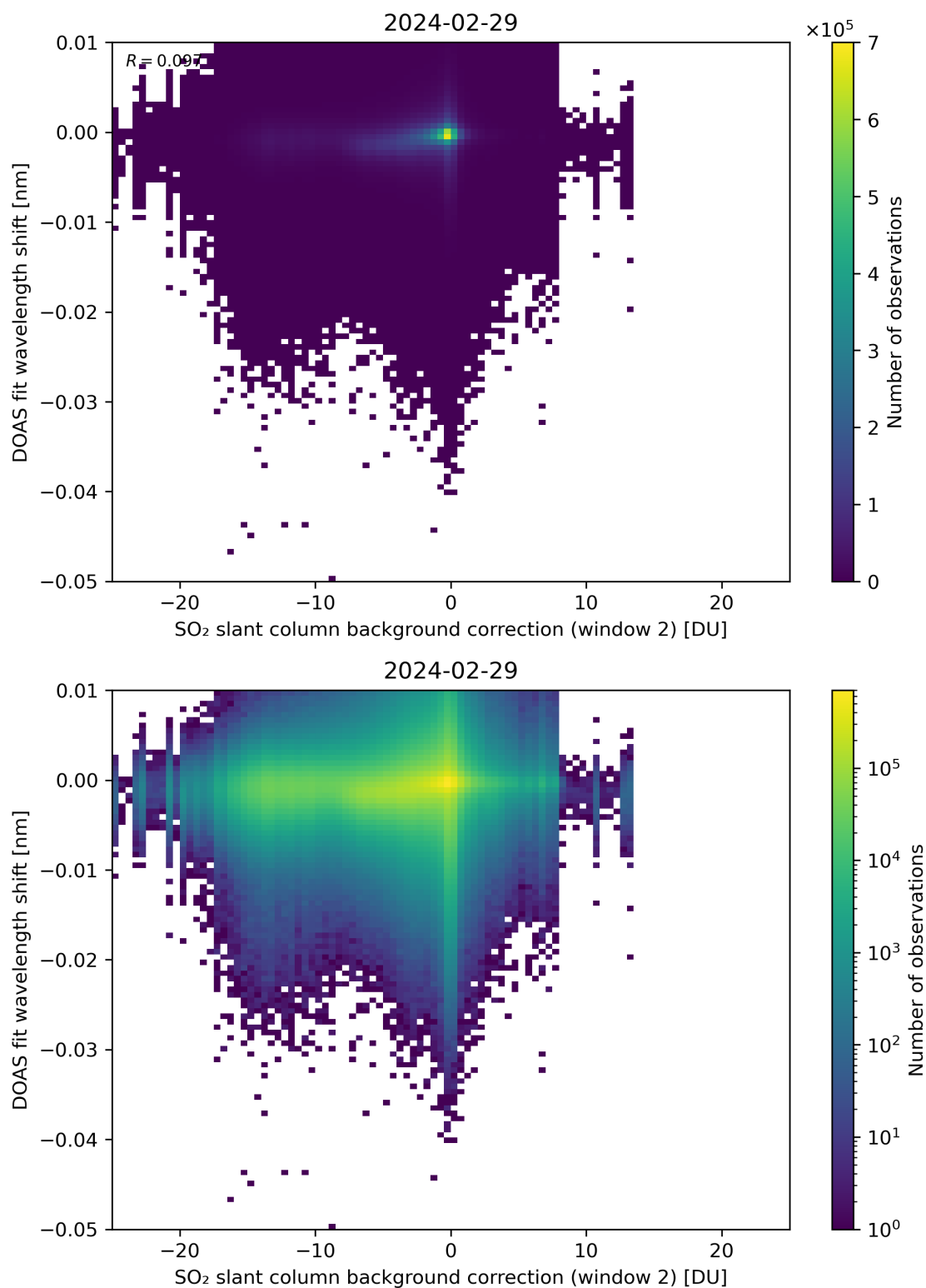
Figure 112: Scatter density plot of “SO 2 slant column background correction (window 2)” against “DOAS fit wavelength shift” for 2024-02-28 to 2024-03-01.
