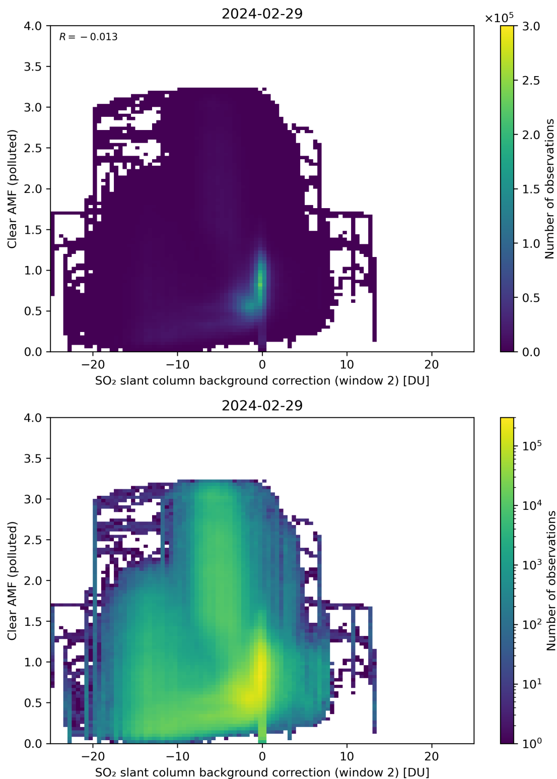
Figure 115: Scatter density plot of “SO 2 slant column background correction (window 2)” against “Clear AMF (polluted)” for 2024-02-28 to 2024-03-01.
