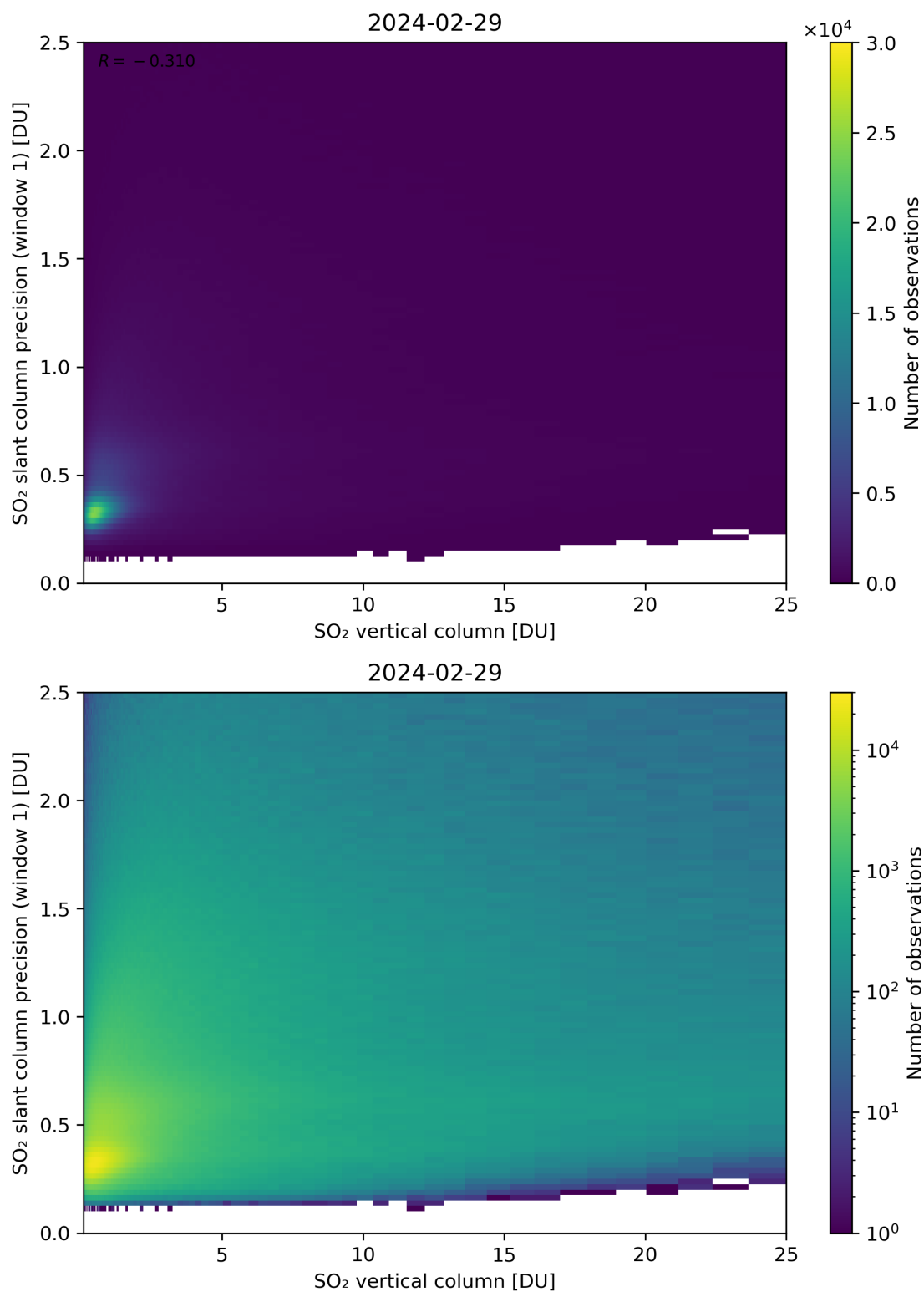
Figure 301: Scatter density plot of “SO 2 vertical column” against “SO 2 slant column precision (window 1)” for 2024-02-28 to 2024-03-01.
