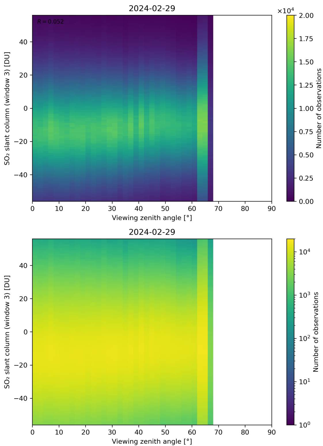
Figure 323: Scatter density plot of “Viewing zenith angle” against “SO 2 slant column (window 3)” for 2024-02-28 to 2024-03-01.
