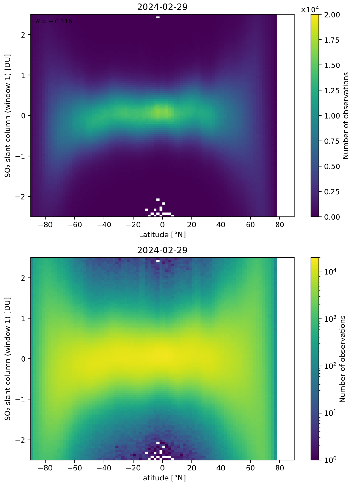
Figure 149: Scatter density plot of “Latitude” against “SO 2 slant column (window 1)” for 2024-02-28 to 2024-03-01.
