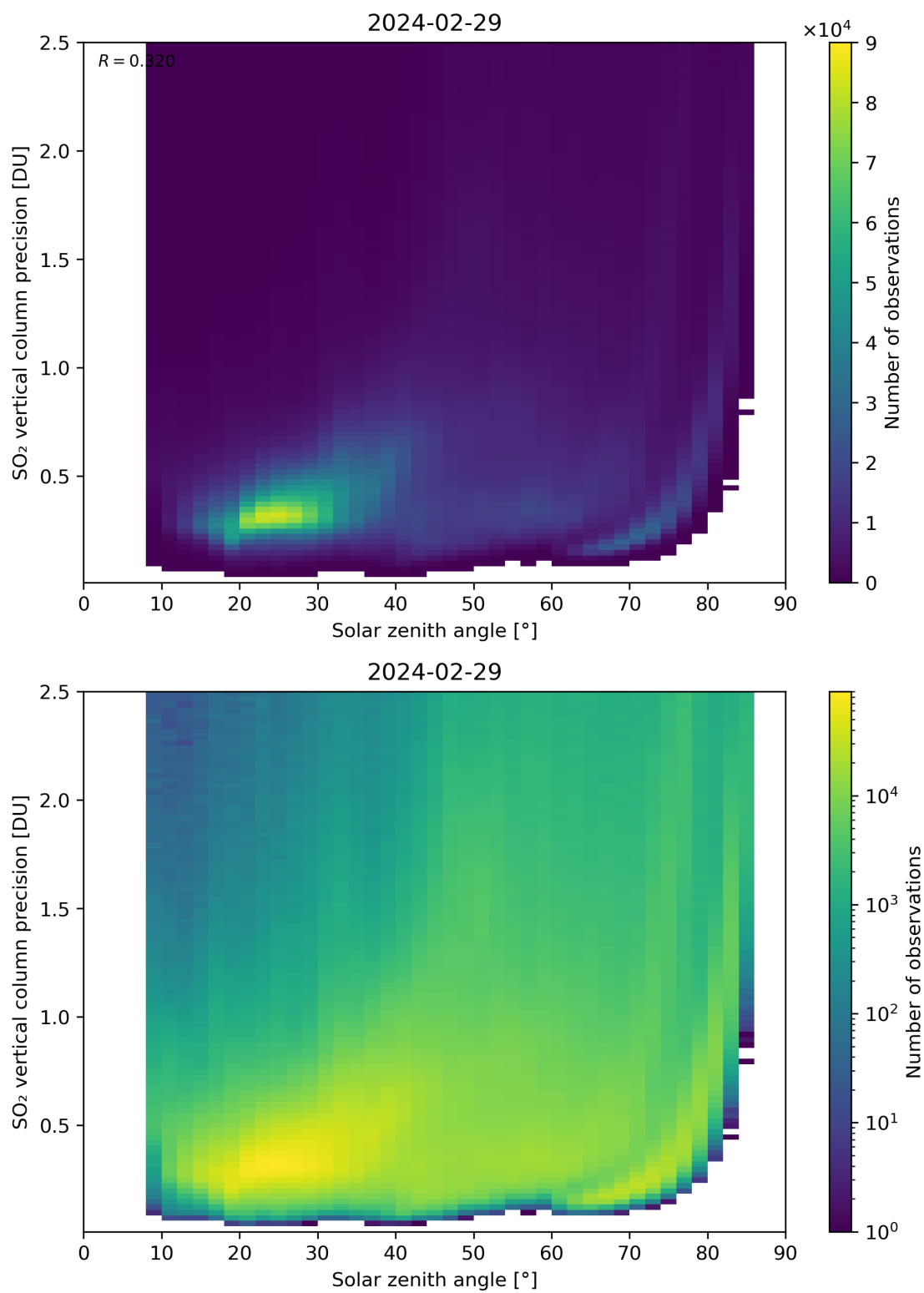
Figure 177: Scatter density plot of “Solar zenith angle” against “SO 2 vertical column precision” for 2024-02-28 to 2024-03-01.
