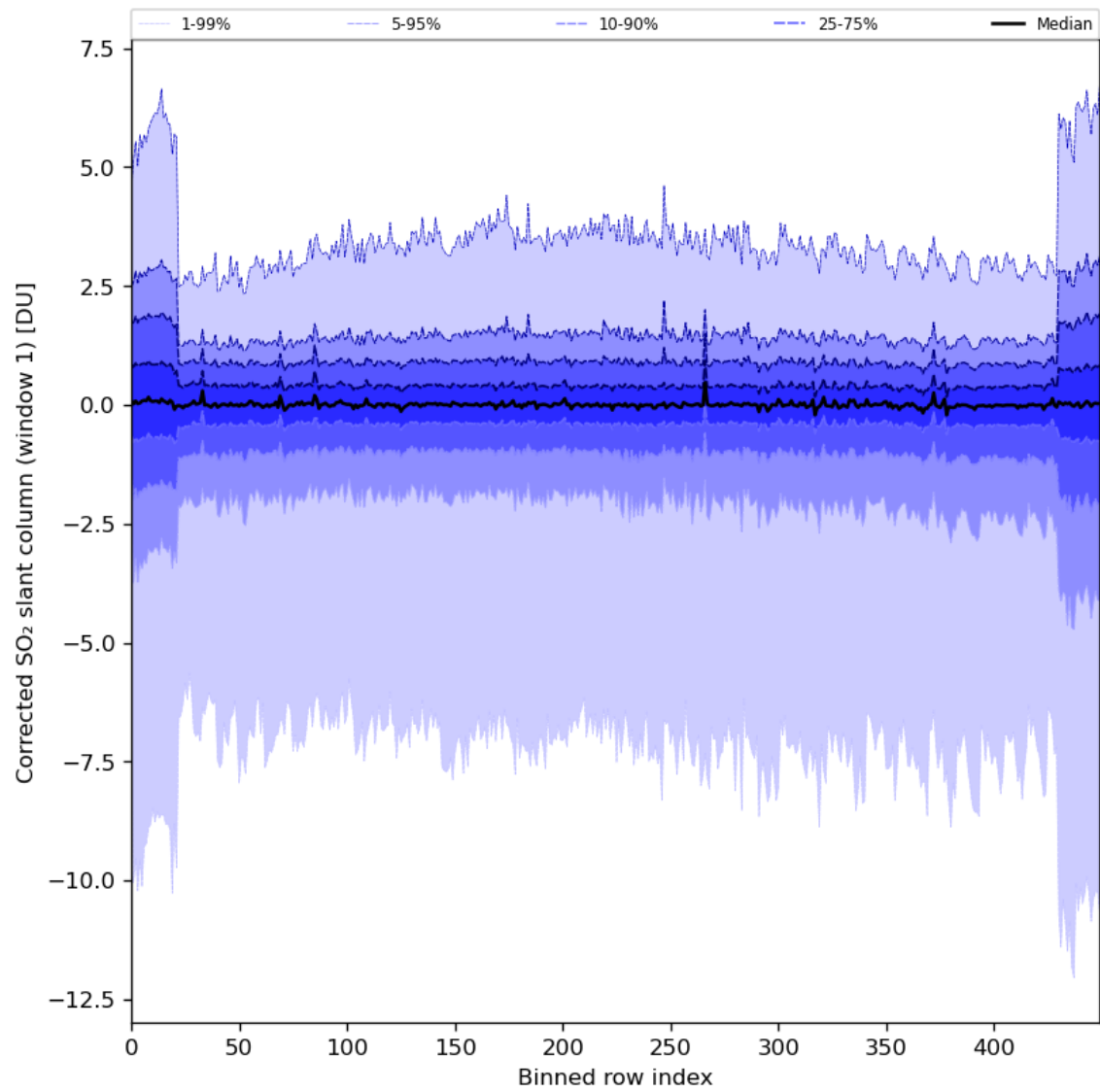
Figure 81: Along track statistics of “Corrected SO 2 slant column (window 1)” for 2024-02-28 to 2024-03-01
