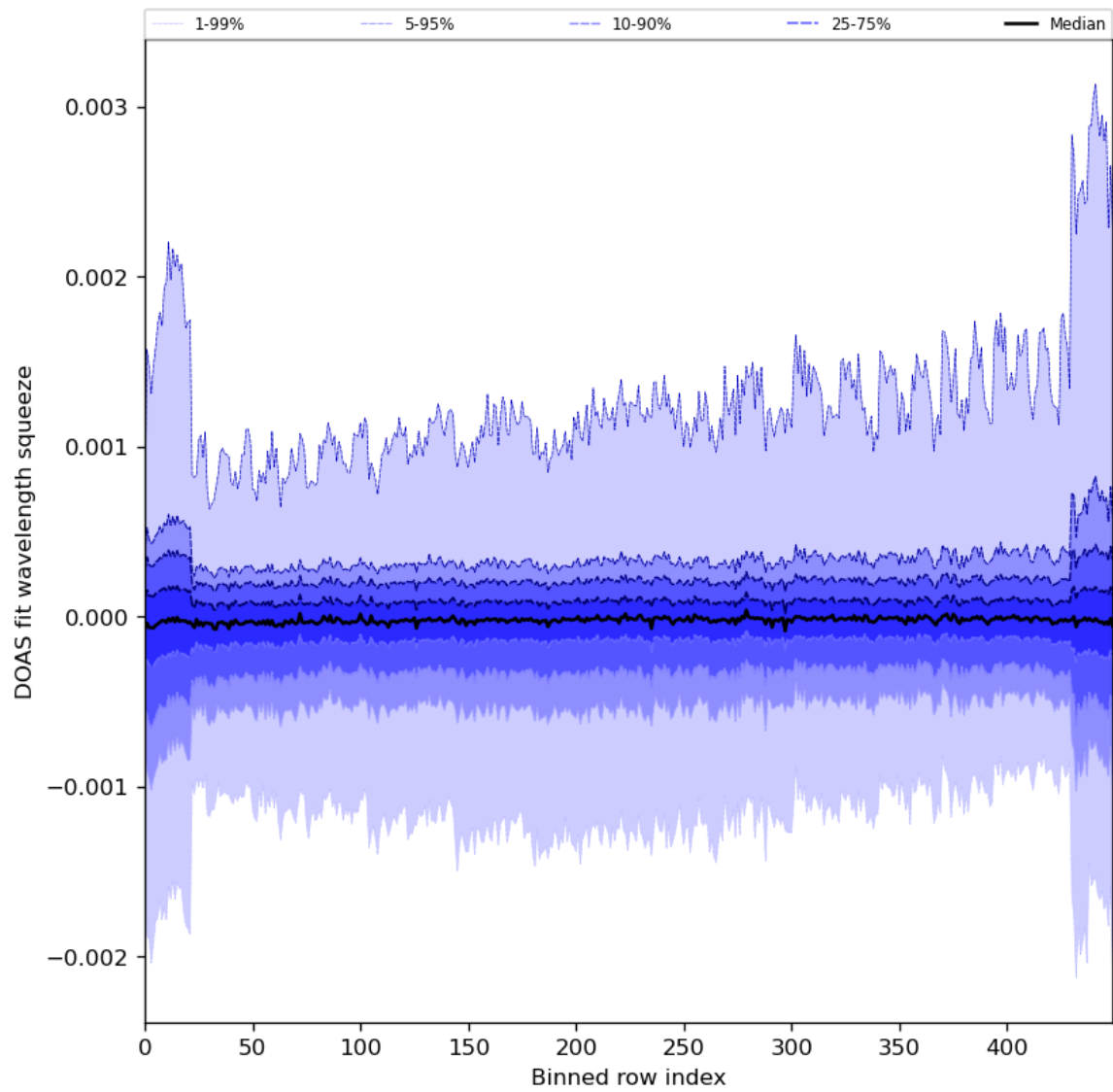
Figure 92: Along track statistics of “DOAS fit wavelength squeeze” for 2024-02-28 to 2024-03-01
