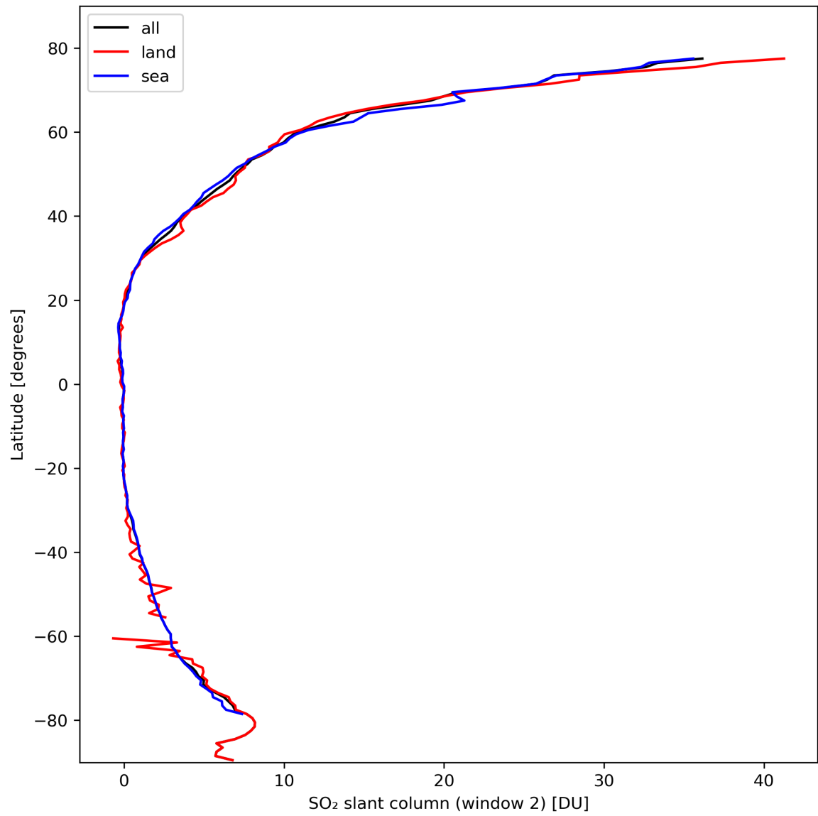
Figure 37: Zonal average of “SO 2 slant column (window 2)” for 2024-02-28 to 2024-03-01.
