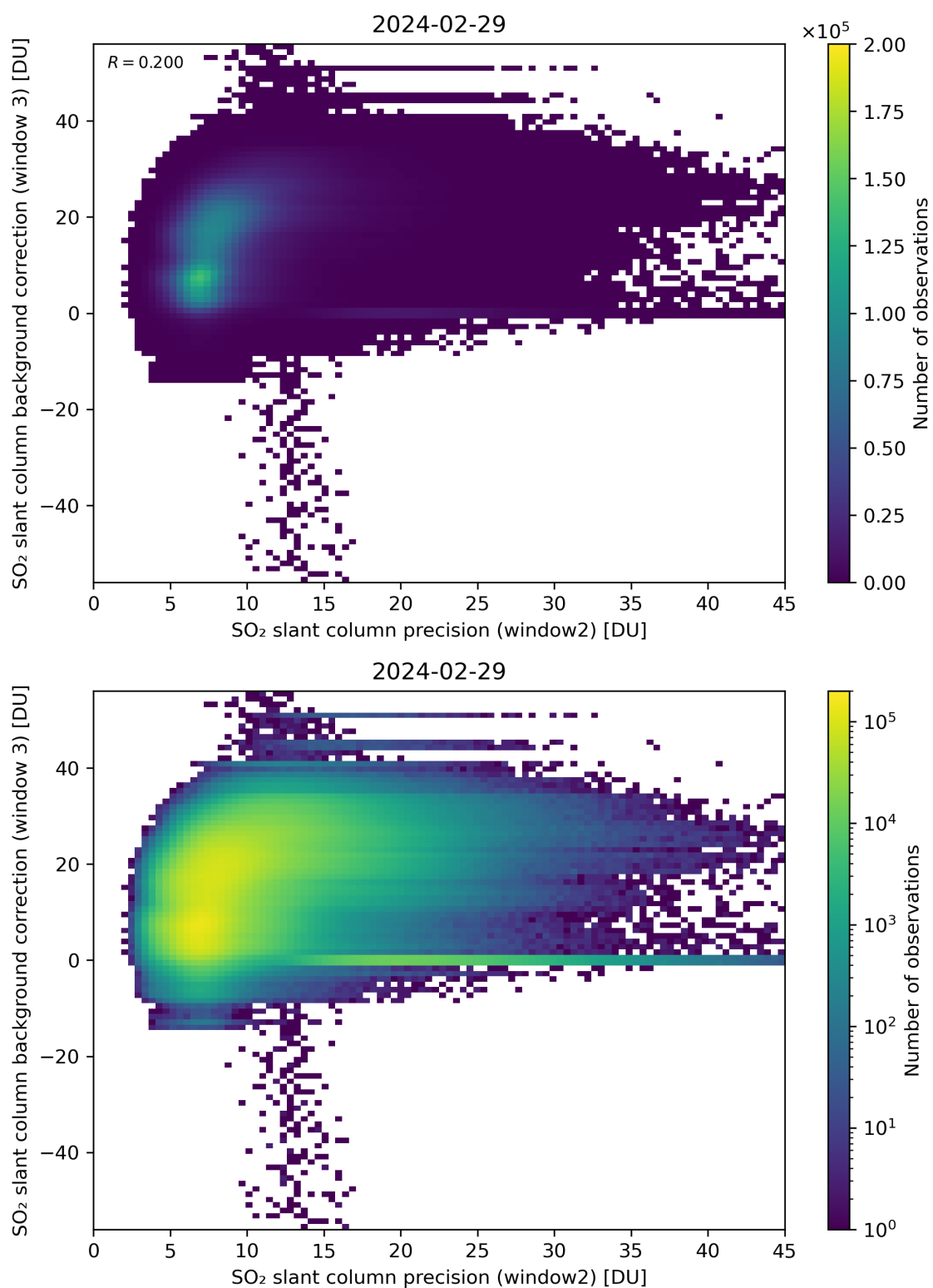
Figure 242: Scatter density plot of “SO 2 slant column precision (window2)” against “SO 2 slant column background correction (window 3)” for 2024-02-28 to 2024-03-01.
