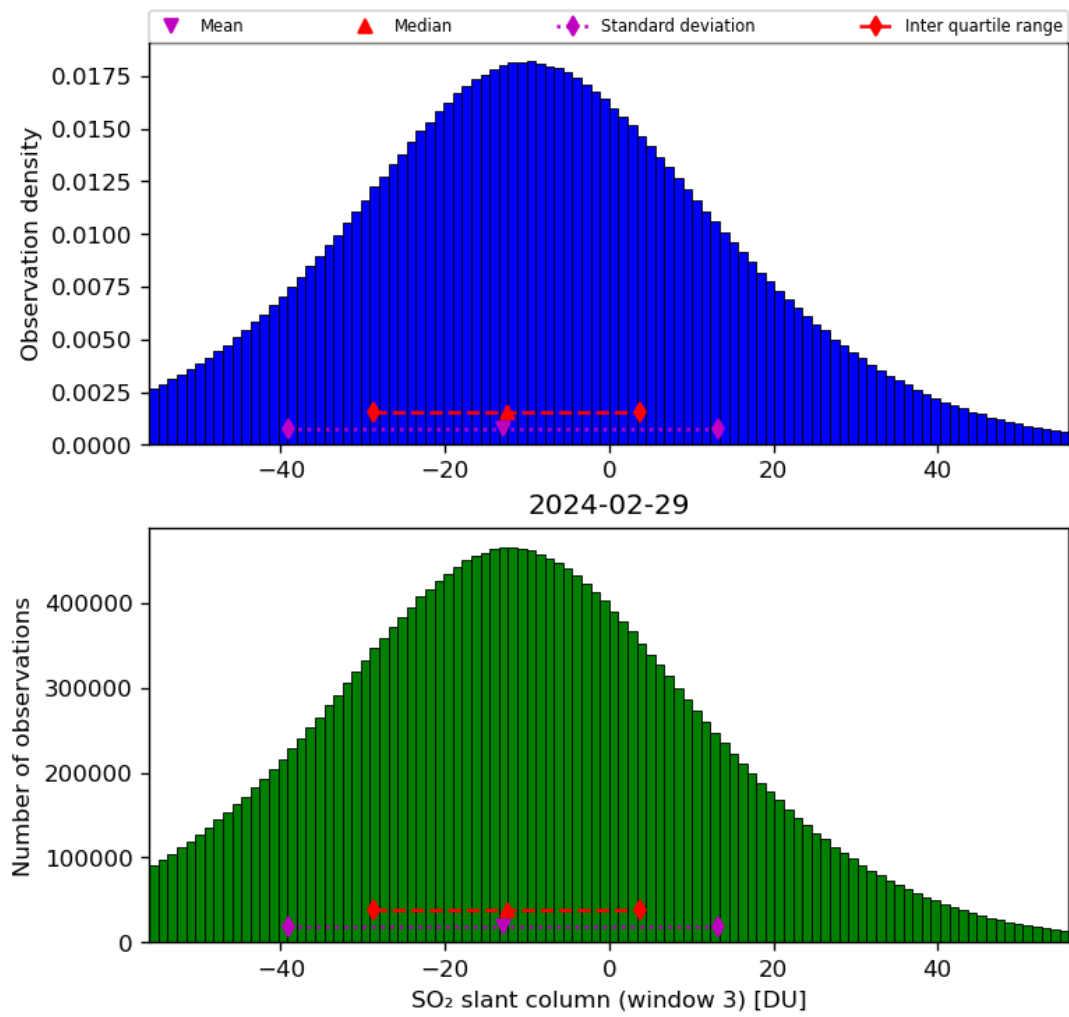
Figure 64: Histogram of “SO 2 slant column (window 3)” for 2024-02-28 to 2024-03-01
