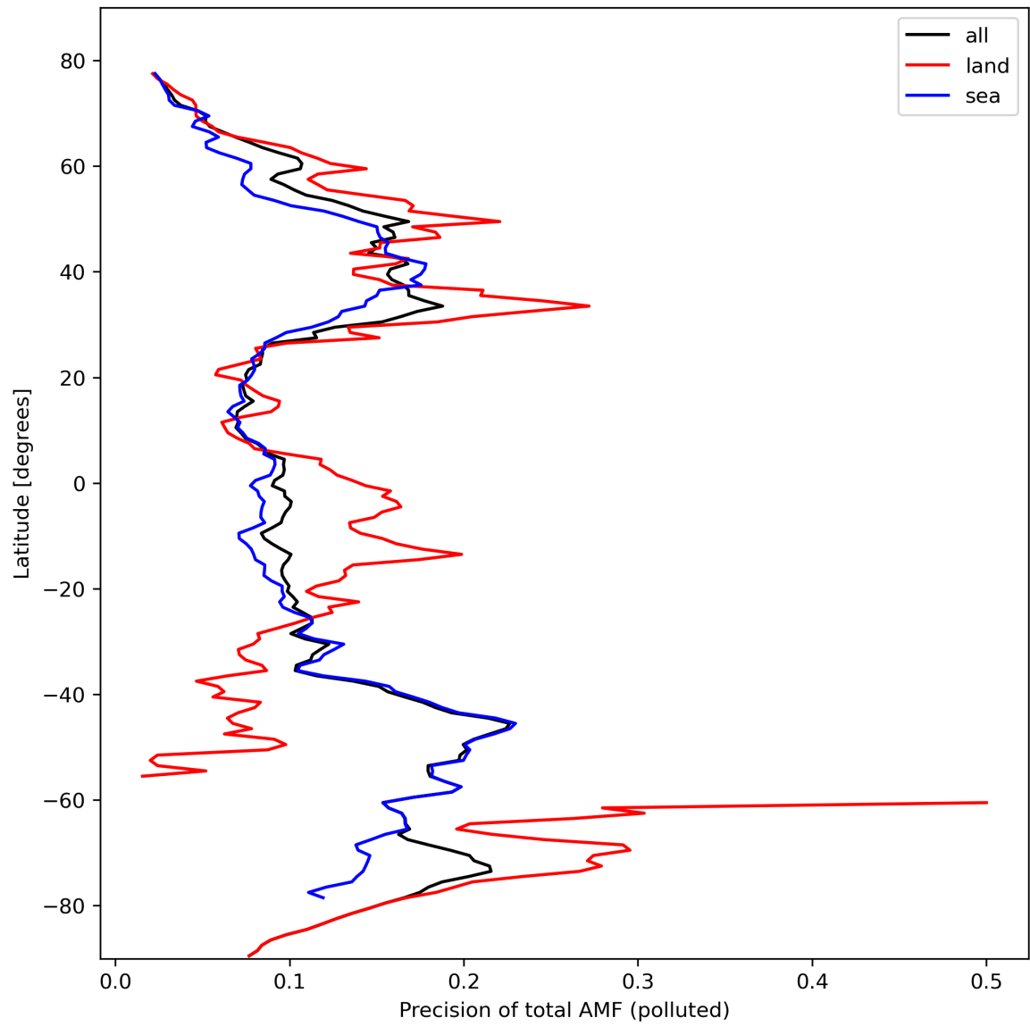
Figure 49: Zonal average of “Precision of total AMF (polluted)” for 2024-02-28 to 2024-03-01.
