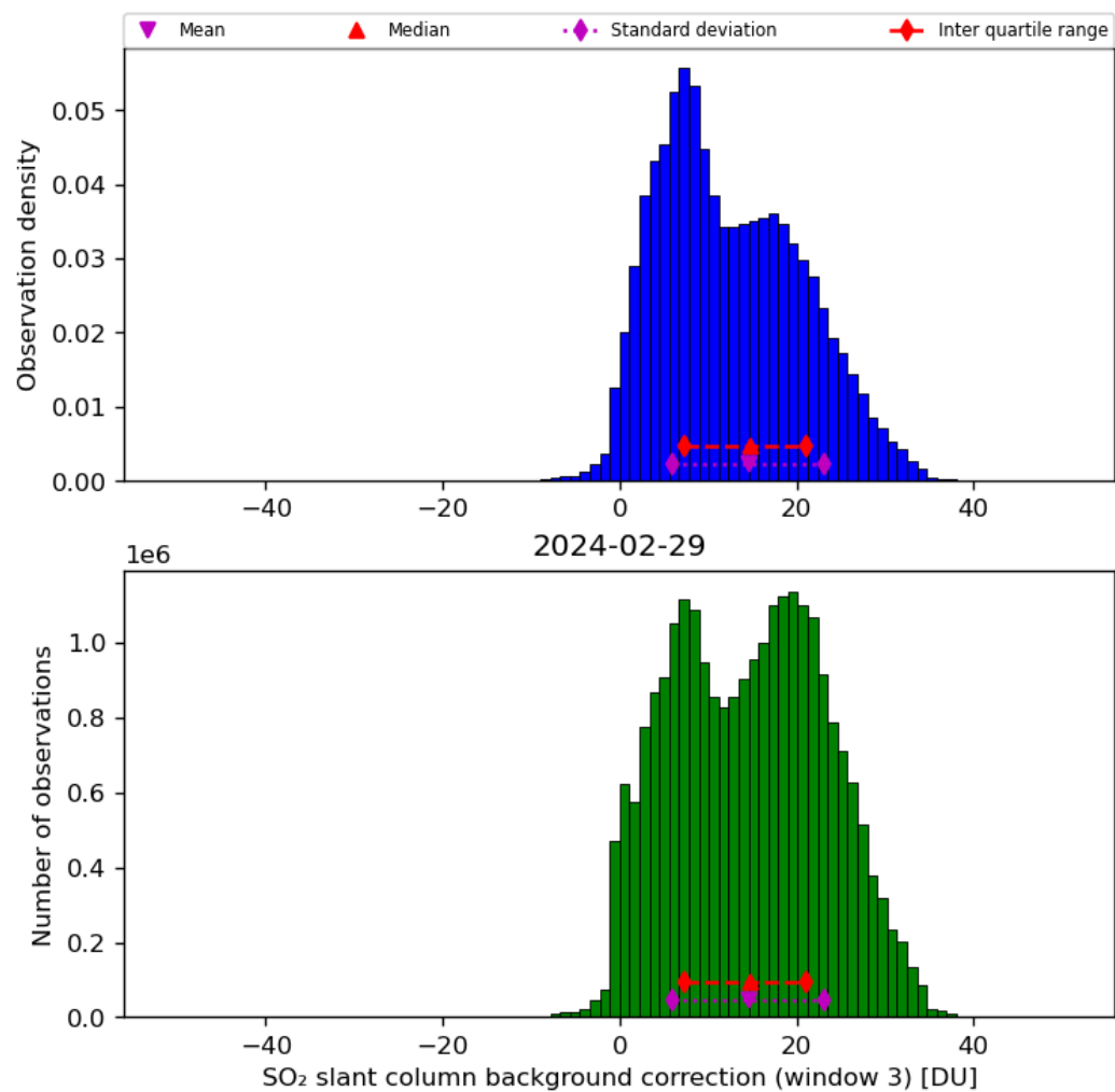
Figure 67: Histogram of “SO 2 slant column background correction (window 3)” for 2024-02-28 to 2024-03-01
