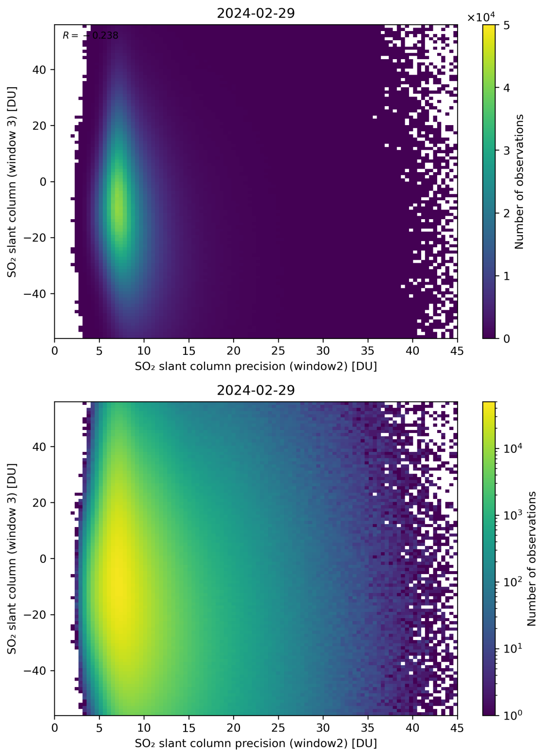
Figure 249: Scatter density plot of “SO 2 slant column precision (window2)” against “SO 2 slant column (window 3)” for 2024-02-28 to 2024-03-01.
