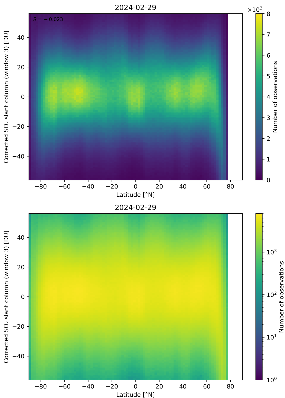
Figure 148: Scatter density plot of “Latitude” against “Corrected SO 2 slant column (window 3)” for 2024-02-28 to 2024-03-01.
