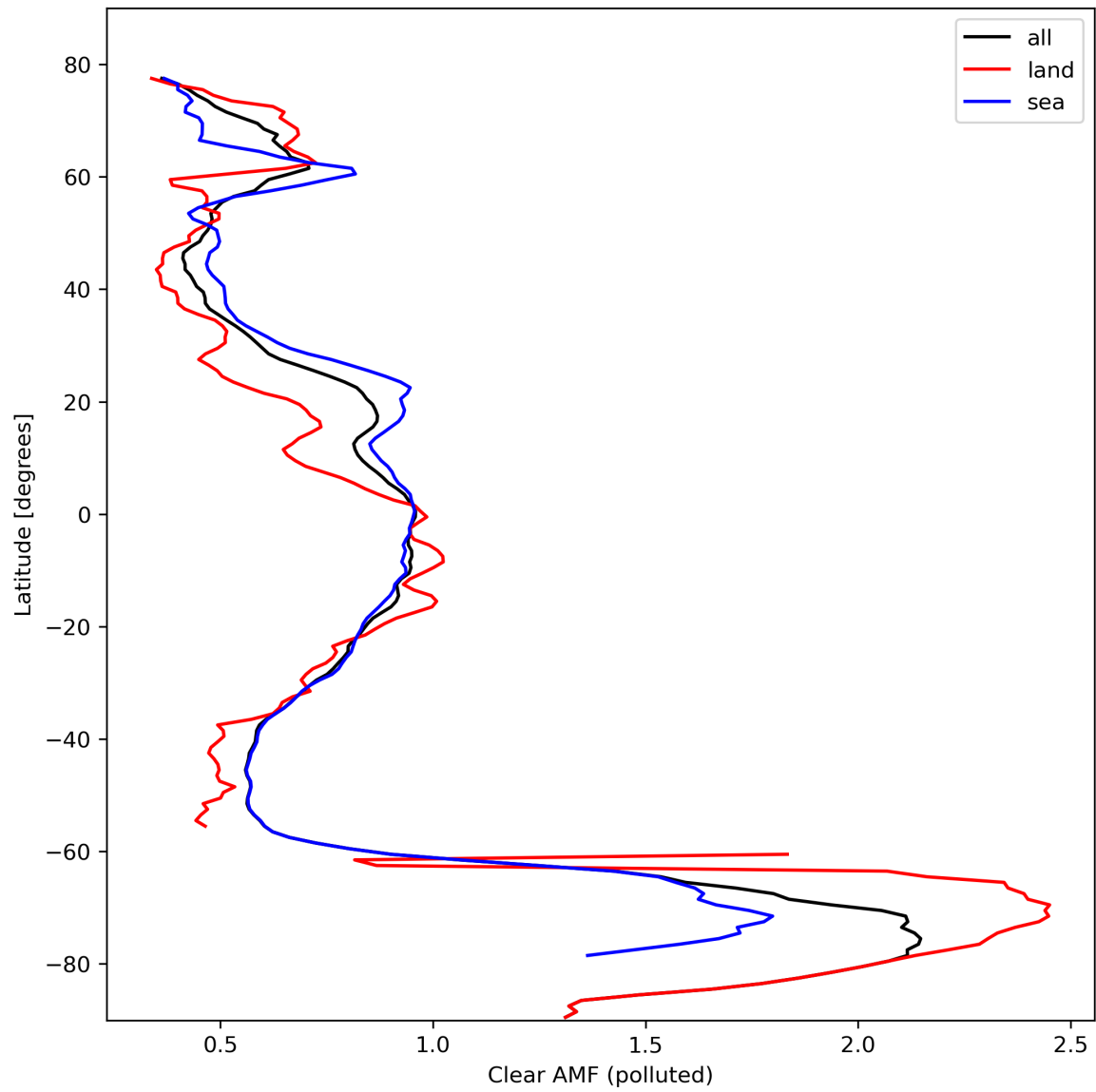
Figure 50: Zonal average of “Clear AMF (polluted)” for 2024-02-28 to 2024-03-01.
