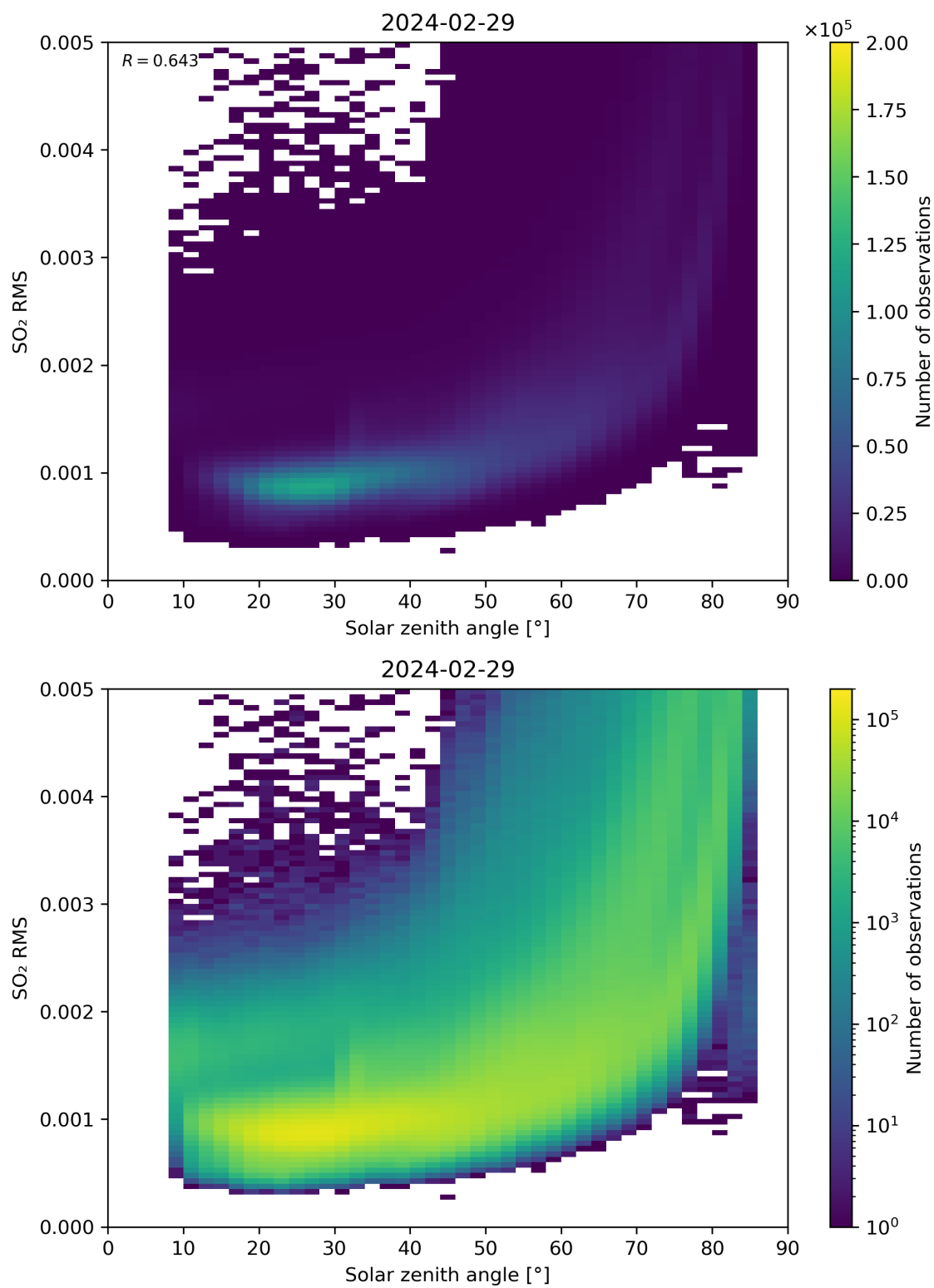
Figure 163: Scatter density plot of “Solar zenith angle” against “SO 2 RMS” for 2024-02-28 to 2024-03-01.
