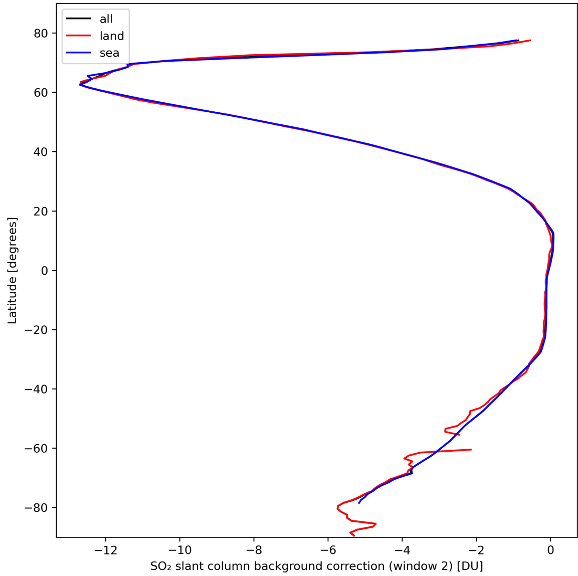
Figure 40: Zonal average of “SO 2 slant column background correction (window 2)” for 2024-02-28 to 2024-03-01.
