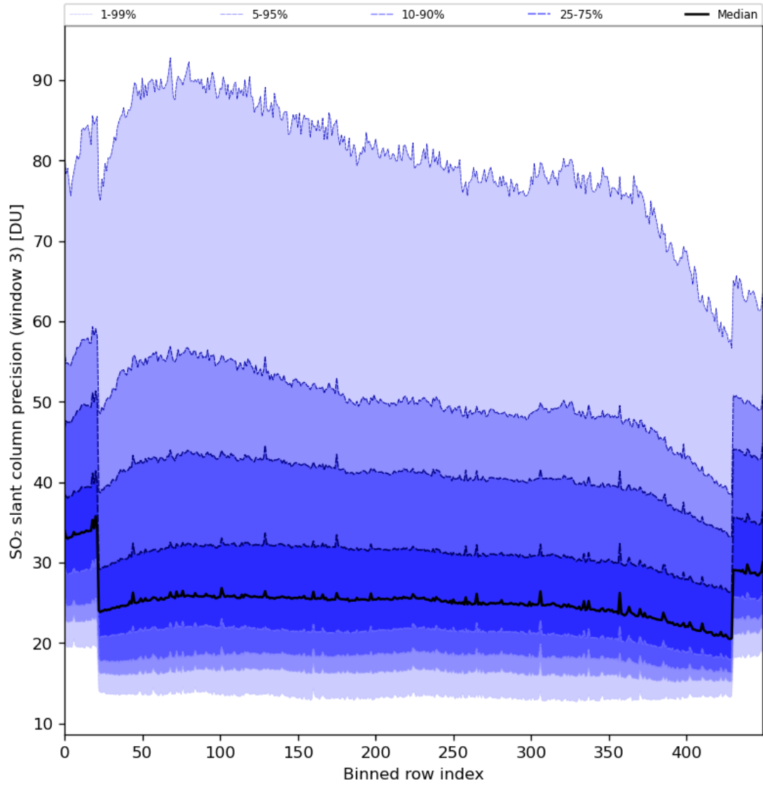
Figure 88: Along track statistics of “SO 2 slant column precision (window 3)” for 2024-02-28 to 2024-03-01
