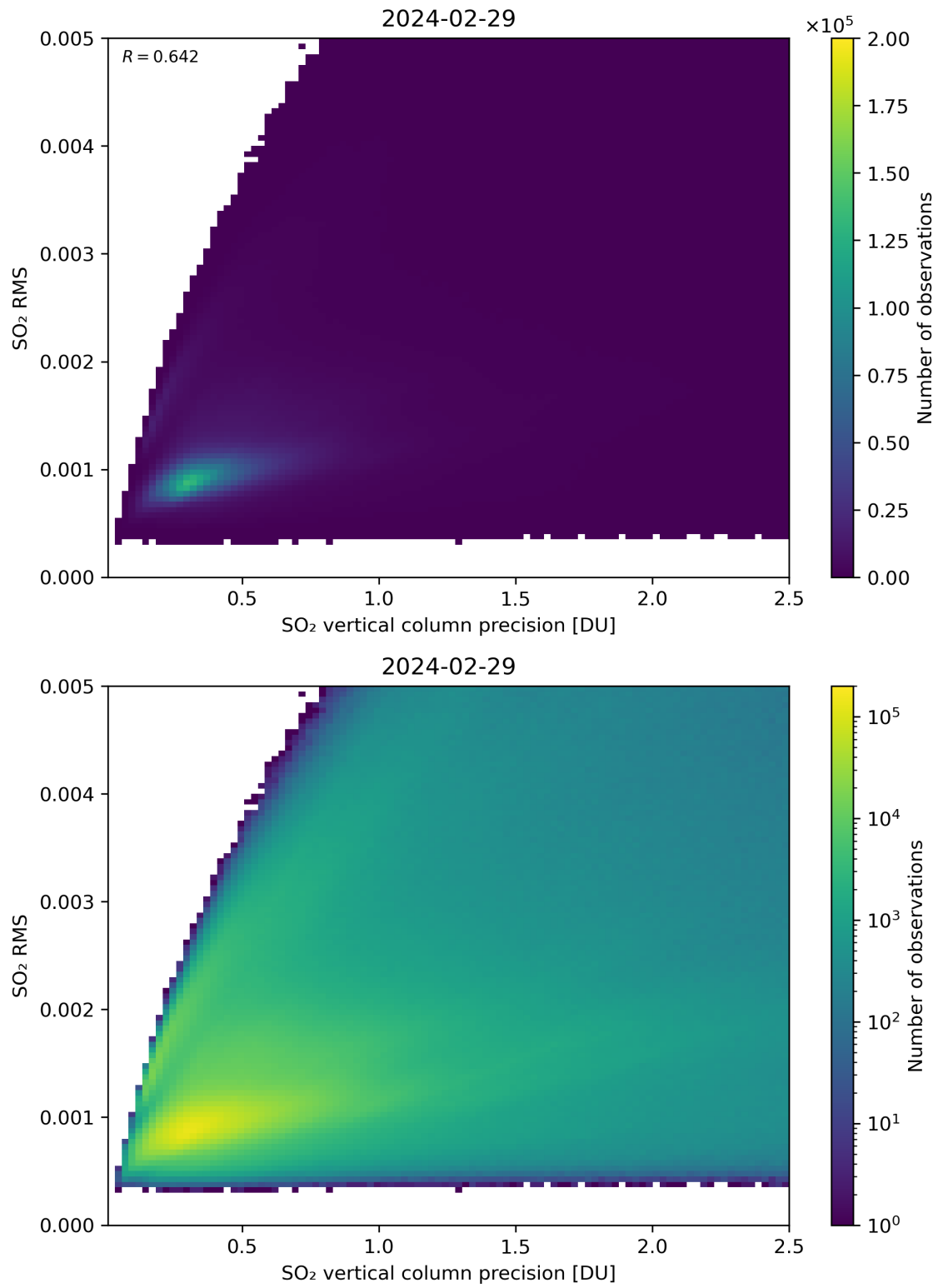
Figure 284: Scatter density plot of “SO 2 vertical column precision” against “SO 2 RMS” for 2024-02-28 to 2024-03-01.
