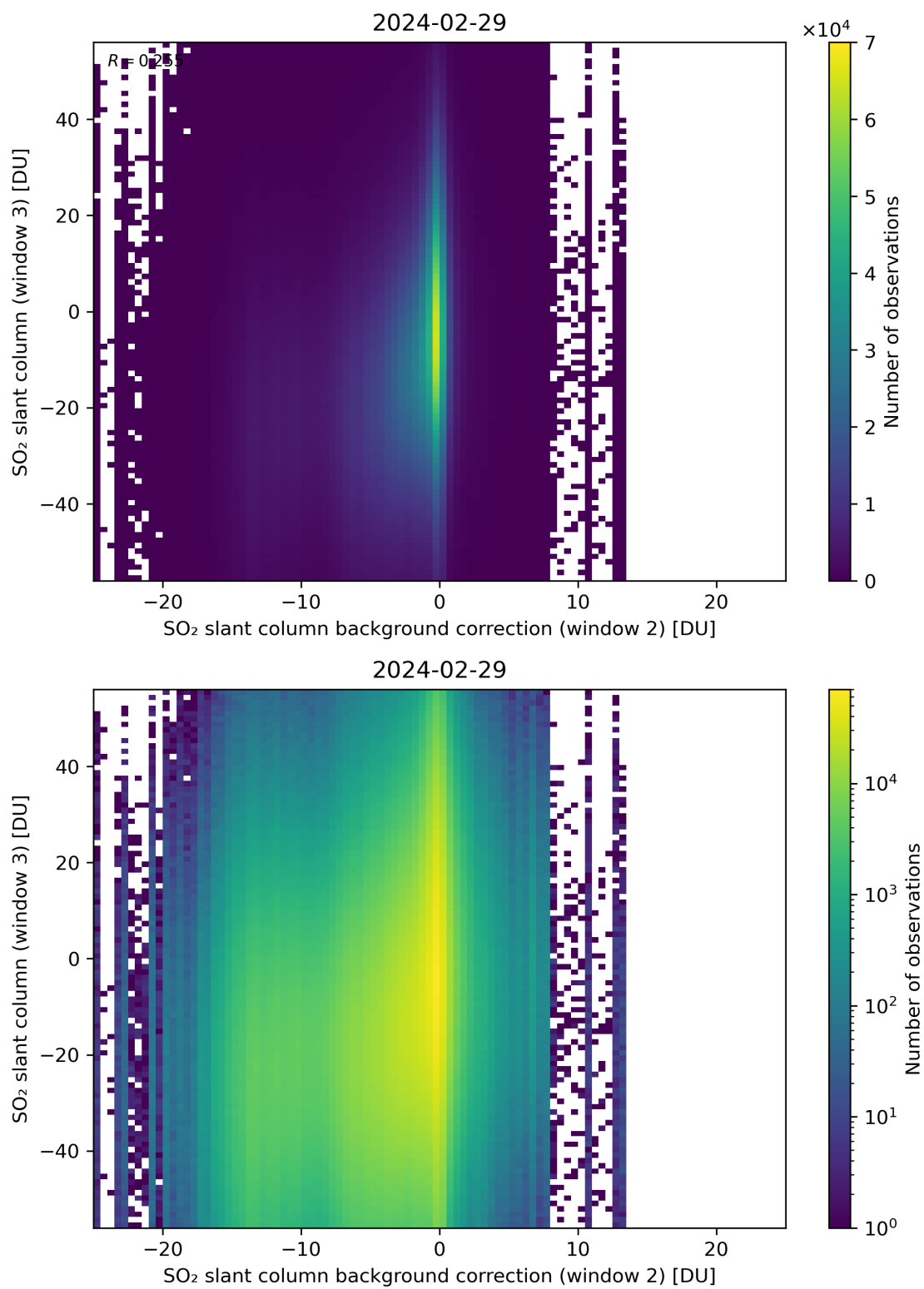
Figure 117: Scatter density plot of “SO 2 slant column background correction (window 2)” against “SO 2 slant column (window 3)” for 2024-02-28 to 2024-03-01.
