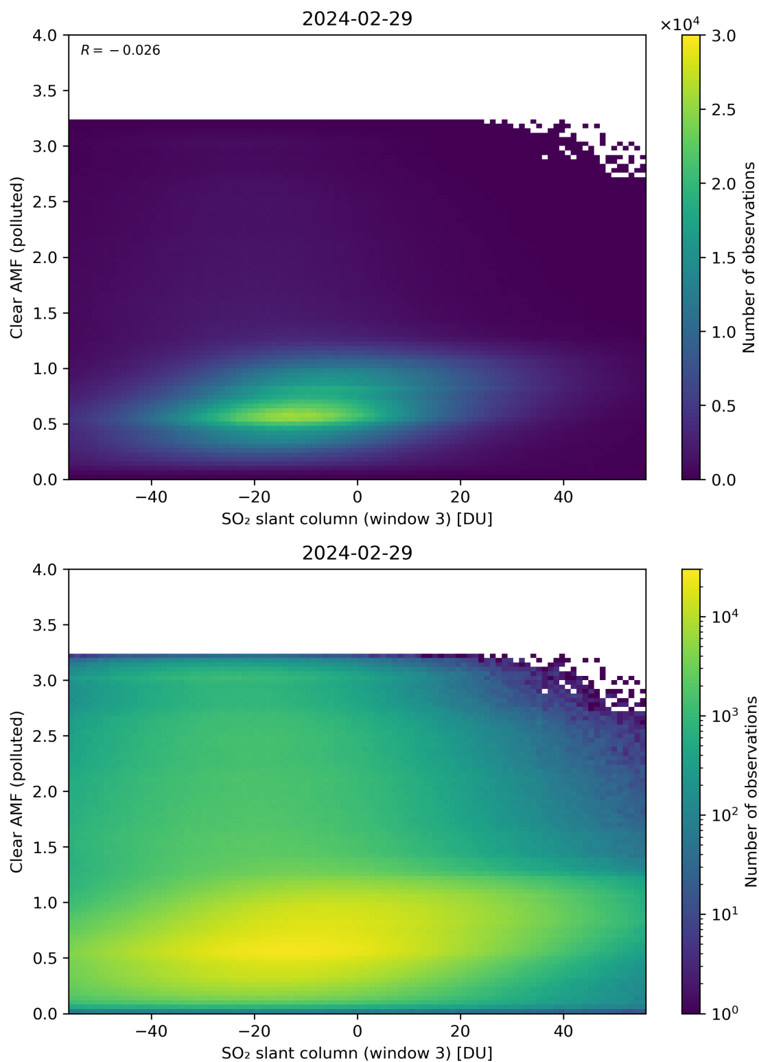
Figure 265: Scatter density plot of “SO 2 slant column (window 3)” against “Clear AMF (polluted)” for 2024-02-28 to 2024-03-01.
