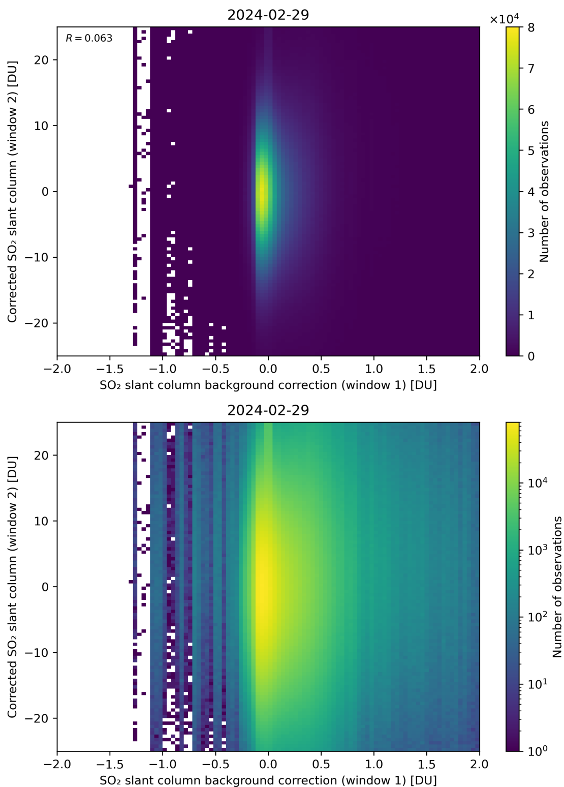
Figure 104: Scatter density plot of “SO 2 slant column background correction (window 1)” against “Corrected SO 2 slant column (window 2)” for 2024-02-28 to 2024-03-01.
