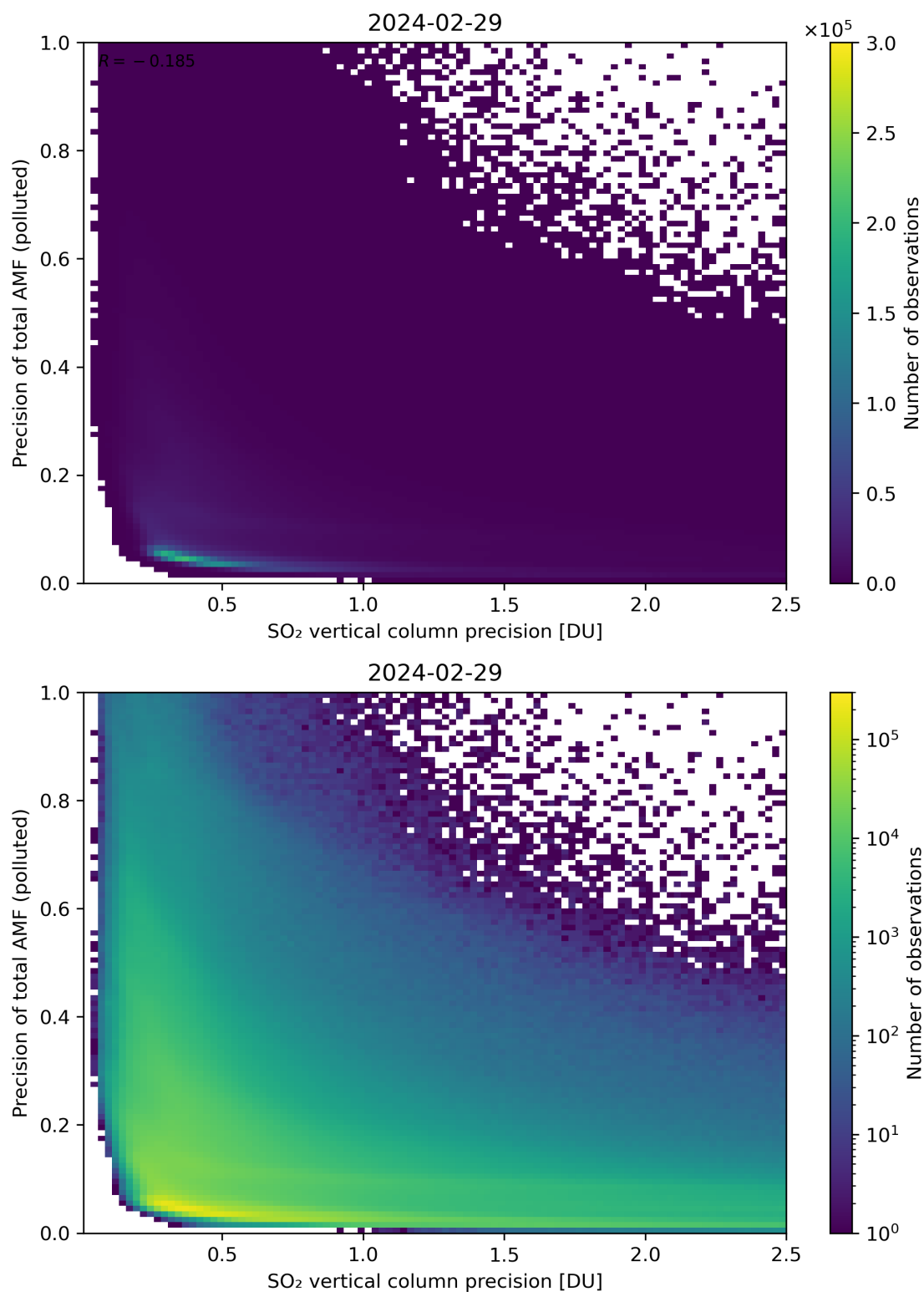
Figure 295: Scatter density plot of “SO 2 vertical column precision” against “Precision of total AMF (polluted)” for 2024-02-28 to 2024-03-01.
