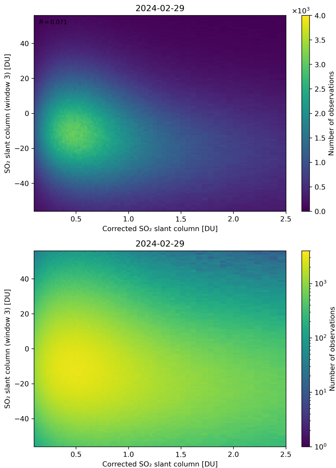
Figure 190: Scatter density plot of “Corrected SO 2 slant column” against “SO 2 slant column (window 3)” for 2024-02-28 to 2024-03-01.
