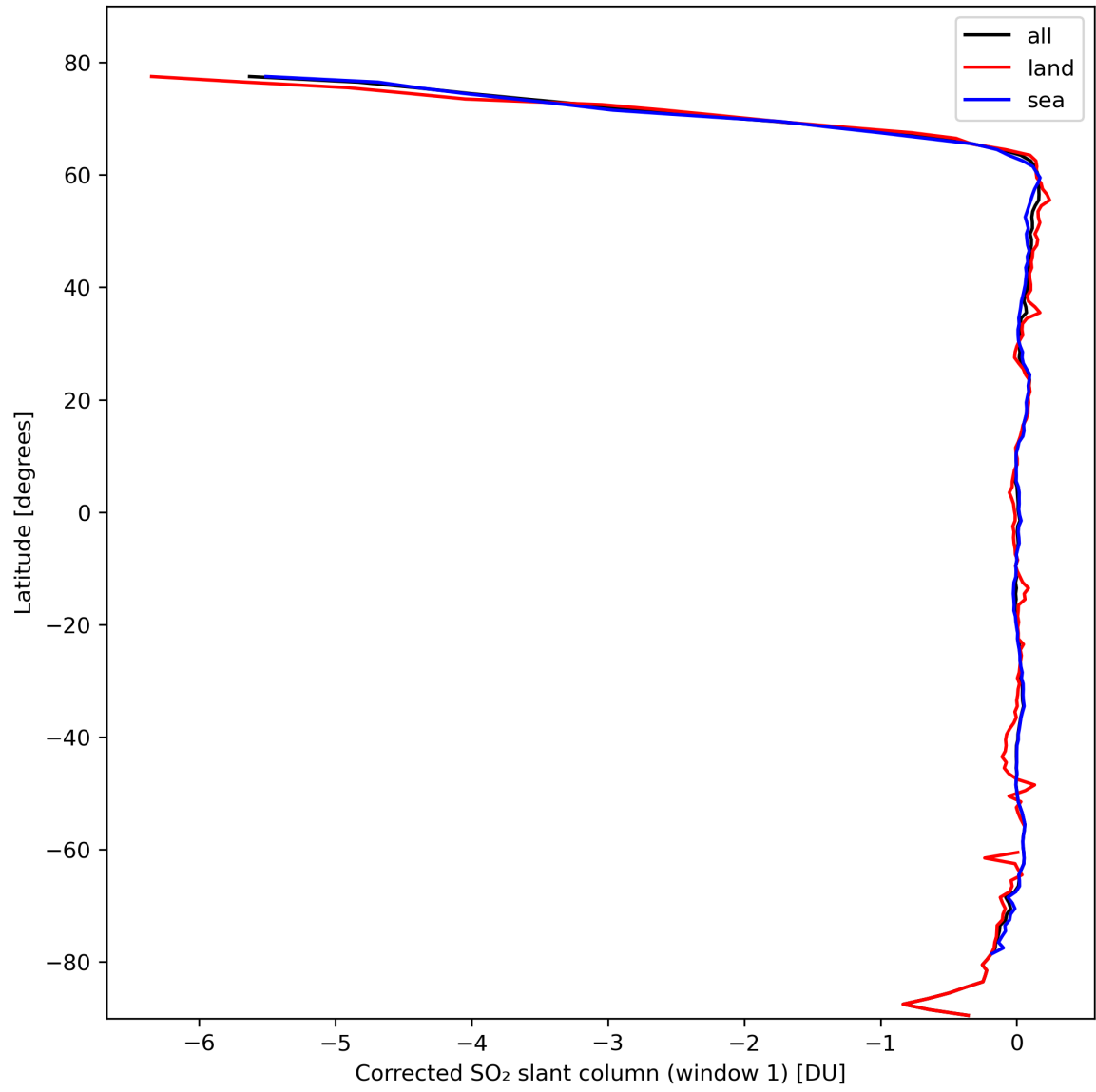
Figure 35: Zonal average of “Corrected SO 2 slant column (window 1)” for 2024-02-28 to 2024-03-01.
