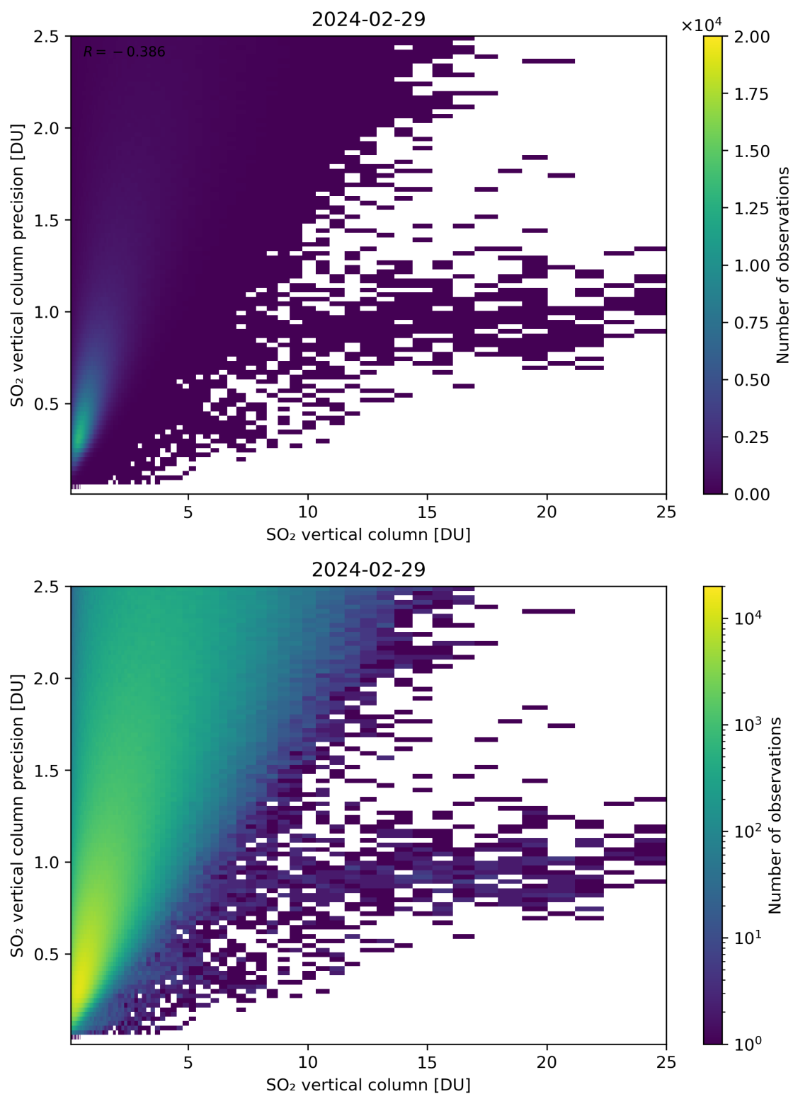
Figure 307: Scatter density plot of “SO 2 vertical column” against “SO 2 vertical column precision” for 2024-02-28 to 2024-03-01.
