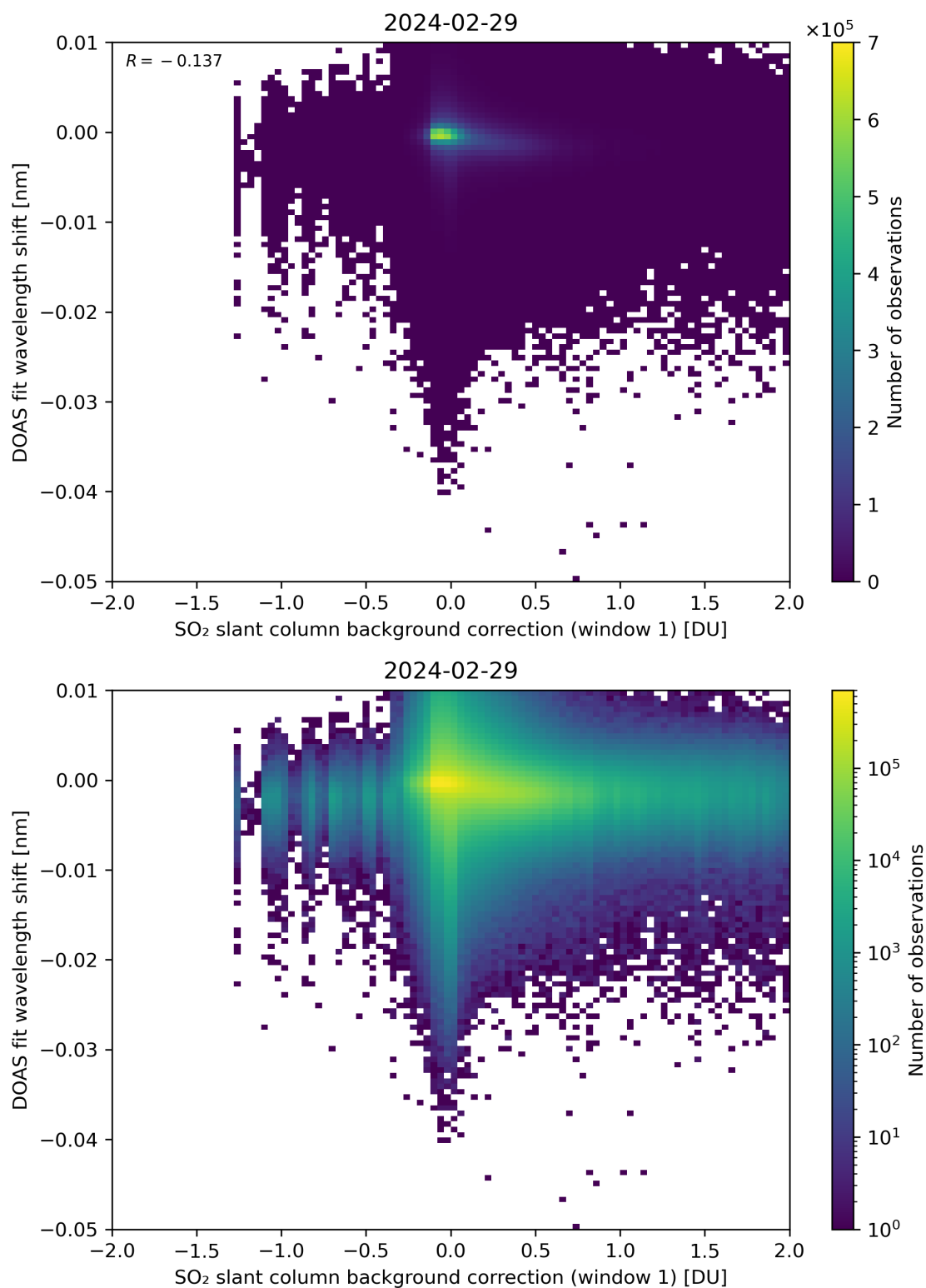
Figure 100: Scatter density plot of “SO 2 slant column background correction (window 1)” against “DOAS fit wavelength shift” for 2024-02-28 to 2024-03-01.
