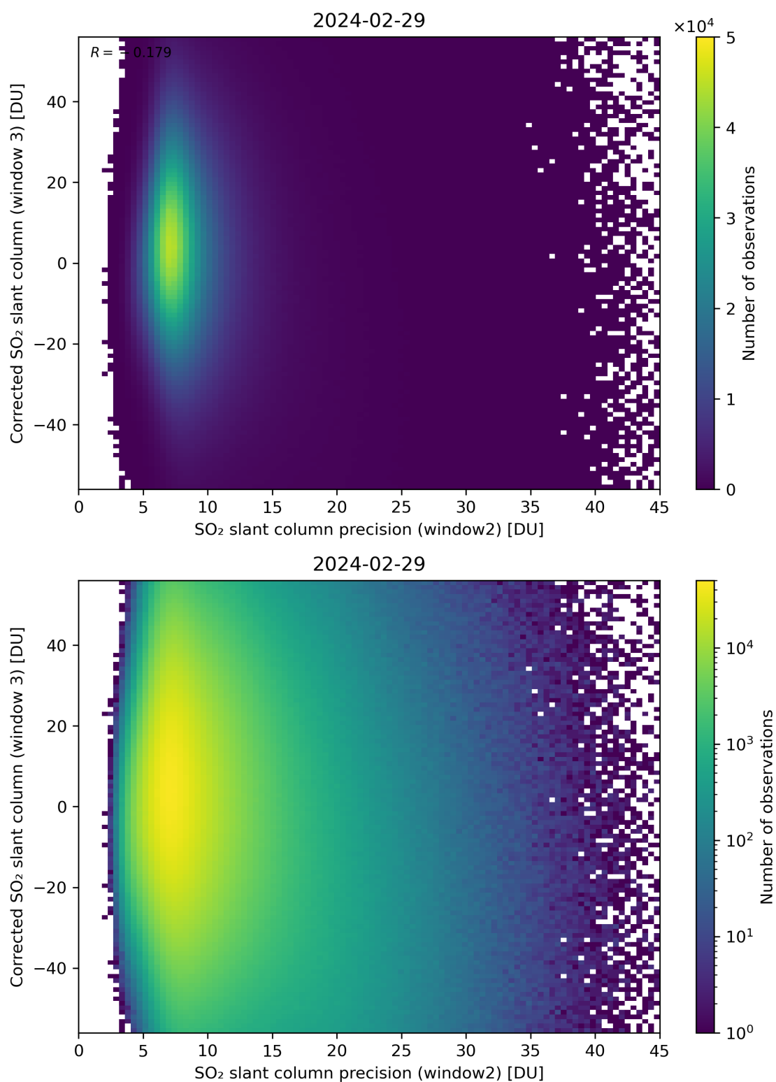
Figure 248: Scatter density plot of “SO 2 slant column precision (window2)” against “Corrected SO 2 slant column (window 3)” for 2024-02-28 to 2024-03-01.
