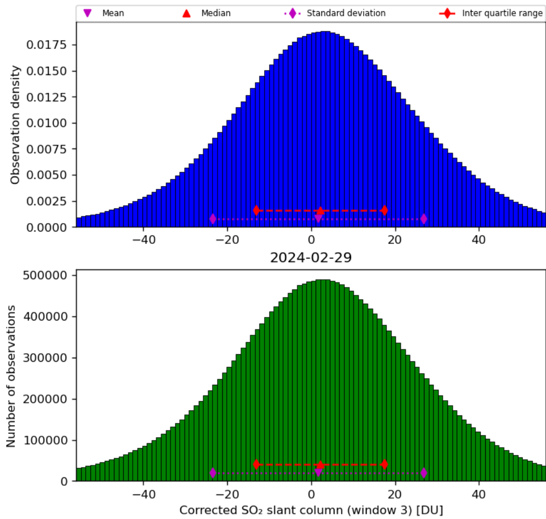
Figure 66: Histogram of “Corrected SO 2 slant column (window 3)” for 2024-02-28 to 2024-03-01
