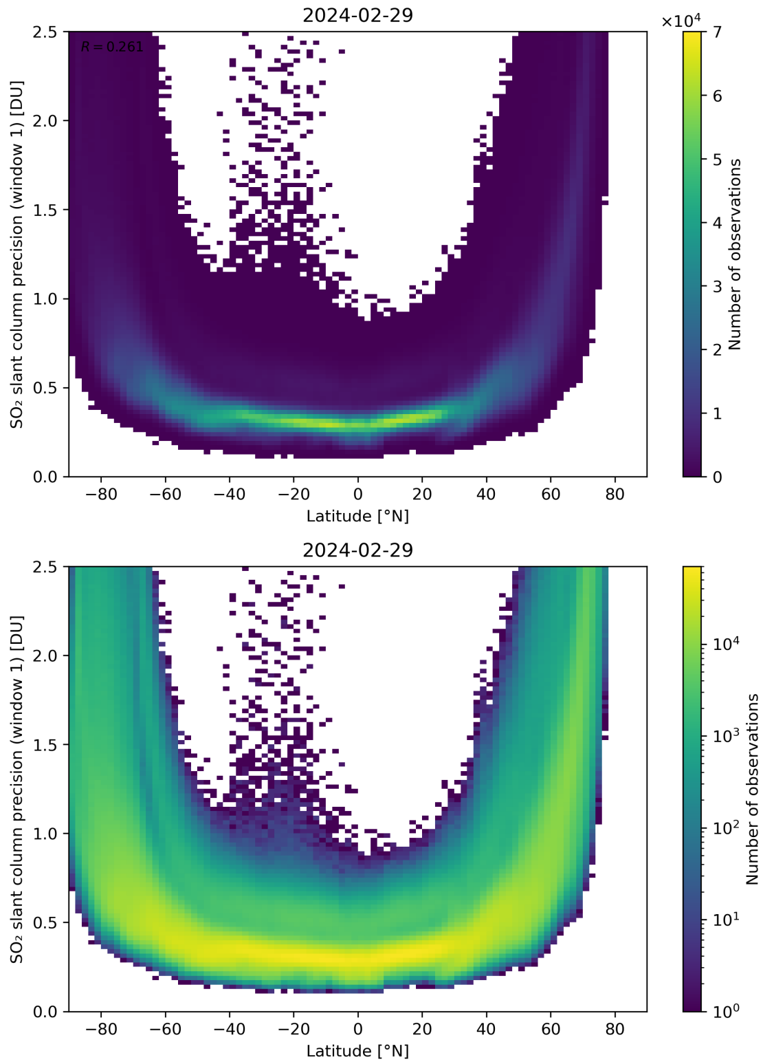
Figure 150: Scatter density plot of “Latitude” against “SO 2 slant column precision (window 1)” for 2024-02-28 to 2024-03-01.
