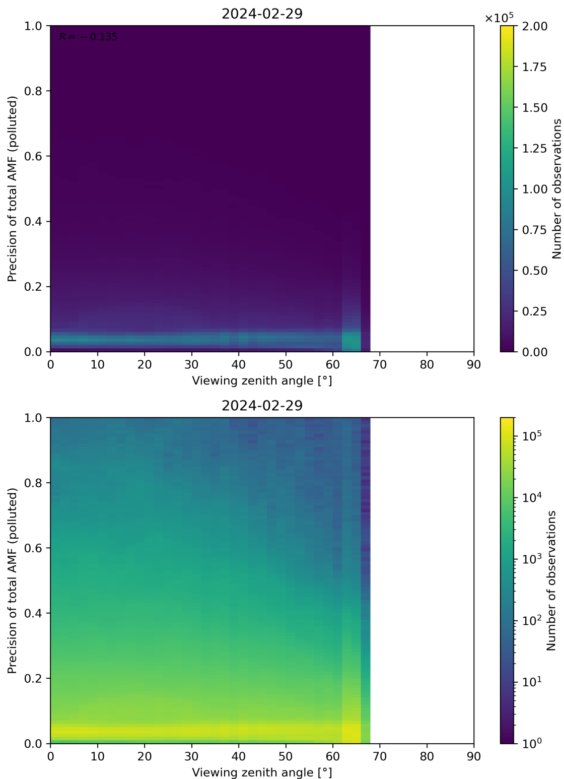
Figure 326: Scatter density plot of “Viewing zenith angle” against “Precision of total AMF (polluted)” for 2024-02-28 to 2024-03-01.
