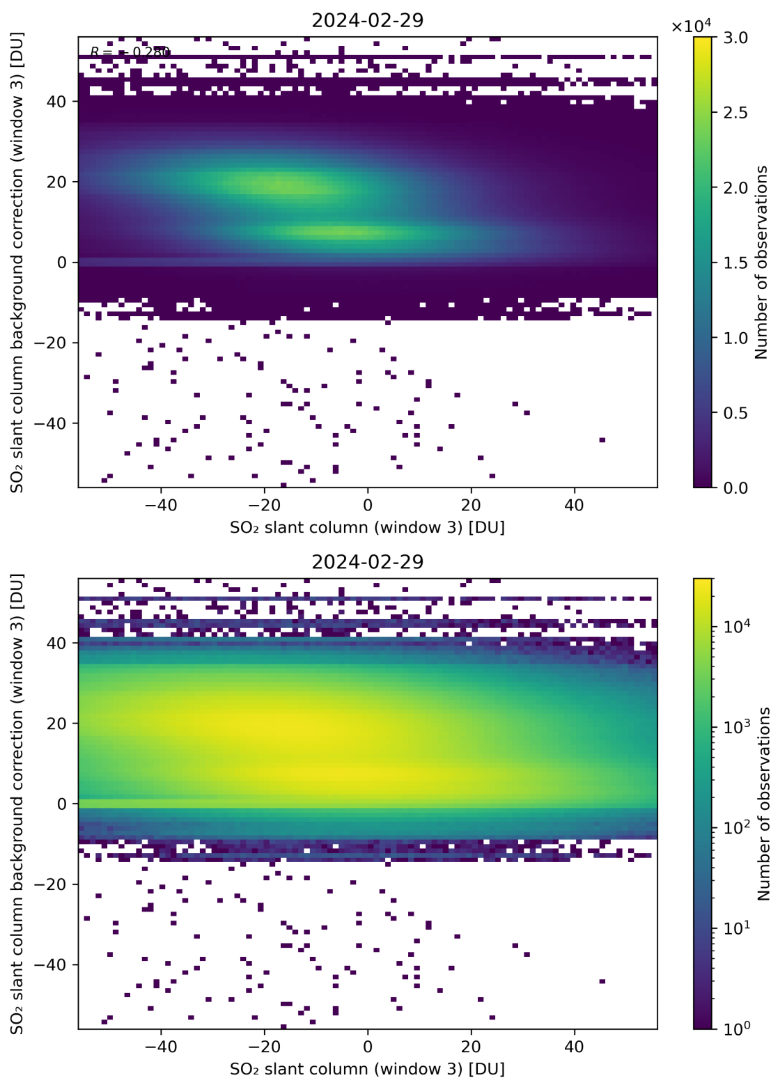
Figure 253: Scatter density plot of “SO 2 slant column (window 3)” against “SO 2 slant column background correction (window 3)” for 2024-02-28 to 2024-03-01.
