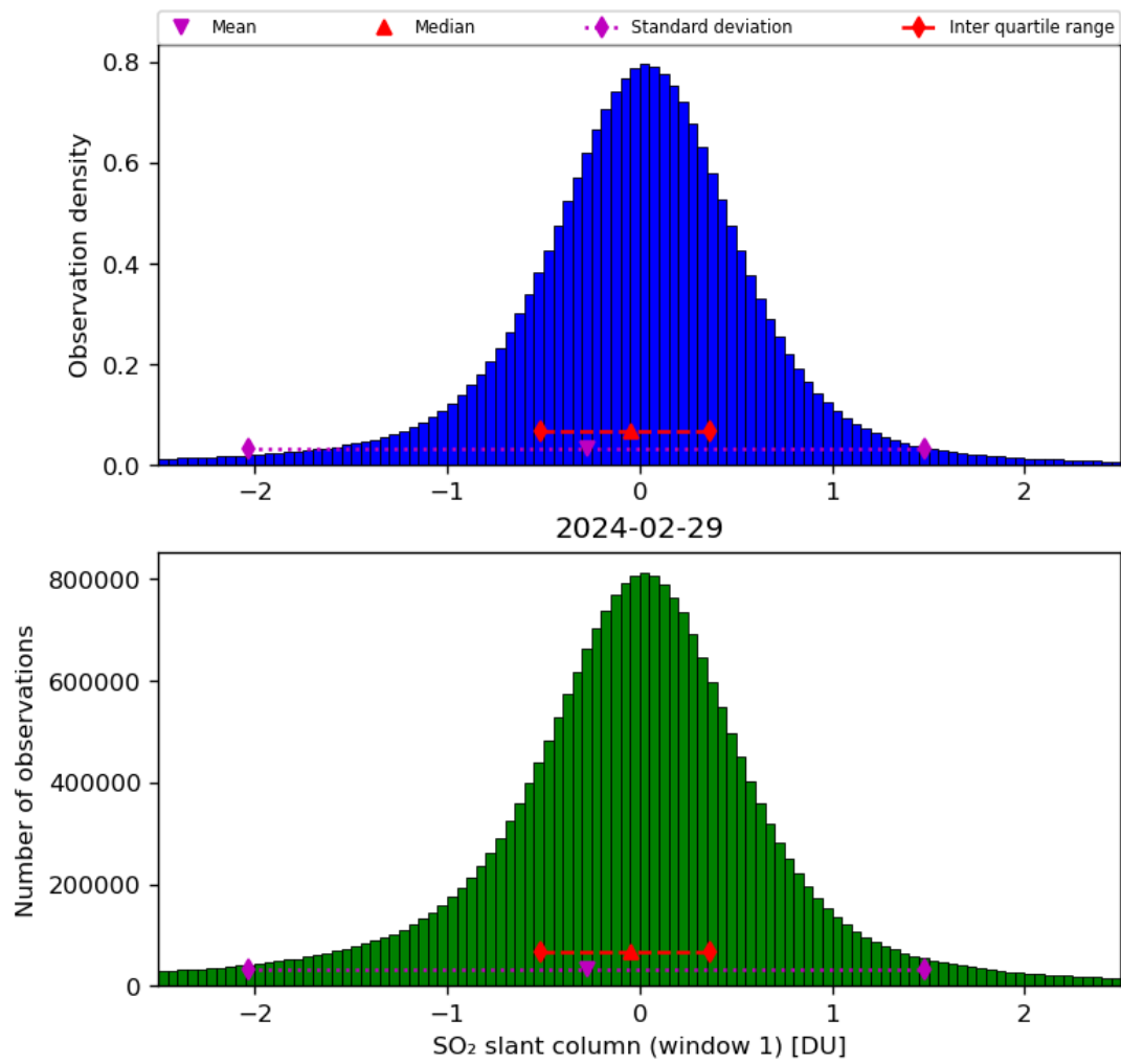
Figure 56: Histogram of “SO 2 slant column (window 1)” for 2024-02-28 to 2024-03-01
