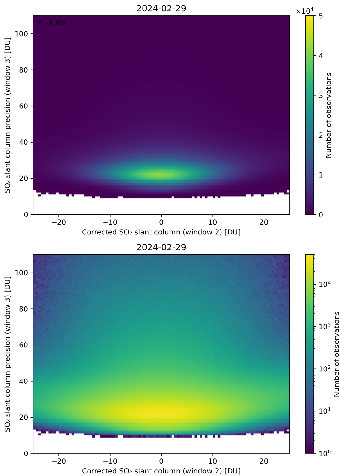
Figure 202: Scatter density plot of “Corrected SO 2 slant column (window 2)” against “SO 2 slant column precision (window 3)” for 2024-02-28 to 2024-03-01.
