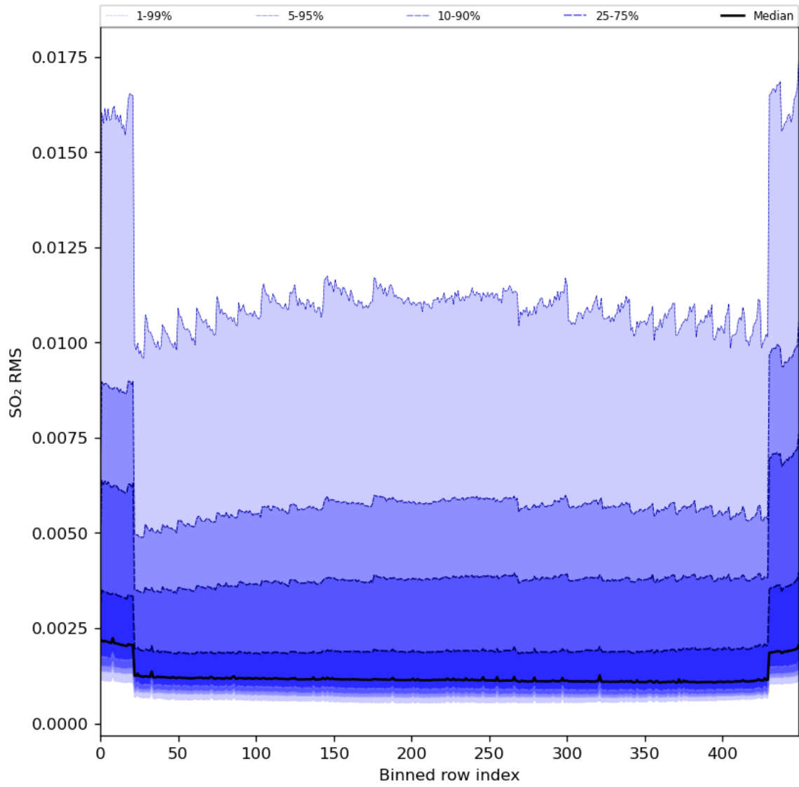
Figure 93: Along track statistics of “SO 2 RMS” for 2024-02-28 to 2024-03-01
