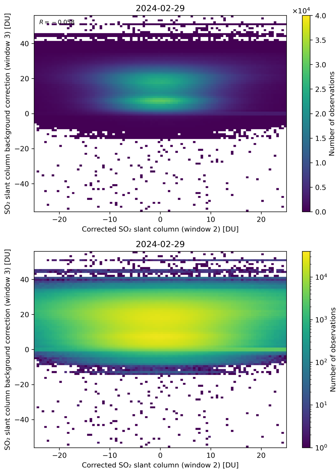
Figure 195: Scatter density plot of “Corrected SO 2 slant column (window 2)” against “SO 2 slant column background correction (window 3)” for 2024-02-28 to 2024-03-01.
