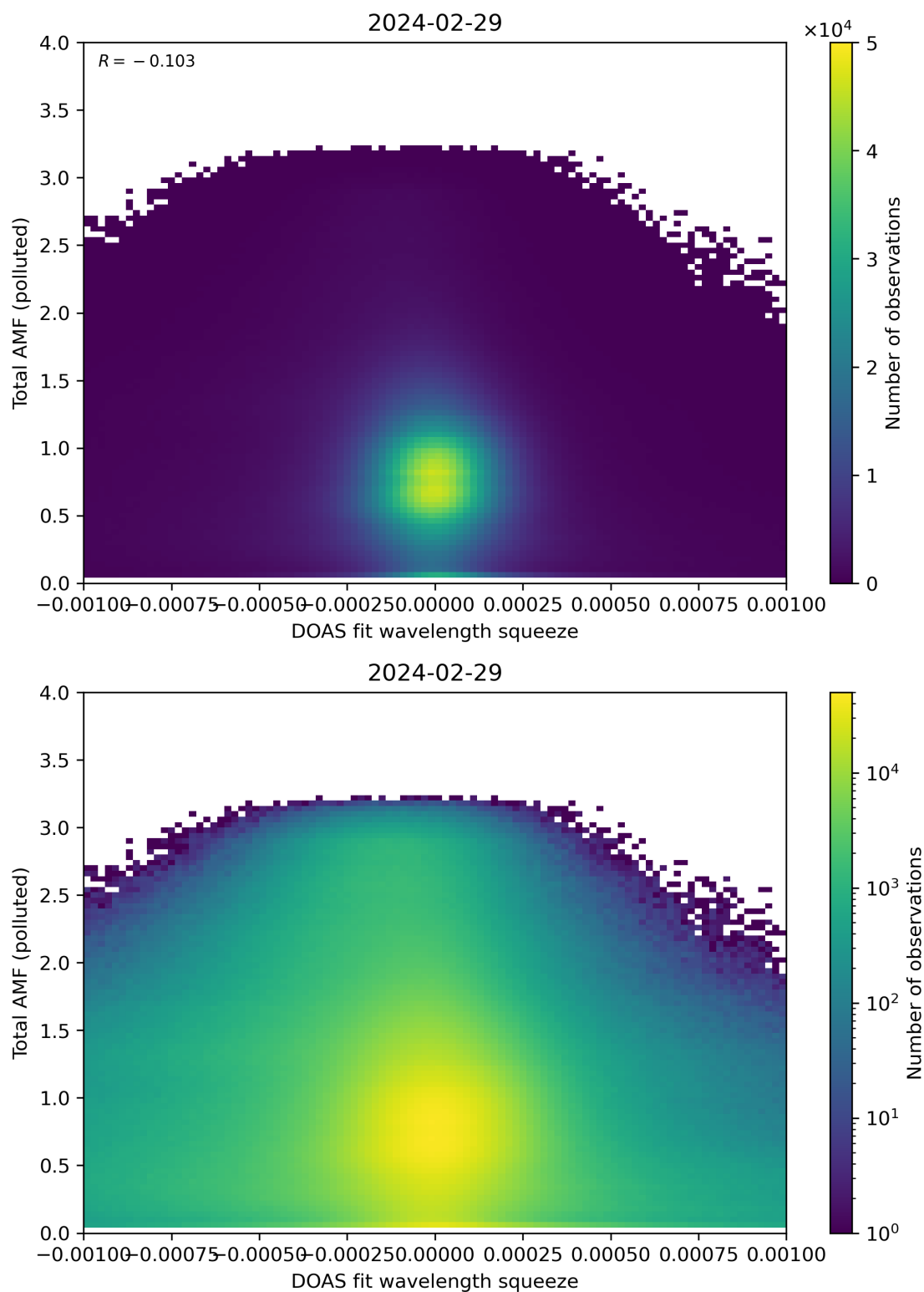
Figure 134: Scatter density plot of “DOAS fit wavelength squeeze” against “Total AMF (polluted)” for 2024-02-28 to 2024-03-01.
