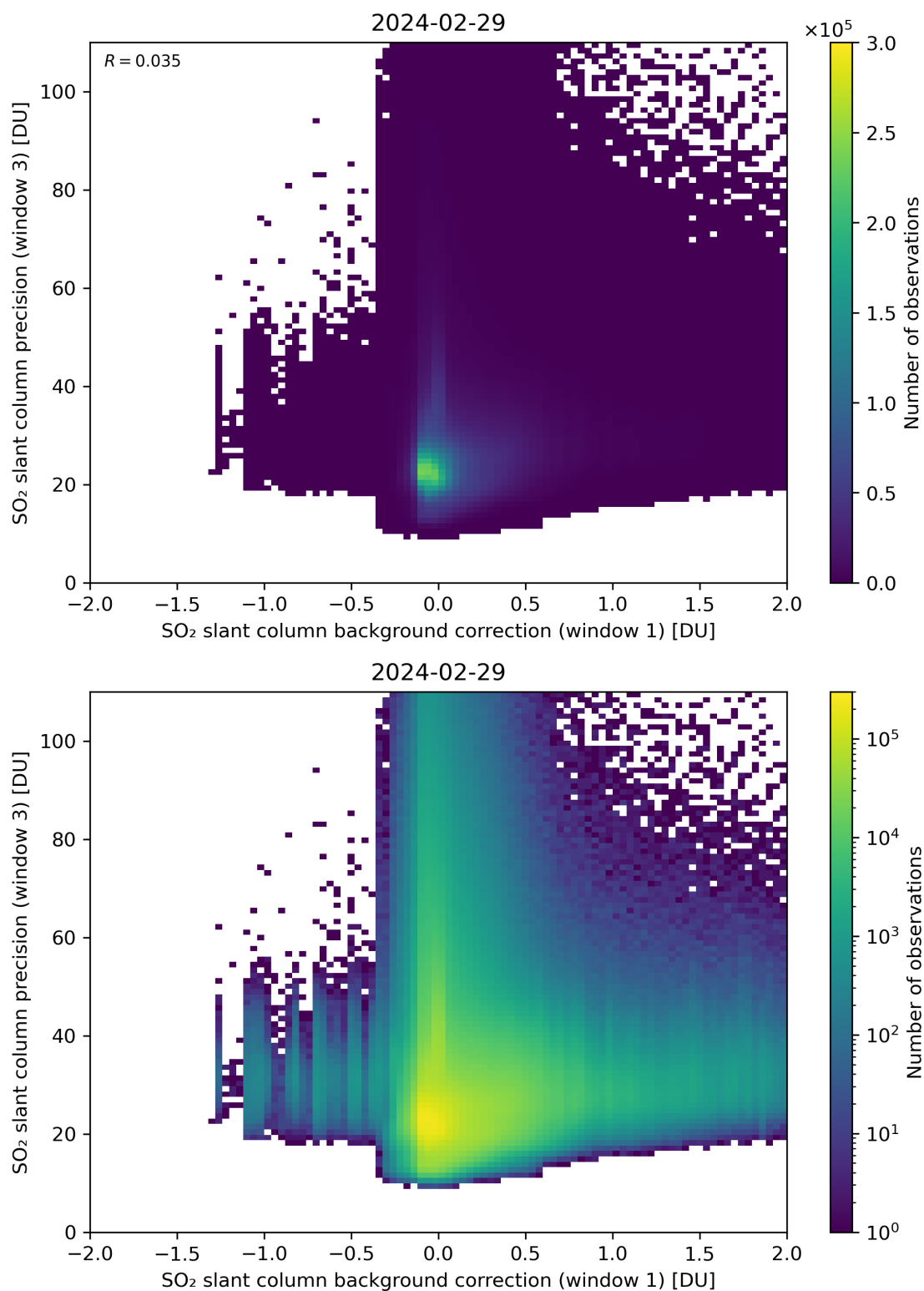
Figure 108: Scatter density plot of “SO 2 slant column background correction (window 1)” against “SO 2 slant column precision (window 3)” for 2024-02-28 to 2024-03-01.
