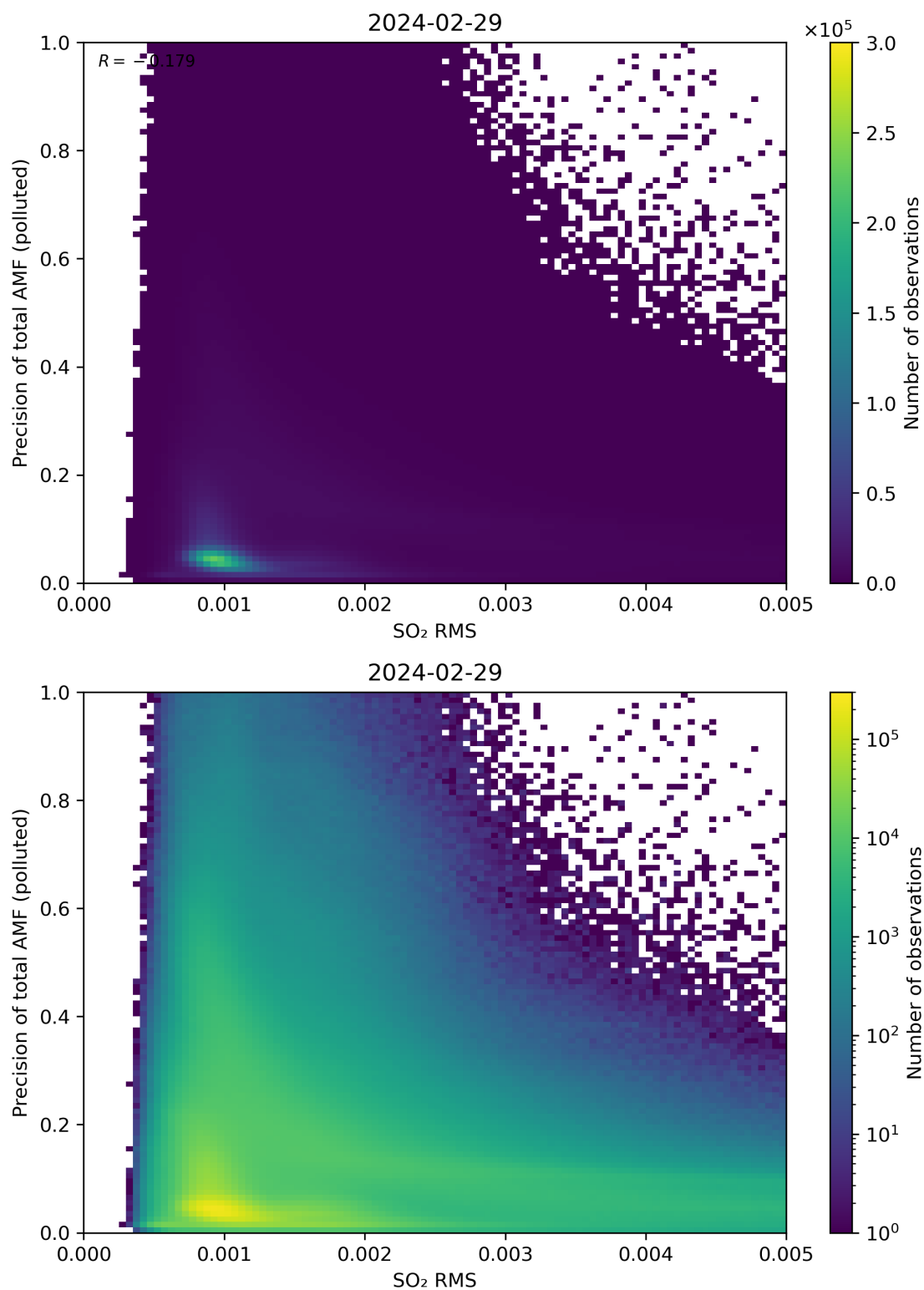
Figure 138: Scatter density plot of “SO 2 RMS” against “Precision of total AMF (polluted)” for 2024-02-28 to 2024-03-01.
