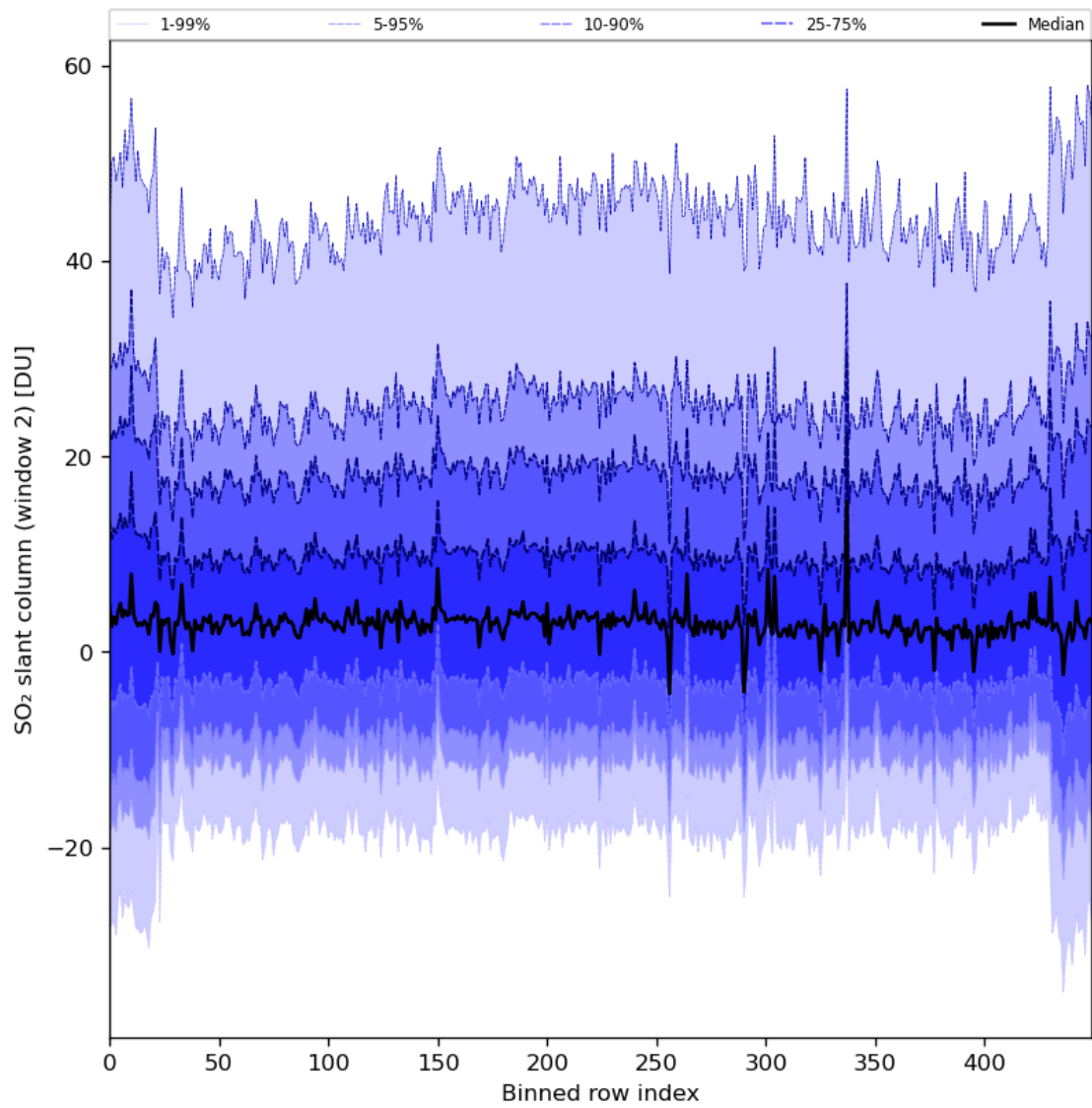
Figure 83: Along track statistics of “SO 2 slant column (window 2)” for 2024-02-28 to 2024-03-01
