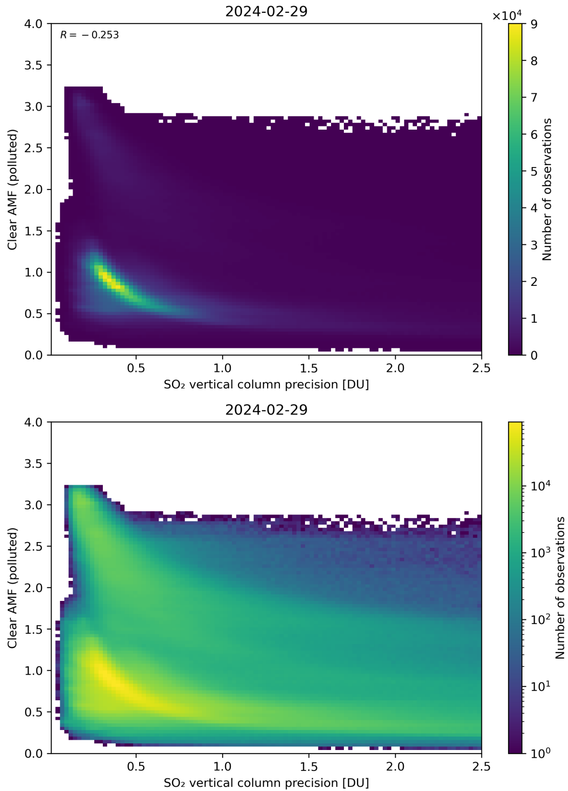
Figure 285: Scatter density plot of “SO 2 vertical column precision” against “Clear AMF (polluted)” for 2024-02-28 to 2024-03-01.
