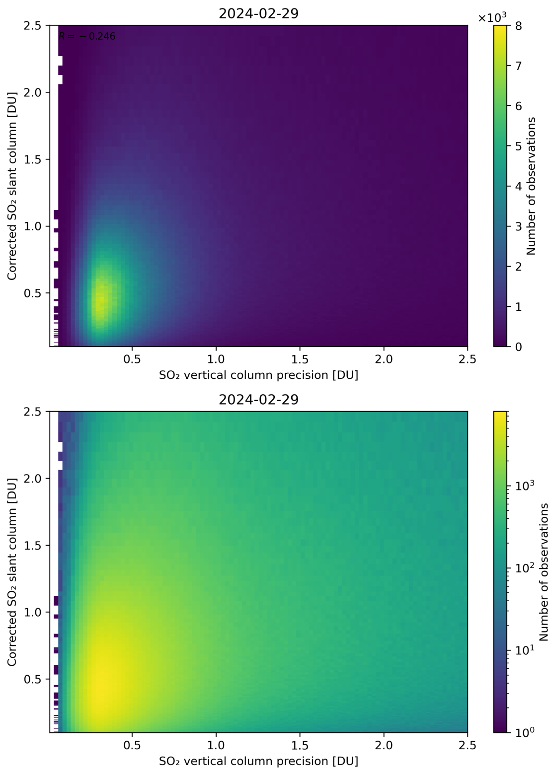
Figure 286: Scatter density plot of “SO 2 vertical column precision” against “Corrected SO 2 slant column” for 2024-02-28 to 2024-03-01.
