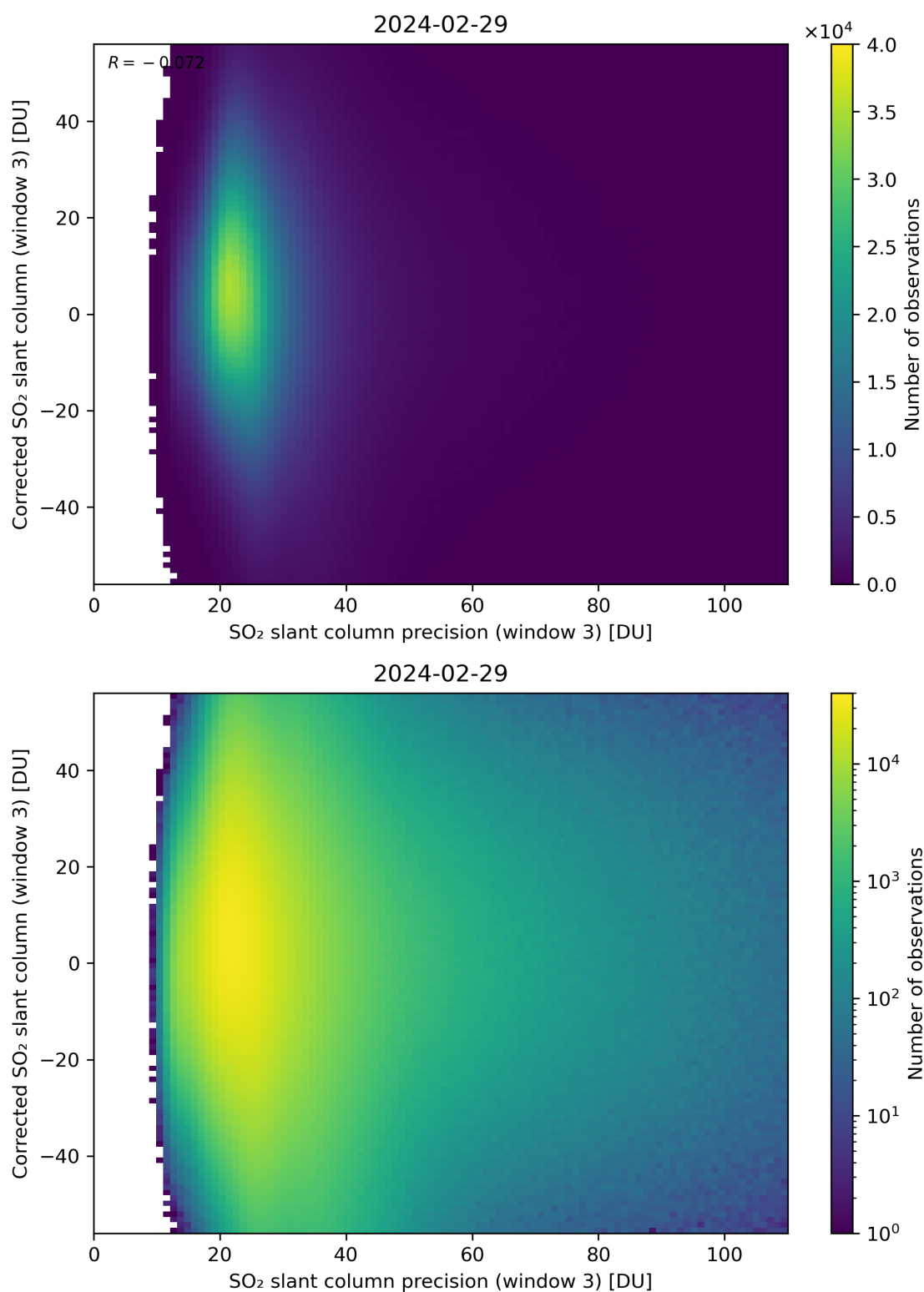
Figure 262: Scatter density plot of “SO 2 slant column precision (window 3)” against “Corrected SO 2 slant column (window 3)” for 2024-02-28 to 2024-03-01.
