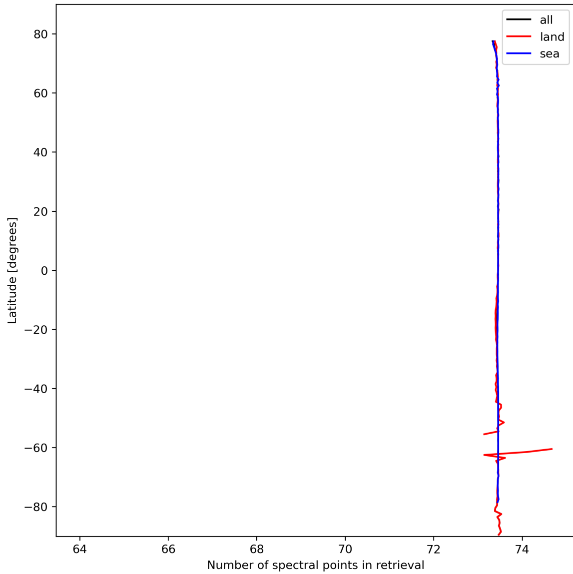
Figure 51: Zonal average of “Number of spectral points in retrieval” for 2024-02-28 to 2024-03-01.
