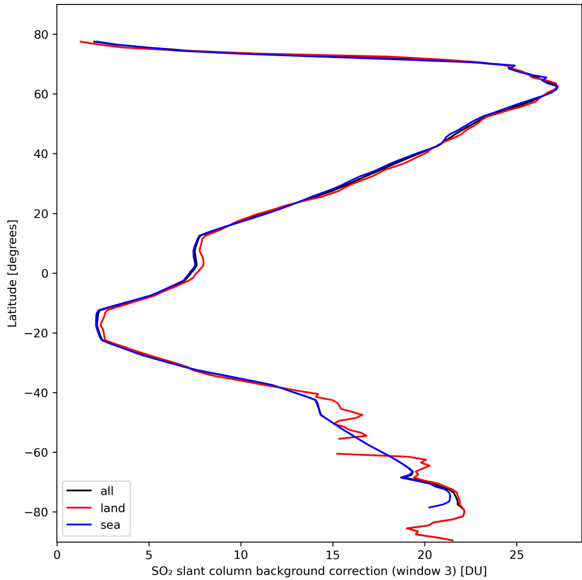
Figure 44: Zonal average of “SO 2 slant column background correction (window 3)” for 2024-02-28 to 2024-03-01.
