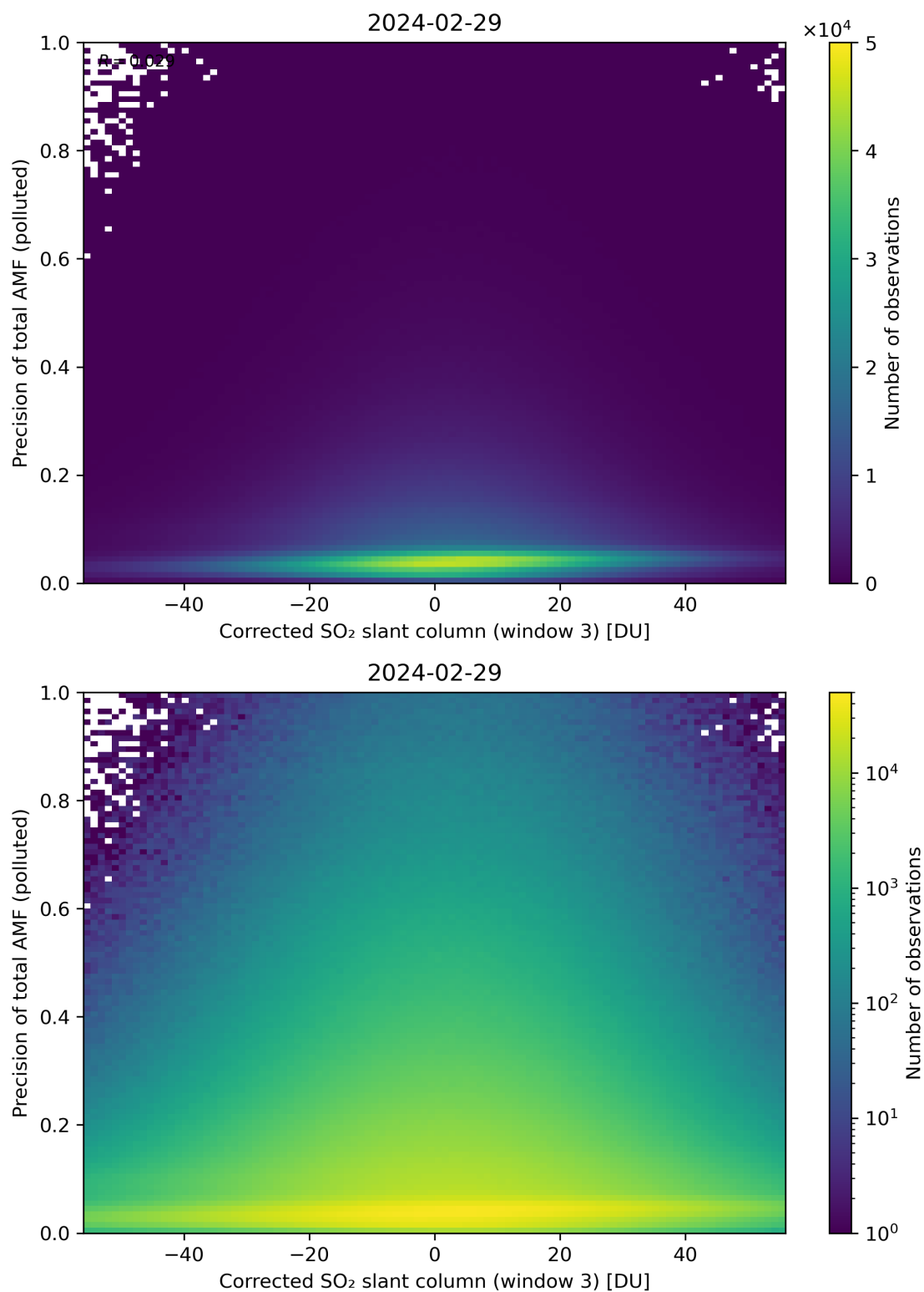
Figure 211: Scatter density plot of “Corrected SO 2 slant column (window 3)” against “Precision of total AMF (polluted)” for 2024-02-28 to 2024-03-01.
