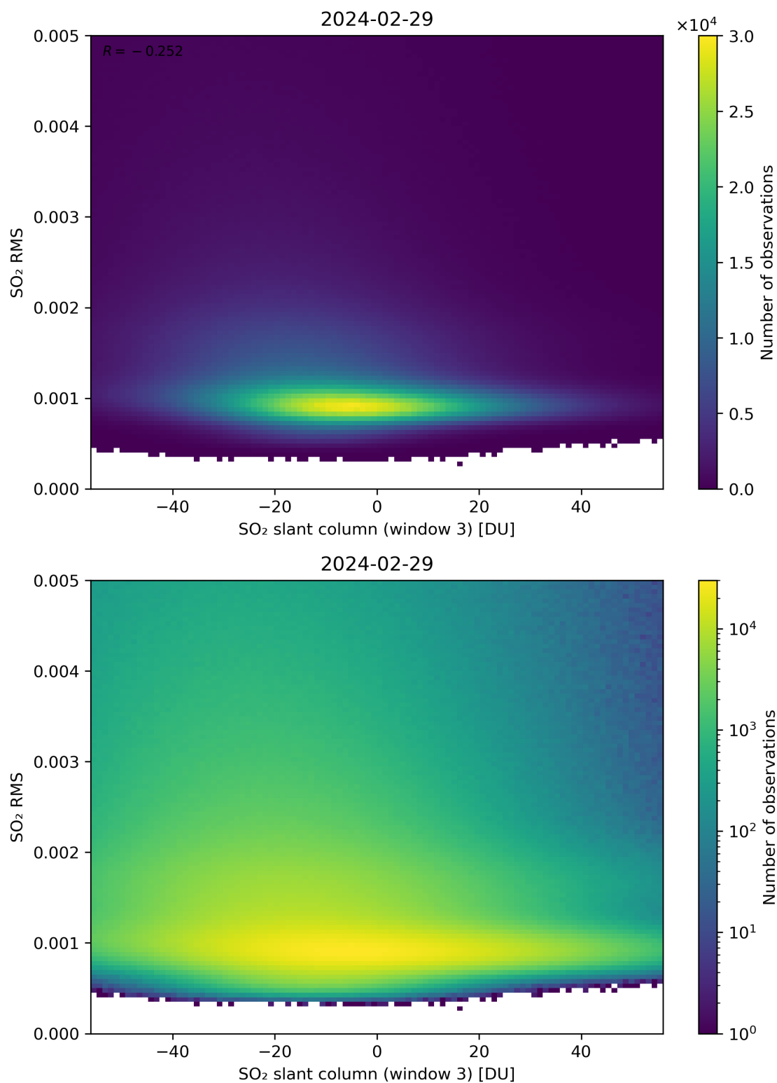
Figure 256: Scatter density plot of “SO 2 slant column (window 3)” against “SO 2 RMS” for 2024-02-28 to 2024-03-01.
