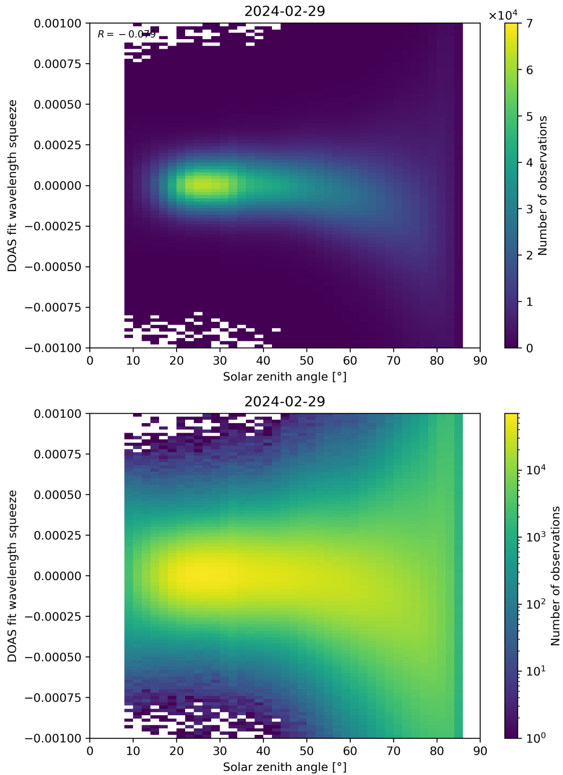
Figure 162: Scatter density plot of “Solar zenith angle” against “DOAS fit wavelength squeeze” for 2024-02-28 to 2024-03-01.
