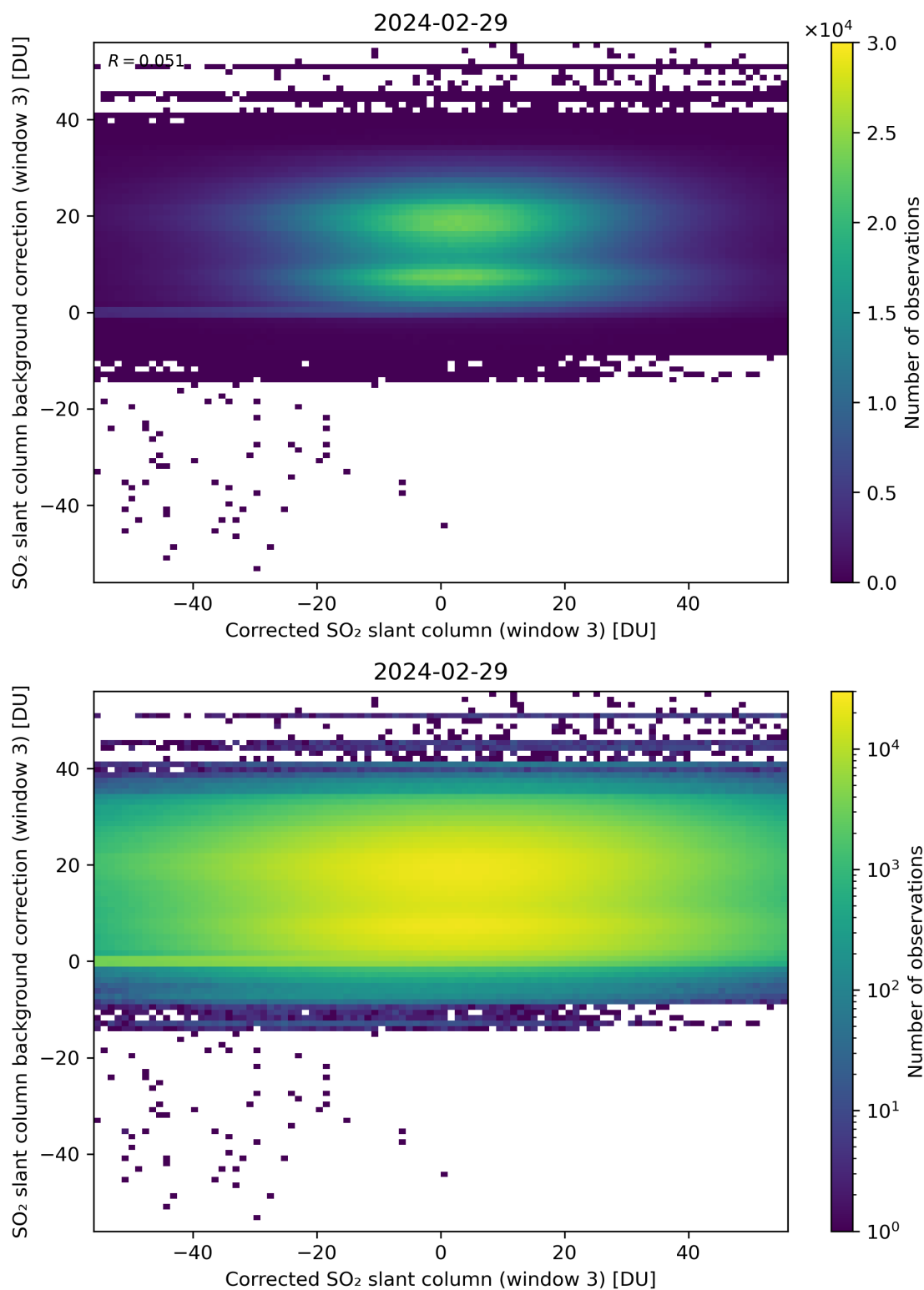
Figure 205: Scatter density plot of “Corrected SO 2 slant column (window 3)” against “SO 2 slant column background correction (window 3)” for 2024-02-28 to 2024-03-01.
