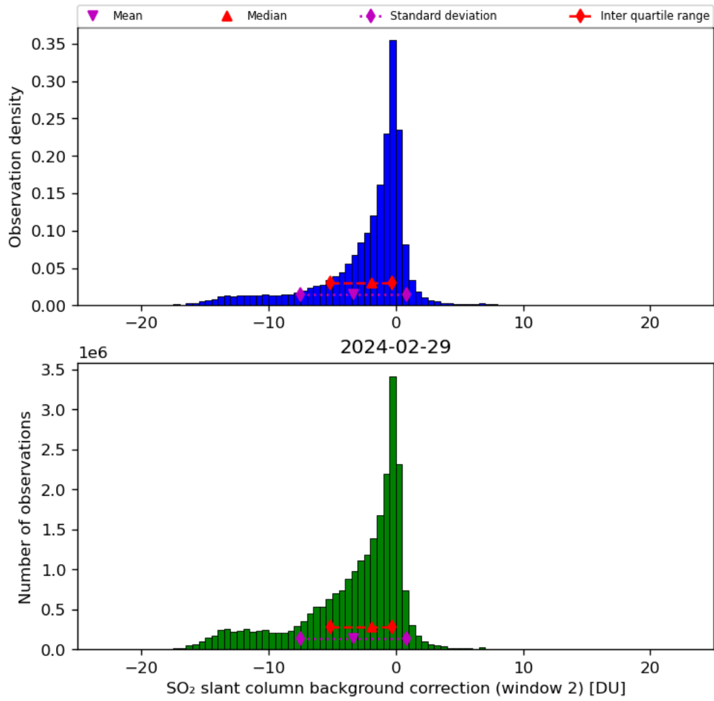
Figure 63: Histogram of “SO 2 slant column background correction (window 2)” for 2024-02-28 to 2024-03-01
