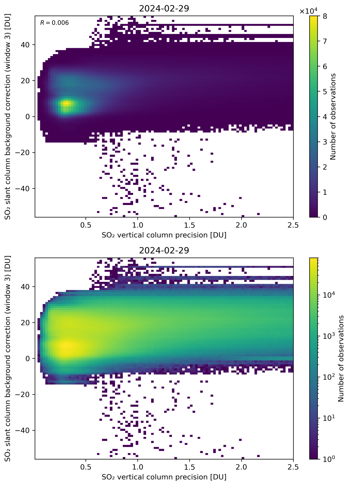
Figure 281: Scatter density plot of “SO 2 vertical column precision” against “SO 2 slant column background correction (window 3)” for 2024-02-28 to 2024-03-01.
