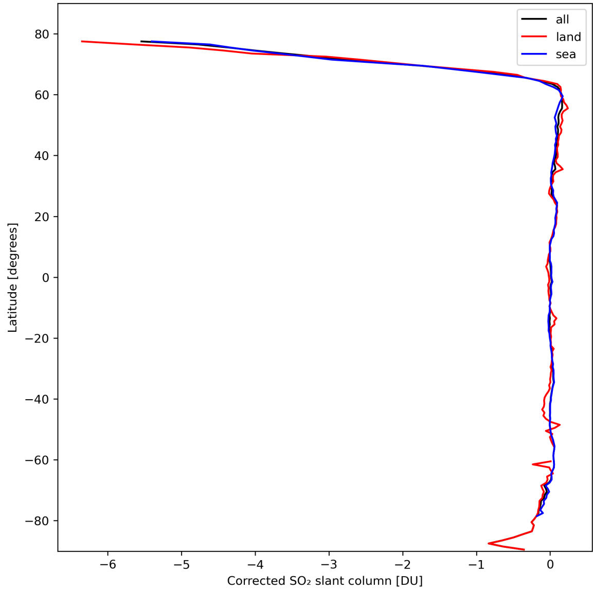
Figure 32: Zonal average of “Corrected SO 2 slant column” for 2024-02-28 to 2024-03-01.
