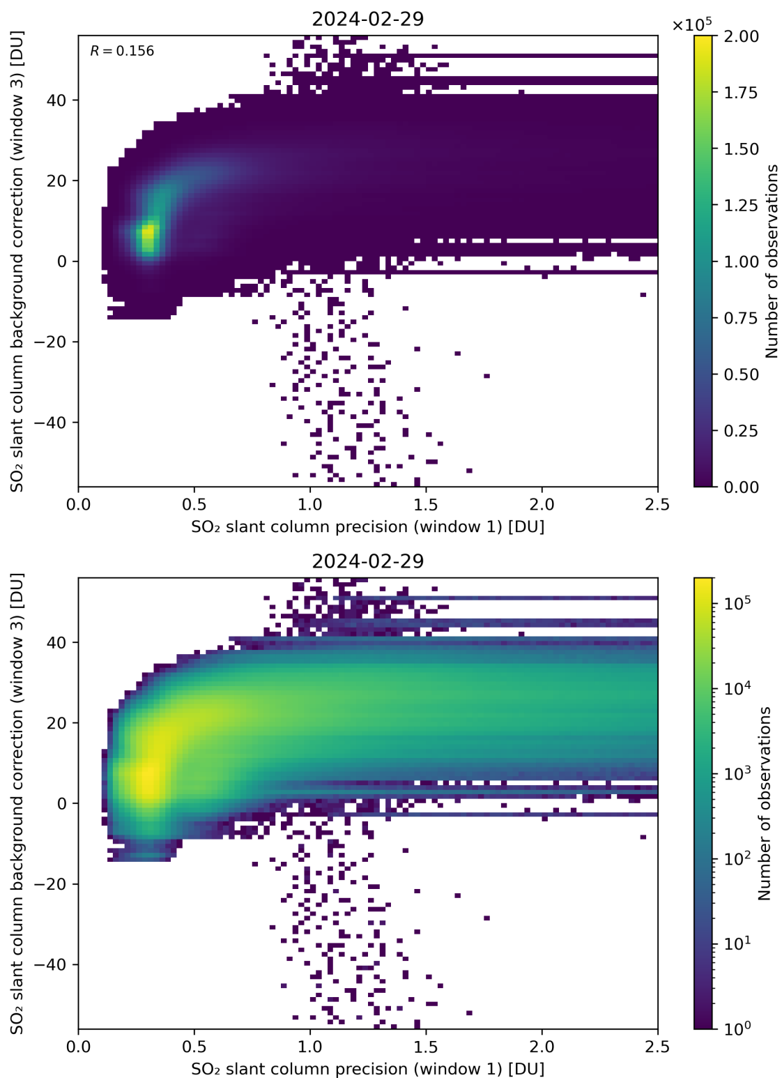
Figure 220: Scatter density plot of “SO 2 slant column precision (window 1)” against “SO 2 slant column background correction (window 3)” for 2024-02-28 to 2024-03-01.
