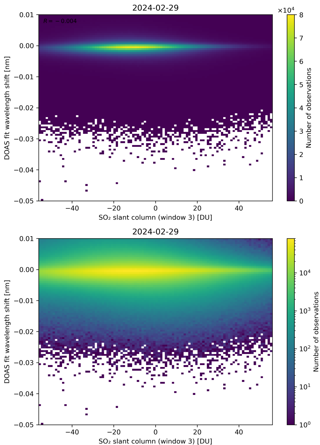
Figure 254: Scatter density plot of “SO 2 slant column (window 3)” against “DOAS fit wavelength shift” for 2024-02-28 to 2024-03-01.
