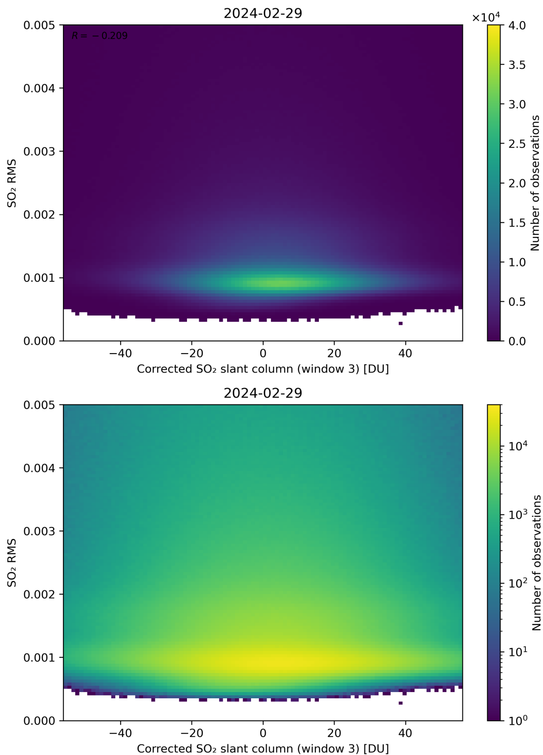
Figure 208: Scatter density plot of “Corrected SO 2 slant column (window 3)” against “SO 2 RMS” for 2024-02-28 to 2024-03-01.
