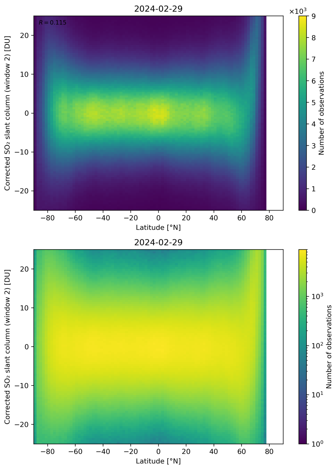
Figure 147: Scatter density plot of “Latitude” against “Corrected SO 2 slant column (window 2)” for 2024-02-28 to 2024-03-01.
