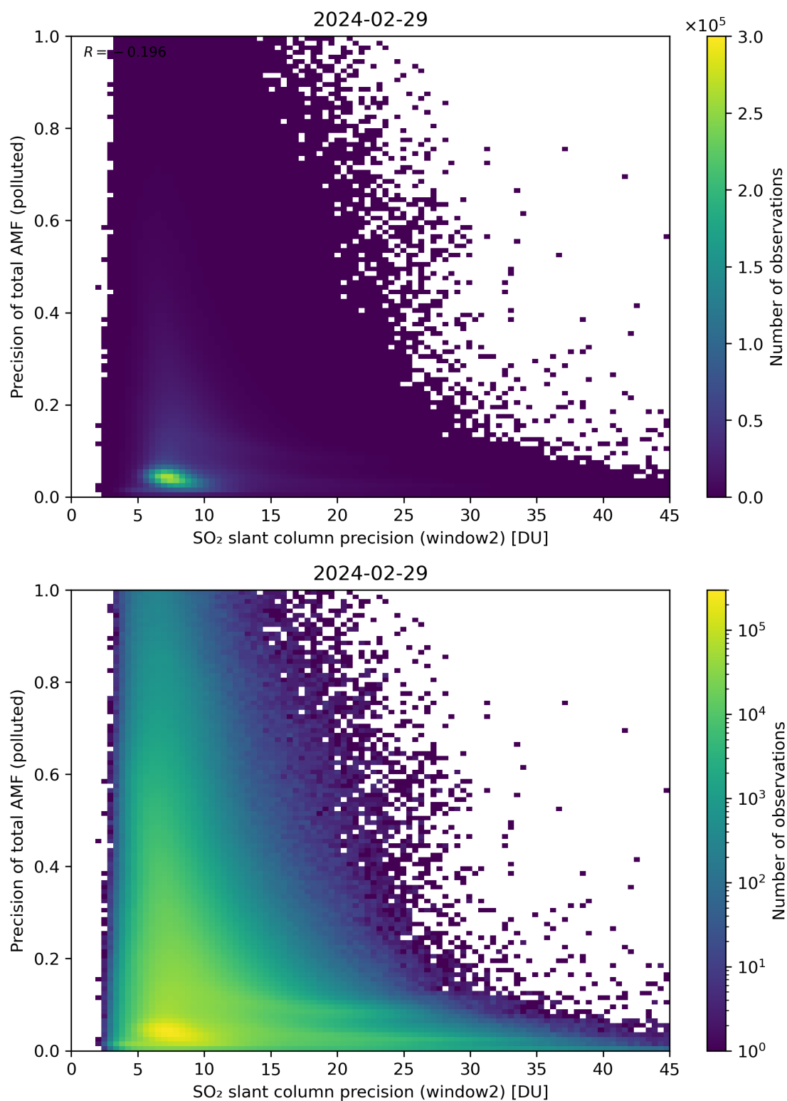
Figure 252: Scatter density plot of “SO 2 slant column precision (window2)” against “Precision of total AMF (polluted)” for 2024-02-28 to 2024-03-01.
