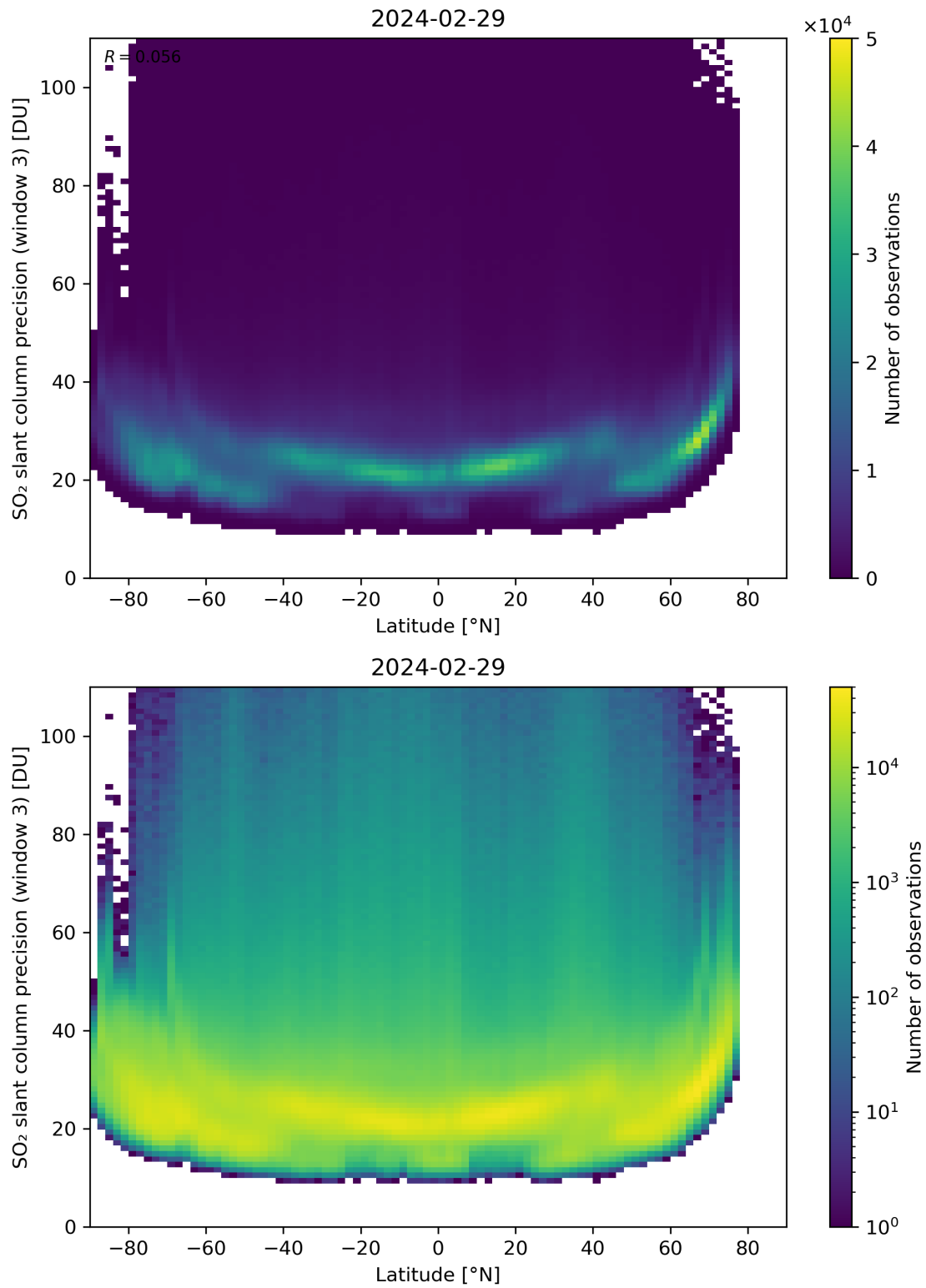
Figure 153: Scatter density plot of “Latitude” against “SO 2 slant column precision (window 3)” for 2024-02-28 to 2024-03-01.
