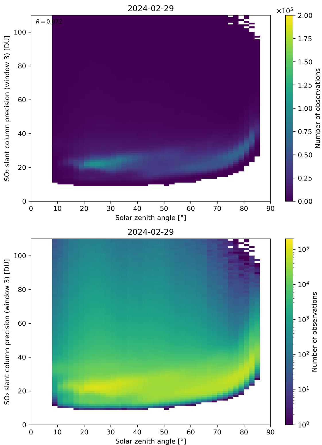
Figure 173: Scatter density plot of “Solar zenith angle” against “SO 2 slant column precision (window 3)” for 2024-02-28 to 2024-03-01.
