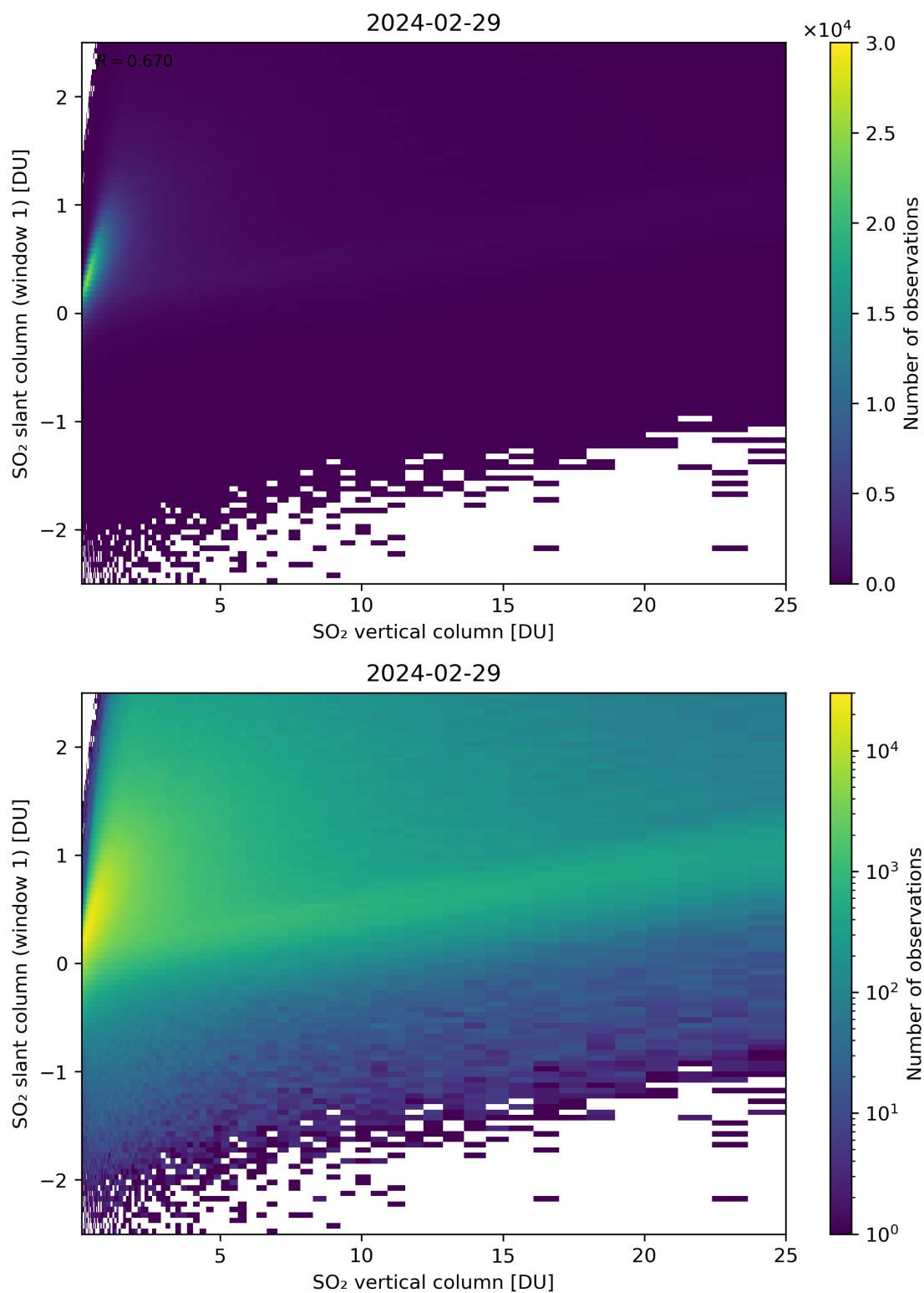
Figure 300: Scatter density plot of “SO 2 vertical column” against “SO 2 slant column (window 1)” for 2024-02-28 to 2024-03-01.
