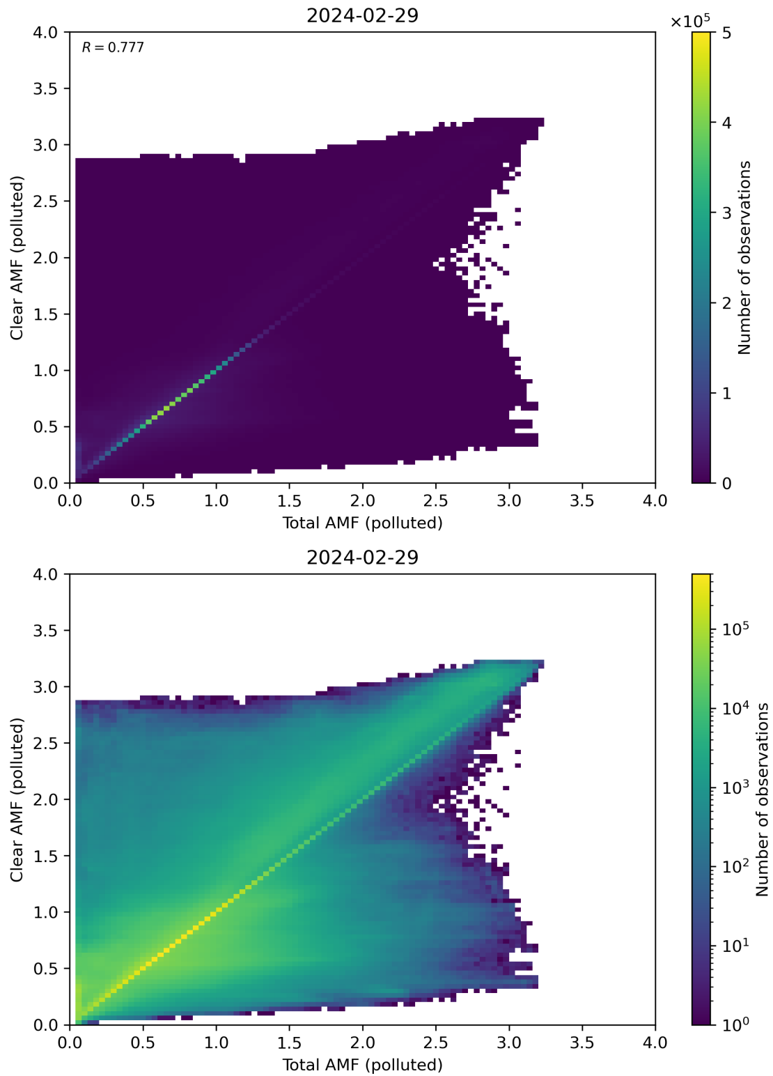
Figure 271: Scatter density plot of “Total AMF (polluted)” against “Clear AMF (polluted)” for 2024-02-28 to 2024-03-01.
