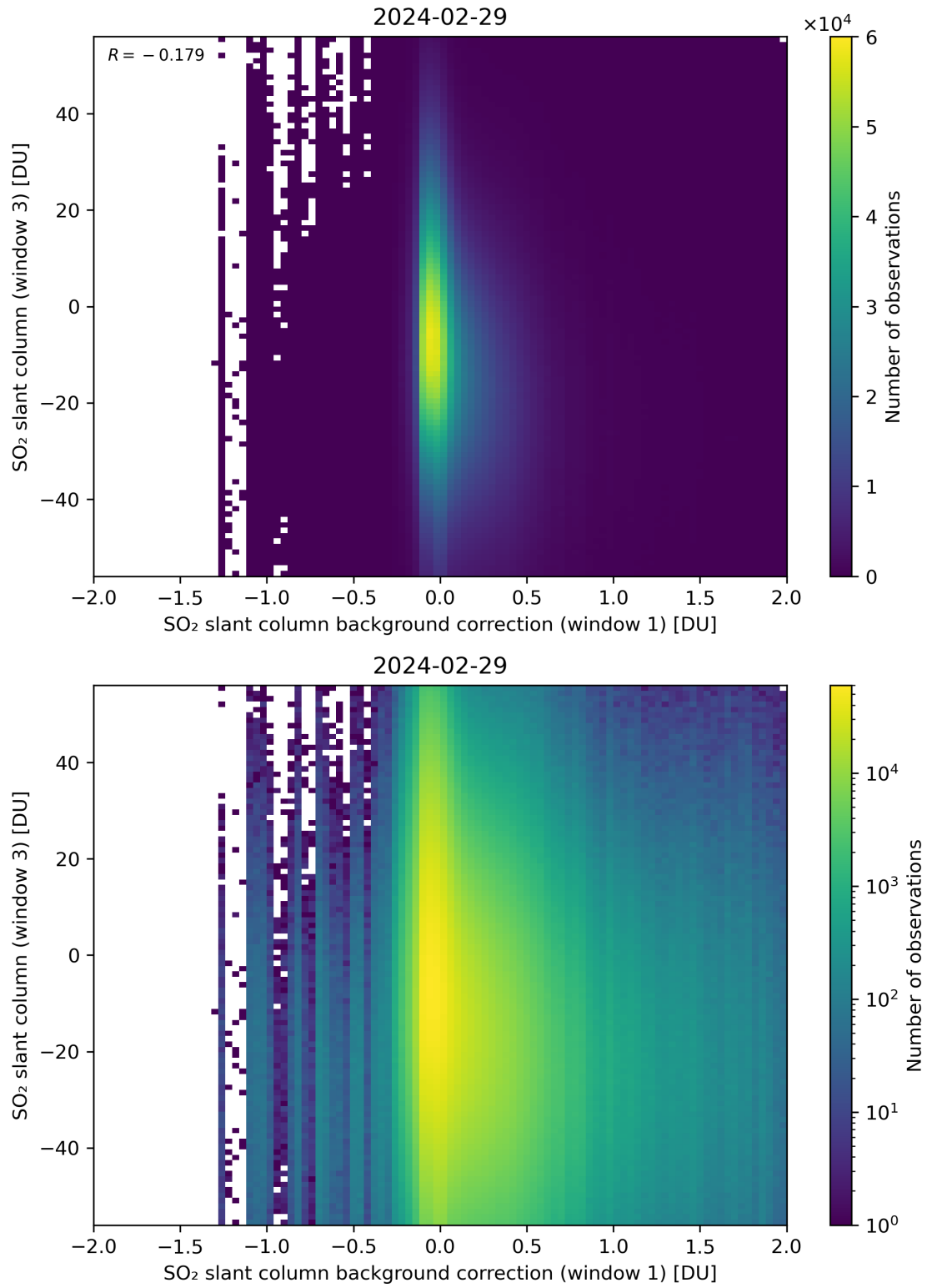
Figure 107: Scatter density plot of “SO 2 slant column background correction (window 1)” against “SO 2 slant column (window 3)” for 2024-02-28 to 2024-03-01.
