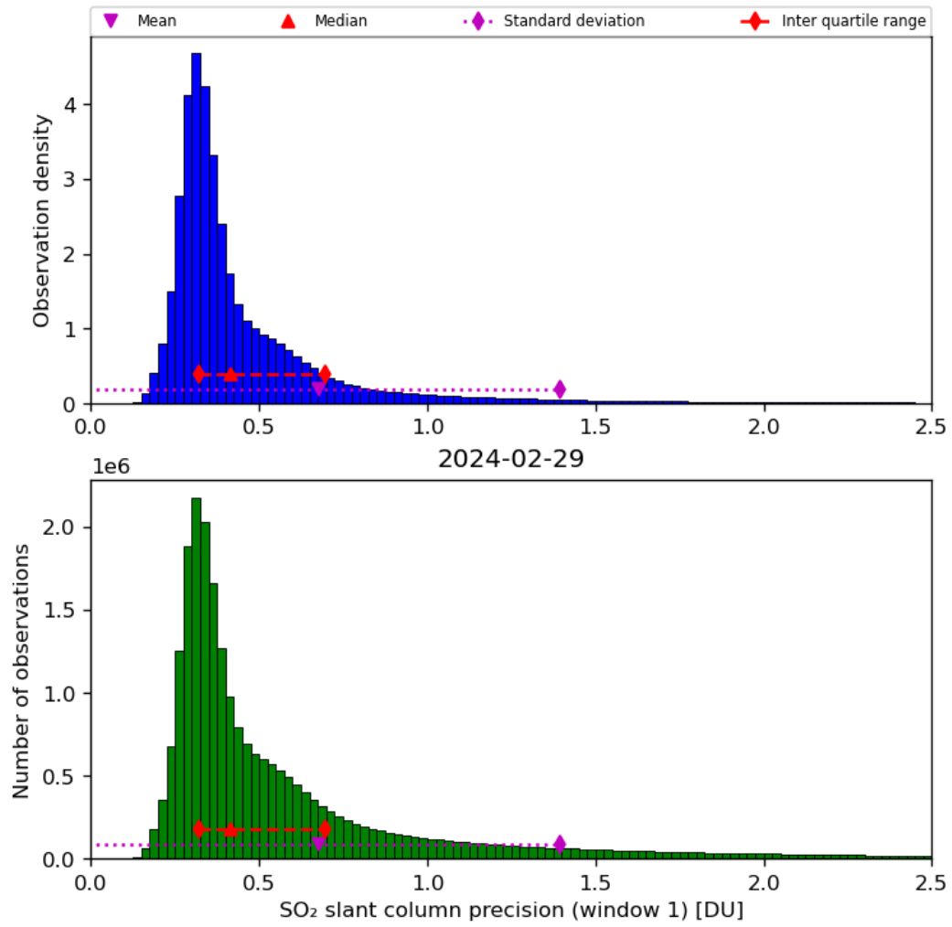
Figure 57: Histogram of “SO 2 slant column precision (window 1)” for 2024-02-28 to 2024-03-01
