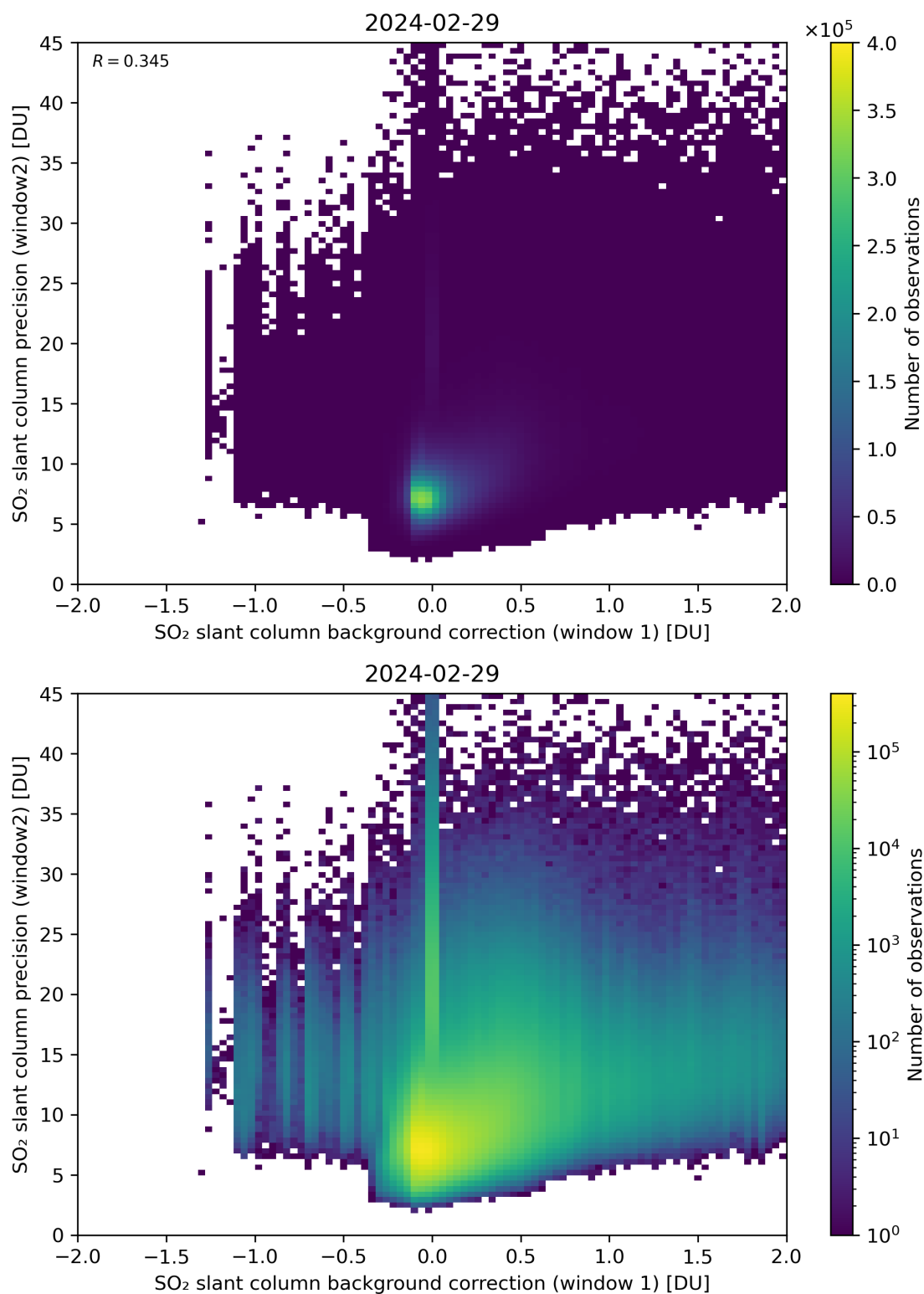
Figure 106: Scatter density plot of “SO 2 slant column background correction (window 1)” against “SO 2 slant column precision (window2)” for 2024-02-28 to 2024-03-01.
