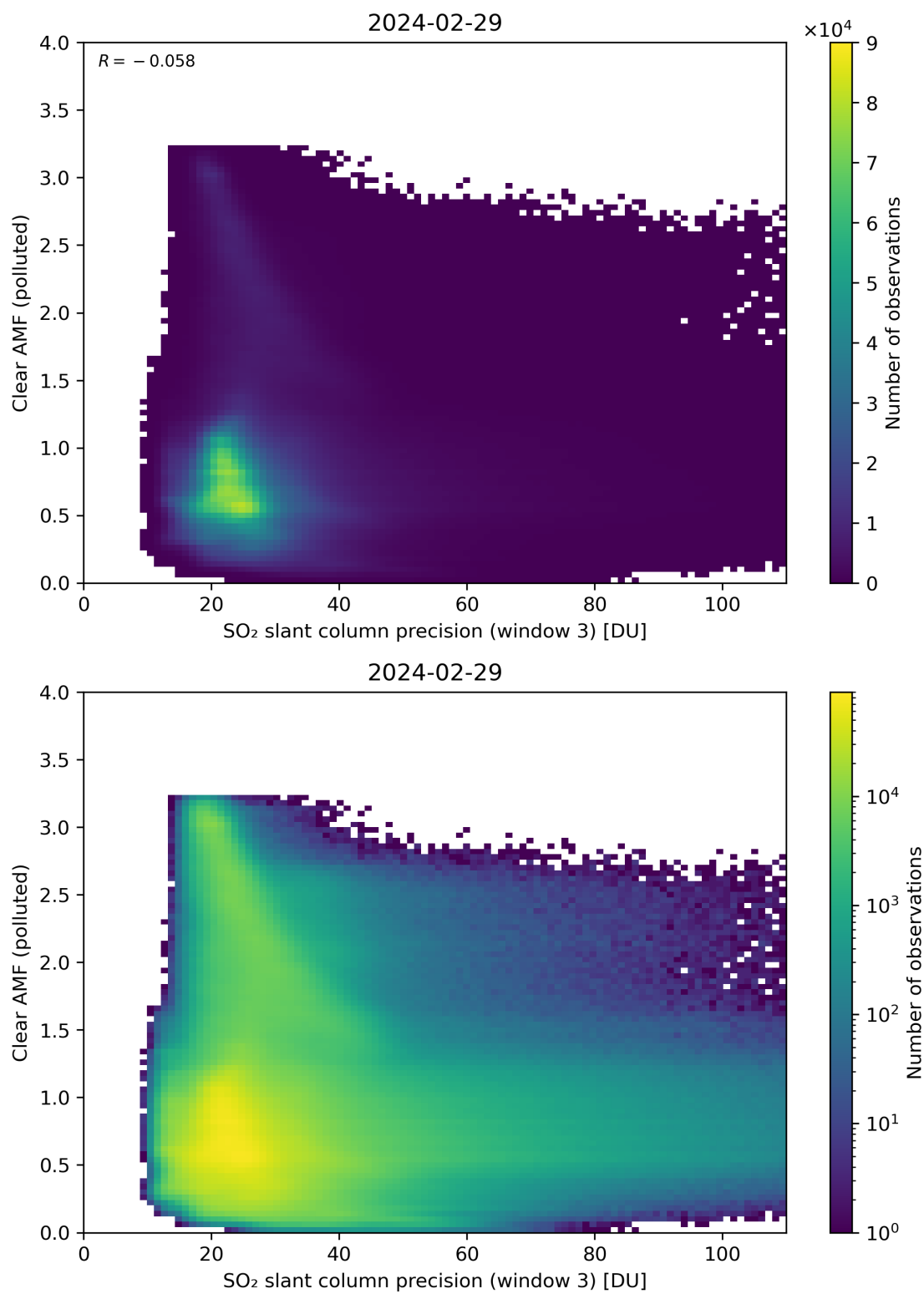
Figure 261: Scatter density plot of “SO 2 slant column precision (window 3)” against “Clear AMF (polluted)” for 2024-02-28 to 2024-03-01.
