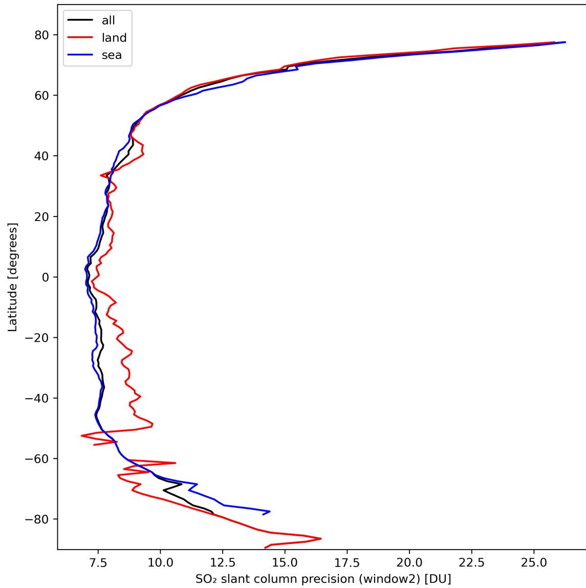
Figure 38: Zonal average of “SO 2 slant column precision (window2)” for 2024-02-28 to 2024-03-01.
