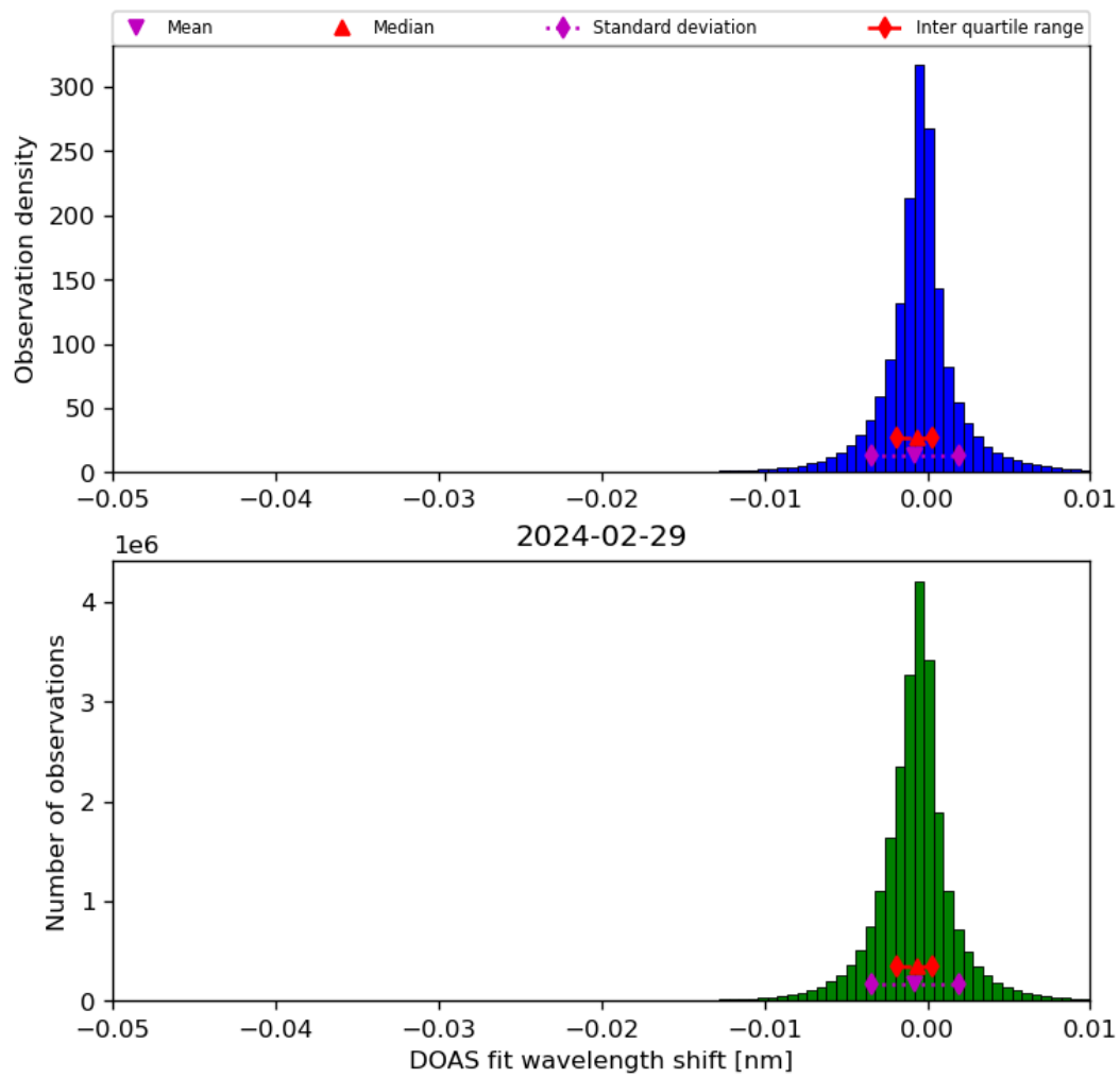
Figure 68: Histogram of “DOAS fit wavelength shift” for 2024-02-28 to 2024-03-01
