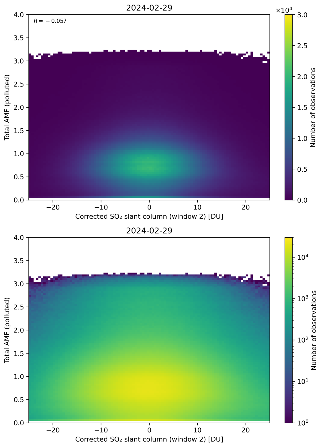
Figure 203: Scatter density plot of “Corrected SO 2 slant column (window 2)” against “Total AMF (polluted)” for 2024-02-28 to 2024-03-01.
