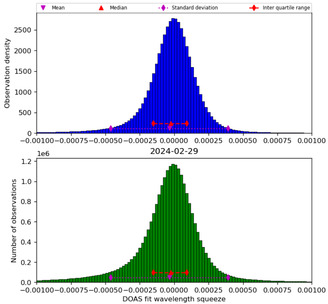
Figure 69: Histogram of “DOAS fit wavelength squeeze” for 2024-02-28 to 2024-03-01
