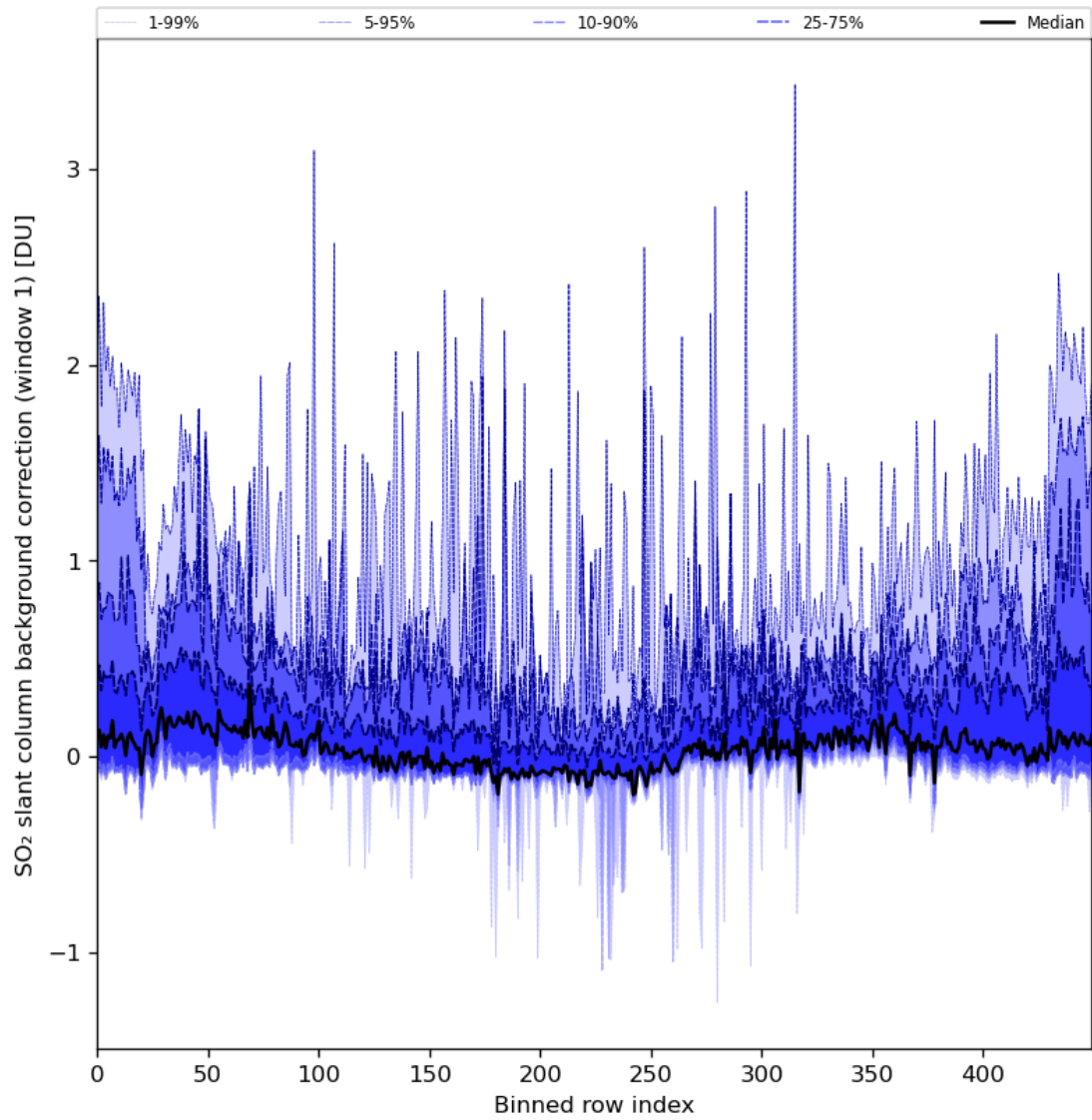
Figure 82: Along track statistics of “SO 2 slant column background correction (window 1)” for 2024-02-28 to 2024-03-01
