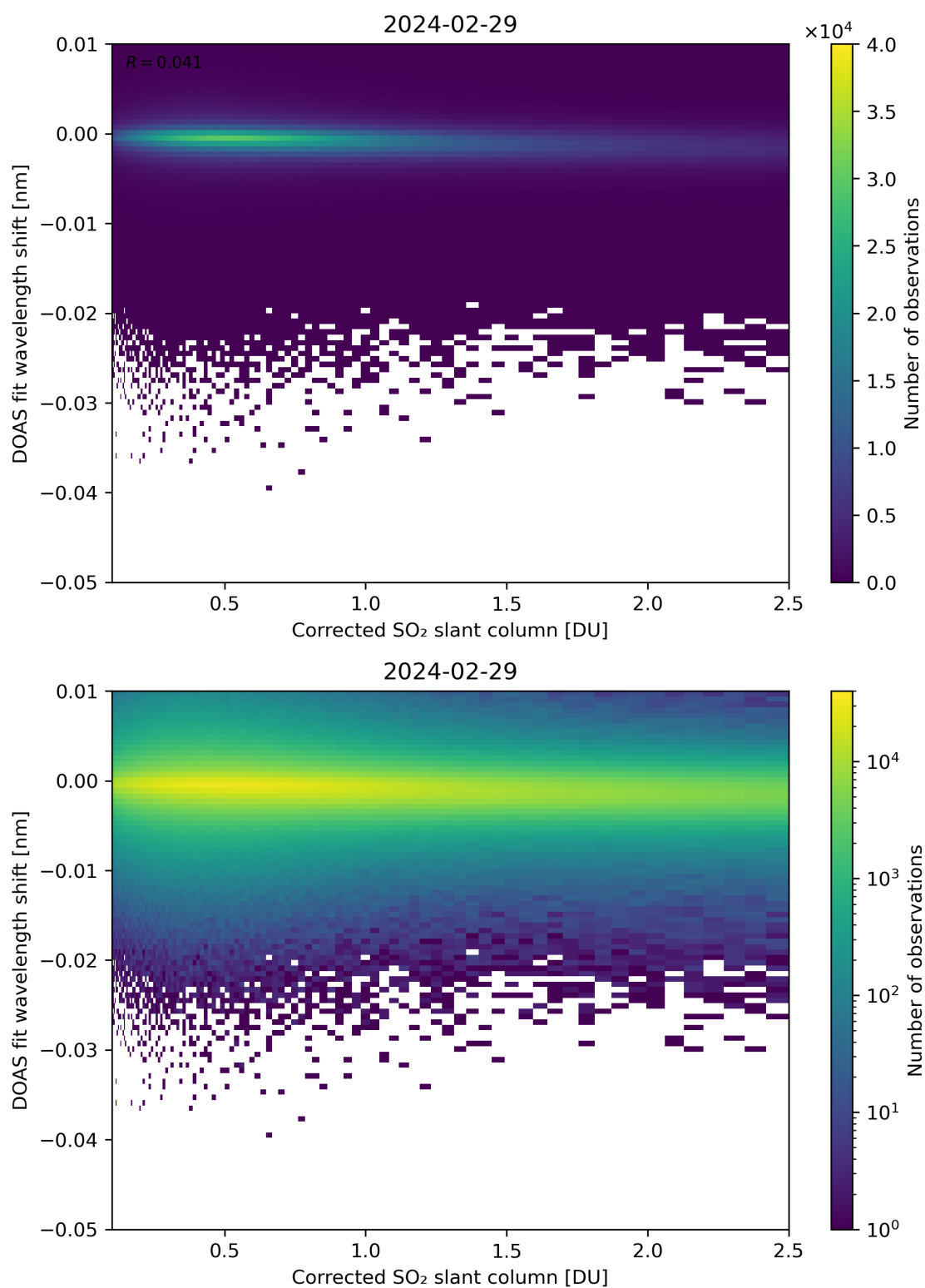
Figure 181: Scatter density plot of “Corrected SO 2 slant column” against “DOAS fit wavelength shift” for 2024-02-28 to 2024-03-01.
