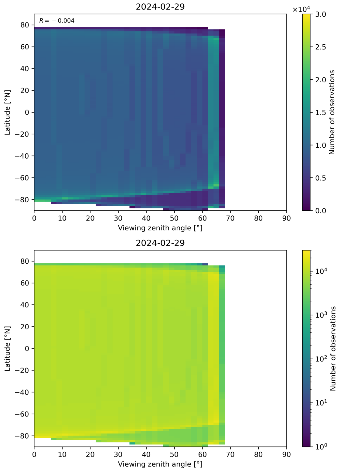
Figure 314: Scatter density plot of “Viewing zenith angle” against “Latitude” for 2024-02-28 to 2024-03-01.
