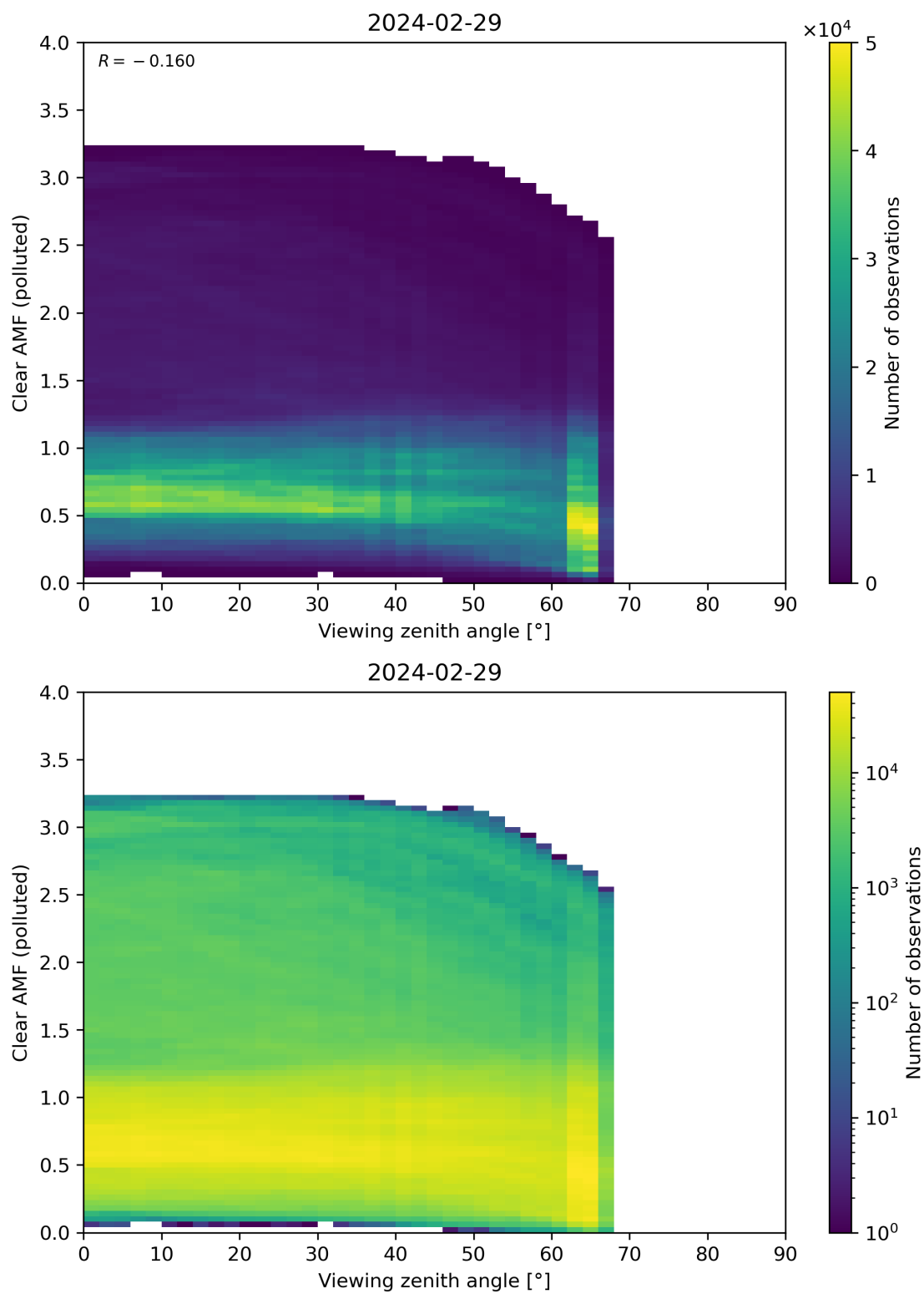
Figure 316: Scatter density plot of “Viewing zenith angle” against “Clear AMF (polluted)” for 2024-02-28 to 2024-03-01.
