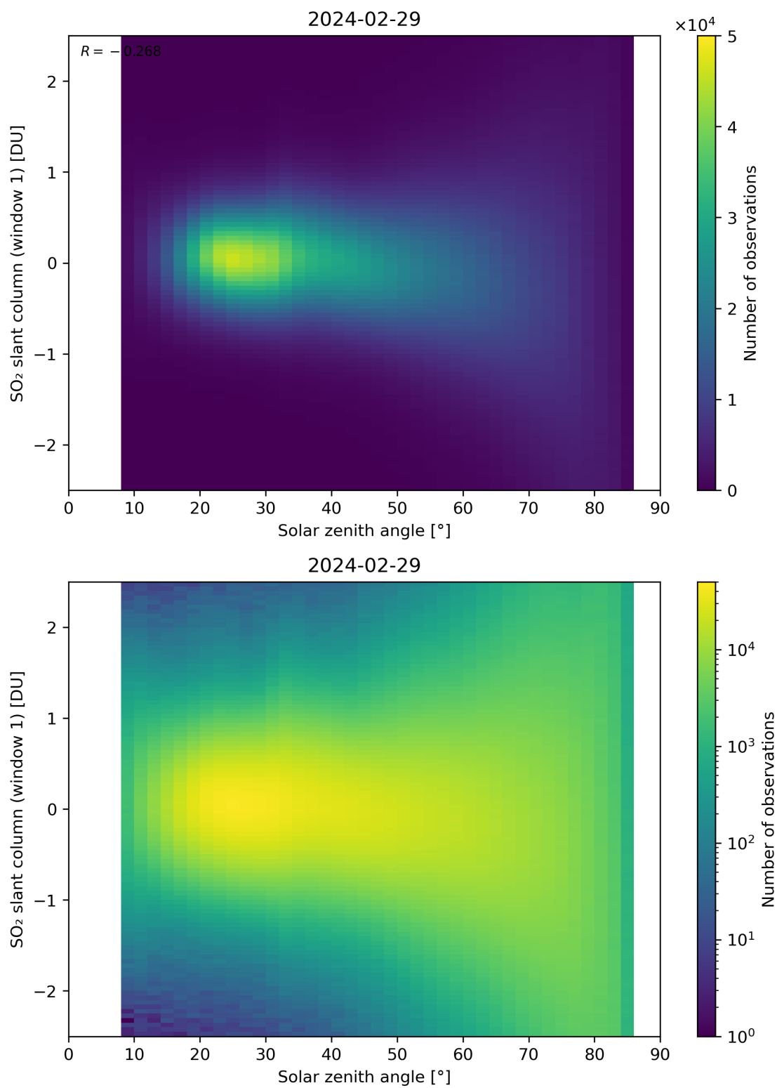
Figure 169: Scatter density plot of “Solar zenith angle” against “SO 2 slant column (window 1)” for 2024-02-28 to 2024-03-01.
