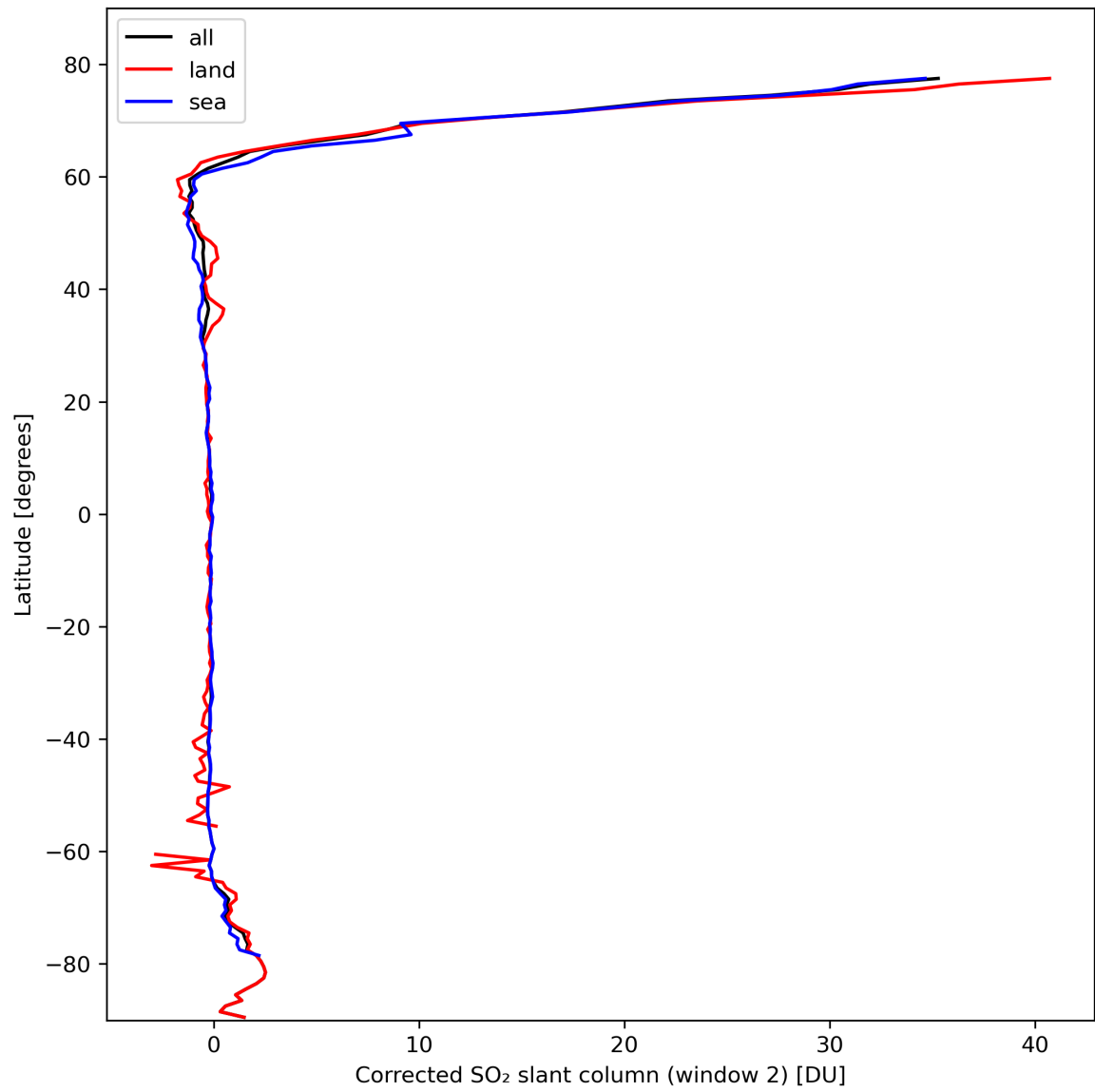
Figure 39: Zonal average of “Corrected SO 2 slant column (window 2)” for 2024-02-28 to 2024-03-01.
