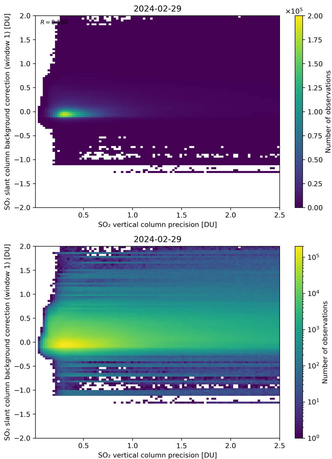
Figure 279: Scatter density plot of “SO 2 vertical column precision” against “SO 2 slant column background correction (window 1)” for 2024-02-28 to 2024-03-01.
