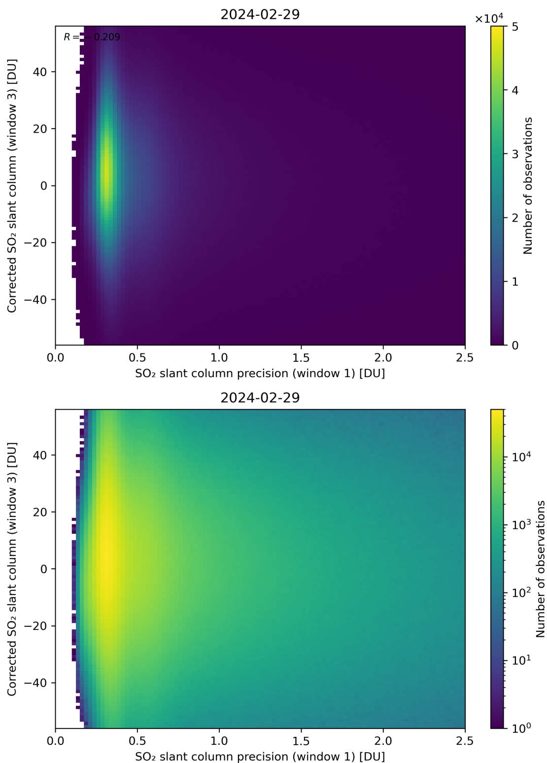
Figure 226: Scatter density plot of “SO 2 slant column precision (window 1)” against “Corrected SO 2 slant column (window 3)” for 2024-02-28 to 2024-03-01.
