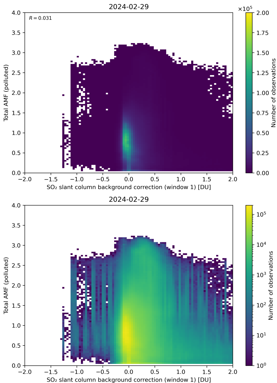
Figure 109: Scatter density plot of “SO 2 slant column background correction (window 1)” against “Total AMF (polluted)” for 2024-02-28 to 2024-03-01.
