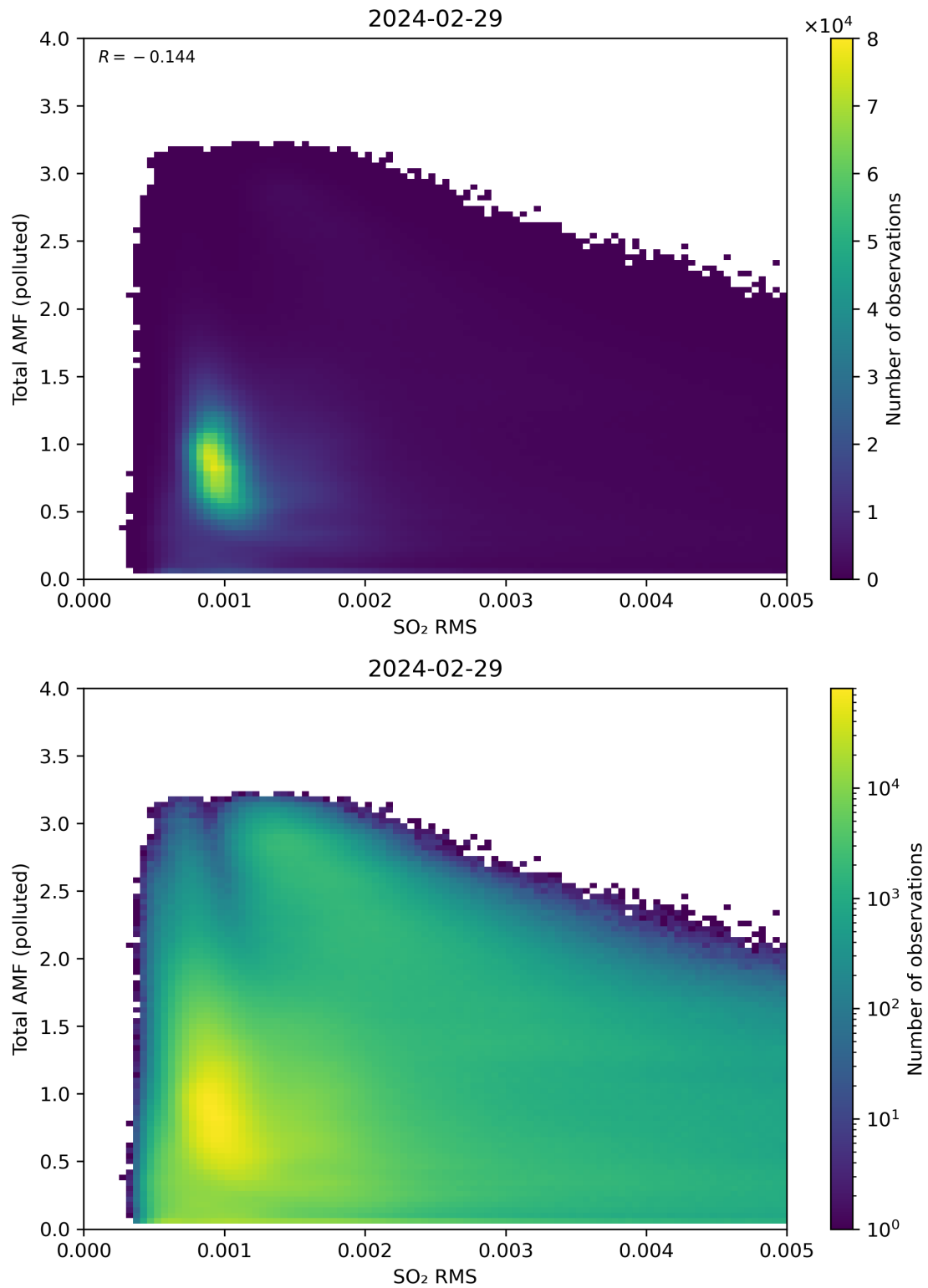
Figure 137: Scatter density plot of “SO 2 RMS” against “Total AMF (polluted)” for 2024-02-28 to 2024-03-01.
