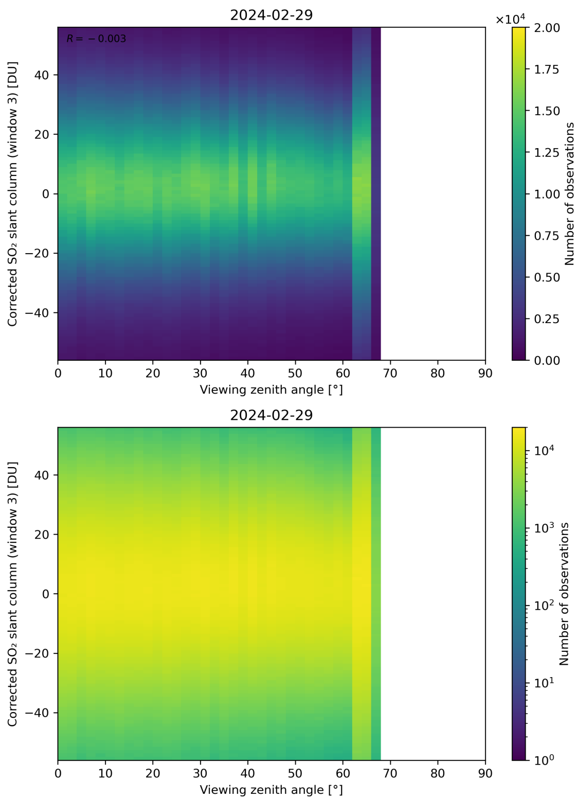
Figure 319: Scatter density plot of “Viewing zenith angle” against “Corrected SO 2 slant column (window 3)” for 2024-02-28 to 2024-03-01.
