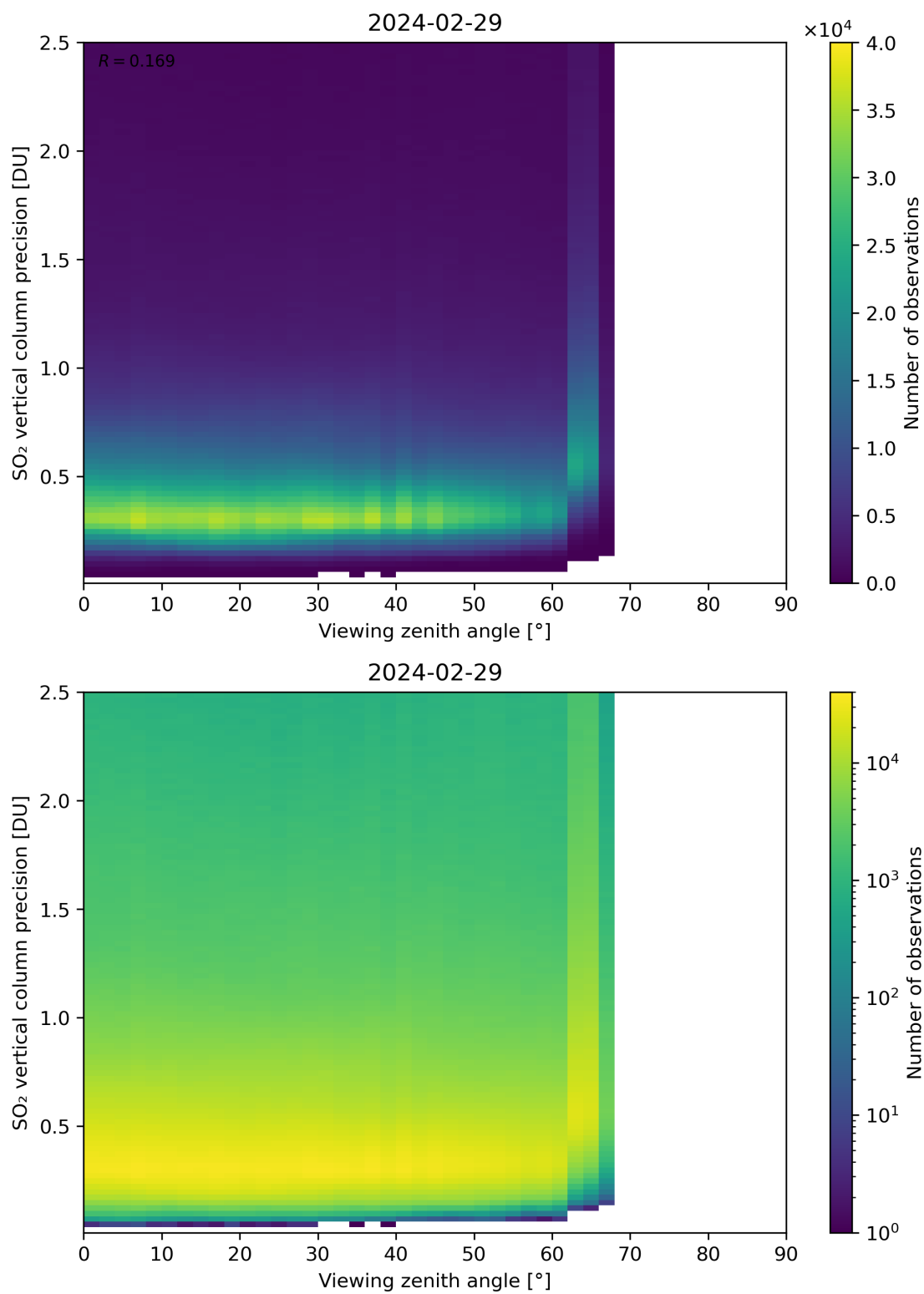
Figure 328: Scatter density plot of “Viewing zenith angle” against “SO 2 vertical column precision” for 2024-02-28 to 2024-03-01.
