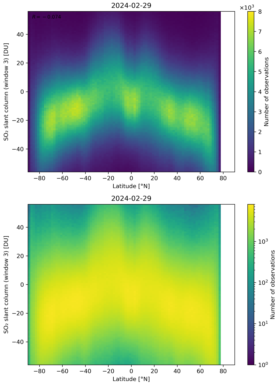
Figure 152: Scatter density plot of “Latitude” against “SO 2 slant column (window 3)” for 2024-02-28 to 2024-03-01.
