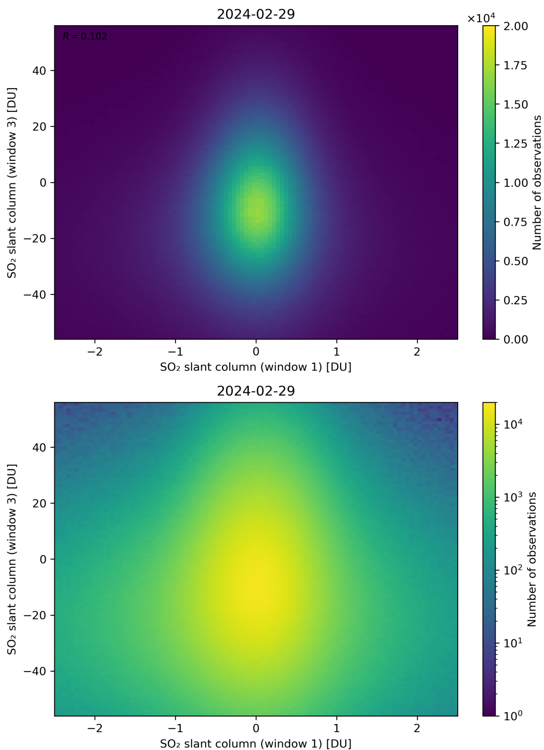
Figure 237: Scatter density plot of “SO 2 slant column (window 1)” against “SO 2 slant column (window 3)” for 2024-02-28 to 2024-03-01.
