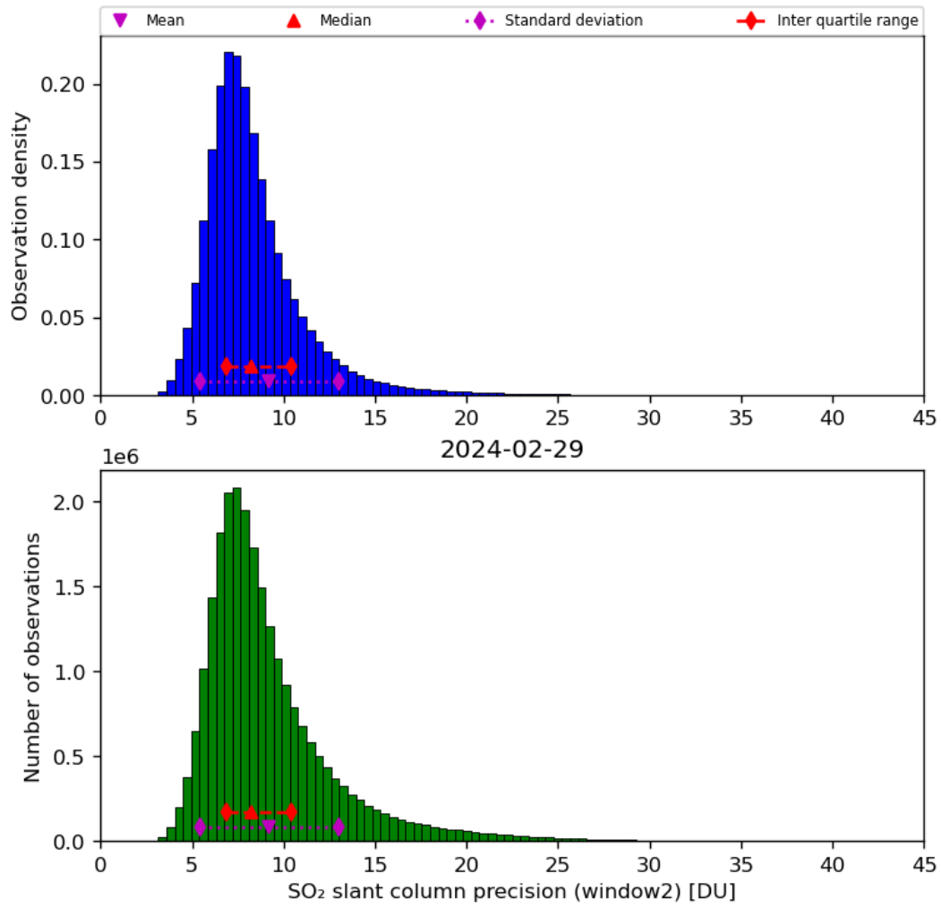
Figure 61: Histogram of “SO 2 slant column precision (window2)” for 2024-02-28 to 2024-03-01
