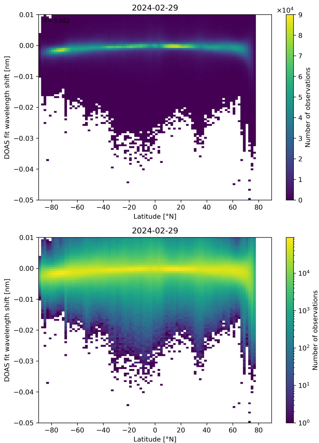
Figure 142: Scatter density plot of “Latitude” against “DOAS fit wavelength shift” for 2024-02-28 to 2024-03-01.
