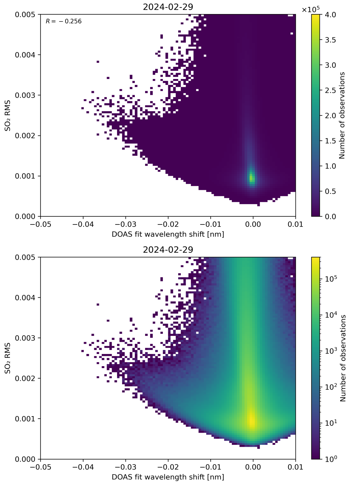
Figure 128: Scatter density plot of “DOAS fit wavelength shift” against “SO 2 RMS” for 2024-02-28 to 2024-03-01.
