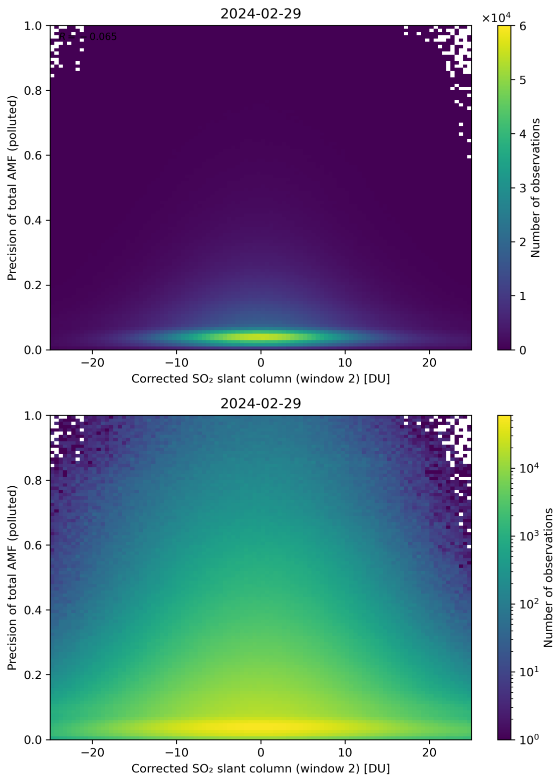
Figure 204: Scatter density plot of “Corrected SO 2 slant column (window 2)” against “Precision of total AMF (polluted)” for 2024-02-28 to 2024-03-01.
