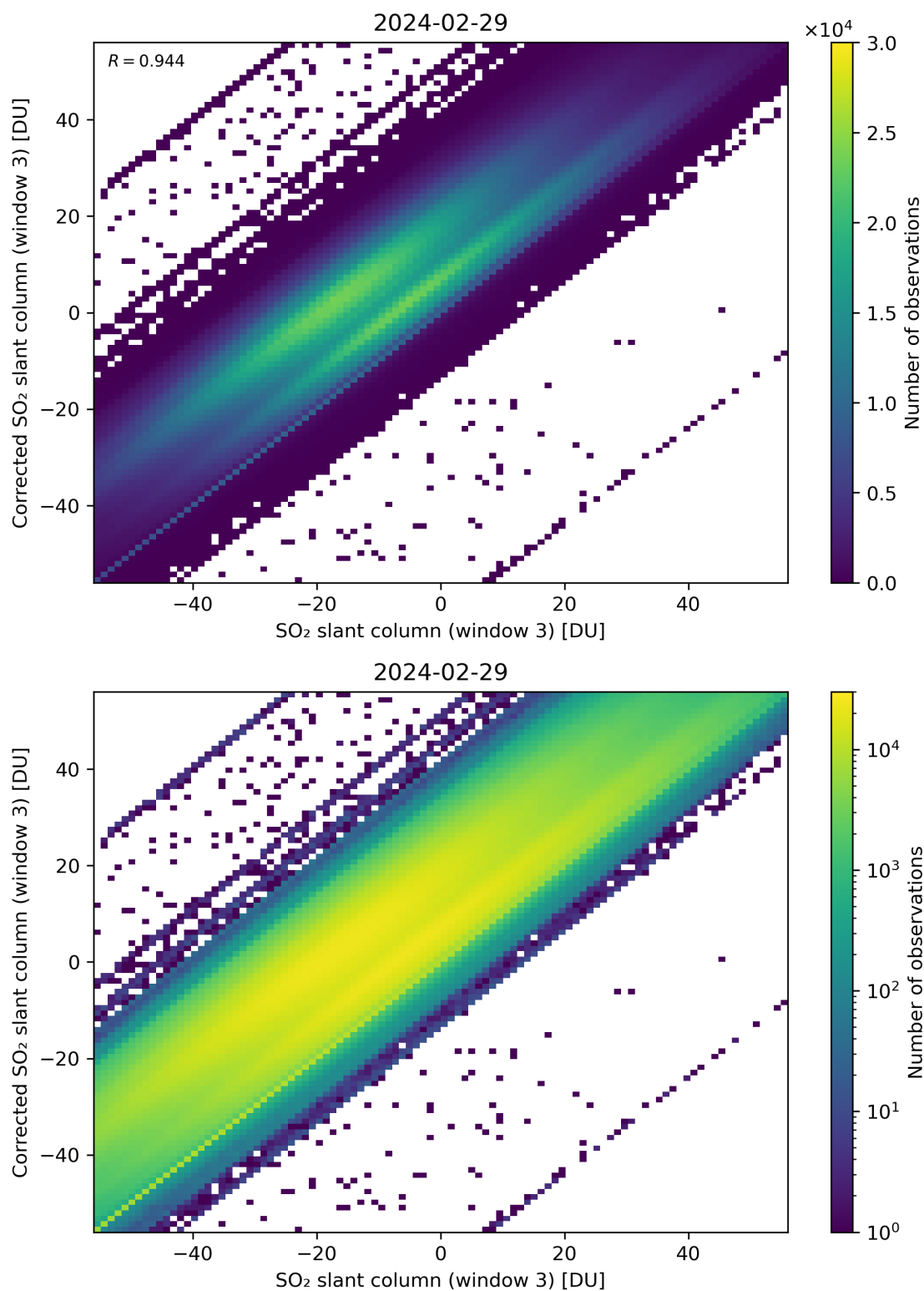
Figure 266: Scatter density plot of “SO 2 slant column (window 3)” against “Corrected SO 2 slant column (window 3)” for 2024-02-28 to 2024-03-01.
