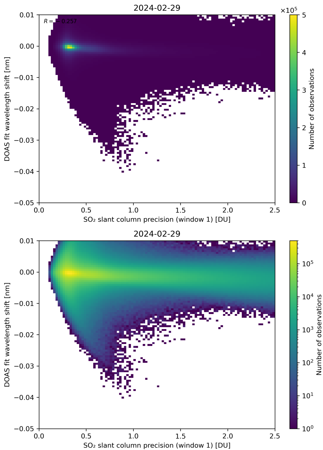
Figure 221: Scatter density plot of “SO 2 slant column precision (window 1)” against “DOAS fit wavelength shift” for 2024-02-28 to 2024-03-01.
