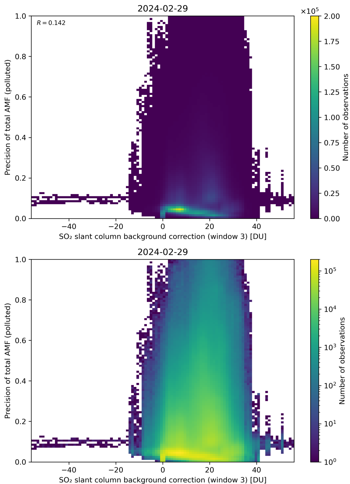
Figure 126: Scatter density plot of “SO 2 slant column background correction (window 3)” against “Precision of total AMF (polluted)” for 2024-02-28 to 2024-03-01.
