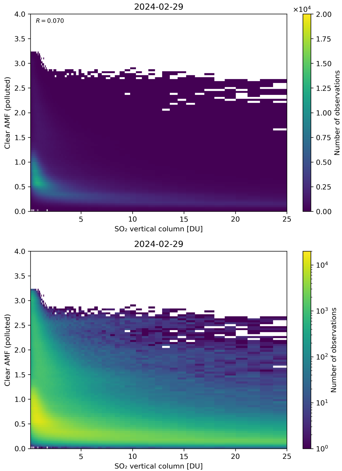
Figure 296: Scatter density plot of “SO 2 vertical column” against “Clear AMF (polluted)” for 2024-02-28 to 2024-03-01.
