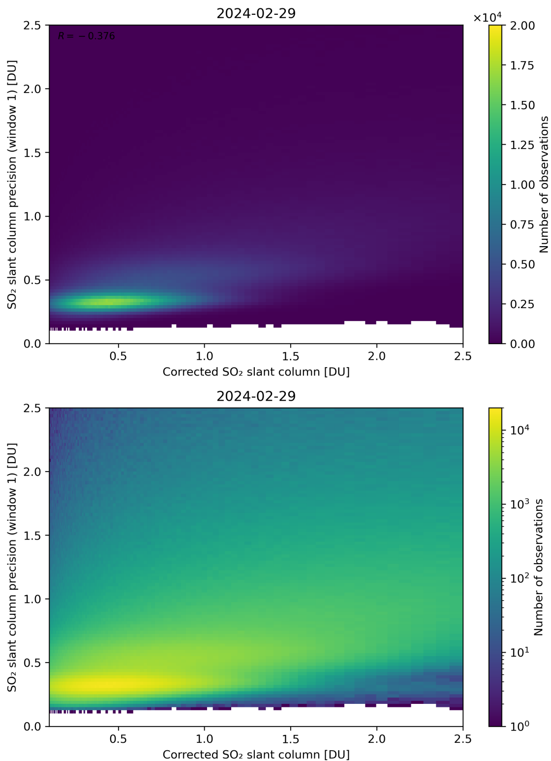
Figure 188: Scatter density plot of “Corrected SO 2 slant column” against “SO 2 slant column precision (window 1)” for 2024-02-28 to 2024-03-01.
