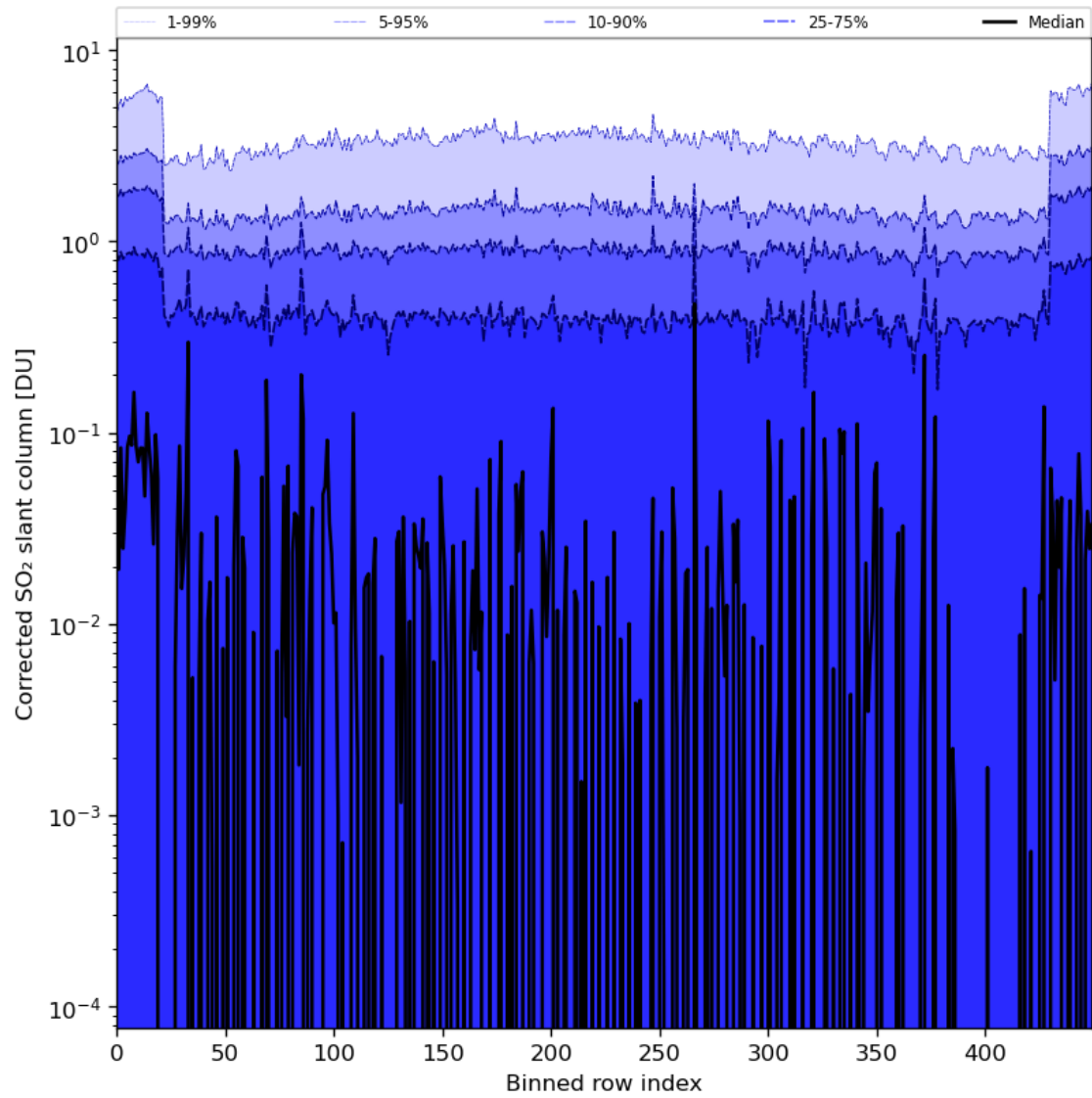
Figure 78: Along track statistics of “Corrected SO 2 slant column” for 2024-02-28 to 2024-03-01
