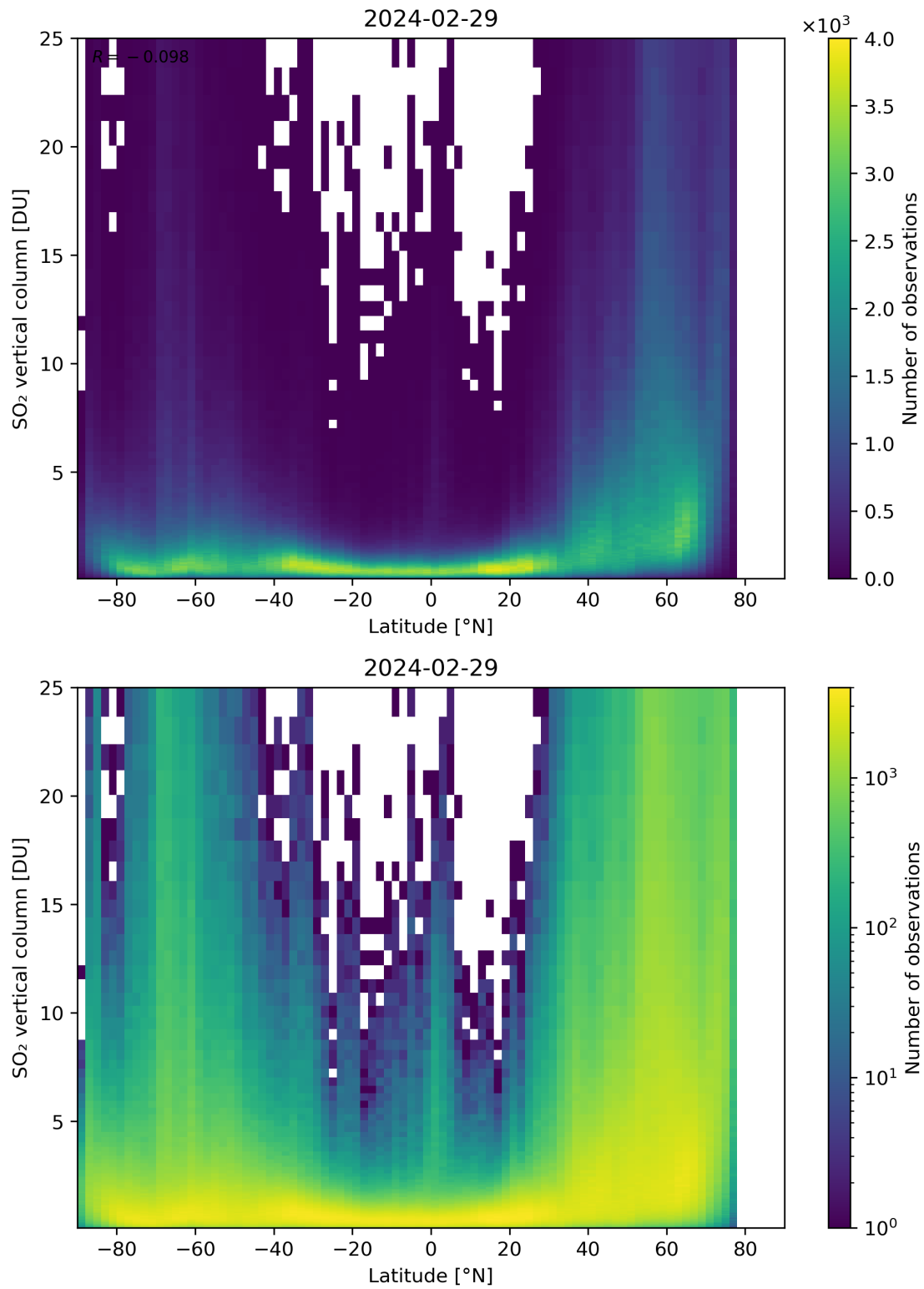
Figure 156: Scatter density plot of “Latitude” against “SO 2 vertical column” for 2024-02-28 to 2024-03-01.
