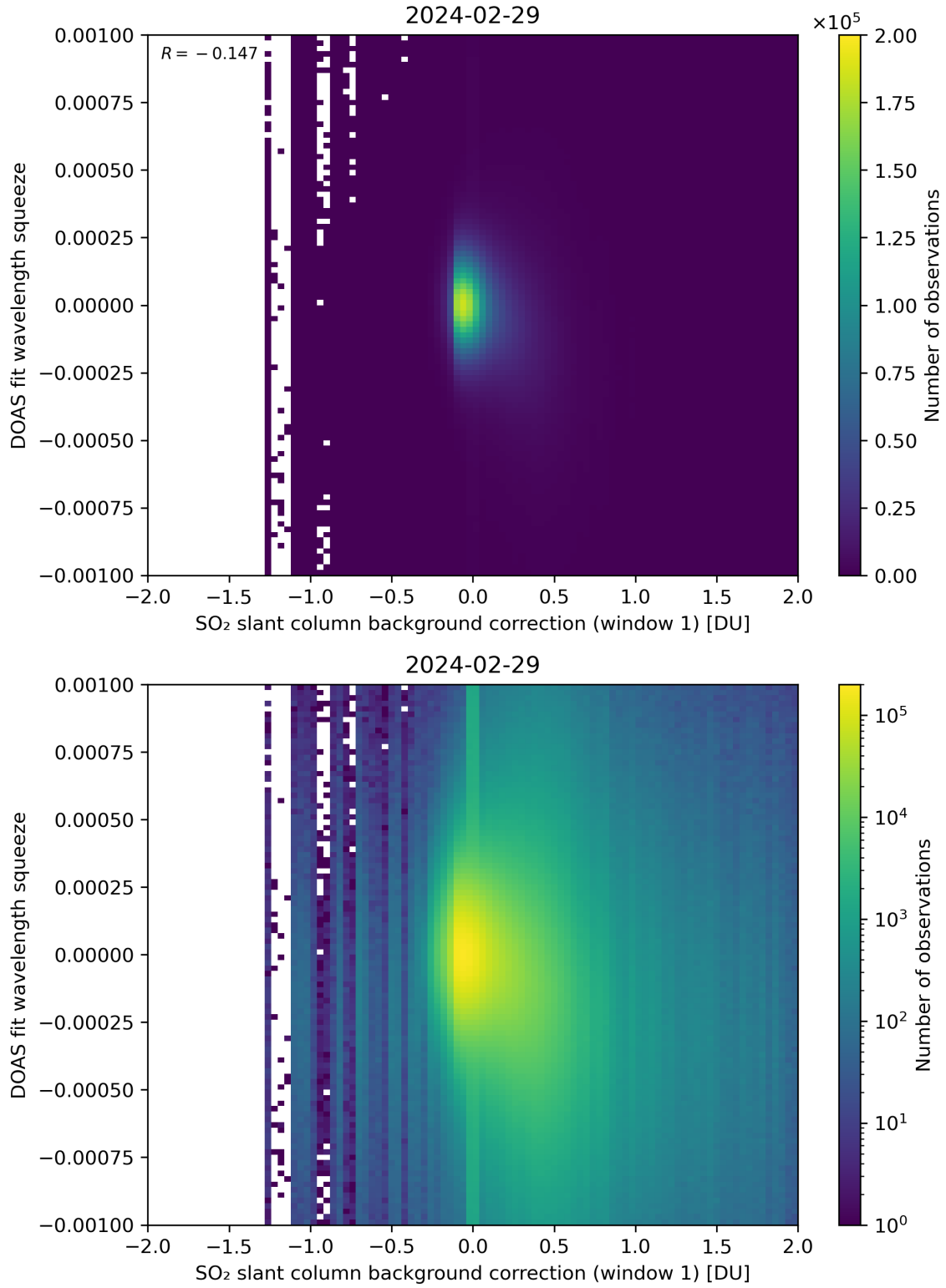
Figure 101: Scatter density plot of “SO 2 slant column background correction (window 1)” against “DOAS fit wavelength squeeze” for 2024-02-28 to 2024-03-01.
