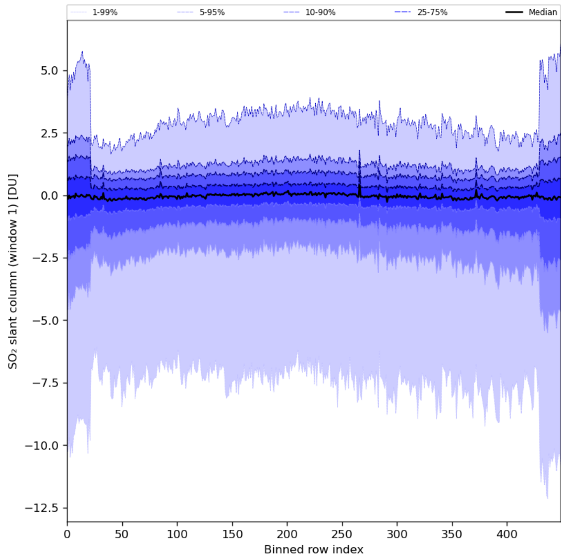
Figure 79: Along track statistics of "SO 2 slant column (window 1)" for 2024-02-28 to 2024-03-01
