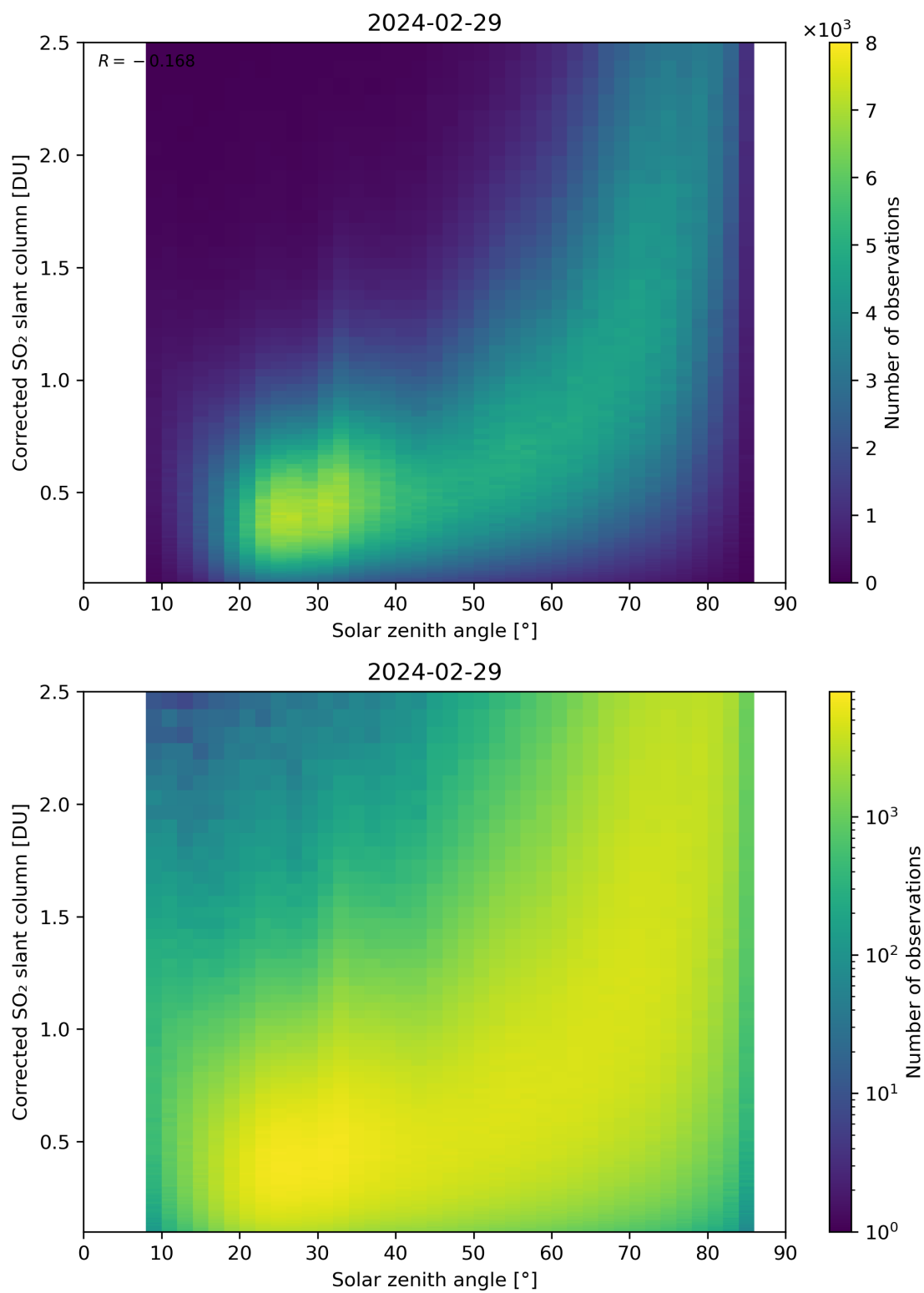
Figure 166: Scatter density plot of “Solar zenith angle” against “Corrected SO 2 slant column” for 2024-02-28 to 2024-03-01.
