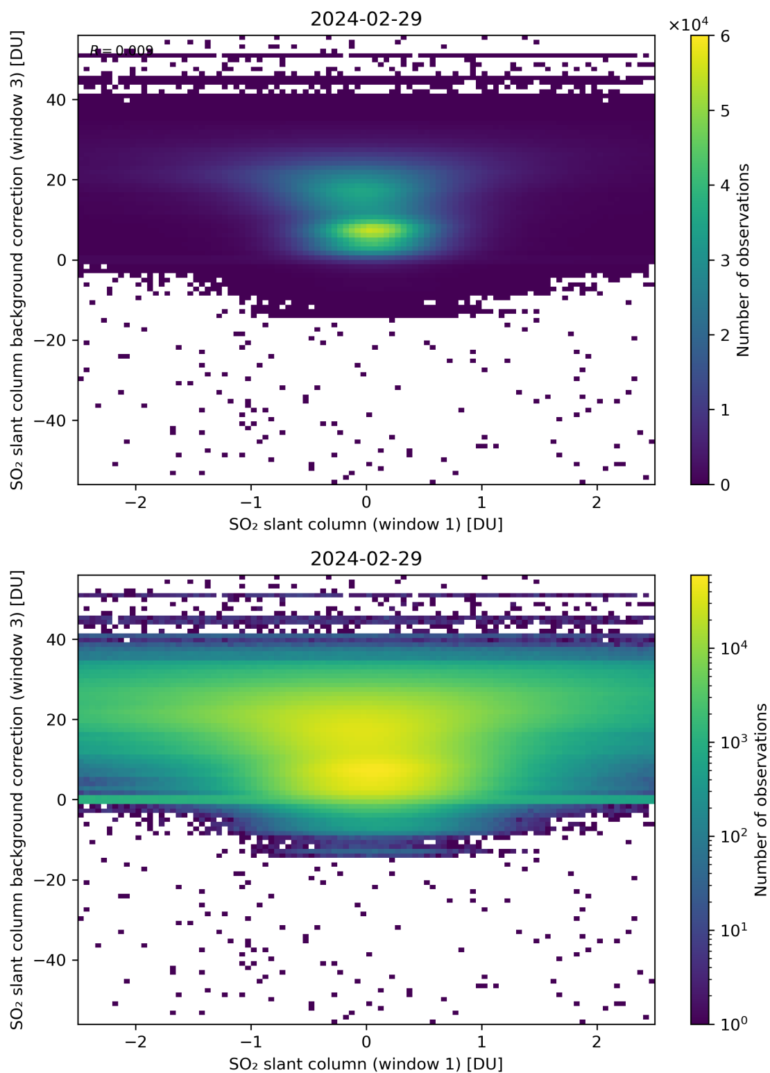
Figure 214: Scatter density plot of “SO 2 slant column (window 1)” against “SO 2 slant column background correction (window 3)” for 2024-02-28 to 2024-03-01.
