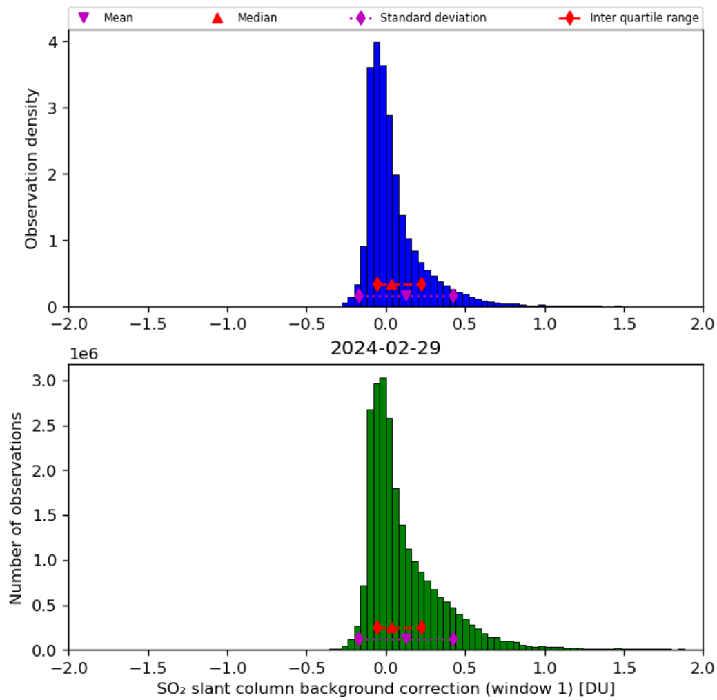
Figure 59: Histogram of “SO 2 slant column background correction (window 1)” for 2024-02-28 to 2024-03-01
