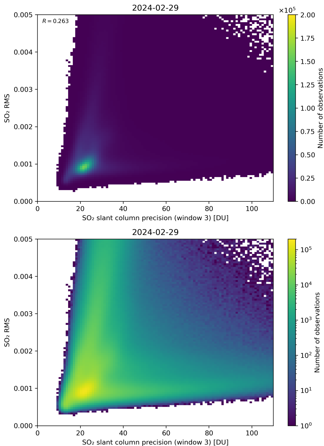
Figure 260: Scatter density plot of “SO 2 slant column precision (window 3)” against “SO 2 RMS” for 2024-02-28 to 2024-03-01.
