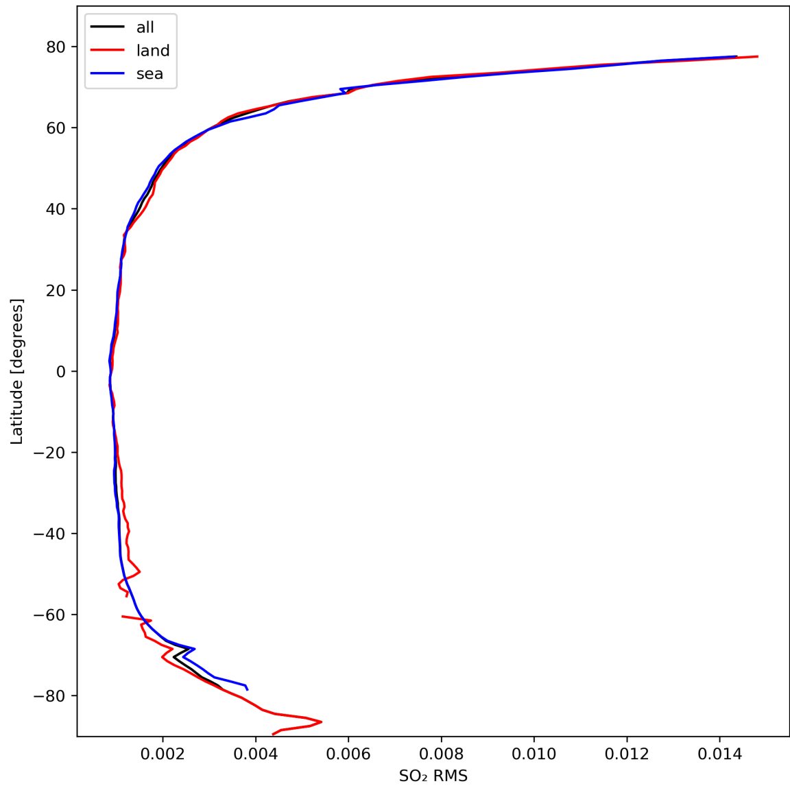
Figure 47: Zonal average of “SO 2 RMS” for 2024-02-28 to 2024-03-01.
