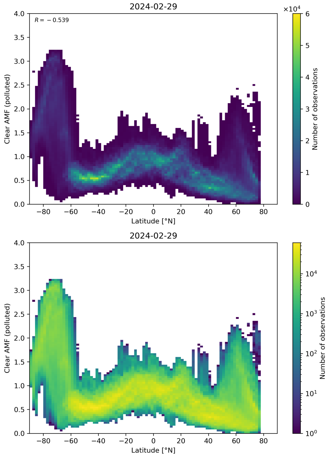
Figure 145: Scatter density plot of “Latitude” against “Clear AMF (polluted)” for 2024-02-28 to 2024-03-01.
