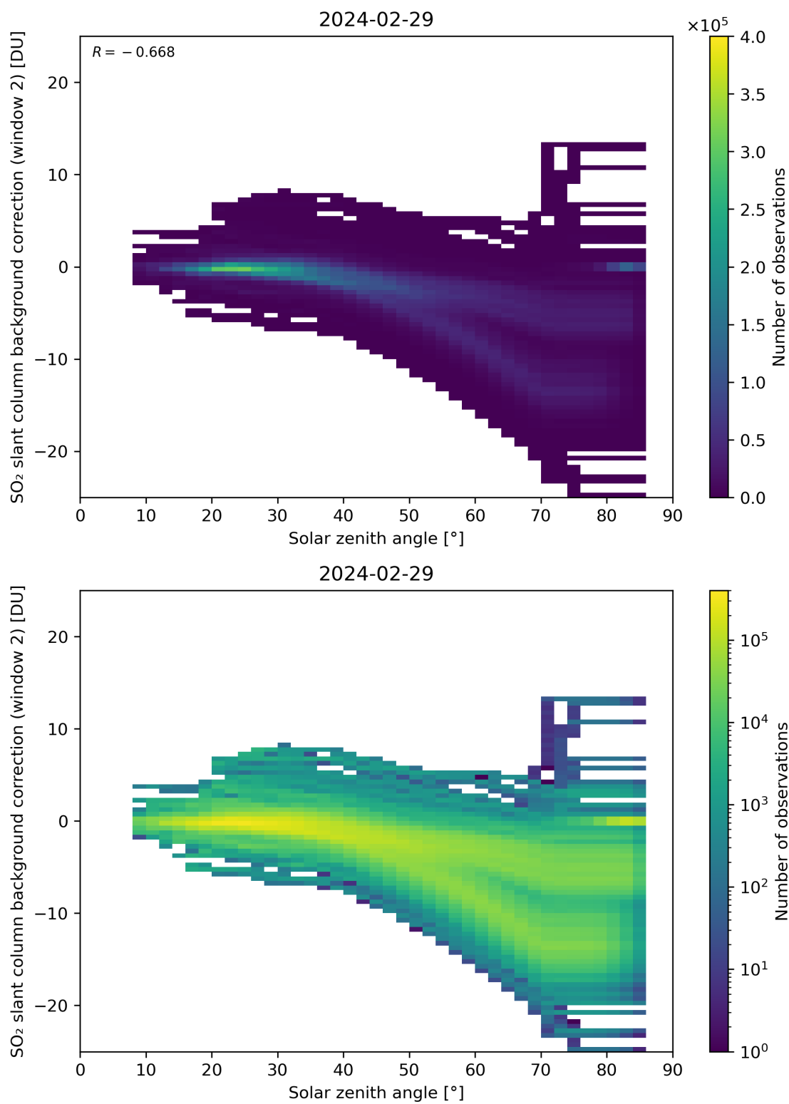
Figure 159: Scatter density plot of “Solar zenith angle” against “SO 2 slant column background correction (window 2)” for 2024-02-28 to 2024-03-01.
