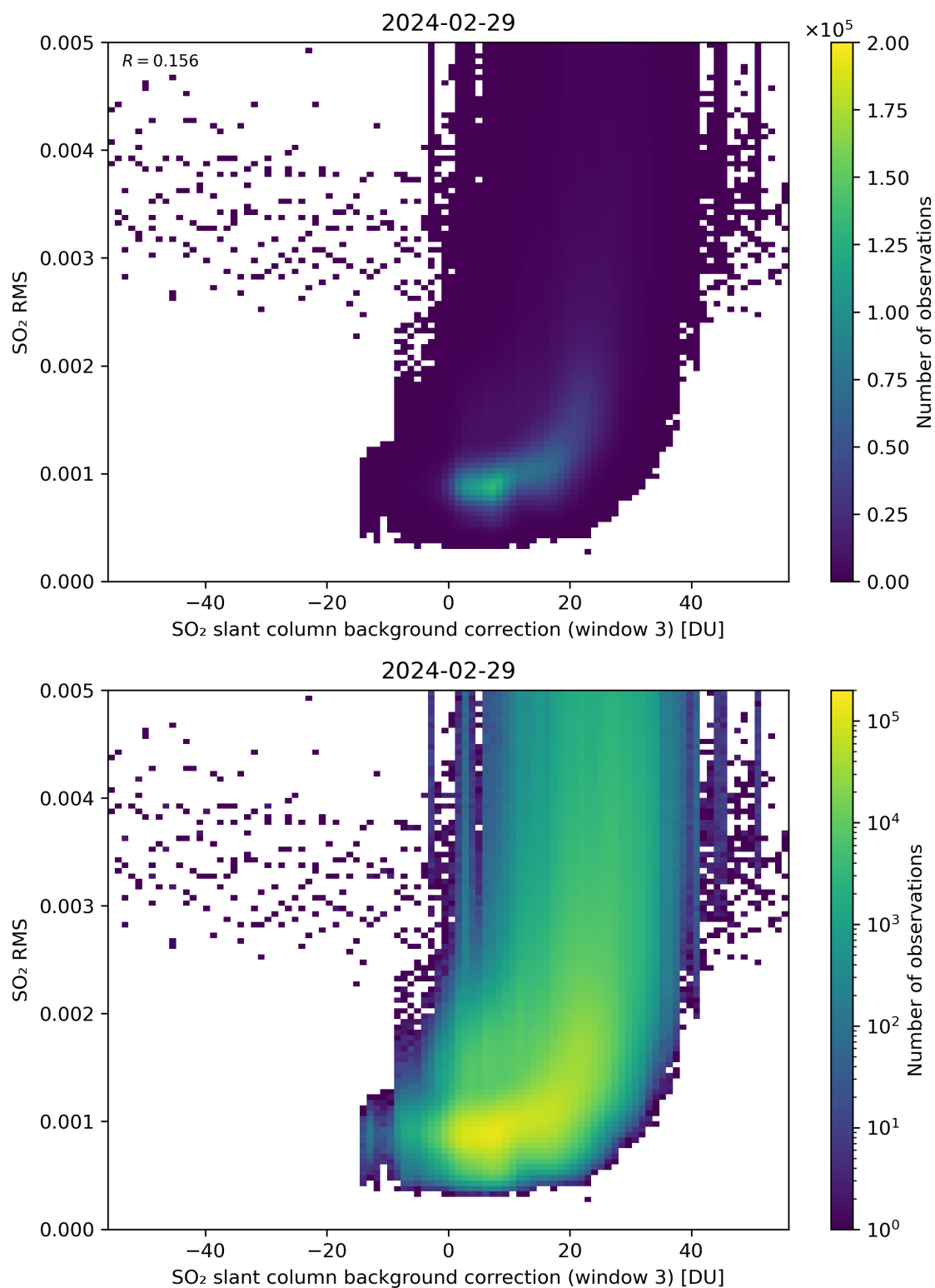
Figure 123: Scatter density plot of “SO 2 slant column background correction (window 3)” against “SO 2 RMS” for 2024-02-28 to 2024-03-01.
