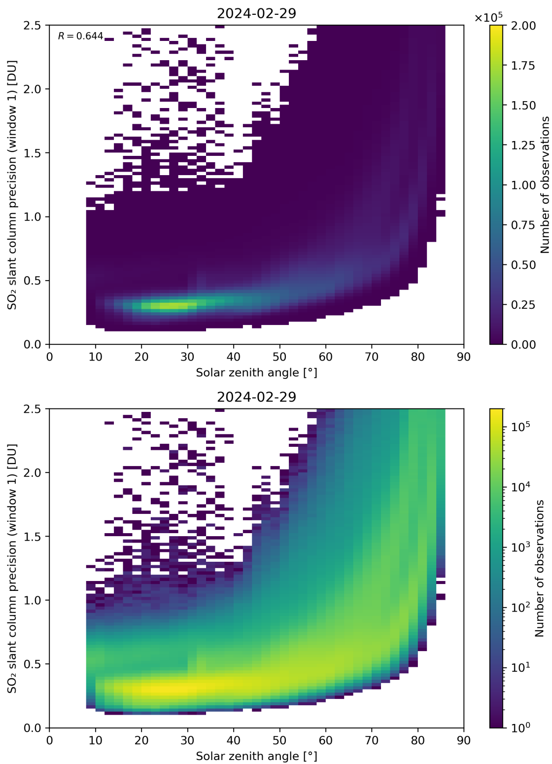
Figure 170: Scatter density plot of “Solar zenith angle” against “SO 2 slant column precision (window 1)” for 2024-02-28 to 2024-03-01.
