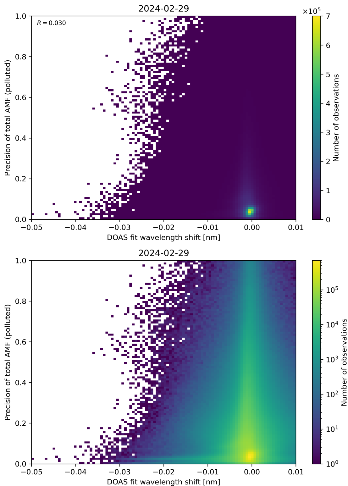
Figure 131: Scatter density plot of “DOAS fit wavelength shift” against “Precision of total AMF (polluted)” for 2024-02-28 to 2024-03-01.
