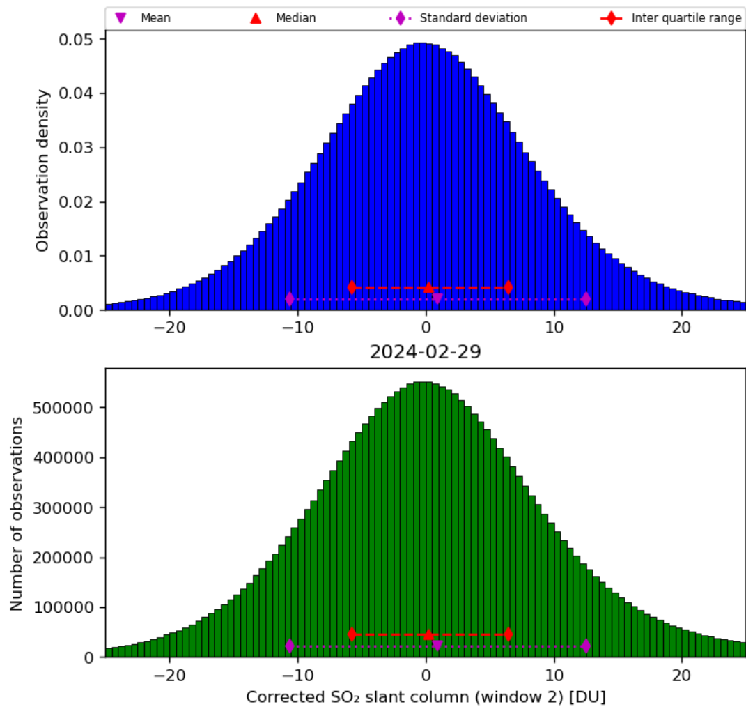
Figure 62: Histogram of “Corrected SO 2 slant column (window 2)” for 2024-02-28 to 2024-03-01
