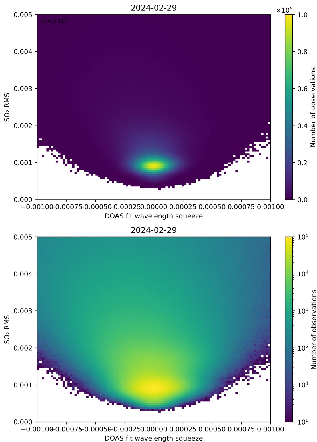
Figure 132: Scatter density plot of “DOAS fit wavelength squeeze” against “SO 2 RMS” for 2024-02-28 to 2024-03-01.
