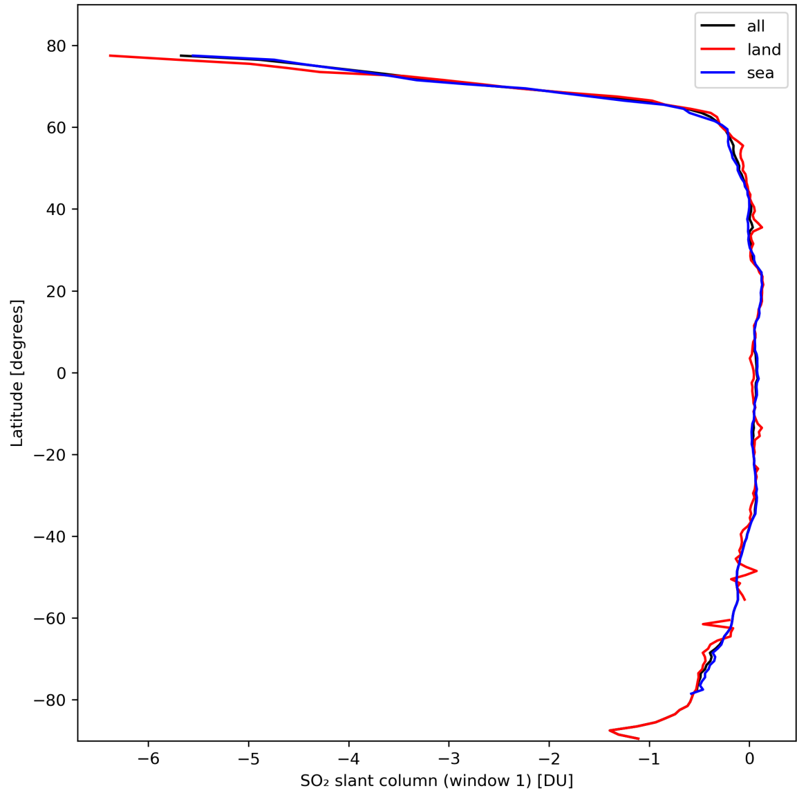
Figure 33: Zonal average of “SO 2 slant column (window 1)” for 2024-02-28 to 2024-03-01.
