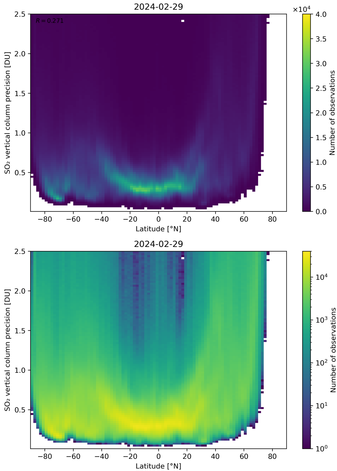
Figure 157: Scatter density plot of “Latitude” against “SO 2 vertical column precision” for 2024-02-28 to 2024-03-01.
