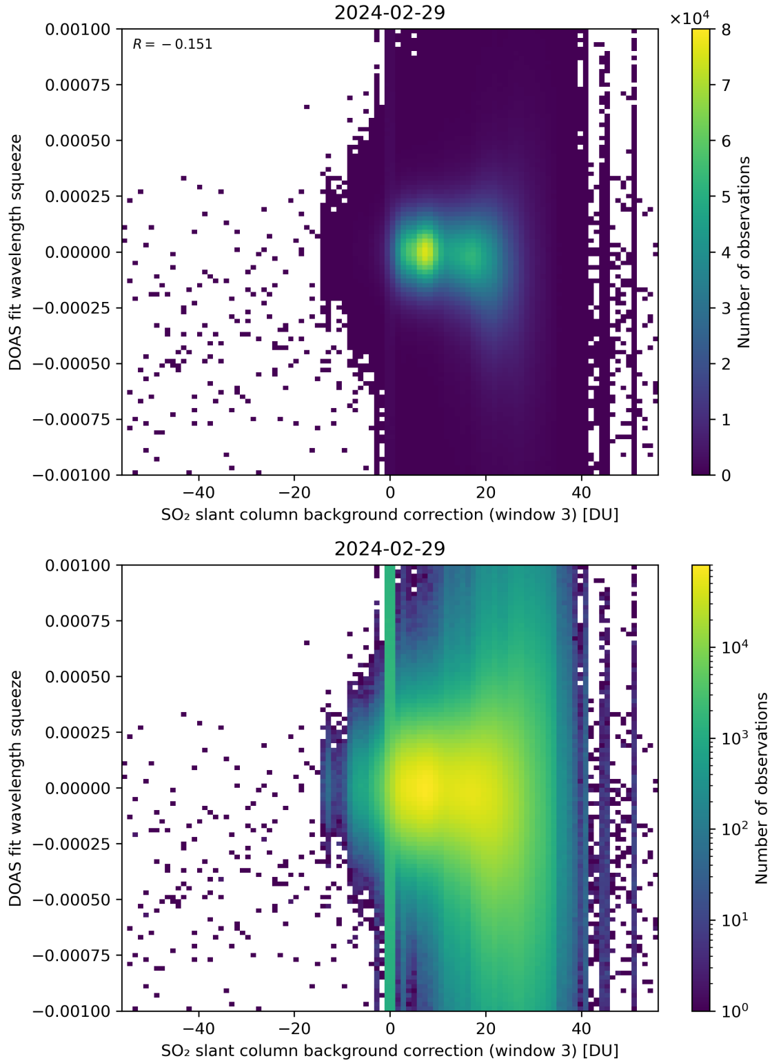
Figure 122: Scatter density plot of “SO 2 slant column background correction (window 3)” against “DOAS fit wavelength squeeze” for 2024-02-28 to 2024-03-01.
