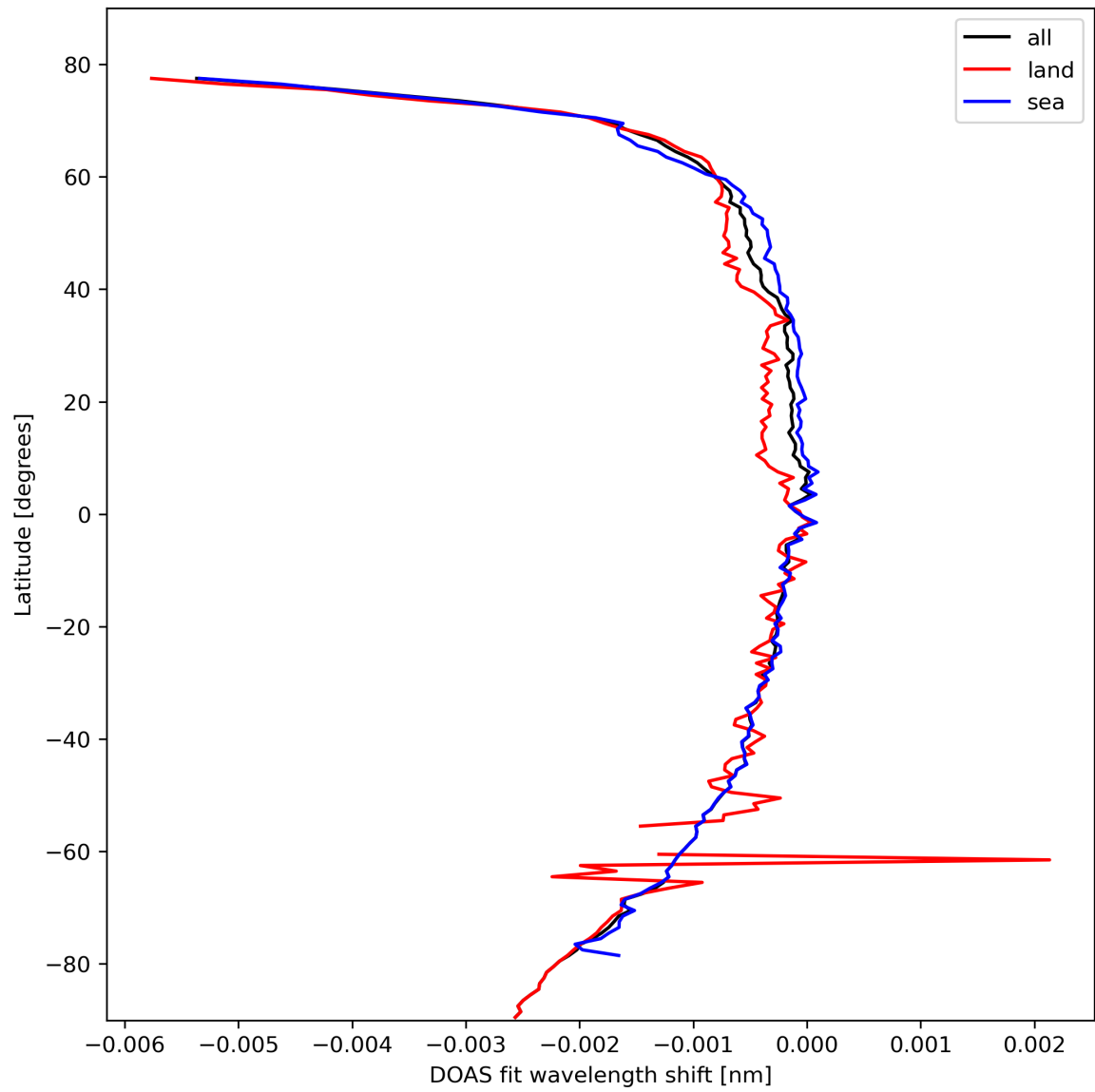
Figure 45: Zonal average of “DOAS fit wavelength shift” for 2024-02-28 to 2024-03-01.
