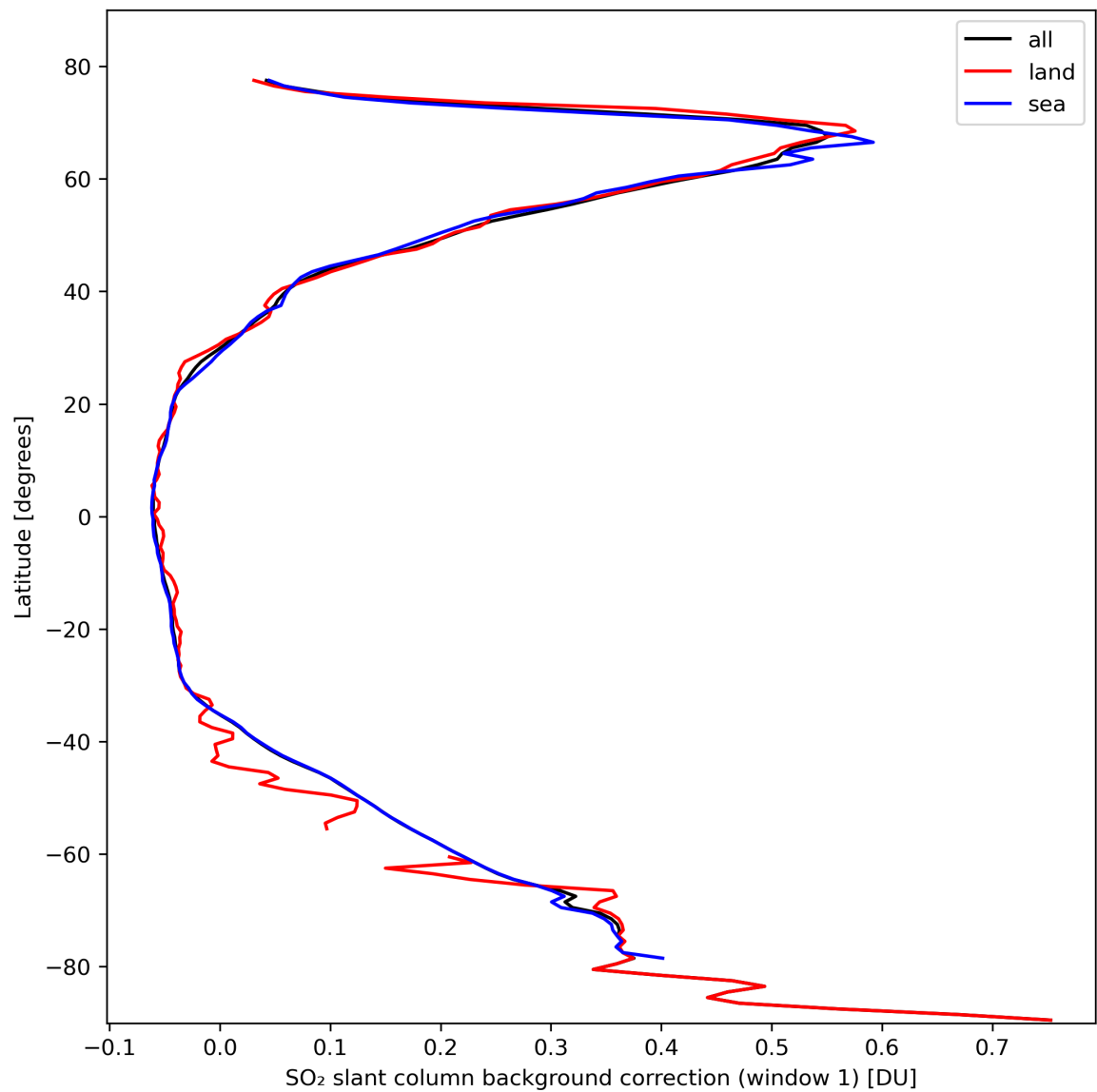
Figure 36: Zonal average of “SO 2 slant column background correction (window 1)” for 2024-02-28 to 2024-03-01.
