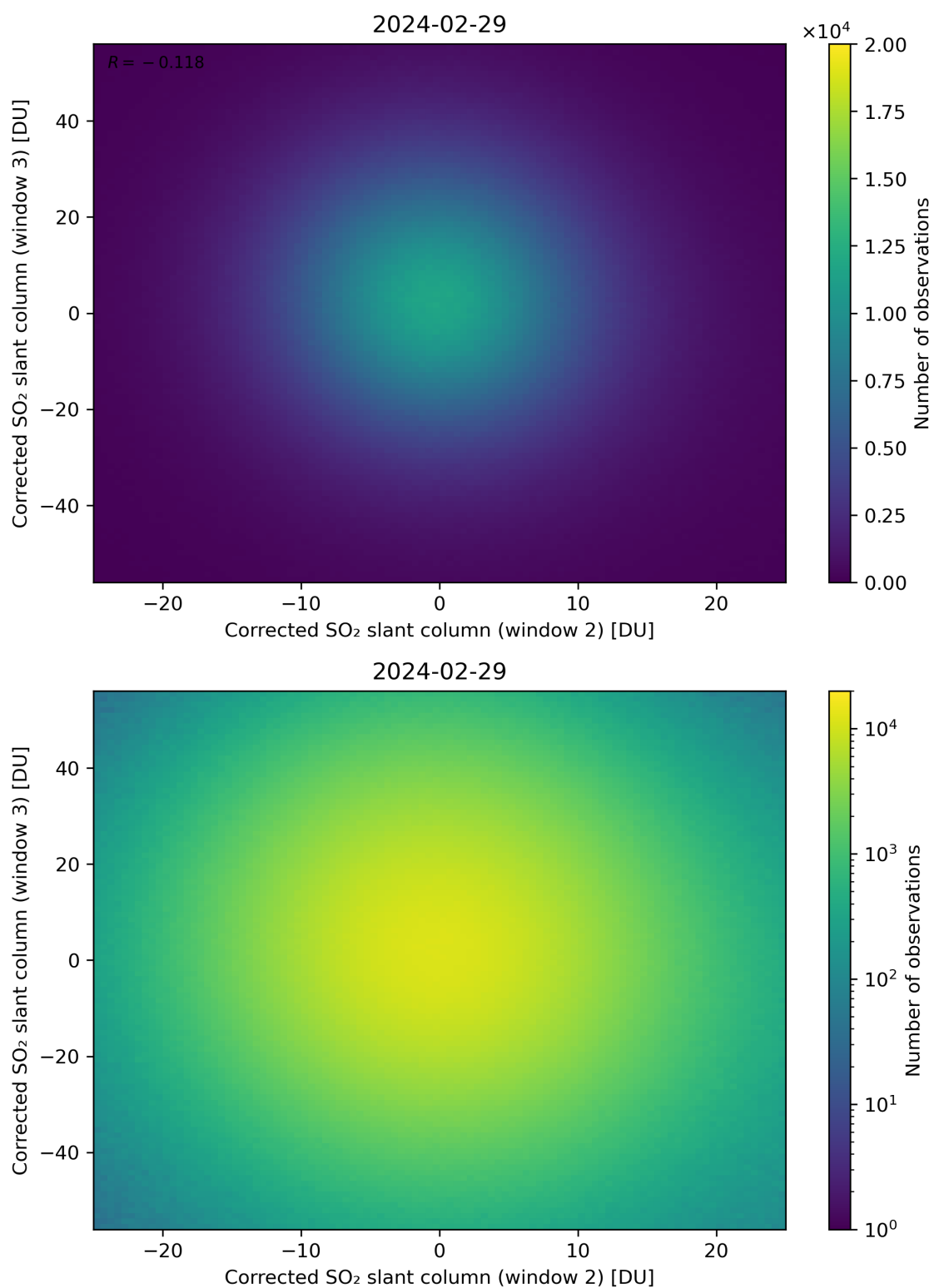
Figure 200: Scatter density plot of “Corrected SO 2 slant column (window 2)” against “Corrected SO 2 slant column (window 3)” for 2024-02-28 to 2024-03-01.
