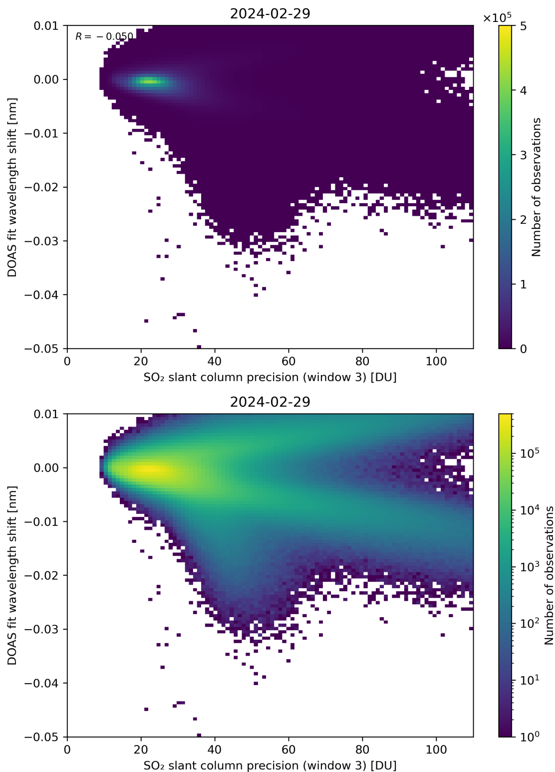
Figure 258: Scatter density plot of “SO 2 slant column precision (window 3)” against “DOAS fit wavelength shift” for 2024-02-28 to 2024-03-01.
