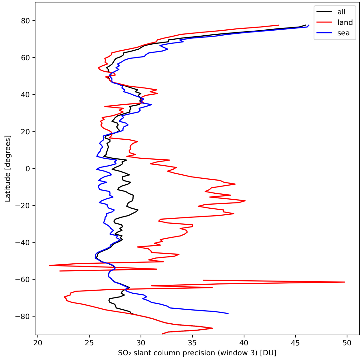
Figure 42: Zonal average of “SO 2 slant column precision (window 3)” for 2024-02-28 to 2024-03-01.
