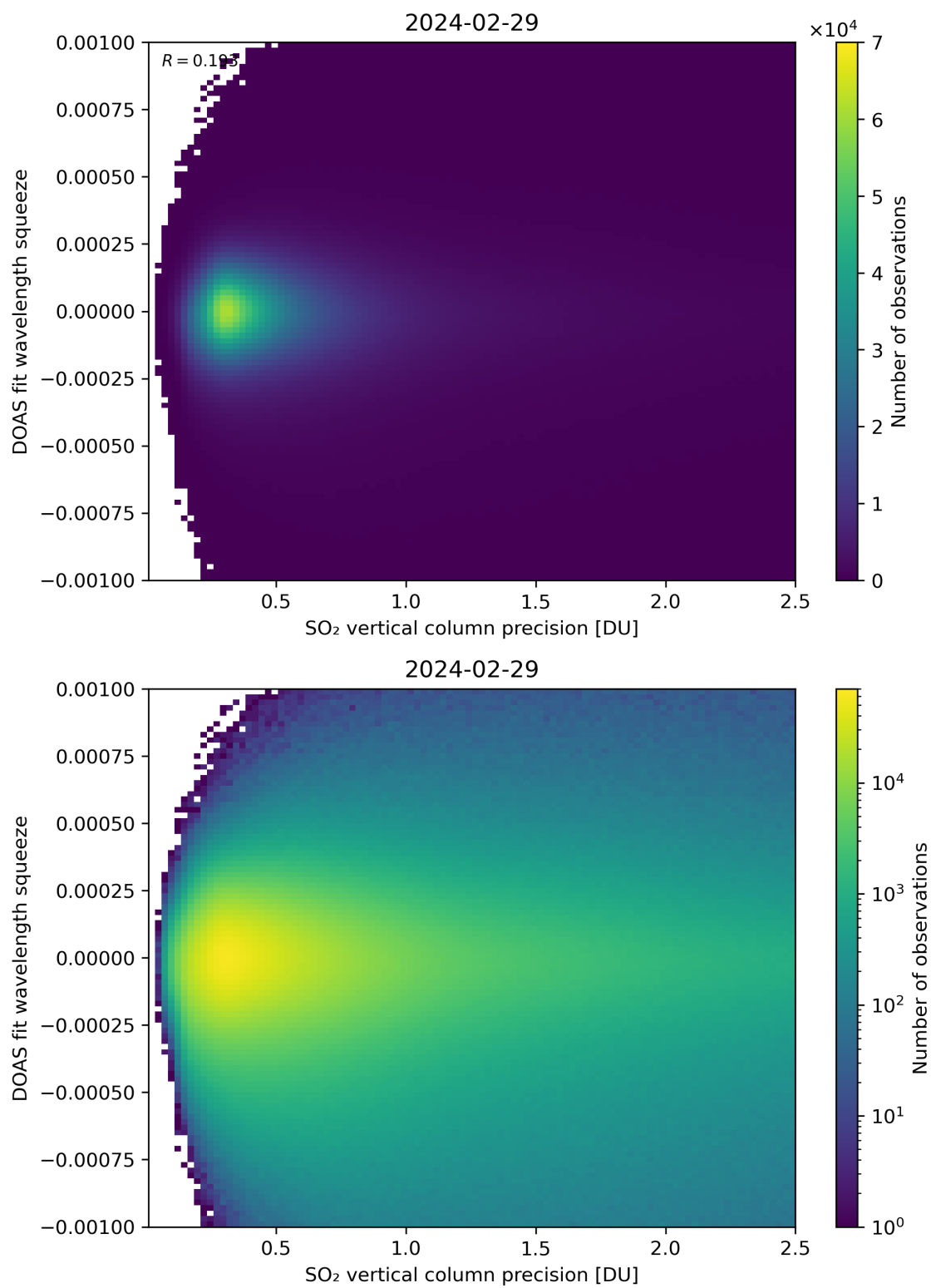
Figure 283: Scatter density plot of “SO 2 vertical column precision” against “DOAS fit wavelength squeeze” for 2024-02-28 to 2024-03-01.
