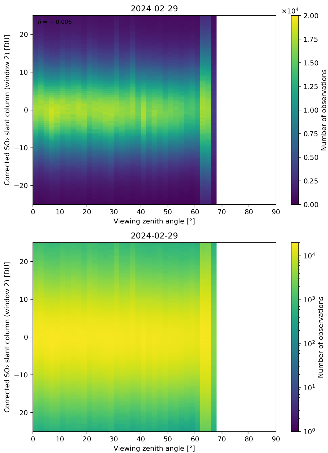
Figure 318: Scatter density plot of “Viewing zenith angle” against “Corrected SO 2 slant column (window 2)” for 2024-02-28 to 2024-03-01.
