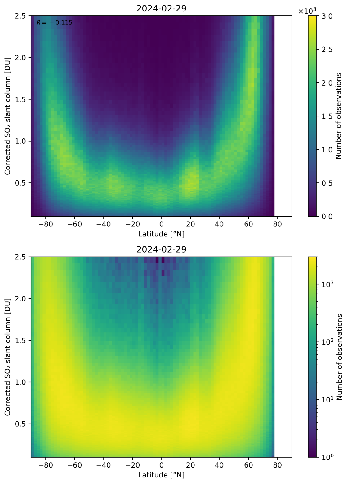
Figure 146: Scatter density plot of “Latitude” against “Corrected SO 2 slant column” for 2024-02-28 to 2024-03-01.
