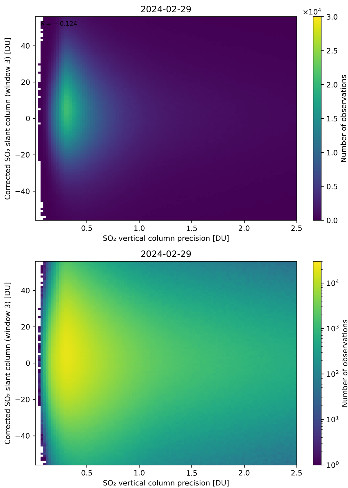
Figure 288: Scatter density plot of “SO 2 vertical column precision” against “Corrected SO 2 slant column (window 3)” for 2024-02-28 to 2024-03-01.
