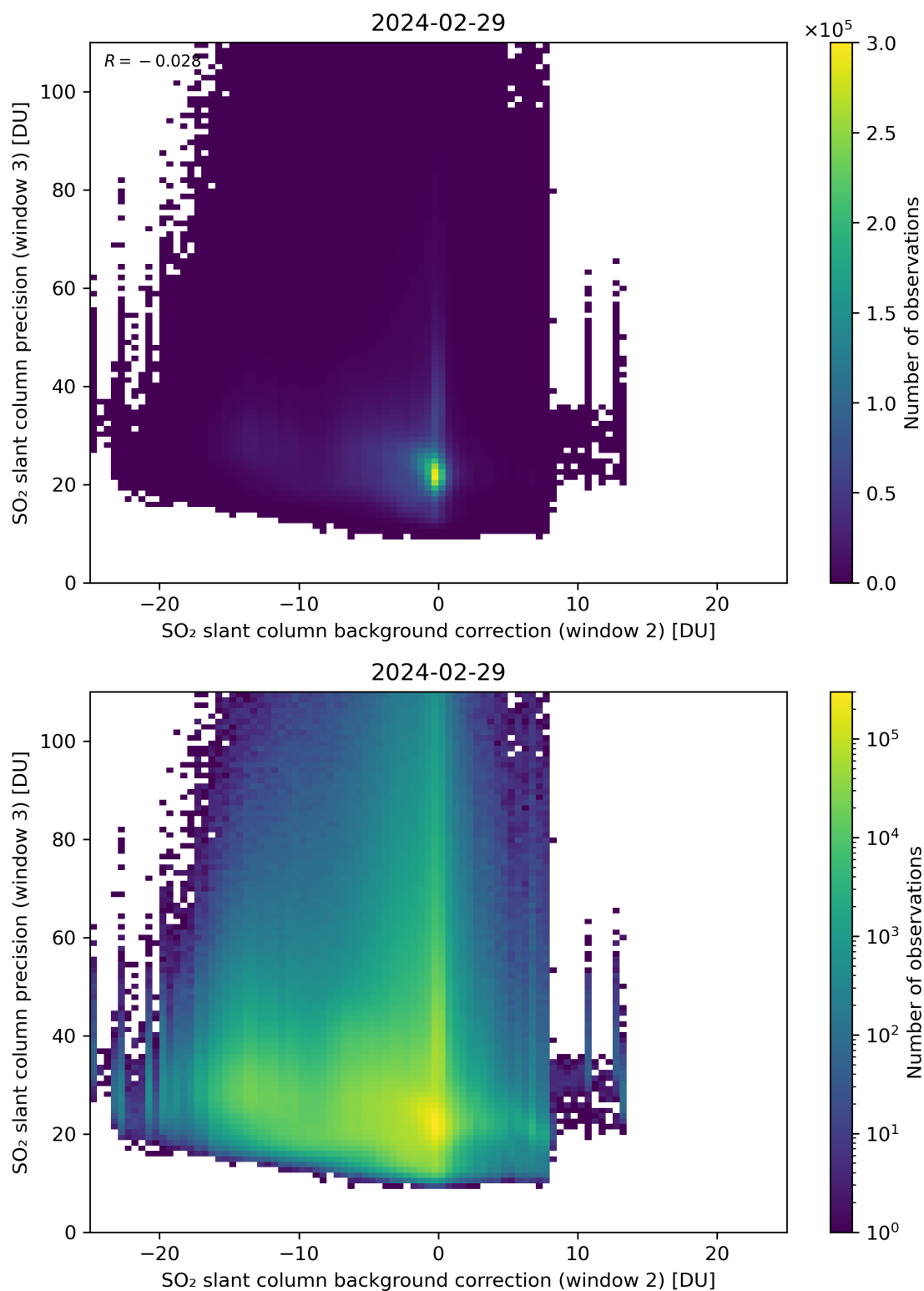
Figure 118: Scatter density plot of “SO 2 slant column background correction (window 2)” against “SO 2 slant column precision (window 3)” for 2024-02-28 to 2024-03-01.
