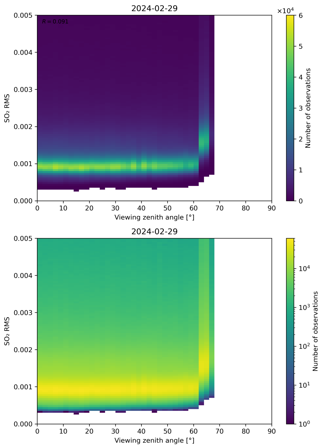
Figure 313: Scatter density plot of “Viewing zenith angle” against “SO 2 RMS” for 2024-02-28 to 2024-03-01.
