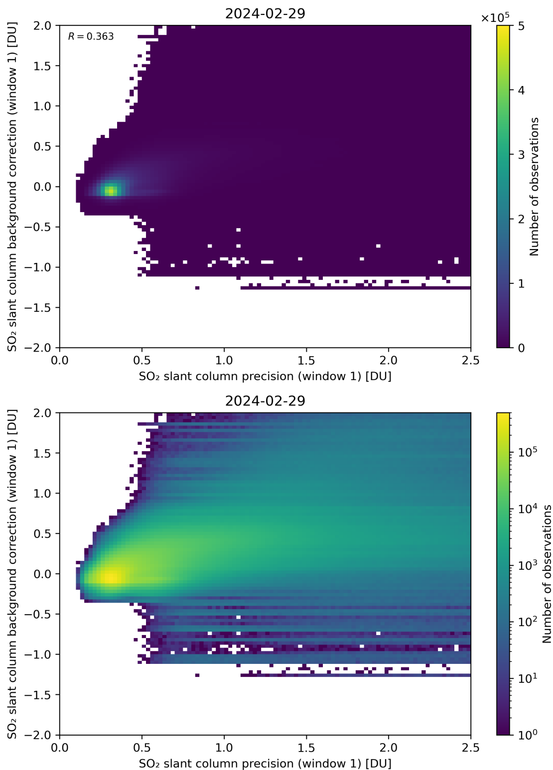
Figure 218: Scatter density plot of “SO 2 slant column precision (window 1)” against “SO 2 slant column background correction (window 1)” for 2024-02-28 to 2024-03-01.
