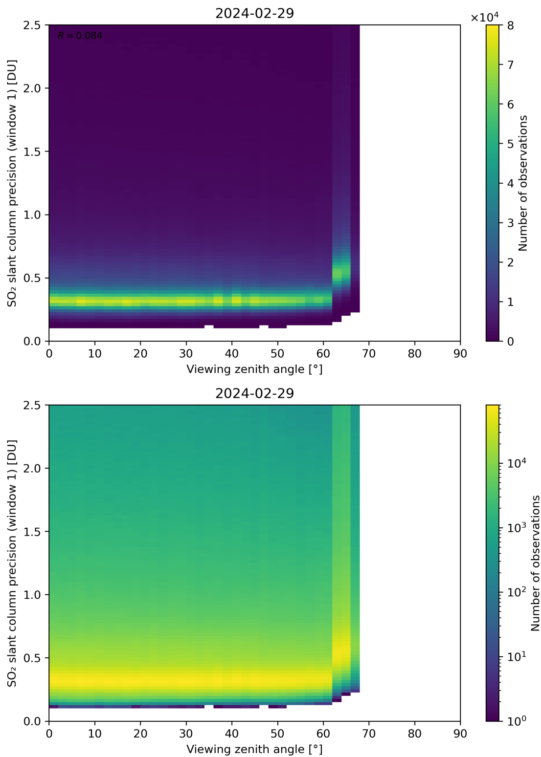
Figure 321: Scatter density plot of “Viewing zenith angle” against “SO 2 slant column precision (window 1)” for 2024-02-28 to 2024-03-01.
