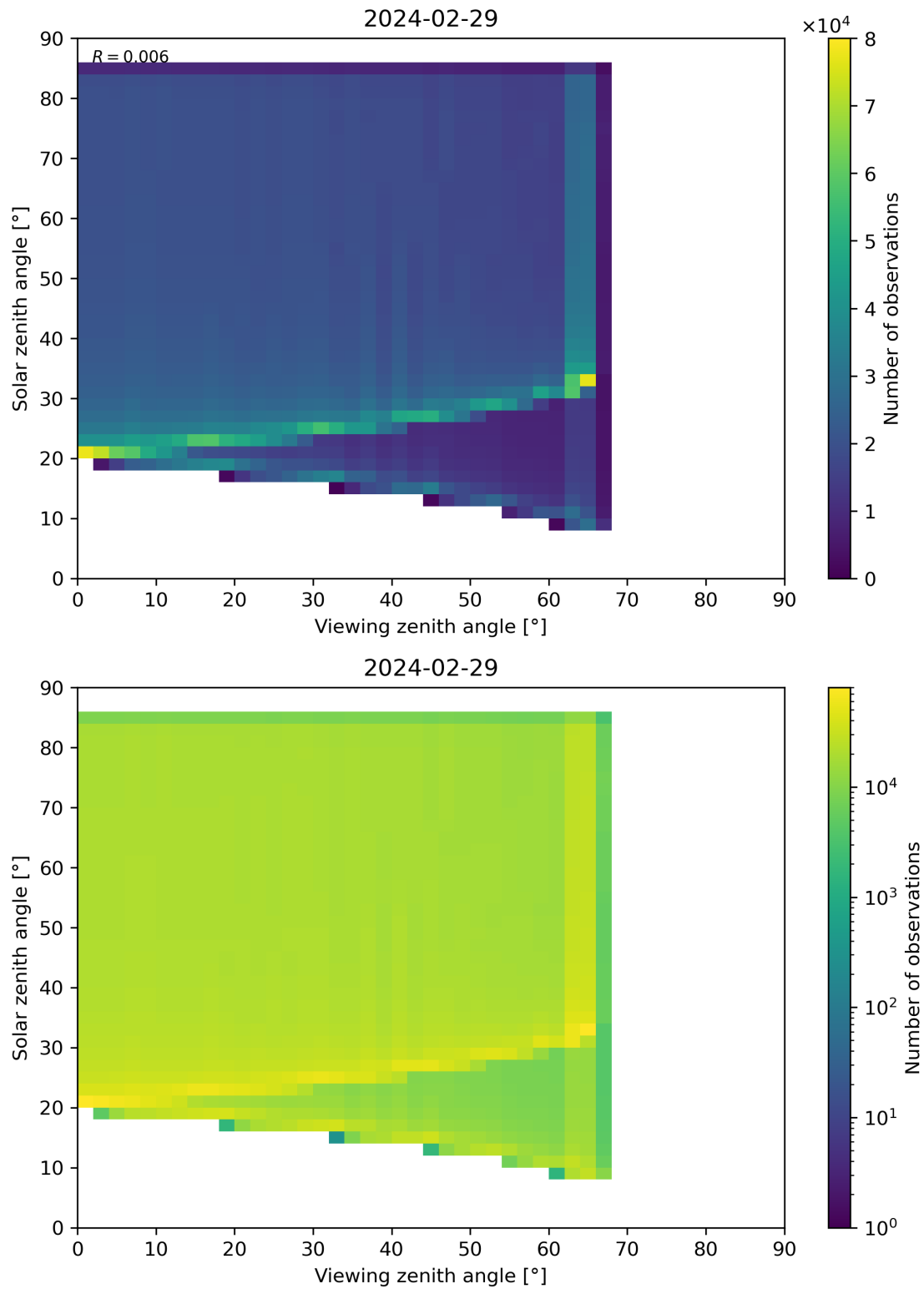
Figure 315: Scatter density plot of “Viewing zenith angle” against “Solar zenith angle” for 2024-02-28 to 2024-03-01.
