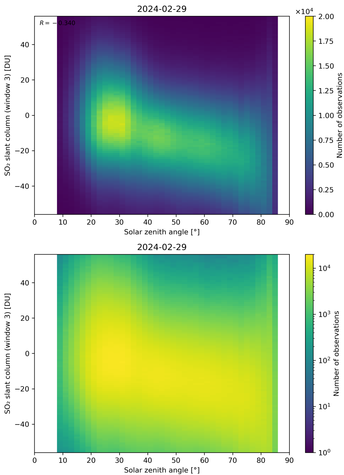
Figure 172: Scatter density plot of “Solar zenith angle” against “SO 2 slant column (window 3)” for 2024-02-28 to 2024-03-01.
