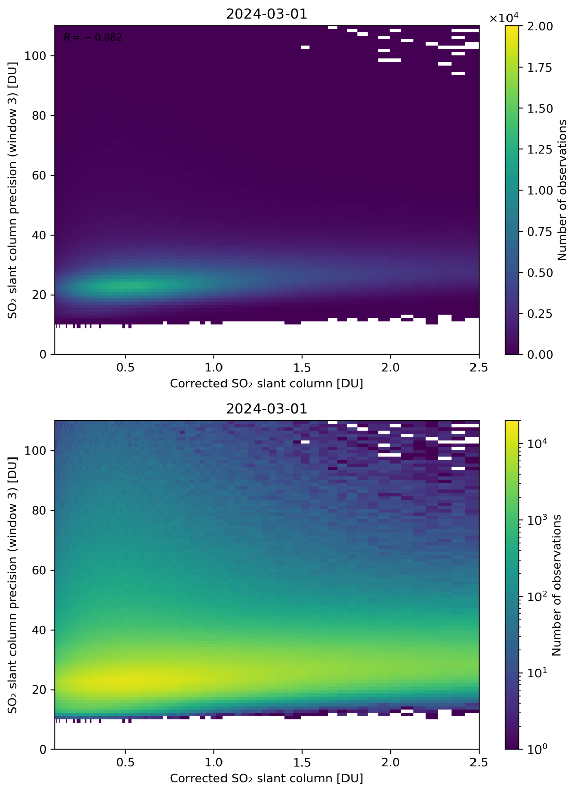
Figure 191: Scatter density plot of “Corrected SO 2 slant column” against “SO 2 slant column precision (window 3)” for 2024-02-29 to 2024-03-02.
