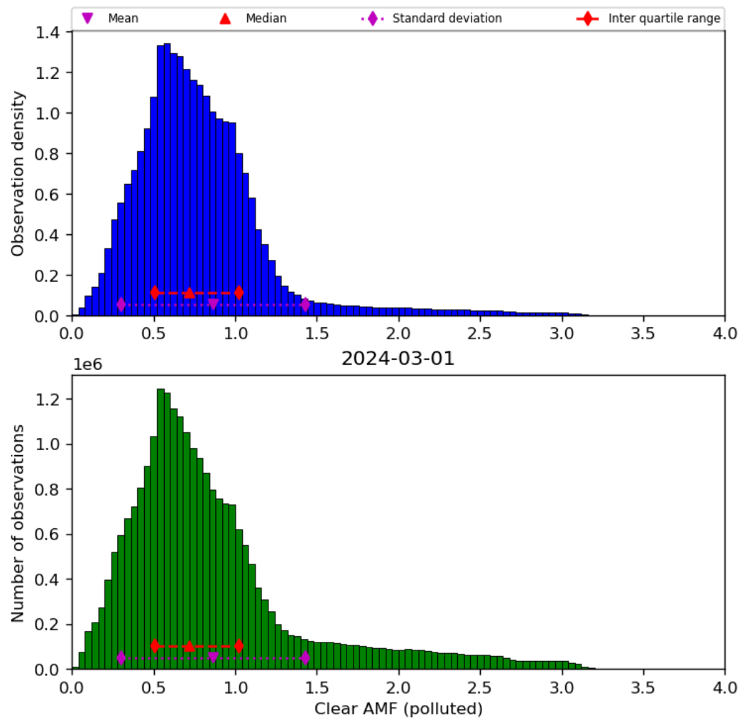
Figure 73: Histogram of “Clear AMF (polluted)” for 2024-02-29 to 2024-03-02
