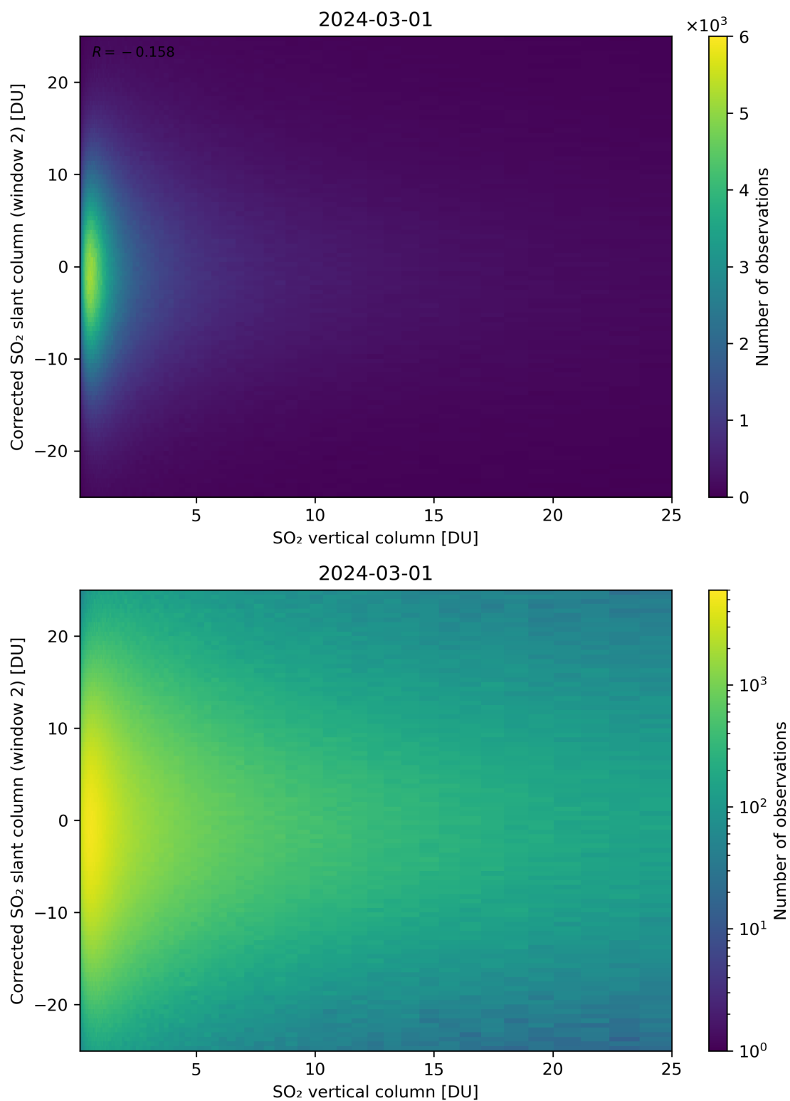
Figure 298: Scatter density plot of “SO 2 vertical column” against “Corrected SO 2 slant column (window 2)” for 2024-02-29 to 2024-03-02.
