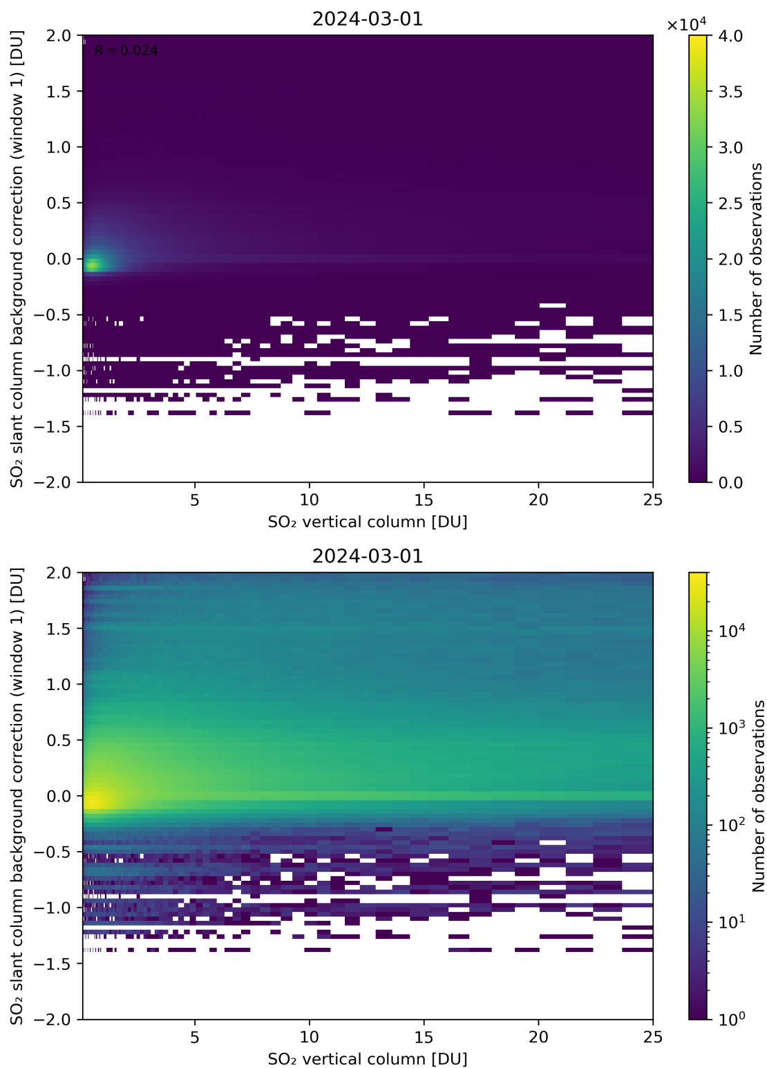
Figure 273: Scatter density plot of “SO 2 vertical column” against “SO 2 slant column background correction (window 1)” for 2024-02-29 to 2024-03-02.
