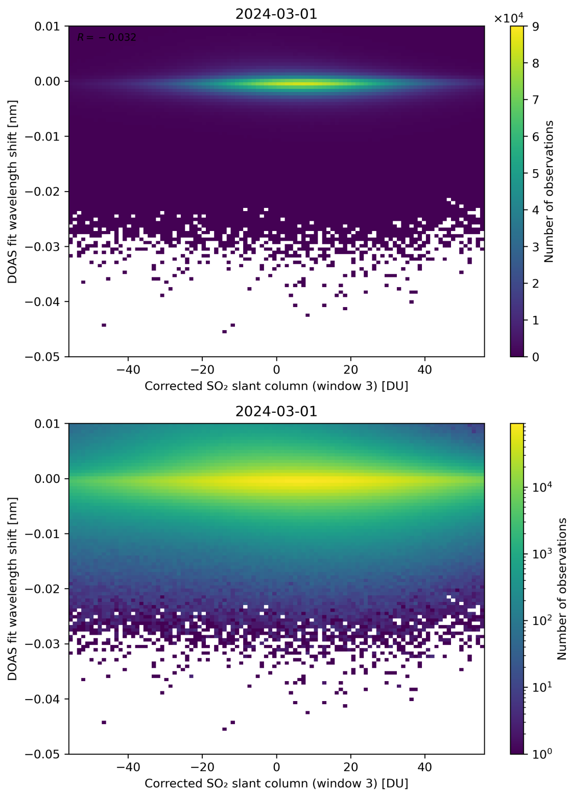
Figure 206: Scatter density plot of “Corrected SO 2 slant column (window 3)” against “DOAS fit wavelength shift” for 2024-02-29 to 2024-03-02.
