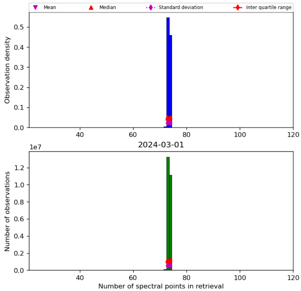
Figure 74: Histogram of “Number of spectral points in retrieval” for 2024-02-29 to 2024-03-02
