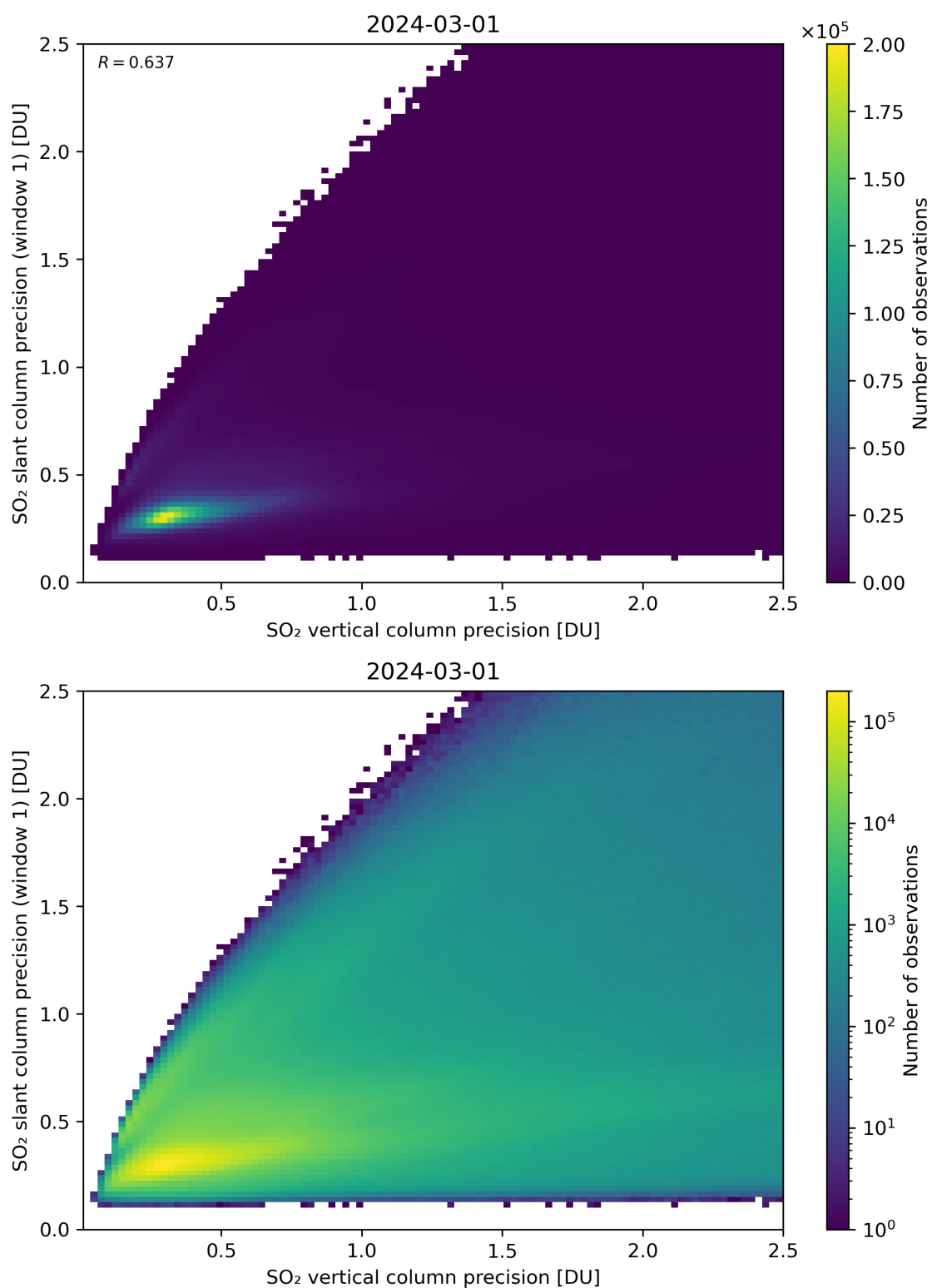
Figure 290: Scatter density plot of “SO 2 vertical column precision” against “SO 2 slant column precision (window 1)” for 2024-02-29 to 2024-03-02.
