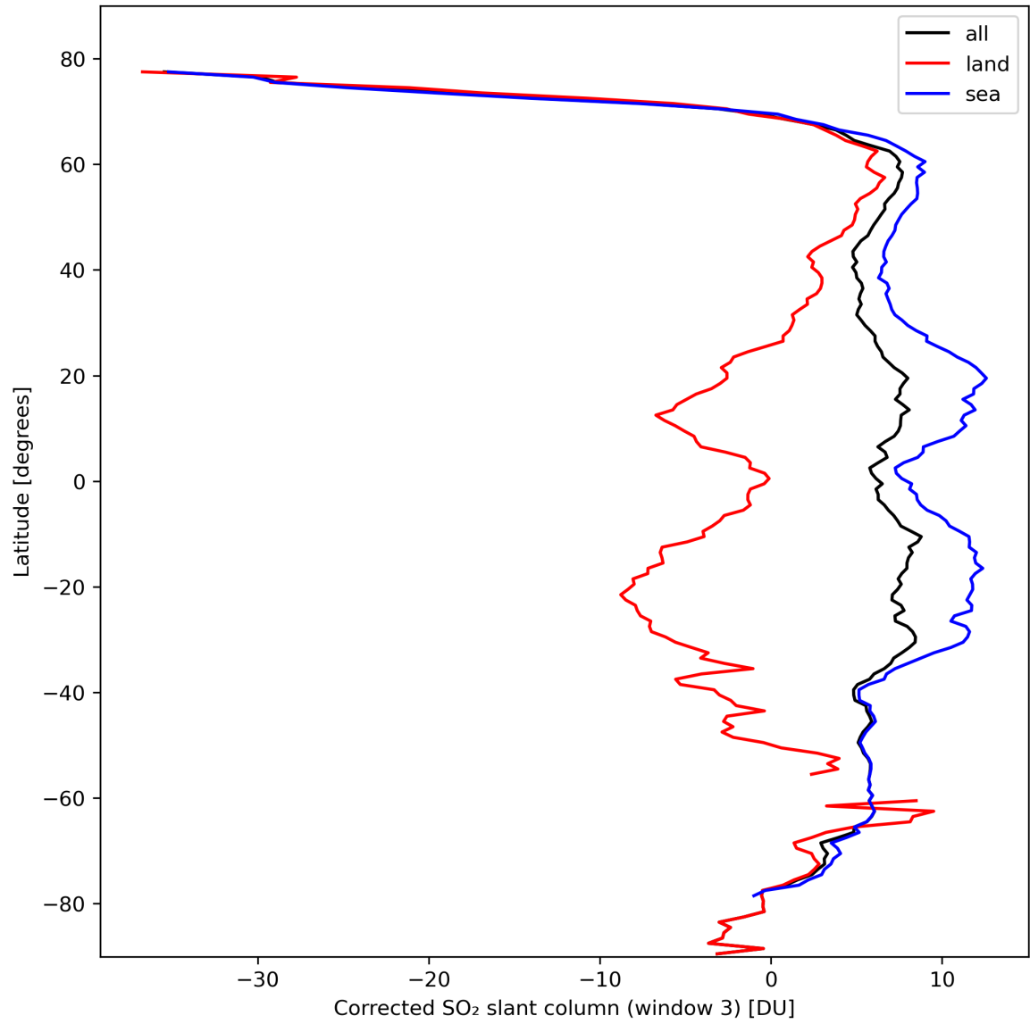
Figure 43: Zonal average of “Corrected SO 2 slant column (window 3)” for 2024-02-29 to 2024-03-02.
