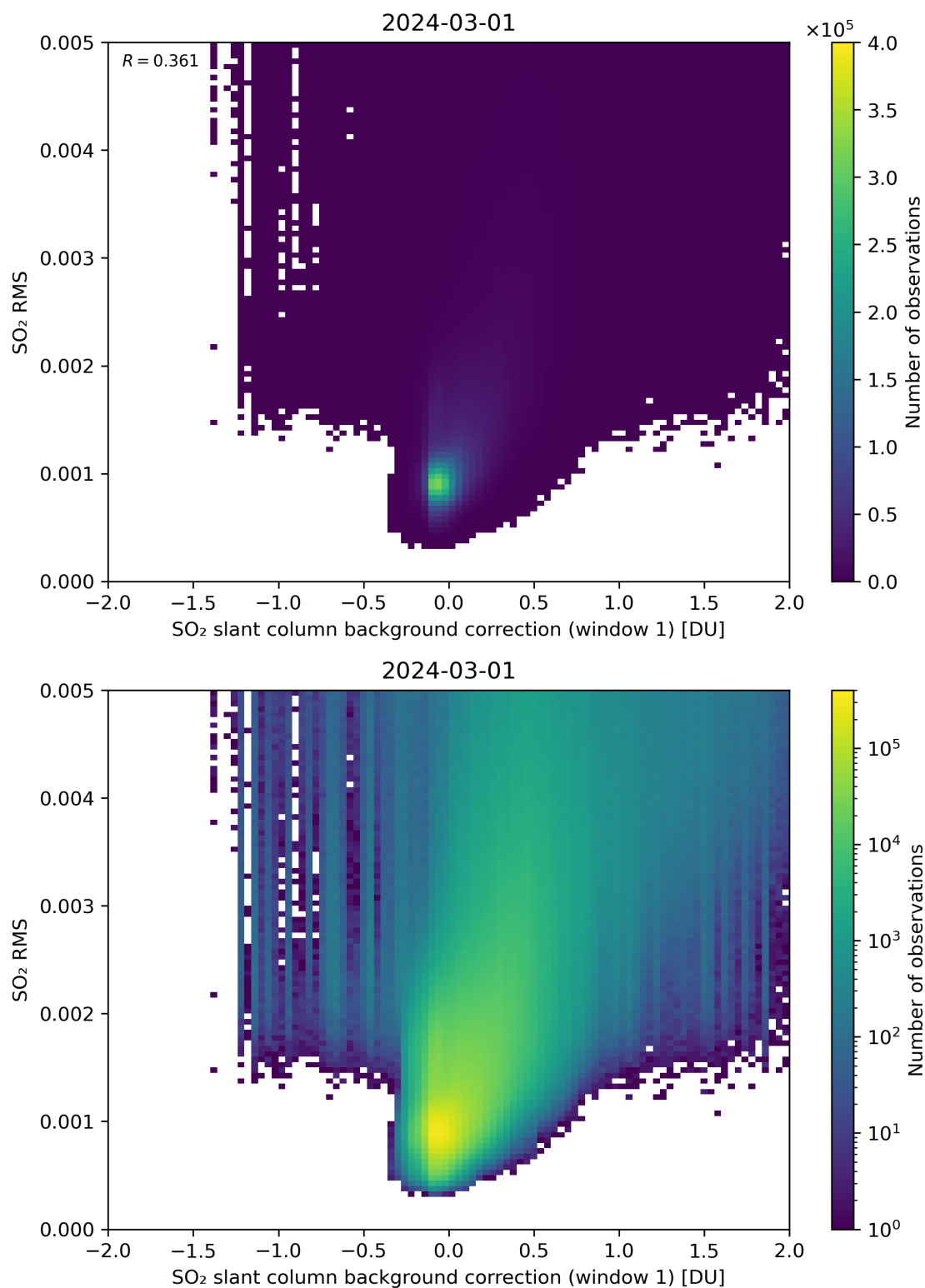
Figure 102: Scatter density plot of “SO 2 slant column background correction (window 1)” against “SO 2 RMS” for 2024-02-29 to 2024-03-02.
