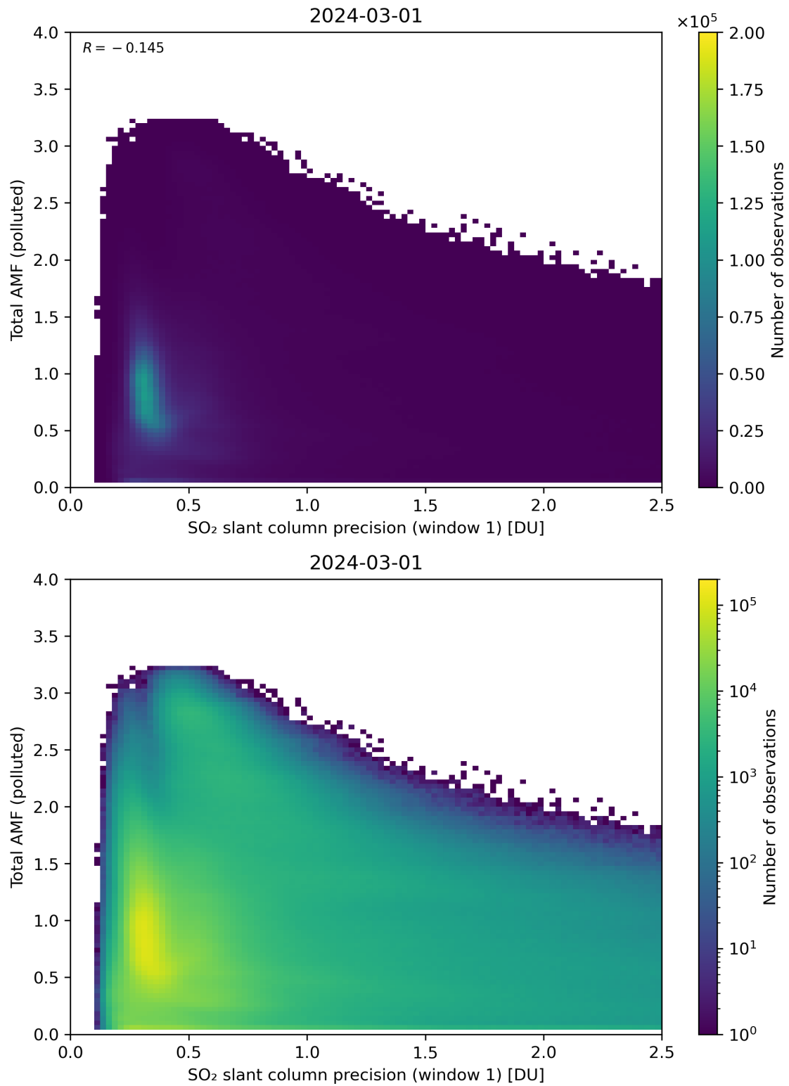
Figure 230: Scatter density plot of “SO 2 slant column precision (window 1)” against “Total AMF (polluted)” for 2024-02-29 to 2024-03-02.
