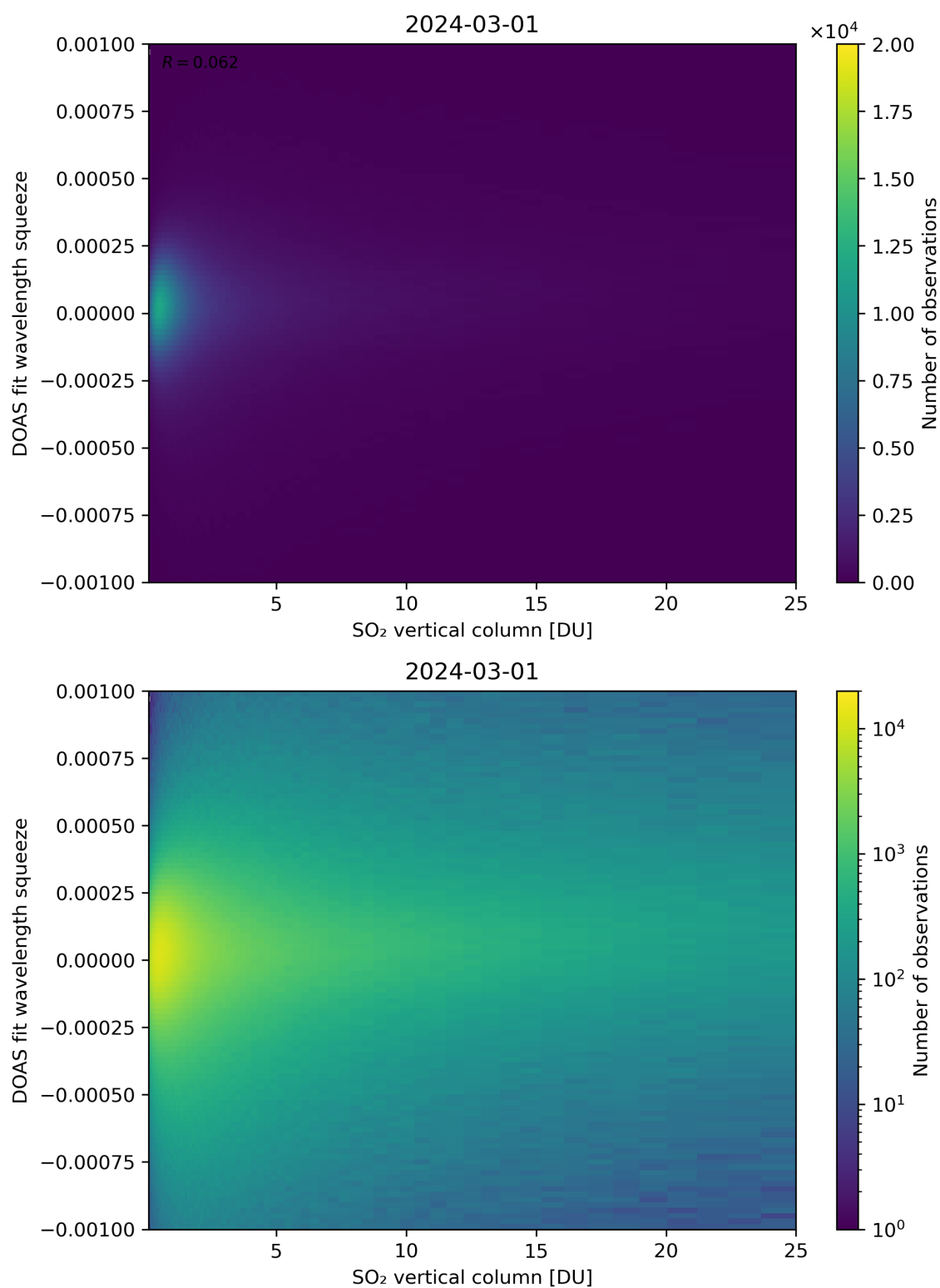
Figure 277: Scatter density plot of “SO 2 vertical column” against “DOAS fit wavelength squeeze” for 2024-02-29 to 2024-03-02.
