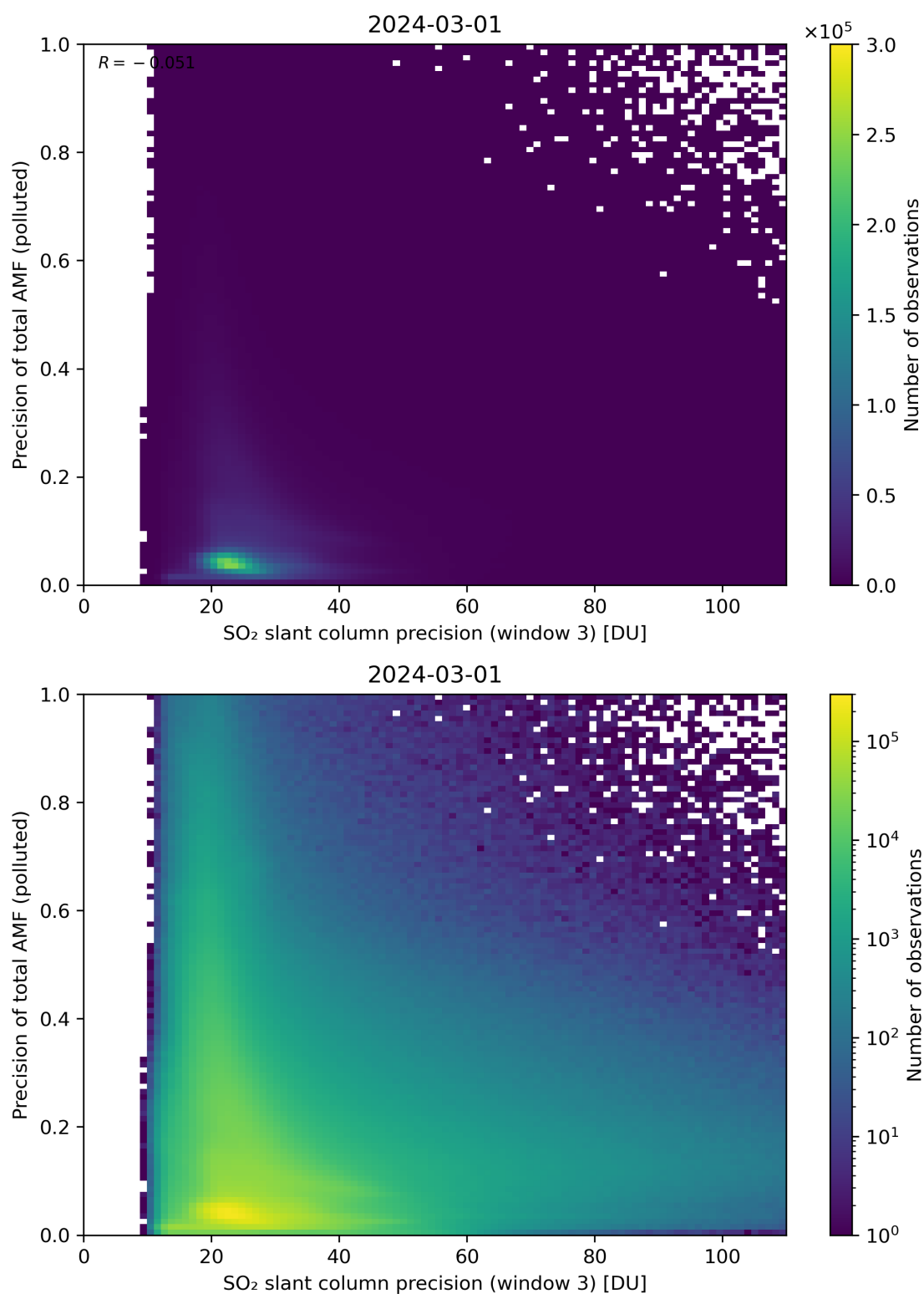
Figure 264: Scatter density plot of “SO 2 slant column precision (window 3)” against “Precision of total AMF (polluted)” for 2024-02-29 to 2024-03-02.
