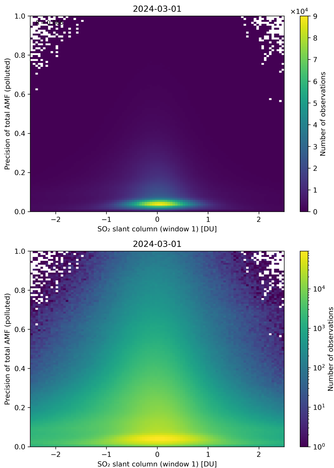
Figure 240: Scatter density plot of “SO 2 slant column (window 1)” against “Precision of total AMF (polluted)” for 2024-02-29 to 2024-03-02.
