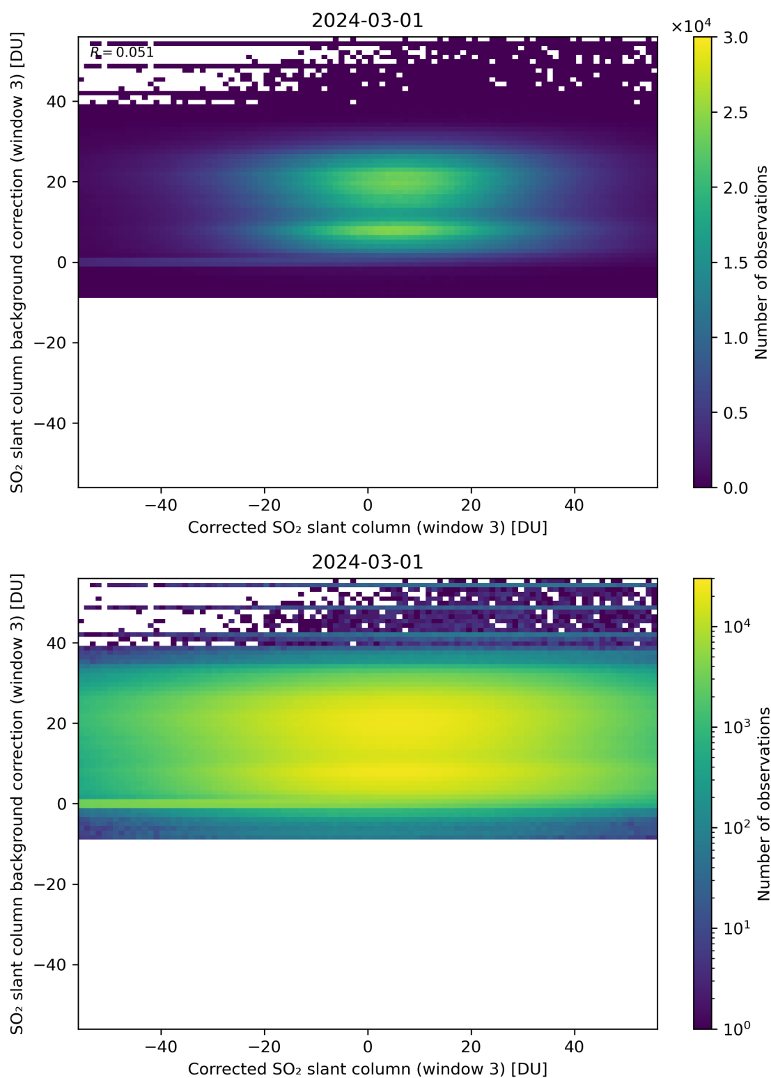
Figure 205: Scatter density plot of “Corrected SO 2 slant column (window 3)” against “SO 2 slant column background correction (window 3)” for 2024-02-29 to 2024-03-02.
