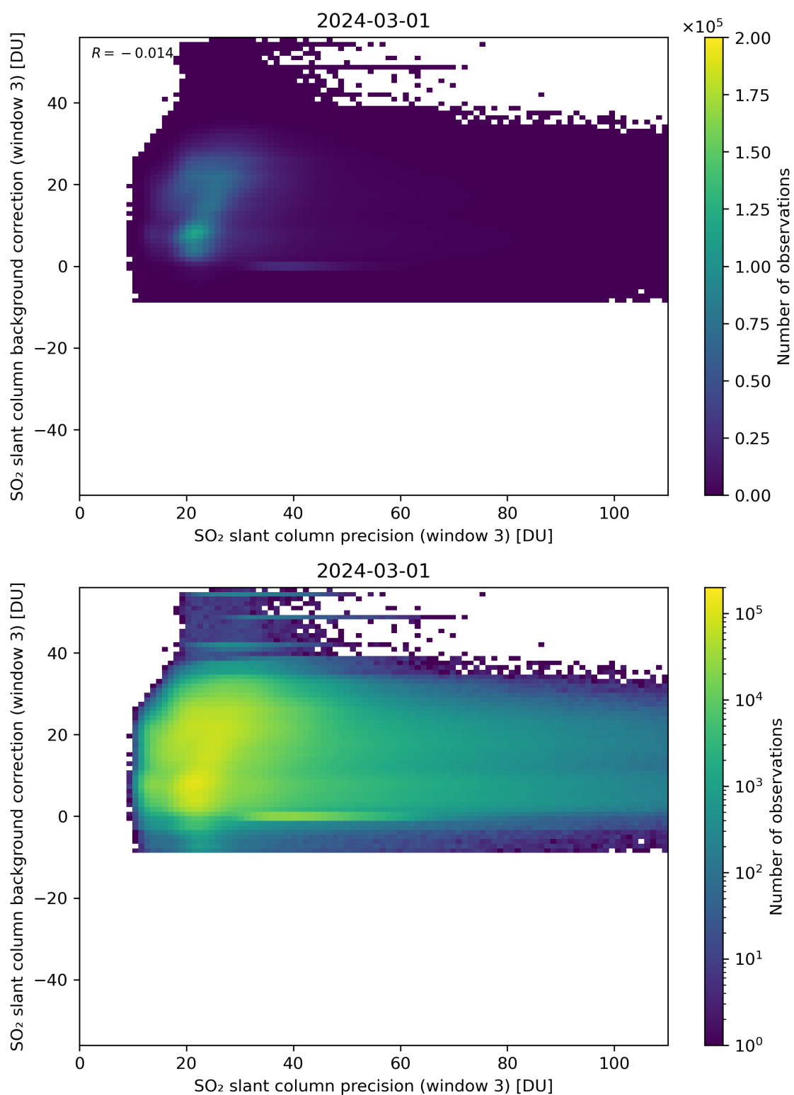
Figure 257: Scatter density plot of “SO 2 slant column precision (window 3)” against “SO 2 slant column background correction (window 3)” for 2024-02-29 to 2024-03-02.
