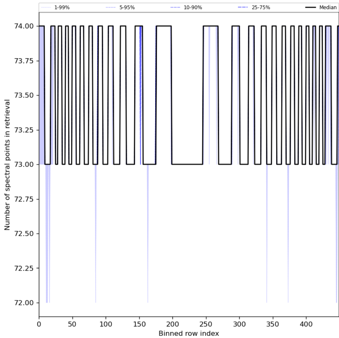
Figure 97: Along track statistics of “Number of spectral points in retrieval” for 2024-02-29 to 2024-03-02
