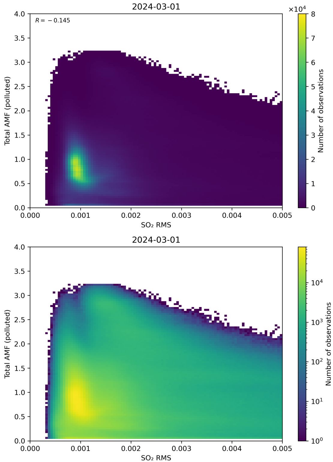
Figure 137: Scatter density plot of “SO 2 RMS” against “Total AMF (polluted)” for 2024-02-29 to 2024-03-02.
