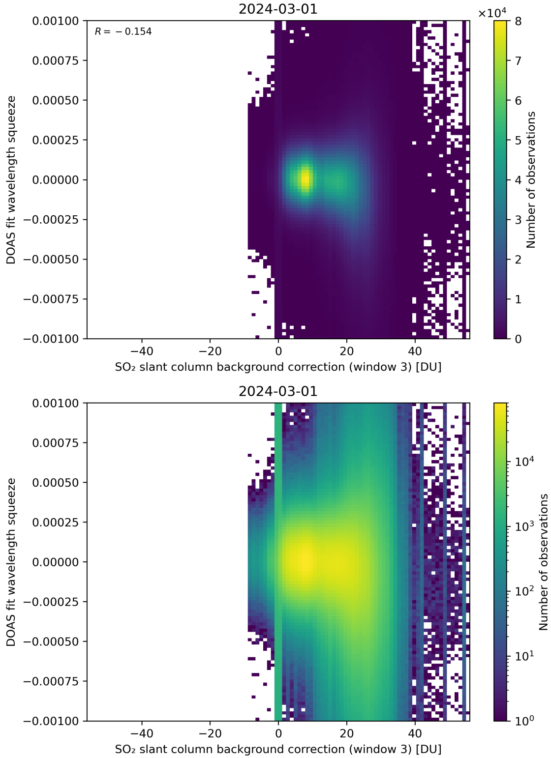
Figure 122: Scatter density plot of “SO 2 slant column background correction (window 3)” against “DOAS fit wavelength squeeze” for 2024-02-29 to 2024-03-02.
