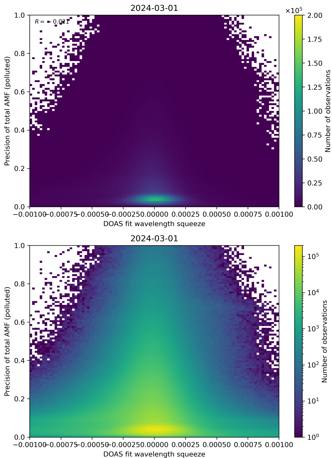
Figure 135: Scatter density plot of “DOAS fit wavelength squeeze” against “Precision of total AMF (polluted)” for 2024-02-29 to 2024-03-02.
