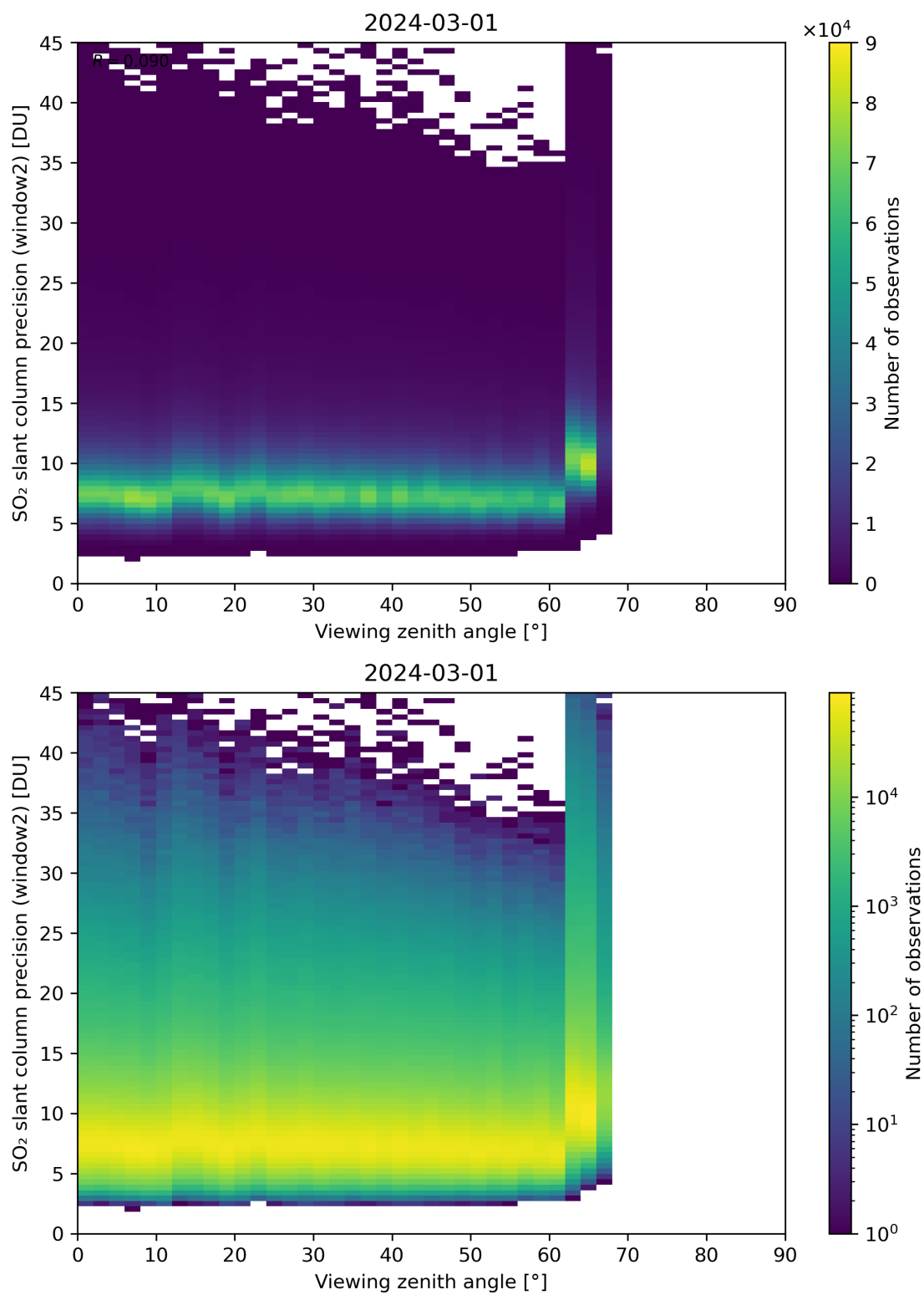
Figure 322: Scatter density plot of “Viewing zenith angle” against “SO 2 slant column precision (window2)” for 2024-02-29 to 2024-03-02.
