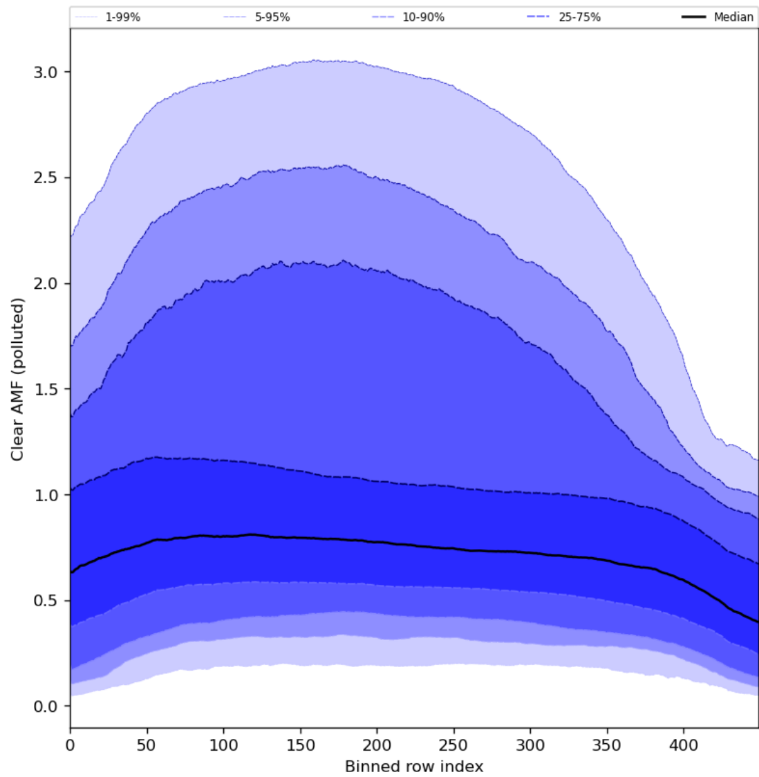
Figure 96: Along track statistics of “Clear AMF (polluted)” for 2024-02-29 to 2024-03-02
