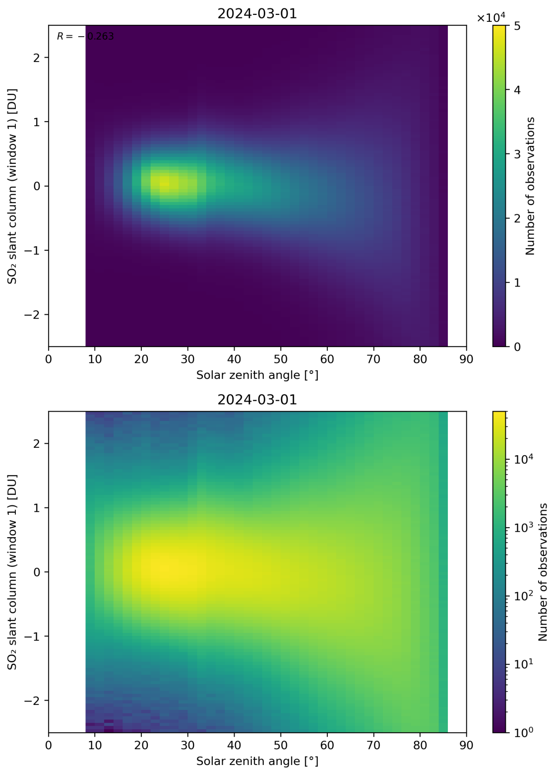
Figure 169: Scatter density plot of “Solar zenith angle” against “SO 2 slant column (window 1)” for 2024-02-29 to 2024-03-02.
