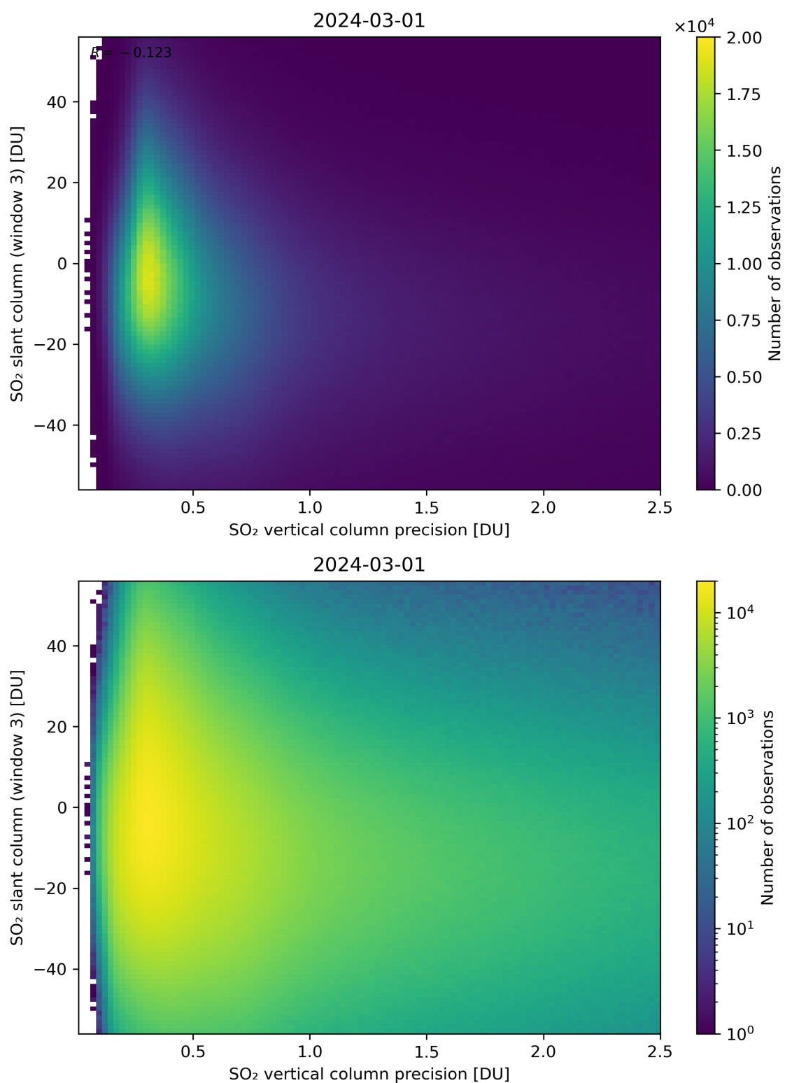
Figure 292: Scatter density plot of “SO 2 vertical column precision” against “SO 2 slant column (window 3)” for 2024-02-29 to 2024-03-02.
