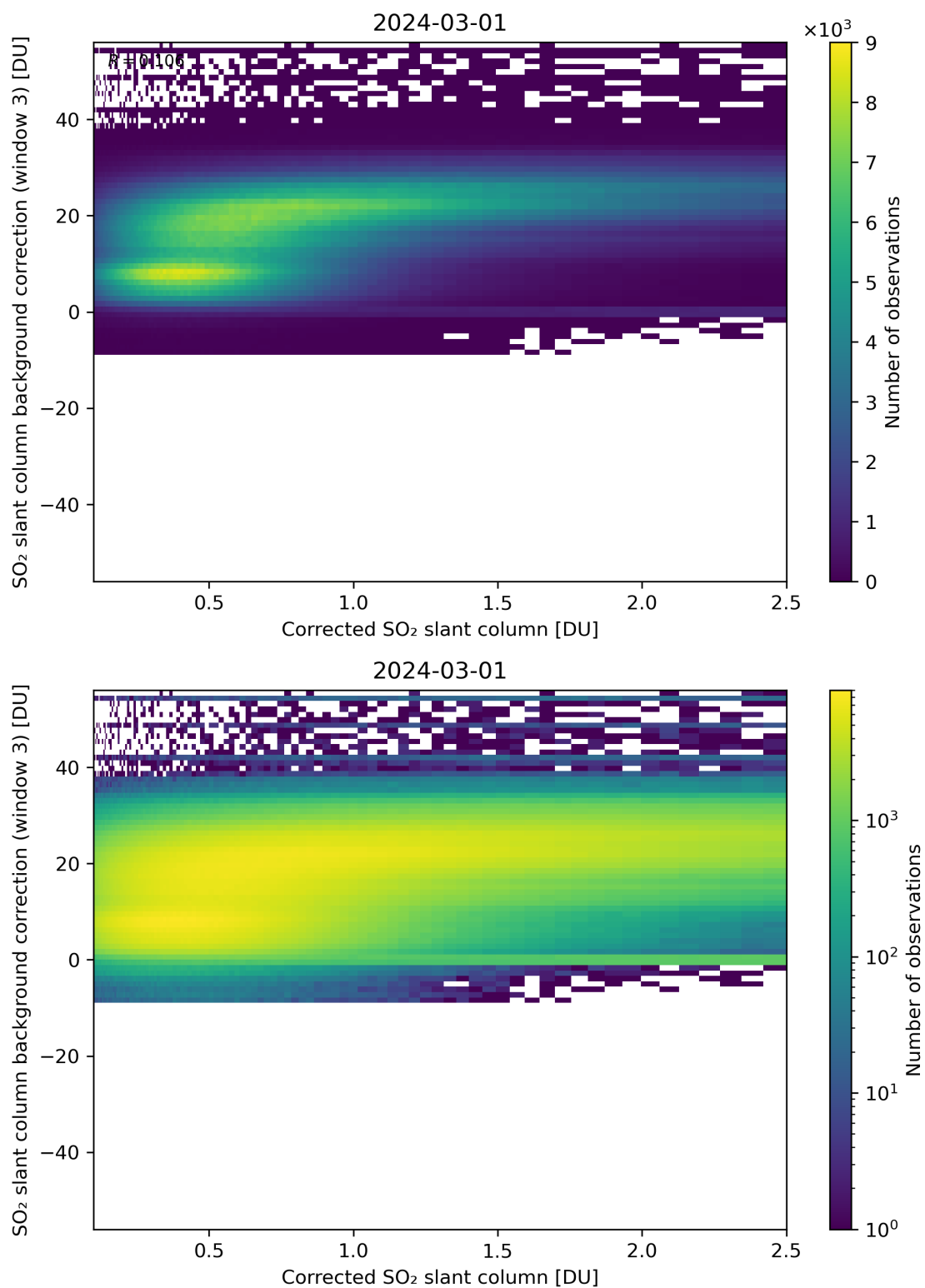
Figure 180: Scatter density plot of “Corrected SO 2 slant column” against “SO 2 slant column background correction (window 3)” for 2024-02-29 to 2024-03-02.
