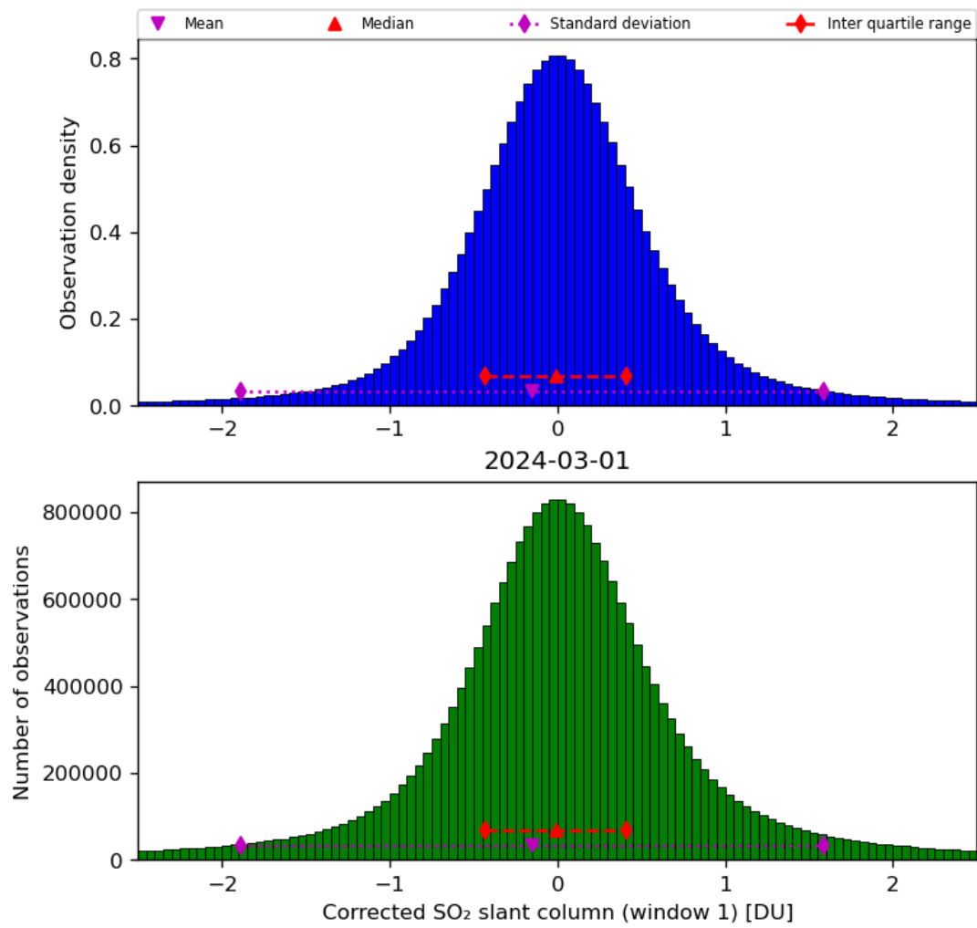
Figure 58: Histogram of “Corrected SO 2 slant column (window 1)” for 2024-02-29 to 2024-03-02
