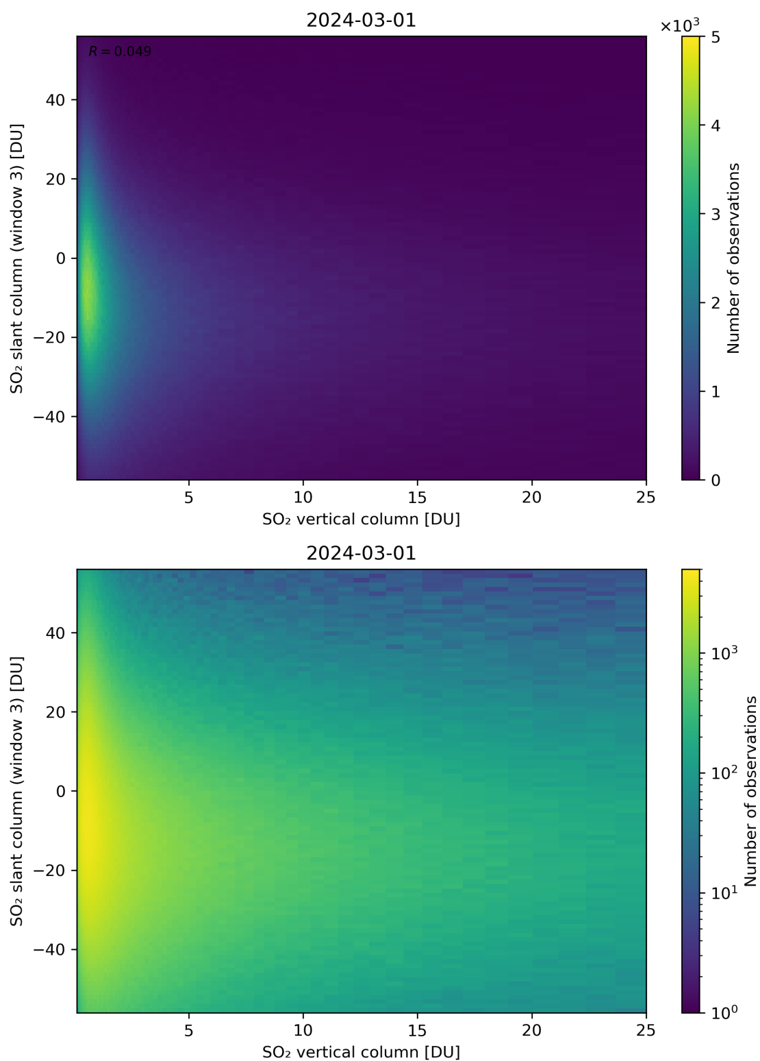
Figure 303: Scatter density plot of “SO 2 vertical column” against “SO 2 slant column (window 3)” for 2024-02-29 to 2024-03-02.
