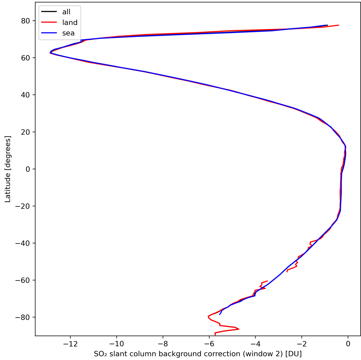
Figure 40: Zonal average of “SO 2 slant column background correction (window 2)” for 2024-02-29 to 2024-03-02.
