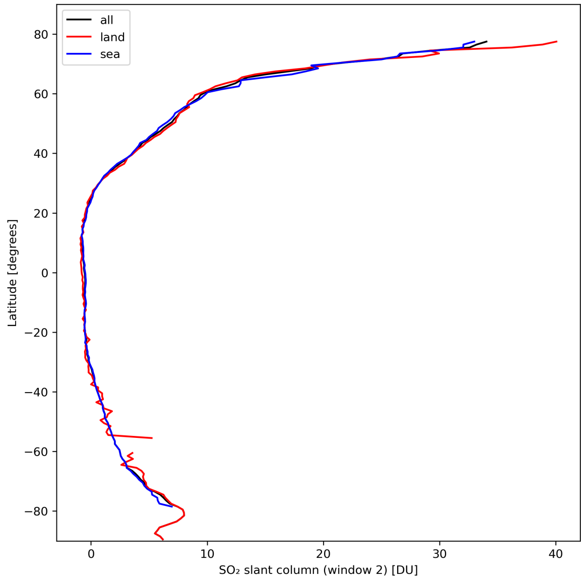
Figure 37: Zonal average of “SO 2 slant column (window 2)” for 2024-02-29 to 2024-03-02.
