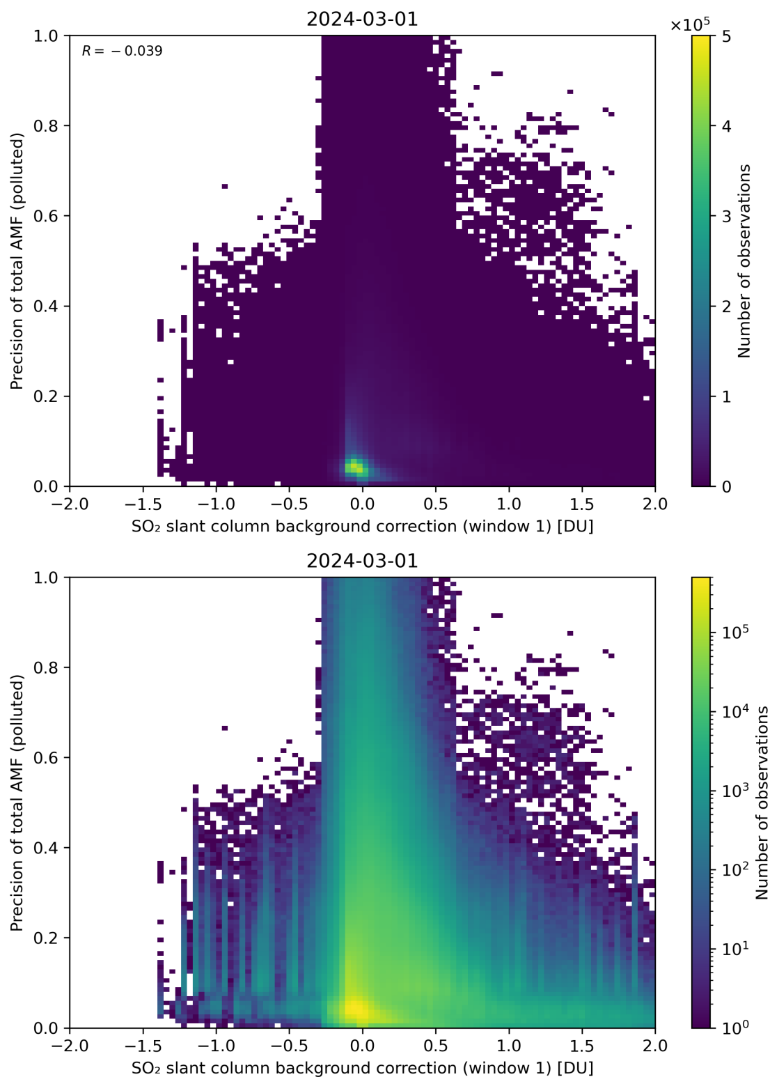
Figure 110: Scatter density plot of “SO 2 slant column background correction (window 1)” against “Precision of total AMF (polluted)” for 2024-02-29 to 2024-03-02.
