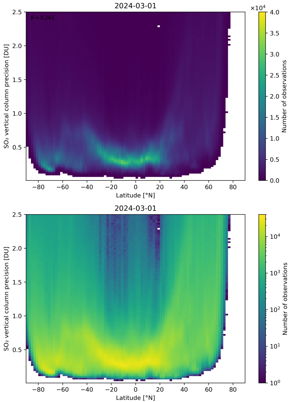
Figure 157: Scatter density plot of “Latitude” against “SO 2 vertical column precision” for 2024-02-29 to 2024-03-02.
