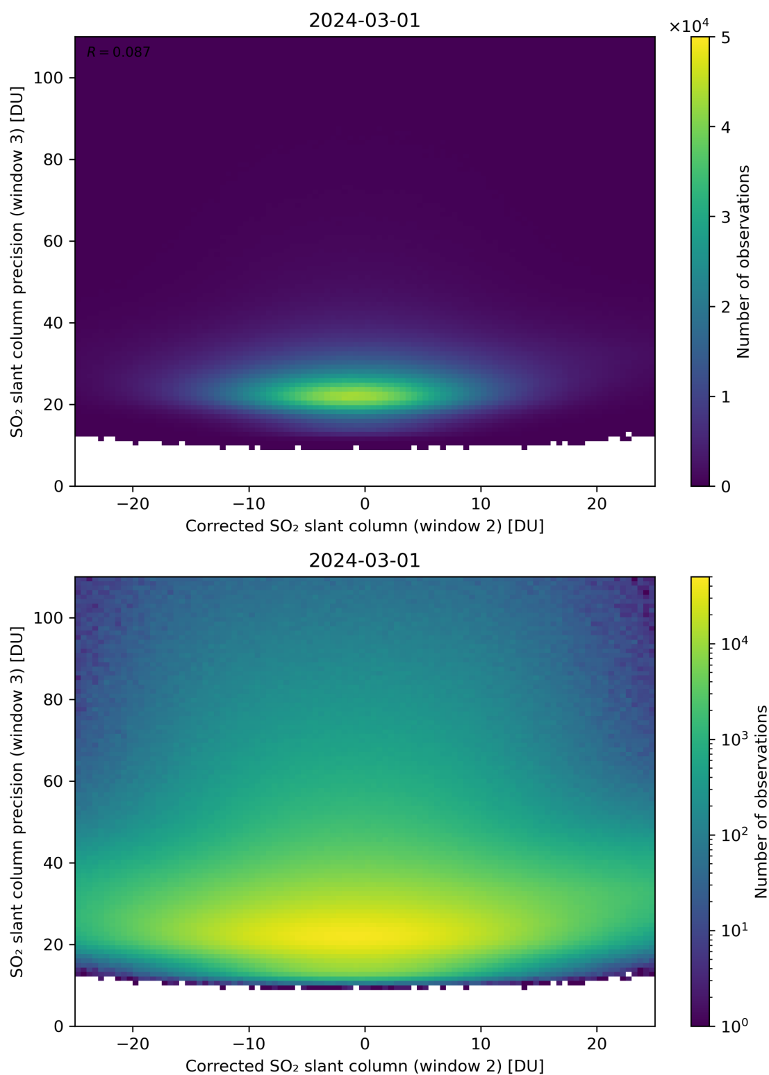
Figure 202: Scatter density plot of “Corrected SO 2 slant column (window 2)” against “SO 2 slant column precision (window 3)” for 2024-02-29 to 2024-03-02.
