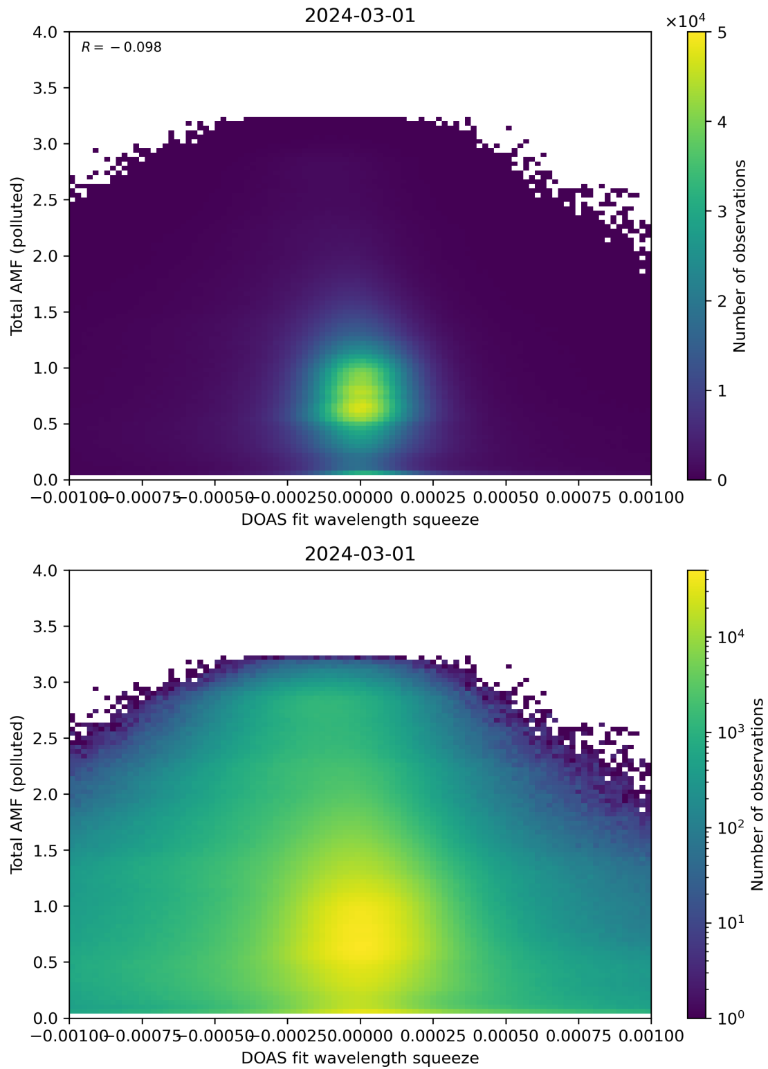
Figure 134: Scatter density plot of “DOAS fit wavelength squeeze” against “Total AMF (polluted)” for 2024-02-29 to 2024-03-02.
