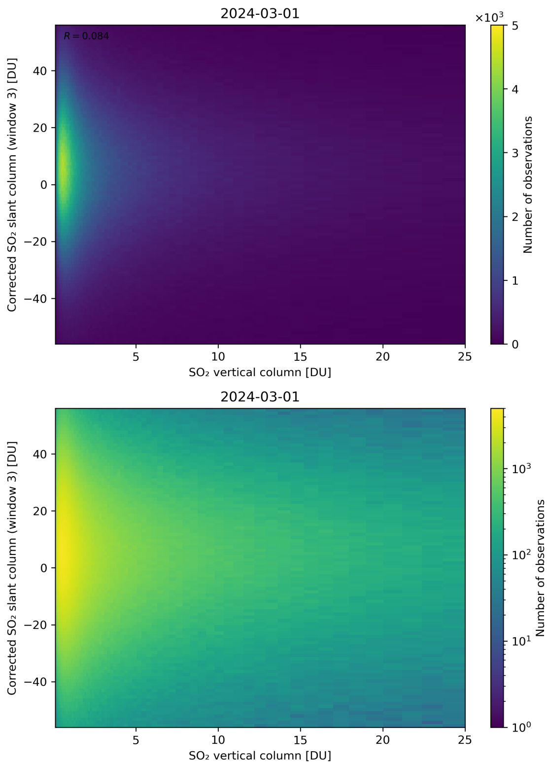
Figure 299: Scatter density plot of “SO 2 vertical column” against “Corrected SO 2 slant column (window 3)” for 2024-02-29 to 2024-03-02.
