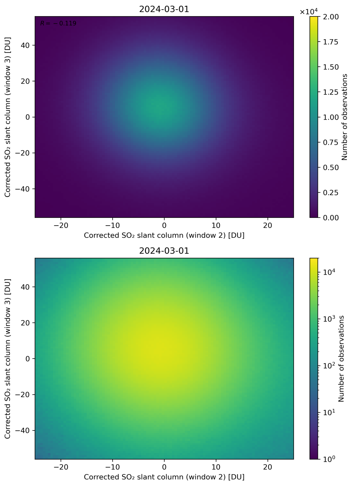
Figure 200: Scatter density plot of “Corrected SO 2 slant column (window 2)” against “Corrected SO 2 slant column (window 3)” for 2024-02-29 to 2024-03-02.
