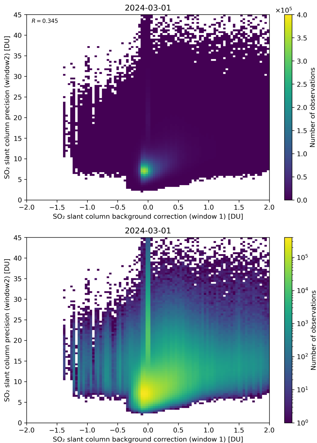
Figure 106: Scatter density plot of “SO 2 slant column background correction (window 1)” against “SO 2 slant column precision (window2)” for 2024-02-29 to 2024-03-02.
