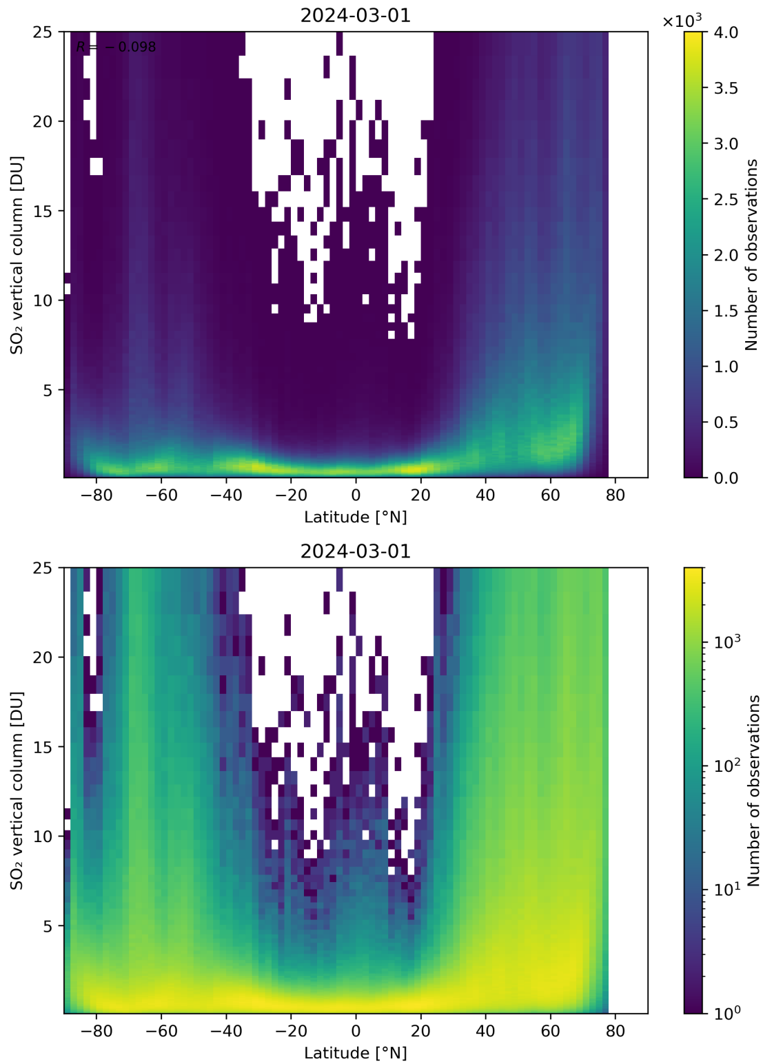
Figure 156: Scatter density plot of “Latitude” against “SO 2 vertical column” for 2024-02-29 to 2024-03-02.
