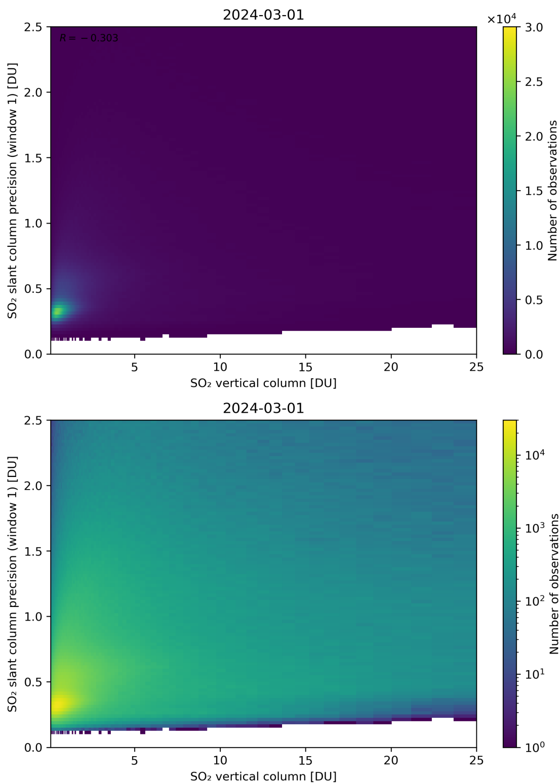
Figure 301: Scatter density plot of “SO 2 vertical column” against “SO 2 slant column precision (window 1)” for 2024-02-29 to 2024-03-02.
