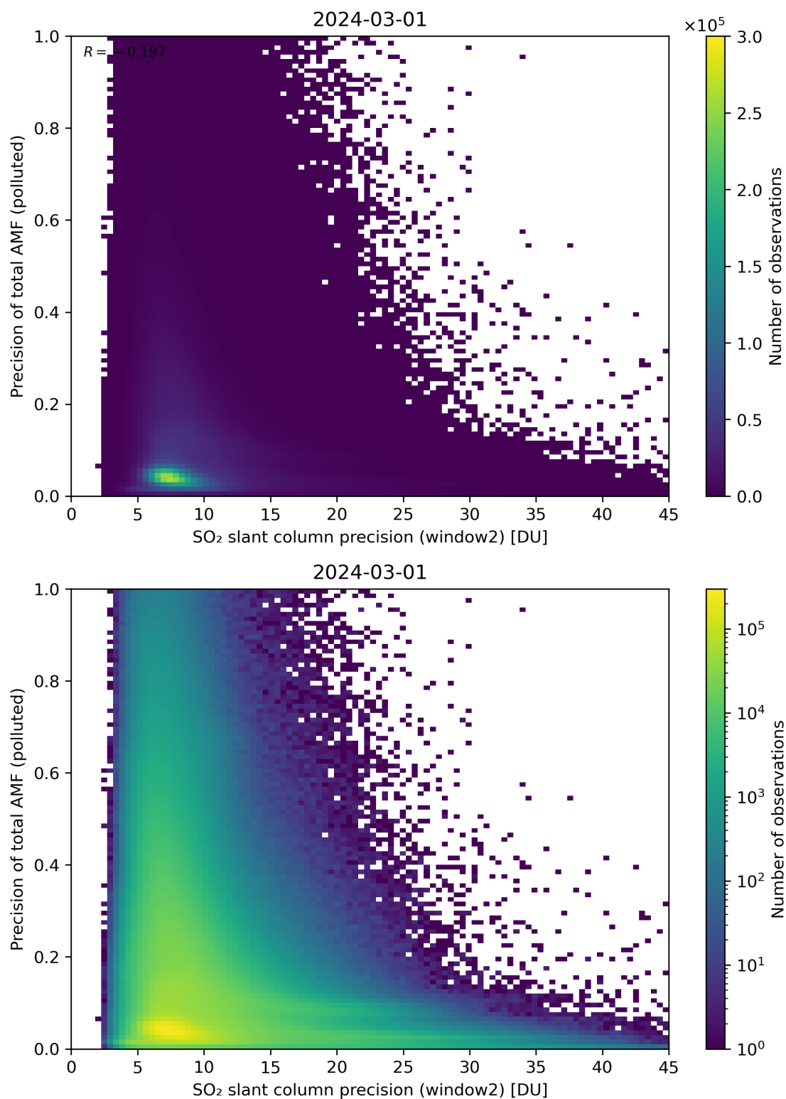
Figure 252: Scatter density plot of “SO 2 slant column precision (window2)” against “Precision of total AMF (polluted)” for 2024-02-29 to 2024-03-02.
