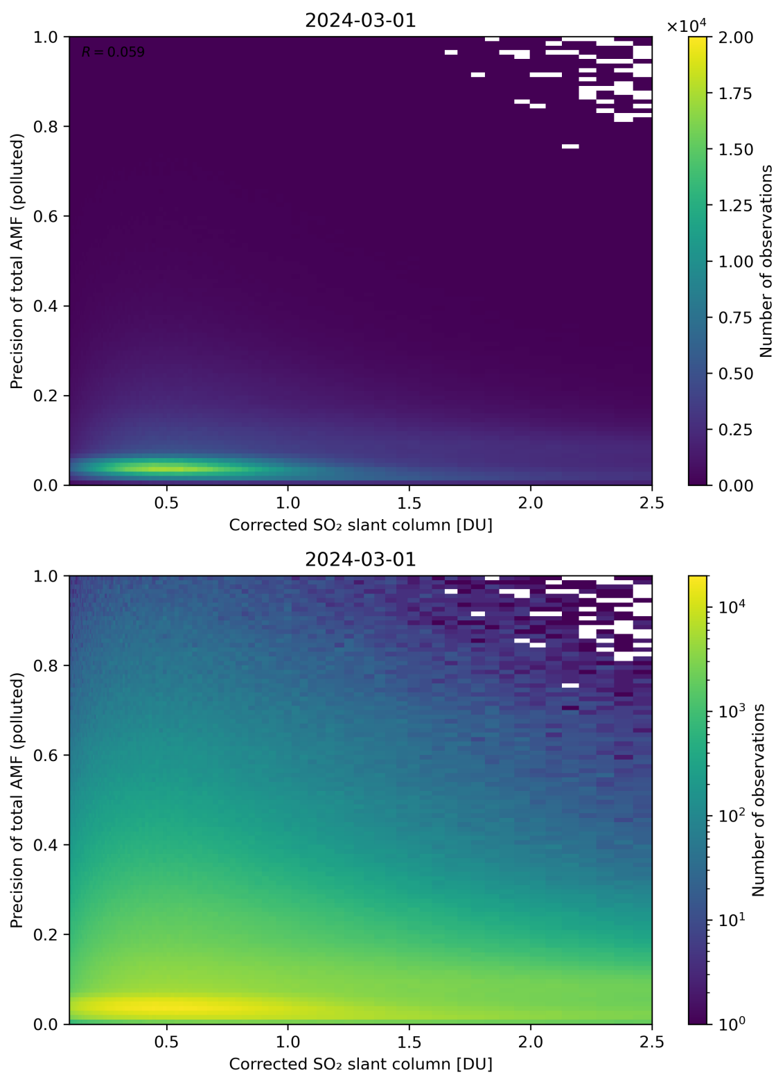
Figure 193: Scatter density plot of “Corrected SO 2 slant column” against “Precision of total AMF (polluted)” for 2024-02-29 to 2024-03-02.
