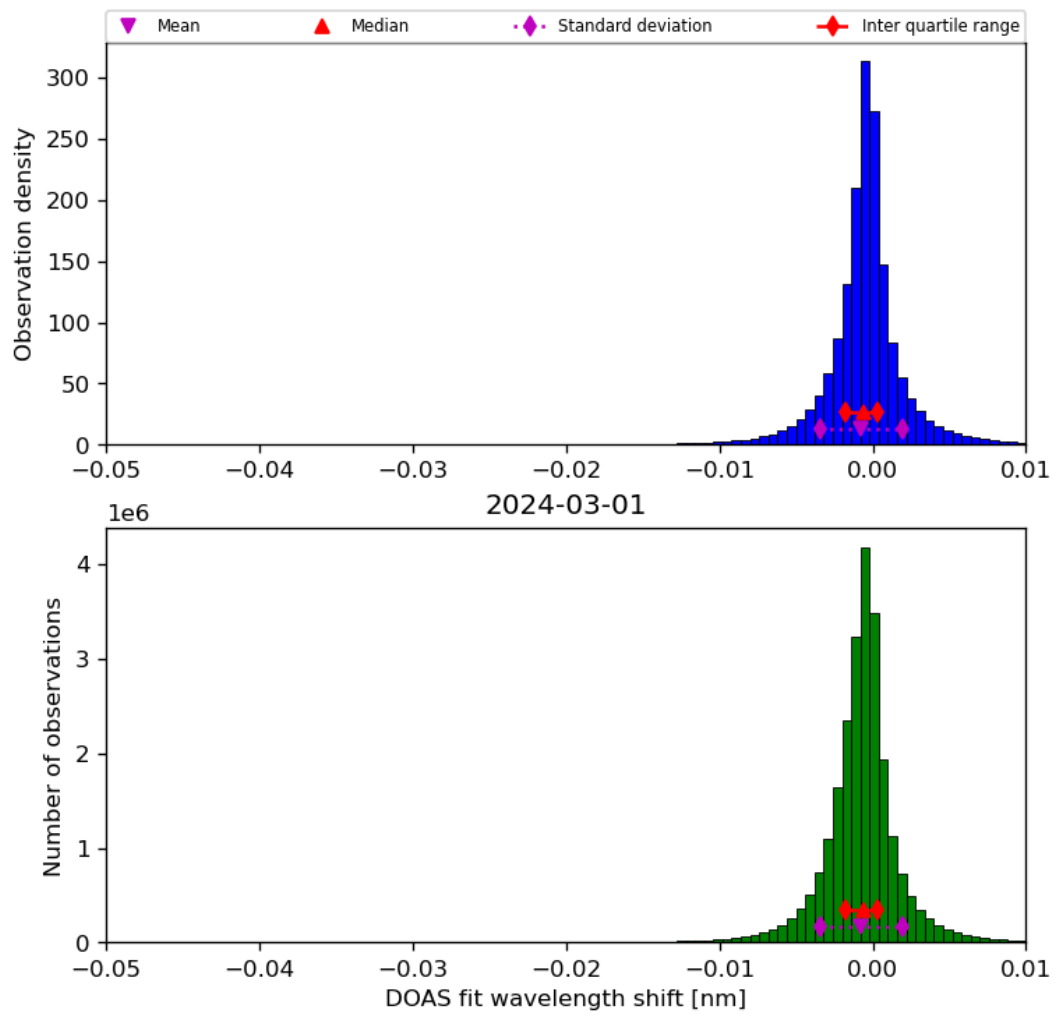
Figure 68: Histogram of “DOAS fit wavelength shift” for 2024-02-29 to 2024-03-02
