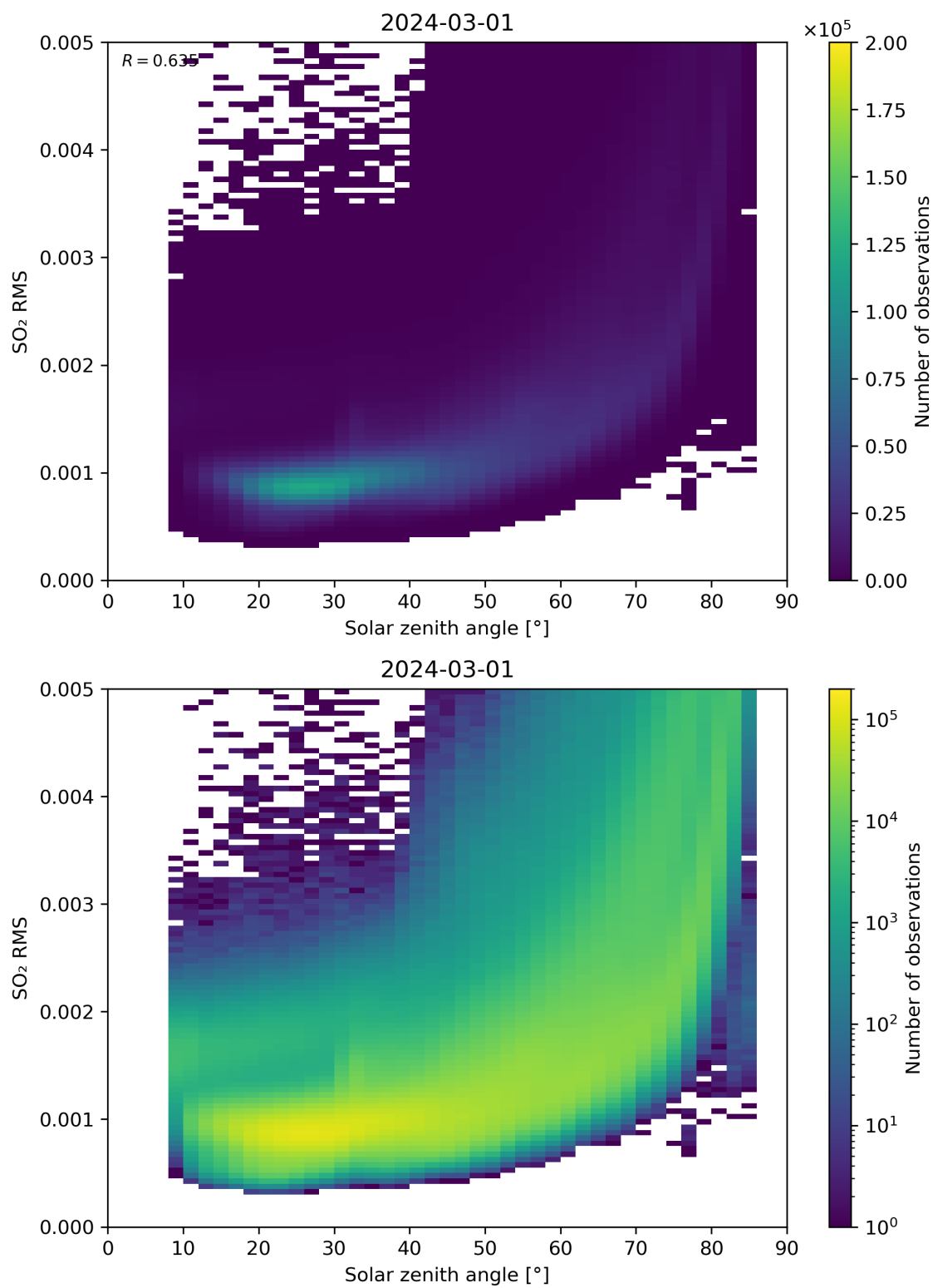
Figure 163: Scatter density plot of “Solar zenith angle” against “SO 2 RMS” for 2024-02-29 to 2024-03-02.
