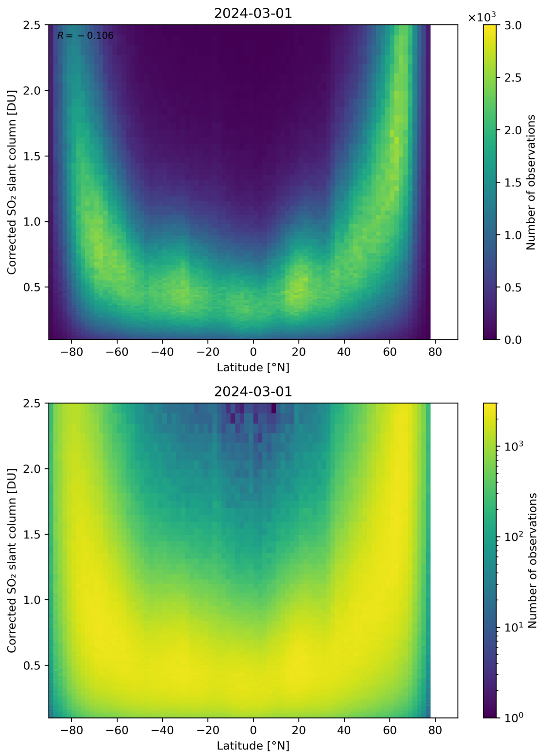
Figure 146: Scatter density plot of “Latitude” against “Corrected SO 2 slant column” for 2024-02-29 to 2024-03-02.
