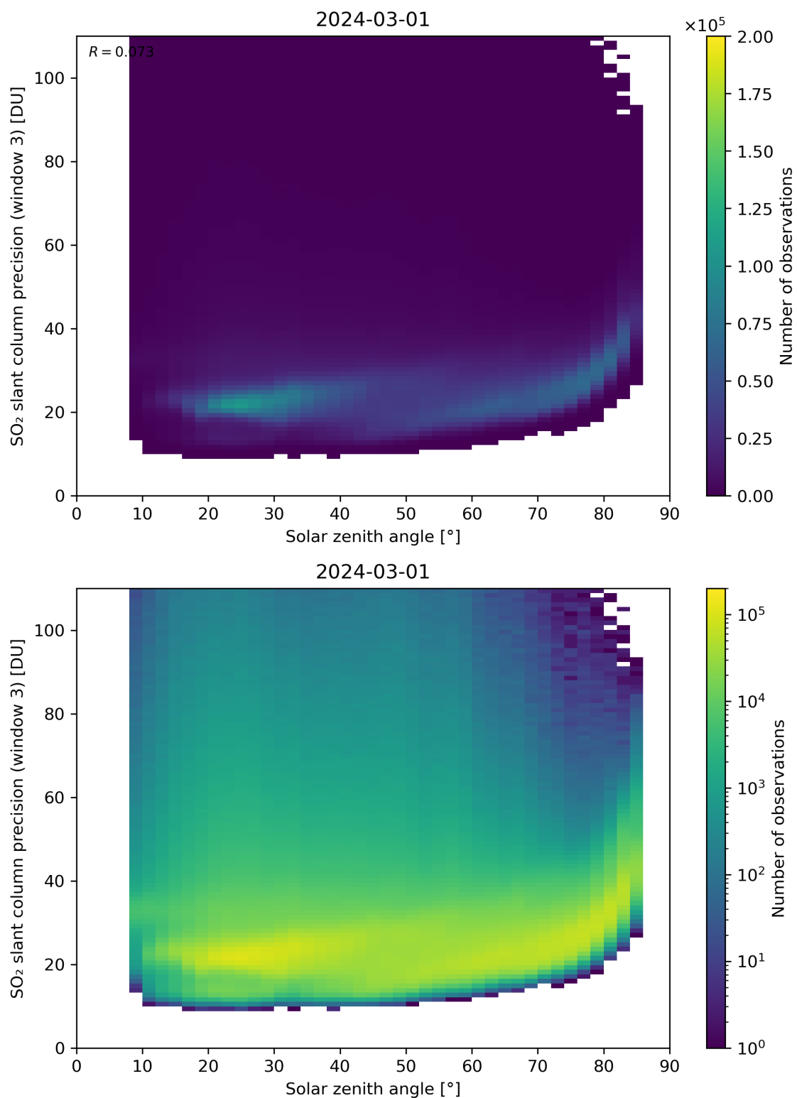
Figure 173: Scatter density plot of “Solar zenith angle” against “SO 2 slant column precision (window 3)” for 2024-02-29 to 2024-03-02.
