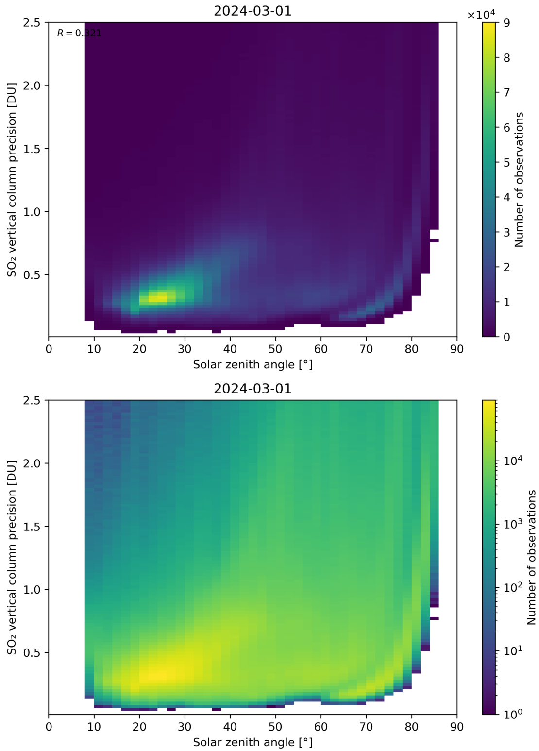
Figure 177: Scatter density plot of “Solar zenith angle” against “SO 2 vertical column precision” for 2024-02-29 to 2024-03-02.
