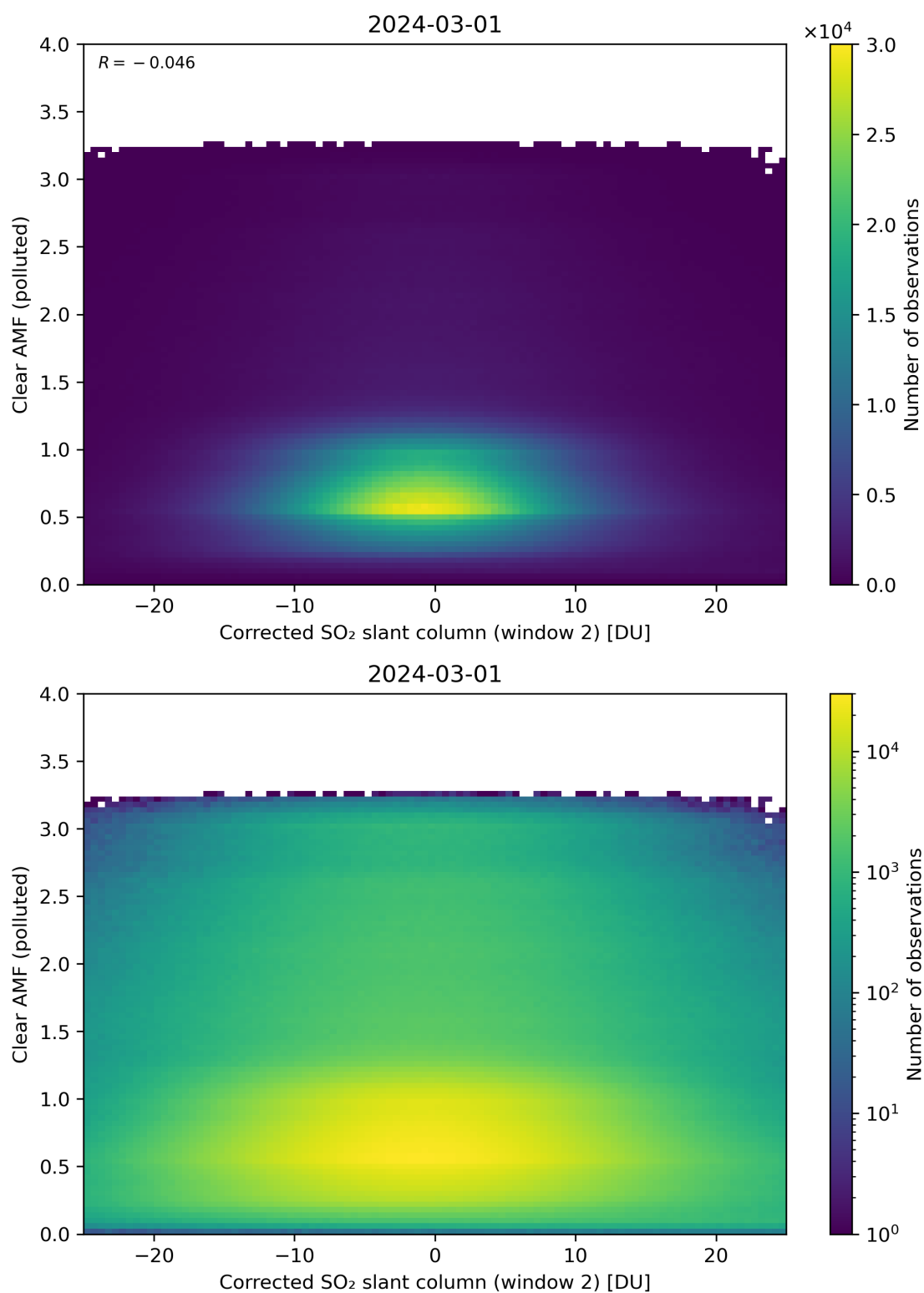
Figure 199: Scatter density plot of “Corrected SO 2 slant column (window 2)” against “Clear AMF (polluted)” for 2024-02-29 to 2024-03-02.
