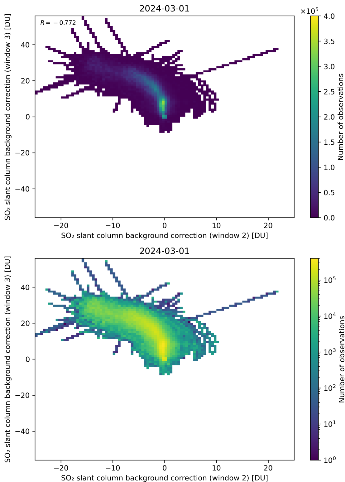
Figure 111: Scatter density plot of “SO 2 slant column background correction (window 2)” against “SO 2 slant column background correction (window 3)” for 2024-02-29 to 2024-03-02.
