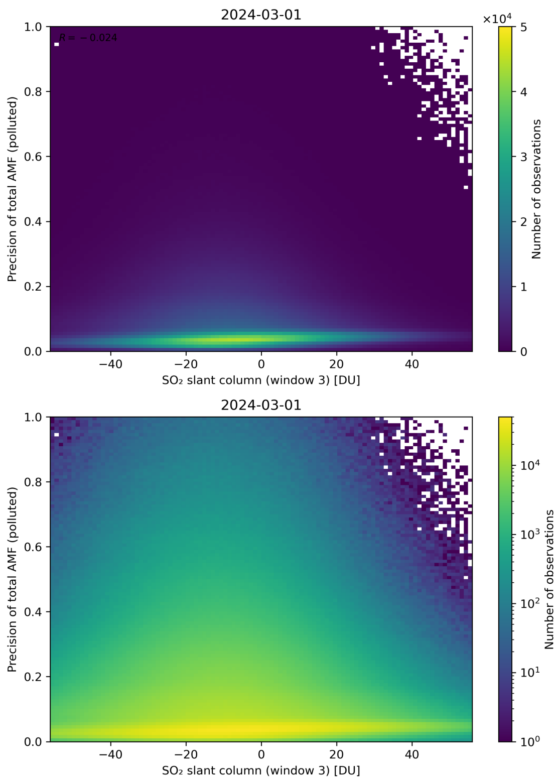
Figure 269: Scatter density plot of “SO 2 slant column (window 3)” against “Precision of total AMF (polluted)” for 2024-02-29 to 2024-03-02.
