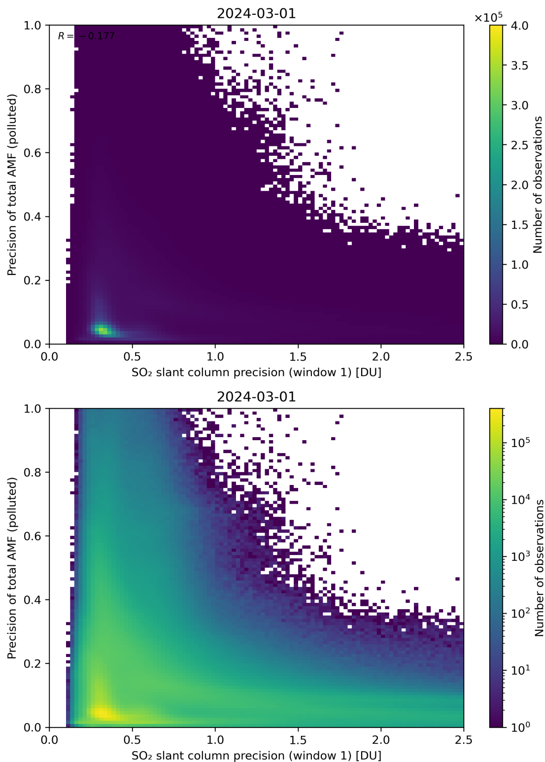
Figure 231: Scatter density plot of “SO 2 slant column precision (window 1)” against “Precision of total AMF (polluted)” for 2024-02-29 to 2024-03-02.
