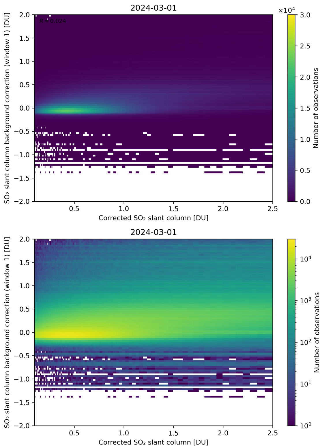
Figure 178: Scatter density plot of “Corrected SO 2 slant column” against “SO 2 slant column background correction (window 1)” for 2024-02-29 to 2024-03-02.
