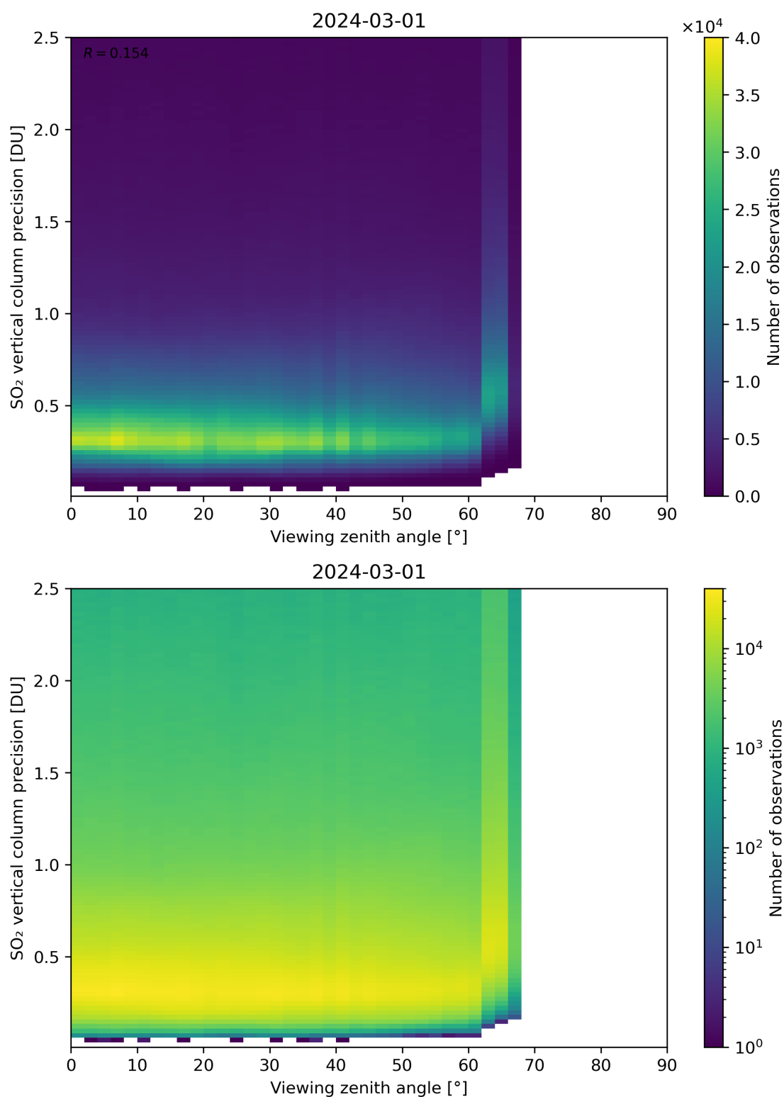
Figure 328: Scatter density plot of “Viewing zenith angle” against “SO 2 vertical column precision” for 2024-02-29 to 2024-03-02.
