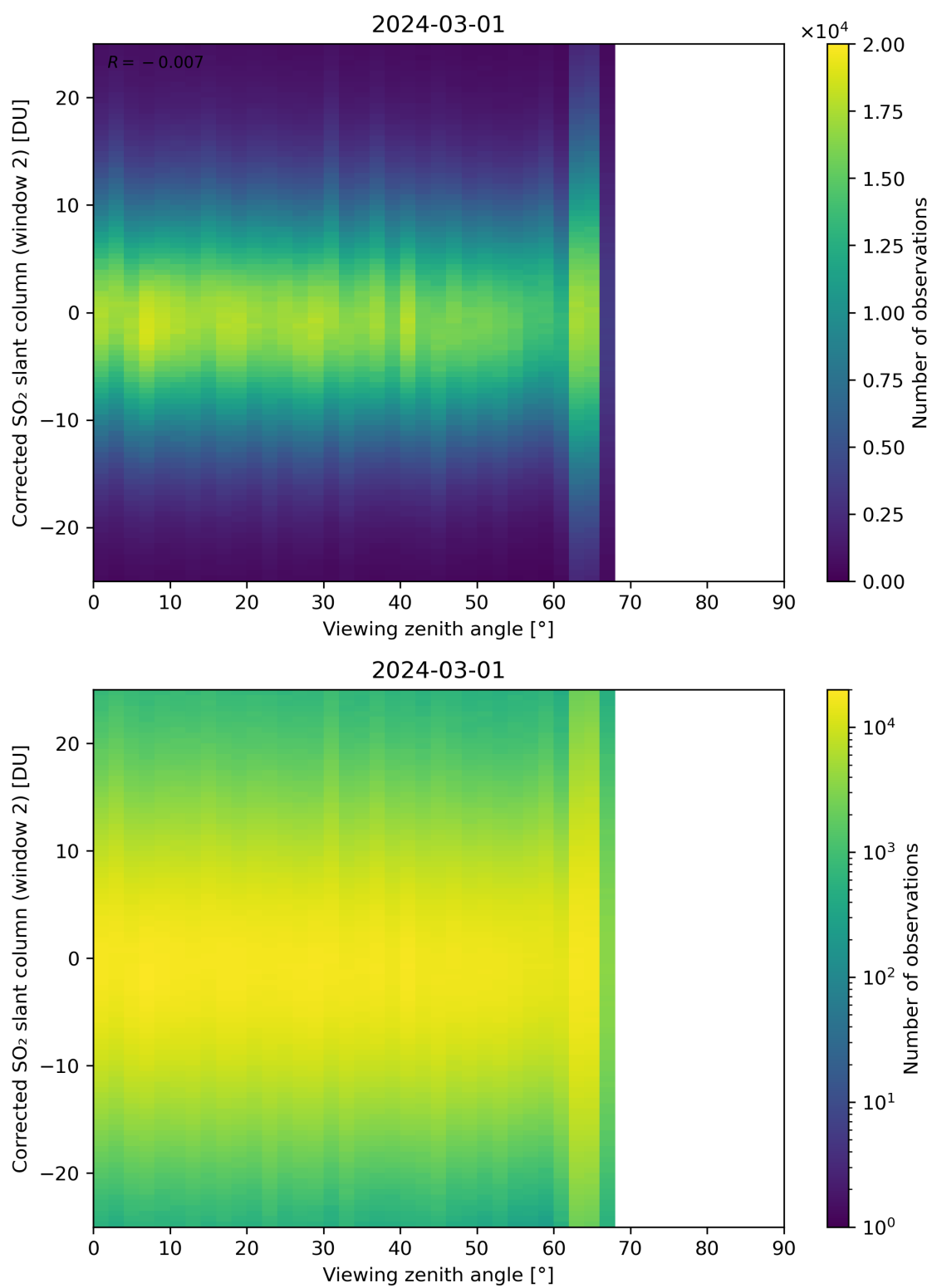
Figure 318: Scatter density plot of “Viewing zenith angle” against “Corrected SO 2 slant column (window 2)” for 2024-02-29 to 2024-03-02.
