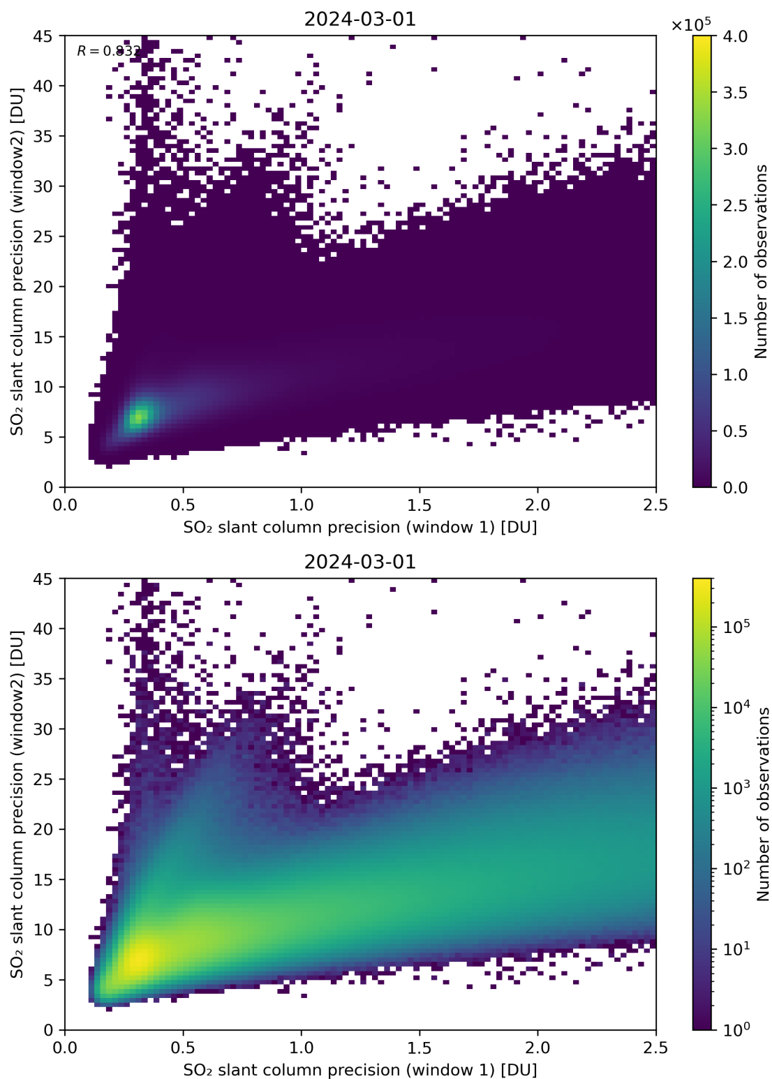
Figure 227: Scatter density plot of “SO 2 slant column precision (window 1)” against “SO 2 slant column precision (window2)” for 2024-02-29 to 2024-03-02.
