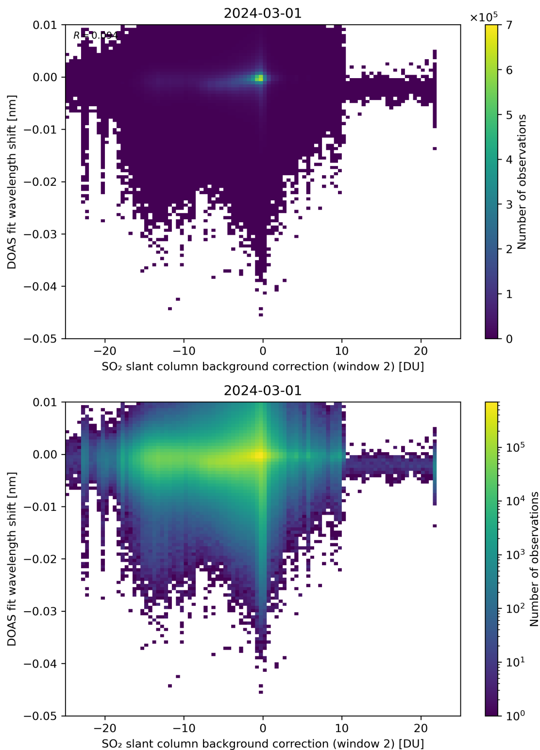
Figure 112: Scatter density plot of “SO 2 slant column background correction (window 2)” against “DOAS fit wavelength shift” for 2024-02-29 to 2024-03-02.
