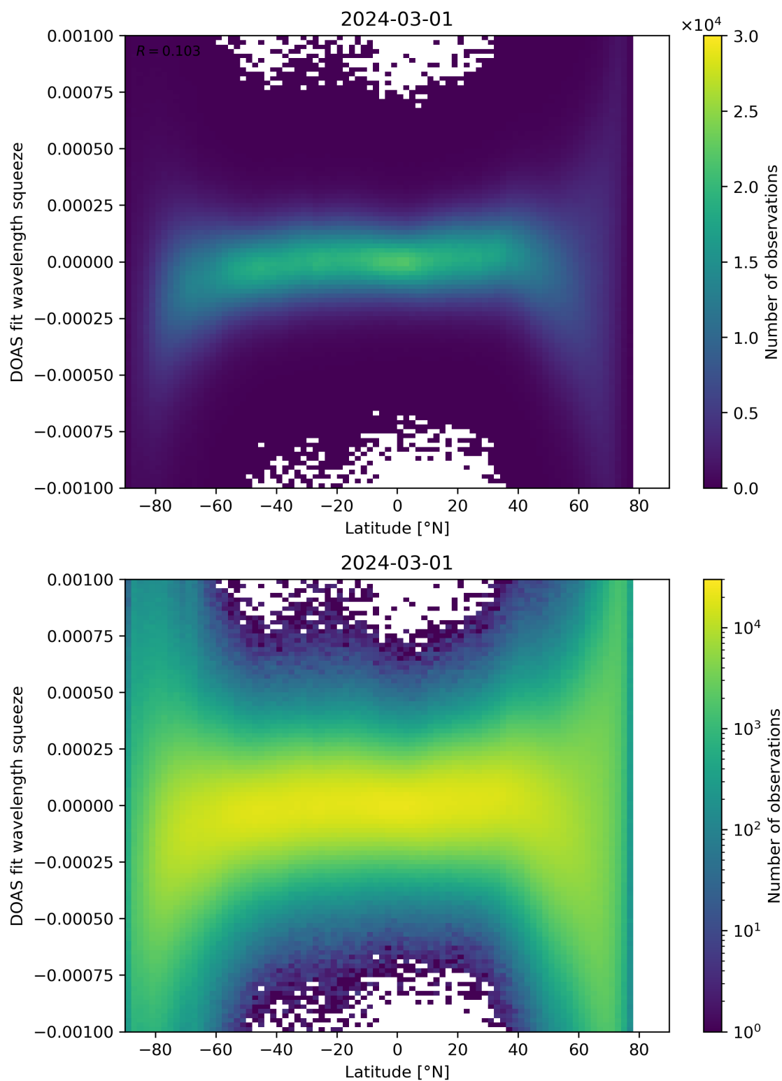
Figure 143: Scatter density plot of “Latitude” against “DOAS fit wavelength squeeze” for 2024-02-29 to 2024-03-02.
