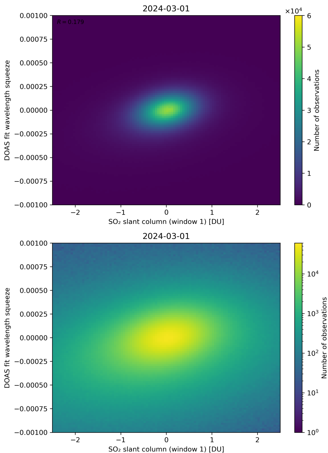
Figure 216: Scatter density plot of “SO 2 slant column (window 1)” against “DOAS fit wavelength squeeze” for 2024-02-29 to 2024-03-02.
