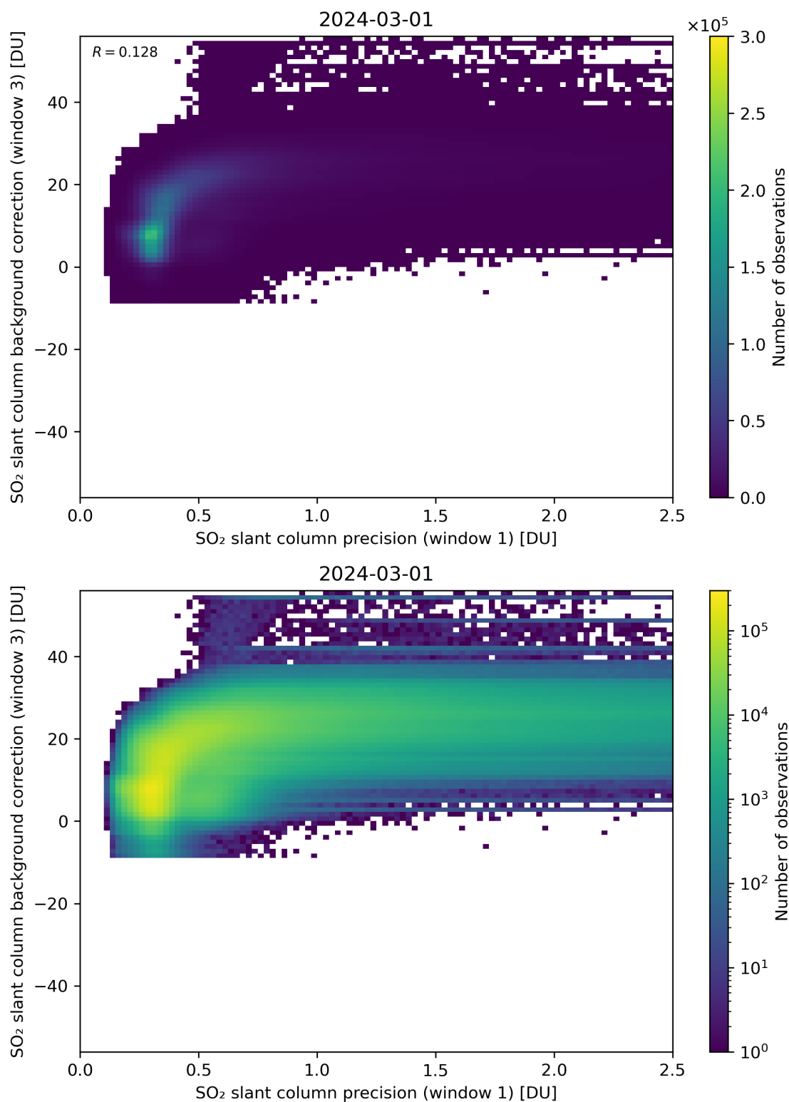
Figure 220: Scatter density plot of “SO 2 slant column precision (window 1)” against “SO 2 slant column background correction (window 3)” for 2024-02-29 to 2024-03-02.
