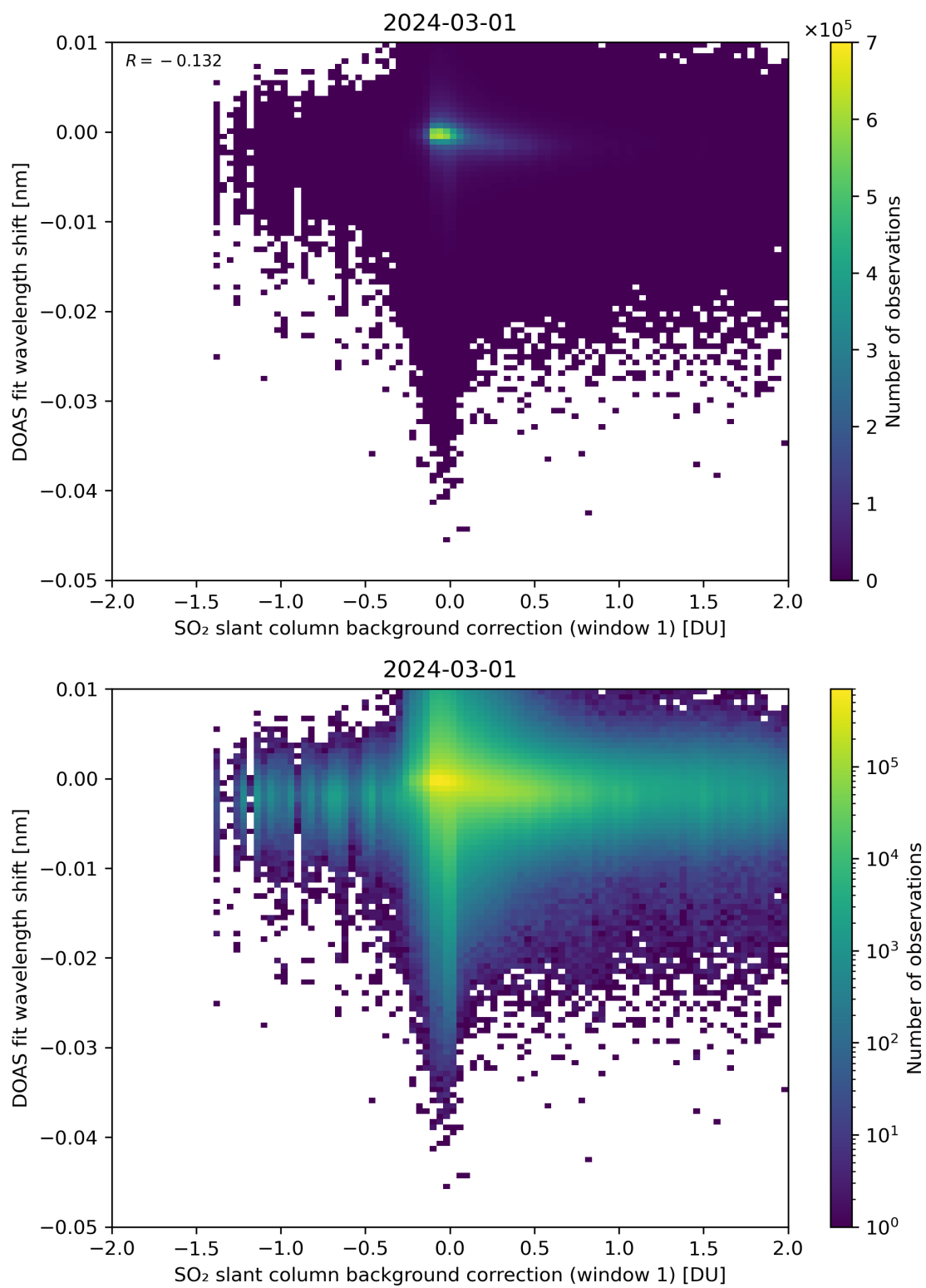
Figure 100: Scatter density plot of “SO 2 slant column background correction (window 1)” against “DOAS fit wavelength shift” for 2024-02-29 to 2024-03-02.
