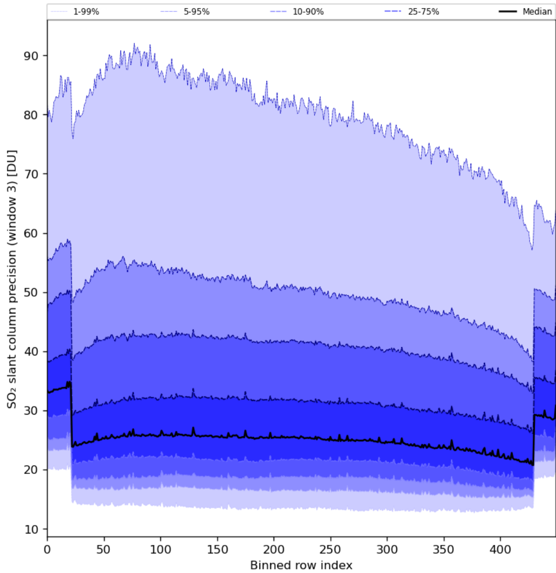
Figure 88: Along track statistics of “SO 2 slant column precision (window 3)” for 2024-02-29 to 2024-03-02
