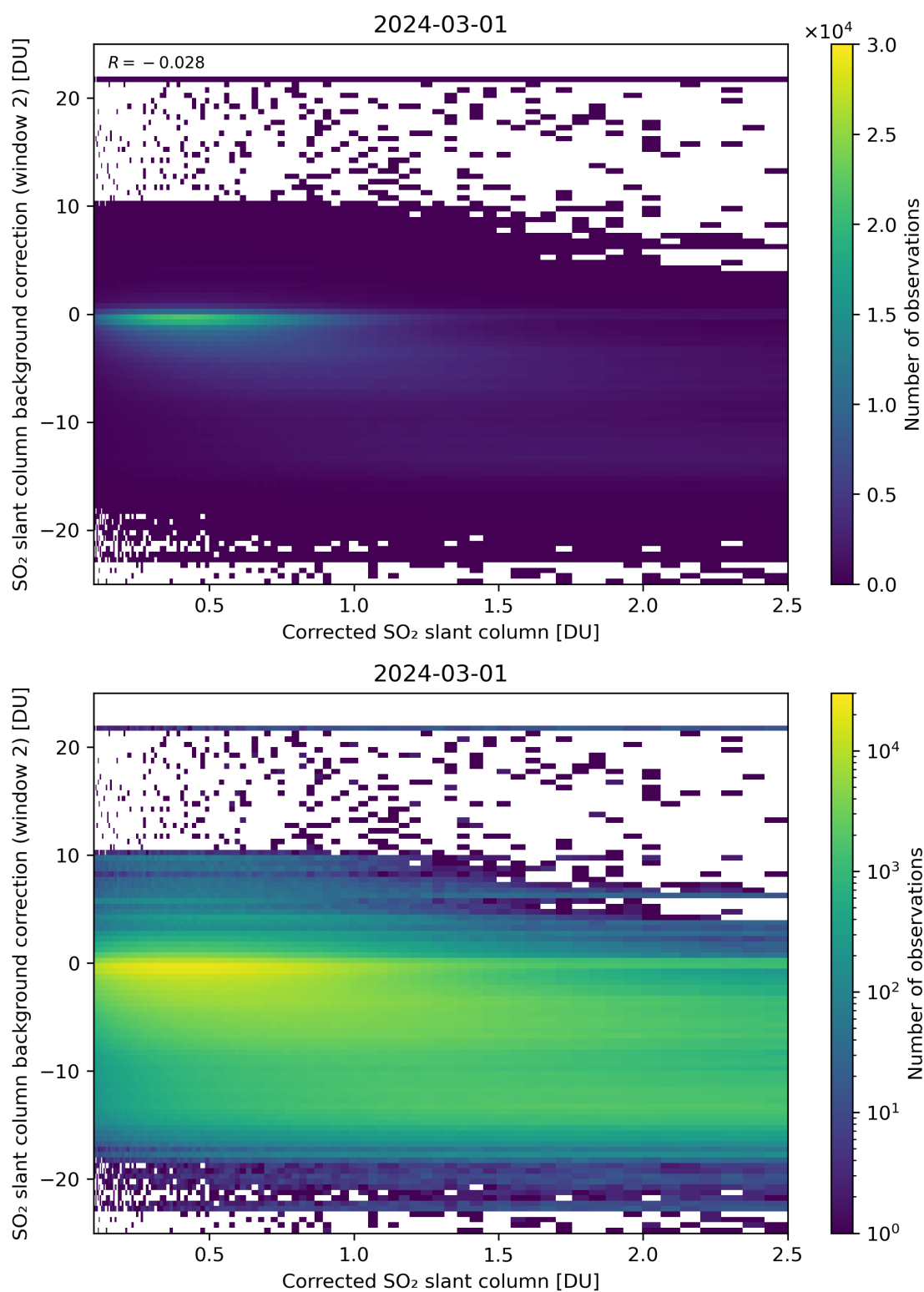
Figure 179: Scatter density plot of “Corrected SO 2 slant column” against “SO 2 slant column background correction (window 2)” for 2024-02-29 to 2024-03-02.
