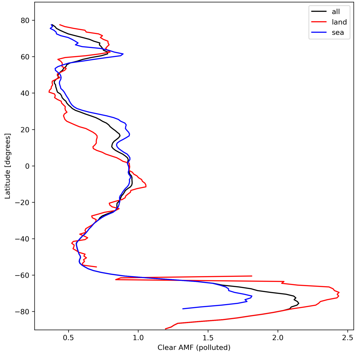
Figure 50: Zonal average of “Clear AMF (polluted)” for 2024-02-29 to 2024-03-02.
