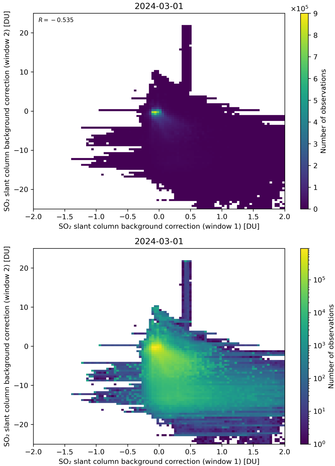
Figure 98: Scatter density plot of “SO 2 slant column background correction (window 1)” against “SO 2 slant column background correction (window 2)” for 2024-02-29 to 2024-03-02.
