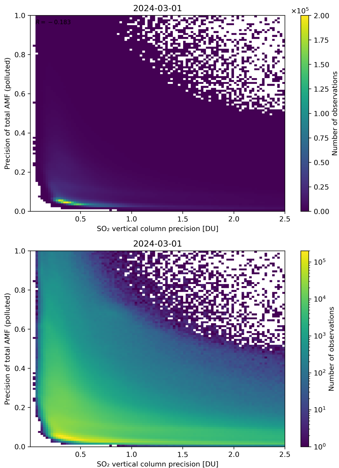
Figure 295: Scatter density plot of “SO 2 vertical column precision” against “Precision of total AMF (polluted)” for 2024-02-29 to 2024-03-02.
