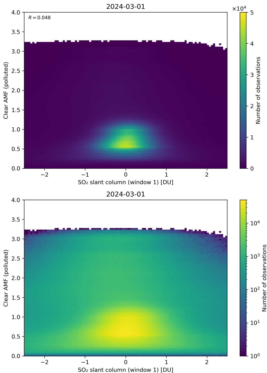
Figure 232: Scatter density plot of “SO 2 slant column (window 1)” against “Clear AMF (polluted)” for 2024-02-29 to 2024-03-02.
