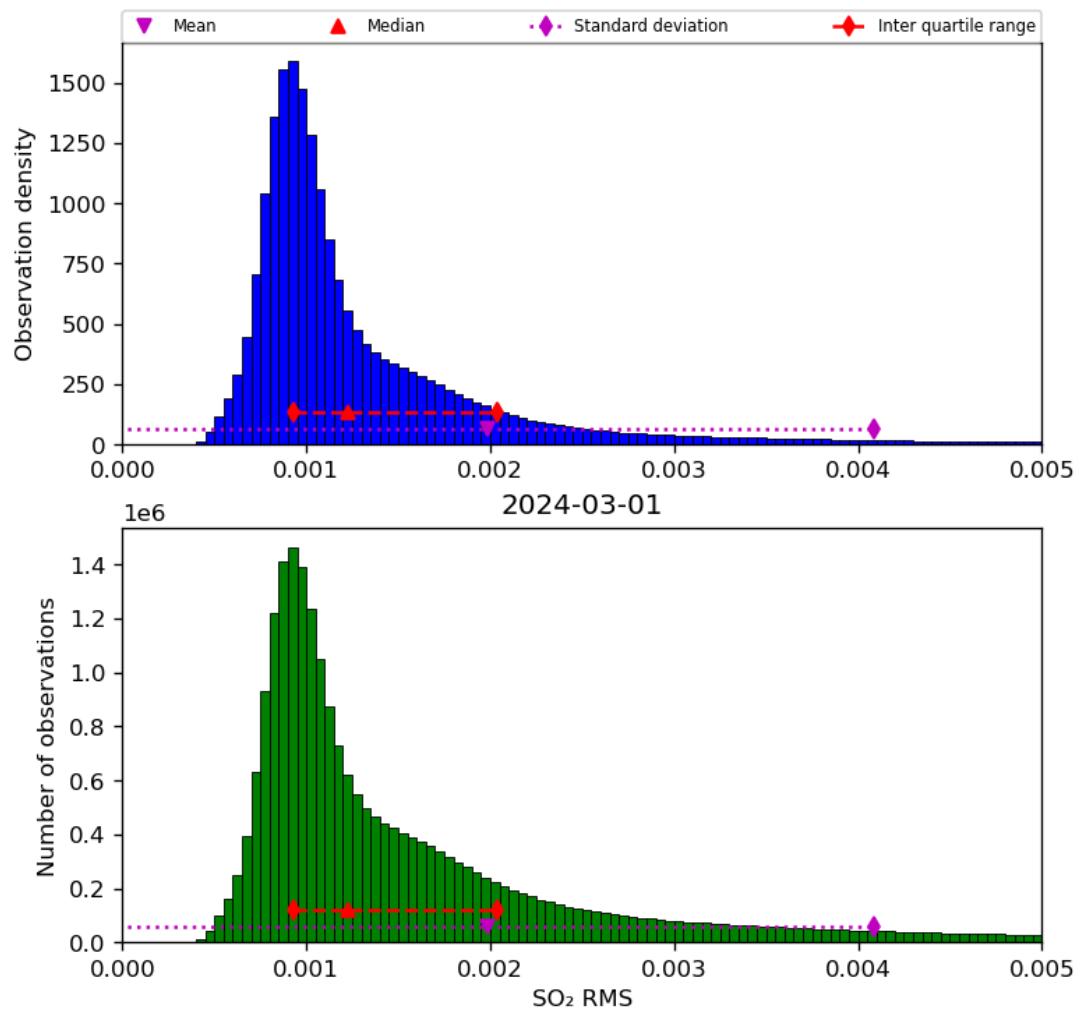
Figure 70: Histogram of “SO 2 RMS” for 2024-02-29 to 2024-03-02
