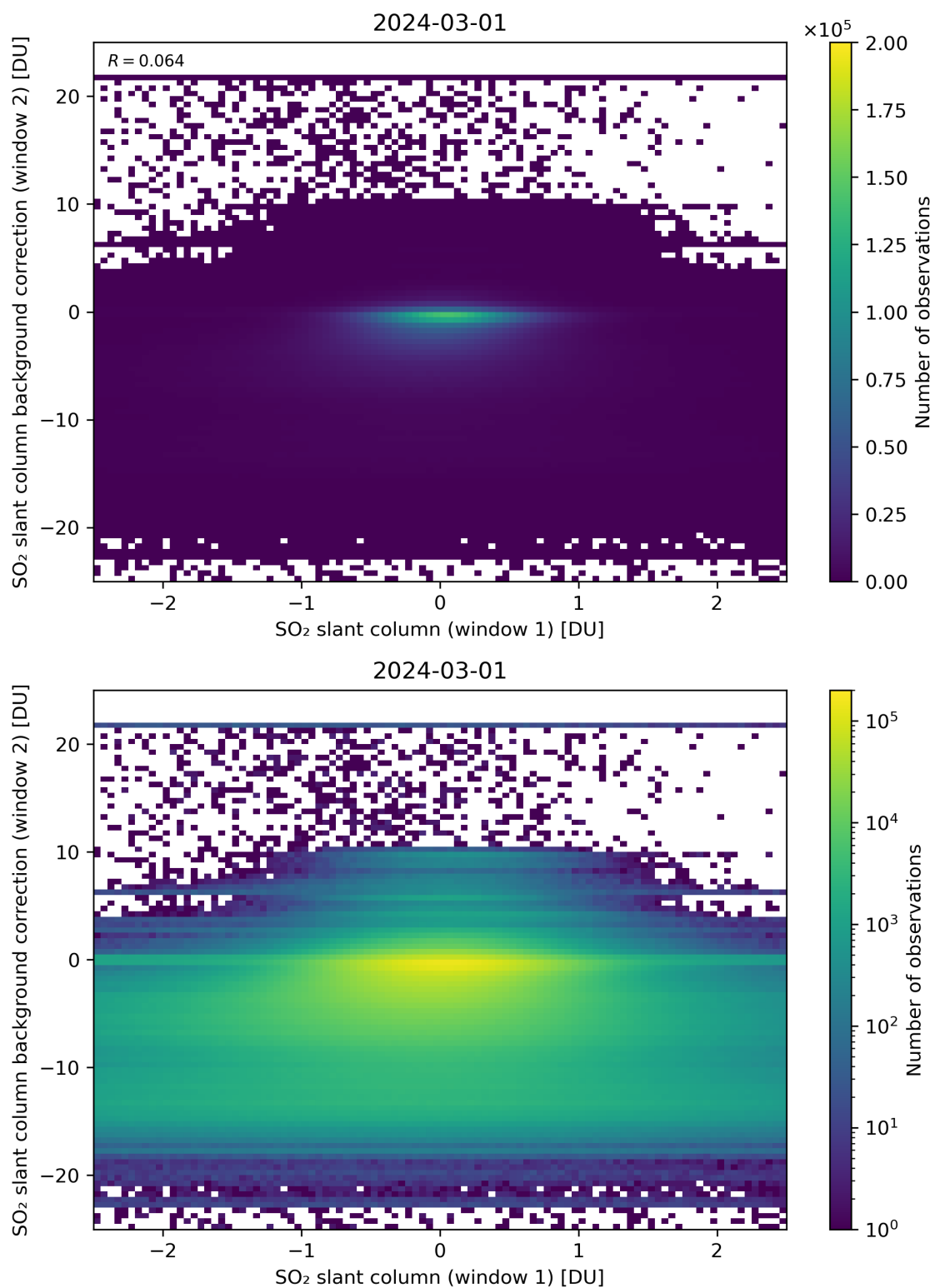
Figure 213: Scatter density plot of “SO 2 slant column (window 1)” against “SO 2 slant column background correction (window 2)” for 2024-02-29 to 2024-03-02.
