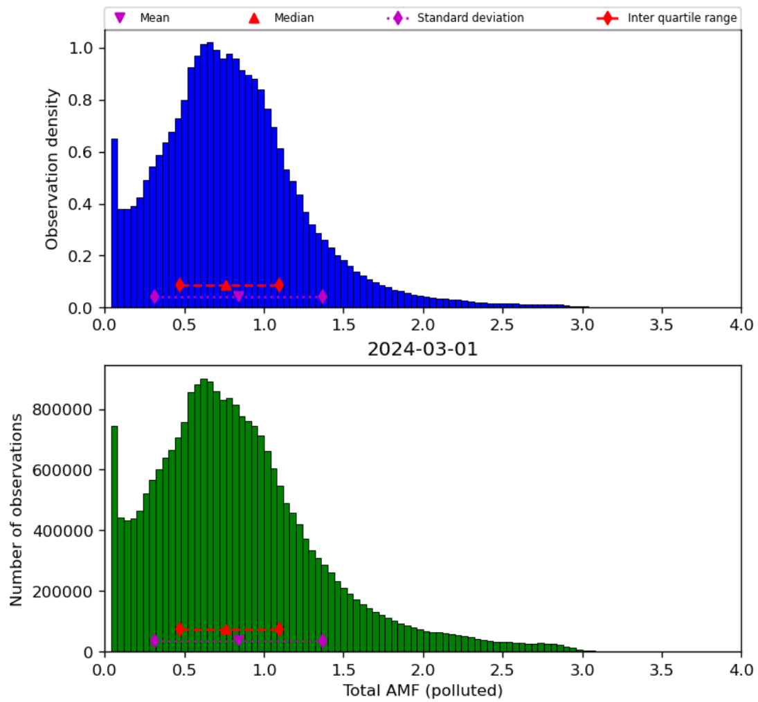
Figure 71: Histogram of “Total AMF (polluted)” for 2024-02-29 to 2024-03-02
