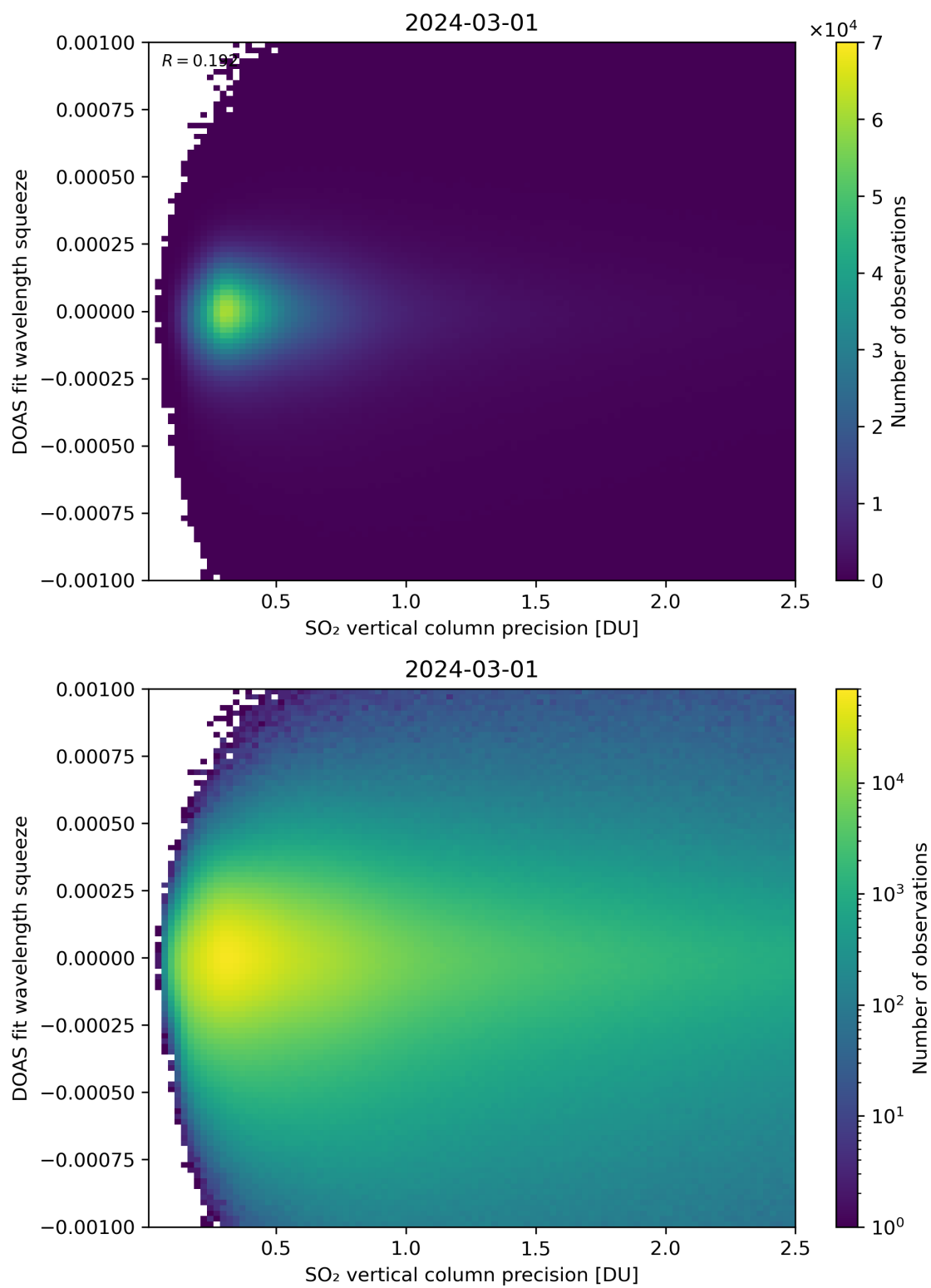
Figure 283: Scatter density plot of “SO 2 vertical column precision” against “DOAS fit wavelength squeeze” for 2024-02-29 to 2024-03-02.
