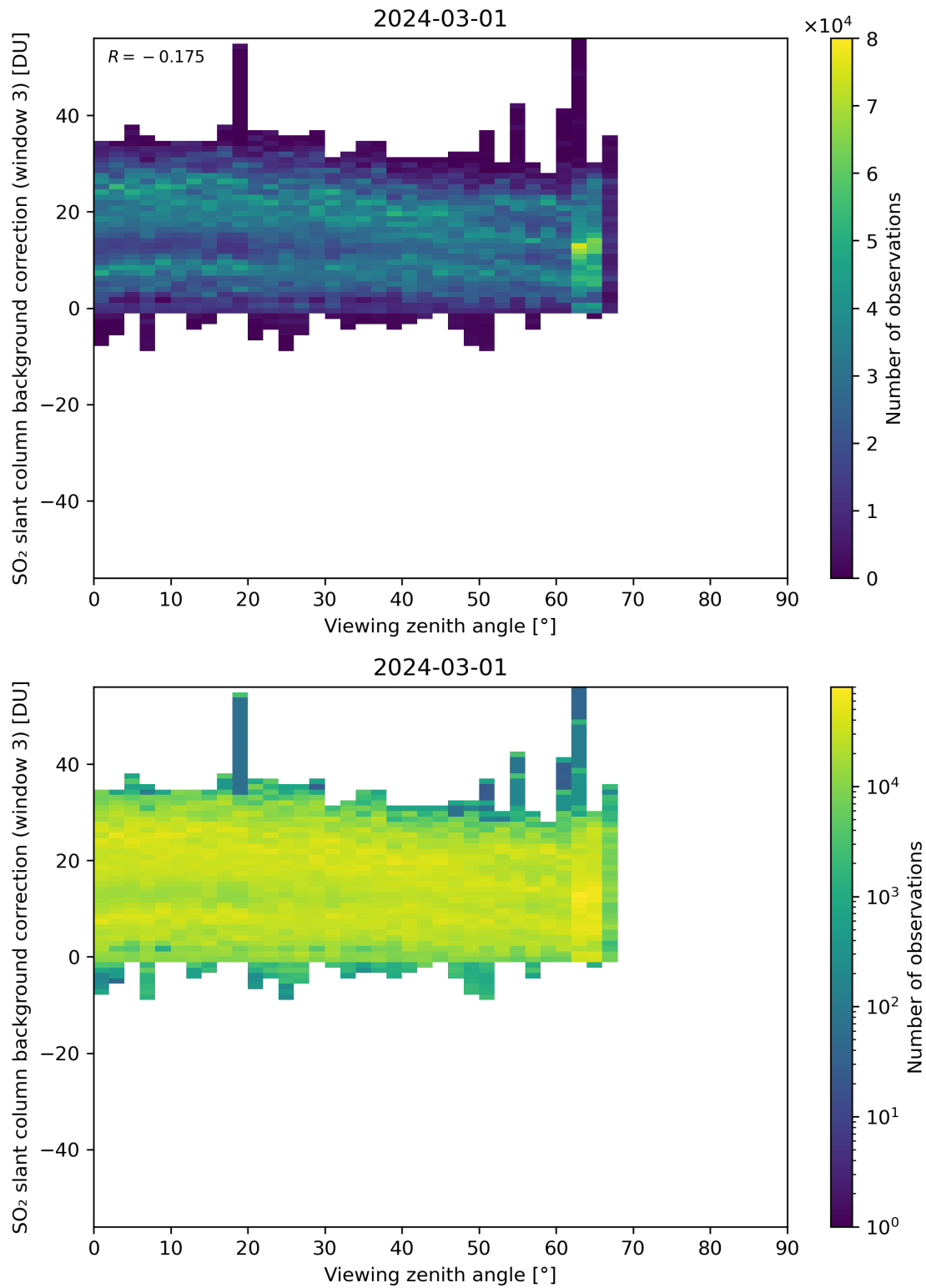
Figure 310: Scatter density plot of “Viewing zenith angle” against “SO 2 slant column background correction (window 3)” for 2024-02-29 to 2024-03-02.
