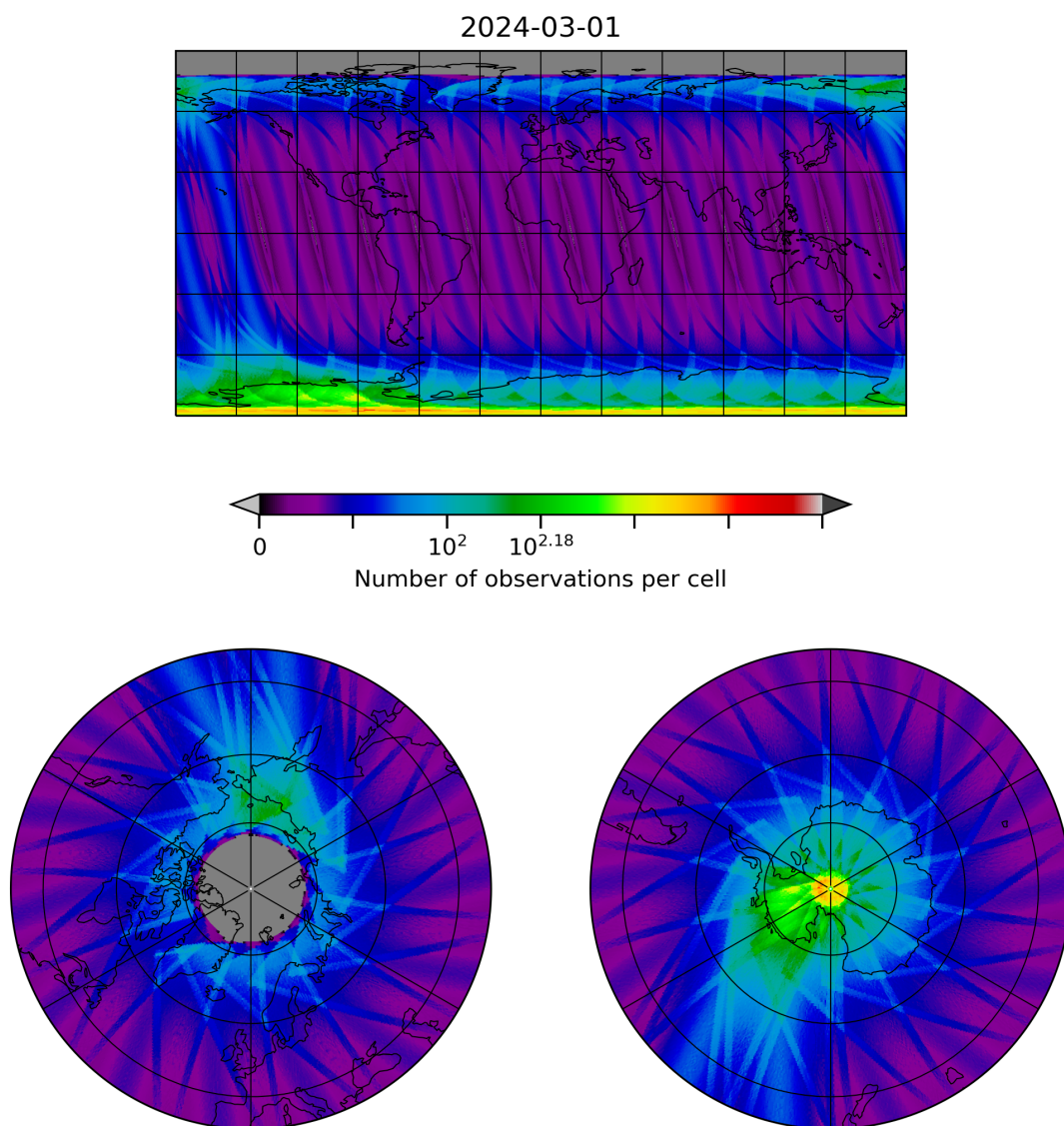
Figure 28: Map of the number of observations for 2024-02-29 to 2024-03-02
