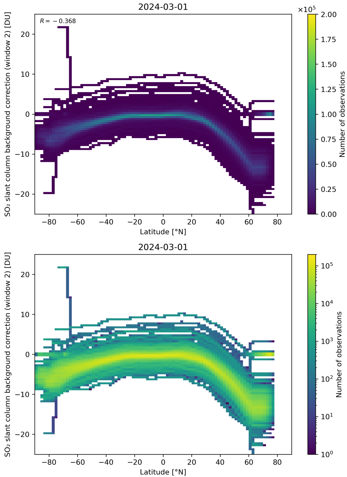
Figure 140: Scatter density plot of “Latitude” against “SO 2 slant column background correction (window 2)” for 2024-02-29 to 2024-03-02.
