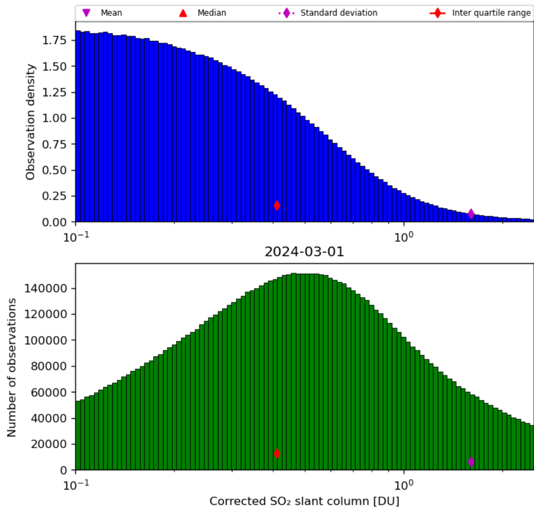
Figure 55: Histogram of “Corrected SO 2 slant column” for 2024-02-29 to 2024-03-02
