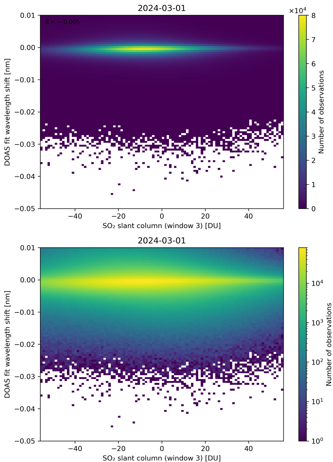
Figure 254: Scatter density plot of “SO 2 slant column (window 3)” against “DOAS fit wavelength shift” for 2024-02-29 to 2024-03-02.
