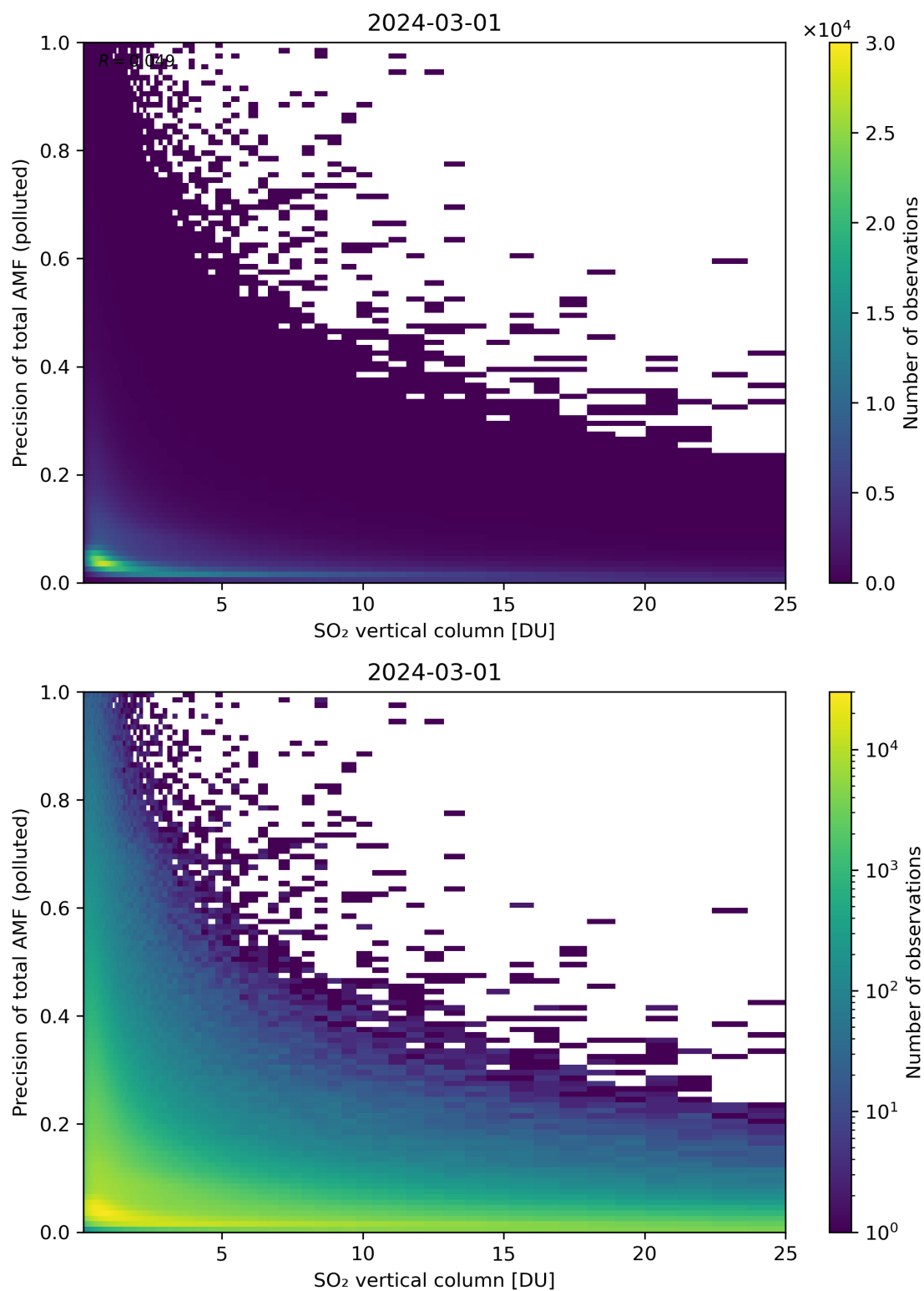
Figure 306: Scatter density plot of “SO 2 vertical column” against “Precision of total AMF (polluted)” for 2024-02-29 to 2024-03-02.
