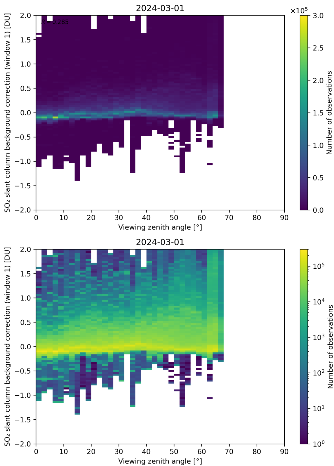
Figure 308: Scatter density plot of “Viewing zenith angle” against “SO 2 slant column background correction (window 1)” for 2024-02-29 to 2024-03-02.
