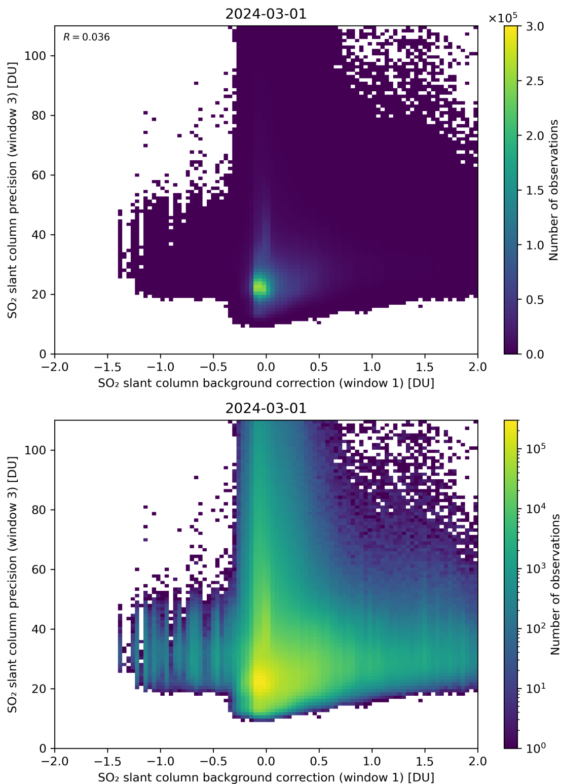
Figure 108: Scatter density plot of “SO 2 slant column background correction (window 1)” against “SO 2 slant column precision (window 3)” for 2024-02-29 to 2024-03-02.
