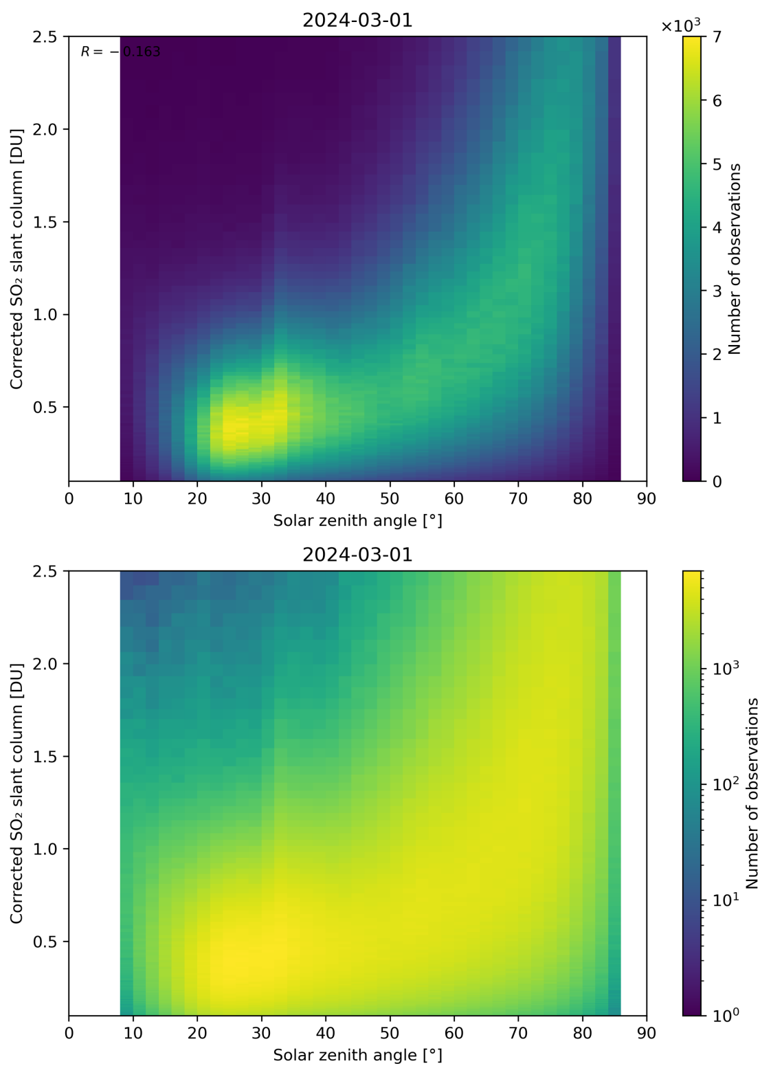
Figure 166: Scatter density plot of “Solar zenith angle” against “Corrected SO 2 slant column” for 2024-02-29 to 2024-03-02.
