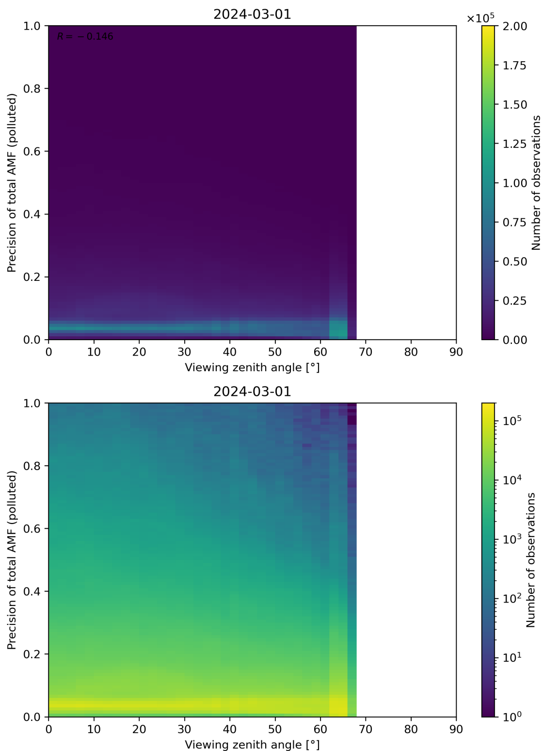
Figure 326: Scatter density plot of “Viewing zenith angle” against “Precision of total AMF (polluted)” for 2024-02-29 to 2024-03-02.
