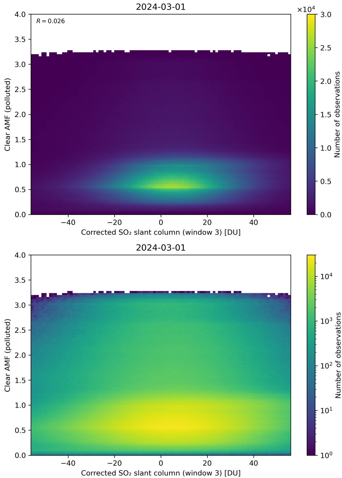
Figure 209: Scatter density plot of “Corrected SO 2 slant column (window 3)” against “Clear AMF (polluted)” for 2024-02-29 to 2024-03-02.
