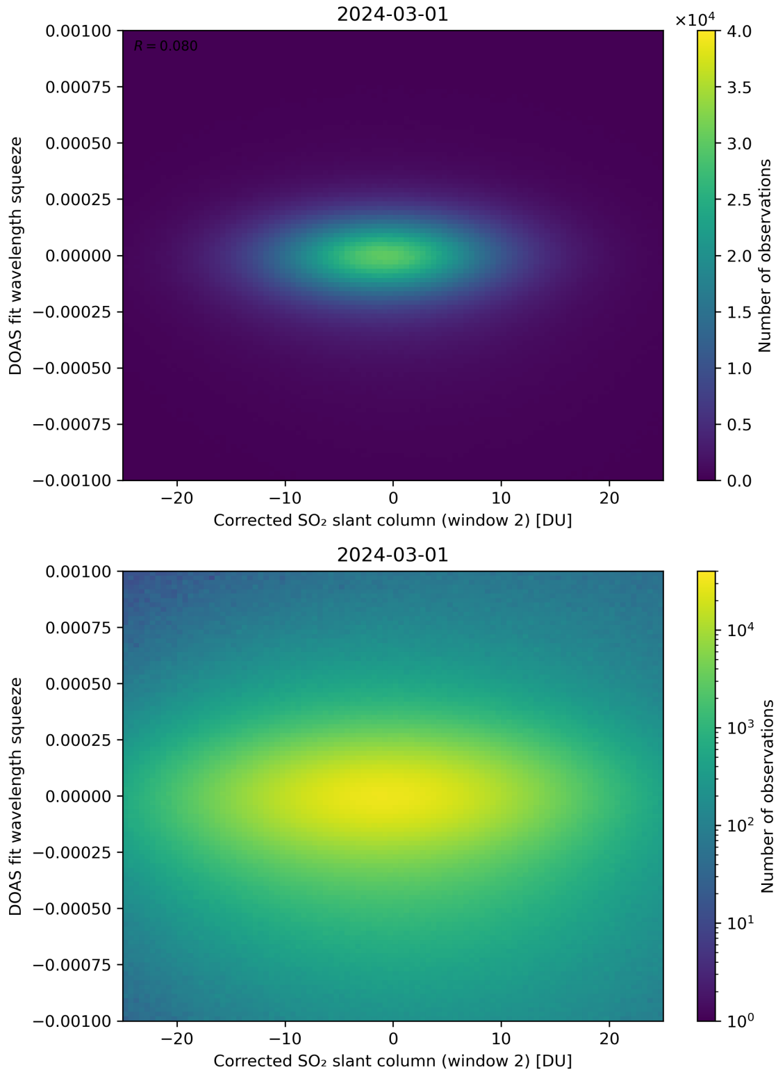
Figure 197: Scatter density plot of “Corrected SO 2 slant column (window 2)” against “DOAS fit wavelength squeeze” for 2024-02-29 to 2024-03-02.
