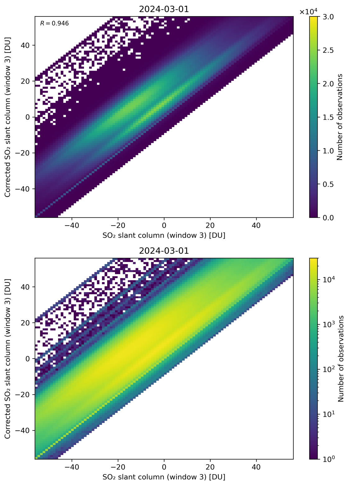
Figure 266: Scatter density plot of “SO 2 slant column (window 3)” against “Corrected SO 2 slant column (window 3)” for 2024-02-29 to 2024-03-02.
