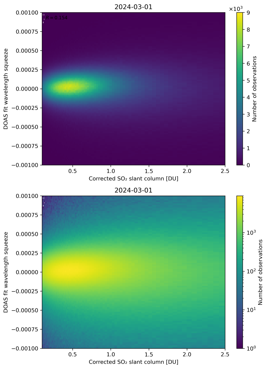
Figure 182: Scatter density plot of “Corrected SO 2 slant column” against “DOAS fit wavelength squeeze” for 2024-02-29 to 2024-03-02.
