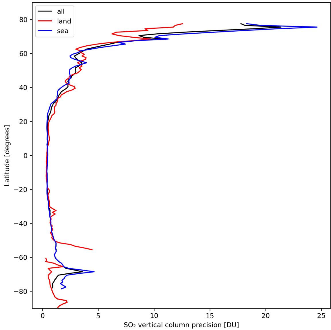
Figure 31: Zonal average of “SO 2 vertical column precision” for 2024-02-29 to 2024-03-02.
