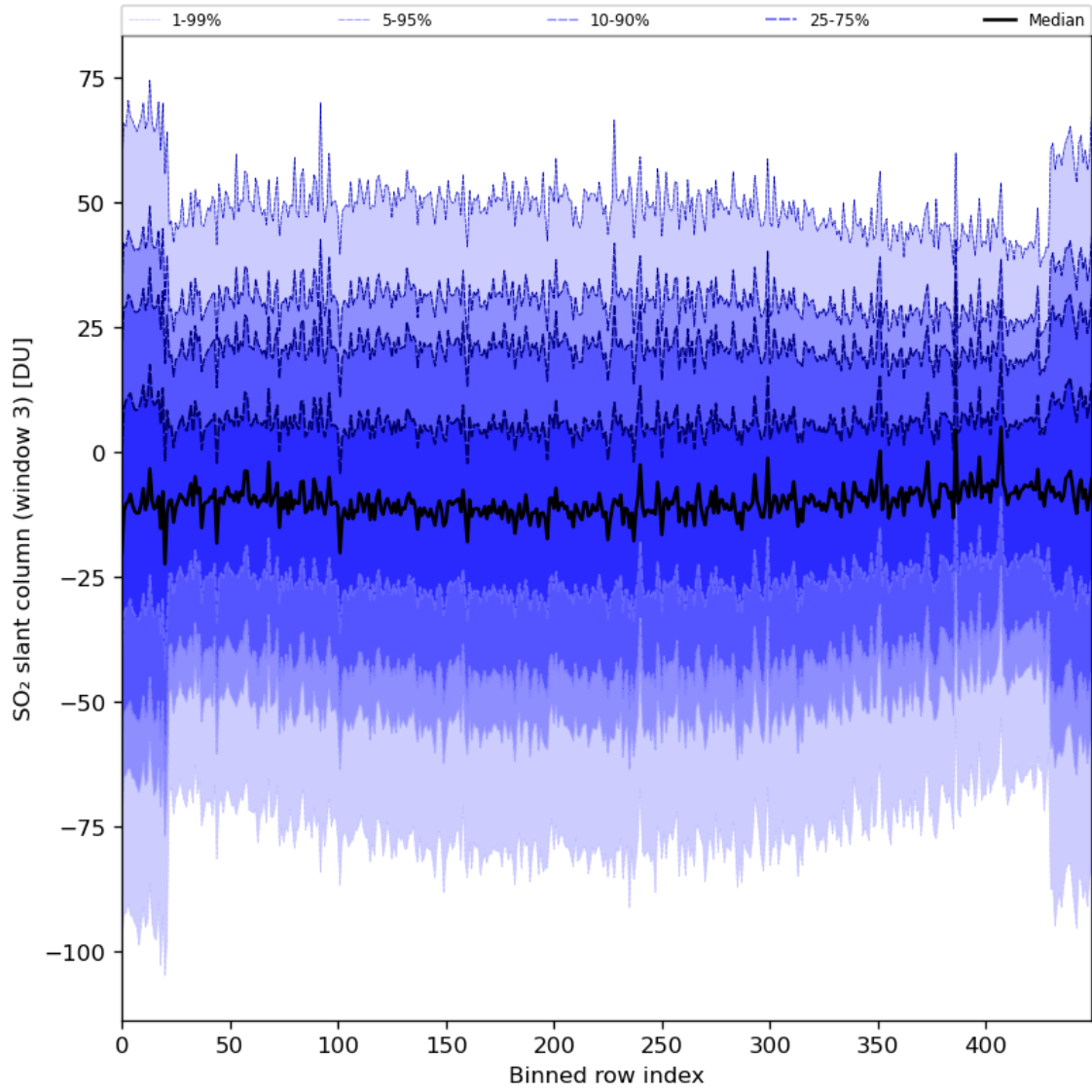
Figure 87: Along track statistics of “SO 2 slant column (window 3)” for 2024-02-29 to 2024-03-02
