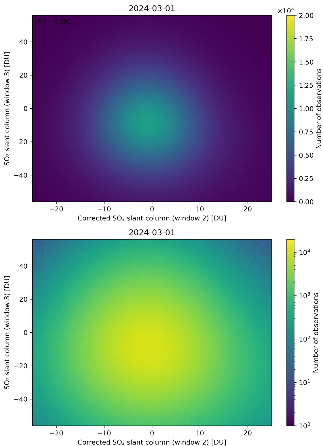
Figure 201: Scatter density plot of “Corrected SO 2 slant column (window 2)” against “SO 2 slant column (window 3)” for 2024-02-29 to 2024-03-02.
