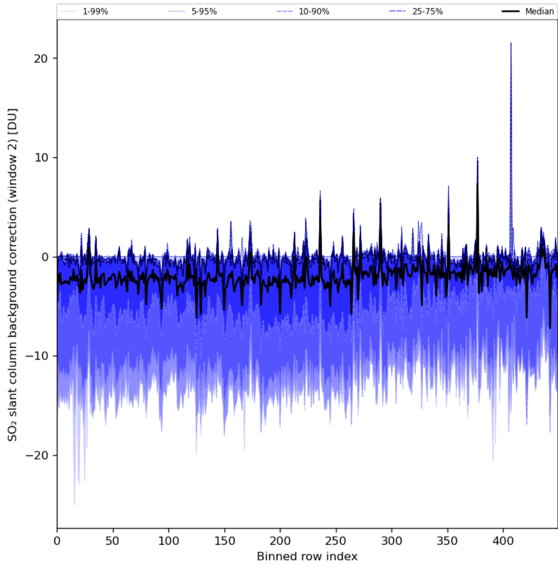
Figure 86: Along track statistics of “SO 2 slant column background correction (window 2)” for 2024-02-29 to 2024-03-02
