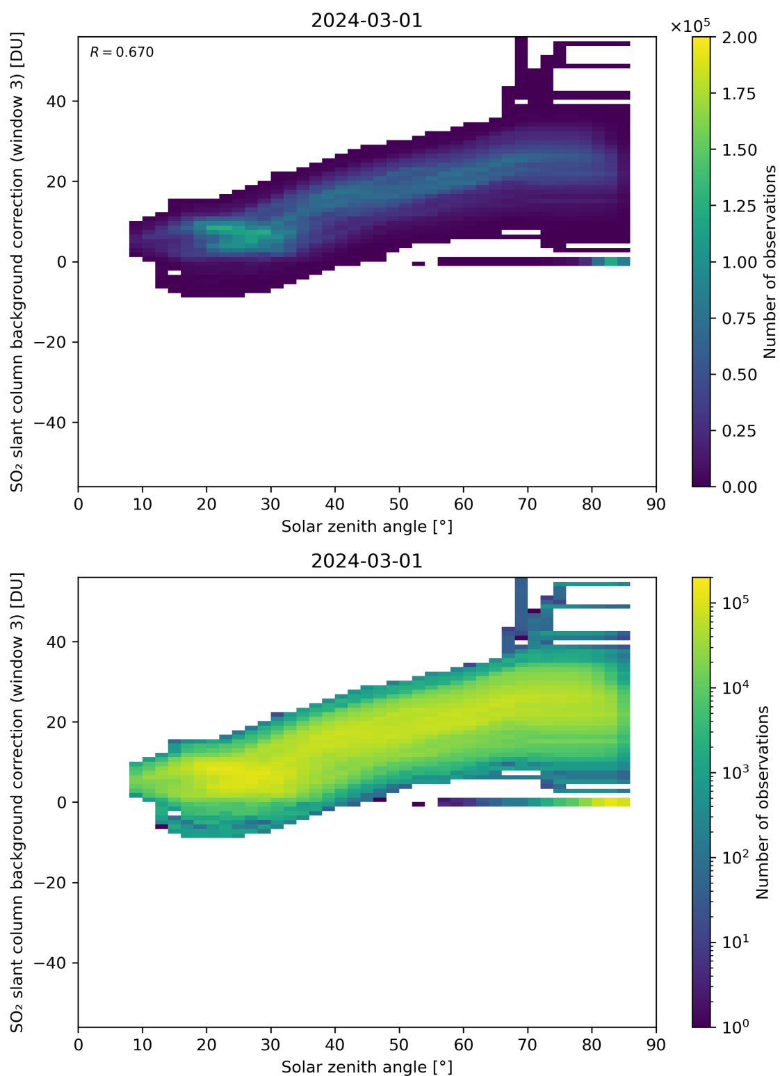
Figure 160: Scatter density plot of “Solar zenith angle” against “SO 2 slant column background correction (window 3)” for 2024-02-29 to 2024-03-02.
