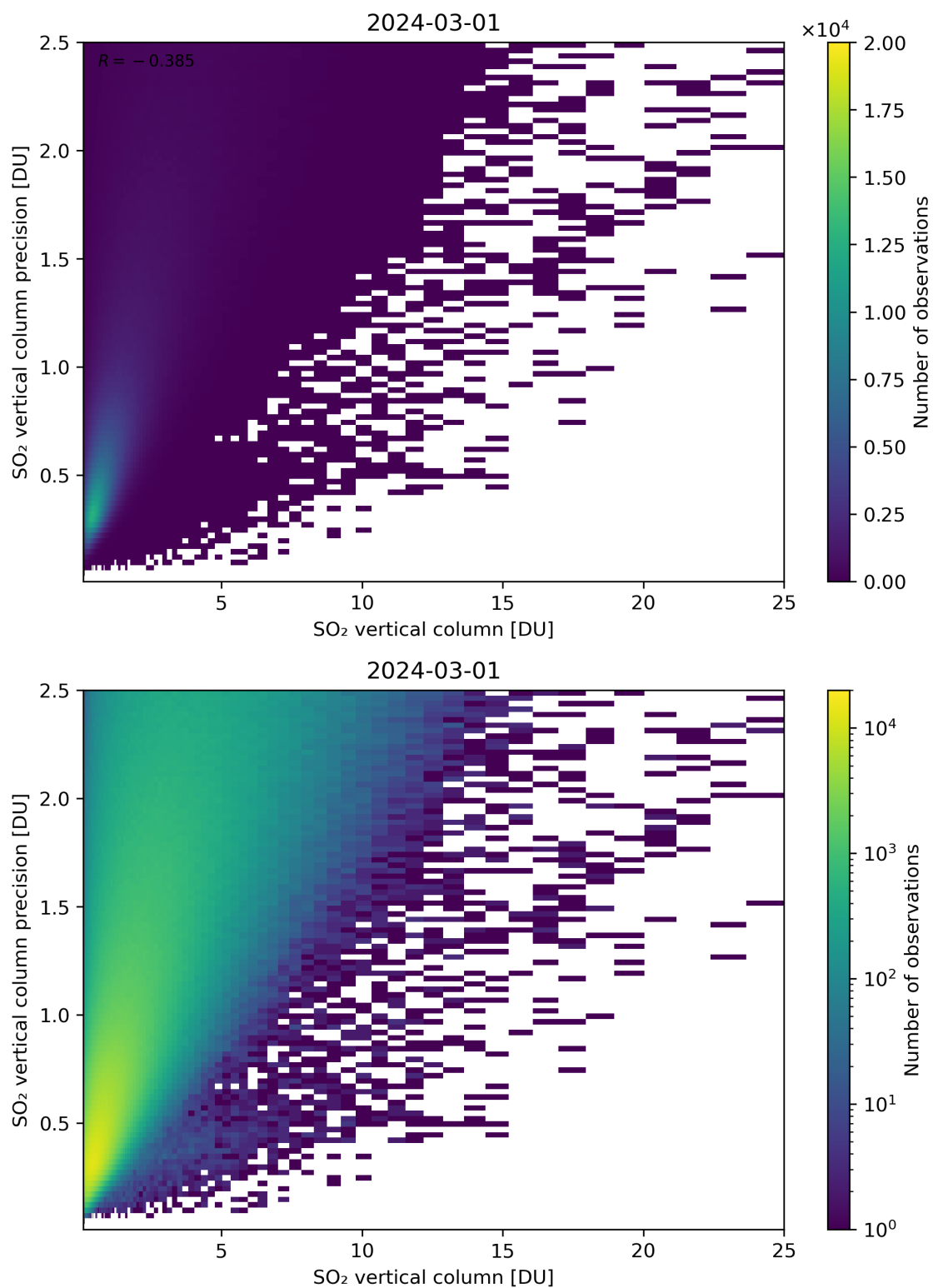
Figure 307: Scatter density plot of “SO 2 vertical column” against “SO 2 vertical column precision” for 2024-02-29 to 2024-03-02.
