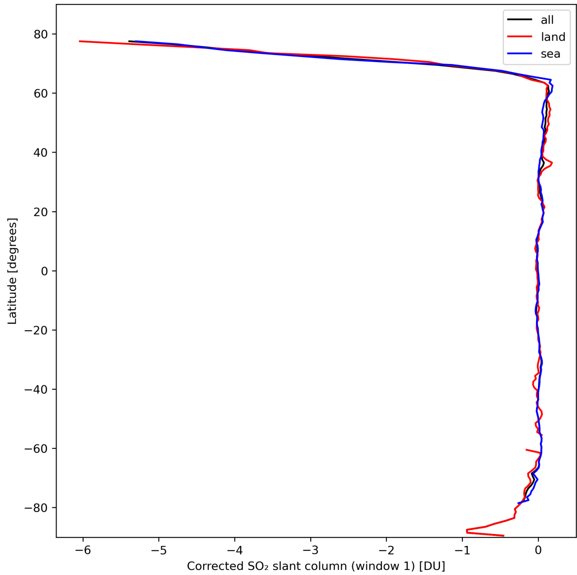
Figure 35: Zonal average of “Corrected SO 2 slant column (window 1)” for 2024-02-29 to 2024-03-02.
