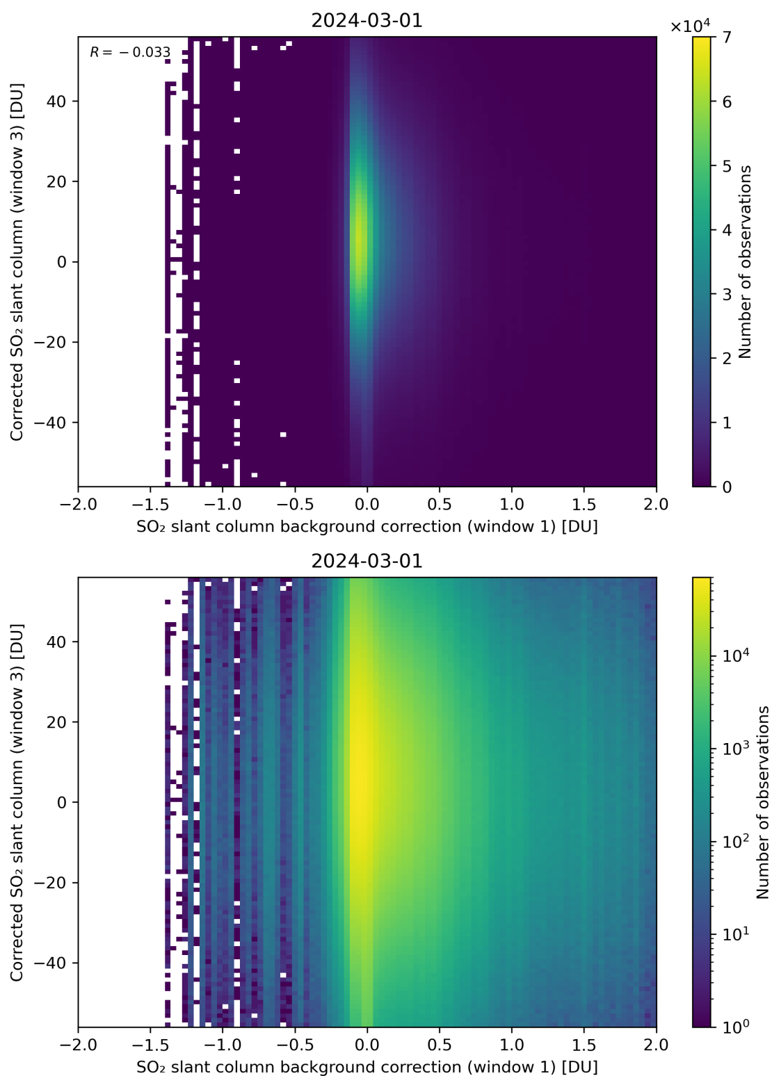
Figure 105: Scatter density plot of “SO 2 slant column background correction (window 1)” against “Corrected SO 2 slant column (window 3)” for 2024-02-29 to 2024-03-02.
