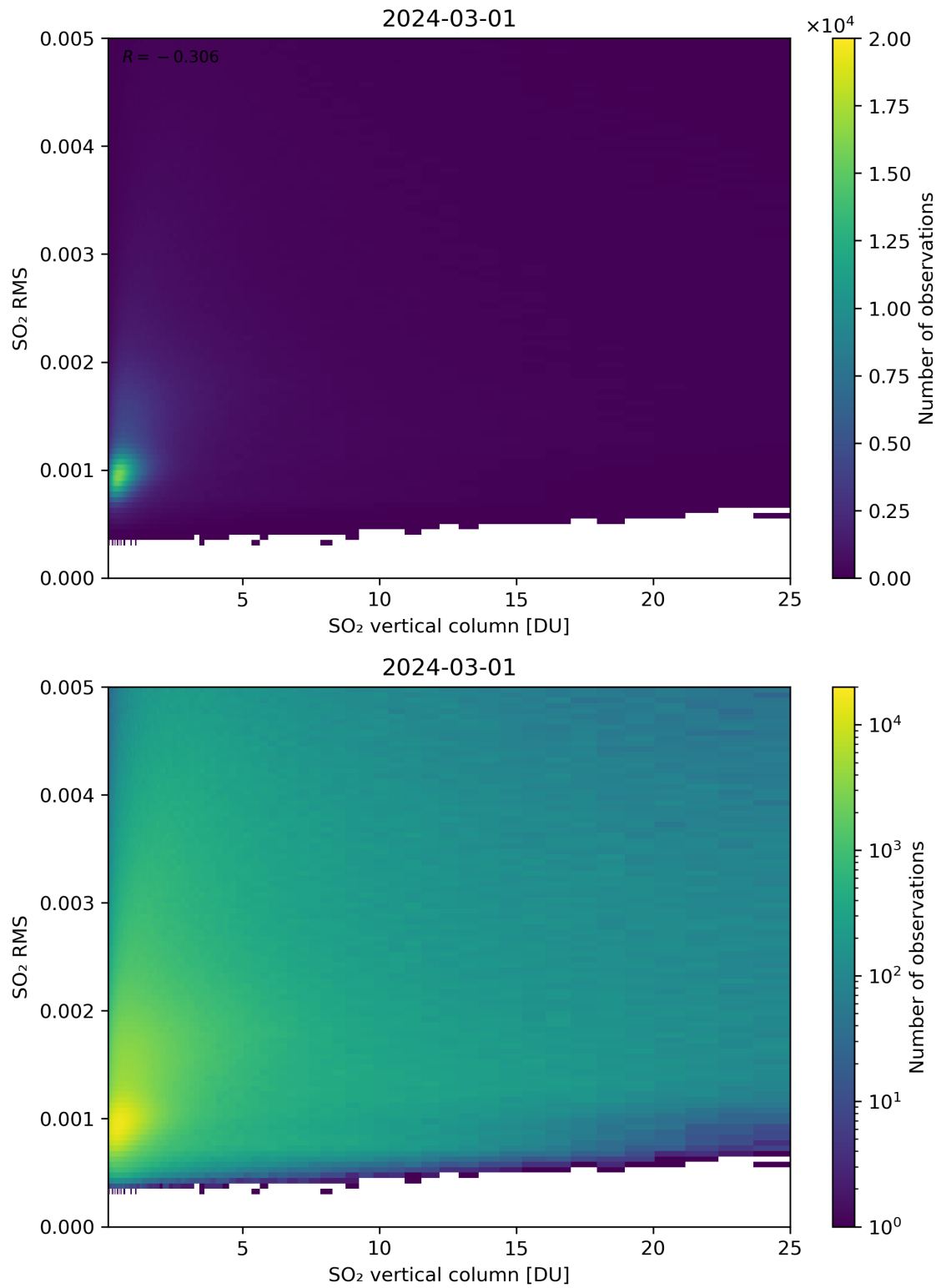
Figure 278: Scatter density plot of “SO 2 vertical column” against “SO 2 RMS” for 2024-02-29 to 2024-03-02.
