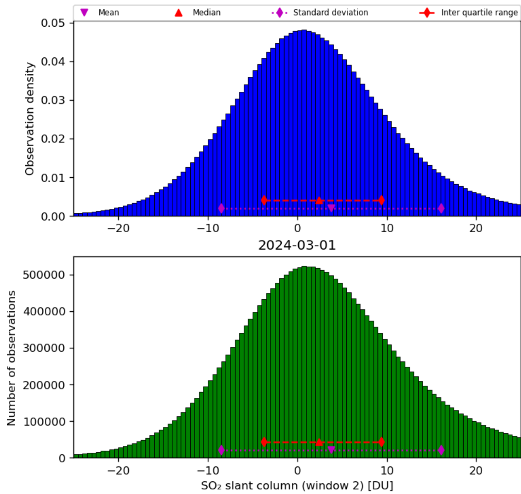
Figure 60: Histogram of “SO 2 slant column (window 2)” for 2024-02-29 to 2024-03-02
