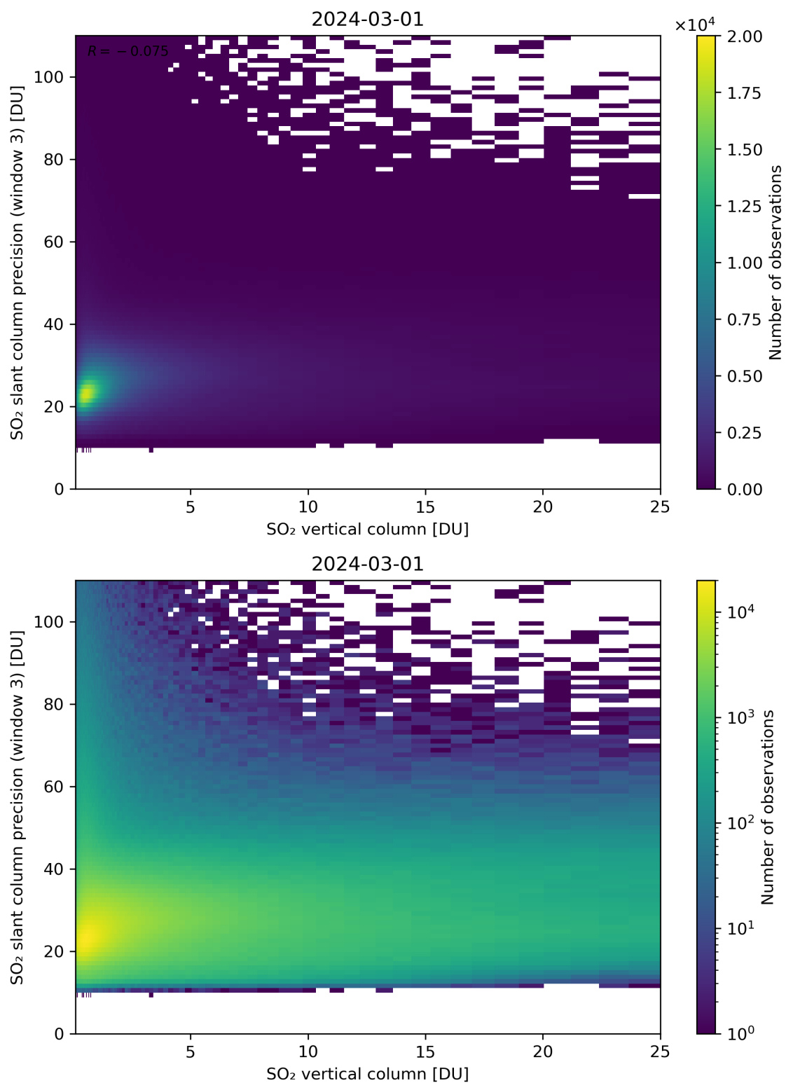
Figure 304: Scatter density plot of “SO 2 vertical column” against “SO 2 slant column precision (window 3)” for 2024-02-29 to 2024-03-02.
