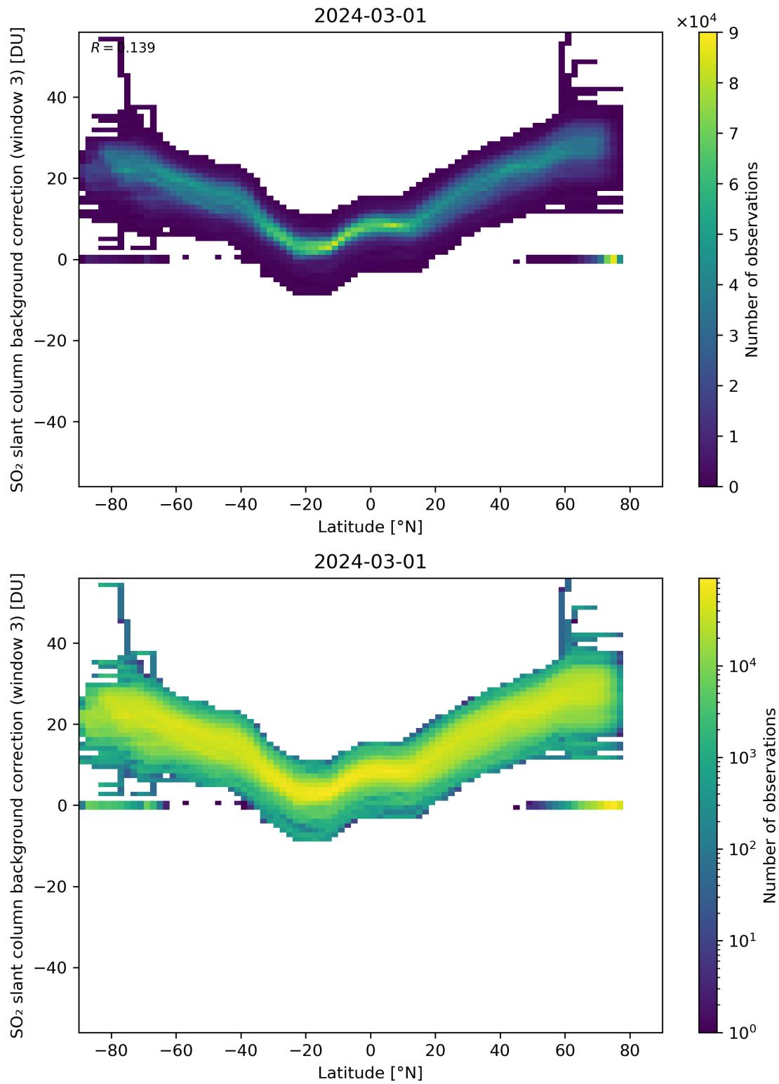
Figure 141: Scatter density plot of “Latitude” against “SO 2 slant column background correction (window 3)” for 2024-02-29 to 2024-03-02.
