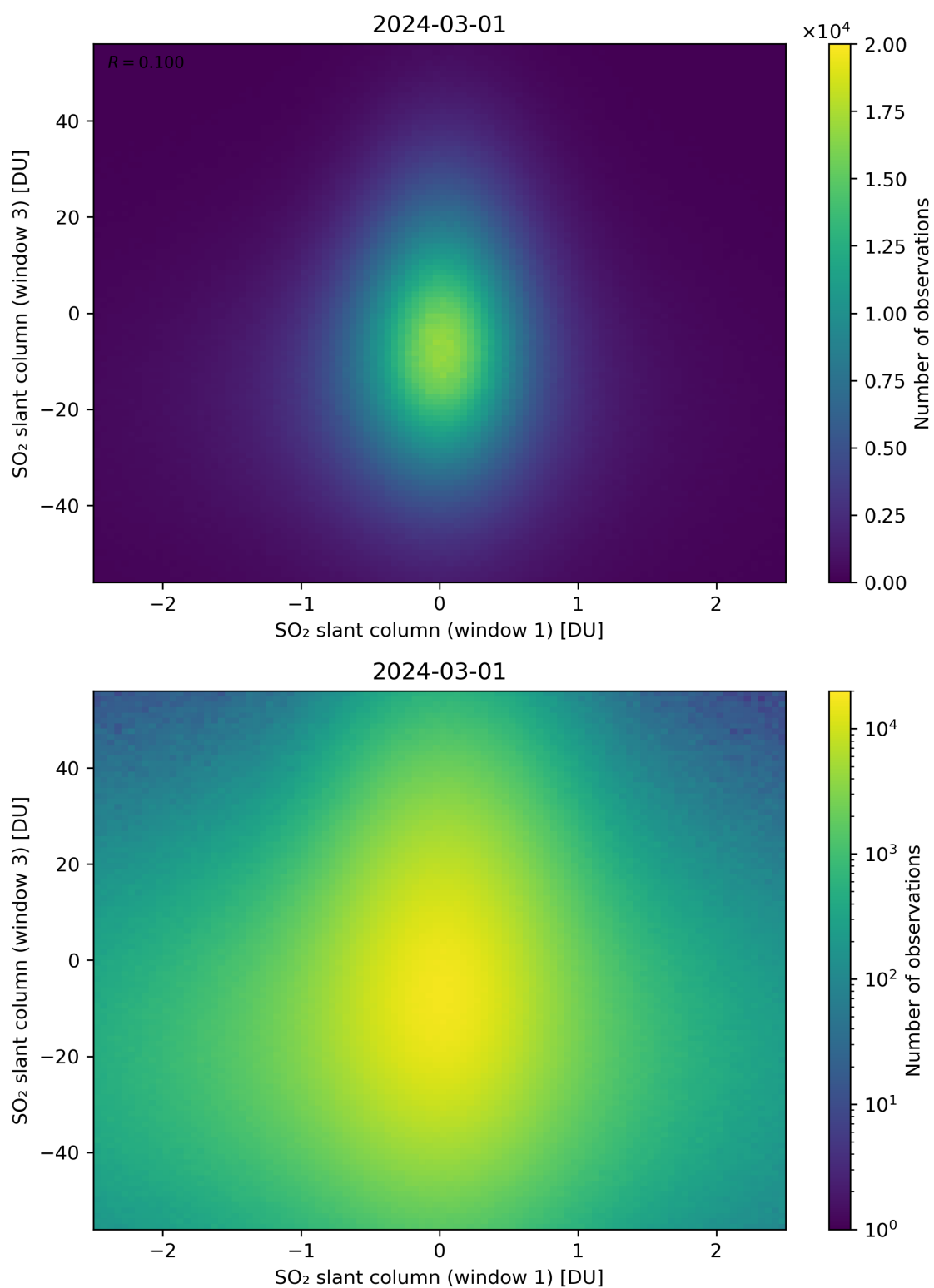
Figure 237: Scatter density plot of “SO 2 slant column (window 1)” against “SO 2 slant column (window 3)” for 2024-02-29 to 2024-03-02.
