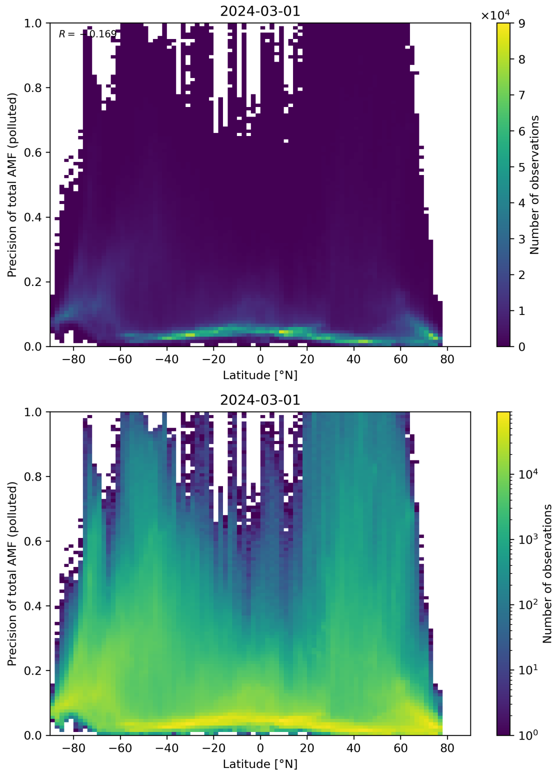
Figure 155: Scatter density plot of “Latitude” against “Precision of total AMF (polluted)” for 2024-02-29 to 2024-03-02.
