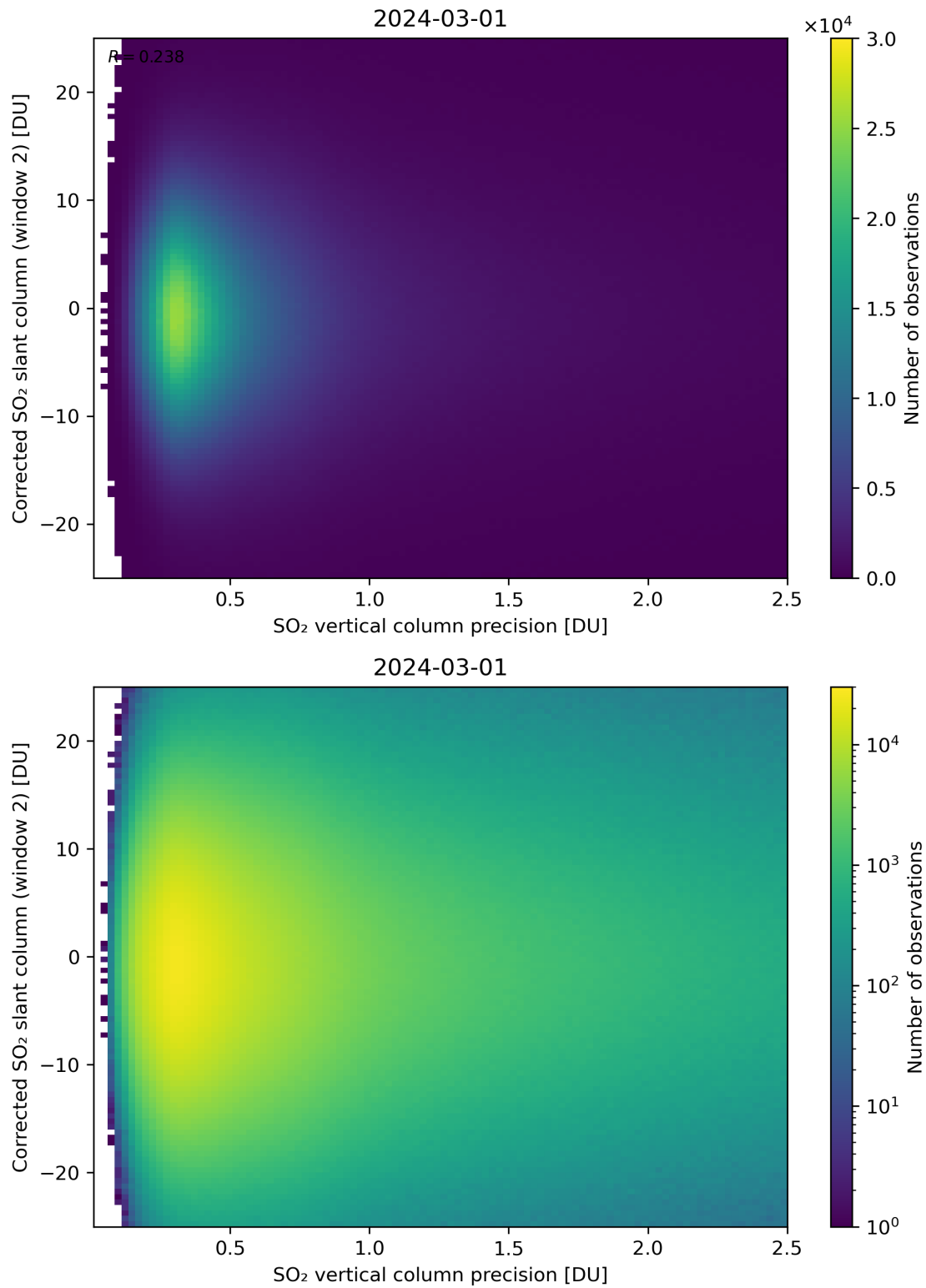
Figure 287: Scatter density plot of “SO 2 vertical column precision” against “Corrected SO 2 slant column (window 2)” for 2024-02-29 to 2024-03-02.
