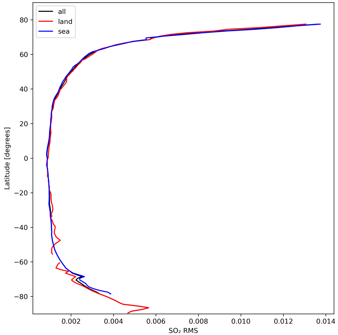
Figure 47: Zonal average of “SO 2 RMS” for 2024-02-29 to 2024-03-02.
