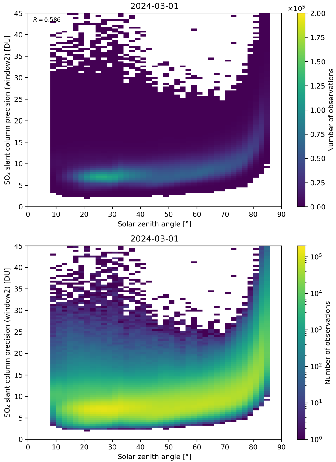
Figure 171: Scatter density plot of “Solar zenith angle” against “SO 2 slant column precision (window2)” for 2024-02-29 to 2024-03-02.
