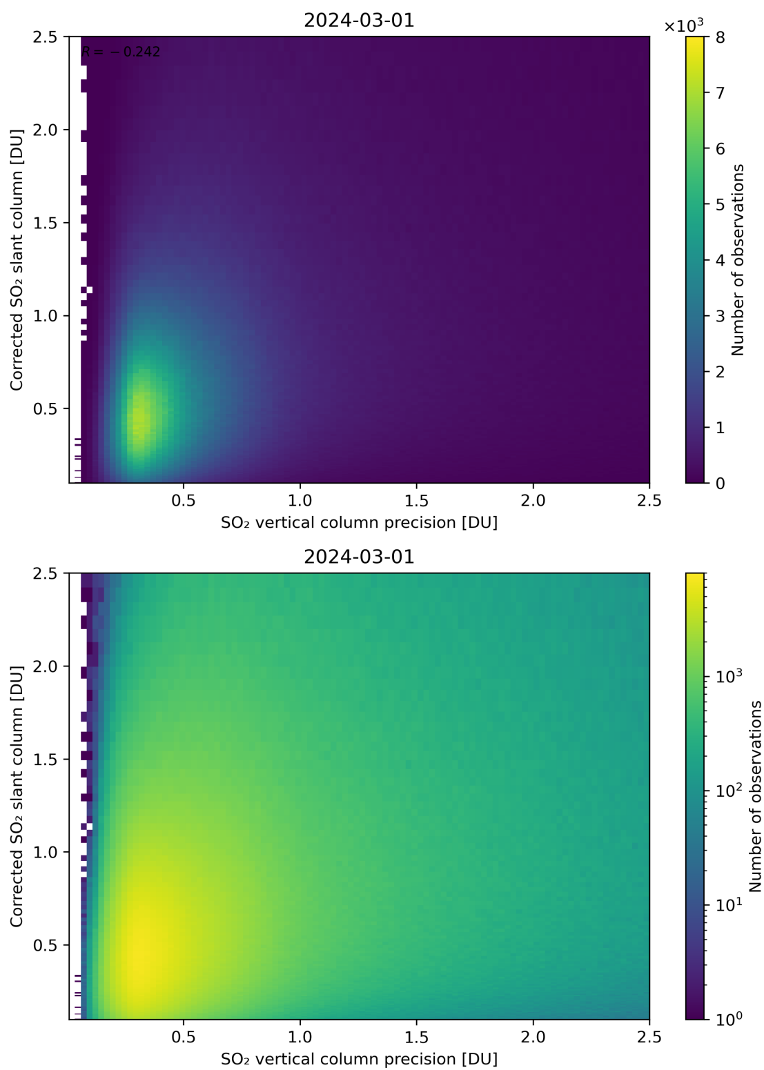
Figure 286: Scatter density plot of “SO 2 vertical column precision” against “Corrected SO 2 slant column” for 2024-02-29 to 2024-03-02.
