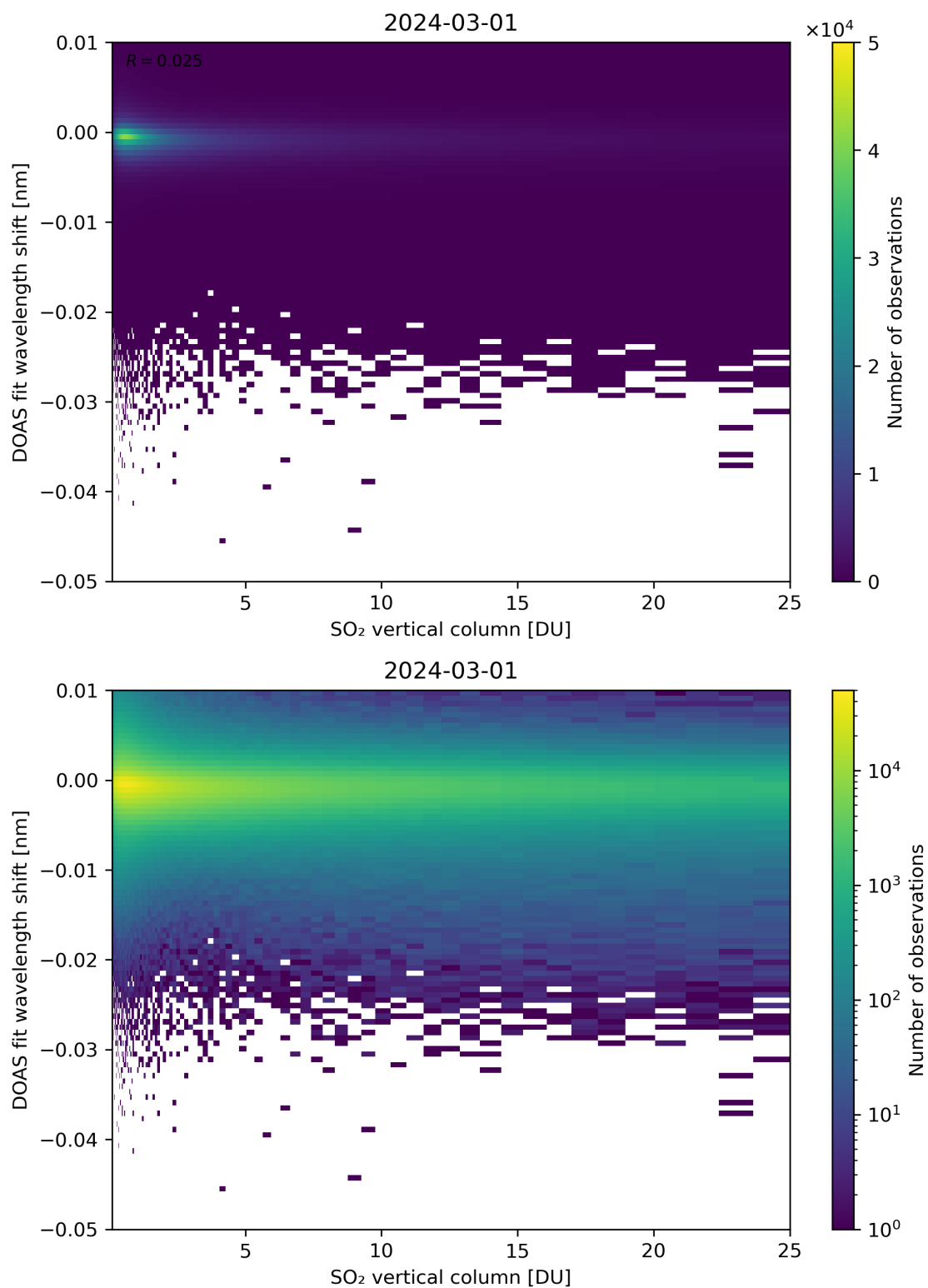
Figure 276: Scatter density plot of “SO 2 vertical column” against “DOAS fit wavelength shift” for 2024-02-29 to 2024-03-02.
