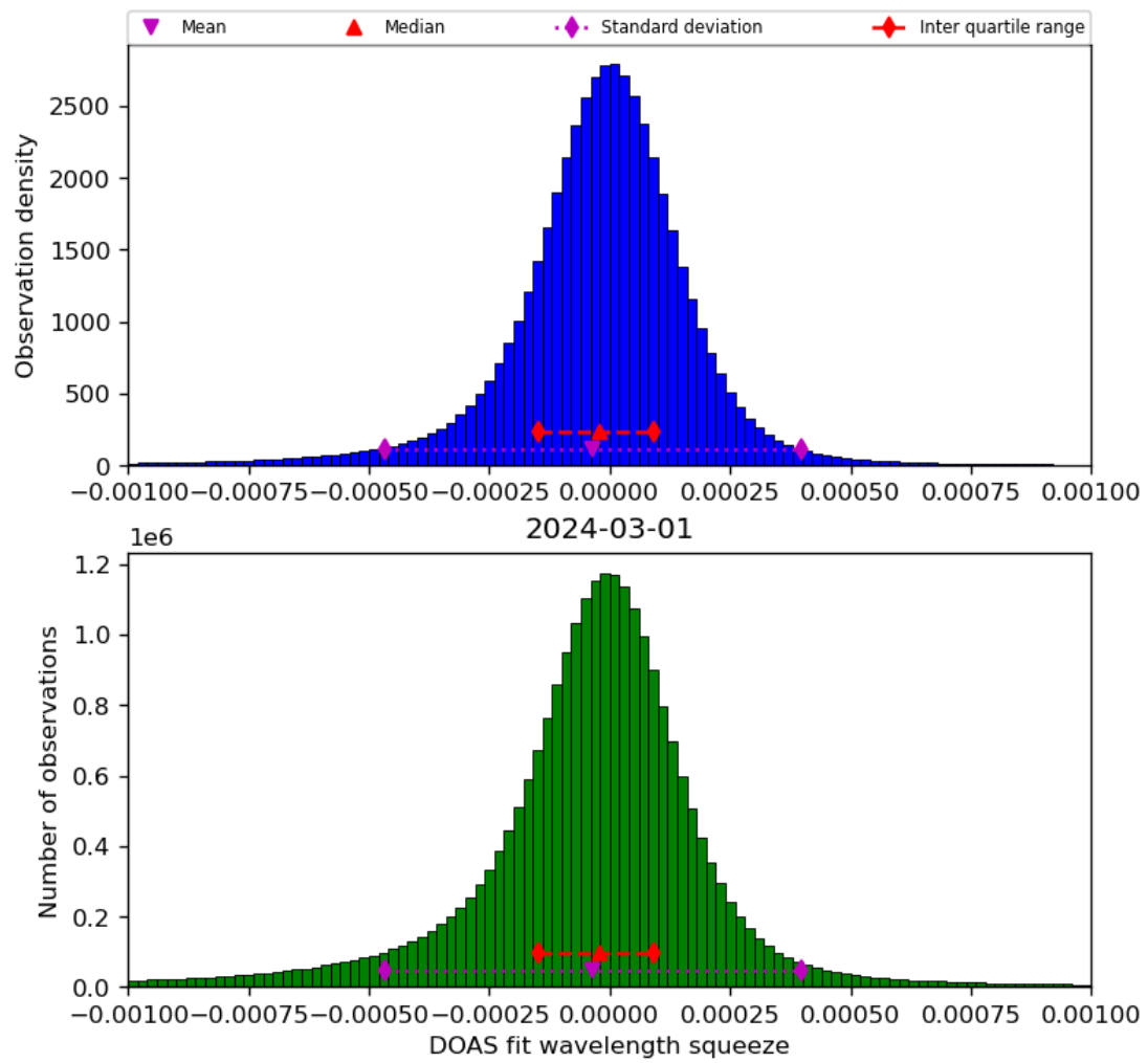
Figure 69: Histogram of “DOAS fit wavelength squeeze” for 2024-02-29 to 2024-03-02
