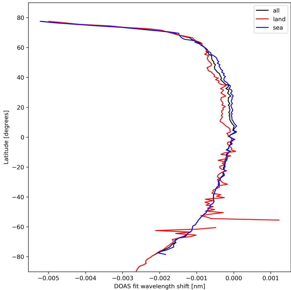
Figure 45: Zonal average of “DOAS fit wavelength shift” for 2024-02-29 to 2024-03-02.
