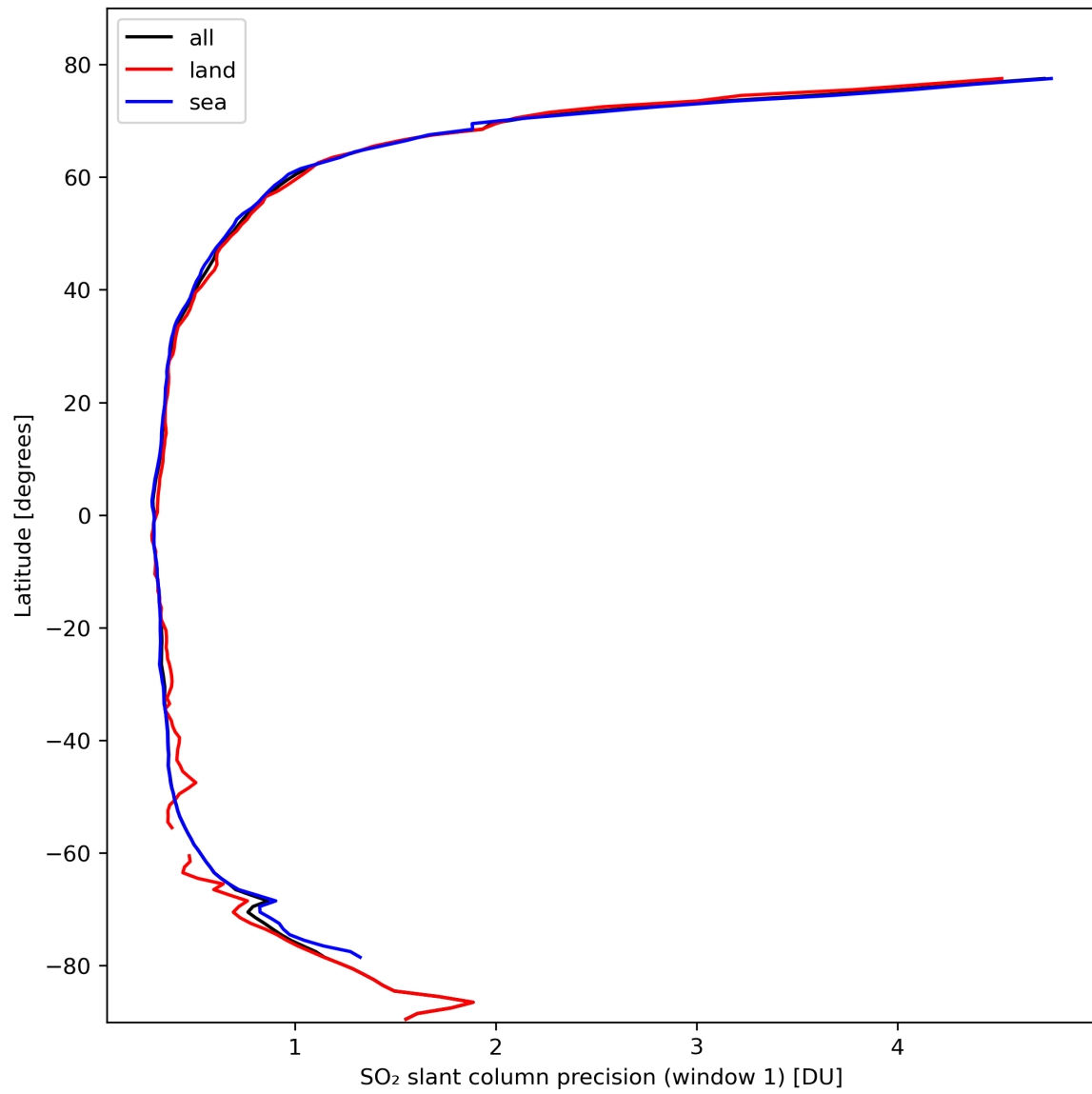
Figure 34: Zonal average of “SO 2 slant column precision (window 1)” for 2024-02-29 to 2024-03-02.
