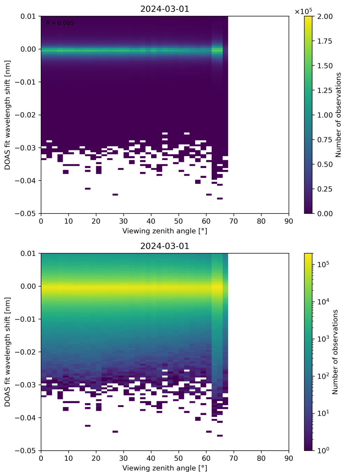
Figure 311: Scatter density plot of “Viewing zenith angle” against “DOAS fit wavelength shift” for 2024-02-29 to 2024-03-02.
