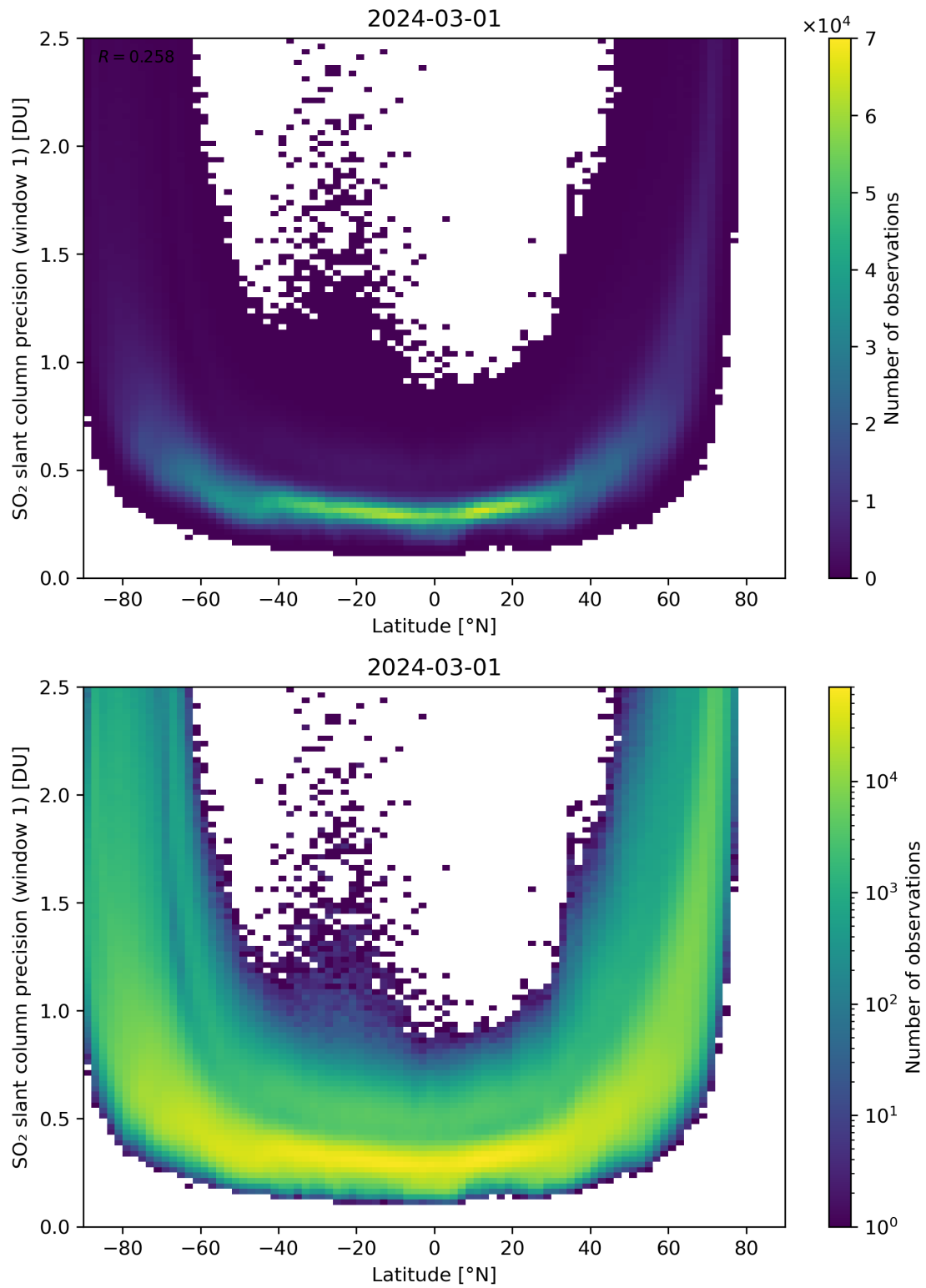
Figure 150: Scatter density plot of “Latitude” against “SO 2 slant column precision (window 1)” for 2024-02-29 to 2024-03-02.
