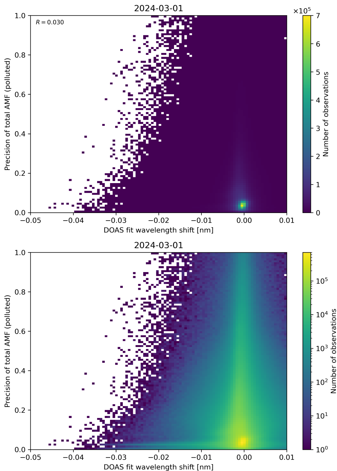
Figure 131: Scatter density plot of “DOAS fit wavelength shift” against “Precision of total AMF (polluted)” for 2024-02-29 to 2024-03-02.
