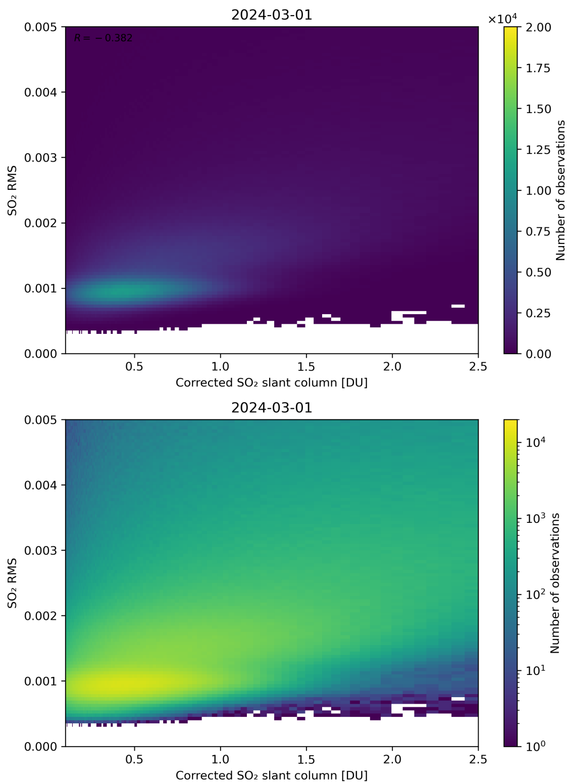
Figure 183: Scatter density plot of “Corrected SO 2 slant column” against “SO 2 RMS” for 2024-02-29 to 2024-03-02.
