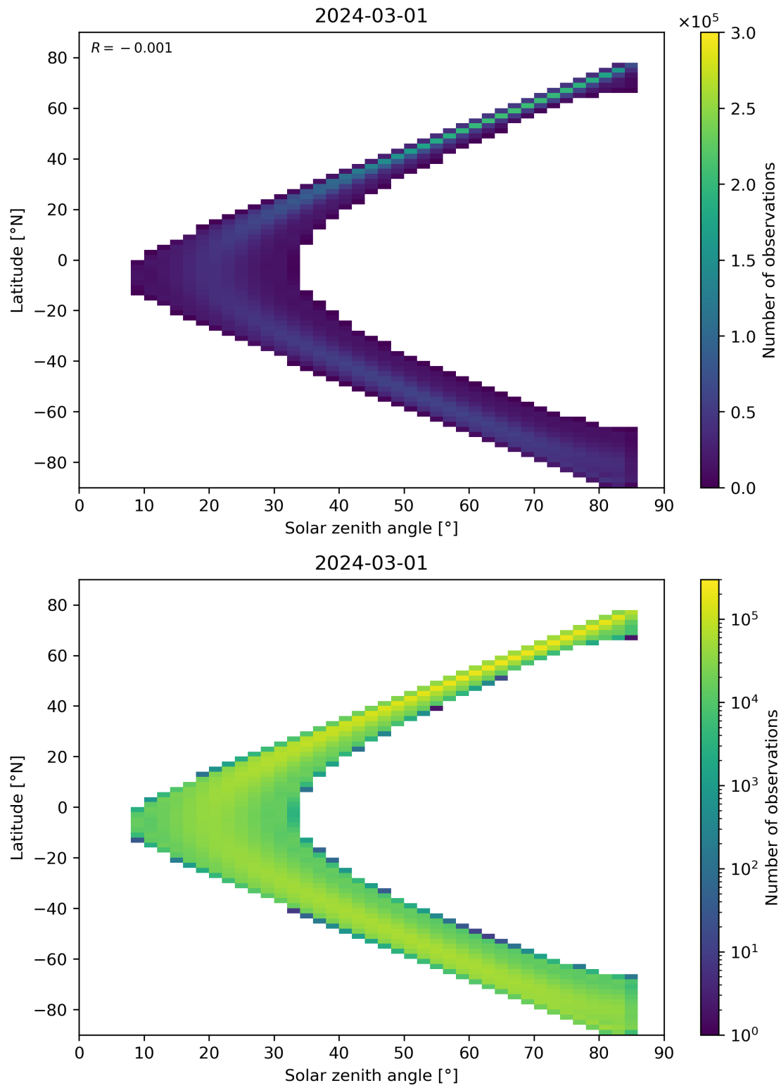
Figure 164: Scatter density plot of “Solar zenith angle” against “Latitude” for 2024-02-29 to 2024-03-02.
