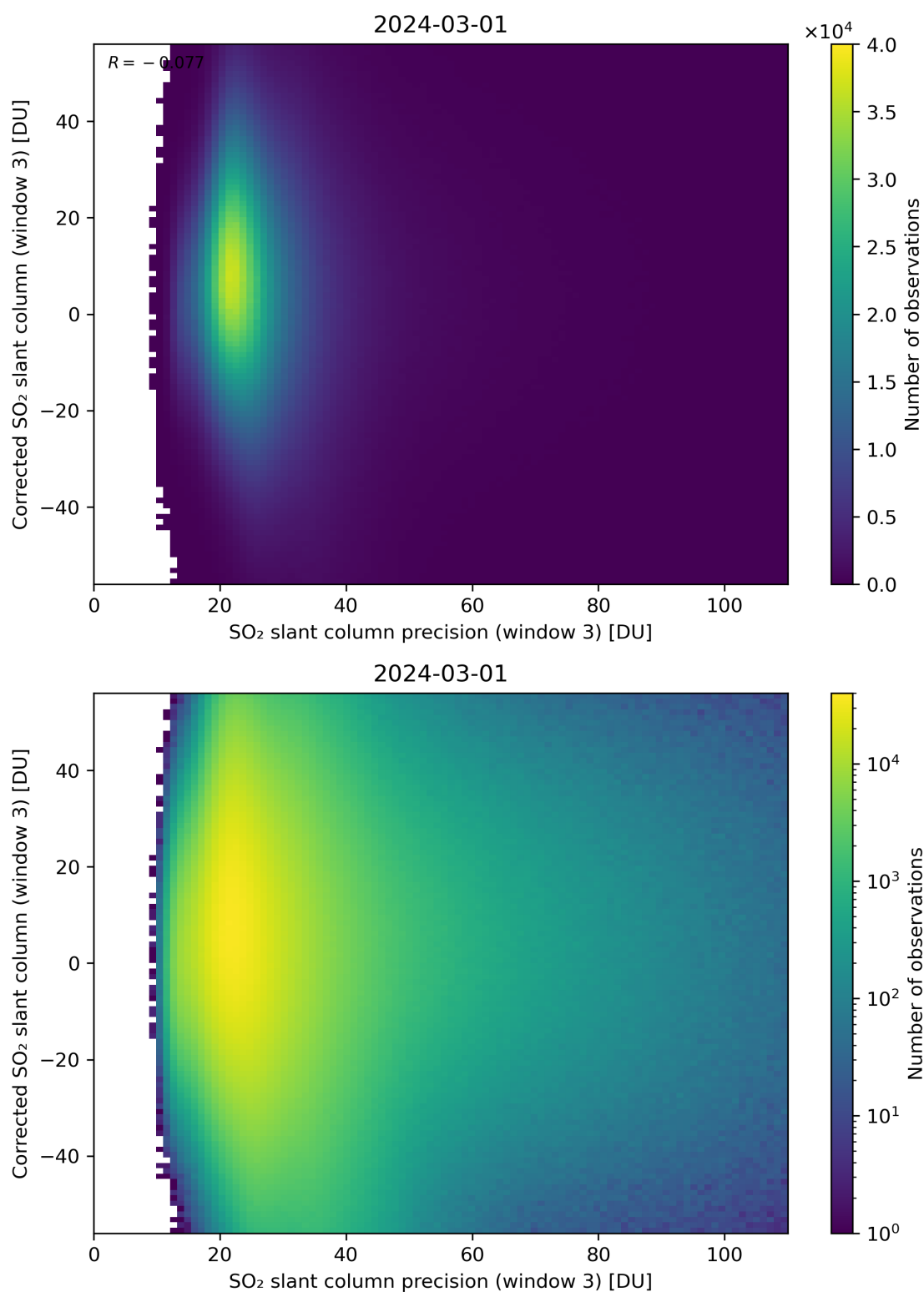
Figure 262: Scatter density plot of “SO 2 slant column precision (window 3)” against “Corrected SO 2 slant column (window 3)” for 2024-02-29 to 2024-03-02.
