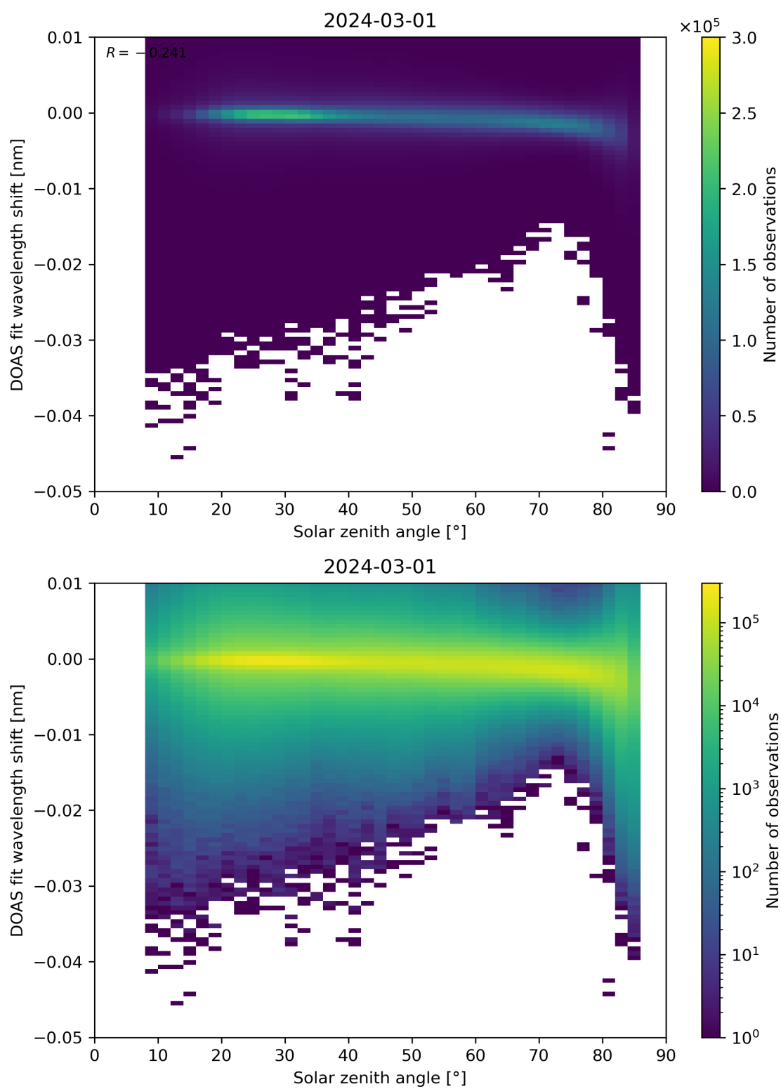
Figure 161: Scatter density plot of “Solar zenith angle” against “DOAS fit wavelength shift” for 2024-02-29 to 2024-03-02.
