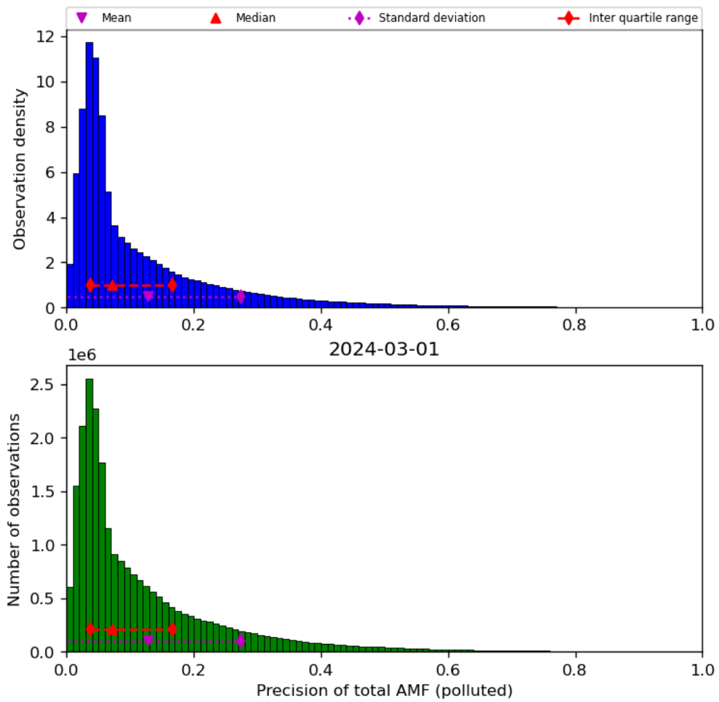
Figure 72: Histogram of “Precision of total AMF (polluted)” for 2024-02-29 to 2024-03-02
