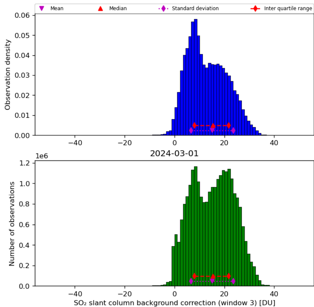
Figure 67: Histogram of “SO 2 slant column background correction (window 3)” for 2024-02-29 to 2024-03-02
