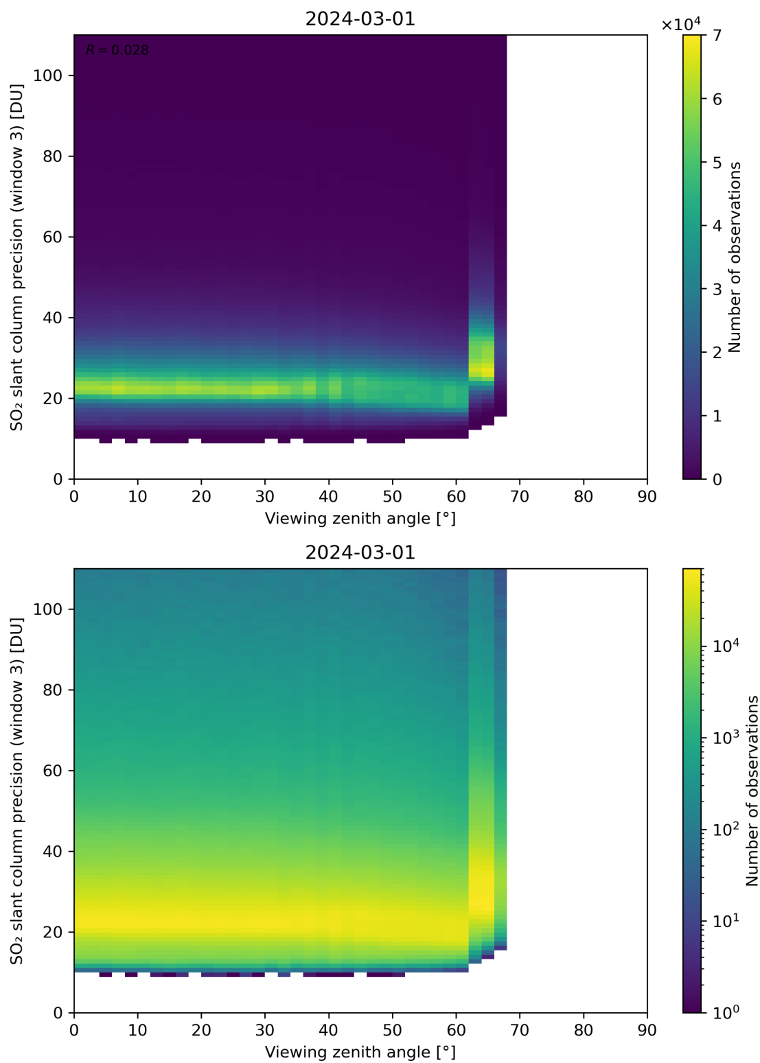
Figure 324: Scatter density plot of “Viewing zenith angle” against “SO 2 slant column precision (window 3)” for 2024-02-29 to 2024-03-02.
