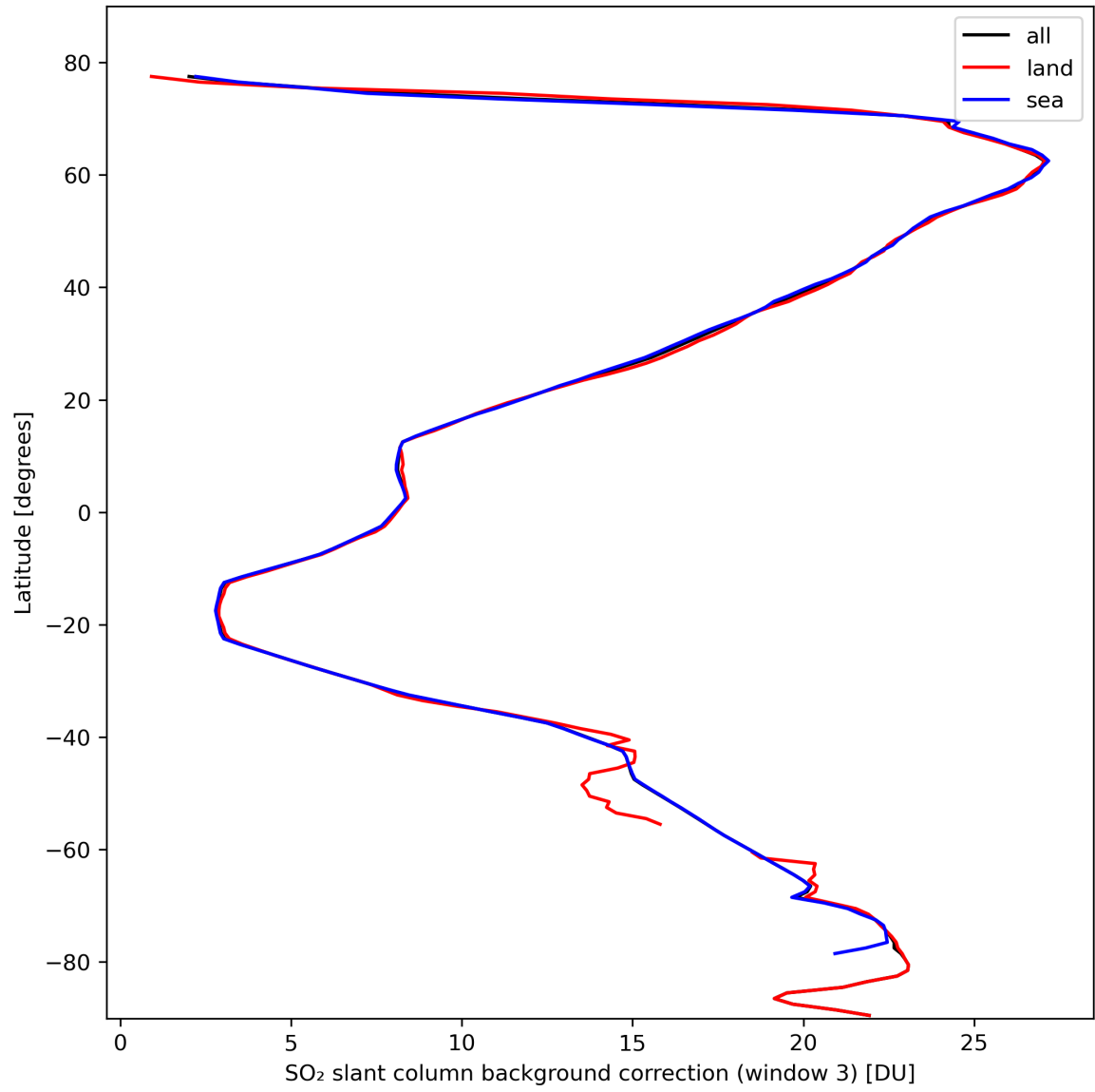
Figure 44: Zonal average of “SO 2 slant column background correction (window 3)” for 2024-02-29 to 2024-03-02.
