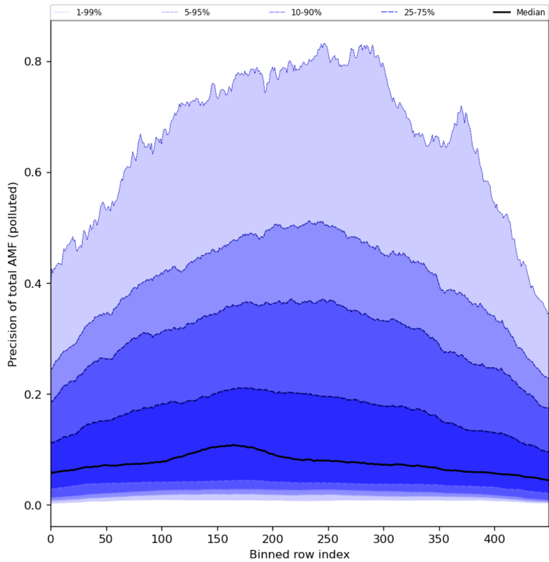
Figure 95: Along track statistics of “Precision of total AMF (polluted)” for 2024-02-29 to 2024-03-02
