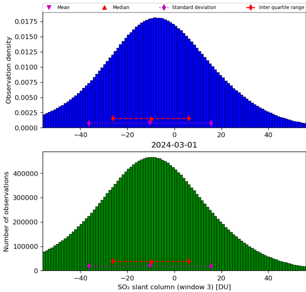
Figure 64: Histogram of “SO 2 slant column (window 3)” for 2024-02-29 to 2024-03-02
