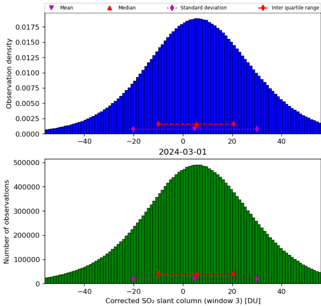
Figure 66: Histogram of “Corrected SO 2 slant column (window 3)” for 2024-02-29 to 2024-03-02
