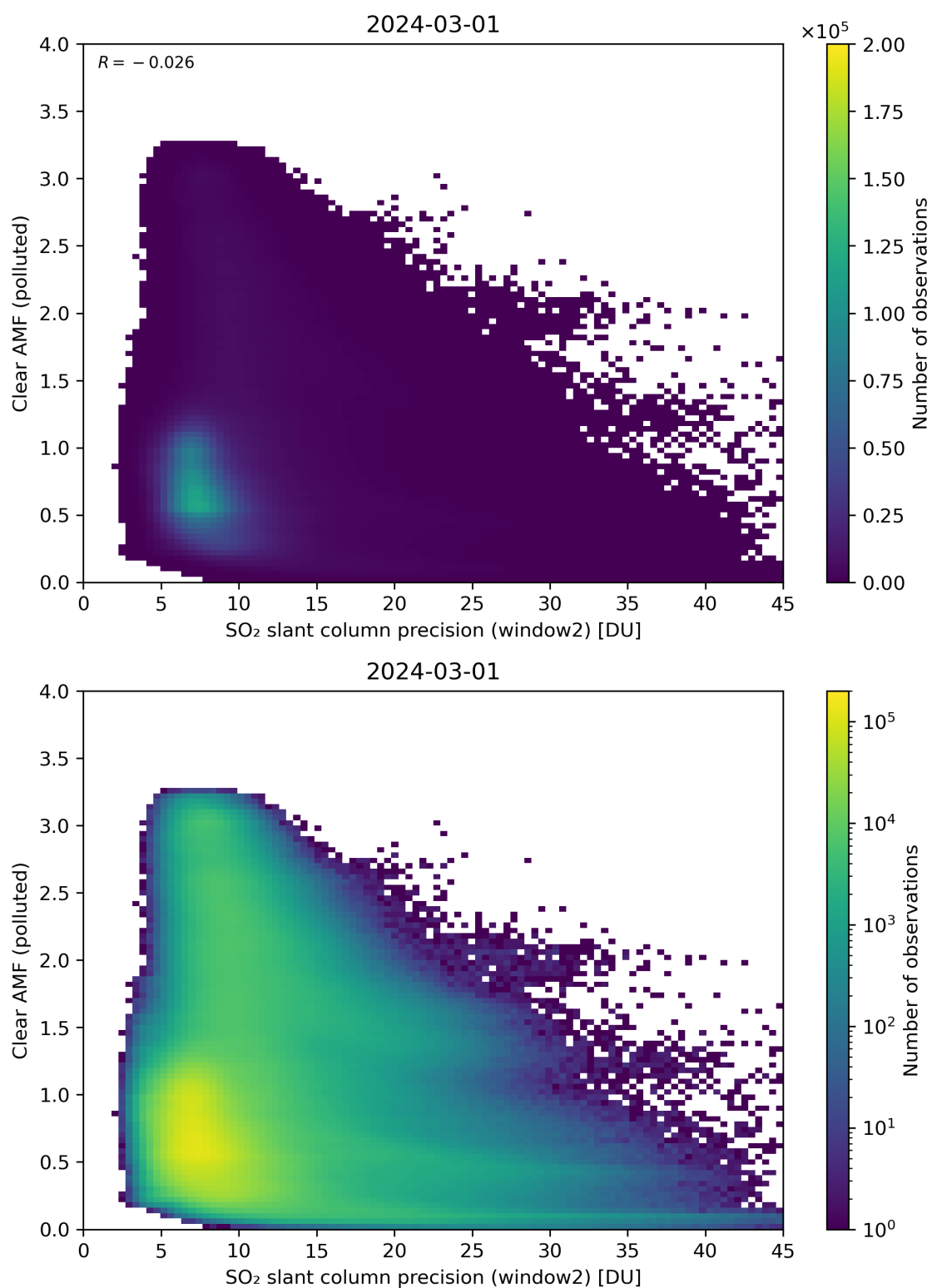
Figure 246: Scatter density plot of “SO 2 slant column precision (window2)” against “Clear AMF (polluted)” for 2024-02-29 to 2024-03-02.
