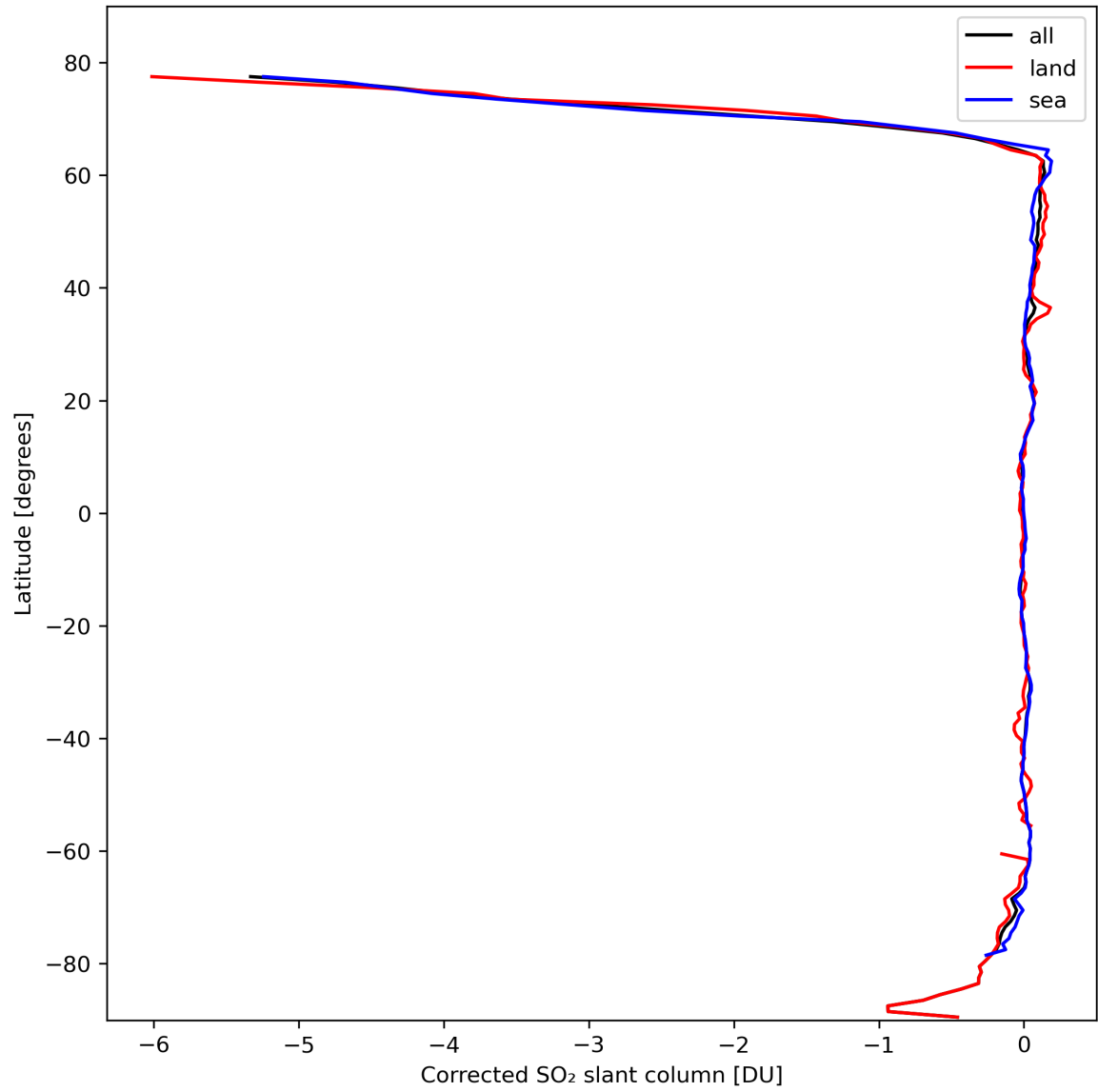
Figure 32: Zonal average of “Corrected SO 2 slant column” for 2024-02-29 to 2024-03-02.
