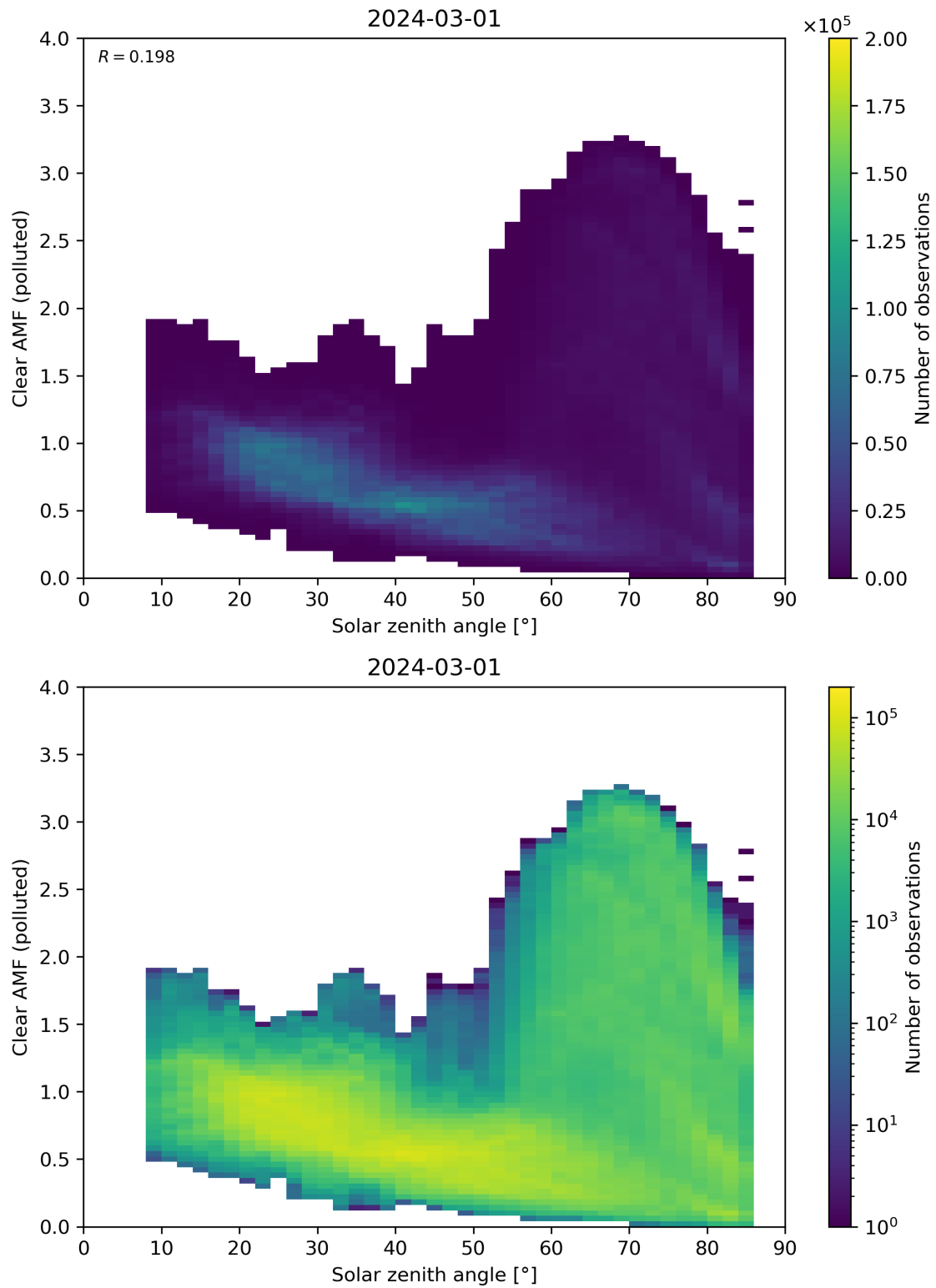
Figure 165: Scatter density plot of “Solar zenith angle” against “Clear AMF (polluted)” for 2024-02-29 to 2024-03-02.
