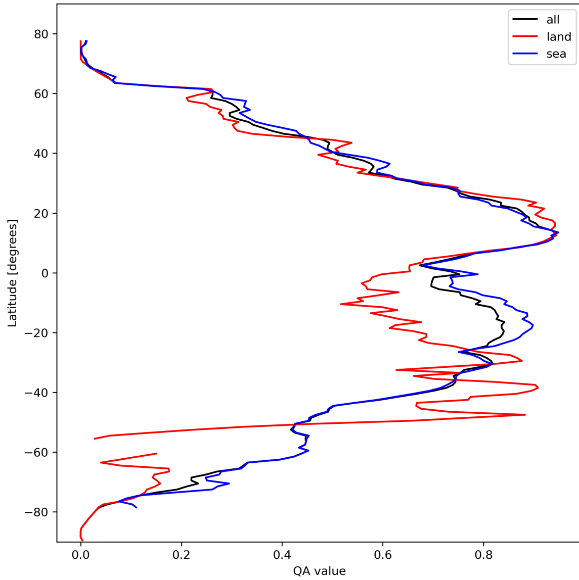
Figure 29: Zonal average of “QA value” for 2024-02-29 to 2024-03-02.
