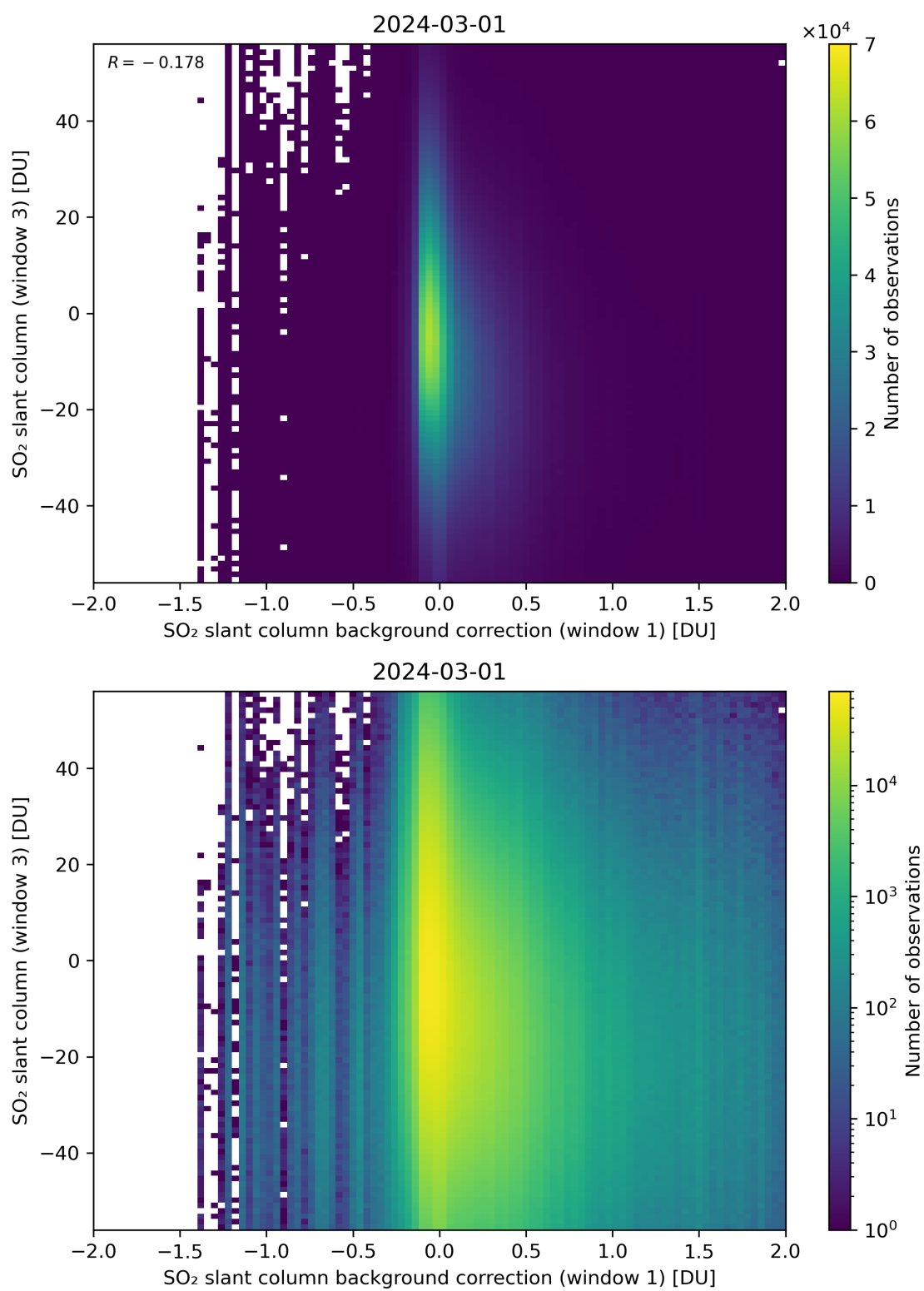
Figure 107: Scatter density plot of “SO 2 slant column background correction (window 1)” against “SO 2 slant column (window 3)” for 2024-02-29 to 2024-03-02.
