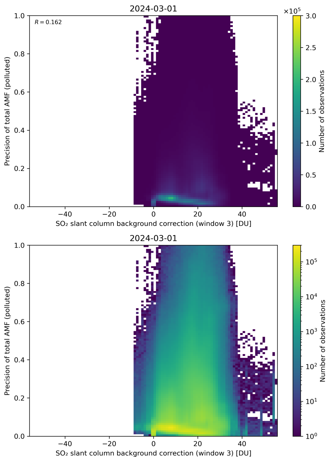
Figure 126: Scatter density plot of “SO 2 slant column background correction (window 3)” against “Precision of total AMF (polluted)” for 2024-02-29 to 2024-03-02.
