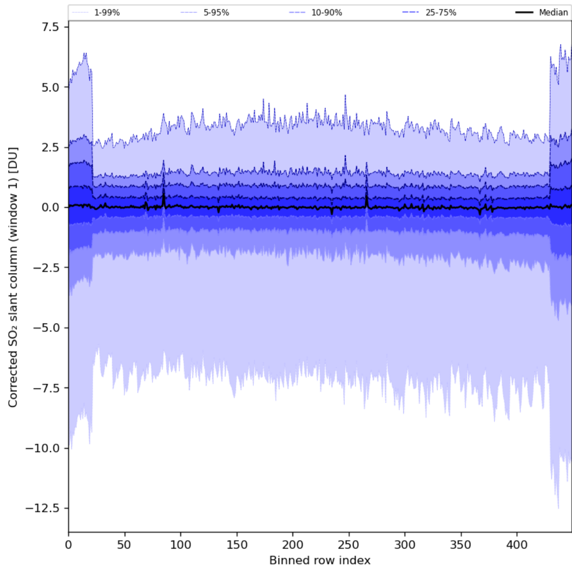
Figure 81: Along track statistics of “Corrected SO 2 slant column (window 1)” for 2024-02-29 to 2024-03-02
