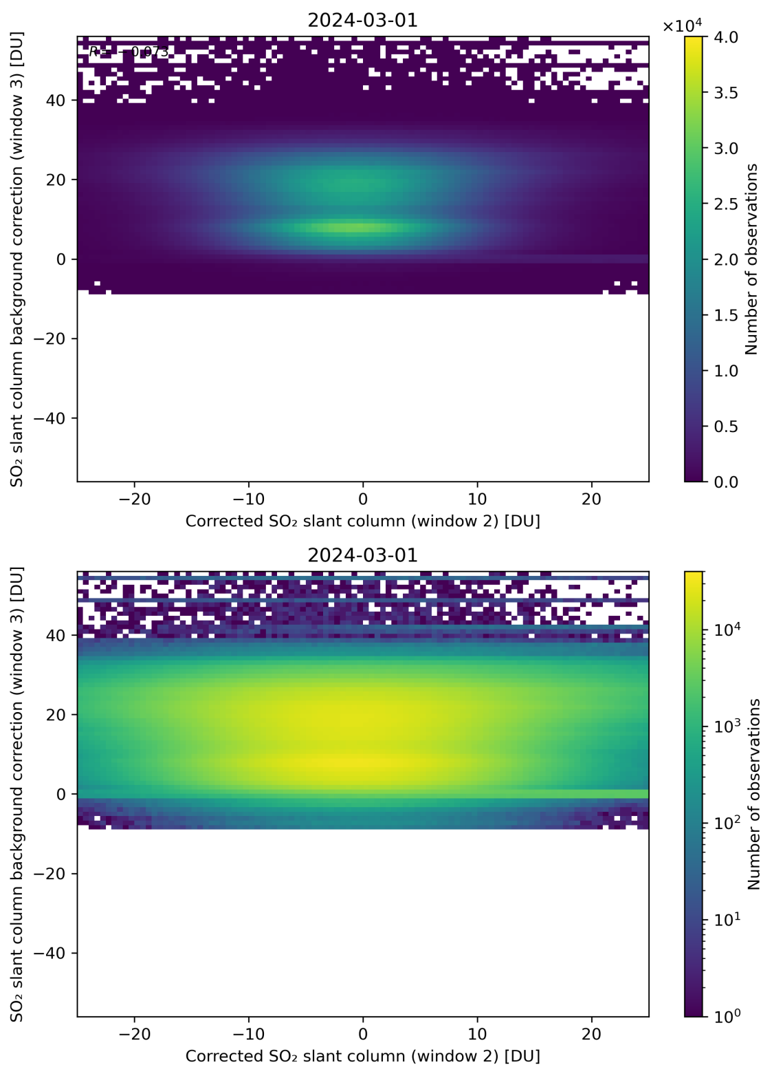
Figure 195: Scatter density plot of “Corrected SO 2 slant column (window 2)” against “SO 2 slant column background correction (window 3)” for 2024-02-29 to 2024-03-02.
