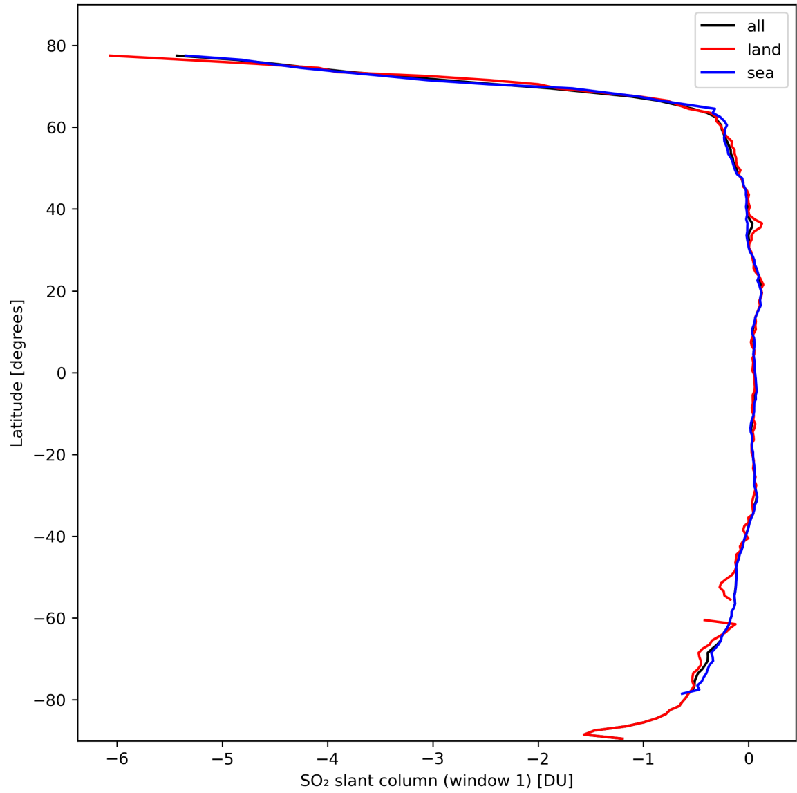
Figure 33: Zonal average of “SO 2 slant column (window 1)” for 2024-02-29 to 2024-03-02.
