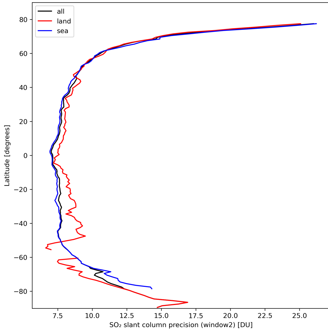
Figure 38: Zonal average of “SO 2 slant column precision (window2)” for 2024-02-29 to 2024-03-02.
