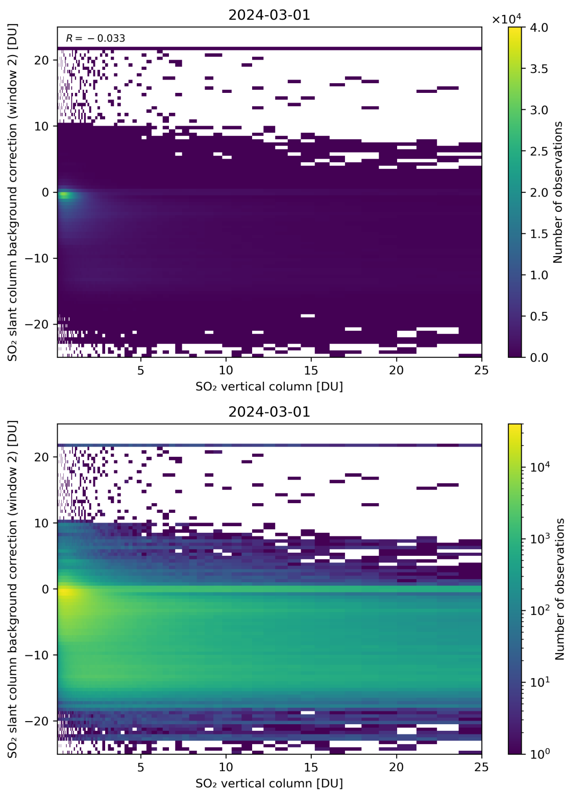
Figure 274: Scatter density plot of “SO 2 vertical column” against “SO 2 slant column background correction (window 2)” for 2024-02-29 to 2024-03-02.
