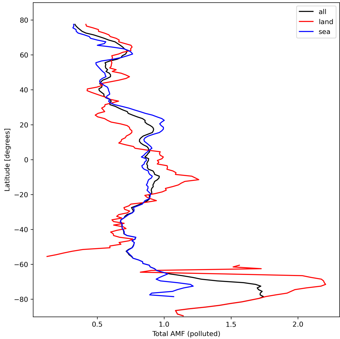
Figure 48: Zonal average of “Total AMF (polluted)” for 2024-02-29 to 2024-03-02.
