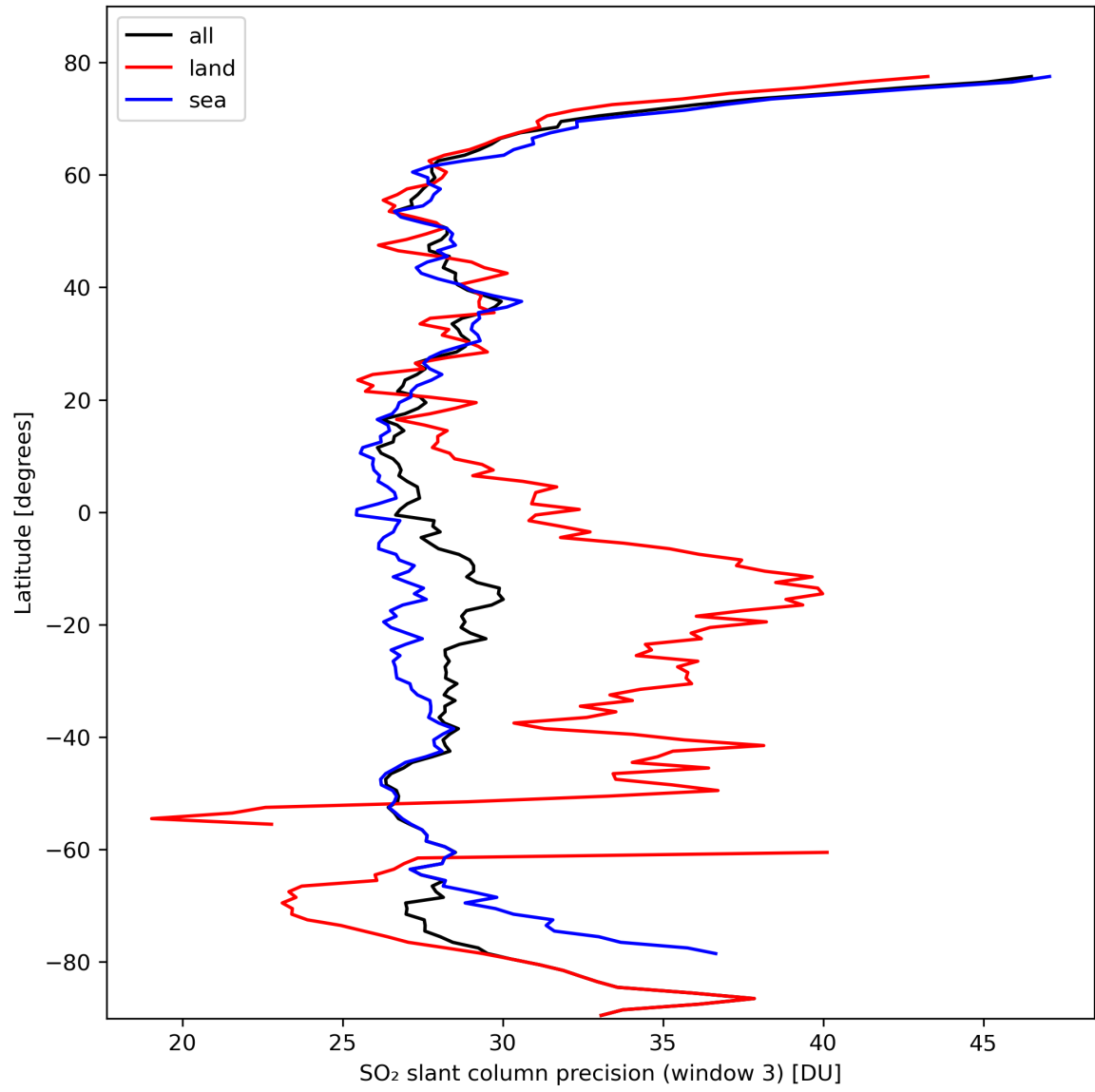
Figure 42: Zonal average of “SO 2 slant column precision (window 3)” for 2024-02-29 to 2024-03-02.
