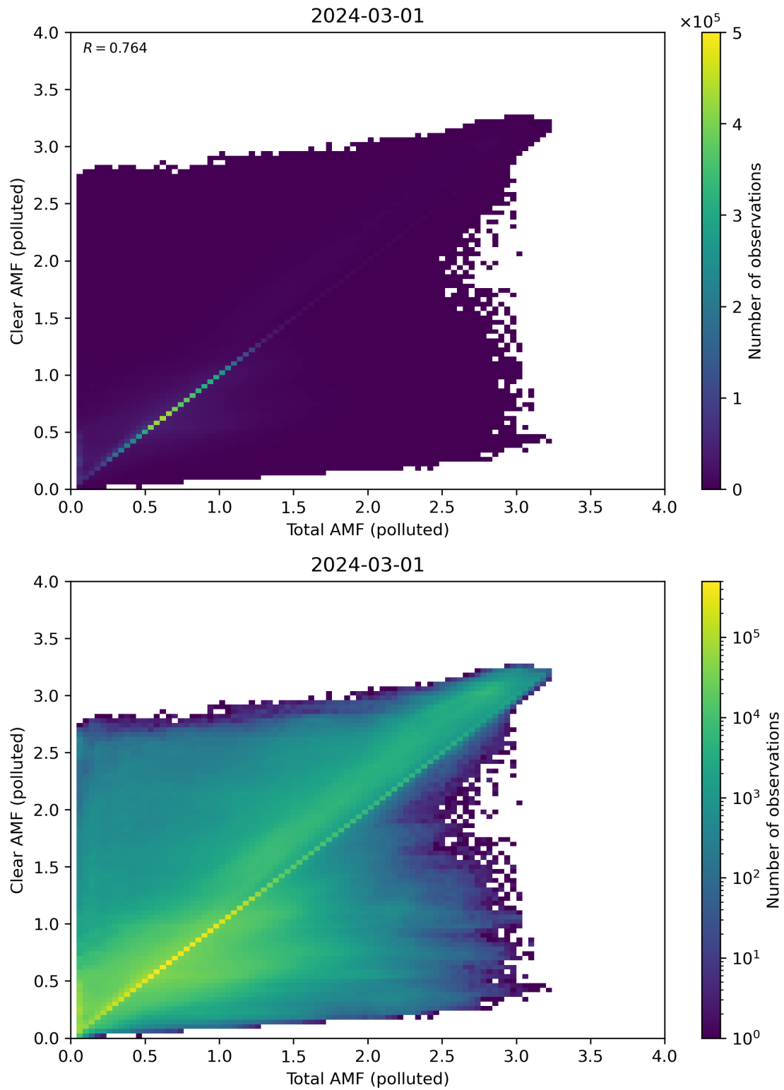
Figure 271: Scatter density plot of “Total AMF (polluted)” against “Clear AMF (polluted)” for 2024-02-29 to 2024-03-02.
