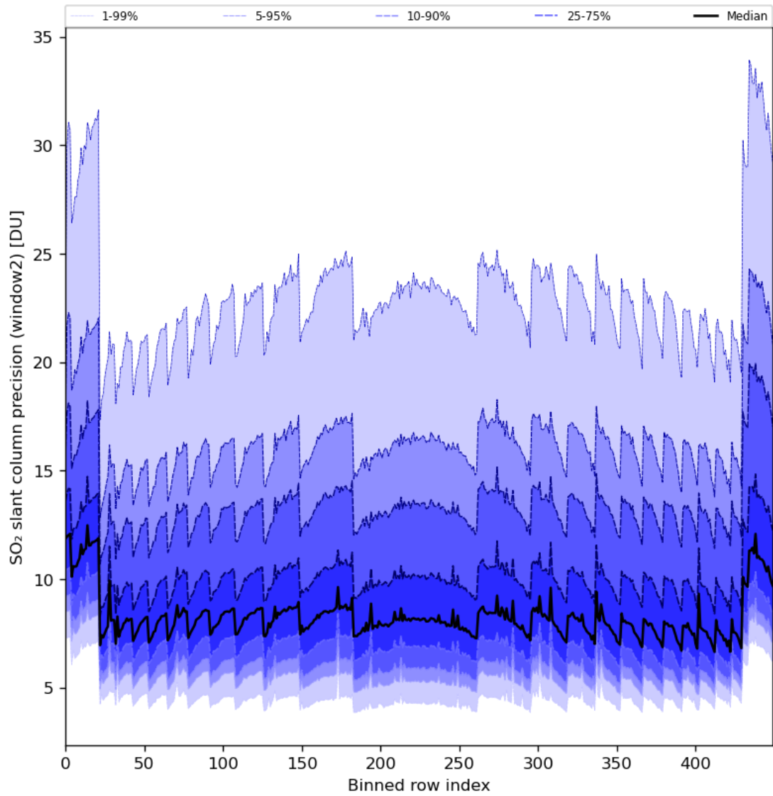
Figure 84: Along track statistics of “SO 2 slant column precision (window2)” for 2024-02-29 to 2024-03-02
