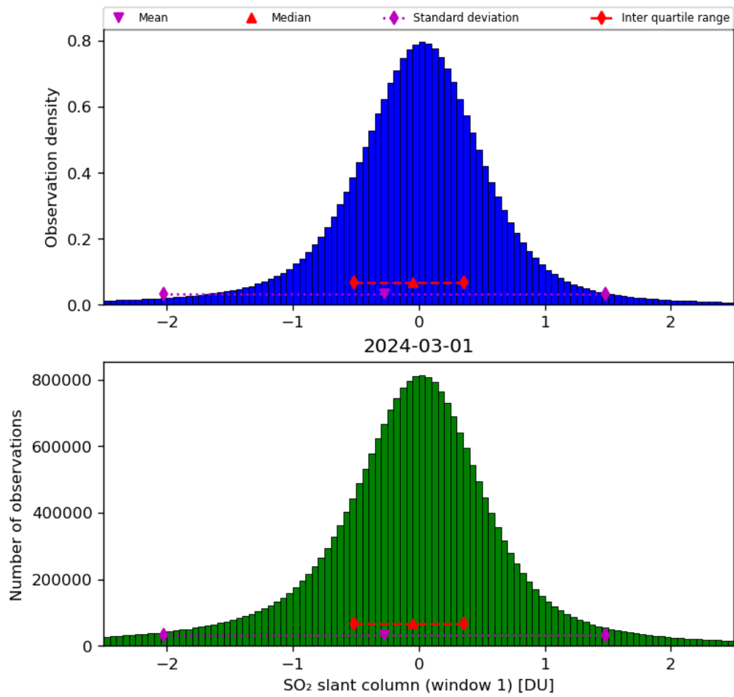
Figure 56: Histogram of “SO 2 slant column (window 1)” for 2024-02-29 to 2024-03-02
