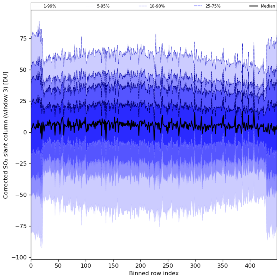
Figure 89: Along track statistics of “Corrected SO 2 slant column (window 3)” for 2024-02-29 to 2024-03-02
