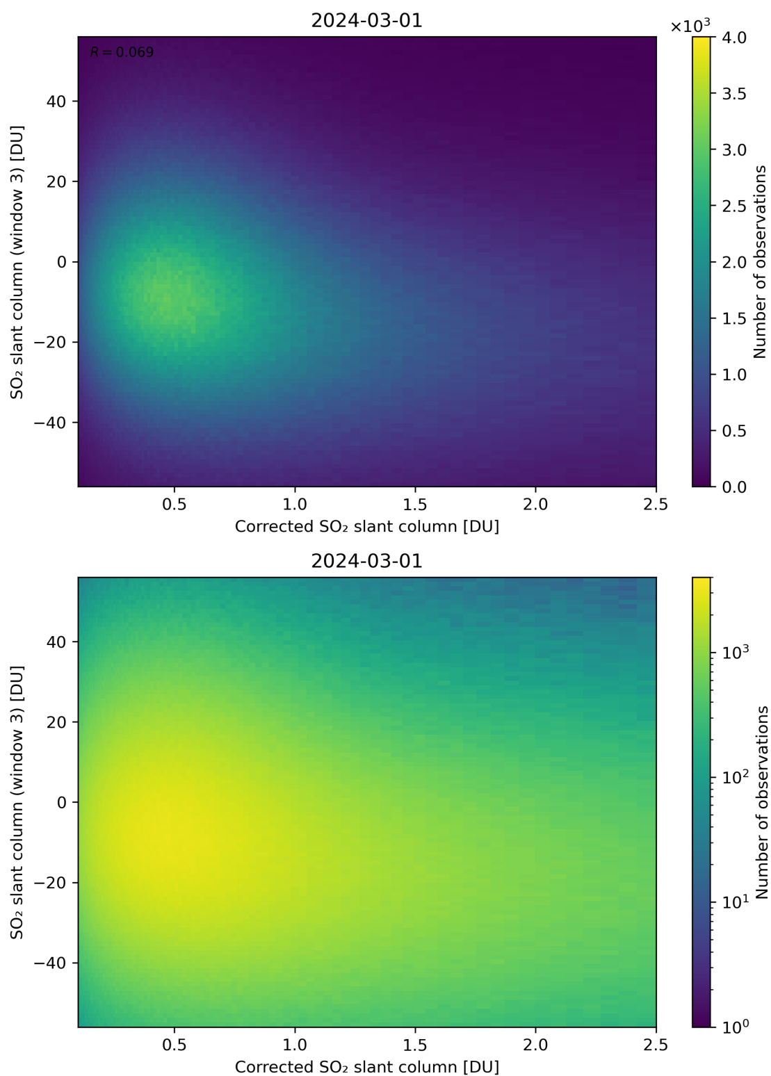
Figure 190: Scatter density plot of “Corrected SO 2 slant column” against “SO 2 slant column (window 3)” for 2024-02-29 to 2024-03-02.
