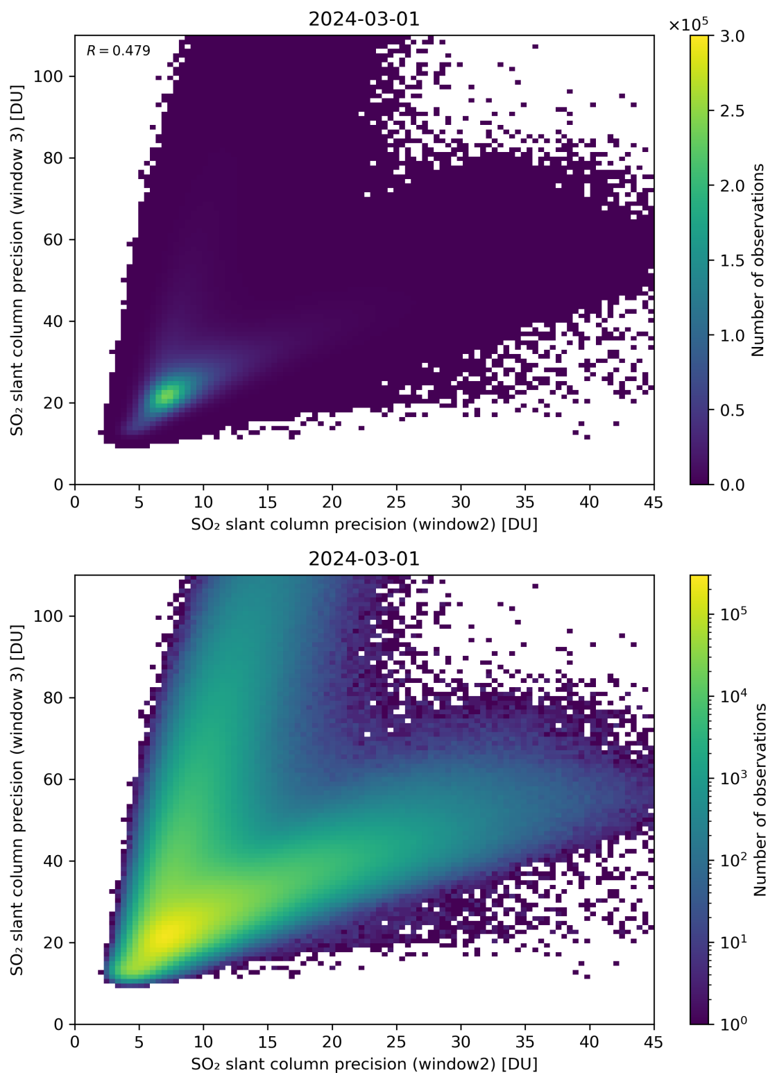
Figure 250: Scatter density plot of “SO 2 slant column precision (window2)” against “SO 2 slant column precision (window 3)” for 2024-02-29 to 2024-03-02.
