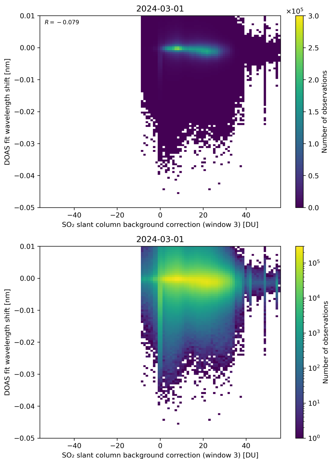
Figure 121: Scatter density plot of “SO 2 slant column background correction (window 3)” against “DOAS fit wavelength shift” for 2024-02-29 to 2024-03-02.
