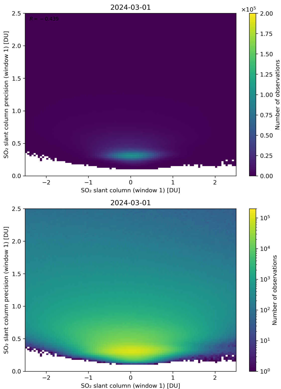
Figure 235: Scatter density plot of “SO 2 slant column (window 1)” against “SO 2 slant column precision (window 1)” for 2024-02-29 to 2024-03-02.
