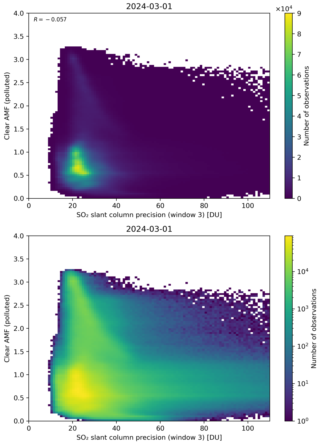
Figure 261: Scatter density plot of “SO 2 slant column precision (window 3)” against “Clear AMF (polluted)” for 2024-02-29 to 2024-03-02.
