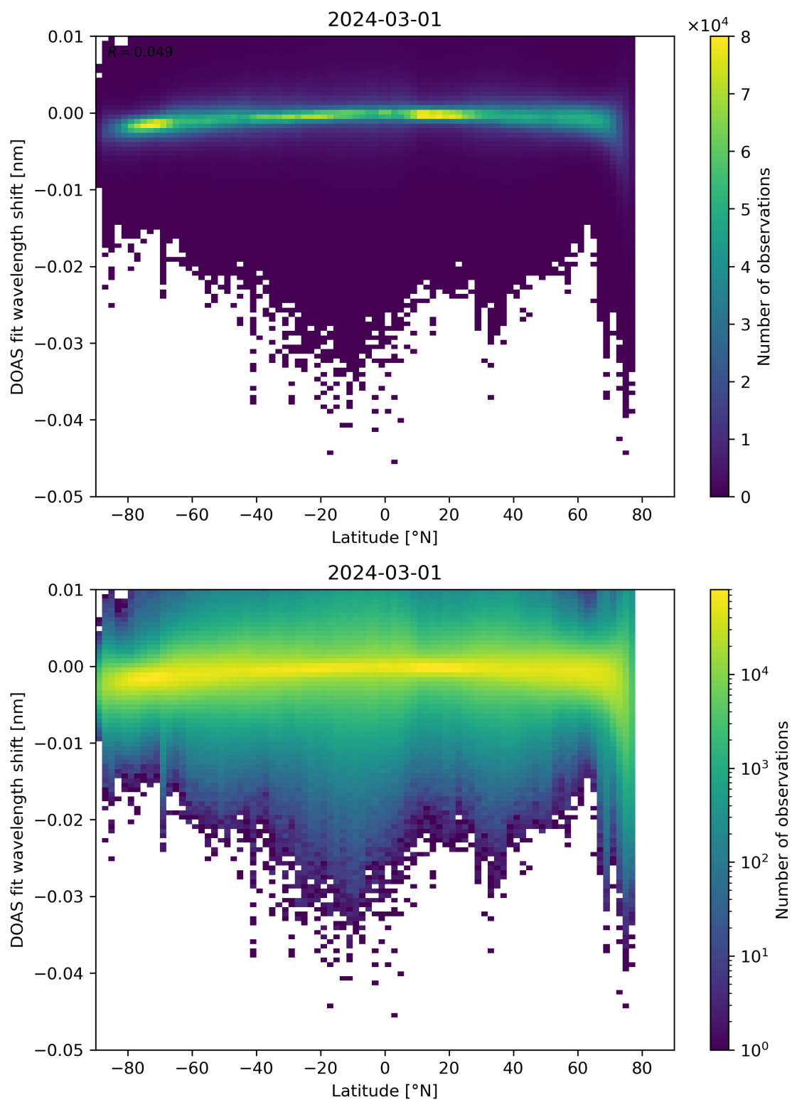
Figure 142: Scatter density plot of “Latitude” against “DOAS fit wavelength shift” for 2024-02-29 to 2024-03-02.
