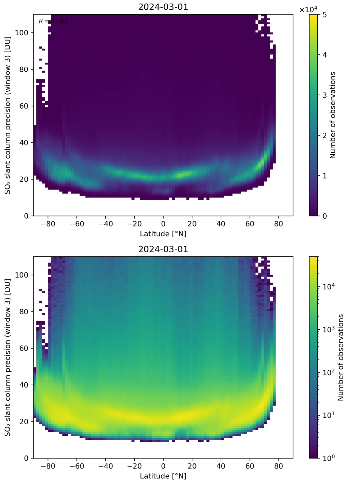
Figure 153: Scatter density plot of “Latitude” against “SO 2 slant column precision (window 3)” for 2024-02-29 to 2024-03-02.
