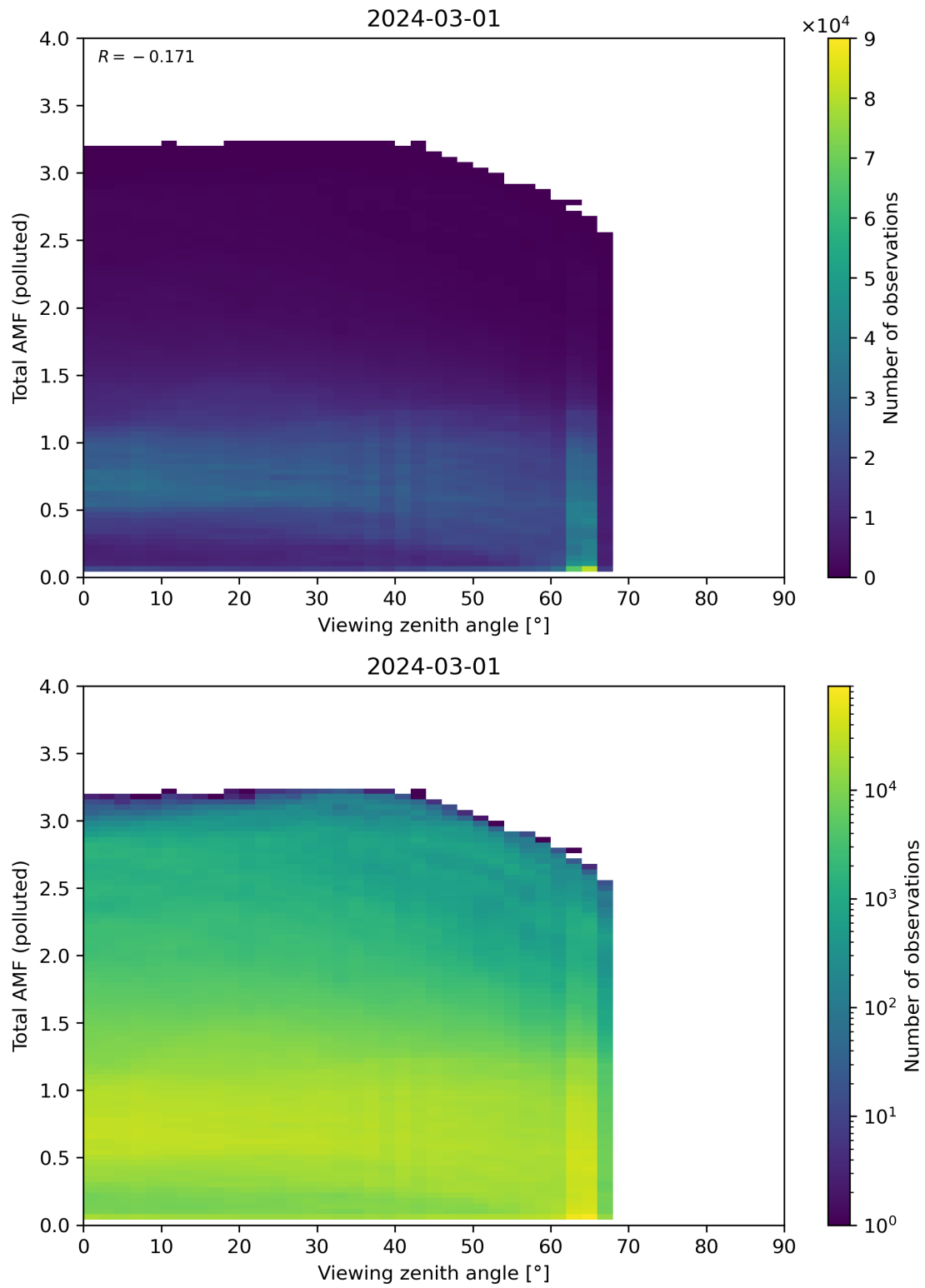
Figure 325: Scatter density plot of “Viewing zenith angle” against “Total AMF (polluted)” for 2024-02-29 to 2024-03-02.
