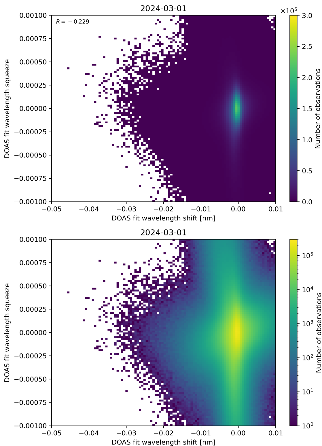
Figure 127: Scatter density plot of “DOAS fit wavelength shift” against “DOAS fit wavelength squeeze” for 2024-02-29 to 2024-03-02.
