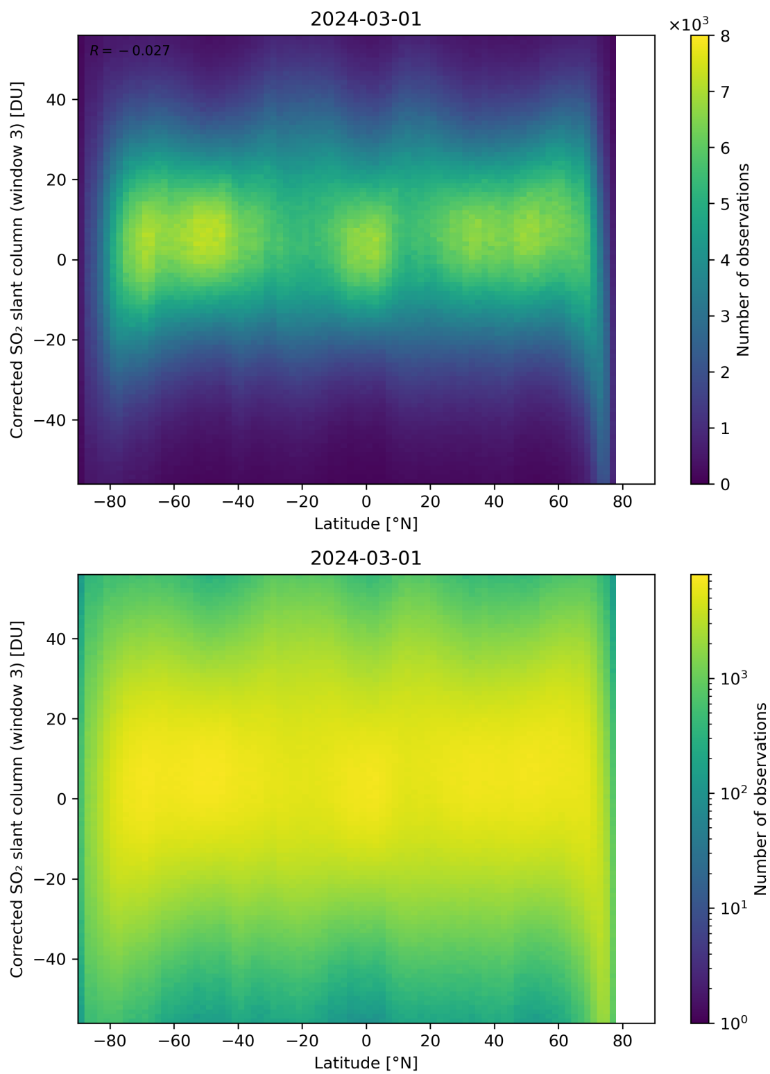
Figure 148: Scatter density plot of “Latitude” against “Corrected SO 2 slant column (window 3)” for 2024-02-29 to 2024-03-02.
