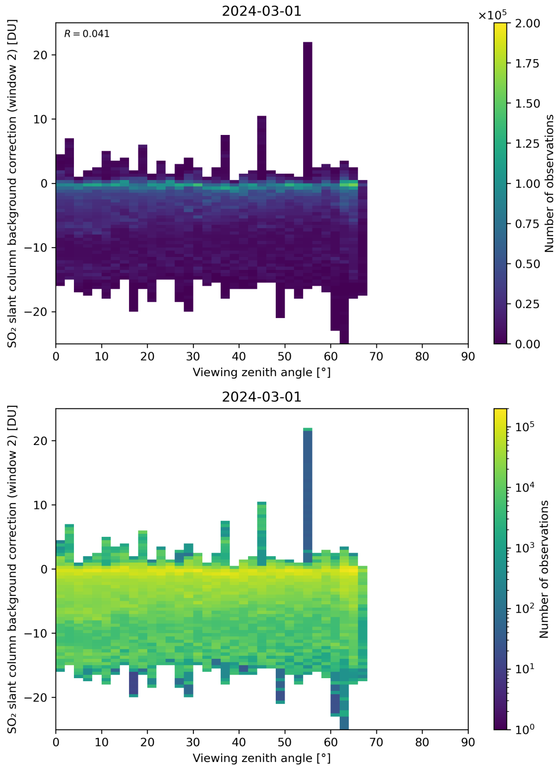
Figure 309: Scatter density plot of “Viewing zenith angle” against “SO 2 slant column background correction (window 2)” for 2024-02-29 to 2024-03-02.
