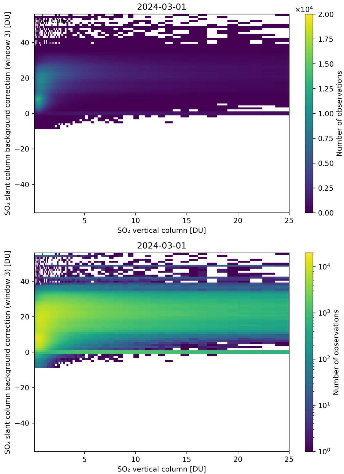
Figure 275: Scatter density plot of “SO 2 vertical column” against “SO 2 slant column background correction (window 3)” for 2024-02-29 to 2024-03-02.
