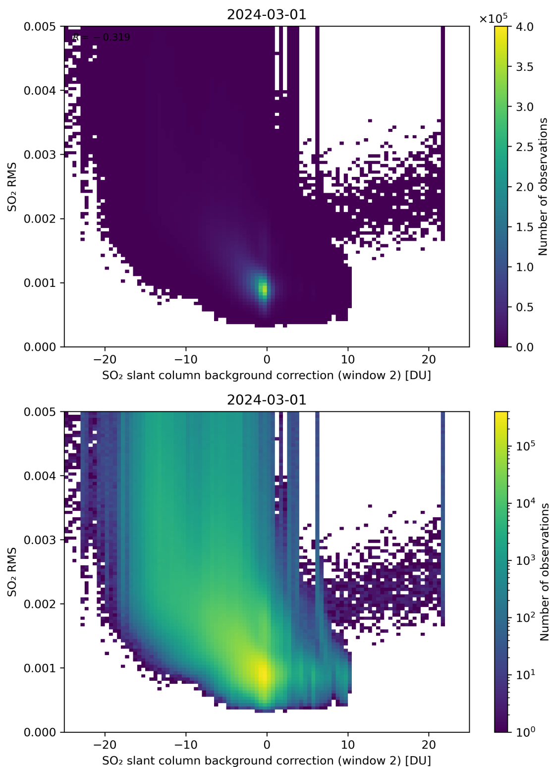
Figure 114: Scatter density plot of “SO 2 slant column background correction (window 2)” against “SO 2 RMS” for 2024-02-29 to 2024-03-02.
