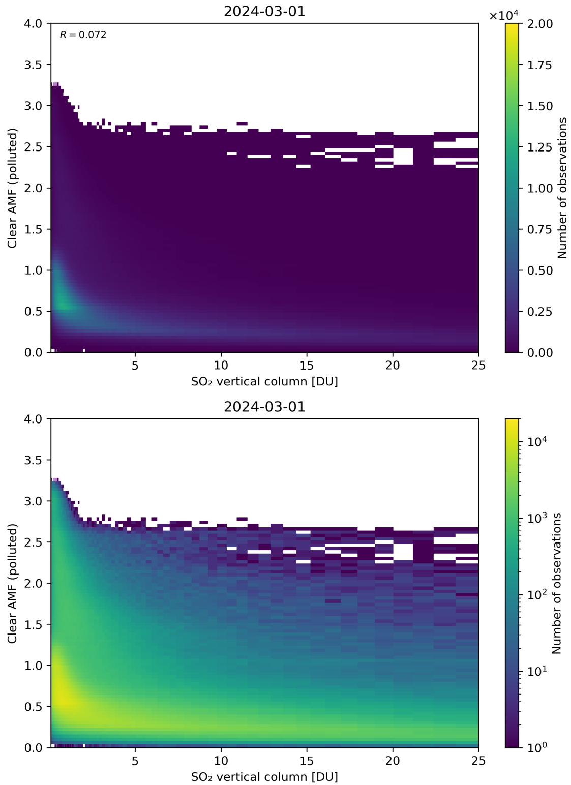
Figure 296: Scatter density plot of “SO 2 vertical column” against “Clear AMF (polluted)” for 2024-02-29 to 2024-03-02.
