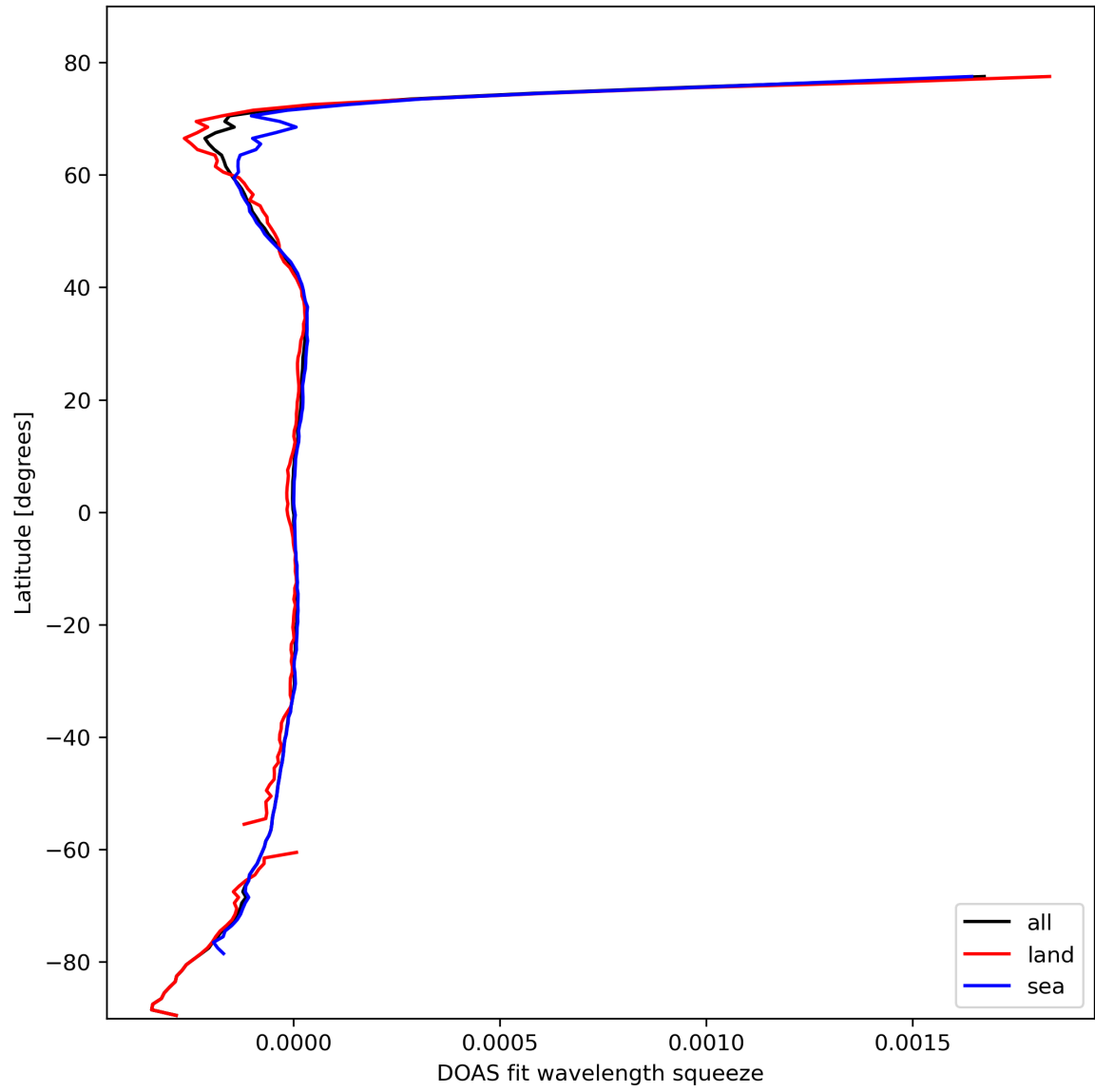
Figure 46: Zonal average of “DOAS fit wavelength squeeze” for 2024-02-29 to 2024-03-02.
