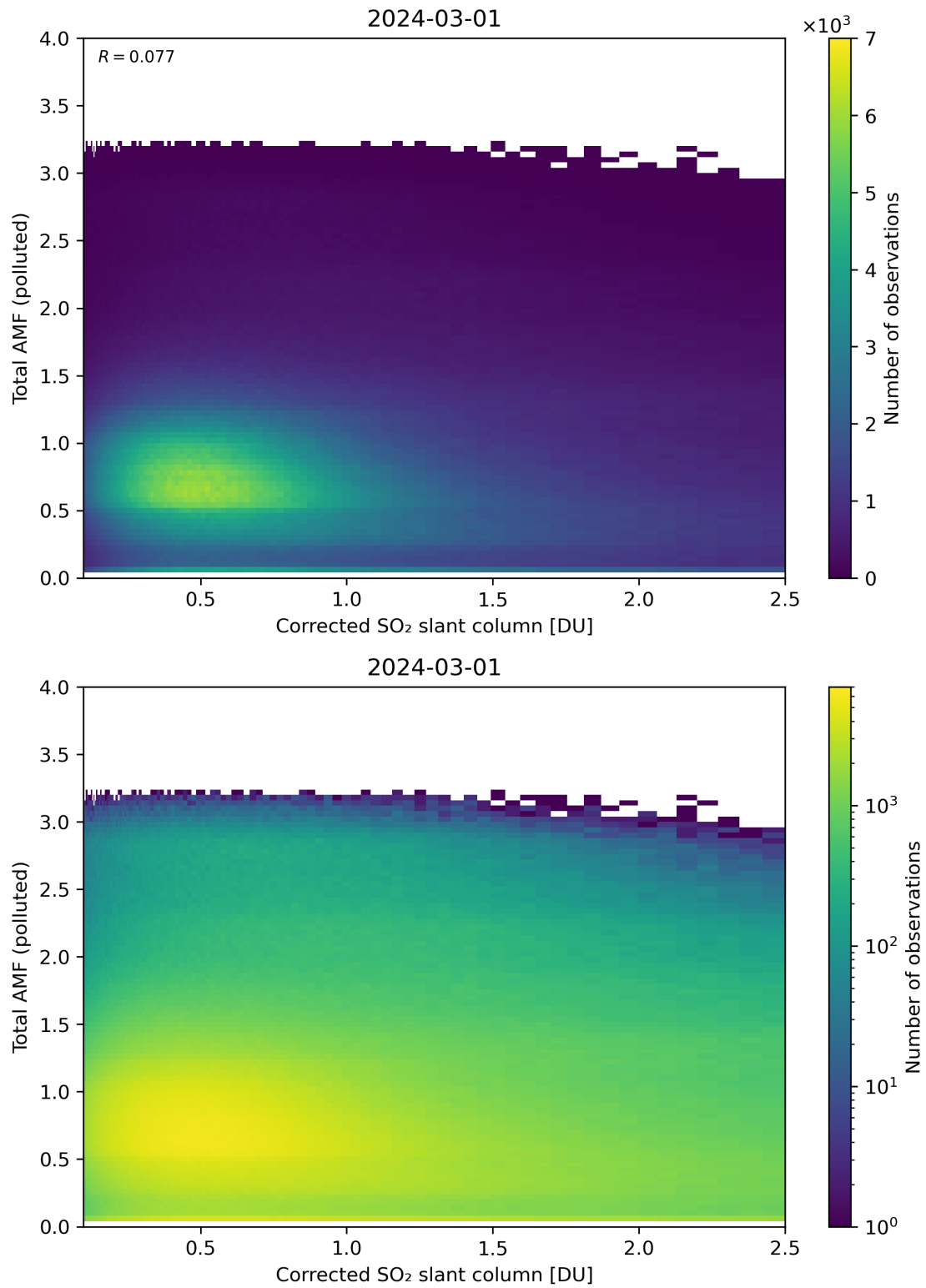
Figure 192: Scatter density plot of “Corrected SO 2 slant column” against “Total AMF (polluted)” for 2024-02-29 to 2024-03-02.
