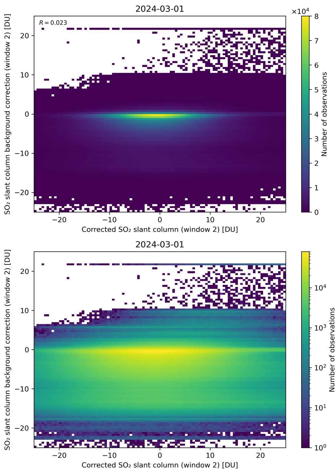
Figure 194: Scatter density plot of “Corrected SO 2 slant column (window 2)” against “SO 2 slant column background correction (window 2)” for 2024-02-29 to 2024-03-02.
