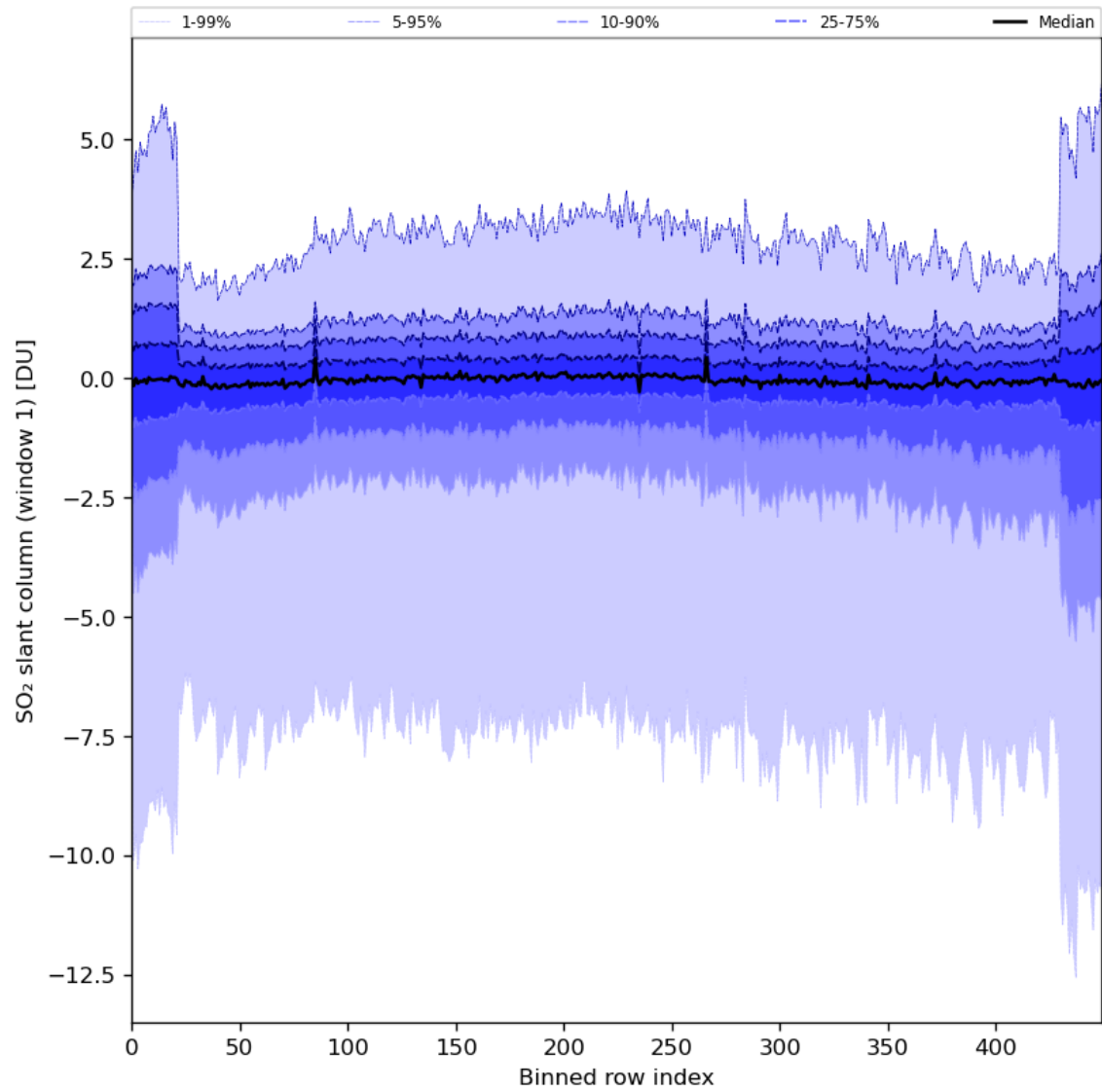
Figure 79: Along track statistics of “SO 2 slant column (window 1)” for 2024-02-29 to 2024-03-02
