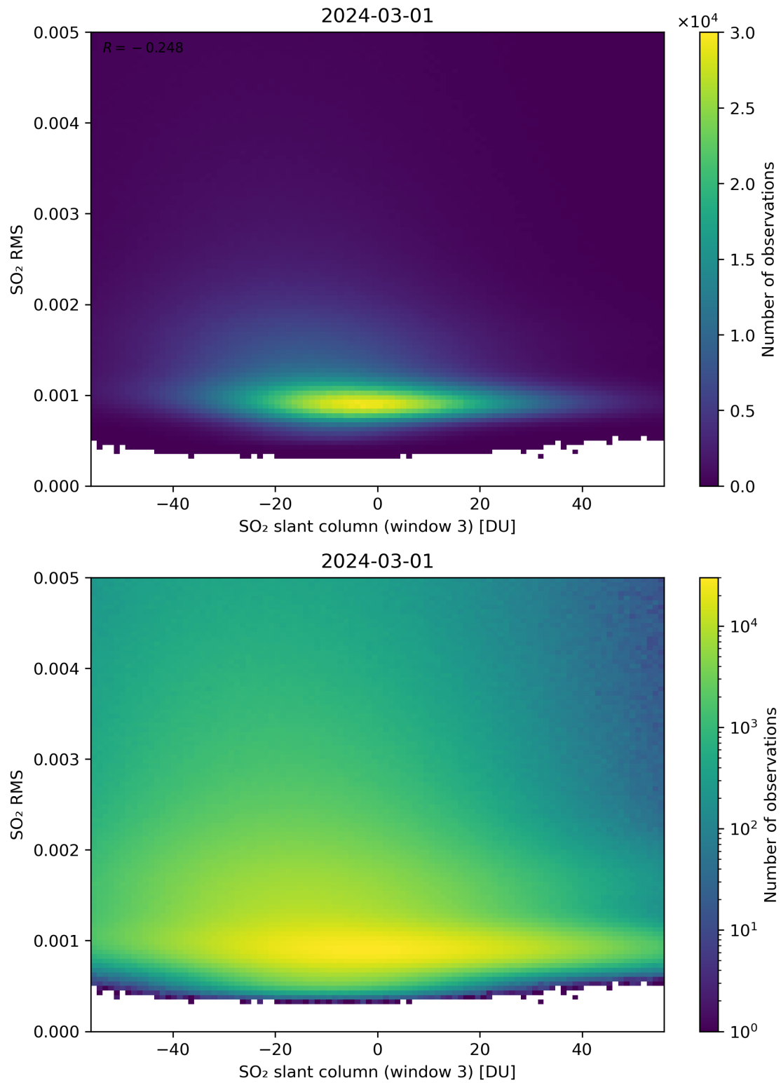
Figure 256: Scatter density plot of “SO 2 slant column (window 3)” against “SO 2 RMS” for 2024-02-29 to 2024-03-02.
