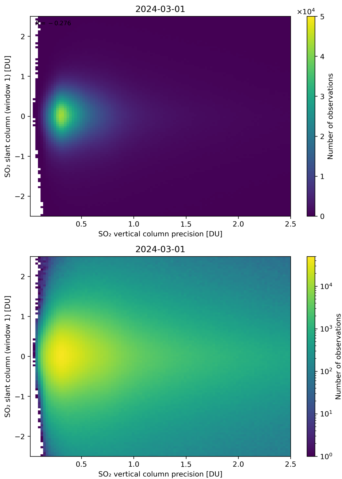
Figure 289: Scatter density plot of “SO 2 vertical column precision” against “SO 2 slant column (window 1)” for 2024-02-29 to 2024-03-02.
