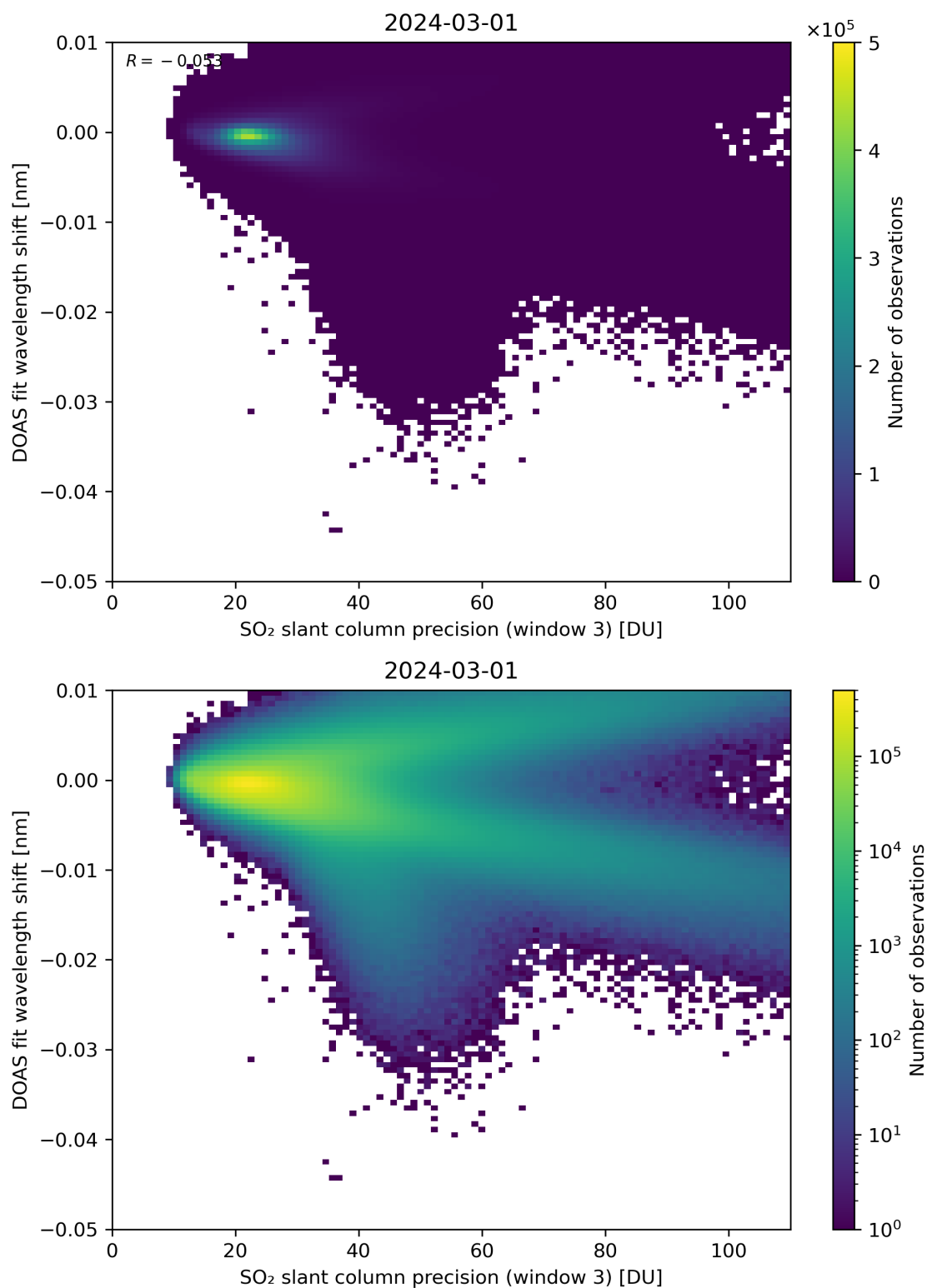
Figure 258: Scatter density plot of “SO 2 slant column precision (window 3)” against “DOAS fit wavelength shift” for 2024-02-29 to 2024-03-02.
