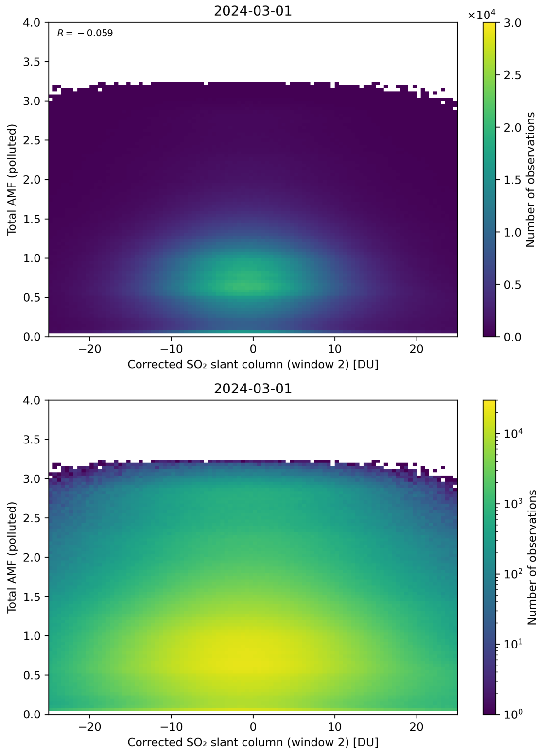
Figure 203: Scatter density plot of “Corrected SO 2 slant column (window 2)” against “Total AMF (polluted)” for 2024-02-29 to 2024-03-02.
