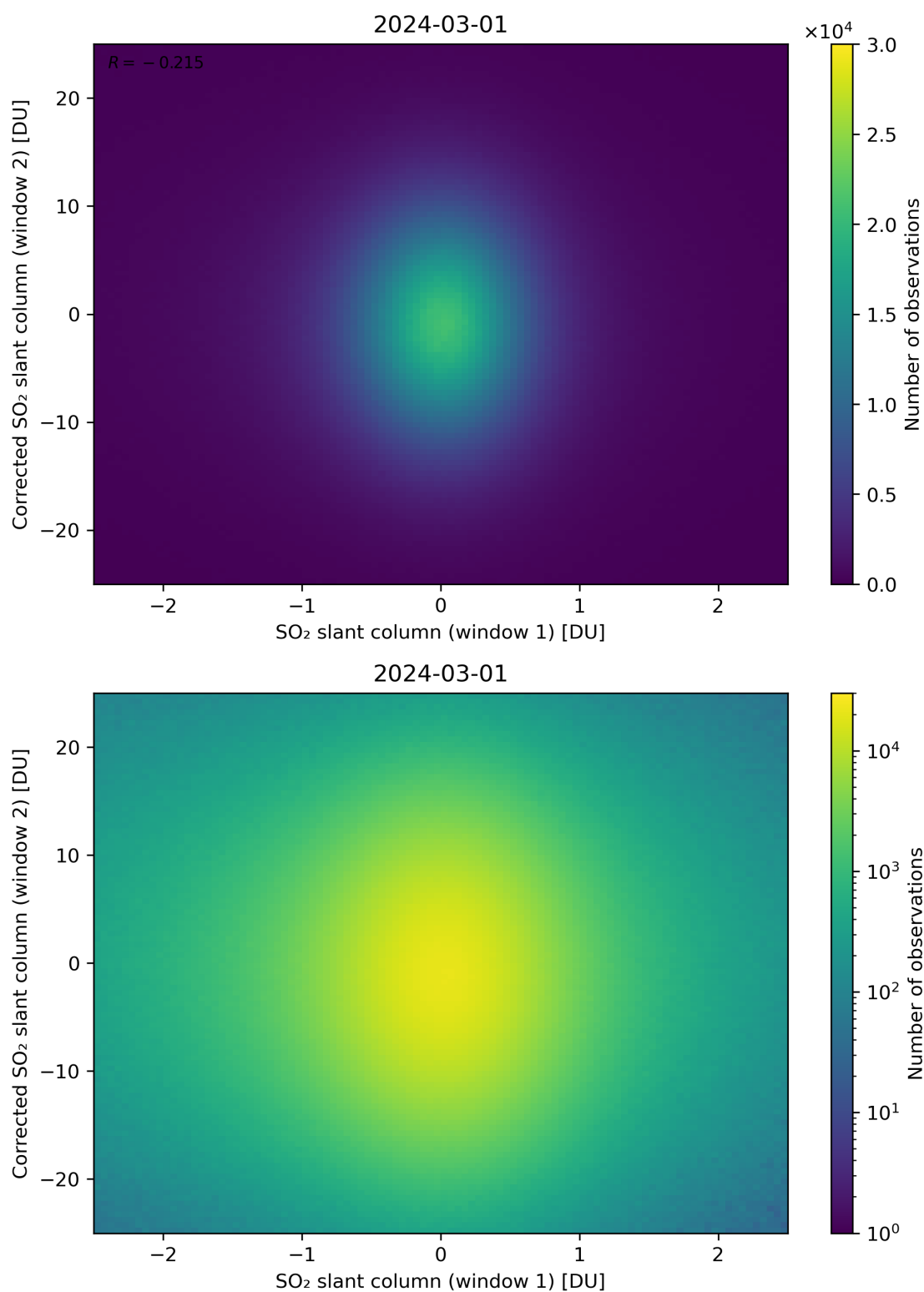
Figure 233: Scatter density plot of “SO 2 slant column (window 1)” against “Corrected SO 2 slant column (window 2)” for 2024-02-29 to 2024-03-02.
