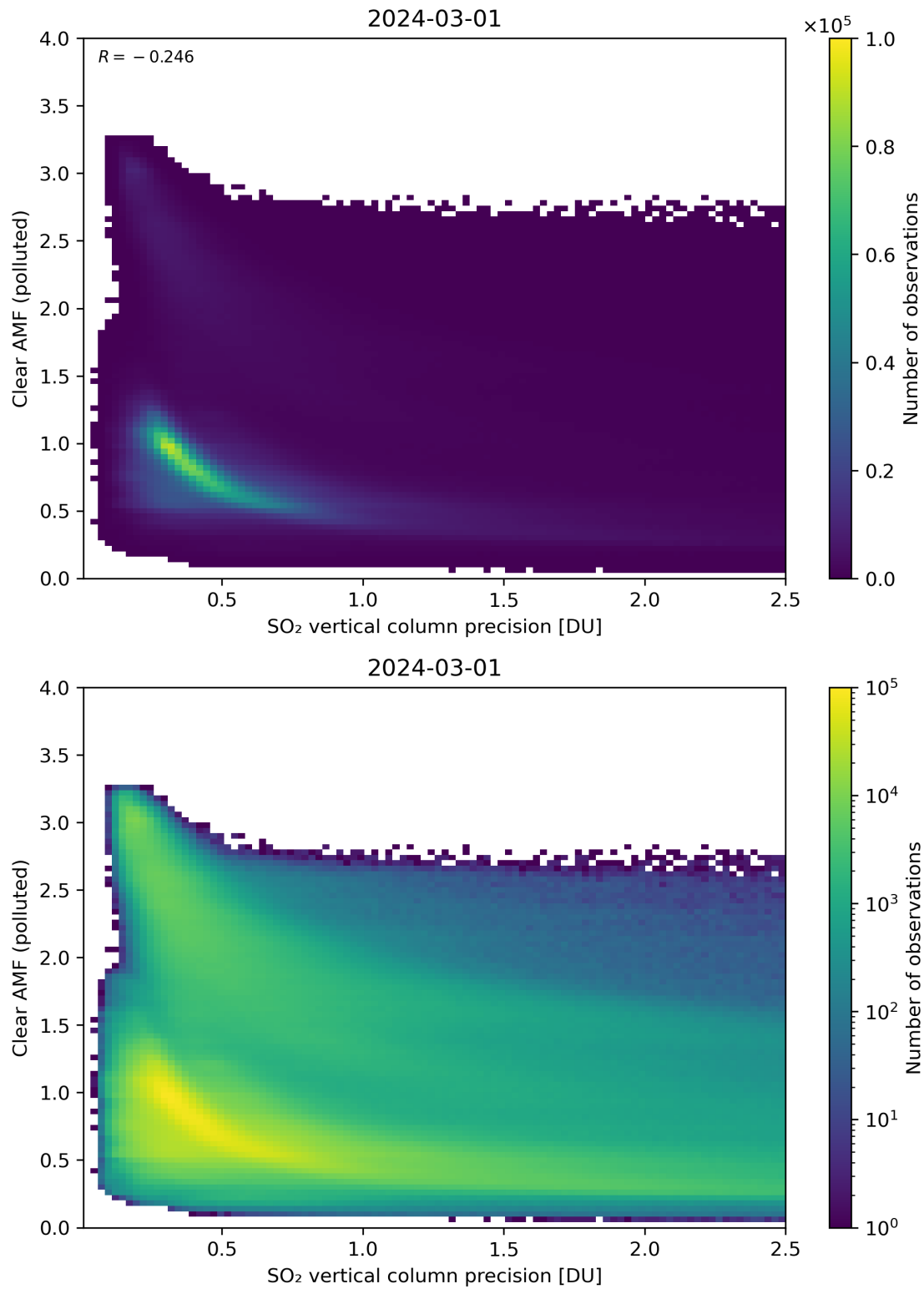
Figure 285: Scatter density plot of “SO 2 vertical column precision” against “Clear AMF (polluted)” for 2024-02-29 to 2024-03-02.
