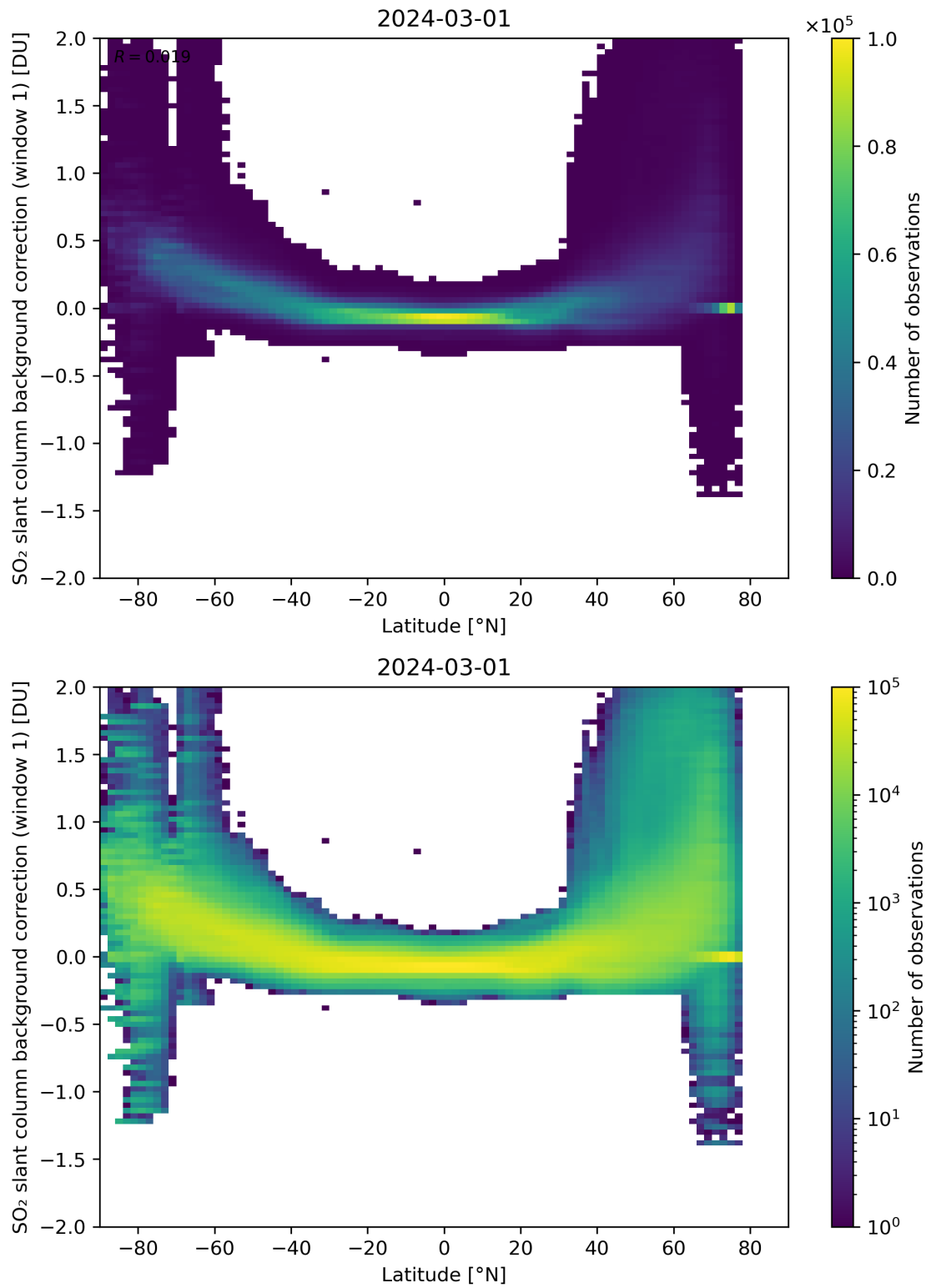
Figure 139: Scatter density plot of “Latitude” against “SO 2 slant column background correction (window 1)” for 2024-02-29 to 2024-03-02.
