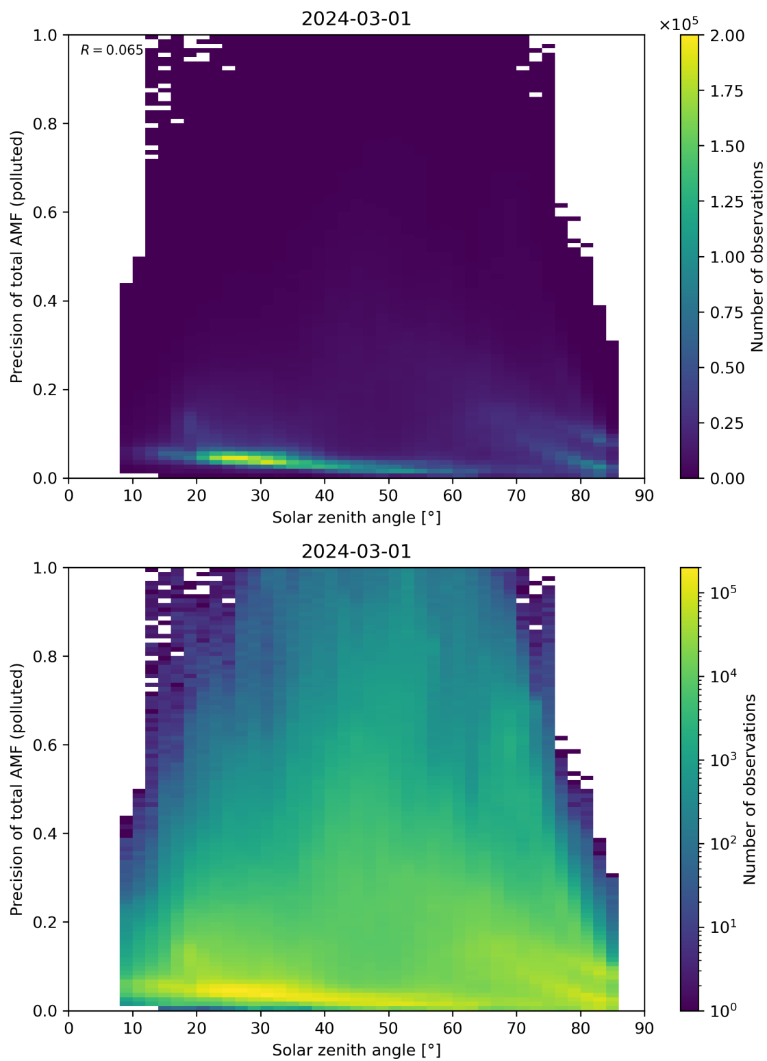
Figure 175: Scatter density plot of “Solar zenith angle” against “Precision of total AMF (polluted)” for 2024-02-29 to 2024-03-02.
