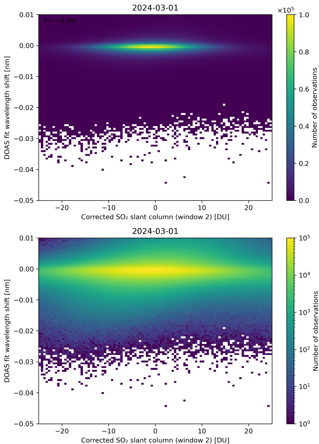
Figure 196: Scatter density plot of “Corrected SO 2 slant column (window 2)” against “DOAS fit wavelength shift” for 2024-02-29 to 2024-03-02.
