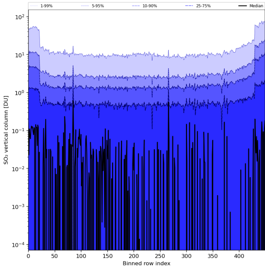
Figure 76: Along track statistics of “SO 2 vertical column” for 2024-02-29 to 2024-03-02
