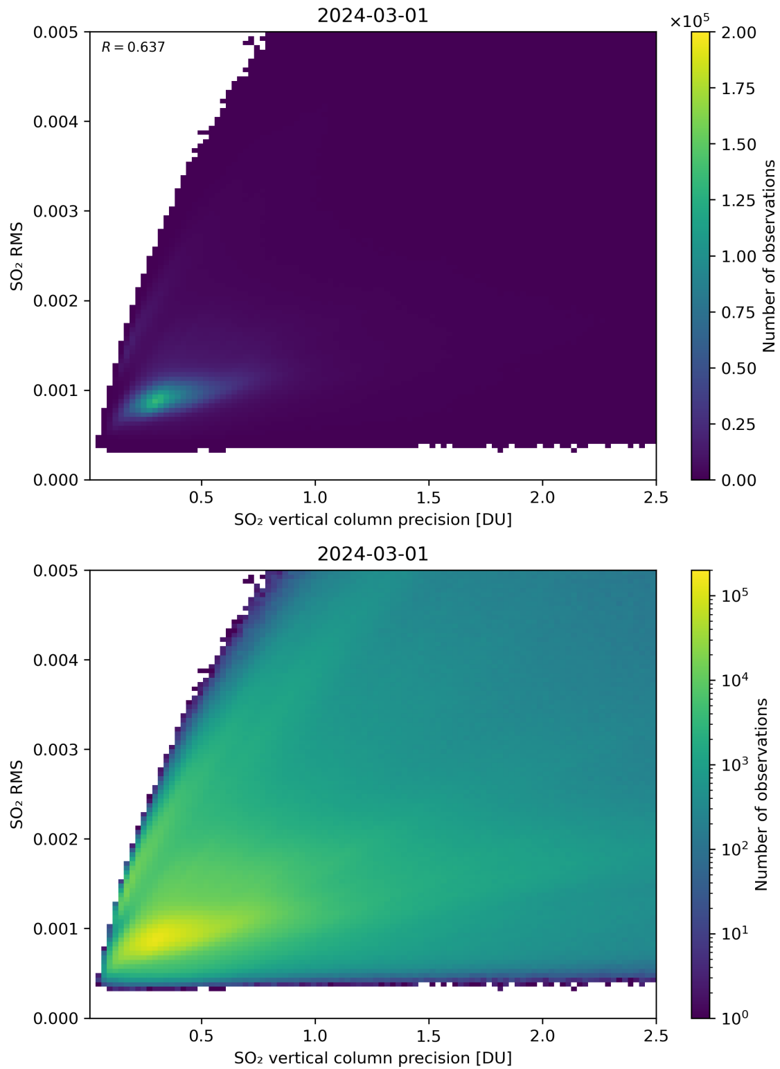
Figure 284: Scatter density plot of “SO 2 vertical column precision” against “SO 2 RMS” for 2024-02-29 to 2024-03-02.
