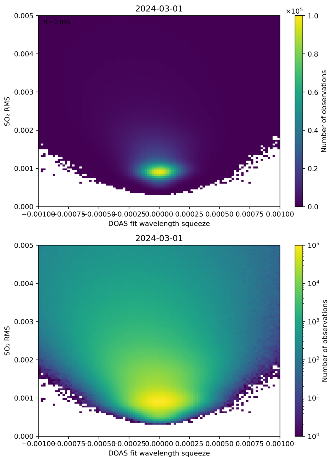
Figure 132: Scatter density plot of “DOAS fit wavelength squeeze” against “SO 2 RMS” for 2024-02-29 to 2024-03-02.
