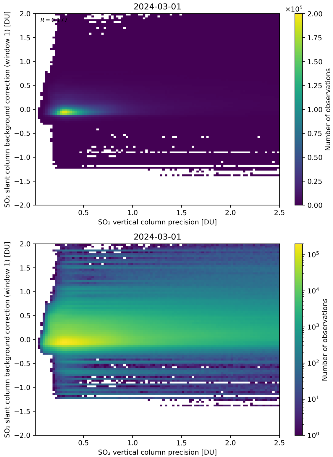
Figure 279: Scatter density plot of “SO 2 vertical column precision” against “SO 2 slant column background correction (window 1)” for 2024-02-29 to 2024-03-02.
