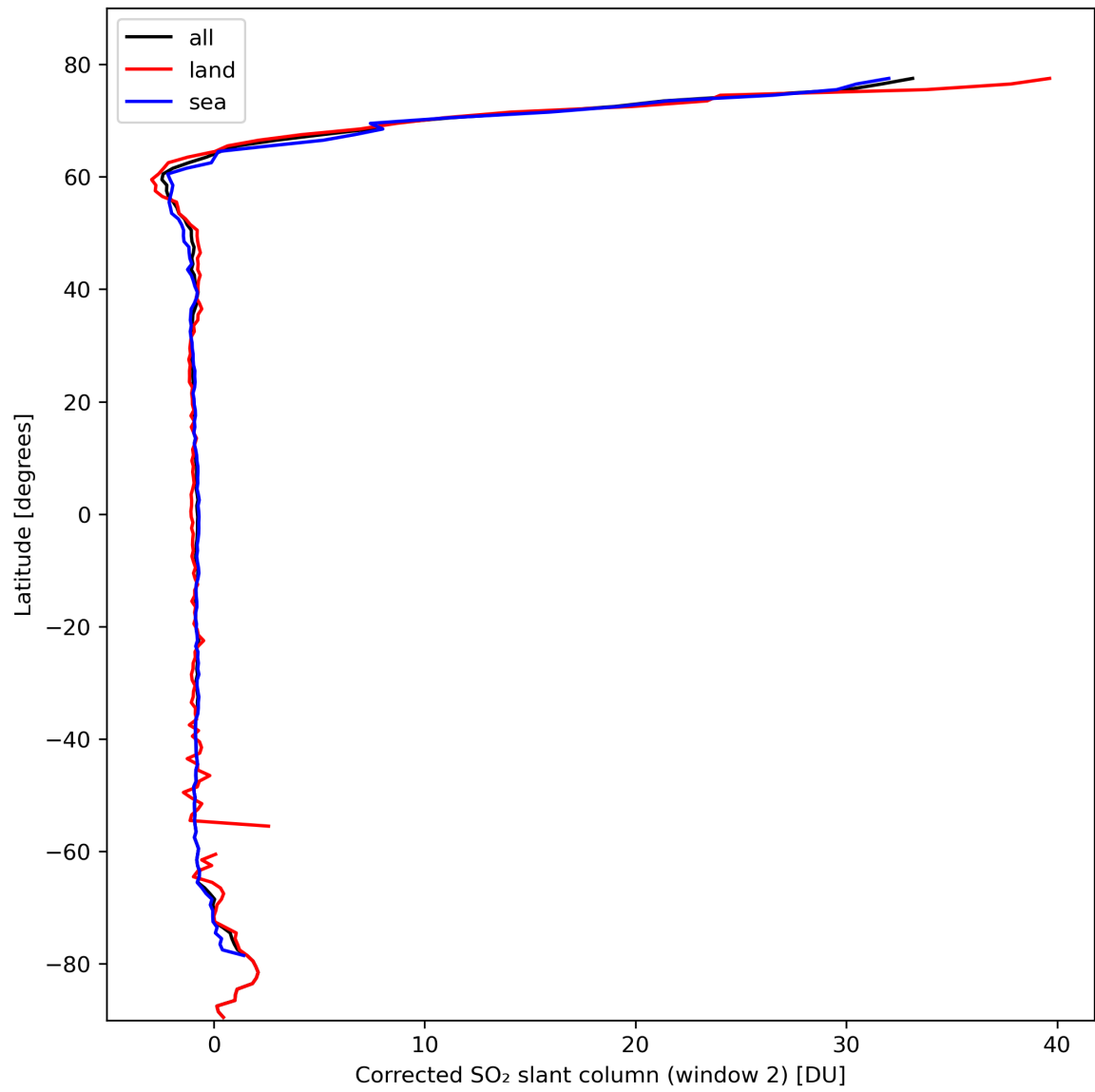
Figure 39: Zonal average of “Corrected SO 2 slant column (window 2)” for 2024-02-29 to 2024-03-02.
