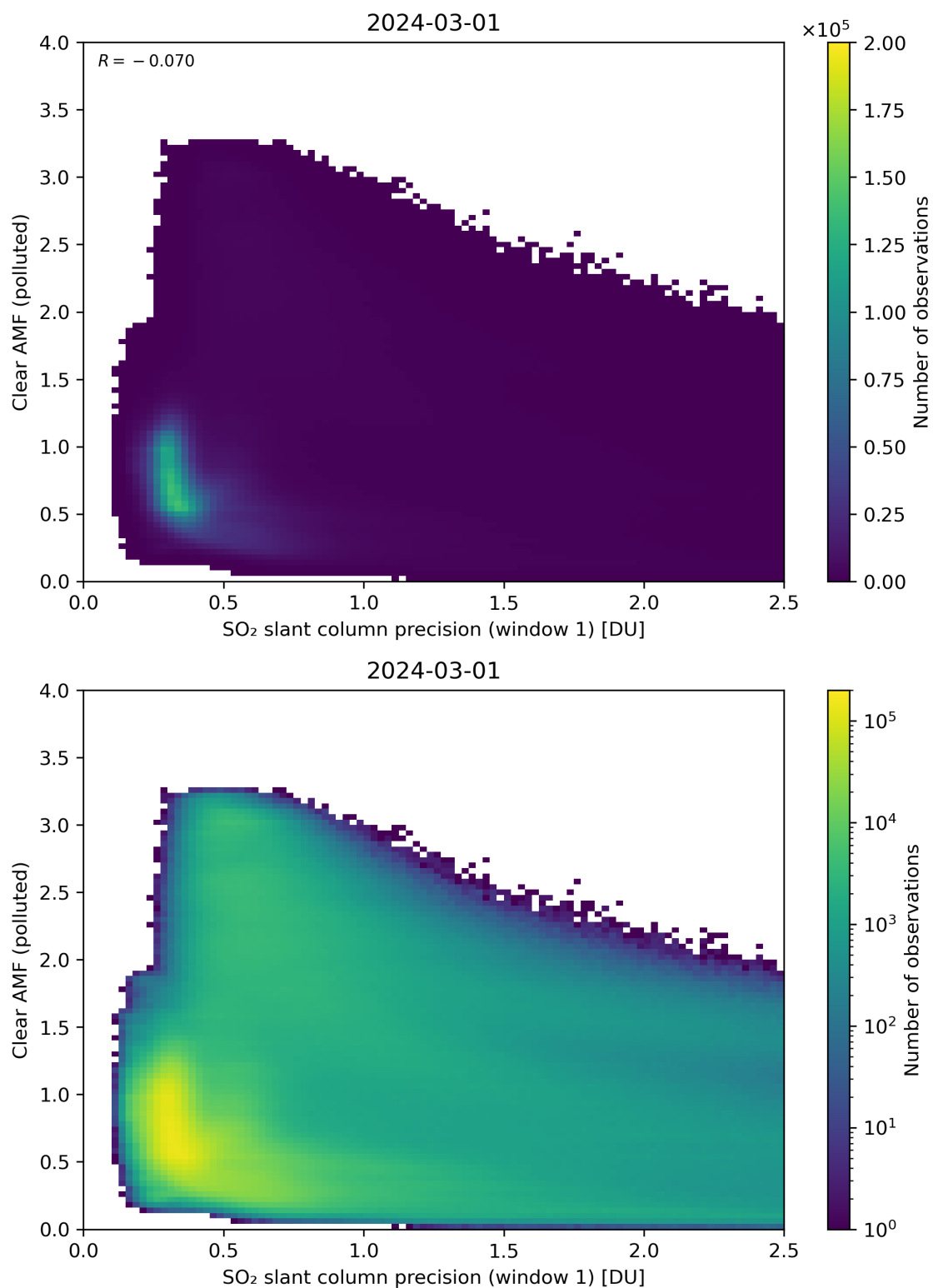
Figure 224: Scatter density plot of “SO 2 slant column precision (window 1)” against “Clear AMF (polluted)” for 2024-02-29 to 2024-03-02.
