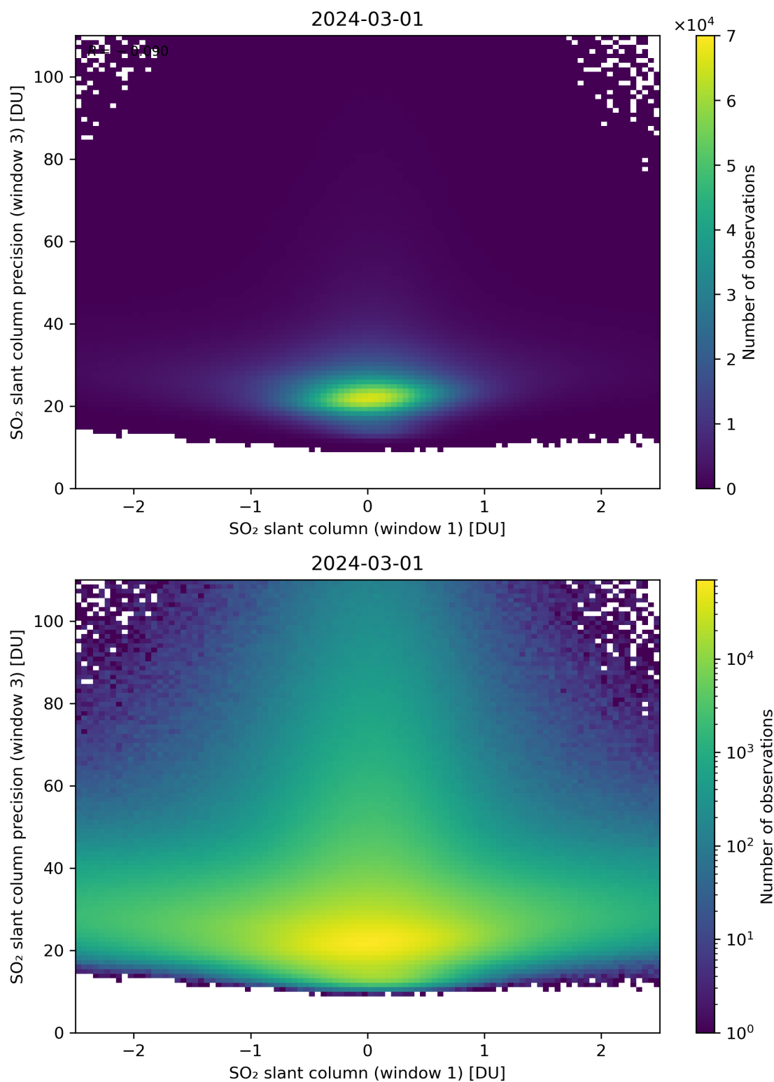
Figure 238: Scatter density plot of “SO 2 slant column (window 1)” against “SO 2 slant column precision (window 3)” for 2024-02-29 to 2024-03-02.
