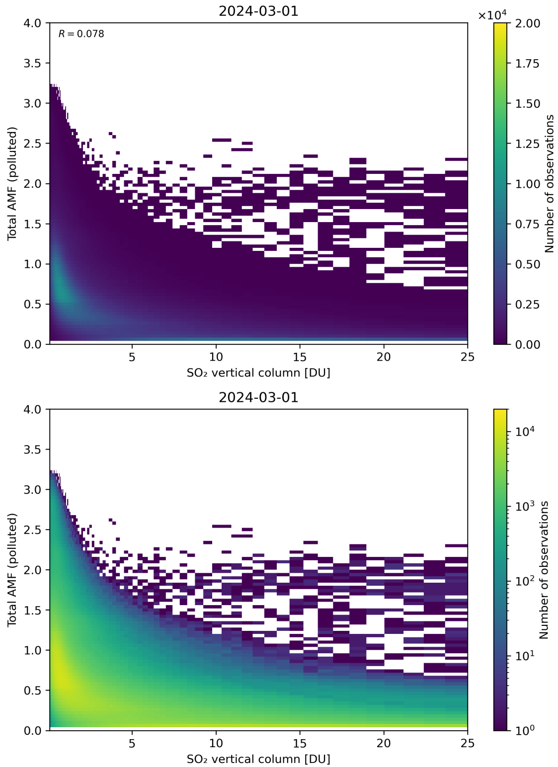
Figure 305: Scatter density plot of “SO 2 vertical column” against “Total AMF (polluted)” for 2024-02-29 to 2024-03-02.
