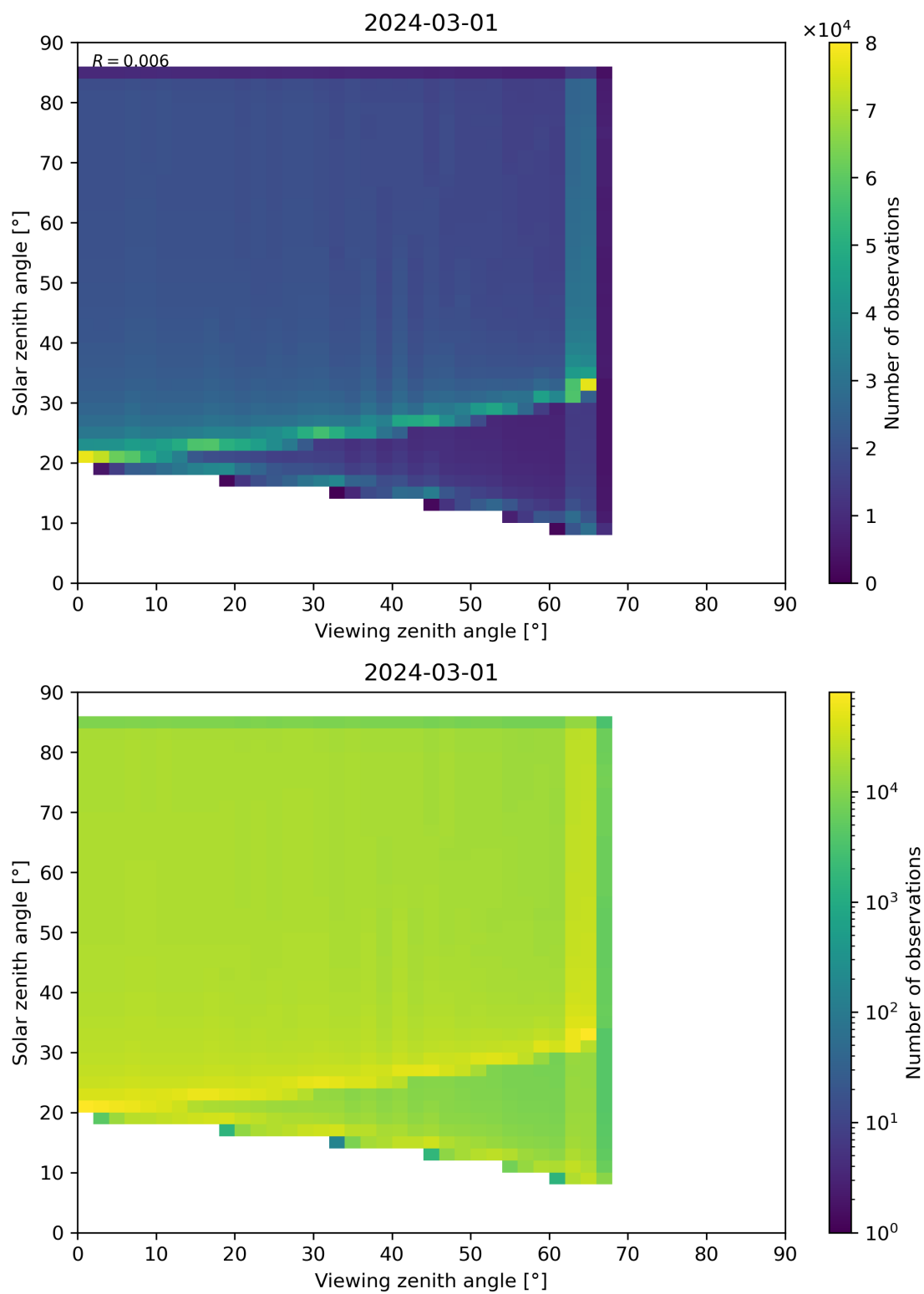
Figure 315: Scatter density plot of “Viewing zenith angle” against “Solar zenith angle” for 2024-02-29 to 2024-03-02.
