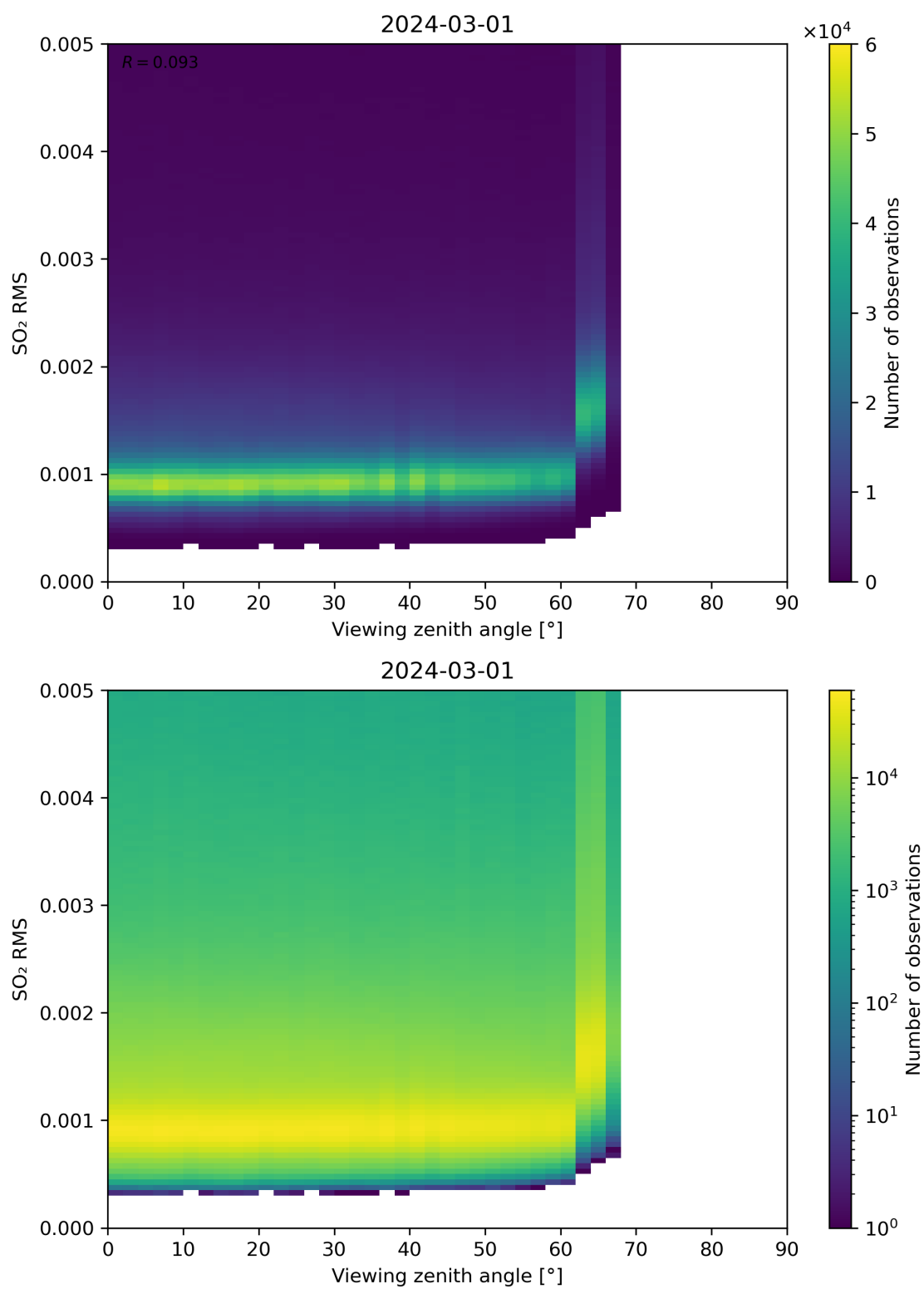
Figure 313: Scatter density plot of “Viewing zenith angle” against “SO 2 RMS” for 2024-02-29 to 2024-03-02.
