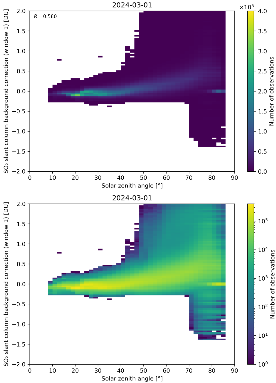
Figure 158: Scatter density plot of “Solar zenith angle” against “SO 2 slant column background correction (window 1)” for 2024-02-29 to 2024-03-02.
