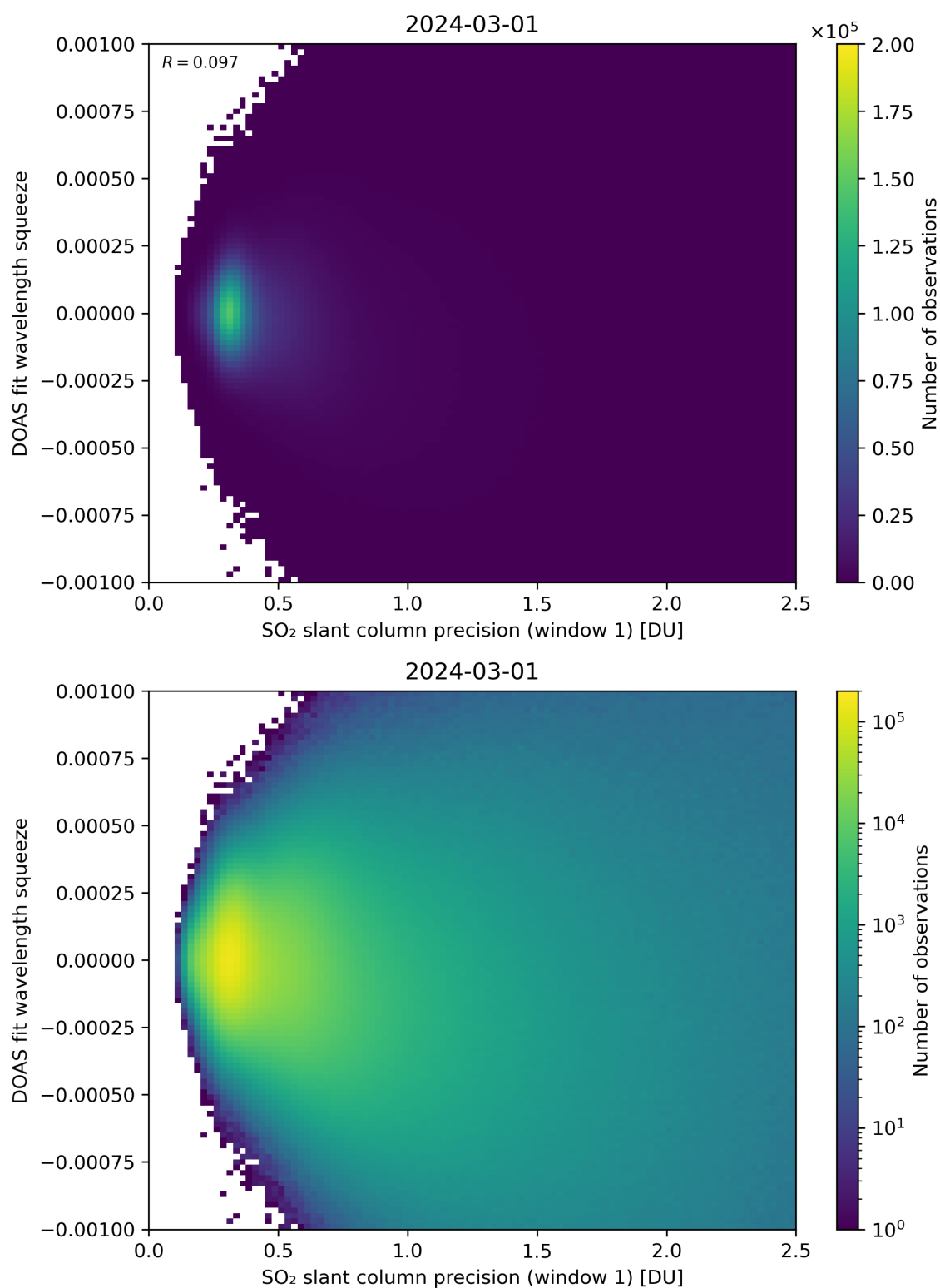
Figure 222: Scatter density plot of “SO 2 slant column precision (window 1)” against “DOAS fit wavelength squeeze” for 2024-02-29 to 2024-03-02.
