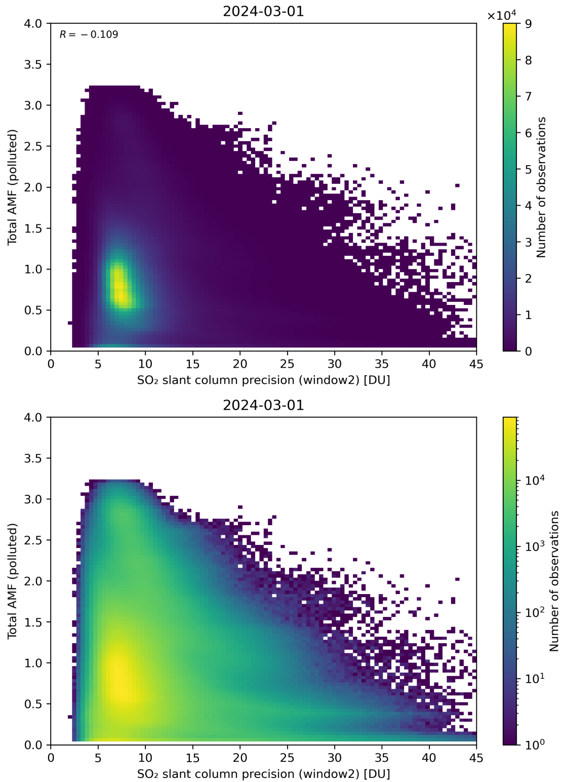
Figure 251: Scatter density plot of “SO 2 slant column precision (window2)” against “Total AMF (polluted)” for 2024-02-29 to 2024-03-02.
