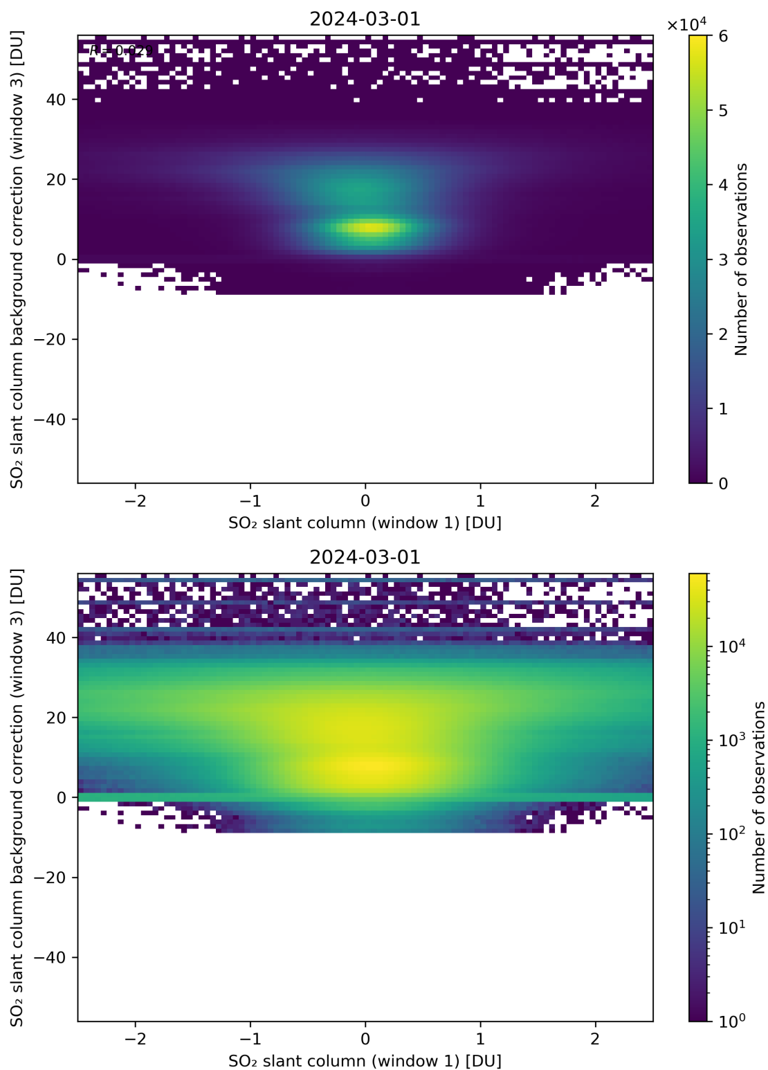
Figure 214: Scatter density plot of “SO 2 slant column (window 1)” against “SO 2 slant column background correction (window 3)” for 2024-02-29 to 2024-03-02.
