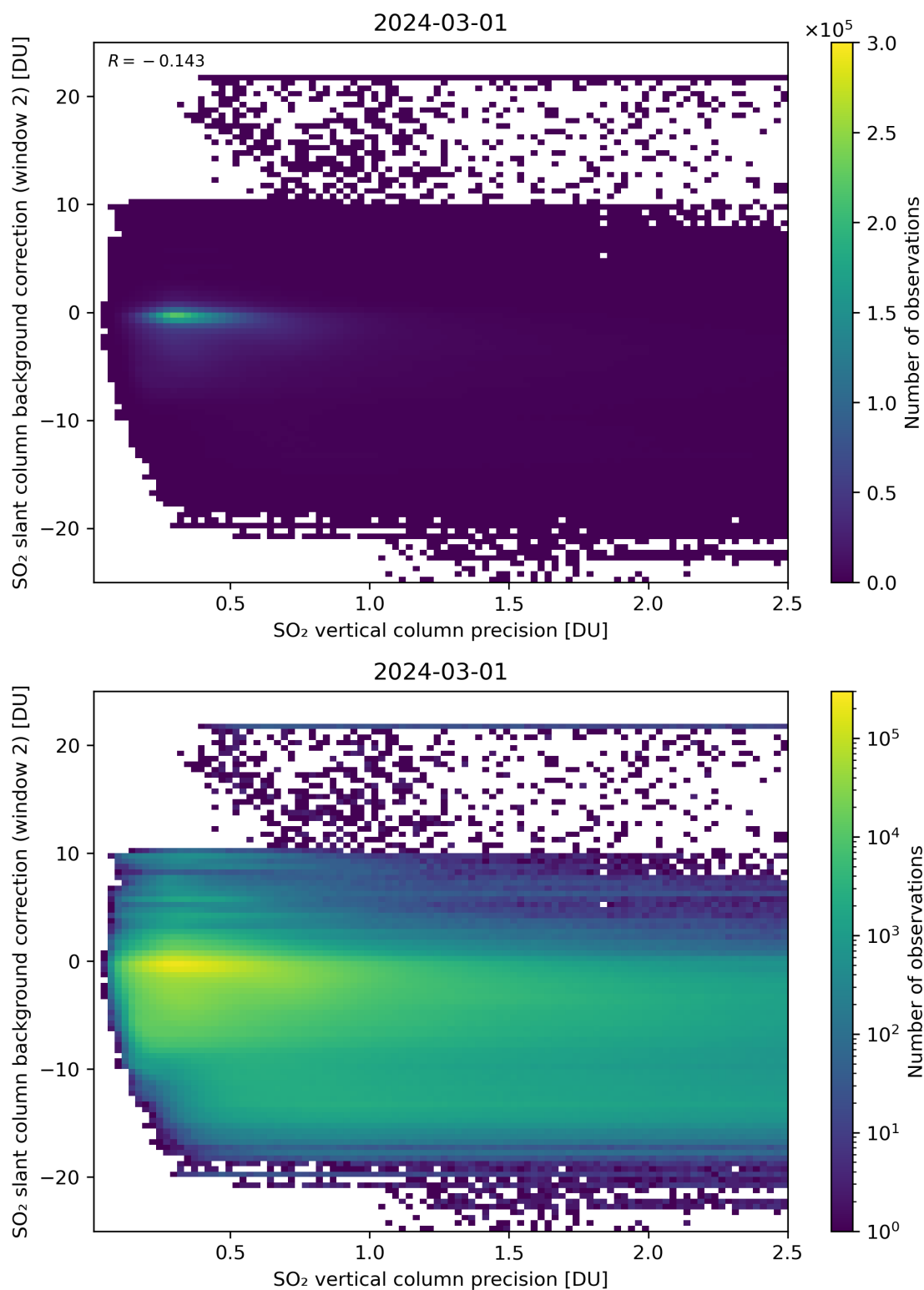
Figure 280: Scatter density plot of “SO 2 vertical column precision” against “SO 2 slant column background correction (window 2)” for 2024-02-29 to 2024-03-02.
