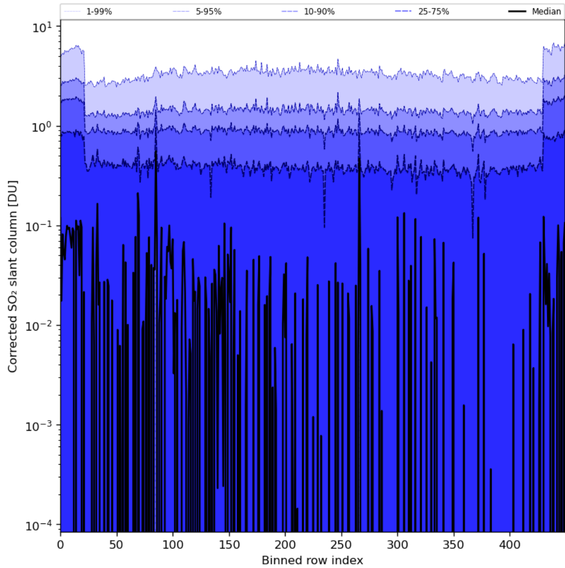
Figure 78: Along track statistics of “Corrected SO 2 slant column” for 2024-02-29 to 2024-03-02
