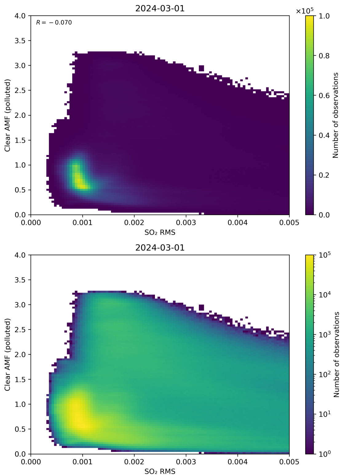
Figure 136: Scatter density plot of “SO 2 RMS” against “Clear AMF (polluted)” for 2024-02-29 to 2024-03-02.
