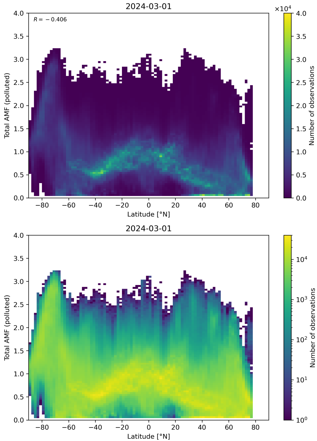
Figure 154: Scatter density plot of “Latitude” against “Total AMF (polluted)” for 2024-02-29 to 2024-03-02.
