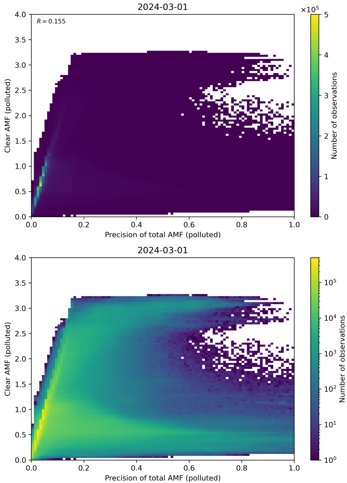
Figure 270: Scatter density plot of “Precision of total AMF (polluted)” against “Clear AMF (polluted)” for 2024-02-29 to 2024-03-02.
