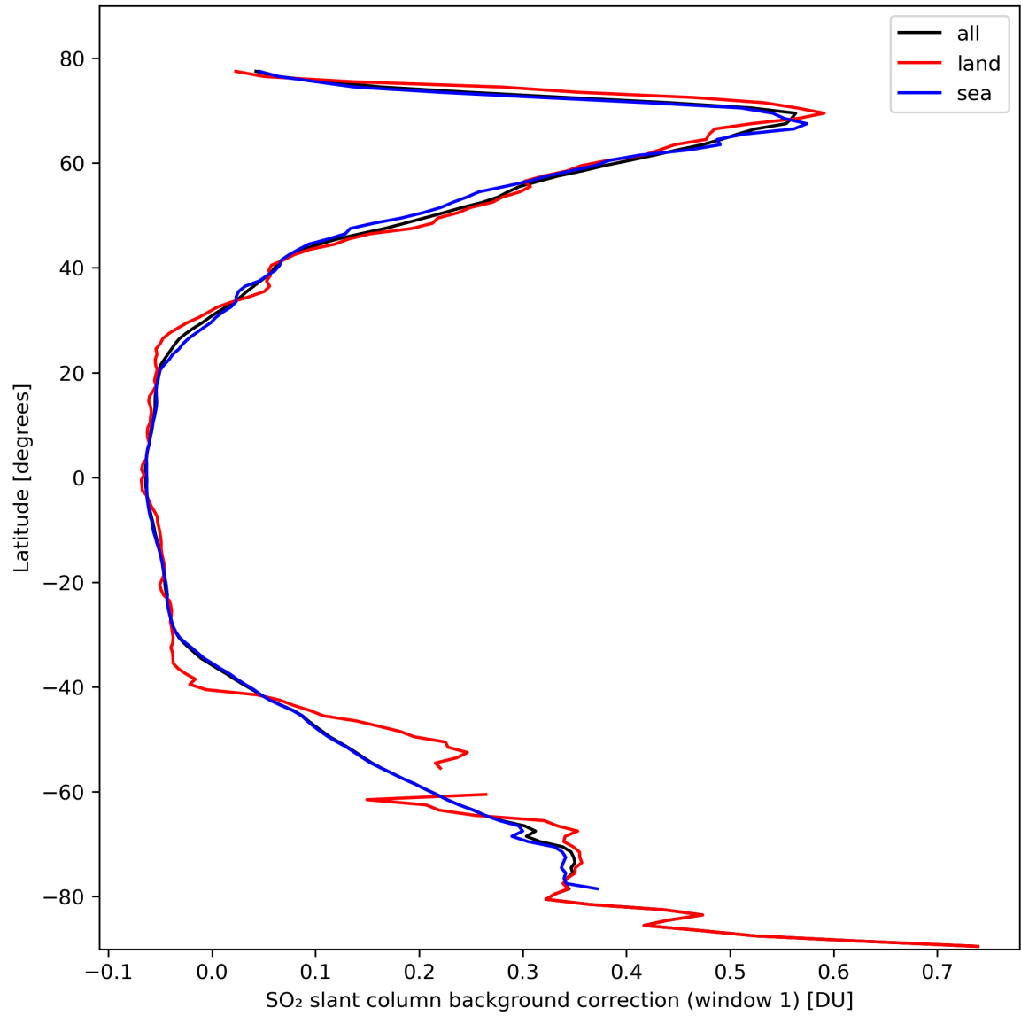
Figure 36: Zonal average of “SO 2 slant column background correction (window 1)” for 2024-02-29 to 2024-03-02.
