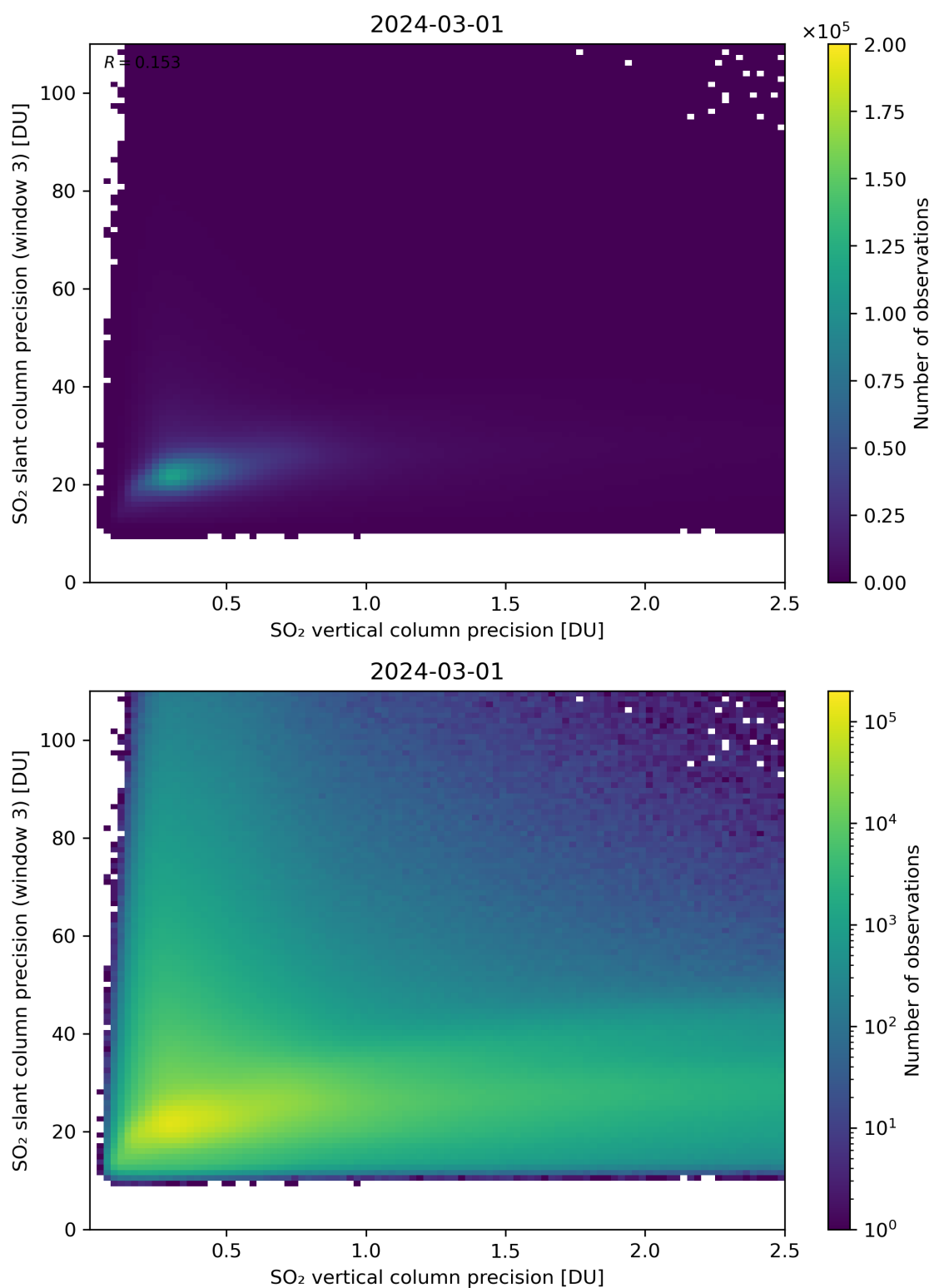
Figure 293: Scatter density plot of “SO 2 vertical column precision” against “SO 2 slant column precision (window 3)” for 2024-02-29 to 2024-03-02.
