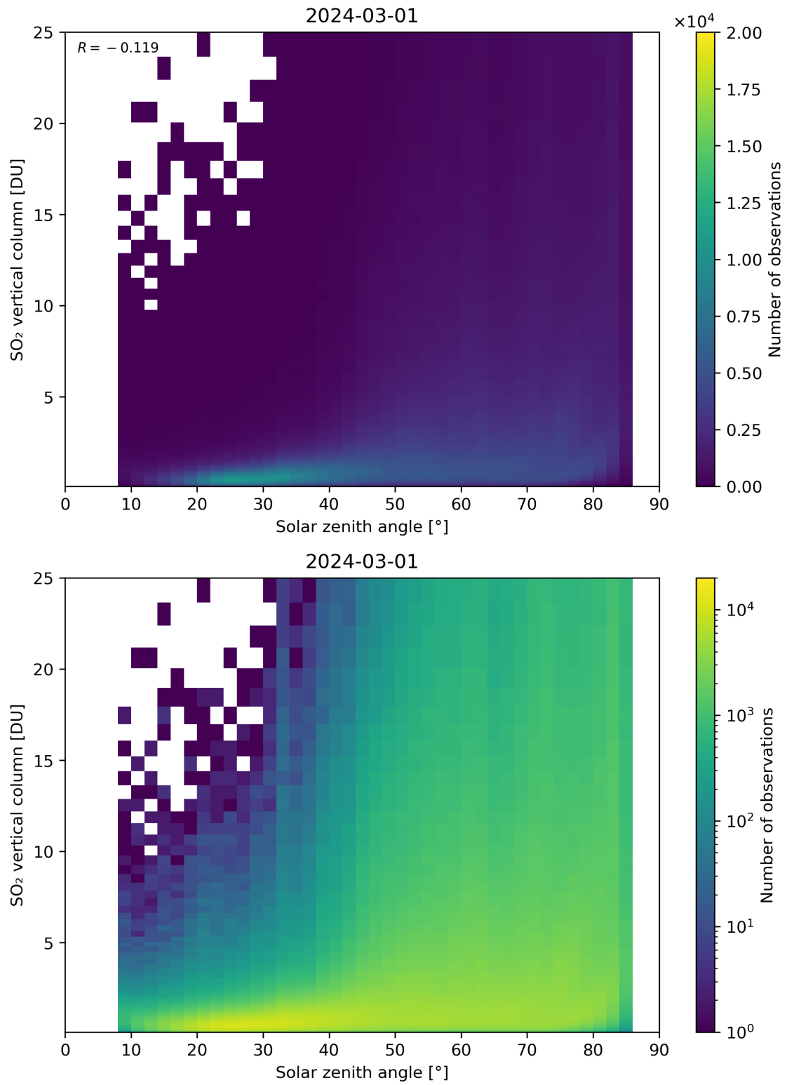
Figure 176: Scatter density plot of “Solar zenith angle” against “SO 2 vertical column” for 2024-02-29 to 2024-03-02.
