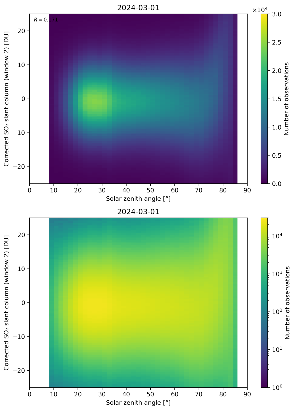
Figure 167: Scatter density plot of “Solar zenith angle” against “Corrected SO 2 slant column (window 2)” for 2024-02-29 to 2024-03-02.
