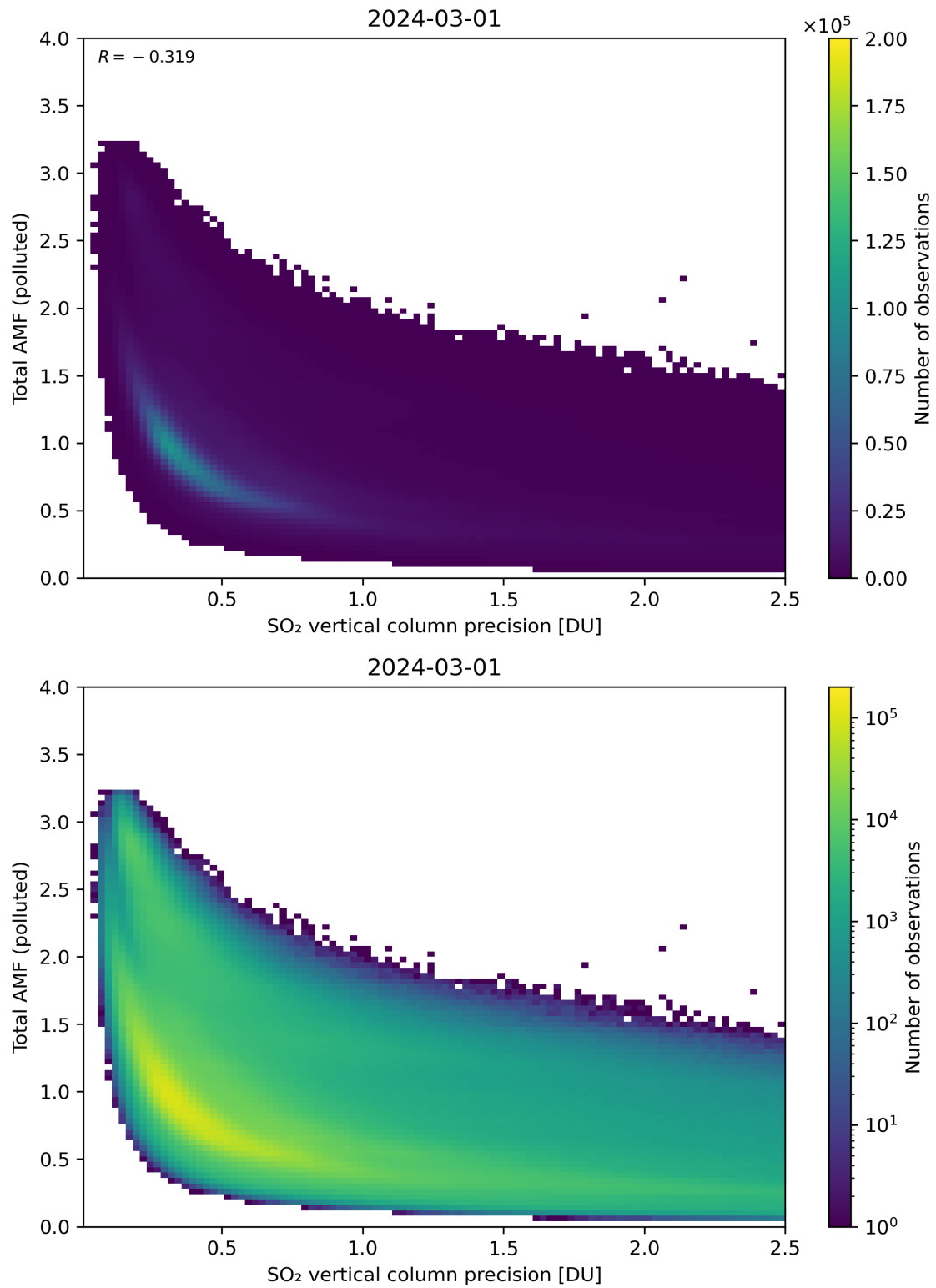
Figure 294: Scatter density plot of “SO 2 vertical column precision” against “Total AMF (polluted)” for 2024-02-29 to 2024-03-02.
