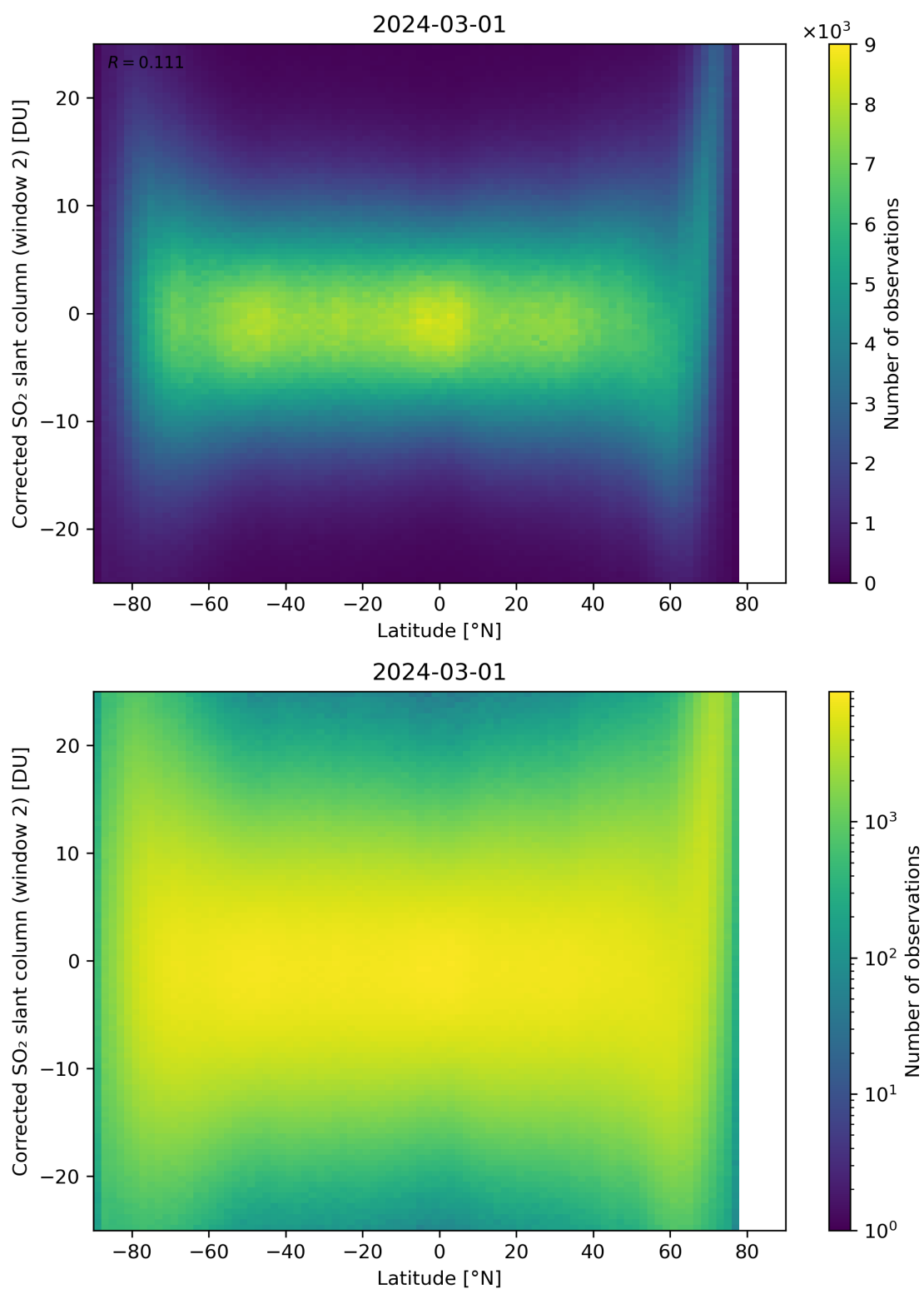
Figure 147: Scatter density plot of “Latitude” against “Corrected SO 2 slant column (window 2)” for 2024-02-29 to 2024-03-02.
