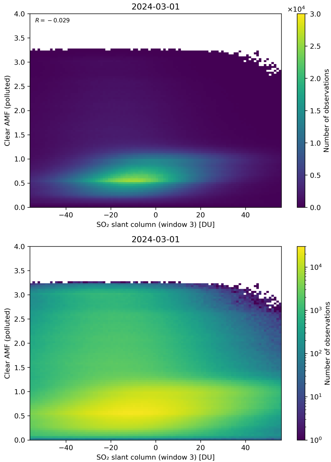
Figure 265: Scatter density plot of “SO 2 slant column (window 3)” against “Clear AMF (polluted)” for 2024-02-29 to 2024-03-02.
