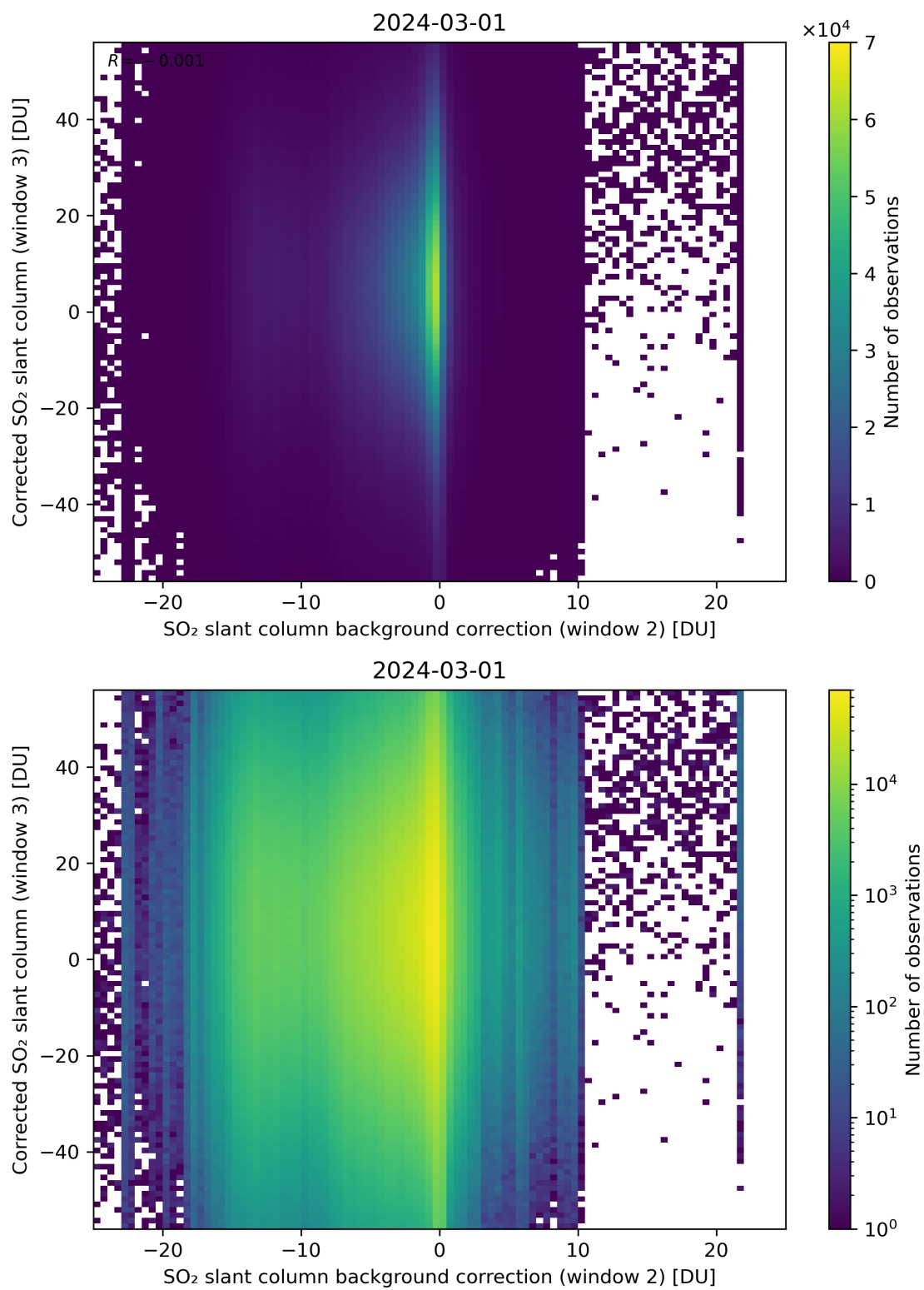
Figure 116: Scatter density plot of “SO 2 slant column background correction (window 2)” against “Corrected SO 2 slant column (window 3)” for 2024-02-29 to 2024-03-02.
