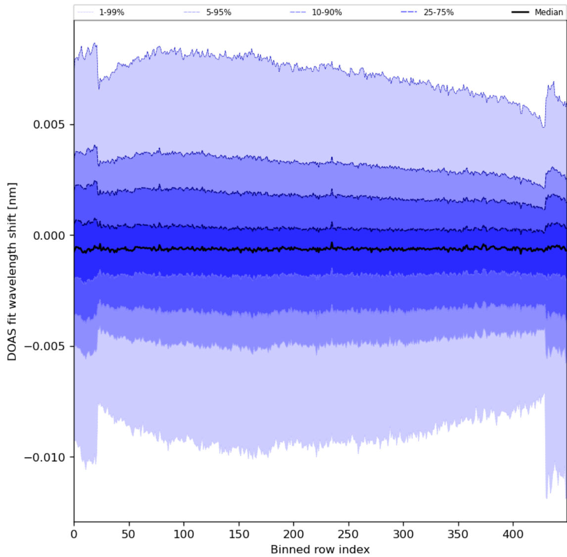
Figure 91: Along track statistics of “DOAS fit wavelength shift” for 2024-02-29 to 2024-03-02
