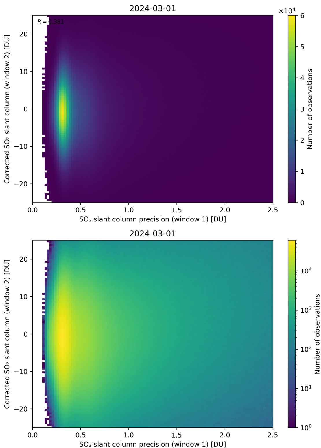
Figure 225: Scatter density plot of “SO 2 slant column precision (window 1)” against “Corrected SO 2 slant column (window 2)” for 2024-02-29 to 2024-03-02.
