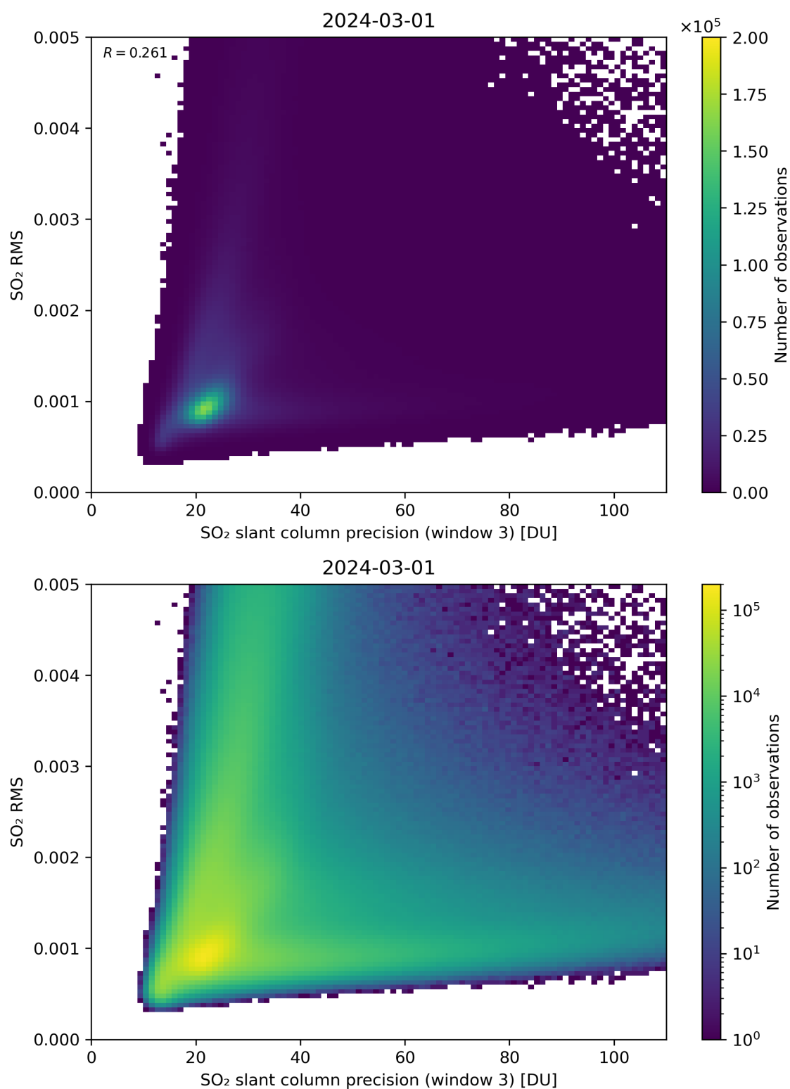
Figure 260: Scatter density plot of “SO 2 slant column precision (window 3)” against “SO 2 RMS” for 2024-02-29 to 2024-03-02.
