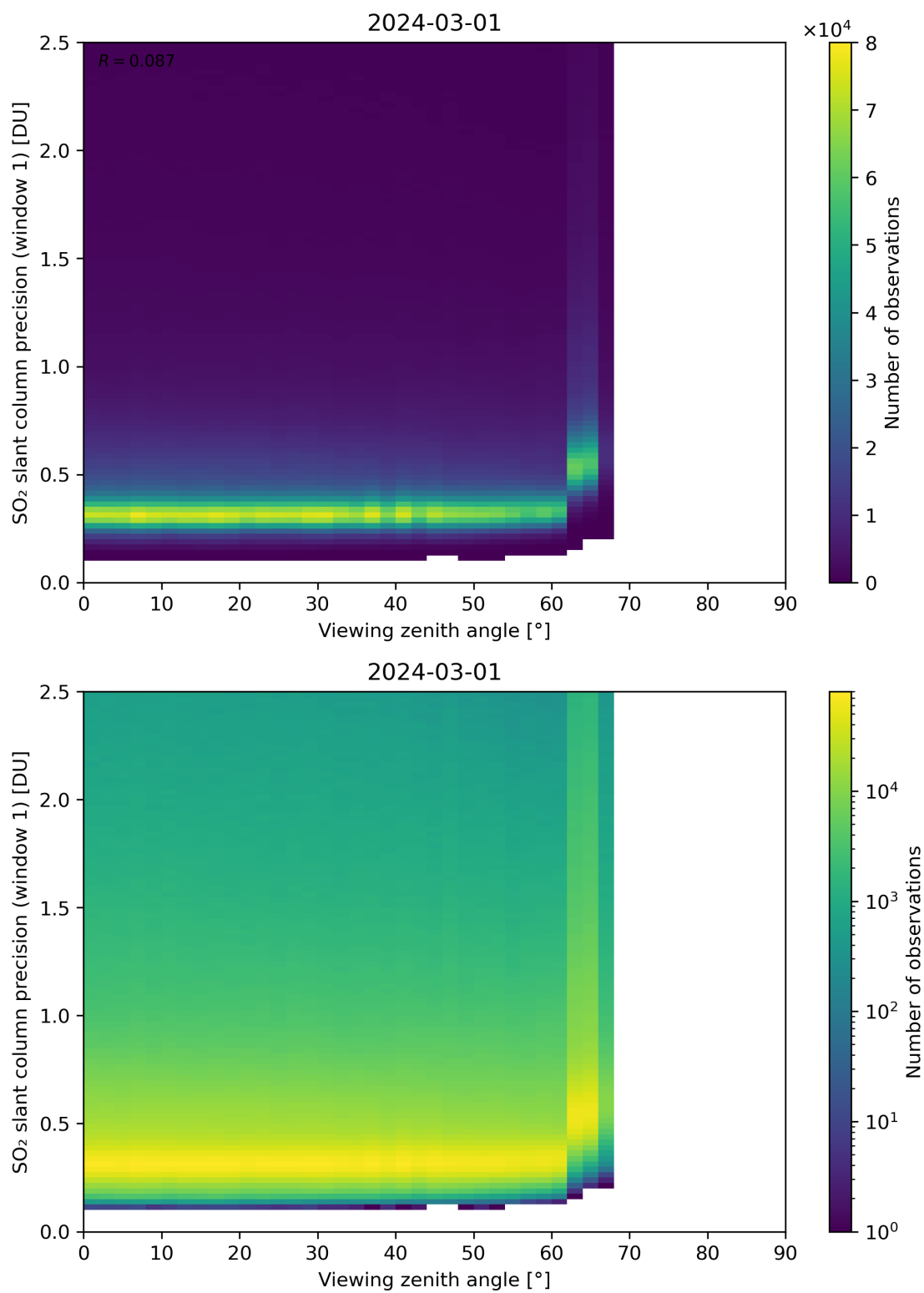
Figure 321: Scatter density plot of “Viewing zenith angle” against “SO 2 slant column precision (window 1)” for 2024-02-29 to 2024-03-02.
