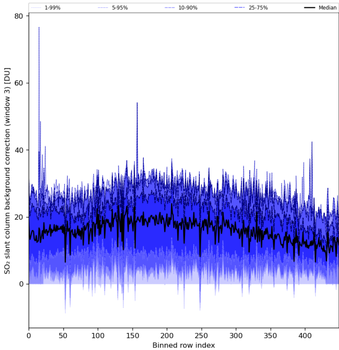
Figure 90: Along track statistics of “SO 2 slant column background correction (window 3)” for 2024-02-29 to 2024-03-02
