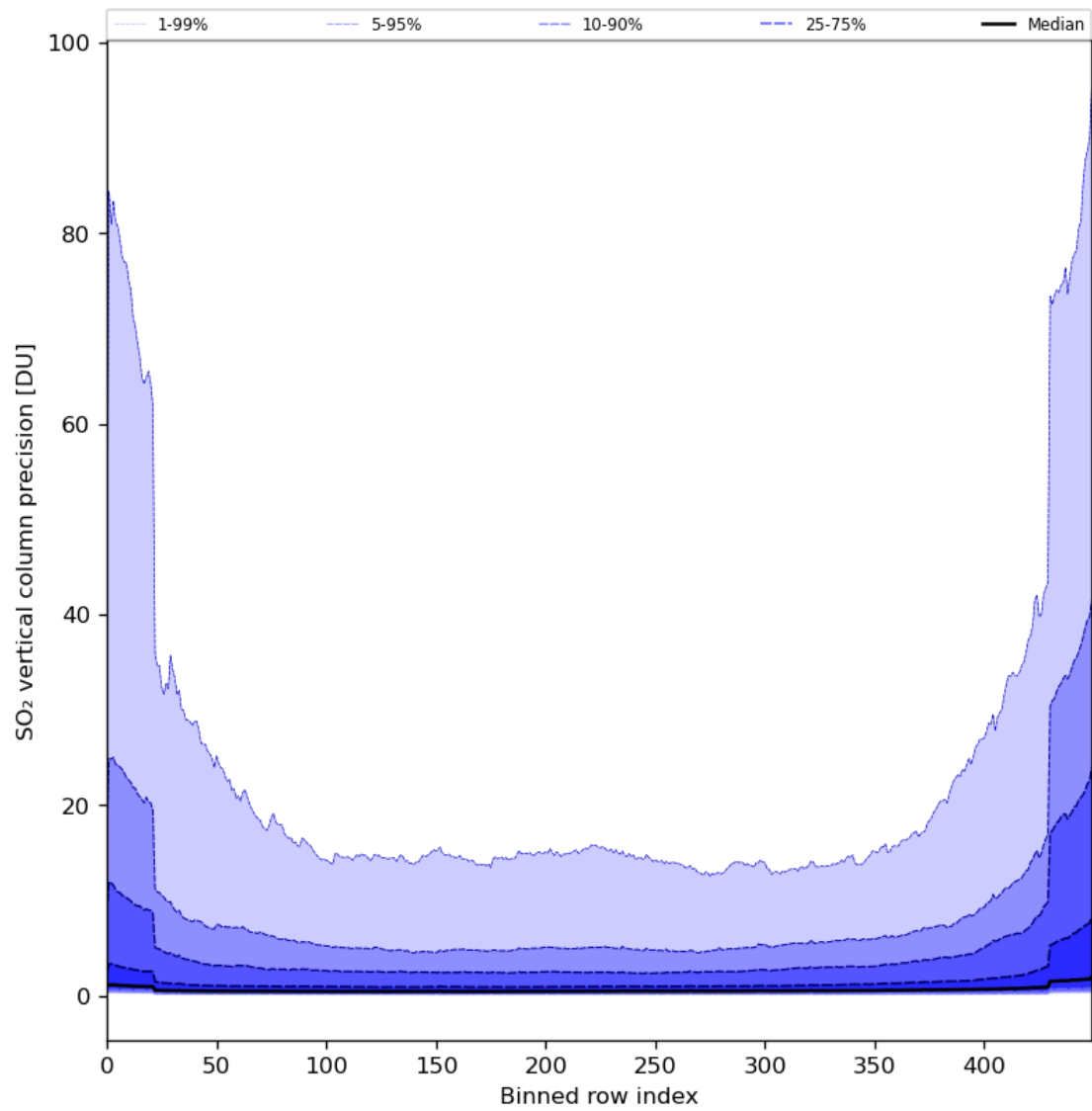
Figure 77: Along track statistics of “SO 2 vertical column precision” for 2024-02-29 to 2024-03-02
