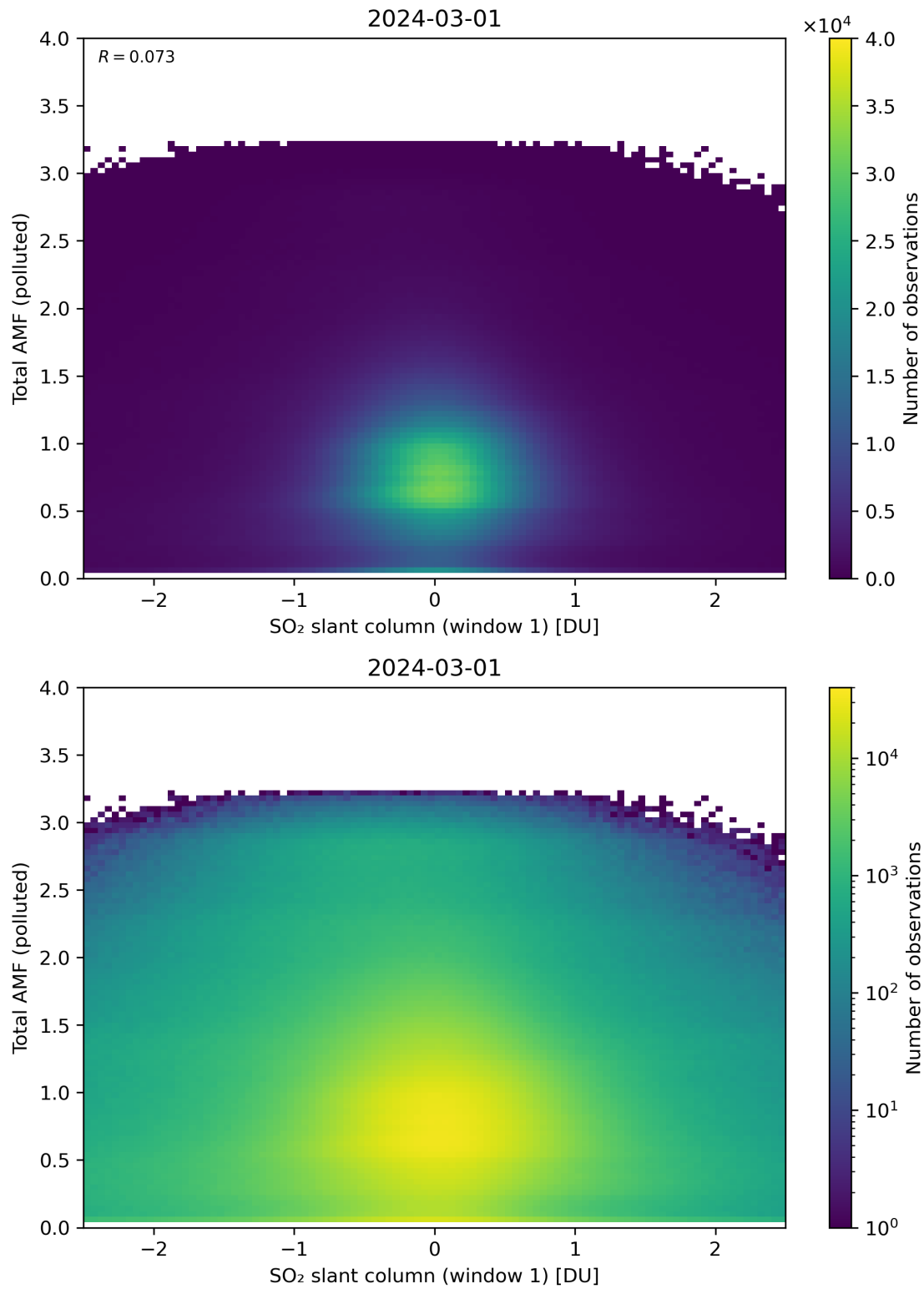
Figure 239: Scatter density plot of “SO 2 slant column (window 1)” against “Total AMF (polluted)” for 2024-02-29 to 2024-03-02.
