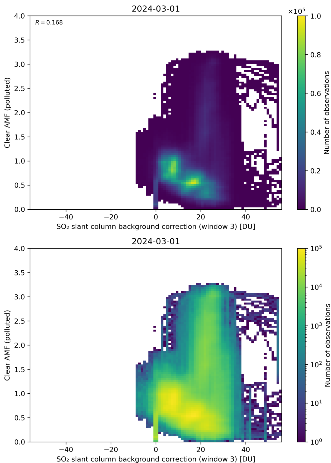
Figure 124: Scatter density plot of “SO 2 slant column background correction (window 3)” against “Clear AMF (polluted)” for 2024-02-29 to 2024-03-02.
