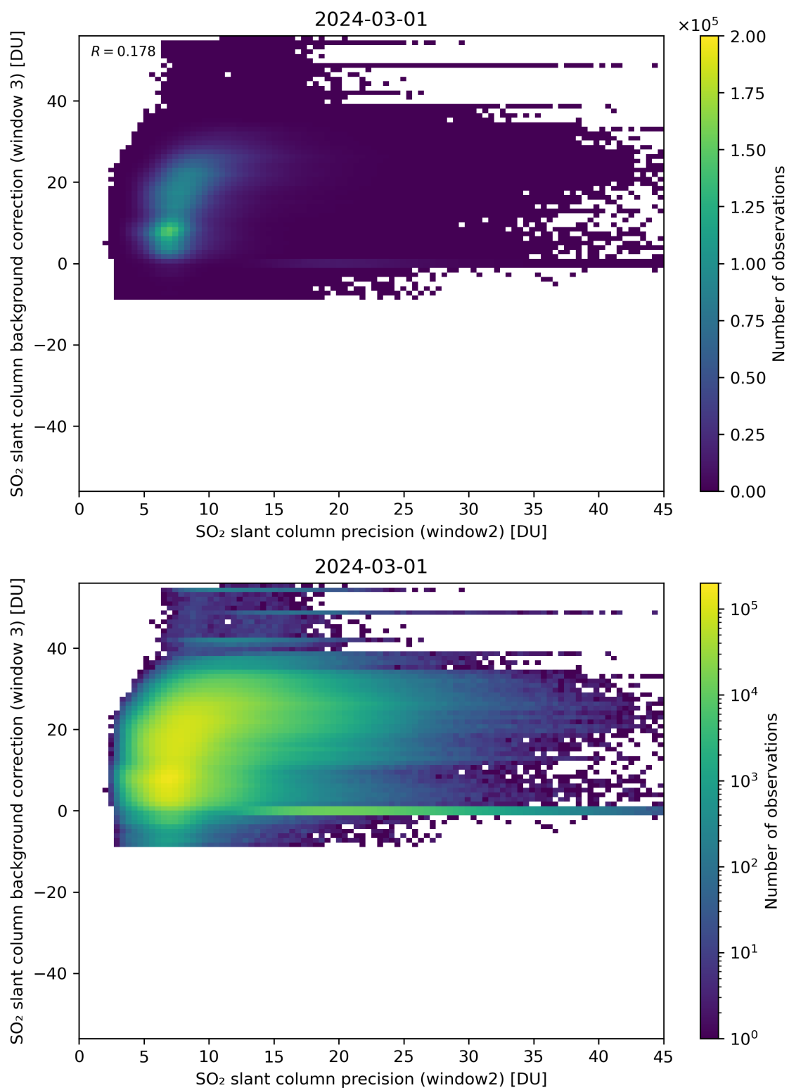
Figure 242: Scatter density plot of “SO 2 slant column precision (window2)” against “SO 2 slant column background correction (window 3)” for 2024-02-29 to 2024-03-02.
