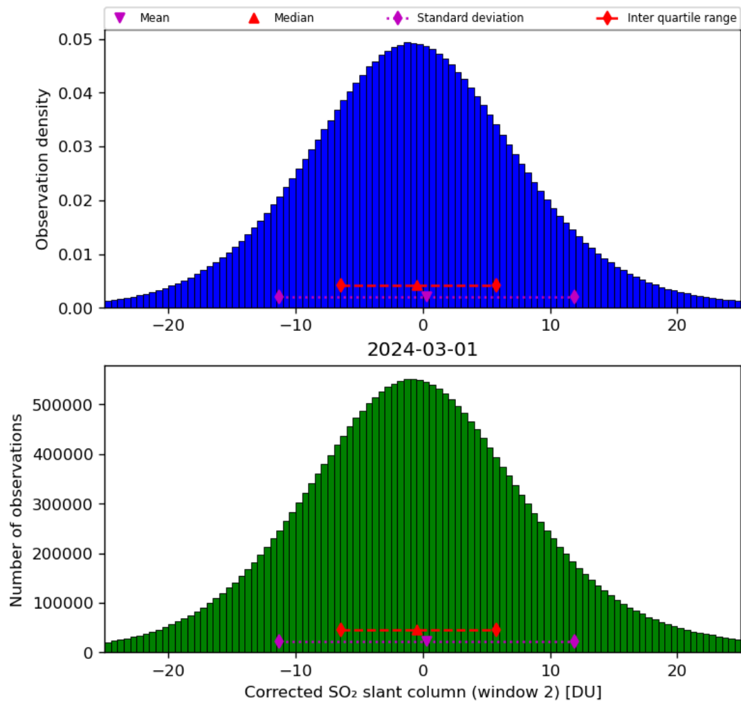
Figure 62: Histogram of “Corrected SO 2 slant column (window 2)” for 2024-02-29 to 2024-03-02
