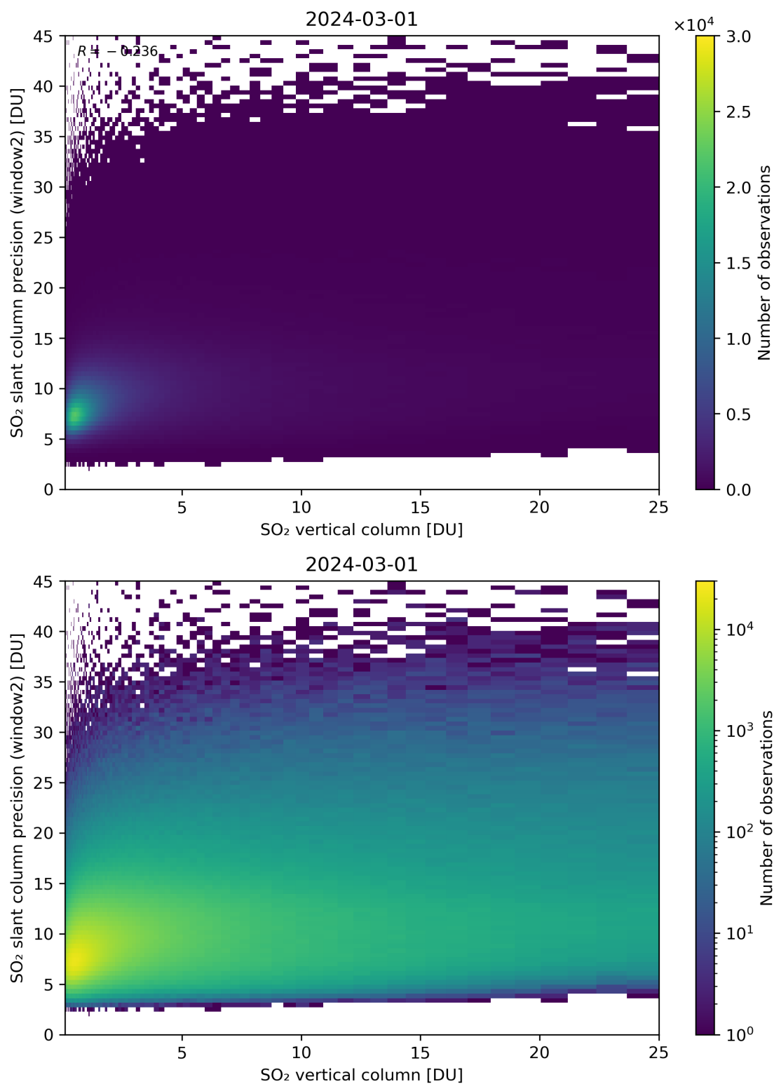
Figure 302: Scatter density plot of “SO 2 vertical column” against “SO 2 slant column precision (window2)” for 2024-02-29 to 2024-03-02.
