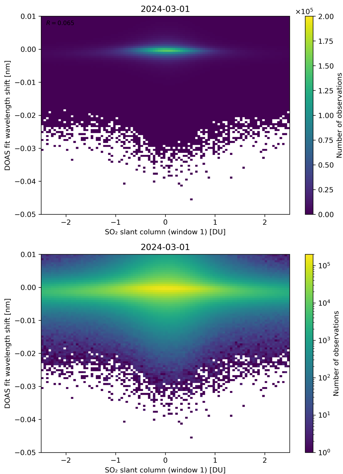
Figure 215: Scatter density plot of “SO 2 slant column (window 1)” against “DOAS fit wavelength shift” for 2024-02-29 to 2024-03-02.
