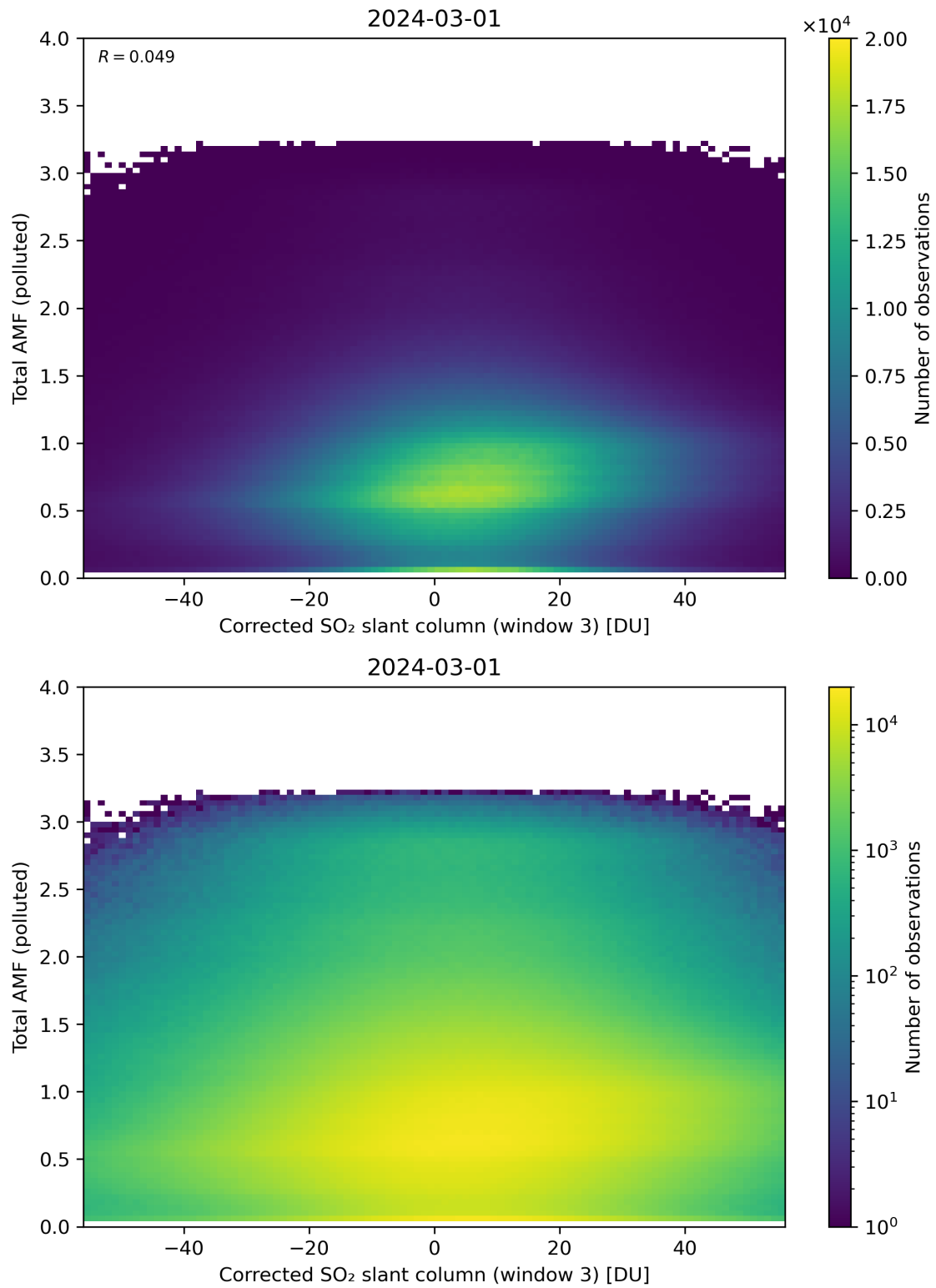
Figure 210: Scatter density plot of “Corrected SO 2 slant column (window 3)” against “Total AMF (polluted)” for 2024-02-29 to 2024-03-02.
