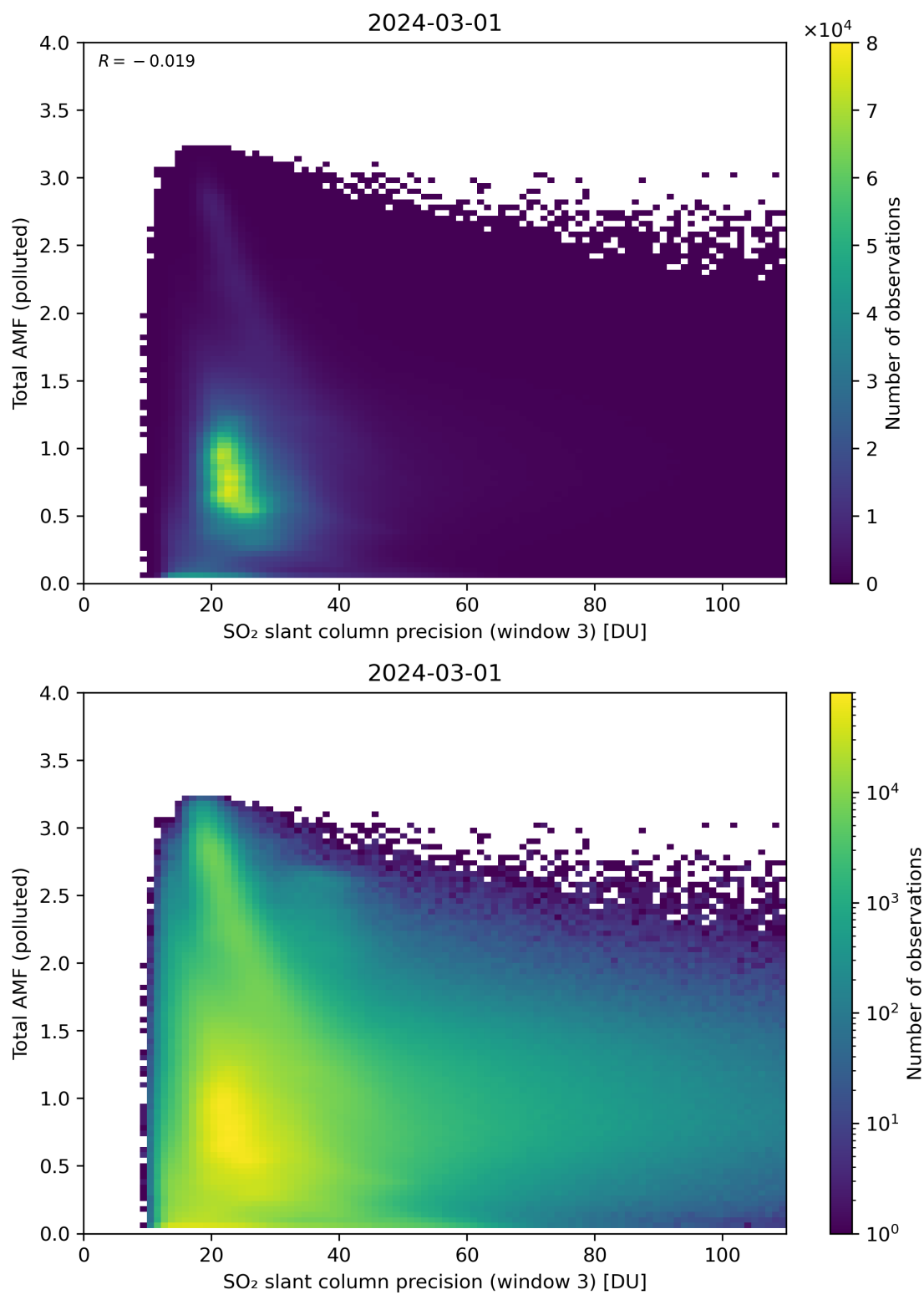
Figure 263: Scatter density plot of “SO 2 slant column precision (window 3)” against “Total AMF (polluted)” for 2024-02-29 to 2024-03-02.
