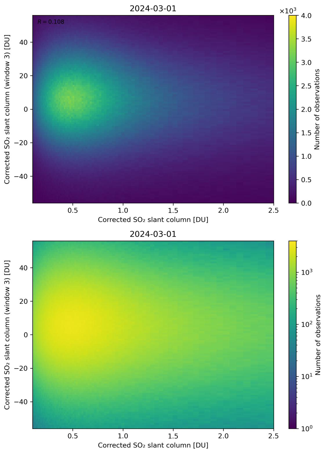
Figure 186: Scatter density plot of “Corrected SO 2 slant column” against “Corrected SO 2 slant column (window 3)” for 2024-02-29 to 2024-03-02.
