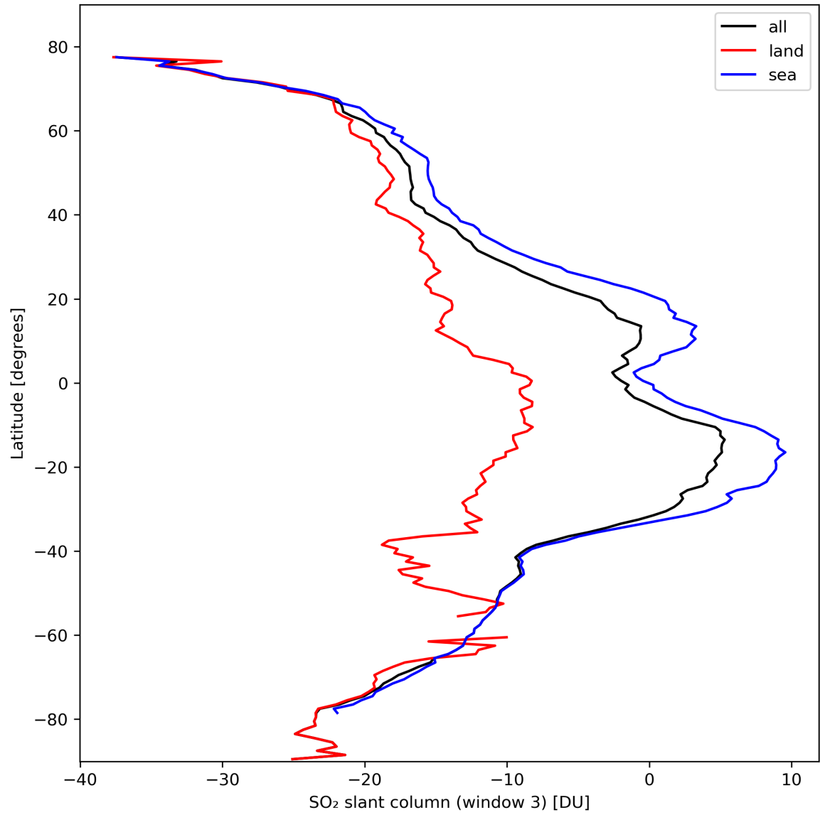
Figure 41: Zonal average of “SO 2 slant column (window 3)” for 2024-02-29 to 2024-03-02.
