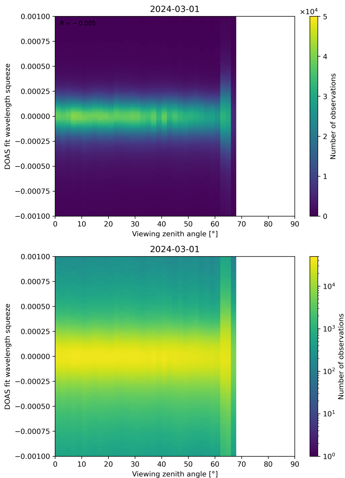
Figure 312: Scatter density plot of “Viewing zenith angle” against “DOAS fit wavelength squeeze” for 2024-02-29 to 2024-03-02.
