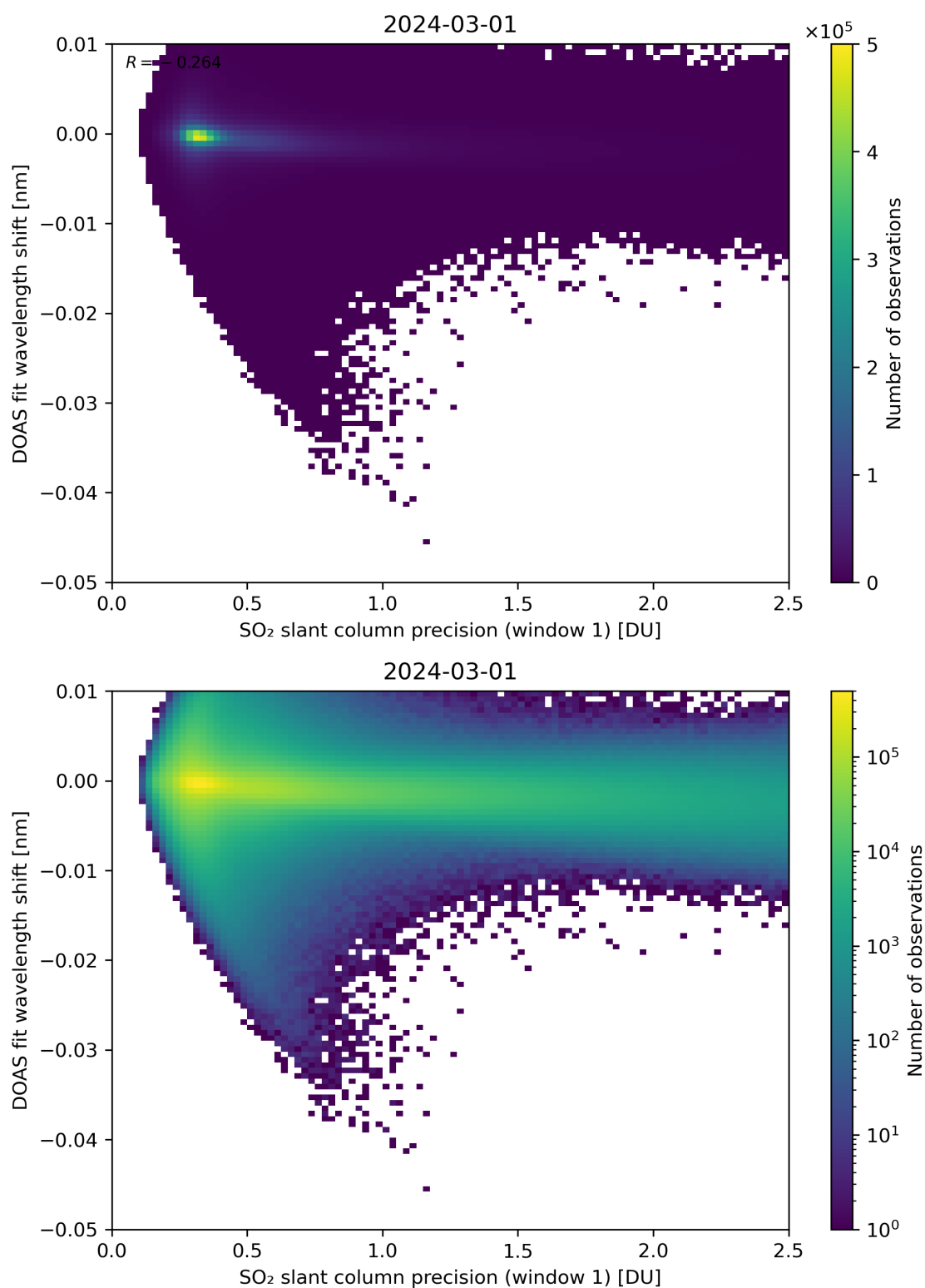
Figure 221: Scatter density plot of “SO 2 slant column precision (window 1)” against “DOAS fit wavelength shift” for 2024-02-29 to 2024-03-02.
