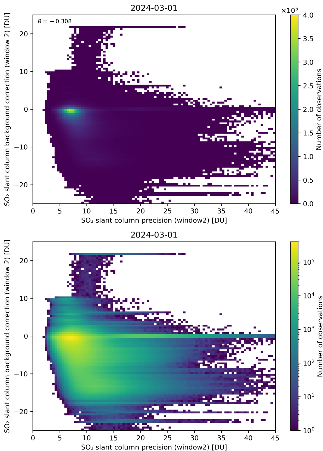
Figure 241: Scatter density plot of “SO 2 slant column precision (window2)” against “SO 2 slant column background correction (window 2)” for 2024-02-29 to 2024-03-02.
