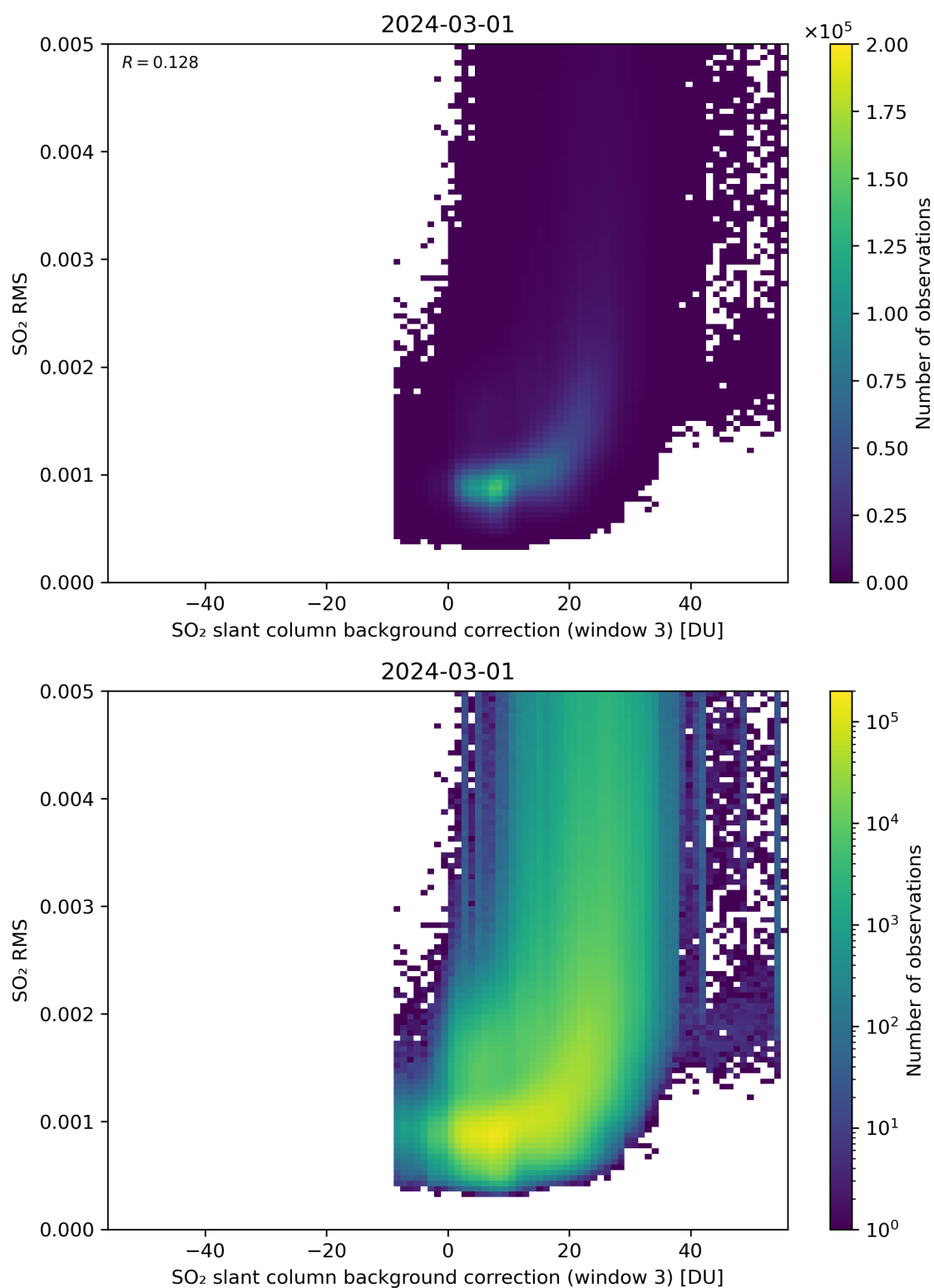
Figure 123: Scatter density plot of “SO 2 slant column background correction (window 3)” against “SO 2 RMS” for 2024-02-29 to 2024-03-02.
