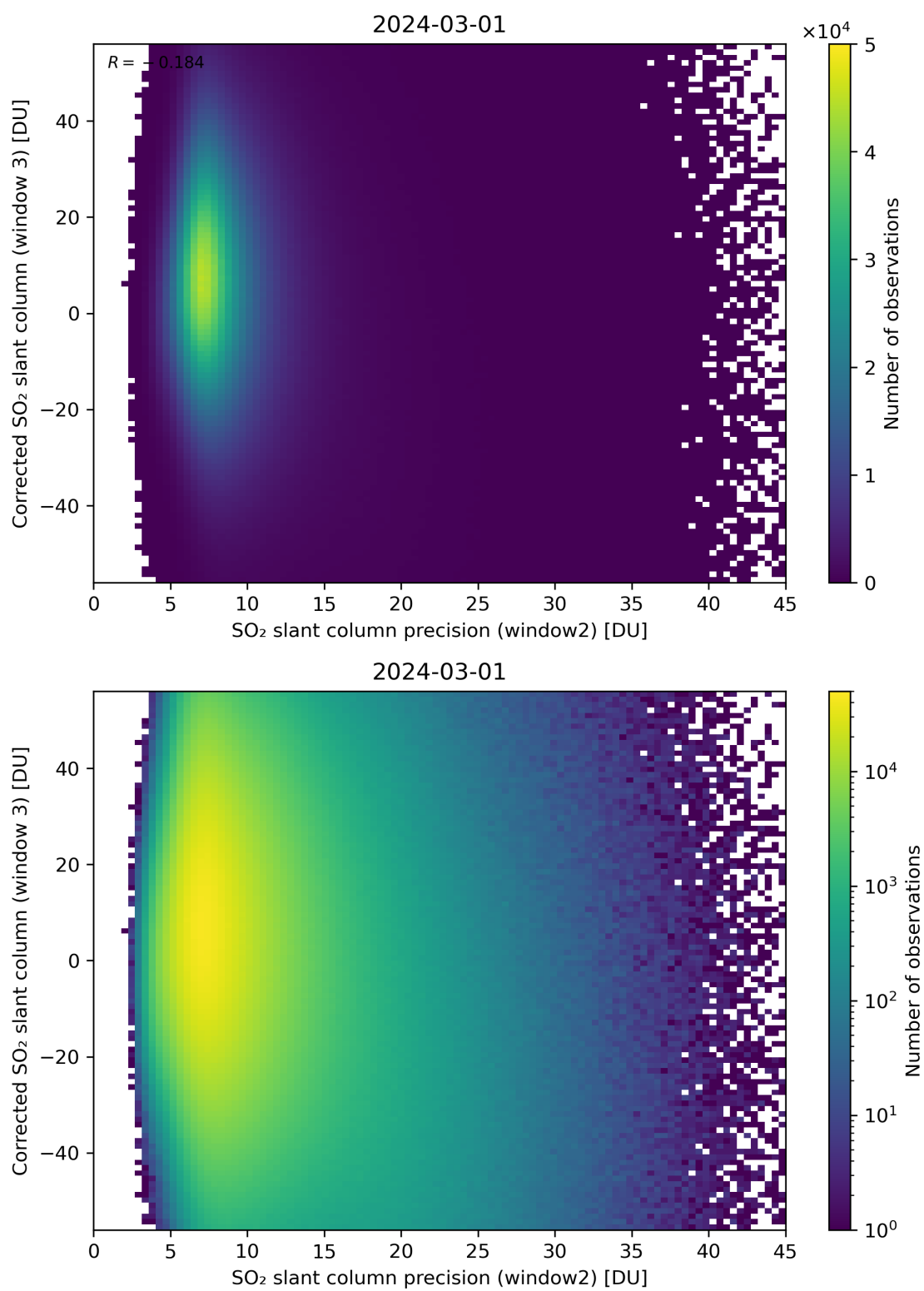
Figure 248: Scatter density plot of “SO 2 slant column precision (window2)” against “Corrected SO 2 slant column (window 3)” for 2024-02-29 to 2024-03-02.
