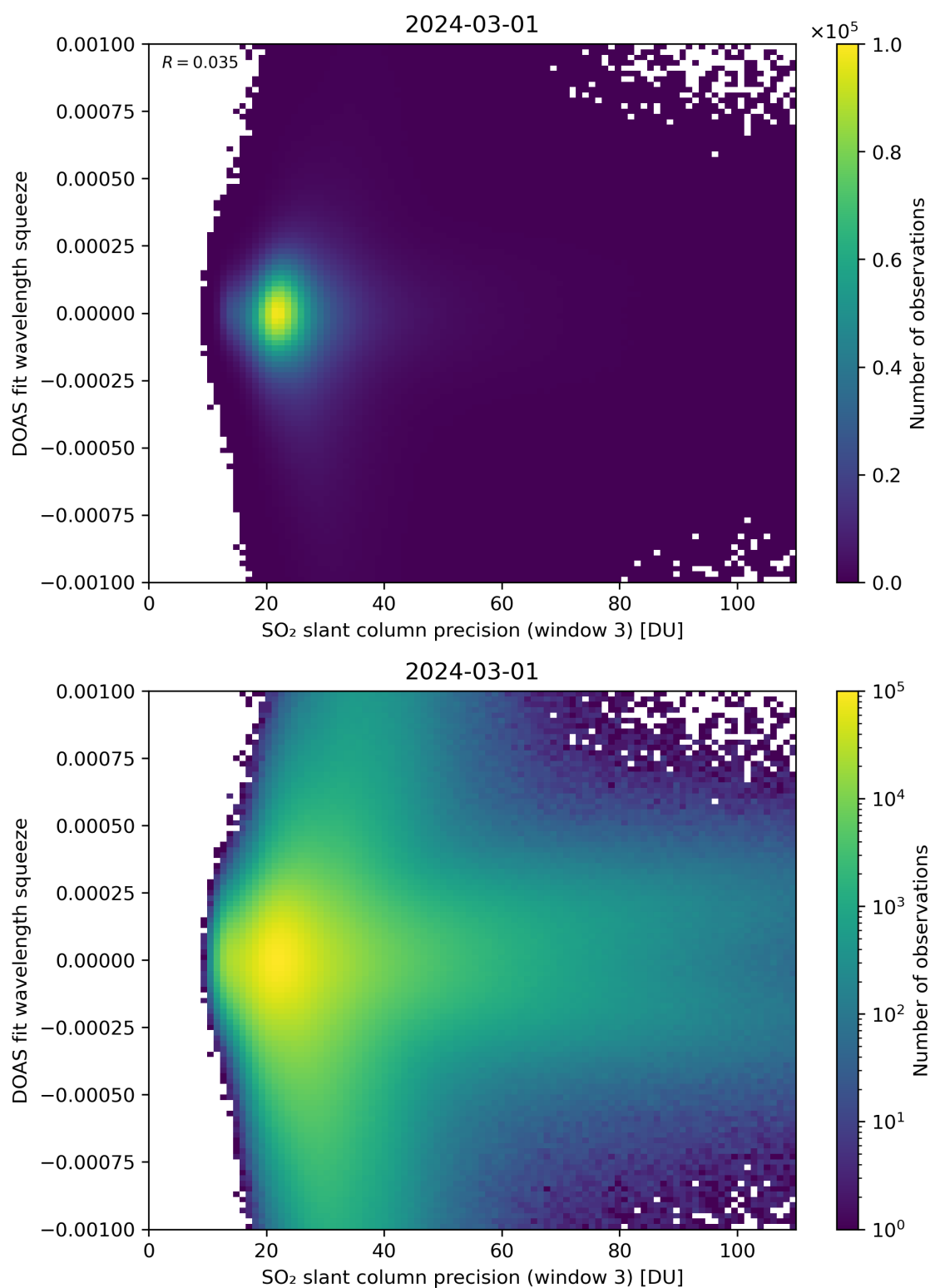
Figure 259: Scatter density plot of “SO 2 slant column precision (window 3)” against “DOAS fit wavelength squeeze” for 2024-02-29 to 2024-03-02.
