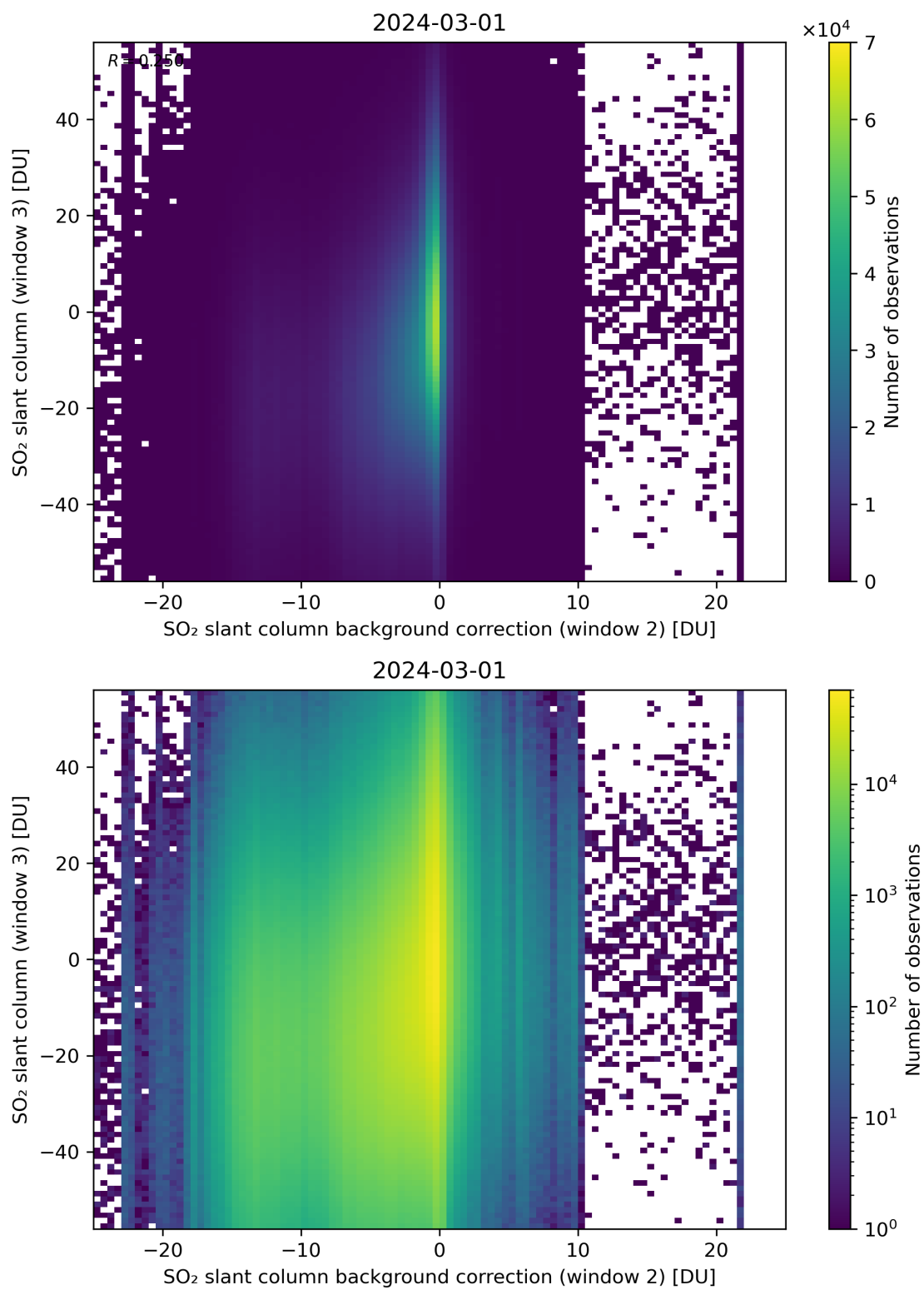
Figure 117: Scatter density plot of “SO 2 slant column background correction (window 2)” against “SO 2 slant column (window 3)” for 2024-02-29 to 2024-03-02.
