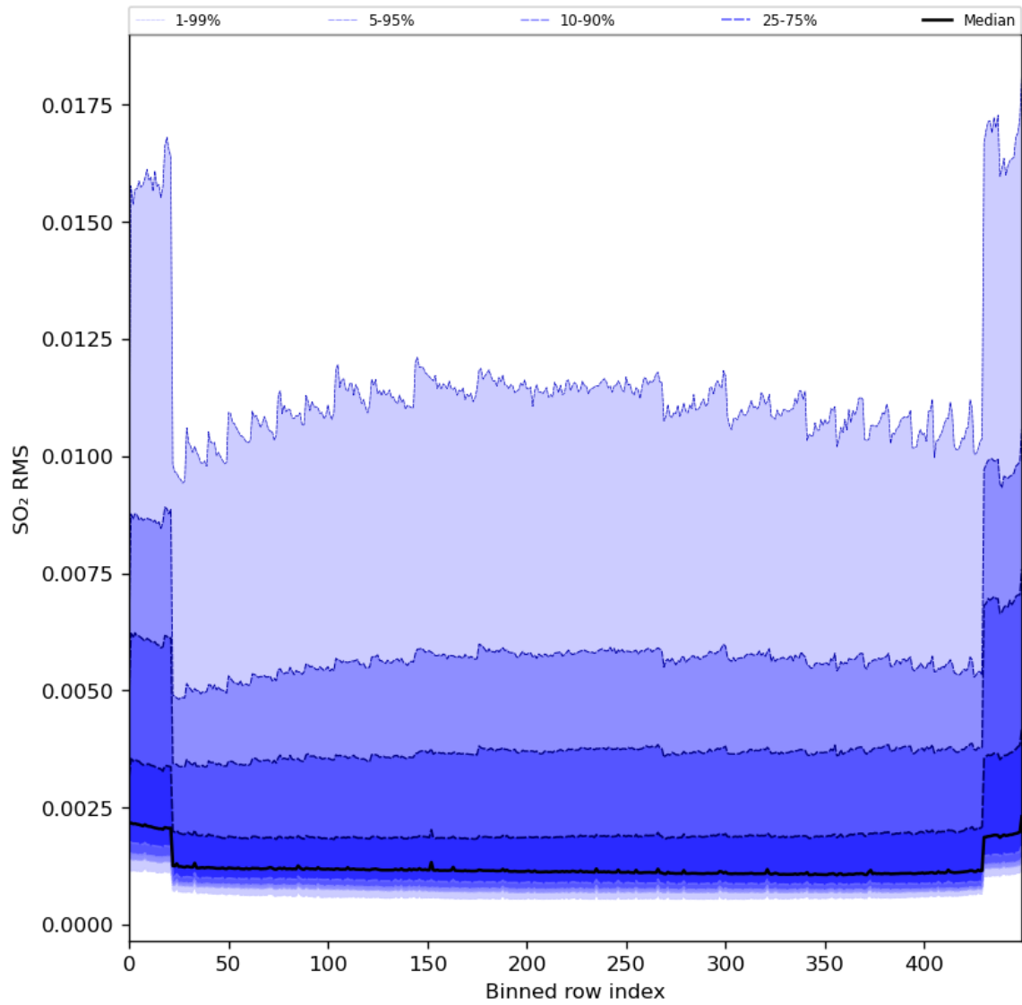
Figure 93: Along track statistics of “SO 2 RMS” for 2024-02-29 to 2024-03-02
