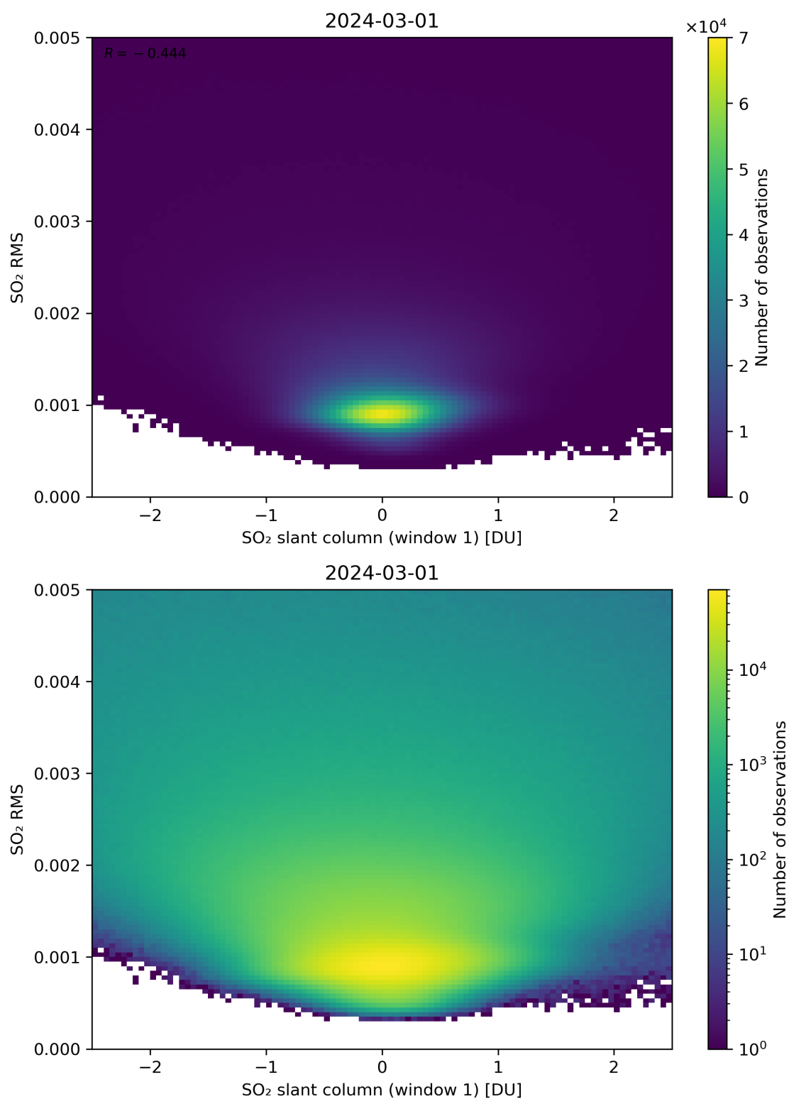
Figure 217: Scatter density plot of “SO 2 slant column (window 1)” against “SO 2 RMS” for 2024-02-29 to 2024-03-02.
