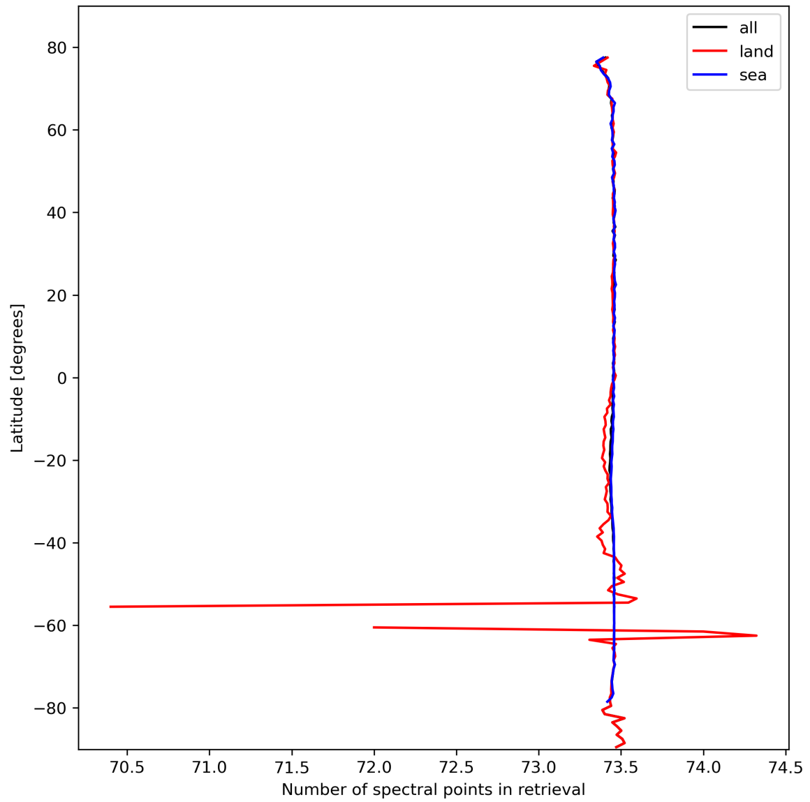
Figure 51: Zonal average of “Number of spectral points in retrieval” for 2024-02-29 to 2024-03-02.
