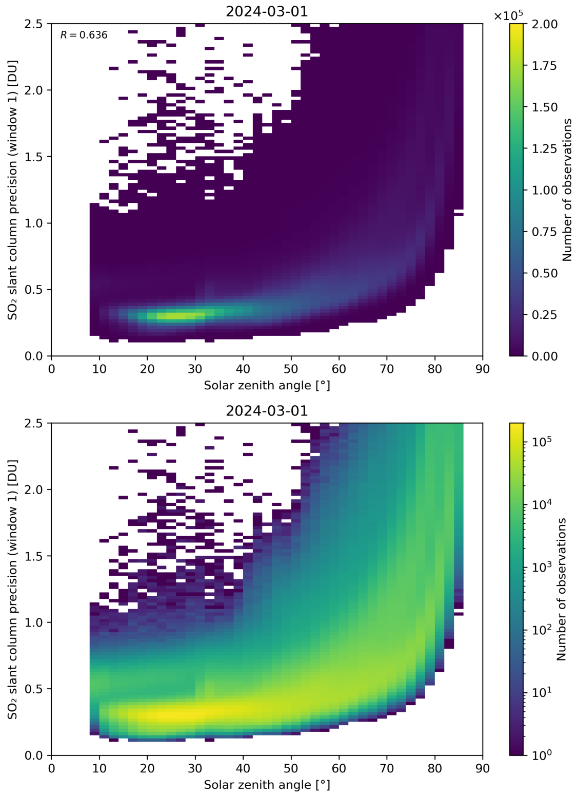
Figure 170: Scatter density plot of “Solar zenith angle” against “SO 2 slant column precision (window 1)” for 2024-02-29 to 2024-03-02.
