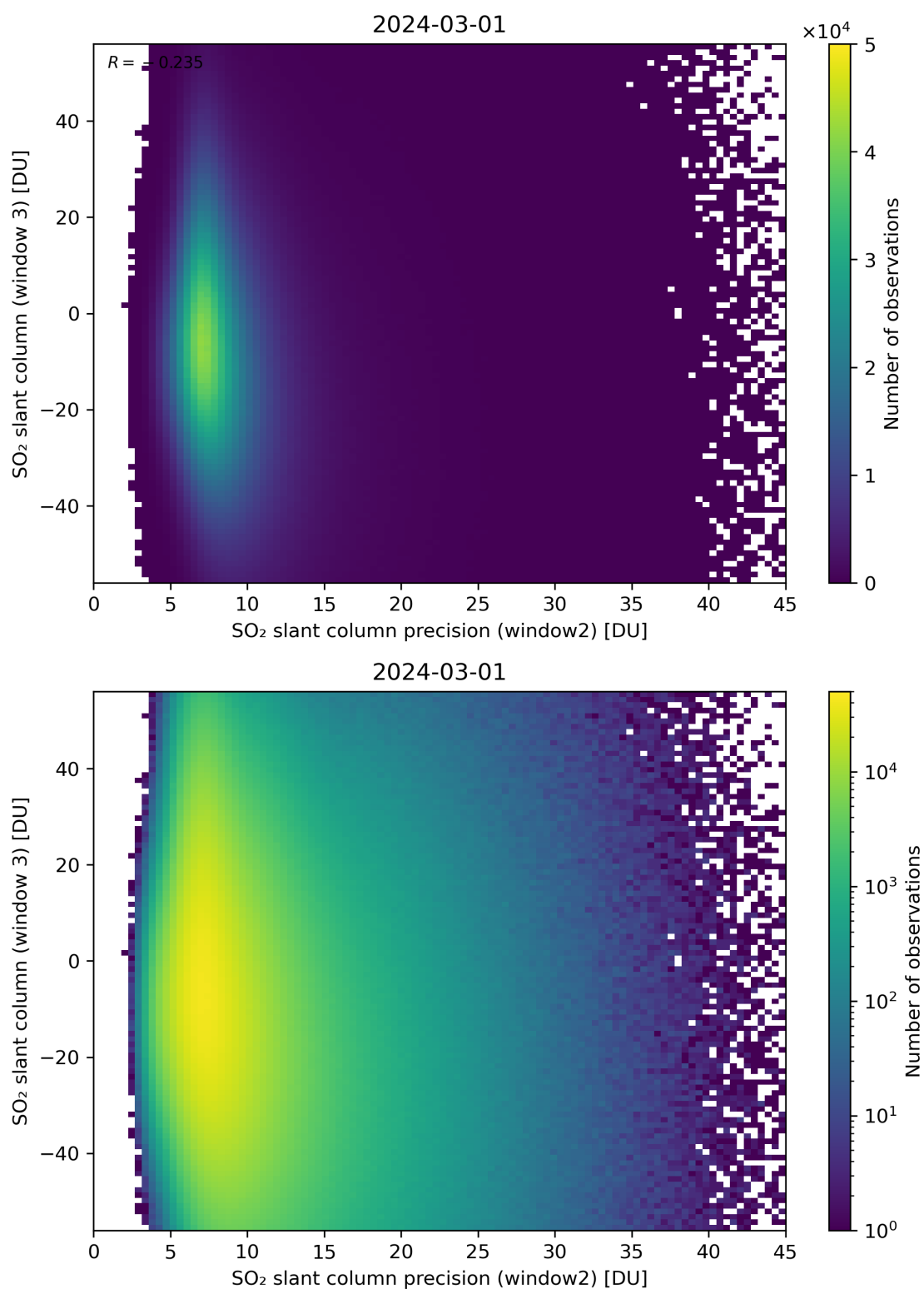
Figure 249: Scatter density plot of “SO 2 slant column precision (window2)” against “SO 2 slant column (window 3)” for 2024-02-29 to 2024-03-02.
