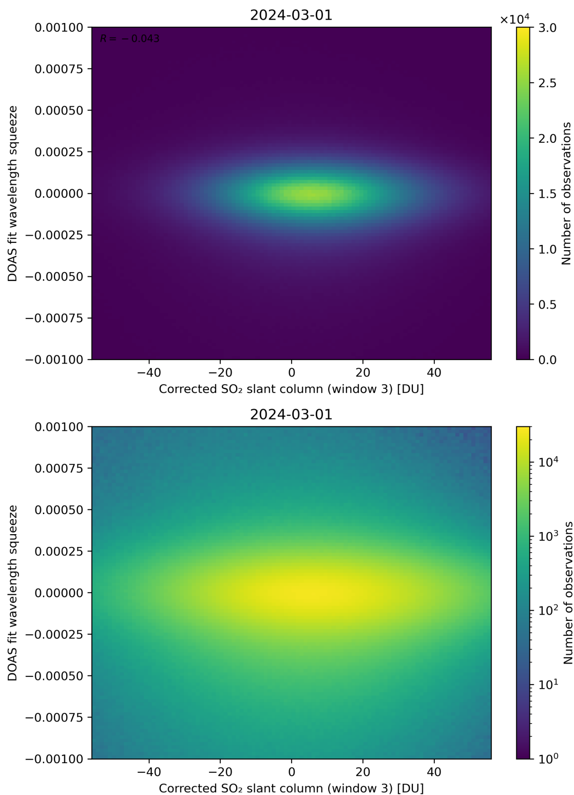
Figure 207: Scatter density plot of “Corrected SO 2 slant column (window 3)” against “DOAS fit wavelength squeeze” for 2024-02-29 to 2024-03-02.
