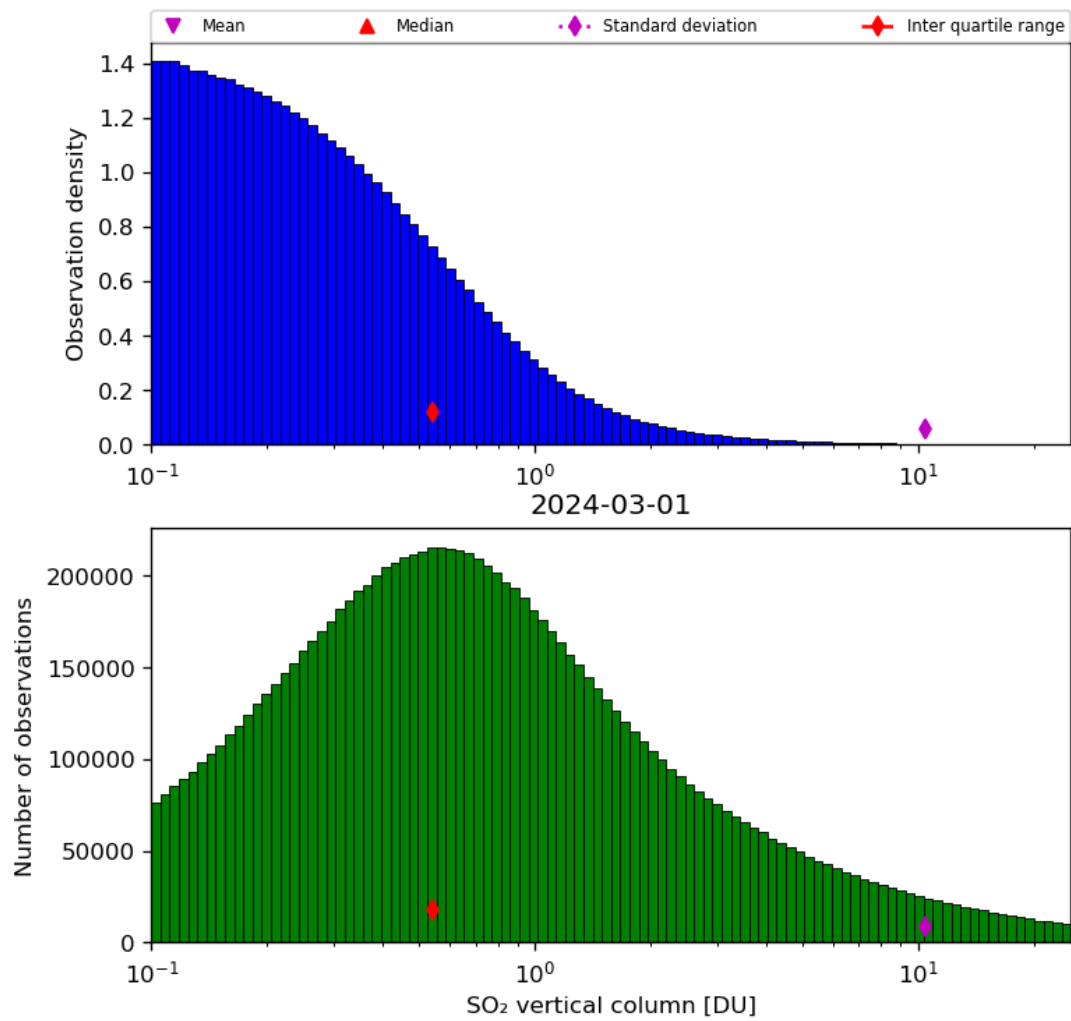
Figure 53: Histogram of “SO 2 vertical column” for 2024-02-29 to 2024-03-02
