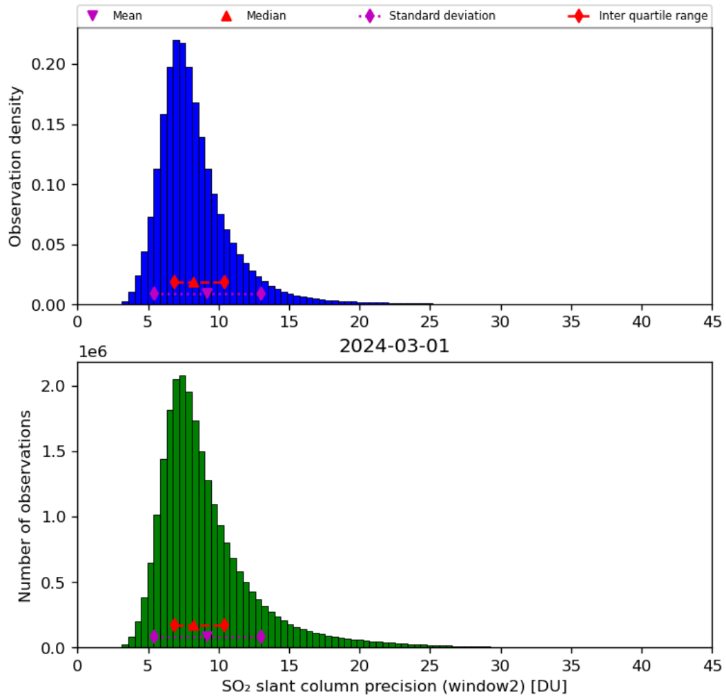
Figure 61: Histogram of “SO 2 slant column precision (window2)” for 2024-02-29 to 2024-03-02
