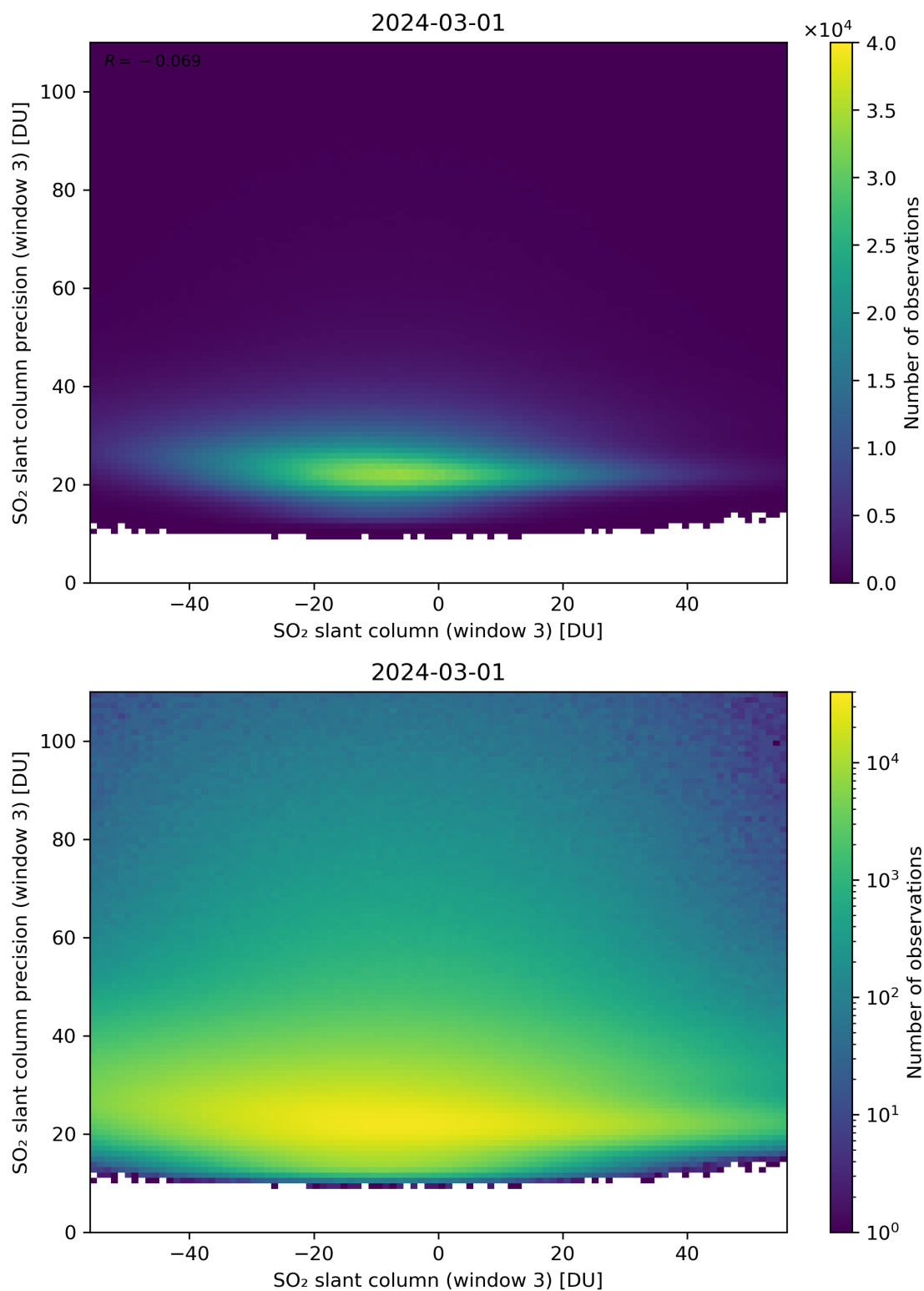
Figure 267: Scatter density plot of “SO 2 slant column (window 3)” against “SO 2 slant column precision (window 3)” for 2024-02-29 to 2024-03-02.
