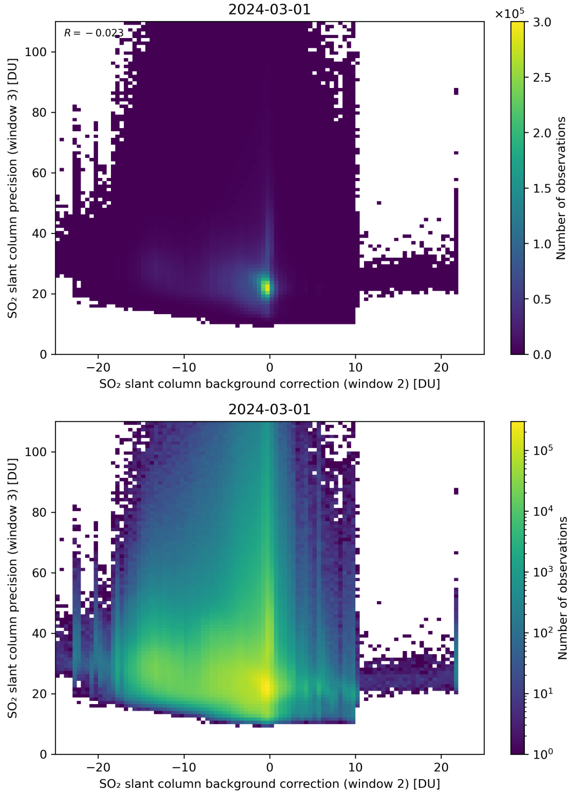
Figure 118: Scatter density plot of “SO 2 slant column background correction (window 2)” against “SO 2 slant column precision (window 3)” for 2024-02-29 to 2024-03-02.
