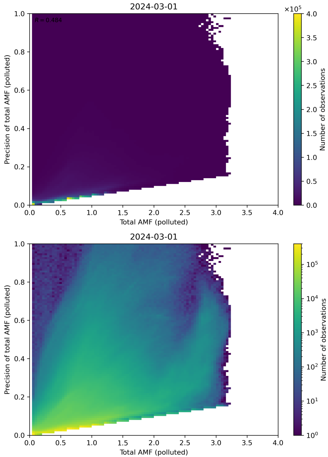
Figure 272: Scatter density plot of “Total AMF (polluted)” against “Precision of total AMF (polluted)” for 2024-02-29 to 2024-03-02.
