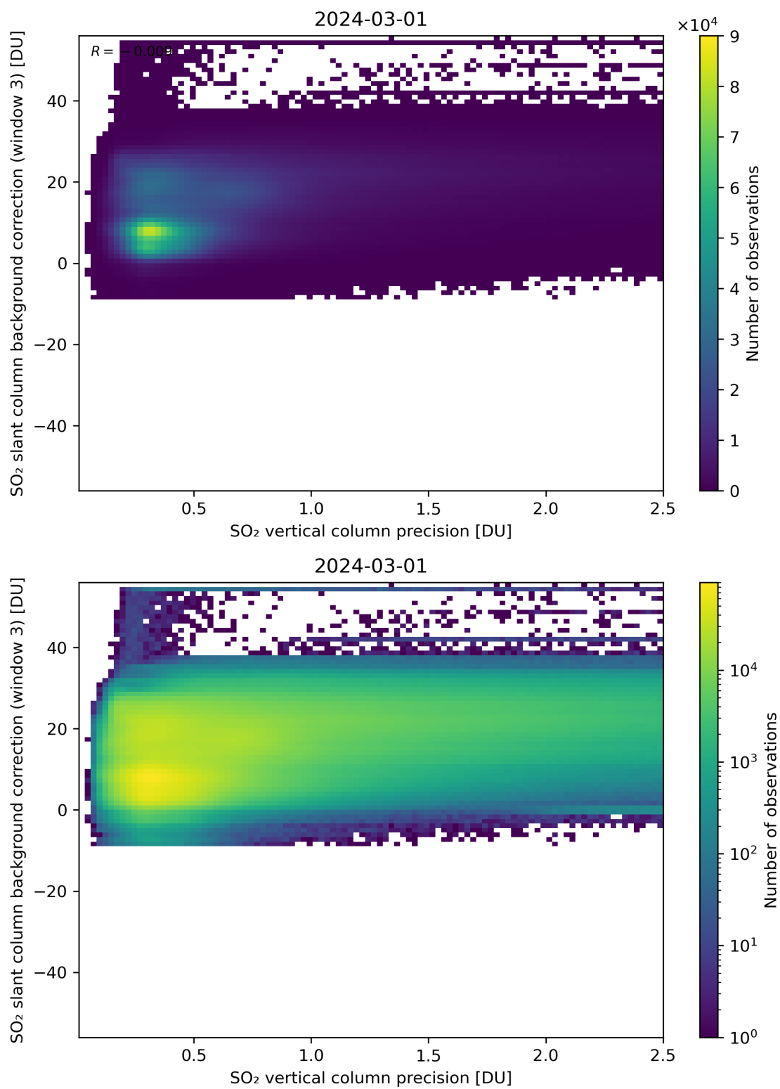
Figure 281: Scatter density plot of “SO 2 vertical column precision” against “SO 2 slant column background correction (window 3)” for 2024-02-29 to 2024-03-02.
