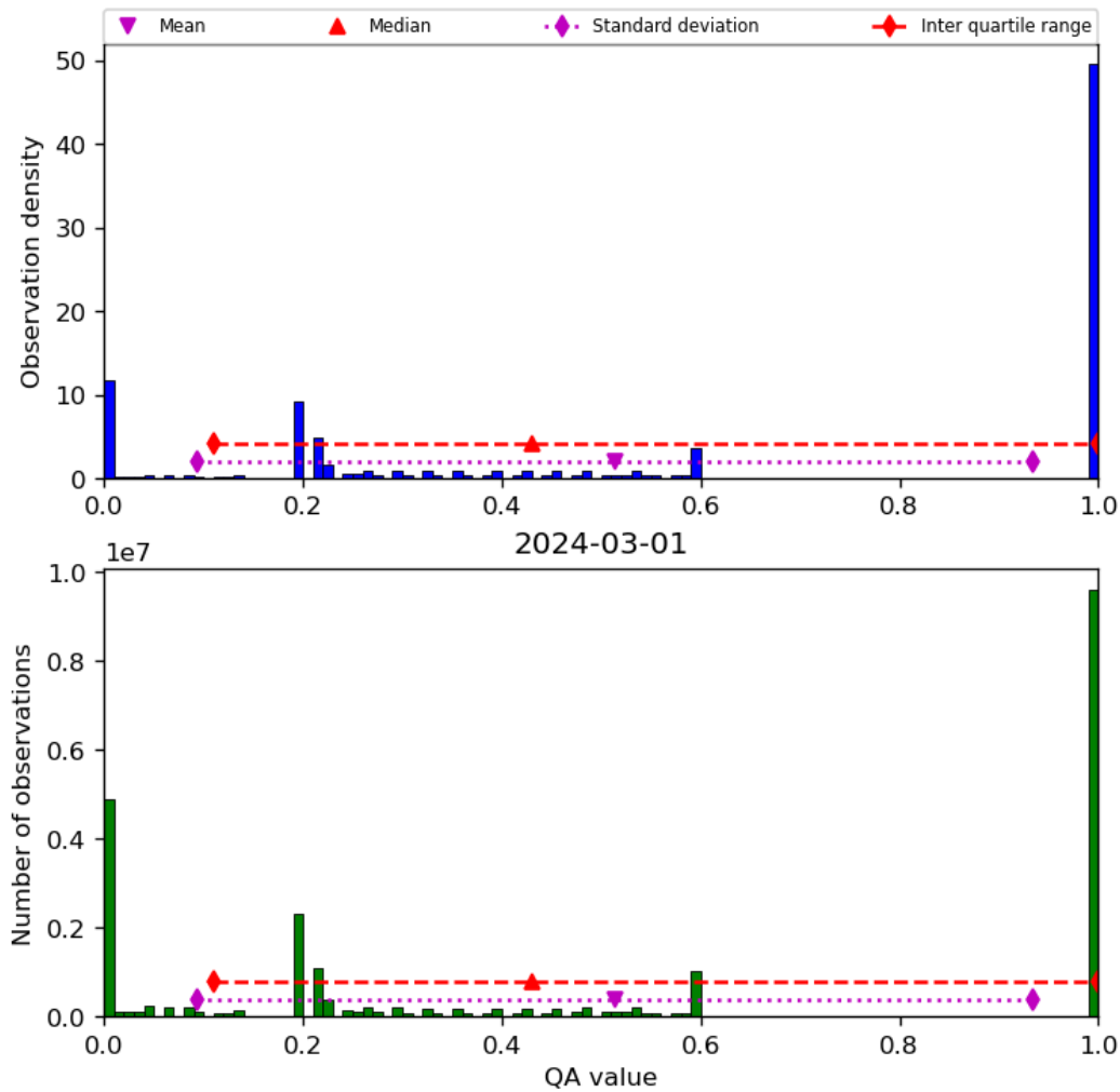
Figure 52: Histogram of “QA value” for 2024-02-29 to 2024-03-02
