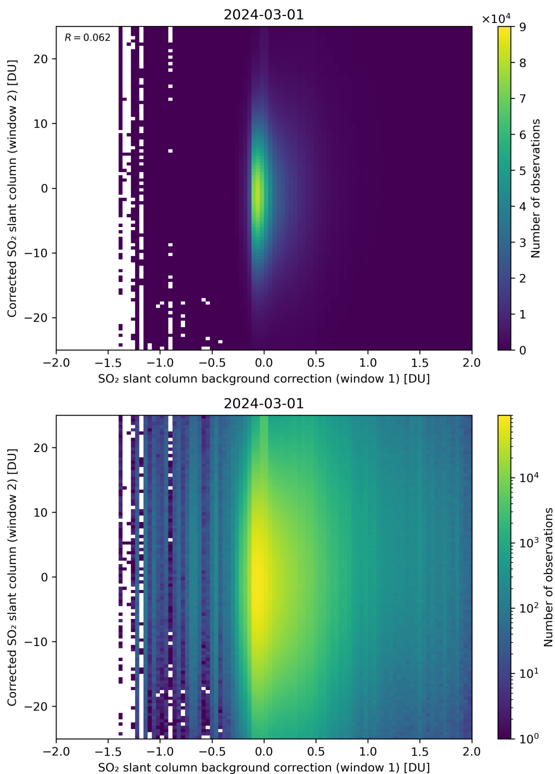
Figure 104: Scatter density plot of “SO 2 slant column background correction (window 1)” against “Corrected SO 2 slant column (window 2)” for 2024-02-29 to 2024-03-02.
