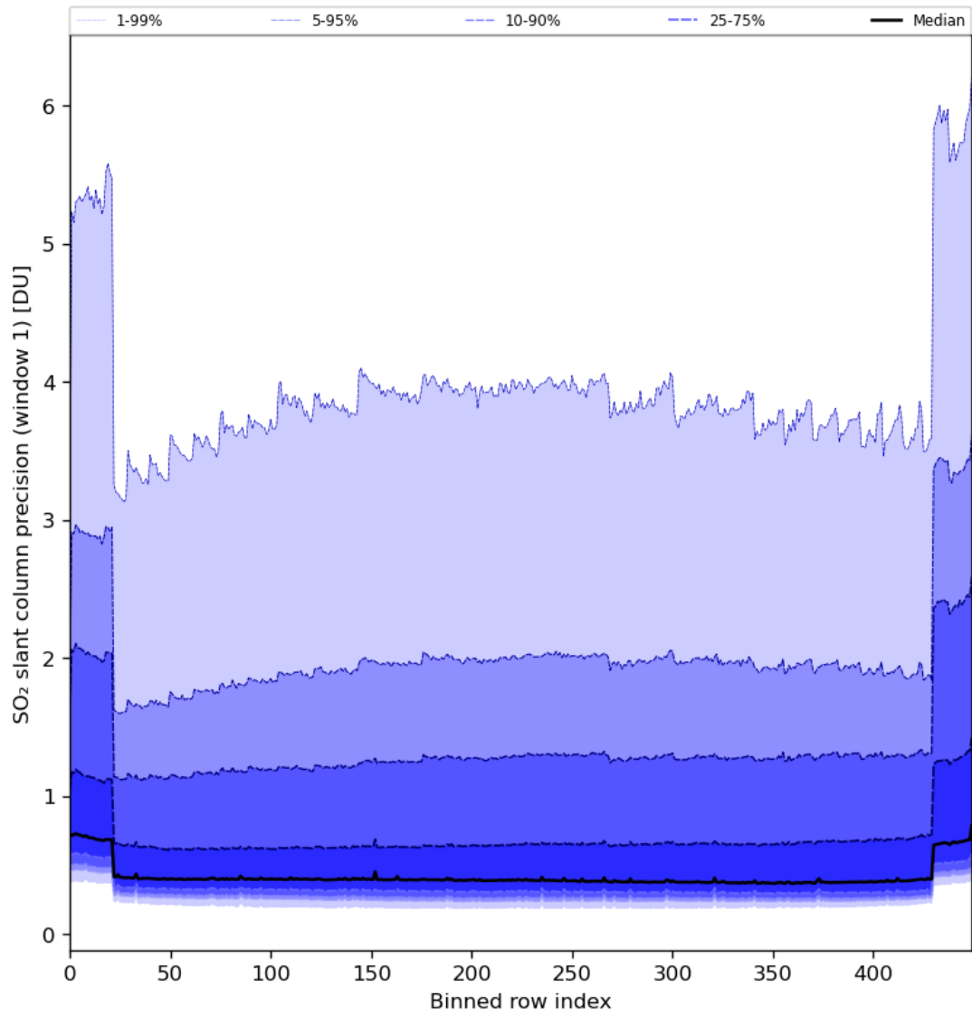
Figure 80: Along track statistics of “SO 2 slant column precision (window 1)” for 2024-02-29 to 2024-03-02
