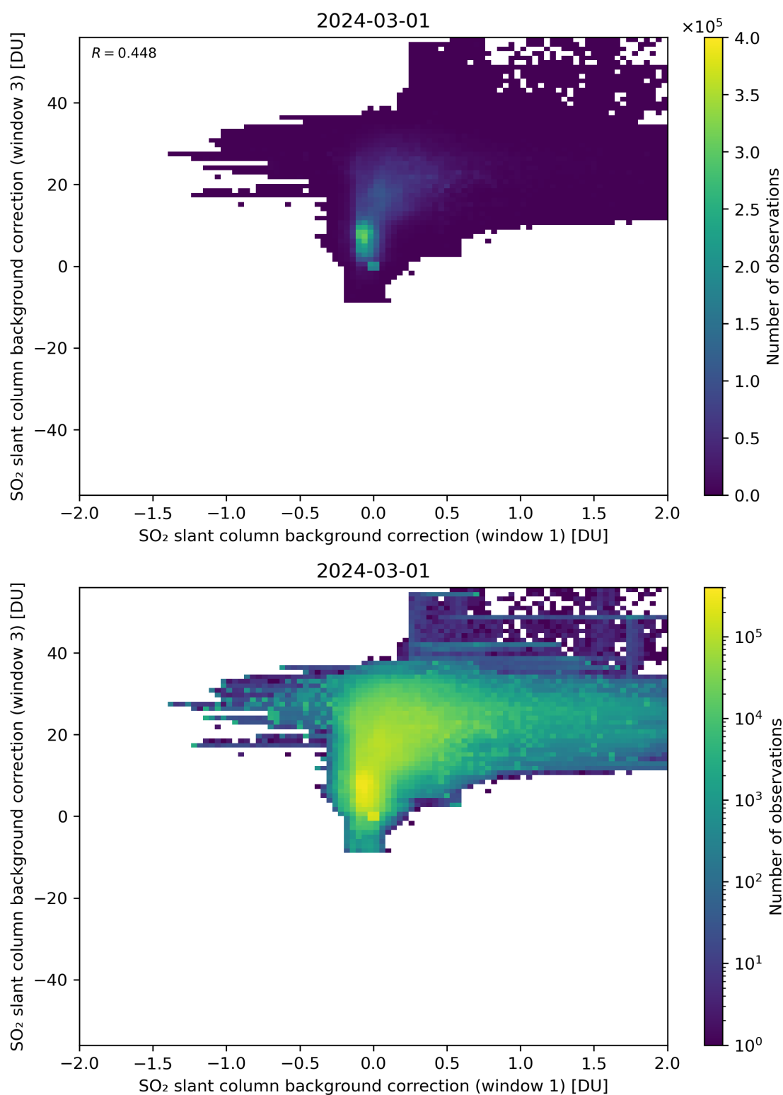
Figure 99: Scatter density plot of “SO 2 slant column background correction (window 1)” against “SO 2 slant column background correction (window 3)” for 2024-02-29 to 2024-03-02.
