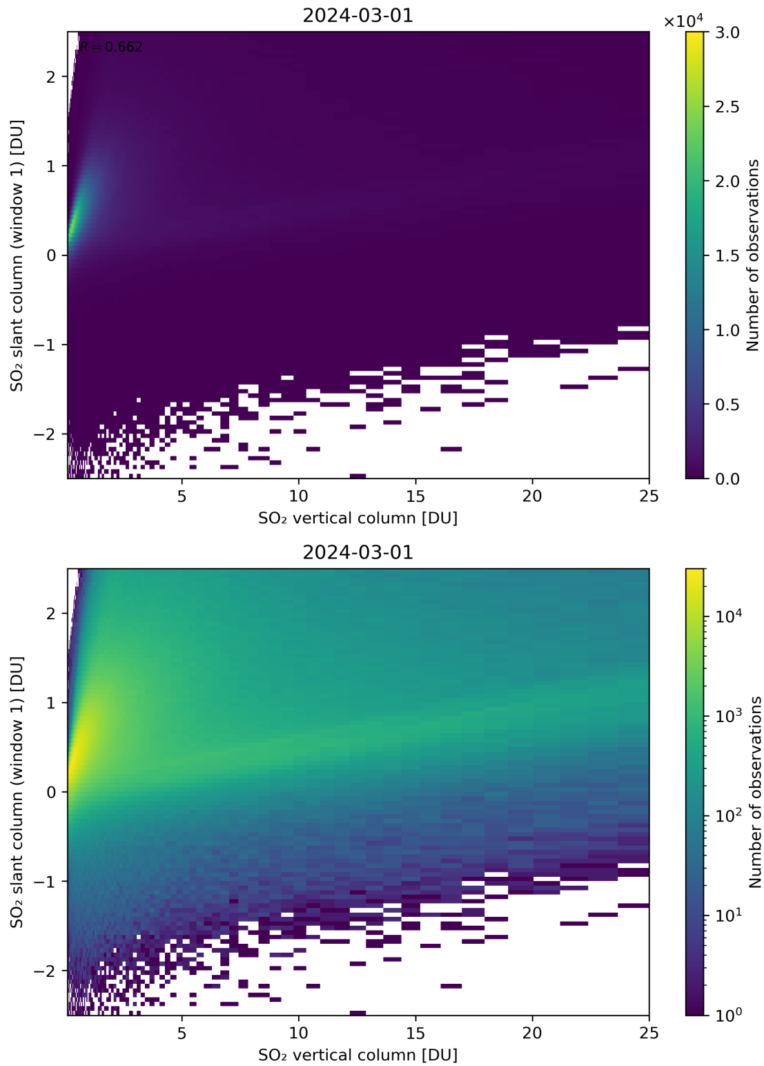
Figure 300: Scatter density plot of “SO 2 vertical column” against “SO 2 slant column (window 1)” for 2024-02-29 to 2024-03-02.
