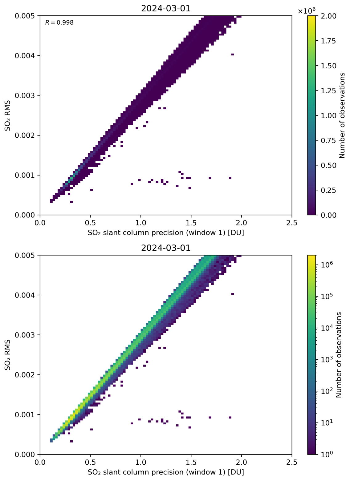
Figure 223: Scatter density plot of “SO 2 slant column precision (window 1)” against “SO 2 RMS” for 2024-02-29 to 2024-03-02.
