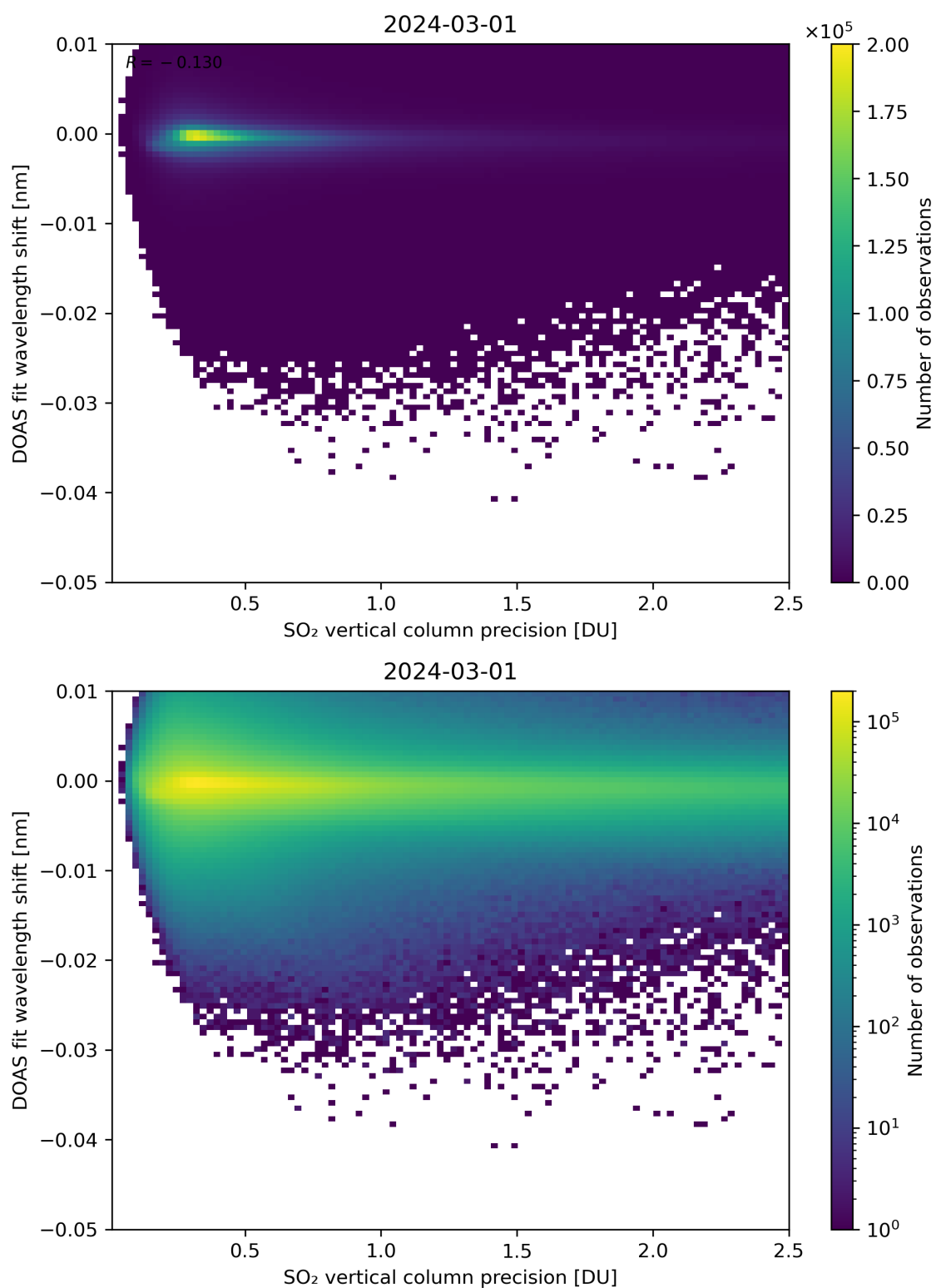
Figure 282: Scatter density plot of “SO 2 vertical column precision” against “DOAS fit wavelength shift” for 2024-02-29 to 2024-03-02.
