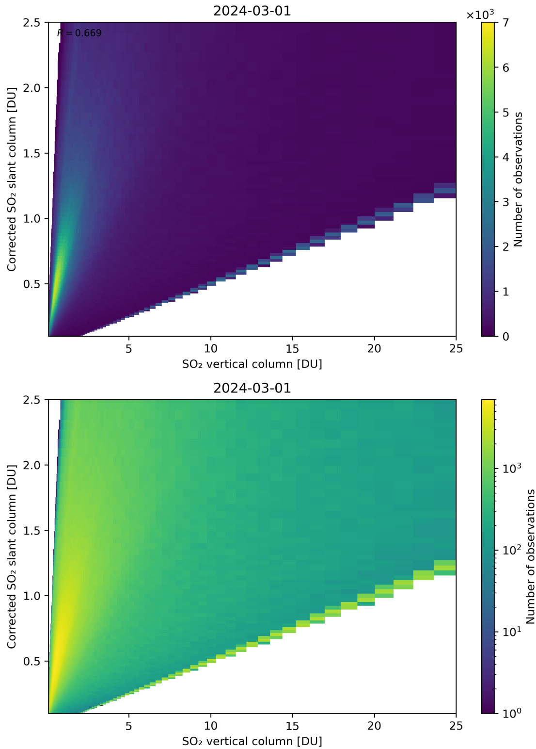
Figure 297: Scatter density plot of “SO 2 vertical column” against “Corrected SO 2 slant column” for 2024-02-29 to 2024-03-02.
