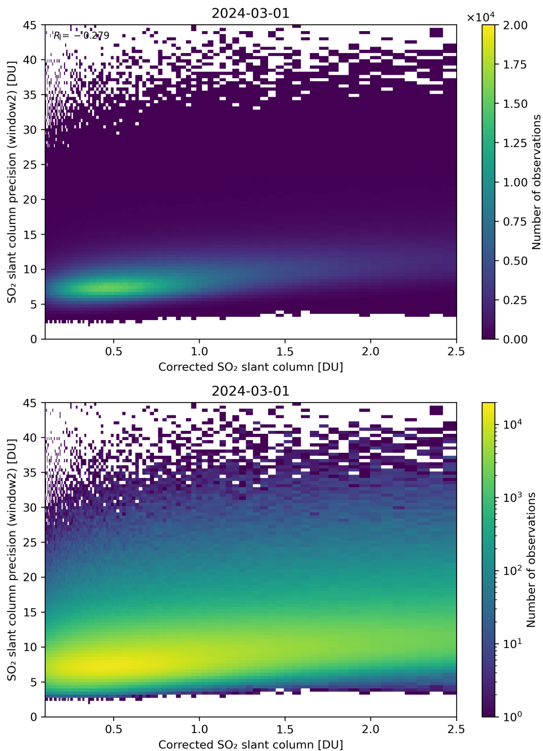
Figure 189: Scatter density plot of “Corrected SO 2 slant column” against “SO 2 slant column precision (window2)” for 2024-02-29 to 2024-03-02.
