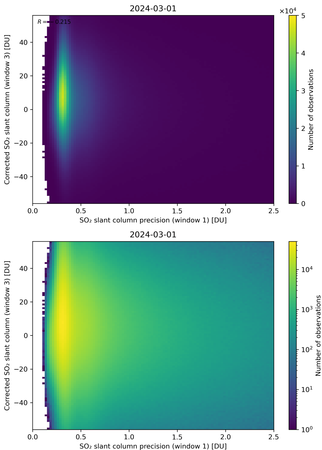
Figure 226: Scatter density plot of “SO 2 slant column precision (window 1)” against “Corrected SO 2 slant column (window 3)” for 2024-02-29 to 2024-03-02.
