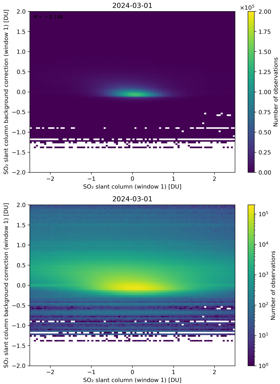
Figure 212: Scatter density plot of “SO 2 slant column (window 1)” against “SO 2 slant column background correction (window 1)” for 2024-02-29 to 2024-03-02.
