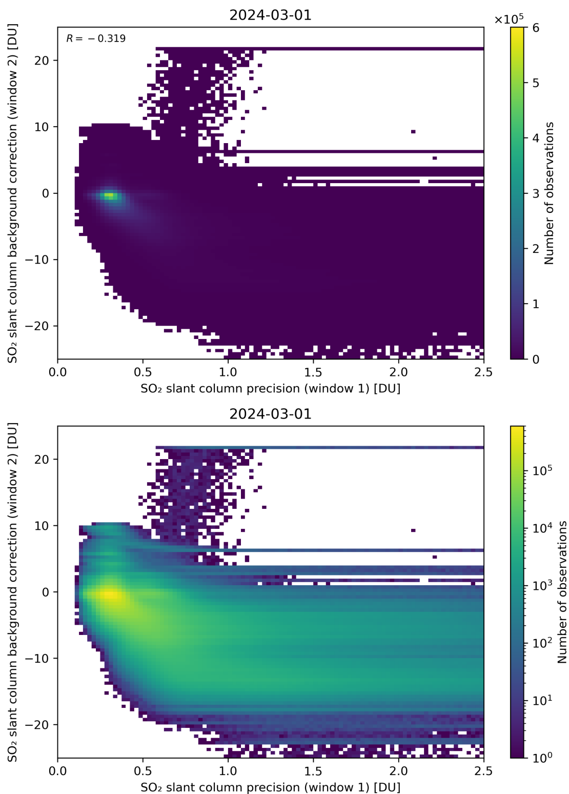
Figure 219: Scatter density plot of “SO 2 slant column precision (window 1)” against “SO 2 slant column background correction (window 2)” for 2024-02-29 to 2024-03-02.
