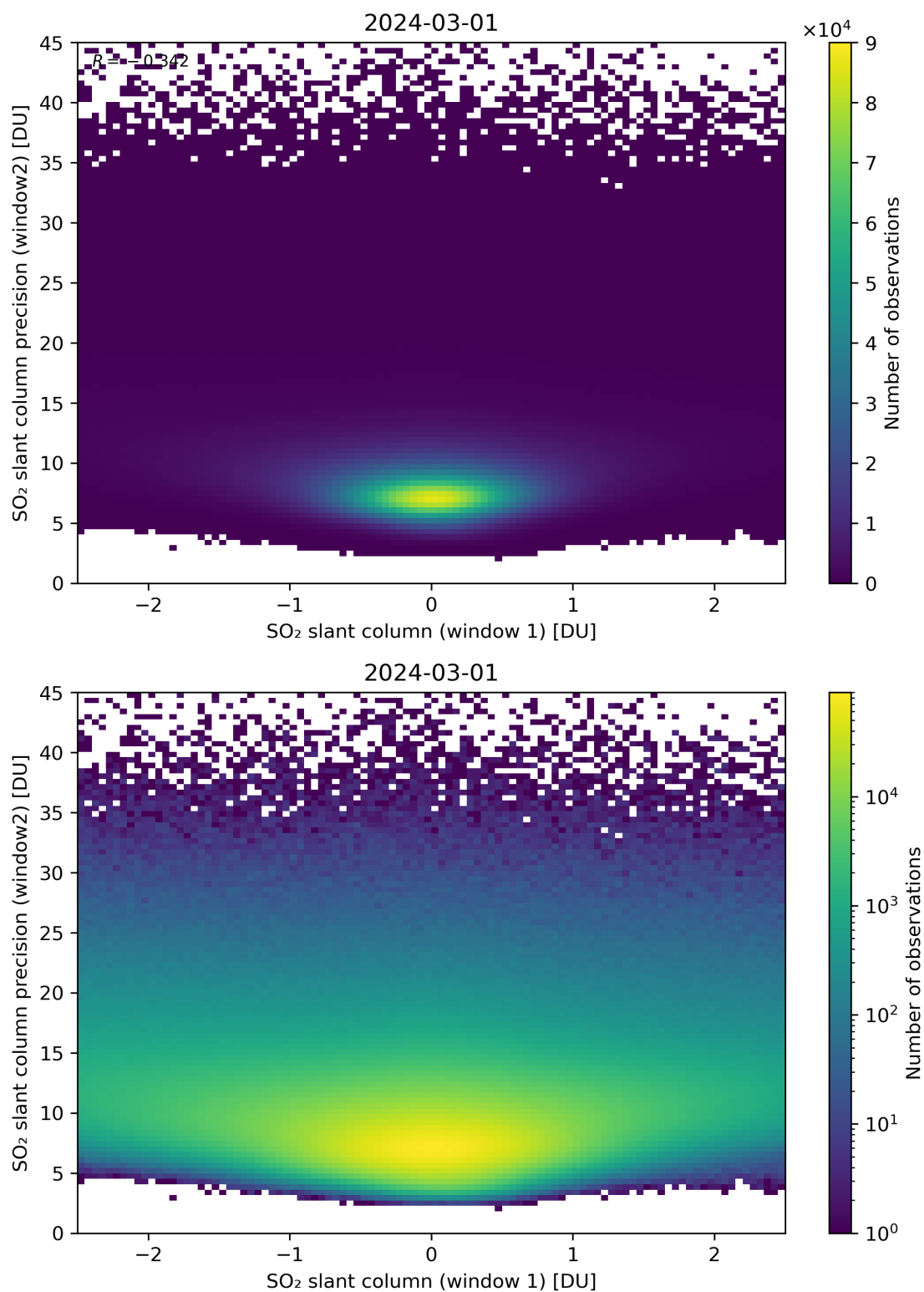
Figure 236: Scatter density plot of “SO 2 slant column (window 1)” against “SO 2 slant column precision (window2)” for 2024-02-29 to 2024-03-02.
