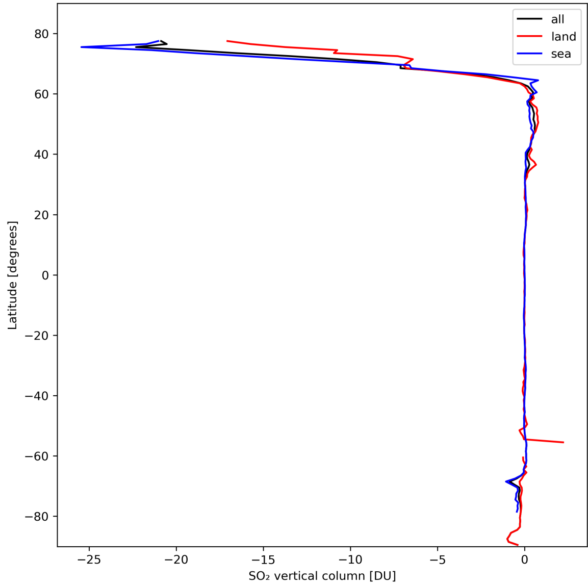
Figure 30: Zonal average of “SO 2 vertical column” for 2024-02-29 to 2024-03-02.
