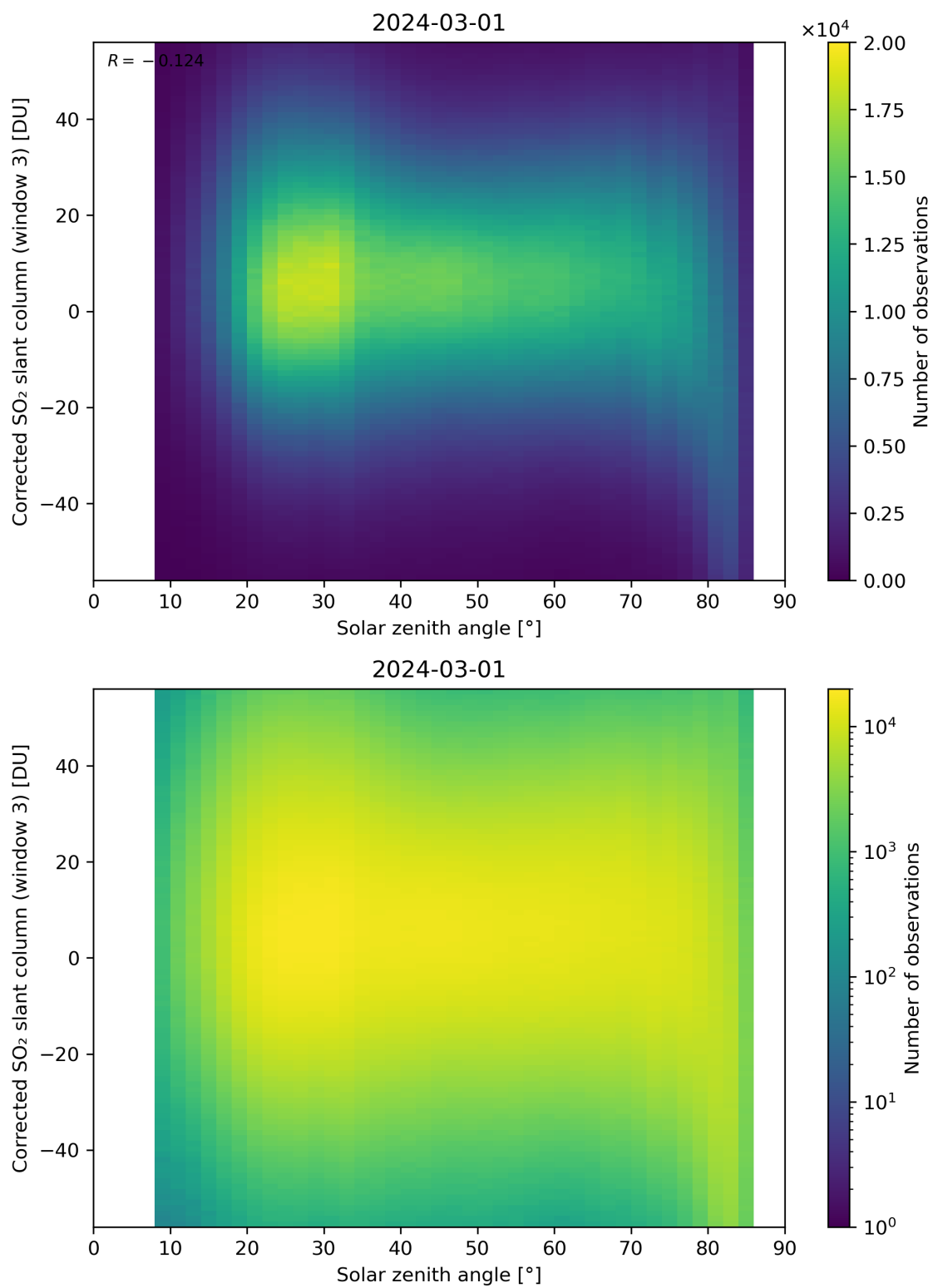
Figure 168: Scatter density plot of “Solar zenith angle” against “Corrected SO 2 slant column (window 3)” for 2024-02-29 to 2024-03-02.
