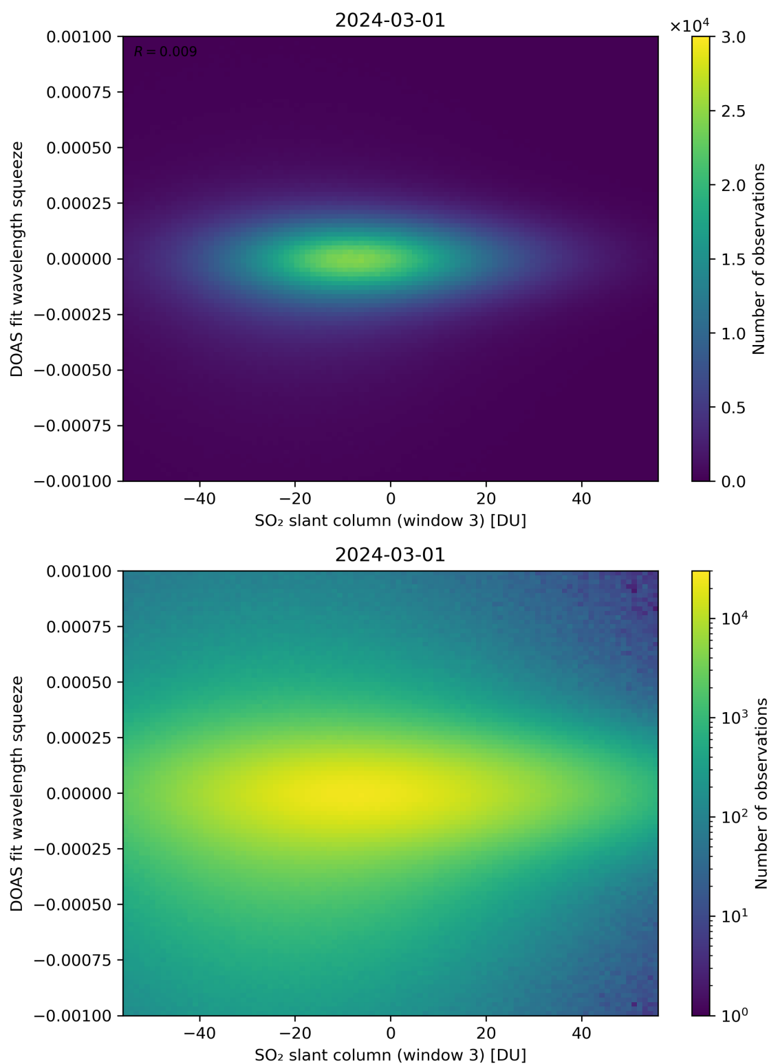
Figure 255: Scatter density plot of “SO 2 slant column (window 3)” against “DOAS fit wavelength squeeze” for 2024-02-29 to 2024-03-02.
