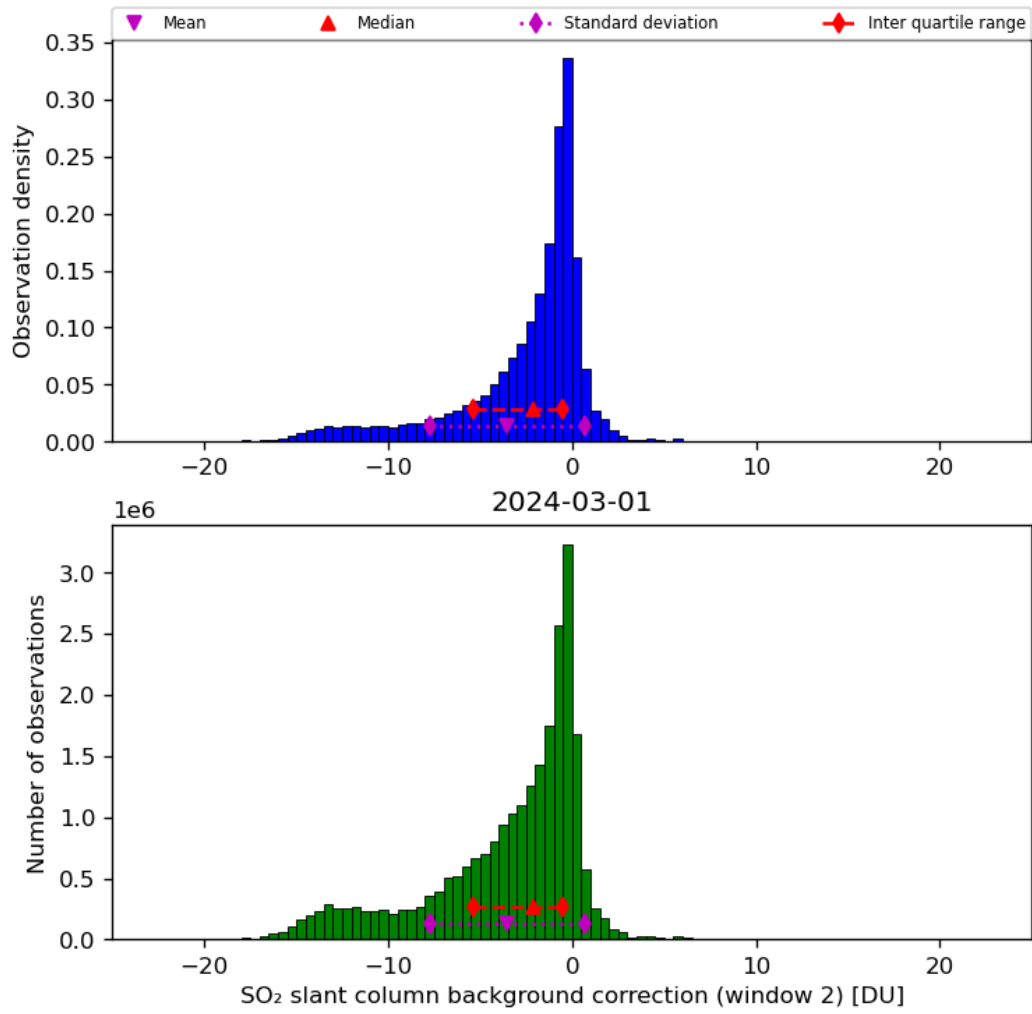
Figure 63: Histogram of “SO 2 slant column background correction (window 2)” for 2024-02-29 to 2024-03-02
