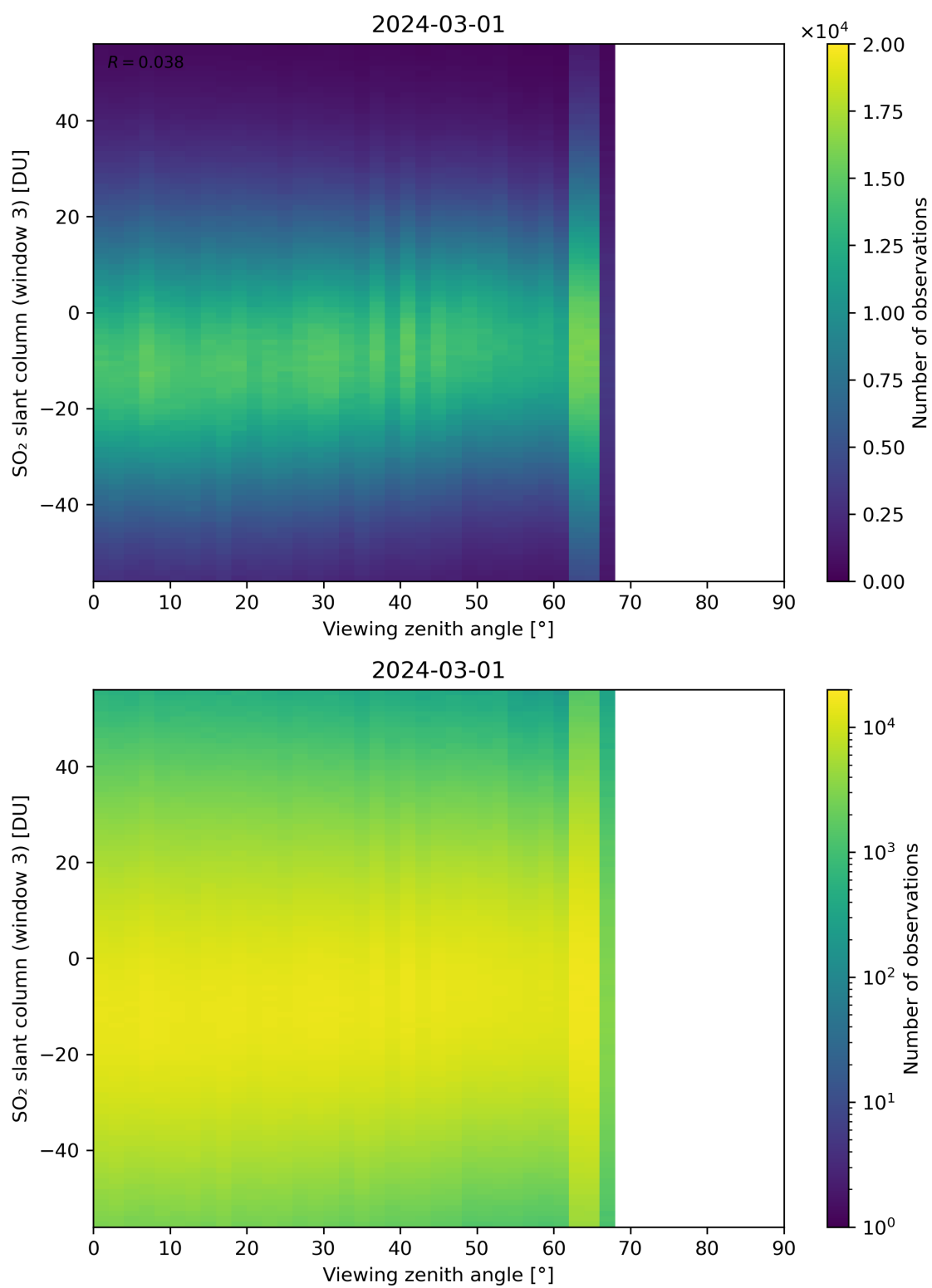
Figure 323: Scatter density plot of “Viewing zenith angle” against “SO 2 slant column (window 3)” for 2024-02-29 to 2024-03-02.
