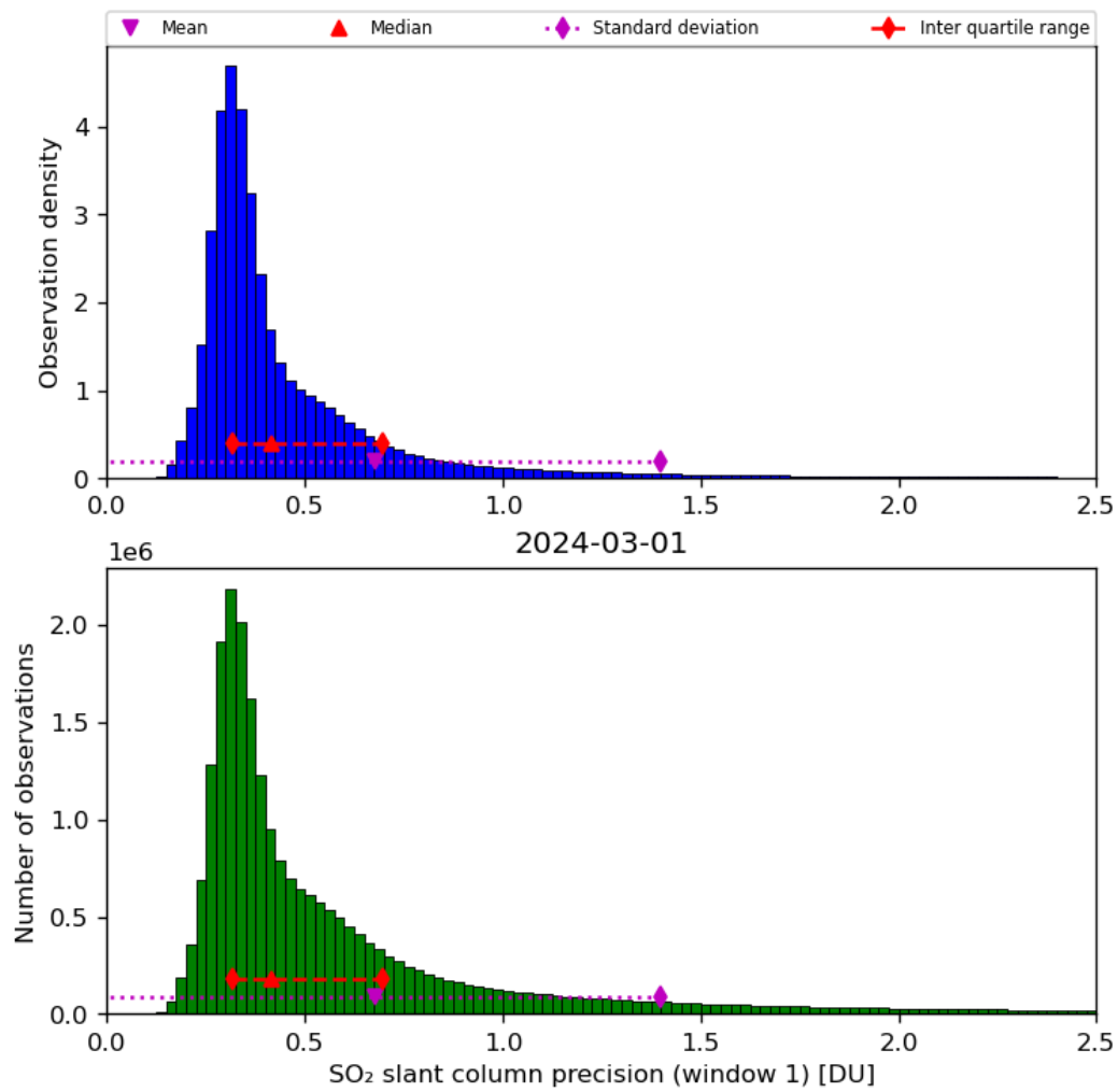
Figure 57: Histogram of “SO 2 slant column precision (window 1)” for 2024-02-29 to 2024-03-02
