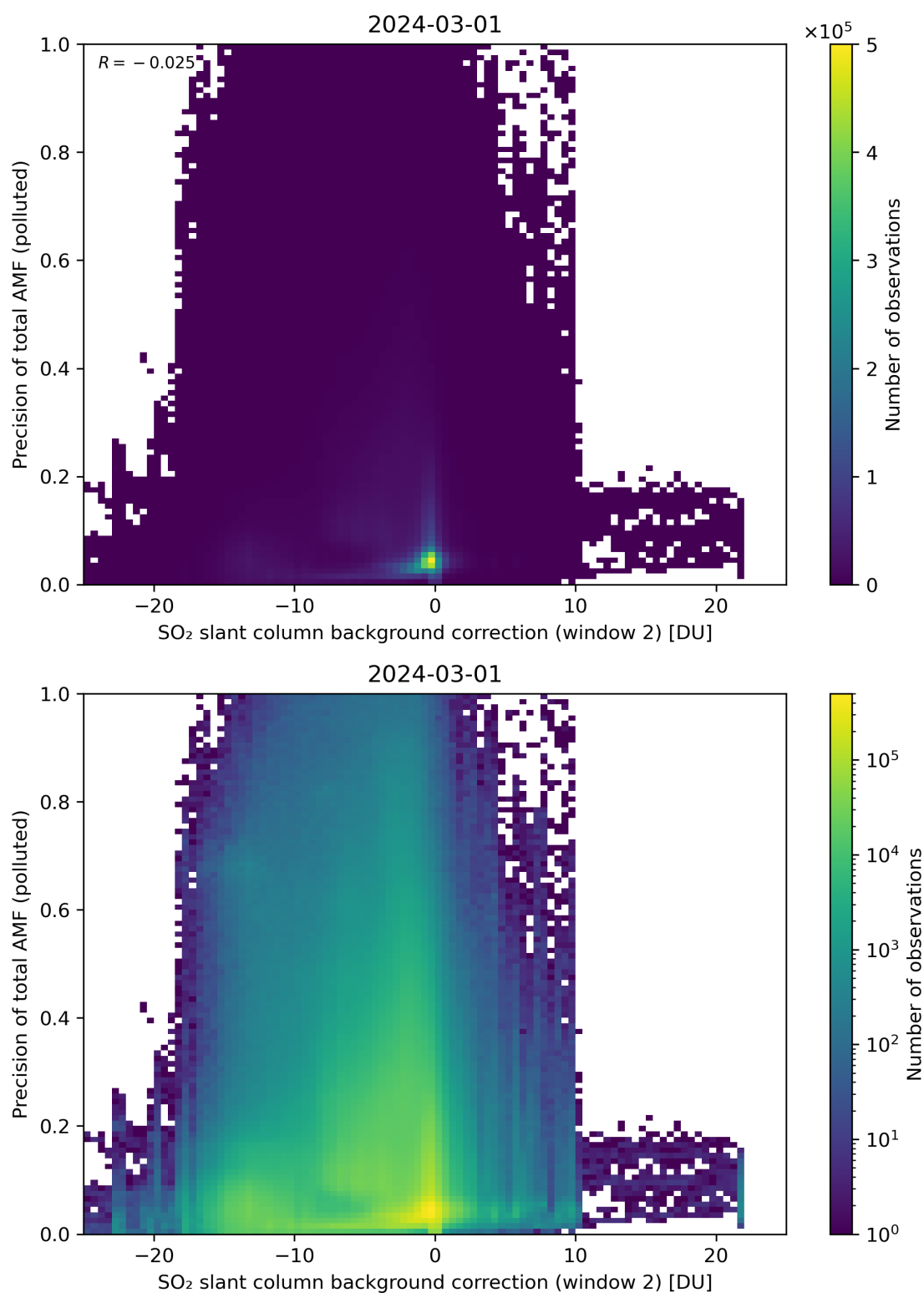
Figure 120: Scatter density plot of “SO 2 slant column background correction (window 2)” against “Precision of total AMF (polluted)” for 2024-02-29 to 2024-03-02.
