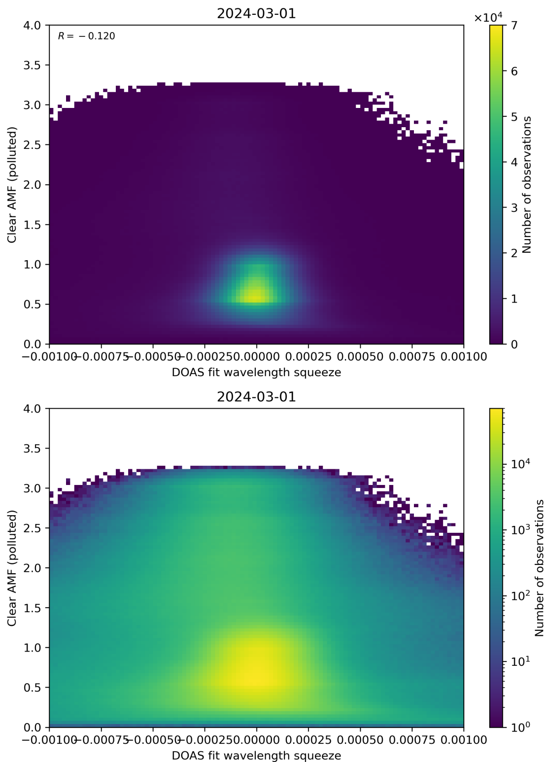
Figure 133: Scatter density plot of “DOAS fit wavelength squeeze” against “Clear AMF (polluted)” for 2024-02-29 to 2024-03-02.
