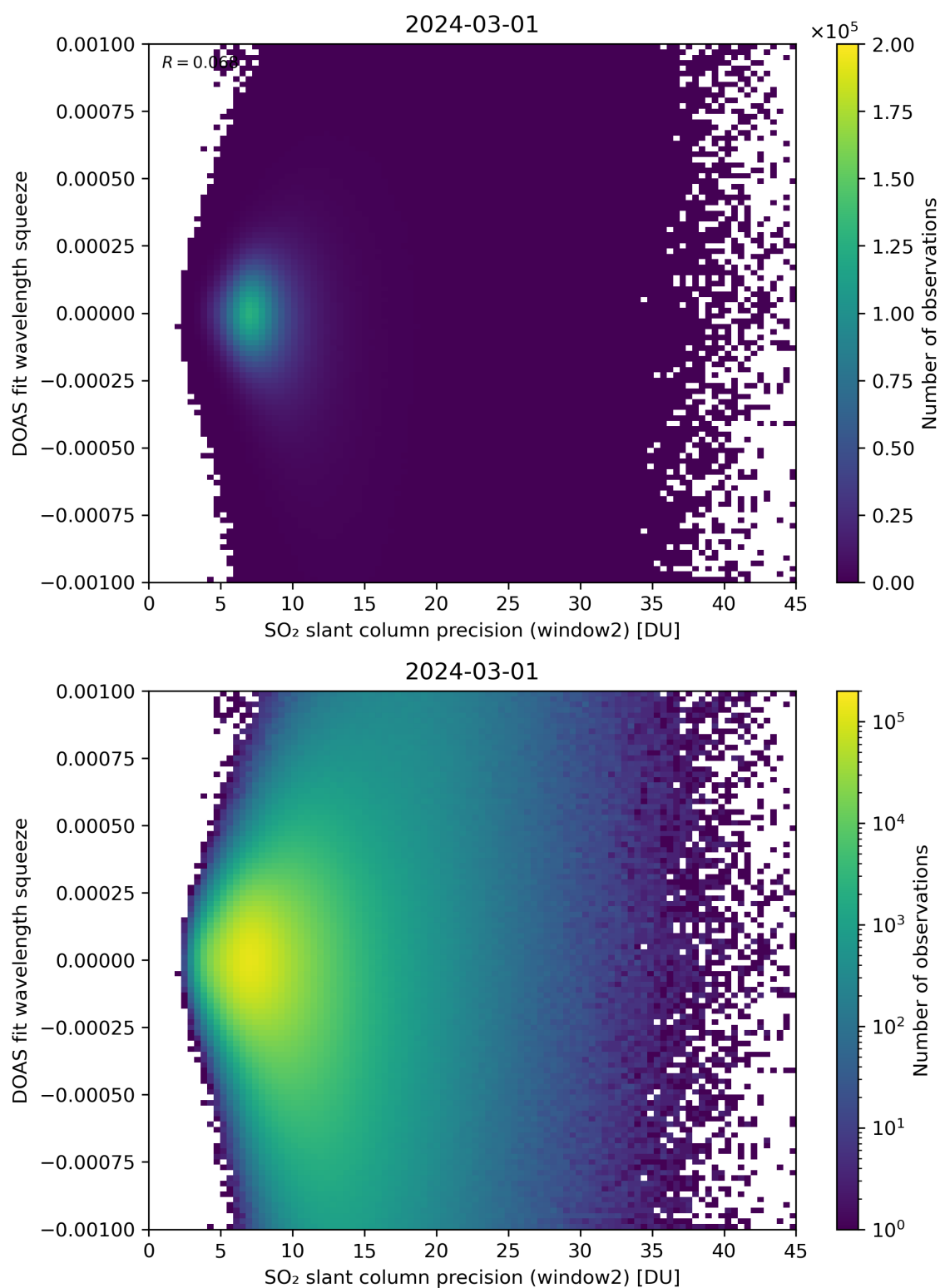
Figure 244: Scatter density plot of “SO 2 slant column precision (window2)” against “DOAS fit wavelength squeeze” for 2024-02-29 to 2024-03-02.
