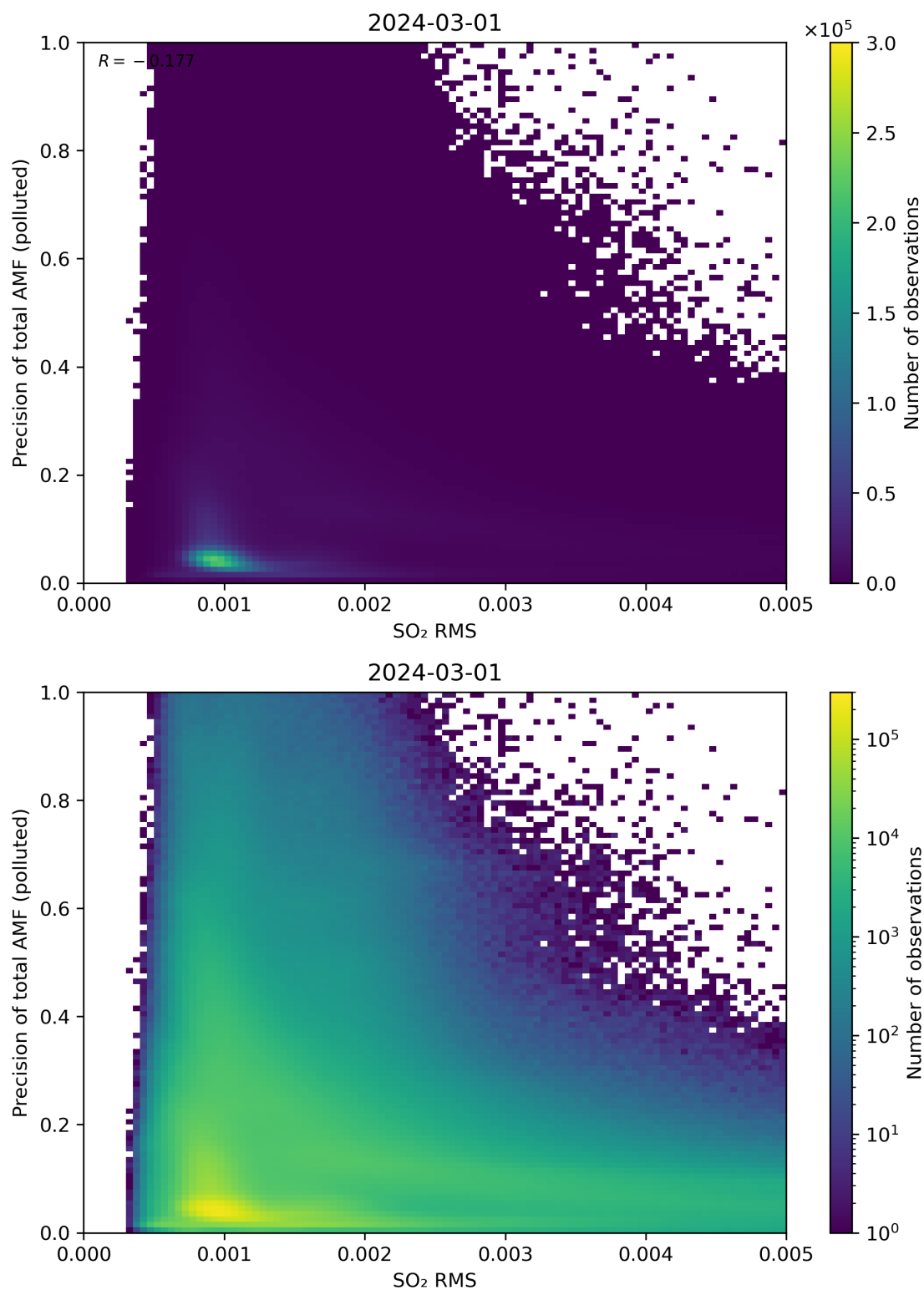
Figure 138: Scatter density plot of “SO 2 RMS” against “Precision of total AMF (polluted)” for 2024-02-29 to 2024-03-02.
