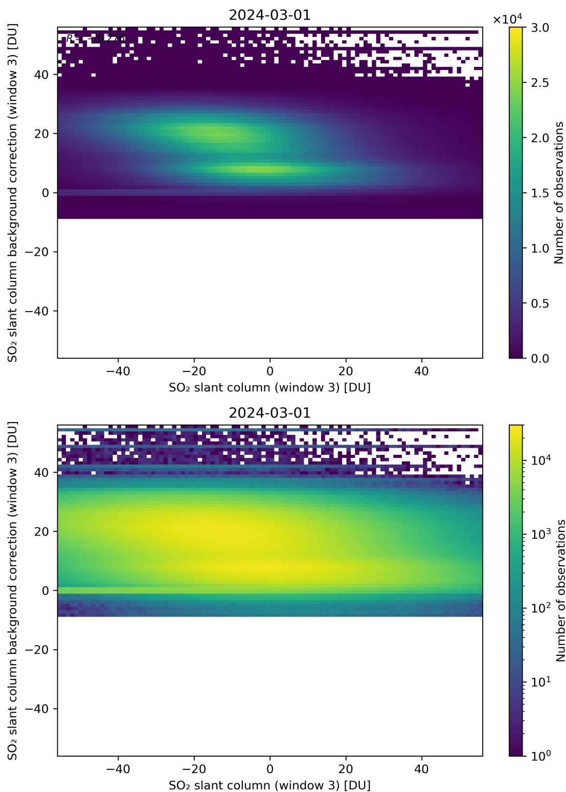
Figure 253: Scatter density plot of “SO 2 slant column (window 3)” against “SO 2 slant column background correction (window 3)” for 2024-02-29 to 2024-03-02.
