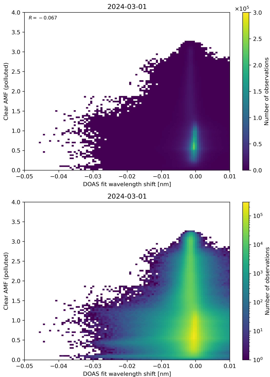
Figure 129: Scatter density plot of “DOAS fit wavelength shift” against “Clear AMF (polluted)” for 2024-02-29 to 2024-03-02.
