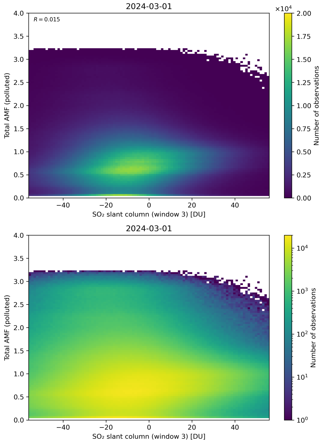
Figure 268: Scatter density plot of “SO 2 slant column (window 3)” against “Total AMF (polluted)” for 2024-02-29 to 2024-03-02.
