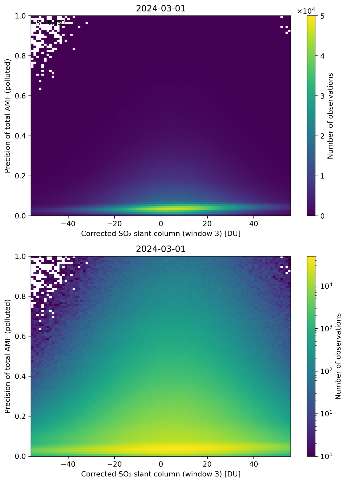
Figure 211: Scatter density plot of “Corrected SO 2 slant column (window 3)” against “Precision of total AMF (polluted)” for 2024-02-29 to 2024-03-02.
