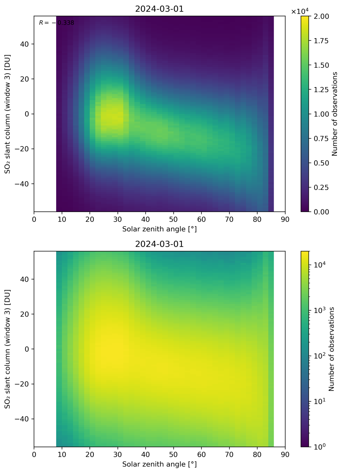
Figure 172: Scatter density plot of “Solar zenith angle” against “SO 2 slant column (window 3)” for 2024-02-29 to 2024-03-02.
