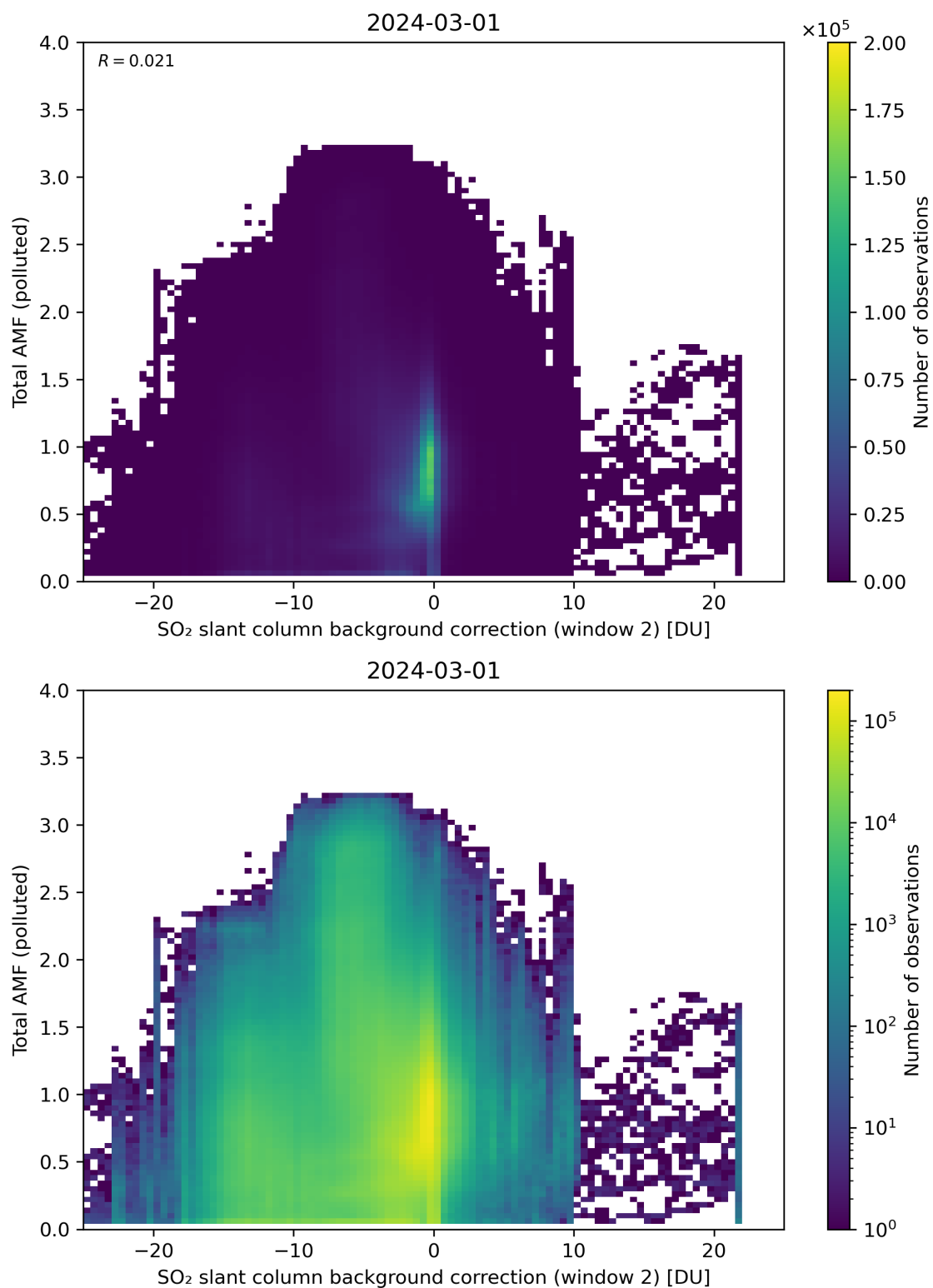
Figure 119: Scatter density plot of “SO 2 slant column background correction (window 2)” against “Total AMF (polluted)” for 2024-02-29 to 2024-03-02.
