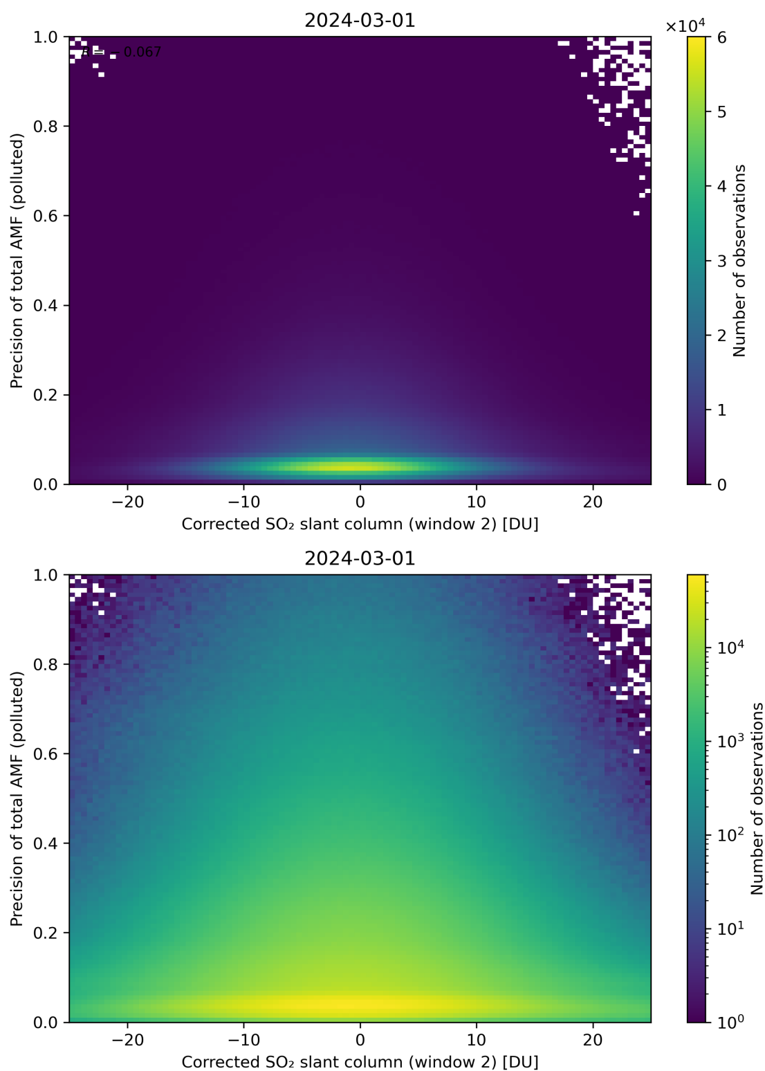
Figure 204: Scatter density plot of “Corrected SO 2 slant column (window 2)” against “Precision of total AMF (polluted)” for 2024-02-29 to 2024-03-02.
