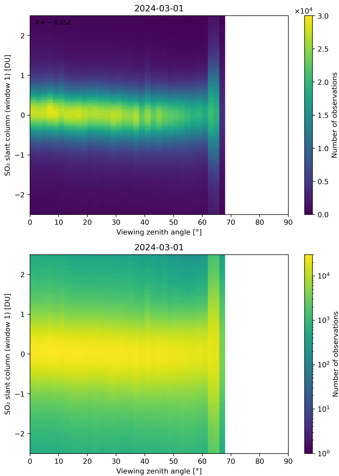
Figure 320: Scatter density plot of “Viewing zenith angle” against “SO 2 slant column (window 1)” for 2024-02-29 to 2024-03-02.
