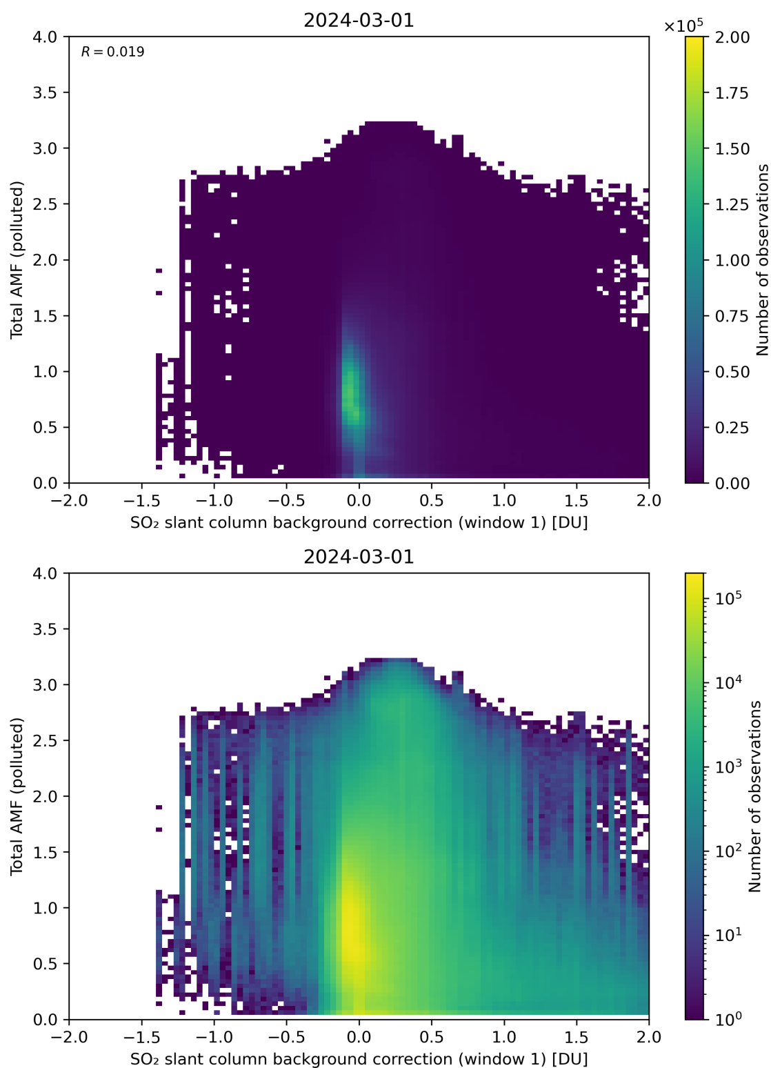
Figure 109: Scatter density plot of “SO 2 slant column background correction (window 1)” against “Total AMF (polluted)” for 2024-02-29 to 2024-03-02.
