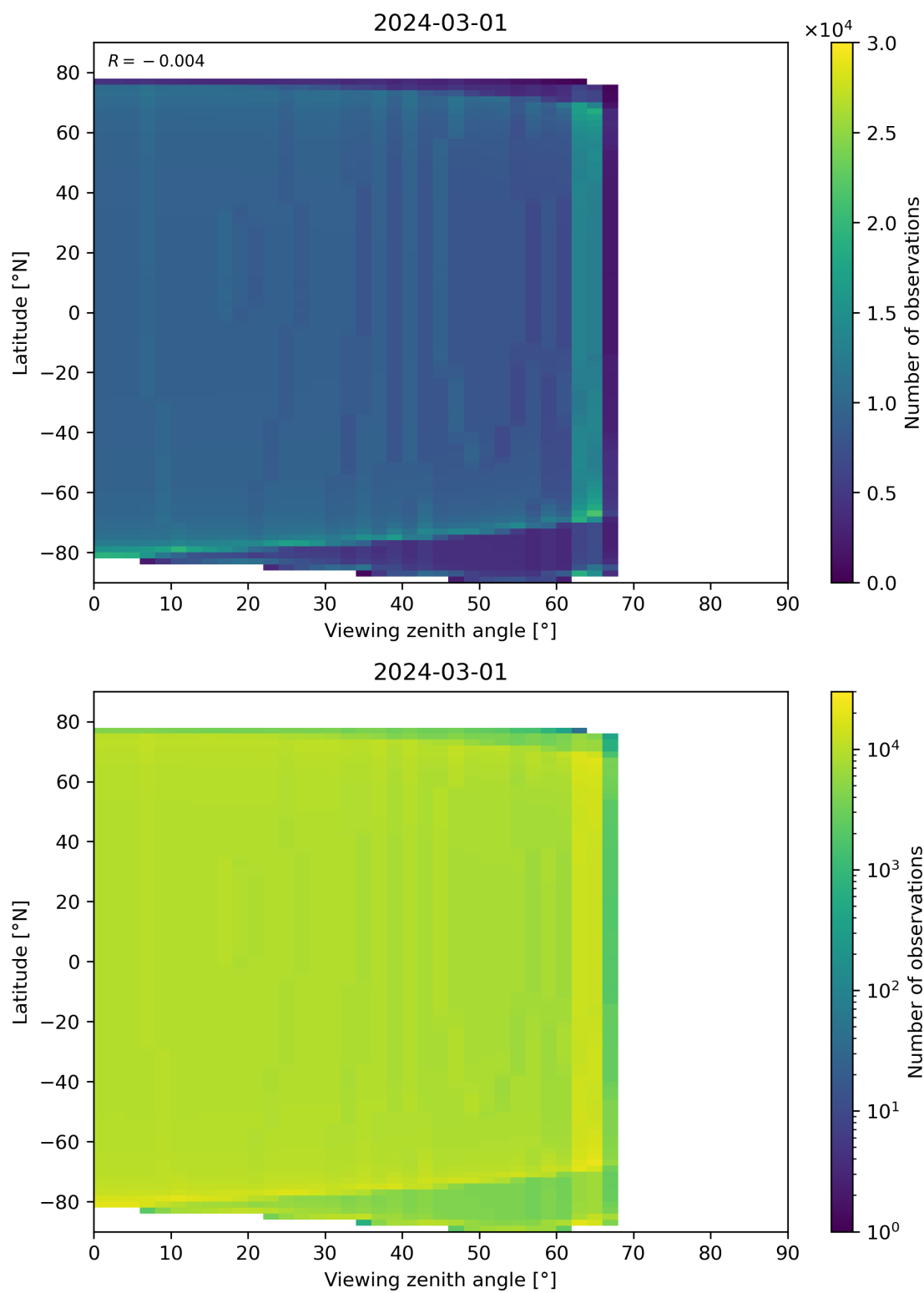
Figure 314: Scatter density plot of “Viewing zenith angle” against “Latitude” for 2024-02-29 to 2024-03-02.
