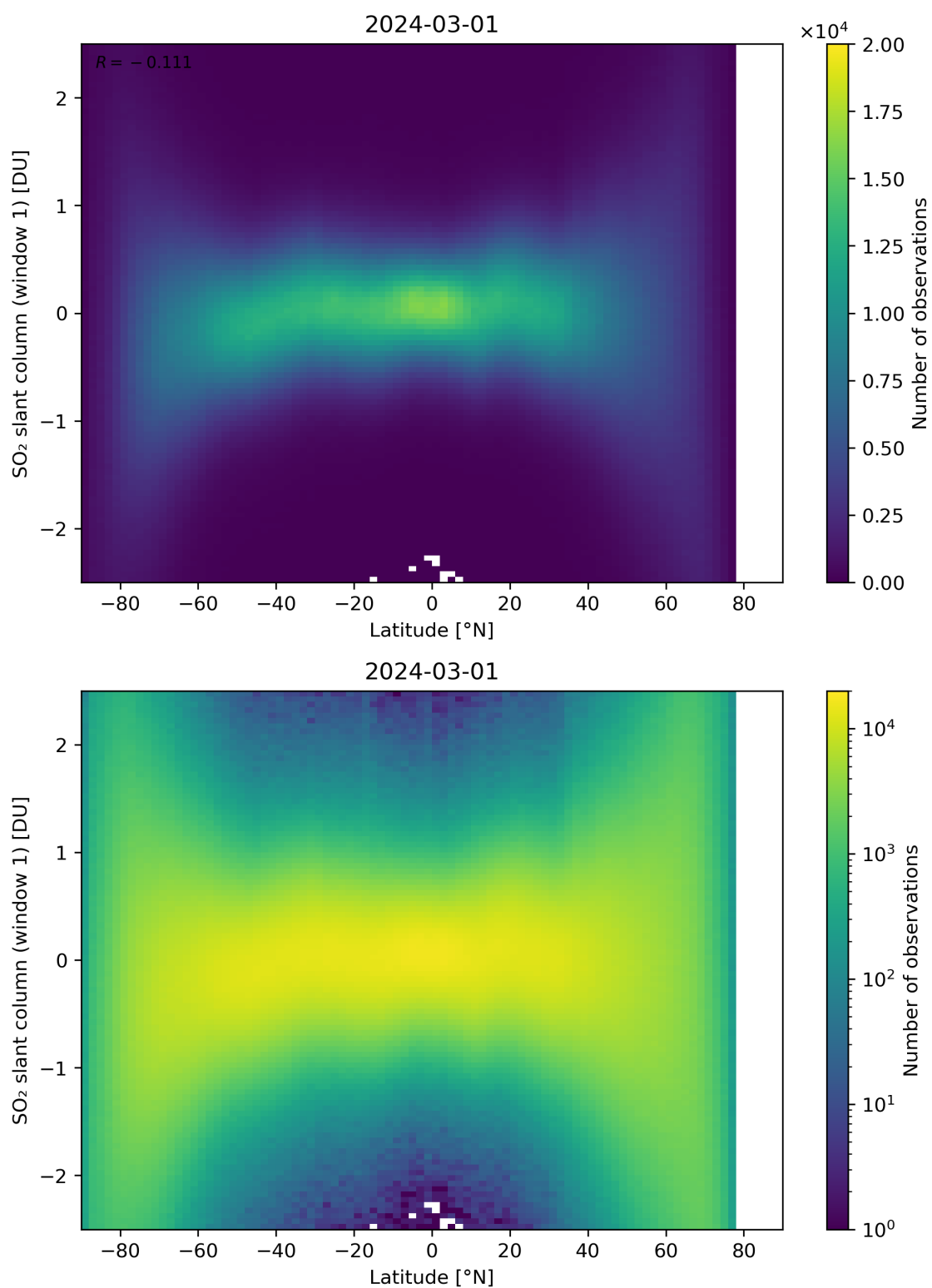
Figure 149: Scatter density plot of “Latitude” against “SO 2 slant column (window 1)” for 2024-02-29 to 2024-03-02.
