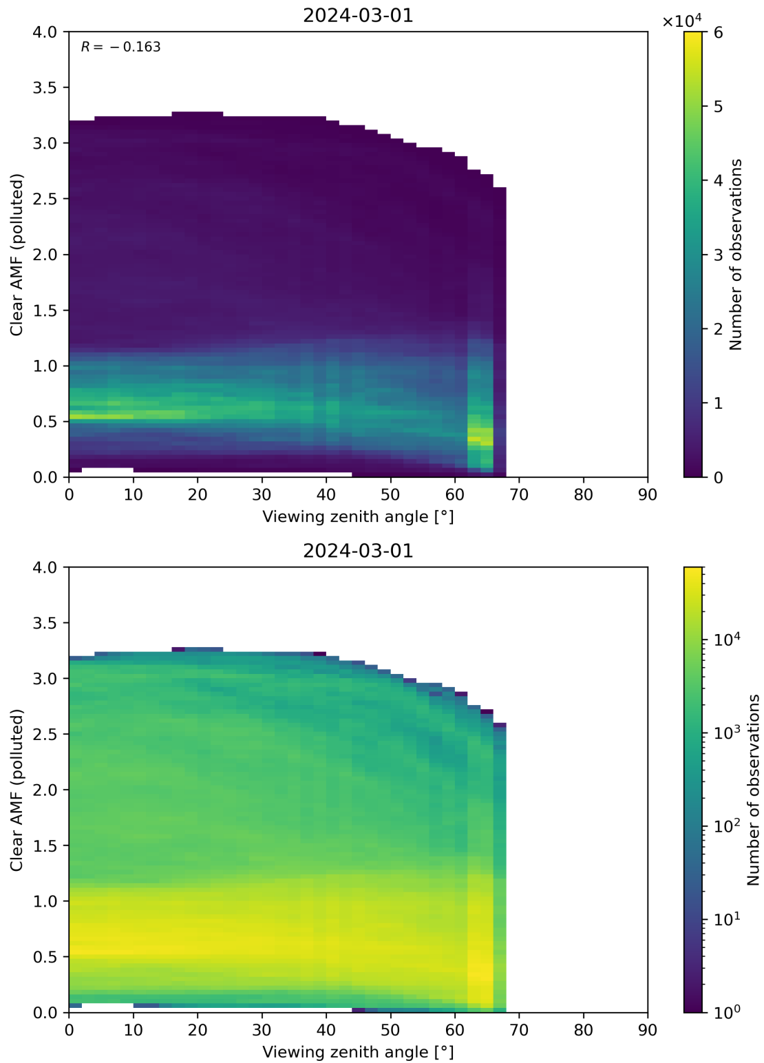
Figure 316: Scatter density plot of “Viewing zenith angle” against “Clear AMF (polluted)” for 2024-02-29 to 2024-03-02.
