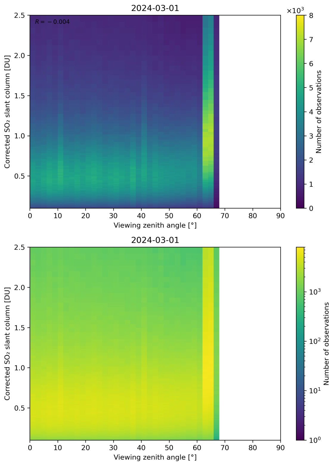
Figure 317: Scatter density plot of “Viewing zenith angle” against “Corrected SO 2 slant column” for 2024-02-29 to 2024-03-02.
