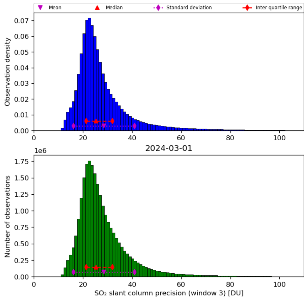
Figure 65: Histogram of “SO 2 slant column precision (window 3)” for 2024-02-29 to 2024-03-02
