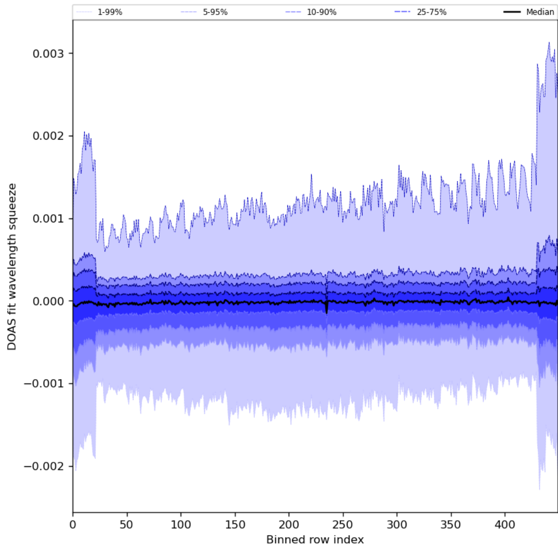
Figure 92: Along track statistics of “DOAS fit wavelength squeeze” for 2024-02-29 to 2024-03-02
