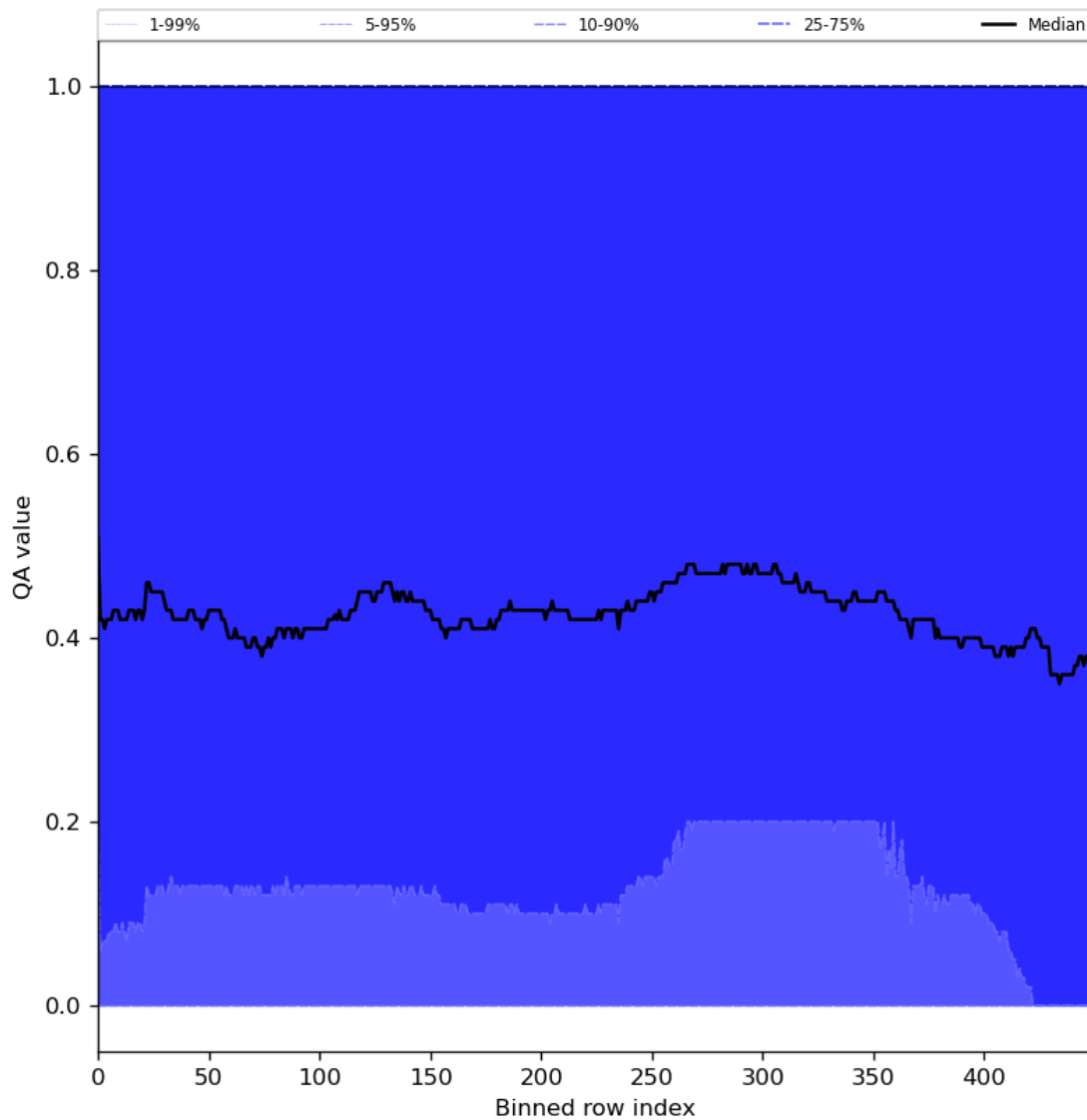
Figure 75: Along track statistics of “QA value” for 2024-02-29 to 2024-03-02
