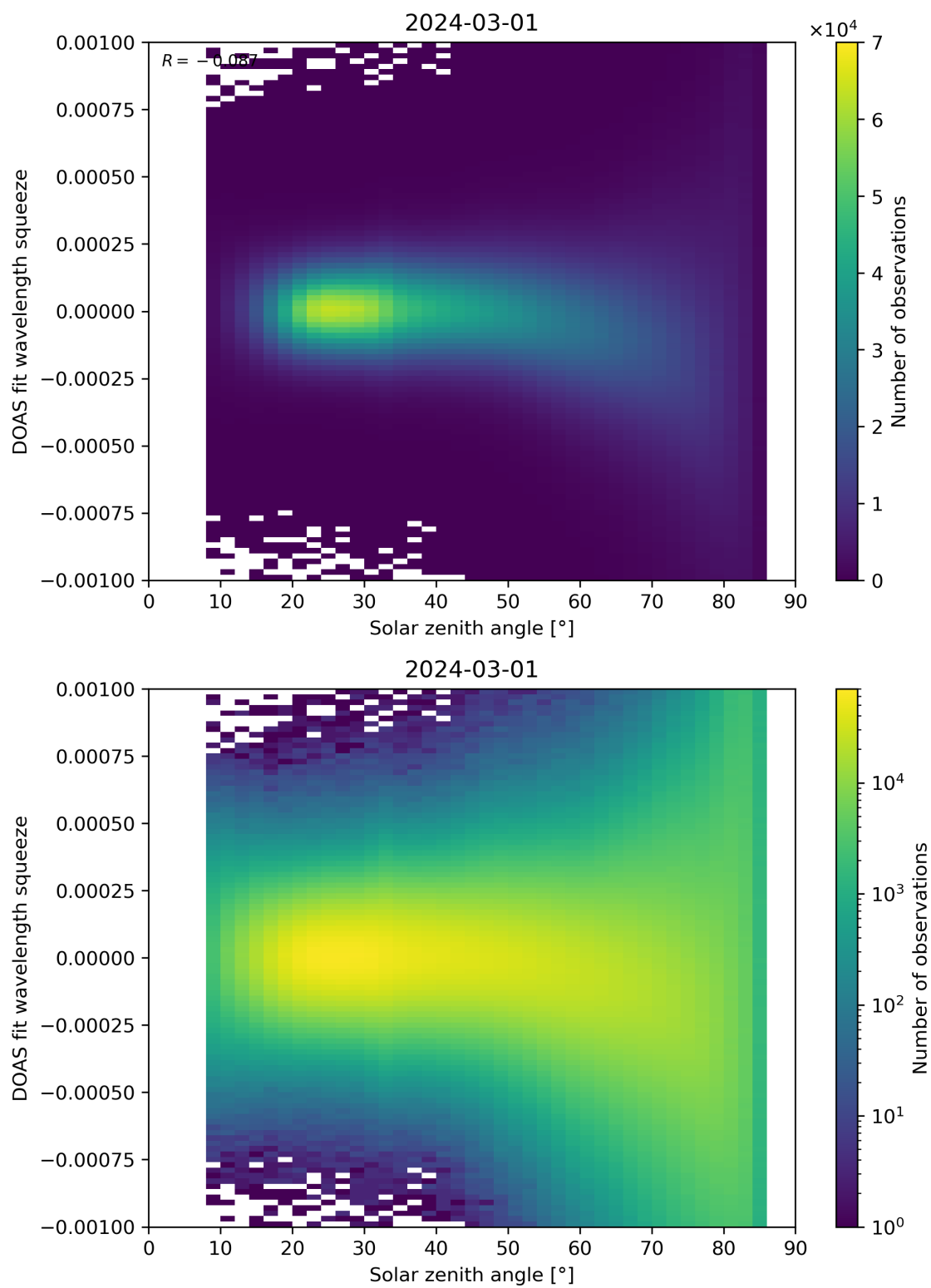
Figure 162: Scatter density plot of “Solar zenith angle” against “DOAS fit wavelength squeeze” for 2024-02-29 to 2024-03-02.
