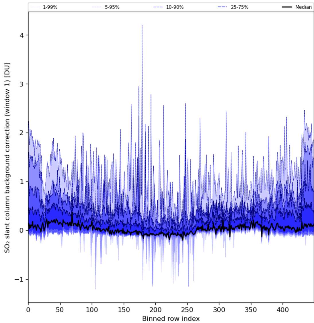
Figure 82: Along track statistics of “SO 2 slant column background correction (window 1)” for 2024-02-29 to 2024-03-02
