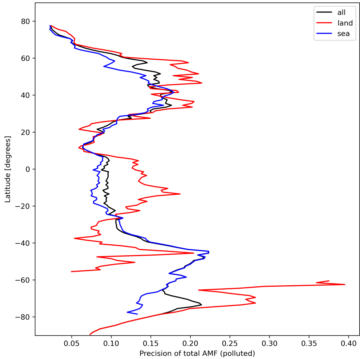
Figure 49: Zonal average of “Precision of total AMF (polluted)” for 2024-02-29 to 2024-03-02.
