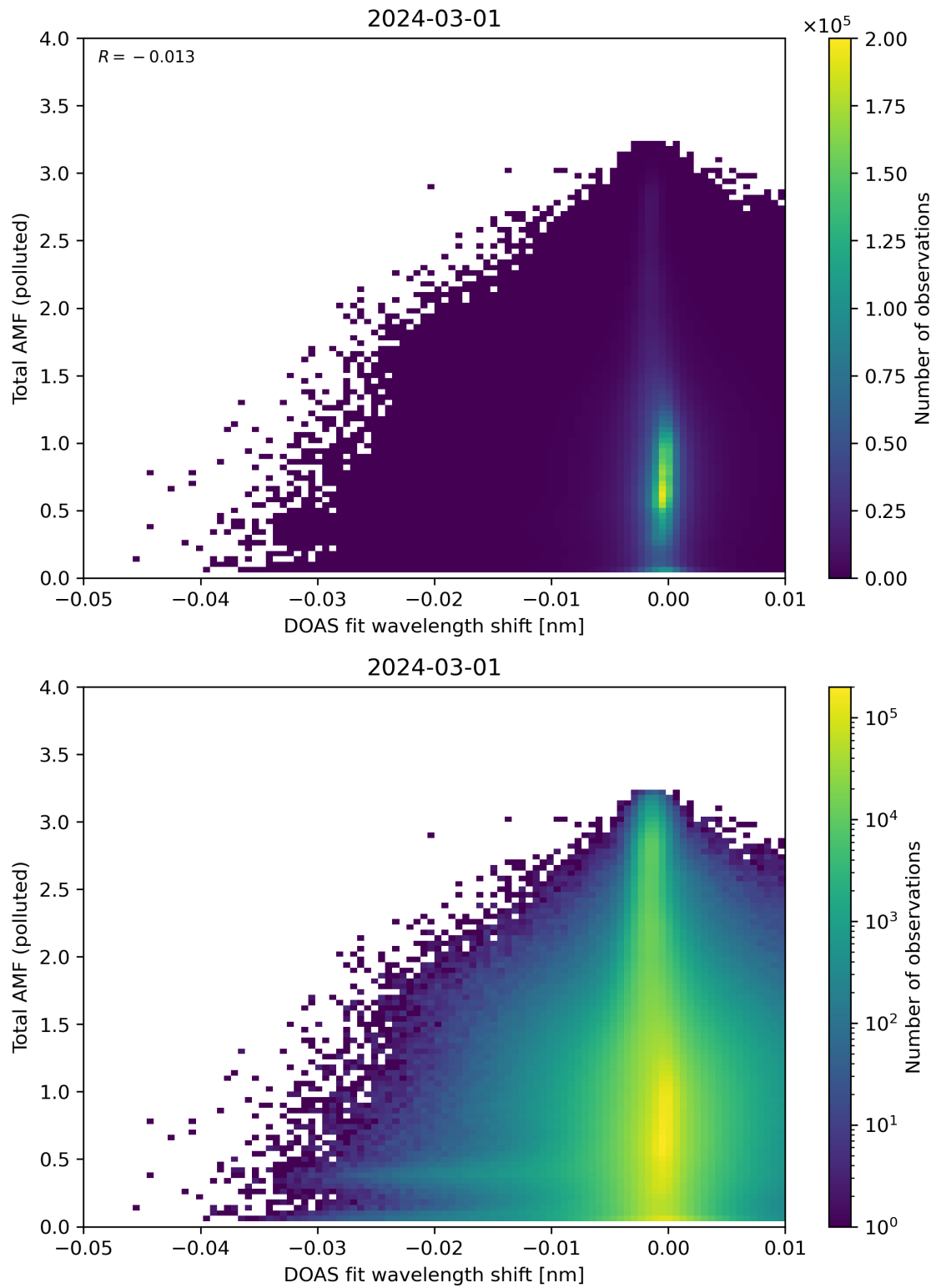
Figure 130: Scatter density plot of “DOAS fit wavelength shift” against “Total AMF (polluted)” for 2024-02-29 to 2024-03-02.
