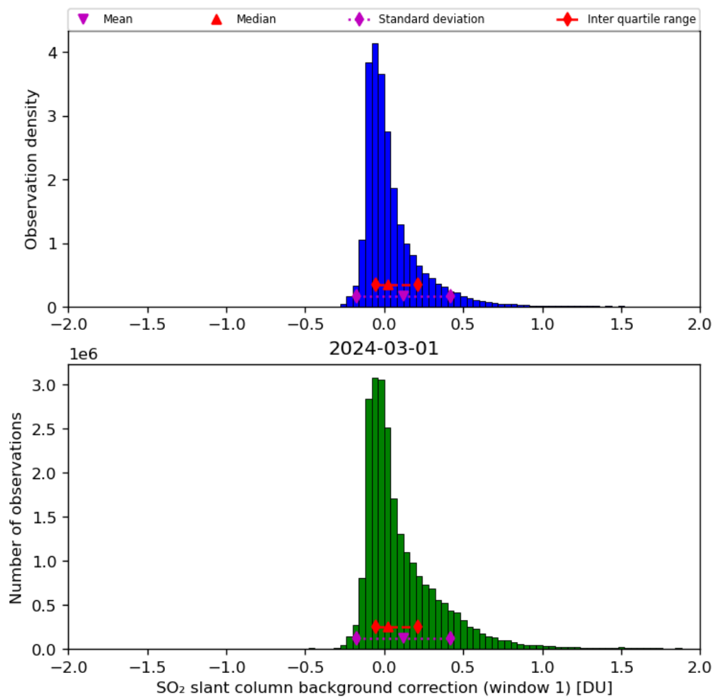
Figure 59: Histogram of “SO 2 slant column background correction (window 1)” for 2024-02-29 to 2024-03-02
