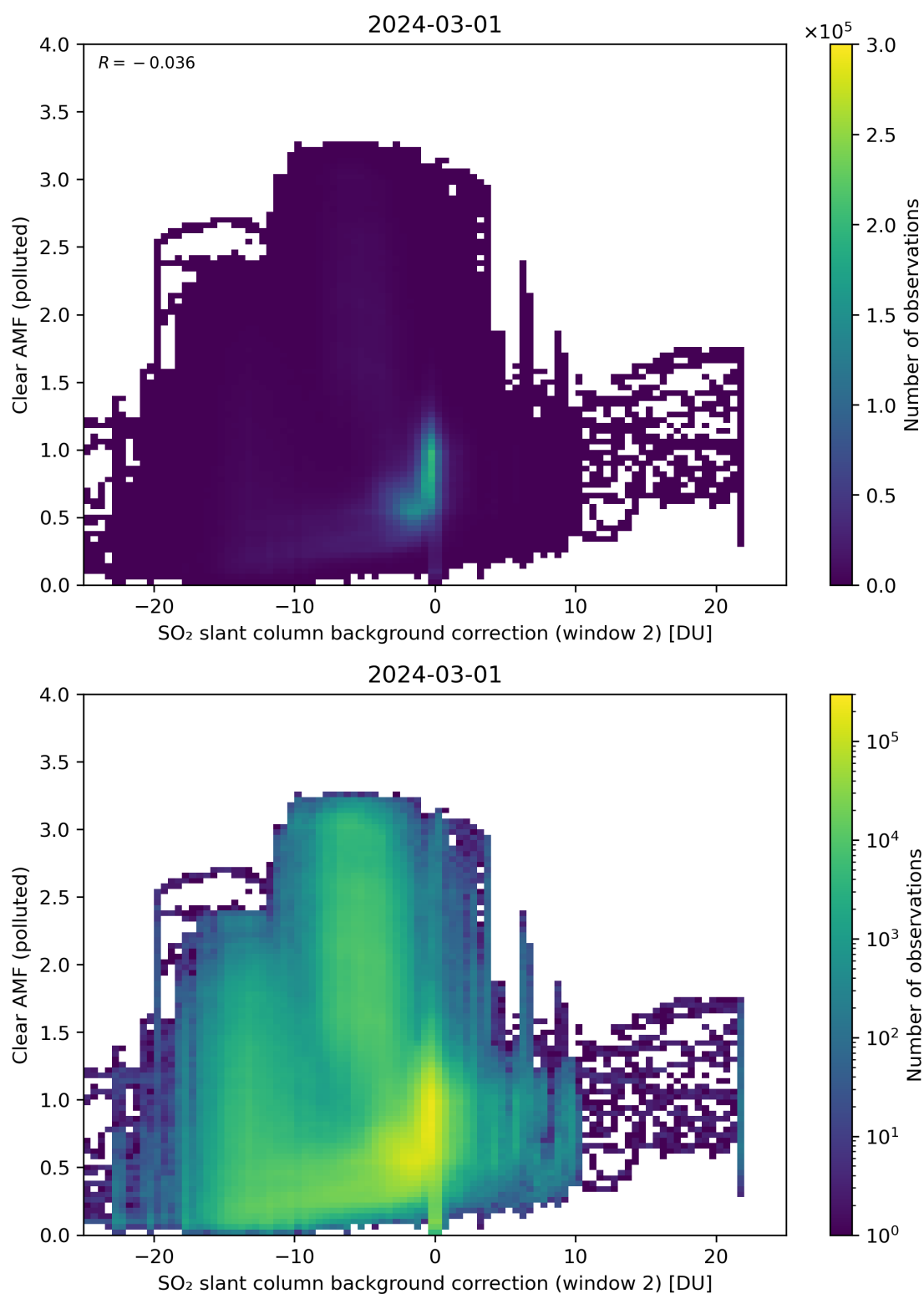
Figure 115: Scatter density plot of “SO 2 slant column background correction (window 2)” against “Clear AMF (polluted)” for 2024-02-29 to 2024-03-02.
