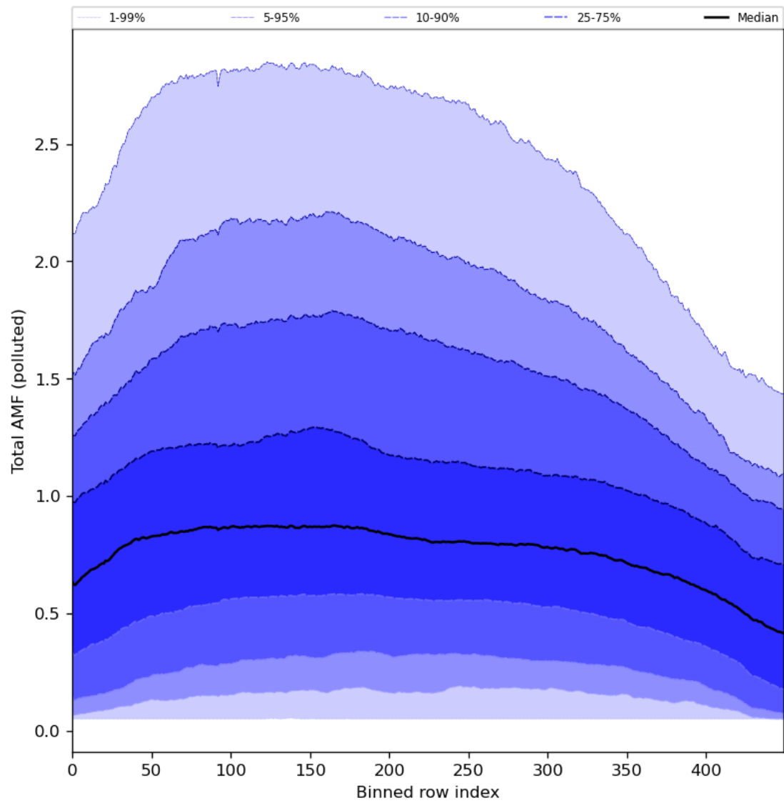
Figure 94: Along track statistics of “Total AMF (polluted)” for 2024-02-29 to 2024-03-02
