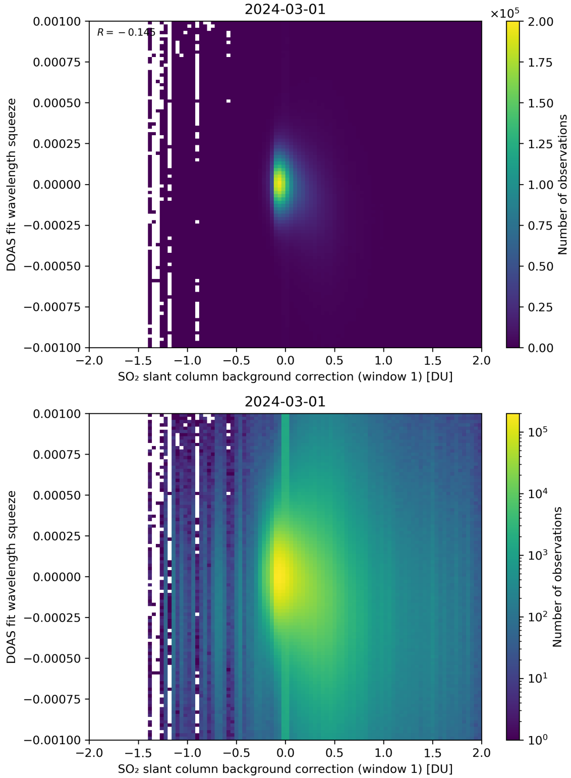
Figure 101: Scatter density plot of “SO 2 slant column background correction (window 1)” against “DOAS fit wavelength squeeze” for 2024-02-29 to 2024-03-02.
