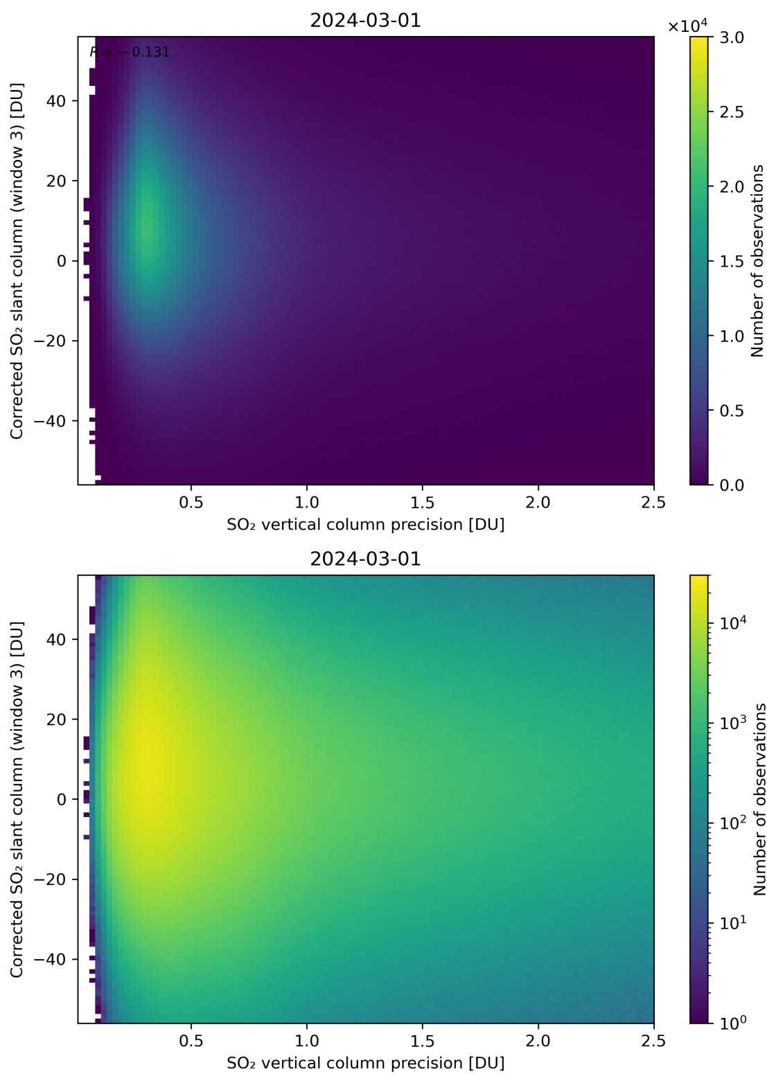
Figure 288: Scatter density plot of “SO 2 vertical column precision” against “Corrected SO 2 slant column (window 3)” for 2024-02-29 to 2024-03-02.
