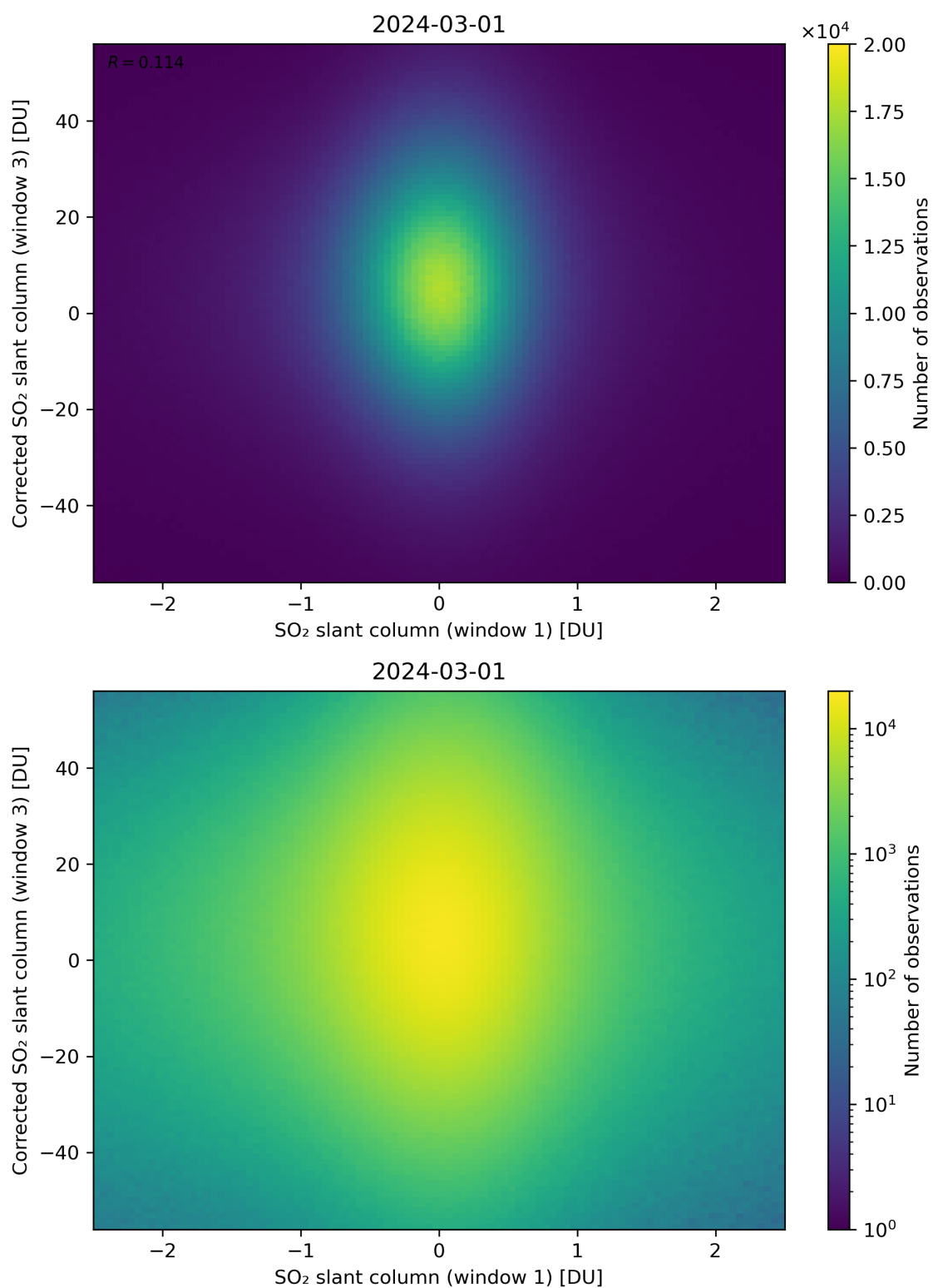
Figure 234: Scatter density plot of “SO 2 slant column (window 1)” against “Corrected SO 2 slant column (window 3)” for 2024-02-29 to 2024-03-02.
