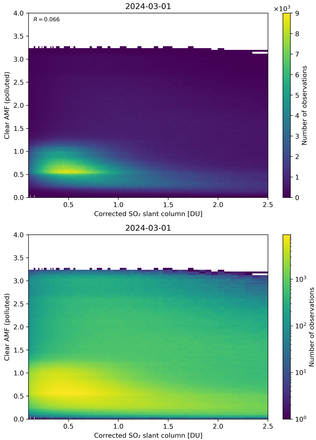
Figure 184: Scatter density plot of “Corrected SO 2 slant column” against “Clear AMF (polluted)” for 2024-02-29 to 2024-03-02.
