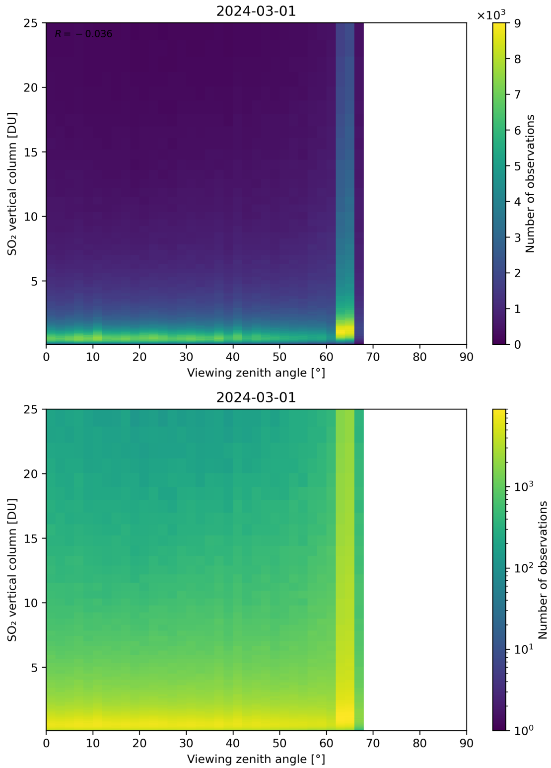
Figure 327: Scatter density plot of “Viewing zenith angle” against “SO 2 vertical column” for 2024-02-29 to 2024-03-02.
