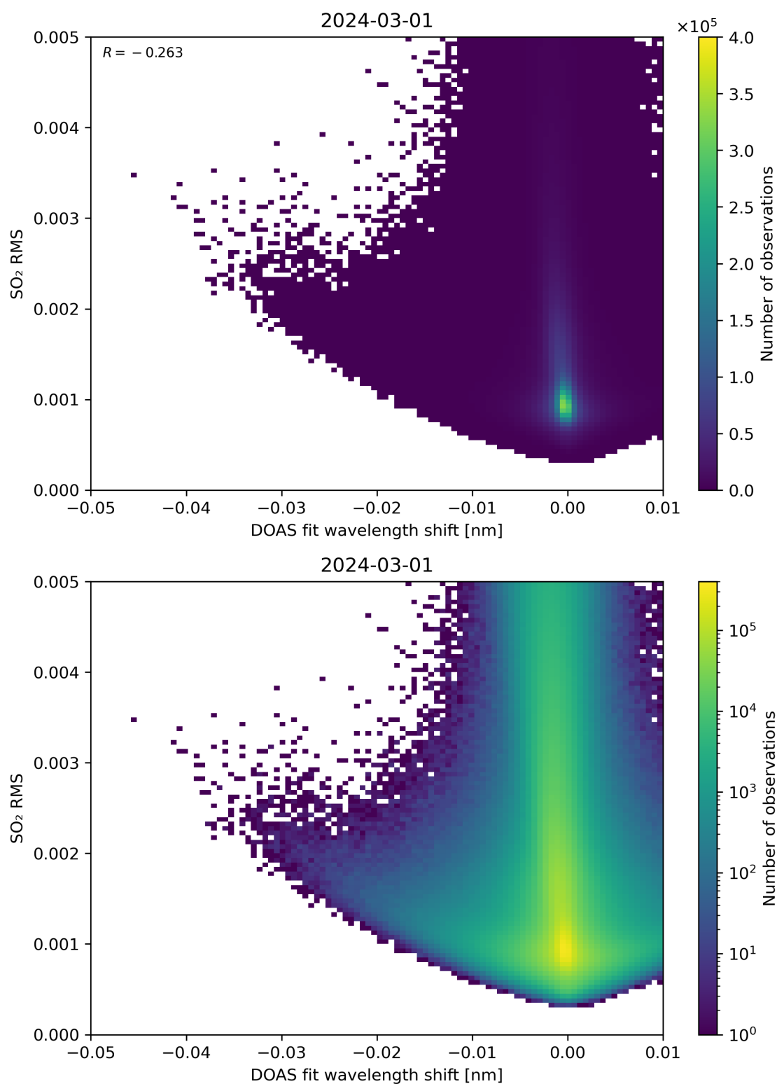
Figure 128: Scatter density plot of “DOAS fit wavelength shift” against “SO 2 RMS” for 2024-02-29 to 2024-03-02.
