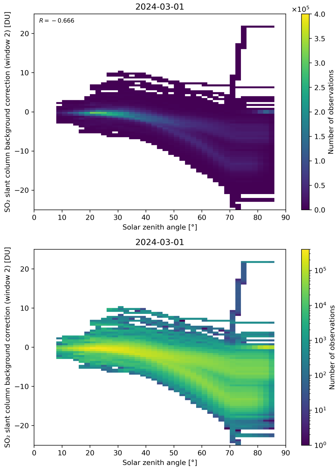
Figure 159: Scatter density plot of “Solar zenith angle” against “SO 2 slant column background correction (window 2)” for 2024-02-29 to 2024-03-02.
