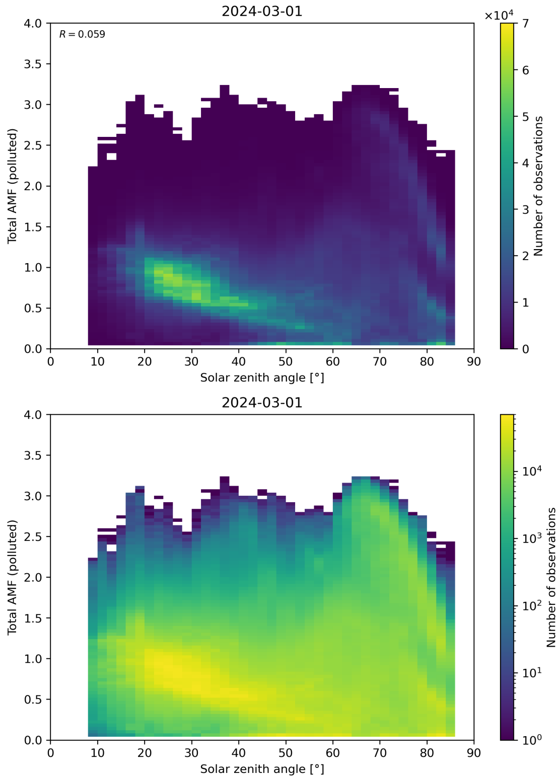
Figure 174: Scatter density plot of “Solar zenith angle” against “Total AMF (polluted)” for 2024-02-29 to 2024-03-02.
