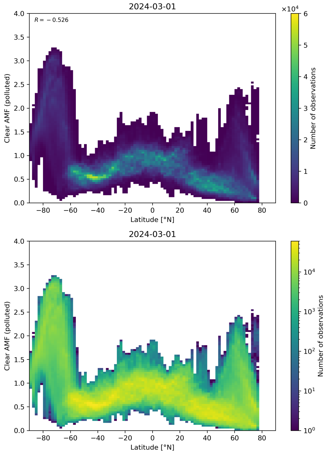
Figure 145: Scatter density plot of “Latitude” against “Clear AMF (polluted)” for 2024-02-29 to 2024-03-02.
