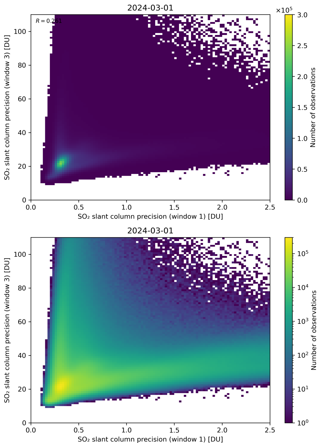
Figure 229: Scatter density plot of “SO 2 slant column precision (window 1)” against “SO 2 slant column precision (window 3)” for 2024-02-29 to 2024-03-02.
