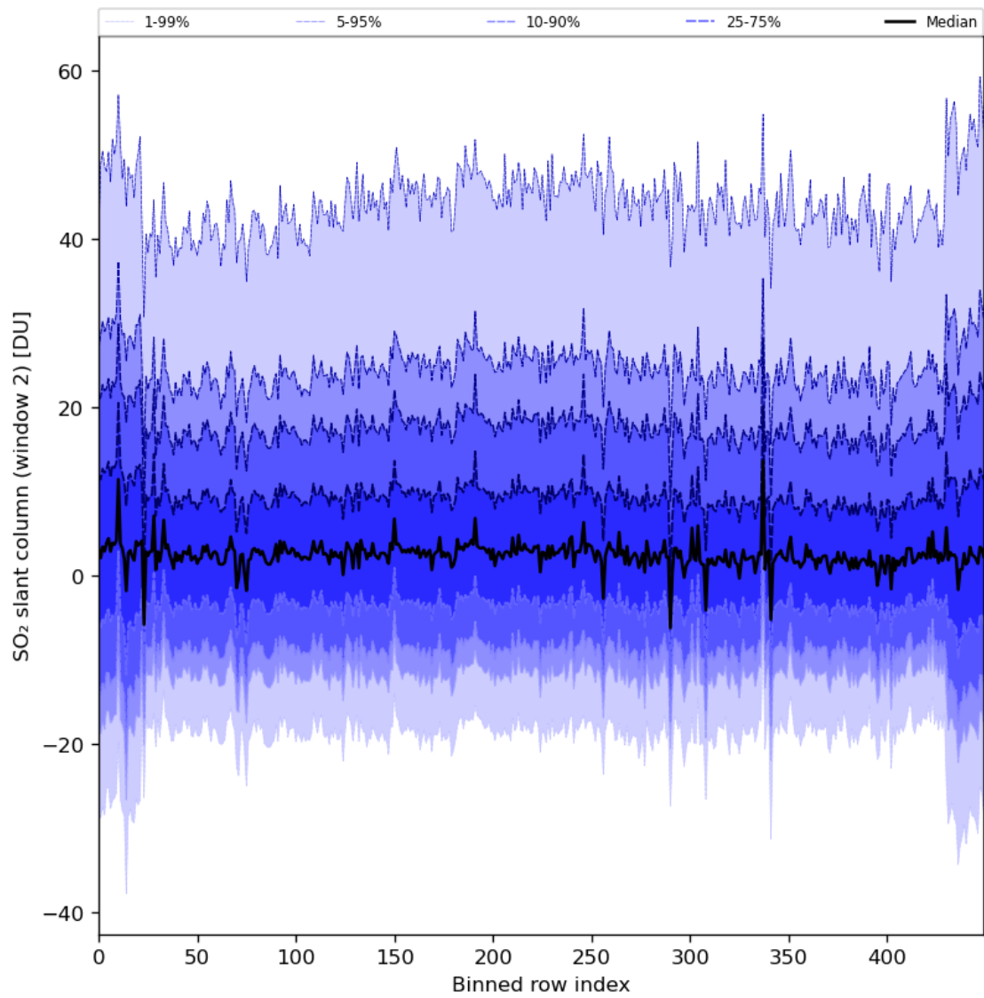
Figure 83: Along track statistics of “SO 2 slant column (window 2)” for 2024-02-29 to 2024-03-02
