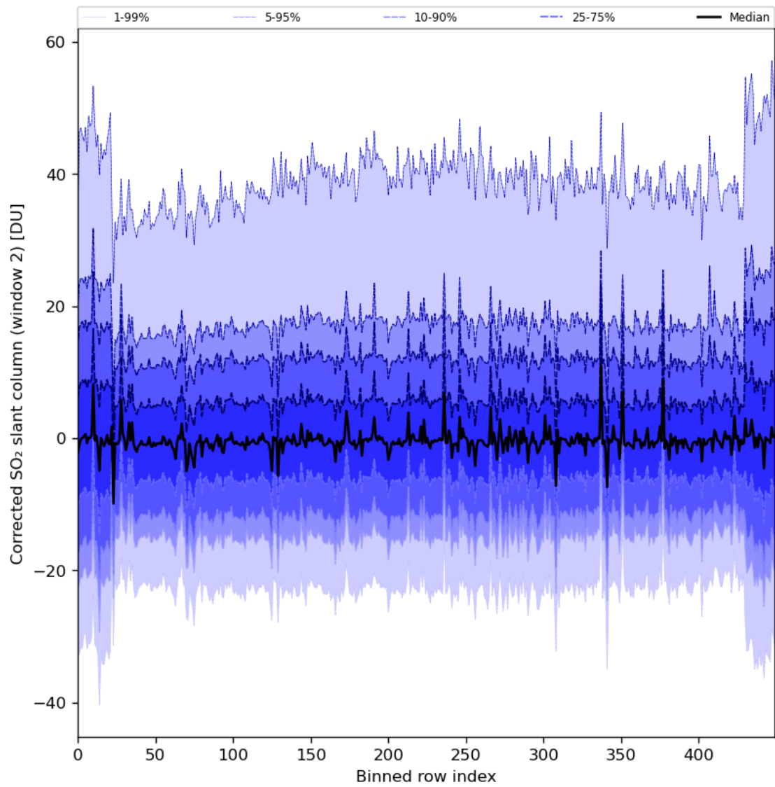
Figure 85: Along track statistics of “Corrected SO 2 slant column (window 2)” for 2024-02-29 to 2024-03-02
