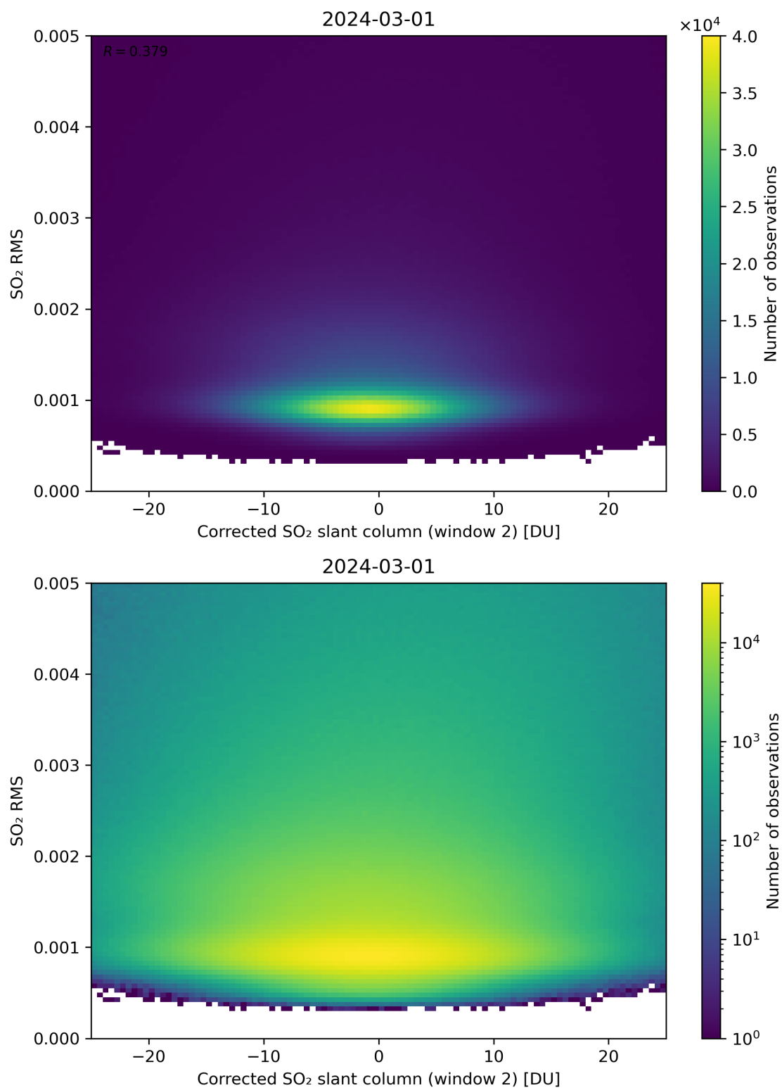
Figure 198: Scatter density plot of “Corrected SO 2 slant column (window 2)” against “SO 2 RMS” for 2024-02-29 to 2024-03-02.
