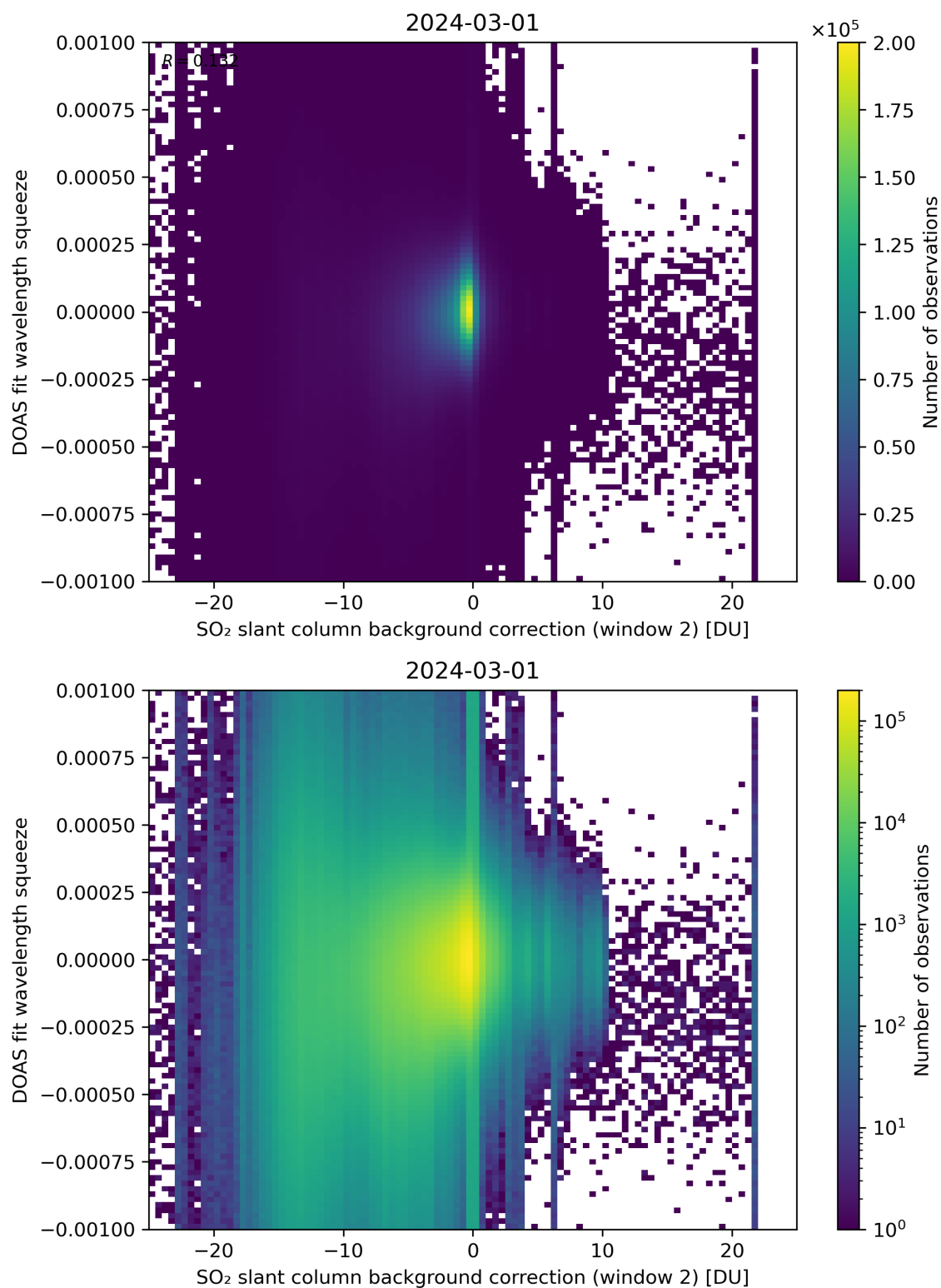
Figure 113: Scatter density plot of “SO 2 slant column background correction (window 2)” against “DOAS fit wavelength squeeze” for 2024-02-29 to 2024-03-02.
