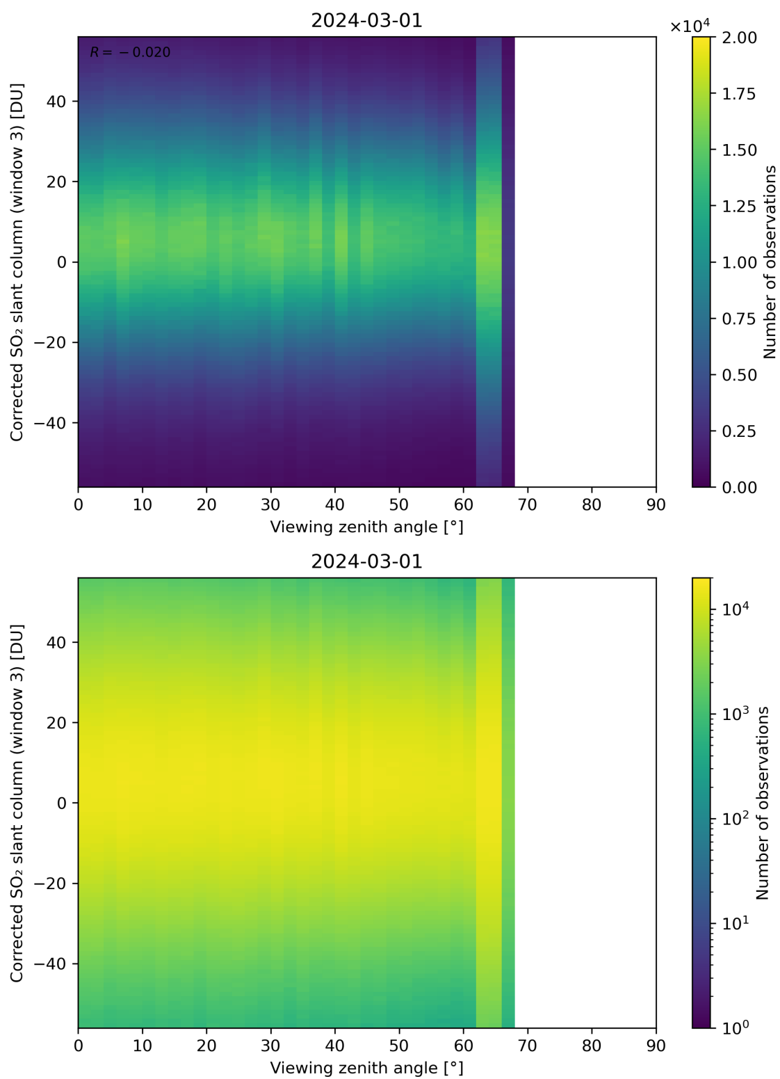
Figure 319: Scatter density plot of “Viewing zenith angle” against “Corrected SO 2 slant column (window 3)” for 2024-02-29 to 2024-03-02.
