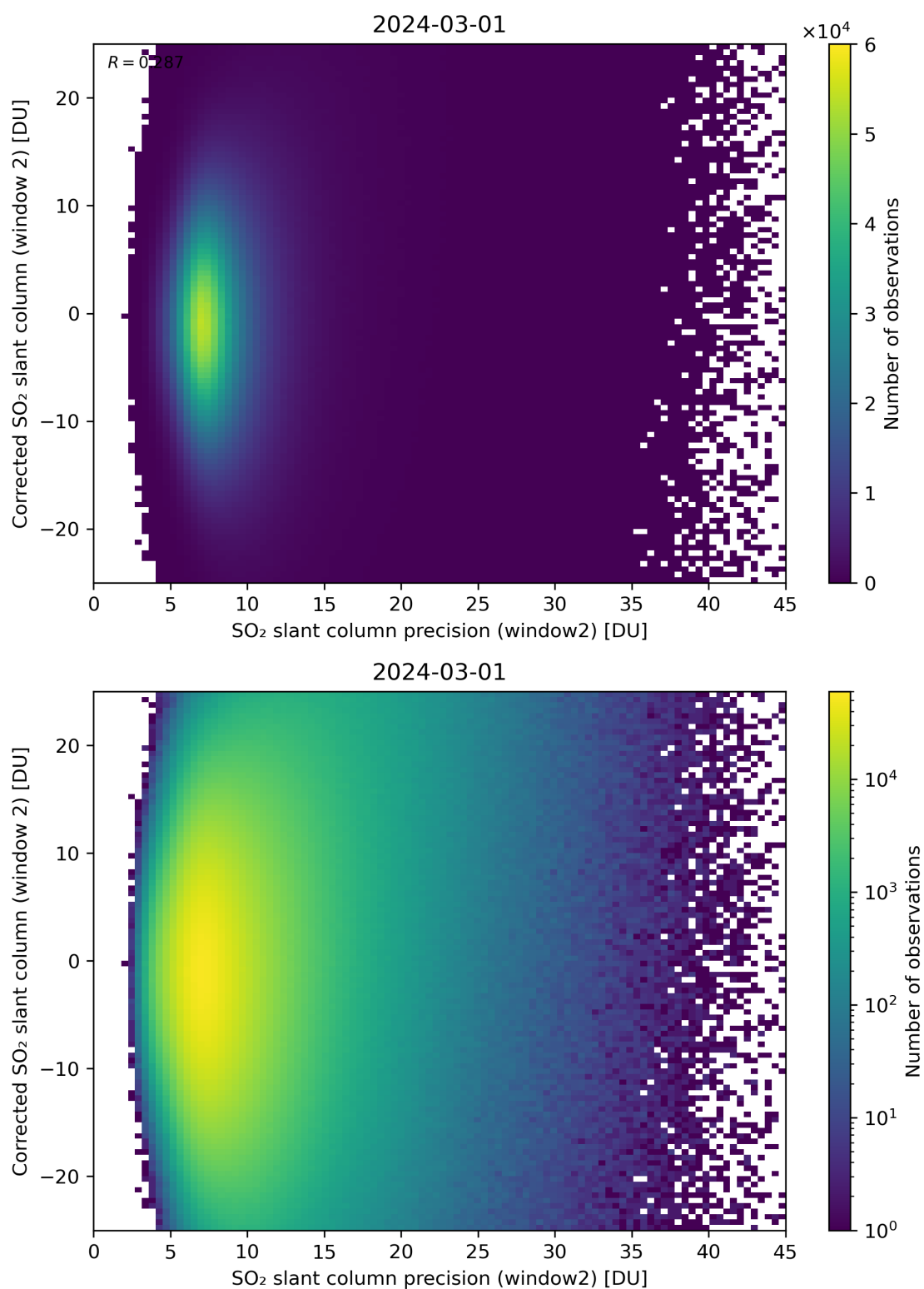
Figure 247: Scatter density plot of “SO 2 slant column precision (window2)” against “Corrected SO 2 slant column (window 2)” for 2024-02-29 to 2024-03-02.
