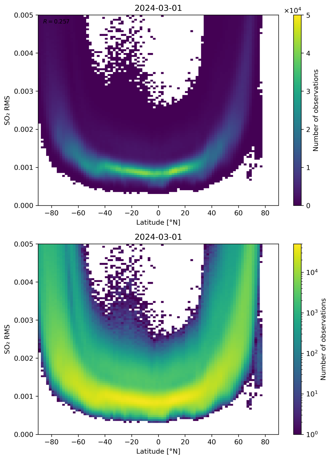
Figure 144: Scatter density plot of “Latitude” against “SO 2 RMS” for 2024-02-29 to 2024-03-02.
