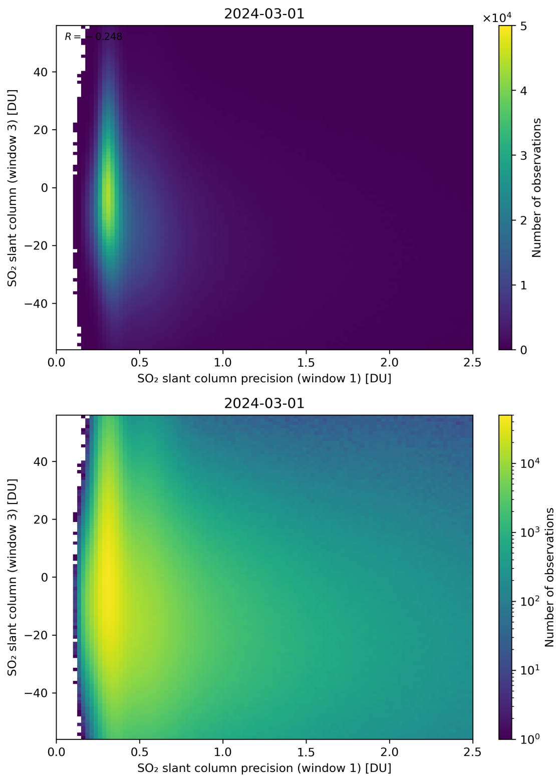
Figure 228: Scatter density plot of “SO 2 slant column precision (window 1)” against “SO 2 slant column (window 3)” for 2024-02-29 to 2024-03-02.
