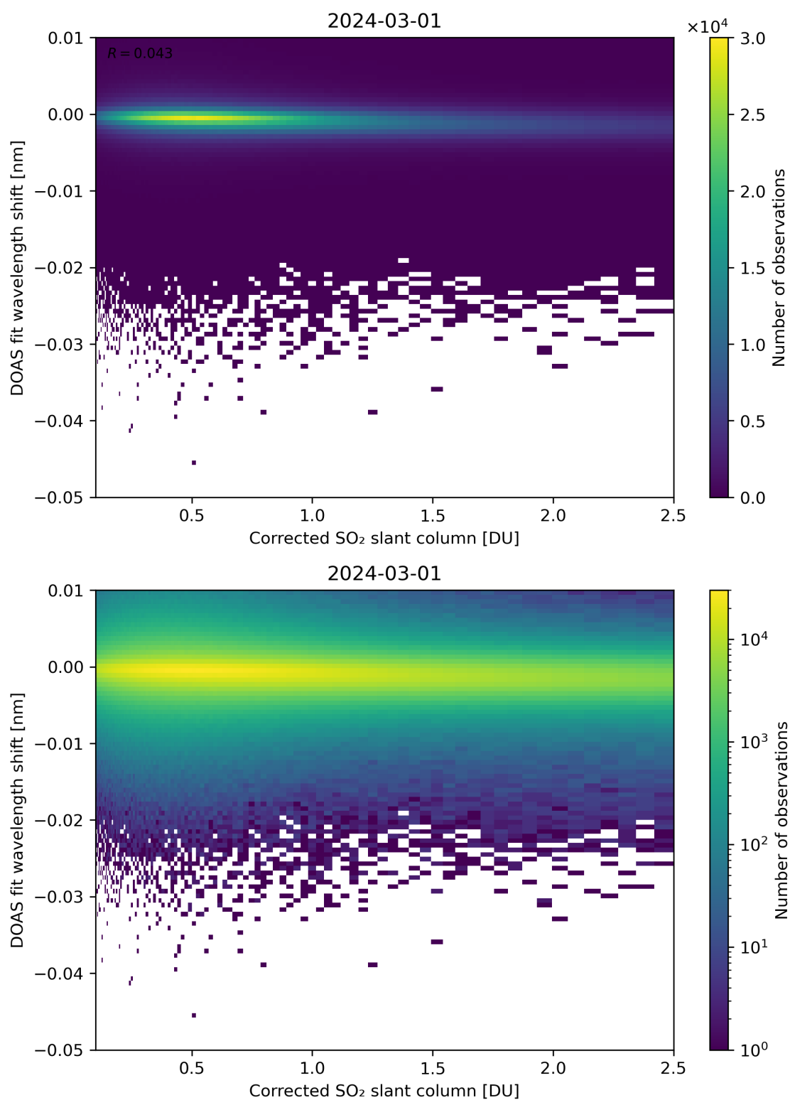
Figure 181: Scatter density plot of “Corrected SO 2 slant column” against “DOAS fit wavelength shift” for 2024-02-29 to 2024-03-02.
