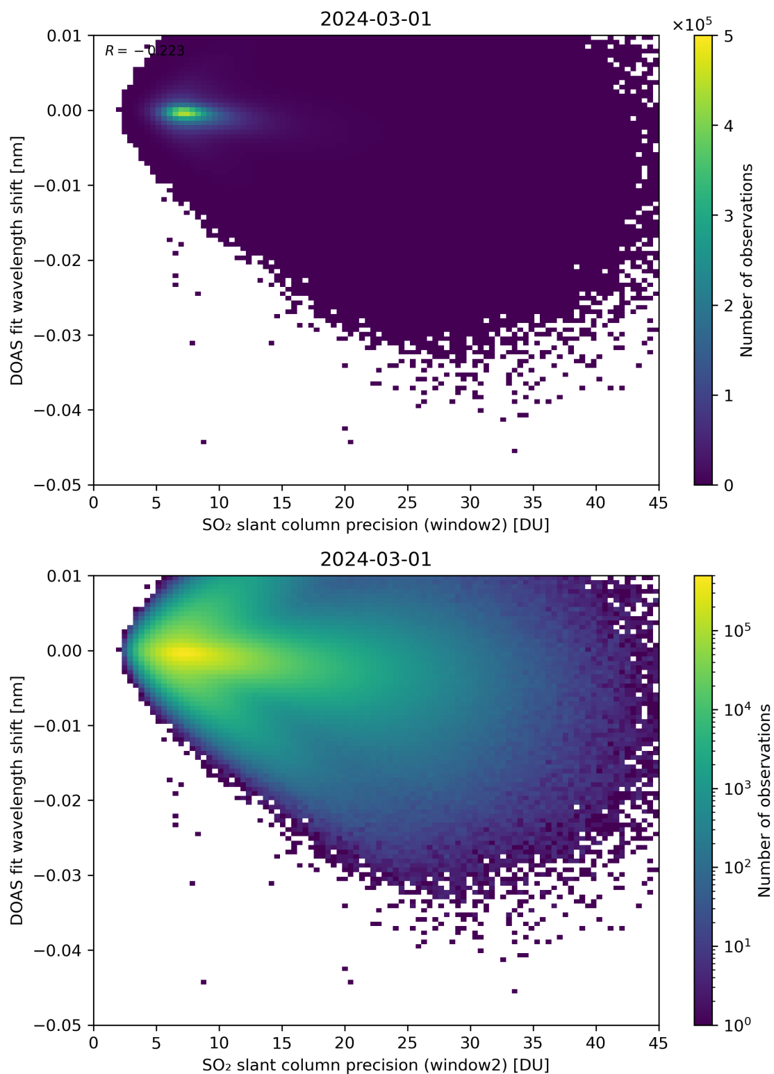
Figure 243: Scatter density plot of “SO 2 slant column precision (window2)” against “DOAS fit wavelength shift” for 2024-02-29 to 2024-03-02.
