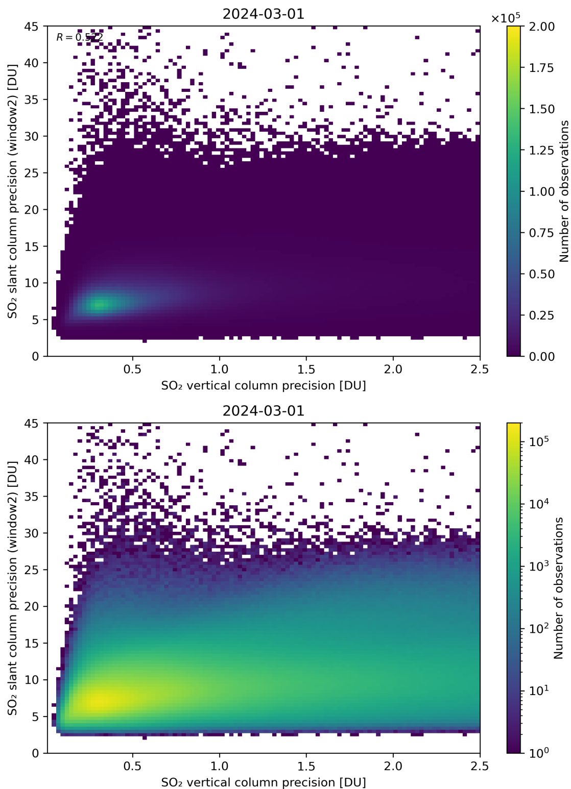
Figure 291: Scatter density plot of “SO 2 vertical column precision” against “SO 2 slant column precision (window2)” for 2024-02-29 to 2024-03-02.
