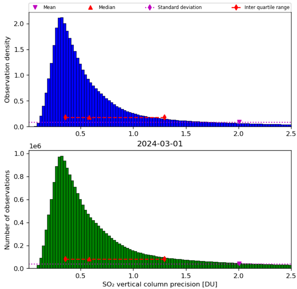
Figure 54: Histogram of “SO 2 vertical column precision” for 2024-02-29 to 2024-03-02
