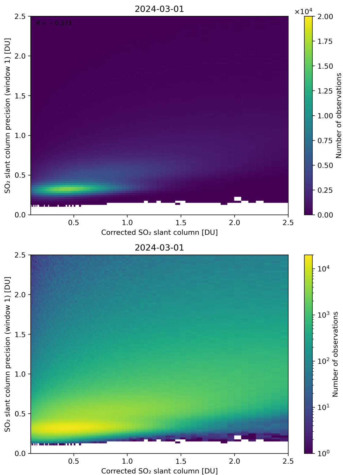
Figure 188: Scatter density plot of “Corrected SO 2 slant column” against “SO 2 slant column precision (window 1)” for 2024-02-29 to 2024-03-02.
