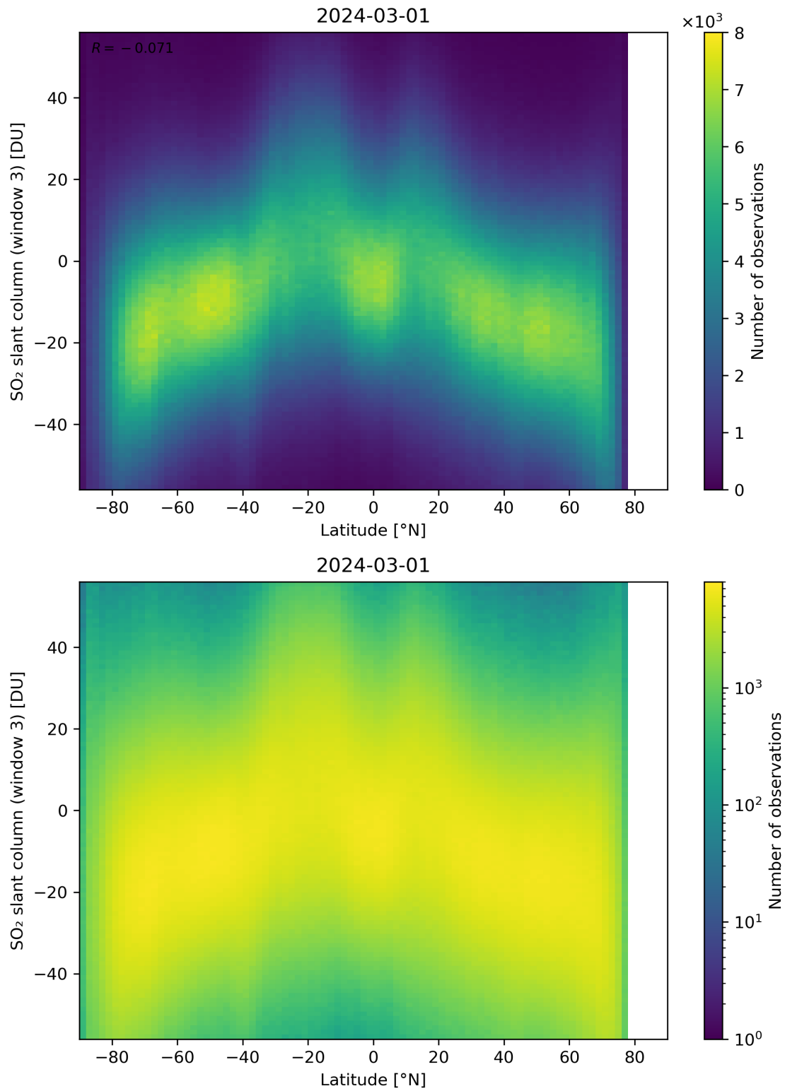
Figure 152: Scatter density plot of “Latitude” against “SO 2 slant column (window 3)” for 2024-02-29 to 2024-03-02.
