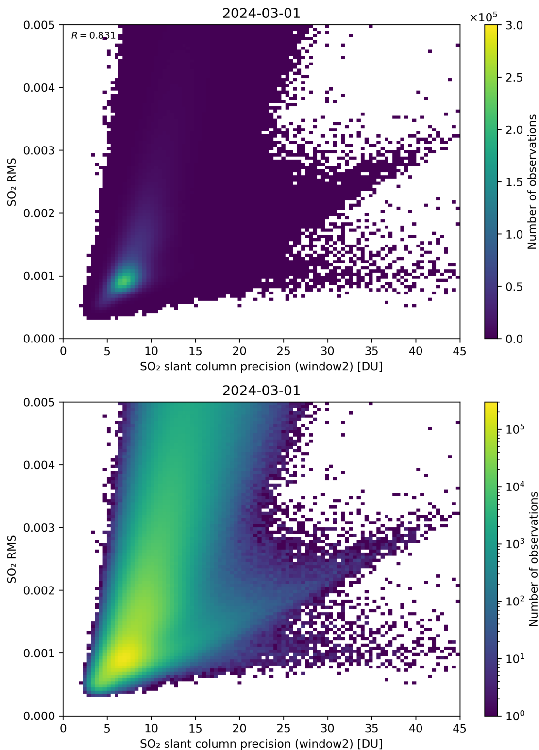
Figure 245: Scatter density plot of “SO 2 slant column precision (window2)” against “SO 2 RMS” for 2024-02-29 to 2024-03-02.
