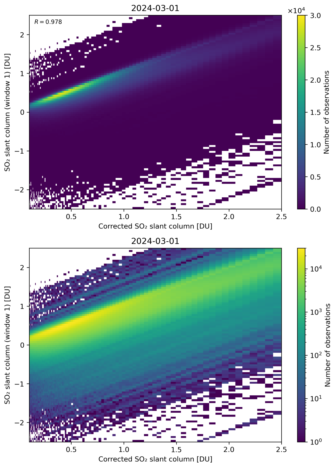
Figure 187: Scatter density plot of “Corrected SO 2 slant column” against “SO 2 slant column (window 1)” for 2024-02-29 to 2024-03-02.
