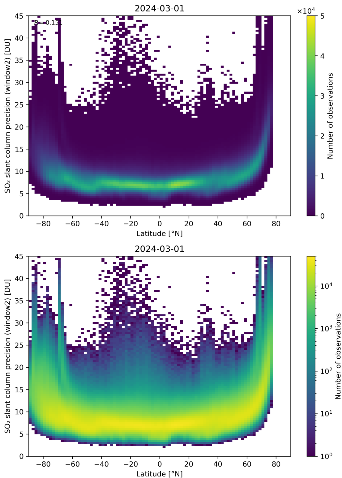
Figure 151: Scatter density plot of “Latitude” against “SO 2 slant column precision (window2)” for 2024-02-29 to 2024-03-02.
