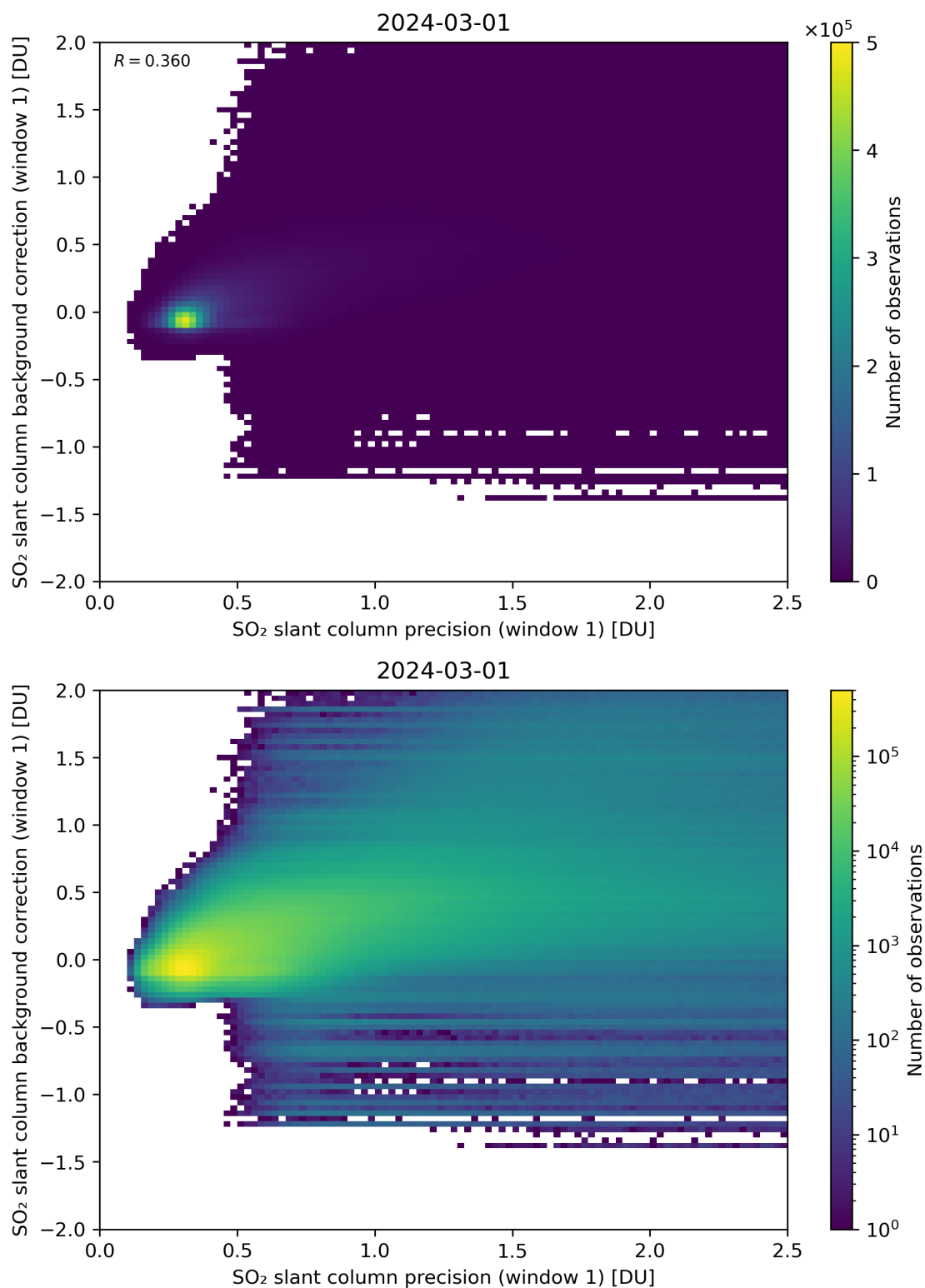
Figure 218: Scatter density plot of “SO 2 slant column precision (window 1)” against “SO 2 slant column background correction (window 1)” for 2024-02-29 to 2024-03-02.
