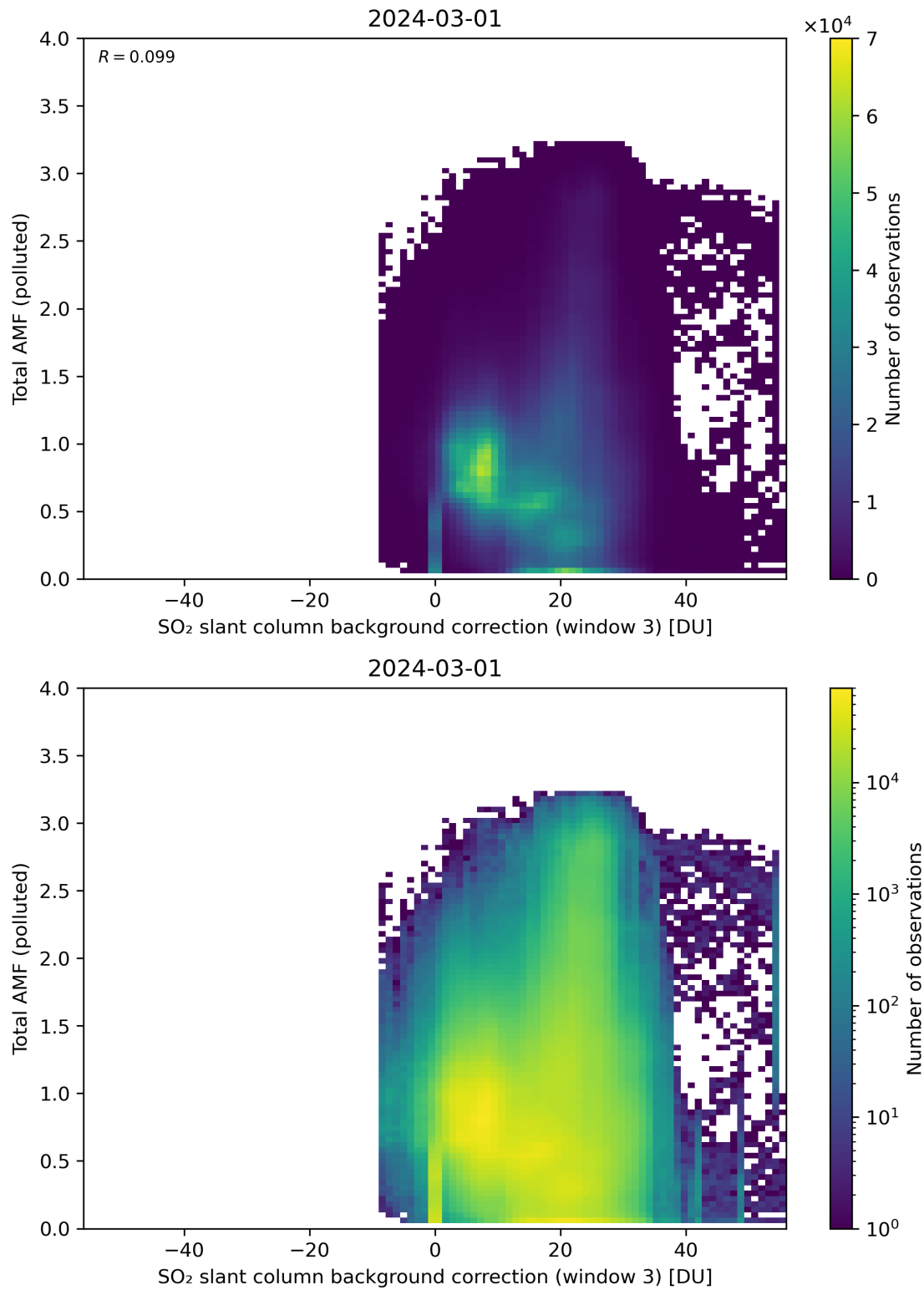
Figure 125: Scatter density plot of “SO 2 slant column background correction (window 3)” against “Total AMF (polluted)” for 2024-02-29 to 2024-03-02.
