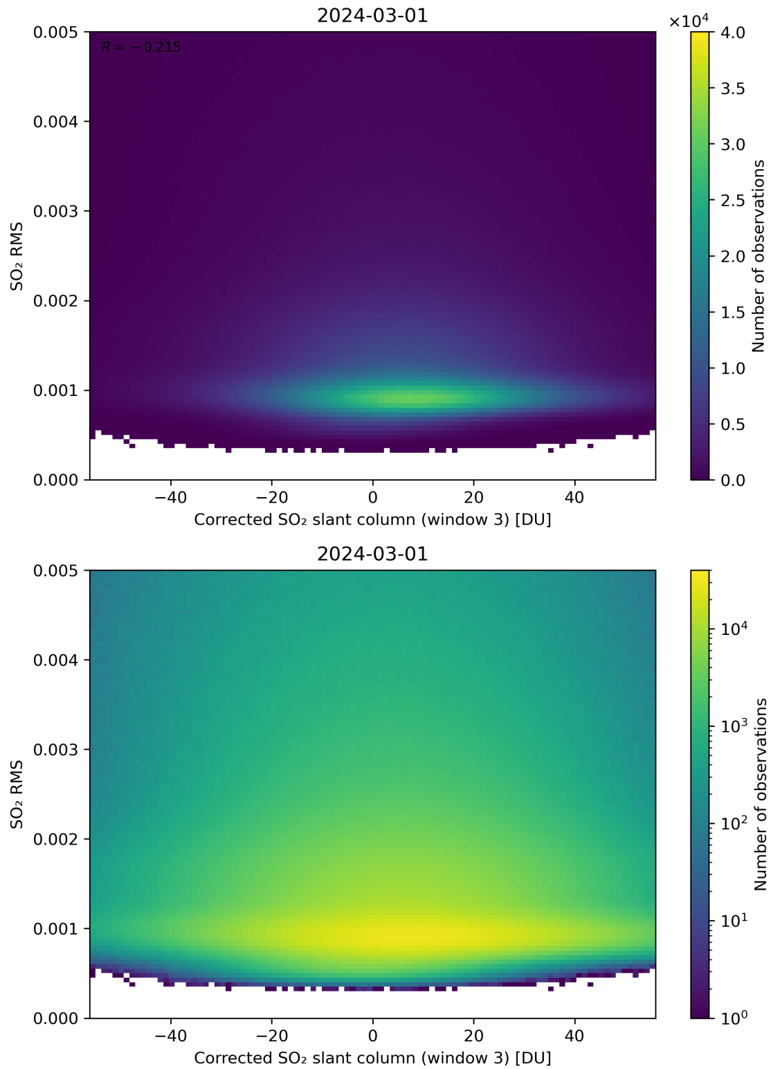
Figure 208: Scatter density plot of “Corrected SO 2 slant column (window 3)” against “SO 2 RMS” for 2024-02-29 to 2024-03-02.
