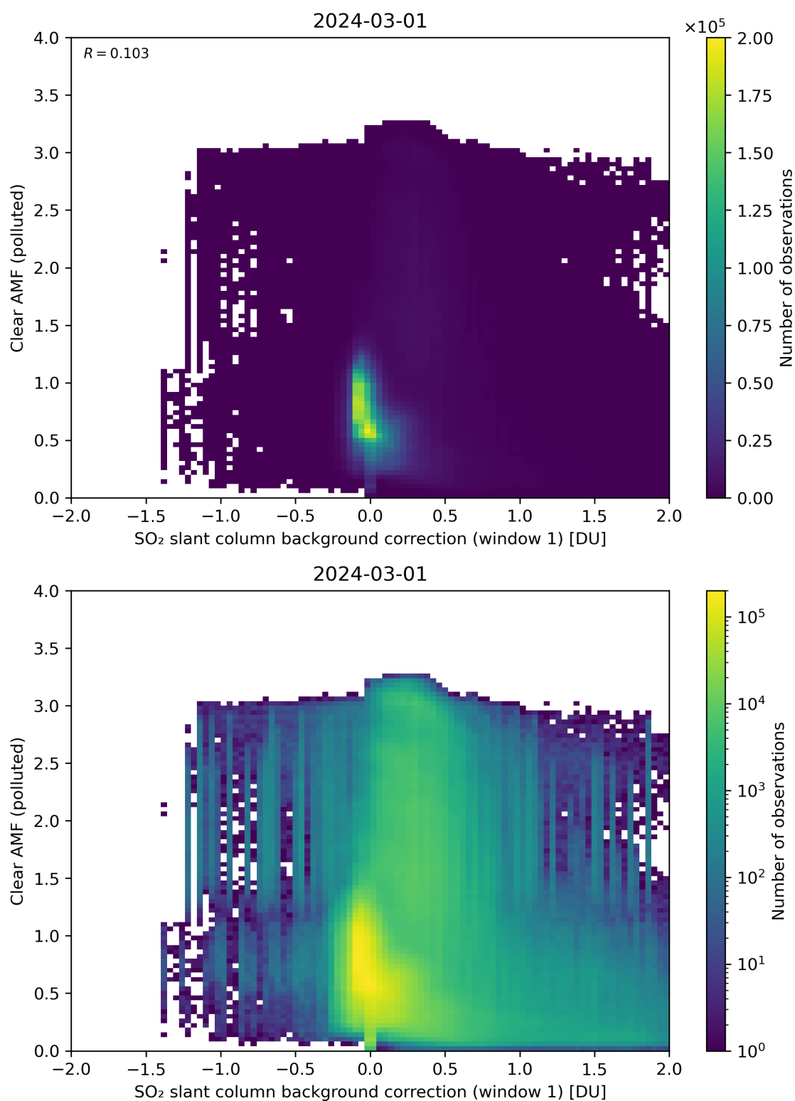
Figure 103: Scatter density plot of “SO 2 slant column background correction (window 1)” against “Clear AMF (polluted)” for 2024-02-29 to 2024-03-02.
