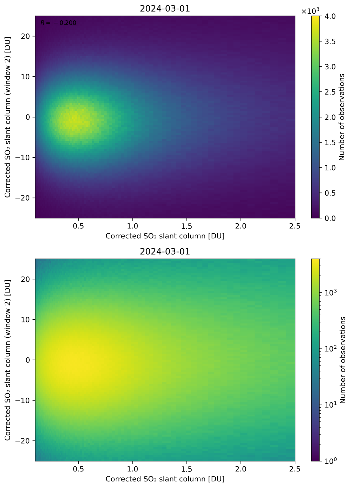
Figure 185: Scatter density plot of “Corrected SO 2 slant column” against “Corrected SO 2 slant column (window 2)” for 2024-02-29 to 2024-03-02.
