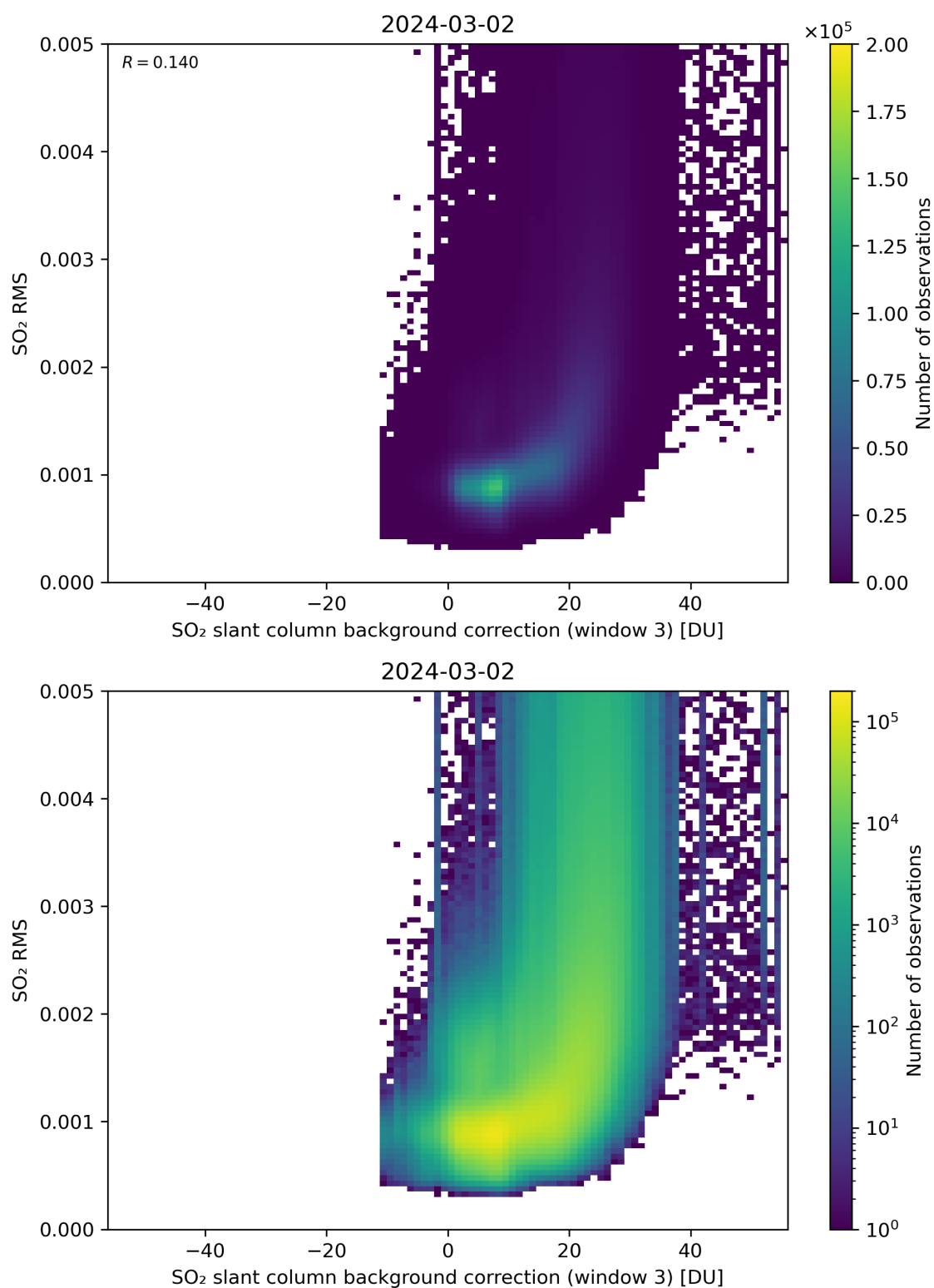
Figure 123: Scatter density plot of “SO 2 slant column background correction (window 3)” against “SO 2 RMS” for 2024-03-01 to 2024-03-03.
