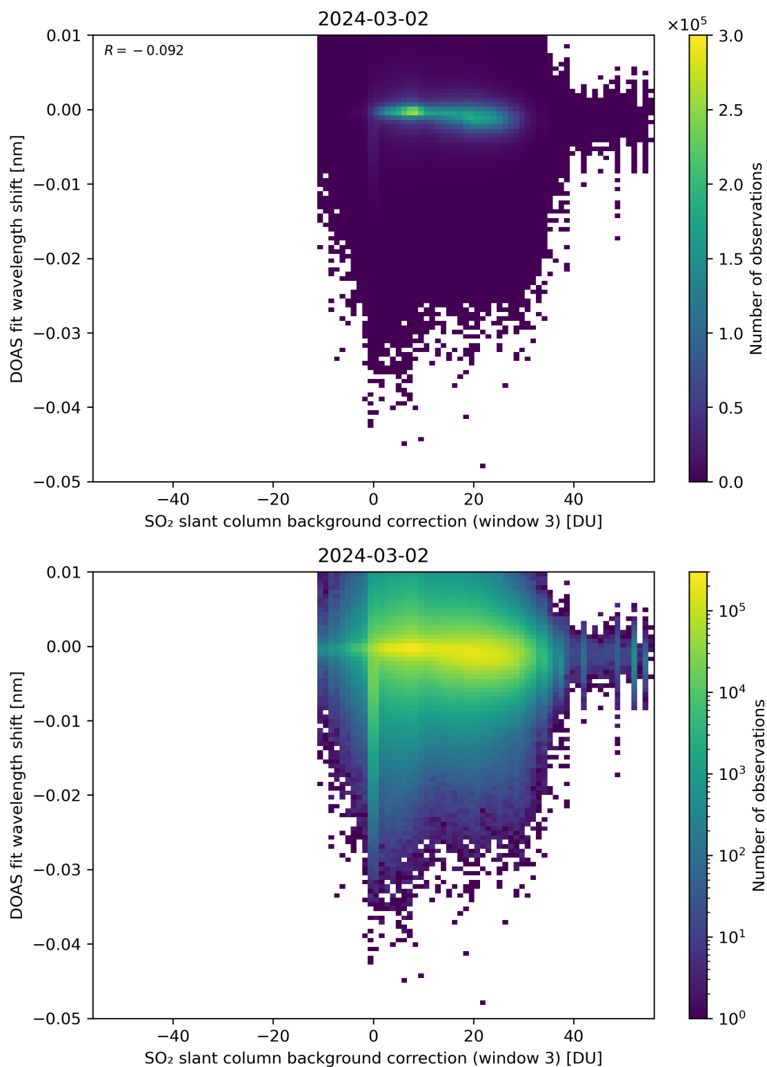
Figure 121: Scatter density plot of “SO 2 slant column background correction (window 3)” against “DOAS fit wavelength shift” for 2024-03-01 to 2024-03-03.
