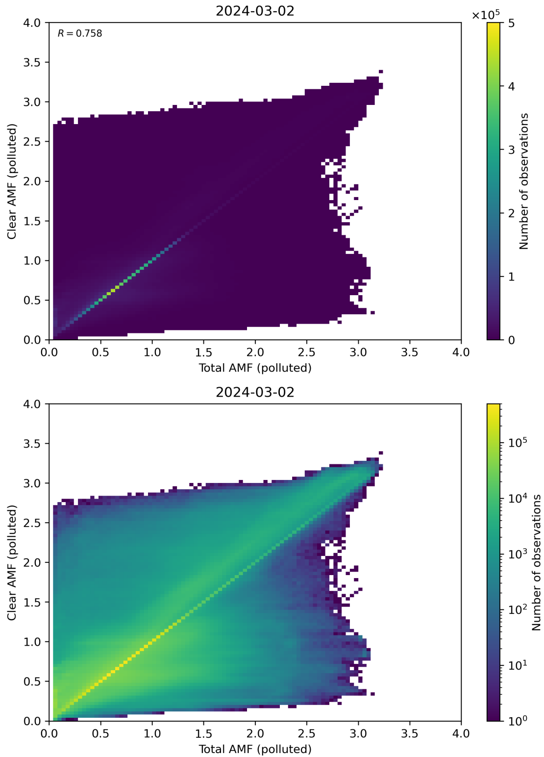
Figure 271: Scatter density plot of “Total AMF (polluted)” against “Clear AMF (polluted)” for 2024-03-01 to 2024-03-03.
