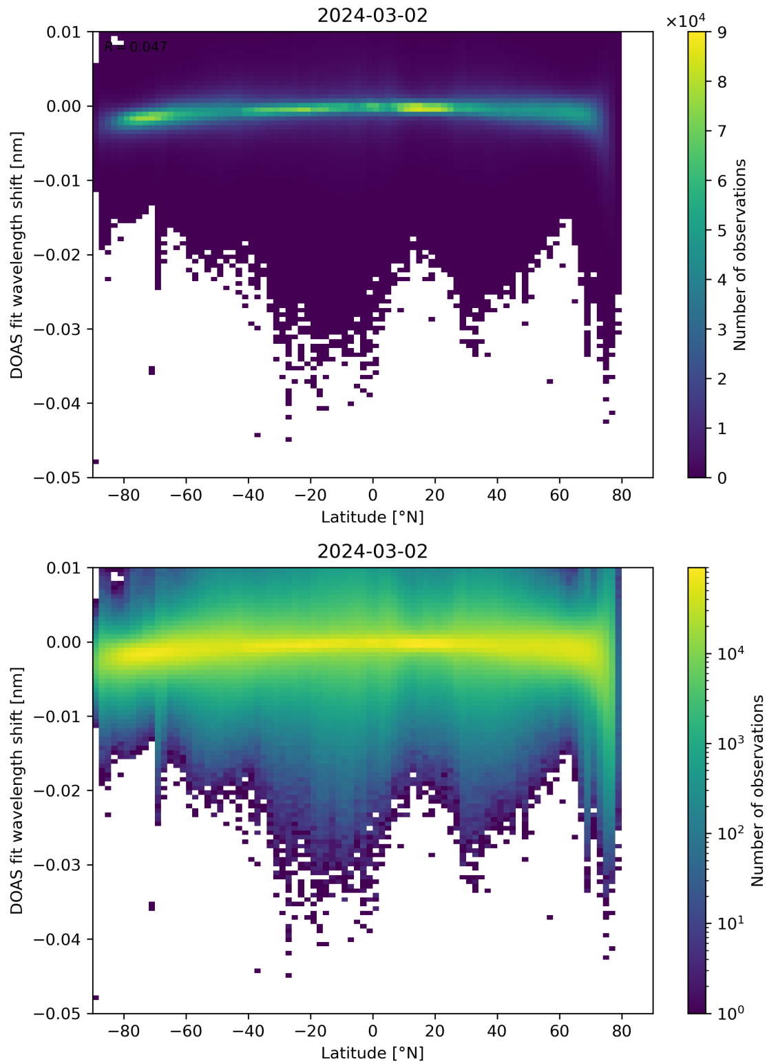
Figure 142: Scatter density plot of “Latitude” against “DOAS fit wavelength shift” for 2024-03-01 to 2024-03-03.
