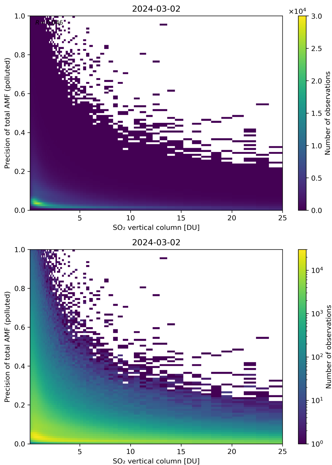
Figure 306: Scatter density plot of “SO 2 vertical column” against “Precision of total AMF (polluted)” for 2024-03-01 to 2024-03-03.
