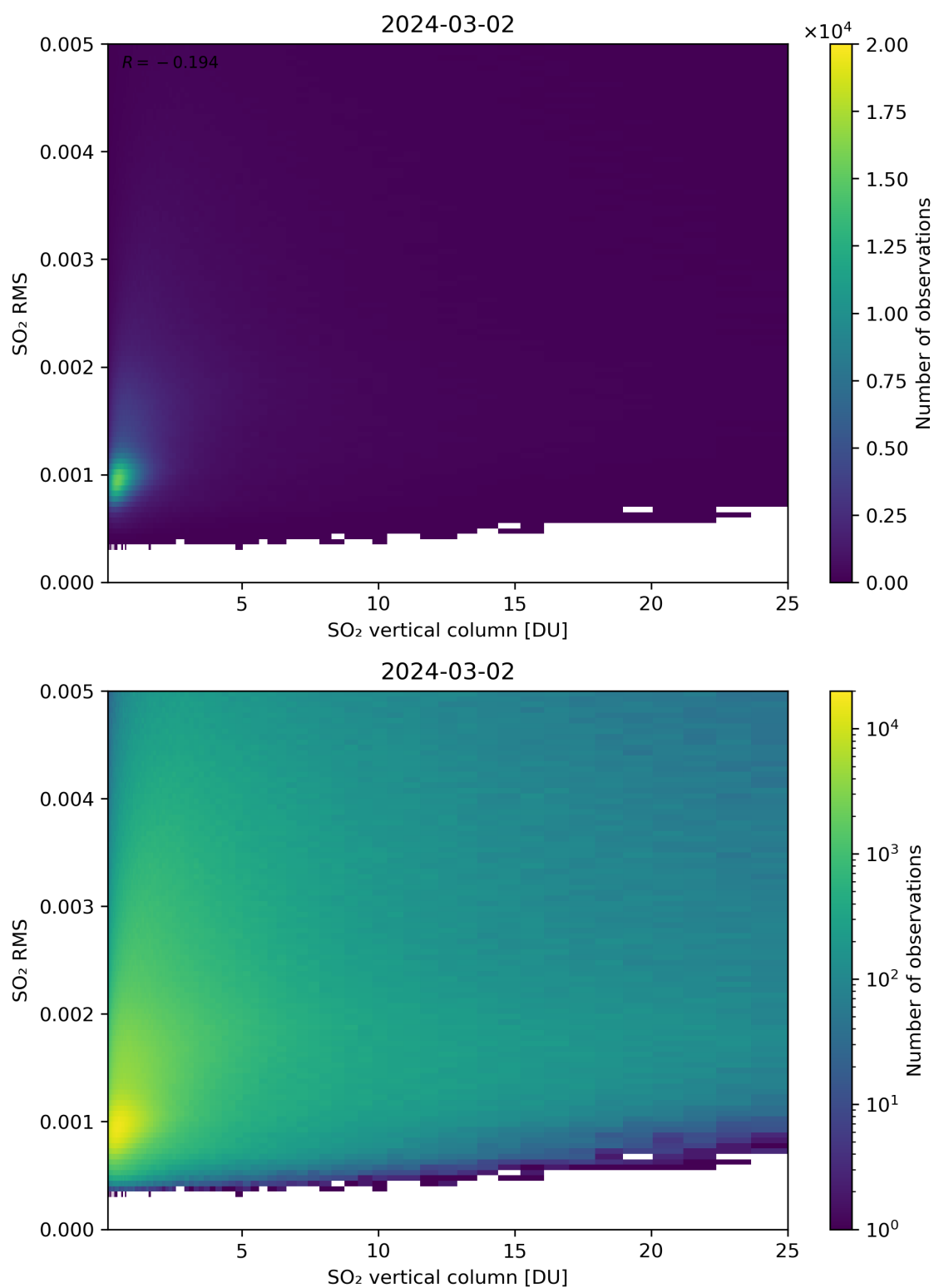
Figure 278: Scatter density plot of “SO 2 vertical column” against “SO 2 RMS” for 2024-03-01 to 2024-03-03.
