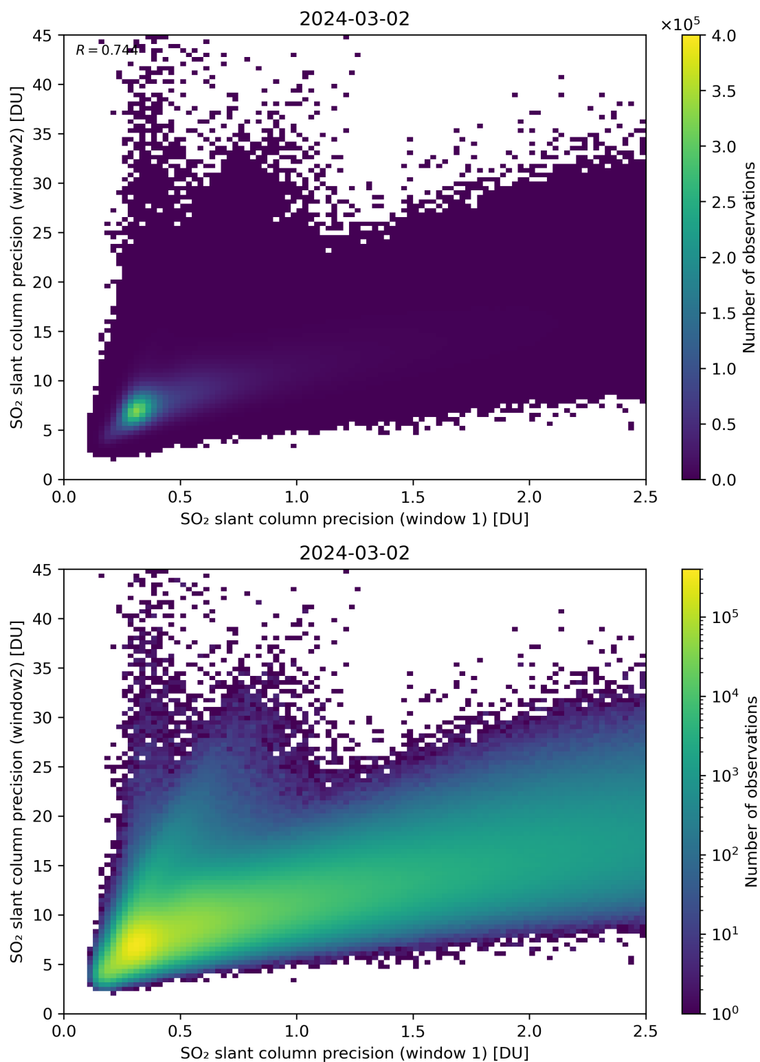
Figure 227: Scatter density plot of “SO 2 slant column precision (window 1)” against “SO 2 slant column precision (window 2)” for 2024-03-01 to 2024-03-03.
