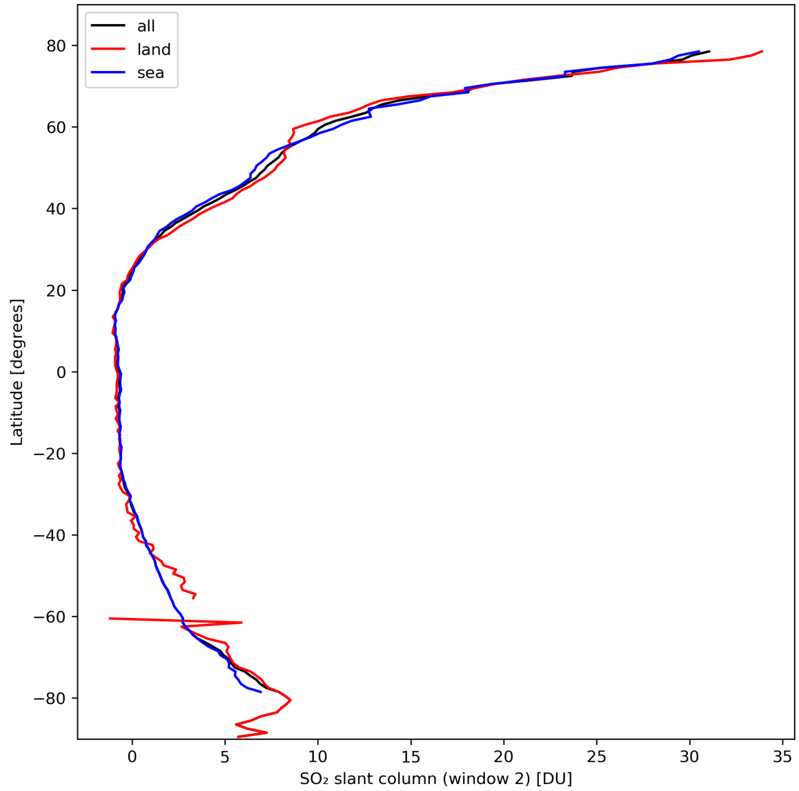
Figure 37: Zonal average of “SO 2 slant column (window 2)” for 2024-03-01 to 2024-03-03.
