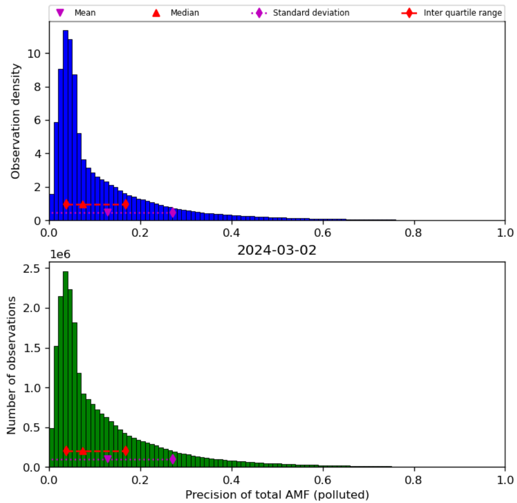
Figure 72: Histogram of “Precision of total AMF (polluted)” for 2024-03-01 to 2024-03-03
