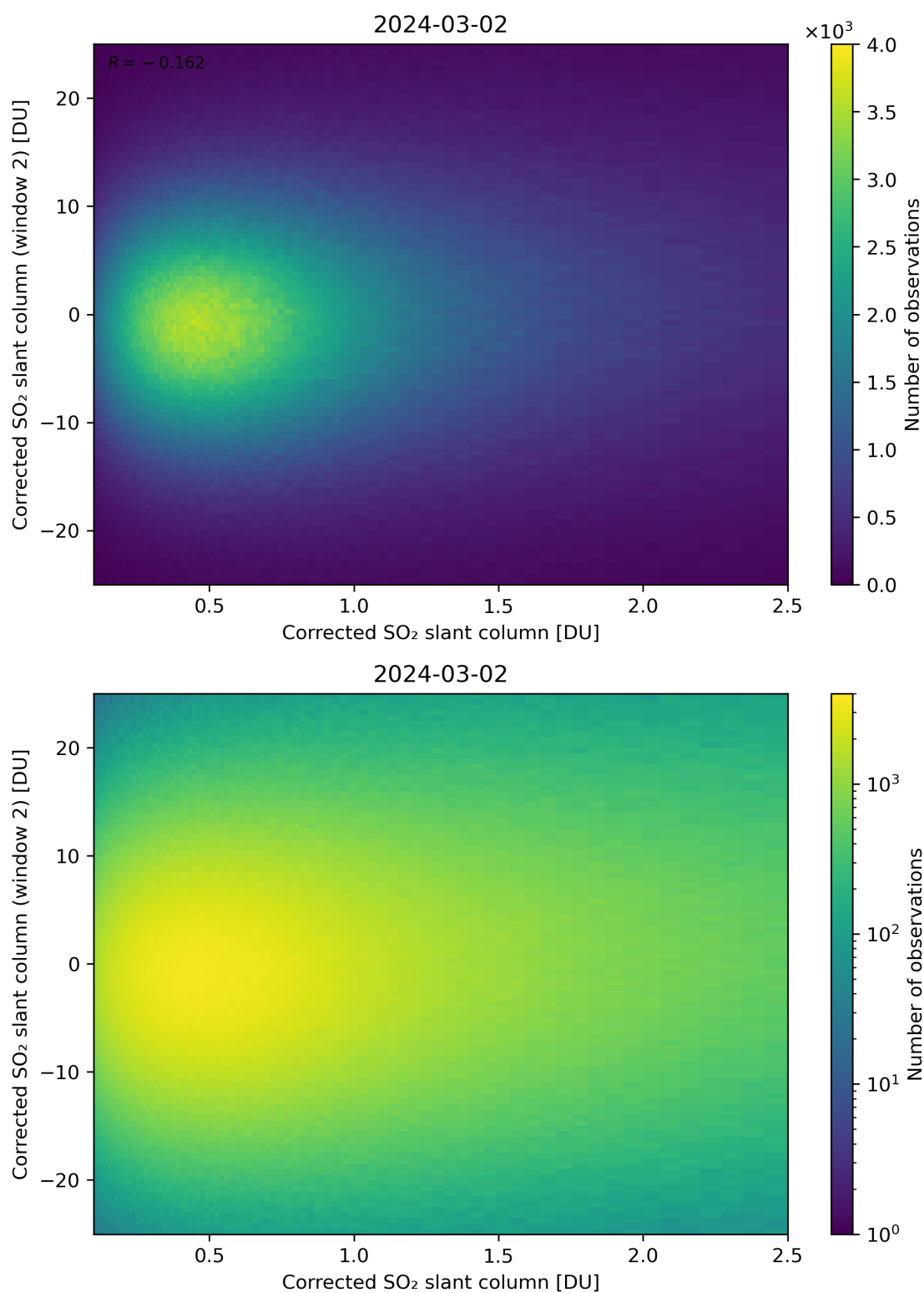
Figure 185: Scatter density plot of “Corrected SO 2 slant column” against “Corrected SO 2 slant column (window 2)” for 2024-03-01 to 2024-03-03.
