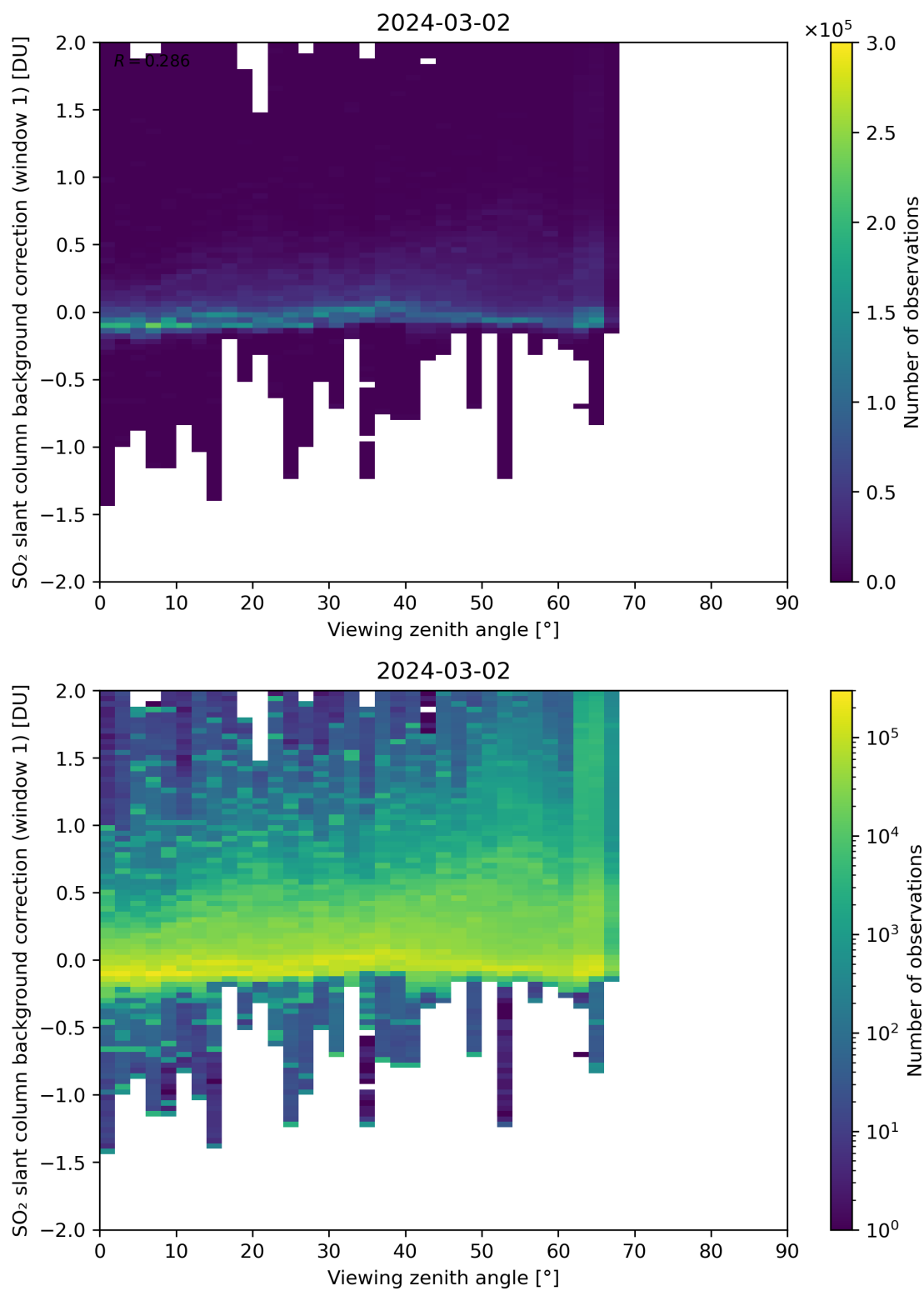
Figure 308: Scatter density plot of “Viewing zenith angle” against “SO 2 slant column background correction (window 1)” for 2024-03-01 to 2024-03-03.
