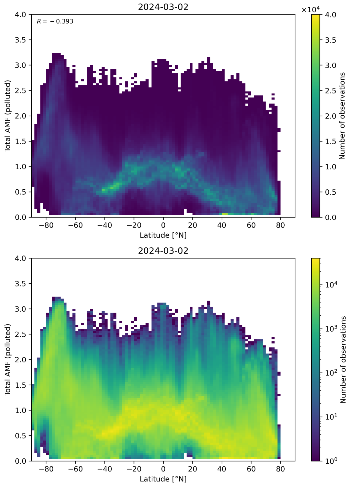
Figure 154: Scatter density plot of “Latitude” against “Total AMF (polluted)” for 2024-03-01 to 2024-03-03.
