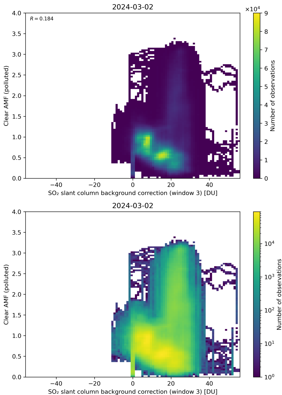
Figure 124: Scatter density plot of “SO 2 slant column background correction (window 3)” against “Clear AMF (polluted)” for 2024-03-01 to 2024-03-03.
