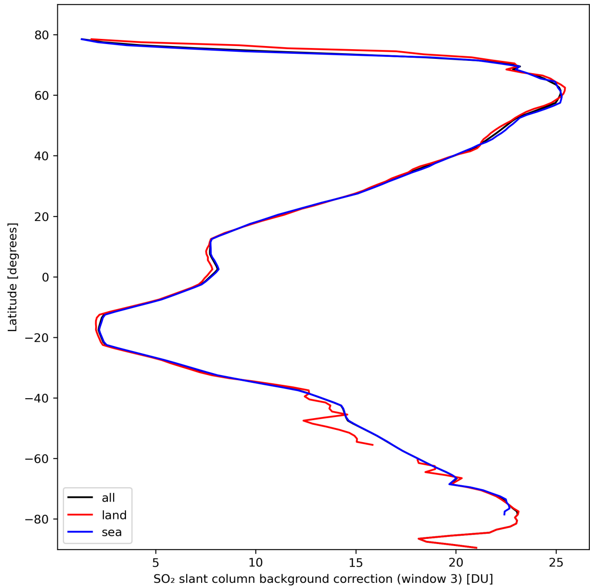
Figure 44: Zonal average of “SO 2 slant column background correction (window 3)” for 2024-03-01 to 2024-03-03.
