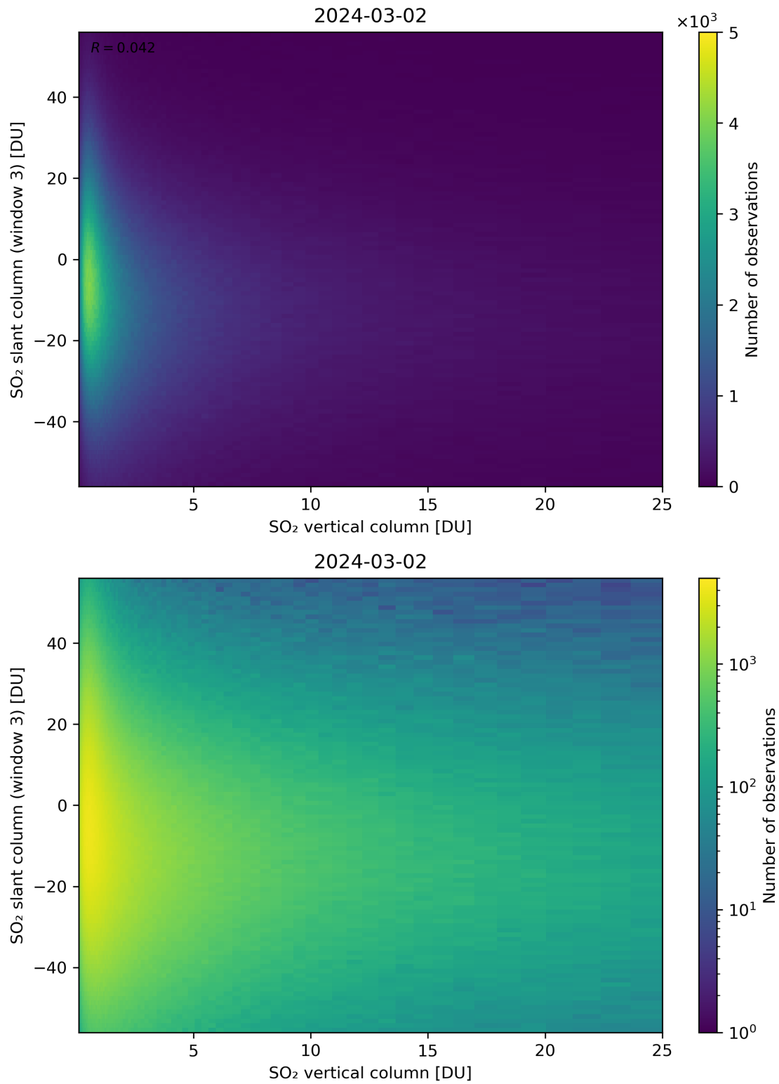
Figure 303: Scatter density plot of “SO 2 vertical column” against “SO 2 slant column (window 3)” for 2024-03-01 to 2024-03-03.
