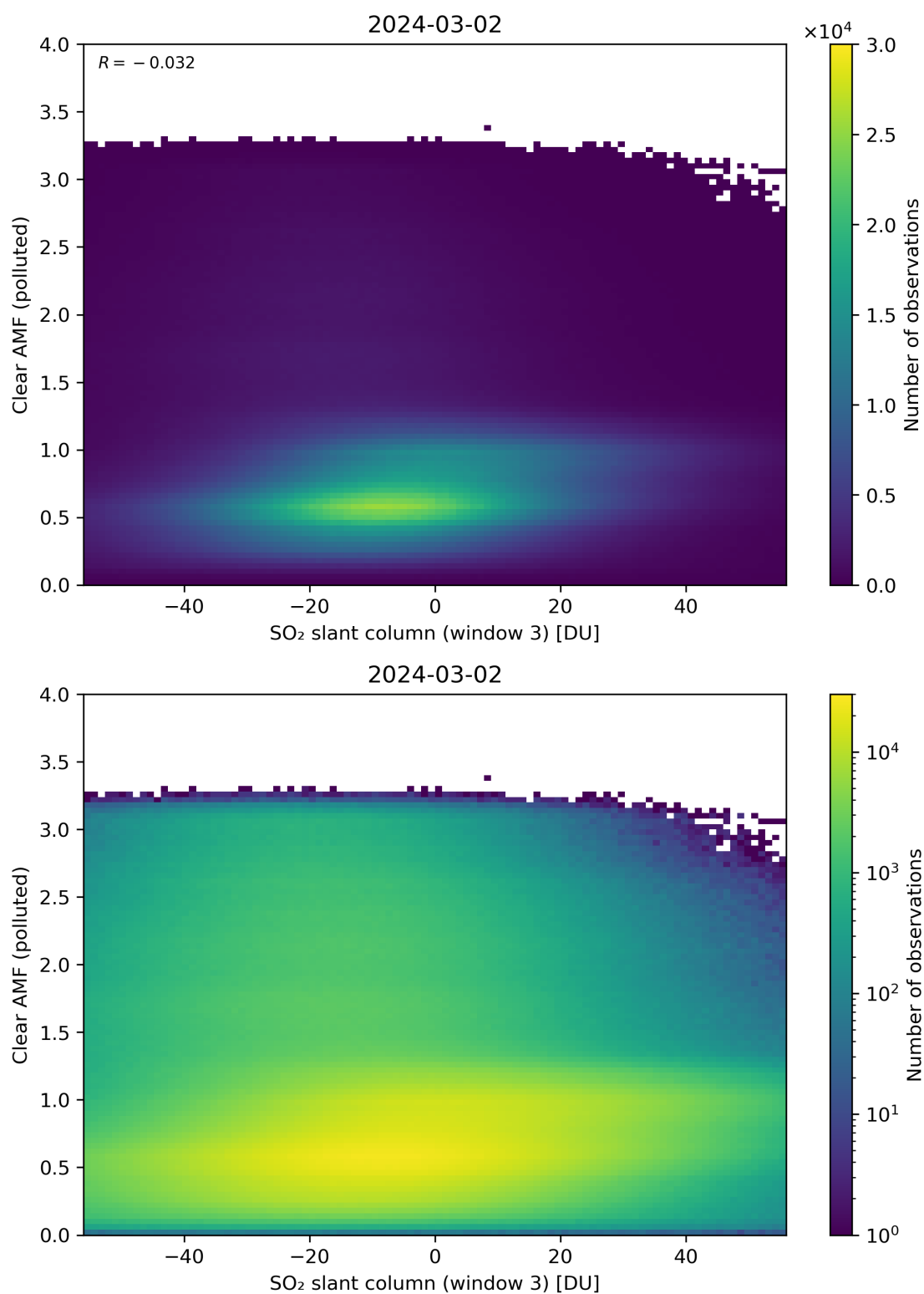
Figure 265: Scatter density plot of “SO 2 slant column (window 3)” against “Clear AMF (polluted)” for 2024-03-01 to 2024-03-03.
