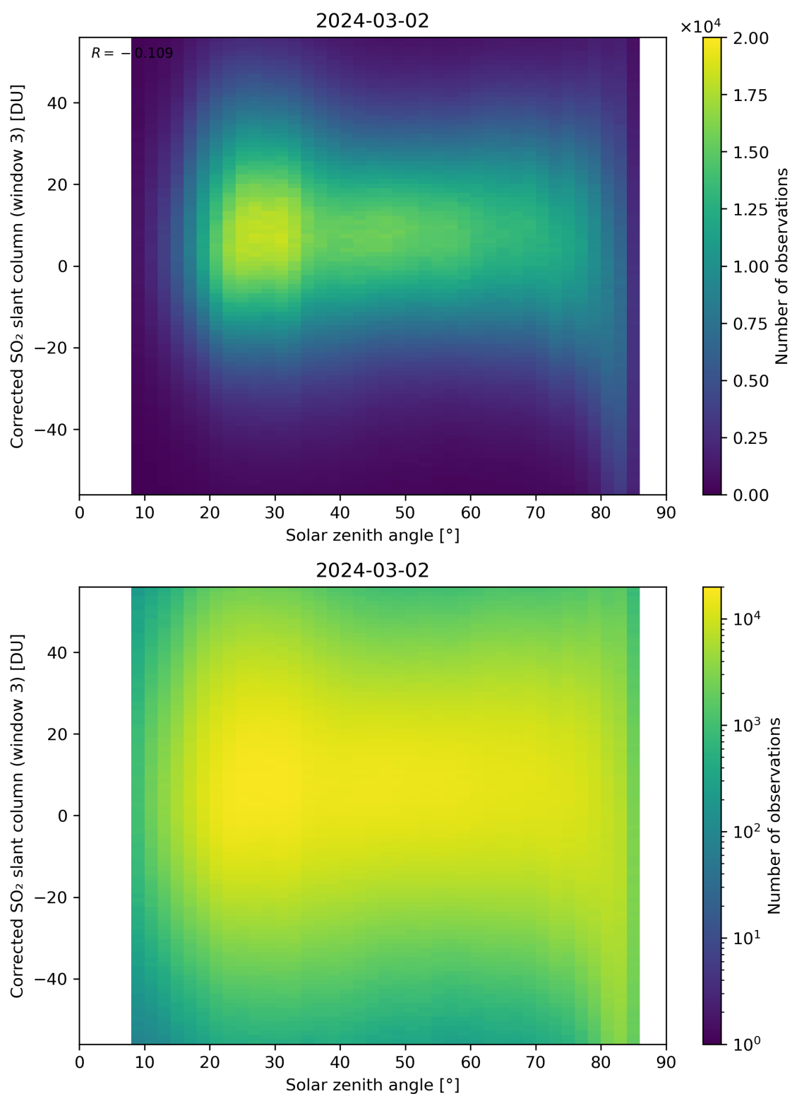
Figure 168: Scatter density plot of “Solar zenith angle” against “Corrected SO 2 slant column (window 3)” for 2024-03-01 to 2024-03-03.
