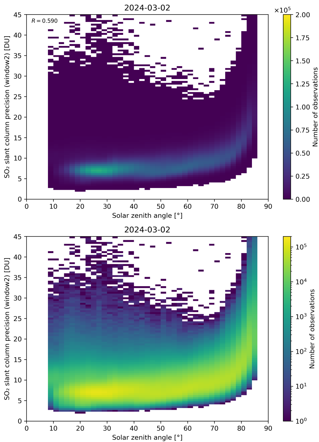
Figure 171: Scatter density plot of “Solar zenith angle” against “SO 2 slant column precision (window2)” for 2024-03-01 to 2024-03-03.
