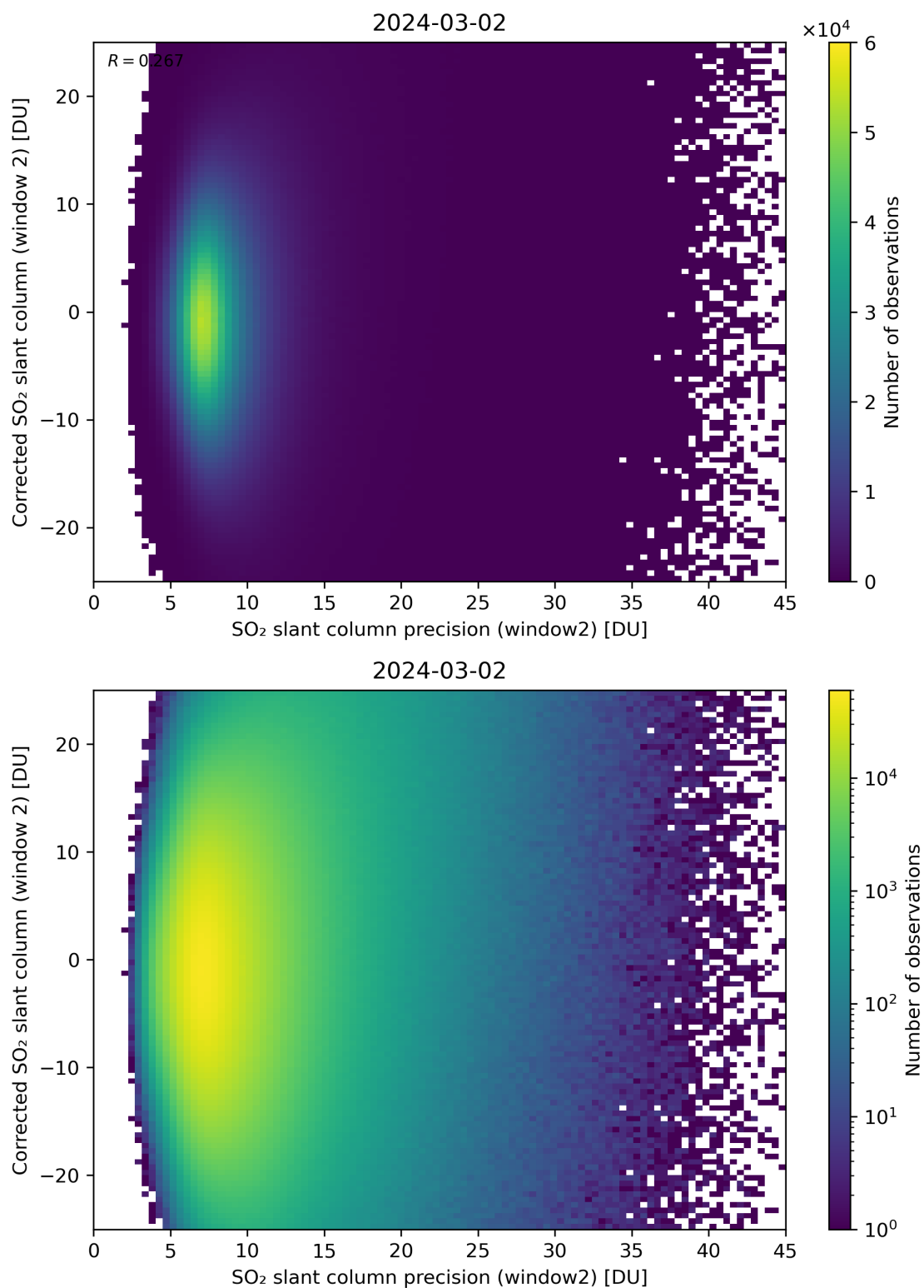
Figure 247: Scatter density plot of “SO 2 slant column precision (window2)” against “Corrected SO 2 slant column (window 2)” for 2024-03-01 to 2024-03-03.
