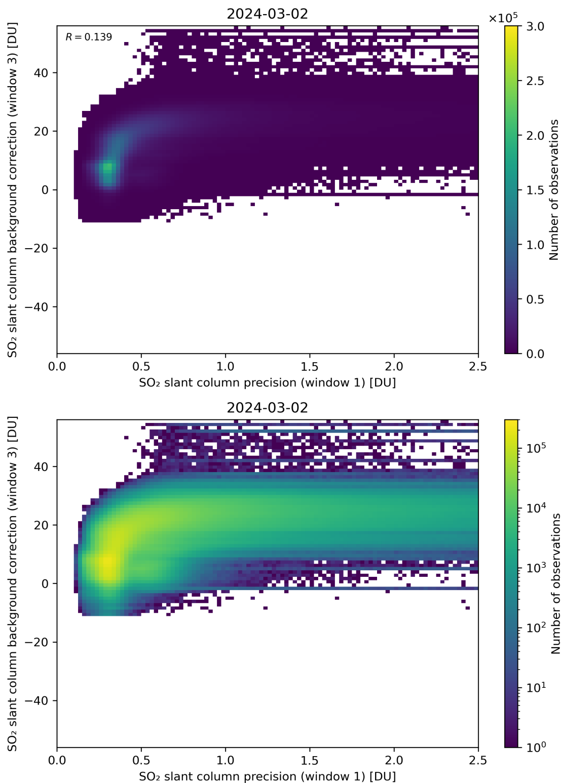
Figure 220: Scatter density plot of “SO 2 slant column precision (window 1)” against “SO 2 slant column background correction (window 3)” for 2024-03-01 to 2024-03-03.
