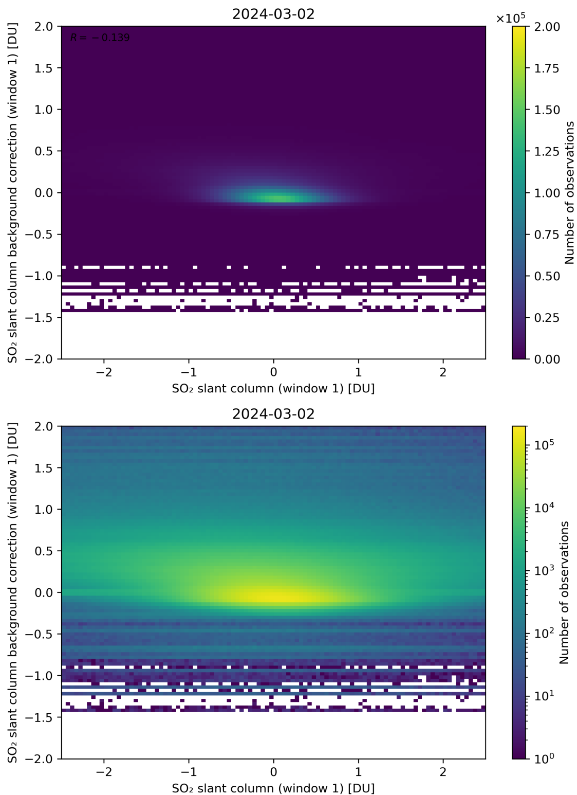
Figure 212: Scatter density plot of “SO 2 slant column (window 1)” against “SO 2 slant column background correction (window 1)” for 2024-03-01 to 2024-03-03.
