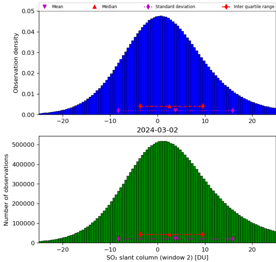
Figure 60: Histogram of “SO 2 slant column (window 2)” for 2024-03-01 to 2024-03-03
