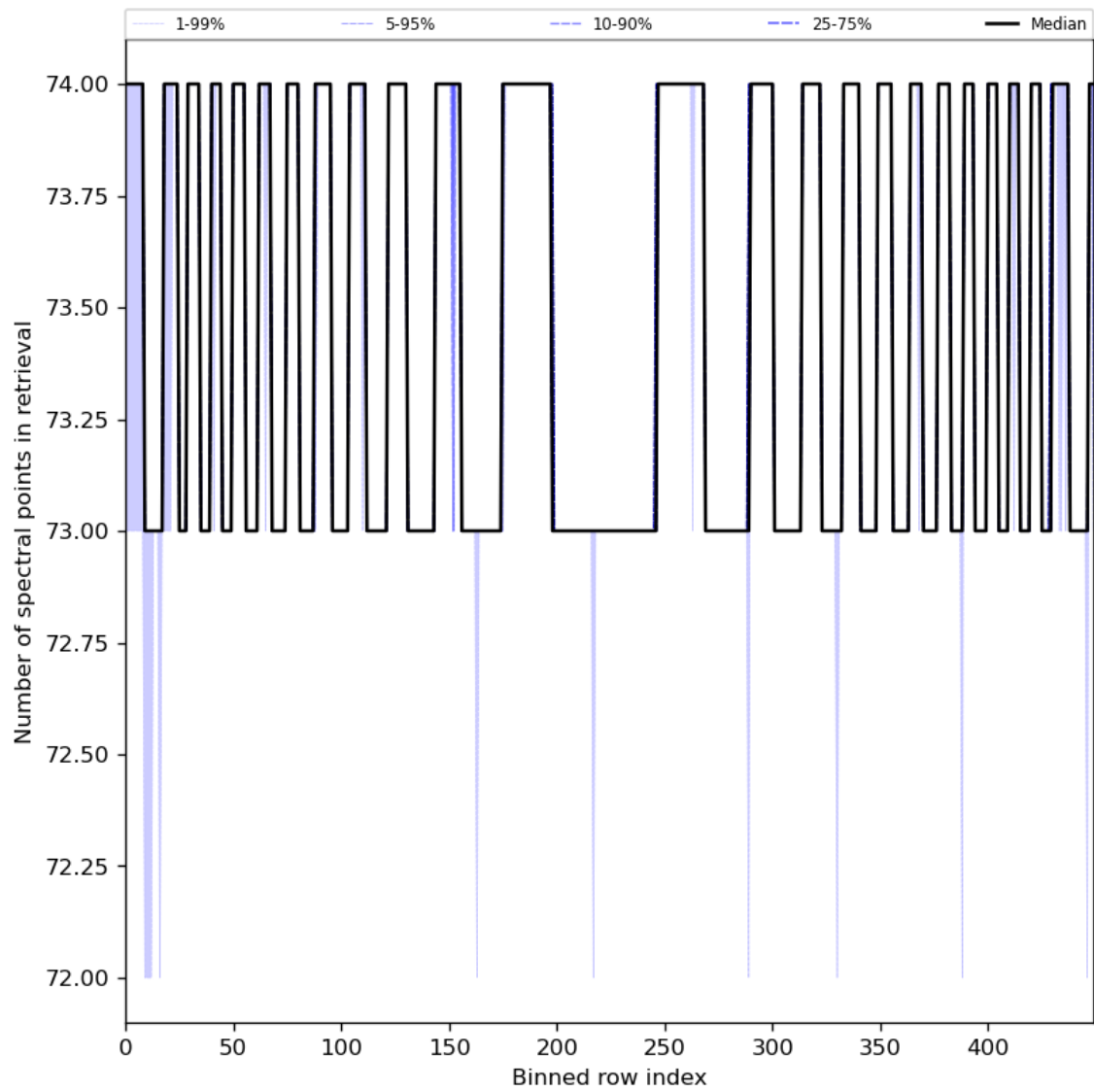
Figure 97: Along track statistics of “Number of spectral points in retrieval” for 2024-03-01 to 2024-03-03
