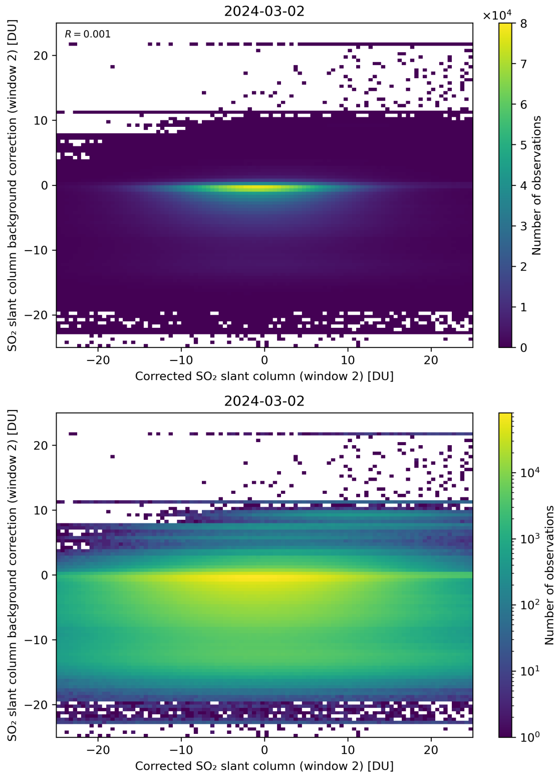
Figure 194: Scatter density plot of “Corrected SO 2 slant column (window 2)” against “SO 2 slant column background correction (window 2)” for 2024-03-01 to 2024-03-03.
