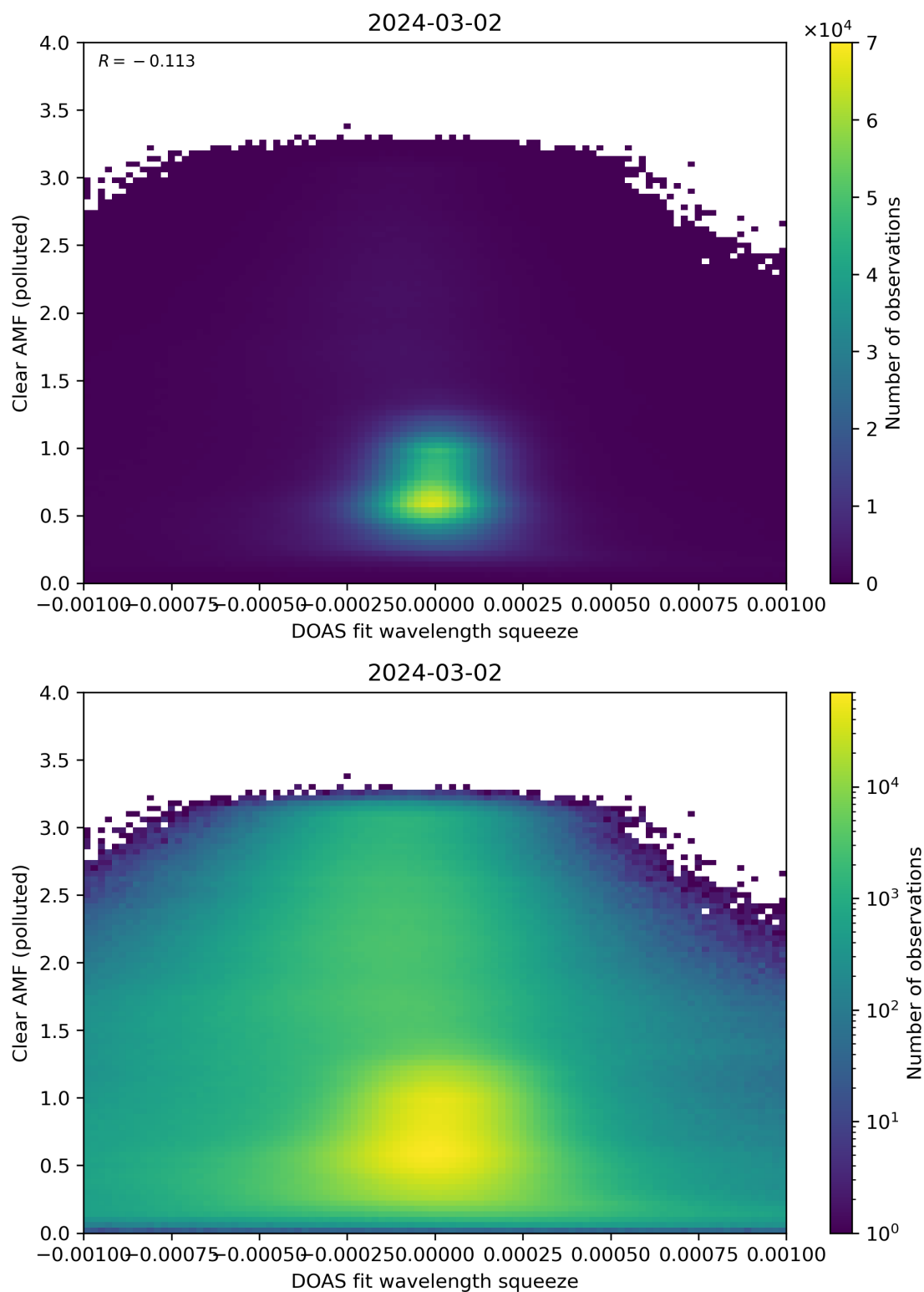
Figure 133: Scatter density plot of “DOAS fit wavelength squeeze” against “Clear AMF (polluted)” for 2024-03-01 to 2024-03-03.
