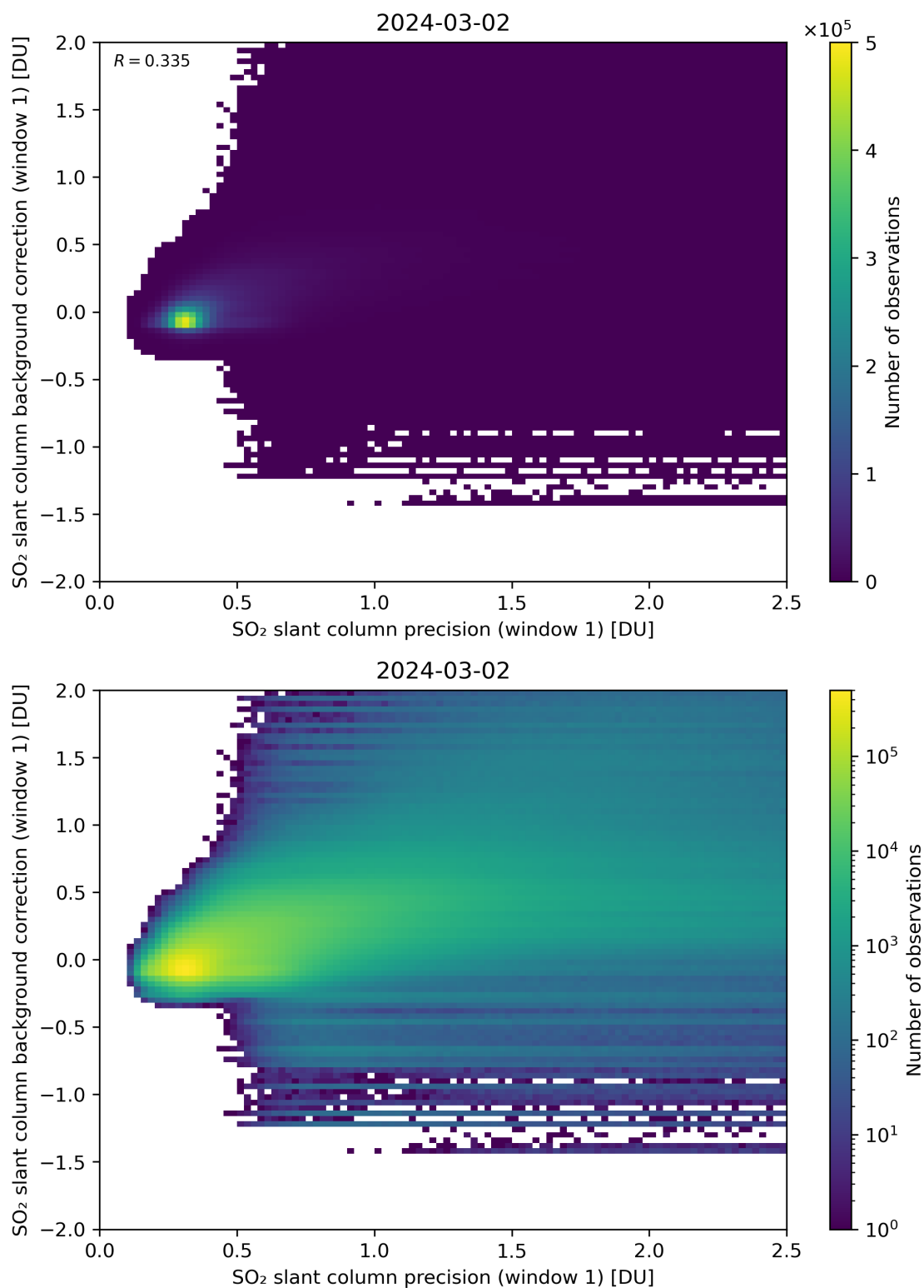
Figure 218: Scatter density plot of “SO 2 slant column precision (window 1)” against “SO 2 slant column background correction (window 1)” for 2024-03-01 to 2024-03-03.
