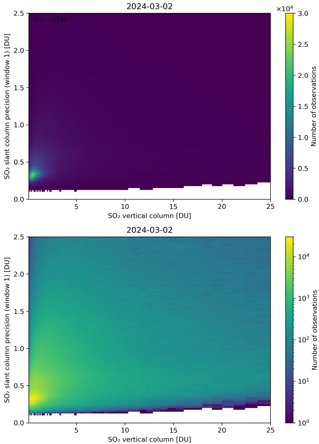
Figure 301: Scatter density plot of “SO 2 vertical column” against “SO 2 slant column precision (window 1)” for 2024-03-01 to 2024-03-03.
