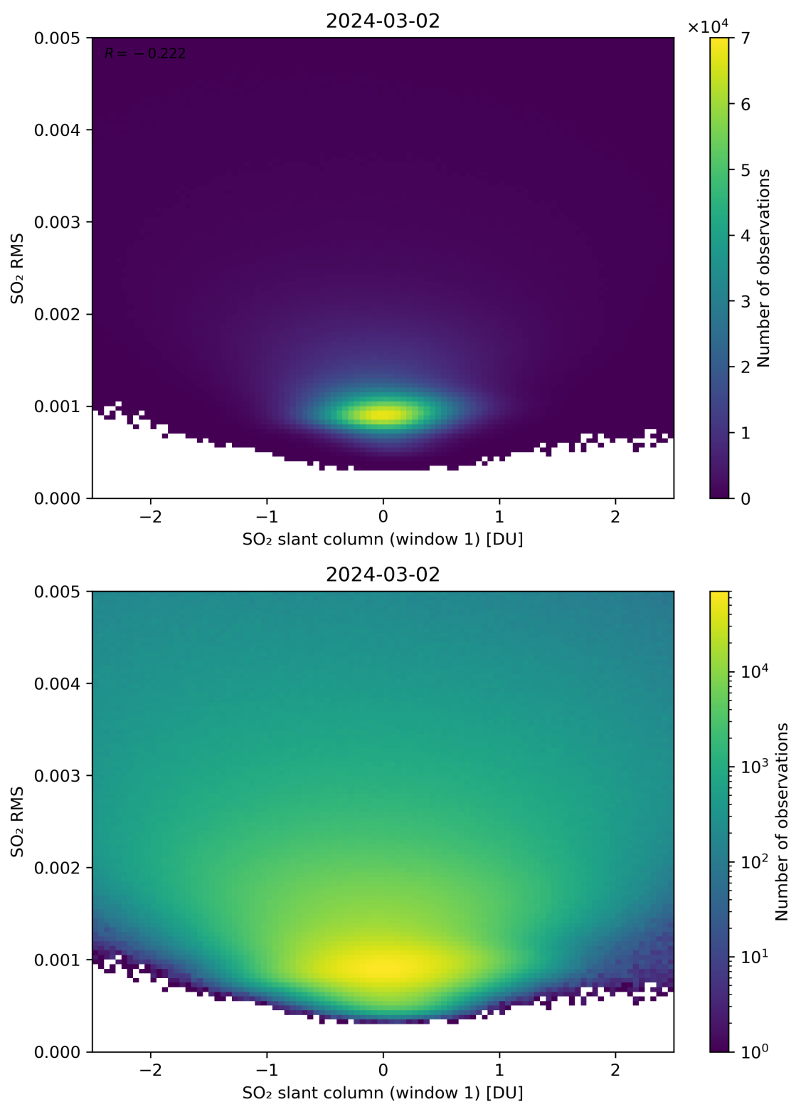
Figure 217: Scatter density plot of “SO 2 slant column (window 1)” against “SO 2 RMS” for 2024-03-01 to 2024-03-03.
