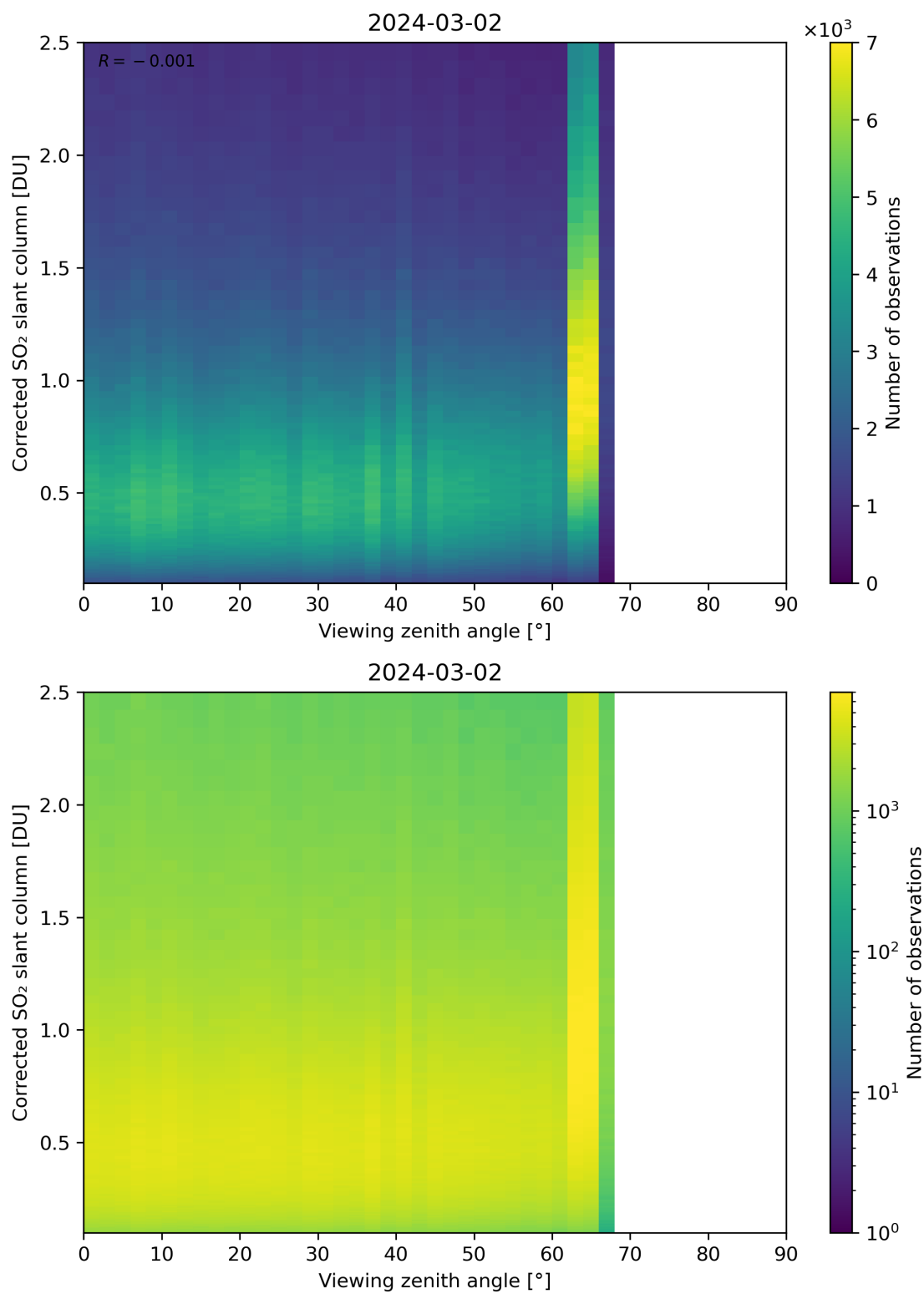
Figure 317: Scatter density plot of “Viewing zenith angle” against “Corrected SO 2 slant column” for 2024-03-01 to 2024-03-03.
