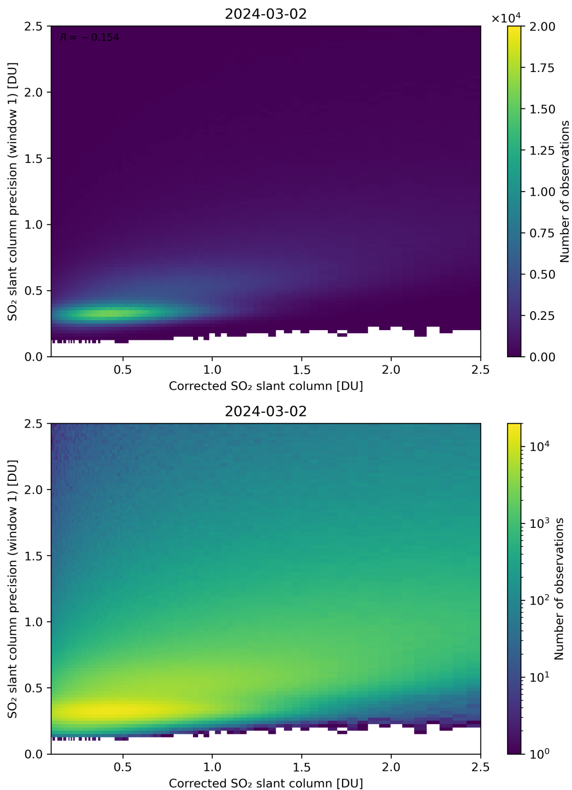
Figure 188: Scatter density plot of “Corrected SO 2 slant column” against “SO 2 slant column precision (window 1)” for 2024-03-01 to 2024-03-03.
