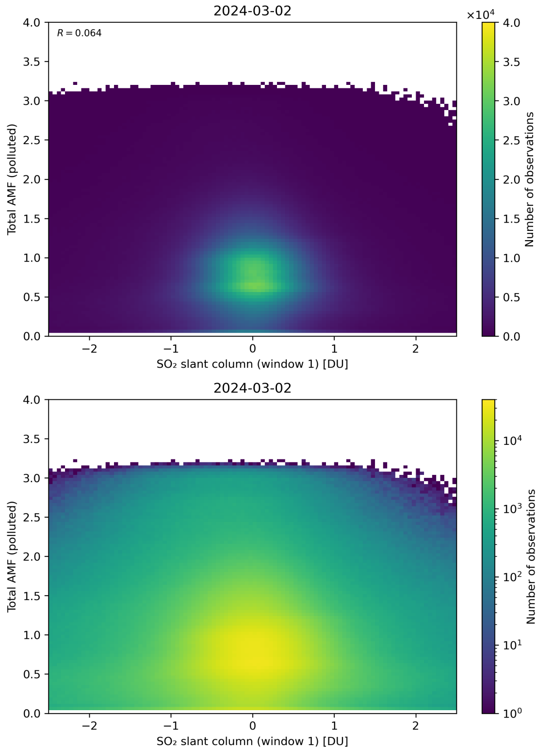
Figure 239: Scatter density plot of “SO 2 slant column (window 1)” against “Total AMF (polluted)” for 2024-03-01 to 2024-03-03.
