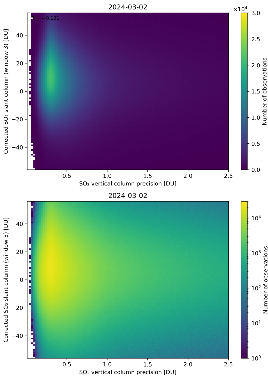
Figure 288: Scatter density plot of “SO 2 vertical column precision” against “Corrected SO 2 slant column (window 3)” for 2024-03-01 to 2024-03-03.
