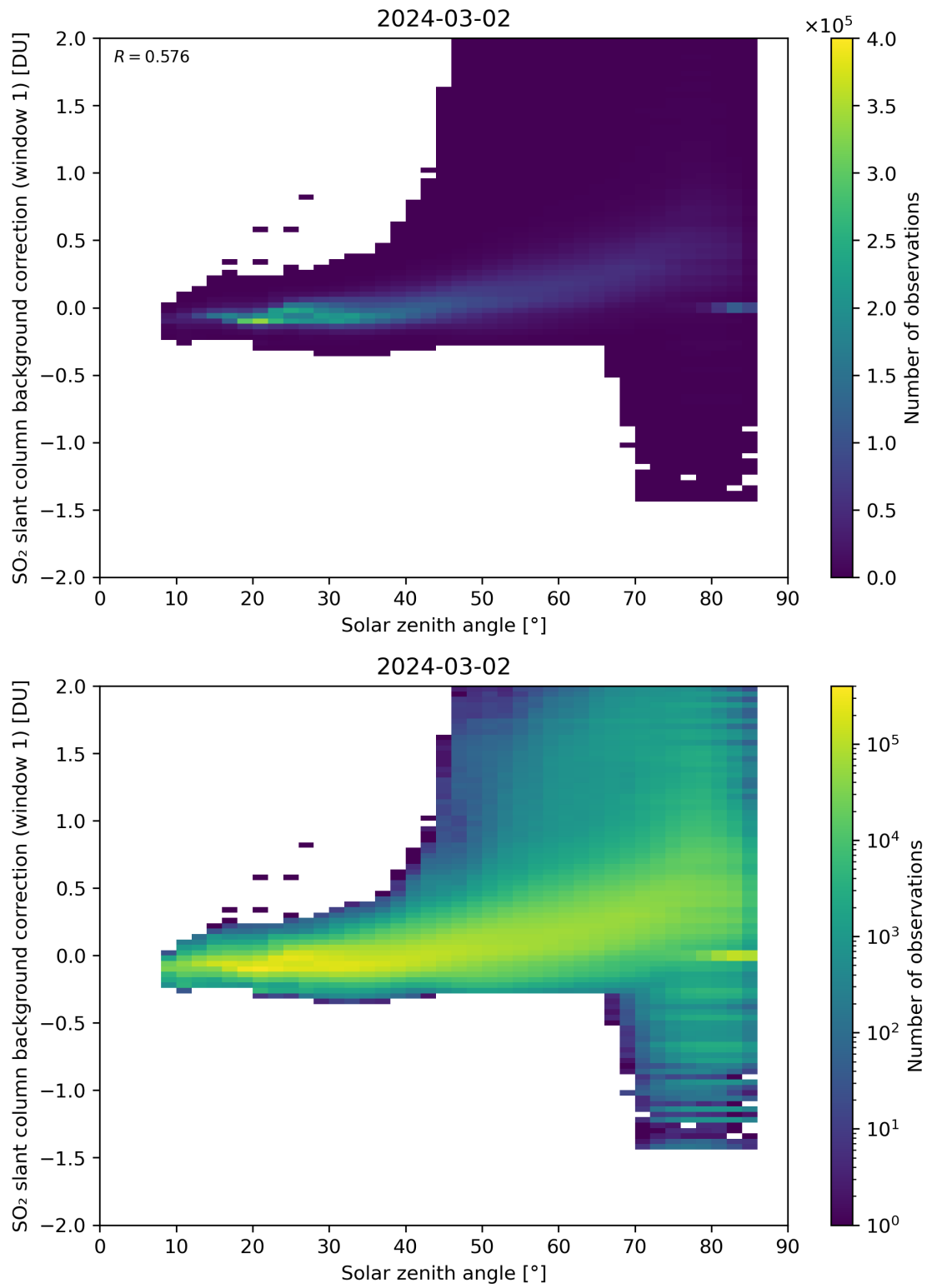
Figure 158: Scatter density plot of “Solar zenith angle” against “SO 2 slant column background correction (window 1)” for 2024-03-01 to 2024-03-03.
