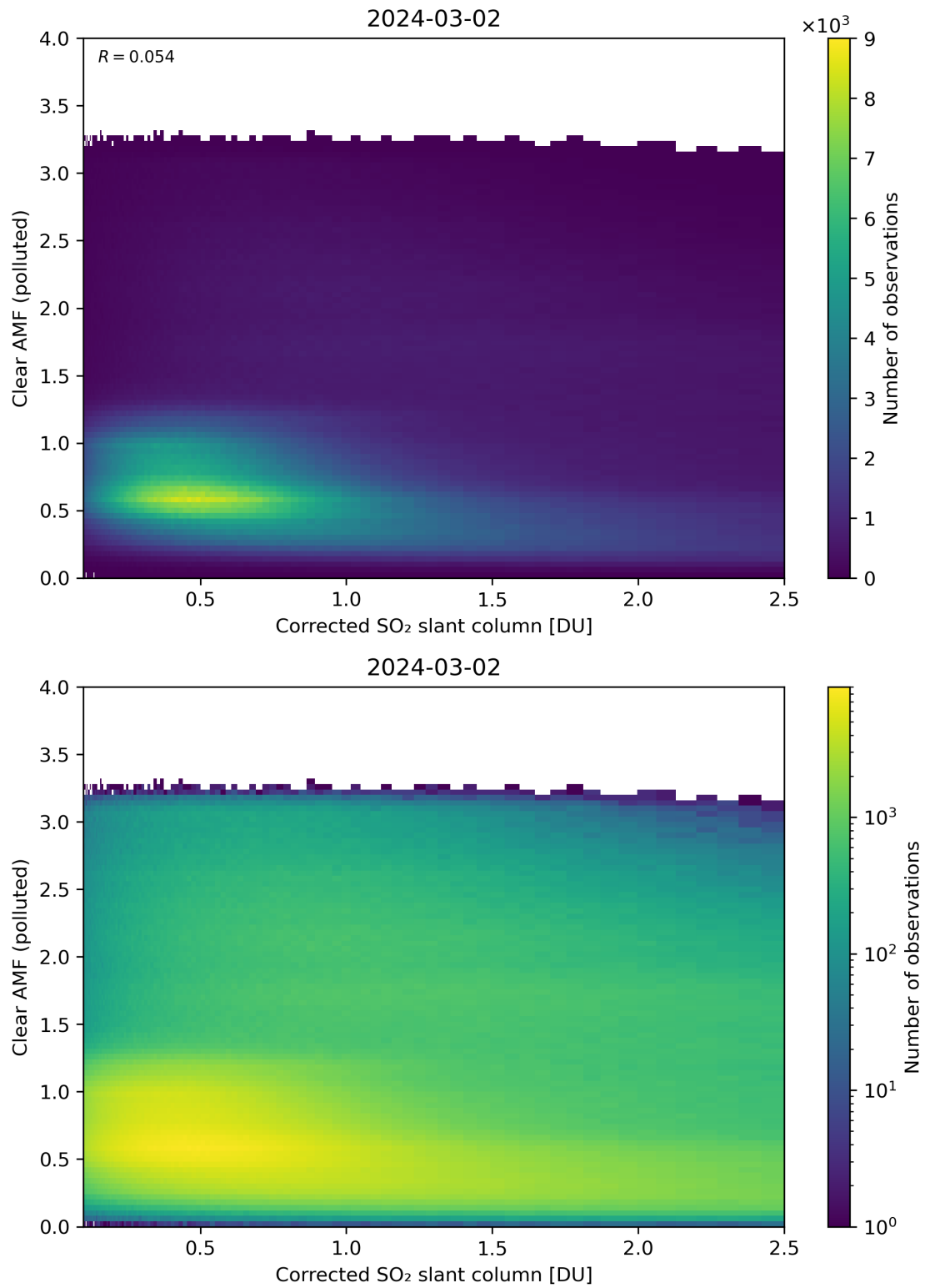
Figure 184: Scatter density plot of “Corrected SO 2 slant column” against “Clear AMF (polluted)” for 2024-03-01 to 2024-03-03.
