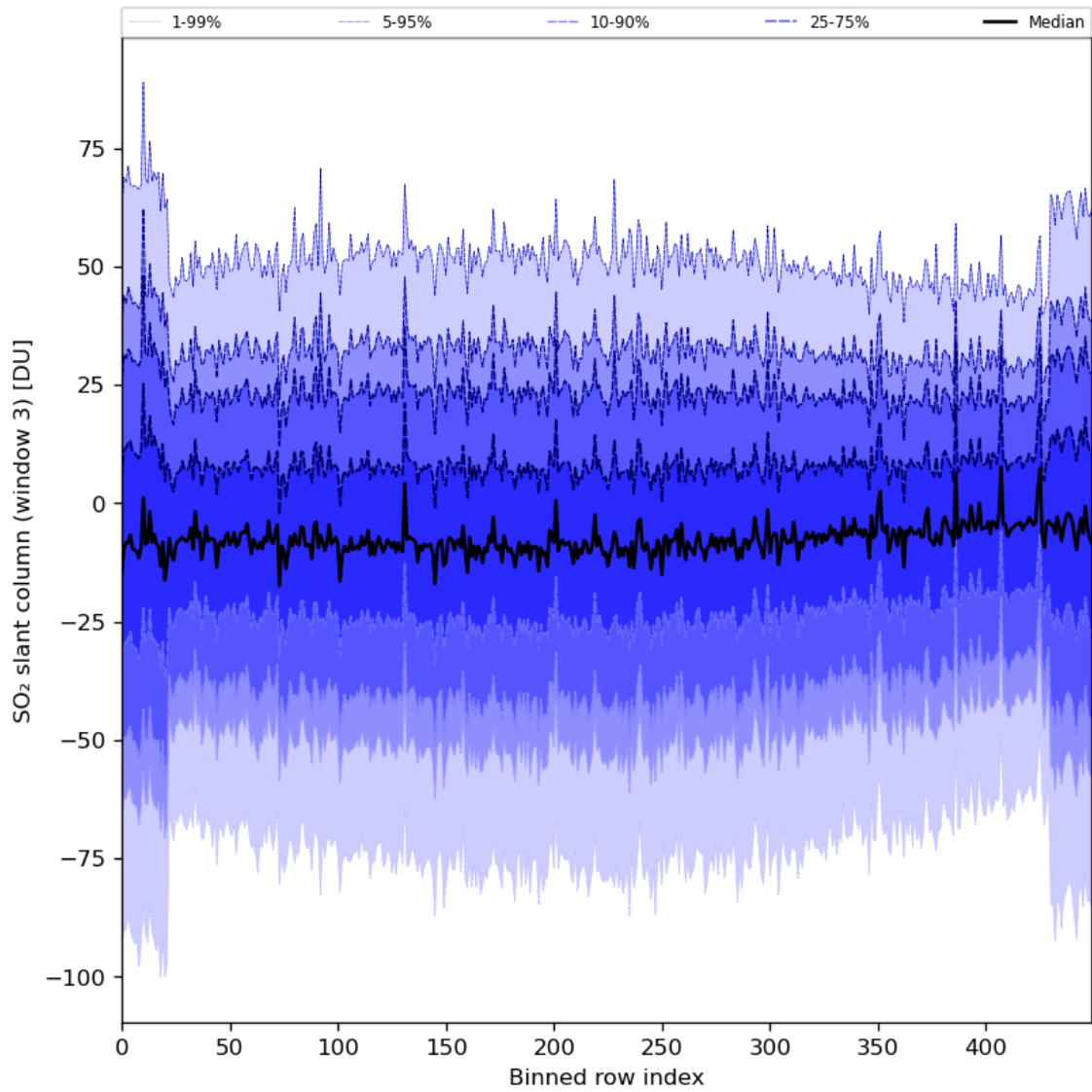
Figure 87: Along track statistics of “SO 2 slant column (window 3)” for 2024-03-01 to 2024-03-03
