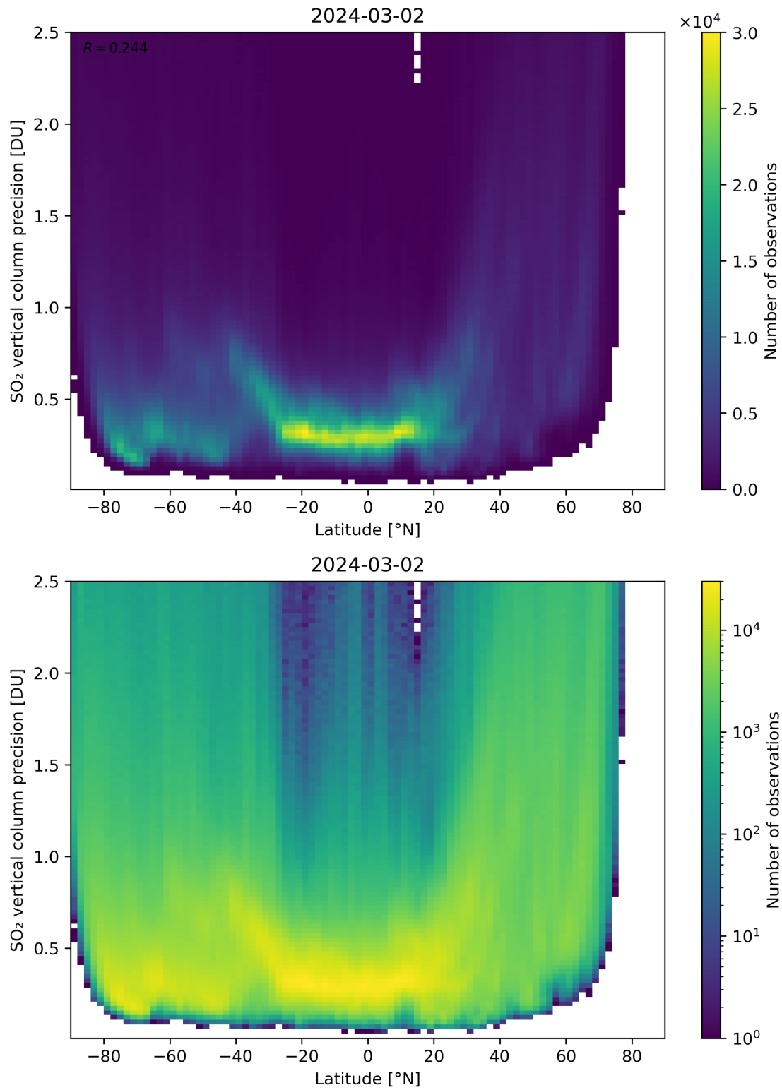
Figure 157: Scatter density plot of “Latitude” against “SO 2 vertical column precision” for 2024-03-01 to 2024-03-03.
