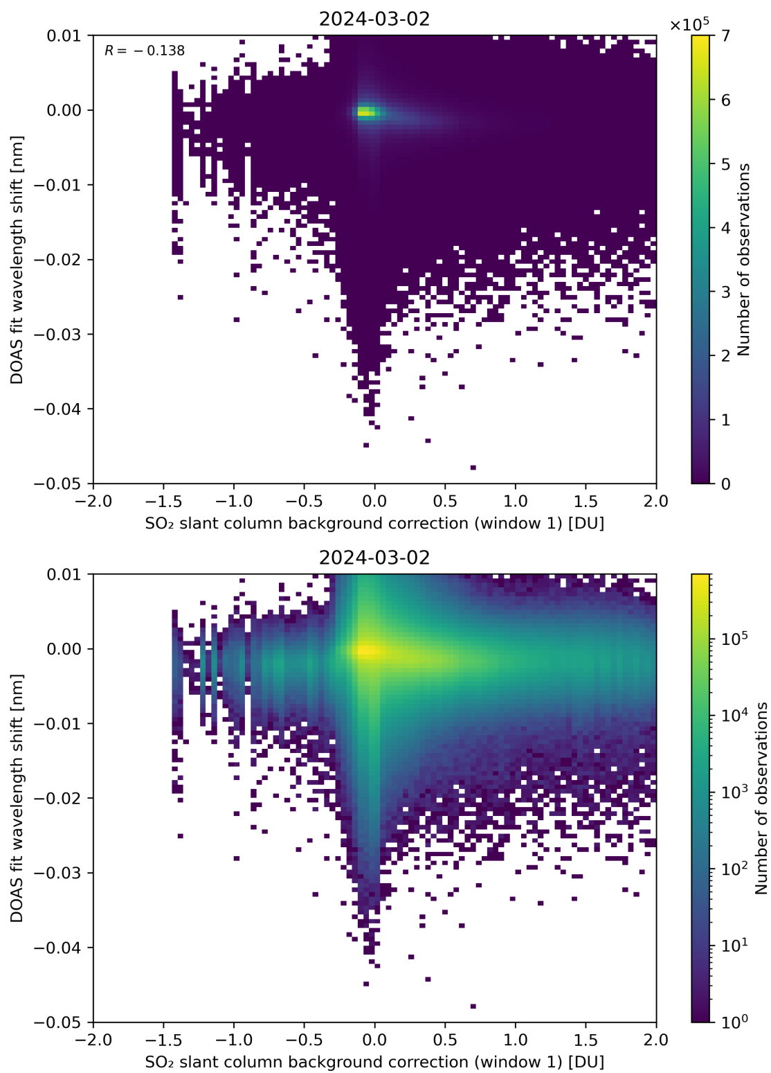
Figure 100: Scatter density plot of “SO 2 slant column background correction (window 1)” against “DOAS fit wavelength shift” for 2024-03-01 to 2024-03-03.
