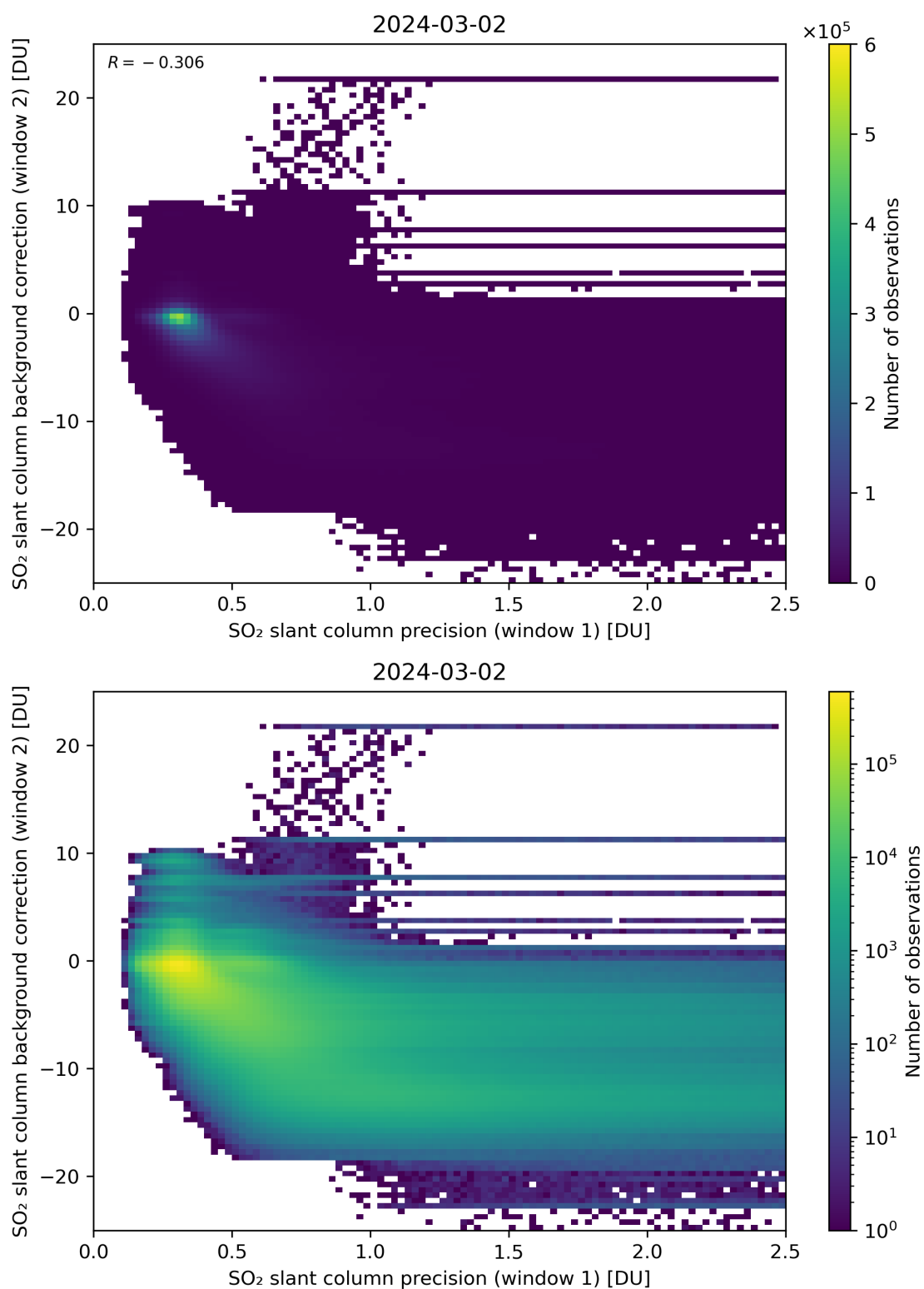
Figure 219: Scatter density plot of “SO 2 slant column precision (window 1)” against “SO 2 slant column background correction (window 2)” for 2024-03-01 to 2024-03-03.
