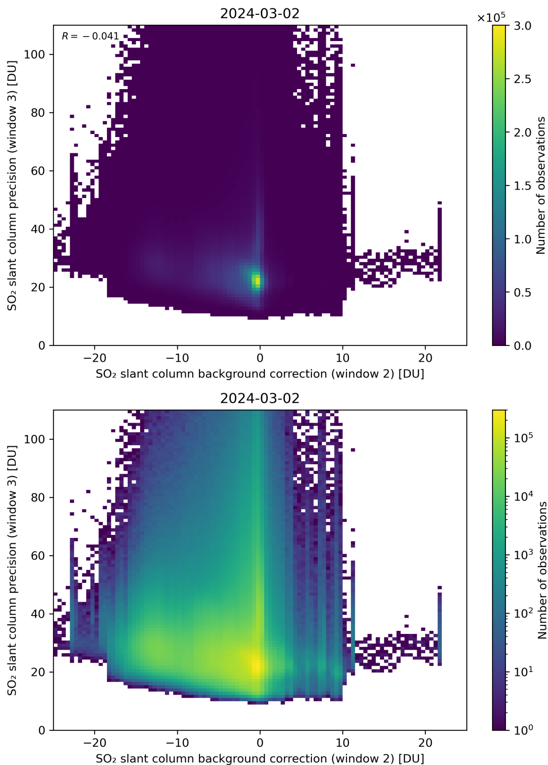
Figure 118: Scatter density plot of “SO 2 slant column background correction (window 2)” against “SO 2 slant column precision (window 3)” for 2024-03-01 to 2024-03-03.
