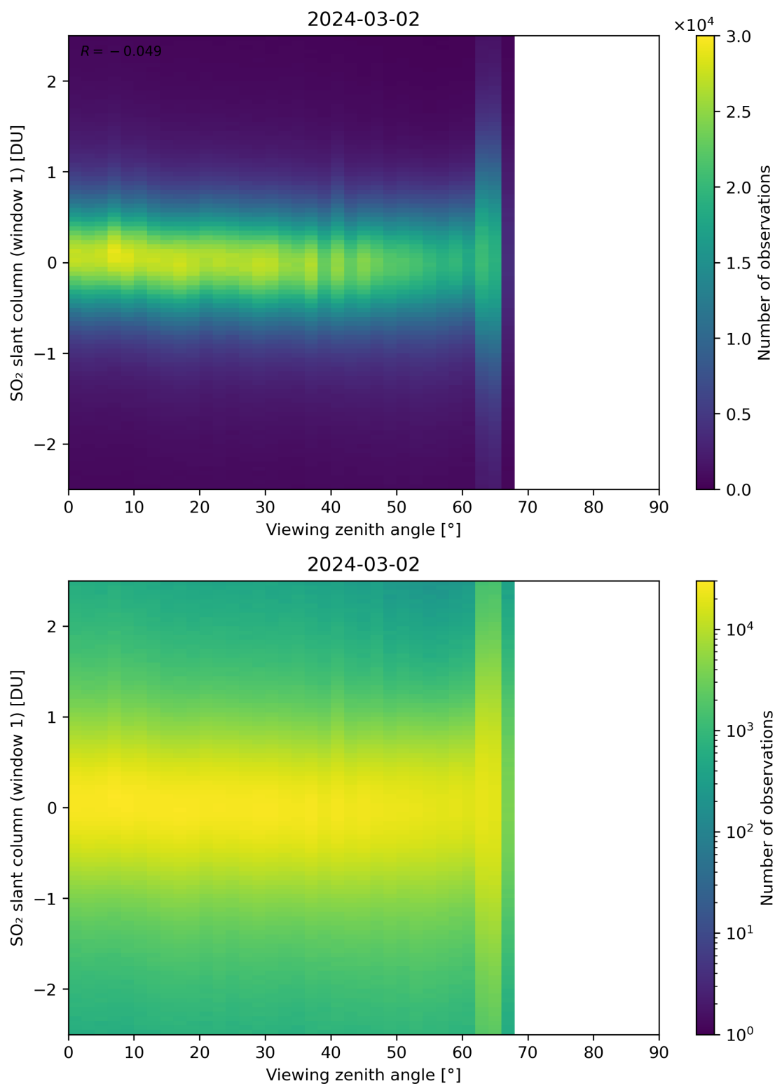
Figure 320: Scatter density plot of “Viewing zenith angle” against “SO 2 slant column (window 1)” for 2024-03-01 to 2024-03-03.
