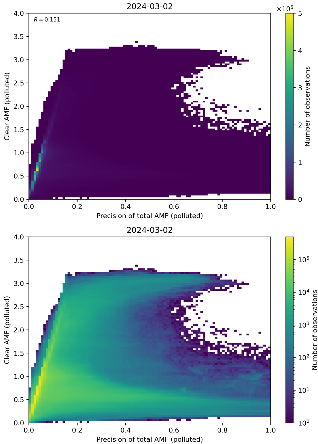
Figure 270: Scatter density plot of “Precision of total AMF (polluted)” against “Clear AMF (polluted)” for 2024-03-01 to 2024-03-03.
