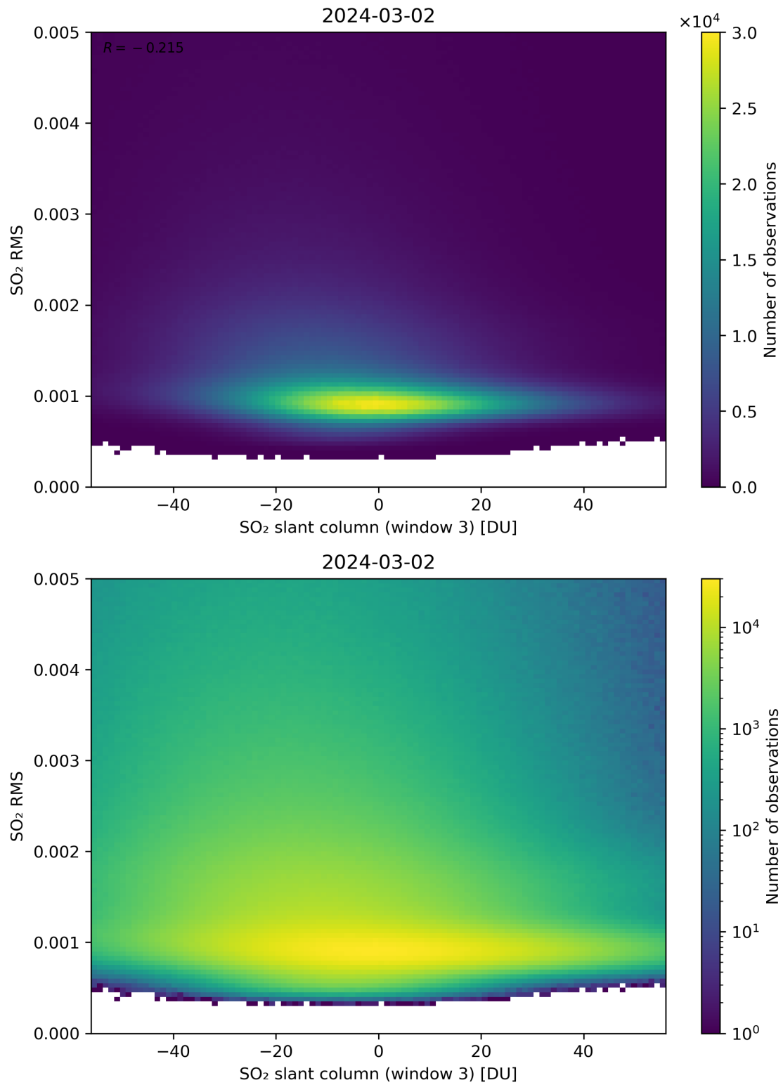
Figure 256: Scatter density plot of “SO 2 slant column (window 3)” against “SO 2 RMS” for 2024-03-01 to 2024-03-03.
