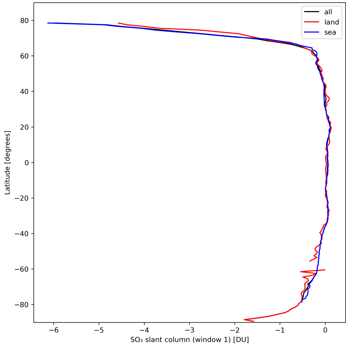
Figure 33: Zonal average of “SO 2 slant column (window 1)” for 2024-03-01 to 2024-03-03.
