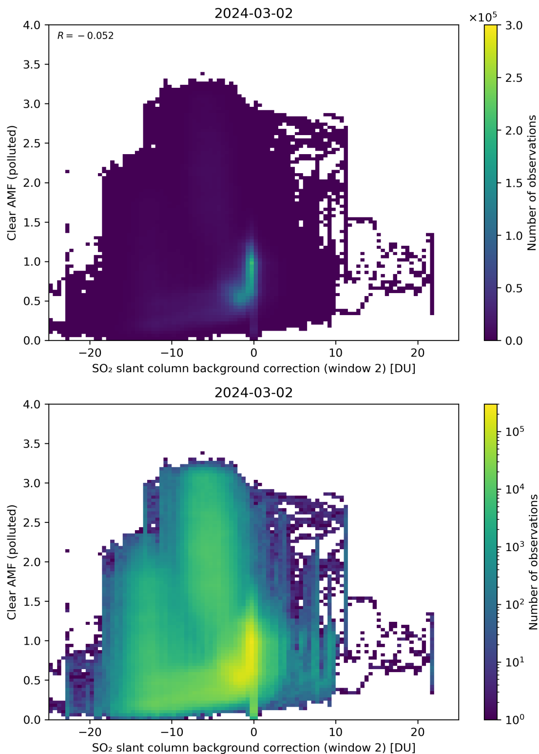
Figure 115: Scatter density plot of “SO 2 slant column background correction (window 2)” against “Clear AMF (polluted)” for 2024-03-01 to 2024-03-03.
