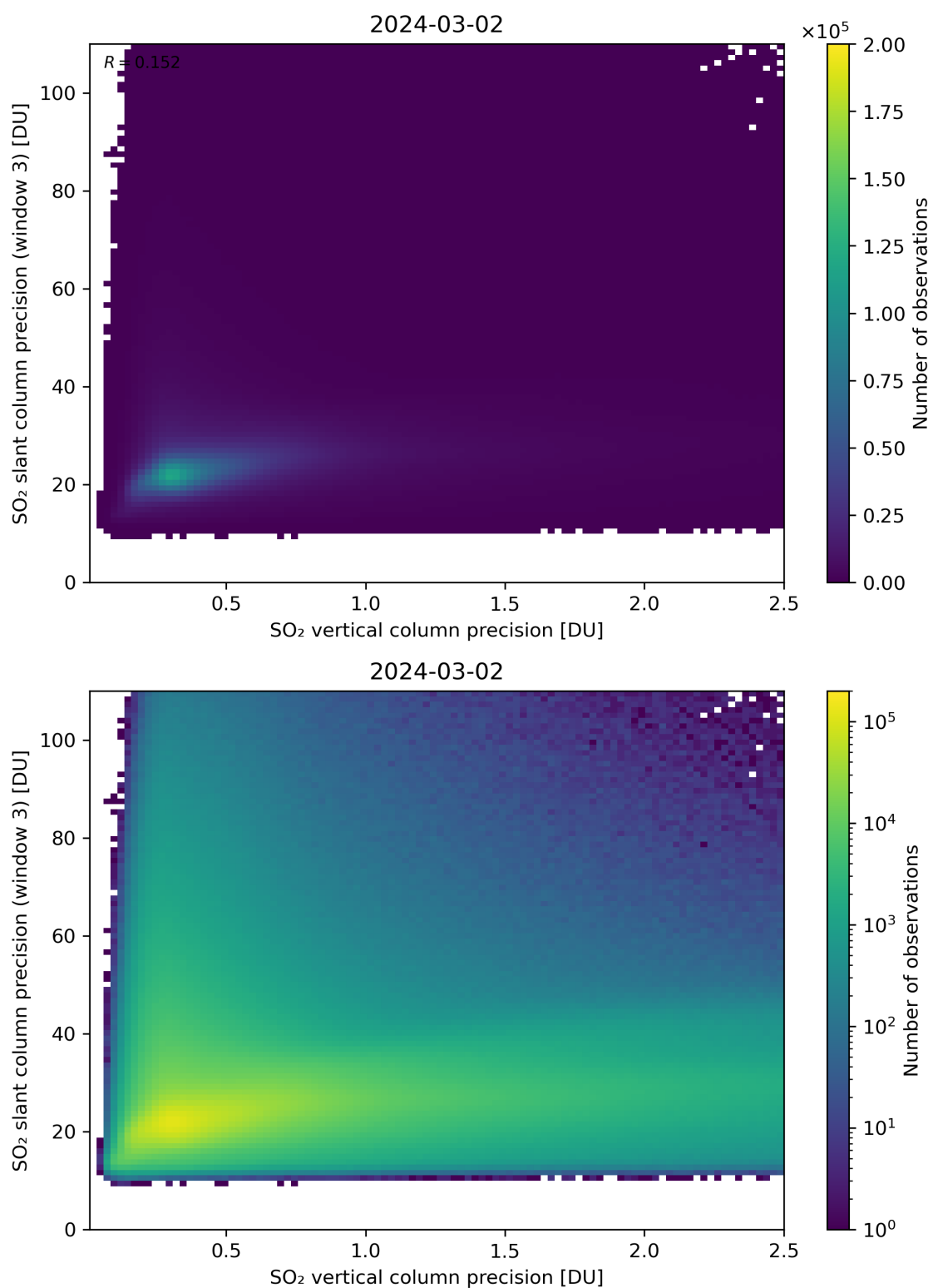
Figure 293: Scatter density plot of “SO 2 vertical column precision” against “SO 2 slant column precision (window 3)” for 2024-03-01 to 2024-03-03.
