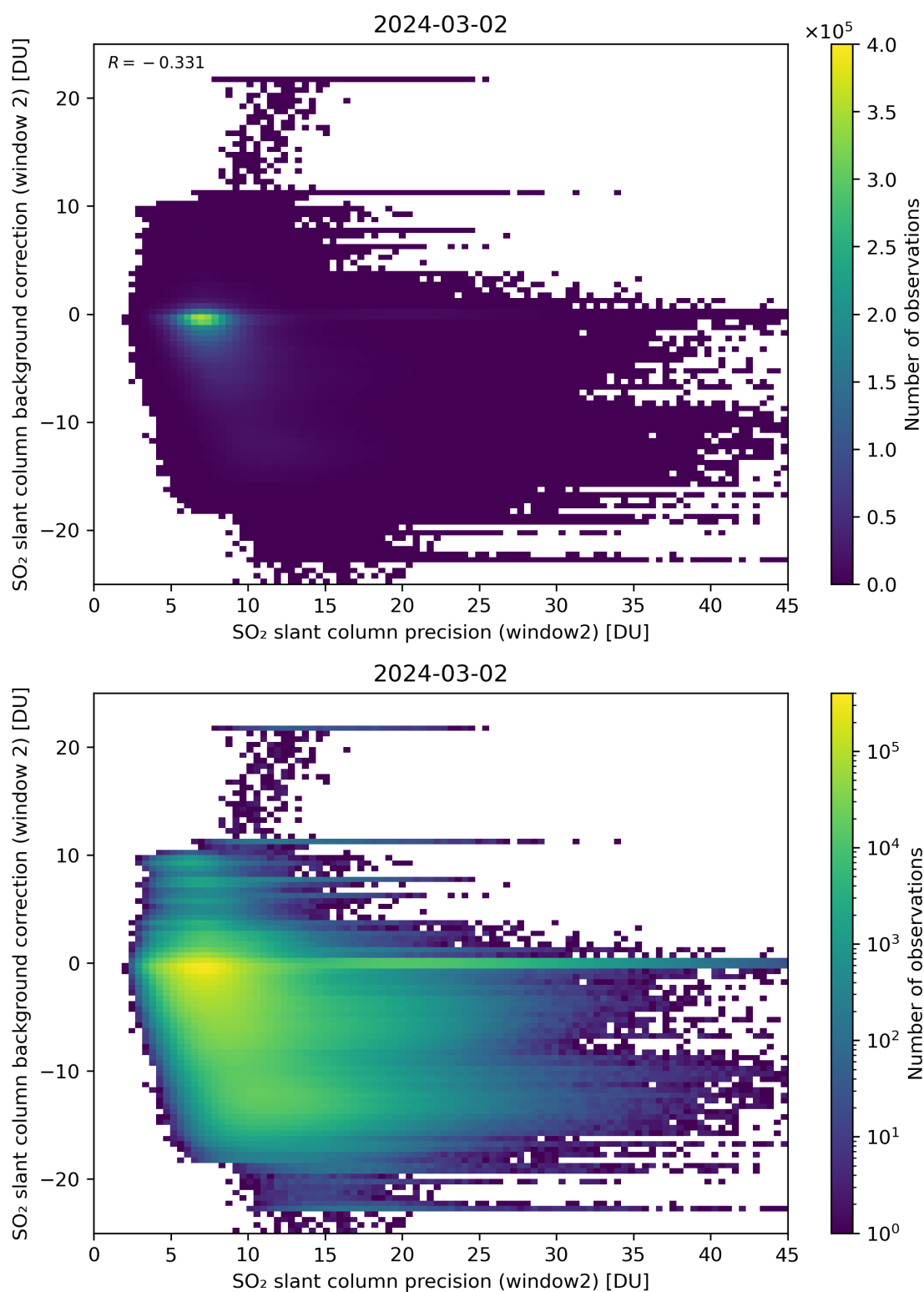
Figure 241: Scatter density plot of “SO 2 slant column precision (window2)” against “SO 2 slant column background correction (window 2)” for 2024-03-01 to 2024-03-03.
