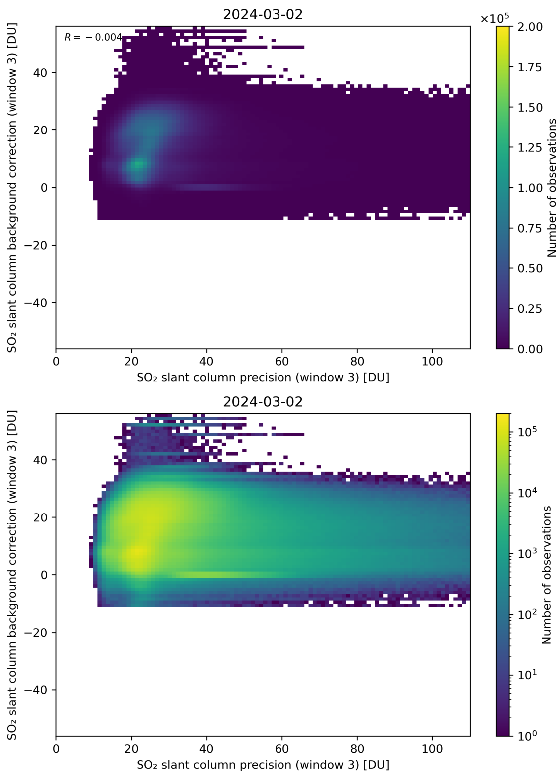
Figure 257: Scatter density plot of “SO 2 slant column precision (window 3)” against “SO 2 slant column background correction (window 3)” for 2024-03-01 to 2024-03-03.
