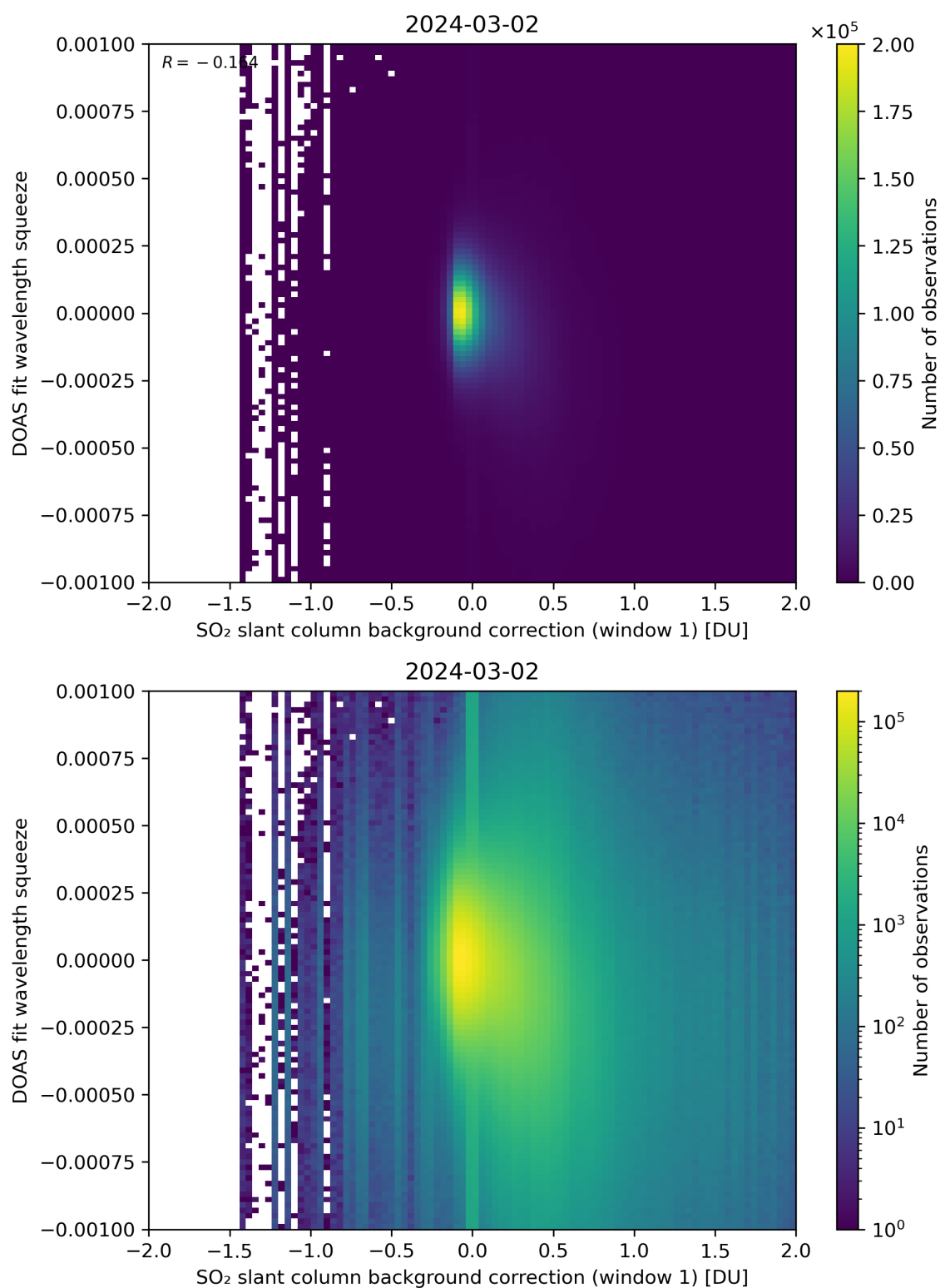
Figure 101: Scatter density plot of “SO 2 slant column background correction (window 1)” against “DOAS fit wavelength squeeze” for 2024-03-01 to 2024-03-03.
