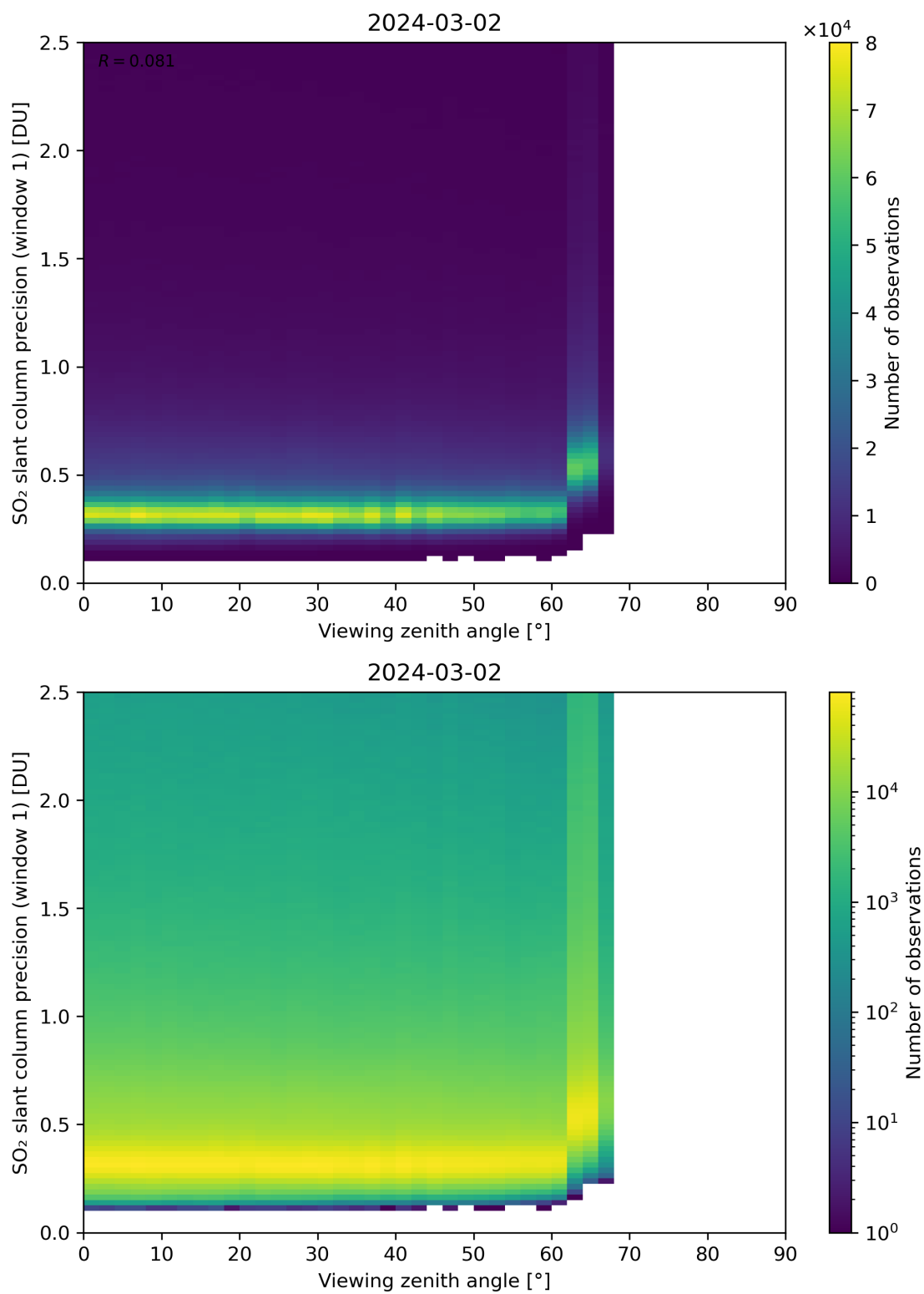
Figure 321: Scatter density plot of “Viewing zenith angle” against “SO 2 slant column precision (window 1)” for 2024-03-01 to 2024-03-03.
