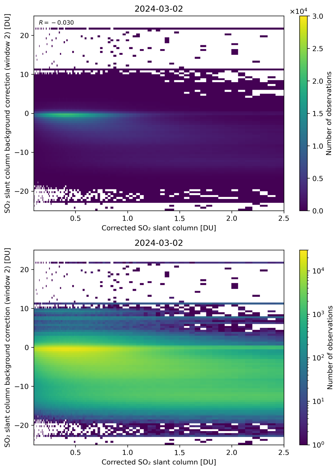
Figure 179: Scatter density plot of “Corrected SO 2 slant column” against “SO 2 slant column background correction (window 2)” for 2024-03-01 to 2024-03-03.
