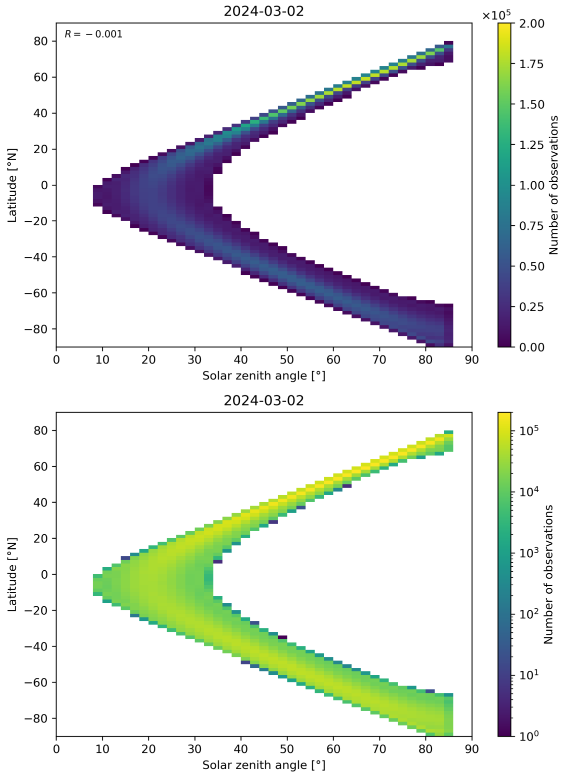
Figure 164: Scatter density plot of “Solar zenith angle” against “Latitude” for 2024-03-01 to 2024-03-03.
