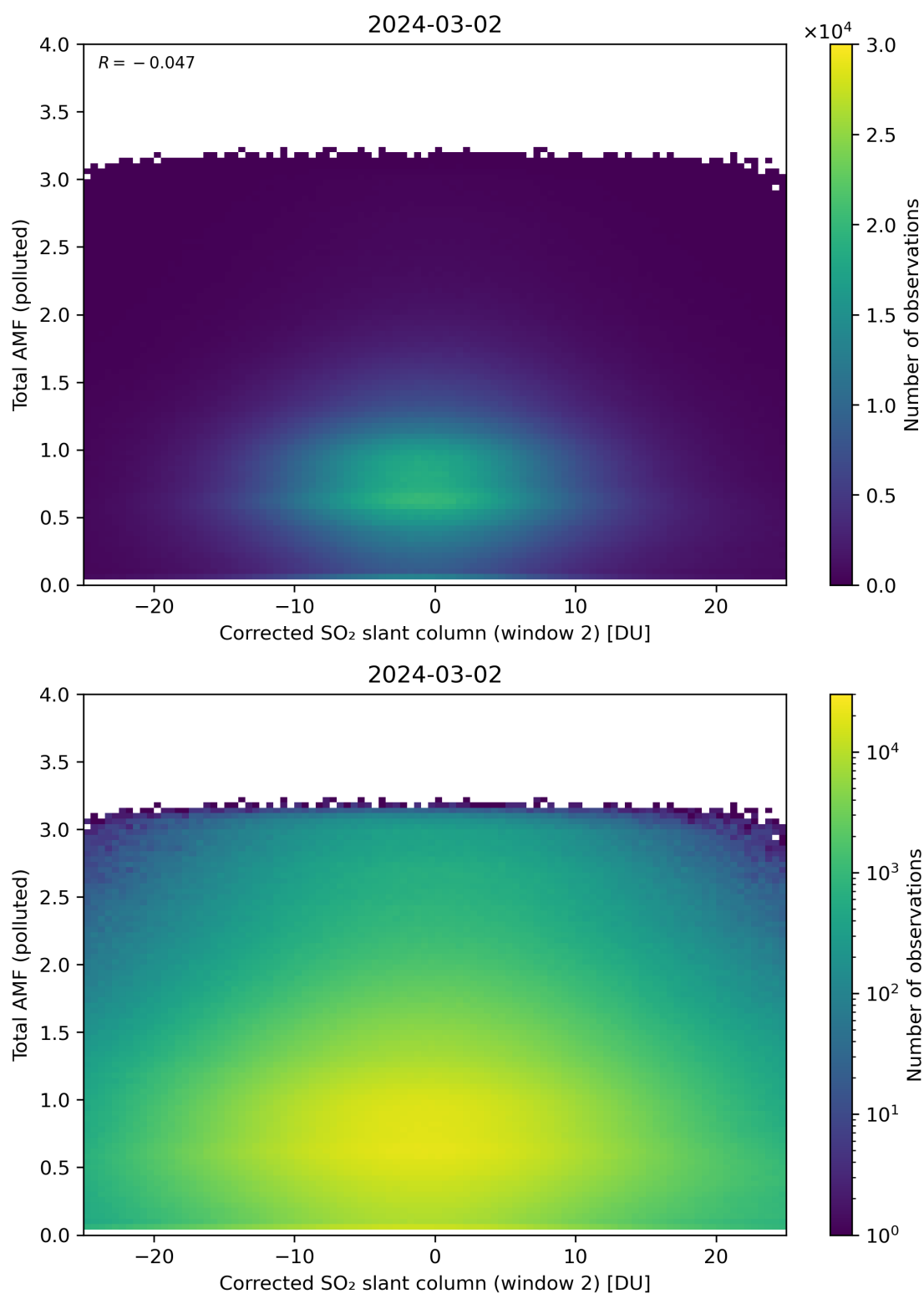
Figure 203: Scatter density plot of “Corrected SO 2 slant column (window 2)” against “Total AMF (polluted)” for 2024-03-01 to 2024-03-03.
