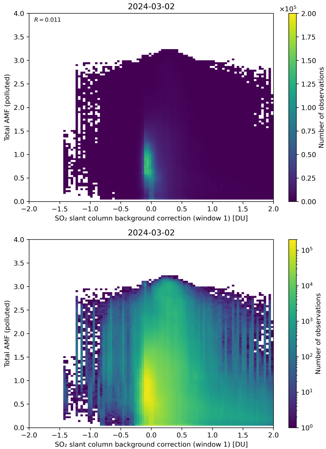
Figure 109: Scatter density plot of “SO 2 slant column background correction (window 1)” against “Total AMF (polluted)” for 2024-03-01 to 2024-03-03.
