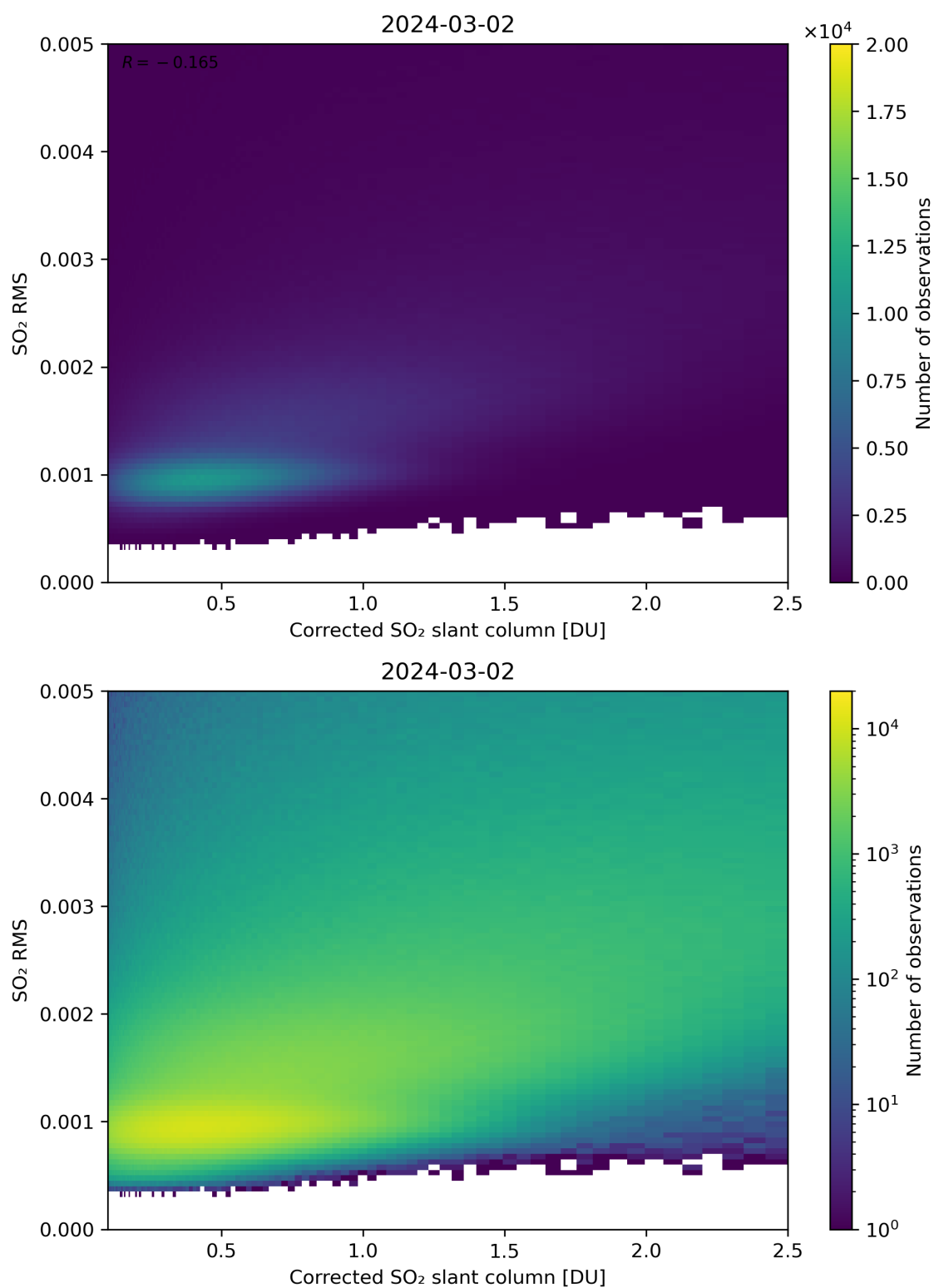
Figure 183: Scatter density plot of “Corrected SO 2 slant column” against “SO 2 RMS” for 2024-03-01 to 2024-03-03.
