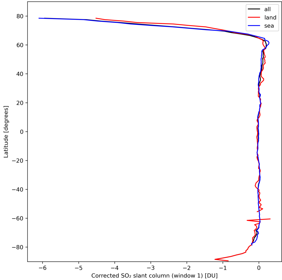
Figure 35: Zonal average of “Corrected SO 2 slant column (window 1)” for 2024-03-01 to 2024-03-03.
