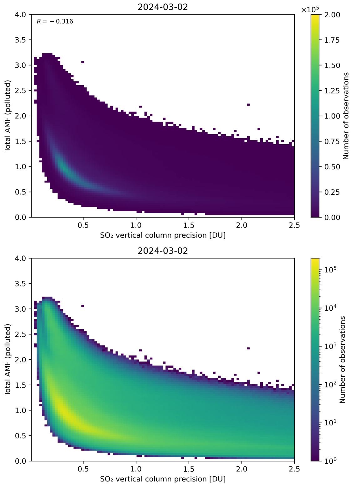
Figure 294: Scatter density plot of “SO 2 vertical column precision” against “Total AMF (polluted)” for 2024-03-01 to 2024-03-03.
