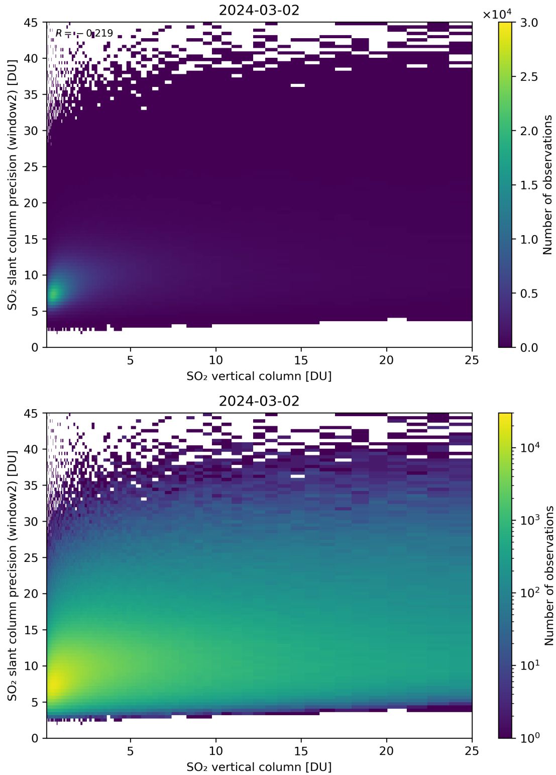
Figure 302: Scatter density plot of “SO 2 vertical column” against “SO 2 slant column precision (window2)” for 2024-03-01 to 2024-03-03.
