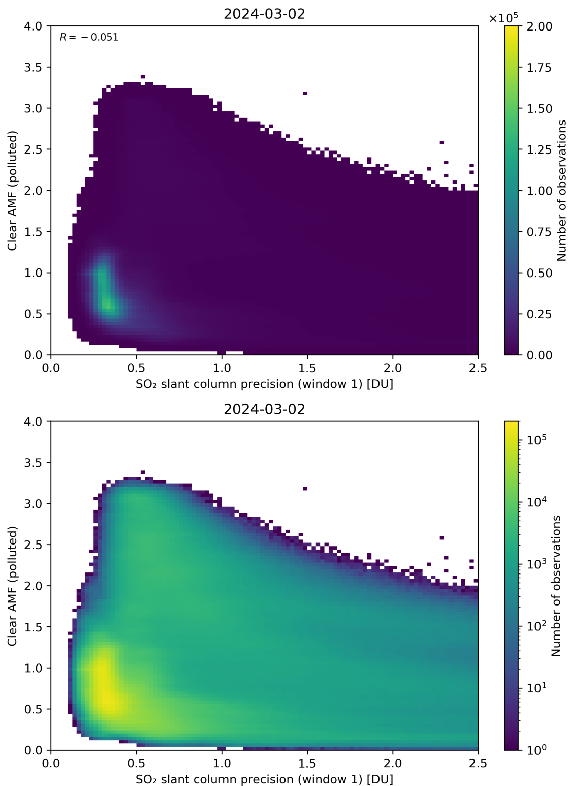
Figure 224: Scatter density plot of “SO 2 slant column precision (window 1)” against “Clear AMF (polluted)” for 2024-03-01 to 2024-03-03.
