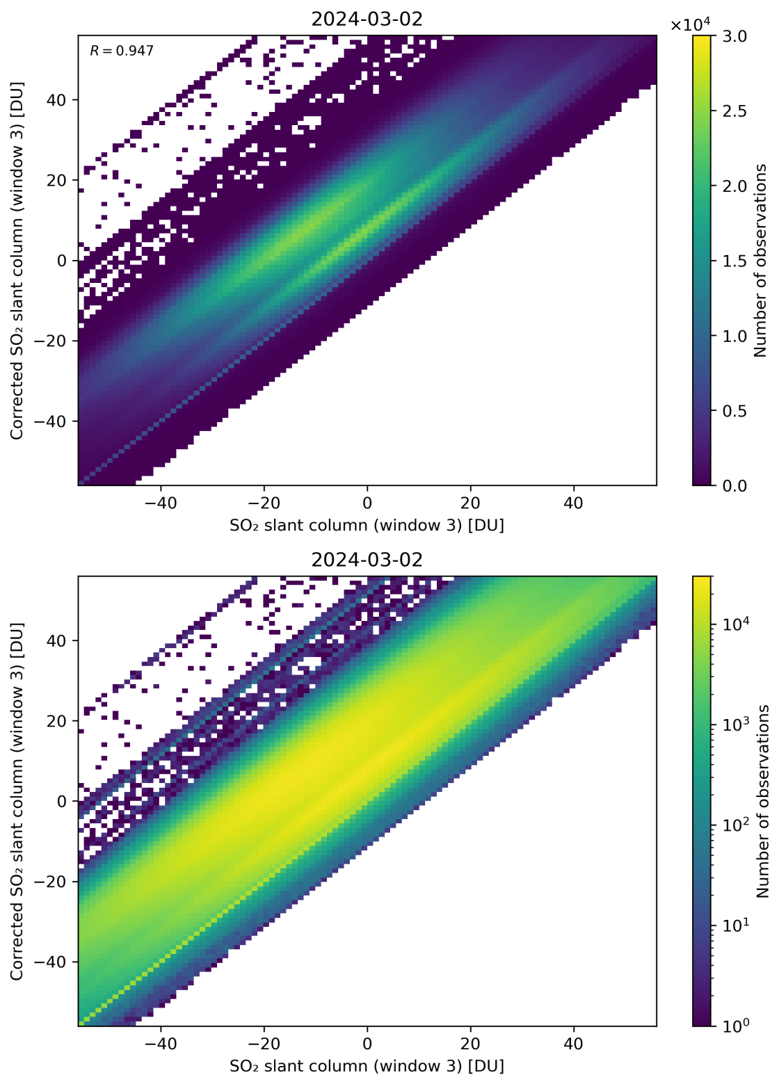
Figure 266: Scatter density plot of “SO 2 slant column (window 3)” against “Corrected SO 2 slant column (window 3)” for 2024-03-01 to 2024-03-03.
