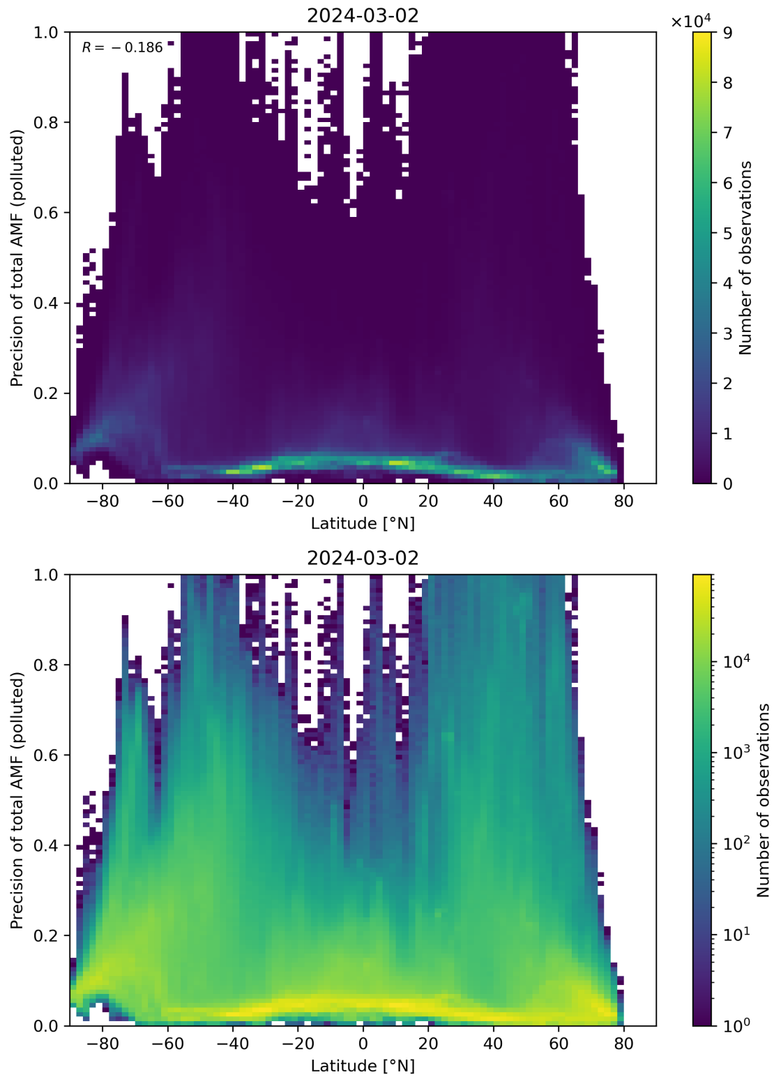
Figure 155: Scatter density plot of “Latitude” against “Precision of total AMF (polluted)” for 2024-03-01 to 2024-03-03.
