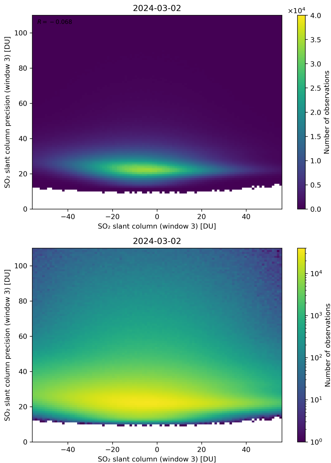
Figure 267: Scatter density plot of “SO 2 slant column (window 3)” against “SO 2 slant column precision (window 3)” for 2024-03-01 to 2024-03-03.
