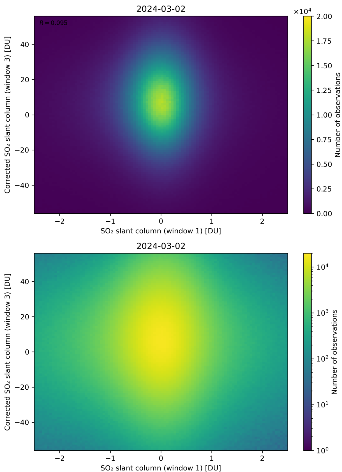
Figure 234: Scatter density plot of “SO 2 slant column (window 1)” against “Corrected SO 2 slant column (window 3)” for 2024-03-01 to 2024-03-03.
