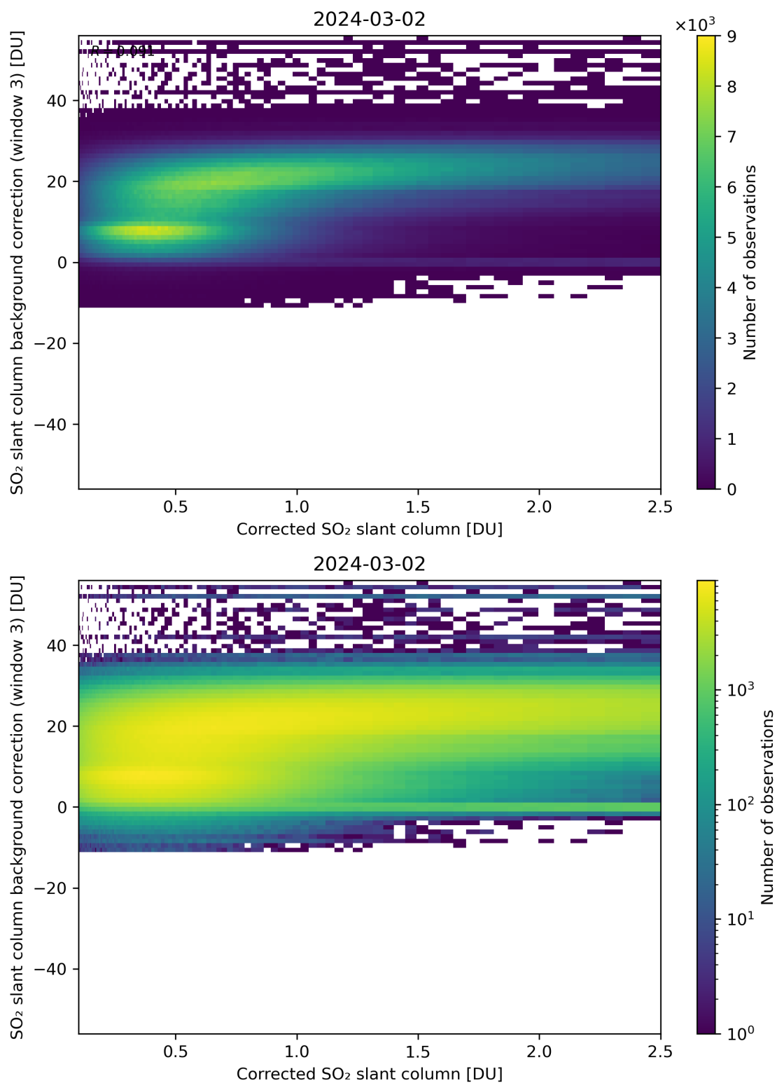
Figure 180: Scatter density plot of “Corrected SO 2 slant column” against “SO 2 slant column background correction (window 3)” for 2024-03-01 to 2024-03-03.
