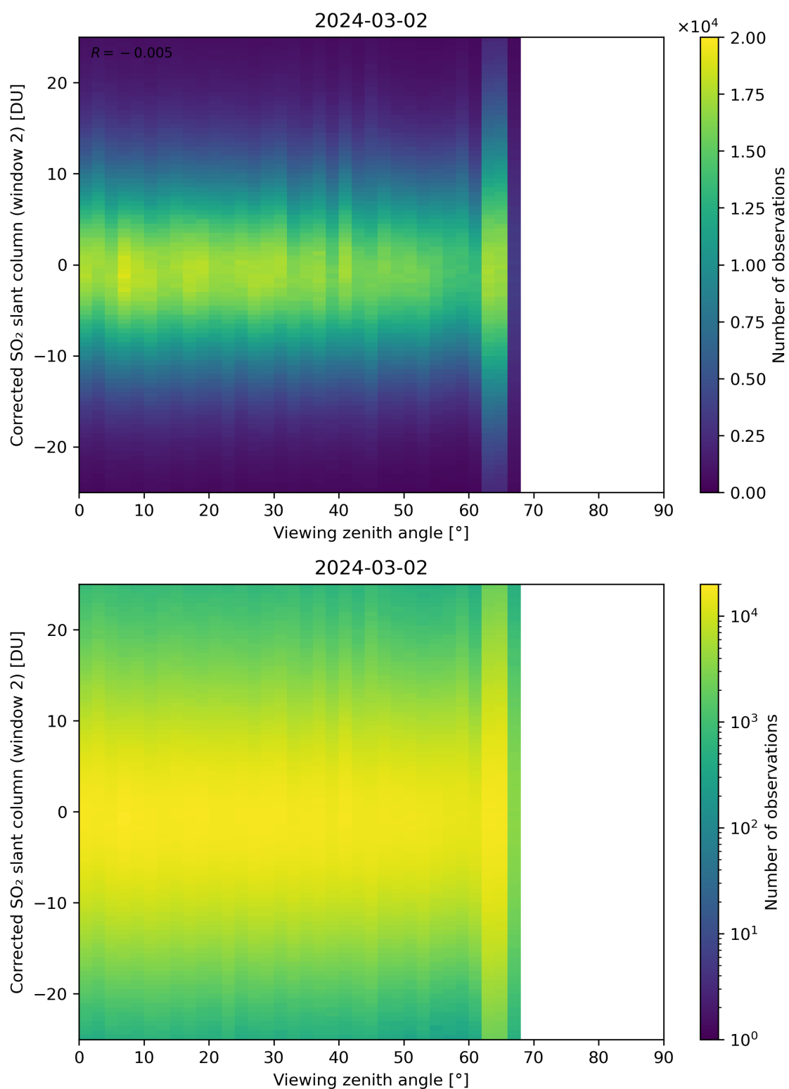
Figure 318: Scatter density plot of “Viewing zenith angle” against “Corrected SO 2 slant column (window 2)” for 2024-03-01 to 2024-03-03.
