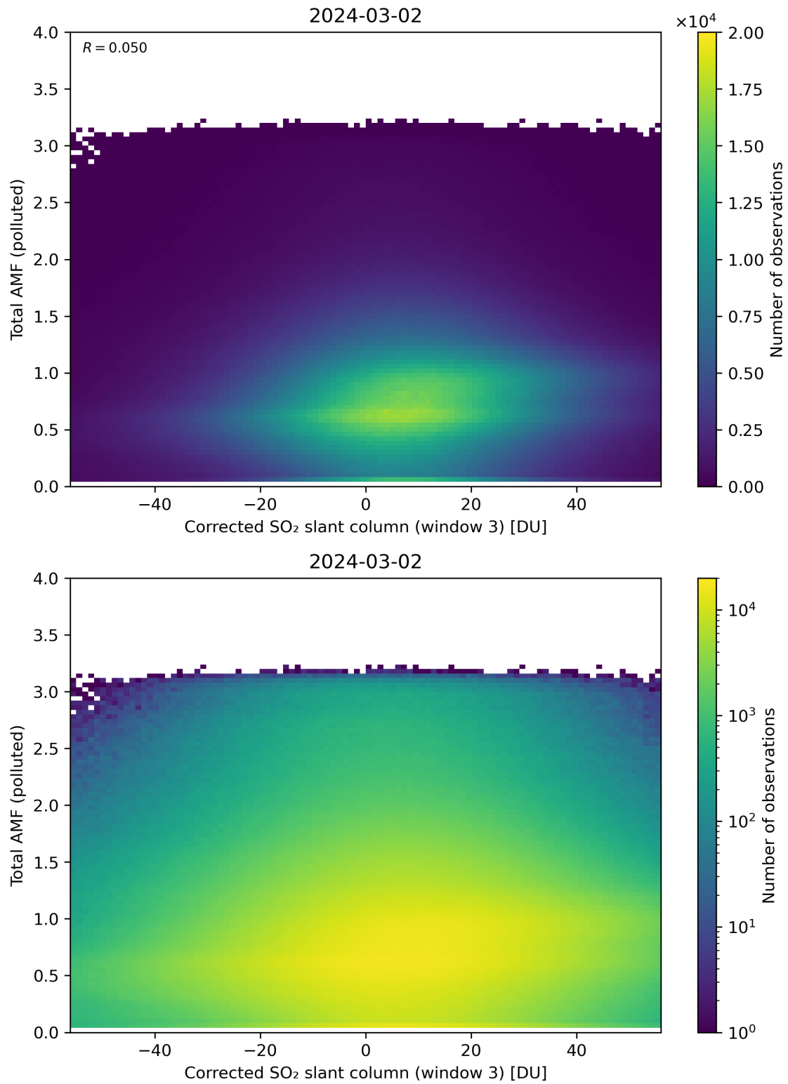
Figure 210: Scatter density plot of “Corrected SO 2 slant column (window 3)” against “Total AMF (polluted)” for 2024-03-01 to 2024-03-03.
