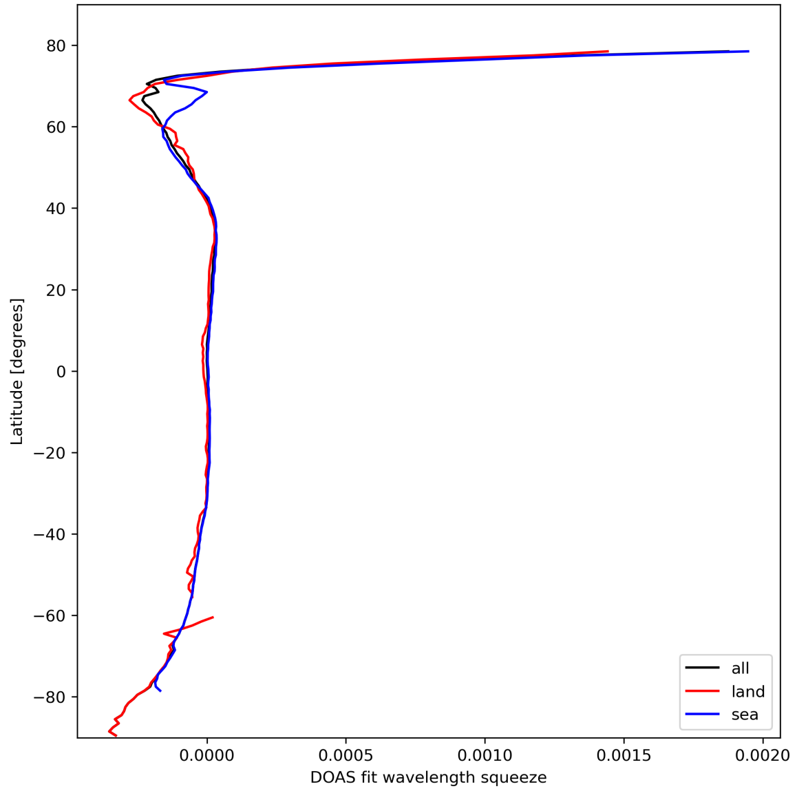
Figure 46: Zonal average of “DOAS fit wavelength squeeze” for 2024-03-01 to 2024-03-03.
