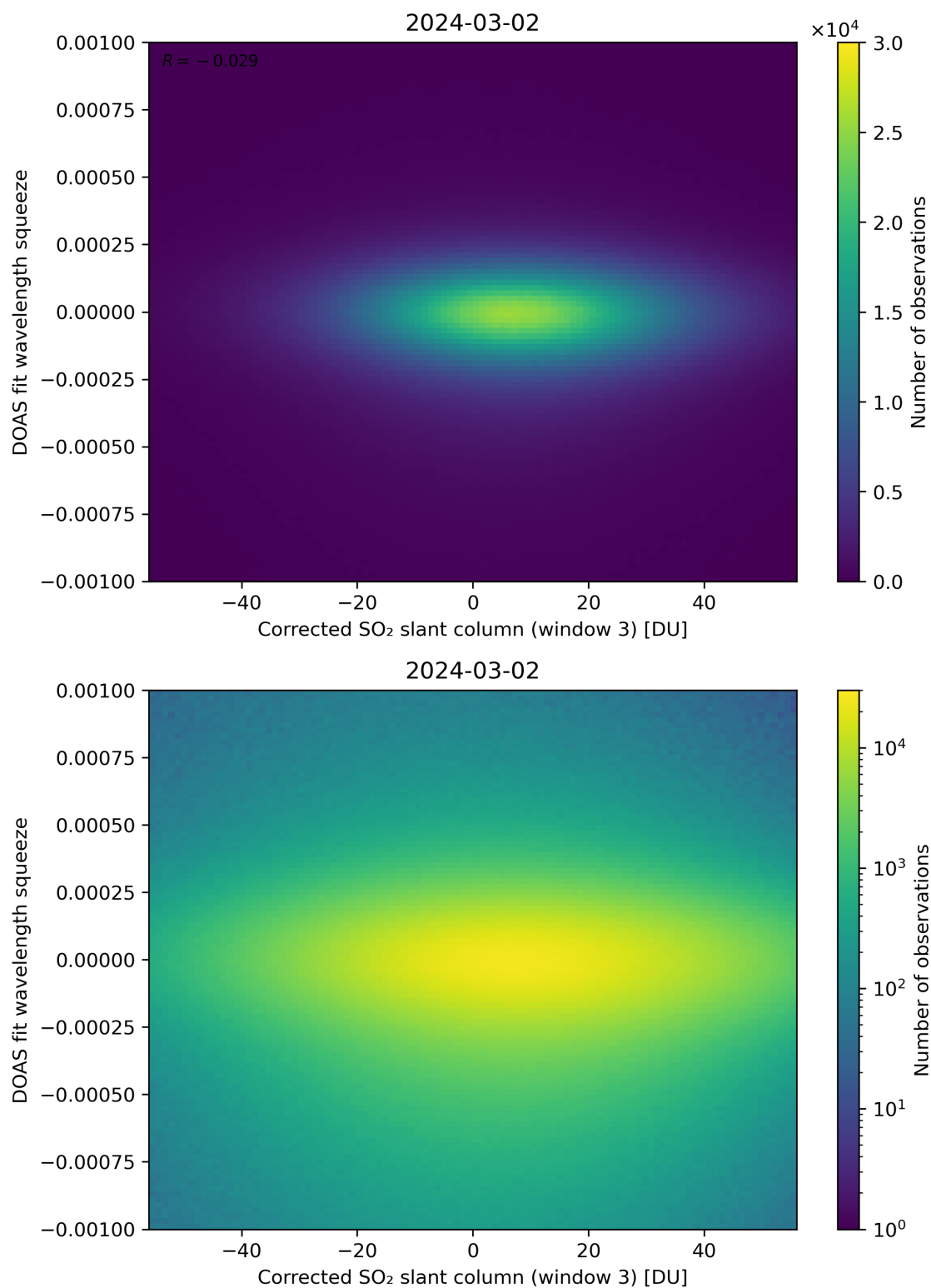
Figure 207: Scatter density plot of “Corrected SO 2 slant column (window 3)” against “DOAS fit wavelength squeeze” for 2024-03-01 to 2024-03-03.
