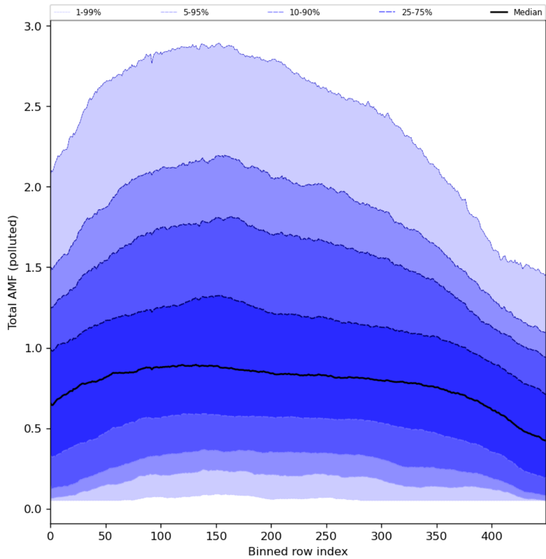
Figure 94: Along track statistics of “Total AMF (polluted)” for 2024-03-01 to 2024-03-03
