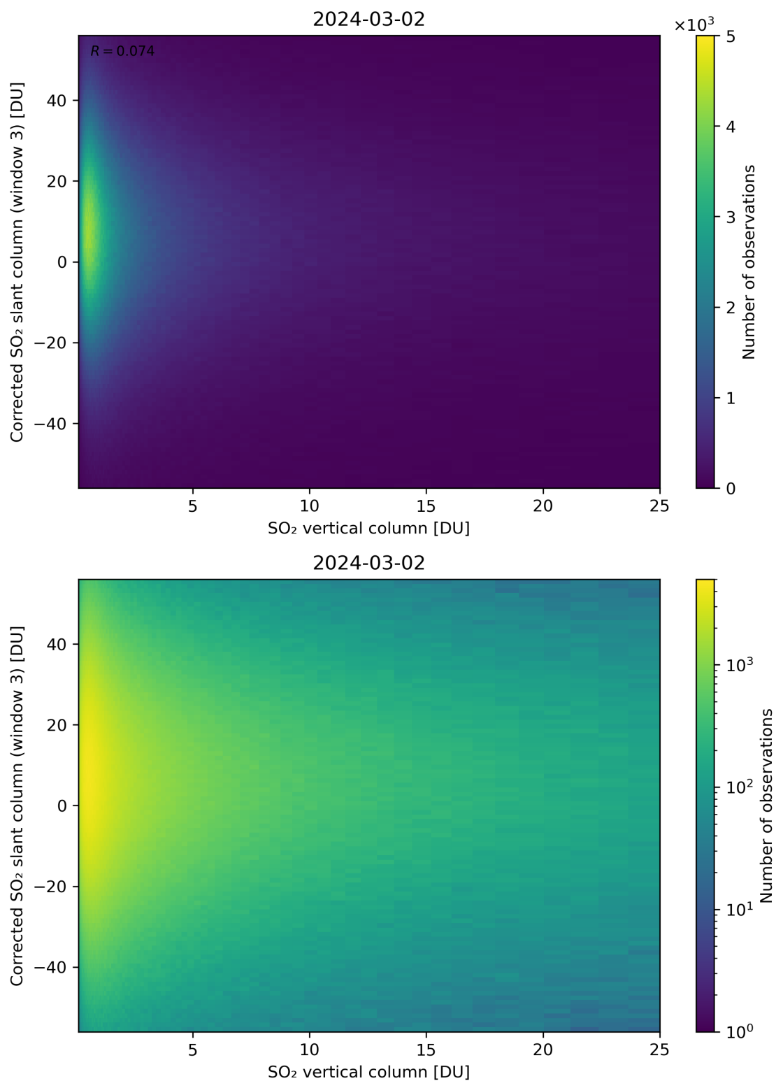
Figure 299: Scatter density plot of “SO 2 vertical column” against “Corrected SO 2 slant column (window 3)” for 2024-03-01 to 2024-03-03.
