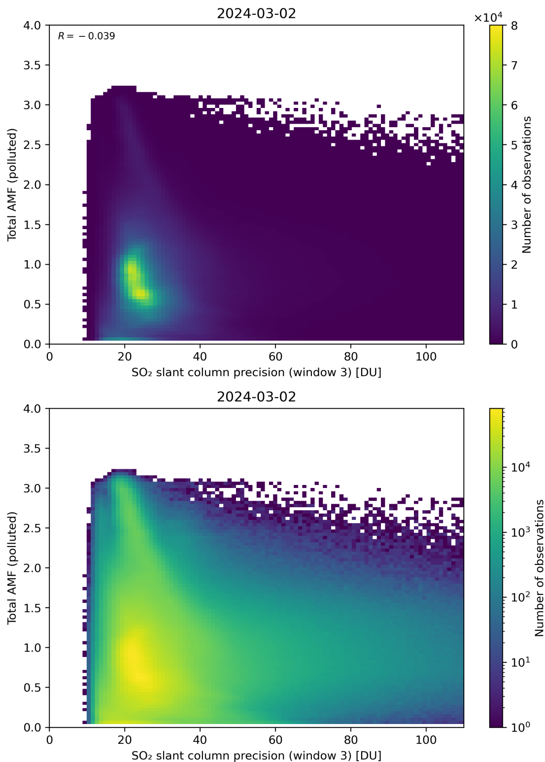
Figure 263: Scatter density plot of “SO 2 slant column precision (window 3)” against “Total AMF (polluted)” for 2024-03-01 to 2024-03-03.
