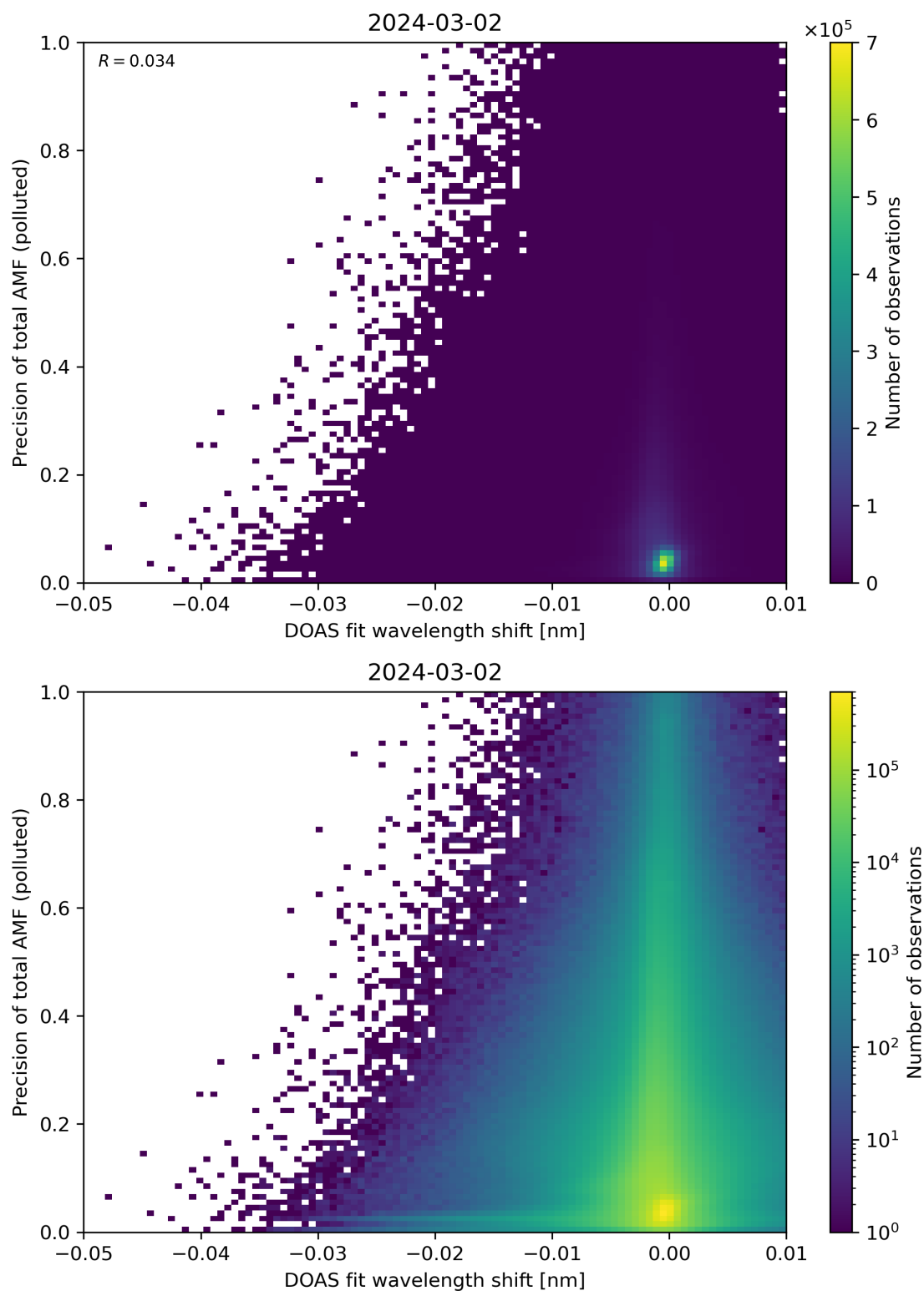
Figure 131: Scatter density plot of “DOAS fit wavelength shift” against “Precision of total AMF (polluted)” for 2024-03-01 to 2024-03-03.
