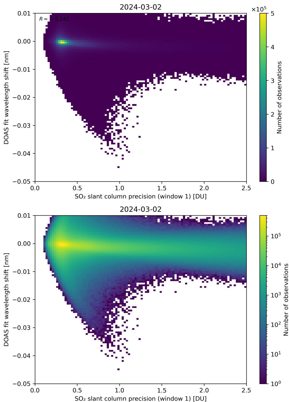
Figure 221: Scatter density plot of “SO 2 slant column precision (window 1)” against “DOAS fit wavelength shift” for 2024-03-01 to 2024-03-03.
