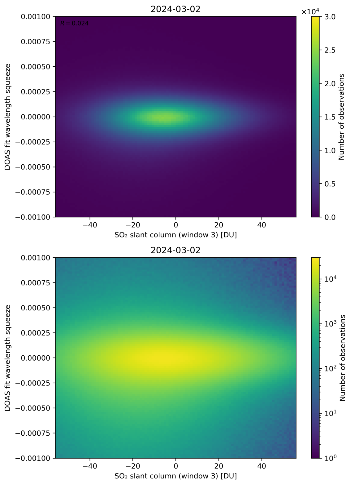
Figure 255: Scatter density plot of “SO 2 slant column (window 3)” against “DOAS fit wavelength squeeze” for 2024-03-01 to 2024-03-03.
