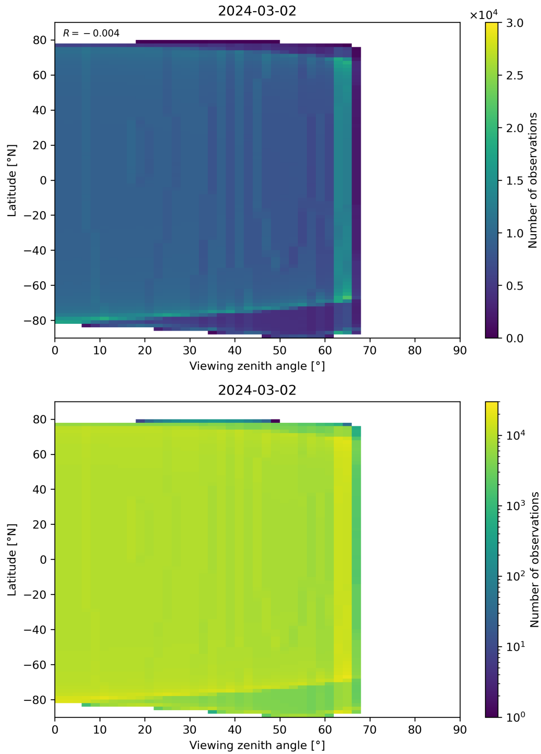
Figure 314: Scatter density plot of “Viewing zenith angle” against “Latitude” for 2024-03-01 to 2024-03-03.
