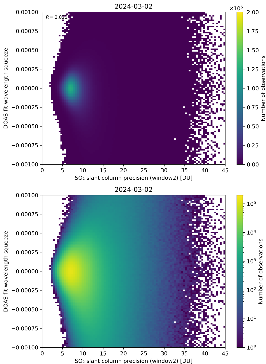
Figure 244: Scatter density plot of “SO 2 slant column precision (window2)” against “DOAS fit wavelength squeeze” for 2024-03-01 to 2024-03-03.
