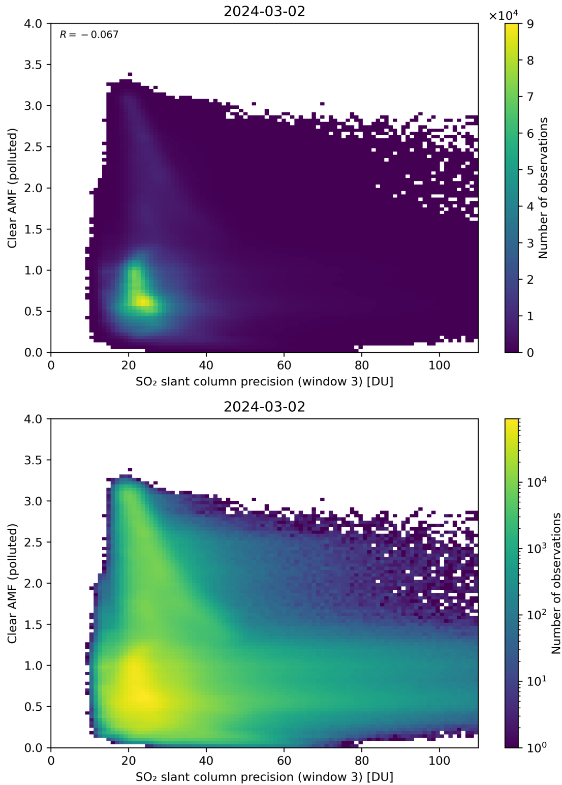
Figure 261: Scatter density plot of “SO 2 slant column precision (window 3)” against “Clear AMF (polluted)” for 2024-03-01 to 2024-03-03.
