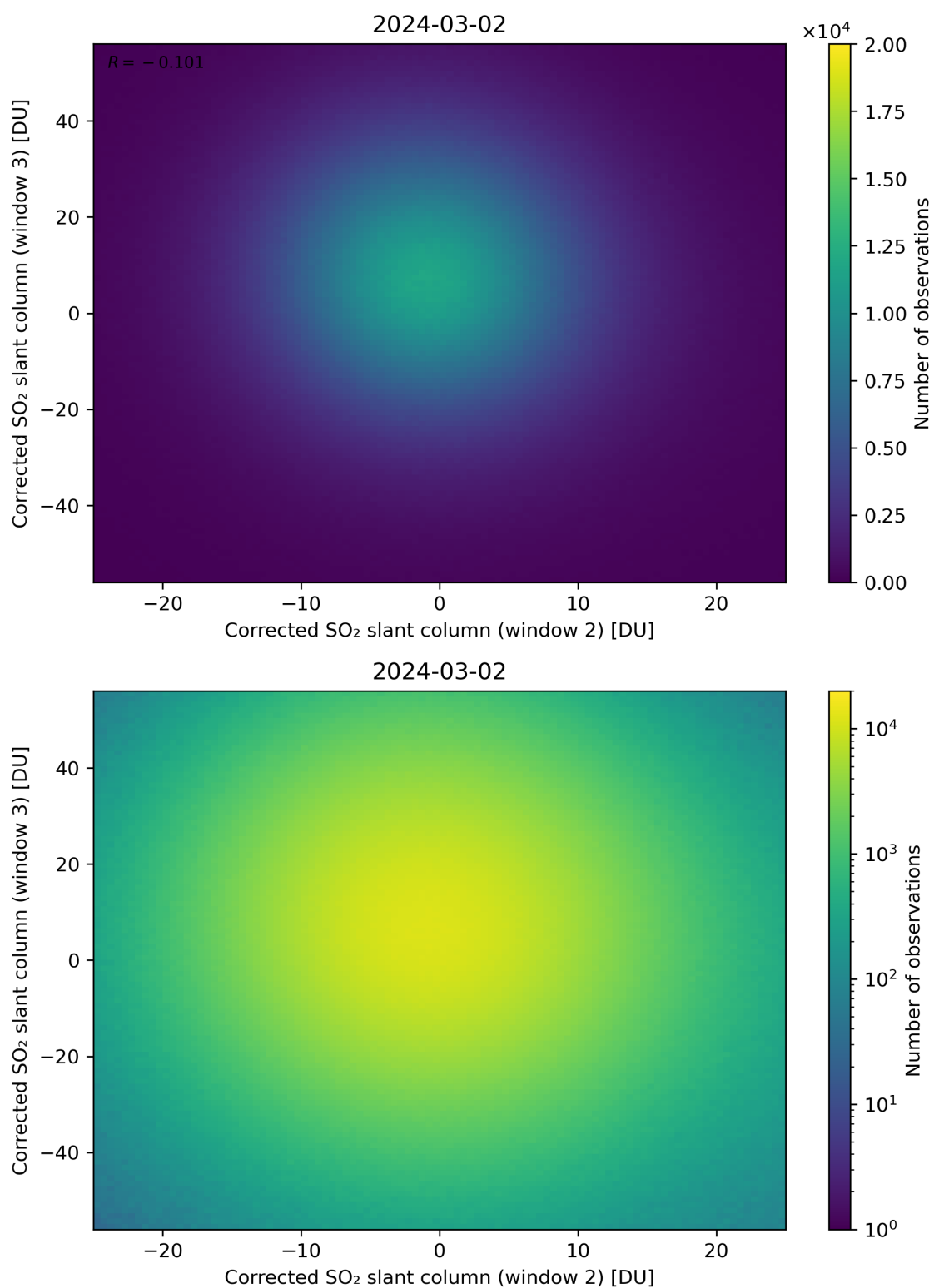
Figure 200: Scatter density plot of “Corrected SO 2 slant column (window 2)” against “Corrected SO 2 slant column (window 3)” for 2024-03-01 to 2024-03-03.
