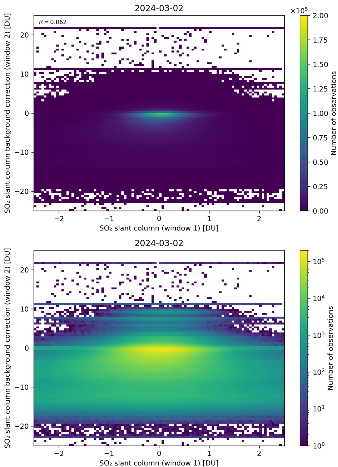
Figure 213: Scatter density plot of “SO 2 slant column (window 1)” against “SO 2 slant column background correction (window 2)” for 2024-03-01 to 2024-03-03.
