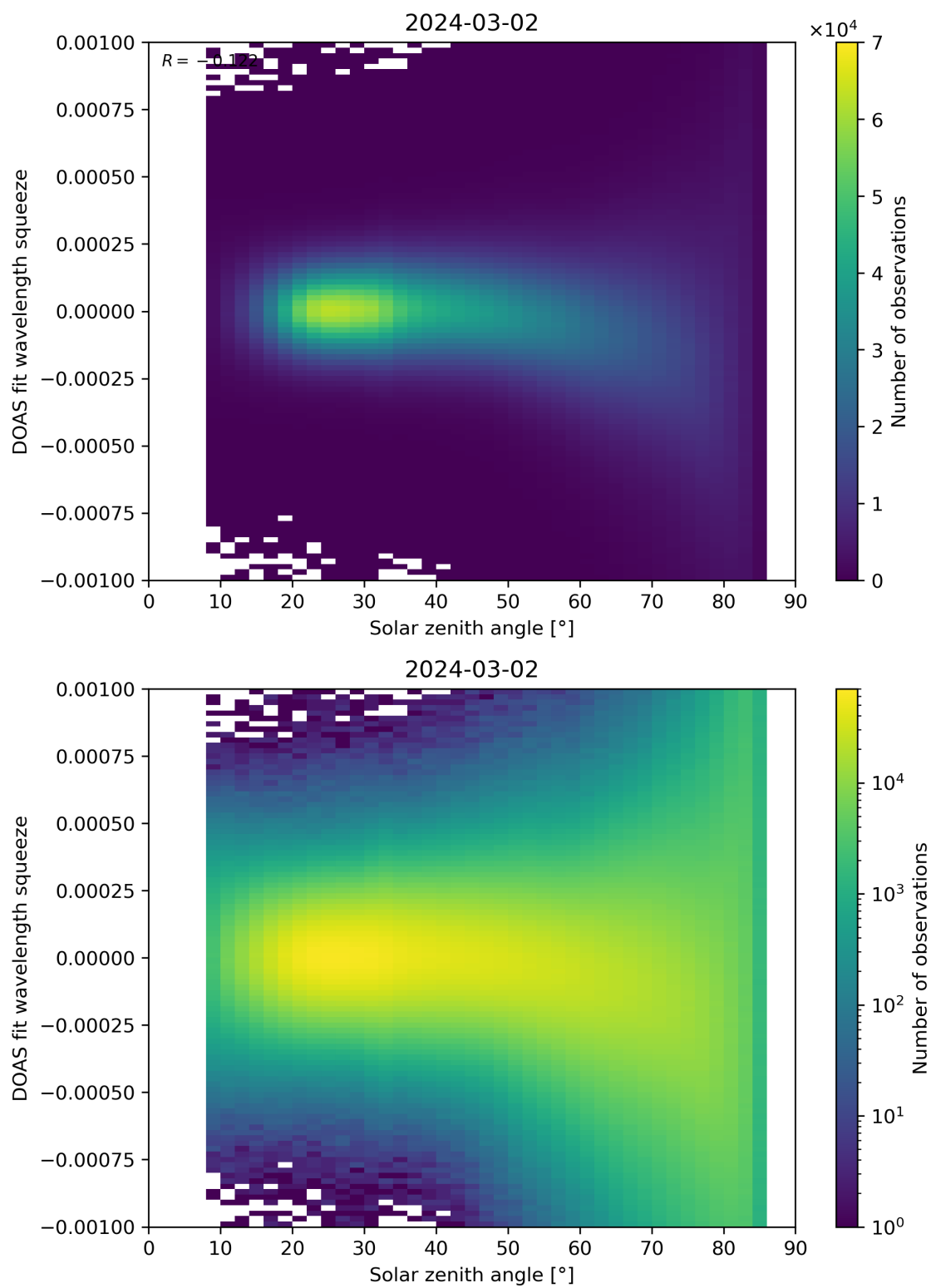
Figure 162: Scatter density plot of “Solar zenith angle” against “DOAS fit wavelength squeeze” for 2024-03-01 to 2024-03-03.
