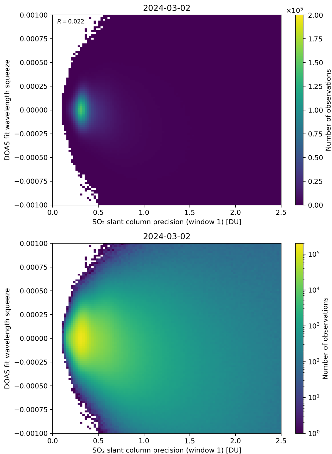
Figure 222: Scatter density plot of “SO 2 slant column precision (window 1)” against “DOAS fit wavelength squeeze” for 2024-03-01 to 2024-03-03.
