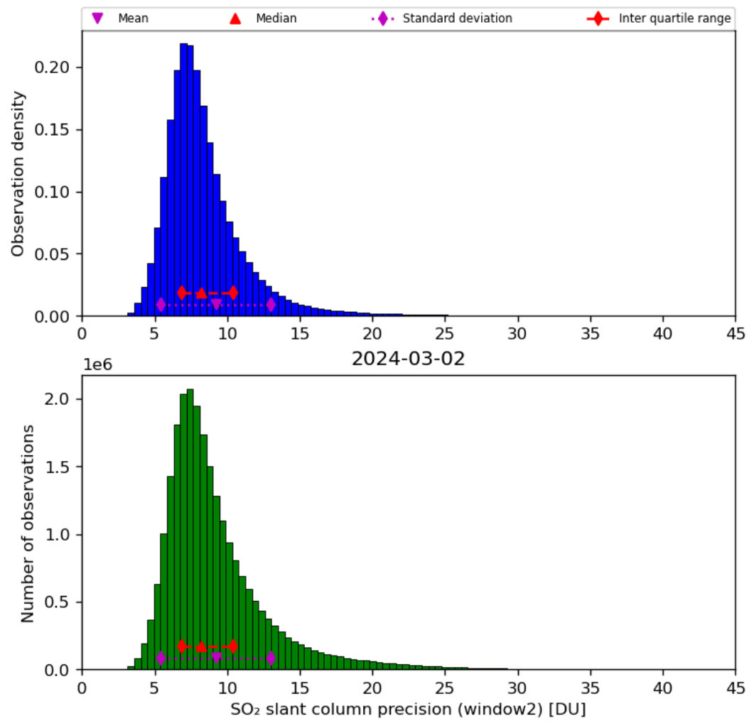
Figure 61: Histogram of “SO 2 slant column precision (window2)” for 2024-03-01 to 2024-03-03
