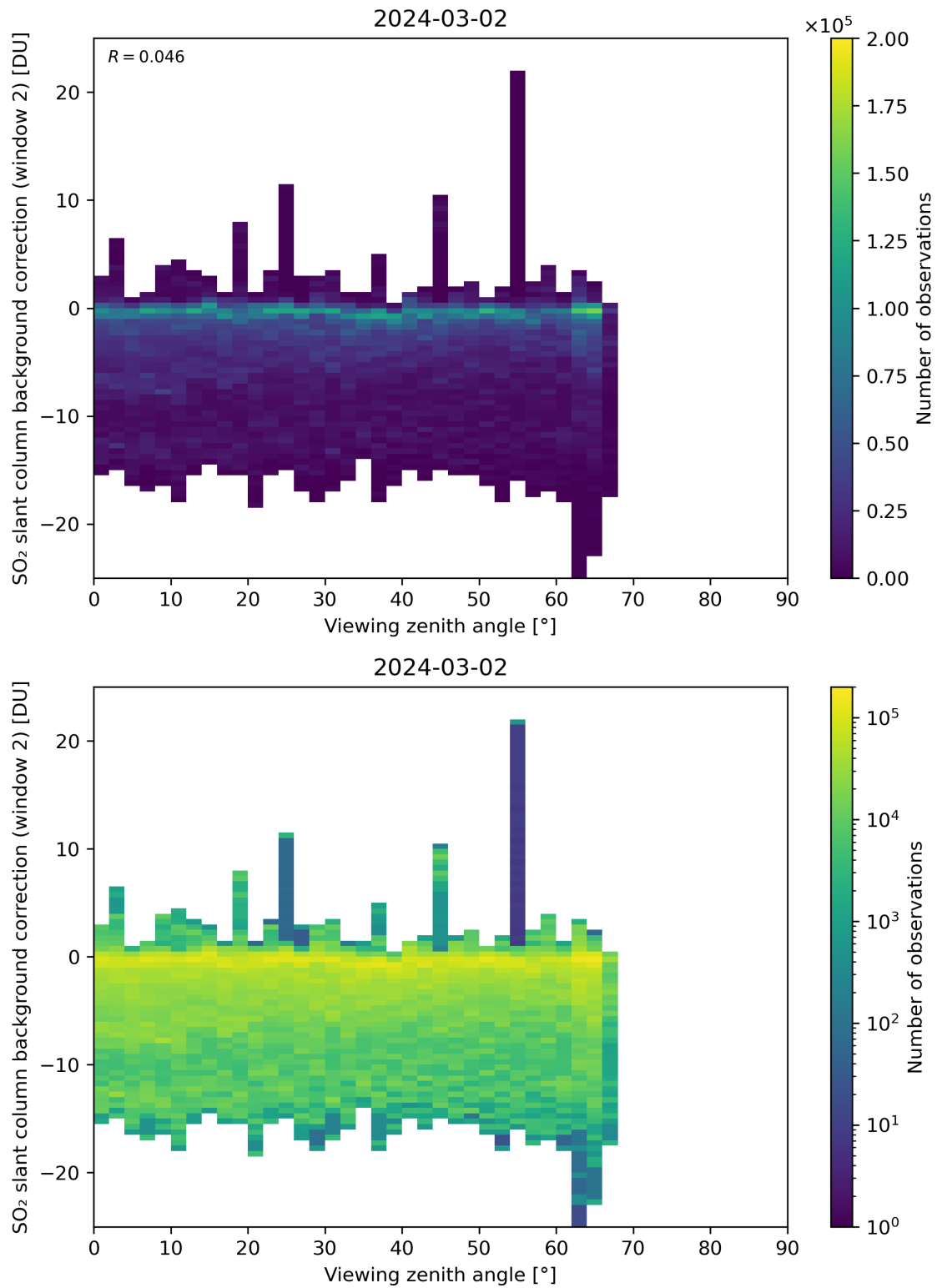
Figure 309: Scatter density plot of “Viewing zenith angle” against “SO 2 slant column background correction (window 2)” for 2024-03-01 to 2024-03-03.
