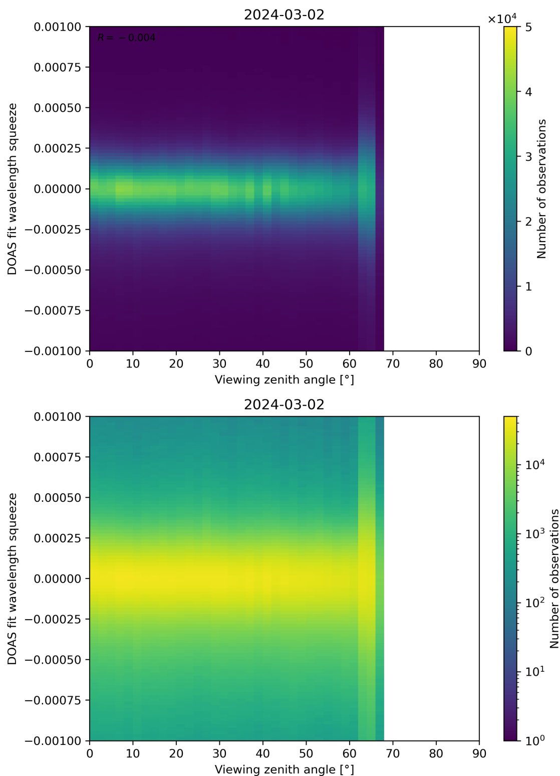
Figure 312: Scatter density plot of “Viewing zenith angle” against “DOAS fit wavelength squeeze” for 2024-03-01 to 2024-03-03.
