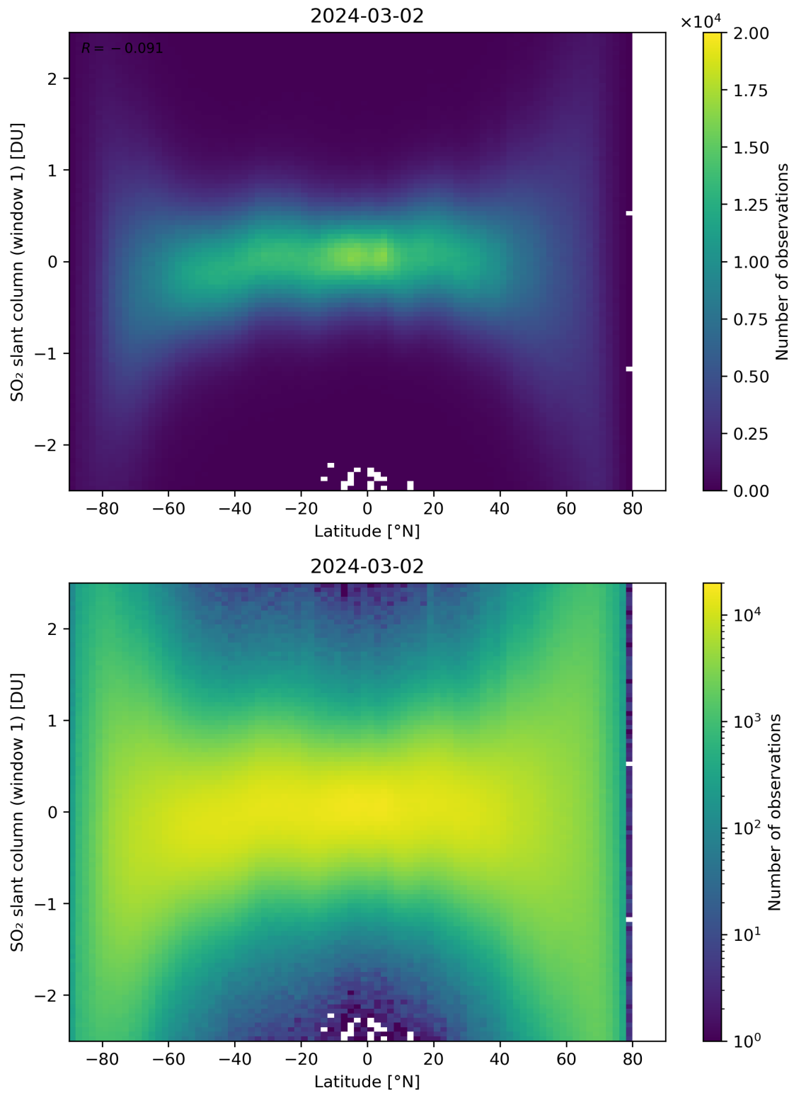
Figure 149: Scatter density plot of “Latitude” against “SO 2 slant column (window 1)” for 2024-03-01 to 2024-03-03.
