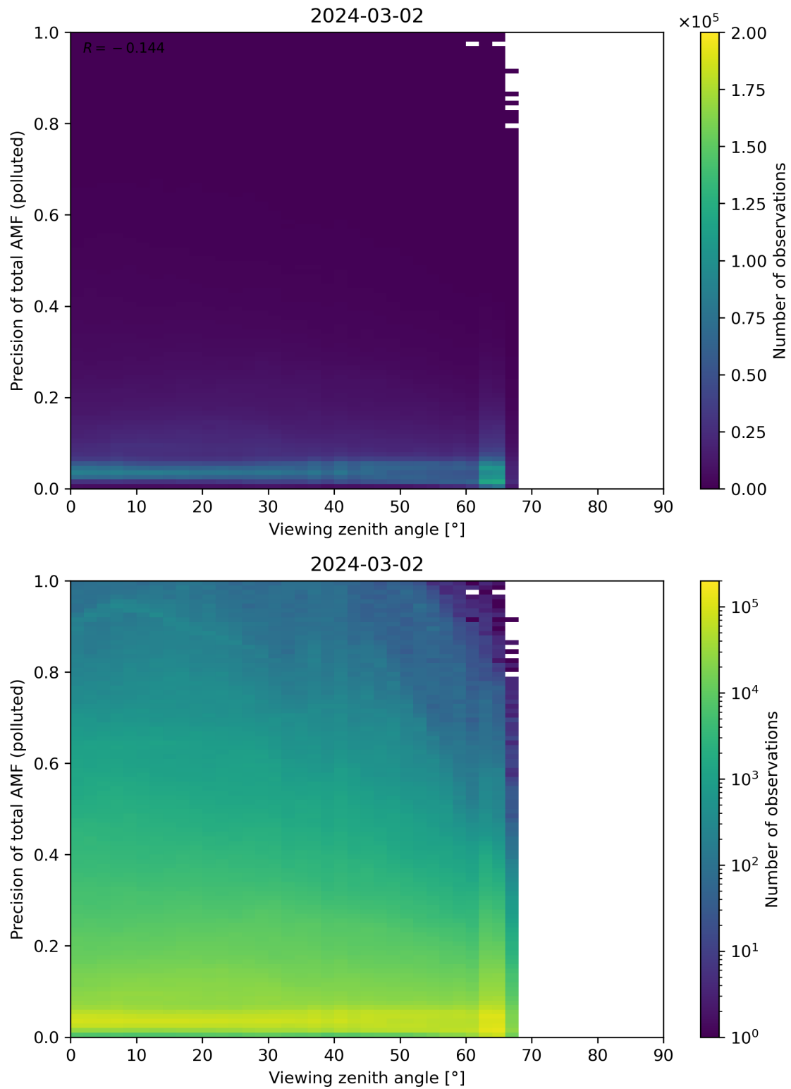
Figure 326: Scatter density plot of “Viewing zenith angle” against “Precision of total AMF (polluted)” for 2024-03-01 to 2024-03-03.
