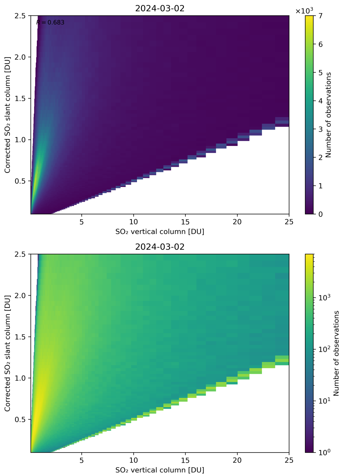
Figure 297: Scatter density plot of “SO 2 vertical column” against “Corrected SO 2 slant column” for 2024-03-01 to 2024-03-03.
