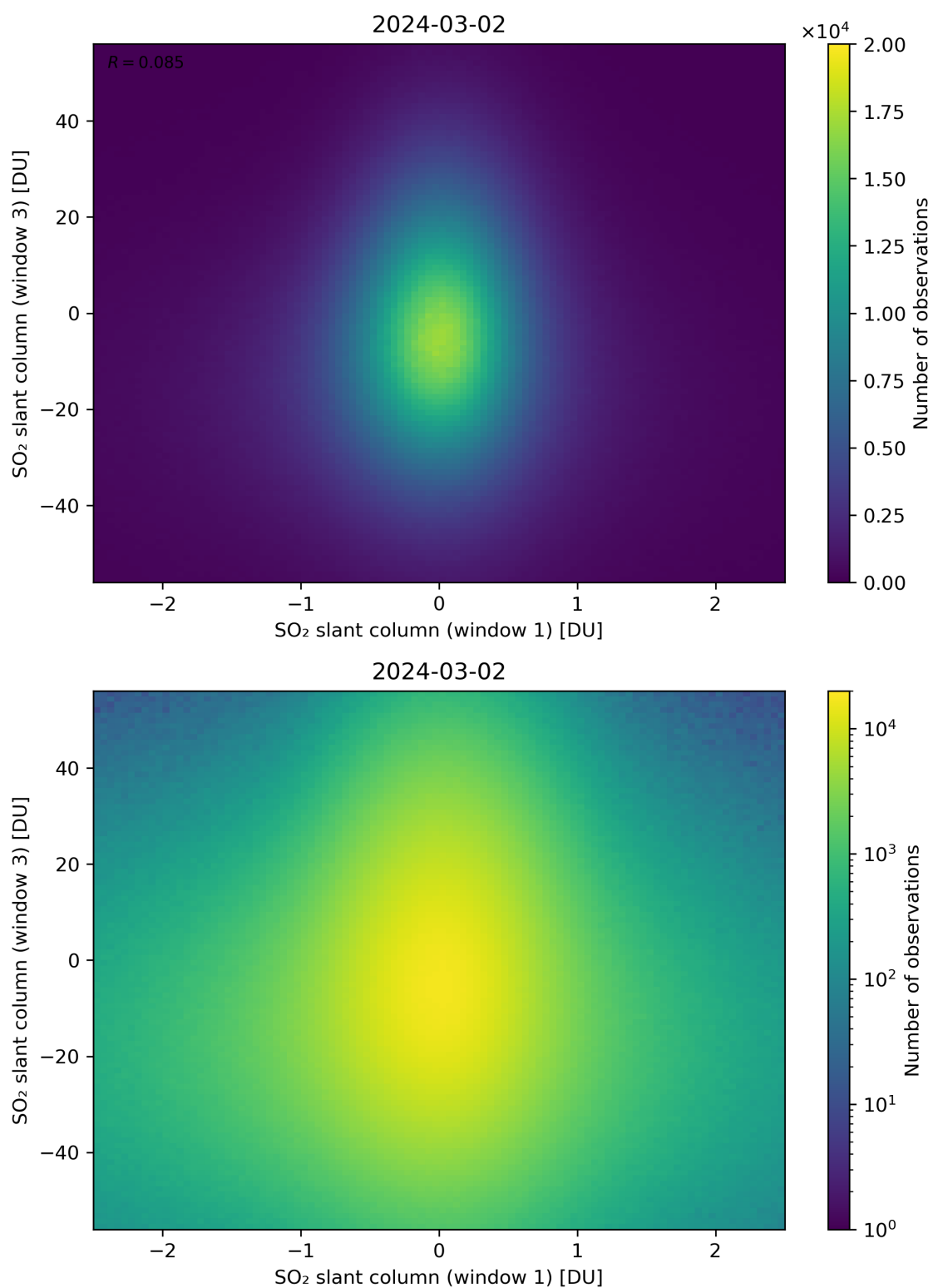
Figure 237: Scatter density plot of “SO 2 slant column (window 1)” against “SO 2 slant column (window 3)” for 2024-03-01 to 2024-03-03.
