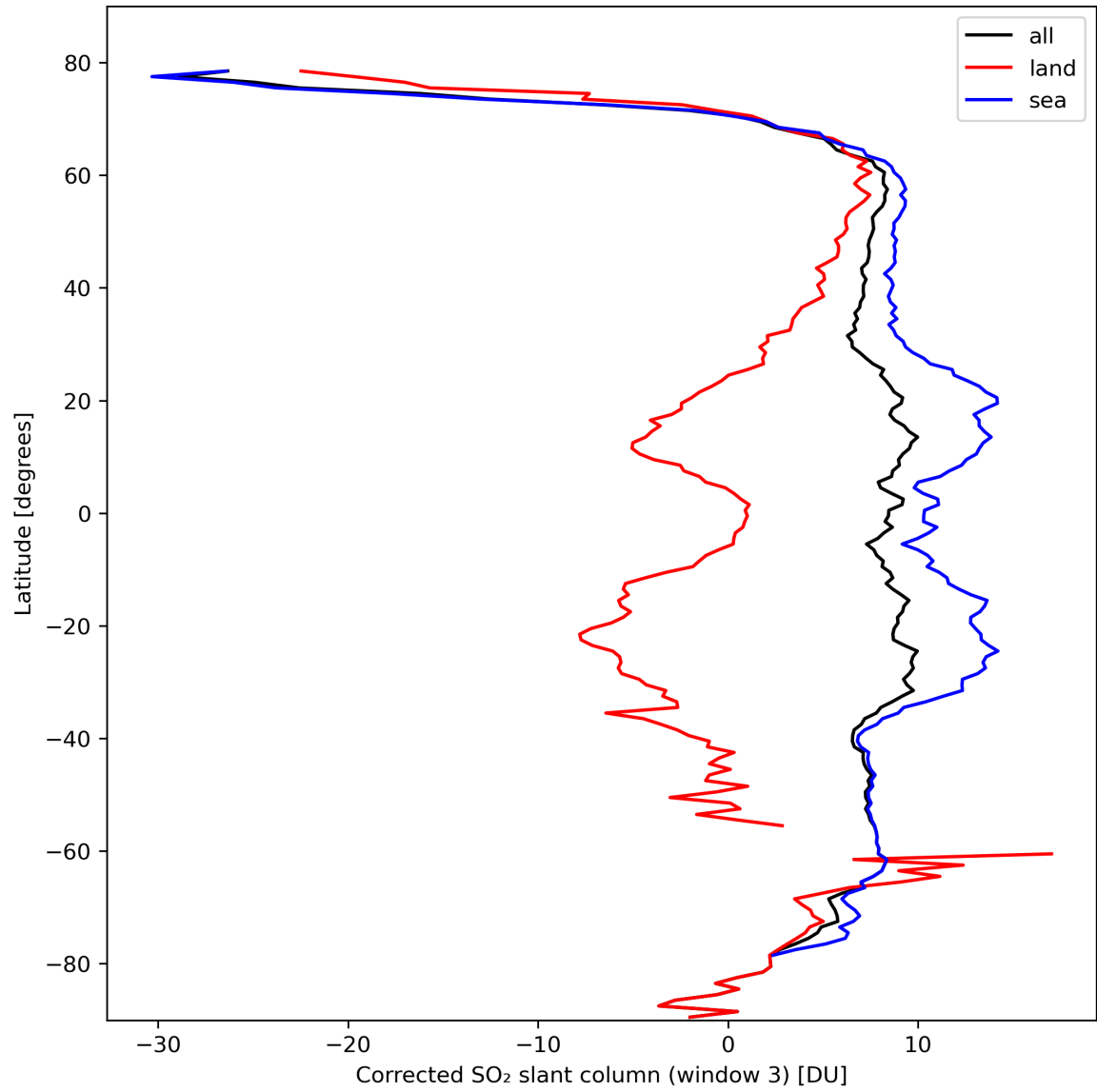
Figure 43: Zonal average of “Corrected SO 2 slant column (window 3)” for 2024-03-01 to 2024-03-03.
