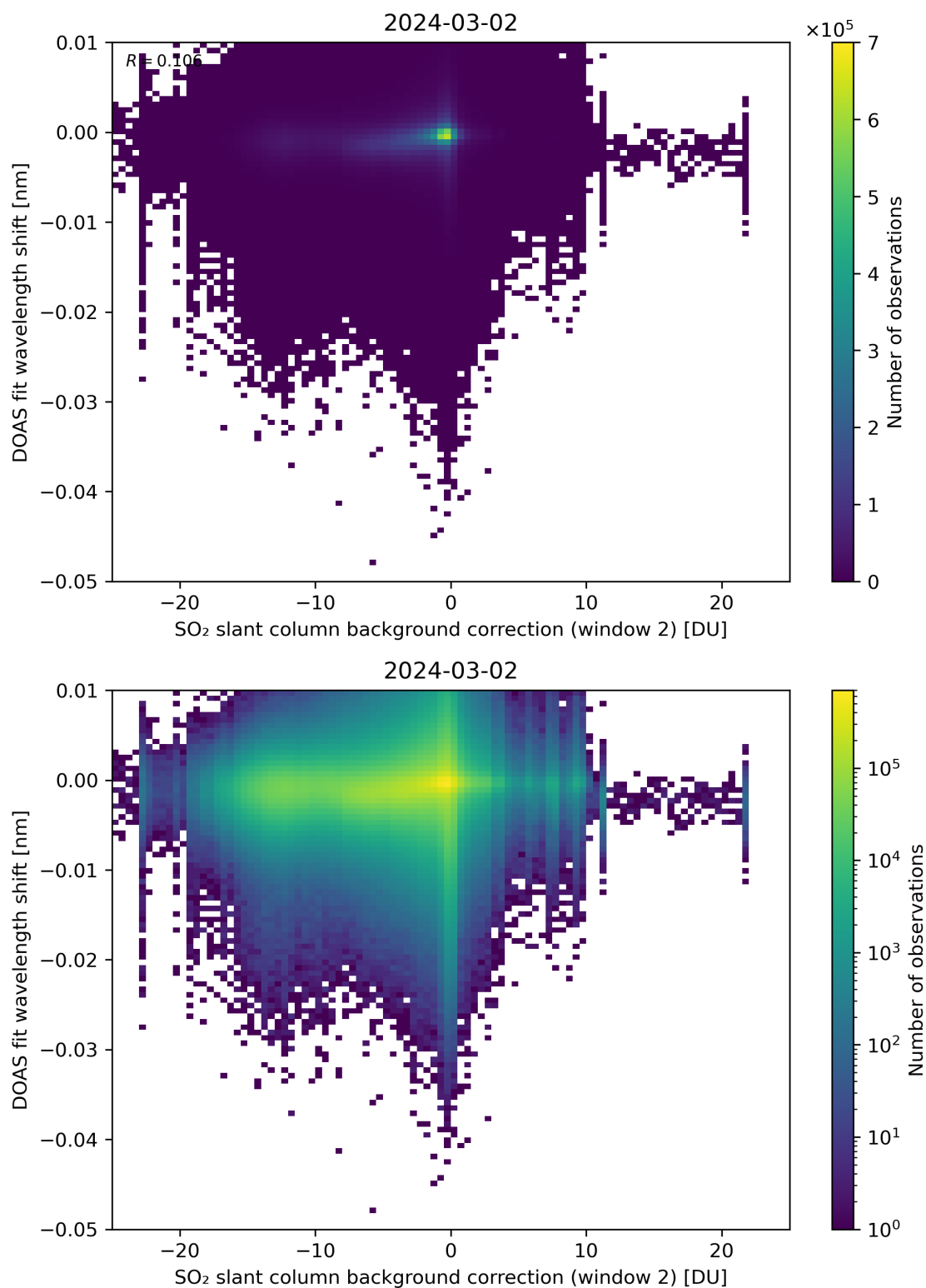
Figure 112: Scatter density plot of “SO 2 slant column background correction (window 2)” against “DOAS fit wavelength shift” for 2024-03-01 to 2024-03-03.
