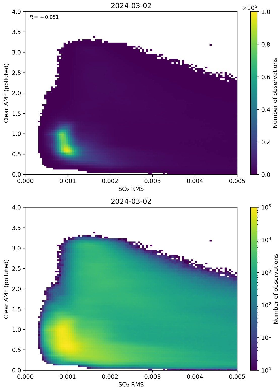
Figure 136: Scatter density plot of “SO 2 RMS” against “Clear AMF (polluted)” for 2024-03-01 to 2024-03-03.
