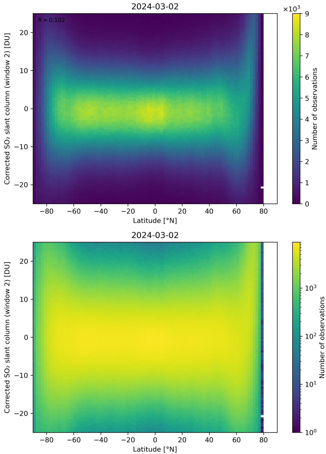
Figure 147: Scatter density plot of “Latitude” against “Corrected SO 2 slant column (window 2)” for 2024-03-01 to 2024-03-03.
