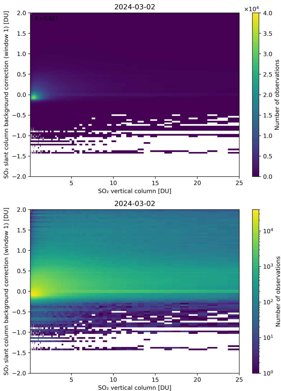
Figure 273: Scatter density plot of “SO 2 vertical column” against “SO 2 slant column background correction (window 1)” for 2024-03-01 to 2024-03-03.
