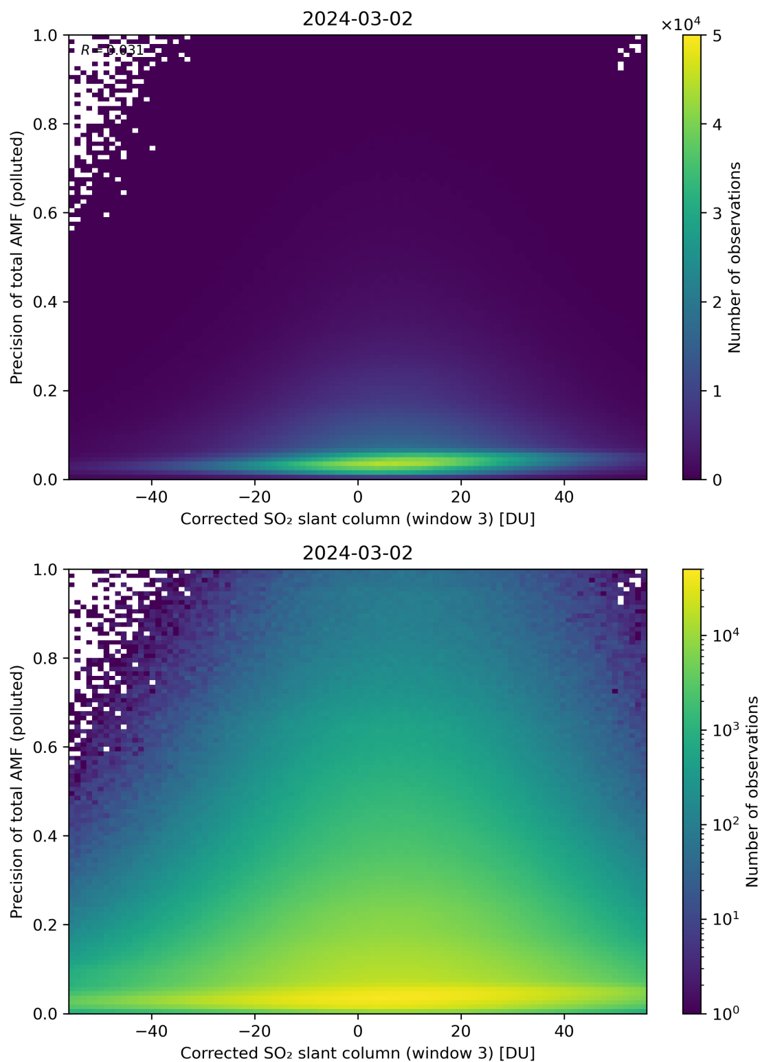
Figure 211: Scatter density plot of “Corrected SO 2 slant column (window 3)” against “Precision of total AMF (polluted)” for 2024-03-01 to 2024-03-03.
