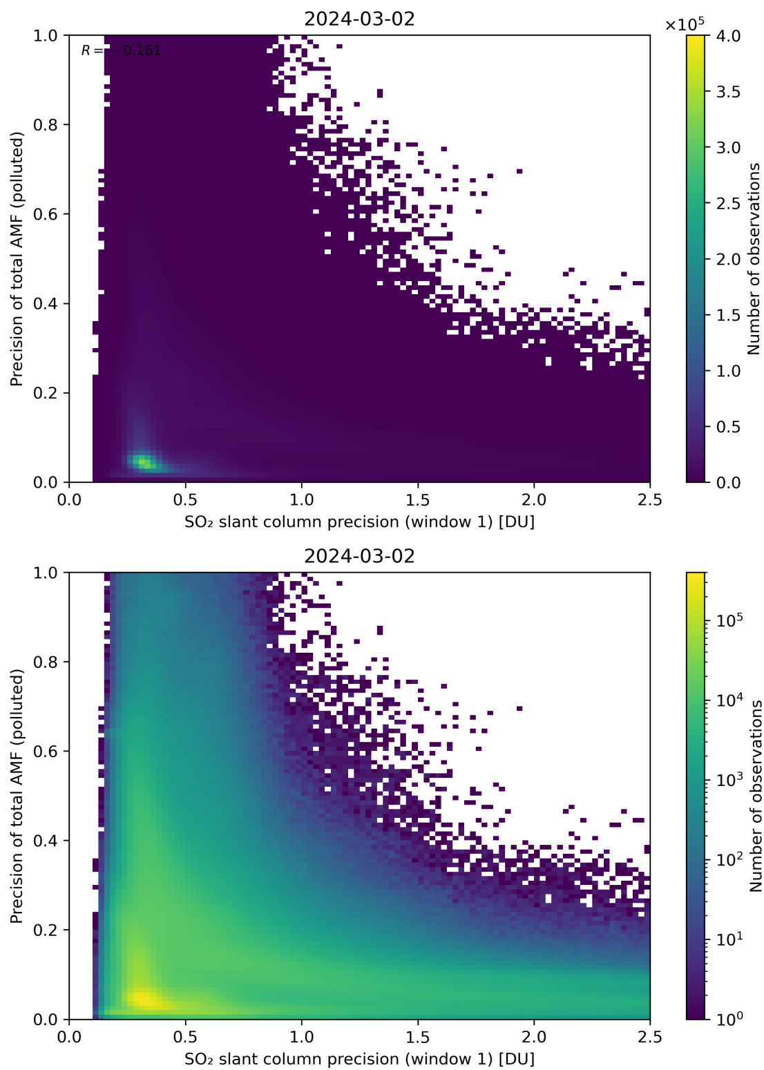
Figure 231: Scatter density plot of “SO 2 slant column precision (window 1)” against “Precision of total AMF (polluted)” for 2024-03-01 to 2024-03-03.
