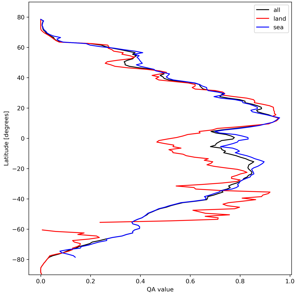
Figure 29: Zonal average of “QA value” for 2024-03-01 to 2024-03-03.
