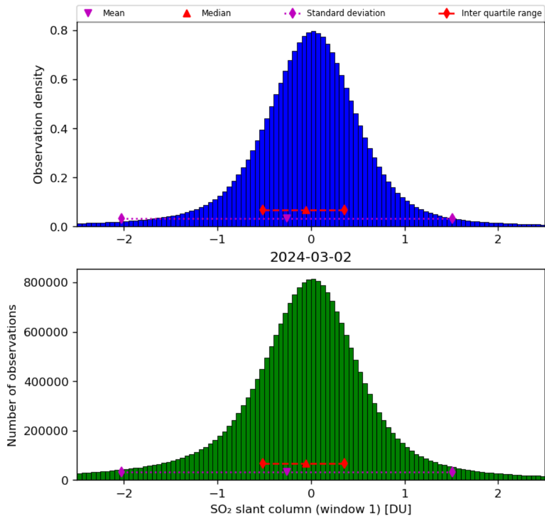
Figure 56: Histogram of “SO 2 slant column (window 1)” for 2024-03-01 to 2024-03-03
