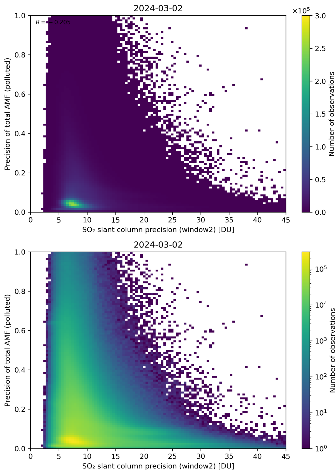
Figure 252: Scatter density plot of “SO 2 slant column precision (window2)” against “Precision of total AMF (polluted)” for 2024-03-01 to 2024-03-03.
