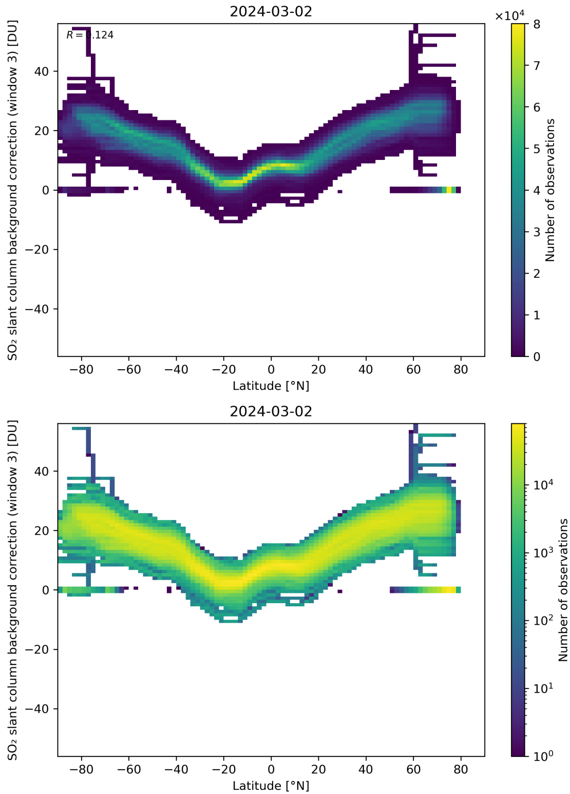
Figure 141: Scatter density plot of “Latitude” against “SO 2 slant column background correction (window 3)” for 2024-03-01 to 2024-03-03.
