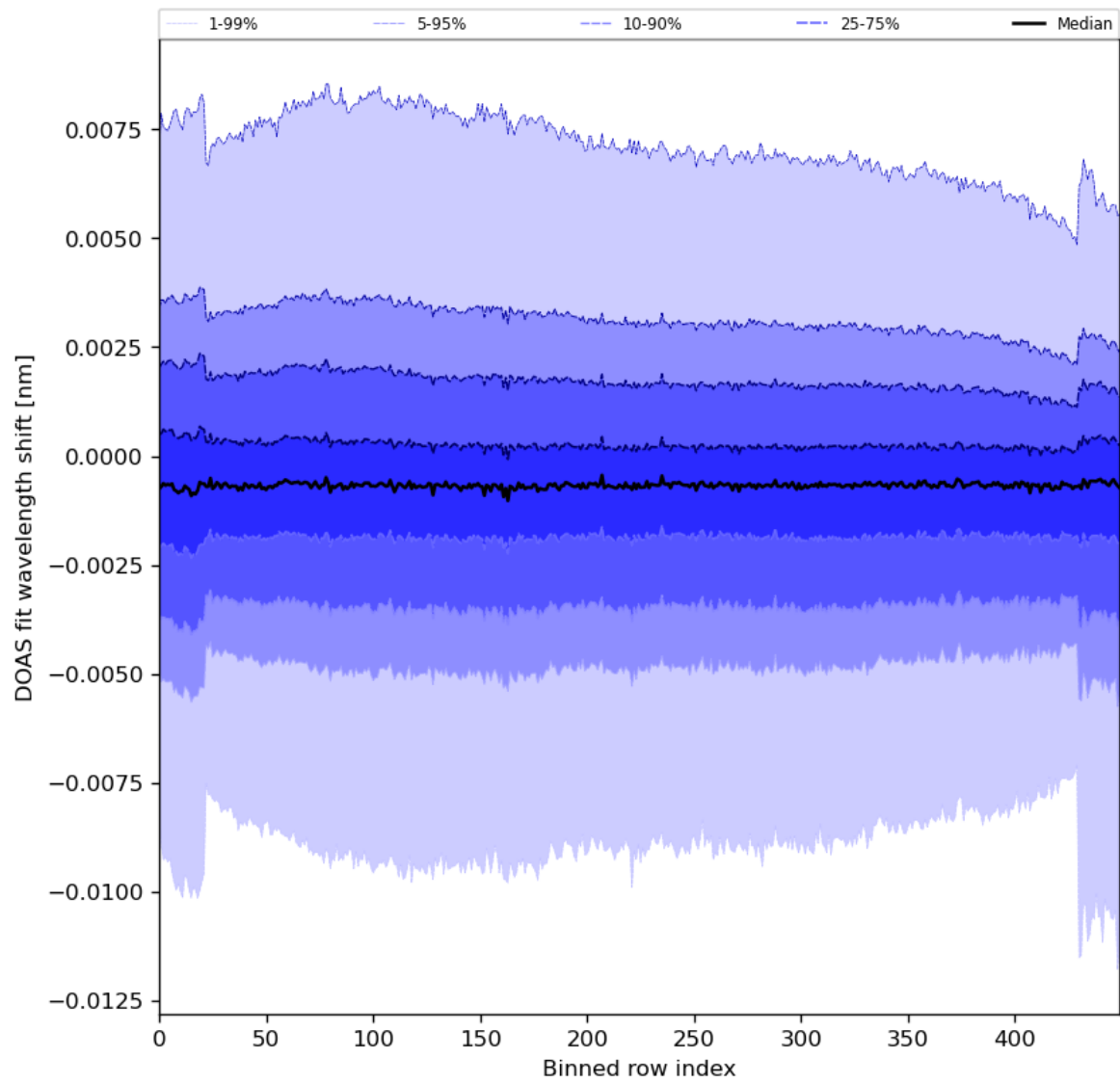
Figure 91: Along track statistics of "DOAS fit wavelength shift" for 2024-03-01 to 2024-03-03
