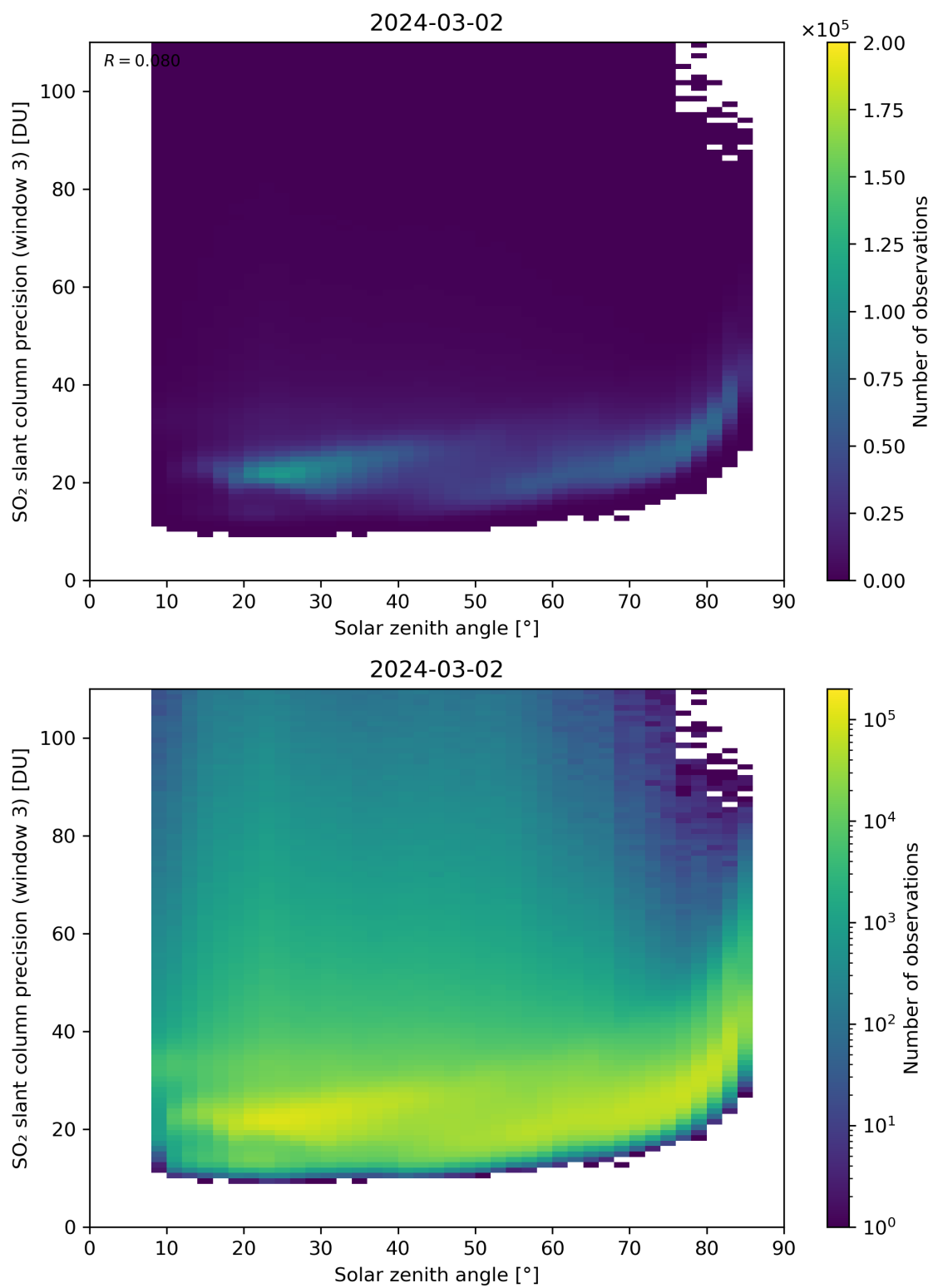
Figure 173: Scatter density plot of “Solar zenith angle” against “SO 2 slant column precision (window 3)” for 2024-03-01 to 2024-03-03.
