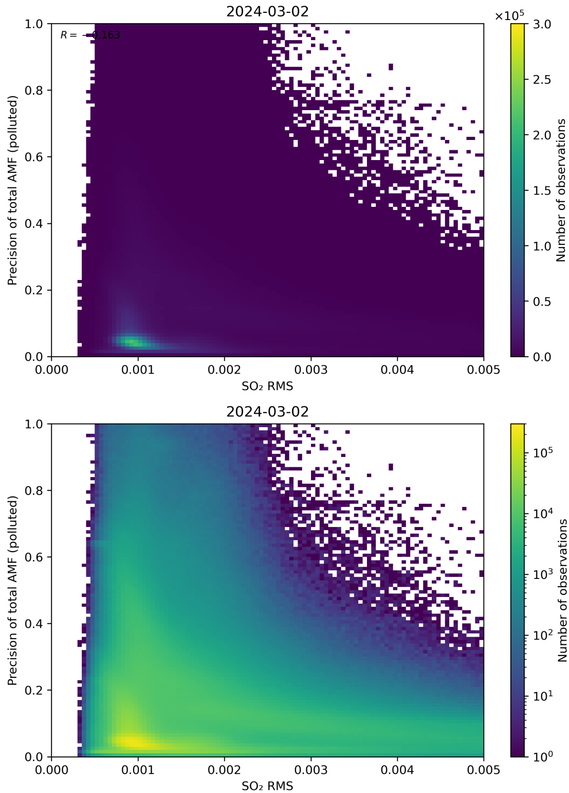
Figure 138: Scatter density plot of “SO 2 RMS” against “Precision of total AMF (polluted)” for 2024-03-01 to 2024-03-03.
