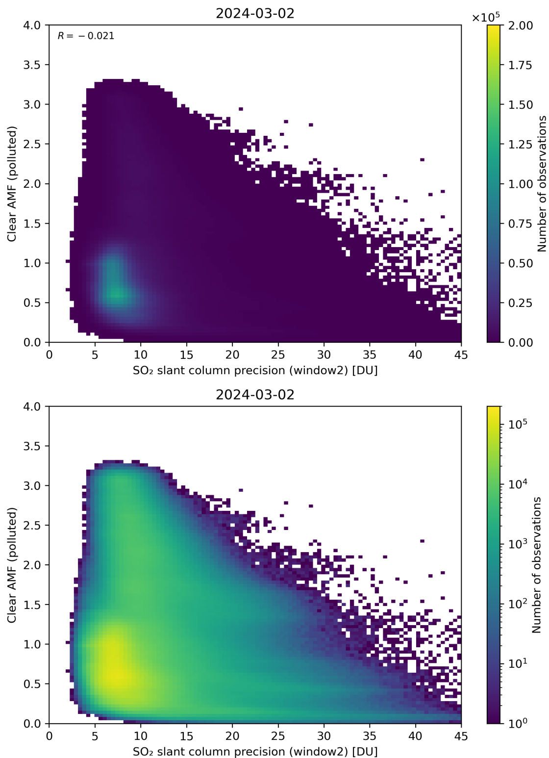
Figure 246: Scatter density plot of “SO 2 slant column precision (window2)” against “Clear AMF (polluted)” for 2024-03-01 to 2024-03-03.
