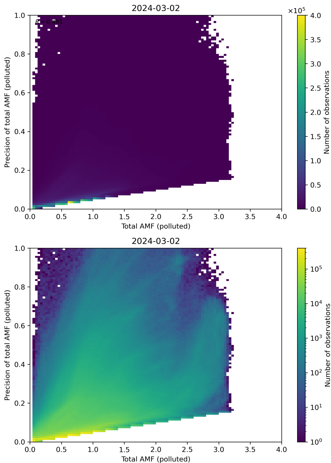
Figure 272: Scatter density plot of “Total AMF (polluted)” against “Precision of total AMF (polluted)” for 2024-03-01 to 2024-03-03.
