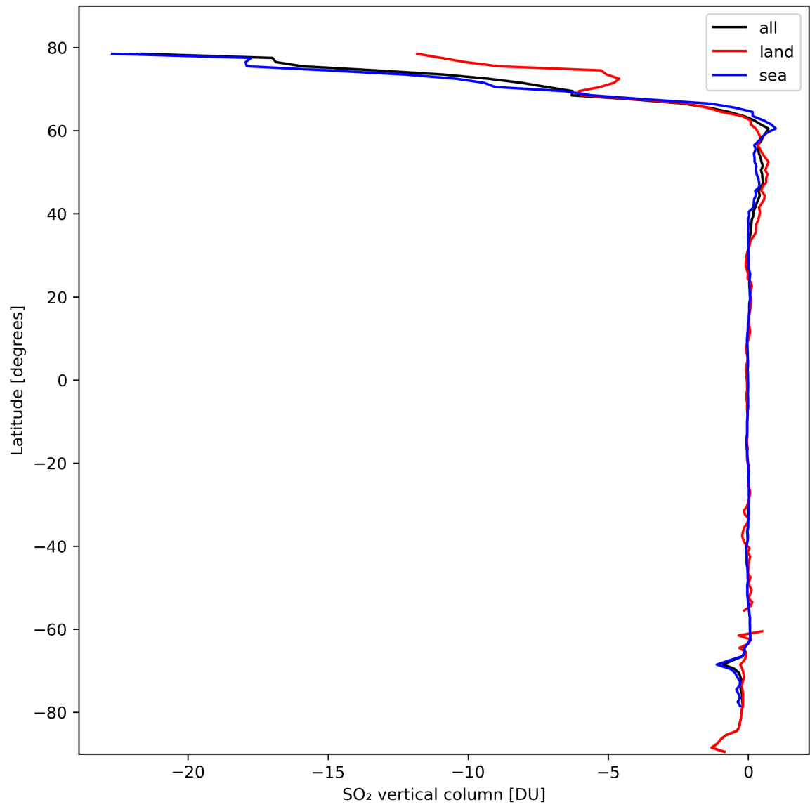
Figure 30: Zonal average of “SO 2 vertical column” for 2024-03-01 to 2024-03-03.
