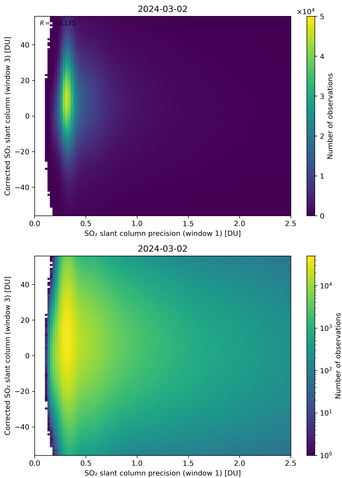
Figure 226: Scatter density plot of “SO 2 slant column precision (window 1)” against “Corrected SO 2 slant column (window 3)” for 2024-03-01 to 2024-03-03.
