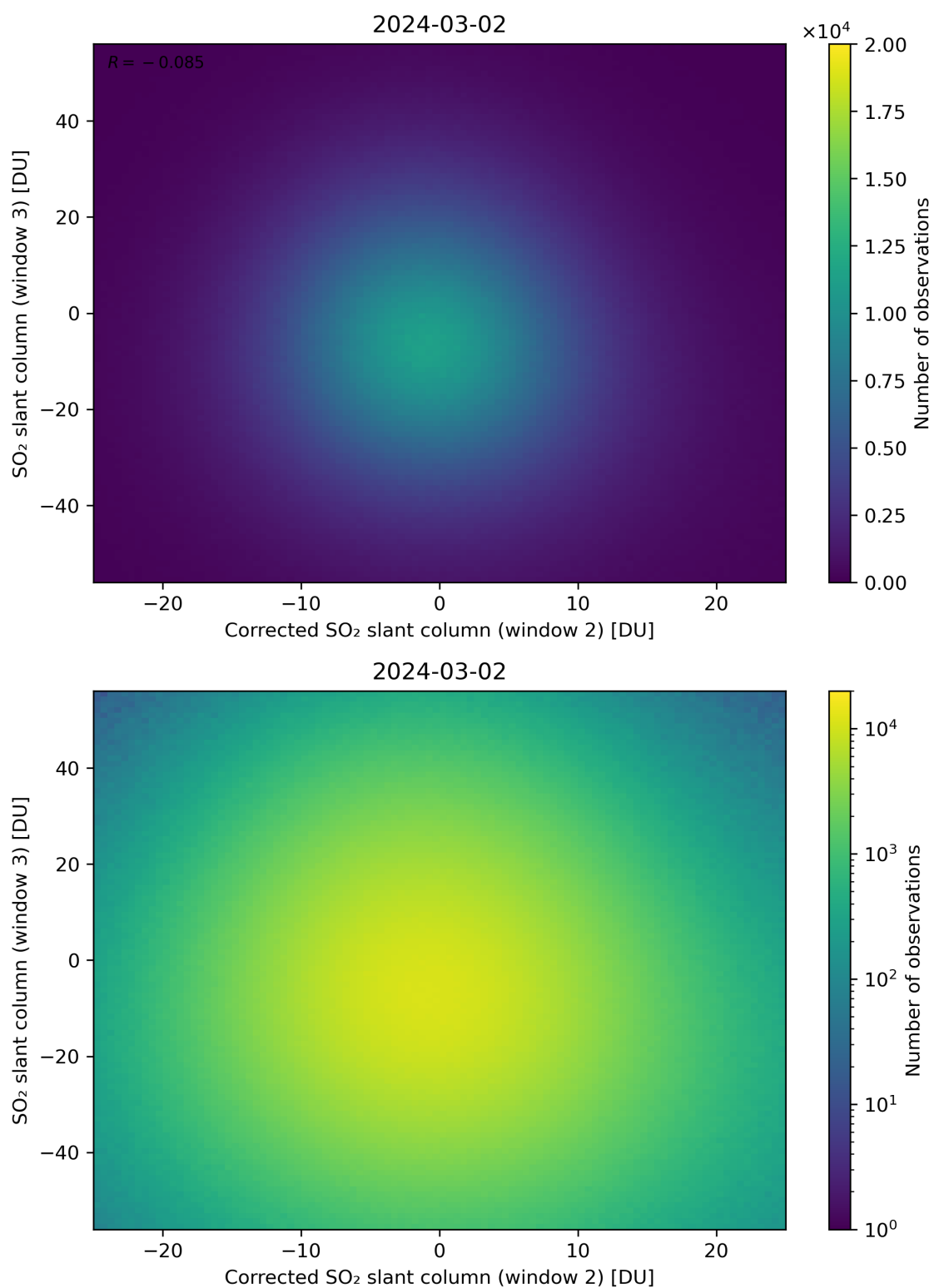
Figure 201: Scatter density plot of “Corrected SO 2 slant column (window 2)” against “SO 2 slant column (window 3)” for 2024-03-01 to 2024-03-03.
