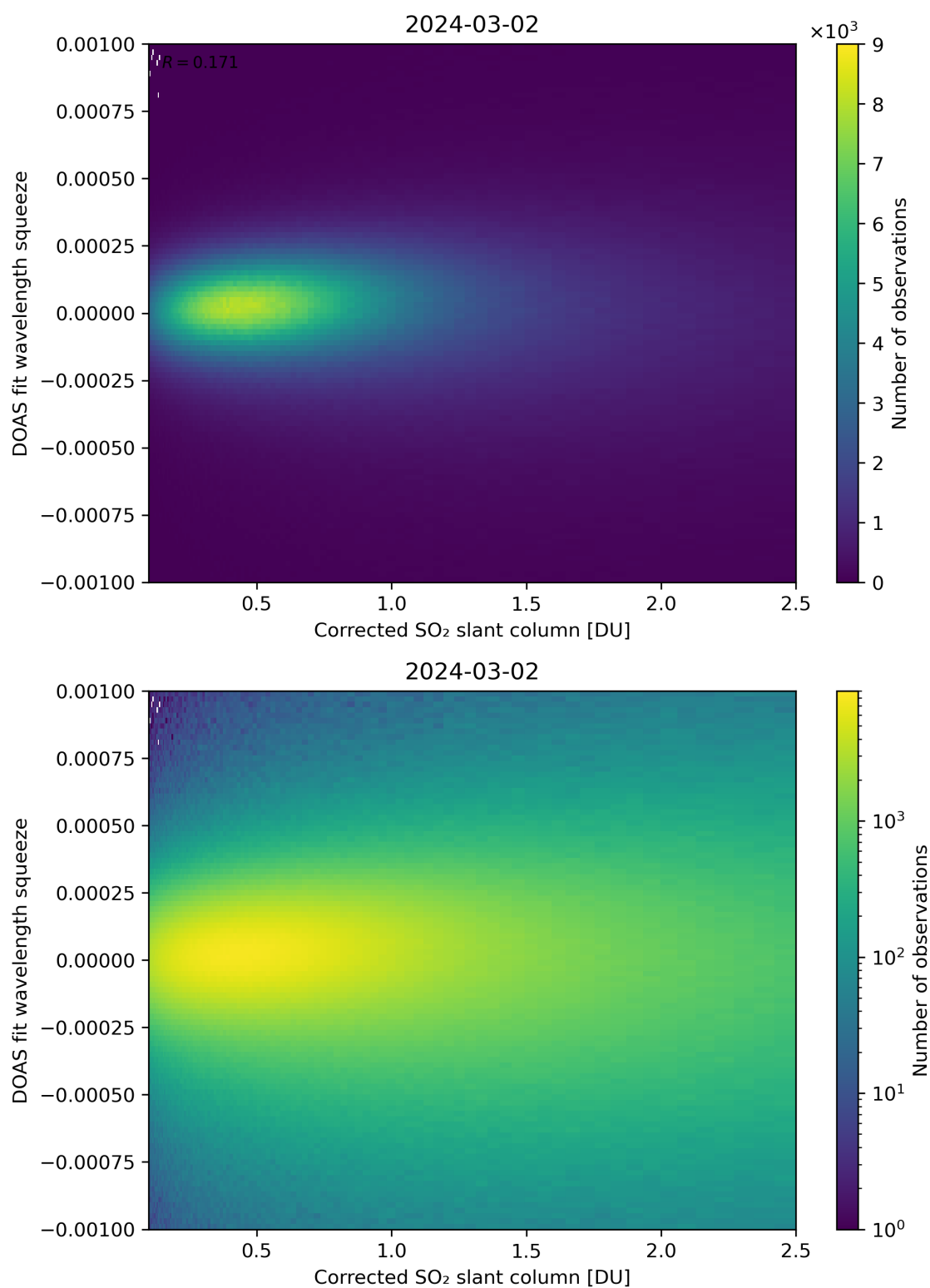
Figure 182: Scatter density plot of “Corrected SO 2 slant column” against “DOAS fit wavelength squeeze” for 2024-03-01 to 2024-03-03.
