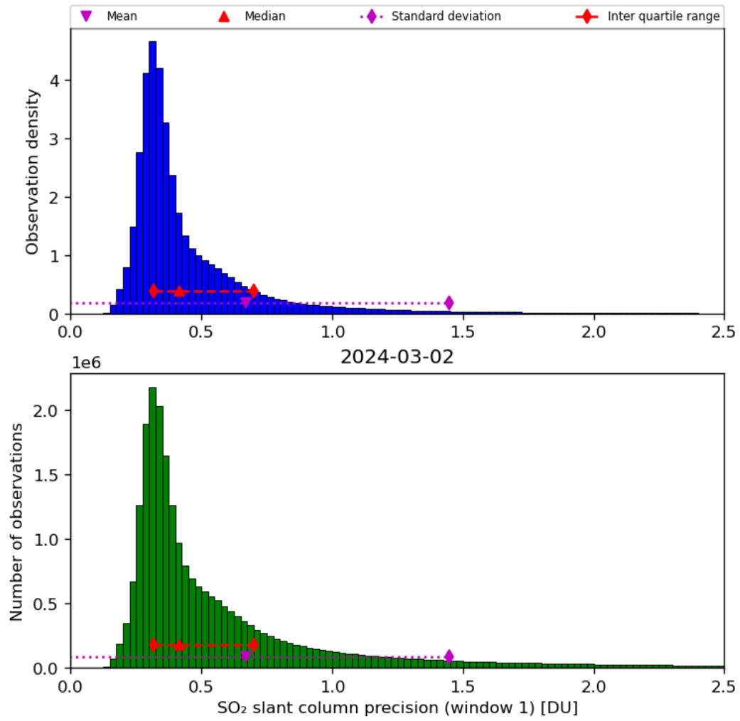
Figure 57: Histogram of “SO 2 slant column precision (window 1)” for 2024-03-01 to 2024-03-03
