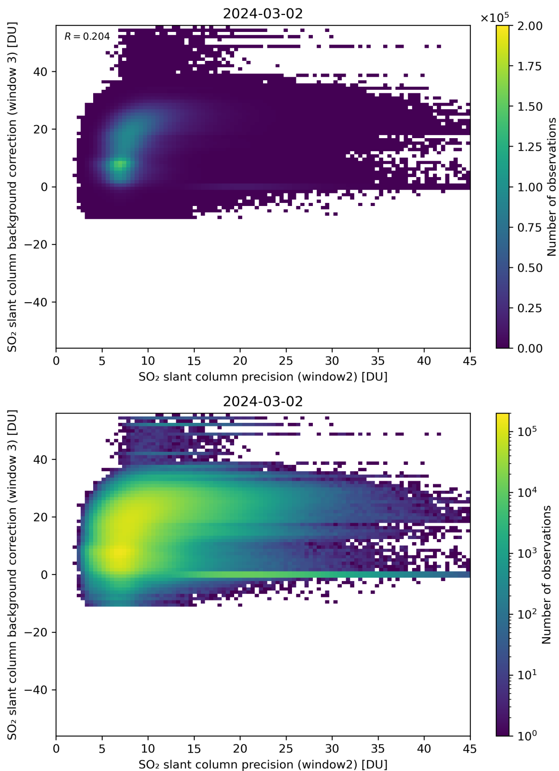
Figure 242: Scatter density plot of “SO 2 slant column precision (window2)” against “SO 2 slant column background correction (window 3)” for 2024-03-01 to 2024-03-03.
