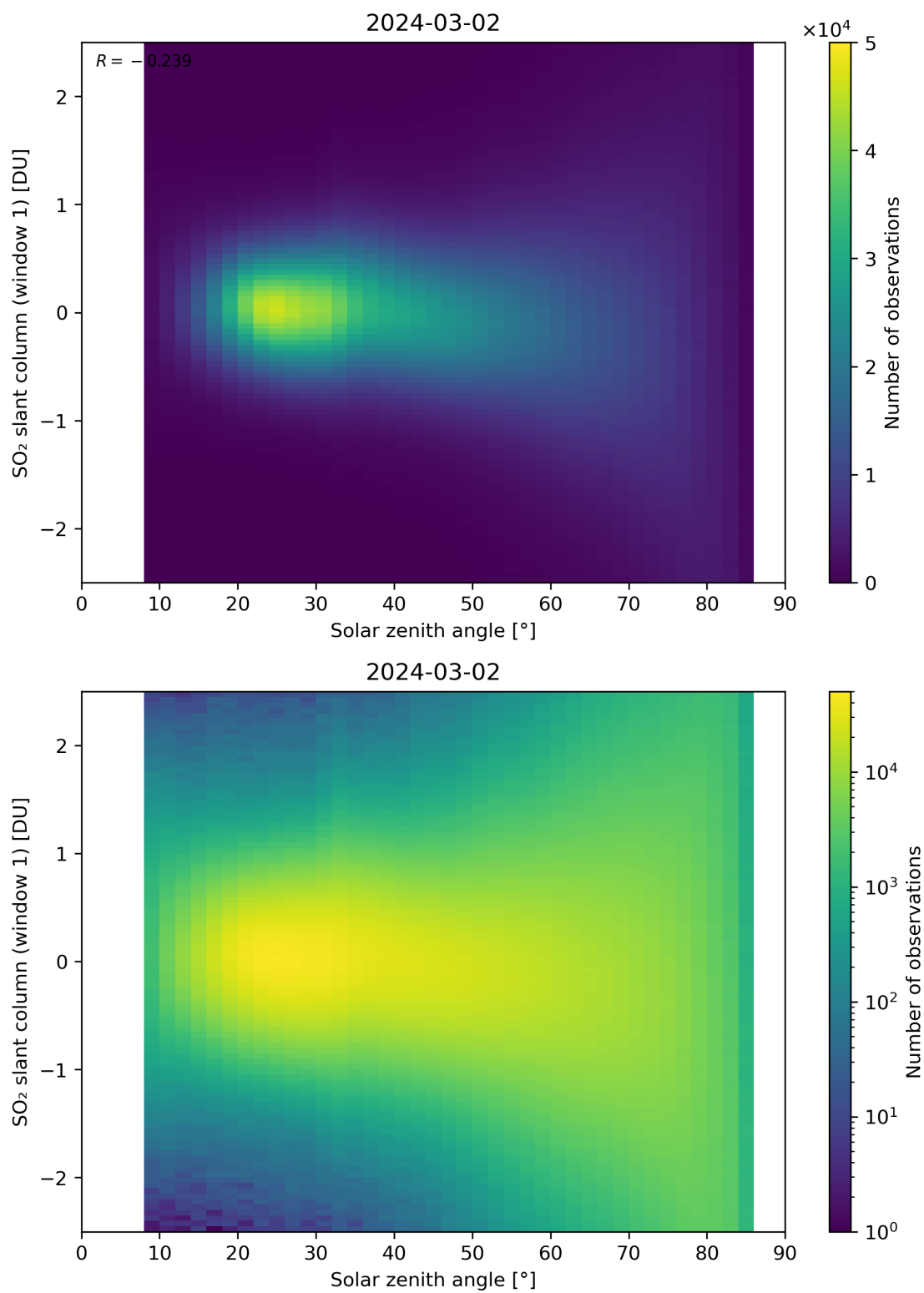
Figure 169: Scatter density plot of “Solar zenith angle” against “SO 2 slant column (window 1)” for 2024-03-01 to 2024-03-03.
