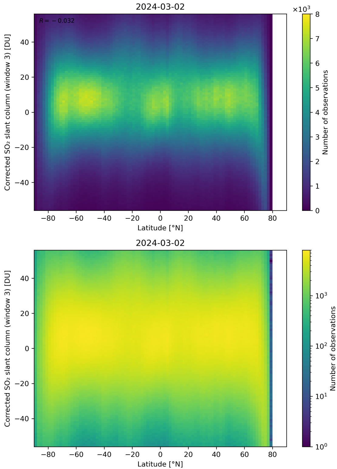
Figure 148: Scatter density plot of “Latitude” against “Corrected SO 2 slant column (window 3)” for 2024-03-01 to 2024-03-03.
