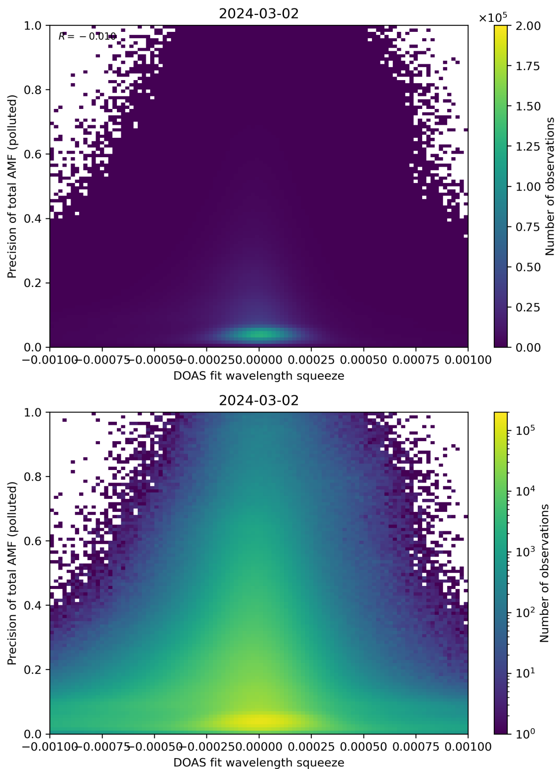
Figure 135: Scatter density plot of “DOAS fit wavelength squeeze” against “Precision of total AMF (polluted)” for 2024-03-01 to 2024-03-03.
