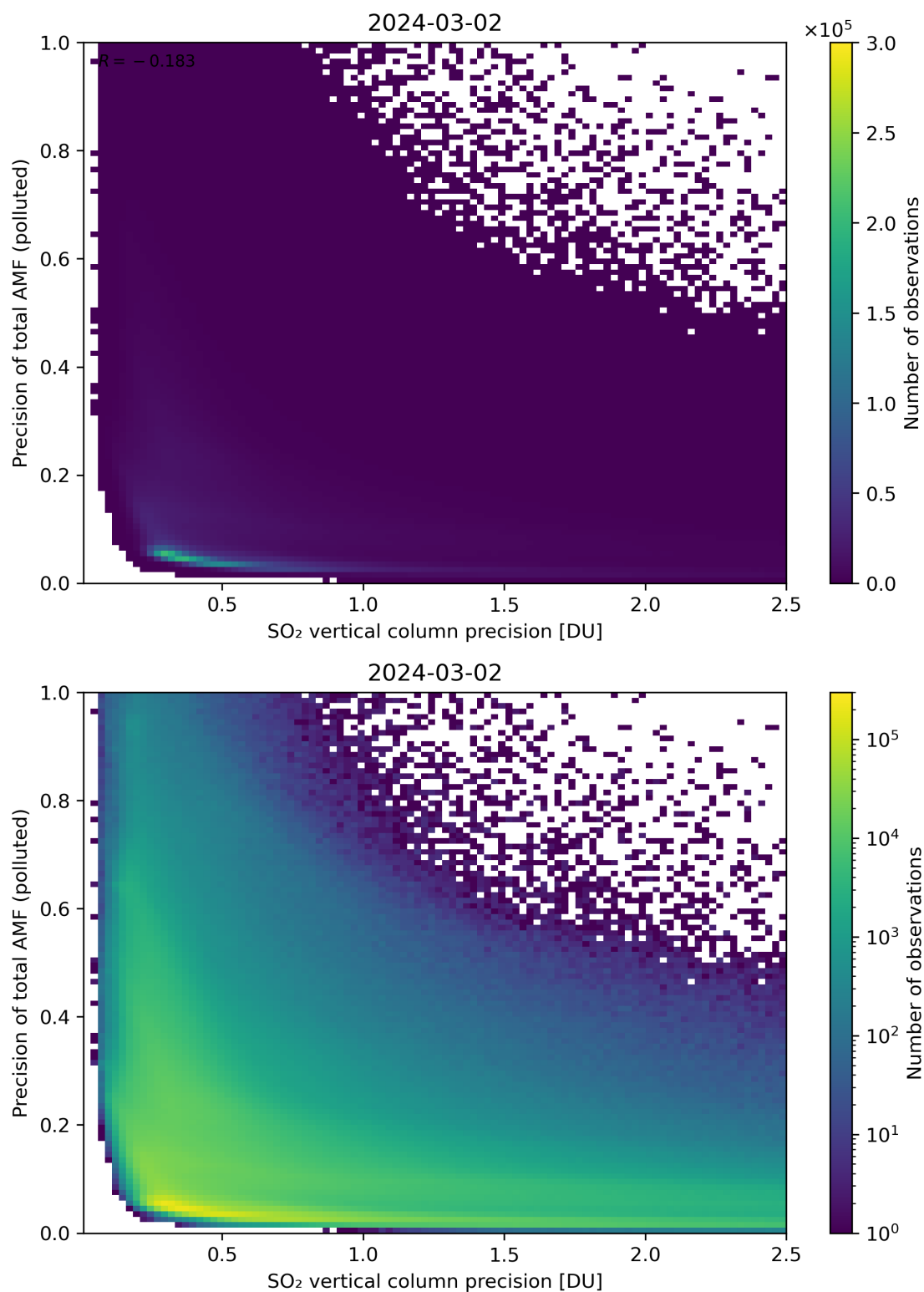
Figure 295: Scatter density plot of “SO 2 vertical column precision” against “Precision of total AMF (polluted)” for 2024-03-01 to 2024-03-03.
