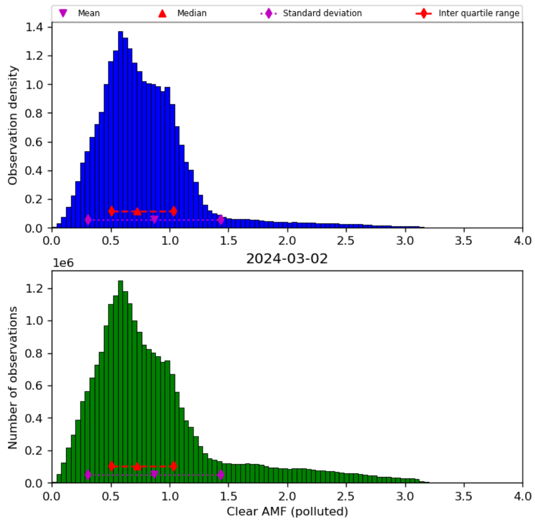
Figure 73: Histogram of “Clear AMF (polluted)” for 2024-03-01 to 2024-03-03
