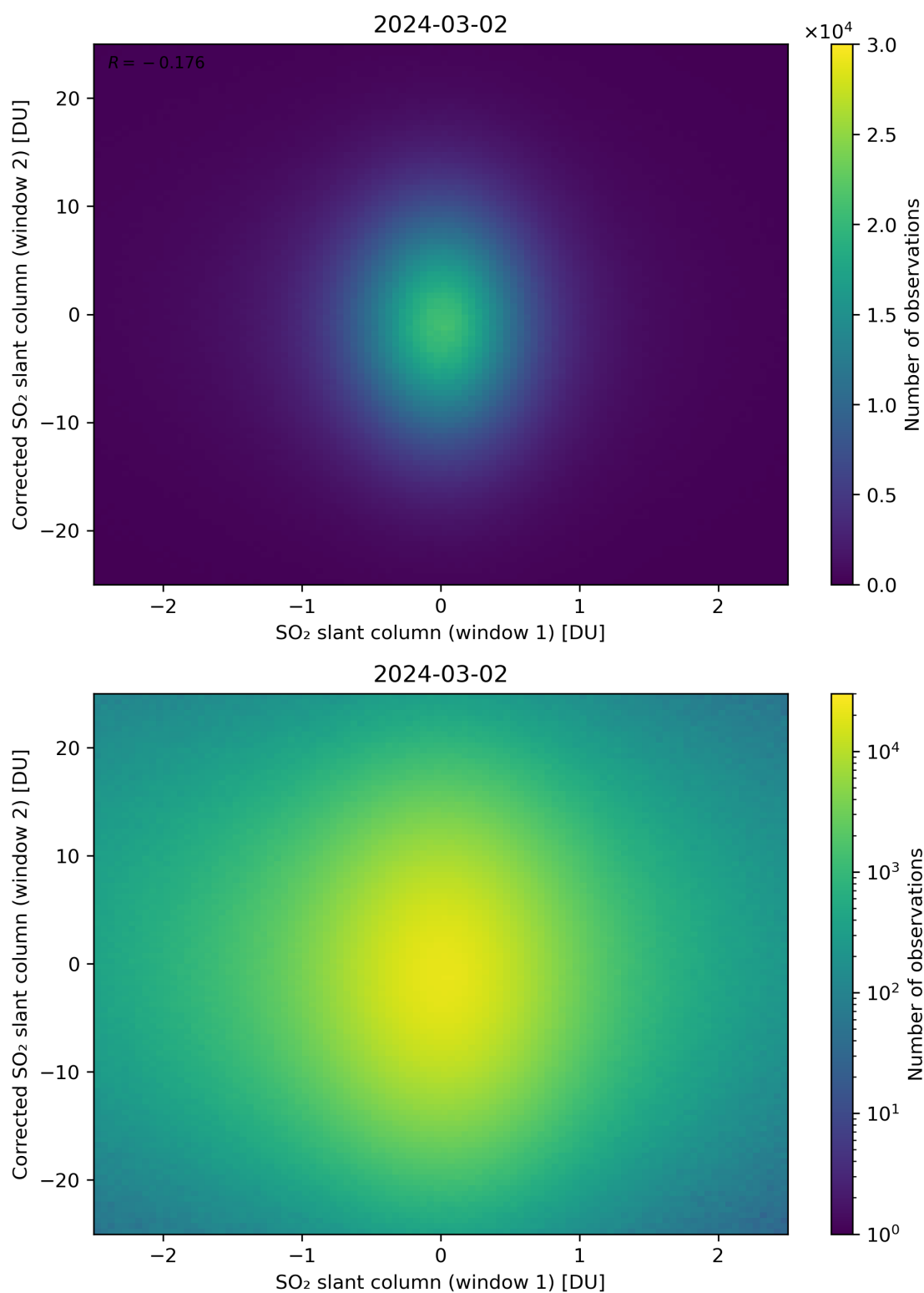
Figure 233: Scatter density plot of “SO 2 slant column (window 1)” against “Corrected SO 2 slant column (window 2)” for 2024-03-01 to 2024-03-03.
