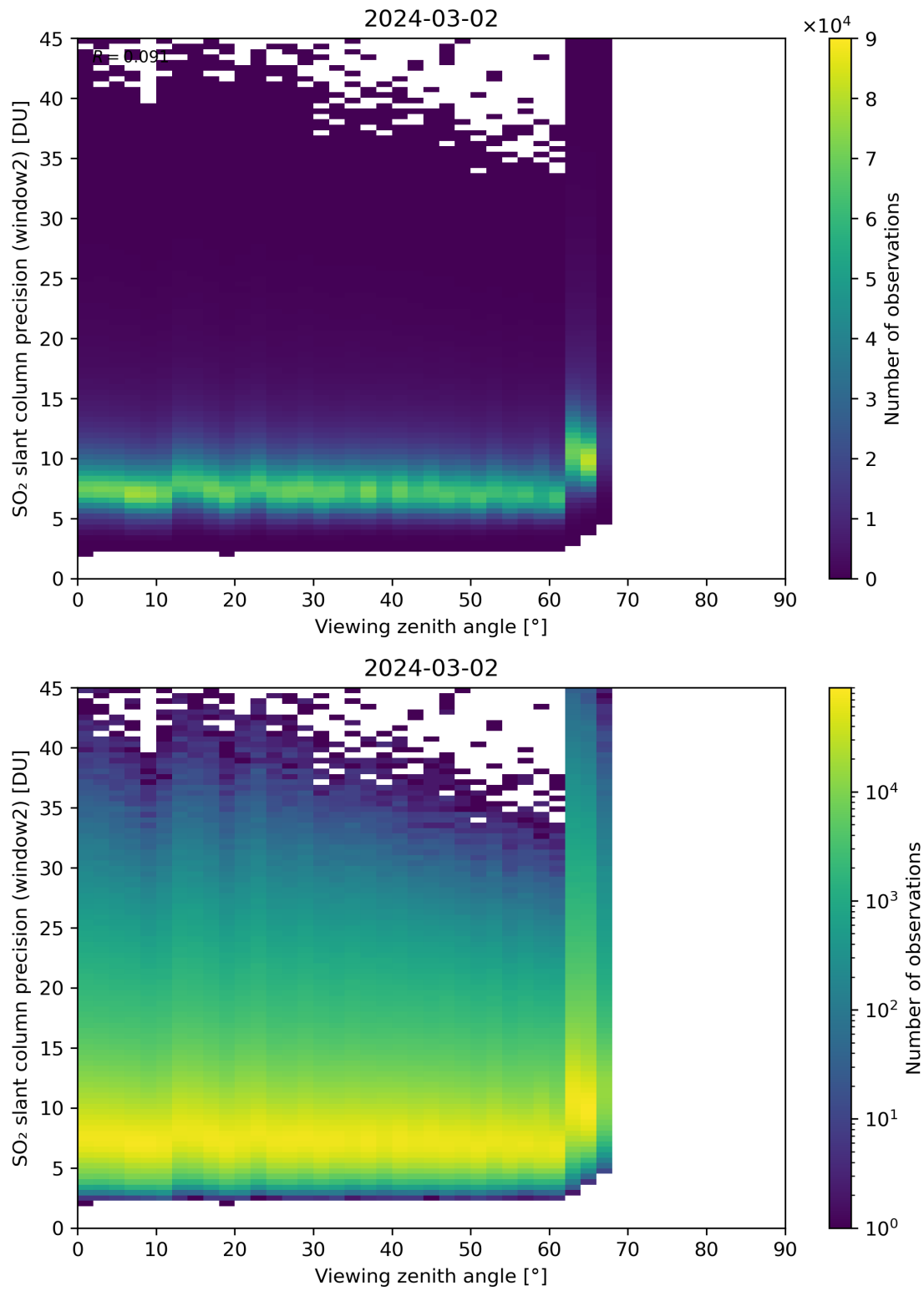
Figure 322: Scatter density plot of “Viewing zenith angle” against “SO 2 slant column precision (window2)” for 2024-03-01 to 2024-03-03.
