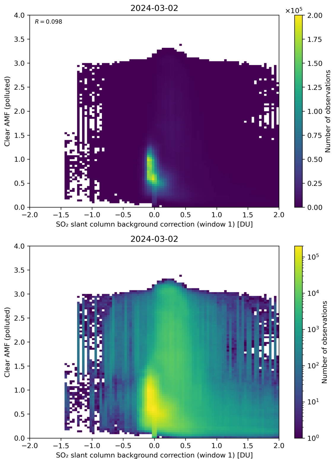
Figure 103: Scatter density plot of “SO 2 slant column background correction (window 1)” against “Clear AMF (polluted)” for 2024-03-01 to 2024-03-03.
