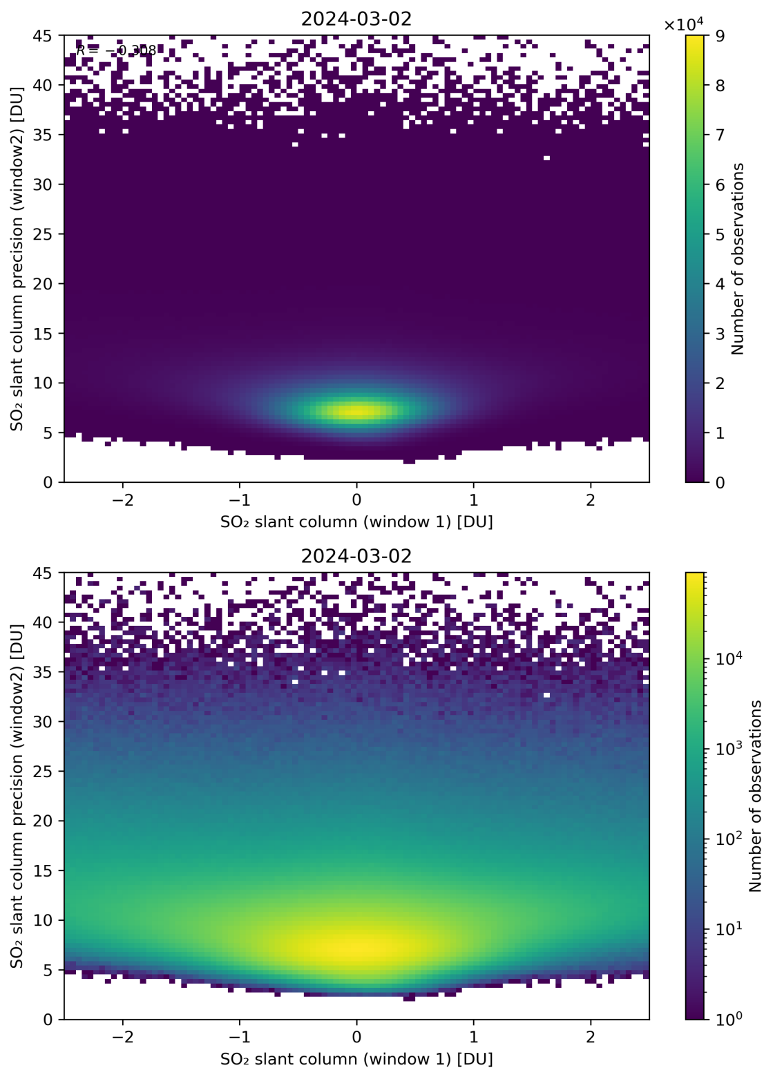
Figure 236: Scatter density plot of “SO 2 slant column (window 1)” against “SO 2 slant column precision (window2)” for 2024-03-01 to 2024-03-03.
