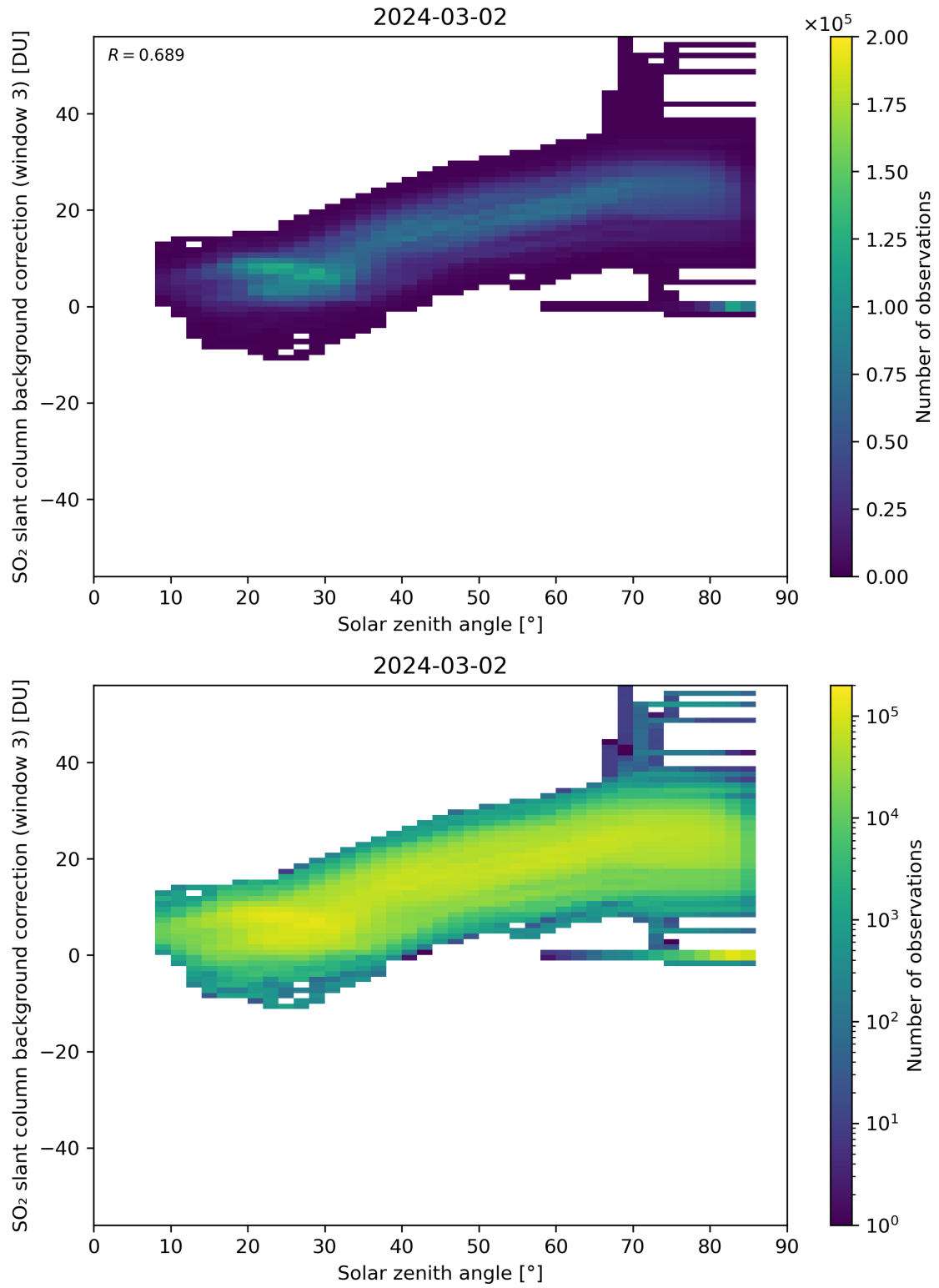
Figure 160: Scatter density plot of “Solar zenith angle” against “SO 2 slant column background correction (window 3)” for 2024-03-01 to 2024-03-03.
