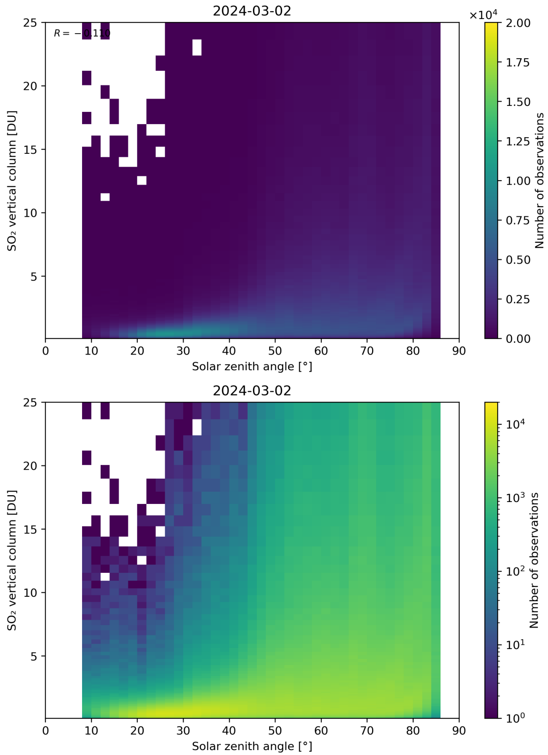
Figure 176: Scatter density plot of “Solar zenith angle” against “SO 2 vertical column” for 2024-03-01 to 2024-03-03.
