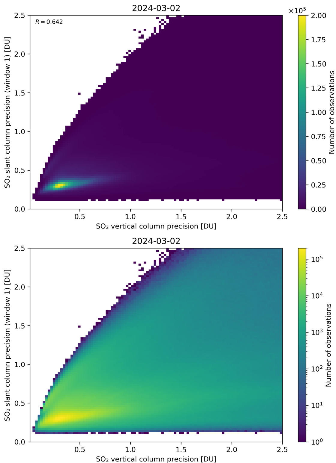
Figure 290: Scatter density plot of “SO 2 vertical column precision” against “SO 2 slant column precision (window 1)” for 2024-03-01 to 2024-03-03.
