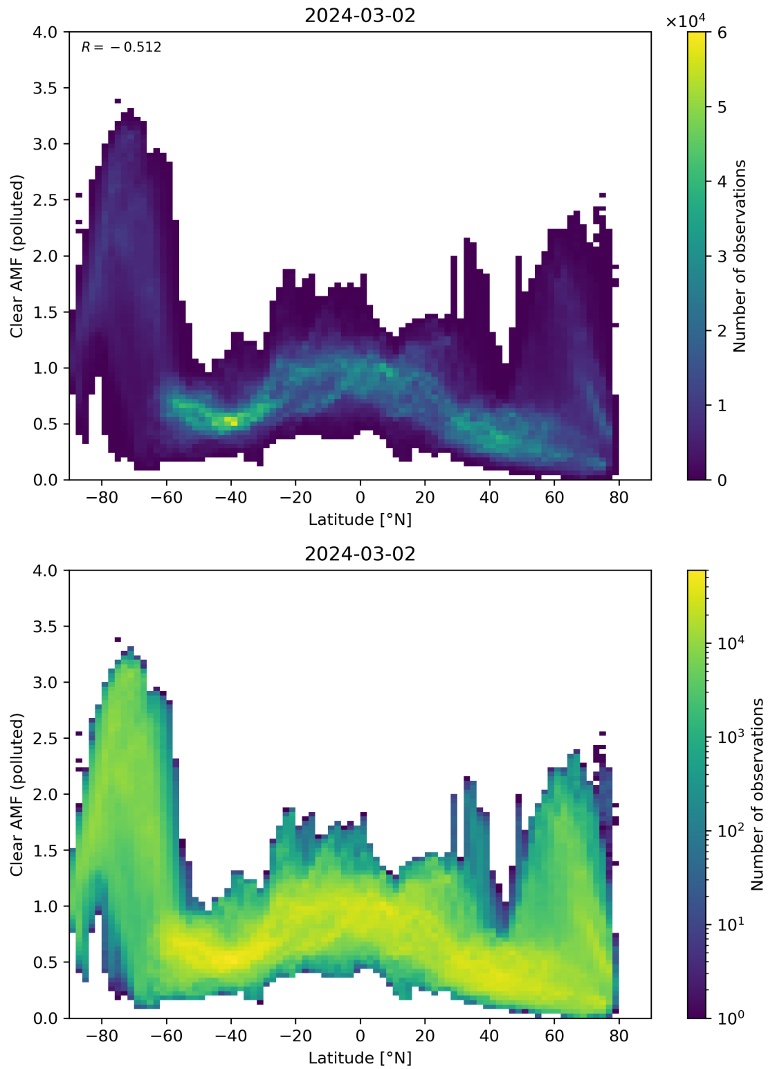
Figure 145: Scatter density plot of “Latitude” against “Clear AMF (polluted)” for 2024-03-01 to 2024-03-03.
