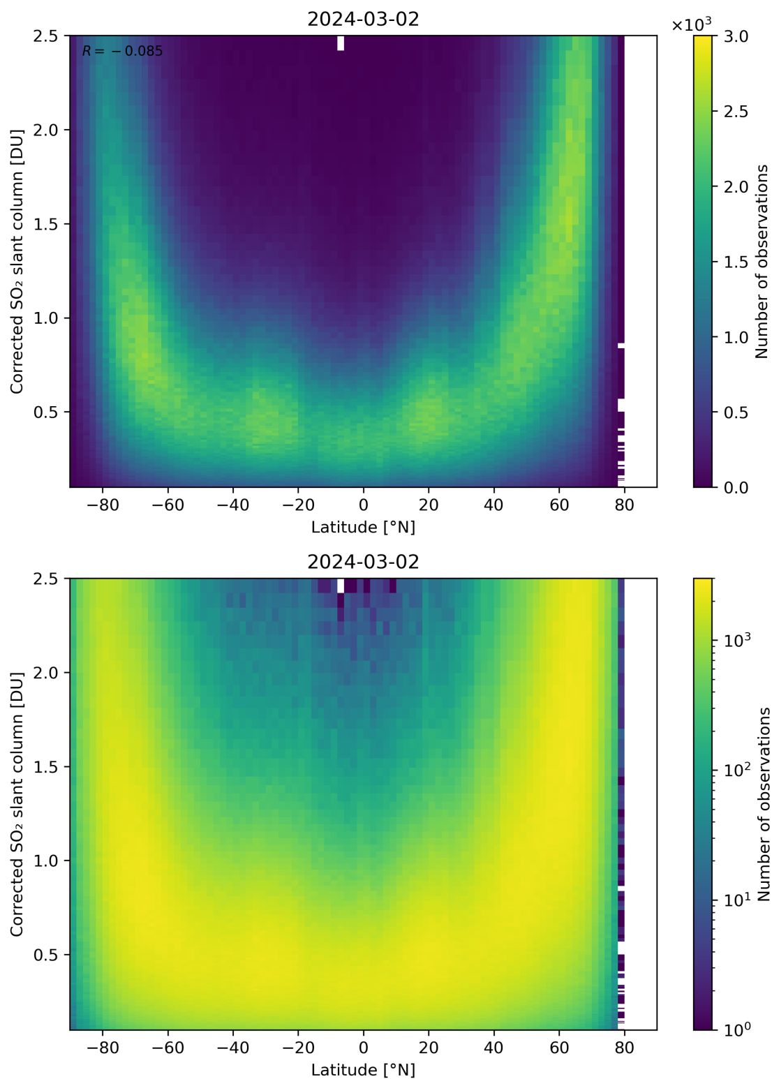
Figure 146: Scatter density plot of “Latitude” against “Corrected SO 2 slant column” for 2024-03-01 to 2024-03-03.
