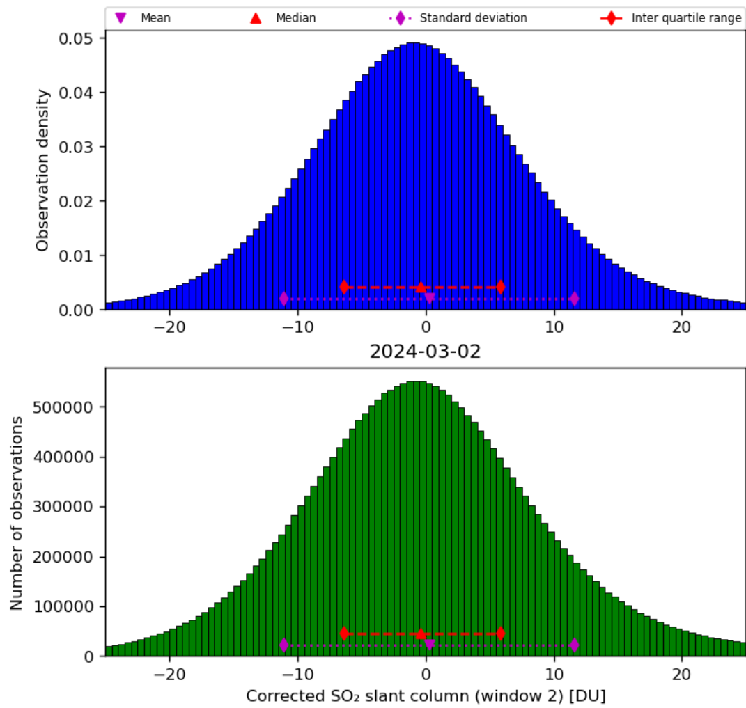
Figure 62: Histogram of “Corrected SO 2 slant column (window 2)” for 2024-03-01 to 2024-03-03
