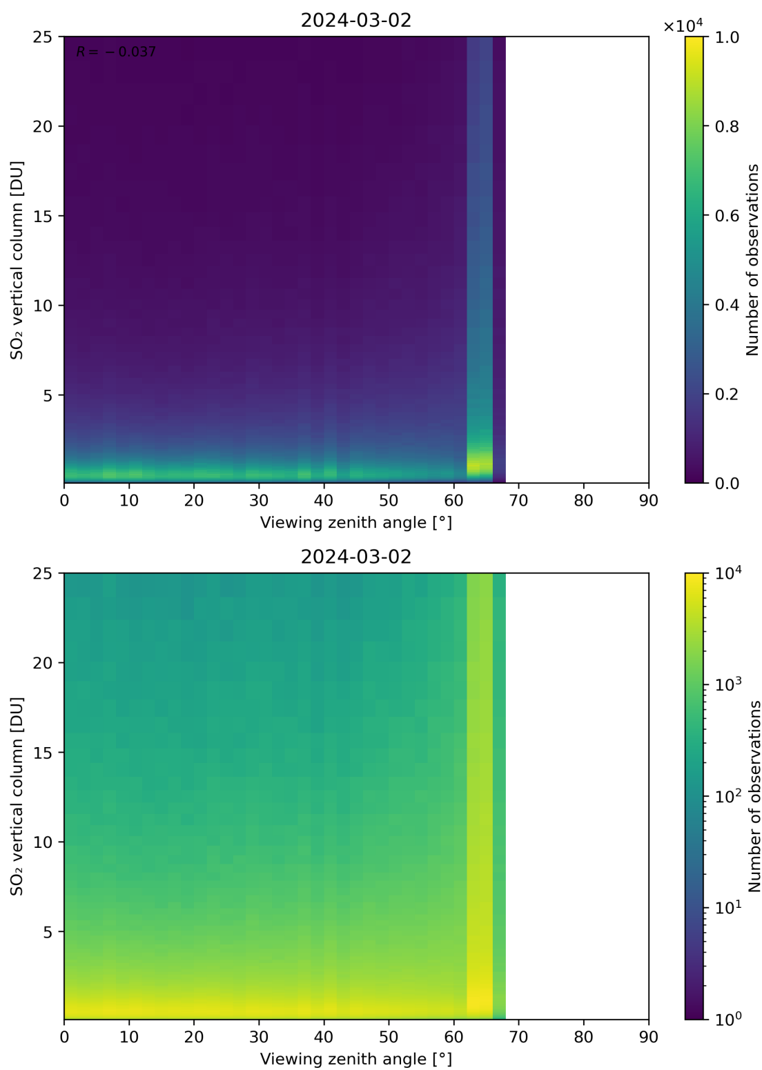
Figure 327: Scatter density plot of “Viewing zenith angle” against “SO 2 vertical column” for 2024-03-01 to 2024-03-03.
