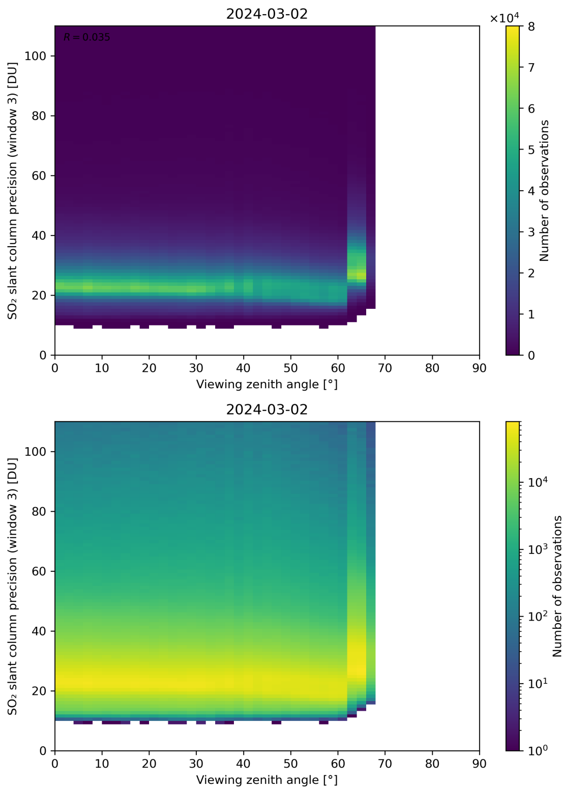
Figure 324: Scatter density plot of “Viewing zenith angle” against “SO 2 slant column precision (window 3)” for 2024-03-01 to 2024-03-03.
