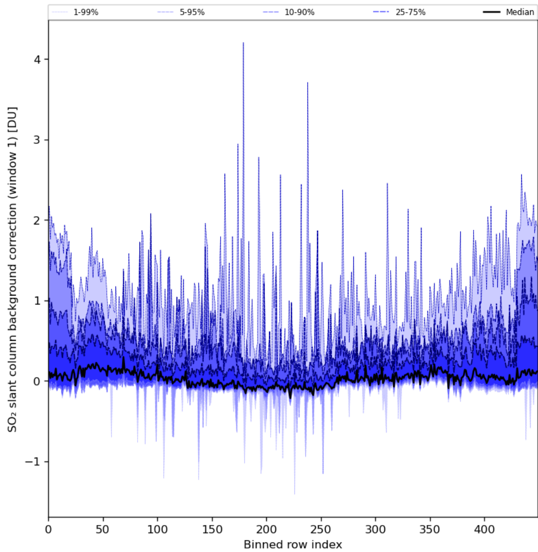
Figure 82: Along track statistics of “SO 2 slant column background correction (window 1)” for 2024-03-01 to 2024-03-03
