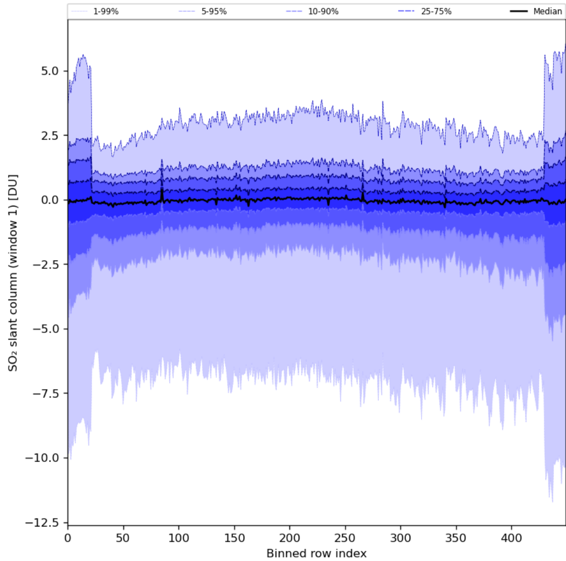
Figure 79: Along track statistics of “SO 2 slant column (window 1)” for 2024-03-01 to 2024-03-03
