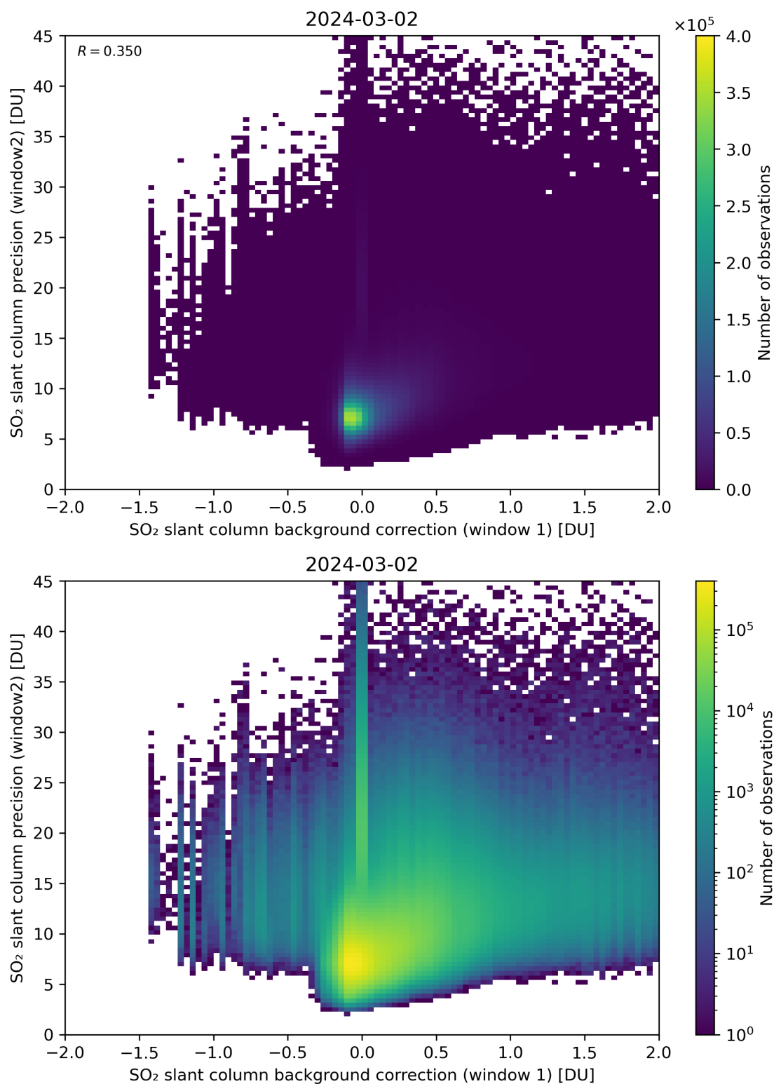
Figure 106: Scatter density plot of “SO 2 slant column background correction (window 1)” against “SO 2 slant column precision (window2)” for 2024-03-01 to 2024-03-03.
