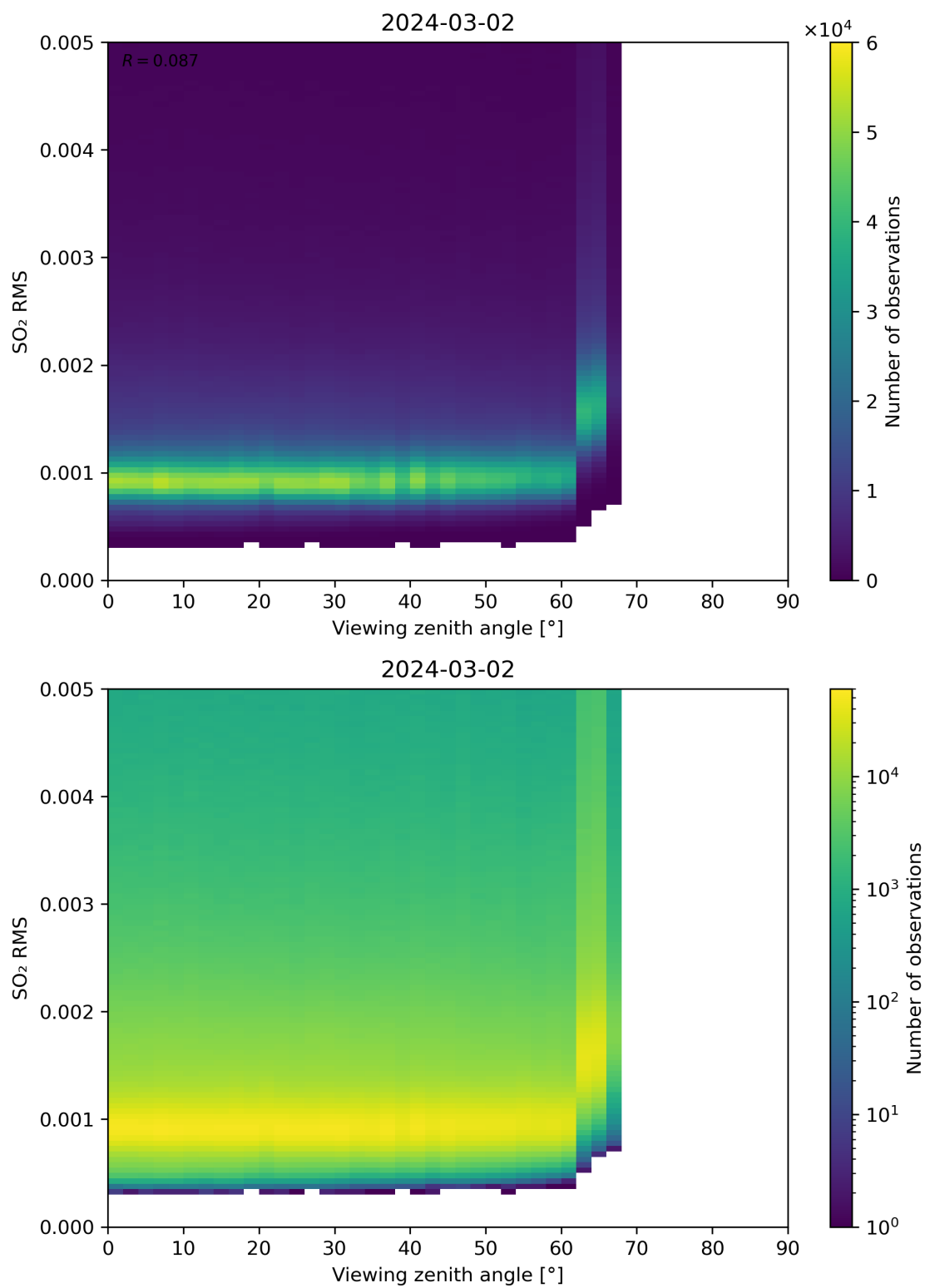
Figure 313: Scatter density plot of “Viewing zenith angle” against “SO 2 RMS” for 2024-03-01 to 2024-03-03.
