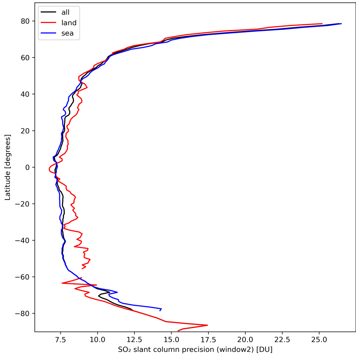
Figure 38: Zonal average of "SO 2 slant column precision (window2)" for 2024-03-01 to 2024-03-03.
