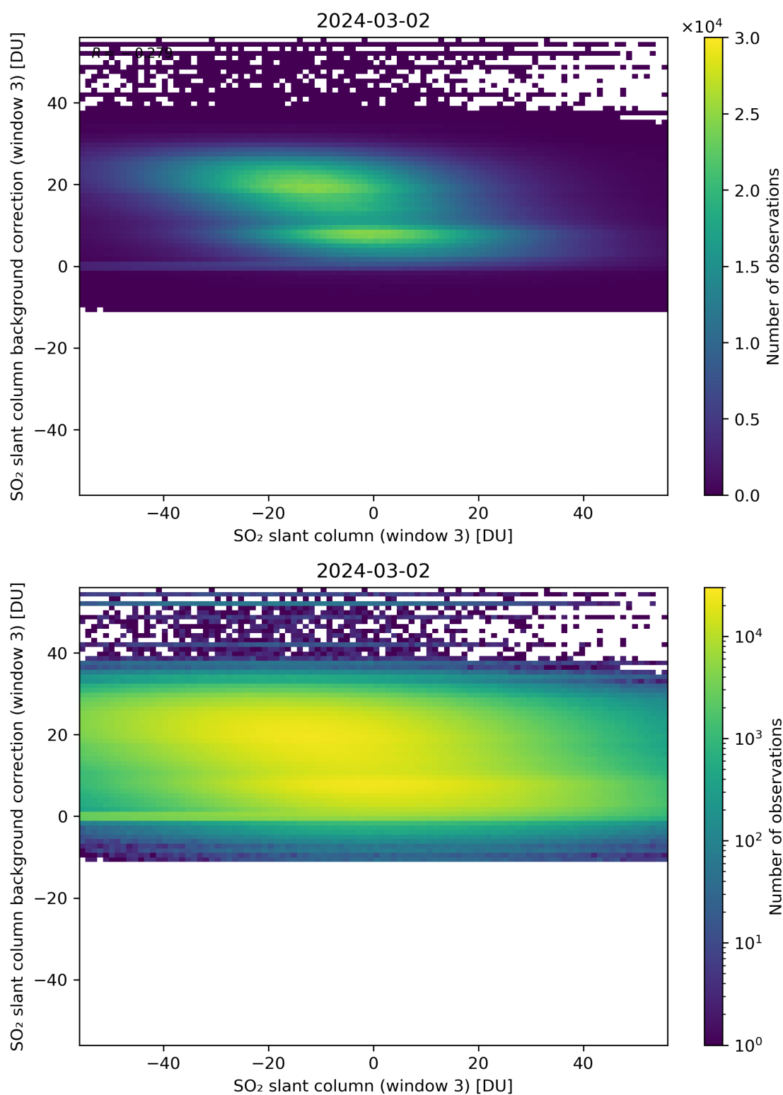
Figure 253: Scatter density plot of “SO 2 slant column (window 3)” against “SO 2 slant column background correction (window 3)” for 2024-03-01 to 2024-03-03.
