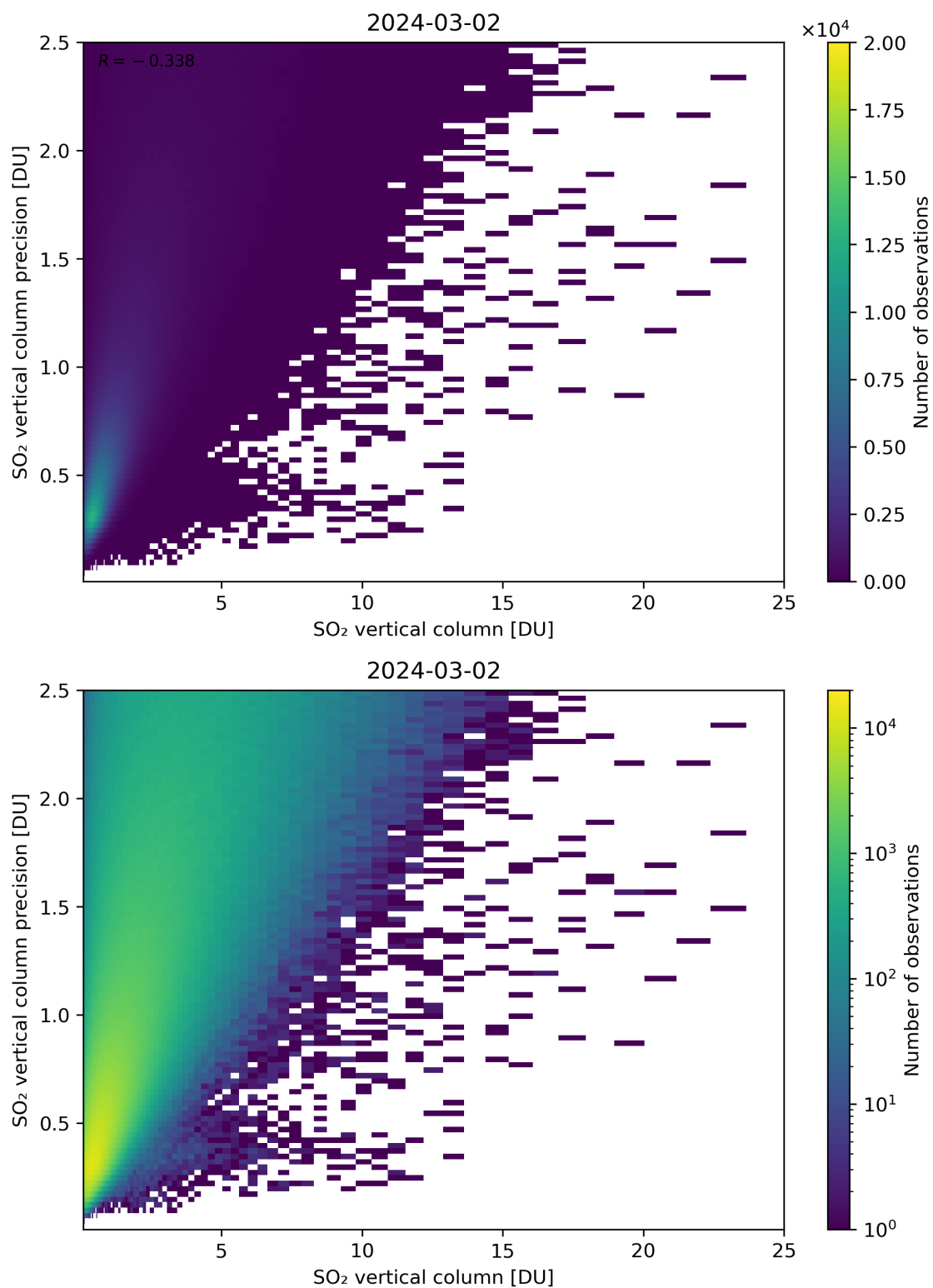
Figure 307: Scatter density plot of “SO 2 vertical column” against “SO 2 vertical column precision” for 2024-03-01 to 2024-03-03.
