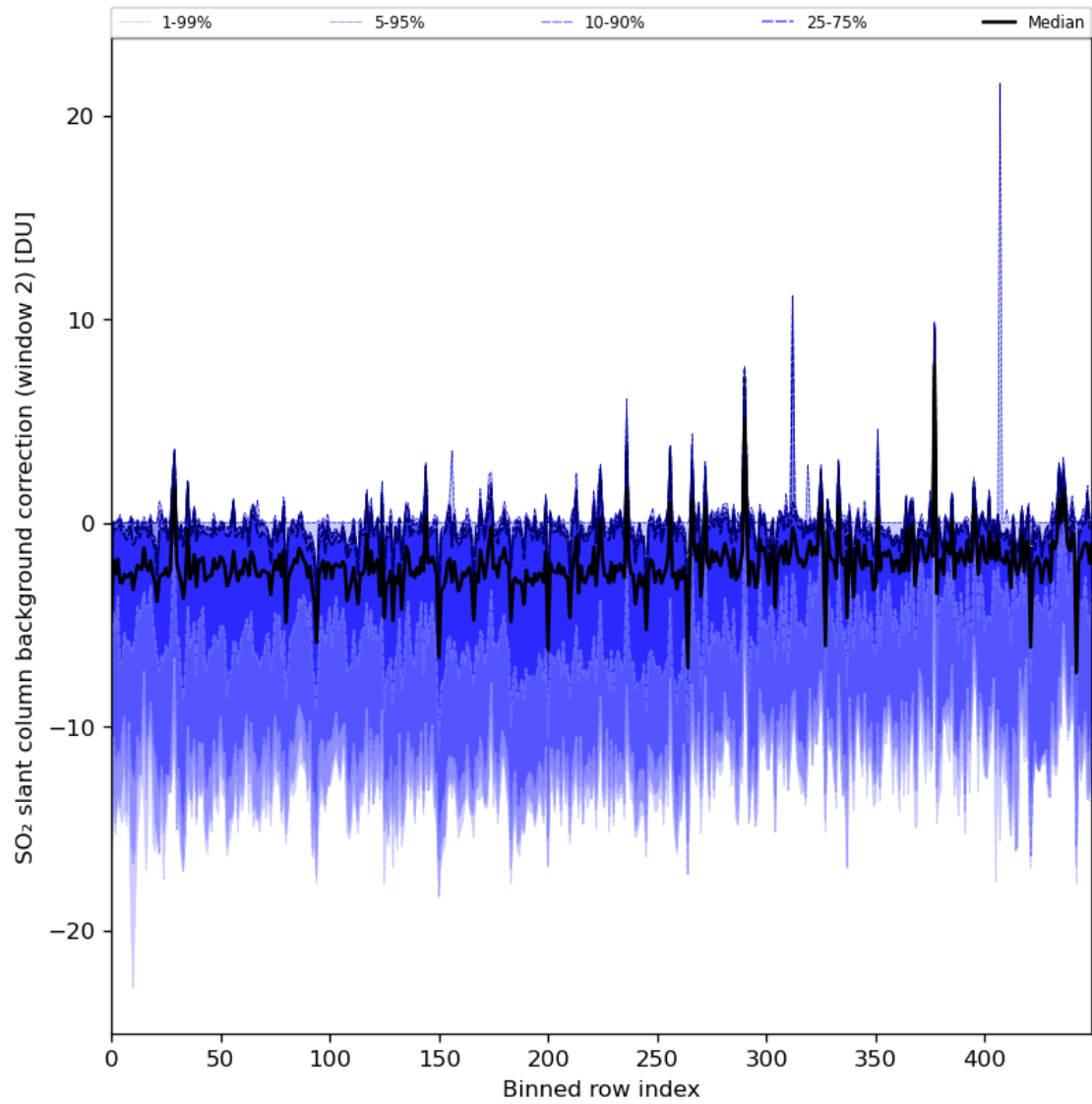
Figure 86: Along track statistics of “SO 2 slant column background correction (window 2)” for 2024-03-01 to 2024-03-03
