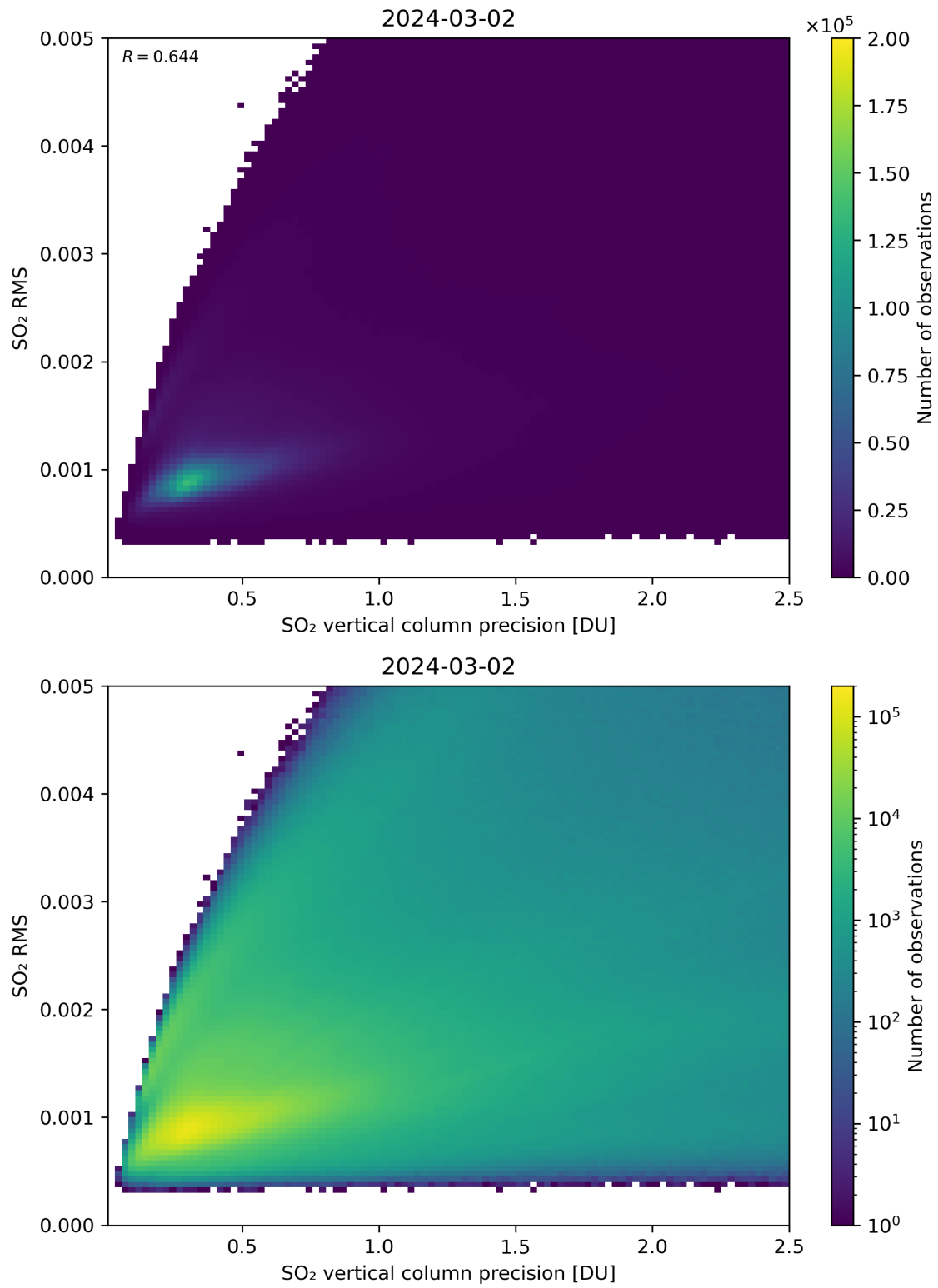
Figure 284: Scatter density plot of “SO 2 vertical column precision” against “SO 2 RMS” for 2024-03-01 to 2024-03-03.
