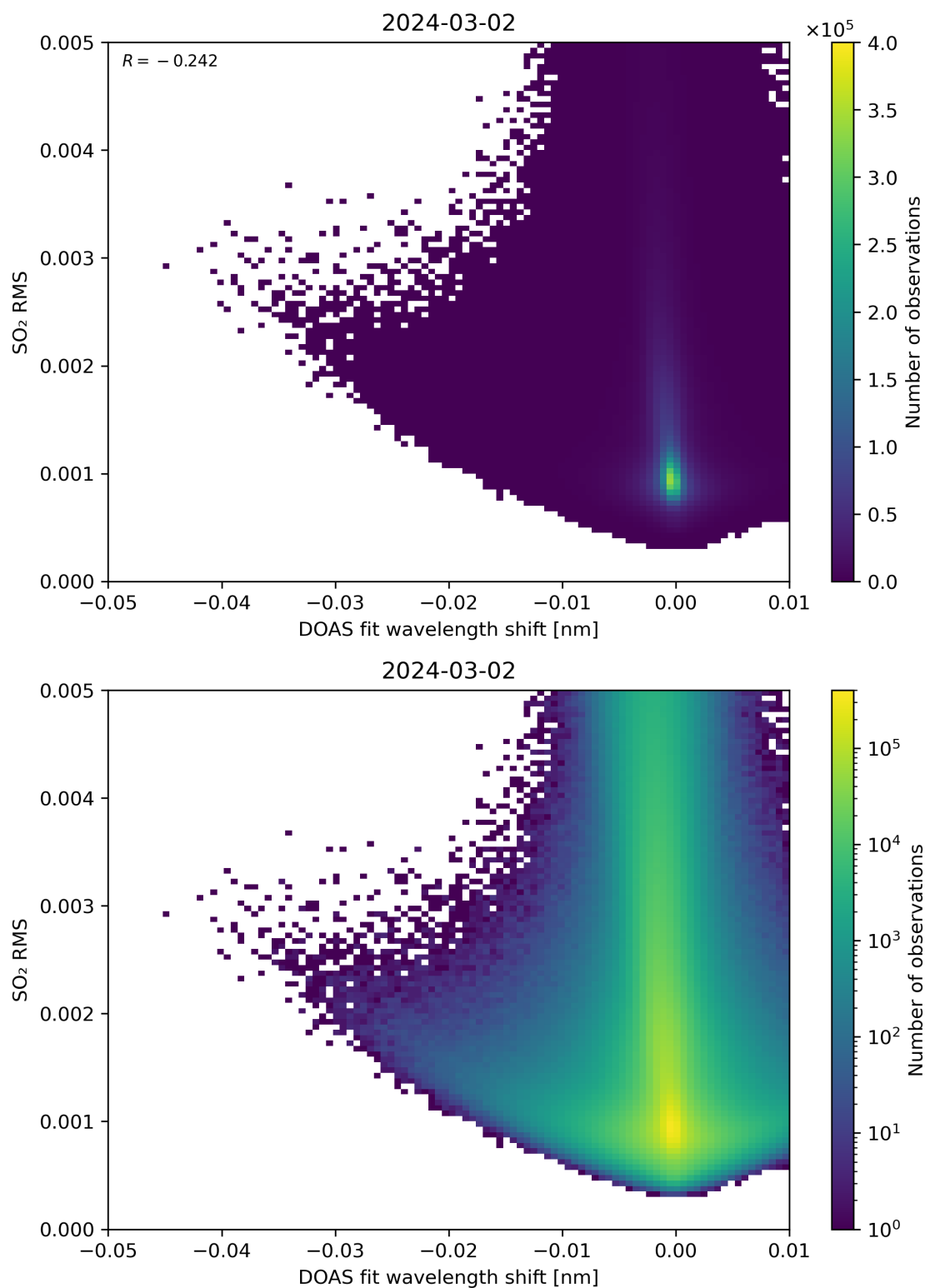
Figure 128: Scatter density plot of “DOAS fit wavelength shift” against “SO 2 RMS” for 2024-03-01 to 2024-03-03.
