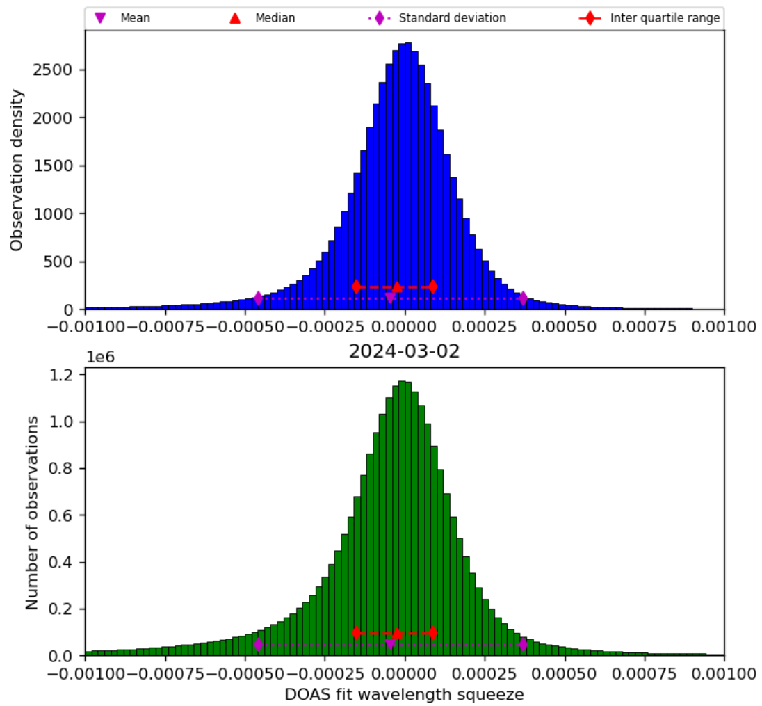
Figure 69: Histogram of “DOAS fit wavelength squeeze” for 2024-03-01 to 2024-03-03
