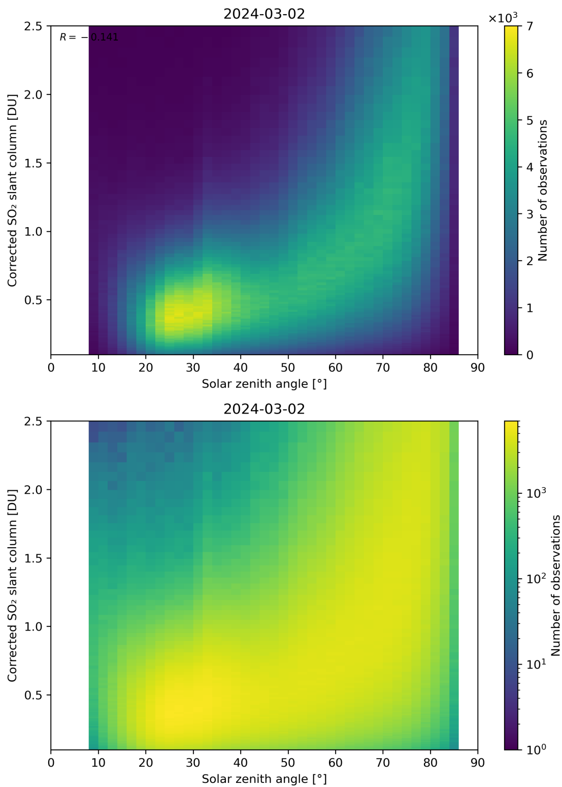
Figure 166: Scatter density plot of “Solar zenith angle” against “Corrected SO 2 slant column” for 2024-03-01 to 2024-03-03.
