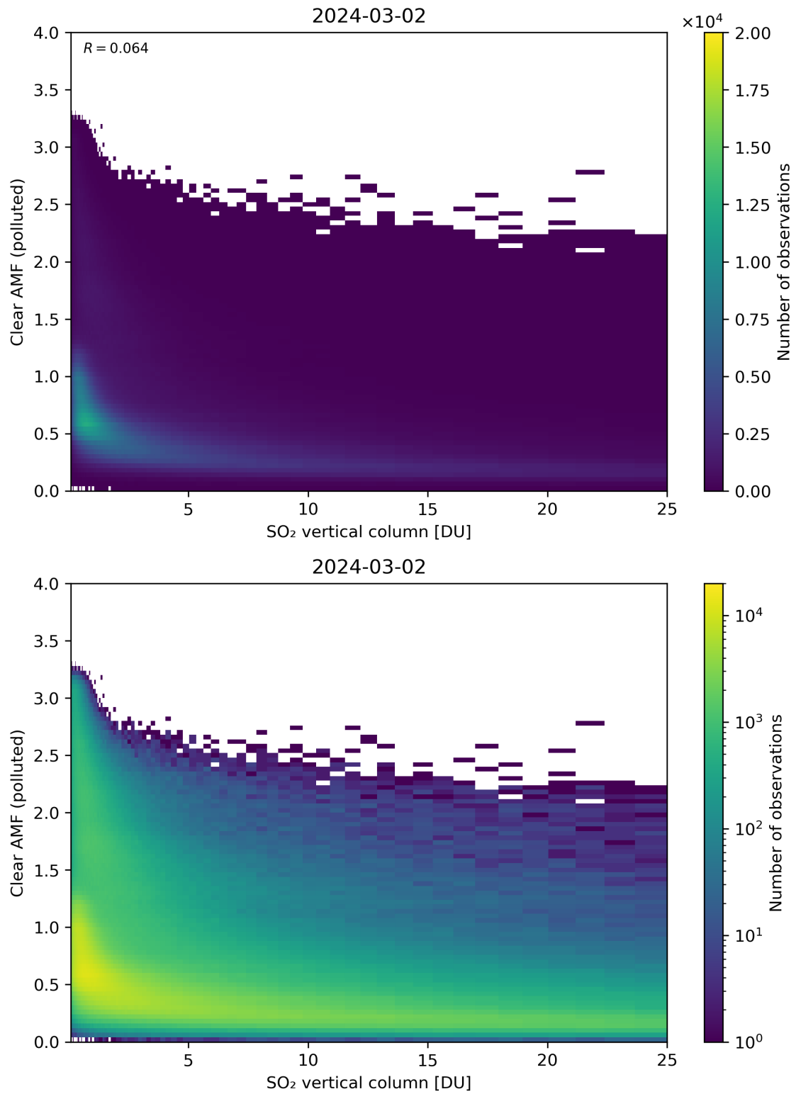
Figure 296: Scatter density plot of “SO 2 vertical column” against “Clear AMF (polluted)” for 2024-03-01 to 2024-03-03.
