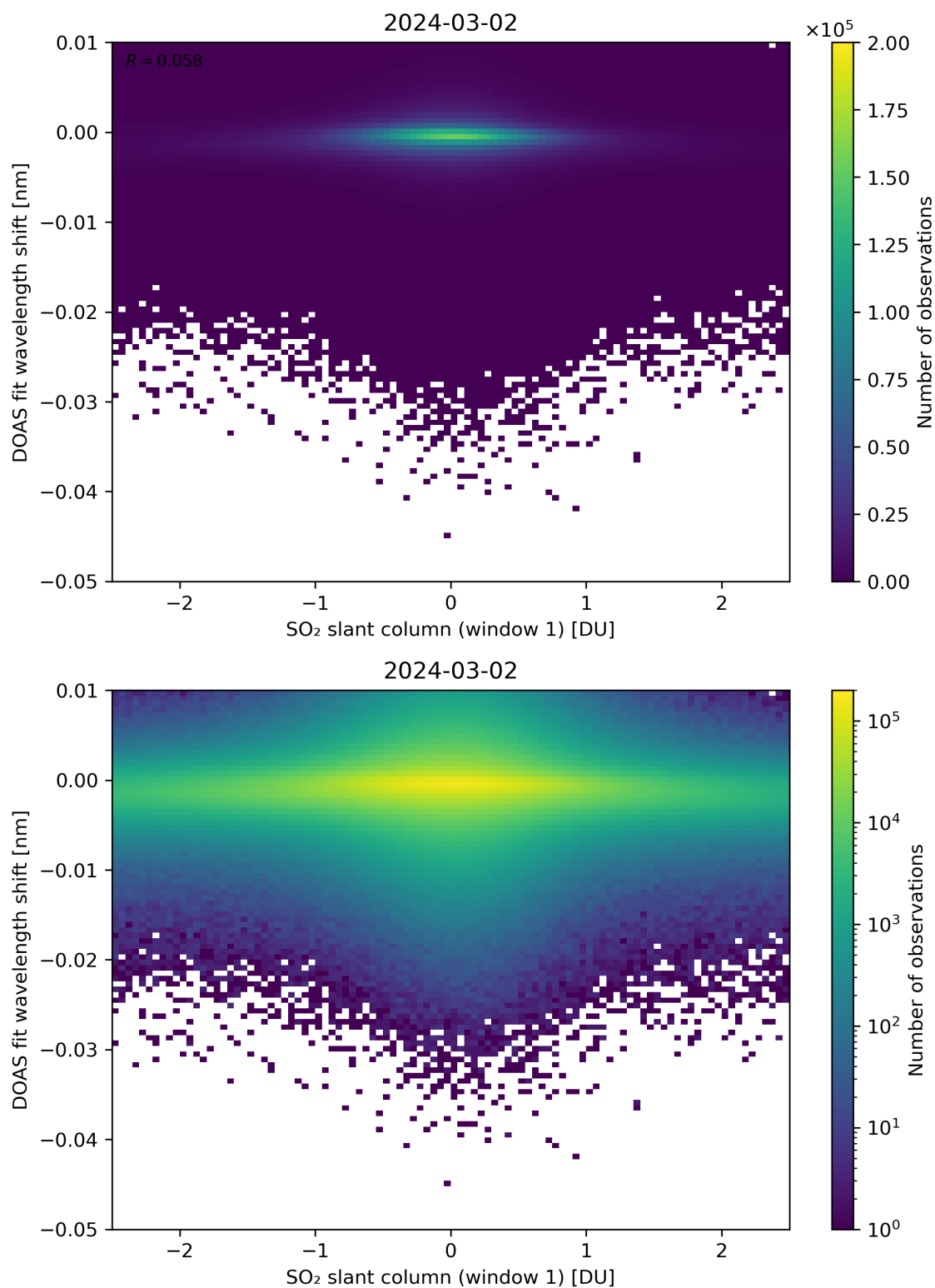
Figure 215: Scatter density plot of “SO 2 slant column (window 1)” against “DOAS fit wavelength shift” for 2024-03-01 to 2024-03-03.
