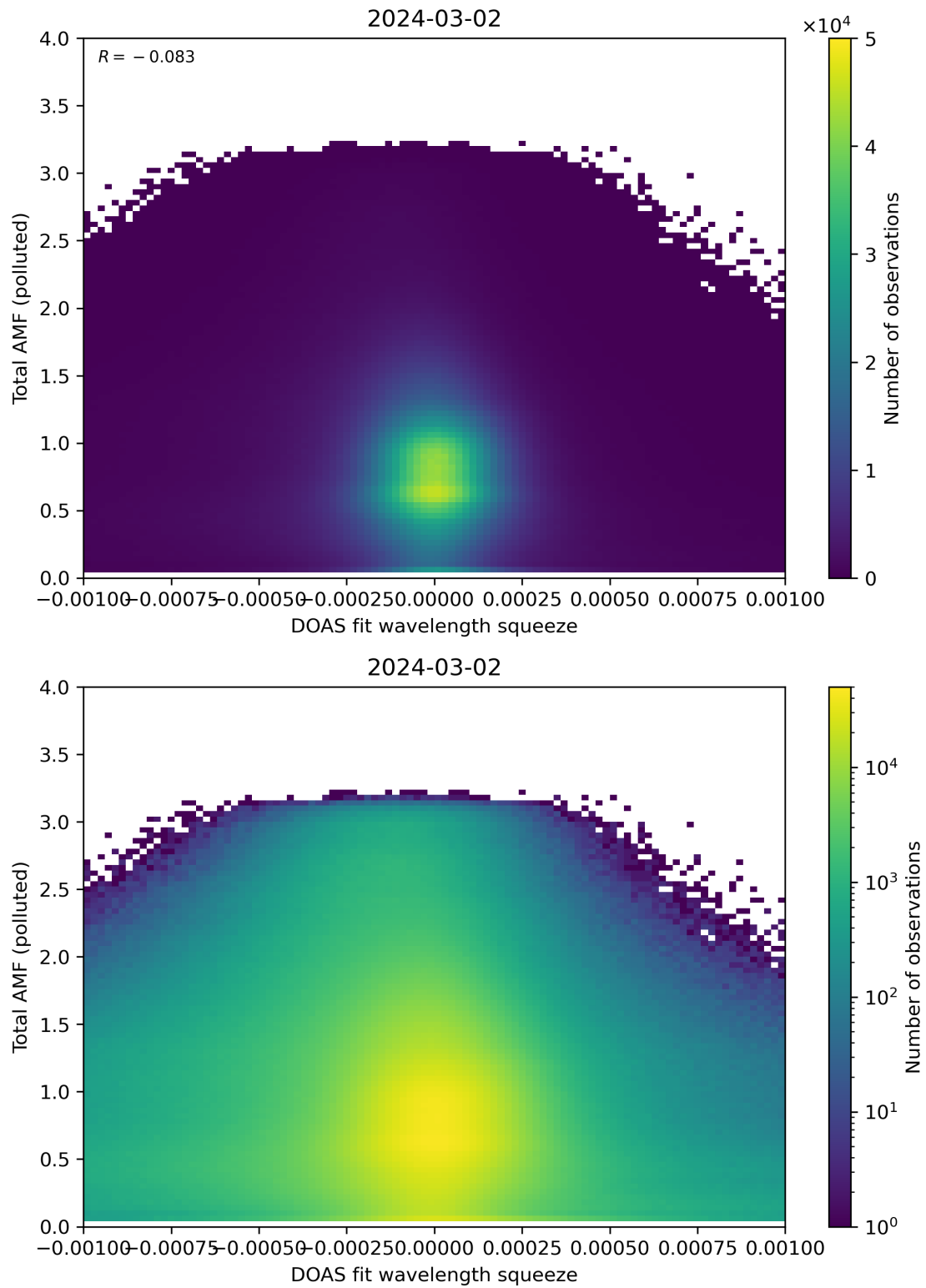
Figure 134: Scatter density plot of “DOAS fit wavelength squeeze” against “Total AMF (polluted)” for 2024-03-01 to 2024-03-03.
