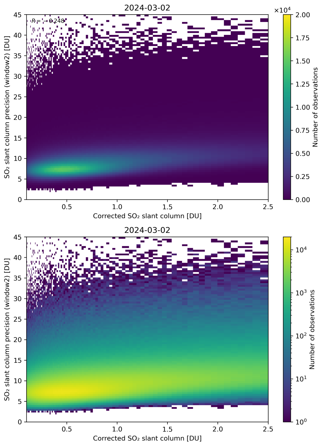
Figure 189: Scatter density plot of “Corrected SO 2 slant column” against “SO 2 slant column precision (window2)” for 2024-03-01 to 2024-03-03.
