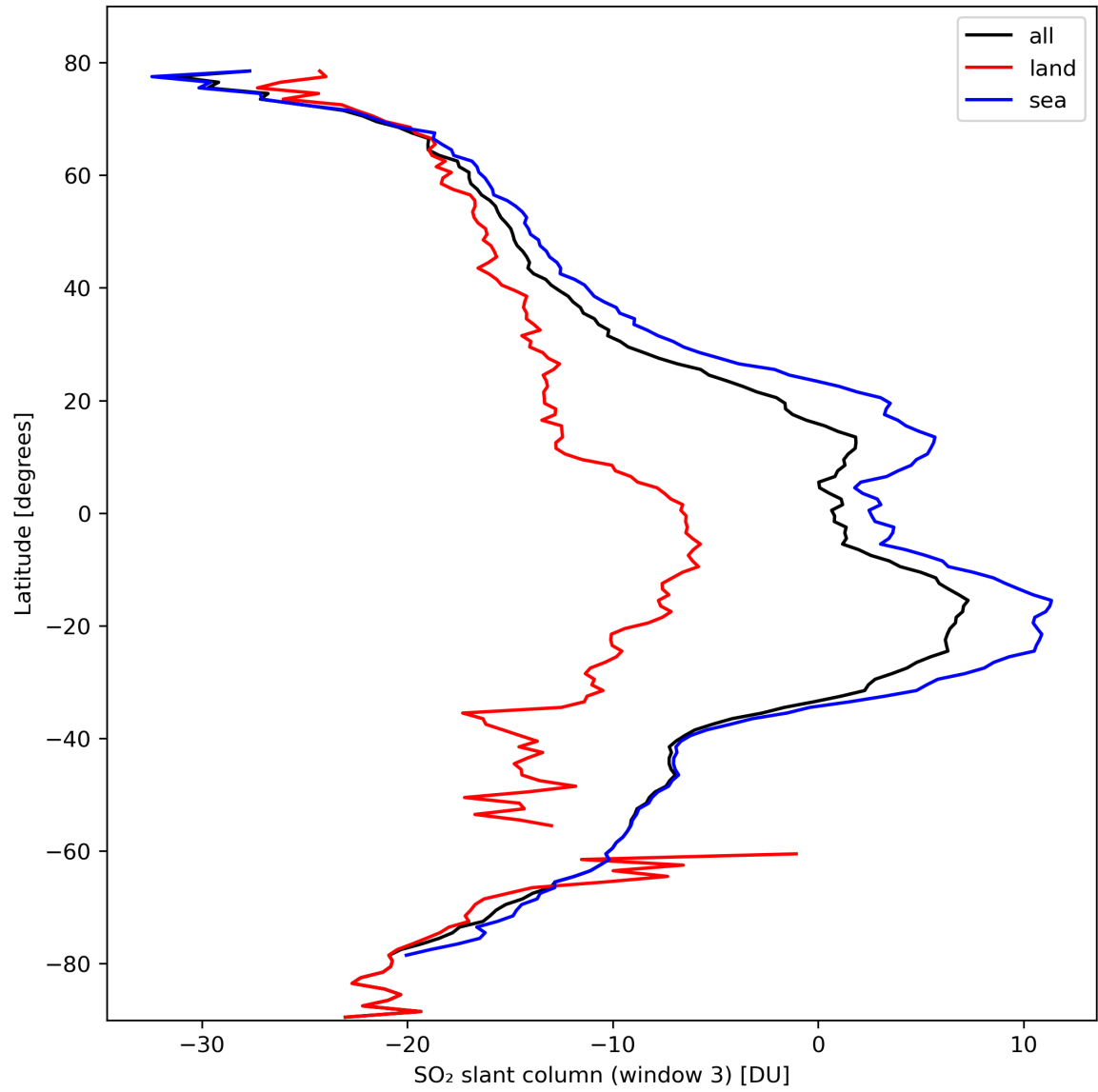
Figure 41: Zonal average of “SO 2 slant column (window 3)” for 2024-03-01 to 2024-03-03.
