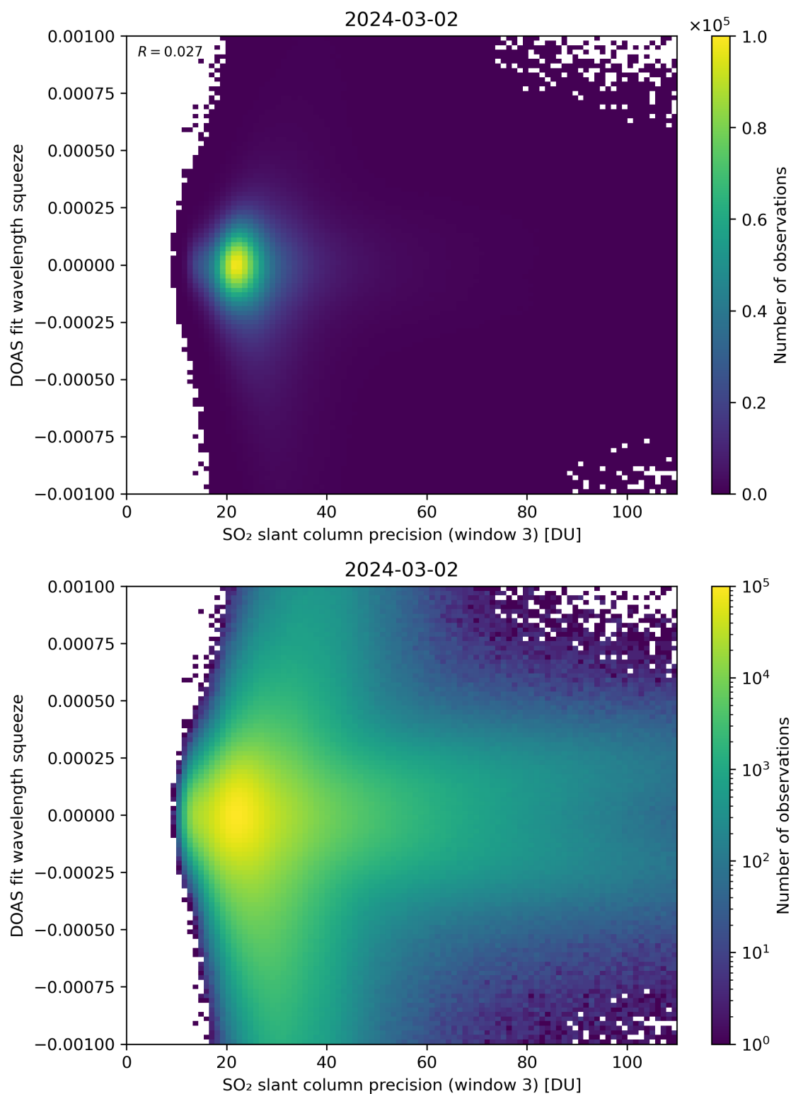
Figure 259: Scatter density plot of “SO 2 slant column precision (window 3)” against “DOAS fit wavelength squeeze” for 2024-03-01 to 2024-03-03.
