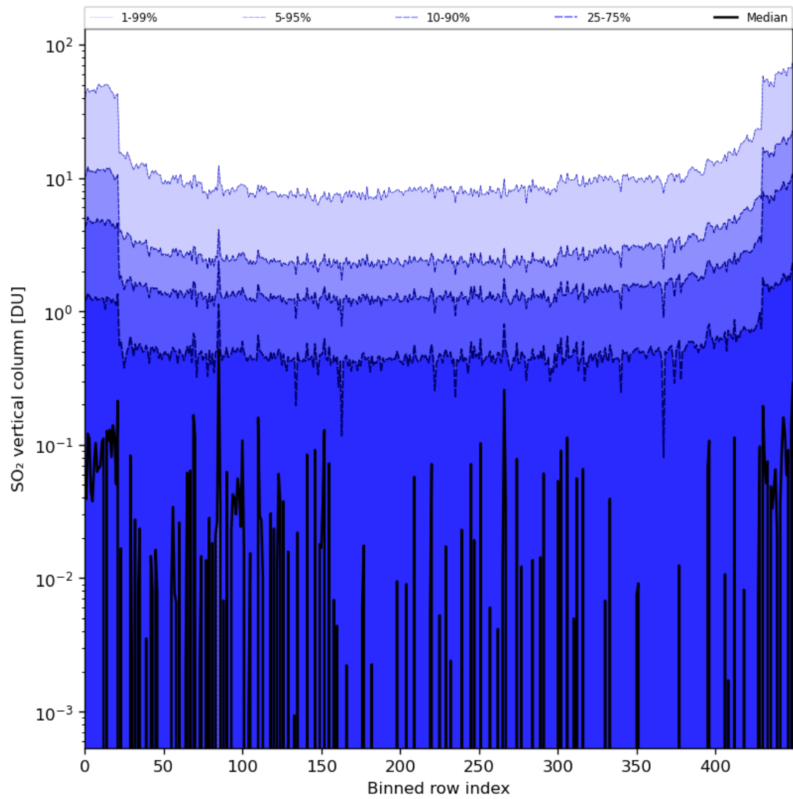
Figure 76: Along track statistics of “SO 2 vertical column” for 2024-03-01 to 2024-03-03
