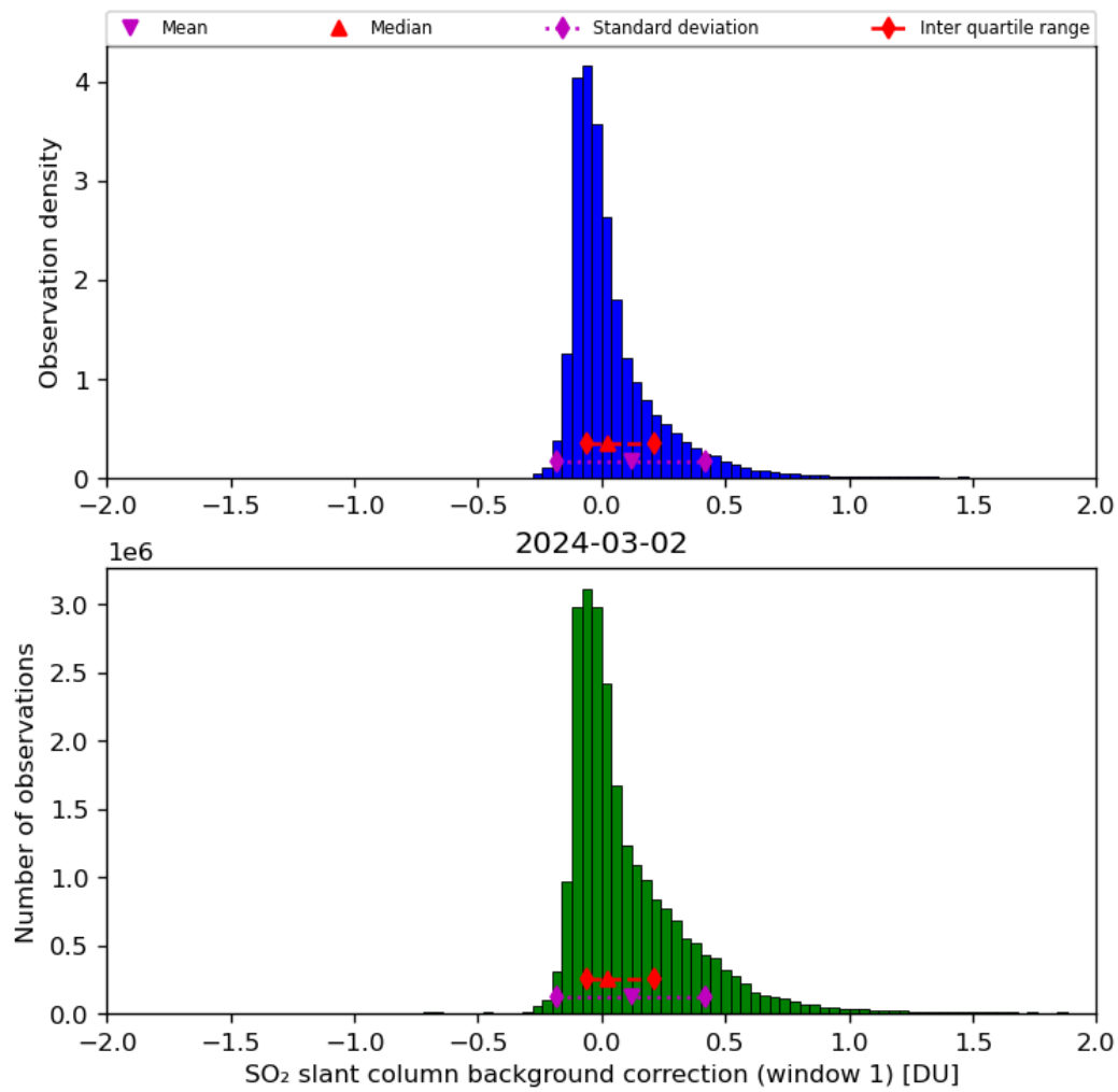
Figure 59: Histogram of “SO 2 slant column background correction (window 1)” for 2024-03-01 to 2024-03-03
