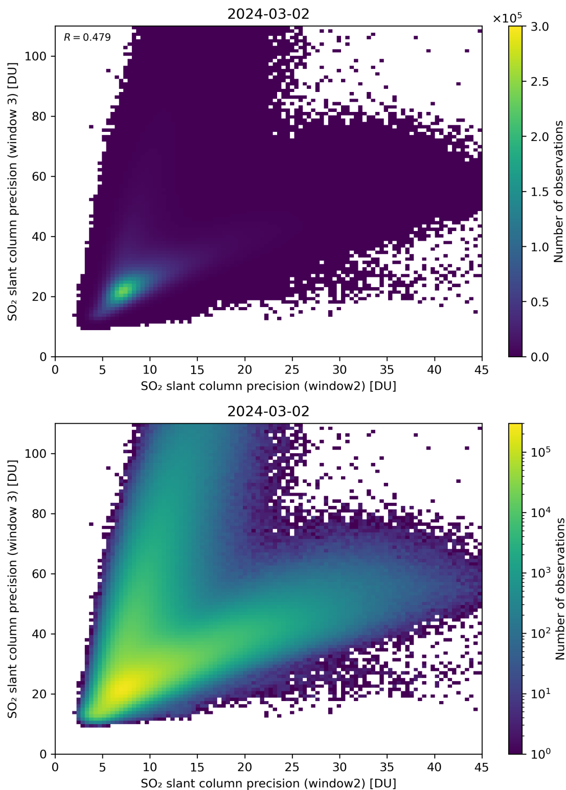
Figure 250: Scatter density plot of “SO 2 slant column precision (window2)” against “SO 2 slant column precision (window 3)” for 2024-03-01 to 2024-03-03.
