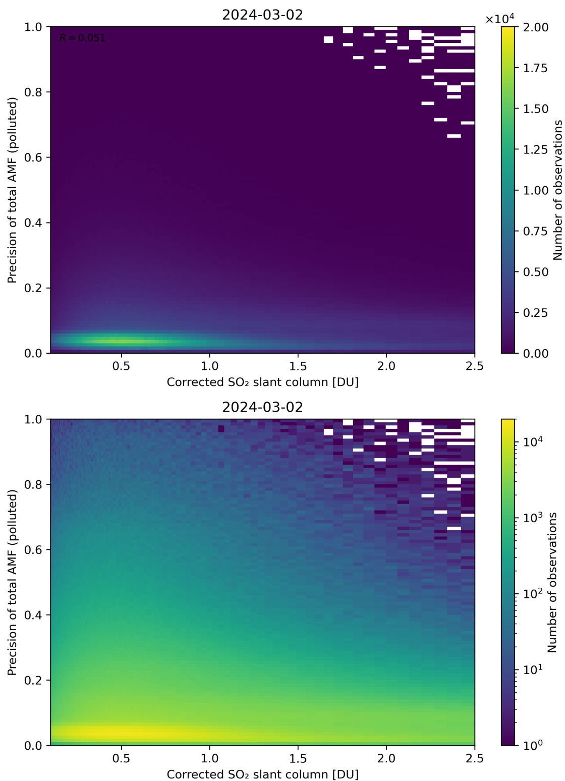
Figure 193: Scatter density plot of “Corrected SO 2 slant column” against “Precision of total AMF (polluted)” for 2024-03-01 to 2024-03-03.
