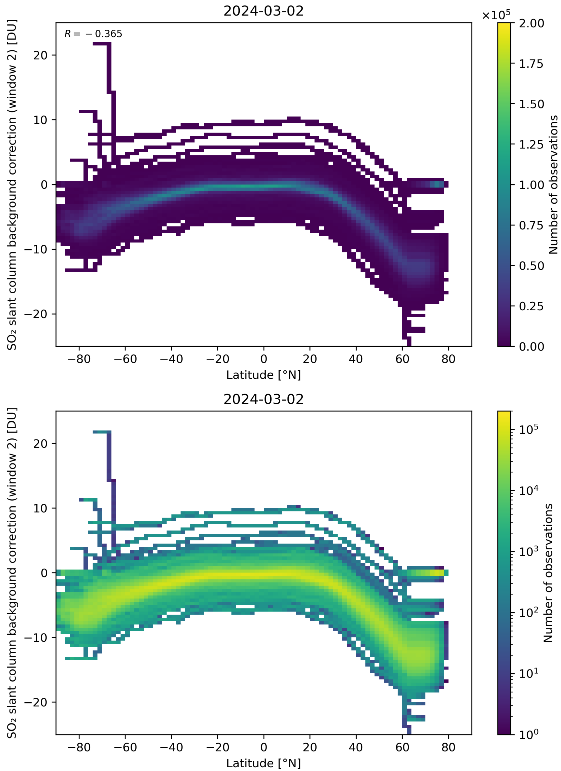
Figure 140: Scatter density plot of “Latitude” against “SO 2 slant column background correction (window 2)” for 2024-03-01 to 2024-03-03.
