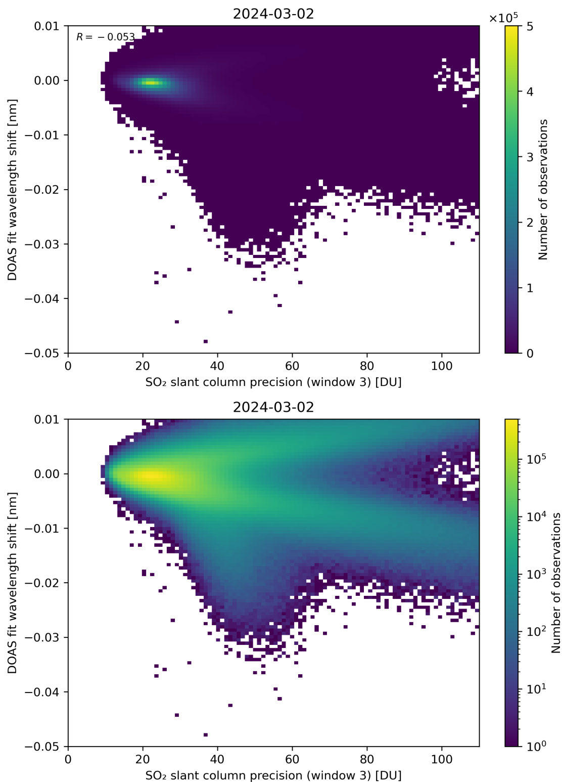
Figure 258: Scatter density plot of “SO 2 slant column precision (window 3)” against “DOAS fit wavelength shift” for 2024-03-01 to 2024-03-03.
