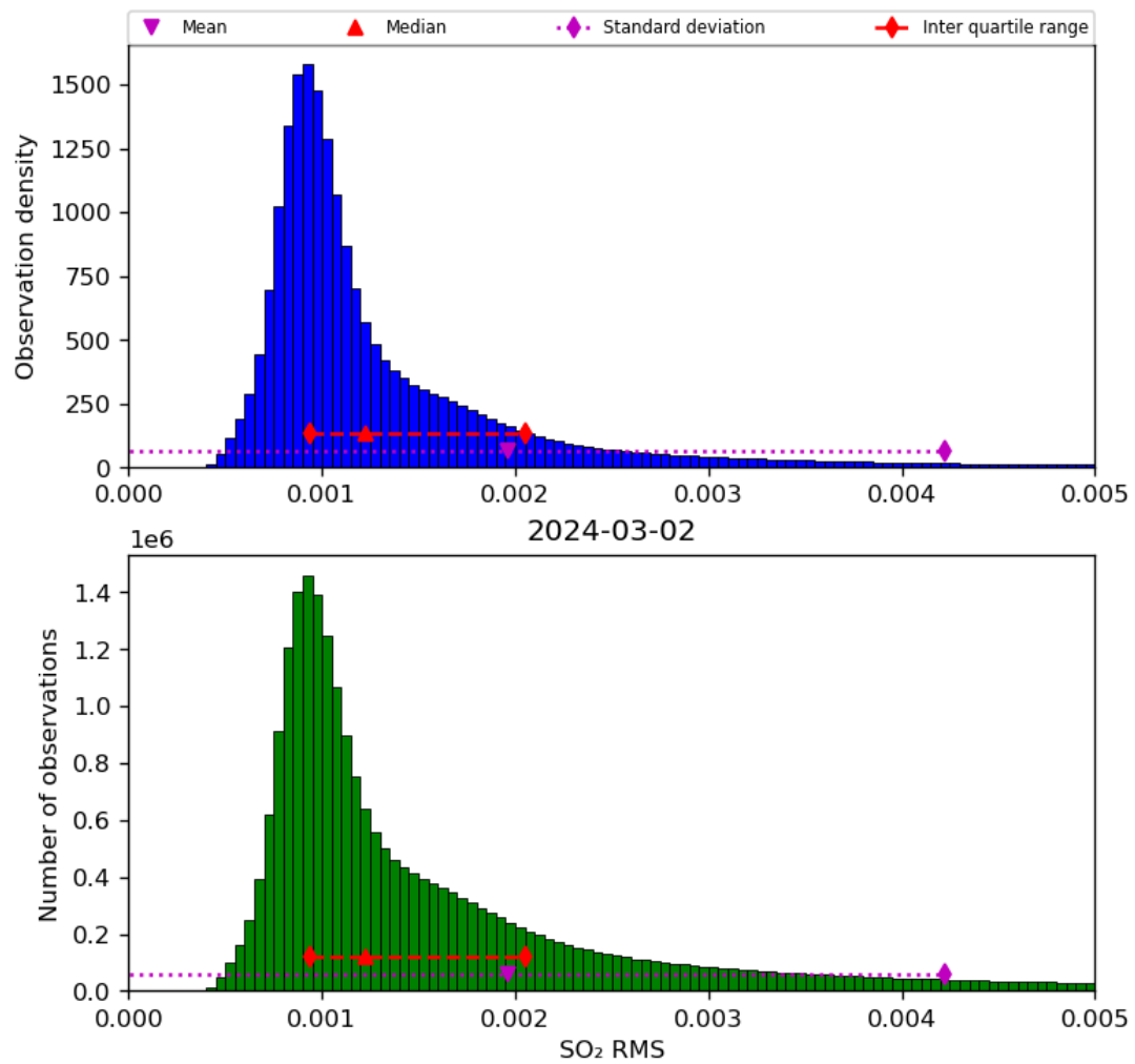
Figure 70: Histogram of “SO 2 RMS” for 2024-03-01 to 2024-03-03
