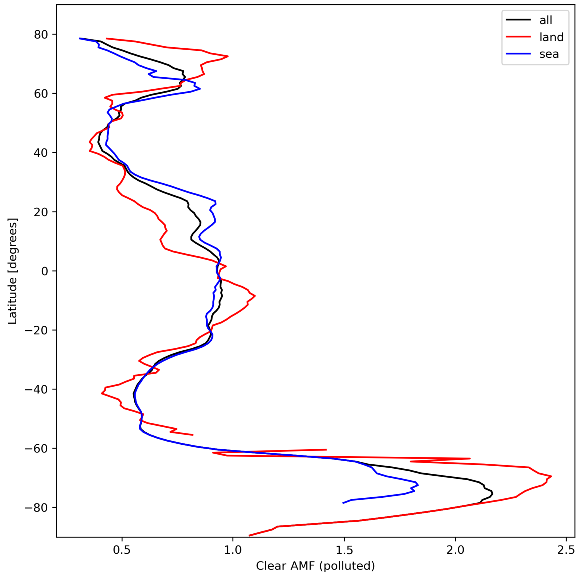
Figure 50: Zonal average of “Clear AMF (polluted)” for 2024-03-01 to 2024-03-03.
