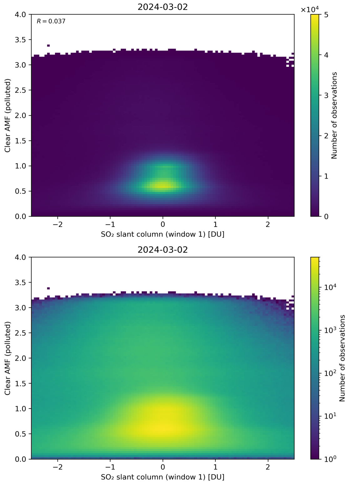
Figure 232: Scatter density plot of “SO 2 slant column (window 1)” against “Clear AMF (polluted)” for 2024-03-01 to 2024-03-03.
