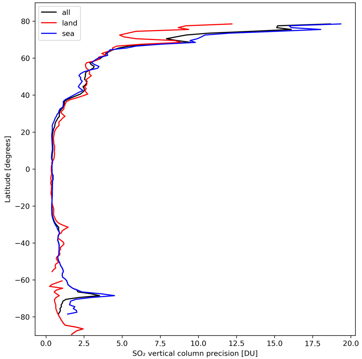
Figure 31: Zonal average of “SO 2 vertical column precision” for 2024-03-01 to 2024-03-03.
