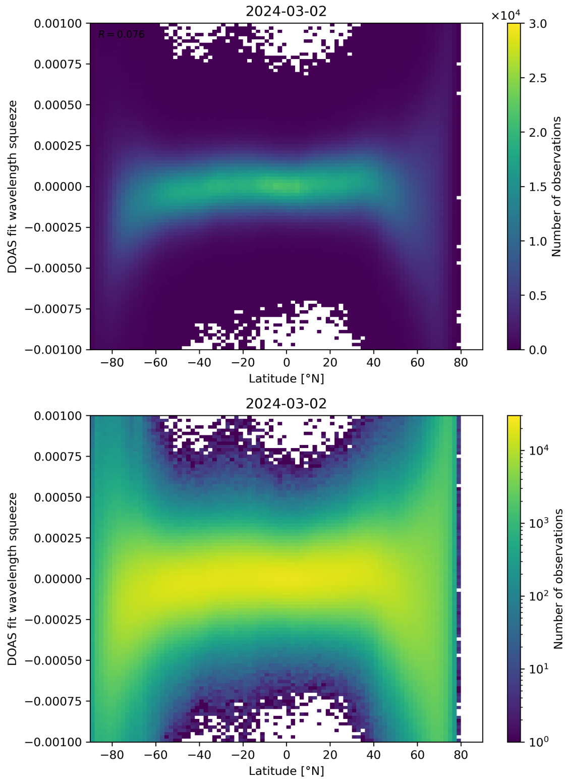
Figure 143: Scatter density plot of “Latitude” against “DOAS fit wavelength squeeze” for 2024-03-01 to 2024-03-03.
