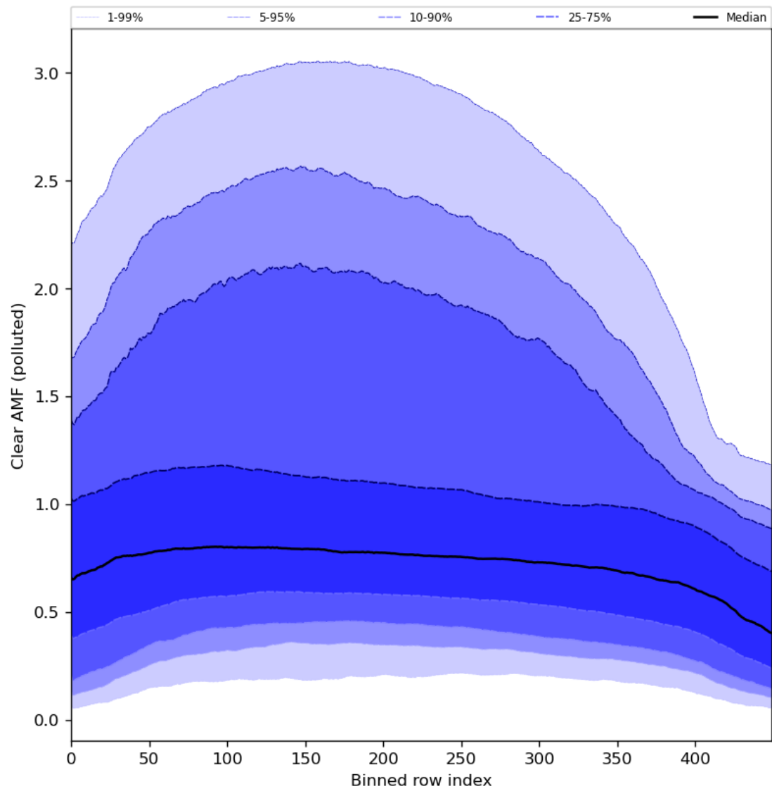
Figure 96: Along track statistics of “Clear AMF (polluted)” for 2024-03-01 to 2024-03-03
