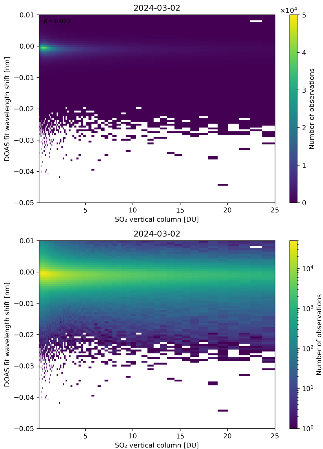
Figure 276: Scatter density plot of “SO 2 vertical column” against “DOAS fit wavelength shift” for 2024-03-01 to 2024-03-03.
