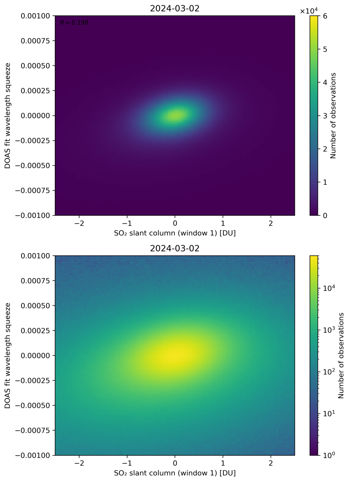
Figure 216: Scatter density plot of “SO 2 slant column (window 1)” against “DOAS fit wavelength squeeze” for 2024-03-01 to 2024-03-03.
