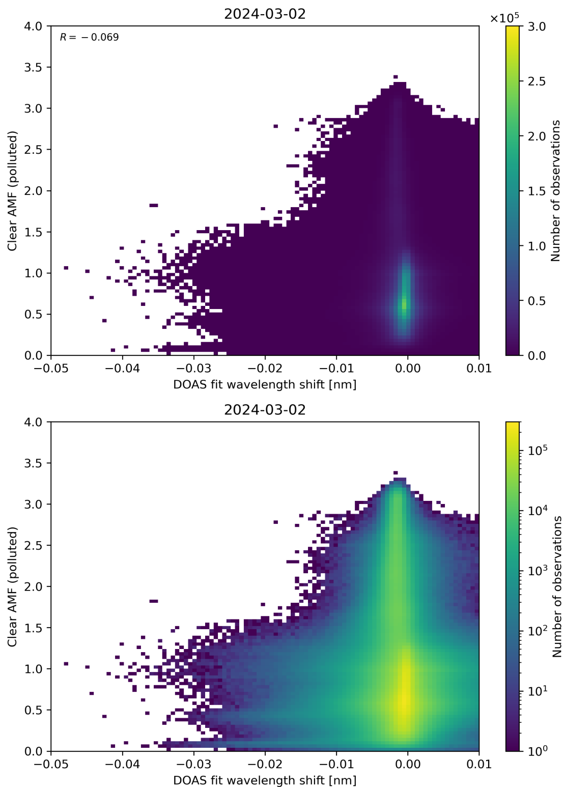
Figure 129: Scatter density plot of “DOAS fit wavelength shift” against “Clear AMF (polluted)” for 2024-03-01 to 2024-03-03.
