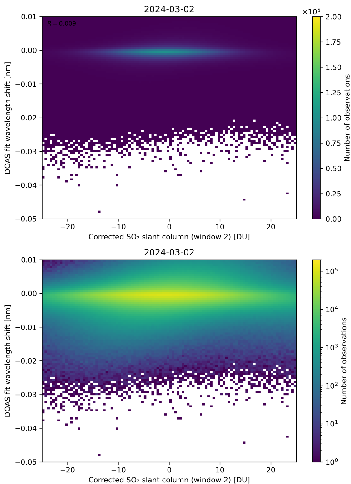
Figure 196: Scatter density plot of “Corrected SO 2 slant column (window 2)” against “DOAS fit wavelength shift” for 2024-03-01 to 2024-03-03.
