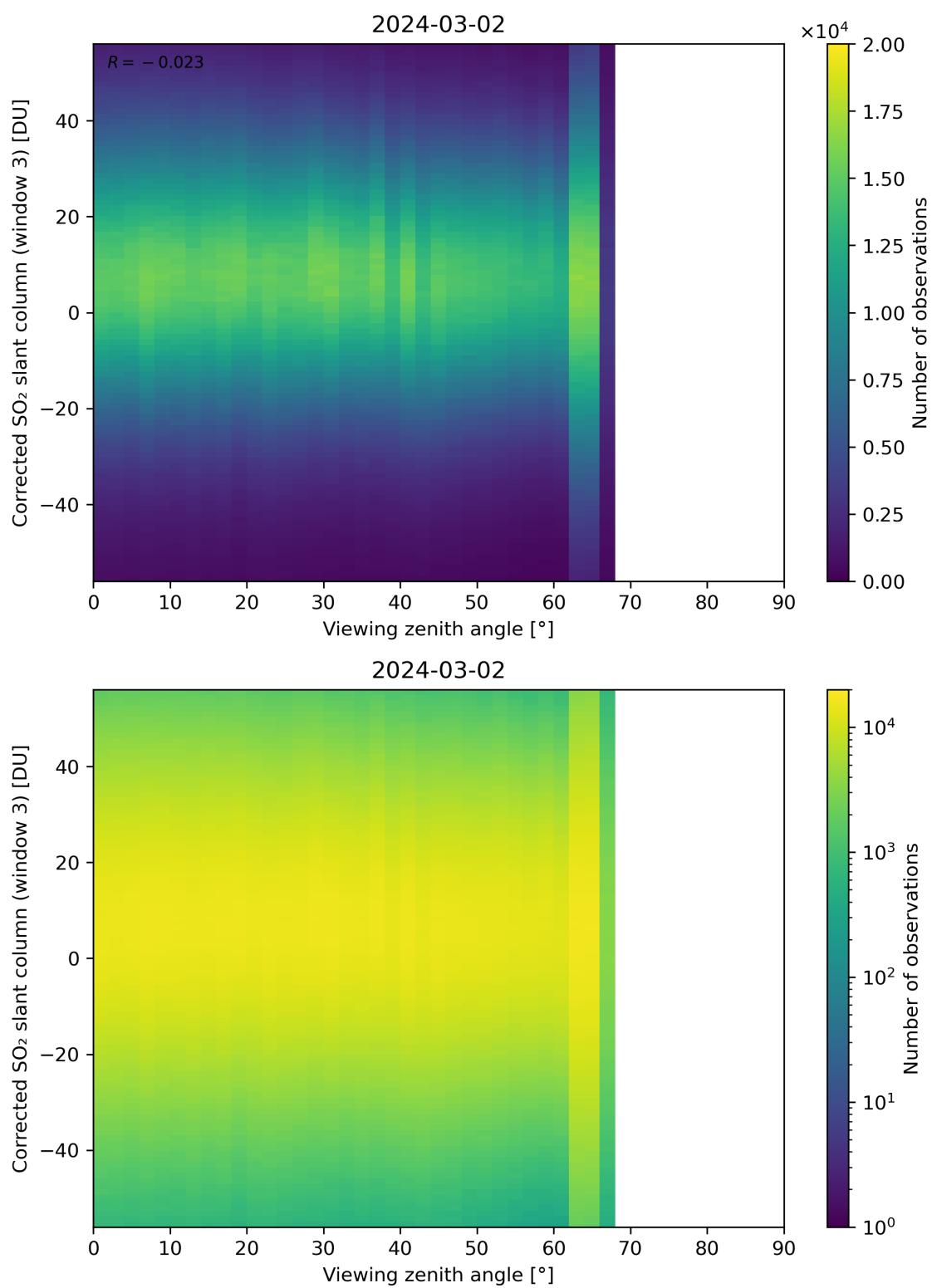
Figure 319: Scatter density plot of “Viewing zenith angle” against “Corrected SO 2 slant column (window 3)” for 2024-03-01 to 2024-03-03.
