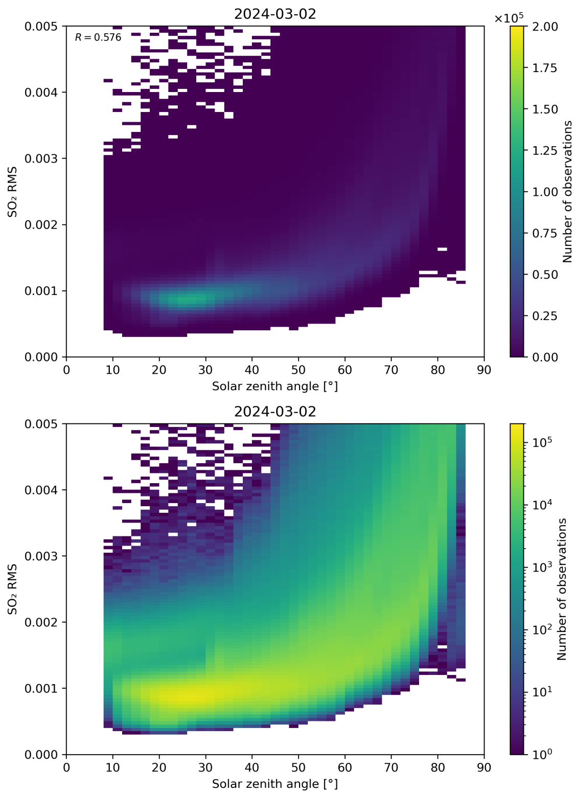
Figure 163: Scatter density plot of “Solar zenith angle” against “SO 2 RMS” for 2024-03-01 to 2024-03-03.
