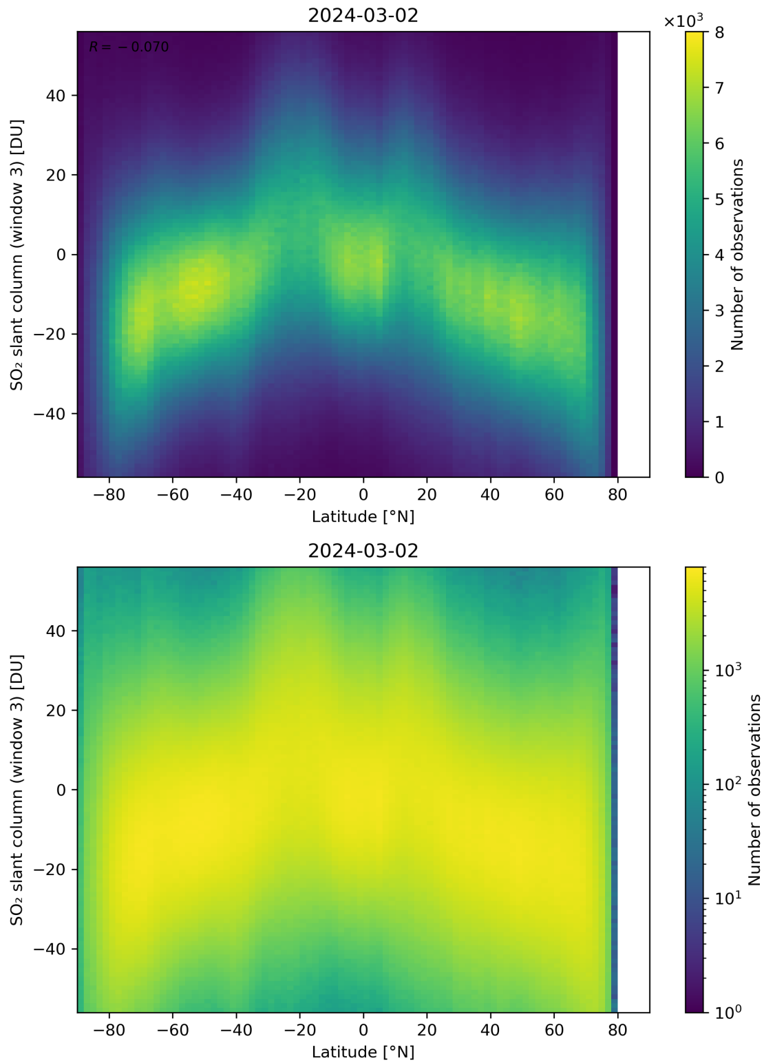
Figure 152: Scatter density plot of “Latitude” against “SO 2 slant column (window 3)” for 2024-03-01 to 2024-03-03.
