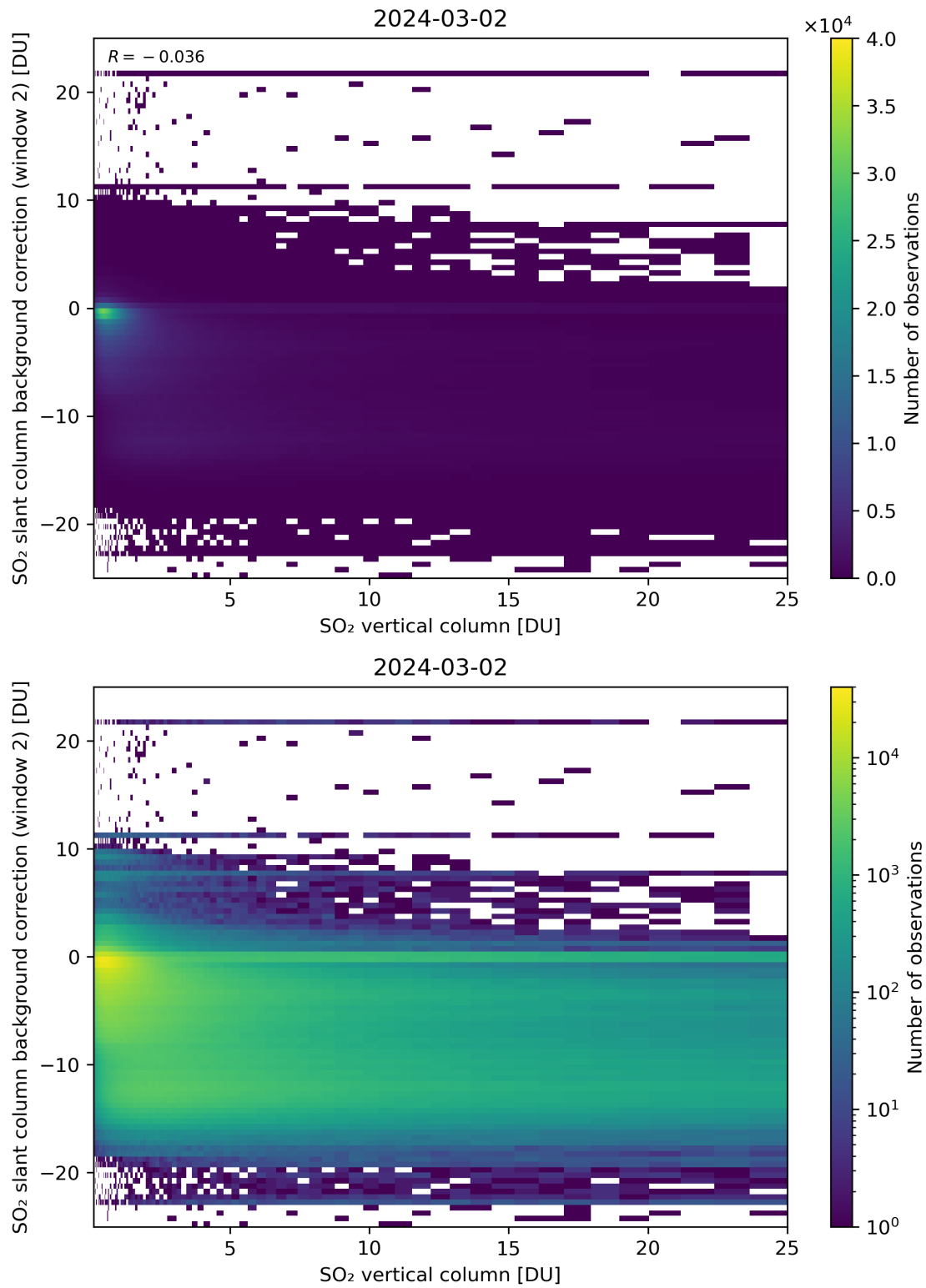
Figure 274: Scatter density plot of “SO 2 vertical column” against “SO 2 slant column background correction (window 2)” for 2024-03-01 to 2024-03-03.
