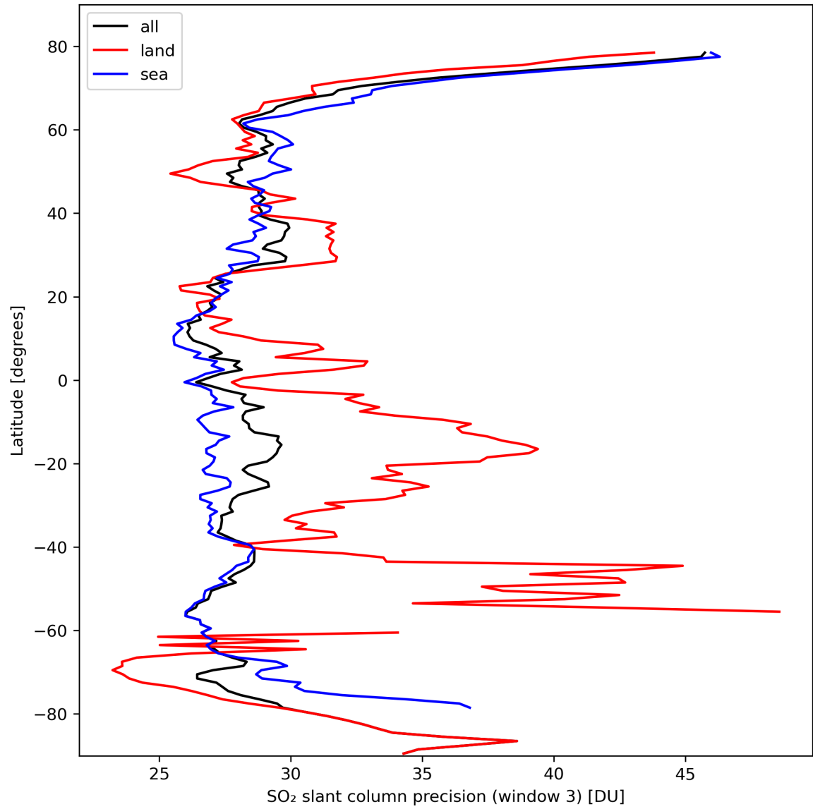
Figure 42: Zonal average of “SO 2 slant column precision (window 3)” for 2024-03-01 to 2024-03-03.
