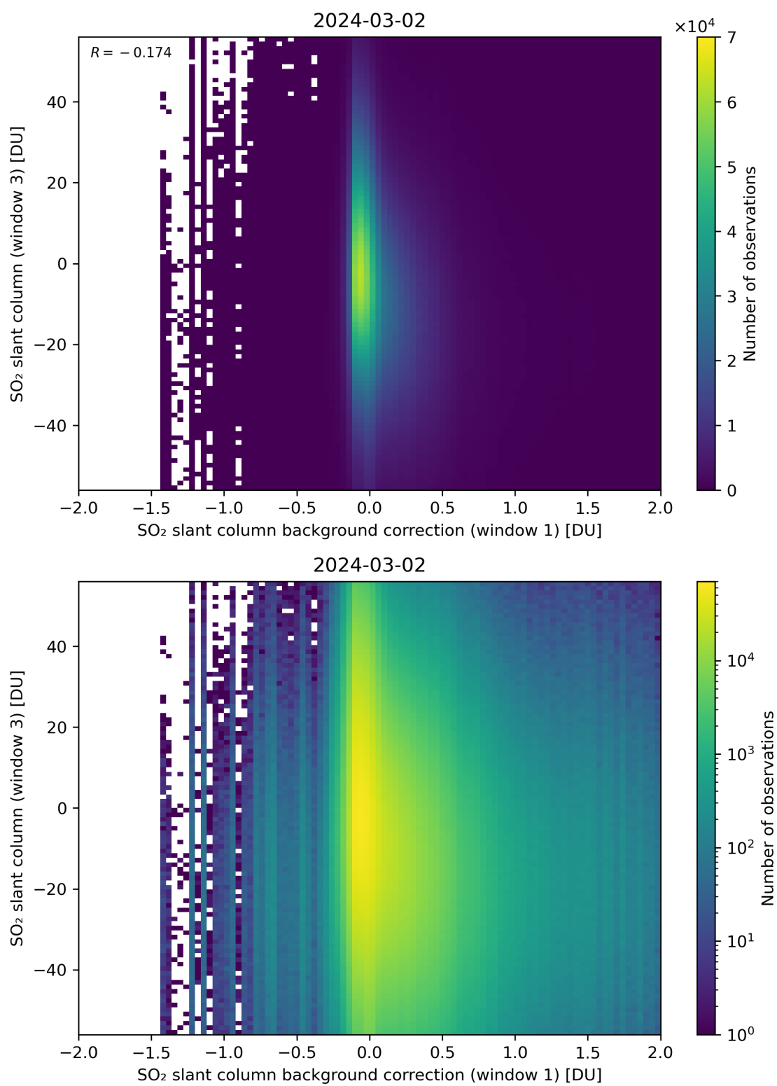
Figure 107: Scatter density plot of “SO 2 slant column background correction (window 1)” against “SO 2 slant column (window 3)” for 2024-03-01 to 2024-03-03.
