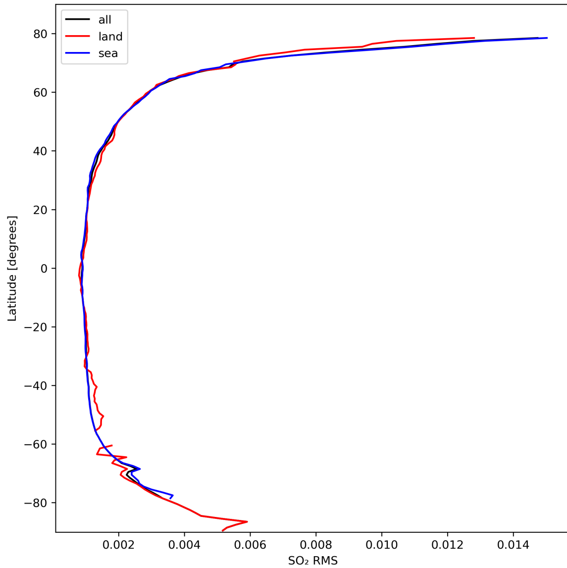
Figure 47: Zonal average of “SO 2 RMS” for 2024-03-01 to 2024-03-03.
