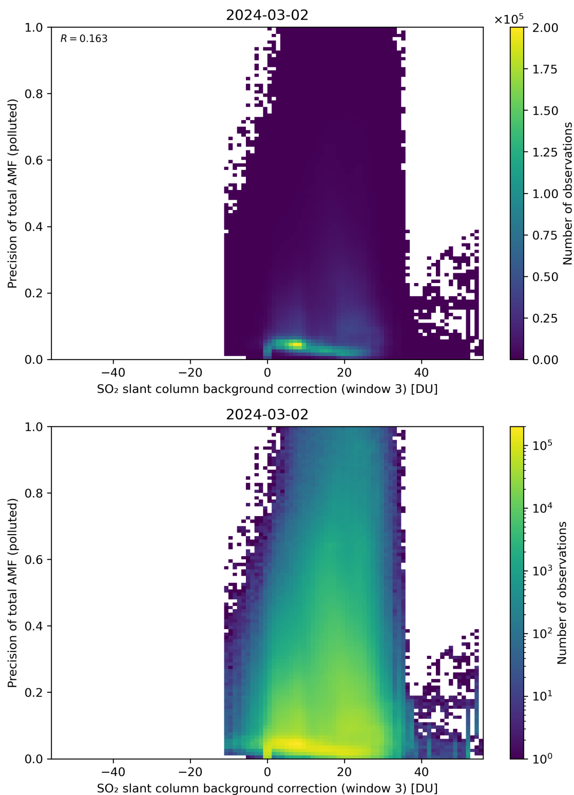
Figure 126: Scatter density plot of “SO 2 slant column background correction (window 3)” against “Precision of total AMF (polluted)” for 2024-03-01 to 2024-03-03.
