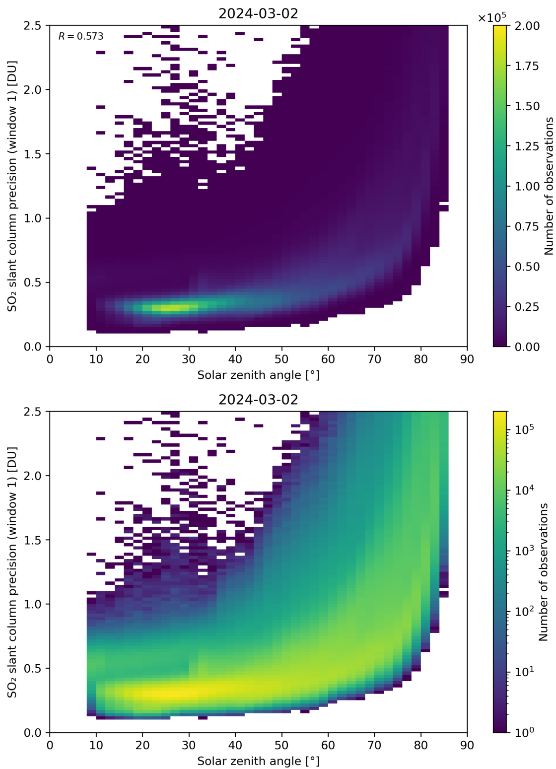
Figure 170: Scatter density plot of “Solar zenith angle” against “SO 2 slant column precision (window 1)” for 2024-03-01 to 2024-03-03.
