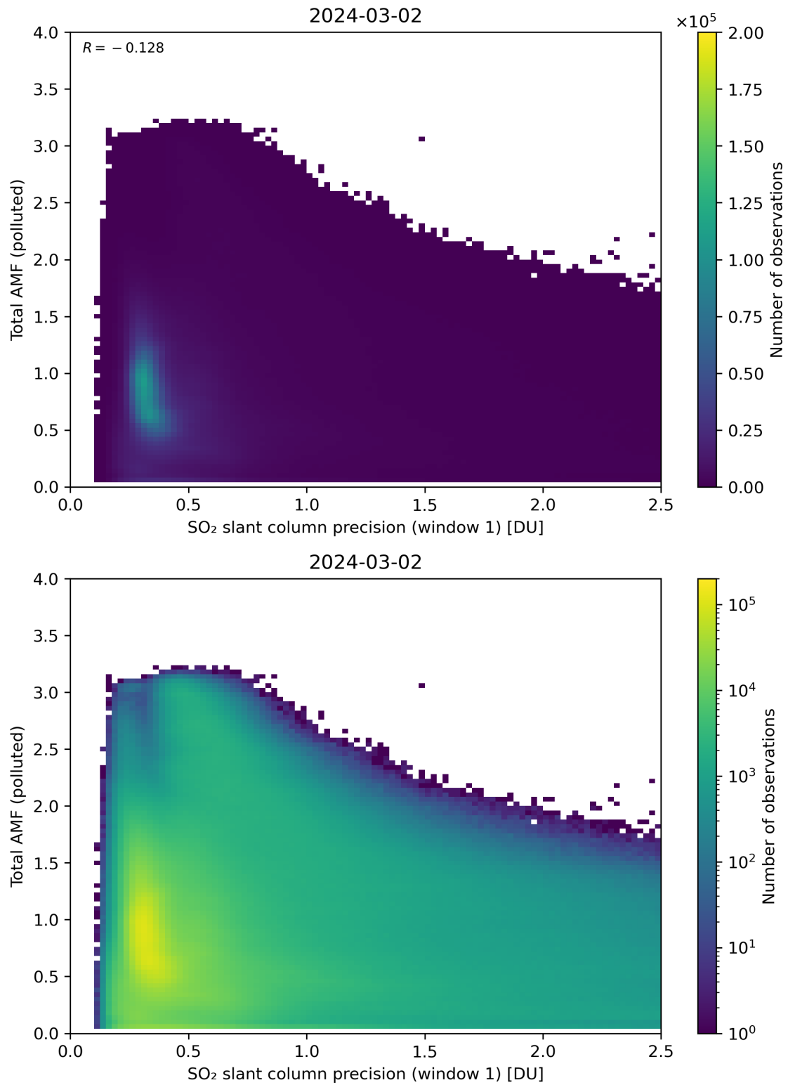
Figure 230: Scatter density plot of “SO 2 slant column precision (window 1)” against “Total AMF (polluted)” for 2024-03-01 to 2024-03-03.
