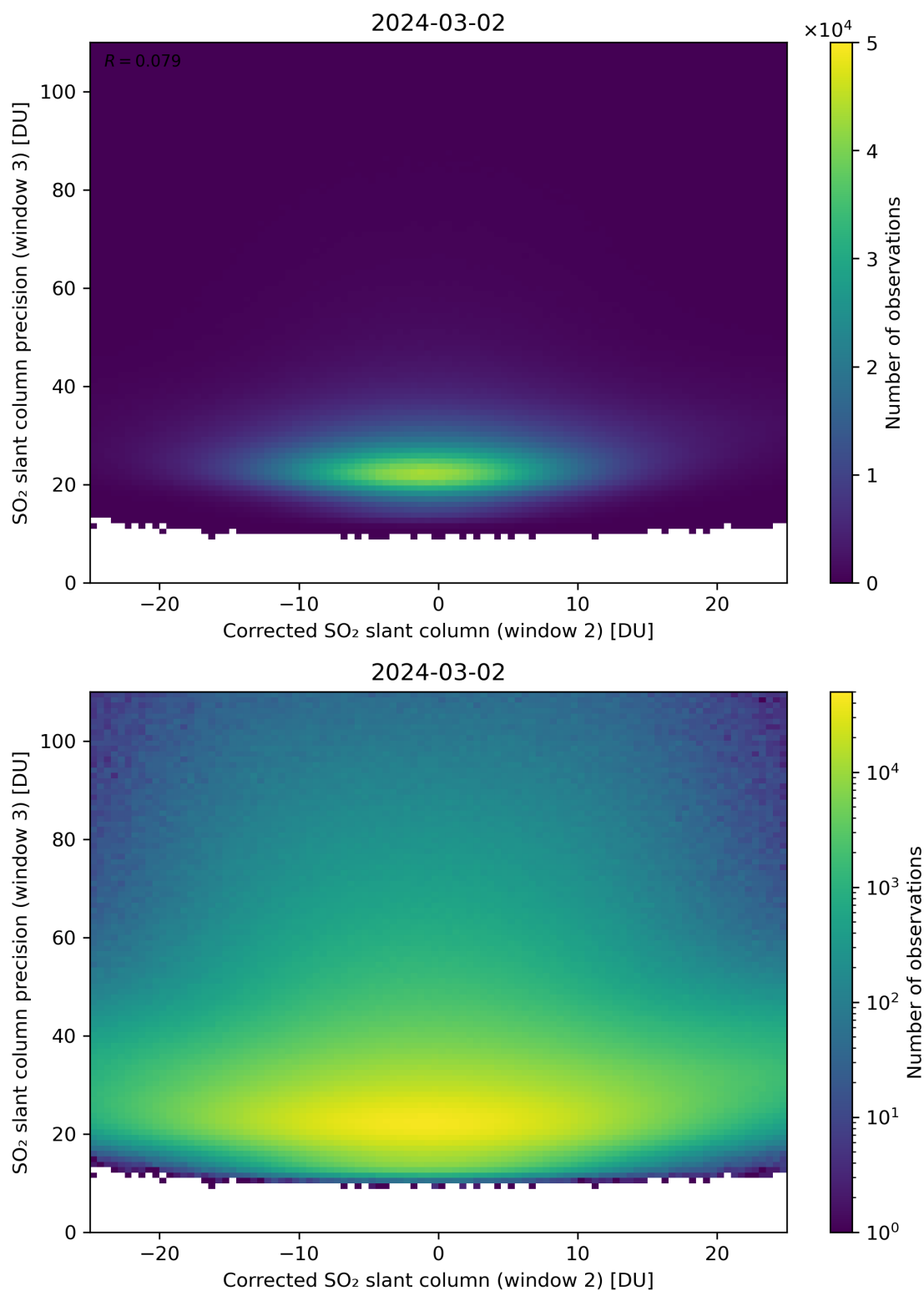
Figure 202: Scatter density plot of “Corrected SO 2 slant column (window 2)” against “SO 2 slant column precision (window 3)” for 2024-03-01 to 2024-03-03.
