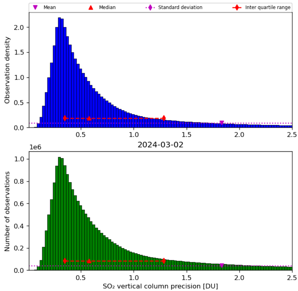
Figure 54: Histogram of “SO 2 vertical column precision” for 2024-03-01 to 2024-03-03
