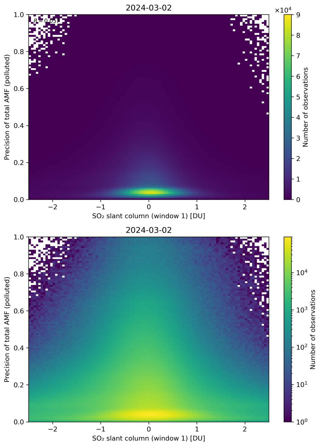
Figure 240: Scatter density plot of “SO 2 slant column (window 1)” against “Precision of total AMF (polluted)” for 2024-03-01 to 2024-03-03.
