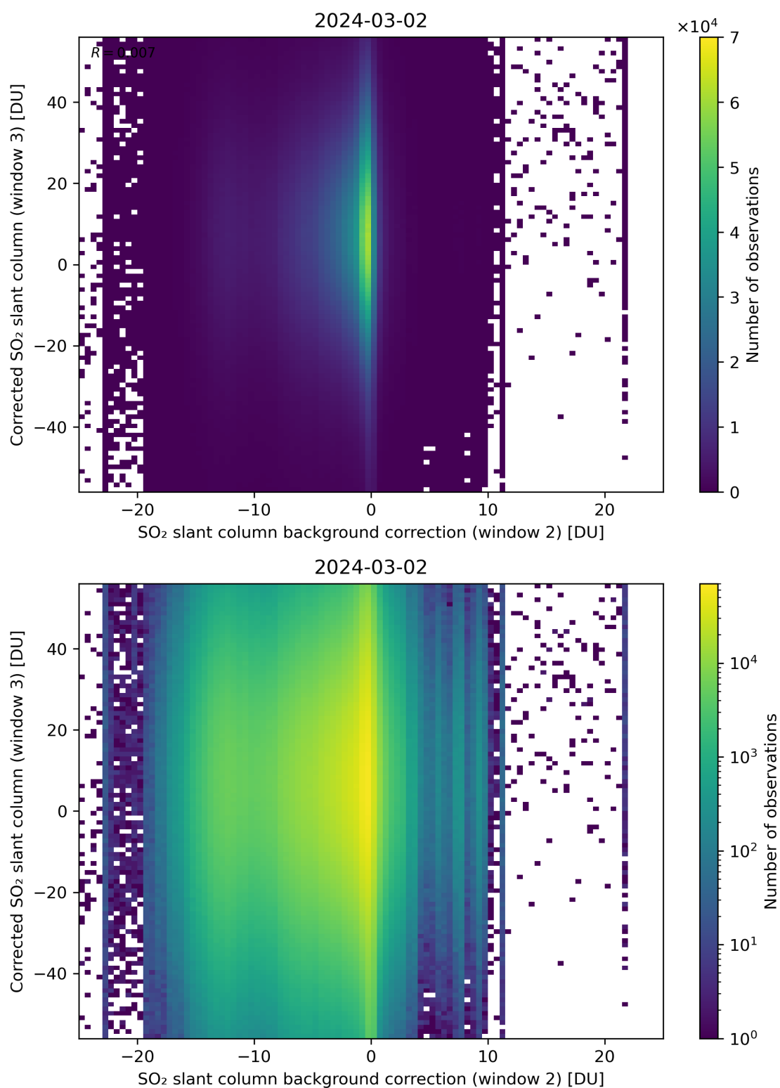
Figure 116: Scatter density plot of “SO 2 slant column background correction (window 2)” against “Corrected SO 2 slant column (window 3)” for 2024-03-01 to 2024-03-03.
