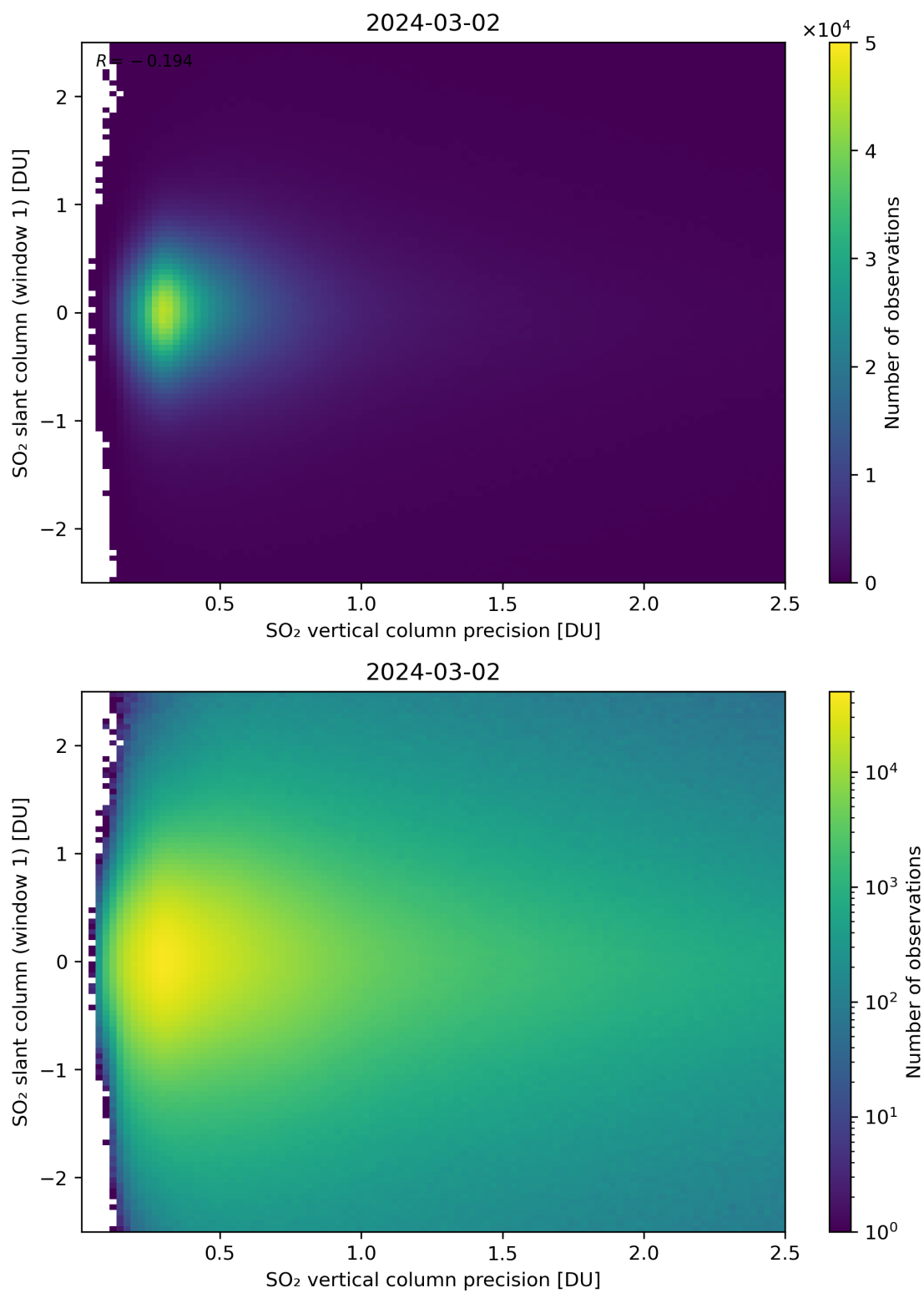
Figure 289: Scatter density plot of “SO 2 vertical column precision” against “SO 2 slant column (window 1)” for 2024-03-01 to 2024-03-03.
