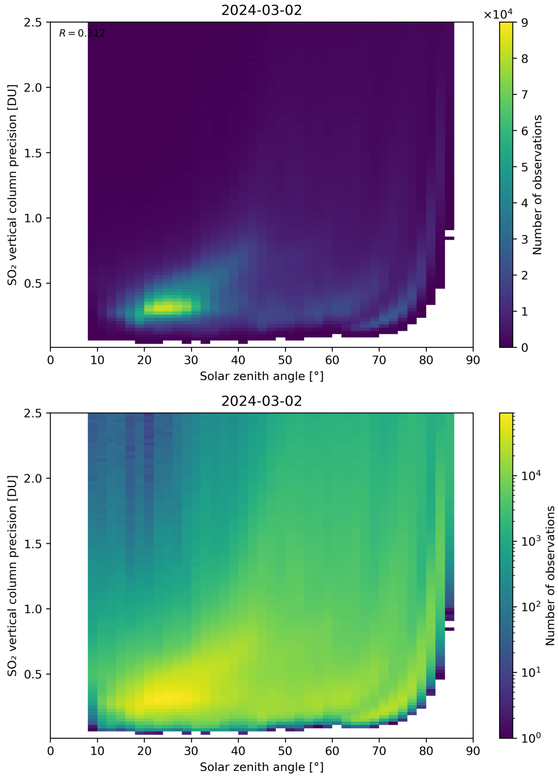
Figure 177: Scatter density plot of “Solar zenith angle” against “SO 2 vertical column precision” for 2024-03-01 to 2024-03-03.
