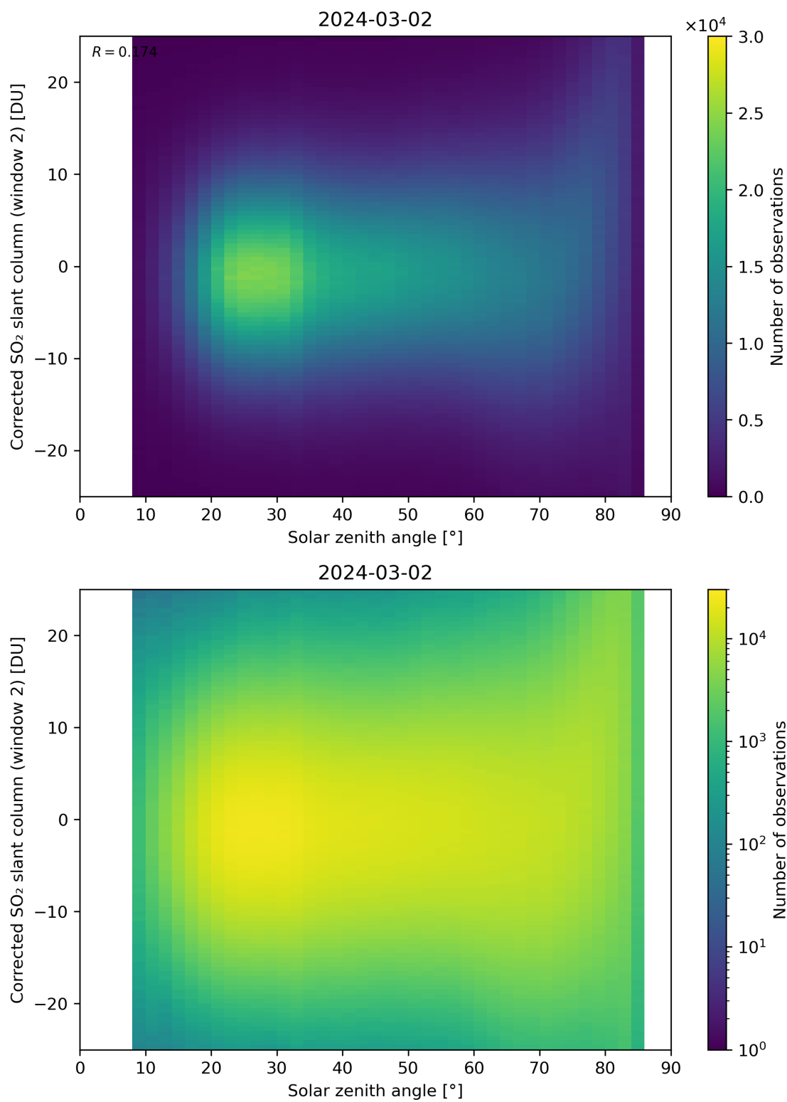
Figure 167: Scatter density plot of “Solar zenith angle” against “Corrected SO 2 slant column (window 2)” for 2024-03-01 to 2024-03-03.
