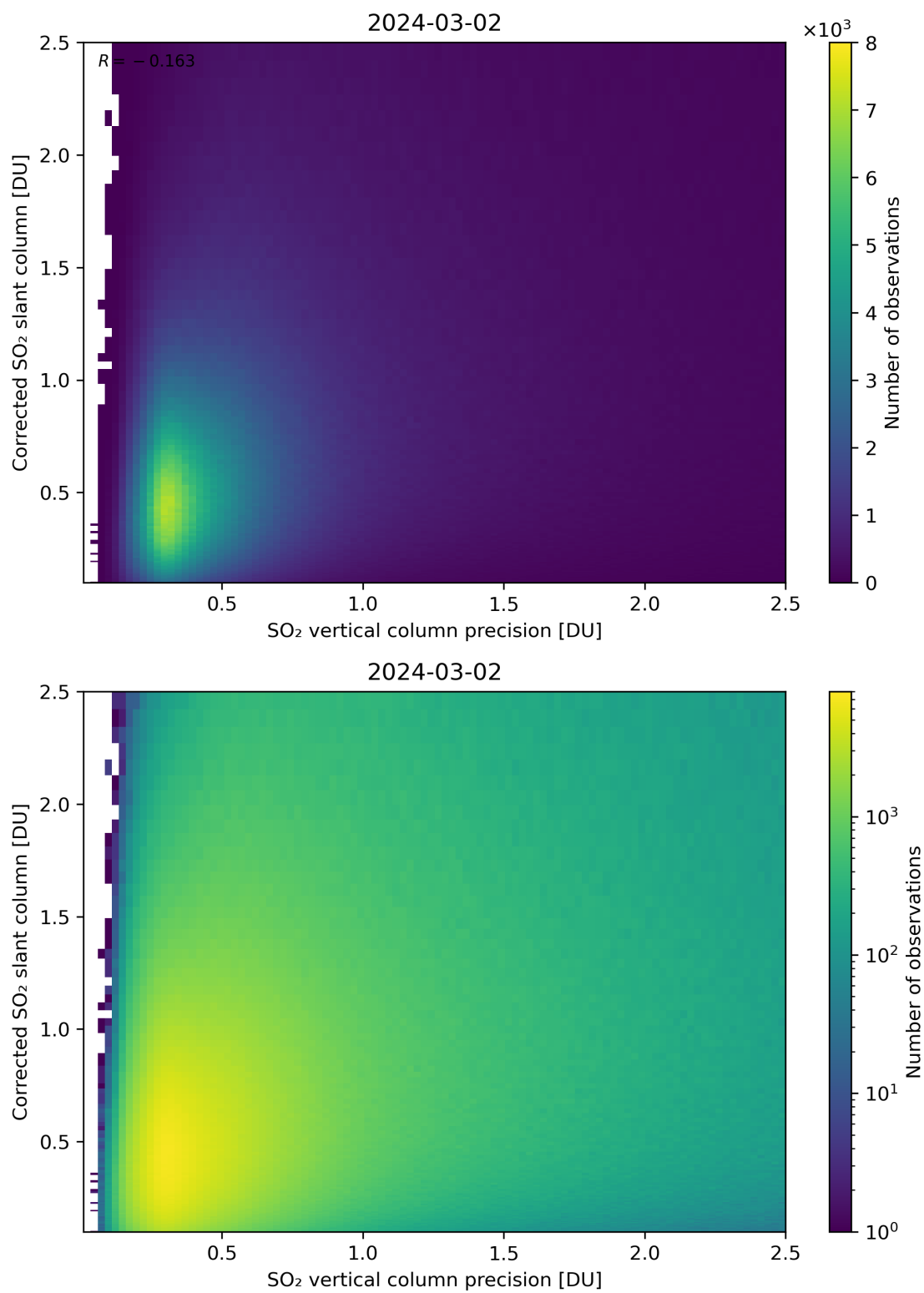
Figure 286: Scatter density plot of “SO 2 vertical column precision” against “Corrected SO 2 slant column” for 2024-03-01 to 2024-03-03.
