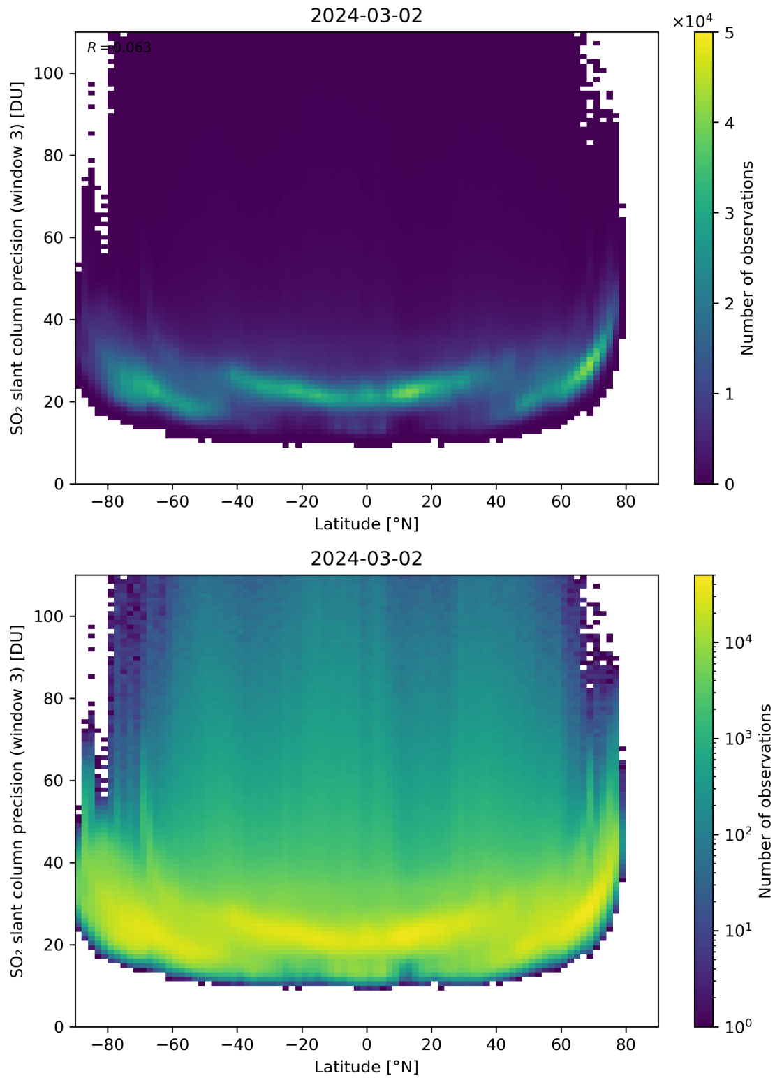
Figure 153: Scatter density plot of “Latitude” against “SO 2 slant column precision (window 3)” for 2024-03-01 to 2024-03-03.
