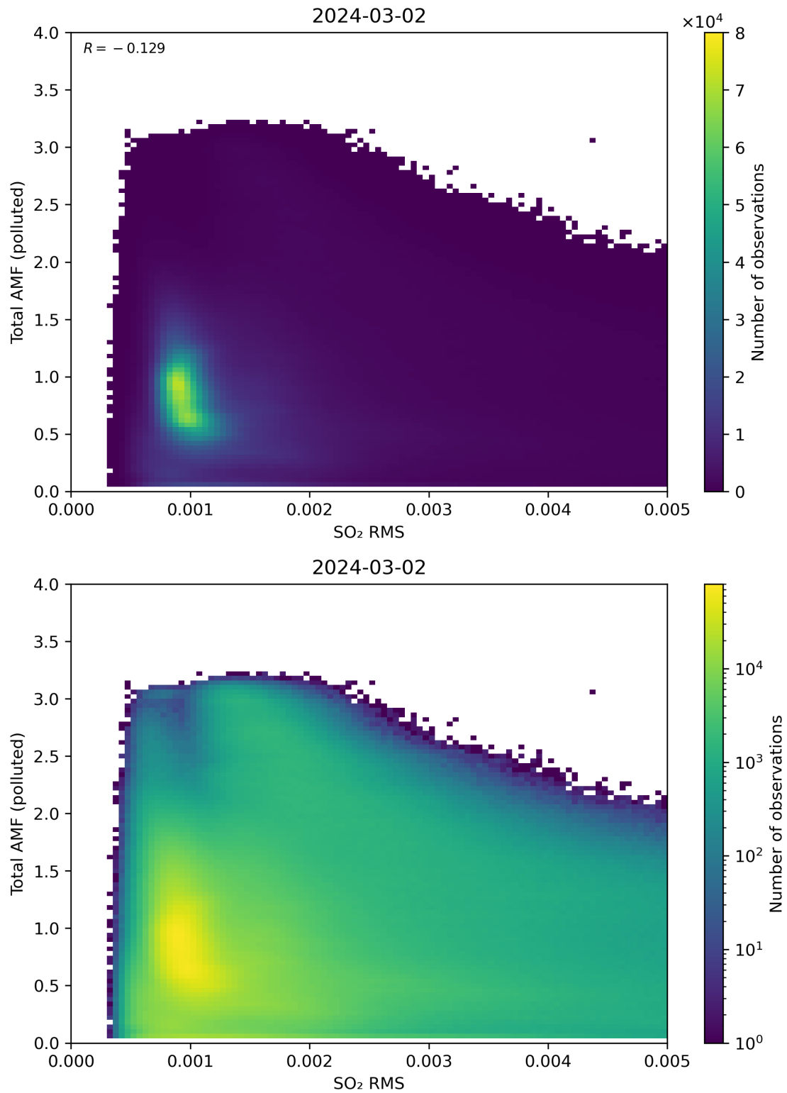
Figure 137: Scatter density plot of “SO 2 RMS” against “Total AMF (polluted)” for 2024-03-01 to 2024-03-03.
