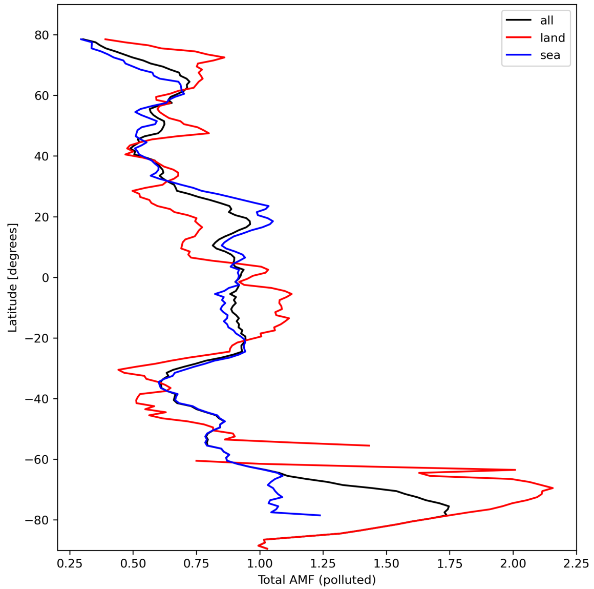
Figure 48: Zonal average of “Total AMF (polluted)” for 2024-03-01 to 2024-03-03.
