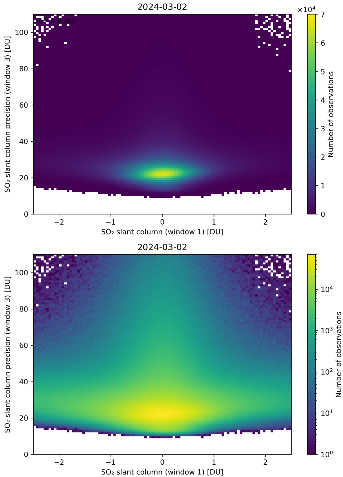
Figure 238: Scatter density plot of “SO 2 slant column (window 1)” against “SO 2 slant column precision (window 3)” for 2024-03-01 to 2024-03-03.
