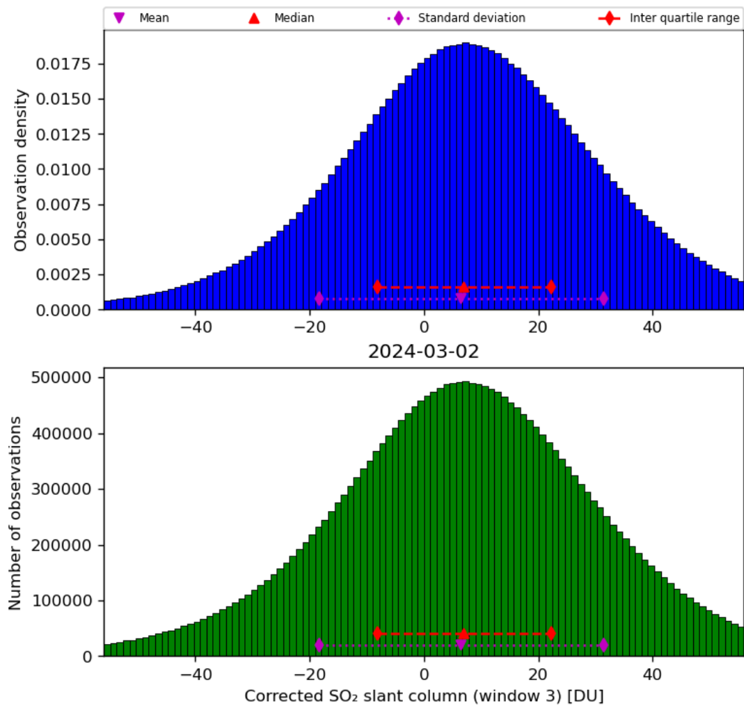
Figure 66: Histogram of “Corrected SO 2 slant column (window 3)” for 2024-03-01 to 2024-03-03
