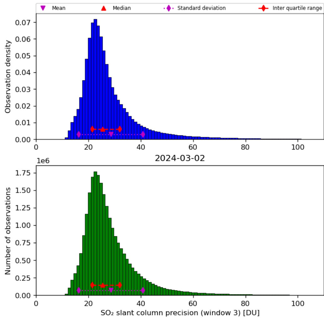
Figure 65: Histogram of “SO 2 slant column precision (window 3)” for 2024-03-01 to 2024-03-03
