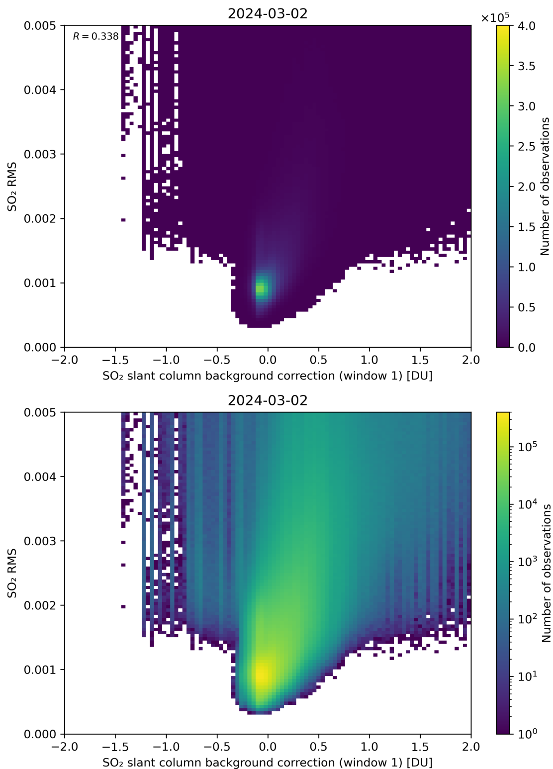
Figure 102: Scatter density plot of “SO 2 slant column background correction (window 1)” against “SO 2 RMS” for 2024-03-01 to 2024-03-03.
