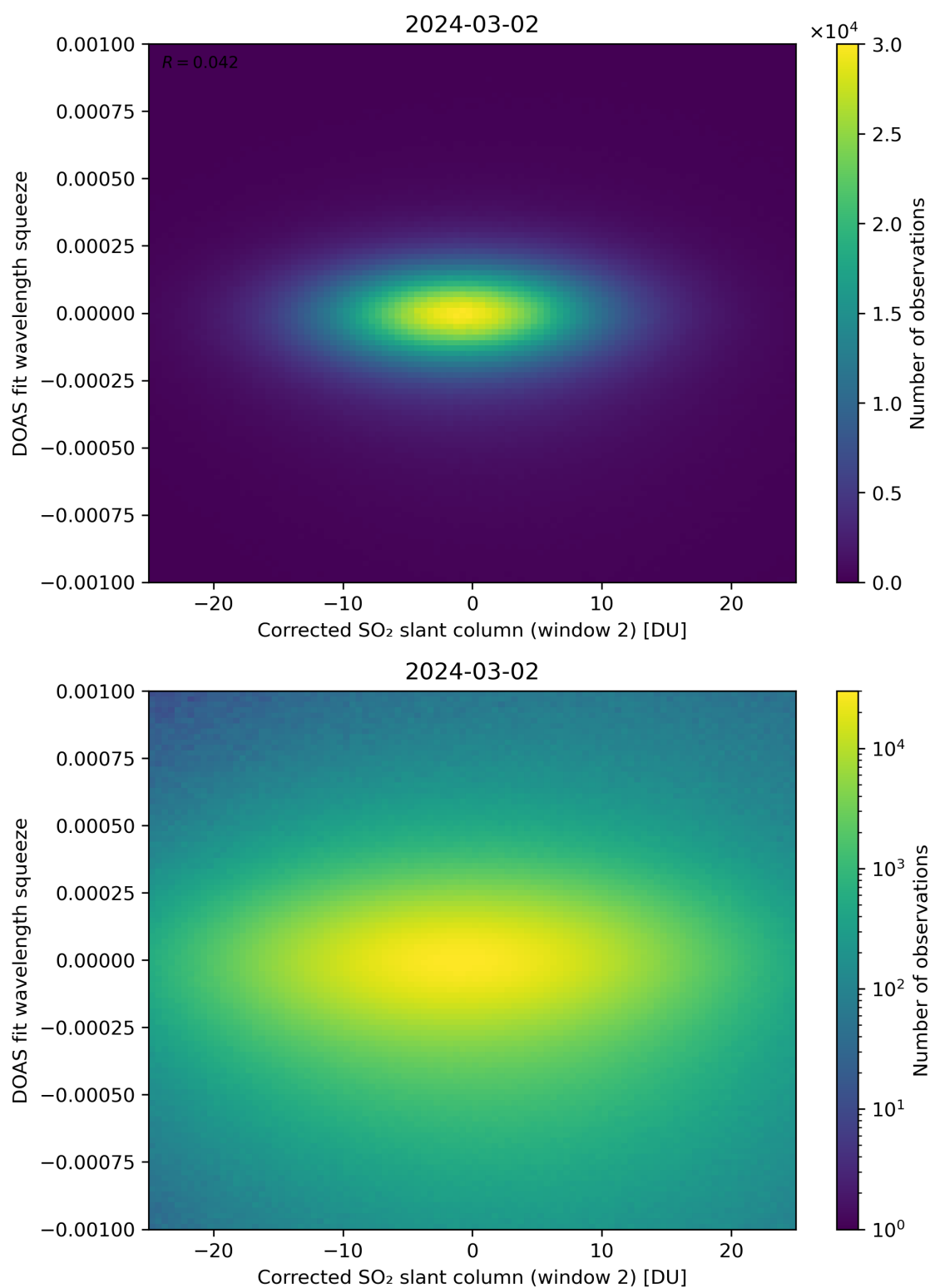
Figure 197: Scatter density plot of “Corrected SO 2 slant column (window 2)” against “DOAS fit wavelength squeeze” for 2024-03-01 to 2024-03-03.
