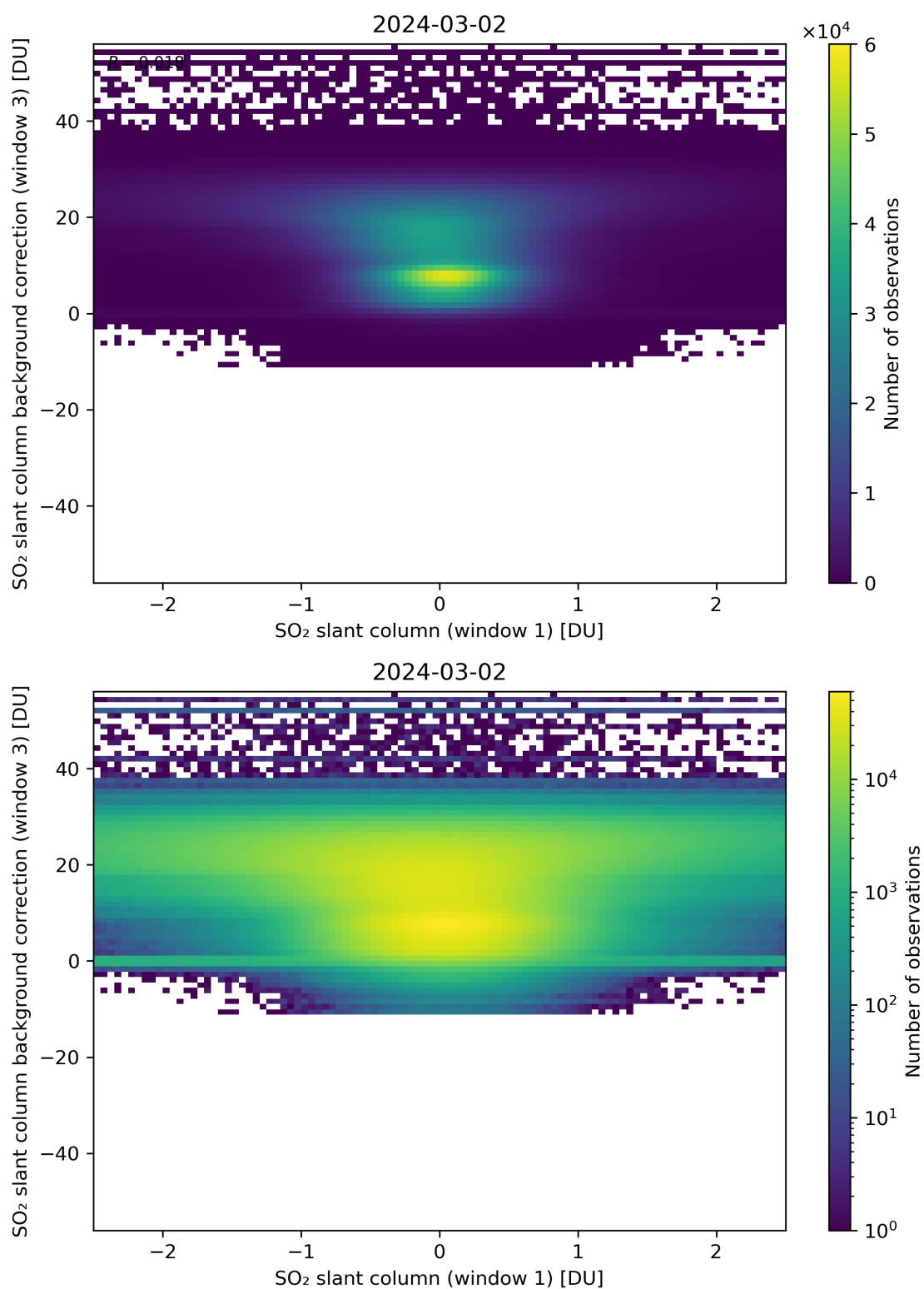
Figure 214: Scatter density plot of “SO 2 slant column (window 1)” against “SO 2 slant column background correction (window 3)” for 2024-03-01 to 2024-03-03.
