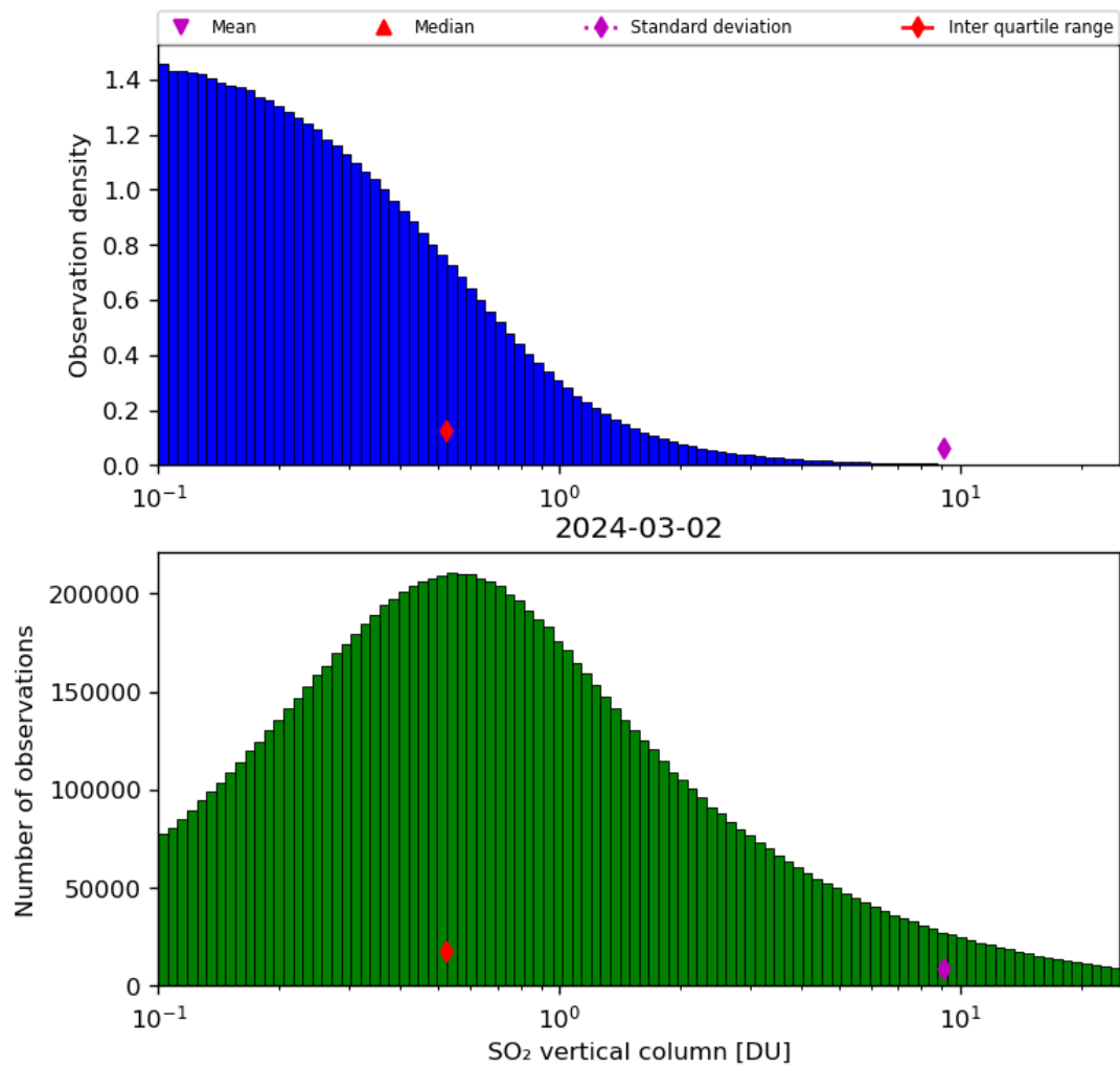
Figure 53: Histogram of “SO 2 vertical column” for 2024-03-01 to 2024-03-03
