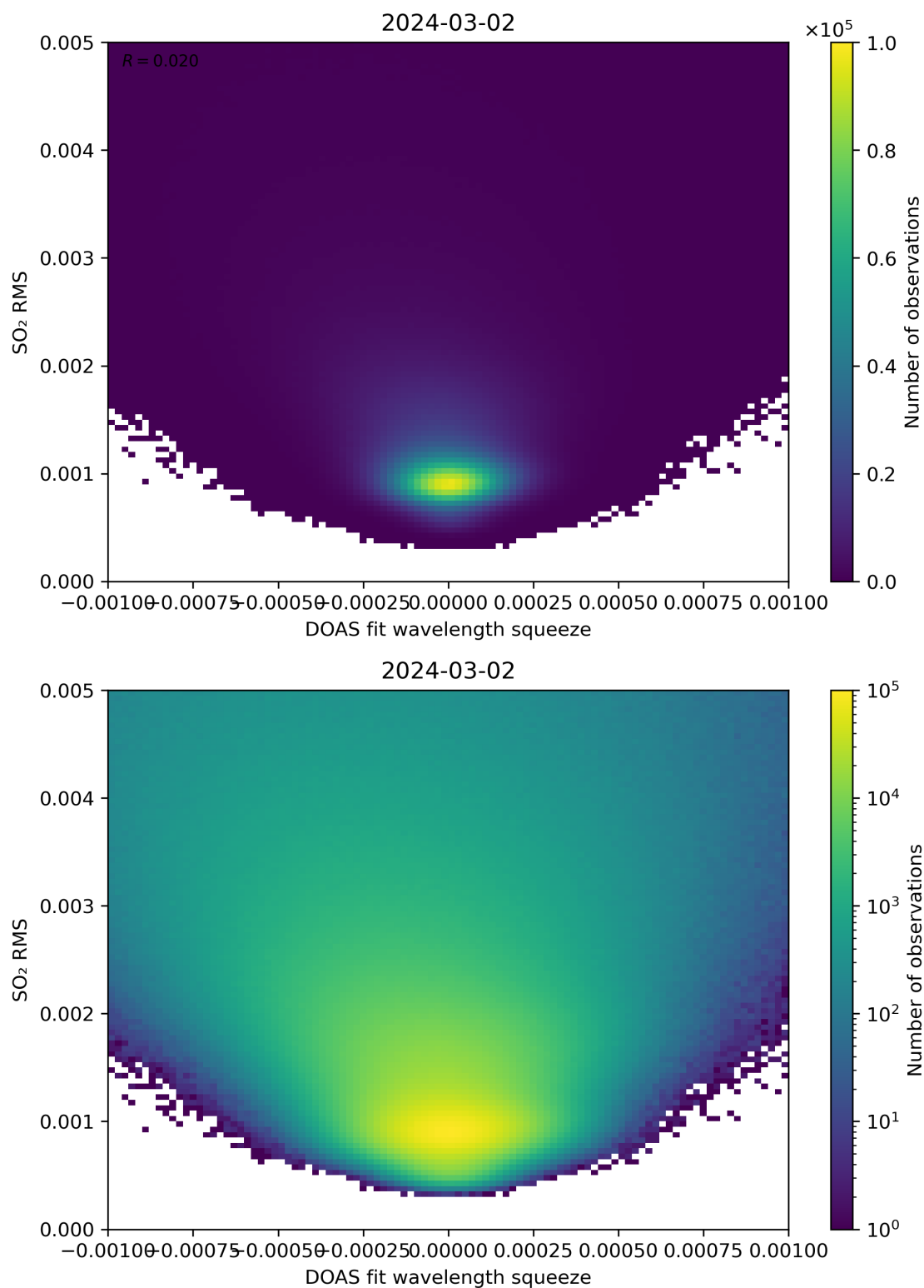
Figure 132: Scatter density plot of “DOAS fit wavelength squeeze” against “SO 2 RMS” for 2024-03-01 to 2024-03-03.
