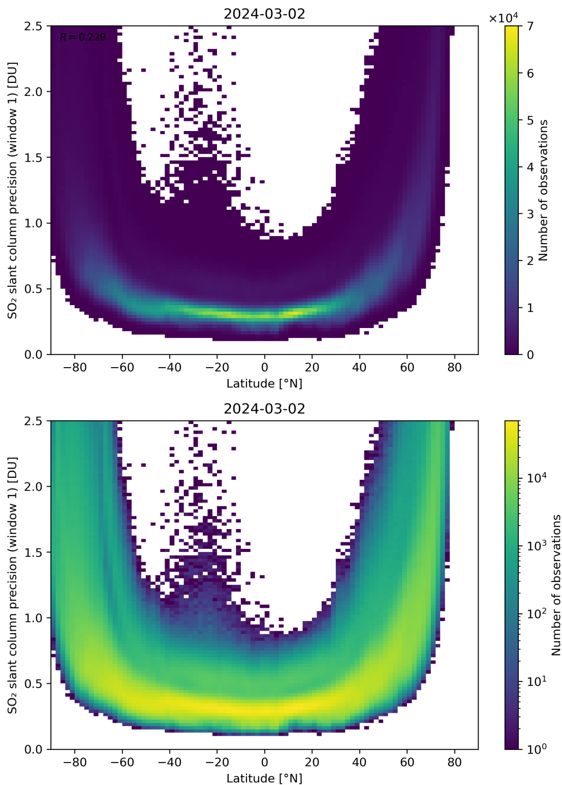
Figure 150: Scatter density plot of “Latitude” against “SO 2 slant column precision (window 1)” for 2024-03-01 to 2024-03-03.
