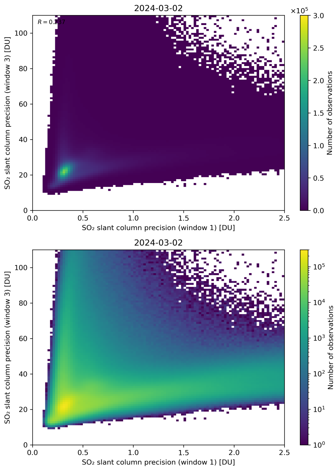
Figure 229: Scatter density plot of “SO 2 slant column precision (window 1)” against “SO 2 slant column precision (window 3)” for 2024-03-01 to 2024-03-03.
