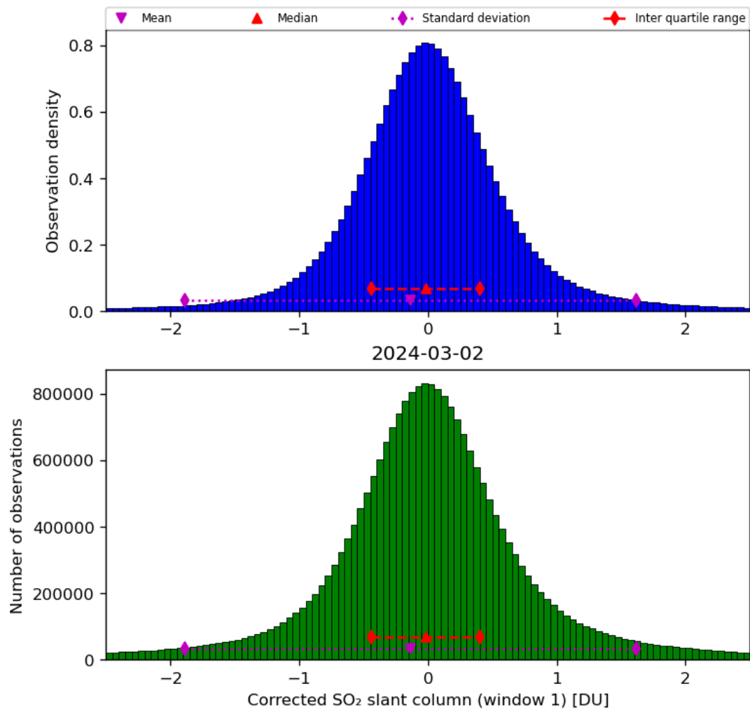
Figure 58: Histogram of “Corrected SO 2 slant column (window 1)” for 2024-03-01 to 2024-03-03
