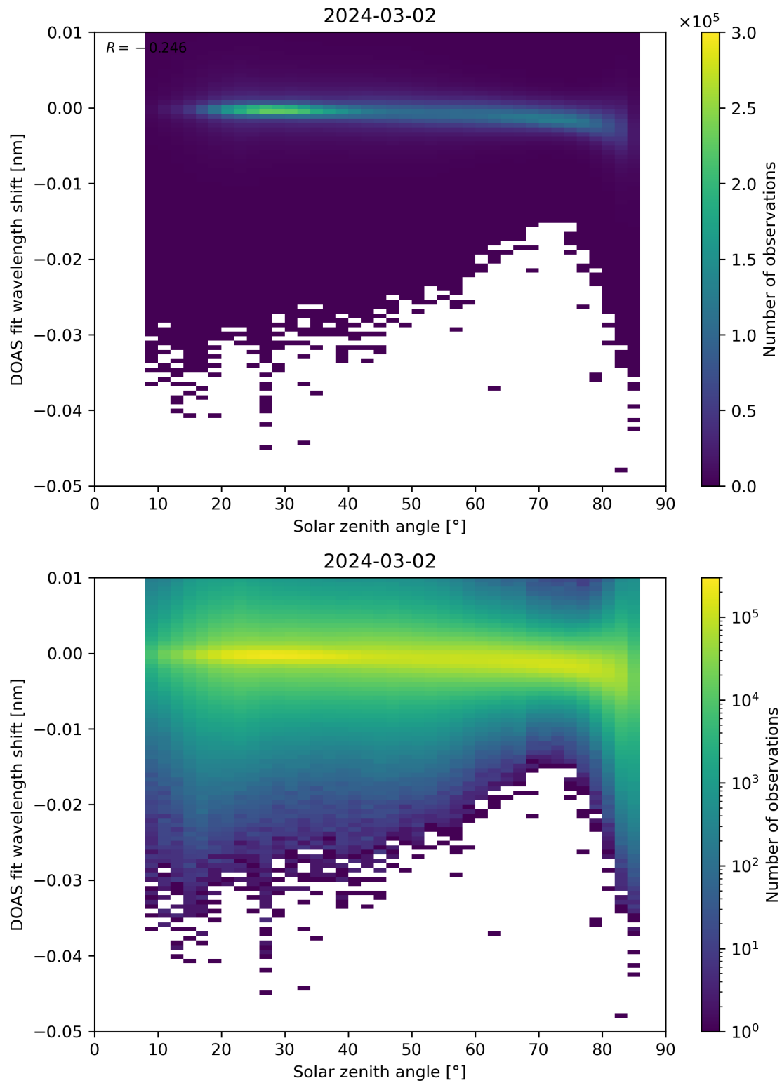
Figure 161: Scatter density plot of “Solar zenith angle” against “DOAS fit wavelength shift” for 2024-03-01 to 2024-03-03.
