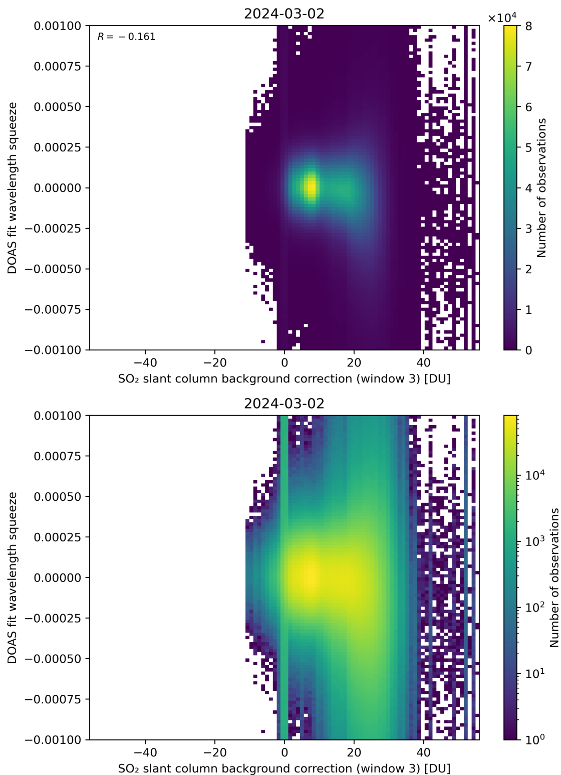
Figure 122: Scatter density plot of “SO 2 slant column background correction (window 3)” against “DOAS fit wavelength squeeze” for 2024-03-01 to 2024-03-03.
