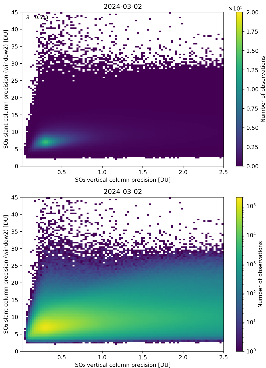
Figure 291: Scatter density plot of “SO 2 vertical column precision” against “SO 2 slant column precision (window2)” for 2024-03-01 to 2024-03-03.
