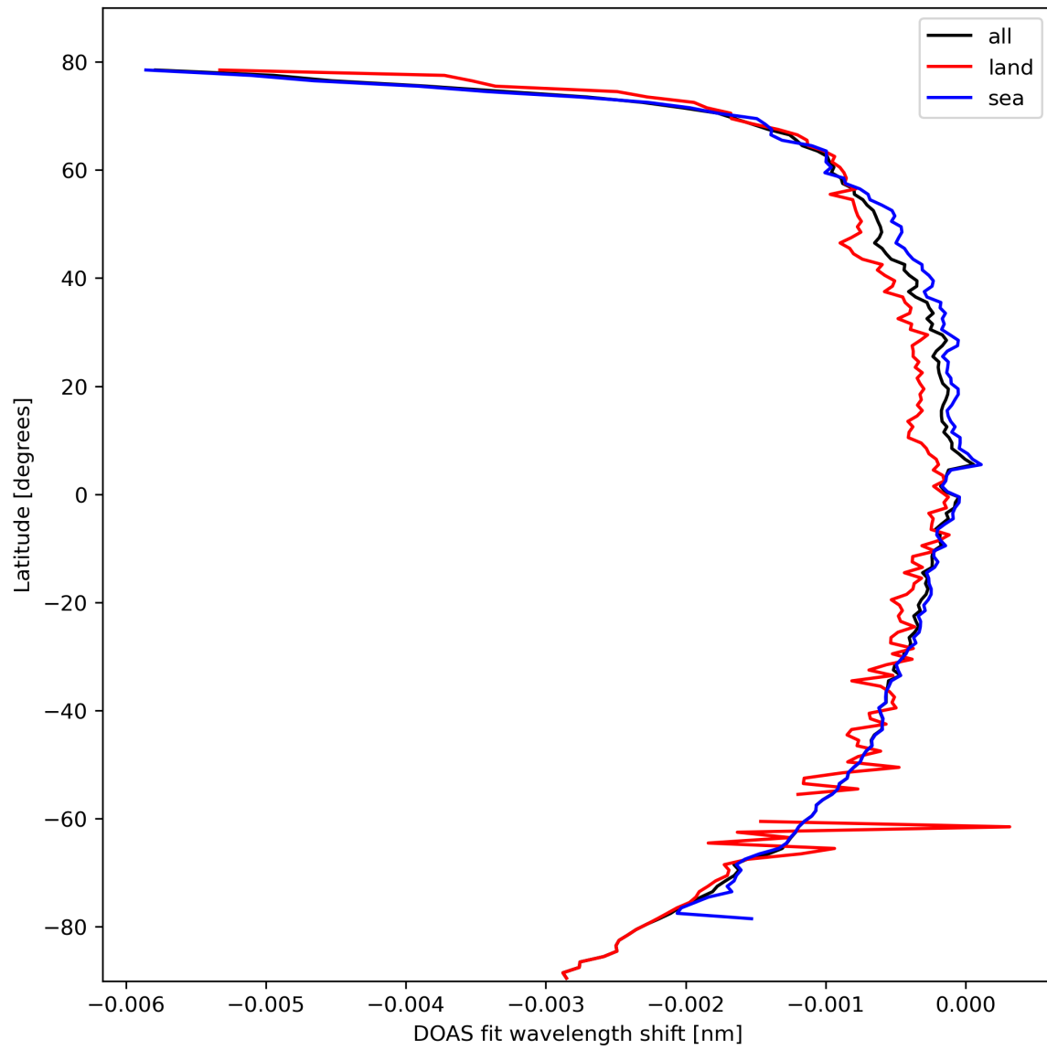
Figure 45: Zonal average of “DOAS fit wavelength shift” for 2024-03-01 to 2024-03-03.
