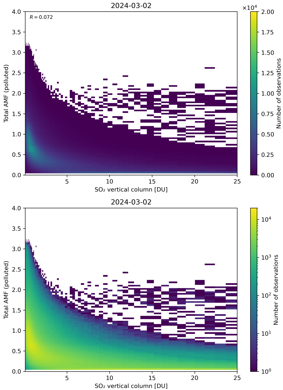
Figure 305: Scatter density plot of “SO 2 vertical column” against “Total AMF (polluted)” for 2024-03-01 to 2024-03-03.
