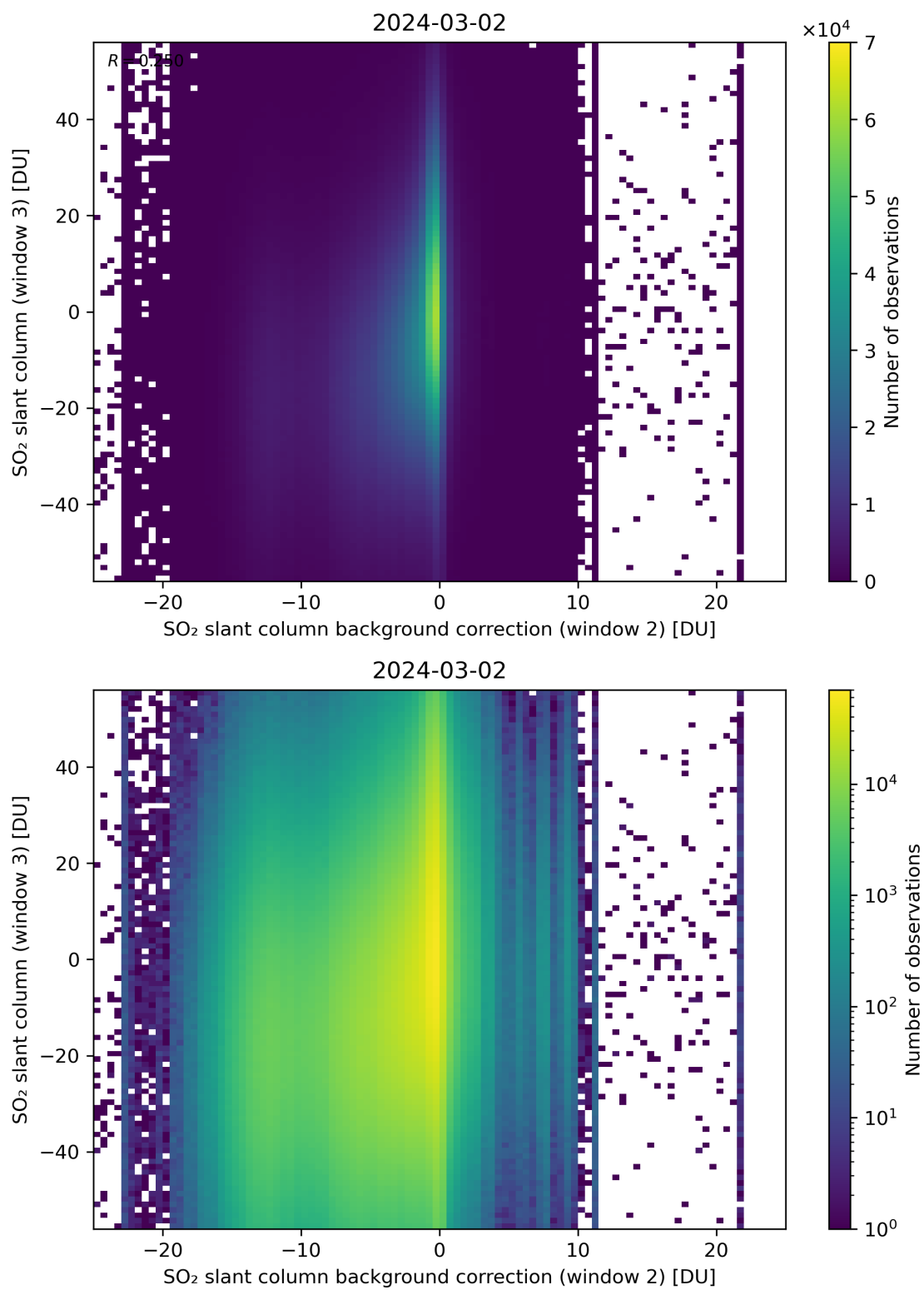
Figure 117: Scatter density plot of “SO 2 slant column background correction (window 2)” against “SO 2 slant column (window 3)” for 2024-03-01 to 2024-03-03.
