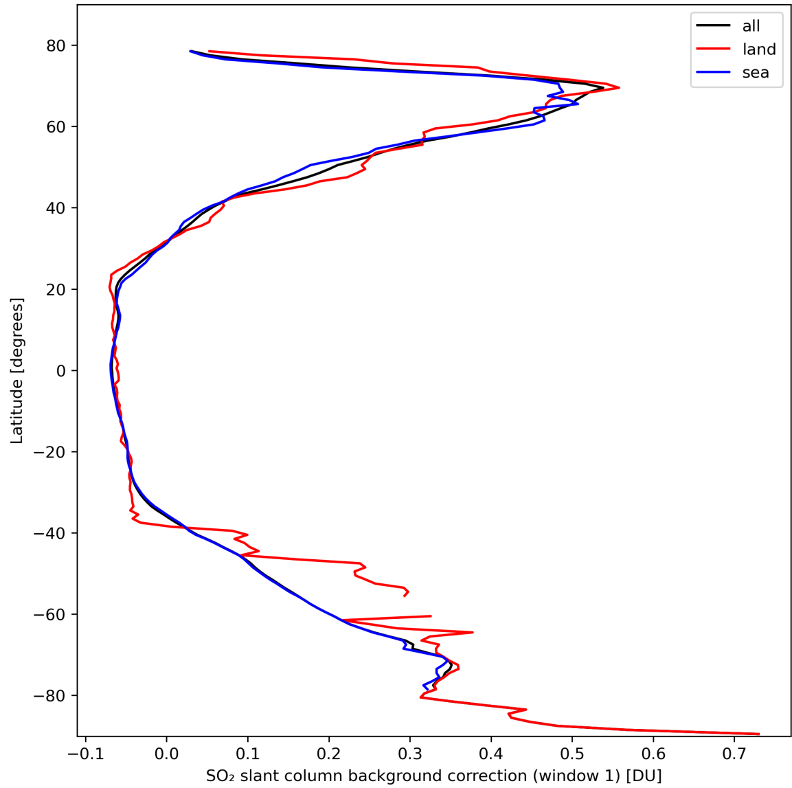
Figure 36: Zonal average of “SO 2 slant column background correction (window 1)” for 2024-03-01 to 2024-03-03.
