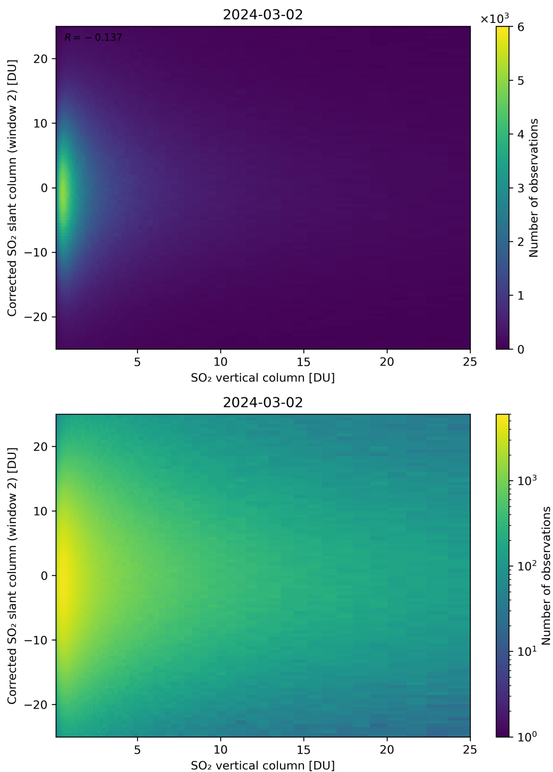
Figure 298: Scatter density plot of “SO 2 vertical column” against “Corrected SO 2 slant column (window 2)” for 2024-03-01 to 2024-03-03.
