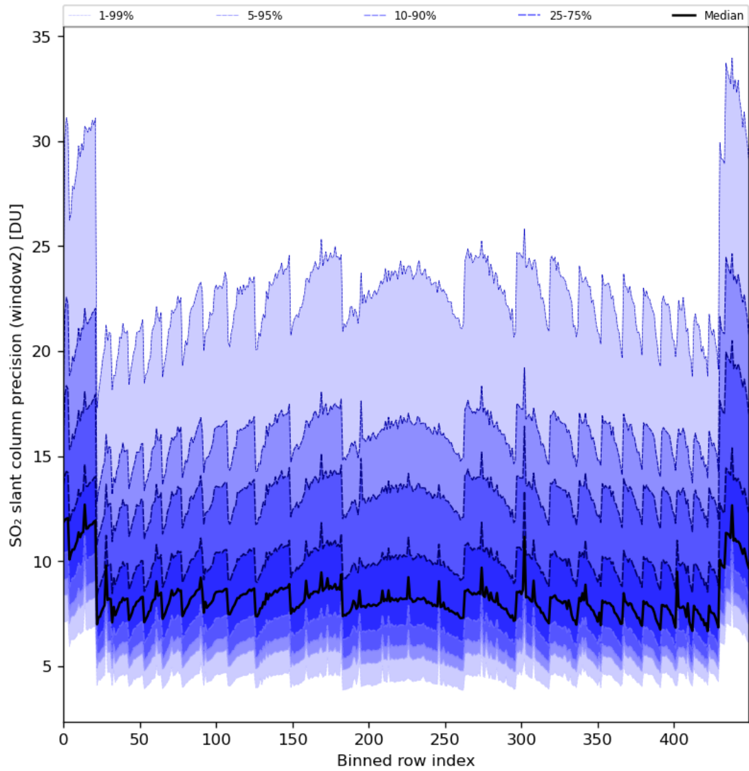
Figure 84: Along track statistics of “SO 2 slant column precision (window2)” for 2024-03-01 to 2024-03-03
