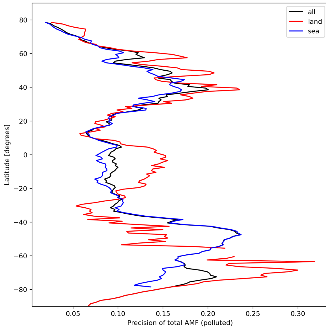
Figure 49: Zonal average of “Precision of total AMF (polluted)” for 2024-03-01 to 2024-03-03.
