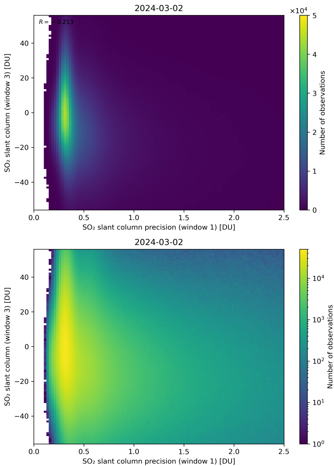
Figure 228: Scatter density plot of “SO 2 slant column precision (window 1)” against “SO 2 slant column (window 3)” for 2024-03-01 to 2024-03-03.
