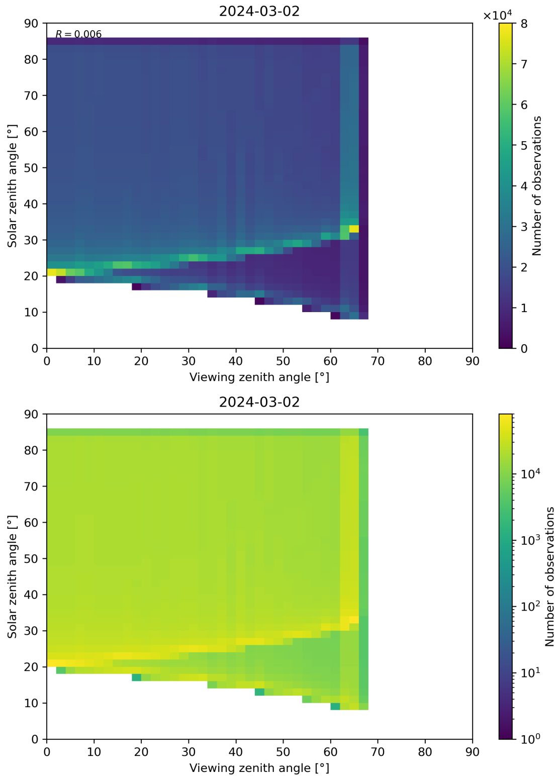
Figure 315: Scatter density plot of “Viewing zenith angle” against “Solar zenith angle” for 2024-03-01 to 2024-03-03.
