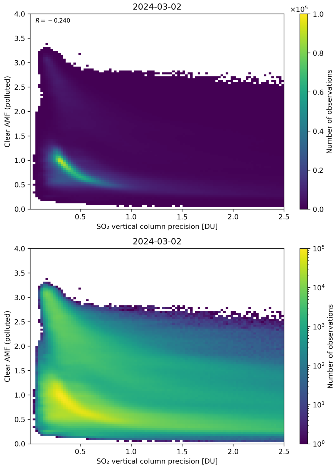
Figure 285: Scatter density plot of “SO 2 vertical column precision” against “Clear AMF (polluted)” for 2024-03-01 to 2024-03-03.
