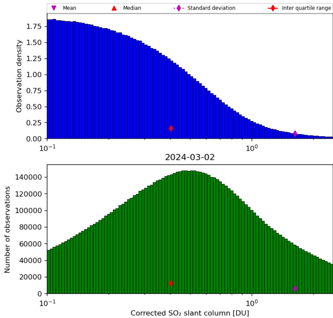
Figure 55: Histogram of “Corrected SO 2 slant column” for 2024-03-01 to 2024-03-03
