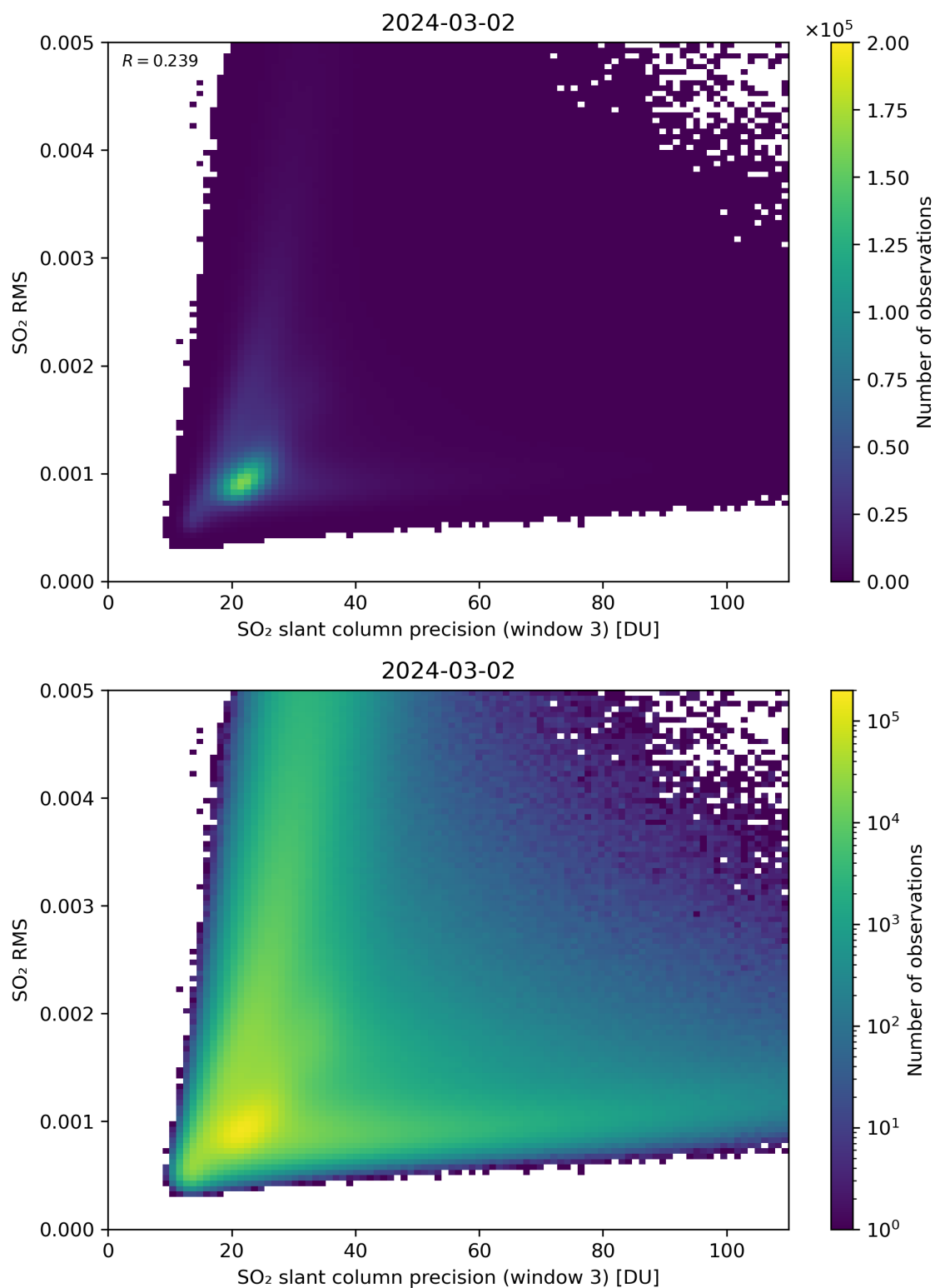
Figure 260: Scatter density plot of “SO 2 slant column precision (window 3)” against “SO 2 RMS” for 2024-03-01 to 2024-03-03.
