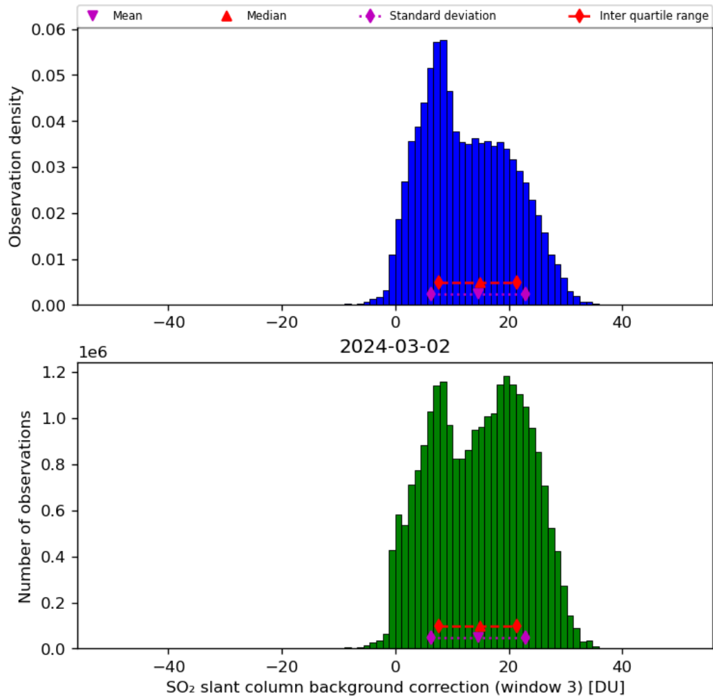
Figure 67: Histogram of “SO 2 slant column background correction (window 3)” for 2024-03-01 to 2024-03-03
