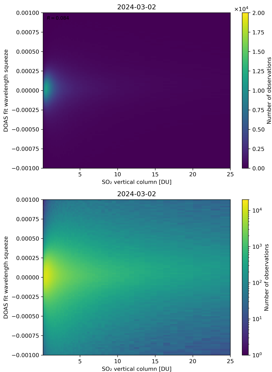
Figure 277: Scatter density plot of “SO 2 vertical column” against “DOAS fit wavelength squeeze” for 2024-03-01 to 2024-03-03.
