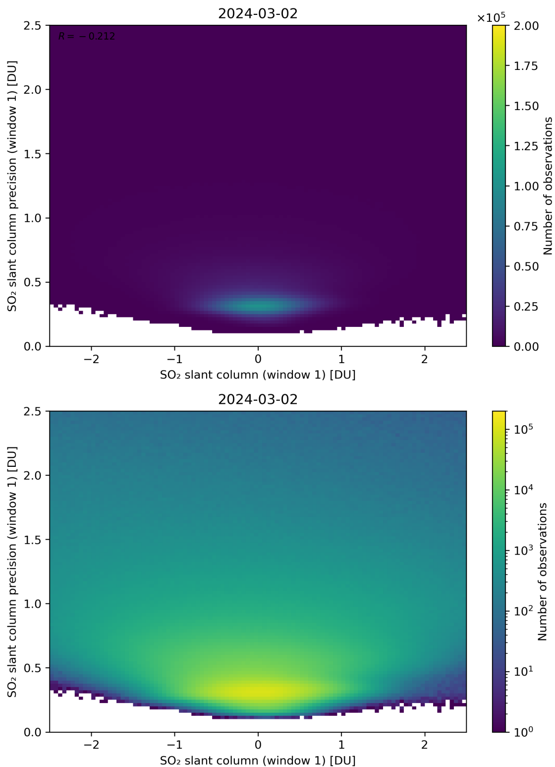
Figure 235: Scatter density plot of “SO 2 slant column (window 1)” against “SO 2 slant column precision (window 1)” for 2024-03-01 to 2024-03-03.
