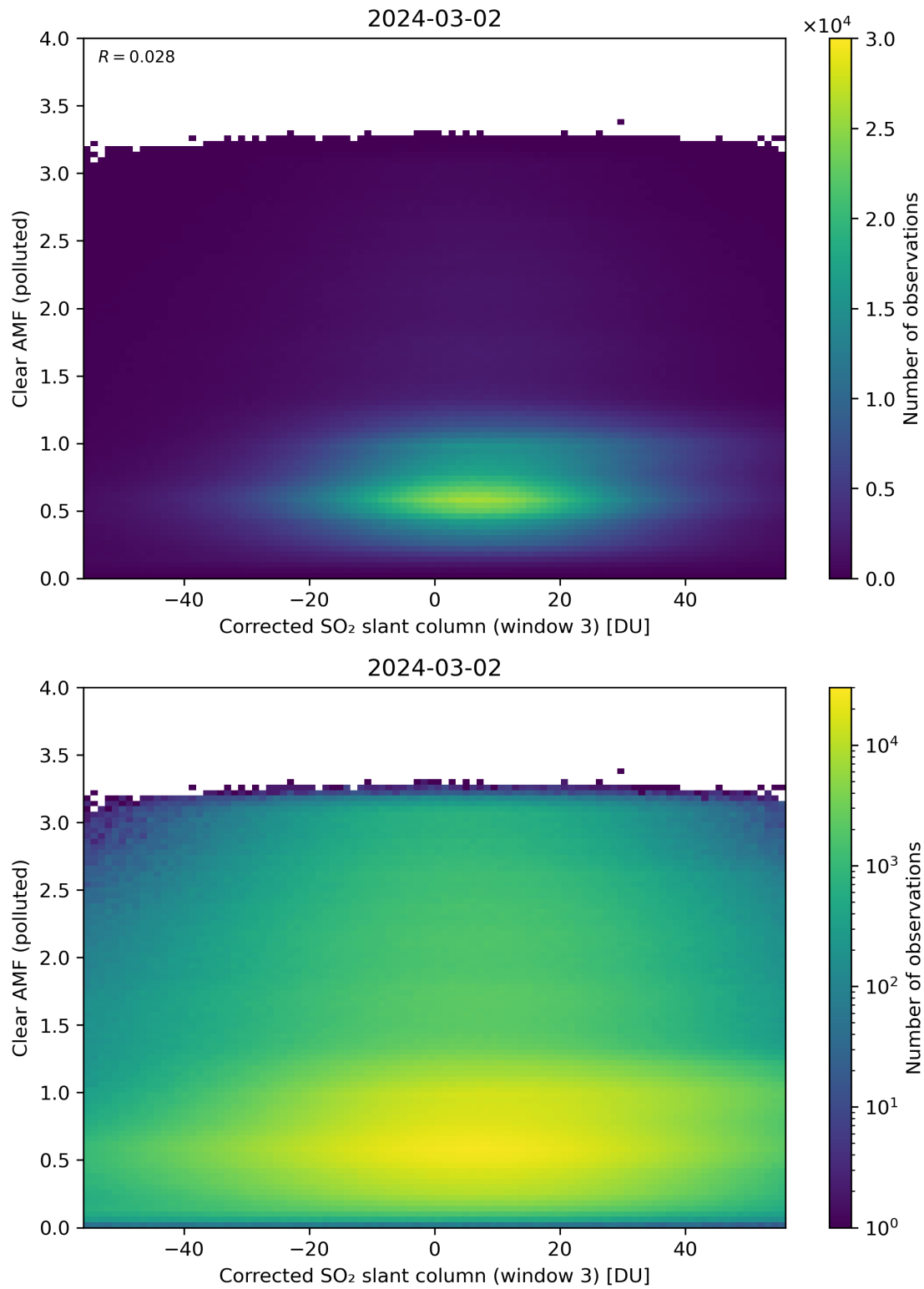
Figure 209: Scatter density plot of “Corrected SO 2 slant column (window 3)” against “Clear AMF (polluted)” for 2024-03-01 to 2024-03-03.
