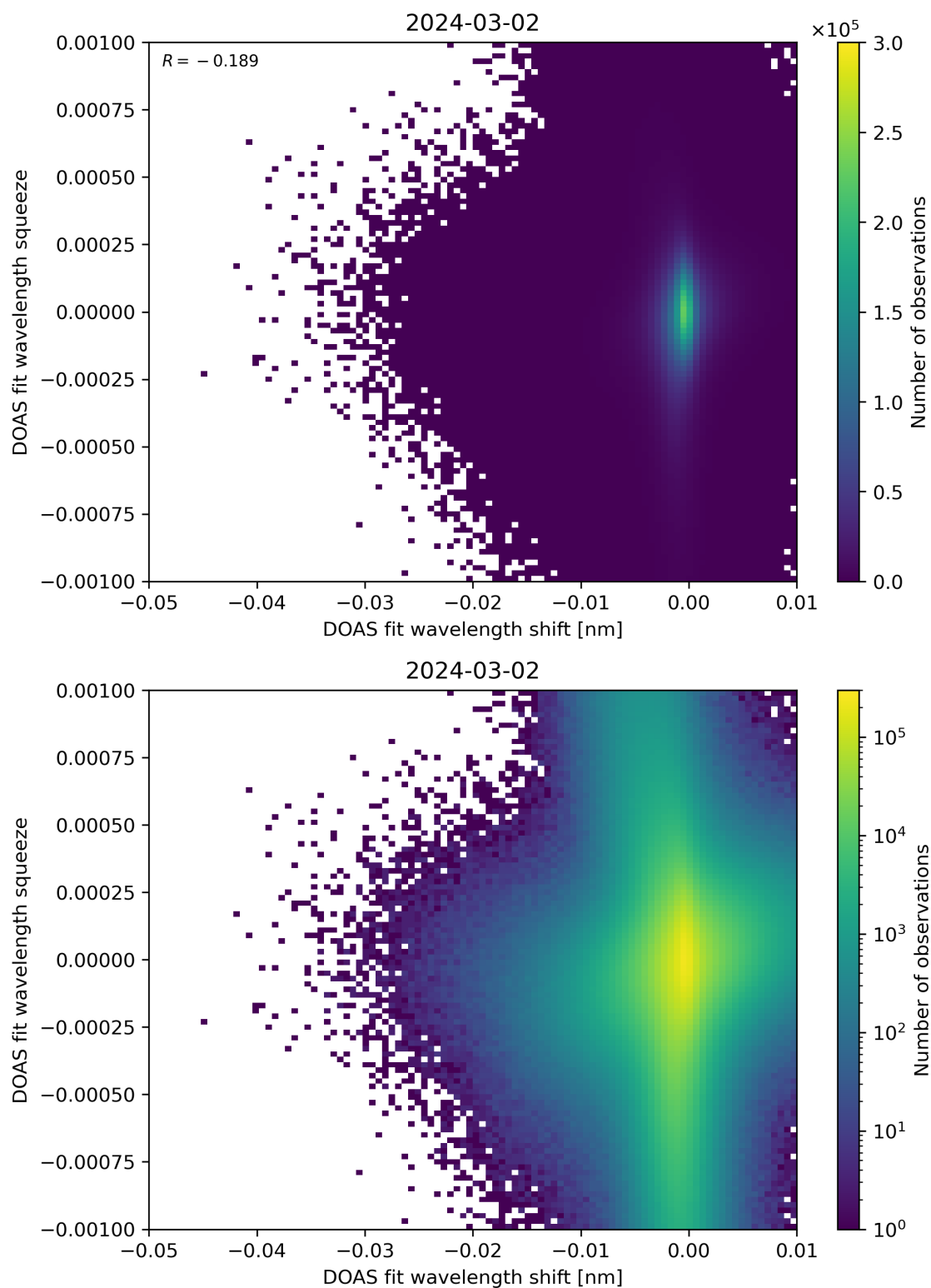
Figure 127: Scatter density plot of “DOAS fit wavelength shift” against “DOAS fit wavelength squeeze” for 2024-03-01 to 2024-03-03.
