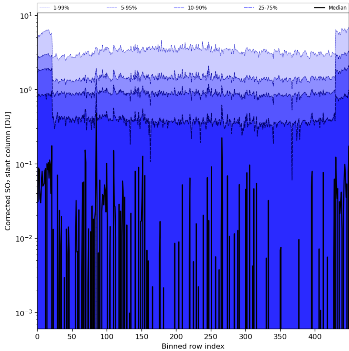
Figure 78: Along track statistics of “Corrected SO 2 slant column” for 2024-03-01 to 2024-03-03
