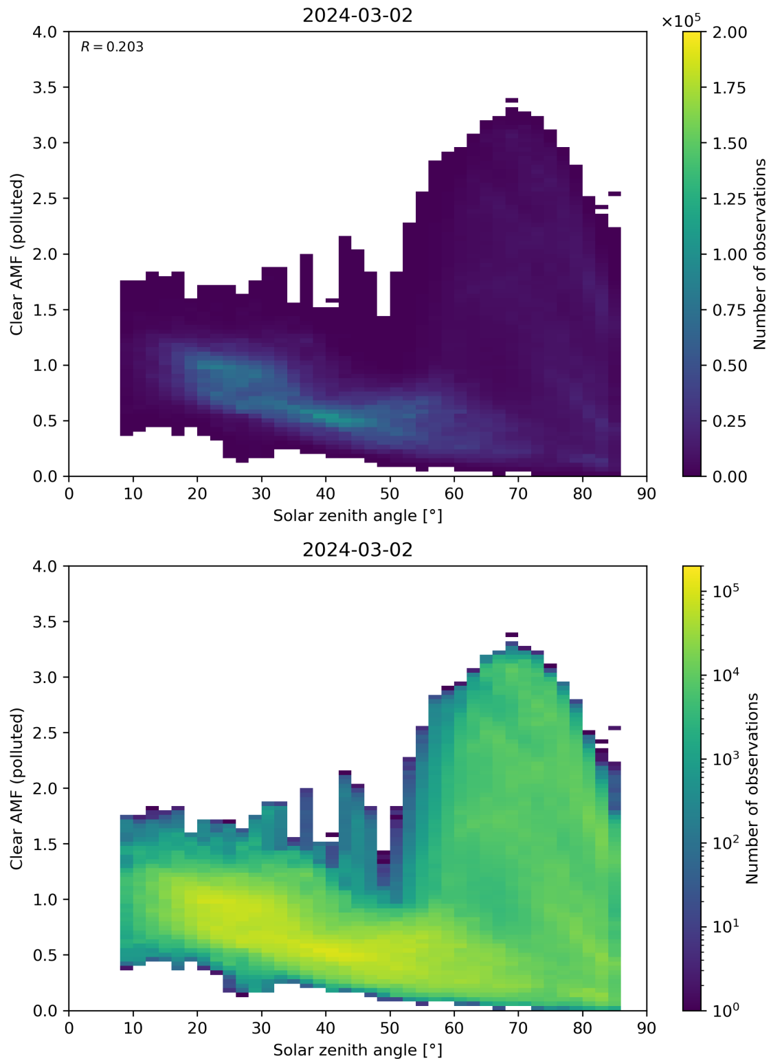
Figure 165: Scatter density plot of “Solar zenith angle” against “Clear AMF (polluted)” for 2024-03-01 to 2024-03-03.
