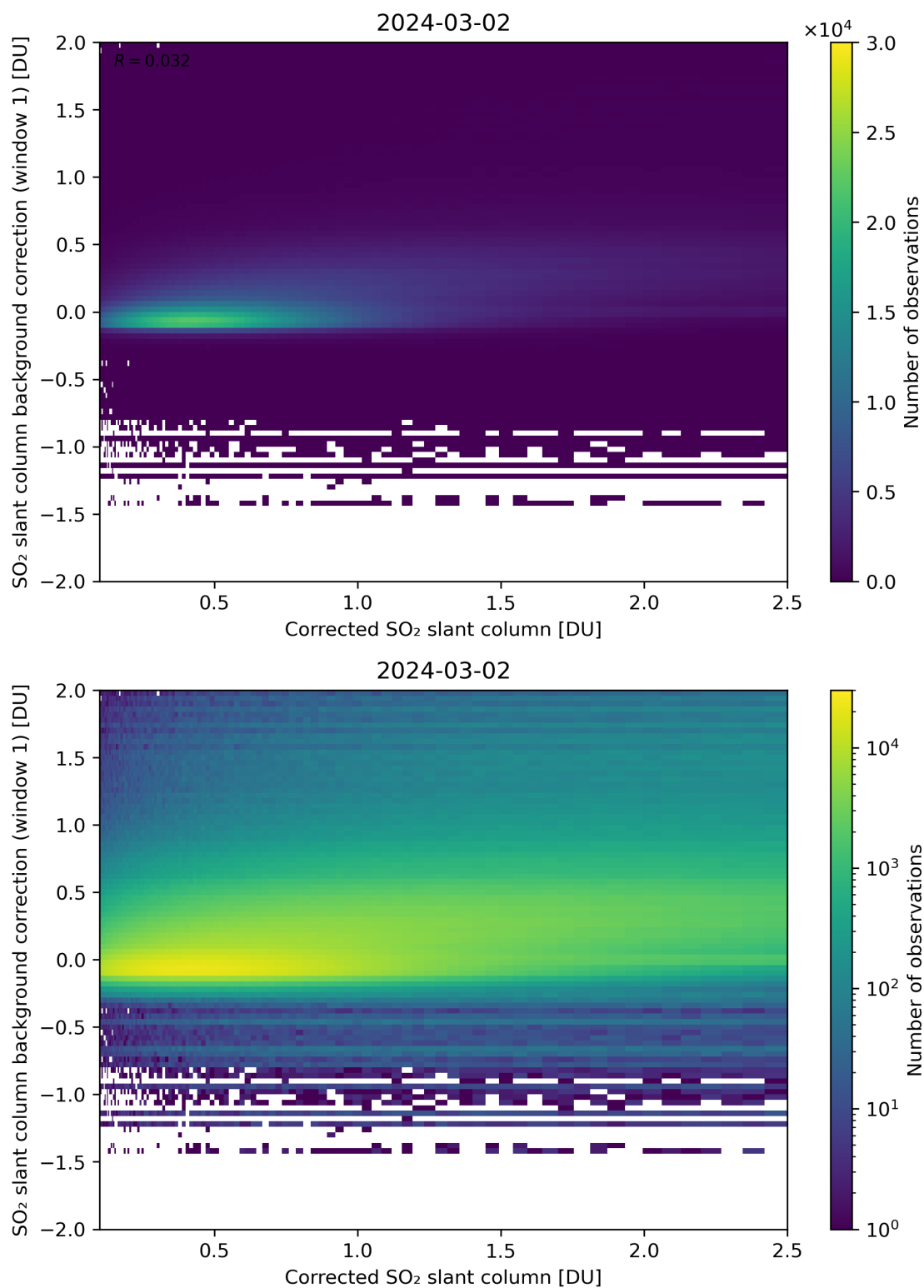
Figure 178: Scatter density plot of “Corrected SO 2 slant column” against “SO 2 slant column background correction (window 1)” for 2024-03-01 to 2024-03-03.
