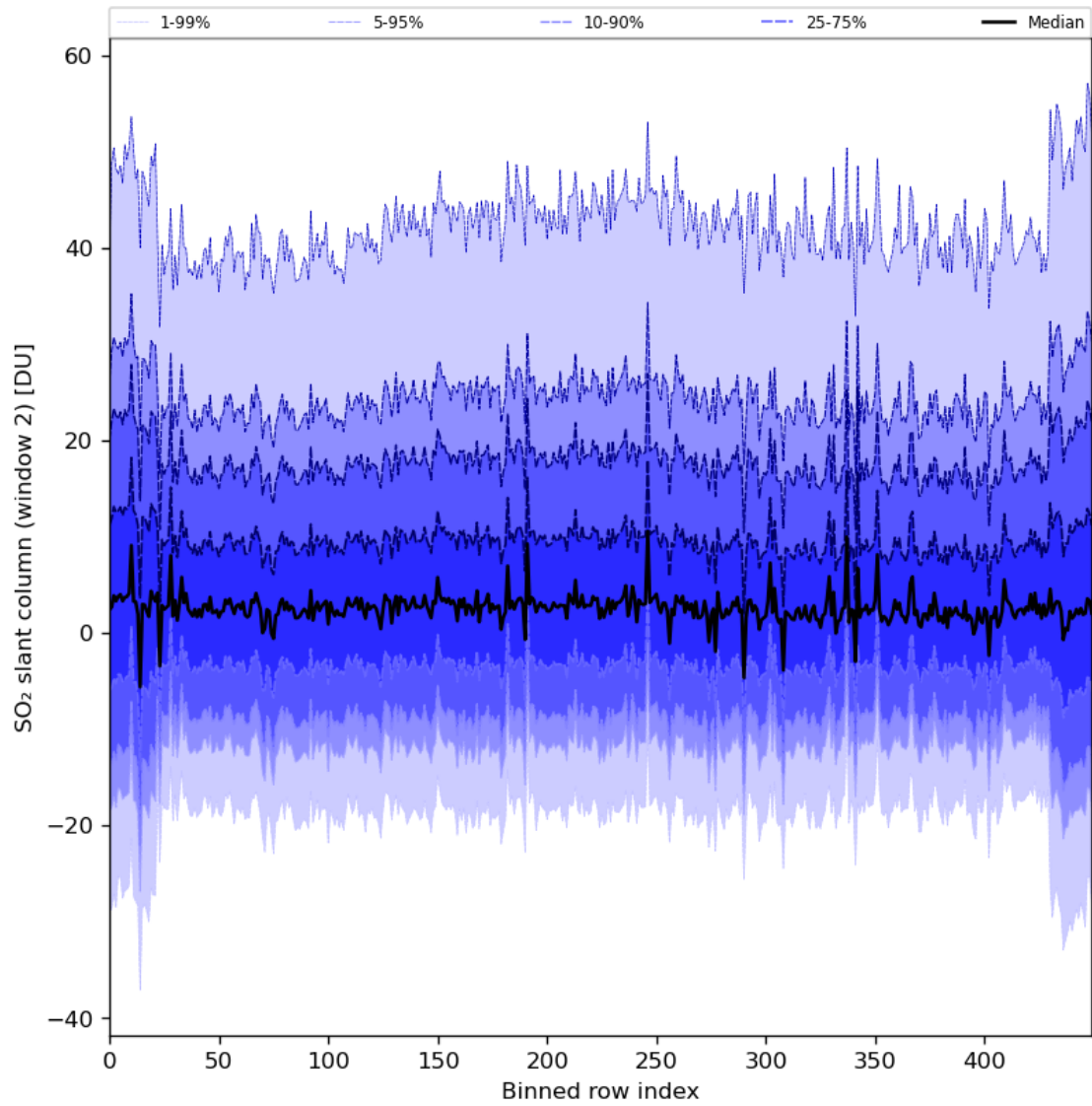
Figure 83: Along track statistics of “SO 2 slant column (window 2)” for 2024-03-01 to 2024-03-03
