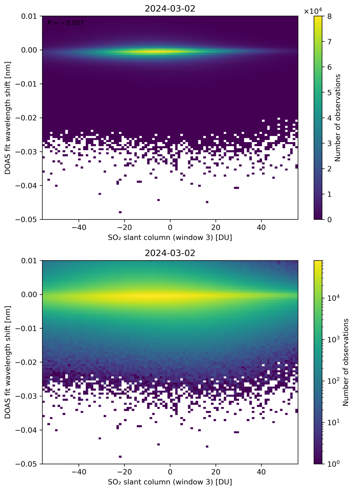
Figure 254: Scatter density plot of “SO 2 slant column (window 3)” against “DOAS fit wavelength shift” for 2024-03-01 to 2024-03-03.
