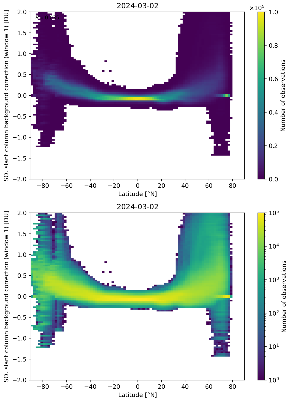
Figure 139: Scatter density plot of “Latitude” against “SO 2 slant column background correction (window 1)” for 2024-03-01 to 2024-03-03.
