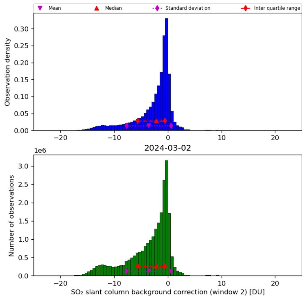
Figure 63: Histogram of “SO 2 slant column background correction (window 2)” for 2024-03-01 to 2024-03-03
