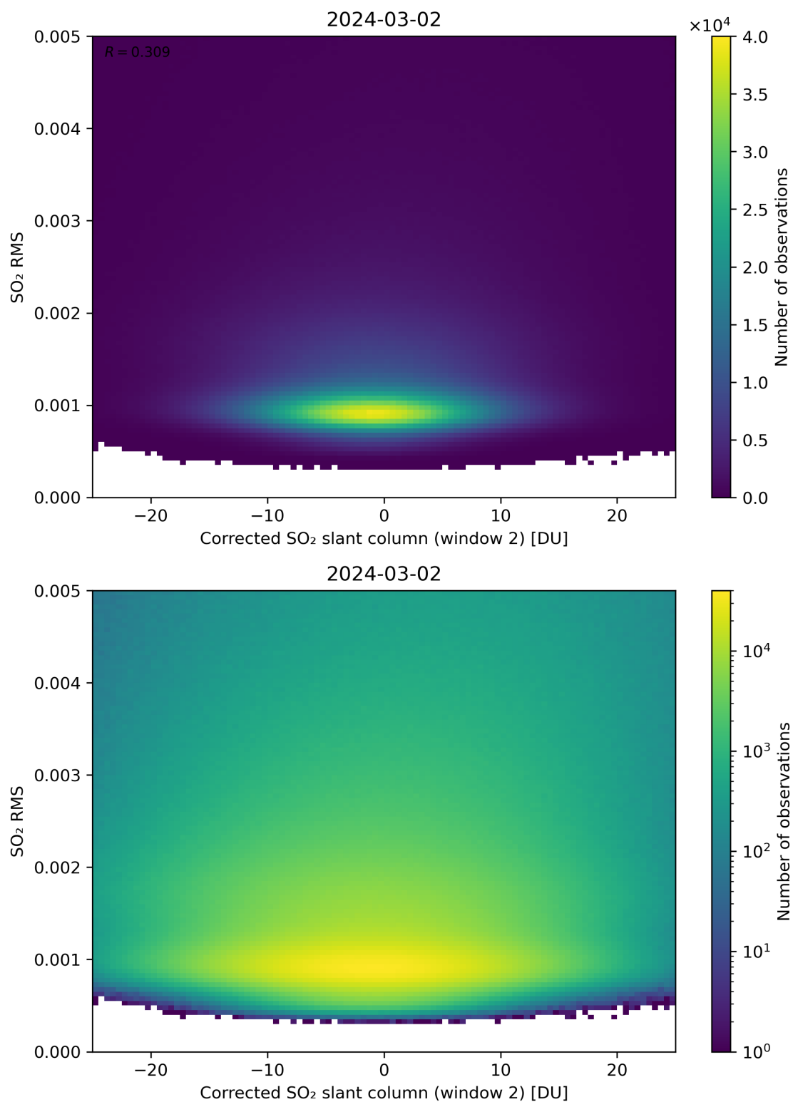
Figure 198: Scatter density plot of “Corrected SO 2 slant column (window 2)” against “SO 2 RMS” for 2024-03-01 to 2024-03-03.
