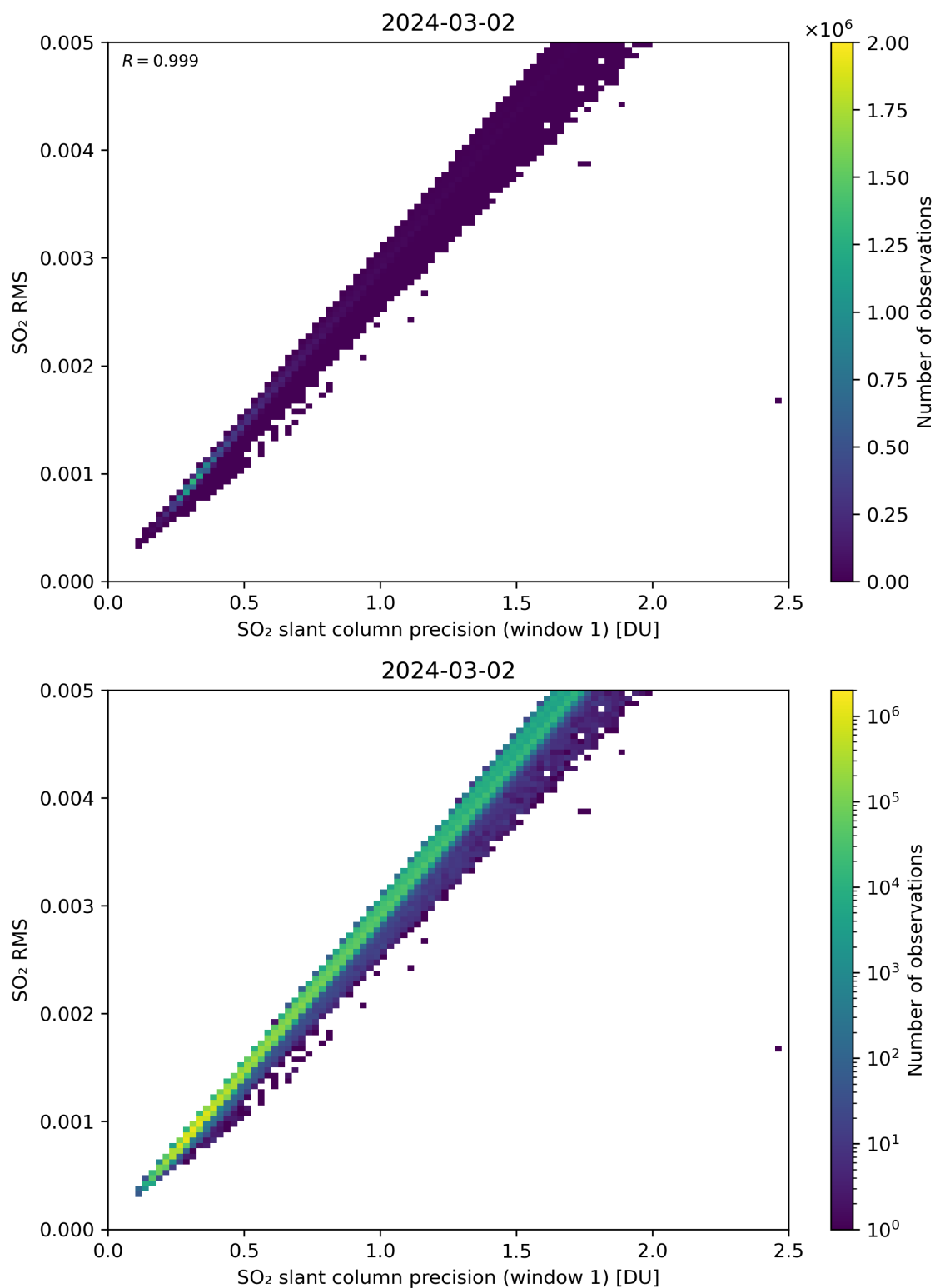
Figure 223: Scatter density plot of “SO 2 slant column precision (window 1)” against “SO 2 RMS” for 2024-03-01 to 2024-03-03.
