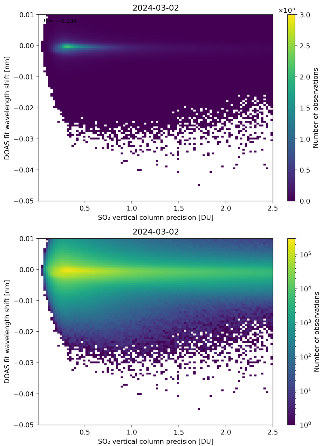
Figure 282: Scatter density plot of “SO 2 vertical column precision” against “DOAS fit wavelength shift” for 2024-03-01 to 2024-03-03.
