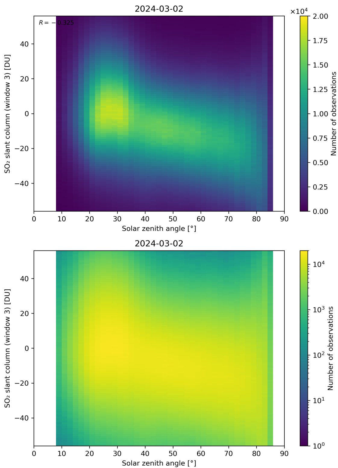
Figure 172: Scatter density plot of “Solar zenith angle” against “SO 2 slant column (window 3)” for 2024-03-01 to 2024-03-03.
