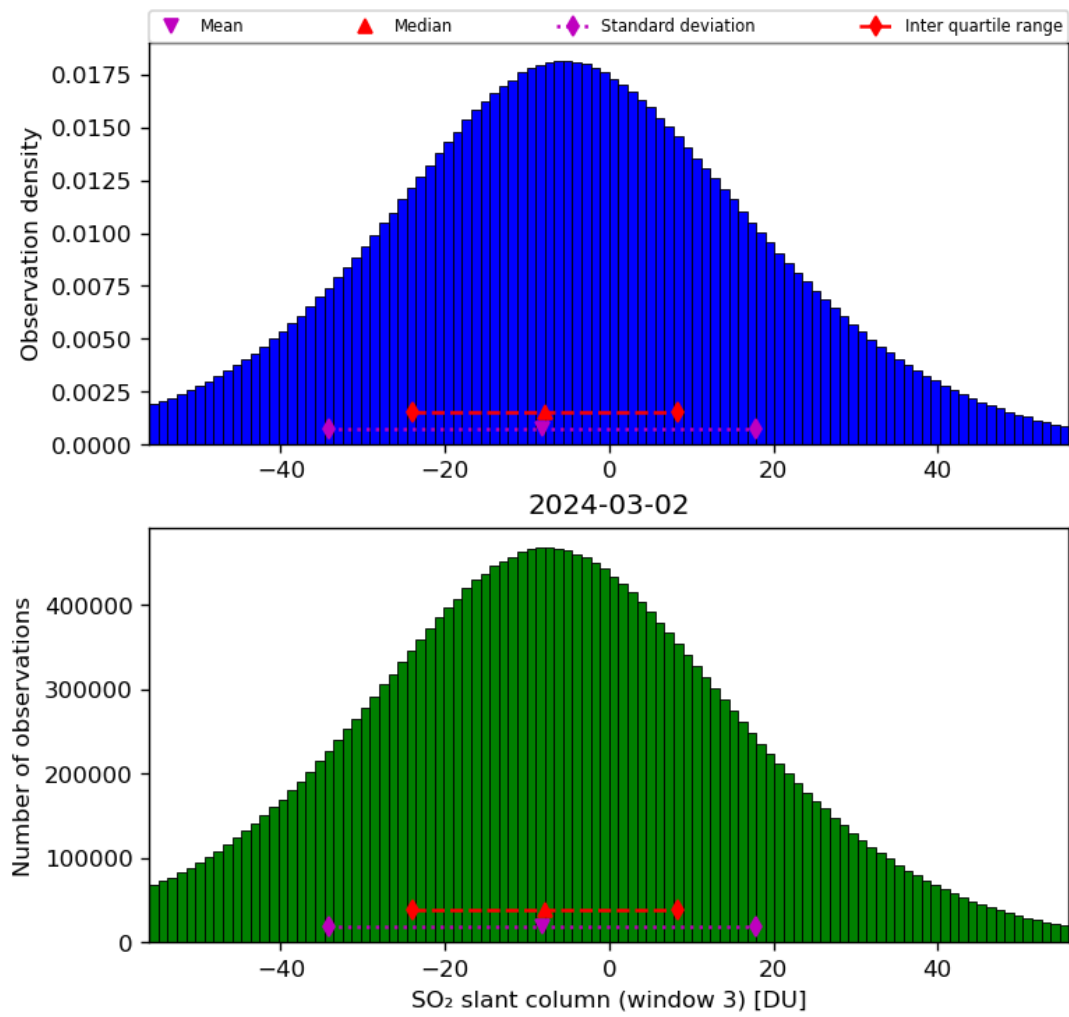
Figure 64: Histogram of “SO 2 slant column (window 3)” for 2024-03-01 to 2024-03-03
