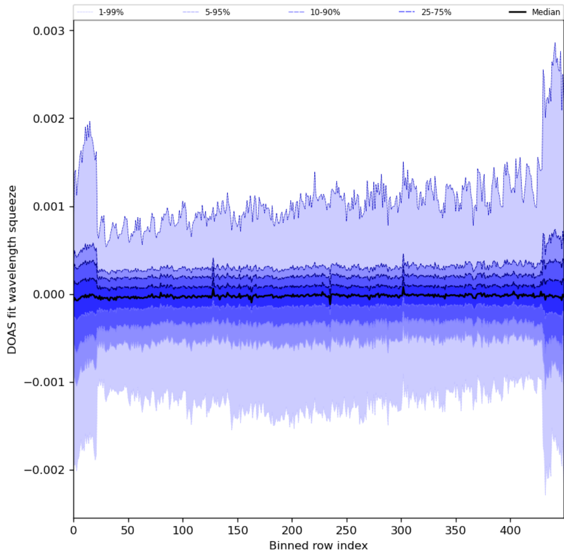
Figure 92: Along track statistics of “DOAS fit wavelength squeeze” for 2024-03-01 to 2024-03-03
