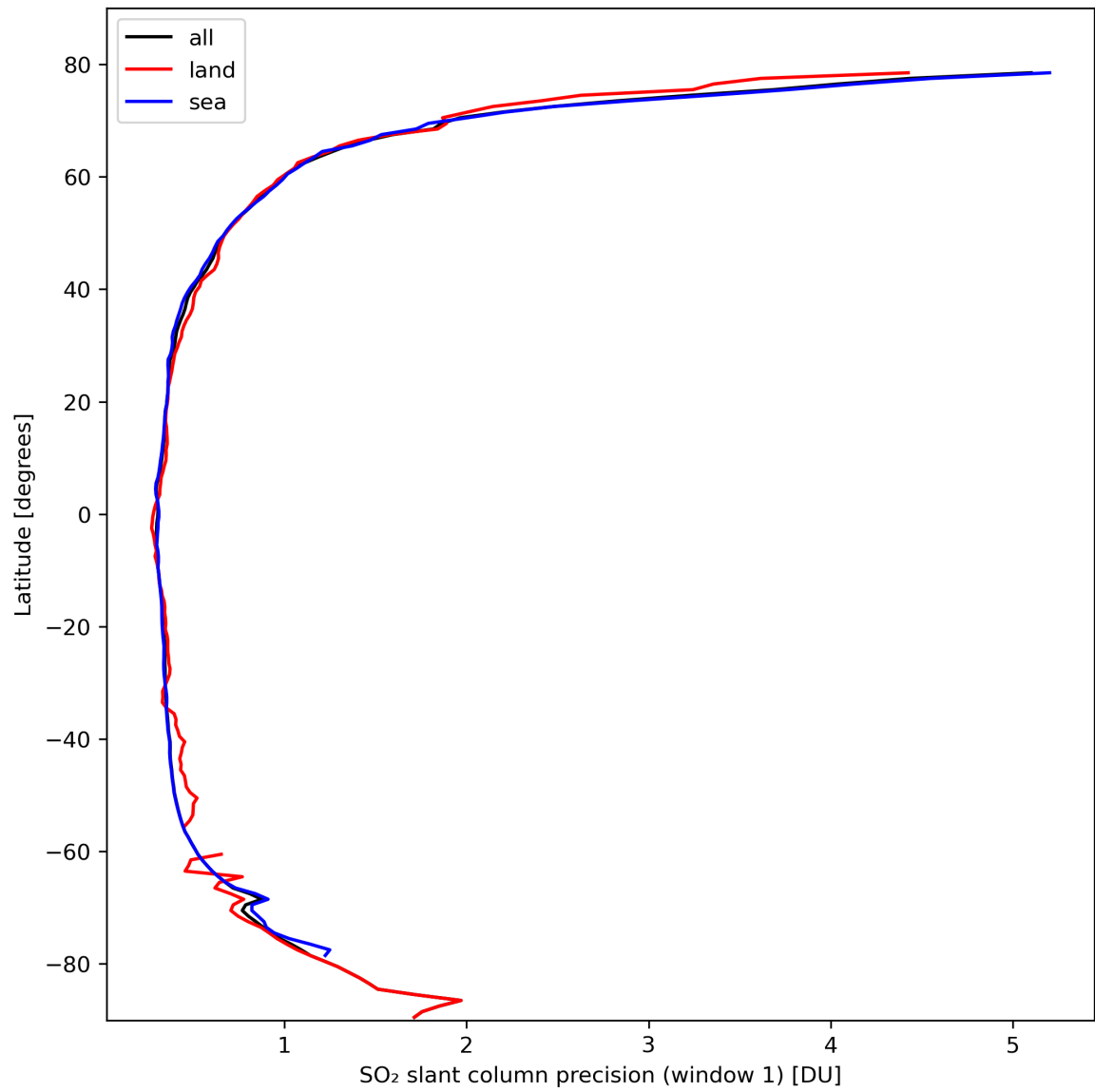
Figure 34: Zonal average of “SO 2 slant column precision (window 1)” for 2024-03-01 to 2024-03-03.
