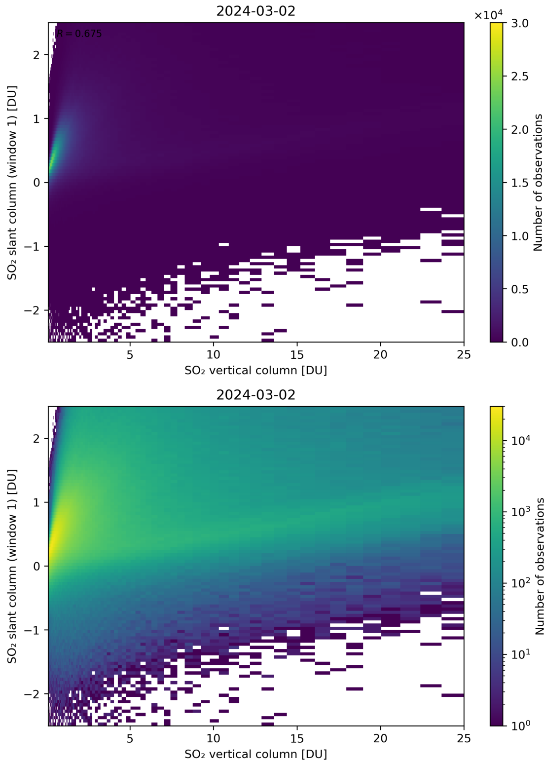
Figure 300: Scatter density plot of “SO 2 vertical column” against “SO 2 slant column (window 1)” for 2024-03-01 to 2024-03-03.
