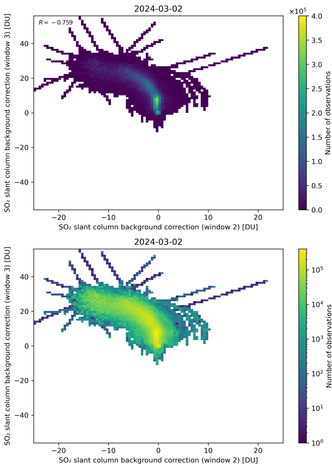
Figure 111: Scatter density plot of “SO 2 slant column background correction (window 2)” against “SO 2 slant column background correction (window 3)” for 2024-03-01 to 2024-03-03.
