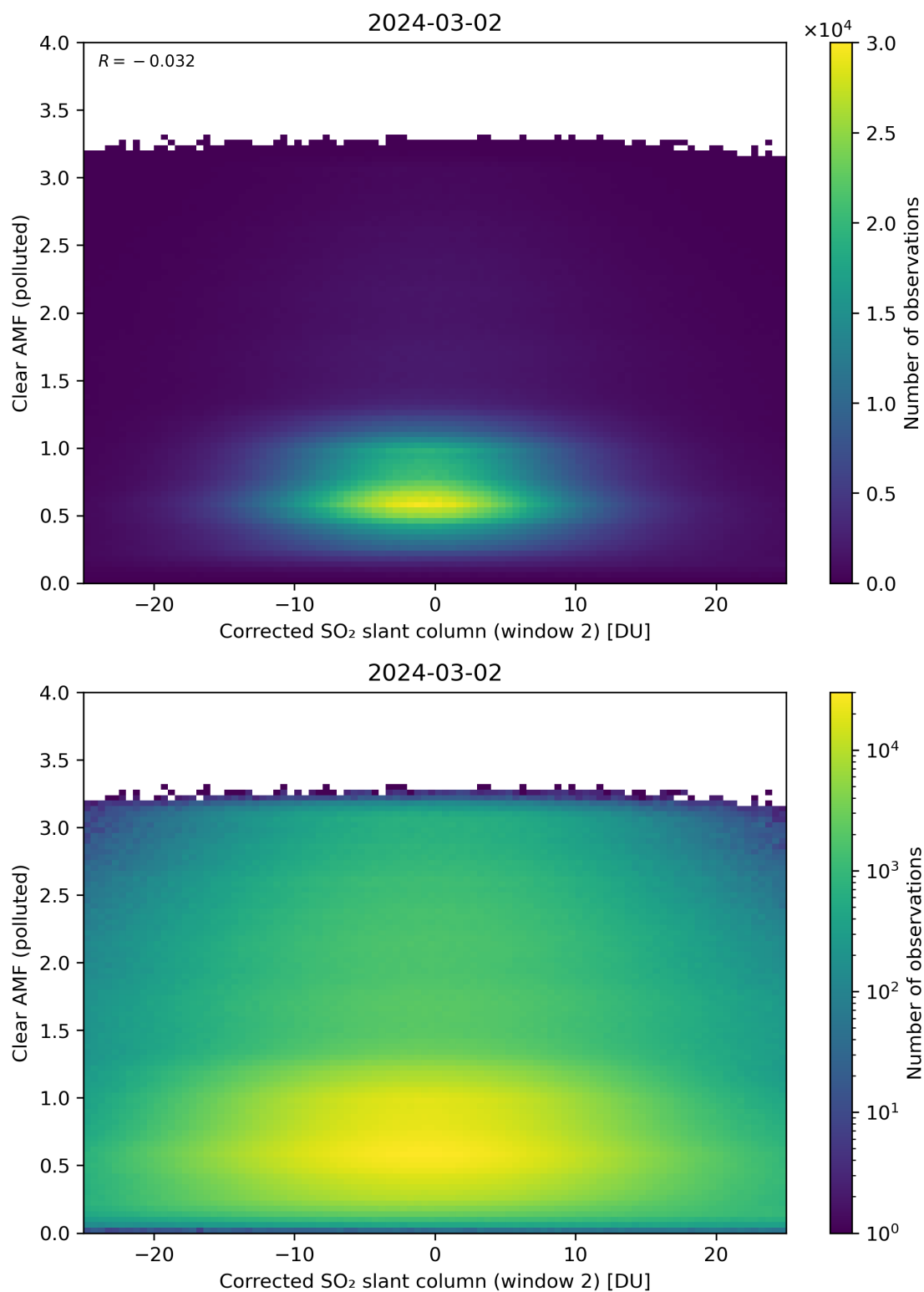
Figure 199: Scatter density plot of “Corrected SO 2 slant column (window 2)” against “Clear AMF (polluted)” for 2024-03-01 to 2024-03-03.
