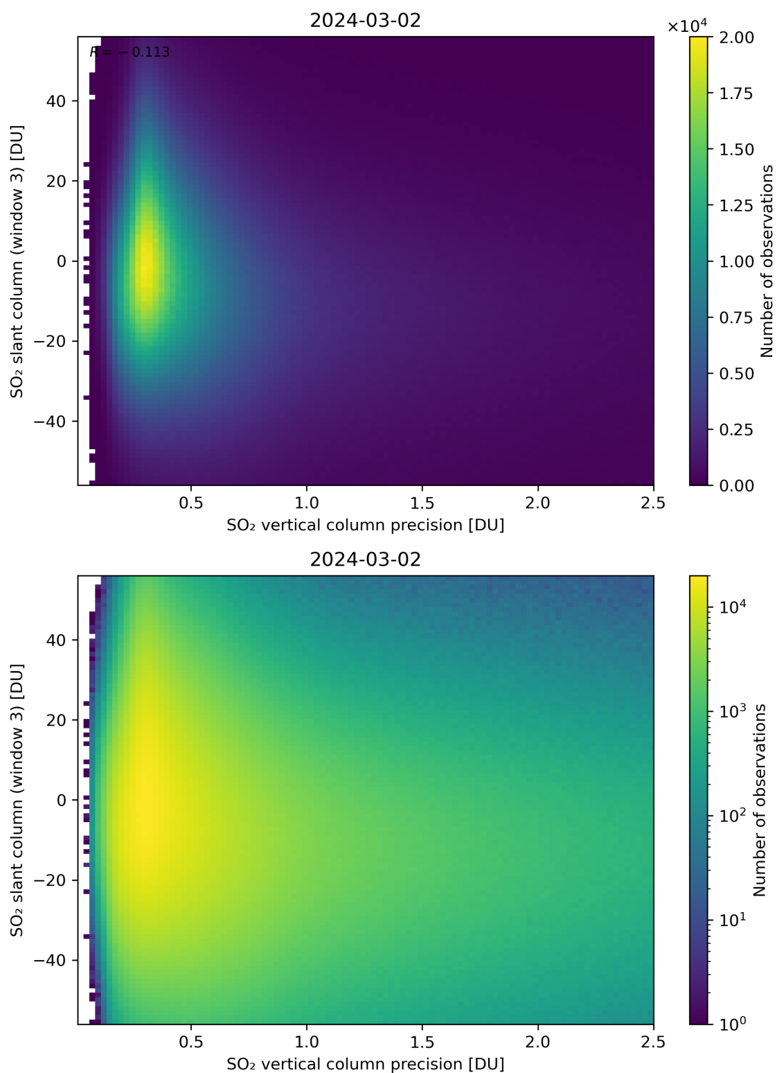
Figure 292: Scatter density plot of “SO 2 vertical column precision” against “SO 2 slant column (window 3)” for 2024-03-01 to 2024-03-03.
