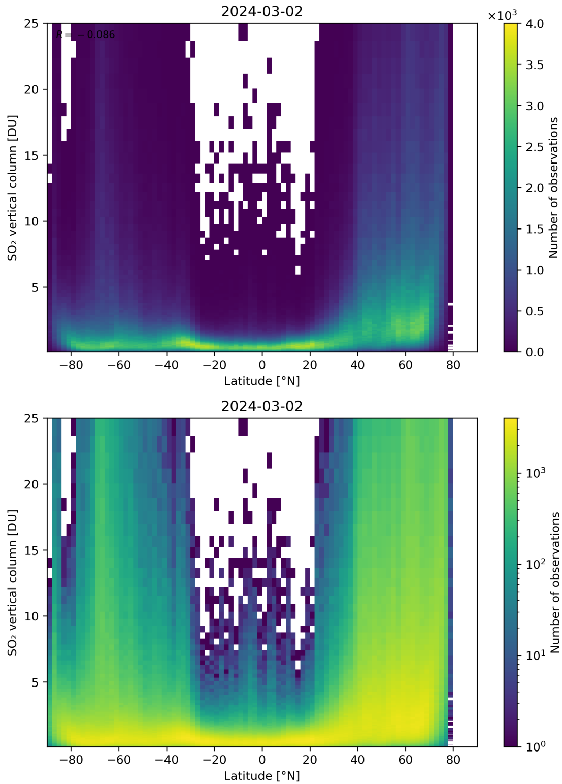
Figure 156: Scatter density plot of “Latitude” against “SO 2 vertical column” for 2024-03-01 to 2024-03-03.
