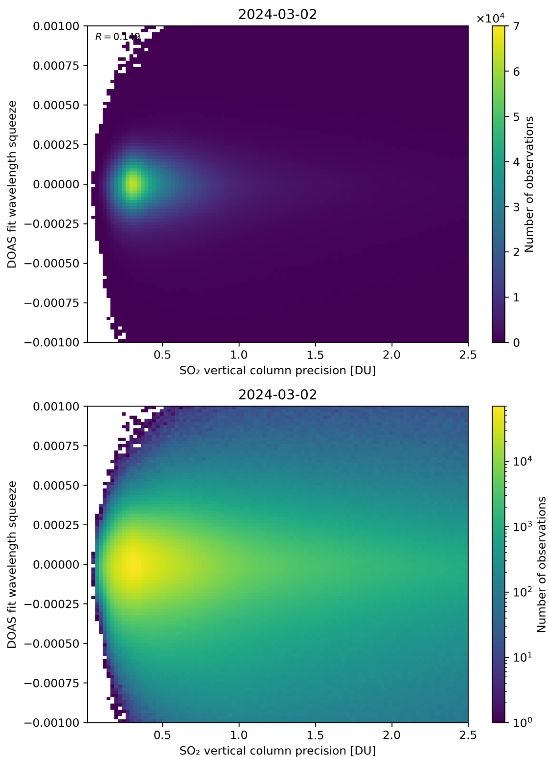
Figure 283: Scatter density plot of “SO 2 vertical column precision” against “DOAS fit wavelength squeeze” for 2024-03-01 to 2024-03-03.
