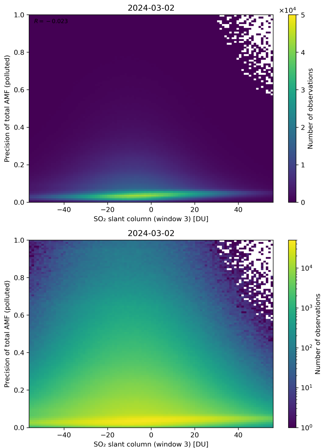
Figure 269: Scatter density plot of “SO 2 slant column (window 3)” against “Precision of total AMF (polluted)” for 2024-03-01 to 2024-03-03.
