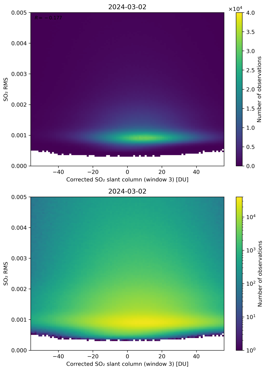
Figure 208: Scatter density plot of “Corrected SO 2 slant column (window 3)” against “SO 2 RMS” for 2024-03-01 to 2024-03-03.
