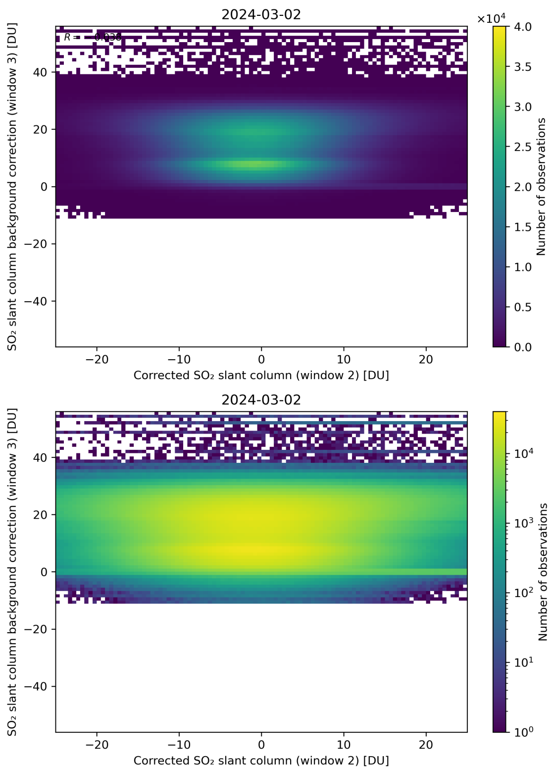
Figure 195: Scatter density plot of “Corrected SO 2 slant column (window 2)” against “SO 2 slant column background correction (window 3)” for 2024-03-01 to 2024-03-03.
