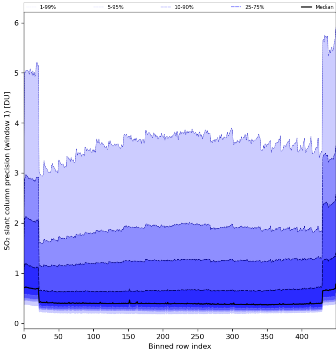
Figure 80: Along track statistics of “SO 2 slant column precision (window 1)” for 2024-03-01 to 2024-03-03
