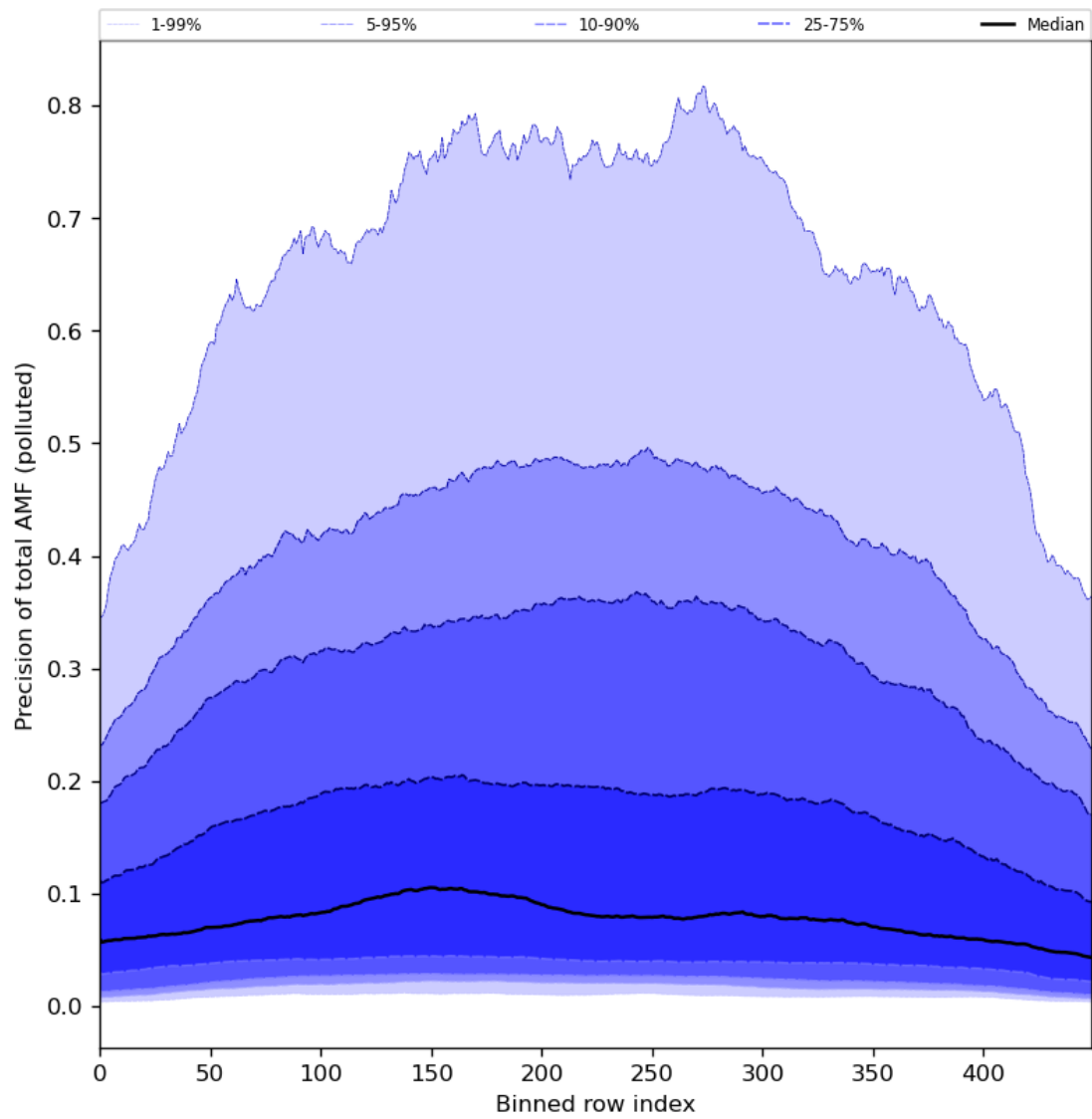
Figure 95: Along track statistics of “Precision of total AMF (polluted)” for 2024-03-01 to 2024-03-03
