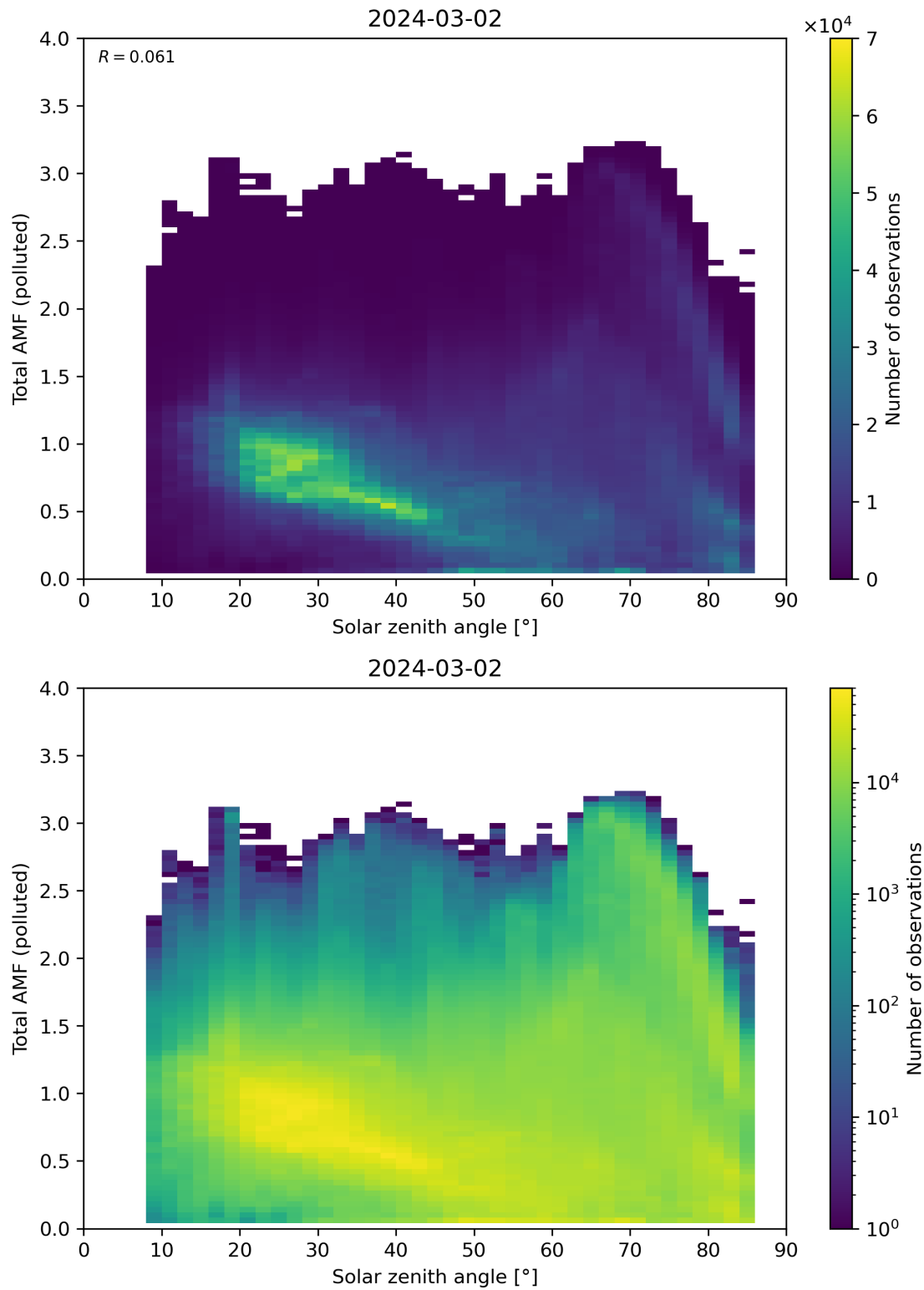
Figure 174: Scatter density plot of “Solar zenith angle” against “Total AMF (polluted)” for 2024-03-01 to 2024-03-03.
