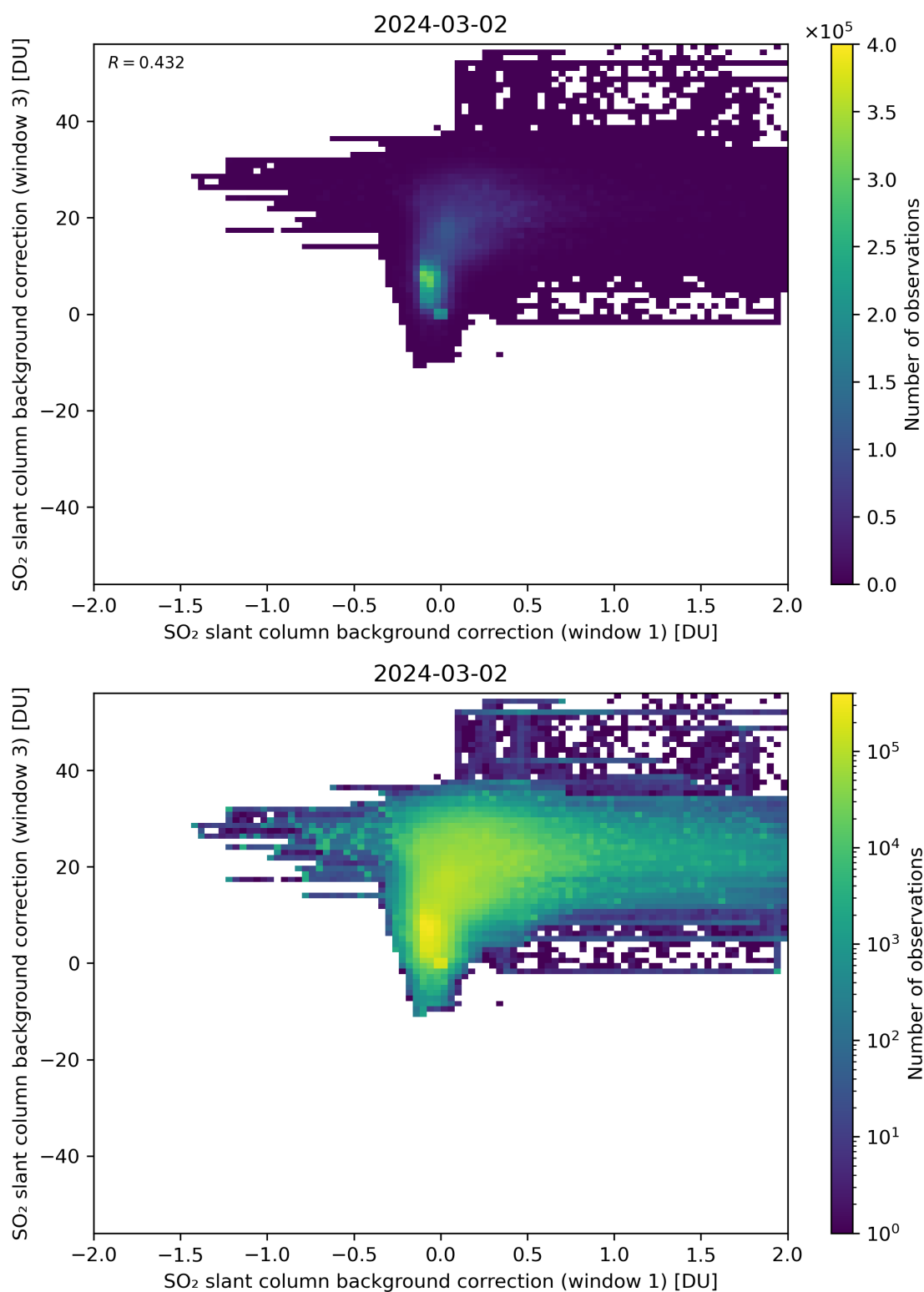
Figure 99: Scatter density plot of “SO 2 slant column background correction (window 1)” against “SO 2 slant column background correction (window 3)” for 2024-03-01 to 2024-03-03.
