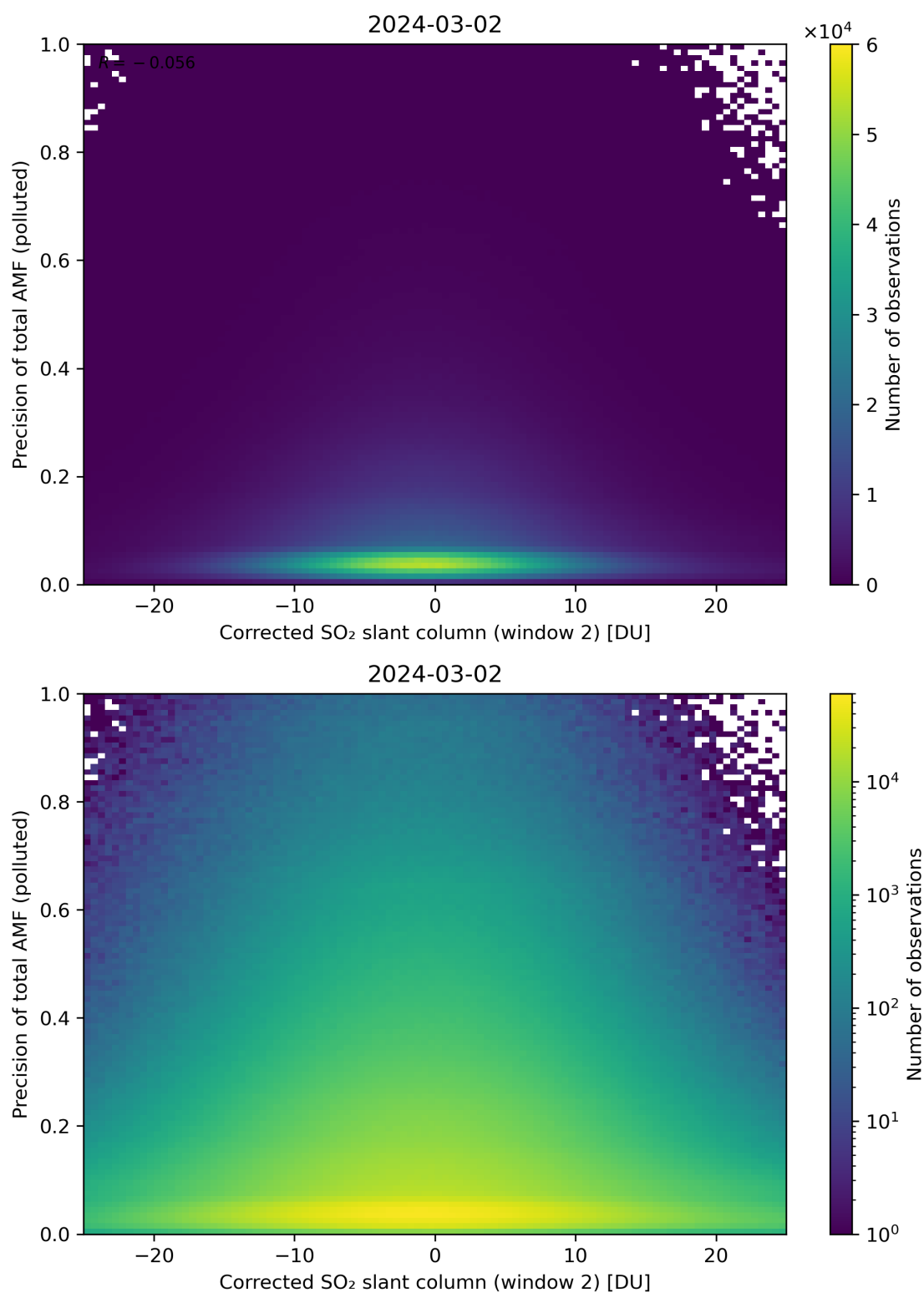
Figure 204: Scatter density plot of “Corrected SO 2 slant column (window 2)” against “Precision of total AMF (polluted)” for 2024-03-01 to 2024-03-03.
