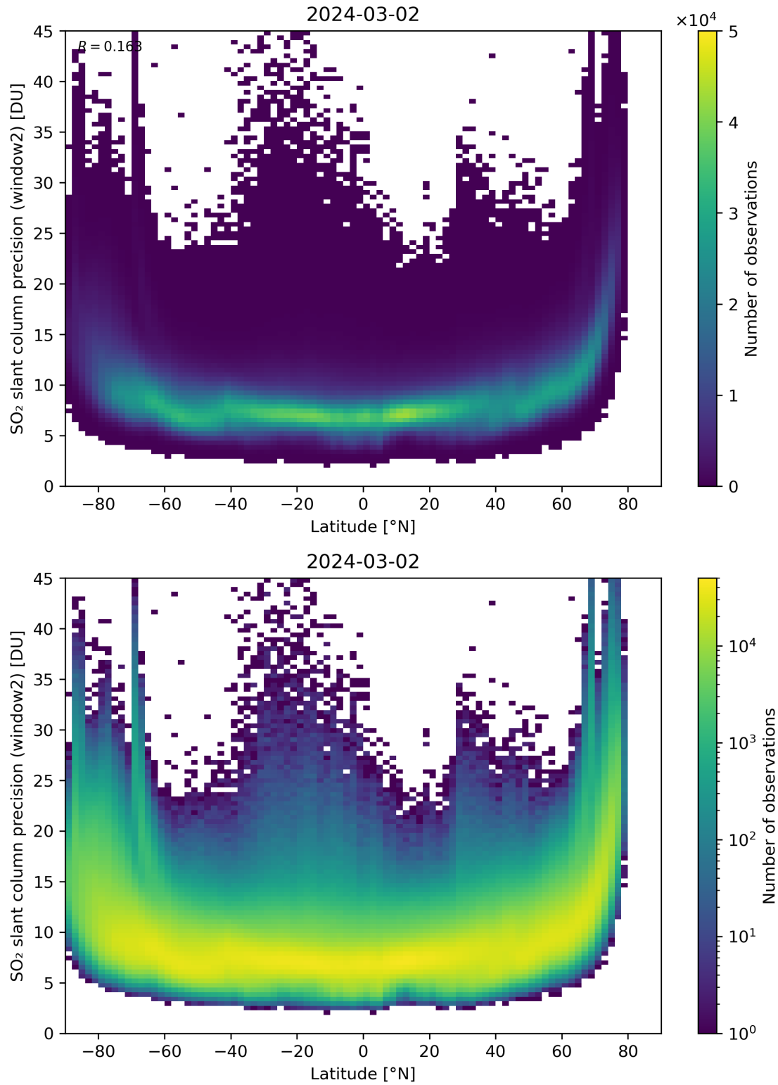
Figure 151: Scatter density plot of “Latitude” against “SO 2 slant column precision (window2)” for 2024-03-01 to 2024-03-03.
