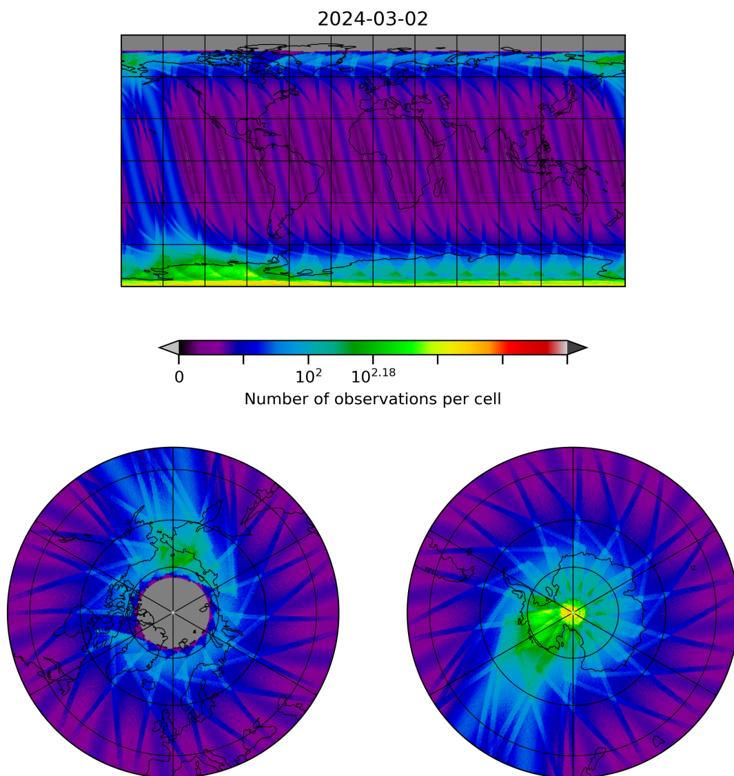
Figure 28: Map of the number of observations for 2024-03-01 to 2024-03-03
