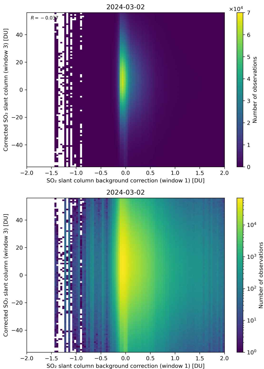
Figure 105: Scatter density plot of “SO 2 slant column background correction (window 1)” against “Corrected SO 2 slant column (window 3)” for 2024-03-01 to 2024-03-03.
