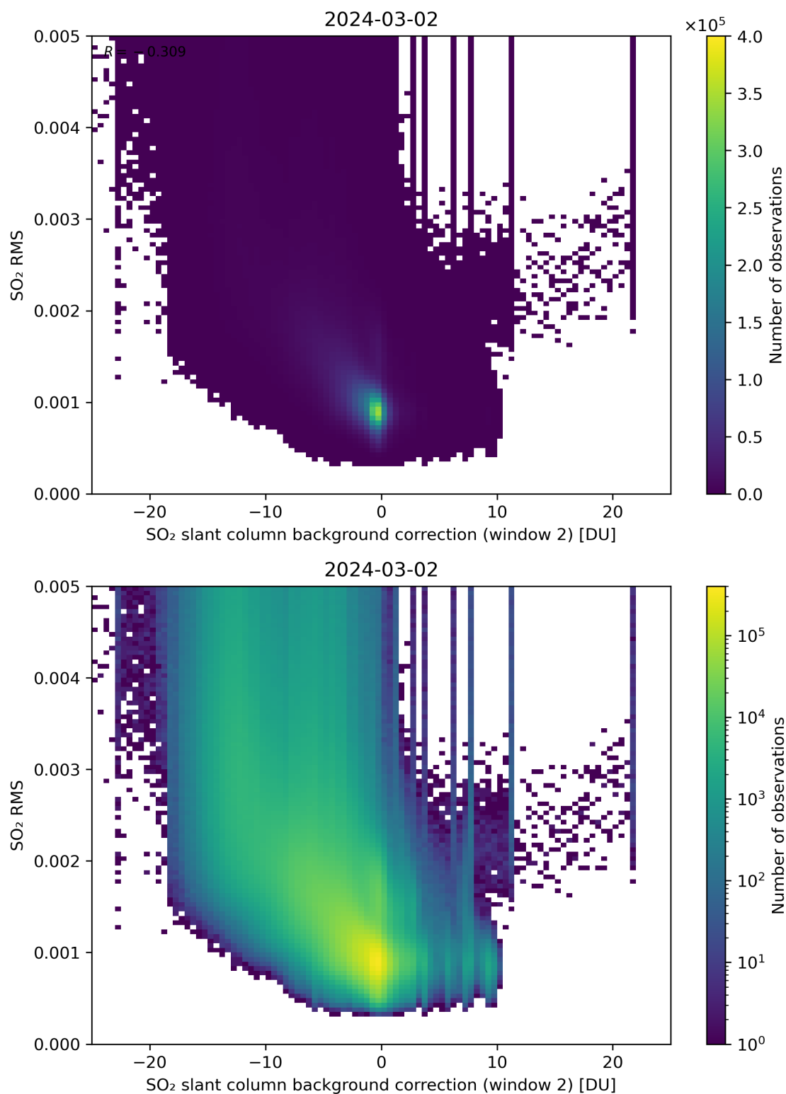
Figure 114: Scatter density plot of “SO 2 slant column background correction (window 2)” against “SO 2 RMS” for 2024-03-01 to 2024-03-03.
