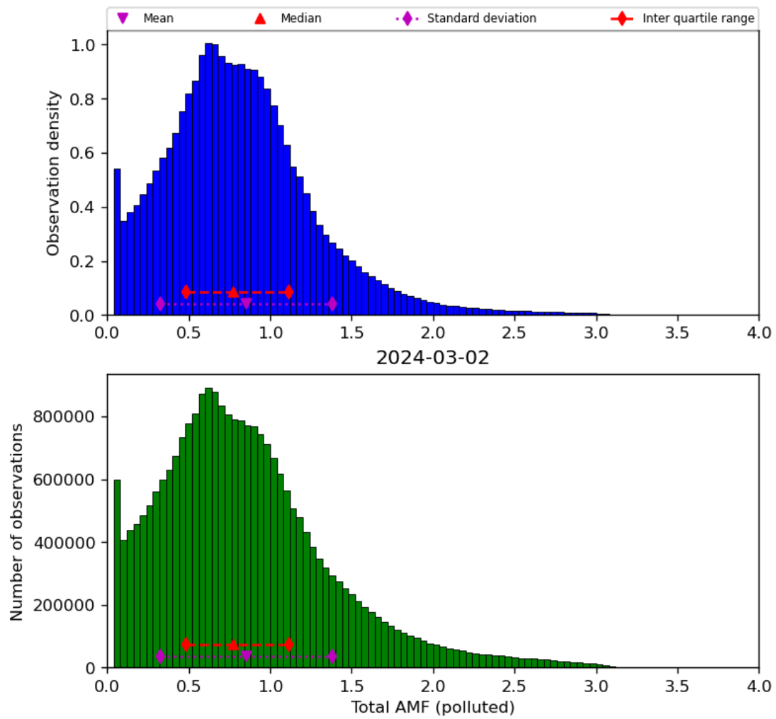
Figure 71: Histogram of “Total AMF (polluted)” for 2024-03-01 to 2024-03-03
