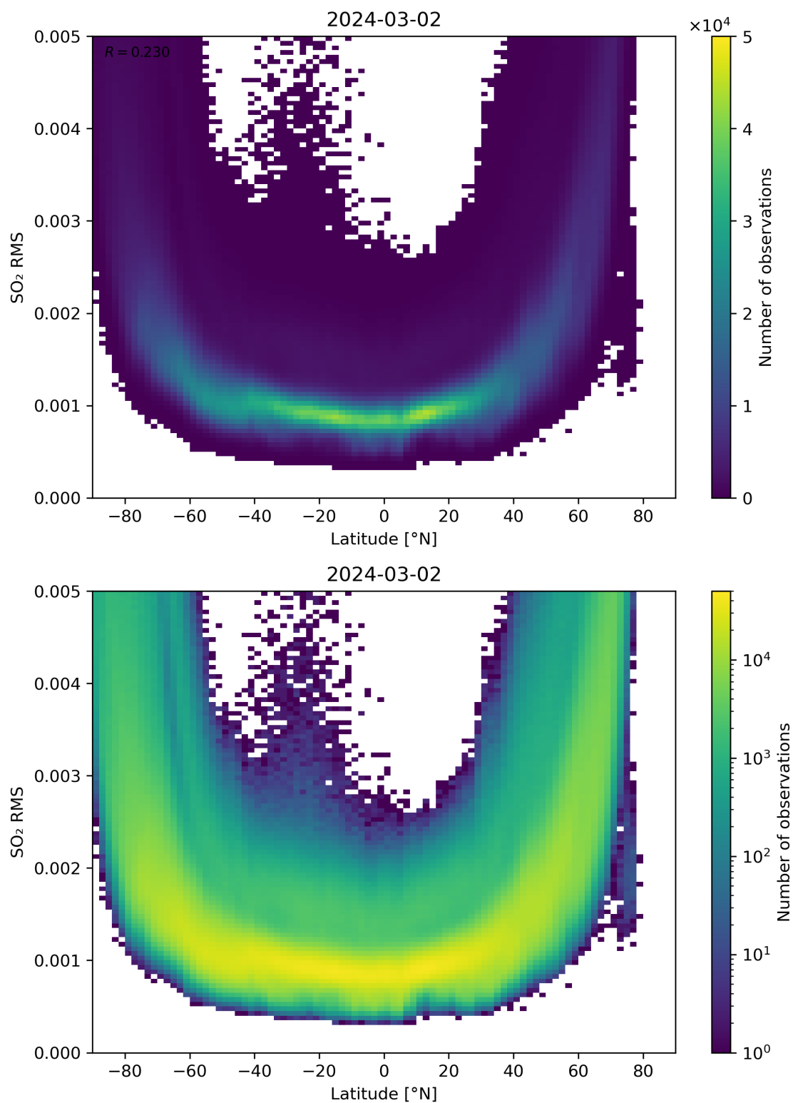
Figure 144: Scatter density plot of “Latitude” against “SO 2 RMS” for 2024-03-01 to 2024-03-03.
