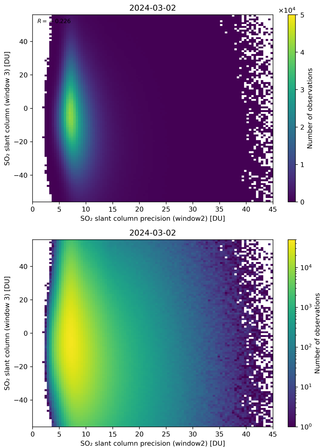
Figure 249: Scatter density plot of “SO 2 slant column precision (window2)” against “SO 2 slant column (window 3)” for 2024-03-01 to 2024-03-03.
