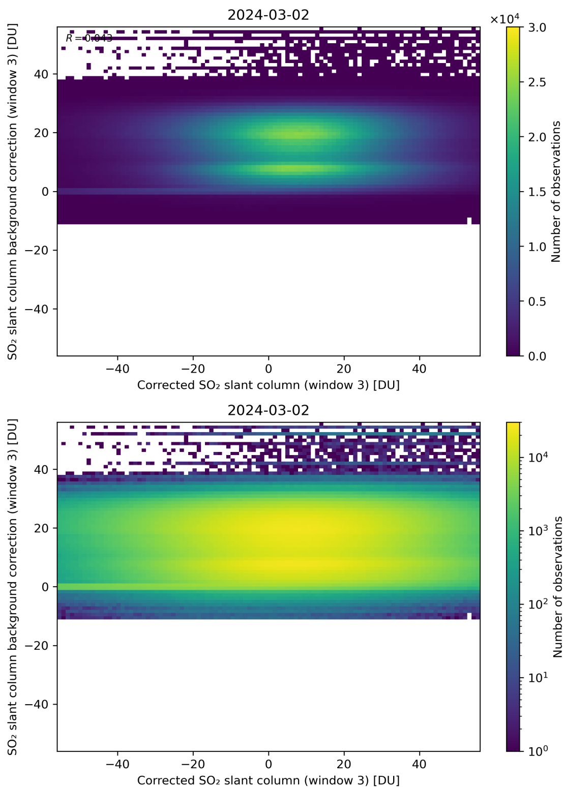
Figure 205: Scatter density plot of “Corrected SO 2 slant column (window 3)” against “SO 2 slant column background correction (window 3)” for 2024-03-01 to 2024-03-03.
