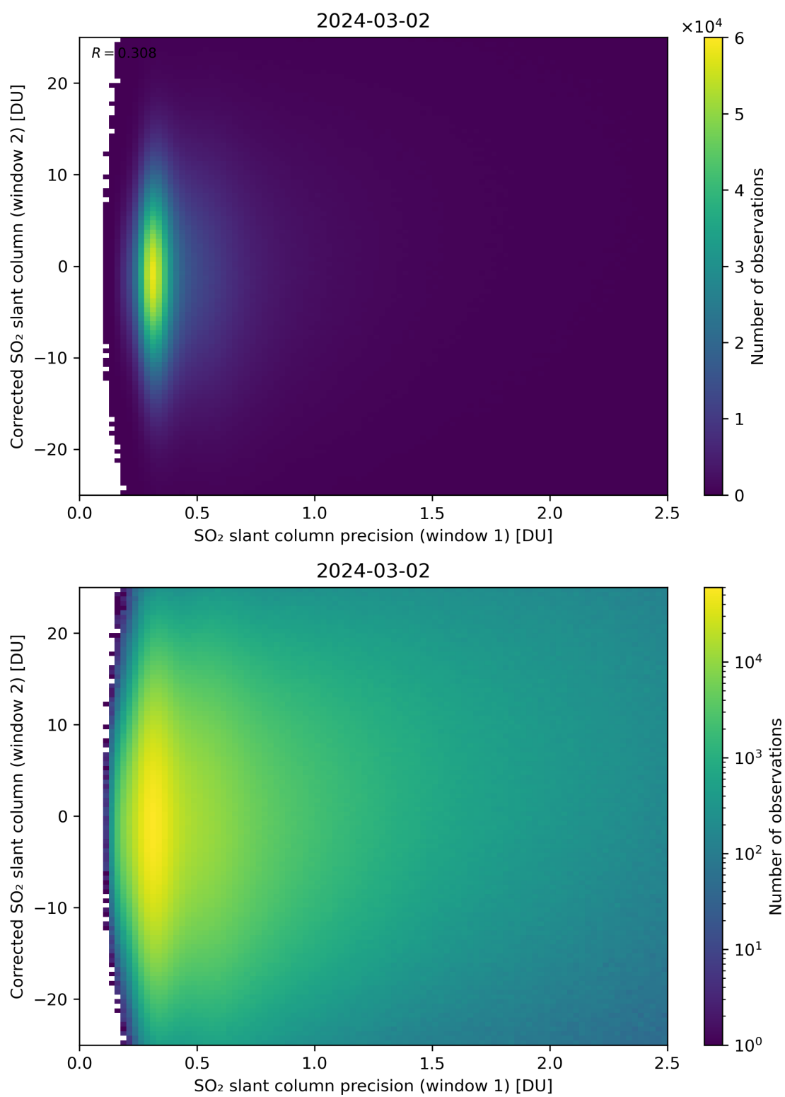
Figure 225: Scatter density plot of “SO 2 slant column precision (window 1)” against “Corrected SO 2 slant column (window 2)” for 2024-03-01 to 2024-03-03.
