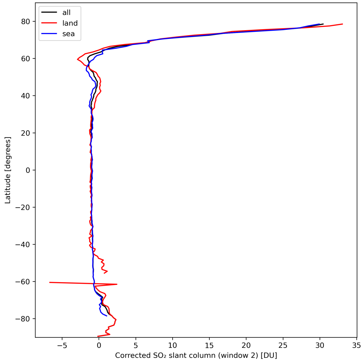
Figure 39: Zonal average of “Corrected SO 2 slant column (window 2)” for 2024-03-01 to 2024-03-03.
