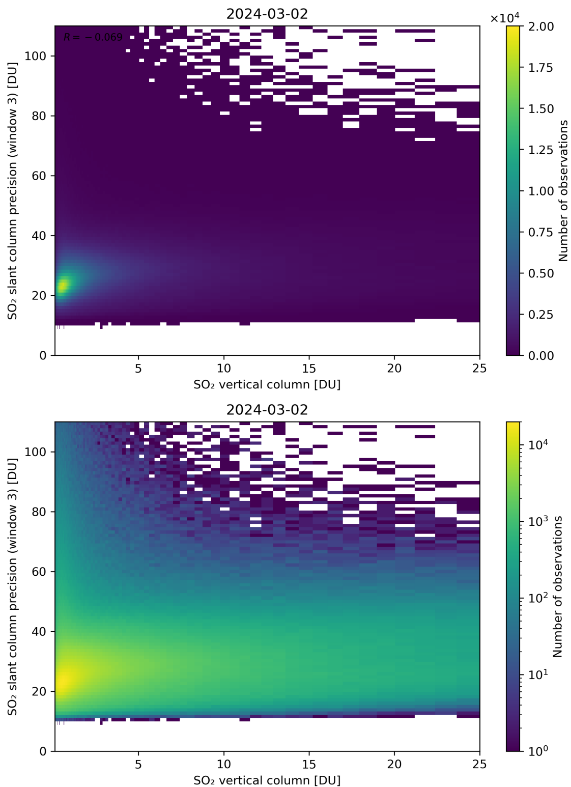
Figure 304: Scatter density plot of “SO 2 vertical column” against “SO 2 slant column precision (window 3)” for 2024-03-01 to 2024-03-03.
