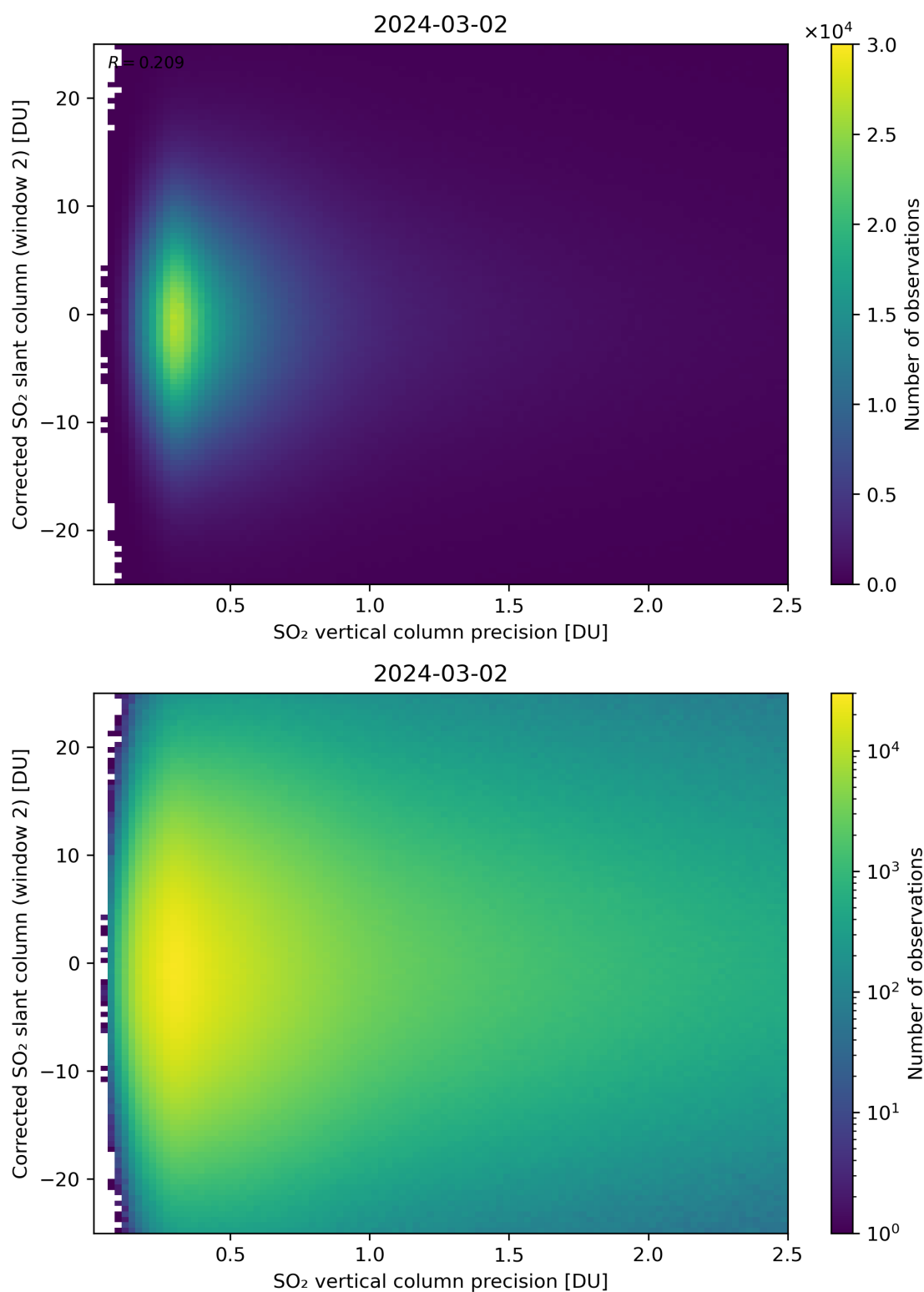
Figure 287: Scatter density plot of “SO 2 vertical column precision” against “Corrected SO 2 slant column (window 2)” for 2024-03-01 to 2024-03-03.
