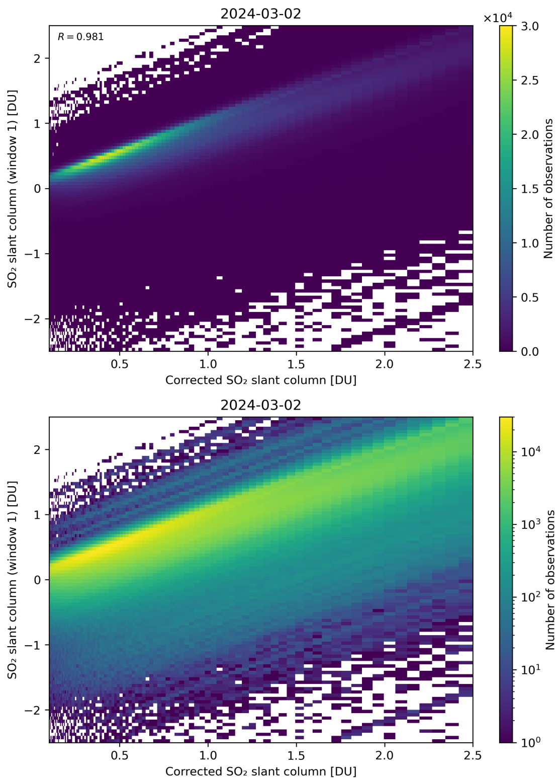
Figure 187: Scatter density plot of “Corrected SO 2 slant column” against “SO 2 slant column (window 1)” for 2024-03-01 to 2024-03-03.
