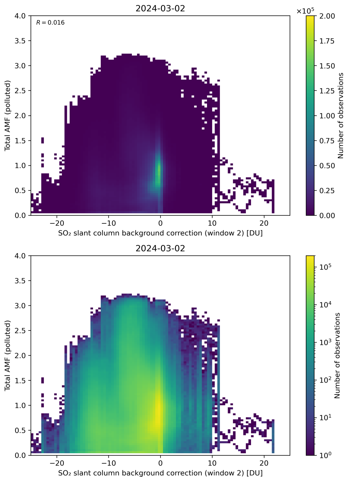
Figure 119: Scatter density plot of “SO 2 slant column background correction (window 2)” against “Total AMF (polluted)” for 2024-03-01 to 2024-03-03.
