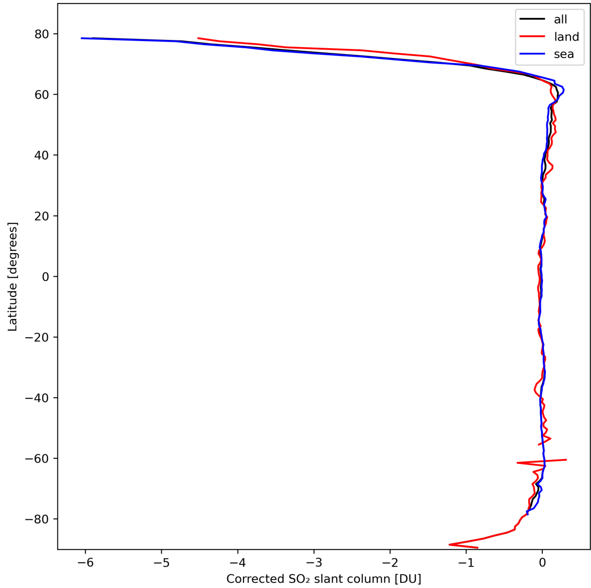
Figure 32: Zonal average of “Corrected SO 2 slant column” for 2024-03-01 to 2024-03-03.
