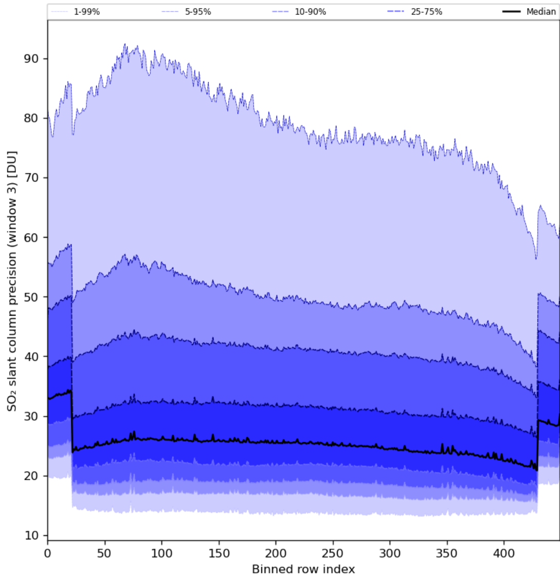
Figure 88: Along track statistics of “SO 2 slant column precision (window 3)” for 2024-03-01 to 2024-03-03
