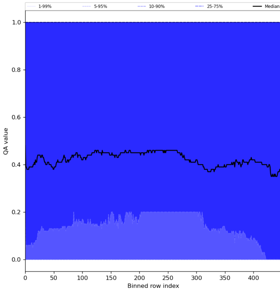
Figure 75: Along track statistics of “QA value” for 2024-03-01 to 2024-03-03
