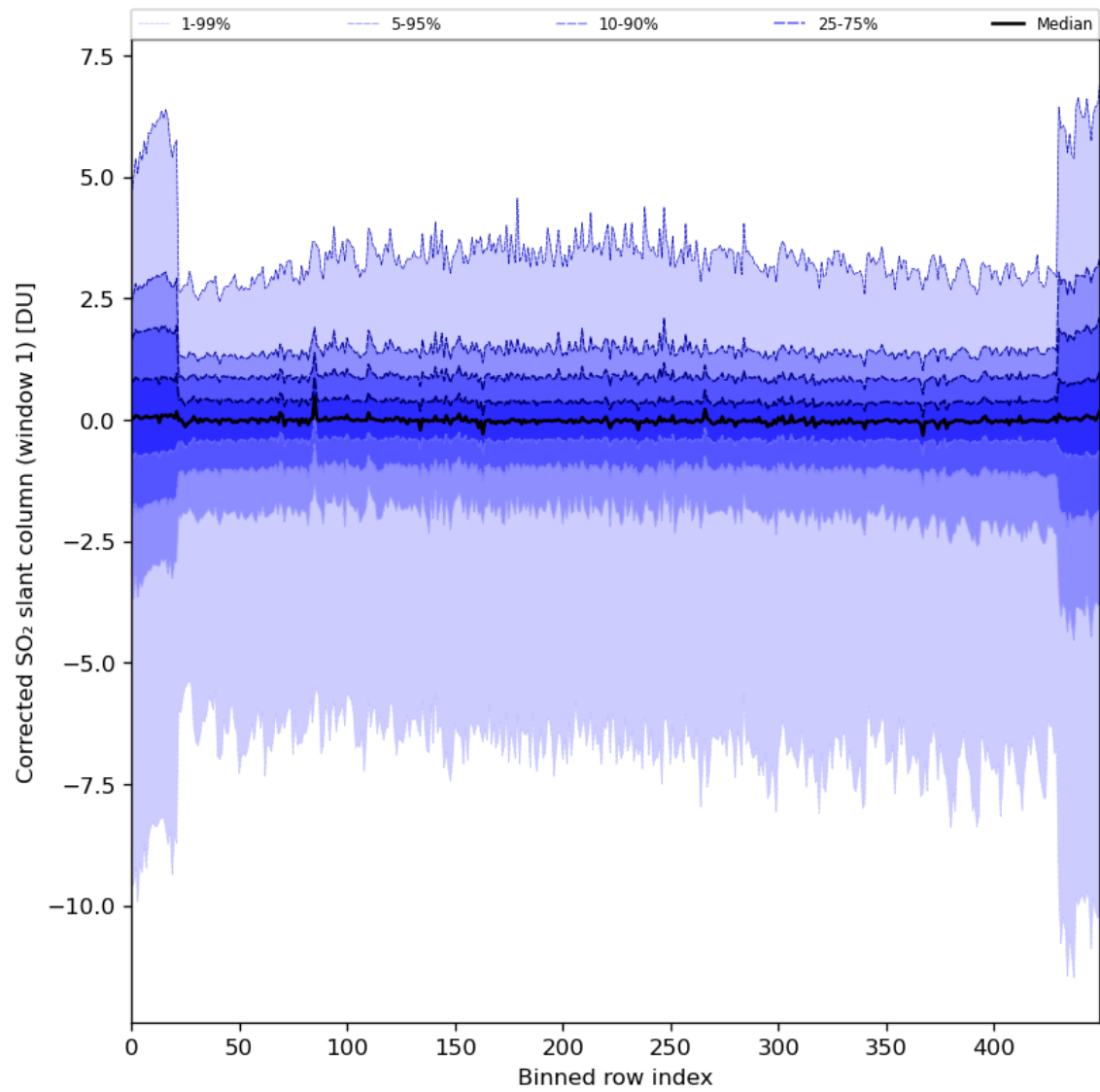
Figure 81: Along track statistics of “Corrected SO 2 slant column (window 1)” for 2024-03-01 to 2024-03-03
