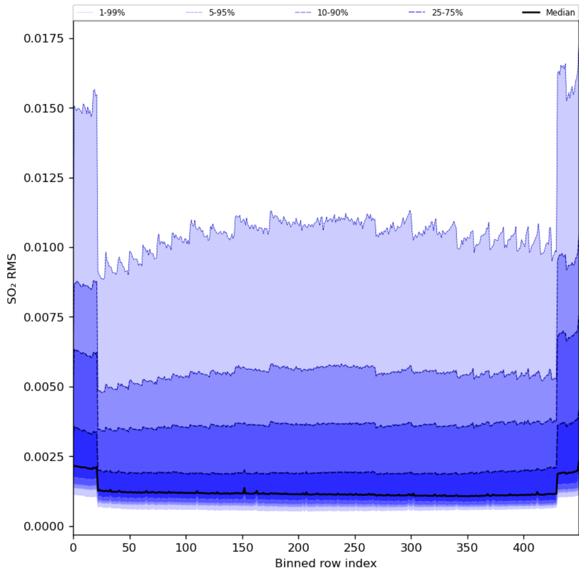
Figure 93: Along track statistics of “SO 2 RMS” for 2024-03-01 to 2024-03-03
