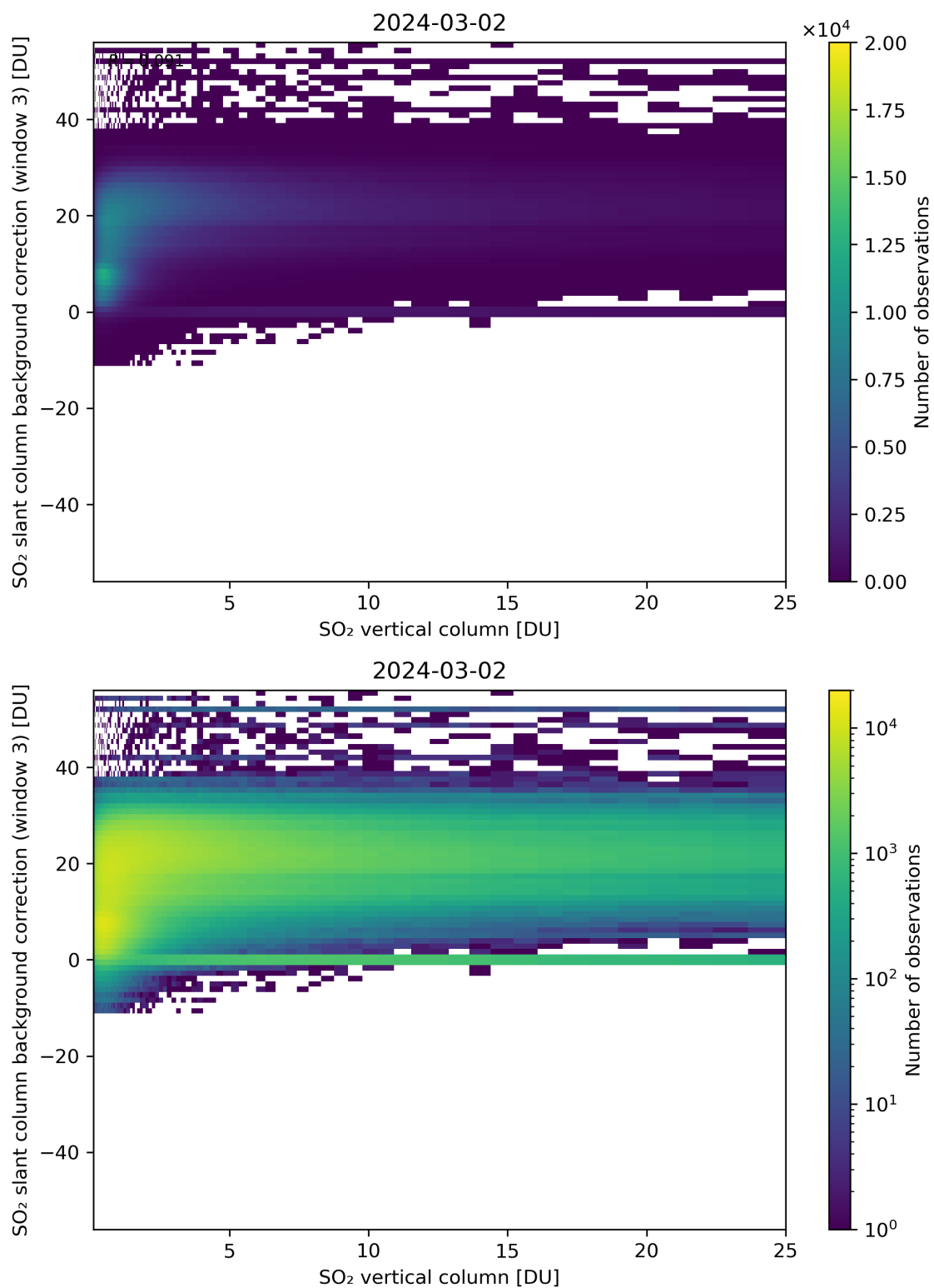
Figure 275: Scatter density plot of “SO 2 vertical column” against “SO 2 slant column background correction (window 3)” for 2024-03-01 to 2024-03-03.
