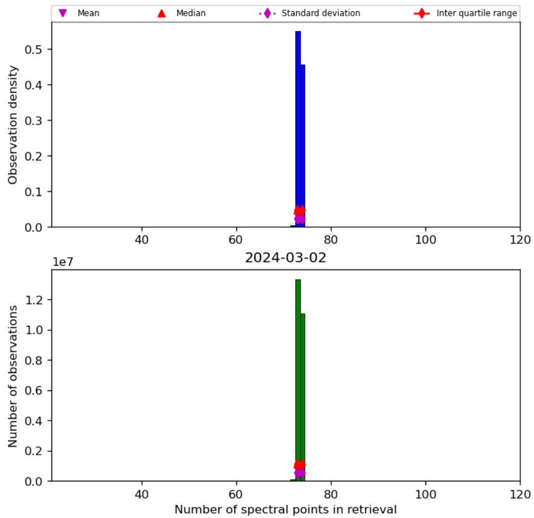
Figure 74: Histogram of “Number of spectral points in retrieval” for 2024-03-01 to 2024-03-03
