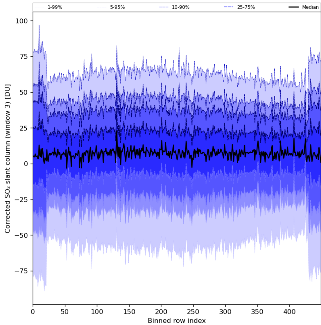
Figure 89: Along track statistics of “Corrected SO 2 slant column (window 3)” for 2024-03-01 to 2024-03-03
