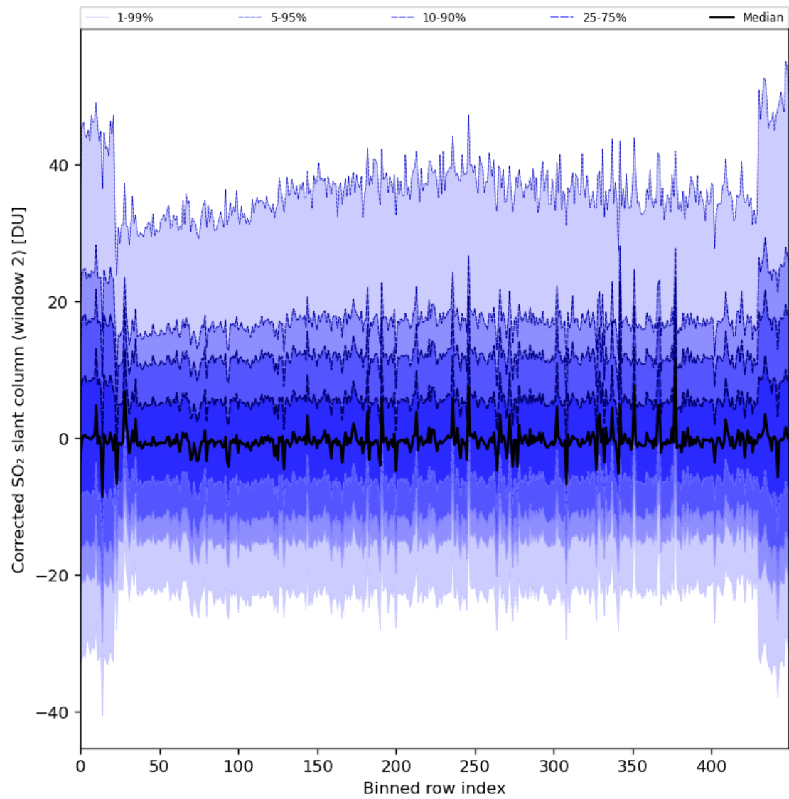
Figure 85: Along track statistics of “Corrected SO 2 slant column (window 2)” for 2024-03-01 to 2024-03-03
