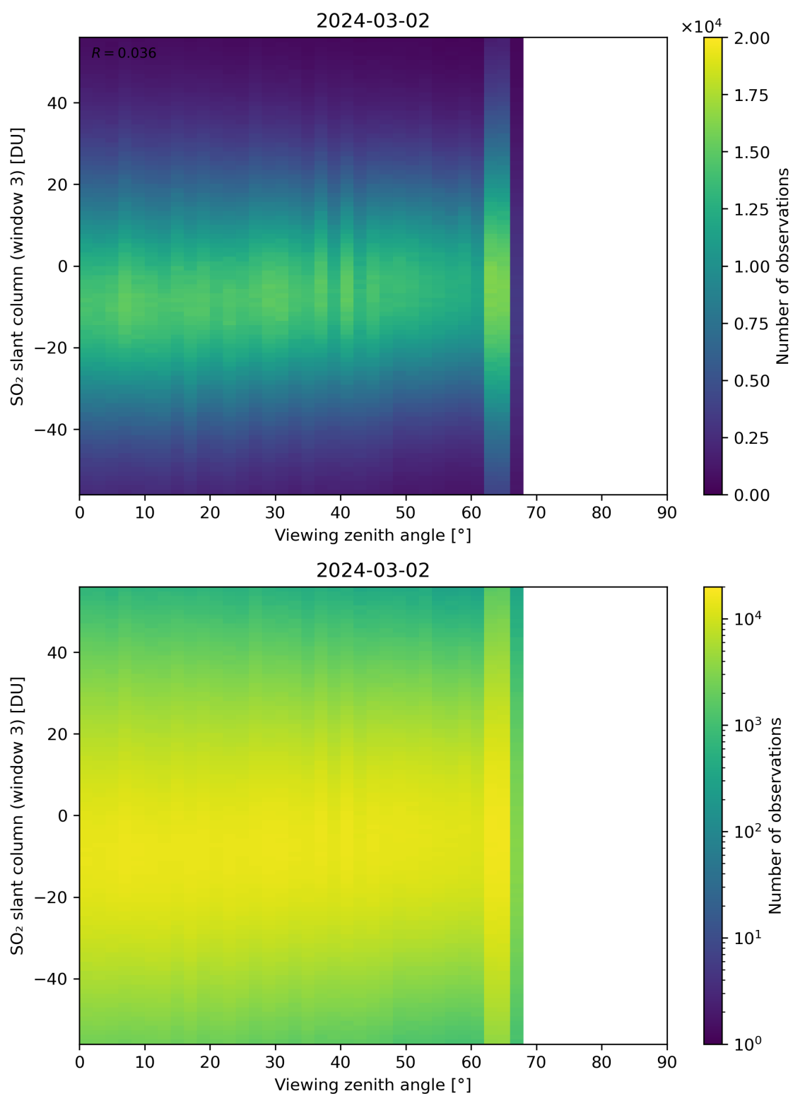
Figure 323: Scatter density plot of “Viewing zenith angle” against “SO 2 slant column (window 3)” for 2024-03-01 to 2024-03-03.
