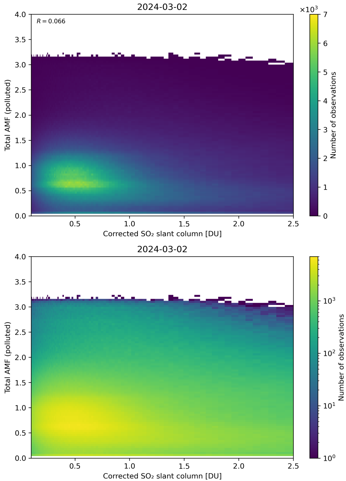
Figure 192: Scatter density plot of “Corrected SO 2 slant column” against “Total AMF (polluted)” for 2024-03-01 to 2024-03-03.
