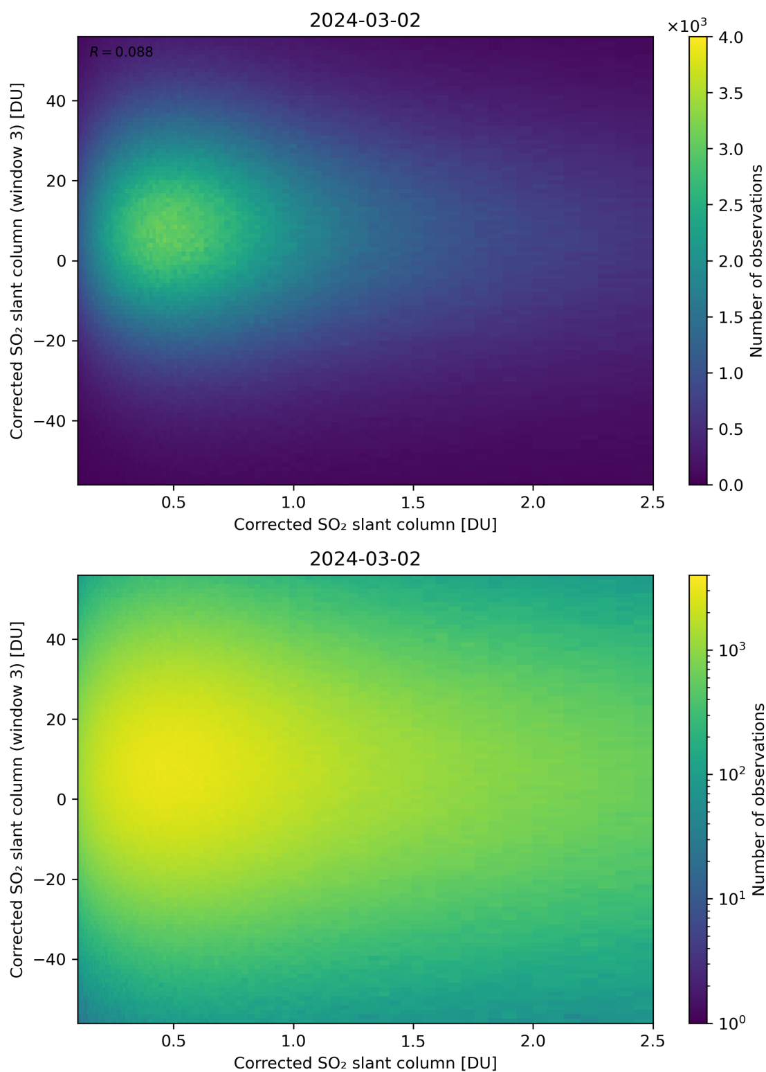
Figure 186: Scatter density plot of “Corrected SO 2 slant column” against “Corrected SO 2 slant column (window 3)” for 2024-03-01 to 2024-03-03.
