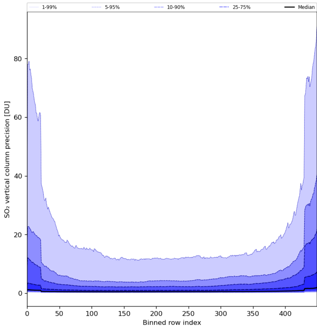
Figure 77: Along track statistics of “SO 2 vertical column precision” for 2024-03-01 to 2024-03-03
