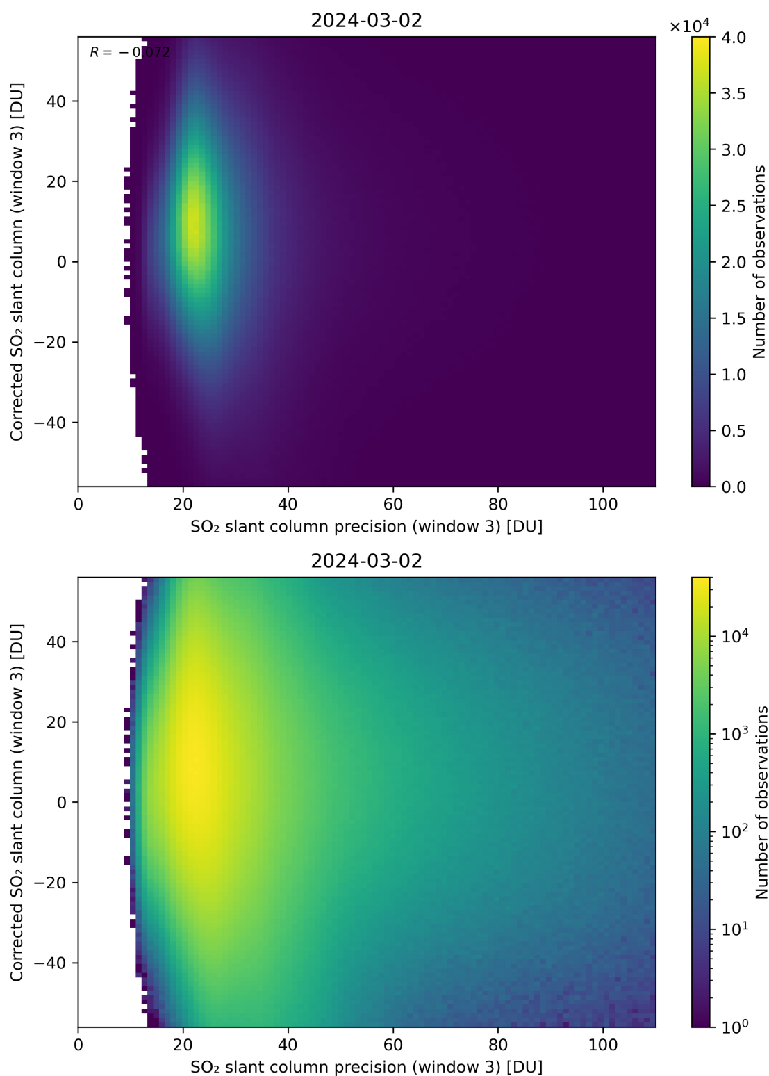
Figure 262: Scatter density plot of “SO 2 slant column precision (window 3)” against “Corrected SO 2 slant column (window 3)” for 2024-03-01 to 2024-03-03.
