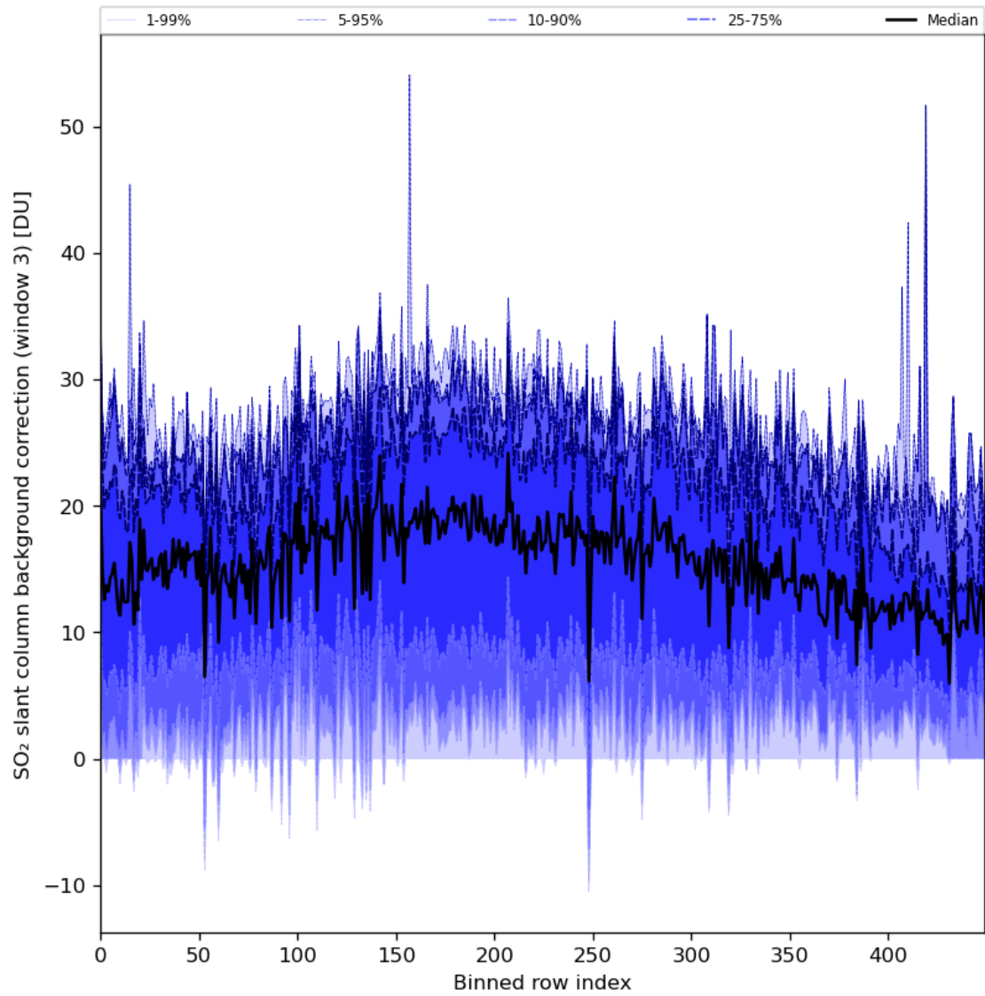
Figure 90: Along track statistics of “SO 2 slant column background correction (window 3)” for 2024-03-01 to 2024-03-03
