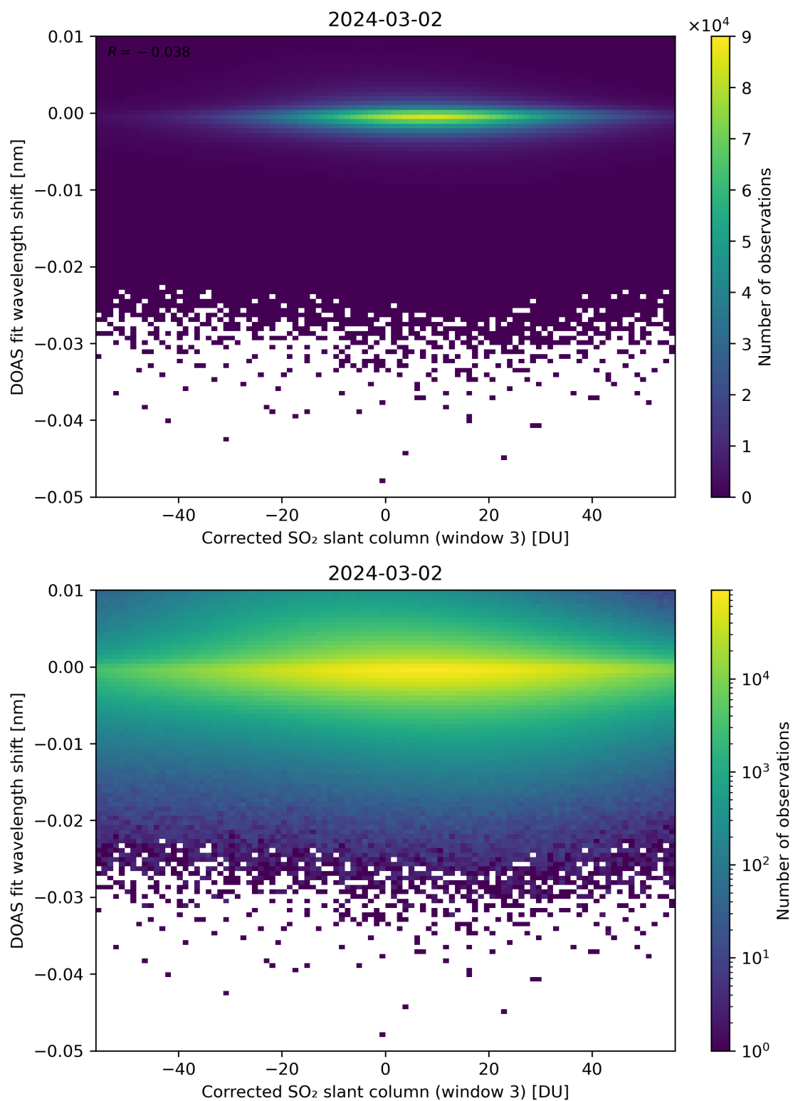
Figure 206: Scatter density plot of “Corrected SO 2 slant column (window 3)” against “DOAS fit wavelength shift” for 2024-03-01 to 2024-03-03.
