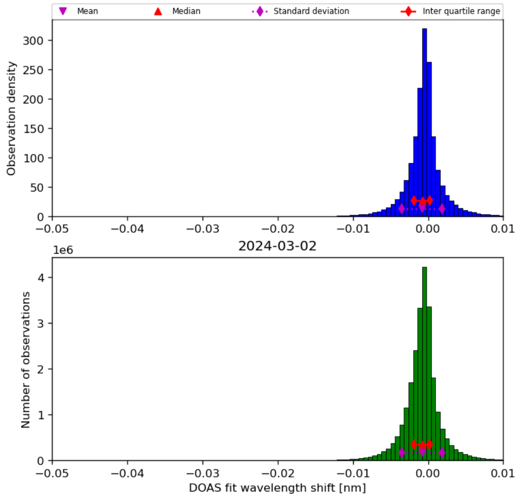
Figure 68: Histogram of “DOAS fit wavelength shift” for 2024-03-01 to 2024-03-03
