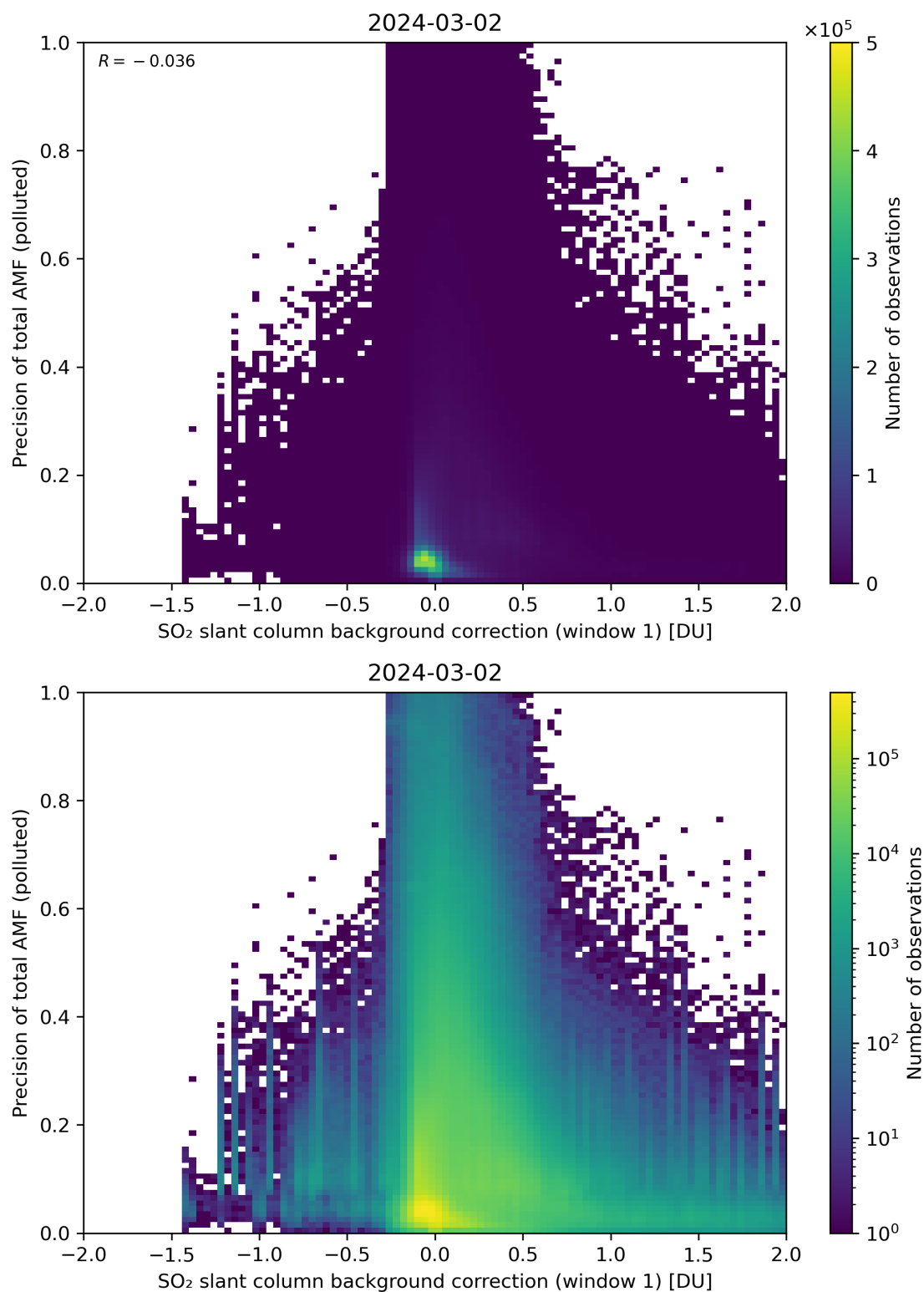
Figure 110: Scatter density plot of “SO 2 slant column background correction (window 1)” against “Precision of total AMF (polluted)” for 2024-03-01 to 2024-03-03.
