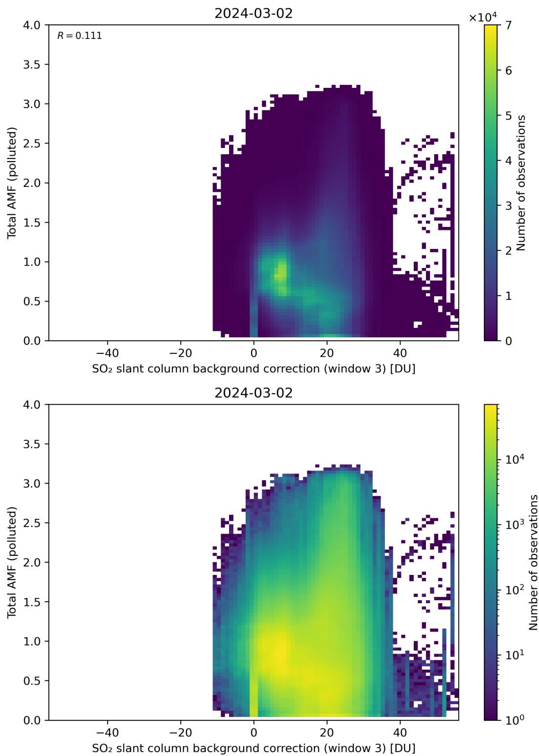
Figure 125: Scatter density plot of “SO 2 slant column background correction (window 3)” against “Total AMF (polluted)” for 2024-03-01 to 2024-03-03.
