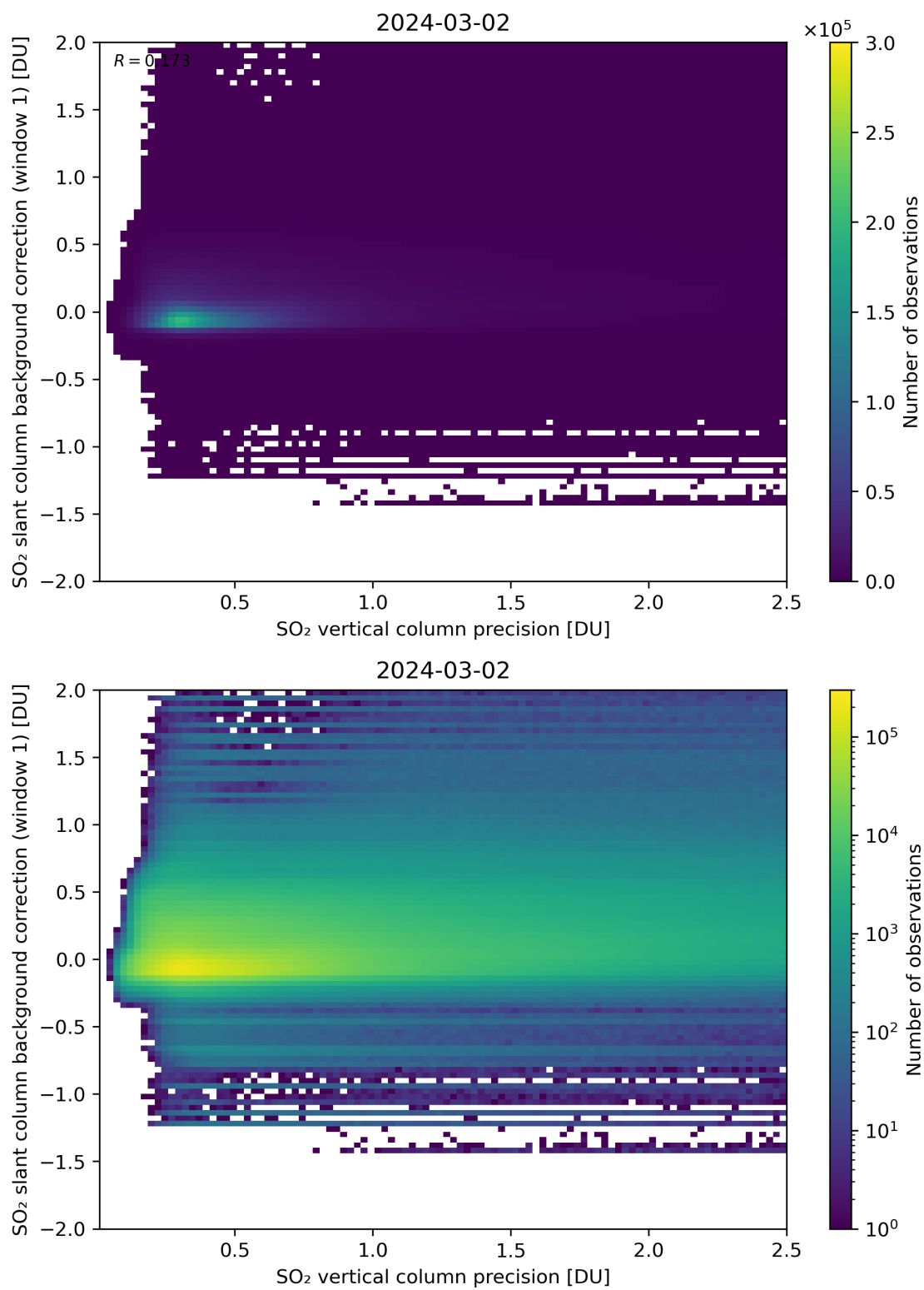
Figure 279: Scatter density plot of “SO 2 vertical column precision” against “SO 2 slant column background correction (window 1)” for 2024-03-01 to 2024-03-03.
