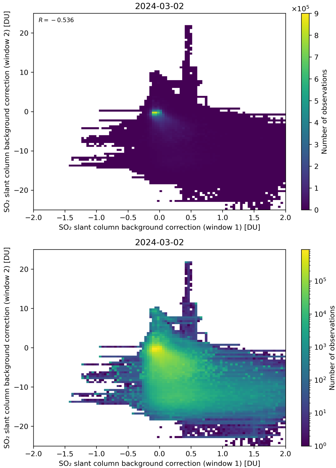
Figure 98: Scatter density plot of “SO 2 slant column background correction (window 1)” against “SO 2 slant column background correction (window 2)” for 2024-03-01 to 2024-03-03.
