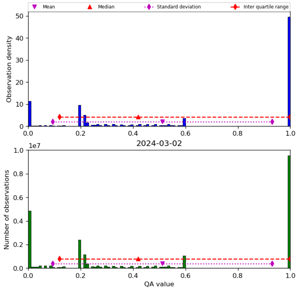
Figure 52: Histogram of “QA value” for 2024-03-01 to 2024-03-03
