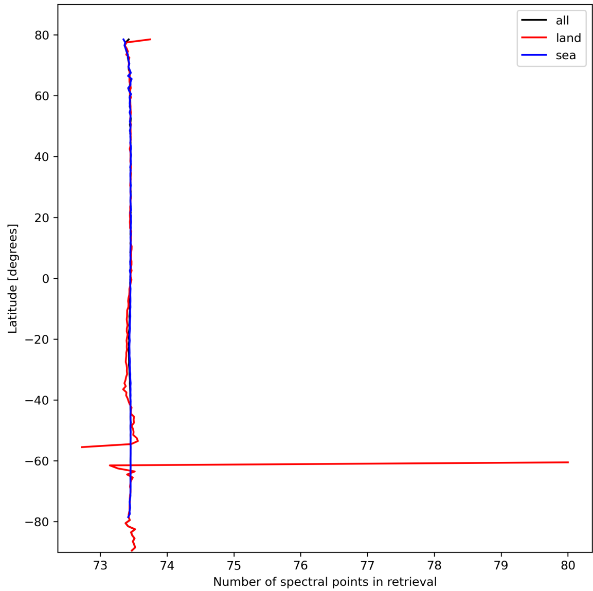
Figure 51: Zonal average of “Number of spectral points in retrieval” for 2024-03-01 to 2024-03-03.
