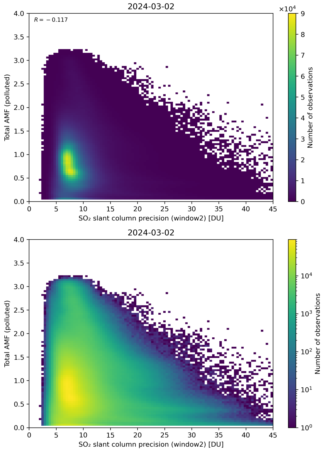
Figure 251: Scatter density plot of “SO 2 slant column precision (window2)” against “Total AMF (polluted)” for 2024-03-01 to 2024-03-03.
