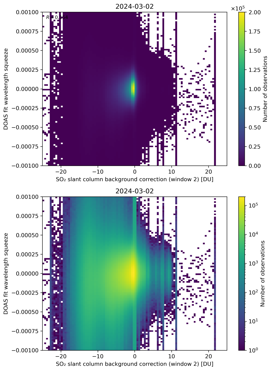
Figure 113: Scatter density plot of “SO 2 slant column background correction (window 2)” against “DOAS fit wavelength squeeze” for 2024-03-01 to 2024-03-03.
