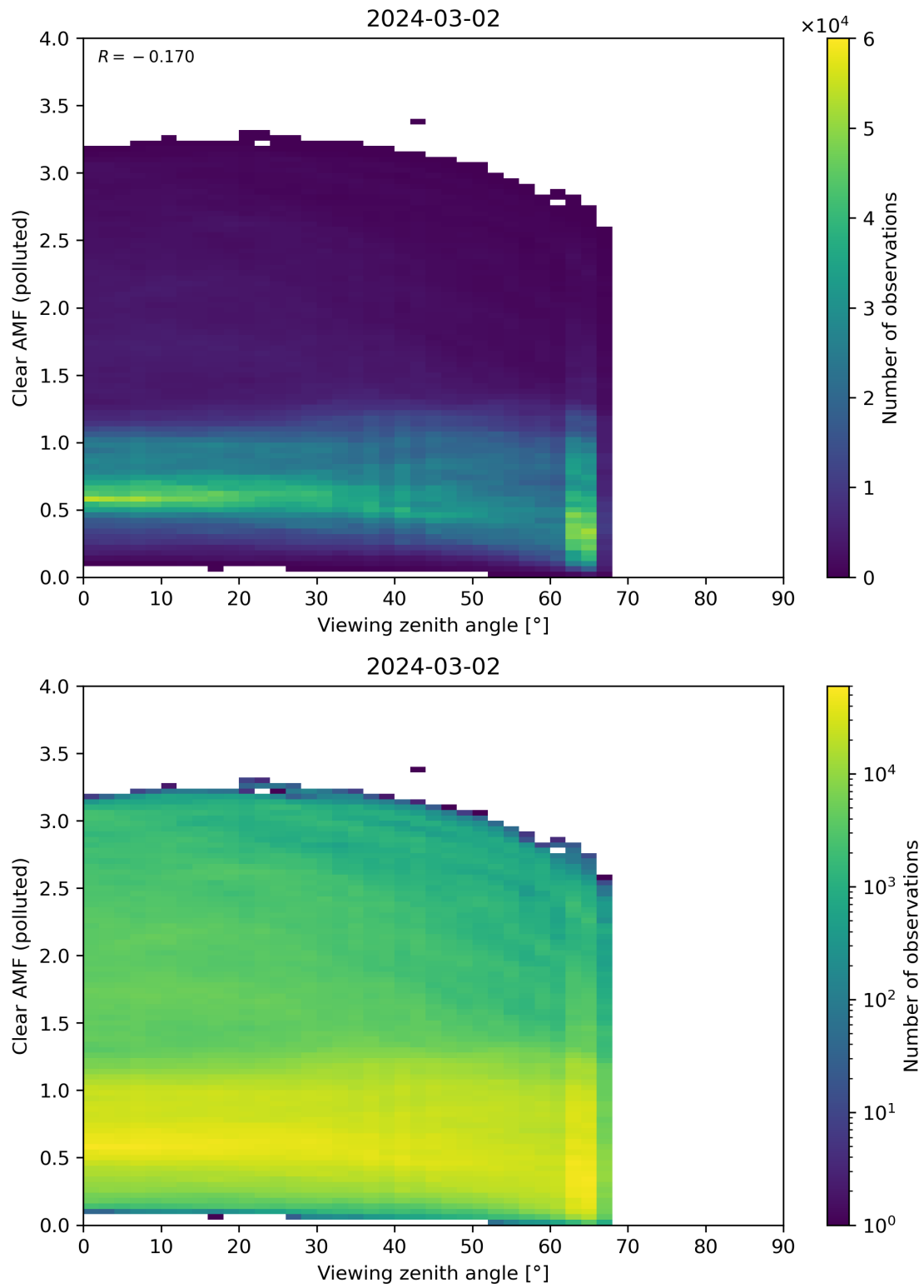
Figure 316: Scatter density plot of “Viewing zenith angle” against “Clear AMF (polluted)” for 2024-03-01 to 2024-03-03.
