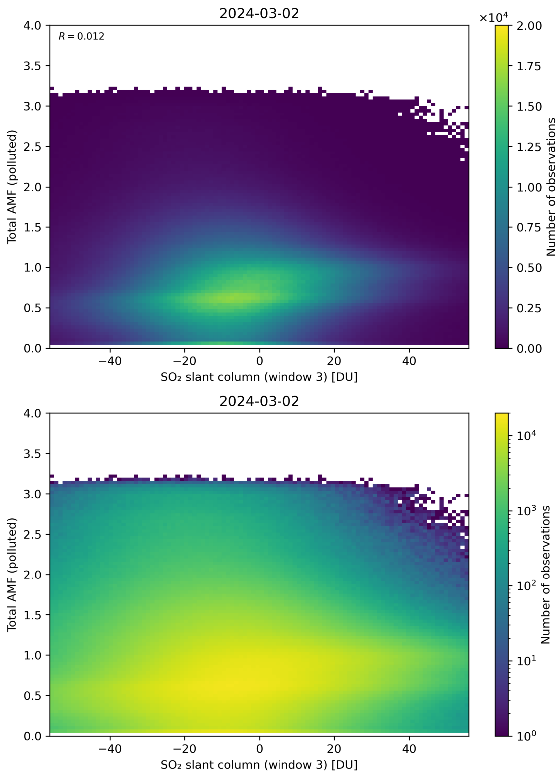
Figure 268: Scatter density plot of “SO 2 slant column (window 3)” against “Total AMF (polluted)” for 2024-03-01 to 2024-03-03.
