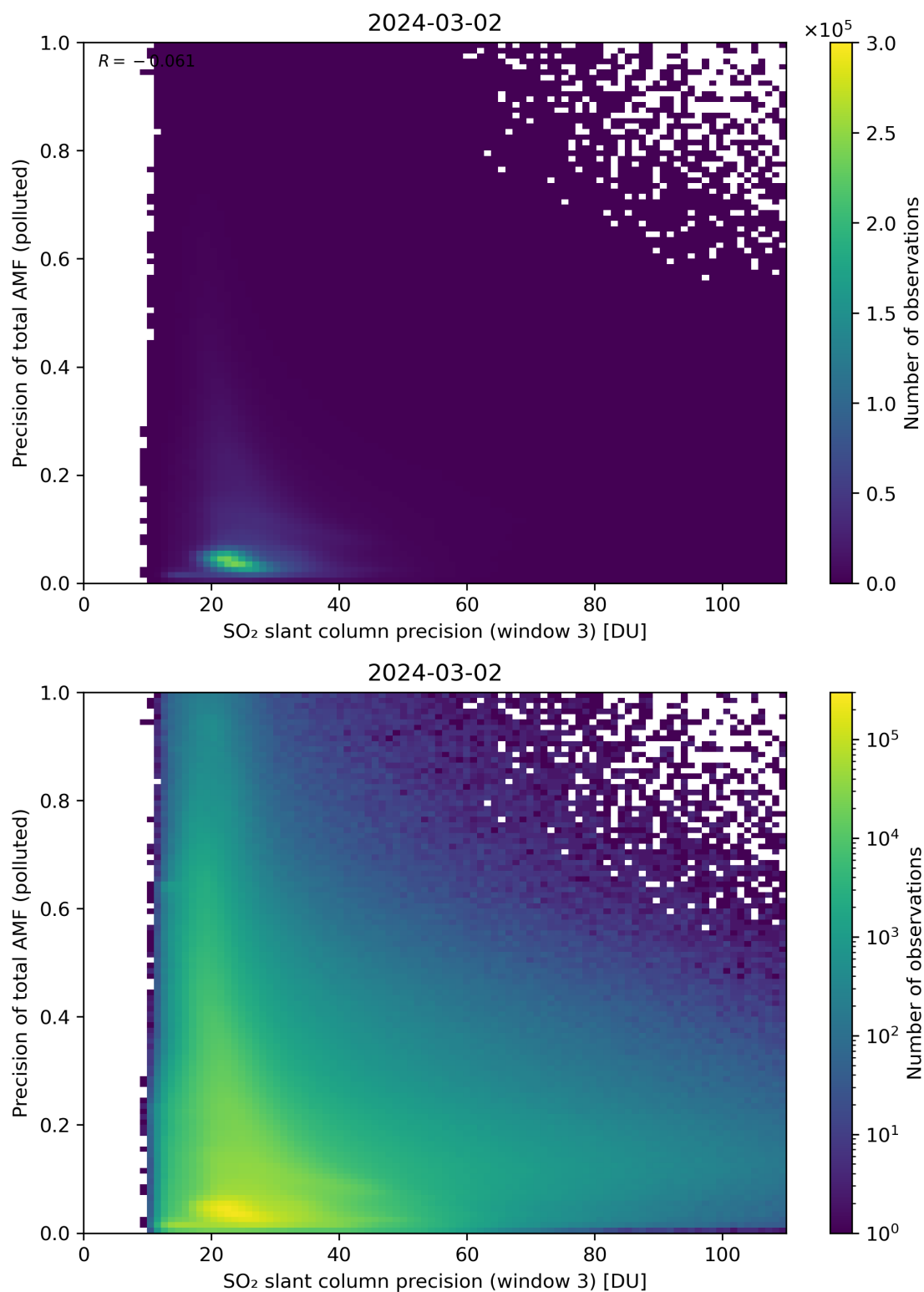
Figure 264: Scatter density plot of “SO 2 slant column precision (window 3)” against “Precision of total AMF (polluted)” for 2024-03-01 to 2024-03-03.
