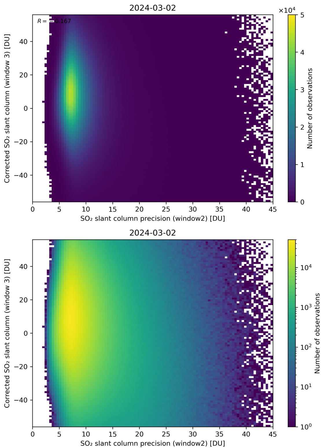
Figure 248: Scatter density plot of “SO 2 slant column precision (window2)” against “Corrected SO 2 slant column (window 3)” for 2024-03-01 to 2024-03-03.
