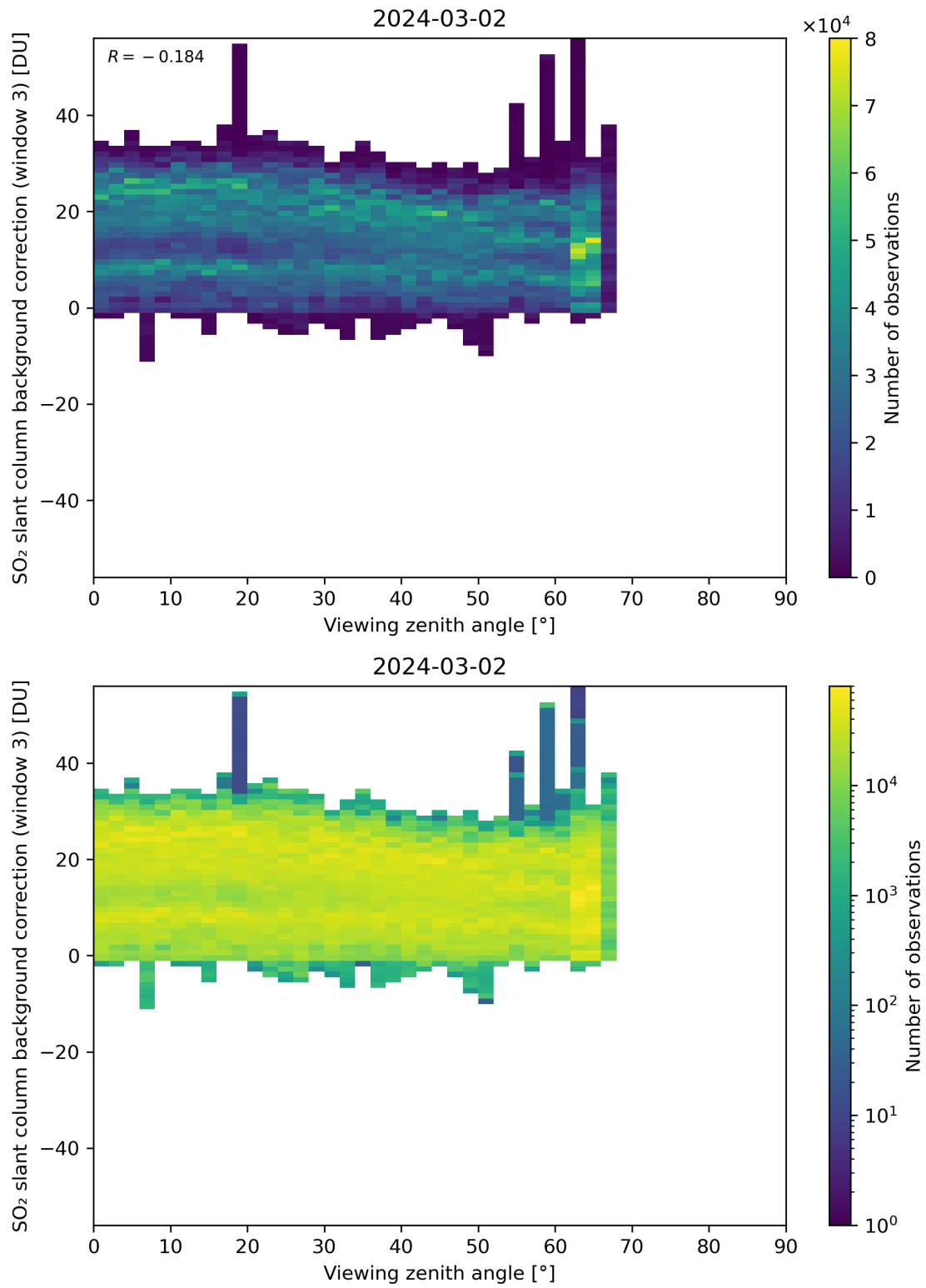
Figure 310: Scatter density plot of “Viewing zenith angle” against “SO 2 slant column background correction (window 3)” for 2024-03-01 to 2024-03-03.
