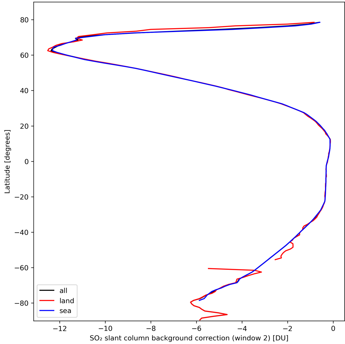
Figure 40: Zonal average of “SO 2 slant column background correction (window 2)” for 2024-03-01 to 2024-03-03.
