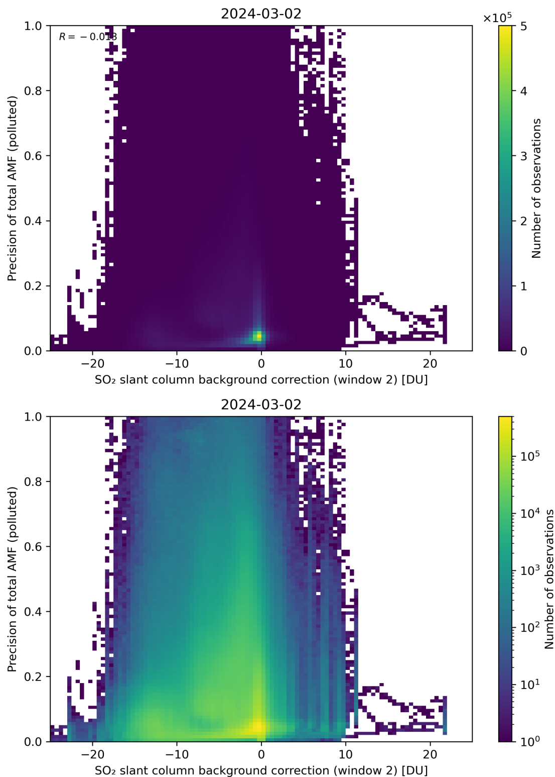
Figure 120: Scatter density plot of “SO 2 slant column background correction (window 2)” against “Precision of total AMF (polluted)” for 2024-03-01 to 2024-03-03.
