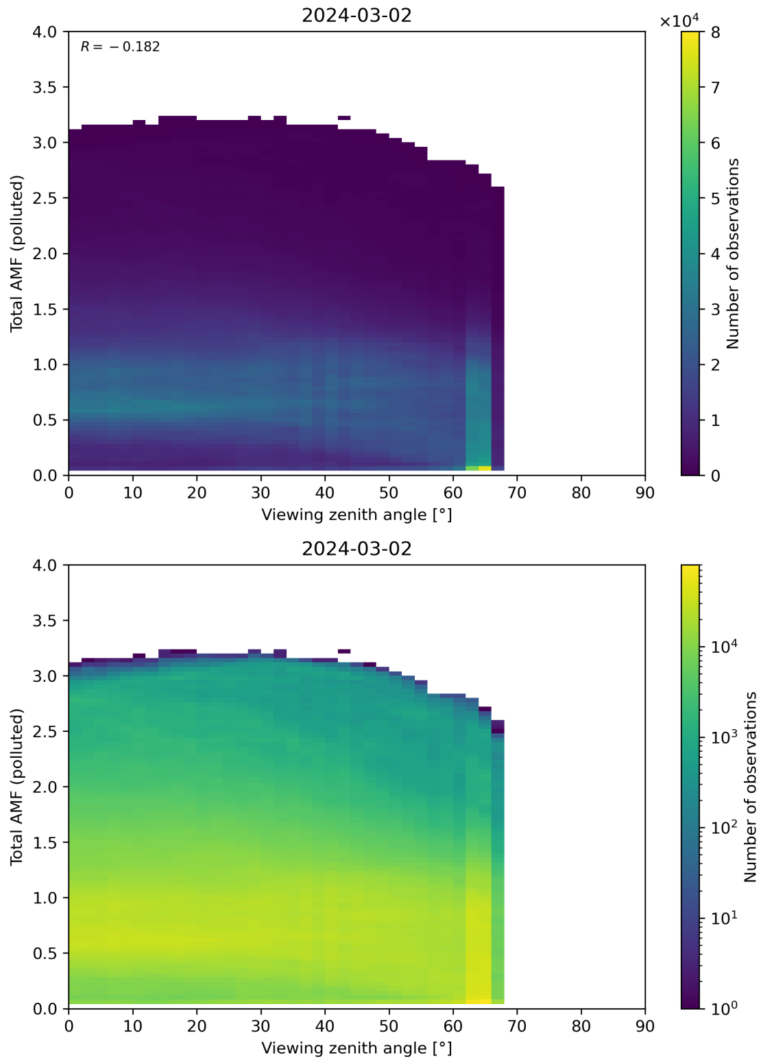
Figure 325: Scatter density plot of “Viewing zenith angle” against “Total AMF (polluted)” for 2024-03-01 to 2024-03-03.
