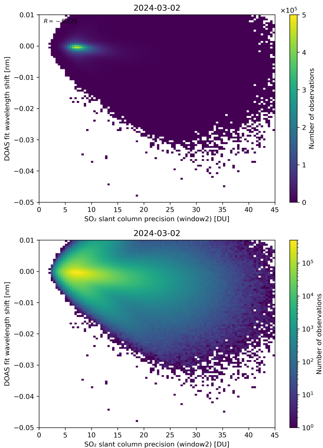
Figure 243: Scatter density plot of “SO 2 slant column precision (window2)” against “DOAS fit wavelength shift” for 2024-03-01 to 2024-03-03.
