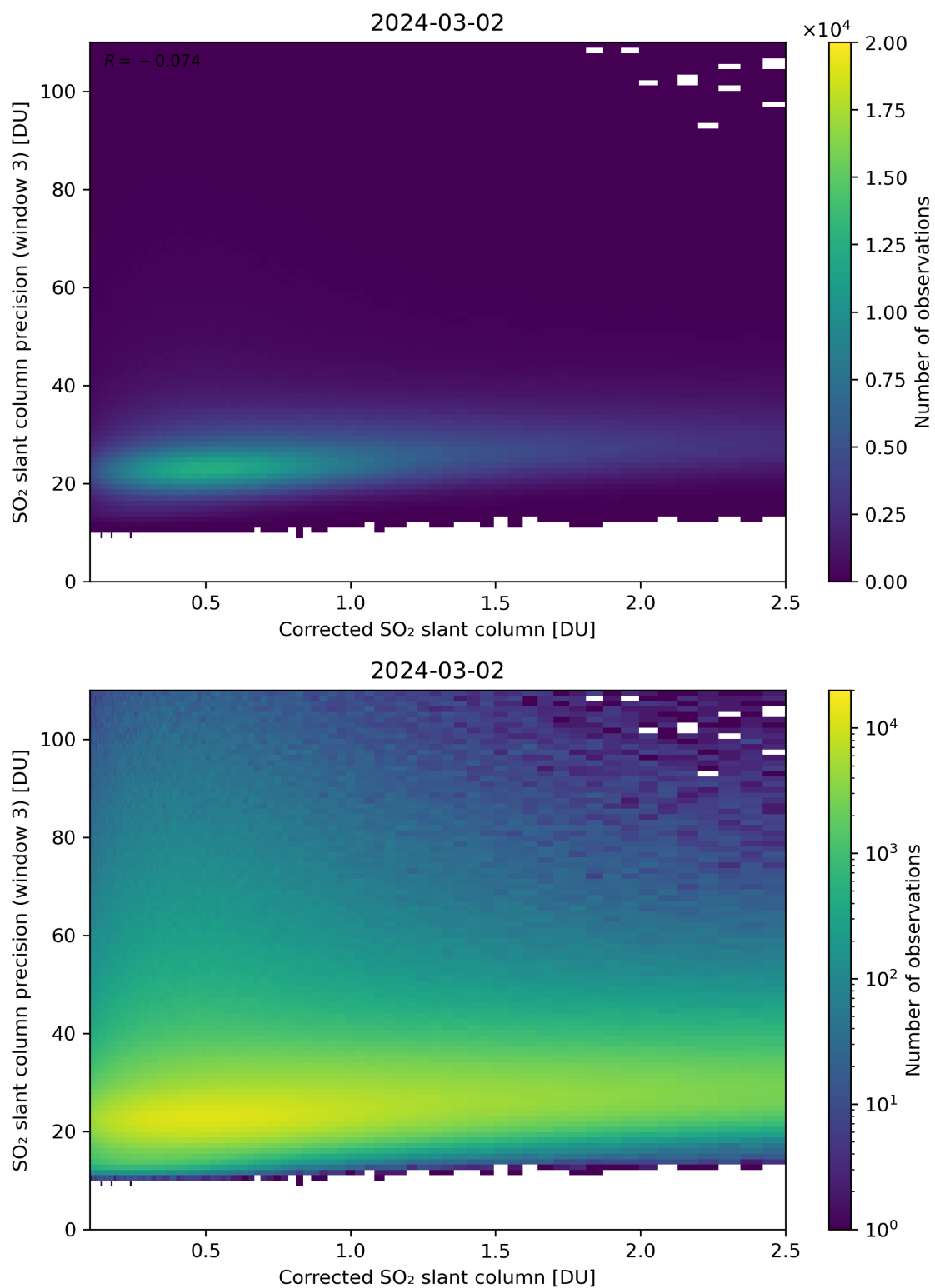
Figure 191: Scatter density plot of “Corrected SO 2 slant column” against “SO 2 slant column precision (window 3)” for 2024-03-01 to 2024-03-03.
