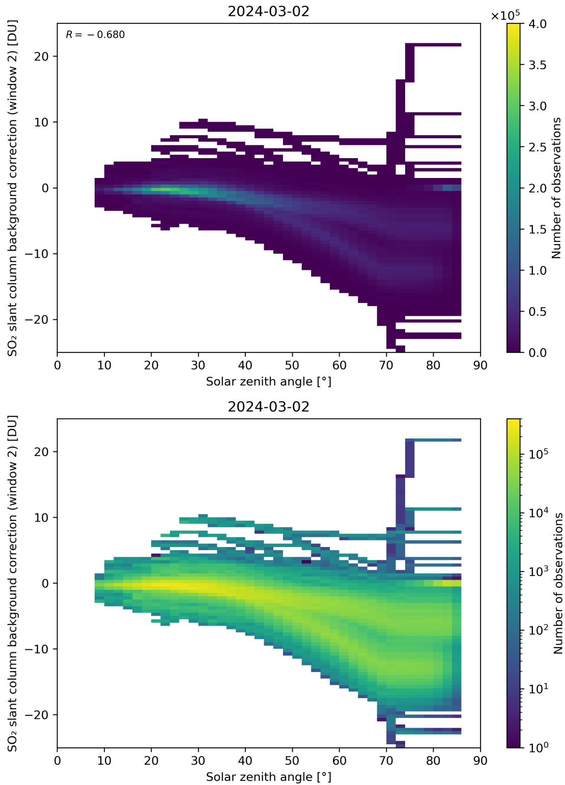
Figure 159: Scatter density plot of “Solar zenith angle” against “SO 2 slant column background correction (window 2)” for 2024-03-01 to 2024-03-03.
