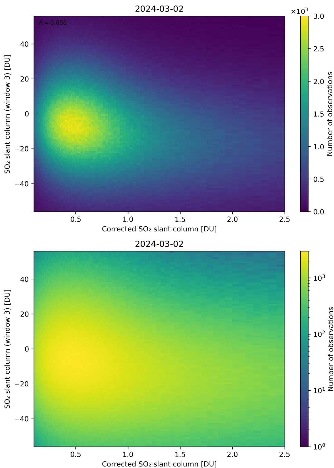
Figure 190: Scatter density plot of “Corrected SO 2 slant column” against “SO 2 slant column (window 3)” for 2024-03-01 to 2024-03-03.
