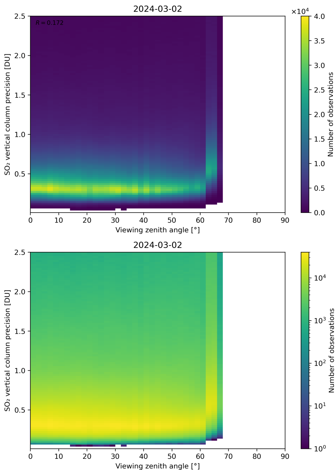
Figure 328: Scatter density plot of “Viewing zenith angle” against “SO 2 vertical column precision” for 2024-03-01 to 2024-03-03.
