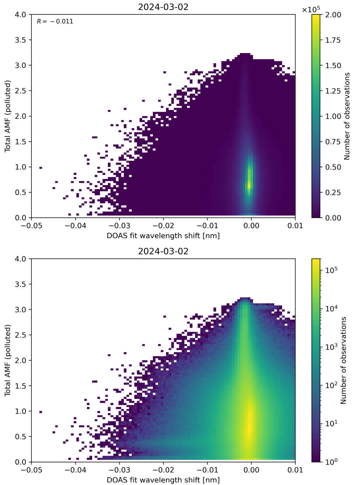
Figure 130: Scatter density plot of “DOAS fit wavelength shift” against “Total AMF (polluted)” for 2024-03-01 to 2024-03-03.
