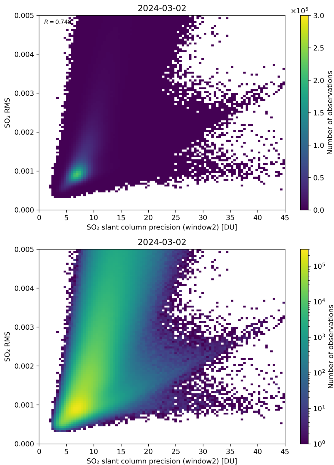
Figure 245: Scatter density plot of “SO 2 slant column precision (window2)” against “SO 2 RMS” for 2024-03-01 to 2024-03-03.
