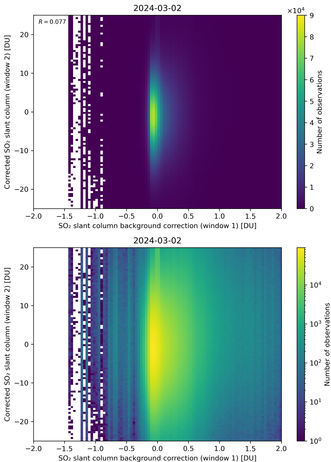
Figure 104: Scatter density plot of “SO 2 slant column background correction (window 1)” against “Corrected SO 2 slant column (window 2)” for 2024-03-01 to 2024-03-03.
