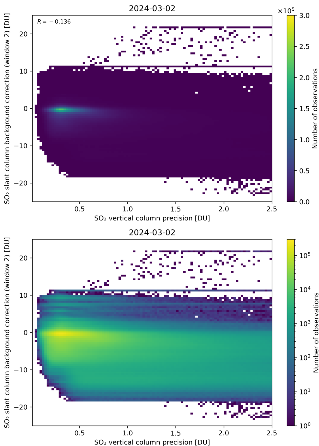
Figure 280: Scatter density plot of “SO 2 vertical column precision” against “SO 2 slant column background correction (window 2)” for 2024-03-01 to 2024-03-03.
