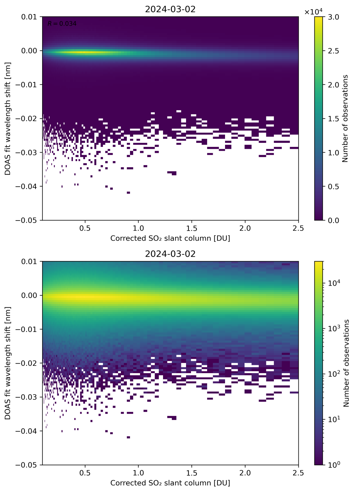
Figure 181: Scatter density plot of “Corrected SO 2 slant column” against “DOAS fit wavelength shift” for 2024-03-01 to 2024-03-03.
