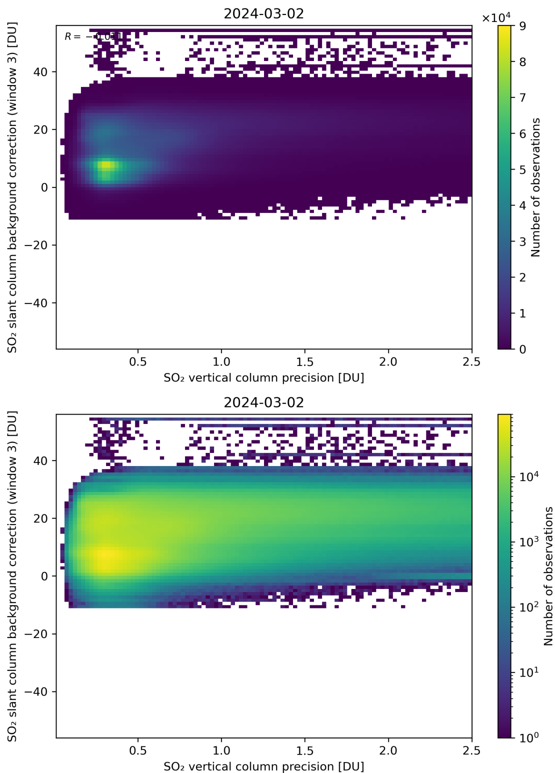
Figure 281: Scatter density plot of “SO 2 vertical column precision” against “SO 2 slant column background correction (window 3)” for 2024-03-01 to 2024-03-03.
