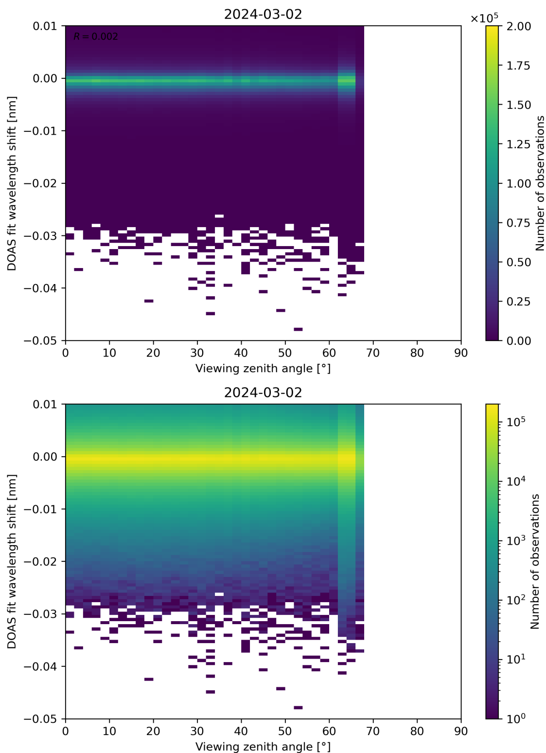
Figure 311: Scatter density plot of “Viewing zenith angle” against “DOAS fit wavelength shift” for 2024-03-01 to 2024-03-03.
