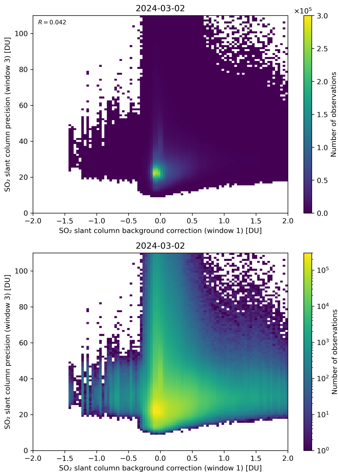
Figure 108: Scatter density plot of “SO 2 slant column background correction (window 1)” against “SO 2 slant column precision (window 3)” for 2024-03-01 to 2024-03-03.
