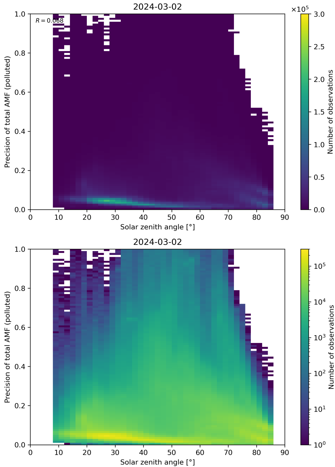
Figure 175: Scatter density plot of “Solar zenith angle” against “Precision of total AMF (polluted)” for 2024-03-01 to 2024-03-03.
