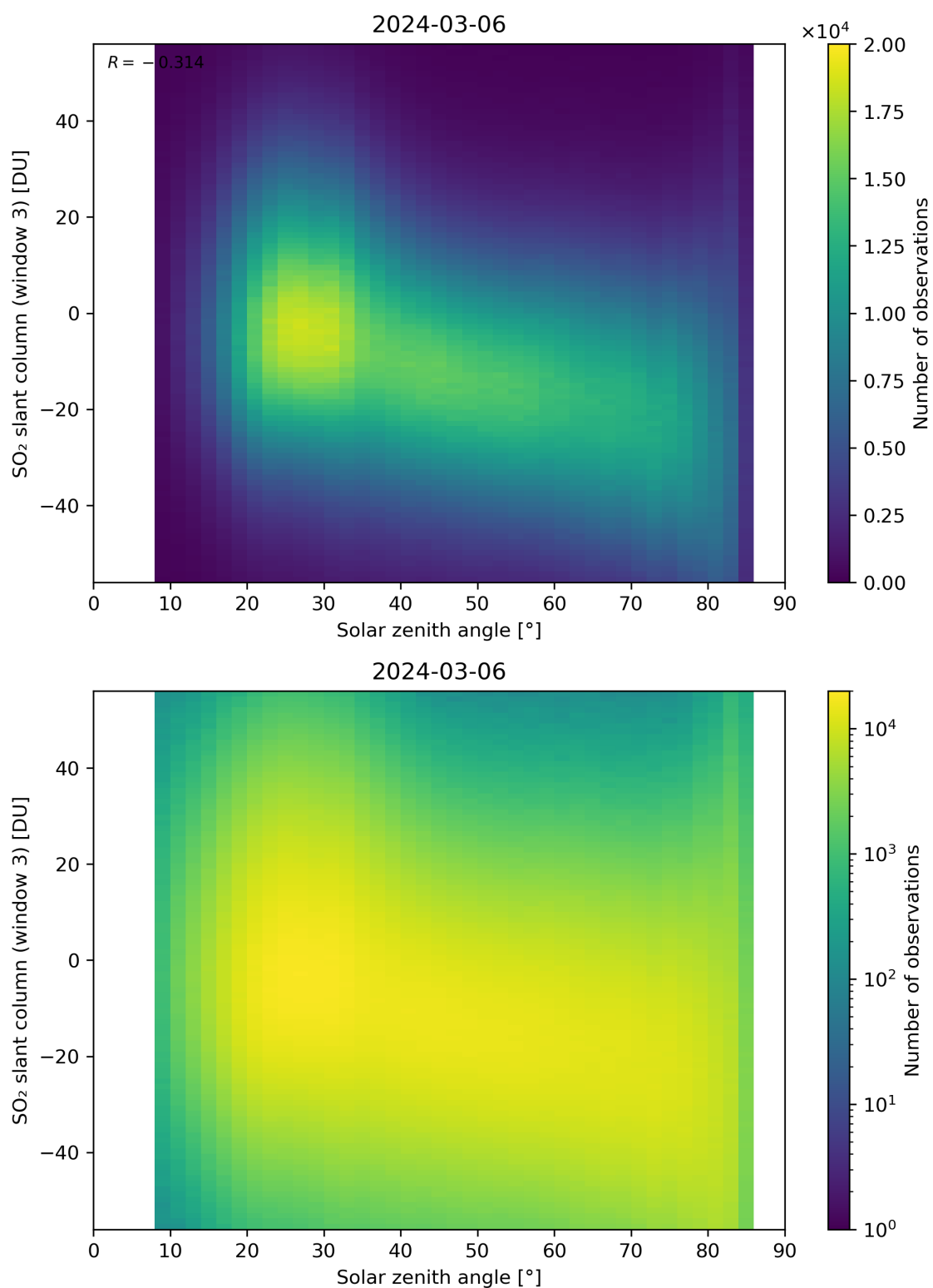
Figure 172: Scatter density plot of “Solar zenith angle” against “SO 2 slant column (window 3)” for 2024-03-05 to 2024-03-07.
