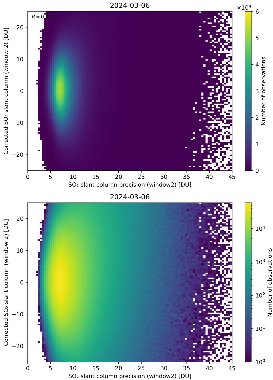
Figure 247: Scatter density plot of “SO 2 slant column precision (window2)” against “Corrected SO 2 slant column (window 2)” for 2024-03-05 to 2024-03-07.
