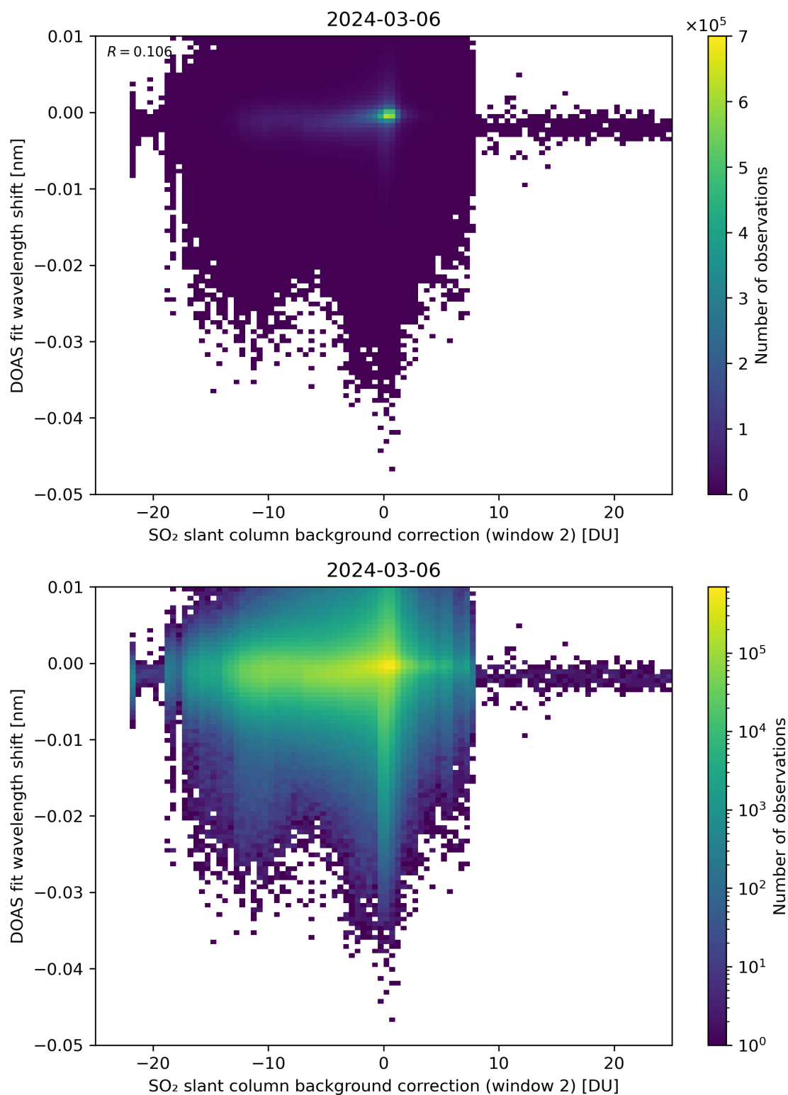
Figure 112: Scatter density plot of “SO 2 slant column background correction (window 2)” against “DOAS fit wavelength shift” for 2024-03-05 to 2024-03-07.
