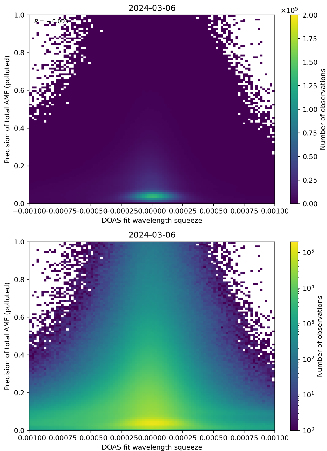
Figure 135: Scatter density plot of “DOAS fit wavelength squeeze” against “Precision of total AMF (polluted)” for 2024-03-05 to 2024-03-07.
