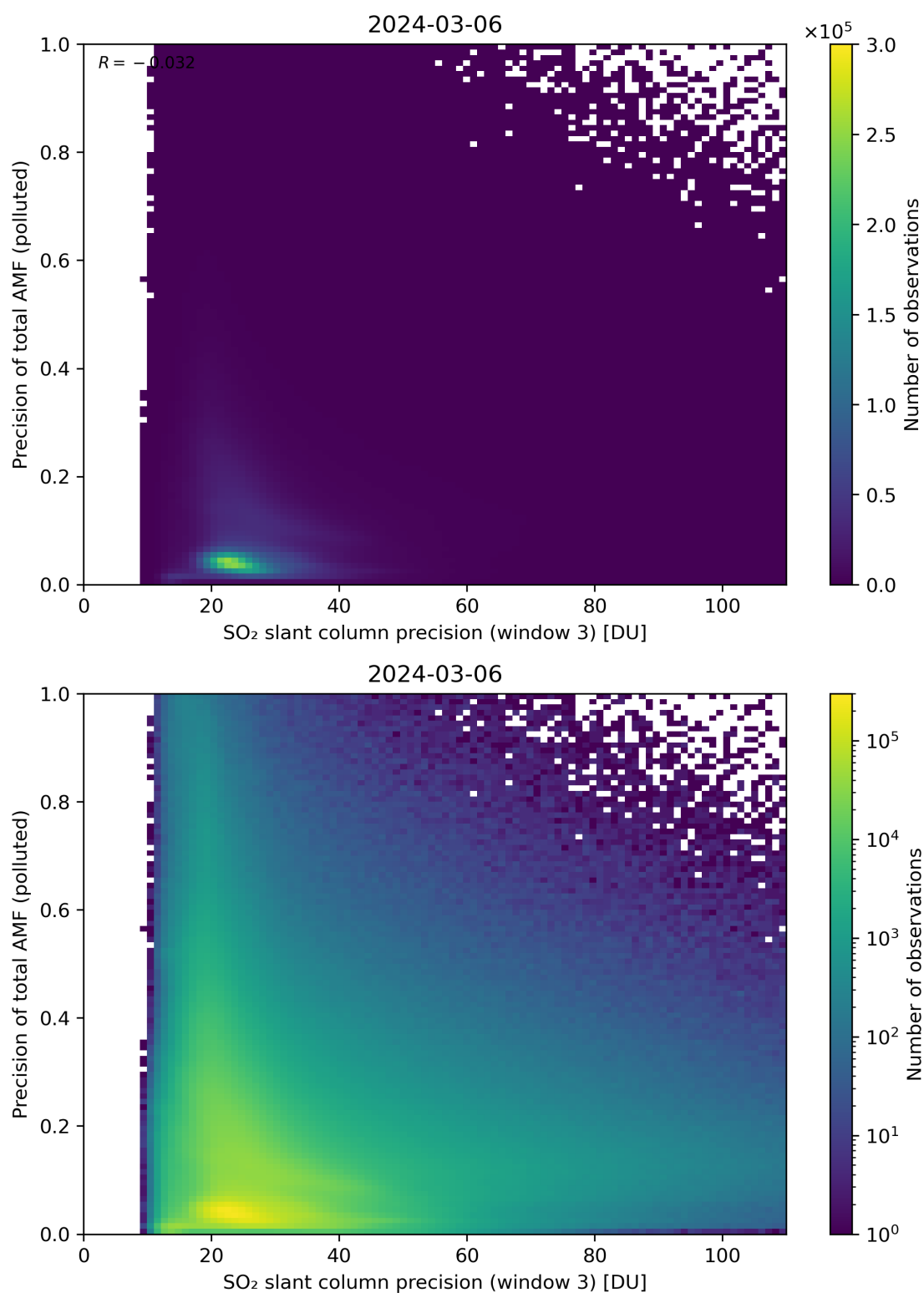
Figure 264: Scatter density plot of “SO 2 slant column precision (window 3)” against “Precision of total AMF (polluted)” for 2024-03-05 to 2024-03-07.
