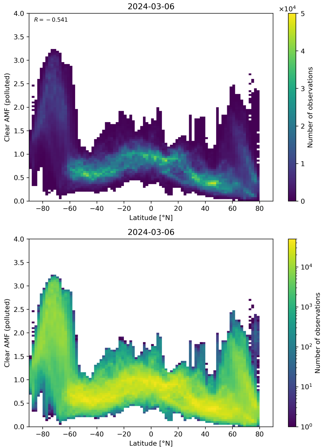
Figure 145: Scatter density plot of “Latitude” against “Clear AMF (polluted)” for 2024-03-05 to 2024-03-07.
