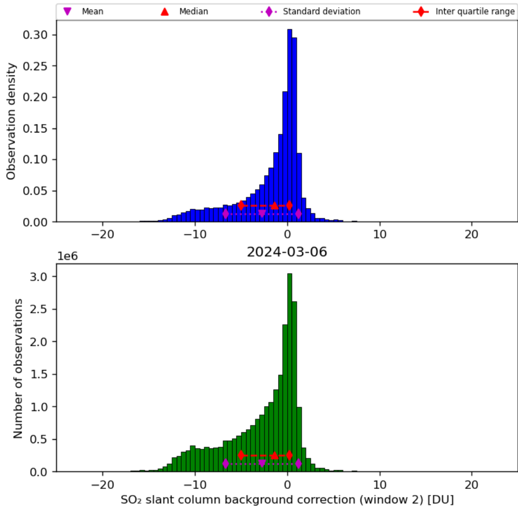
Figure 63: Histogram of “SO 2 slant column background correction (window 2)” for 2024-03-05 to 2024-03-07
