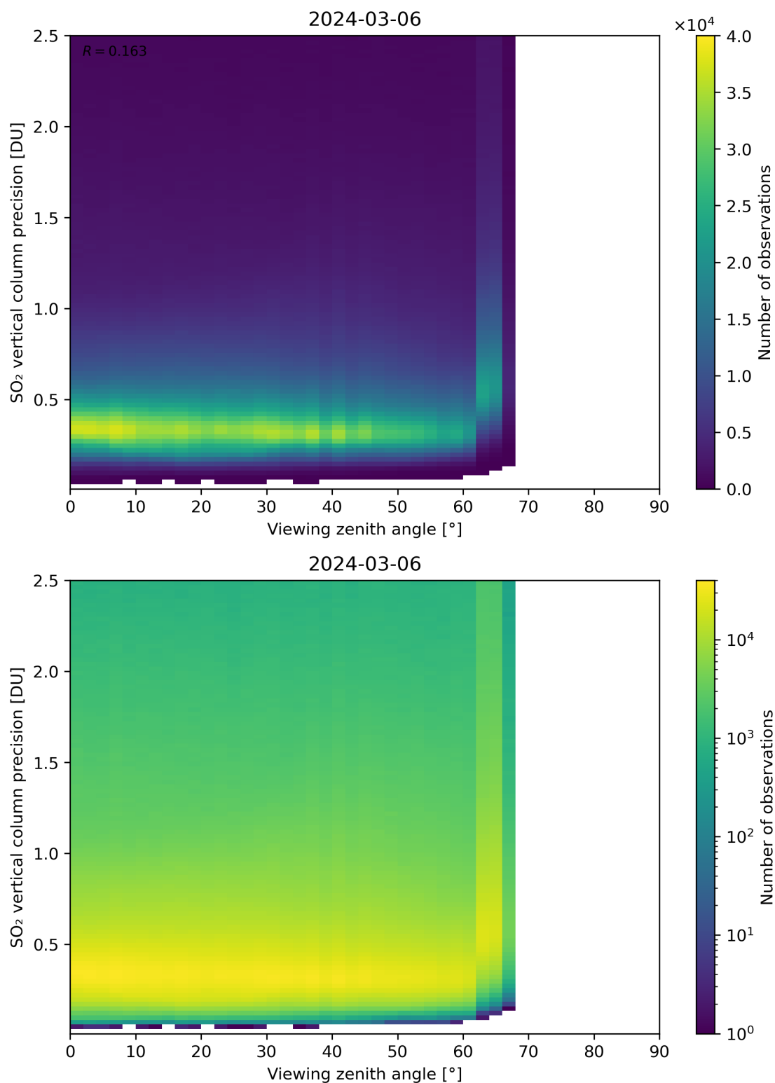
Figure 328: Scatter density plot of “Viewing zenith angle” against “SO 2 vertical column precision” for 2024-03-05 to 2024-03-07.
