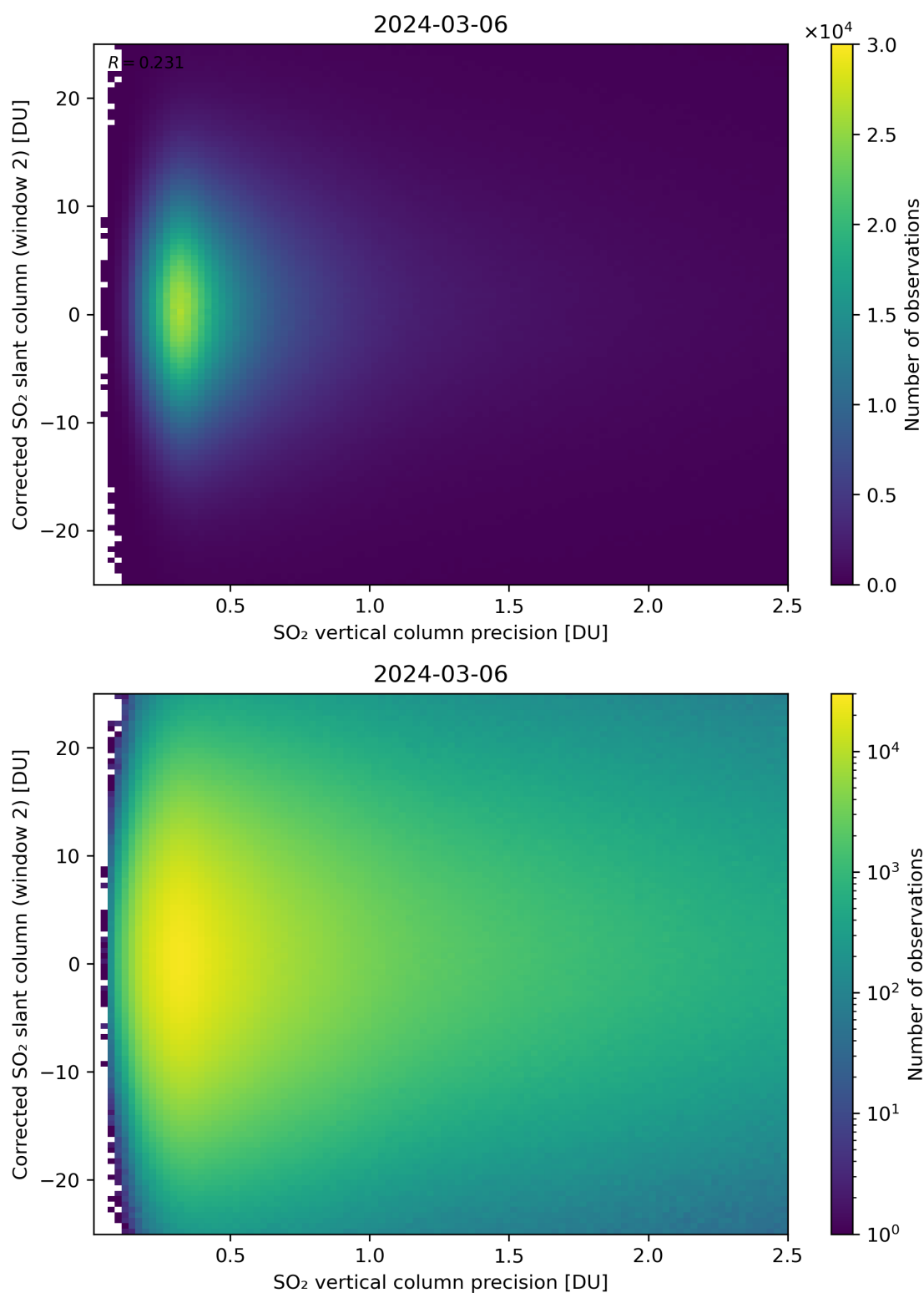
Figure 287: Scatter density plot of “SO 2 vertical column precision” against “Corrected SO 2 slant column (window 2)” for 2024-03-05 to 2024-03-07.
