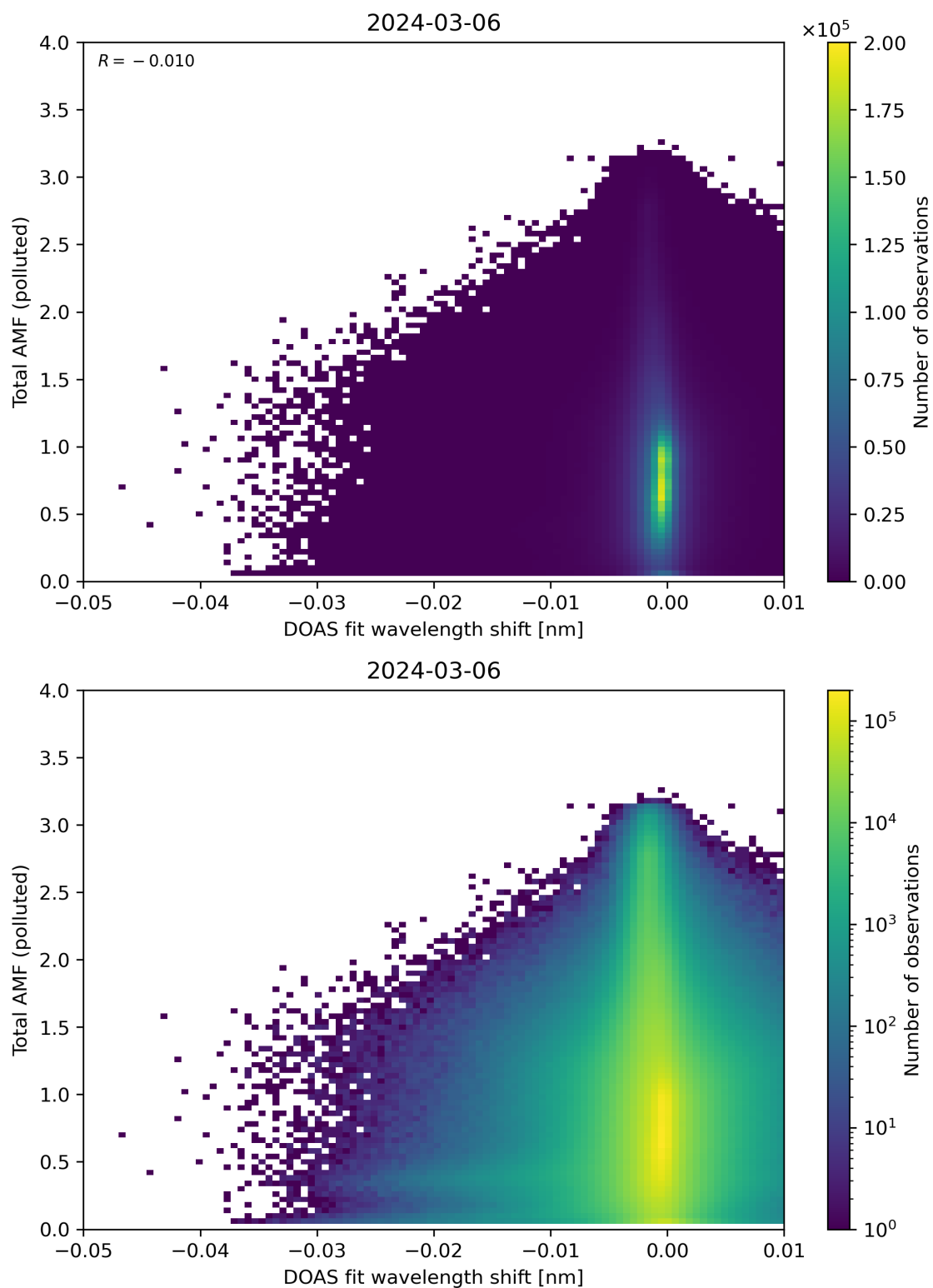
Figure 130: Scatter density plot of “DOAS fit wavelength shift” against “Total AMF (polluted)” for 2024-03-05 to 2024-03-07.
