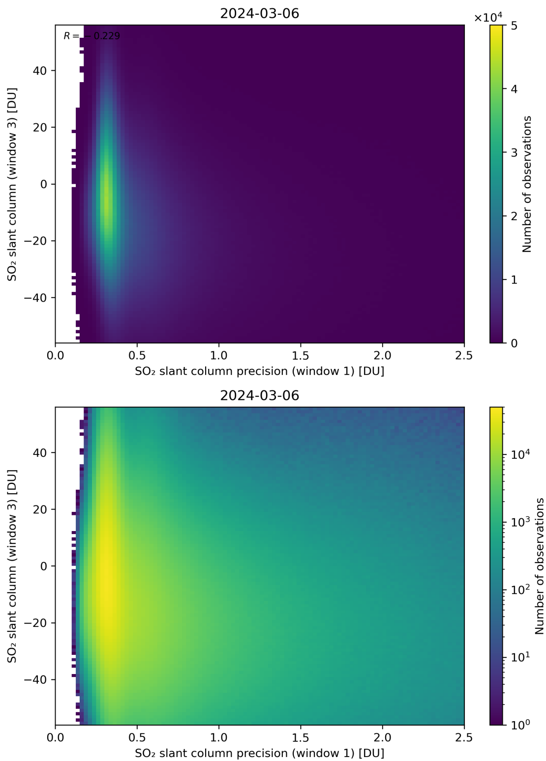
Figure 228: Scatter density plot of “SO 2 slant column precision (window 1)” against “SO 2 slant column (window 3)” for 2024-03-05 to 2024-03-07.
