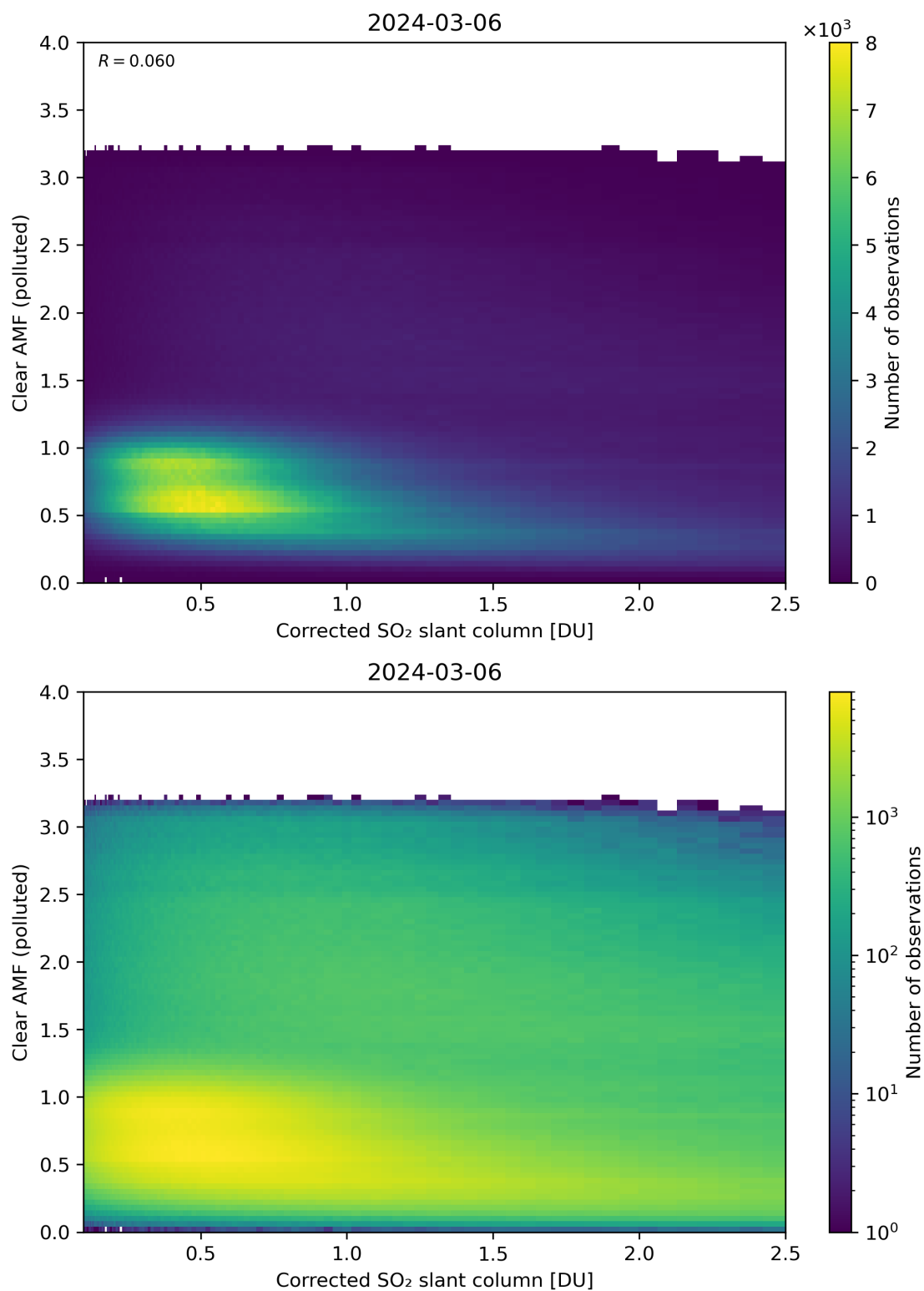
Figure 184: Scatter density plot of “Corrected SO 2 slant column” against “Clear AMF (polluted)” for 2024-03-05 to 2024-03-07.
