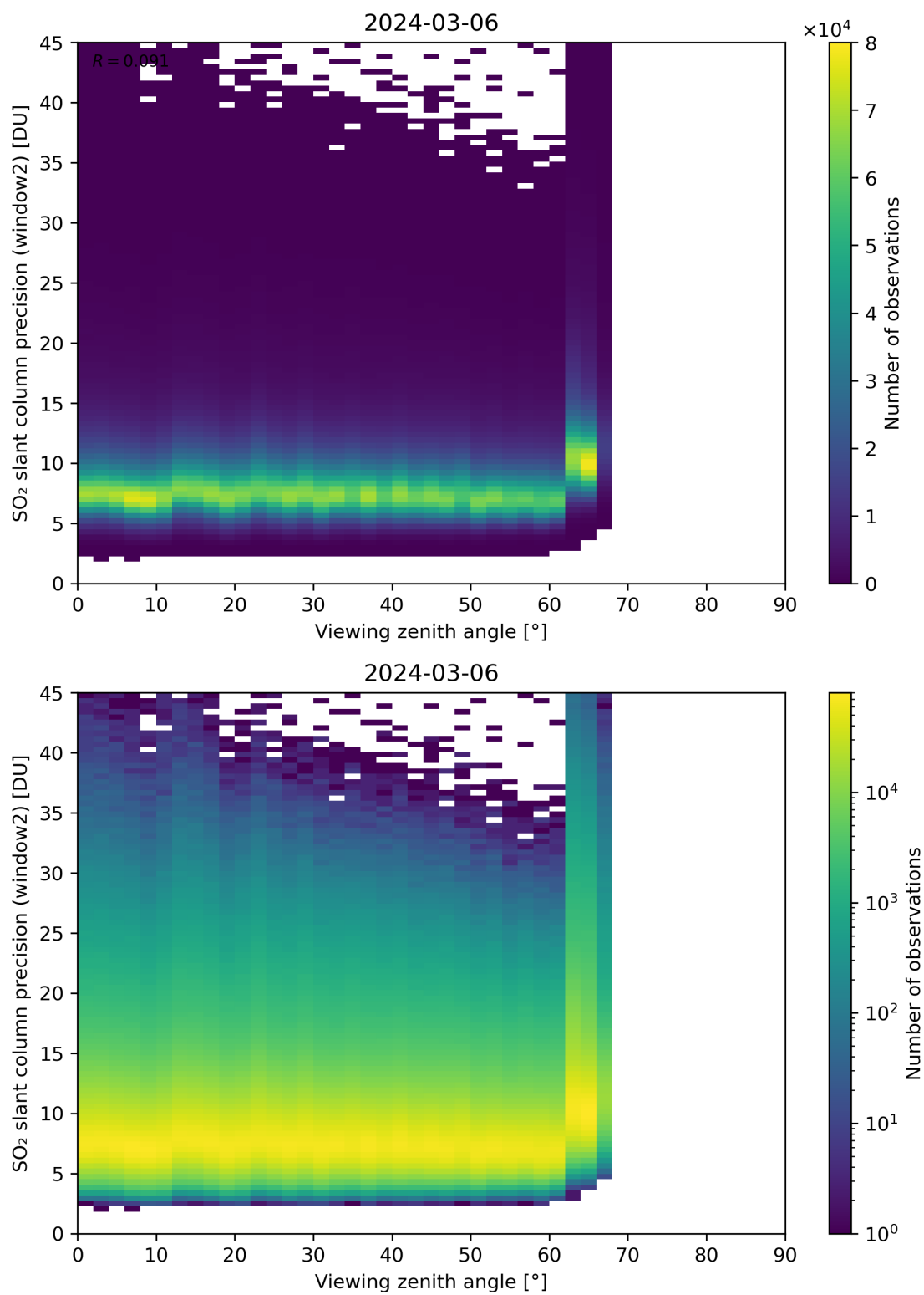
Figure 322: Scatter density plot of “Viewing zenith angle” against “SO 2 slant column precision (window2)” for 2024-03-05 to 2024-03-07.
