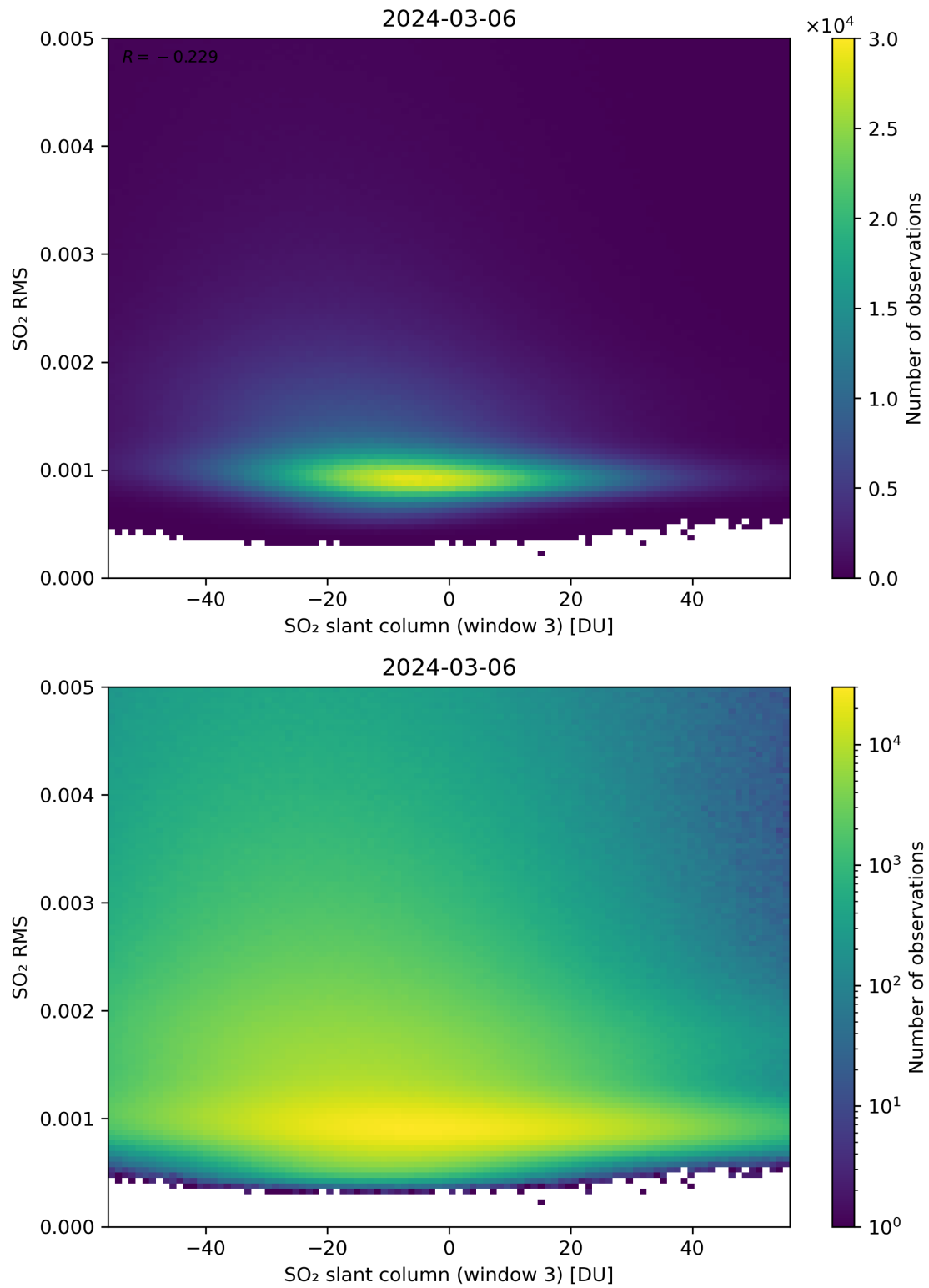
Figure 256: Scatter density plot of “SO 2 slant column (window 3)” against “SO 2 RMS” for 2024-03-05 to 2024-03-07.
