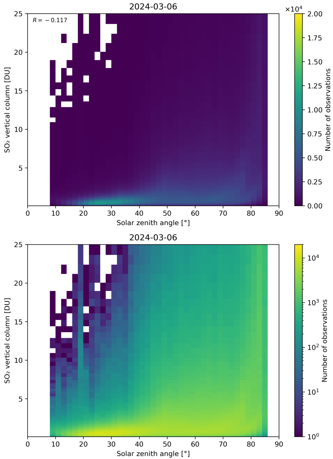
Figure 176: Scatter density plot of “Solar zenith angle” against “SO 2 vertical column” for 2024-03-05 to 2024-03-07.
