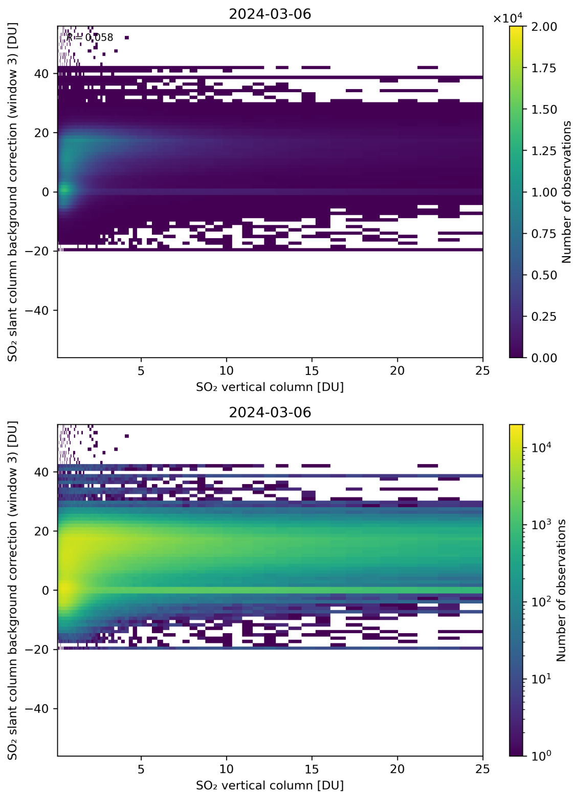
Figure 275: Scatter density plot of “SO 2 vertical column” against “SO 2 slant column background correction (window 3)” for 2024-03-05 to 2024-03-07.
