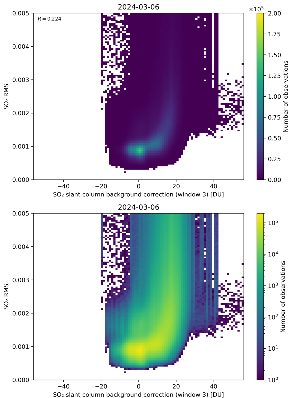
Figure 123: Scatter density plot of “SO 2 slant column background correction (window 3)” against “SO 2 RMS” for 2024-03-05 to 2024-03-07.
