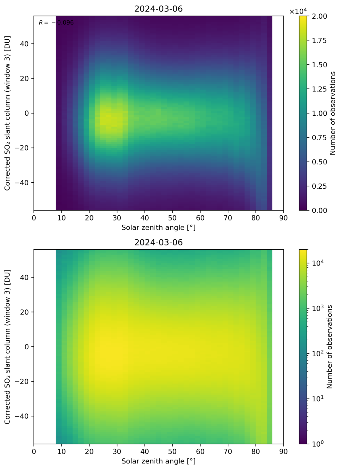
Figure 168: Scatter density plot of “Solar zenith angle” against “Corrected SO 2 slant column (window 3)” for 2024-03-05 to 2024-03-07.
