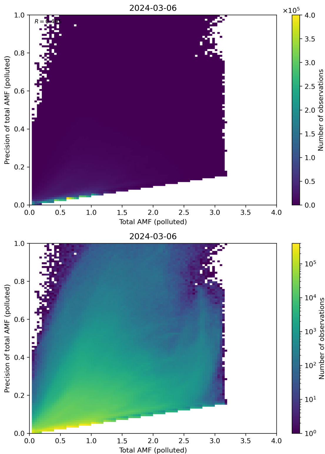
Figure 272: Scatter density plot of “Total AMF (polluted)” against “Precision of total AMF (polluted)” for 2024-03-05 to 2024-03-07.
