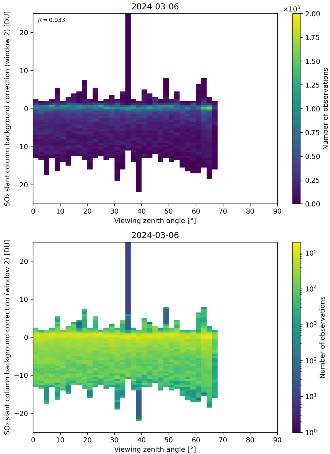
Figure 309: Scatter density plot of “Viewing zenith angle” against “SO 2 slant column background correction (window 2)” for 2024-03-05 to 2024-03-07.
