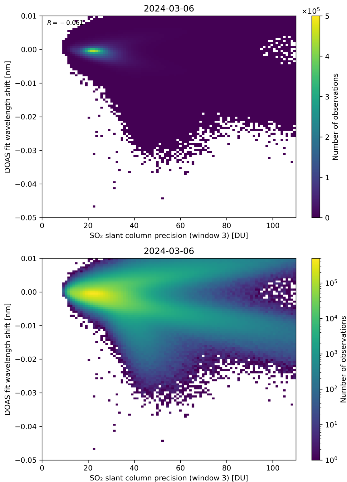
Figure 258: Scatter density plot of “SO 2 slant column precision (window 3)” against “DOAS fit wavelength shift” for 2024-03-05 to 2024-03-07.
