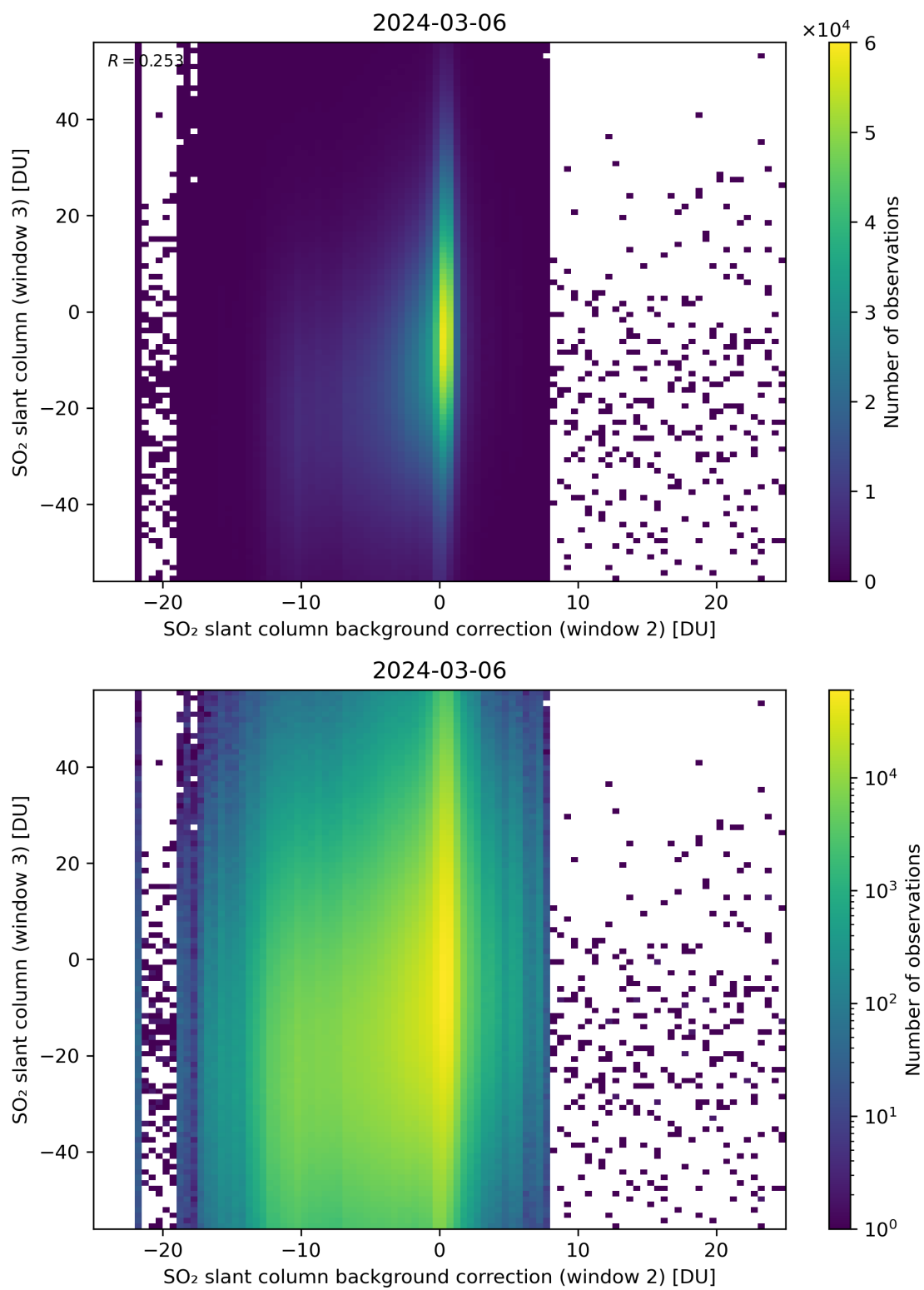
Figure 117: Scatter density plot of “SO 2 slant column background correction (window 2)” against “SO 2 slant column (window 3)” for 2024-03-05 to 2024-03-07.
