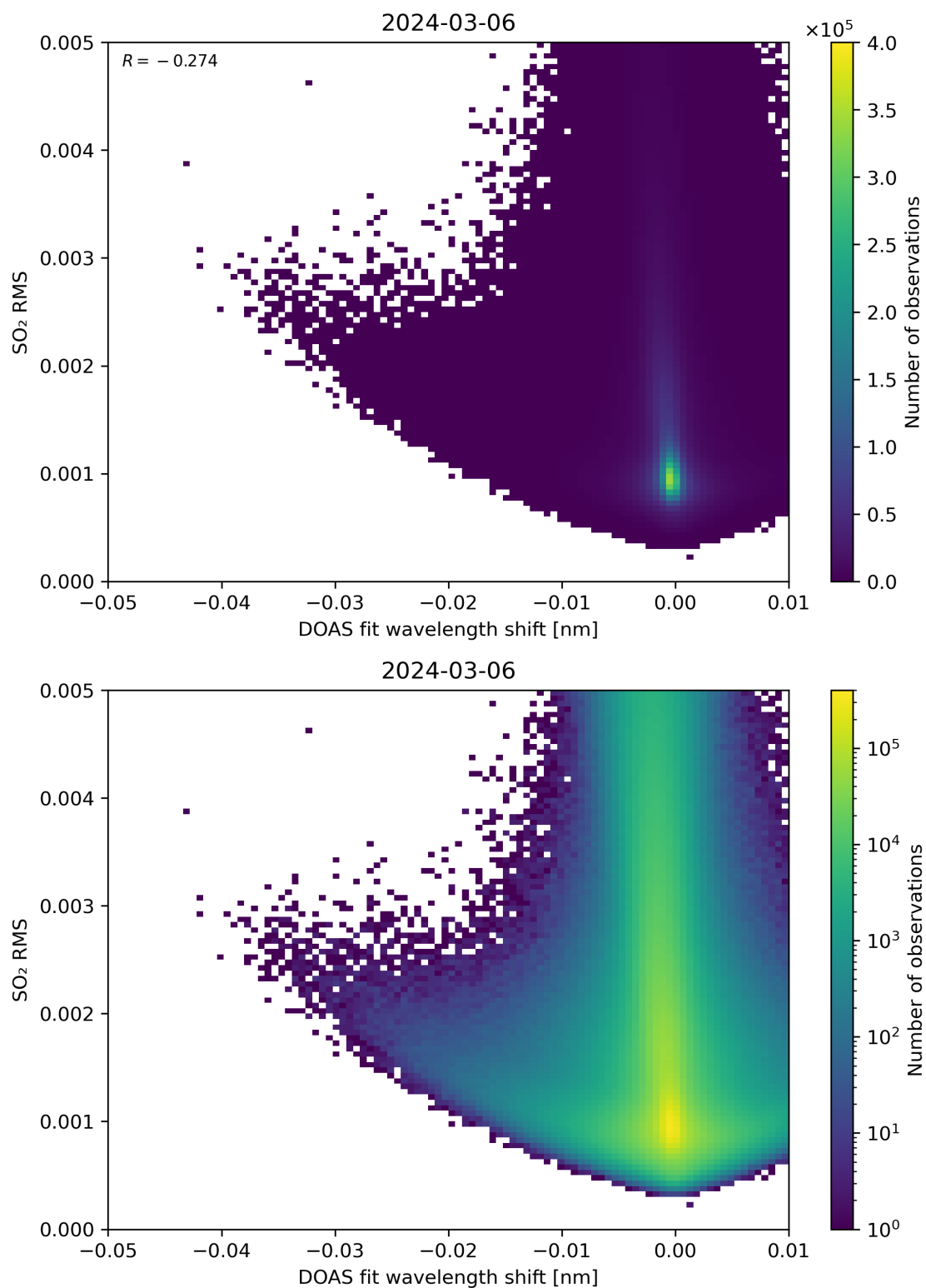
Figure 128: Scatter density plot of “DOAS fit wavelength shift” against “SO 2 RMS” for 2024-03-05 to 2024-03-07.
