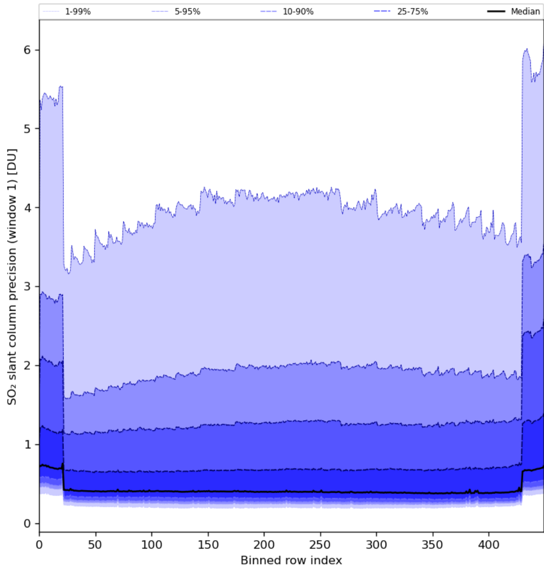
Figure 80: Along track statistics of “SO 2 slant column precision (window 1)” for 2024-03-05 to 2024-03-07
