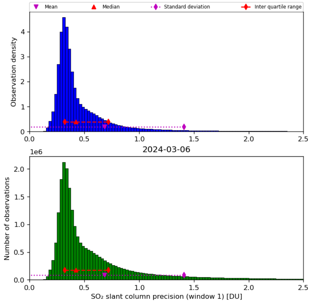
Figure 57: Histogram of “SO 2 slant column precision (window 1)” for 2024-03-05 to 2024-03-07
