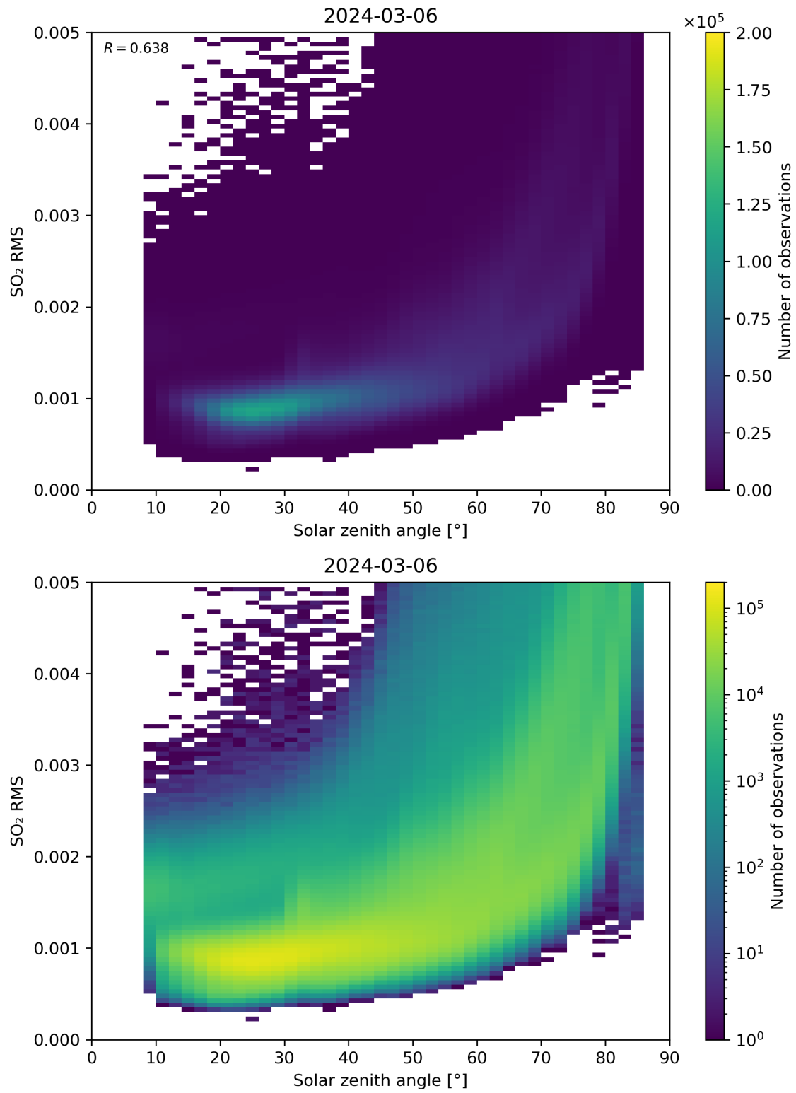
Figure 163: Scatter density plot of “Solar zenith angle” against “SO 2 RMS” for 2024-03-05 to 2024-03-07.
