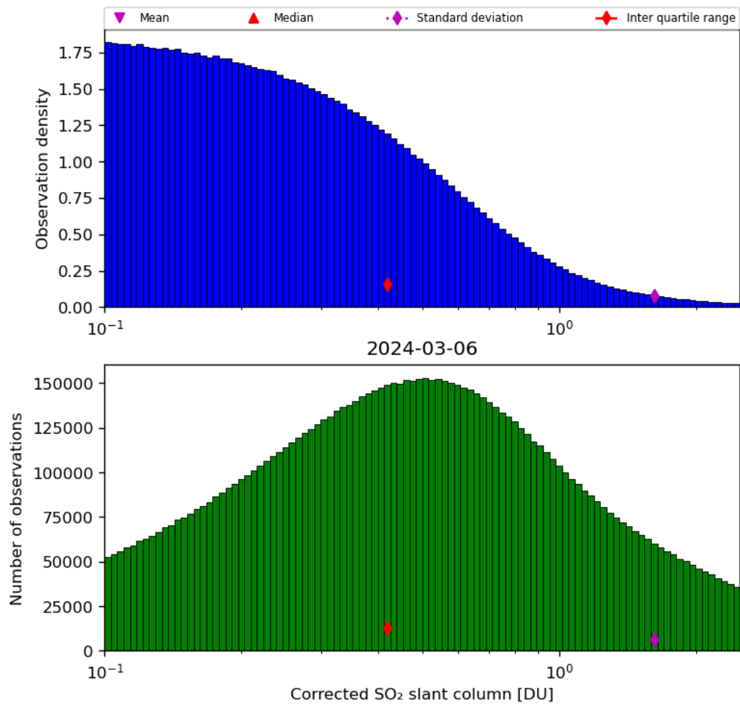
Figure 55: Histogram of “Corrected SO 2 slant column” for 2024-03-05 to 2024-03-07
