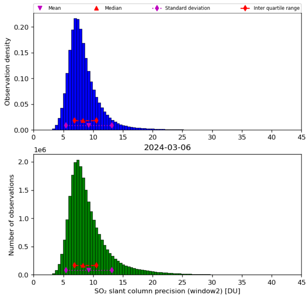
Figure 61: Histogram of “SO 2 slant column precision (window2)” for 2024-03-05 to 2024-03-07
