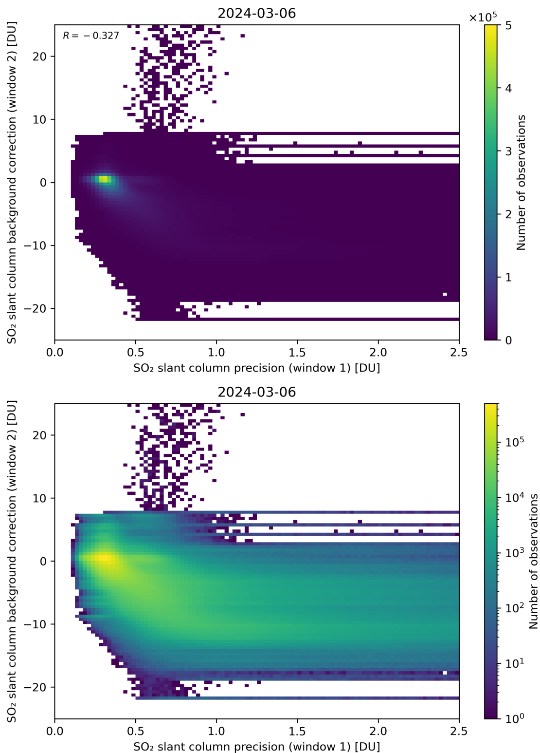
Figure 219: Scatter density plot of “SO 2 slant column precision (window 1)” against “SO 2 slant column background correction (window 2)” for 2024-03-05 to 2024-03-07.
