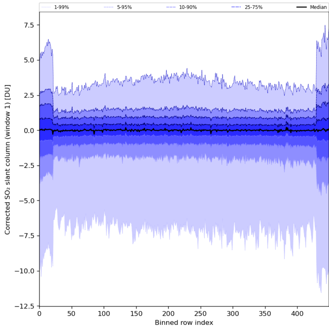
Figure 81: Along track statistics of “Corrected SO 2 slant column (window 1)” for 2024-03-05 to 2024-03-07
