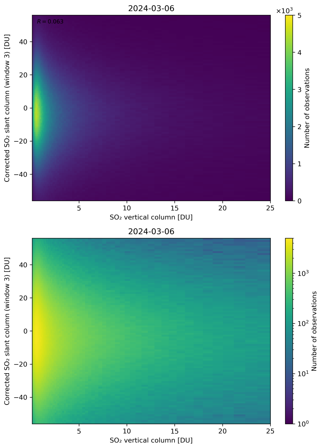
Figure 299: Scatter density plot of “SO 2 vertical column” against “Corrected SO 2 slant column (window 3)” for 2024-03-05 to 2024-03-07.
