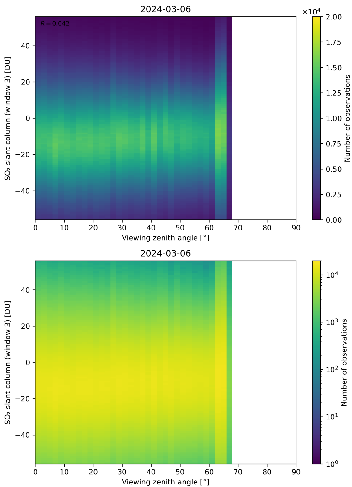
Figure 323: Scatter density plot of “Viewing zenith angle” against “SO 2 slant column (window 3)” for 2024-03-05 to 2024-03-07.
