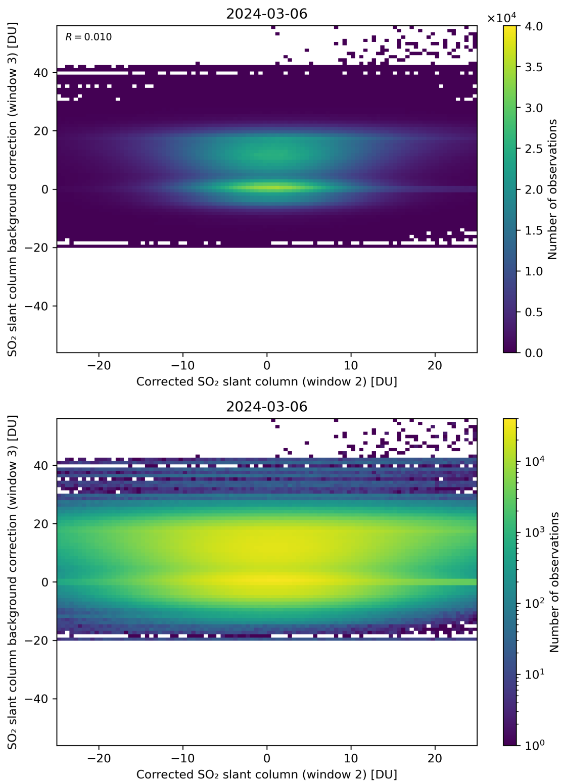
Figure 195: Scatter density plot of “Corrected SO 2 slant column (window 2)” against “SO 2 slant column background correction (window 3)” for 2024-03-05 to 2024-03-07.
