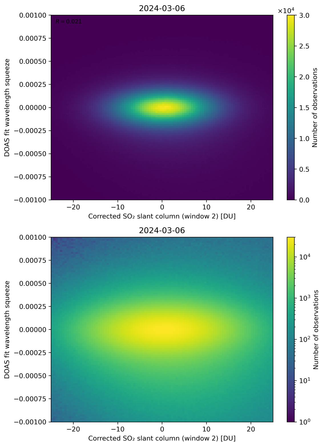
Figure 197: Scatter density plot of “Corrected SO 2 slant column (window 2)” against “DOAS fit wavelength squeeze” for 2024-03-05 to 2024-03-07.
