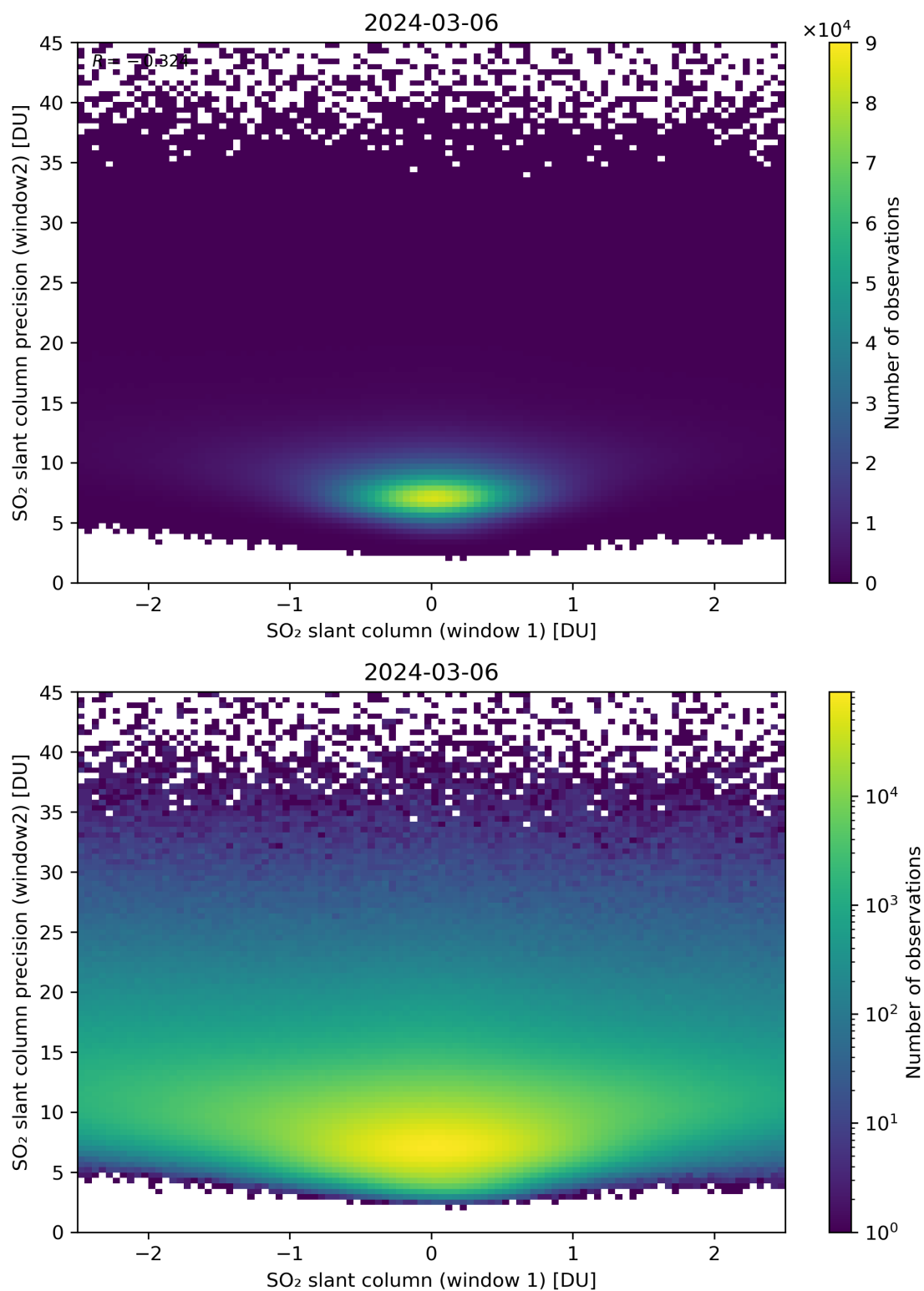
Figure 236: Scatter density plot of “SO 2 slant column (window 1)” against “SO 2 slant column precision (window2)” for 2024-03-05 to 2024-03-07.
