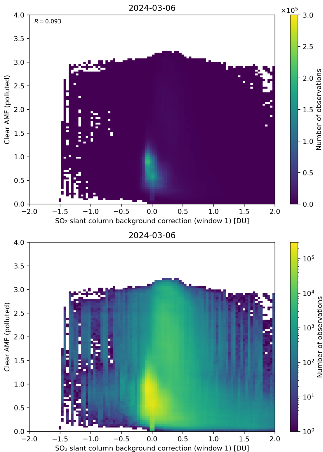
Figure 103: Scatter density plot of “SO 2 slant column background correction (window 1)” against “Clear AMF (polluted)” for 2024-03-05 to 2024-03-07.
