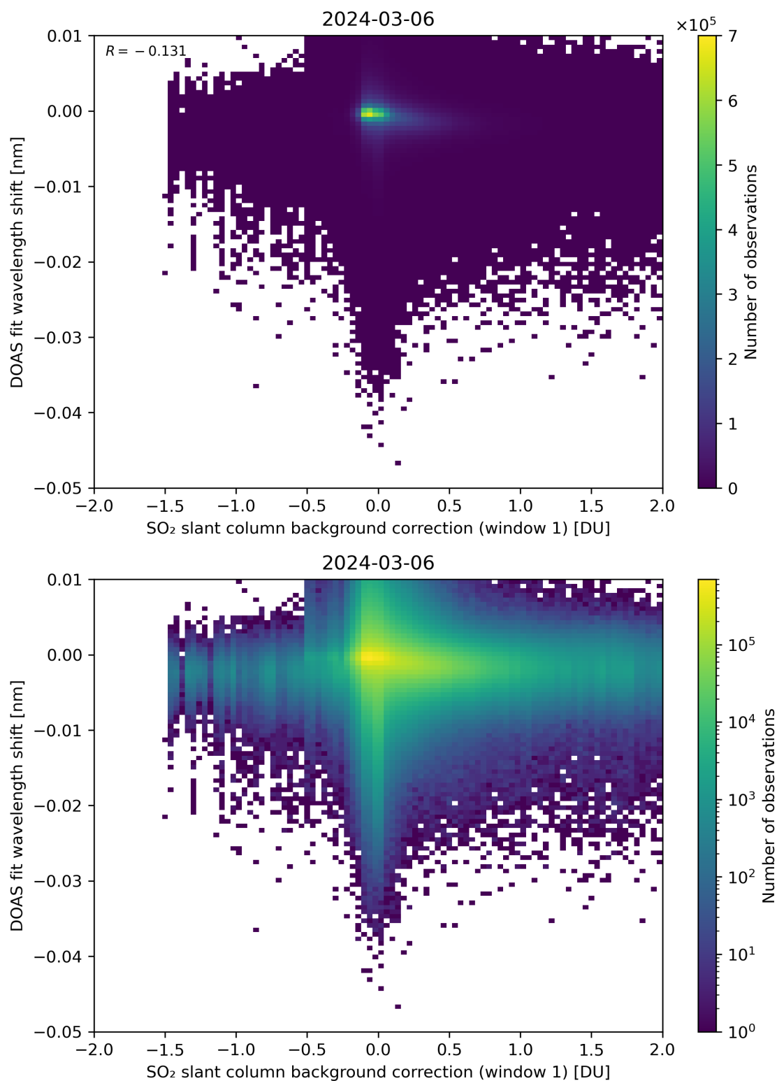
Figure 100: Scatter density plot of “SO 2 slant column background correction (window 1)” against “DOAS fit wavelength shift” for 2024-03-05 to 2024-03-07.
