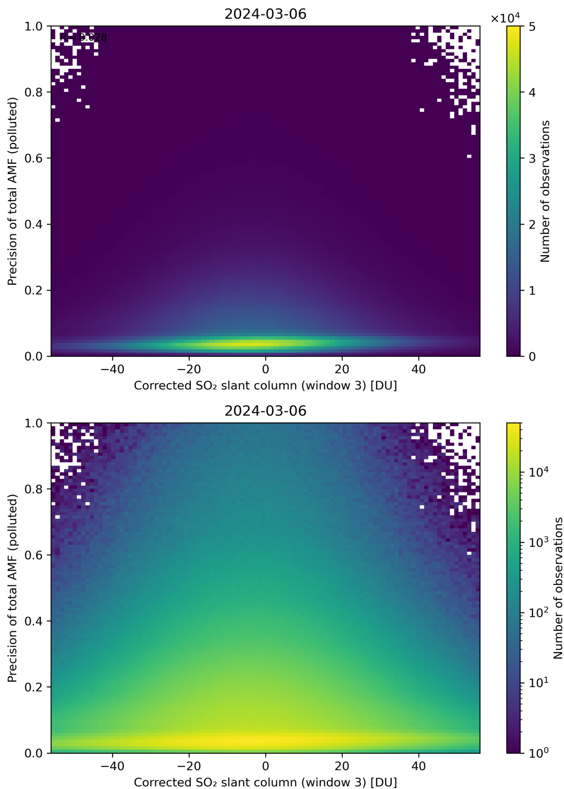
Figure 211: Scatter density plot of “Corrected SO 2 slant column (window 3)” against “Precision of total AMF (polluted)” for 2024-03-05 to 2024-03-07.
