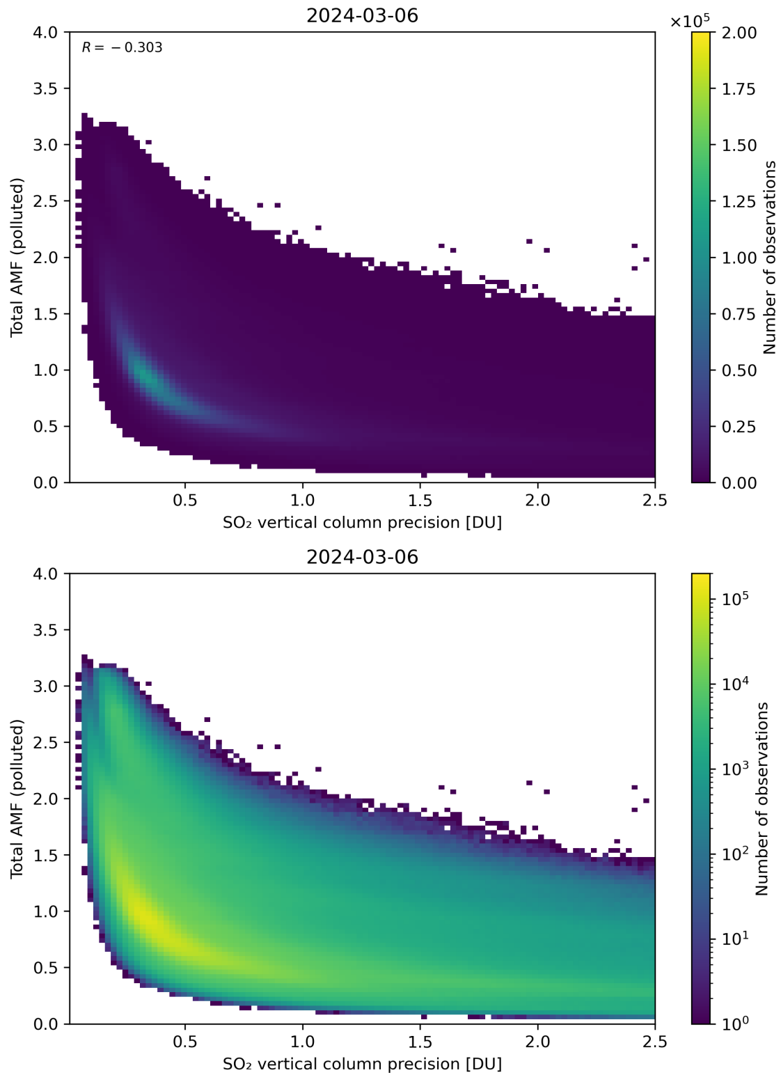
Figure 294: Scatter density plot of “SO 2 vertical column precision” against “Total AMF (polluted)” for 2024-03-05 to 2024-03-07.
