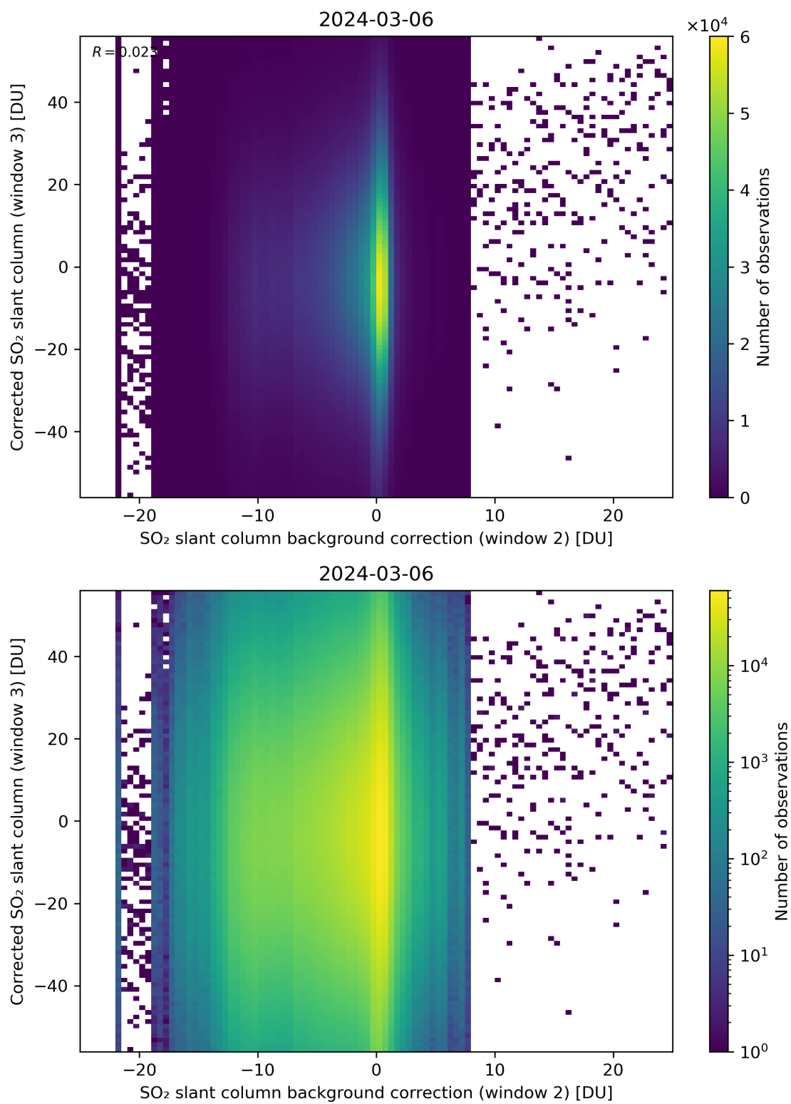
Figure 116: Scatter density plot of “SO 2 slant column background correction (window 2)” against “Corrected SO 2 slant column (window 3)” for 2024-03-05 to 2024-03-07.
