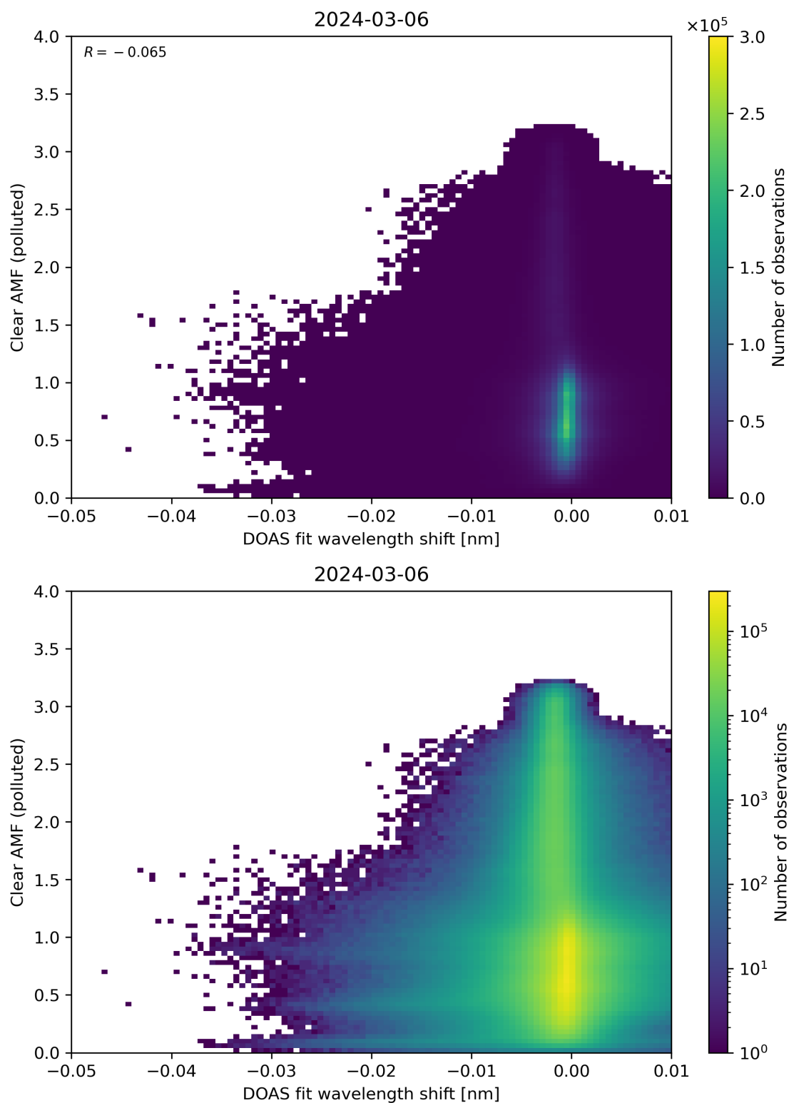
Figure 129: Scatter density plot of “DOAS fit wavelength shift” against “Clear AMF (polluted)” for 2024-03-05 to 2024-03-07.
