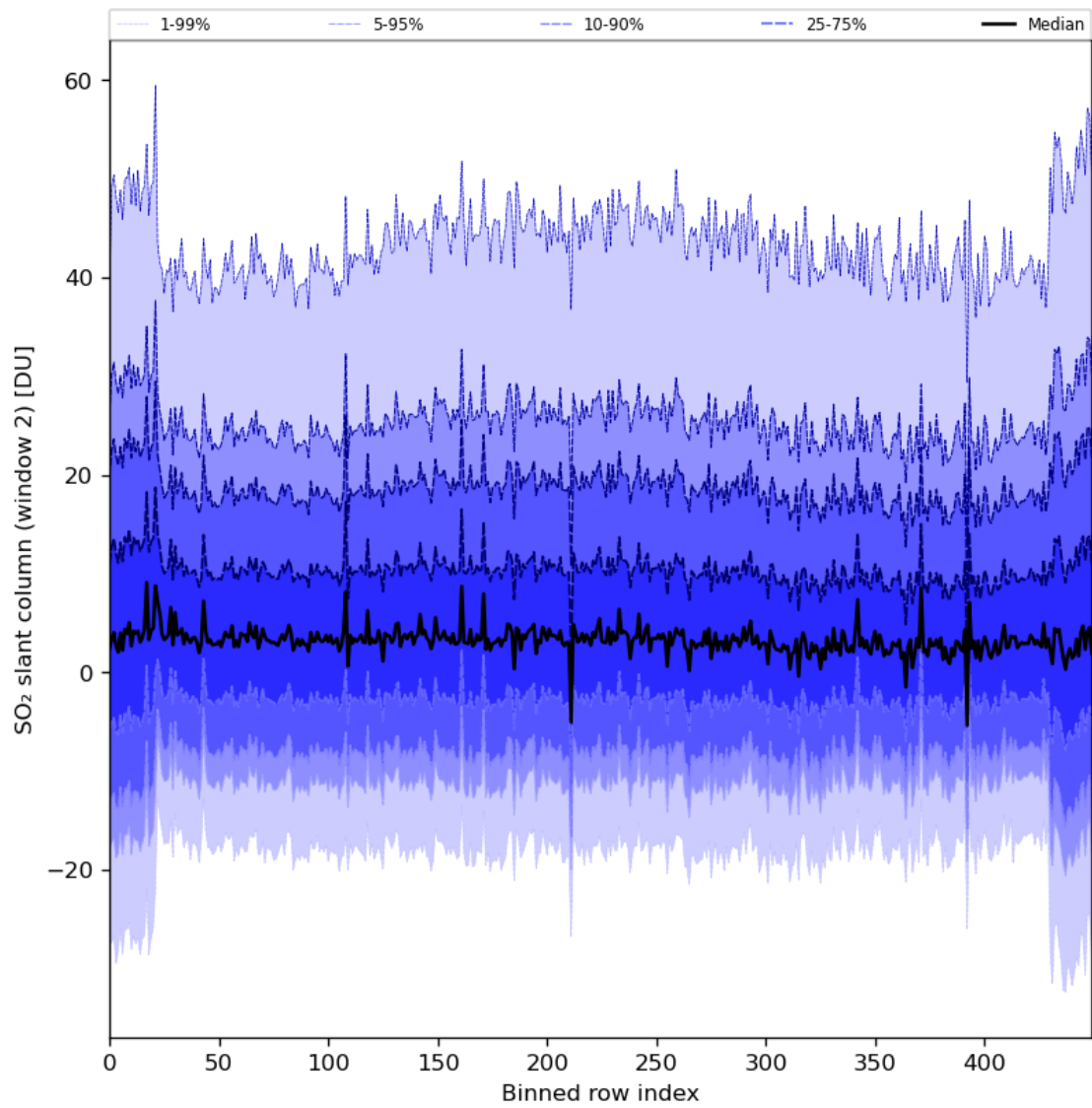
Figure 83: Along track statistics of “SO 2 slant column (window 2)” for 2024-03-05 to 2024-03-07
