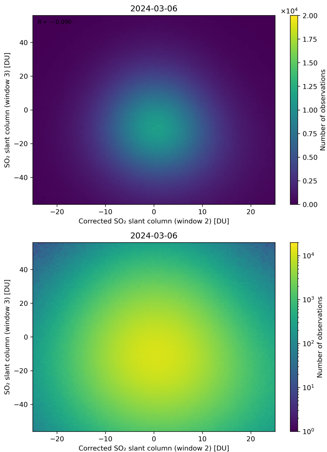
Figure 201: Scatter density plot of “Corrected SO 2 slant column (window 2)” against “SO 2 slant column (window 3)” for 2024-03-05 to 2024-03-07.
