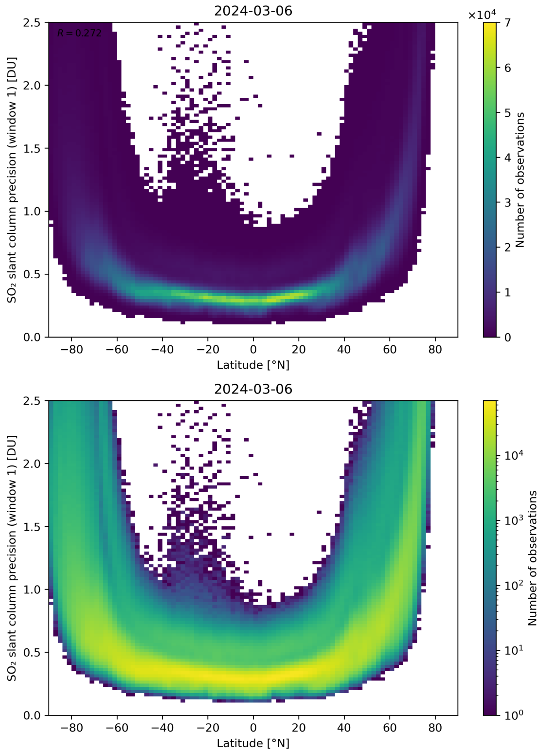
Figure 150: Scatter density plot of “Latitude” against “SO 2 slant column precision (window 1)” for 2024-03-05 to 2024-03-07.
