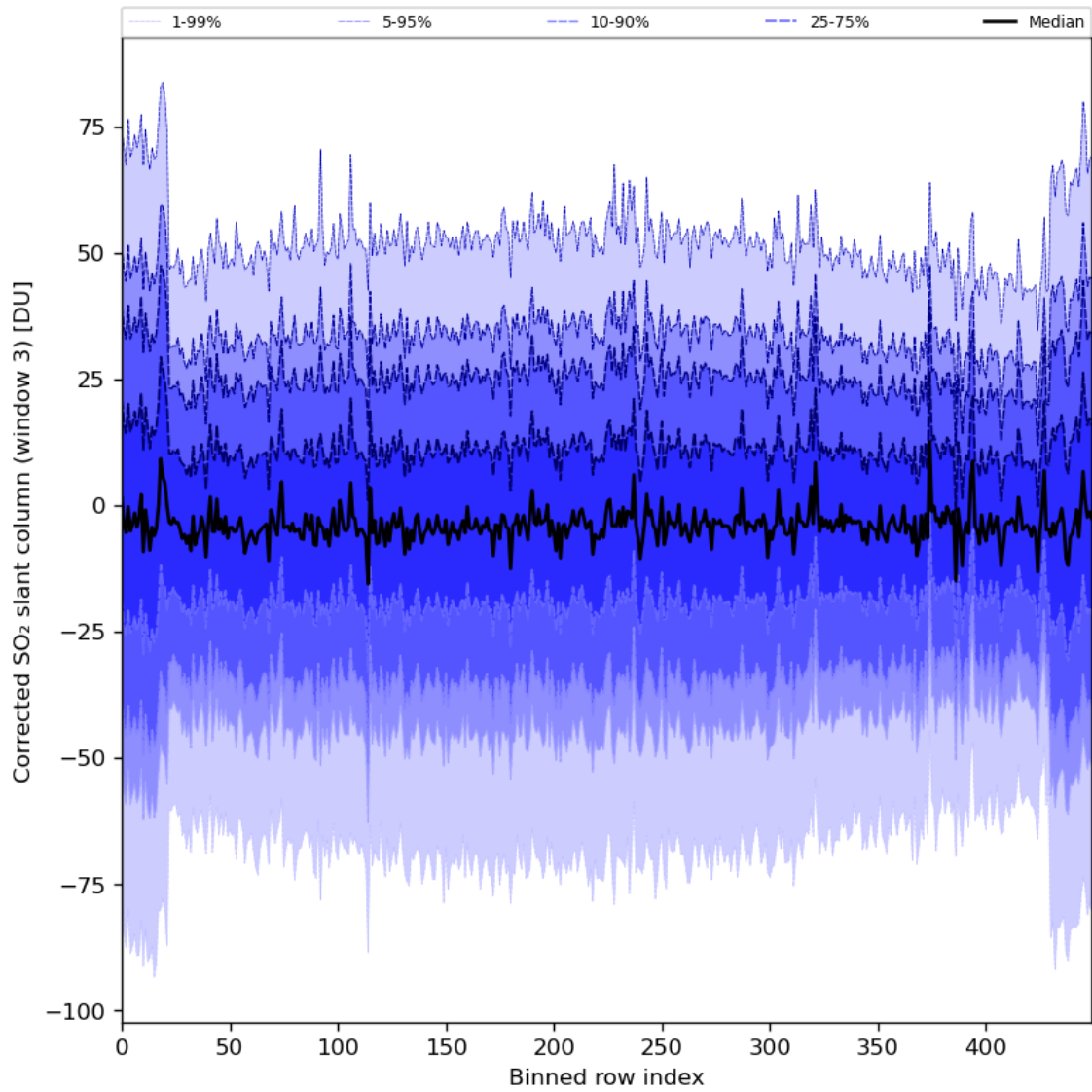
Figure 89: Along track statistics of “Corrected SO 2 slant column (window 3)” for 2024-03-05 to 2024-03-07
