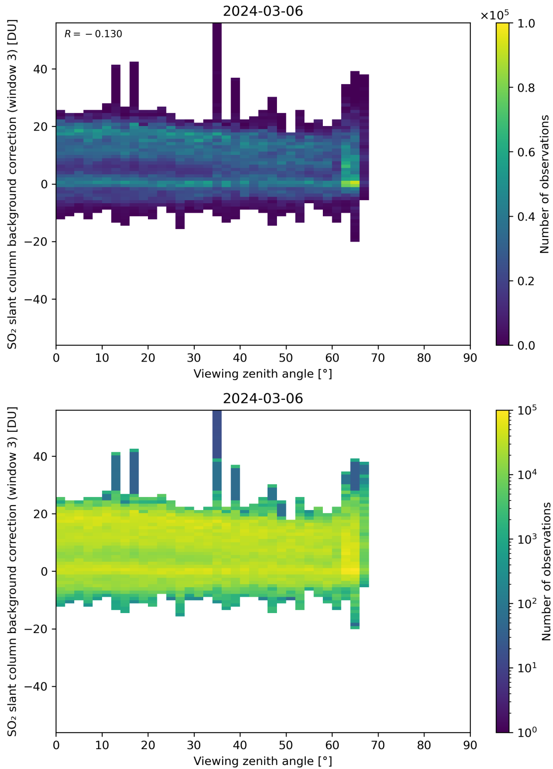
Figure 310: Scatter density plot of “Viewing zenith angle” against “SO 2 slant column background correction (window 3)” for 2024-03-05 to 2024-03-07.
