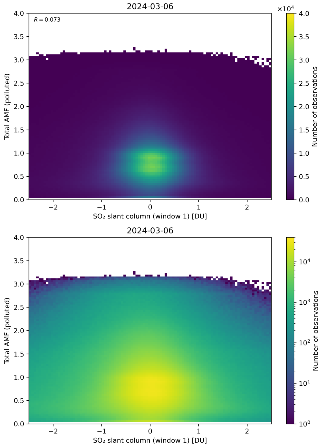
Figure 239: Scatter density plot of “SO 2 slant column (window 1)” against “Total AMF (polluted)” for 2024-03-05 to 2024-03-07.
