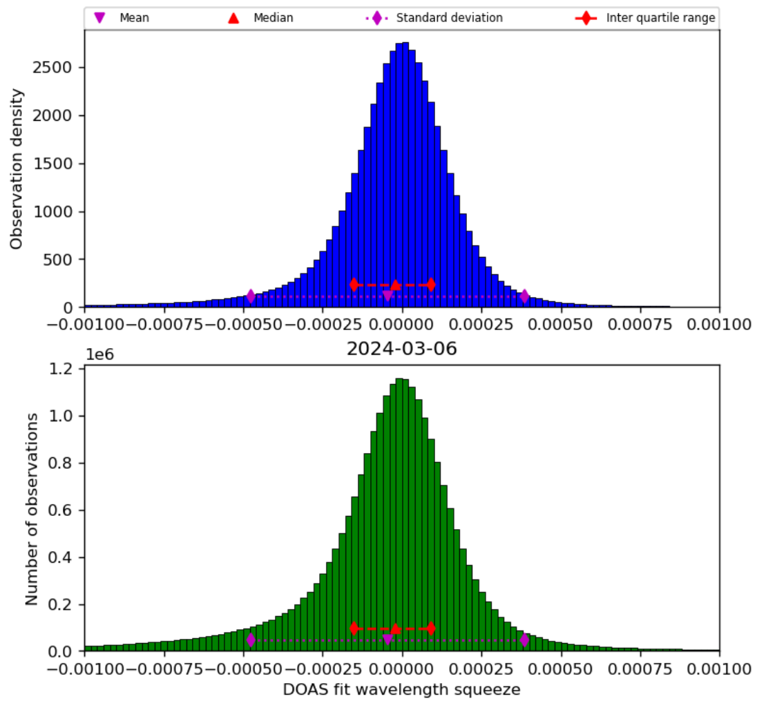
Figure 69: Histogram of “DOAS fit wavelength squeeze” for 2024-03-05 to 2024-03-07
