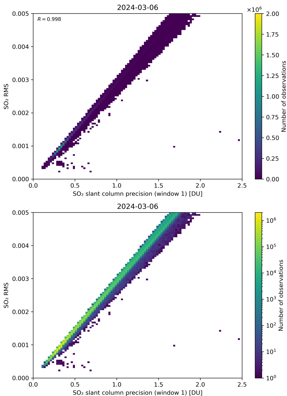
Figure 223: Scatter density plot of “SO 2 slant column precision (window 1)” against “SO 2 RMS” for 2024-03-05 to 2024-03-07.
