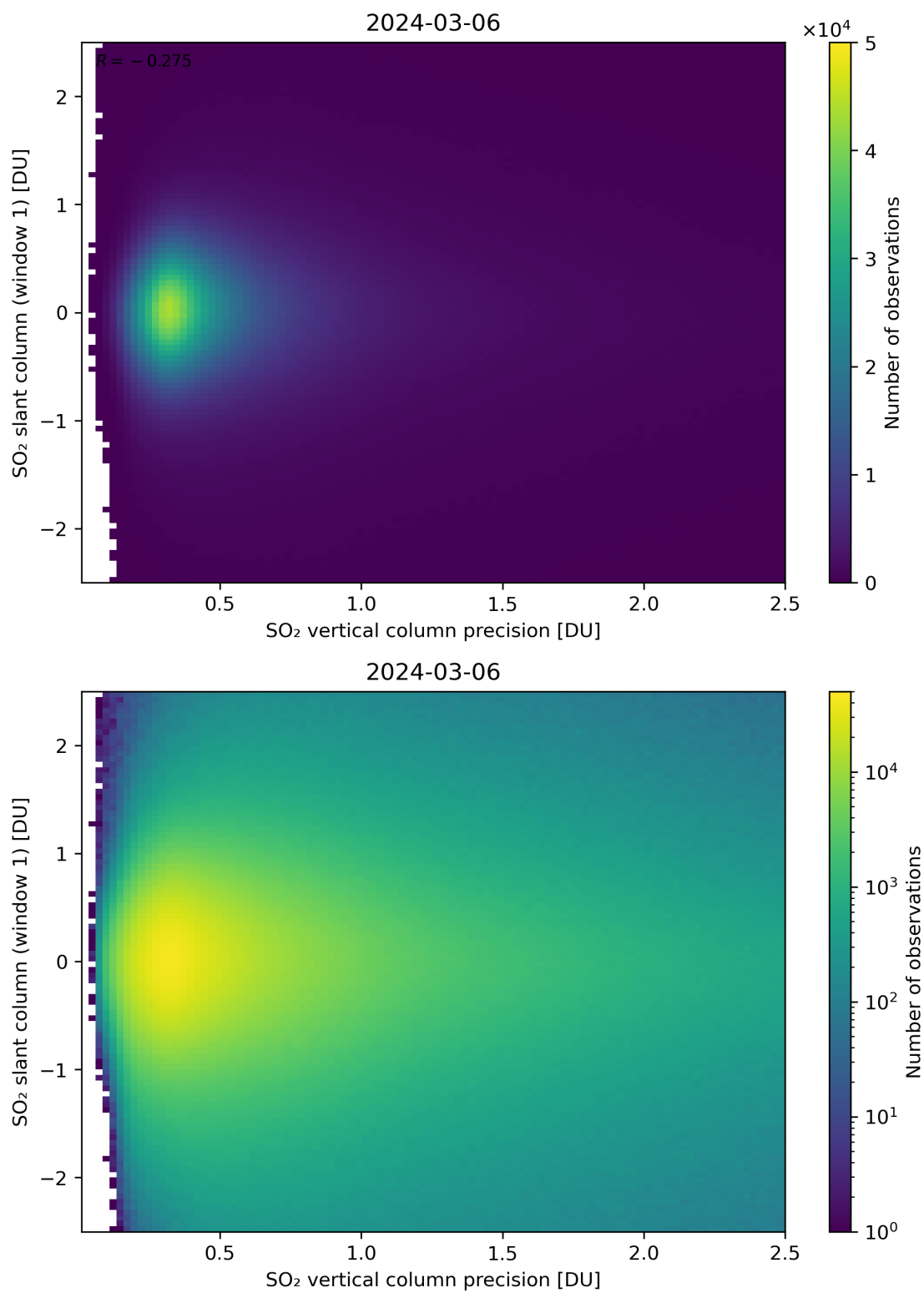
Figure 289: Scatter density plot of “SO 2 vertical column precision” against “SO 2 slant column (window 1)” for 2024-03-05 to 2024-03-07.
