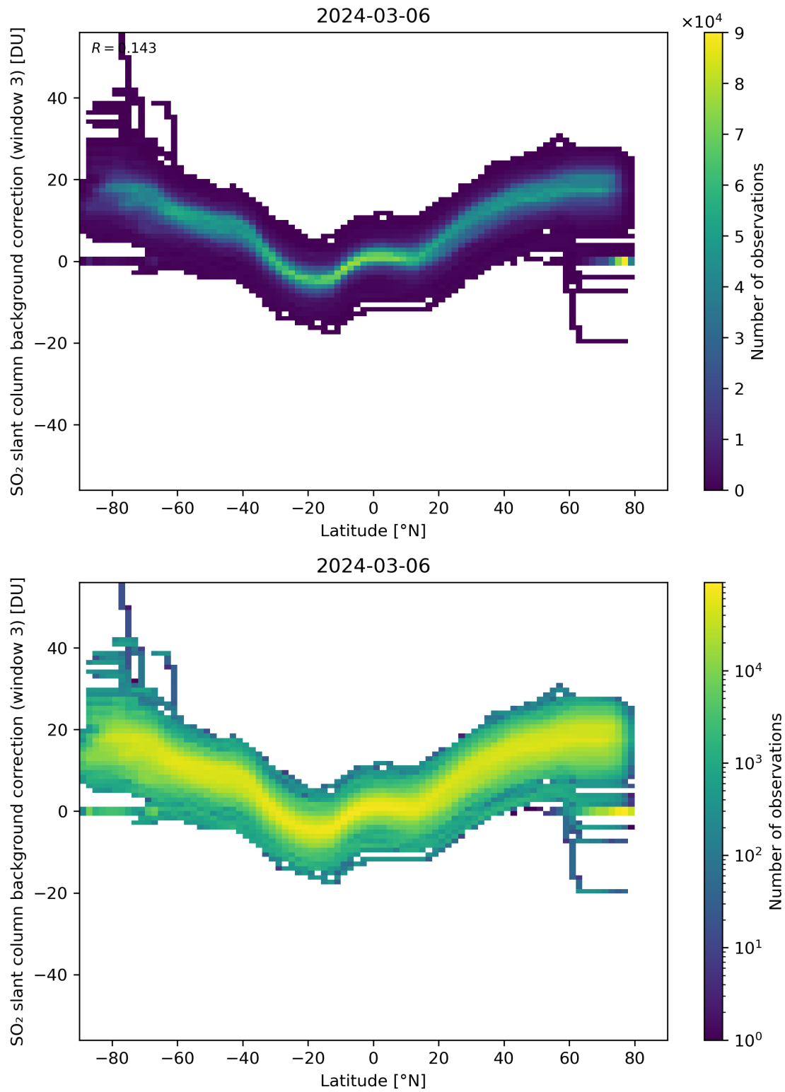
Figure 141: Scatter density plot of “Latitude” against “SO 2 slant column background correction (window 3)” for 2024-03-05 to 2024-03-07.
