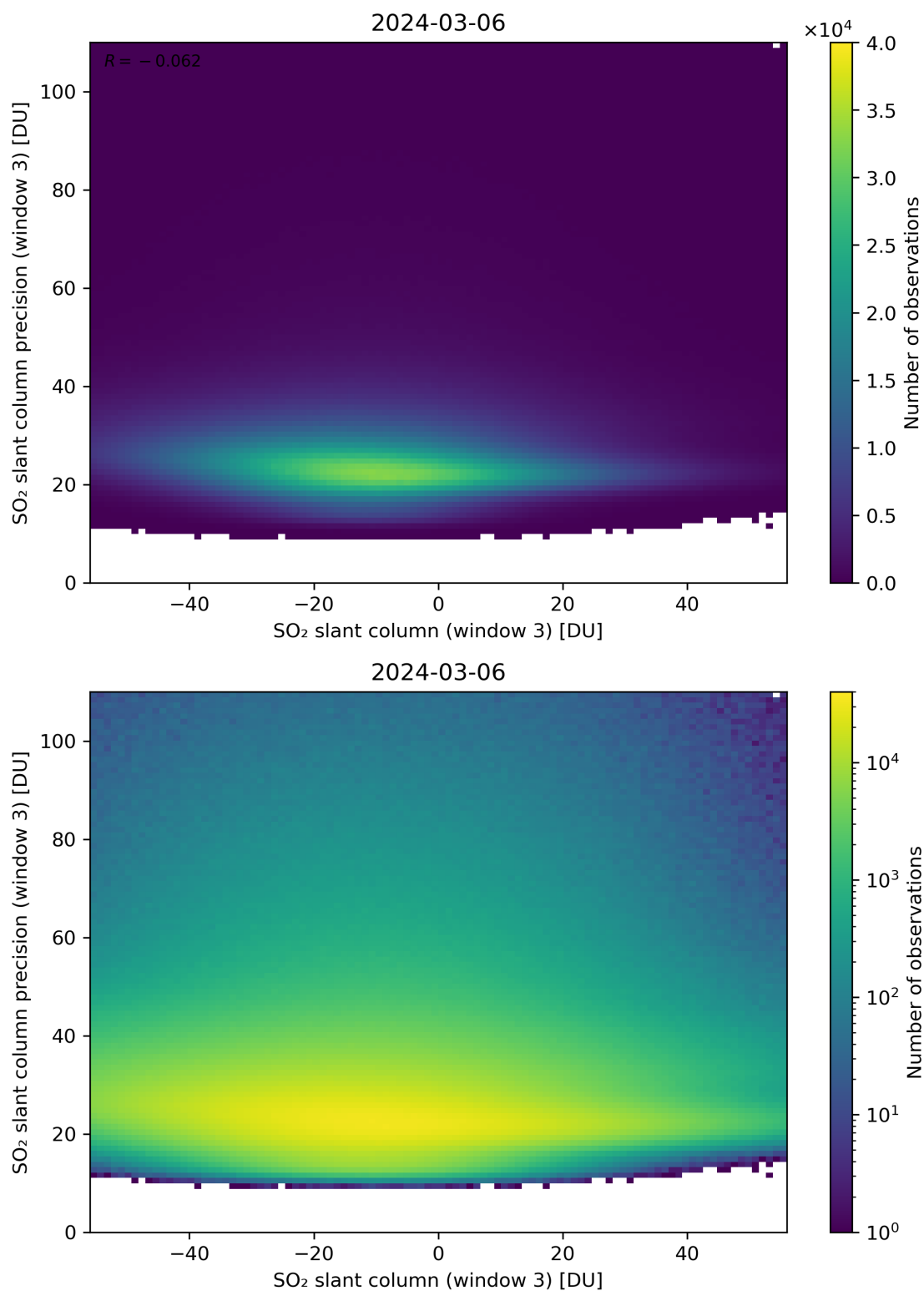
Figure 267: Scatter density plot of “SO 2 slant column (window 3)” against “SO 2 slant column precision (window 3)” for 2024-03-05 to 2024-03-07.
