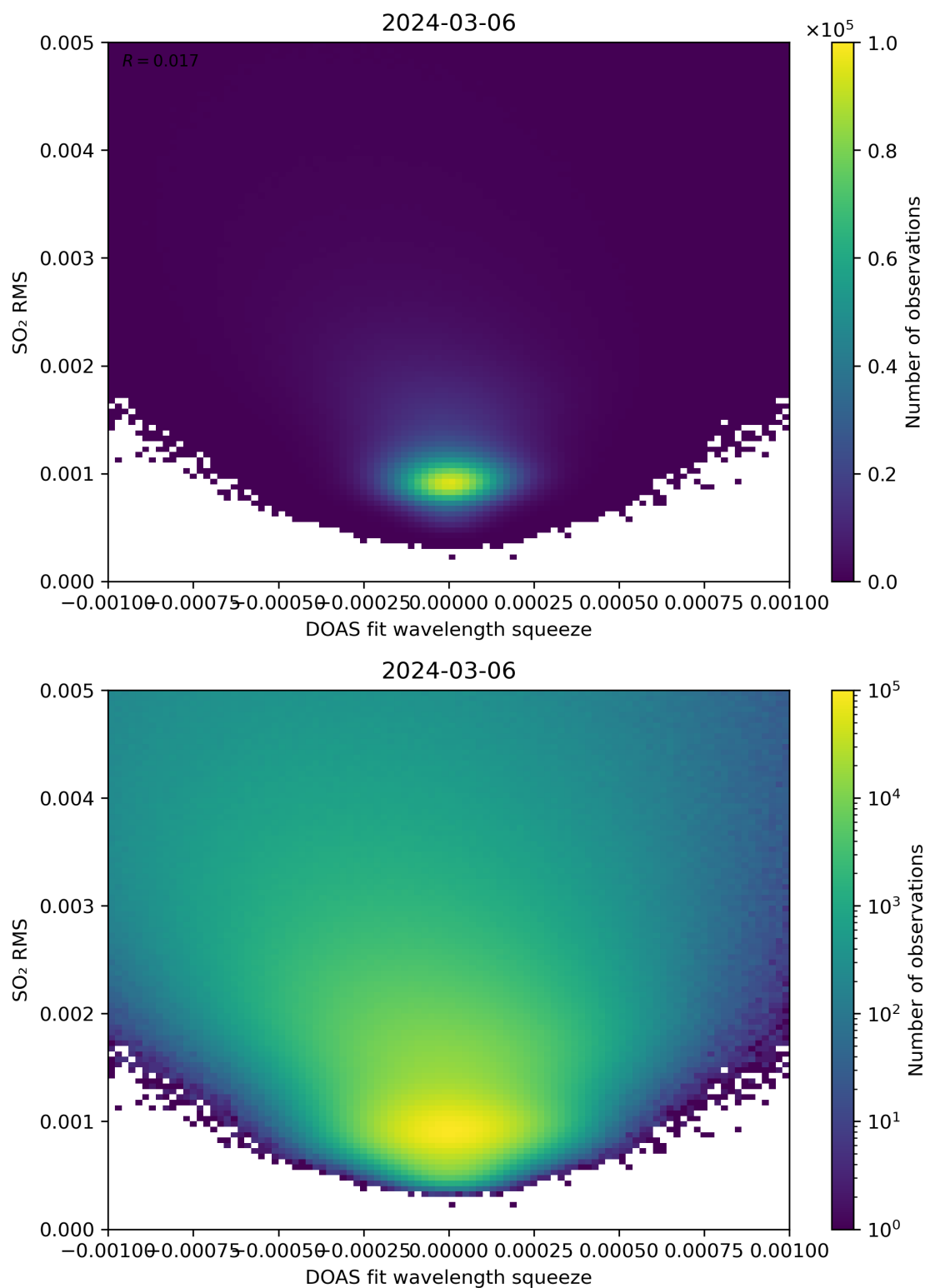
Figure 132: Scatter density plot of “DOAS fit wavelength squeeze” against “SO 2 RMS” for 2024-03-05 to 2024-03-07.
