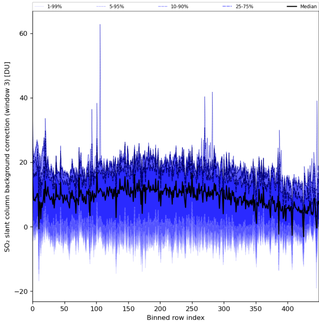
Figure 90: Along track statistics of “SO 2 slant column background correction (window 3)” for 2024-03-05 to 2024-03-07
