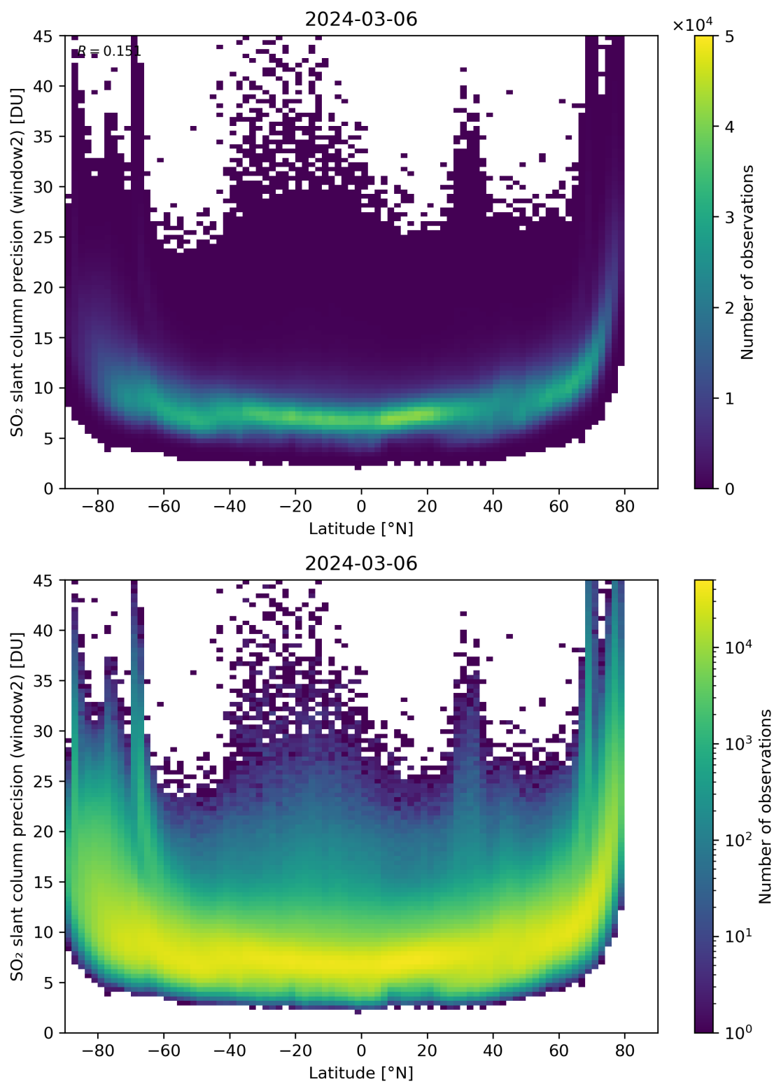
Figure 151: Scatter density plot of “Latitude” against “SO 2 slant column precision (window2)” for 2024-03-05 to 2024-03-07.
