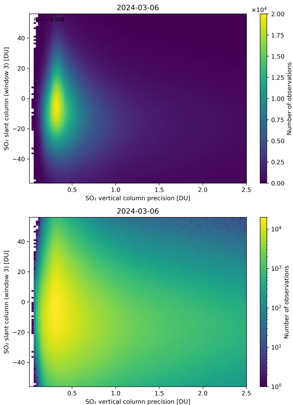
Figure 292: Scatter density plot of “SO 2 vertical column precision” against “SO 2 slant column (window 3)” for 2024-03-05 to 2024-03-07.
