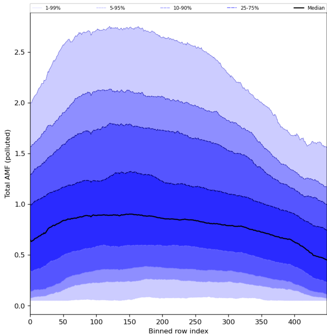
Figure 94: Along track statistics of “Total AMF (polluted)” for 2024-03-05 to 2024-03-07
