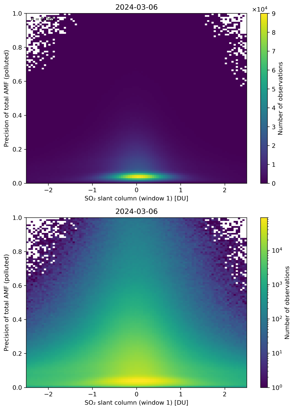
Figure 240: Scatter density plot of “SO 2 slant column (window 1)” against “Precision of total AMF (polluted)” for 2024-03-05 to 2024-03-07.
