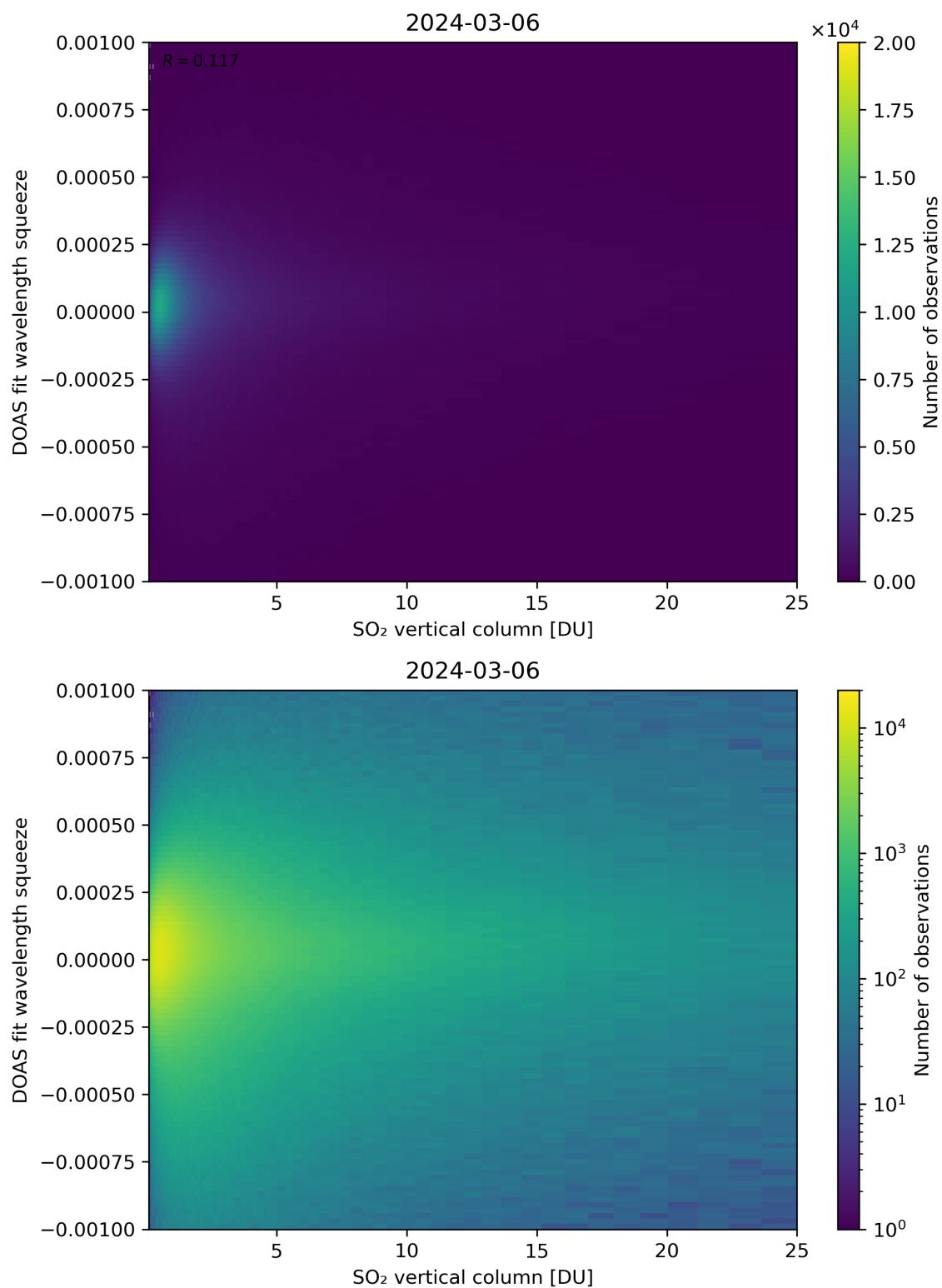
Figure 277: Scatter density plot of “SO 2 vertical column” against “DOAS fit wavelength squeeze” for 2024-03-05 to 2024-03-07.
