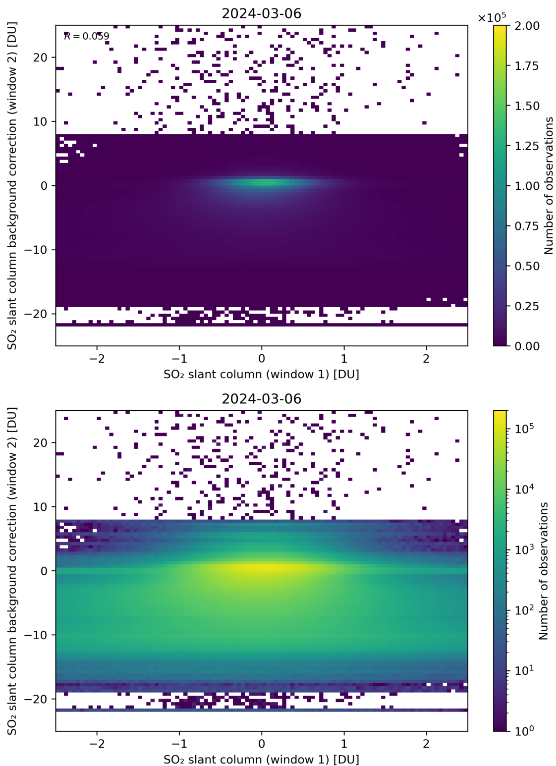
Figure 213: Scatter density plot of “SO 2 slant column (window 1)” against “SO 2 slant column background correction (window 2)” for 2024-03-05 to 2024-03-07.
