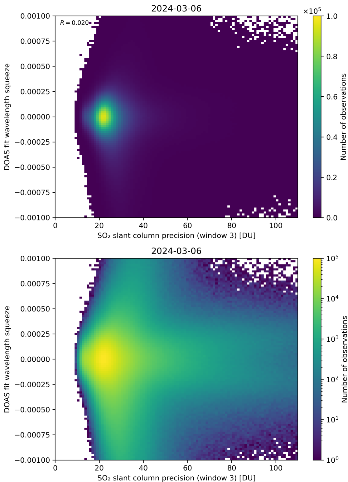
Figure 259: Scatter density plot of “SO 2 slant column precision (window 3)” against “DOAS fit wavelength squeeze” for 2024-03-05 to 2024-03-07.
