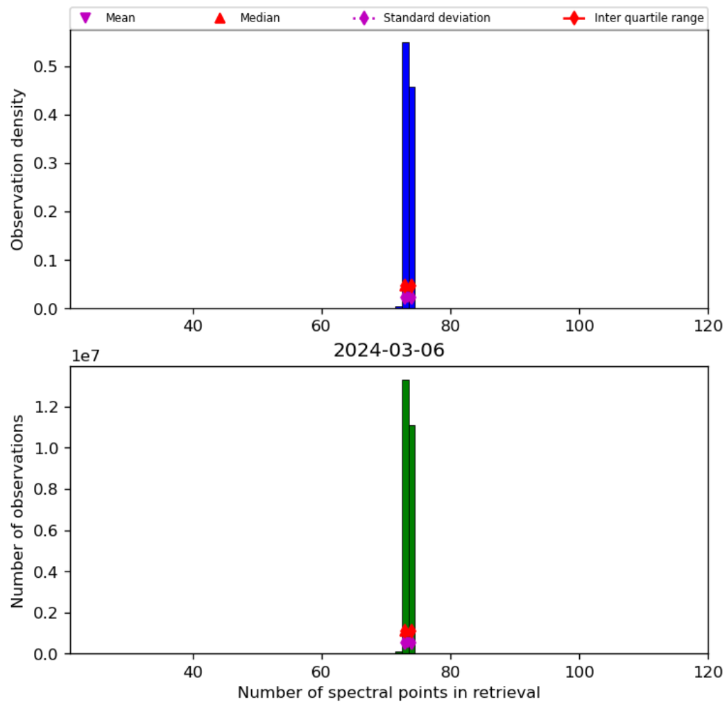
Figure 74: Histogram of “Number of spectral points in retrieval” for 2024-03-05 to 2024-03-07
