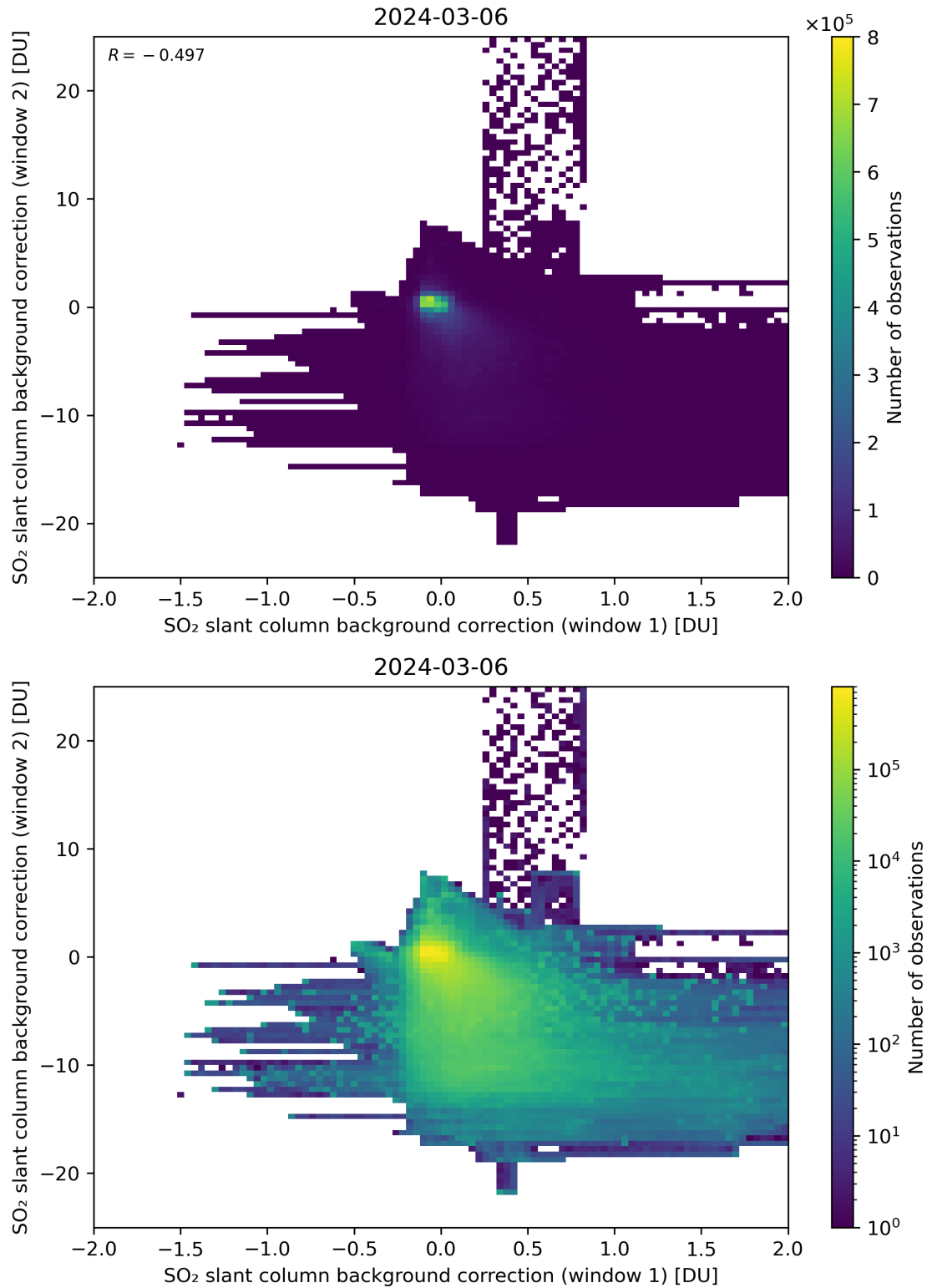
Figure 98: Scatter density plot of “SO 2 slant column background correction (window 1)” against “SO 2 slant column background correction (window 2)” for 2024-03-05 to 2024-03-07.
