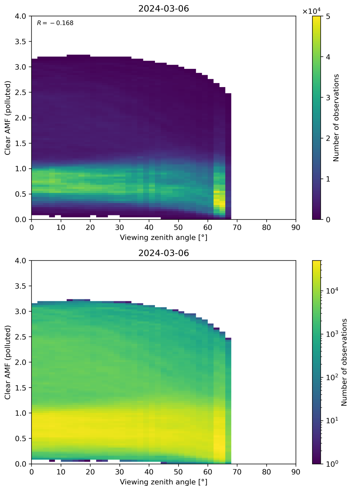
Figure 316: Scatter density plot of “Viewing zenith angle” against “Clear AMF (polluted)” for 2024-03-05 to 2024-03-07.
