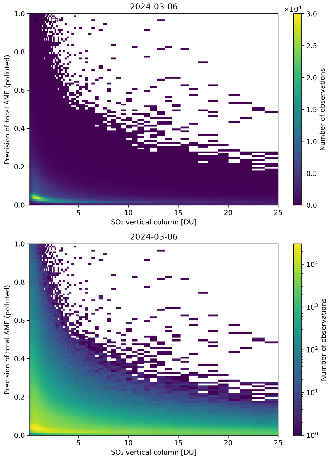
Figure 306: Scatter density plot of “SO 2 vertical column” against “Precision of total AMF (polluted)” for 2024-03-05 to 2024-03-07.
