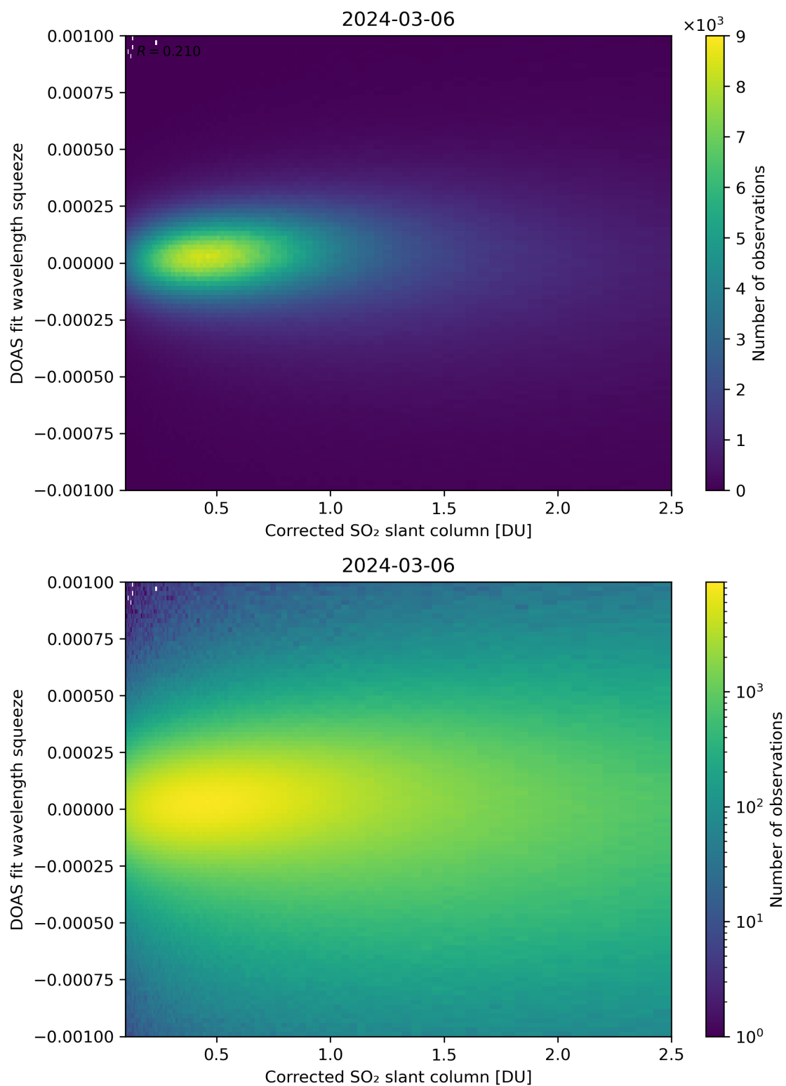
Figure 182: Scatter density plot of “Corrected SO 2 slant column” against “DOAS fit wavelength squeeze” for 2024-03-05 to 2024-03-07.
