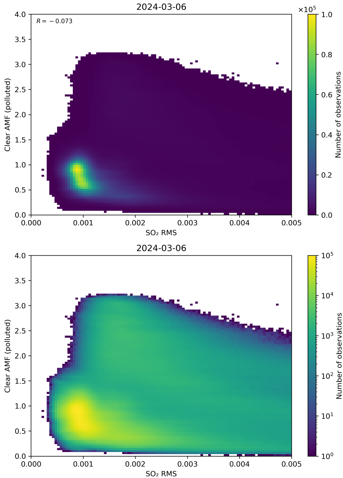
Figure 136: Scatter density plot of “SO 2 RMS” against “Clear AMF (polluted)” for 2024-03-05 to 2024-03-07.
