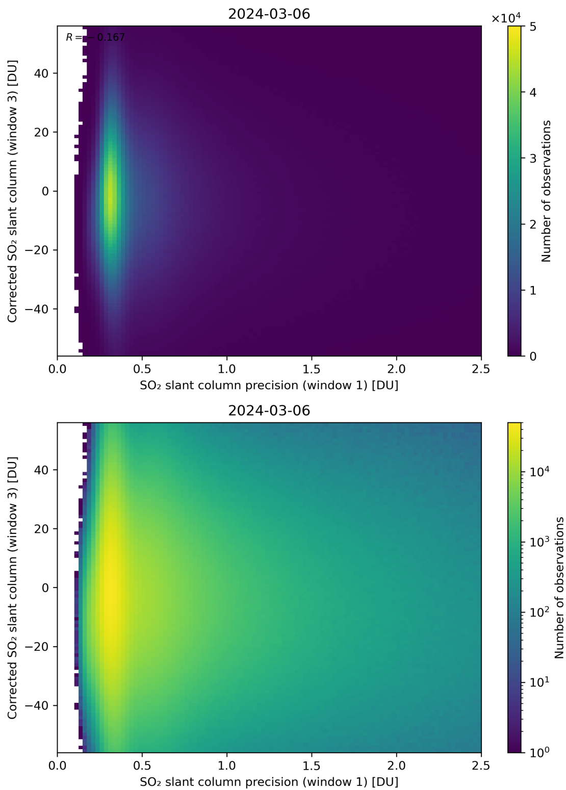
Figure 226: Scatter density plot of “SO 2 slant column precision (window 1)” against “Corrected SO 2 slant column (window 3)” for 2024-03-05 to 2024-03-07.
