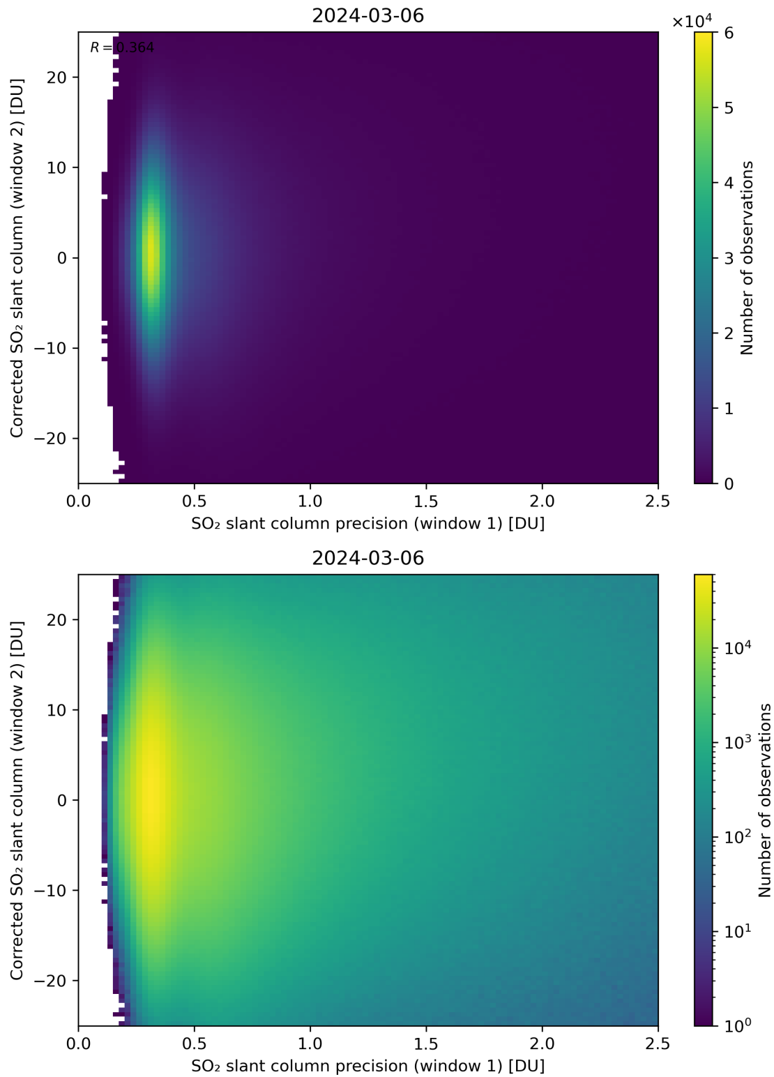
Figure 225: Scatter density plot of “SO 2 slant column precision (window 1)” against “Corrected SO 2 slant column (window 2)” for 2024-03-05 to 2024-03-07.
