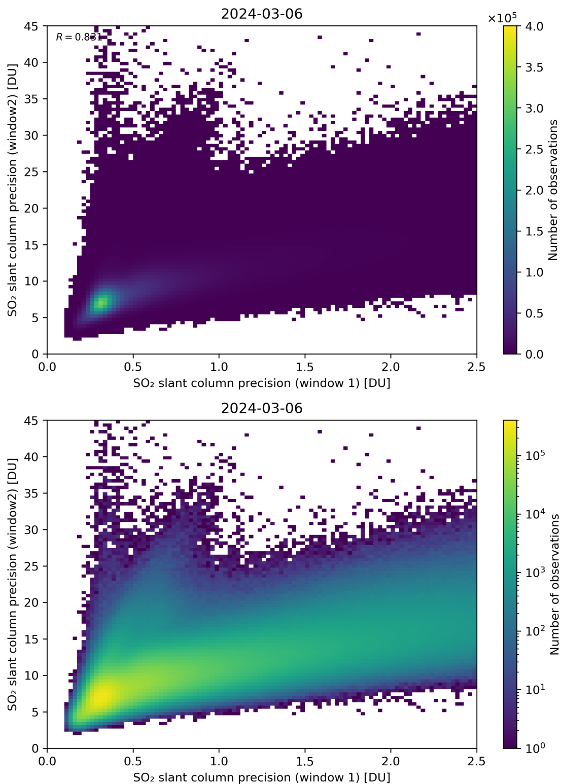
Figure 227: Scatter density plot of “SO 2 slant column precision (window 1)” against “SO 2 slant column precision (window2)” for 2024-03-05 to 2024-03-07.
