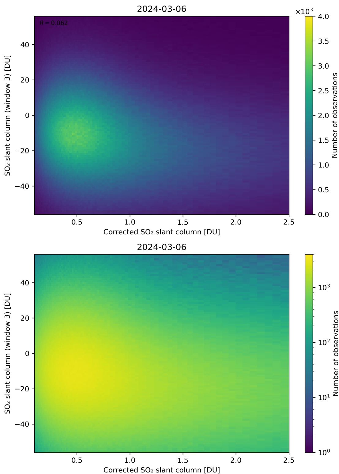
Figure 190: Scatter density plot of “Corrected SO 2 slant column” against “SO 2 slant column (window 3)” for 2024-03-05 to 2024-03-07.
