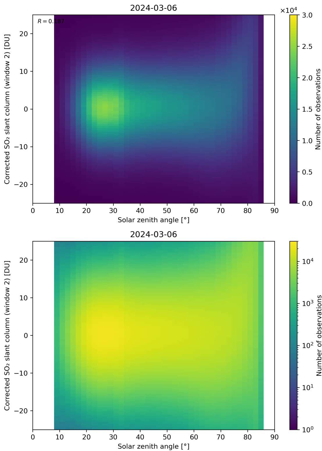
Figure 167: Scatter density plot of “Solar zenith angle” against “Corrected SO 2 slant column (window 2)” for 2024-03-05 to 2024-03-07.
