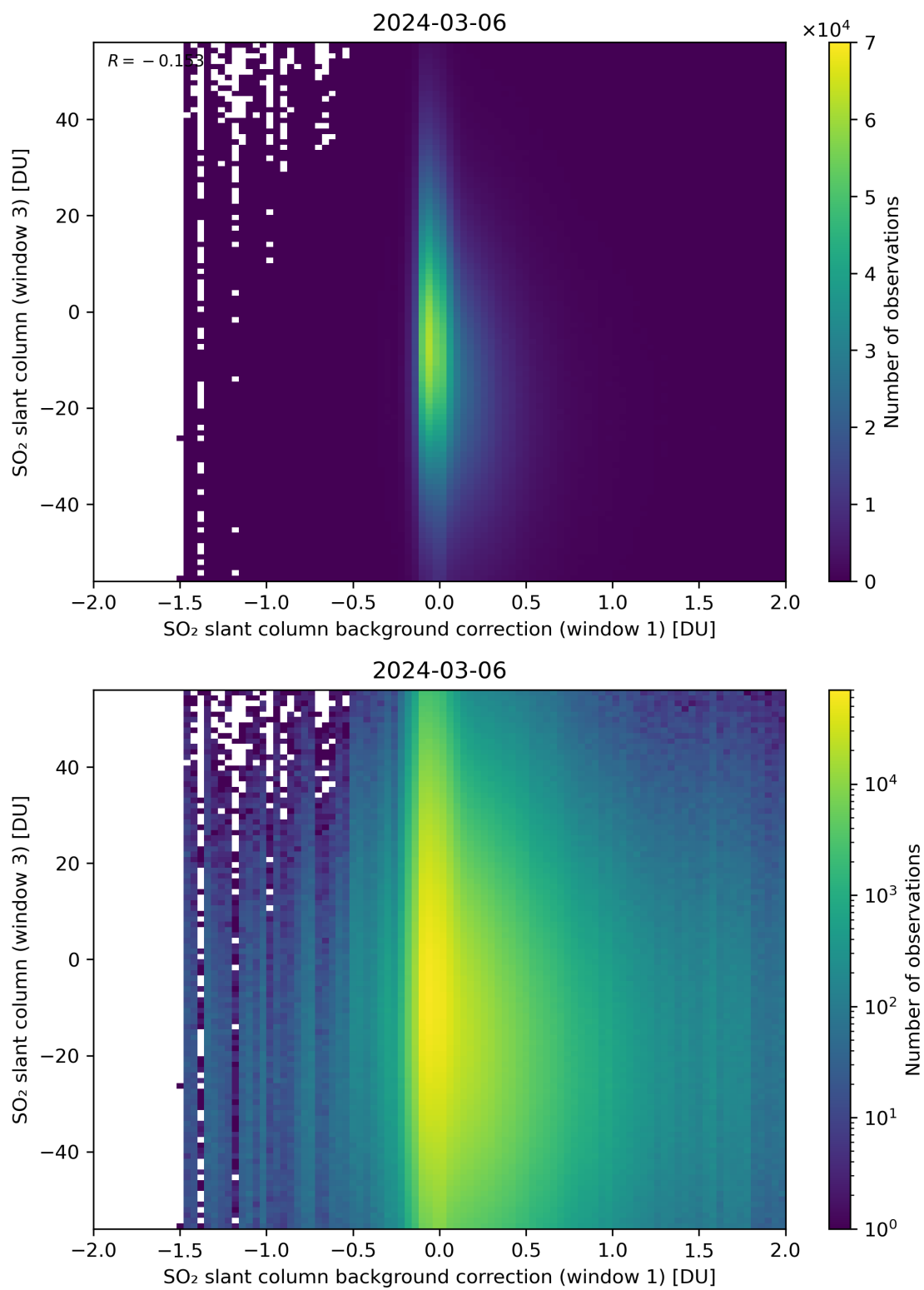
Figure 107: Scatter density plot of “SO 2 slant column background correction (window 1)” against “SO 2 slant column (window 3)” for 2024-03-05 to 2024-03-07.
