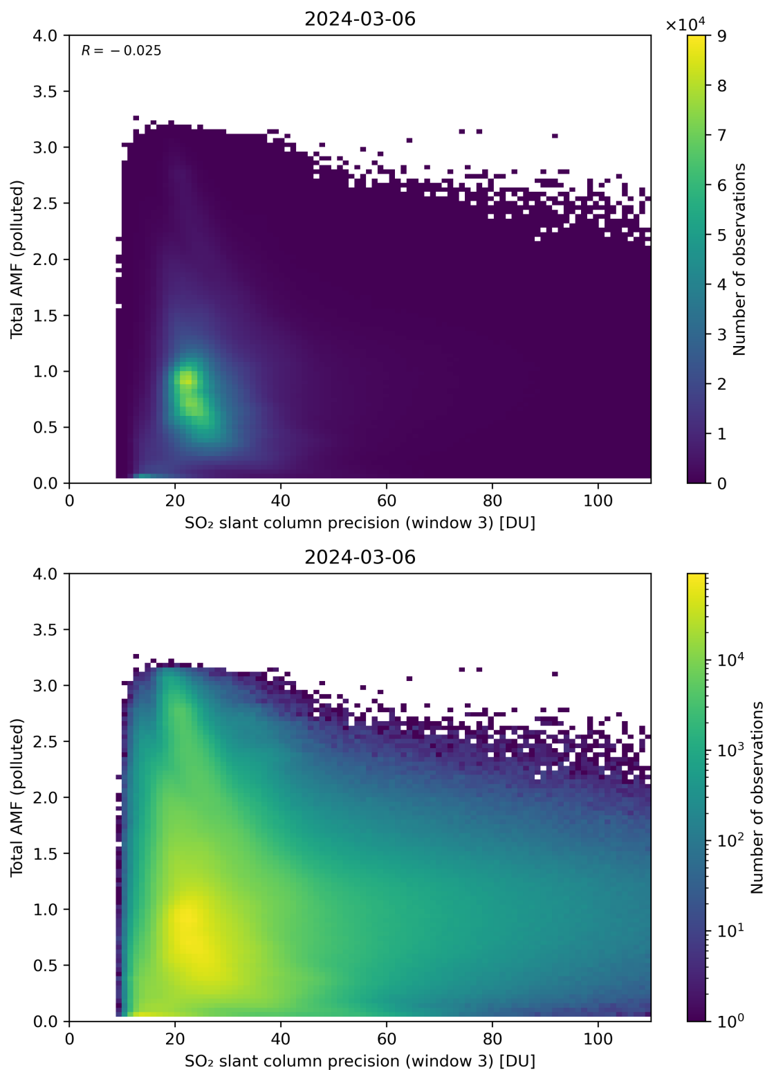
Figure 263: Scatter density plot of “SO 2 slant column precision (window 3)” against “Total AMF (polluted)” for 2024-03-05 to 2024-03-07.
