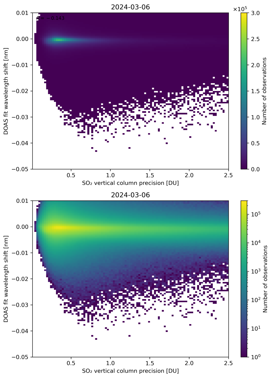
Figure 282: Scatter density plot of “SO 2 vertical column precision” against “DOAS fit wavelength shift” for 2024-03-05 to 2024-03-07.
