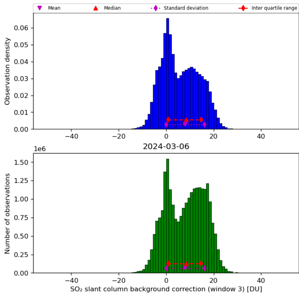
Figure 67: Histogram of “SO 2 slant column background correction (window 3)” for 2024-03-05 to 2024-03-07
