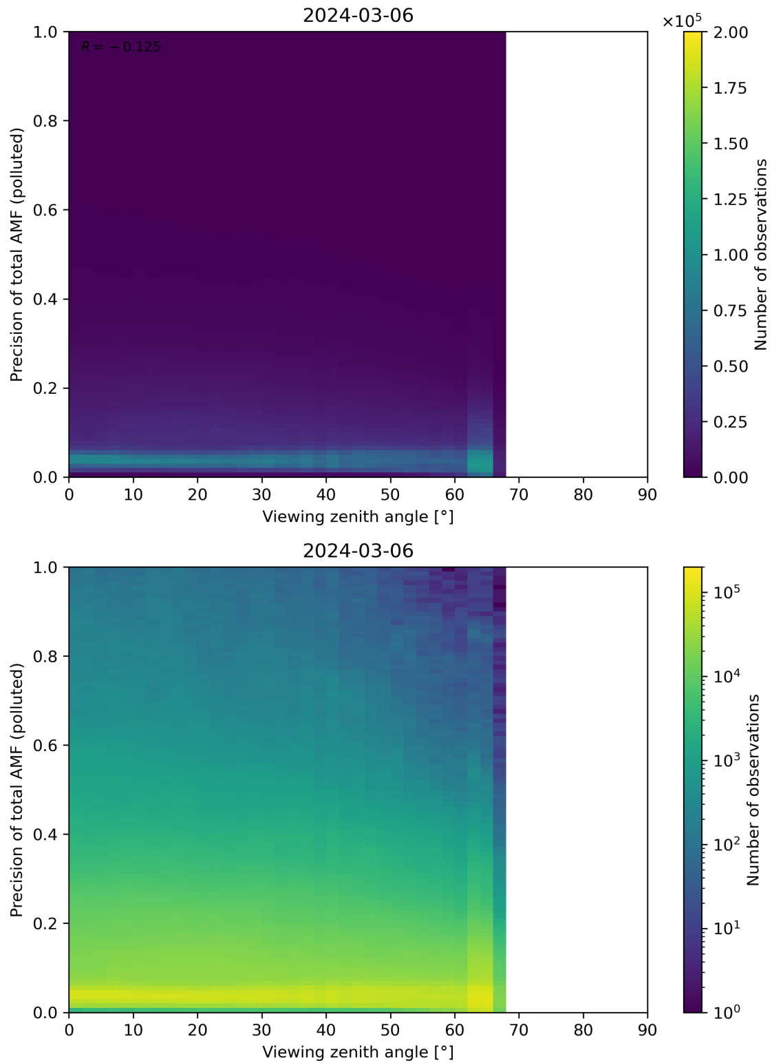
Figure 326: Scatter density plot of “Viewing zenith angle” against “Precision of total AMF (polluted)” for 2024-03-05 to 2024-03-07.
