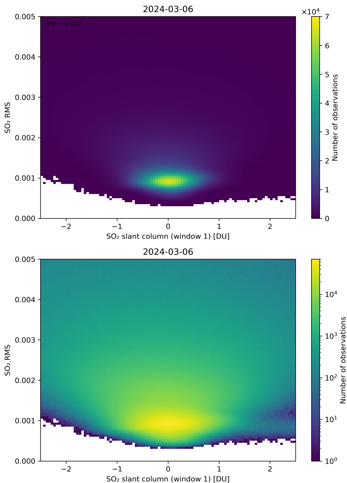
Figure 217: Scatter density plot of “SO 2 slant column (window 1)” against “SO 2 RMS” for 2024-03-05 to 2024-03-07.
