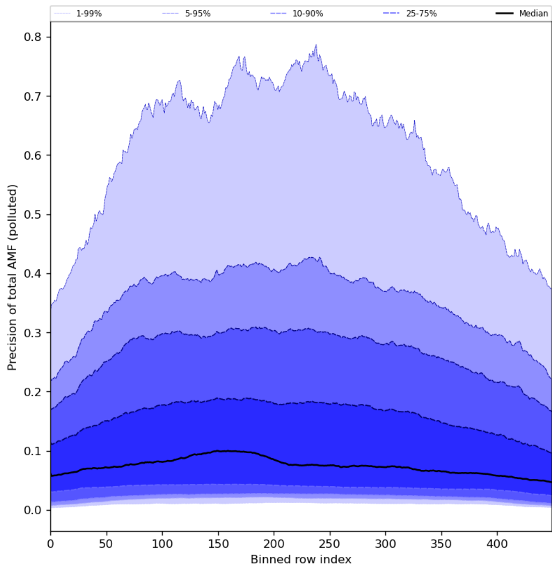
Figure 95: Along track statistics of “Precision of total AMF (polluted)” for 2024-03-05 to 2024-03-07
