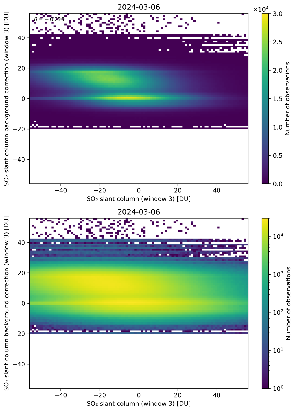
Figure 253: Scatter density plot of “SO 2 slant column (window 3)” against “SO 2 slant column background correction (window 3)” for 2024-03-05 to 2024-03-07.
