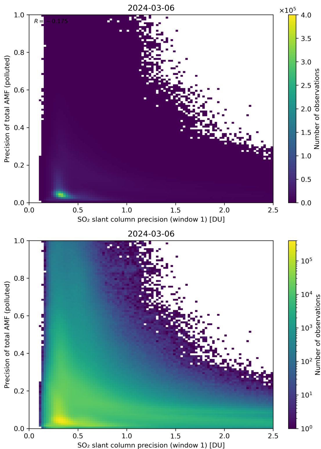
Figure 231: Scatter density plot of “SO 2 slant column precision (window 1)” against “Precision of total AMF (polluted)” for 2024-03-05 to 2024-03-07.
