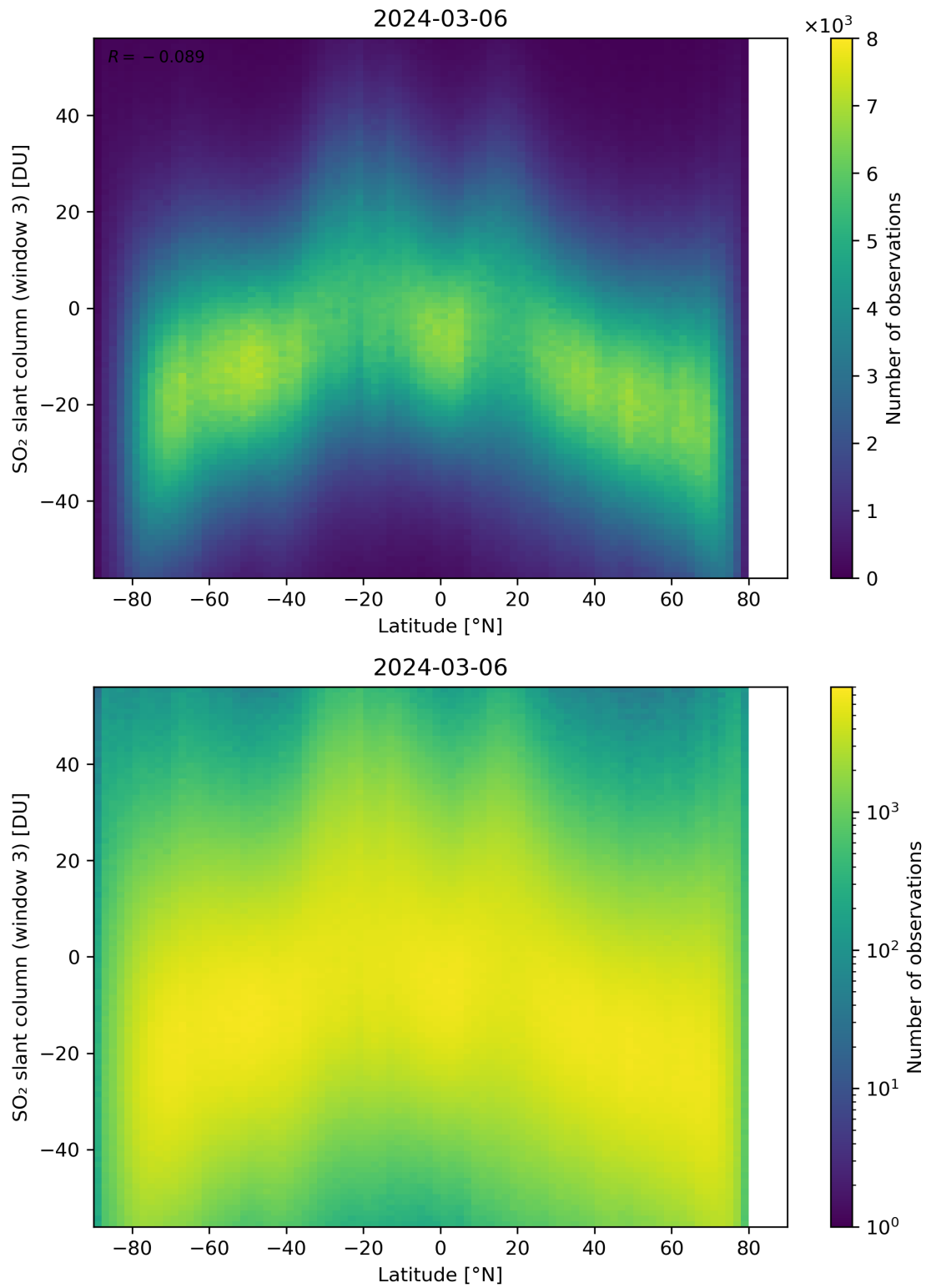
Figure 152: Scatter density plot of “Latitude” against “SO 2 slant column (window 3)” for 2024-03-05 to 2024-03-07.
