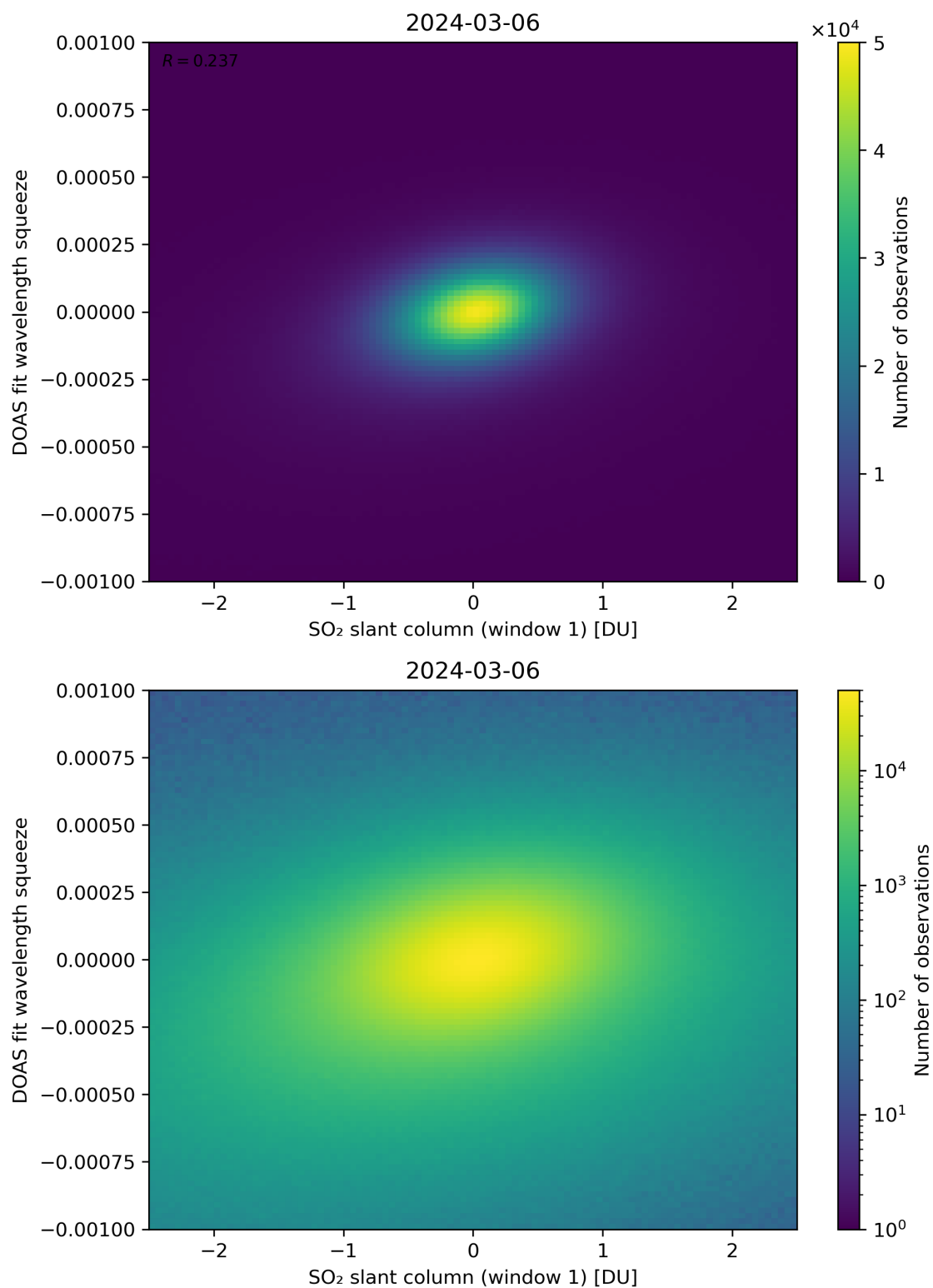
Figure 216: Scatter density plot of “SO 2 slant column (window 1)” against “DOAS fit wavelength squeeze” for 2024-03-05 to 2024-03-07.
