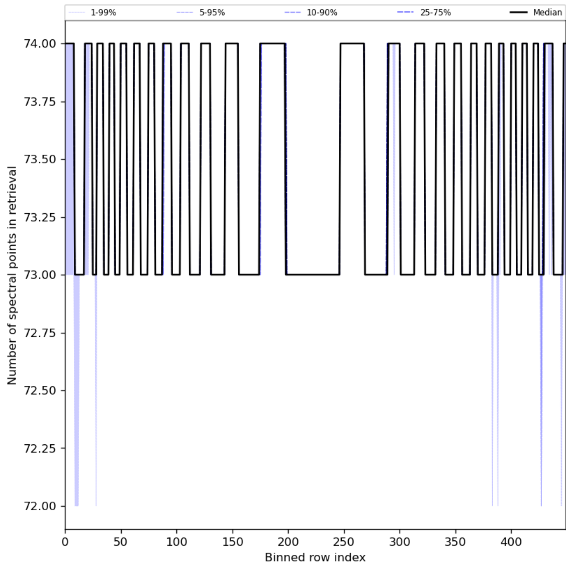
Figure 97: Along track statistics of “Number of spectral points in retrieval” for 2024-03-05 to 2024-03-07
