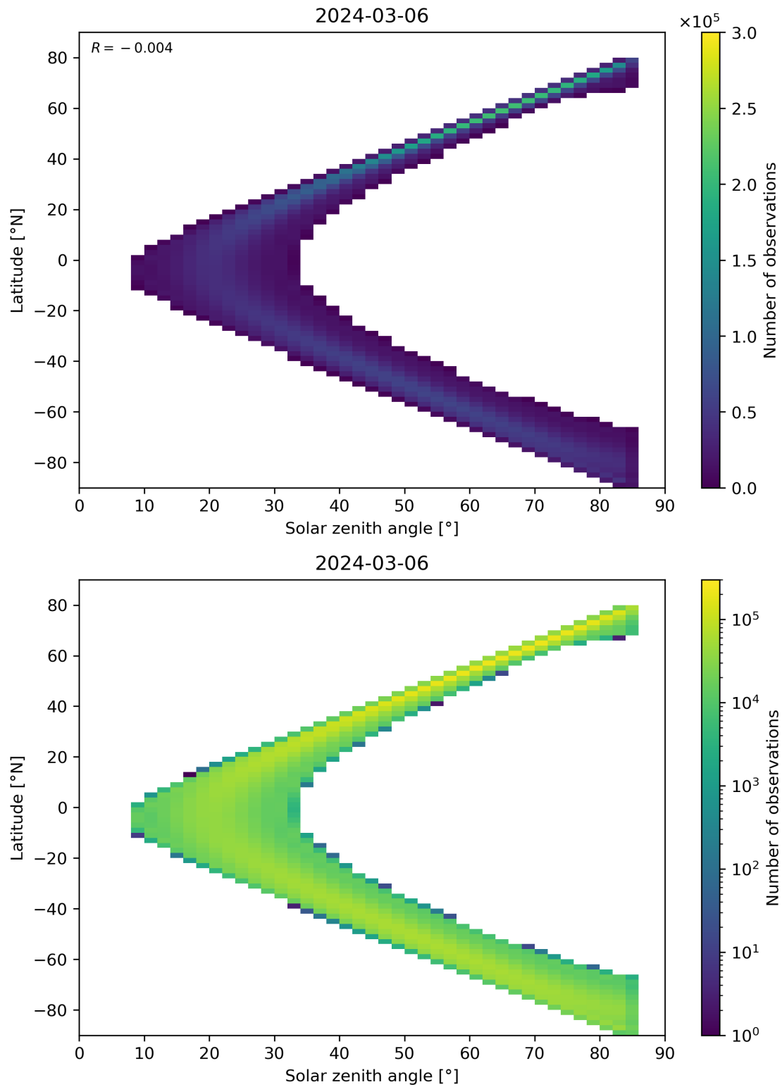
Figure 164: Scatter density plot of “Solar zenith angle” against “Latitude” for 2024-03-05 to 2024-03-07.
