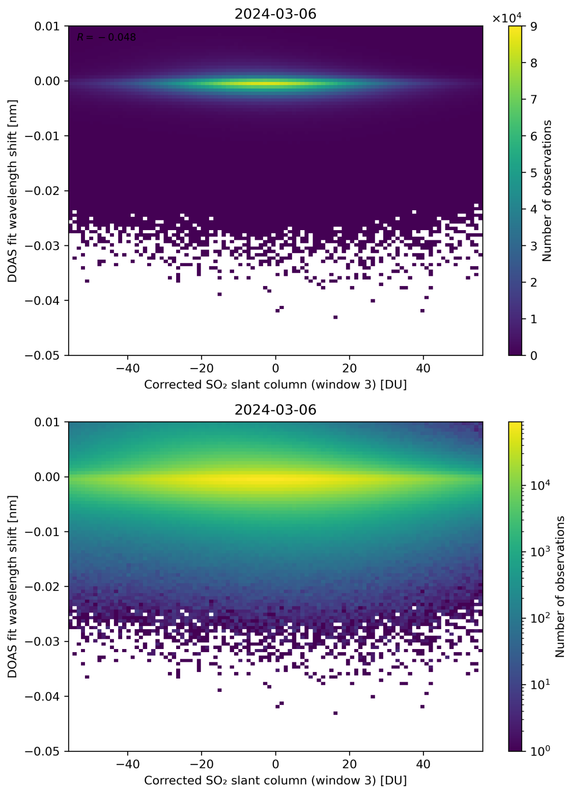
Figure 206: Scatter density plot of “Corrected SO 2 slant column (window 3)” against “DOAS fit wavelength shift” for 2024-03-05 to 2024-03-07.
