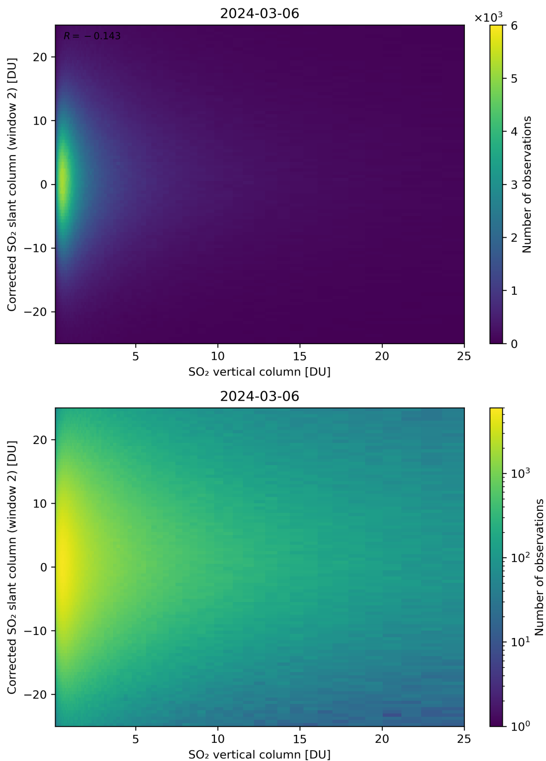
Figure 298: Scatter density plot of “SO 2 vertical column” against “Corrected SO 2 slant column (window 2)” for 2024-03-05 to 2024-03-07.
