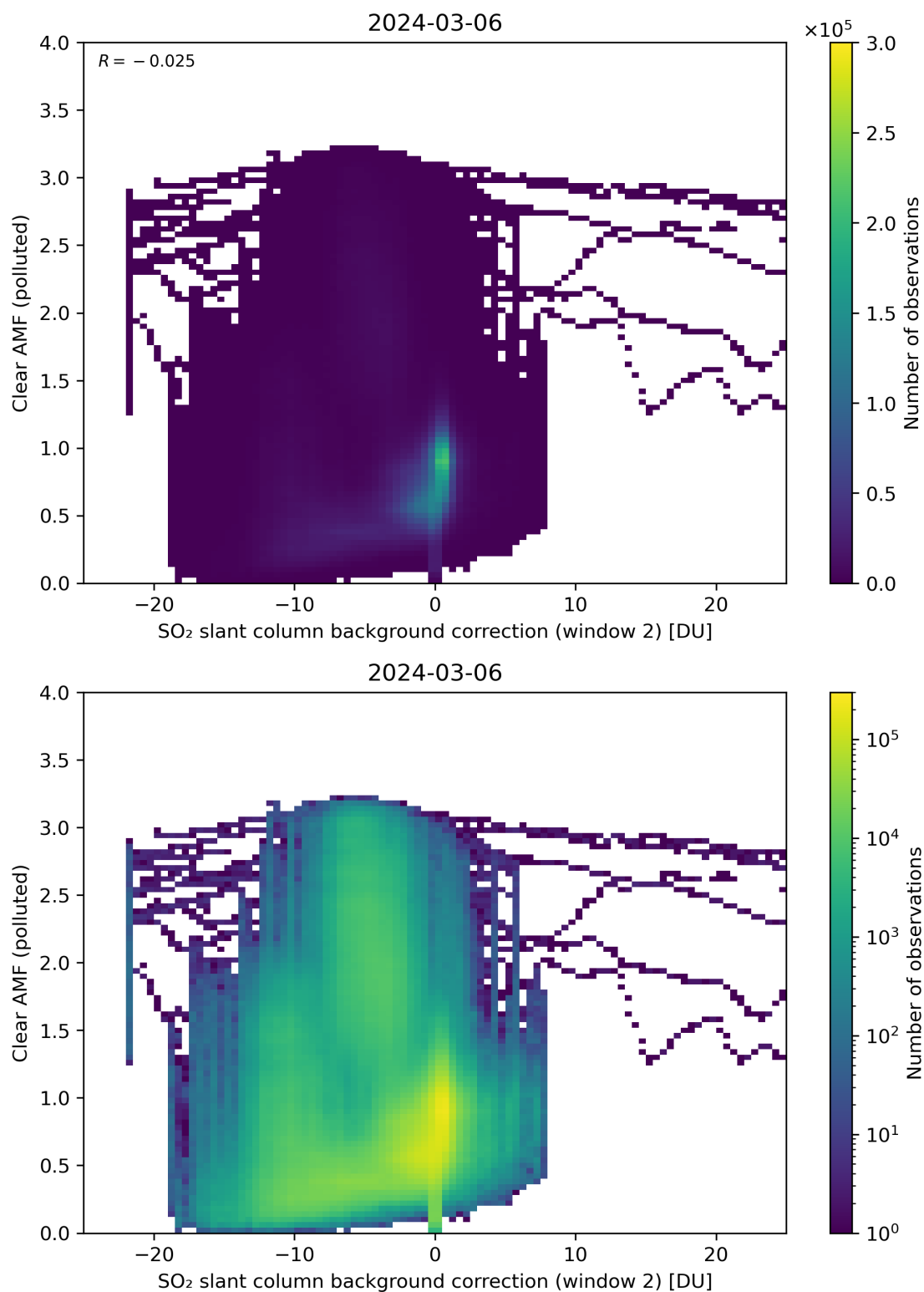
Figure 115: Scatter density plot of “SO 2 slant column background correction (window 2)” against “Clear AMF (polluted)” for 2024-03-05 to 2024-03-07.
