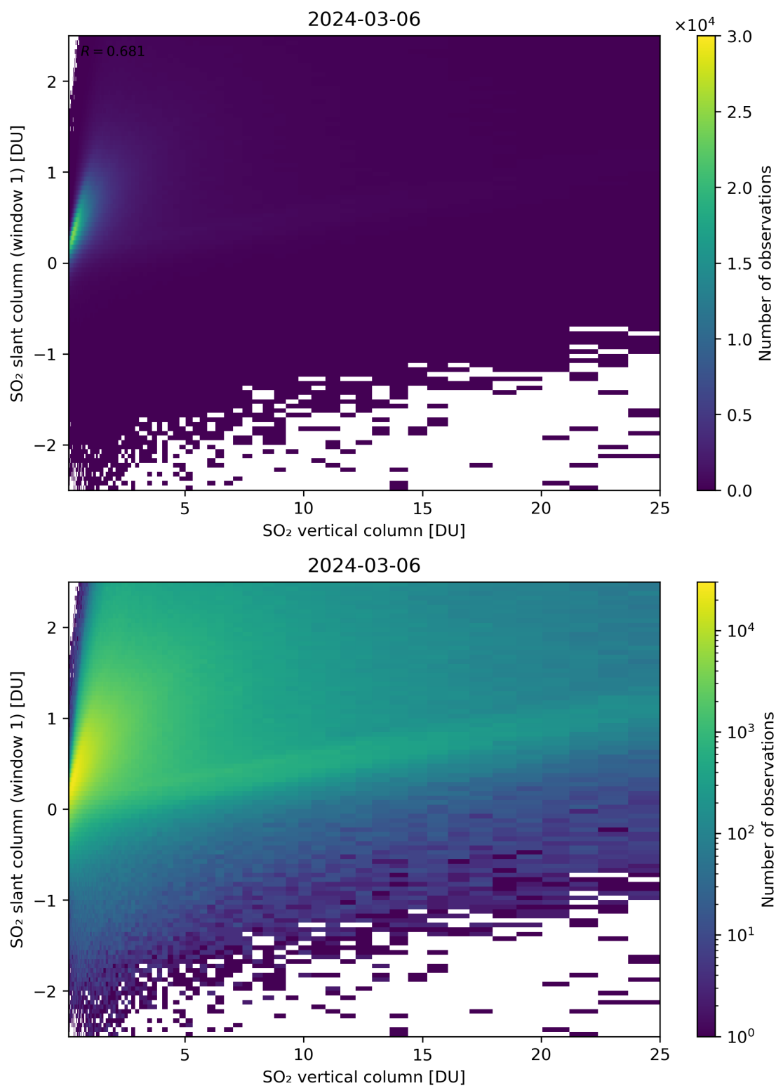
Figure 300: Scatter density plot of “SO 2 vertical column” against “SO 2 slant column (window 1)” for 2024-03-05 to 2024-03-07.
