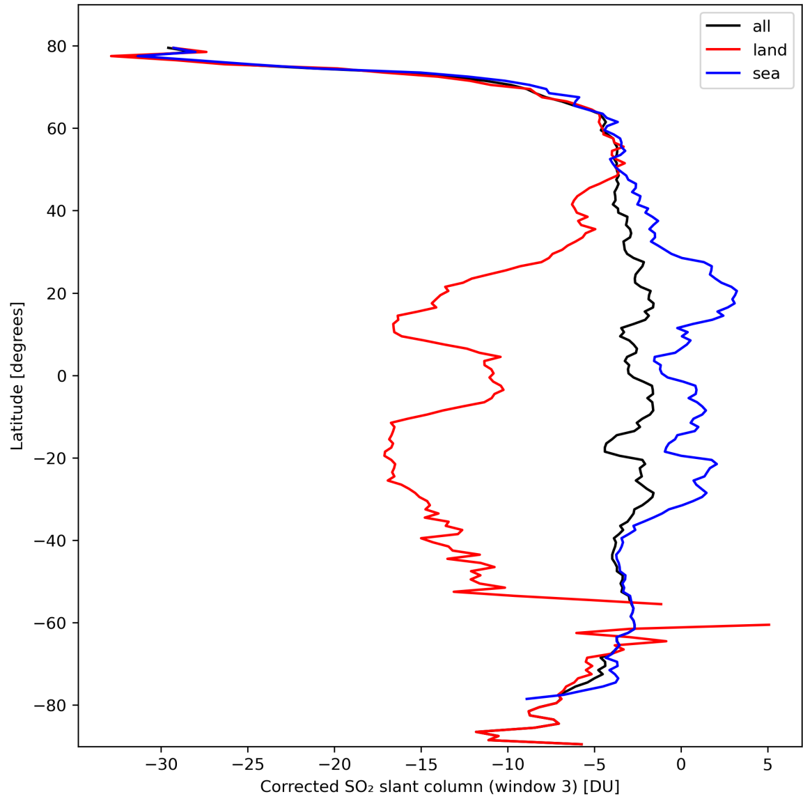
Figure 43: Zonal average of “Corrected SO 2 slant column (window 3)” for 2024-03-05 to 2024-03-07.
