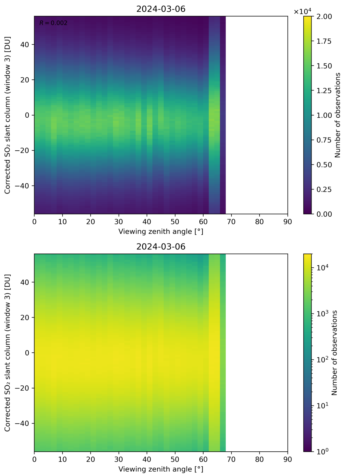
Figure 319: Scatter density plot of “Viewing zenith angle” against “Corrected SO 2 slant column (window 3)” for 2024-03-05 to 2024-03-07.
