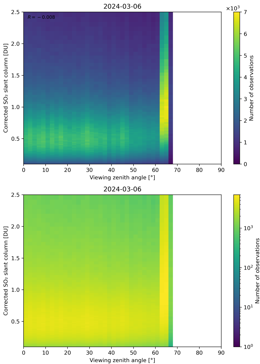
Figure 317: Scatter density plot of “Viewing zenith angle” against “Corrected SO 2 slant column” for 2024-03-05 to 2024-03-07.
