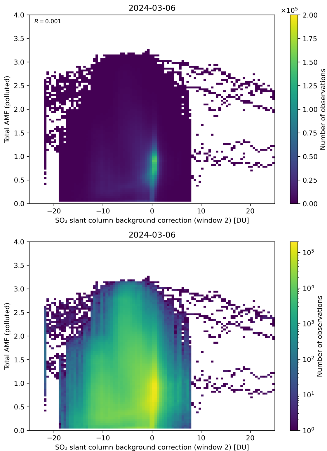
Figure 119: Scatter density plot of “SO 2 slant column background correction (window 2)” against “Total AMF (polluted)” for 2024-03-05 to 2024-03-07.
