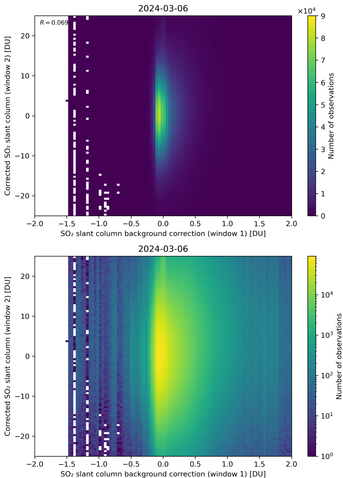
Figure 104: Scatter density plot of “SO 2 slant column background correction (window 1)” against “Corrected SO 2 slant column (window 2)” for 2024-03-05 to 2024-03-07.
