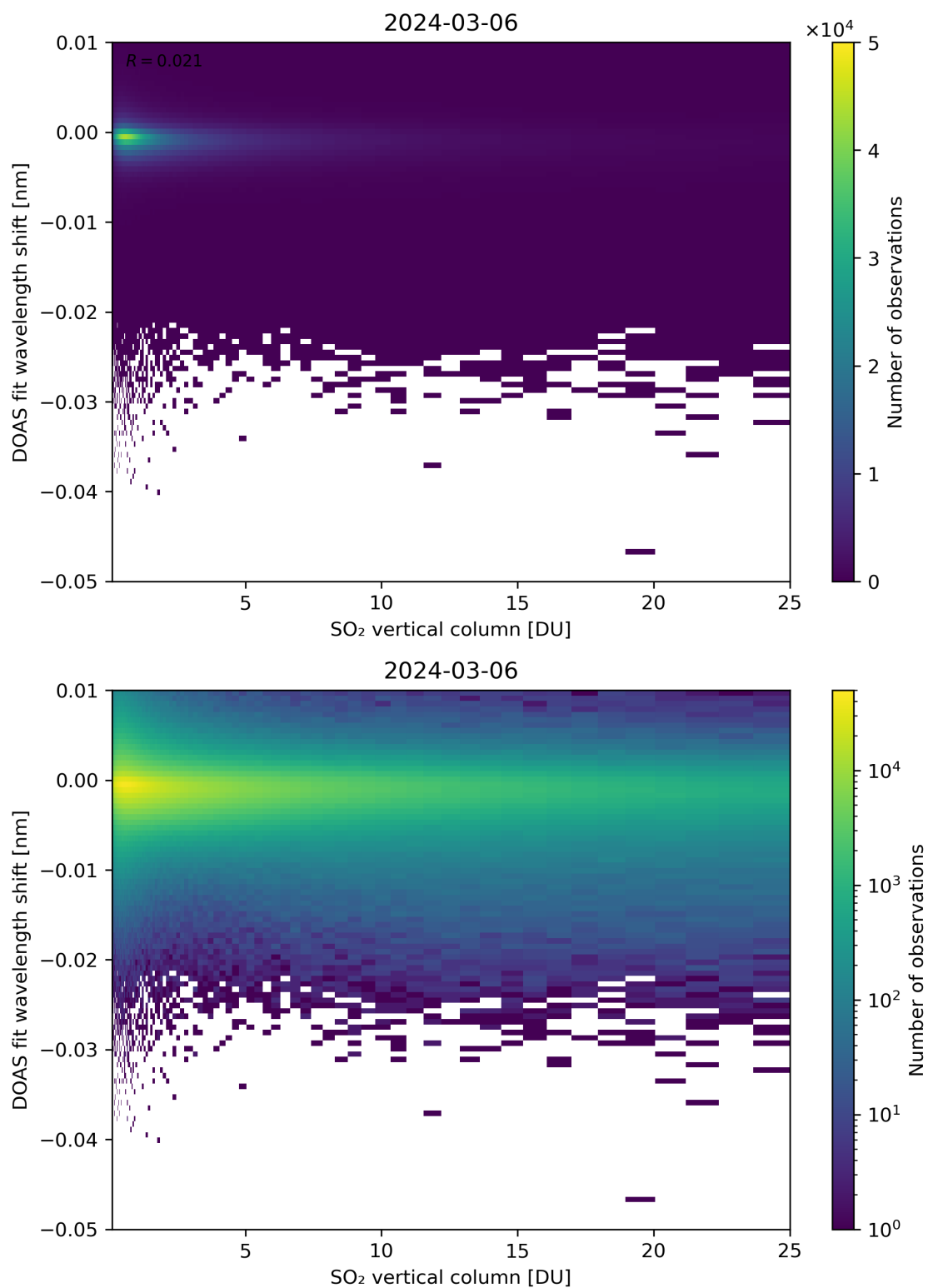
Figure 276: Scatter density plot of “SO 2 vertical column” against “DOAS fit wavelength shift” for 2024-03-05 to 2024-03-07.
