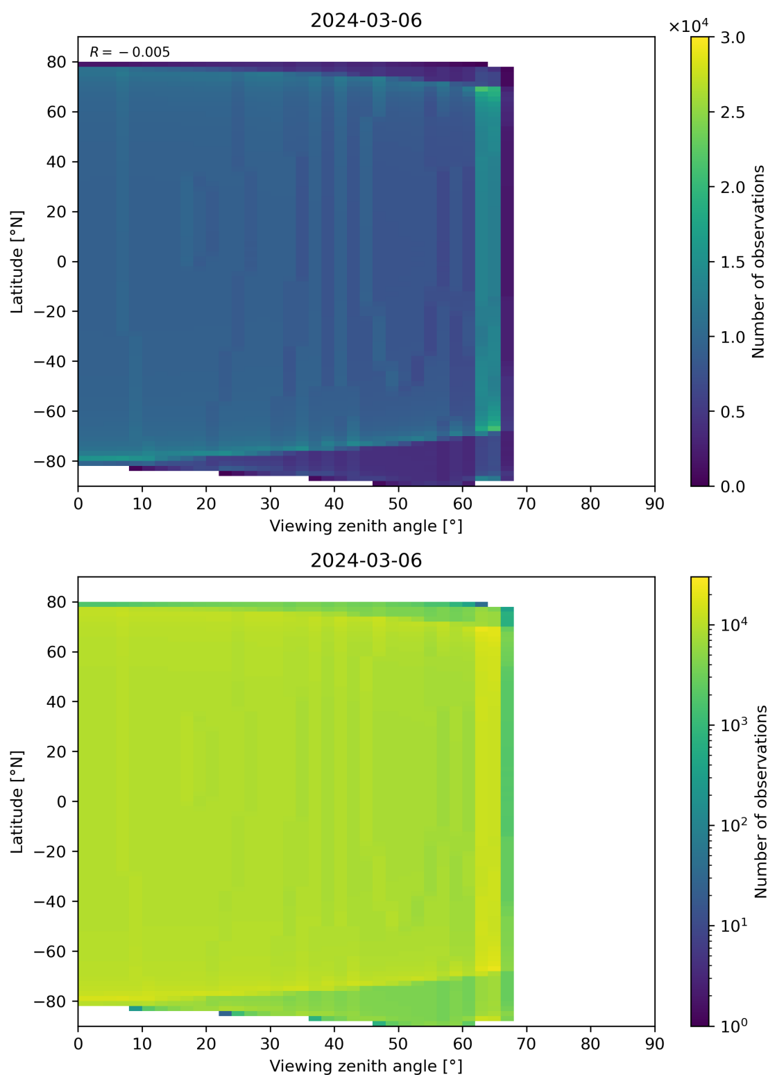
Figure 314: Scatter density plot of “Viewing zenith angle” against “Latitude” for 2024-03-05 to 2024-03-07.
