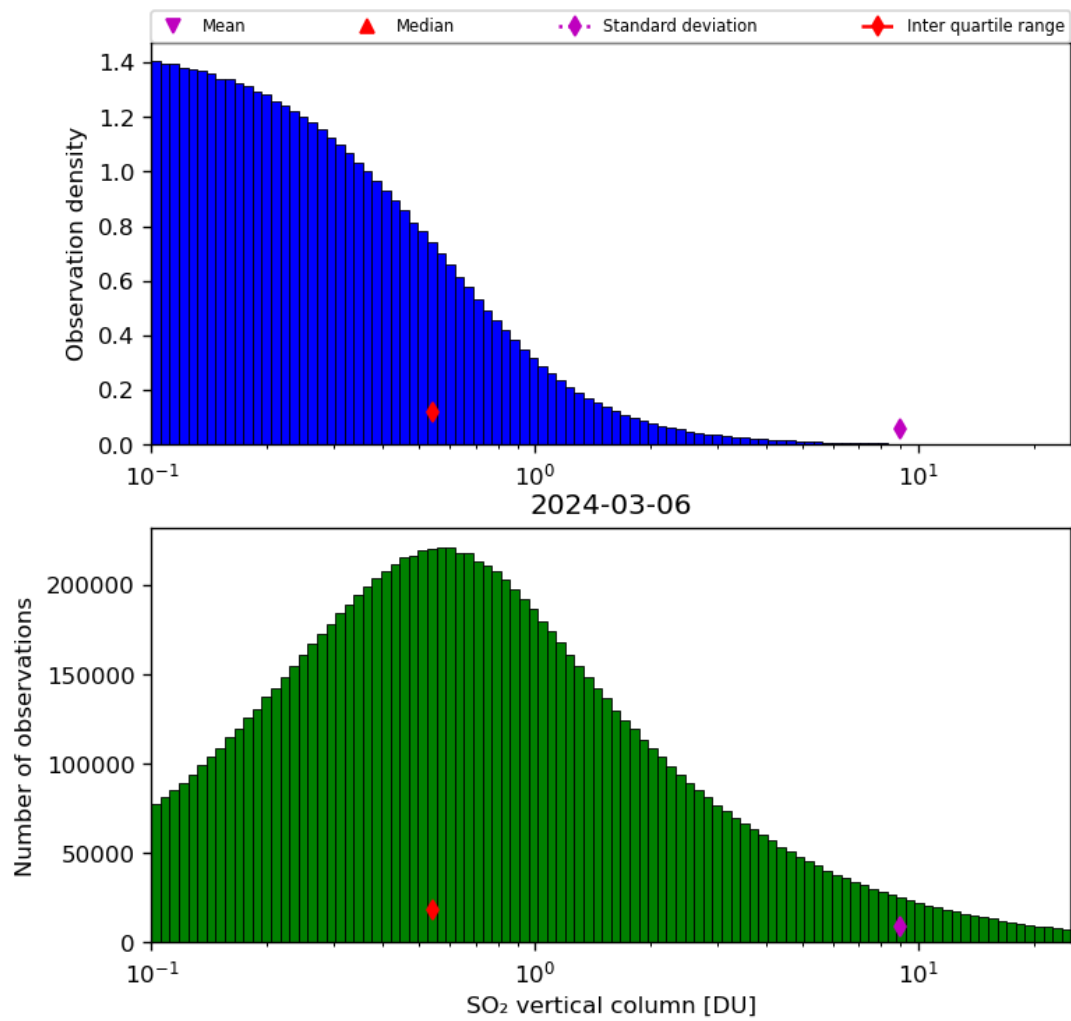
Figure 53: Histogram of “SO 2 vertical column” for 2024-03-05 to 2024-03-07
