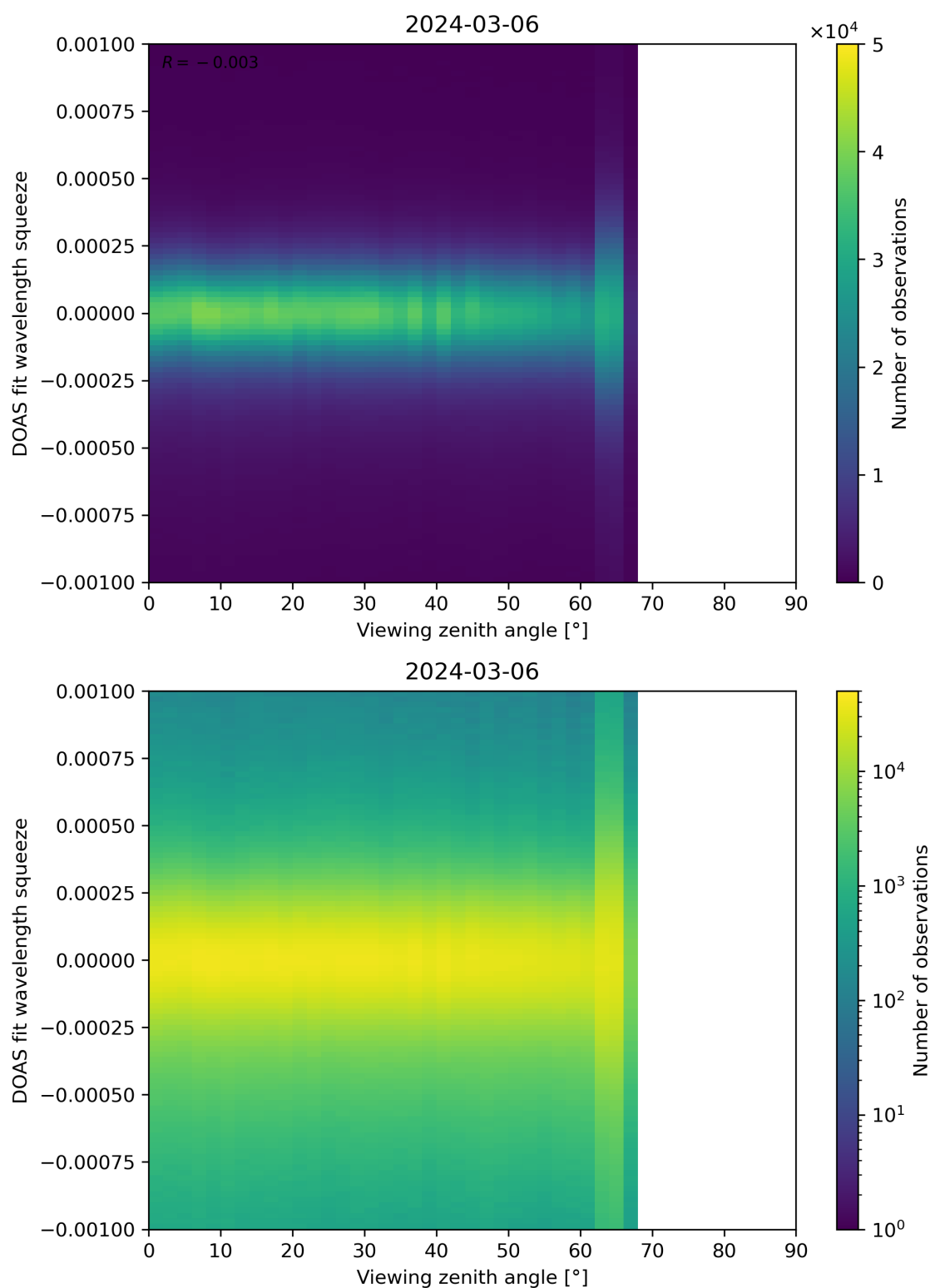
Figure 312: Scatter density plot of “Viewing zenith angle” against “DOAS fit wavelength squeeze” for 2024-03-05 to 2024-03-07.
