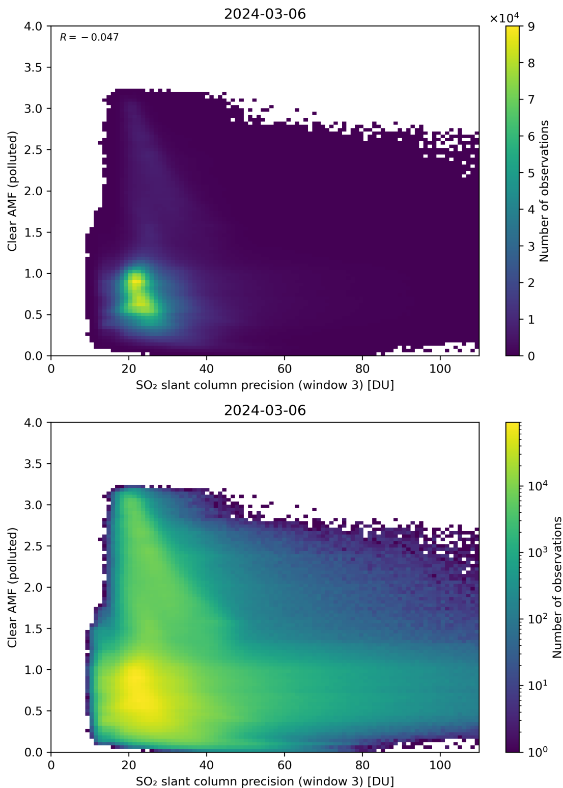
Figure 261: Scatter density plot of “SO 2 slant column precision (window 3)” against “Clear AMF (polluted)” for 2024-03-05 to 2024-03-07.
