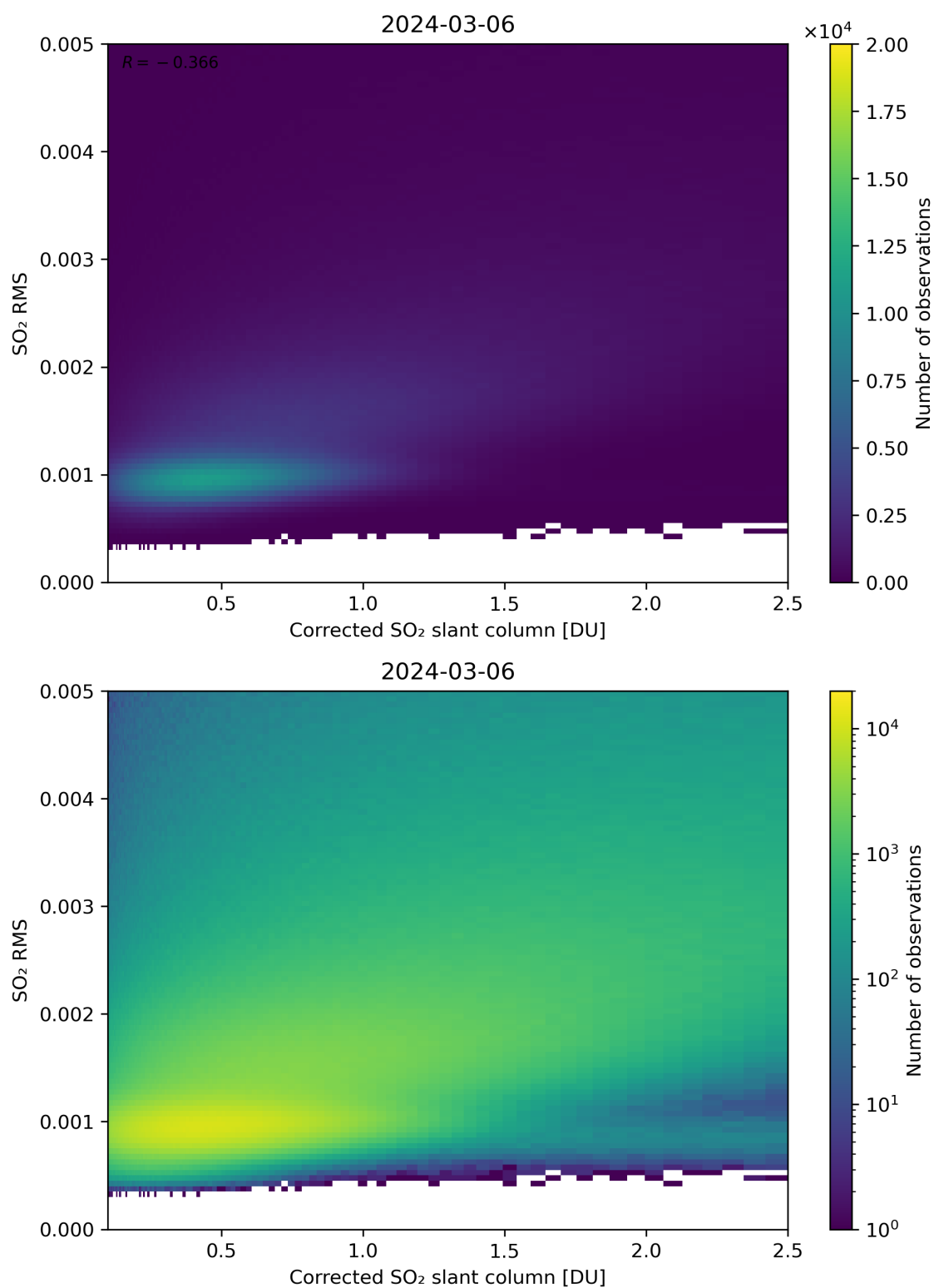
Figure 183: Scatter density plot of “Corrected SO 2 slant column” against “SO 2 RMS” for 2024-03-05 to 2024-03-07.
