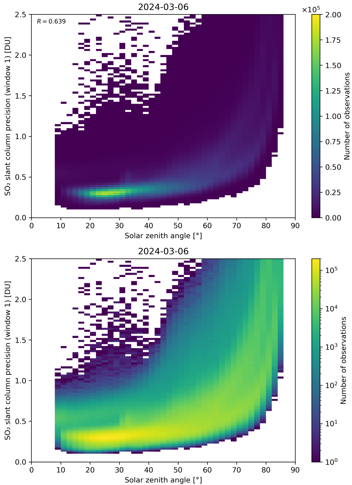
Figure 170: Scatter density plot of “Solar zenith angle” against “SO 2 slant column precision (window 1)” for 2024-03-05 to 2024-03-07.
