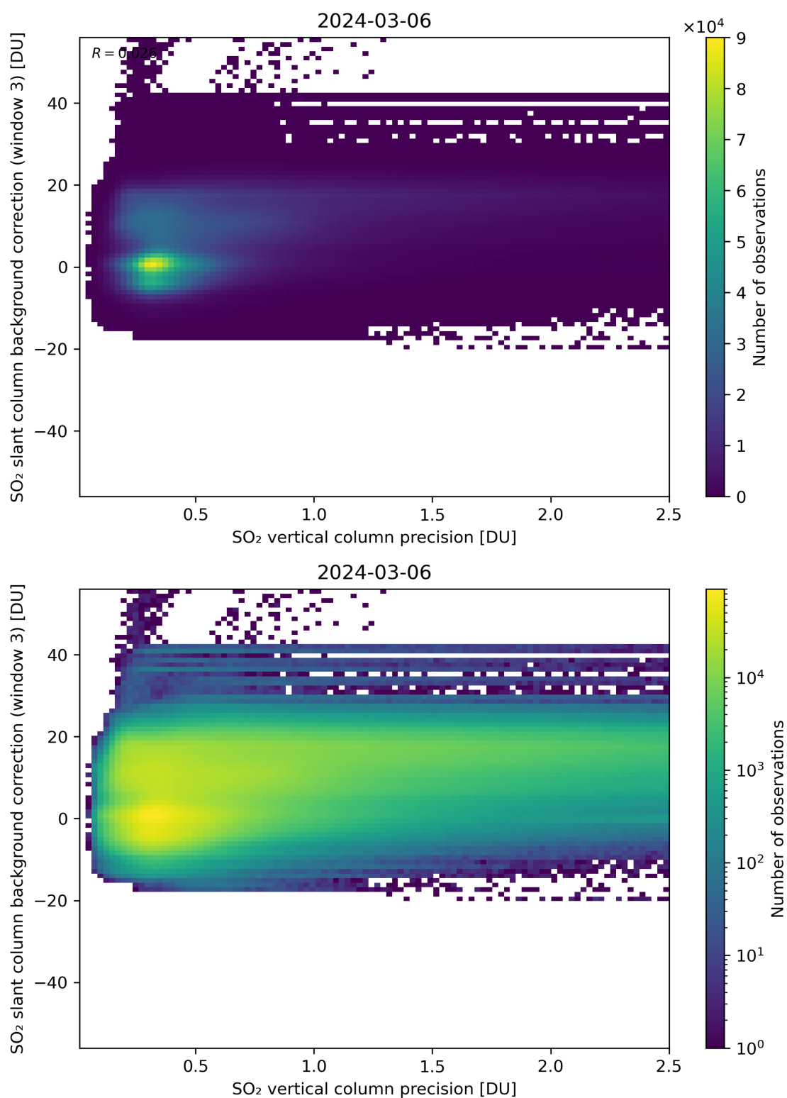
Figure 281: Scatter density plot of “SO 2 vertical column precision” against “SO 2 slant column background correction (window 3)” for 2024-03-05 to 2024-03-07.
