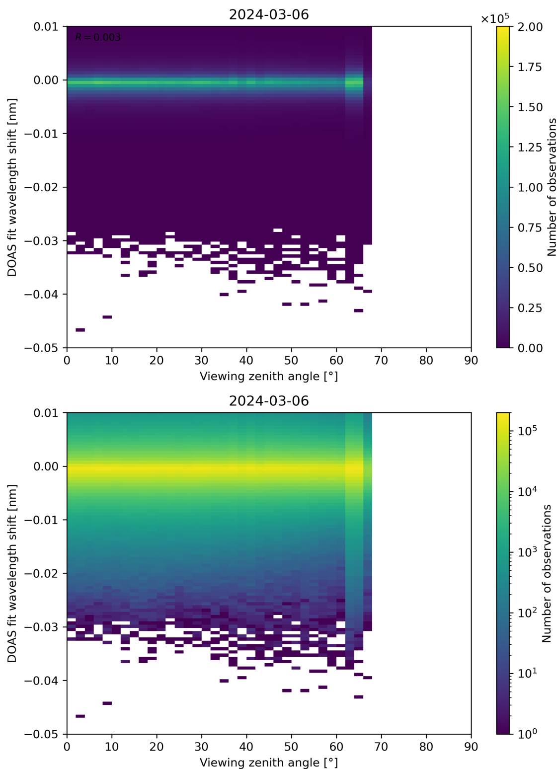
Figure 311: Scatter density plot of “Viewing zenith angle” against “DOAS fit wavelength shift” for 2024-03-05 to 2024-03-07.
