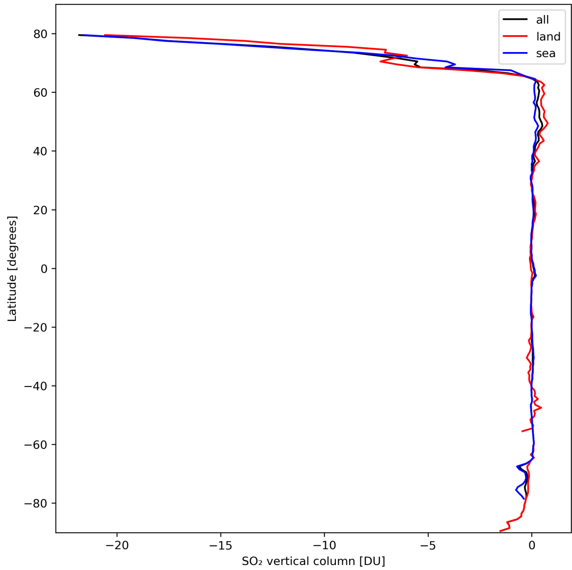
Figure 30: Zonal average of “SO 2 vertical column” for 2024-03-05 to 2024-03-07.
