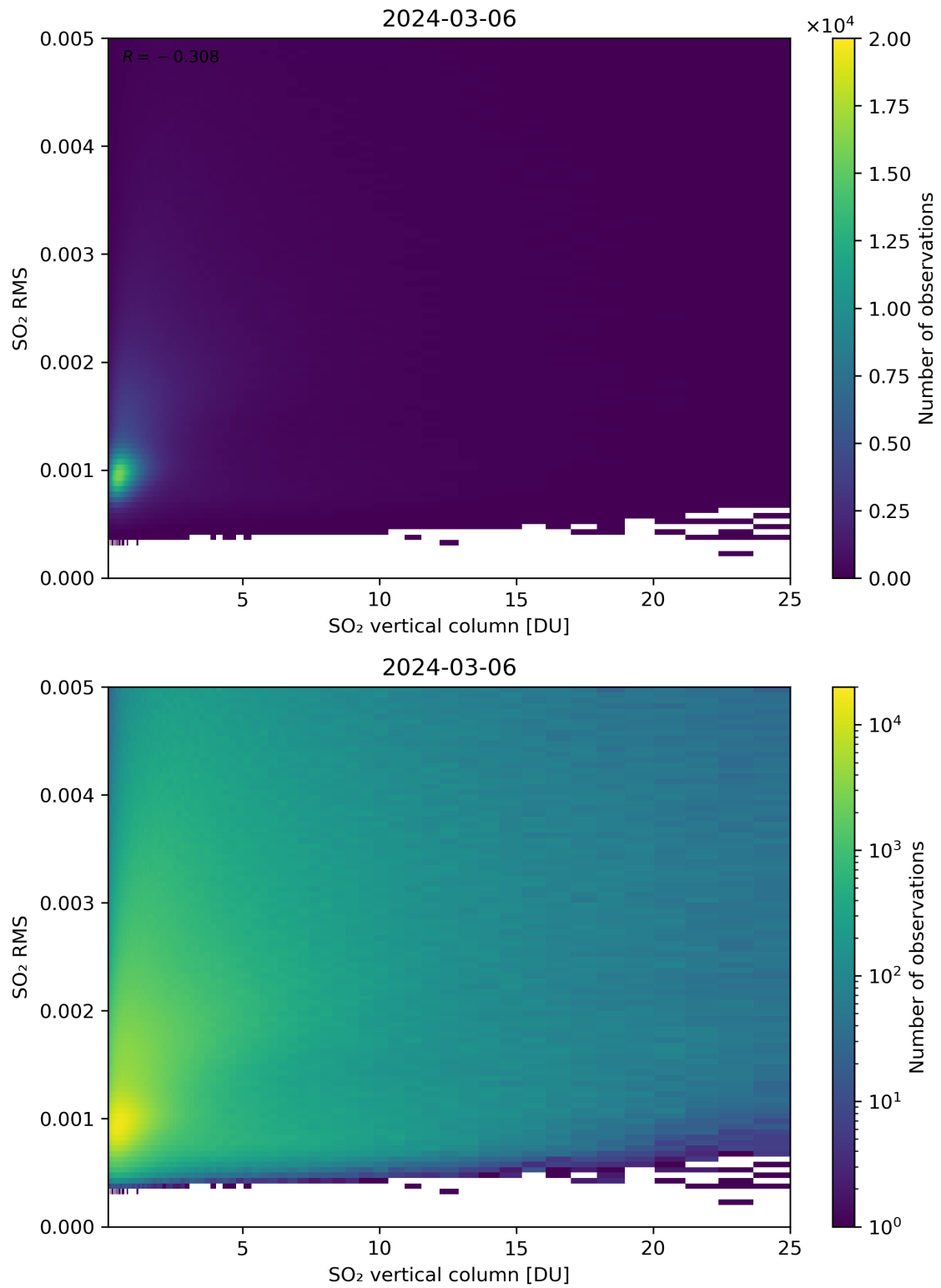
Figure 278: Scatter density plot of “SO 2 vertical column” against “SO 2 RMS” for 2024-03-05 to 2024-03-07.
