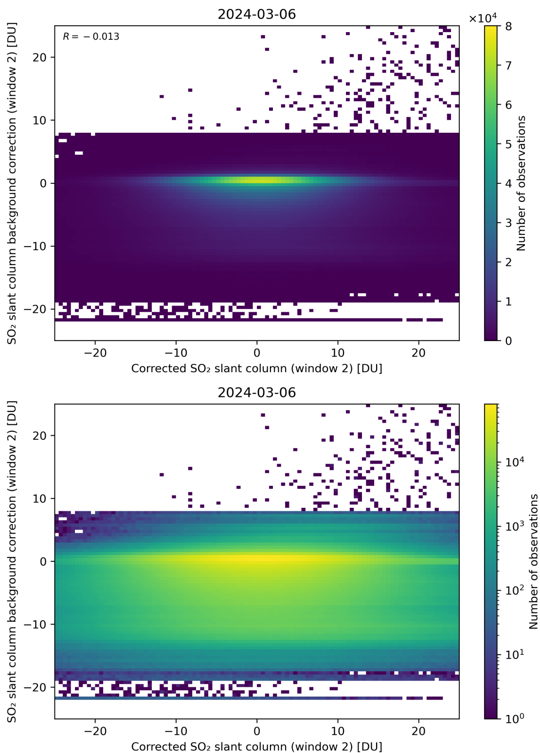
Figure 194: Scatter density plot of “Corrected SO 2 slant column (window 2)” against “SO 2 slant column background correction (window 2)” for 2024-03-05 to 2024-03-07.
