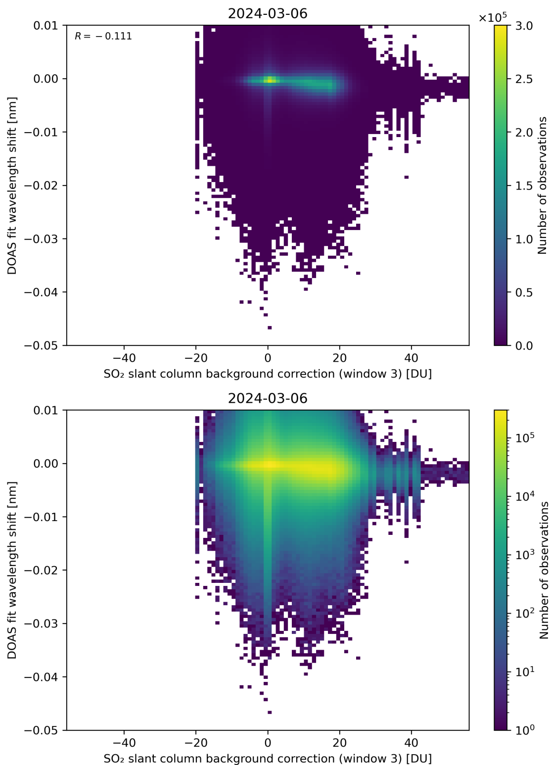
Figure 121: Scatter density plot of “SO 2 slant column background correction (window 3)” against “DOAS fit wavelength shift” for 2024-03-05 to 2024-03-07.
