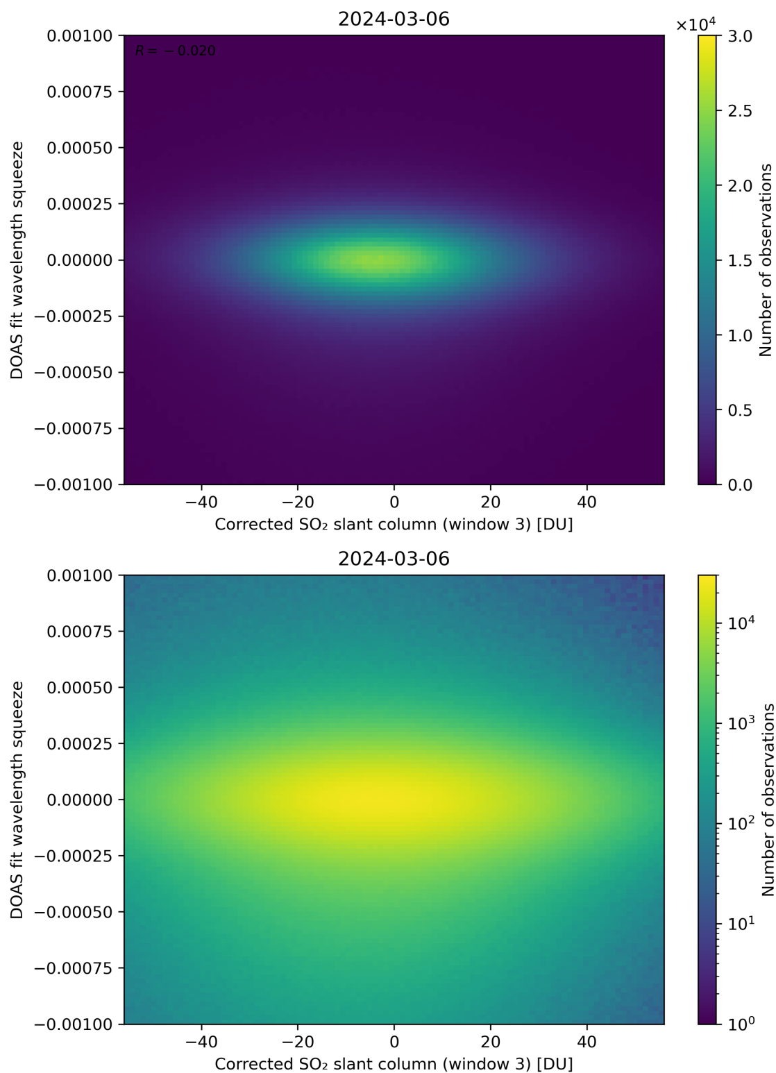
Figure 207: Scatter density plot of “Corrected SO 2 slant column (window 3)” against “DOAS fit wavelength squeeze” for 2024-03-05 to 2024-03-07.
