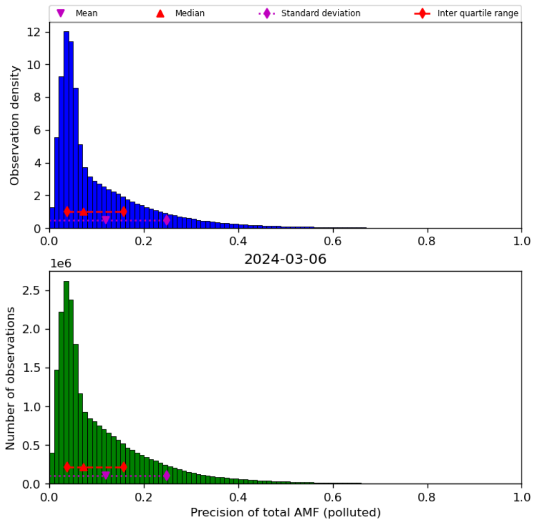
Figure 72: Histogram of “Precision of total AMF (polluted)” for 2024-03-05 to 2024-03-07
