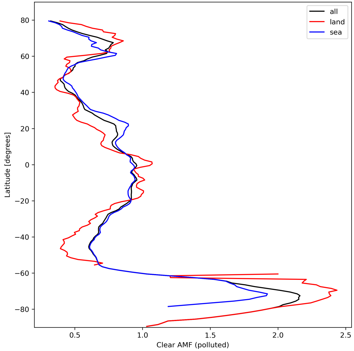
Figure 50: Zonal average of “Clear AMF (polluted)” for 2024-03-05 to 2024-03-07.
