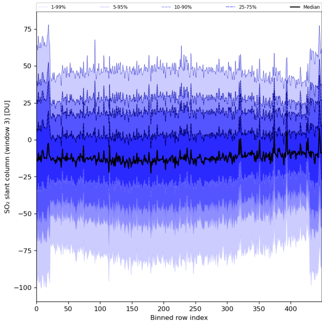
Figure 87: Along track statistics of “SO 2 slant column (window 3)” for 2024-03-05 to 2024-03-07
