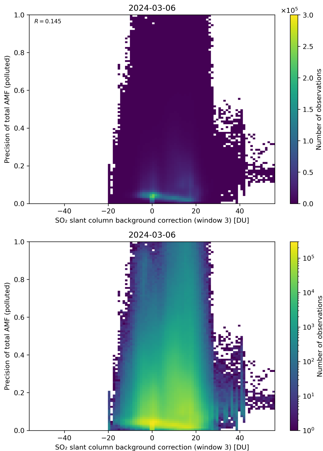
Figure 126: Scatter density plot of “SO 2 slant column background correction (window 3)” against “Precision of total AMF (polluted)” for 2024-03-05 to 2024-03-07.
