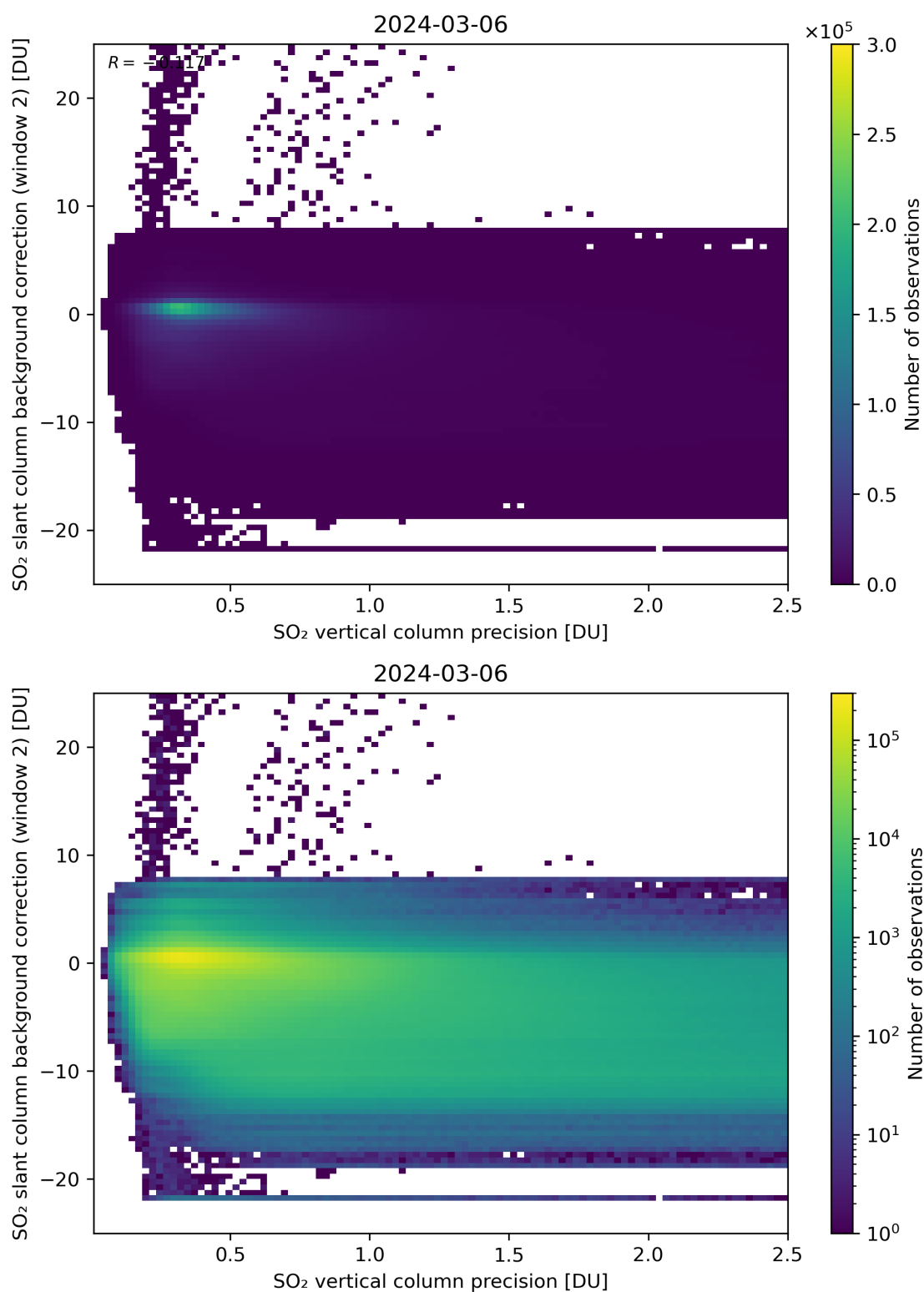
Figure 280: Scatter density plot of “SO 2 vertical column precision” against “SO 2 slant column background correction (window 2)” for 2024-03-05 to 2024-03-07.
