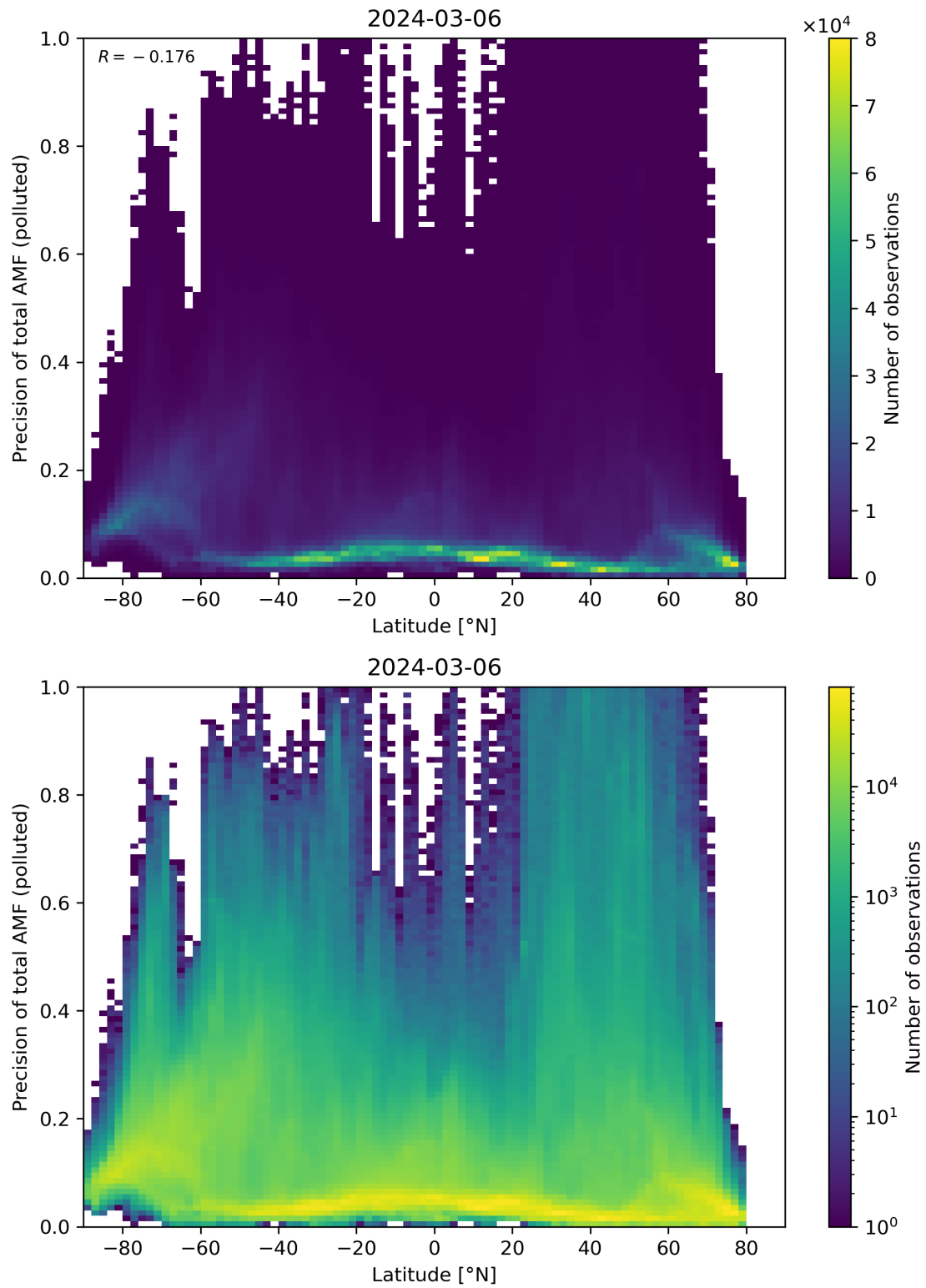
Figure 155: Scatter density plot of “Latitude” against “Precision of total AMF (polluted)” for 2024-03-05 to 2024-03-07.
