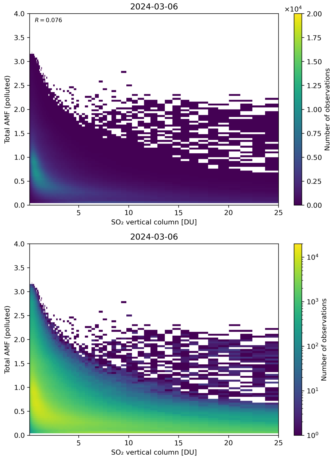
Figure 305: Scatter density plot of “SO 2 vertical column” against “Total AMF (polluted)” for 2024-03-05 to 2024-03-07.
