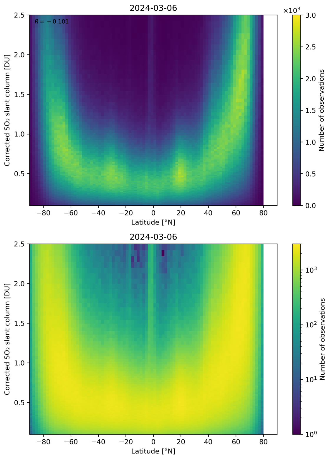
Figure 146: Scatter density plot of “Latitude” against “Corrected SO 2 slant column” for 2024-03-05 to 2024-03-07.
