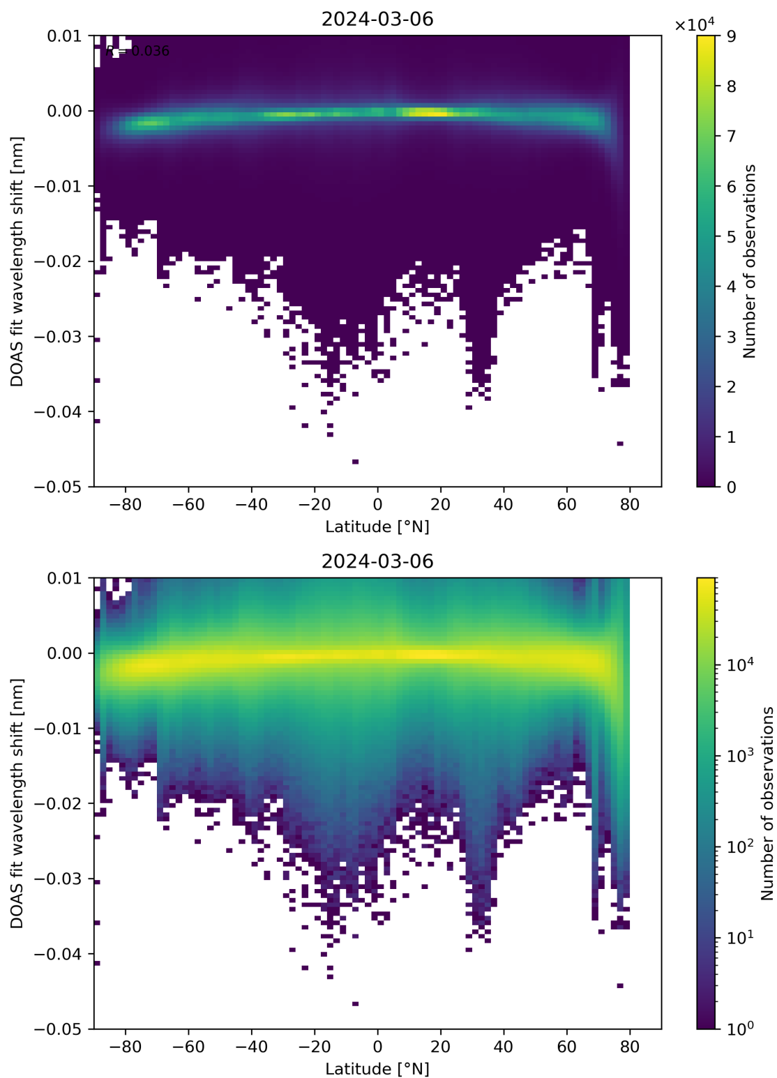
Figure 142: Scatter density plot of “Latitude” against “DOAS fit wavelength shift” for 2024-03-05 to 2024-03-07.
