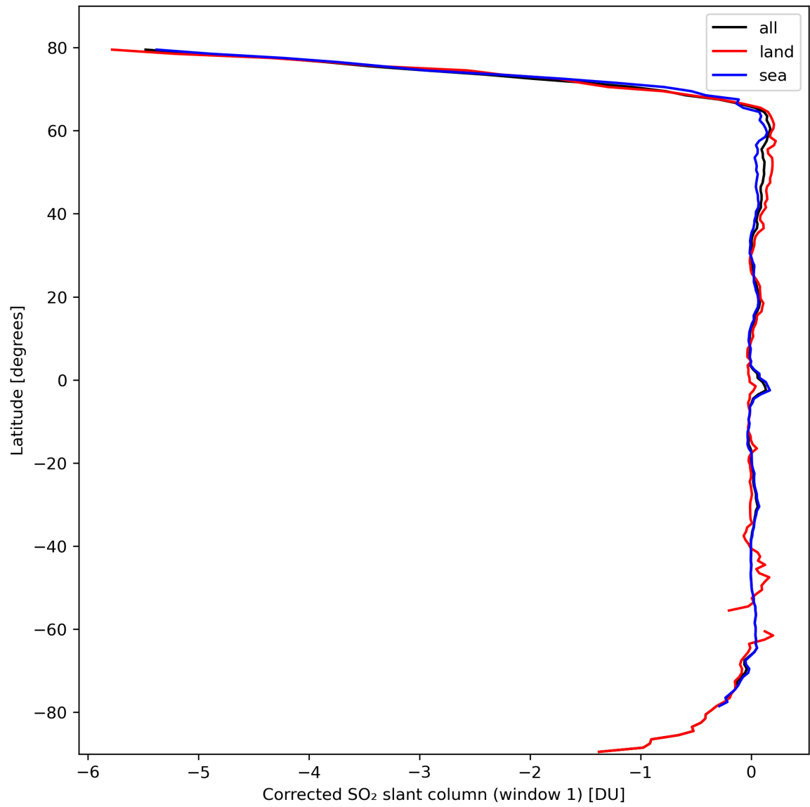
Figure 35: Zonal average of “Corrected SO 2 slant column (window 1)” for 2024-03-05 to 2024-03-07.
