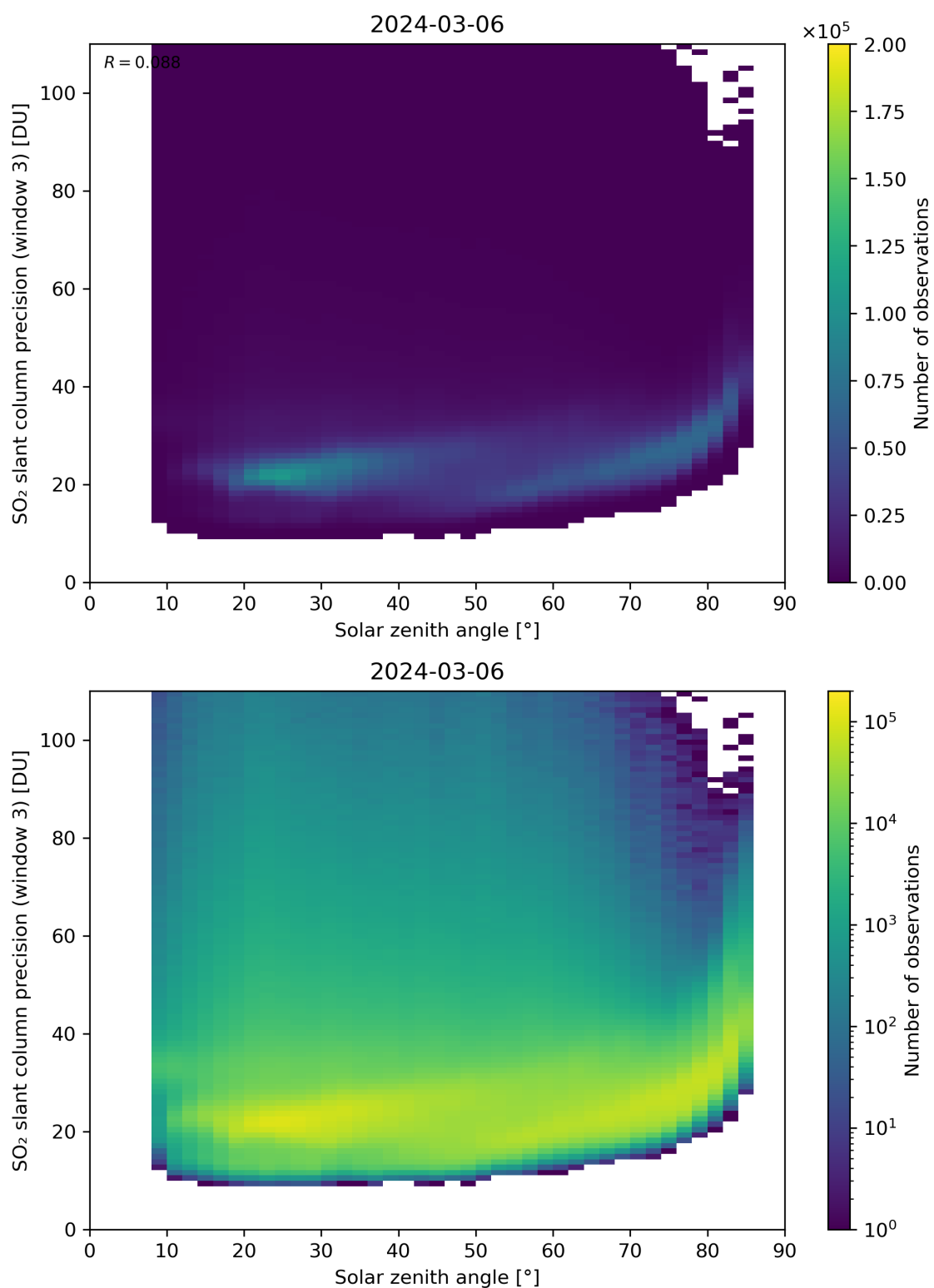
Figure 173: Scatter density plot of “Solar zenith angle” against “SO 2 slant column precision (window 3)” for 2024-03-05 to 2024-03-07.
