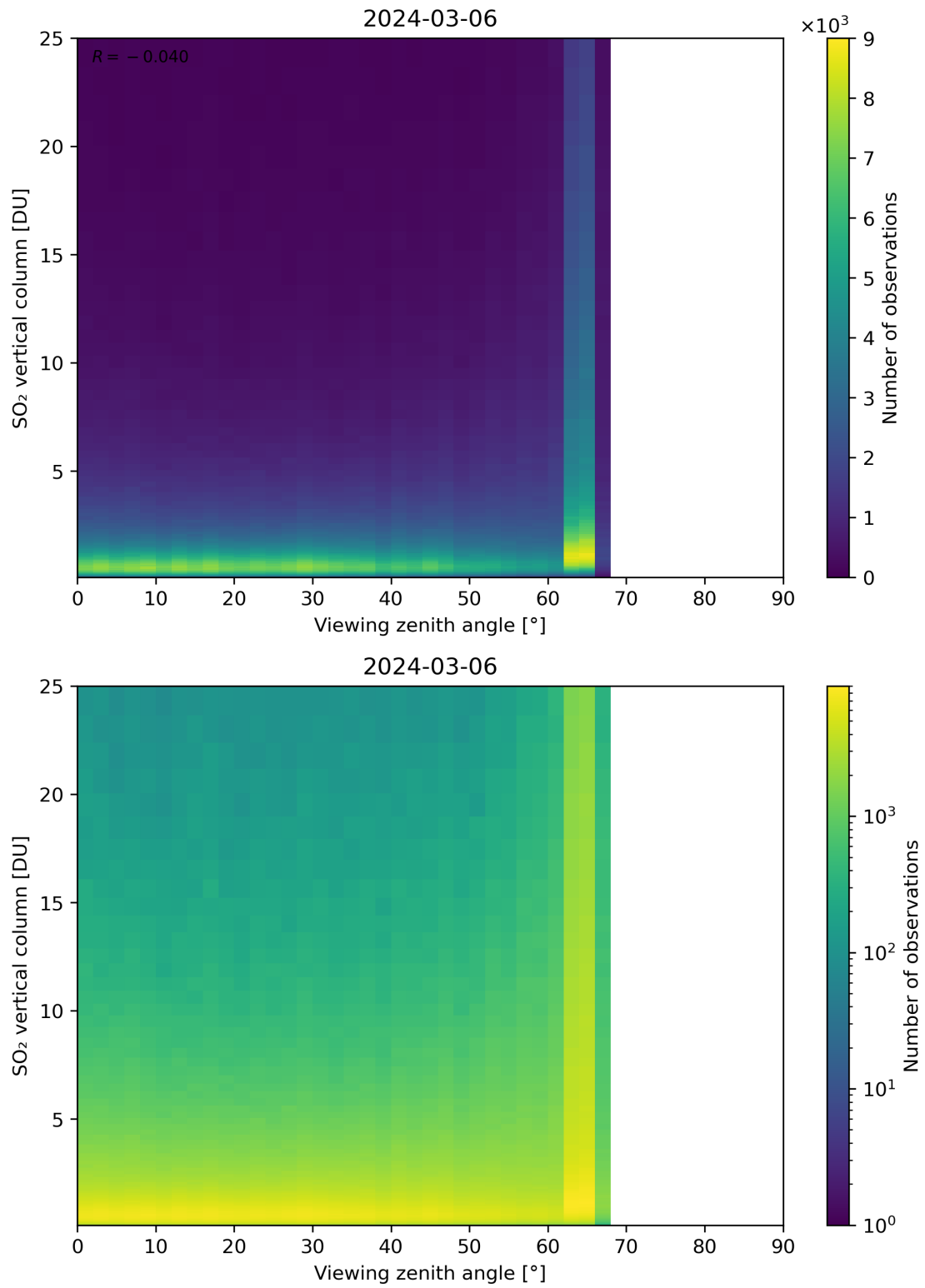
Figure 327: Scatter density plot of “Viewing zenith angle” against “SO 2 vertical column” for 2024-03-05 to 2024-03-07.
