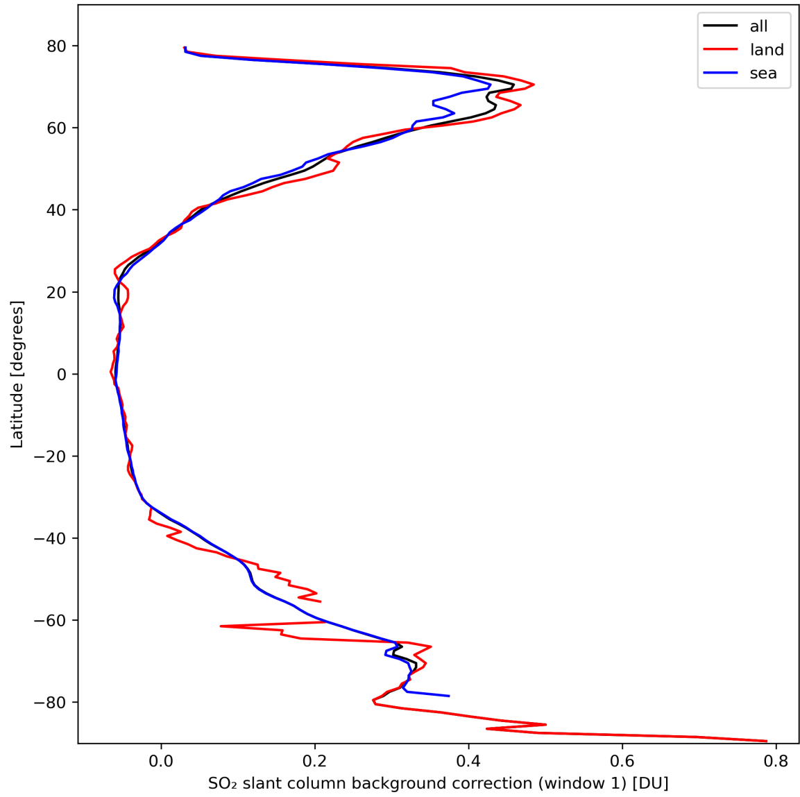
Figure 36: Zonal average of “SO 2 slant column background correction (window 1)” for 2024-03-05 to 2024-03-07.
