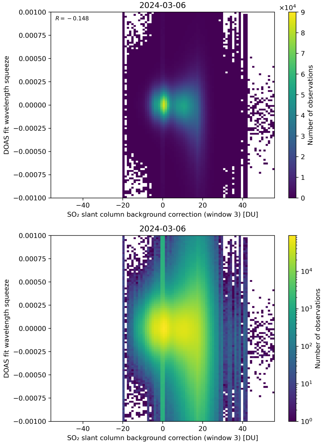
Figure 122: Scatter density plot of “SO 2 slant column background correction (window 3)” against “DOAS fit wavelength squeeze” for 2024-03-05 to 2024-03-07.
