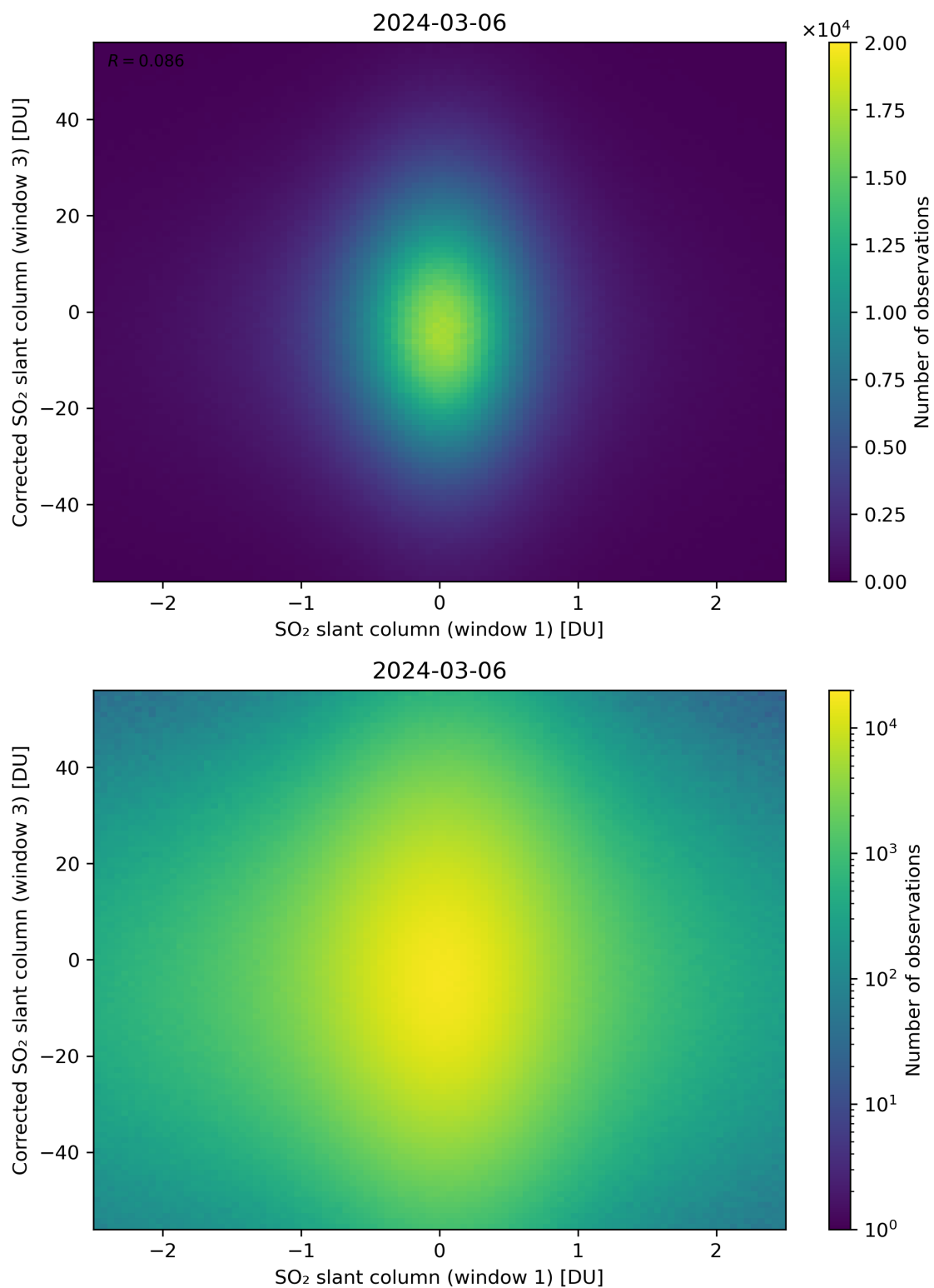
Figure 234: Scatter density plot of “SO 2 slant column (window 1)” against “Corrected SO 2 slant column (window 3)” for 2024-03-05 to 2024-03-07.
