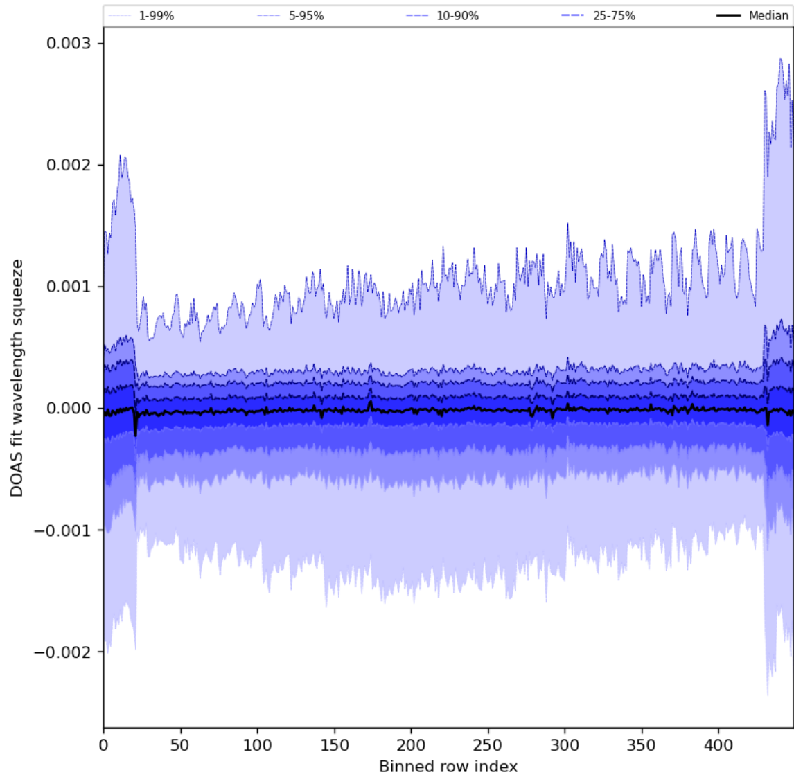
Figure 92: Along track statistics of “DOAS fit wavelength squeeze” for 2024-03-05 to 2024-03-07
