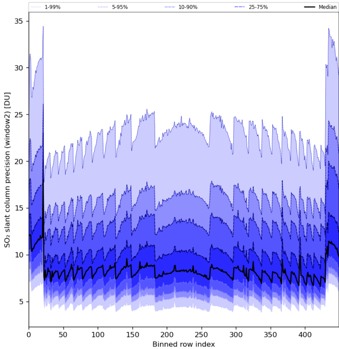
Figure 84: Along track statistics of “SO 2 slant column precision (window2)” for 2024-03-05 to 2024-03-07
