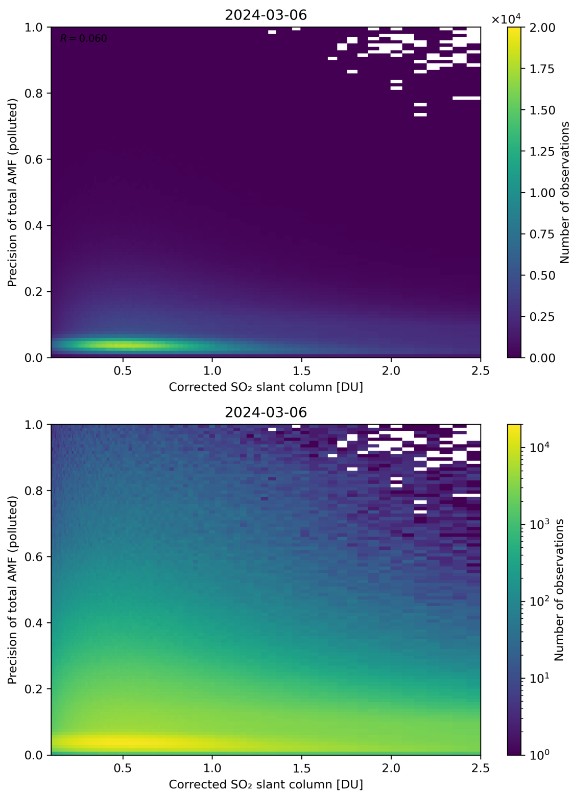
Figure 193: Scatter density plot of “Corrected SO 2 slant column” against “Precision of total AMF (polluted)” for 2024-03-05 to 2024-03-07.
