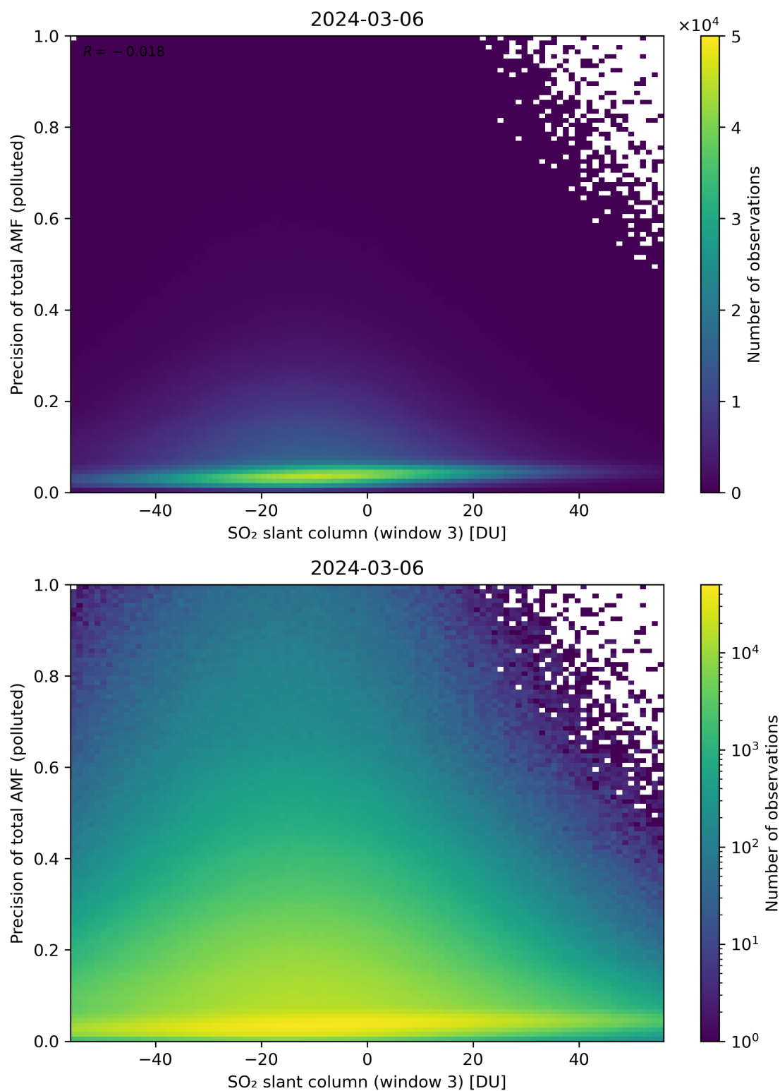
Figure 269: Scatter density plot of “SO 2 slant column (window 3)” against “Precision of total AMF (polluted)” for 2024-03-05 to 2024-03-07.
