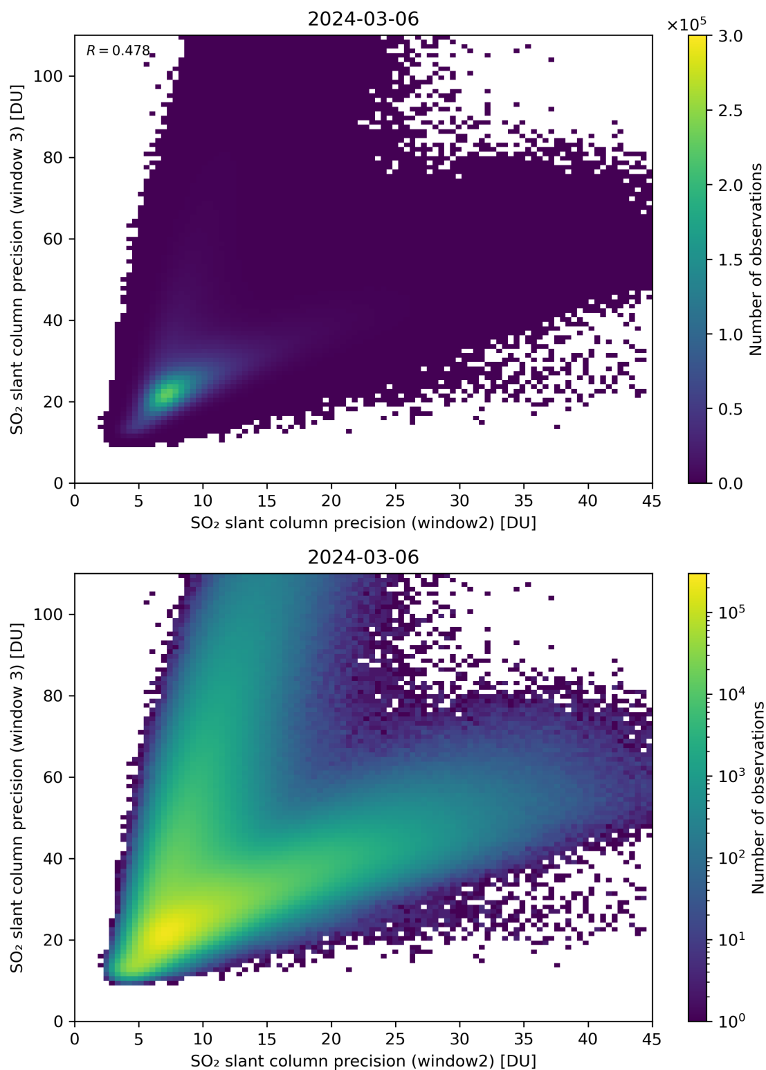
Figure 250: Scatter density plot of “SO 2 slant column precision (window2)” against “SO 2 slant column precision (window 3)” for 2024-03-05 to 2024-03-07.
