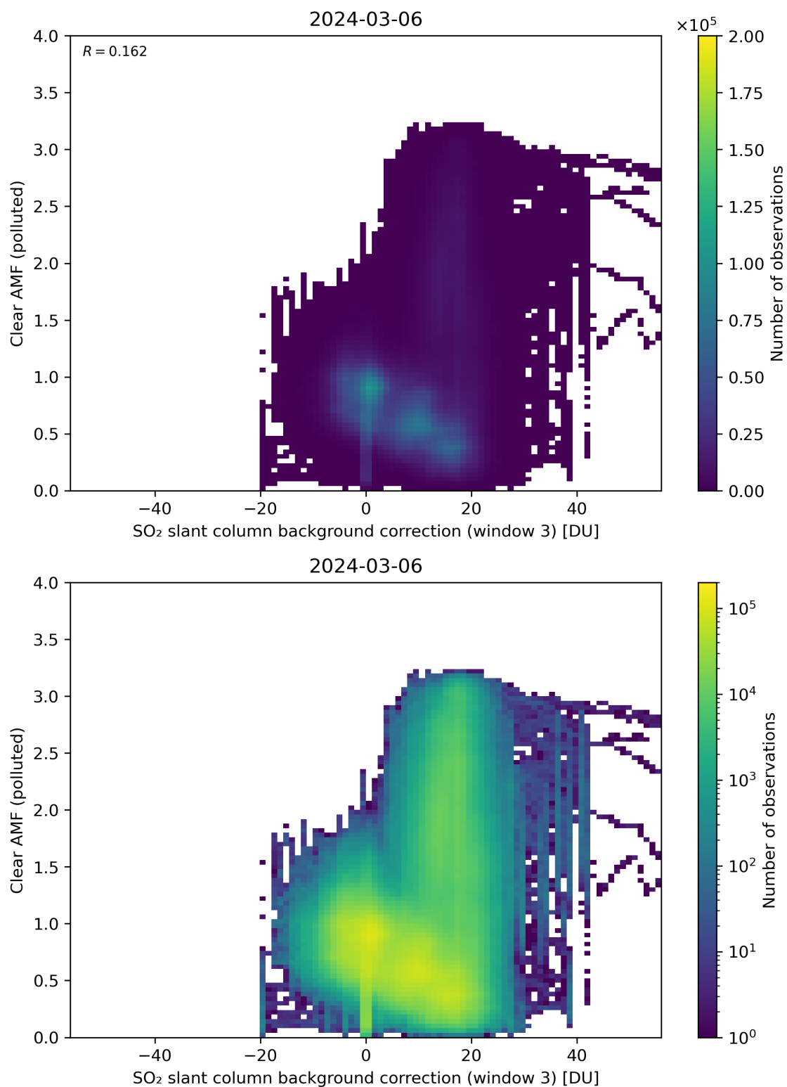
Figure 124: Scatter density plot of “SO 2 slant column background correction (window 3)” against “Clear AMF (polluted)” for 2024-03-05 to 2024-03-07.
