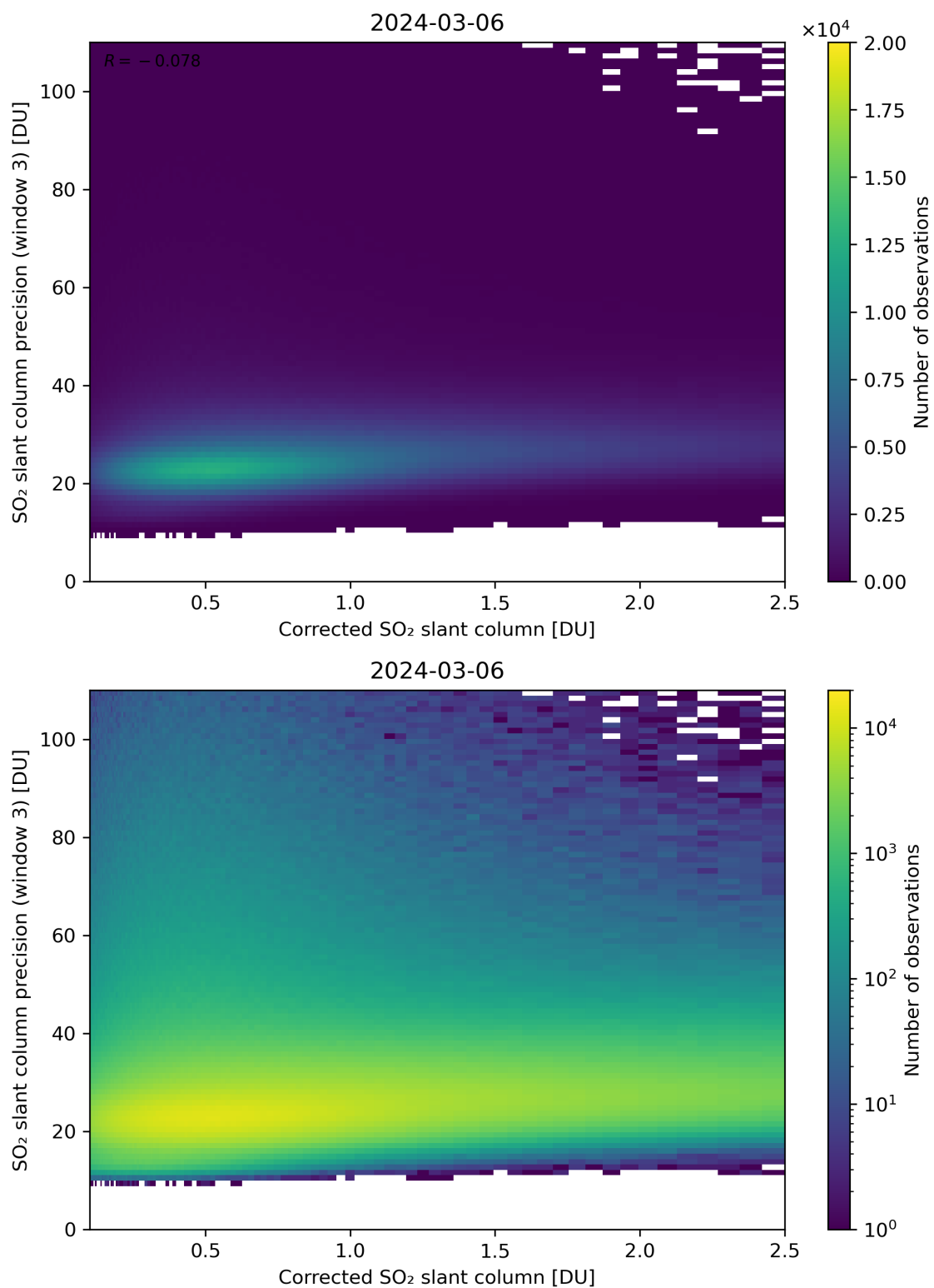
Figure 191: Scatter density plot of “Corrected SO 2 slant column” against “SO 2 slant column precision (window 3)” for 2024-03-05 to 2024-03-07.
