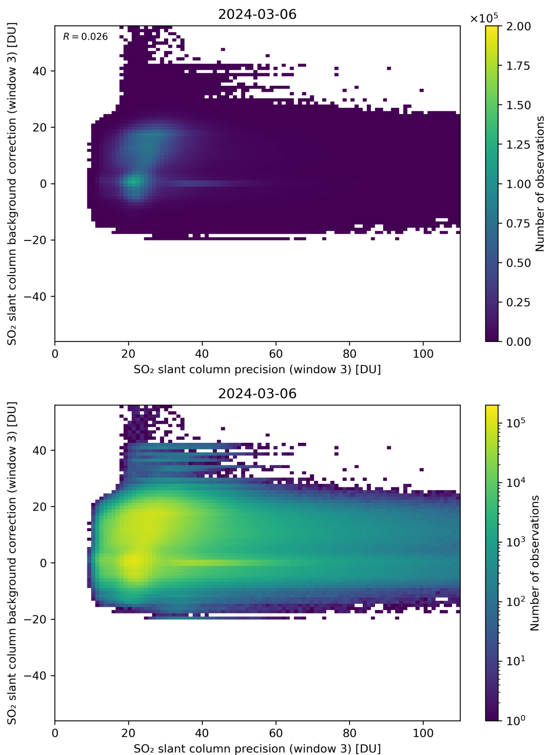
Figure 257: Scatter density plot of “SO 2 slant column precision (window 3)” against “SO 2 slant column background correction (window 3)” for 2024-03-05 to 2024-03-07.
