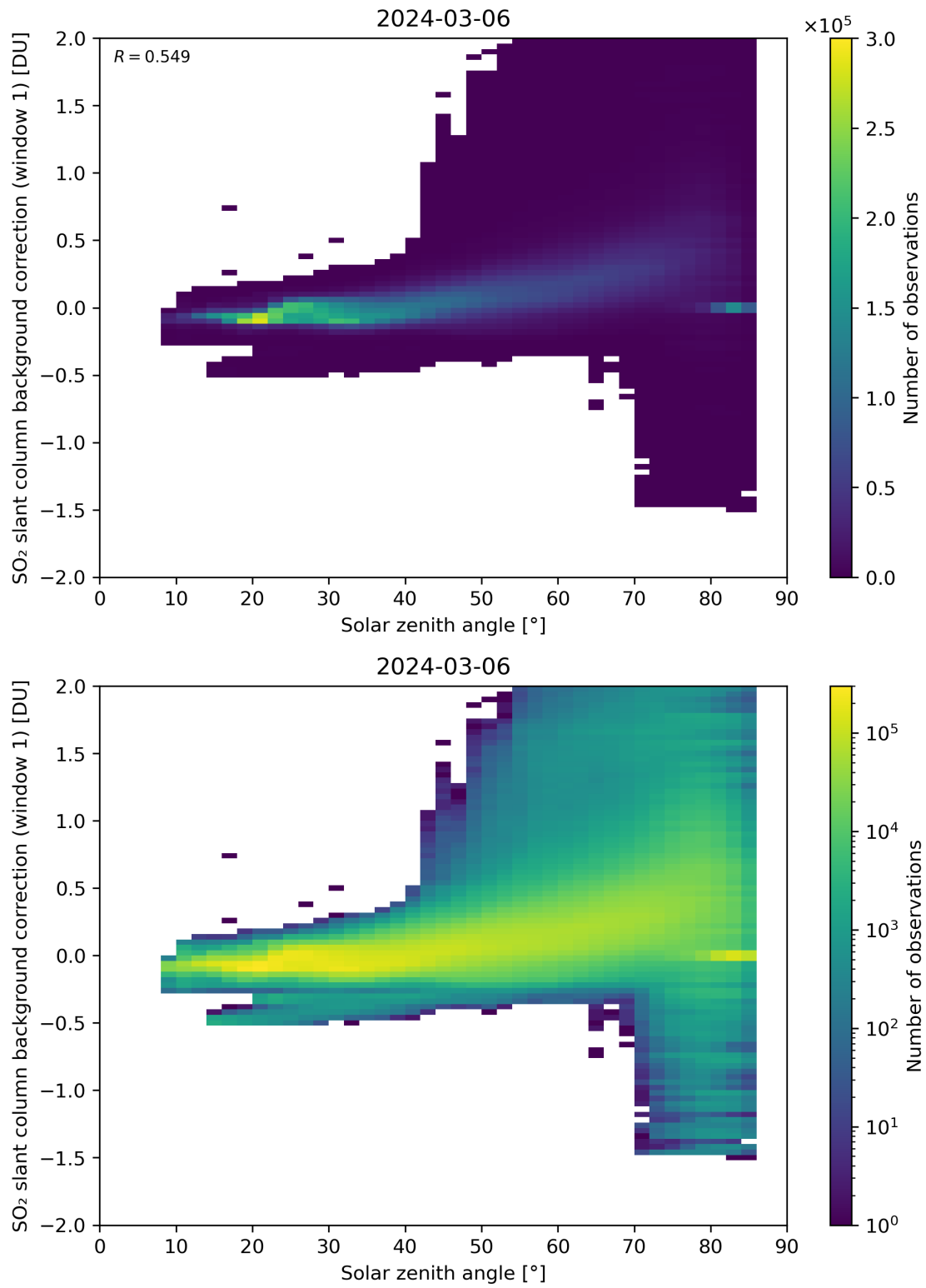
Figure 158: Scatter density plot of “Solar zenith angle” against “SO 2 slant column background correction (window 1)” for 2024-03-05 to 2024-03-07.
