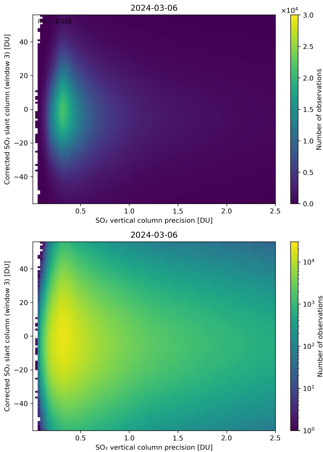
Figure 288: Scatter density plot of “SO 2 vertical column precision” against “Corrected SO 2 slant column (window 3)” for 2024-03-05 to 2024-03-07.
