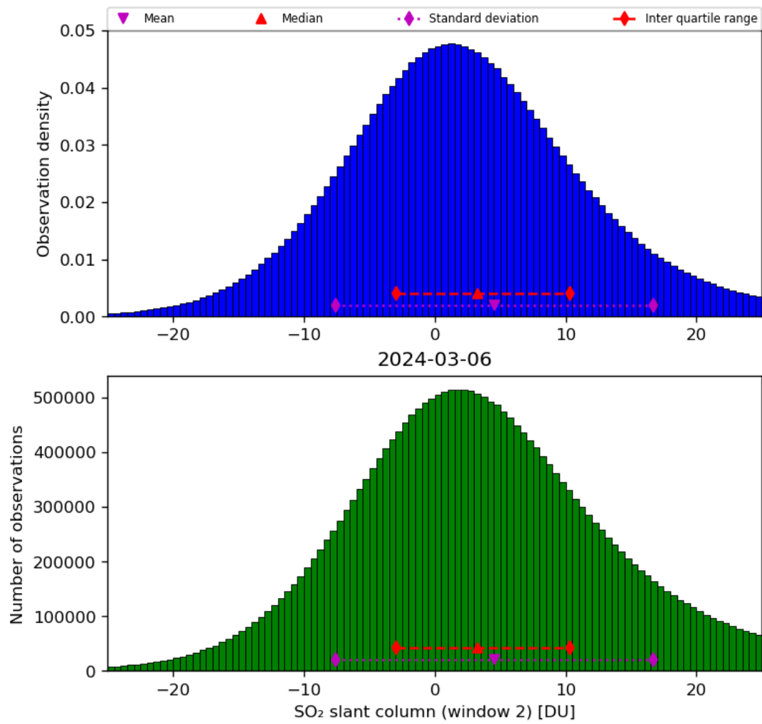
Figure 60: Histogram of “SO 2 slant column (window 2)” for 2024-03-05 to 2024-03-07
