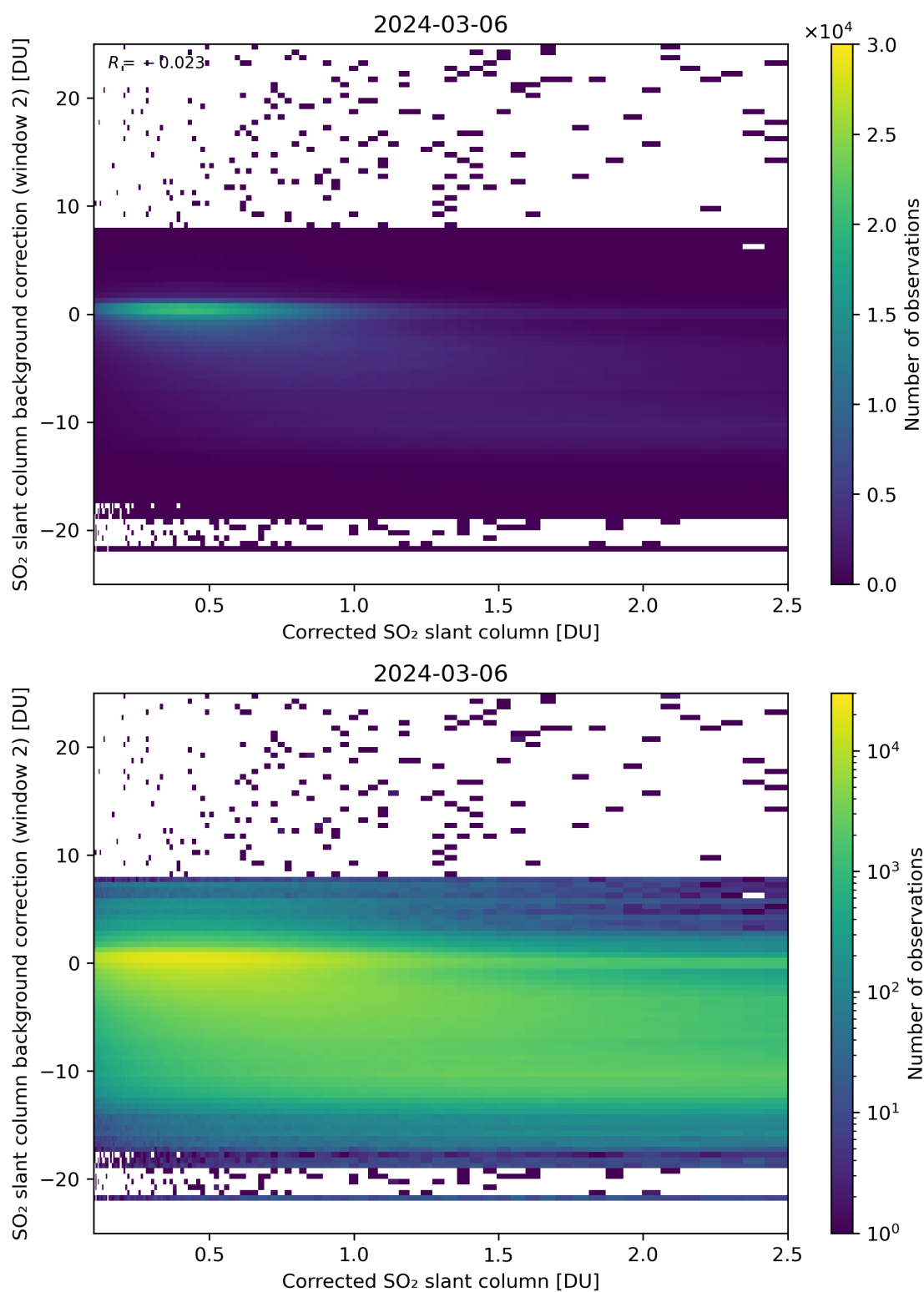
Figure 179: Scatter density plot of “Corrected SO 2 slant column” against “SO 2 slant column background correction (window 2)” for 2024-03-05 to 2024-03-07.
