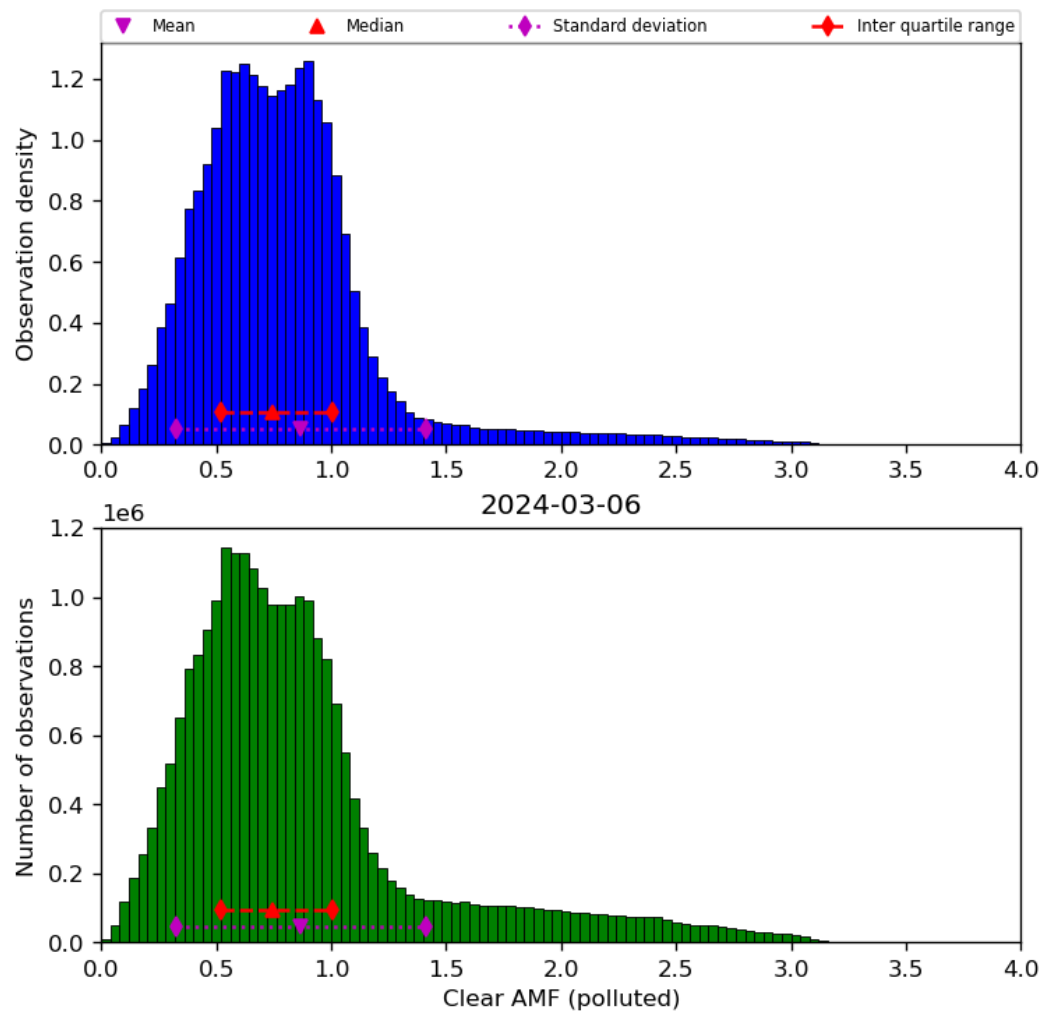
Figure 73: Histogram of “Clear AMF (polluted)” for 2024-03-05 to 2024-03-07
