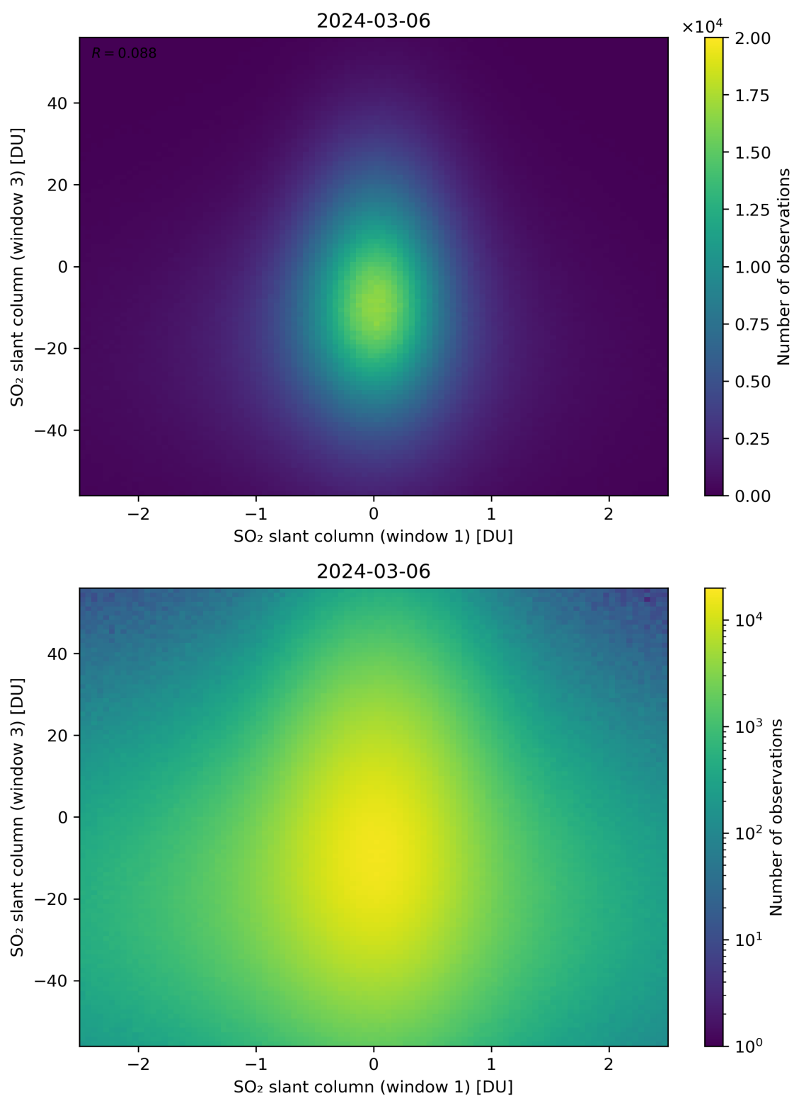
Figure 237: Scatter density plot of “SO 2 slant column (window 1)” against “SO 2 slant column (window 3)” for 2024-03-05 to 2024-03-07.
