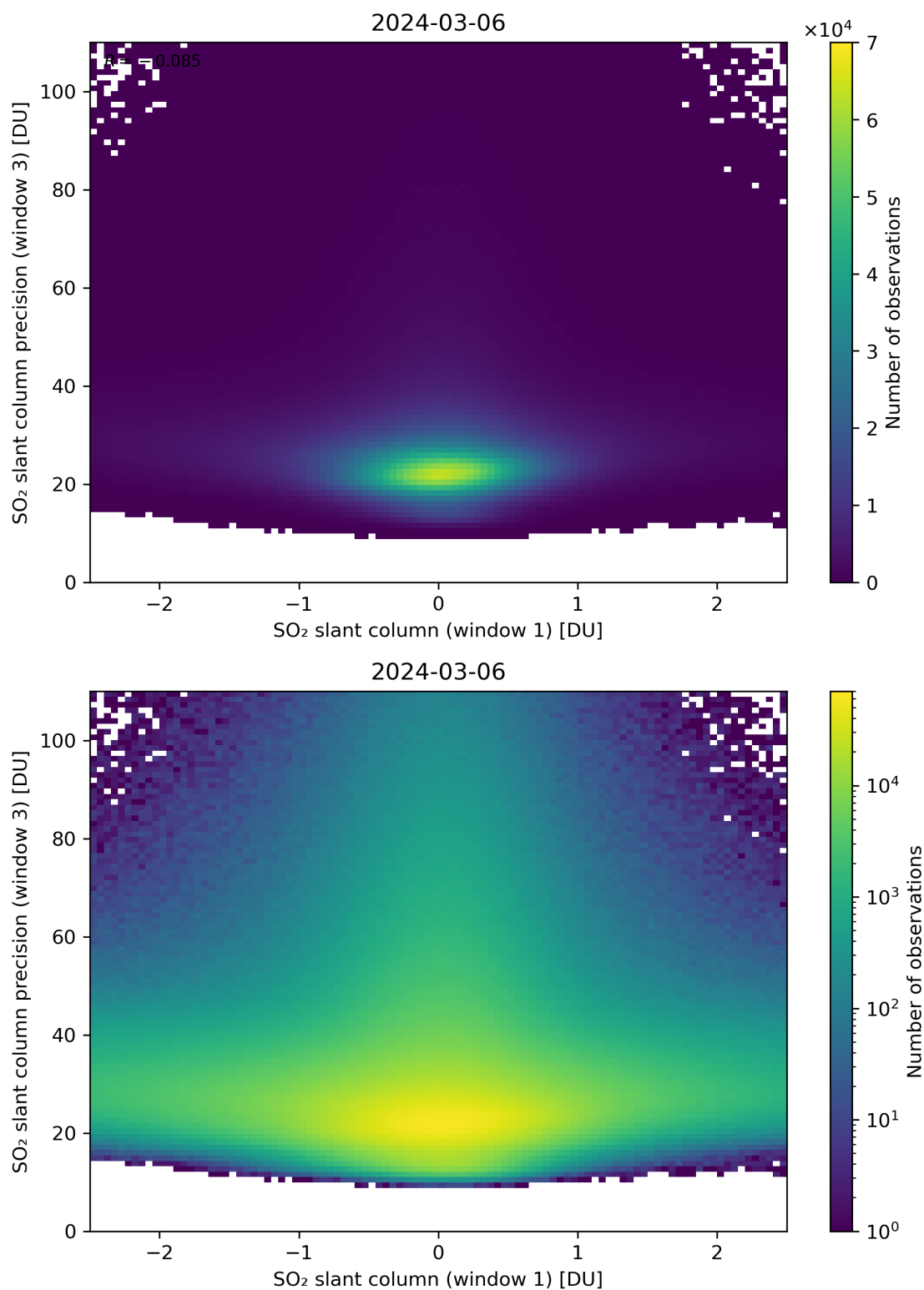
Figure 238: Scatter density plot of “SO 2 slant column (window 1)” against “SO 2 slant column precision (window 3)” for 2024-03-05 to 2024-03-07.
