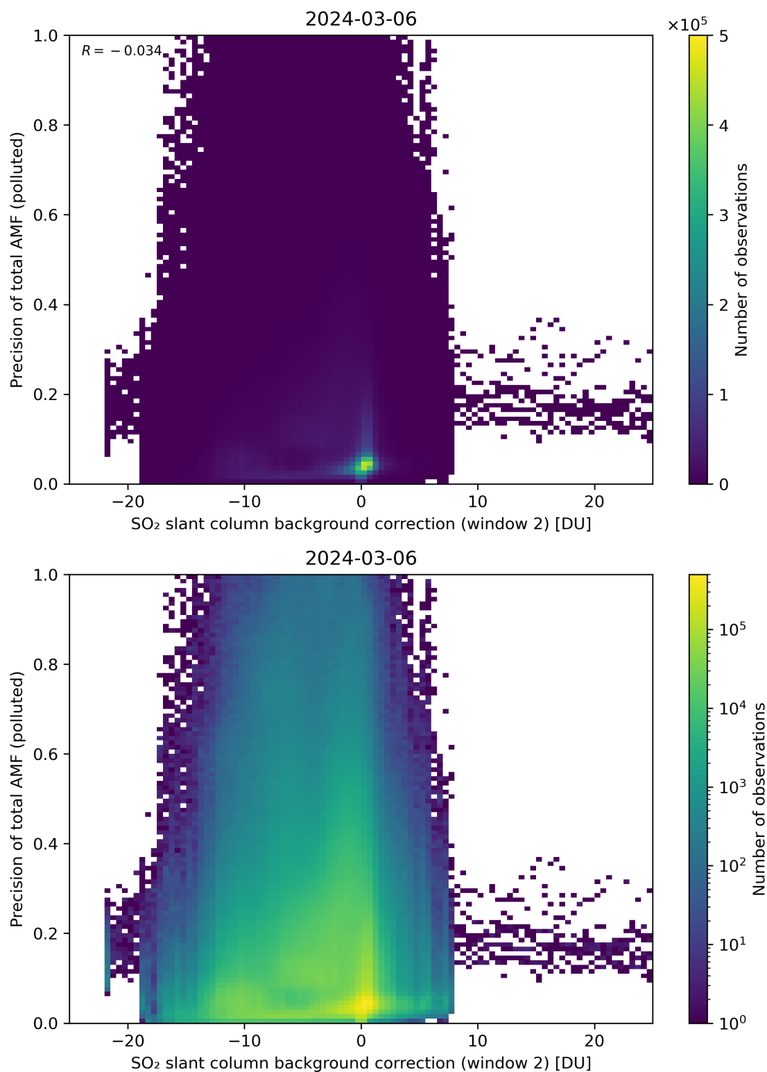
Figure 120: Scatter density plot of “SO 2 slant column background correction (window 2)” against “Precision of total AMF (polluted)” for 2024-03-05 to 2024-03-07.
