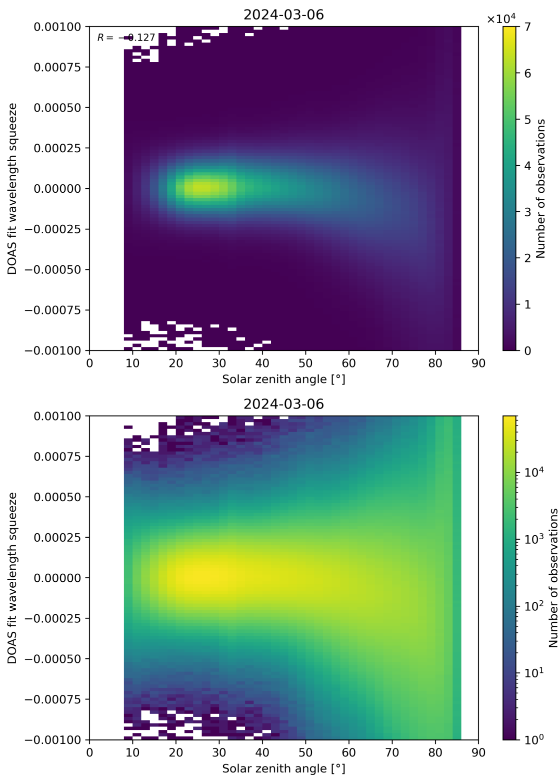
Figure 162: Scatter density plot of “Solar zenith angle” against “DOAS fit wavelength squeeze” for 2024-03-05 to 2024-03-07.
