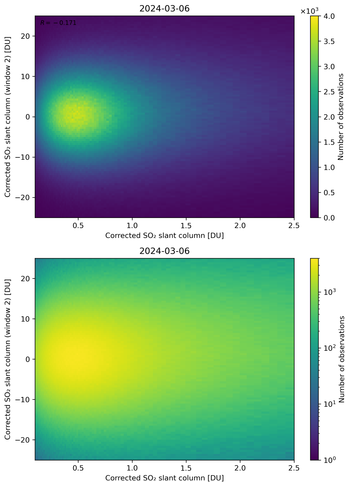
Figure 185: Scatter density plot of “Corrected SO 2 slant column” against “Corrected SO 2 slant column (window 2)” for 2024-03-05 to 2024-03-07.
