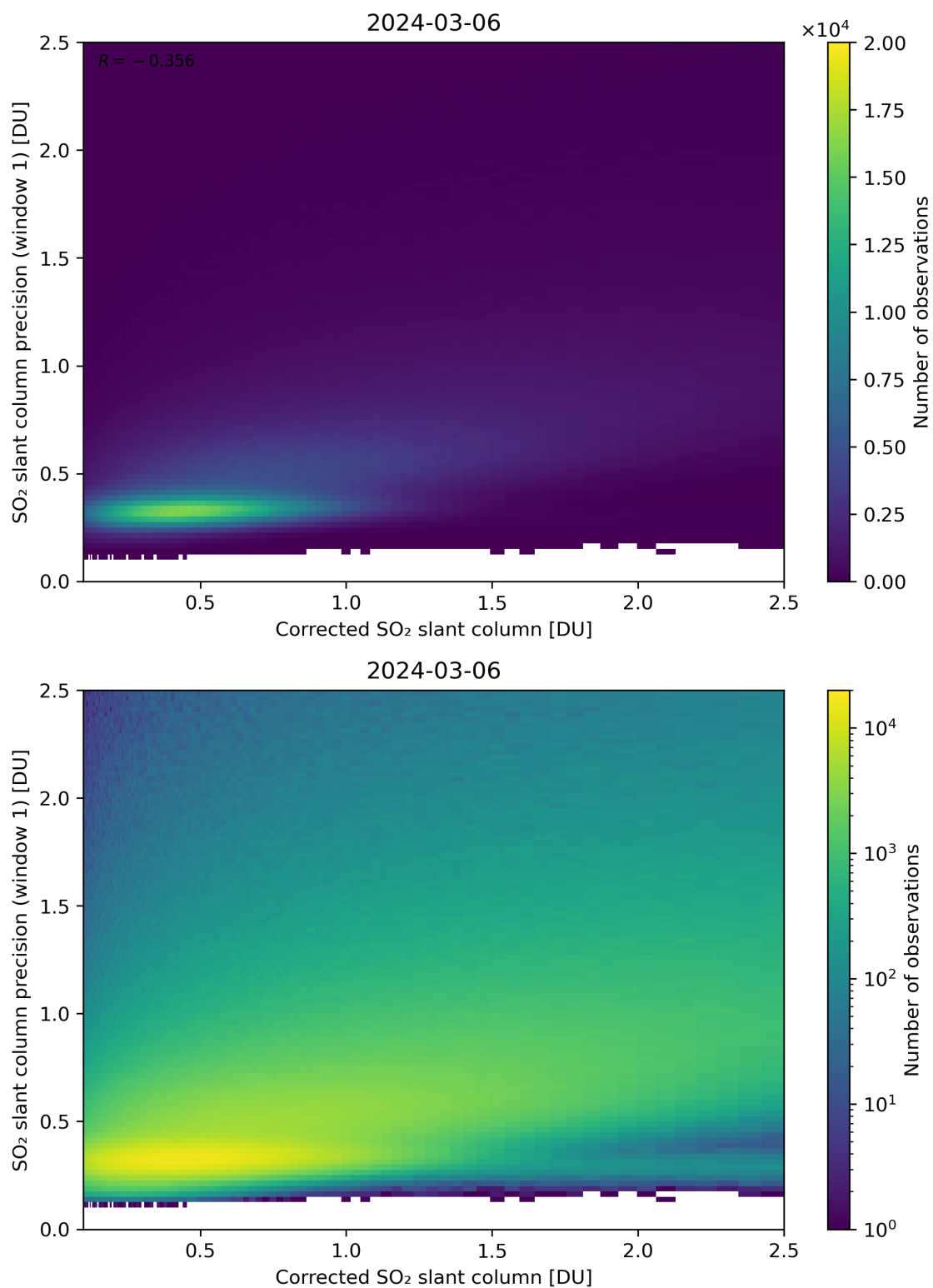
Figure 188: Scatter density plot of “Corrected SO 2 slant column” against “SO 2 slant column precision (window 1)” for 2024-03-05 to 2024-03-07.
