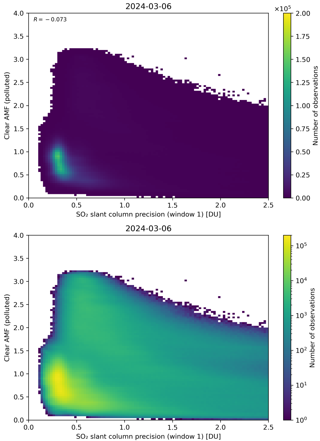
Figure 224: Scatter density plot of “SO 2 slant column precision (window 1)” against “Clear AMF (polluted)” for 2024-03-05 to 2024-03-07.
