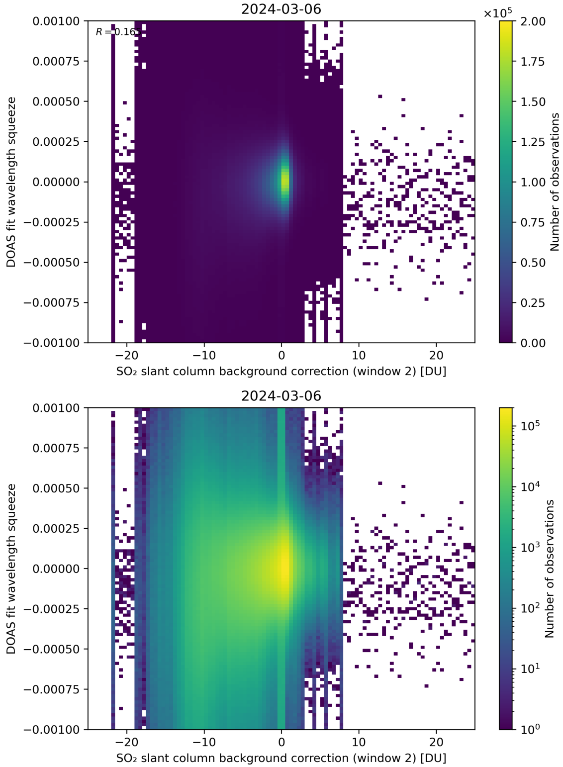
Figure 113: Scatter density plot of “SO 2 slant column background correction (window 2)” against “DOAS fit wavelength squeeze” for 2024-03-05 to 2024-03-07.
