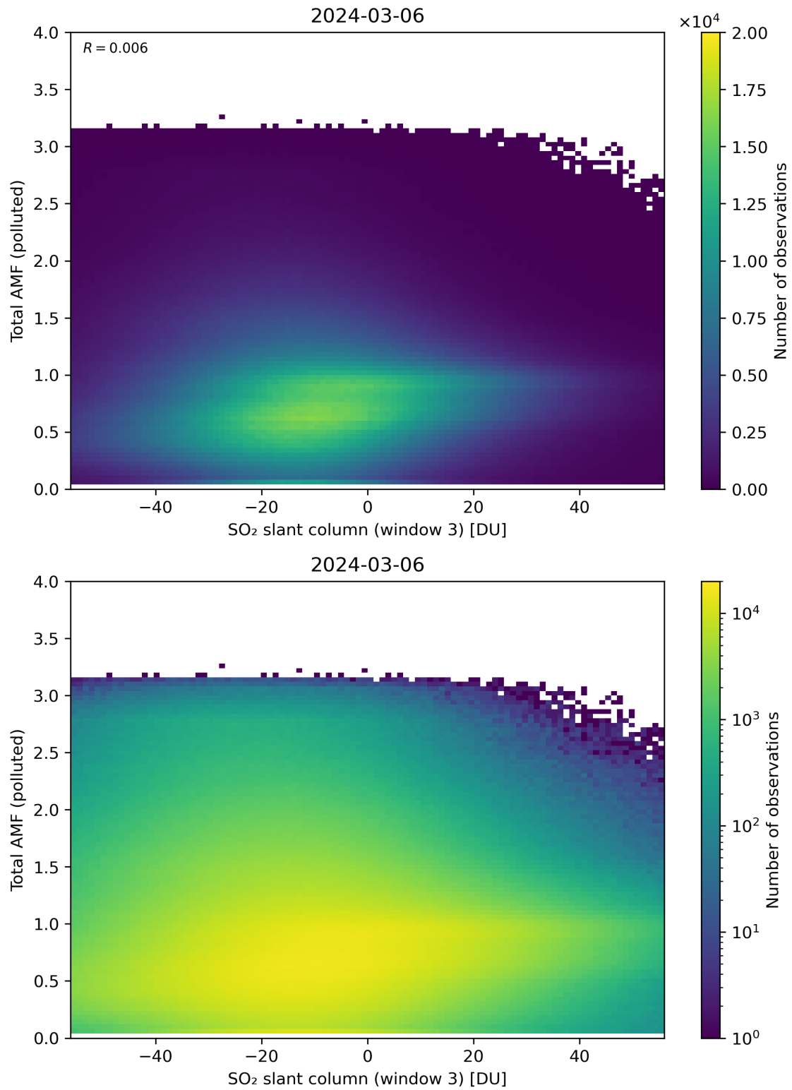
Figure 268: Scatter density plot of “SO 2 slant column (window 3)” against “Total AMF (polluted)” for 2024-03-05 to 2024-03-07.
