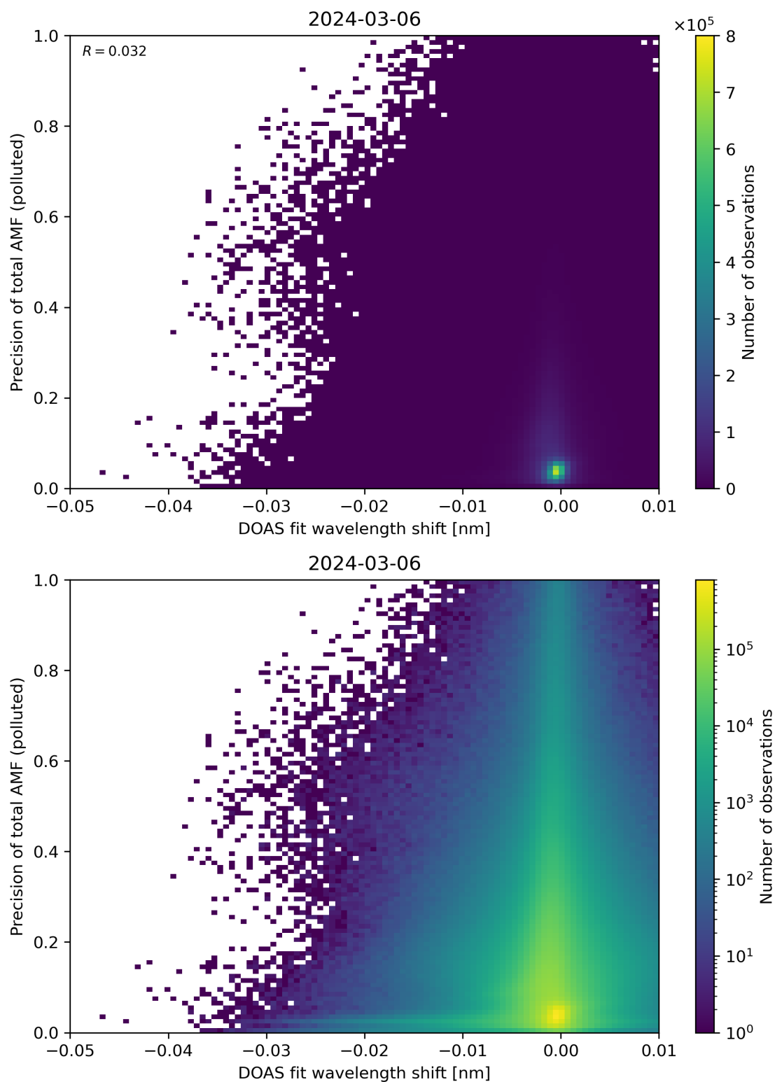
Figure 131: Scatter density plot of “DOAS fit wavelength shift” against “Precision of total AMF (polluted)” for 2024-03-05 to 2024-03-07.
