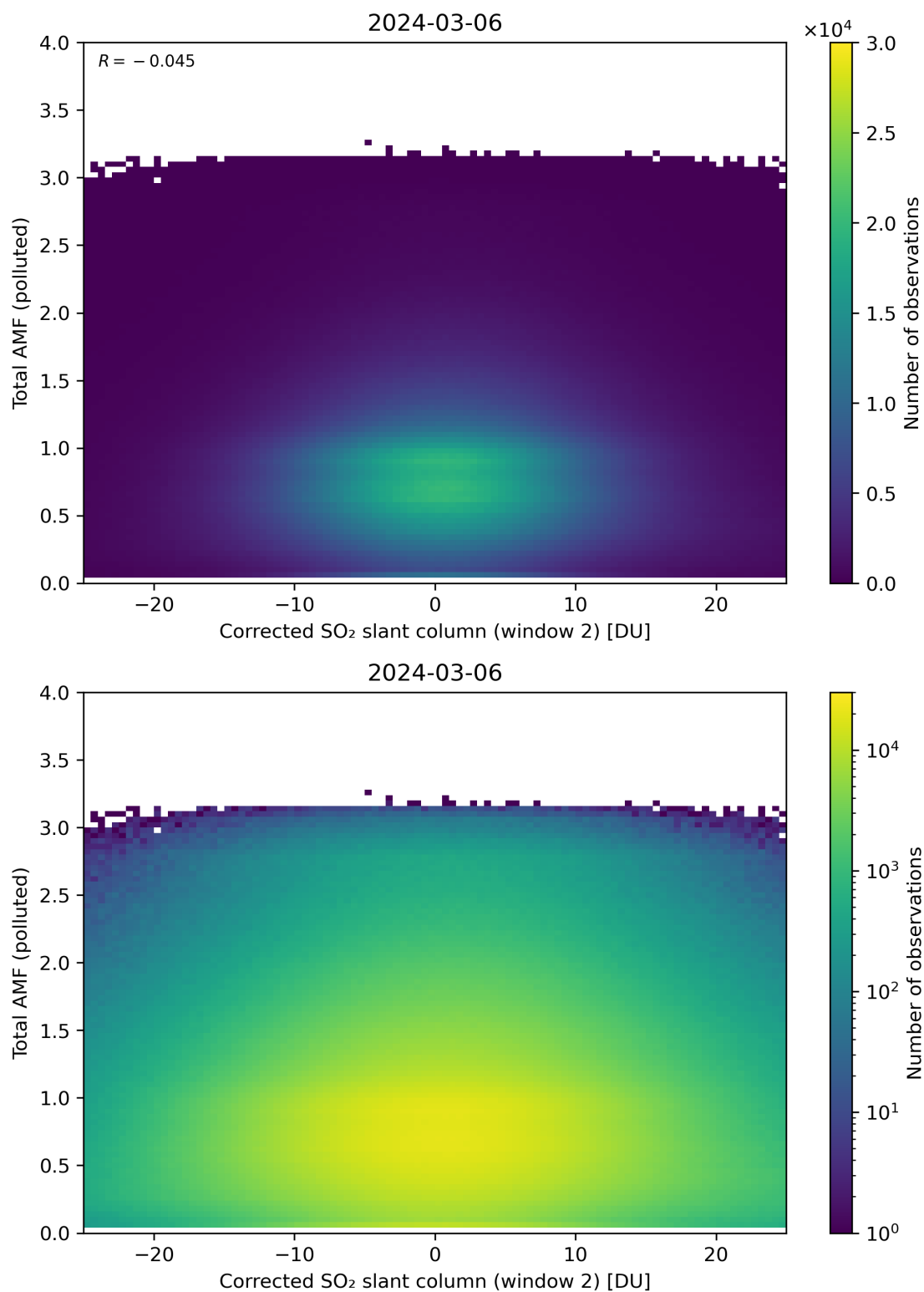
Figure 203: Scatter density plot of “Corrected SO 2 slant column (window 2)” against “Total AMF (polluted)” for 2024-03-05 to 2024-03-07.
