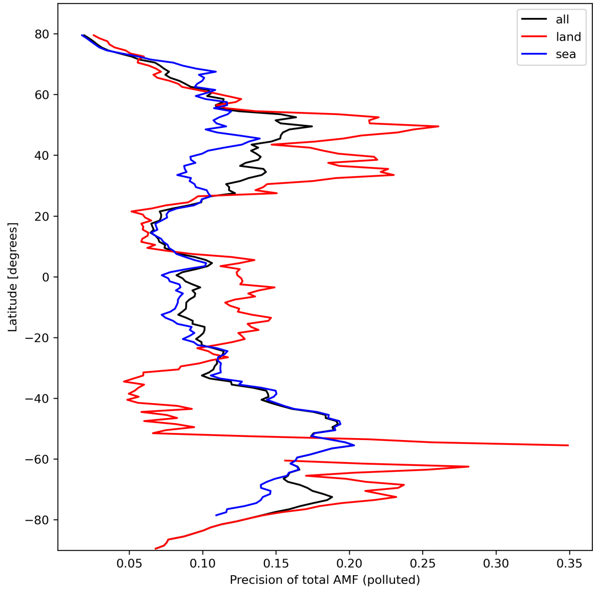
Figure 49: Zonal average of “Precision of total AMF (polluted)” for 2024-03-05 to 2024-03-07.
