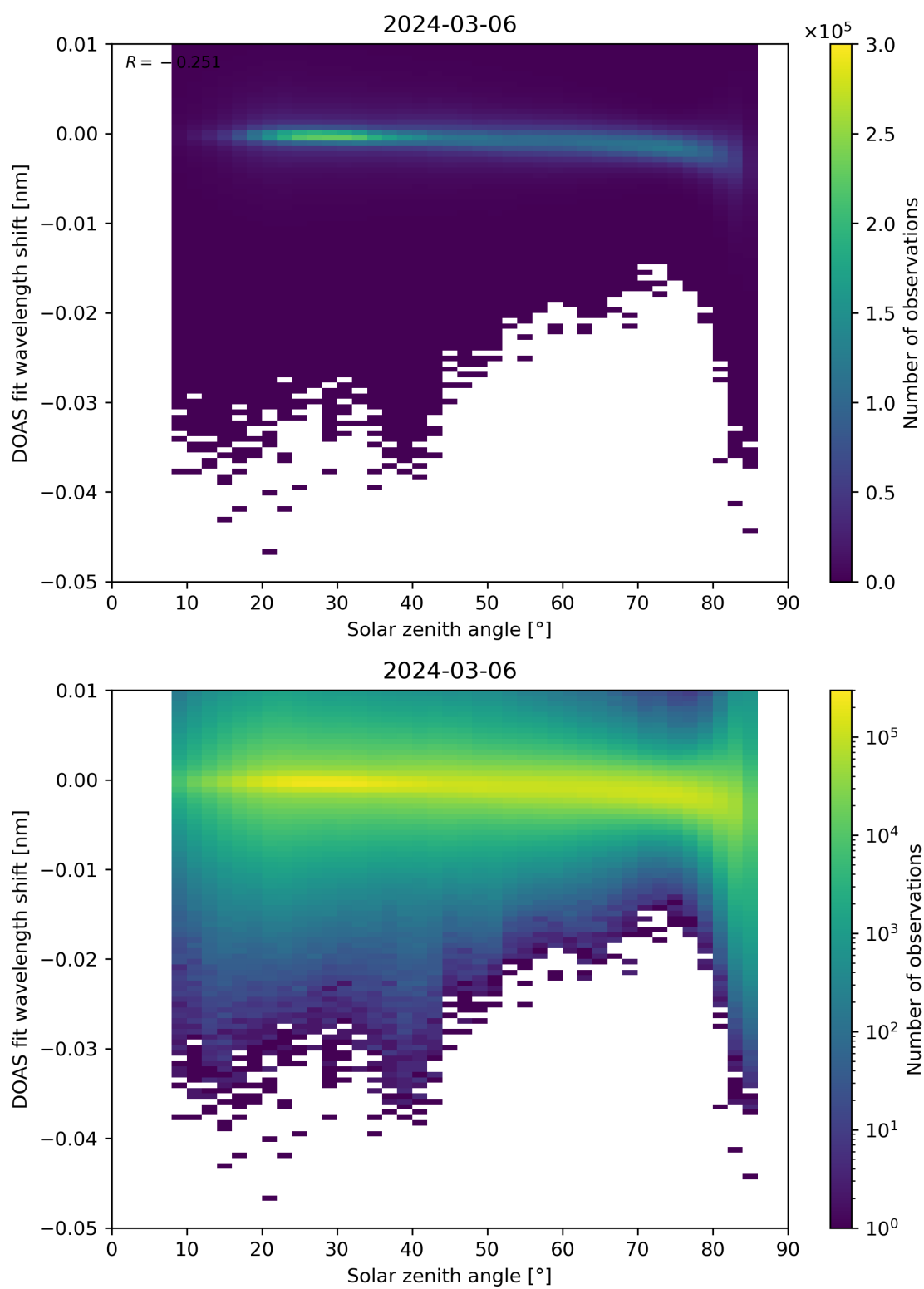
Figure 161: Scatter density plot of “Solar zenith angle” against “DOAS fit wavelength shift” for 2024-03-05 to 2024-03-07.
