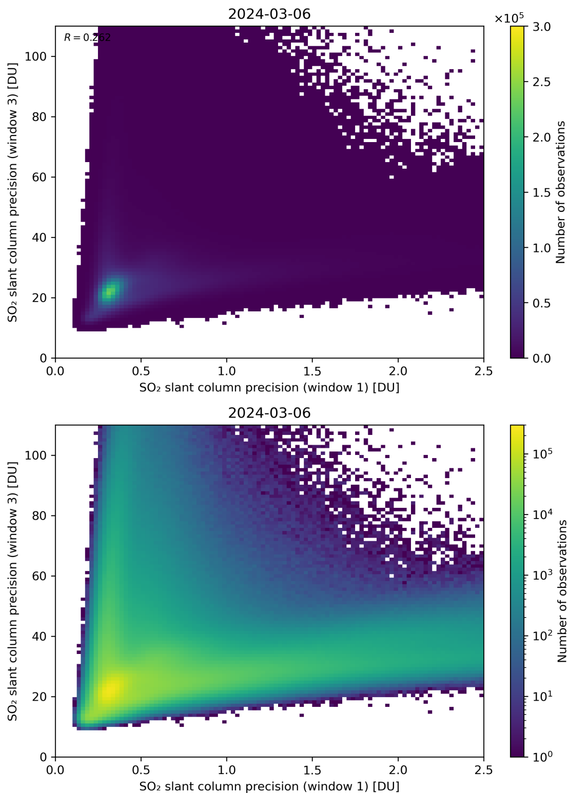
Figure 229: Scatter density plot of “SO 2 slant column precision (window 1)” against “SO 2 slant column precision (window 3)” for 2024-03-05 to 2024-03-07.
