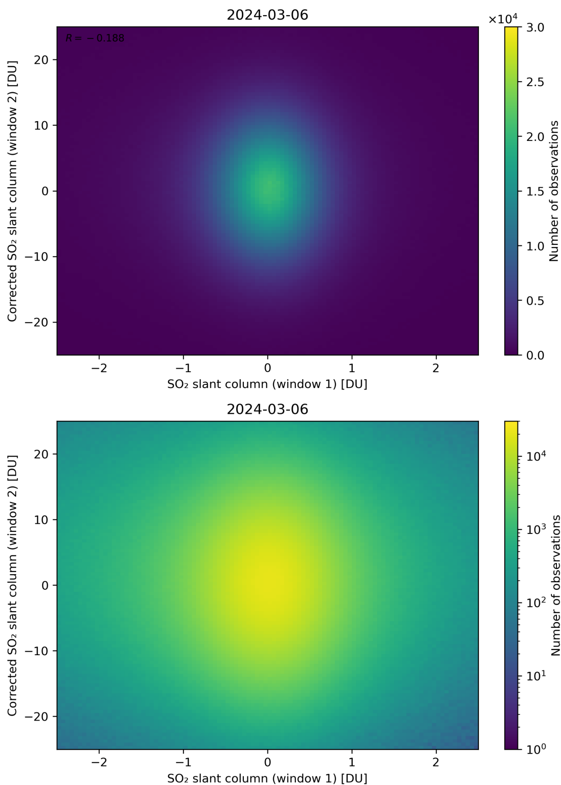
Figure 233: Scatter density plot of “SO 2 slant column (window 1)” against “Corrected SO 2 slant column (window 2)” for 2024-03-05 to 2024-03-07.
