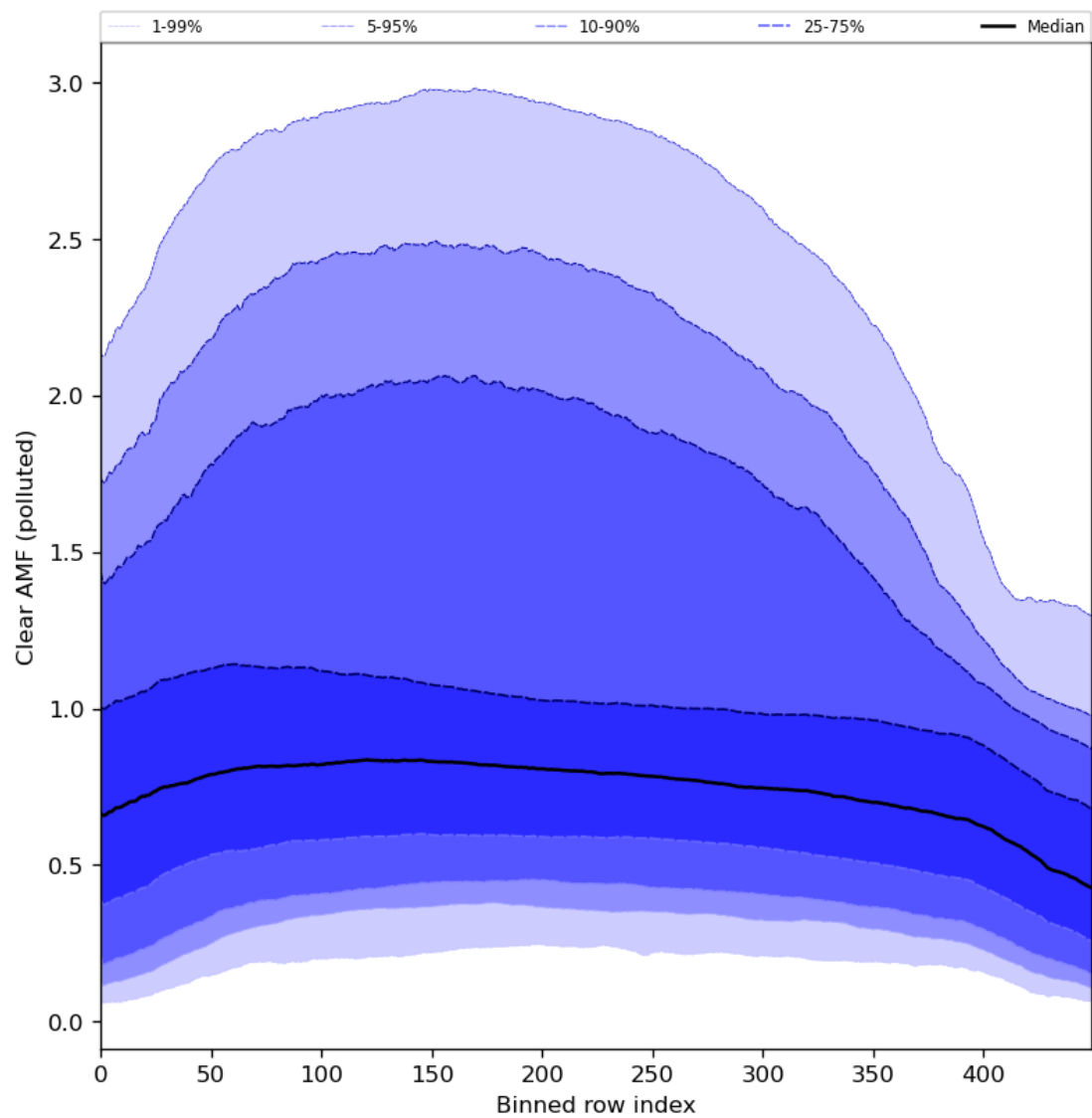
Figure 96: Along track statistics of “Clear AMF (polluted)” for 2024-03-05 to 2024-03-07
