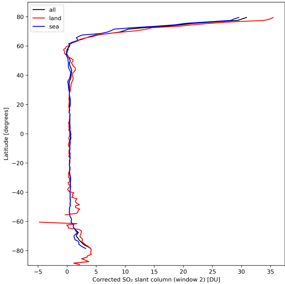
Figure 39: Zonal average of “Corrected SO 2 slant column (window 2)” for 2024-03-05 to 2024-03-07.
