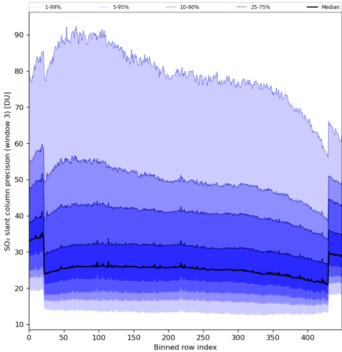
Figure 88: Along track statistics of “SO 2 slant column precision (window 3)” for 2024-03-05 to 2024-03-07
