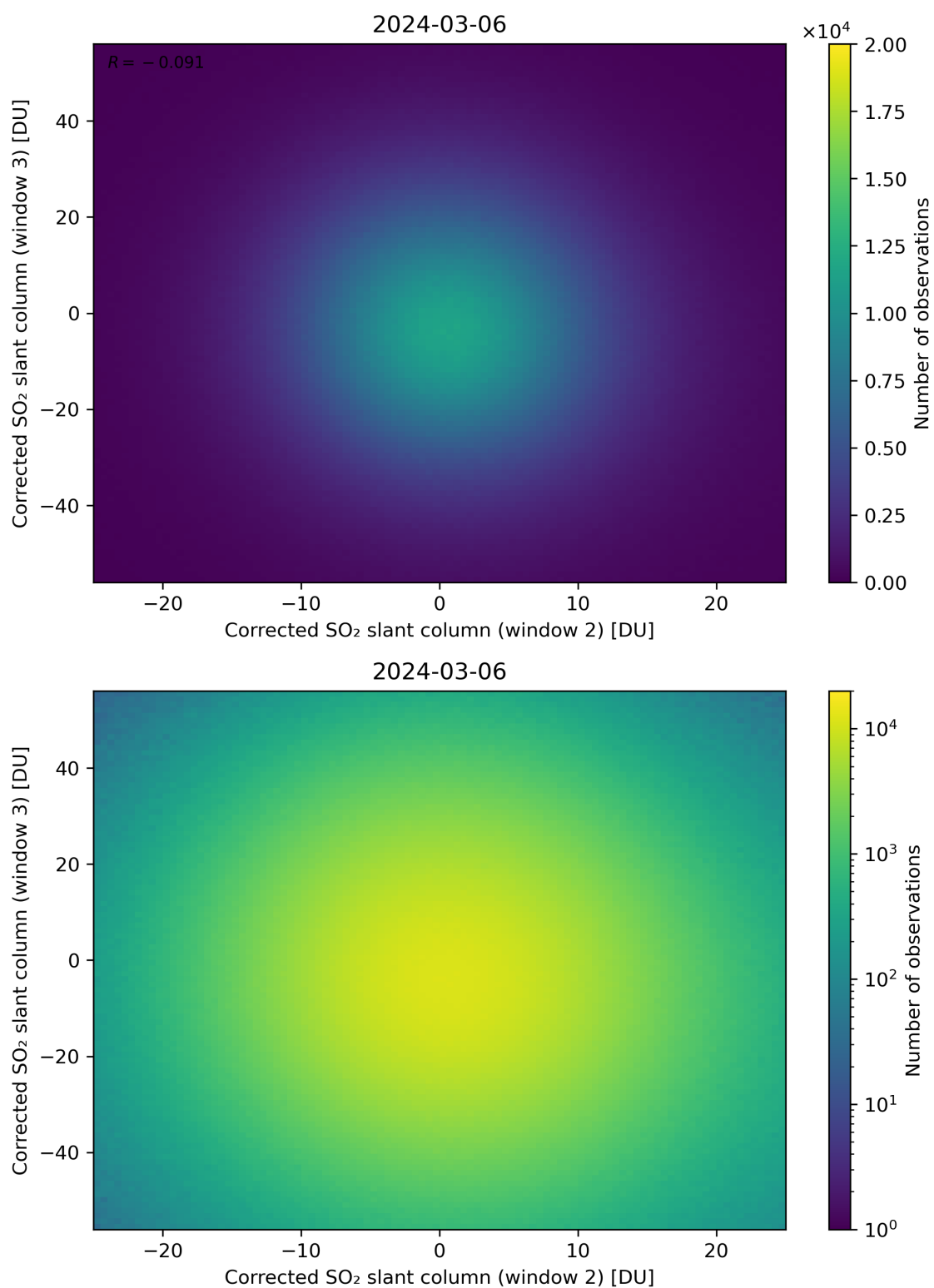
Figure 200: Scatter density plot of “Corrected SO 2 slant column (window 2)” against “Corrected SO 2 slant column (window 3)” for 2024-03-05 to 2024-03-07.
