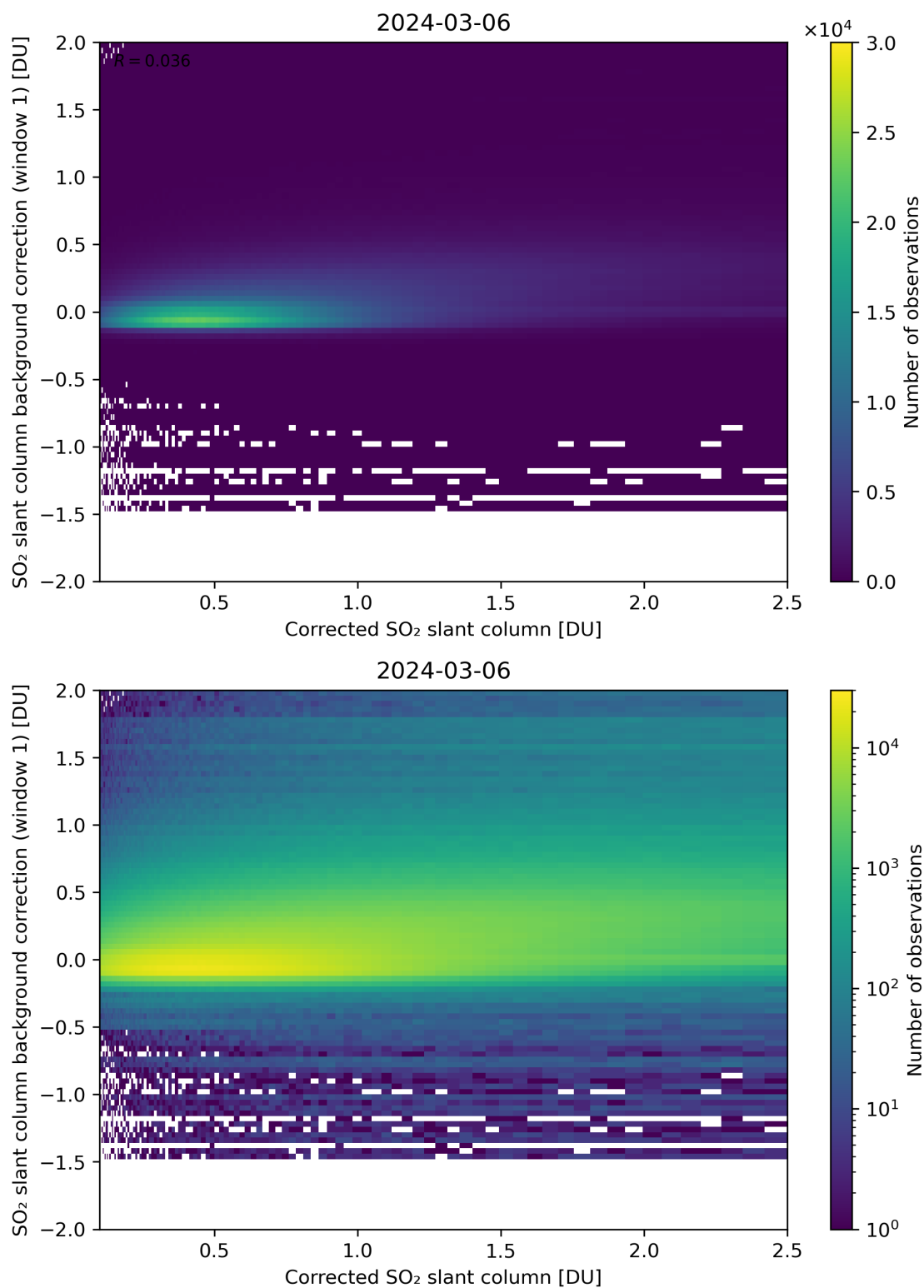
Figure 178: Scatter density plot of “Corrected SO 2 slant column” against “SO 2 slant column background correction (window 1)” for 2024-03-05 to 2024-03-07.
