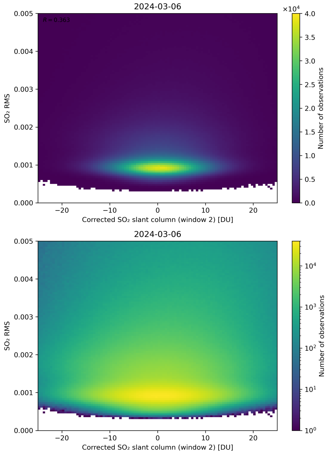
Figure 198: Scatter density plot of “Corrected SO 2 slant column (window 2)” against “SO 2 RMS” for 2024-03-05 to 2024-03-07.
