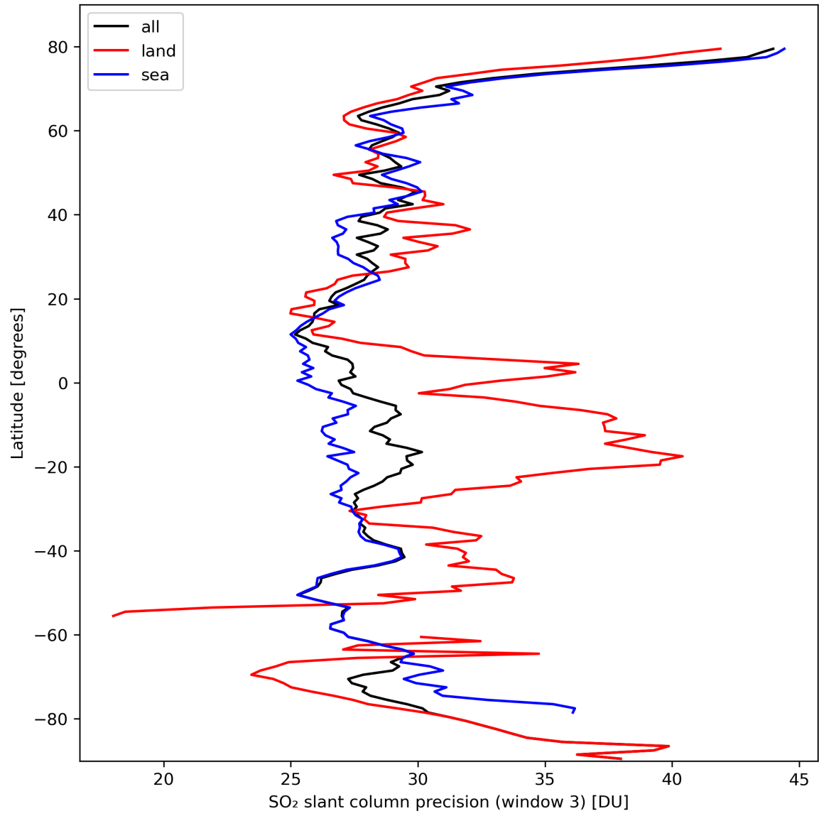
Figure 42: Zonal average of “SO 2 slant column precision (window 3)” for 2024-03-05 to 2024-03-07.
