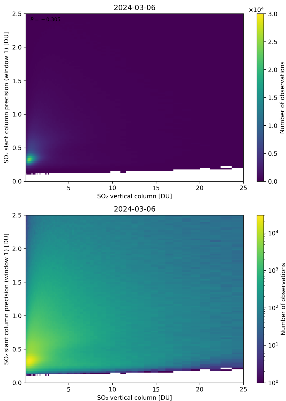
Figure 301: Scatter density plot of “SO 2 vertical column” against “SO 2 slant column precision (window 1)” for 2024-03-05 to 2024-03-07.
