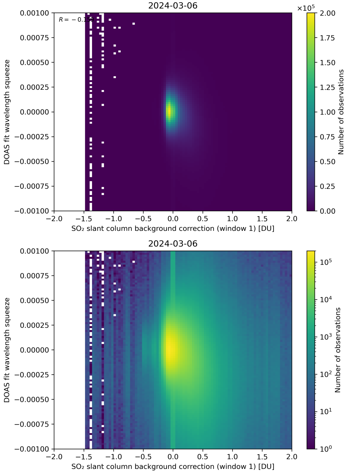
Figure 101: Scatter density plot of “SO 2 slant column background correction (window 1)” against “DOAS fit wavelength squeeze” for 2024-03-05 to 2024-03-07.
