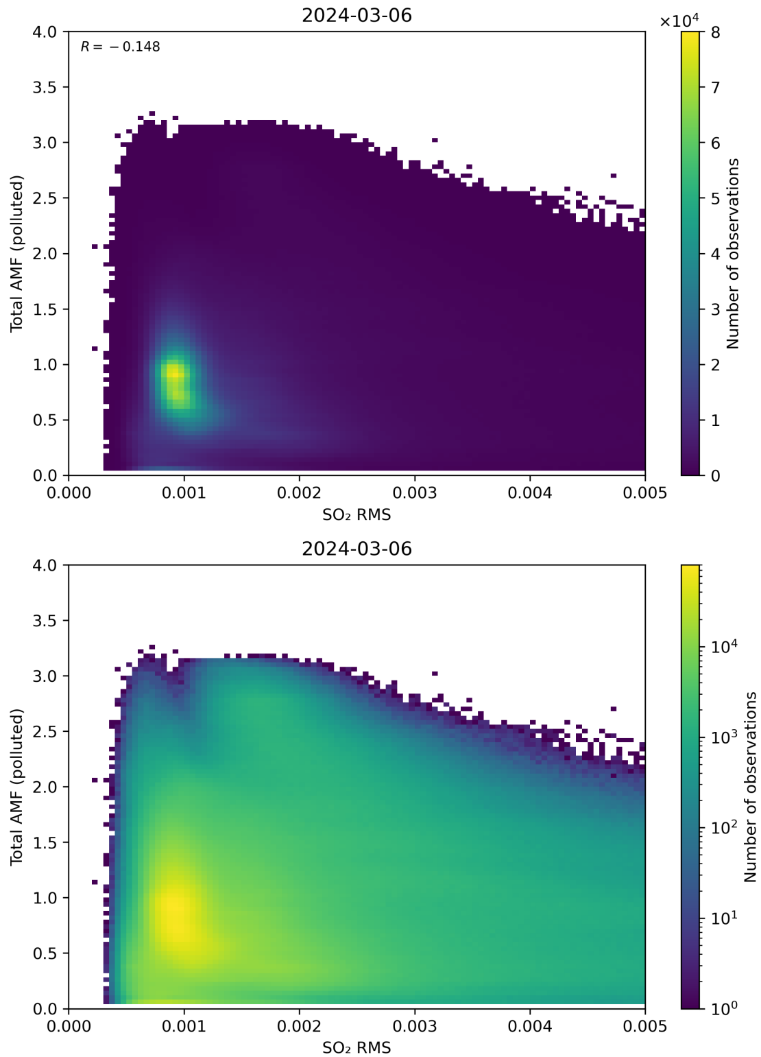
Figure 137: Scatter density plot of “SO 2 RMS” against “Total AMF (polluted)” for 2024-03-05 to 2024-03-07.
