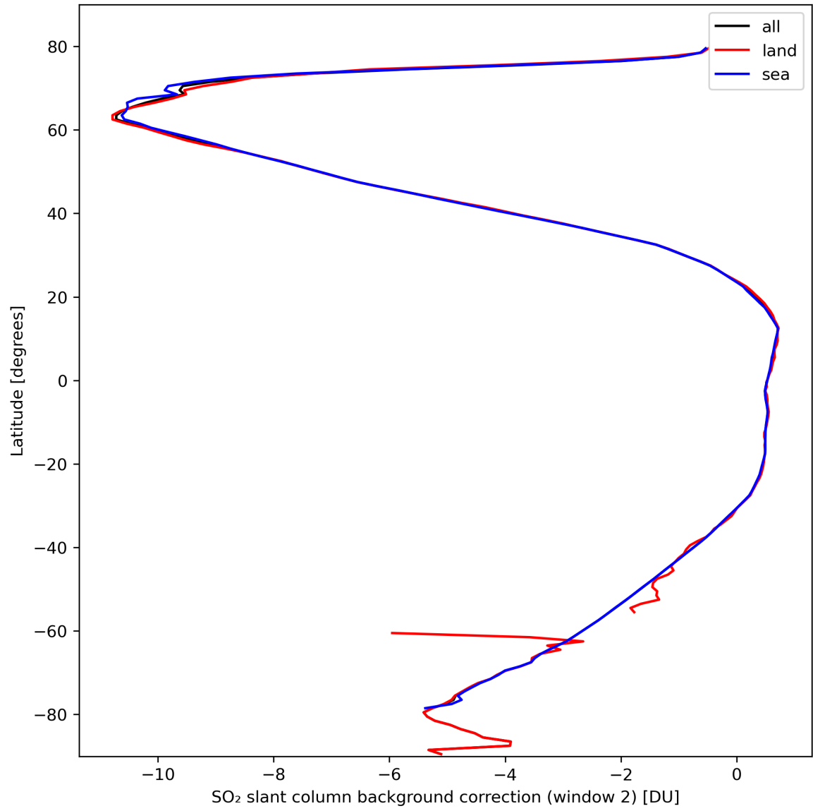
Figure 40: Zonal average of “SO 2 slant column background correction (window 2)” for 2024-03-05 to 2024-03-07.
