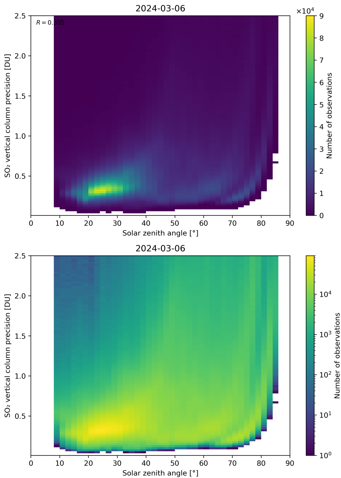
Figure 177: Scatter density plot of “Solar zenith angle” against “SO 2 vertical column precision” for 2024-03-05 to 2024-03-07.
