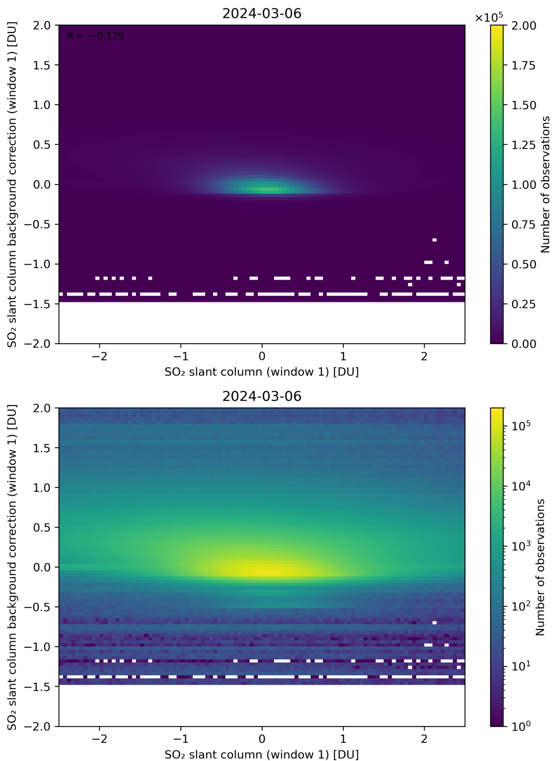
Figure 212: Scatter density plot of “SO 2 slant column (window 1)” against “SO 2 slant column background correction (window 1)” for 2024-03-05 to 2024-03-07.
