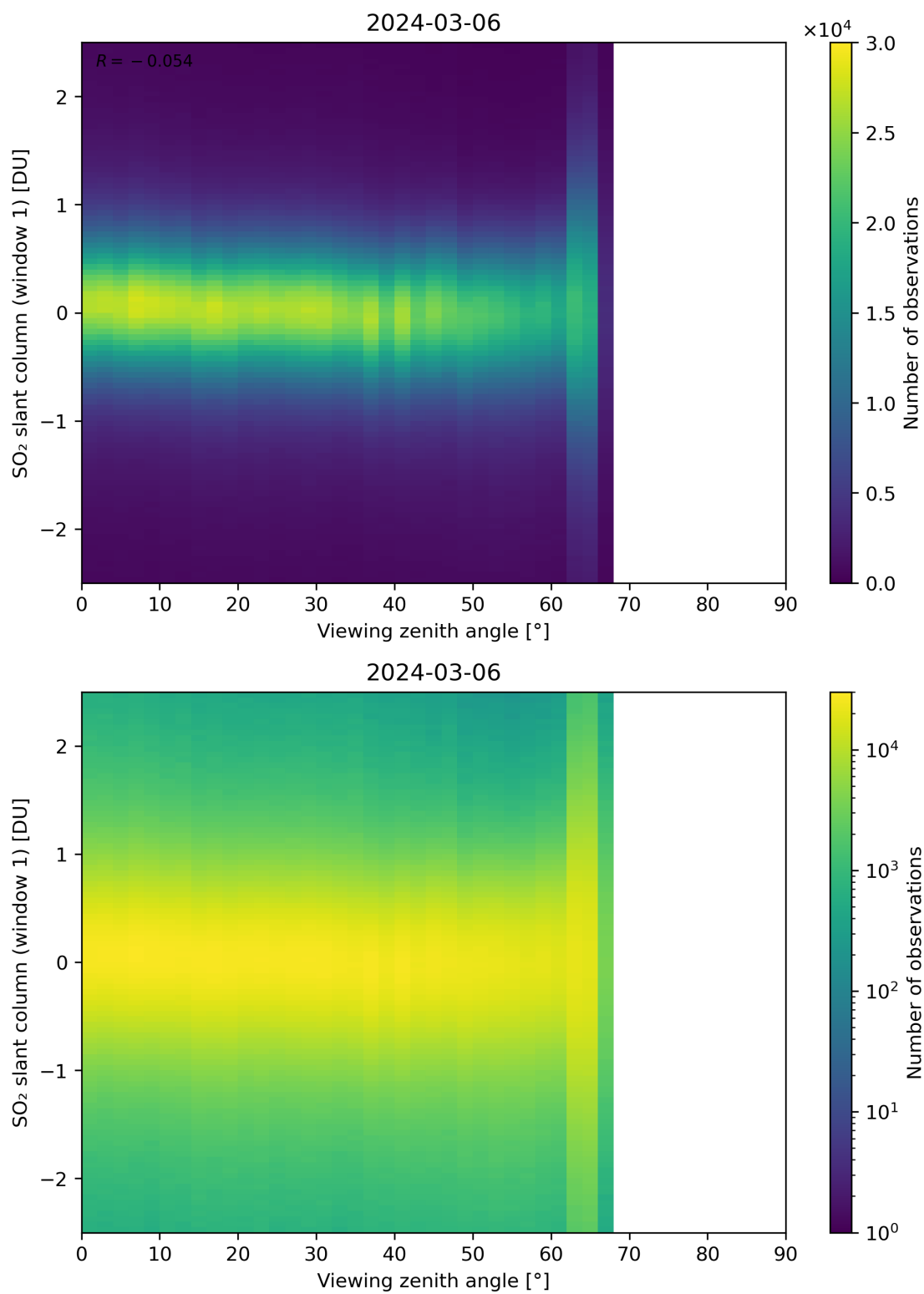
Figure 320: Scatter density plot of “Viewing zenith angle” against “SO 2 slant column (window 1)” for 2024-03-05 to 2024-03-07.
