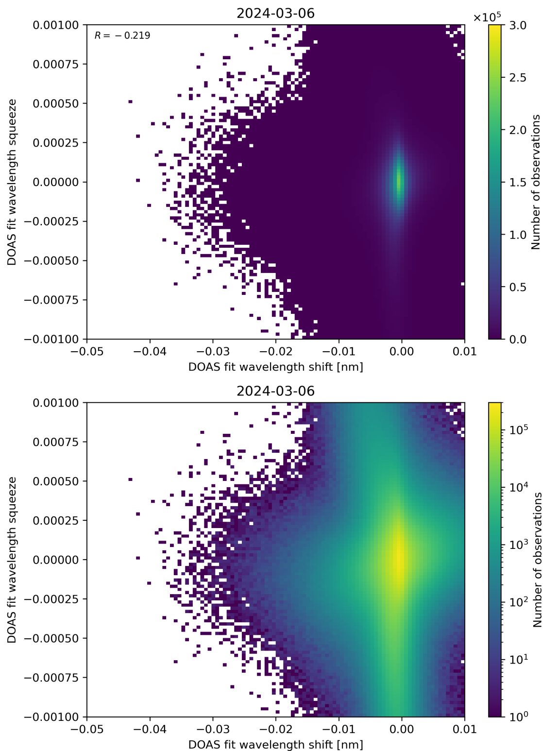
Figure 127: Scatter density plot of “DOAS fit wavelength shift” against “DOAS fit wavelength squeeze” for 2024-03-05 to 2024-03-07.
