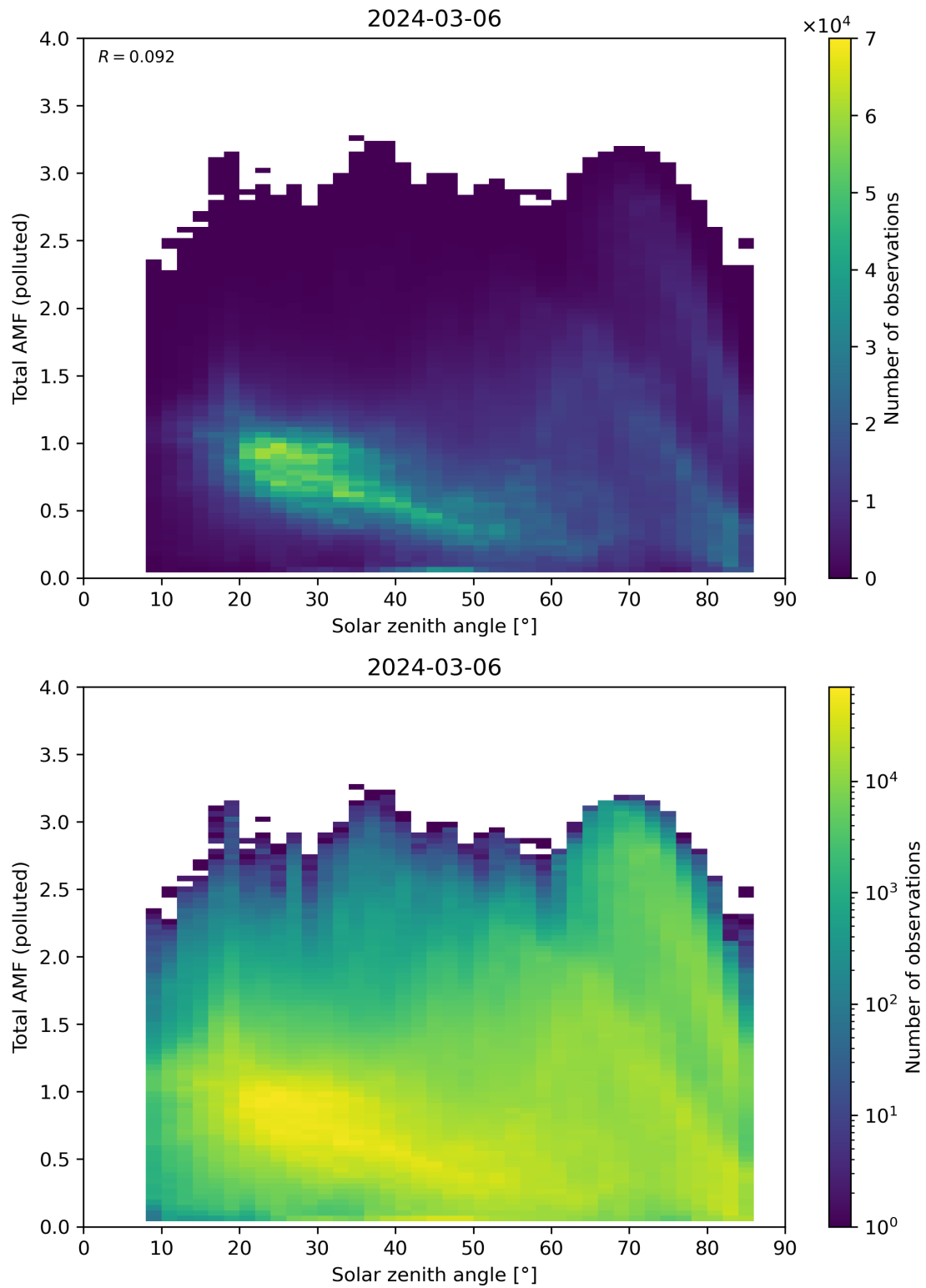
Figure 174: Scatter density plot of “Solar zenith angle” against “Total AMF (polluted)” for 2024-03-05 to 2024-03-07.
