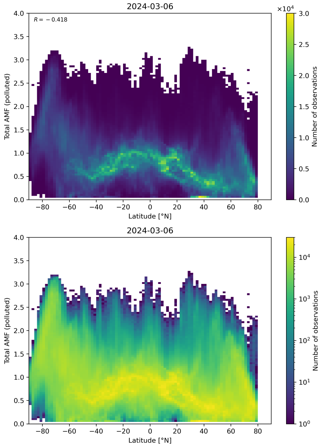
Figure 154: Scatter density plot of “Latitude” against “Total AMF (polluted)” for 2024-03-05 to 2024-03-07.
