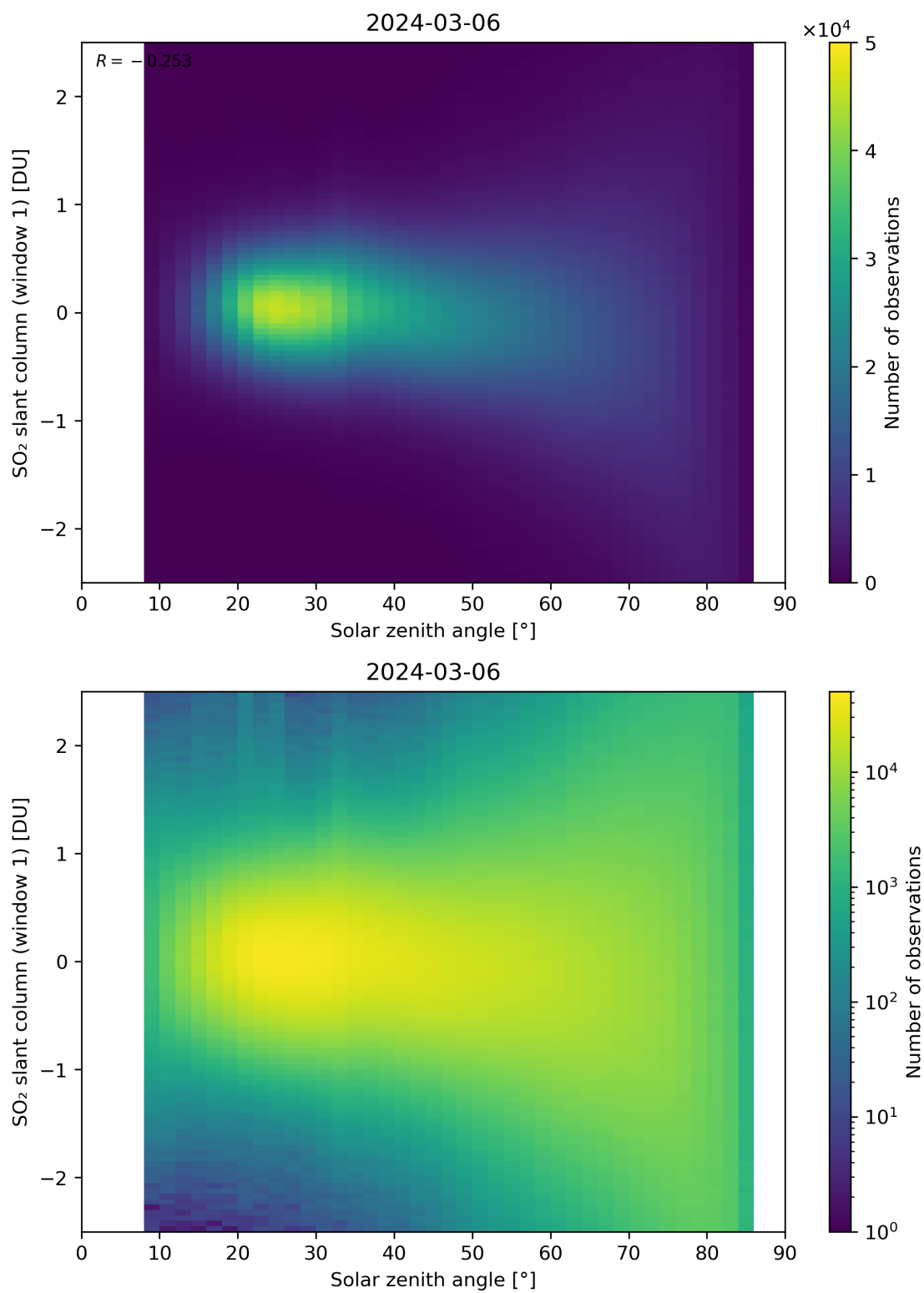
Figure 169: Scatter density plot of “Solar zenith angle” against “SO 2 slant column (window 1)” for 2024-03-05 to 2024-03-07.
