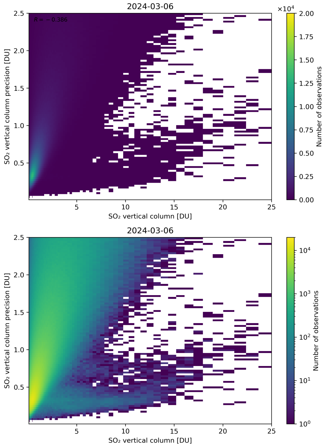
Figure 307: Scatter density plot of “SO 2 vertical column” against “SO 2 vertical column precision” for 2024-03-05 to 2024-03-07.
