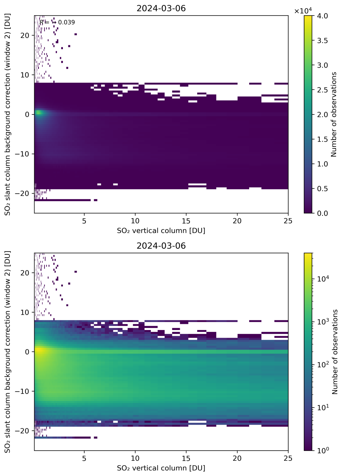
Figure 274: Scatter density plot of “SO 2 vertical column” against “SO 2 slant column background correction (window 2)” for 2024-03-05 to 2024-03-07.
