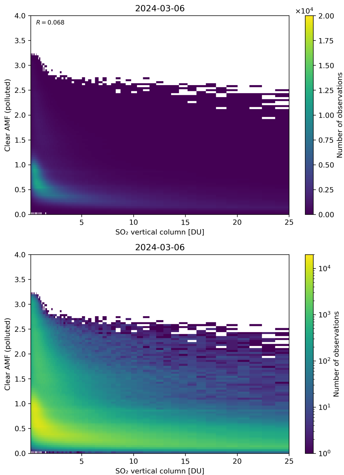
Figure 296: Scatter density plot of “SO 2 vertical column” against “Clear AMF (polluted)” for 2024-03-05 to 2024-03-07.
