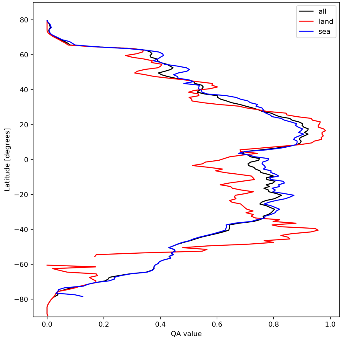
Figure 29: Zonal average of “QA value” for 2024-03-05 to 2024-03-07.
