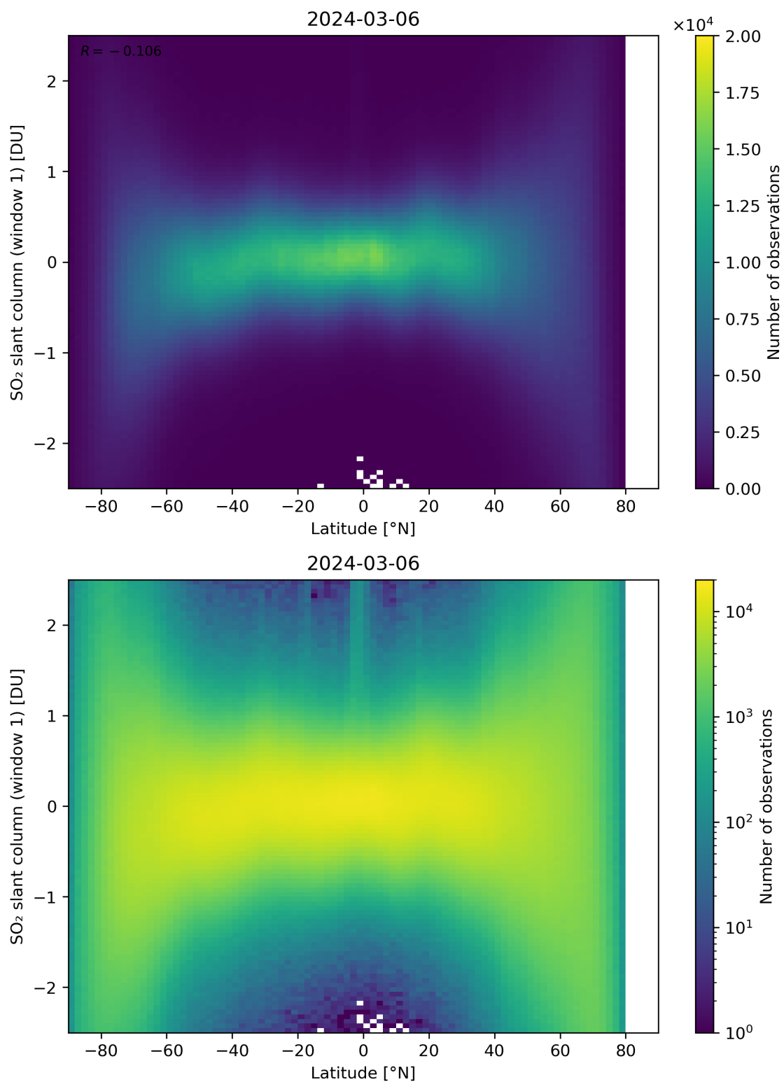
Figure 149: Scatter density plot of “Latitude” against “SO 2 slant column (window 1)” for 2024-03-05 to 2024-03-07.
