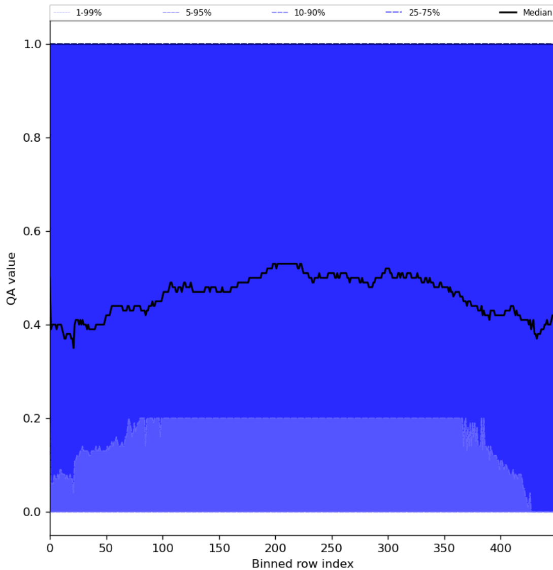
Figure 75: Along track statistics of “QA value” for 2024-03-05 to 2024-03-07
