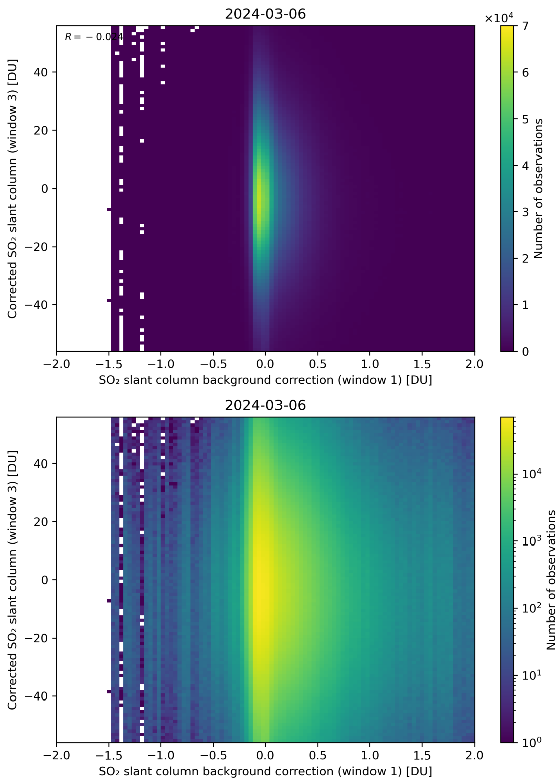
Figure 105: Scatter density plot of “SO 2 slant column background correction (window 1)” against “Corrected SO 2 slant column (window 3)” for 2024-03-05 to 2024-03-07.
