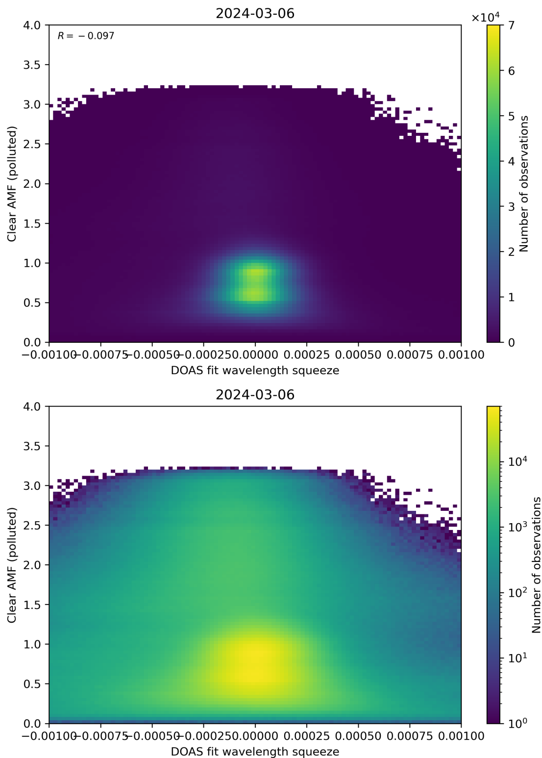
Figure 133: Scatter density plot of “DOAS fit wavelength squeeze” against “Clear AMF (polluted)” for 2024-03-05 to 2024-03-07.
