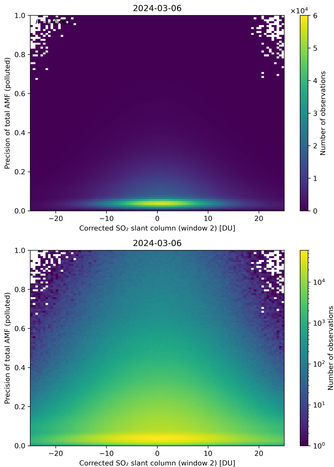
Figure 204: Scatter density plot of “Corrected SO 2 slant column (window 2)” against “Precision of total AMF (polluted)” for 2024-03-05 to 2024-03-07.
