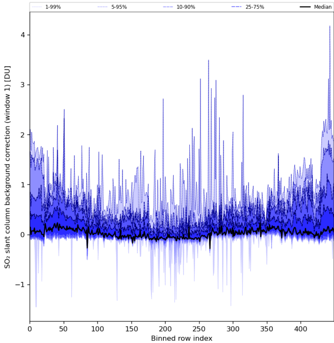
Figure 82: Along track statistics of “SO 2 slant column background correction (window 1)” for 2024-03-05 to 2024-03-07
