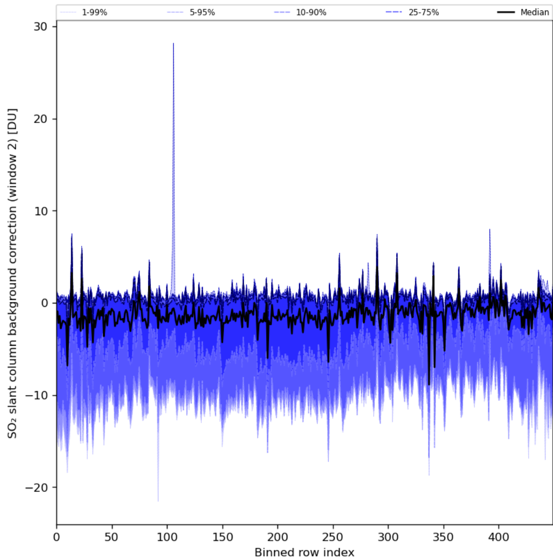
Figure 86: Along track statistics of “SO 2 slant column background correction (window 2)” for 2024-03-05 to 2024-03-07
