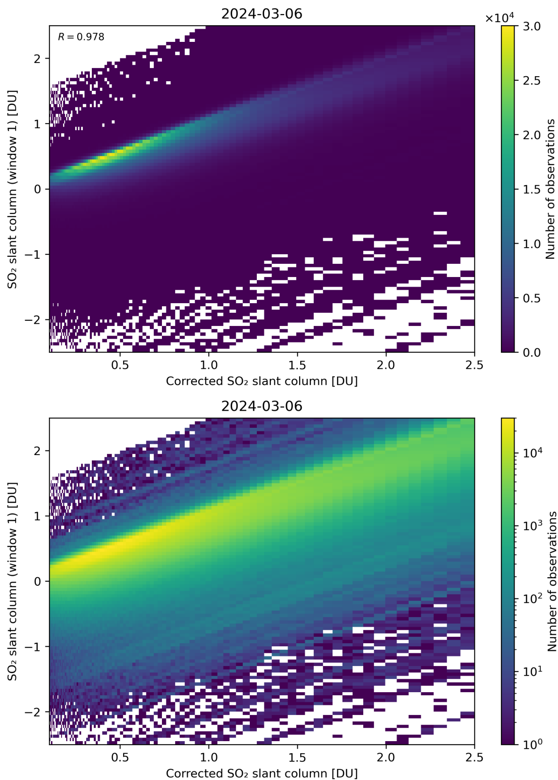
Figure 187: Scatter density plot of “Corrected SO 2 slant column” against “SO 2 slant column (window 1)” for 2024-03-05 to 2024-03-07.
