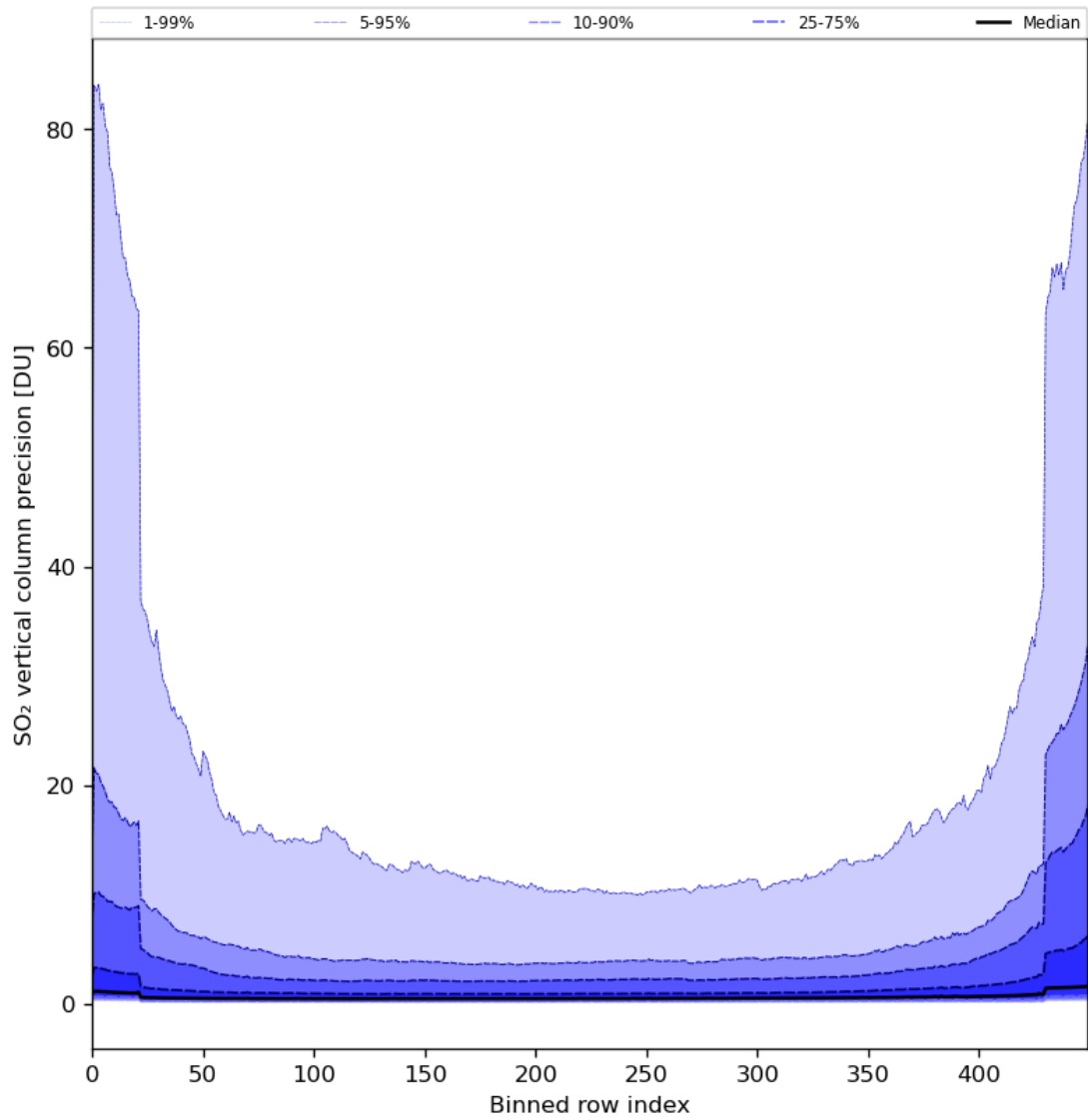
Figure 77: Along track statistics of “SO 2 vertical column precision” for 2024-03-05 to 2024-03-07
