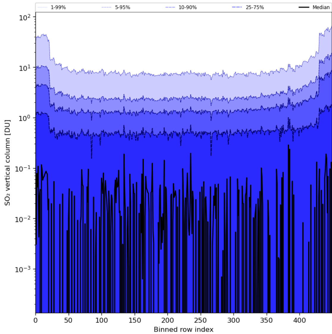
Figure 76: Along track statistics of “SO 2 vertical column” for 2024-03-05 to 2024-03-07
