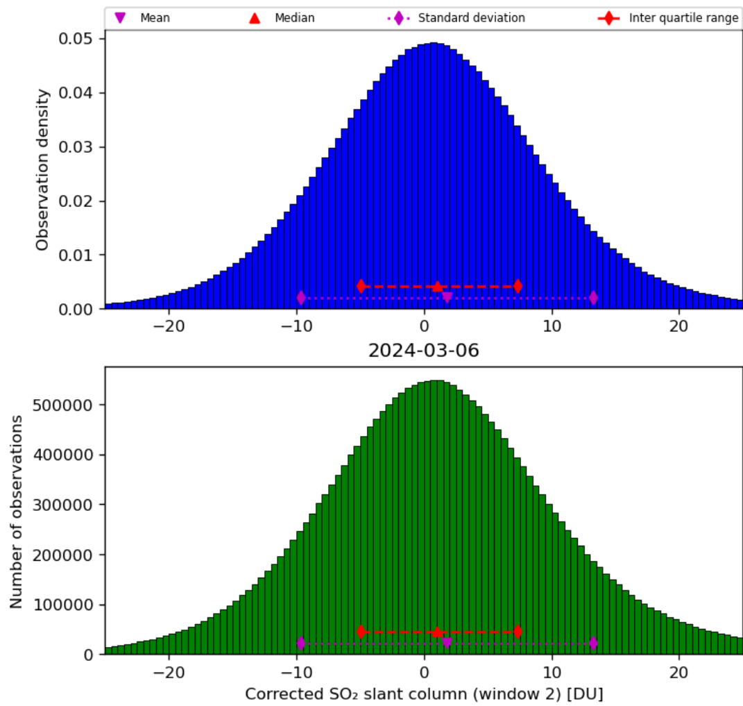
Figure 62: Histogram of “Corrected SO 2 slant column (window 2)” for 2024-03-05 to 2024-03-07
