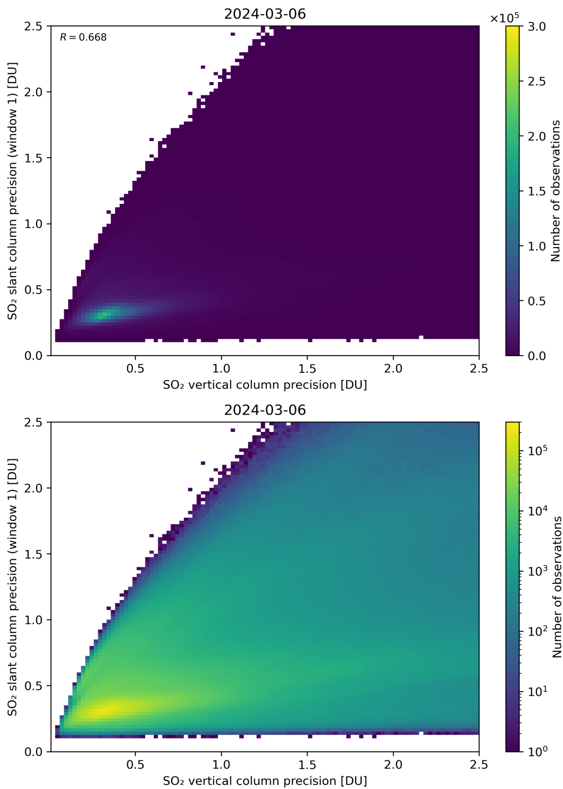
Figure 290: Scatter density plot of “SO 2 vertical column precision” against “SO 2 slant column precision (window 1)” for 2024-03-05 to 2024-03-07.
