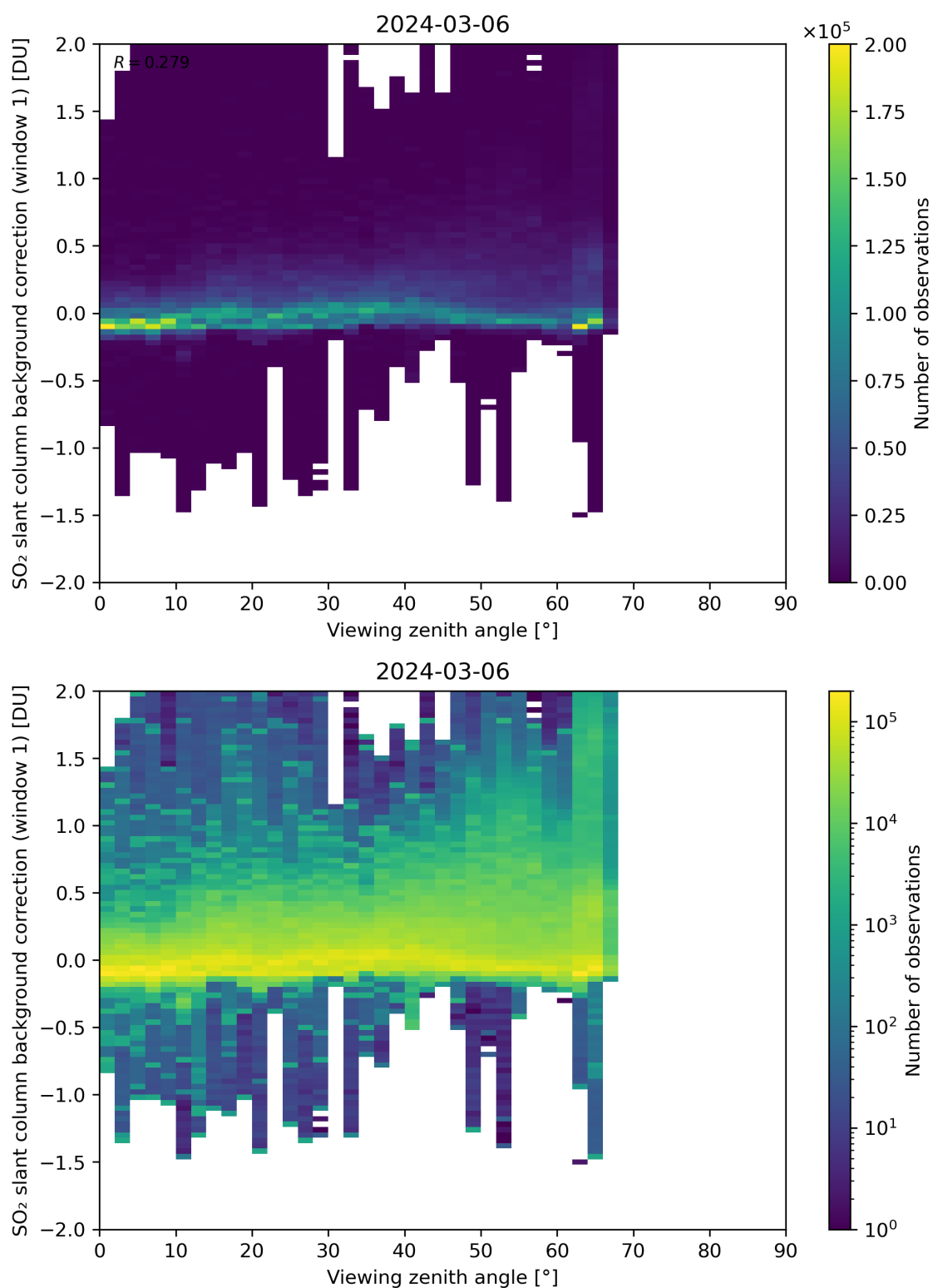
Figure 308: Scatter density plot of “Viewing zenith angle” against “SO 2 slant column background correction (window 1)” for 2024-03-05 to 2024-03-07.
