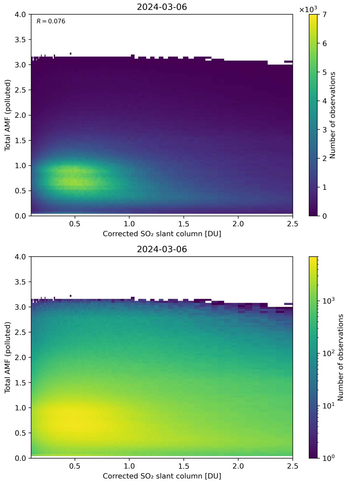
Figure 192: Scatter density plot of “Corrected SO 2 slant column” against “Total AMF (polluted)” for 2024-03-05 to 2024-03-07.
