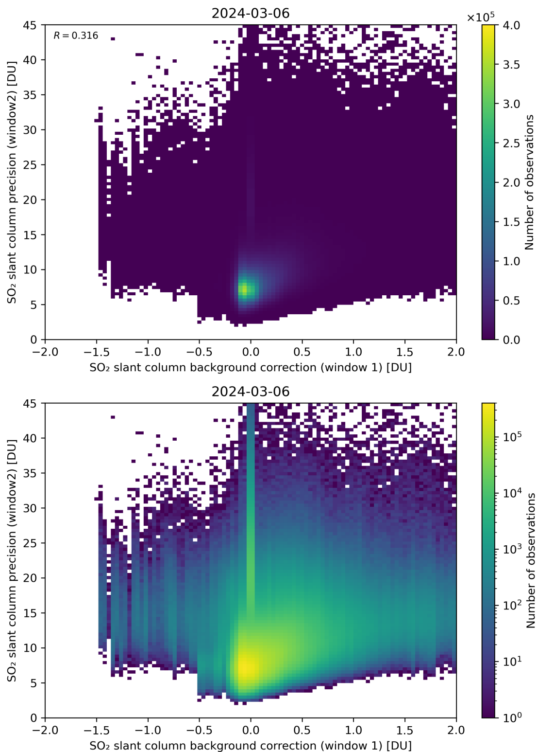
Figure 106: Scatter density plot of “SO 2 slant column background correction (window 1)” against “SO 2 slant column precision (window2)” for 2024-03-05 to 2024-03-07.
