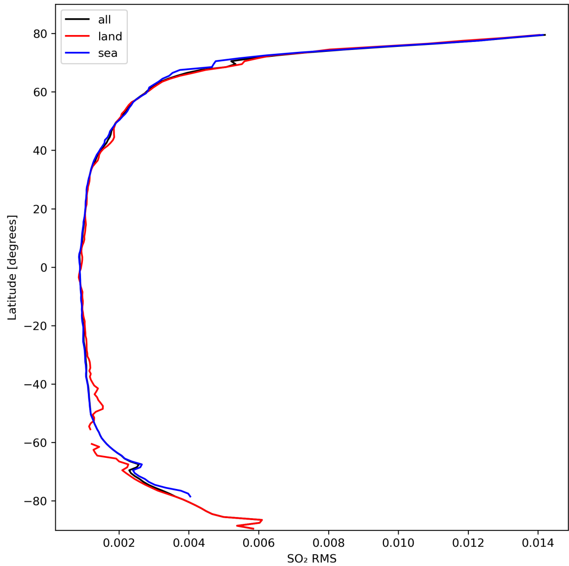
Figure 47: Zonal average of “SO 2 RMS” for 2024-03-05 to 2024-03-07.
