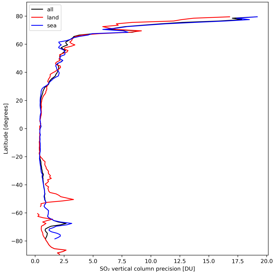
Figure 31: Zonal average of “SO 2 vertical column precision” for 2024-03-05 to 2024-03-07.
