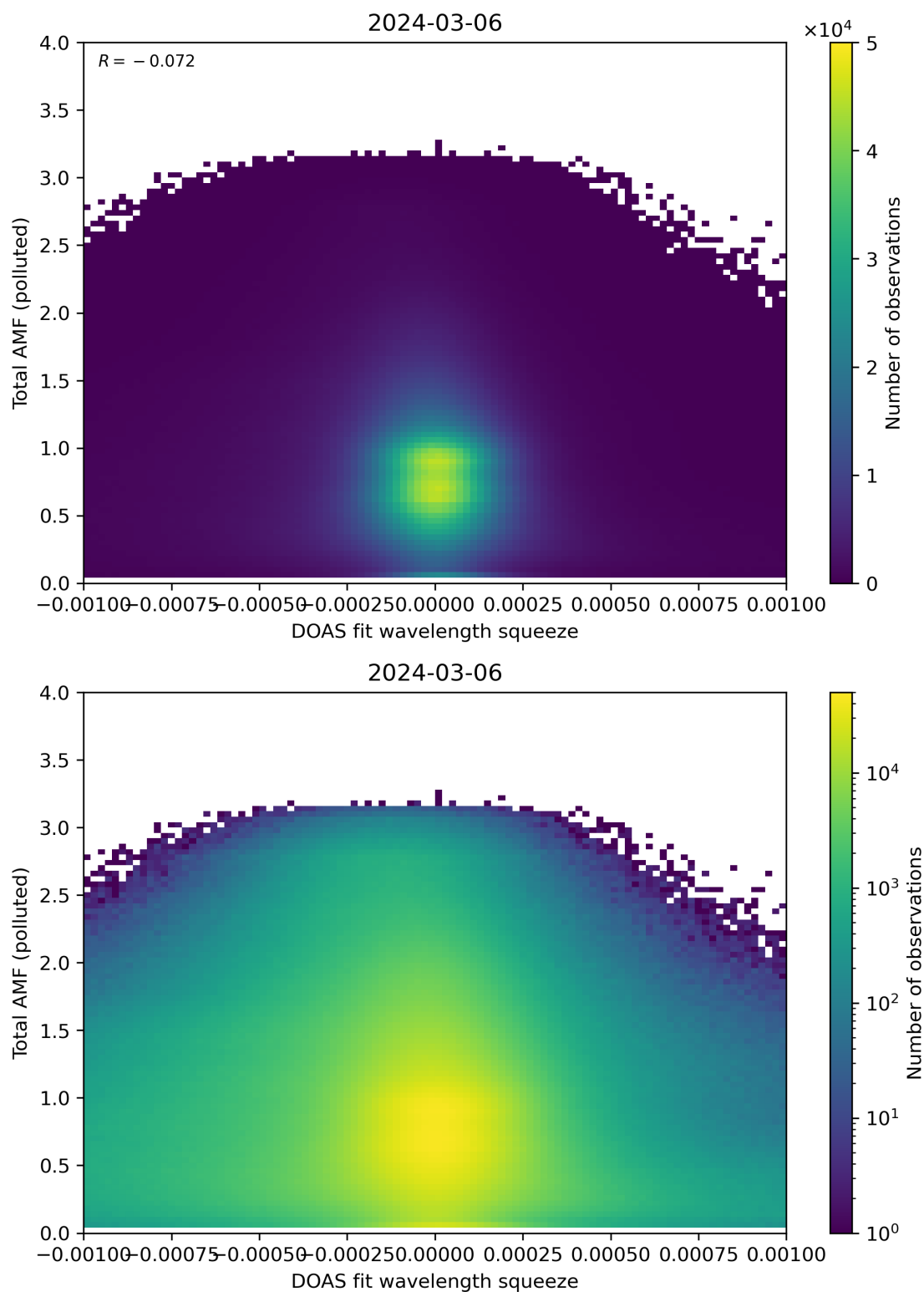
Figure 134: Scatter density plot of “DOAS fit wavelength squeeze” against “Total AMF (polluted)” for 2024-03-05 to 2024-03-07.
