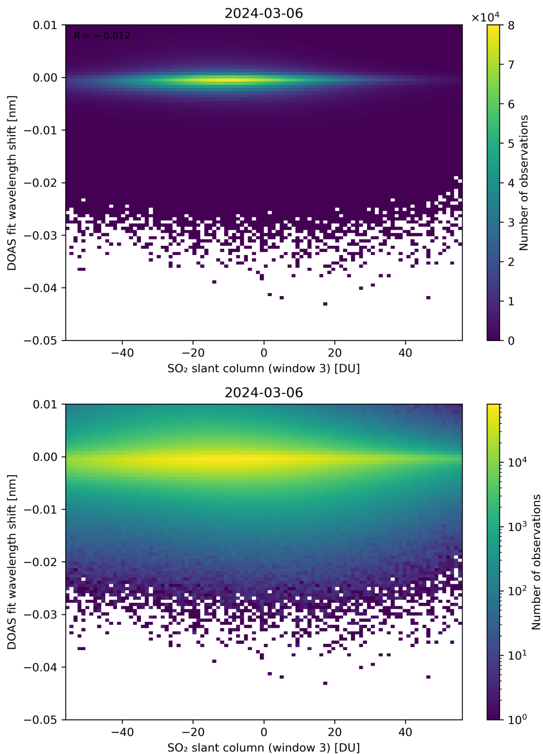
Figure 254: Scatter density plot of “SO 2 slant column (window 3)” against “DOAS fit wavelength shift” for 2024-03-05 to 2024-03-07.
