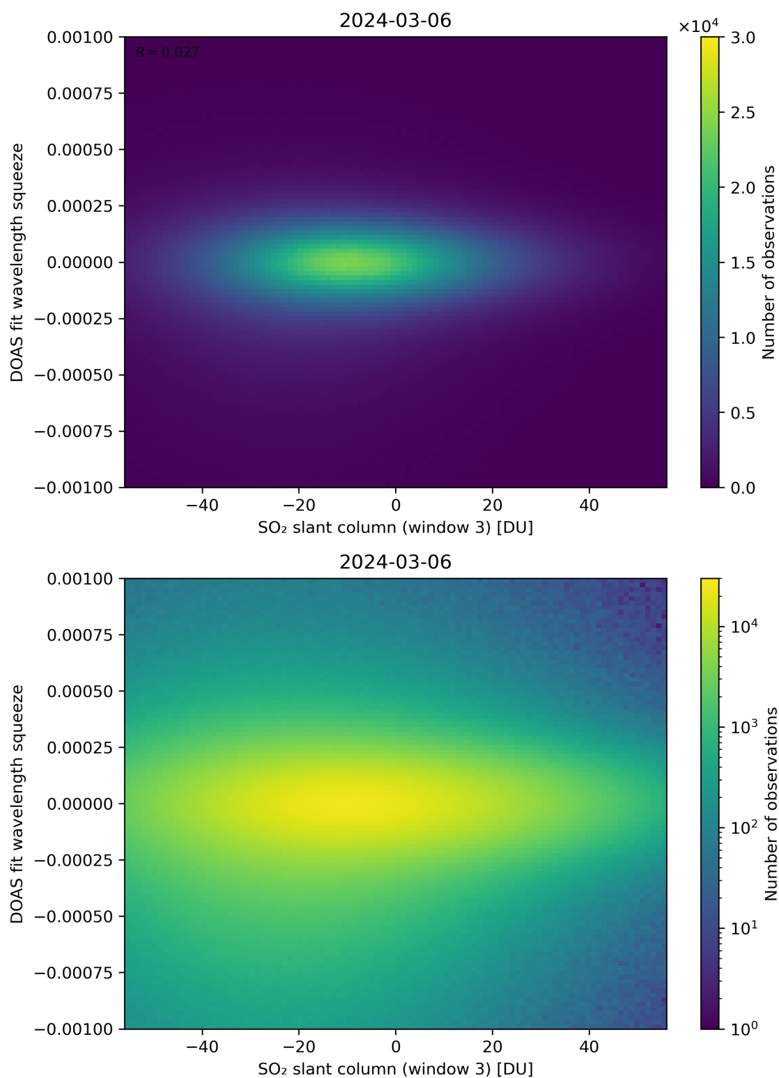
Figure 255: Scatter density plot of “SO 2 slant column (window 3)” against “DOAS fit wavelength squeeze” for 2024-03-05 to 2024-03-07.
