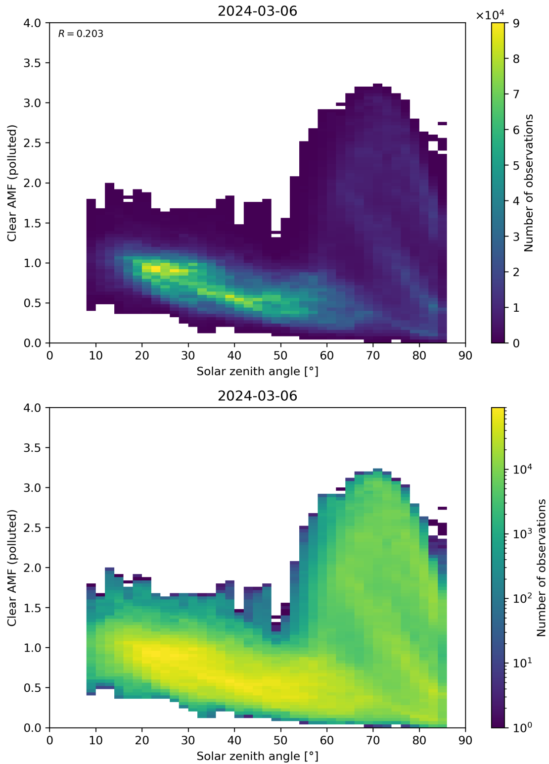
Figure 165: Scatter density plot of “Solar zenith angle” against “Clear AMF (polluted)” for 2024-03-05 to 2024-03-07.
