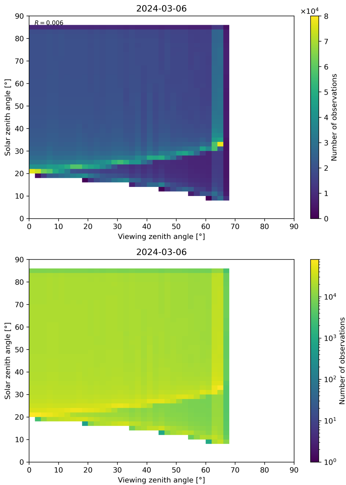
Figure 315: Scatter density plot of “Viewing zenith angle” against “Solar zenith angle” for 2024-03-05 to 2024-03-07.
