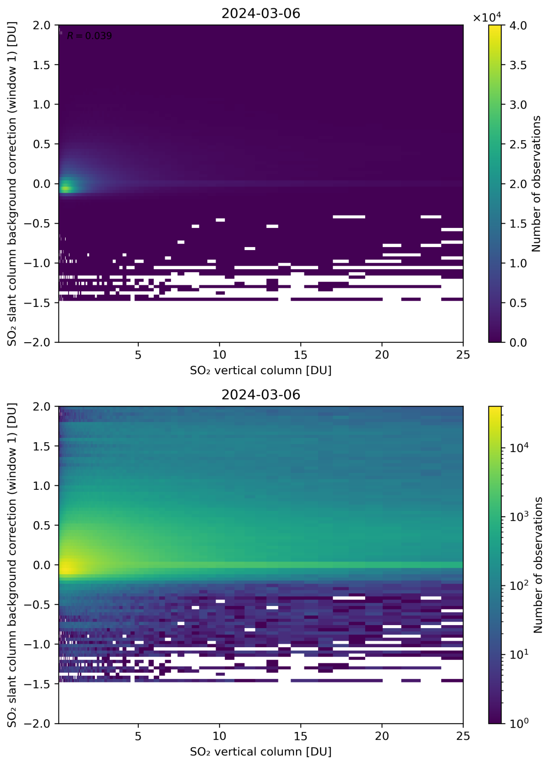
Figure 273: Scatter density plot of “SO 2 vertical column” against “SO 2 slant column background correction (window 1)” for 2024-03-05 to 2024-03-07.
