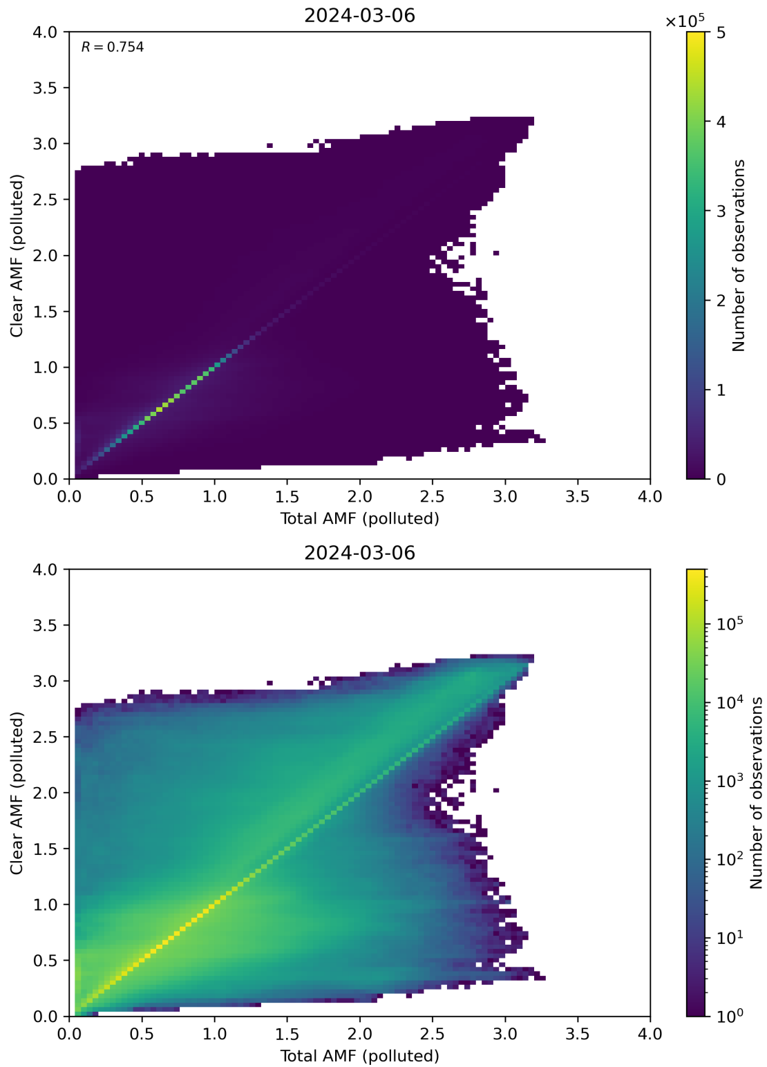
Figure 271: Scatter density plot of “Total AMF (polluted)” against “Clear AMF (polluted)” for 2024-03-05 to 2024-03-07.
