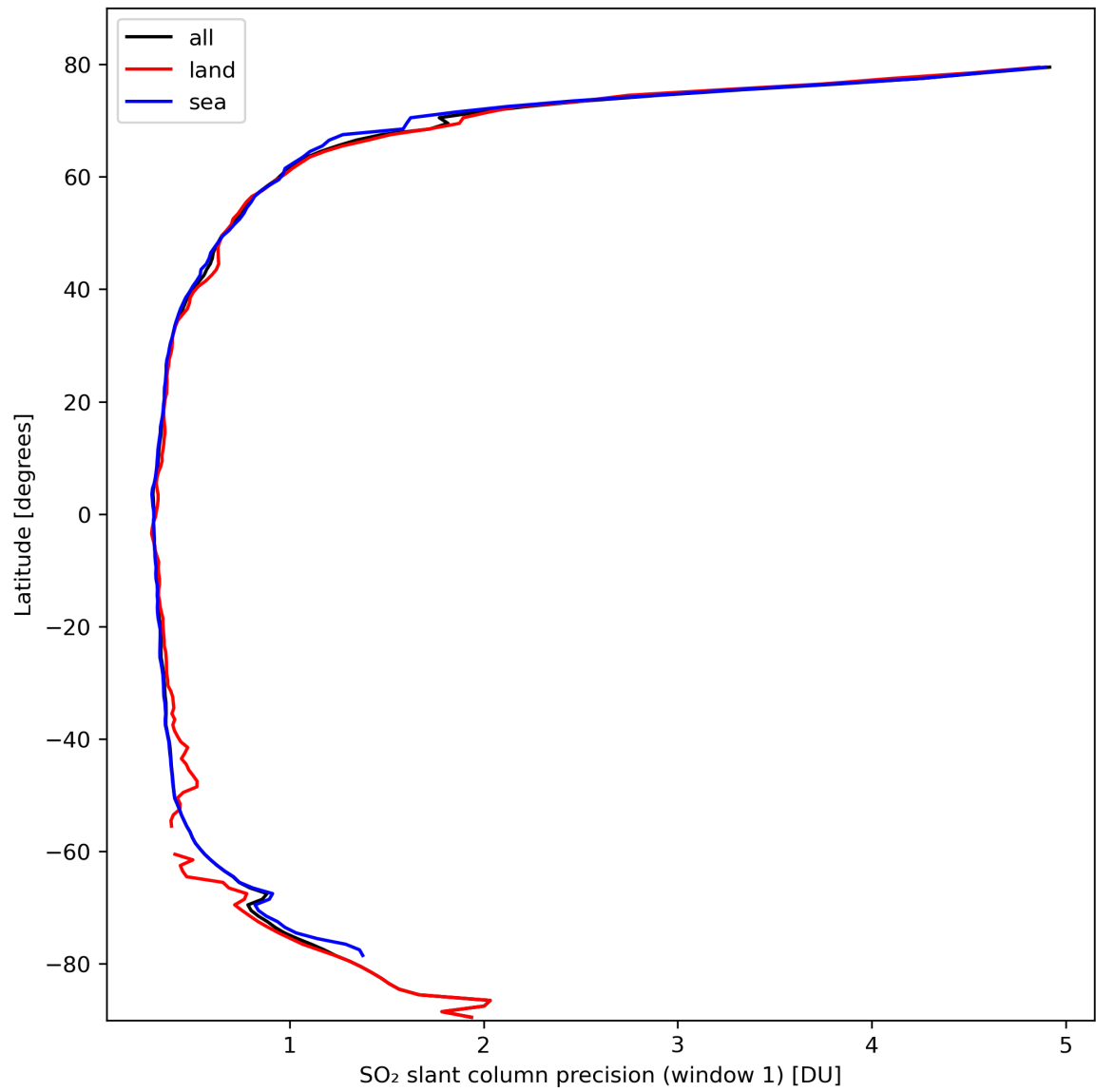
Figure 34: Zonal average of “SO 2 slant column precision (window 1)” for 2024-03-05 to 2024-03-07.
