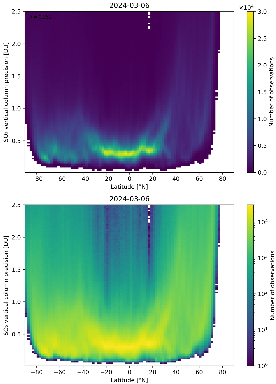
Figure 157: Scatter density plot of “Latitude” against “SO 2 vertical column precision” for 2024-03-05 to 2024-03-07.
