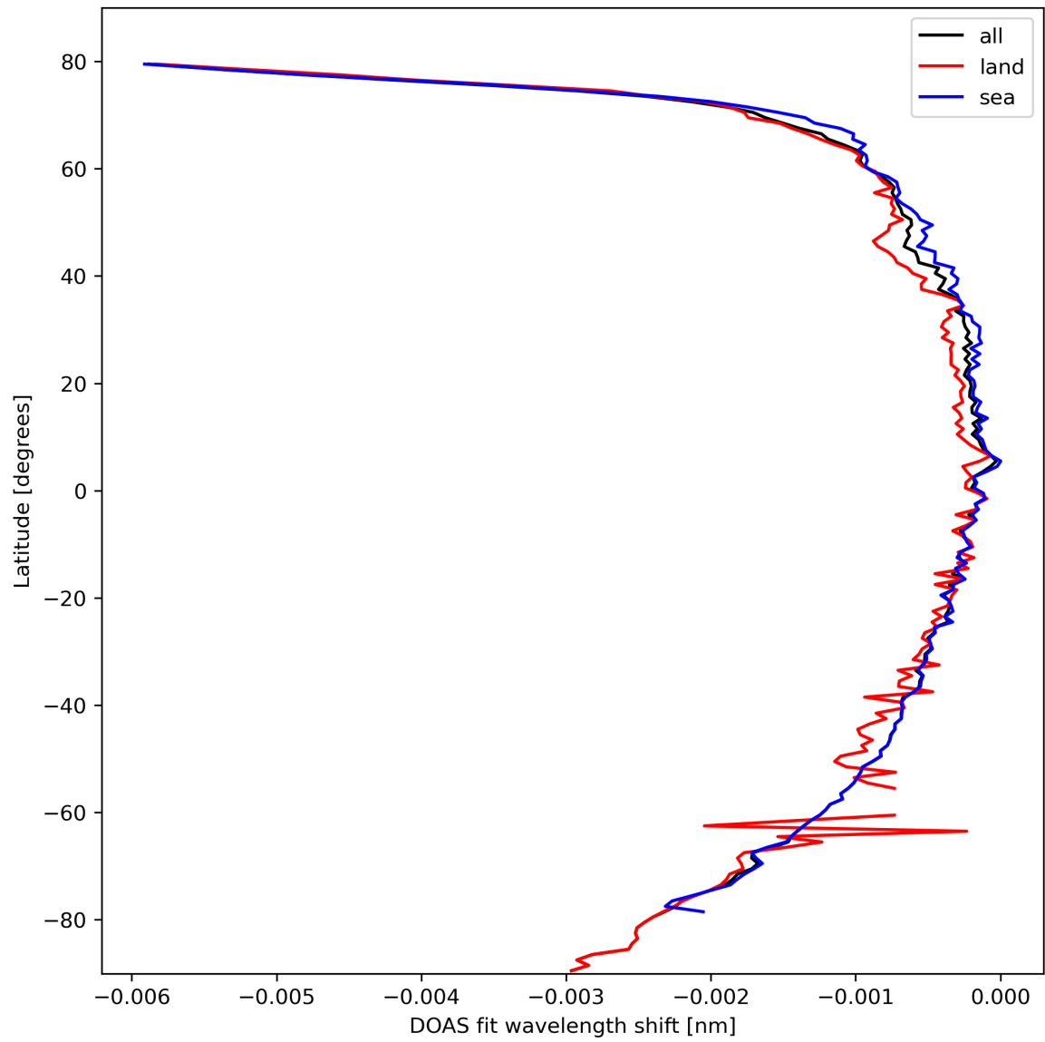
Figure 45: Zonal average of “DOAS fit wavelength shift” for 2024-03-05 to 2024-03-07.
