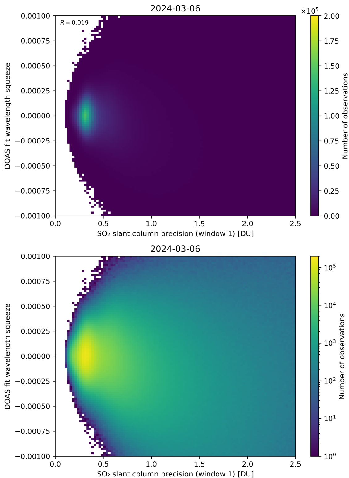
Figure 222: Scatter density plot of “SO 2 slant column precision (window 1)” against “DOAS fit wavelength squeeze” for 2024-03-05 to 2024-03-07.
