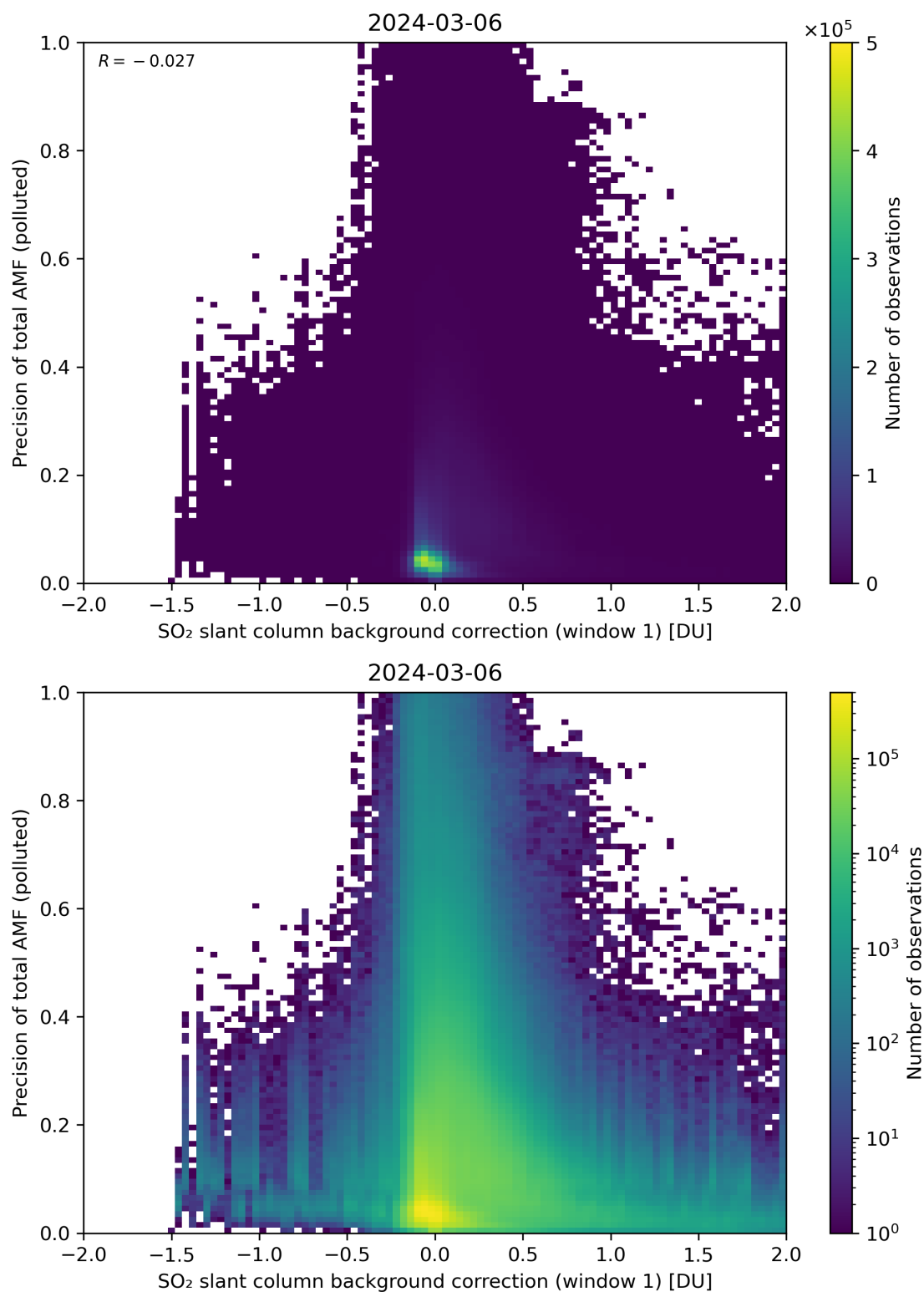
Figure 110: Scatter density plot of “SO 2 slant column background correction (window 1)” against “Precision of total AMF (polluted)” for 2024-03-05 to 2024-03-07.
