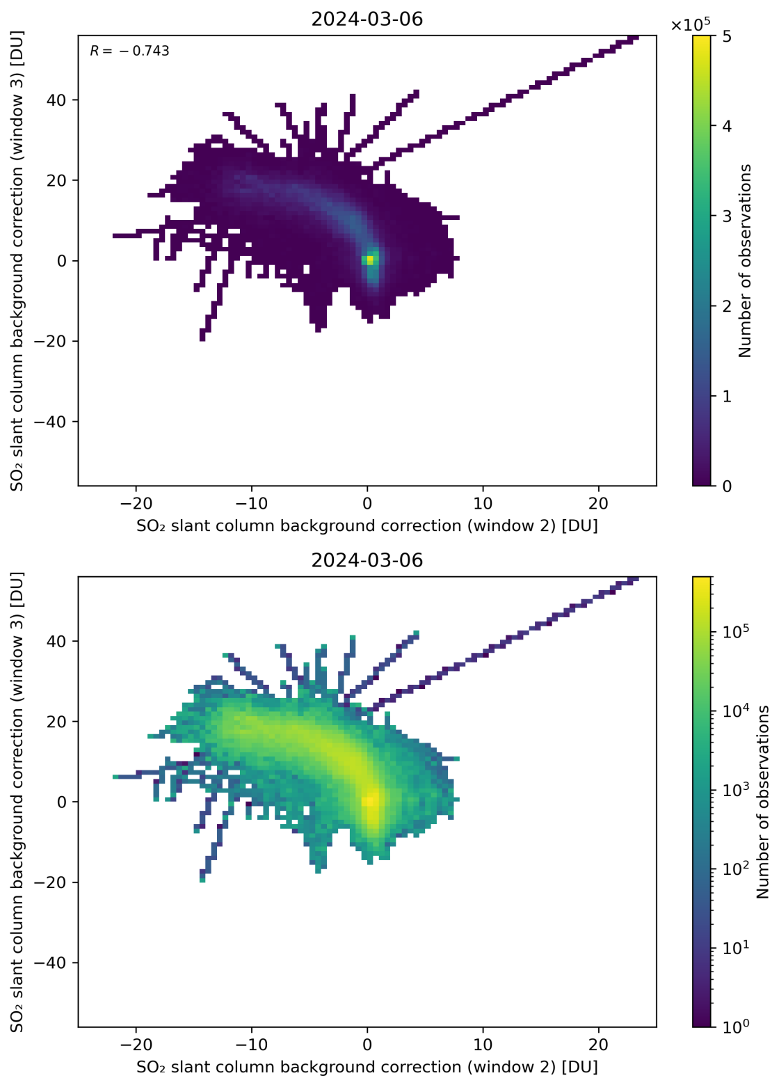
Figure 111: Scatter density plot of “SO 2 slant column background correction (window 2)” against “SO 2 slant column background correction (window 3)” for 2024-03-05 to 2024-03-07.
