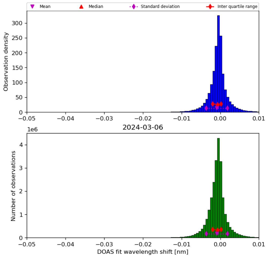
Figure 68: Histogram of “DOAS fit wavelength shift” for 2024-03-05 to 2024-03-07
