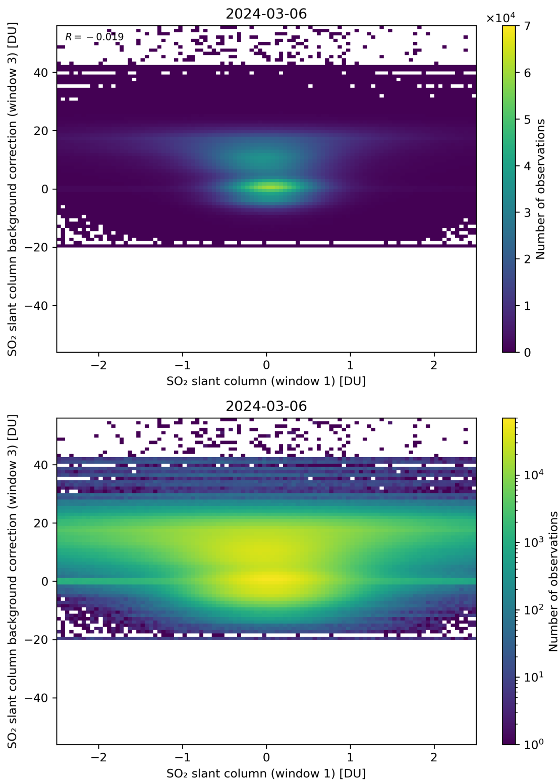
Figure 214: Scatter density plot of “SO 2 slant column (window 1)” against “SO 2 slant column background correction (window 3)” for 2024-03-05 to 2024-03-07.
