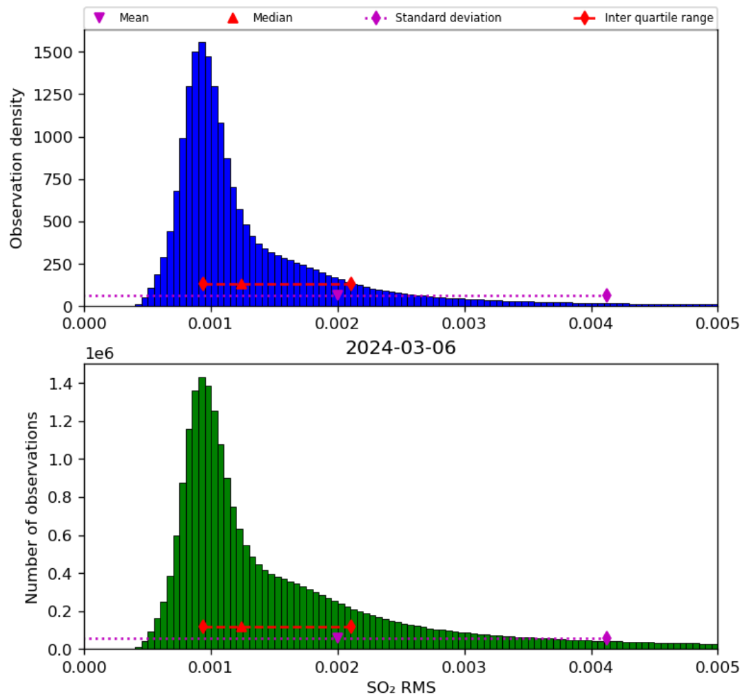
Figure 70: Histogram of “SO 2 RMS” for 2024-03-05 to 2024-03-07
