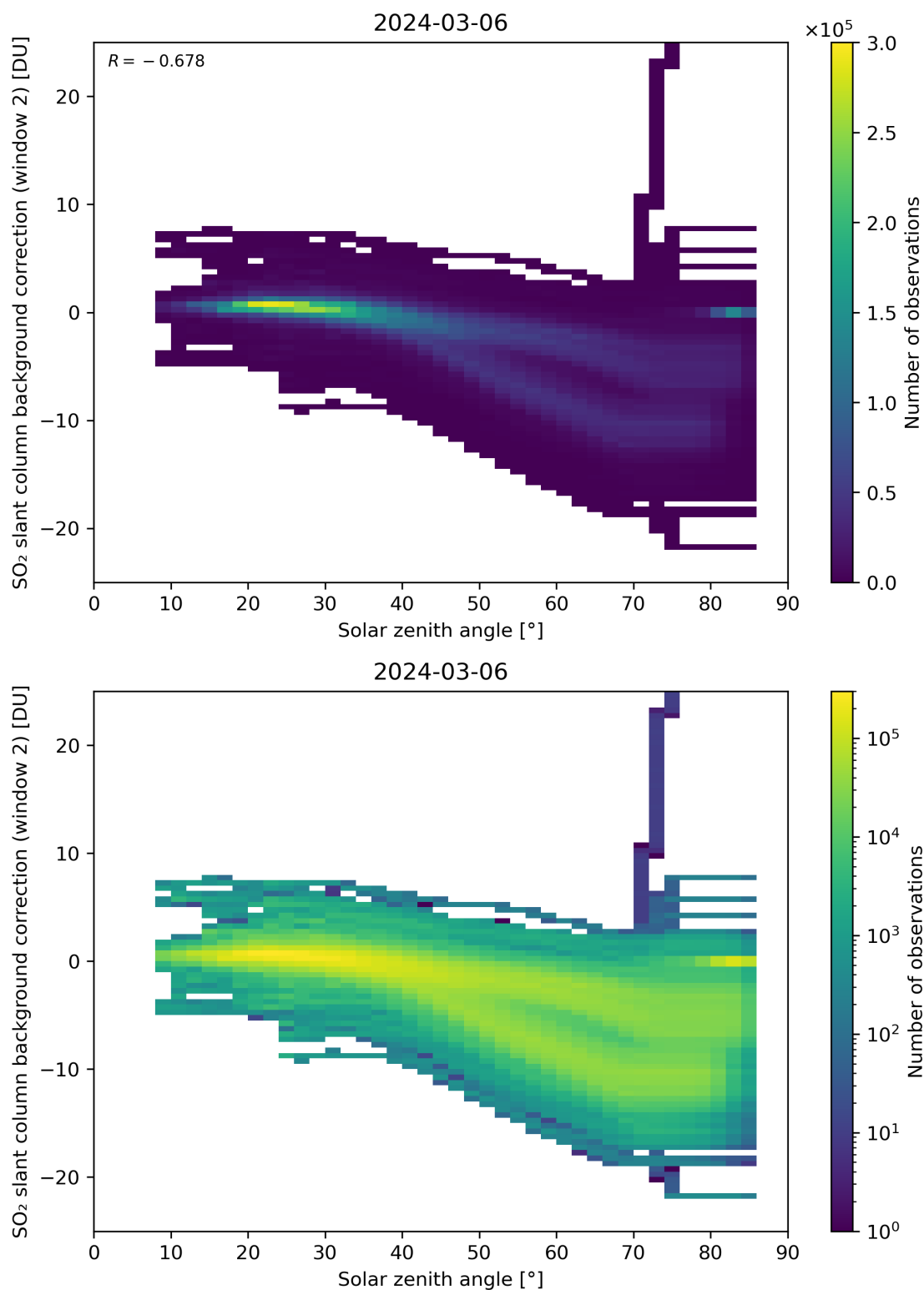
Figure 159: Scatter density plot of “Solar zenith angle” against “SO 2 slant column background correction (window 2)” for 2024-03-05 to 2024-03-07.
