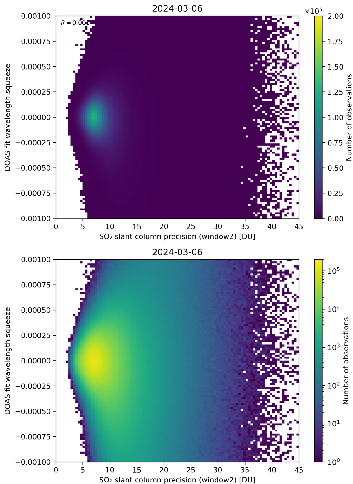
Figure 244: Scatter density plot of “SO 2 slant column precision (window2)” against “DOAS fit wavelength squeeze” for 2024-03-05 to 2024-03-07.
