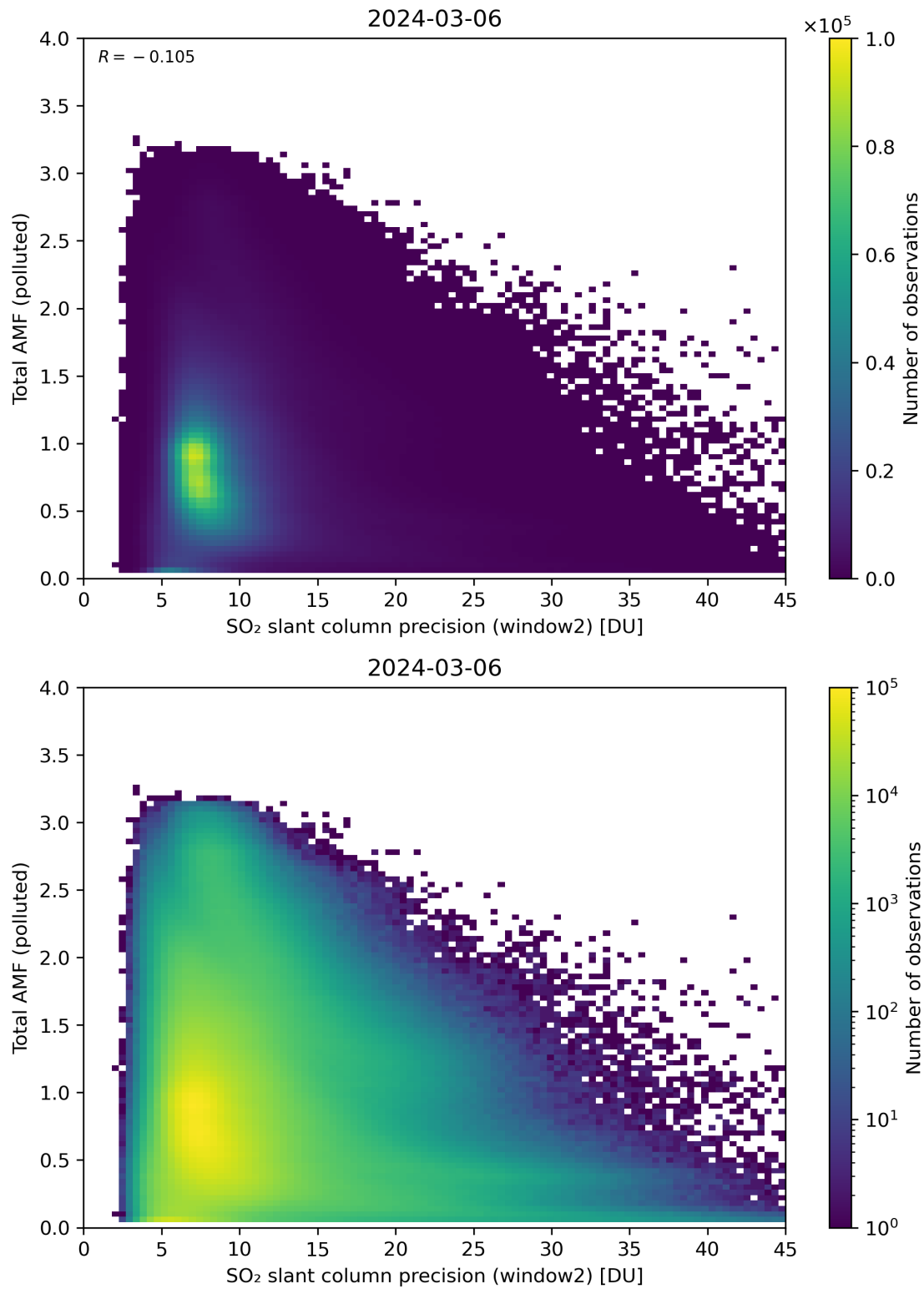
Figure 251: Scatter density plot of “SO 2 slant column precision (window2)” against “Total AMF (polluted)” for 2024-03-05 to 2024-03-07.
