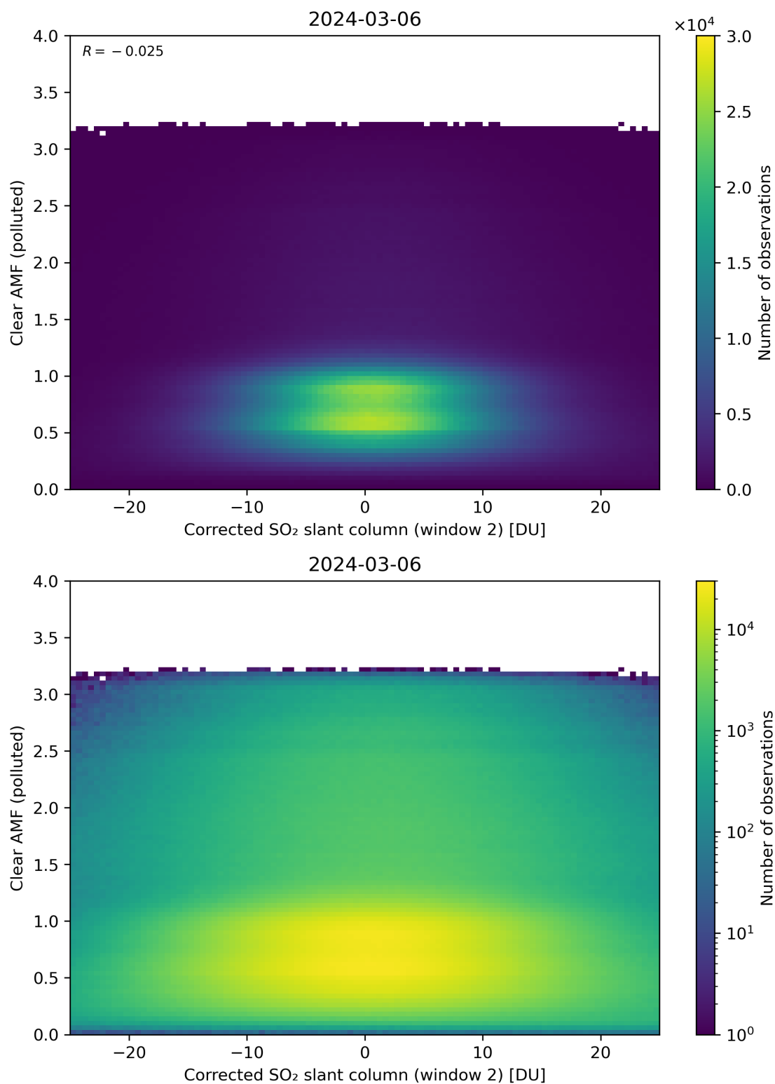
Figure 199: Scatter density plot of “Corrected SO 2 slant column (window 2)” against “Clear AMF (polluted)” for 2024-03-05 to 2024-03-07.
