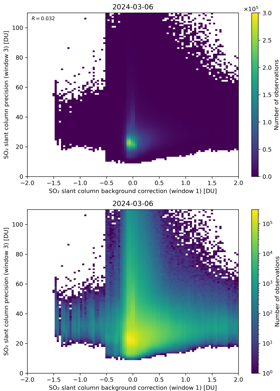
Figure 108: Scatter density plot of “SO 2 slant column background correction (window 1)” against “SO 2 slant column precision (window 3)” for 2024-03-05 to 2024-03-07.
