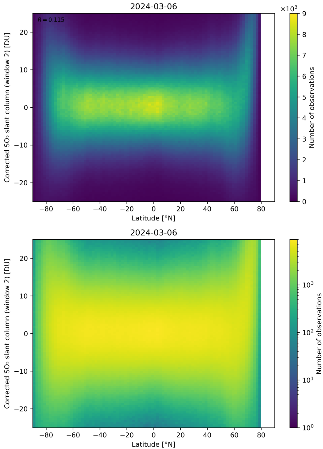
Figure 147: Scatter density plot of “Latitude” against “Corrected SO 2 slant column (window 2)” for 2024-03-05 to 2024-03-07.
