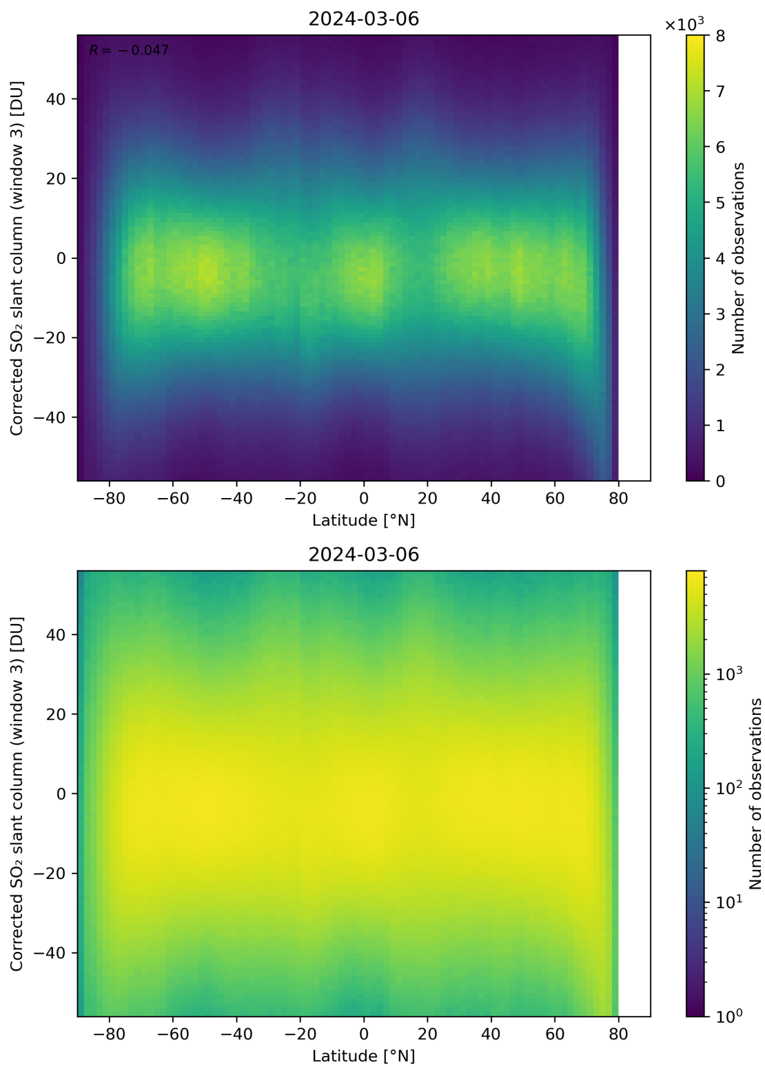
Figure 148: Scatter density plot of “Latitude” against “Corrected SO 2 slant column (window 3)” for 2024-03-05 to 2024-03-07.
