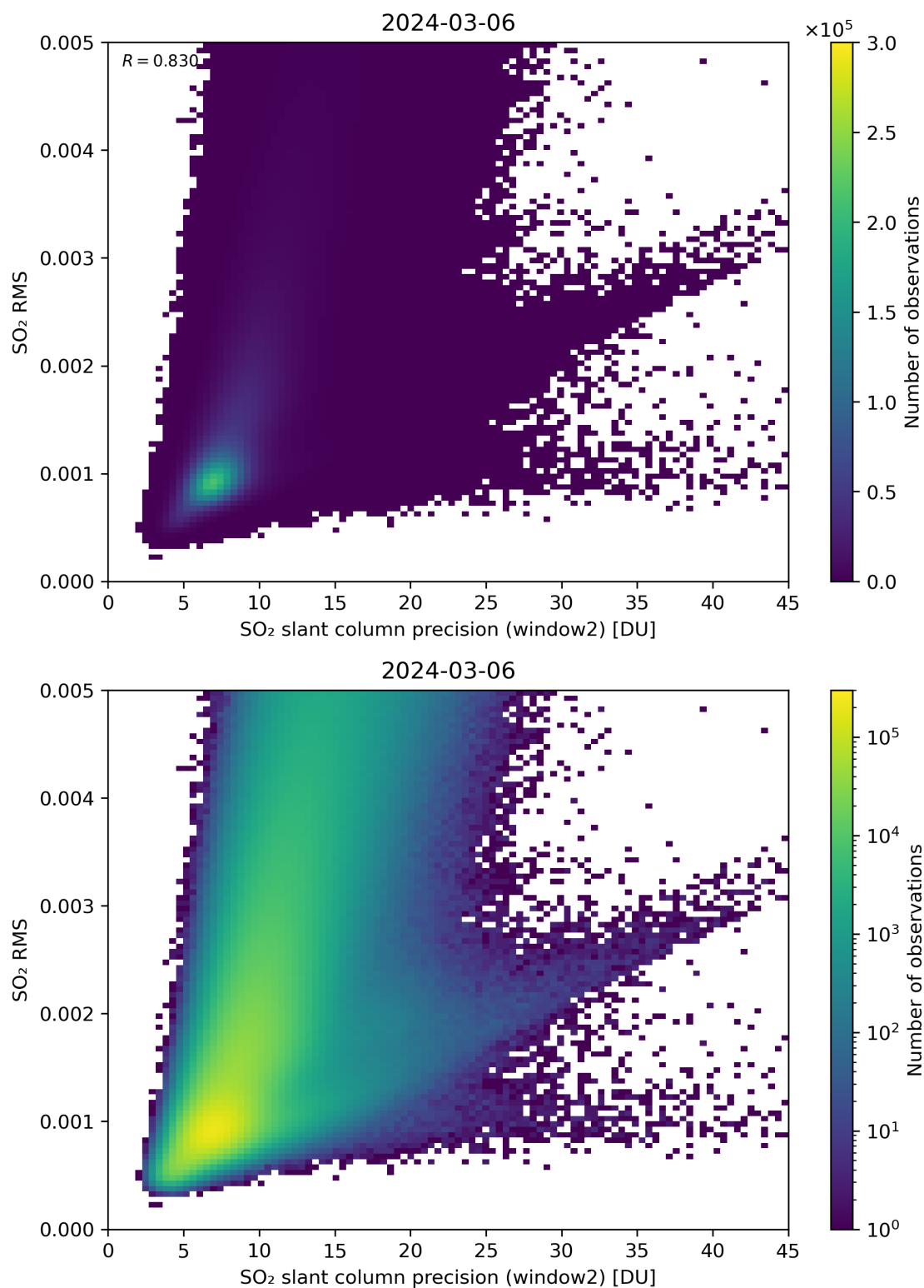
Figure 245: Scatter density plot of “SO 2 slant column precision (window2)” against “SO 2 RMS” for 2024-03-05 to 2024-03-07.
