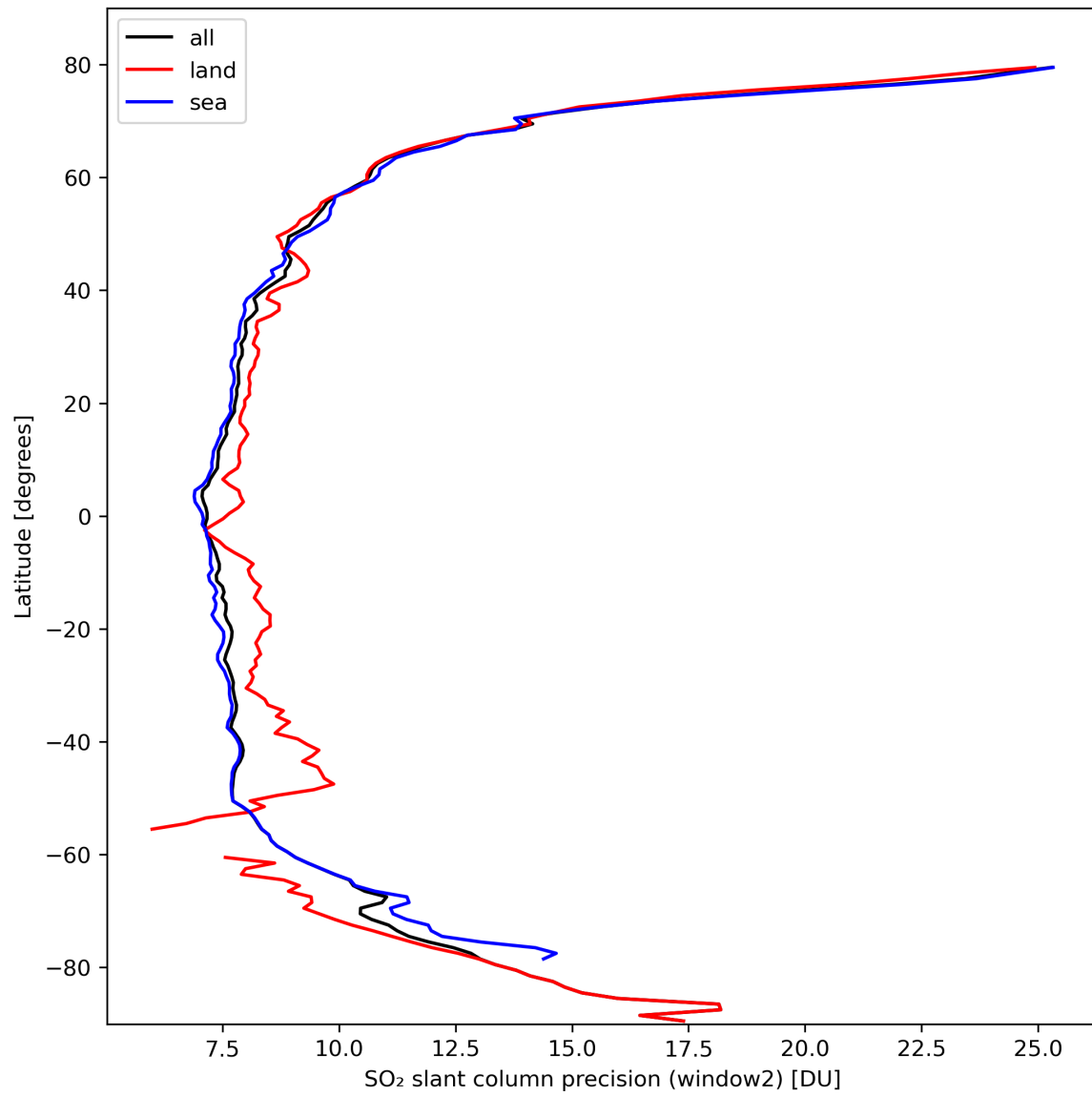
Figure 38: Zonal average of “SO 2 slant column precision (window2)” for 2024-03-05 to 2024-03-07.
