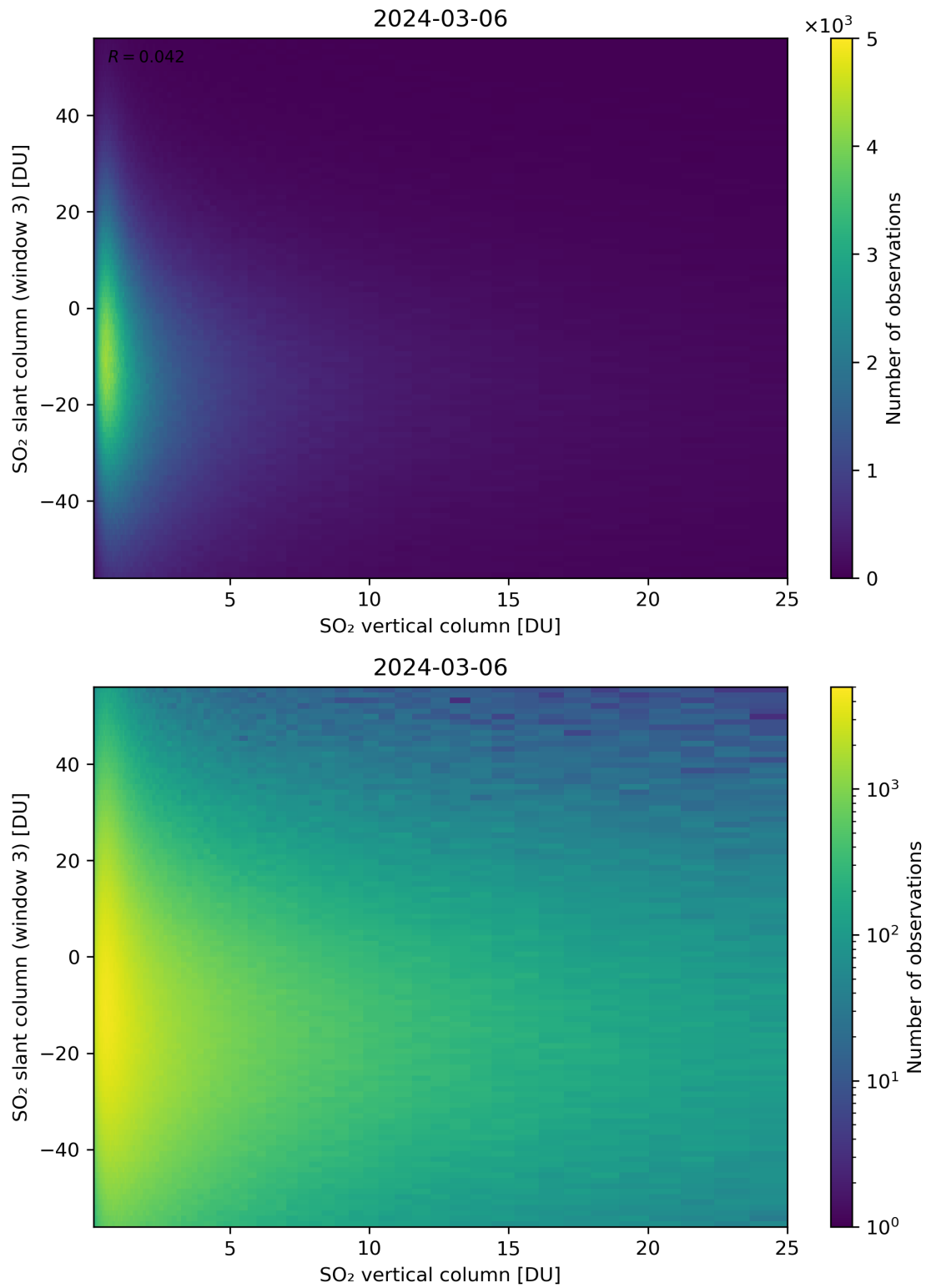
Figure 303: Scatter density plot of “SO 2 vertical column” against “SO 2 slant column (window 3)” for 2024-03-05 to 2024-03-07.
