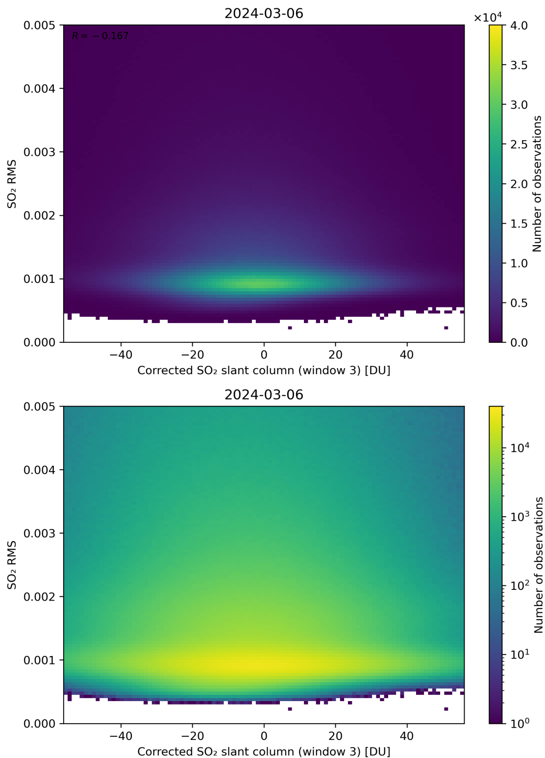
Figure 208: Scatter density plot of “Corrected SO 2 slant column (window 3)” against “SO 2 RMS” for 2024-03-05 to 2024-03-07.
