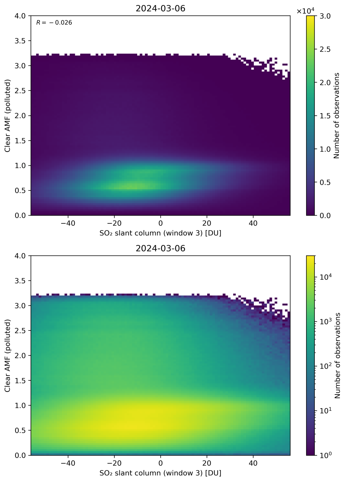
Figure 265: Scatter density plot of “SO 2 slant column (window 3)” against “Clear AMF (polluted)” for 2024-03-05 to 2024-03-07.
