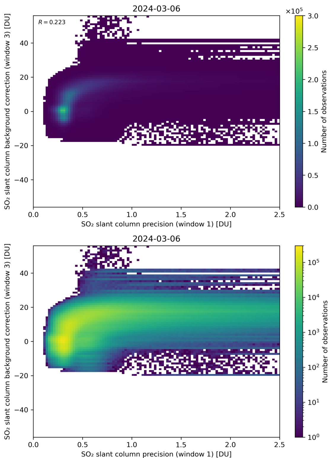
Figure 220: Scatter density plot of “SO 2 slant column precision (window 1)” against “SO 2 slant column background correction (window 3)” for 2024-03-05 to 2024-03-07.
