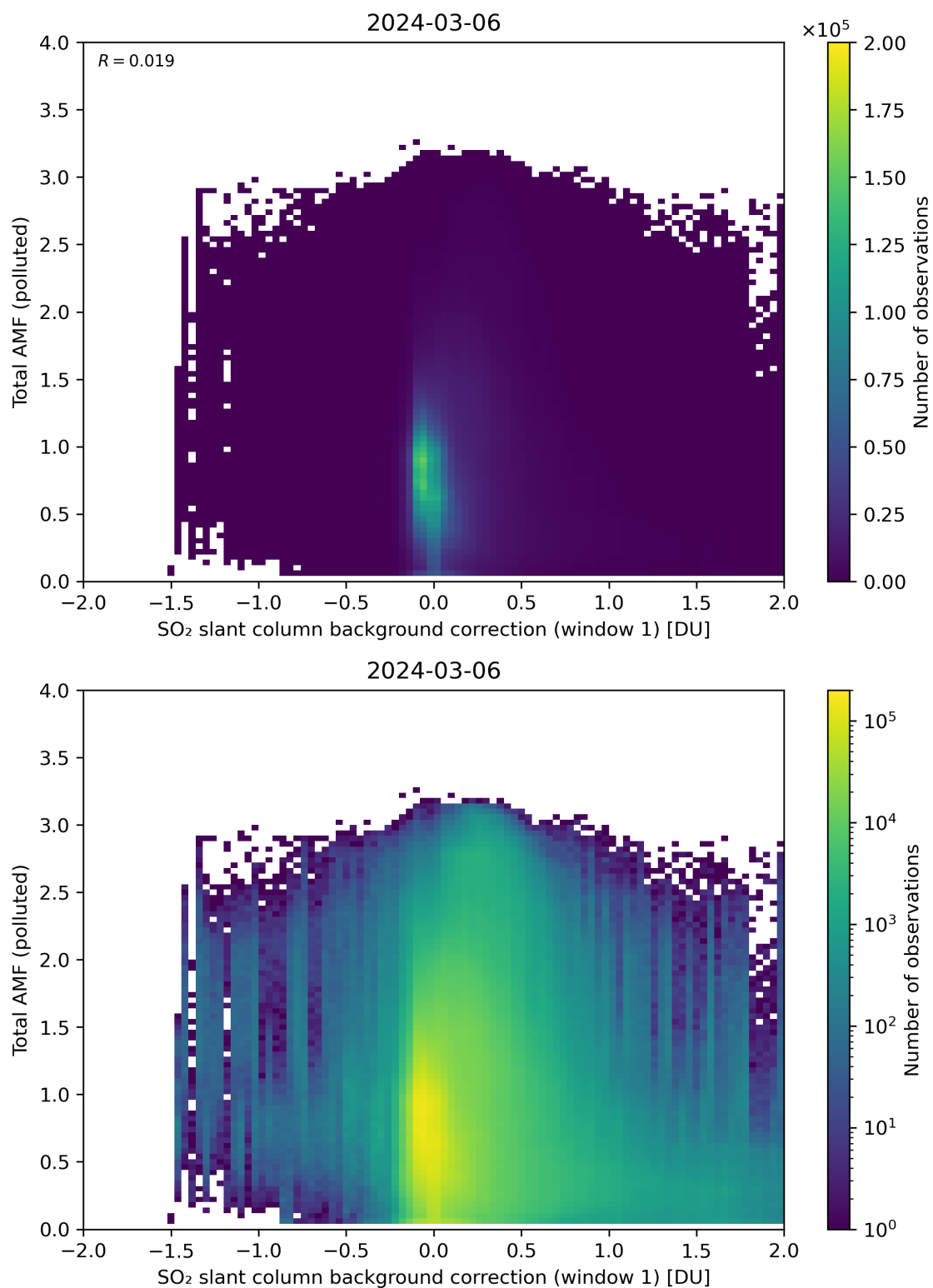
Figure 109: Scatter density plot of “SO 2 slant column background correction (window 1)” against “Total AMF (polluted)” for 2024-03-05 to 2024-03-07.
