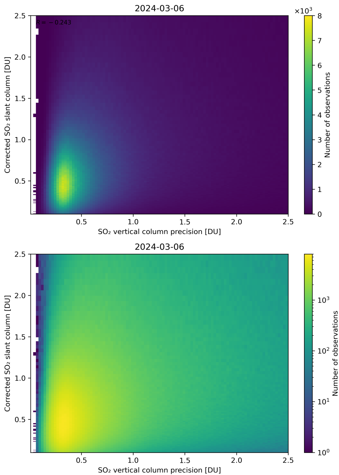
Figure 286: Scatter density plot of “SO 2 vertical column precision” against “Corrected SO 2 slant column” for 2024-03-05 to 2024-03-07.
