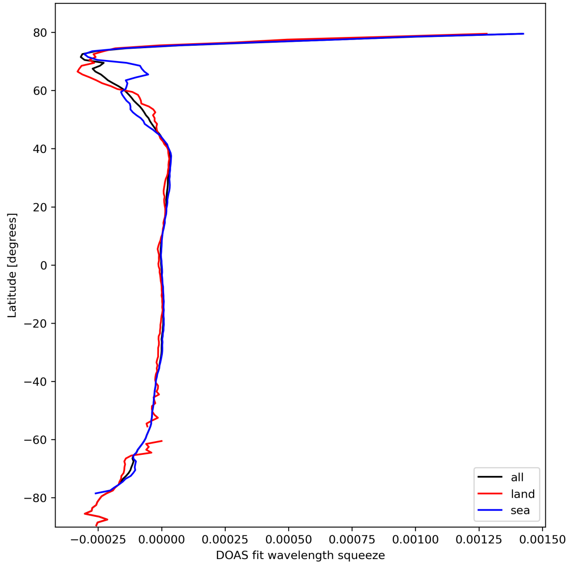
Figure 46: Zonal average of “DOAS fit wavelength squeeze” for 2024-03-05 to 2024-03-07.
