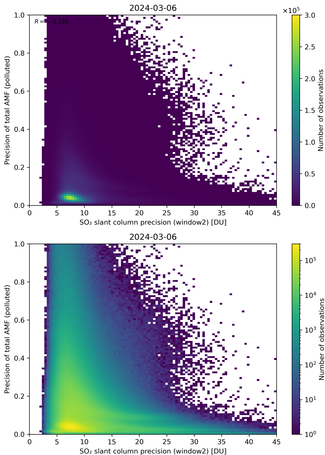
Figure 252: Scatter density plot of “SO 2 slant column precision (window2)” against “Precision of total AMF (polluted)” for 2024-03-05 to 2024-03-07.
