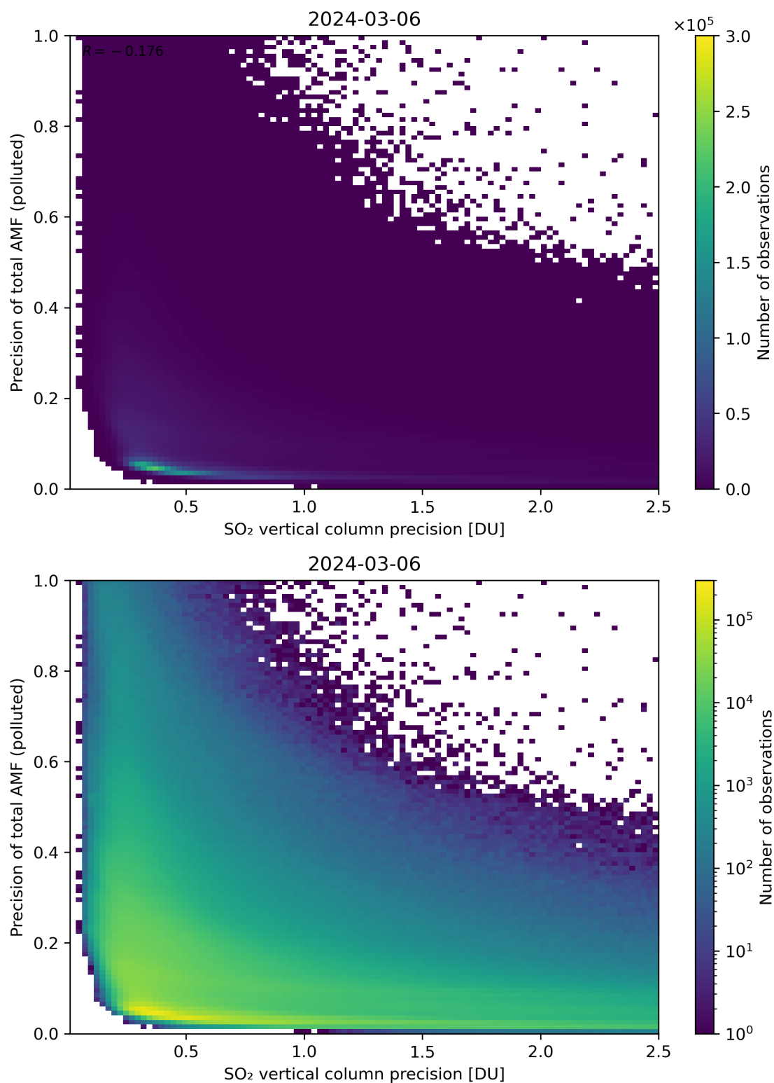
Figure 295: Scatter density plot of “SO 2 vertical column precision” against “Precision of total AMF (polluted)” for 2024-03-05 to 2024-03-07.
