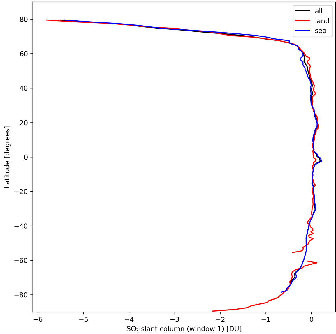
Figure 33: Zonal average of “SO 2 slant column (window 1)” for 2024-03-05 to 2024-03-07.
