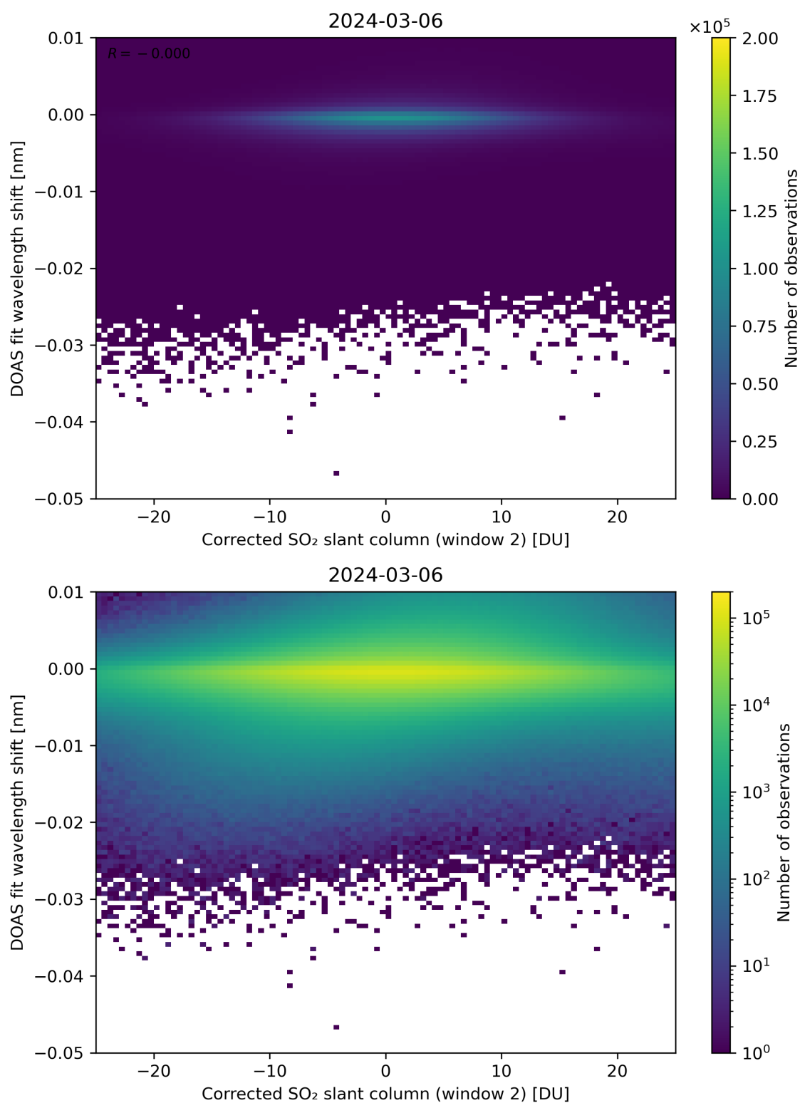
Figure 196: Scatter density plot of “Corrected SO 2 slant column (window 2)” against “DOAS fit wavelength shift” for 2024-03-05 to 2024-03-07.
