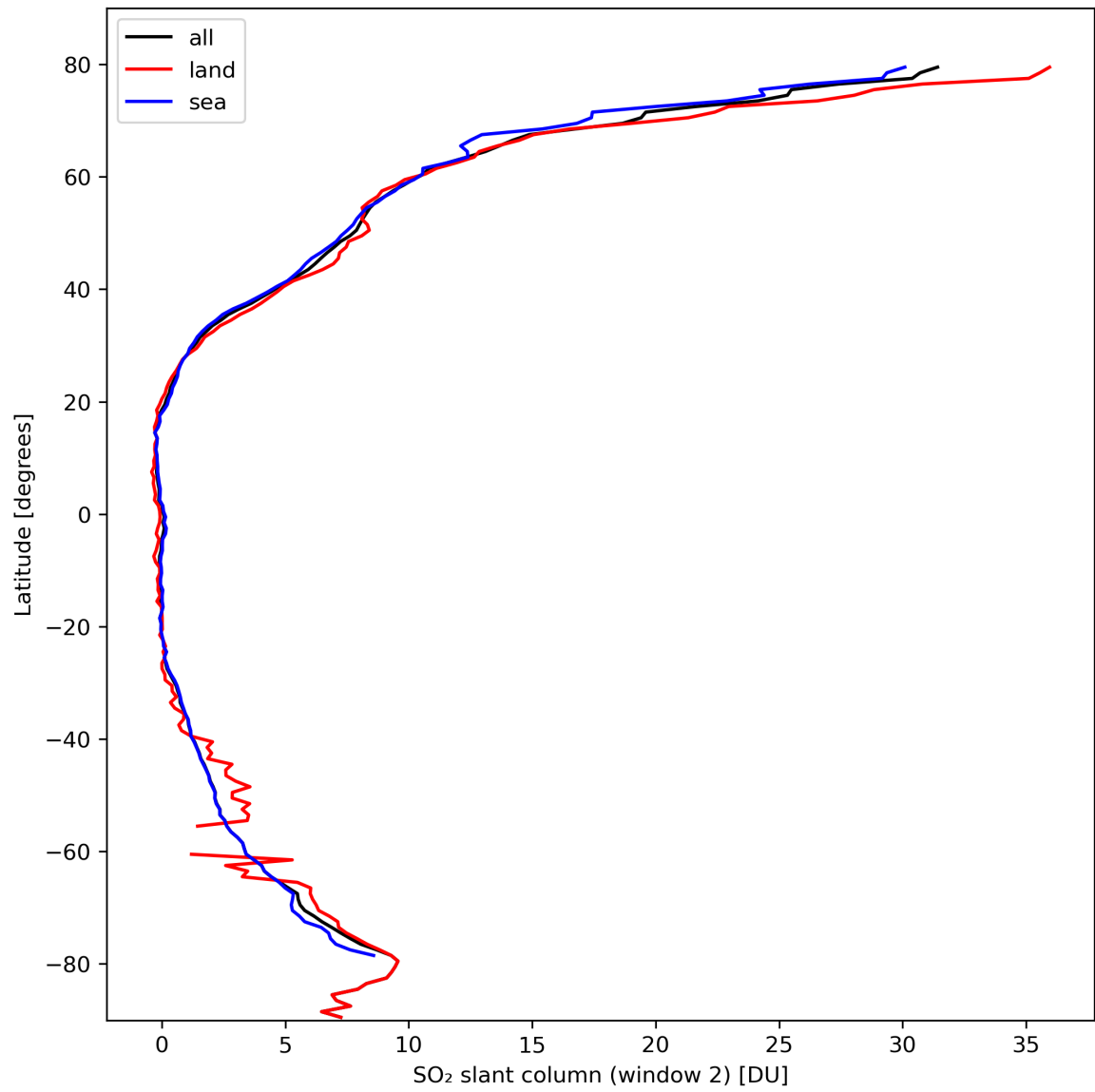
Figure 37: Zonal average of “SO 2 slant column (window 2)” for 2024-03-05 to 2024-03-07.
