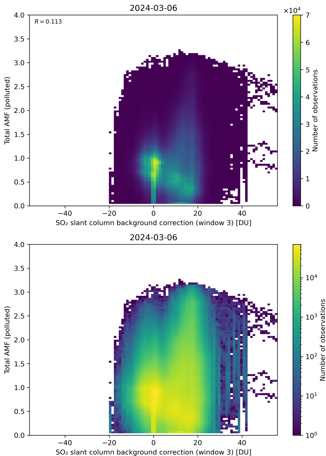
Figure 125: Scatter density plot of “SO 2 slant column background correction (window 3)” against “Total AMF (polluted)” for 2024-03-05 to 2024-03-07.
