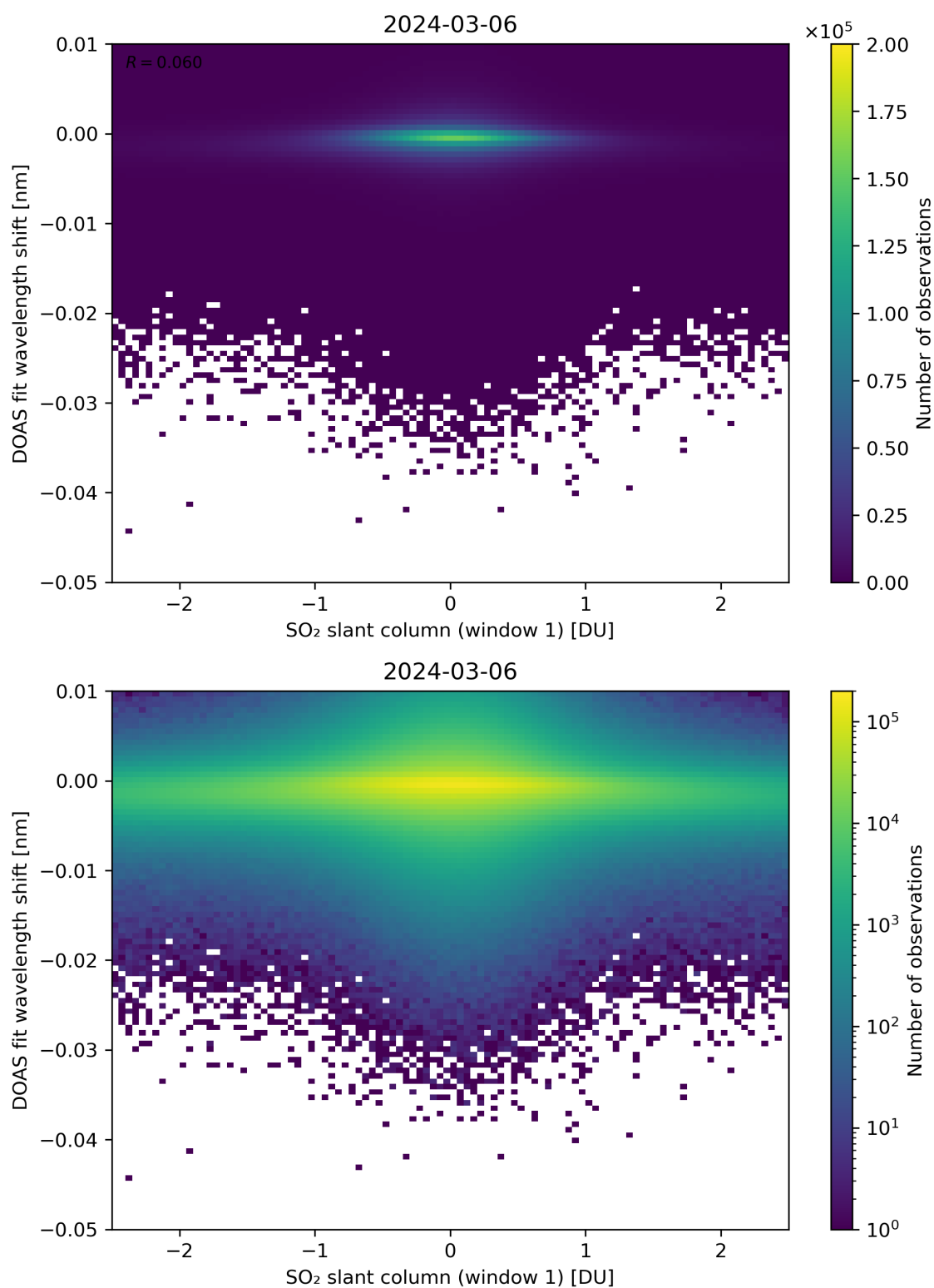
Figure 215: Scatter density plot of “SO 2 slant column (window 1)” against “DOAS fit wavelength shift” for 2024-03-05 to 2024-03-07.
