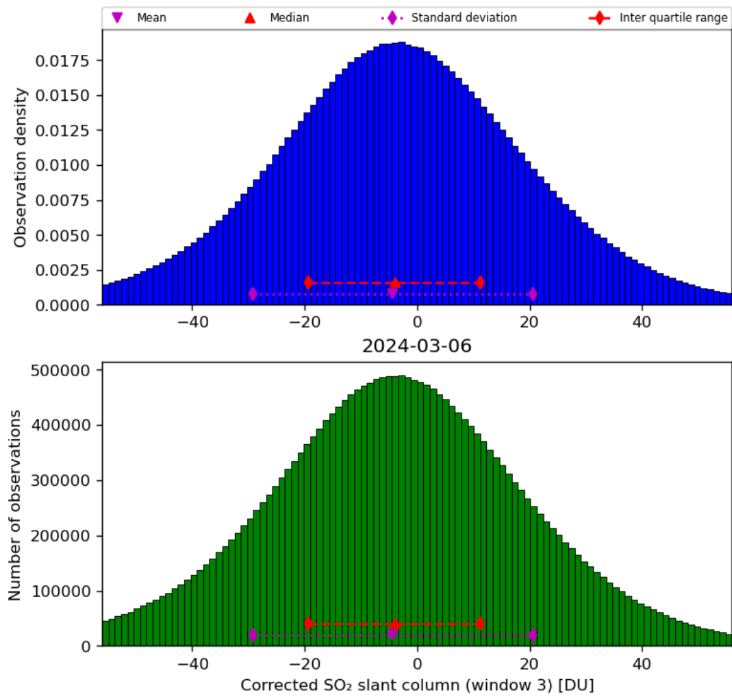
Figure 66: Histogram of “Corrected SO 2 slant column (window 3)” for 2024-03-05 to 2024-03-07
