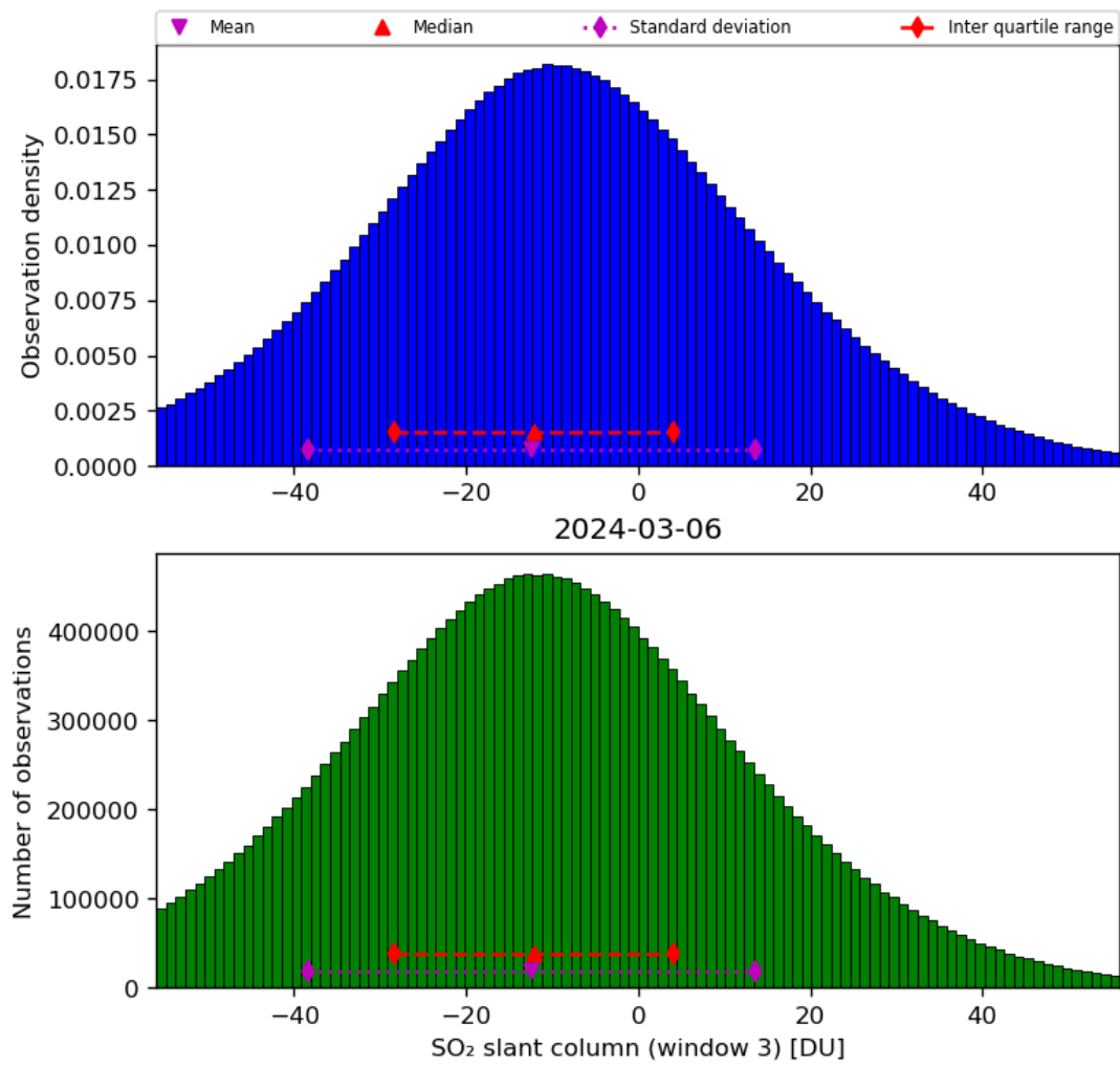
Figure 64: Histogram of “SO 2 slant column (window 3)” for 2024-03-05 to 2024-03-07
