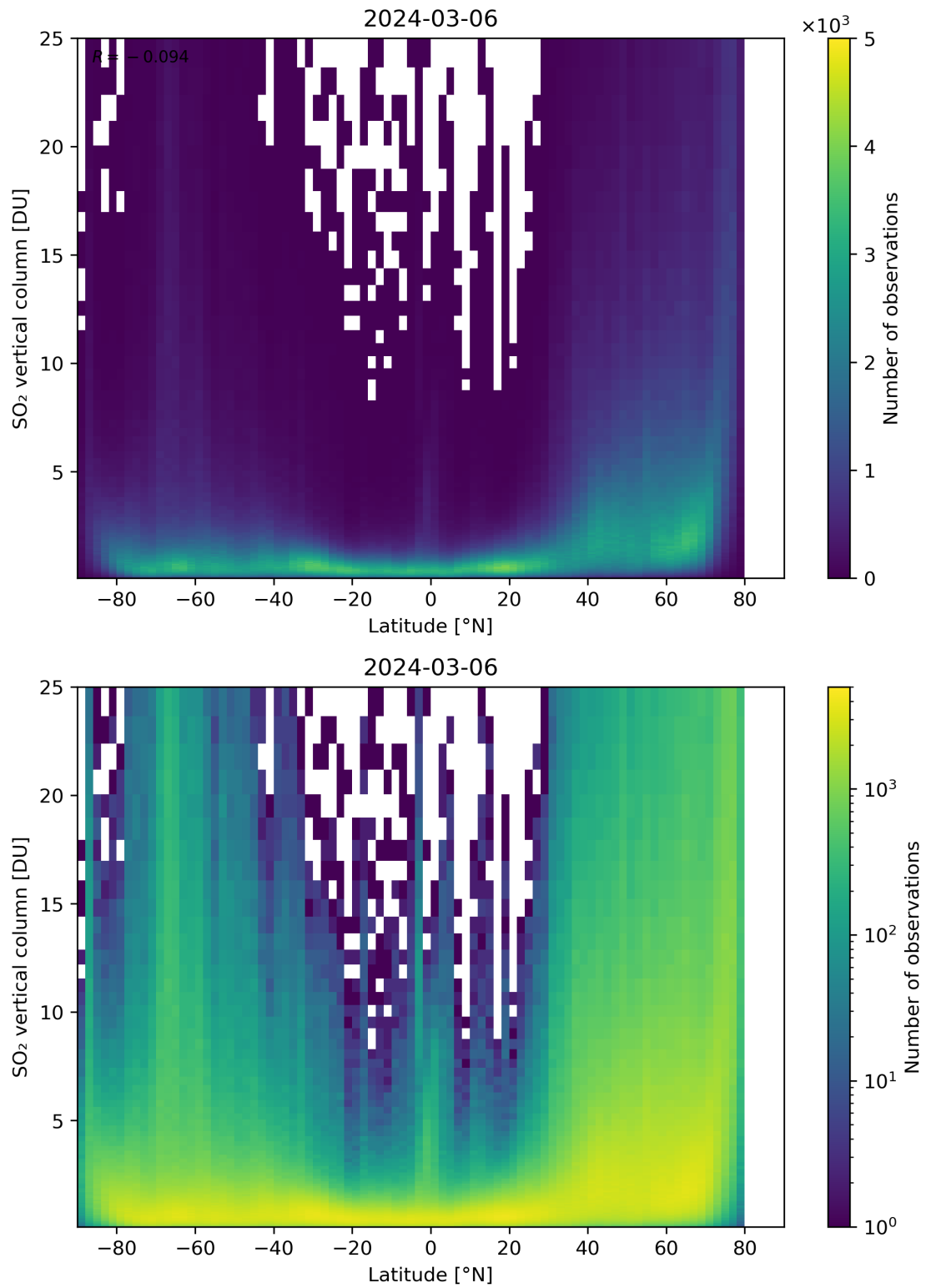
Figure 156: Scatter density plot of “Latitude” against “SO 2 vertical column” for 2024-03-05 to 2024-03-07.
