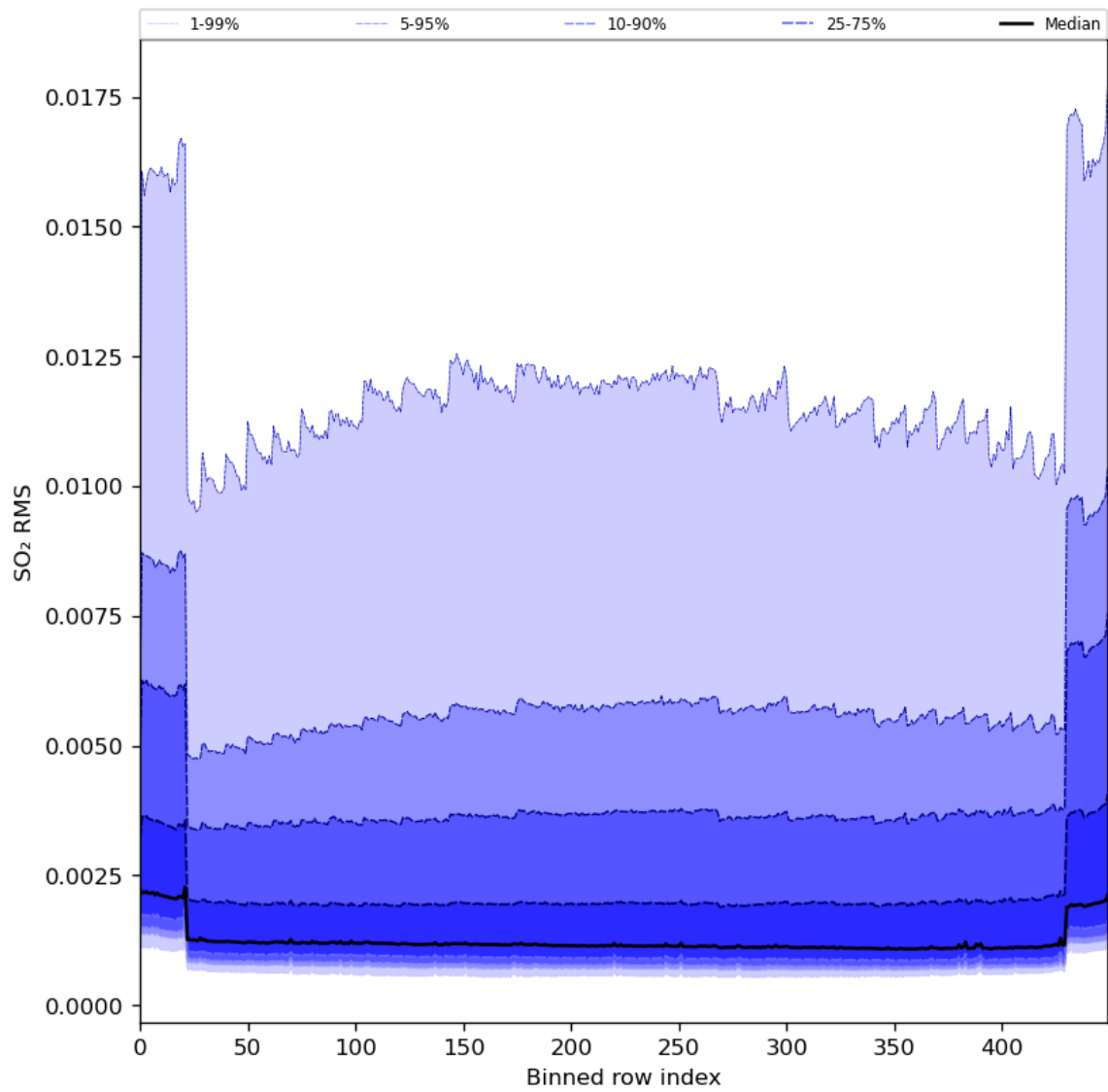
Figure 93: Along track statistics of “SO 2 RMS” for 2024-03-05 to 2024-03-07
