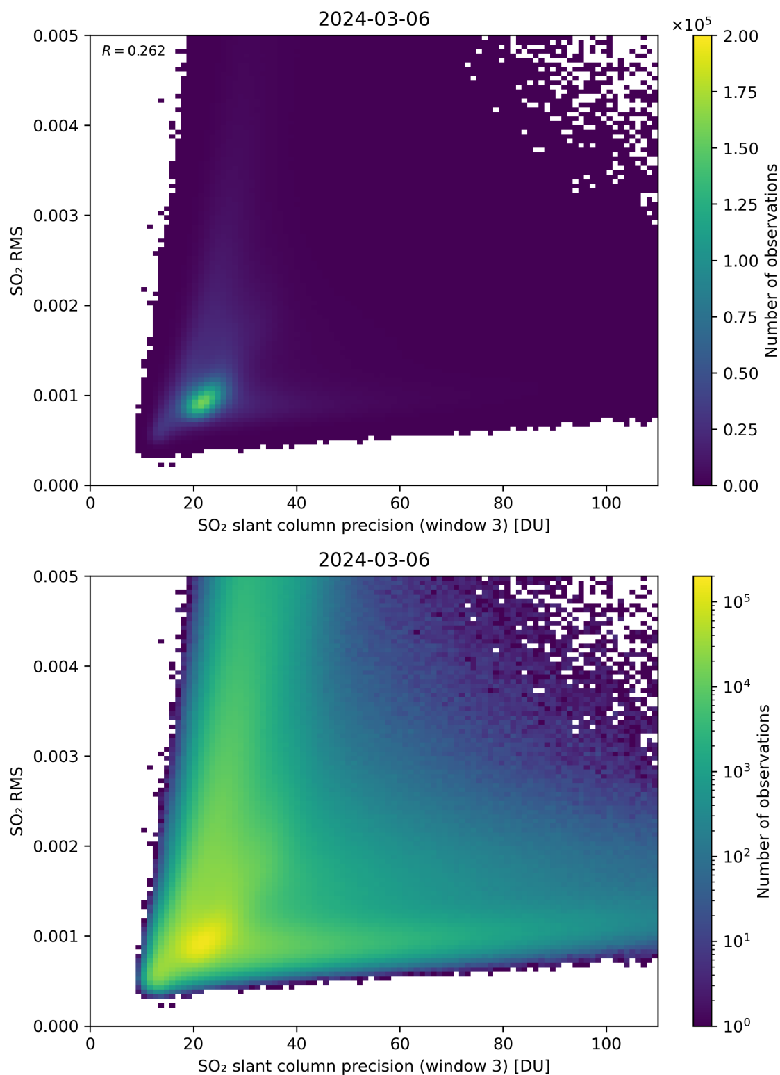
Figure 260: Scatter density plot of “SO 2 slant column precision (window 3)” against “SO 2 RMS” for 2024-03-05 to 2024-03-07.
