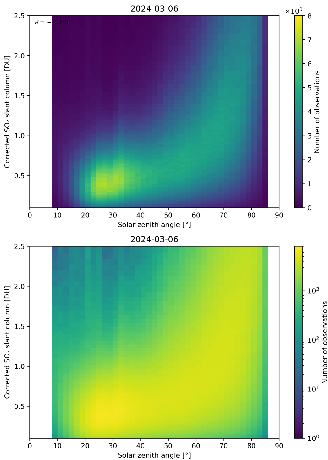
Figure 166: Scatter density plot of “Solar zenith angle” against “Corrected SO 2 slant column” for 2024-03-05 to 2024-03-07.
