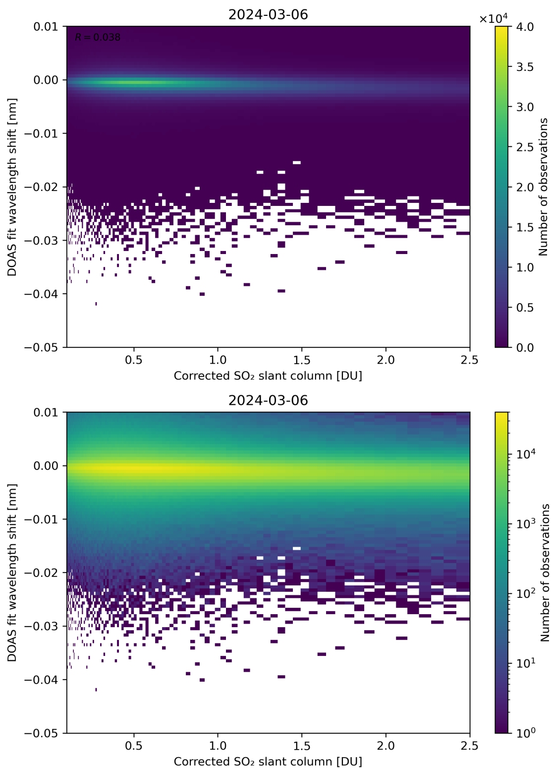
Figure 181: Scatter density plot of “Corrected SO 2 slant column” against “DOAS fit wavelength shift” for 2024-03-05 to 2024-03-07.
