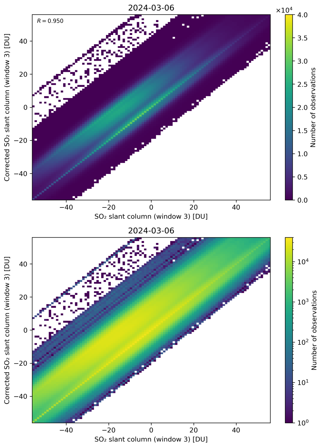
Figure 266: Scatter density plot of “SO 2 slant column (window 3)” against “Corrected SO 2 slant column (window 3)” for 2024-03-05 to 2024-03-07.
