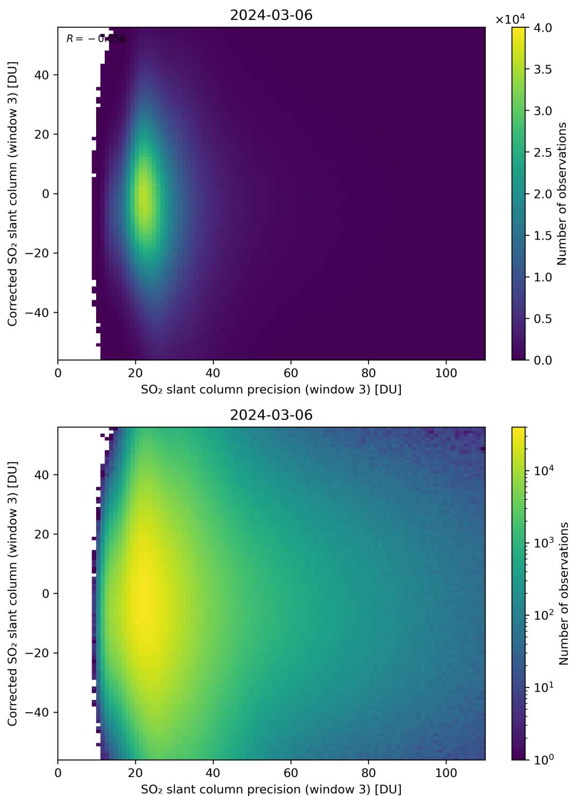
Figure 262: Scatter density plot of “SO 2 slant column precision (window 3)” against “Corrected SO 2 slant column (window 3)” for 2024-03-05 to 2024-03-07.
