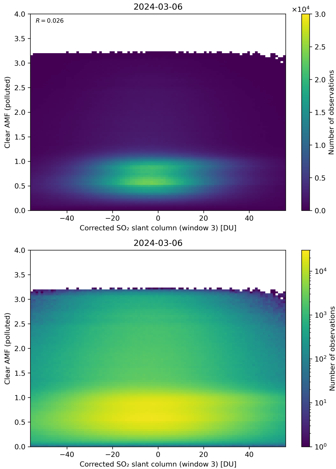
Figure 209: Scatter density plot of “Corrected SO 2 slant column (window 3)” against “Clear AMF (polluted)” for 2024-03-05 to 2024-03-07.
