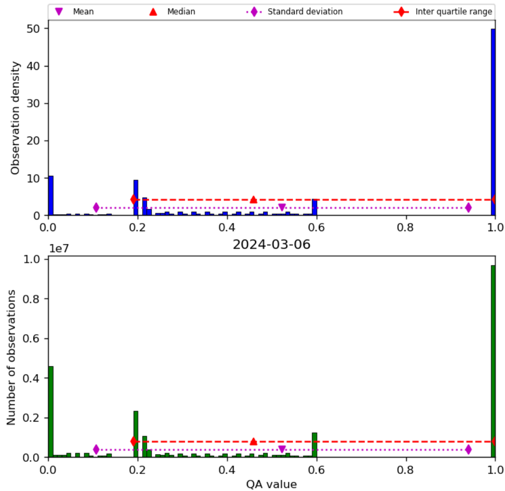
Figure 52: Histogram of “QA value” for 2024-03-05 to 2024-03-07
