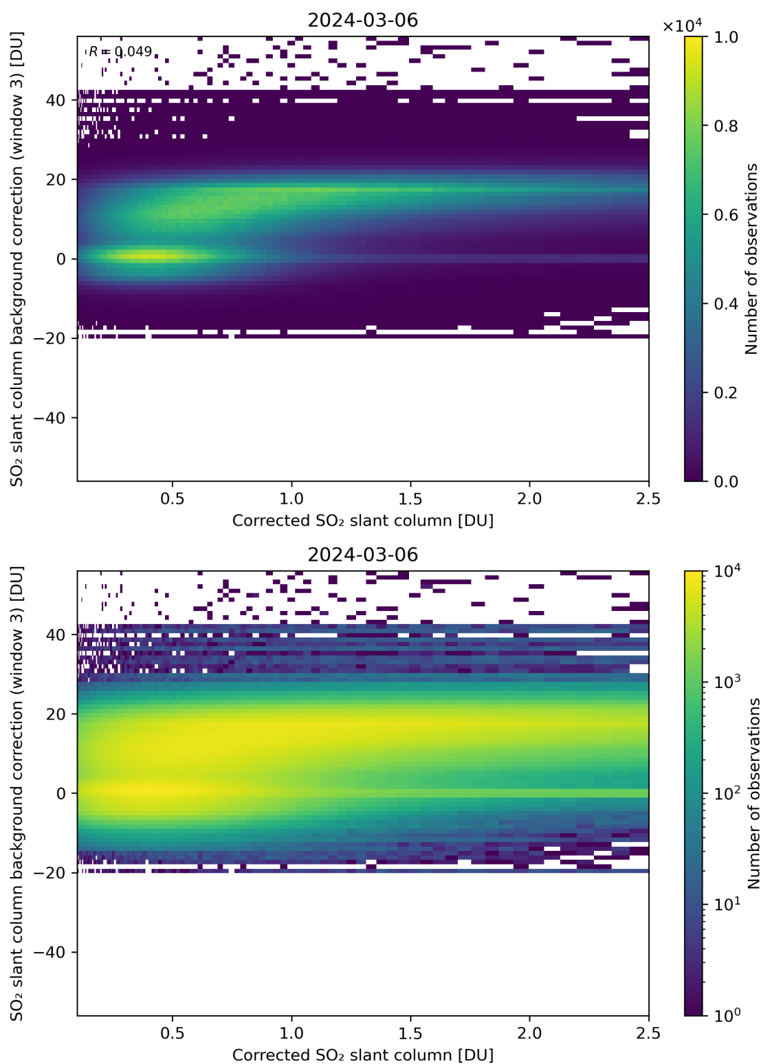
Figure 180: Scatter density plot of “Corrected SO 2 slant column” against “SO 2 slant column background correction (window 3)” for 2024-03-05 to 2024-03-07.
