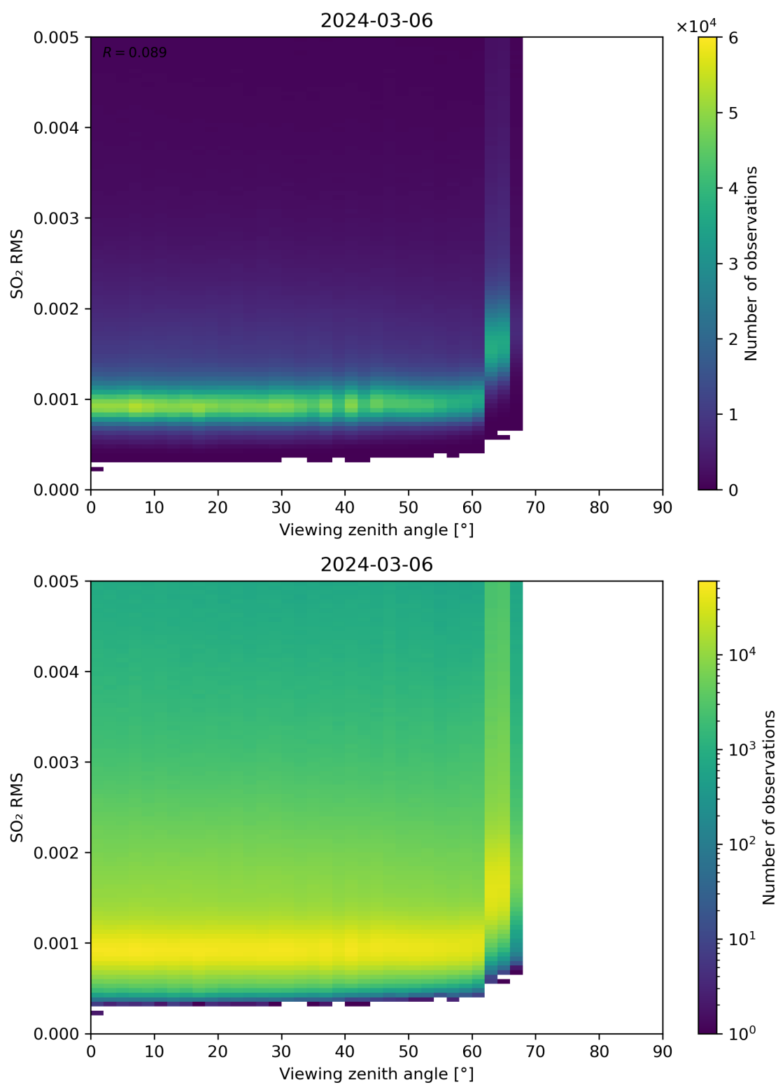
Figure 313: Scatter density plot of “Viewing zenith angle” against “SO 2 RMS” for 2024-03-05 to 2024-03-07.
