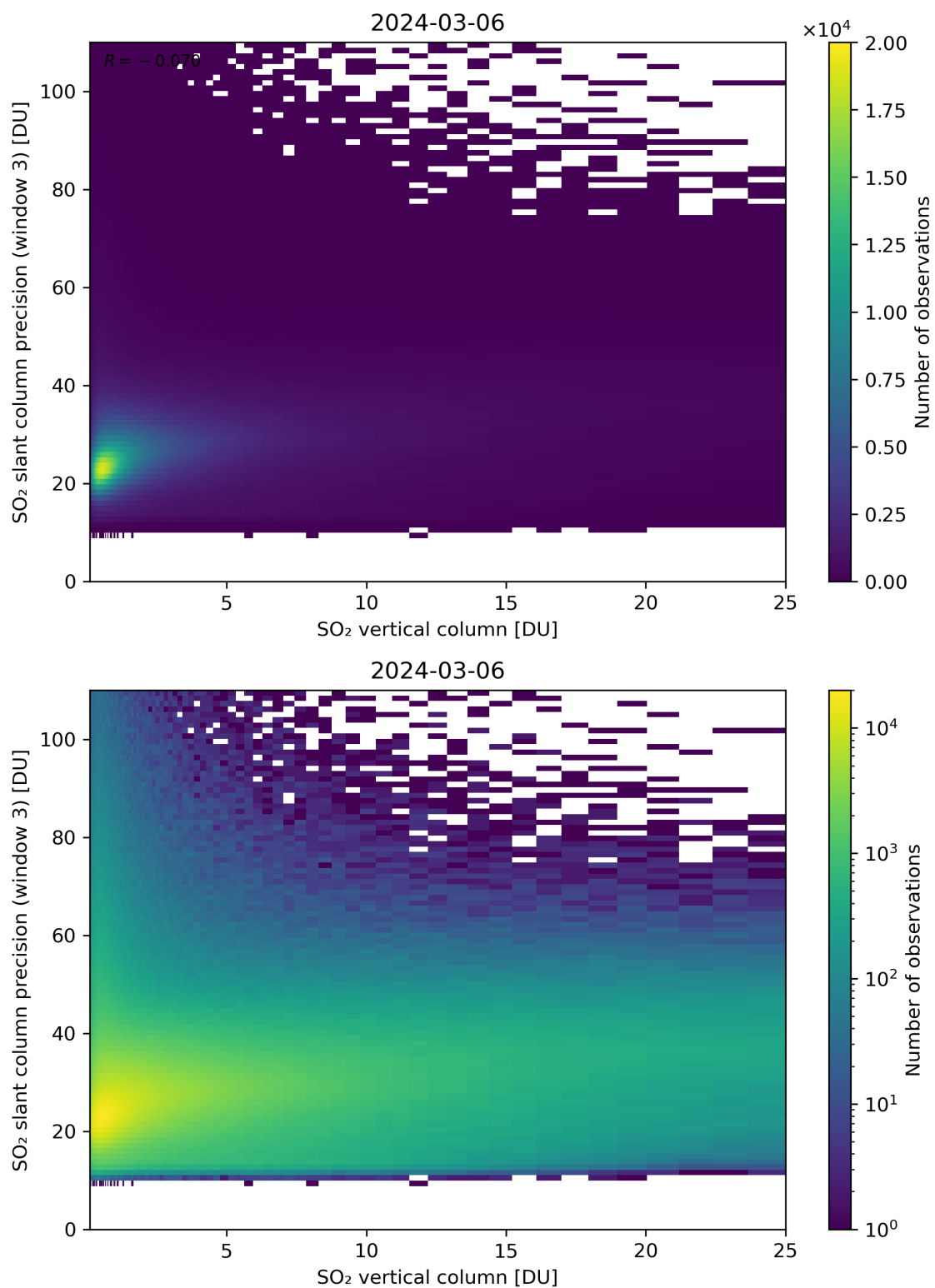
Figure 304: Scatter density plot of “SO 2 vertical column” against “SO 2 slant column precision (window 3)” for 2024-03-05 to 2024-03-07.
