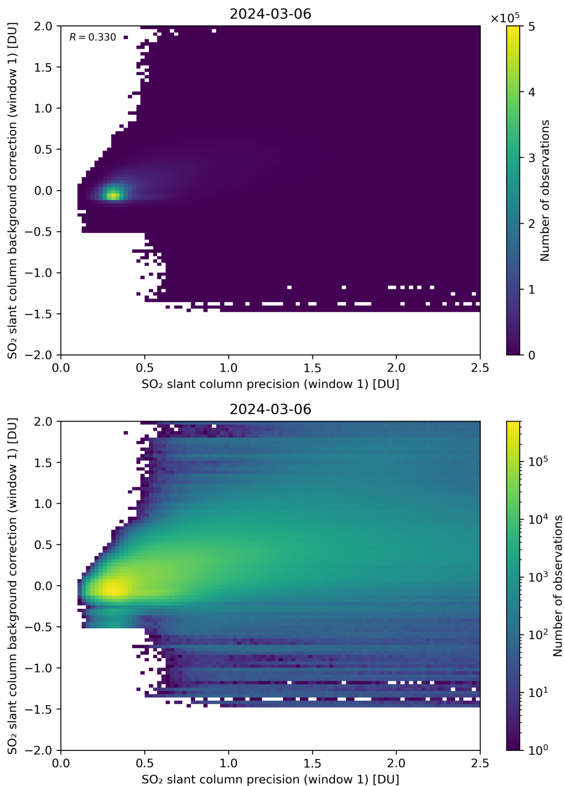
Figure 218: Scatter density plot of “SO 2 slant column precision (window 1)” against “SO 2 slant column background correction (window 1)” for 2024-03-05 to 2024-03-07.
