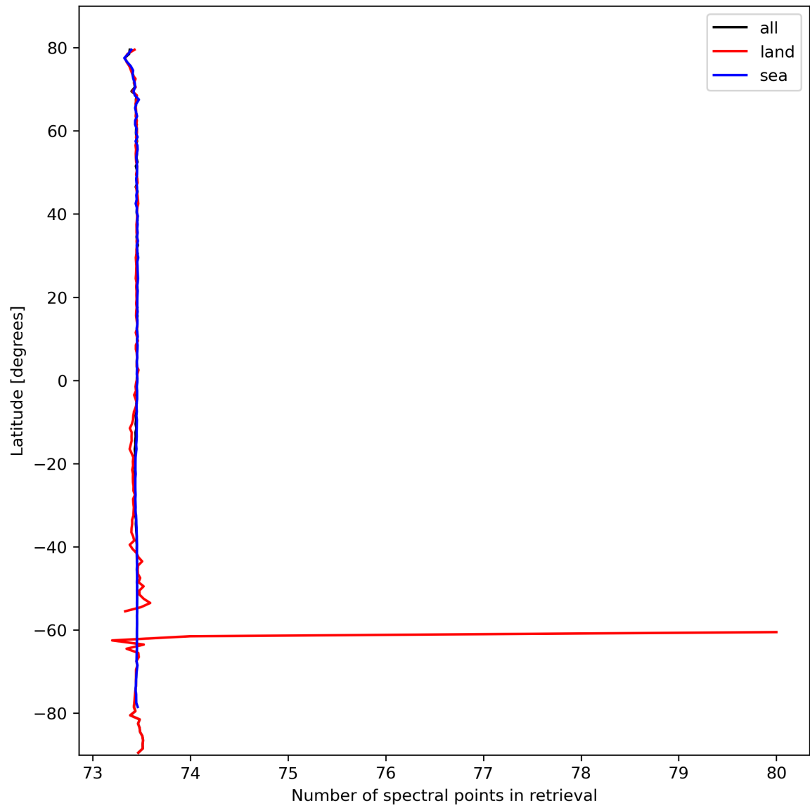
Figure 51: Zonal average of “Number of spectral points in retrieval” for 2024-03-05 to 2024-03-07.
