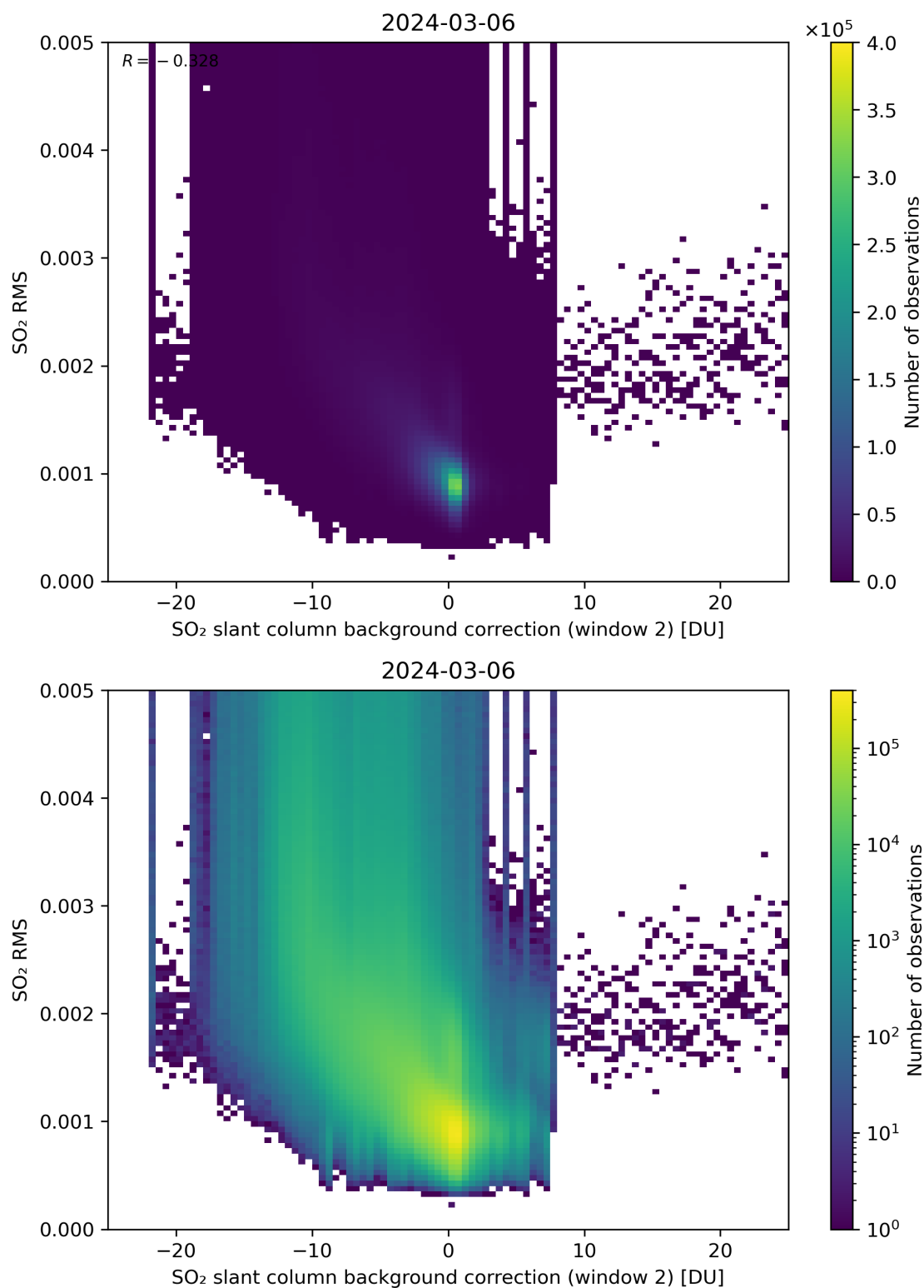
Figure 114: Scatter density plot of “SO 2 slant column background correction (window 2)” against “SO 2 RMS” for 2024-03-05 to 2024-03-07.
