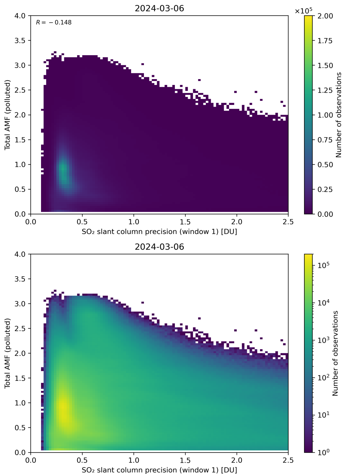
Figure 230: Scatter density plot of “SO 2 slant column precision (window 1)” against “Total AMF (polluted)” for 2024-03-05 to 2024-03-07.
