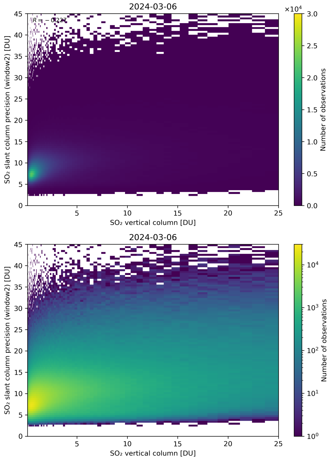
Figure 302: Scatter density plot of “SO 2 vertical column” against “SO 2 slant column precision (window2)” for 2024-03-05 to 2024-03-07.
