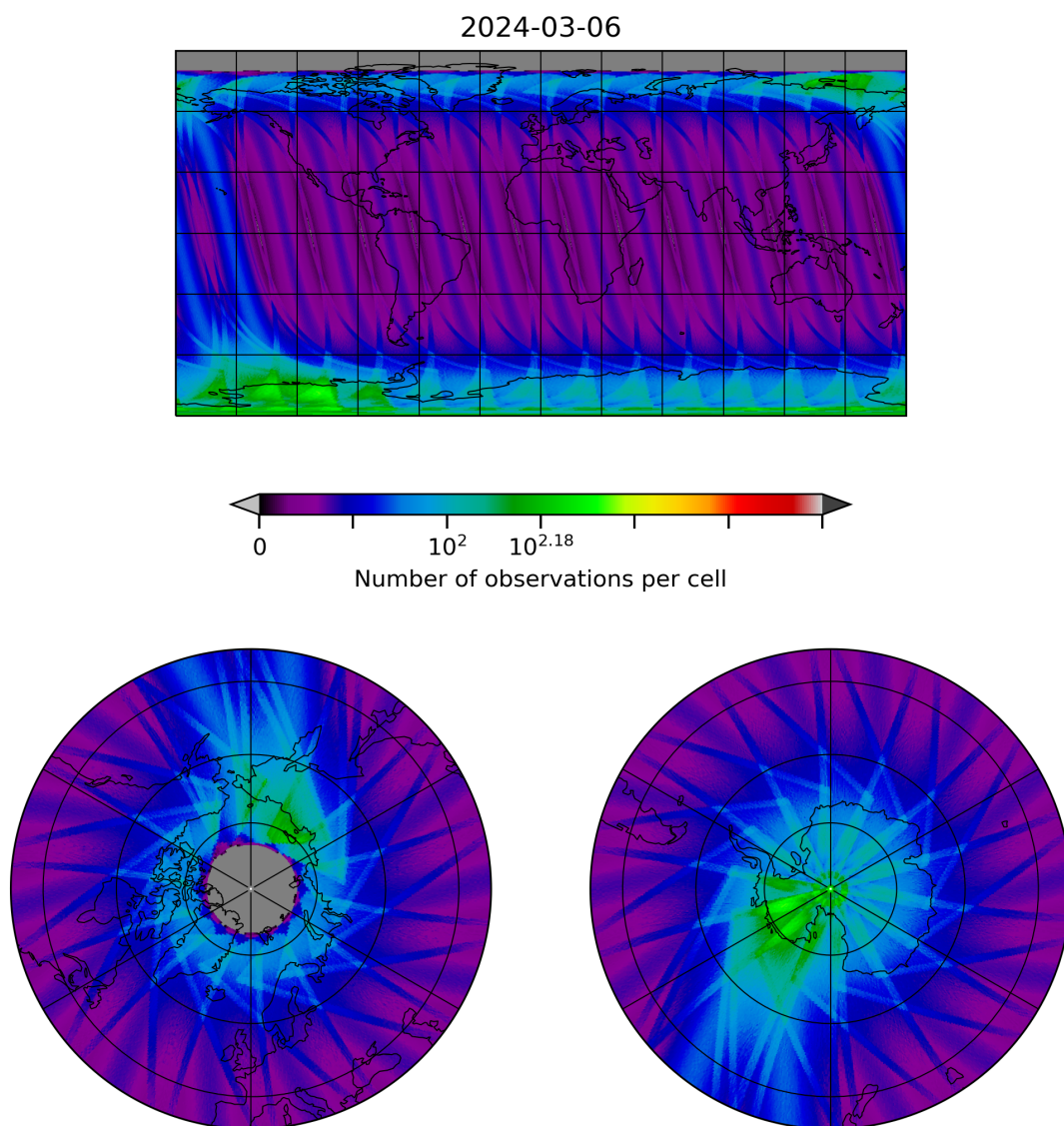
Figure 28: Map of the number of observations for 2024-03-05 to 2024-03-07
