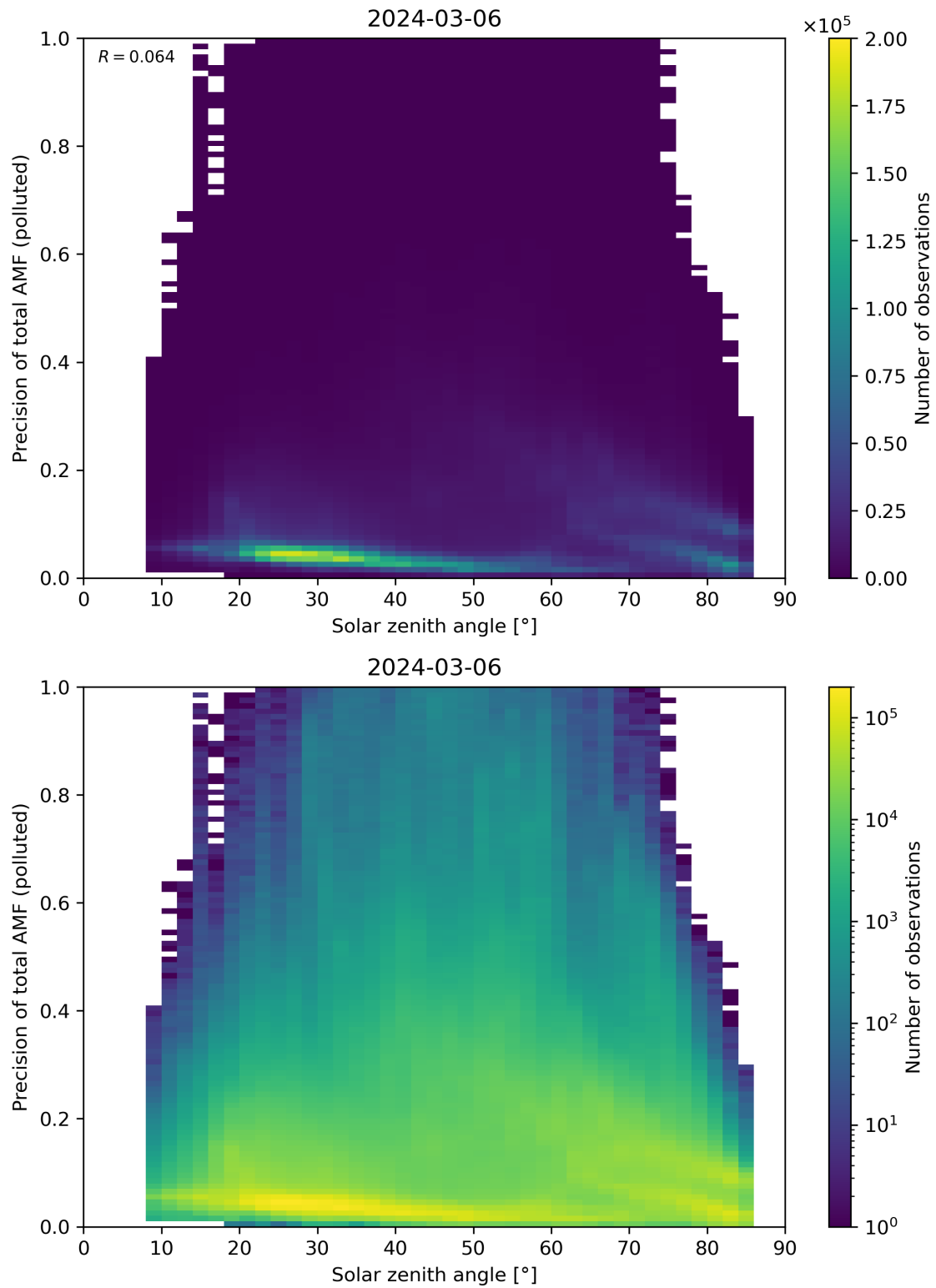
Figure 175: Scatter density plot of “Solar zenith angle” against “Precision of total AMF (polluted)” for 2024-03-05 to 2024-03-07.
