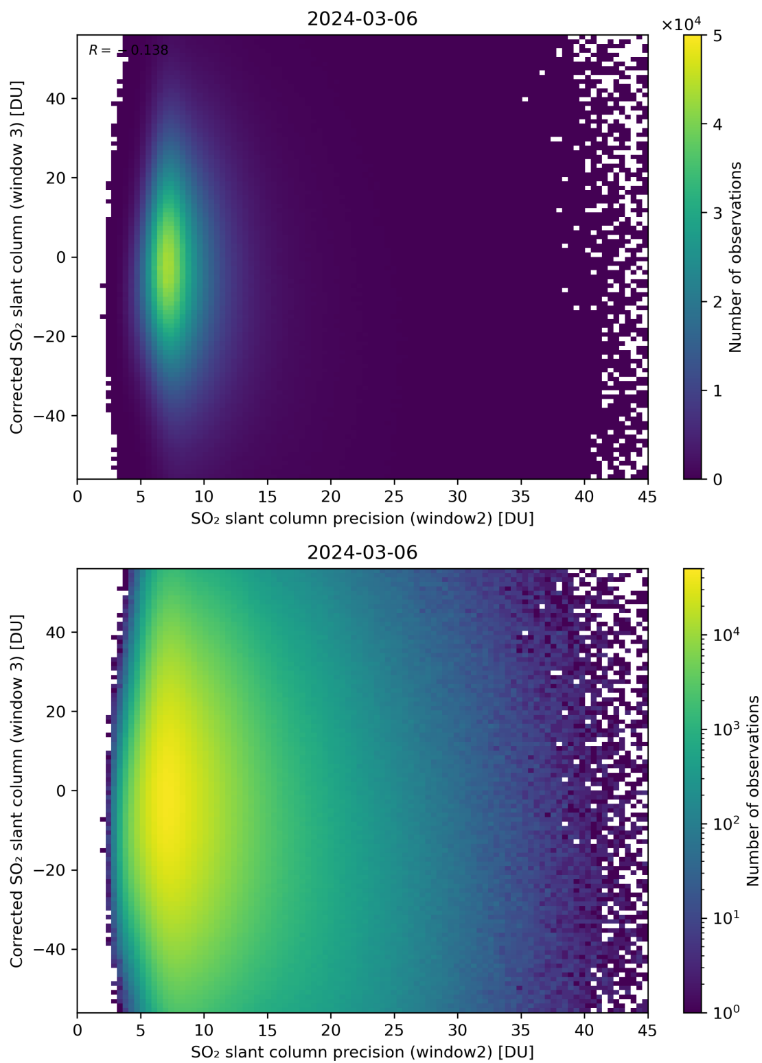
Figure 248: Scatter density plot of “SO 2 slant column precision (window2)” against “Corrected SO 2 slant column (window 3)” for 2024-03-05 to 2024-03-07.
