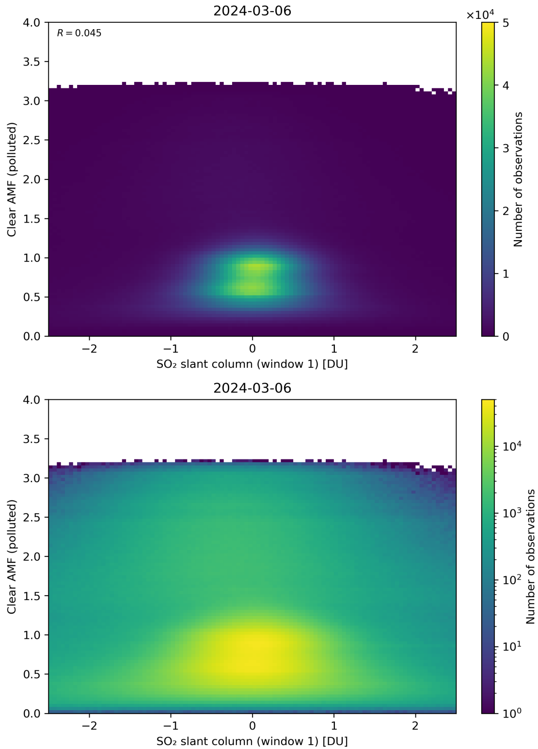
Figure 232: Scatter density plot of “SO 2 slant column (window 1)” against “Clear AMF (polluted)” for 2024-03-05 to 2024-03-07.
