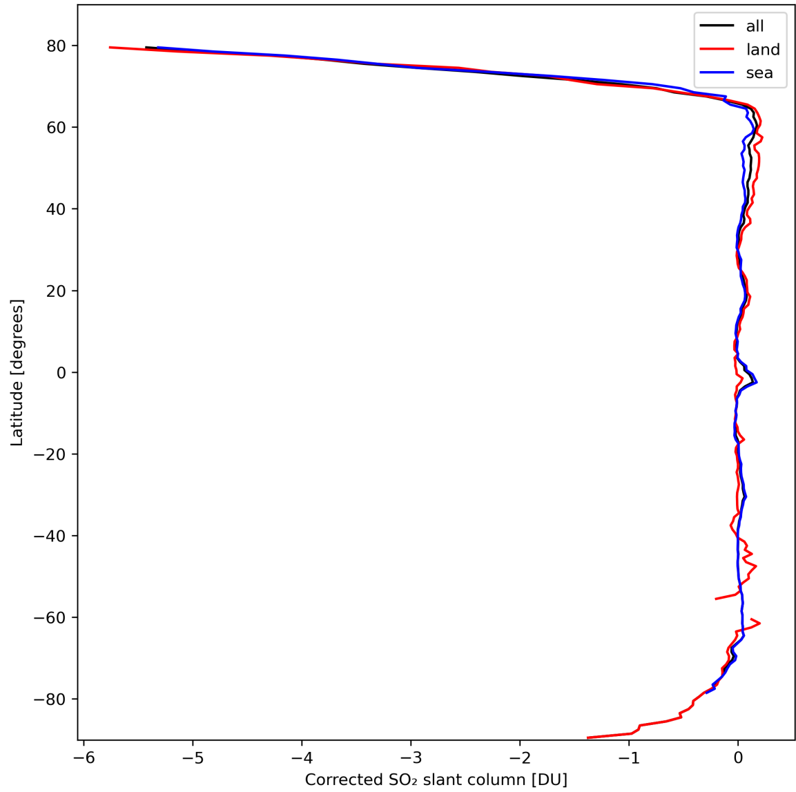
Figure 32: Zonal average of “Corrected SO 2 slant column” for 2024-03-05 to 2024-03-07.
