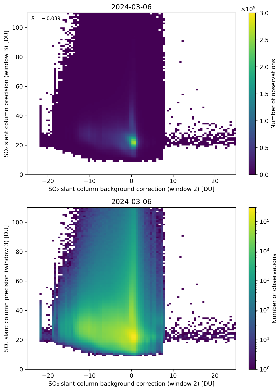
Figure 118: Scatter density plot of “SO 2 slant column background correction (window 2)” against “SO 2 slant column precision (window 3)” for 2024-03-05 to 2024-03-07.
