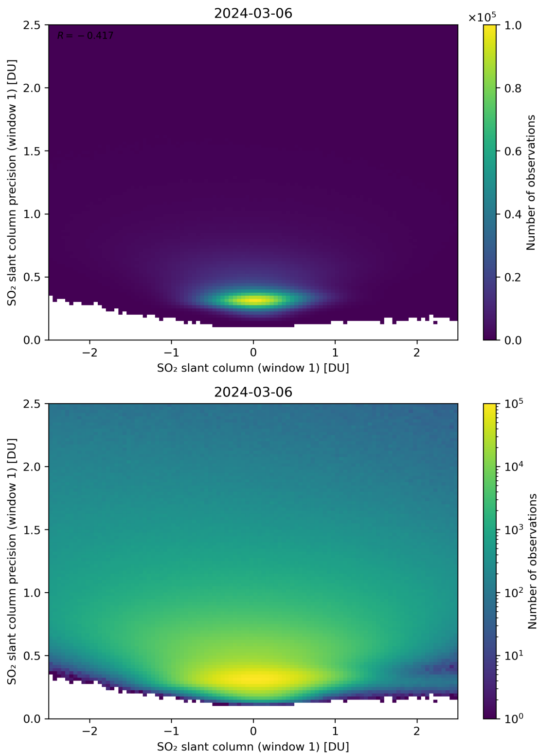
Figure 235: Scatter density plot of “SO 2 slant column (window 1)” against “SO 2 slant column precision (window 1)” for 2024-03-05 to 2024-03-07.
