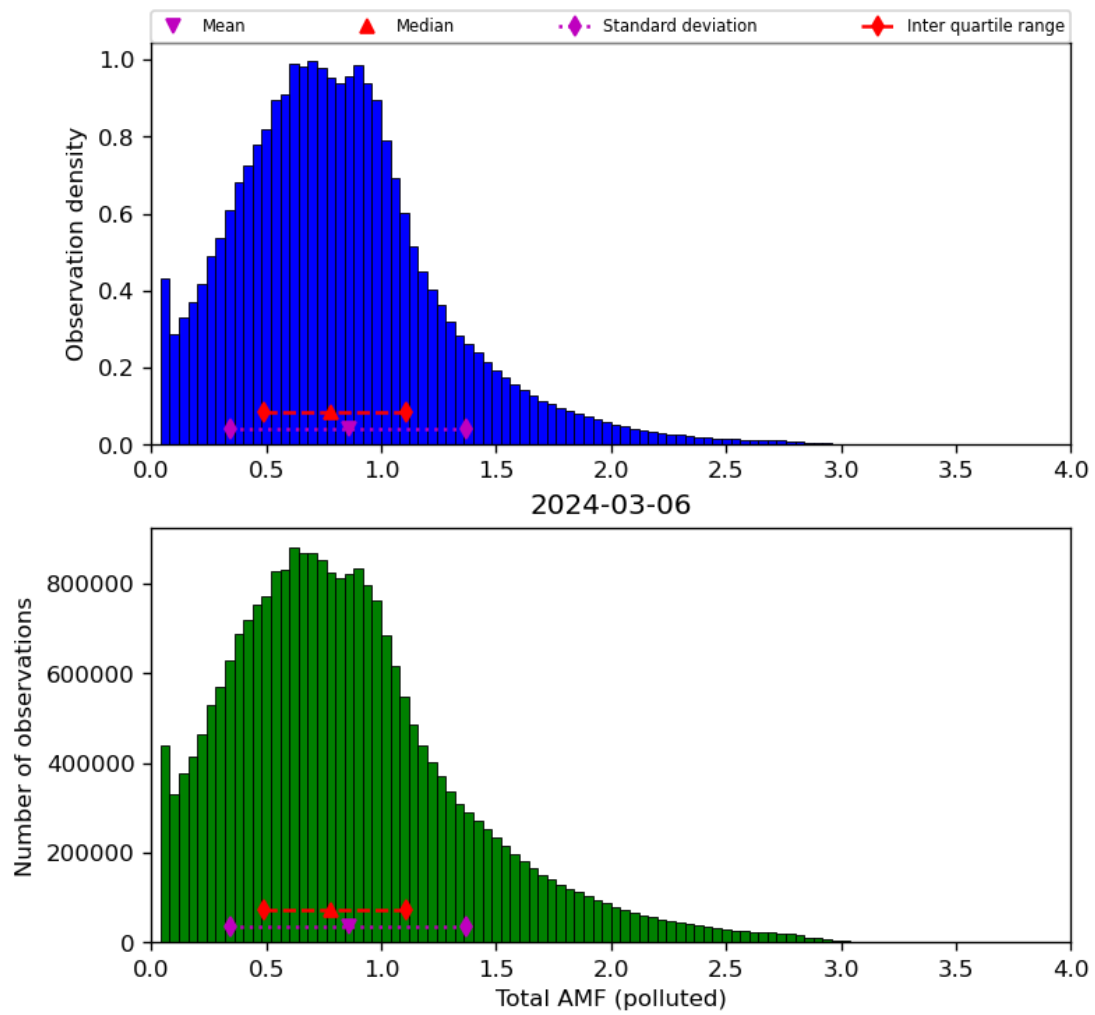
Figure 71: Histogram of “Total AMF (polluted)” for 2024-03-05 to 2024-03-07
