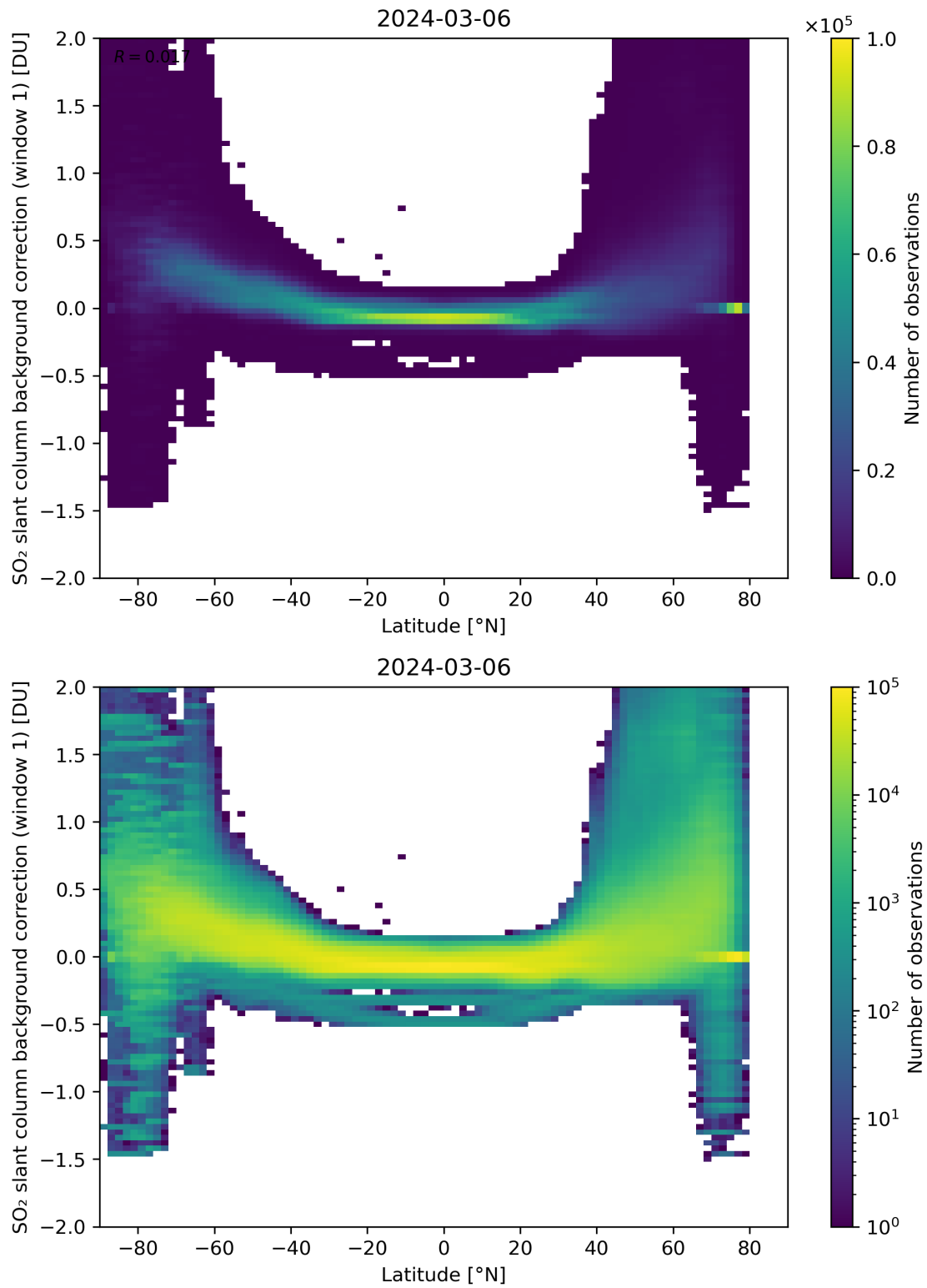
Figure 139: Scatter density plot of “Latitude” against “SO 2 slant column background correction (window 1)” for 2024-03-05 to 2024-03-07.
