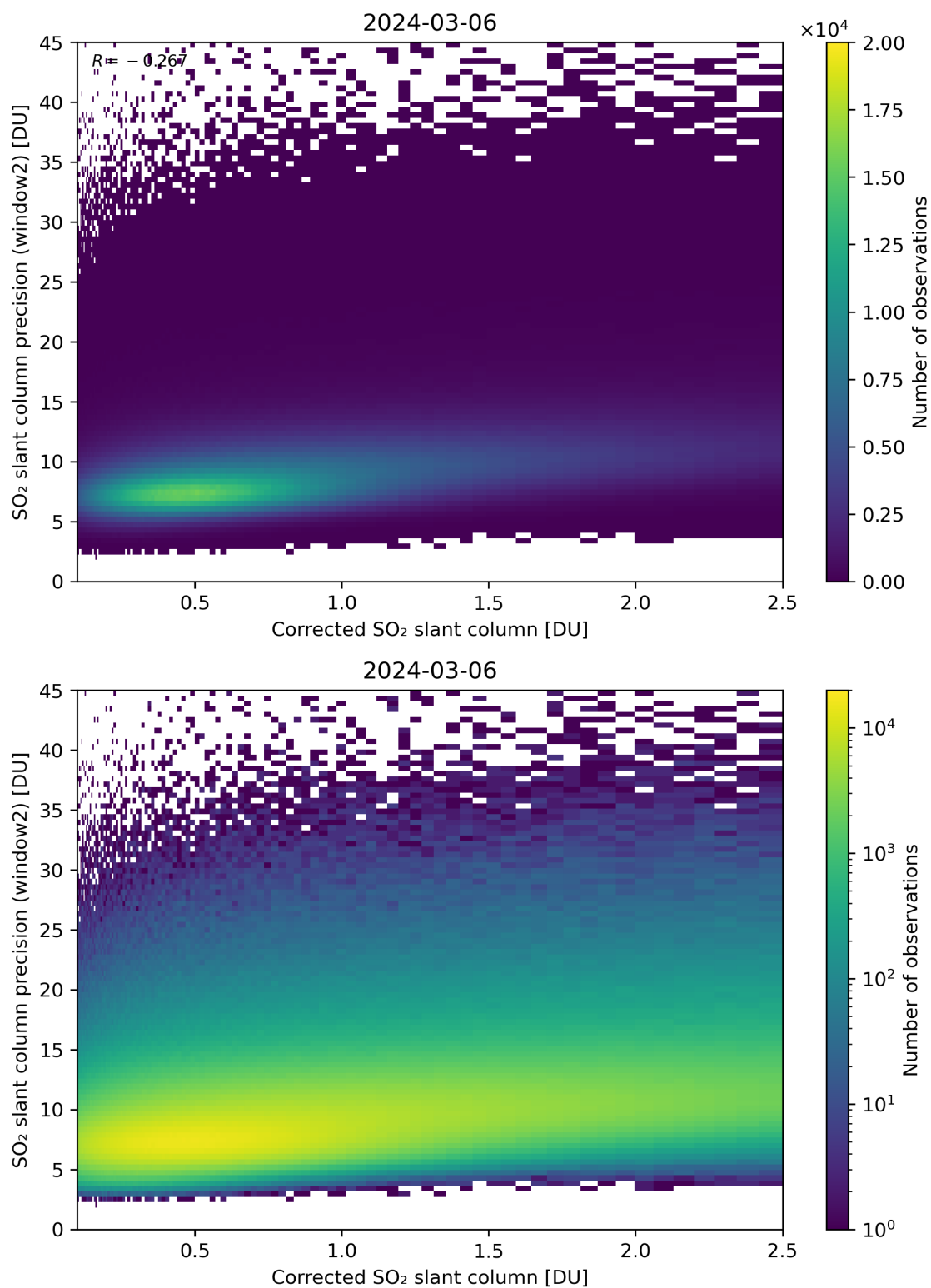
Figure 189: Scatter density plot of “Corrected SO 2 slant column” against “SO 2 slant column precision (window2)” for 2024-03-05 to 2024-03-07.
