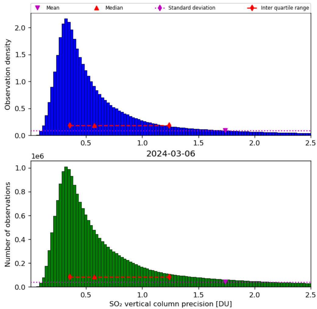
Figure 54: Histogram of “SO 2 vertical column precision” for 2024-03-05 to 2024-03-07
