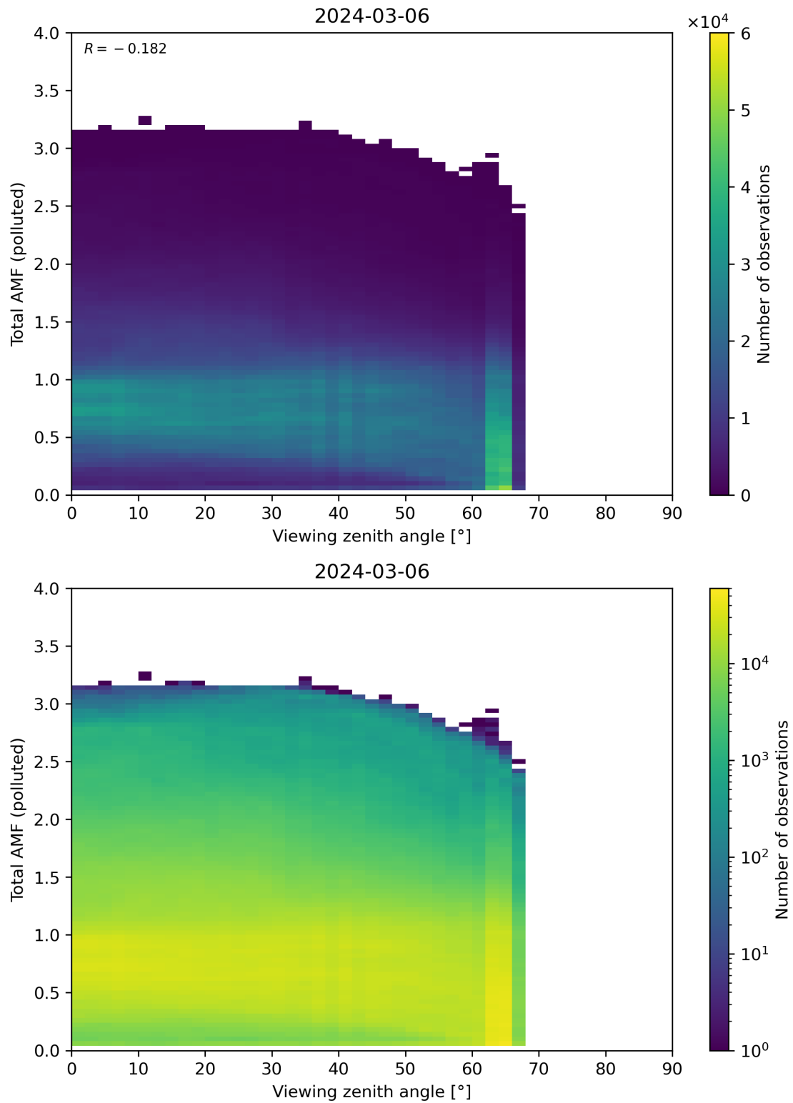
Figure 325: Scatter density plot of “Viewing zenith angle” against “Total AMF (polluted)” for 2024-03-05 to 2024-03-07.
