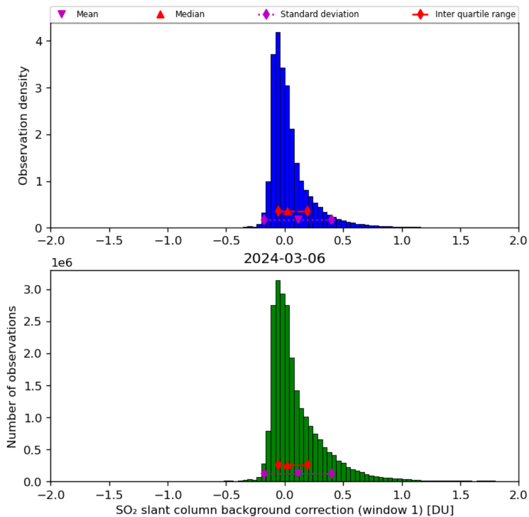
Figure 59: Histogram of “SO 2 slant column background correction (window 1)” for 2024-03-05 to 2024-03-07
