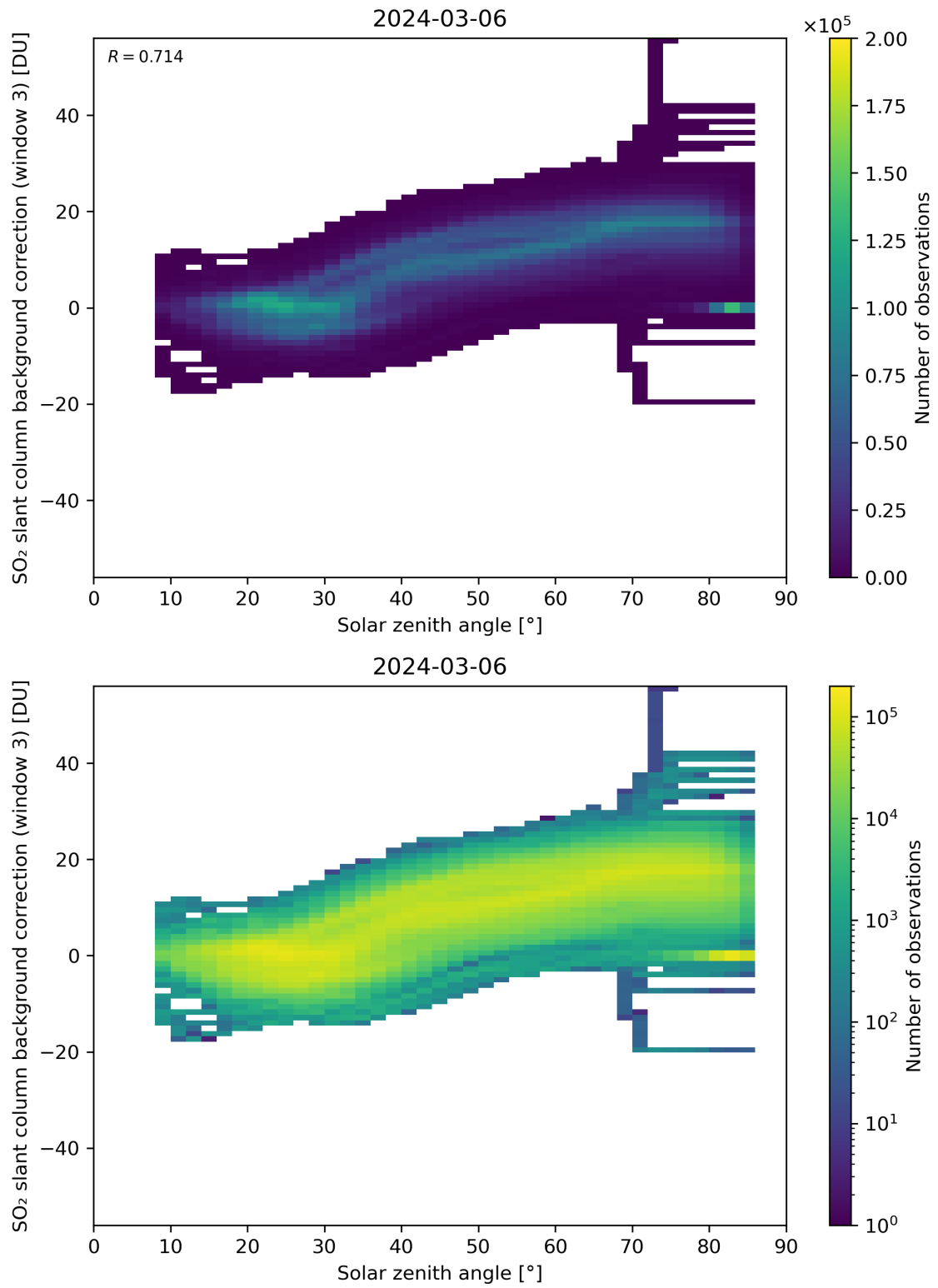
Figure 160: Scatter density plot of “Solar zenith angle” against “SO 2 slant column background correction (window 3)” for 2024-03-05 to 2024-03-07.
