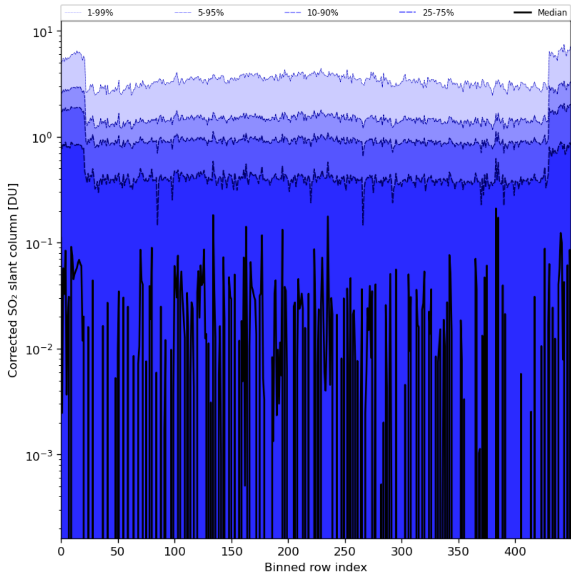
Figure 78: Along track statistics of “Corrected SO 2 slant column” for 2024-03-05 to 2024-03-07
