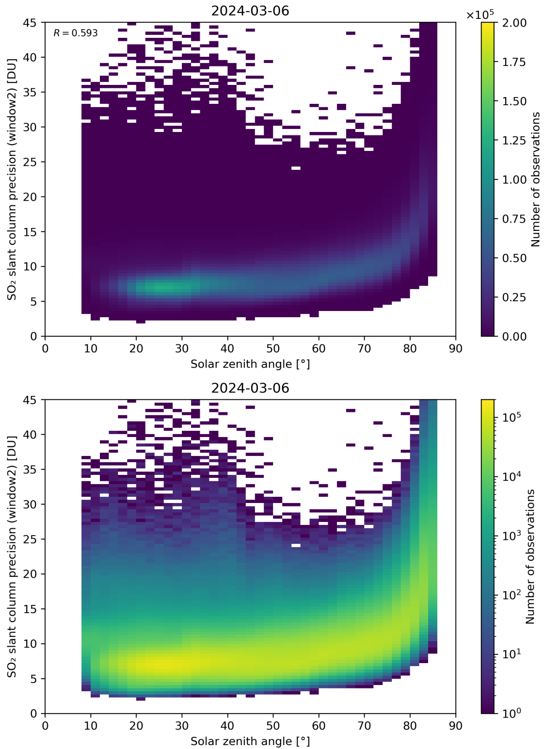
Figure 171: Scatter density plot of “Solar zenith angle” against “SO 2 slant column precision (window2)” for 2024-03-05 to 2024-03-07.
