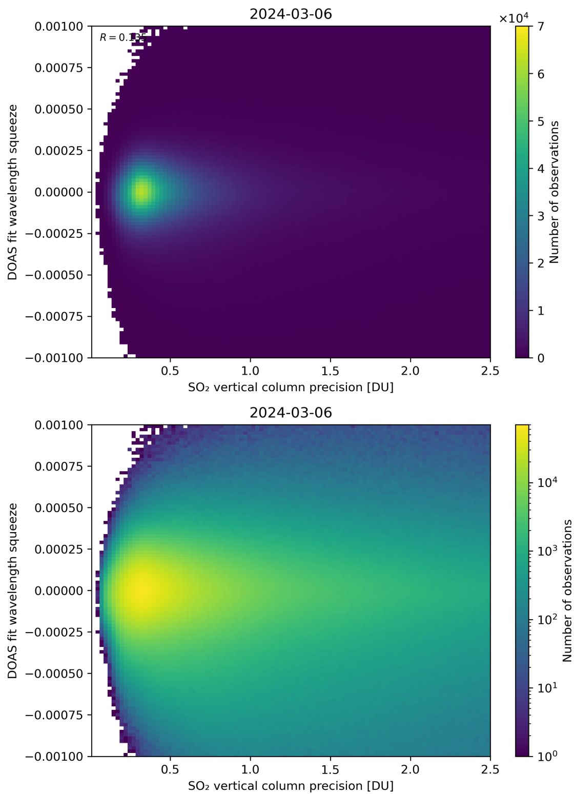
Figure 283: Scatter density plot of “SO 2 vertical column precision” against “DOAS fit wavelength squeeze” for 2024-03-05 to 2024-03-07.
