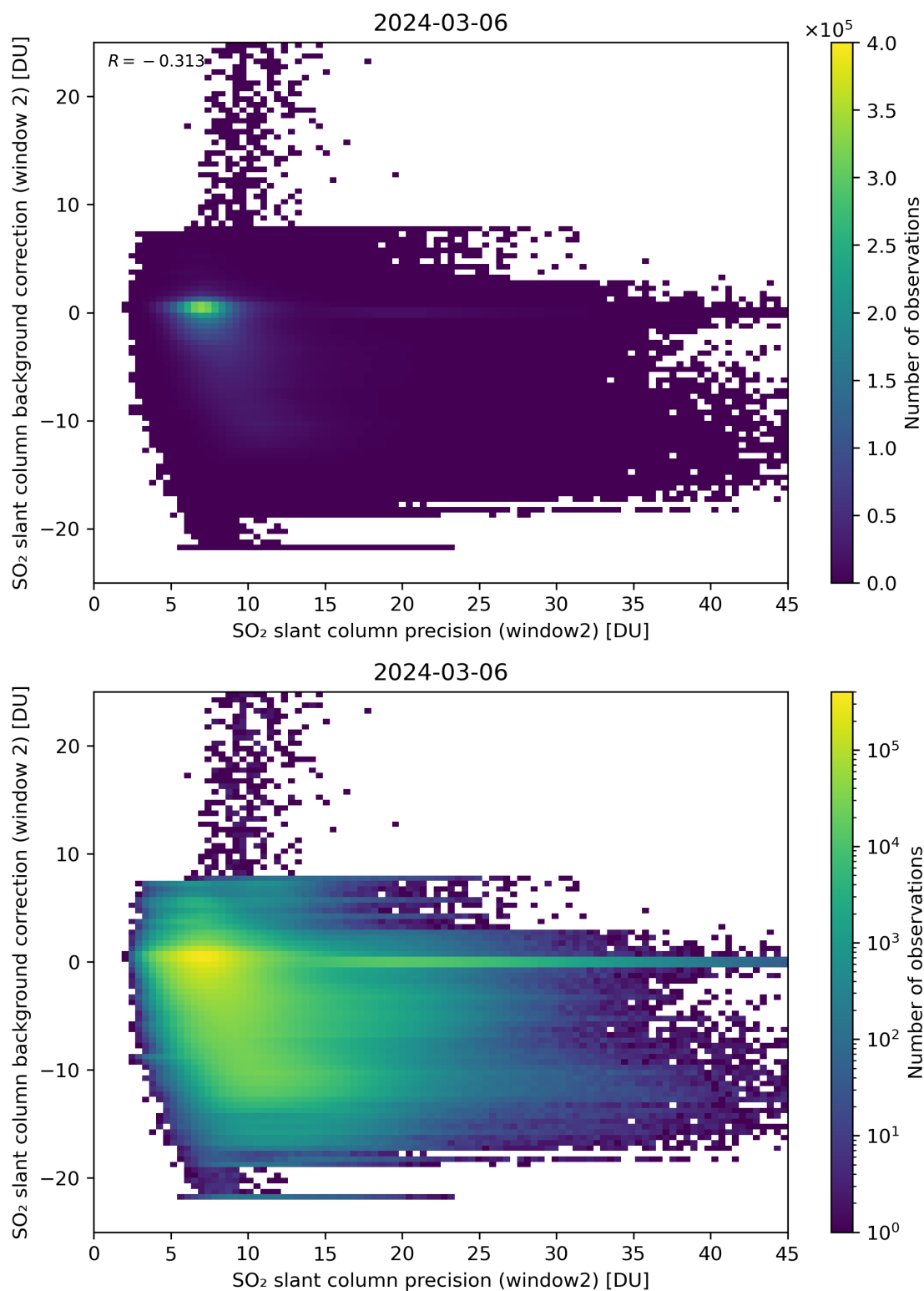
Figure 241: Scatter density plot of “SO 2 slant column precision (window2)” against “SO 2 slant column background correction (window 2)” for 2024-03-05 to 2024-03-07.
