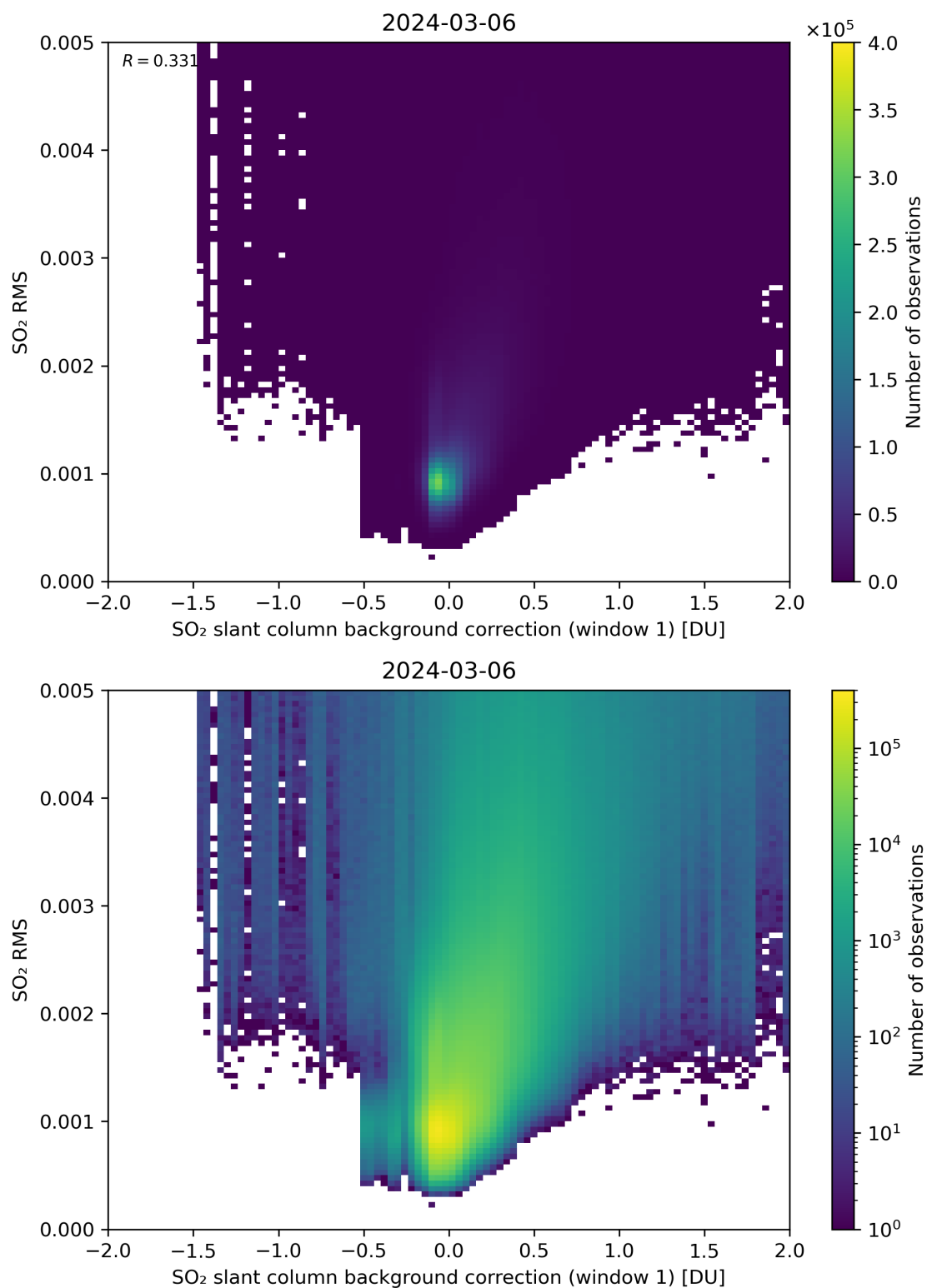
Figure 102: Scatter density plot of “SO 2 slant column background correction (window 1)” against “SO 2 RMS” for 2024-03-05 to 2024-03-07.
