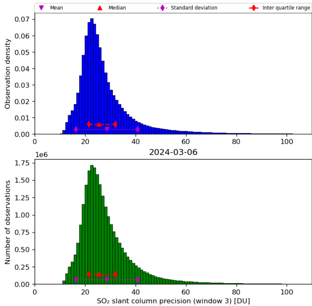
Figure 65: Histogram of “SO 2 slant column precision (window 3)” for 2024-03-05 to 2024-03-07
