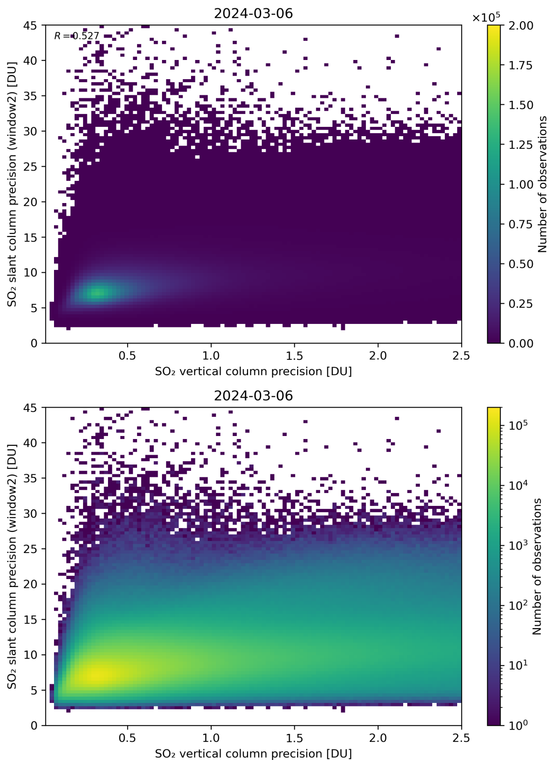
Figure 291: Scatter density plot of “SO 2 vertical column precision” against “SO 2 slant column precision (window2)” for 2024-03-05 to 2024-03-07.
