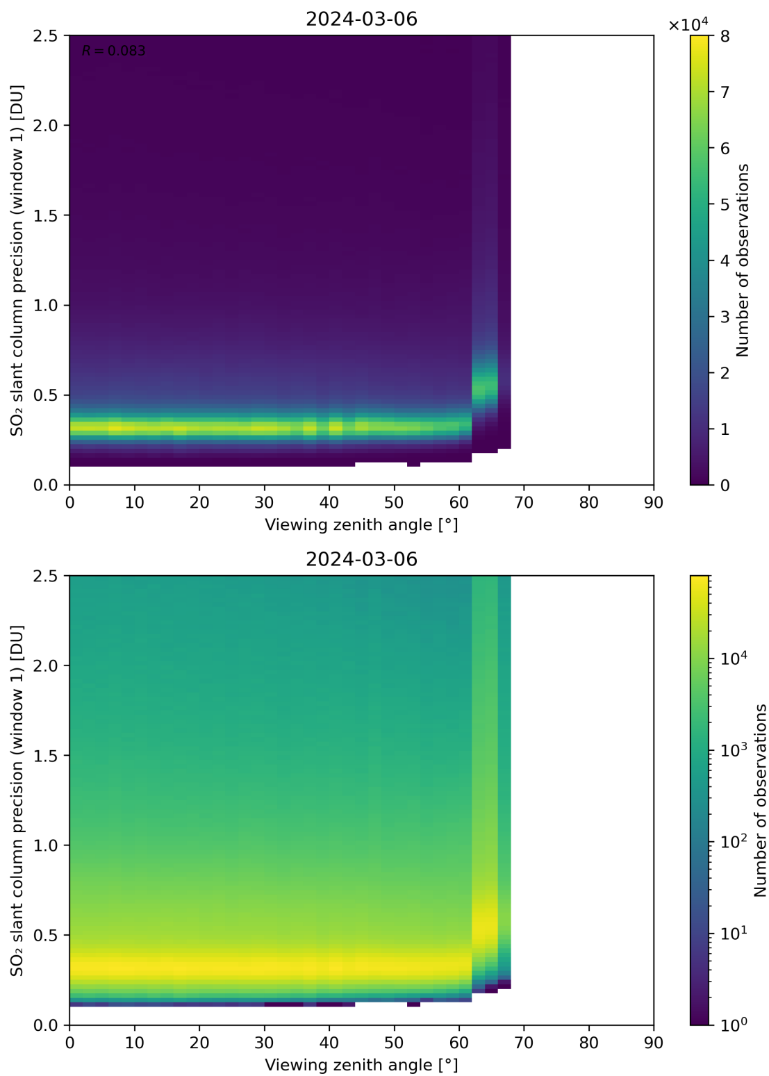
Figure 321: Scatter density plot of “Viewing zenith angle” against “SO 2 slant column precision (window 1)” for 2024-03-05 to 2024-03-07.
