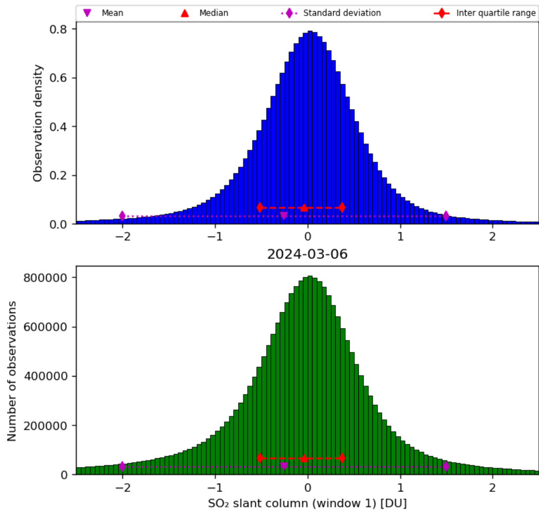
Figure 56: Histogram of “SO 2 slant column (window 1)” for 2024-03-05 to 2024-03-07
