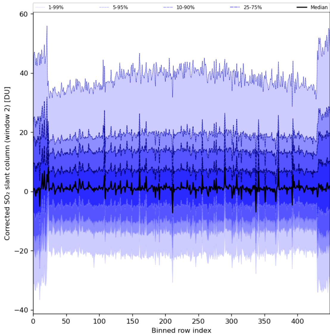
Figure 85: Along track statistics of “Corrected SO 2 slant column (window 2)” for 2024-03-05 to 2024-03-07
