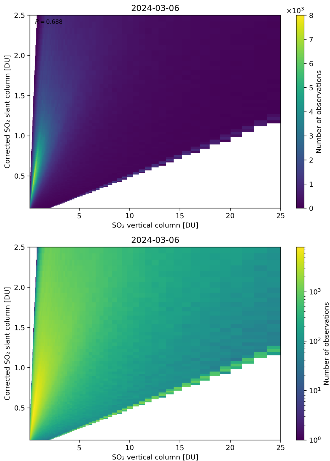
Figure 297: Scatter density plot of “SO 2 vertical column” against “Corrected SO 2 slant column” for 2024-03-05 to 2024-03-07.
