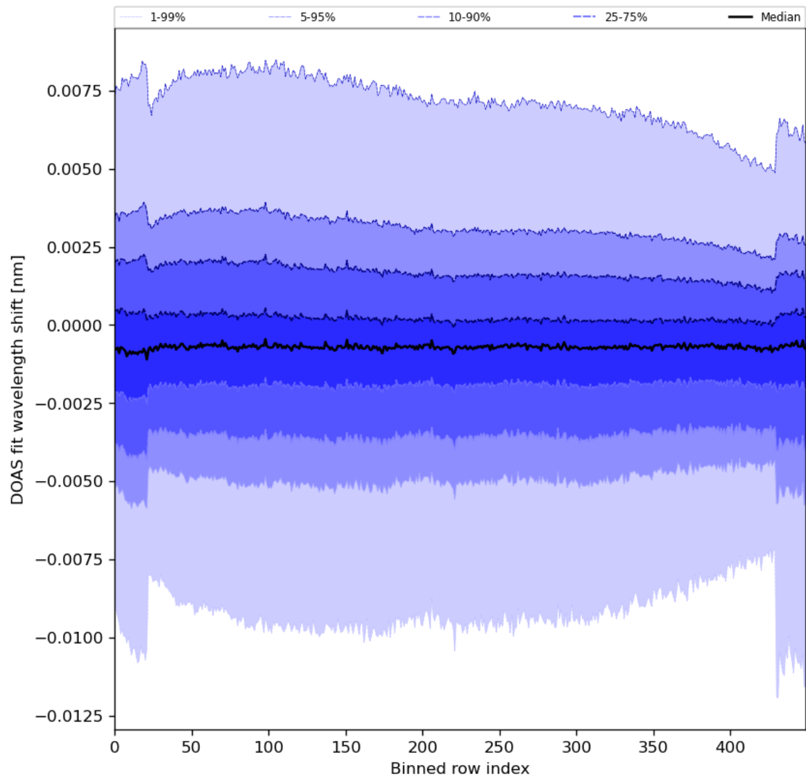
Figure 91: Along track statistics of “DOAS fit wavelength shift” for 2024-03-05 to 2024-03-07
