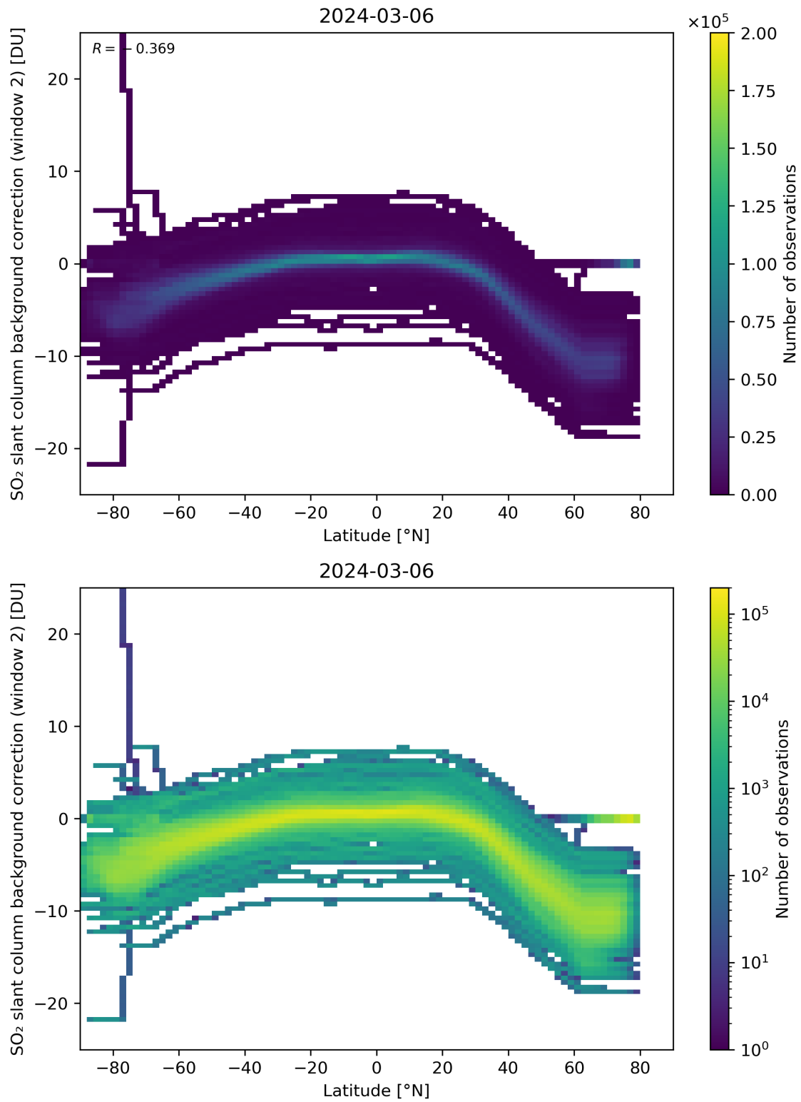
Figure 140: Scatter density plot of “Latitude” against “SO 2 slant column background correction (window 2)” for 2024-03-05 to 2024-03-07.
