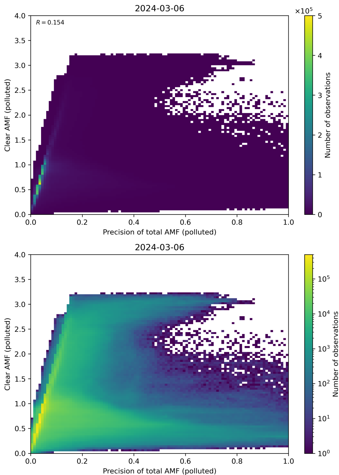
Figure 270: Scatter density plot of “Precision of total AMF (polluted)” against “Clear AMF (polluted)” for 2024-03-05 to 2024-03-07.
