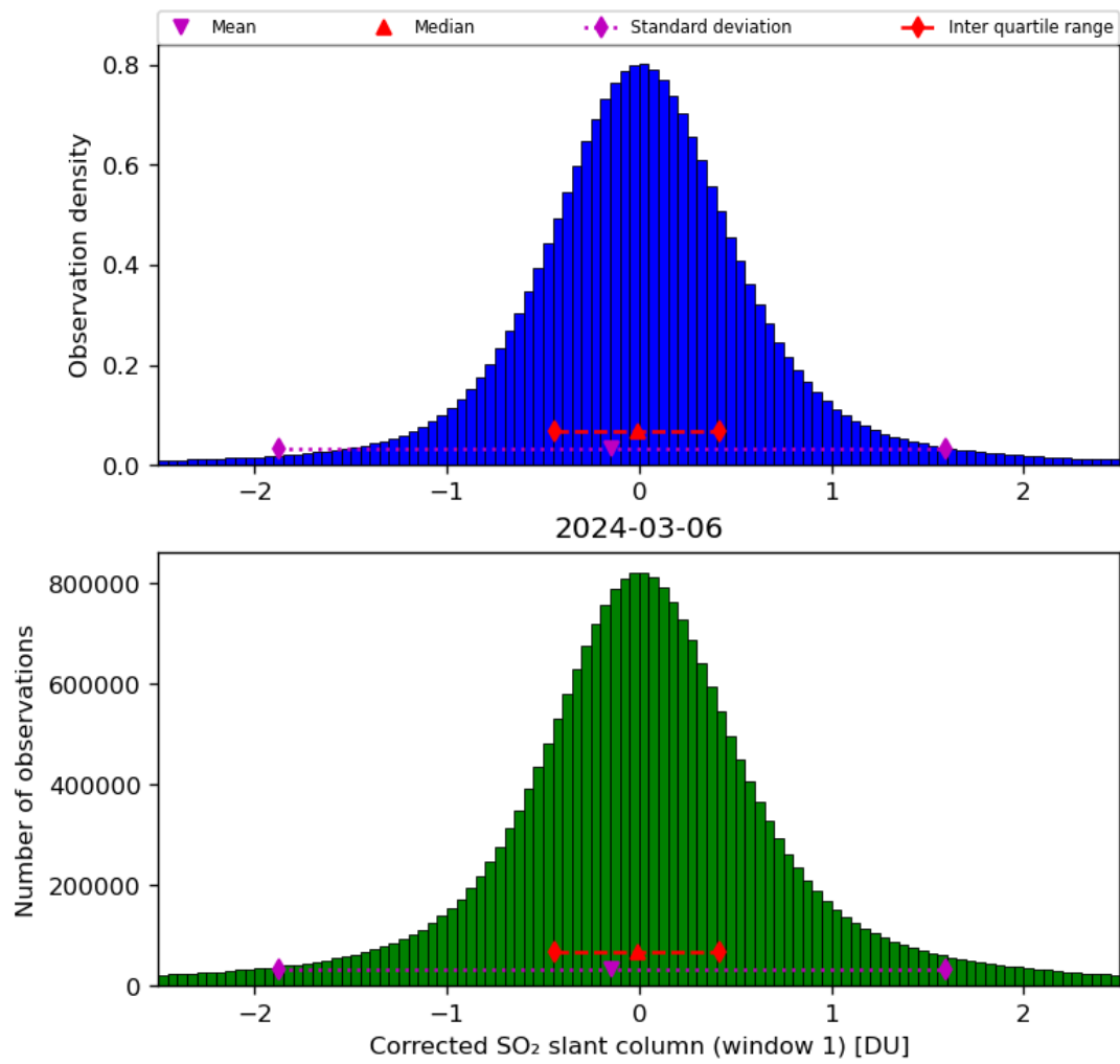
Figure 58: Histogram of “Corrected SO 2 slant column (window 1)” for 2024-03-05 to 2024-03-07
