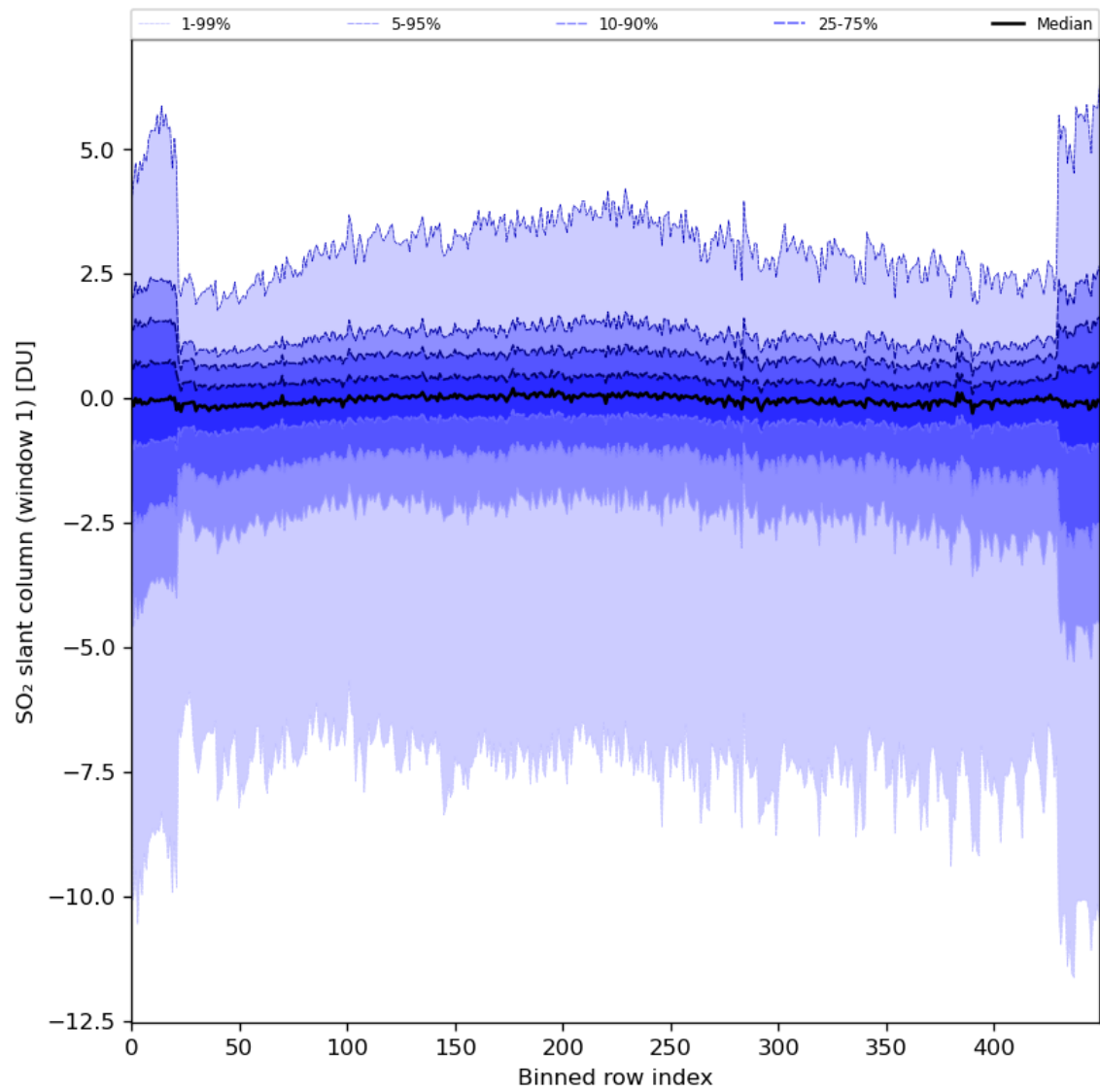
Figure 79: Along track statistics of "SO 2 slant column (window 1)" for 2024-03-05 to 2024-03-07
