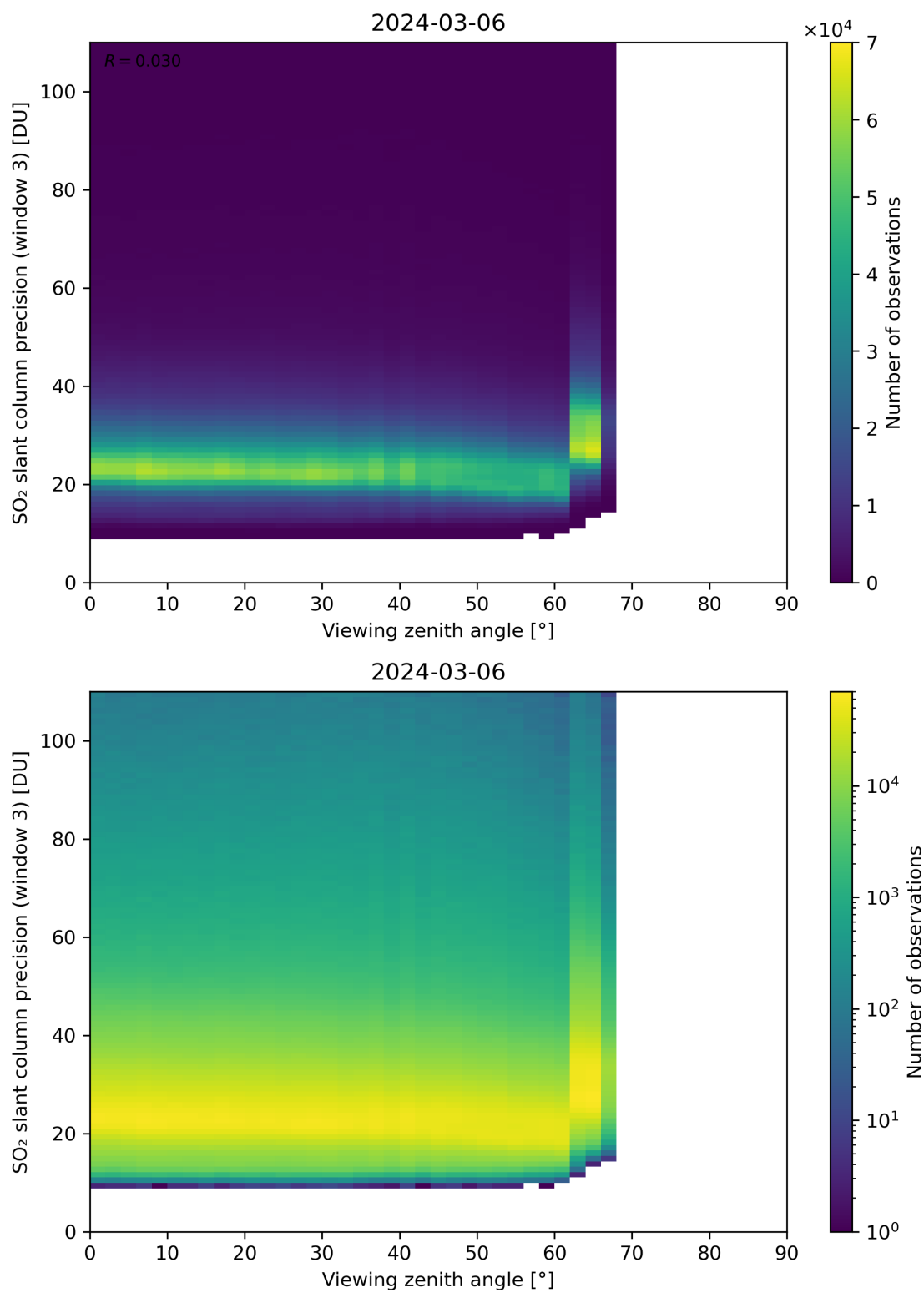
Figure 324: Scatter density plot of “Viewing zenith angle” against “SO 2 slant column precision (window 3)” for 2024-03-05 to 2024-03-07.
