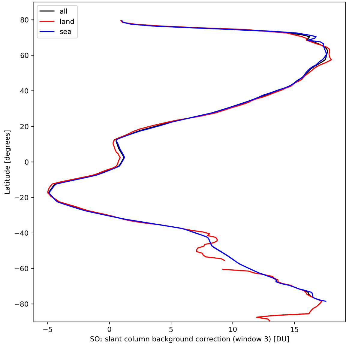
Figure 44: Zonal average of “SO 2 slant column background correction (window 3)” for 2024-03-05 to 2024-03-07.
