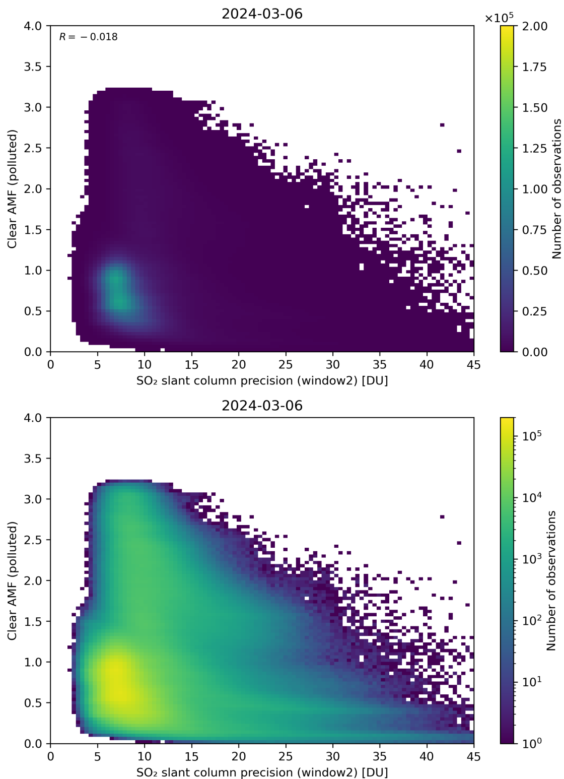
Figure 246: Scatter density plot of “SO 2 slant column precision (window2)” against “Clear AMF (polluted)” for 2024-03-05 to 2024-03-07.
