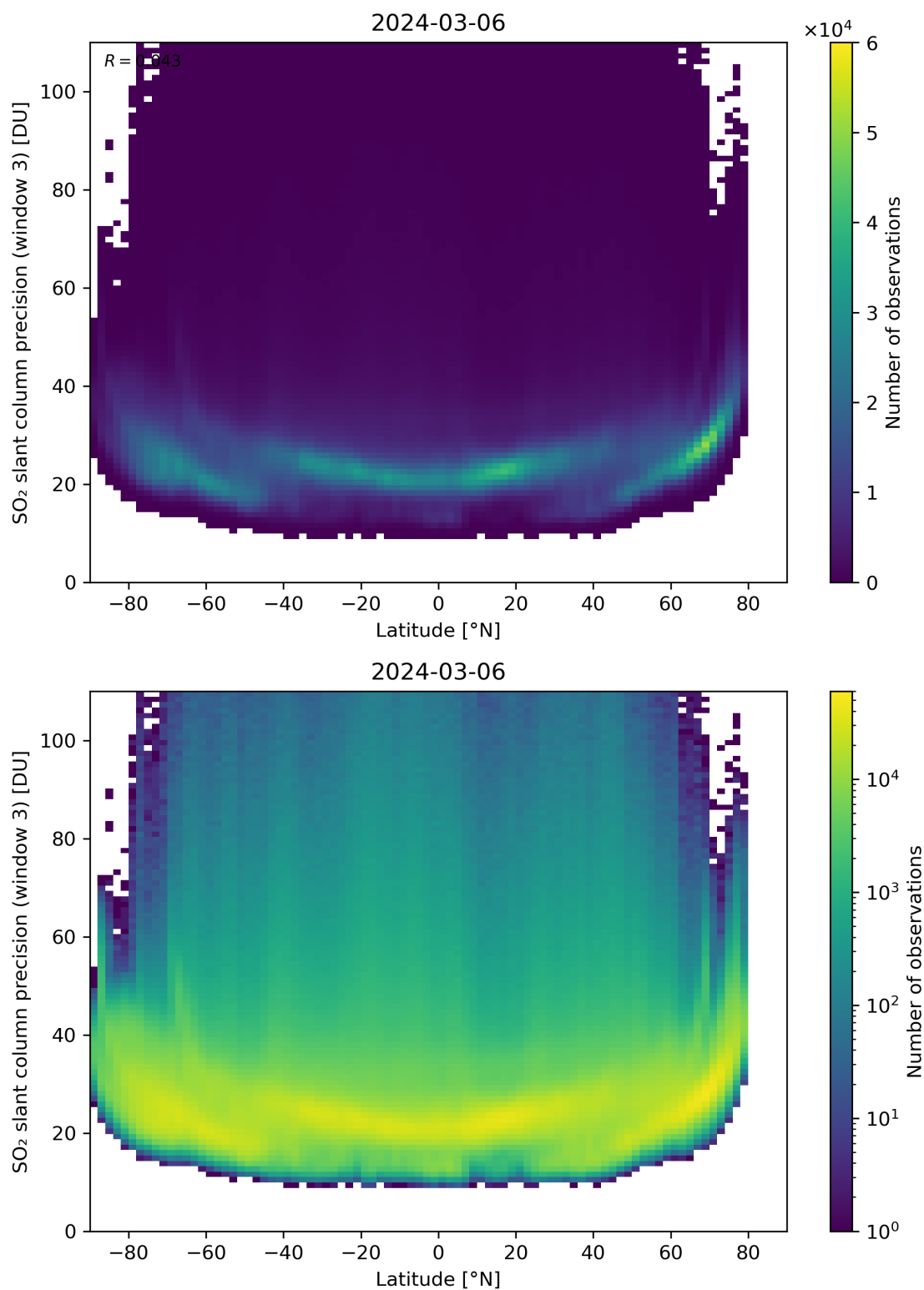
Figure 153: Scatter density plot of “Latitude” against “SO 2 slant column precision (window 3)” for 2024-03-05 to 2024-03-07.
