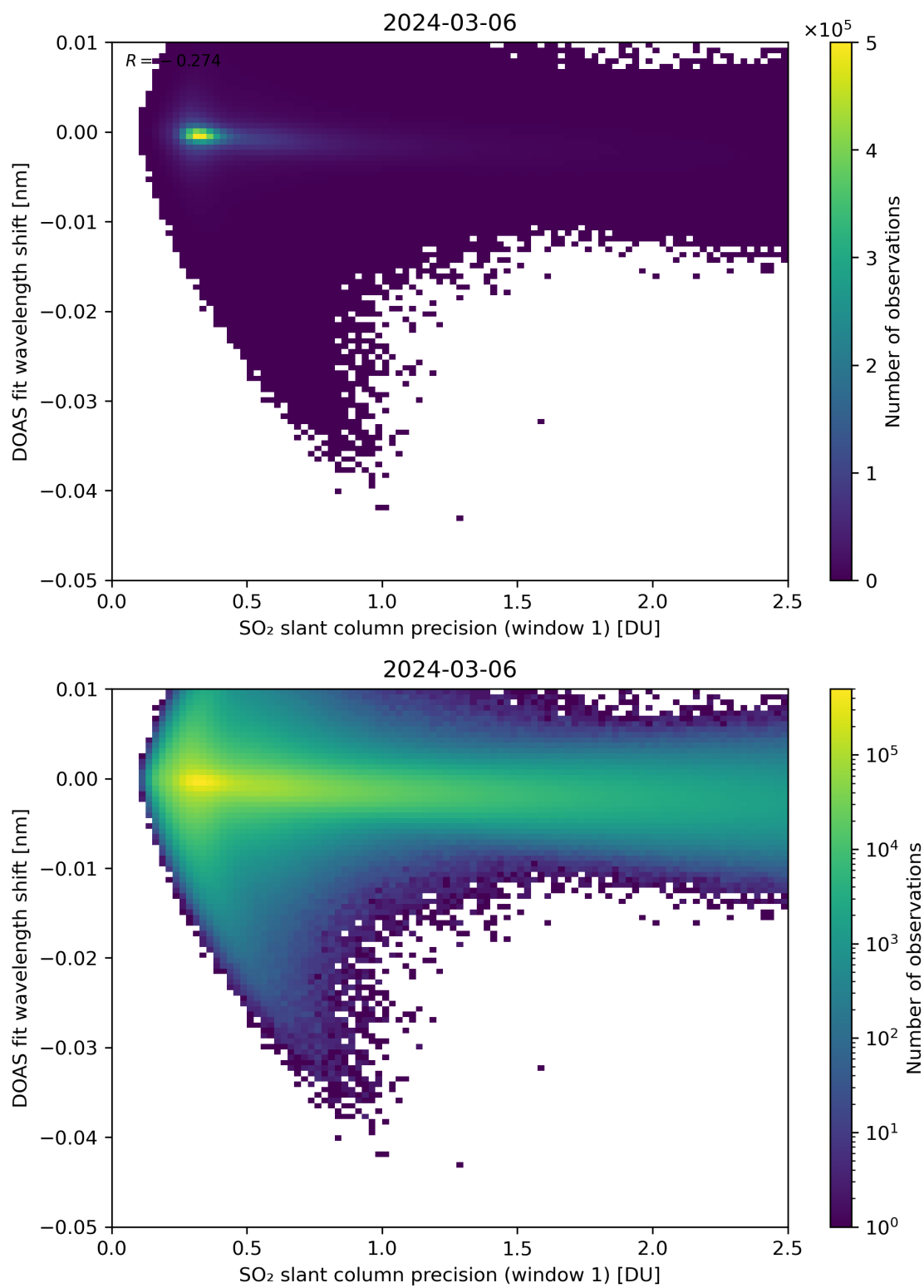
Figure 221: Scatter density plot of “SO 2 slant column precision (window 1)” against “DOAS fit wavelength shift” for 2024-03-05 to 2024-03-07.
