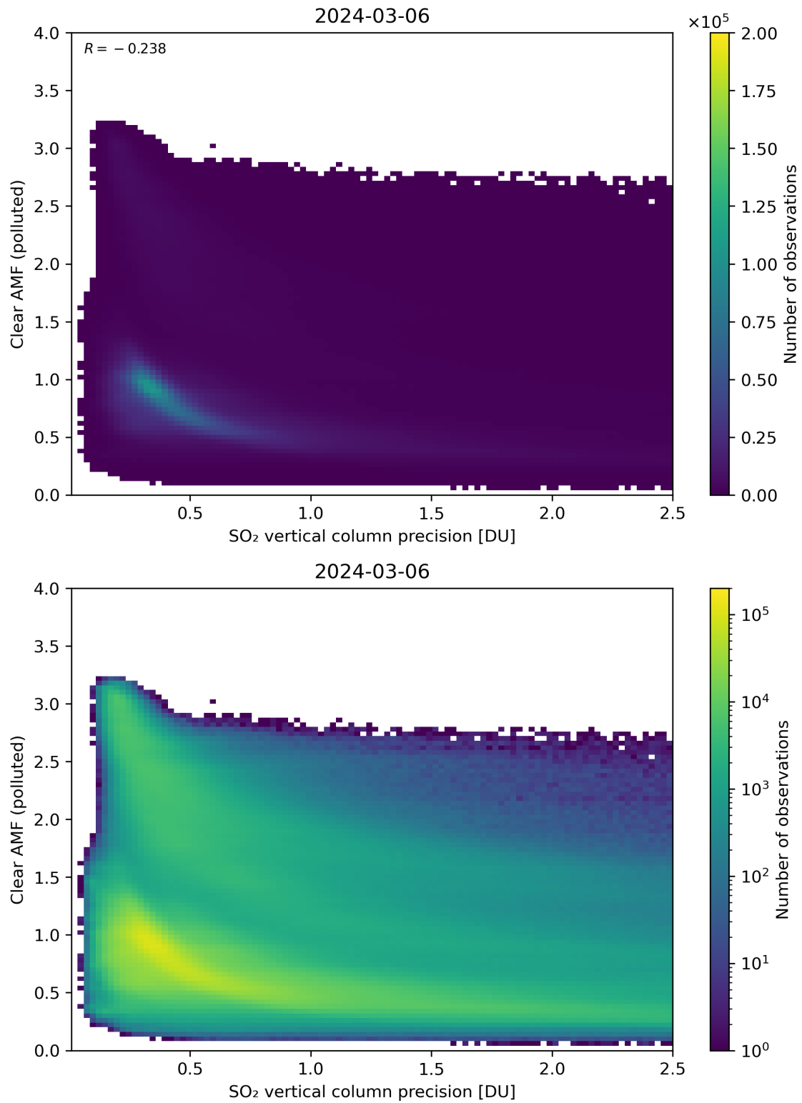
Figure 285: Scatter density plot of “SO 2 vertical column precision” against “Clear AMF (polluted)” for 2024-03-05 to 2024-03-07.
