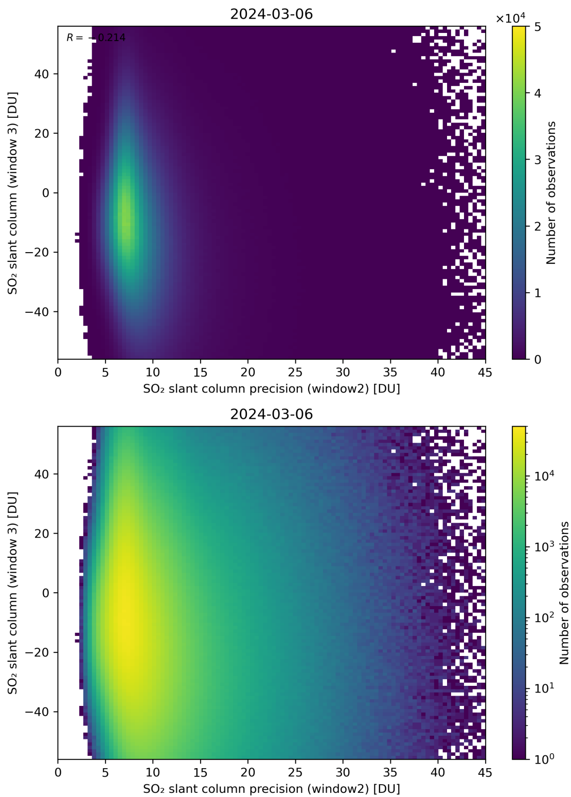
Figure 249: Scatter density plot of “SO 2 slant column precision (window2)” against “SO 2 slant column (window 3)” for 2024-03-05 to 2024-03-07.
