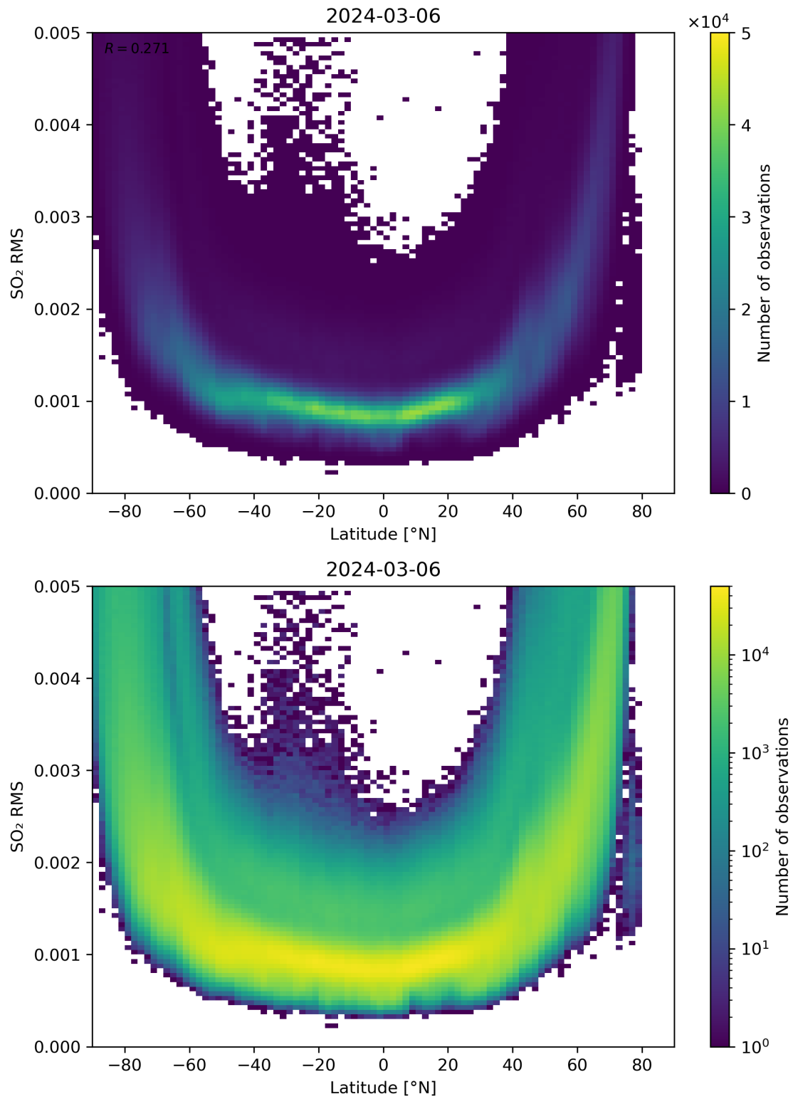
Figure 144: Scatter density plot of “Latitude” against “SO 2 RMS” for 2024-03-05 to 2024-03-07.
