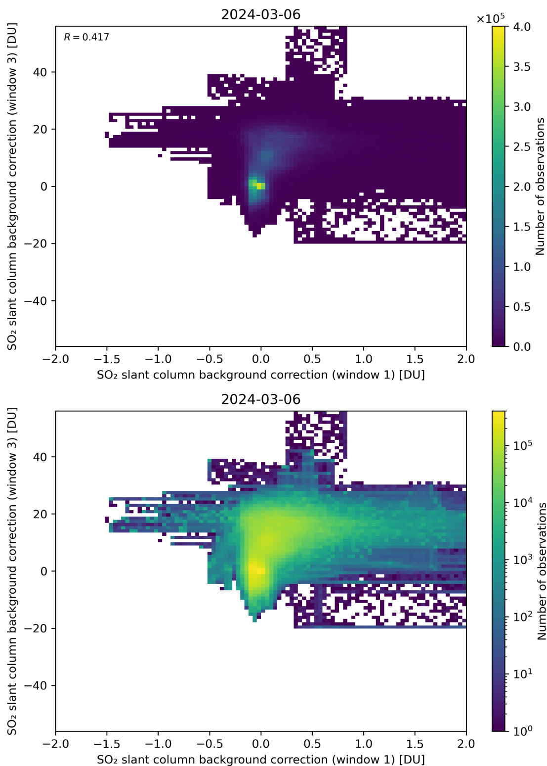
Figure 99: Scatter density plot of “SO 2 slant column background correction (window 1)” against “SO 2 slant column background correction (window 3)” for 2024-03-05 to 2024-03-07.
