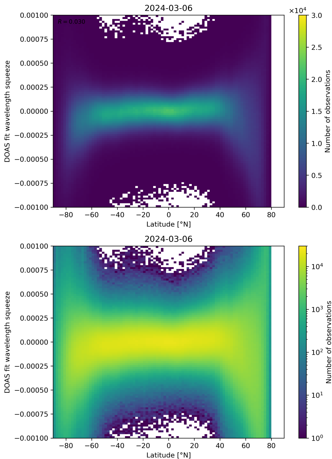
Figure 143: Scatter density plot of “Latitude” against “DOAS fit wavelength squeeze” for 2024-03-05 to 2024-03-07.
