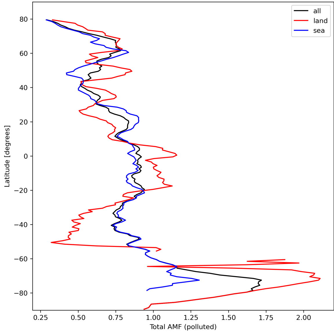
Figure 48: Zonal average of “Total AMF (polluted)” for 2024-03-05 to 2024-03-07.
