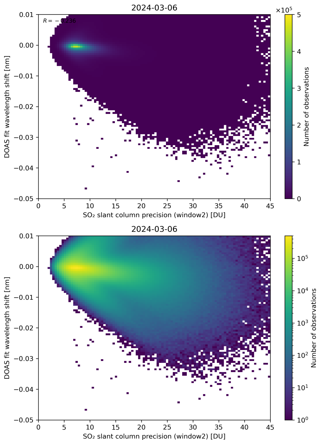
Figure 243: Scatter density plot of “SO 2 slant column precision (window2)” against “DOAS fit wavelength shift” for 2024-03-05 to 2024-03-07.
