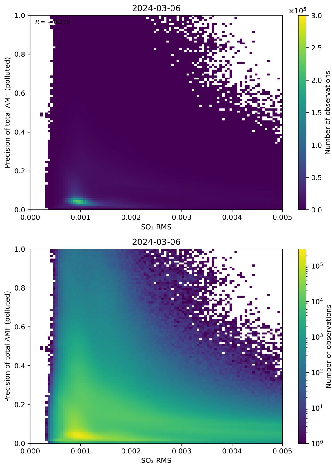
Figure 138: Scatter density plot of “SO 2 RMS” against “Precision of total AMF (polluted)” for 2024-03-05 to 2024-03-07.
