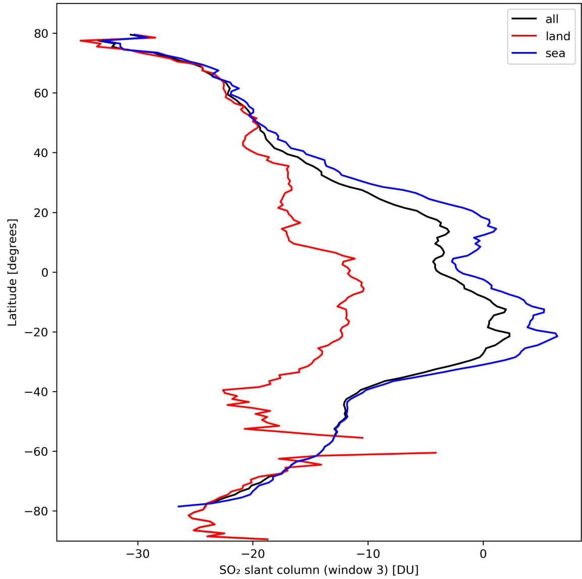
Figure 41: Zonal average of “SO 2 slant column (window 3)” for 2024-03-05 to 2024-03-07.
