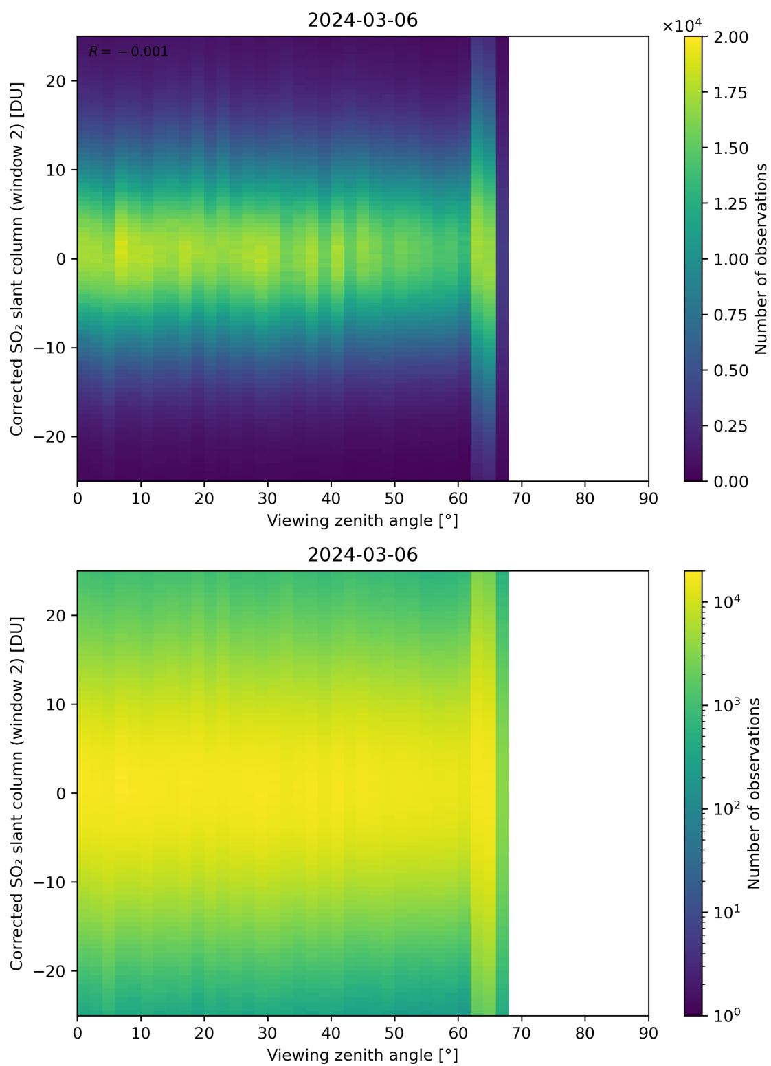
Figure 318: Scatter density plot of “Viewing zenith angle” against “Corrected SO 2 slant column (window 2)” for 2024-03-05 to 2024-03-07.
