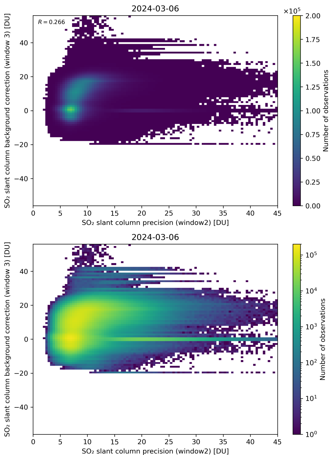
Figure 242: Scatter density plot of “SO 2 slant column precision (window2)” against “SO 2 slant column background correction (window 3)” for 2024-03-05 to 2024-03-07.
