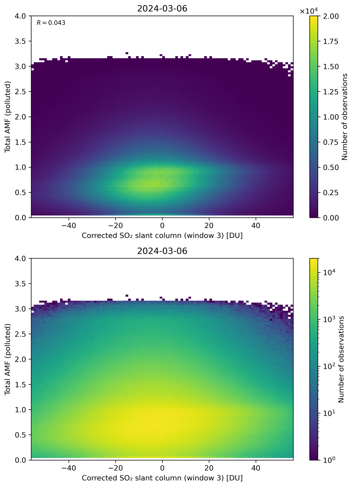
Figure 210: Scatter density plot of “Corrected SO 2 slant column (window 3)” against “Total AMF (polluted)” for 2024-03-05 to 2024-03-07.
