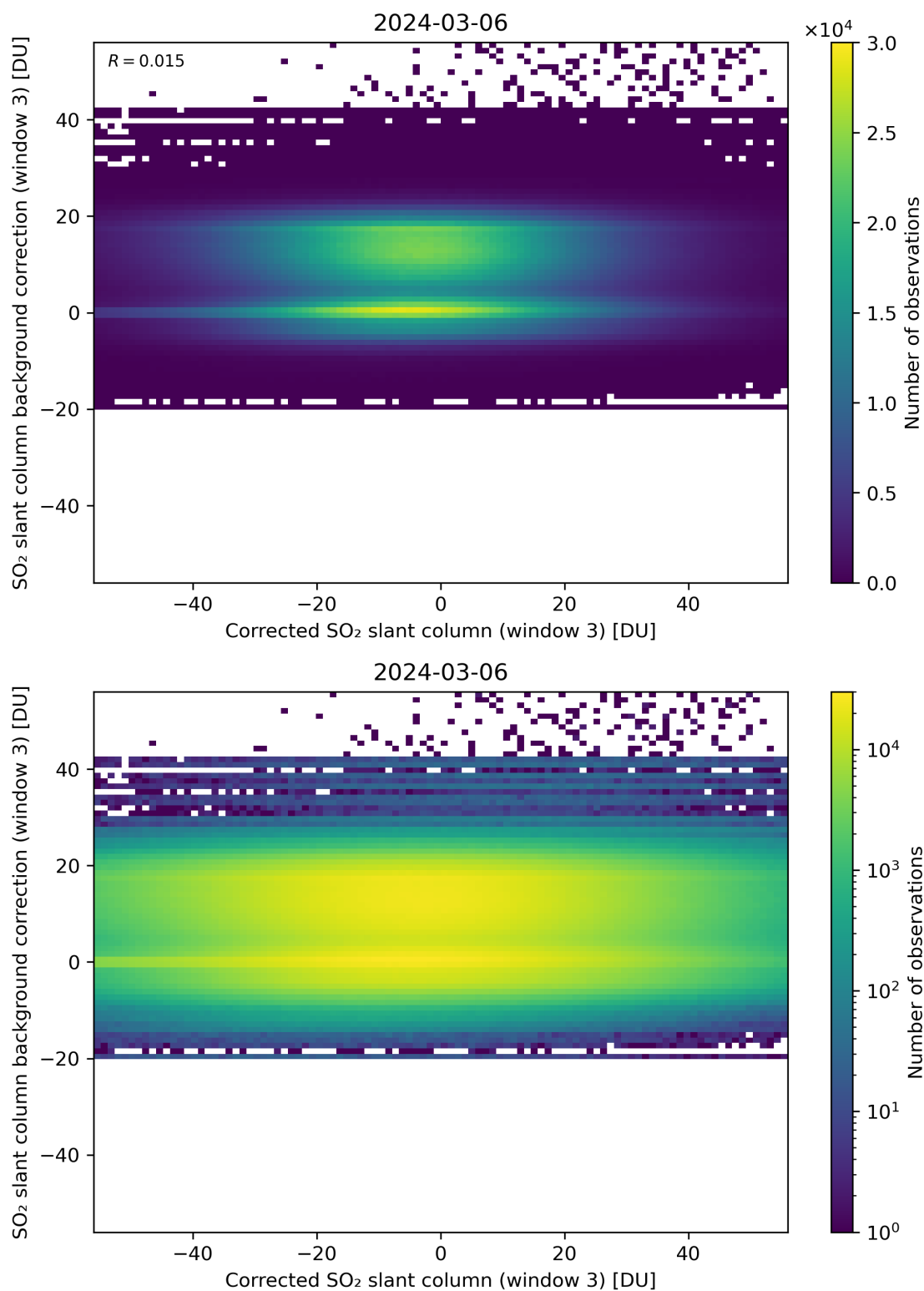
Figure 205: Scatter density plot of “Corrected SO 2 slant column (window 3)” against “SO 2 slant column background correction (window 3)” for 2024-03-05 to 2024-03-07.
