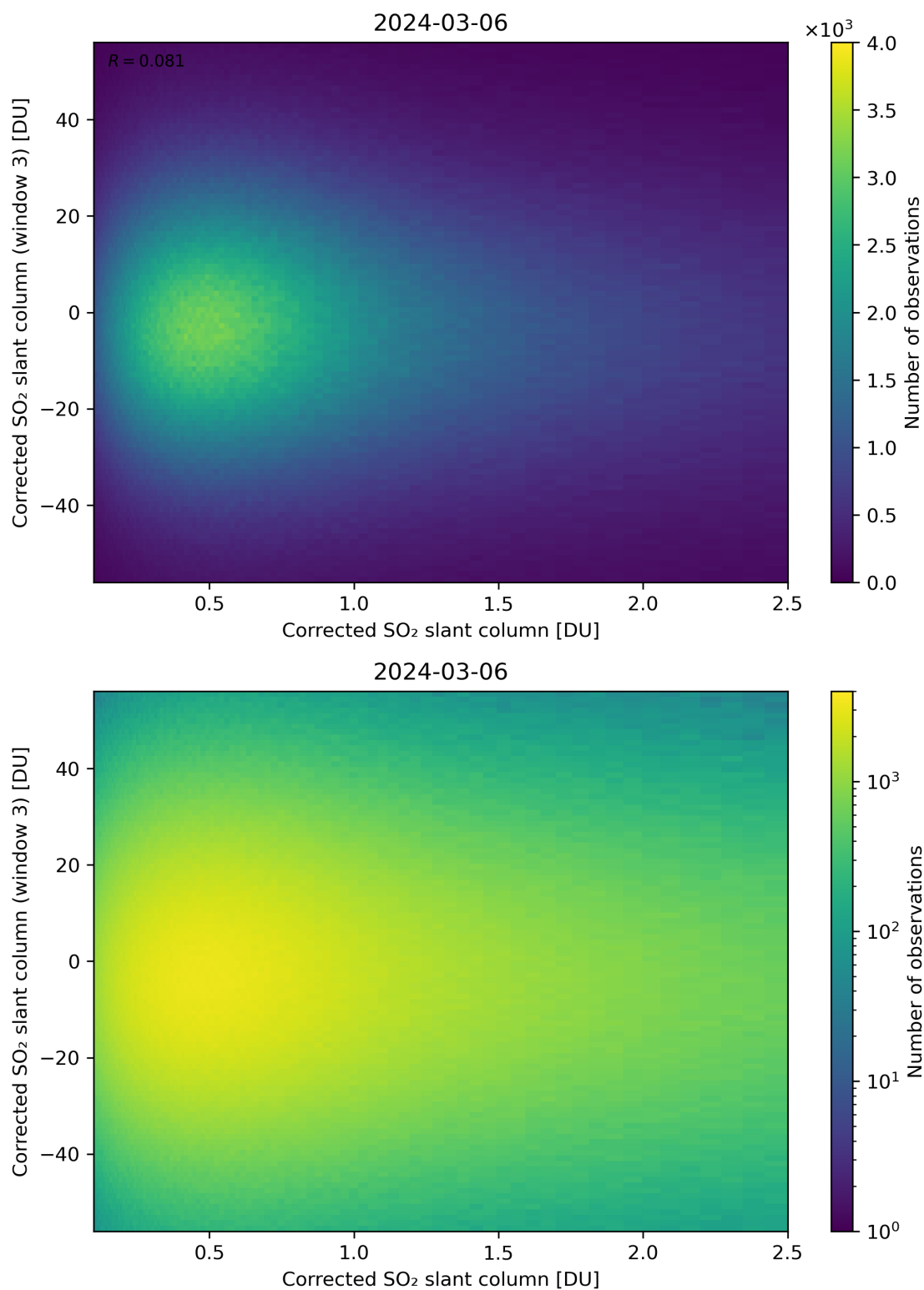
Figure 186: Scatter density plot of “Corrected SO 2 slant column” against “Corrected SO 2 slant column (window 3)” for 2024-03-05 to 2024-03-07.
