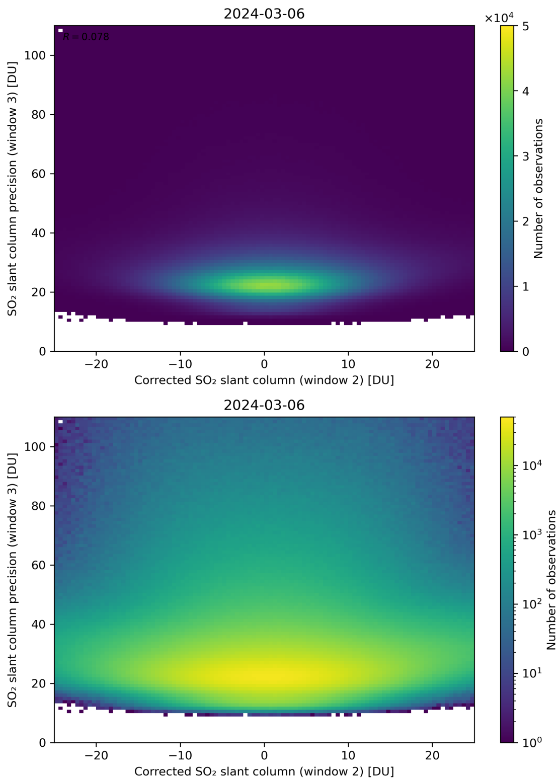
Figure 202: Scatter density plot of “Corrected SO 2 slant column (window 2)” against “SO 2 slant column precision (window 3)” for 2024-03-05 to 2024-03-07.
