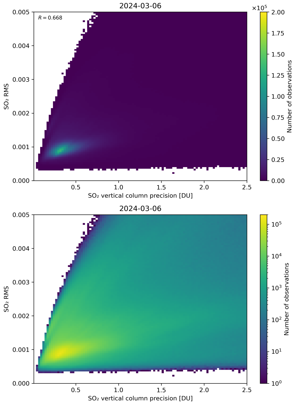
Figure 284: Scatter density plot of “SO 2 vertical column precision” against “SO 2 RMS” for 2024-03-05 to 2024-03-07.
