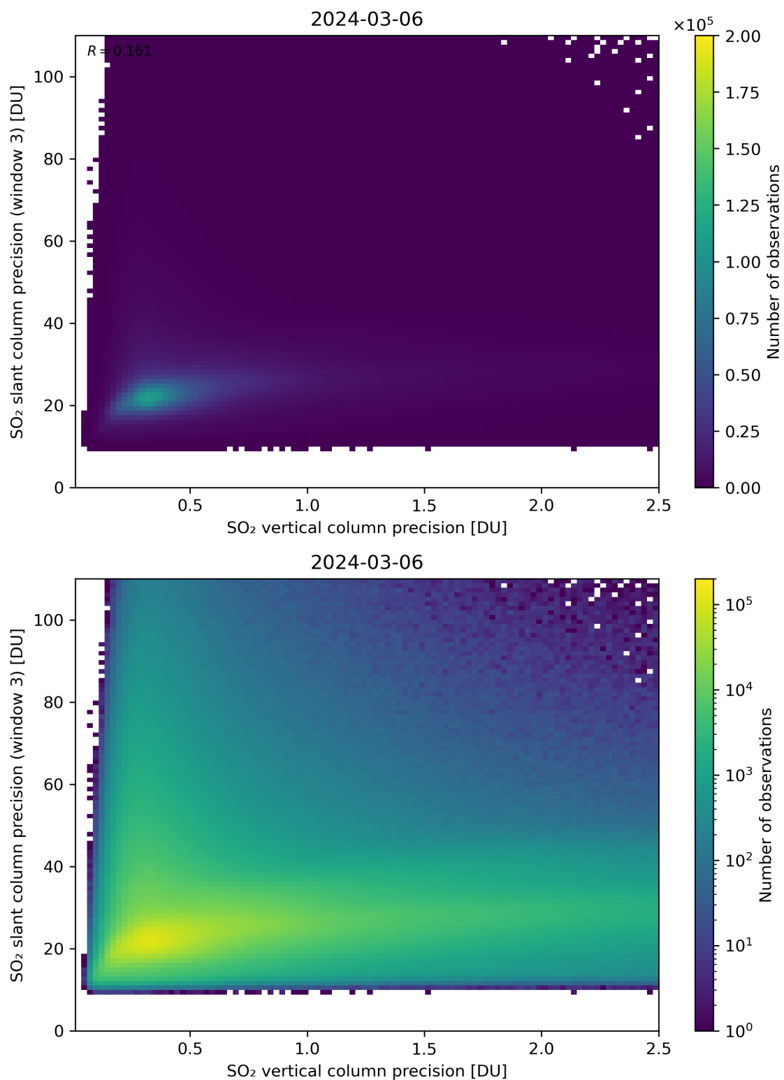
Figure 293: Scatter density plot of “SO 2 vertical column precision” against “SO 2 slant column precision (window 3)” for 2024-03-05 to 2024-03-07.
