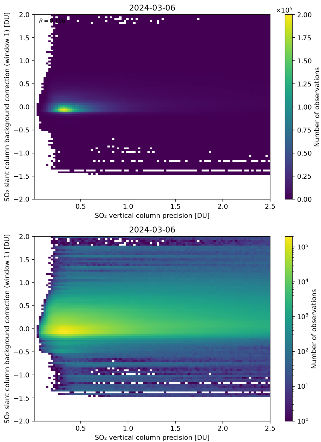
Figure 279: Scatter density plot of “SO 2 vertical column precision” against “SO 2 slant column background correction (window 1)” for 2024-03-05 to 2024-03-07.
