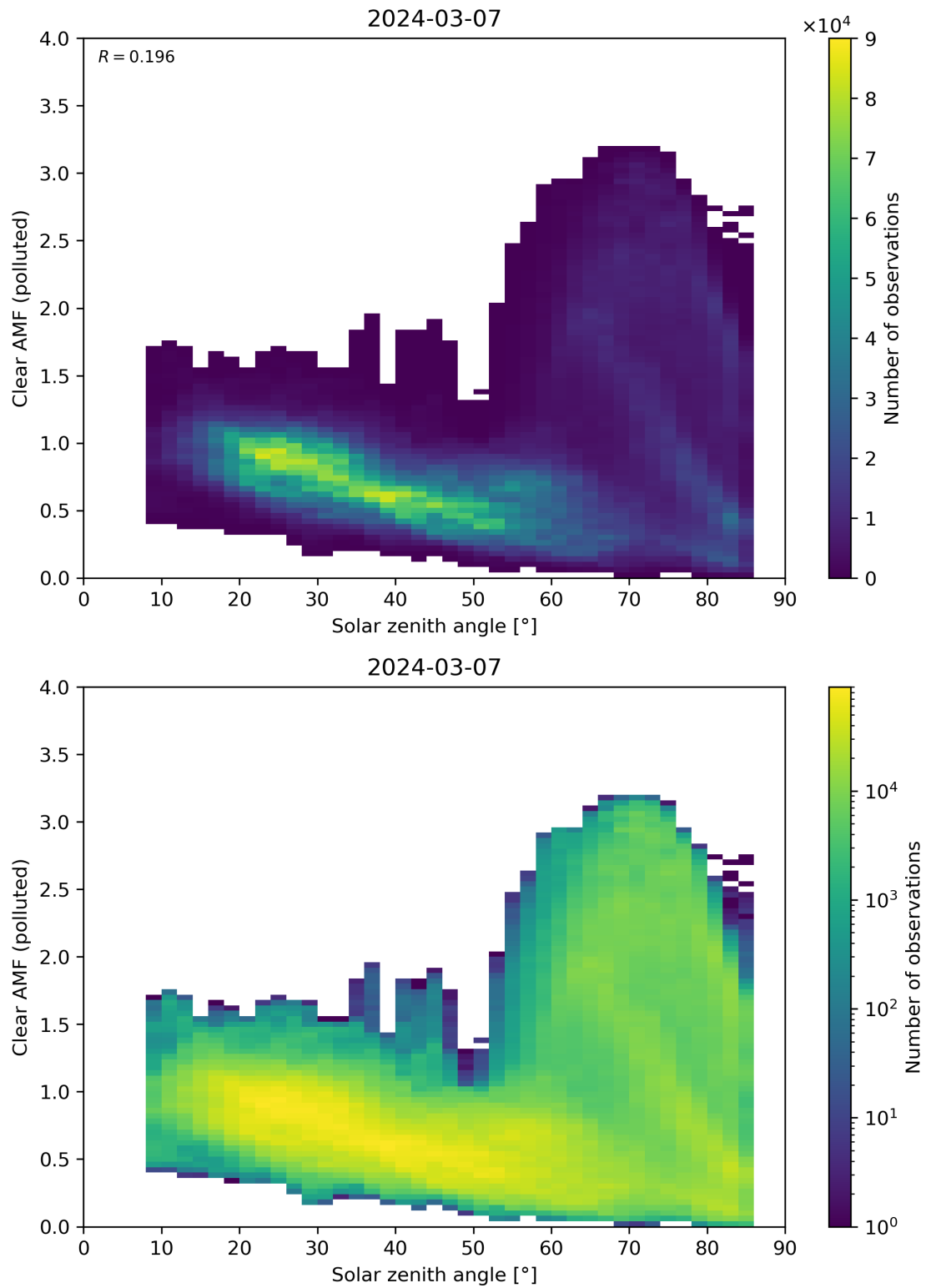
Figure 165: Scatter density plot of “Solar zenith angle” against “Clear AMF (polluted)” for 2024-03-06 to 2024-03-08.
