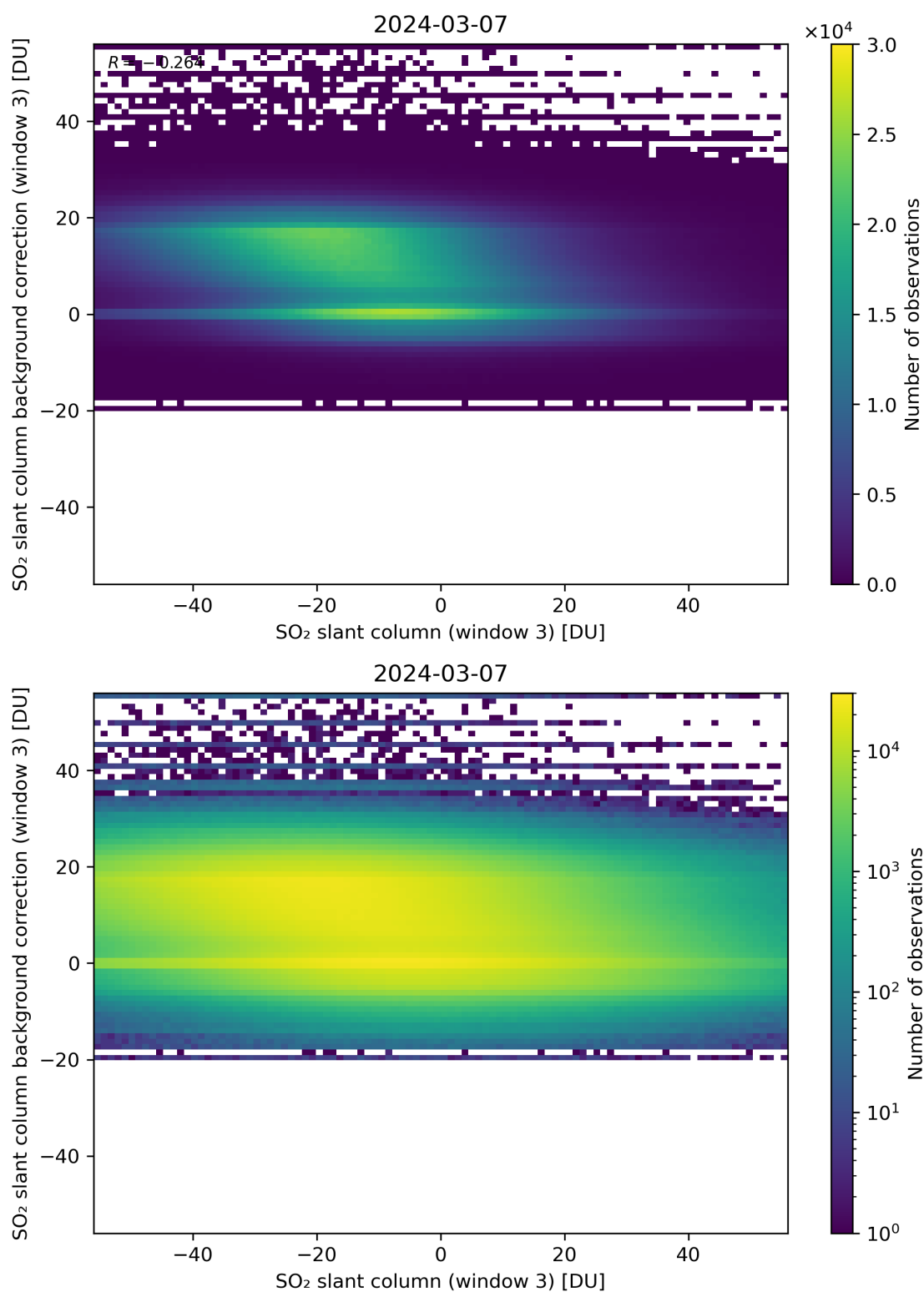
Figure 253: Scatter density plot of “SO 2 slant column (window 3)” against “SO 2 slant column background correction (window 3)” for 2024-03-06 to 2024-03-08.
