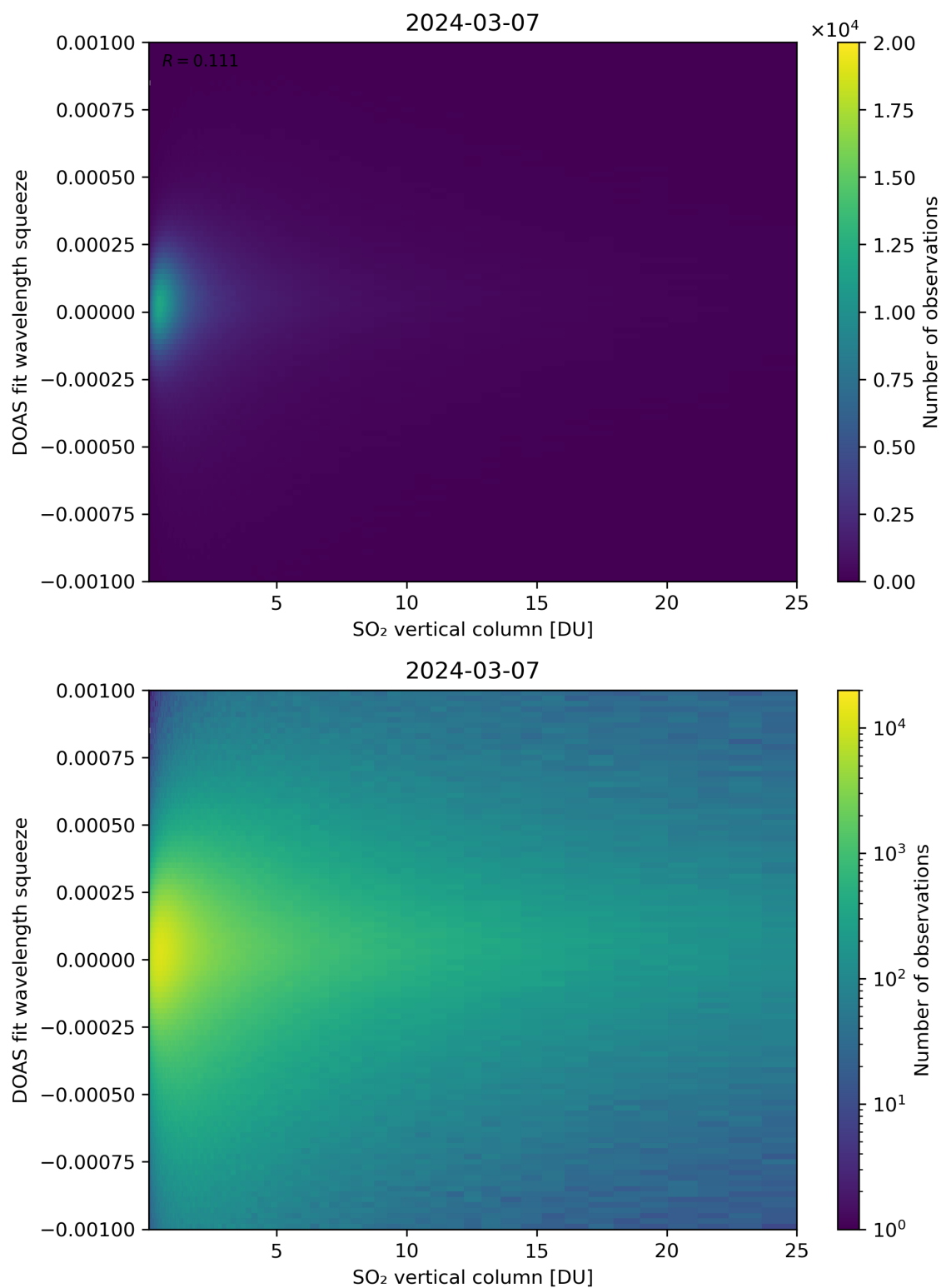
Figure 277: Scatter density plot of “SO 2 vertical column” against “DOAS fit wavelength squeeze” for 2024-03-06 to 2024-03-08.
