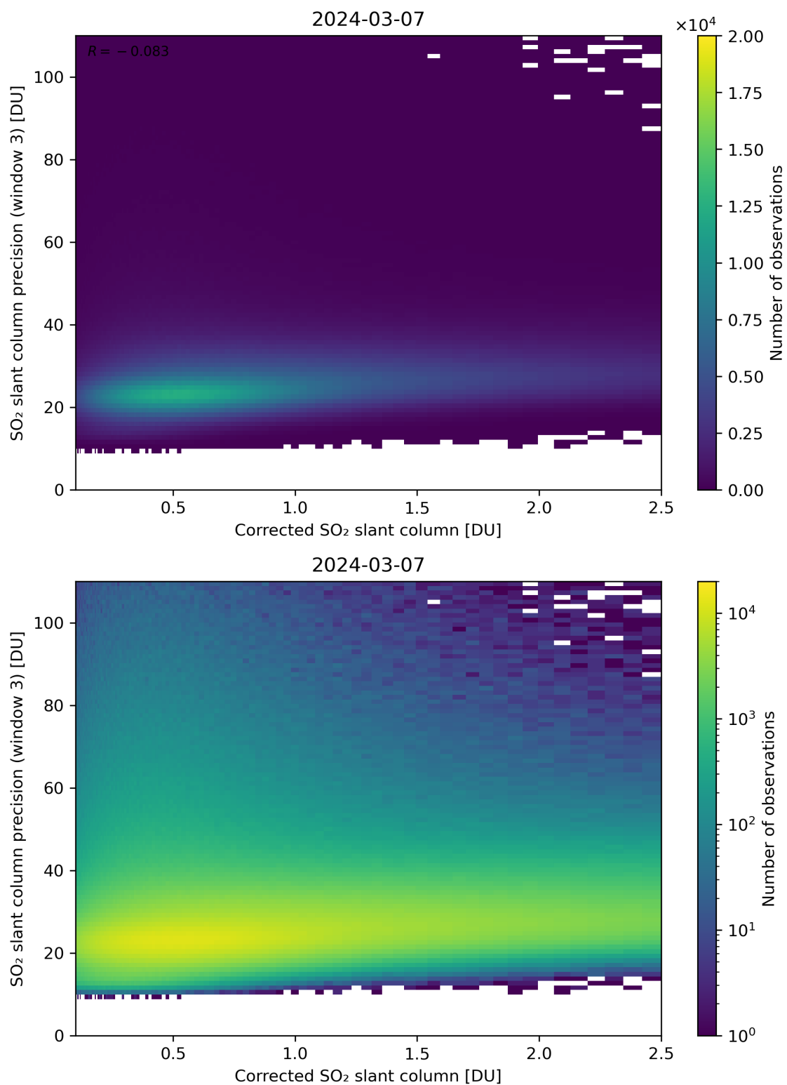
Figure 191: Scatter density plot of “Corrected SO 2 slant column” against “SO 2 slant column precision (window 3)” for 2024-03-06 to 2024-03-08.
