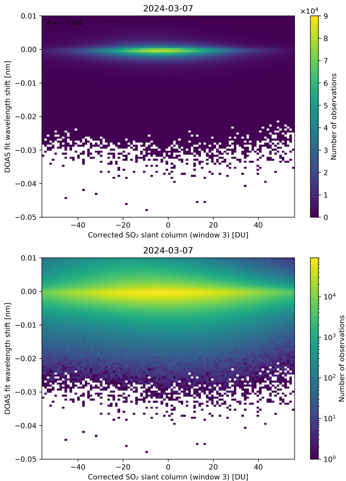
Figure 206: Scatter density plot of “Corrected SO 2 slant column (window 3)” against “DOAS fit wavelength shift” for 2024-03-06 to 2024-03-08.
