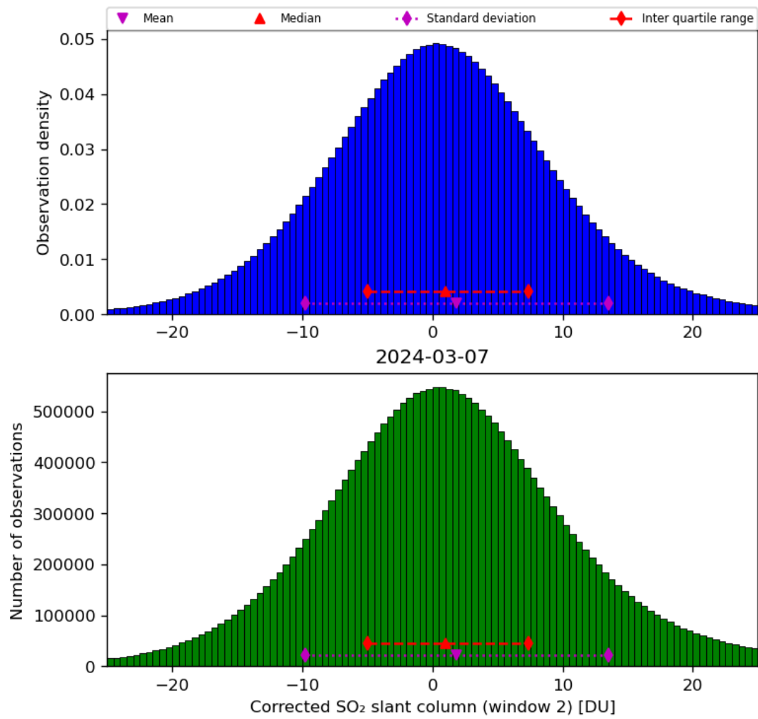
Figure 62: Histogram of “Corrected SO 2 slant column (window 2)” for 2024-03-06 to 2024-03-08
