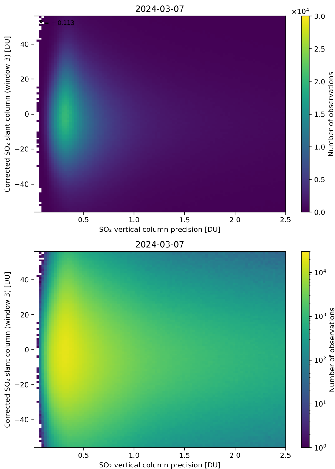
Figure 288: Scatter density plot of “SO 2 vertical column precision” against “Corrected SO 2 slant column (window 3)” for 2024-03-06 to 2024-03-08.
