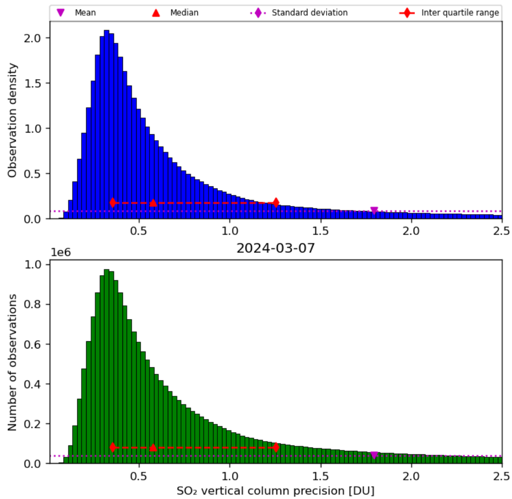
Figure 54: Histogram of “SO 2 vertical column precision” for 2024-03-06 to 2024-03-08
