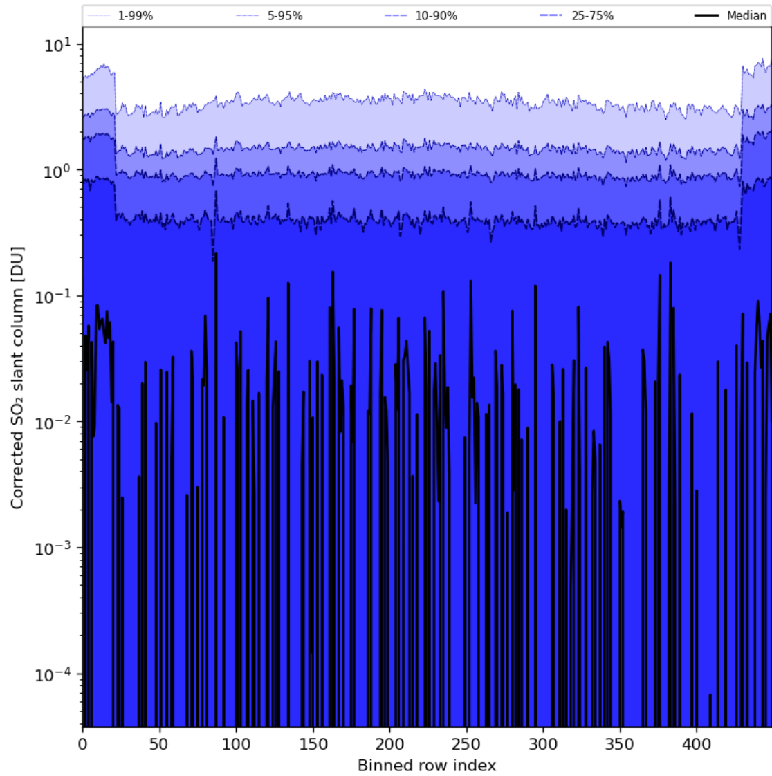
Figure 78: Along track statistics of “Corrected SO 2 slant column” for 2024-03-06 to 2024-03-08
