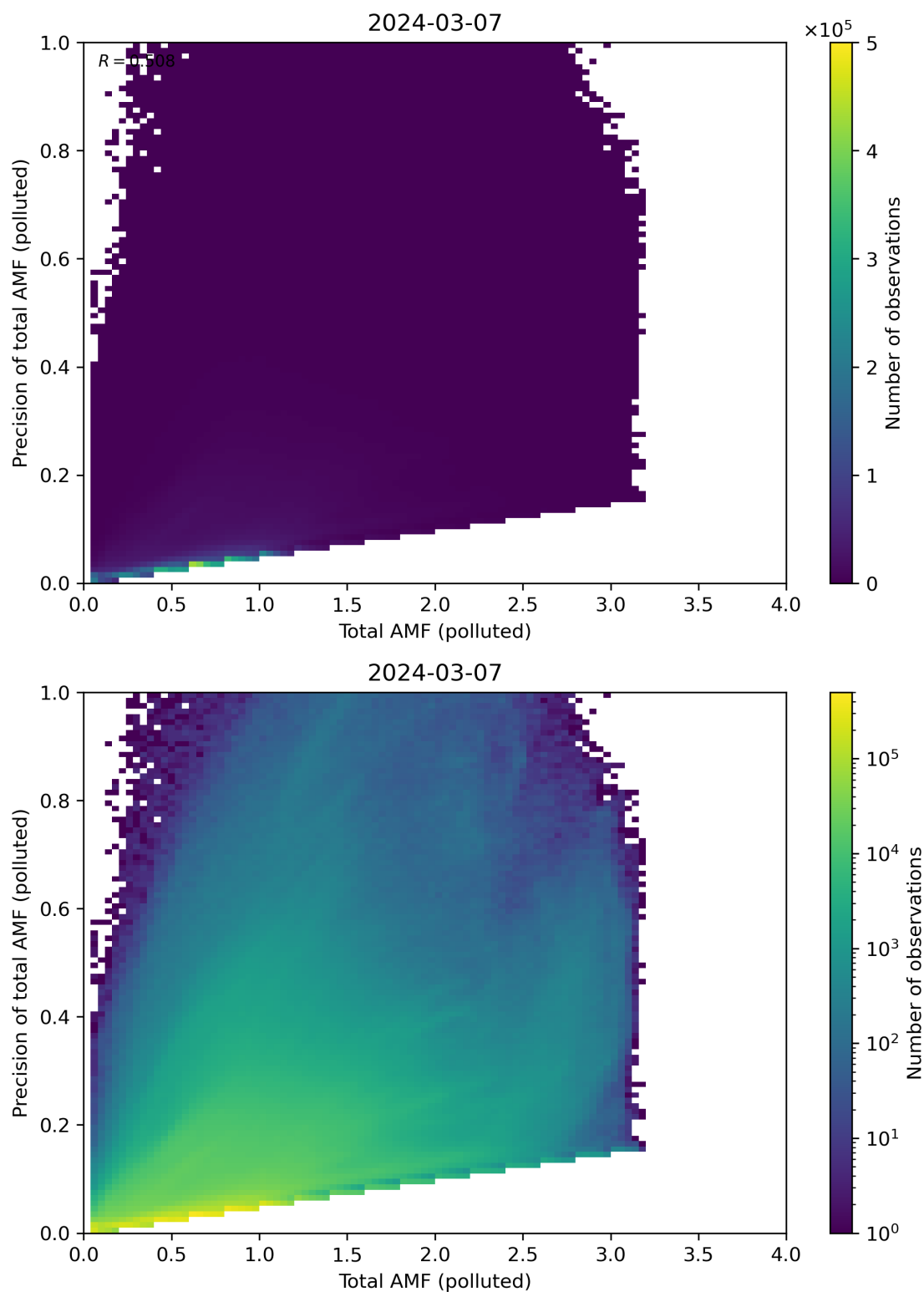
Figure 272: Scatter density plot of “Total AMF (polluted)” against “Precision of total AMF (polluted)” for 2024-03-06 to 2024-03-08.
