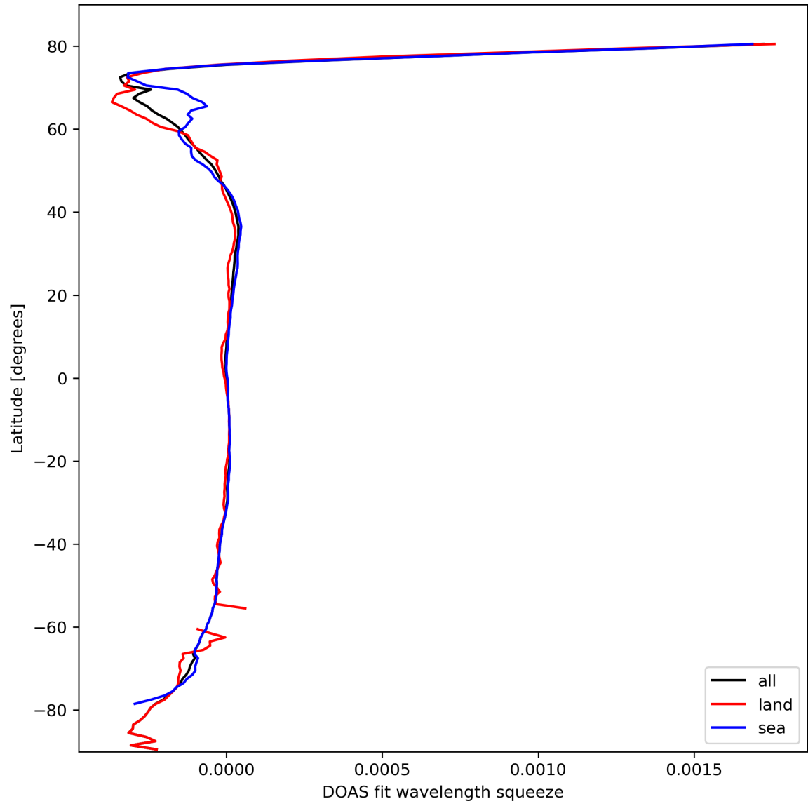
Figure 46: Zonal average of “DOAS fit wavelength squeeze” for 2024-03-06 to 2024-03-08.
