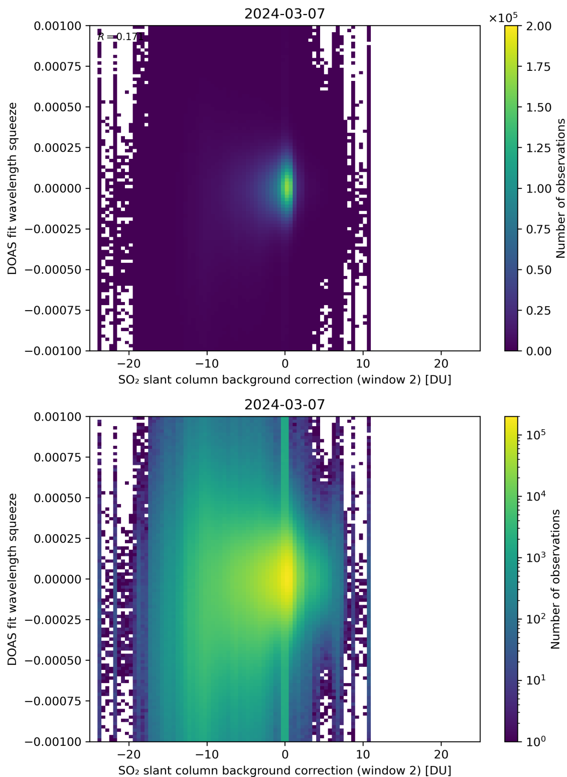
Figure 113: Scatter density plot of “SO 2 slant column background correction (window 2)” against “DOAS fit wavelength squeeze” for 2024-03-06 to 2024-03-08.
