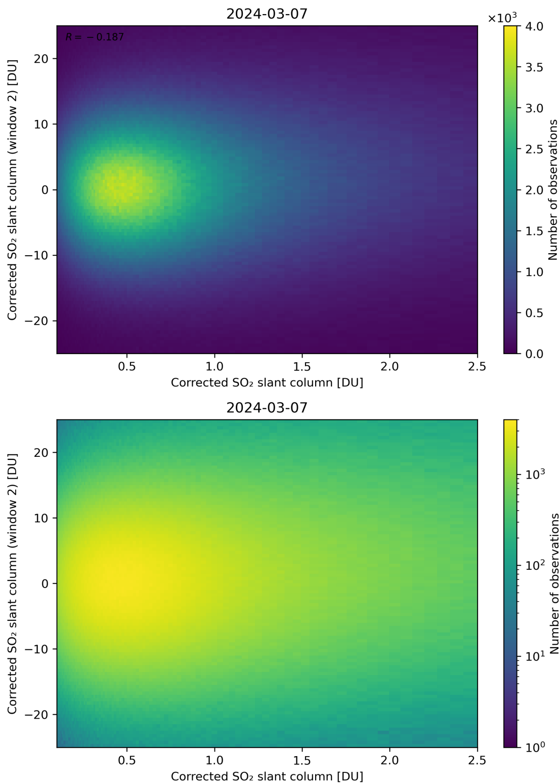
Figure 185: Scatter density plot of “Corrected SO 2 slant column” against “Corrected SO 2 slant column (window 2)” for 2024-03-06 to 2024-03-08.
