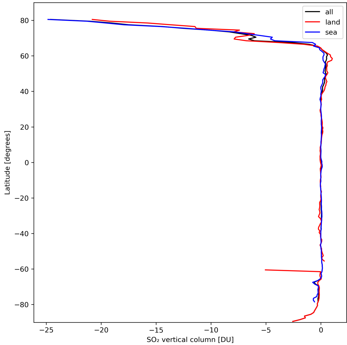
Figure 30: Zonal average of “SO 2 vertical column” for 2024-03-06 to 2024-03-08.
