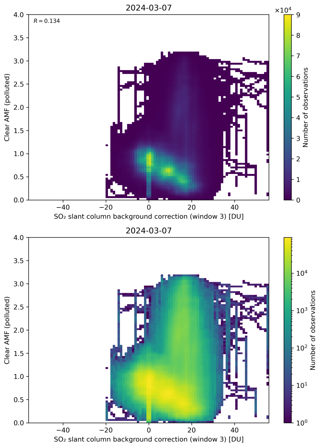
Figure 124: Scatter density plot of “SO 2 slant column background correction (window 3)” against “Clear AMF (polluted)” for 2024-03-06 to 2024-03-08.
