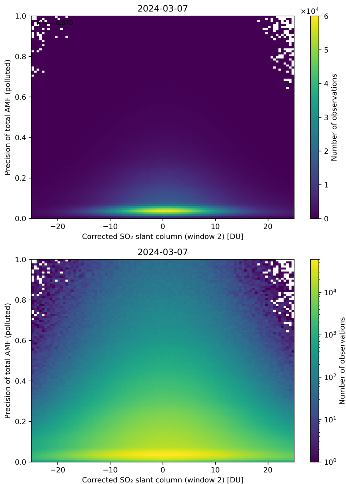
Figure 204: Scatter density plot of “Corrected SO 2 slant column (window 2)” against “Precision of total AMF (polluted)” for 2024-03-06 to 2024-03-08.
