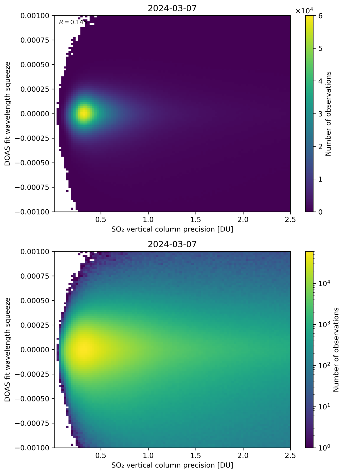
Figure 283: Scatter density plot of “SO 2 vertical column precision” against “DOAS fit wavelength squeeze” for 2024-03-06 to 2024-03-08.
