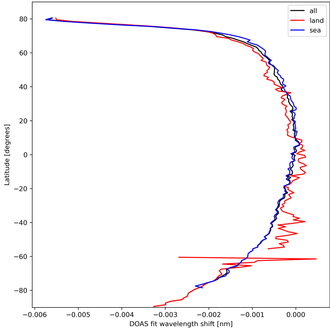
Figure 45: Zonal average of “DOAS fit wavelength shift” for 2024-03-06 to 2024-03-08.
