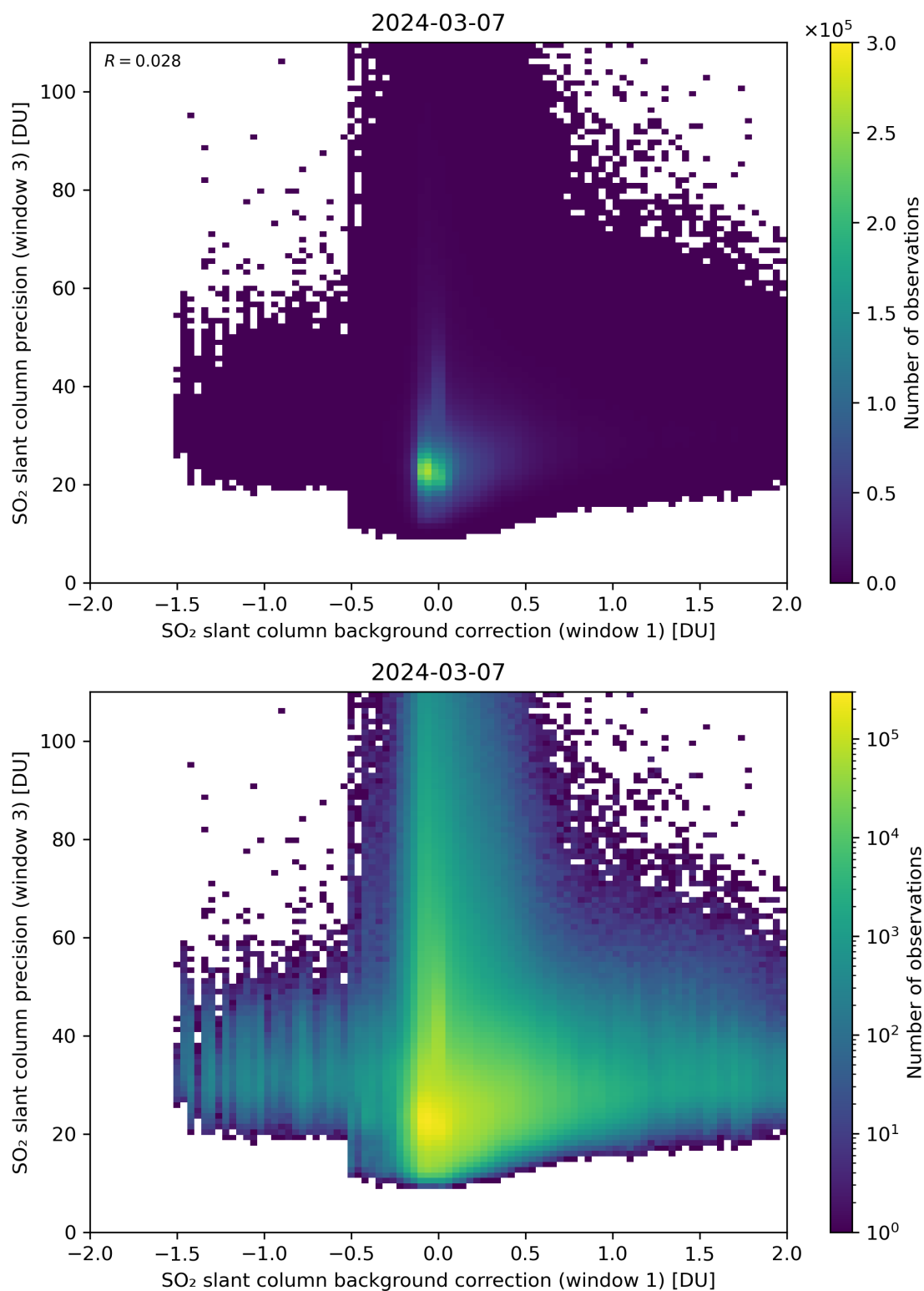
Figure 108: Scatter density plot of “SO 2 slant column background correction (window 1)” against “SO 2 slant column precision (window 3)” for 2024-03-06 to 2024-03-08.
