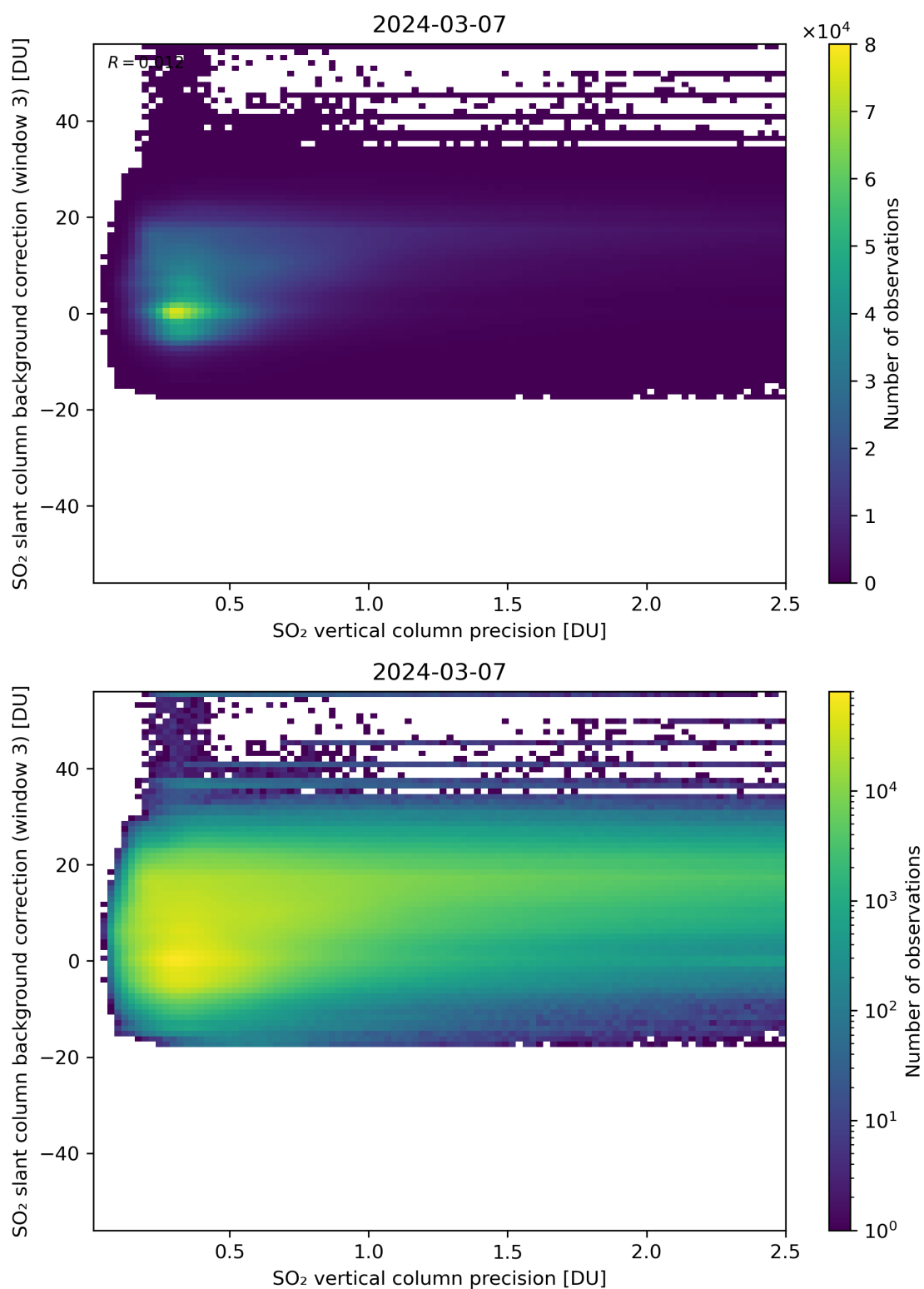
Figure 281: Scatter density plot of “SO 2 vertical column precision” against “SO 2 slant column background correction (window 3)” for 2024-03-06 to 2024-03-08.
