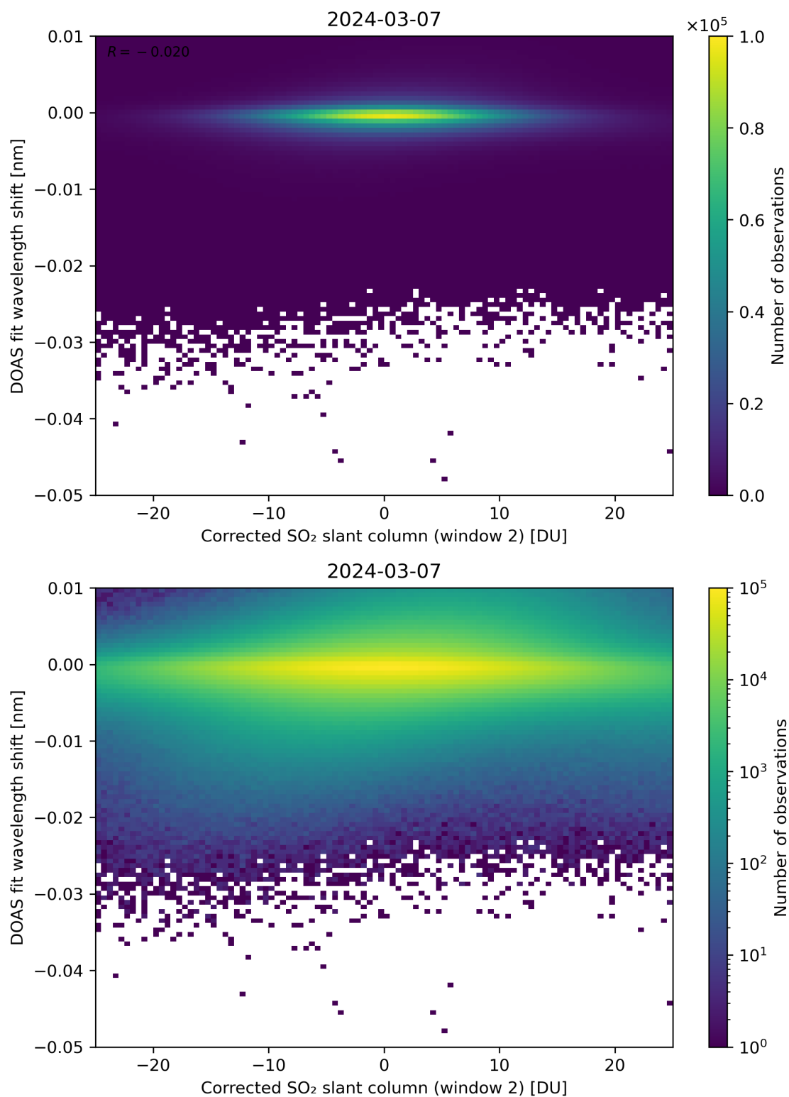
Figure 196: Scatter density plot of “Corrected SO 2 slant column (window 2)” against “DOAS fit wavelength shift” for 2024-03-06 to 2024-03-08.
