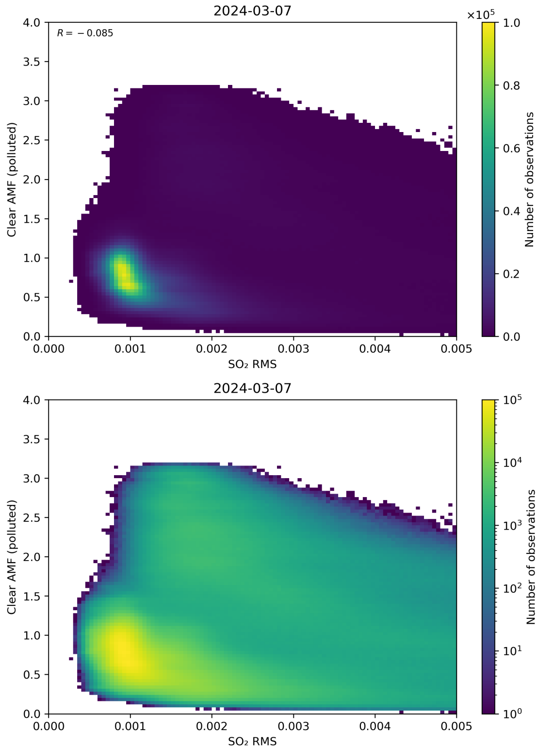
Figure 136: Scatter density plot of “SO 2 RMS” against “Clear AMF (polluted)” for 2024-03-06 to 2024-03-08.
