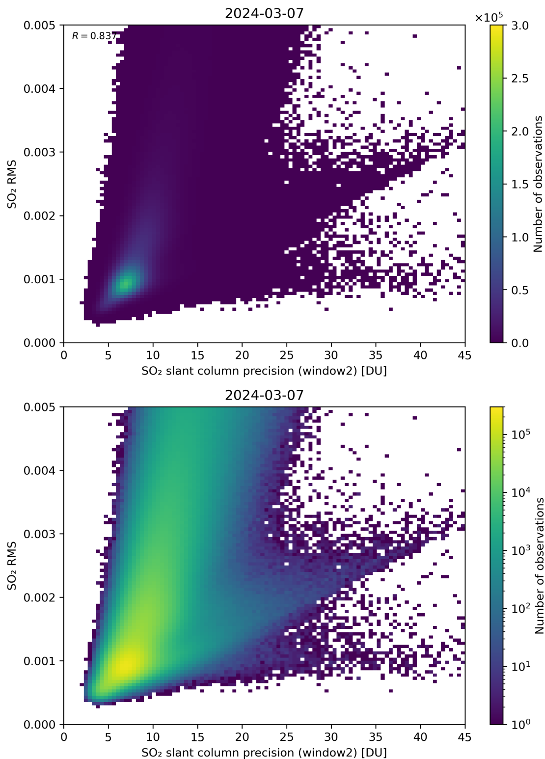
Figure 245: Scatter density plot of “SO 2 slant column precision (window2)” against “SO 2 RMS” for 2024-03-06 to 2024-03-08.
