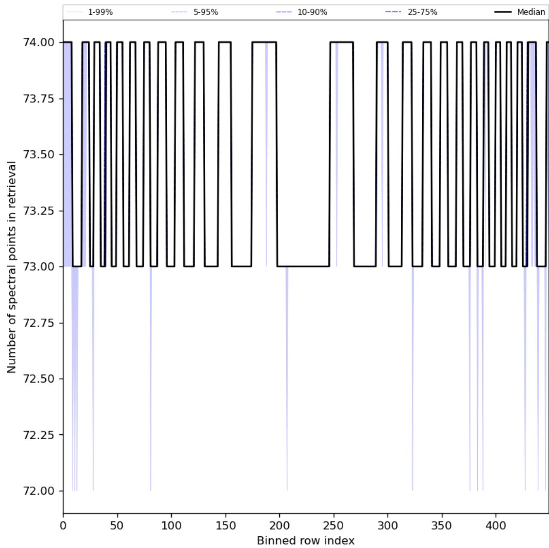
Figure 97: Along track statistics of “Number of spectral points in retrieval” for 2024-03-06 to 2024-03-08
