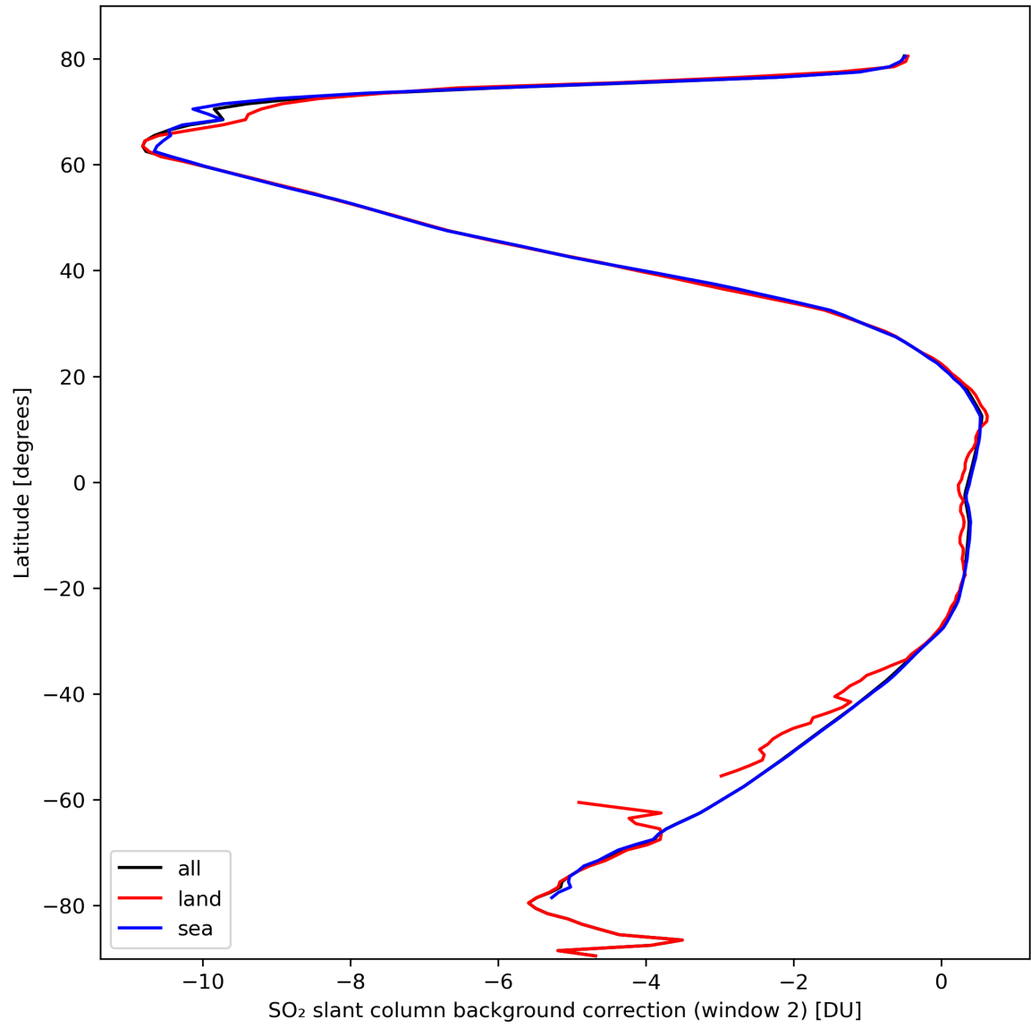
Figure 40: Zonal average of “SO 2 slant column background correction (window 2)” for 2024-03-06 to 2024-03-08.
