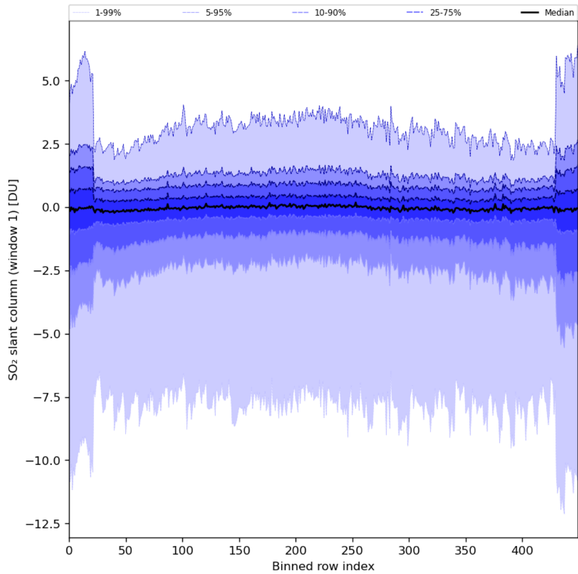
Figure 79: Along track statistics of “SO 2 slant column (window 1)” for 2024-03-06 to 2024-03-08
