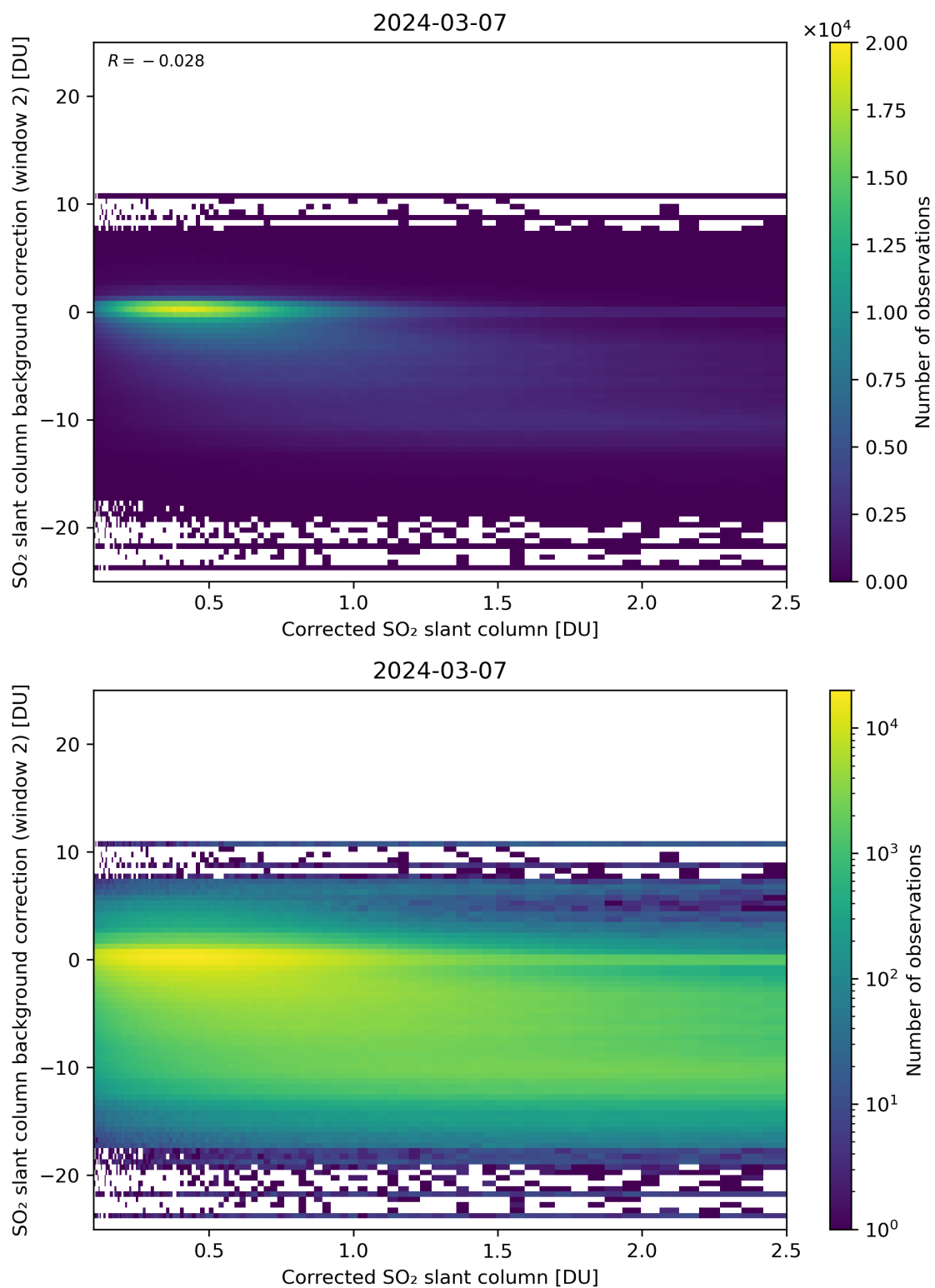
Figure 179: Scatter density plot of “Corrected SO 2 slant column” against “SO 2 slant column background correction (window 2)” for 2024-03-06 to 2024-03-08.
