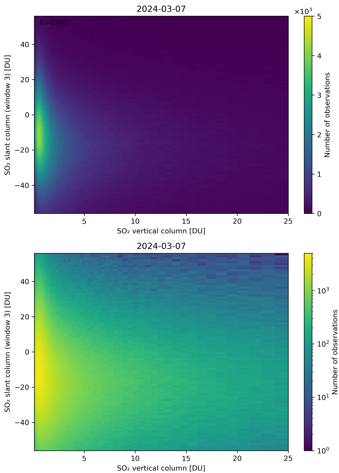
Figure 303: Scatter density plot of “SO 2 vertical column” against “SO 2 slant column (window 3)” for 2024-03-06 to 2024-03-08.
