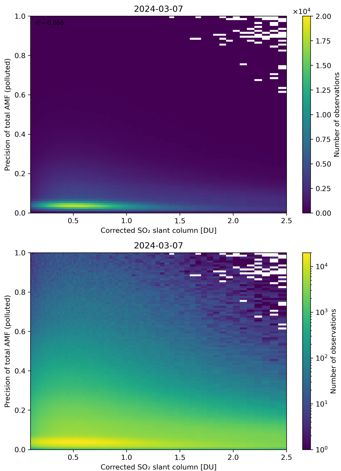
Figure 193: Scatter density plot of “Corrected SO 2 slant column” against “Precision of total AMF (polluted)” for 2024-03-06 to 2024-03-08.
