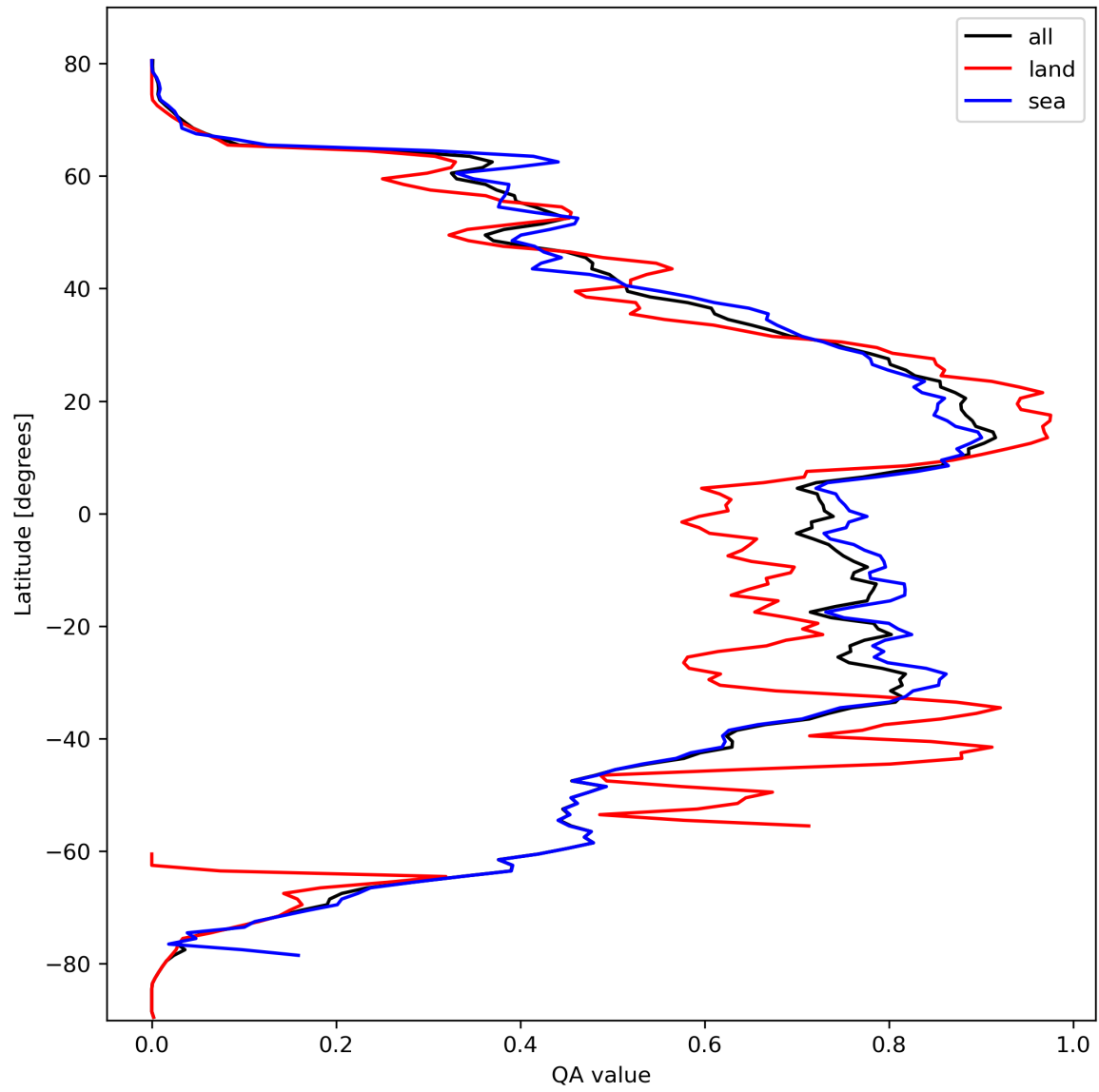
Figure 29: Zonal average of “QA value” for 2024-03-06 to 2024-03-08.
