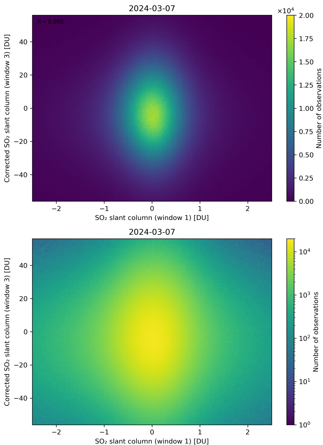
Figure 234: Scatter density plot of “SO 2 slant column (window 1)” against “Corrected SO 2 slant column (window 3)” for 2024-03-06 to 2024-03-08.
