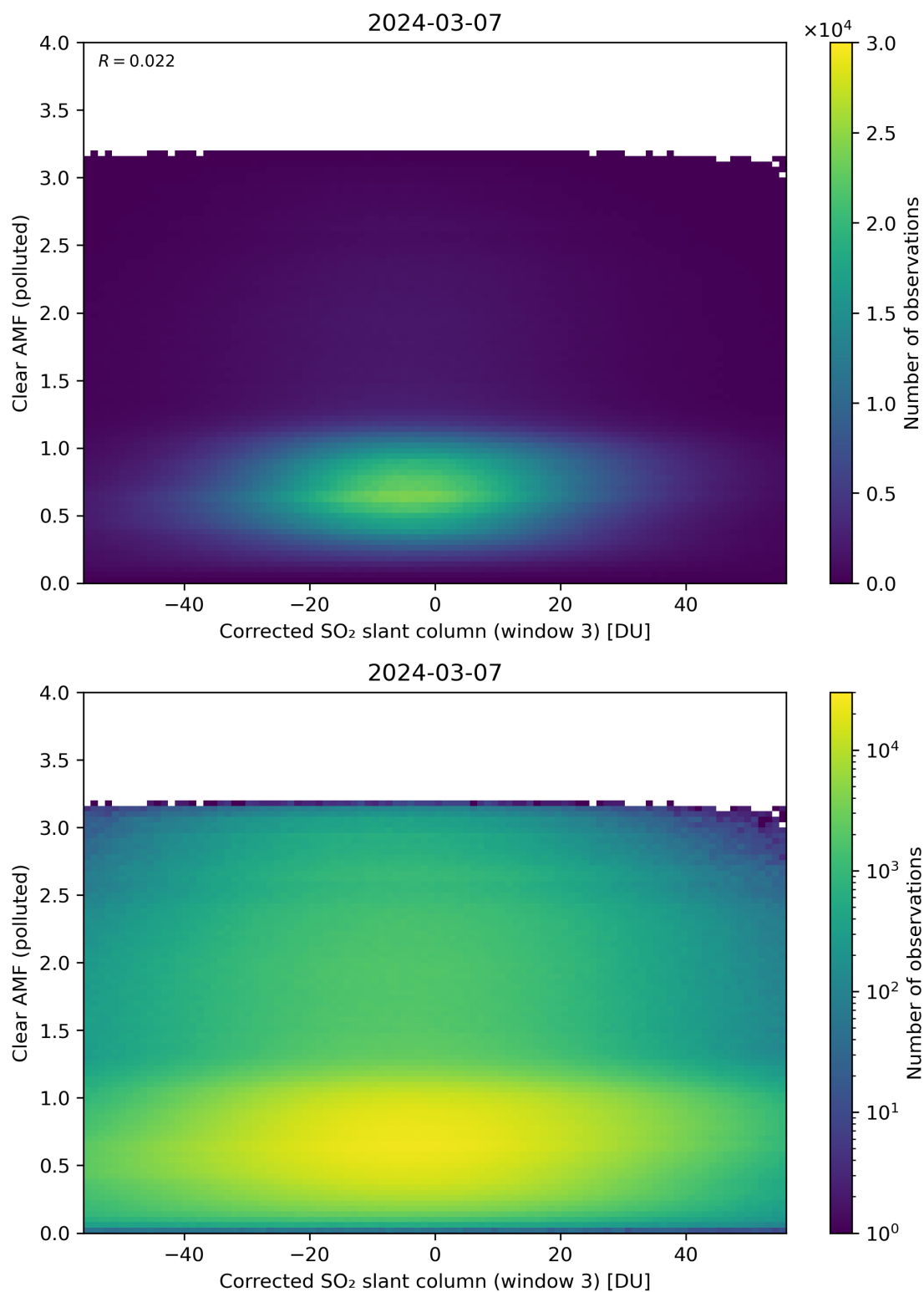
Figure 209: Scatter density plot of “Corrected SO 2 slant column (window 3)” against “Clear AMF (polluted)” for 2024-03-06 to 2024-03-08.
