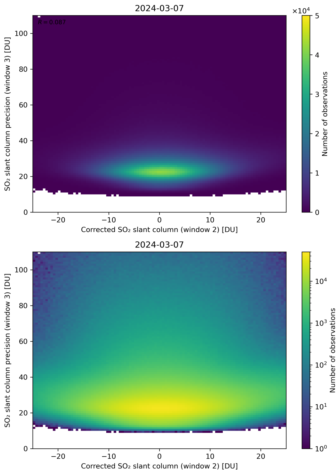
Figure 202: Scatter density plot of “Corrected SO 2 slant column (window 2)” against “SO 2 slant column precision (window 3)” for 2024-03-06 to 2024-03-08.
