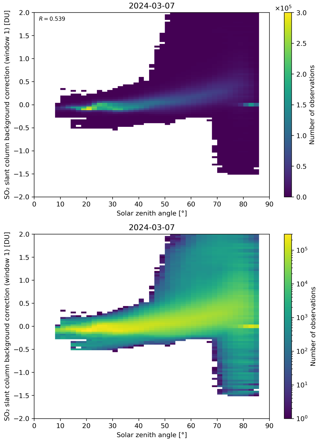
Figure 158: Scatter density plot of “Solar zenith angle” against “SO 2 slant column background correction (window 1)” for 2024-03-06 to 2024-03-08.
