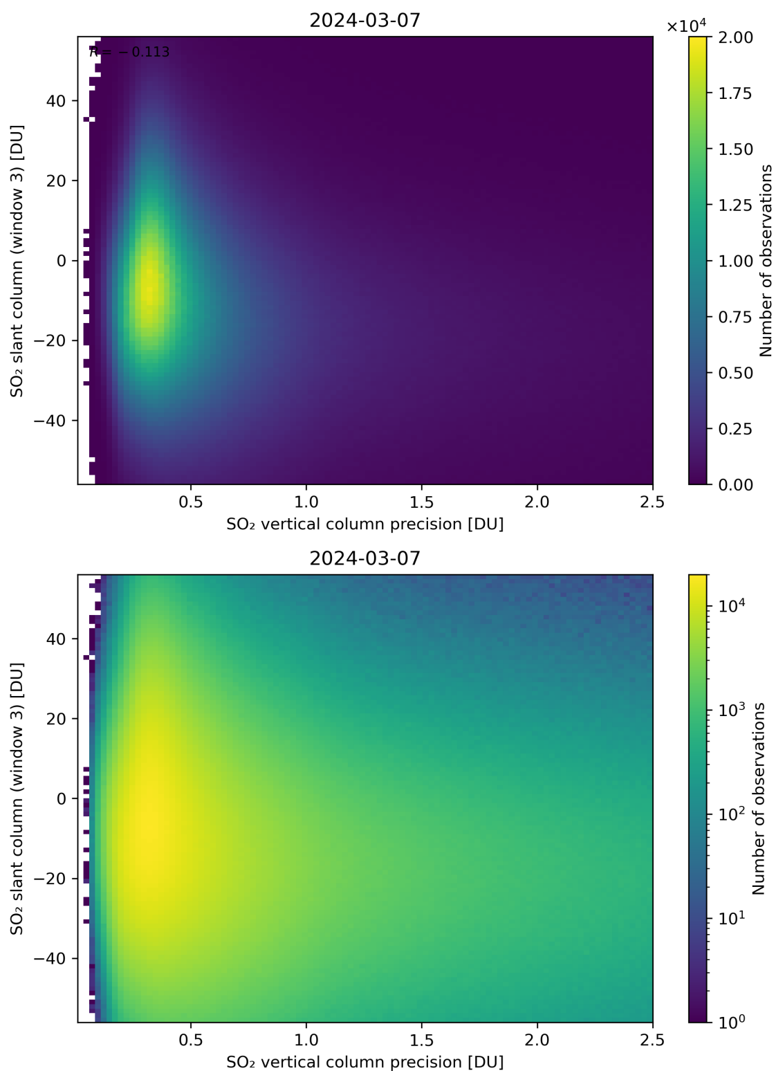
Figure 292: Scatter density plot of “SO 2 vertical column precision” against “SO 2 slant column (window 3)” for 2024-03-06 to 2024-03-08.
