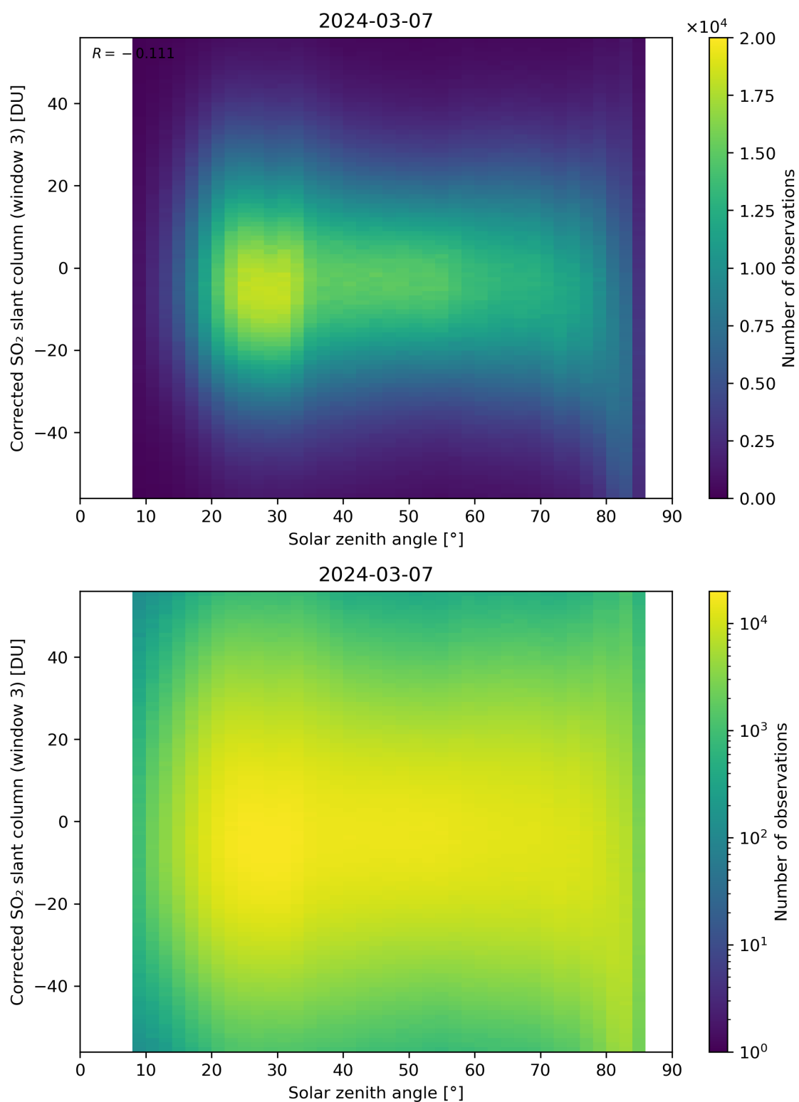
Figure 168: Scatter density plot of “Solar zenith angle” against “Corrected SO 2 slant column (window 3)” for 2024-03-06 to 2024-03-08.
