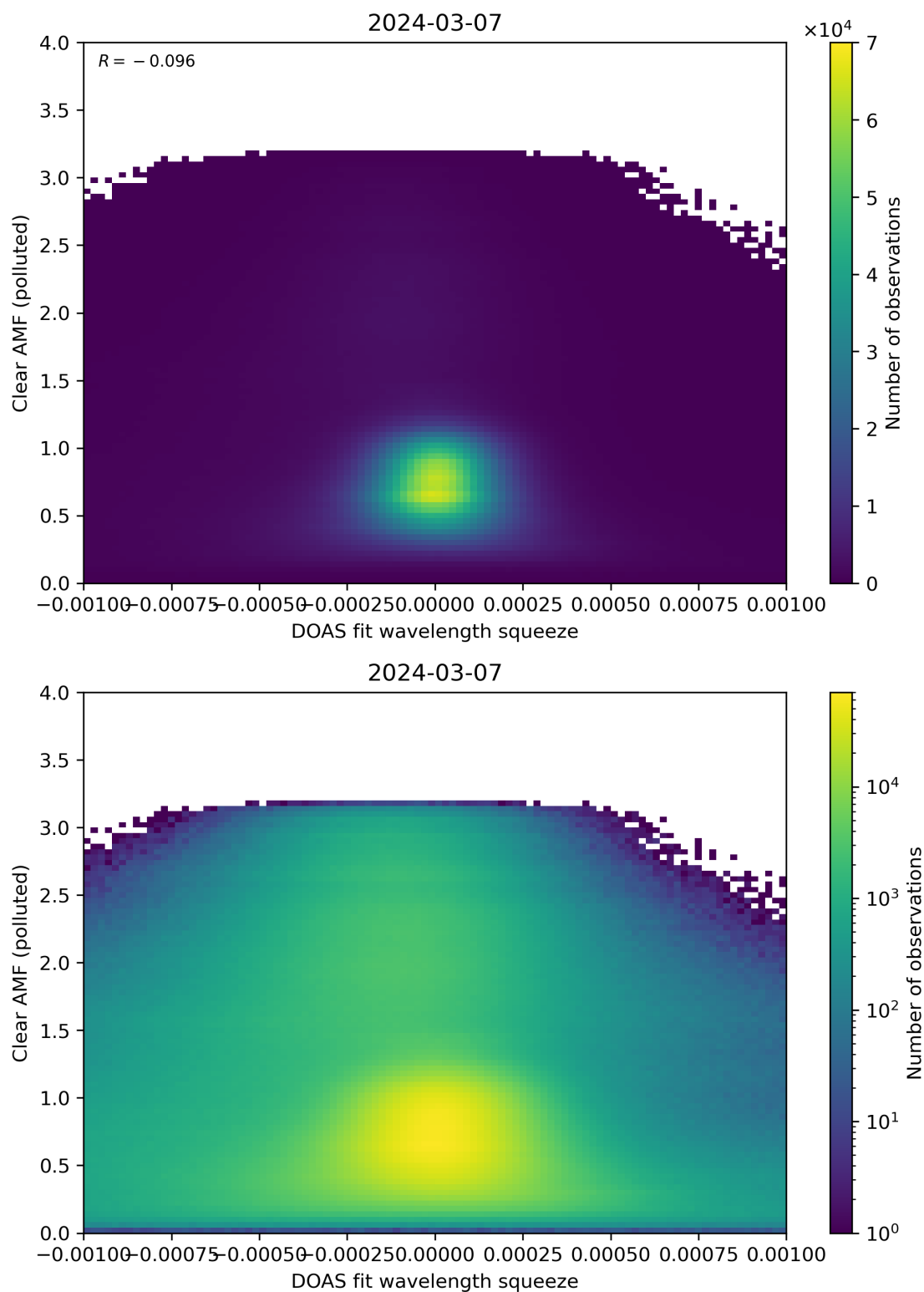
Figure 133: Scatter density plot of “DOAS fit wavelength squeeze” against “Clear AMF (polluted)” for 2024-03-06 to 2024-03-08.
