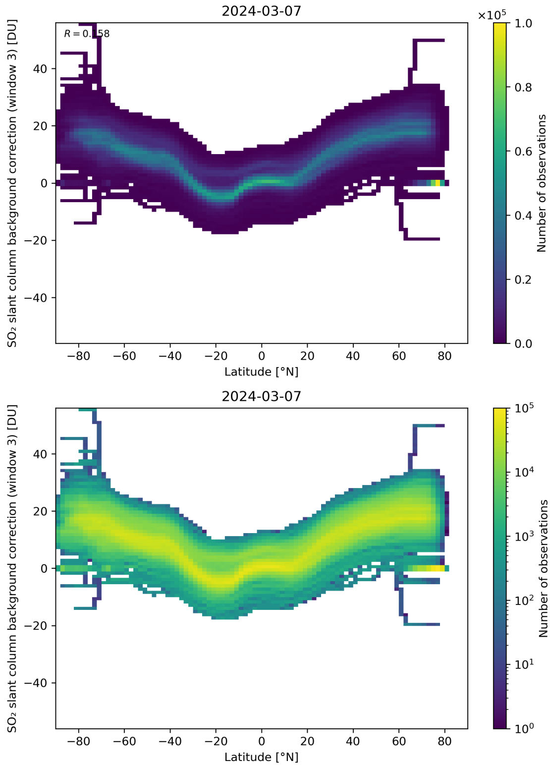
Figure 141: Scatter density plot of “Latitude” against “SO 2 slant column background correction (window 3)” for 2024-03-06 to 2024-03-08.
