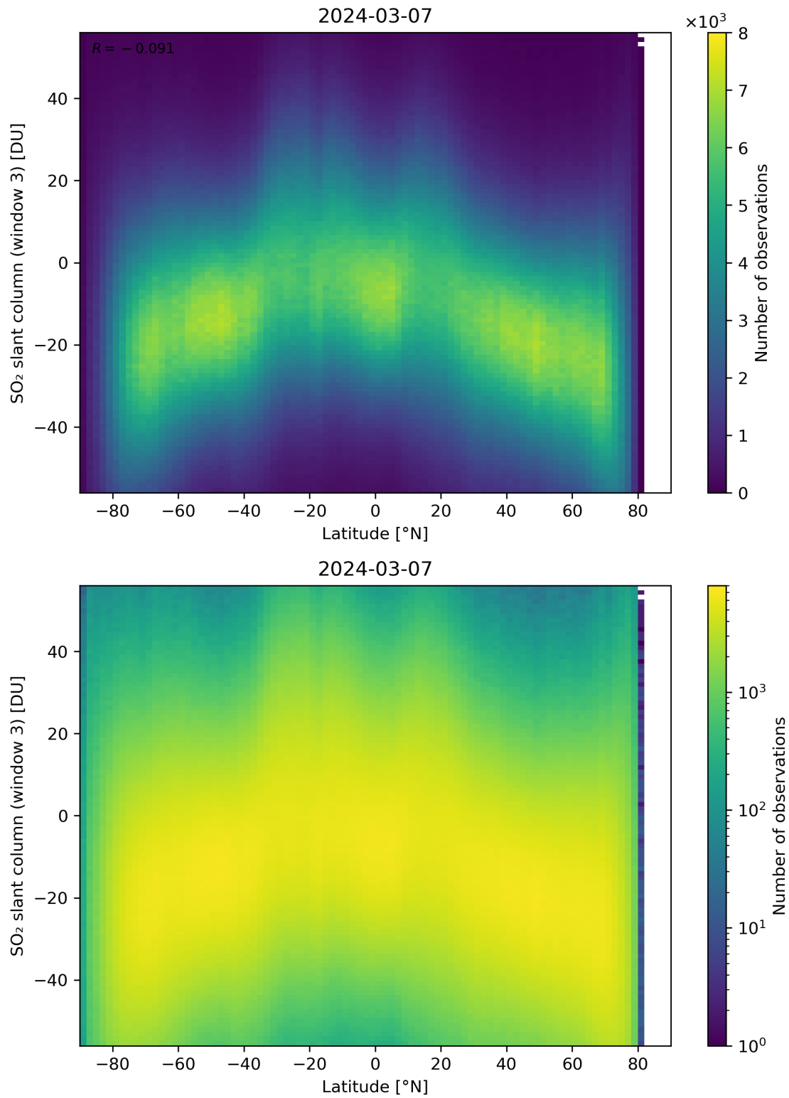
Figure 152: Scatter density plot of “Latitude” against “SO 2 slant column (window 3)” for 2024-03-06 to 2024-03-08.
