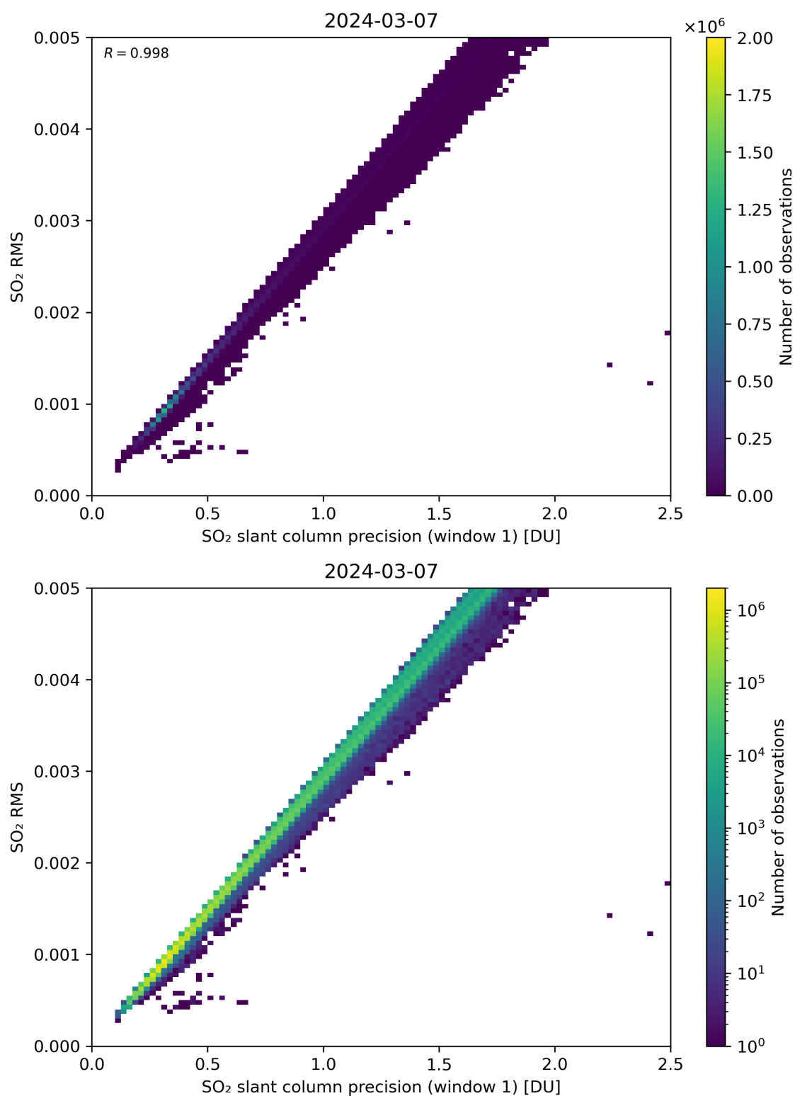
Figure 223: Scatter density plot of “SO 2 slant column precision (window 1)” against “SO 2 RMS” for 2024-03-06 to 2024-03-08.
