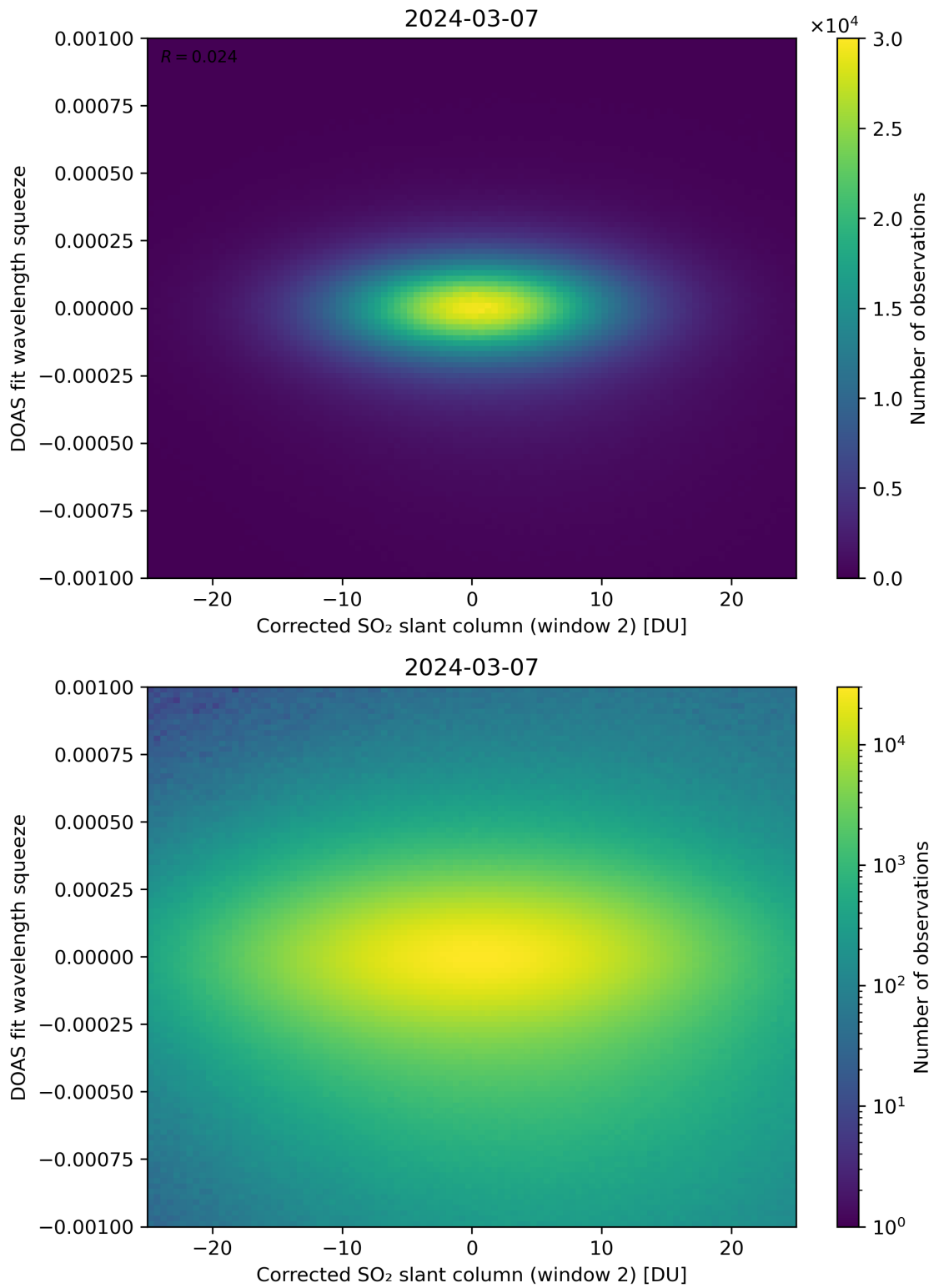
Figure 197: Scatter density plot of “Corrected SO 2 slant column (window 2)” against “DOAS fit wavelength squeeze” for 2024-03-06 to 2024-03-08.
