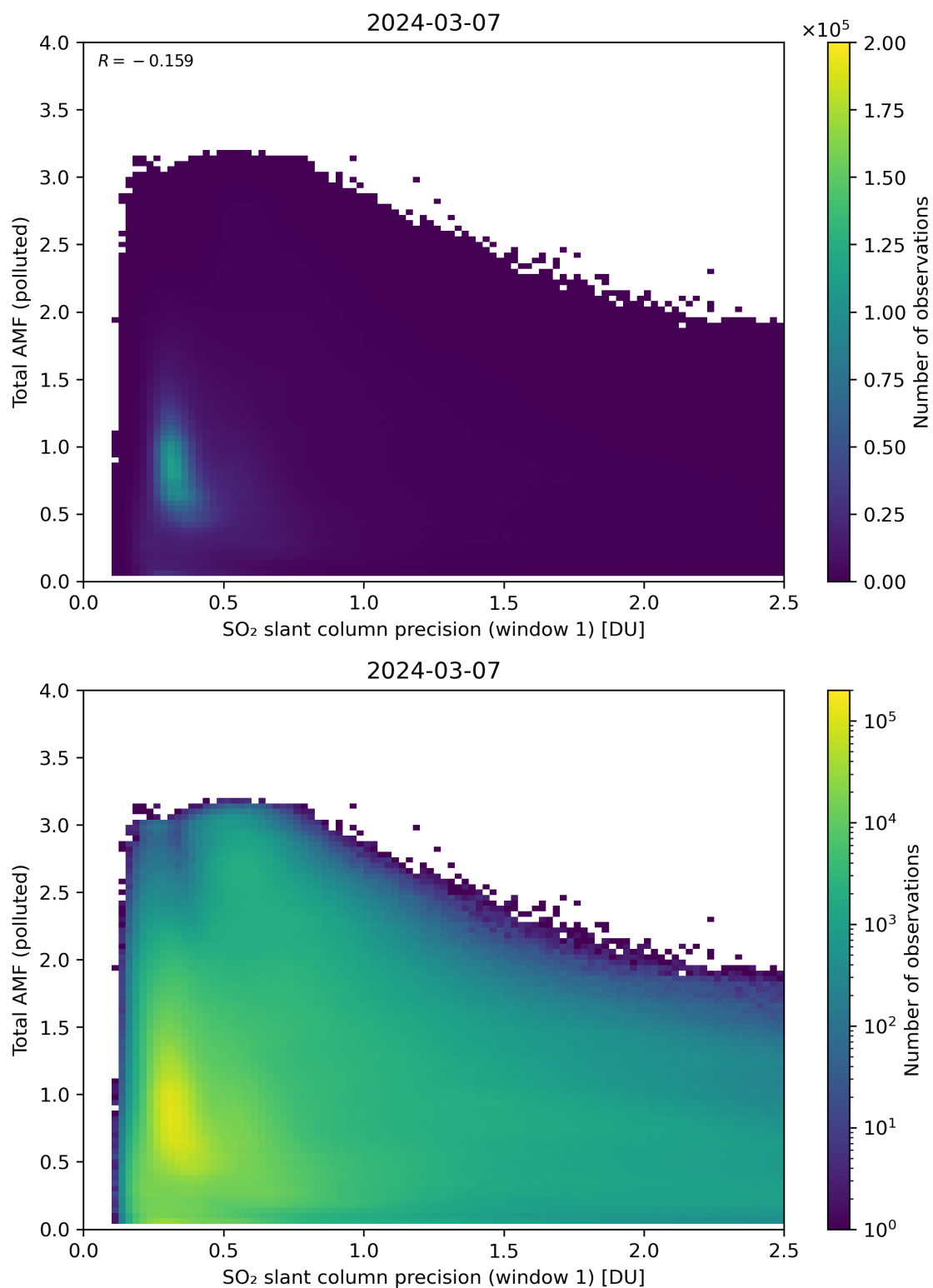
Figure 230: Scatter density plot of “SO 2 slant column precision (window 1)” against “Total AMF (polluted)” for 2024-03-06 to 2024-03-08.
