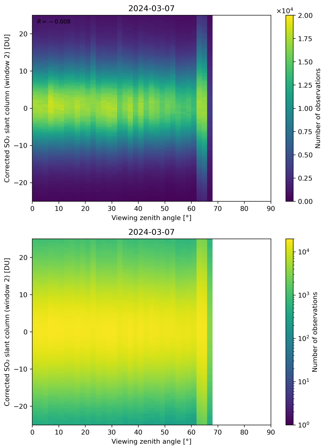
Figure 318: Scatter density plot of “Viewing zenith angle” against “Corrected SO 2 slant column (window 2)” for 2024-03-06 to 2024-03-08.
