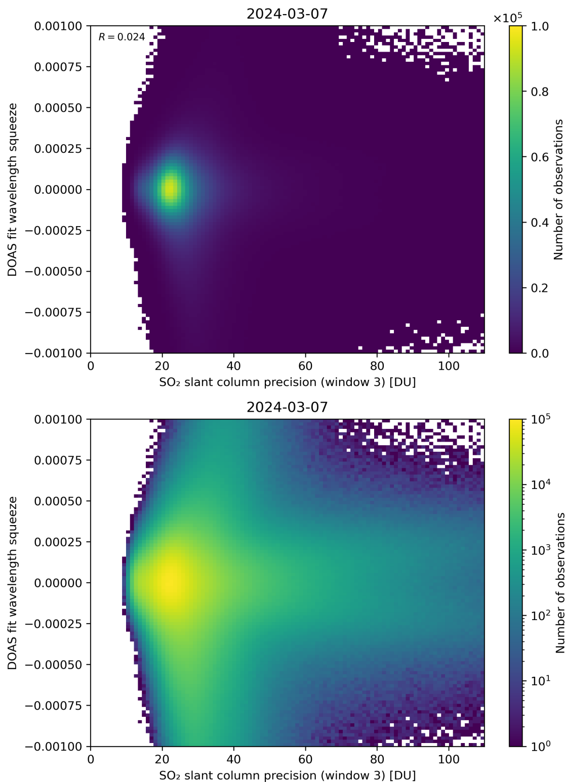
Figure 259: Scatter density plot of “SO 2 slant column precision (window 3)” against “DOAS fit wavelength squeeze” for 2024-03-06 to 2024-03-08.
