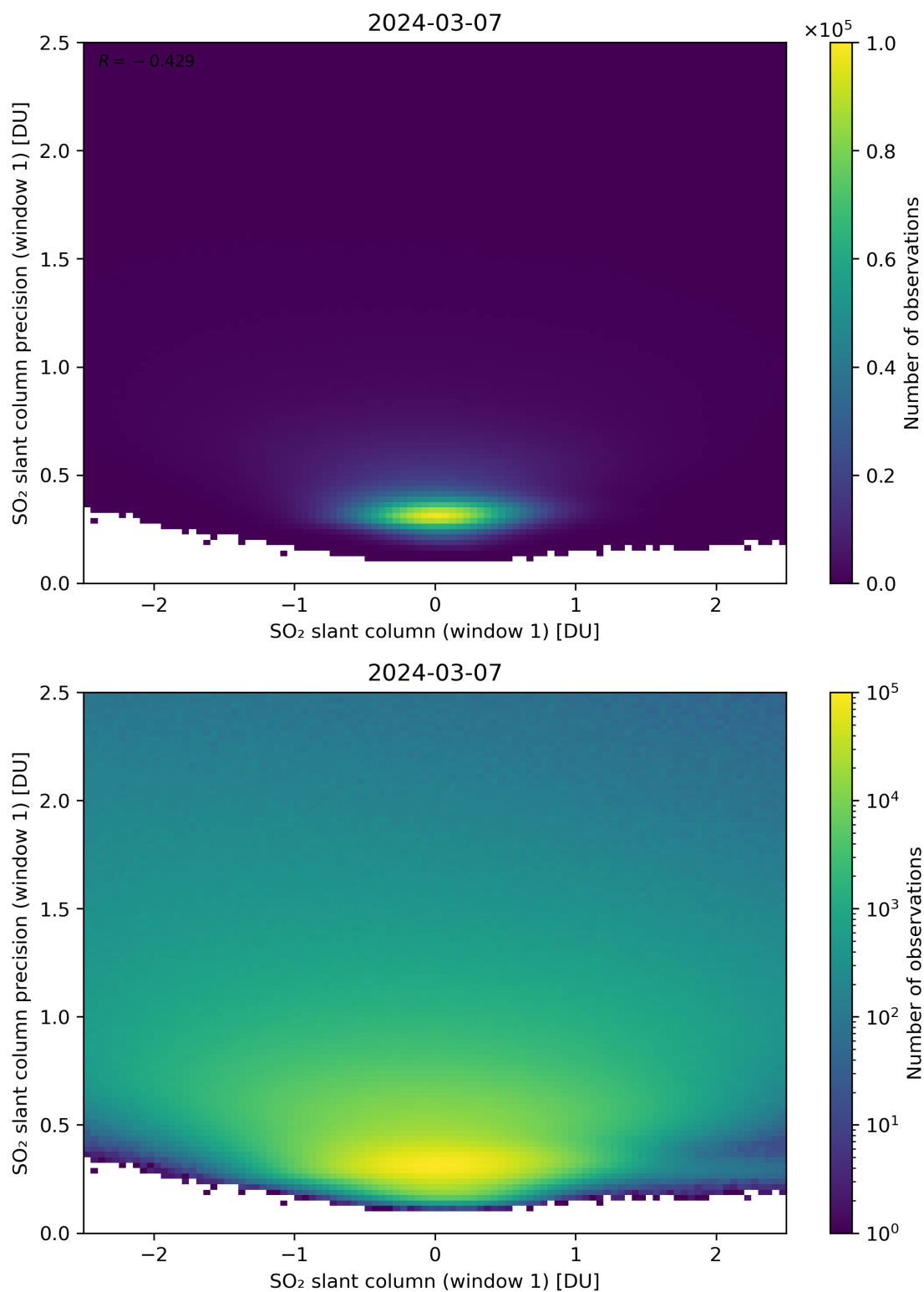
Figure 235: Scatter density plot of “SO 2 slant column (window 1)” against “SO 2 slant column precision (window 1)” for 2024-03-06 to 2024-03-08.
