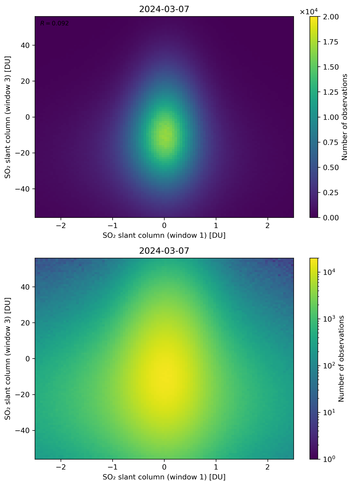
Figure 237: Scatter density plot of “SO 2 slant column (window 1)” against “SO 2 slant column (window 3)” for 2024-03-06 to 2024-03-08.
