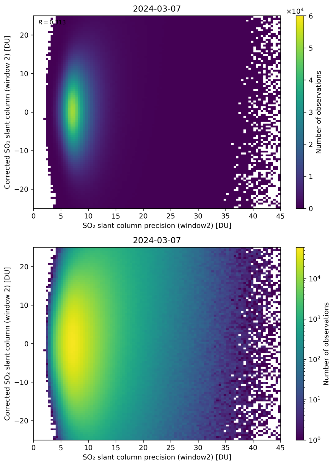
Figure 247: Scatter density plot of “SO 2 slant column precision (window2)” against “Corrected SO 2 slant column (window 2)” for 2024-03-06 to 2024-03-08.
