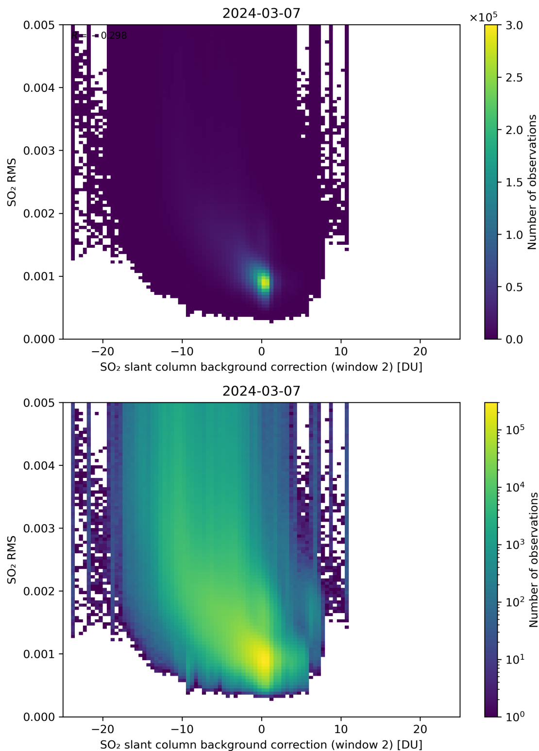
Figure 114: Scatter density plot of “SO 2 slant column background correction (window 2)” against “SO 2 RMS” for 2024-03-06 to 2024-03-08.
