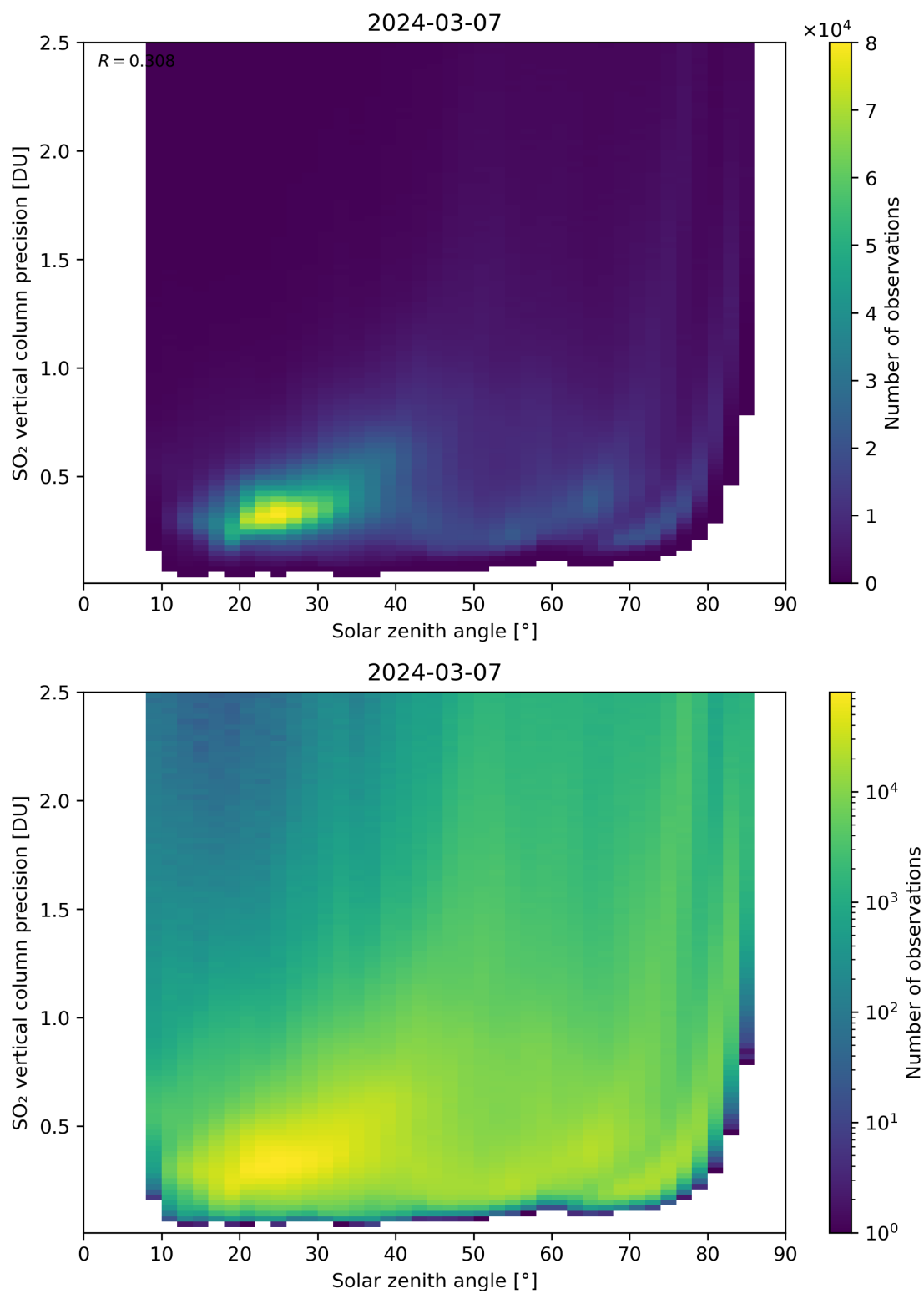
Figure 177: Scatter density plot of “Solar zenith angle” against “SO 2 vertical column precision” for 2024-03-06 to 2024-03-08.
