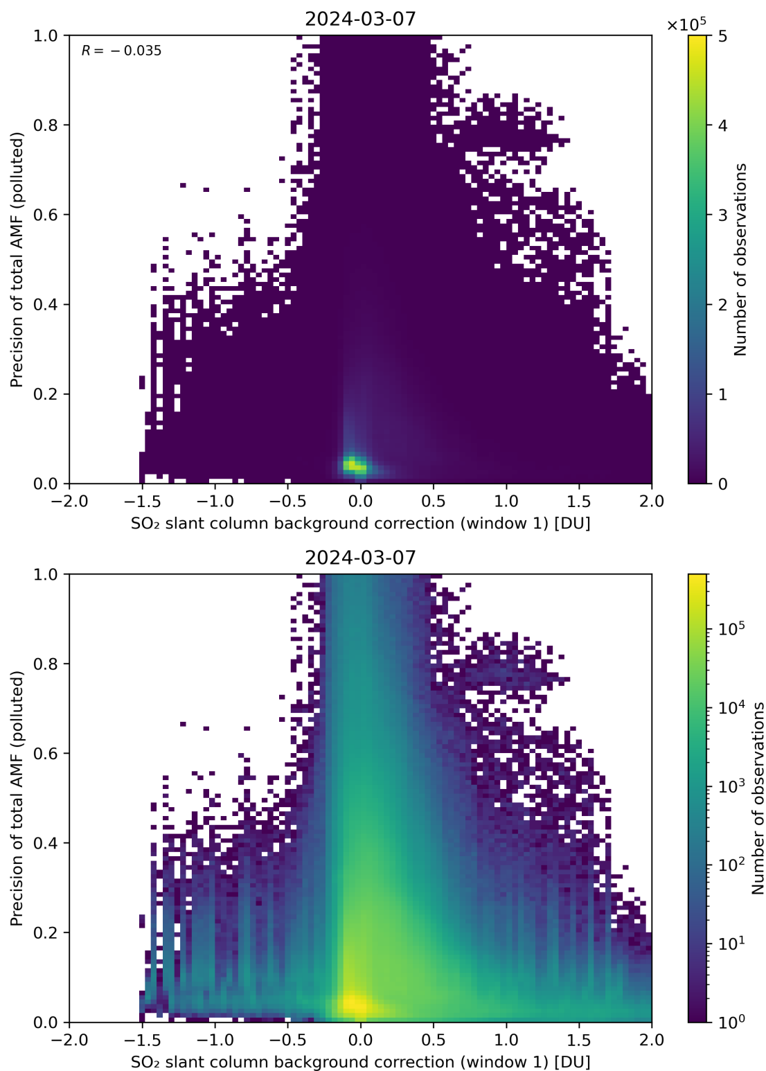
Figure 110: Scatter density plot of “SO 2 slant column background correction (window 1)” against “Precision of total AMF (polluted)” for 2024-03-06 to 2024-03-08.
