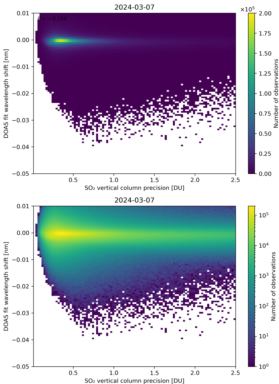
Figure 282: Scatter density plot of “SO 2 vertical column precision” against “DOAS fit wavelength shift” for 2024-03-06 to 2024-03-08.
