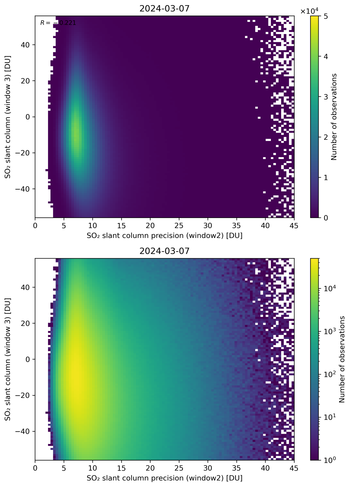
Figure 249: Scatter density plot of “SO 2 slant column precision (window2)” against “SO 2 slant column (window 3)” for 2024-03-06 to 2024-03-08.
