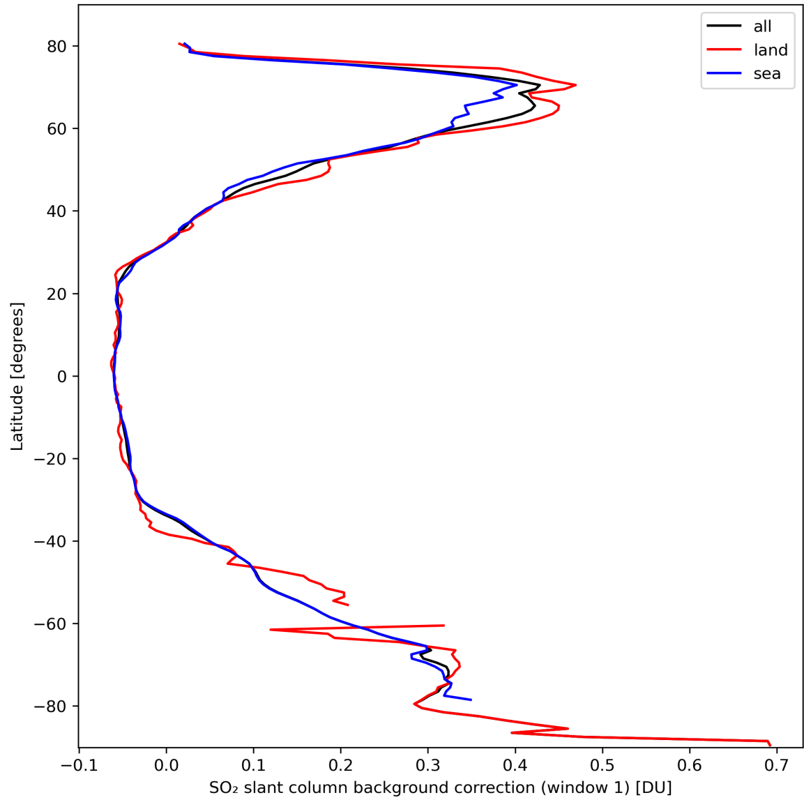
Figure 36: Zonal average of “SO 2 slant column background correction (window 1)” for 2024-03-06 to 2024-03-08.
