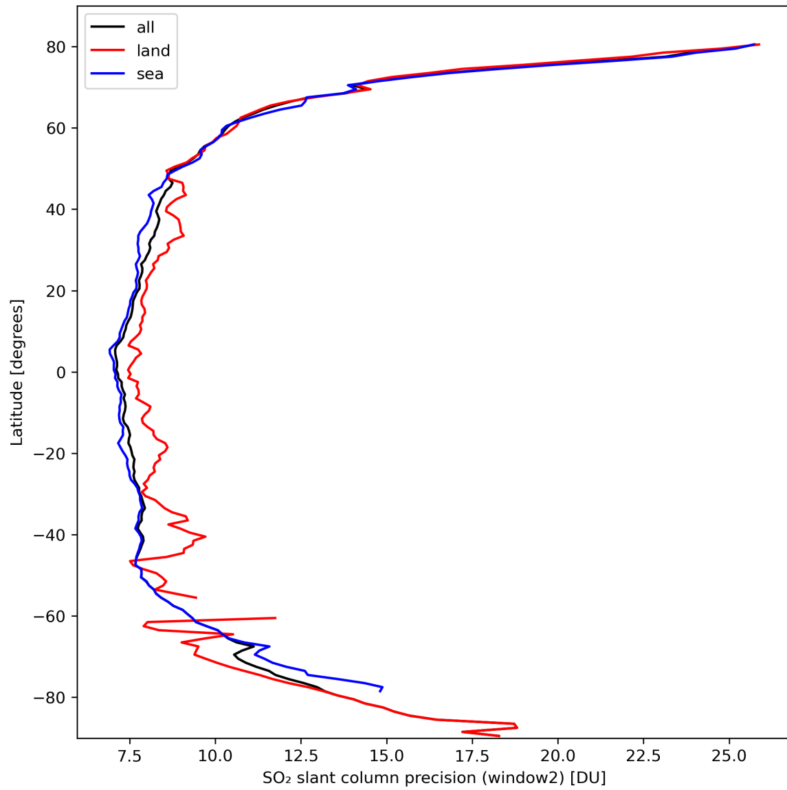
Figure 38: Zonal average of “SO 2 slant column precision (window2)” for 2024-03-06 to 2024-03-08.
