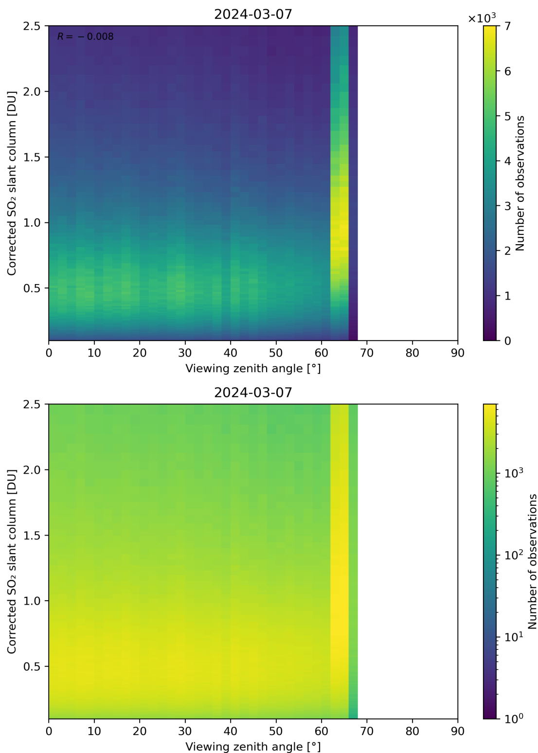
Figure 317: Scatter density plot of “Viewing zenith angle” against “Corrected SO 2 slant column” for 2024-03-06 to 2024-03-08.
