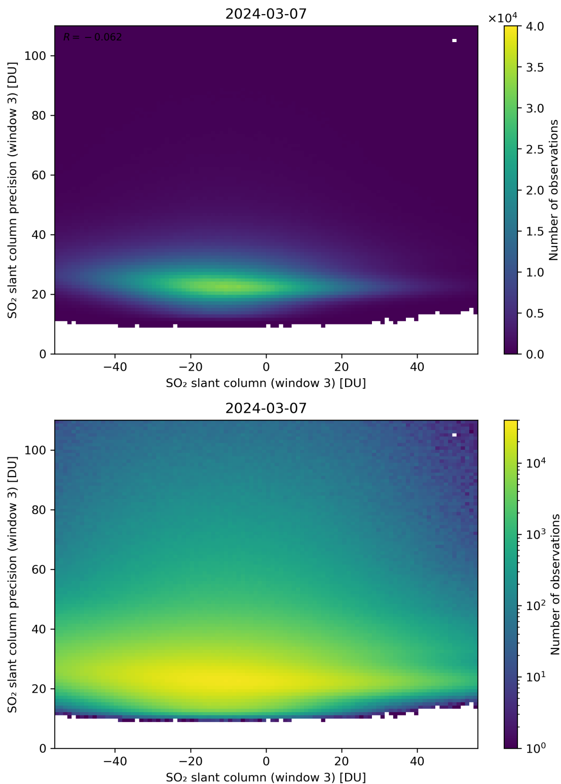
Figure 267: Scatter density plot of “SO 2 slant column (window 3)” against “SO 2 slant column precision (window 3)” for 2024-03-06 to 2024-03-08.
