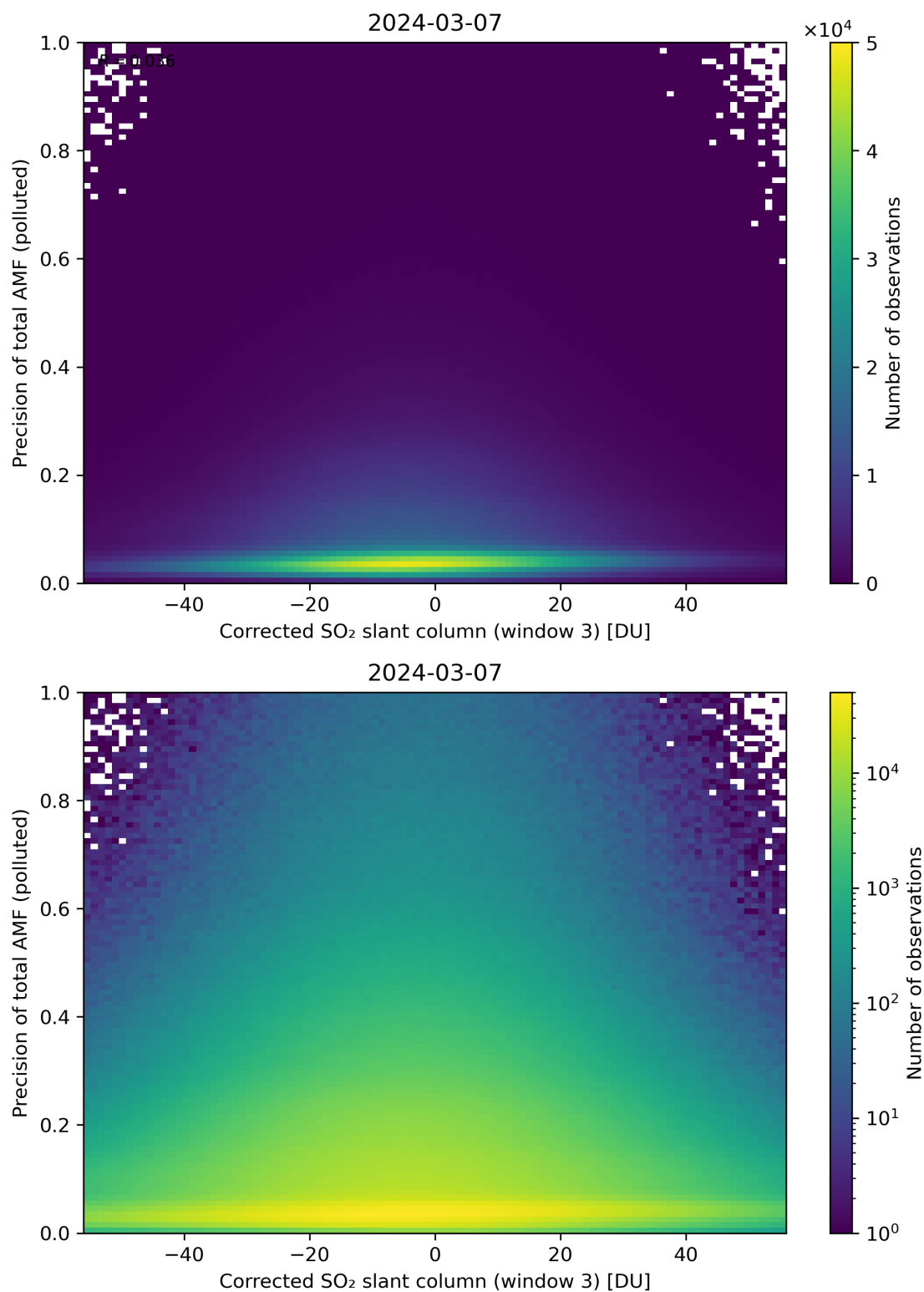
Figure 211: Scatter density plot of “Corrected SO 2 slant column (window 3)” against “Precision of total AMF (polluted)” for 2024-03-06 to 2024-03-08.
