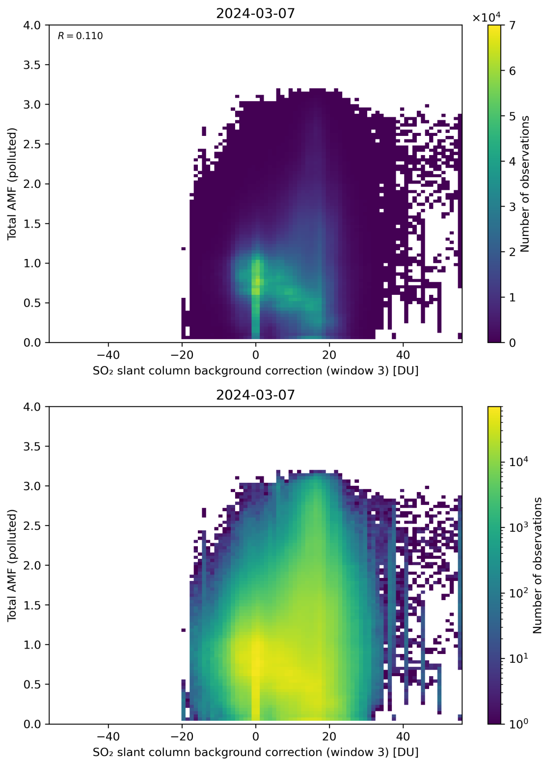
Figure 125: Scatter density plot of “SO 2 slant column background correction (window 3)” against “Total AMF (polluted)” for 2024-03-06 to 2024-03-08.
