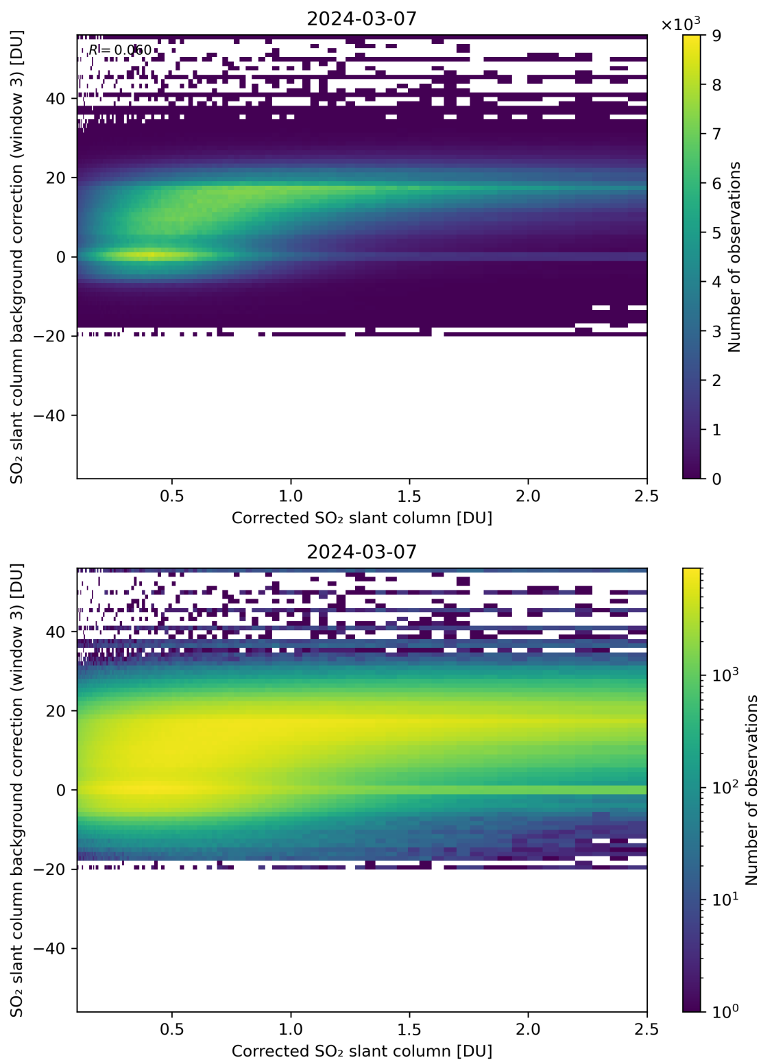
Figure 180: Scatter density plot of “Corrected SO 2 slant column” against “SO 2 slant column background correction (window 3)” for 2024-03-06 to 2024-03-08.
