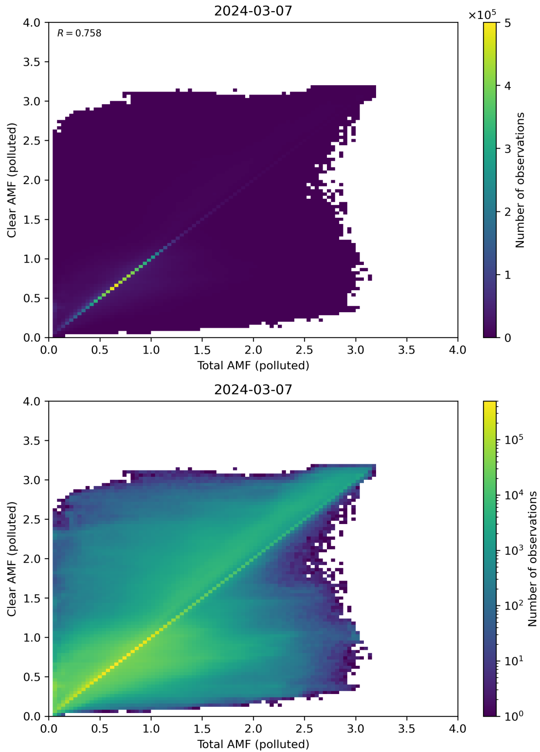
Figure 271: Scatter density plot of “Total AMF (polluted)” against “Clear AMF (polluted)” for 2024-03-06 to 2024-03-08.
