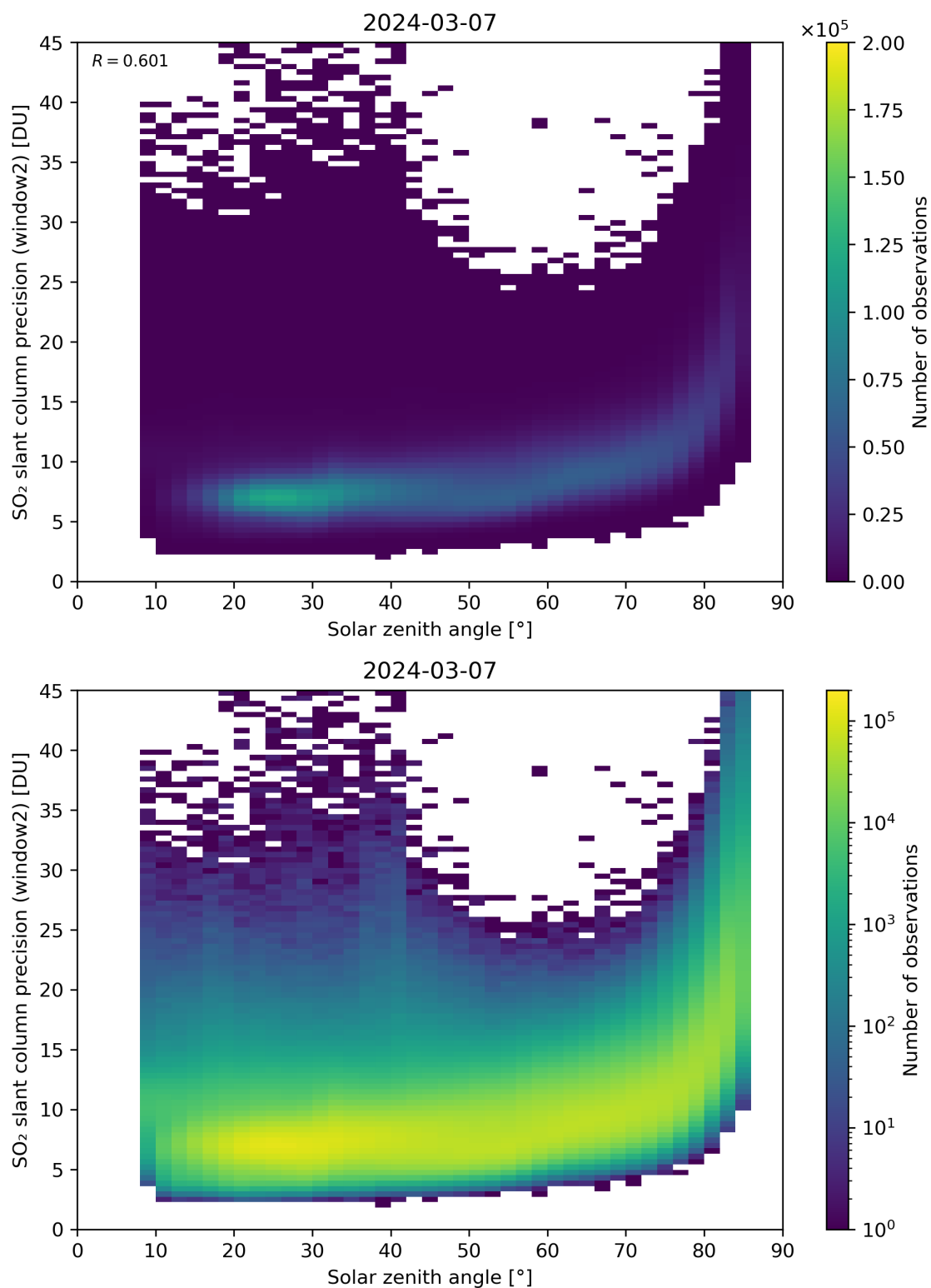
Figure 171: Scatter density plot of “Solar zenith angle” against “SO 2 slant column precision (window2)” for 2024-03-06 to 2024-03-08.
