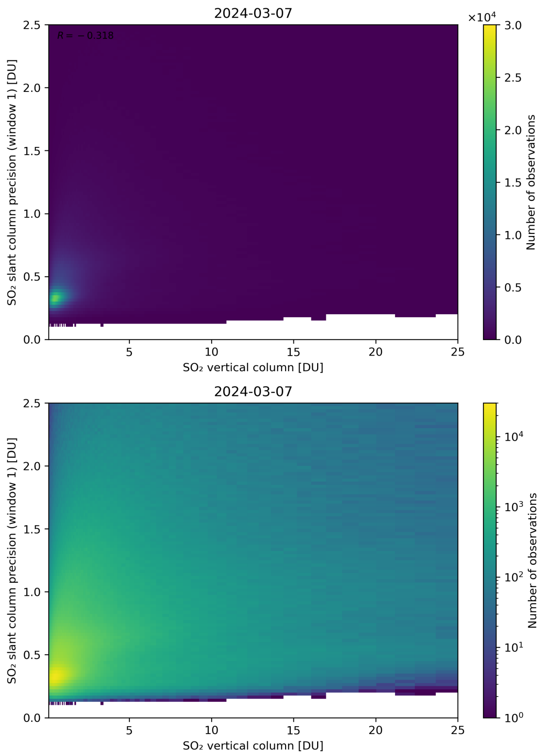
Figure 301: Scatter density plot of “SO 2 vertical column” against “SO 2 slant column precision (window 1)” for 2024-03-06 to 2024-03-08.
