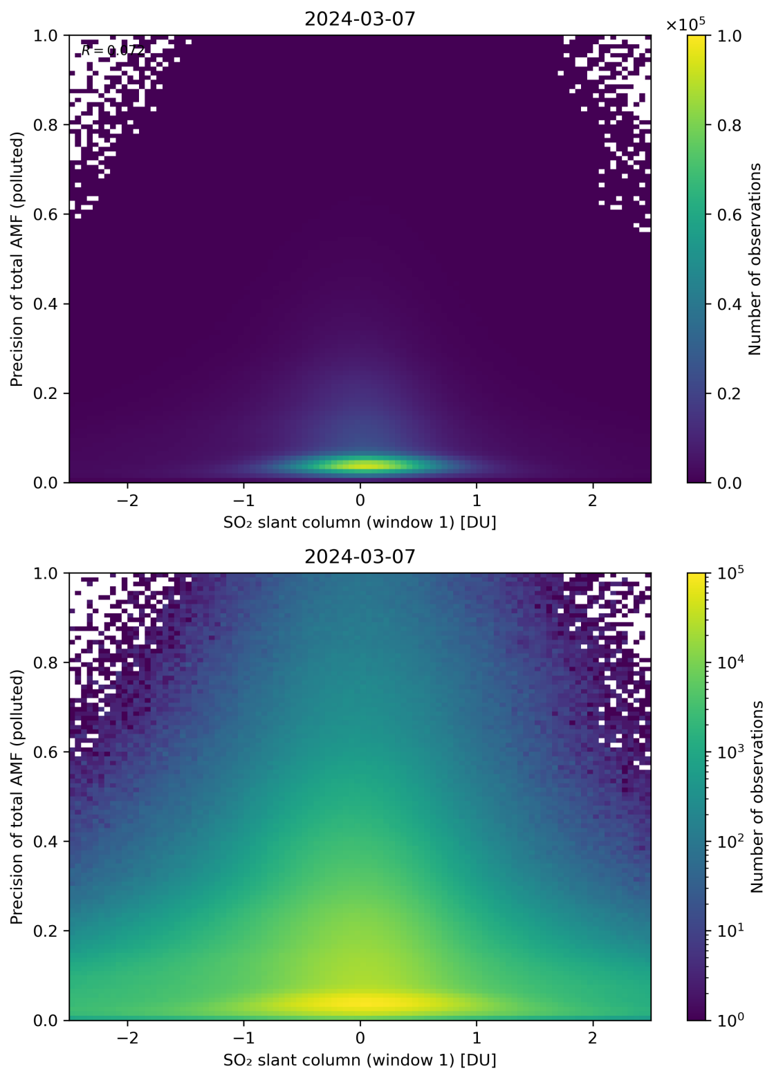
Figure 240: Scatter density plot of “SO 2 slant column (window 1)” against “Precision of total AMF (polluted)” for 2024-03-06 to 2024-03-08.
