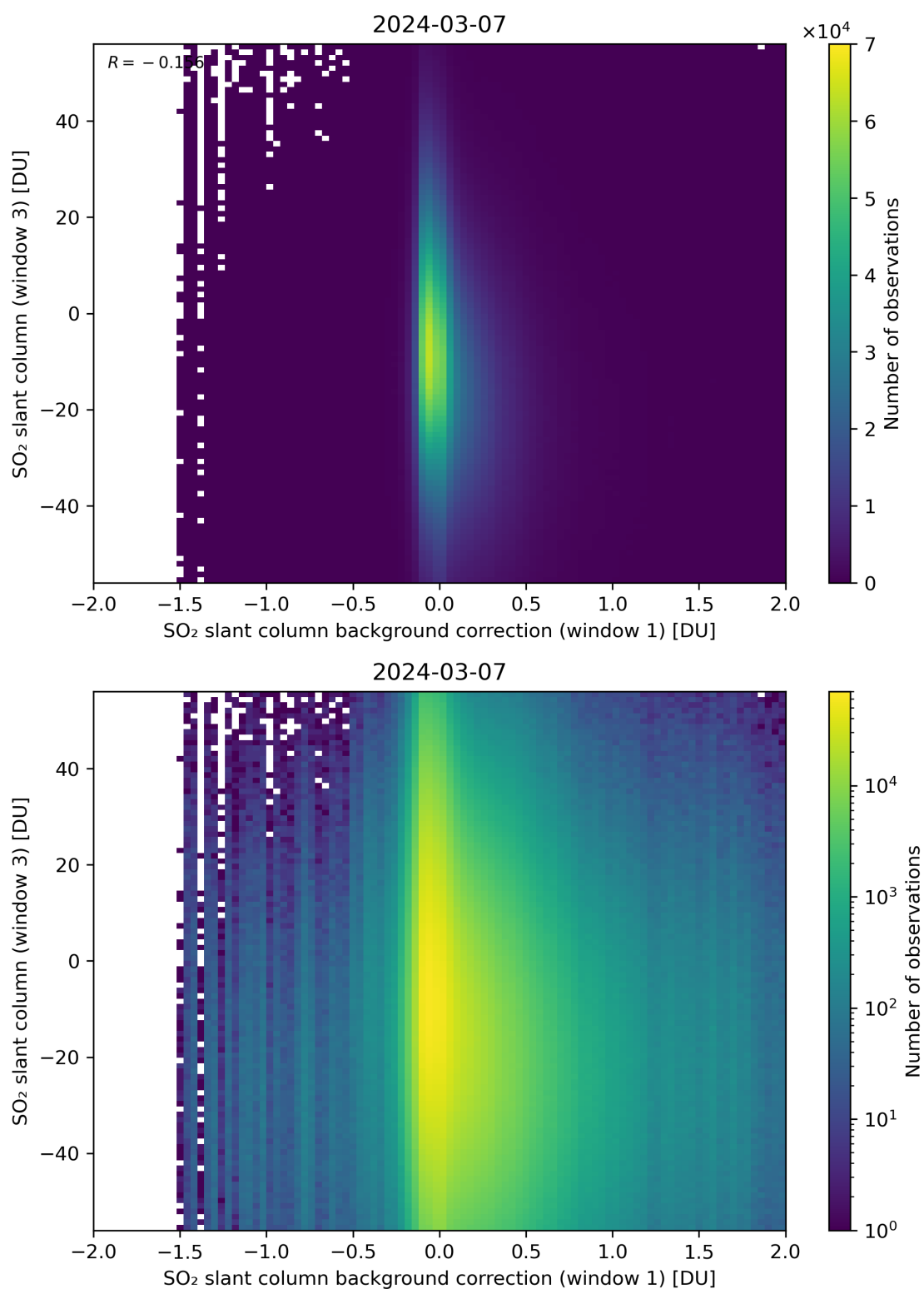
Figure 107: Scatter density plot of “SO 2 slant column background correction (window 1)” against “SO 2 slant column (window 3)” for 2024-03-06 to 2024-03-08.
