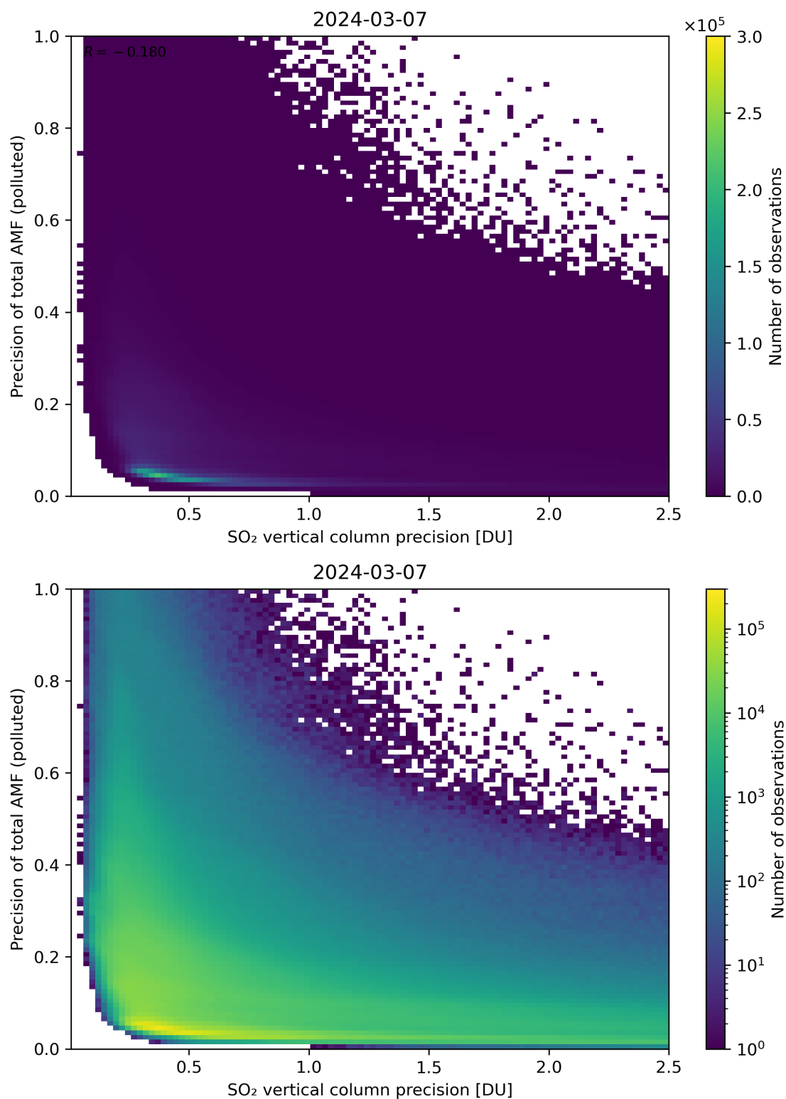
Figure 295: Scatter density plot of “SO 2 vertical column precision” against “Precision of total AMF (polluted)” for 2024-03-06 to 2024-03-08.
