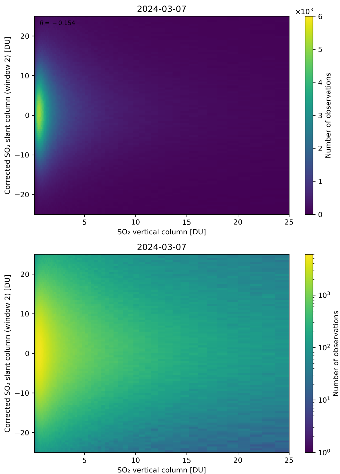
Figure 298: Scatter density plot of “SO 2 vertical column” against “Corrected SO 2 slant column (window 2)” for 2024-03-06 to 2024-03-08.
