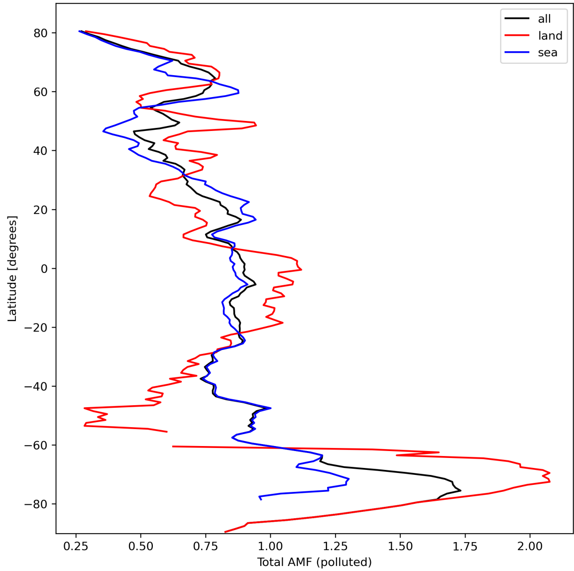
Figure 48: Zonal average of “Total AMF (polluted)” for 2024-03-06 to 2024-03-08.
