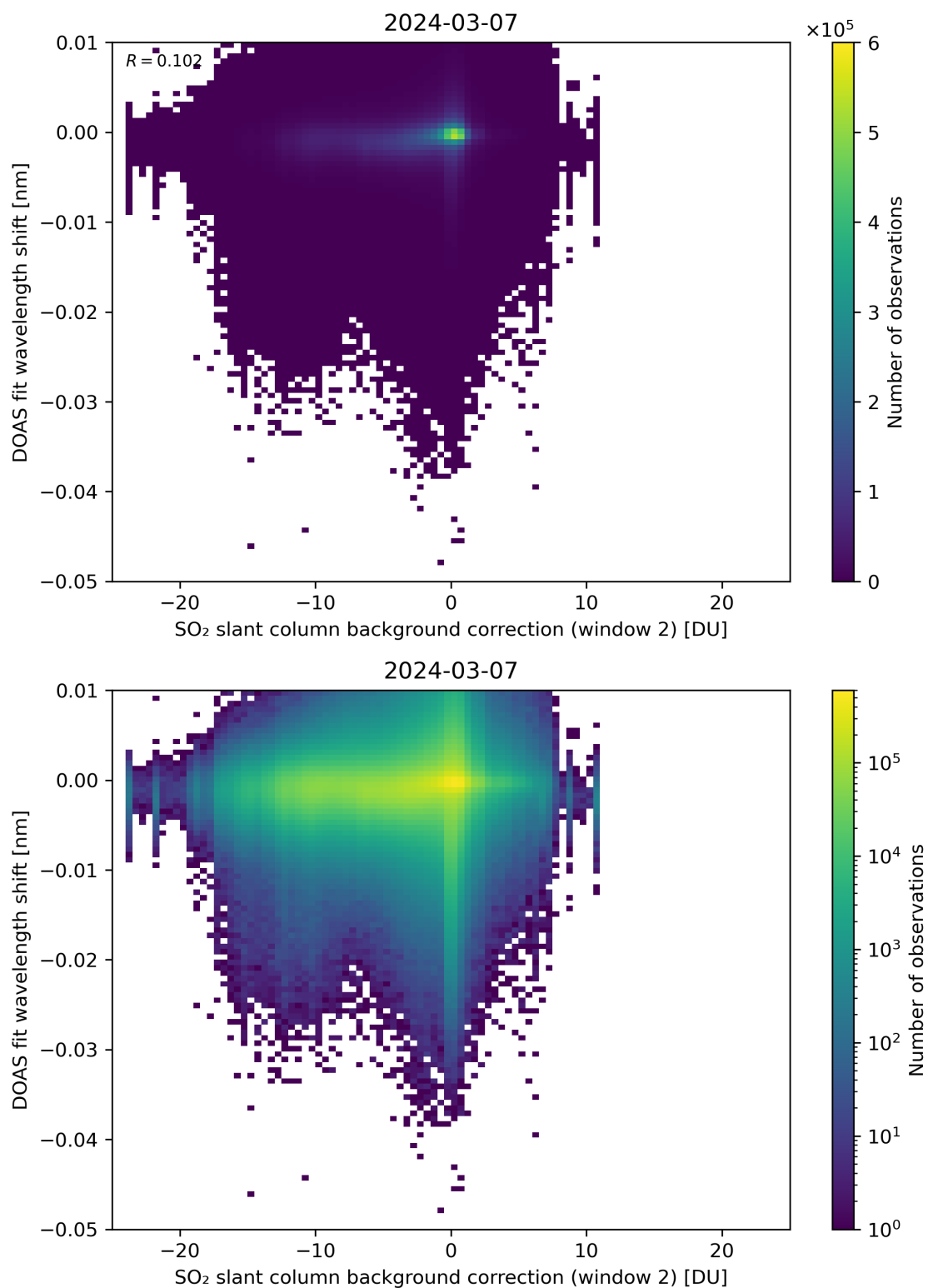
Figure 112: Scatter density plot of “SO 2 slant column background correction (window 2)” against “DOAS fit wavelength shift” for 2024-03-06 to 2024-03-08.
