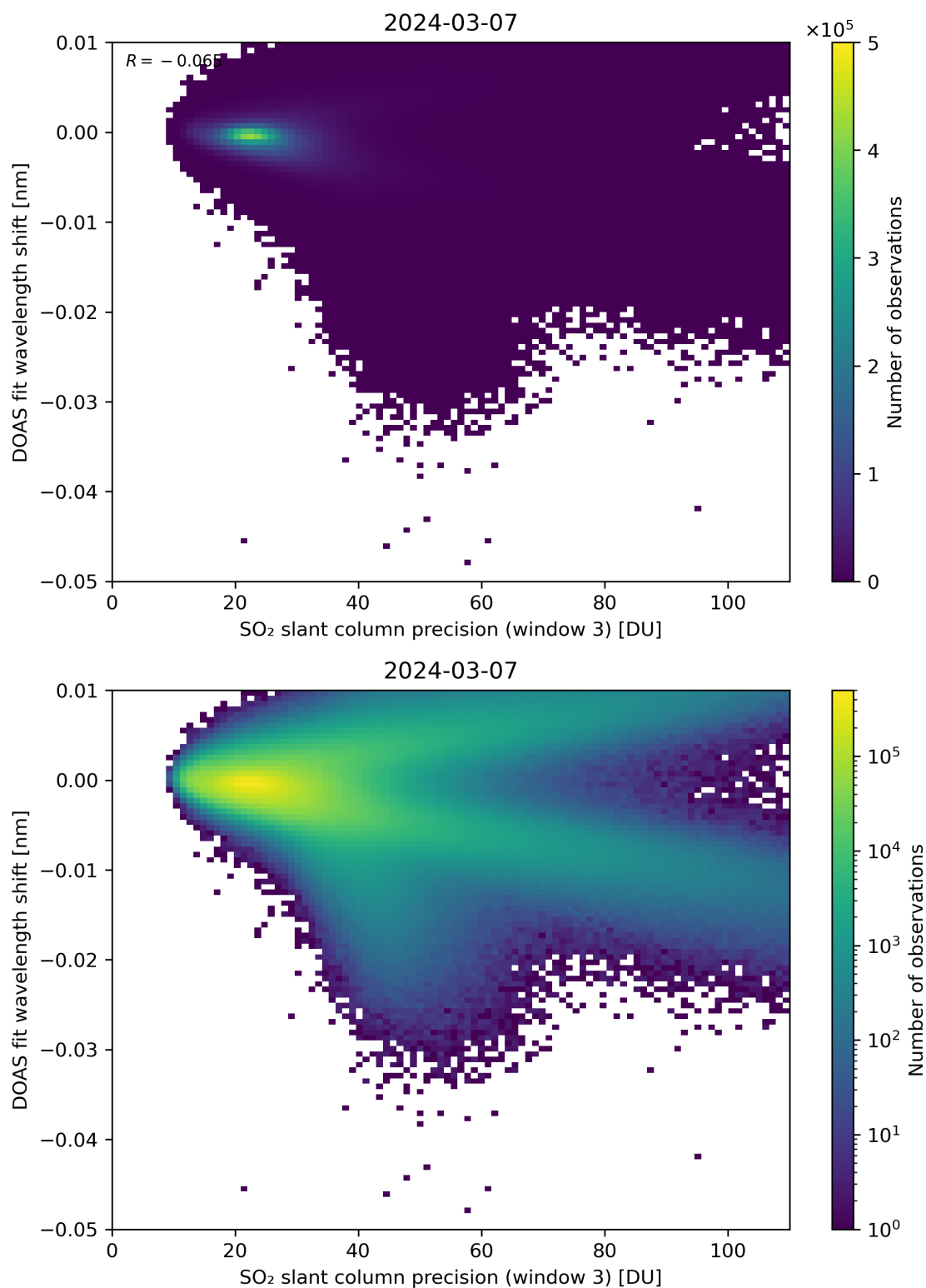
Figure 258: Scatter density plot of “SO 2 slant column precision (window 3)” against “DOAS fit wavelength shift” for 2024-03-06 to 2024-03-08.
