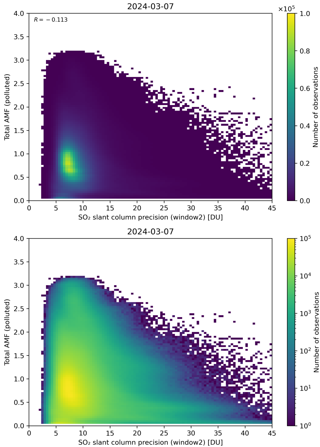
Figure 251: Scatter density plot of “SO 2 slant column precision (window2)” against “Total AMF (polluted)” for 2024-03-06 to 2024-03-08.
