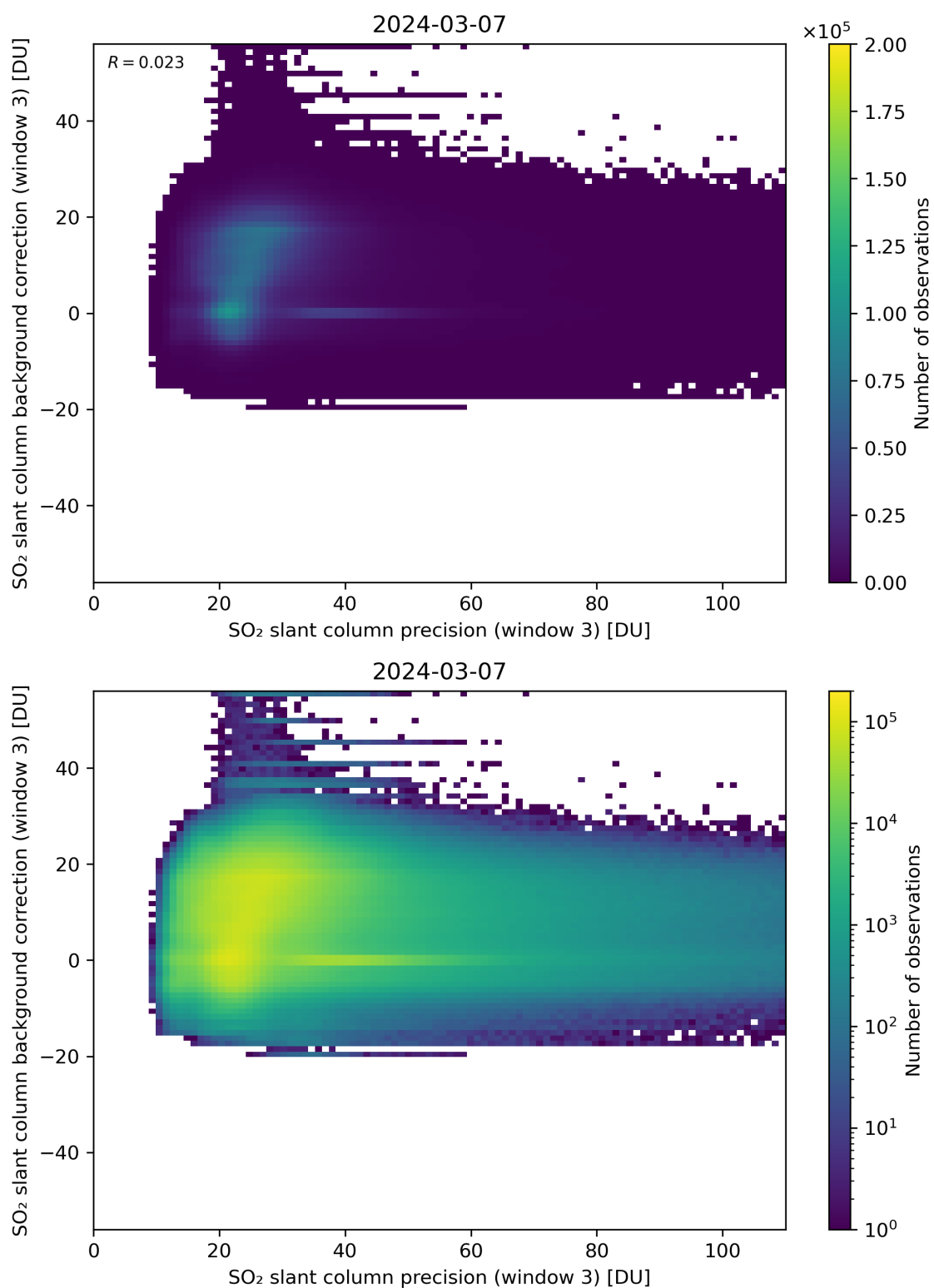
Figure 257: Scatter density plot of “SO 2 slant column precision (window 3)” against “SO 2 slant column background correction (window 3)” for 2024-03-06 to 2024-03-08.
