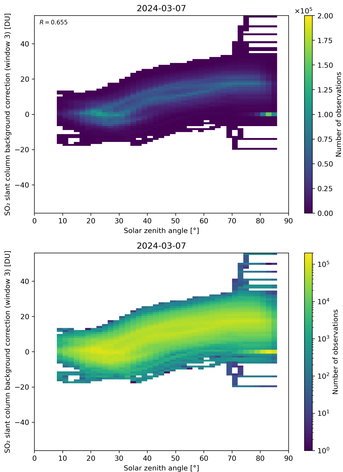
Figure 160: Scatter density plot of “Solar zenith angle” against “SO 2 slant column background correction (window 3)” for 2024-03-06 to 2024-03-08.
