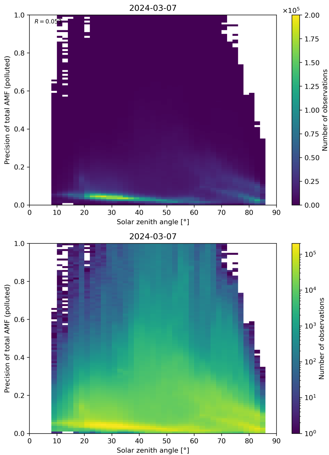
Figure 175: Scatter density plot of “Solar zenith angle” against “Precision of total AMF (polluted)” for 2024-03-06 to 2024-03-08.
