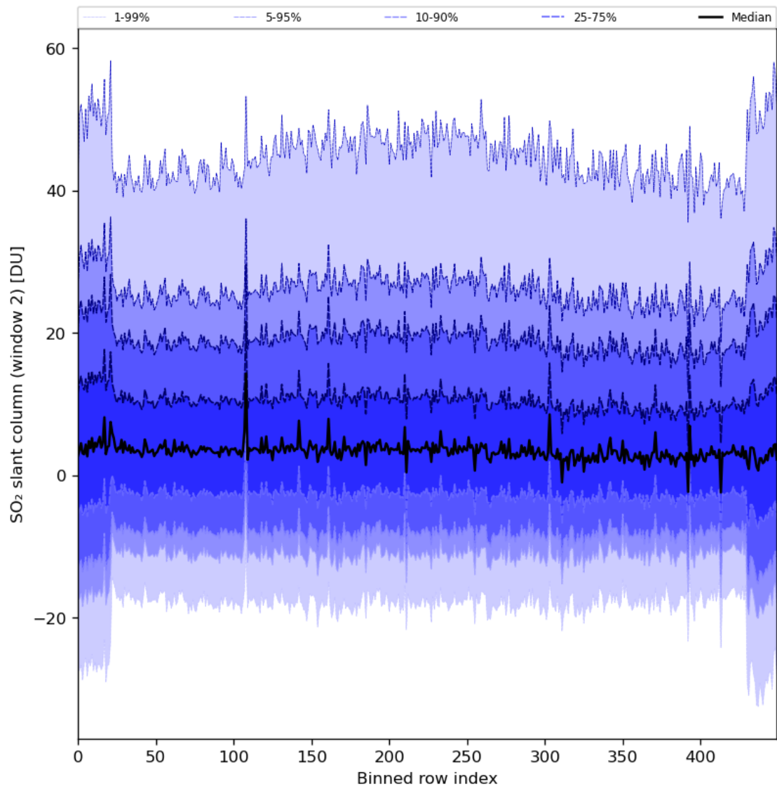
Figure 83: Along track statistics of “SO 2 slant column (window 2)” for 2024-03-06 to 2024-03-08
