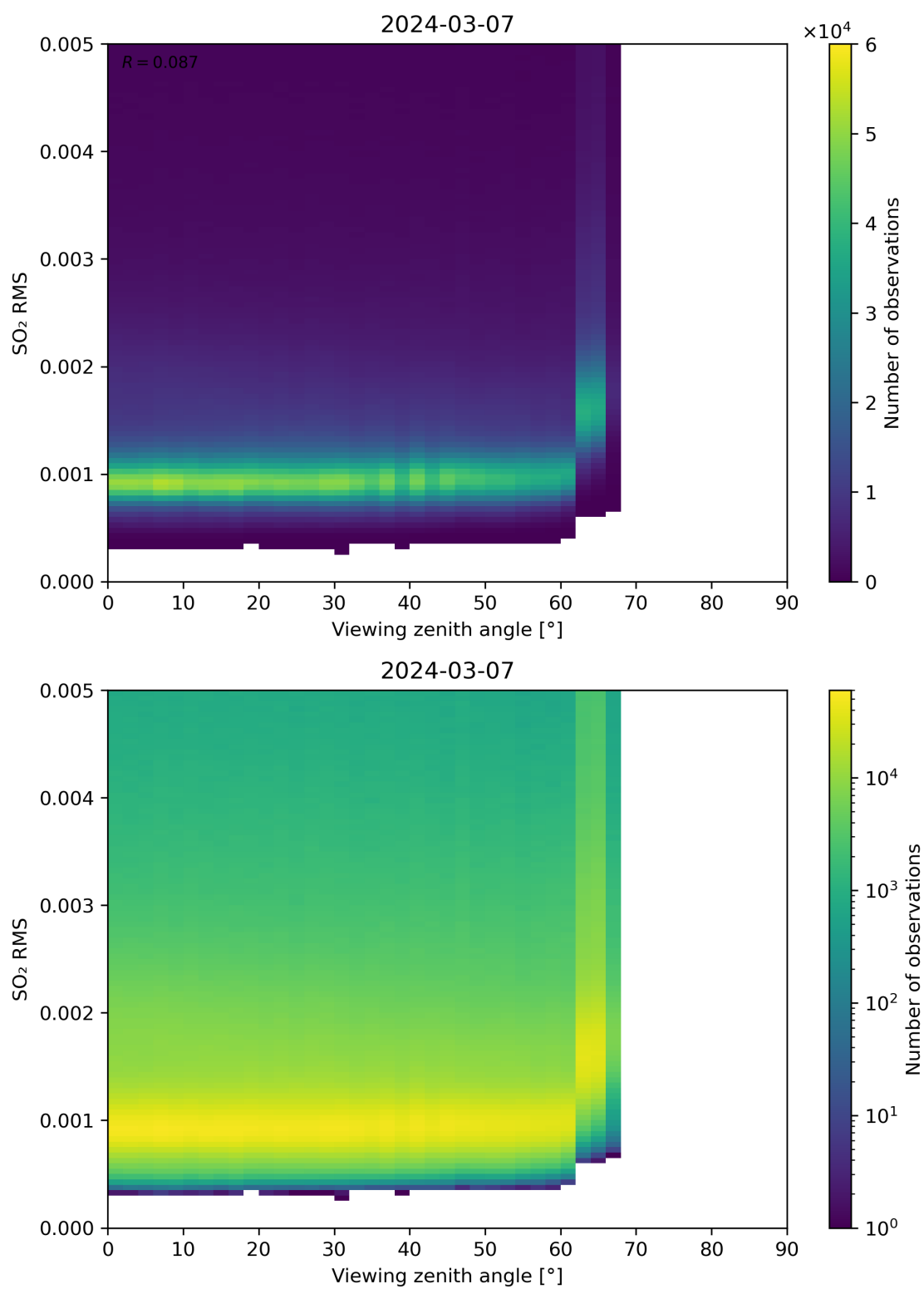
Figure 313: Scatter density plot of “Viewing zenith angle” against “SO 2 RMS” for 2024-03-06 to 2024-03-08.
