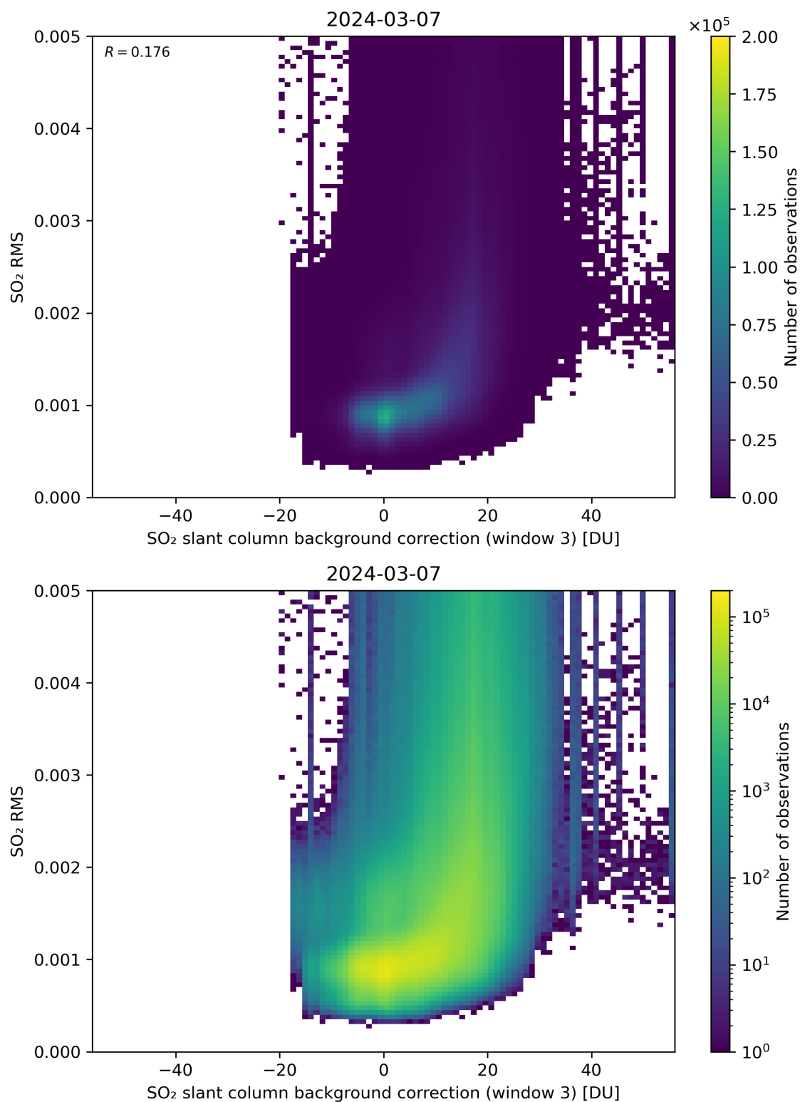
Figure 123: Scatter density plot of “SO 2 slant column background correction (window 3)” against “SO 2 RMS” for 2024-03-06 to 2024-03-08.
