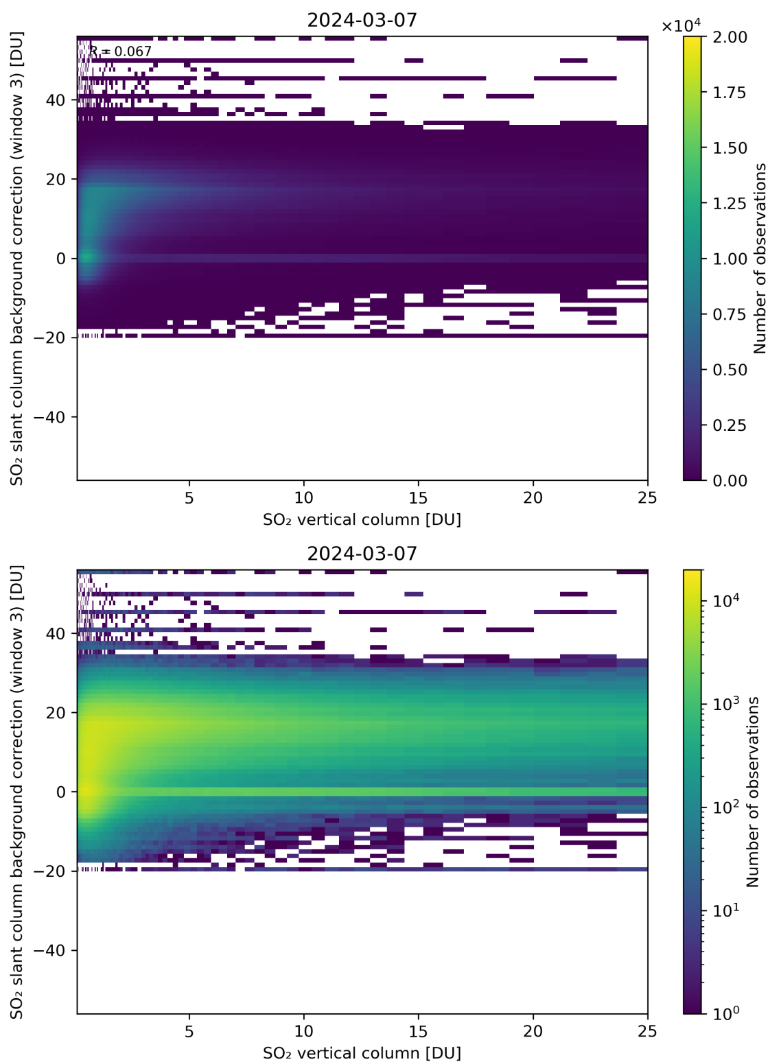
Figure 275: Scatter density plot of “SO 2 vertical column” against “SO 2 slant column background correction (window 3)” for 2024-03-06 to 2024-03-08.
