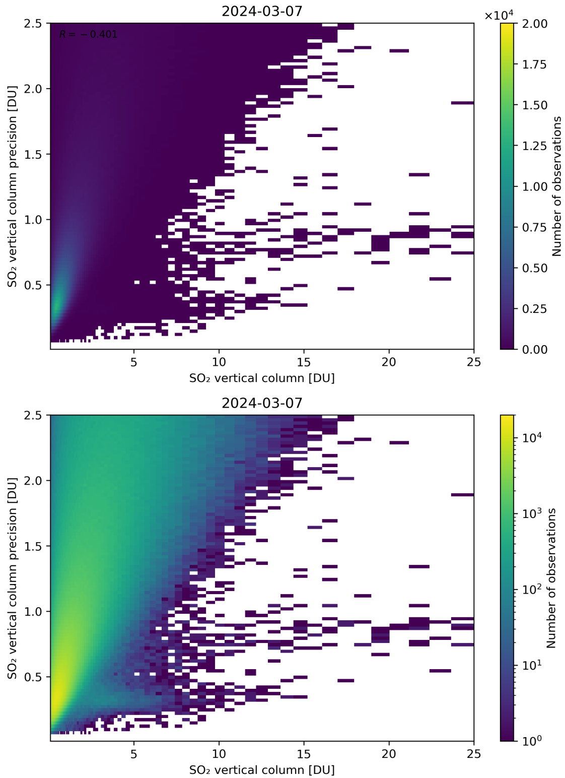
Figure 307: Scatter density plot of “SO 2 vertical column” against “SO 2 vertical column precision” for 2024-03-06 to 2024-03-08.
