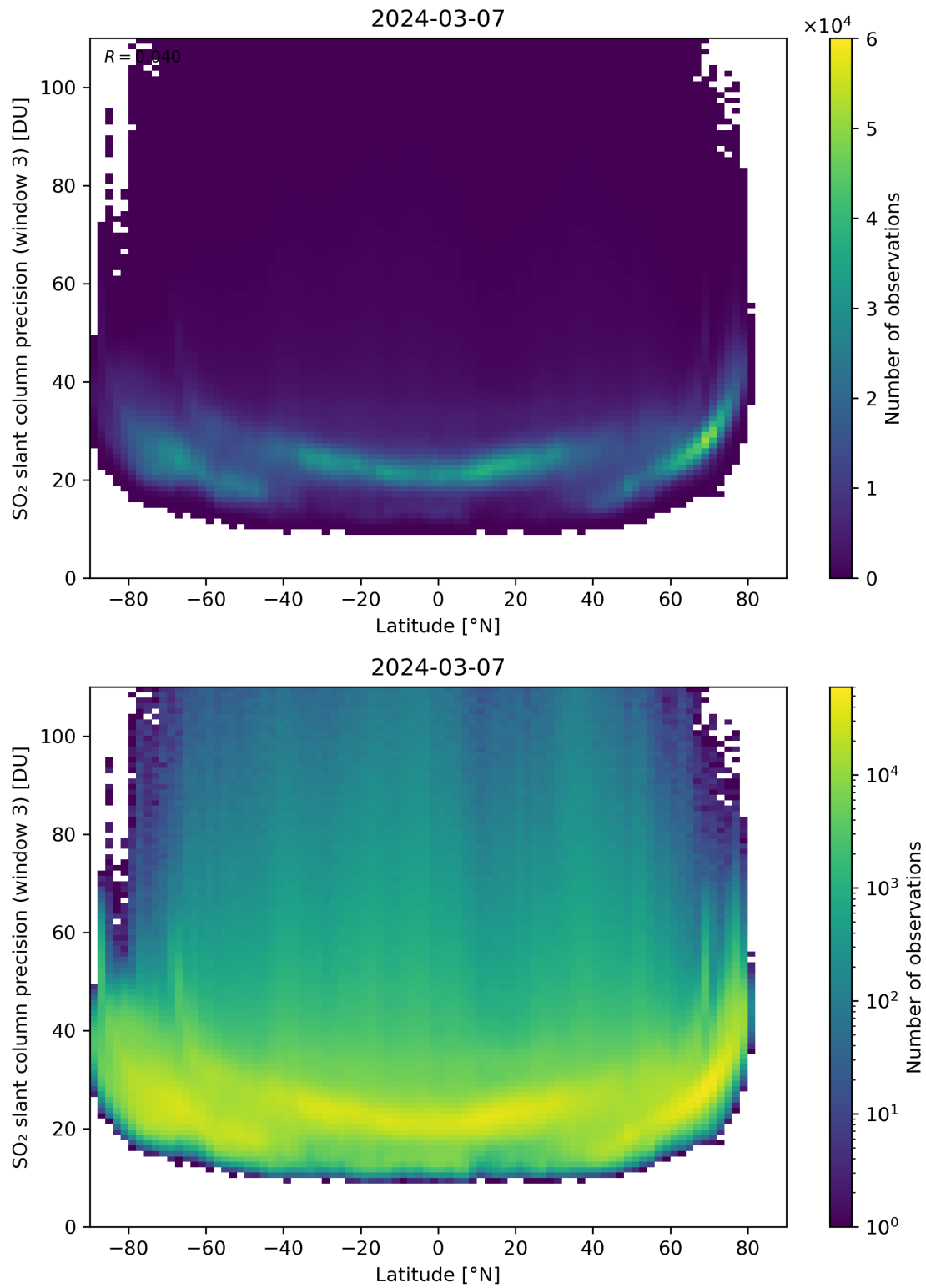
Figure 153: Scatter density plot of “Latitude” against “SO 2 slant column precision (window 3)” for 2024-03-06 to 2024-03-08.
