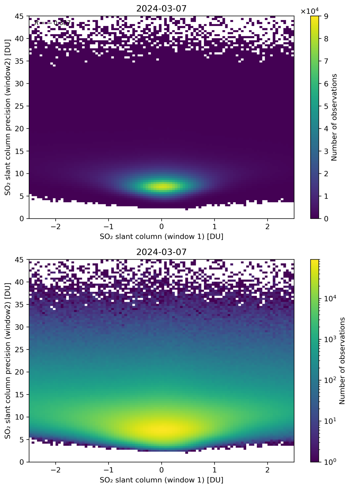
Figure 236: Scatter density plot of “SO 2 slant column (window 1)” against “SO 2 slant column precision (window2)” for 2024-03-06 to 2024-03-08.
