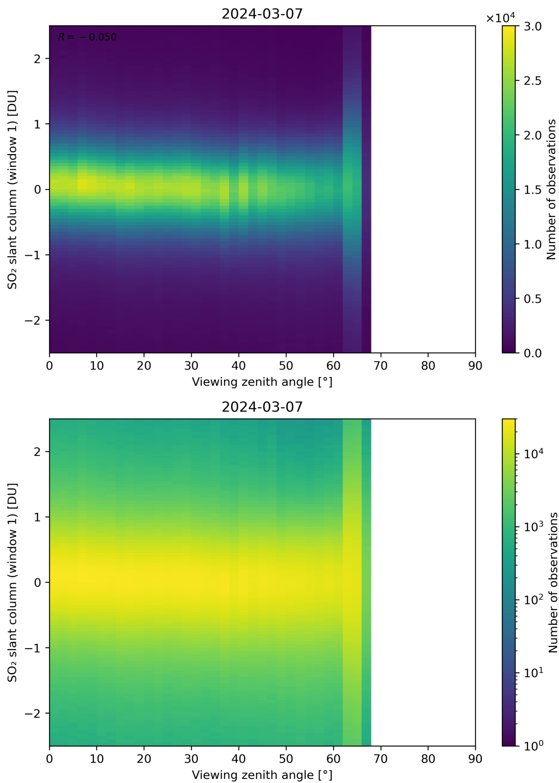
Figure 320: Scatter density plot of “Viewing zenith angle” against “SO 2 slant column (window 1)” for 2024-03-06 to 2024-03-08.
