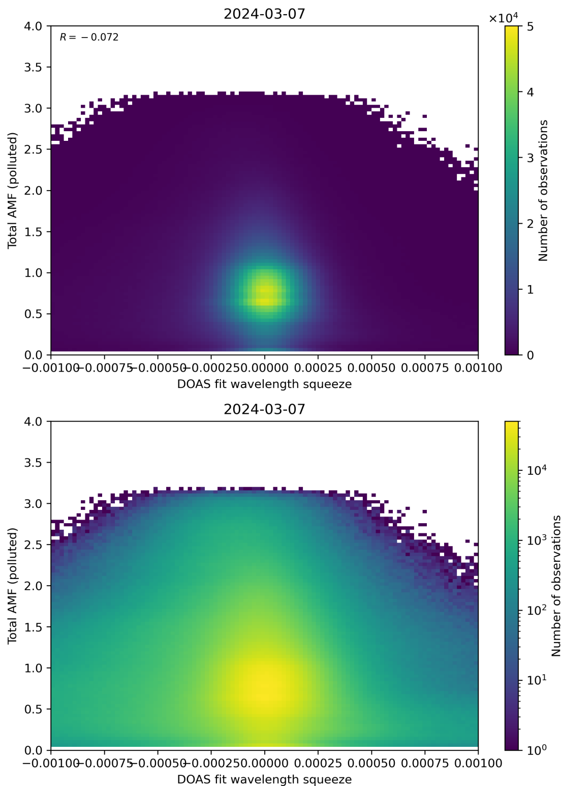
Figure 134: Scatter density plot of “DOAS fit wavelength squeeze” against “Total AMF (polluted)” for 2024-03-06 to 2024-03-08.
