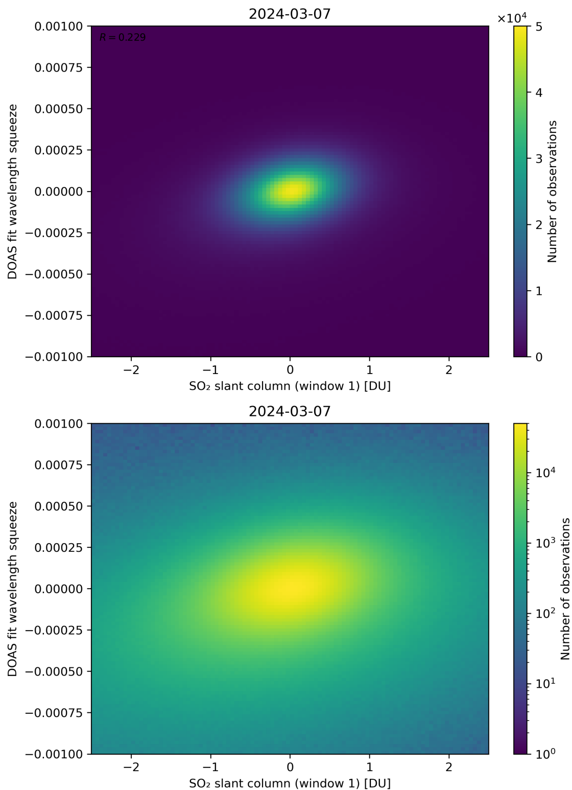
Figure 216: Scatter density plot of “SO 2 slant column (window 1)” against “DOAS fit wavelength squeeze” for 2024-03-06 to 2024-03-08.
