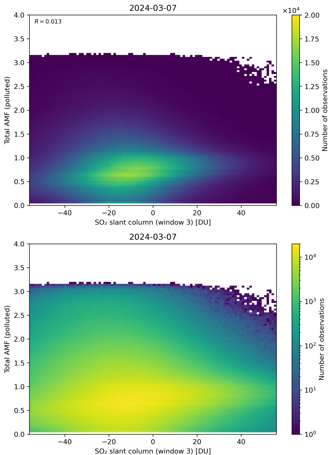
Figure 268: Scatter density plot of “SO 2 slant column (window 3)” against “Total AMF (polluted)” for 2024-03-06 to 2024-03-08.
