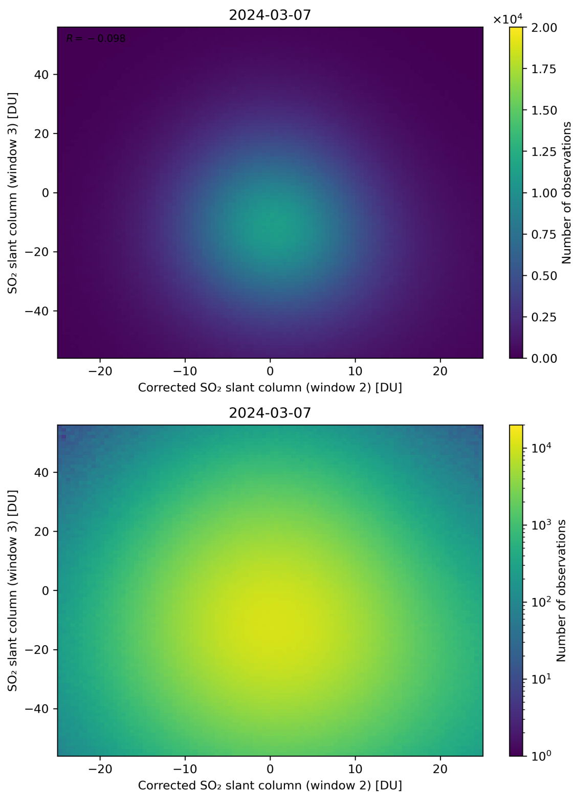
Figure 201: Scatter density plot of “Corrected SO 2 slant column (window 2)” against “SO 2 slant column (window 3)” for 2024-03-06 to 2024-03-08.
