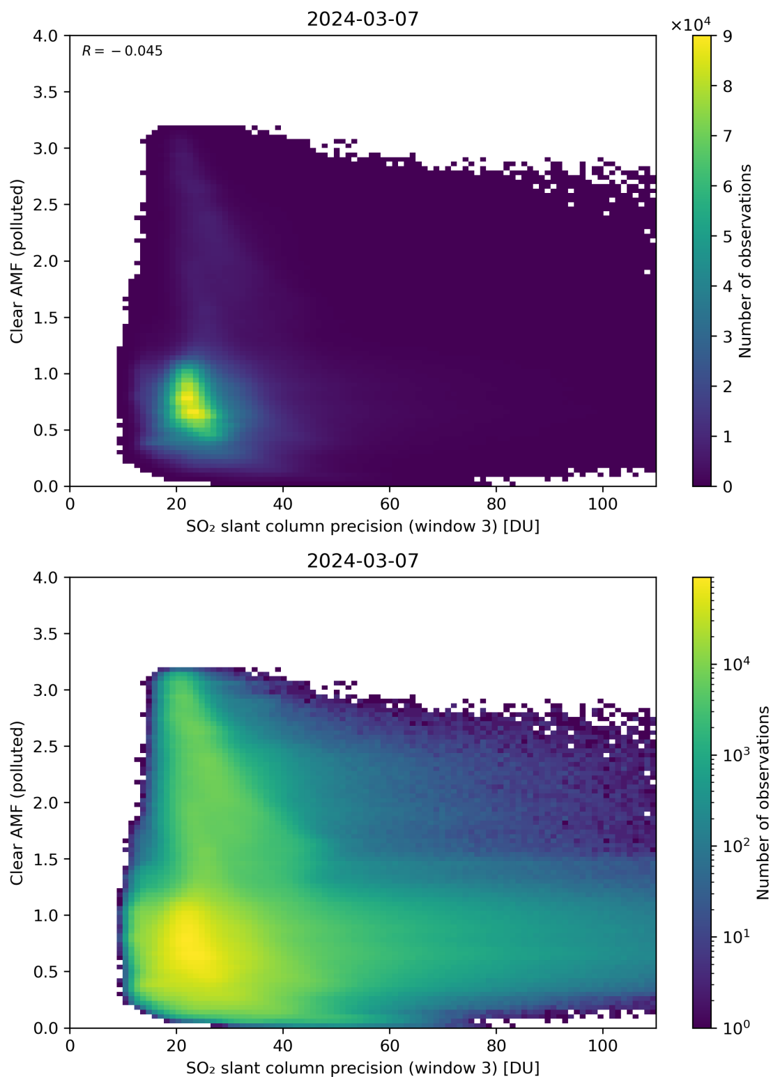
Figure 261: Scatter density plot of “SO 2 slant column precision (window 3)” against “Clear AMF (polluted)” for 2024-03-06 to 2024-03-08.
