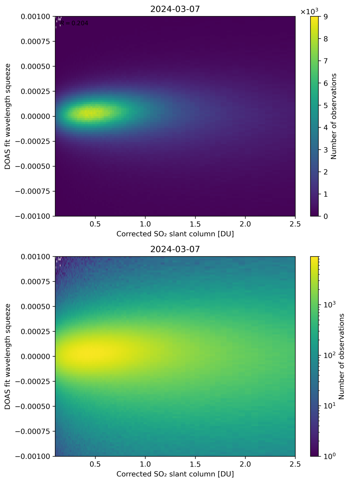
Figure 182: Scatter density plot of “Corrected SO 2 slant column” against “DOAS fit wavelength squeeze” for 2024-03-06 to 2024-03-08.
