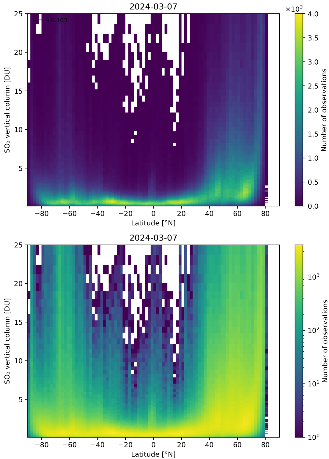
Figure 156: Scatter density plot of “Latitude” against “SO 2 vertical column” for 2024-03-06 to 2024-03-08.
