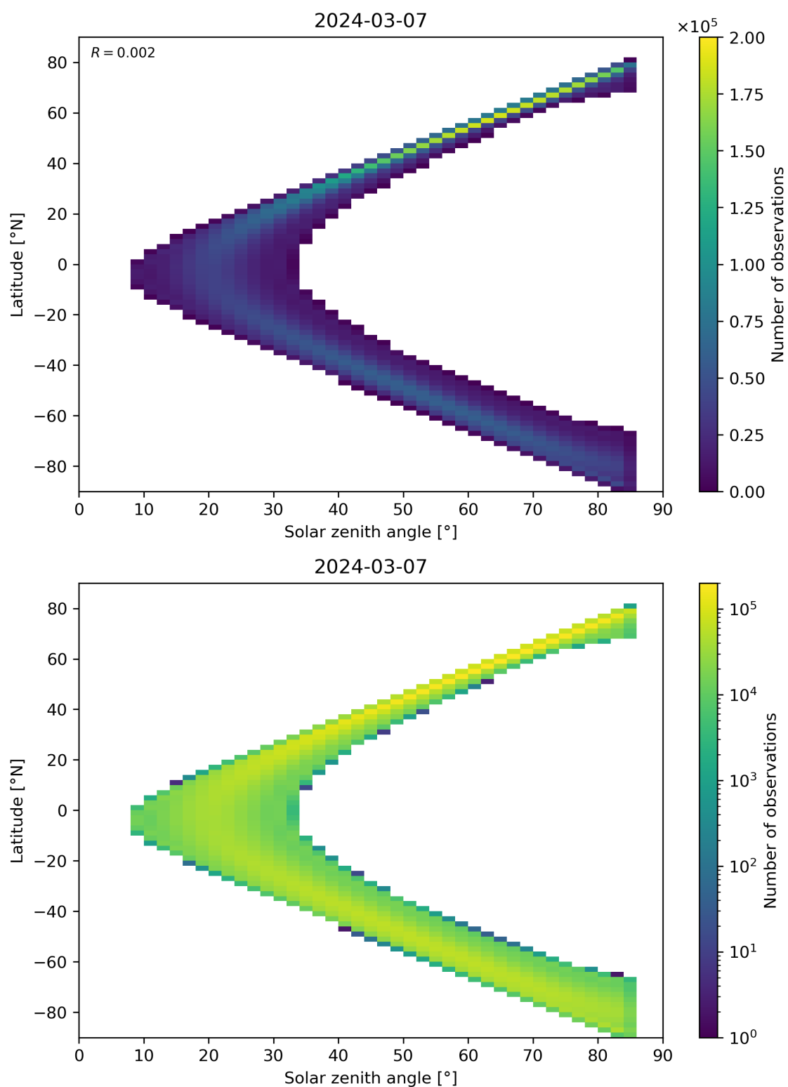
Figure 164: Scatter density plot of “Solar zenith angle” against “Latitude” for 2024-03-06 to 2024-03-08.
