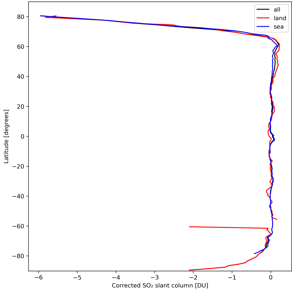
Figure 32: Zonal average of “Corrected SO 2 slant column” for 2024-03-06 to 2024-03-08.
