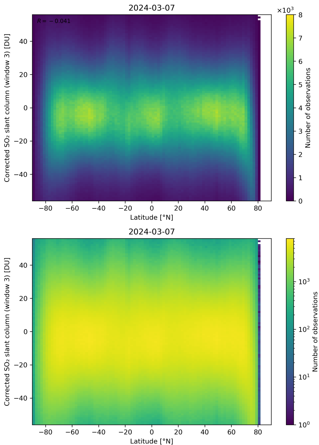
Figure 148: Scatter density plot of “Latitude” against “Corrected SO 2 slant column (window 3)” for 2024-03-06 to 2024-03-08.
