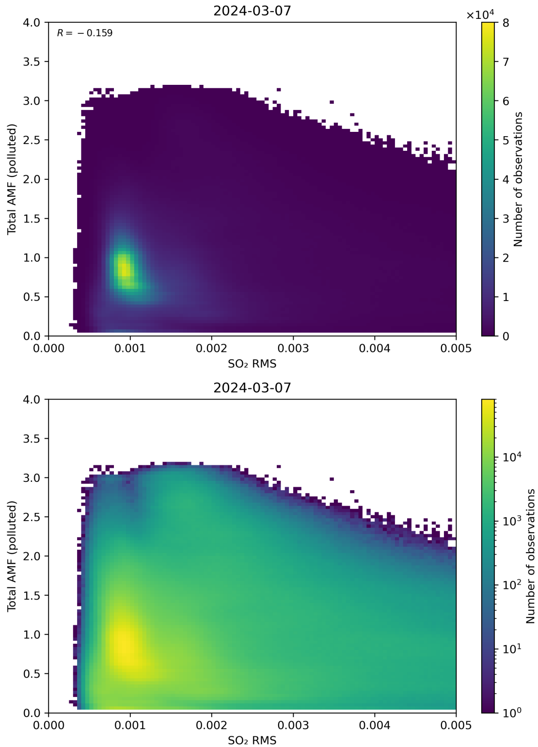
Figure 137: Scatter density plot of “SO 2 RMS” against “Total AMF (polluted)” for 2024-03-06 to 2024-03-08.
