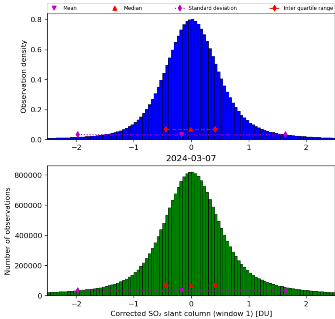
Figure 58: Histogram of “Corrected SO 2 slant column (window 1)” for 2024-03-06 to 2024-03-08
