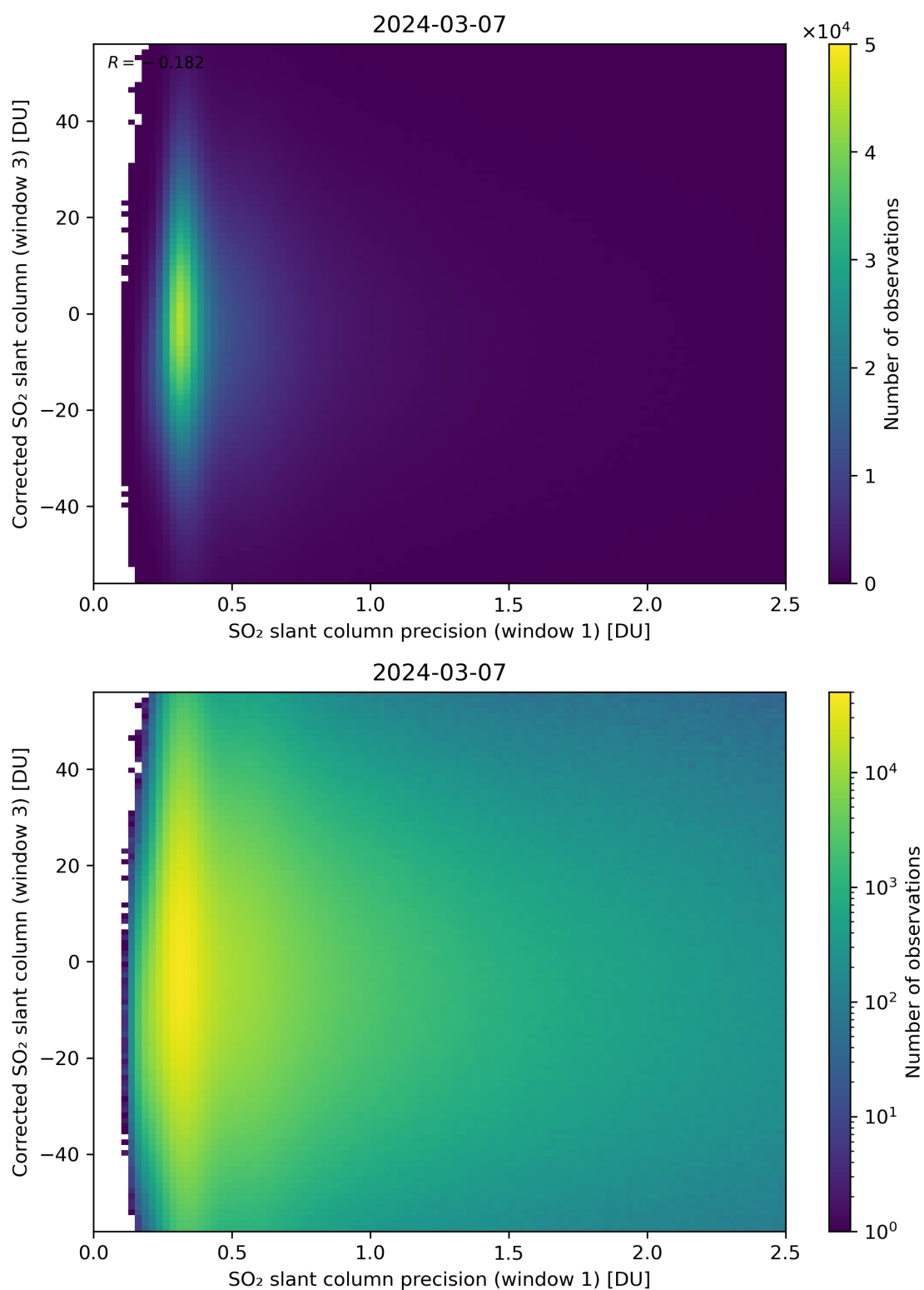
Figure 226: Scatter density plot of “SO 2 slant column precision (window 1)” against “Corrected SO 2 slant column (window 3)” for 2024-03-06 to 2024-03-08.
