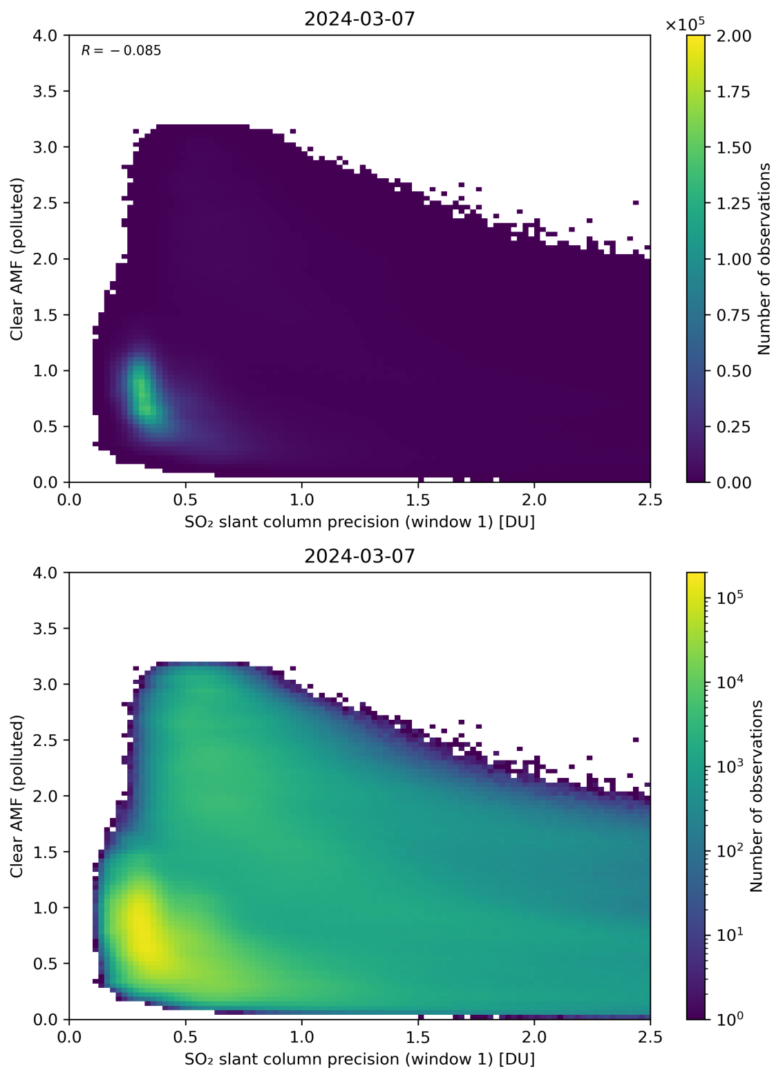
Figure 224: Scatter density plot of “SO 2 slant column precision (window 1)” against “Clear AMF (polluted)” for 2024-03-06 to 2024-03-08.
