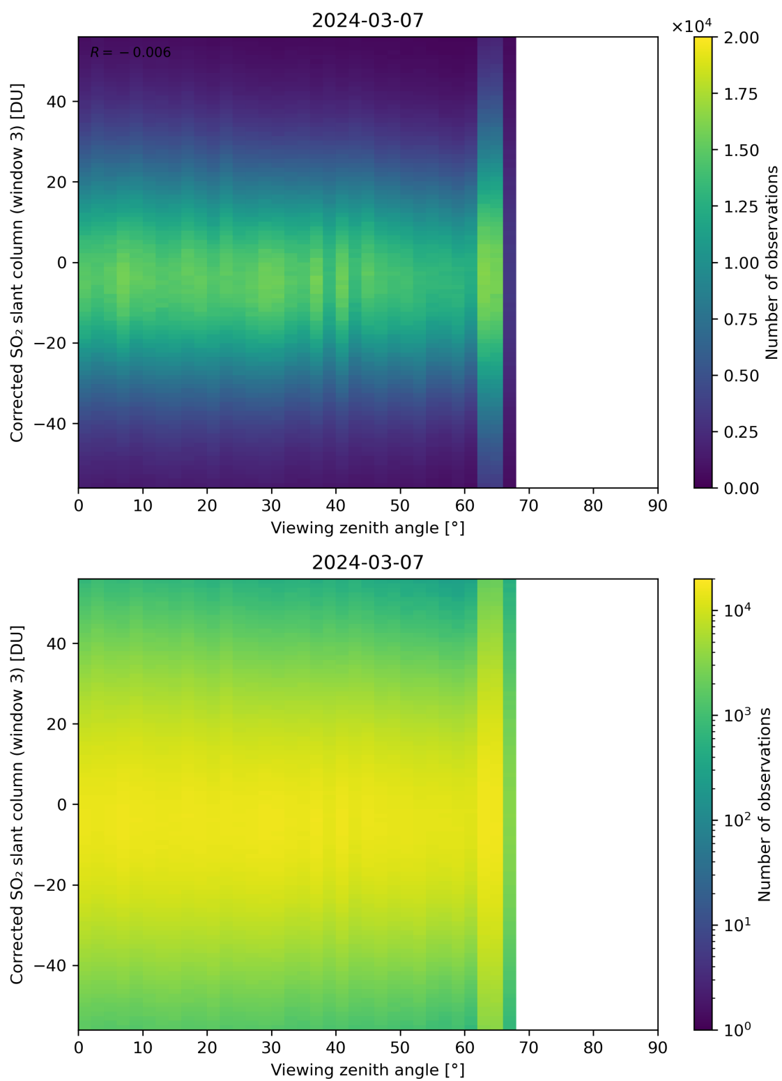
Figure 319: Scatter density plot of “Viewing zenith angle” against “Corrected SO 2 slant column (window 3)” for 2024-03-06 to 2024-03-08.
