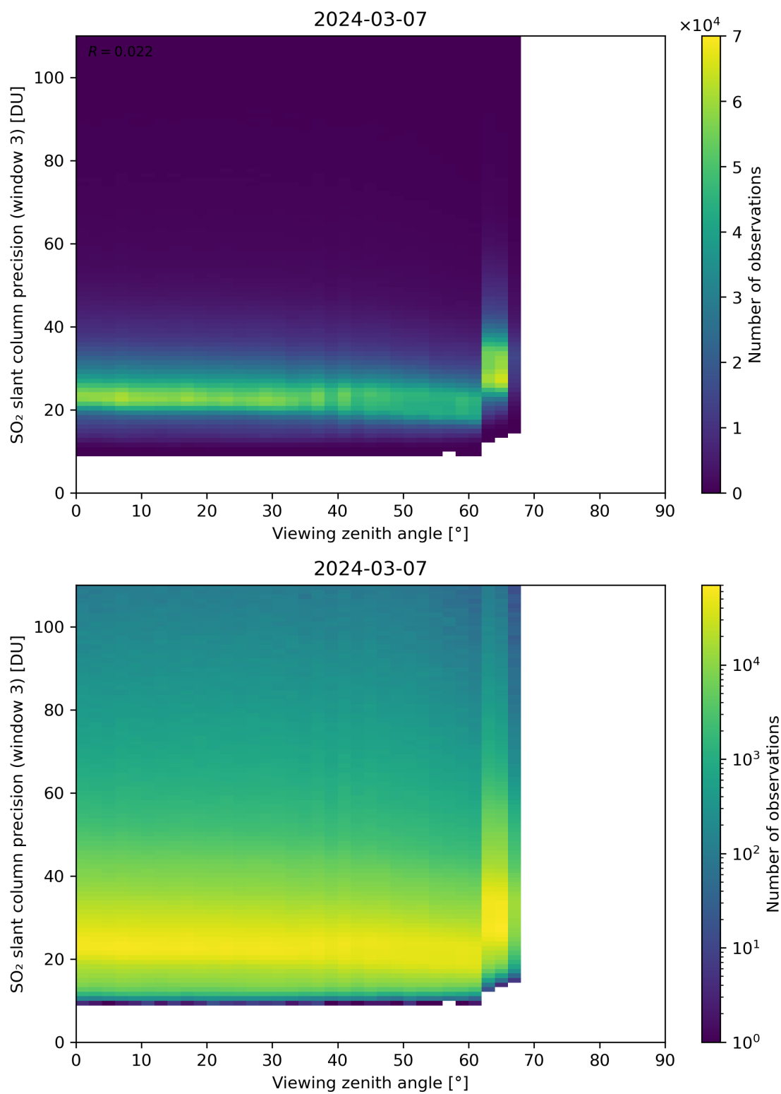
Figure 324: Scatter density plot of “Viewing zenith angle” against “SO 2 slant column precision (window 3)” for 2024-03-06 to 2024-03-08.
