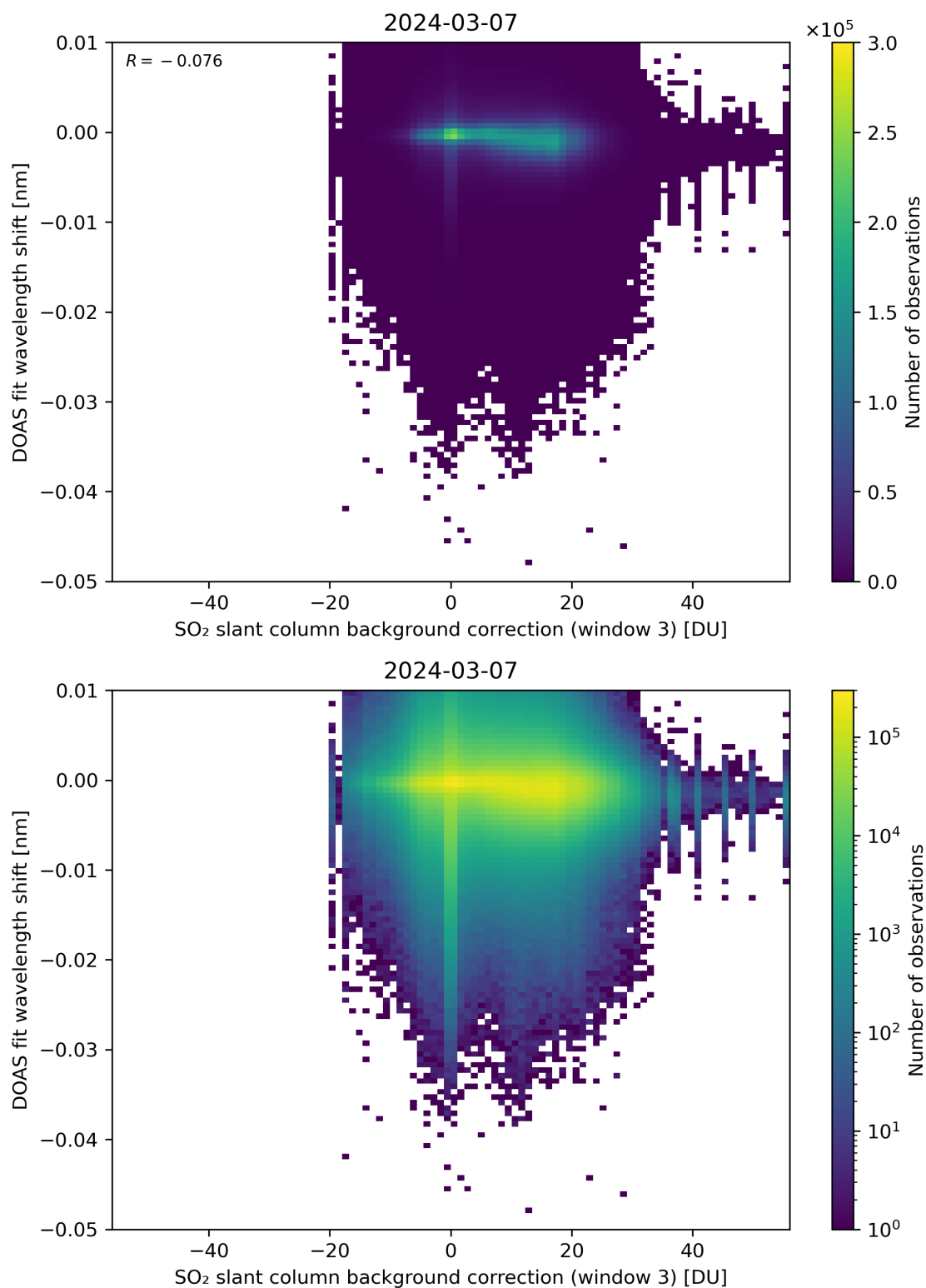
Figure 121: Scatter density plot of “SO 2 slant column background correction (window 3)” against “DOAS fit wavelength shift” for 2024-03-06 to 2024-03-08.
