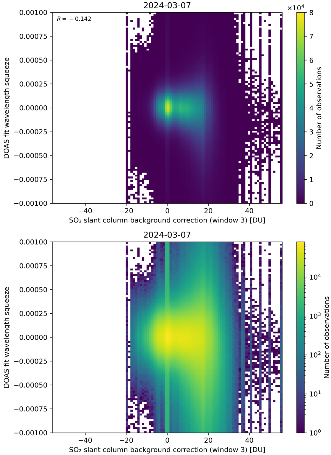
Figure 122: Scatter density plot of “SO 2 slant column background correction (window 3)” against “DOAS fit wavelength squeeze” for 2024-03-06 to 2024-03-08.
