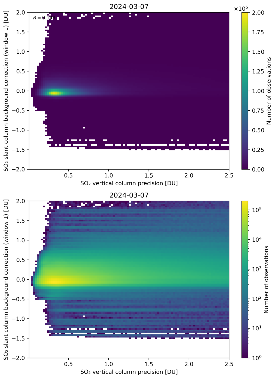
Figure 279: Scatter density plot of “SO 2 vertical column precision” against “SO 2 slant column background correction (window 1)” for 2024-03-06 to 2024-03-08.
