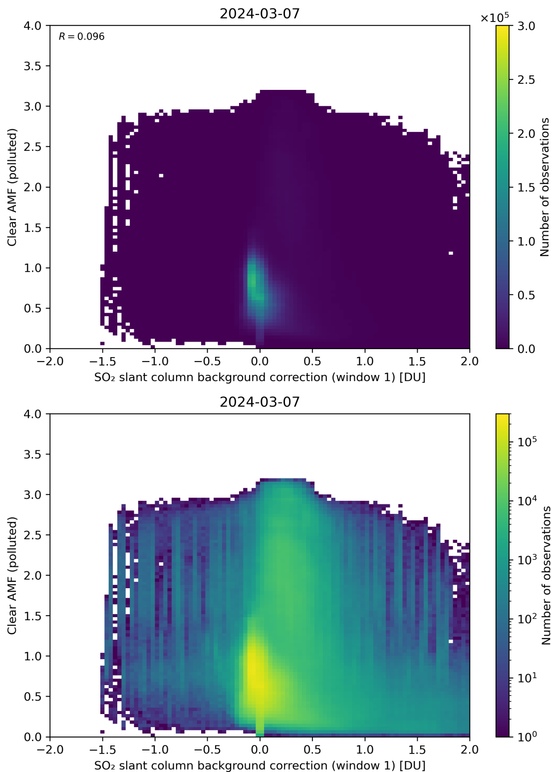
Figure 103: Scatter density plot of “SO 2 slant column background correction (window 1)” against “Clear AMF (polluted)” for 2024-03-06 to 2024-03-08.
