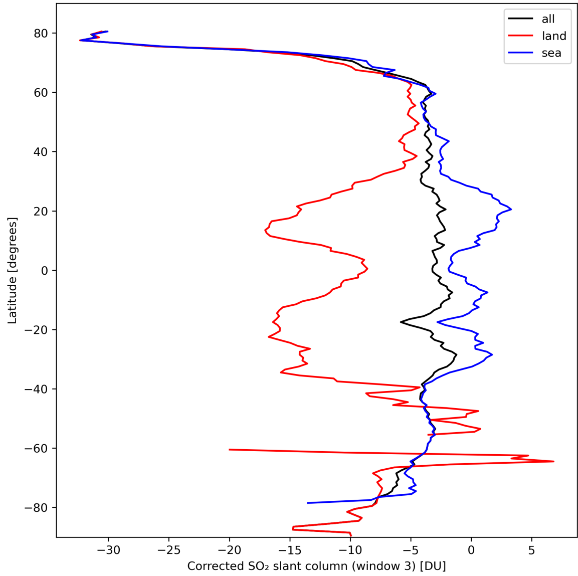
Figure 43: Zonal average of “Corrected SO 2 slant column (window 3)” for 2024-03-06 to 2024-03-08.
