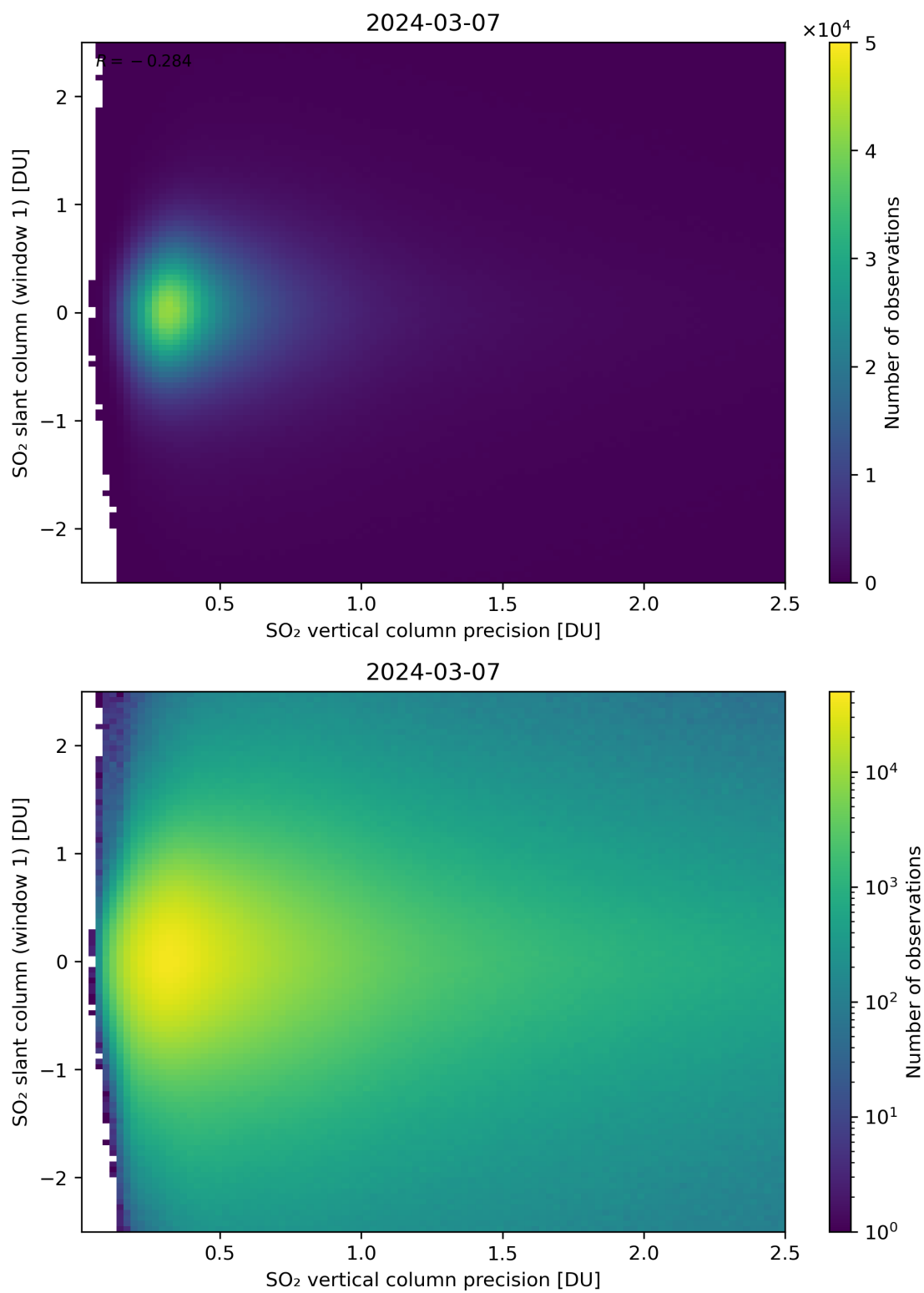
Figure 289: Scatter density plot of “SO 2 vertical column precision” against “SO 2 slant column (window 1)” for 2024-03-06 to 2024-03-08.
