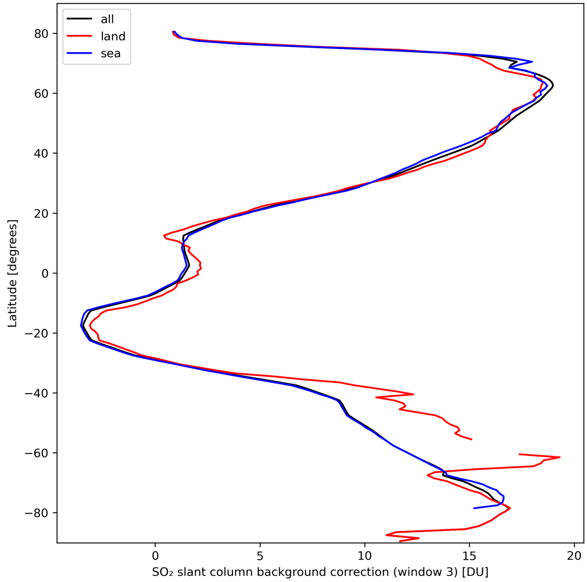
Figure 44: Zonal average of “SO 2 slant column background correction (window 3)” for 2024-03-06 to 2024-03-08.
