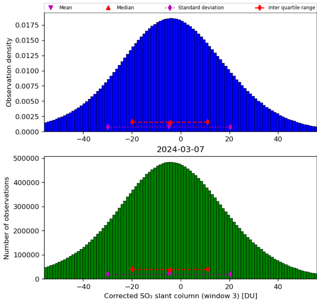
Figure 66: Histogram of "Corrected SO 2 slant column (window 3)" for 2024-03-06 to 2024-03-08
