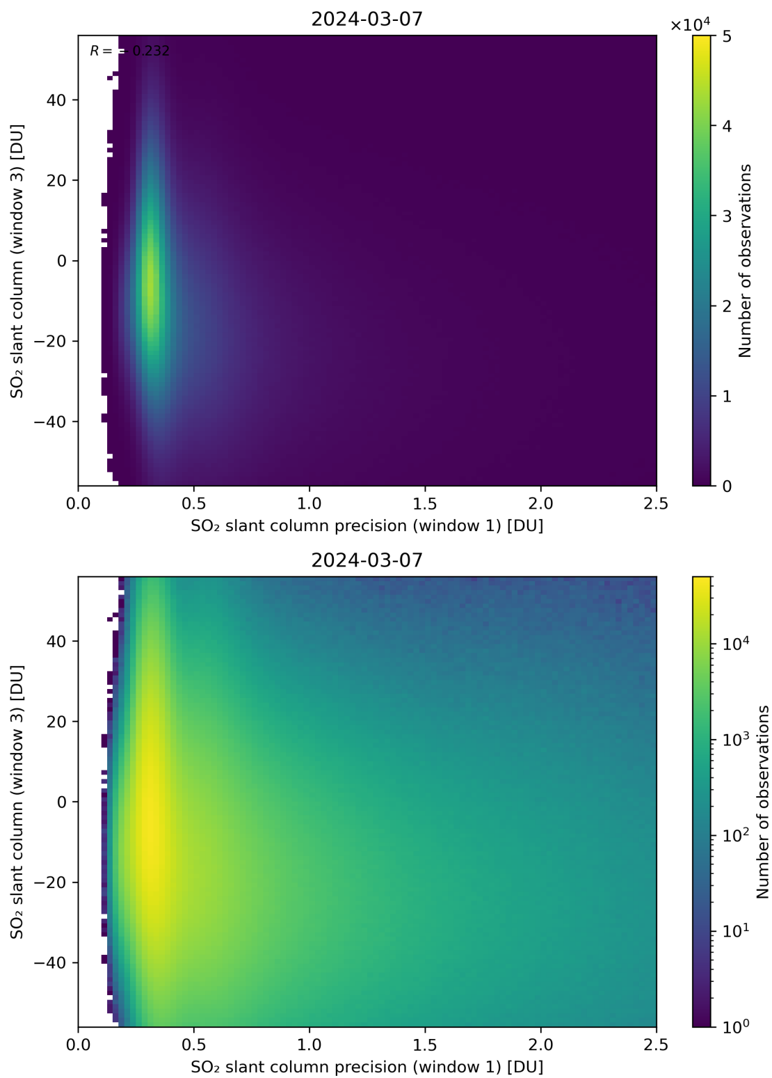
Figure 228: Scatter density plot of “SO 2 slant column precision (window 1)” against “SO 2 slant column (window 3)” for 2024-03-06 to 2024-03-08.
