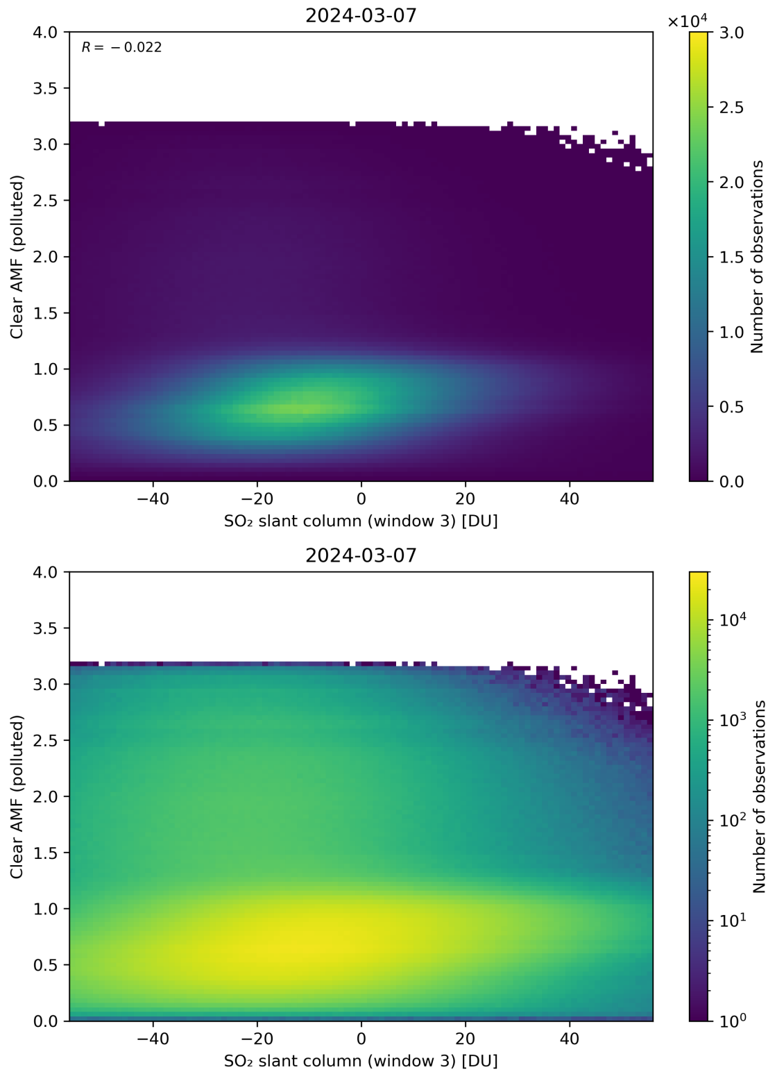
Figure 265: Scatter density plot of “SO 2 slant column (window 3)” against “Clear AMF (polluted)” for 2024-03-06 to 2024-03-08.
