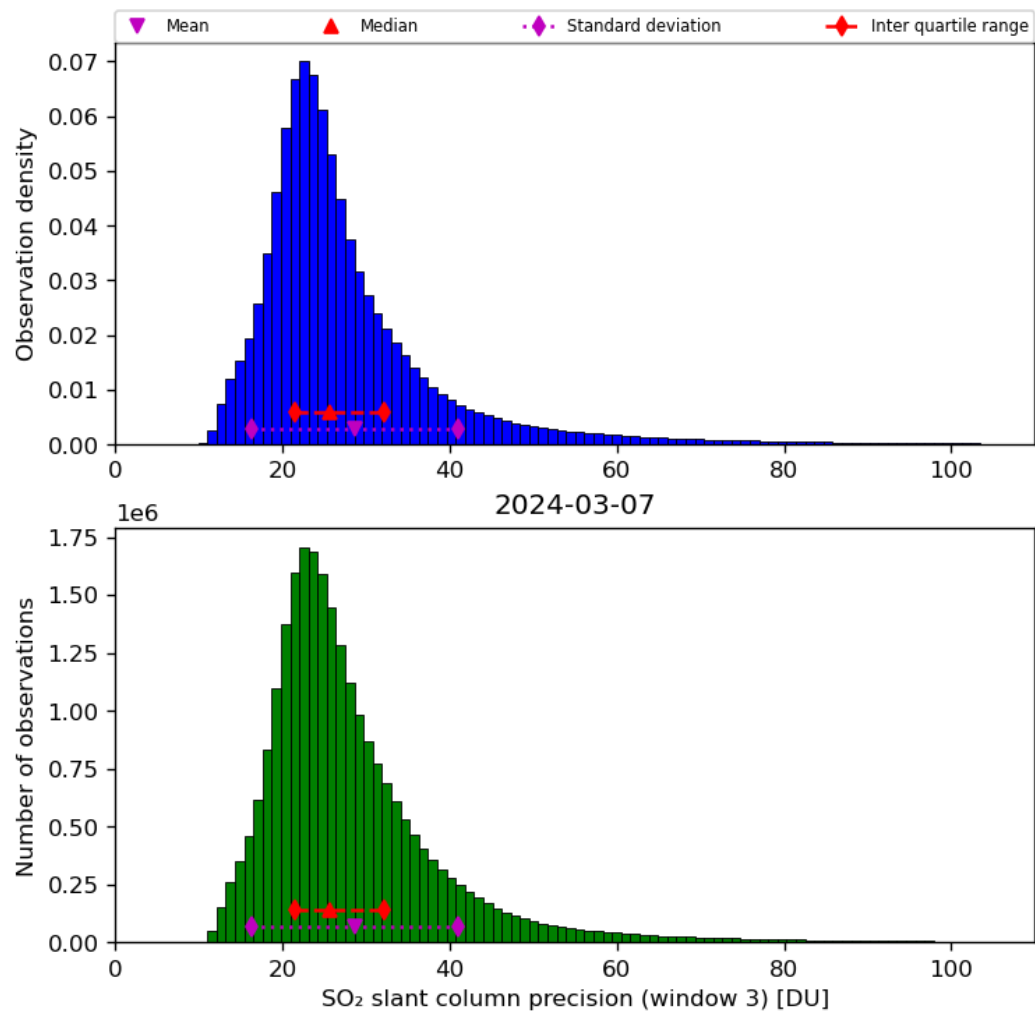
Figure 65: Histogram of “SO 2 slant column precision (window 3)” for 2024-03-06 to 2024-03-08
