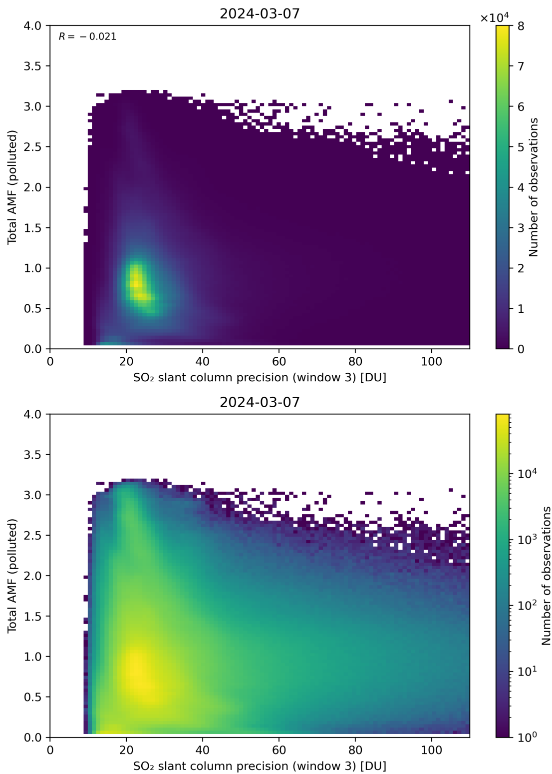
Figure 263: Scatter density plot of “SO 2 slant column precision (window 3)” against “Total AMF (polluted)” for 2024-03-06 to 2024-03-08.
