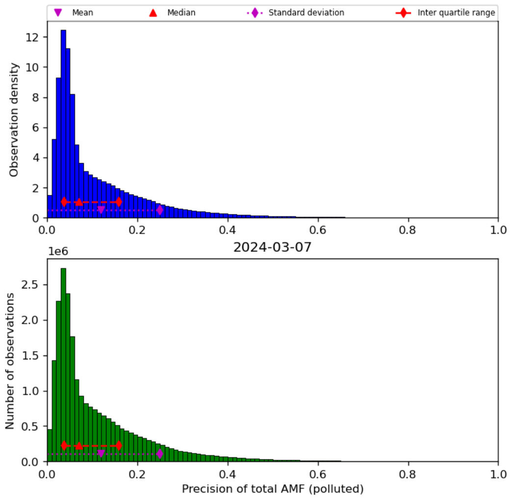
Figure 72: Histogram of “Precision of total AMF (polluted)” for 2024-03-06 to 2024-03-08
