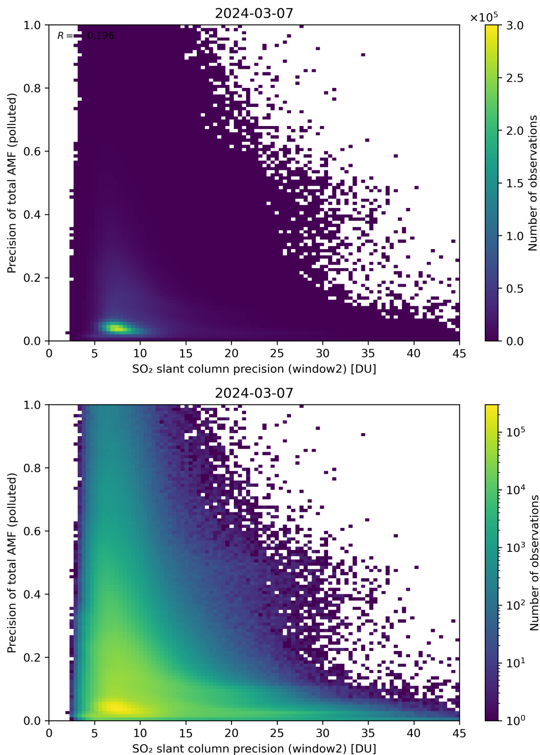
Figure 252: Scatter density plot of “SO 2 slant column precision (window2)” against “Precision of total AMF (polluted)” for 2024-03-06 to 2024-03-08.
