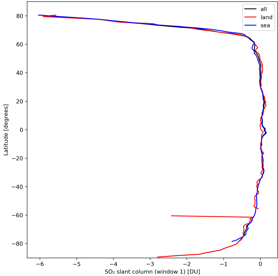
Figure 33: Zonal average of “SO 2 slant column (window 1)” for 2024-03-06 to 2024-03-08.
