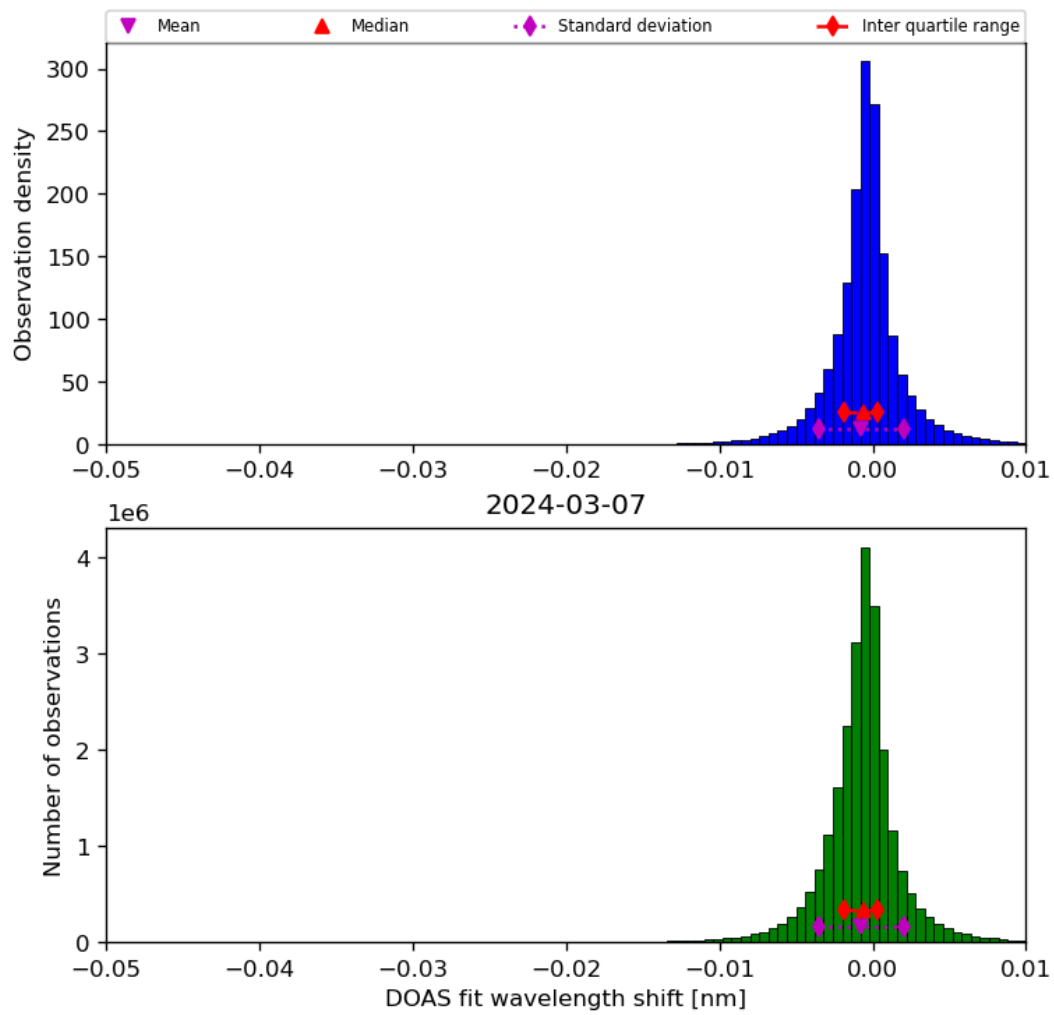
Figure 68: Histogram of “DOAS fit wavelength shift” for 2024-03-06 to 2024-03-08
