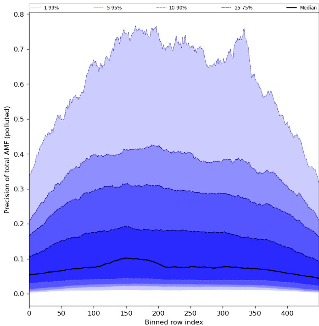
Figure 95: Along track statistics of “Precision of total AMF (polluted)” for 2024-03-06 to 2024-03-08
