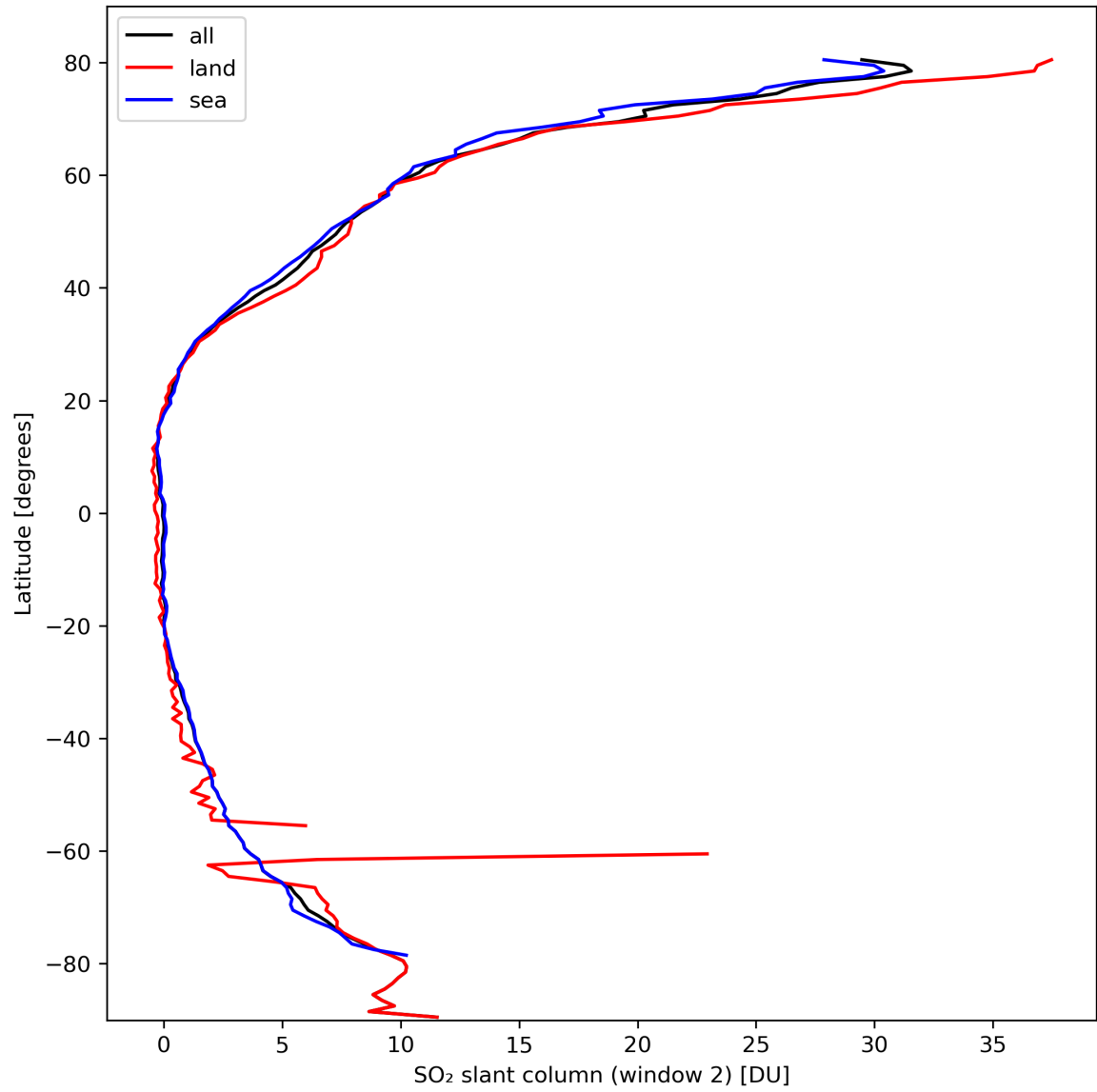
Figure 37: Zonal average of “SO 2 slant column (window 2)” for 2024-03-06 to 2024-03-08.
