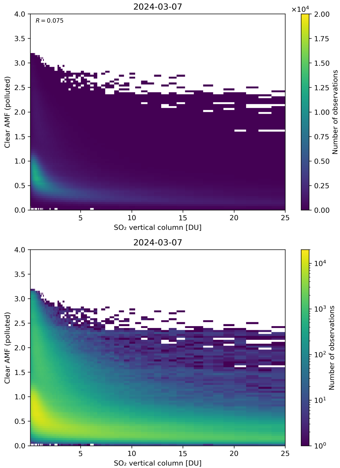
Figure 296: Scatter density plot of “SO 2 vertical column” against “Clear AMF (polluted)” for 2024-03-06 to 2024-03-08.
