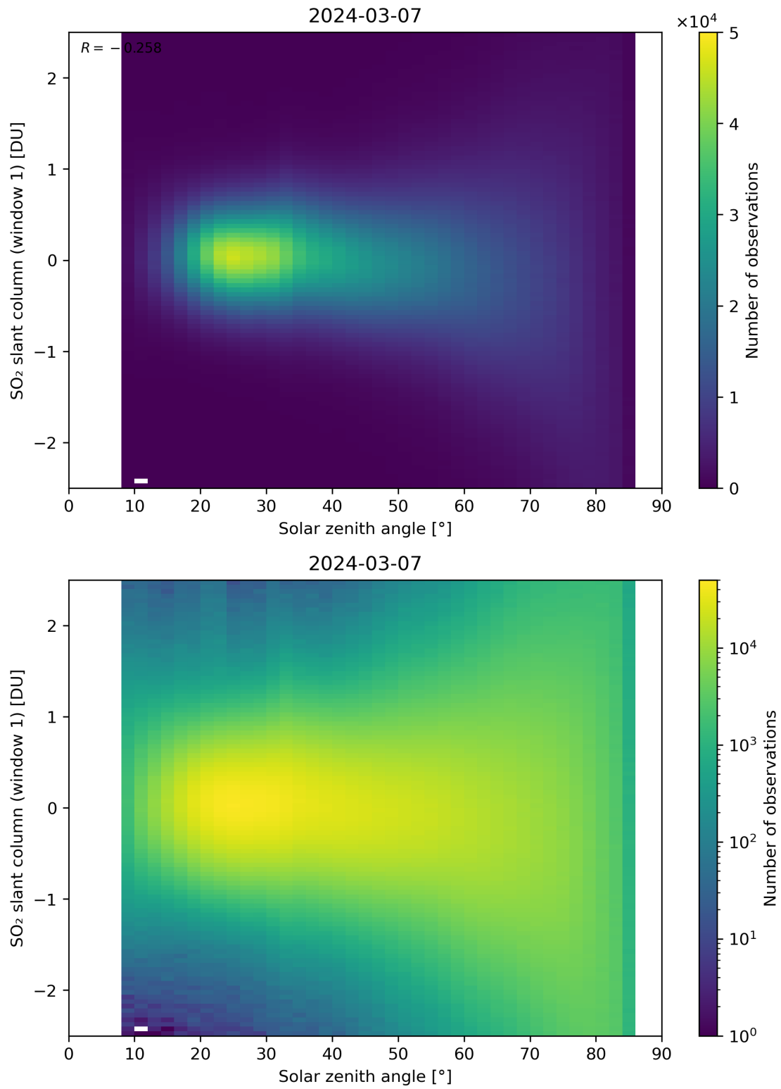
Figure 169: Scatter density plot of “Solar zenith angle” against “SO 2 slant column (window 1)” for 2024-03-06 to 2024-03-08.
