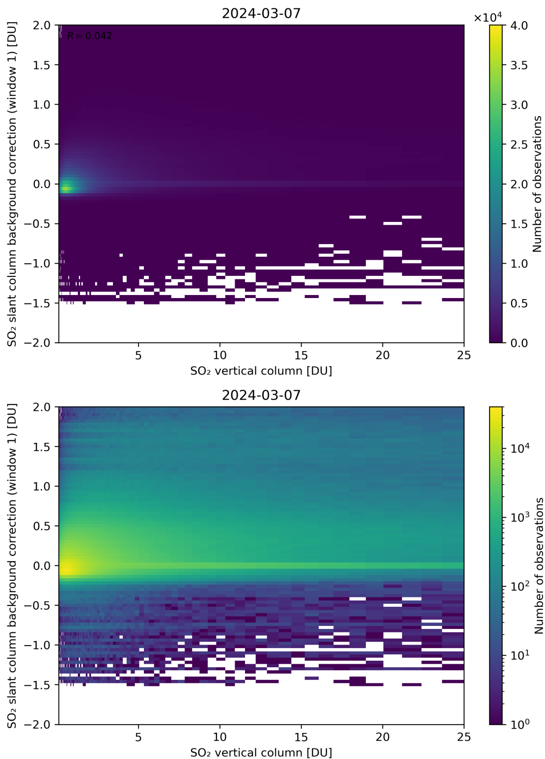
Figure 273: Scatter density plot of “SO 2 vertical column” against “SO 2 slant column background correction (window 1)” for 2024-03-06 to 2024-03-08.
