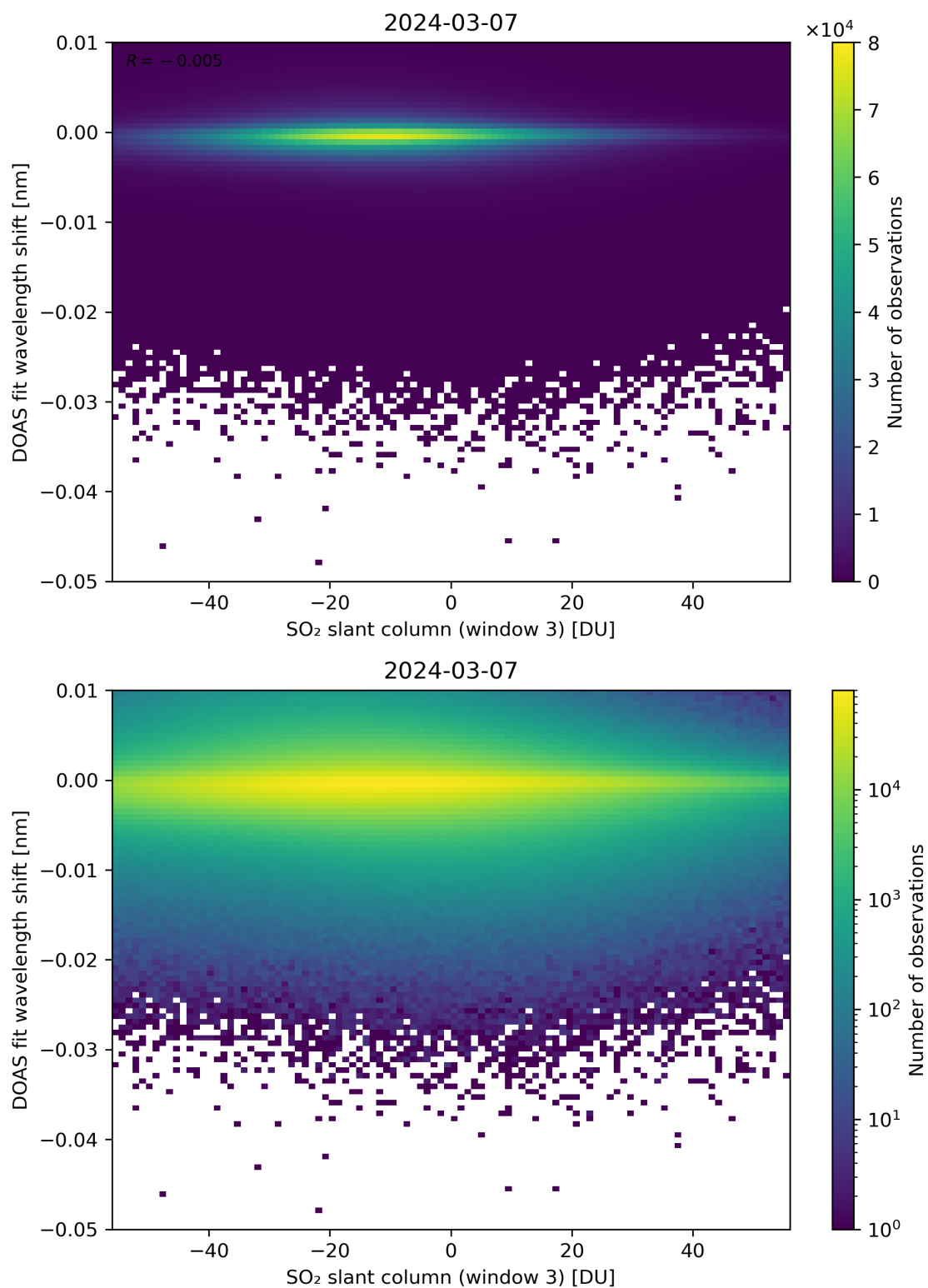
Figure 254: Scatter density plot of “SO 2 slant column (window 3)” against “DOAS fit wavelength shift” for 2024-03-06 to 2024-03-08.
