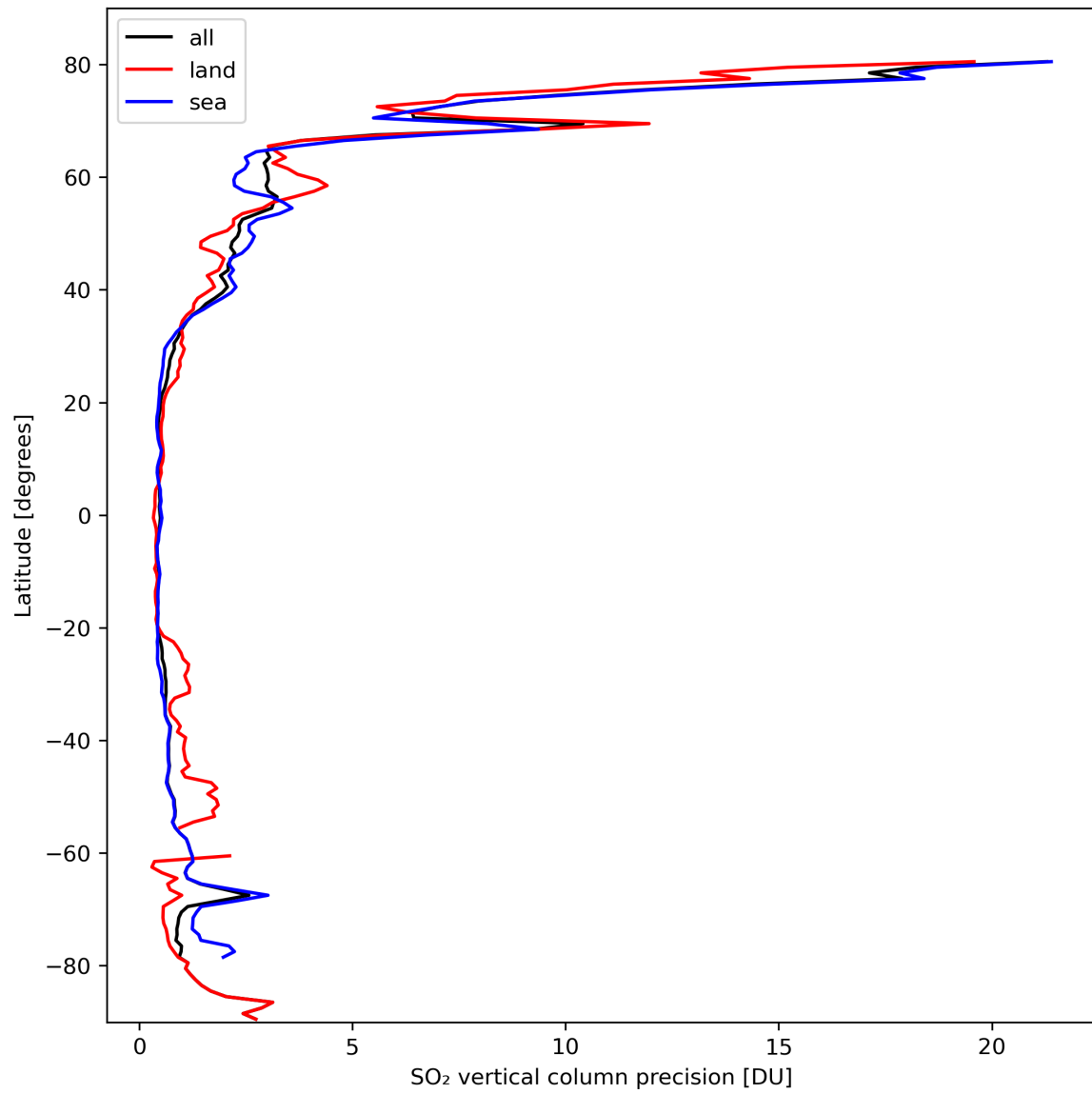
Figure 31: Zonal average of “SO 2 vertical column precision” for 2024-03-06 to 2024-03-08.
