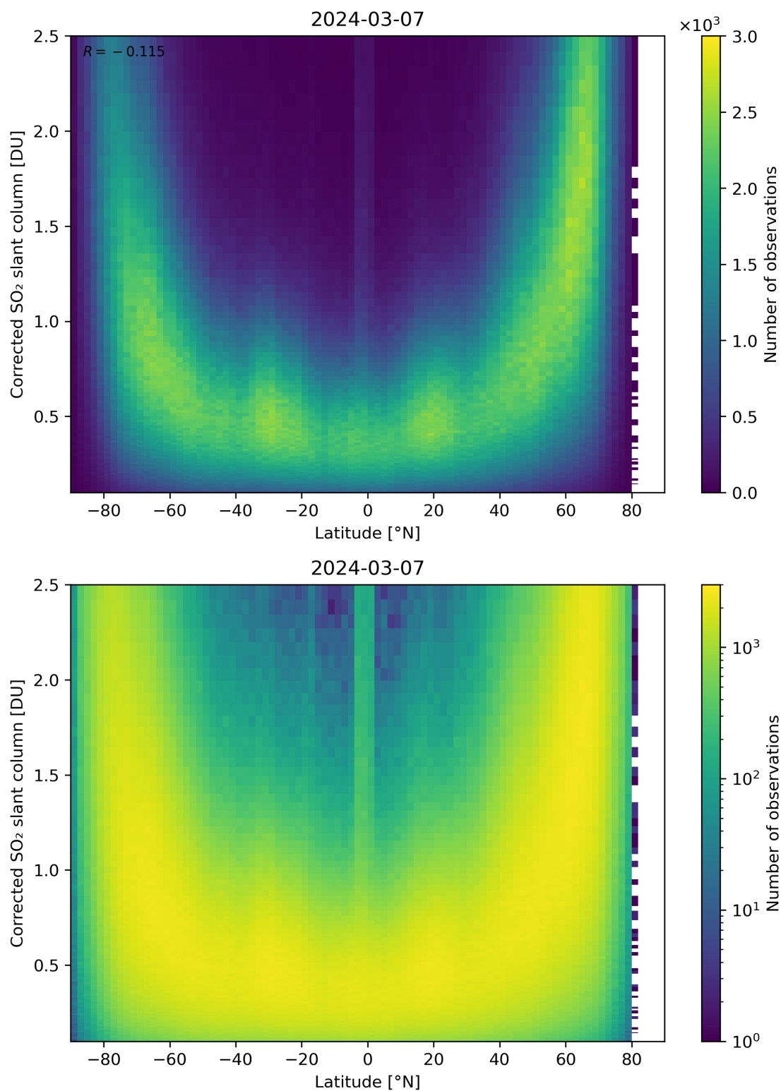
Figure 146: Scatter density plot of “Latitude” against “Corrected SO 2 slant column” for 2024-03-06 to 2024-03-08.
