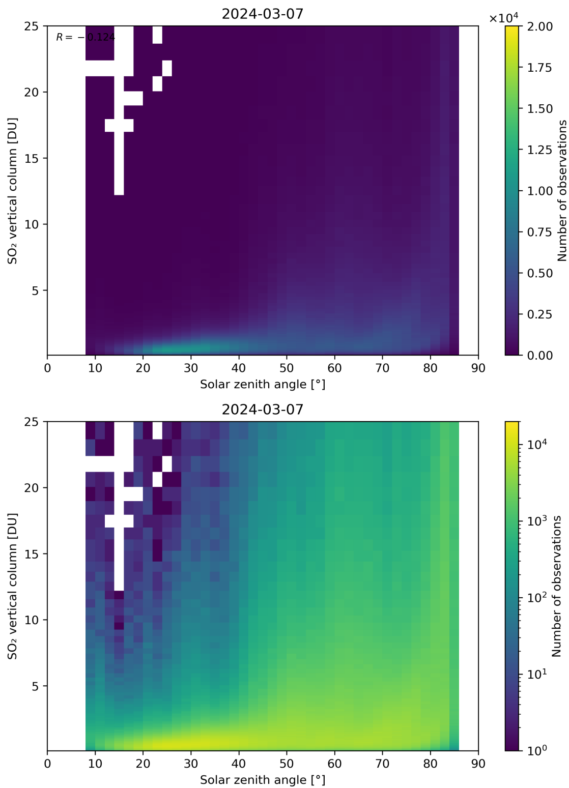
Figure 176: Scatter density plot of “Solar zenith angle” against “SO 2 vertical column” for 2024-03-06 to 2024-03-08.
