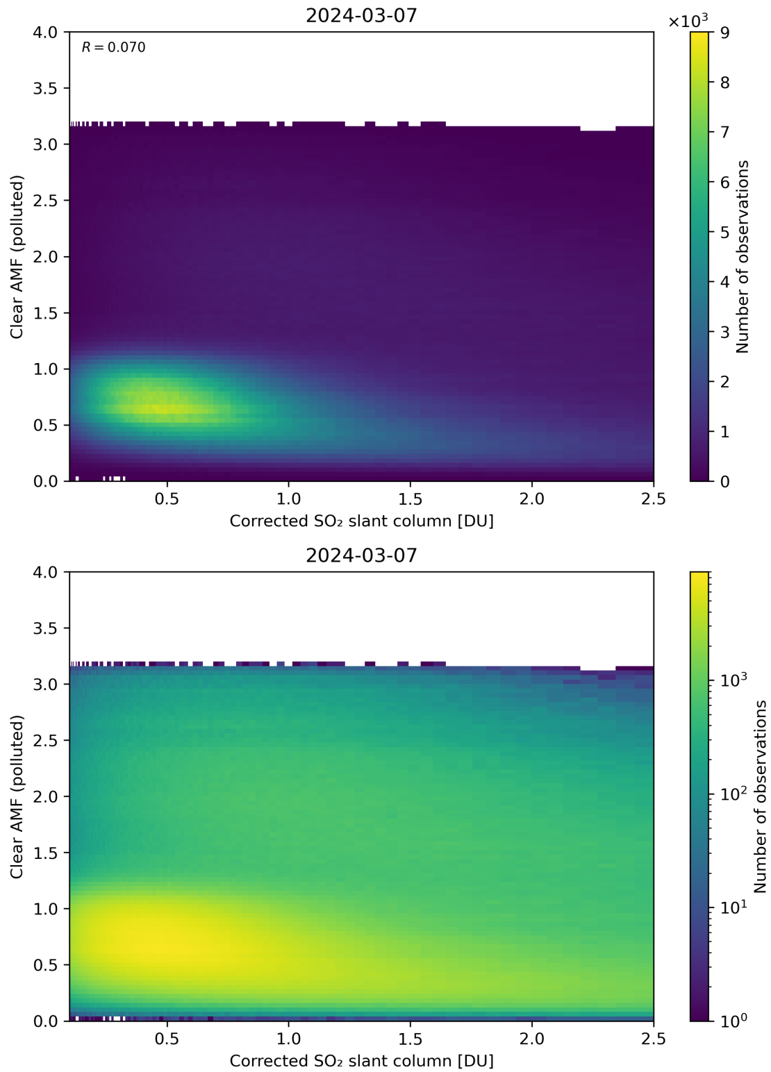
Figure 184: Scatter density plot of “Corrected SO 2 slant column” against “Clear AMF (polluted)” for 2024-03-06 to 2024-03-08.
