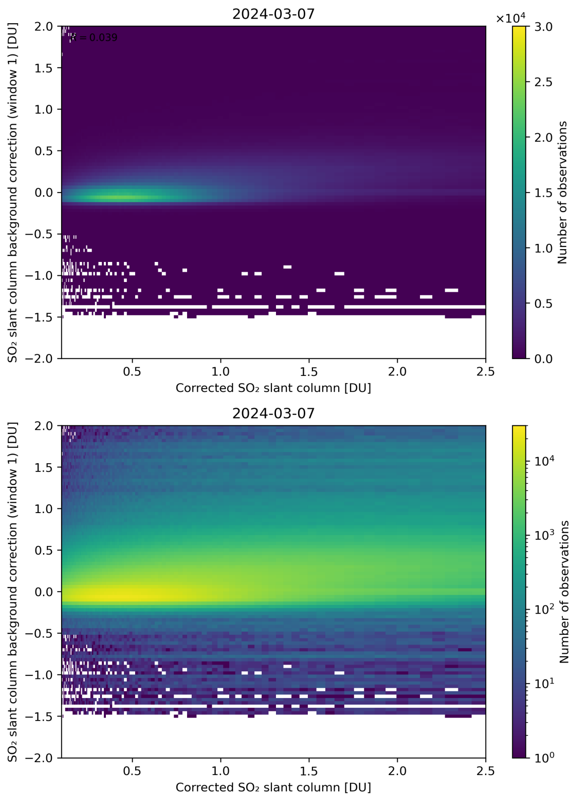
Figure 178: Scatter density plot of “Corrected SO 2 slant column” against “SO 2 slant column background correction (window 1)” for 2024-03-06 to 2024-03-08.
