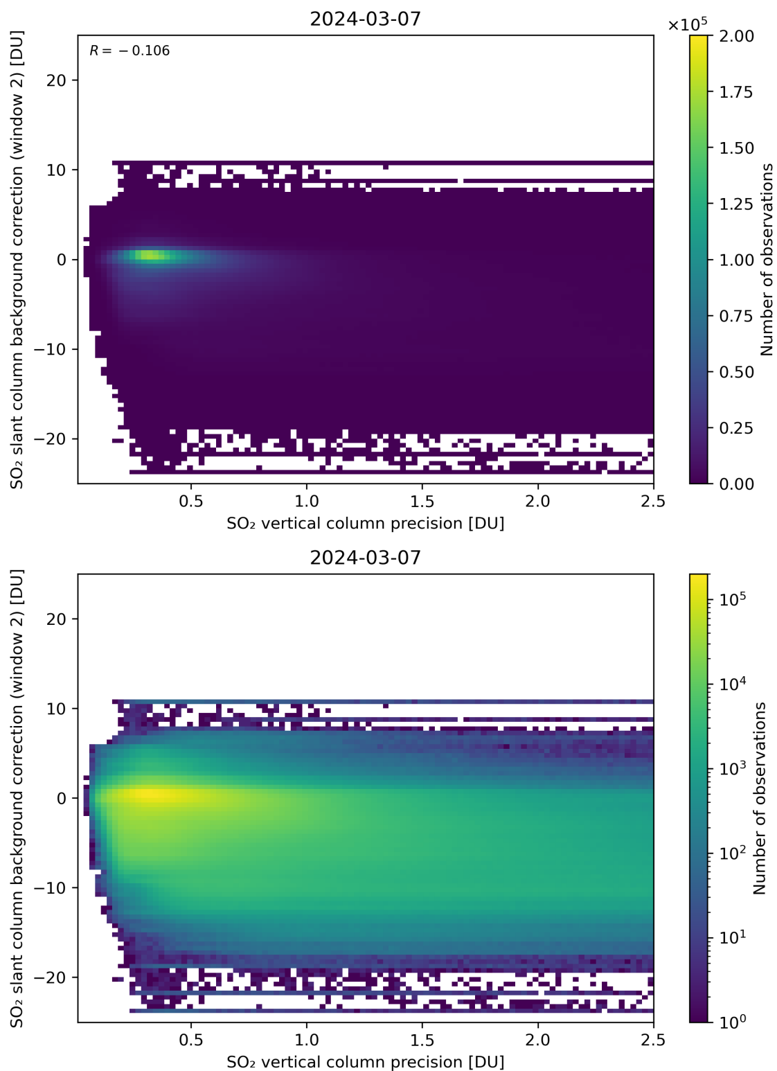
Figure 280: Scatter density plot of “SO 2 vertical column precision” against “SO 2 slant column background correction (window 2)” for 2024-03-06 to 2024-03-08.
