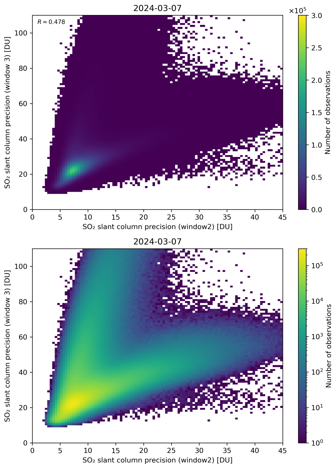
Figure 250: Scatter density plot of “SO 2 slant column precision (window2)” against “SO 2 slant column precision (window 3)” for 2024-03-06 to 2024-03-08.
