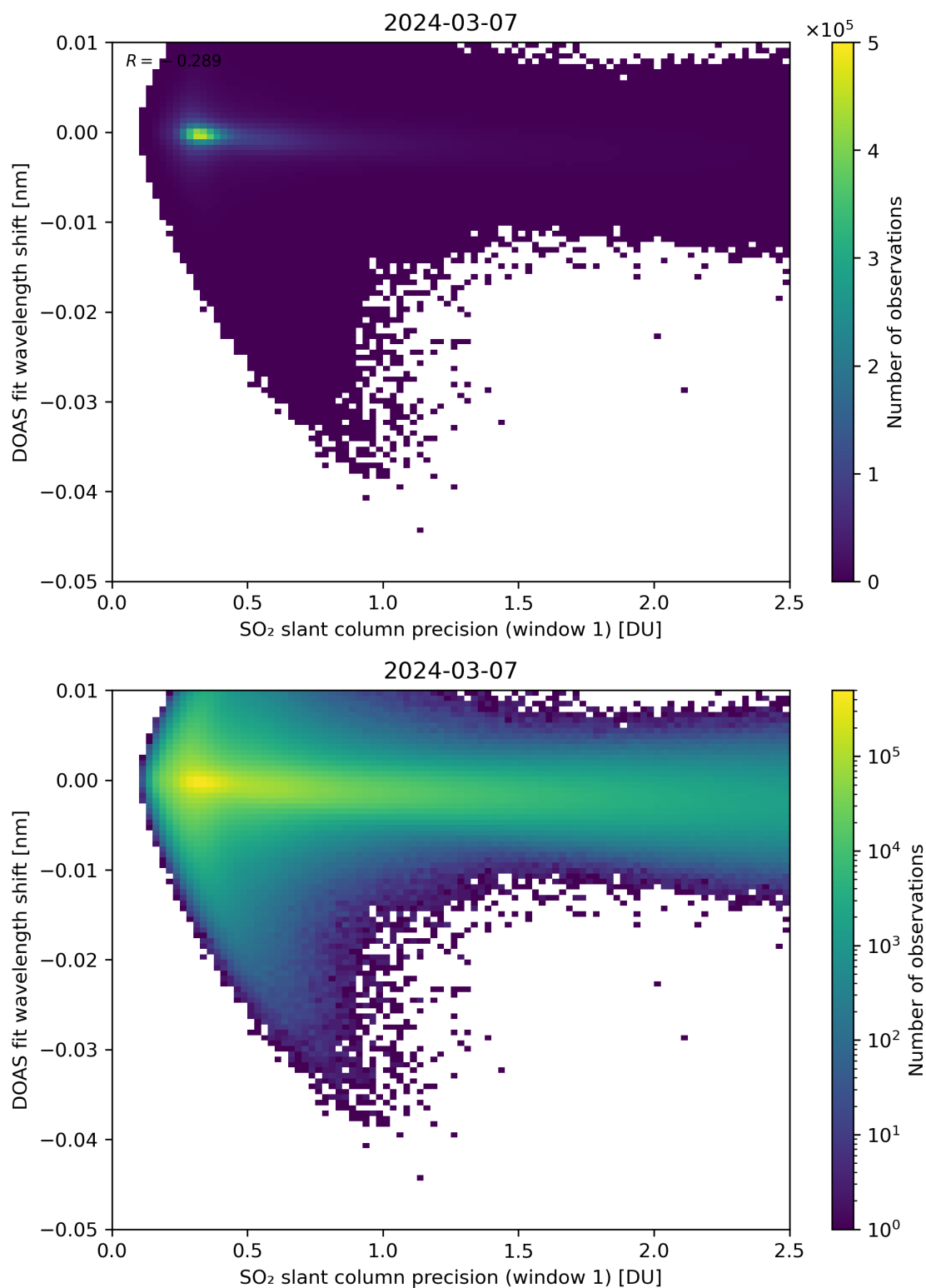
Figure 221: Scatter density plot of “SO 2 slant column precision (window 1)” against “DOAS fit wavelength shift” for 2024-03-06 to 2024-03-08.
