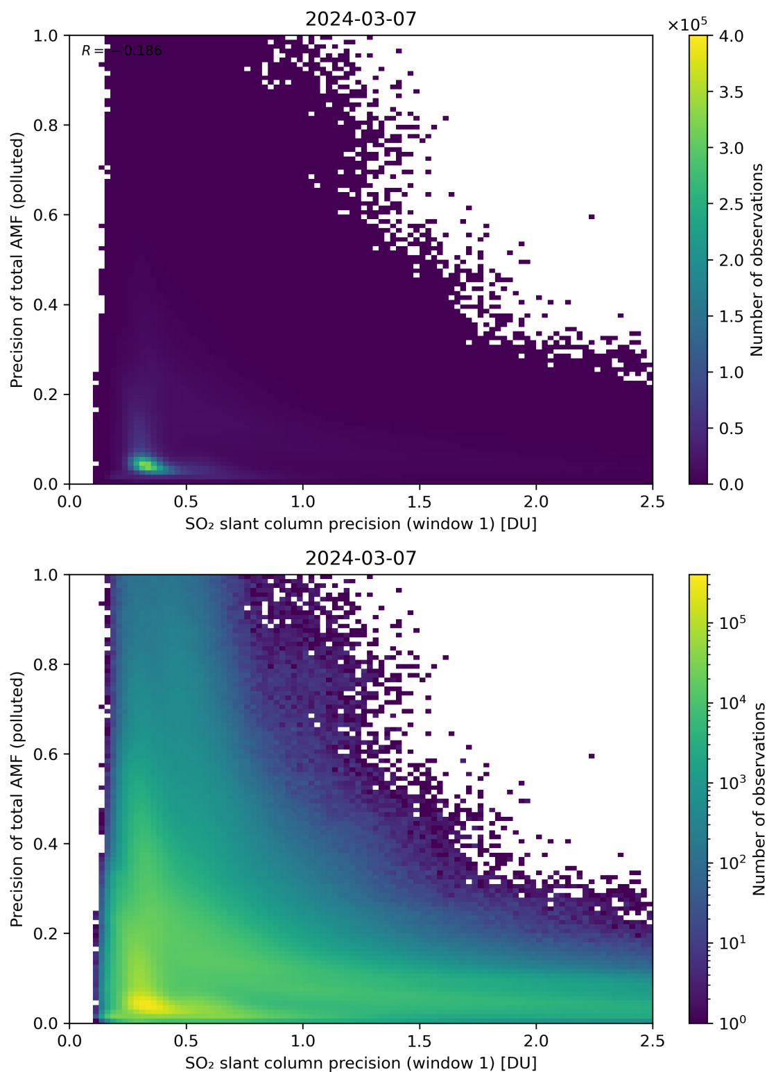
Figure 231: Scatter density plot of “SO 2 slant column precision (window 1)” against “Precision of total AMF (polluted)” for 2024-03-06 to 2024-03-08.
