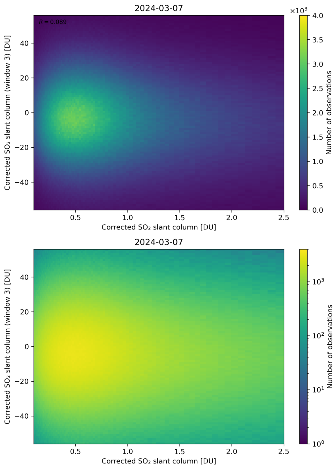
Figure 186: Scatter density plot of “Corrected SO 2 slant column” against “Corrected SO 2 slant column (window 3)” for 2024-03-06 to 2024-03-08.
