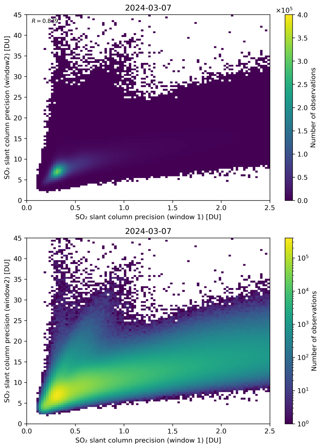
Figure 227: Scatter density plot of “SO 2 slant column precision (window 1)” against “SO 2 slant column precision (window2)” for 2024-03-06 to 2024-03-08.
