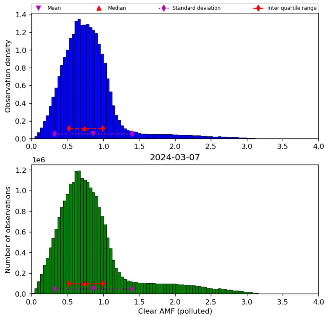
Figure 73: Histogram of “Clear AMF (polluted)” for 2024-03-06 to 2024-03-08
