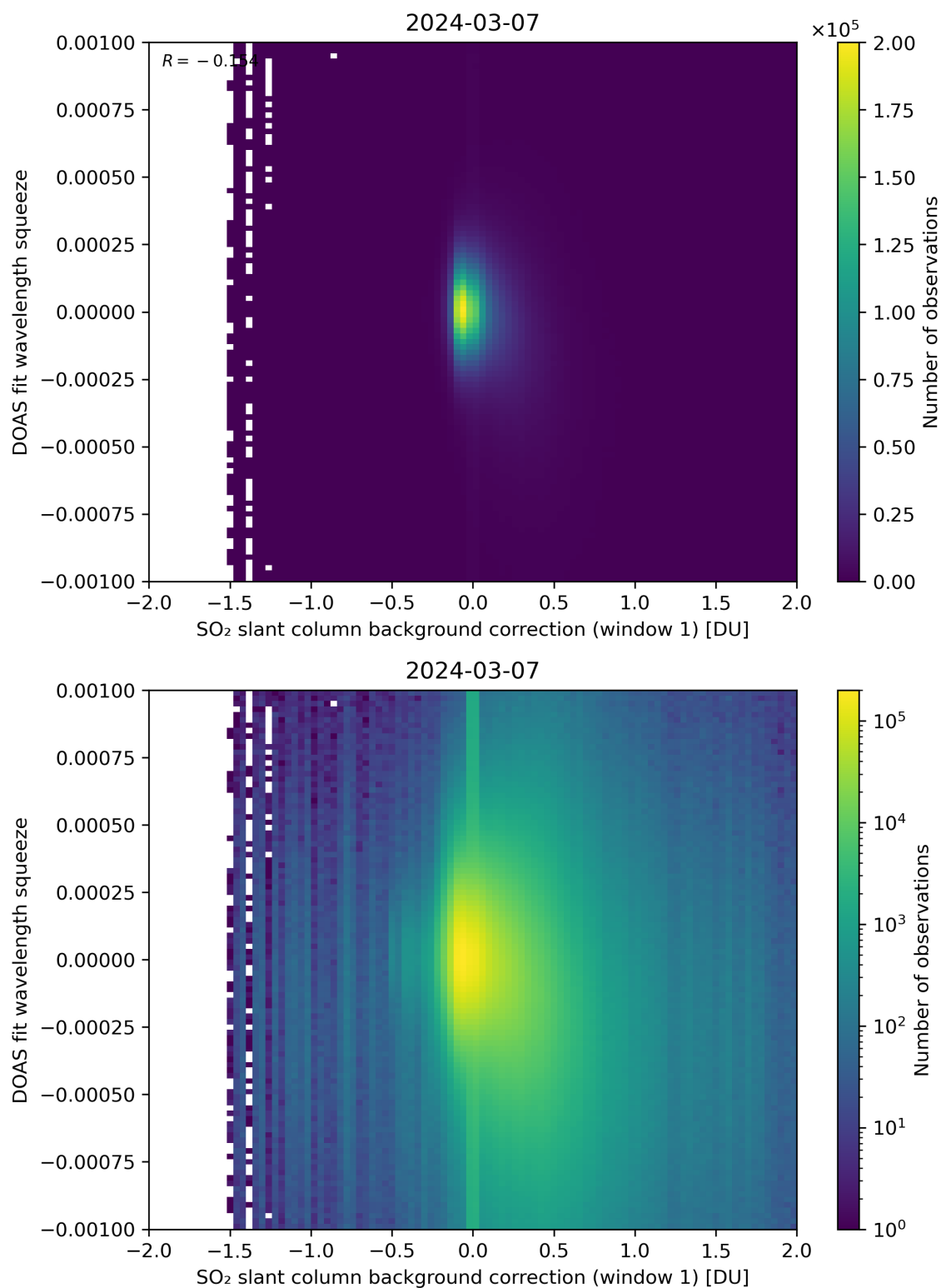
Figure 101: Scatter density plot of “SO 2 slant column background correction (window 1)” against “DOAS fit wavelength squeeze” for 2024-03-06 to 2024-03-08.
