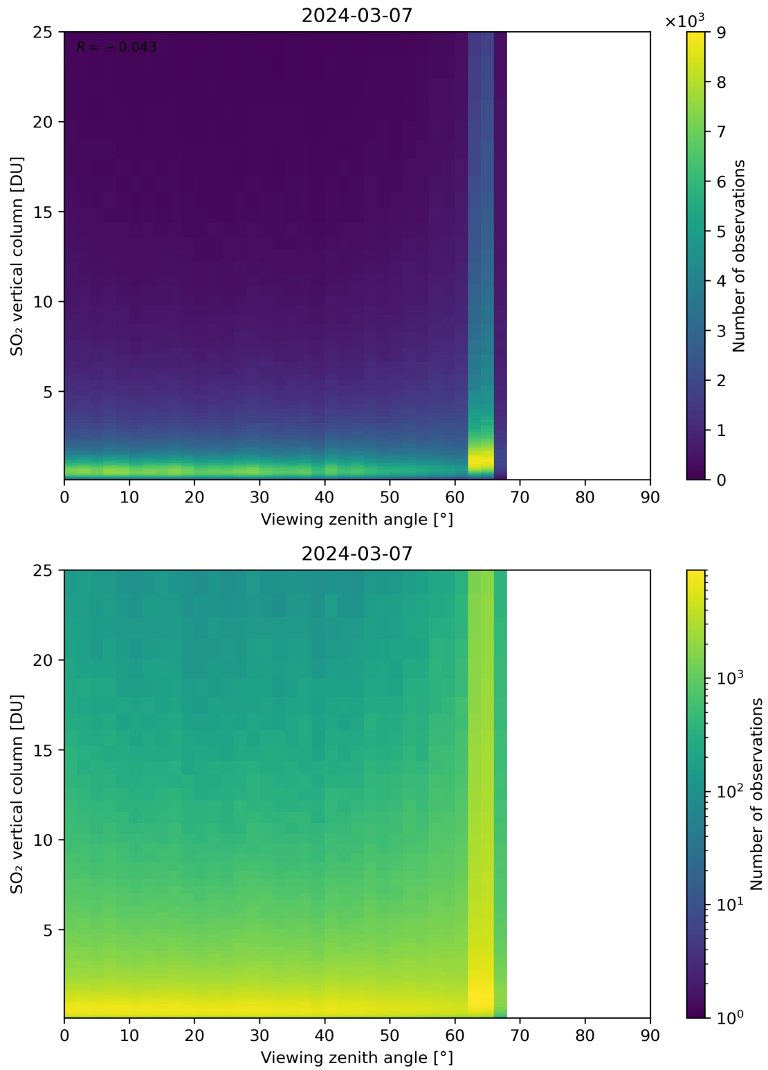
Figure 327: Scatter density plot of “Viewing zenith angle” against “SO 2 vertical column” for 2024-03-06 to 2024-03-08.
