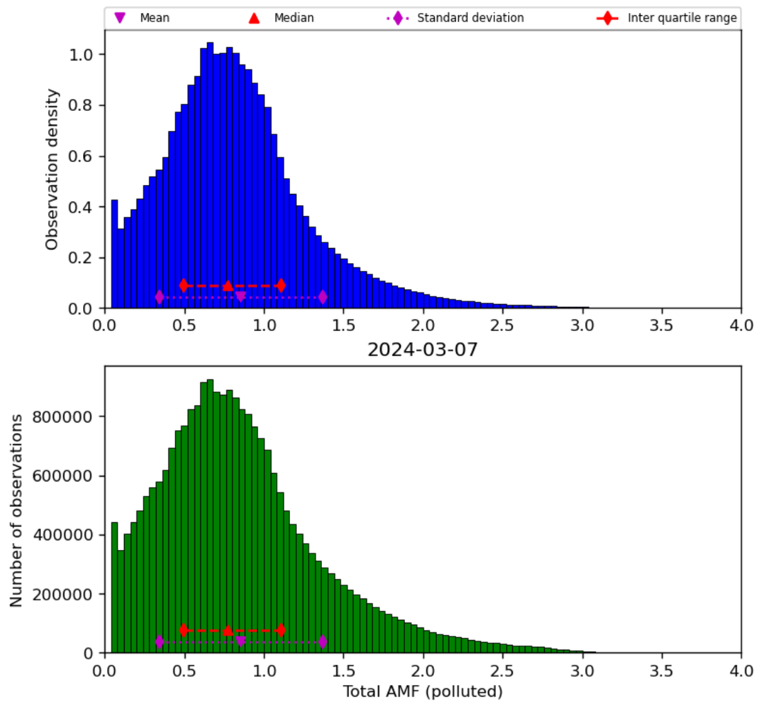
Figure 71: Histogram of “Total AMF (polluted)” for 2024-03-06 to 2024-03-08
