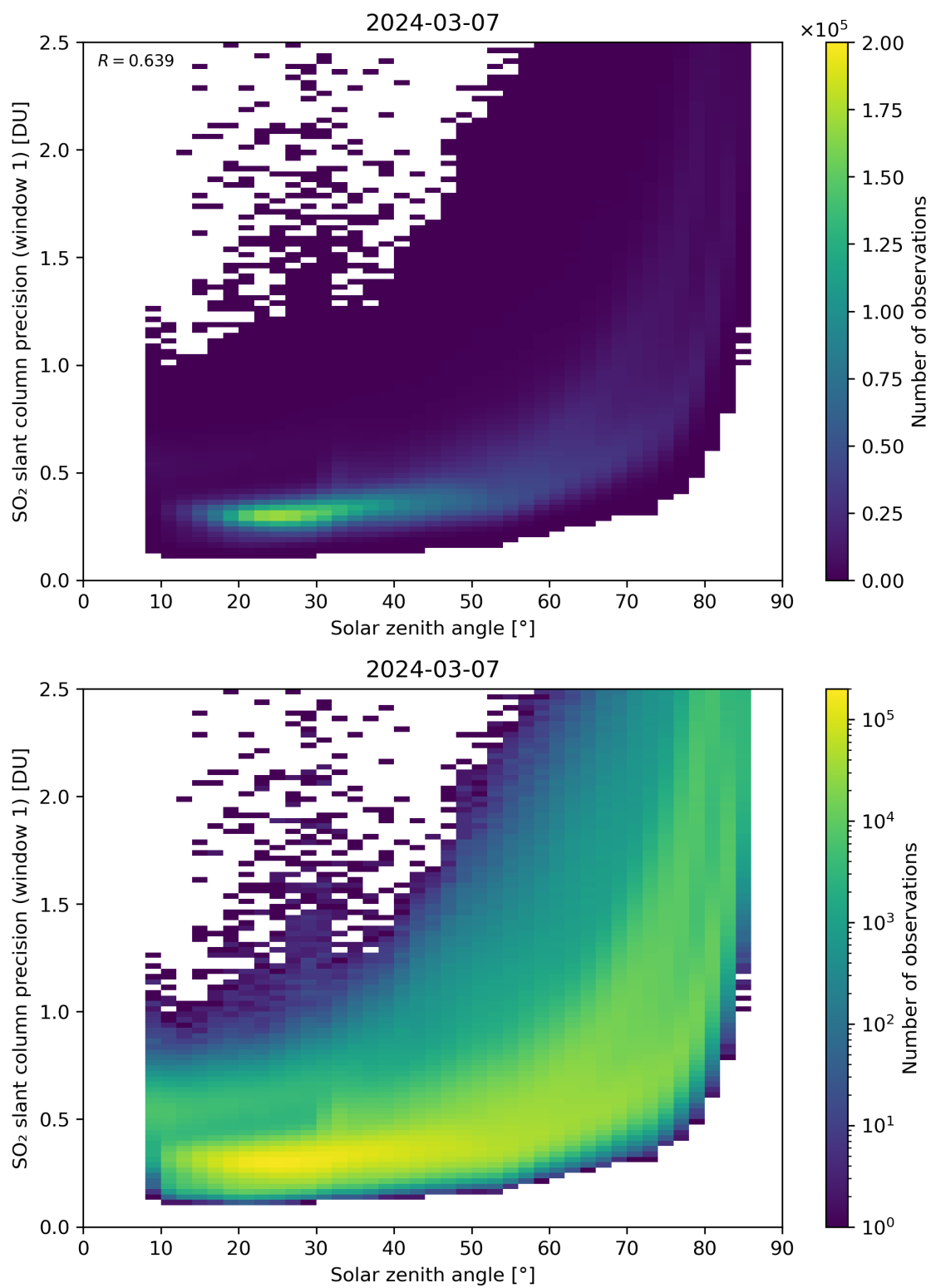
Figure 170: Scatter density plot of “Solar zenith angle” against “SO 2 slant column precision (window 1)” for 2024-03-06 to 2024-03-08.
