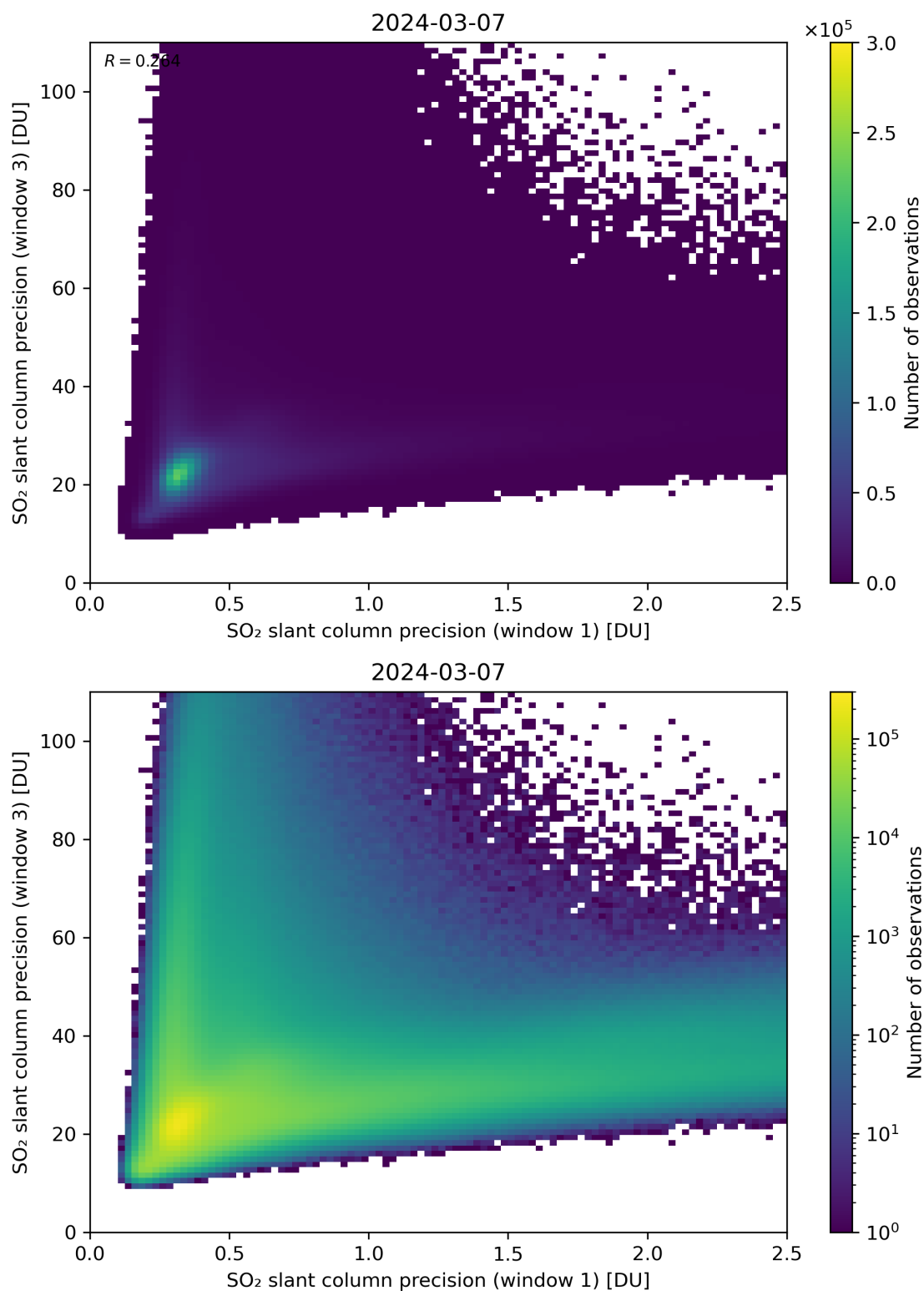
Figure 229: Scatter density plot of “SO 2 slant column precision (window 1)” against “SO 2 slant column precision (window 3)” for 2024-03-06 to 2024-03-08.
