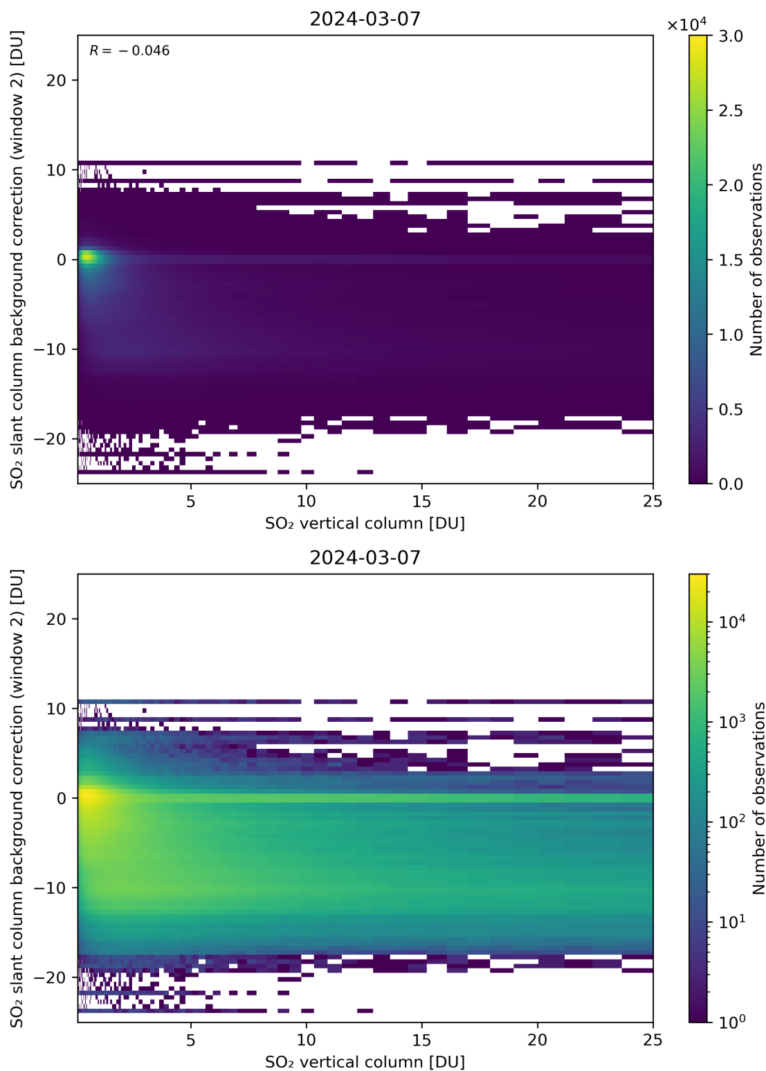
Figure 274: Scatter density plot of “SO 2 vertical column” against “SO 2 slant column background correction (window 2)” for 2024-03-06 to 2024-03-08.
