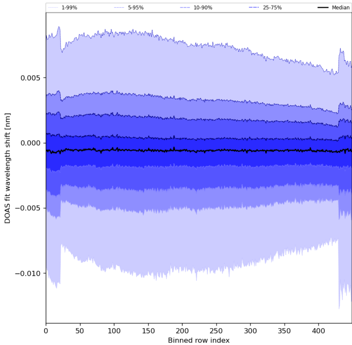
Figure 91: Along track statistics of “DOAS fit wavelength shift” for 2024-03-06 to 2024-03-08
