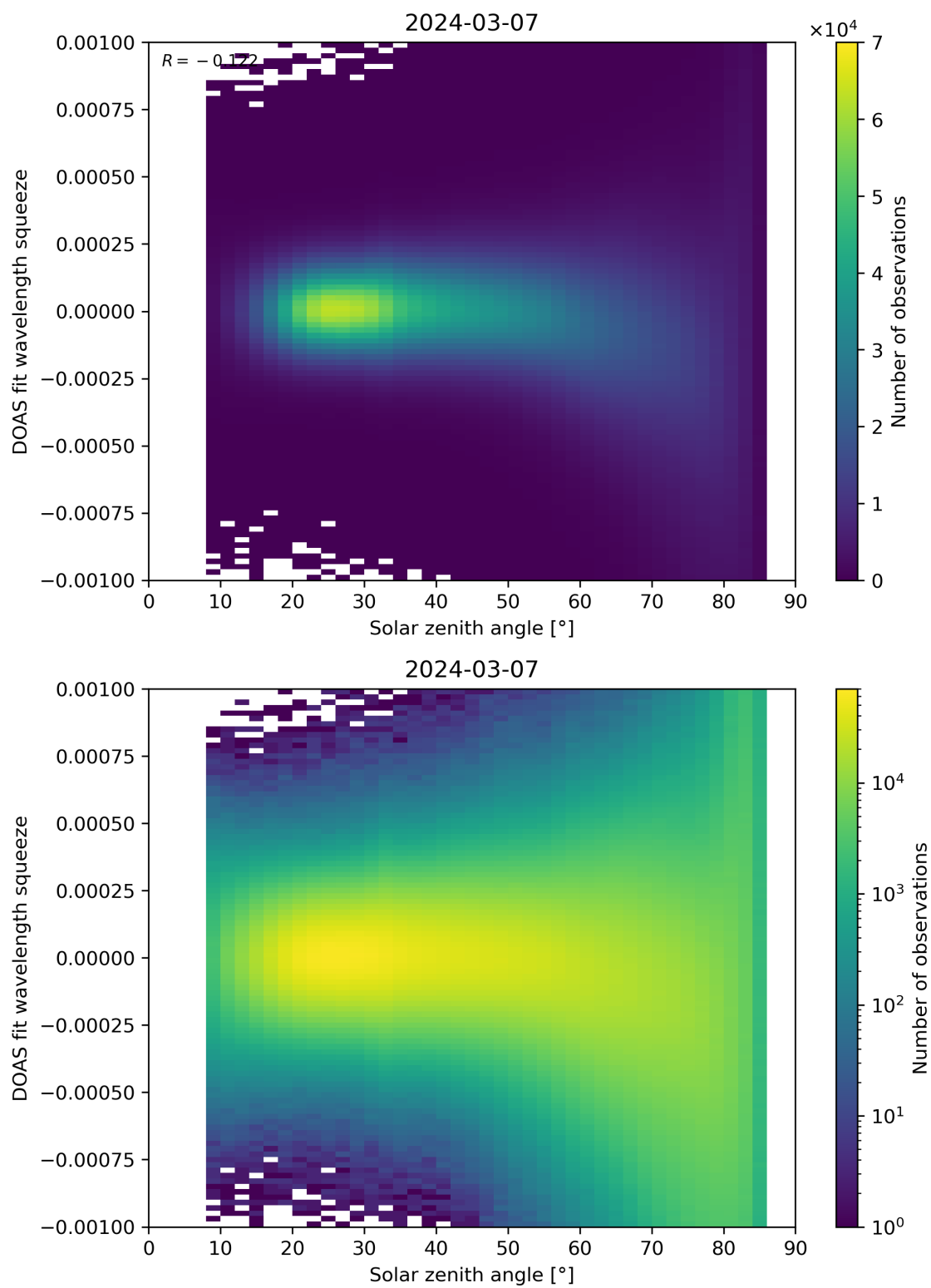
Figure 162: Scatter density plot of “Solar zenith angle” against “DOAS fit wavelength squeeze” for 2024-03-06 to 2024-03-08.
