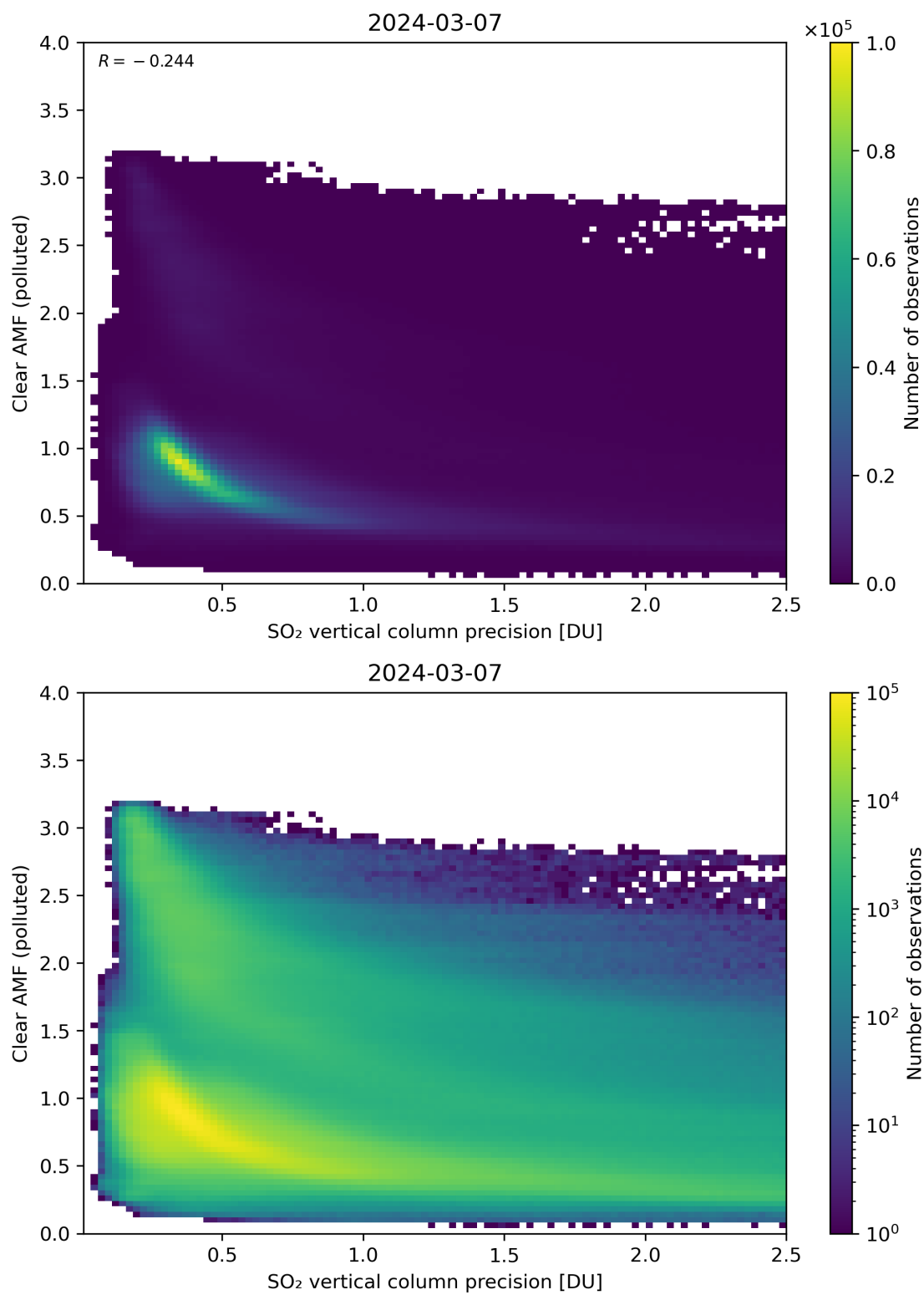
Figure 285: Scatter density plot of “SO 2 vertical column precision” against “Clear AMF (polluted)” for 2024-03-06 to 2024-03-08.
