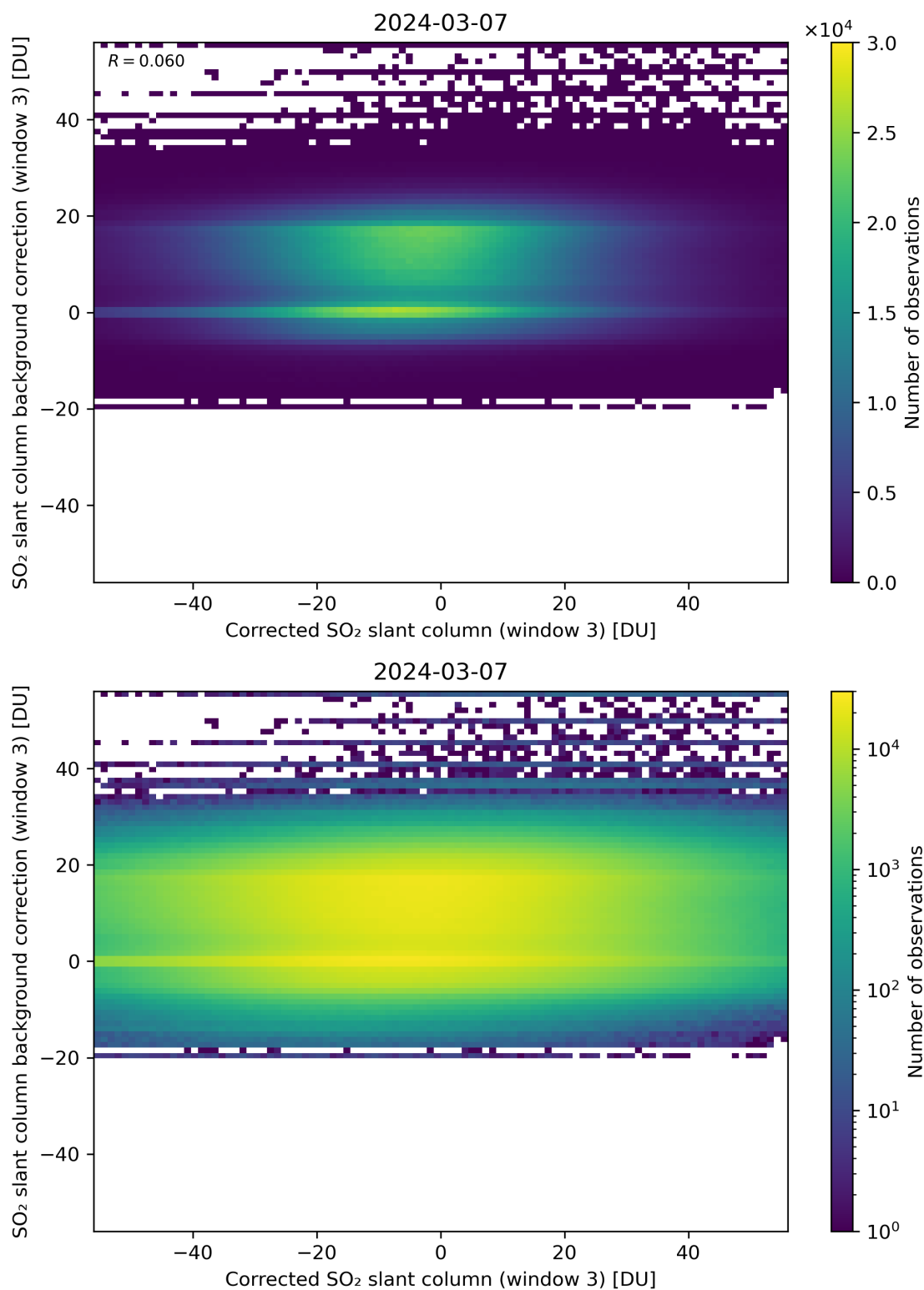
Figure 205: Scatter density plot of “Corrected SO 2 slant column (window 3)” against “SO 2 slant column background correction (window 3)” for 2024-03-06 to 2024-03-08.
