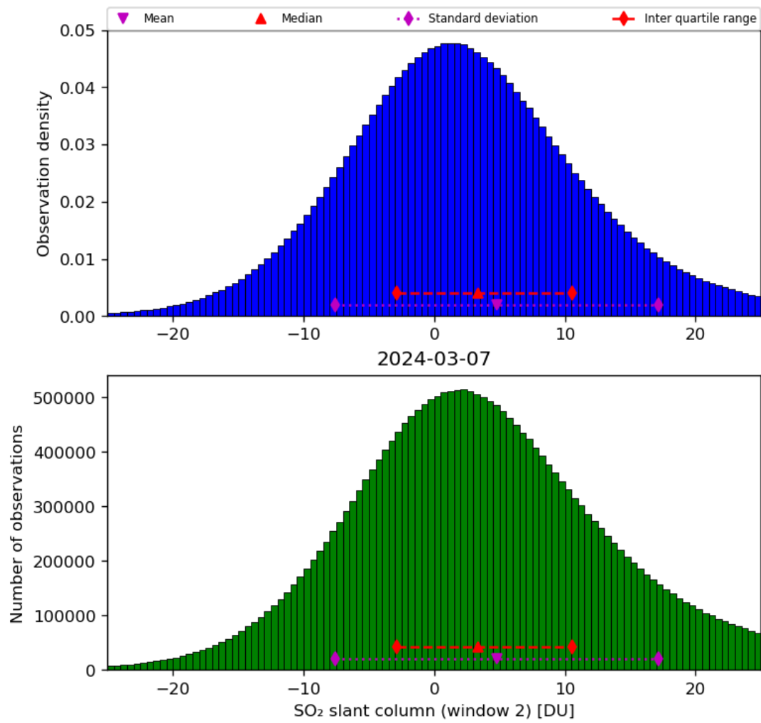
Figure 60: Histogram of “SO 2 slant column (window 2)” for 2024-03-06 to 2024-03-08
