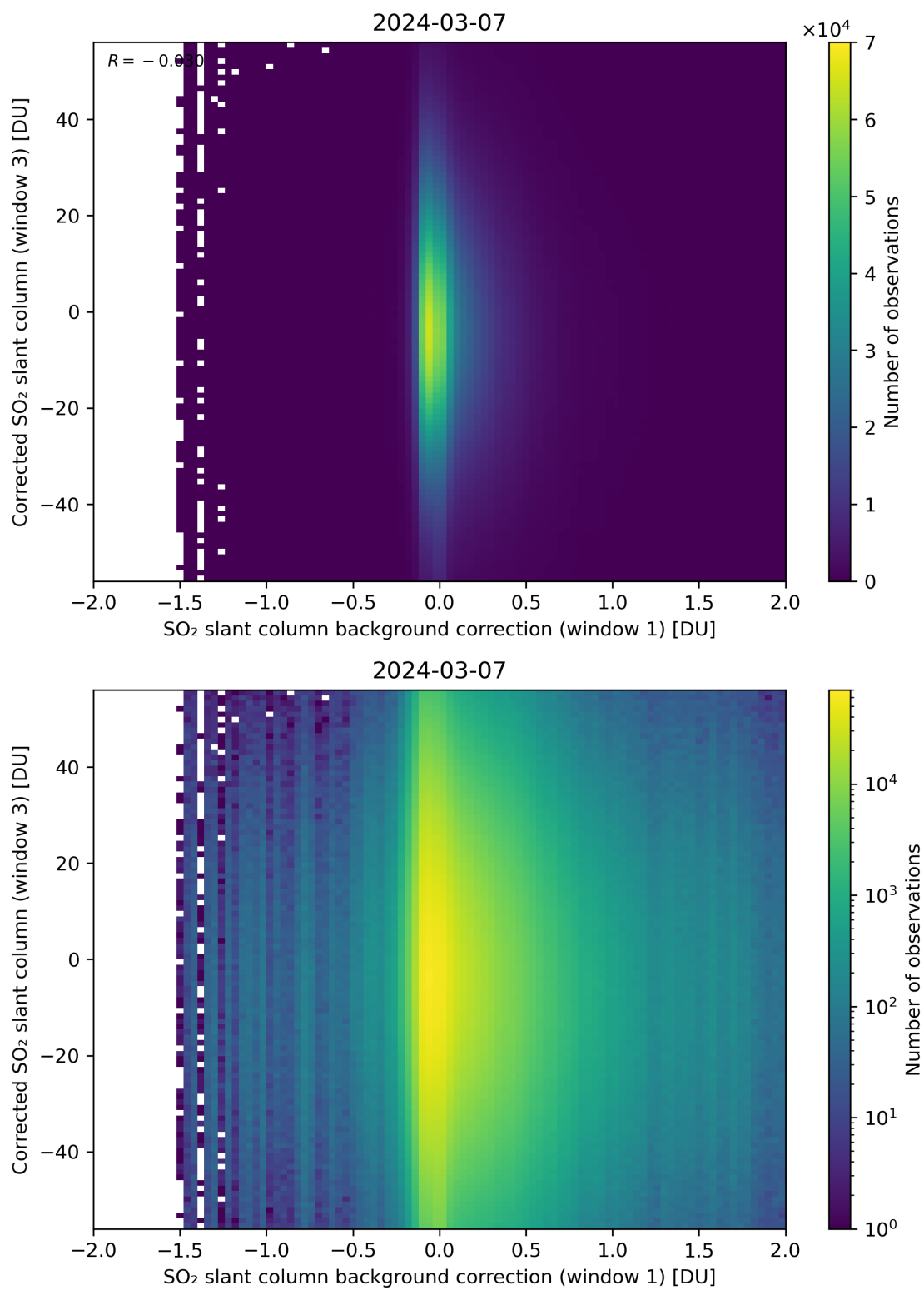
Figure 105: Scatter density plot of “SO 2 slant column background correction (window 1)” against “Corrected SO 2 slant column (window 3)” for 2024-03-06 to 2024-03-08.
