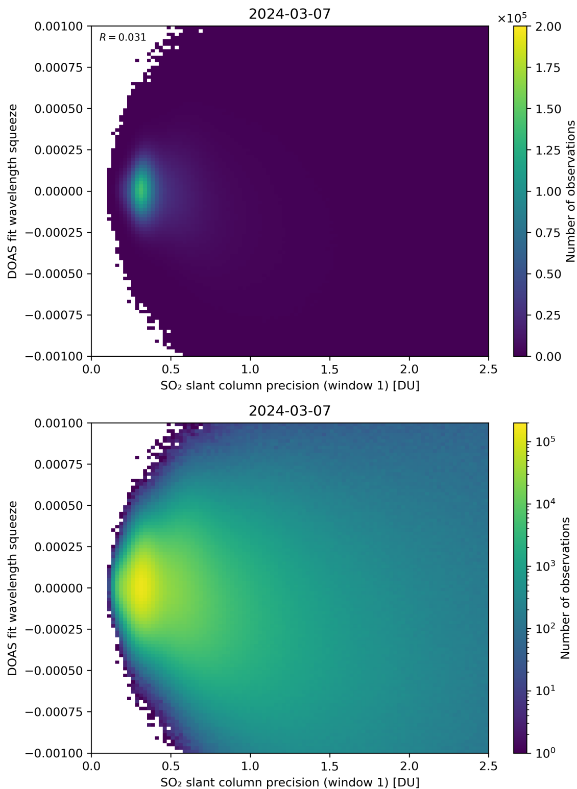
Figure 222: Scatter density plot of “SO 2 slant column precision (window 1)” against “DOAS fit wavelength squeeze” for 2024-03-06 to 2024-03-08.
