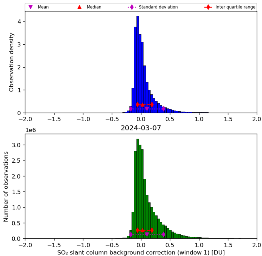
Figure 59: Histogram of “SO 2 slant column background correction (window 1)” for 2024-03-06 to 2024-03-08
