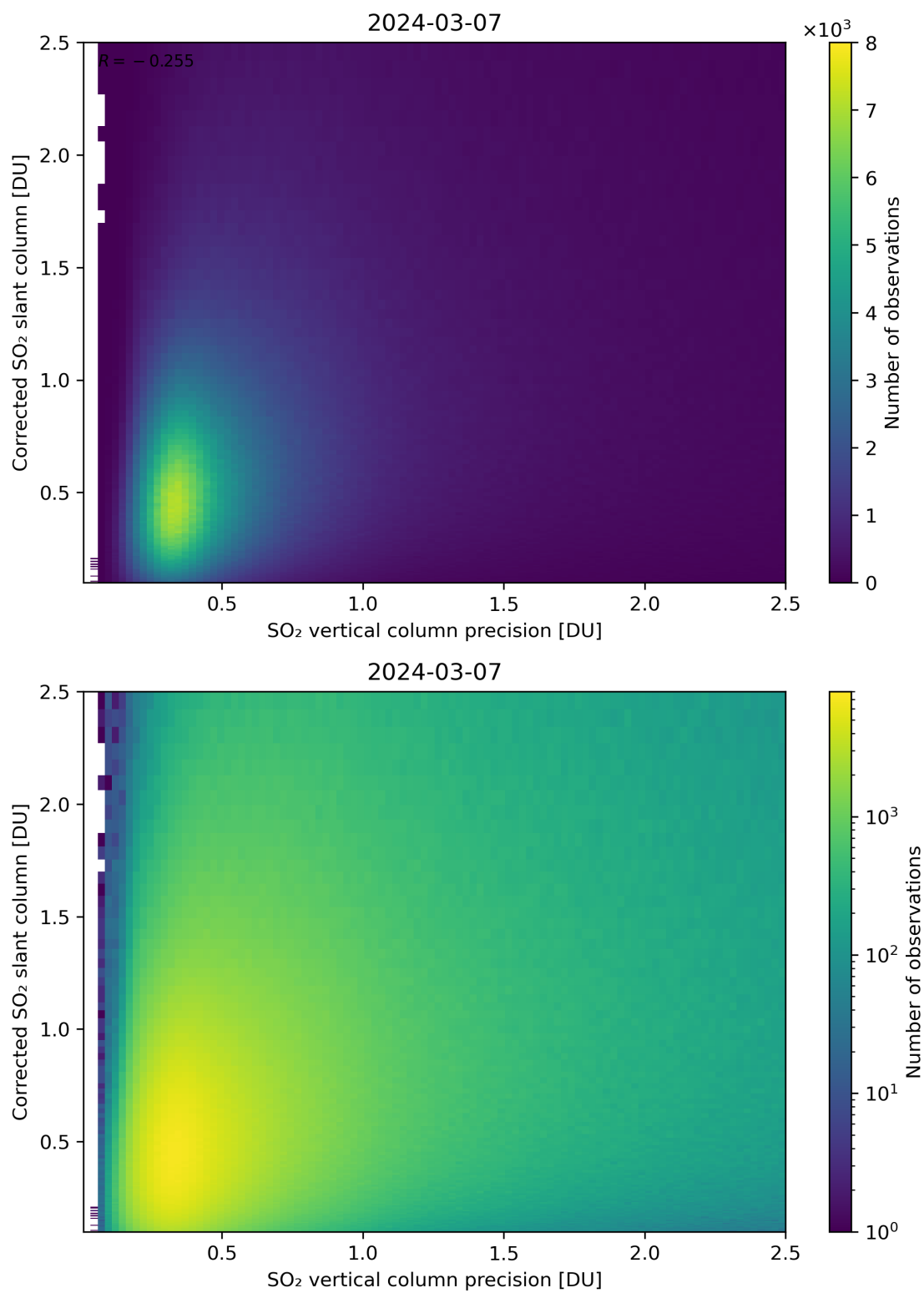
Figure 286: Scatter density plot of “SO 2 vertical column precision” against “Corrected SO 2 slant column” for 2024-03-06 to 2024-03-08.
