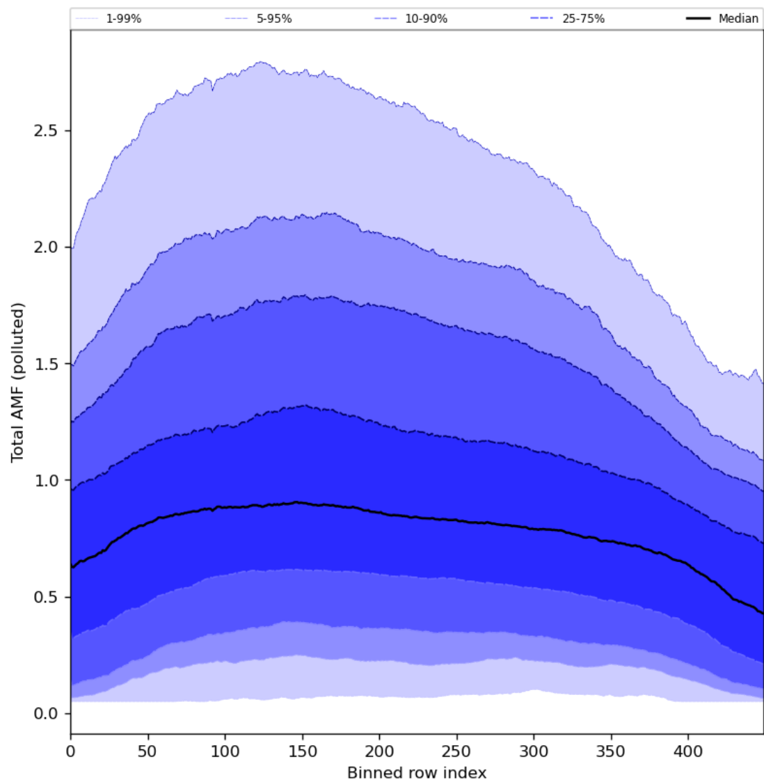
Figure 94: Along track statistics of “Total AMF (polluted)” for 2024-03-06 to 2024-03-08
