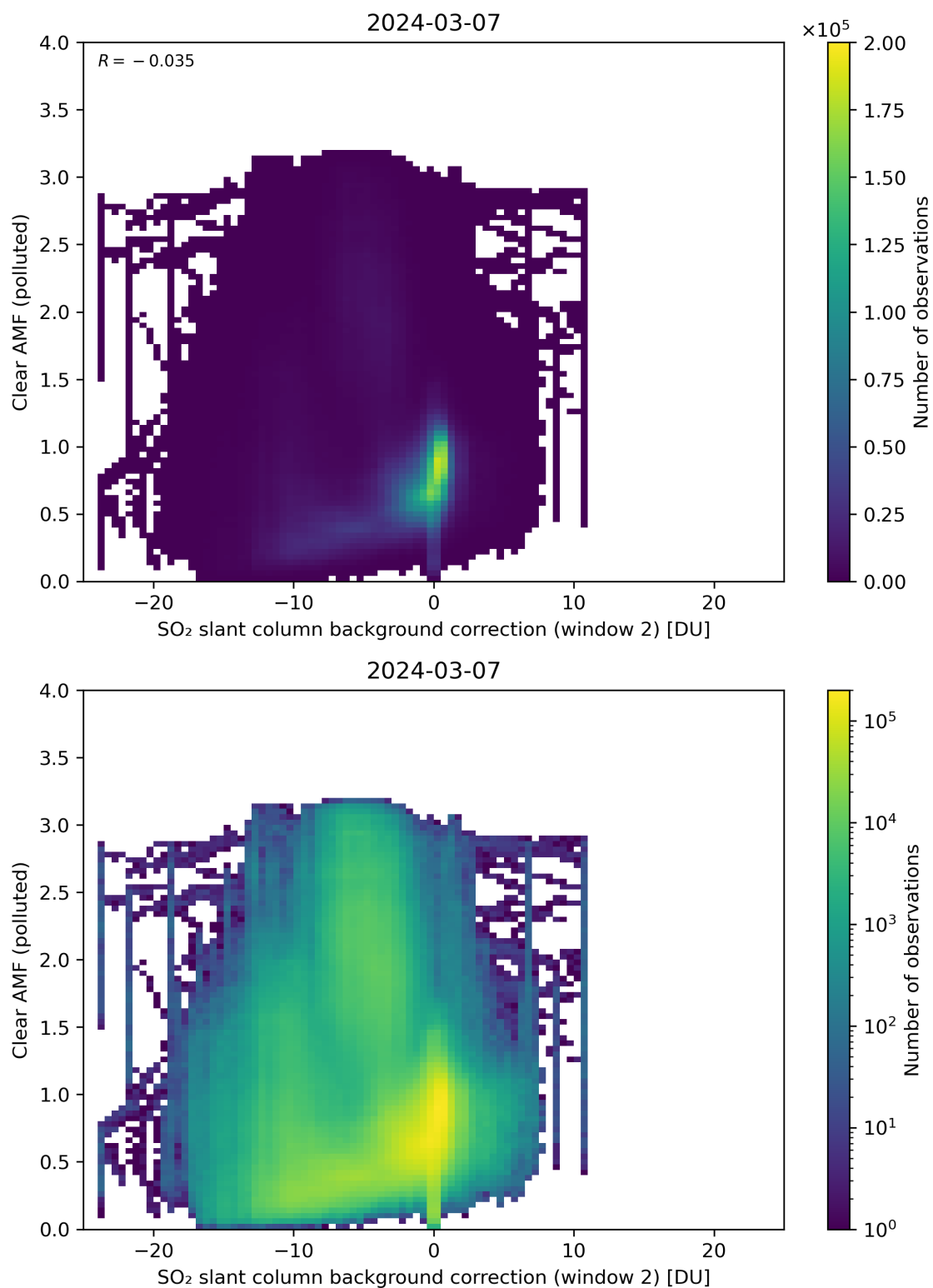
Figure 115: Scatter density plot of “SO 2 slant column background correction (window 2)” against “Clear AMF (polluted)” for 2024-03-06 to 2024-03-08.
