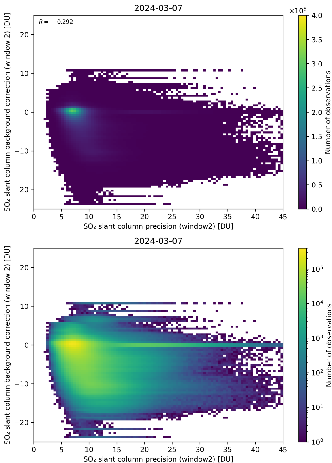
Figure 241: Scatter density plot of “SO 2 slant column precision (window2)” against “SO 2 slant column background correction (window 2)” for 2024-03-06 to 2024-03-08.
