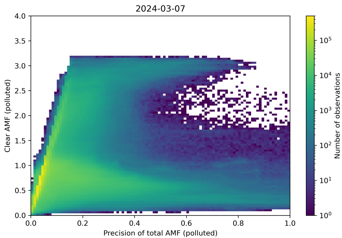
Figure 270: Scatter density plot of “Precision of total AMF (polluted)” against “Clear AMF (polluted)” for 2024-03-06 to 2024-03-08.
