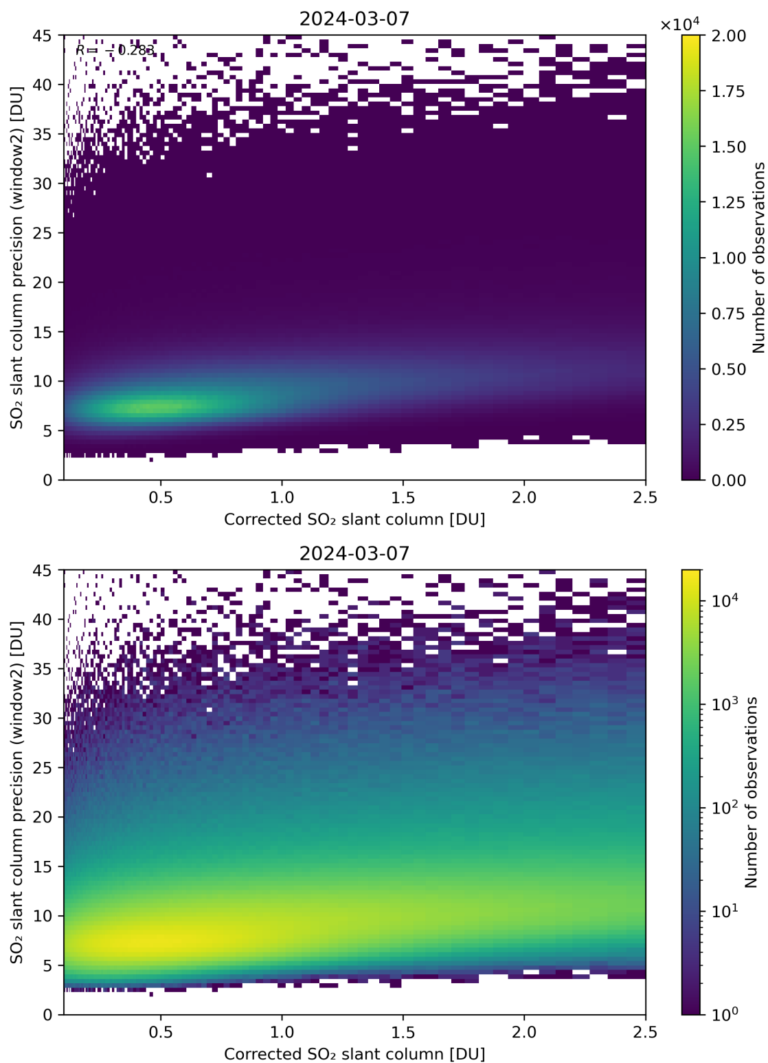
Figure 189: Scatter density plot of “Corrected SO 2 slant column” against “SO 2 slant column precision (window2)” for 2024-03-06 to 2024-03-08.
