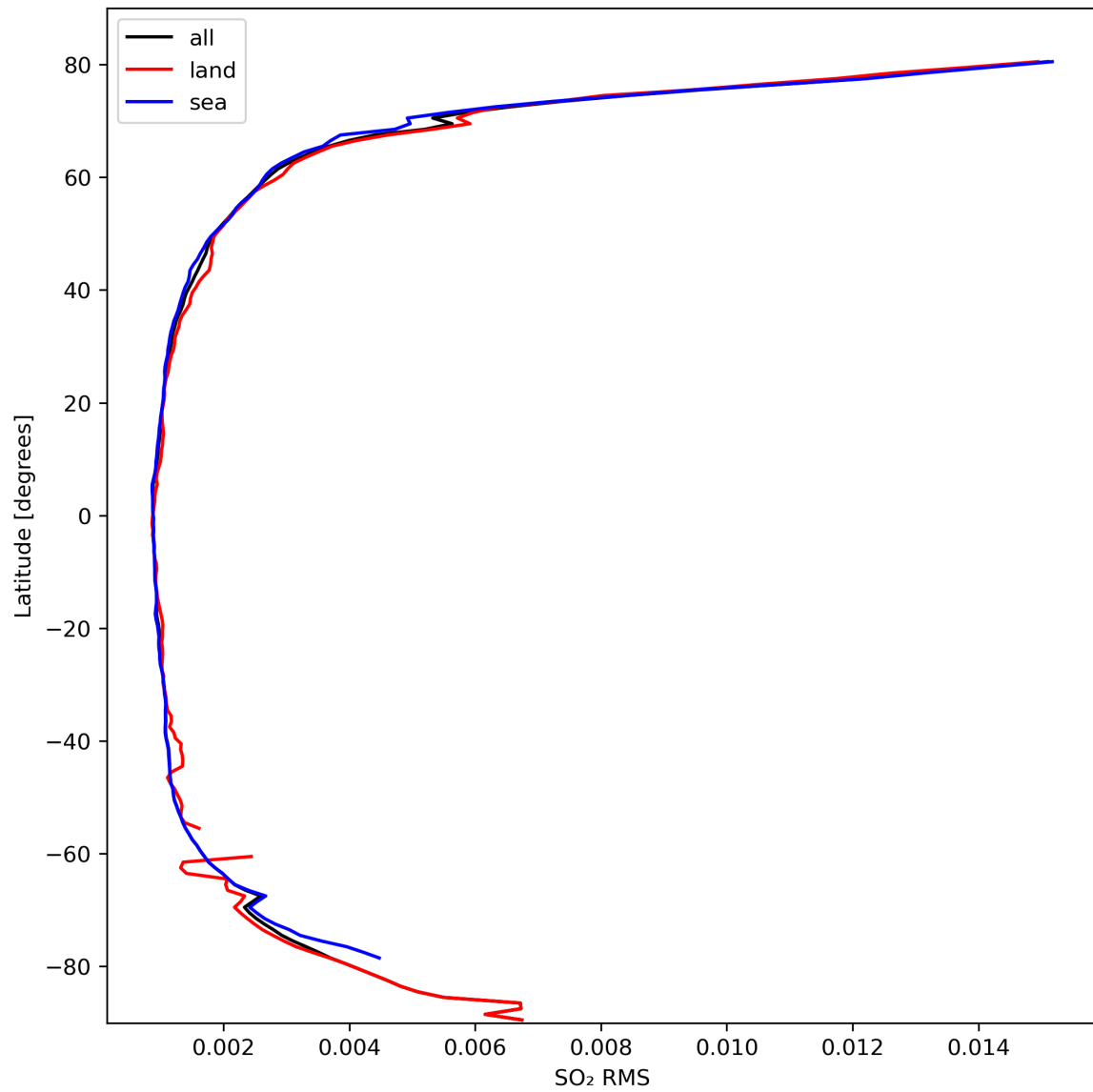
Figure 47: Zonal average of “SO 2 RMS” for 2024-03-06 to 2024-03-08.
