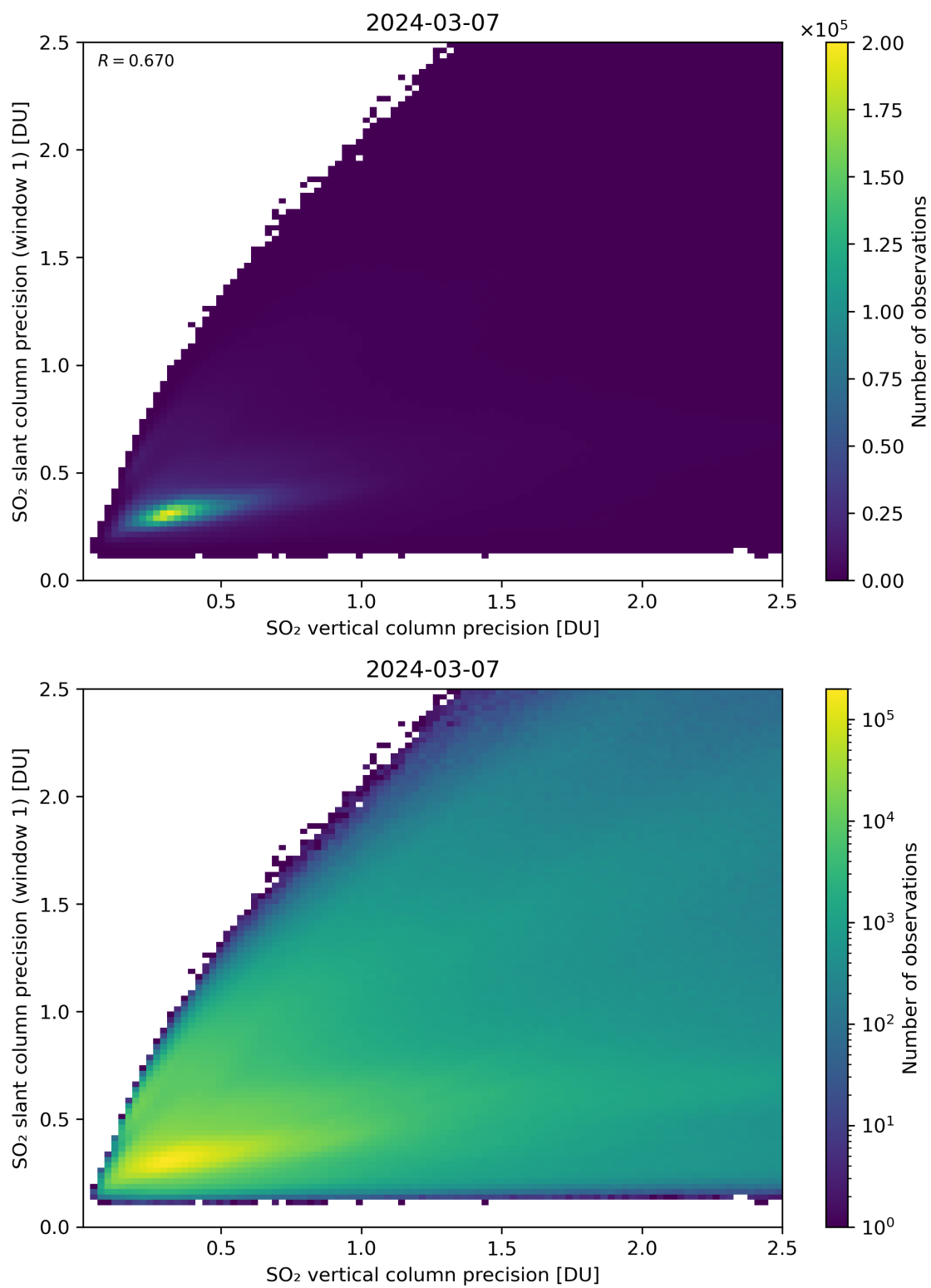
Figure 290: Scatter density plot of “SO 2 vertical column precision” against “SO 2 slant column precision (window 1)” for 2024-03-06 to 2024-03-08.
