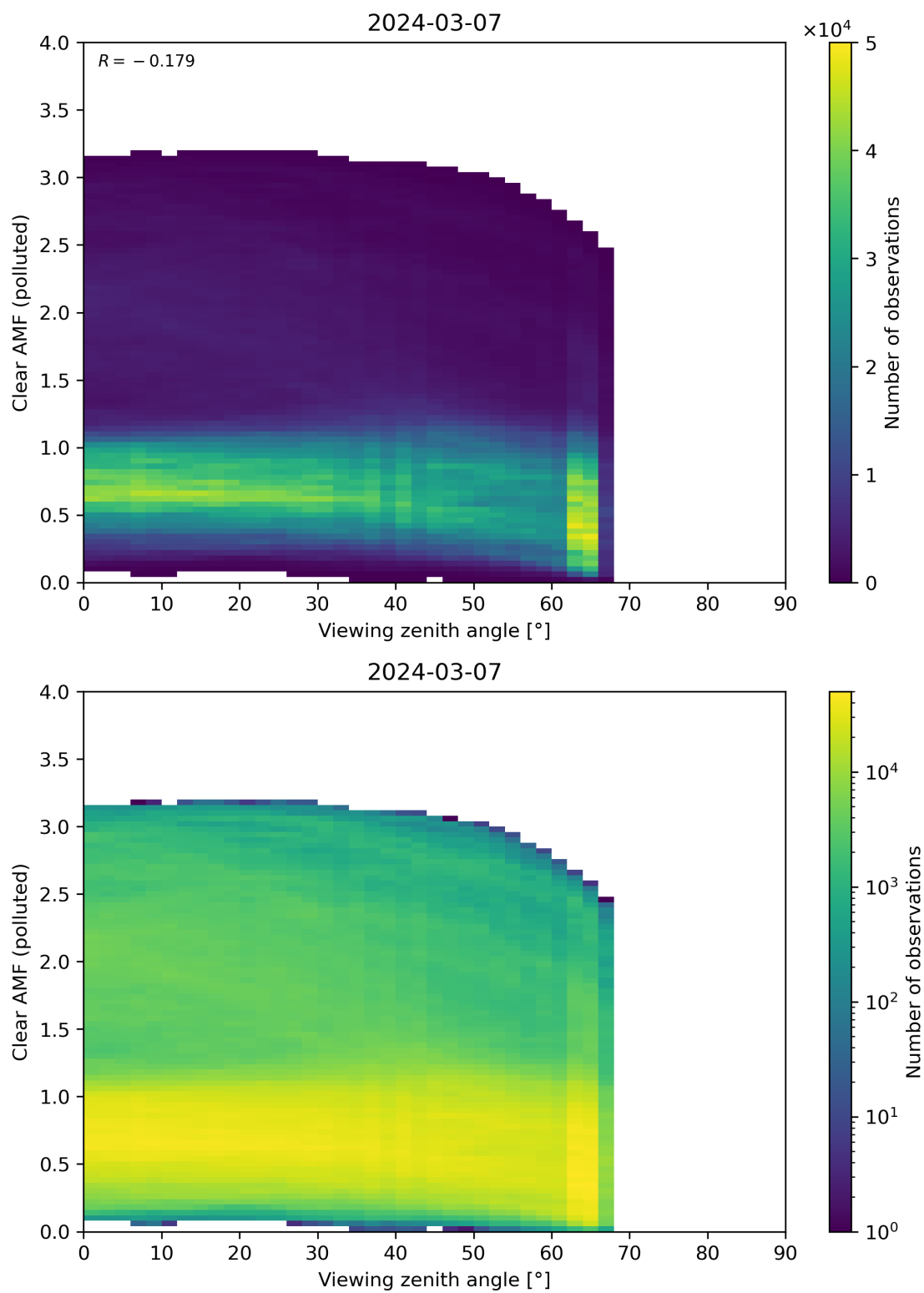
Figure 316: Scatter density plot of “Viewing zenith angle” against “Clear AMF (polluted)” for 2024-03-06 to 2024-03-08.
