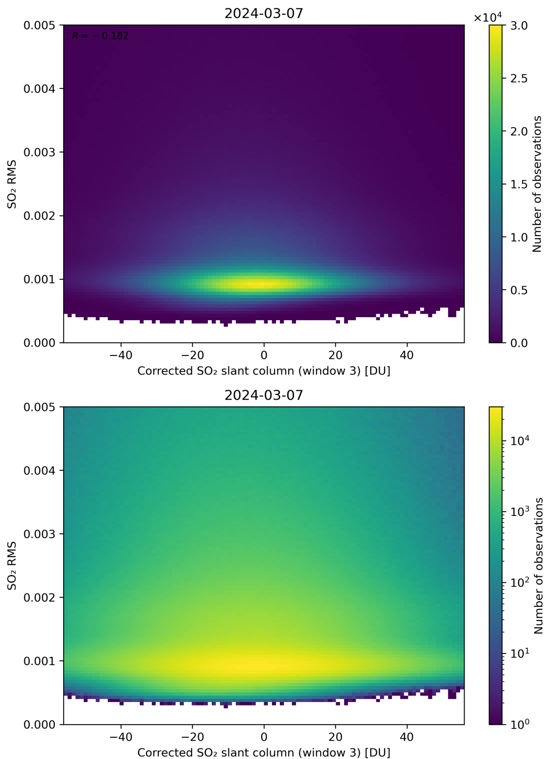
Figure 208: Scatter density plot of “Corrected SO 2 slant column (window 3)” against “SO 2 RMS” for 2024-03-06 to 2024-03-08.
