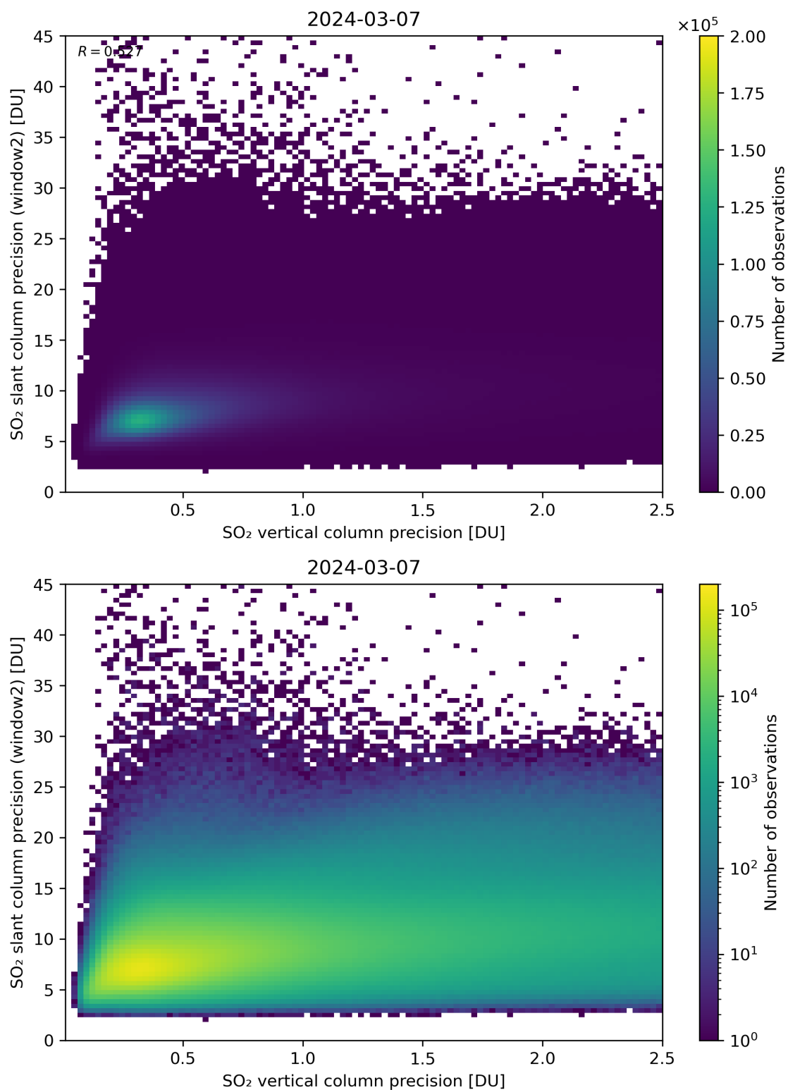
Figure 291: Scatter density plot of “SO 2 vertical column precision” against “SO 2 slant column precision (window2)” for 2024-03-06 to 2024-03-08.
