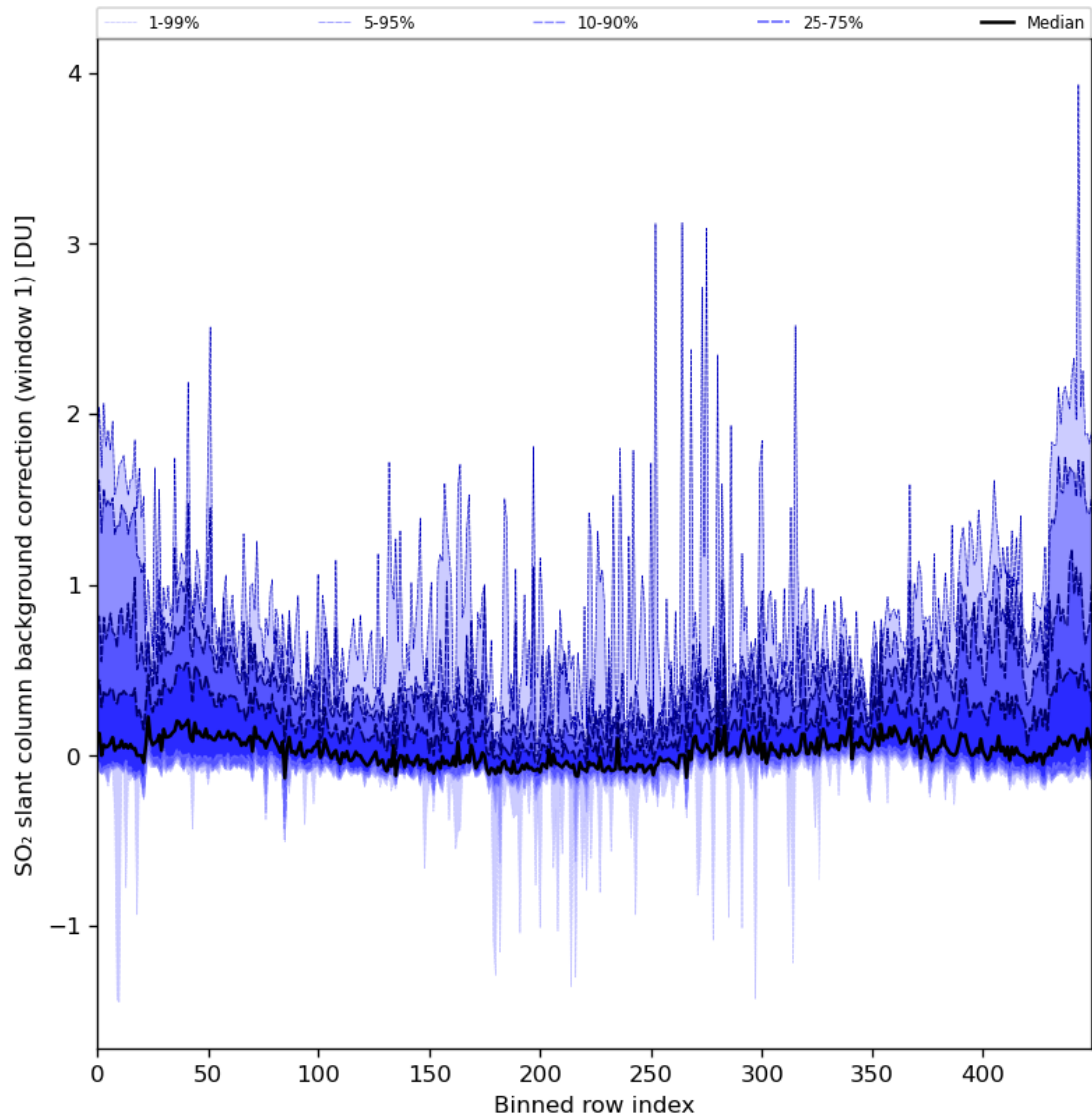
Figure 82: Along track statistics of “SO 2 slant column background correction (window 1)” for 2024-03-06 to 2024-03-08
