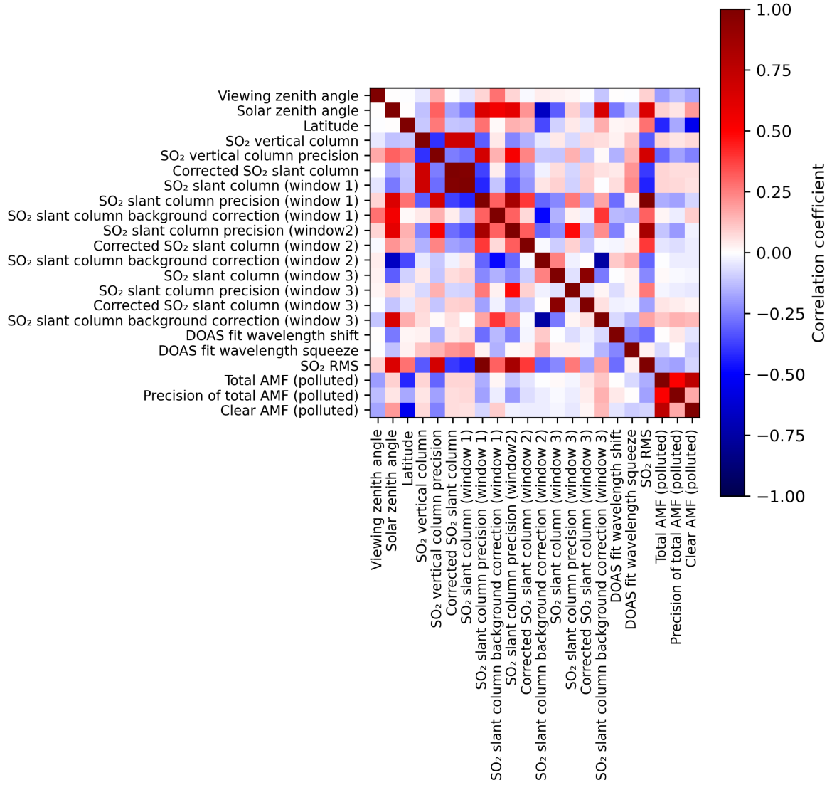
Figure 2: Map of correlation matrix for 2024-03-06 to 2024-03-08.
