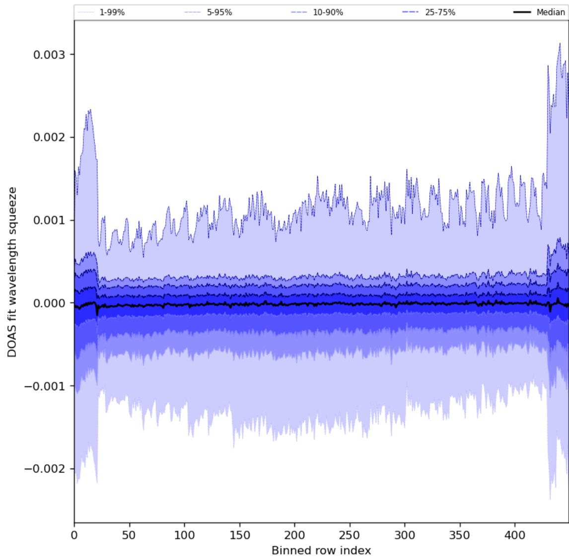
Figure 92: Along track statistics of “DOAS fit wavelength squeeze” for 2024-03-06 to 2024-03-08
