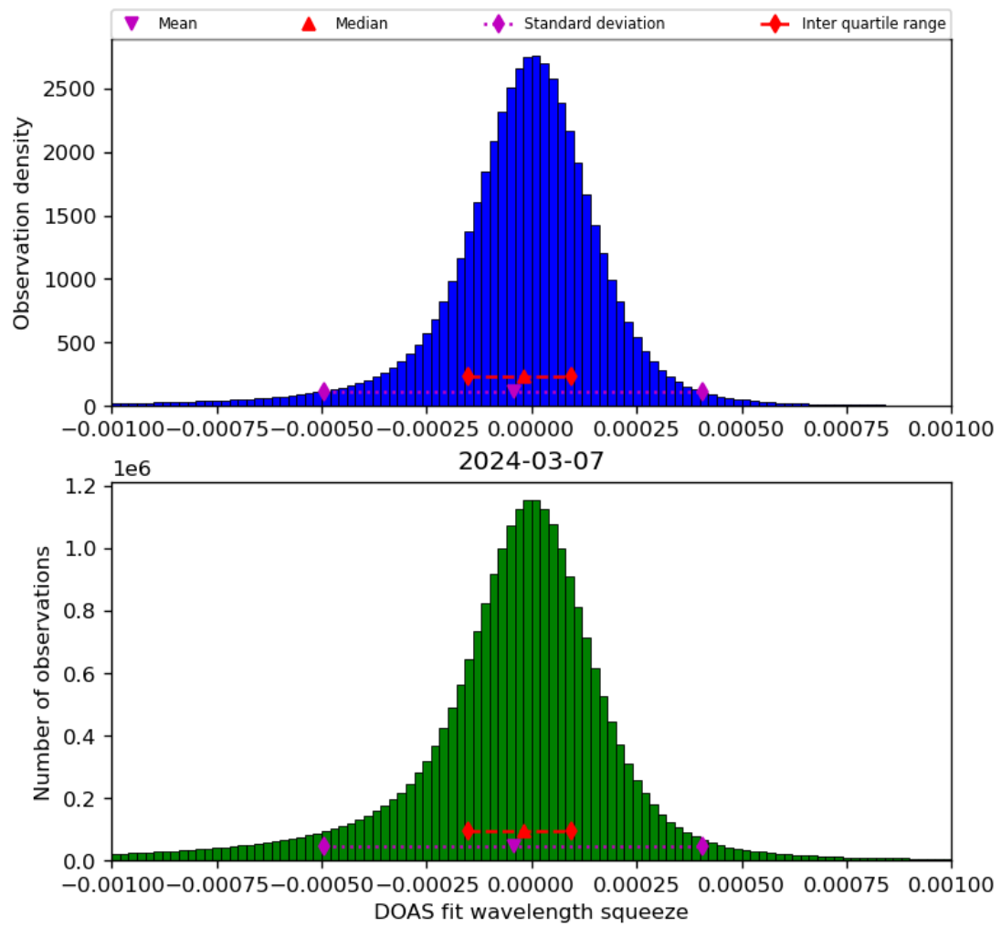
Figure 69: Histogram of “DOAS fit wavelength squeeze” for 2024-03-06 to 2024-03-08
