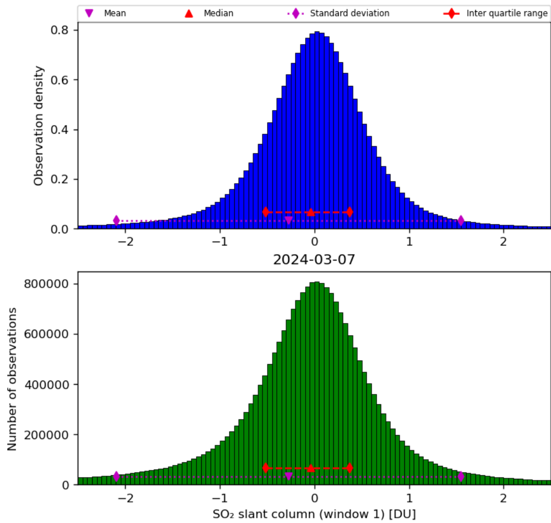
Figure 56: Histogram of “SO 2 slant column (window 1)” for 2024-03-06 to 2024-03-08
