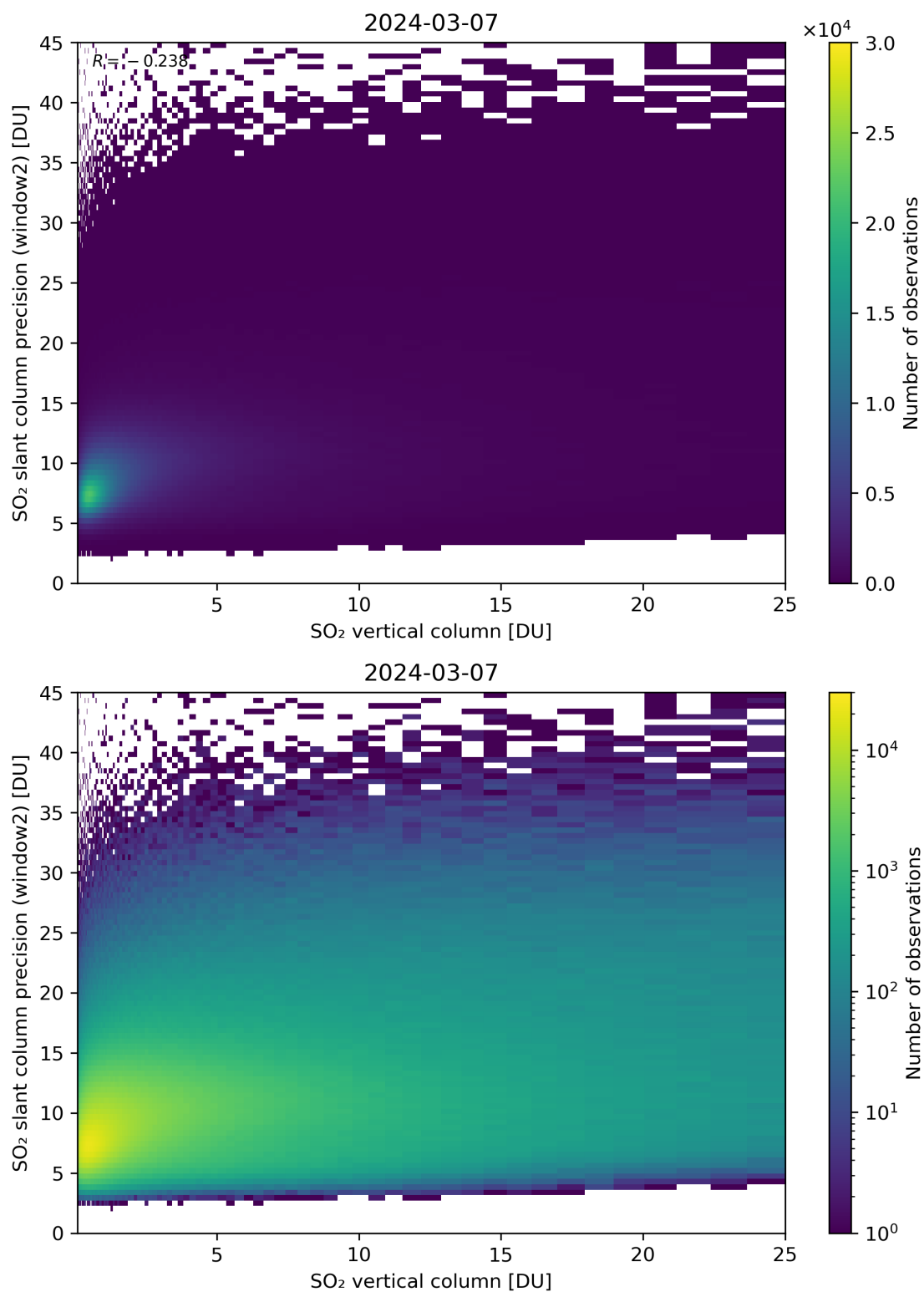
Figure 302: Scatter density plot of “SO 2 vertical column” against “SO 2 slant column precision (window2)” for 2024-03-06 to 2024-03-08.
