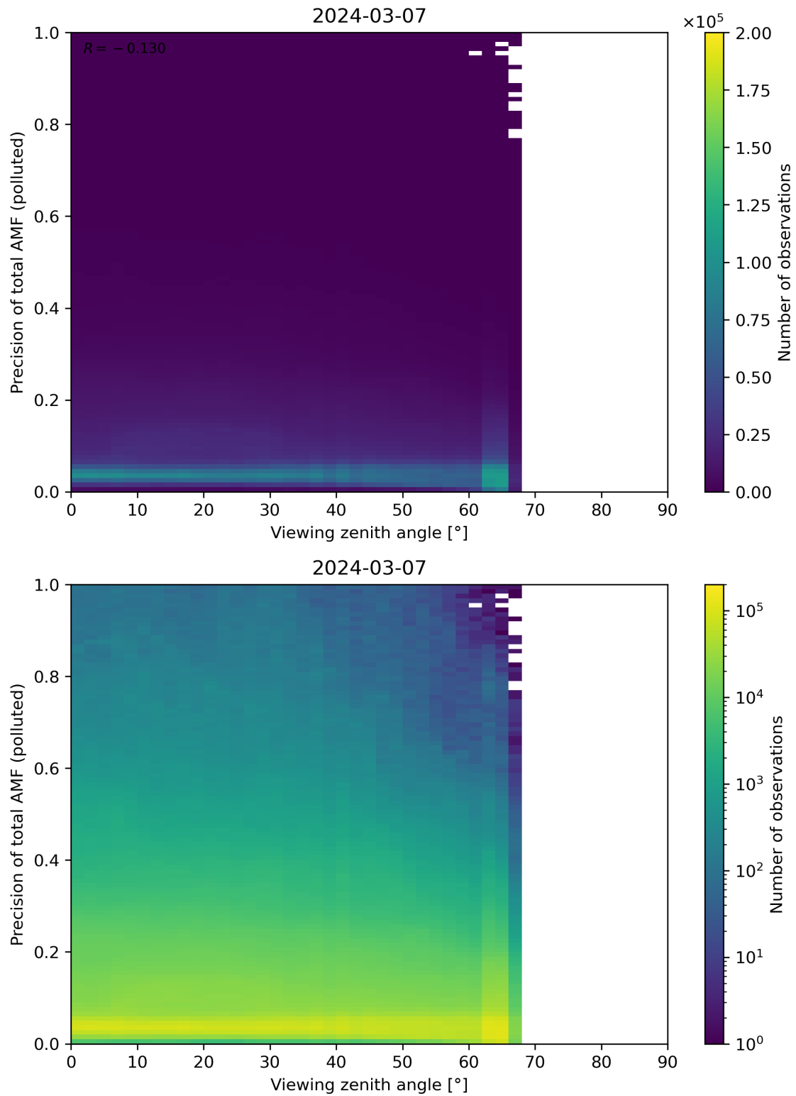
Figure 326: Scatter density plot of “Viewing zenith angle” against “Precision of total AMF (polluted)” for 2024-03-06 to 2024-03-08.
