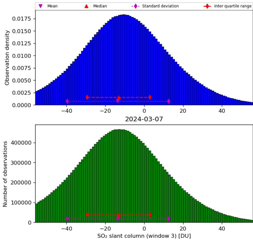
Figure 64: Histogram of “SO 2 slant column (window 3)” for 2024-03-06 to 2024-03-08
