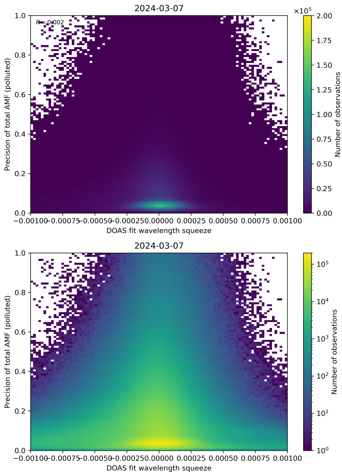
Figure 135: Scatter density plot of “DOAS fit wavelength squeeze” against “Precision of total AMF (polluted)” for 2024-03-06 to 2024-03-08.
