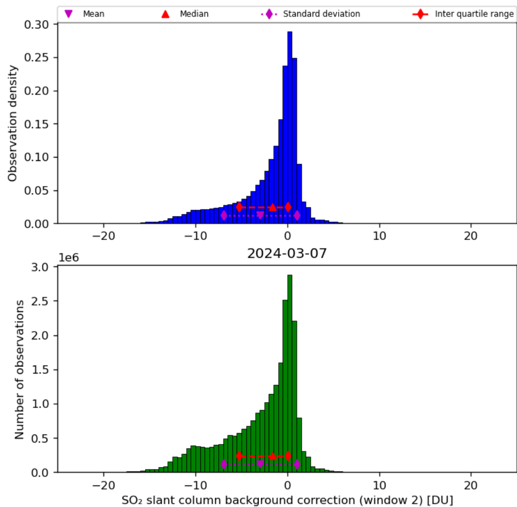
Figure 63: Histogram of “SO 2 slant column background correction (window 2)” for 2024-03-06 to 2024-03-08
