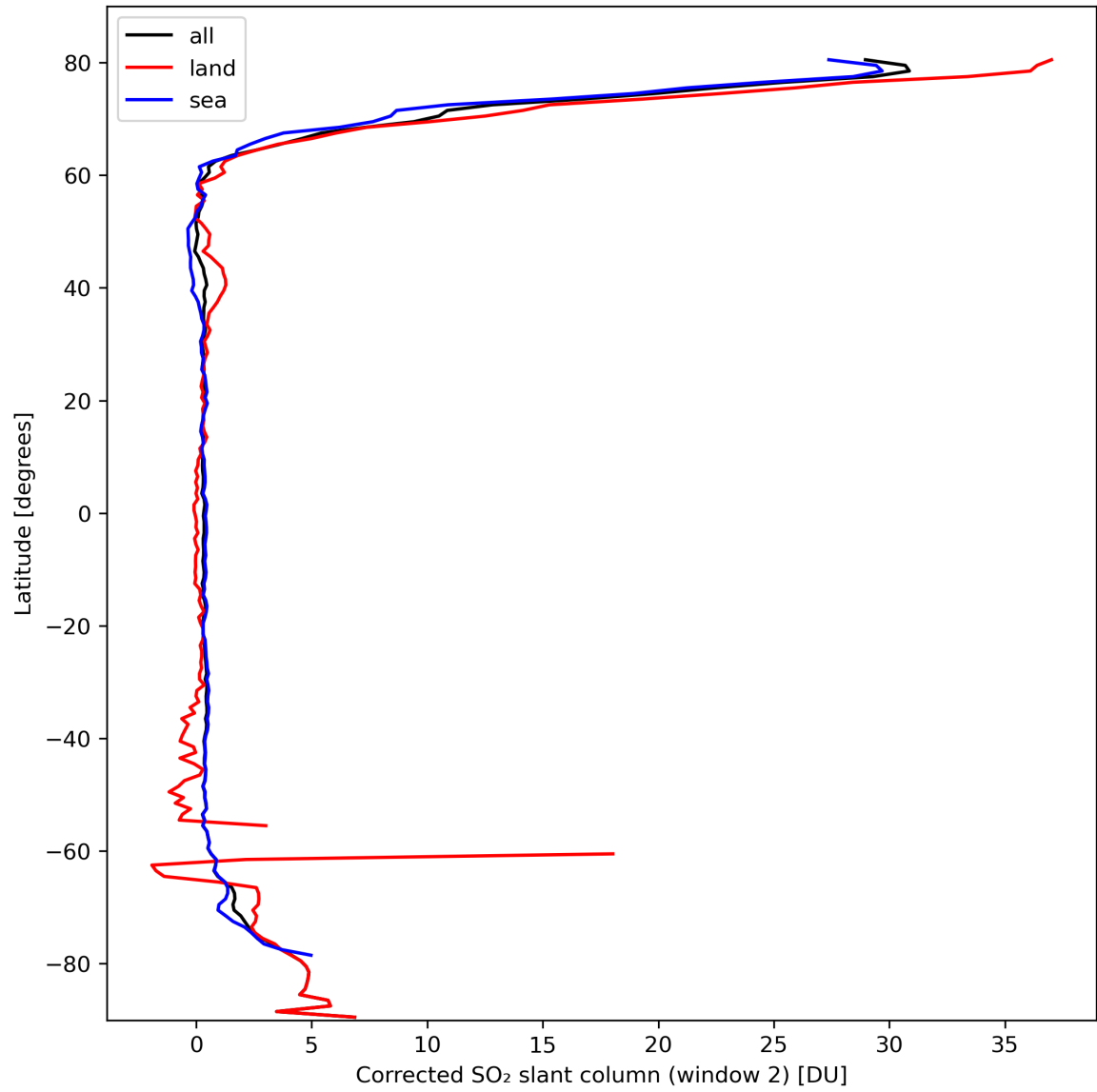
Figure 39: Zonal average of “Corrected SO 2 slant column (window 2)” for 2024-03-06 to 2024-03-08.
