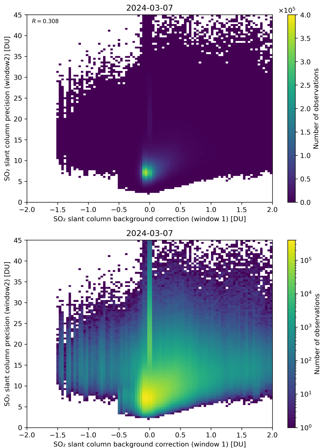
Figure 106: Scatter density plot of “SO 2 slant column background correction (window 1)” against “SO 2 slant column precision (window2)” for 2024-03-06 to 2024-03-08.
