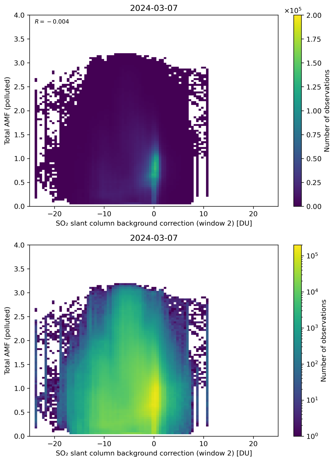
Figure 119: Scatter density plot of “SO 2 slant column background correction (window 2)” against “Total AMF (polluted)” for 2024-03-06 to 2024-03-08.
