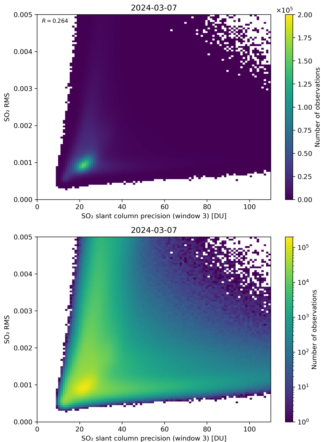
Figure 260: Scatter density plot of “SO 2 slant column precision (window 3)” against “SO 2 RMS” for 2024-03-06 to 2024-03-08.
