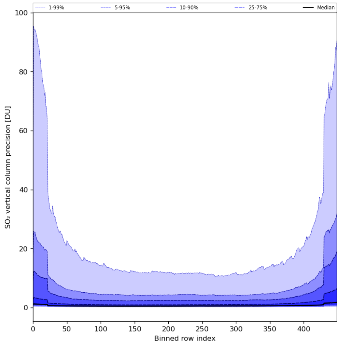
Figure 77: Along track statistics of “SO 2 vertical column precision” for 2024-03-06 to 2024-03-08
