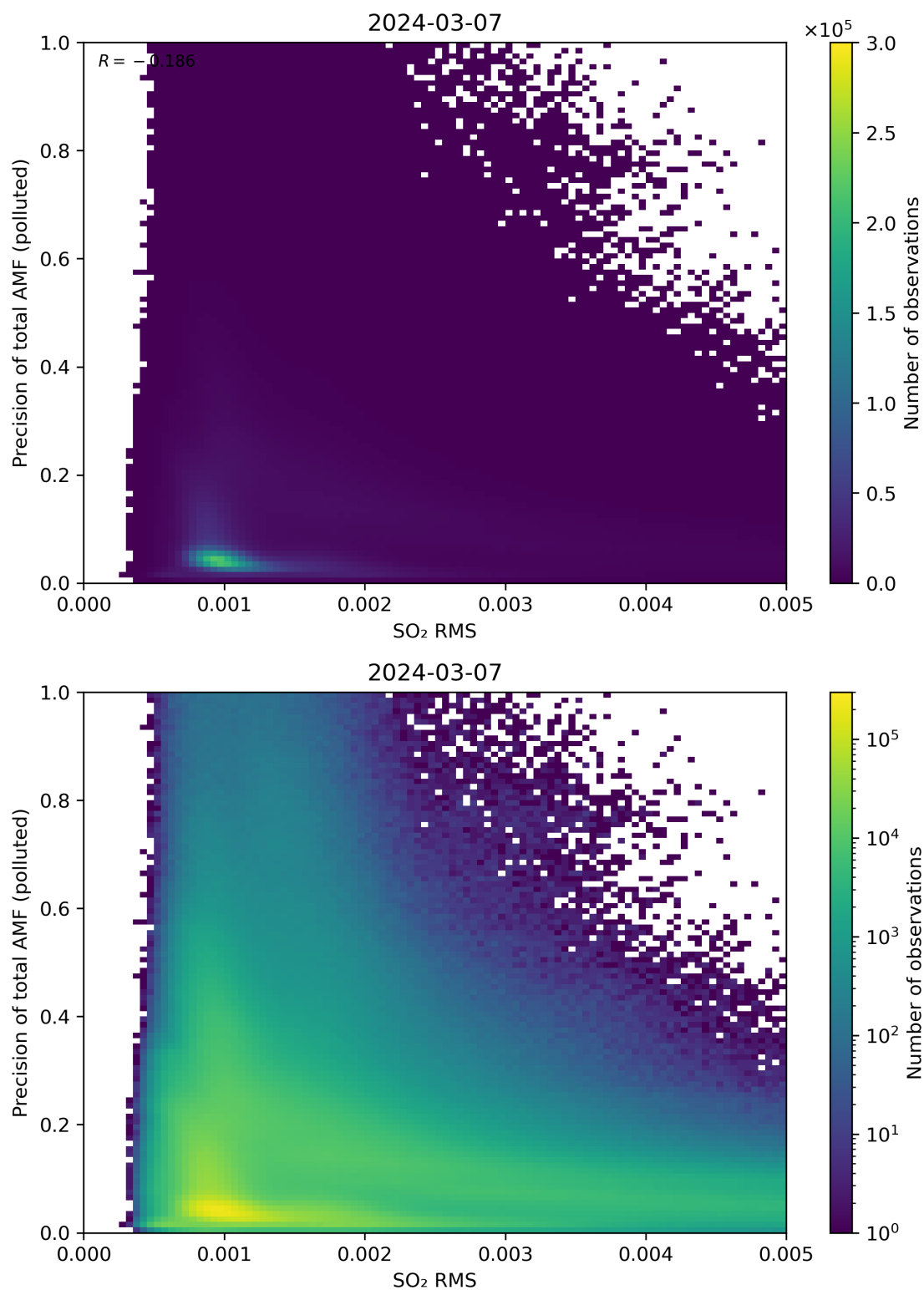
Figure 138: Scatter density plot of “SO 2 RMS” against “Precision of total AMF (polluted)” for 2024-03-06 to 2024-03-08.
