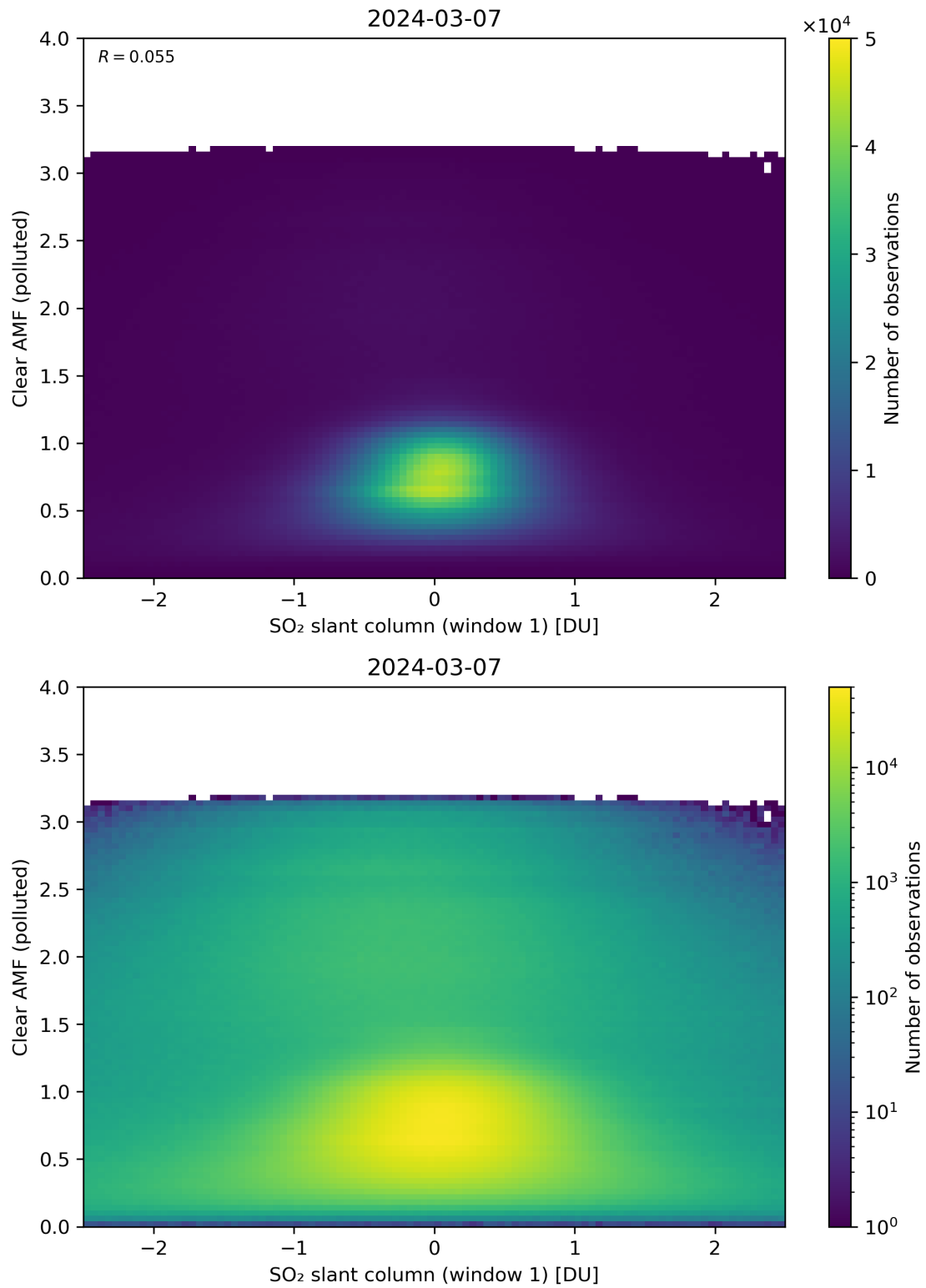
Figure 232: Scatter density plot of “SO 2 slant column (window 1)” against “Clear AMF (polluted)” for 2024-03-06 to 2024-03-08.
