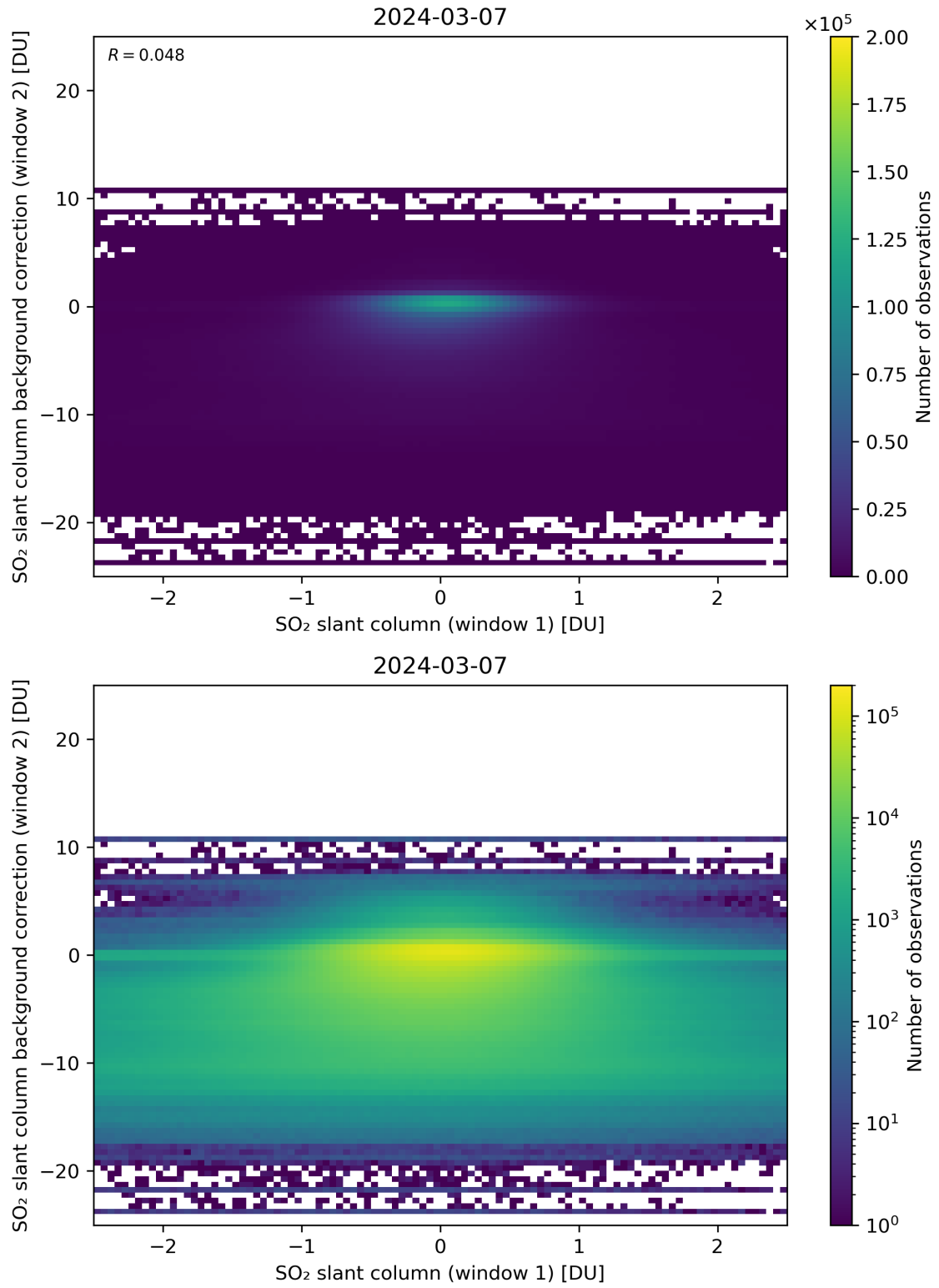
Figure 213: Scatter density plot of “SO 2 slant column (window 1)” against “SO 2 slant column background correction (window 2)” for 2024-03-06 to 2024-03-08.
