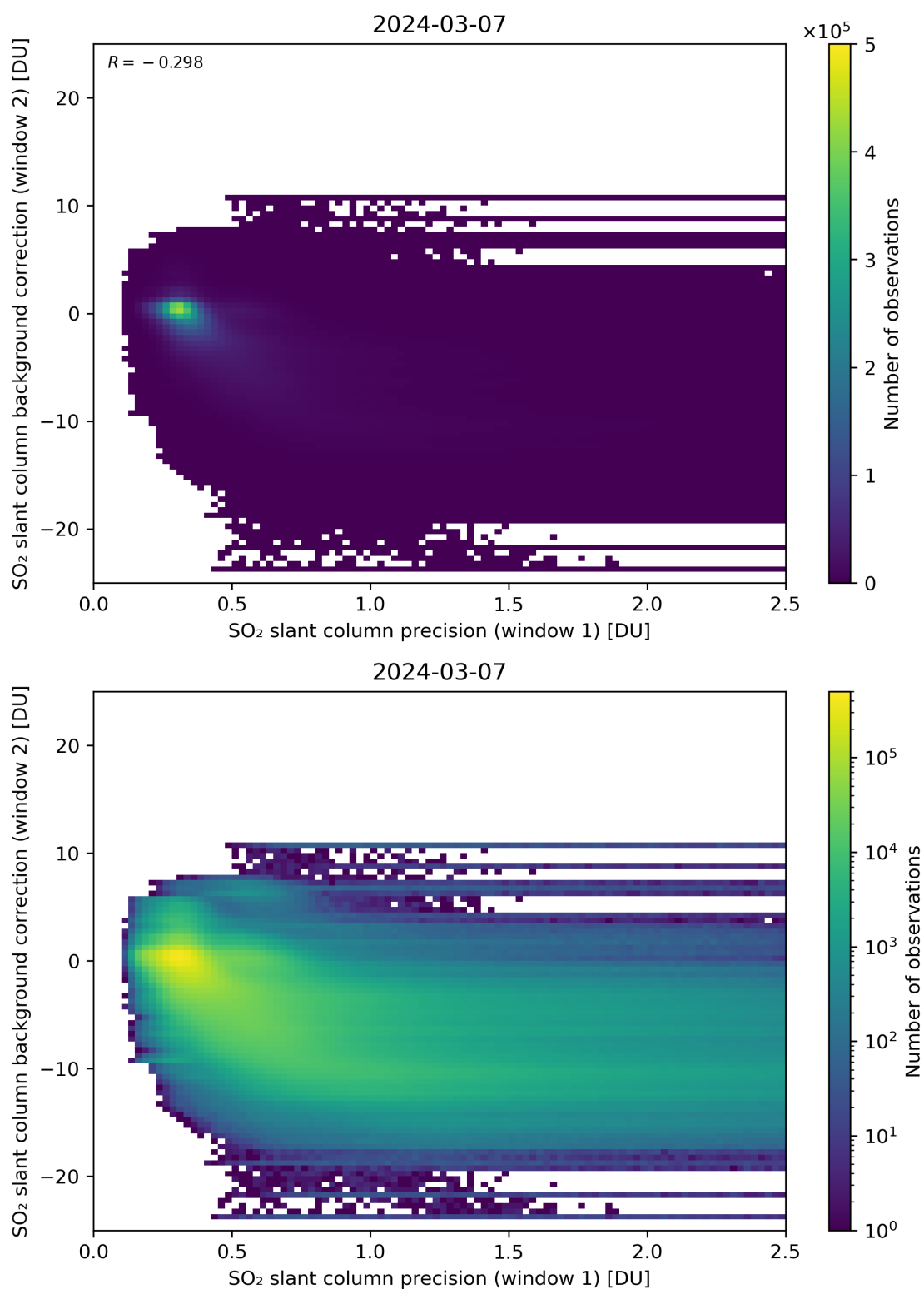
Figure 219: Scatter density plot of “SO 2 slant column precision (window 1)” against “SO 2 slant column background correction (window 2)” for 2024-03-06 to 2024-03-08.
