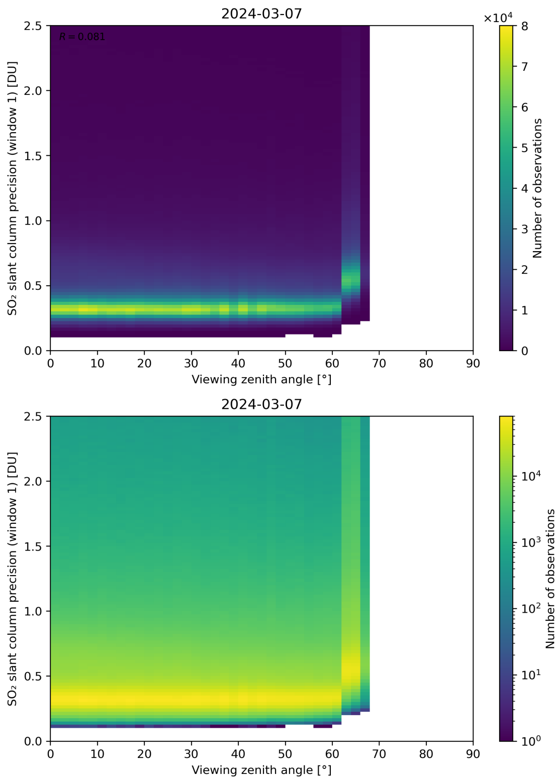
Figure 321: Scatter density plot of “Viewing zenith angle” against “SO 2 slant column precision (window 1)” for 2024-03-06 to 2024-03-08.
