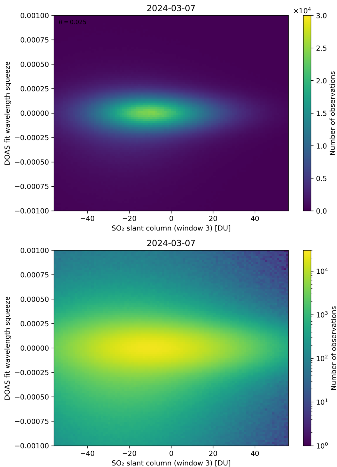
Figure 255: Scatter density plot of “SO 2 slant column (window 3)” against “DOAS fit wavelength squeeze” for 2024-03-06 to 2024-03-08.
