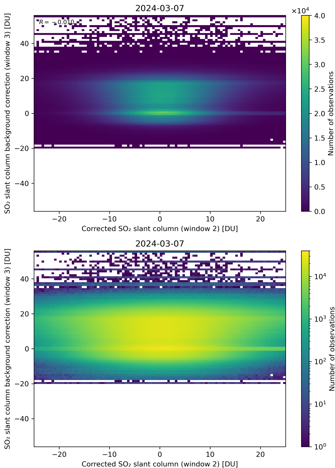
Figure 195: Scatter density plot of “Corrected SO 2 slant column (window 2)” against “SO 2 slant column background correction (window 3)” for 2024-03-06 to 2024-03-08.
