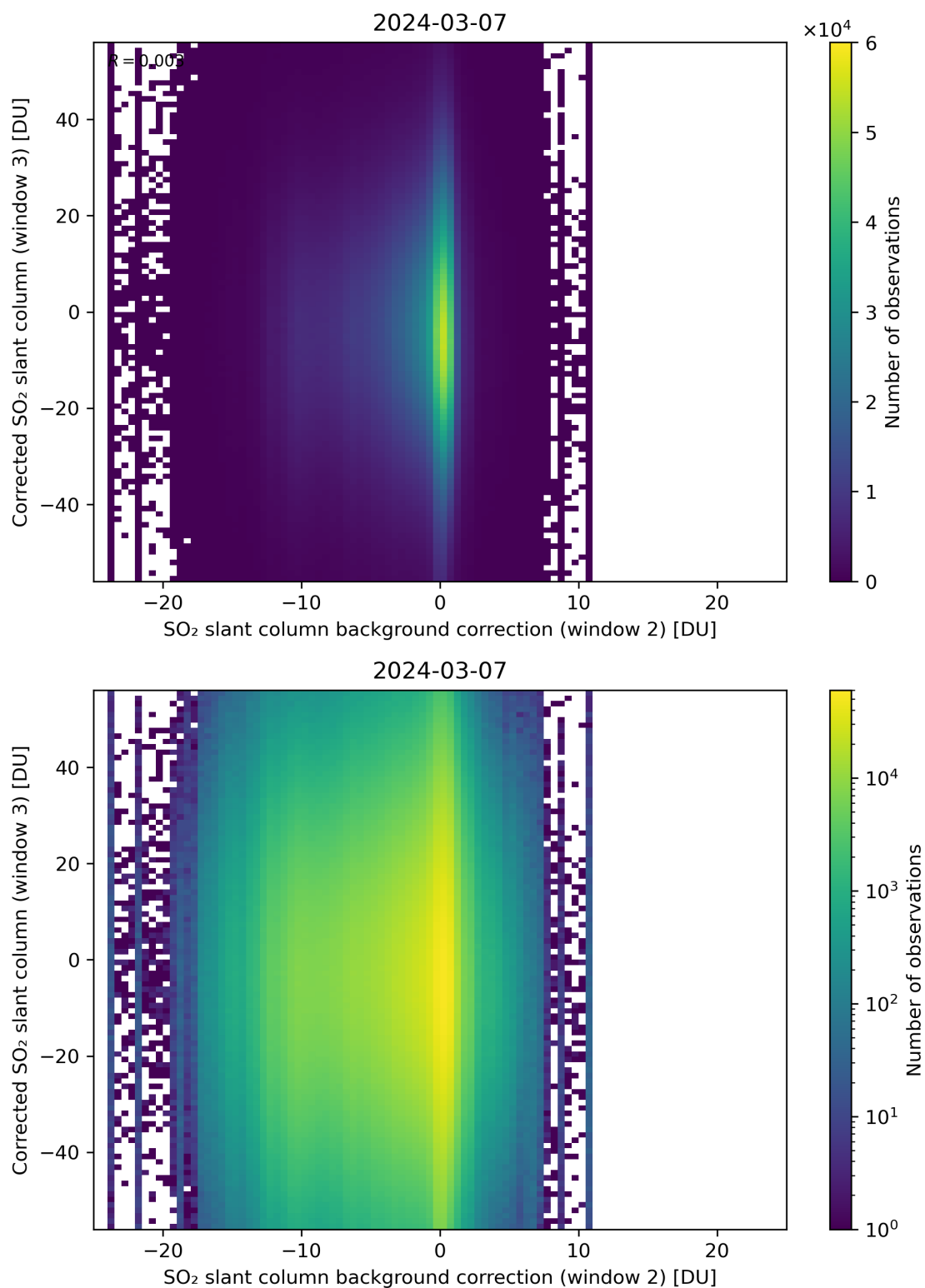
Figure 116: Scatter density plot of “SO 2 slant column background correction (window 2)” against “Corrected SO 2 slant column (window 3)” for 2024-03-06 to 2024-03-08.
