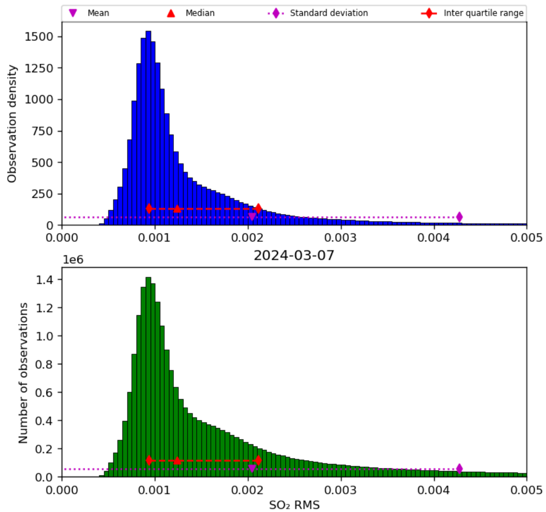
Figure 70: Histogram of “SO 2 RMS” for 2024-03-06 to 2024-03-08
