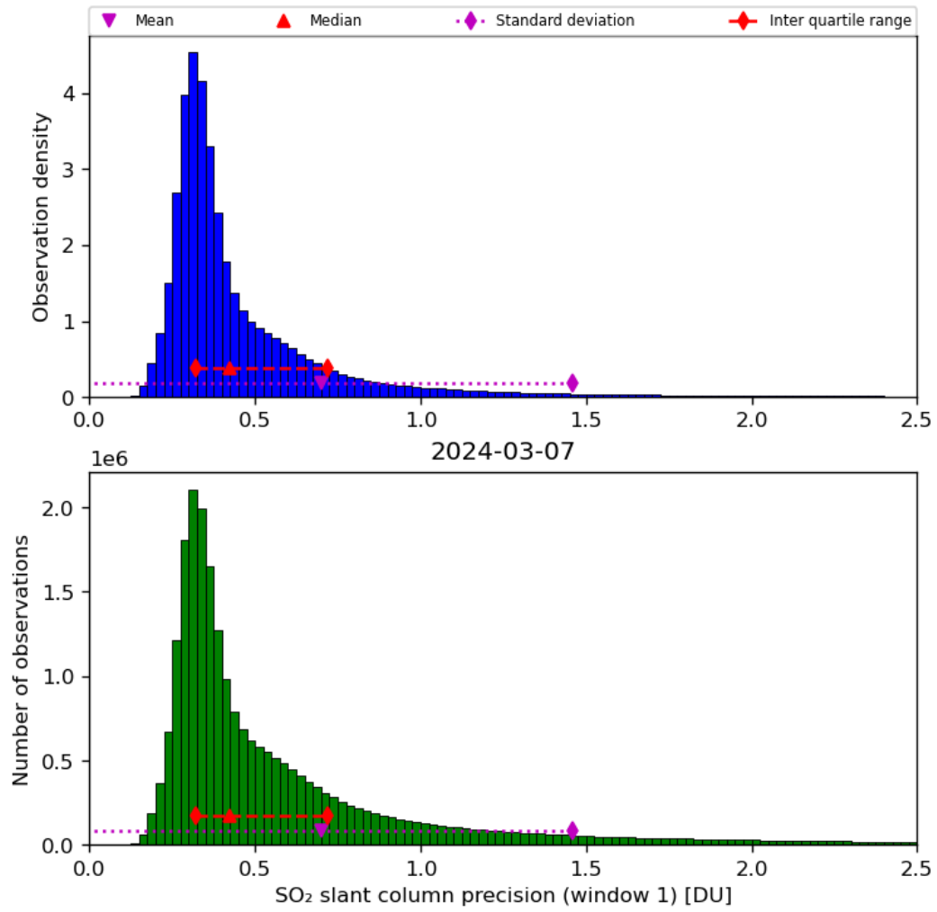
Figure 57: Histogram of “SO 2 slant column precision (window 1)” for 2024-03-06 to 2024-03-08
