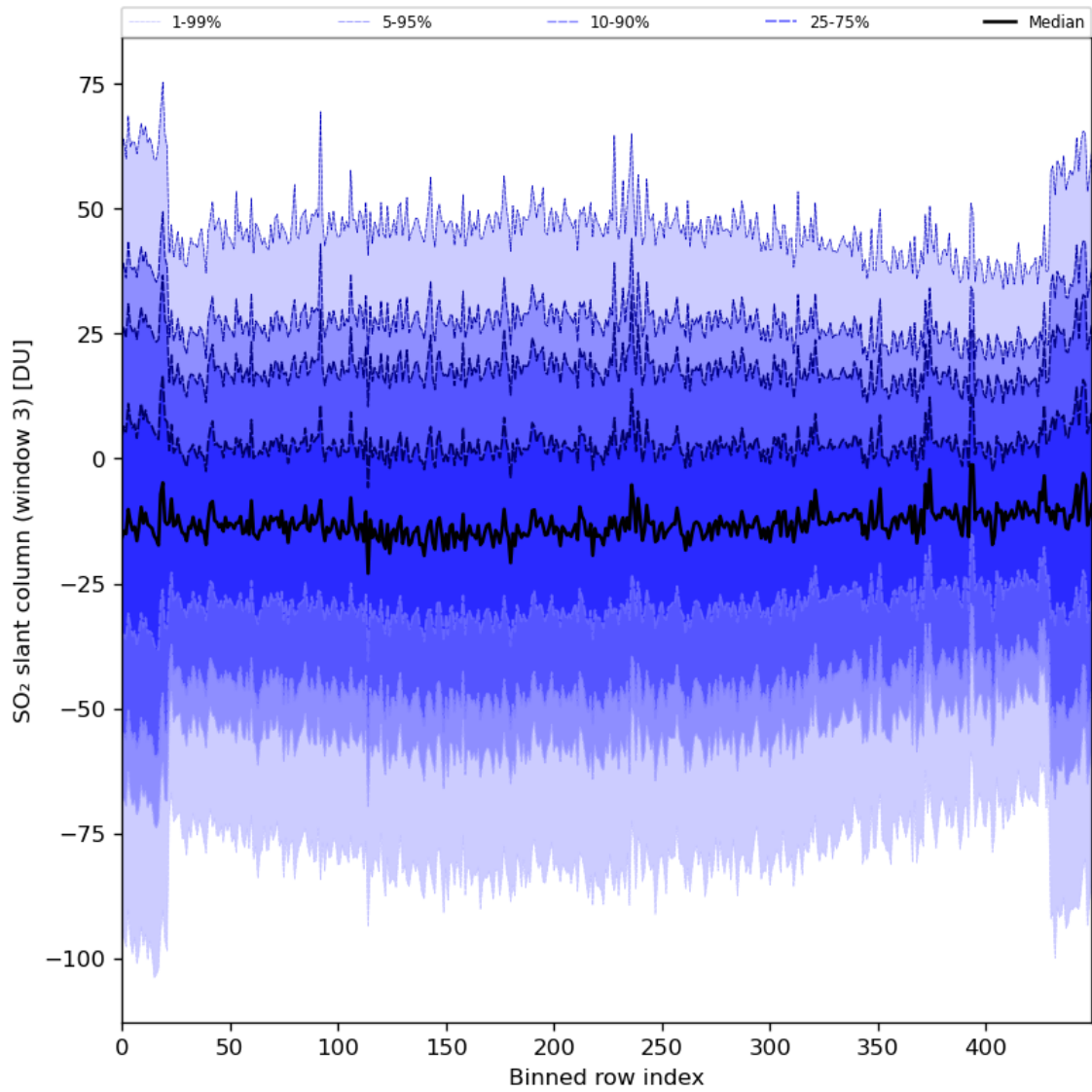
Figure 87: Along track statistics of “SO 2 slant column (window 3)” for 2024-03-06 to 2024-03-08
