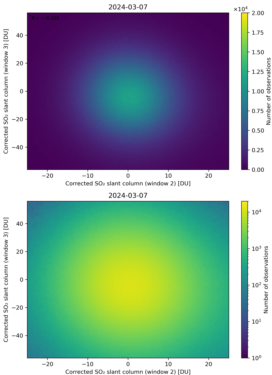
Figure 200: Scatter density plot of “Corrected SO 2 slant column (window 2)” against “Corrected SO 2 slant column (window 3)” for 2024-03-06 to 2024-03-08.
