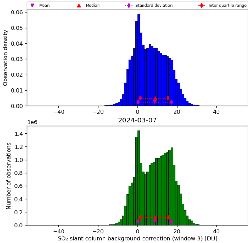
Figure 67: Histogram of “SO 2 slant column background correction (window 3)” for 2024-03-06 to 2024-03-08
