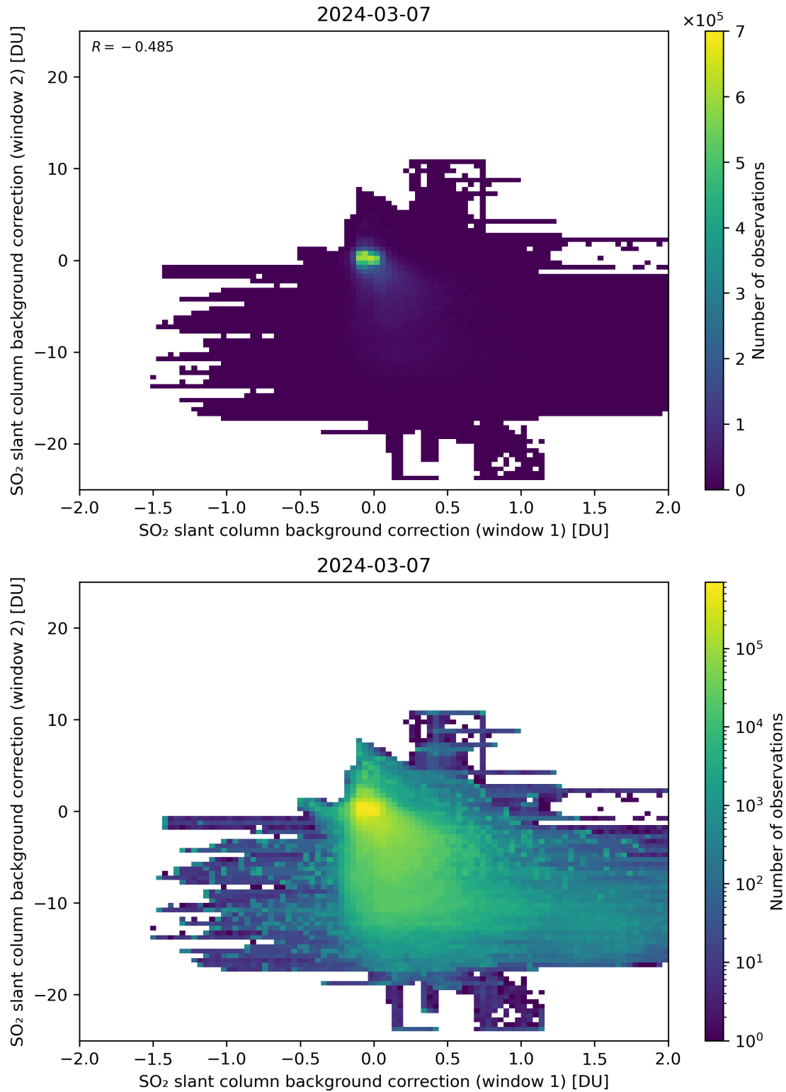
Figure 98: Scatter density plot of “SO 2 slant column background correction (window 1)” against “SO 2 slant column background correction (window 2)” for 2024-03-06 to 2024-03-08.
