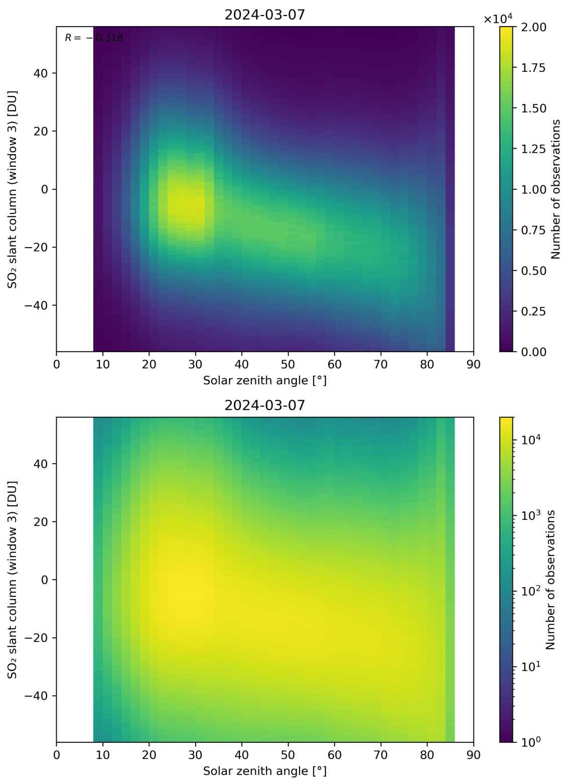
Figure 172: Scatter density plot of “Solar zenith angle” against “SO 2 slant column (window 3)” for 2024-03-06 to 2024-03-08.
