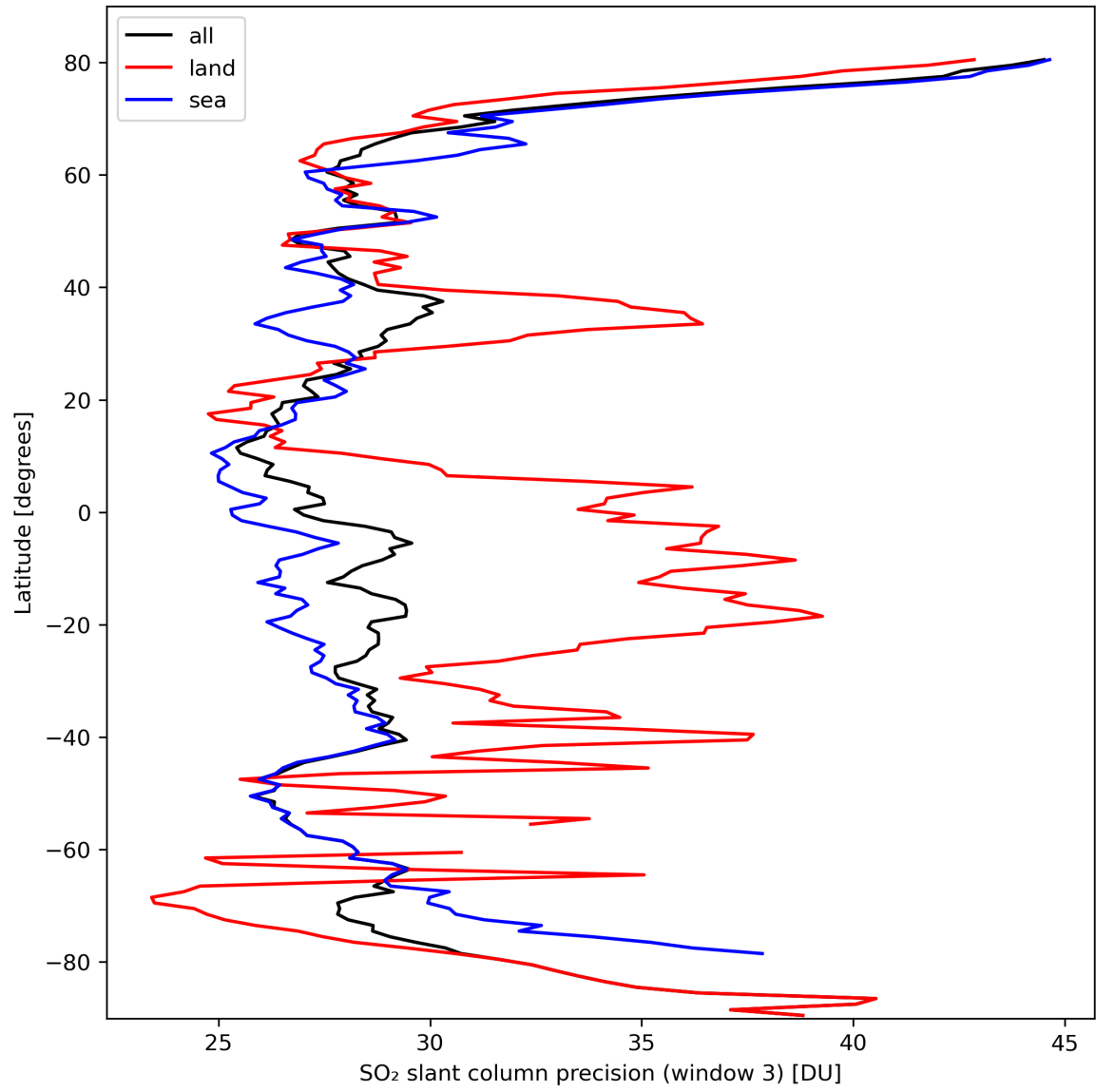
Figure 42: Zonal average of “SO 2 slant column precision (window 3)” for 2024-03-06 to 2024-03-08.
