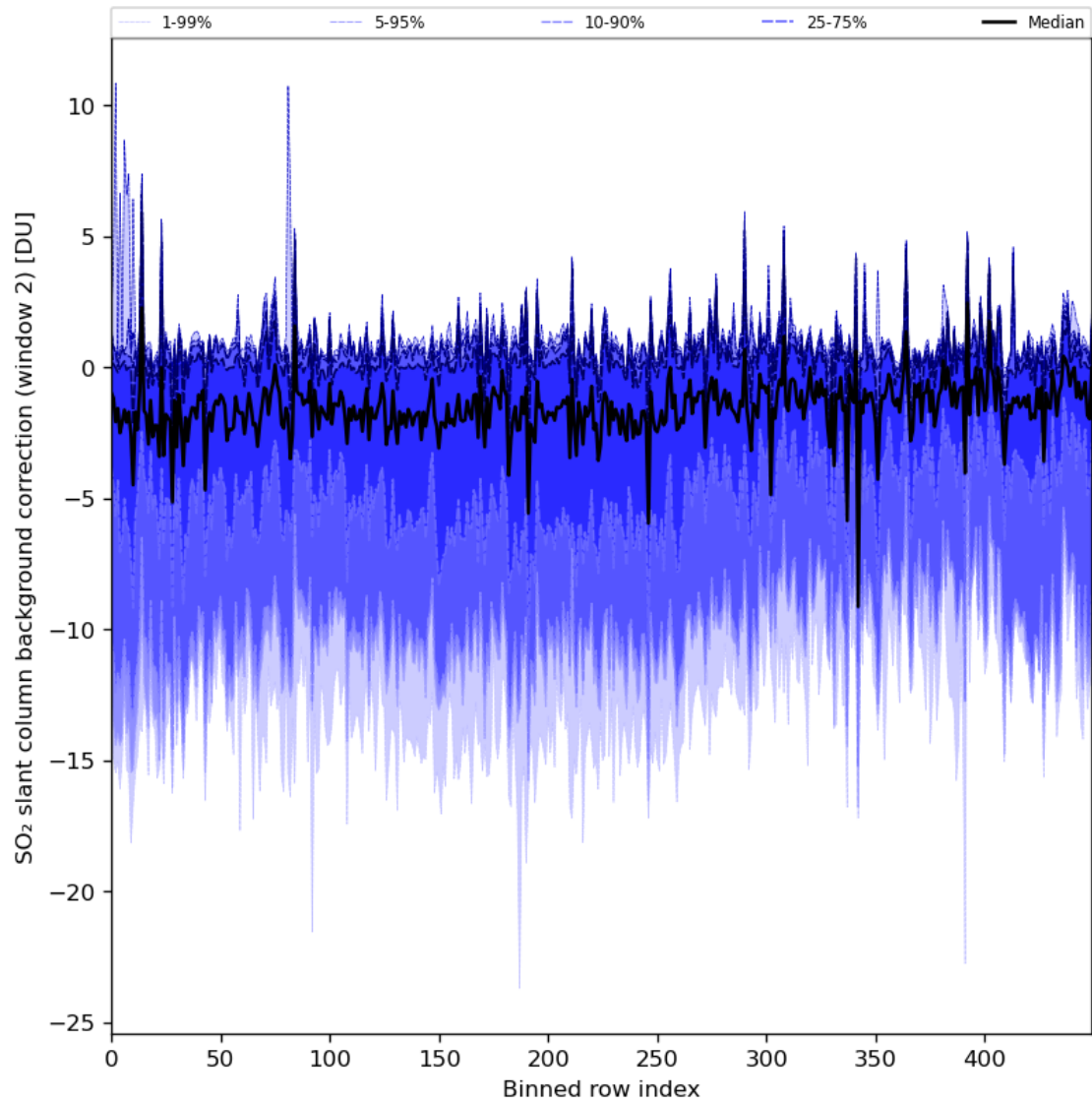
Figure 86: Along track statistics of “SO 2 slant column background correction (window 2)” for 2024-03-06 to 2024-03-08
