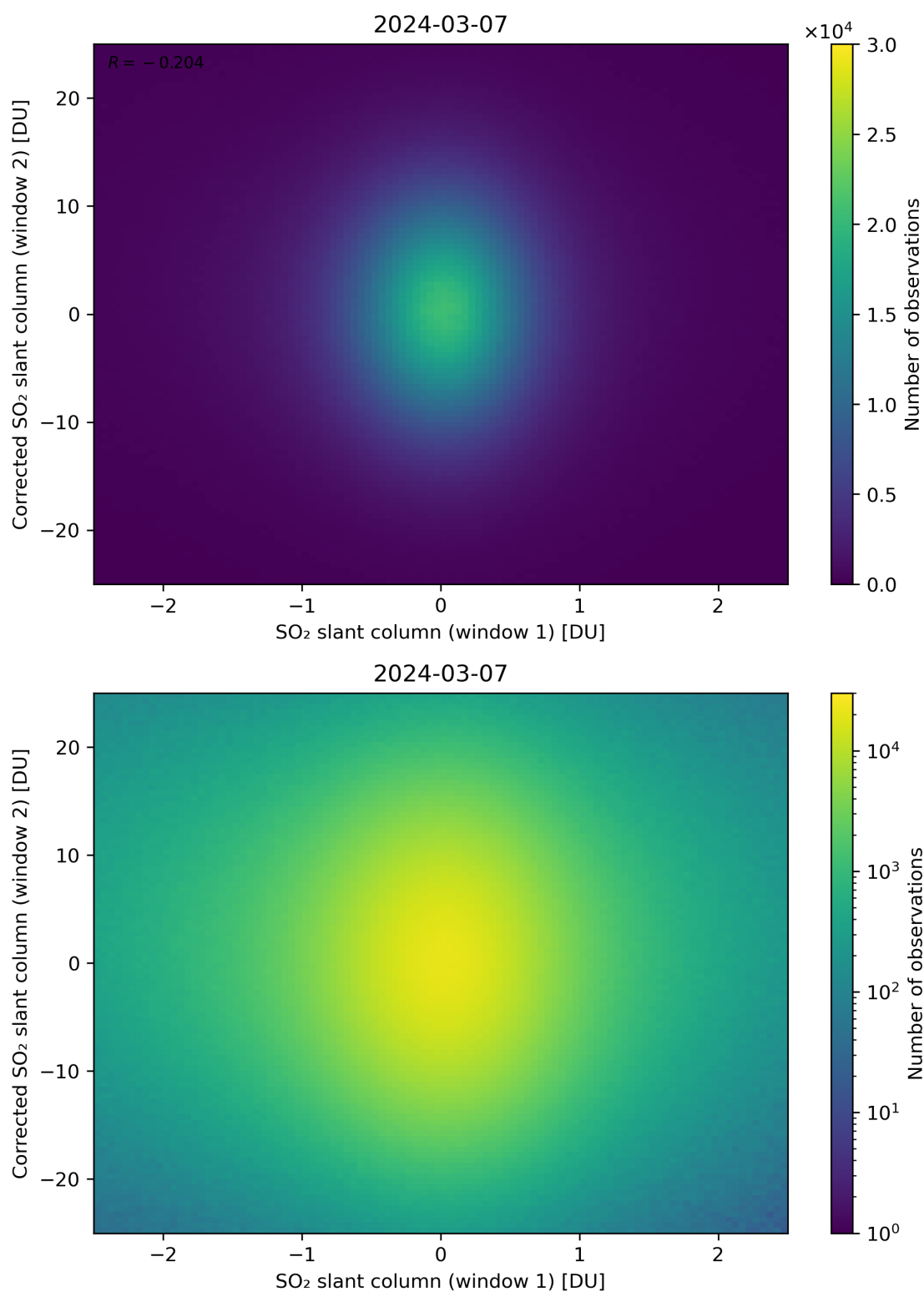
Figure 233: Scatter density plot of “SO 2 slant column (window 1)” against “Corrected SO 2 slant column (window 2)” for 2024-03-06 to 2024-03-08.
