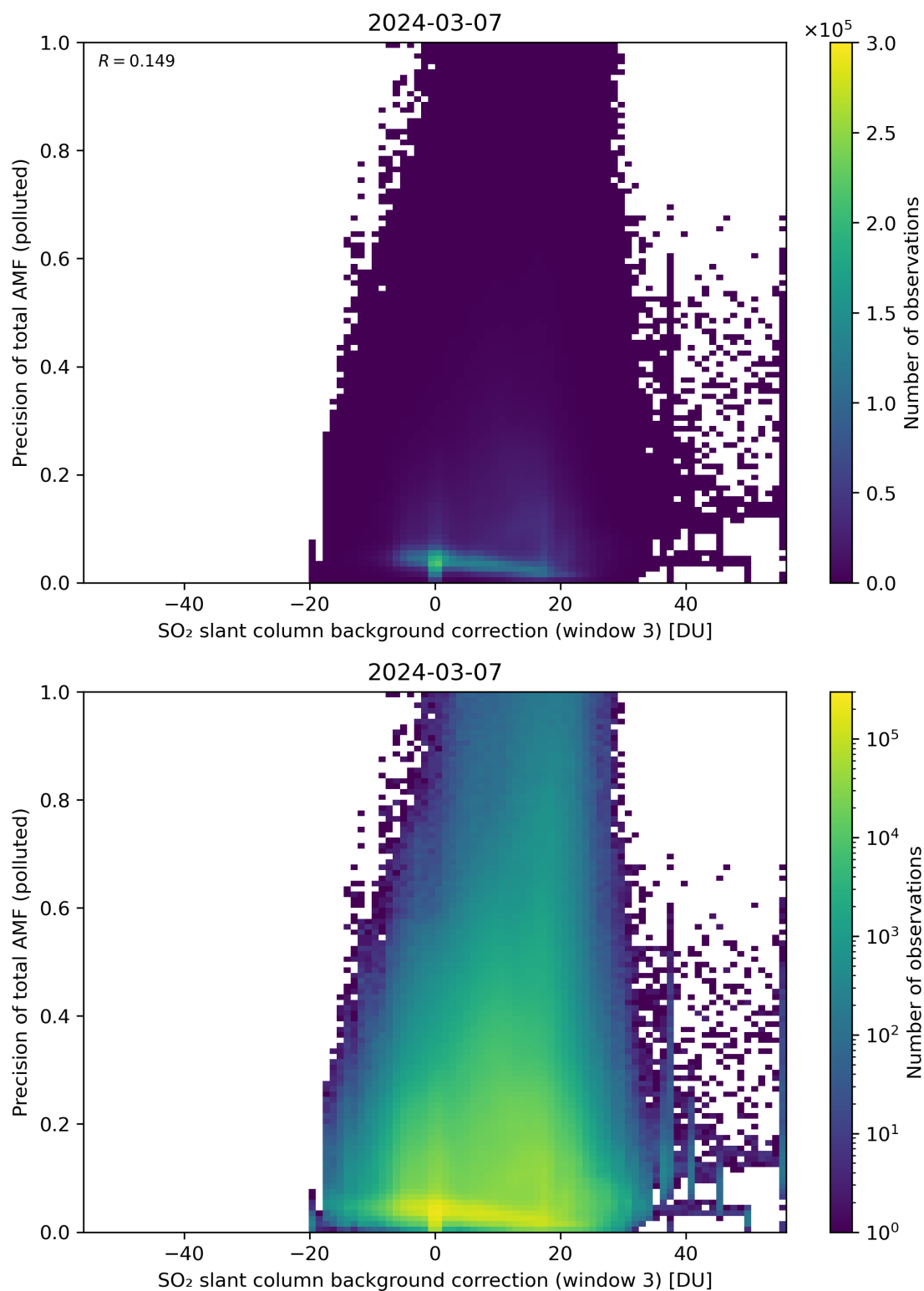
Figure 126: Scatter density plot of “SO 2 slant column background correction (window 3)” against “Precision of total AMF (polluted)” for 2024-03-06 to 2024-03-08.
