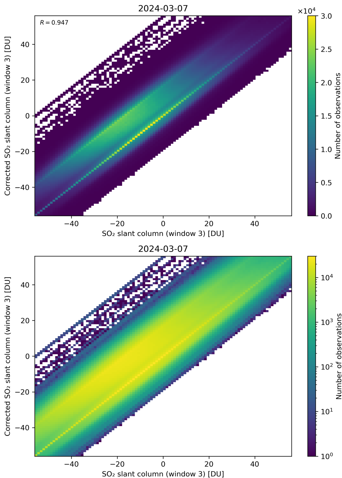
Figure 266: Scatter density plot of “SO 2 slant column (window 3)” against “Corrected SO 2 slant column (window 3)” for 2024-03-06 to 2024-03-08.
