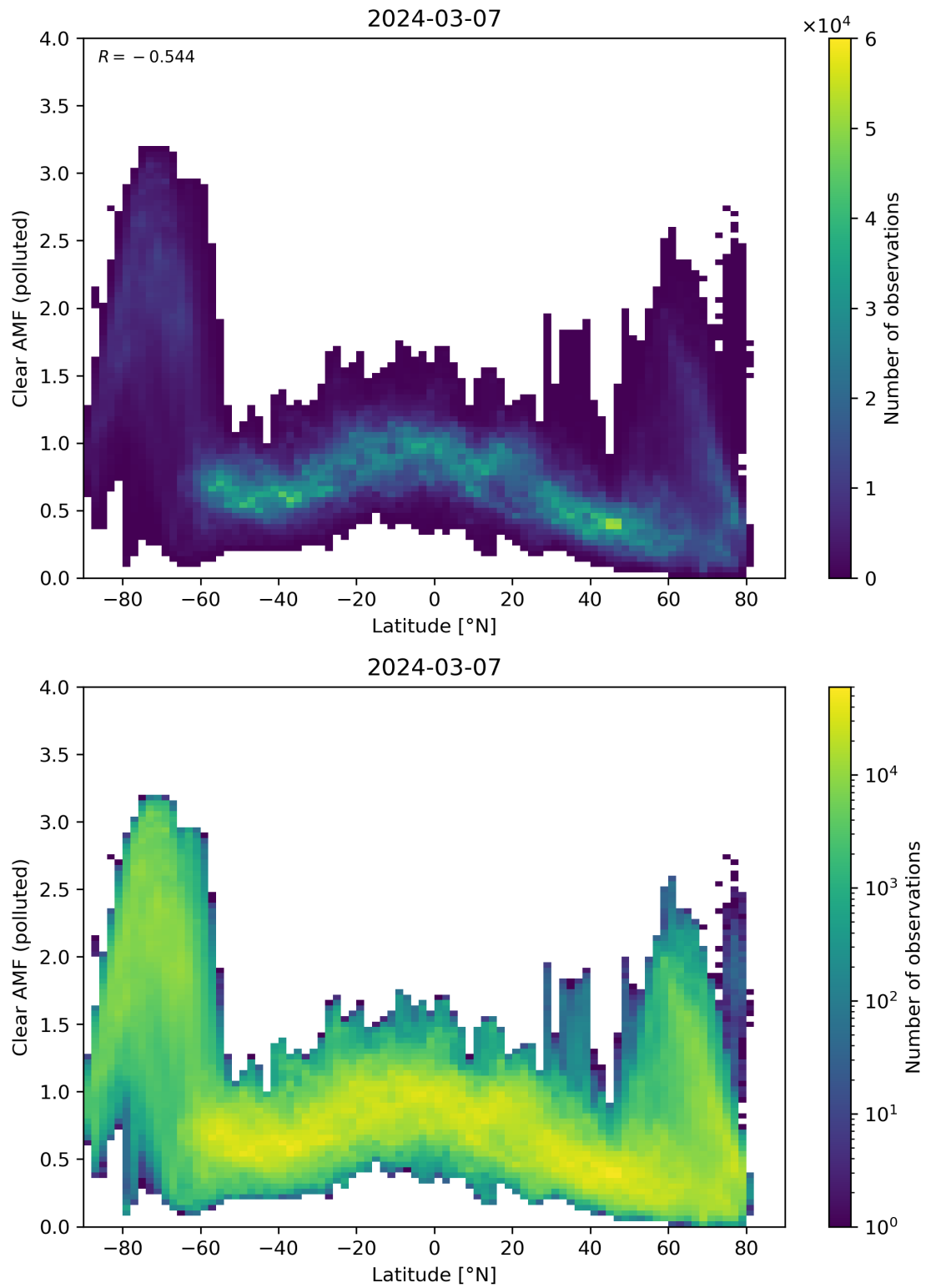
Figure 145: Scatter density plot of “Latitude” against “Clear AMF (polluted)” for 2024-03-06 to 2024-03-08.
