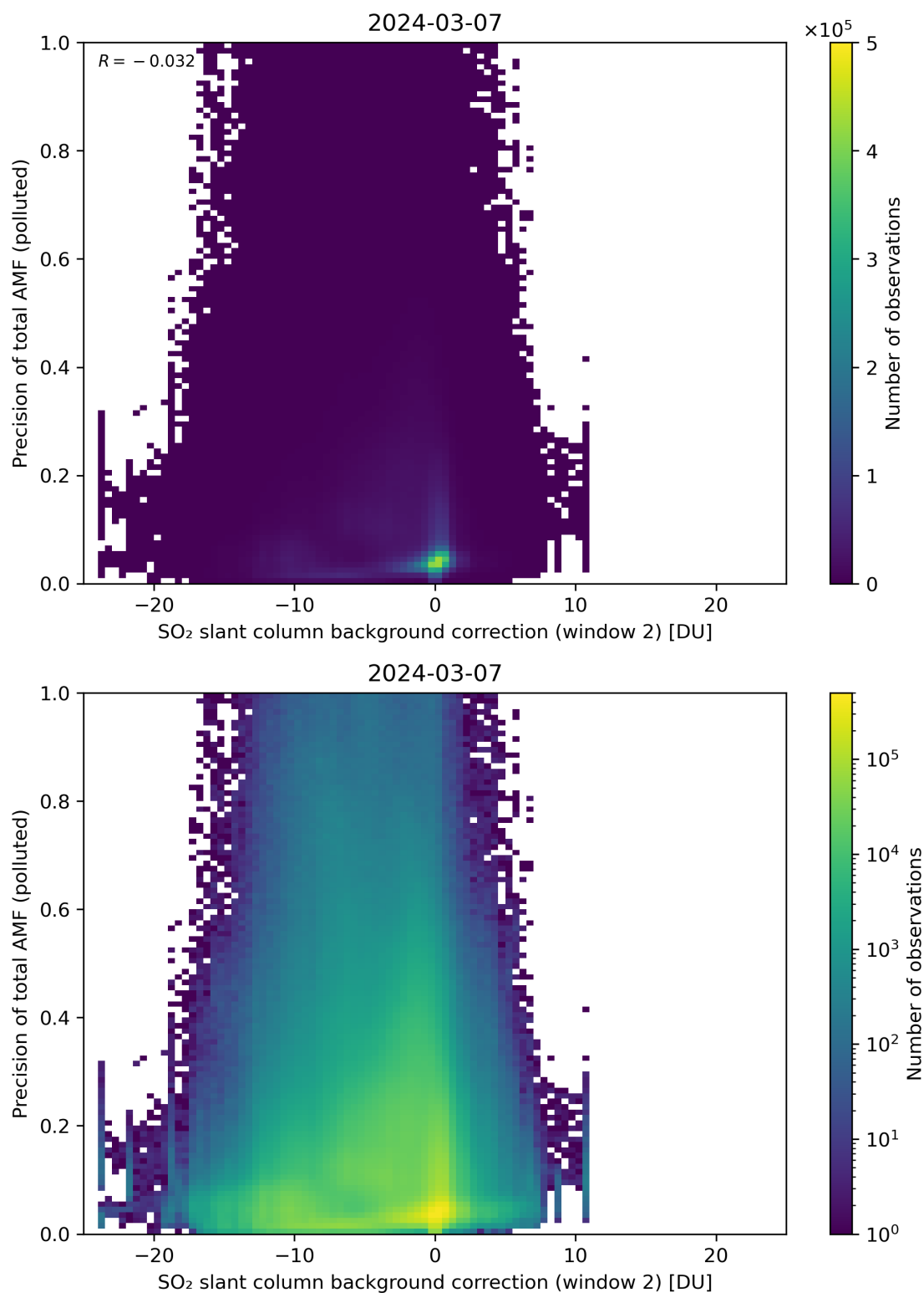
Figure 120: Scatter density plot of “SO 2 slant column background correction (window 2)” against “Precision of total AMF (polluted)” for 2024-03-06 to 2024-03-08.
