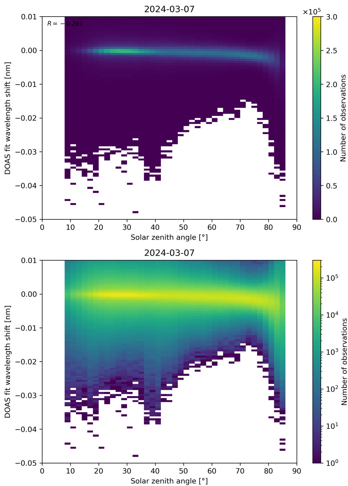
Figure 161: Scatter density plot of “Solar zenith angle” against “DOAS fit wavelength shift” for 2024-03-06 to 2024-03-08.
