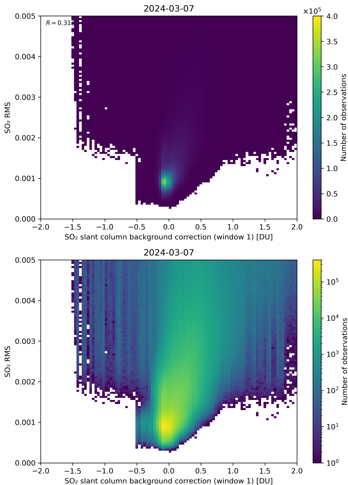
Figure 102: Scatter density plot of “SO 2 slant column background correction (window 1)” against “SO 2 RMS” for 2024-03-06 to 2024-03-08.
