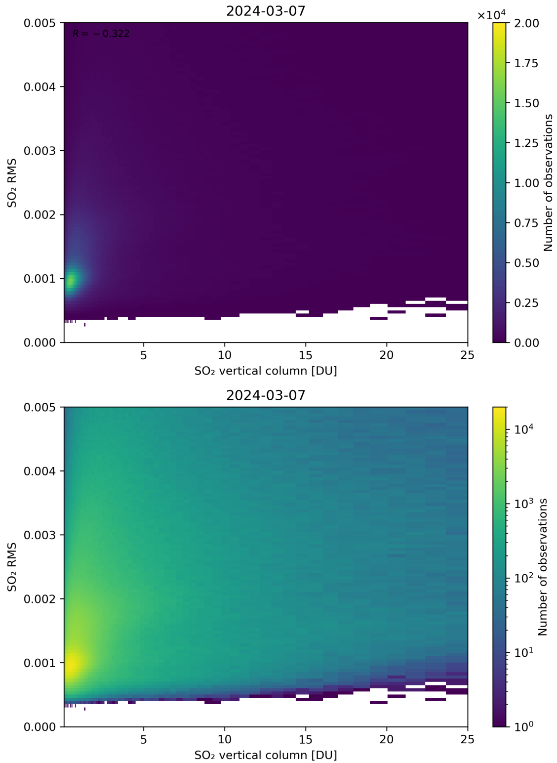
Figure 278: Scatter density plot of “SO 2 vertical column” against “SO 2 RMS” for 2024-03-06 to 2024-03-08.
