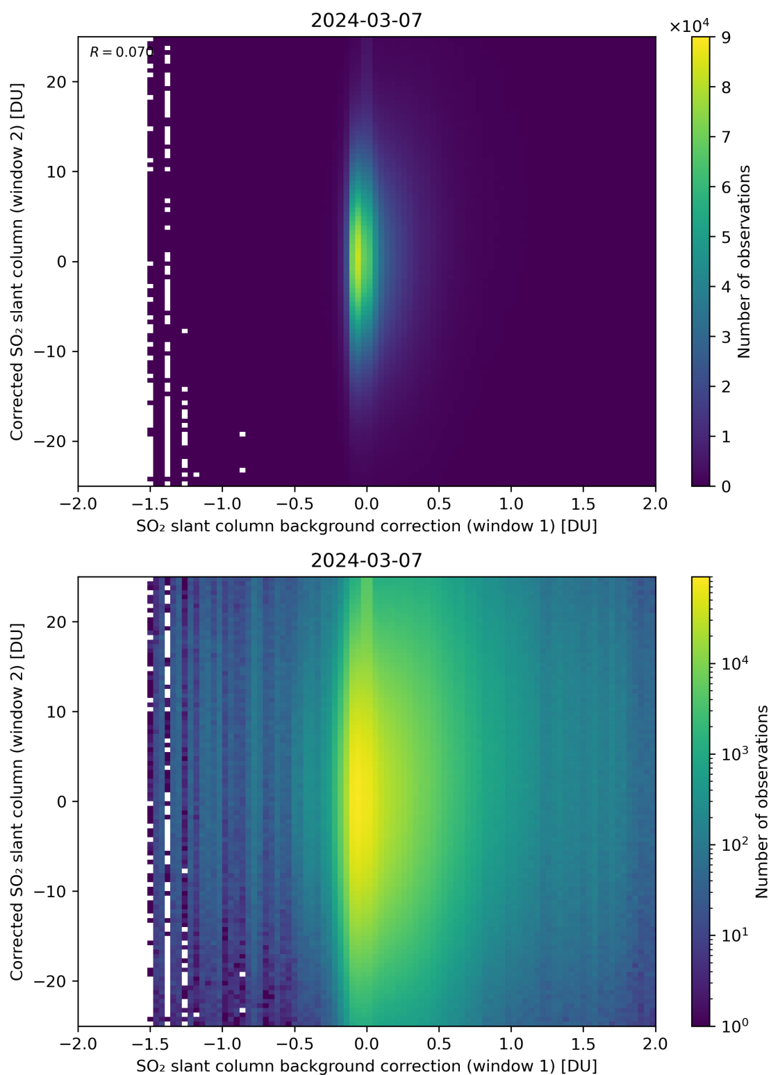
Figure 104: Scatter density plot of “SO 2 slant column background correction (window 1)” against “Corrected SO 2 slant column (window 2)” for 2024-03-06 to 2024-03-08.
