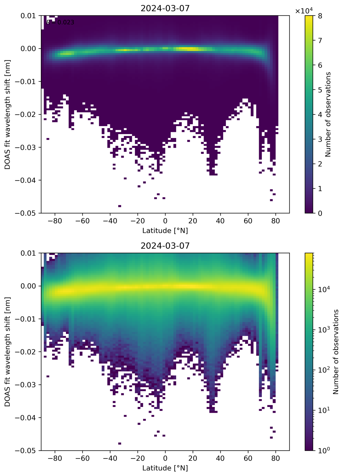
Figure 142: Scatter density plot of “Latitude” against “DOAS fit wavelength shift” for 2024-03-06 to 2024-03-08.
