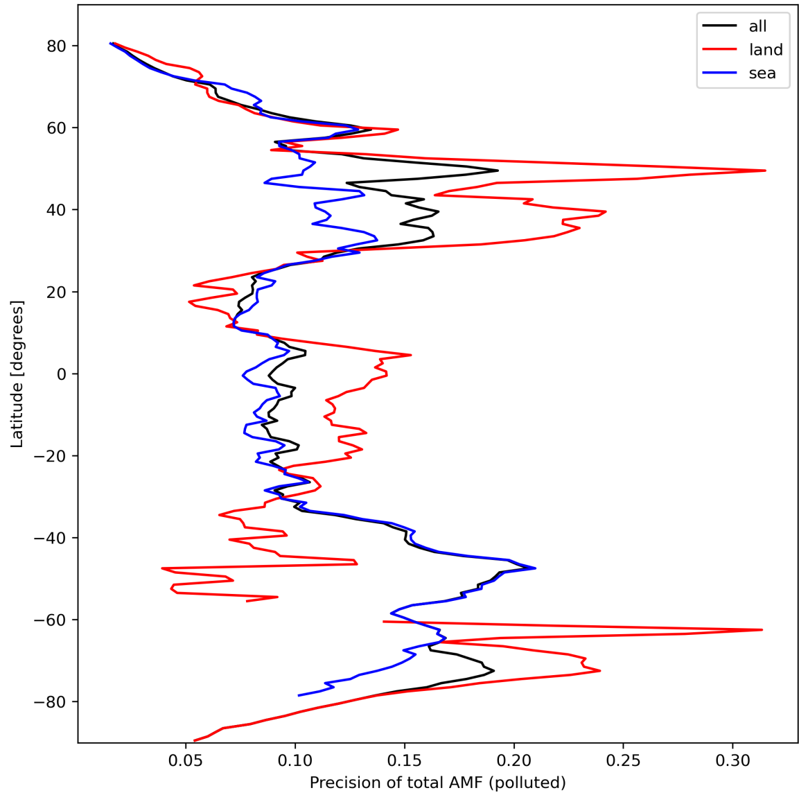
Figure 49: Zonal average of “Precision of total AMF (polluted)” for 2024-03-06 to 2024-03-08.
