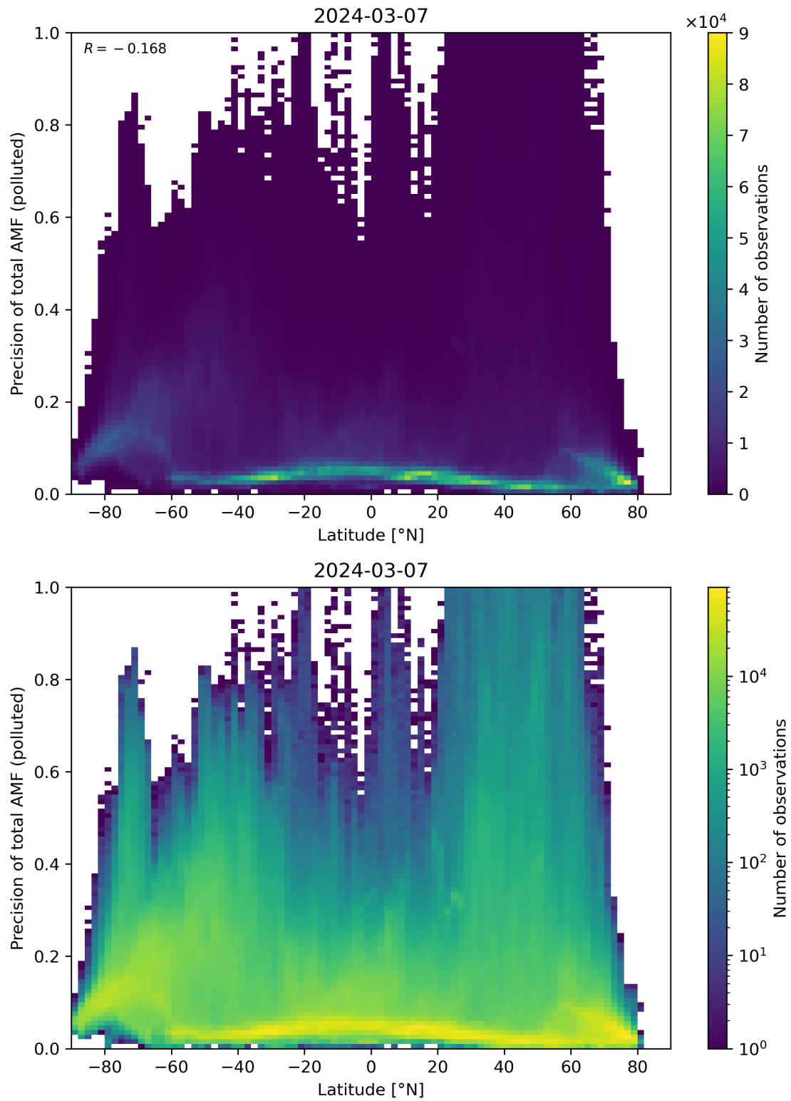
Figure 155: Scatter density plot of “Latitude” against “Precision of total AMF (polluted)” for 2024-03-06 to 2024-03-08.
