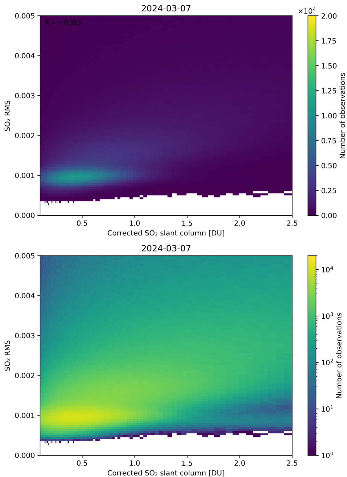
Figure 183: Scatter density plot of “Corrected SO 2 slant column” against “SO 2 RMS” for 2024-03-06 to 2024-03-08.
