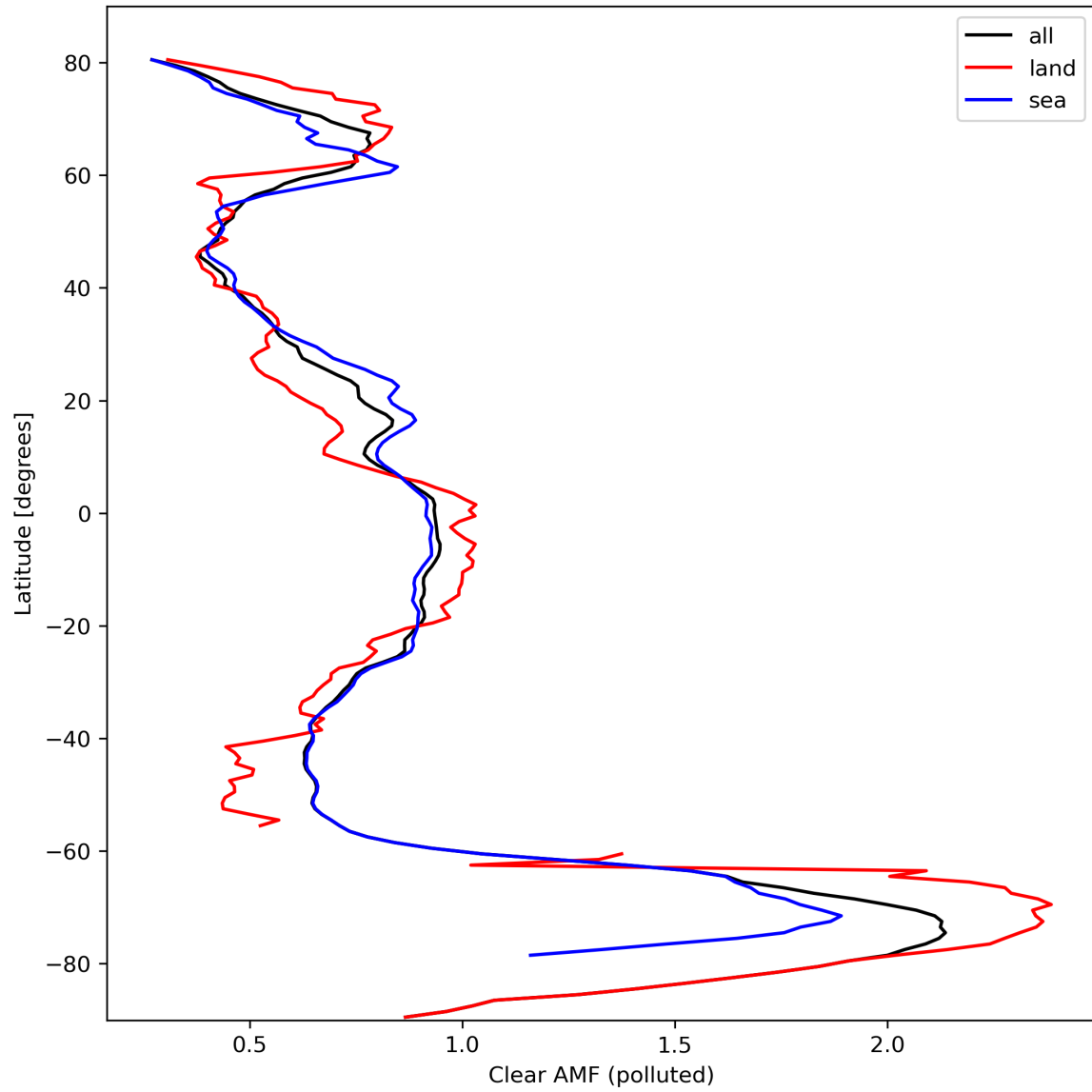
Figure 50: Zonal average of “Clear AMF (polluted)” for 2024-03-06 to 2024-03-08.
