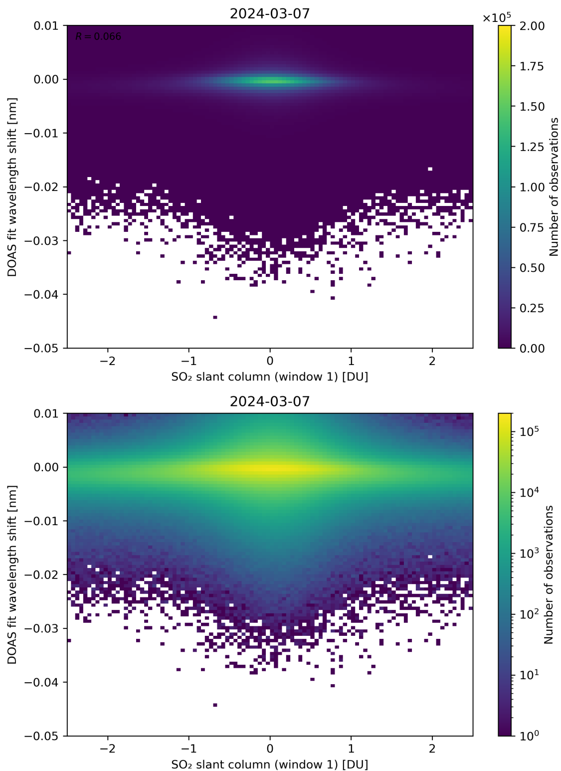
Figure 215: Scatter density plot of “SO 2 slant column (window 1)” against “DOAS fit wavelength shift” for 2024-03-06 to 2024-03-08.
