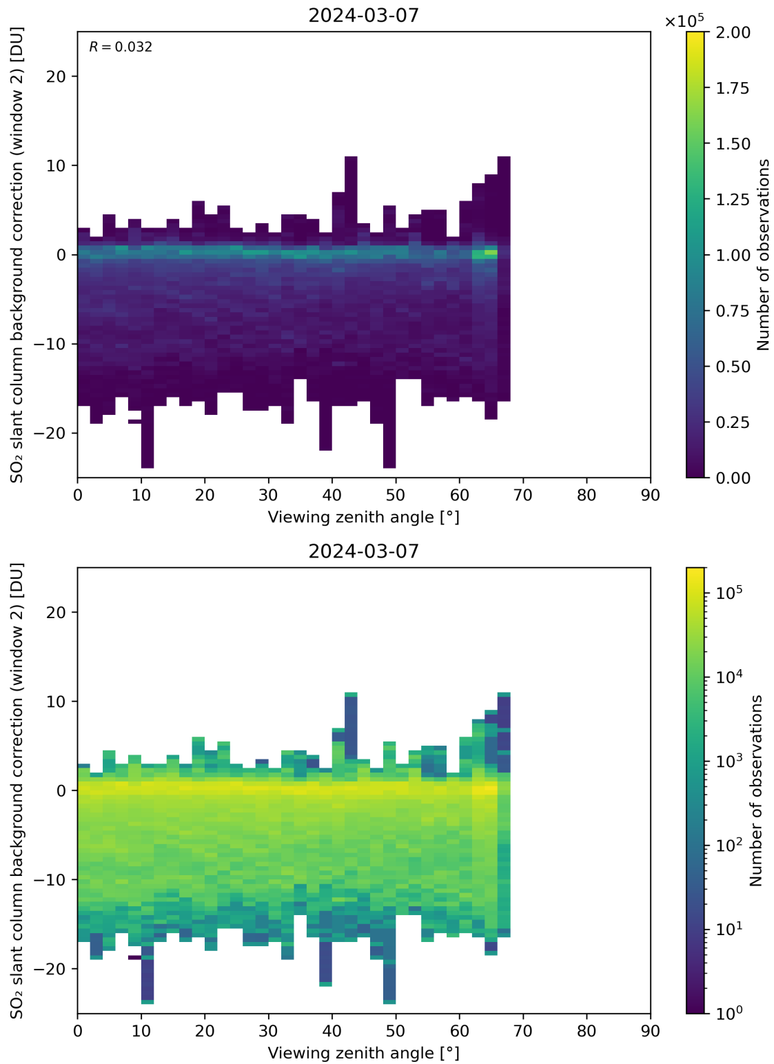
Figure 309: Scatter density plot of “Viewing zenith angle” against “SO 2 slant column background correction (window 2)” for 2024-03-06 to 2024-03-08.
