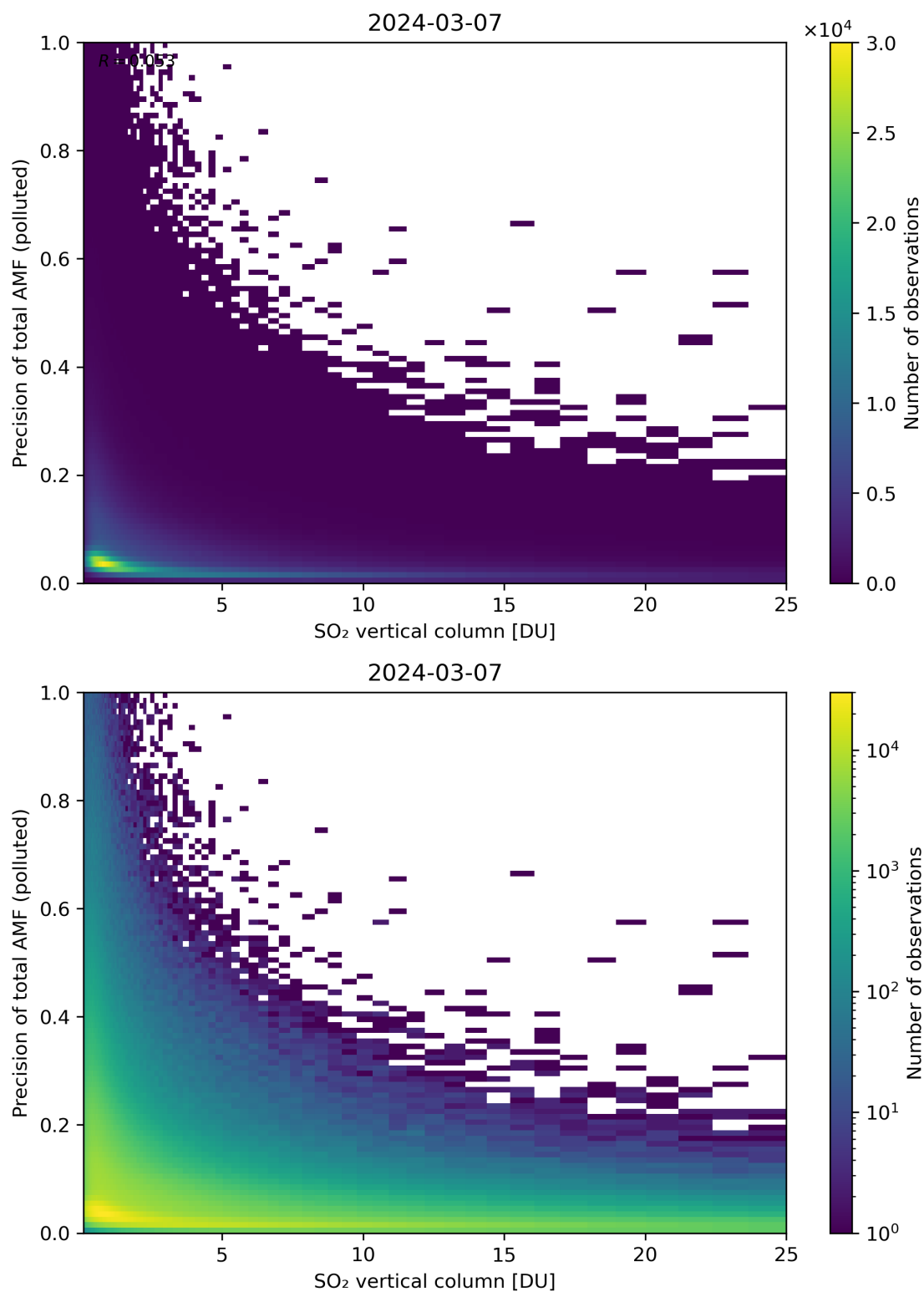
Figure 306: Scatter density plot of “SO 2 vertical column” against “Precision of total AMF (polluted)” for 2024-03-06 to 2024-03-08.
