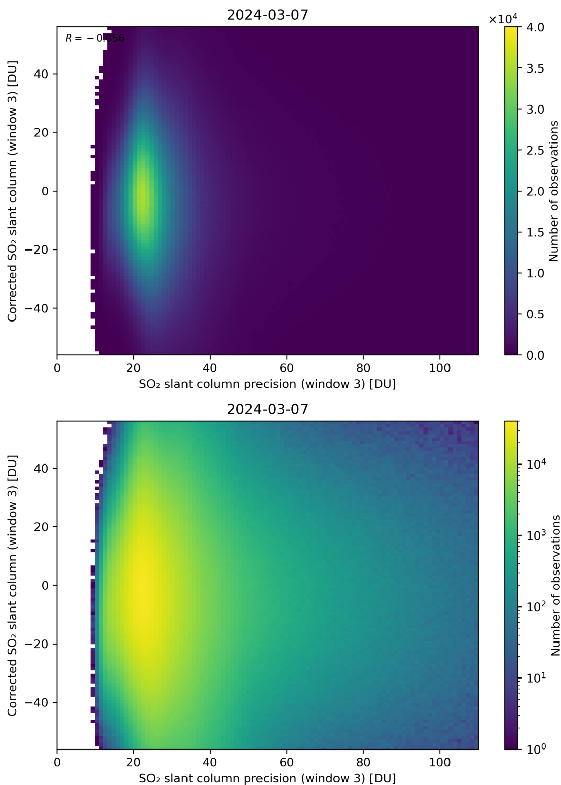
Figure 262: Scatter density plot of “SO 2 slant column precision (window 3)” against “Corrected SO 2 slant column (window 3)” for 2024-03-06 to 2024-03-08.
