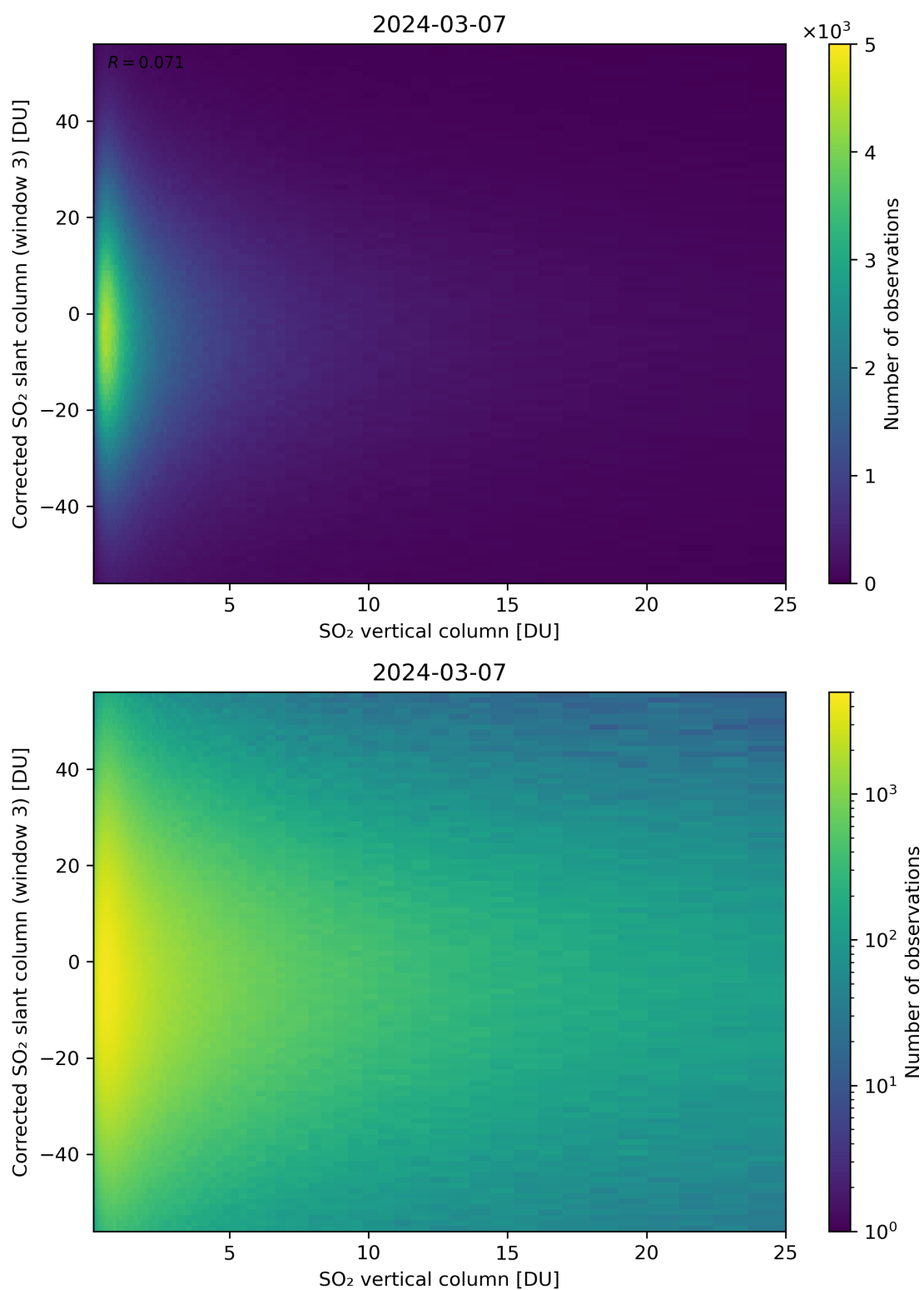
Figure 299: Scatter density plot of “SO 2 vertical column” against “Corrected SO 2 slant column (window 3)” for 2024-03-06 to 2024-03-08.
