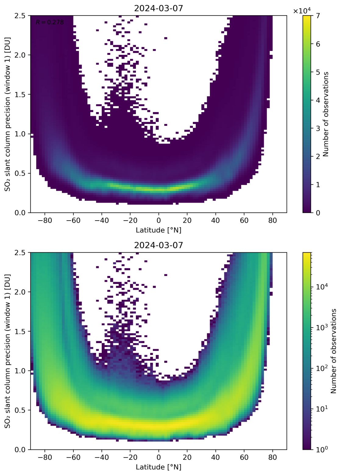
Figure 150: Scatter density plot of “Latitude” against “SO 2 slant column precision (window 1)” for 2024-03-06 to 2024-03-08.
