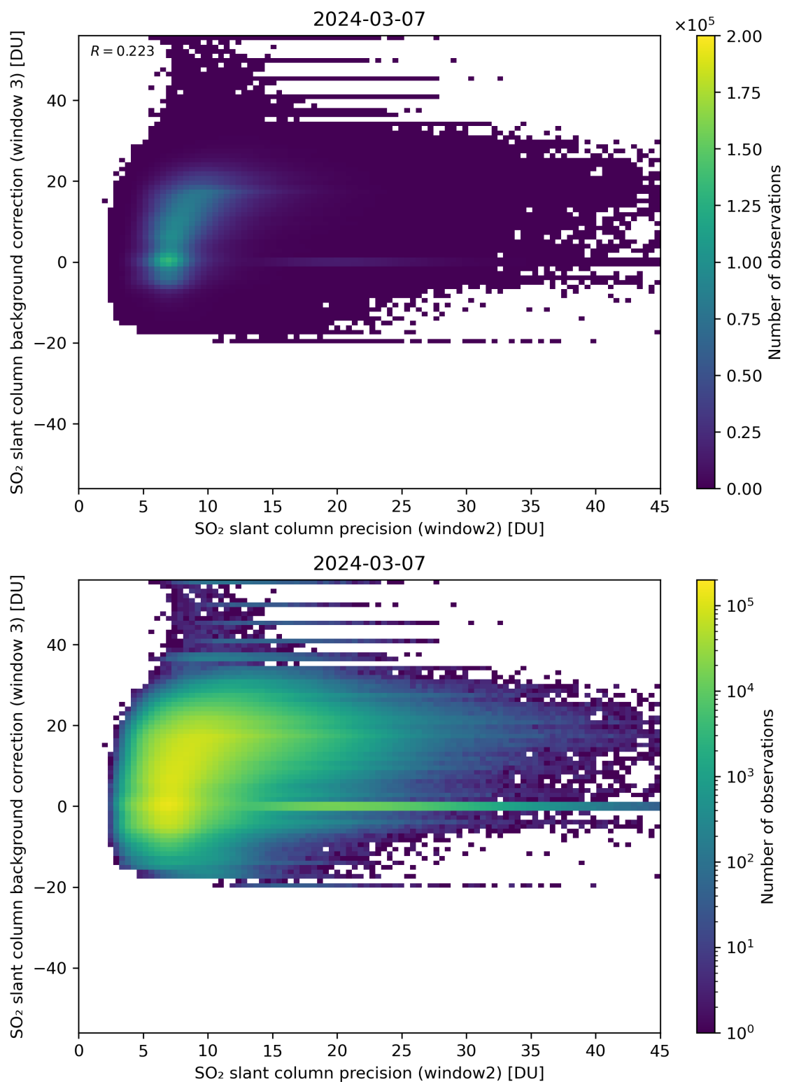
Figure 242: Scatter density plot of “SO 2 slant column precision (window2)” against “SO 2 slant column background correction (window 3)” for 2024-03-06 to 2024-03-08.
