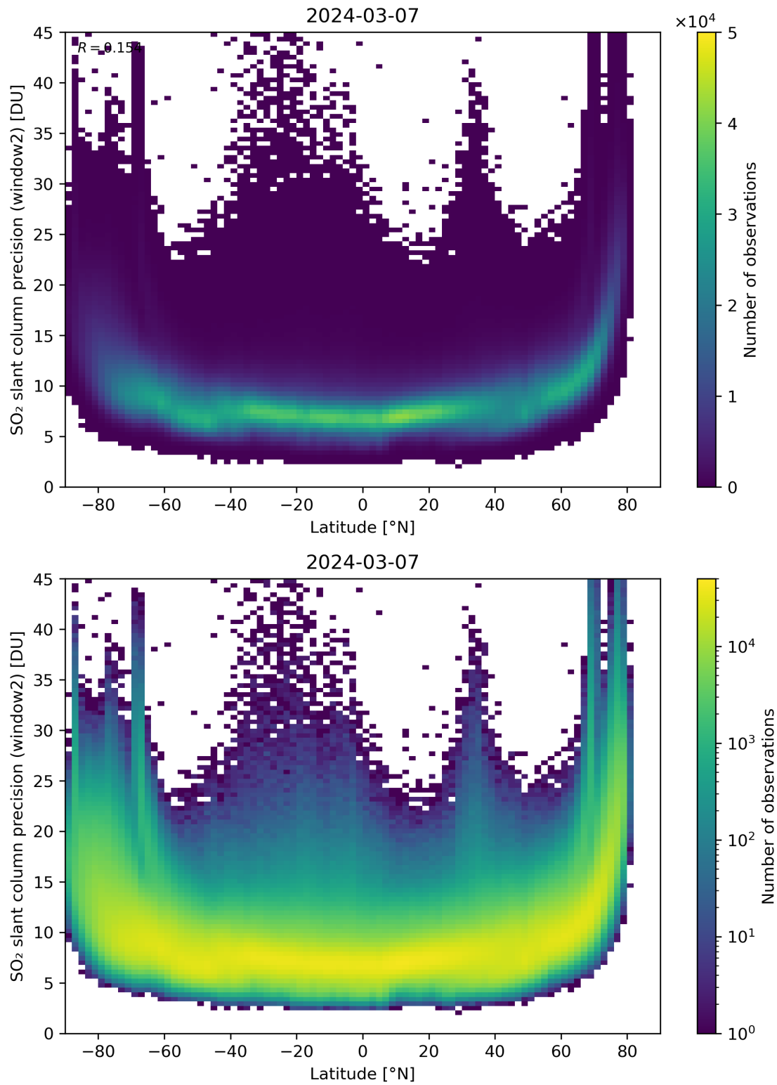
Figure 151: Scatter density plot of “Latitude” against “SO 2 slant column precision (window2)” for 2024-03-06 to 2024-03-08.
