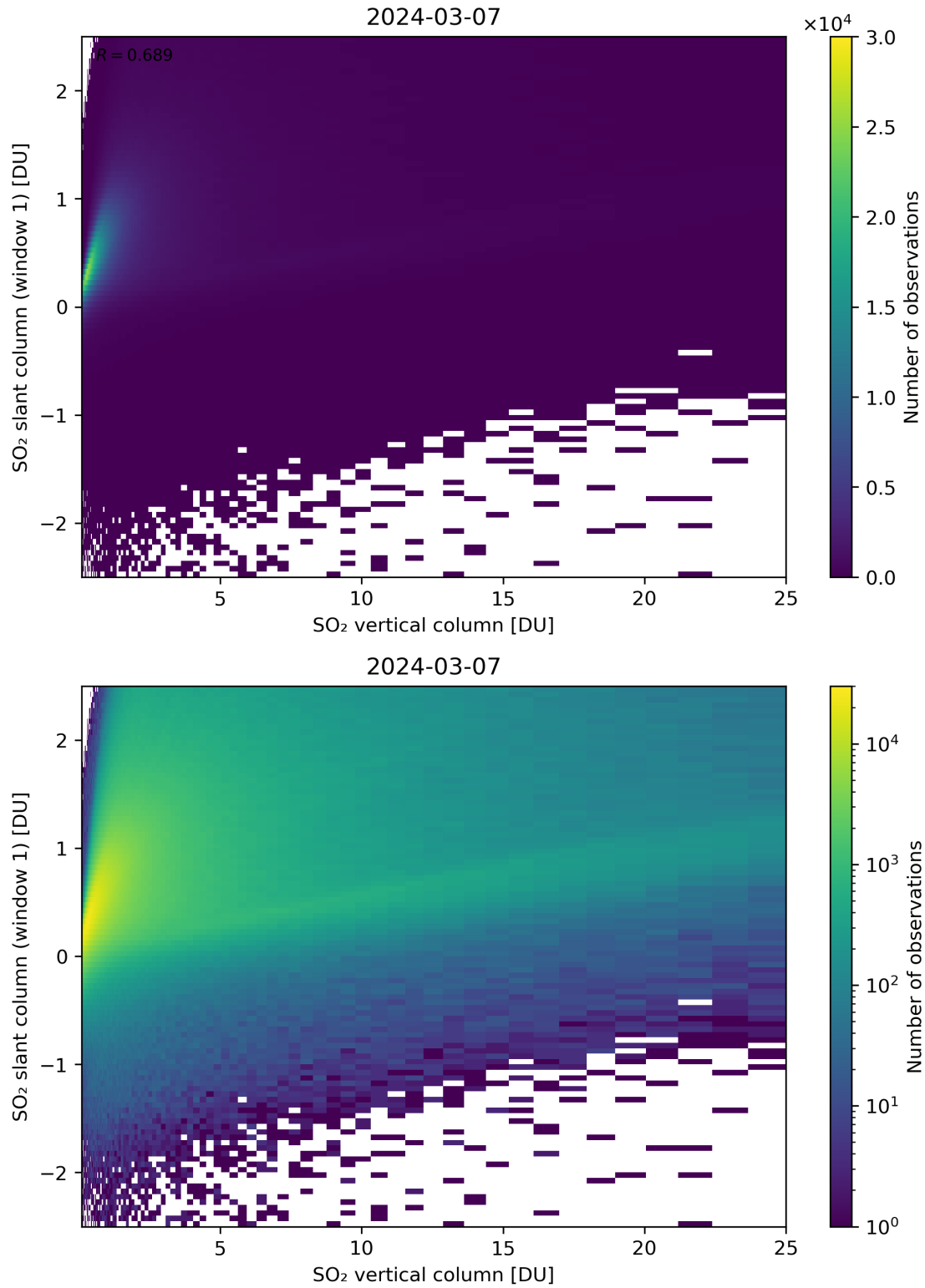
Figure 300: Scatter density plot of “SO 2 vertical column” against “SO 2 slant column (window 1)” for 2024-03-06 to 2024-03-08.
