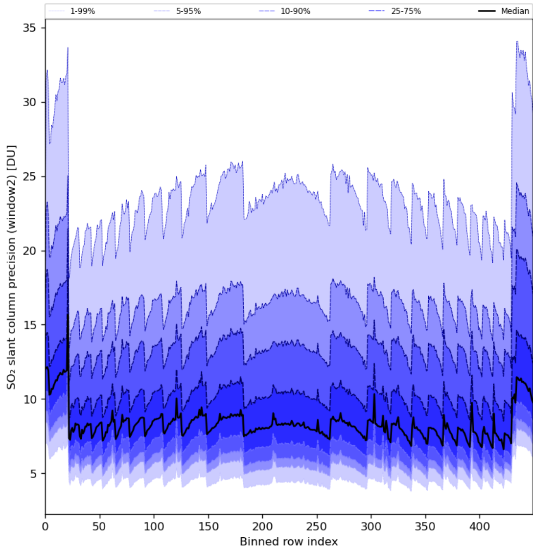
Figure 84: Along track statistics of “SO 2 slant column precision (window2)” for 2024-03-06 to 2024-03-08
