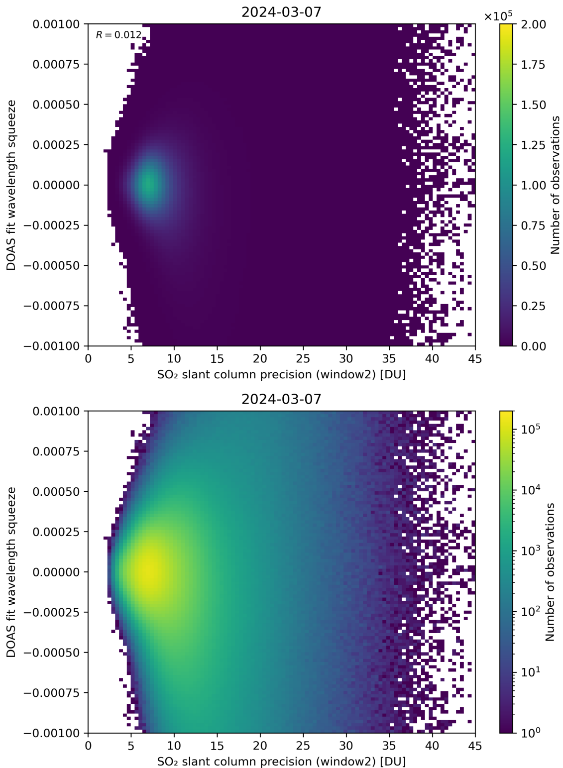
Figure 244: Scatter density plot of “SO 2 slant column precision (window2)” against “DOAS fit wavelength squeeze” for 2024-03-06 to 2024-03-08.
