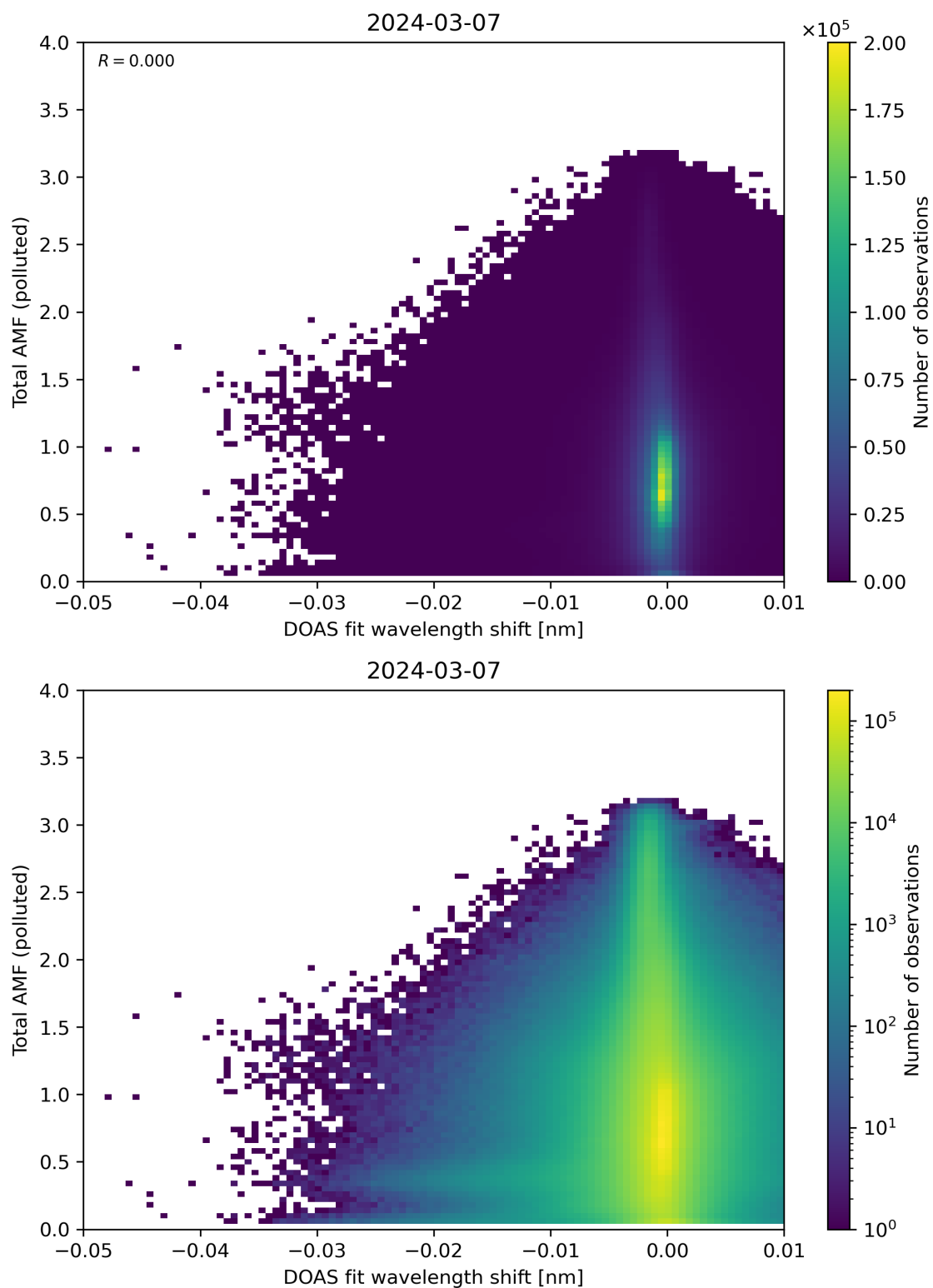
Figure 130: Scatter density plot of “DOAS fit wavelength shift” against “Total AMF (polluted)” for 2024-03-06 to 2024-03-08.
