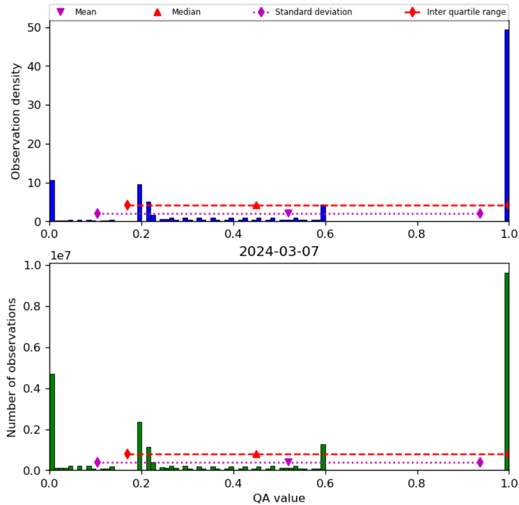
Figure 52: Histogram of “QA value” for 2024-03-06 to 2024-03-08
