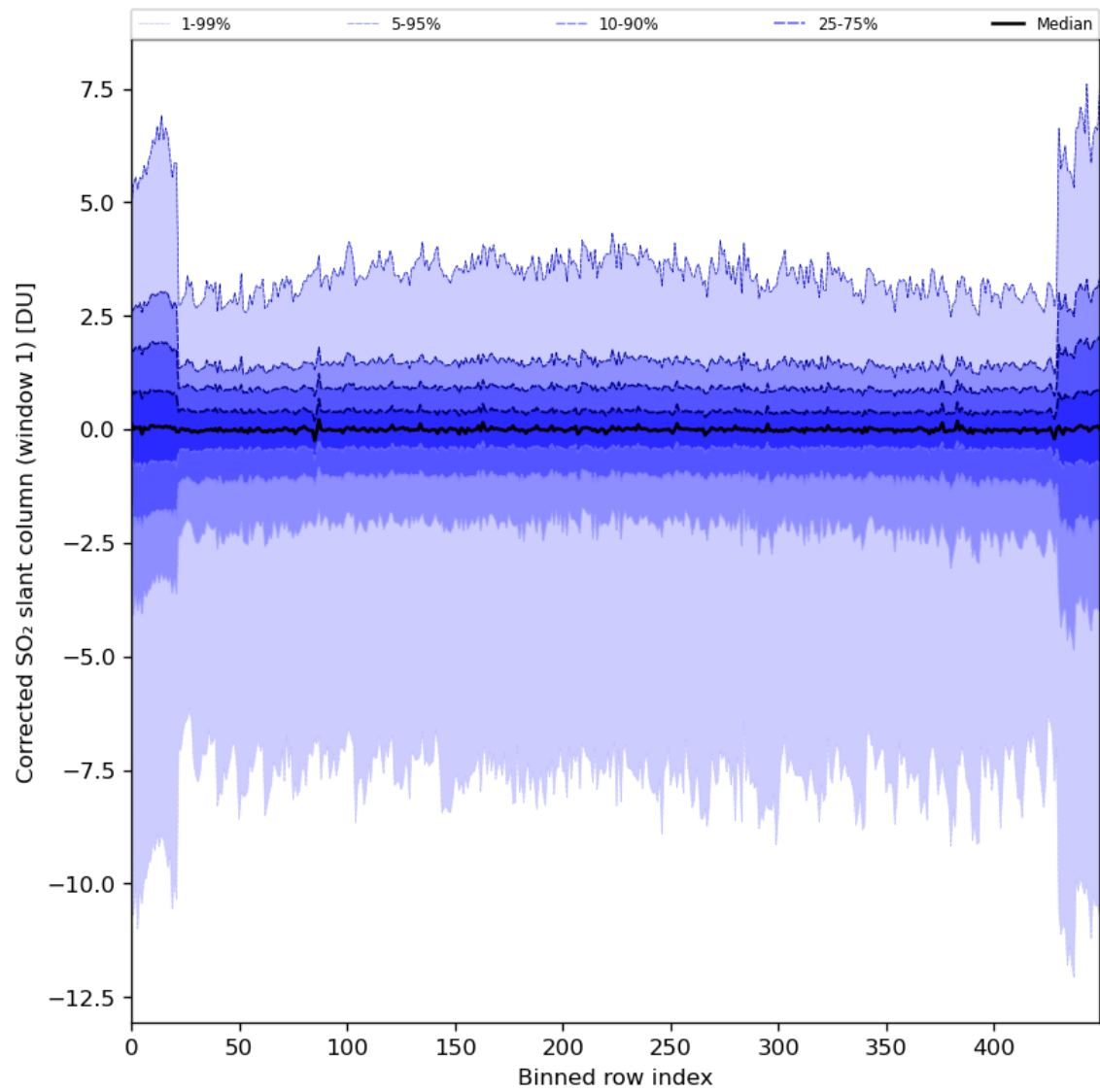
Figure 81: Along track statistics of “Corrected SO 2 slant column (window 1)” for 2024-03-06 to 2024-03-08
