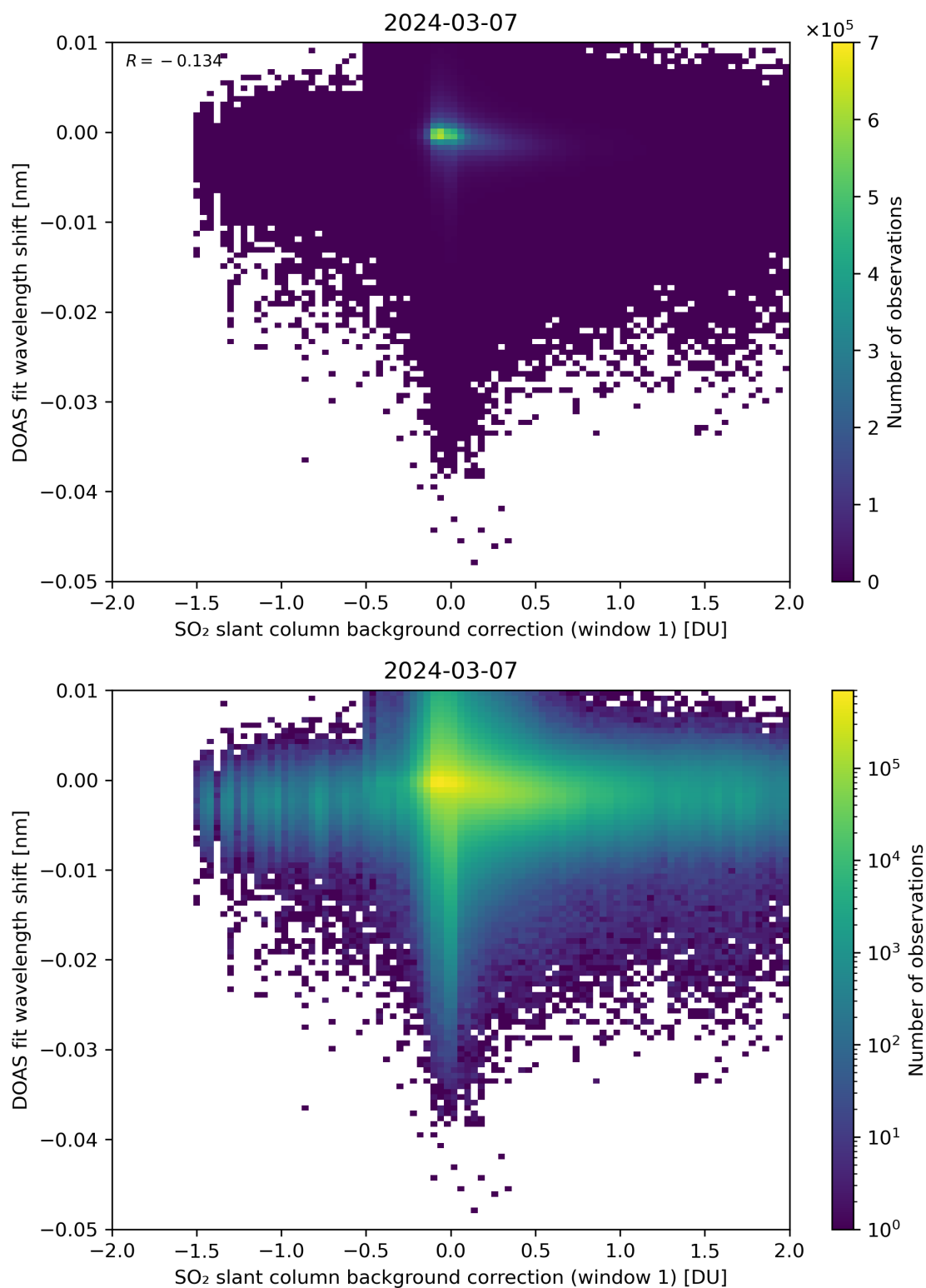
Figure 100: Scatter density plot of “SO 2 slant column background correction (window 1)” against “DOAS fit wavelength shift” for 2024-03-06 to 2024-03-08.
