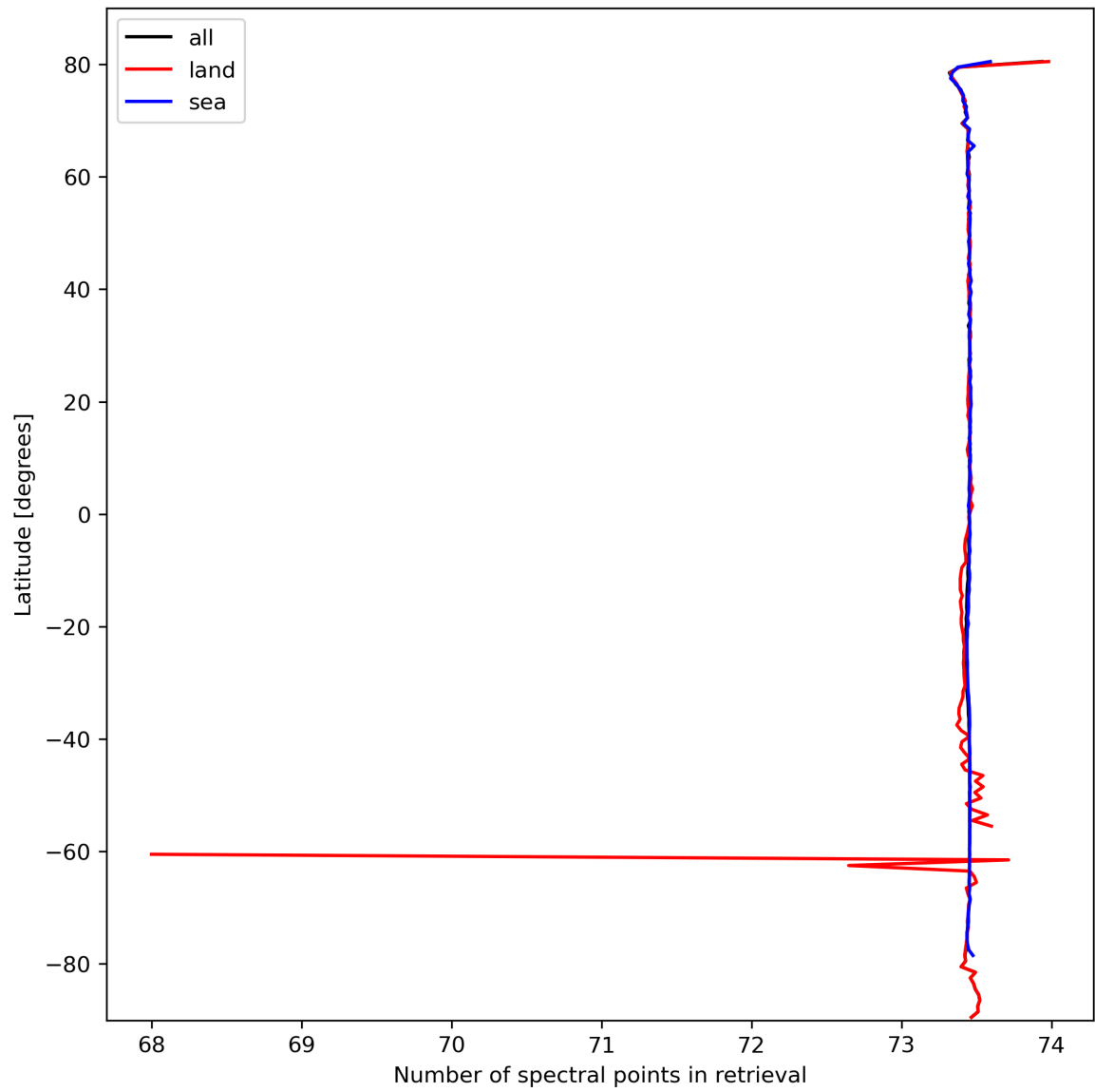
Figure 51: Zonal average of “Number of spectral points in retrieval” for 2024-03-06 to 2024-03-08.
