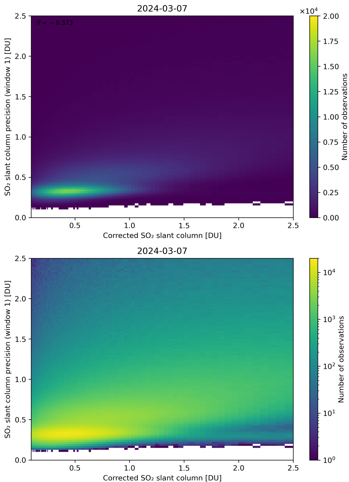
Figure 188: Scatter density plot of “Corrected SO 2 slant column” against “SO 2 slant column precision (window 1)” for 2024-03-06 to 2024-03-08.
