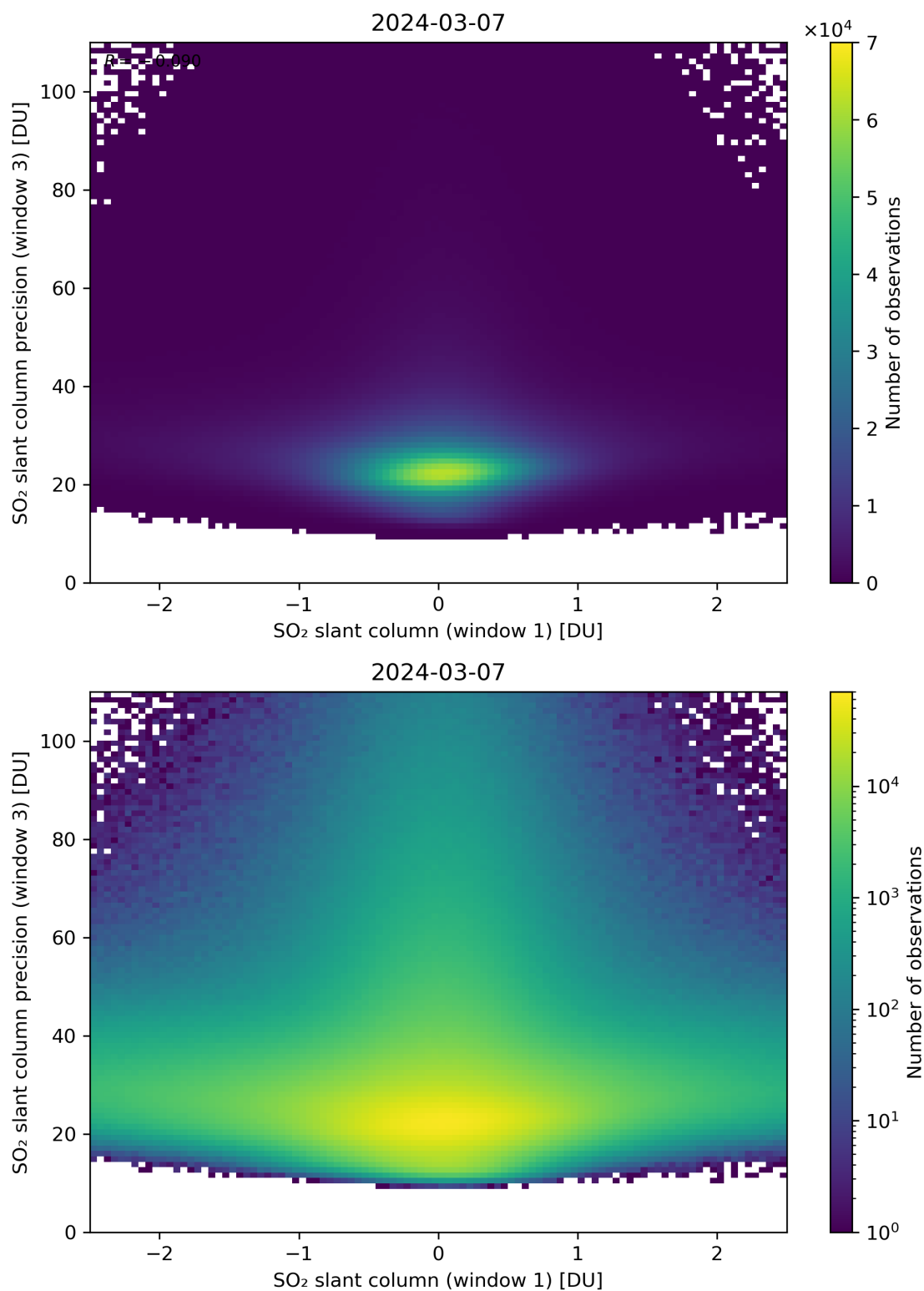
Figure 238: Scatter density plot of “SO 2 slant column (window 1)” against “SO 2 slant column precision (window 3)” for 2024-03-06 to 2024-03-08.
