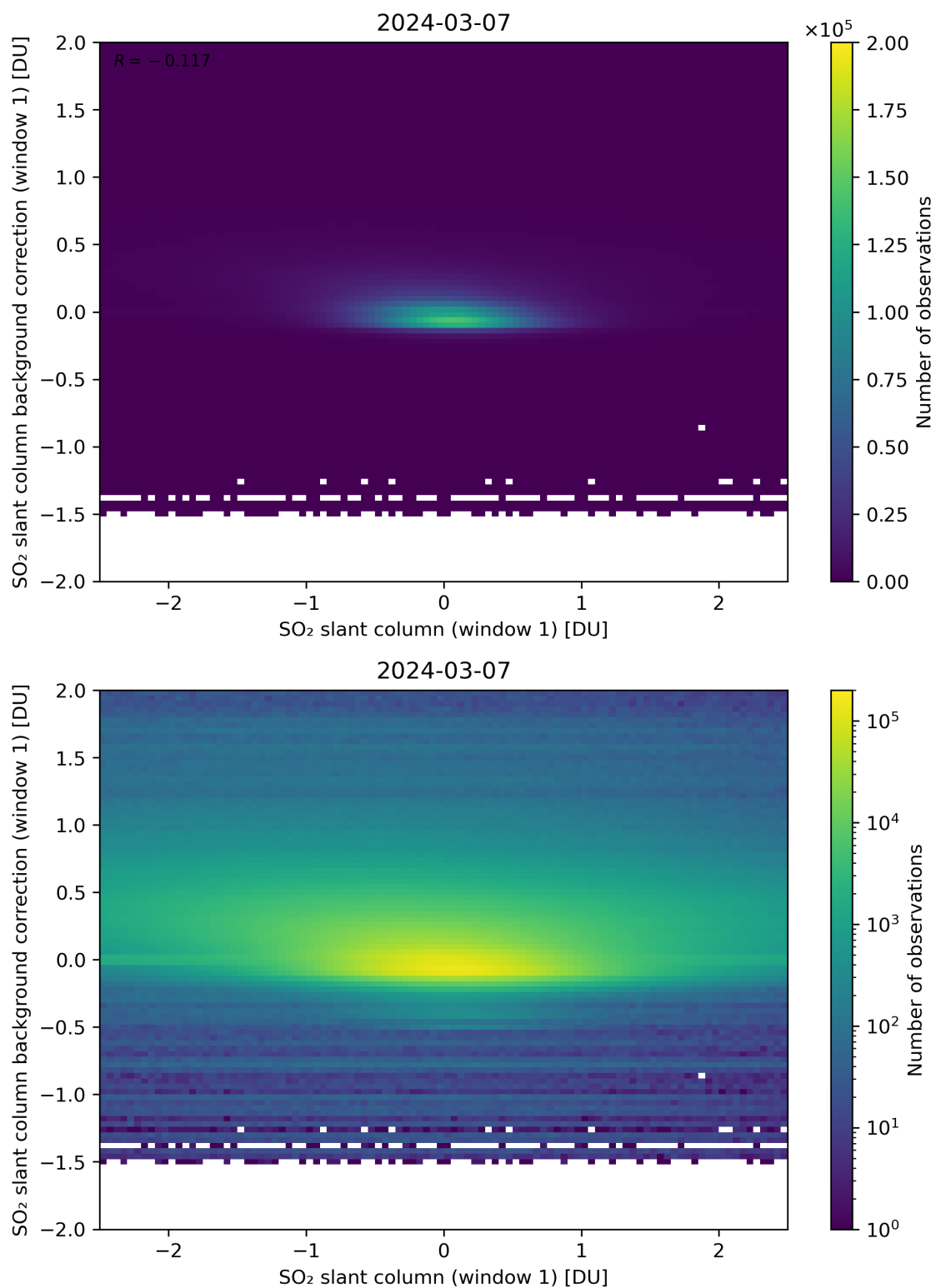
Figure 212: Scatter density plot of “SO 2 slant column (window 1)” against “SO 2 slant column background correction (window 1)” for 2024-03-06 to 2024-03-08.
