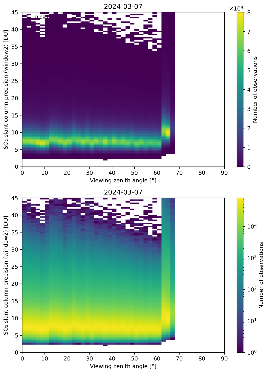
Figure 322: Scatter density plot of “Viewing zenith angle” against “SO 2 slant column precision (window2)” for 2024-03-06 to 2024-03-08.
