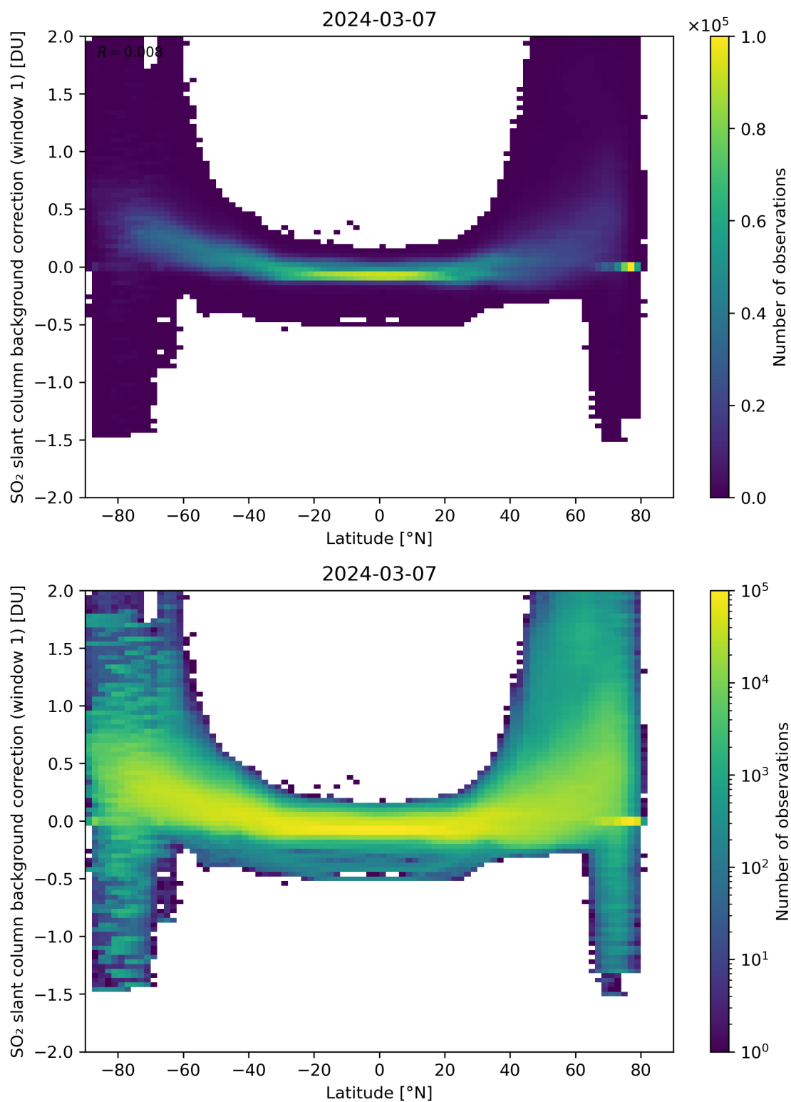
Figure 139: Scatter density plot of “Latitude” against “SO 2 slant column background correction (window 1)” for 2024-03-06 to 2024-03-08.
