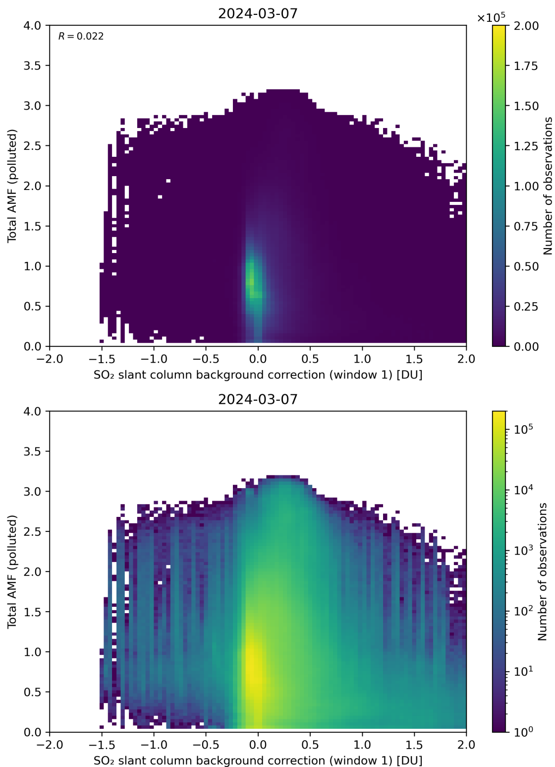
Figure 109: Scatter density plot of “SO 2 slant column background correction (window 1)” against “Total AMF (polluted)” for 2024-03-06 to 2024-03-08.
