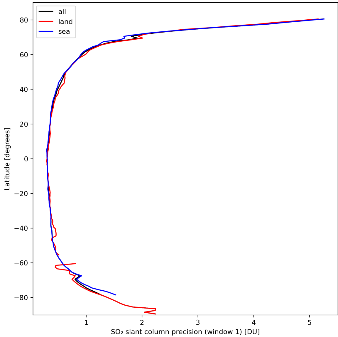
Figure 34: Zonal average of “SO 2 slant column precision (window 1)” for 2024-03-06 to 2024-03-08.
