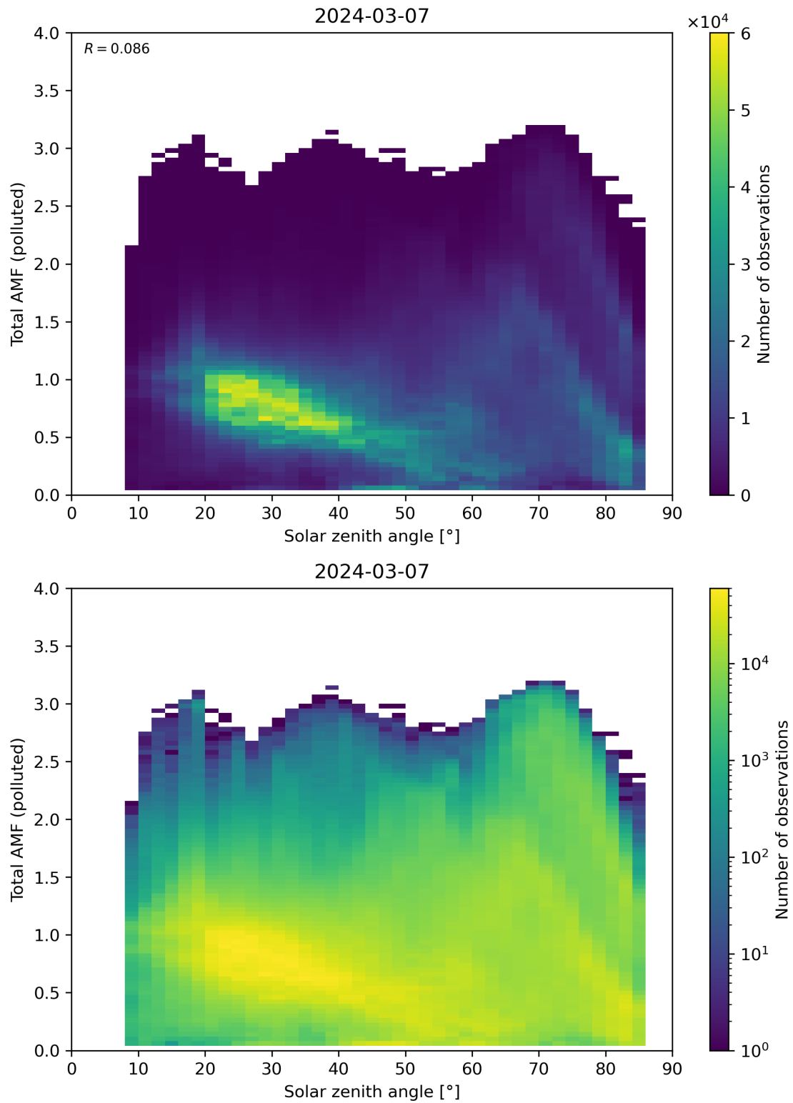
Figure 174: Scatter density plot of “Solar zenith angle” against “Total AMF (polluted)” for 2024-03-06 to 2024-03-08.
