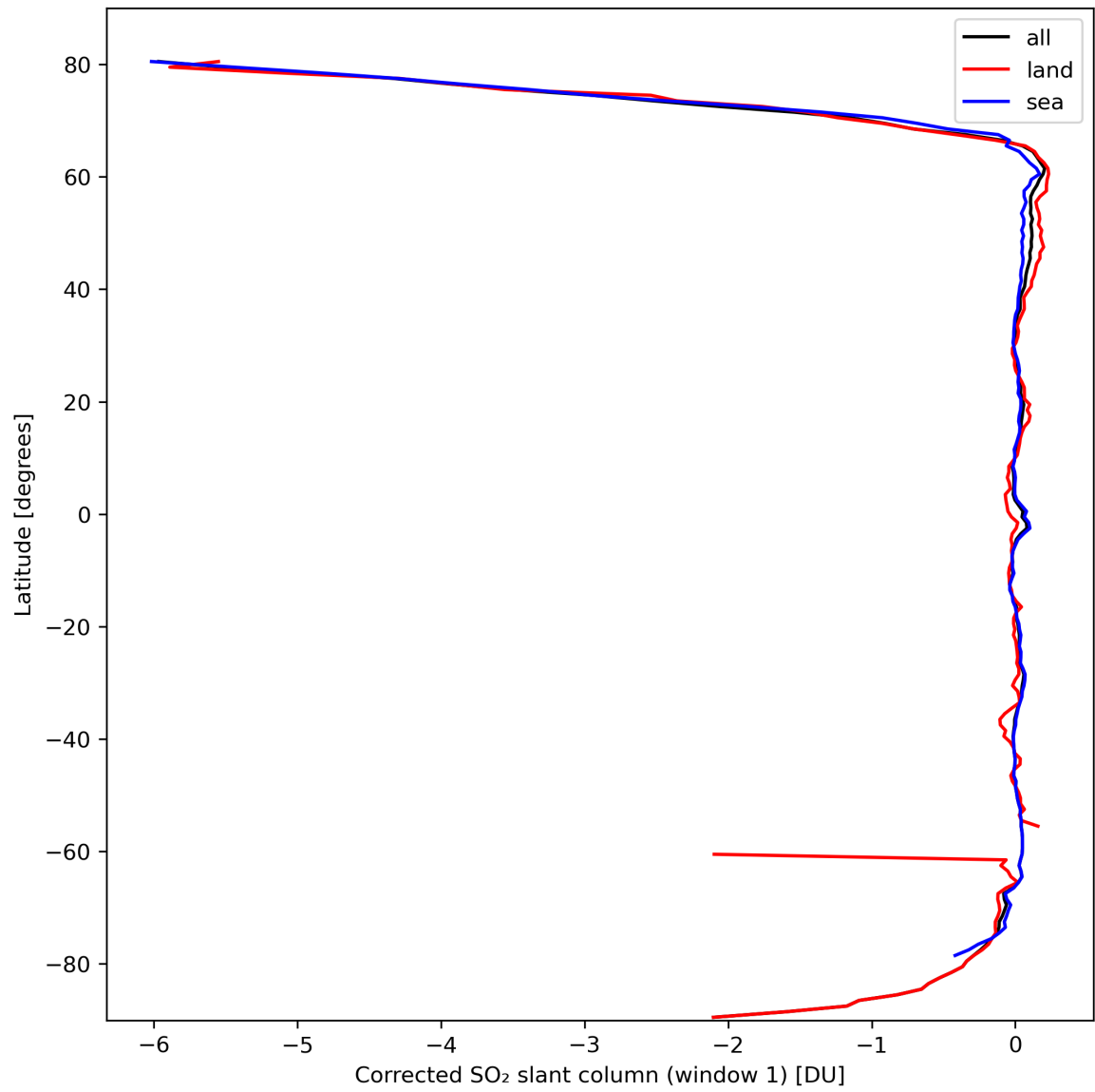
Figure 35: Zonal average of “Corrected SO 2 slant column (window 1)” for 2024-03-06 to 2024-03-08.
