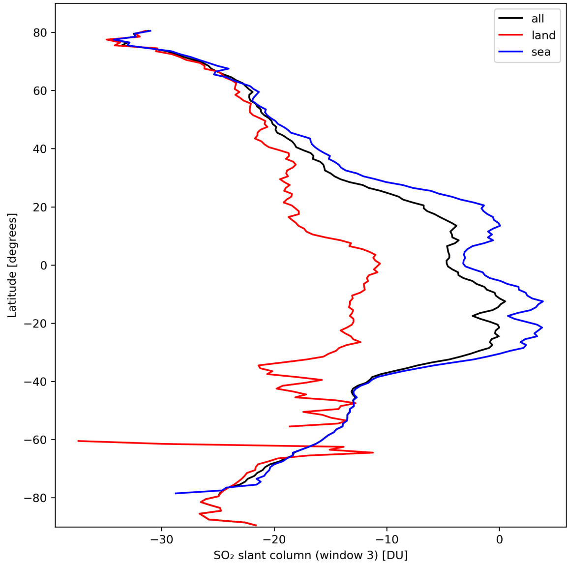
Figure 41: Zonal average of “SO 2 slant column (window 3)” for 2024-03-06 to 2024-03-08.
