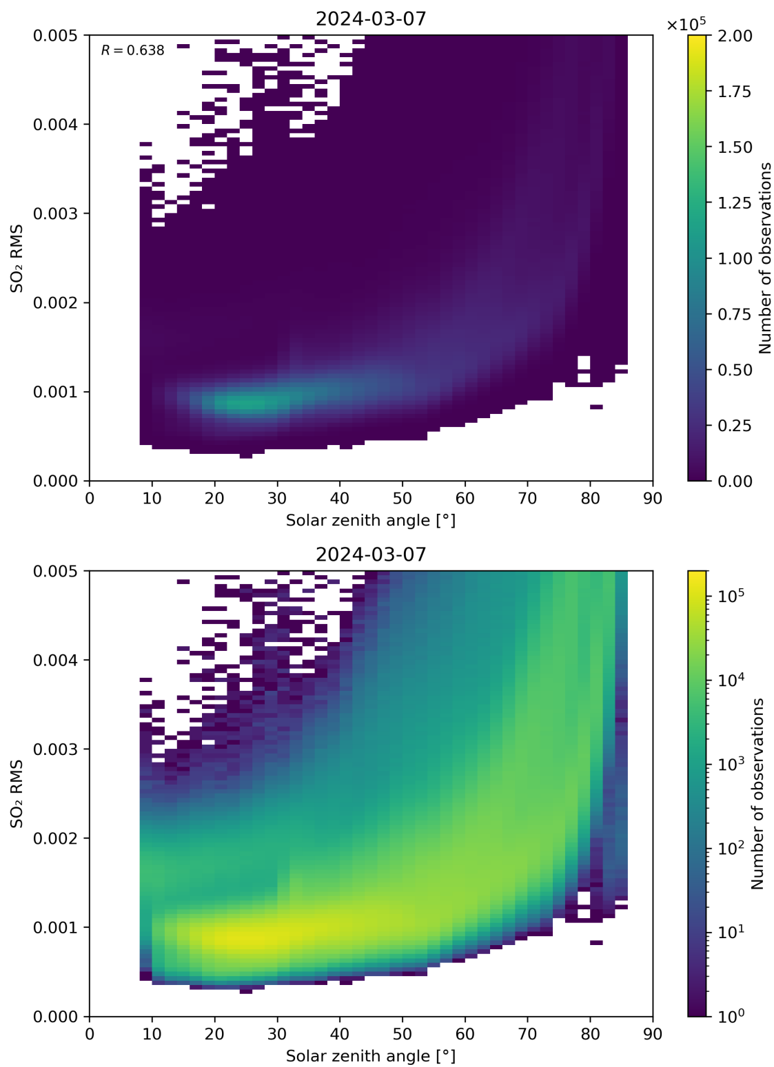
Figure 163: Scatter density plot of “Solar zenith angle” against “SO 2 RMS” for 2024-03-06 to 2024-03-08.
