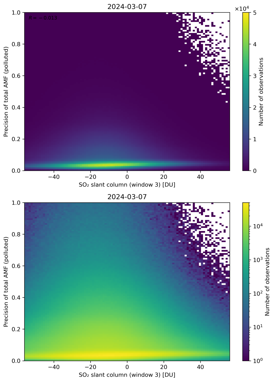
Figure 269: Scatter density plot of “SO 2 slant column (window 3)” against “Precision of total AMF (polluted)” for 2024-03-06 to 2024-03-08.
