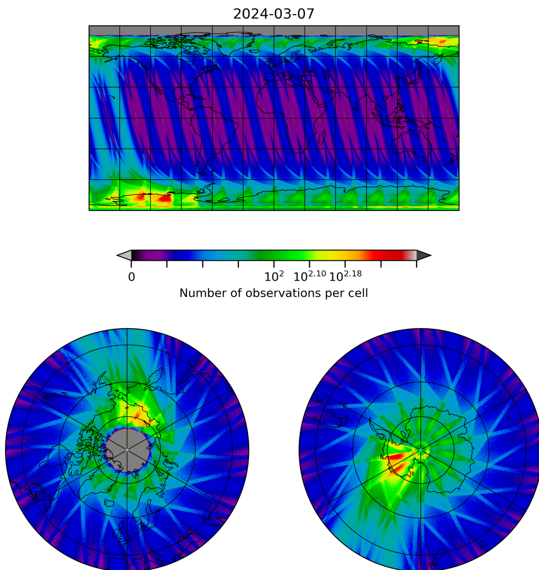
Figure 28: Map of the number of observations for 2024-03-06 to 2024-03-08
