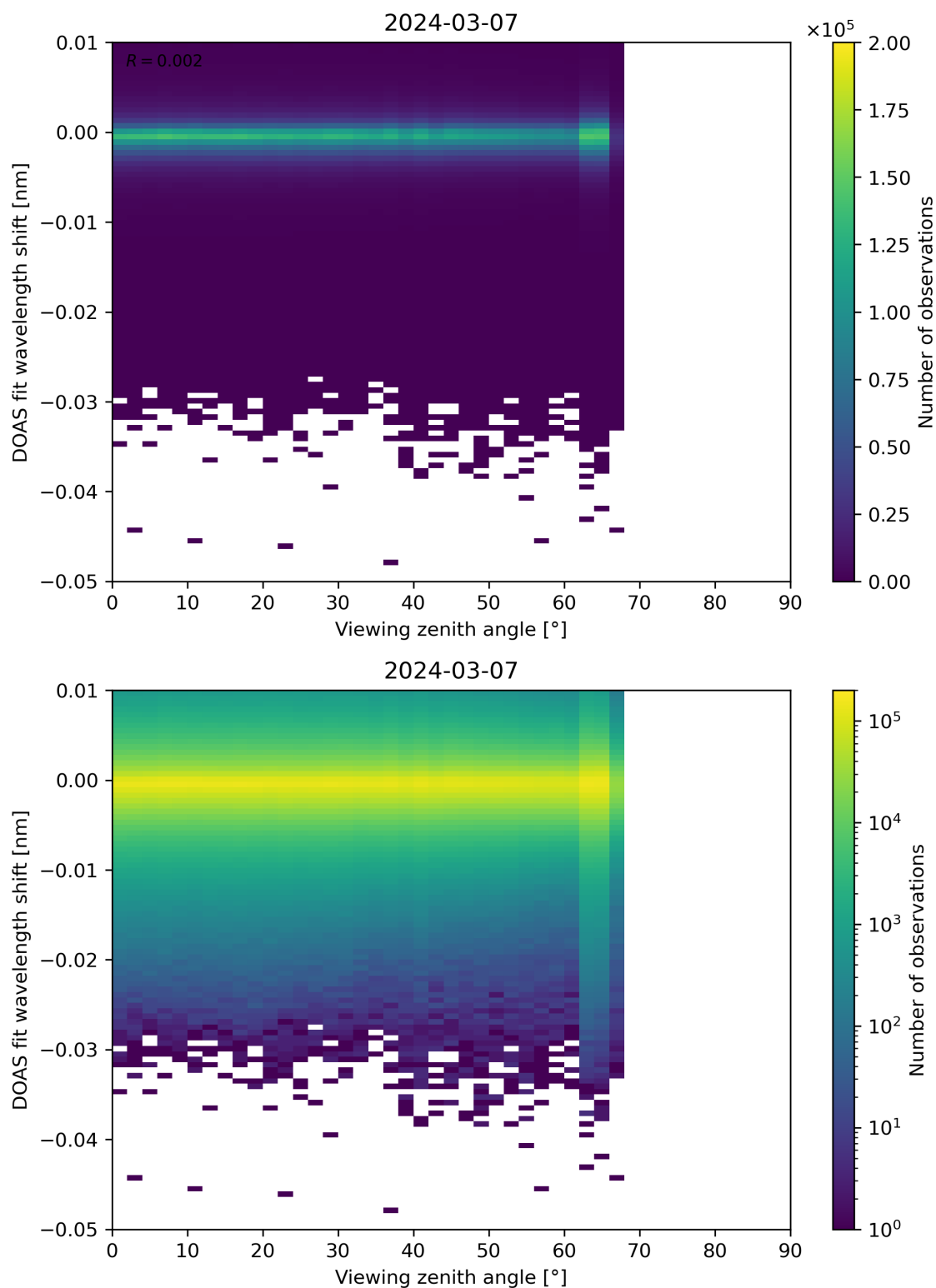
Figure 311: Scatter density plot of “Viewing zenith angle” against “DOAS fit wavelength shift” for 2024-03-06 to 2024-03-08.
