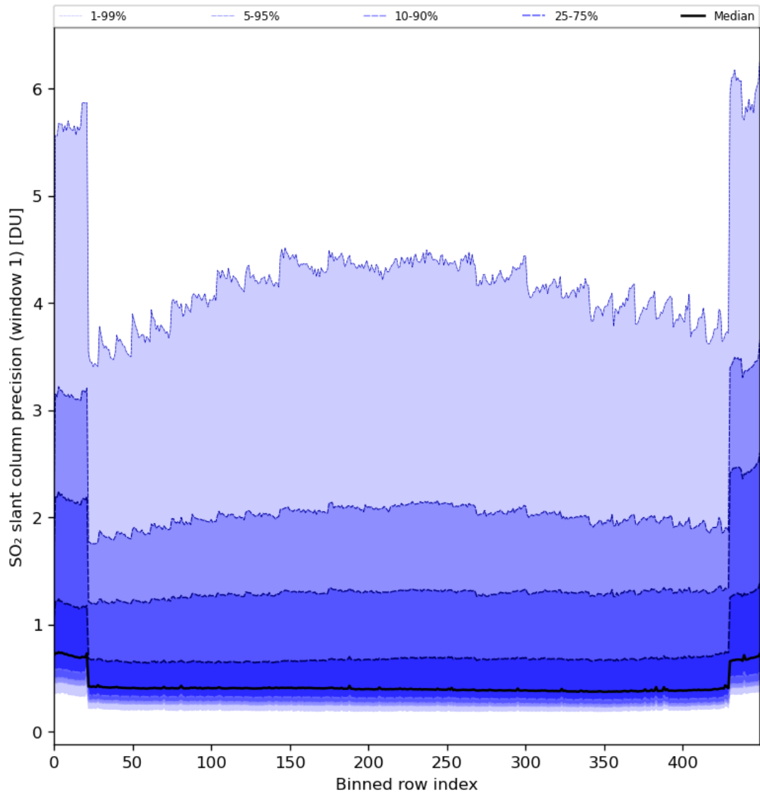
Figure 80: Along track statistics of “SO 2 slant column precision (window 1)” for 2024-03-06 to 2024-03-08
