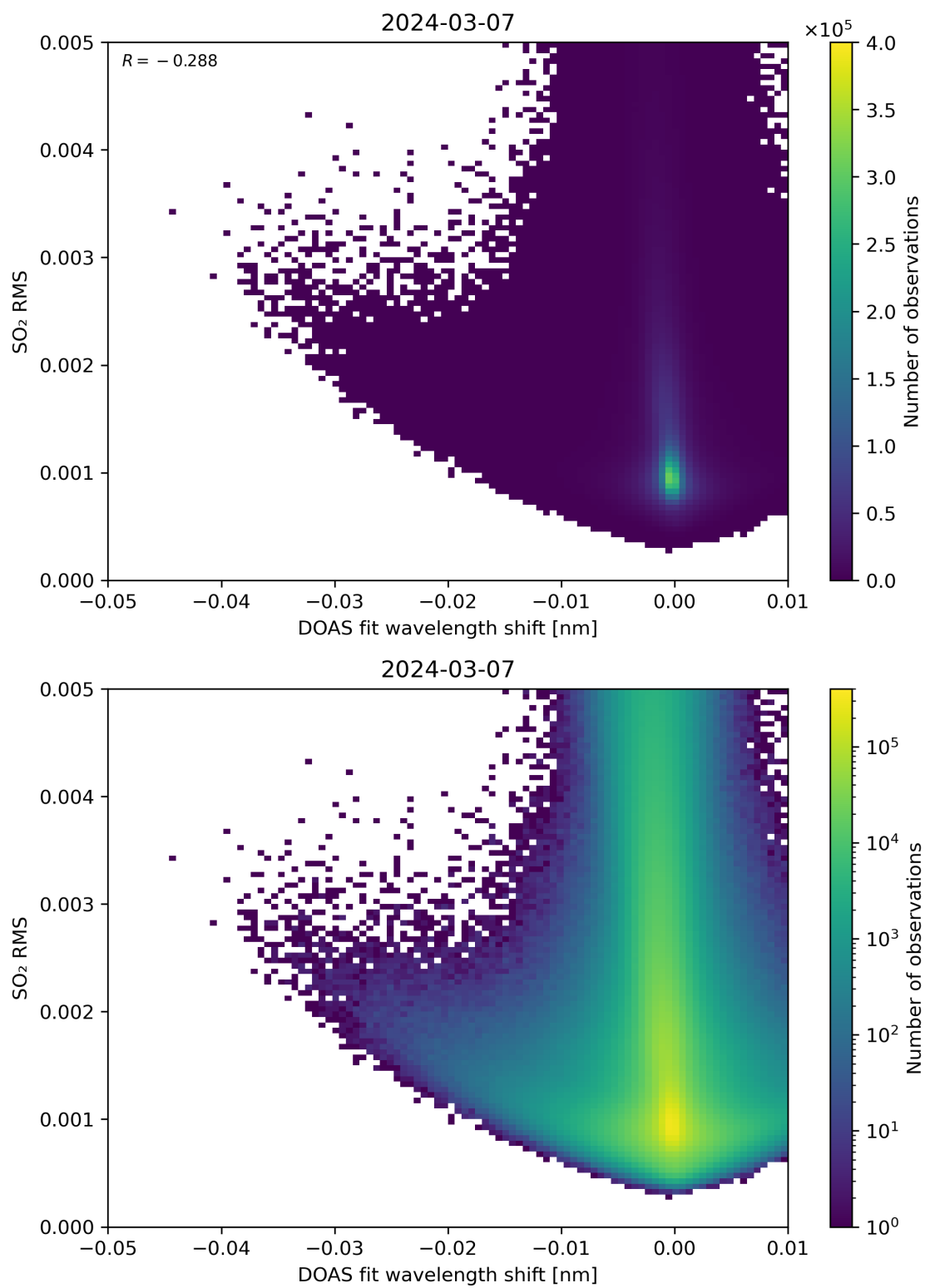
Figure 128: Scatter density plot of “DOAS fit wavelength shift” against “SO 2 RMS” for 2024-03-06 to 2024-03-08.
