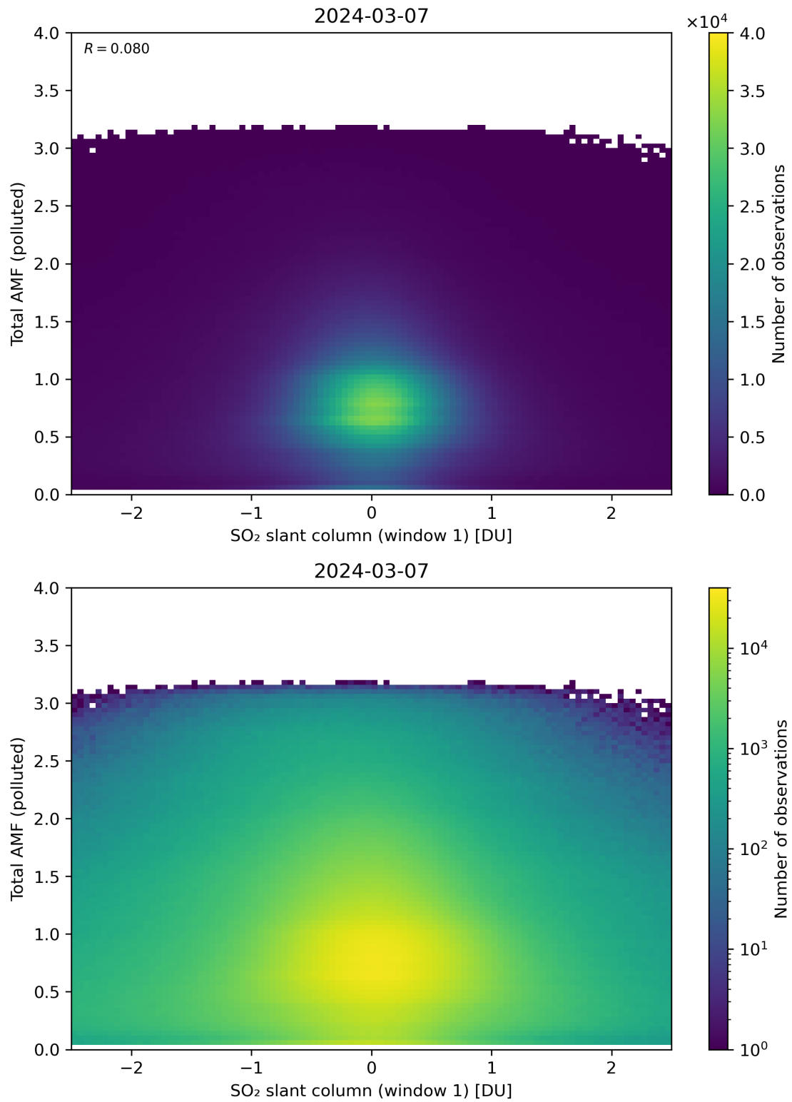
Figure 239: Scatter density plot of “SO 2 slant column (window 1)” against “Total AMF (polluted)” for 2024-03-06 to 2024-03-08.
