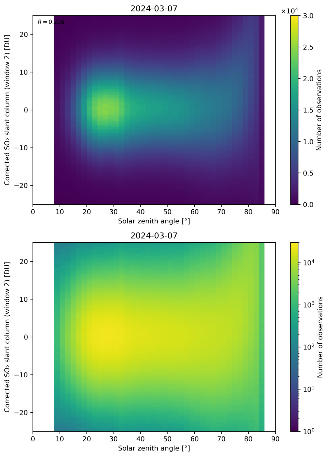
Figure 167: Scatter density plot of “Solar zenith angle” against “Corrected SO 2 slant column (window 2)” for 2024-03-06 to 2024-03-08.
