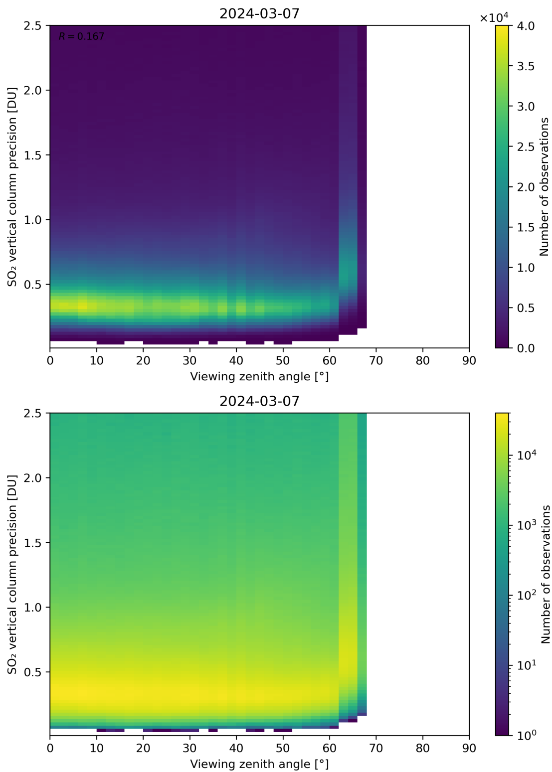
Figure 328: Scatter density plot of “Viewing zenith angle” against “SO 2 vertical column precision” for 2024-03-06 to 2024-03-08.
