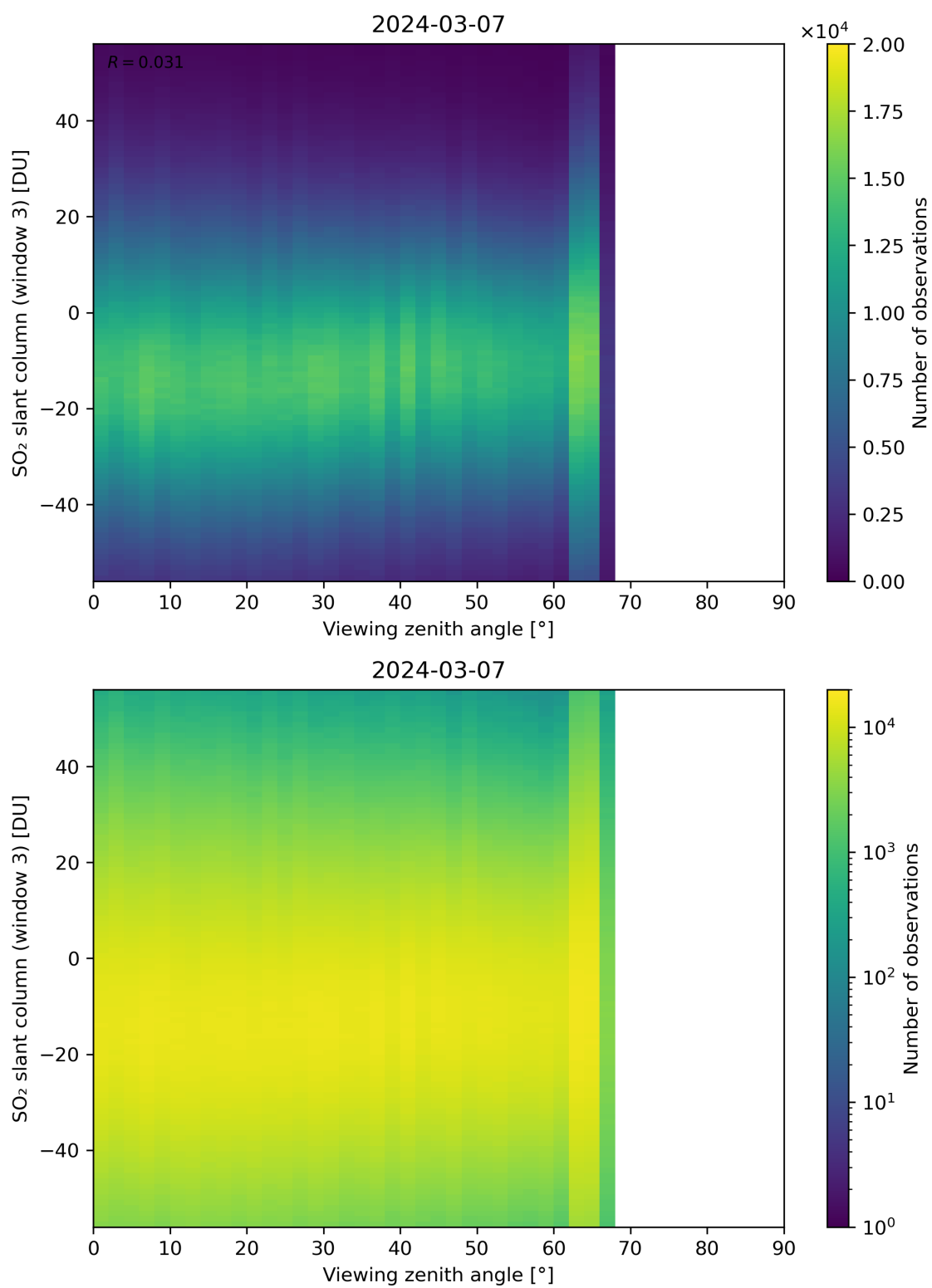
Figure 323: Scatter density plot of “Viewing zenith angle” against “SO 2 slant column (window 3)” for 2024-03-06 to 2024-03-08.
