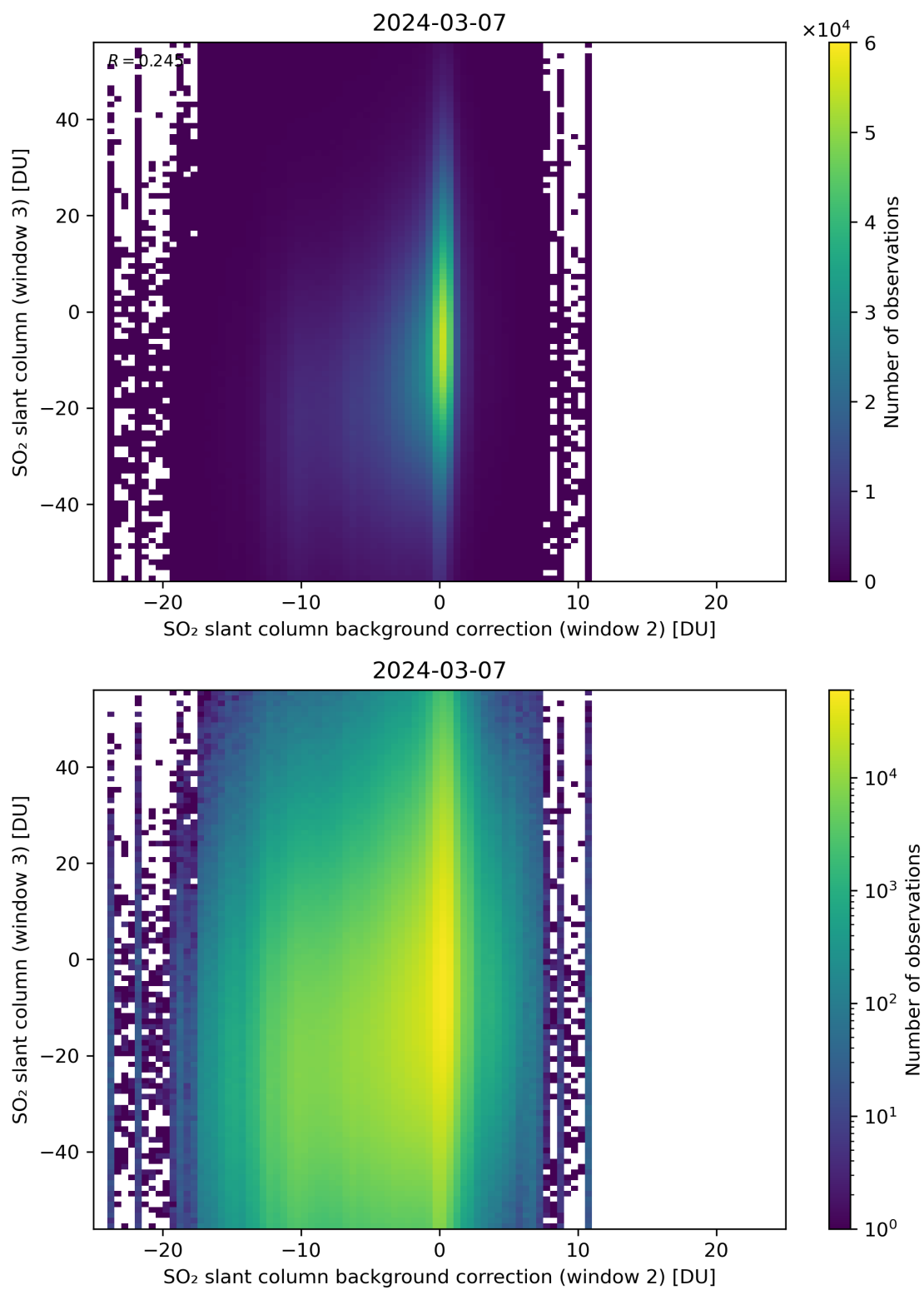
Figure 117: Scatter density plot of “SO 2 slant column background correction (window 2)” against “SO 2 slant column (window 3)” for 2024-03-06 to 2024-03-08.
