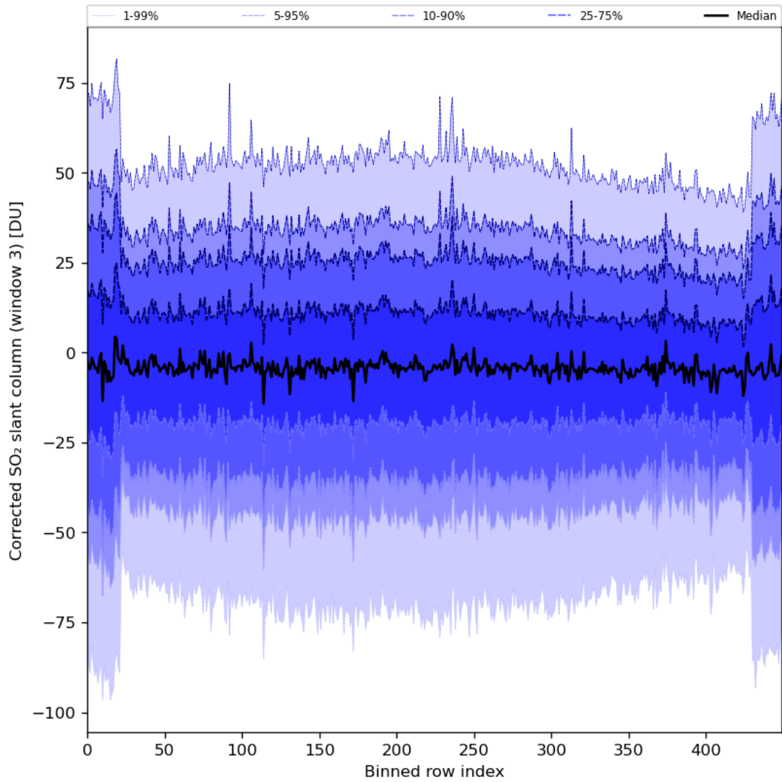
Figure 89: Along track statistics of "Corrected SO 2 slant column (window 3)" for 2024-03-06 to 2024-03-08
