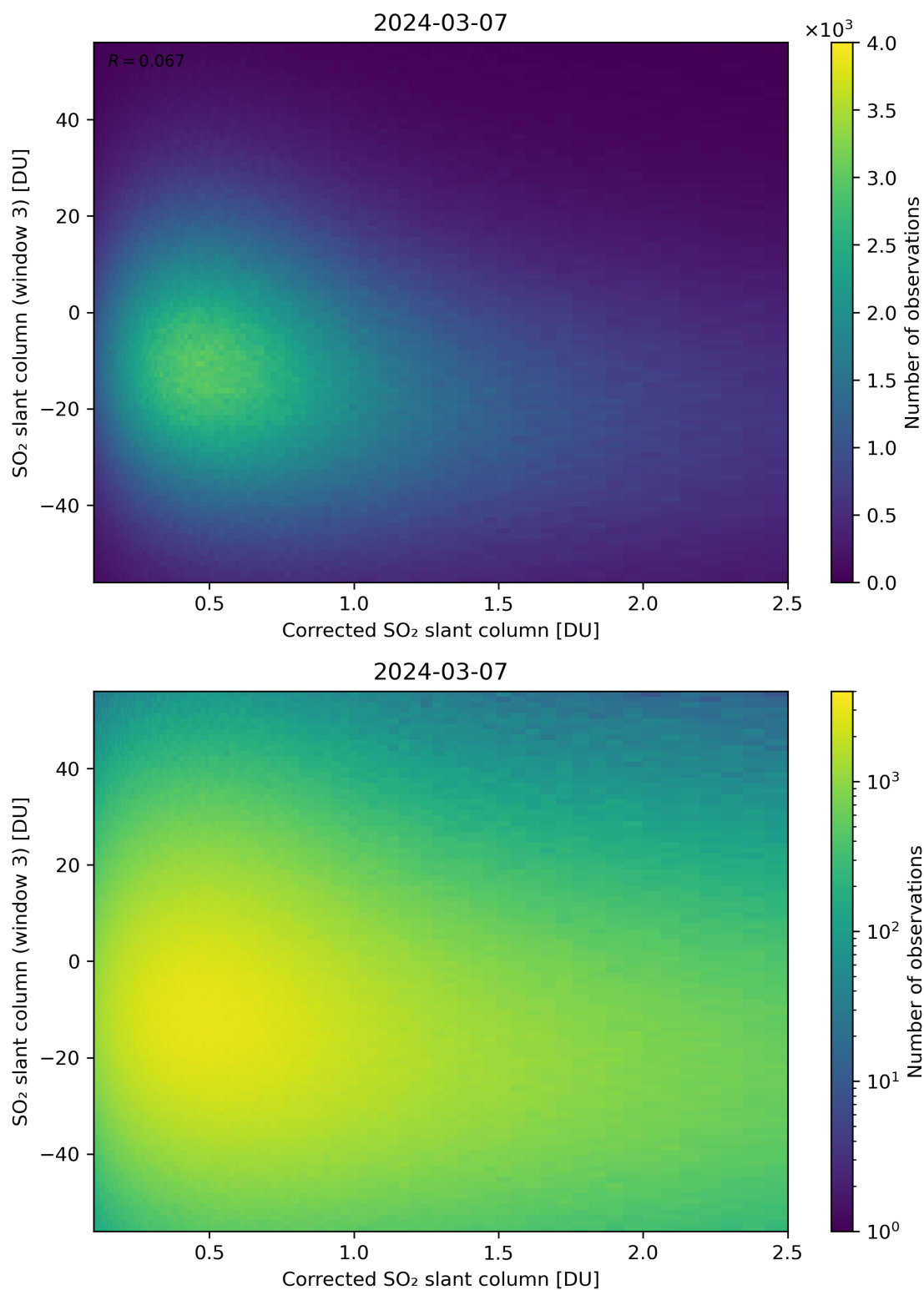
Figure 190: Scatter density plot of “Corrected SO 2 slant column” against “SO 2 slant column (window 3)” for 2024-03-06 to 2024-03-08.
