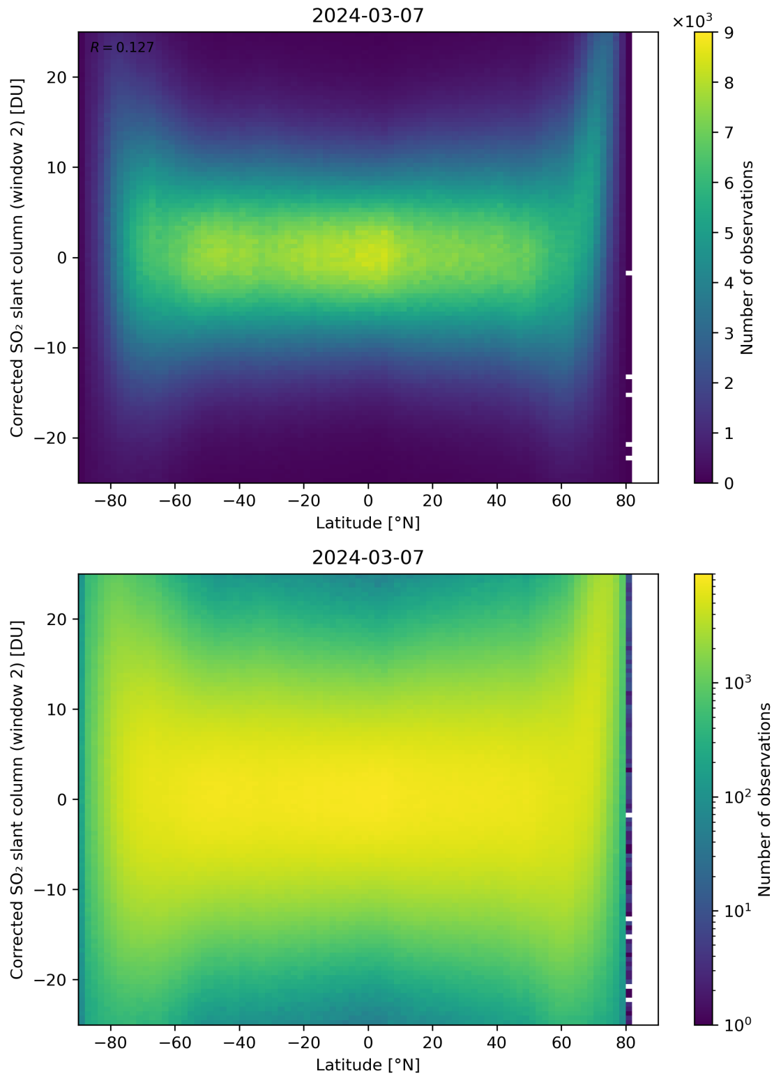
Figure 147: Scatter density plot of “Latitude” against “Corrected SO 2 slant column (window 2)” for 2024-03-06 to 2024-03-08.
