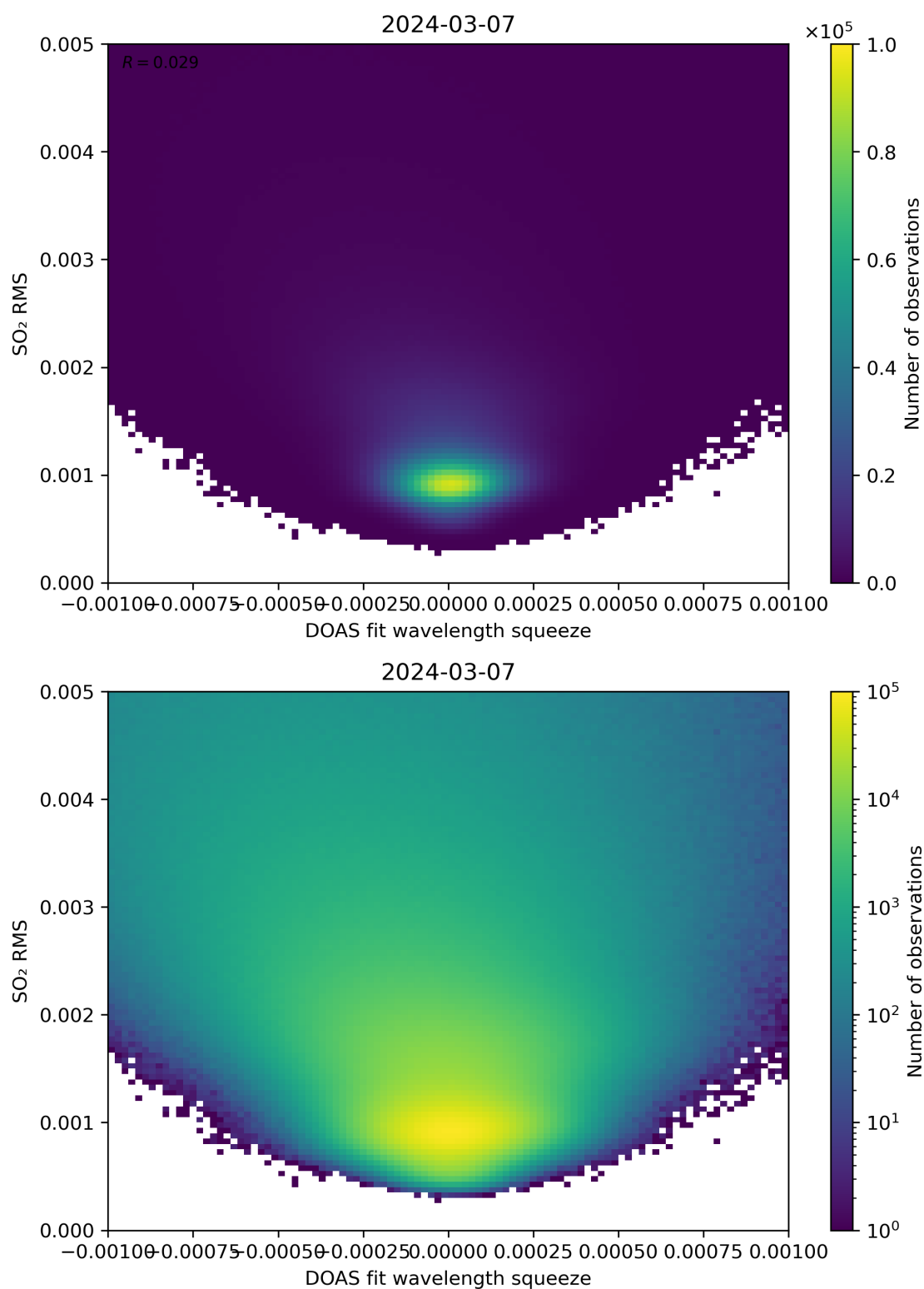
Figure 132: Scatter density plot of “DOAS fit wavelength squeeze” against “SO 2 RMS” for 2024-03-06 to 2024-03-08.
