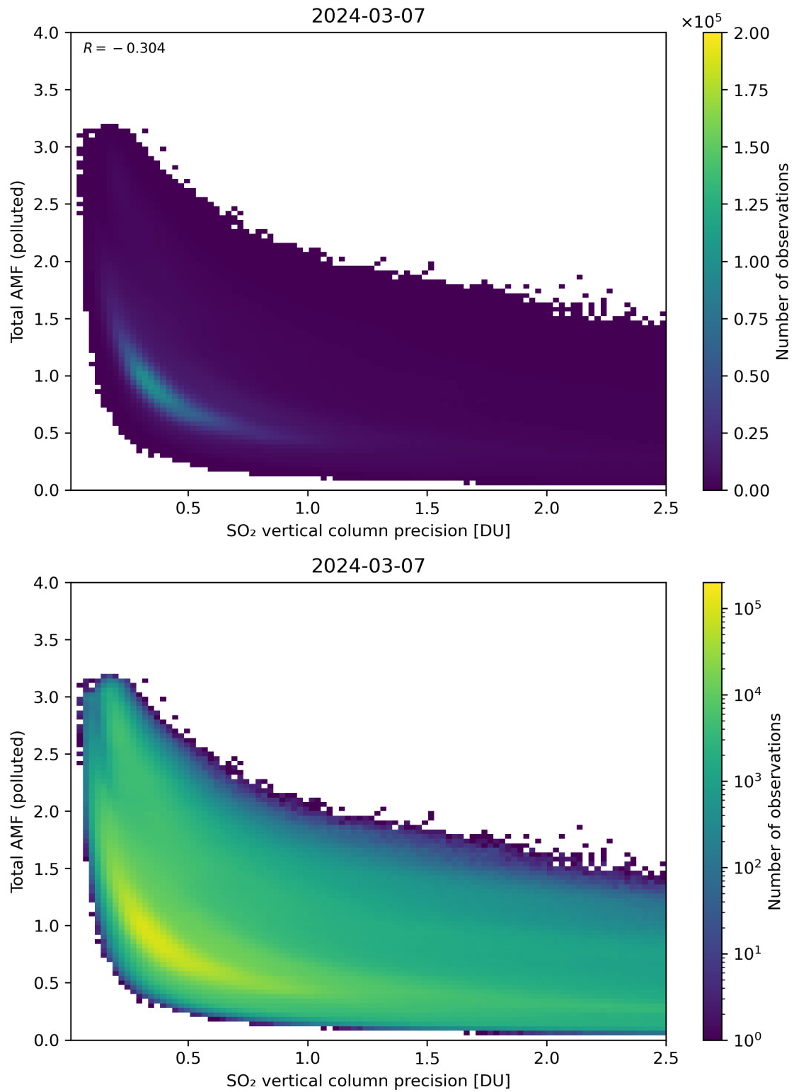
Figure 294: Scatter density plot of “SO 2 vertical column precision” against “Total AMF (polluted)” for 2024-03-06 to 2024-03-08.
