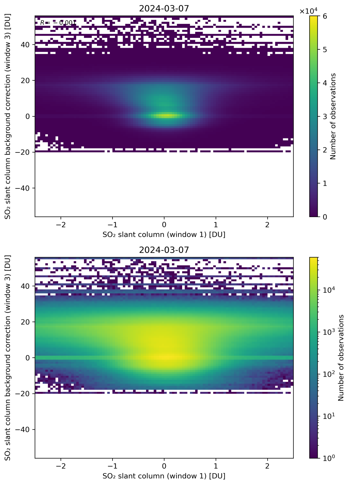
Figure 214: Scatter density plot of “SO 2 slant column (window 1)” against “SO 2 slant column background correction (window 3)” for 2024-03-06 to 2024-03-08.
