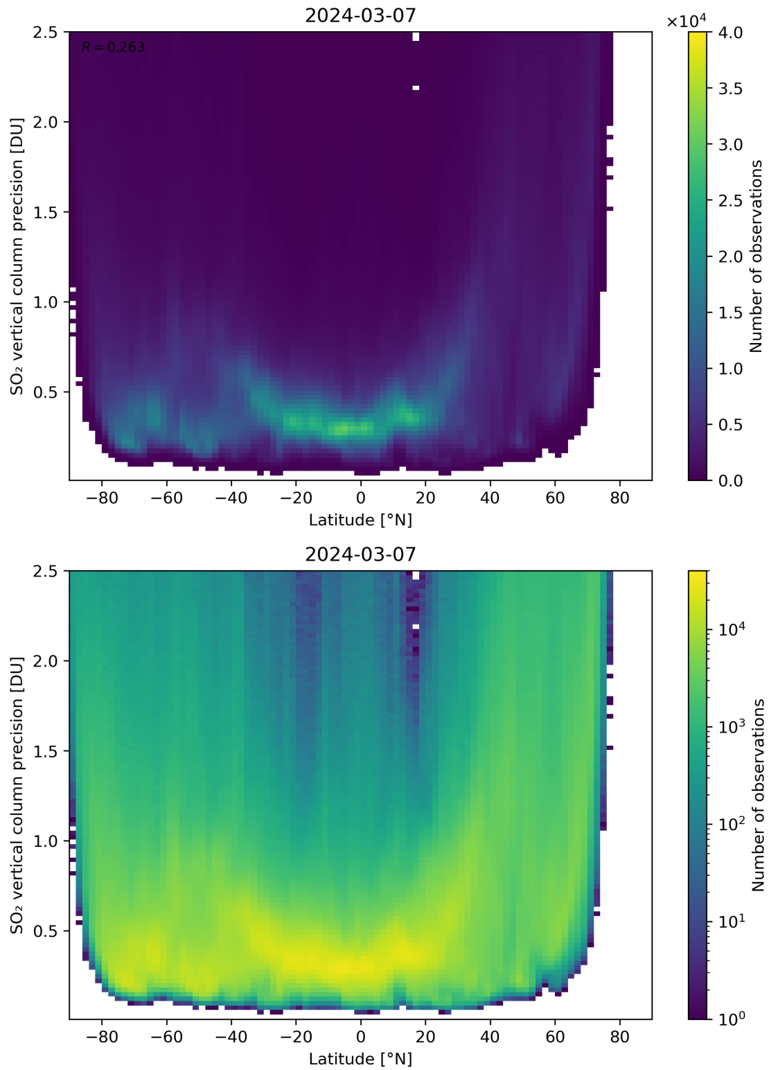
Figure 157: Scatter density plot of “Latitude” against “SO 2 vertical column precision” for 2024-03-06 to 2024-03-08.
