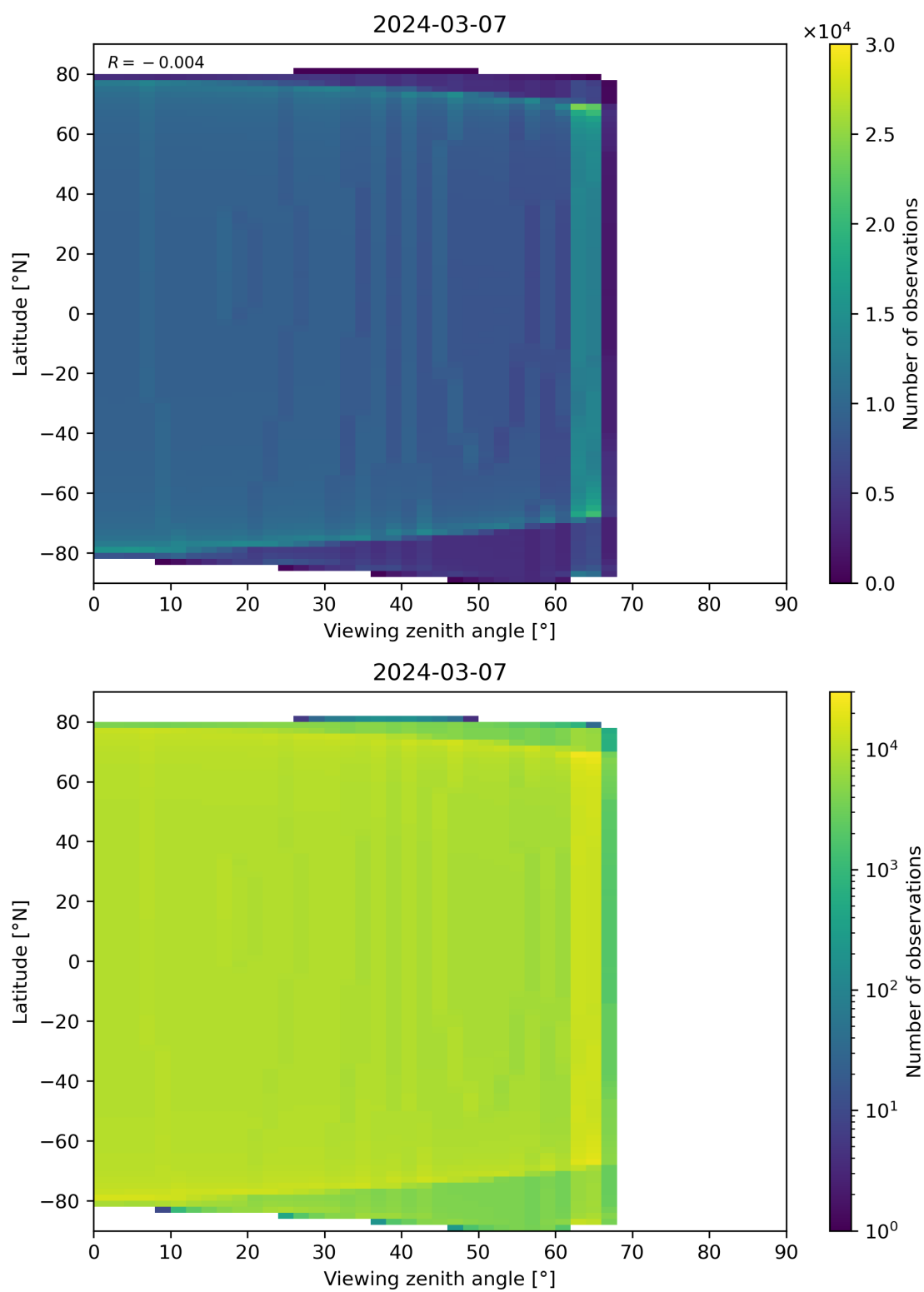
Figure 314: Scatter density plot of “Viewing zenith angle” against “Latitude” for 2024-03-06 to 2024-03-08.
