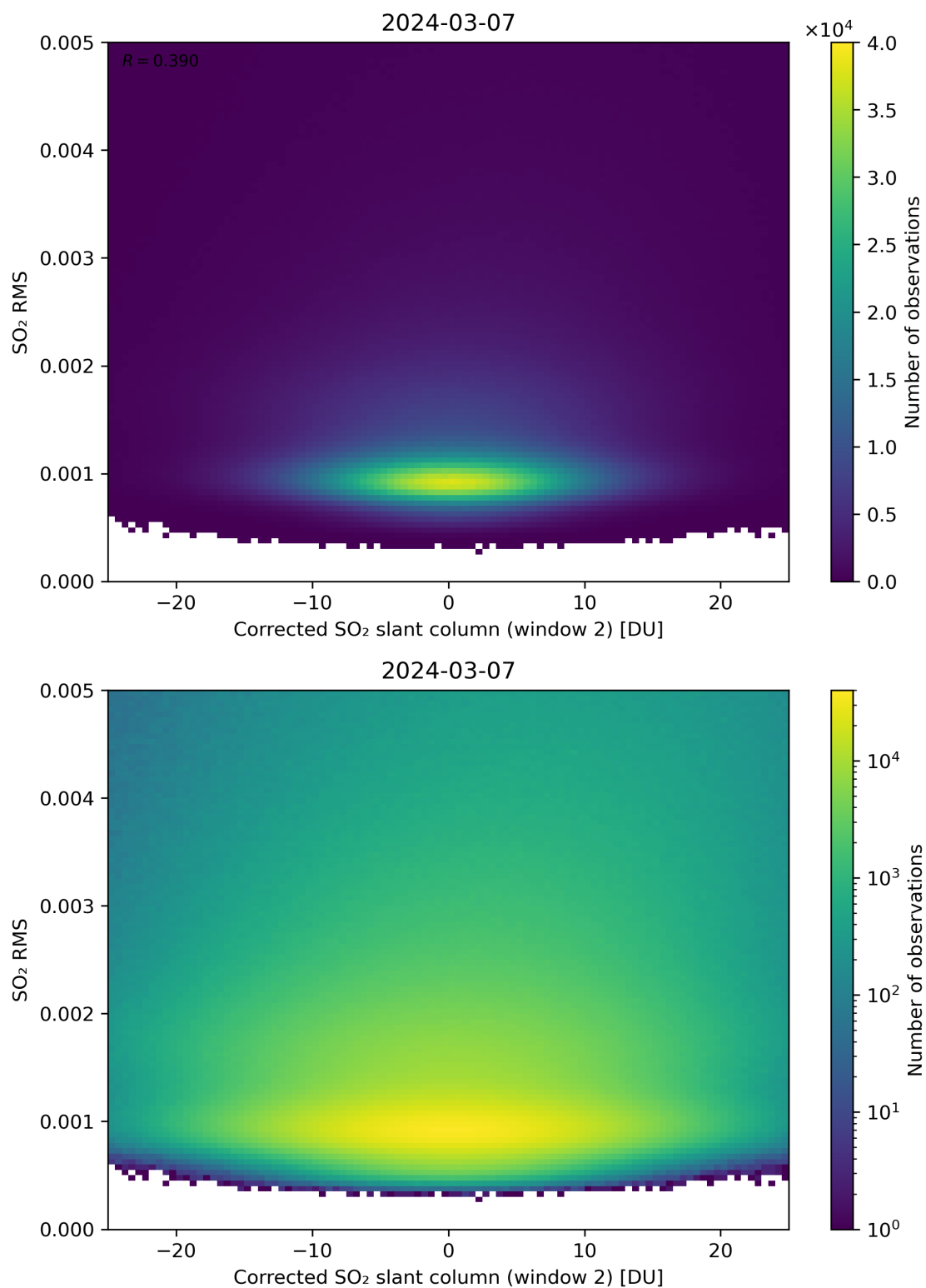
Figure 198: Scatter density plot of “Corrected SO 2 slant column (window 2)” against “SO 2 RMS” for 2024-03-06 to 2024-03-08.
