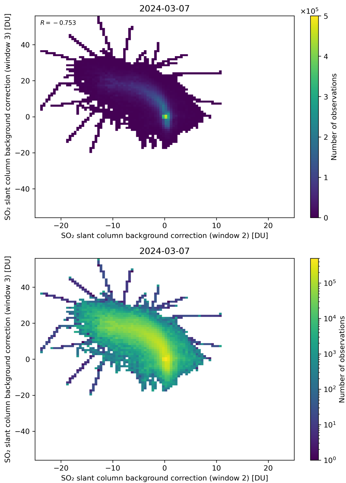
Figure 111: Scatter density plot of “SO 2 slant column background correction (window 2)” against “SO 2 slant column background correction (window 3)” for 2024-03-06 to 2024-03-08.
