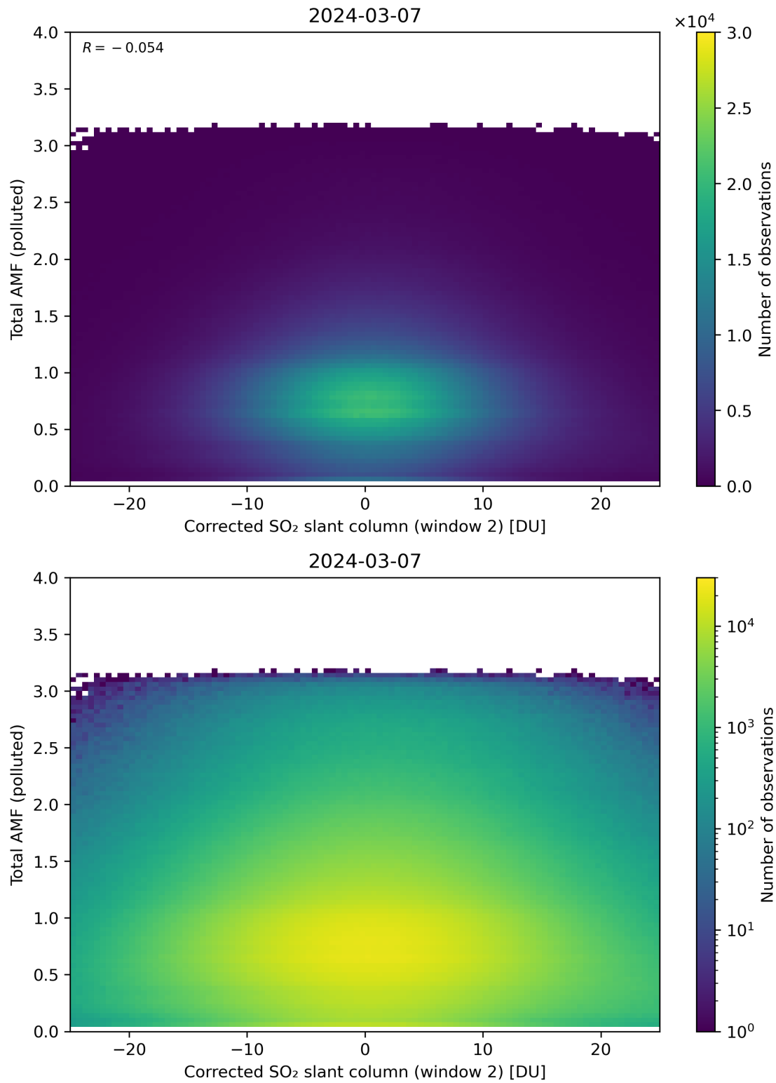
Figure 203: Scatter density plot of “Corrected SO 2 slant column (window 2)” against “Total AMF (polluted)” for 2024-03-06 to 2024-03-08.
