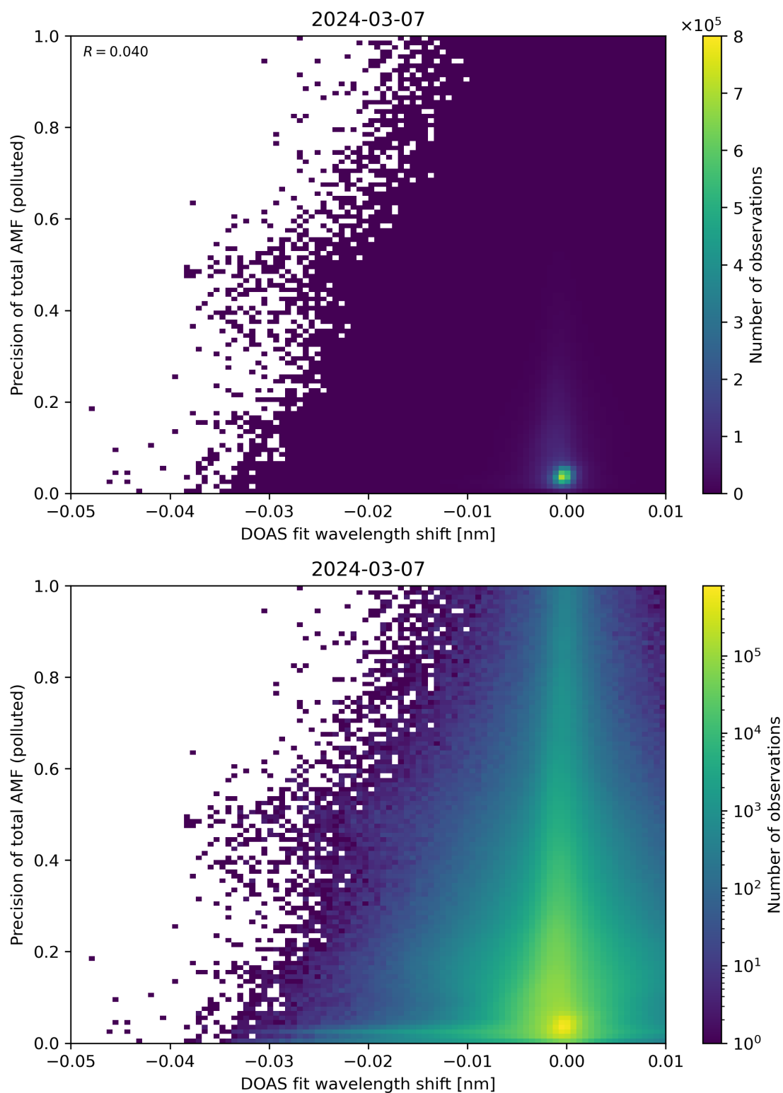
Figure 131: Scatter density plot of “DOAS fit wavelength shift” against “Precision of total AMF (polluted)” for 2024-03-06 to 2024-03-08.
