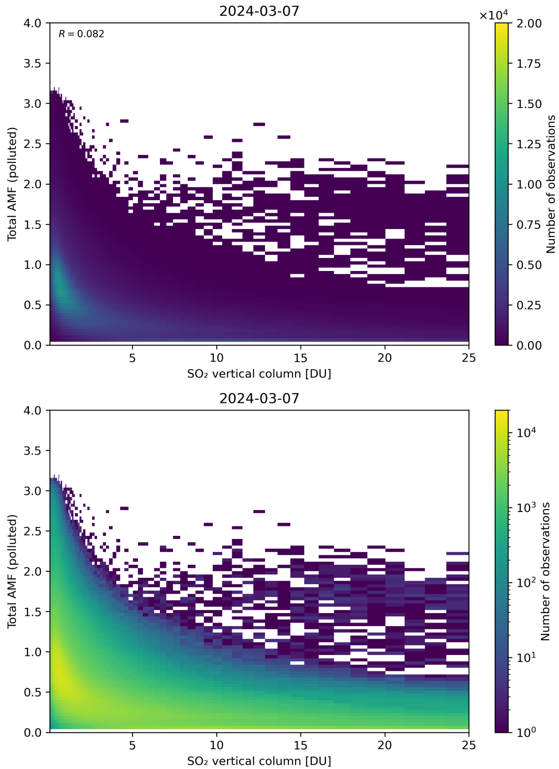
Figure 305: Scatter density plot of “SO 2 vertical column” against “Total AMF (polluted)” for 2024-03-06 to 2024-03-08.
