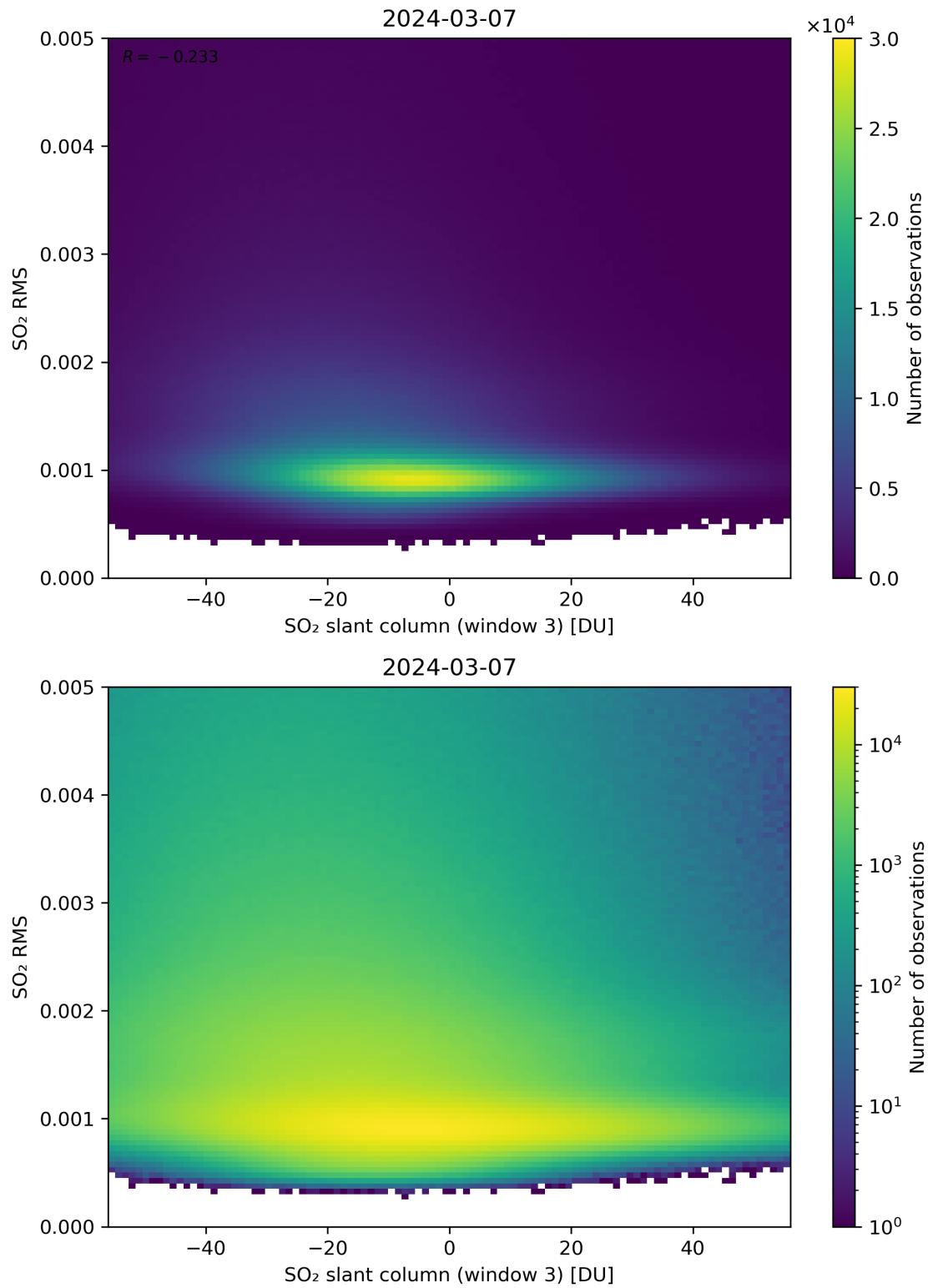
Figure 256: Scatter density plot of “SO 2 slant column (window 3)” against “SO 2 RMS” for 2024-03-06 to 2024-03-08.
