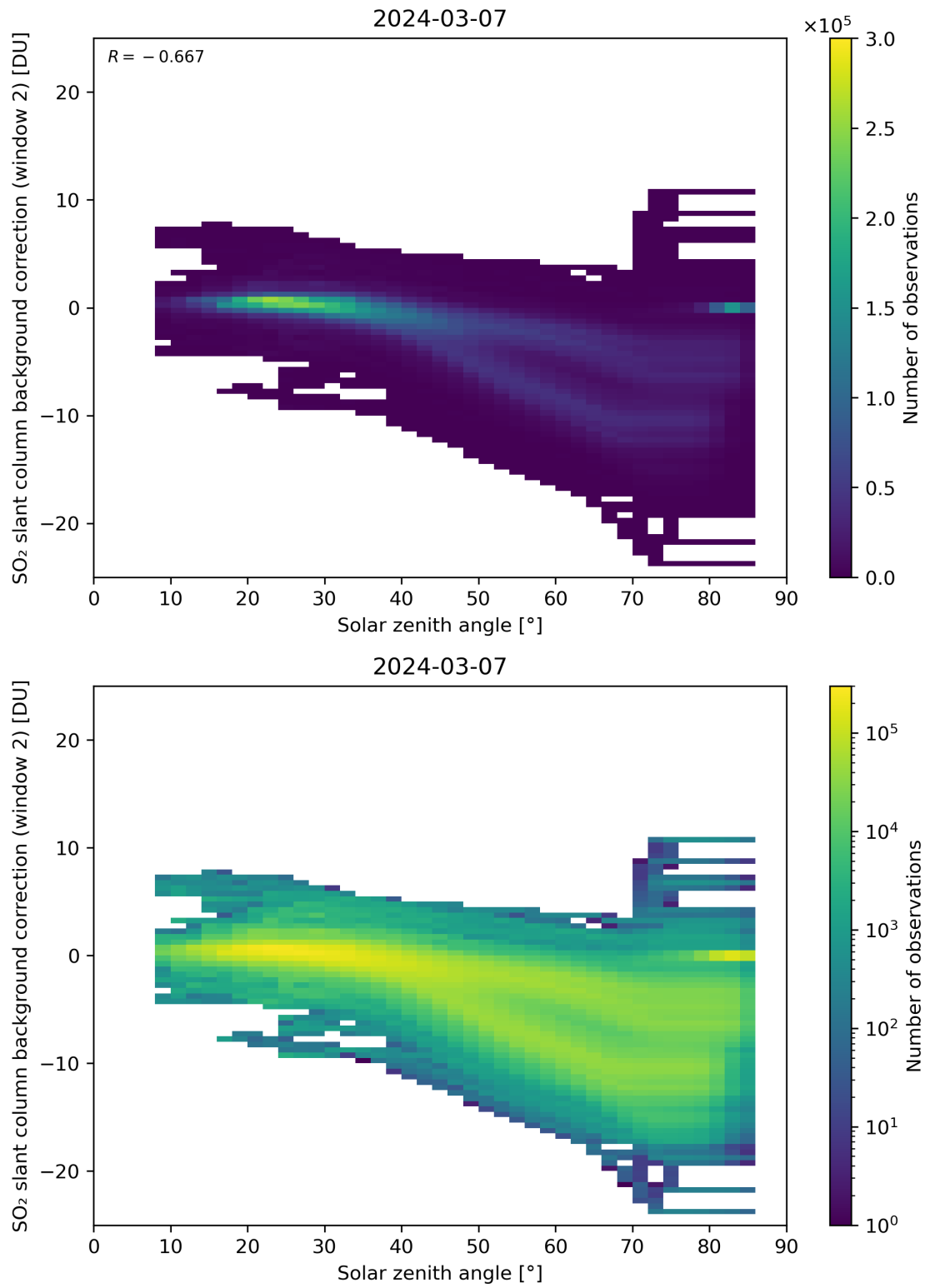
Figure 159: Scatter density plot of “Solar zenith angle” against “SO 2 slant column background correction (window 2)” for 2024-03-06 to 2024-03-08.
