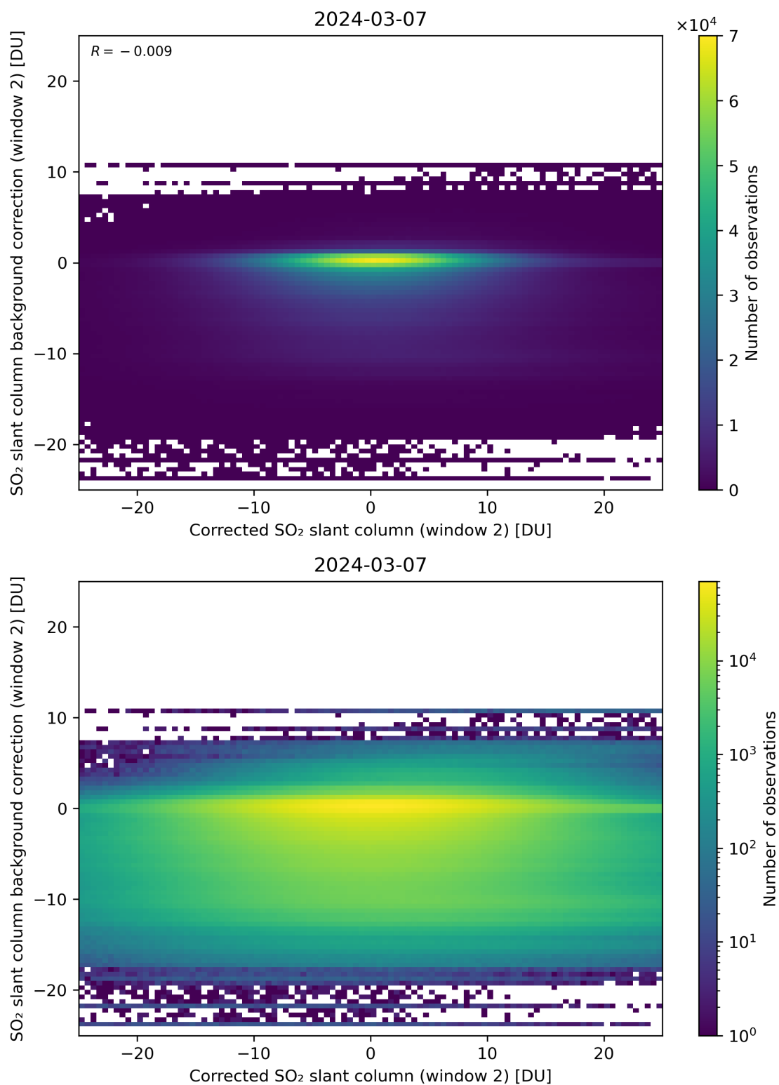
Figure 194: Scatter density plot of “Corrected SO 2 slant column (window 2)” against “SO 2 slant column background correction (window 2)” for 2024-03-06 to 2024-03-08.
