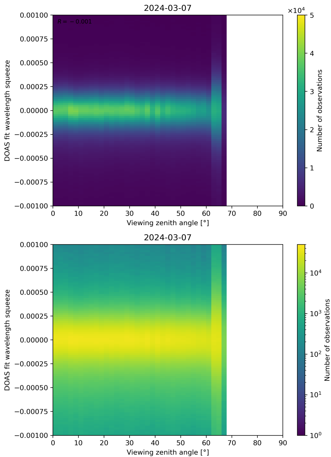
Figure 312: Scatter density plot of “Viewing zenith angle” against “DOAS fit wavelength squeeze” for 2024-03-06 to 2024-03-08.
