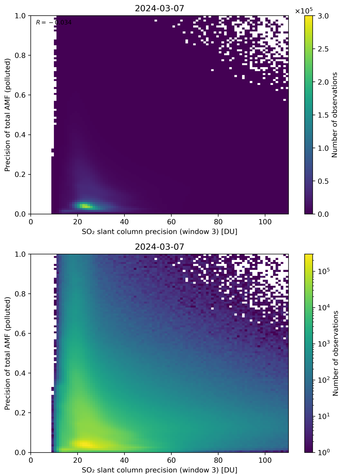
Figure 264: Scatter density plot of “SO 2 slant column precision (window 3)” against “Precision of total AMF (polluted)” for 2024-03-06 to 2024-03-08.
