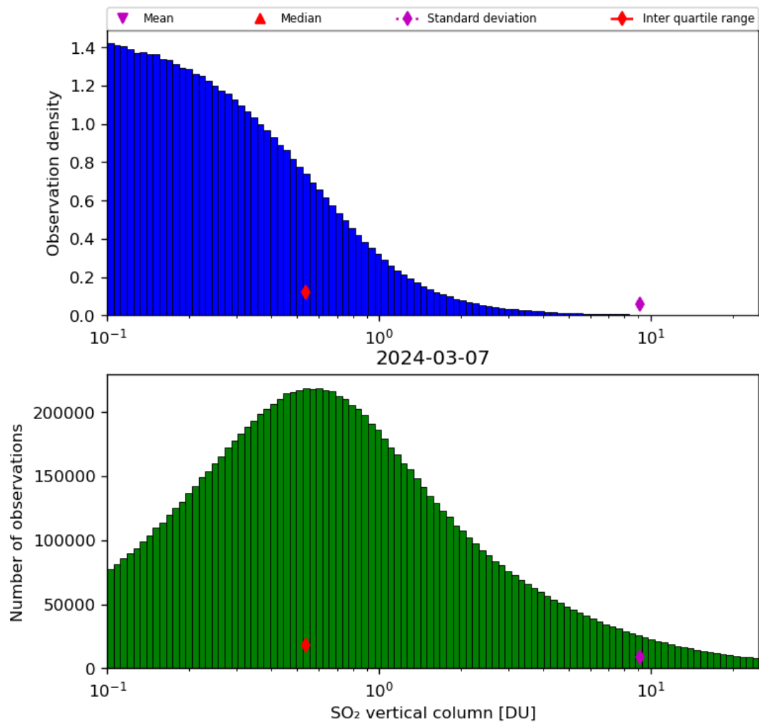
Figure 53: Histogram of “SO 2 vertical column” for 2024-03-06 to 2024-03-08
