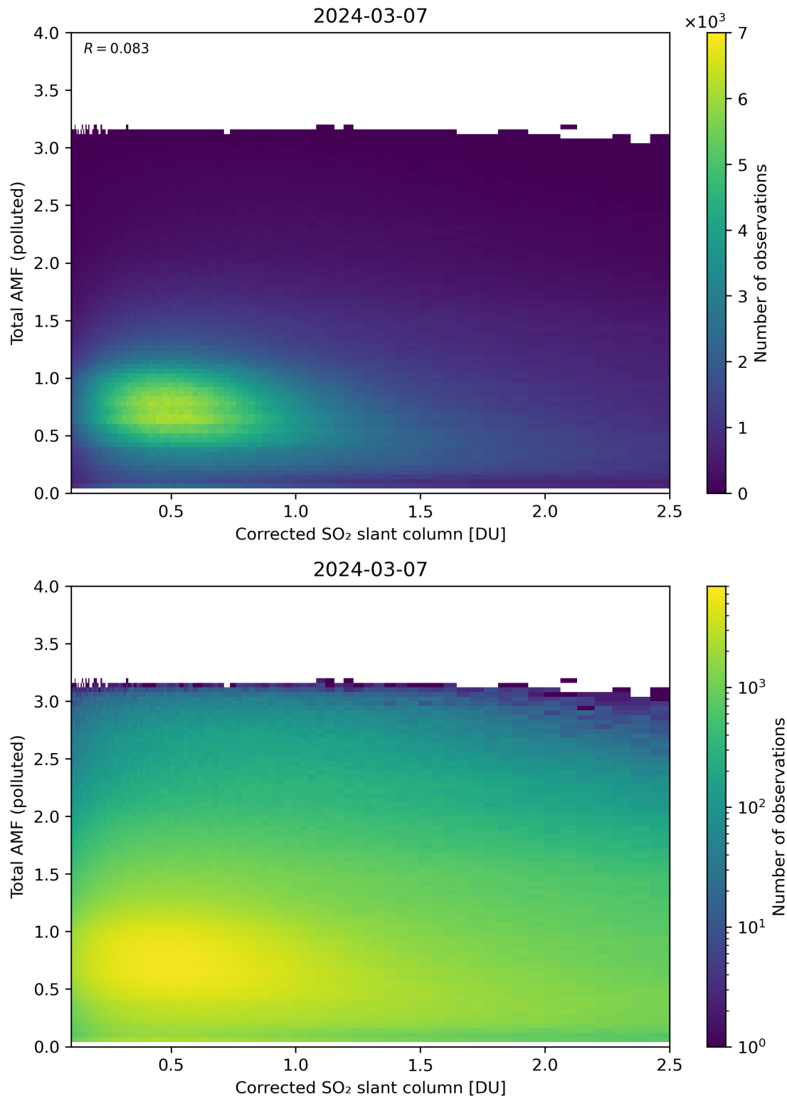
Figure 192: Scatter density plot of “Corrected SO 2 slant column” against “Total AMF (polluted)” for 2024-03-06 to 2024-03-08.
