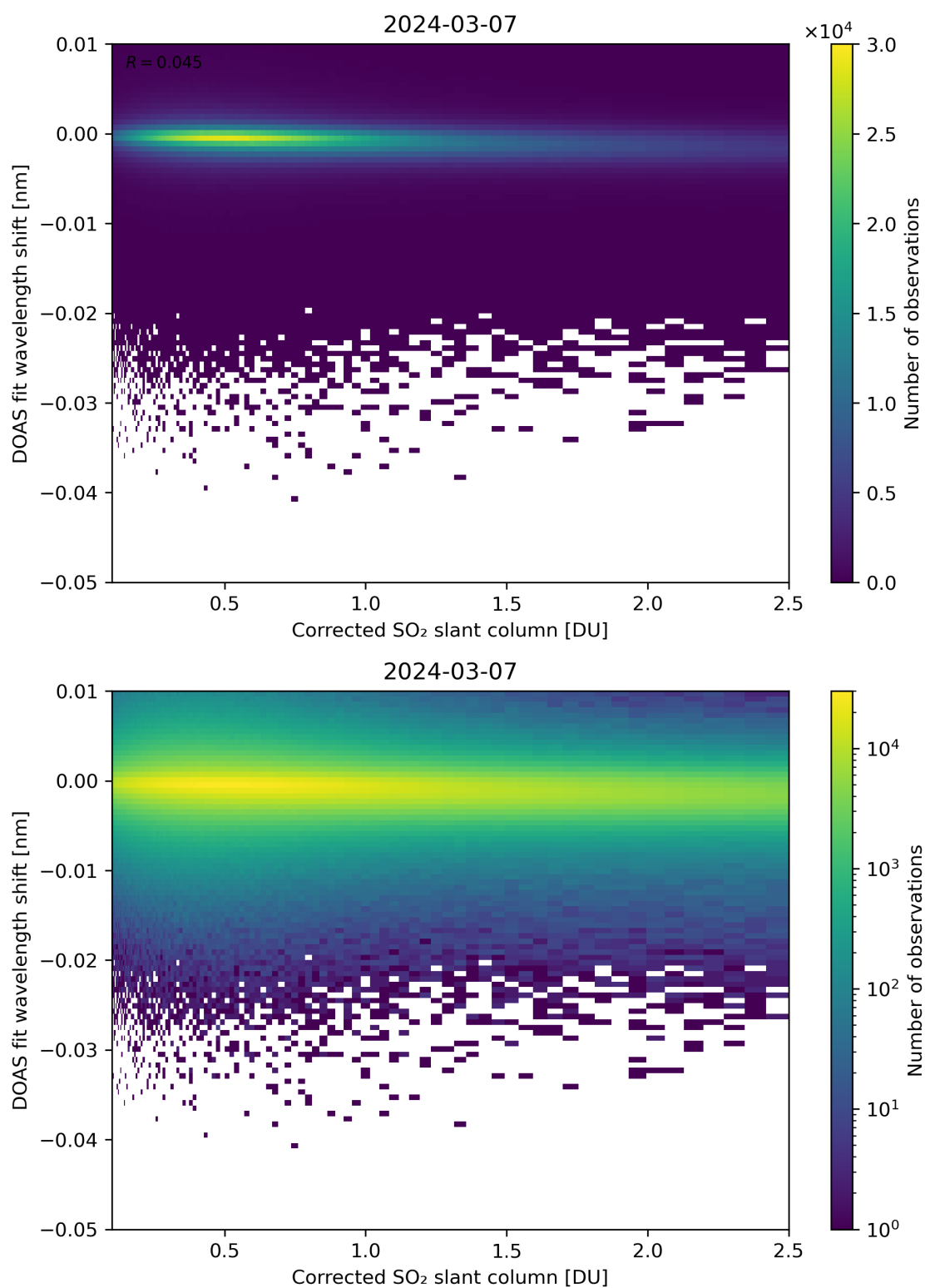
Figure 181: Scatter density plot of “Corrected SO 2 slant column” against “DOAS fit wavelength shift” for 2024-03-06 to 2024-03-08.
