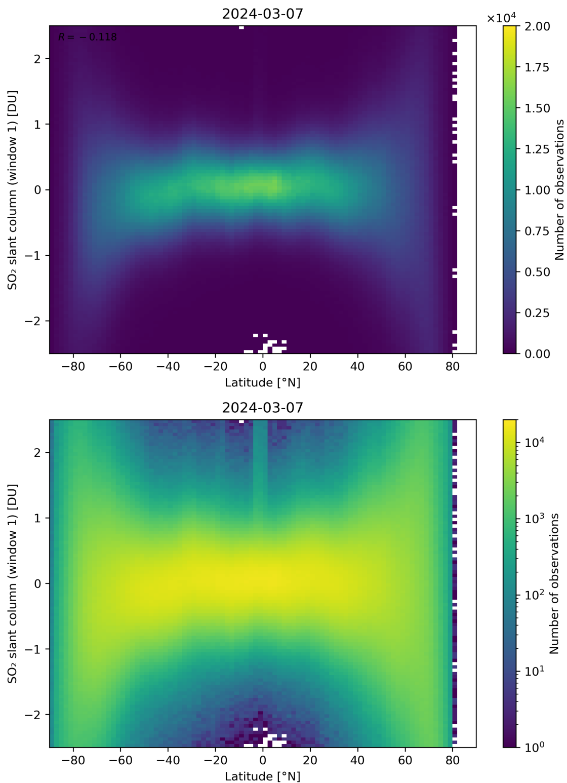
Figure 149: Scatter density plot of “Latitude” against “SO 2 slant column (window 1)” for 2024-03-06 to 2024-03-08.
