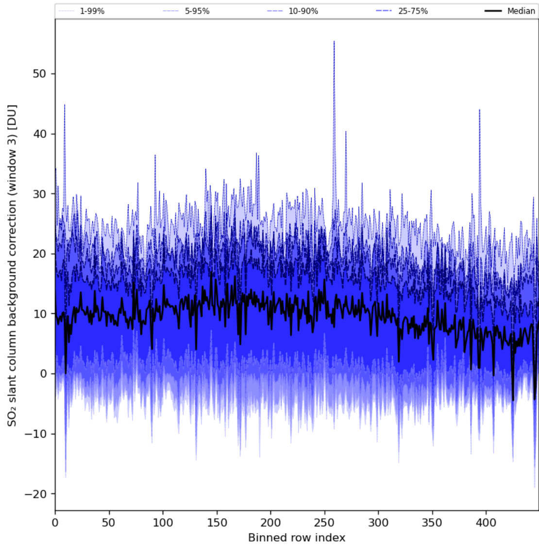
Figure 90: Along track statistics of “SO 2 slant column background correction (window 3)” for 2024-03-06 to 2024-03-08
