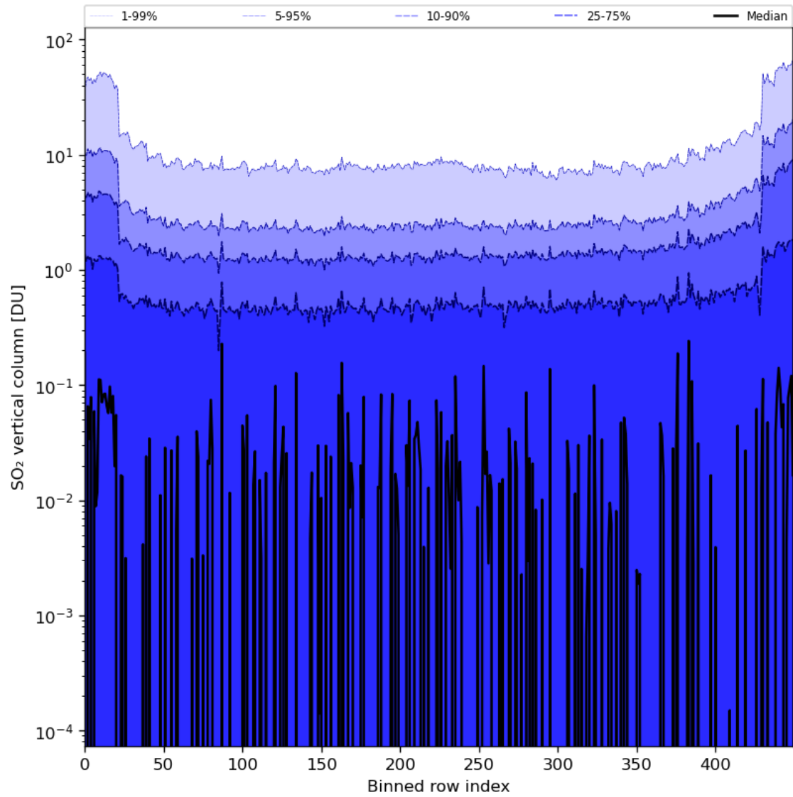
Figure 76: Along track statistics of “SO 2 vertical column” for 2024-03-06 to 2024-03-08
