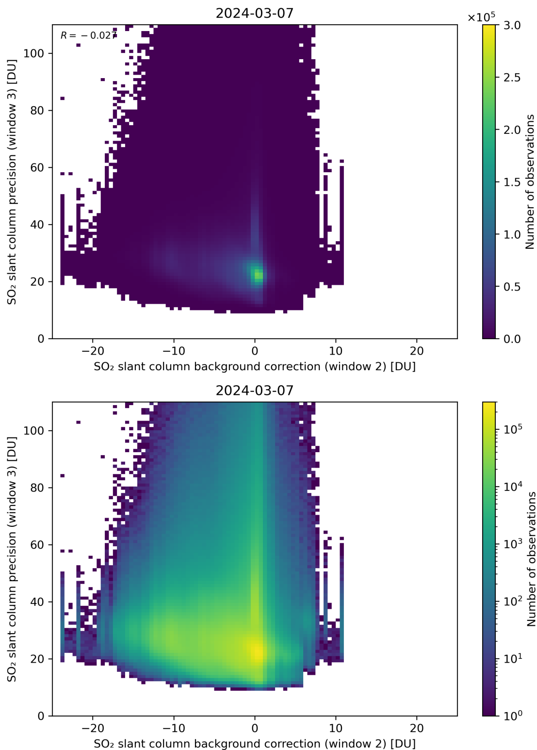
Figure 118: Scatter density plot of “SO 2 slant column background correction (window 2)” against “SO 2 slant column precision (window 3)” for 2024-03-06 to 2024-03-08.
