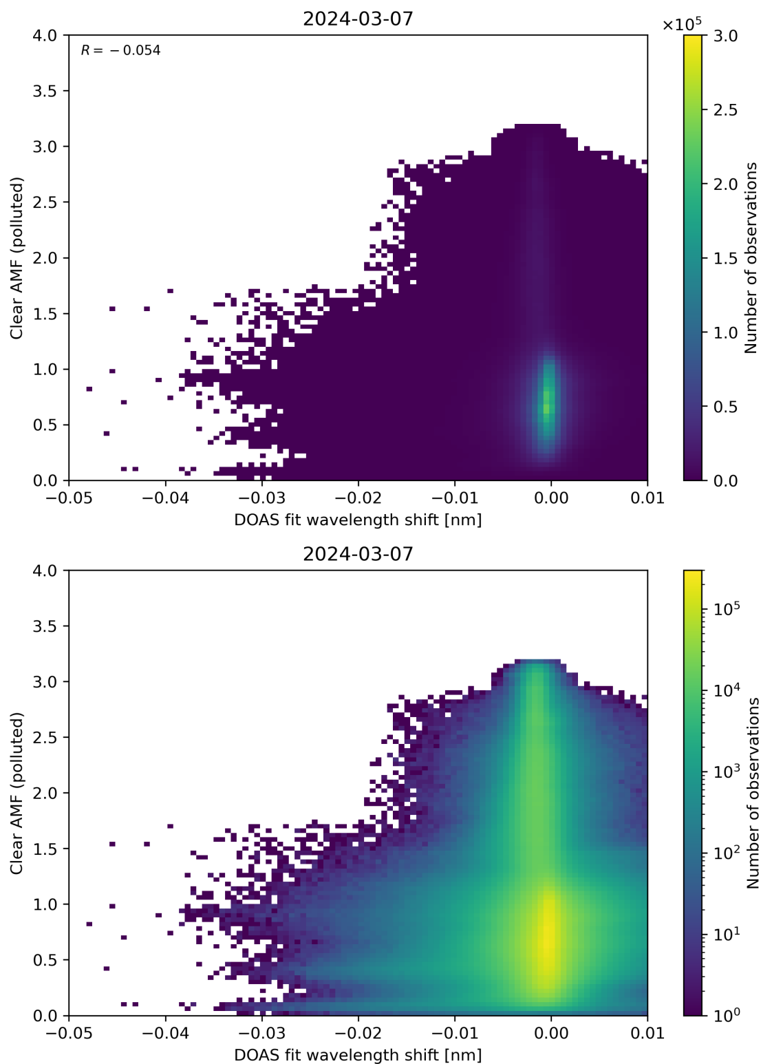
Figure 129: Scatter density plot of “DOAS fit wavelength shift” against “Clear AMF (polluted)” for 2024-03-06 to 2024-03-08.
