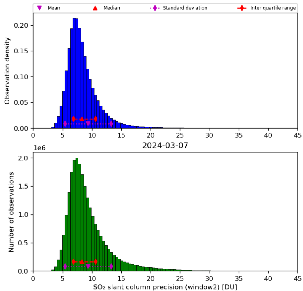
Figure 61: Histogram of “SO 2 slant column precision (window2)” for 2024-03-06 to 2024-03-08
