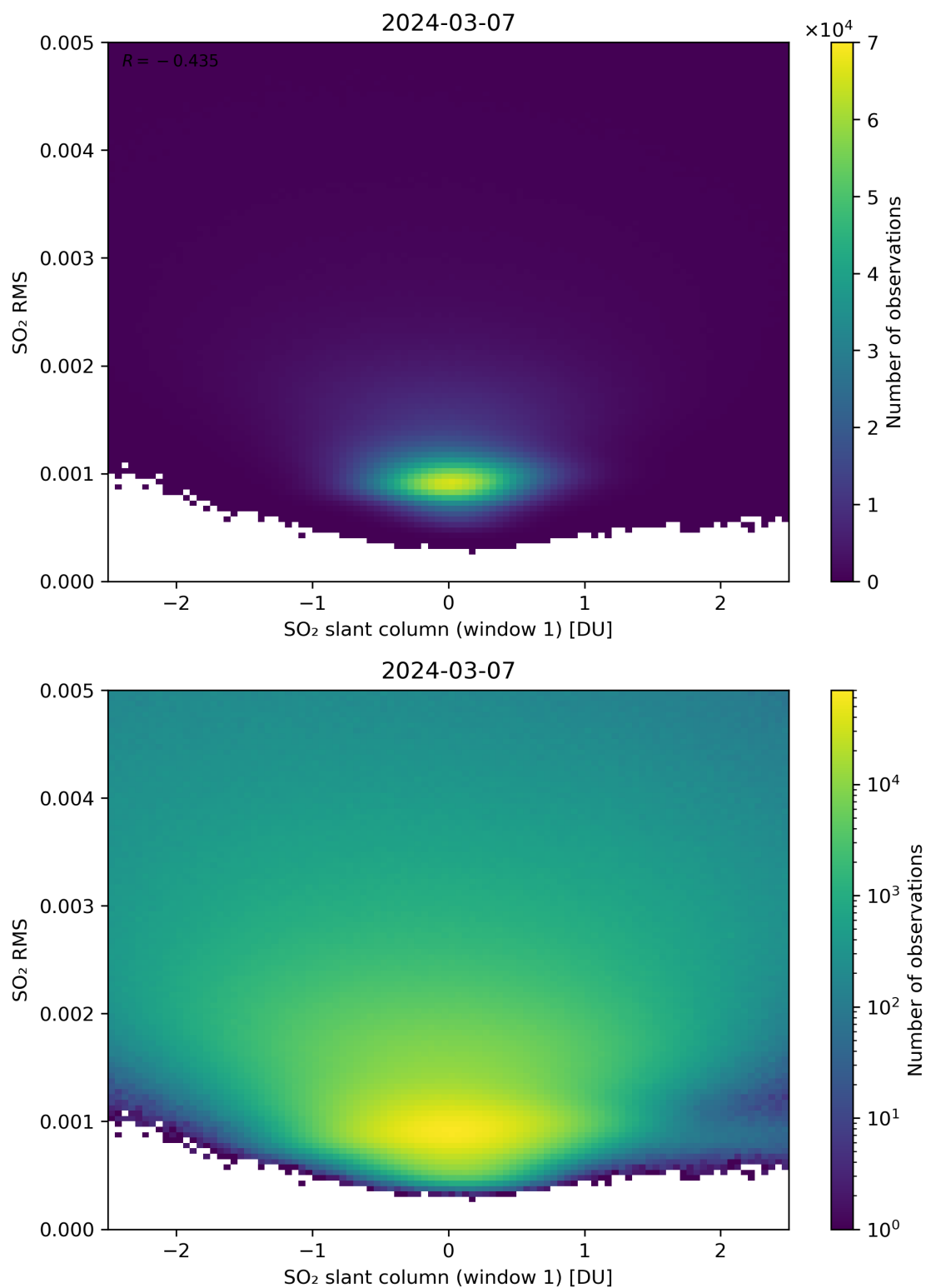
Figure 217: Scatter density plot of “SO 2 slant column (window 1)” against “SO 2 RMS” for 2024-03-06 to 2024-03-08.
