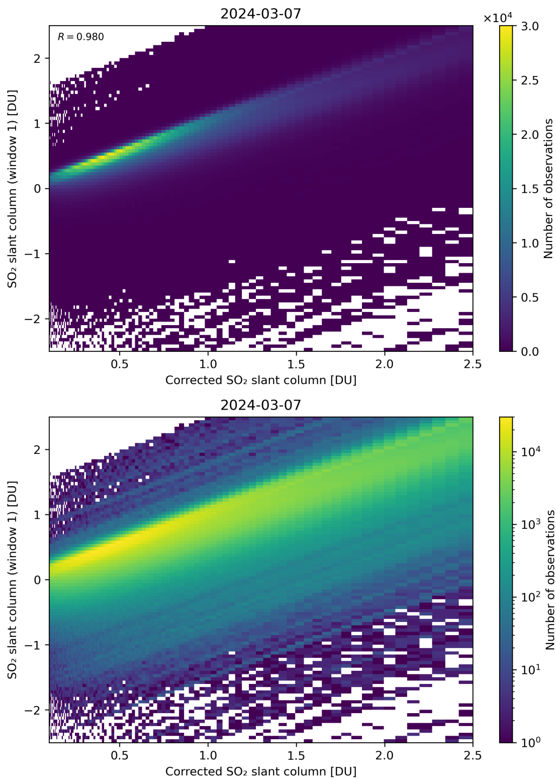
Figure 187: Scatter density plot of “Corrected SO 2 slant column” against “SO 2 slant column (window 1)” for 2024-03-06 to 2024-03-08.
