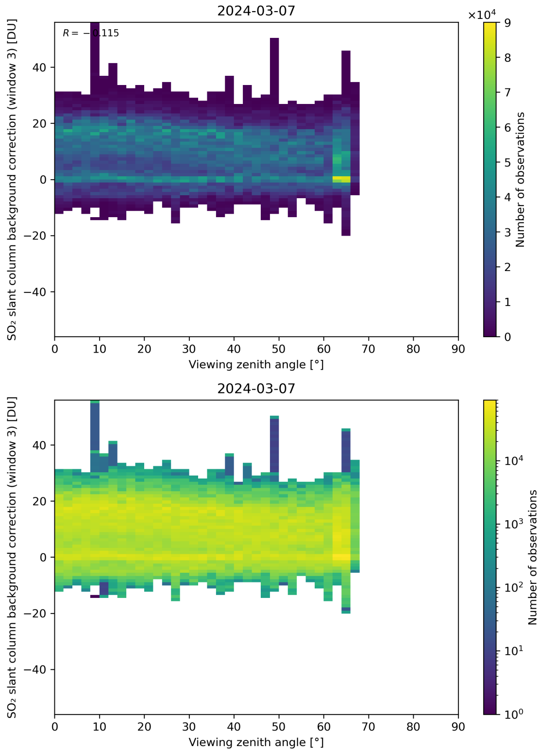
Figure 310: Scatter density plot of “Viewing zenith angle” against “SO 2 slant column background correction (window 3)” for 2024-03-06 to 2024-03-08.
