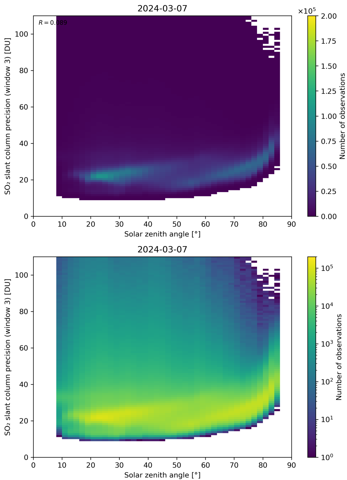
Figure 173: Scatter density plot of “Solar zenith angle” against “SO 2 slant column precision (window 3)” for 2024-03-06 to 2024-03-08.
