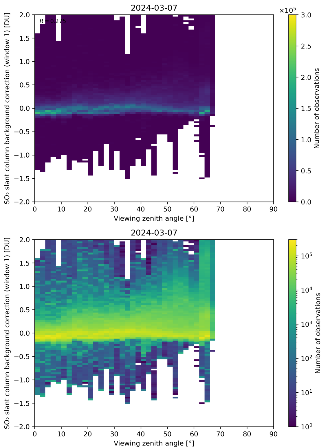
Figure 308: Scatter density plot of “Viewing zenith angle” against “SO 2 slant column background correction (window 1)” for 2024-03-06 to 2024-03-08.
