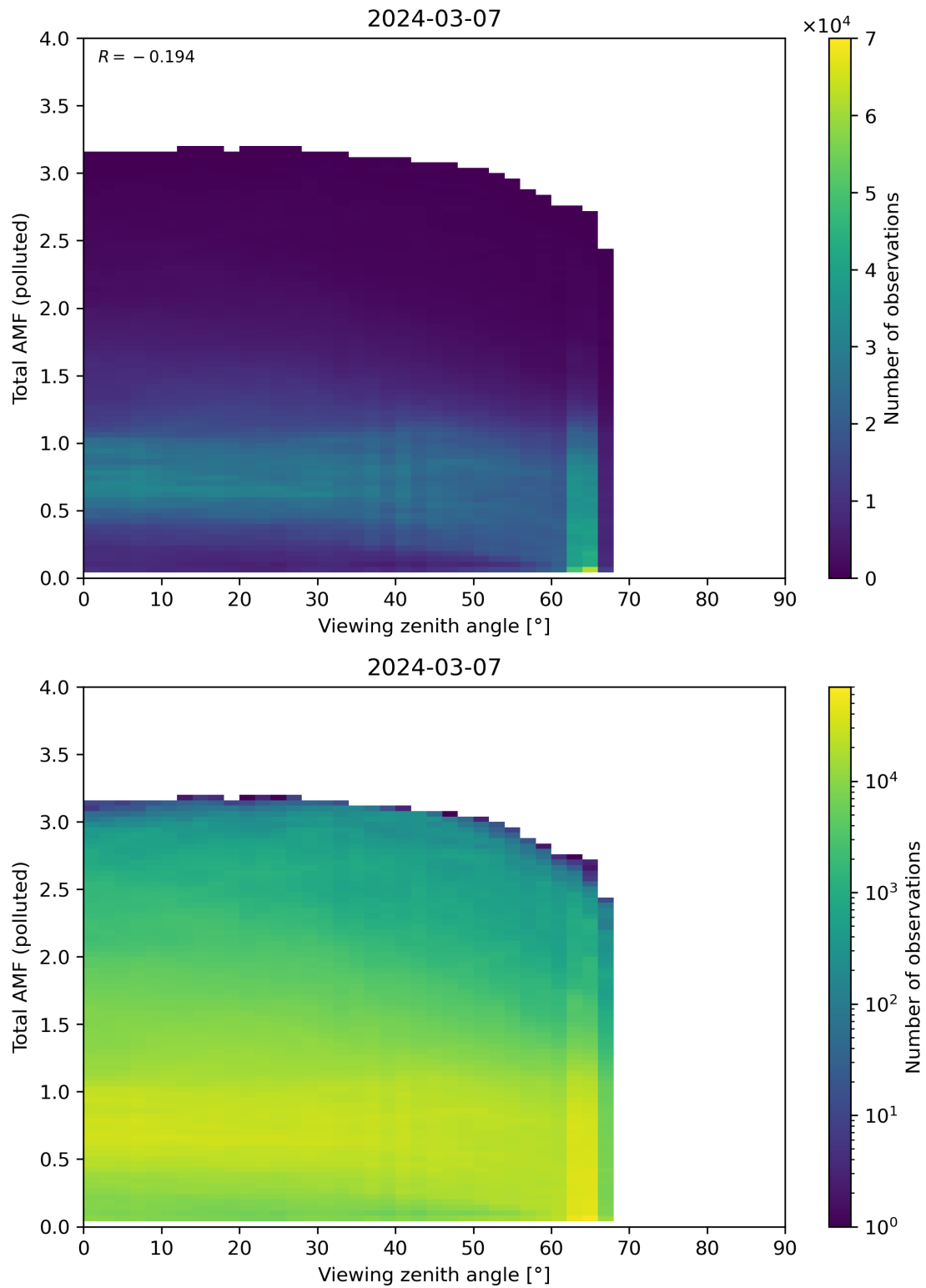
Figure 325: Scatter density plot of “Viewing zenith angle” against “Total AMF (polluted)” for 2024-03-06 to 2024-03-08.
