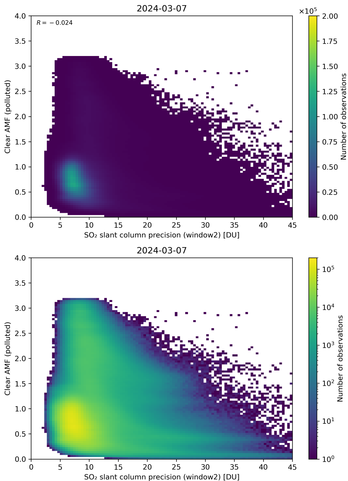
Figure 246: Scatter density plot of “SO 2 slant column precision (window2)” against “Clear AMF (polluted)” for 2024-03-06 to 2024-03-08.
