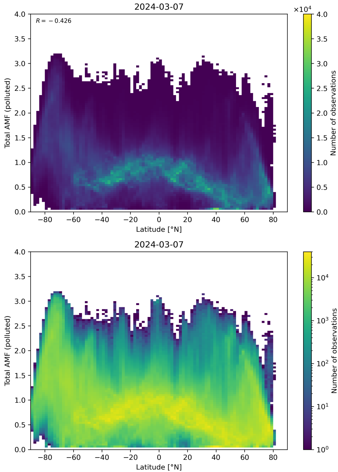
Figure 154: Scatter density plot of “Latitude” against “Total AMF (polluted)” for 2024-03-06 to 2024-03-08.
