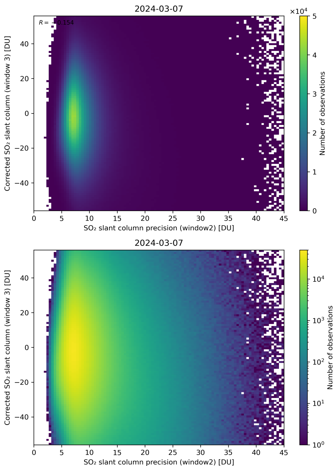
Figure 248: Scatter density plot of “SO 2 slant column precision (window2)” against “Corrected SO 2 slant column (window 3)” for 2024-03-06 to 2024-03-08.
