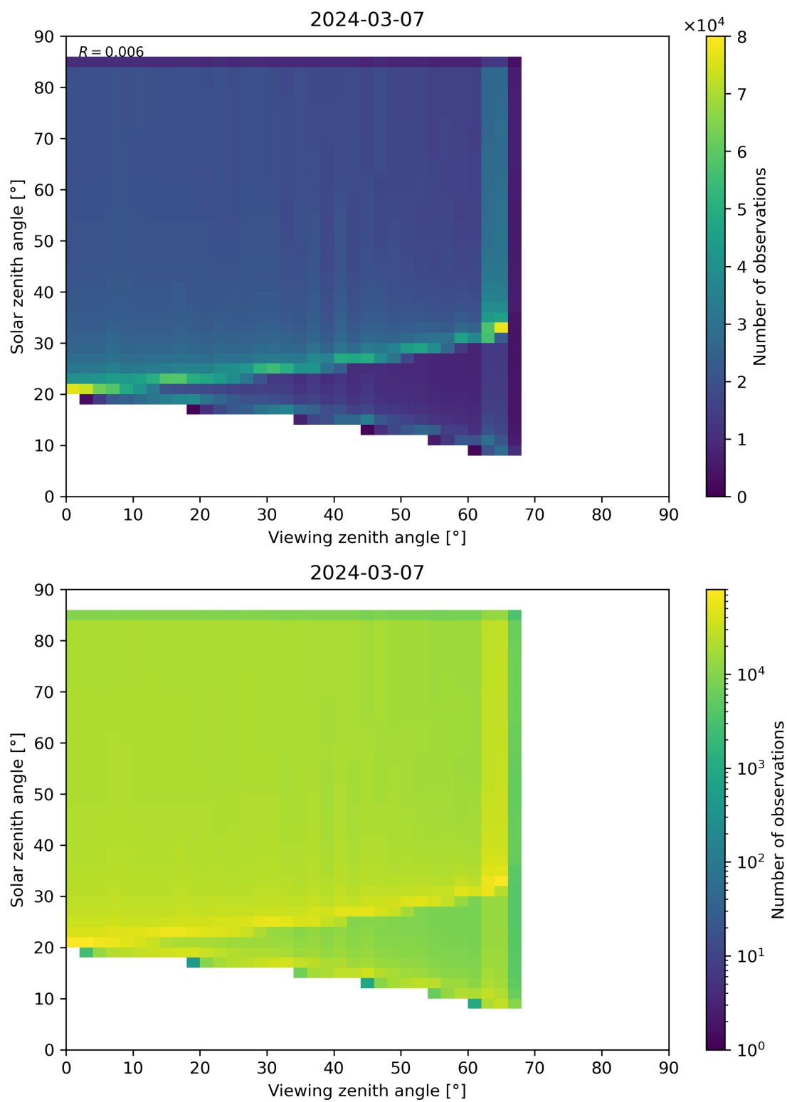
Figure 315: Scatter density plot of “Viewing zenith angle” against “Solar zenith angle” for 2024-03-06 to 2024-03-08.
