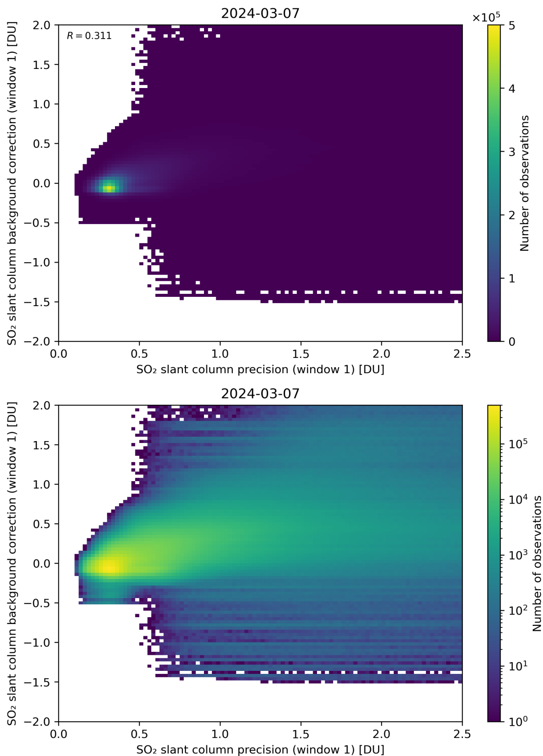
Figure 218: Scatter density plot of “SO 2 slant column precision (window 1)” against “SO 2 slant column background correction (window 1)” for 2024-03-06 to 2024-03-08.
