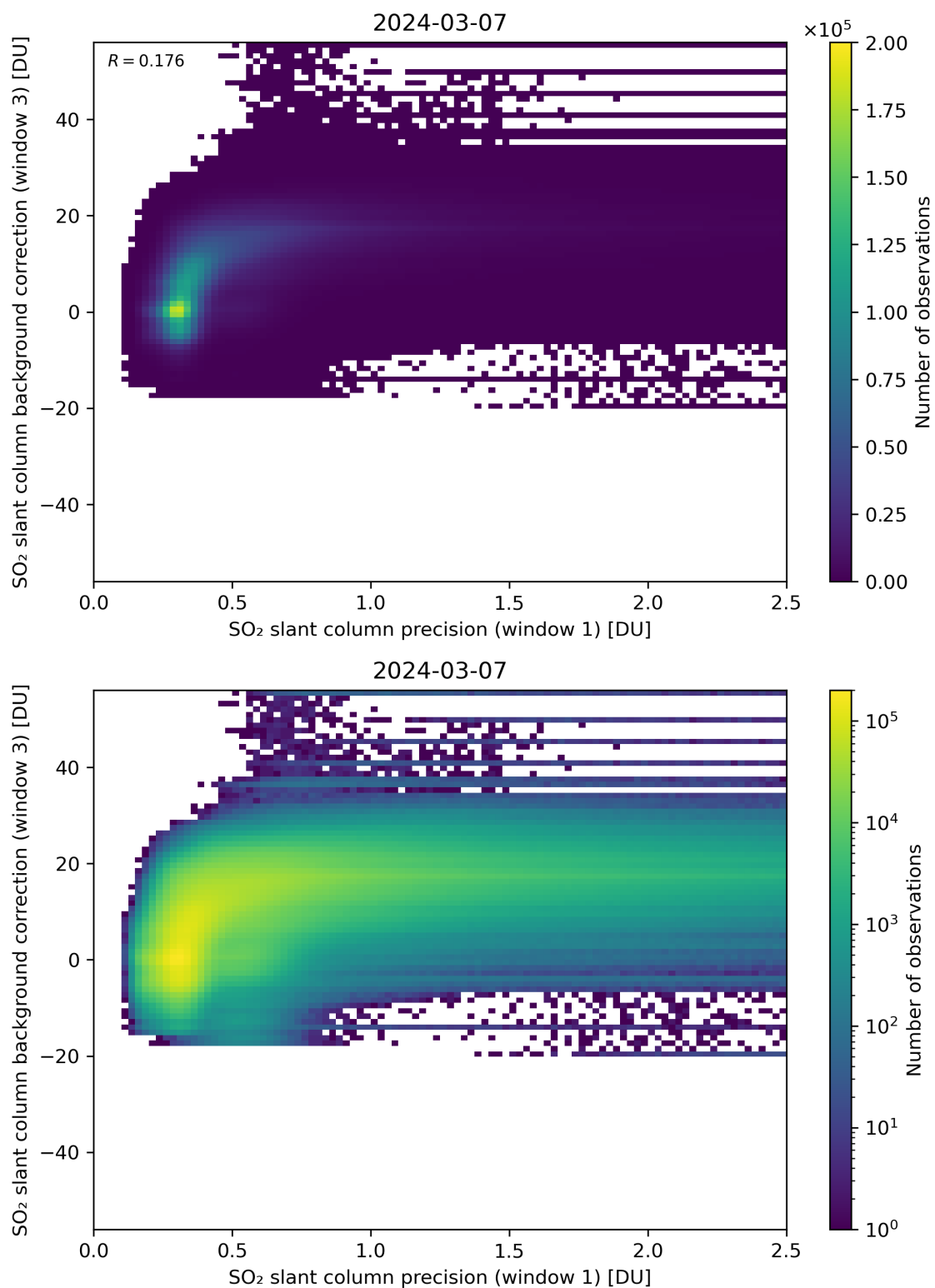
Figure 220: Scatter density plot of “SO 2 slant column precision (window 1)” against “SO 2 slant column background correction (window 3)” for 2024-03-06 to 2024-03-08.
