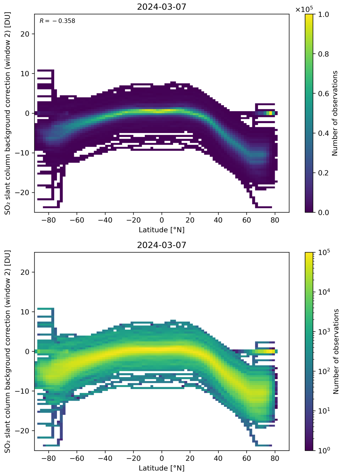
Figure 140: Scatter density plot of “Latitude” against “SO 2 slant column background correction (window 2)” for 2024-03-06 to 2024-03-08.
