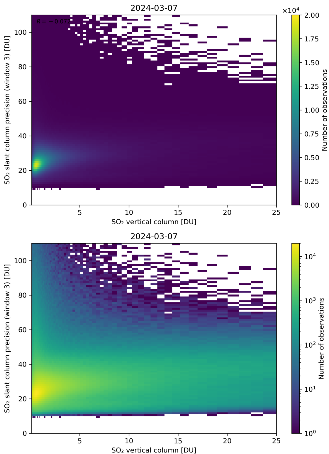
Figure 304: Scatter density plot of “SO 2 vertical column” against “SO 2 slant column precision (window 3)” for 2024-03-06 to 2024-03-08.
