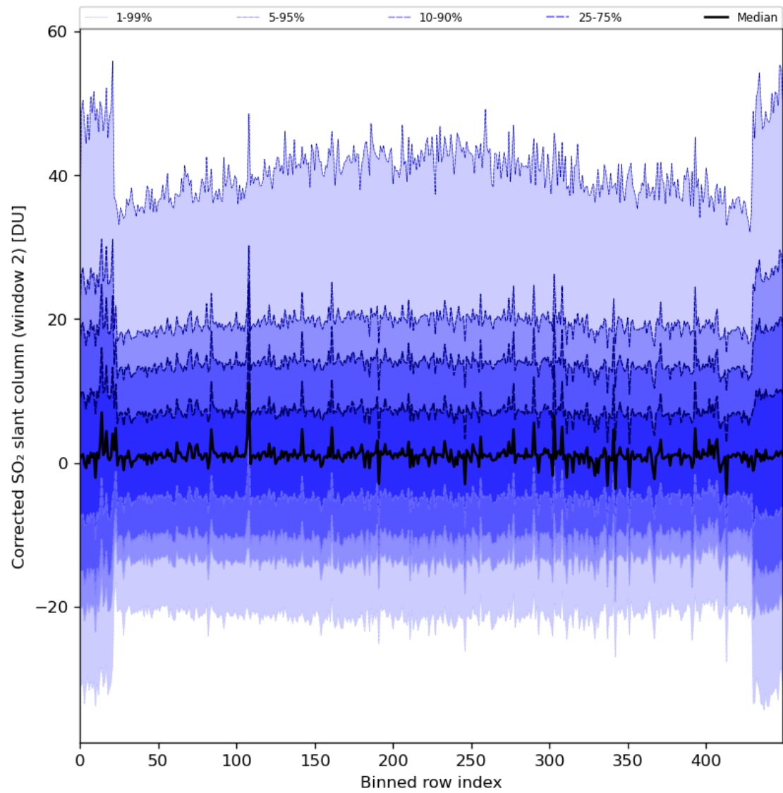
Figure 85: Along track statistics of “Corrected SO 2 slant column (window 2)” for 2024-03-06 to 2024-03-08
