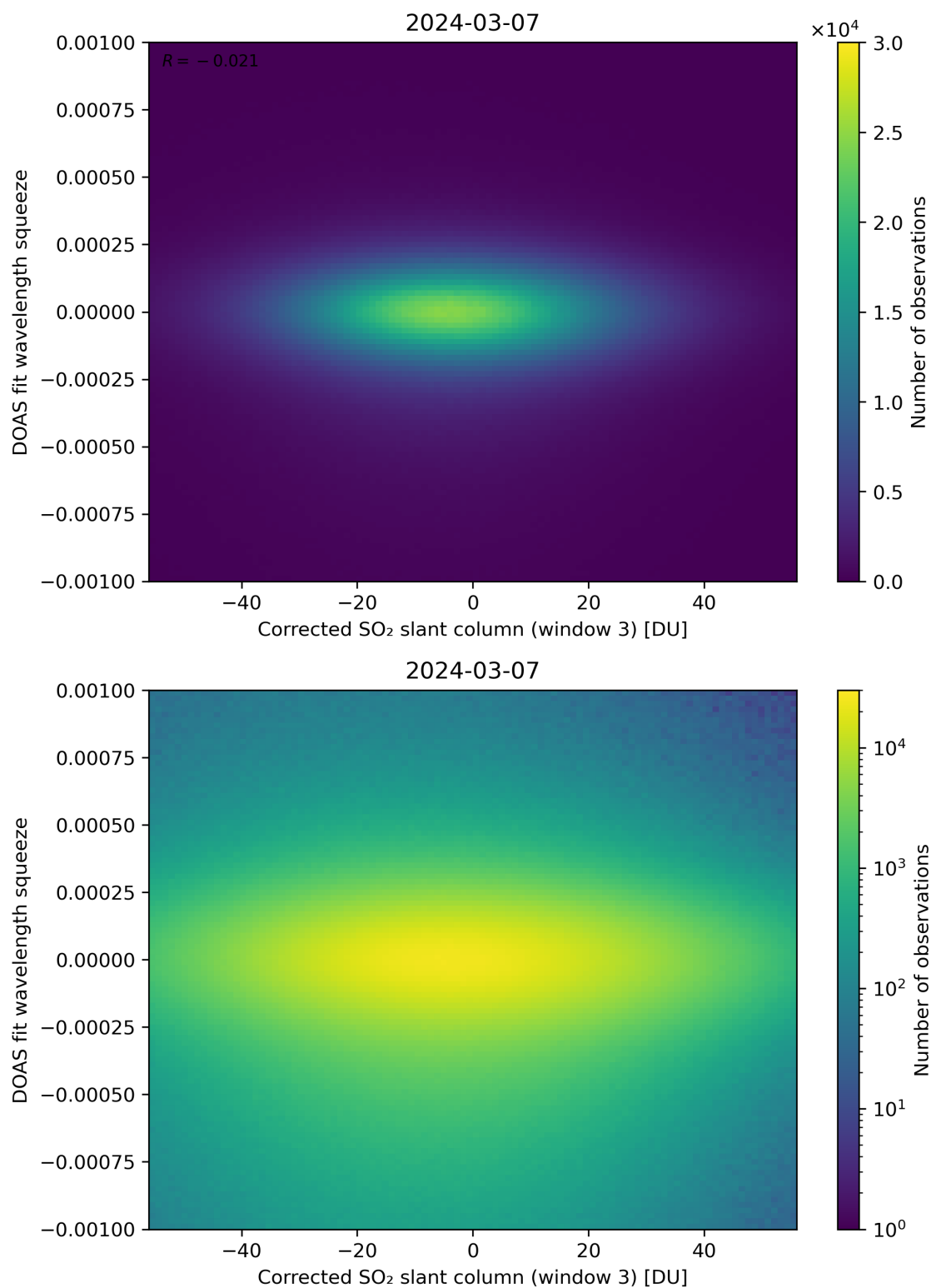
Figure 207: Scatter density plot of “Corrected SO 2 slant column (window 3)” against “DOAS fit wavelength squeeze” for 2024-03-06 to 2024-03-08.
