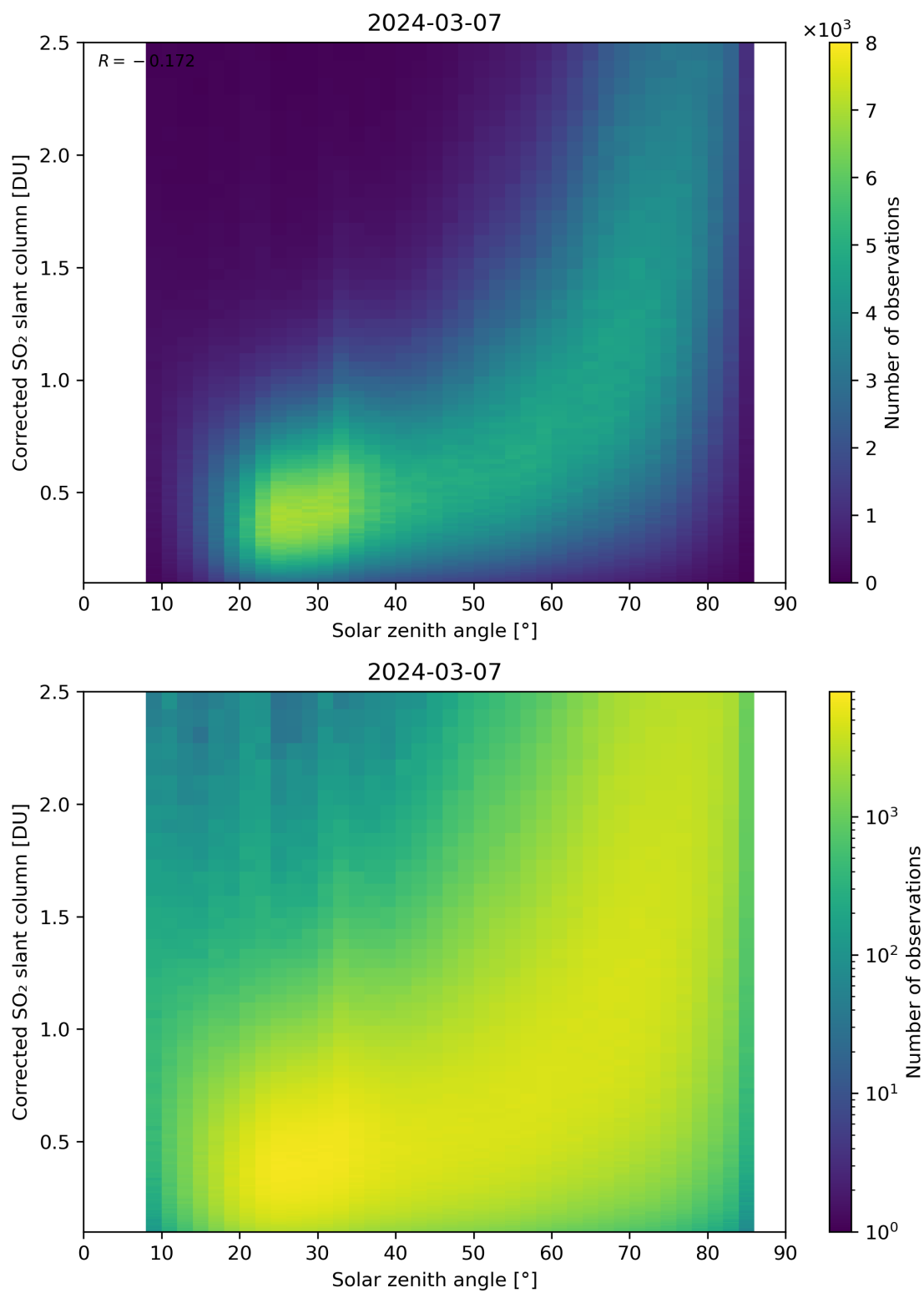
Figure 166: Scatter density plot of “Solar zenith angle” against “Corrected SO 2 slant column” for 2024-03-06 to 2024-03-08.
