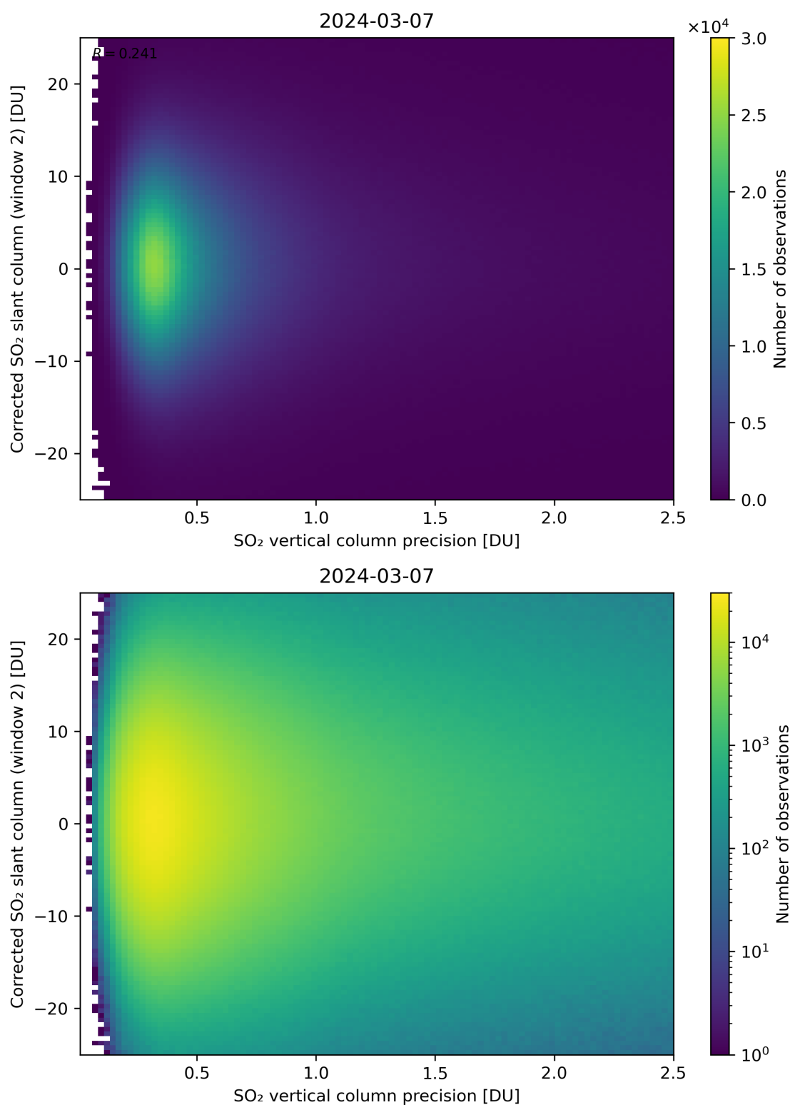
Figure 287: Scatter density plot of “SO 2 vertical column precision” against “Corrected SO 2 slant column (window 2)” for 2024-03-06 to 2024-03-08.
