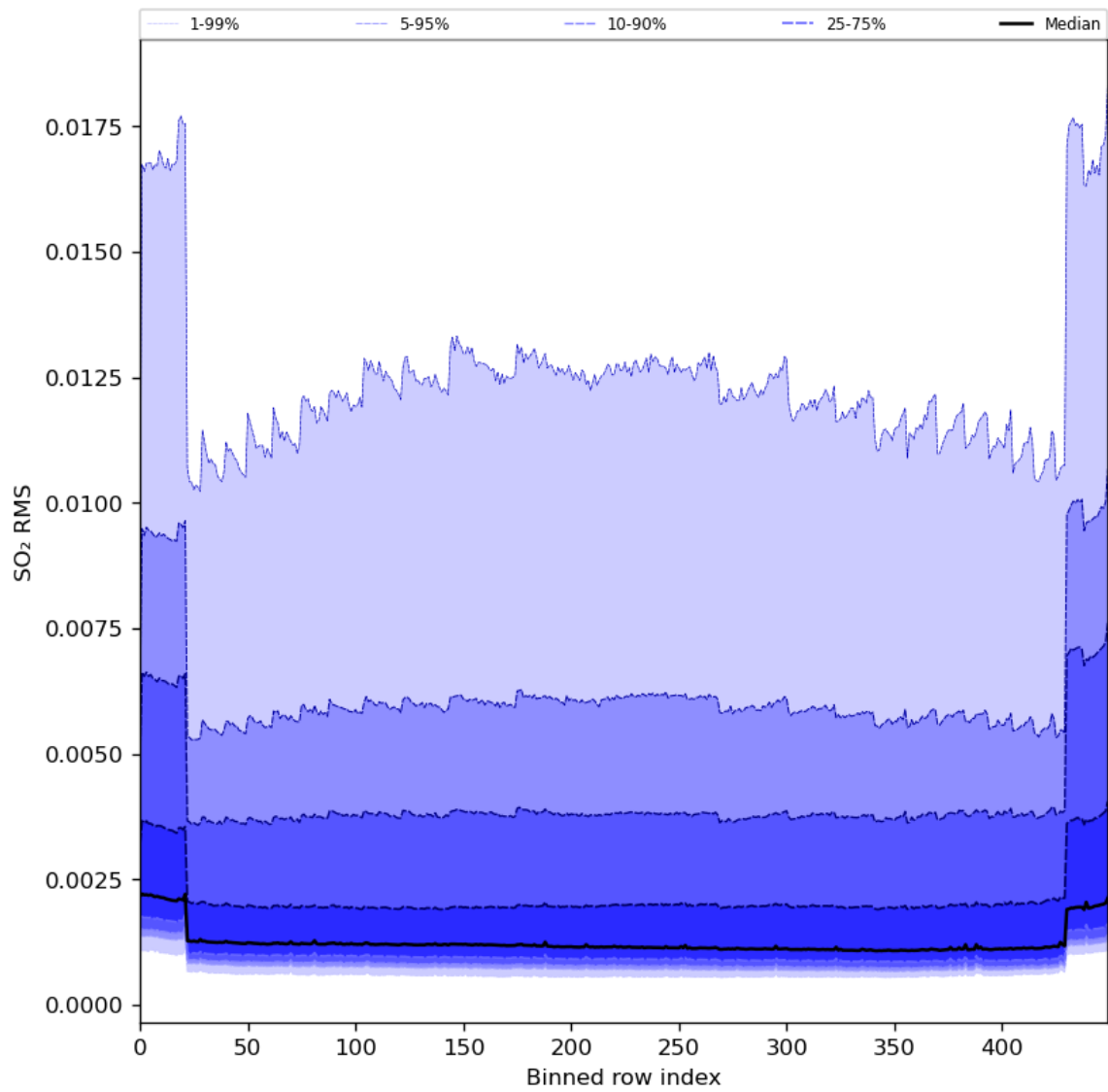
Figure 93: Along track statistics of “SO 2 RMS” for 2024-03-06 to 2024-03-08
