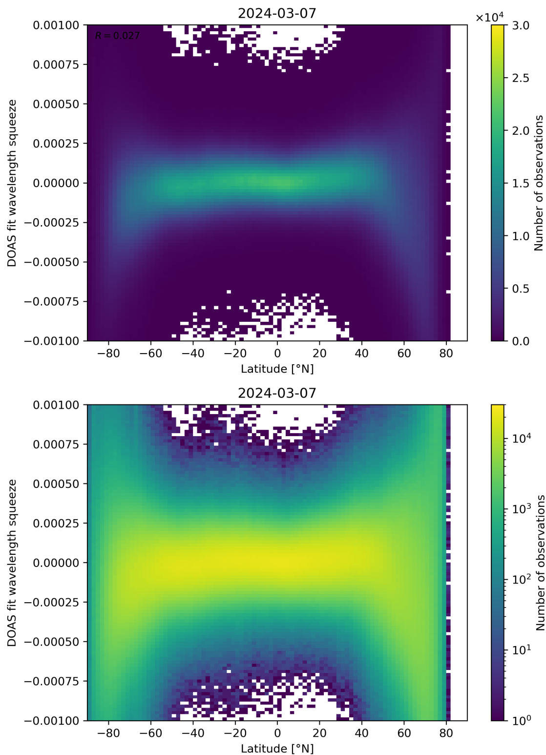
Figure 143: Scatter density plot of “Latitude” against “DOAS fit wavelength squeeze” for 2024-03-06 to 2024-03-08.
