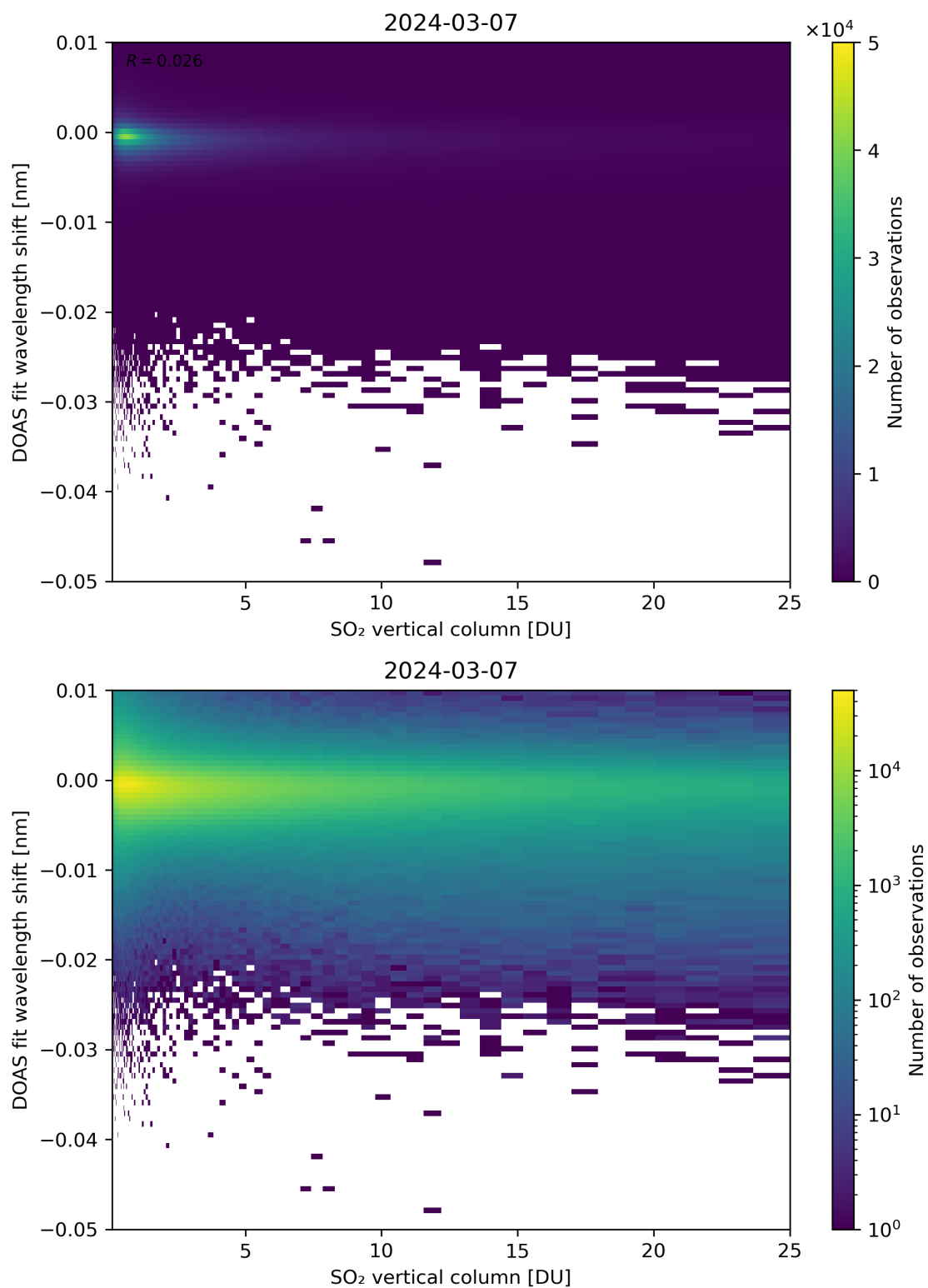
Figure 276: Scatter density plot of “SO 2 vertical column” against “DOAS fit wavelength shift” for 2024-03-06 to 2024-03-08.
