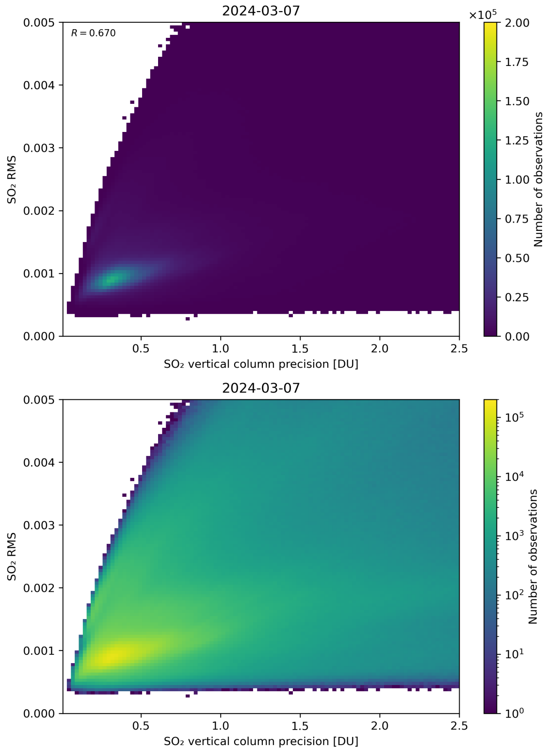
Figure 284: Scatter density plot of “SO 2 vertical column precision” against “SO 2 RMS” for 2024-03-06 to 2024-03-08.
