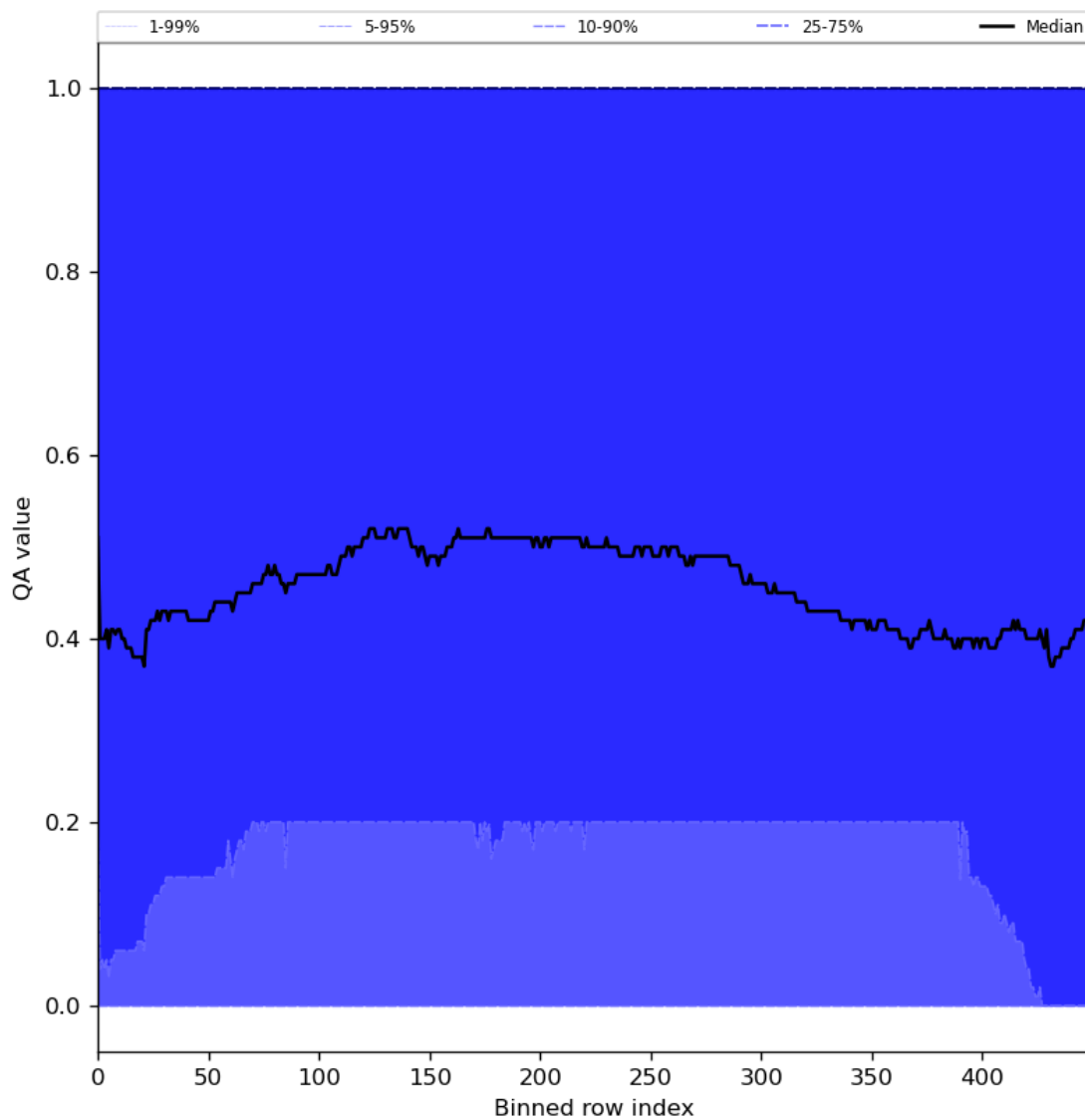
Figure 75: Along track statistics of “QA value” for 2024-03-06 to 2024-03-08
