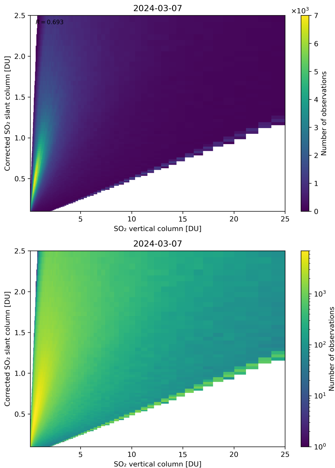
Figure 297: Scatter density plot of “SO 2 vertical column” against “Corrected SO 2 slant column” for 2024-03-06 to 2024-03-08.
