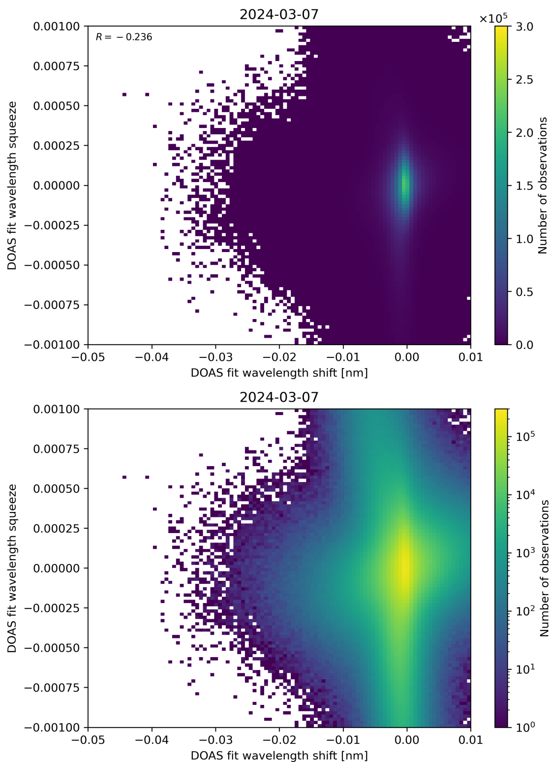
Figure 127: Scatter density plot of “DOAS fit wavelength shift” against “DOAS fit wavelength squeeze” for 2024-03-06 to 2024-03-08.
