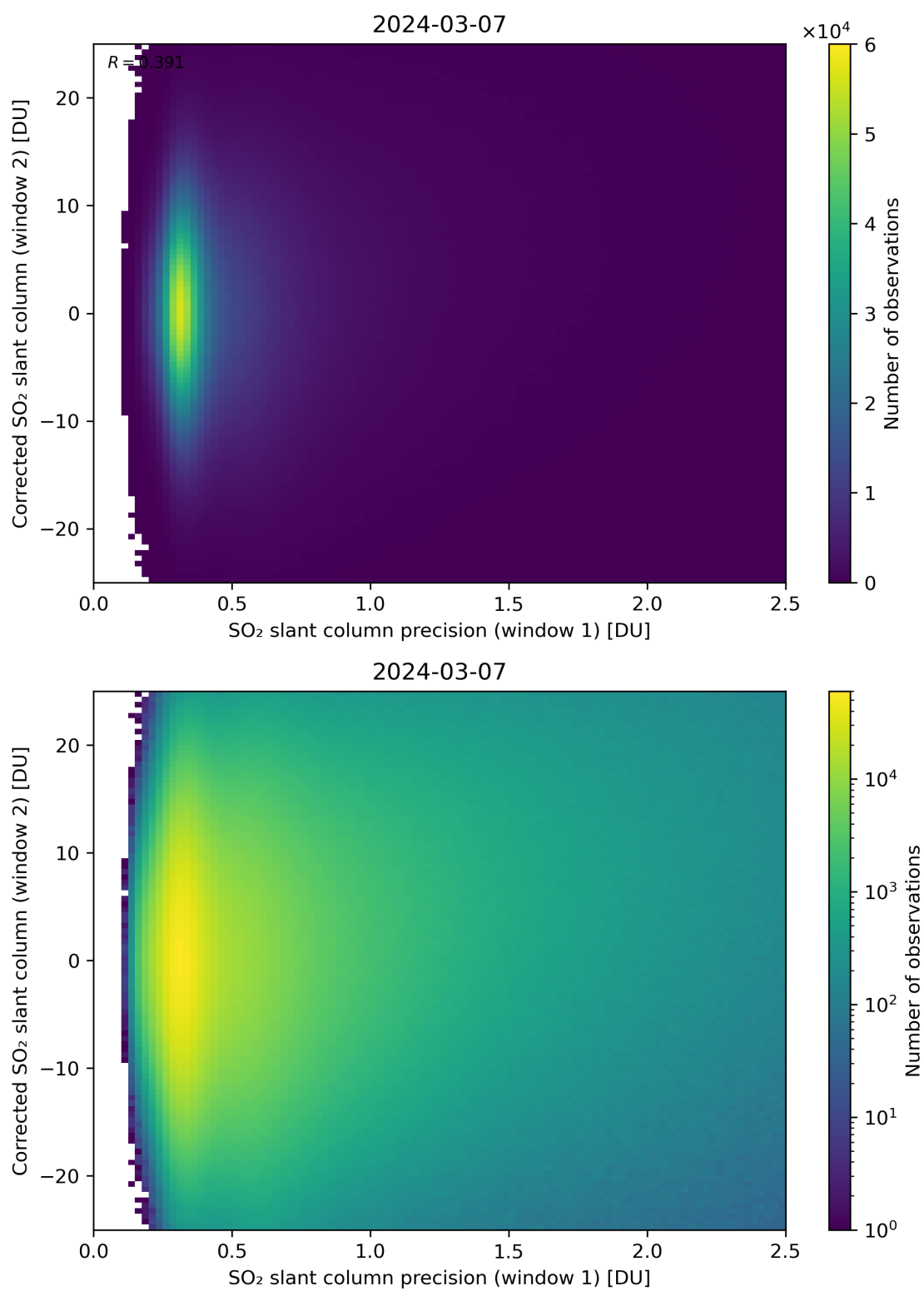
Figure 225: Scatter density plot of “SO 2 slant column precision (window 1)” against “Corrected SO 2 slant column (window 2)” for 2024-03-06 to 2024-03-08.
