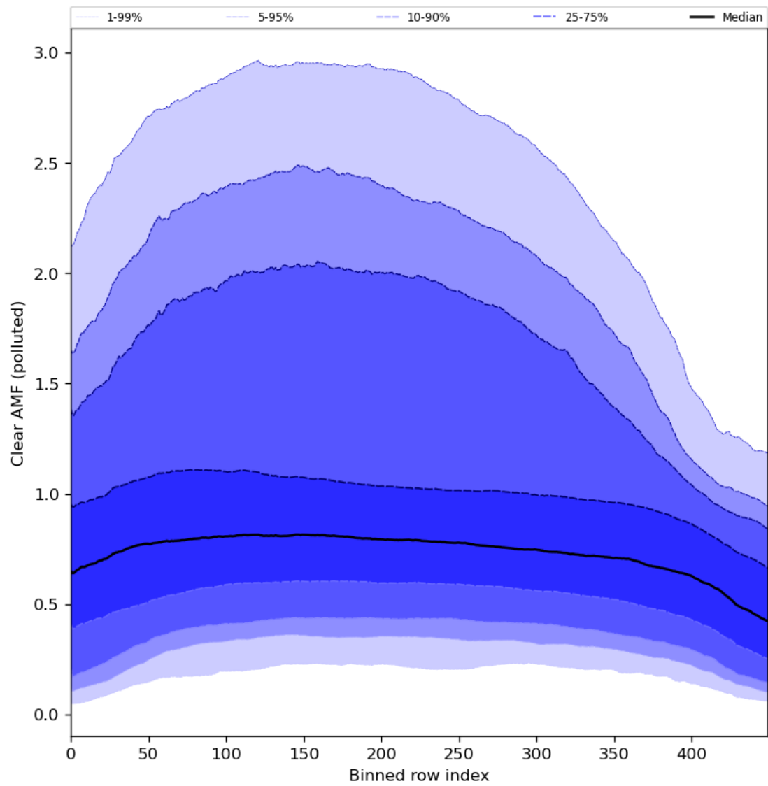
Figure 96: Along track statistics of “Clear AMF (polluted)” for 2024-03-06 to 2024-03-08
