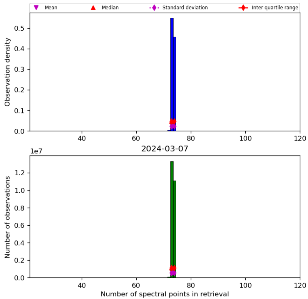
Figure 74: Histogram of “Number of spectral points in retrieval” for 2024-03-06 to 2024-03-08
