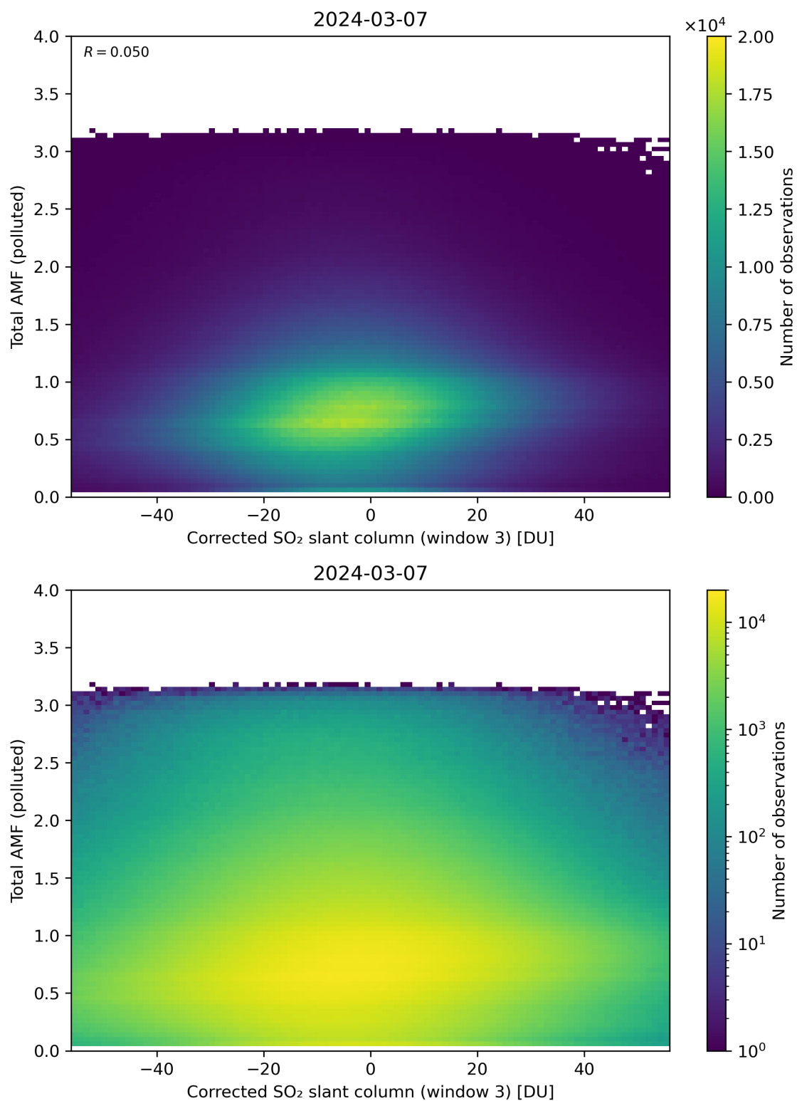
Figure 210: Scatter density plot of “Corrected SO 2 slant column (window 3)” against “Total AMF (polluted)” for 2024-03-06 to 2024-03-08.
