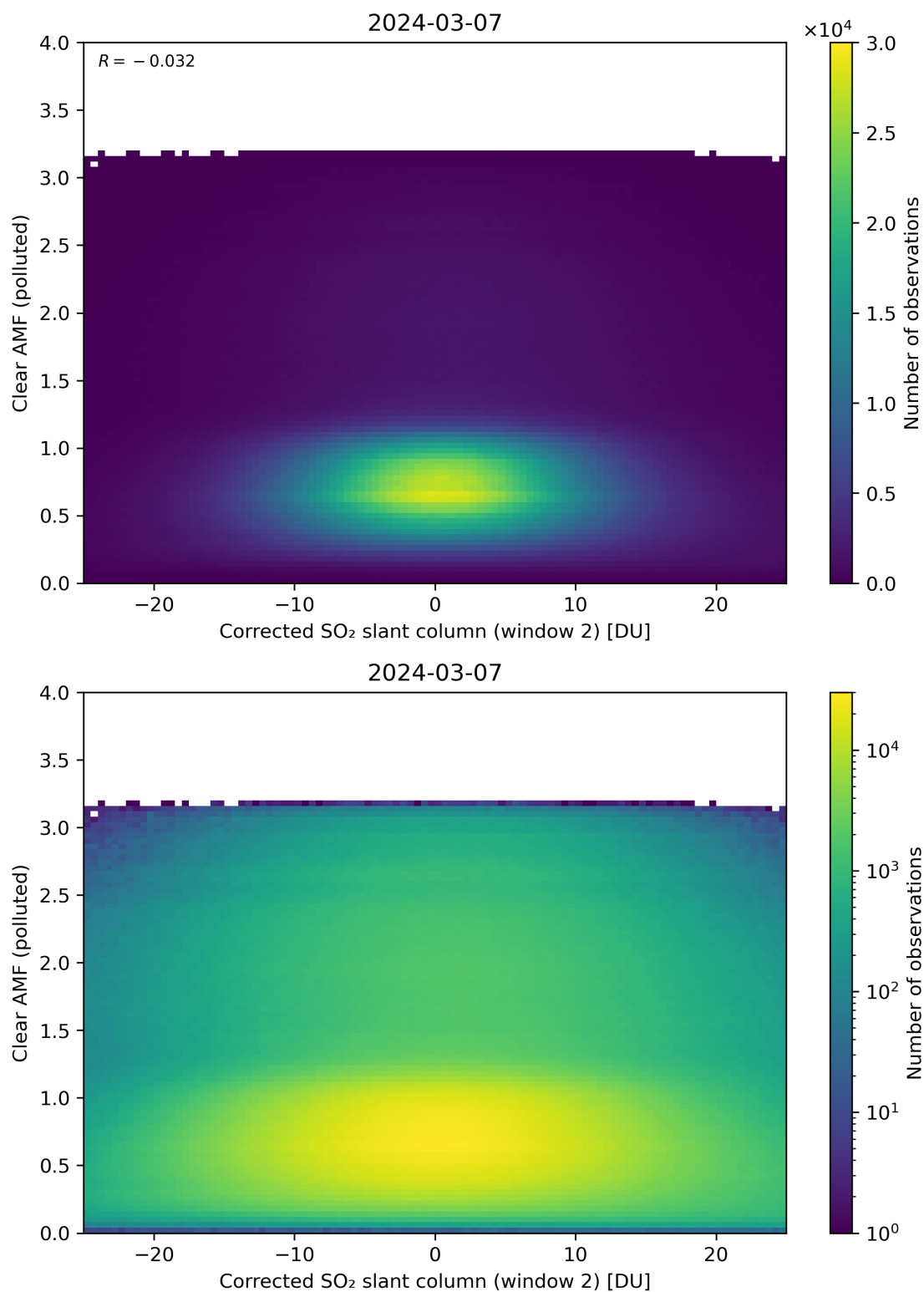
Figure 199: Scatter density plot of “Corrected SO 2 slant column (window 2)” against “Clear AMF (polluted)” for 2024-03-06 to 2024-03-08.
