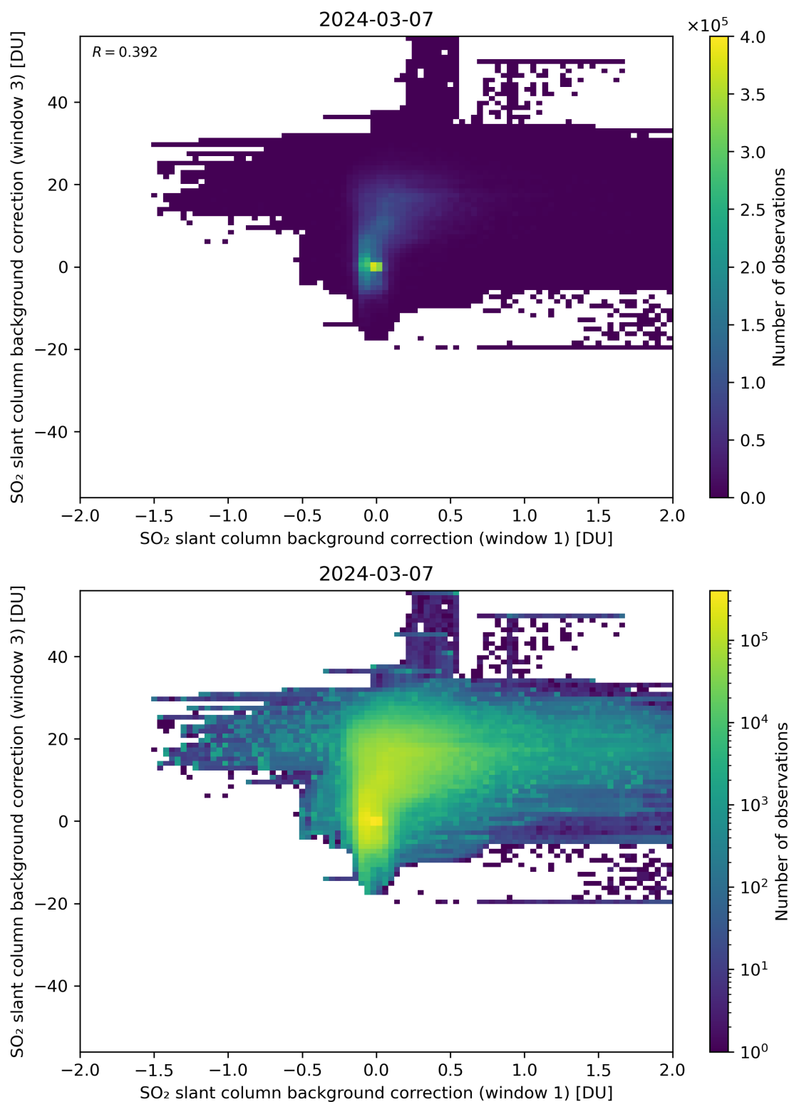
Figure 99: Scatter density plot of “SO 2 slant column background correction (window 1)” against “SO 2 slant column background correction (window 3)” for 2024-03-06 to 2024-03-08.
