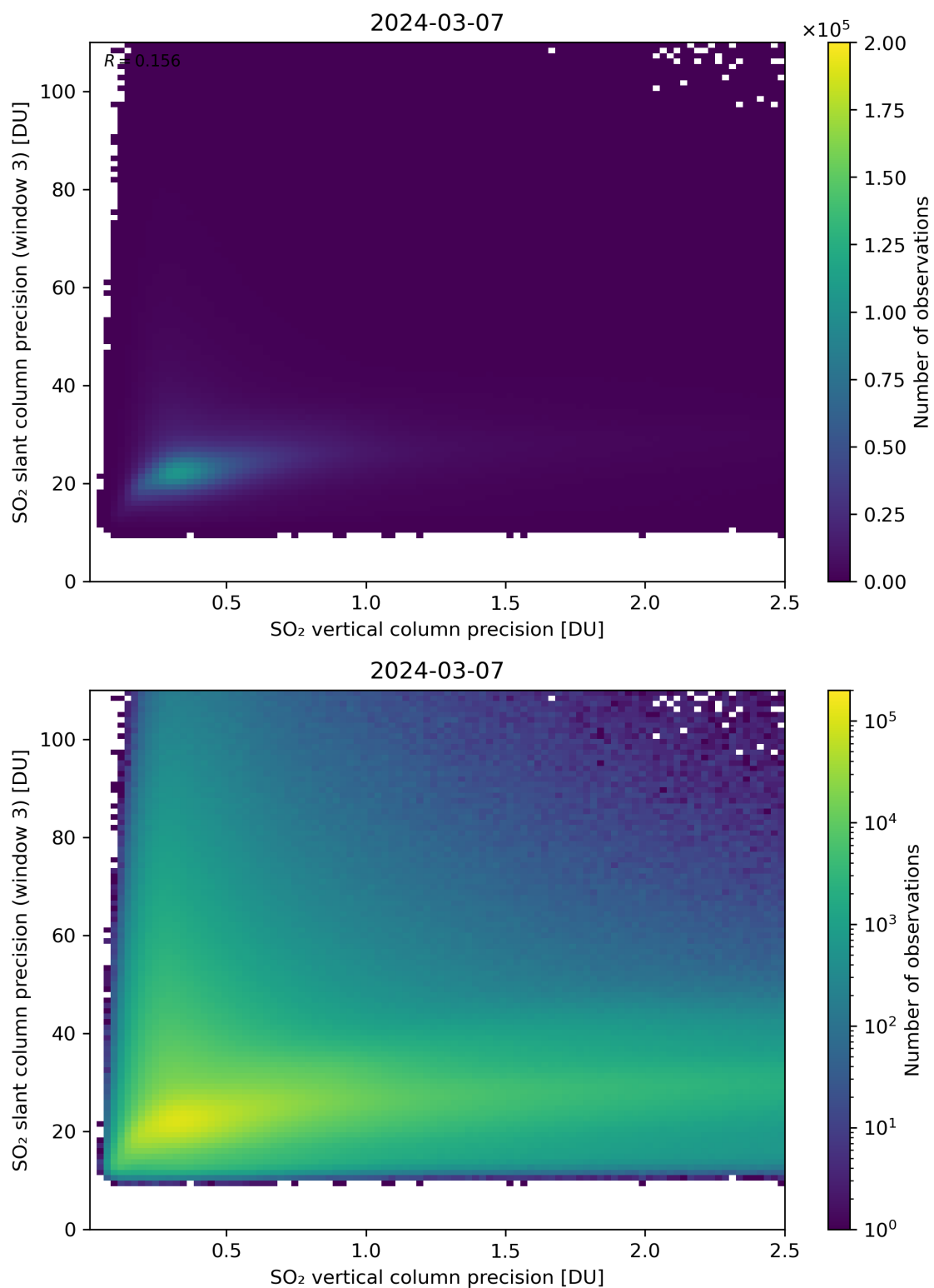
Figure 293: Scatter density plot of “SO 2 vertical column precision” against “SO 2 slant column precision (window 3)” for 2024-03-06 to 2024-03-08.
