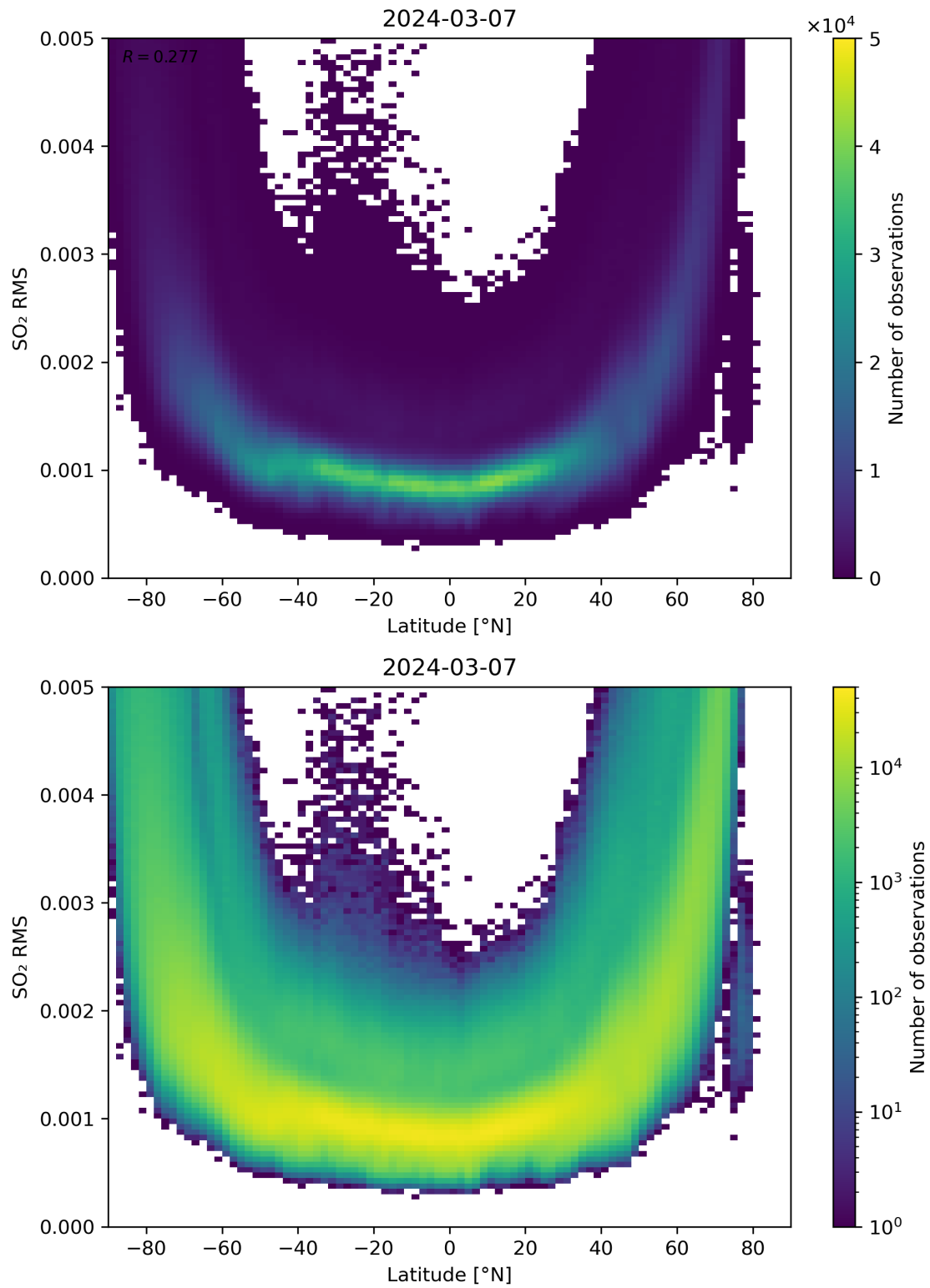
Figure 144: Scatter density plot of “Latitude” against “SO 2 RMS” for 2024-03-06 to 2024-03-08.
