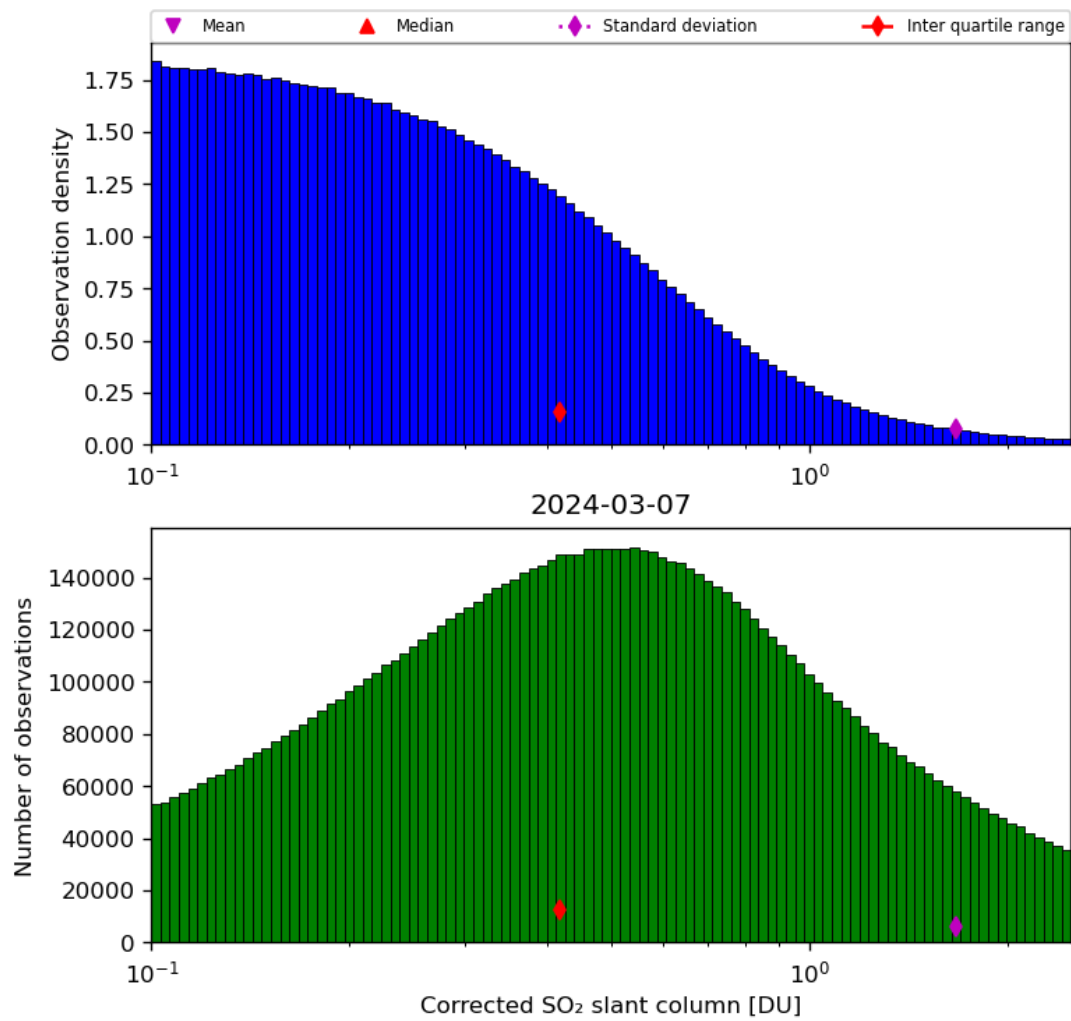
Figure 55: Histogram of “Corrected SO 2 slant column” for 2024-03-06 to 2024-03-08
