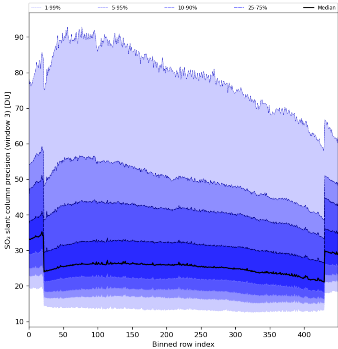
Figure 88: Along track statistics of “SO 2 slant column precision (window 3)” for 2024-03-06 to 2024-03-08
