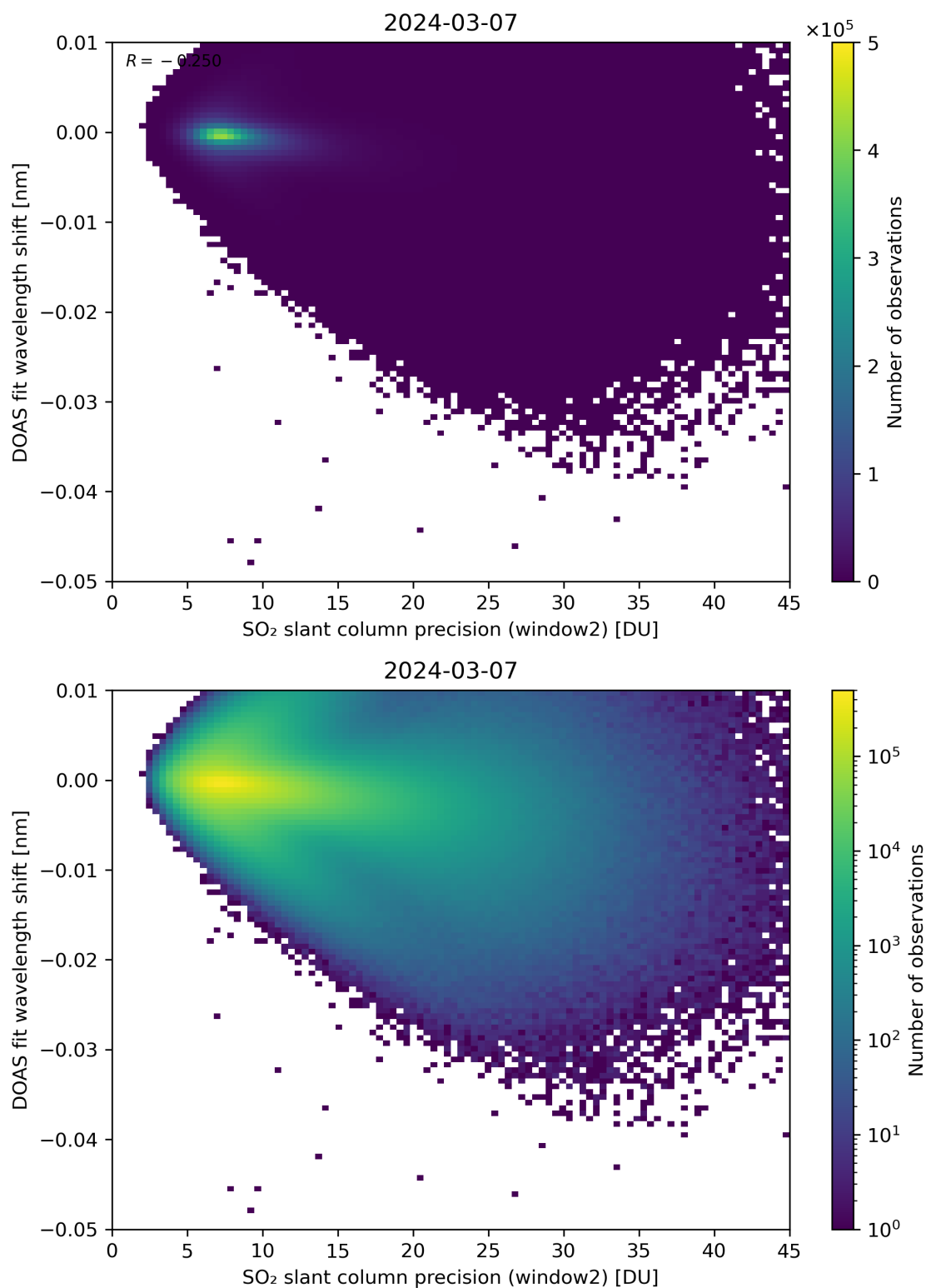
Figure 243: Scatter density plot of “SO 2 slant column precision (window2)” against “DOAS fit wavelength shift” for 2024-03-06 to 2024-03-08.
