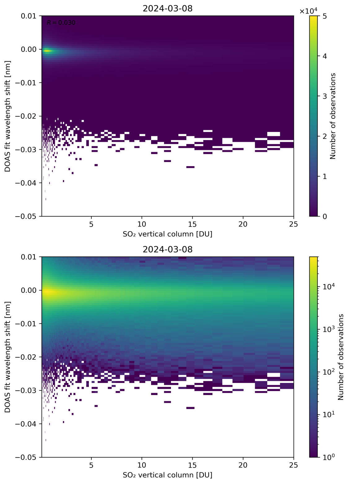
Figure 276: Scatter density plot of “SO 2 vertical column” against “DOAS fit wavelength shift” for 2024-03-07 to 2024-03-09.
