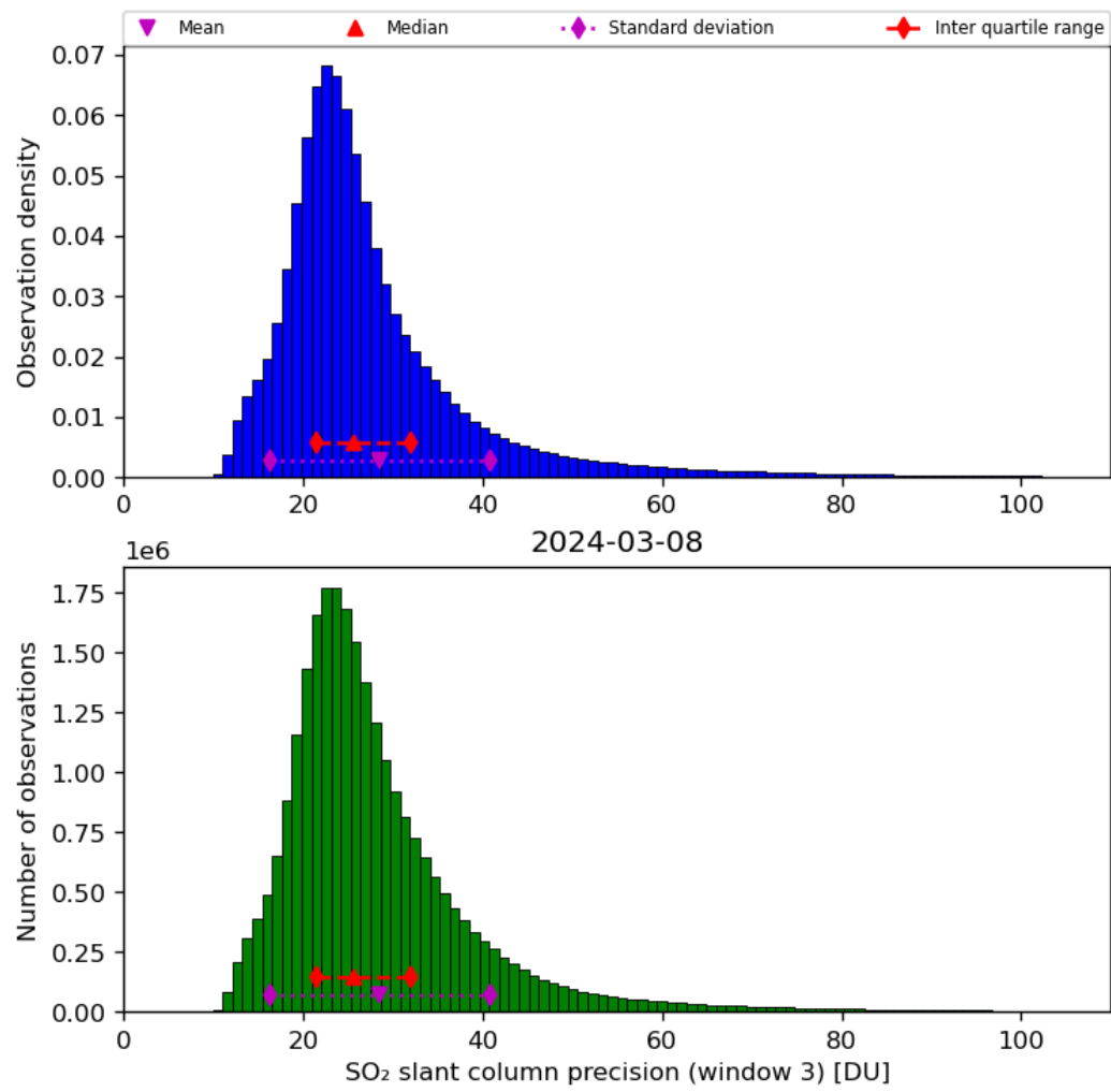
Figure 65: Histogram of “SO 2 slant column precision (window 3)” for 2024-03-07 to 2024-03-09
