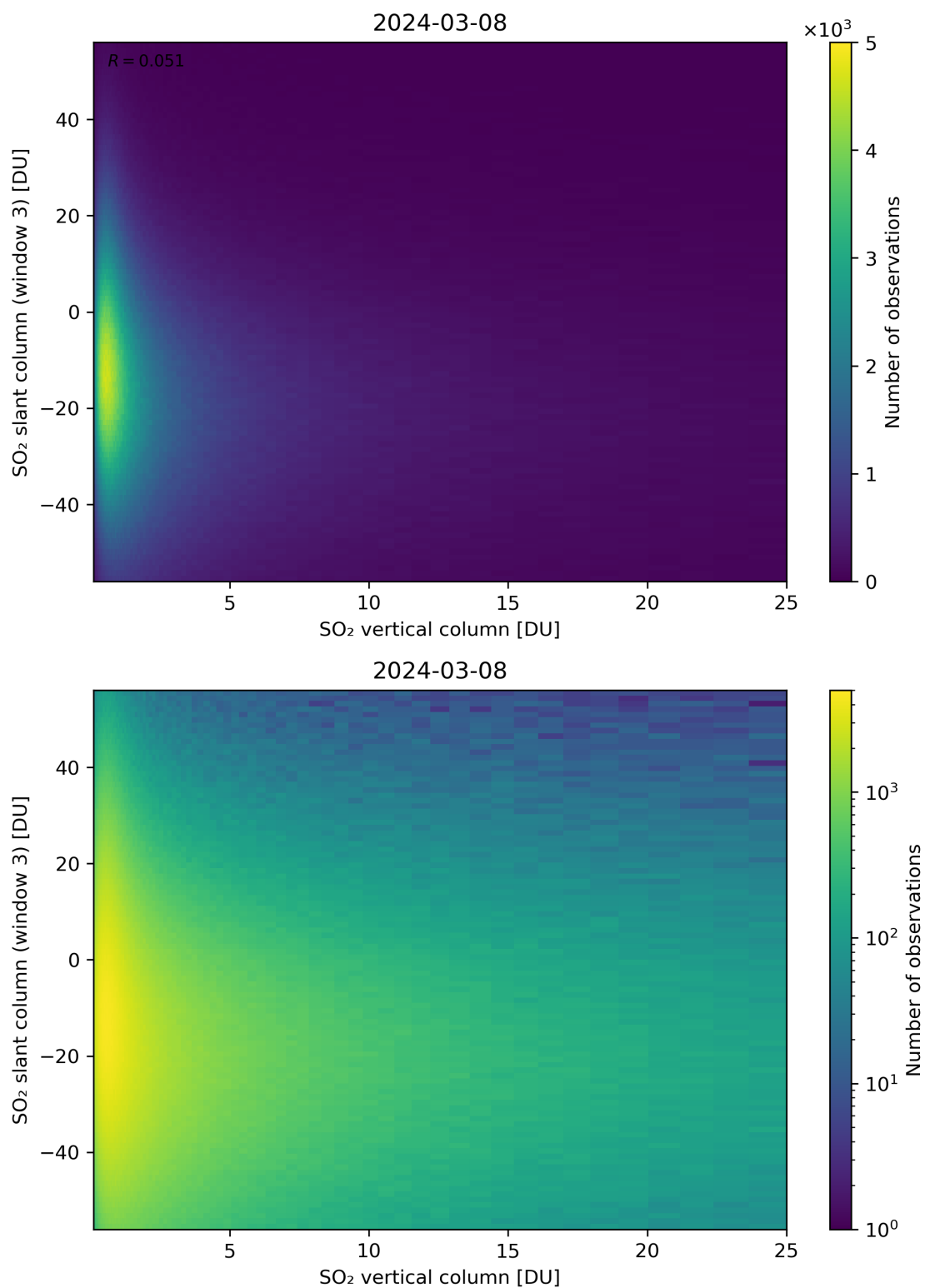
Figure 303: Scatter density plot of “SO 2 vertical column” against “SO 2 slant column (window 3)” for 2024-03-07 to 2024-03-09.
