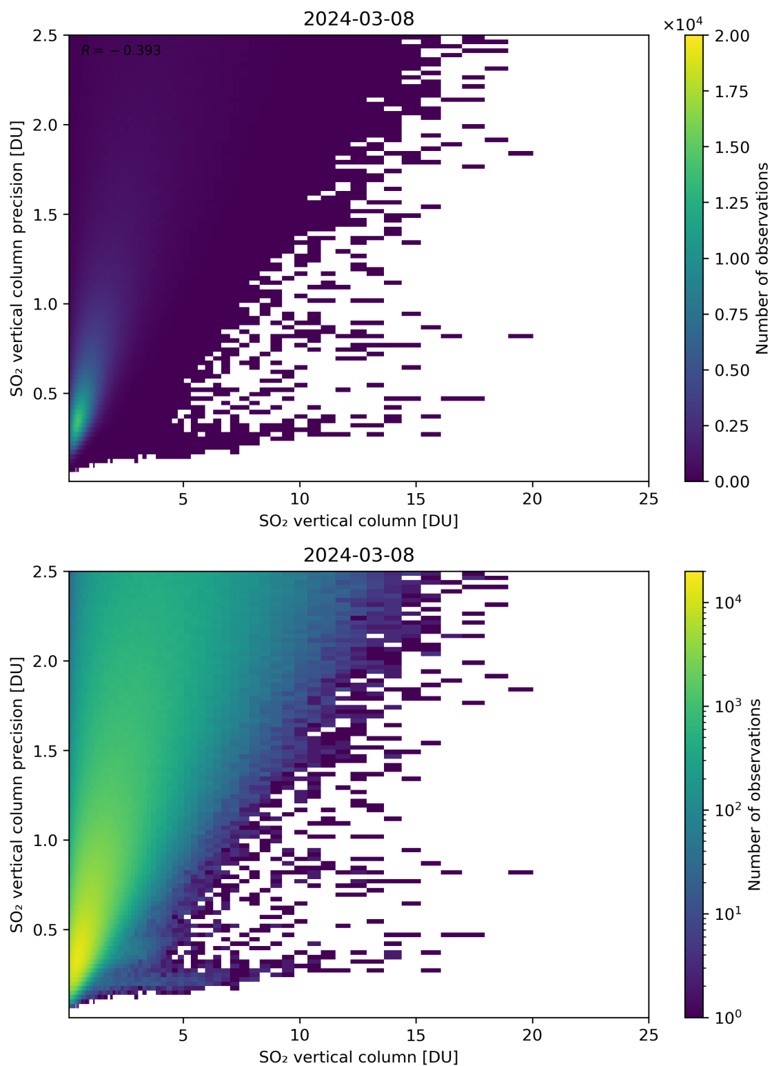
Figure 307: Scatter density plot of “SO 2 vertical column” against “SO 2 vertical column precision” for 2024-03-07 to 2024-03-09.
