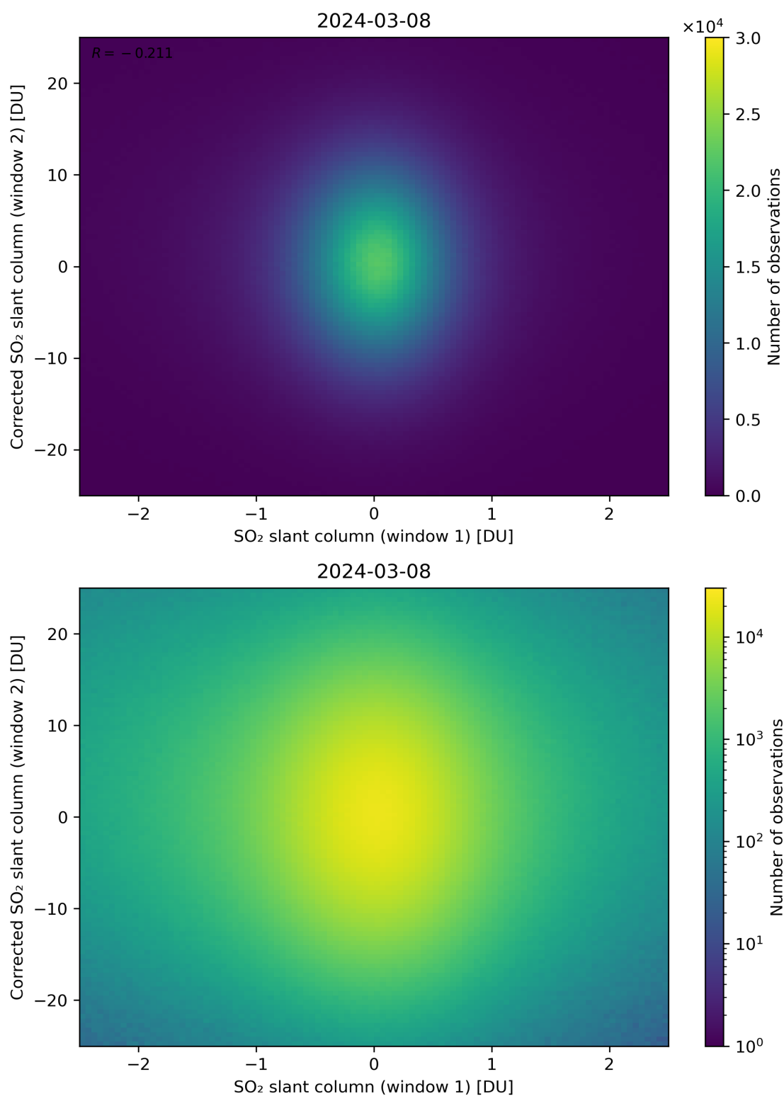
Figure 233: Scatter density plot of “SO 2 slant column (window 1)” against “Corrected SO 2 slant column (window 2)” for 2024-03-07 to 2024-03-09.
