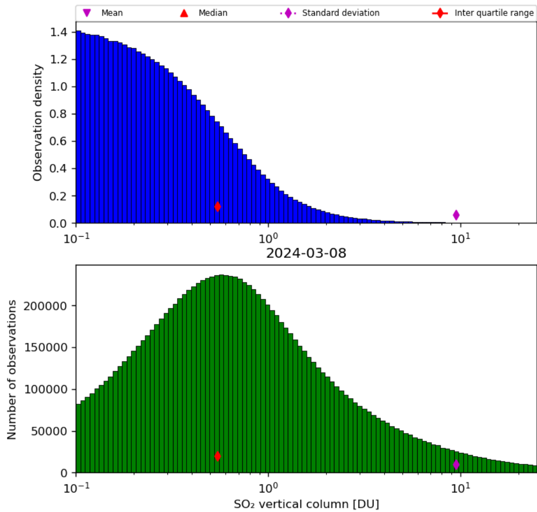
Figure 53: Histogram of “SO 2 vertical column” for 2024-03-07 to 2024-03-09
