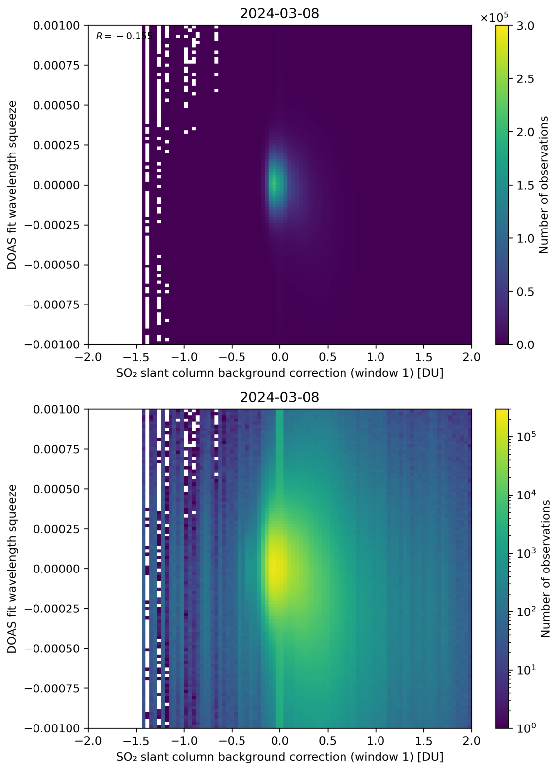
Figure 101: Scatter density plot of “SO 2 slant column background correction (window 1)” against “DOAS fit wavelength squeeze” for 2024-03-07 to 2024-03-09.
