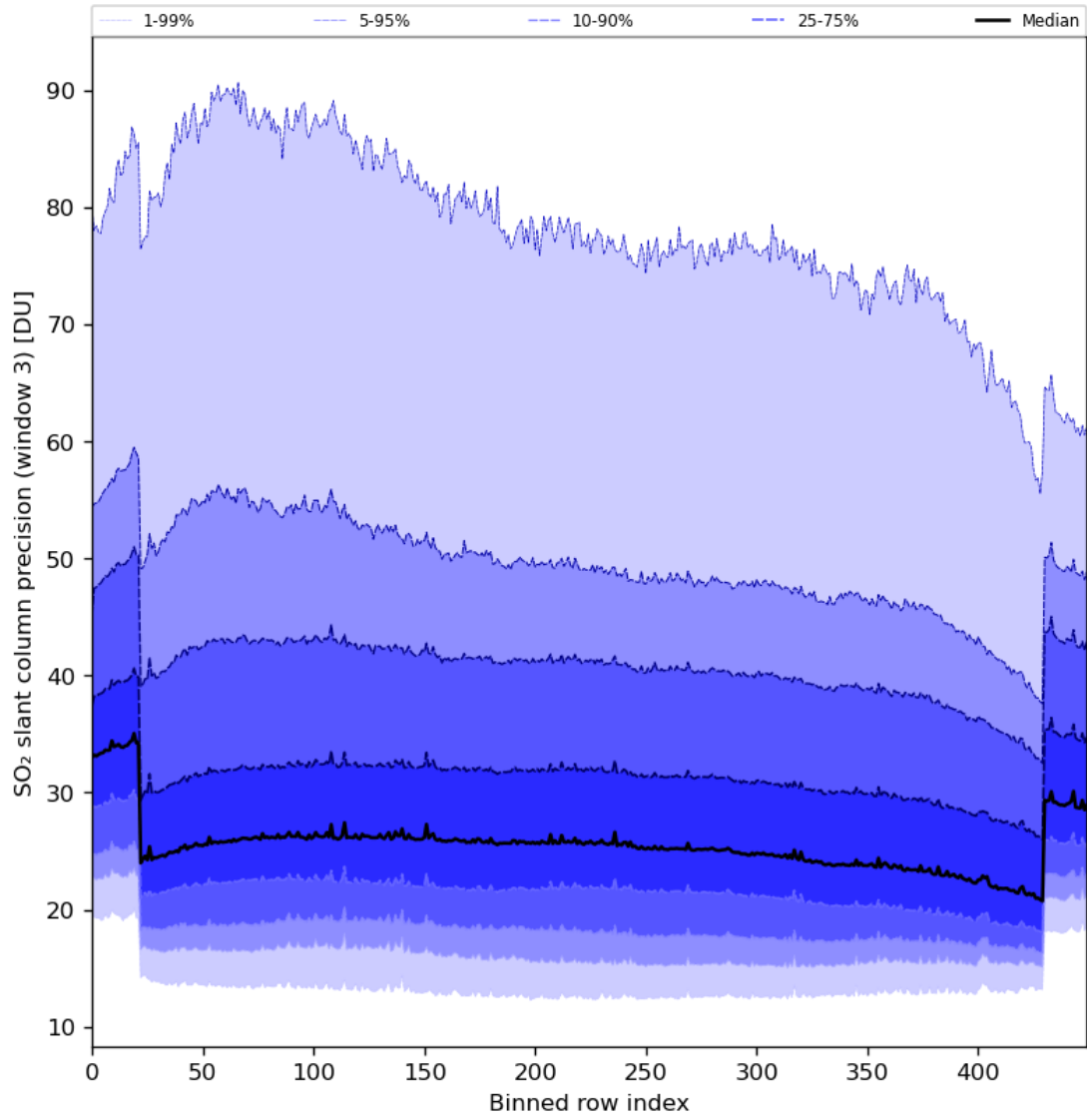
Figure 88: Along track statistics of “SO 2 slant column precision (window 3)” for 2024-03-07 to 2024-03-09
