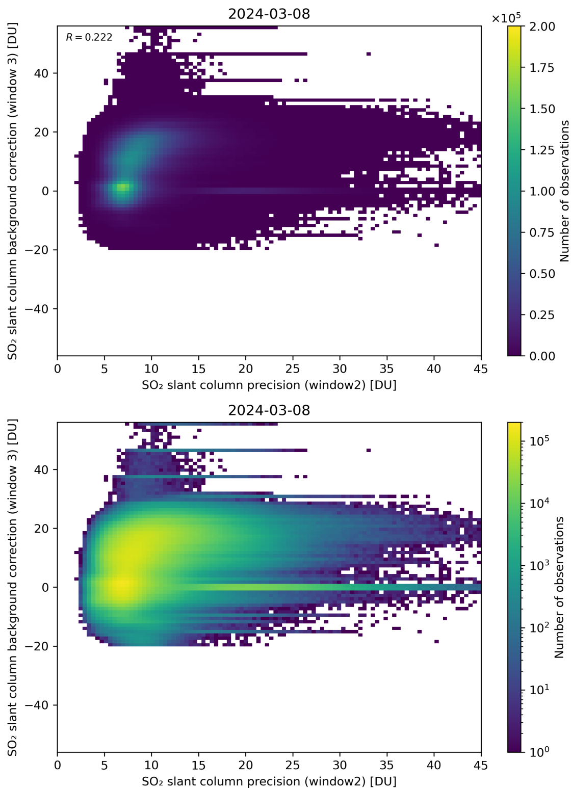
Figure 242: Scatter density plot of “SO 2 slant column precision (window2)” against “SO 2 slant column background correction (window 3)” for 2024-03-07 to 2024-03-09.
