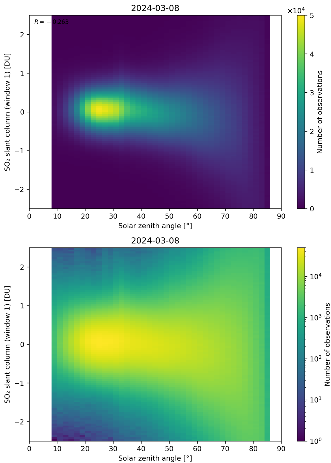
Figure 169: Scatter density plot of “Solar zenith angle” against “SO 2 slant column (window 1)” for 2024-03-07 to 2024-03-09.
