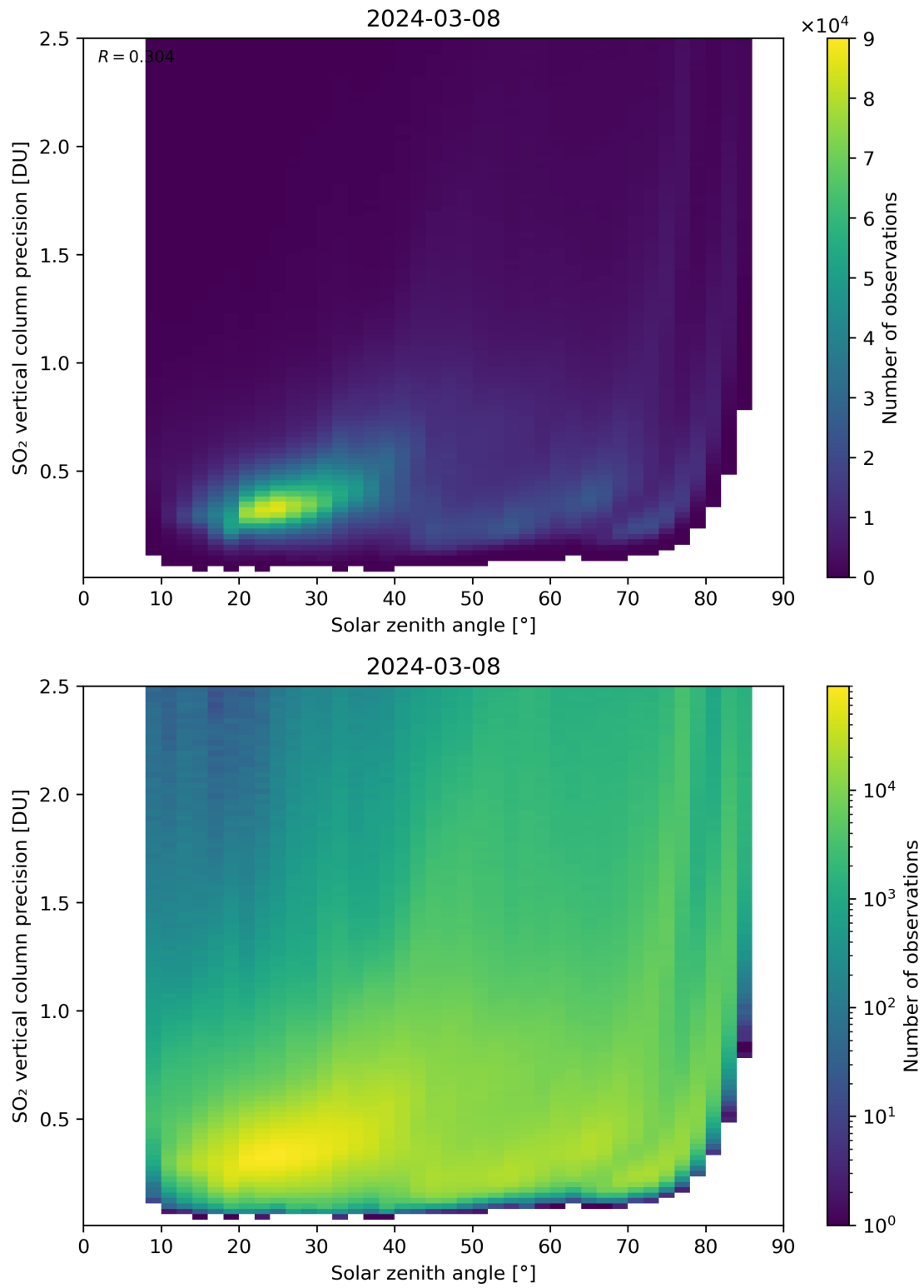
Figure 177: Scatter density plot of “Solar zenith angle” against “SO 2 vertical column precision” for 2024-03-07 to 2024-03-09.
