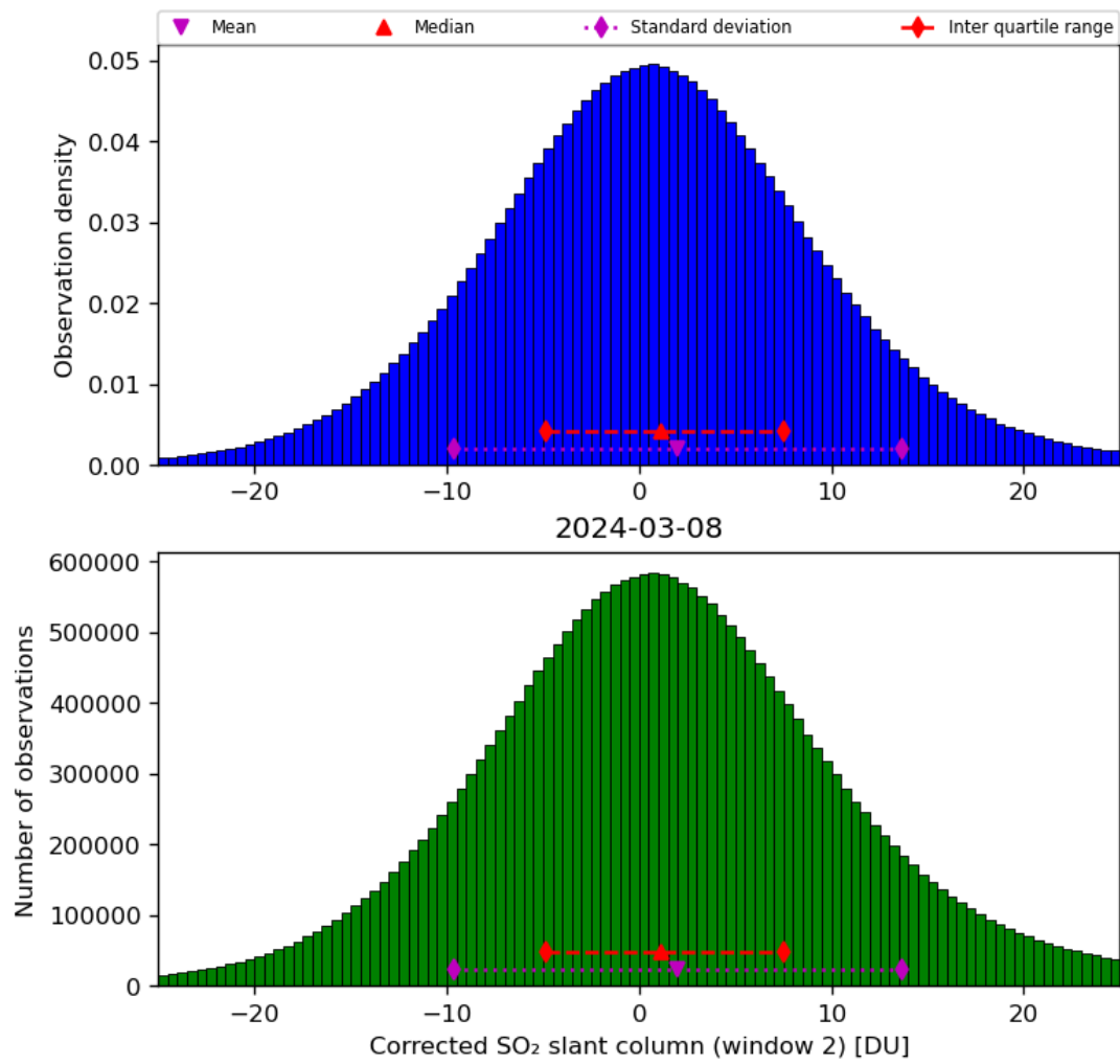
Figure 62: Histogram of “Corrected SO 2 slant column (window 2)” for 2024-03-07 to 2024-03-09
