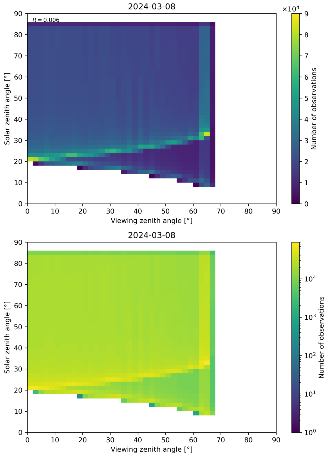
Figure 315: Scatter density plot of “Viewing zenith angle” against “Solar zenith angle” for 2024-03-07 to 2024-03-09.
