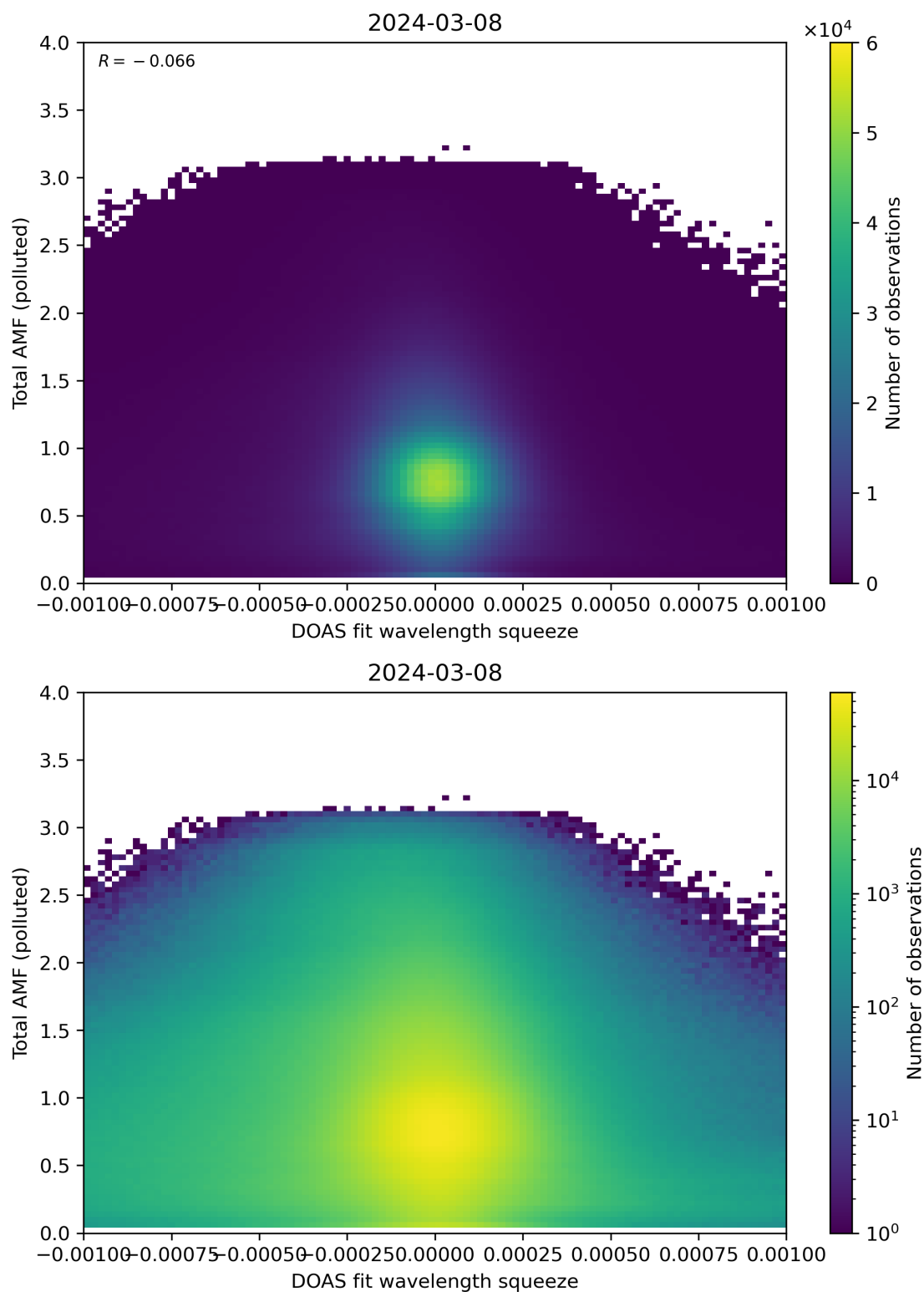
Figure 134: Scatter density plot of “DOAS fit wavelength squeeze” against “Total AMF (polluted)” for 2024-03-07 to 2024-03-09.
