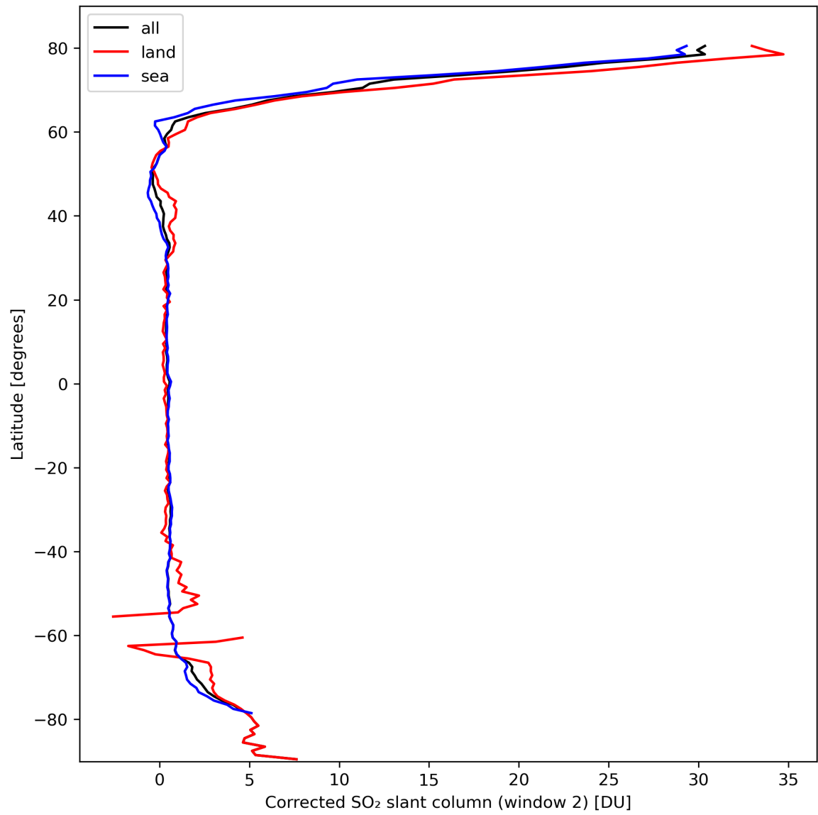
Figure 39: Zonal average of “Corrected SO 2 slant column (window 2)” for 2024-03-07 to 2024-03-09.
