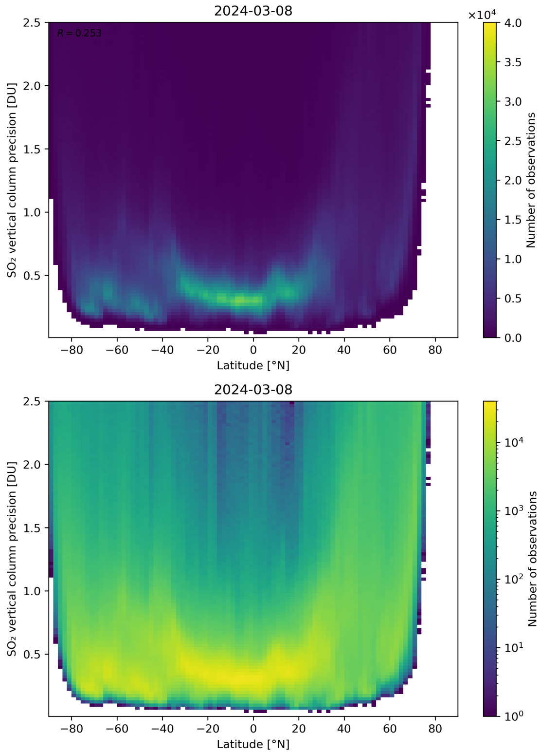
Figure 157: Scatter density plot of “Latitude” against “SO 2 vertical column precision” for 2024-03-07 to 2024-03-09.
