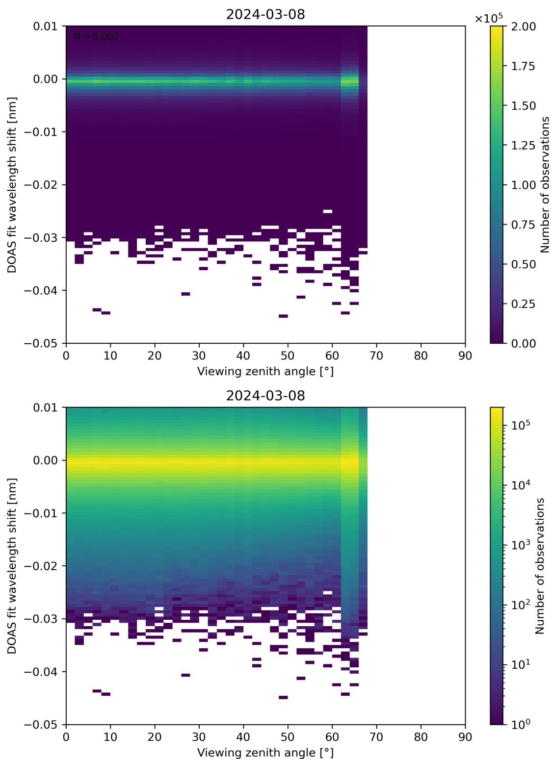
Figure 311: Scatter density plot of “Viewing zenith angle” against “DOAS fit wavelength shift” for 2024-03-07 to 2024-03-09.
