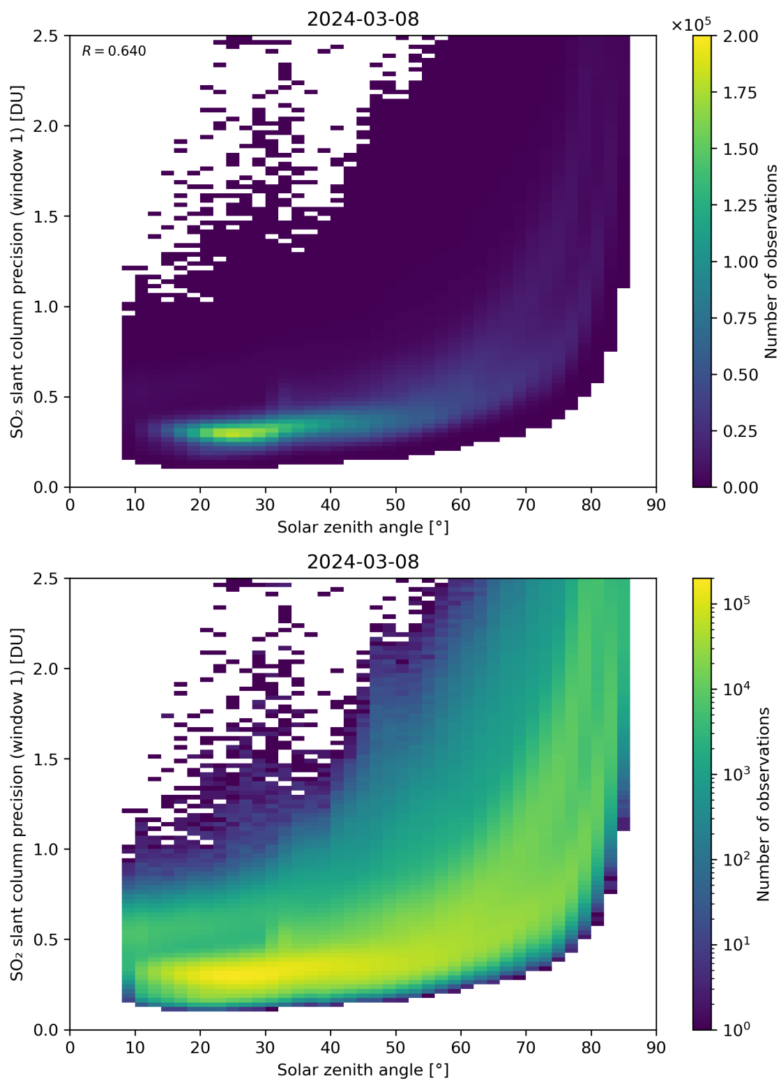
Figure 170: Scatter density plot of “Solar zenith angle” against “SO 2 slant column precision (window 1)” for 2024-03-07 to 2024-03-09.
