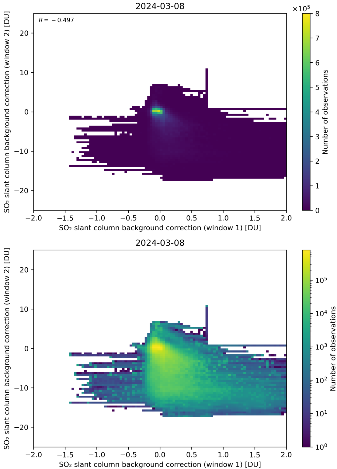
Figure 98: Scatter density plot of “SO 2 slant column background correction (window 1)” against “SO 2 slant column background correction (window 2)” for 2024-03-07 to 2024-03-09.
