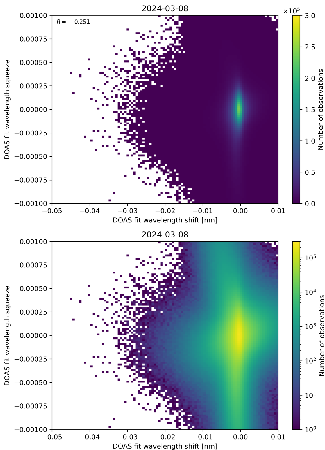
Figure 127: Scatter density plot of “DOAS fit wavelength shift” against “DOAS fit wavelength squeeze” for 2024-03-07 to 2024-03-09.
