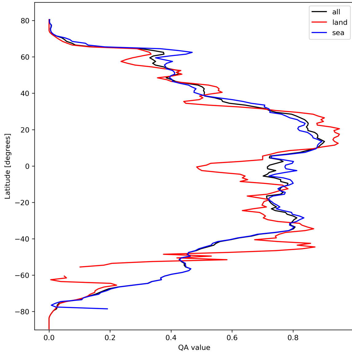
Figure 29: Zonal average of “QA value” for 2024-03-07 to 2024-03-09.
