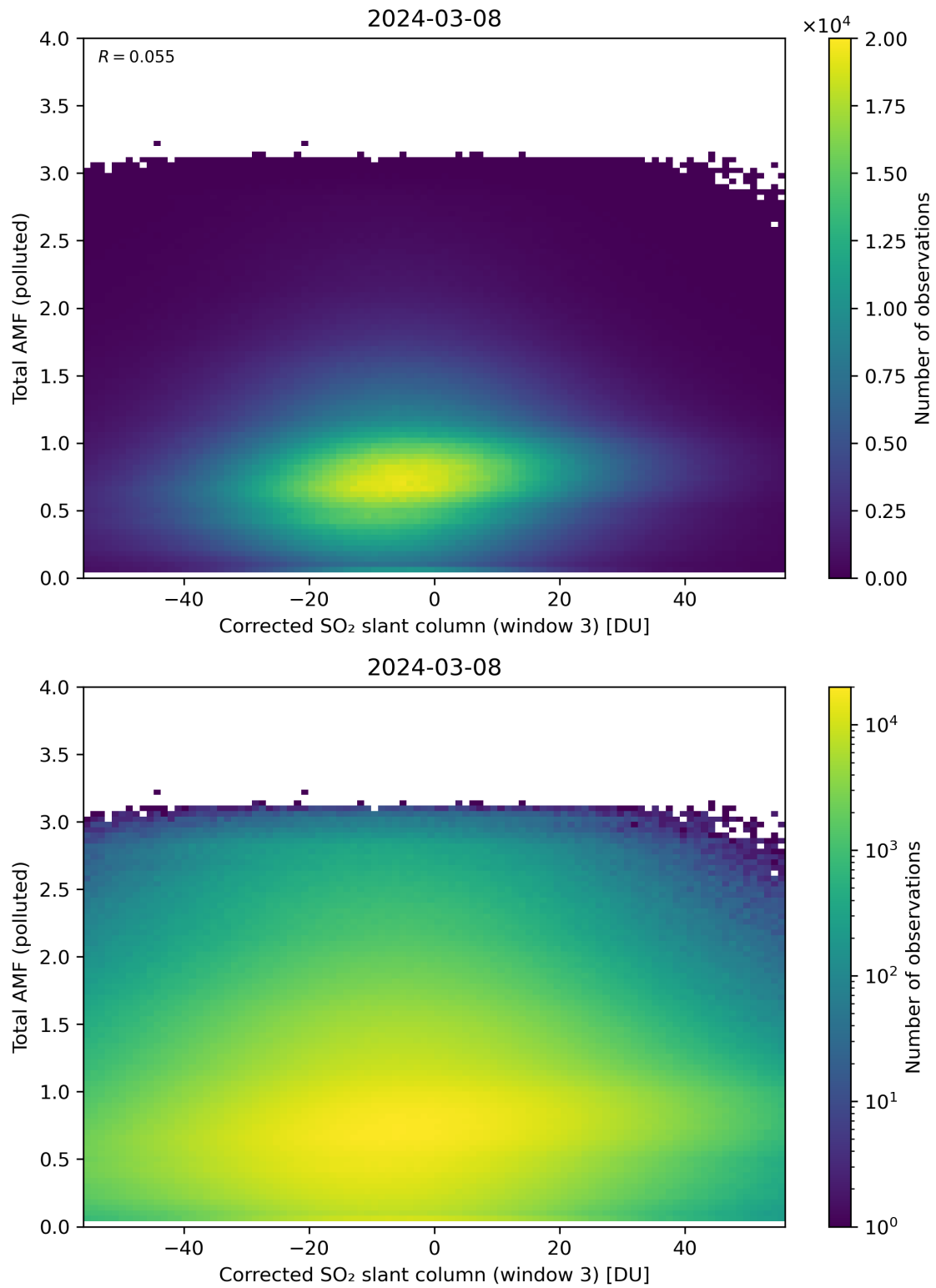
Figure 210: Scatter density plot of “Corrected SO 2 slant column (window 3)” against “Total AMF (polluted)” for 2024-03-07 to 2024-03-09.
