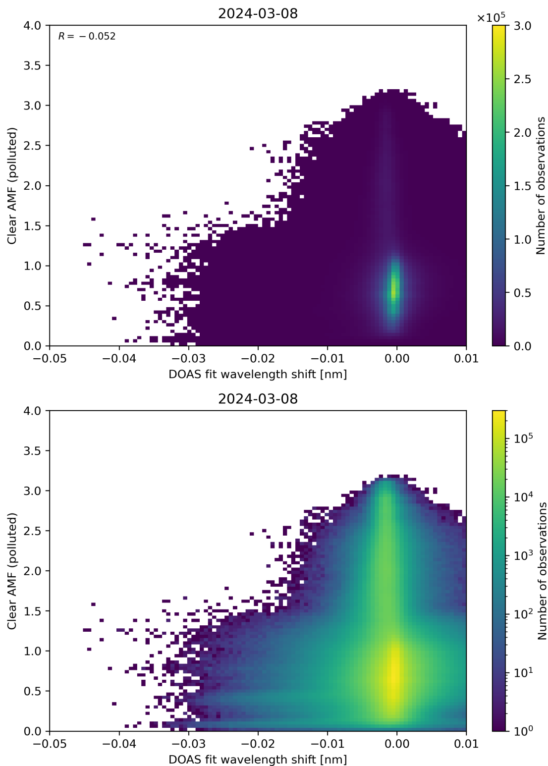
Figure 129: Scatter density plot of “DOAS fit wavelength shift” against “Clear AMF (polluted)” for 2024-03-07 to 2024-03-09.
