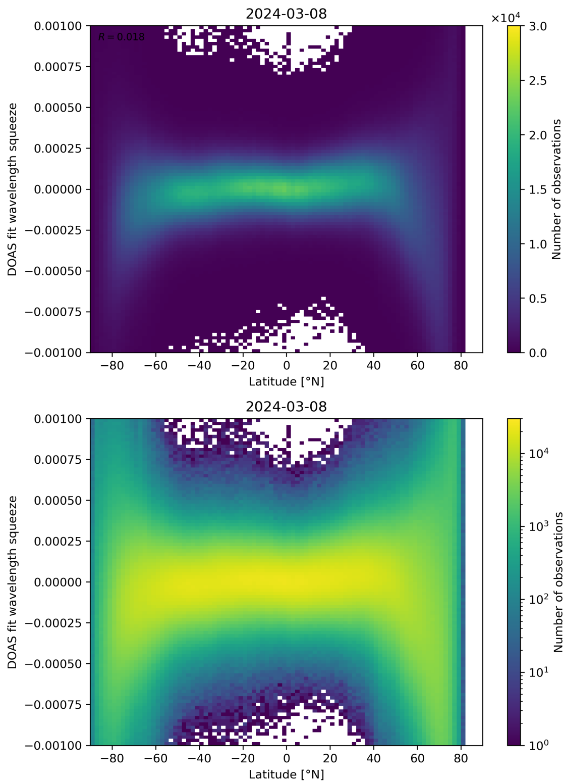
Figure 143: Scatter density plot of “Latitude” against “DOAS fit wavelength squeeze” for 2024-03-07 to 2024-03-09.
