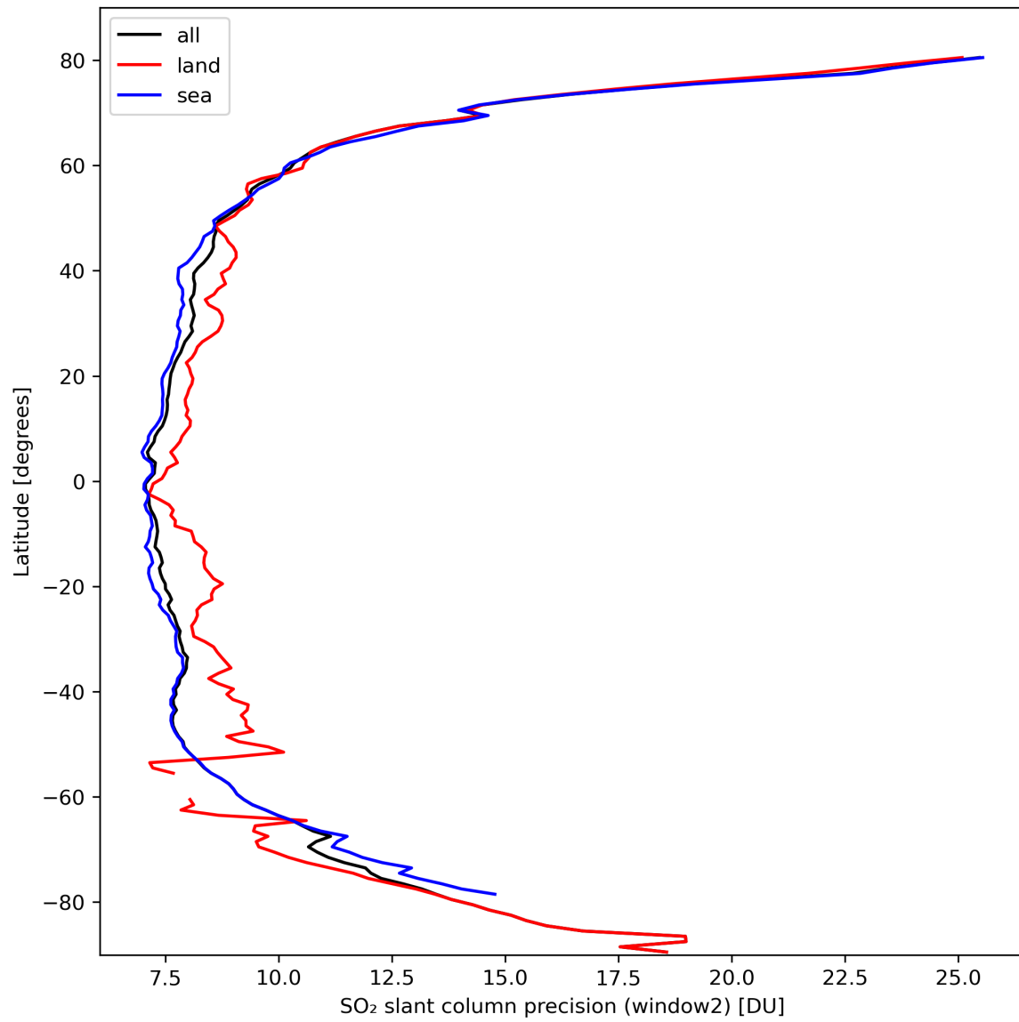
Figure 38: Zonal average of “SO 2 slant column precision (window2)” for 2024-03-07 to 2024-03-09.
