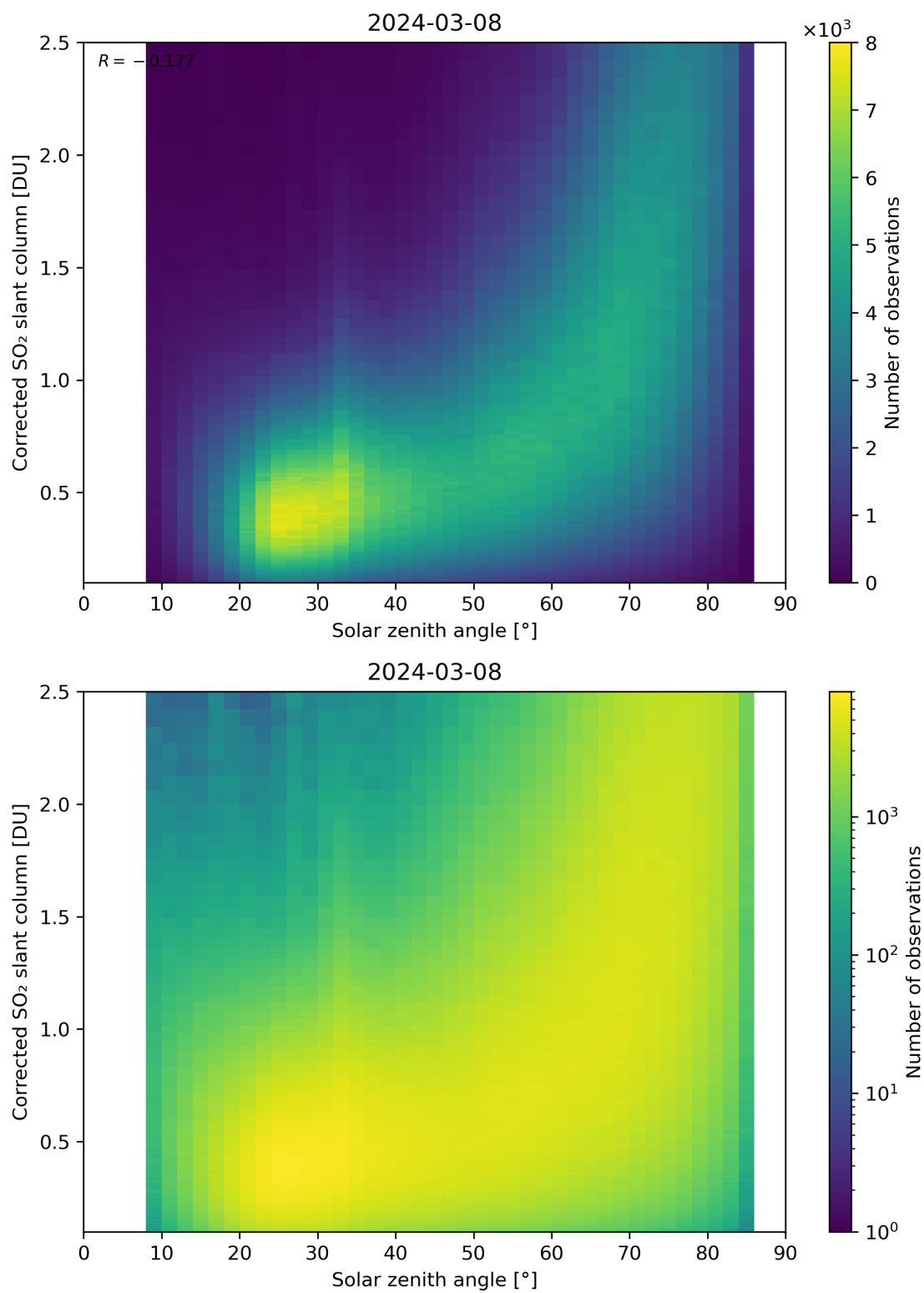
Figure 166: Scatter density plot of “Solar zenith angle” against “Corrected SO 2 slant column” for 2024-03-07 to 2024-03-09.
