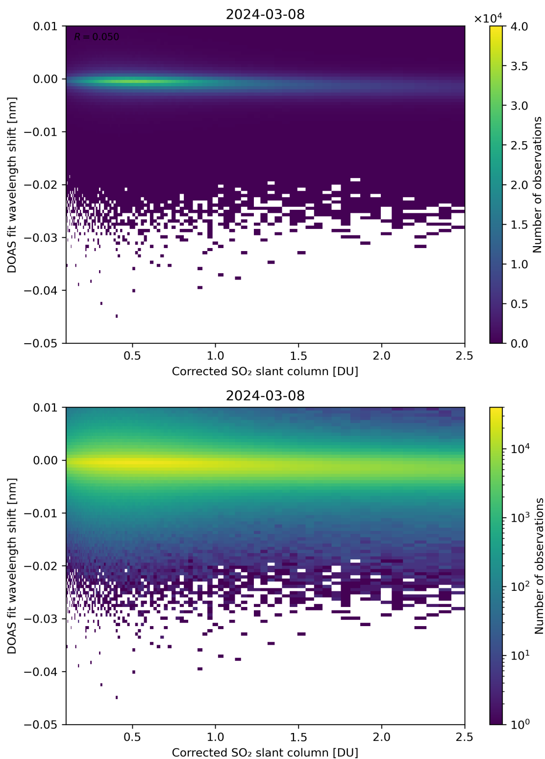
Figure 181: Scatter density plot of “Corrected SO 2 slant column” against “DOAS fit wavelength shift” for 2024-03-07 to 2024-03-09.
