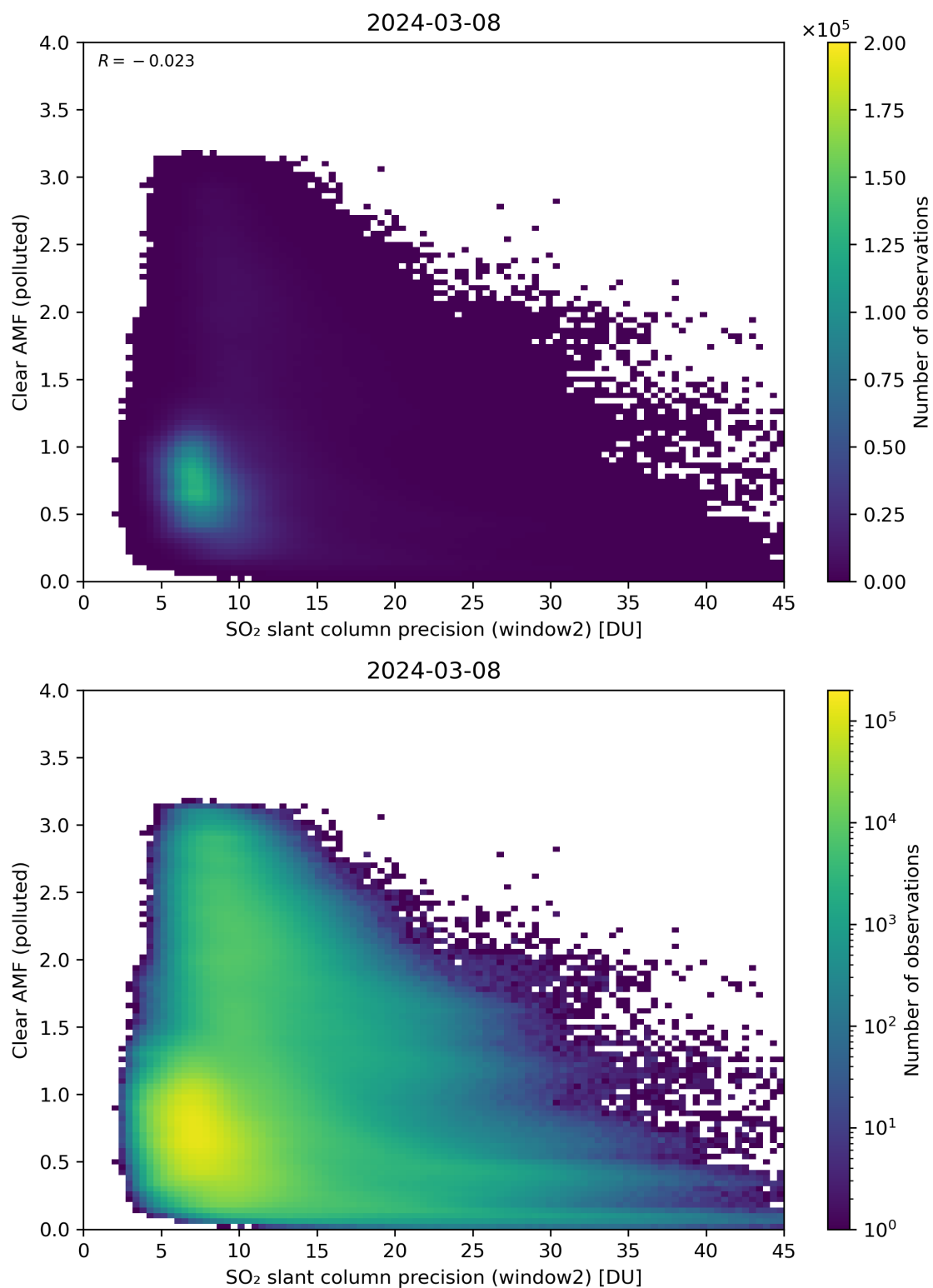
Figure 246: Scatter density plot of “SO 2 slant column precision (window2)” against “Clear AMF (polluted)” for 2024-03-07 to 2024-03-09.
