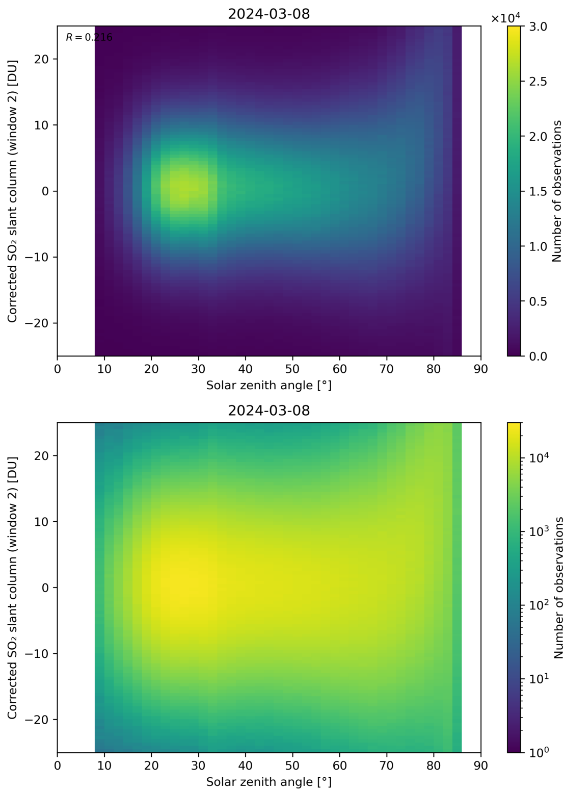
Figure 167: Scatter density plot of “Solar zenith angle” against “Corrected SO 2 slant column (window 2)” for 2024-03-07 to 2024-03-09.
