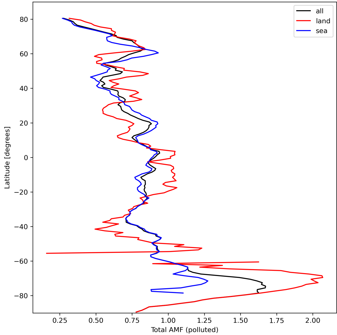
Figure 48: Zonal average of “Total AMF (polluted)” for 2024-03-07 to 2024-03-09.
