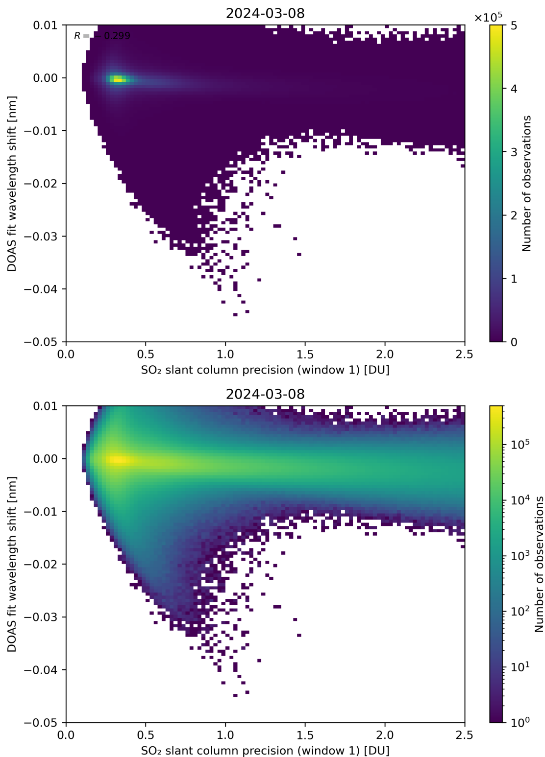
Figure 221: Scatter density plot of “SO 2 slant column precision (window 1)” against “DOAS fit wavelength shift” for 2024-03-07 to 2024-03-09.
