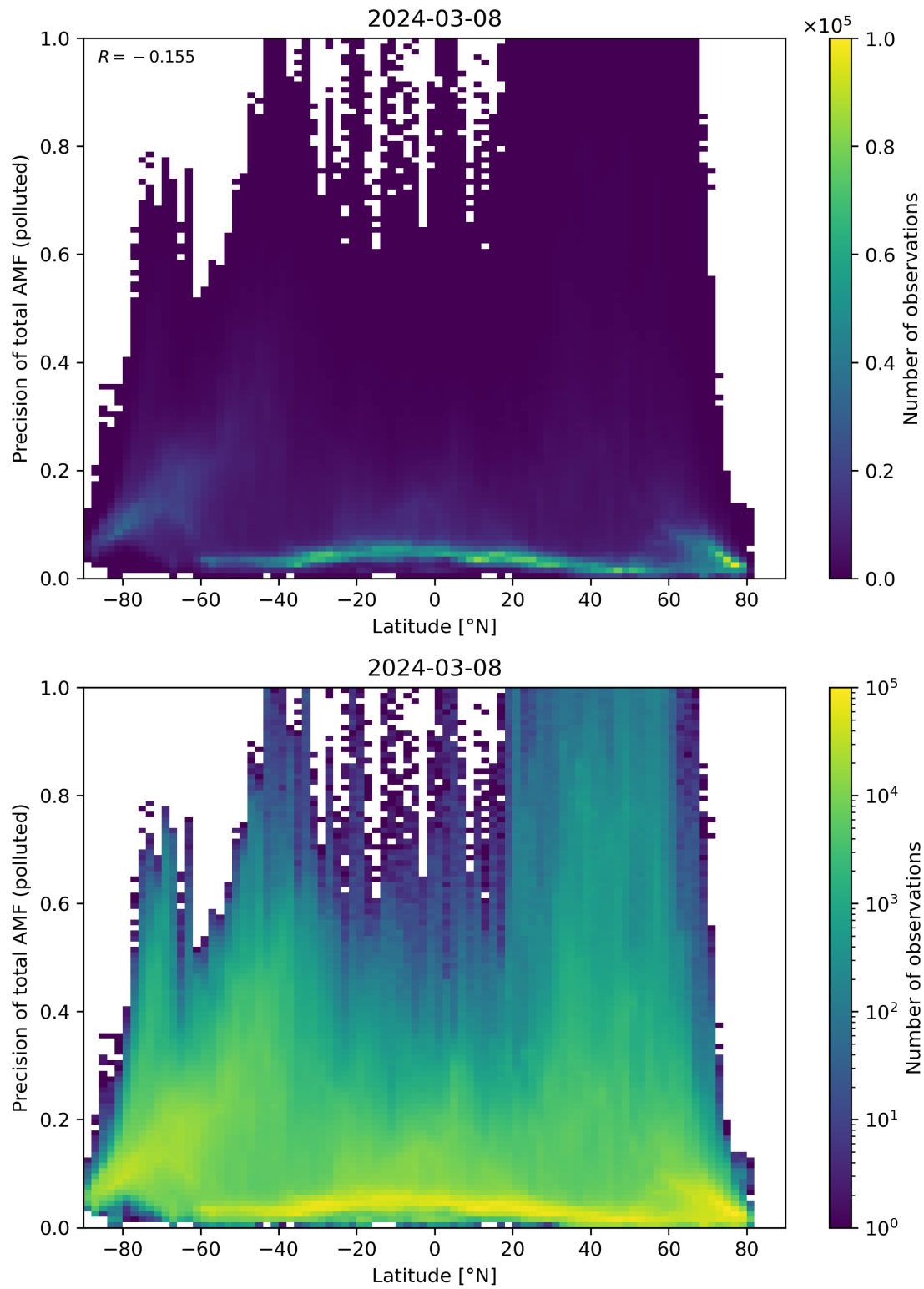
Figure 155: Scatter density plot of “Latitude” against “Precision of total AMF (polluted)” for 2024-03-07 to 2024-03-09.
