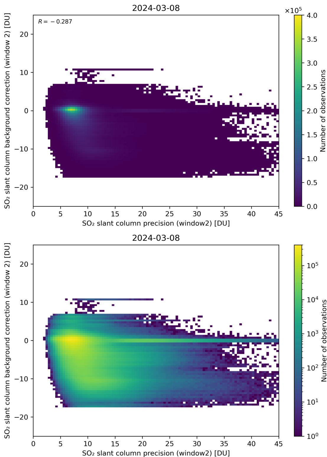
Figure 241: Scatter density plot of “SO 2 slant column precision (window2)” against “SO 2 slant column background correction (window 2)” for 2024-03-07 to 2024-03-09.
