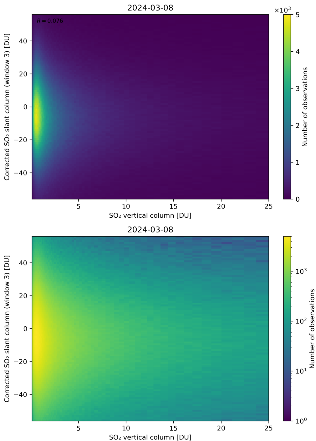
Figure 299: Scatter density plot of “SO 2 vertical column” against “Corrected SO 2 slant column (window 3)” for 2024-03-07 to 2024-03-09.
