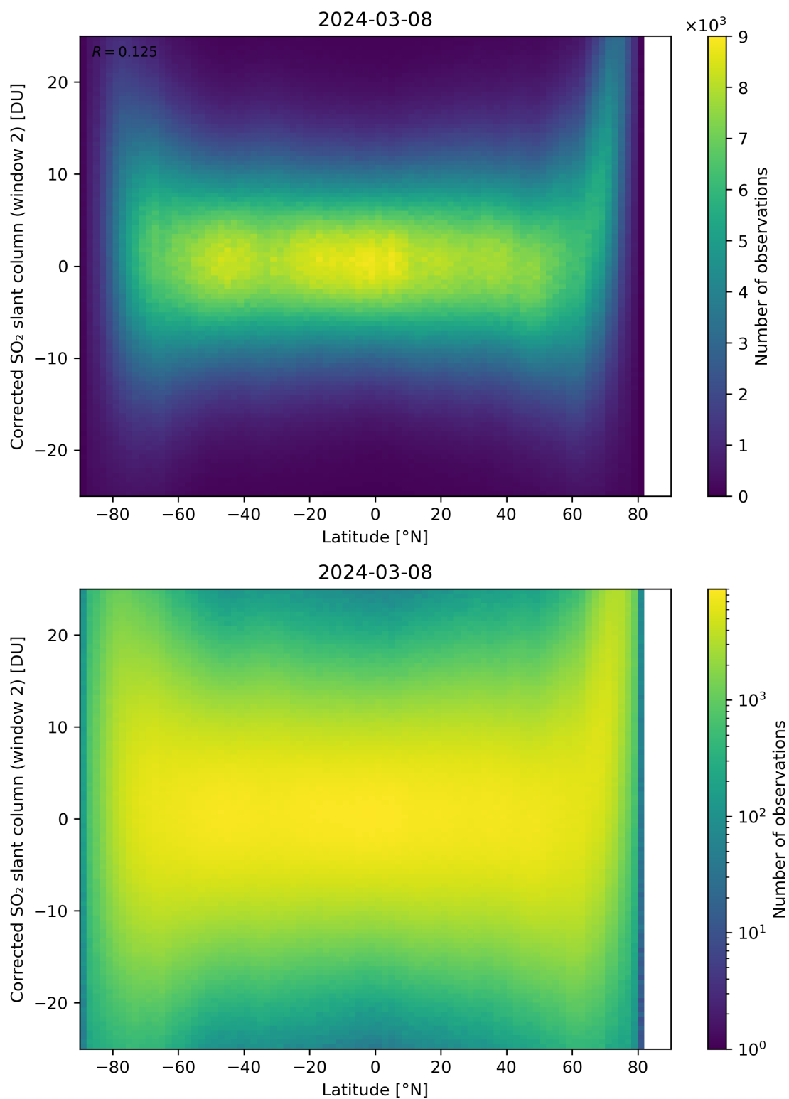
Figure 147: Scatter density plot of “Latitude” against “Corrected SO 2 slant column (window 2)” for 2024-03-07 to 2024-03-09.
