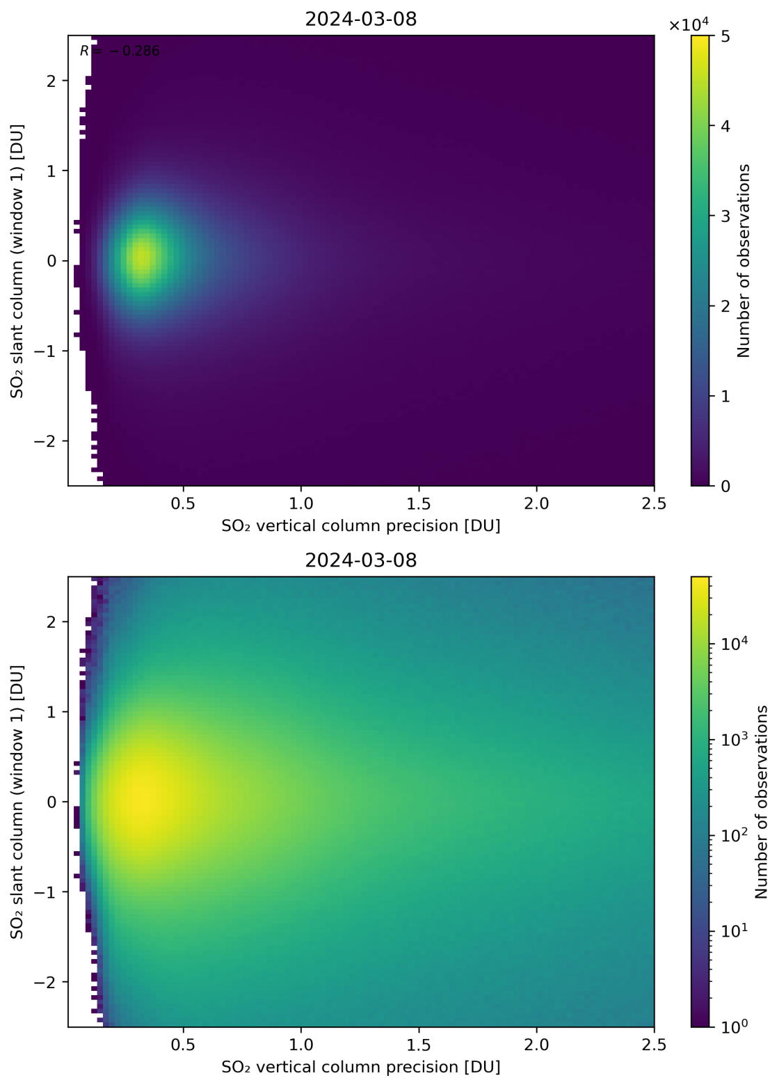
Figure 289: Scatter density plot of “SO 2 vertical column precision” against “SO 2 slant column (window 1)” for 2024-03-07 to 2024-03-09.
