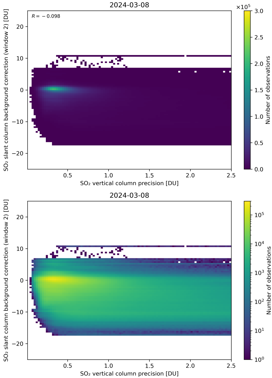
Figure 280: Scatter density plot of “SO 2 vertical column precision” against “SO 2 slant column background correction (window 2)” for 2024-03-07 to 2024-03-09.
