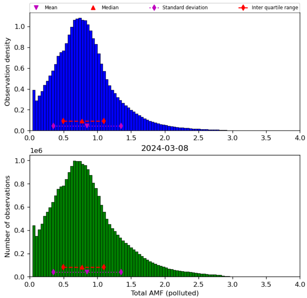
Figure 71: Histogram of “Total AMF (polluted)” for 2024-03-07 to 2024-03-09
