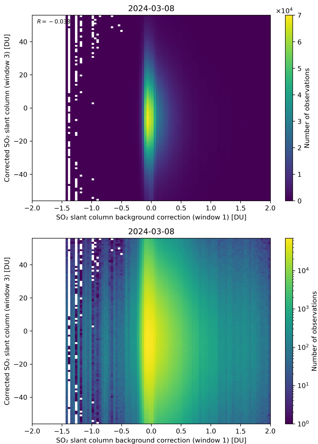
Figure 105: Scatter density plot of “SO 2 slant column background correction (window 1)” against “Corrected SO 2 slant column (window 3)” for 2024-03-07 to 2024-03-09.
