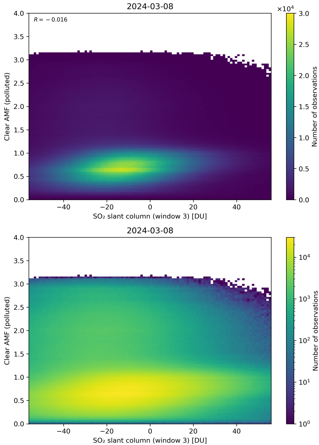
Figure 265: Scatter density plot of “SO 2 slant column (window 3)” against “Clear AMF (polluted)” for 2024-03-07 to 2024-03-09.
