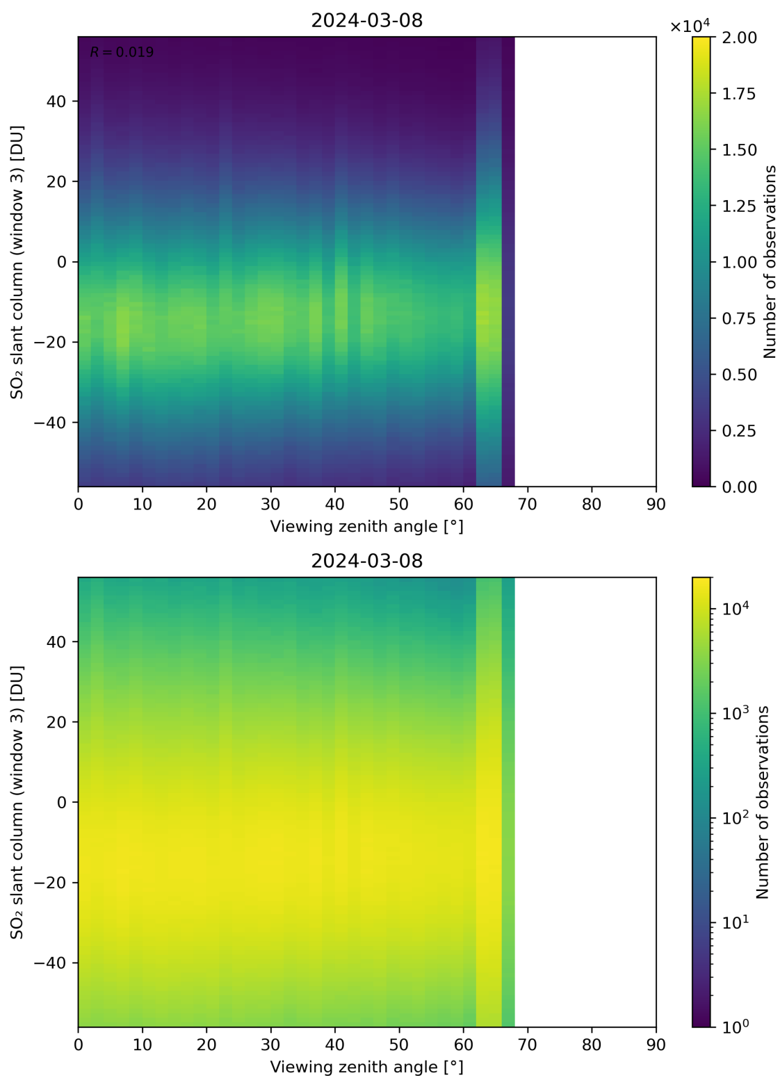
Figure 323: Scatter density plot of “Viewing zenith angle” against “SO 2 slant column (window 3)” for 2024-03-07 to 2024-03-09.
