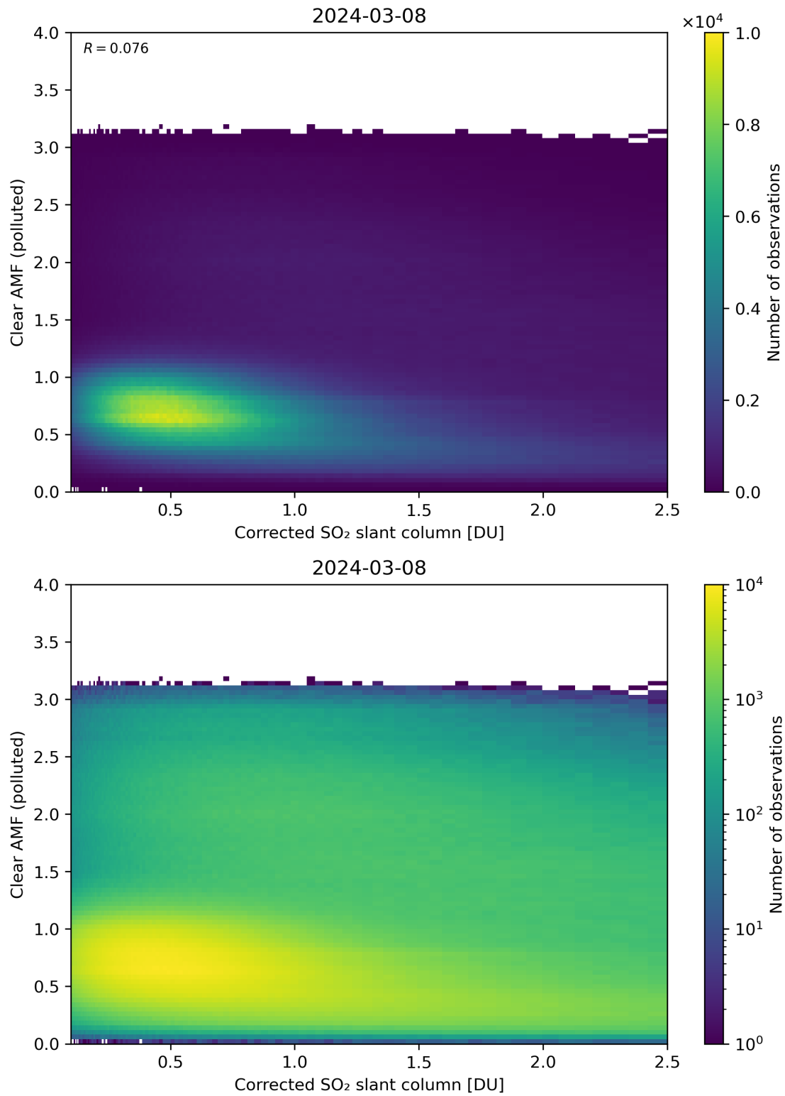
Figure 184: Scatter density plot of “Corrected SO 2 slant column” against “Clear AMF (polluted)” for 2024-03-07 to 2024-03-09.
