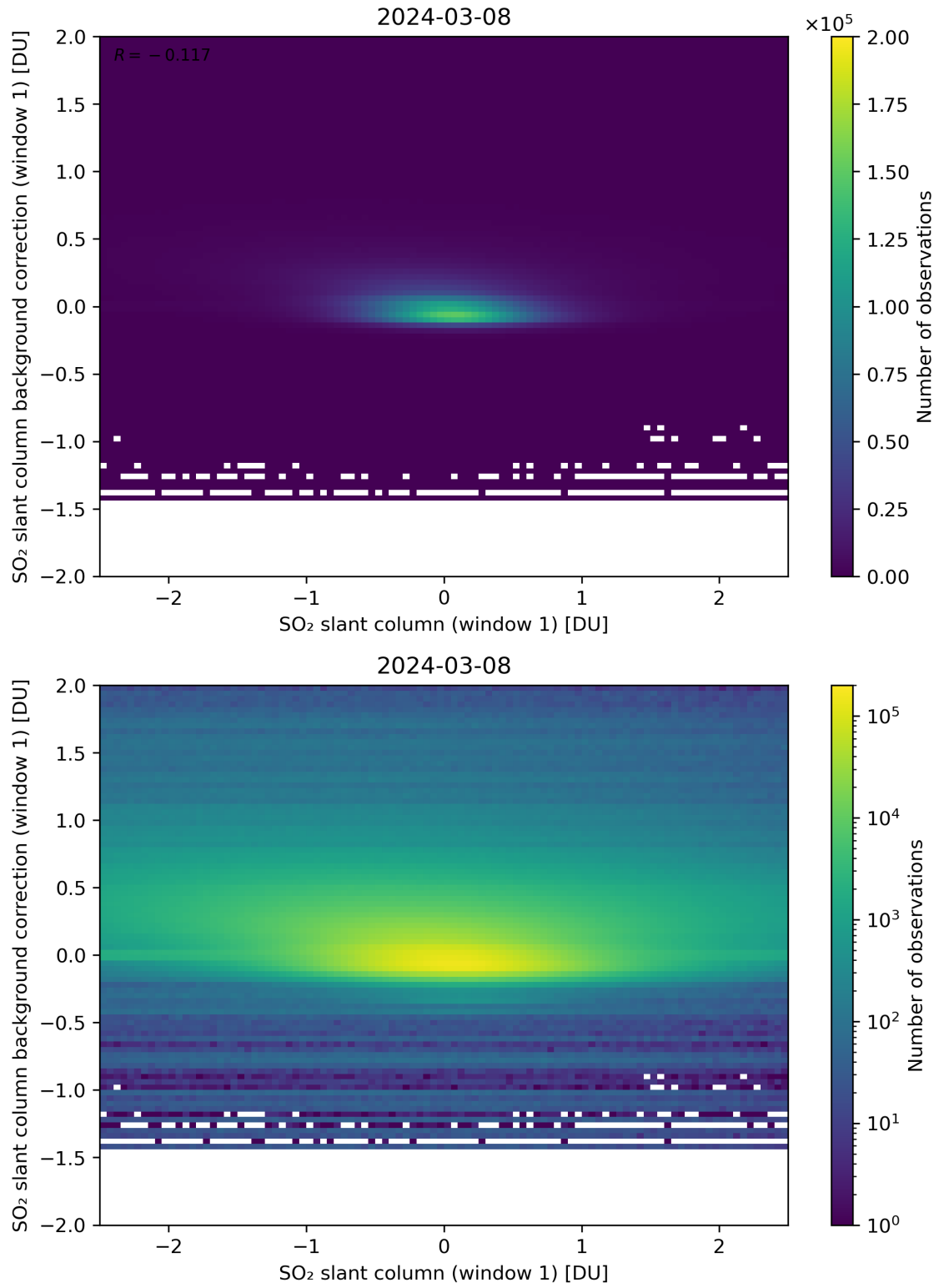
Figure 212: Scatter density plot of “SO 2 slant column (window 1)” against “SO 2 slant column background correction (window 1)” for 2024-03-07 to 2024-03-09.
