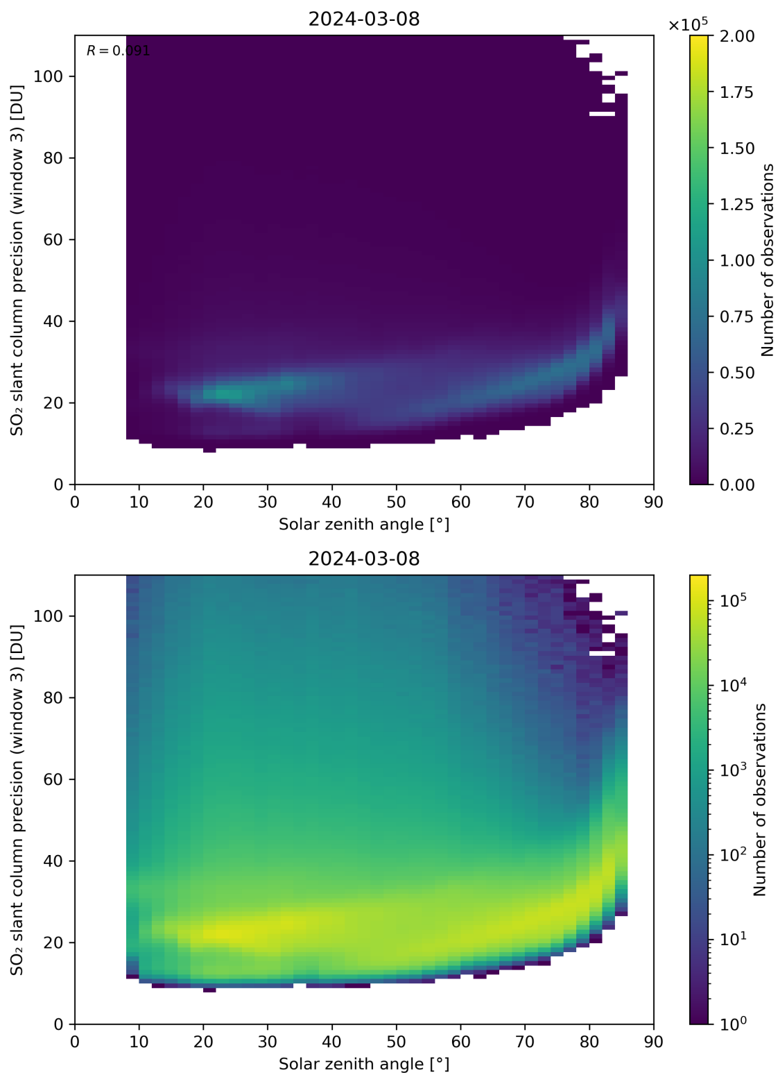
Figure 173: Scatter density plot of “Solar zenith angle” against “SO 2 slant column precision (window 3)” for 2024-03-07 to 2024-03-09.
