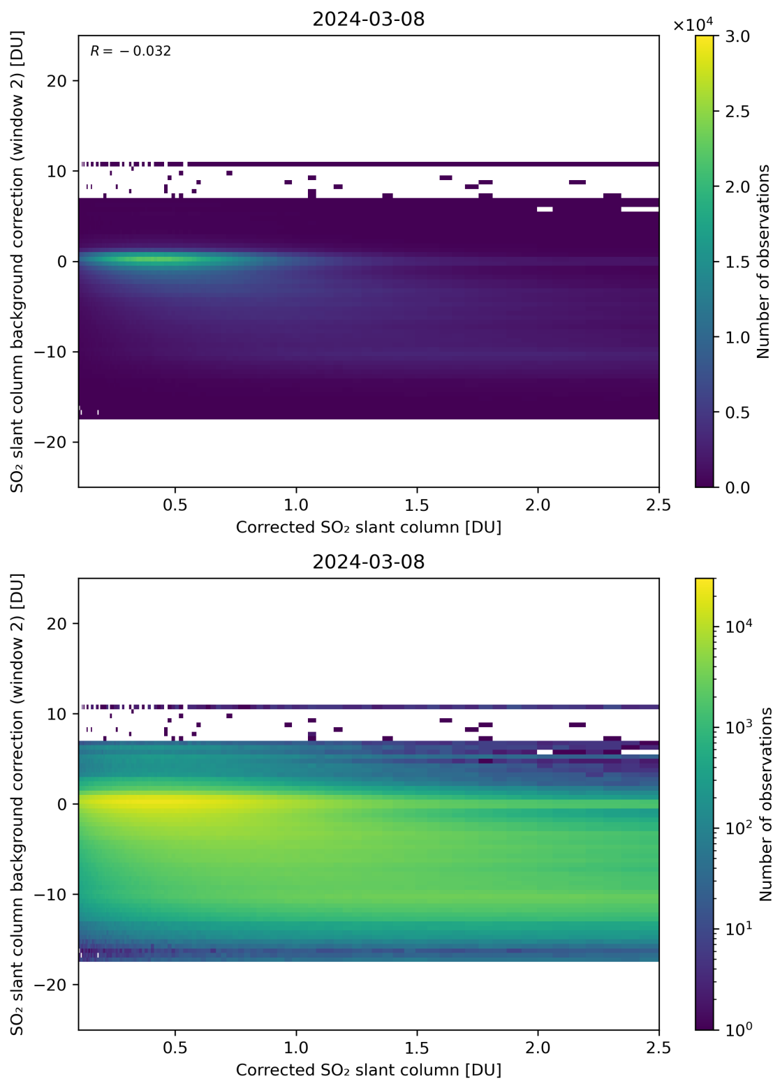
Figure 179: Scatter density plot of “Corrected SO 2 slant column” against “SO 2 slant column background correction (window 2)” for 2024-03-07 to 2024-03-09.
