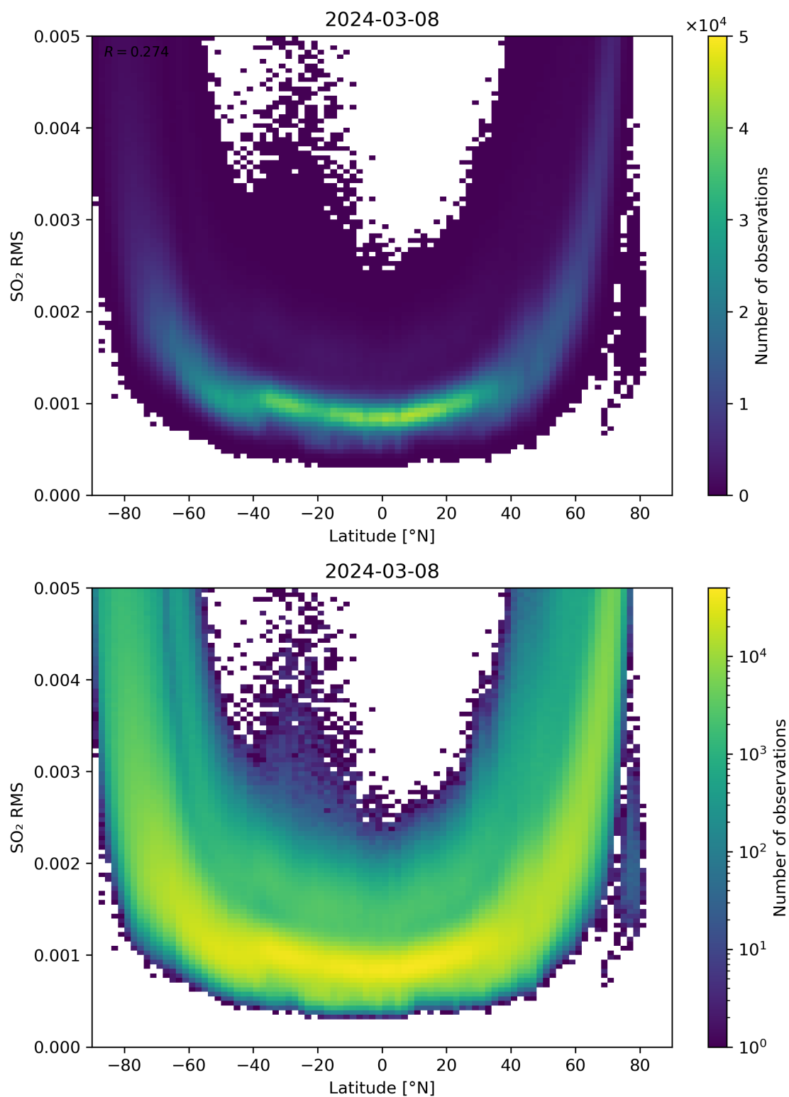
Figure 144: Scatter density plot of “Latitude” against “SO 2 RMS” for 2024-03-07 to 2024-03-09.
