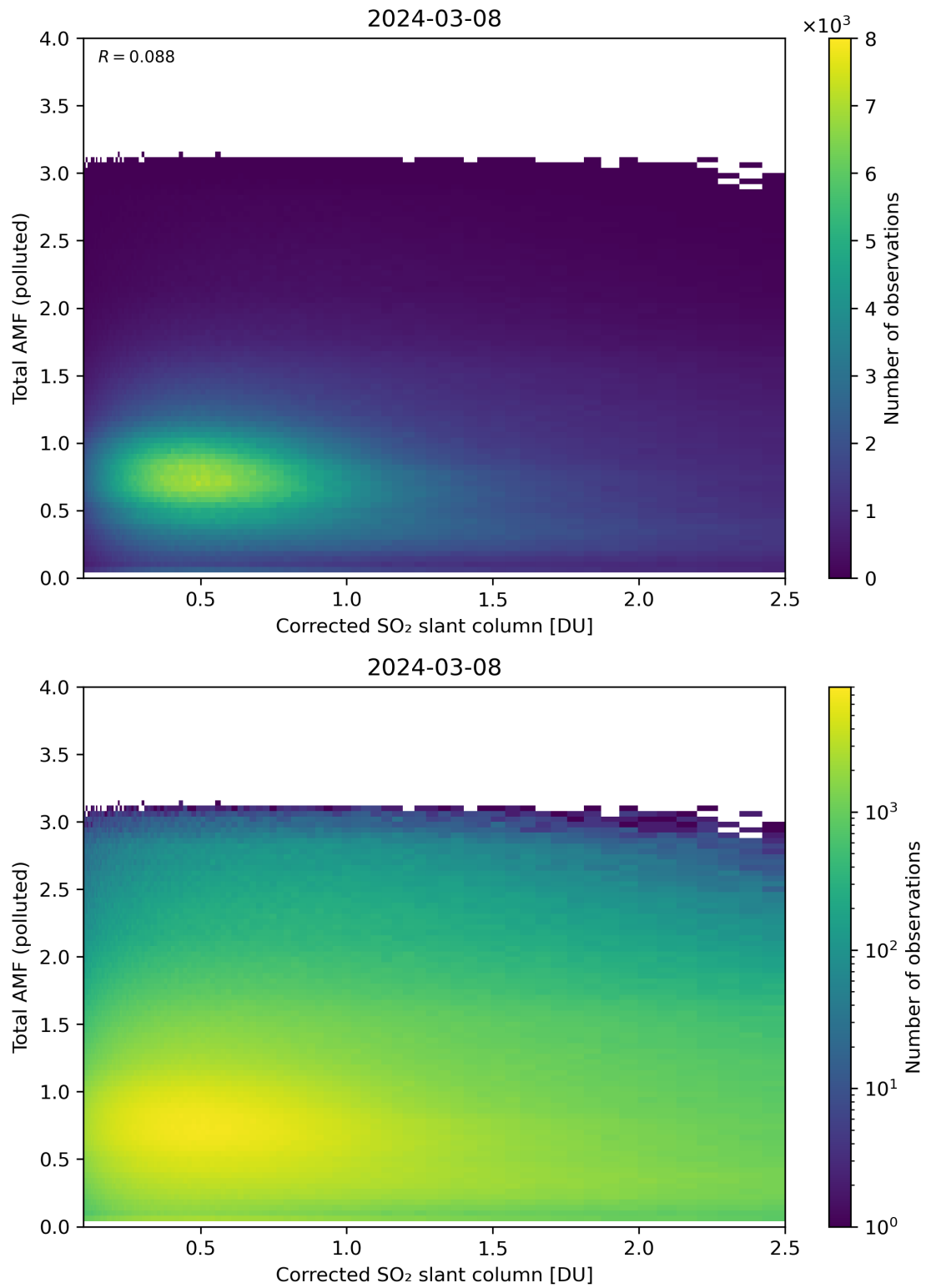
Figure 192: Scatter density plot of “Corrected SO 2 slant column” against “Total AMF (polluted)” for 2024-03-07 to 2024-03-09.
