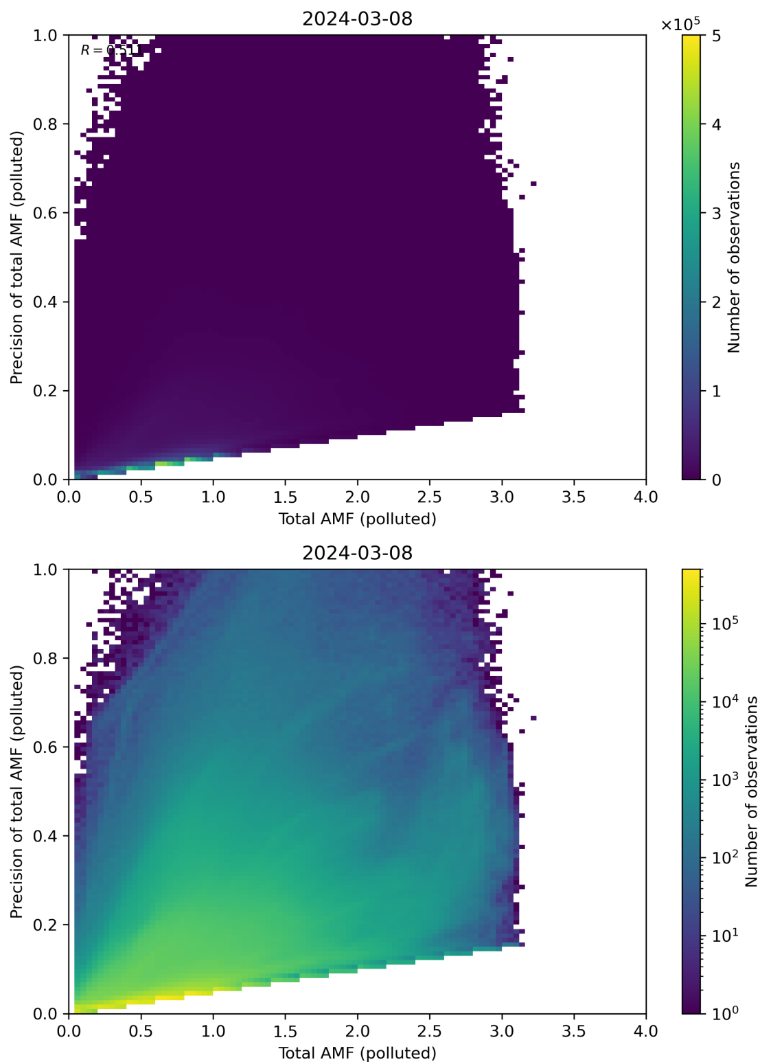
Figure 272: Scatter density plot of “Total AMF (polluted)” against “Precision of total AMF (polluted)” for 2024-03-07 to 2024-03-09.
