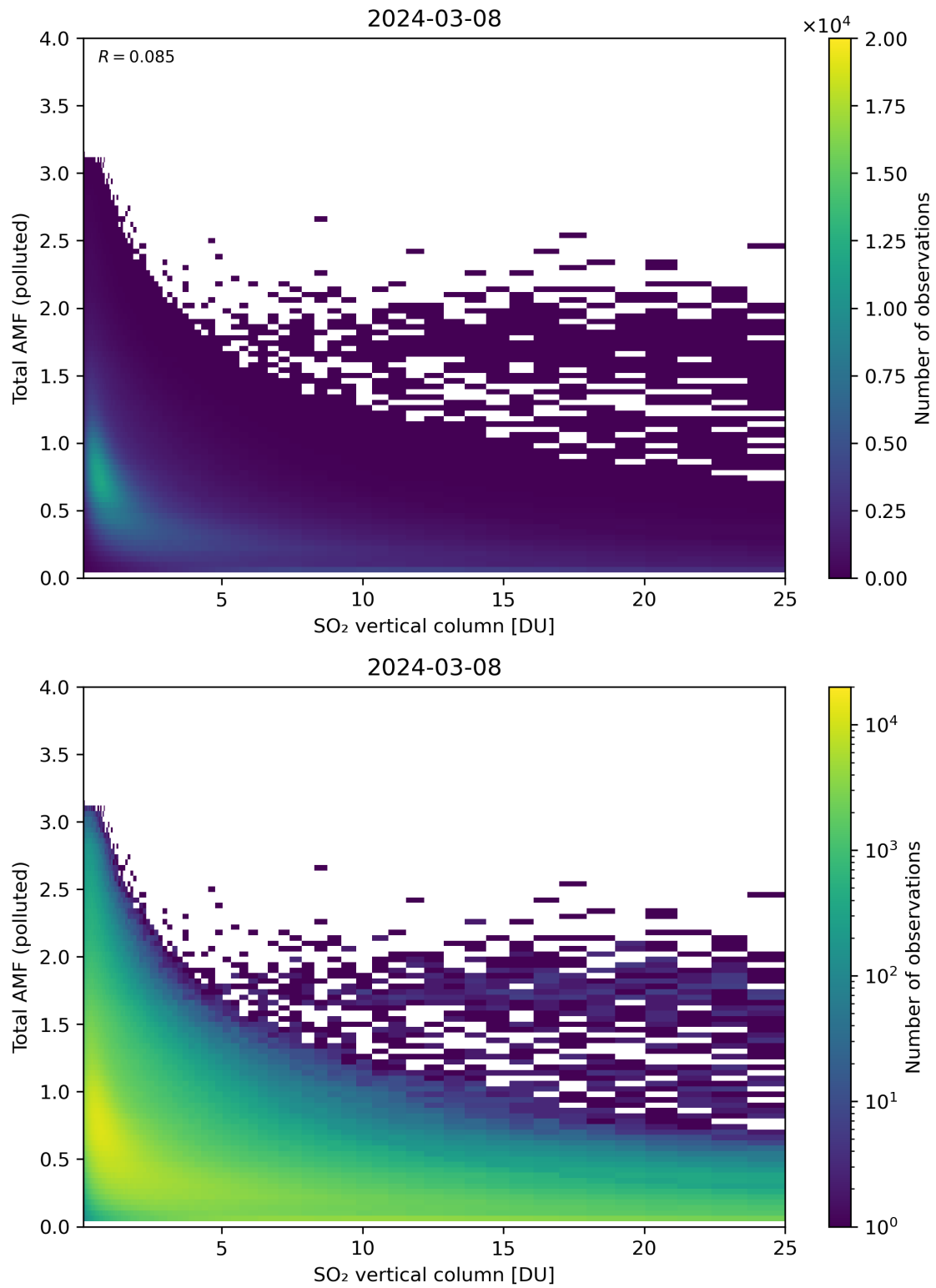
Figure 305: Scatter density plot of “SO 2 vertical column” against “Total AMF (polluted)” for 2024-03-07 to 2024-03-09.
