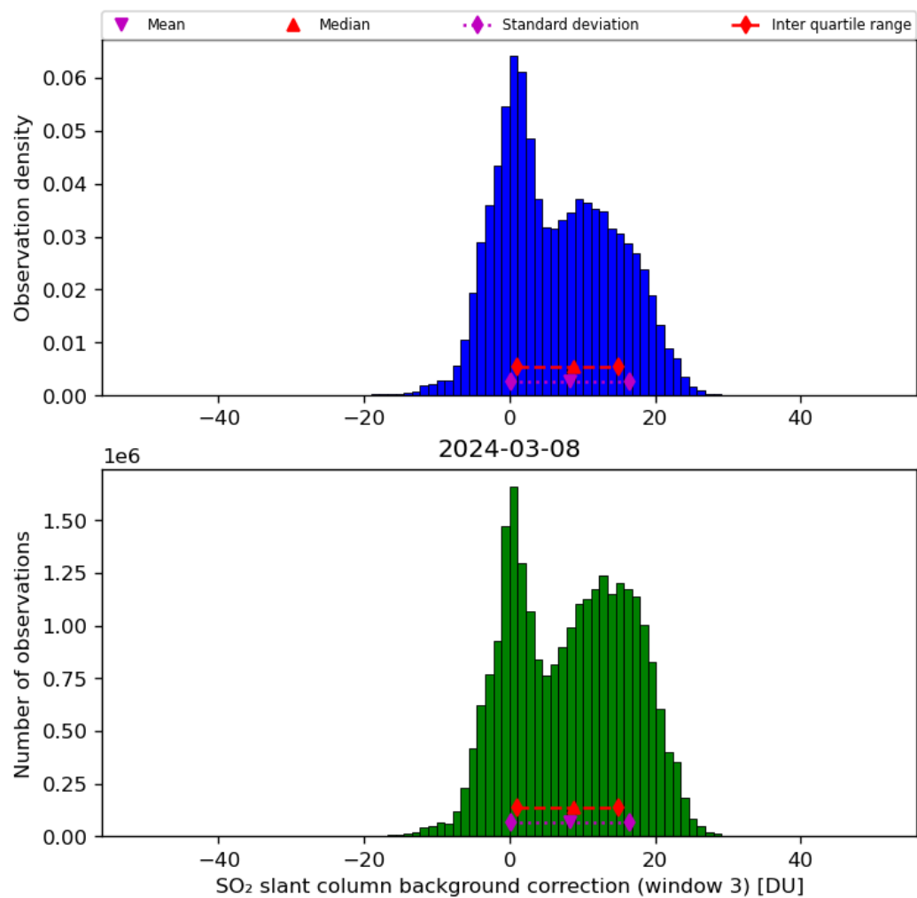
Figure 67: Histogram of “SO 2 slant column background correction (window 3)” for 2024-03-07 to 2024-03-09
