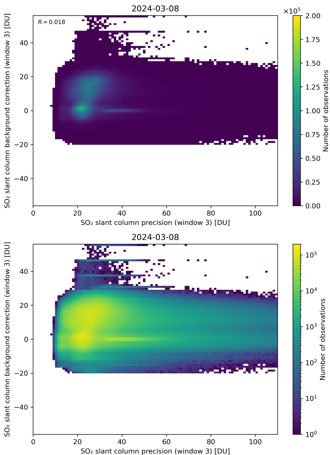
Figure 257: Scatter density plot of “SO 2 slant column precision (window 3)” against “SO 2 slant column background correction (window 3)” for 2024-03-07 to 2024-03-09.
