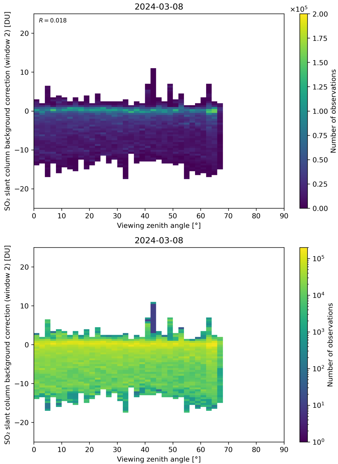
Figure 309: Scatter density plot of “Viewing zenith angle” against “SO 2 slant column background correction (window 2)” for 2024-03-07 to 2024-03-09.
