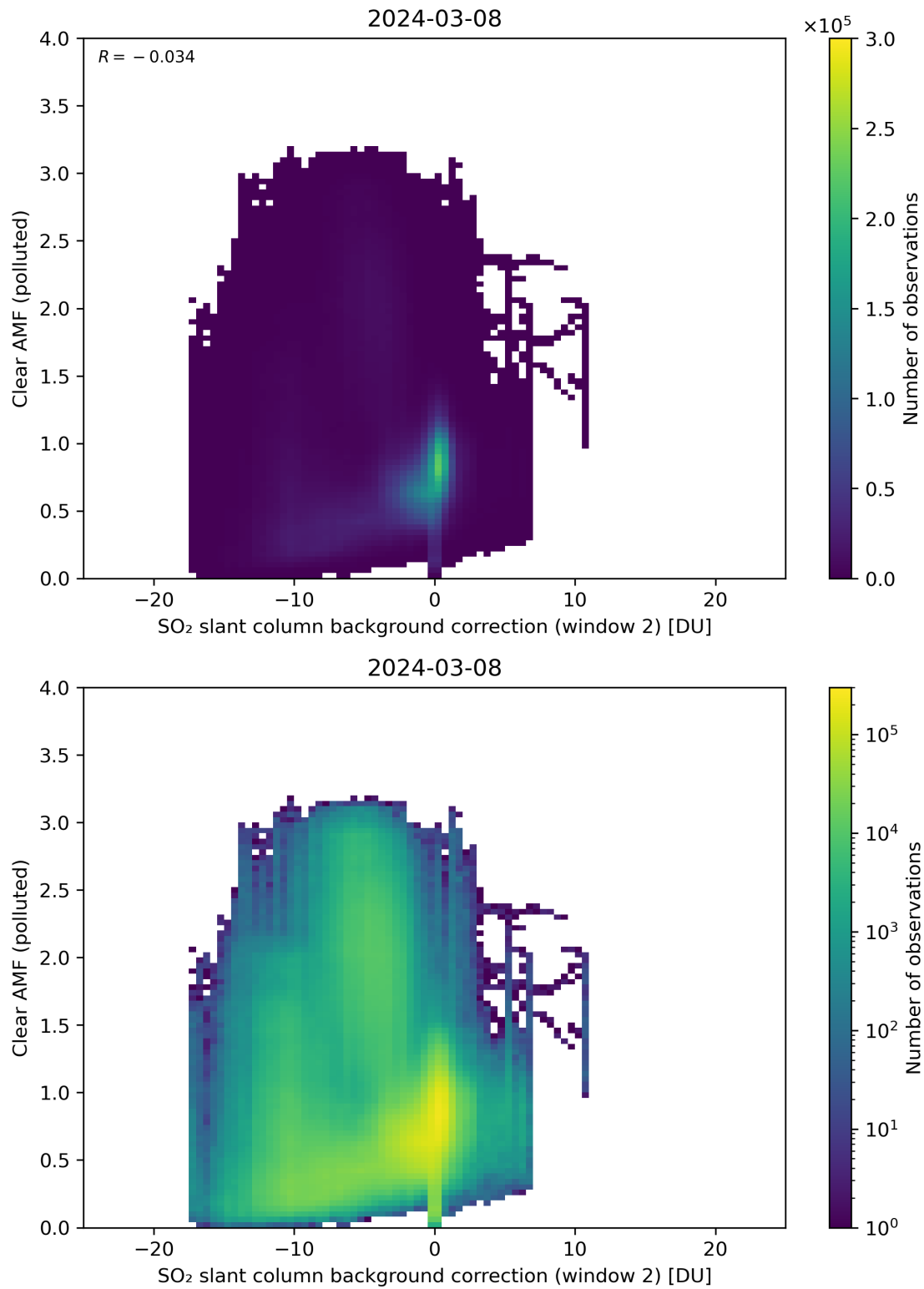
Figure 115: Scatter density plot of “SO 2 slant column background correction (window 2)” against “Clear AMF (polluted)” for 2024-03-07 to 2024-03-09.
