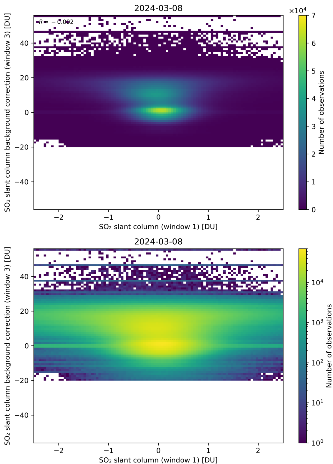
Figure 214: Scatter density plot of “SO 2 slant column (window 1)” against “SO 2 slant column background correction (window 3)” for 2024-03-07 to 2024-03-09.
