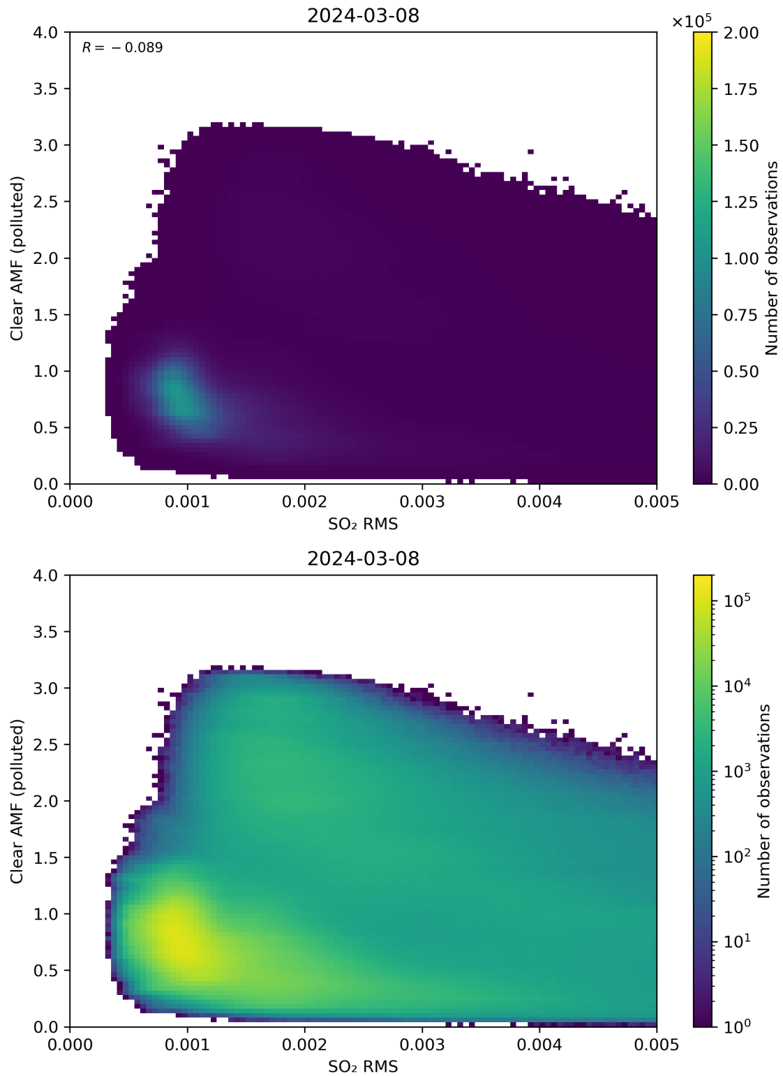
Figure 136: Scatter density plot of “SO 2 RMS” against “Clear AMF (polluted)” for 2024-03-07 to 2024-03-09.
