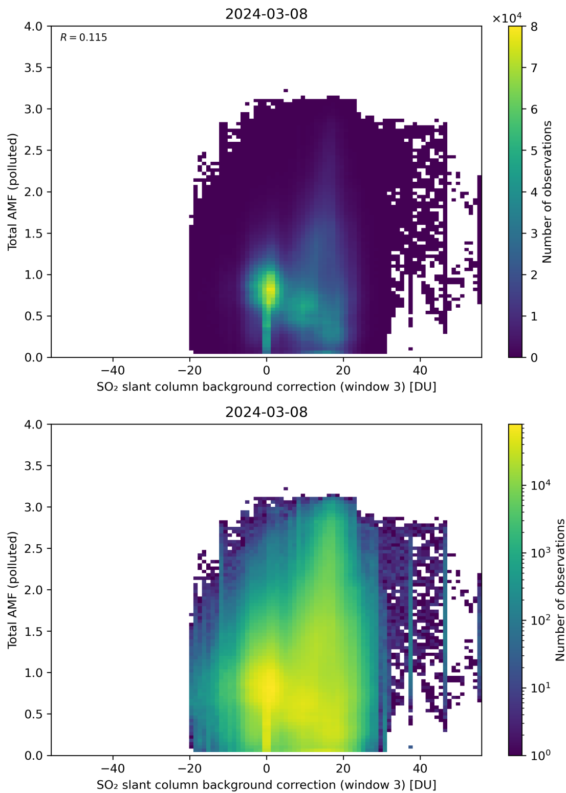
Figure 125: Scatter density plot of “SO 2 slant column background correction (window 3)” against “Total AMF (polluted)” for 2024-03-07 to 2024-03-09.
