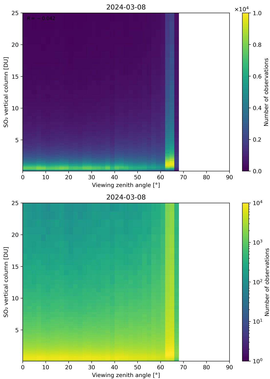
Figure 327: Scatter density plot of “Viewing zenith angle” against “SO 2 vertical column” for 2024-03-07 to 2024-03-09.
