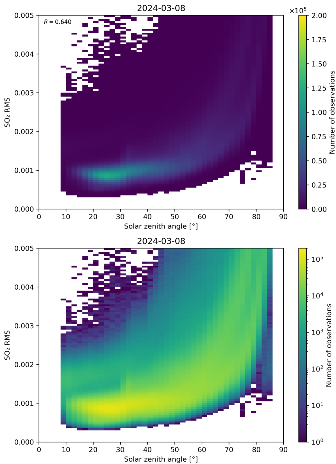
Figure 163: Scatter density plot of “Solar zenith angle” against “SO 2 RMS” for 2024-03-07 to 2024-03-09.
