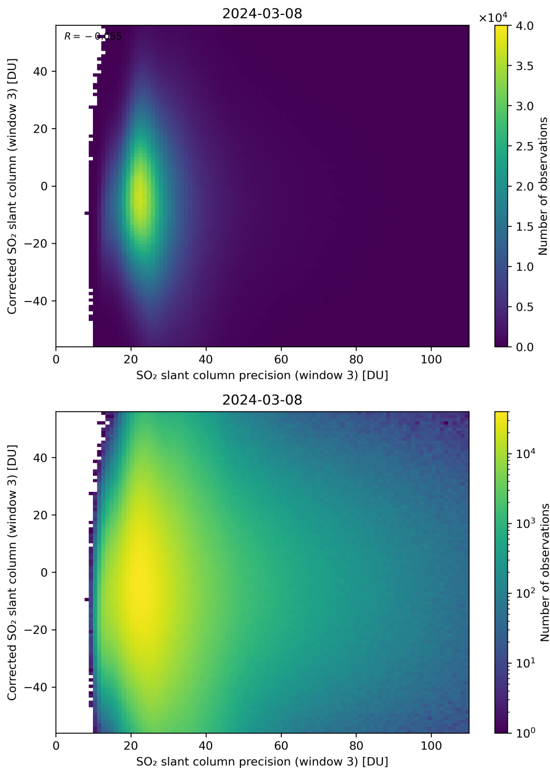
Figure 262: Scatter density plot of “SO 2 slant column precision (window 3)” against “Corrected SO 2 slant column (window 3)” for 2024-03-07 to 2024-03-09.
