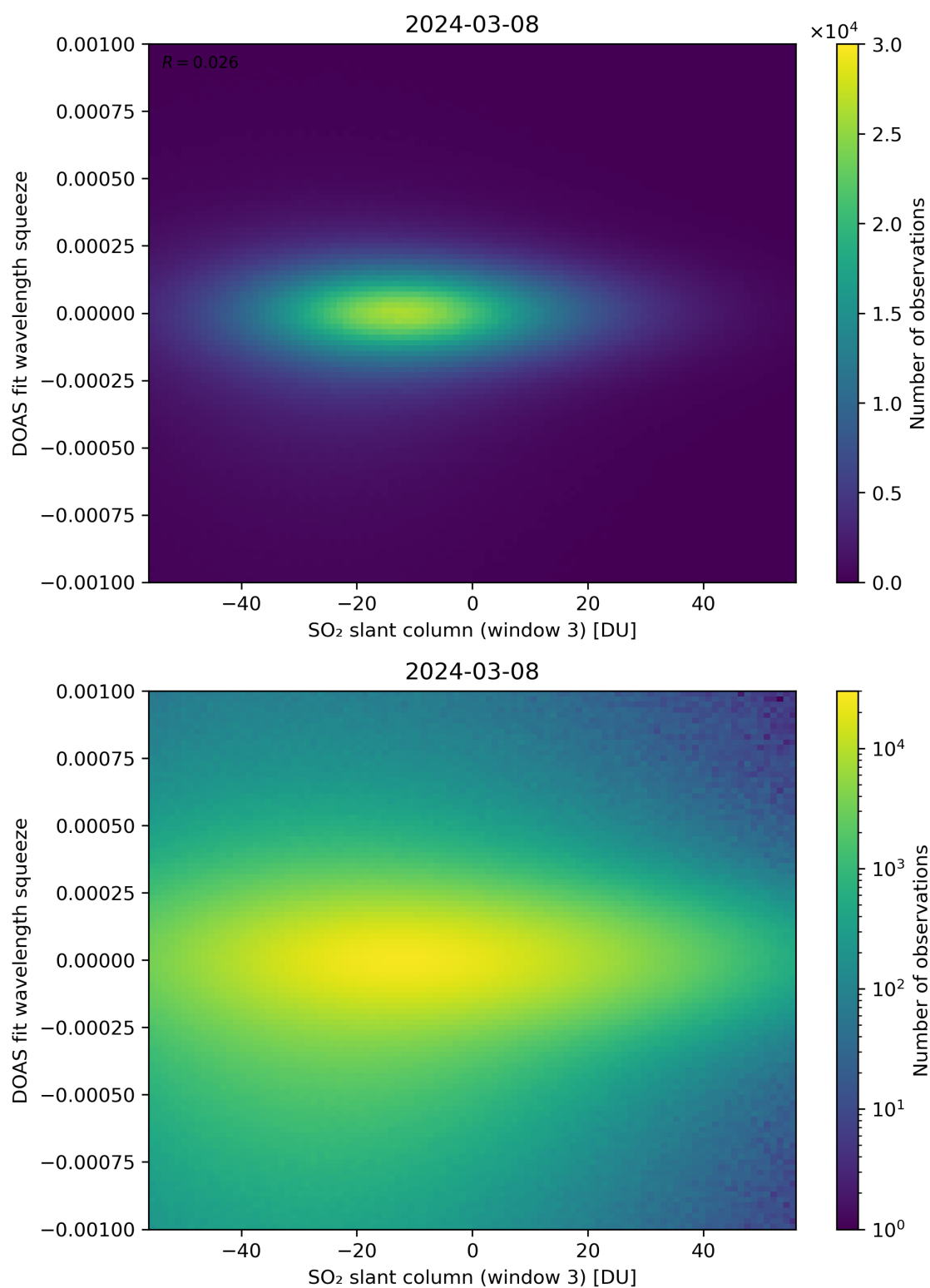
Figure 255: Scatter density plot of “SO 2 slant column (window 3)” against “DOAS fit wavelength squeeze” for 2024-03-07 to 2024-03-09.
