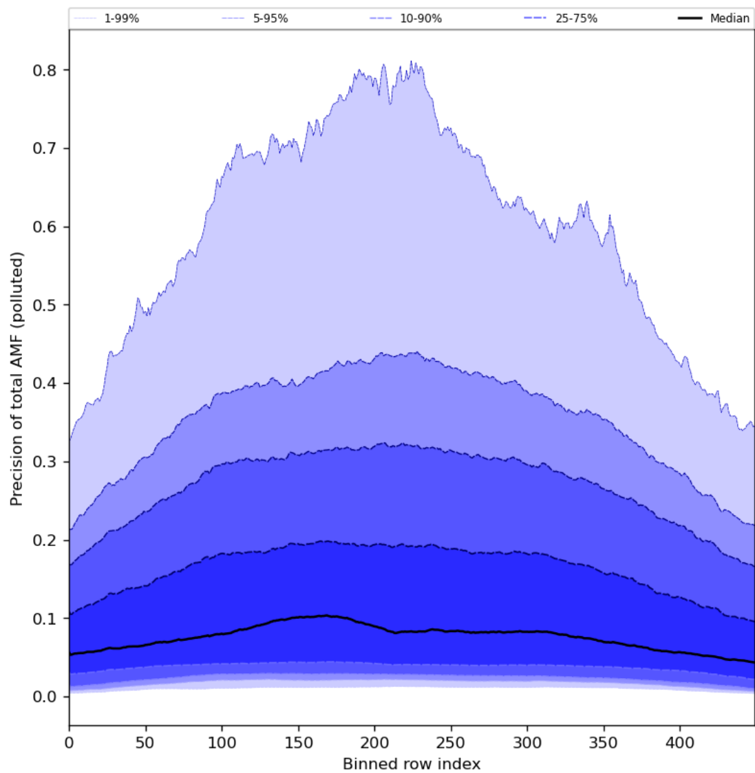
Figure 95: Along track statistics of “Precision of total AMF (polluted)” for 2024-03-07 to 2024-03-09
