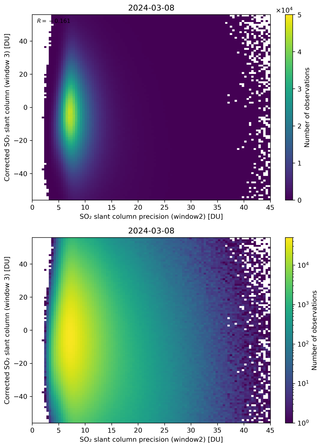
Figure 248: Scatter density plot of “SO 2 slant column precision (window2)” against “Corrected SO 2 slant column (window 3)” for 2024-03-07 to 2024-03-09.
