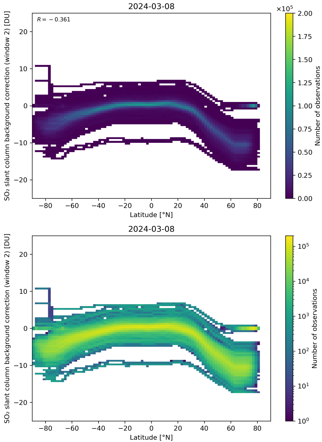
Figure 140: Scatter density plot of “Latitude” against “SO 2 slant column background correction (window 2)” for 2024-03-07 to 2024-03-09.
