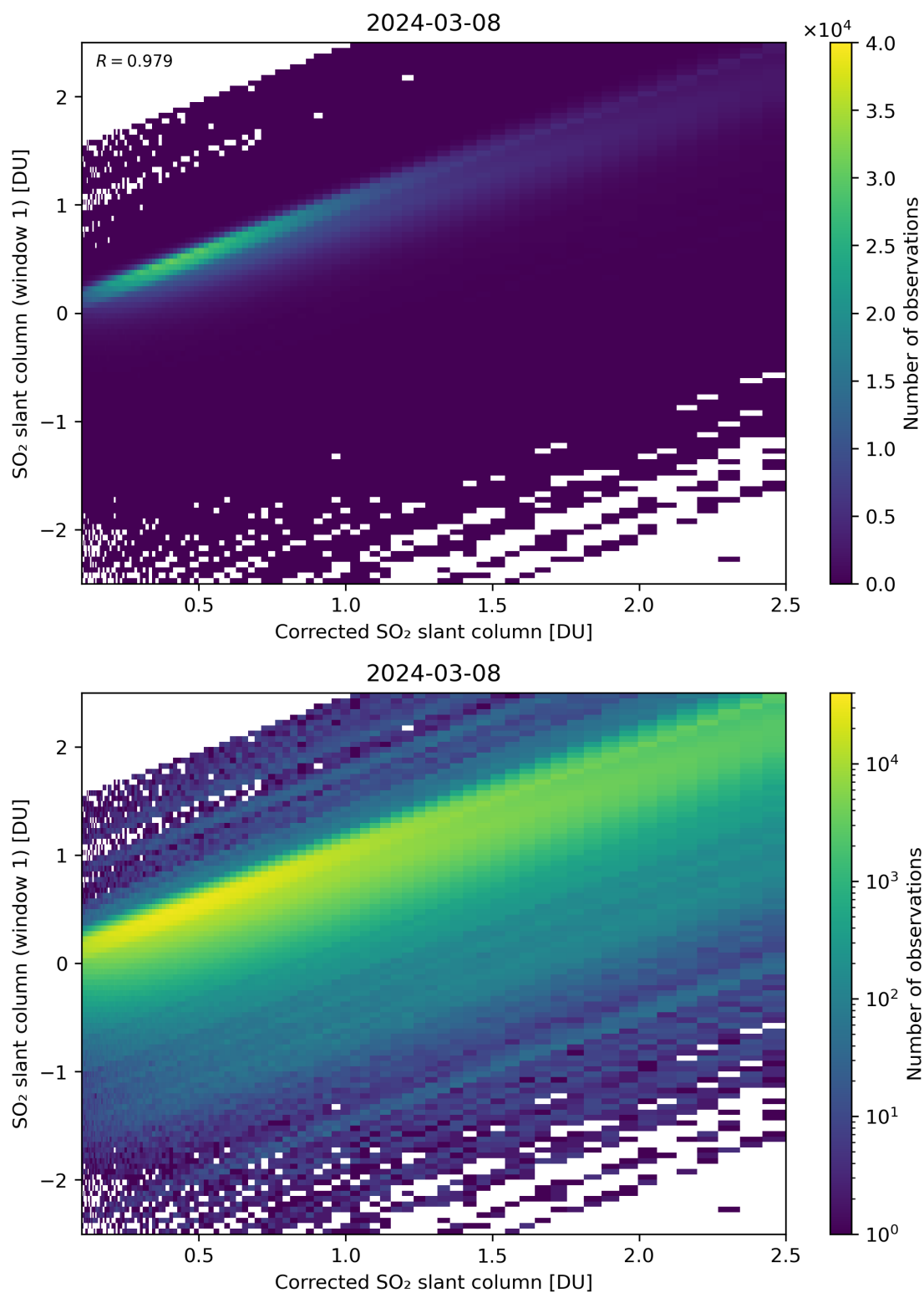
Figure 187: Scatter density plot of “Corrected SO 2 slant column” against “SO 2 slant column (window 1)” for 2024-03-07 to 2024-03-09.
