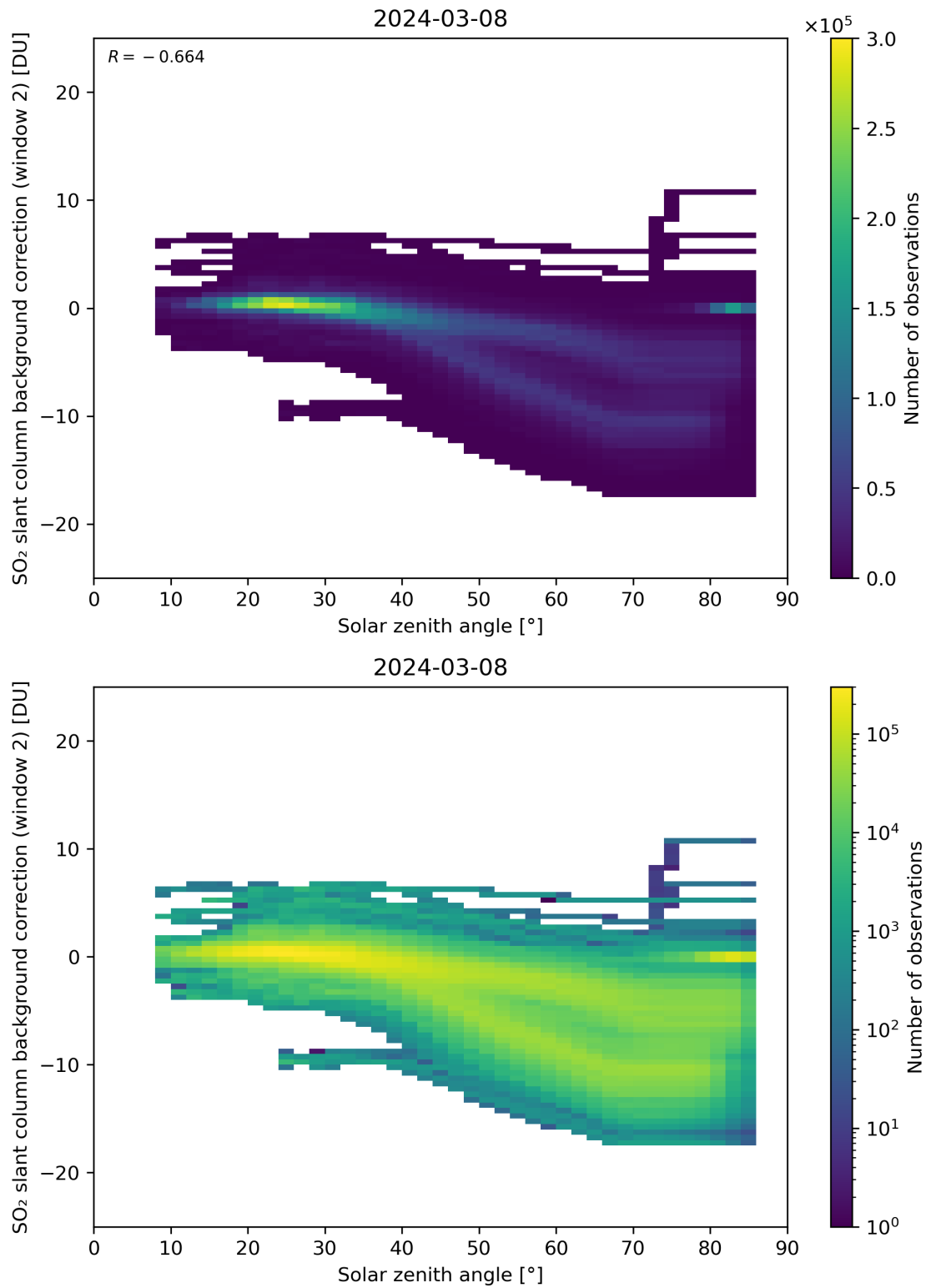
Figure 159: Scatter density plot of “Solar zenith angle” against “SO 2 slant column background correction (window 2)” for 2024-03-07 to 2024-03-09.
