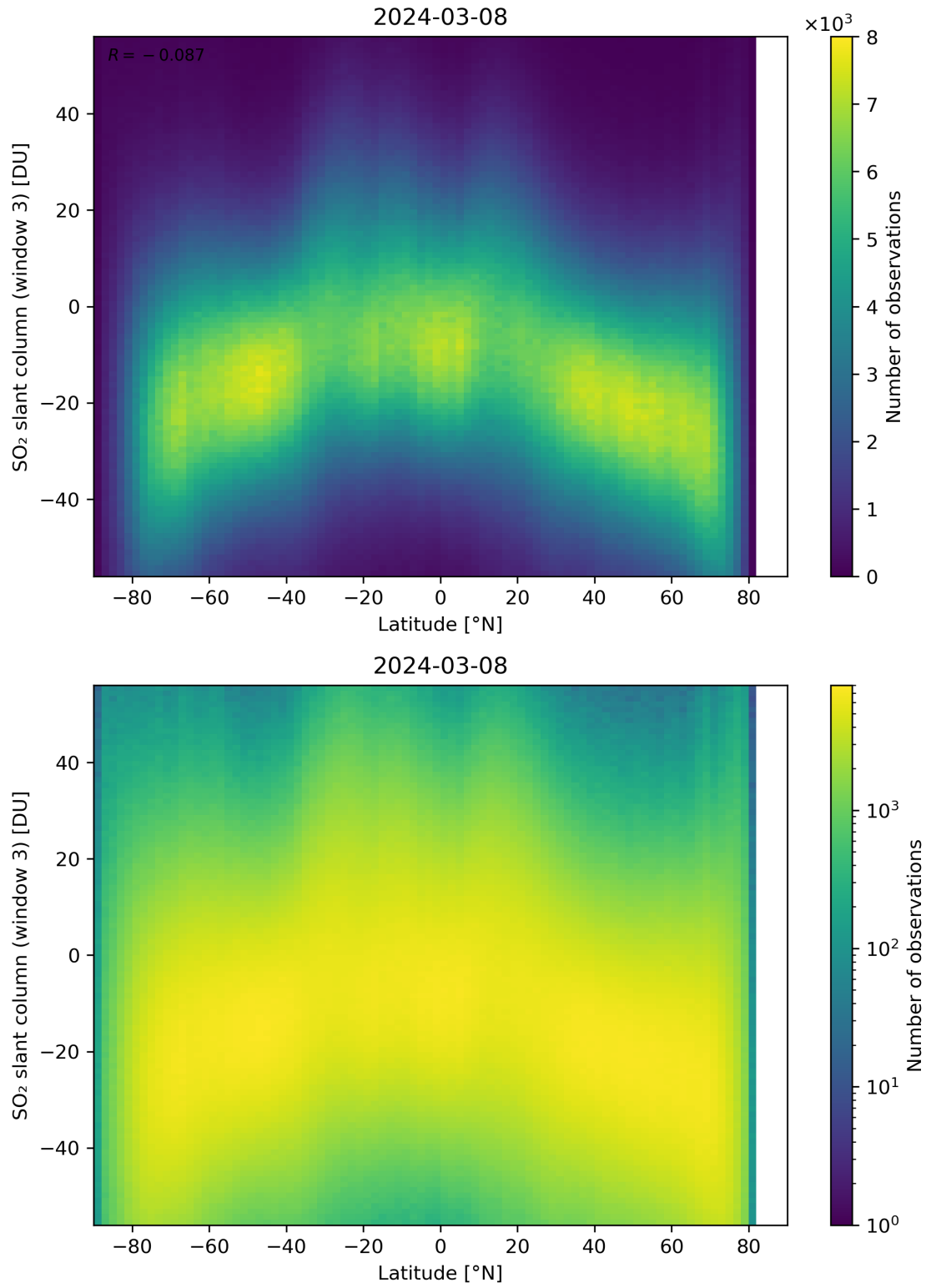
Figure 152: Scatter density plot of “Latitude” against “SO 2 slant column (window 3)” for 2024-03-07 to 2024-03-09.
