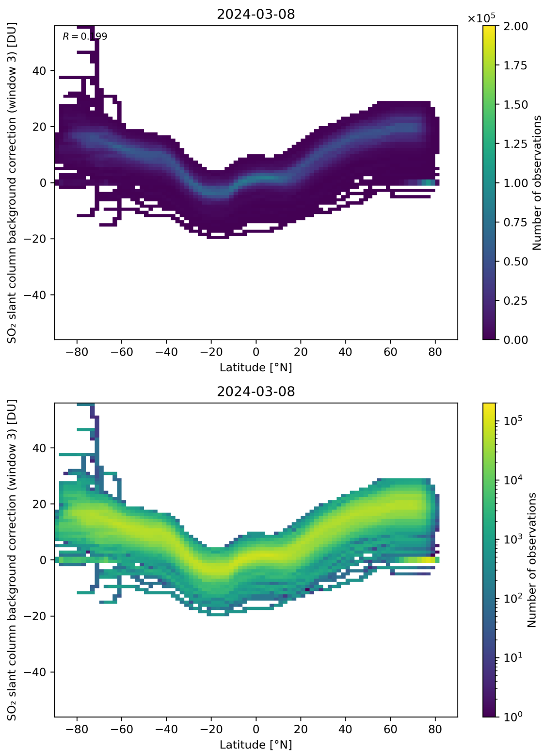
Figure 141: Scatter density plot of “Latitude” against “SO 2 slant column background correction (window 3)” for 2024-03-07 to 2024-03-09.
