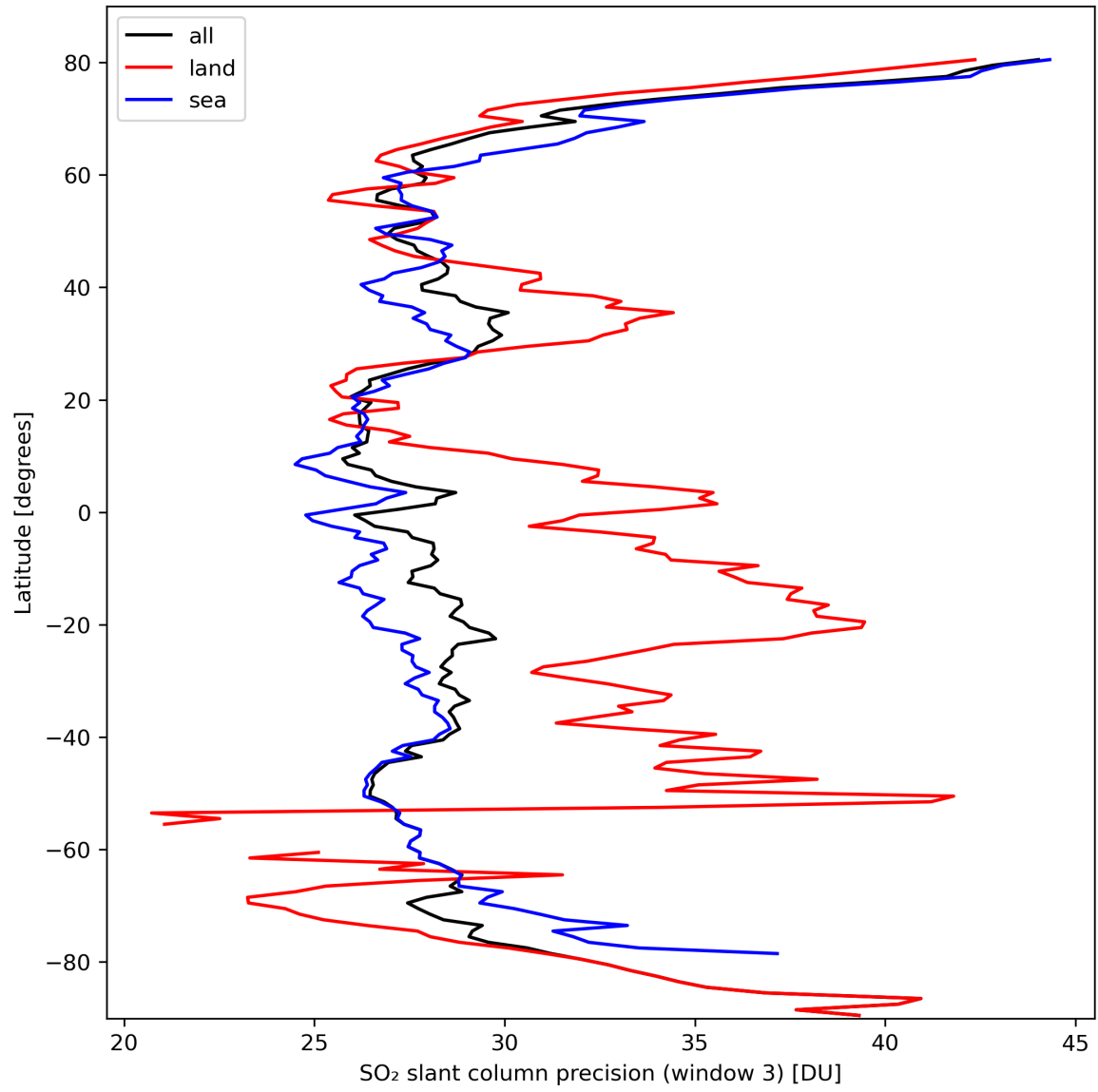
Figure 42: Zonal average of “SO 2 slant column precision (window 3)” for 2024-03-07 to 2024-03-09.
