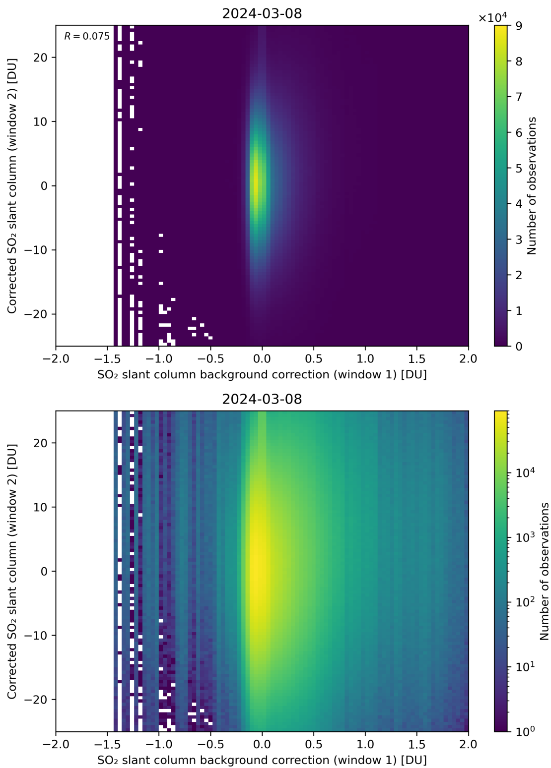
Figure 104: Scatter density plot of “SO 2 slant column background correction (window 1)” against “Corrected SO 2 slant column (window 2)” for 2024-03-07 to 2024-03-09.
