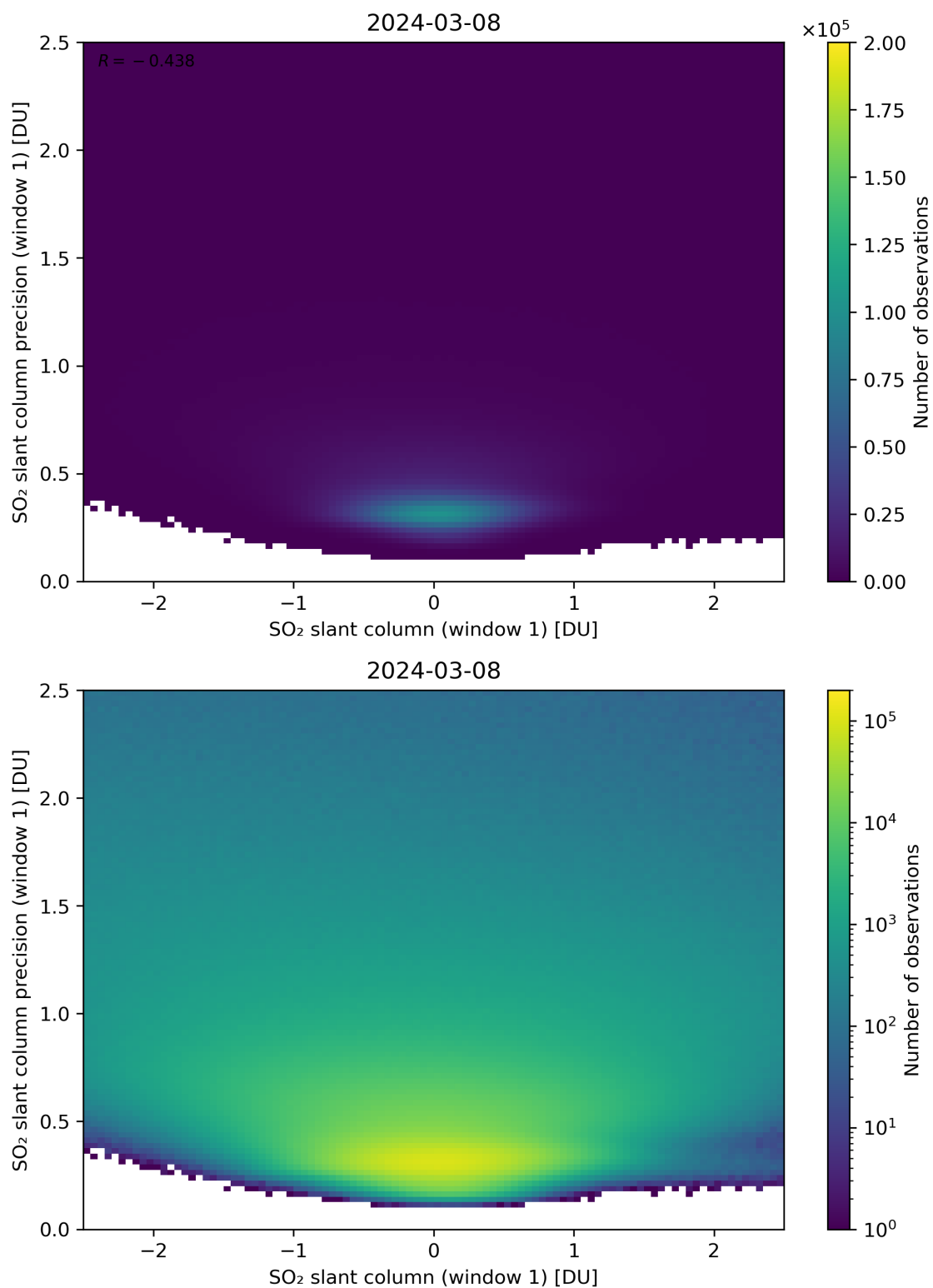
Figure 235: Scatter density plot of “SO 2 slant column (window 1)” against “SO 2 slant column precision (window 1)” for 2024-03-07 to 2024-03-09.
