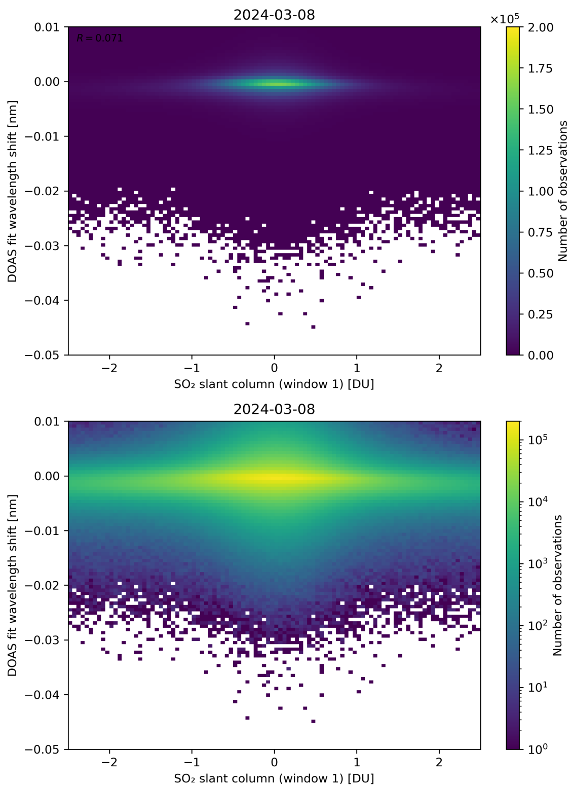
Figure 215: Scatter density plot of “SO 2 slant column (window 1)” against “DOAS fit wavelength shift” for 2024-03-07 to 2024-03-09.
