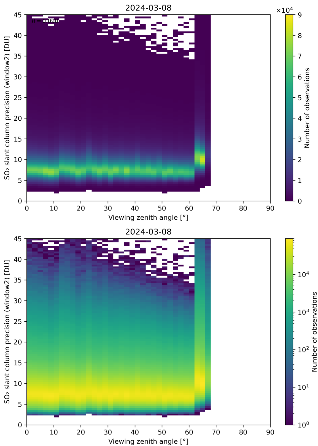
Figure 322: Scatter density plot of “Viewing zenith angle” against “SO 2 slant column precision (window2)” for 2024-03-07 to 2024-03-09.
