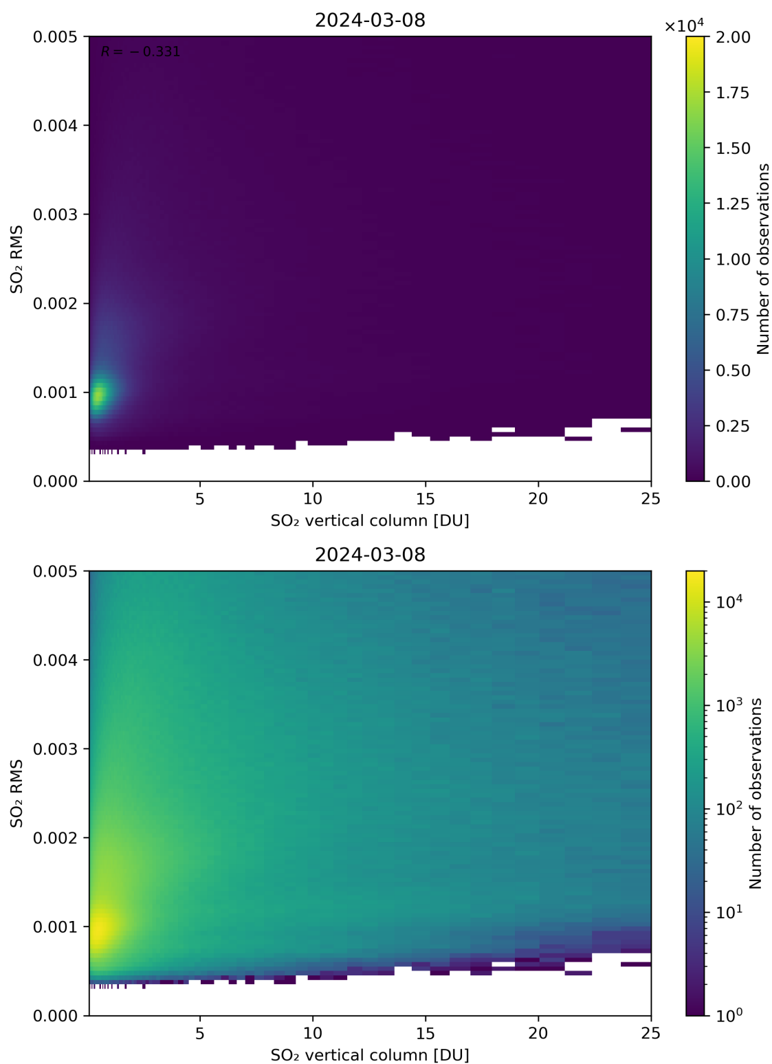
Figure 278: Scatter density plot of “SO 2 vertical column” against “SO 2 RMS” for 2024-03-07 to 2024-03-09.
