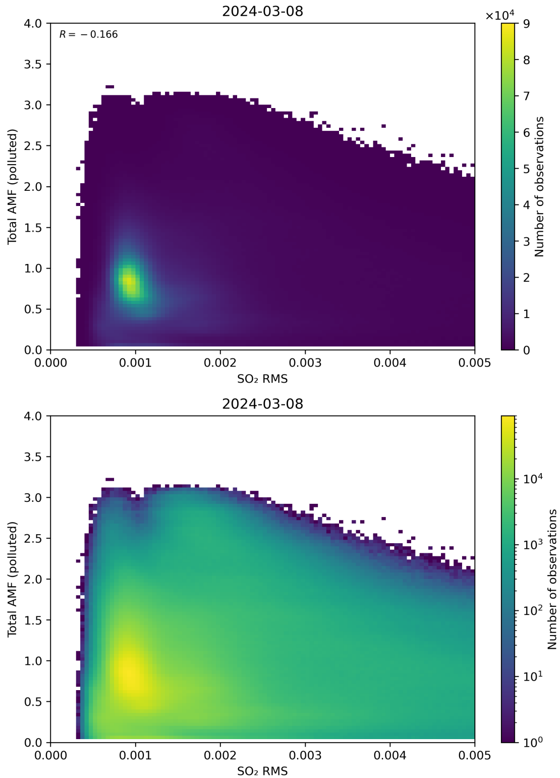
Figure 137: Scatter density plot of “SO 2 RMS” against “Total AMF (polluted)” for 2024-03-07 to 2024-03-09.
