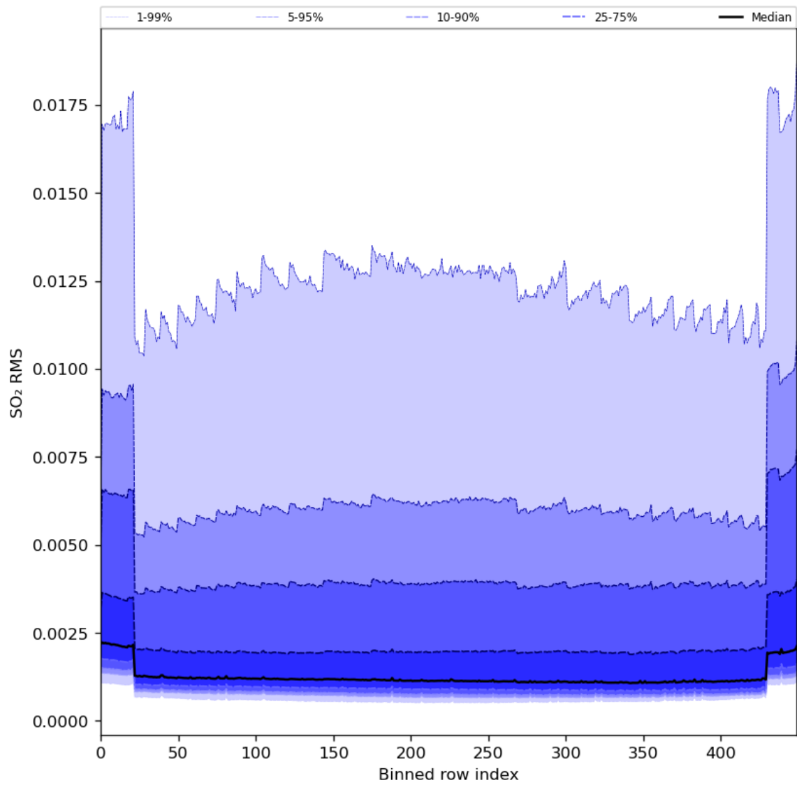
Figure 93: Along track statistics of “SO 2 RMS” for 2024-03-07 to 2024-03-09
