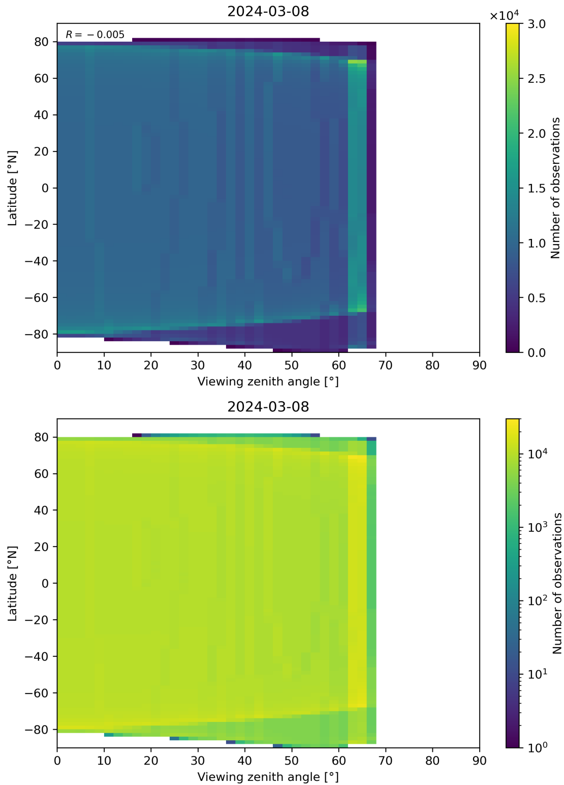
Figure 314: Scatter density plot of “Viewing zenith angle” against “Latitude” for 2024-03-07 to 2024-03-09.
