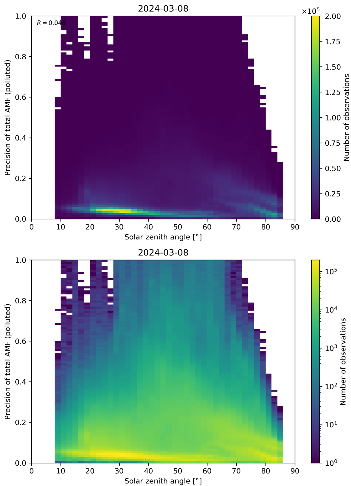
Figure 175: Scatter density plot of “Solar zenith angle” against “Precision of total AMF (polluted)” for 2024-03-07 to 2024-03-09.
