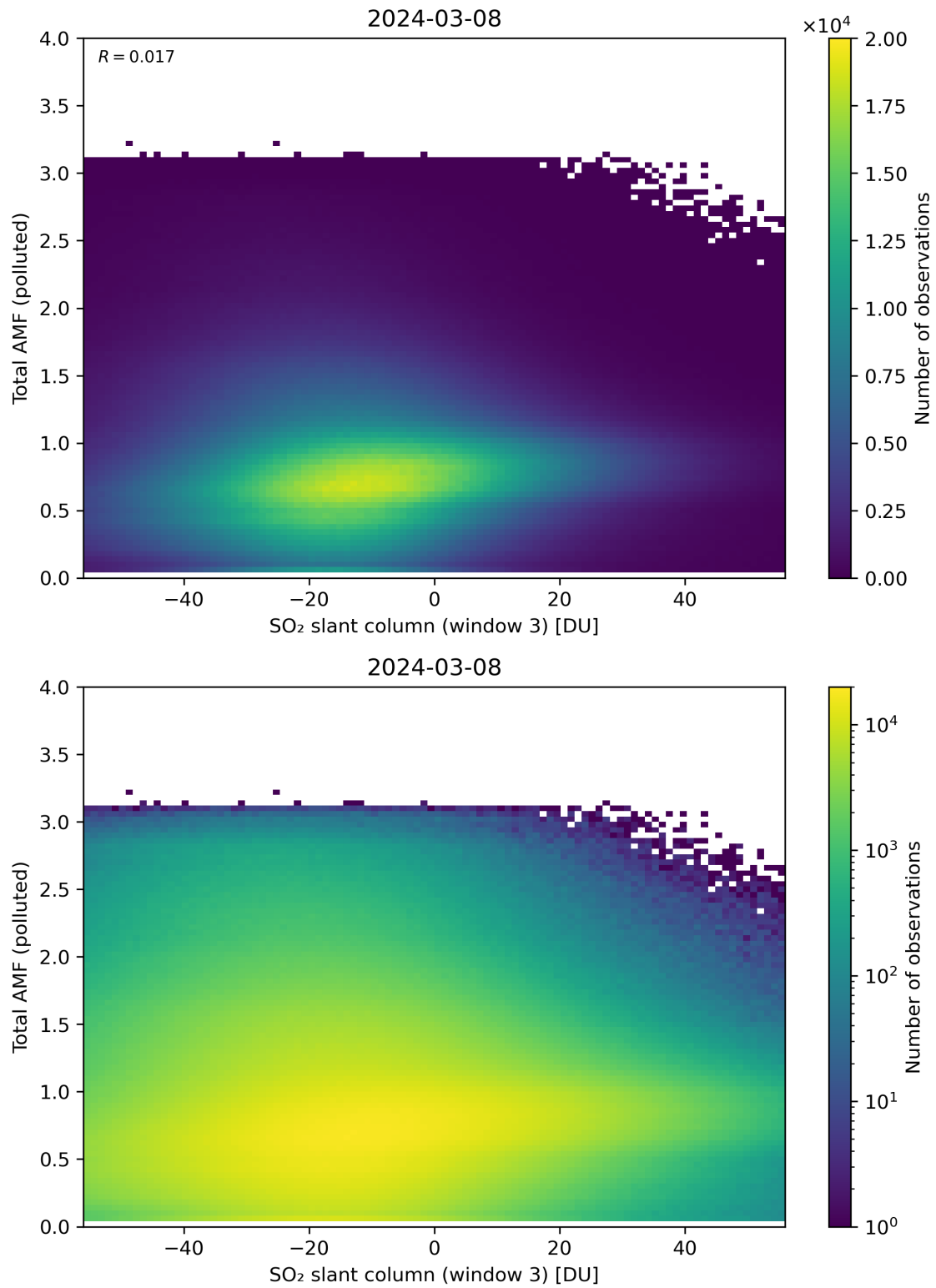
Figure 268: Scatter density plot of “SO 2 slant column (window 3)” against “Total AMF (polluted)” for 2024-03-07 to 2024-03-09.
