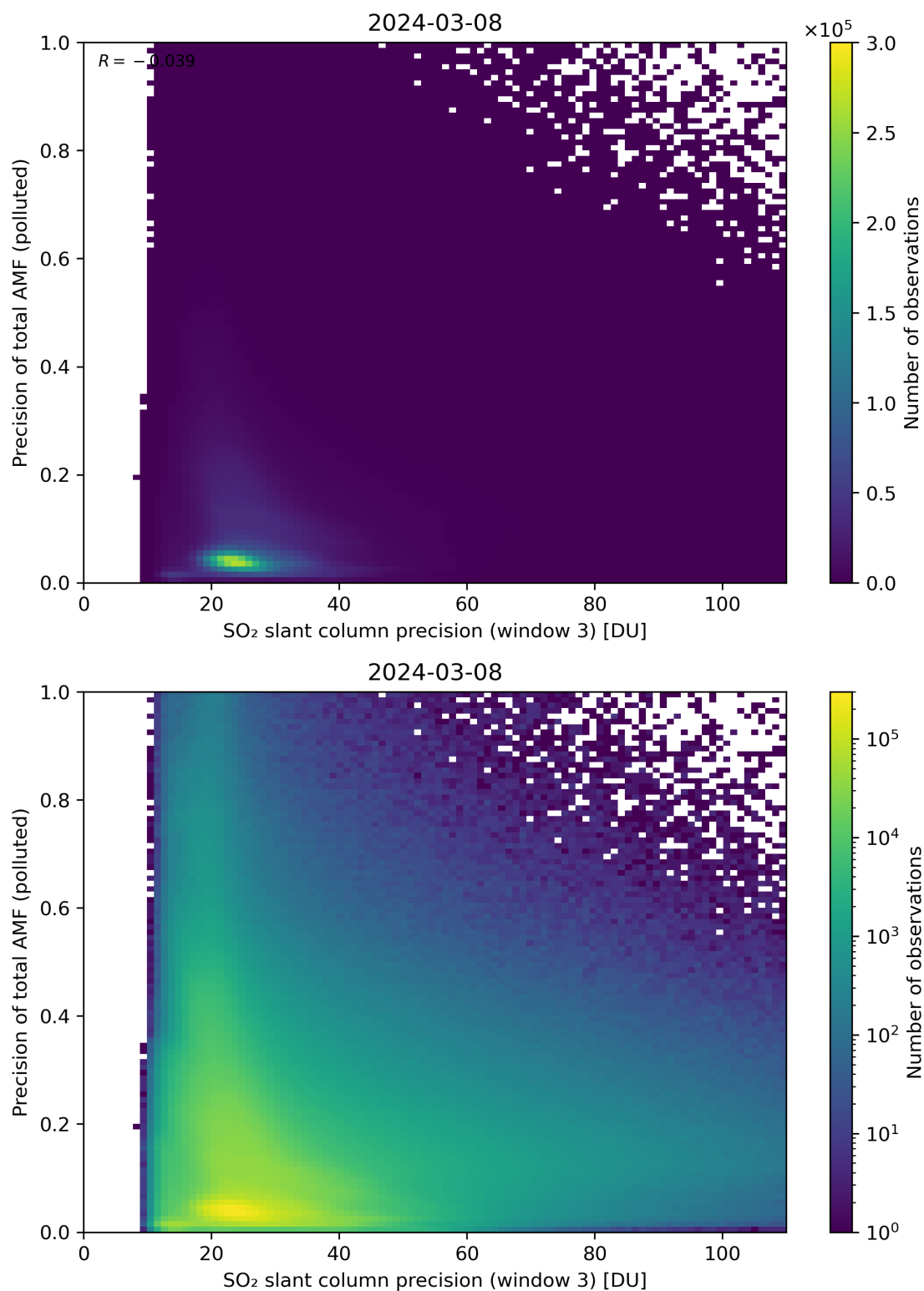
Figure 264: Scatter density plot of “SO 2 slant column precision (window 3)” against “Precision of total AMF (polluted)” for 2024-03-07 to 2024-03-09.
