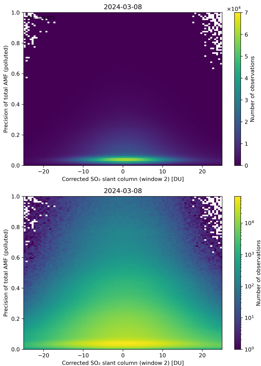
Figure 204: Scatter density plot of “Corrected SO 2 slant column (window 2)” against “Precision of total AMF (polluted)” for 2024-03-07 to 2024-03-09.
