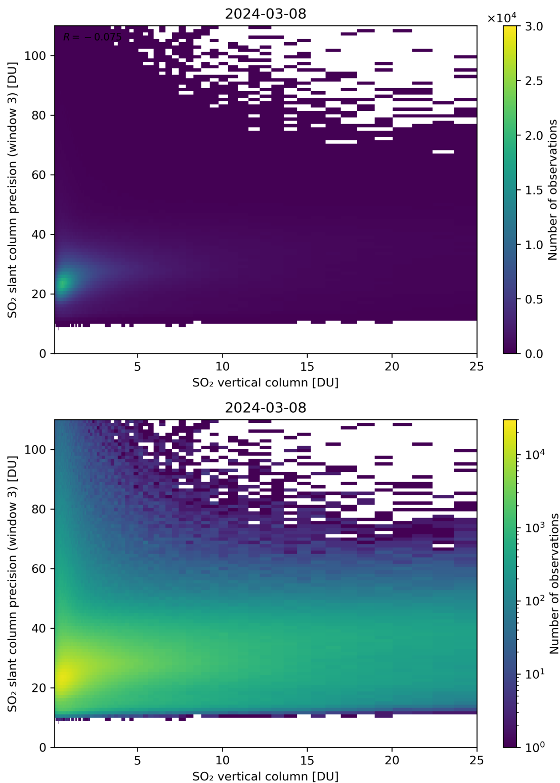
Figure 304: Scatter density plot of “SO 2 vertical column” against “SO 2 slant column precision (window 3)” for 2024-03-07 to 2024-03-09.
