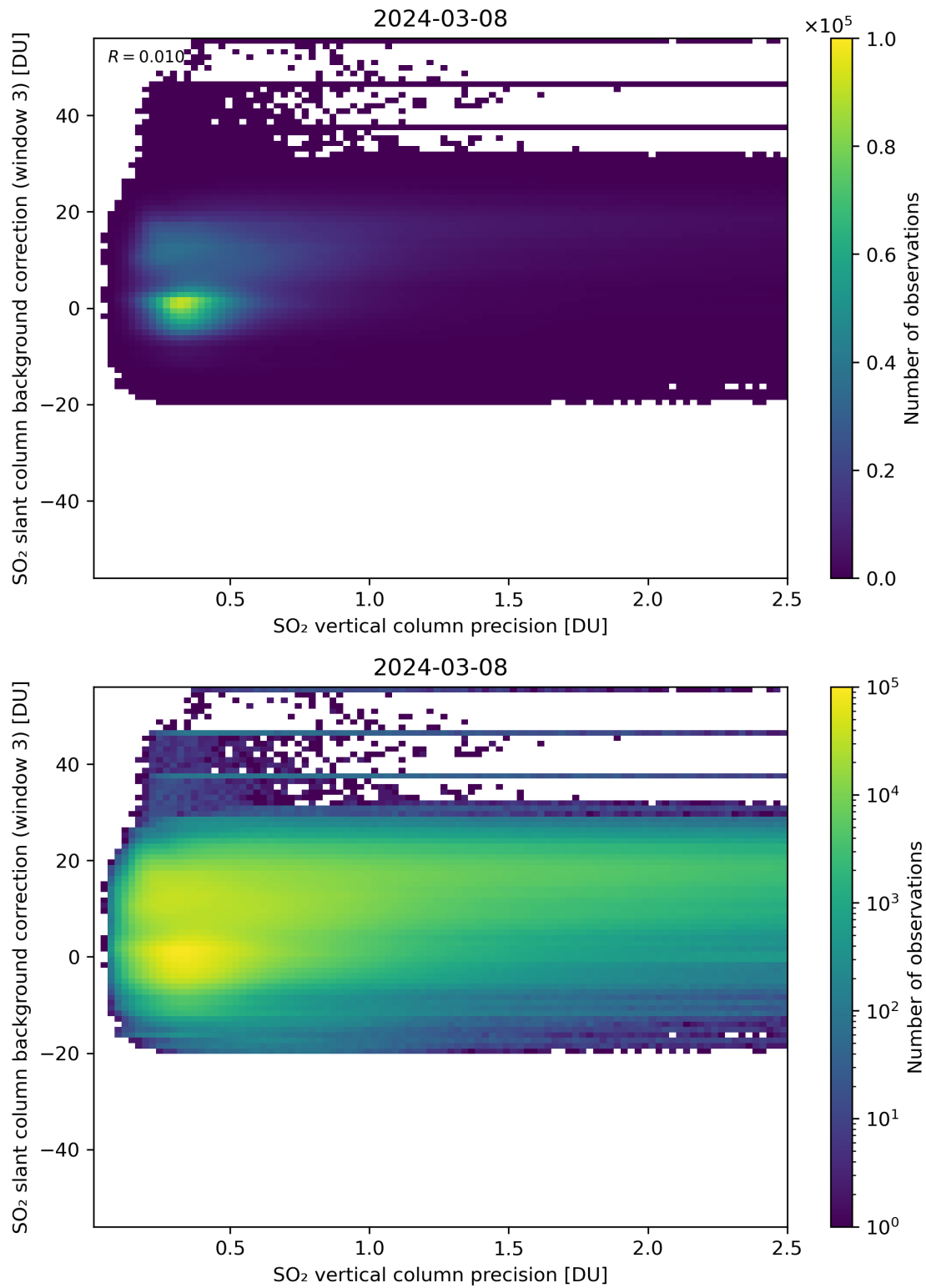
Figure 281: Scatter density plot of “SO 2 vertical column precision” against “SO 2 slant column background correction (window 3)” for 2024-03-07 to 2024-03-09.
