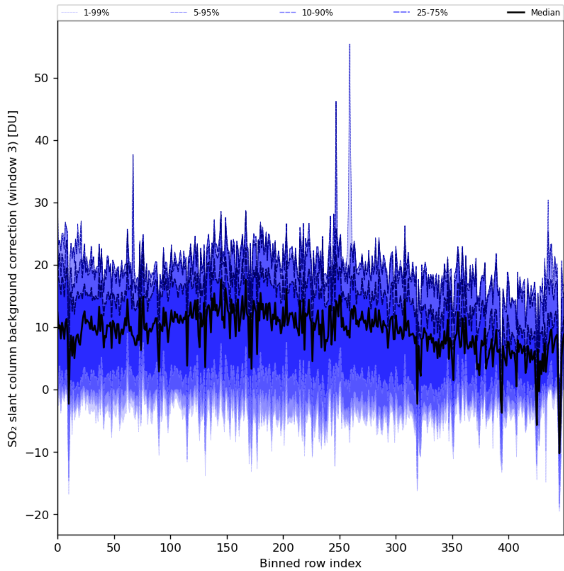
Figure 90: Along track statistics of “SO 2 slant column background correction (window 3)” for 2024-03-07 to 2024-03-09
