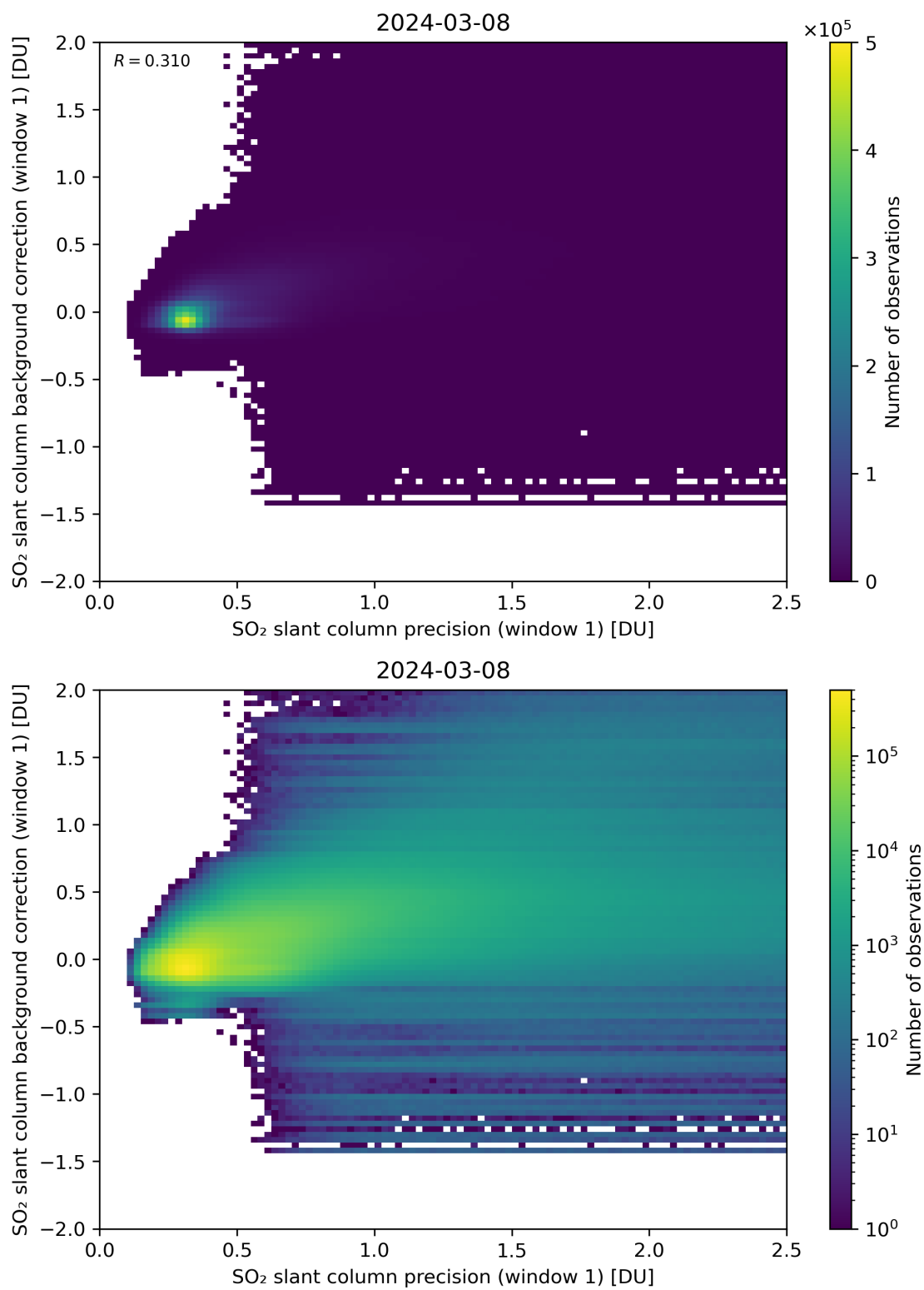
Figure 218: Scatter density plot of “SO 2 slant column precision (window 1)” against “SO 2 slant column background correction (window 1)” for 2024-03-07 to 2024-03-09.
