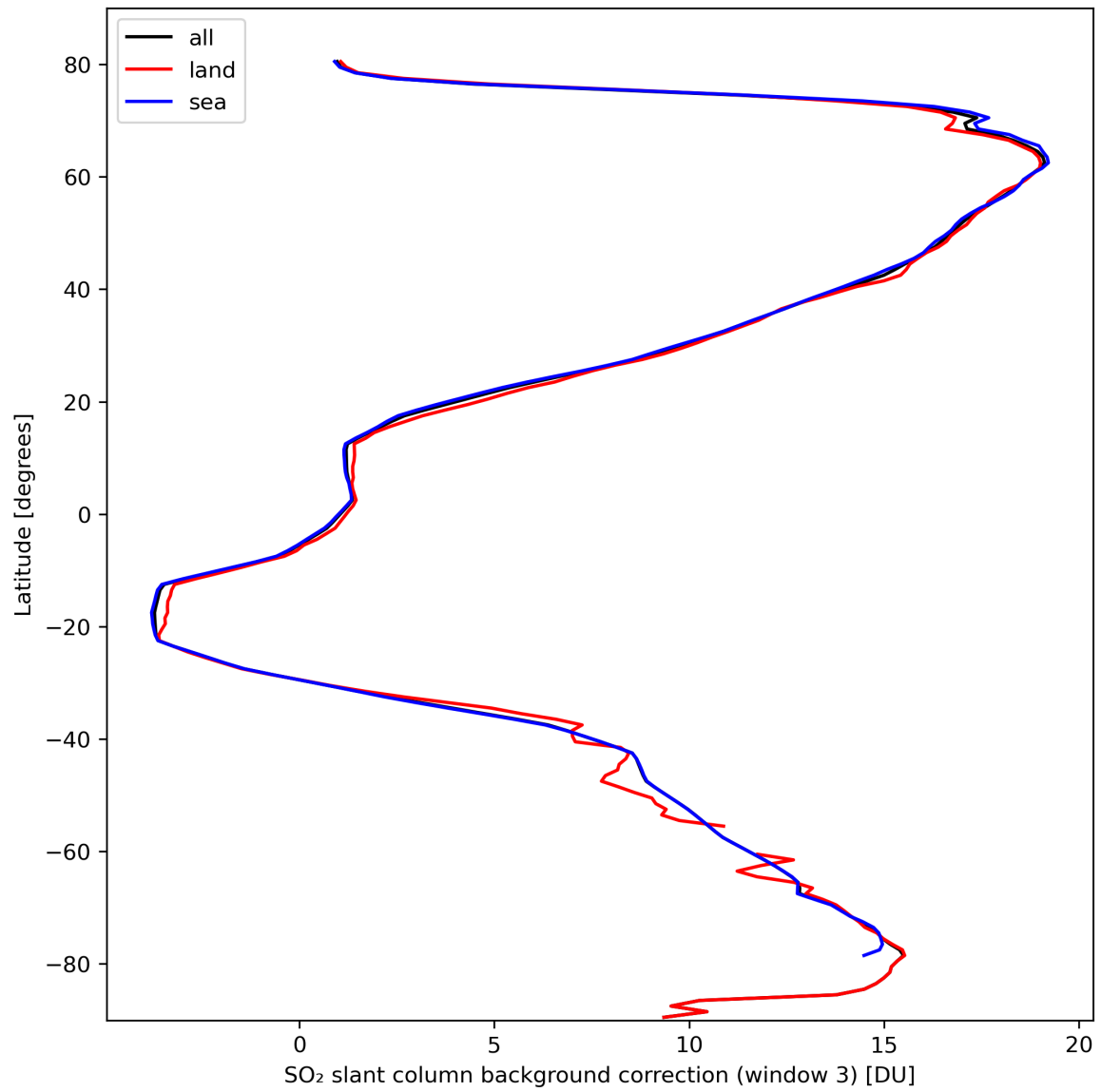
Figure 44: Zonal average of “SO 2 slant column background correction (window 3)” for 2024-03-07 to 2024-03-09.
