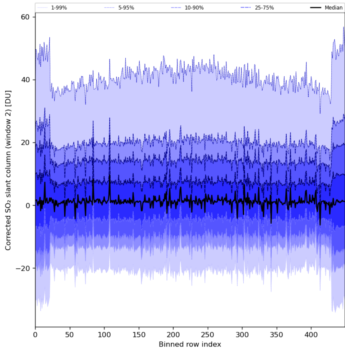
Figure 85: Along track statistics of “Corrected SO 2 slant column (window 2)” for 2024-03-07 to 2024-03-09
