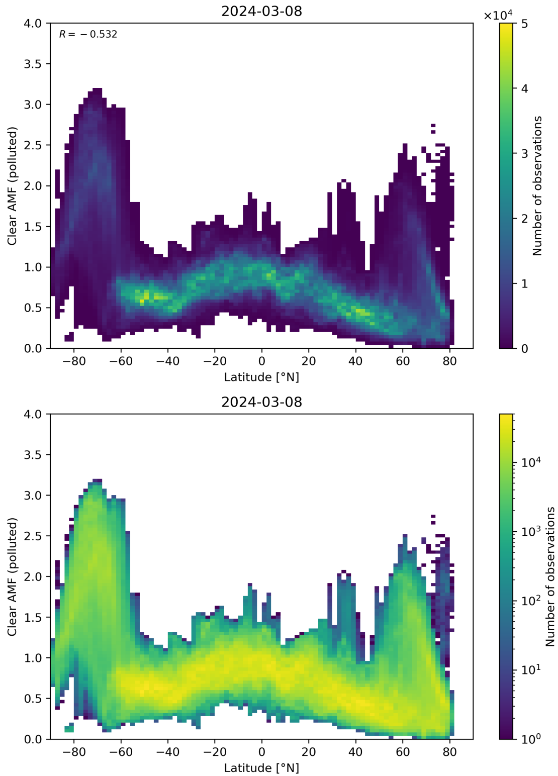
Figure 145: Scatter density plot of “Latitude” against “Clear AMF (polluted)” for 2024-03-07 to 2024-03-09.
