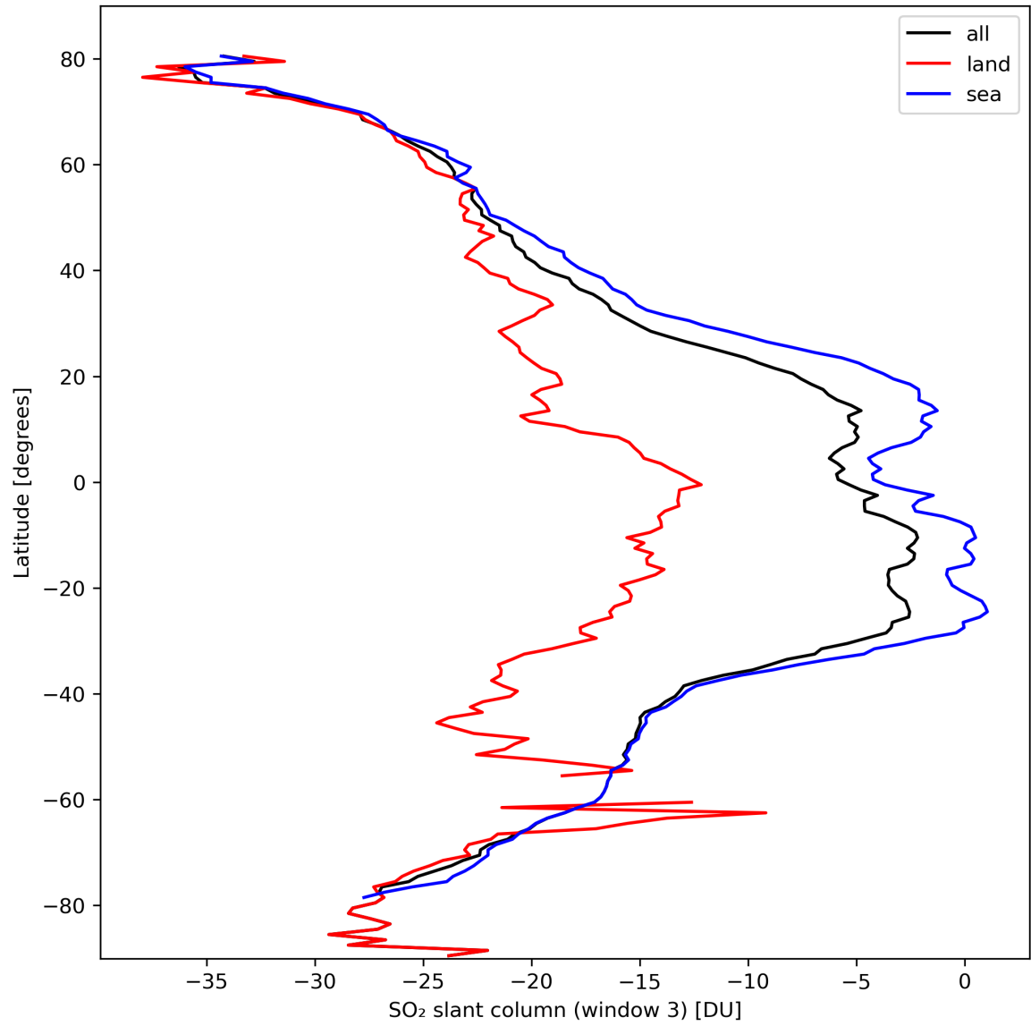
Figure 41: Zonal average of “SO 2 slant column (window 3)” for 2024-03-07 to 2024-03-09.
