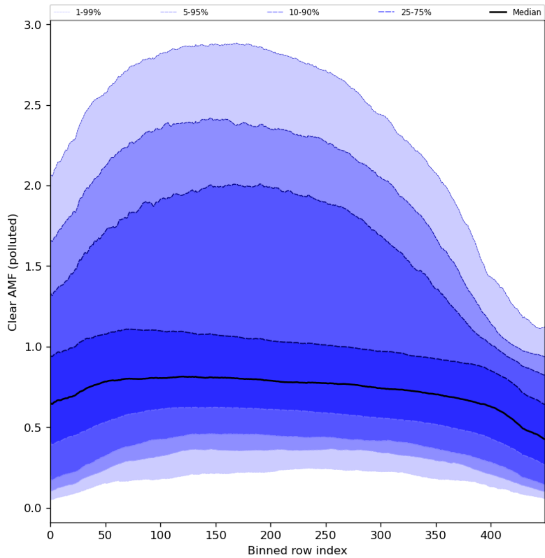
Figure 96: Along track statistics of “Clear AMF (polluted)” for 2024-03-07 to 2024-03-09
