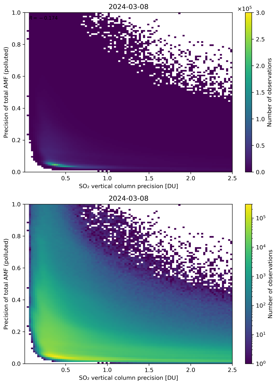
Figure 295: Scatter density plot of “SO 2 vertical column precision” against “Precision of total AMF (polluted)” for 2024-03-07 to 2024-03-09.
