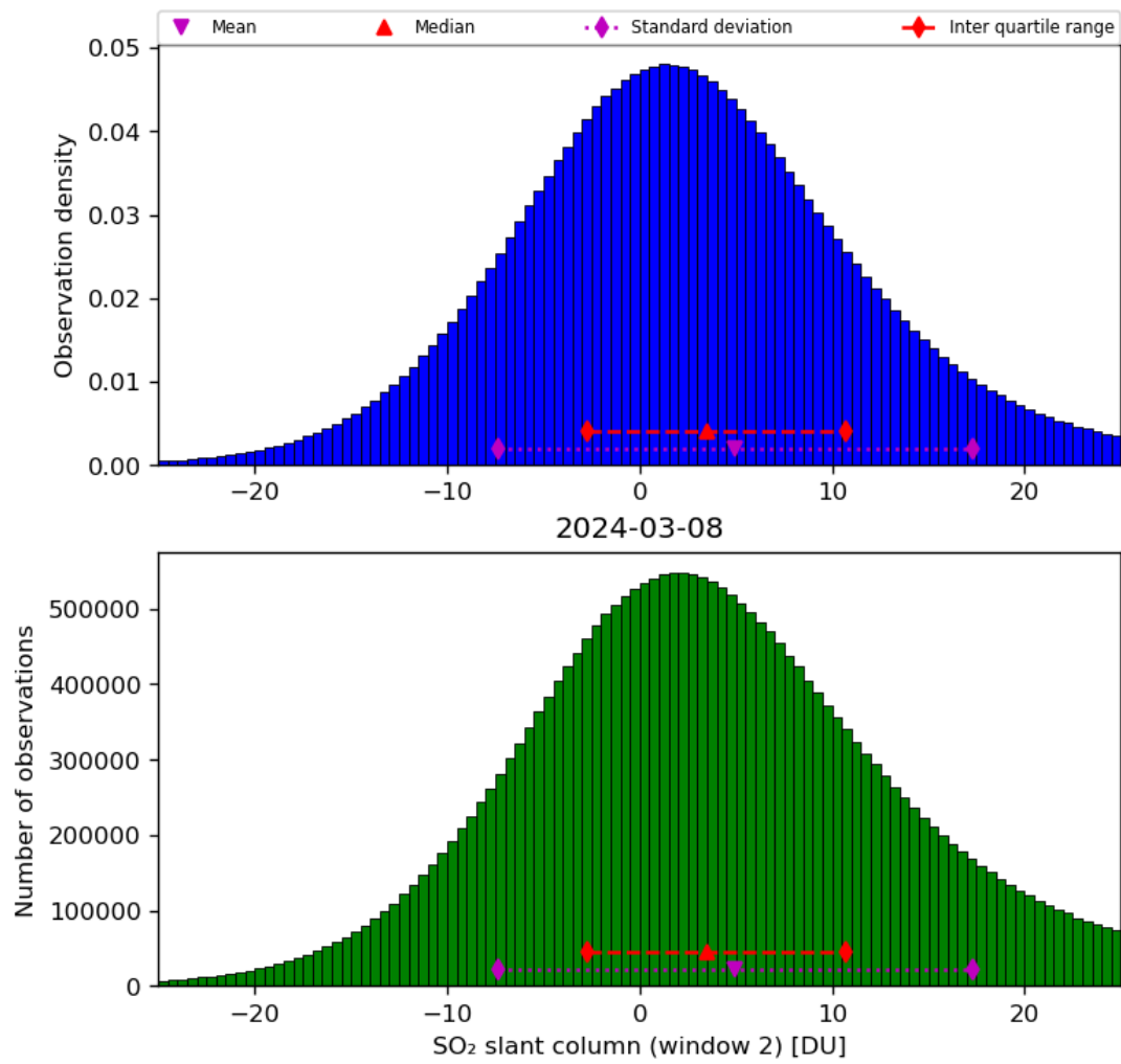
Figure 60: Histogram of “SO 2 slant column (window 2)” for 2024-03-07 to 2024-03-09
