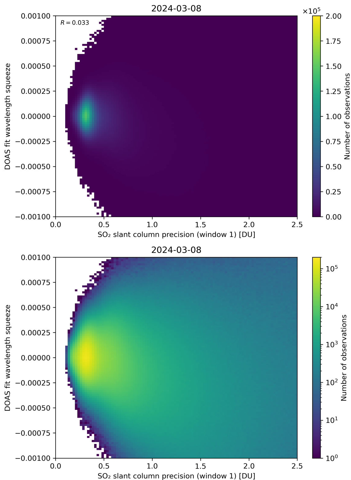
Figure 222: Scatter density plot of “SO 2 slant column precision (window 1)” against “DOAS fit wavelength squeeze” for 2024-03-07 to 2024-03-09.
