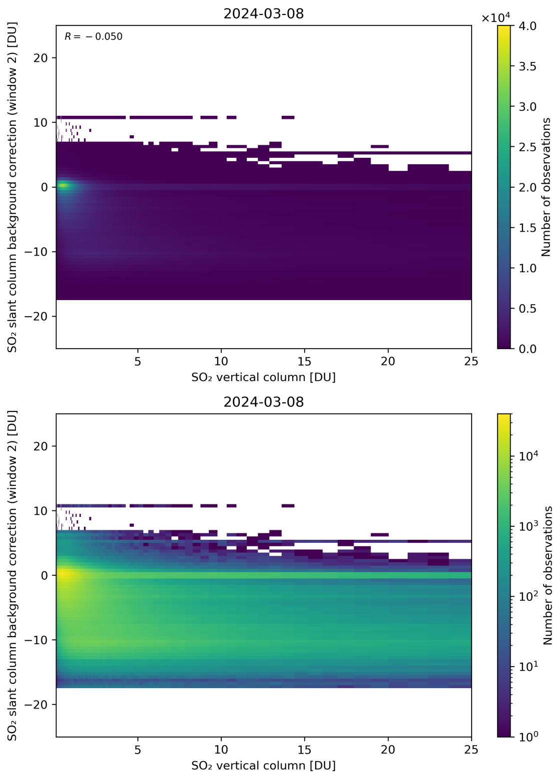
Figure 274: Scatter density plot of “SO 2 vertical column” against “SO 2 slant column background correction (window 2)” for 2024-03-07 to 2024-03-09.
