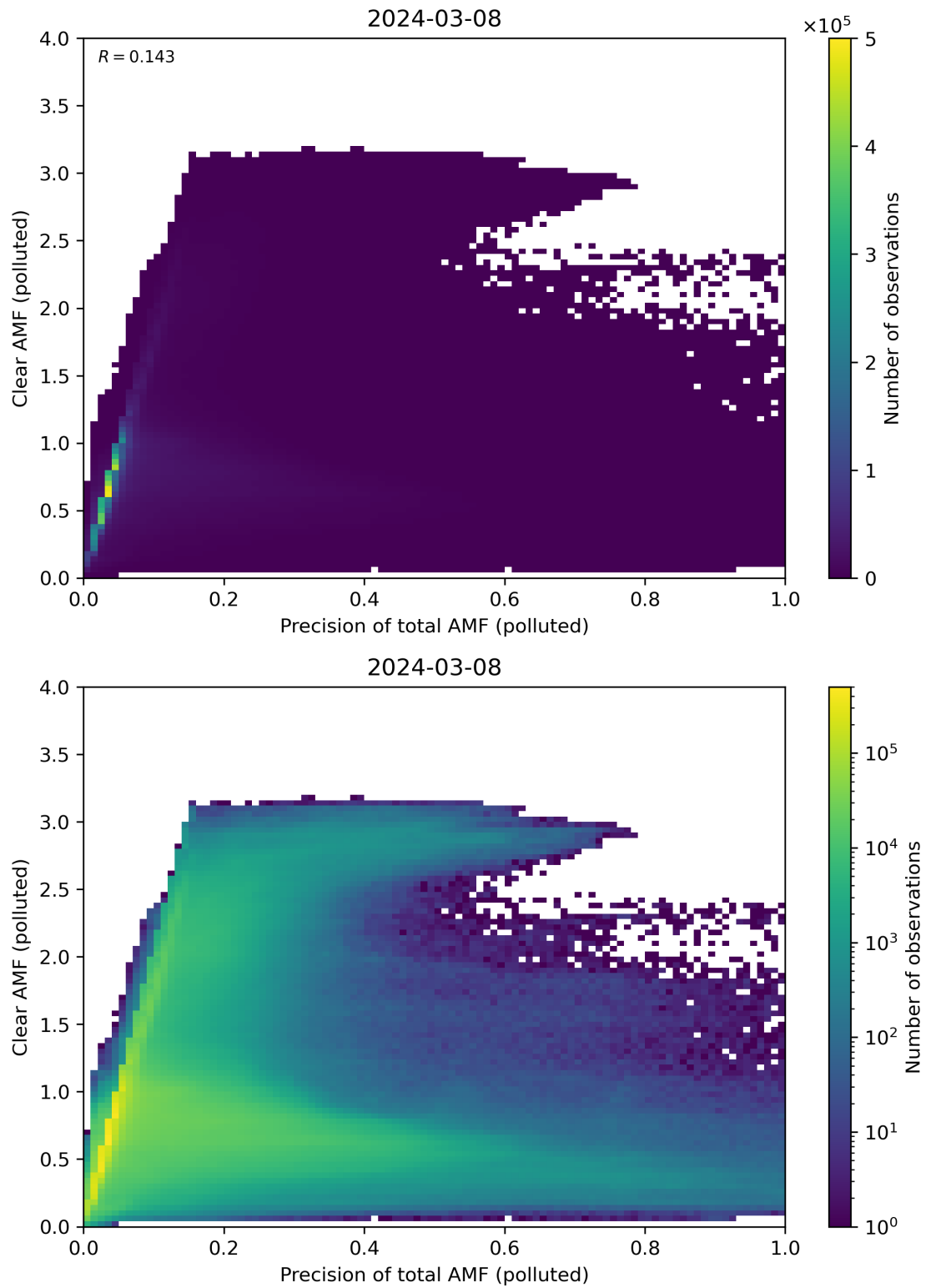
Figure 270: Scatter density plot of “Precision of total AMF (polluted)” against “Clear AMF (polluted)” for 2024-03-07 to 2024-03-09.
