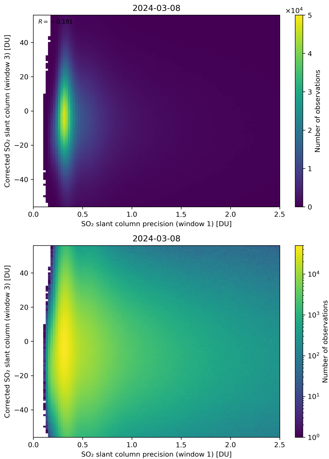
Figure 226: Scatter density plot of “SO 2 slant column precision (window 1)” against “Corrected SO 2 slant column (window 3)” for 2024-03-07 to 2024-03-09.
