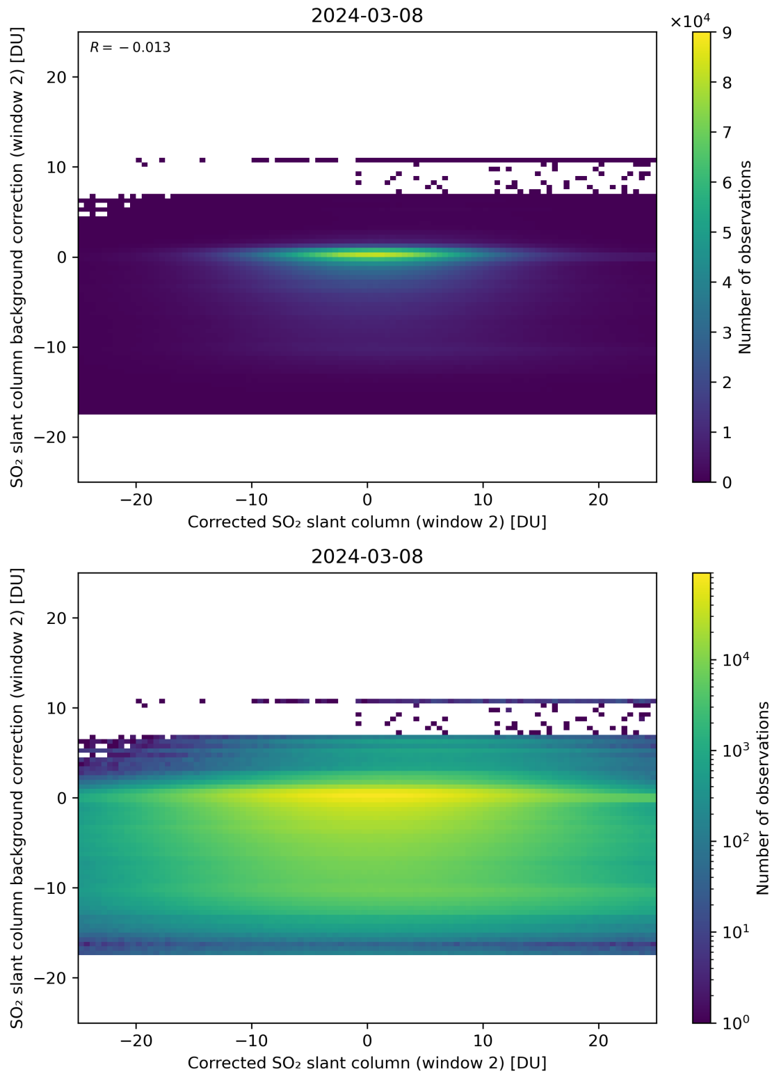
Figure 194: Scatter density plot of “Corrected SO 2 slant column (window 2)” against “SO 2 slant column background correction (window 2)” for 2024-03-07 to 2024-03-09.
