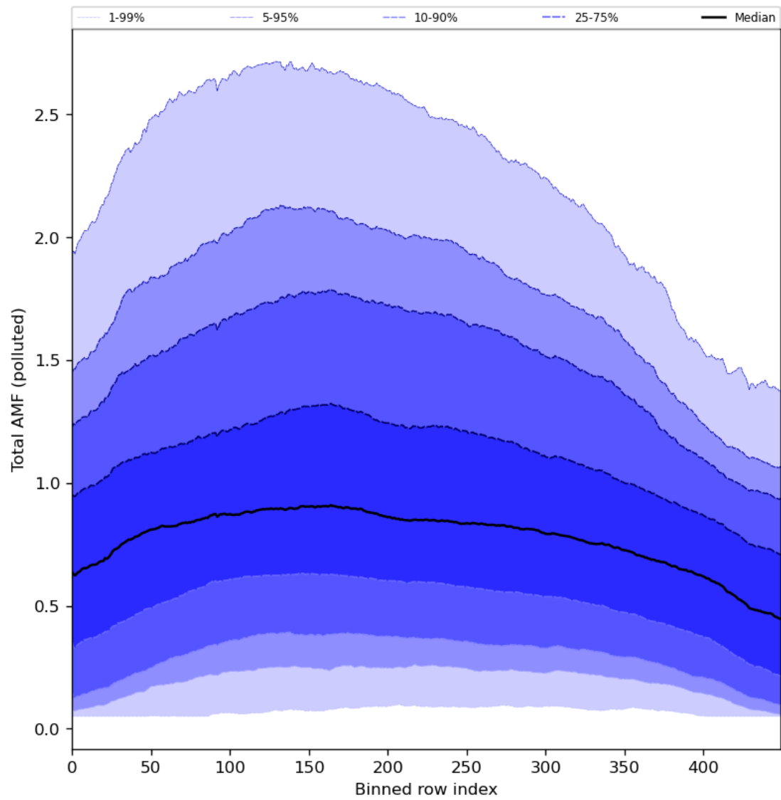
Figure 94: Along track statistics of “Total AMF (polluted)” for 2024-03-07 to 2024-03-09
