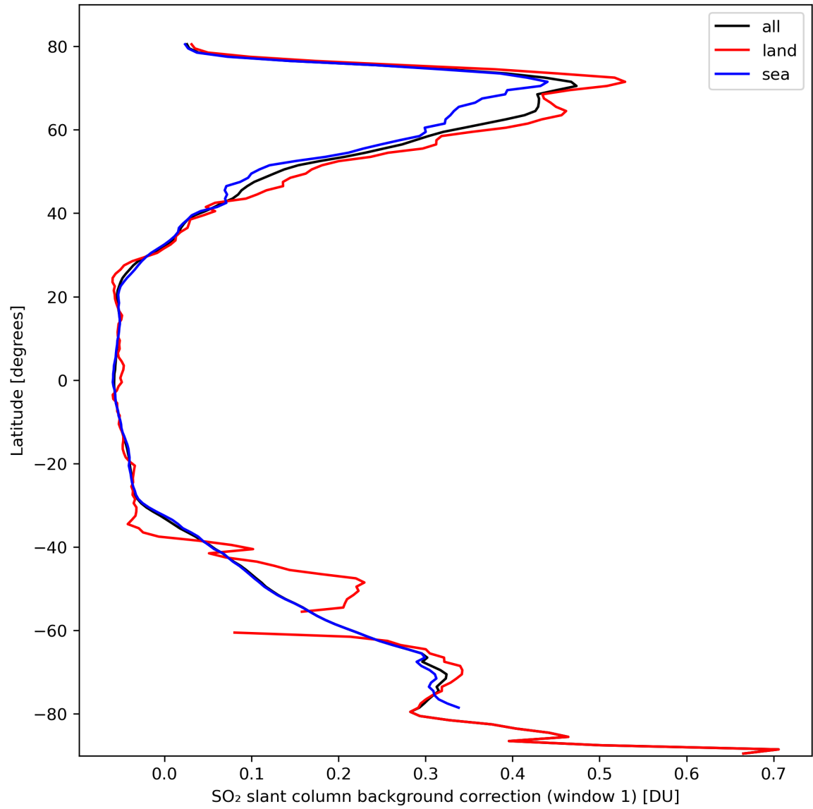
Figure 36: Zonal average of “SO 2 slant column background correction (window 1)” for 2024-03-07 to 2024-03-09.
