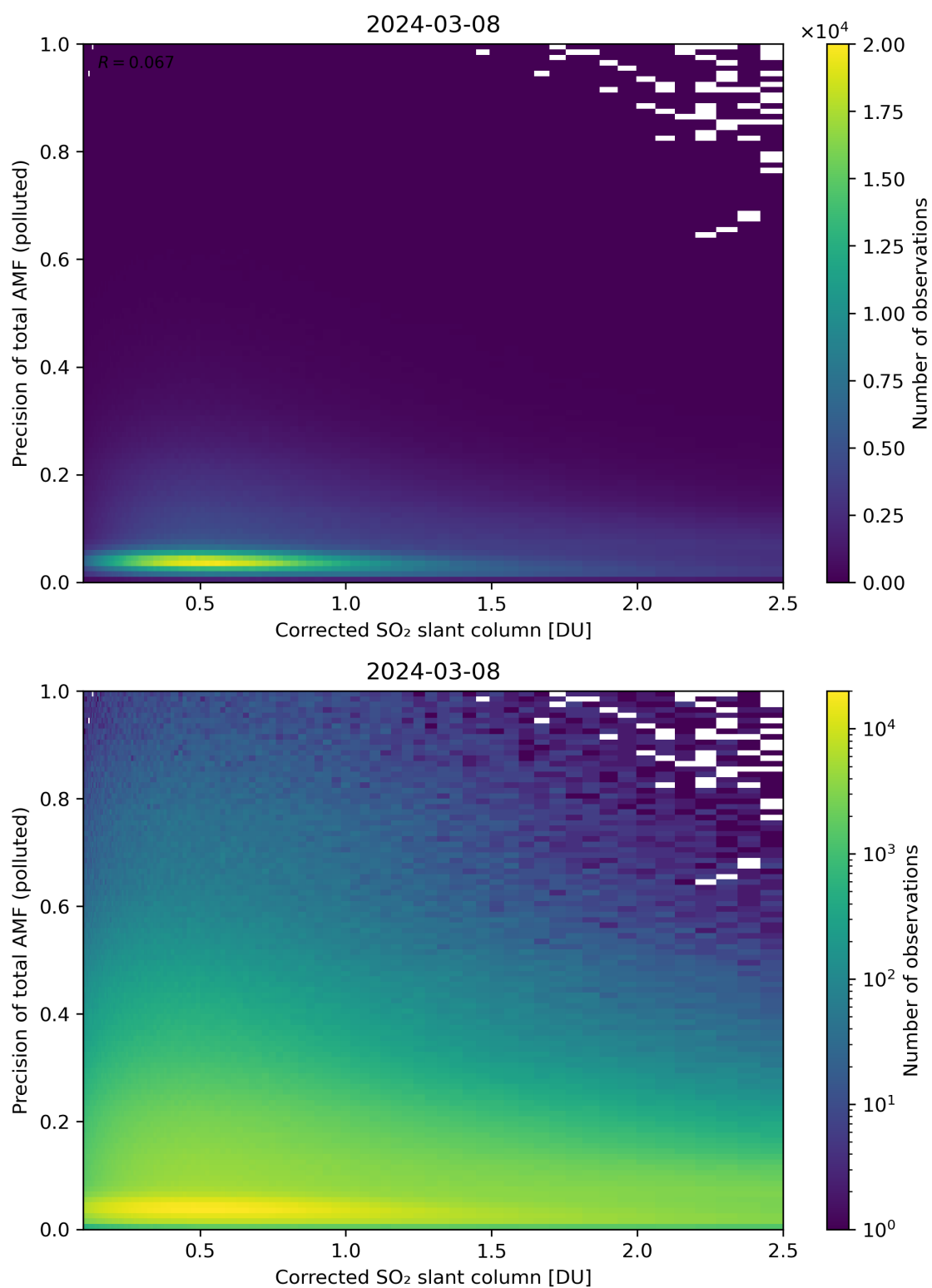
Figure 193: Scatter density plot of “Corrected SO 2 slant column” against “Precision of total AMF (polluted)” for 2024-03-07 to 2024-03-09.
