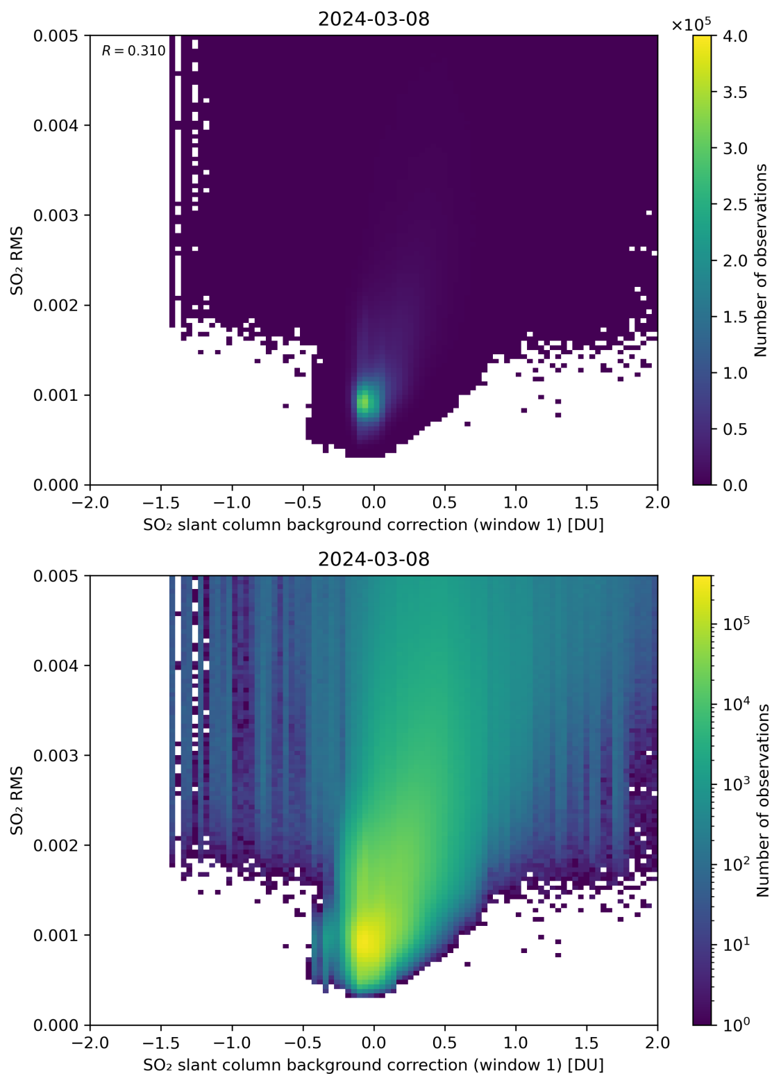
Figure 102: Scatter density plot of “SO 2 slant column background correction (window 1)” against “SO 2 RMS” for 2024-03-07 to 2024-03-09.
