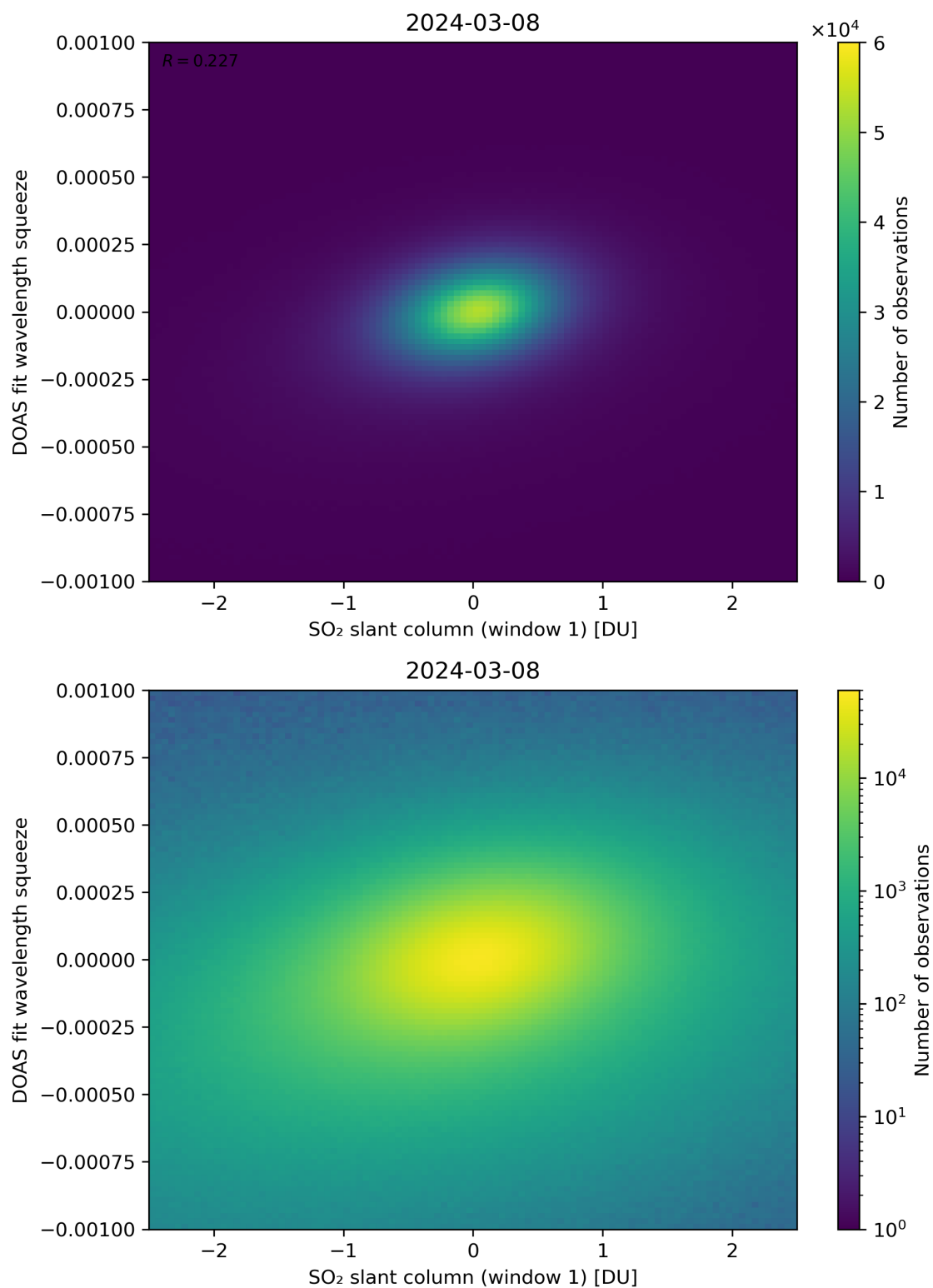
Figure 216: Scatter density plot of “SO 2 slant column (window 1)” against “DOAS fit wavelength squeeze” for 2024-03-07 to 2024-03-09.
