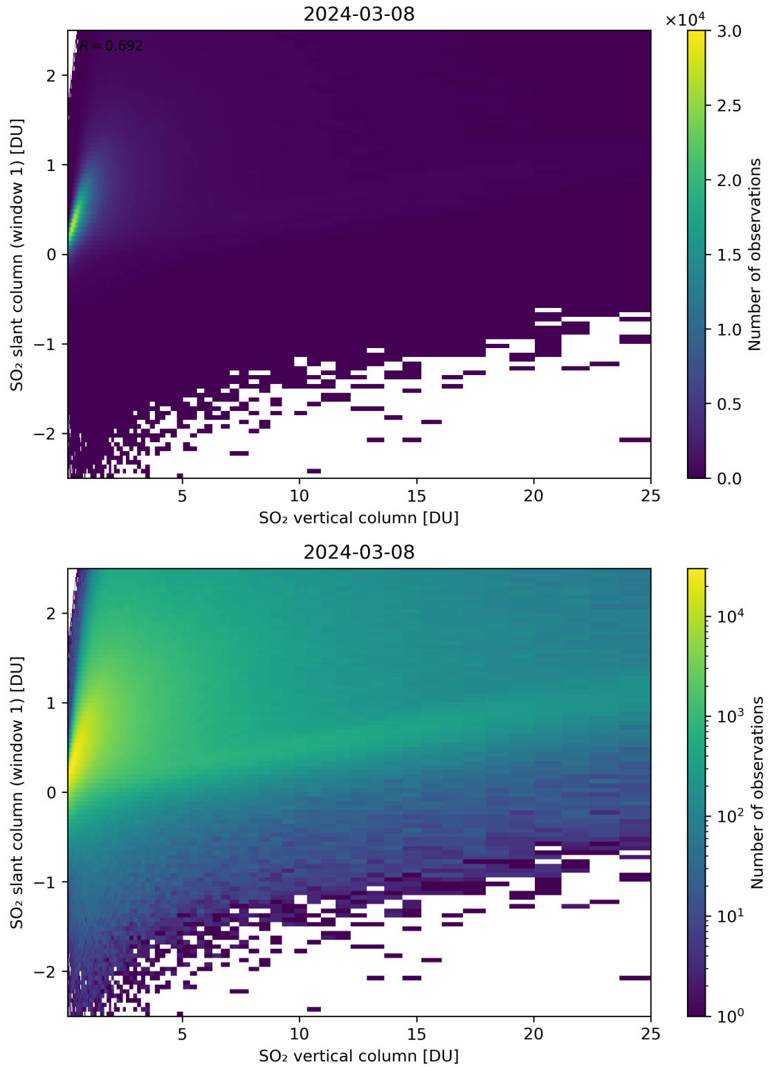
Figure 300: Scatter density plot of “SO 2 vertical column” against “SO 2 slant column (window 1)” for 2024-03-07 to 2024-03-09.
