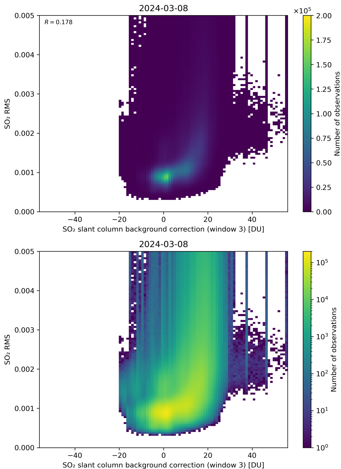
Figure 123: Scatter density plot of “SO 2 slant column background correction (window 3)” against “SO 2 RMS” for 2024-03-07 to 2024-03-09.
