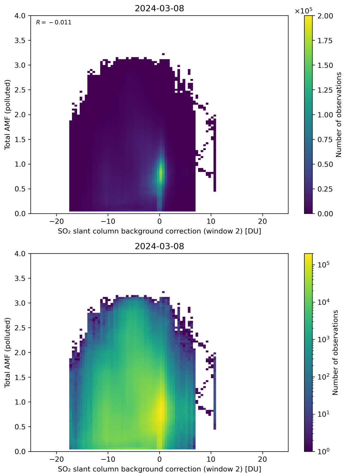
Figure 119: Scatter density plot of “SO 2 slant column background correction (window 2)” against “Total AMF (polluted)” for 2024-03-07 to 2024-03-09.
