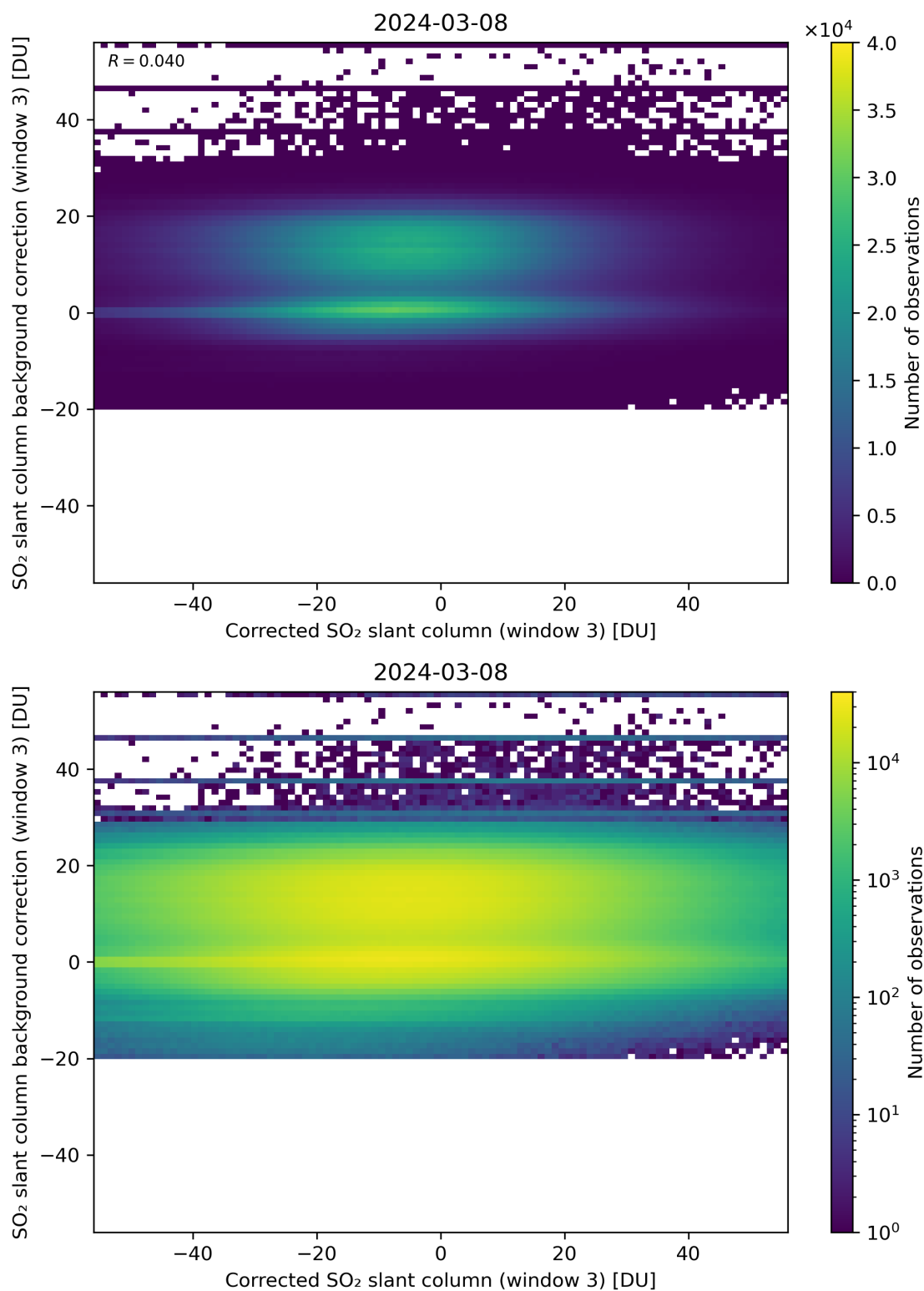
Figure 205: Scatter density plot of “Corrected SO 2 slant column (window 3)” against “SO 2 slant column background correction (window 3)” for 2024-03-07 to 2024-03-09.
