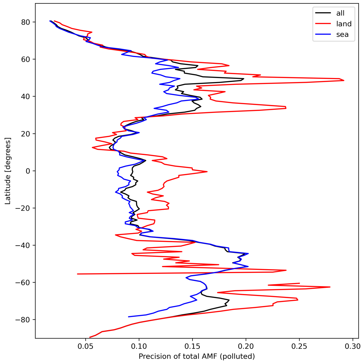
Figure 49: Zonal average of “Precision of total AMF (polluted)” for 2024-03-07 to 2024-03-09.
