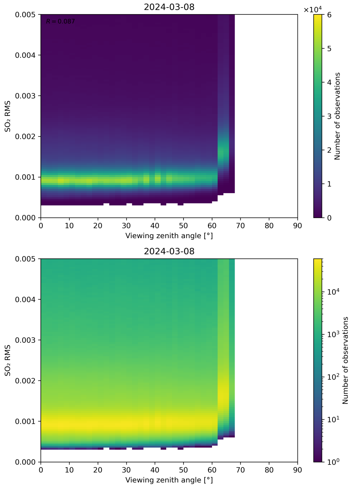
Figure 313: Scatter density plot of “Viewing zenith angle” against “SO 2 RMS” for 2024-03-07 to 2024-03-09.
