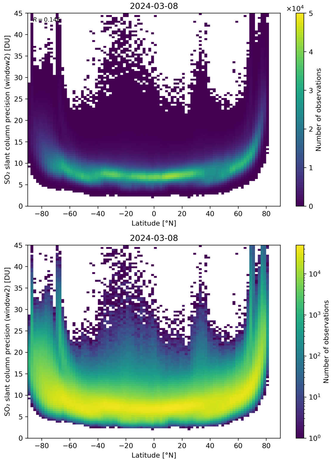
Figure 151: Scatter density plot of “Latitude” against “SO 2 slant column precision (window2)” for 2024-03-07 to 2024-03-09.
