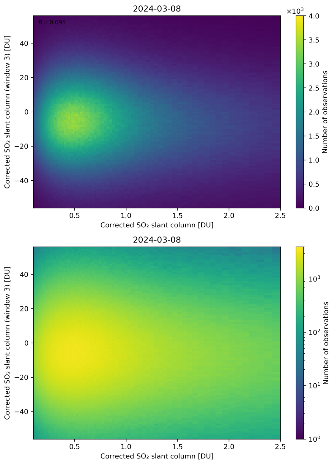
Figure 186: Scatter density plot of “Corrected SO 2 slant column” against “Corrected SO 2 slant column (window 3)” for 2024-03-07 to 2024-03-09.
