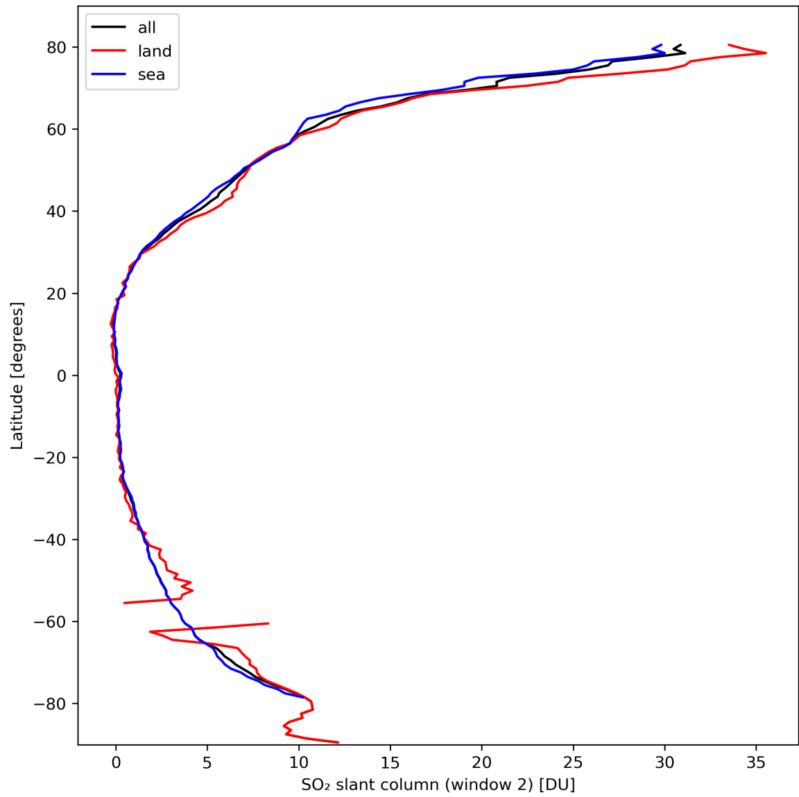
Figure 37: Zonal average of “SO 2 slant column (window 2)” for 2024-03-07 to 2024-03-09.
