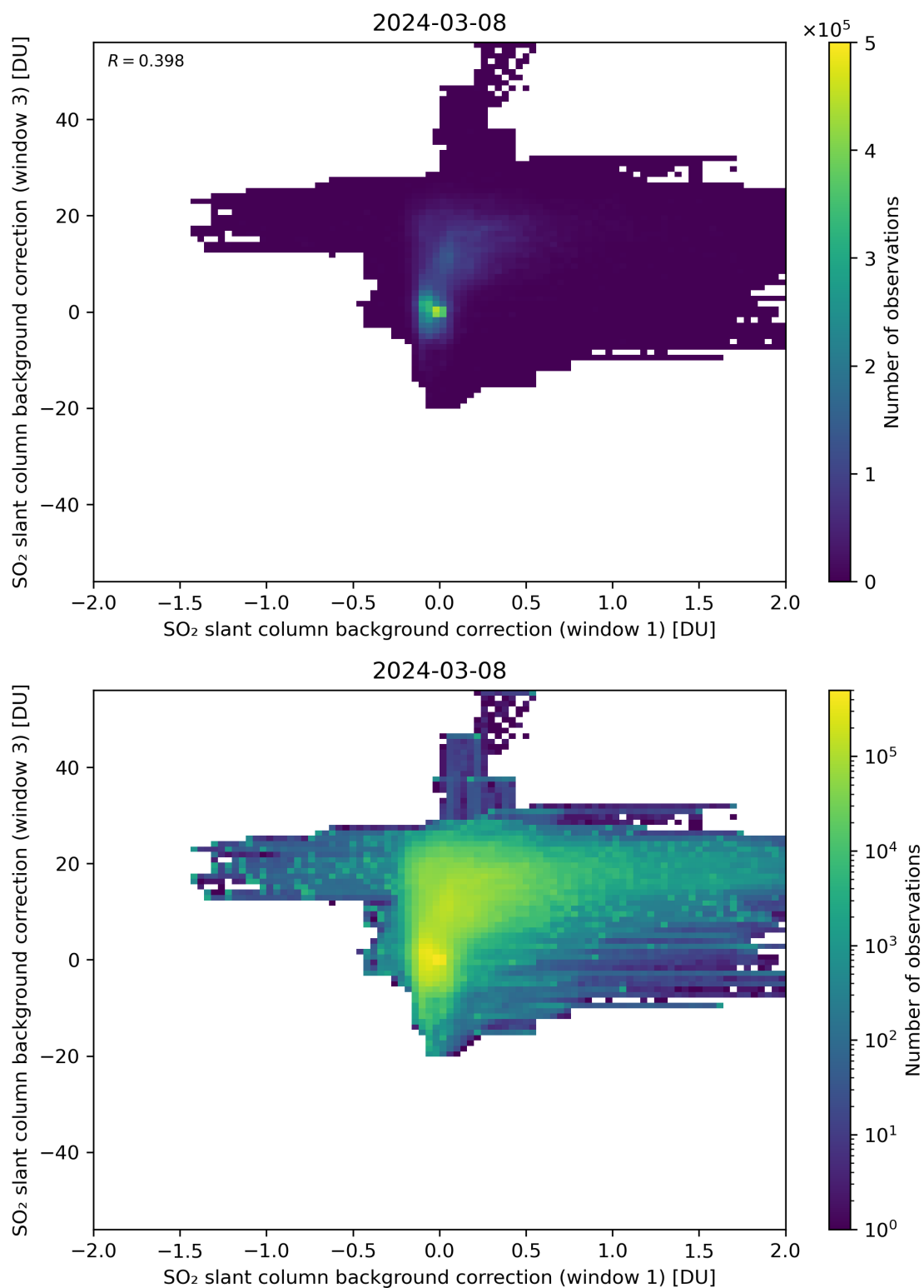
Figure 99: Scatter density plot of “SO 2 slant column background correction (window 1)” against “SO 2 slant column background correction (window 3)” for 2024-03-07 to 2024-03-09.
