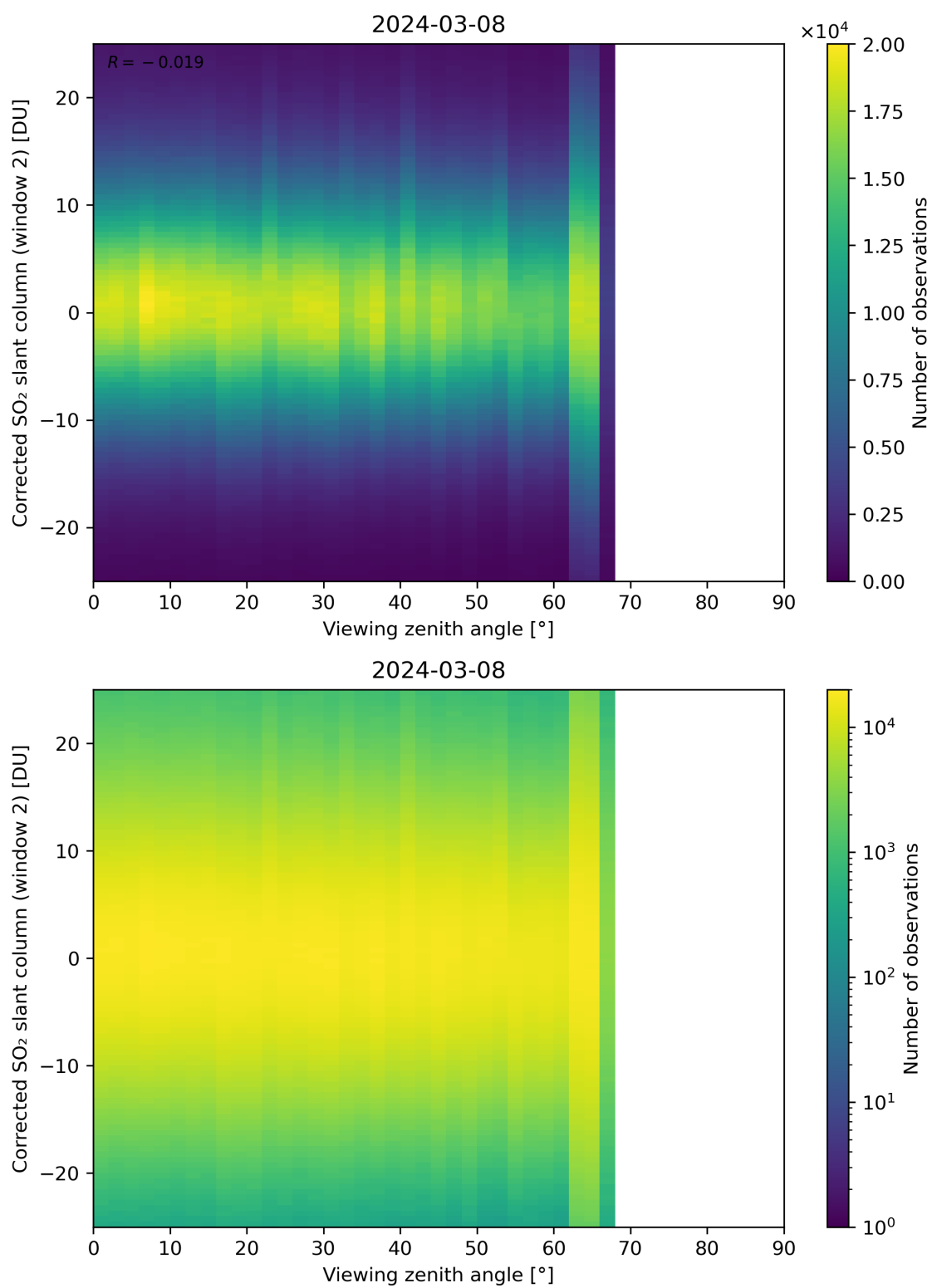
Figure 318: Scatter density plot of “Viewing zenith angle” against “Corrected SO 2 slant column (window 2)” for 2024-03-07 to 2024-03-09.
