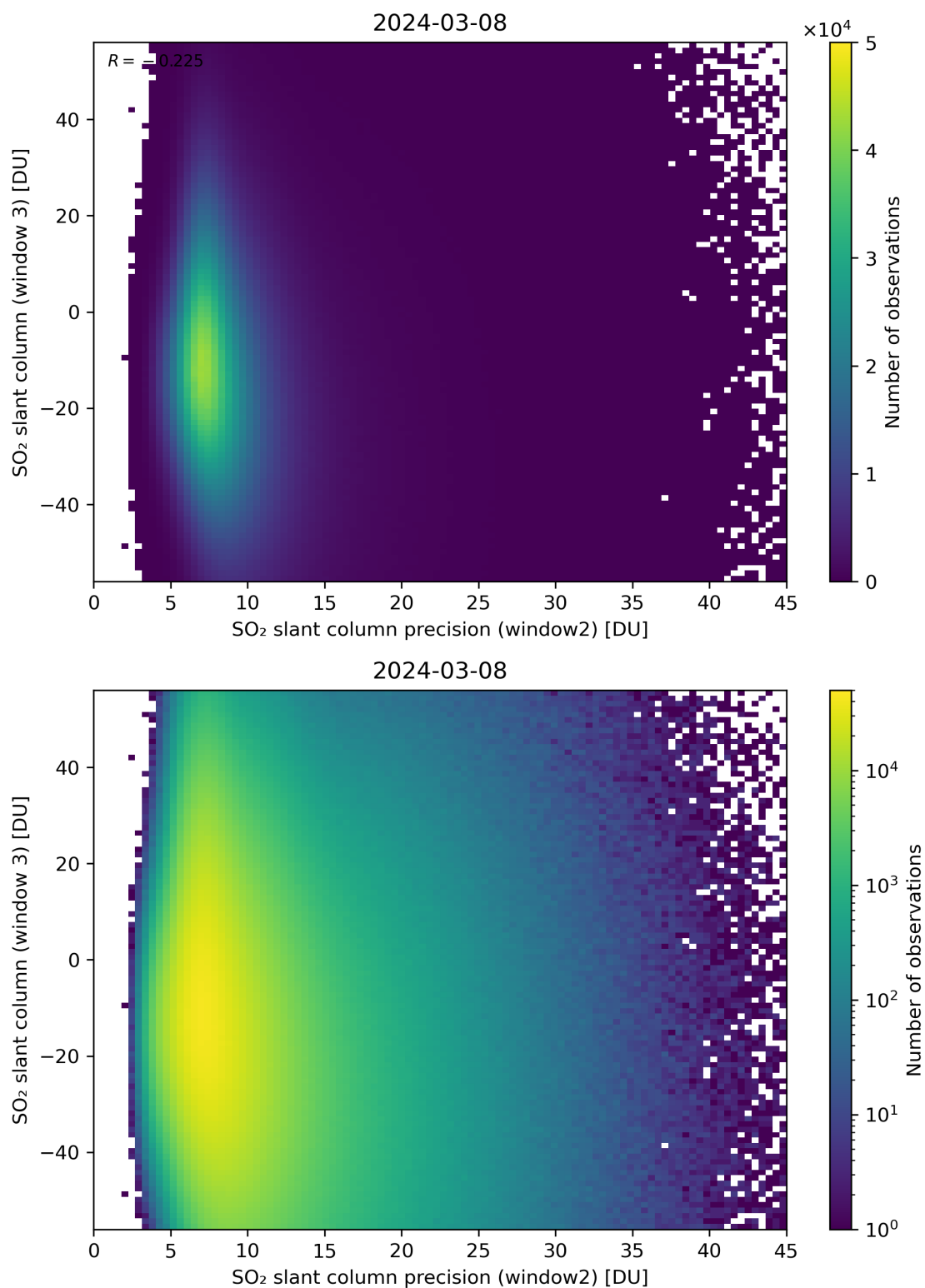
Figure 249: Scatter density plot of “SO 2 slant column precision (window2)” against “SO 2 slant column (window 3)” for 2024-03-07 to 2024-03-09.
