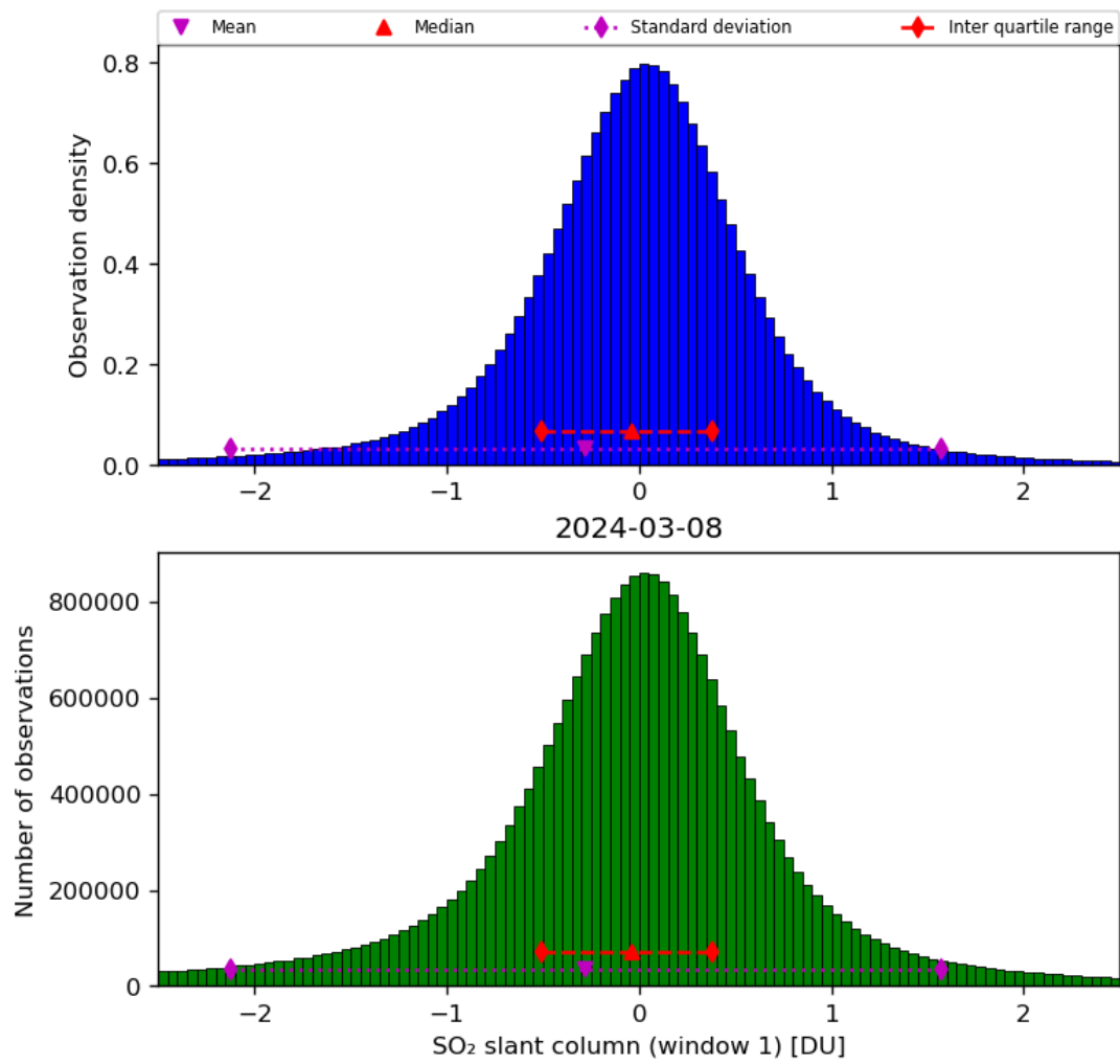
Figure 56: Histogram of “SO 2 slant column (window 1)” for 2024-03-07 to 2024-03-09
