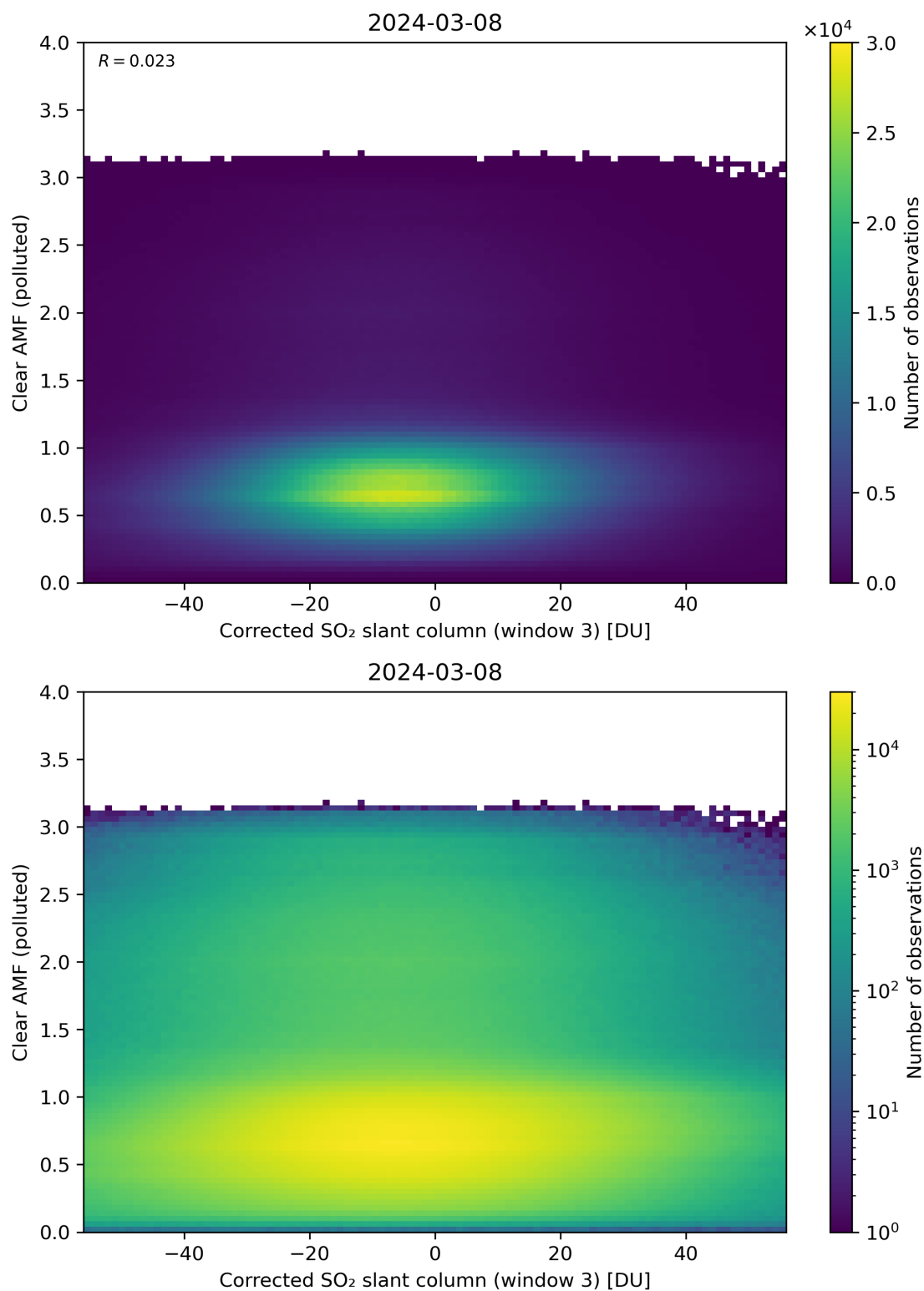
Figure 209: Scatter density plot of “Corrected SO 2 slant column (window 3)” against “Clear AMF (polluted)” for 2024-03-07 to 2024-03-09.
