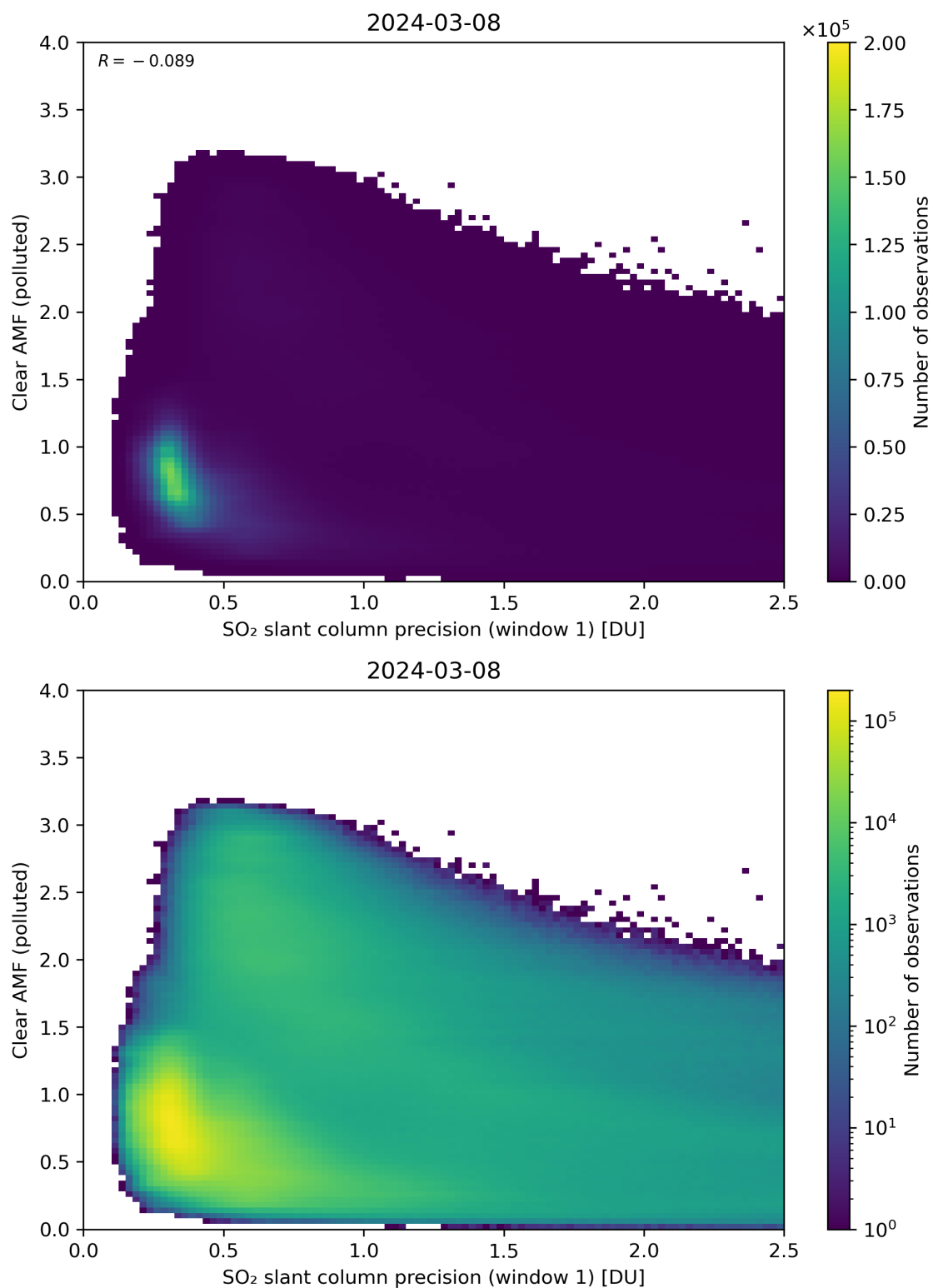
Figure 224: Scatter density plot of “SO 2 slant column precision (window 1)” against “Clear AMF (polluted)” for 2024-03-07 to 2024-03-09.
