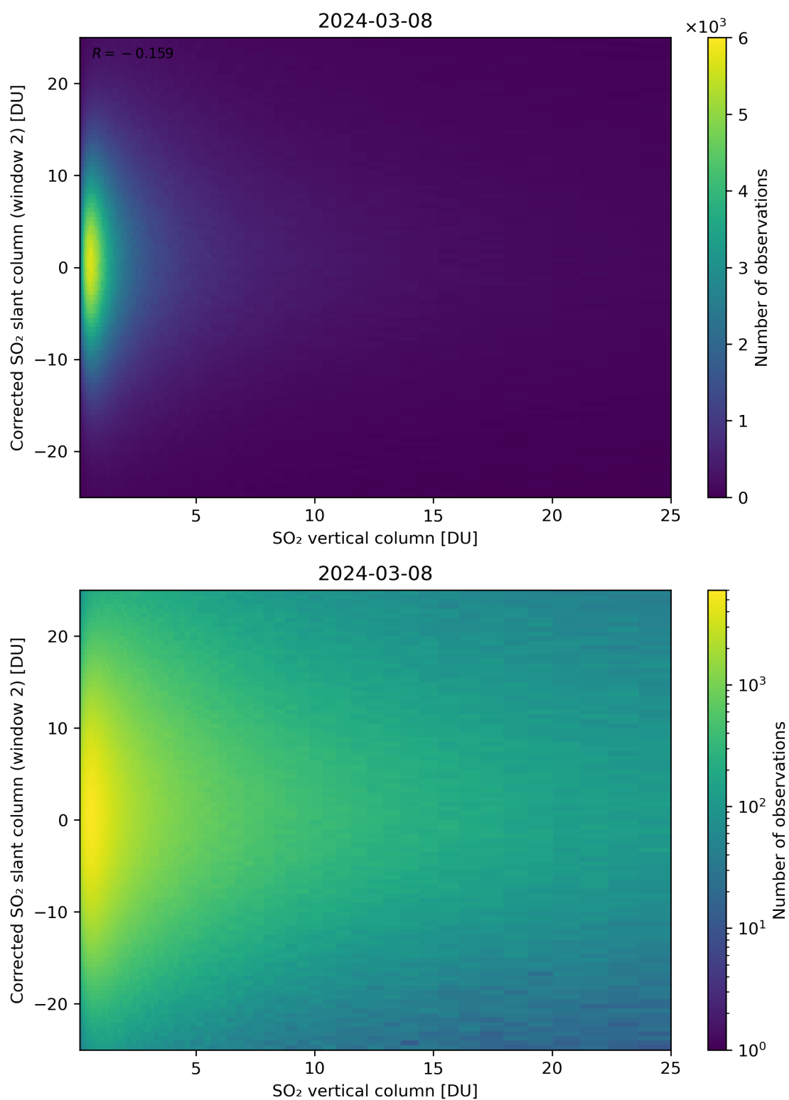
Figure 298: Scatter density plot of “SO 2 vertical column” against “Corrected SO 2 slant column (window 2)” for 2024-03-07 to 2024-03-09.
