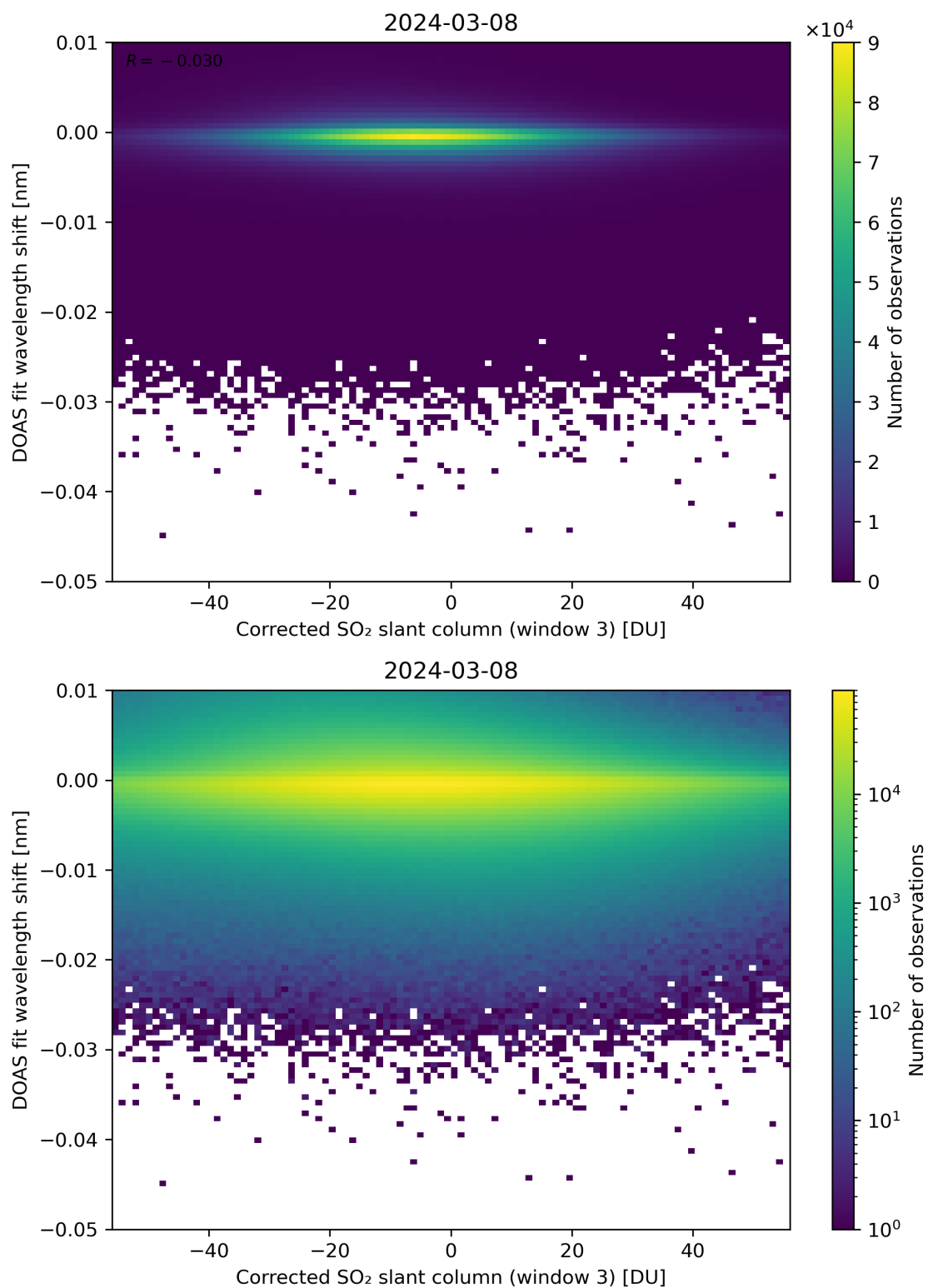
Figure 206: Scatter density plot of “Corrected SO 2 slant column (window 3)” against “DOAS fit wavelength shift” for 2024-03-07 to 2024-03-09.
