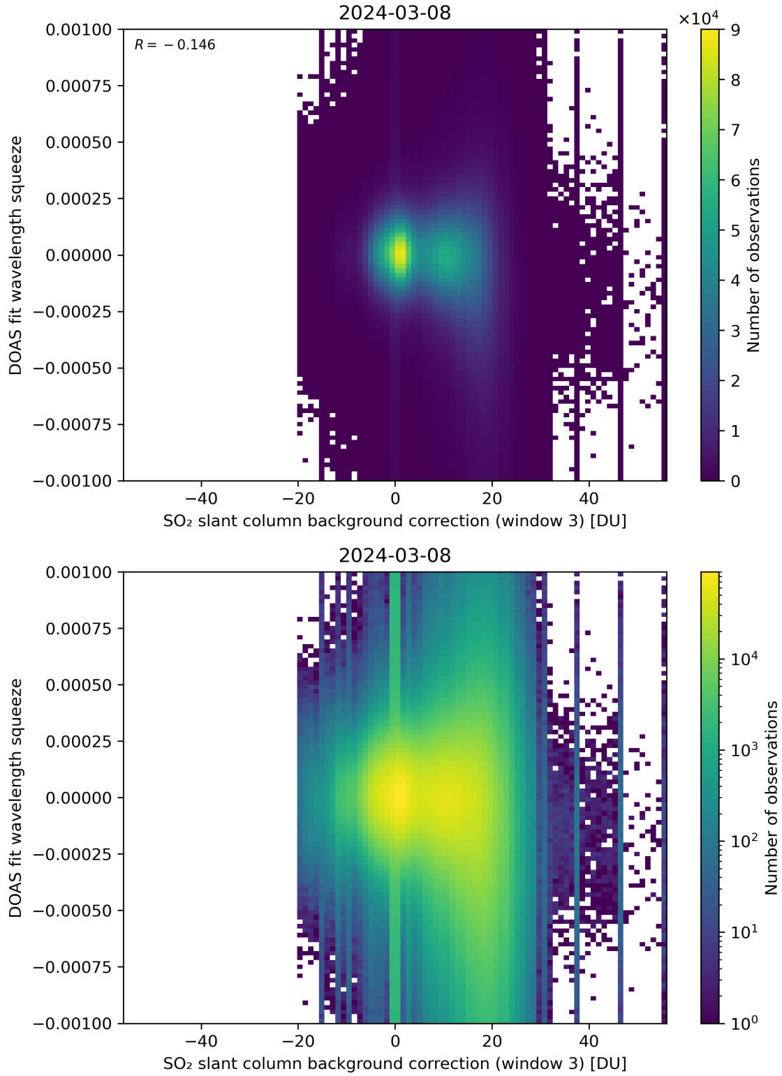
Figure 122: Scatter density plot of “SO 2 slant column background correction (window 3)” against “DOAS fit wavelength squeeze” for 2024-03-07 to 2024-03-09.
