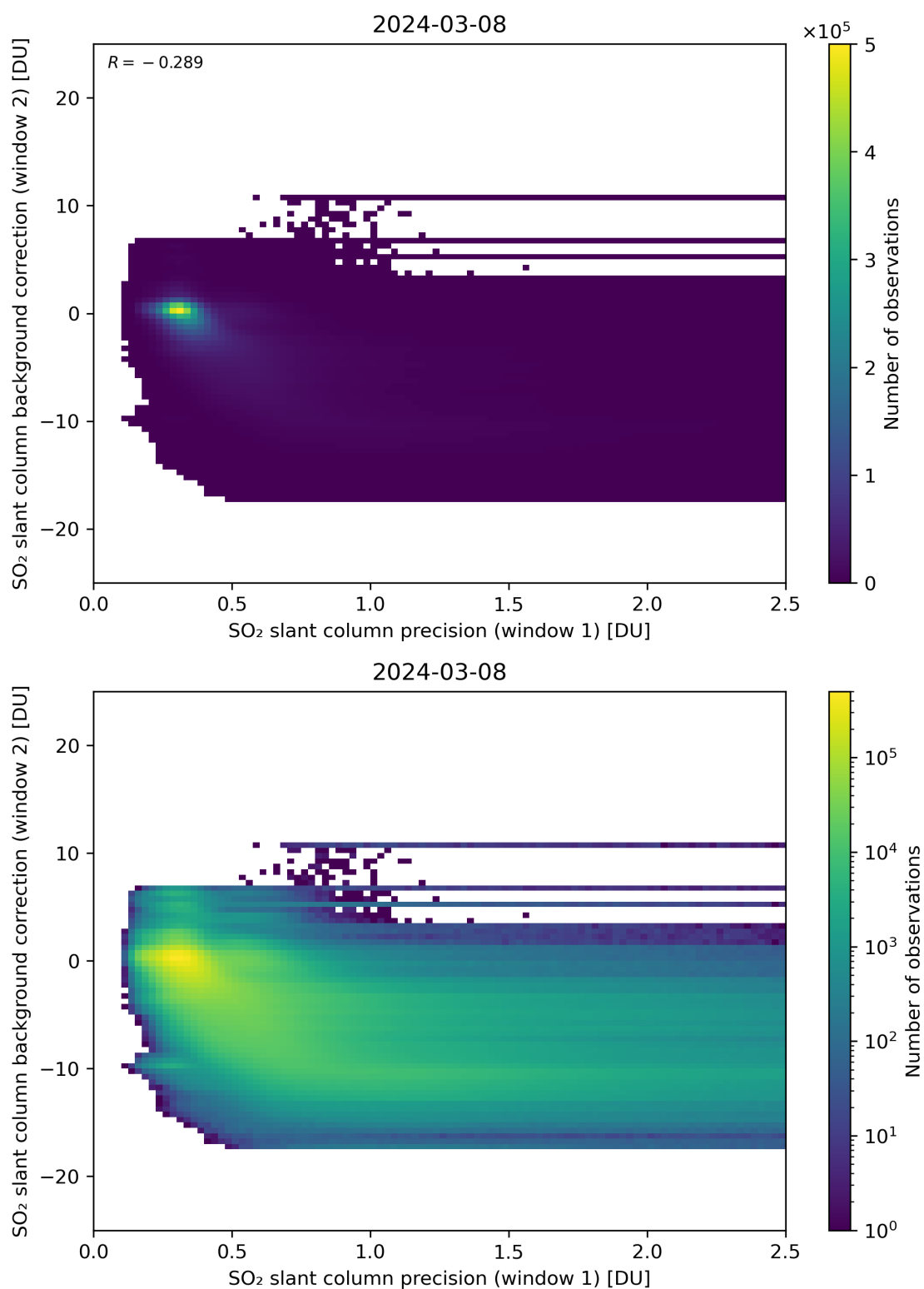
Figure 219: Scatter density plot of “SO 2 slant column precision (window 1)” against “SO 2 slant column background correction (window 2)” for 2024-03-07 to 2024-03-09.
