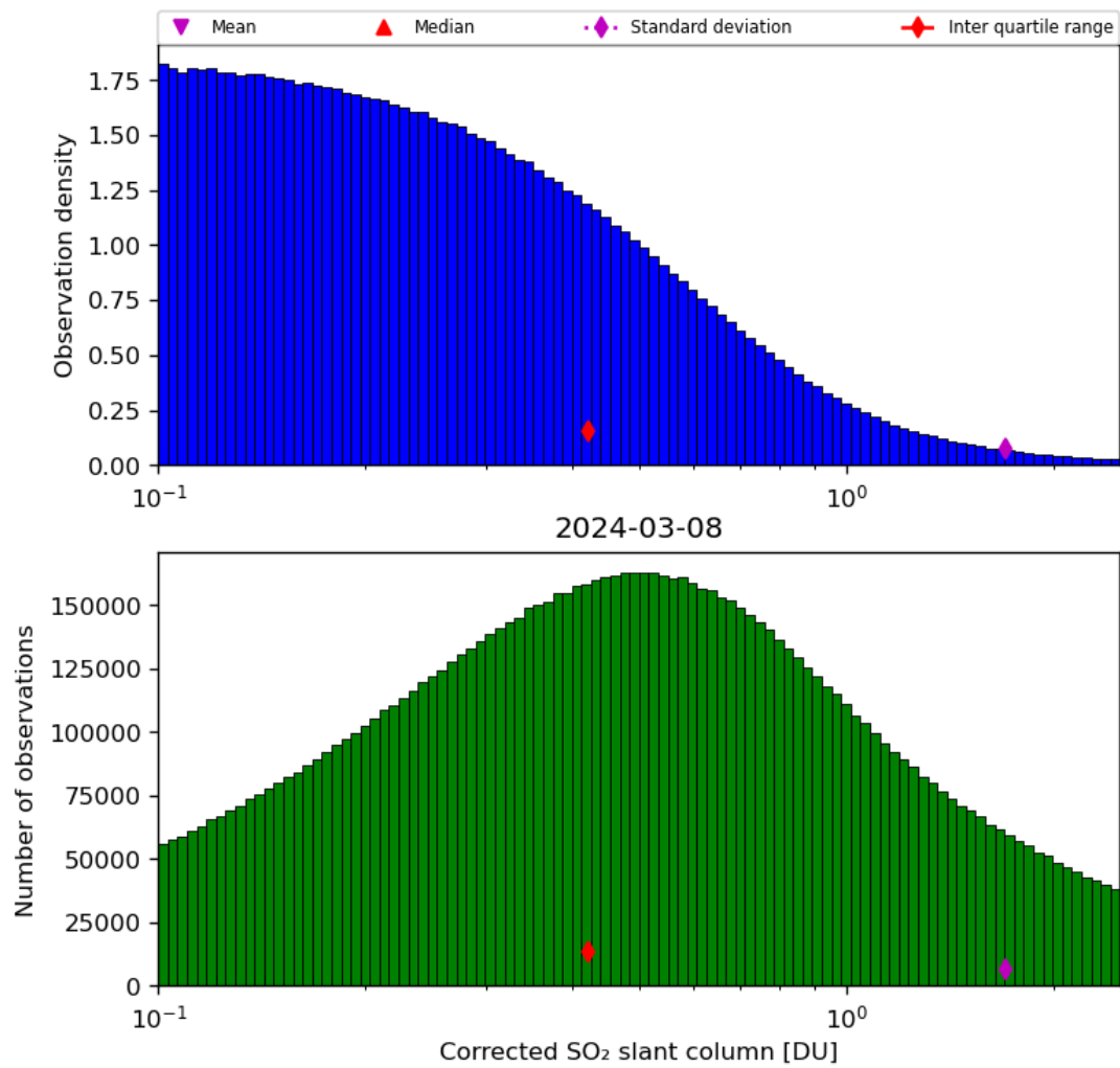
Figure 55: Histogram of “Corrected SO 2 slant column” for 2024-03-07 to 2024-03-09
