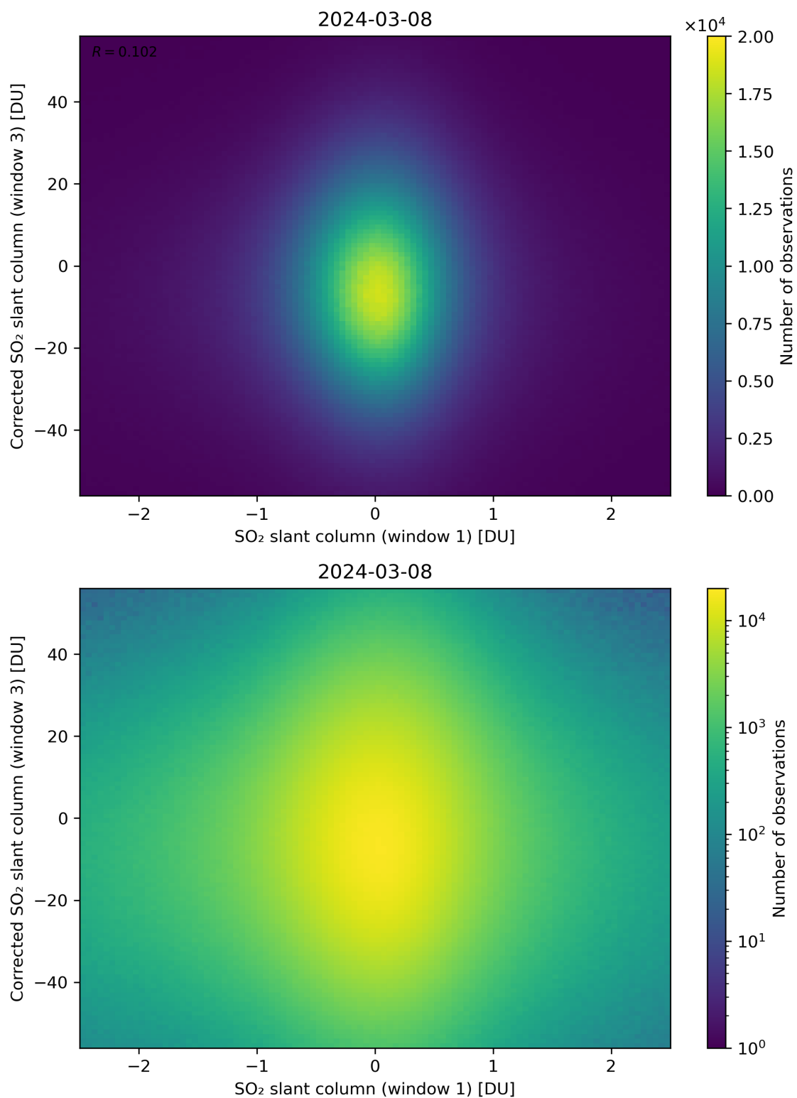
Figure 234: Scatter density plot of “SO 2 slant column (window 1)” against “Corrected SO 2 slant column (window 3)” for 2024-03-07 to 2024-03-09.
