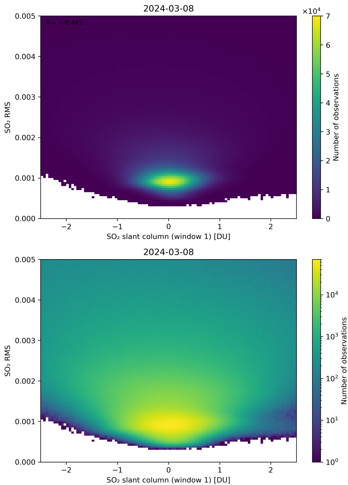
Figure 217: Scatter density plot of “SO 2 slant column (window 1)” against “SO 2 RMS” for 2024-03-07 to 2024-03-09.
