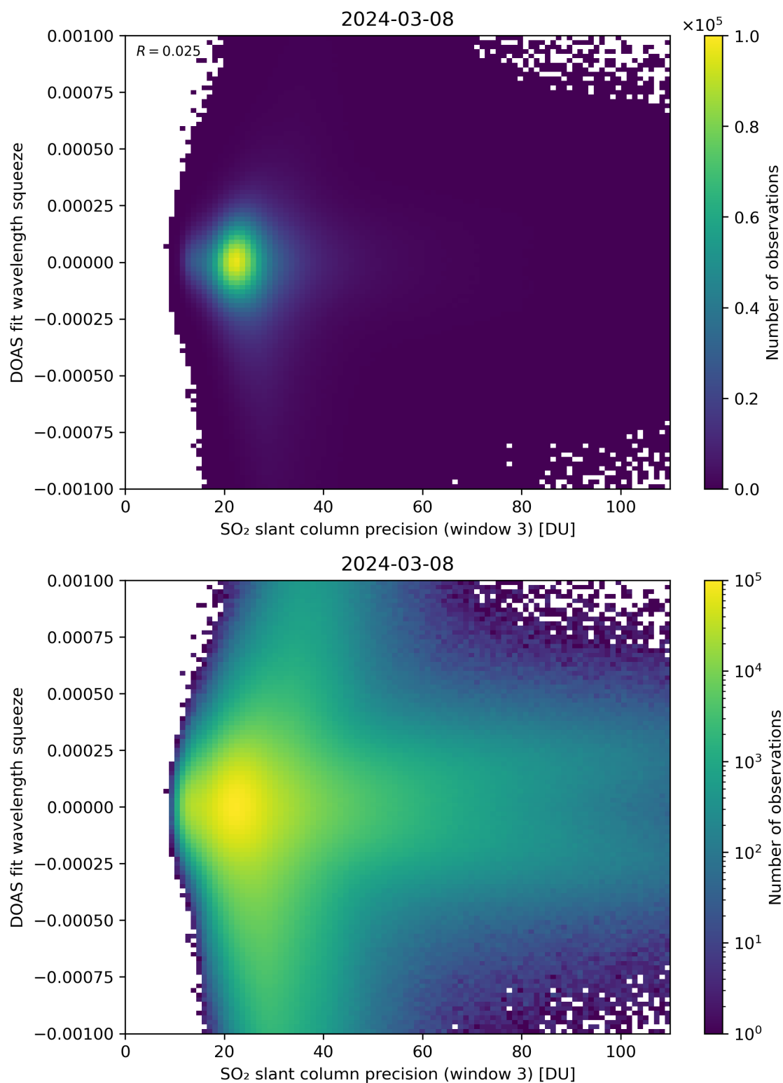
Figure 259: Scatter density plot of “SO 2 slant column precision (window 3)” against “DOAS fit wavelength squeeze” for 2024-03-07 to 2024-03-09.
