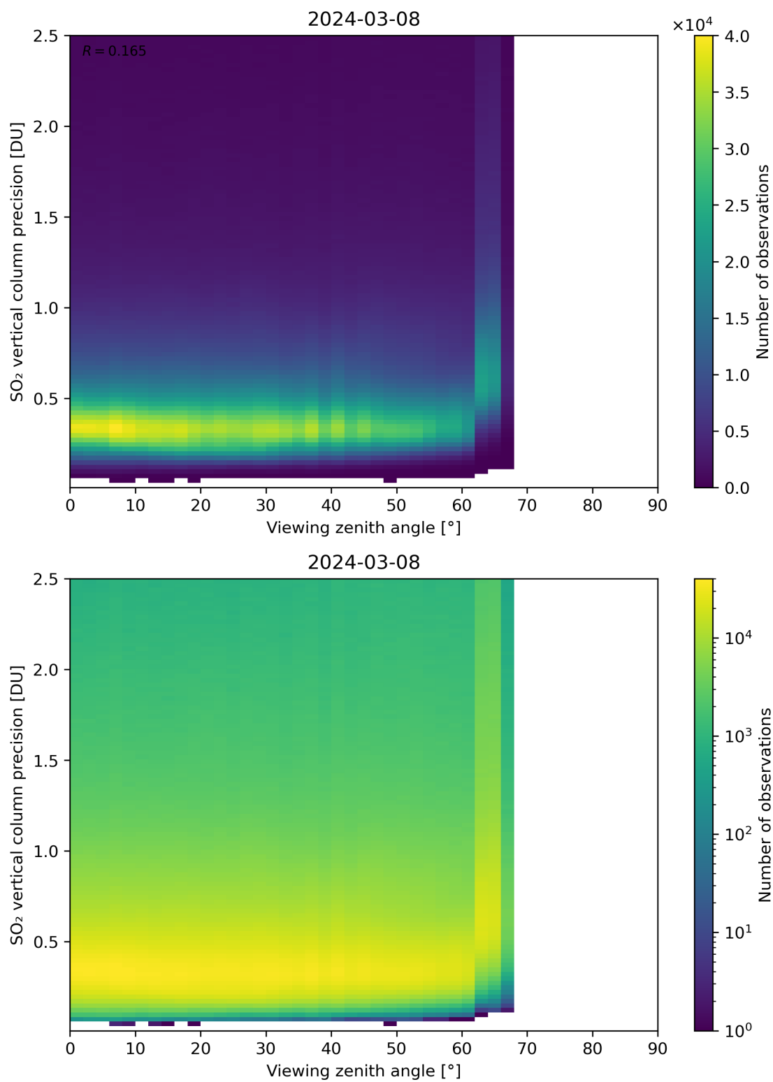
Figure 328: Scatter density plot of “Viewing zenith angle” against “SO 2 vertical column precision” for 2024-03-07 to 2024-03-09.
