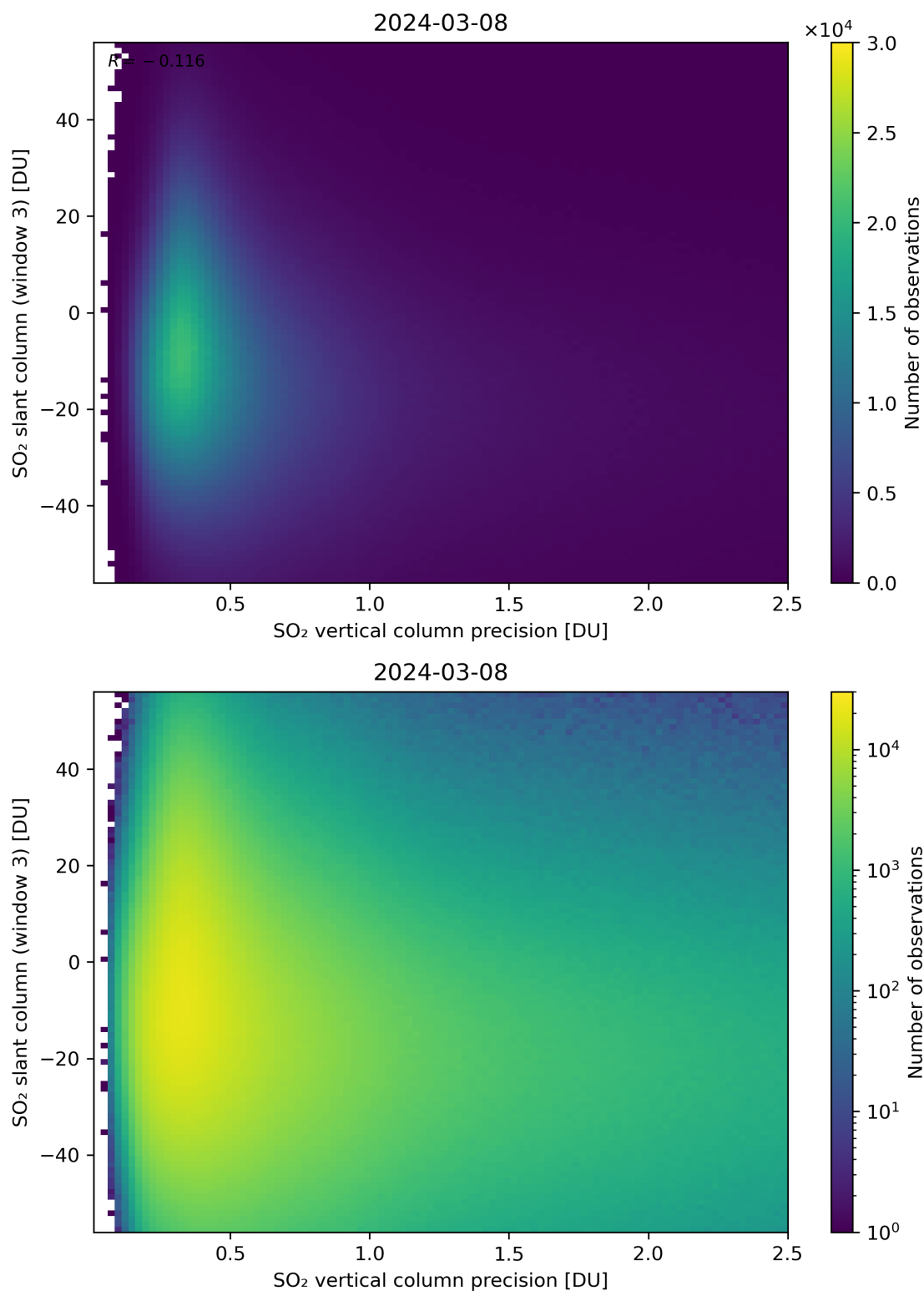
Figure 292: Scatter density plot of “SO 2 vertical column precision” against “SO 2 slant column (window 3)” for 2024-03-07 to 2024-03-09.
