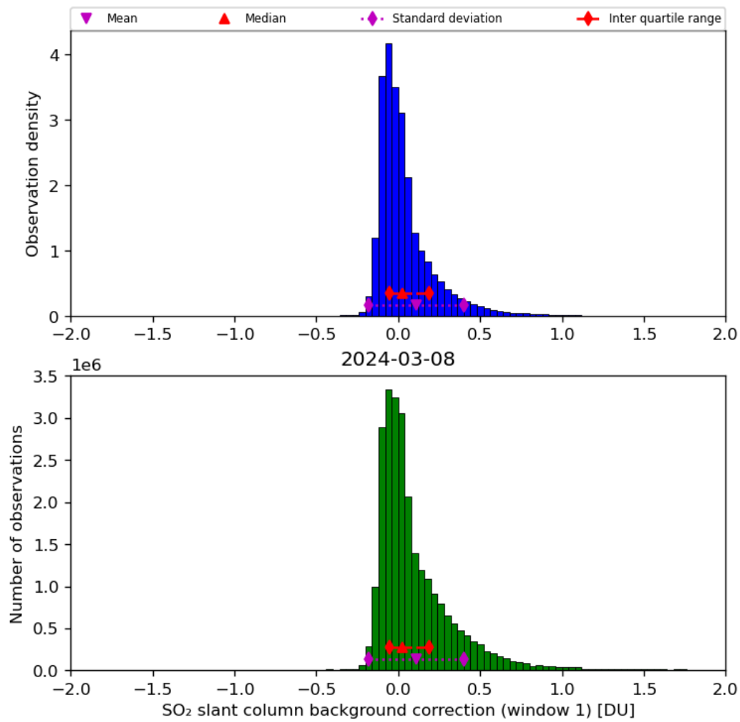
Figure 59: Histogram of “SO 2 slant column background correction (window 1)” for 2024-03-07 to 2024-03-09
