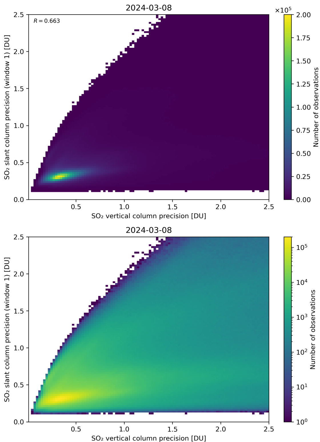
Figure 290: Scatter density plot of “SO 2 vertical column precision” against “SO 2 slant column precision (window 1)” for 2024-03-07 to 2024-03-09.
