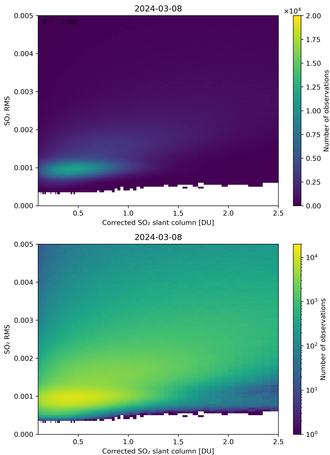
Figure 183: Scatter density plot of “Corrected SO 2 slant column” against “SO 2 RMS” for 2024-03-07 to 2024-03-09.
