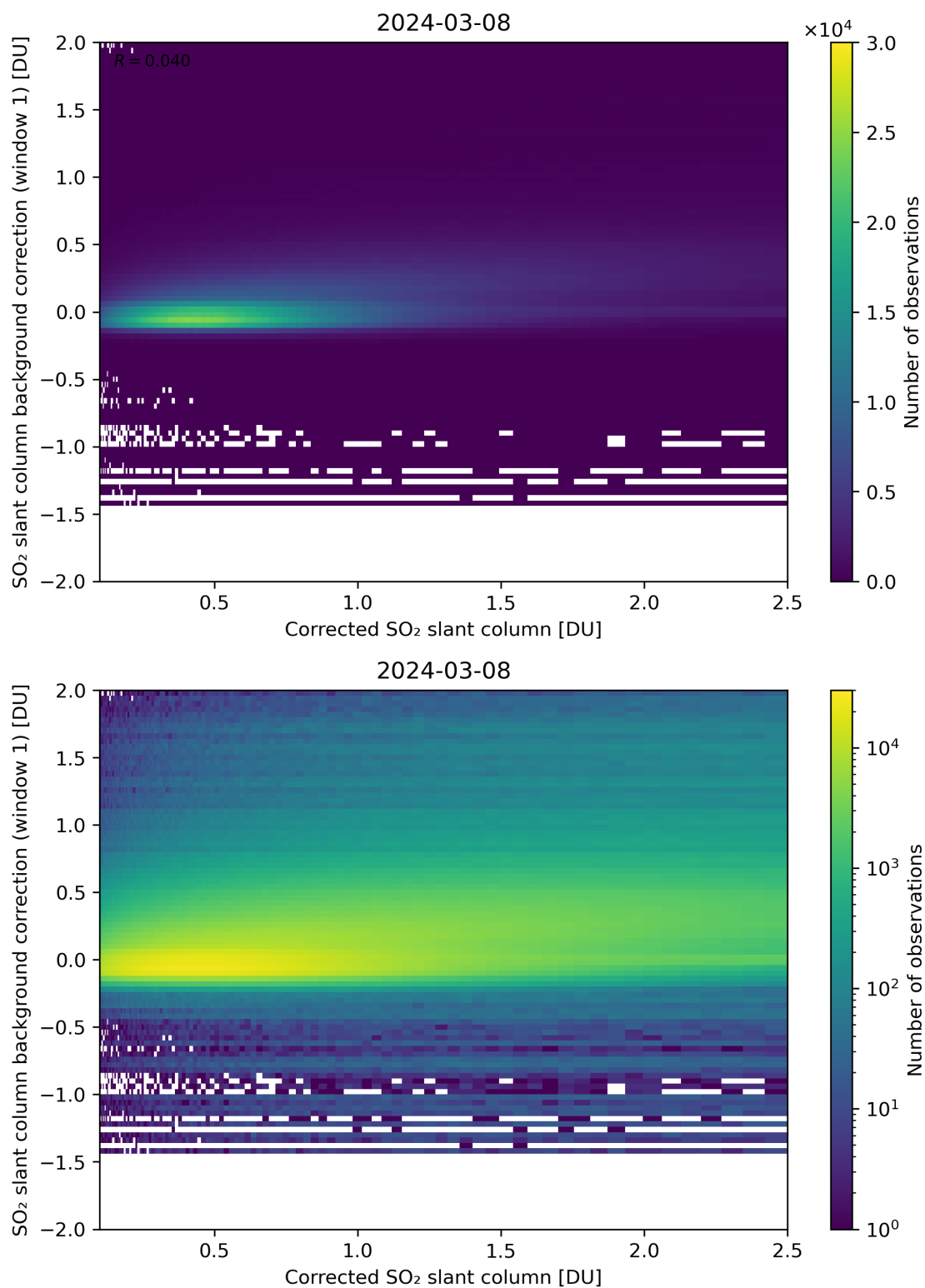
Figure 178: Scatter density plot of “Corrected SO 2 slant column” against “SO 2 slant column background correction (window 1)” for 2024-03-07 to 2024-03-09.
