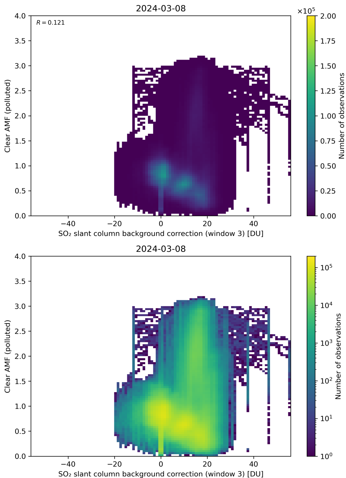
Figure 124: Scatter density plot of “SO 2 slant column background correction (window 3)” against “Clear AMF (polluted)” for 2024-03-07 to 2024-03-09.
