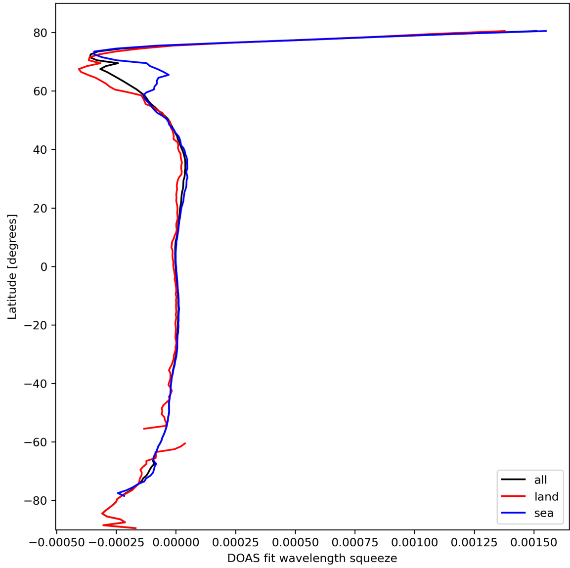
Figure 46: Zonal average of “DOAS fit wavelength squeeze” for 2024-03-07 to 2024-03-09.
