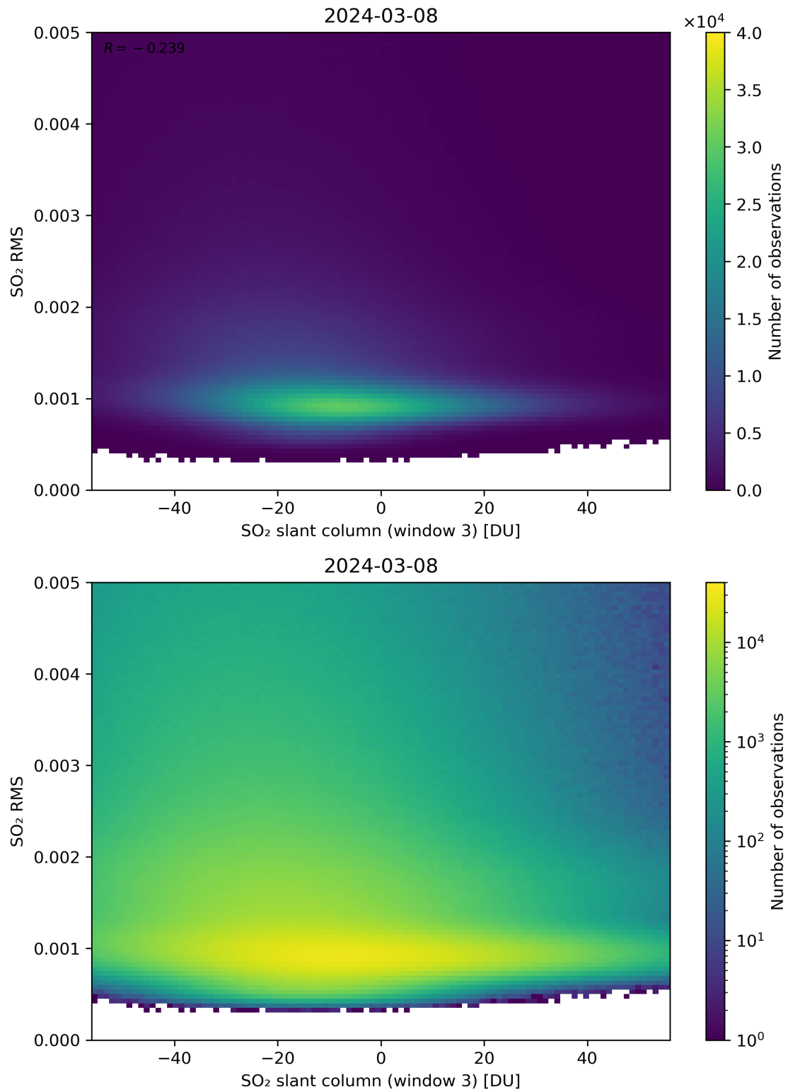
Figure 256: Scatter density plot of “SO 2 slant column (window 3)” against “SO 2 RMS” for 2024-03-07 to 2024-03-09.
