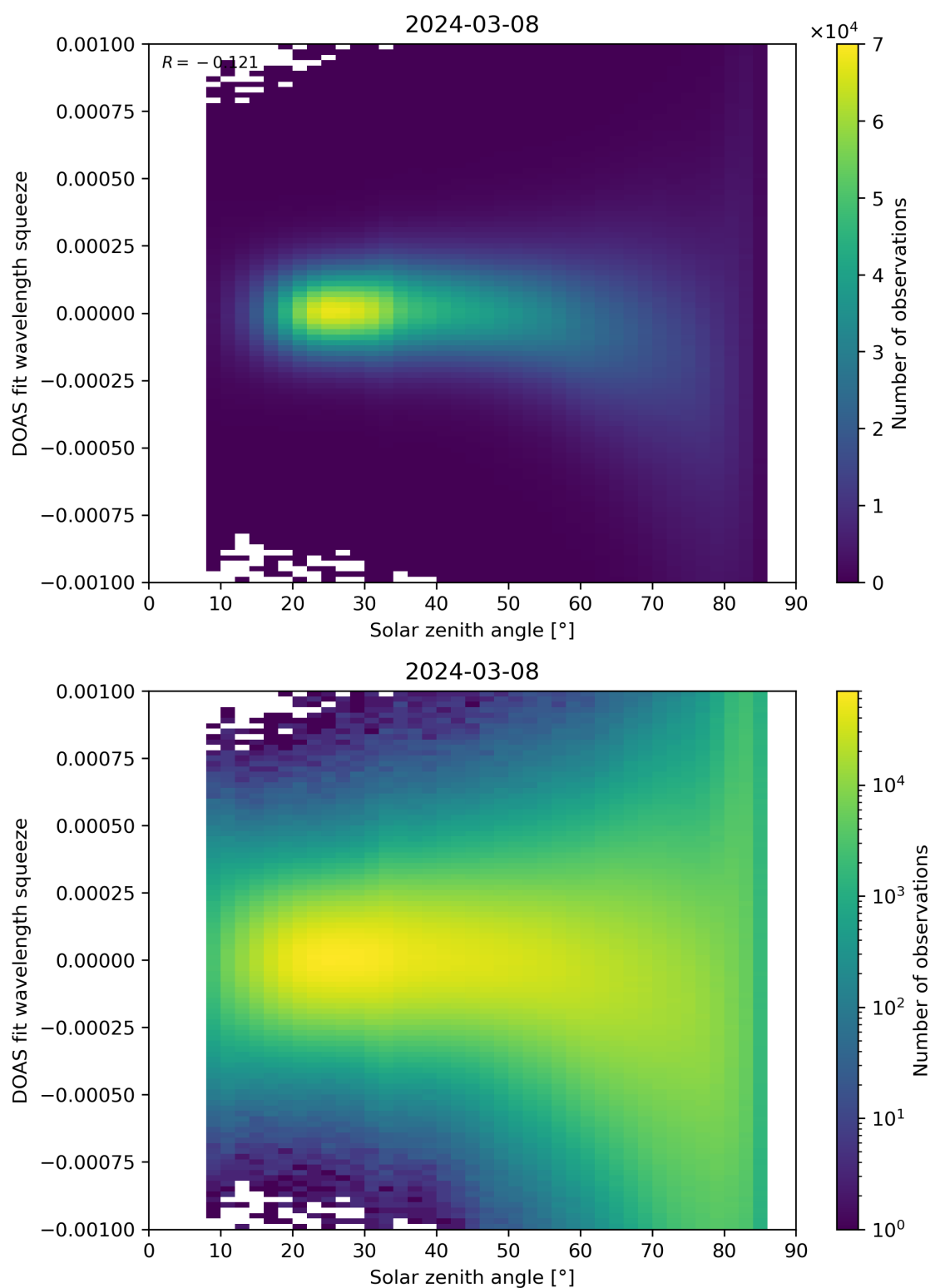
Figure 162: Scatter density plot of “Solar zenith angle” against “DOAS fit wavelength squeeze” for 2024-03-07 to 2024-03-09.
