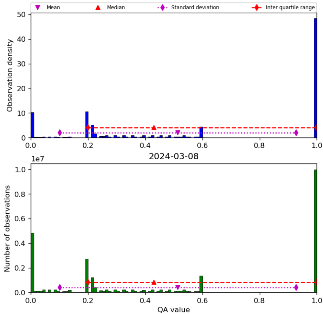
Figure 52: Histogram of “QA value” for 2024-03-07 to 2024-03-09
