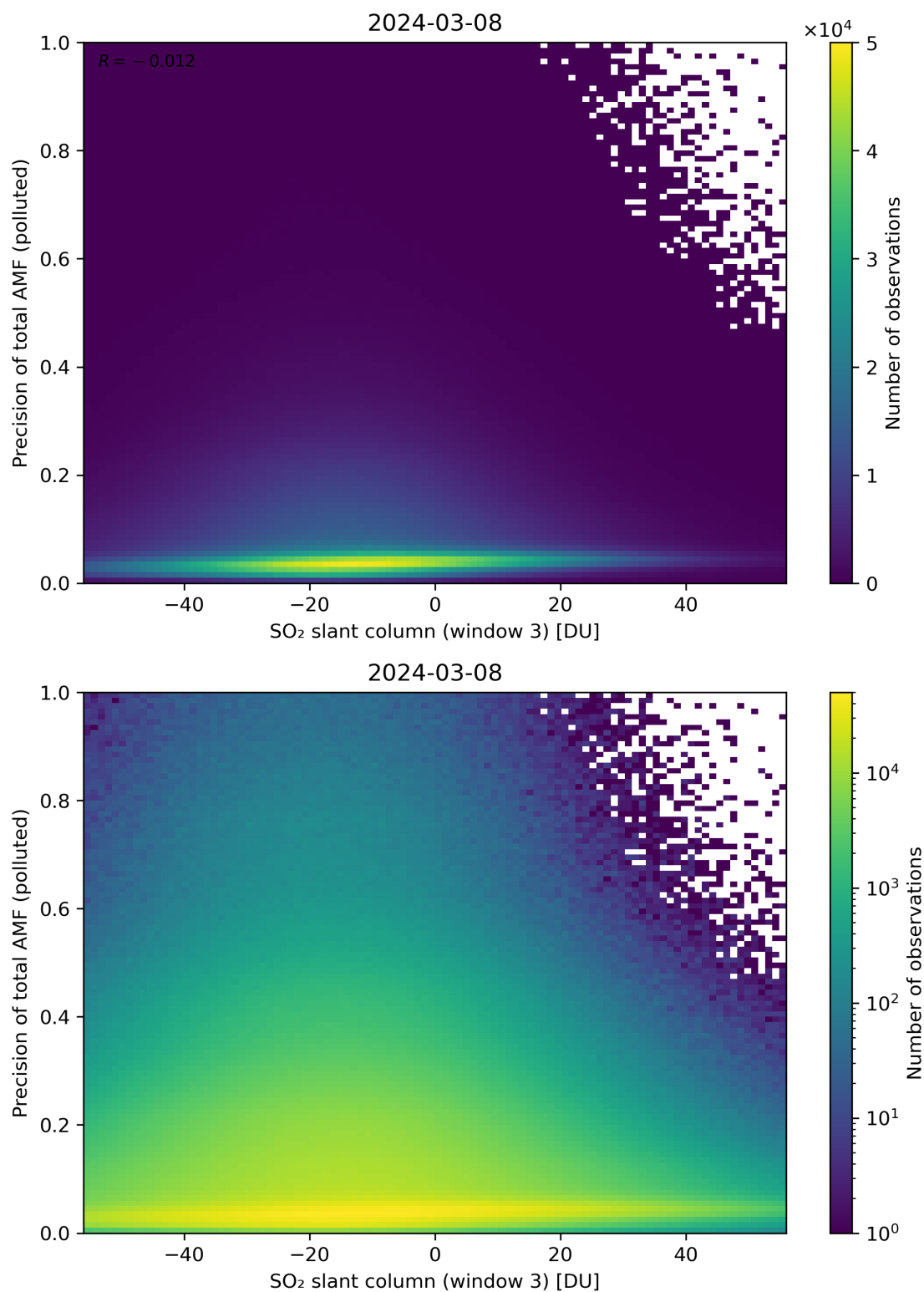
Figure 269: Scatter density plot of “SO 2 slant column (window 3)” against “Precision of total AMF (polluted)” for 2024-03-07 to 2024-03-09.
