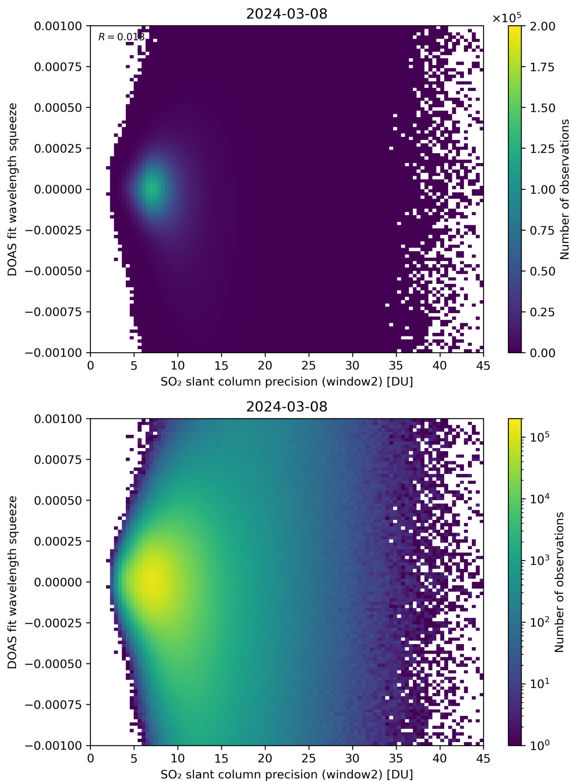
Figure 244: Scatter density plot of “SO 2 slant column precision (window2)” against “DOAS fit wavelength squeeze” for 2024-03-07 to 2024-03-09.
