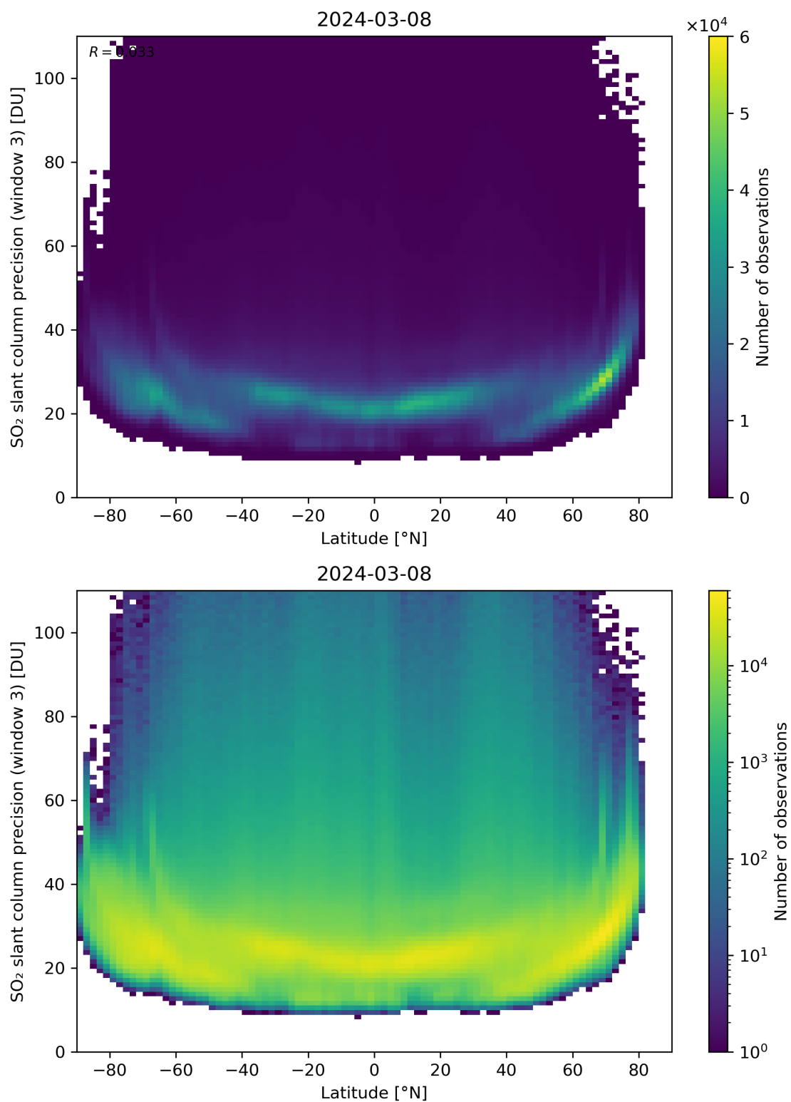
Figure 153: Scatter density plot of “Latitude” against “SO 2 slant column precision (window 3)” for 2024-03-07 to 2024-03-09.
