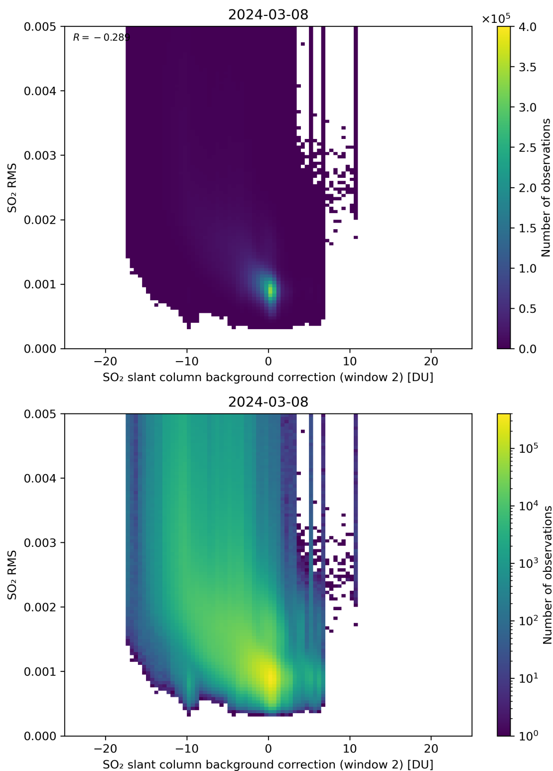
Figure 114: Scatter density plot of “SO 2 slant column background correction (window 2)” against “SO 2 RMS” for 2024-03-07 to 2024-03-09.
