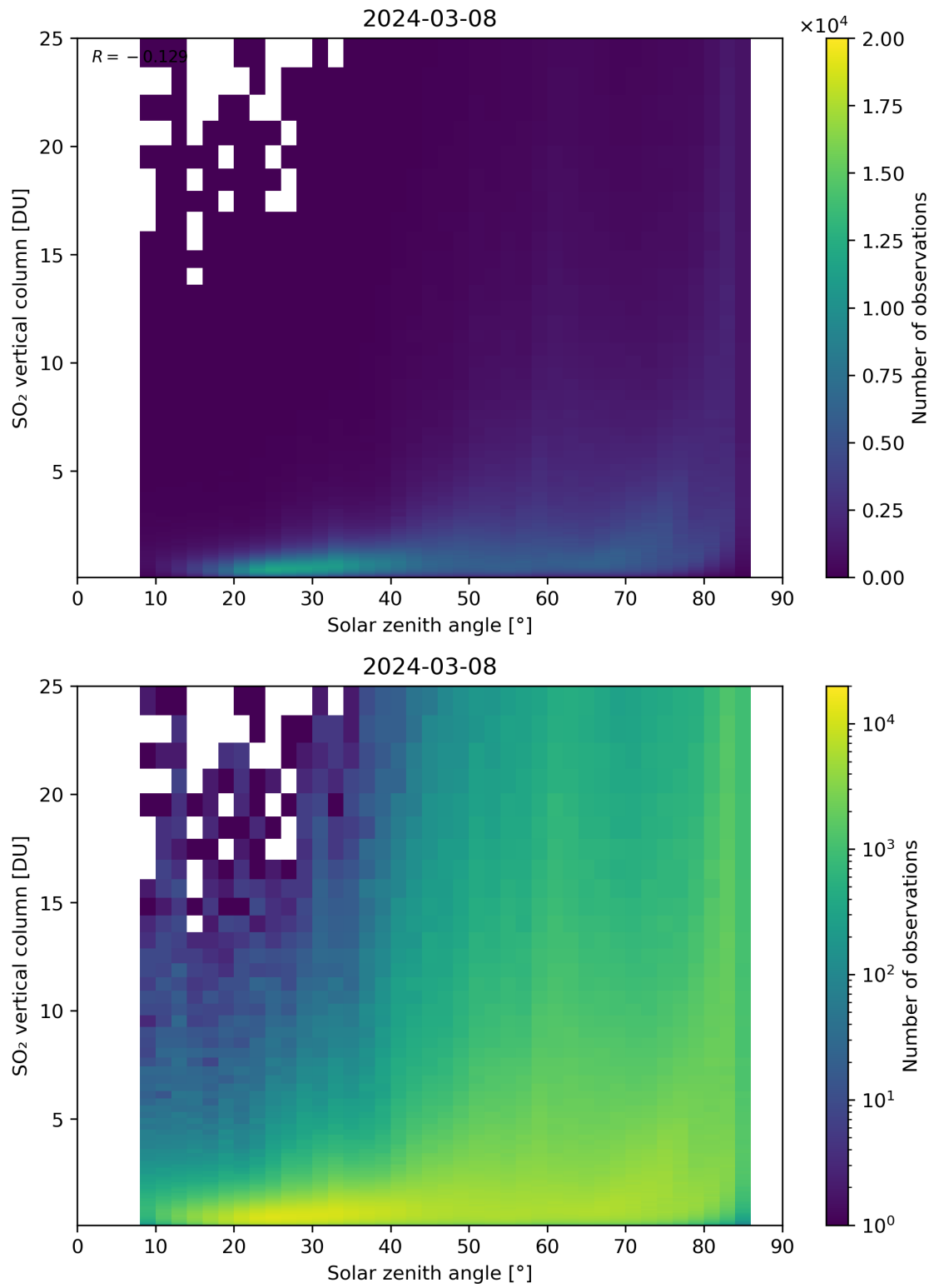
Figure 176: Scatter density plot of “Solar zenith angle” against “SO 2 vertical column” for 2024-03-07 to 2024-03-09.
