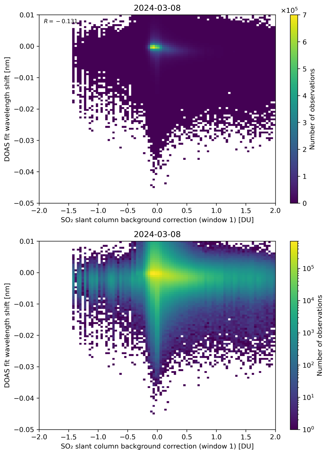
Figure 100: Scatter density plot of “SO 2 slant column background correction (window 1)” against “DOAS fit wavelength shift” for 2024-03-07 to 2024-03-09.
