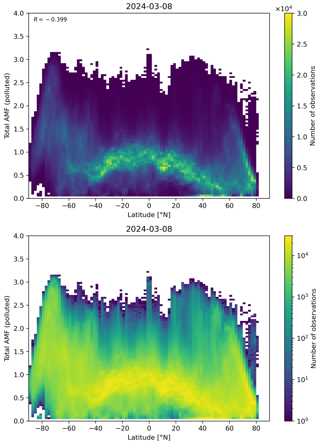
Figure 154: Scatter density plot of “Latitude” against “Total AMF (polluted)” for 2024-03-07 to 2024-03-09.
