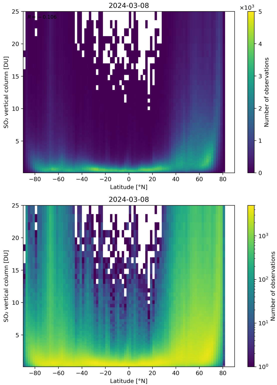
Figure 156: Scatter density plot of “Latitude” against “SO 2 vertical column” for 2024-03-07 to 2024-03-09.
