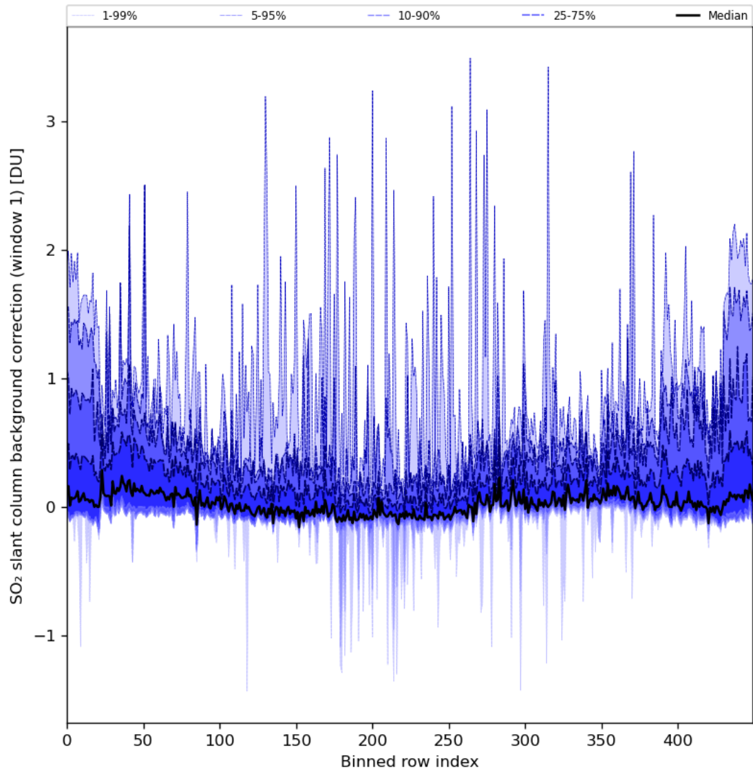
Figure 82: Along track statistics of “SO 2 slant column background correction (window 1)” for 2024-03-07 to 2024-03-09
