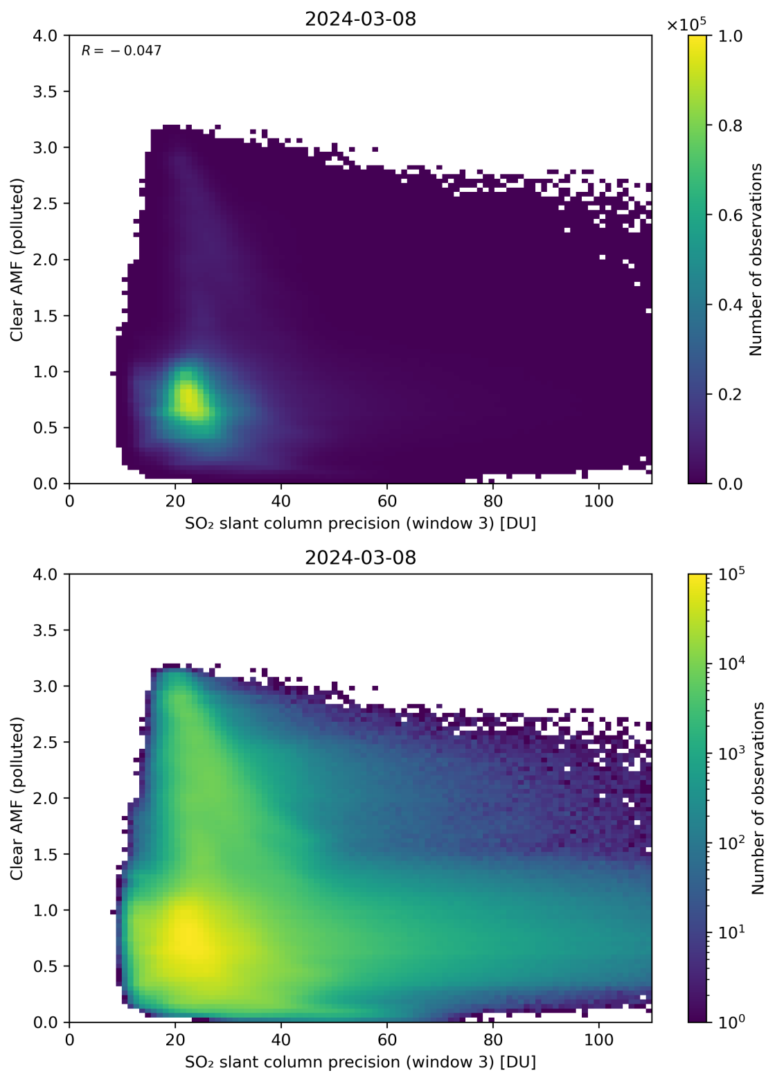
Figure 261: Scatter density plot of “SO 2 slant column precision (window 3)” against “Clear AMF (polluted)” for 2024-03-07 to 2024-03-09.
