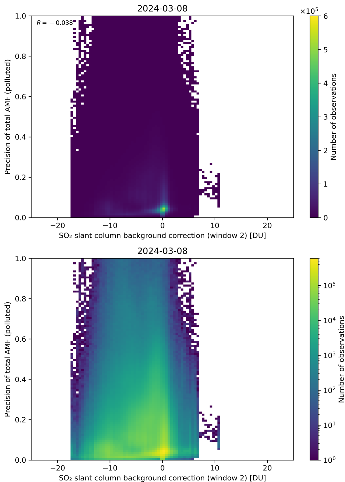
Figure 120: Scatter density plot of “SO 2 slant column background correction (window 2)” against “Precision of total AMF (polluted)” for 2024-03-07 to 2024-03-09.
