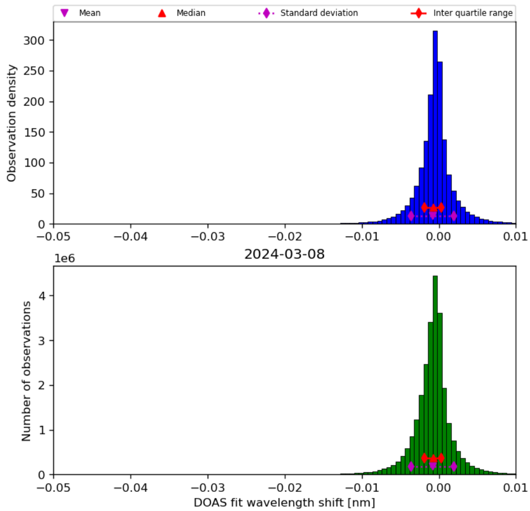
Figure 68: Histogram of “DOAS fit wavelength shift” for 2024-03-07 to 2024-03-09
