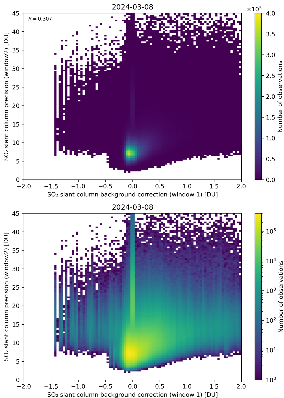
Figure 106: Scatter density plot of “SO 2 slant column background correction (window 1)” against “SO 2 slant column precision (window2)” for 2024-03-07 to 2024-03-09.
