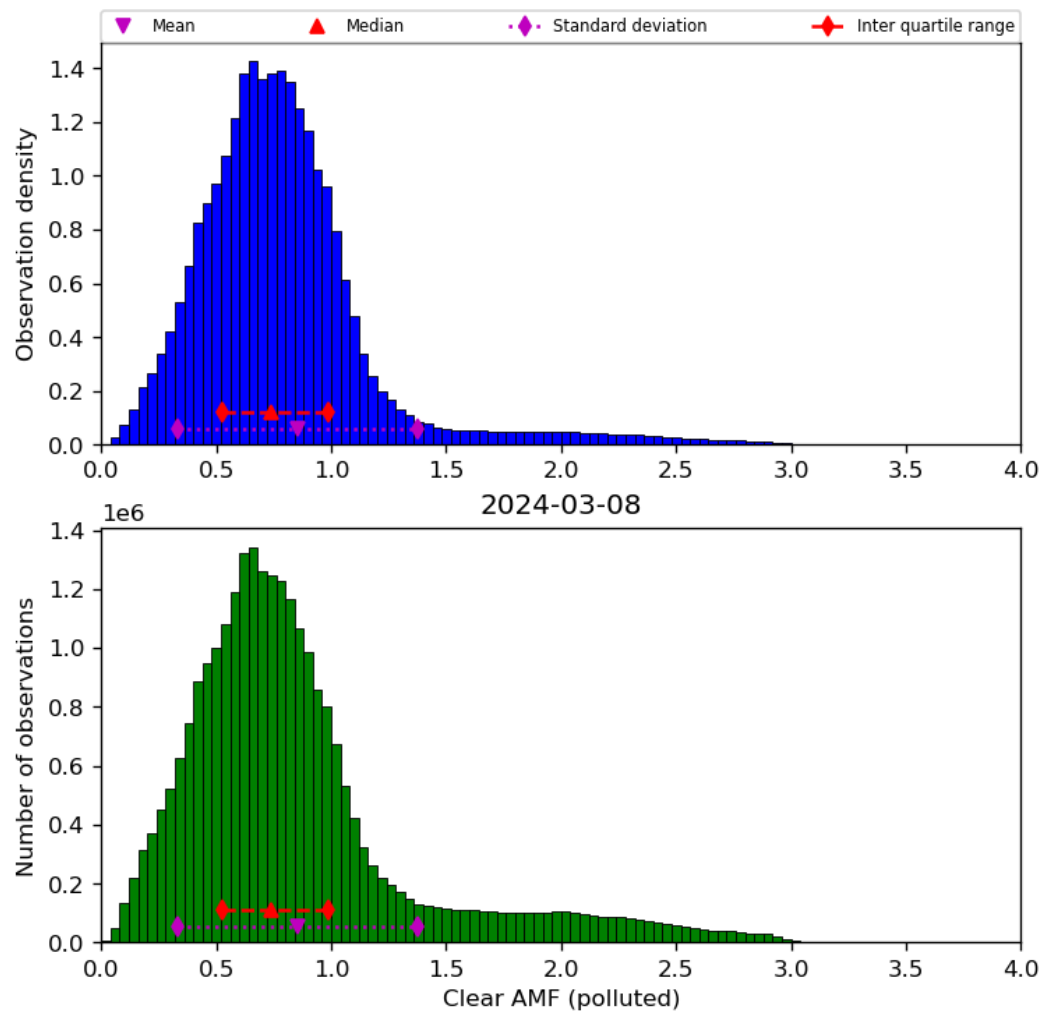
Figure 73: Histogram of "Clear AMF (polluted)" for 2024-03-07 to 2024-03-09
