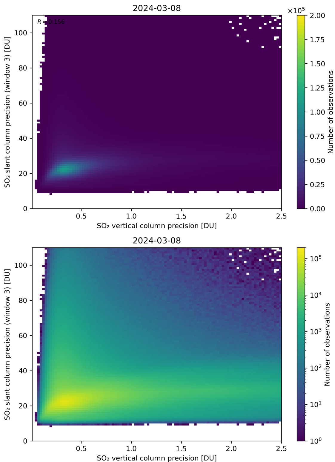
Figure 293: Scatter density plot of “SO 2 vertical column precision” against “SO 2 slant column precision (window 3)” for 2024-03-07 to 2024-03-09.
