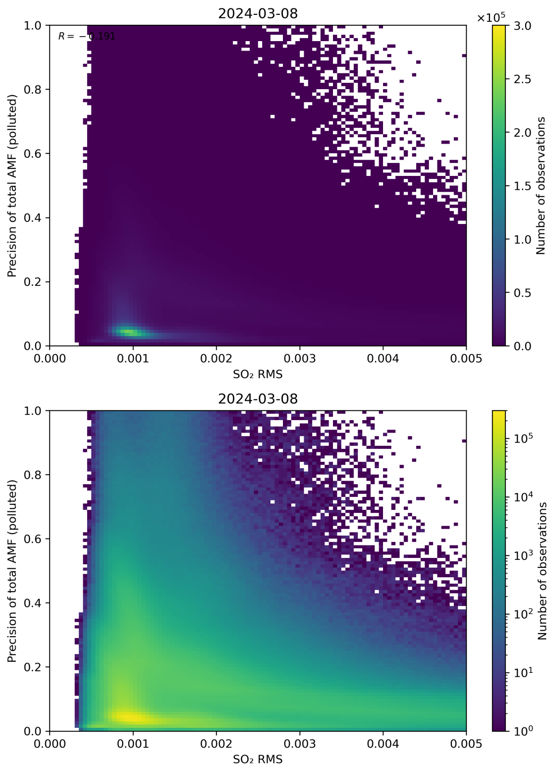
Figure 138: Scatter density plot of “SO 2 RMS” against “Precision of total AMF (polluted)” for 2024-03-07 to 2024-03-09.
