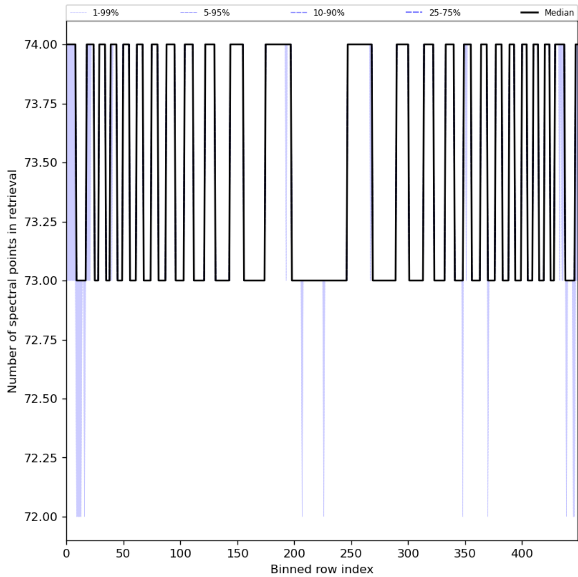
Figure 97: Along track statistics of “Number of spectral points in retrieval” for 2024-03-07 to 2024-03-09
