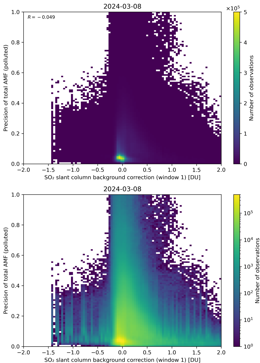
Figure 110: Scatter density plot of “SO 2 slant column background correction (window 1)” against “Precision of total AMF (polluted)” for 2024-03-07 to 2024-03-09.
