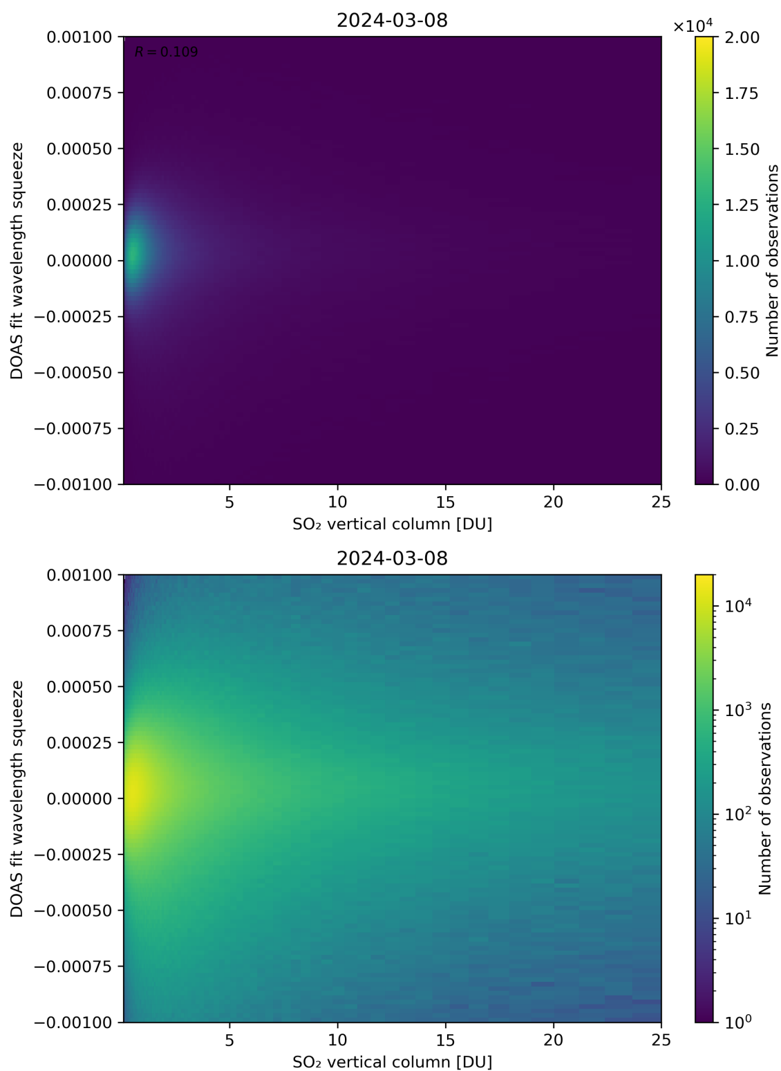
Figure 277: Scatter density plot of “SO 2 vertical column” against “DOAS fit wavelength squeeze” for 2024-03-07 to 2024-03-09.
