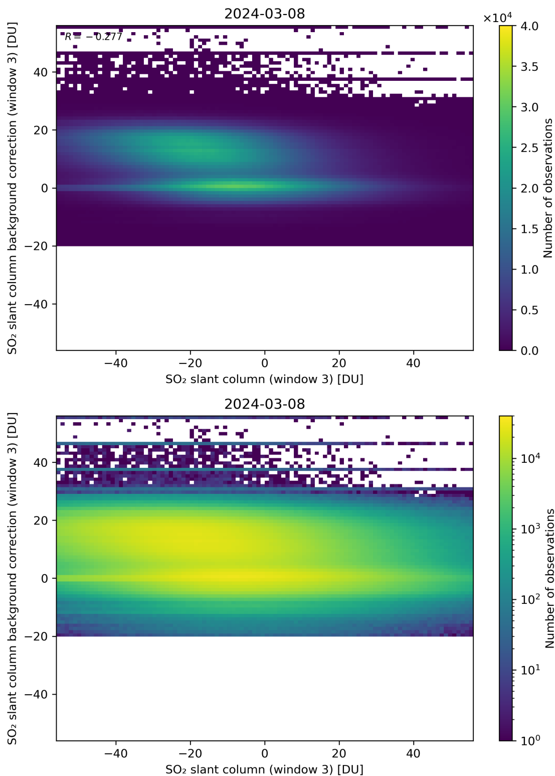
Figure 253: Scatter density plot of “SO 2 slant column (window 3)” against “SO 2 slant column background correction (window 3)” for 2024-03-07 to 2024-03-09.
