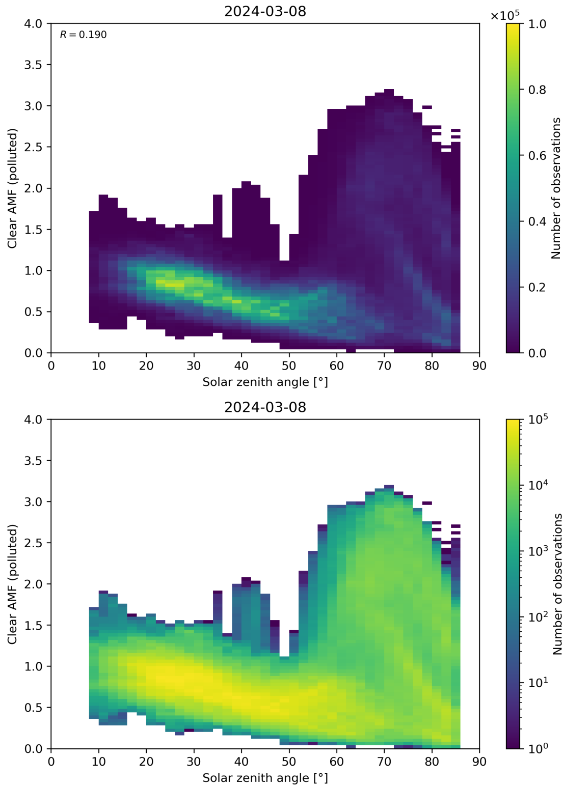
Figure 165: Scatter density plot of “Solar zenith angle” against “Clear AMF (polluted)” for 2024-03-07 to 2024-03-09.
