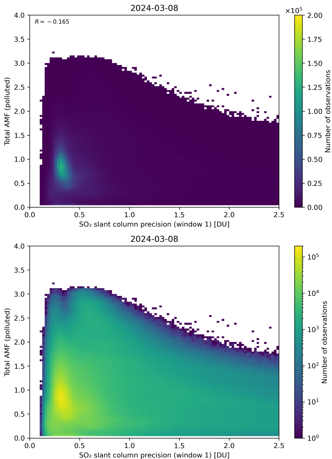
Figure 230: Scatter density plot of “SO 2 slant column precision (window 1)” against “Total AMF (polluted)” for 2024-03-07 to 2024-03-09.
