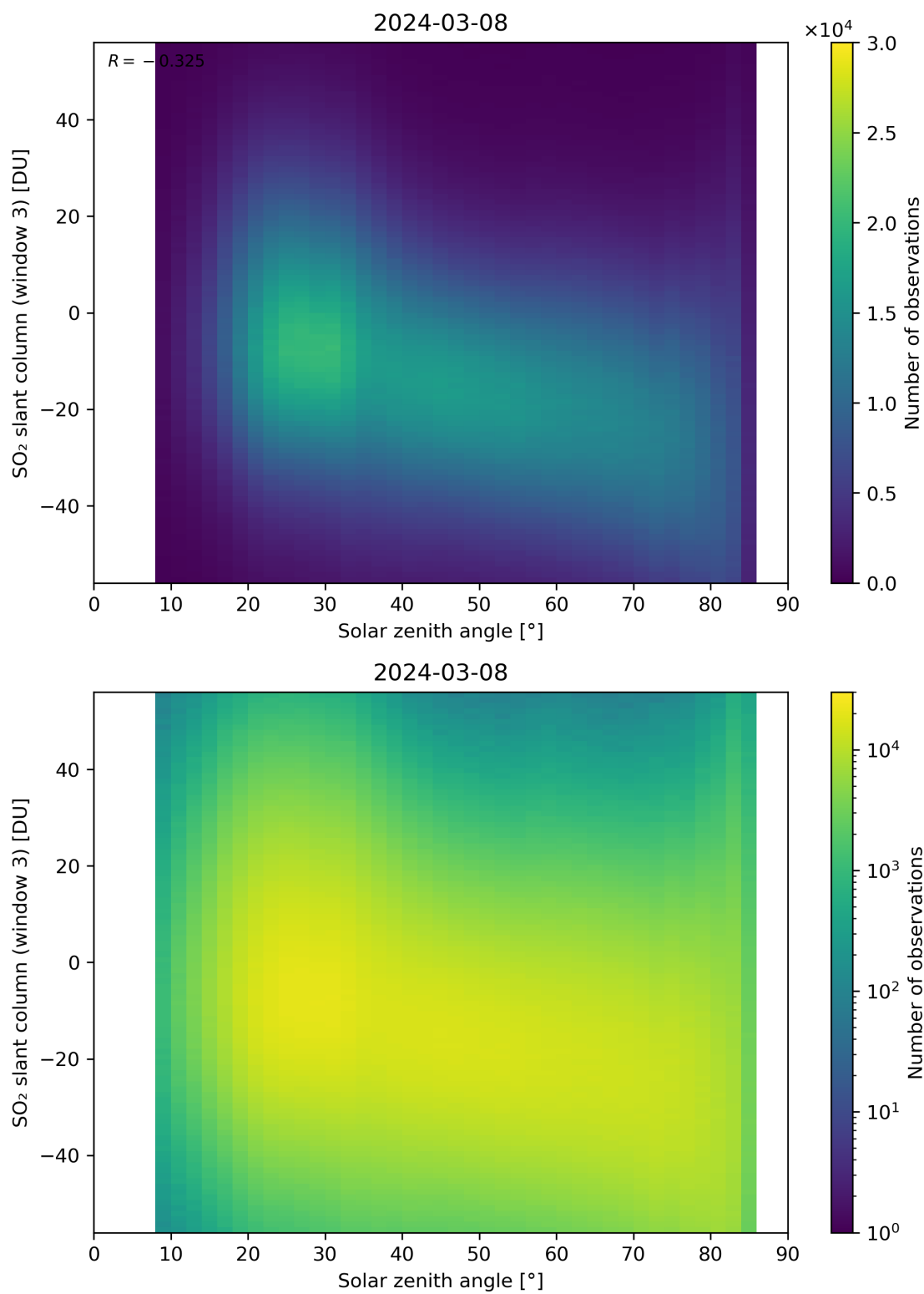
Figure 172: Scatter density plot of “Solar zenith angle” against “SO 2 slant column (window 3)” for 2024-03-07 to 2024-03-09.
