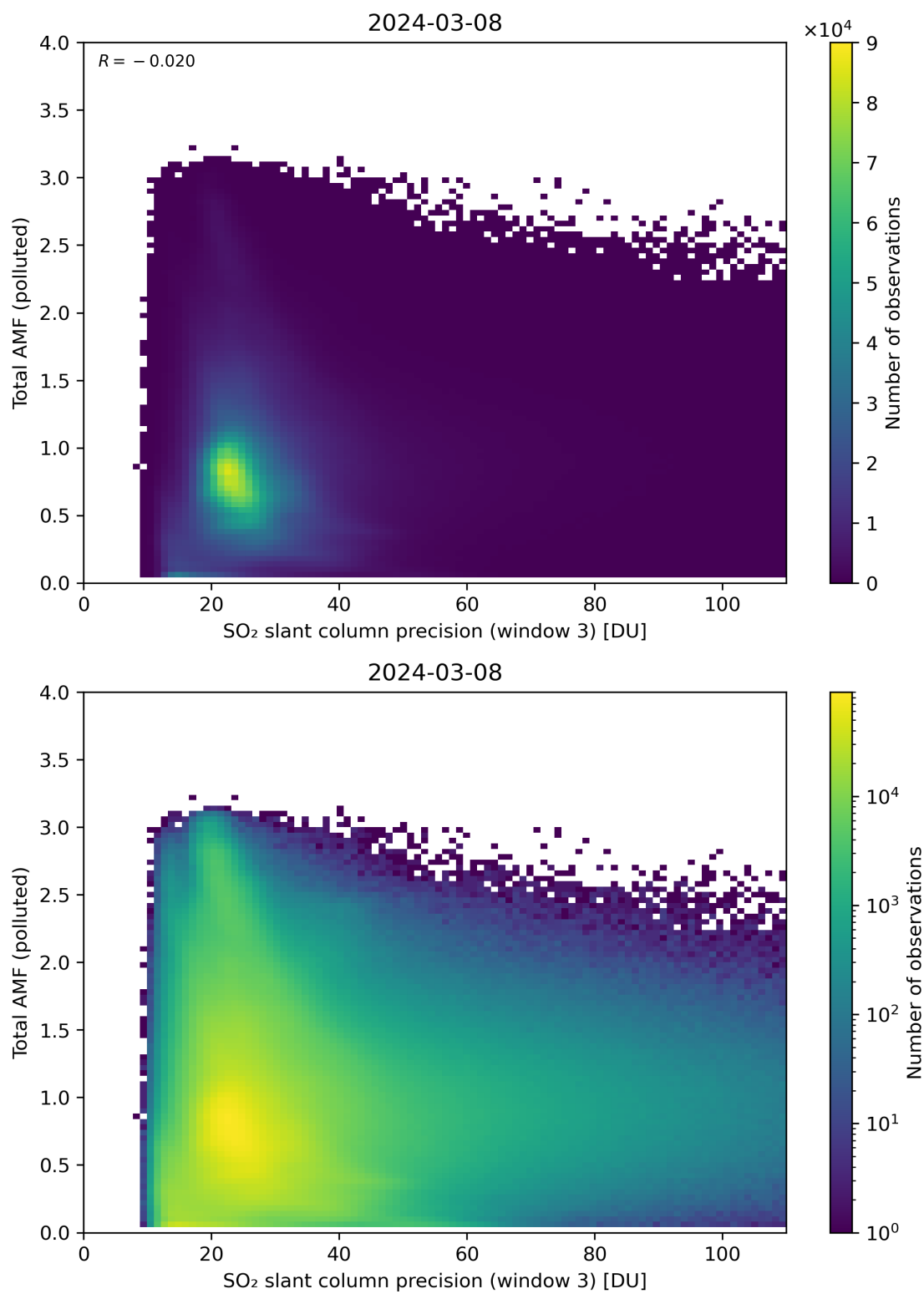
Figure 263: Scatter density plot of “SO 2 slant column precision (window 3)” against “Total AMF (polluted)” for 2024-03-07 to 2024-03-09.
