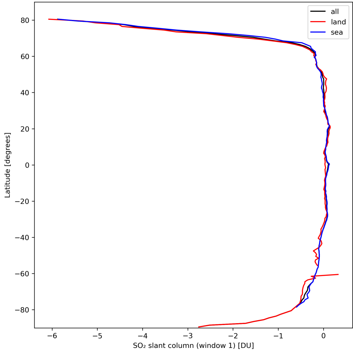
Figure 33: Zonal average of “SO 2 slant column (window 1)” for 2024-03-07 to 2024-03-09.
