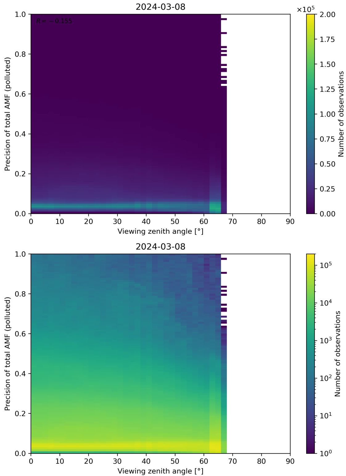
Figure 326: Scatter density plot of “Viewing zenith angle” against “Precision of total AMF (polluted)” for 2024-03-07 to 2024-03-09.
