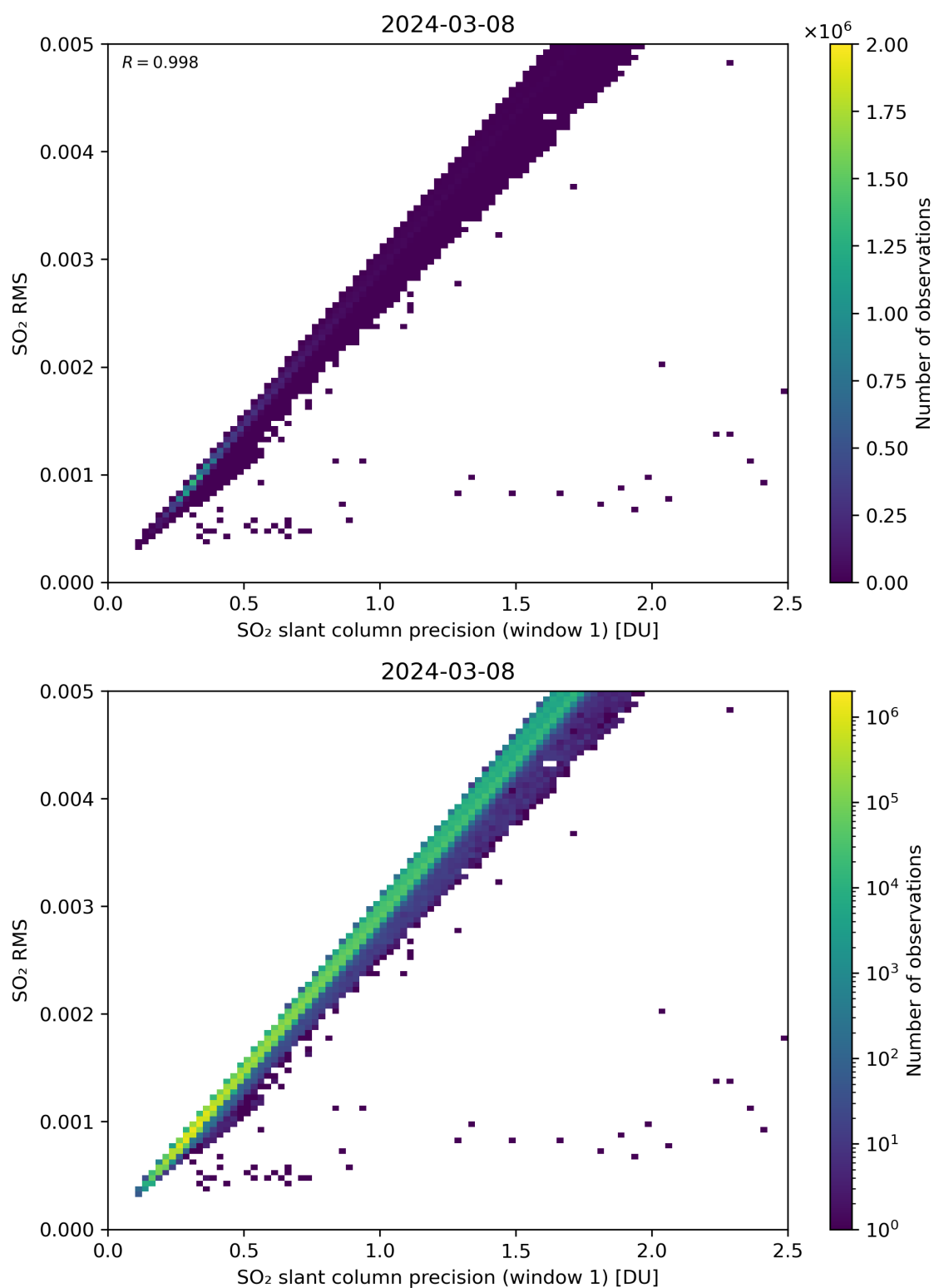
Figure 223: Scatter density plot of “SO 2 slant column precision (window 1)” against “SO 2 RMS” for 2024-03-07 to 2024-03-09.
