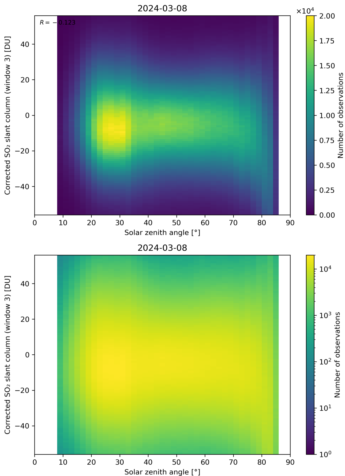
Figure 168: Scatter density plot of “Solar zenith angle” against “Corrected SO 2 slant column (window 3)” for 2024-03-07 to 2024-03-09.
