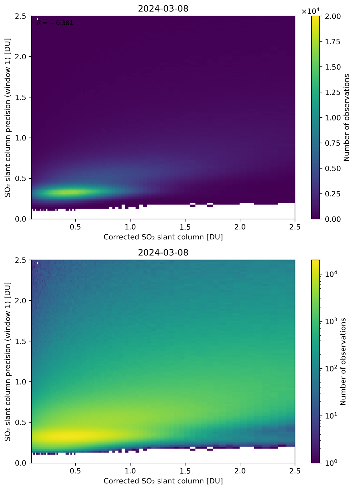
Figure 188: Scatter density plot of “Corrected SO 2 slant column” against “SO 2 slant column precision (window 1)” for 2024-03-07 to 2024-03-09.
