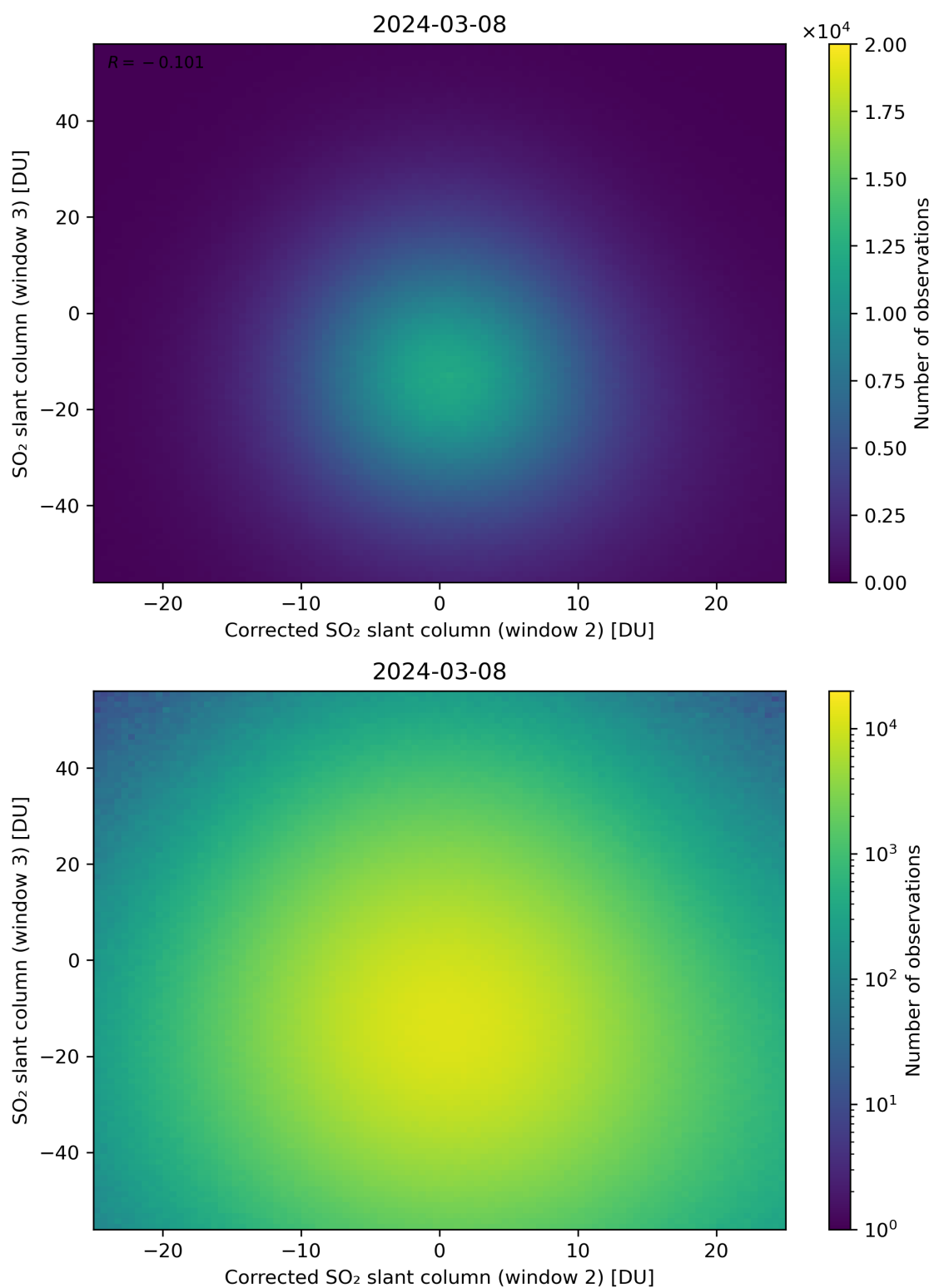
Figure 201: Scatter density plot of “Corrected SO 2 slant column (window 2)” against “SO 2 slant column (window 3)” for 2024-03-07 to 2024-03-09.
