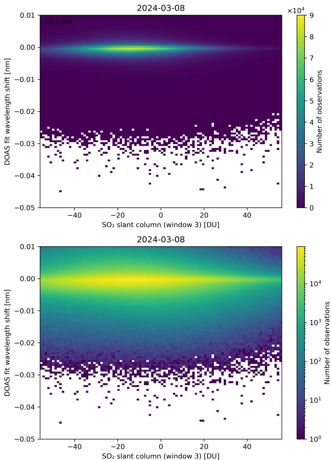
Figure 254: Scatter density plot of “SO 2 slant column (window 3)” against “DOAS fit wavelength shift” for 2024-03-07 to 2024-03-09.
