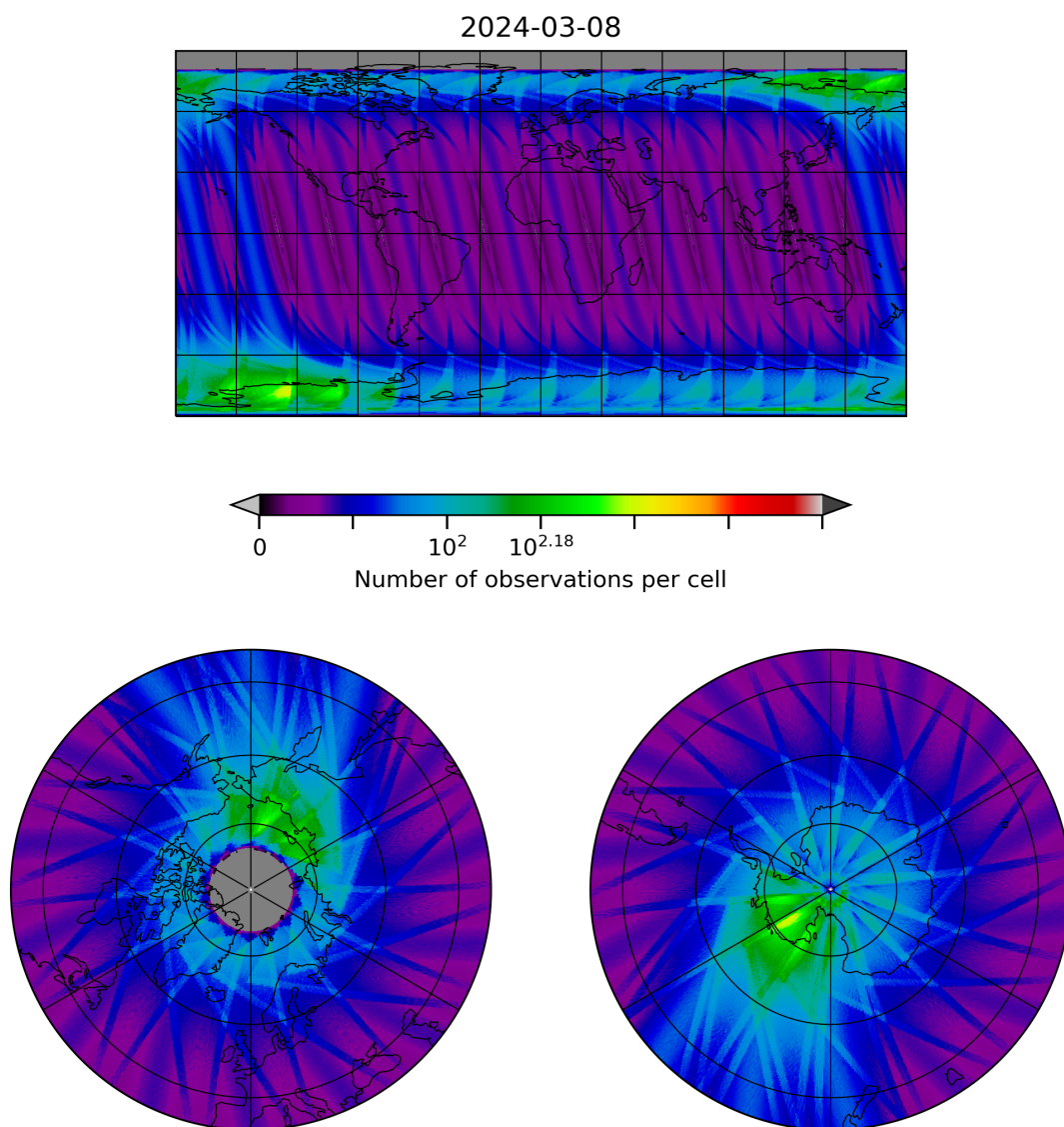
Figure 28: Map of the number of observations for 2024-03-07 to 2024-03-09
