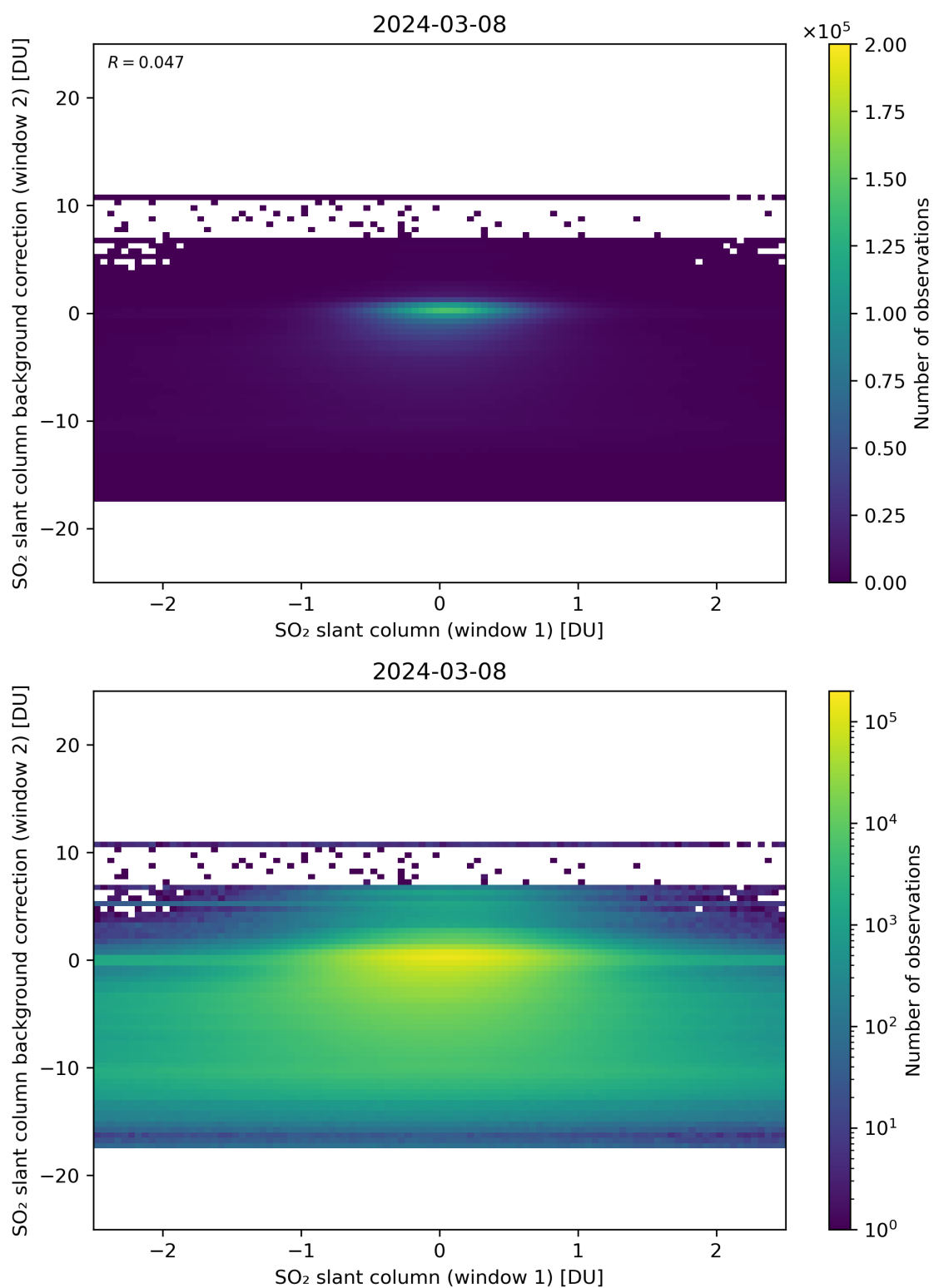
Figure 213: Scatter density plot of “SO 2 slant column (window 1)” against “SO 2 slant column background correction (window 2)” for 2024-03-07 to 2024-03-09.
