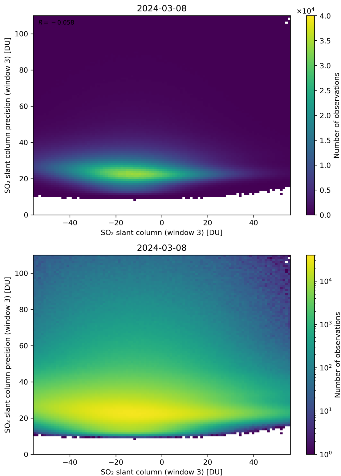
Figure 267: Scatter density plot of “SO 2 slant column (window 3)” against “SO 2 slant column precision (window 3)” for 2024-03-07 to 2024-03-09.
