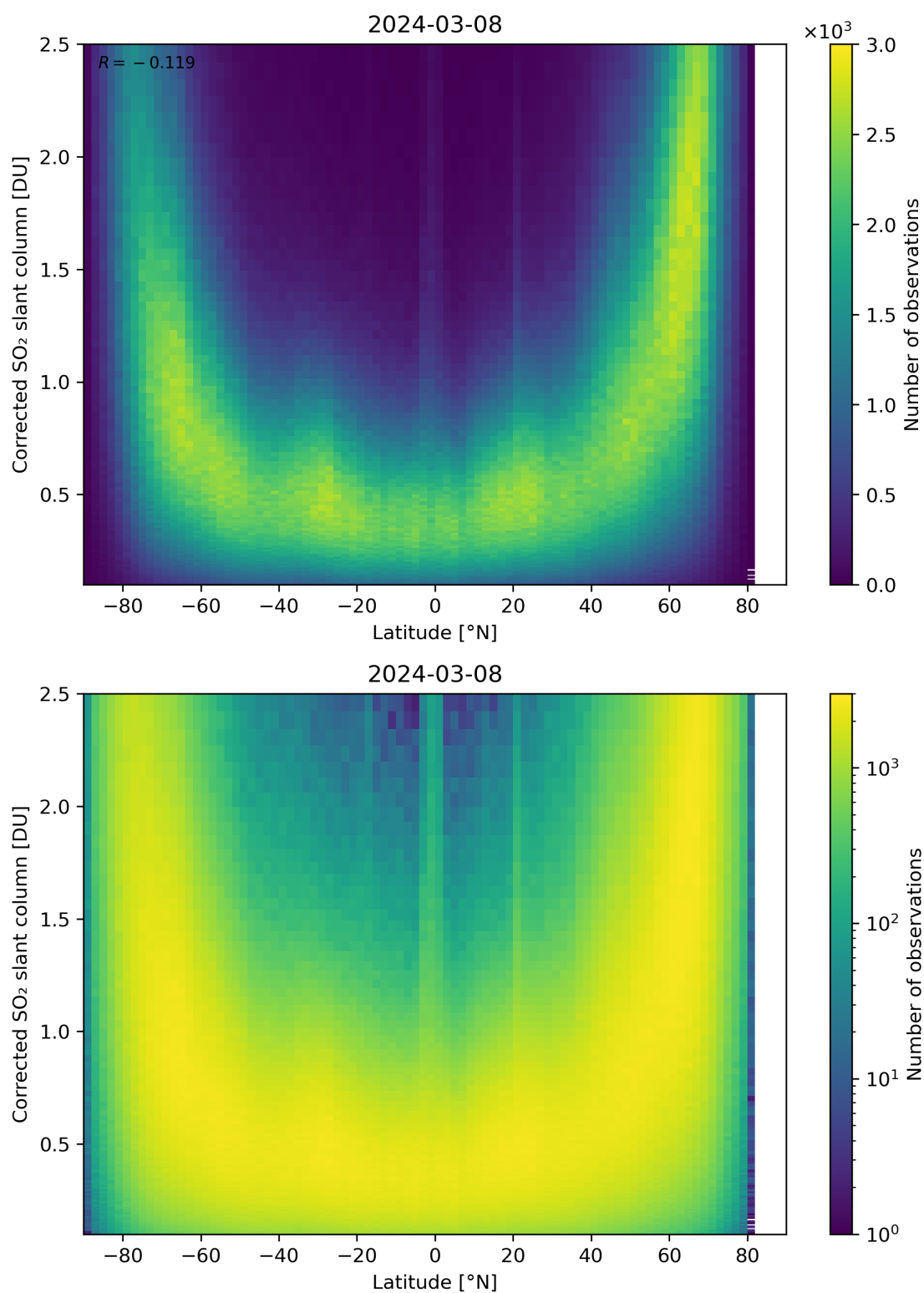
Figure 146: Scatter density plot of “Latitude” against “Corrected SO 2 slant column” for 2024-03-07 to 2024-03-09.
