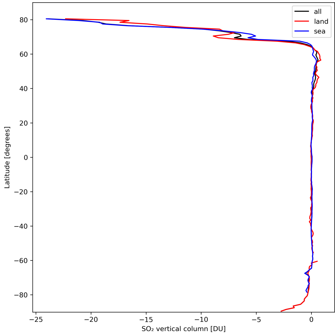
Figure 30: Zonal average of “SO 2 vertical column” for 2024-03-07 to 2024-03-09.
