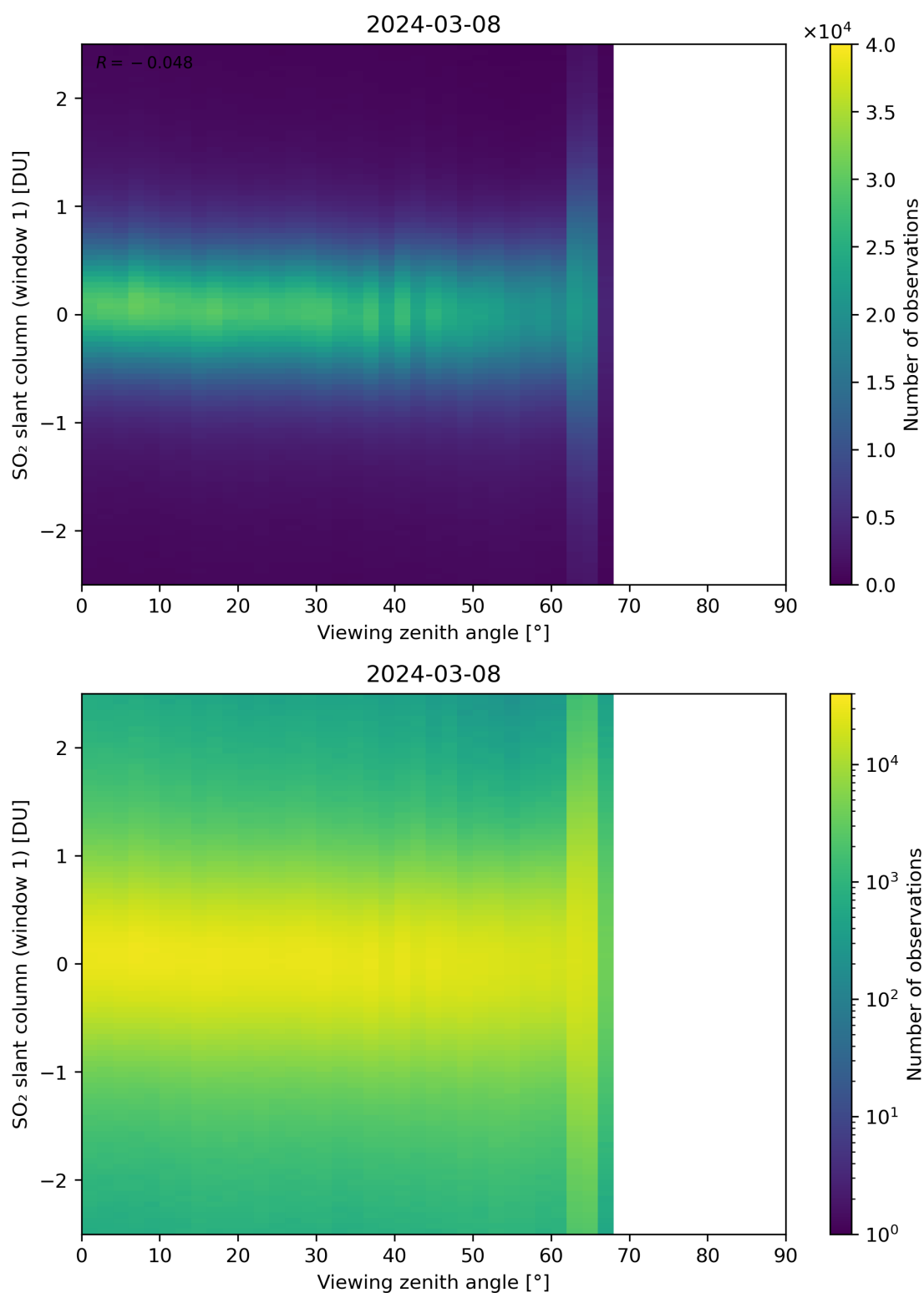
Figure 320: Scatter density plot of “Viewing zenith angle” against “SO 2 slant column (window 1)” for 2024-03-07 to 2024-03-09.
