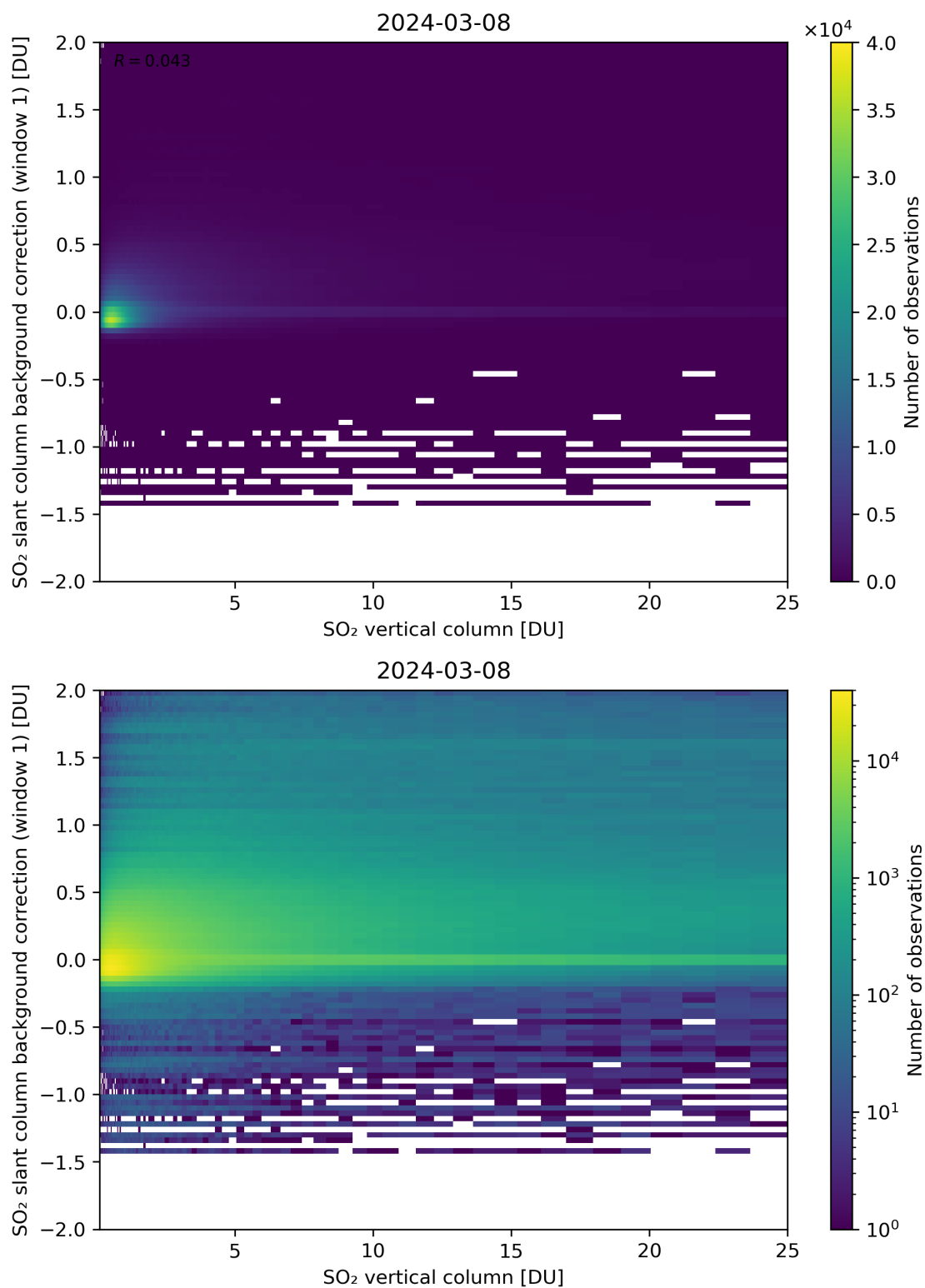
Figure 273: Scatter density plot of “SO 2 vertical column” against “SO 2 slant column background correction (window 1)” for 2024-03-07 to 2024-03-09.
