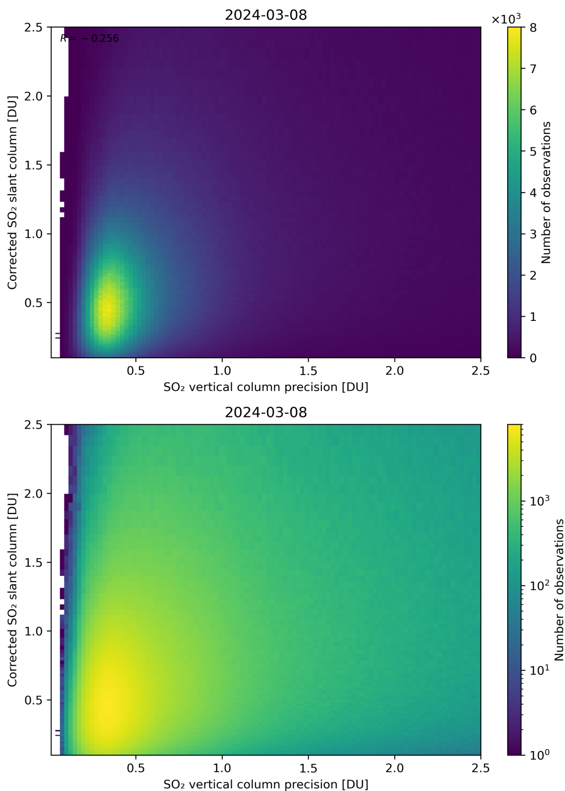
Figure 286: Scatter density plot of “SO 2 vertical column precision” against “Corrected SO 2 slant column” for 2024-03-07 to 2024-03-09.
