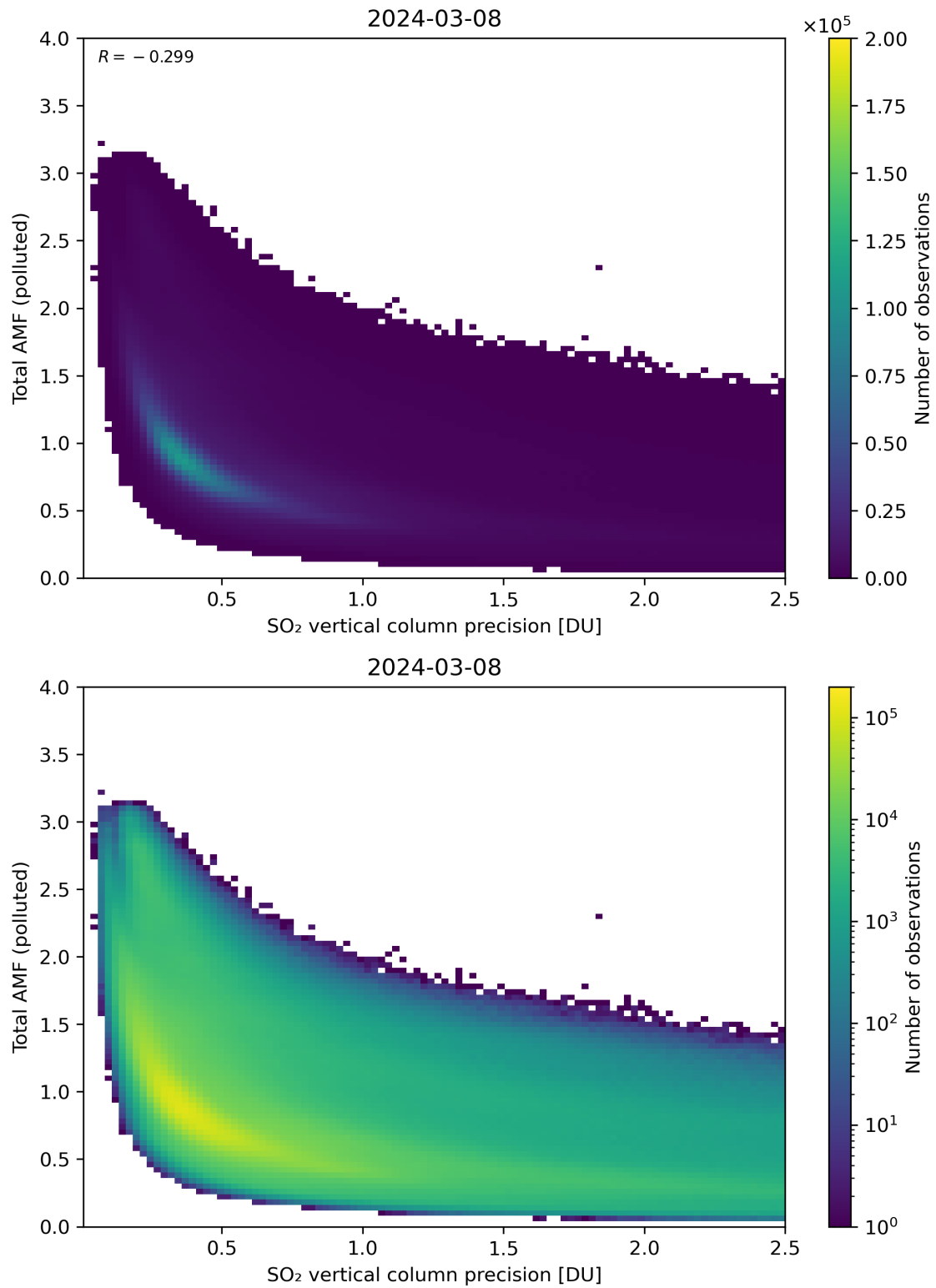
Figure 294: Scatter density plot of “SO 2 vertical column precision” against “Total AMF (polluted)” for 2024-03-07 to 2024-03-09.
