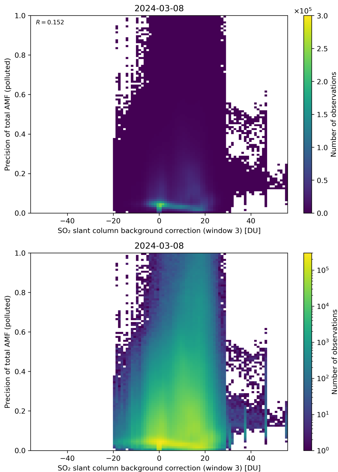
Figure 126: Scatter density plot of “SO 2 slant column background correction (window 3)” against “Precision of total AMF (polluted)” for 2024-03-07 to 2024-03-09.
