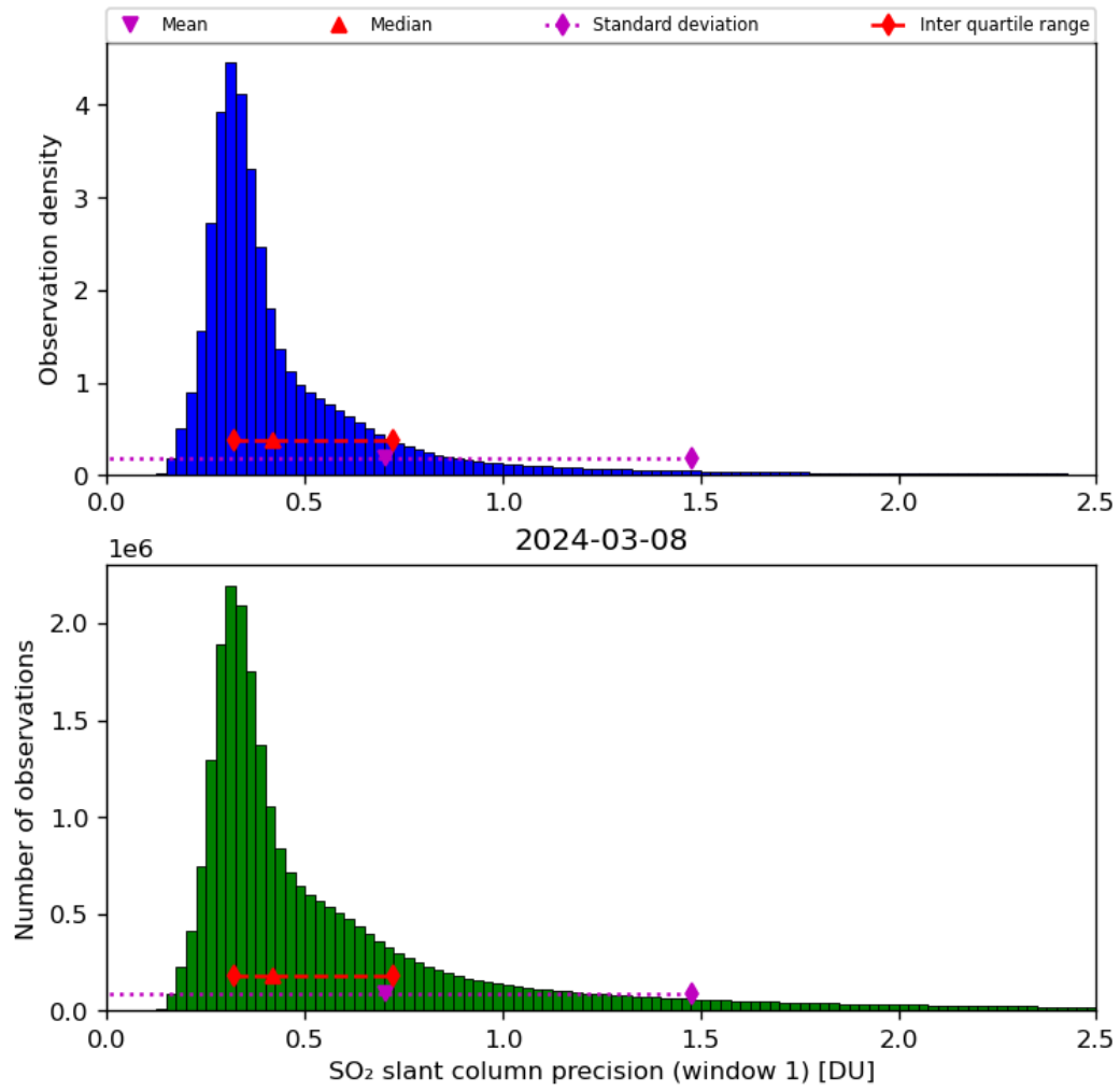
Figure 57: Histogram of “SO 2 slant column precision (window 1)” for 2024-03-07 to 2024-03-09
