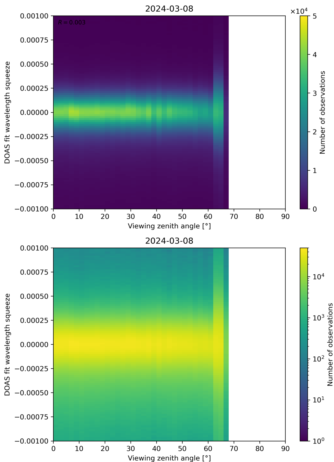
Figure 312: Scatter density plot of “Viewing zenith angle” against “DOAS fit wavelength squeeze” for 2024-03-07 to 2024-03-09.
