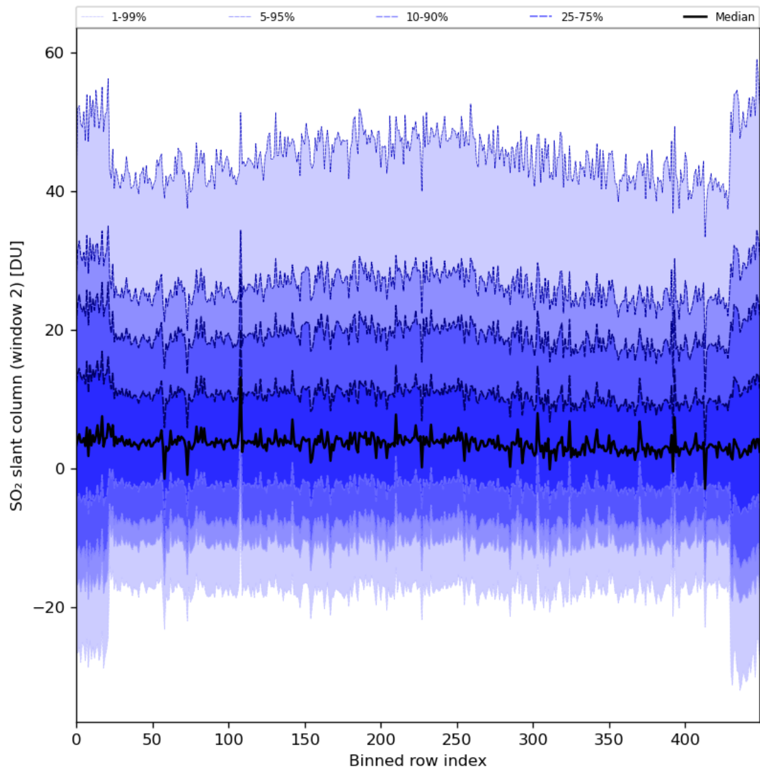
Figure 83: Along track statistics of “SO 2 slant column (window 2)” for 2024-03-07 to 2024-03-09
