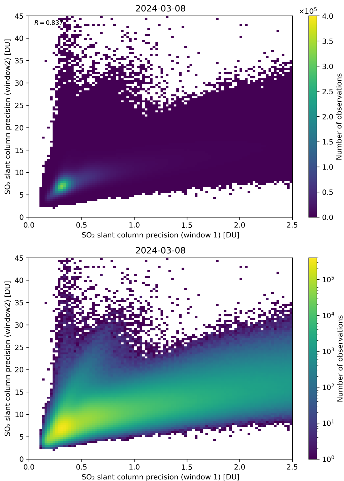
Figure 227: Scatter density plot of “SO 2 slant column precision (window 1)” against “SO 2 slant column precision (window2)” for 2024-03-07 to 2024-03-09.
