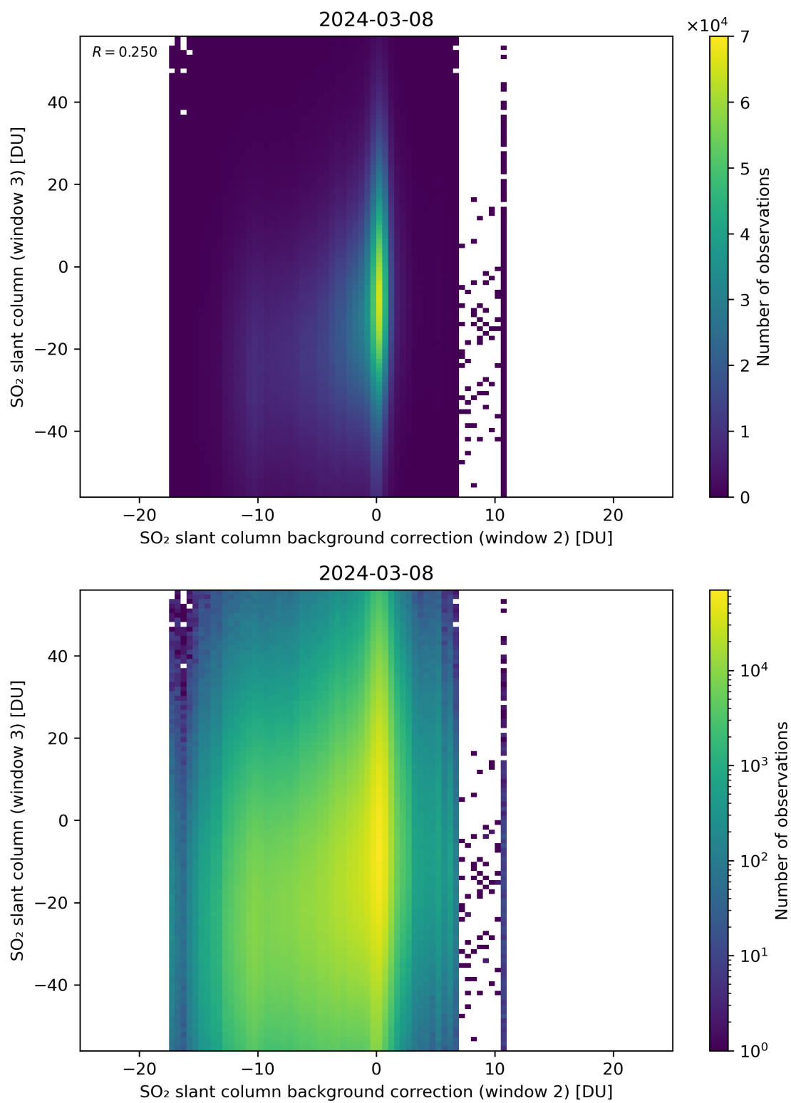
Figure 117: Scatter density plot of “SO 2 slant column background correction (window 2)” against “SO 2 slant column (window 3)” for 2024-03-07 to 2024-03-09.
