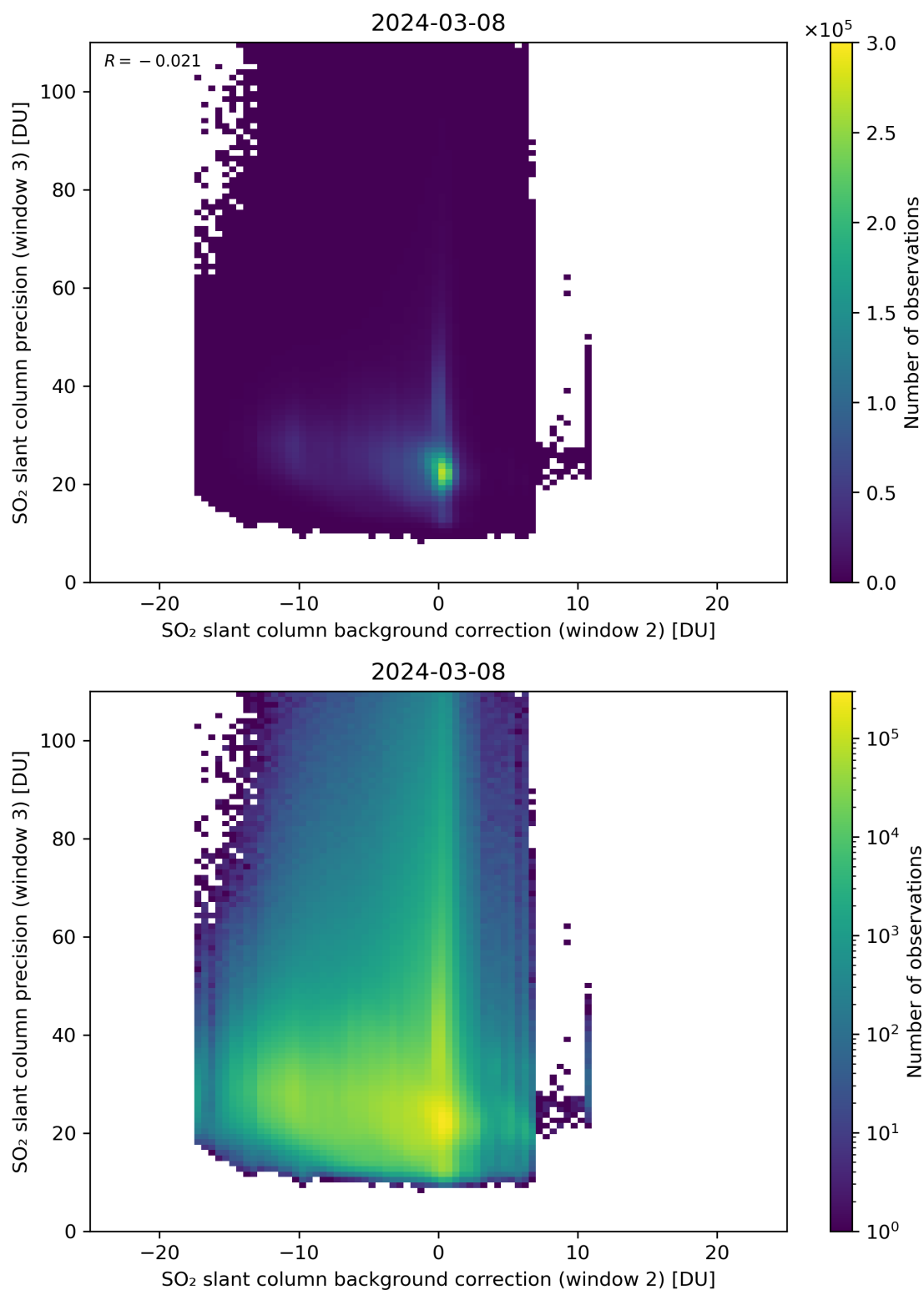
Figure 118: Scatter density plot of “SO 2 slant column background correction (window 2)” against “SO 2 slant column precision (window 3)” for 2024-03-07 to 2024-03-09.
