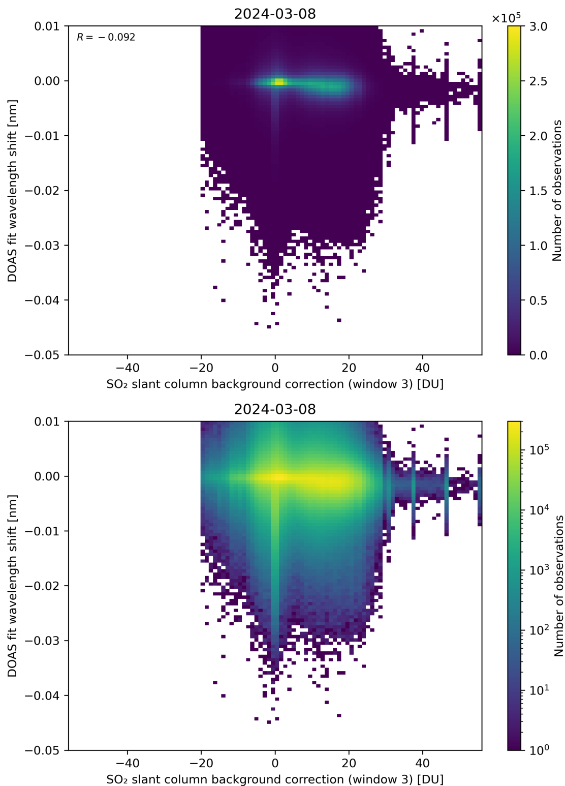
Figure 121: Scatter density plot of “SO 2 slant column background correction (window 3)” against “DOAS fit wavelength shift” for 2024-03-07 to 2024-03-09.
