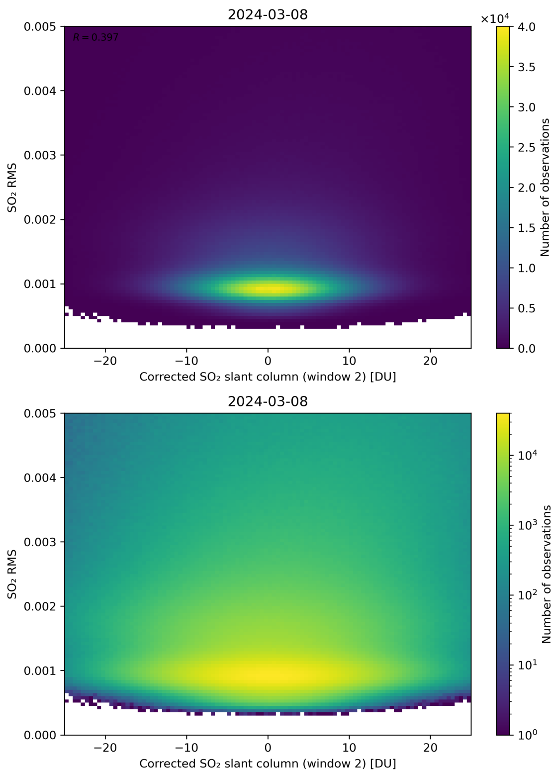
Figure 198: Scatter density plot of “Corrected SO 2 slant column (window 2)” against “SO 2 RMS” for 2024-03-07 to 2024-03-09.
