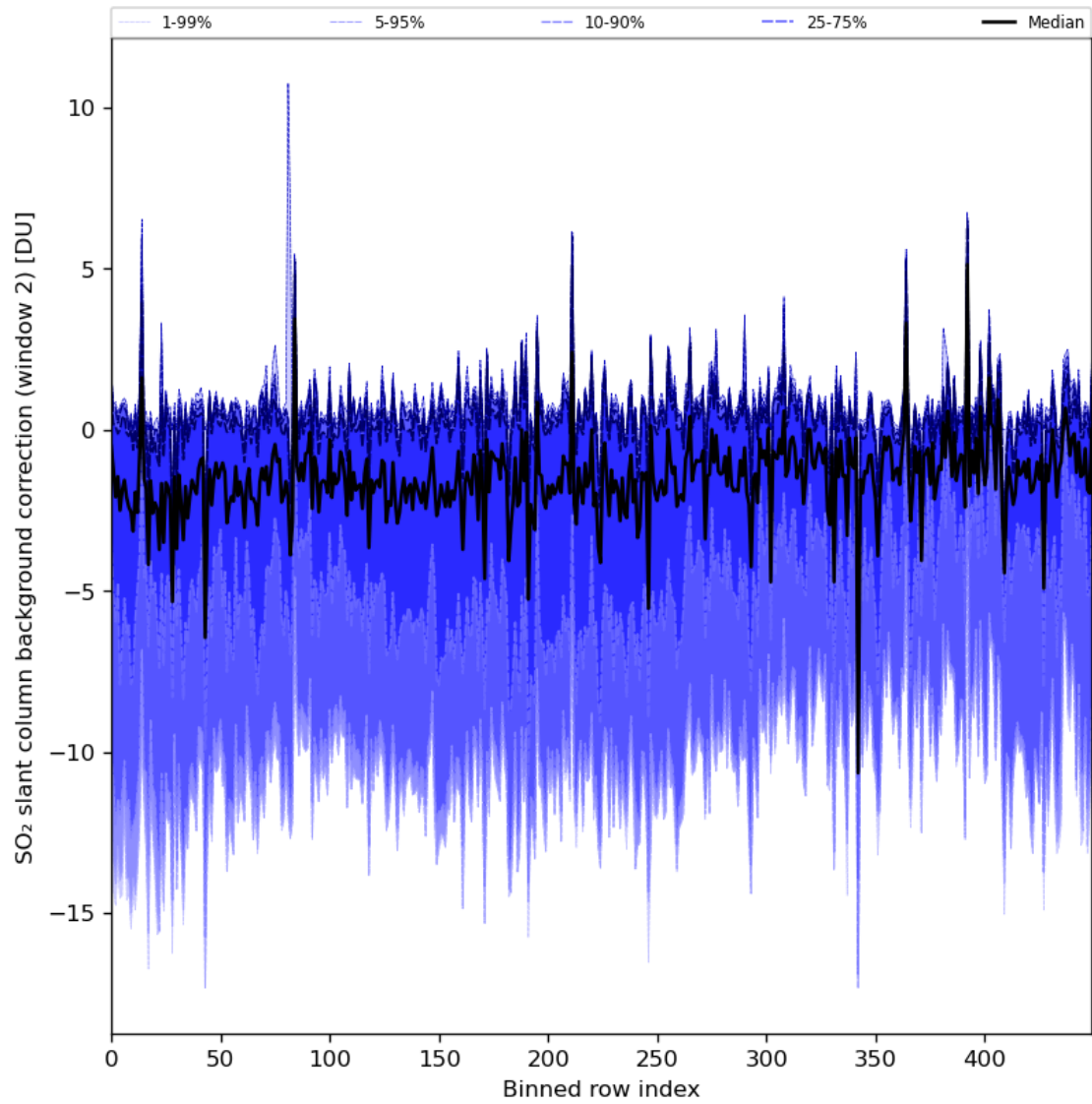
Figure 86: Along track statistics of “SO 2 slant column background correction (window 2)” for 2024-03-07 to 2024-03-09
