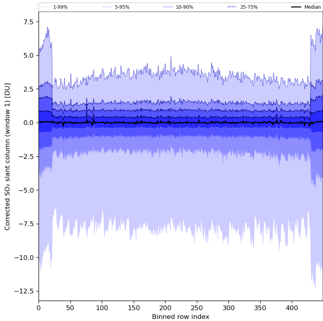
Figure 81: Along track statistics of “Corrected SO 2 slant column (window 1)” for 2024-03-07 to 2024-03-09
