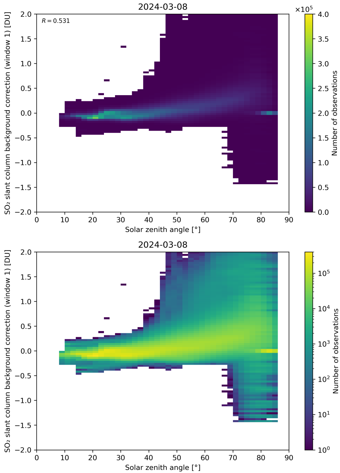
Figure 158: Scatter density plot of “Solar zenith angle” against “SO 2 slant column background correction (window 1)” for 2024-03-07 to 2024-03-09.
