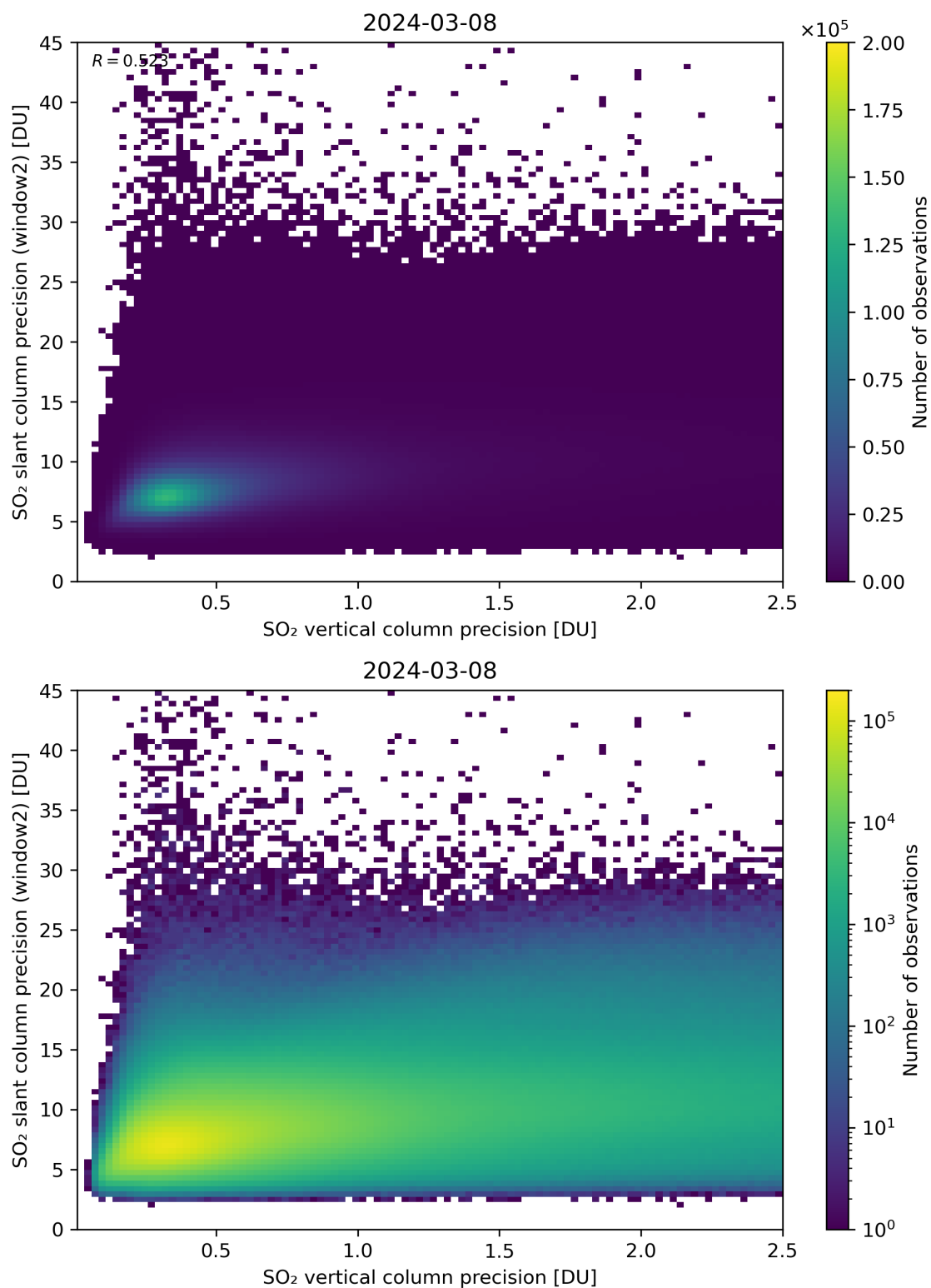
Figure 291: Scatter density plot of “SO 2 vertical column precision” against “SO 2 slant column precision (window2)” for 2024-03-07 to 2024-03-09.
