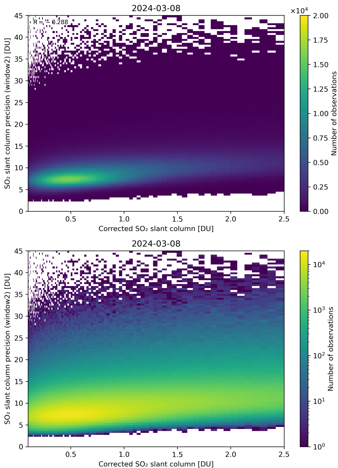
Figure 189: Scatter density plot of “Corrected SO 2 slant column” against “SO 2 slant column precision (window2)” for 2024-03-07 to 2024-03-09.
