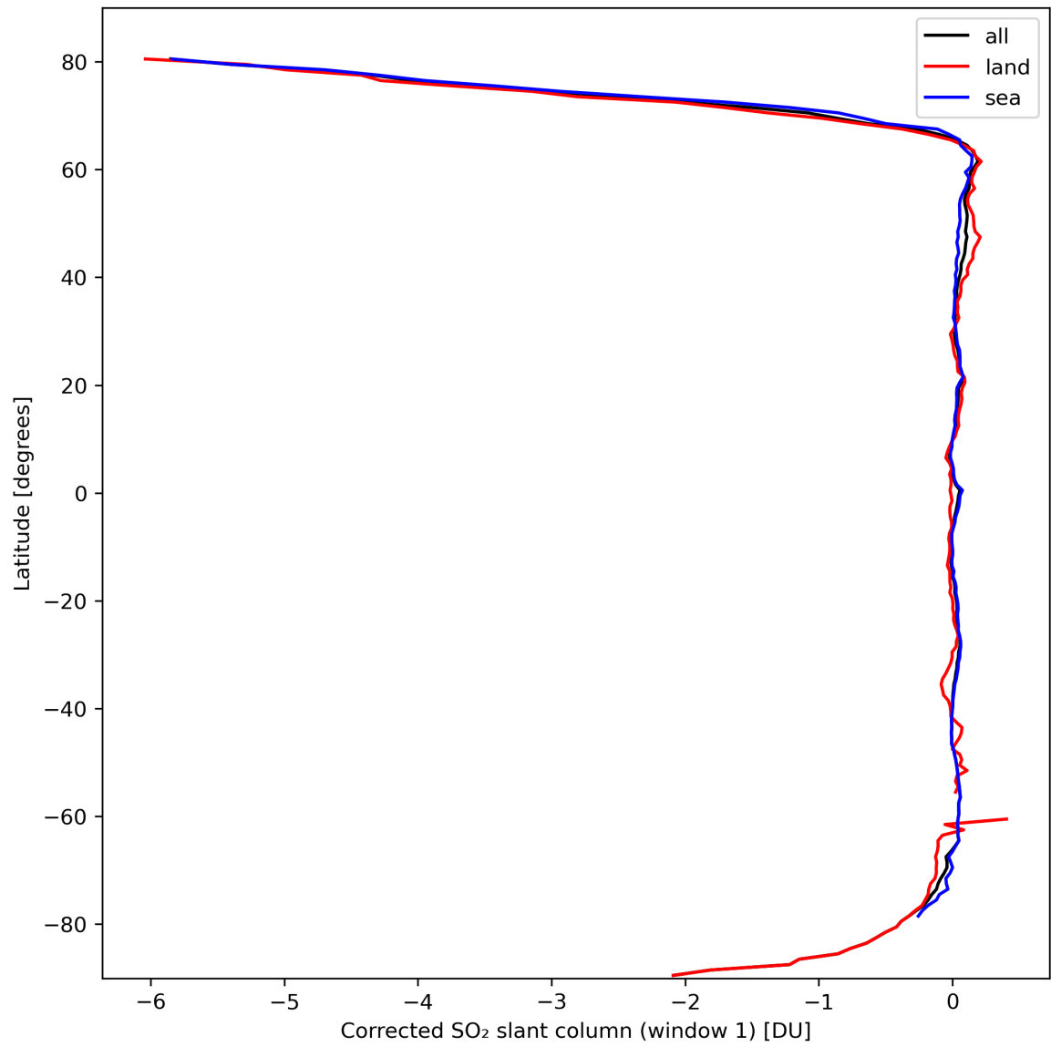
Figure 35: Zonal average of “Corrected SO 2 slant column (window 1)” for 2024-03-07 to 2024-03-09.
