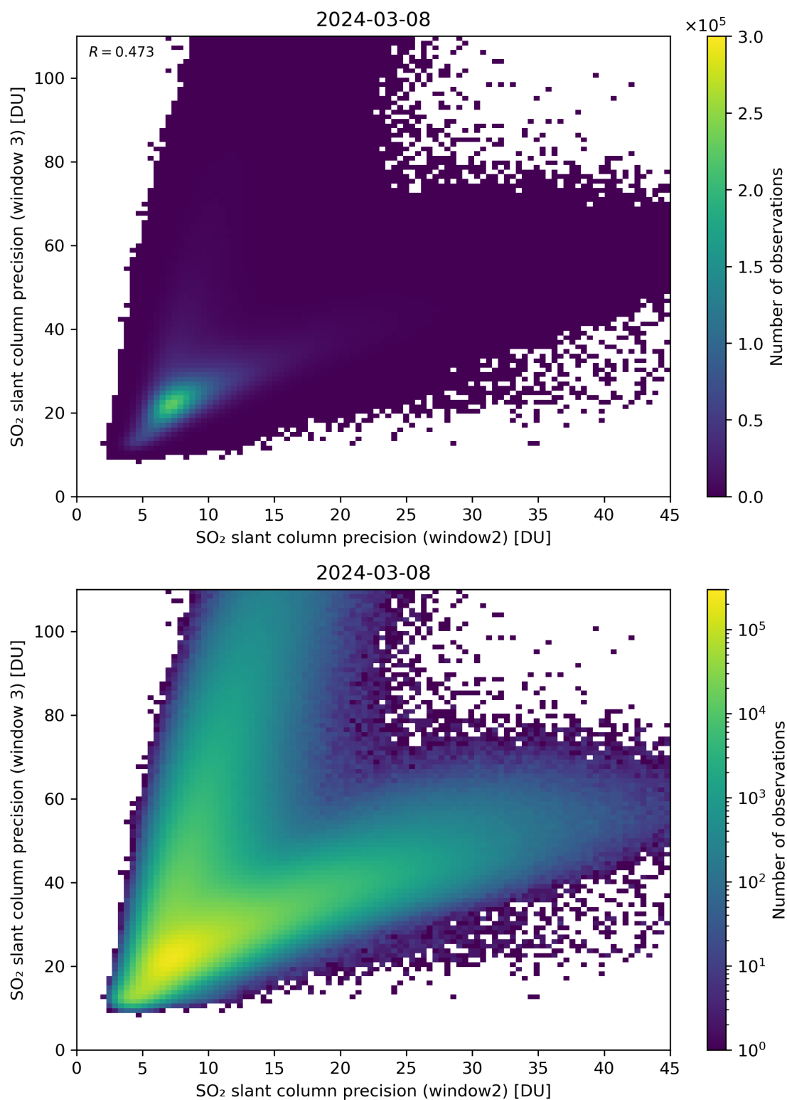
Figure 250: Scatter density plot of “SO 2 slant column precision (window2)” against “SO 2 slant column precision (window 3)” for 2024-03-07 to 2024-03-09.
