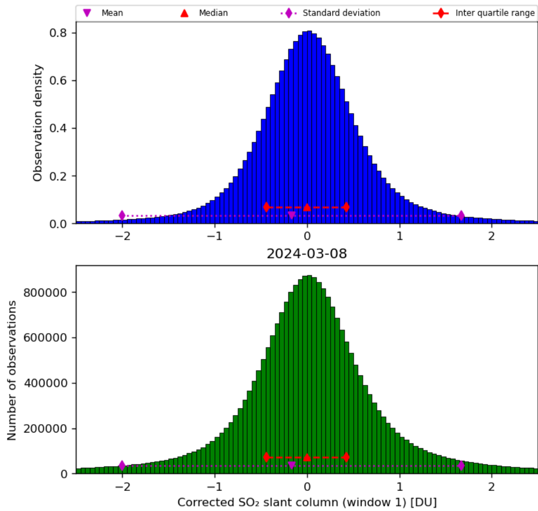
Figure 58: Histogram of “Corrected SO 2 slant column (window 1)” for 2024-03-07 to 2024-03-09
