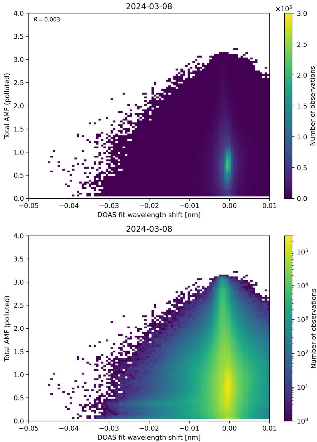
Figure 130: Scatter density plot of “DOAS fit wavelength shift” against “Total AMF (polluted)” for 2024-03-07 to 2024-03-09.
