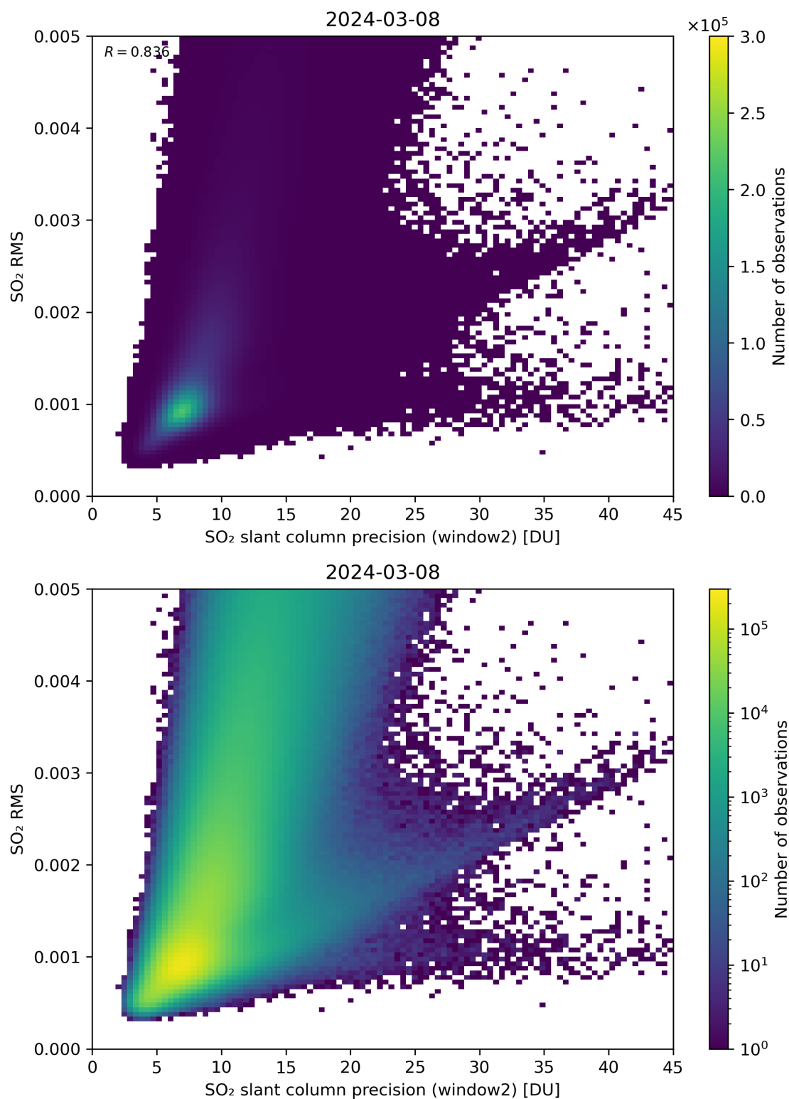
Figure 245: Scatter density plot of “SO 2 slant column precision (window2)” against “SO 2 RMS” for 2024-03-07 to 2024-03-09.
