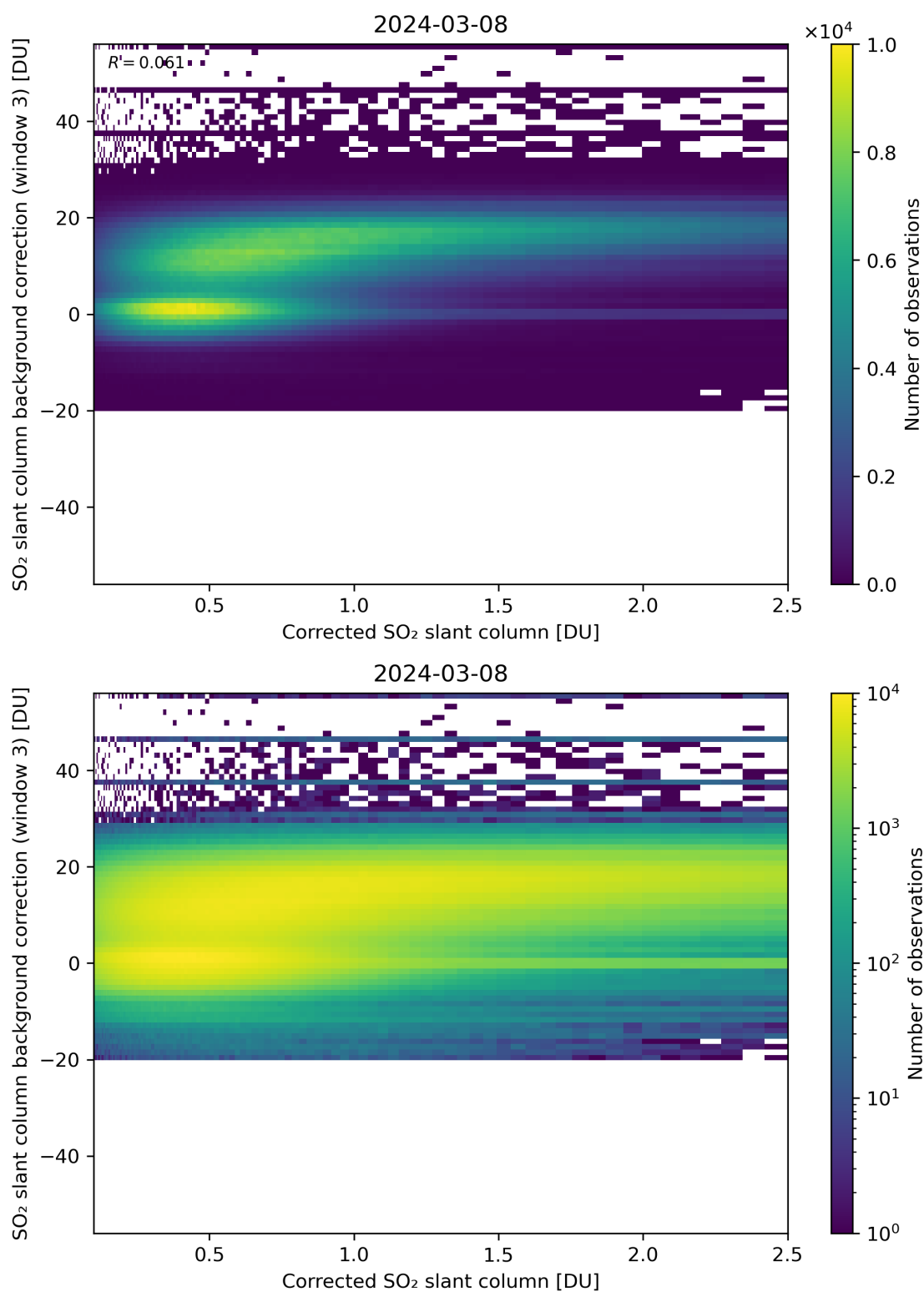
Figure 180: Scatter density plot of “Corrected SO 2 slant column” against “SO 2 slant column background correction (window 3)” for 2024-03-07 to 2024-03-09.
