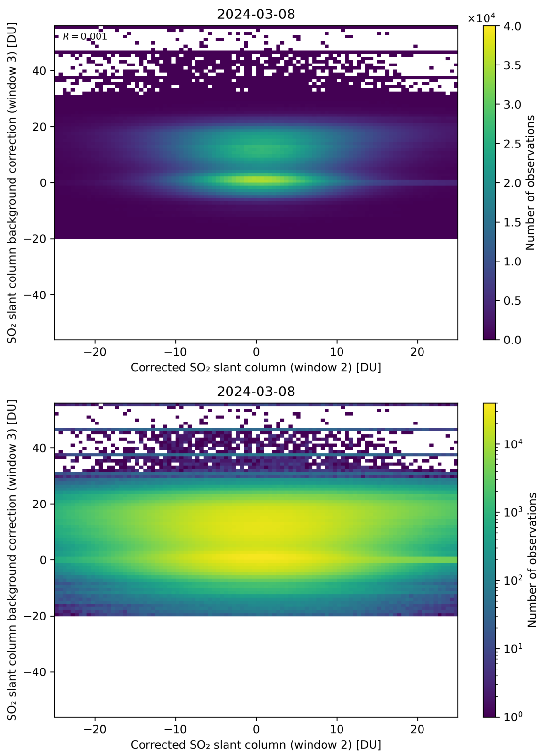
Figure 195: Scatter density plot of “Corrected SO 2 slant column (window 2)” against “SO 2 slant column background correction (window 3)” for 2024-03-07 to 2024-03-09.
