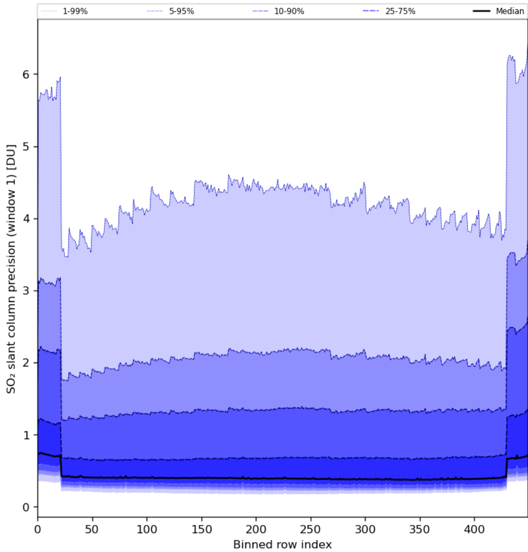
Figure 80: Along track statistics of “SO 2 slant column precision (window 1)” for 2024-03-07 to 2024-03-09
