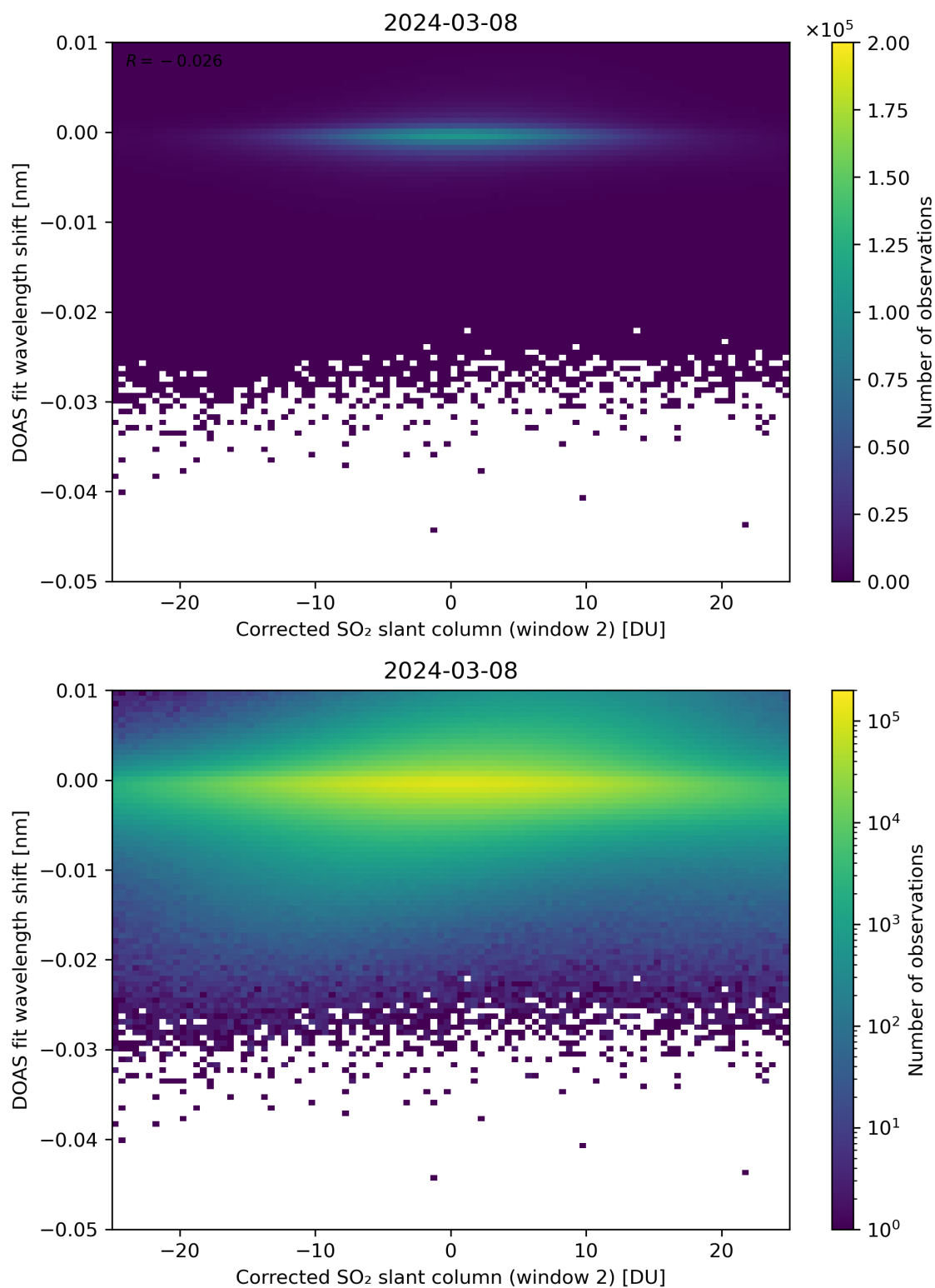
Figure 196: Scatter density plot of “Corrected SO 2 slant column (window 2)” against “DOAS fit wavelength shift” for 2024-03-07 to 2024-03-09.
