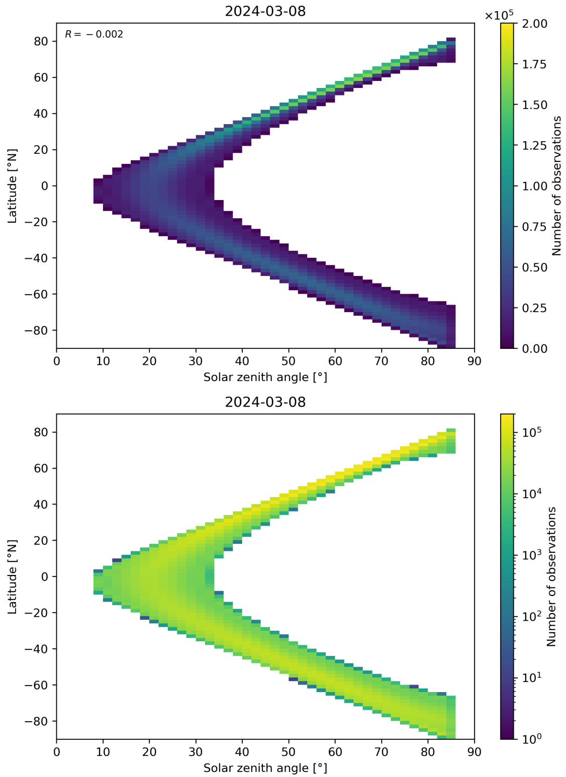
Figure 164: Scatter density plot of “Solar zenith angle” against “Latitude” for 2024-03-07 to 2024-03-09.
