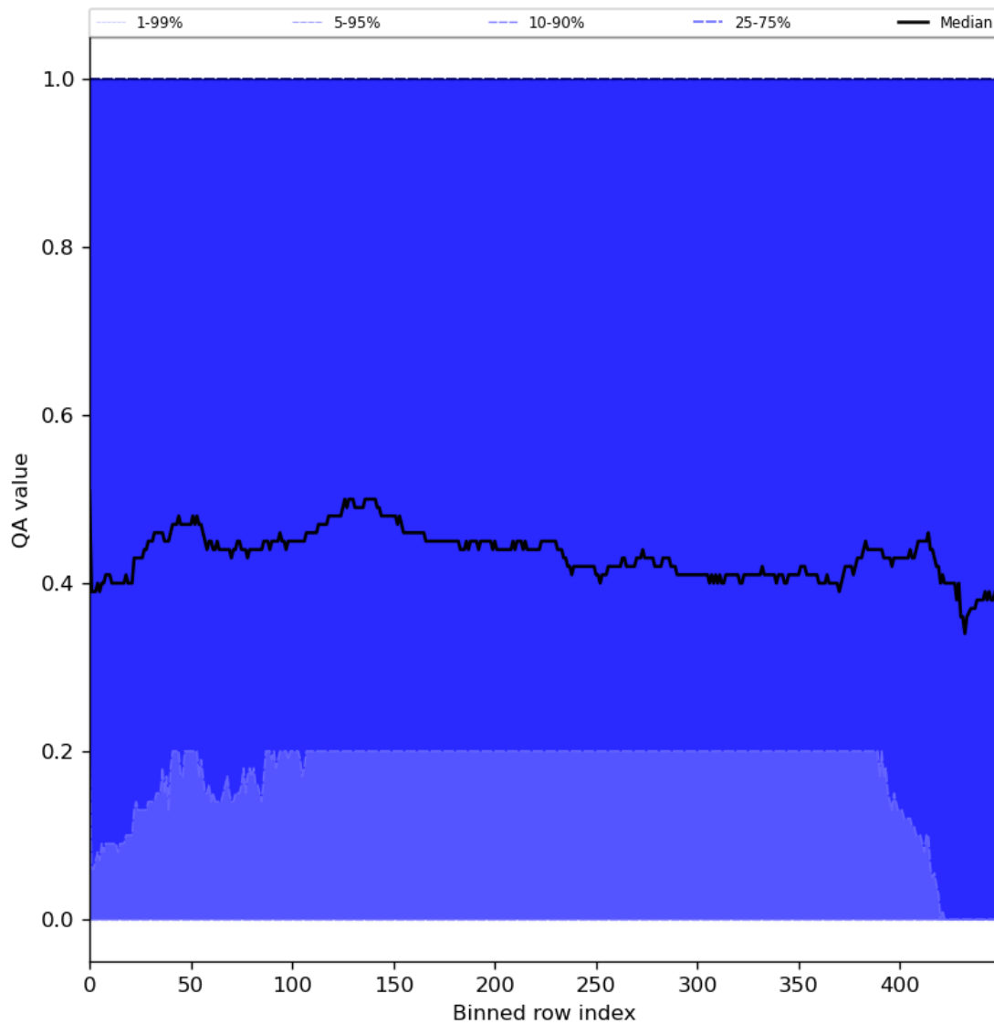
Figure 75: Along track statistics of “QA value” for 2024-03-07 to 2024-03-09
