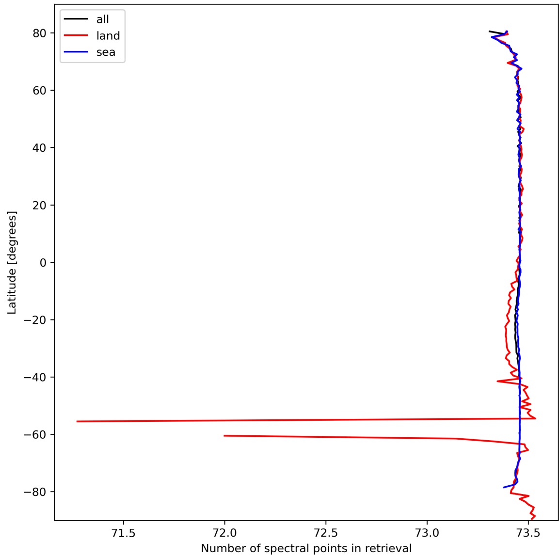
Figure 51: Zonal average of “Number of spectral points in retrieval” for 2024-03-07 to 2024-03-09.
