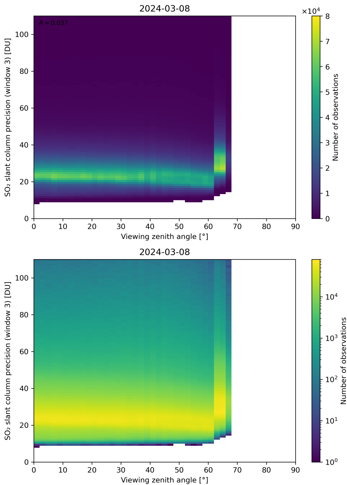
Figure 324: Scatter density plot of “Viewing zenith angle” against “SO 2 slant column precision (window 3)” for 2024-03-07 to 2024-03-09.
