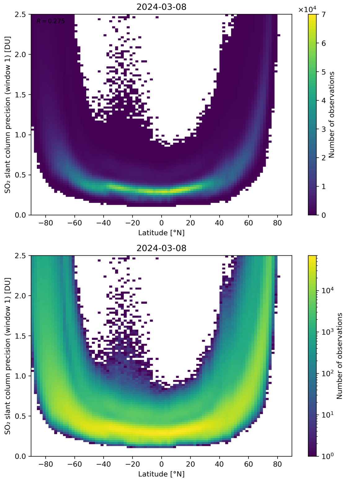
Figure 150: Scatter density plot of “Latitude” against “SO 2 slant column precision (window 1)” for 2024-03-07 to 2024-03-09.
