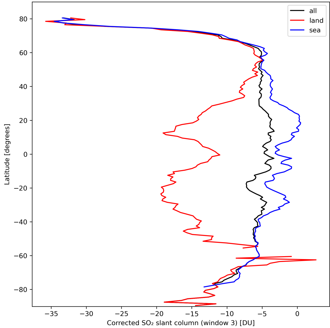
Figure 43: Zonal average of “Corrected SO 2 slant column (window 3)” for 2024-03-07 to 2024-03-09.
