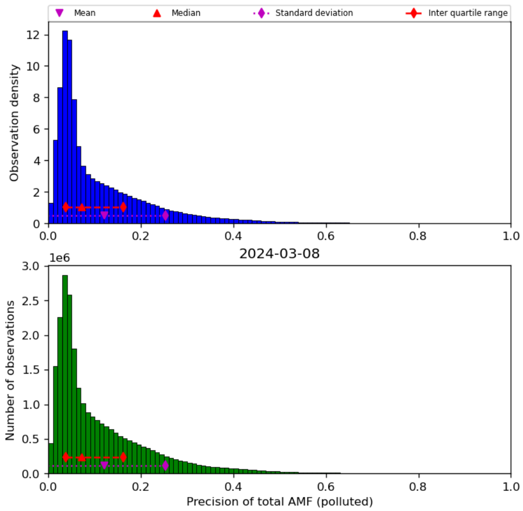
Figure 72: Histogram of “Precision of total AMF (polluted)” for 2024-03-07 to 2024-03-09
