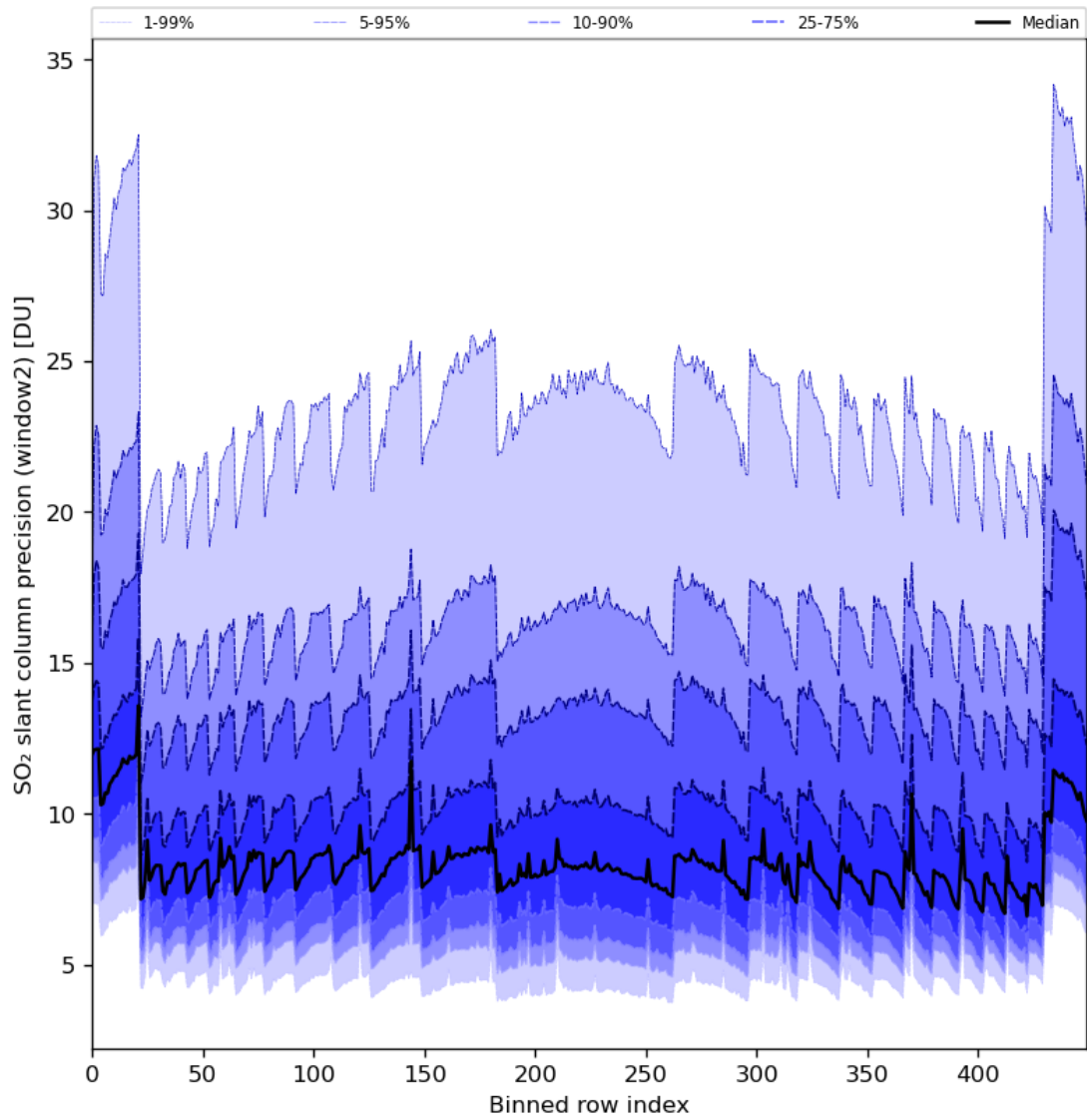
Figure 84: Along track statistics of “SO 2 slant column precision (window2)” for 2024-03-07 to 2024-03-09
