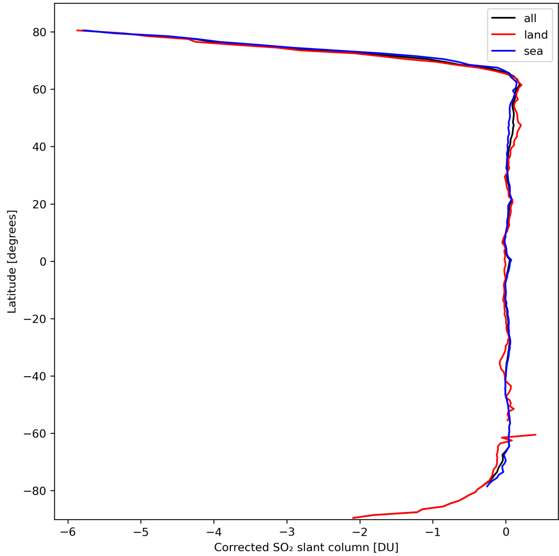
Figure 32: Zonal average of “Corrected SO 2 slant column” for 2024-03-07 to 2024-03-09.
