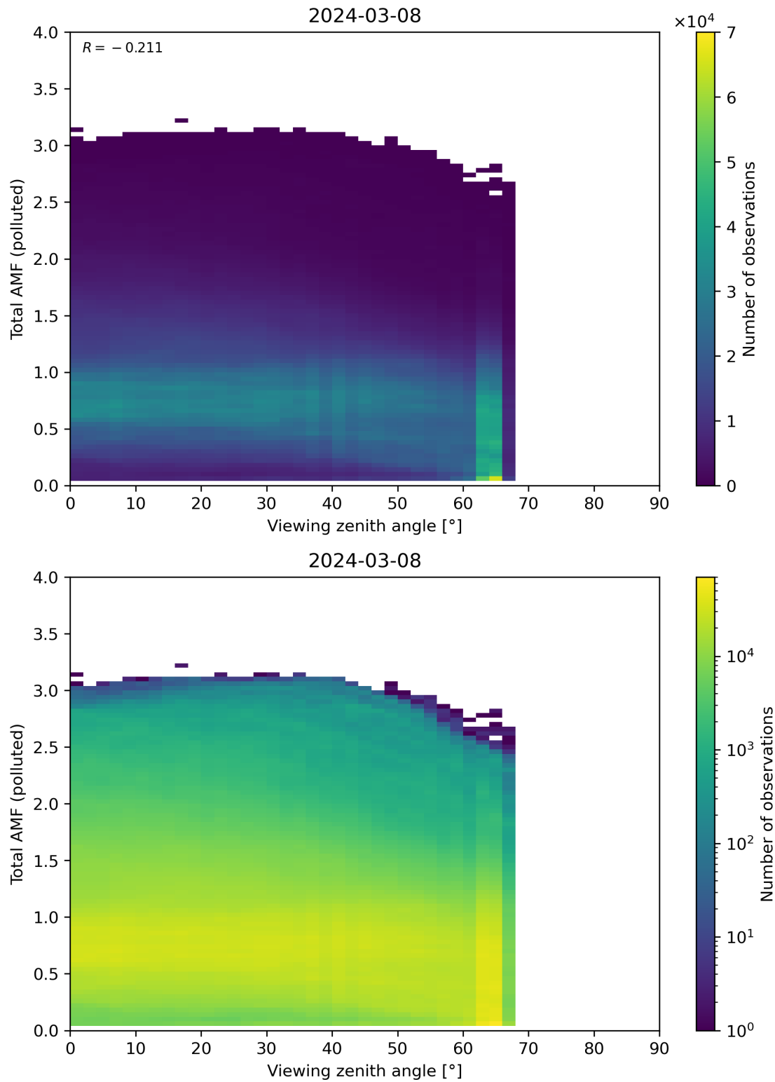
Figure 325: Scatter density plot of “Viewing zenith angle” against “Total AMF (polluted)” for 2024-03-07 to 2024-03-09.
