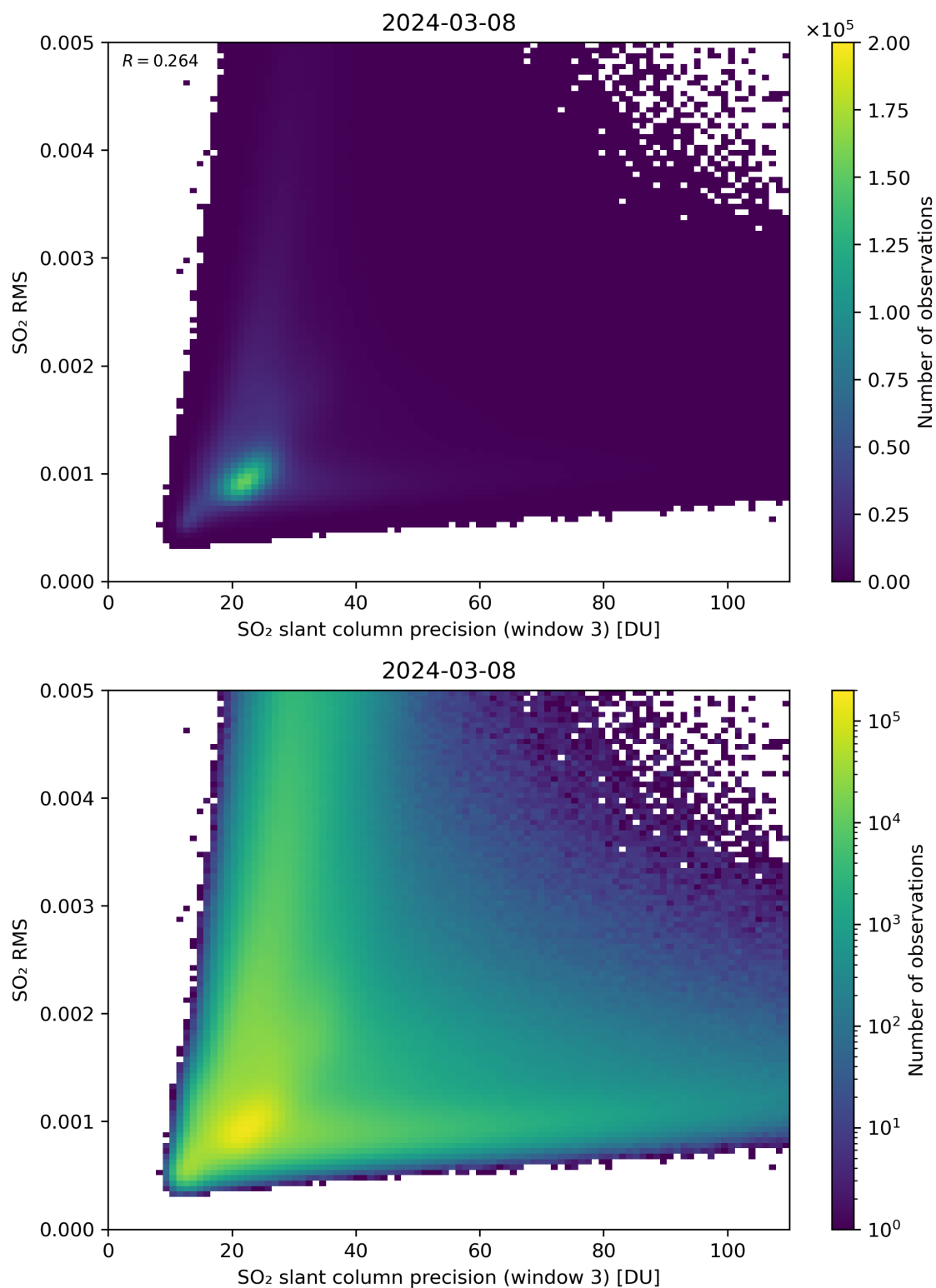
Figure 260: Scatter density plot of “SO 2 slant column precision (window 3)” against “SO 2 RMS” for 2024-03-07 to 2024-03-09.
