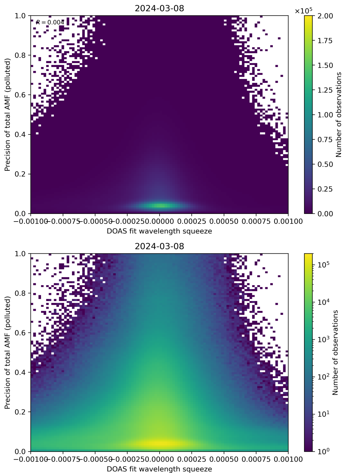
Figure 135: Scatter density plot of “DOAS fit wavelength squeeze” against “Precision of total AMF (polluted)” for 2024-03-07 to 2024-03-09.
