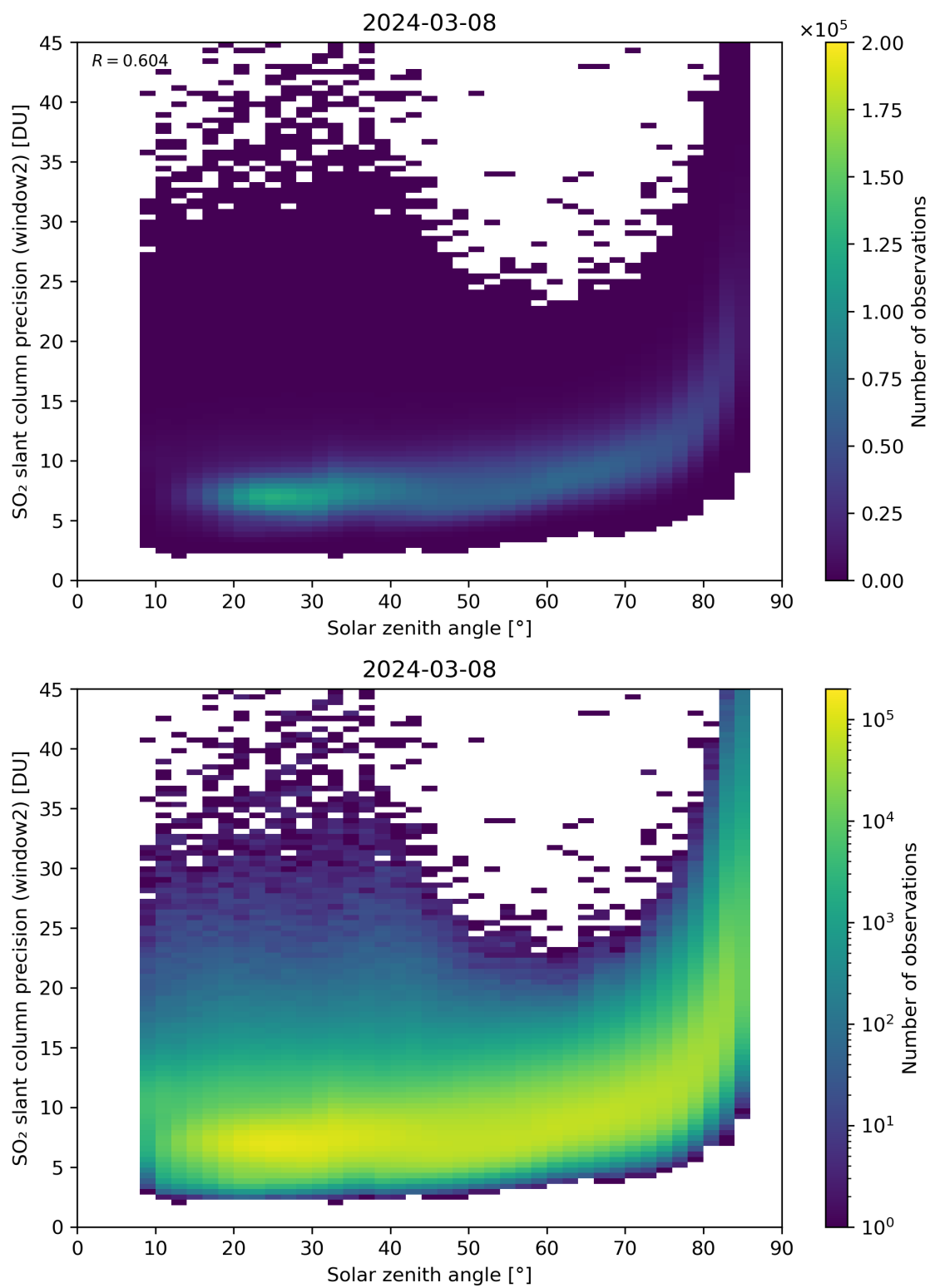
Figure 171: Scatter density plot of “Solar zenith angle” against “SO 2 slant column precision (window2)” for 2024-03-07 to 2024-03-09.
