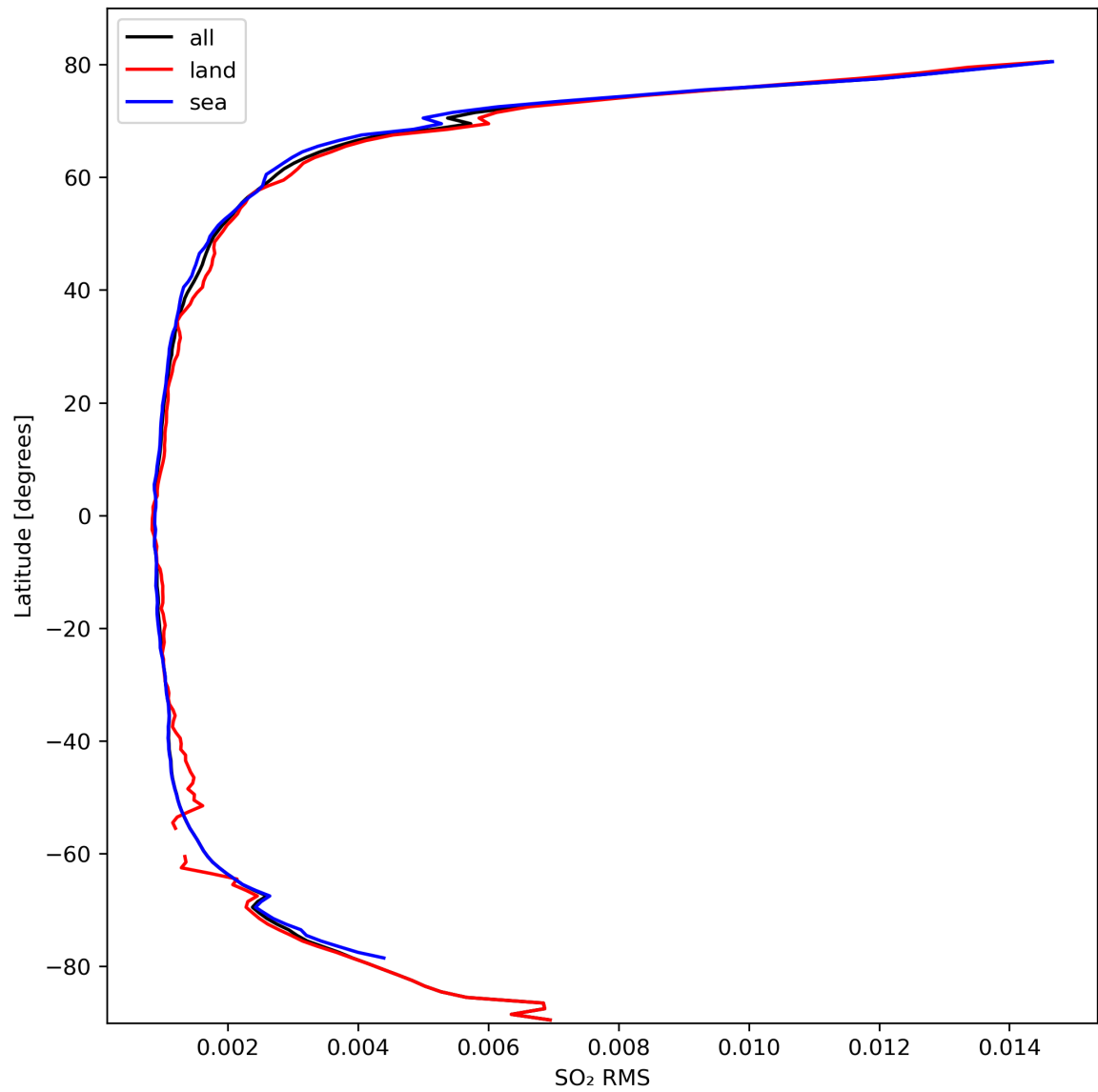
Figure 47: Zonal average of “SO 2 RMS” for 2024-03-07 to 2024-03-09.
