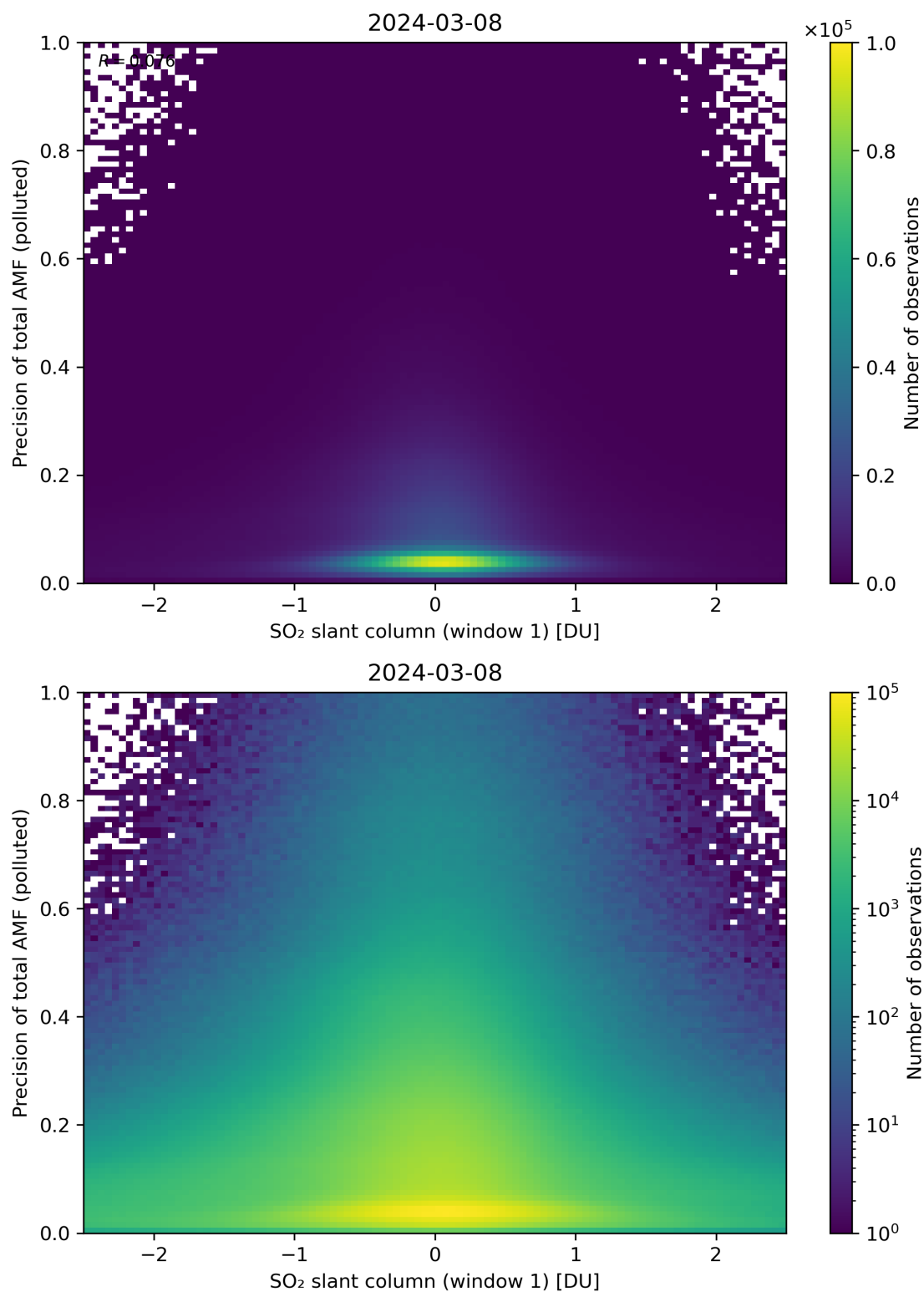
Figure 240: Scatter density plot of “SO 2 slant column (window 1)” against “Precision of total AMF (polluted)” for 2024-03-07 to 2024-03-09.
