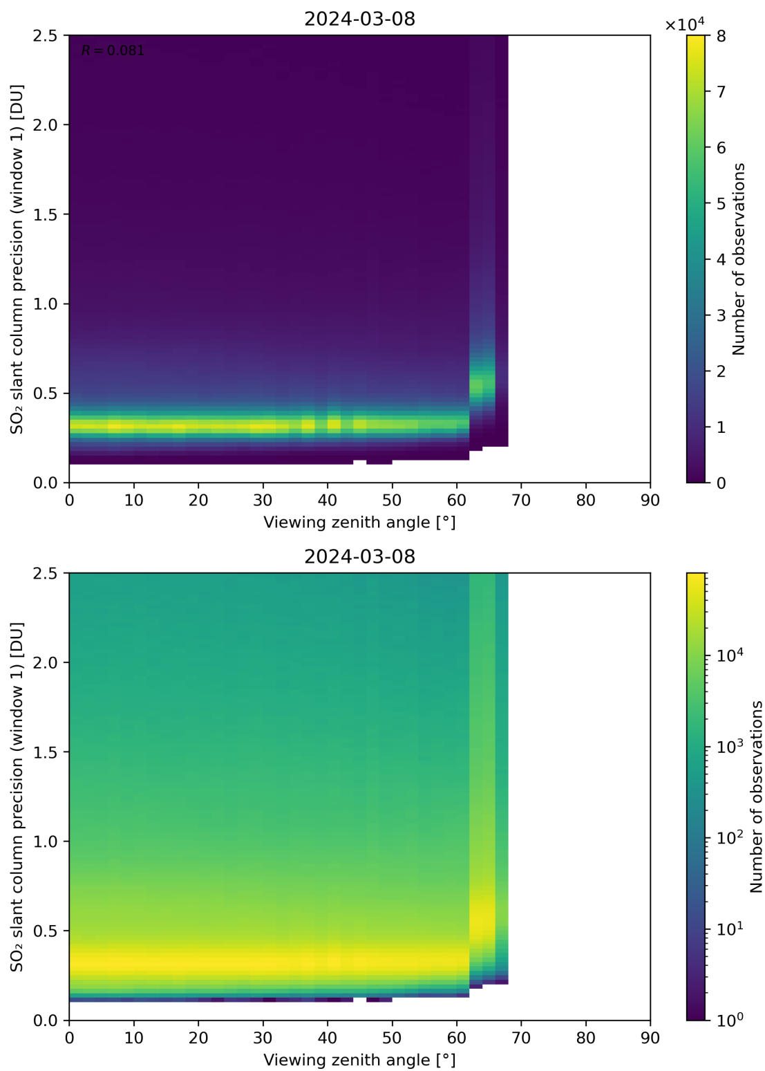
Figure 321: Scatter density plot of “Viewing zenith angle” against “SO 2 slant column precision (window 1)” for 2024-03-07 to 2024-03-09.
