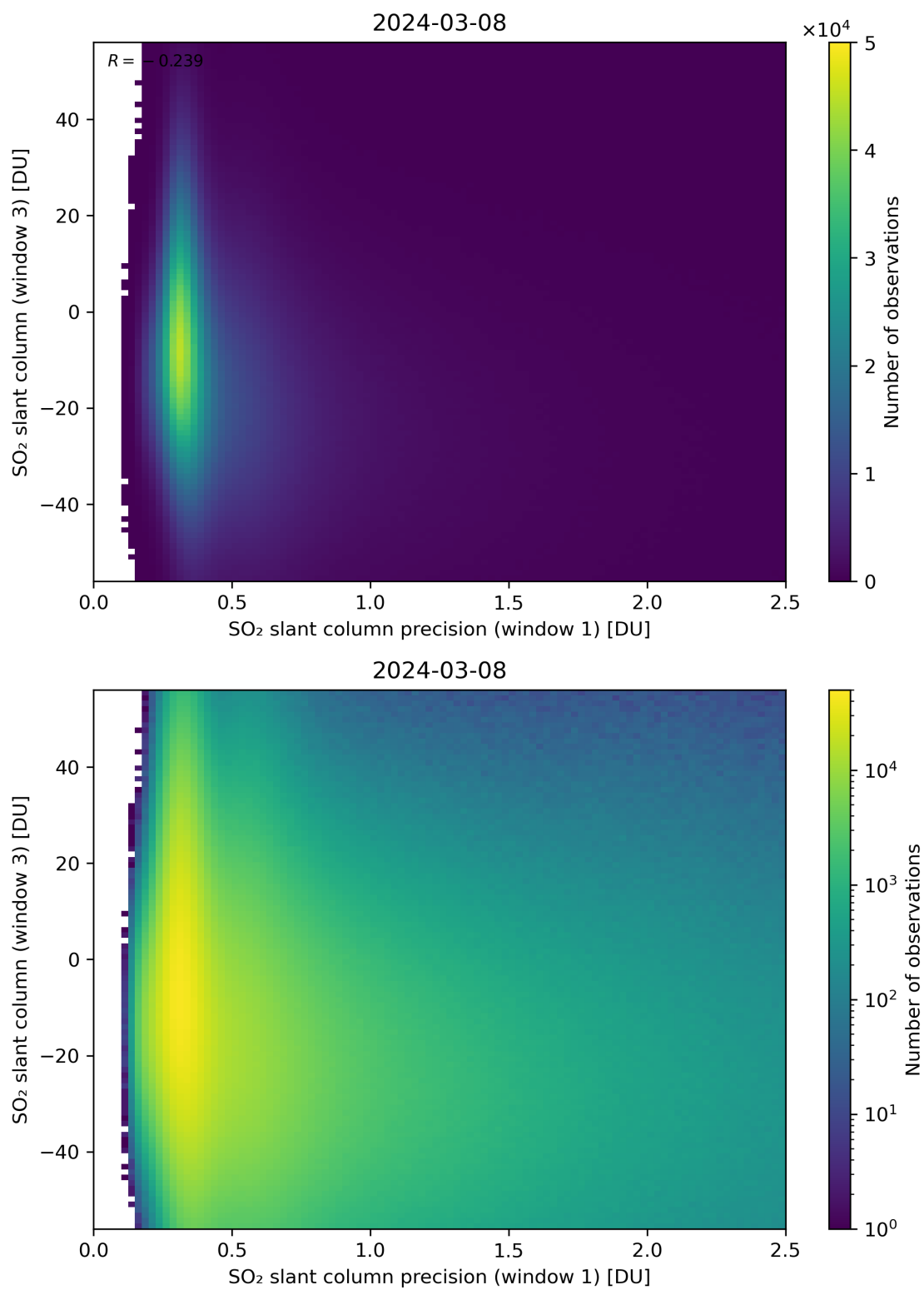
Figure 228: Scatter density plot of “SO 2 slant column precision (window 1)” against “SO 2 slant column (window 3)” for 2024-03-07 to 2024-03-09.
