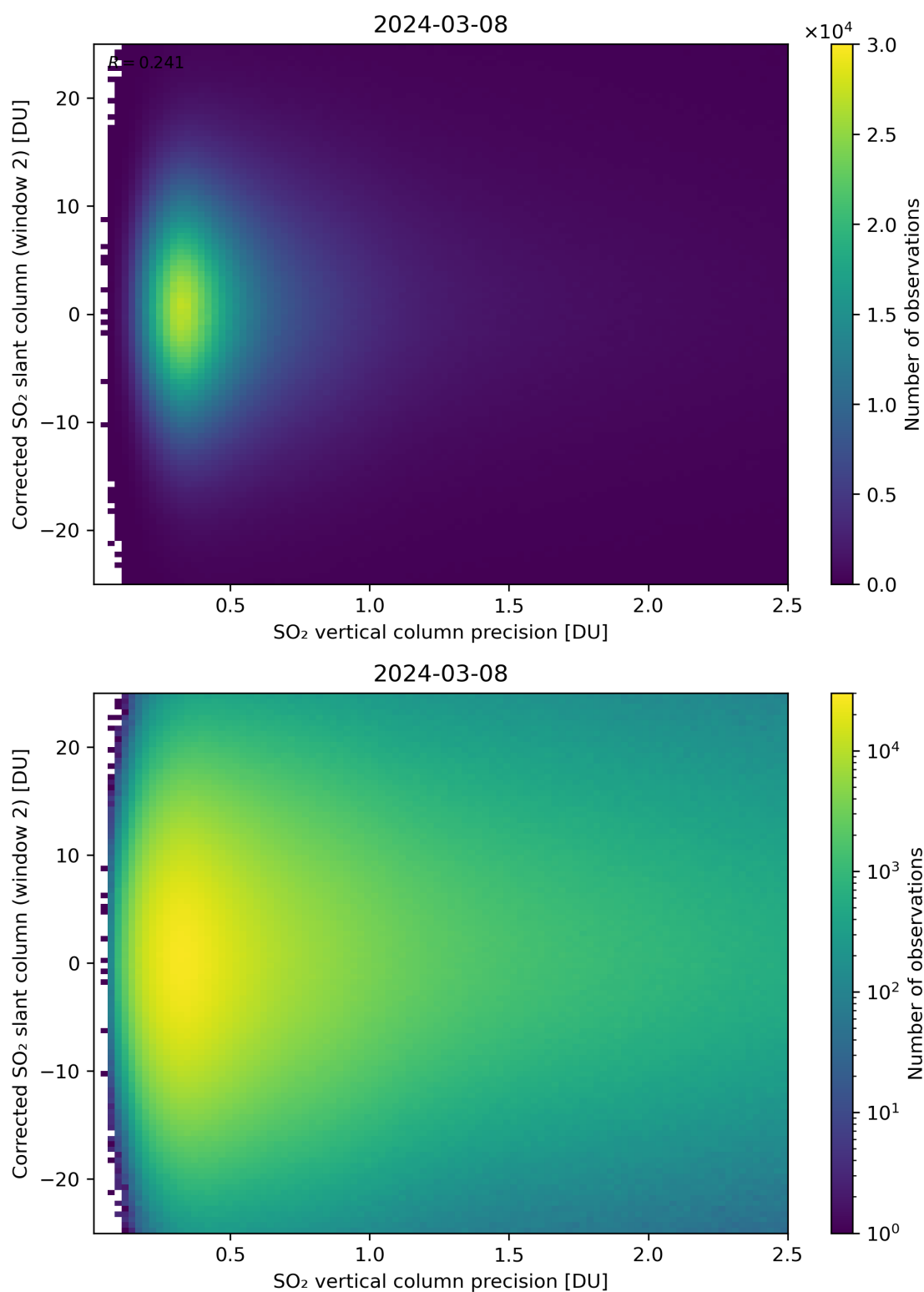
Figure 287: Scatter density plot of “SO 2 vertical column precision” against “Corrected SO 2 slant column (window 2)” for 2024-03-07 to 2024-03-09.
