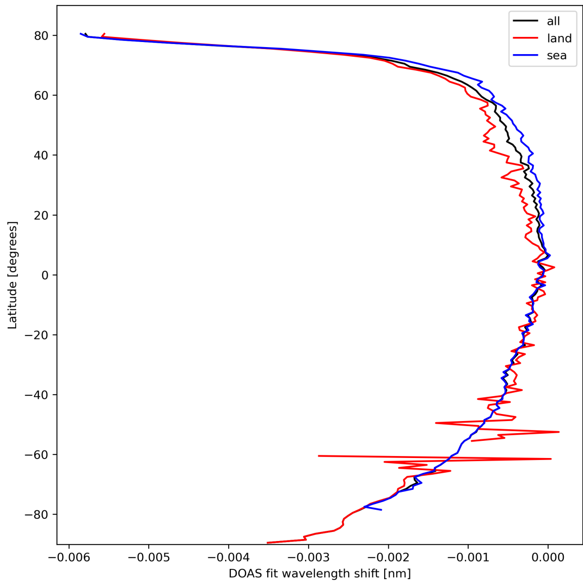
Figure 45: Zonal average of “DOAS fit wavelength shift” for 2024-03-07 to 2024-03-09.
