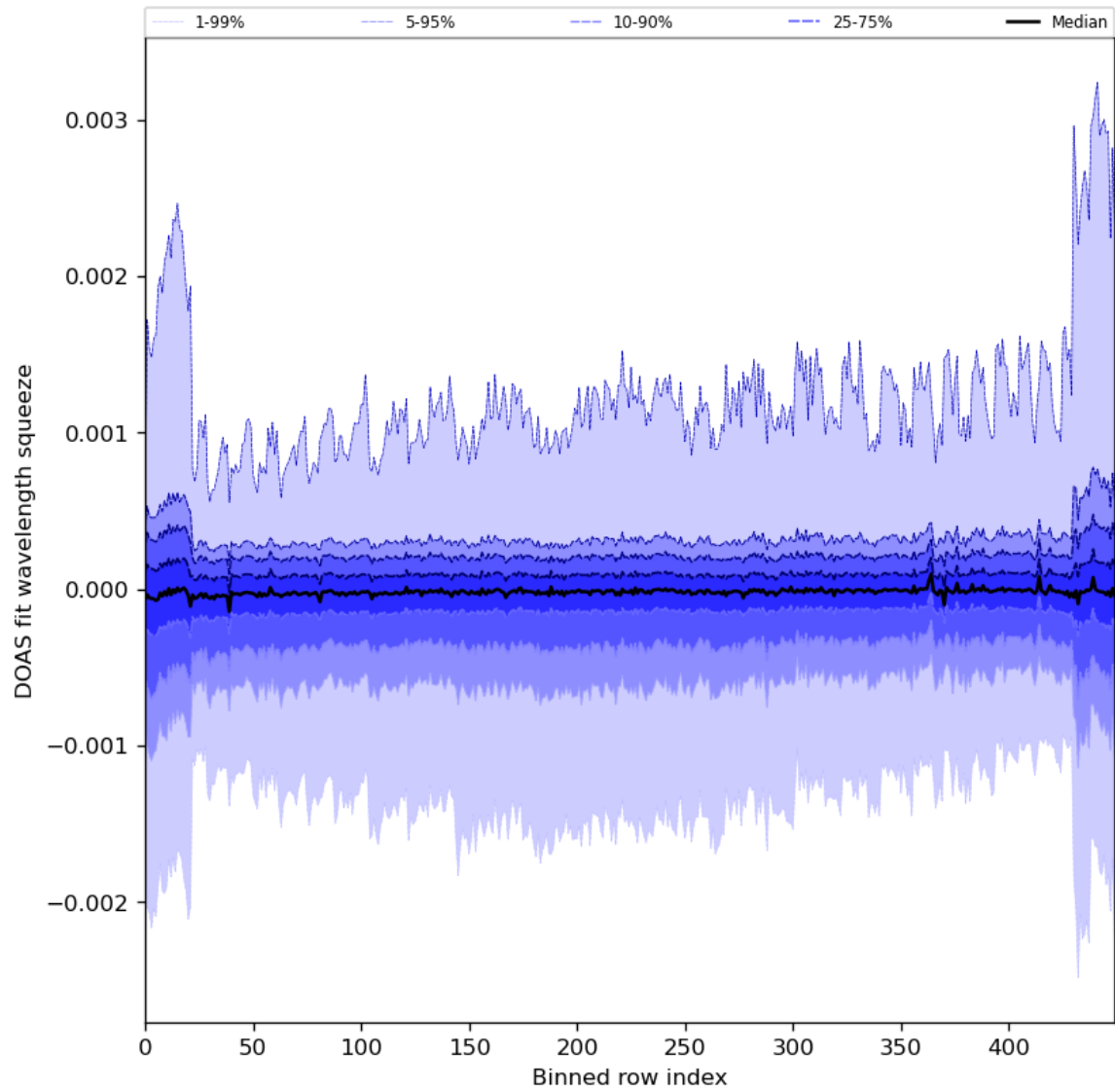
Figure 92: Along track statistics of “DOAS fit wavelength squeeze” for 2024-03-07 to 2024-03-09
