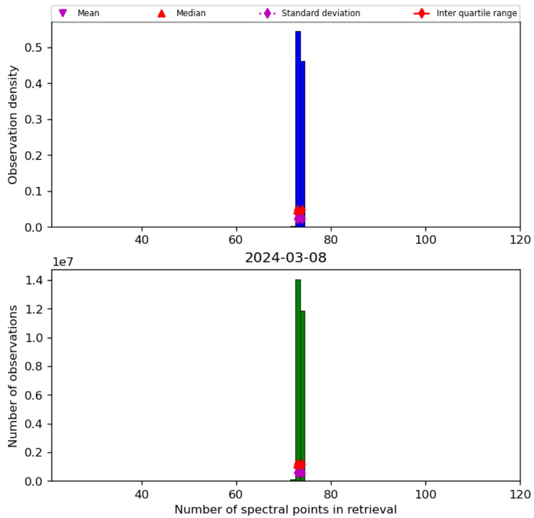
Figure 74: Histogram of “Number of spectral points in retrieval” for 2024-03-07 to 2024-03-09
