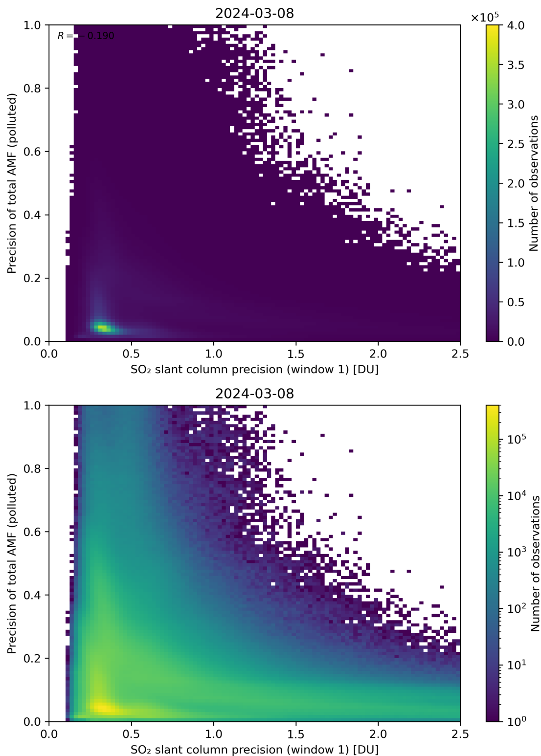
Figure 231: Scatter density plot of “SO 2 slant column precision (window 1)” against “Precision of total AMF (polluted)” for 2024-03-07 to 2024-03-09.
