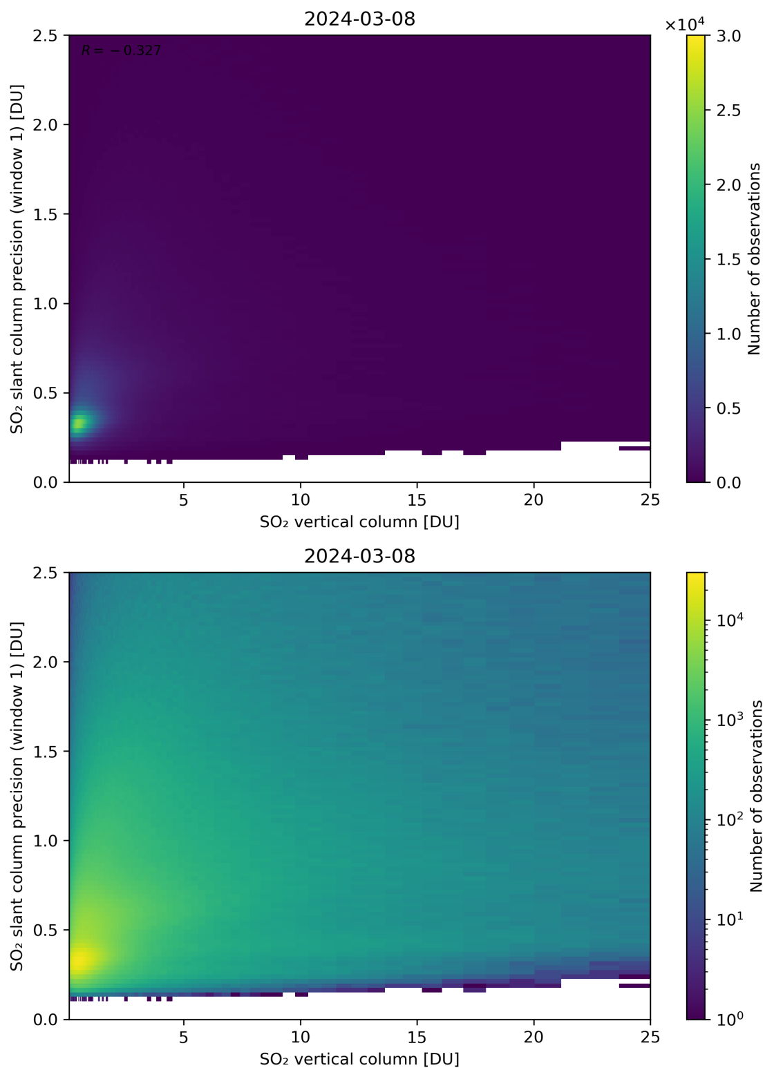
Figure 301: Scatter density plot of “SO 2 vertical column” against “SO 2 slant column precision (window 1)” for 2024-03-07 to 2024-03-09.
