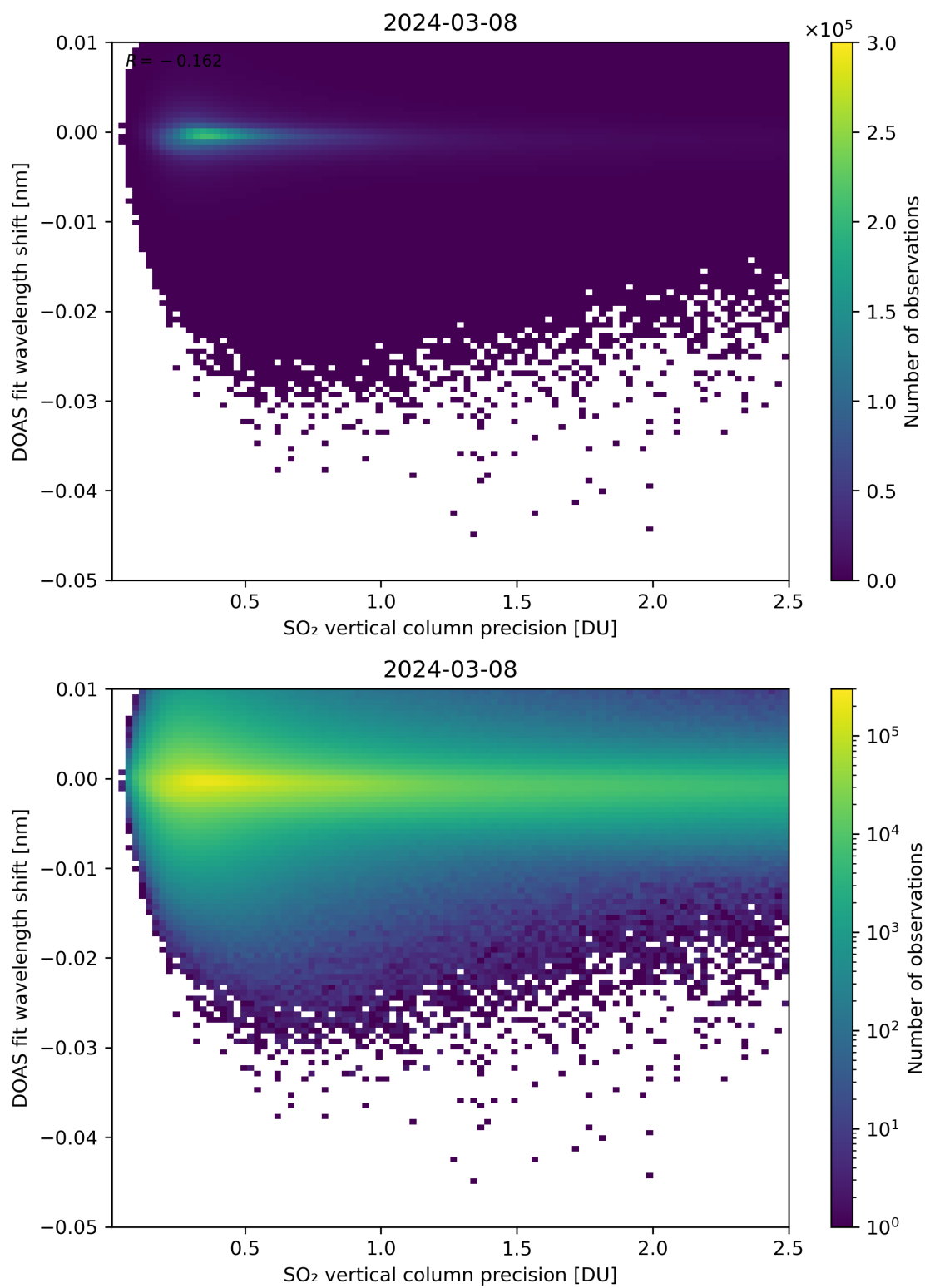
Figure 282: Scatter density plot of “SO 2 vertical column precision” against “DOAS fit wavelength shift” for 2024-03-07 to 2024-03-09.
