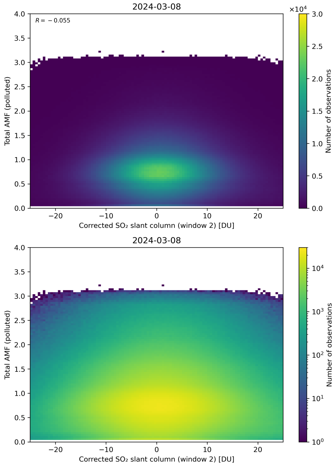
Figure 203: Scatter density plot of “Corrected SO 2 slant column (window 2)” against “Total AMF (polluted)” for 2024-03-07 to 2024-03-09.
