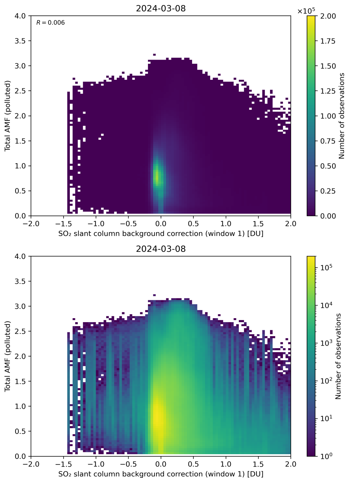
Figure 109: Scatter density plot of “SO 2 slant column background correction (window 1)” against “Total AMF (polluted)” for 2024-03-07 to 2024-03-09.
