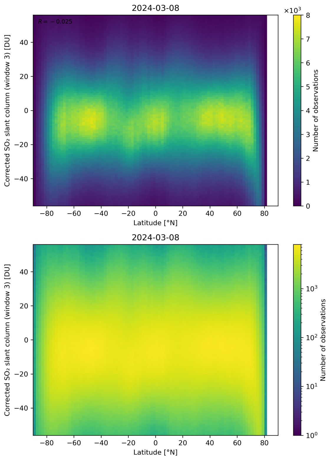
Figure 148: Scatter density plot of “Latitude” against “Corrected SO 2 slant column (window 3)” for 2024-03-07 to 2024-03-09.
