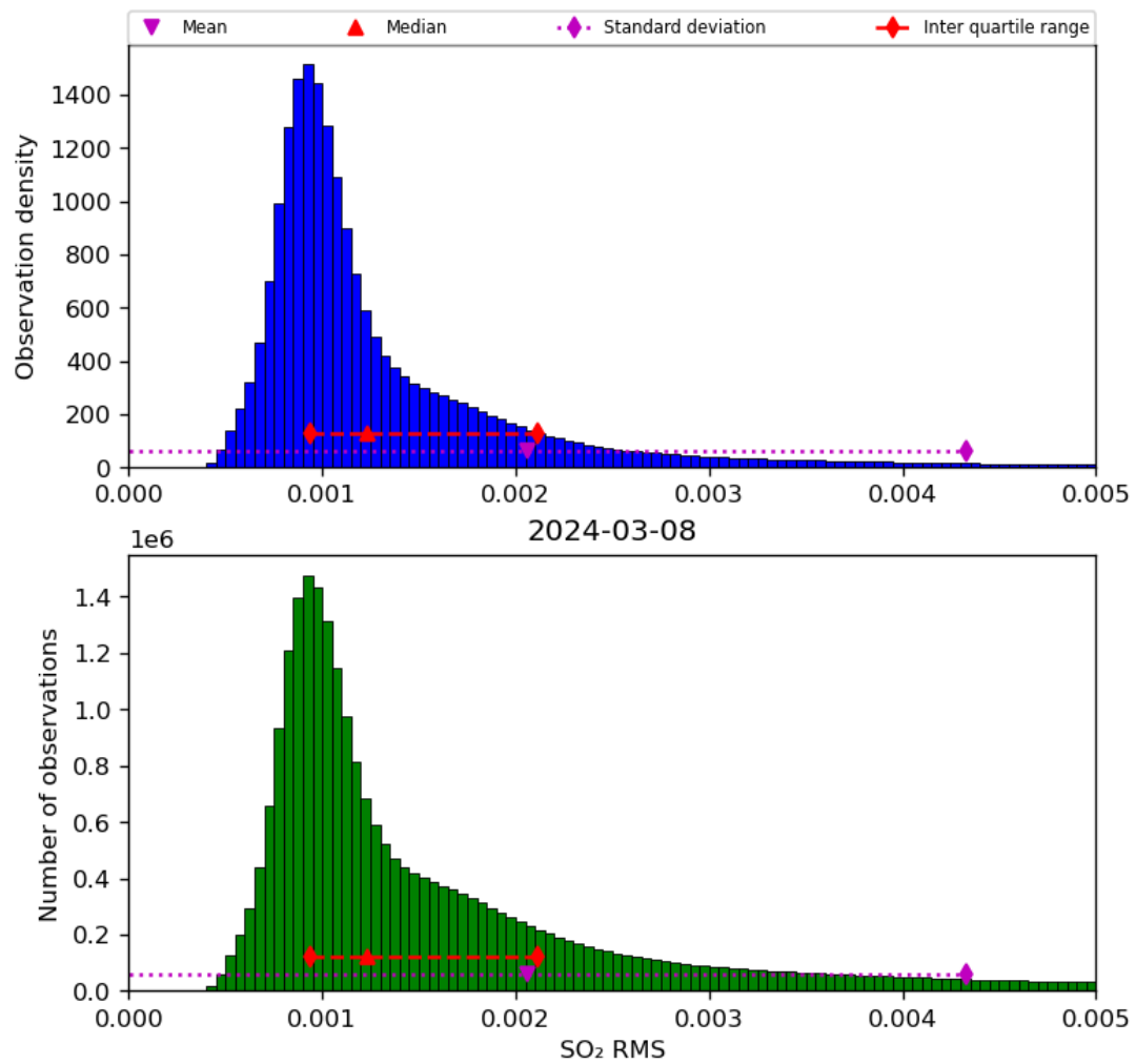
Figure 70: Histogram of “SO 2 RMS” for 2024-03-07 to 2024-03-09
