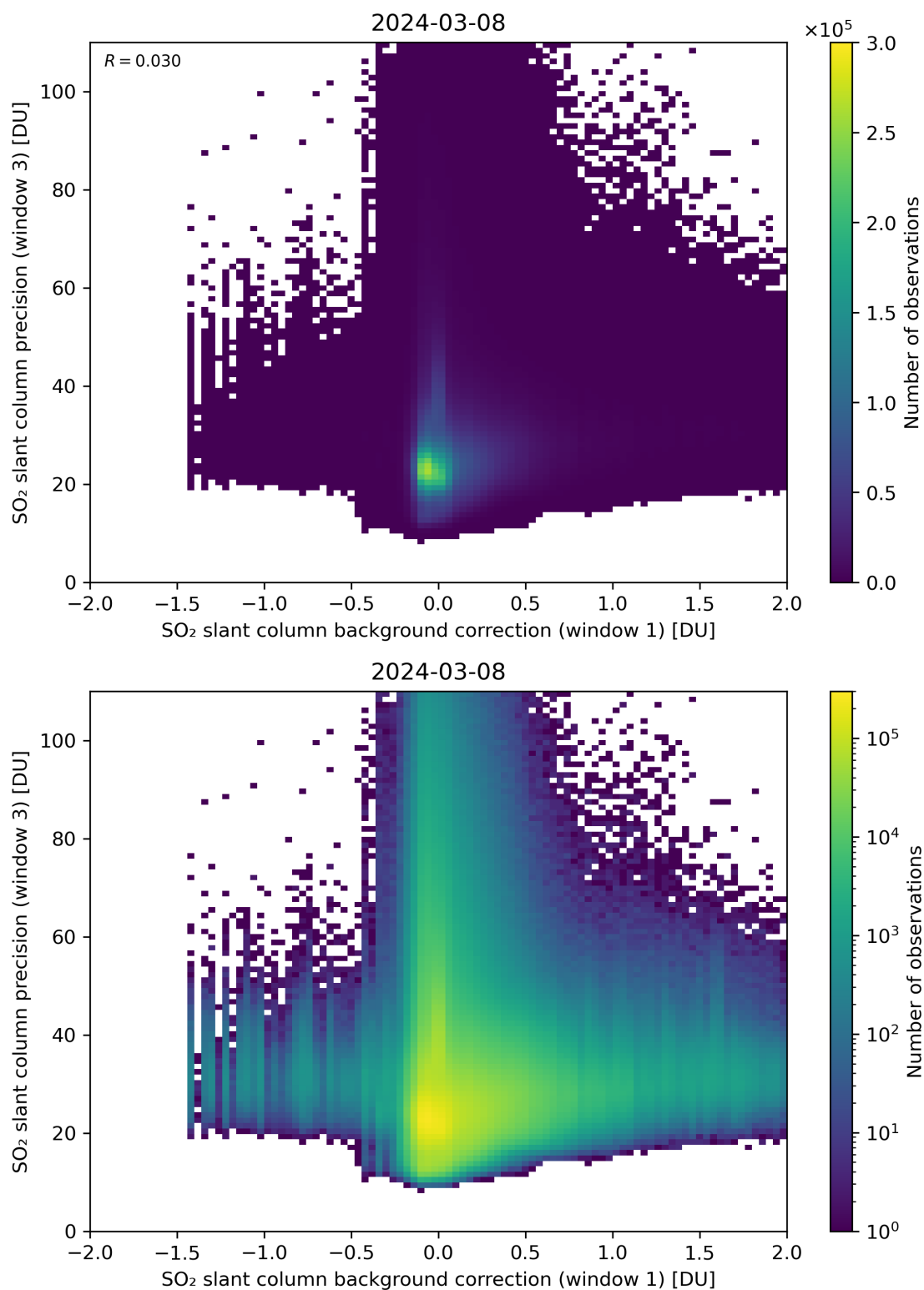
Figure 108: Scatter density plot of “SO 2 slant column background correction (window 1)” against “SO 2 slant column precision (window 3)” for 2024-03-07 to 2024-03-09.
