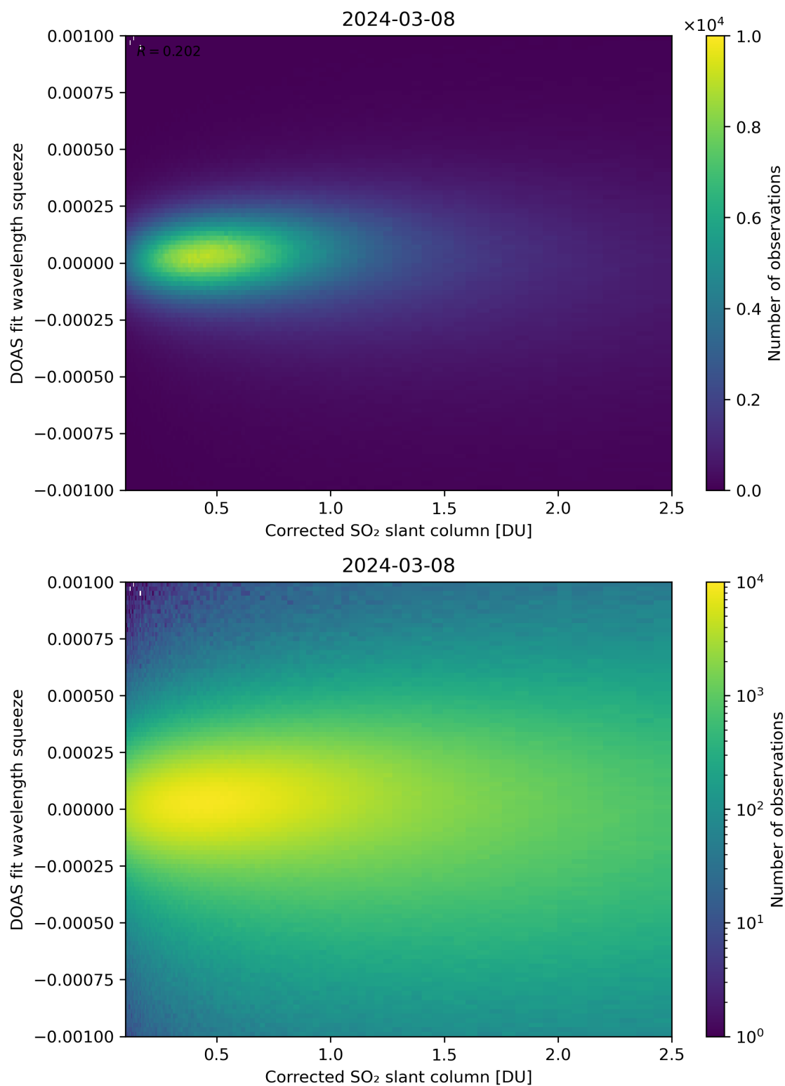
Figure 182: Scatter density plot of “Corrected SO 2 slant column” against “DOAS fit wavelength squeeze” for 2024-03-07 to 2024-03-09.
