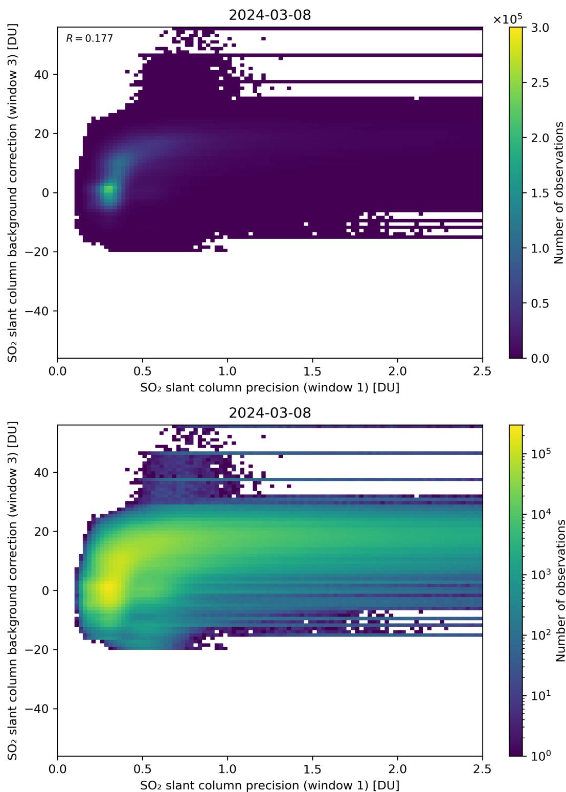
Figure 220: Scatter density plot of “SO 2 slant column precision (window 1)” against “SO 2 slant column background correction (window 3)” for 2024-03-07 to 2024-03-09.
