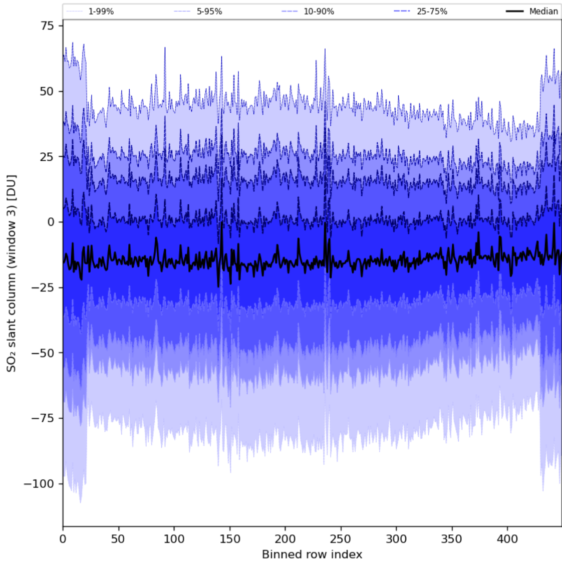
Figure 87: Along track statistics of “SO 2 slant column (window 3)” for 2024-03-07 to 2024-03-09
