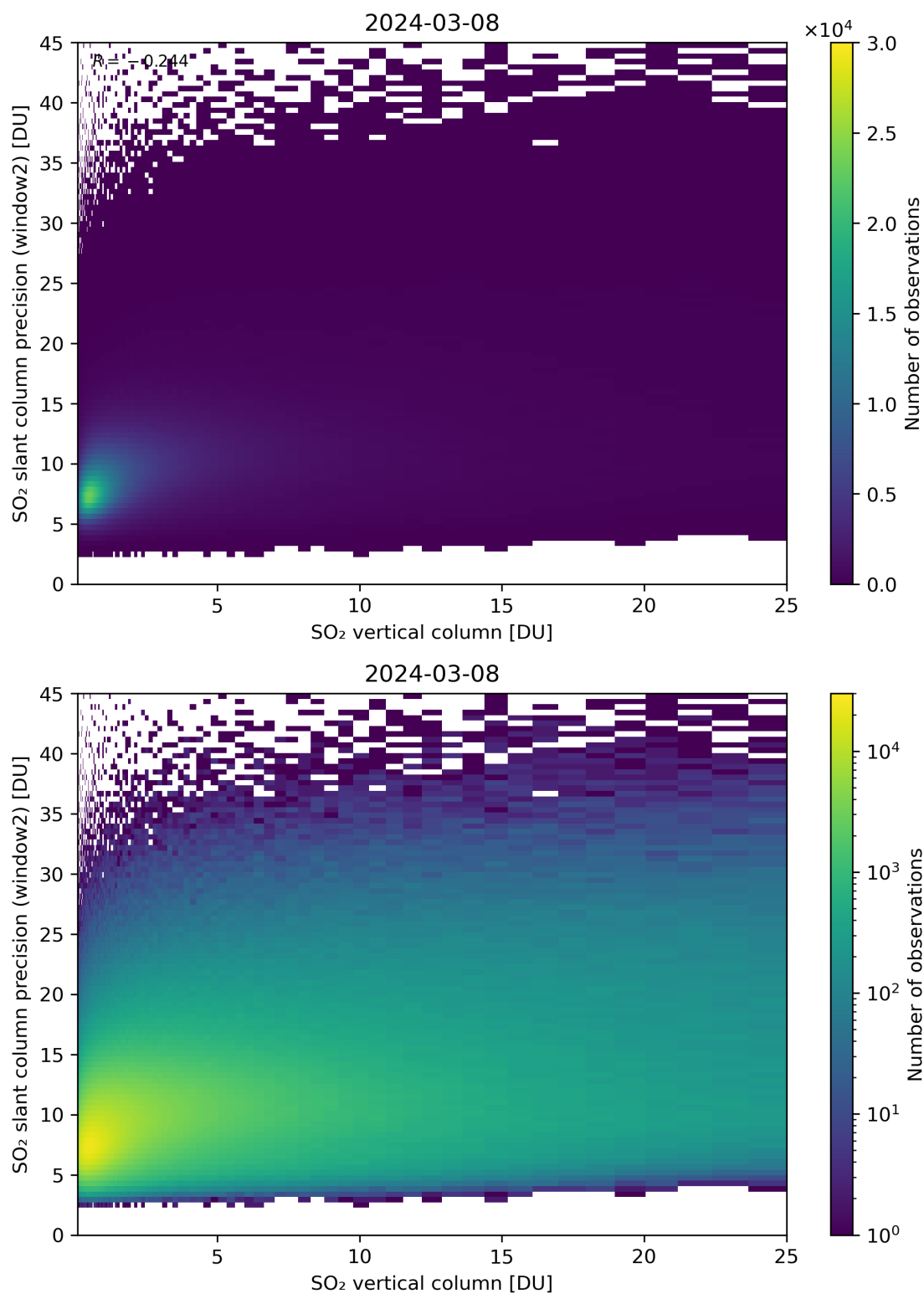
Figure 302: Scatter density plot of “SO 2 vertical column” against “SO 2 slant column precision (window2)” for 2024-03-07 to 2024-03-09.
