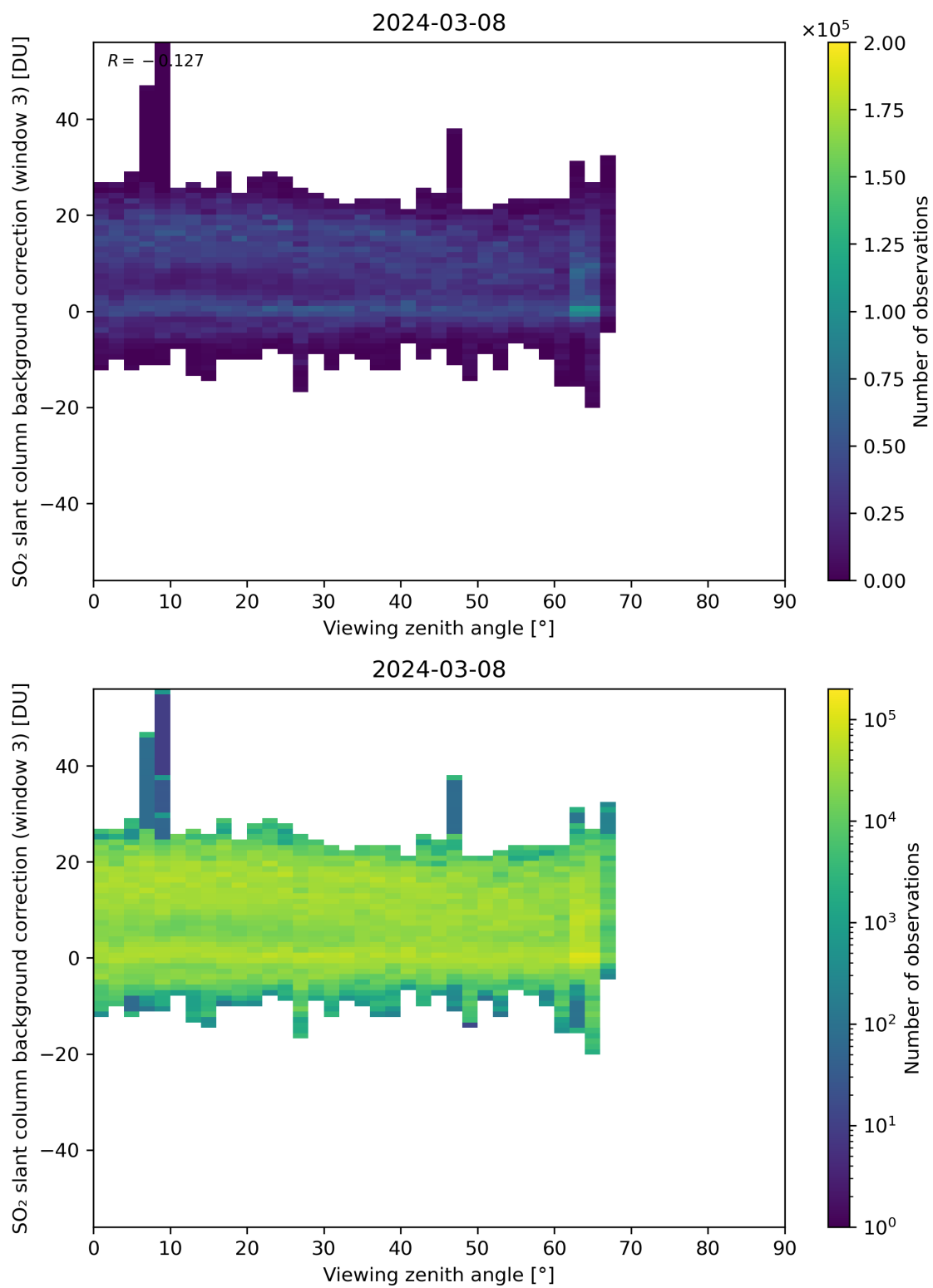
Figure 310: Scatter density plot of “Viewing zenith angle” against “SO 2 slant column background correction (window 3)” for 2024-03-07 to 2024-03-09.
