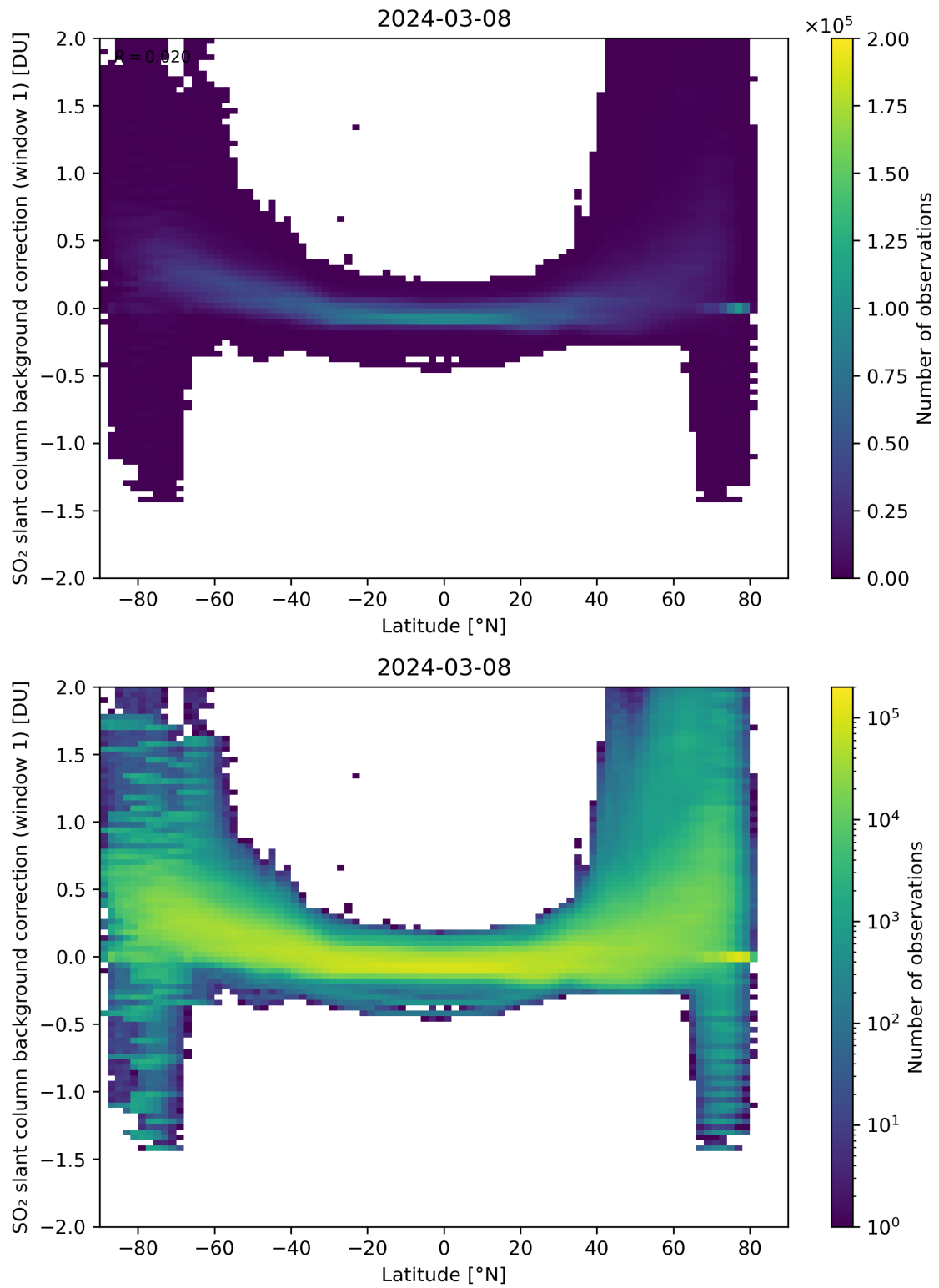
Figure 139: Scatter density plot of “Latitude” against “SO 2 slant column background correction (window 1)” for 2024-03-07 to 2024-03-09.
