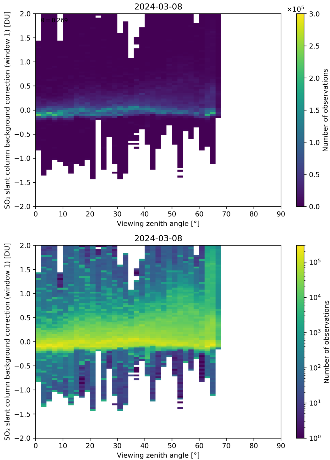
Figure 308: Scatter density plot of “Viewing zenith angle” against “SO 2 slant column background correction (window 1)” for 2024-03-07 to 2024-03-09.
