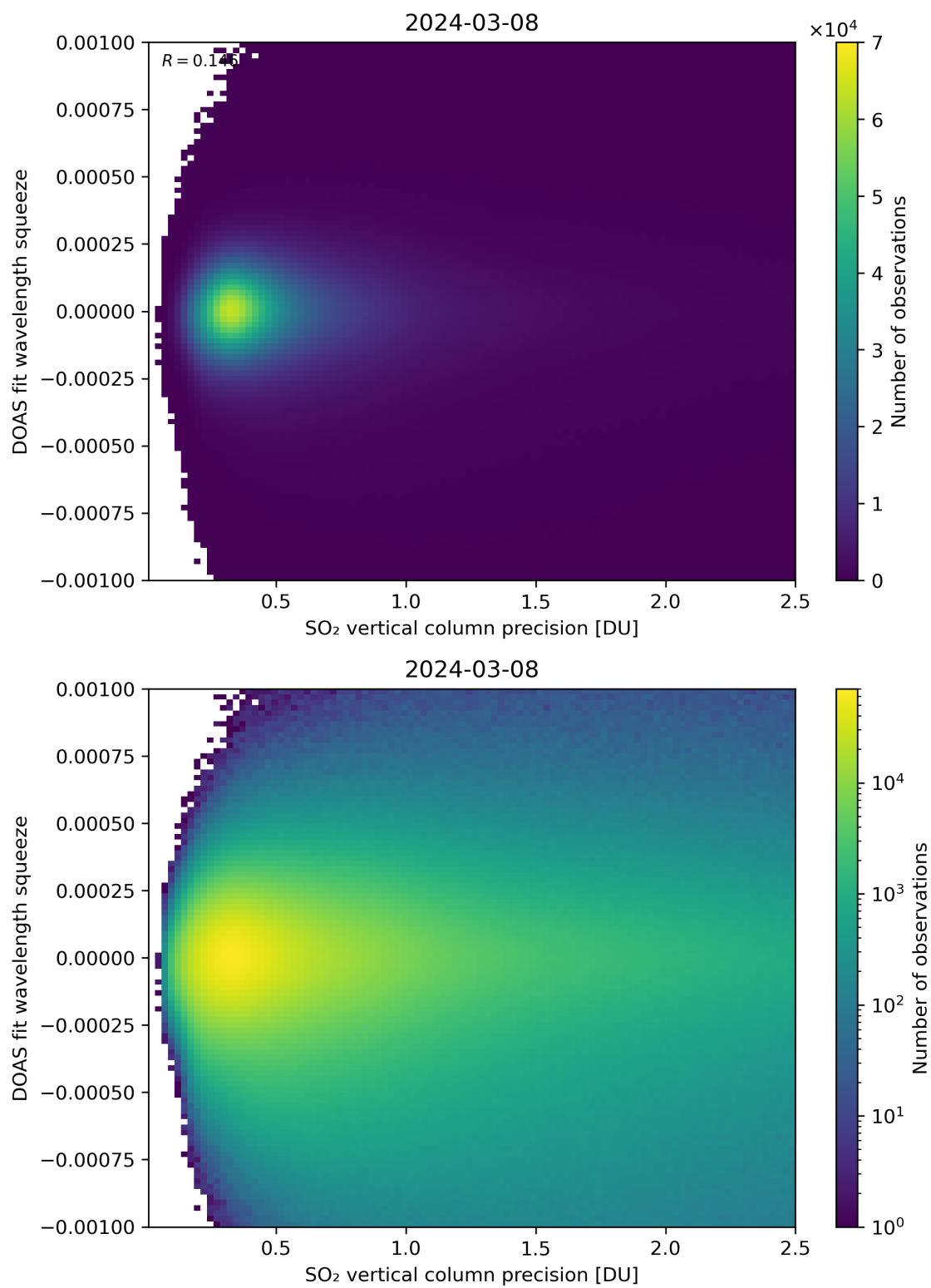
Figure 283: Scatter density plot of “SO 2 vertical column precision” against “DOAS fit wavelength squeeze” for 2024-03-07 to 2024-03-09.
