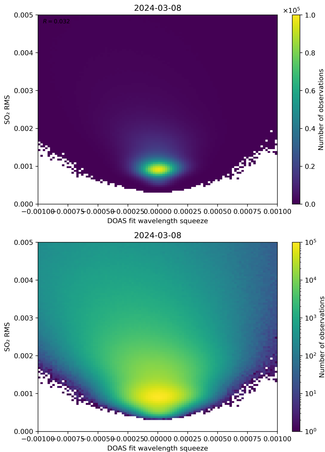
Figure 132: Scatter density plot of “DOAS fit wavelength squeeze” against “SO 2 RMS” for 2024-03-07 to 2024-03-09.
