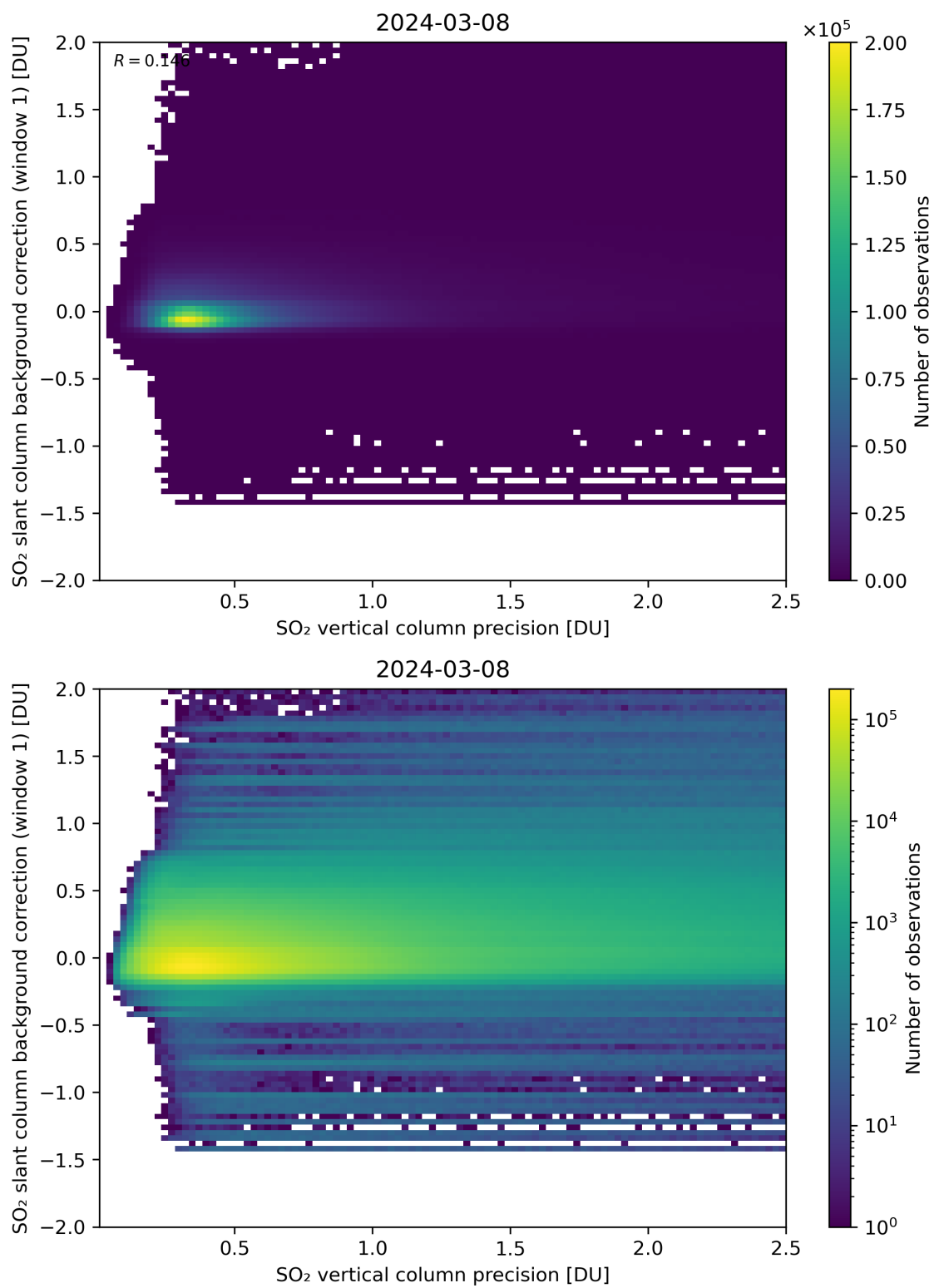
Figure 279: Scatter density plot of “SO 2 vertical column precision” against “SO 2 slant column background correction (window 1)” for 2024-03-07 to 2024-03-09.
