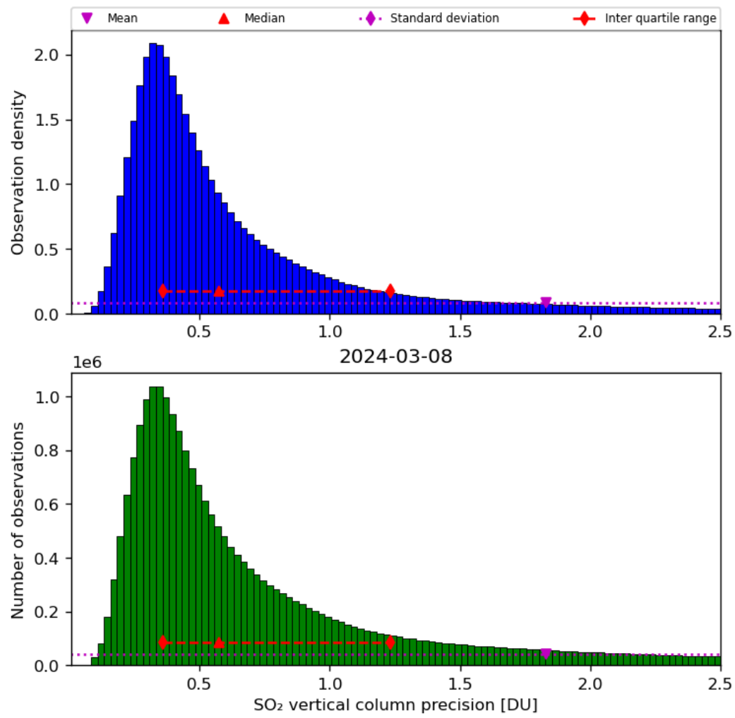
Figure 54: Histogram of “SO 2 vertical column precision” for 2024-03-07 to 2024-03-09
