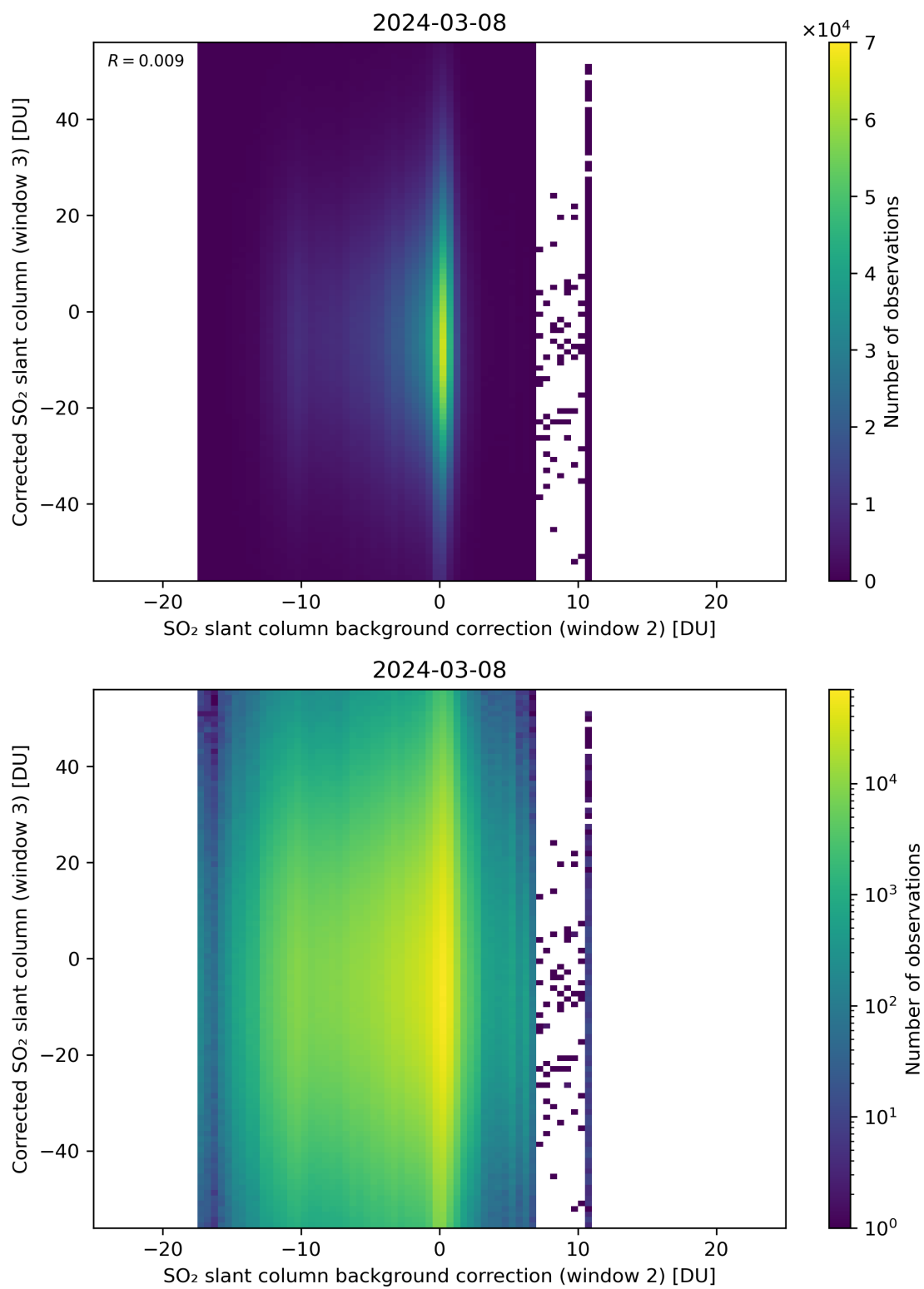
Figure 116: Scatter density plot of “SO 2 slant column background correction (window 2)” against “Corrected SO 2 slant column (window 3)” for 2024-03-07 to 2024-03-09.
