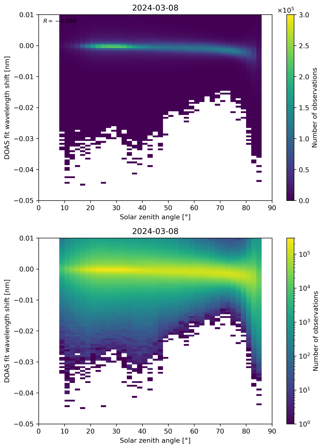
Figure 161: Scatter density plot of “Solar zenith angle” against “DOAS fit wavelength shift” for 2024-03-07 to 2024-03-09.
