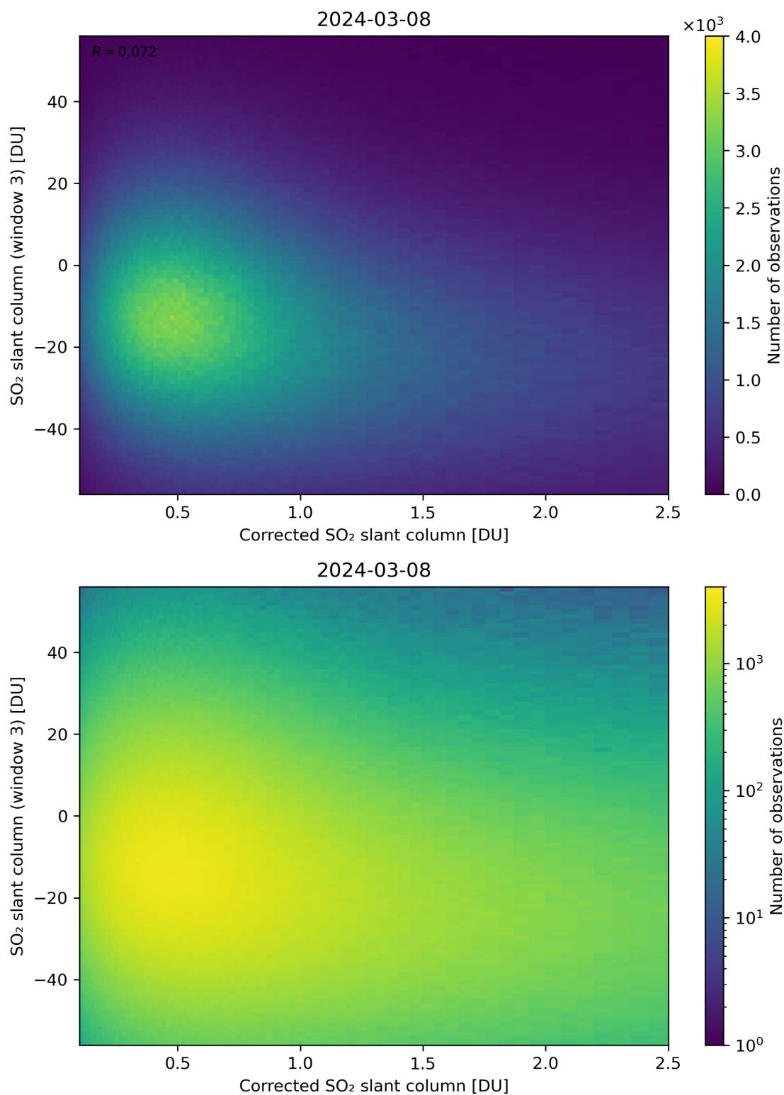
Figure 190: Scatter density plot of “Corrected SO 2 slant column” against “SO 2 slant column (window 3)” for 2024-03-07 to 2024-03-09.
