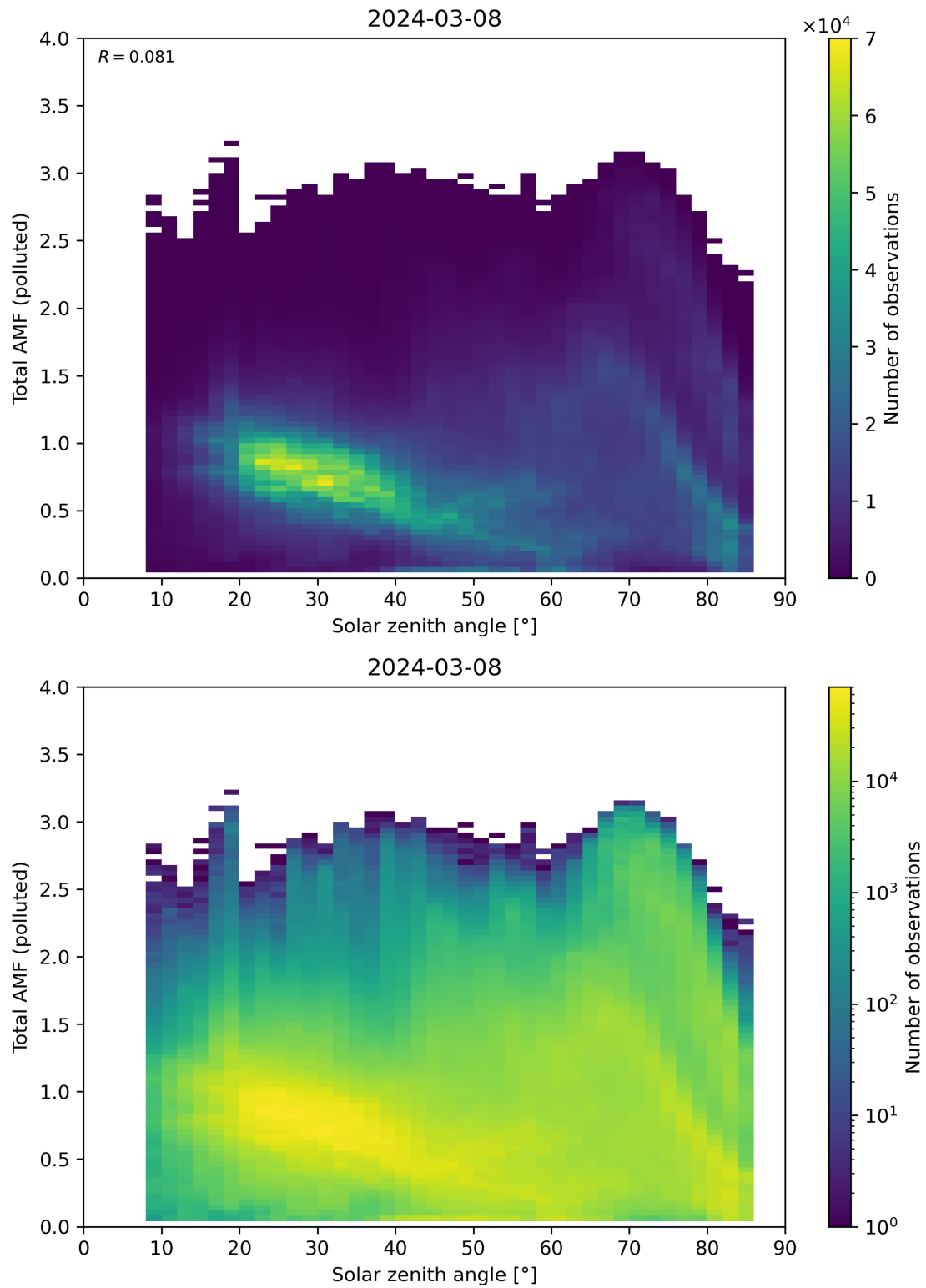
Figure 174: Scatter density plot of “Solar zenith angle” against “Total AMF (polluted)” for 2024-03-07 to 2024-03-09.
