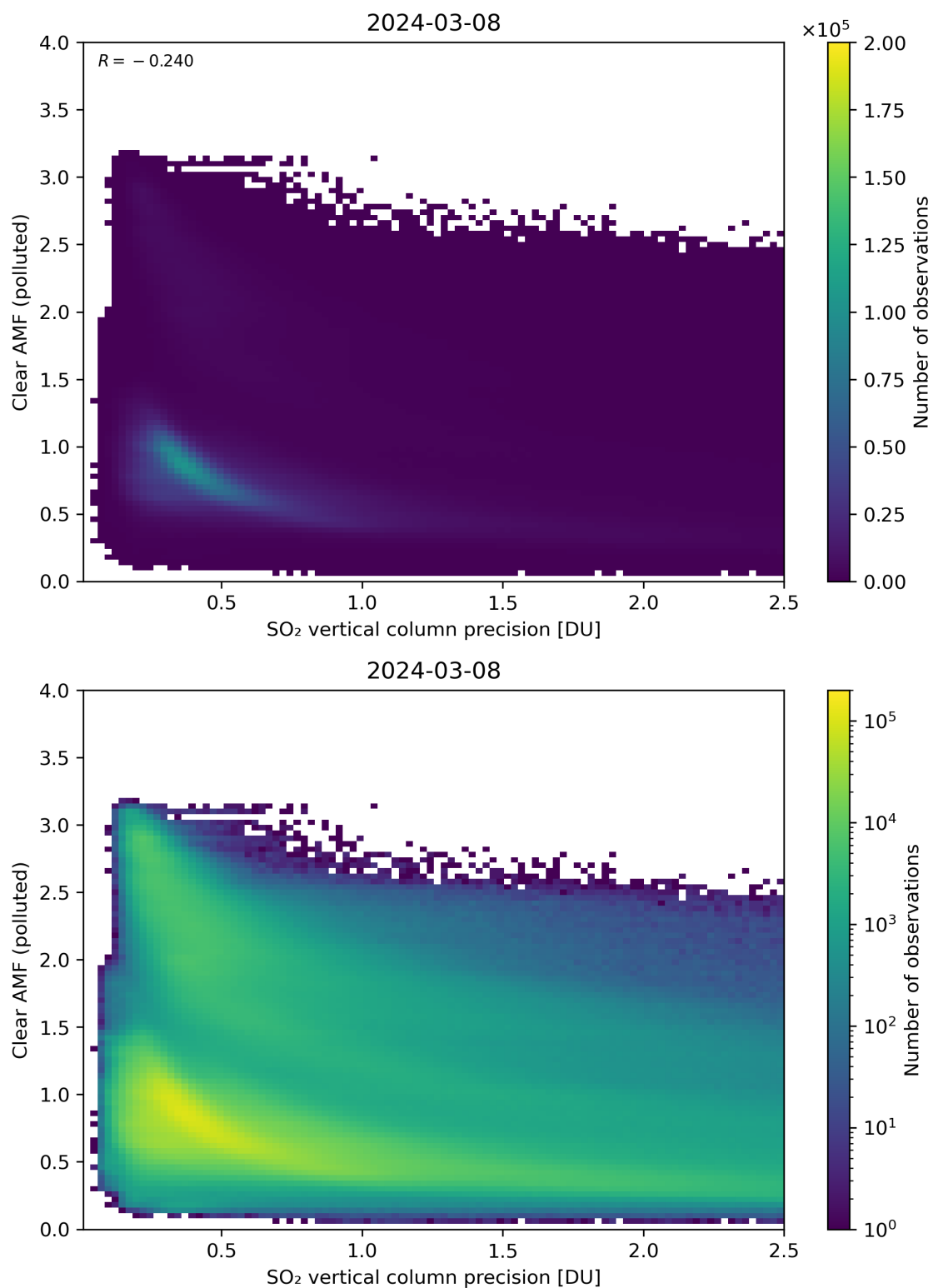
Figure 285: Scatter density plot of “SO 2 vertical column precision” against “Clear AMF (polluted)” for 2024-03-07 to 2024-03-09.
