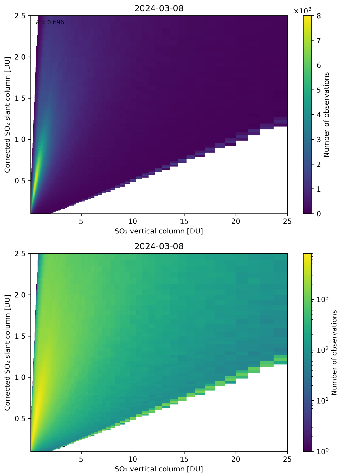
Figure 297: Scatter density plot of “SO 2 vertical column” against “Corrected SO 2 slant column” for 2024-03-07 to 2024-03-09.
