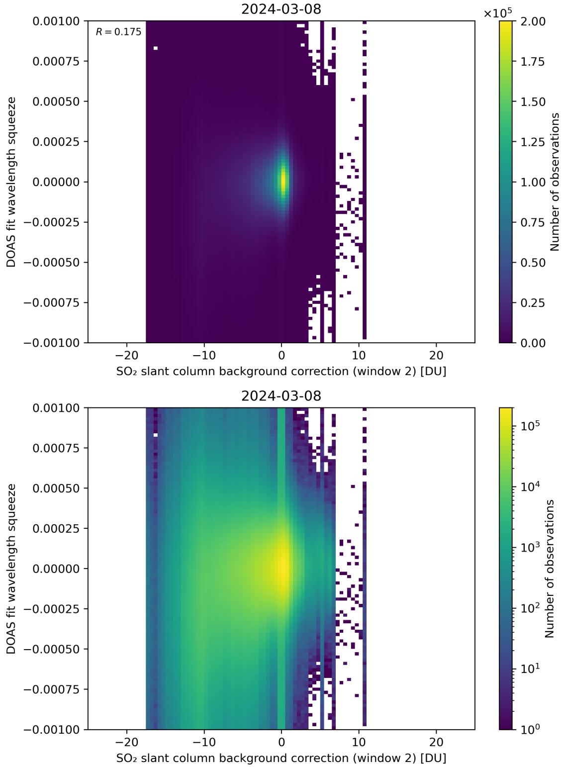
Figure 113: Scatter density plot of “SO 2 slant column background correction (window 2)” against “DOAS fit wavelength squeeze” for 2024-03-07 to 2024-03-09.
