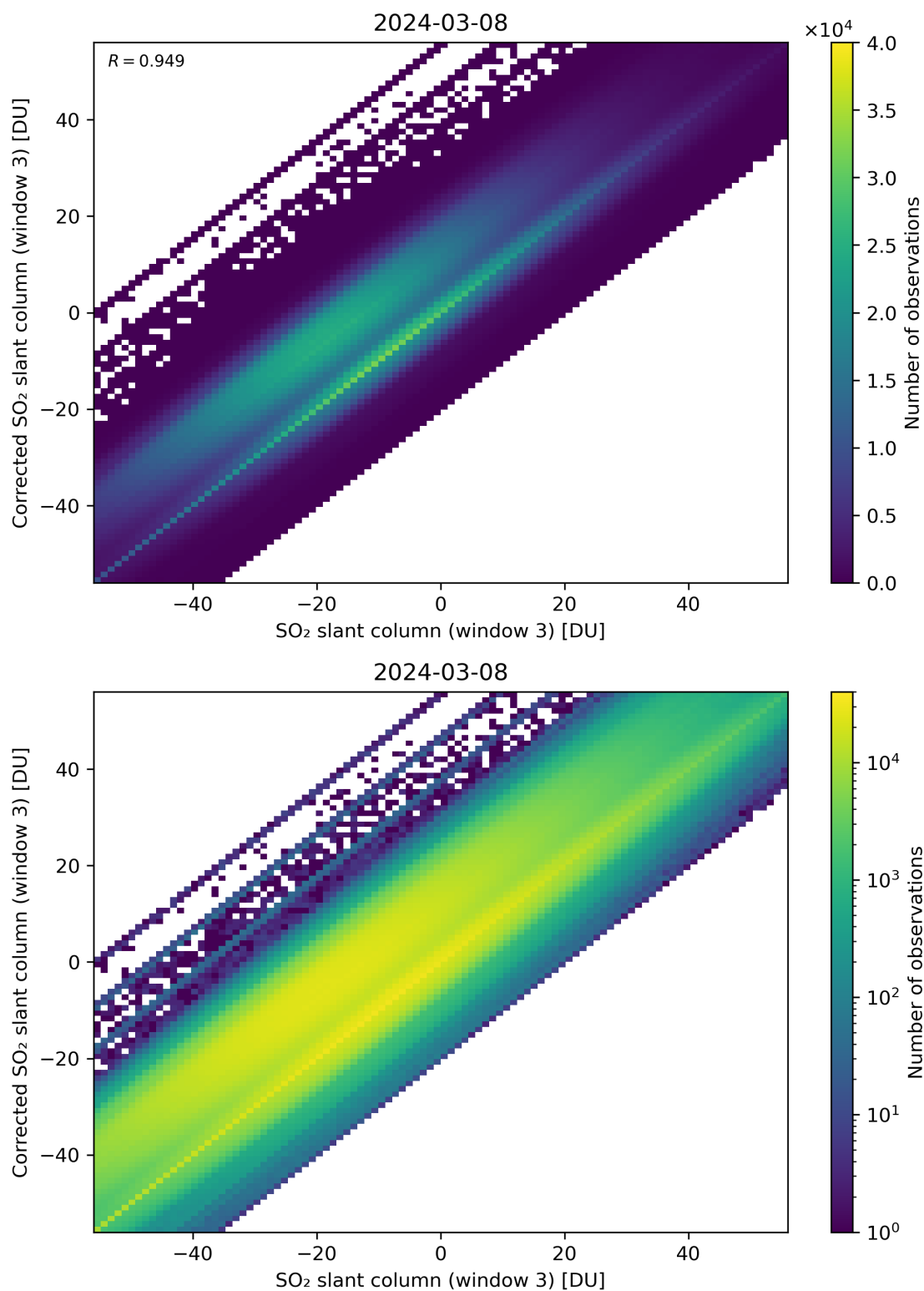
Figure 266: Scatter density plot of “SO 2 slant column (window 3)” against “Corrected SO 2 slant column (window 3)” for 2024-03-07 to 2024-03-09.
