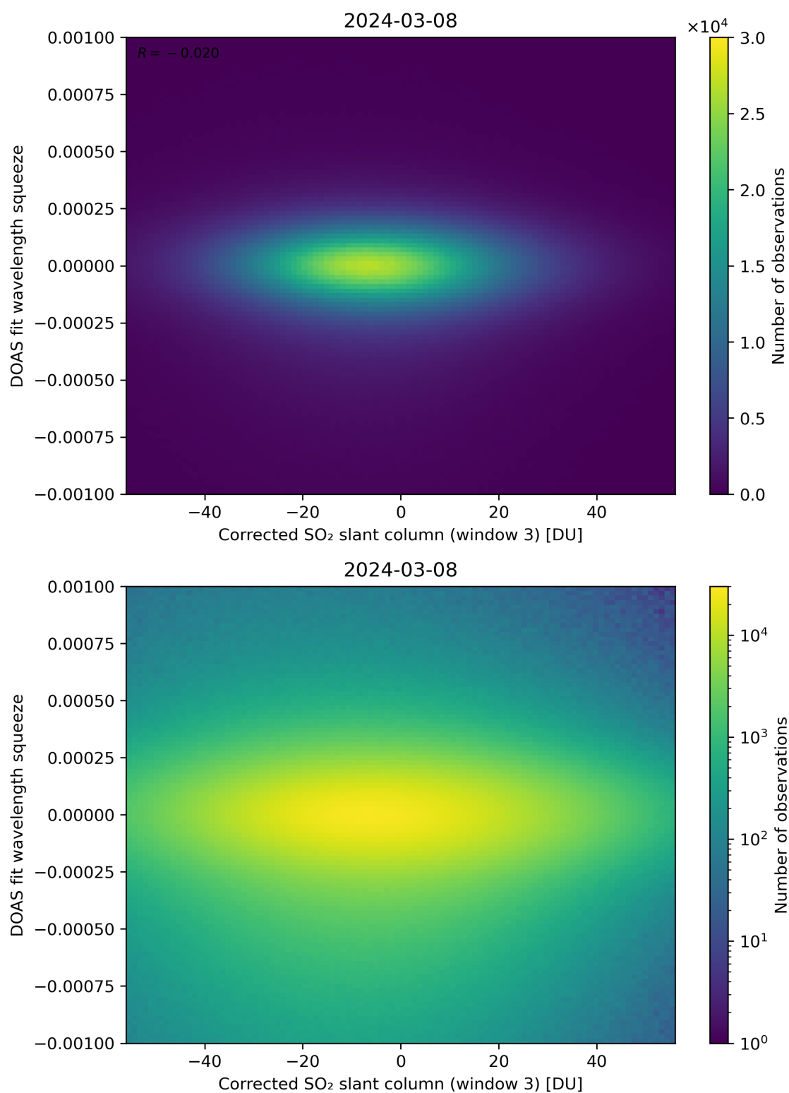
Figure 207: Scatter density plot of “Corrected SO 2 slant column (window 3)” against “DOAS fit wavelength squeeze” for 2024-03-07 to 2024-03-09.
