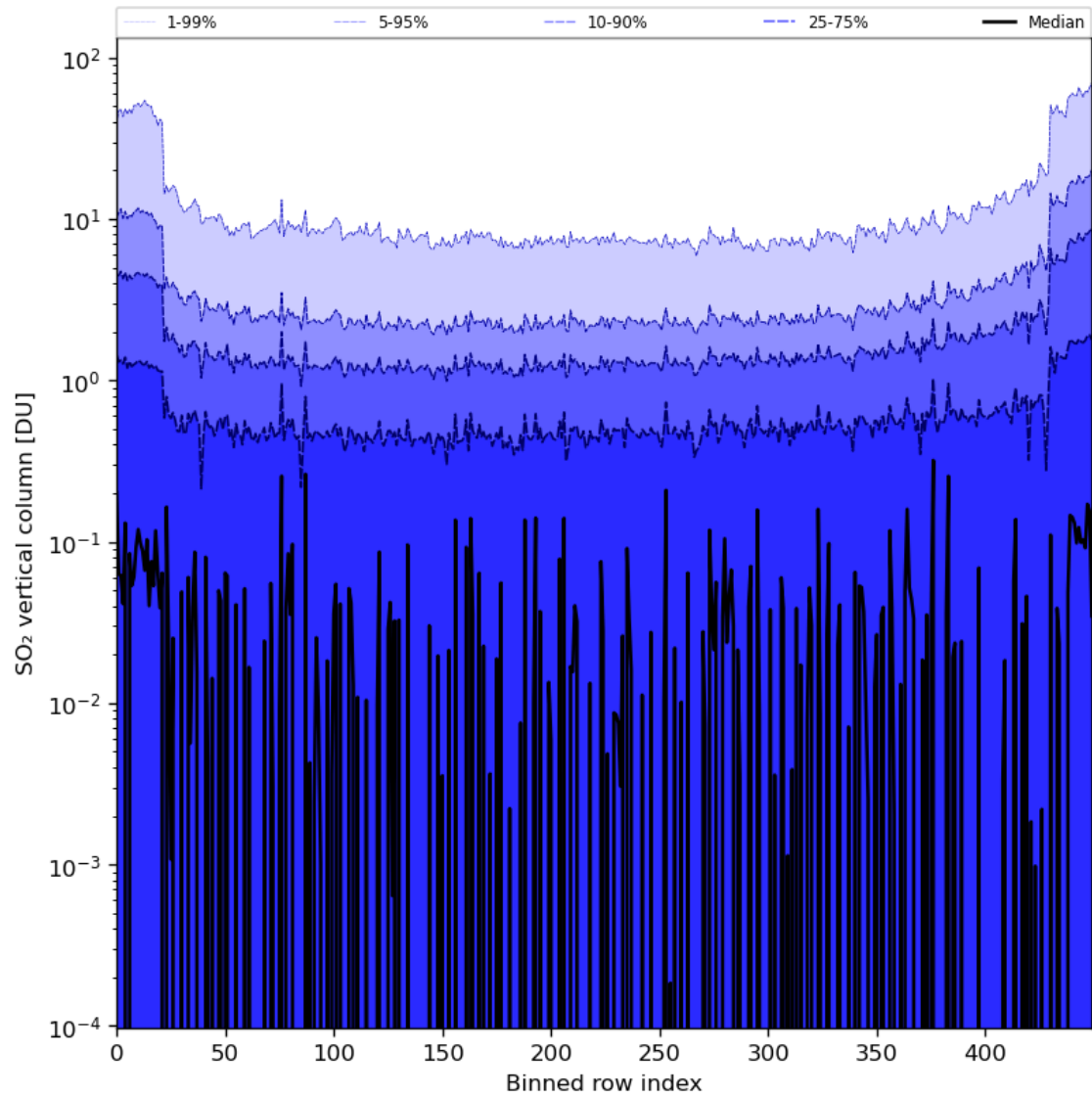
Figure 76: Along track statistics of “SO 2 vertical column” for 2024-03-07 to 2024-03-09
