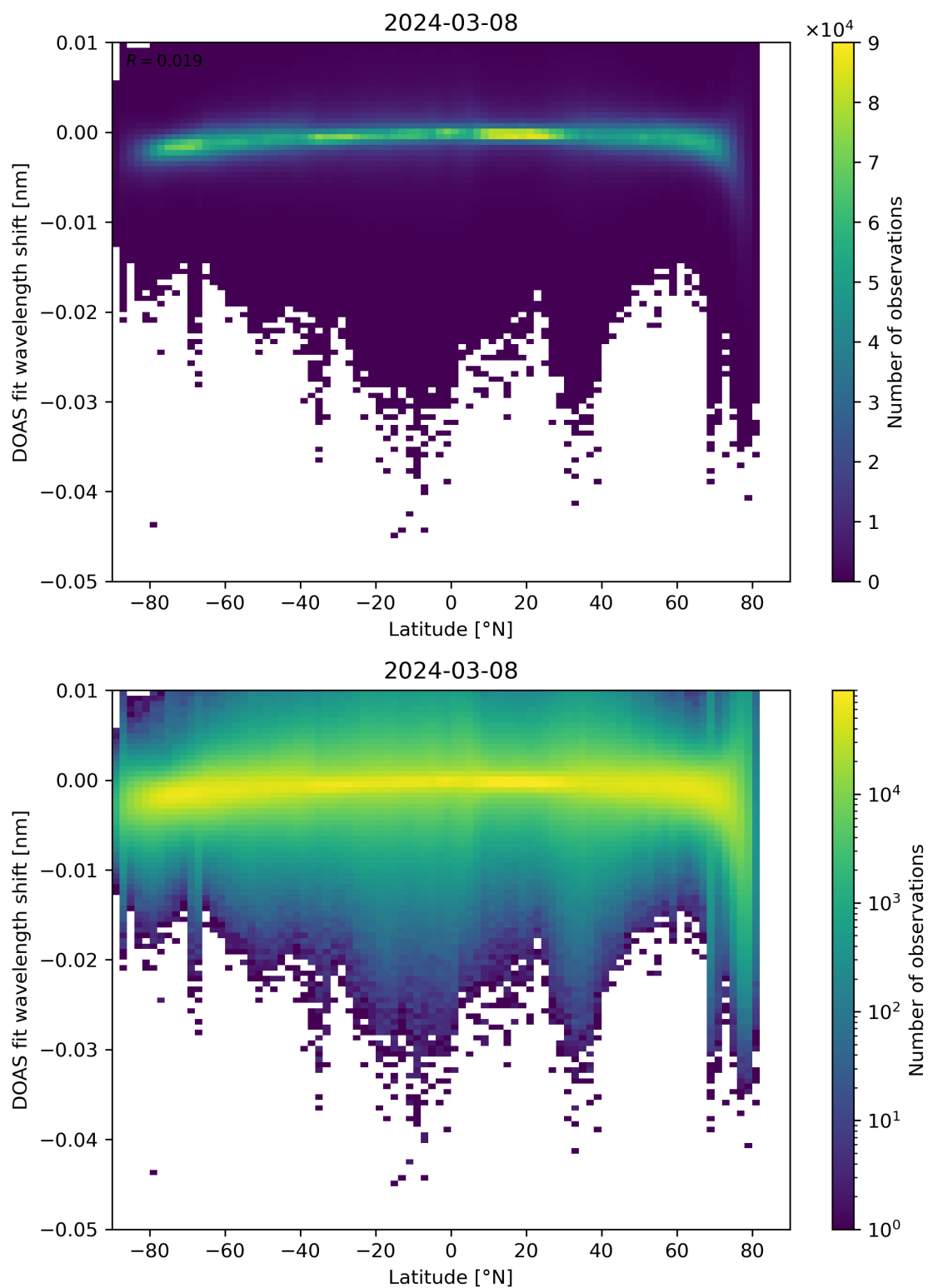
Figure 142: Scatter density plot of “Latitude” against “DOAS fit wavelength shift” for 2024-03-07 to 2024-03-09.
