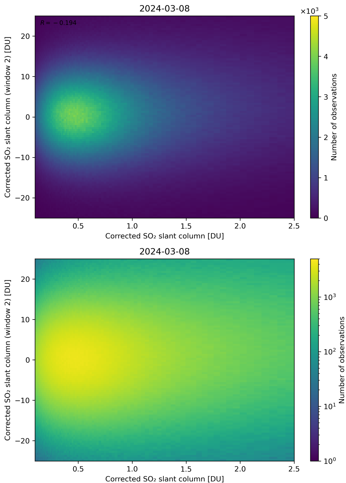
Figure 185: Scatter density plot of “Corrected SO 2 slant column” against “Corrected SO 2 slant column (window 2)” for 2024-03-07 to 2024-03-09.
