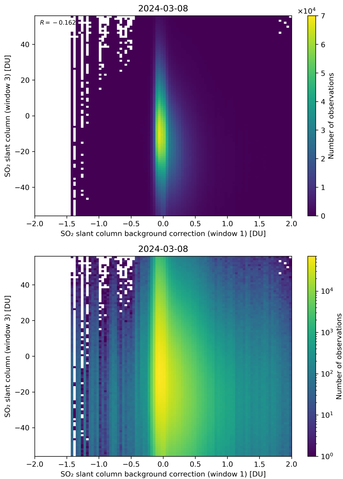
Figure 107: Scatter density plot of “SO 2 slant column background correction (window 1)” against “SO 2 slant column (window 3)” for 2024-03-07 to 2024-03-09.
