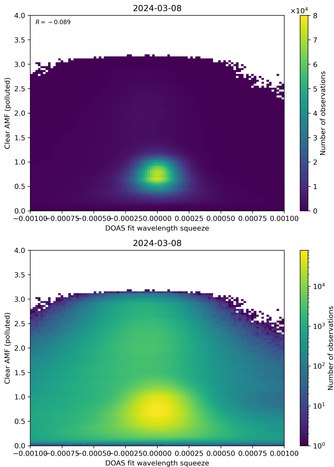
Figure 133: Scatter density plot of “DOAS fit wavelength squeeze” against “Clear AMF (polluted)” for 2024-03-07 to 2024-03-09.
