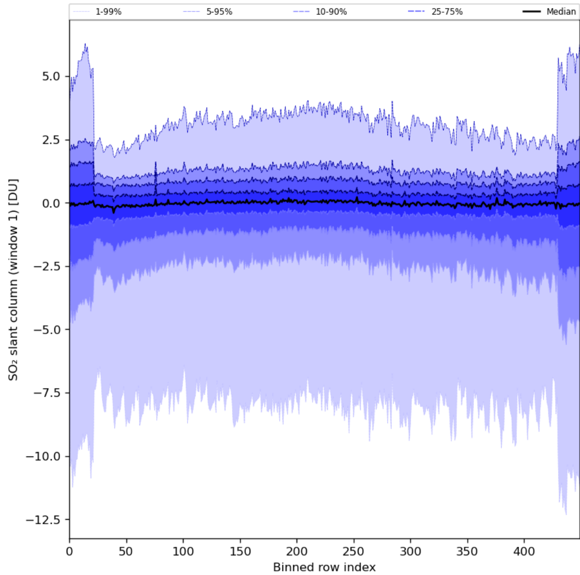
Figure 79: Along track statistics of “SO 2 slant column (window 1)” for 2024-03-07 to 2024-03-09
