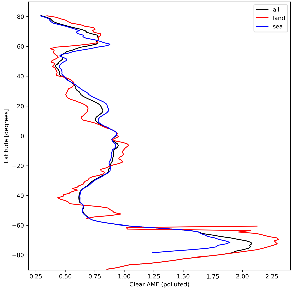
Figure 50: Zonal average of “Clear AMF (polluted)” for 2024-03-07 to 2024-03-09.
