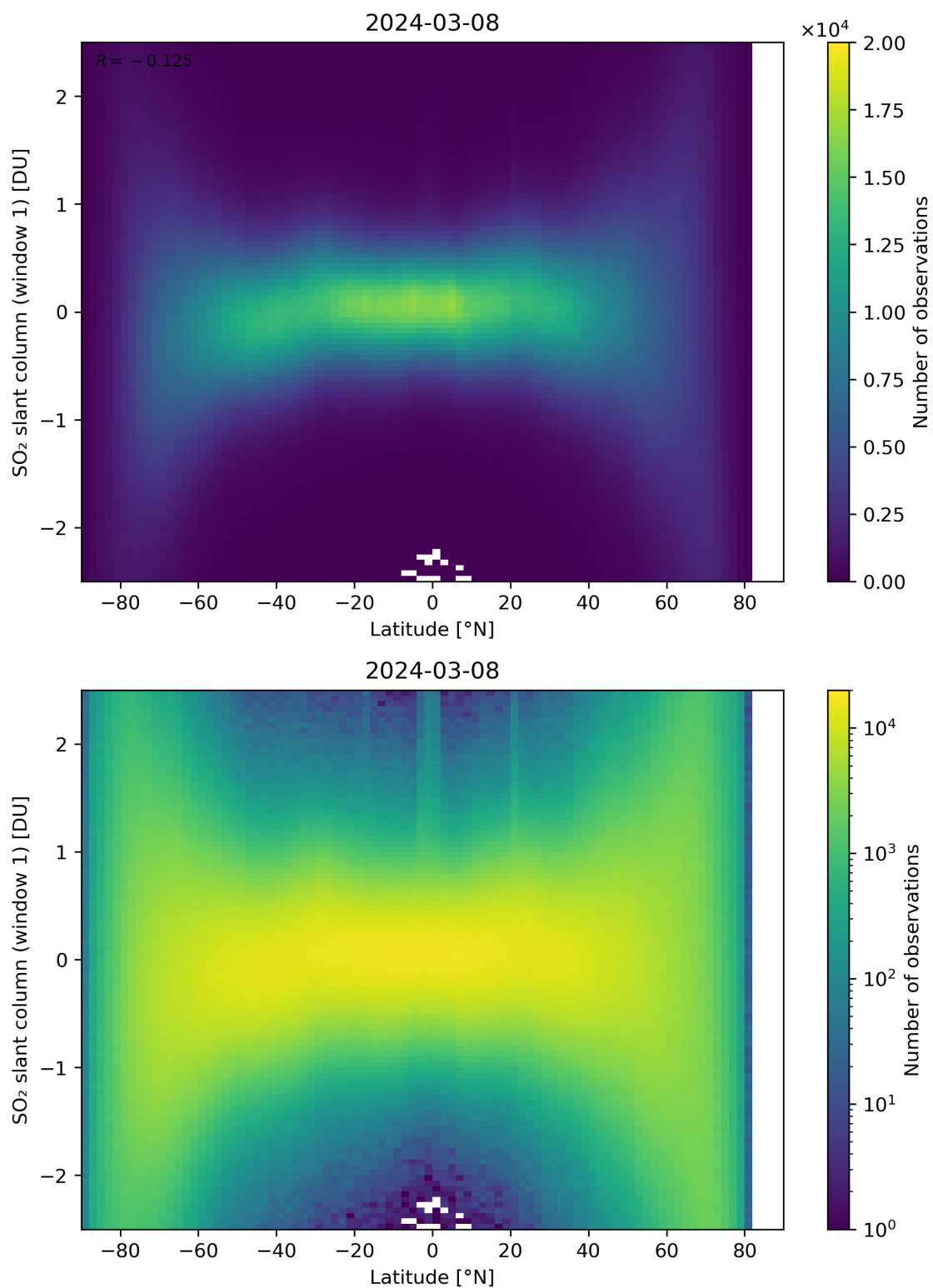
Figure 149: Scatter density plot of “Latitude” against “SO 2 slant column (window 1)” for 2024-03-07 to 2024-03-09.
