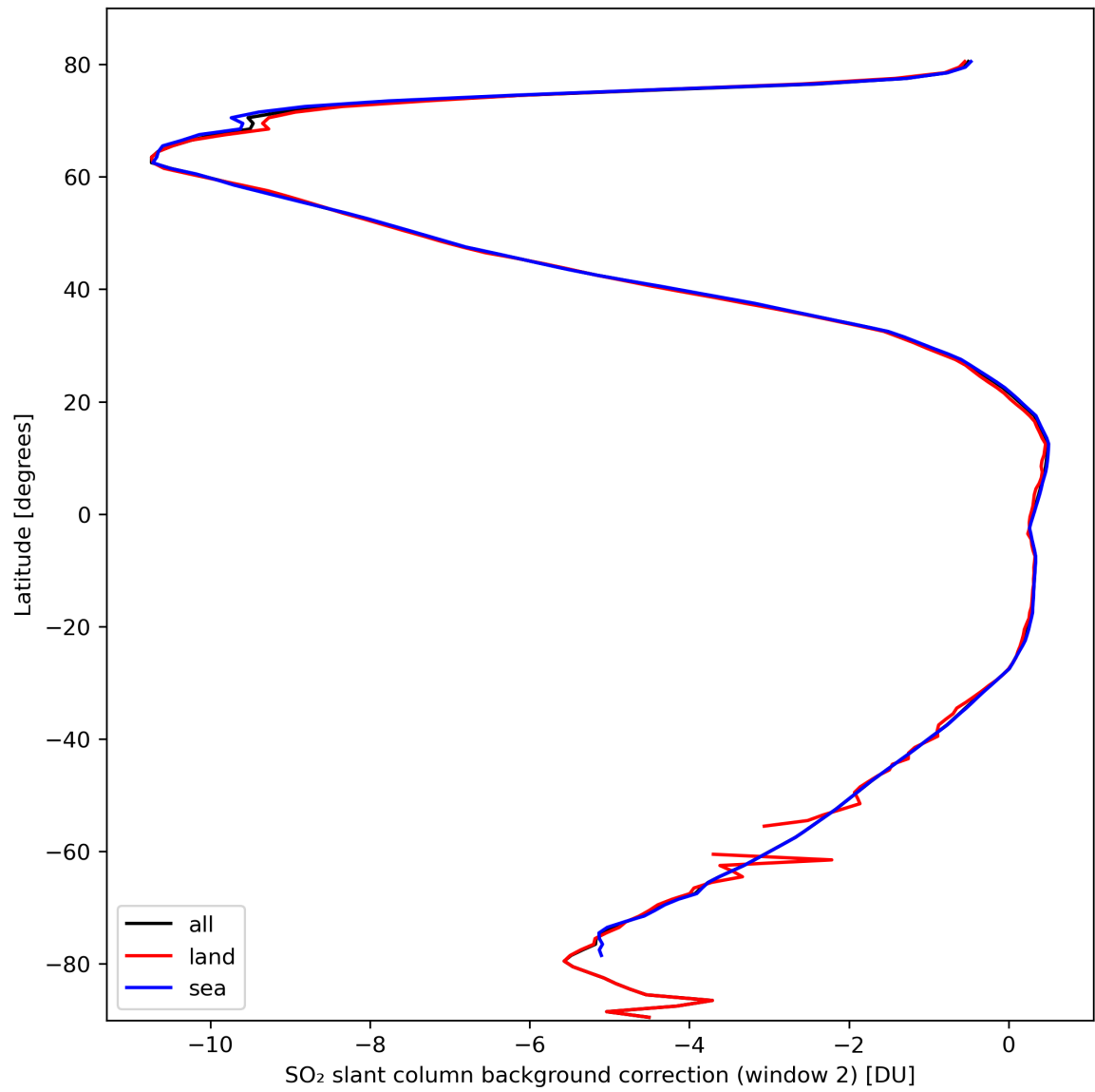
Figure 40: Zonal average of "SO 2 slant column background correction (window 2)" for 2024-03-07 to 2024-03-09.
