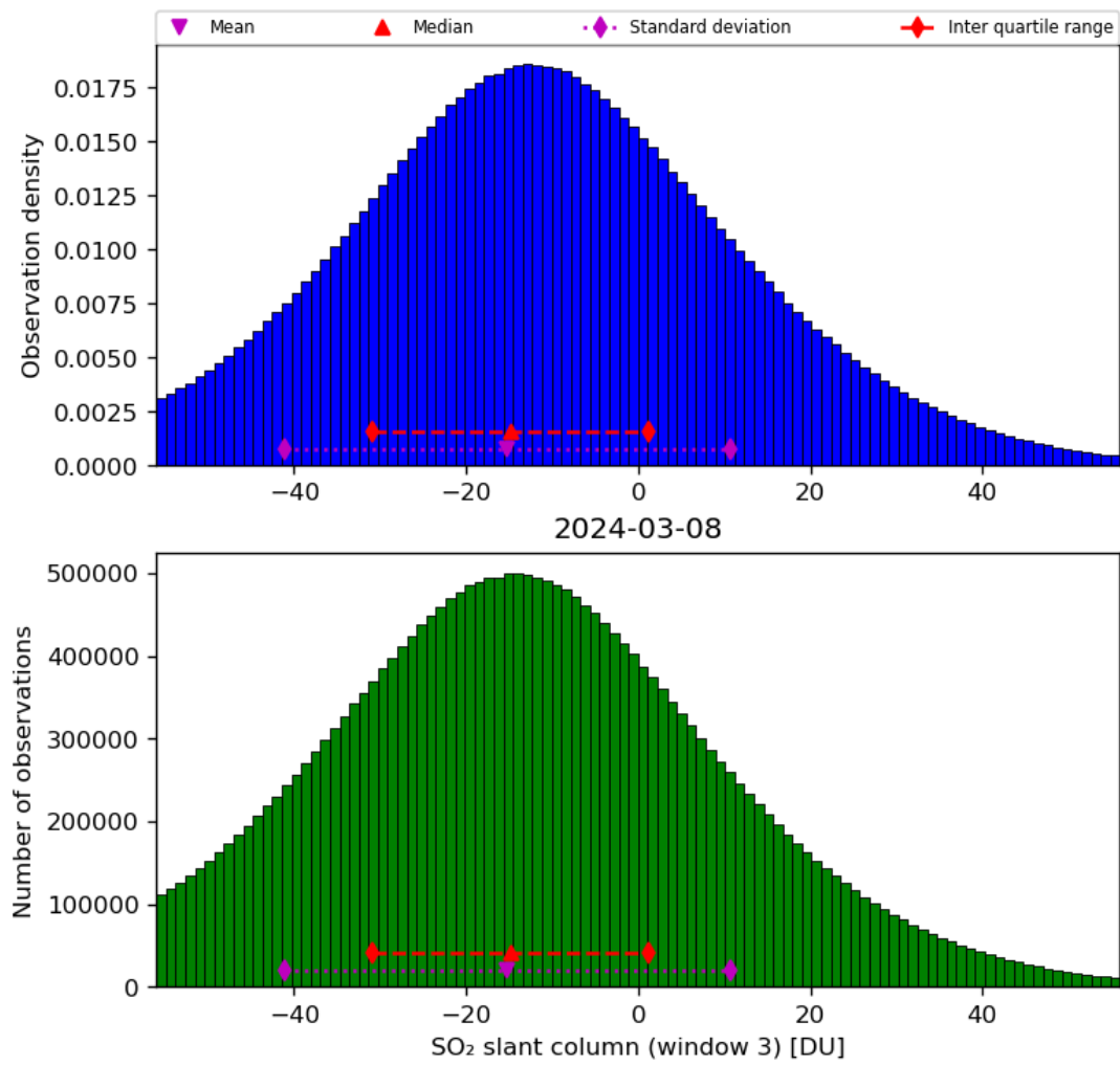
Figure 64: Histogram of “SO 2 slant column (window 3)” for 2024-03-07 to 2024-03-09
