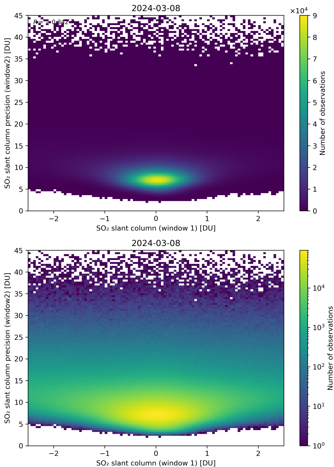
Figure 236: Scatter density plot of “SO 2 slant column (window 1)” against “SO 2 slant column precision (window2)” for 2024-03-07 to 2024-03-09.
