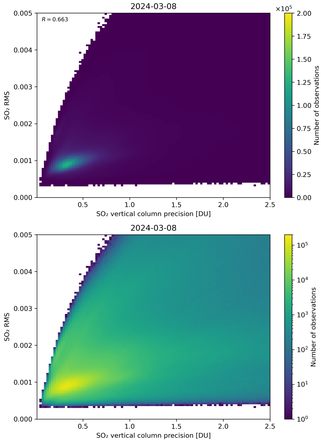
Figure 284: Scatter density plot of “SO 2 vertical column precision” against “SO 2 RMS” for 2024-03-07 to 2024-03-09.
