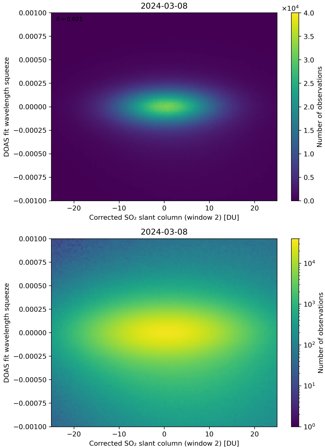
Figure 197: Scatter density plot of “Corrected SO 2 slant column (window 2)” against “DOAS fit wavelength squeeze” for 2024-03-07 to 2024-03-09.
