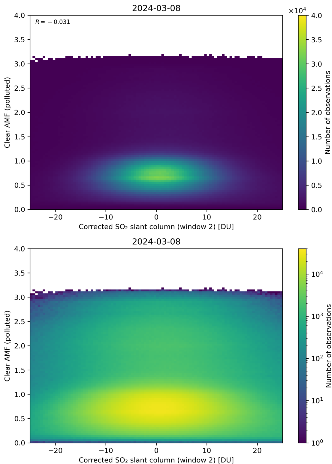
Figure 199: Scatter density plot of “Corrected SO 2 slant column (window 2)” against “Clear AMF (polluted)” for 2024-03-07 to 2024-03-09.
