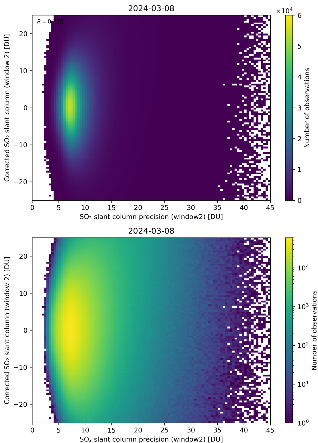
Figure 247: Scatter density plot of “SO 2 slant column precision (window2)” against “Corrected SO 2 slant column (window 2)” for 2024-03-07 to 2024-03-09.
