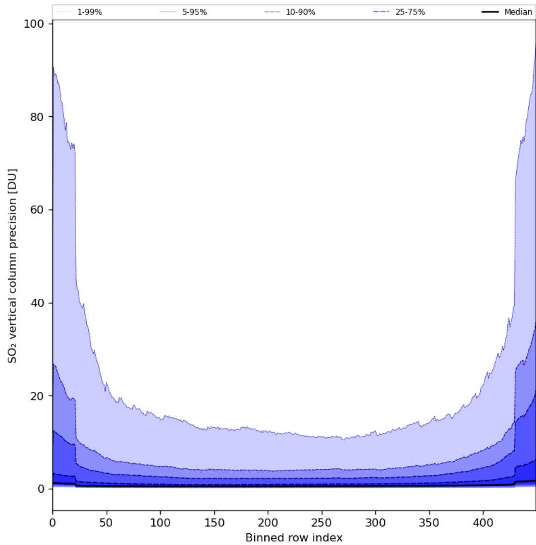
Figure 77: Along track statistics of “SO 2 vertical column precision” for 2024-03-07 to 2024-03-09
