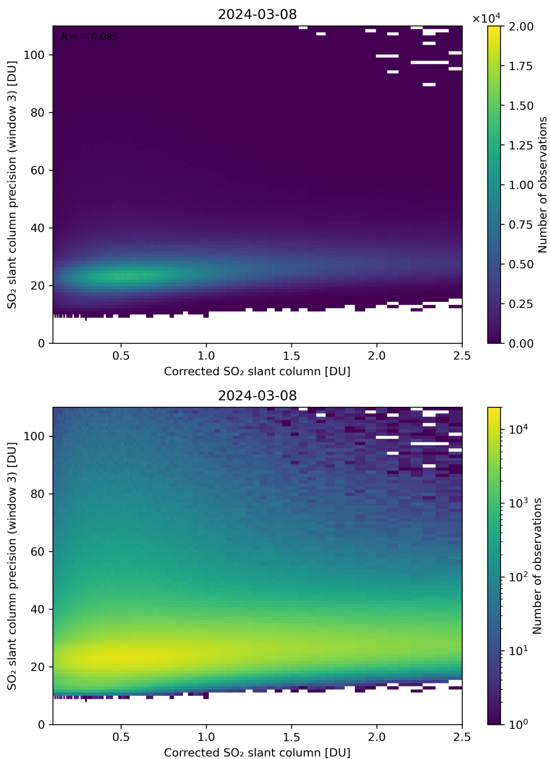
Figure 191: Scatter density plot of “Corrected SO 2 slant column” against “SO 2 slant column precision (window 3)” for 2024-03-07 to 2024-03-09.
