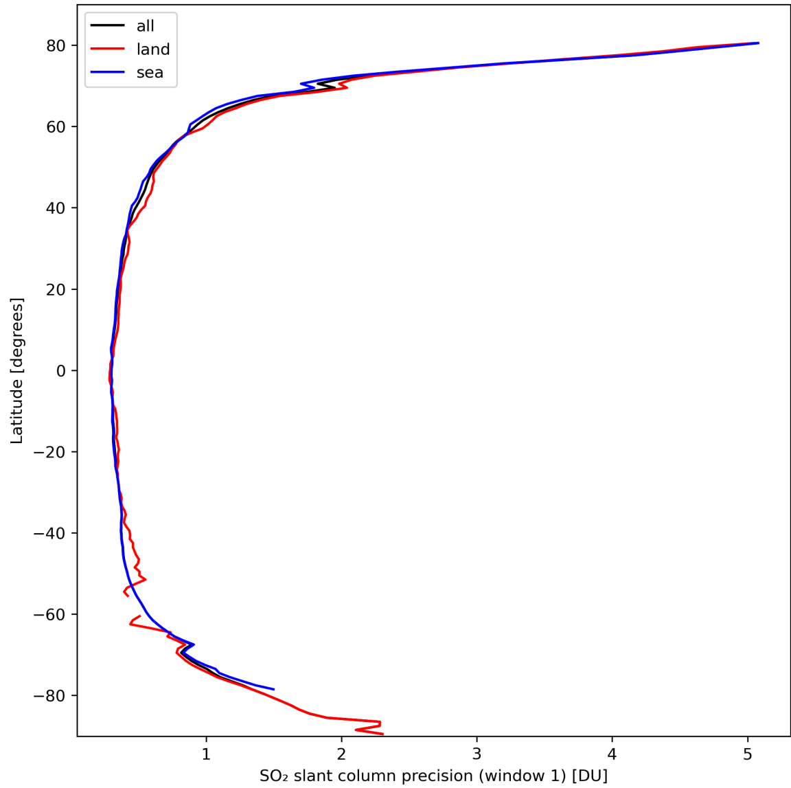
Figure 34: Zonal average of “SO 2 slant column precision (window 1)” for 2024-03-07 to 2024-03-09.
