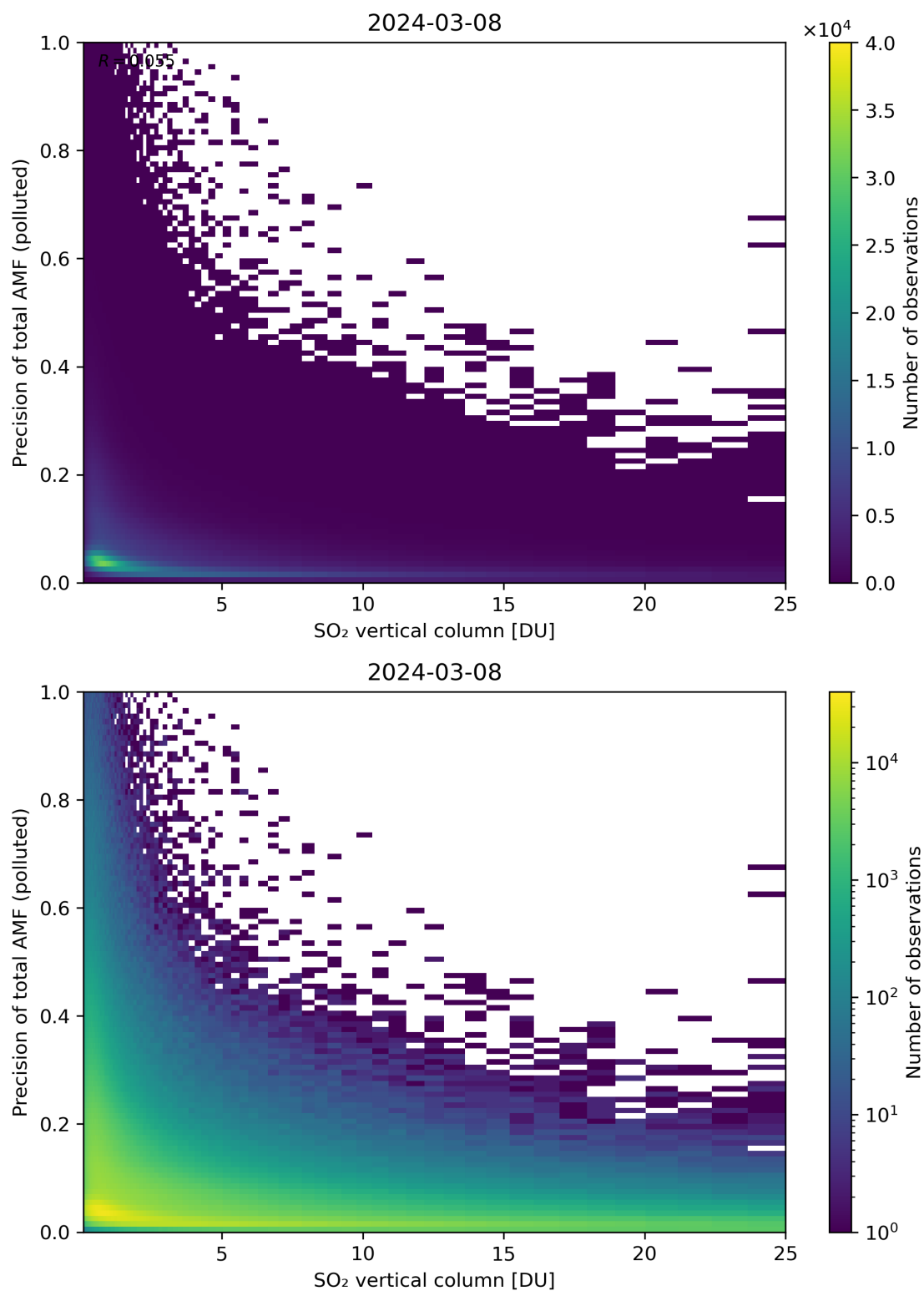
Figure 306: Scatter density plot of “SO 2 vertical column” against “Precision of total AMF (polluted)” for 2024-03-07 to 2024-03-09.
