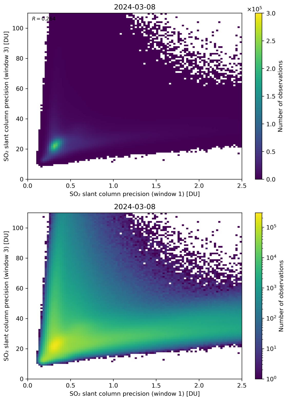
Figure 229: Scatter density plot of “SO 2 slant column precision (window 1)” against “SO 2 slant column precision (window 3)” for 2024-03-07 to 2024-03-09.
