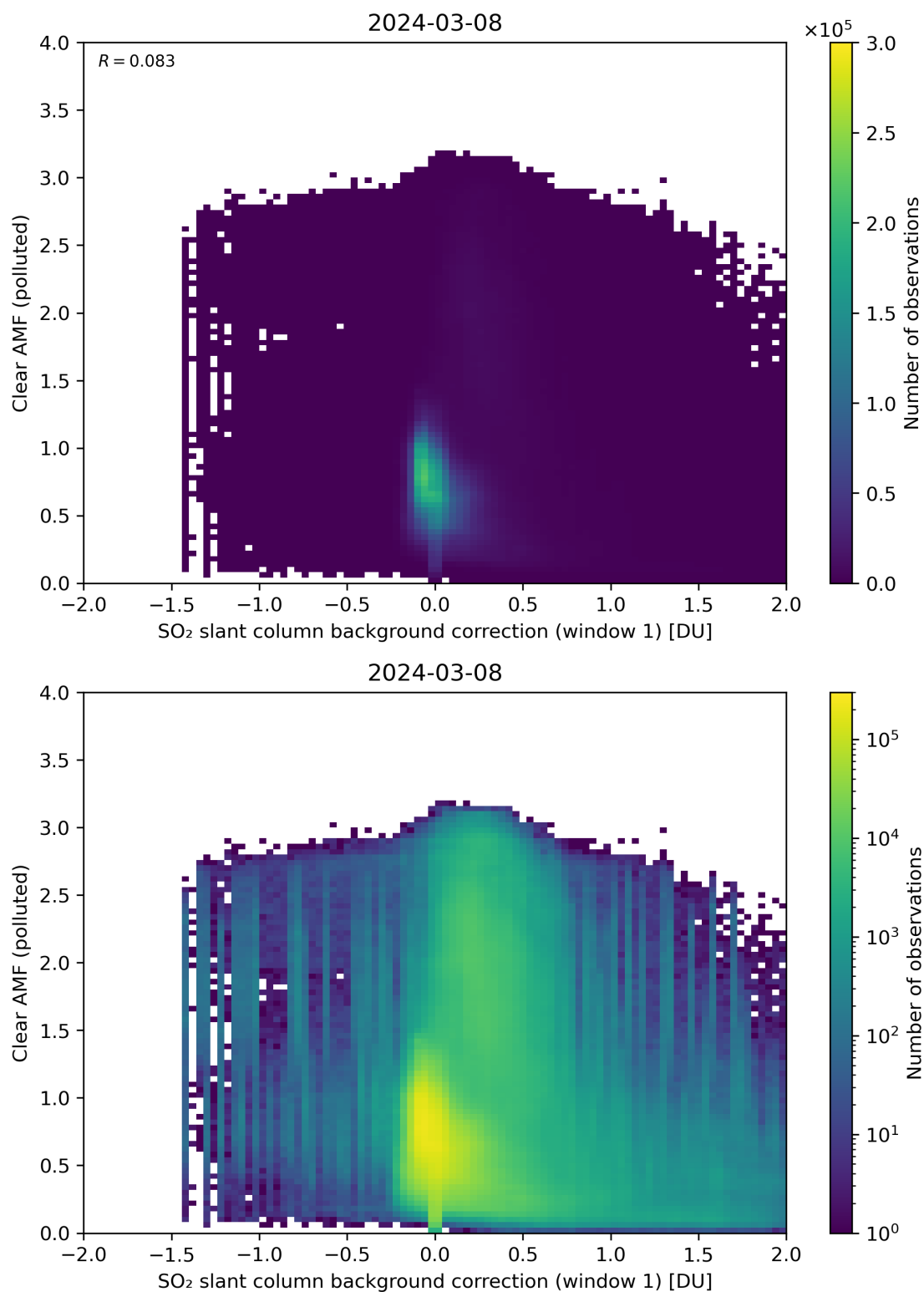
Figure 103: Scatter density plot of “SO 2 slant column background correction (window 1)” against “Clear AMF (polluted)” for 2024-03-07 to 2024-03-09.
