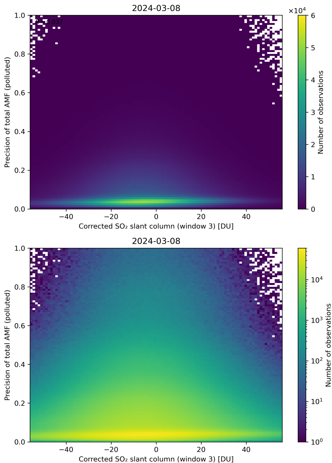
Figure 211: Scatter density plot of “Corrected SO 2 slant column (window 3)” against “Precision of total AMF (polluted)” for 2024-03-07 to 2024-03-09.
