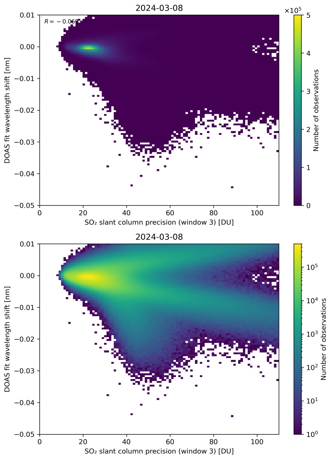
Figure 258: Scatter density plot of “SO 2 slant column precision (window 3)” against “DOAS fit wavelength shift” for 2024-03-07 to 2024-03-09.
