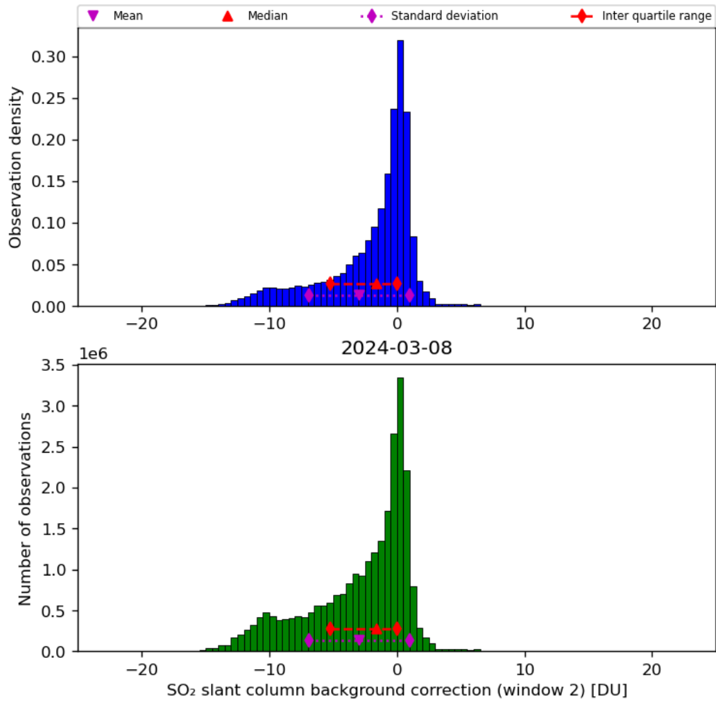
Figure 63: Histogram of “SO 2 slant column background correction (window 2)” for 2024-03-07 to 2024-03-09
