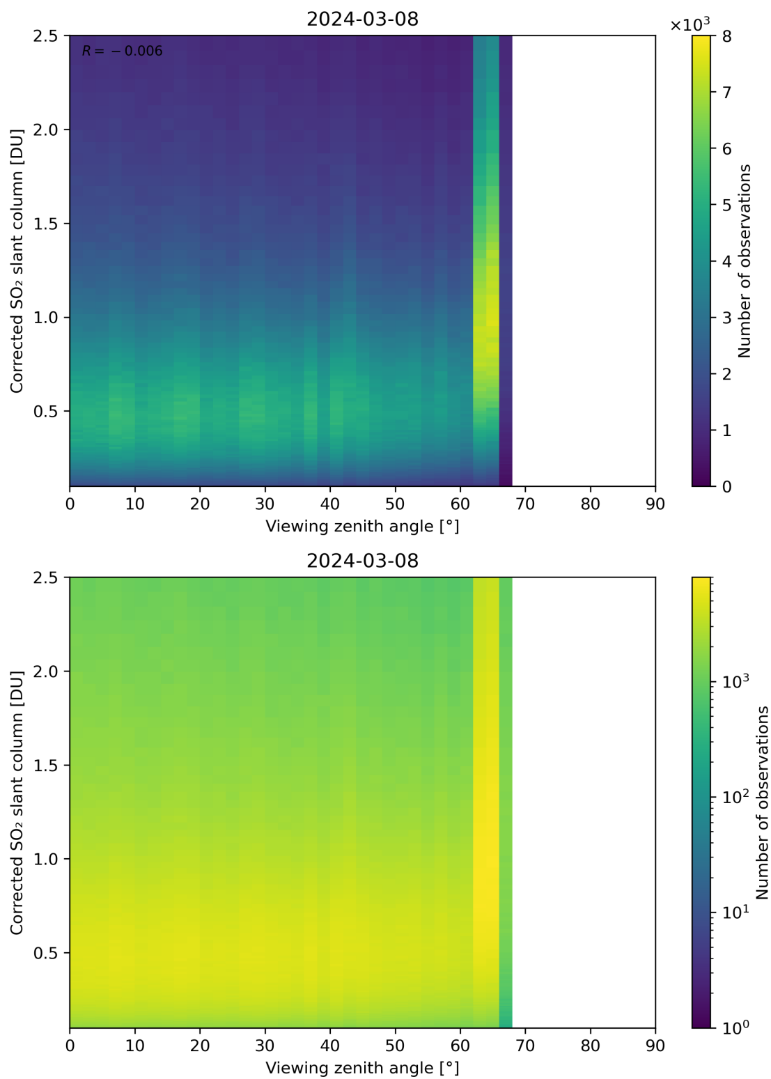
Figure 317: Scatter density plot of “Viewing zenith angle” against “Corrected SO 2 slant column” for 2024-03-07 to 2024-03-09.
