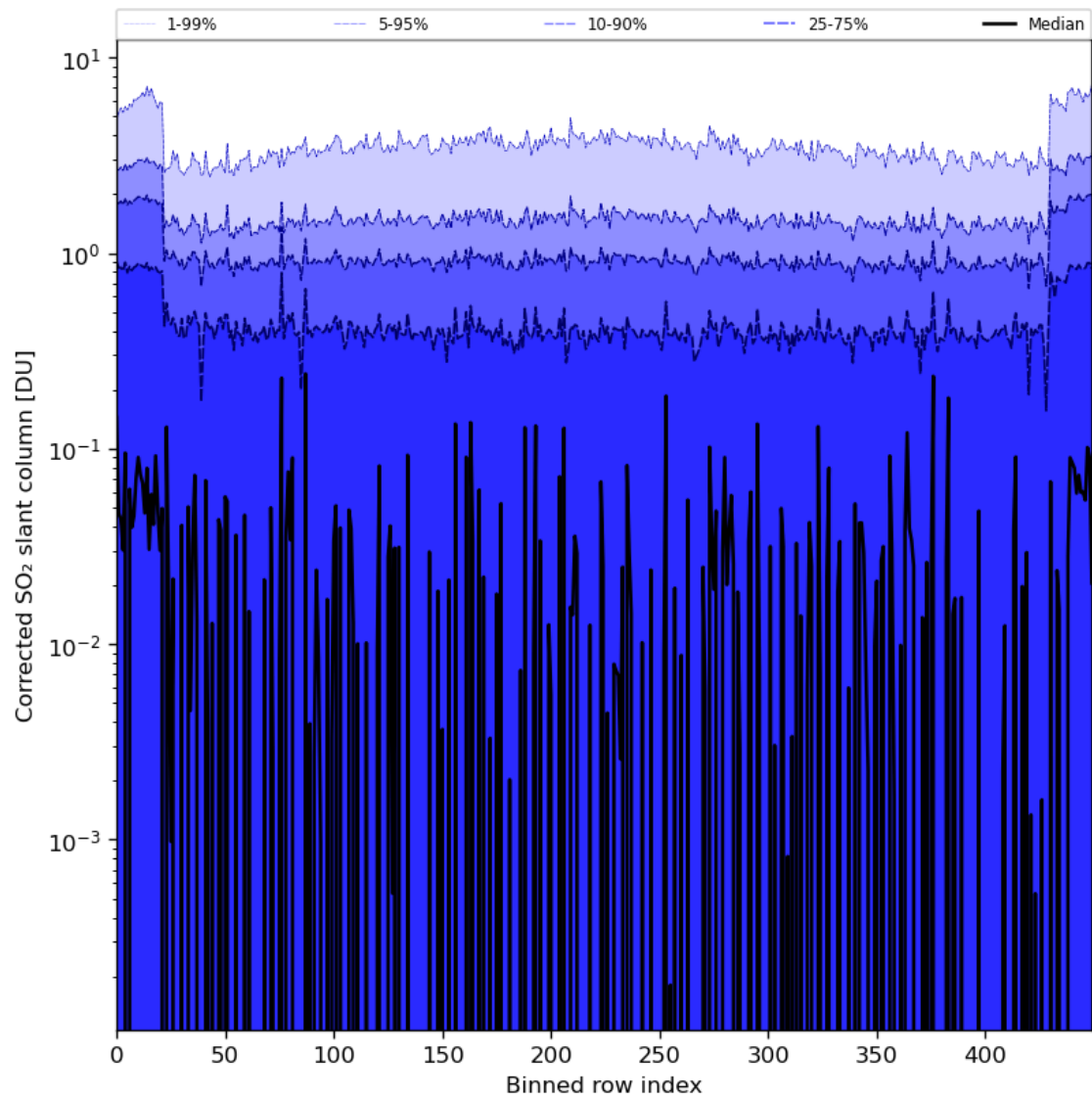
Figure 78: Along track statistics of “Corrected SO 2 slant column” for 2024-03-07 to 2024-03-09
