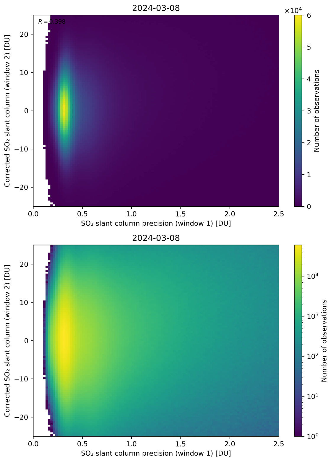
Figure 225: Scatter density plot of “SO 2 slant column precision (window 1)” against “Corrected SO 2 slant column (window 2)” for 2024-03-07 to 2024-03-09.
