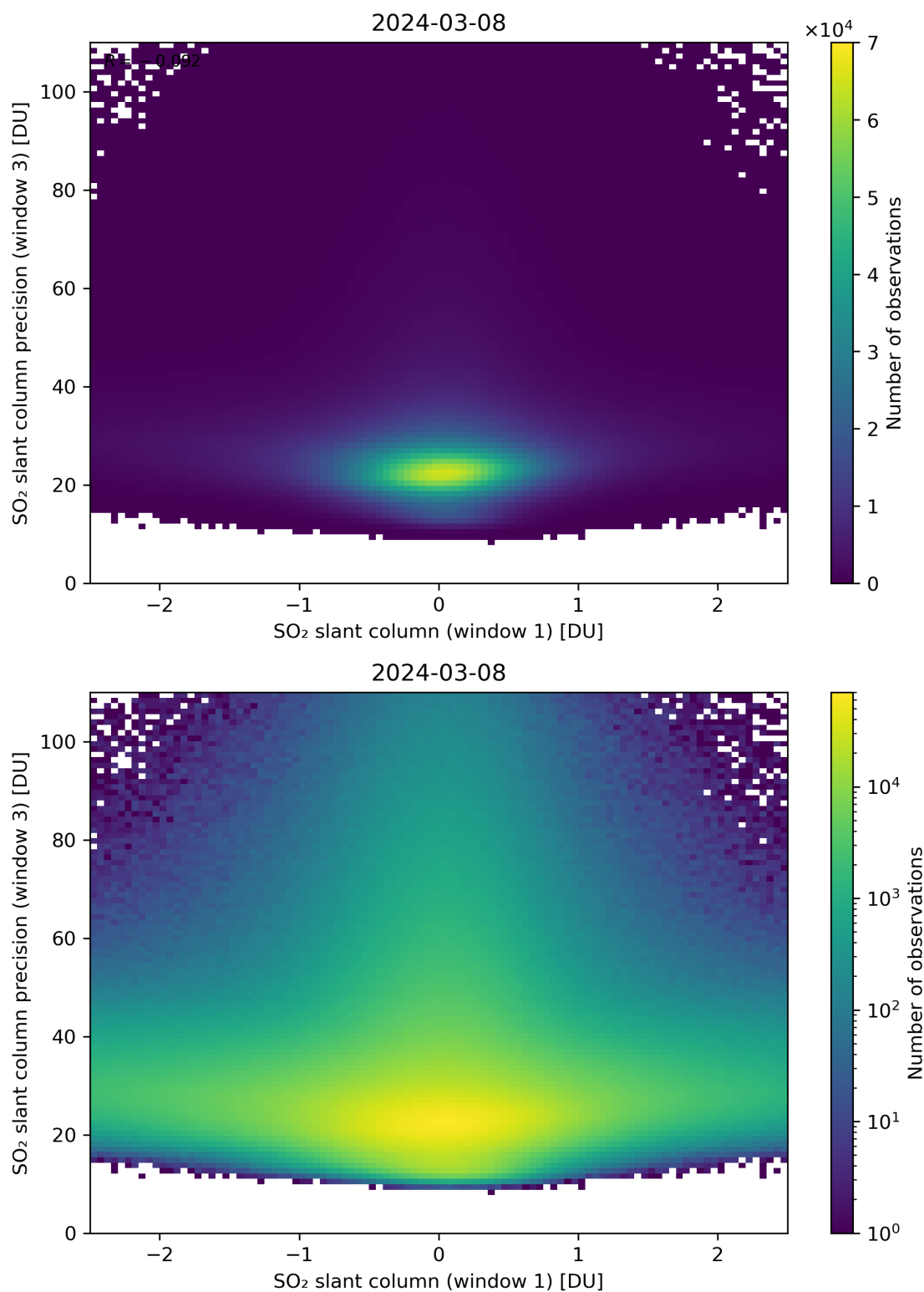
Figure 238: Scatter density plot of “SO 2 slant column (window 1)” against “SO 2 slant column precision (window 3)” for 2024-03-07 to 2024-03-09.
