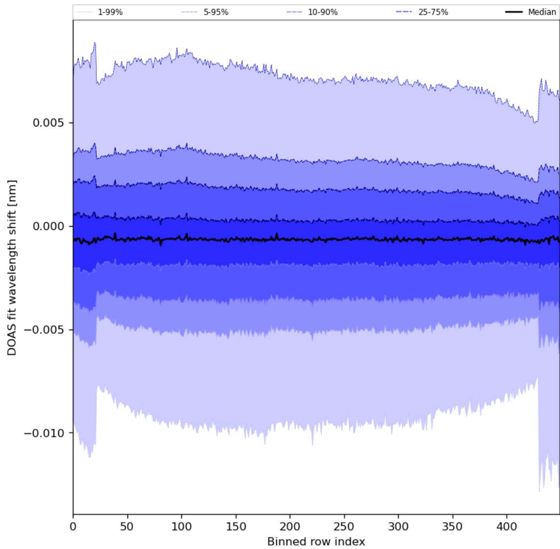
Figure 91: Along track statistics of “DOAS fit wavelength shift” for 2024-03-07 to 2024-03-09
