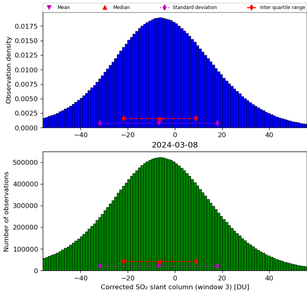
Figure 66: Histogram of “Corrected SO 2 slant column (window 3)” for 2024-03-07 to 2024-03-09
