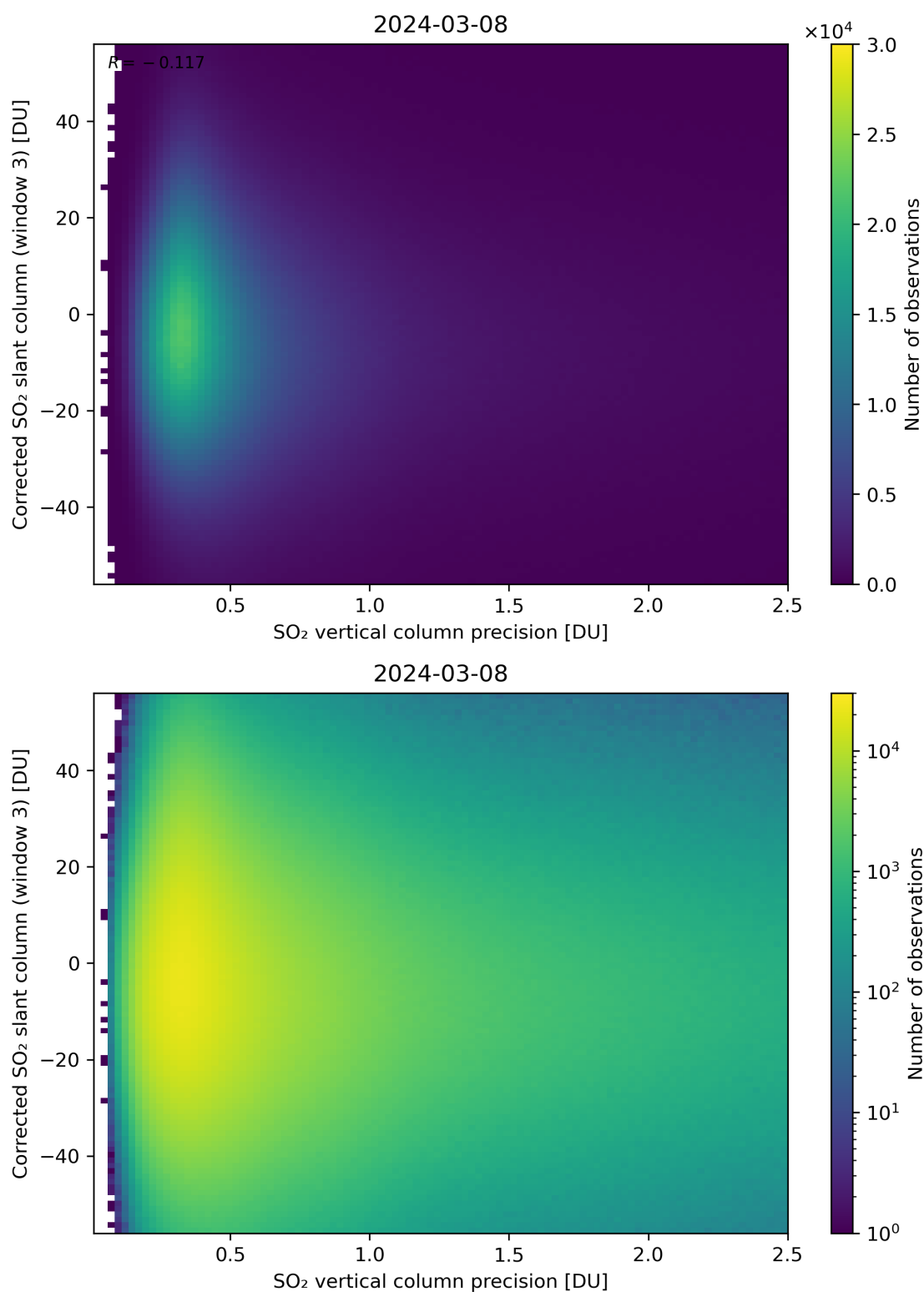
Figure 288: Scatter density plot of “SO 2 vertical column precision” against “Corrected SO 2 slant column (window 3)” for 2024-03-07 to 2024-03-09.
