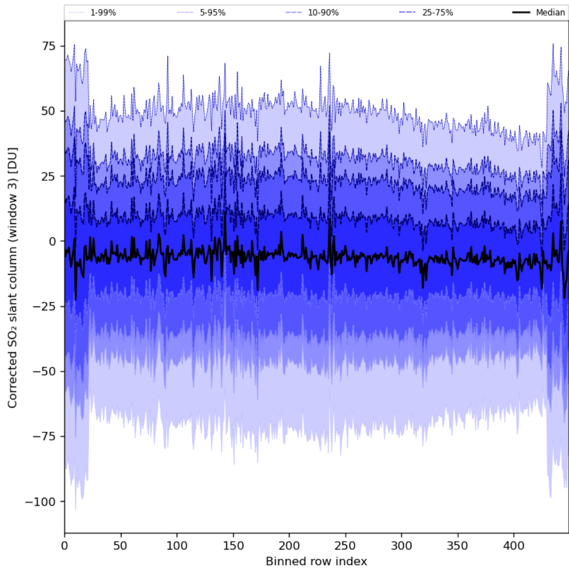
Figure 89: Along track statistics of “Corrected SO 2 slant column (window 3)” for 2024-03-07 to 2024-03-09
