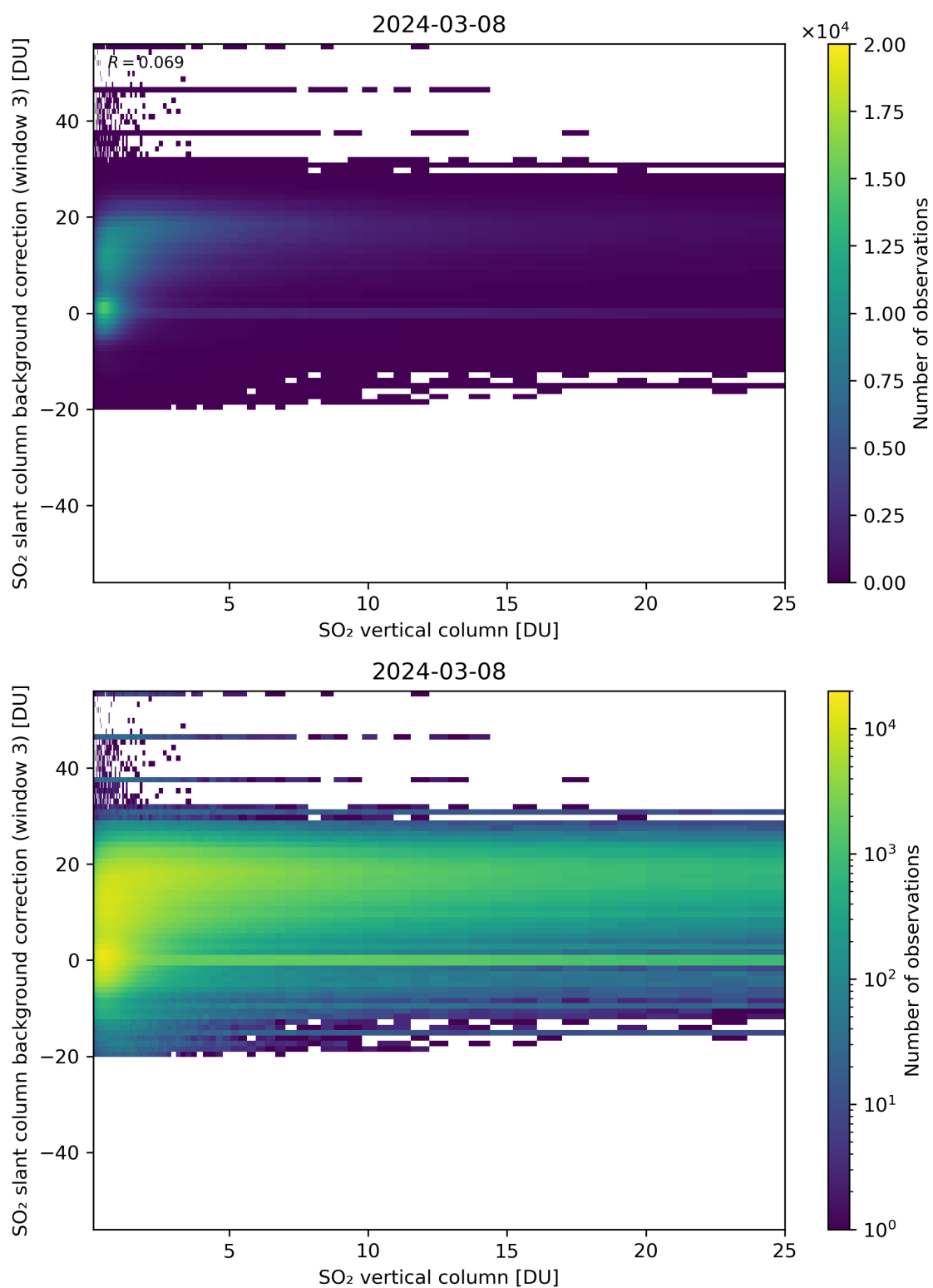
Figure 275: Scatter density plot of “SO 2 vertical column” against “SO 2 slant column background correction (window 3)” for 2024-03-07 to 2024-03-09.
