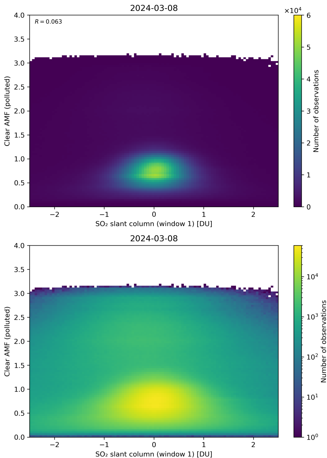
Figure 232: Scatter density plot of “SO 2 slant column (window 1)” against “Clear AMF (polluted)” for 2024-03-07 to 2024-03-09.
