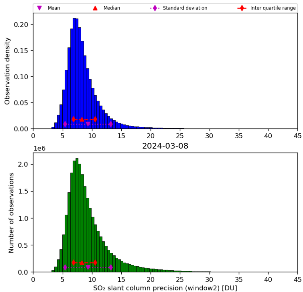
Figure 61: Histogram of “SO 2 slant column precision (window2)” for 2024-03-07 to 2024-03-09
