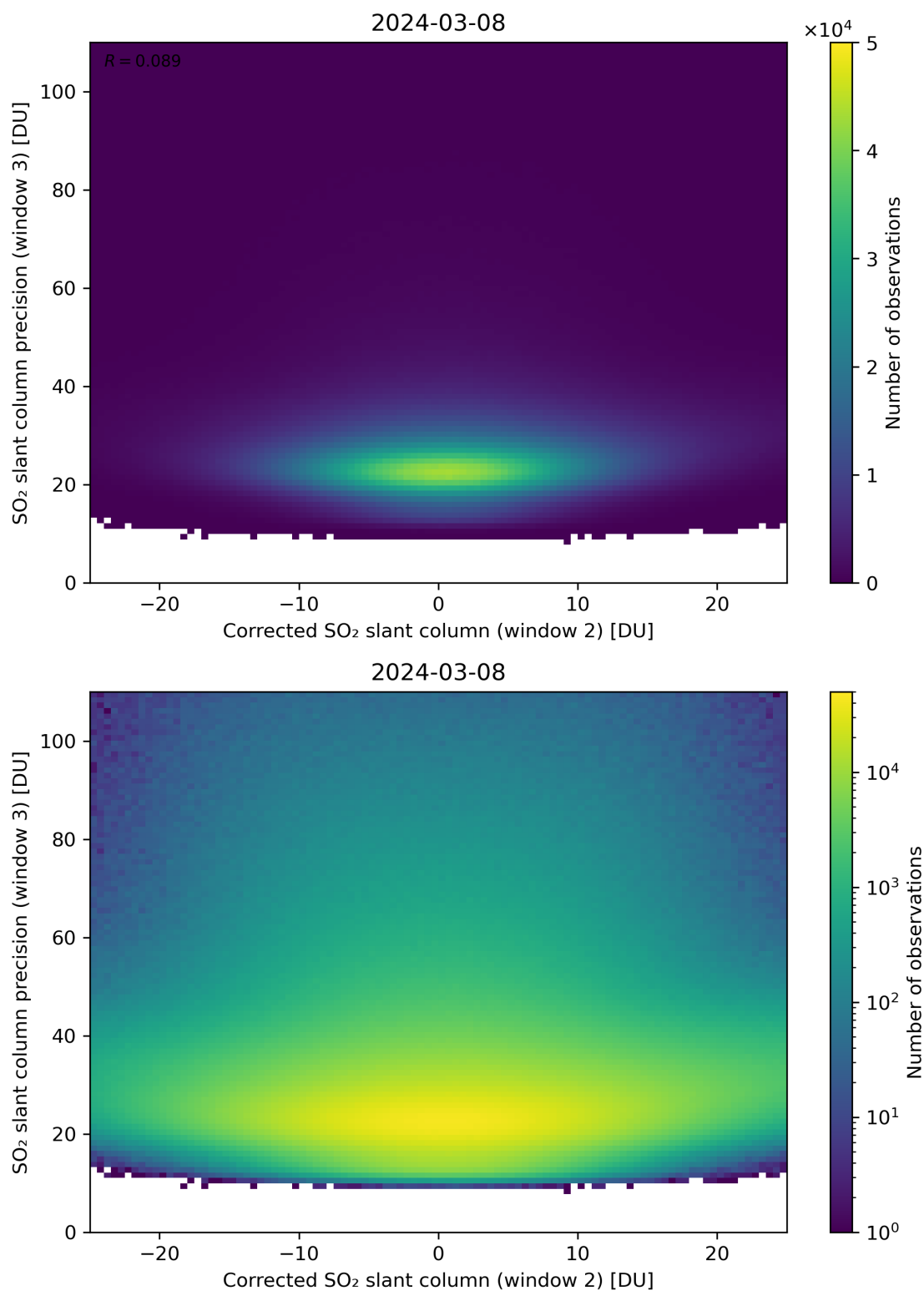
Figure 202: Scatter density plot of “Corrected SO 2 slant column (window 2)” against “SO 2 slant column precision (window 3)” for 2024-03-07 to 2024-03-09.
