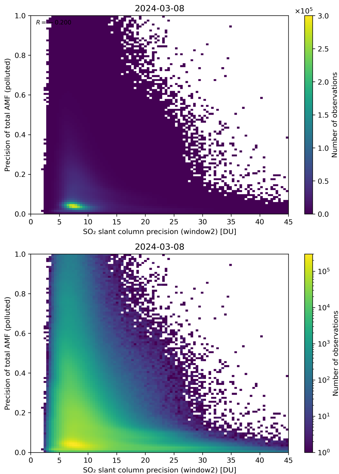
Figure 252: Scatter density plot of “SO 2 slant column precision (window2)” against “Precision of total AMF (polluted)” for 2024-03-07 to 2024-03-09.
