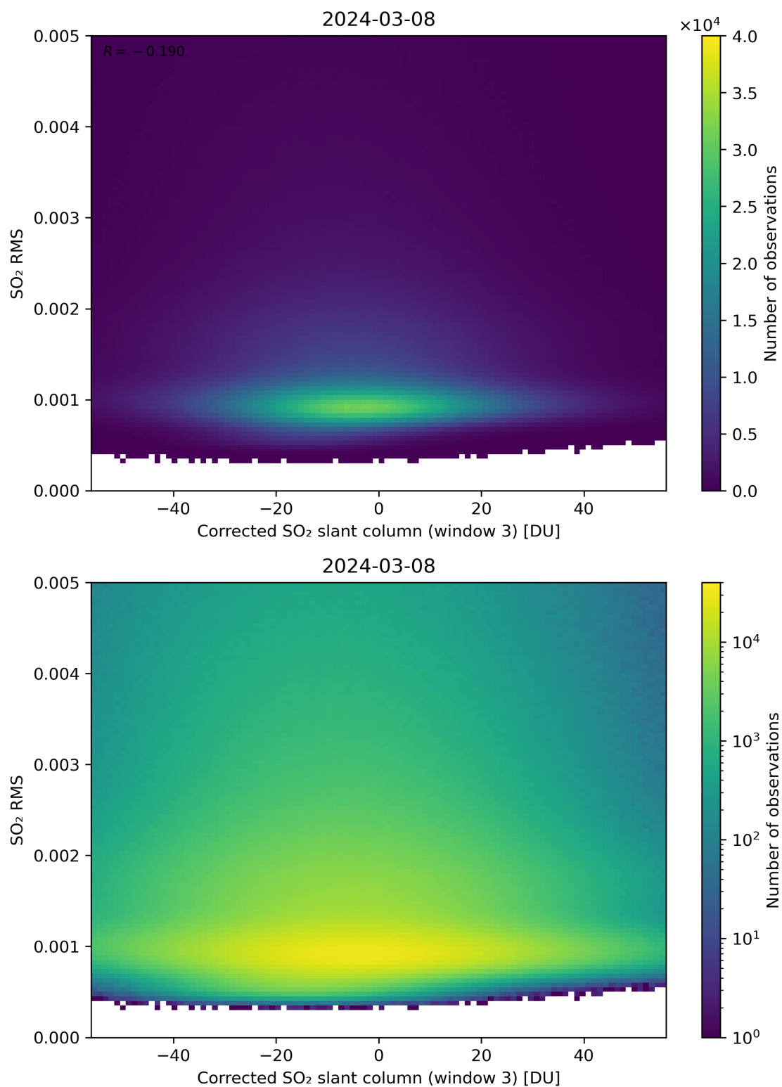
Figure 208: Scatter density plot of “Corrected SO 2 slant column (window 3)” against “SO 2 RMS” for 2024-03-07 to 2024-03-09.
