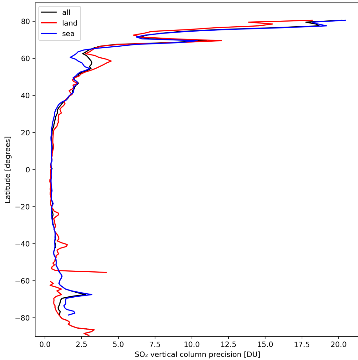
Figure 31: Zonal average of “SO 2 vertical column precision” for 2024-03-07 to 2024-03-09.
