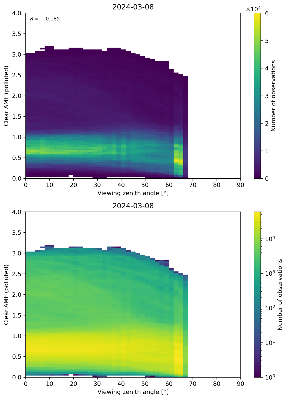
Figure 316: Scatter density plot of “Viewing zenith angle” against “Clear AMF (polluted)” for 2024-03-07 to 2024-03-09.
