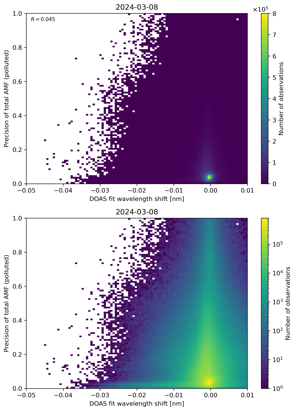
Figure 131: Scatter density plot of “DOAS fit wavelength shift” against “Precision of total AMF (polluted)” for 2024-03-07 to 2024-03-09.
