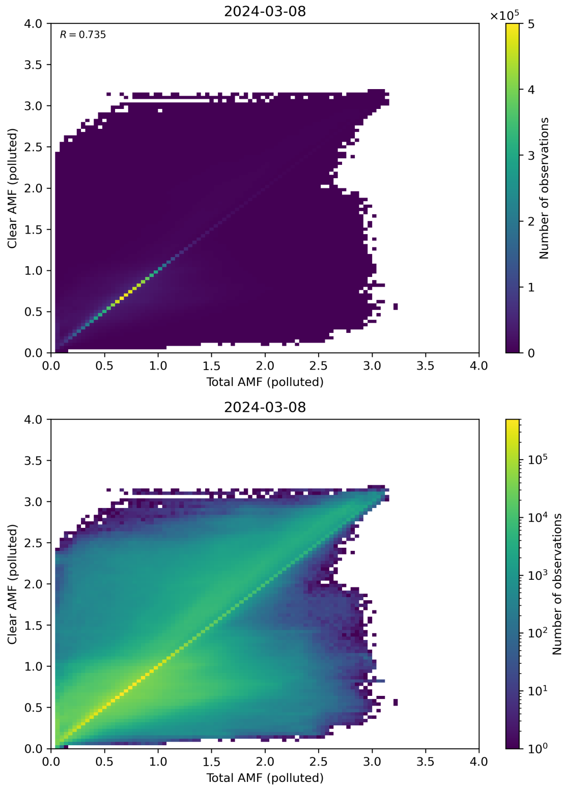
Figure 271: Scatter density plot of “Total AMF (polluted)” against “Clear AMF (polluted)” for 2024-03-07 to 2024-03-09.
