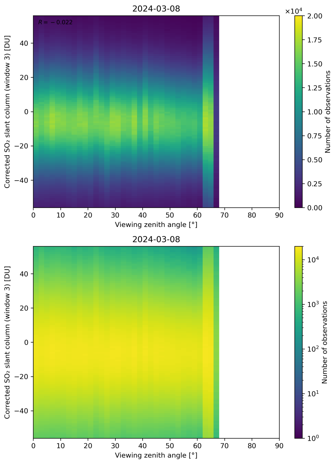
Figure 319: Scatter density plot of “Viewing zenith angle” against “Corrected SO 2 slant column (window 3)” for 2024-03-07 to 2024-03-09.
