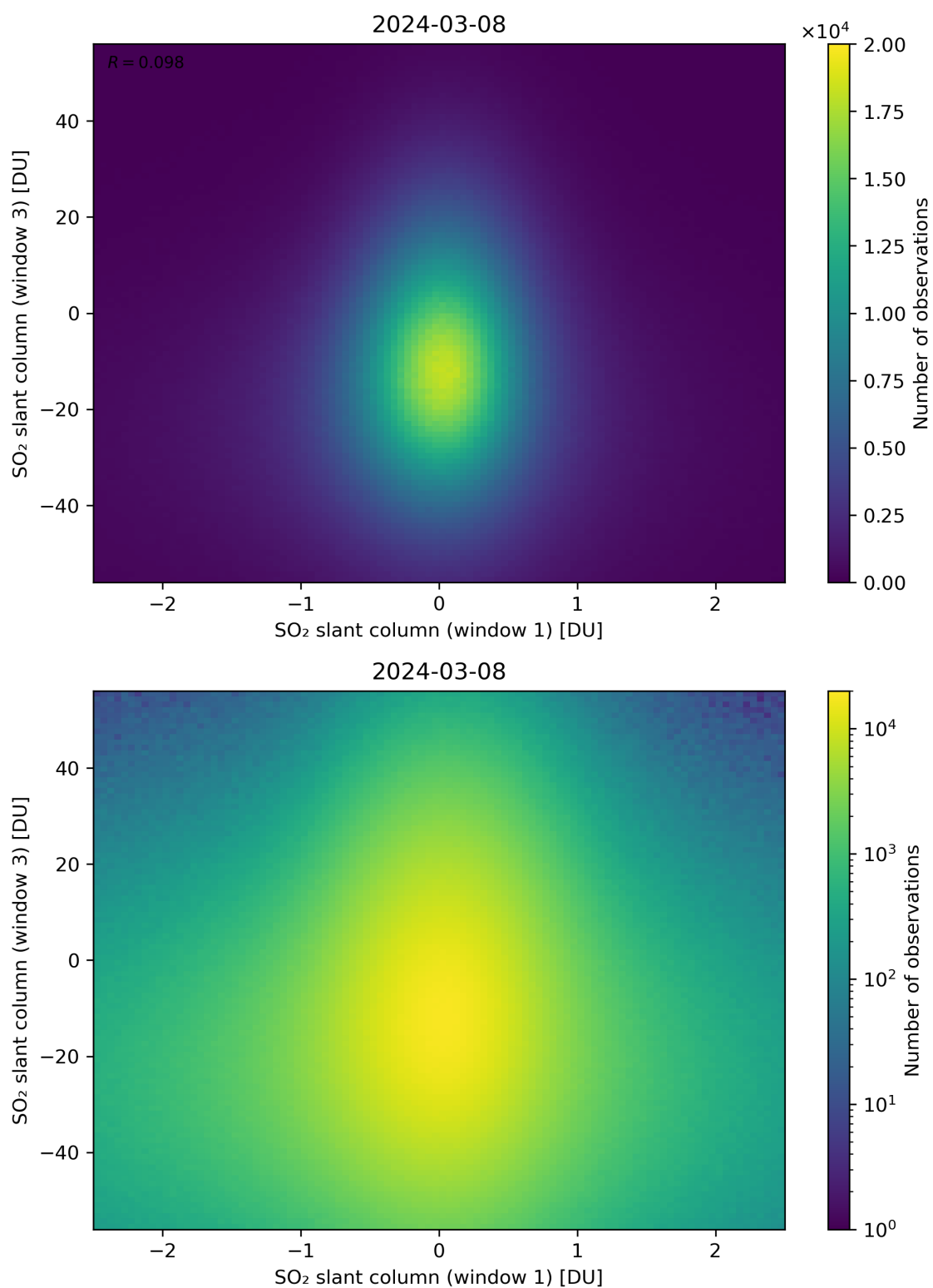
Figure 237: Scatter density plot of “SO 2 slant column (window 1)” against “SO 2 slant column (window 3)” for 2024-03-07 to 2024-03-09.
