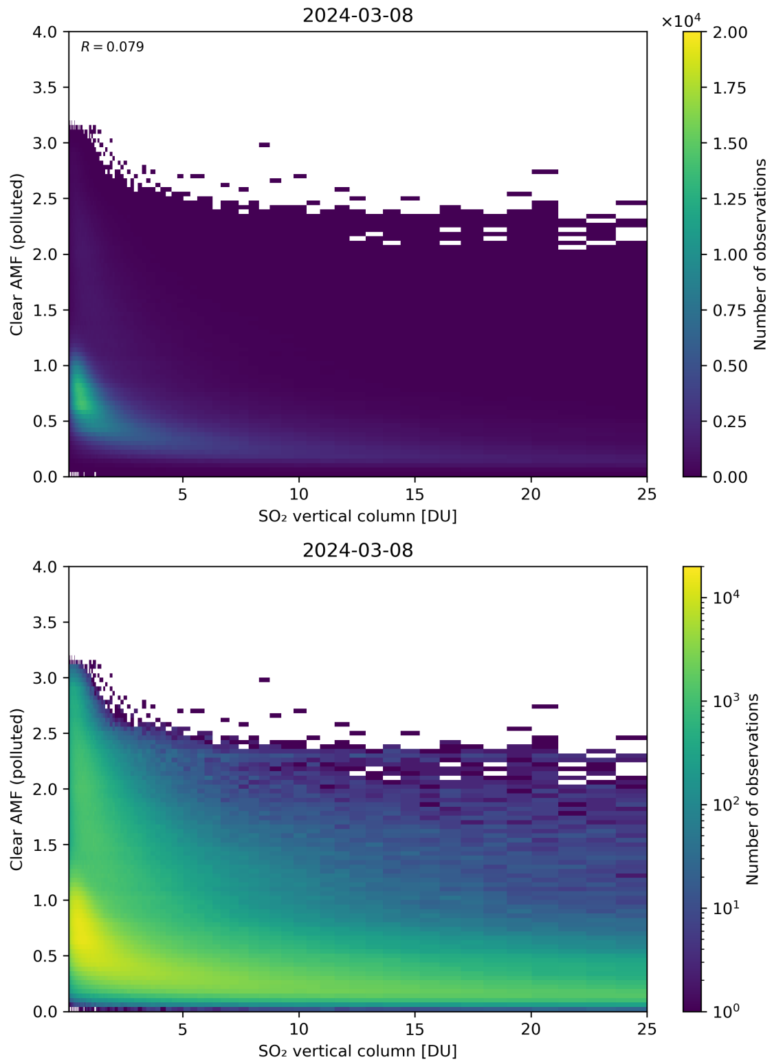
Figure 296: Scatter density plot of “SO 2 vertical column” against “Clear AMF (polluted)” for 2024-03-07 to 2024-03-09.
