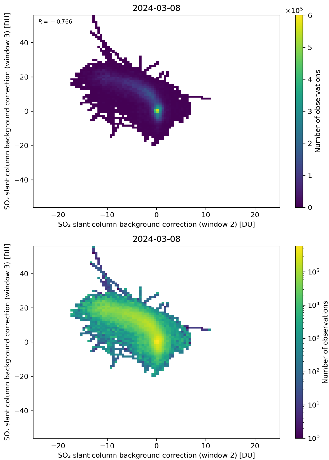
Figure 111: Scatter density plot of “SO 2 slant column background correction (window 2)” against “SO 2 slant column background correction (window 3)” for 2024-03-07 to 2024-03-09.
