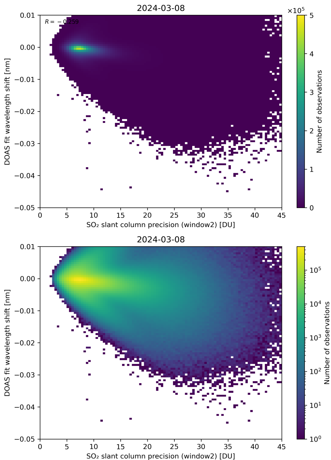
Figure 243: Scatter density plot of “SO 2 slant column precision (window2)” against “DOAS fit wavelength shift” for 2024-03-07 to 2024-03-09.
