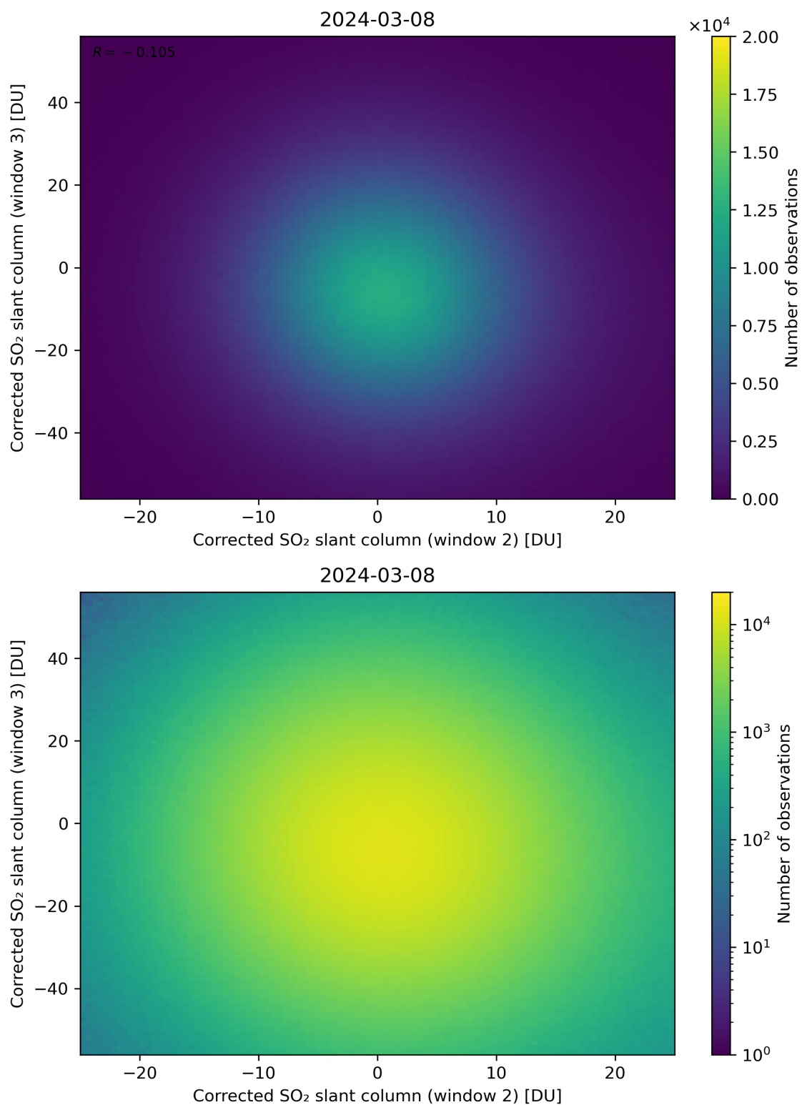
Figure 200: Scatter density plot of “Corrected SO 2 slant column (window 2)” against “Corrected SO 2 slant column (window 3)” for 2024-03-07 to 2024-03-09.
