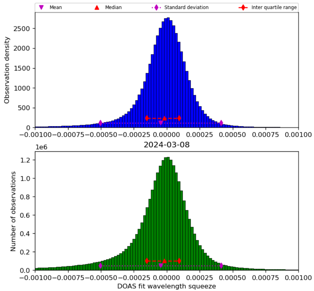
Figure 69: Histogram of “DOAS fit wavelength squeeze” for 2024-03-07 to 2024-03-09
