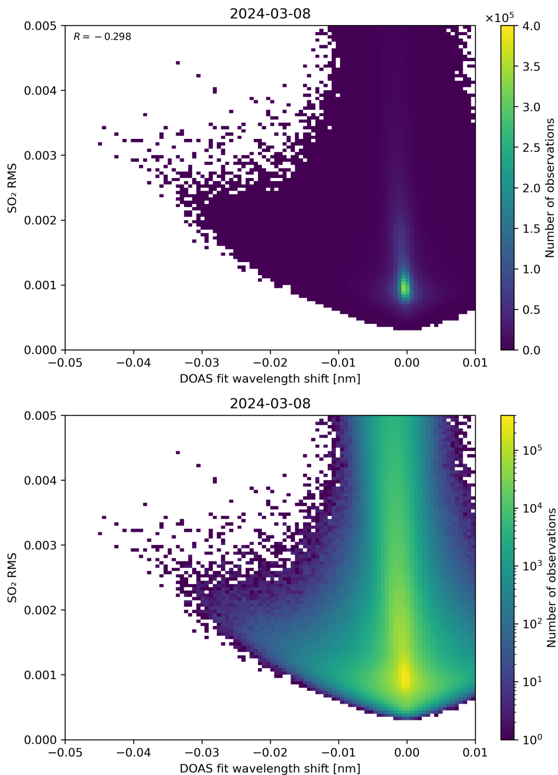
Figure 128: Scatter density plot of “DOAS fit wavelength shift” against “SO 2 RMS” for 2024-03-07 to 2024-03-09.
