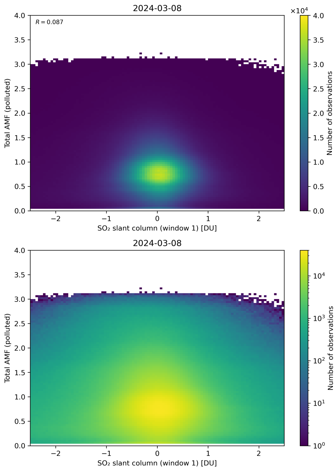
Figure 239: Scatter density plot of “SO 2 slant column (window 1)” against “Total AMF (polluted)” for 2024-03-07 to 2024-03-09.
