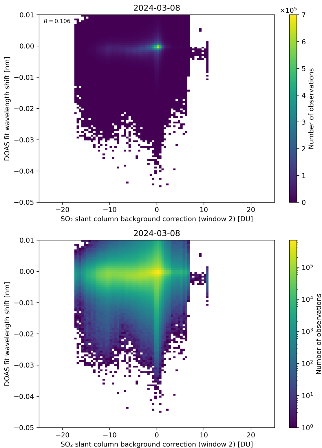
Figure 112: Scatter density plot of “SO 2 slant column background correction (window 2)” against “DOAS fit wavelength shift” for 2024-03-07 to 2024-03-09.
