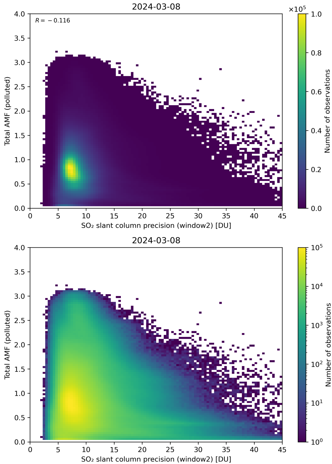
Figure 251: Scatter density plot of “SO 2 slant column precision (window2)” against “Total AMF (polluted)” for 2024-03-07 to 2024-03-09.
