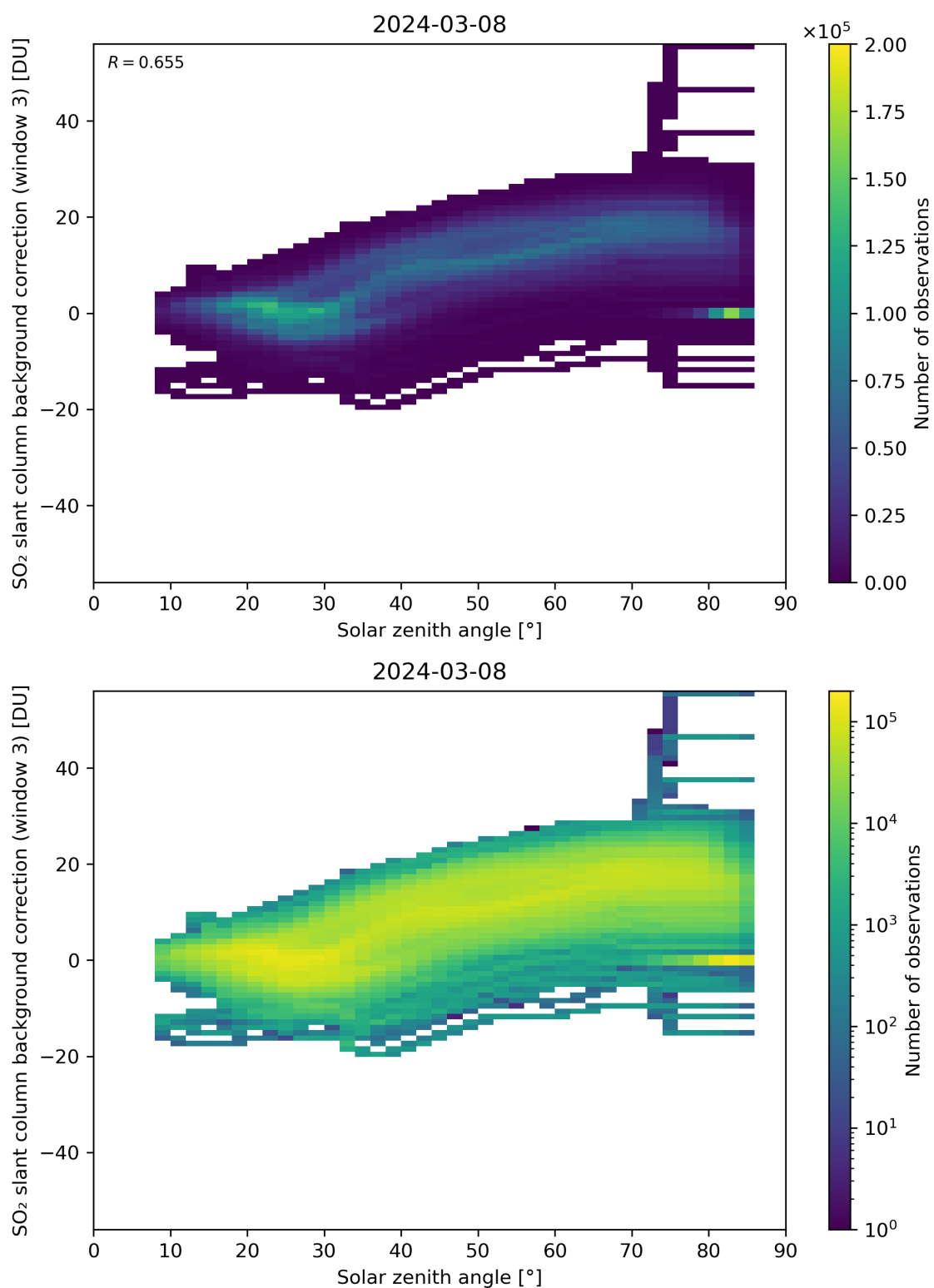
Figure 160: Scatter density plot of “Solar zenith angle” against “SO 2 slant column background correction (window 3)” for 2024-03-07 to 2024-03-09.
