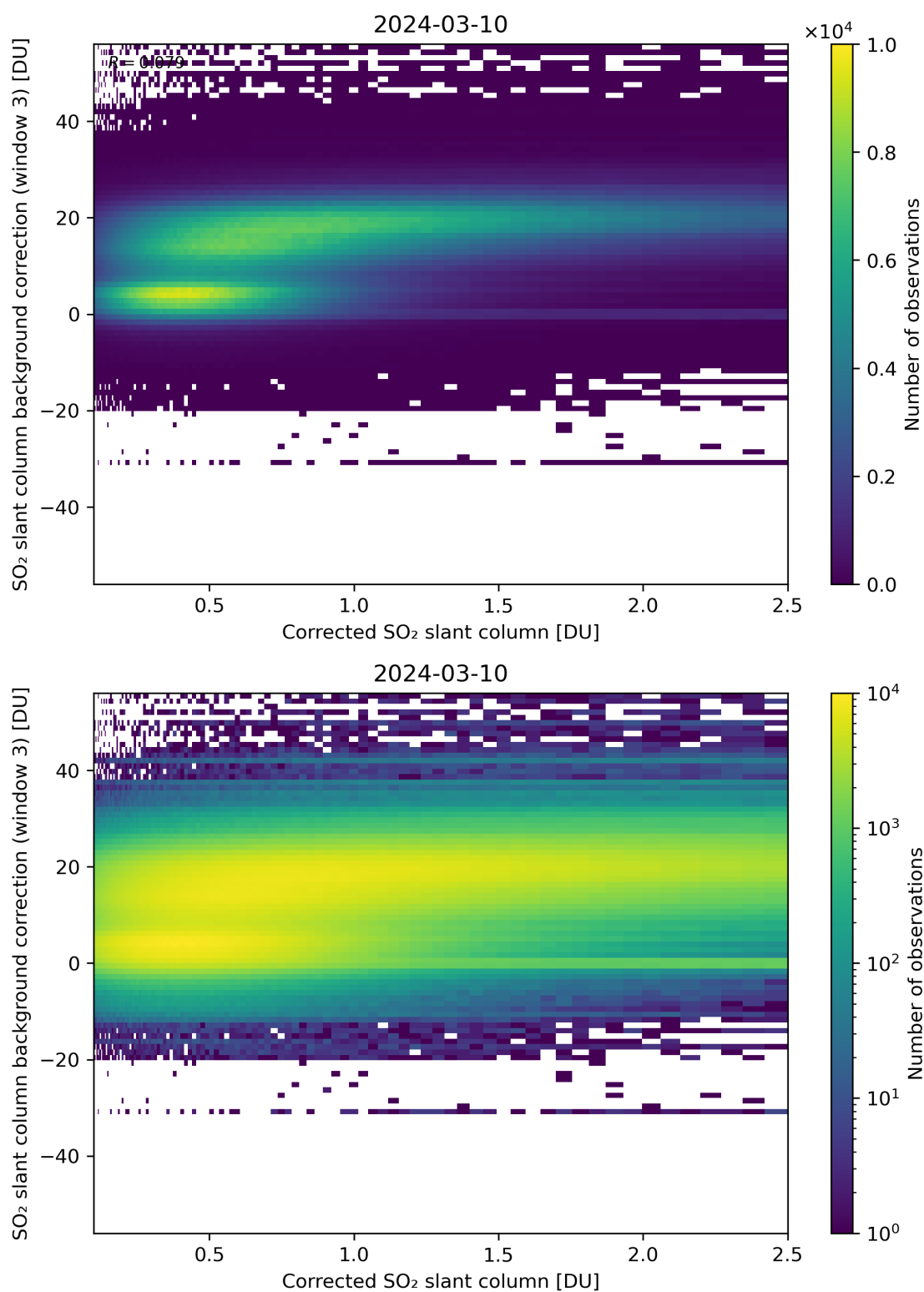
Figure 180: Scatter density plot of “Corrected SO 2 slant column” against “SO 2 slant column background correction (window 3)” for 2024-03-09 to 2024-03-11.
