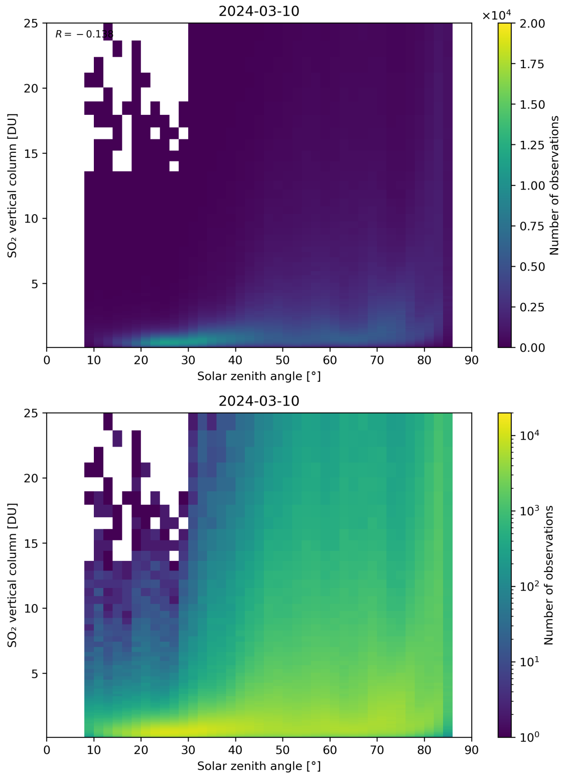
Figure 176: Scatter density plot of “Solar zenith angle” against “SO 2 vertical column” for 2024-03-09 to 2024-03-11.
