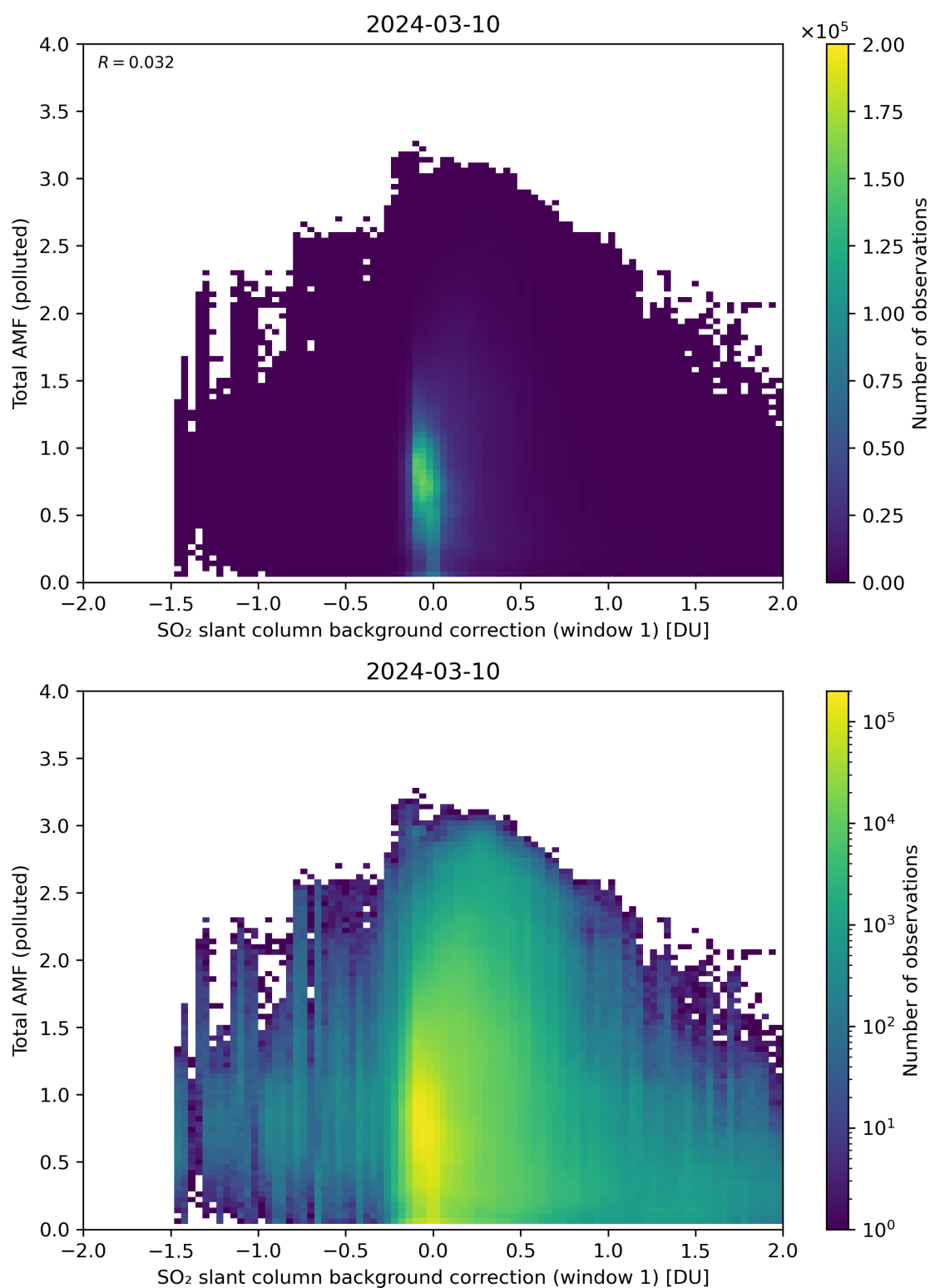
Figure 109: Scatter density plot of “SO 2 slant column background correction (window 1)” against “Total AMF (polluted)” for 2024-03-09 to 2024-03-11.
