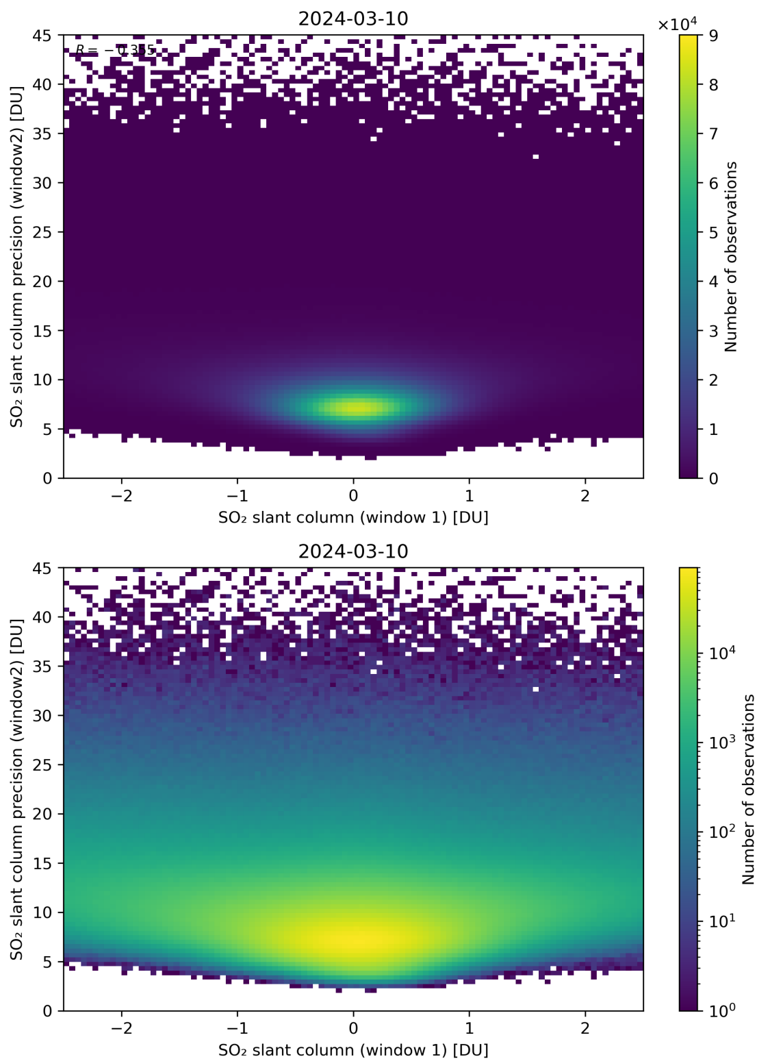
Figure 236: Scatter density plot of “SO 2 slant column (window 1)” against “SO 2 slant column precision (window2)” for 2024-03-09 to 2024-03-11.
