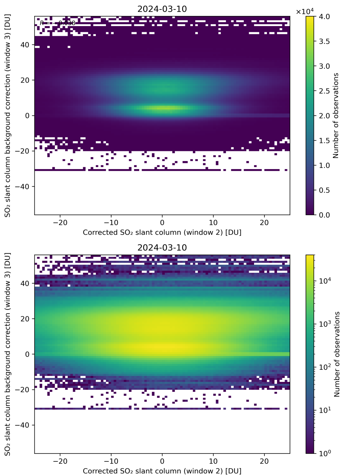
Figure 195: Scatter density plot of “Corrected SO 2 slant column (window 2)” against “SO 2 slant column background correction (window 3)” for 2024-03-09 to 2024-03-11.
