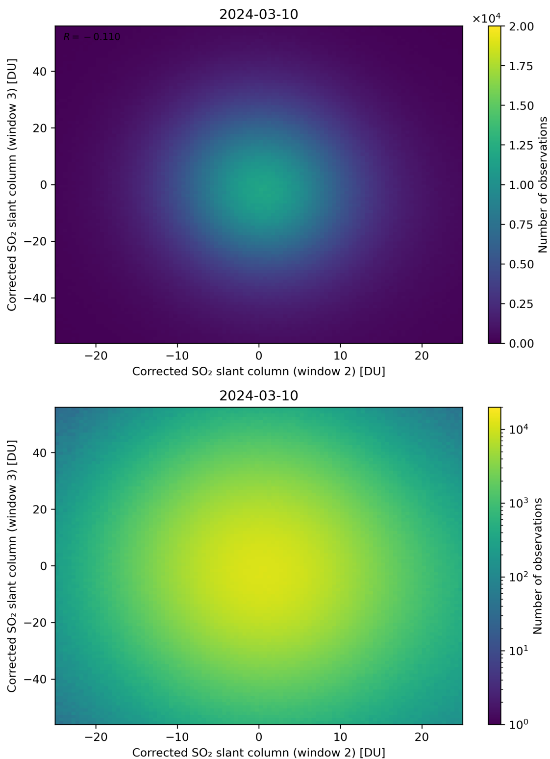
Figure 200: Scatter density plot of “Corrected SO 2 slant column (window 2)” against “Corrected SO 2 slant column (window 3)” for 2024-03-09 to 2024-03-11.
