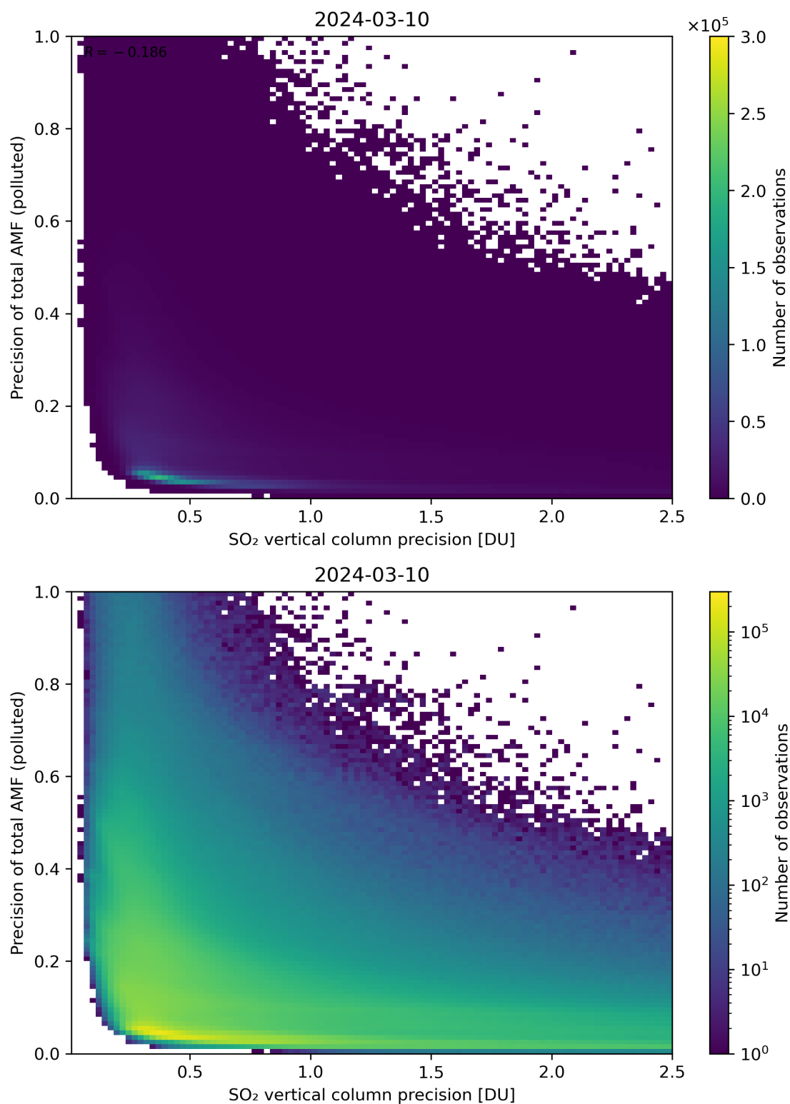
Figure 295: Scatter density plot of “SO 2 vertical column precision” against “Precision of total AMF (polluted)” for 2024-03-09 to 2024-03-11.
