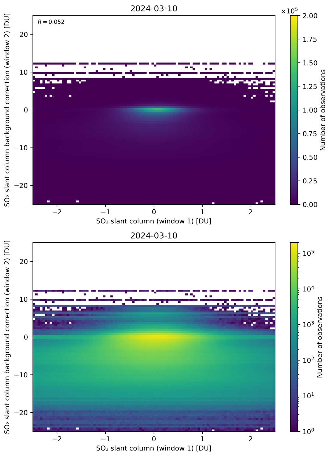
Figure 213: Scatter density plot of “SO 2 slant column (window 1)” against “SO 2 slant column background correction (window 2)” for 2024-03-09 to 2024-03-11.
