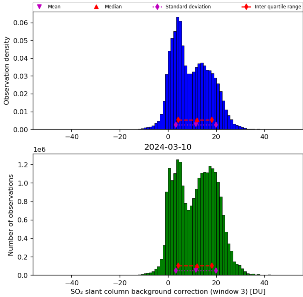
Figure 67: Histogram of “SO 2 slant column background correction (window 3)” for 2024-03-09 to 2024-03-11
