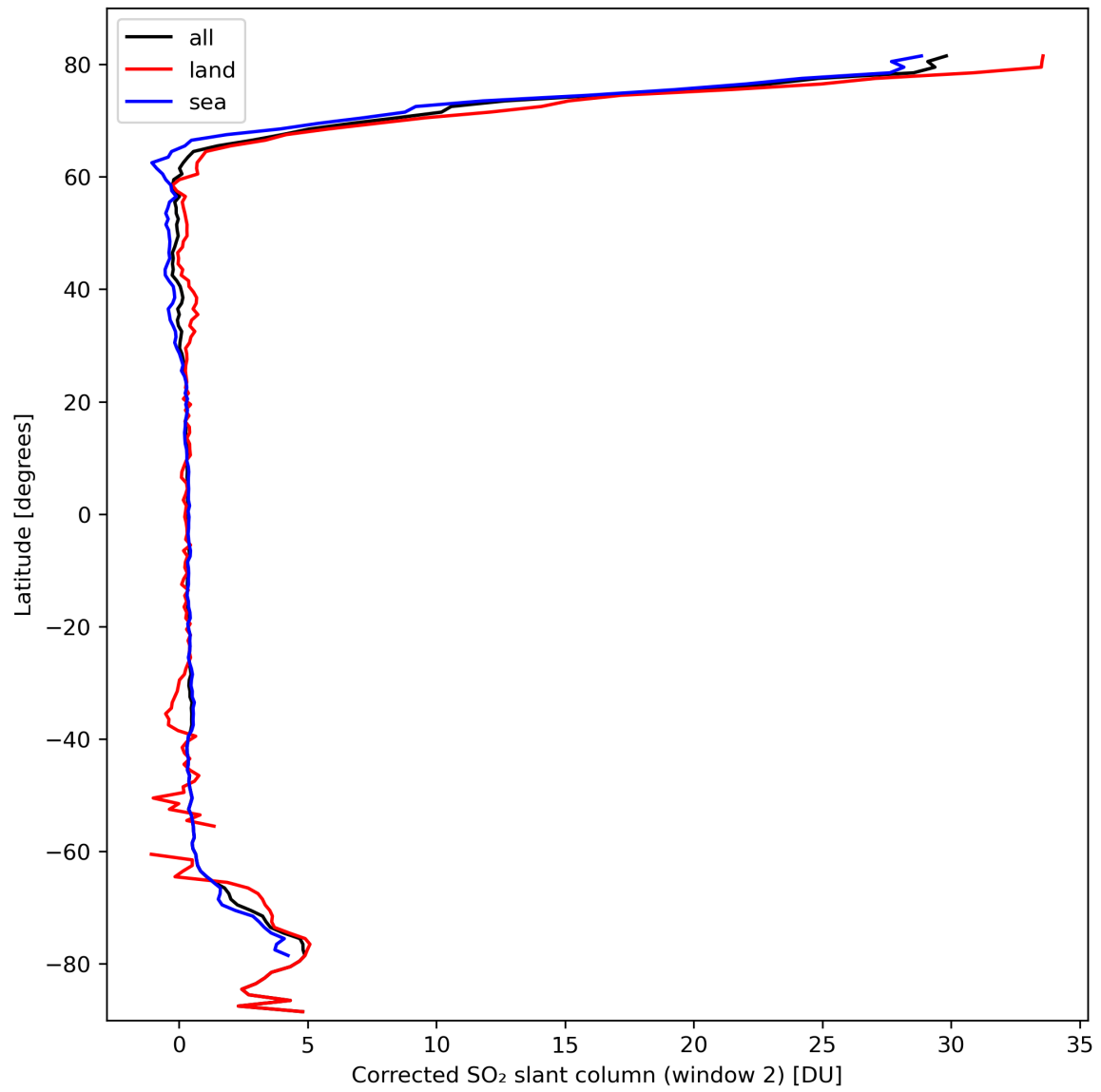
Figure 39: Zonal average of “Corrected SO 2 slant column (window 2)” for 2024-03-09 to 2024-03-11.
