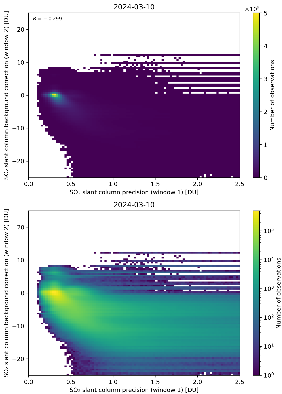
Figure 219: Scatter density plot of “SO 2 slant column precision (window 1)” against “SO 2 slant column background correction (window 2)” for 2024-03-09 to 2024-03-11.
