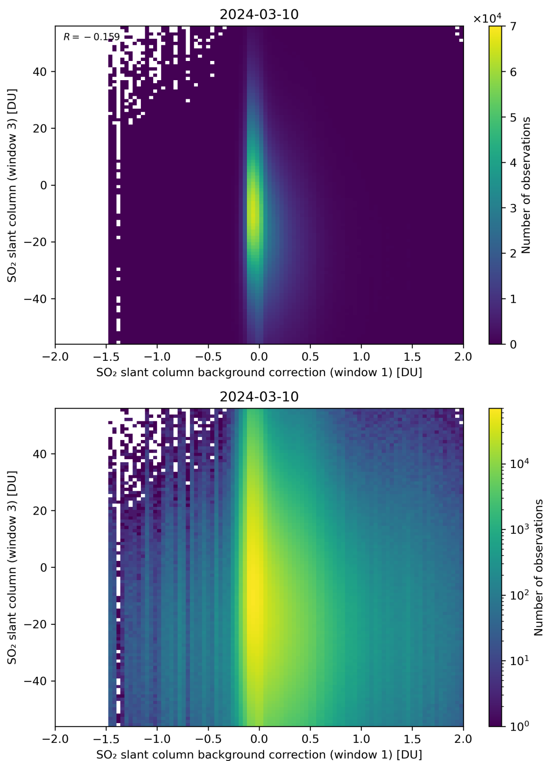
Figure 107: Scatter density plot of “SO 2 slant column background correction (window 1)” against “SO 2 slant column (window 3)” for 2024-03-09 to 2024-03-11.
