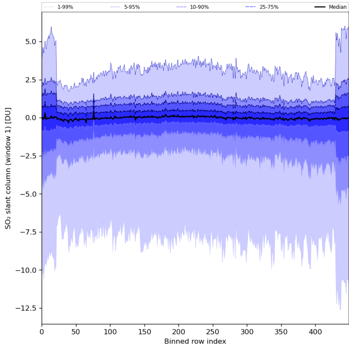
Figure 79: Along track statistics of “SO 2 slant column (window 1)” for 2024-03-09 to 2024-03-11
