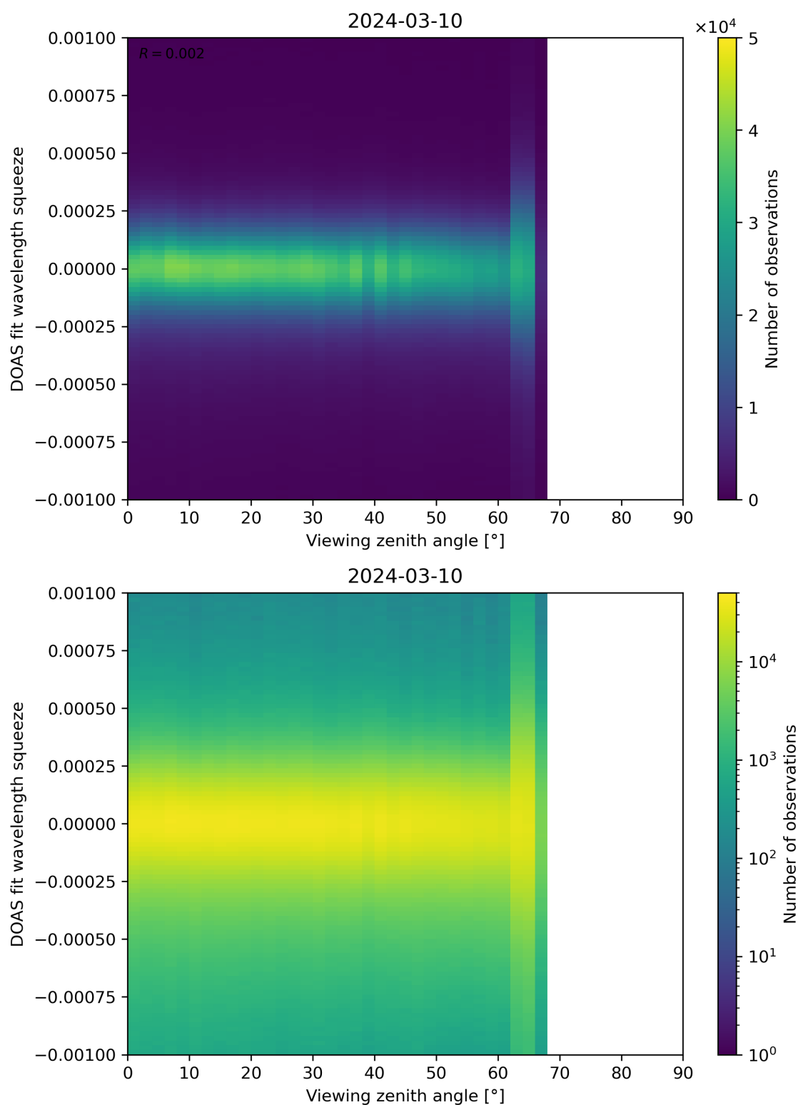
Figure 312: Scatter density plot of “Viewing zenith angle” against “DOAS fit wavelength squeeze” for 2024-03-09 to 2024-03-11.
