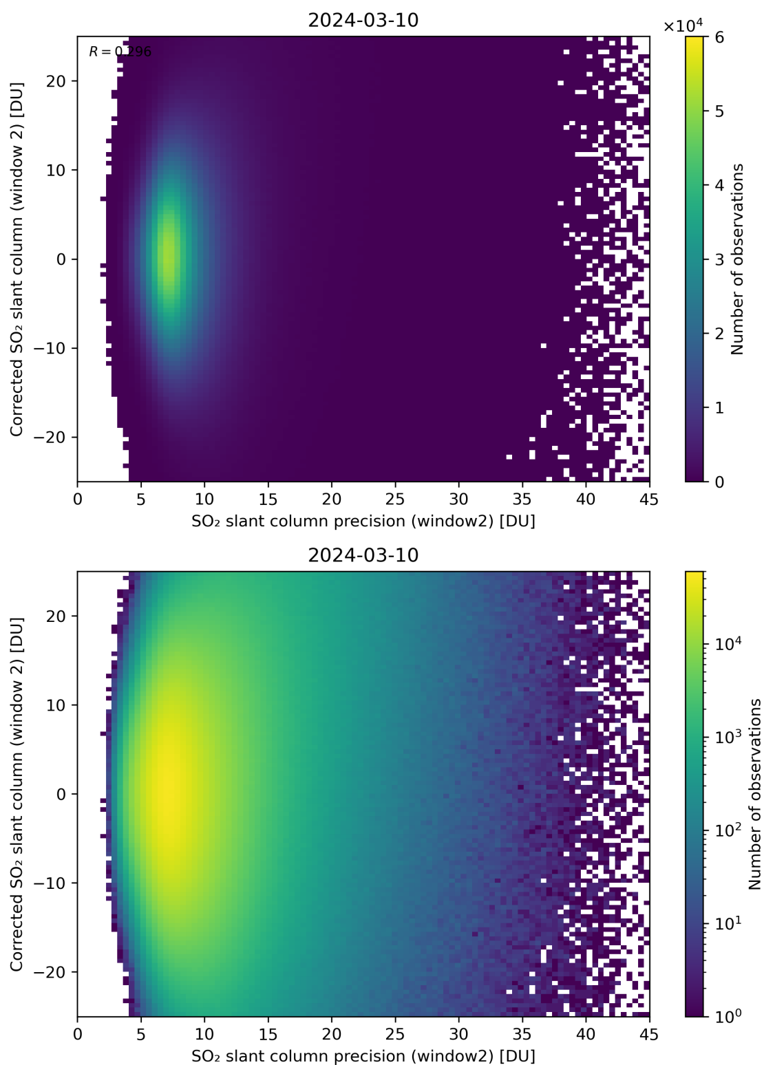
Figure 247: Scatter density plot of “SO 2 slant column precision (window2)” against “Corrected SO 2 slant column (window 2)” for 2024-03-09 to 2024-03-11.
