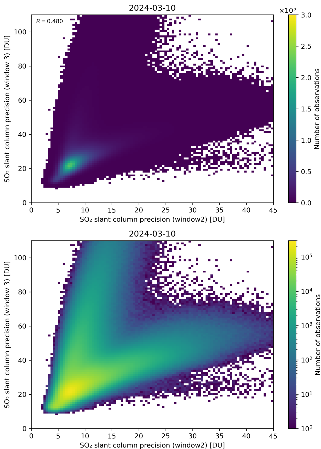
Figure 250: Scatter density plot of “SO 2 slant column precision (window2)” against “SO 2 slant column precision (window 3)” for 2024-03-09 to 2024-03-11.
