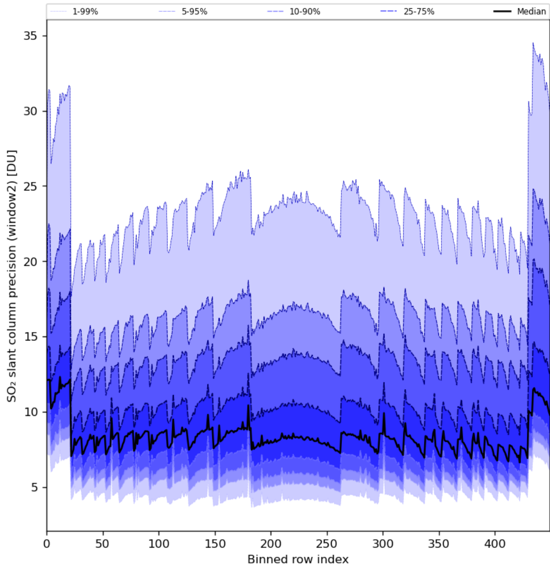
Figure 84: Along track statistics of “SO 2 slant column precision (window2)” for 2024-03-09 to 2024-03-11
