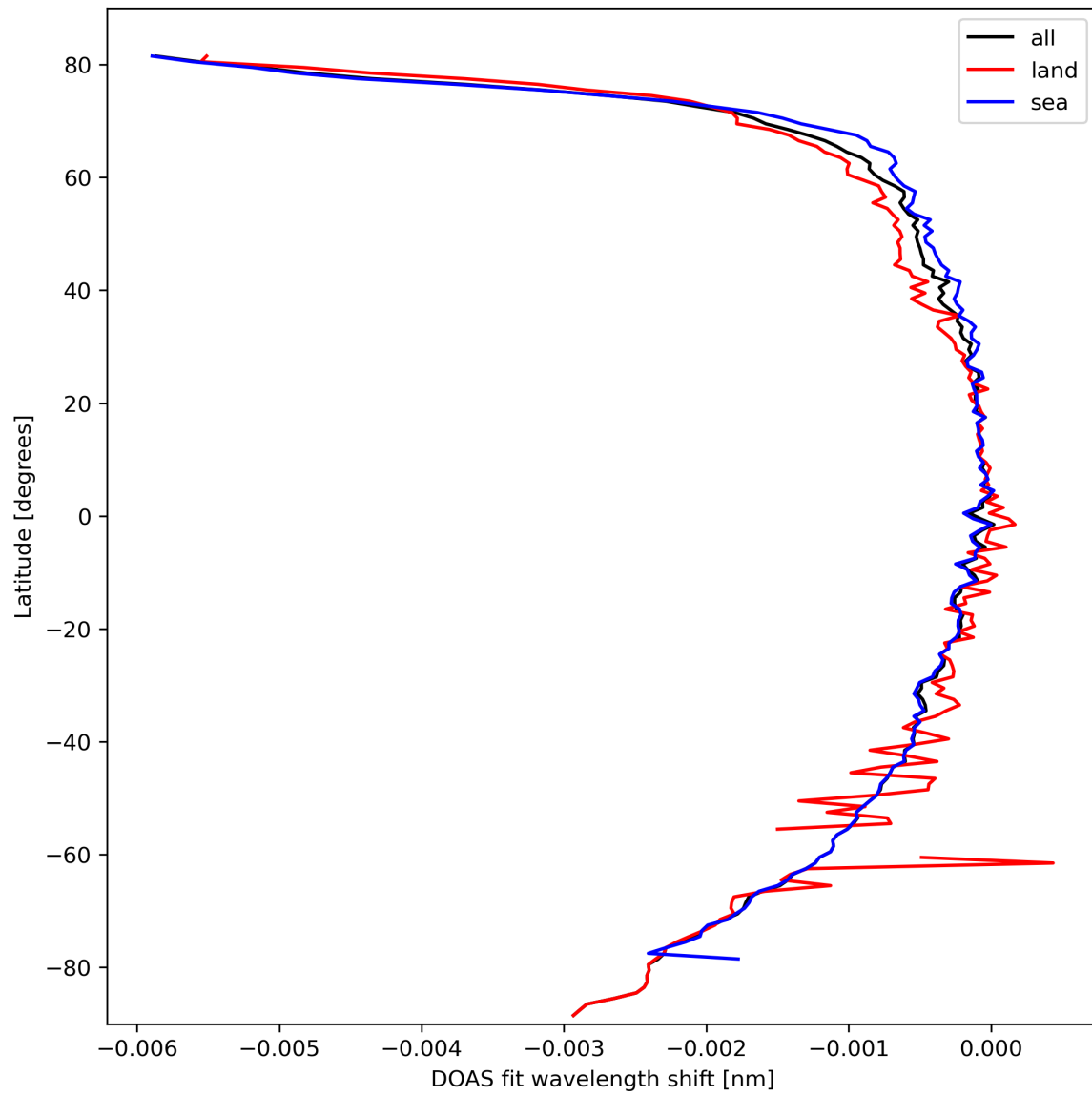
Figure 45: Zonal average of “DOAS fit wavelength shift” for 2024-03-09 to 2024-03-11.
