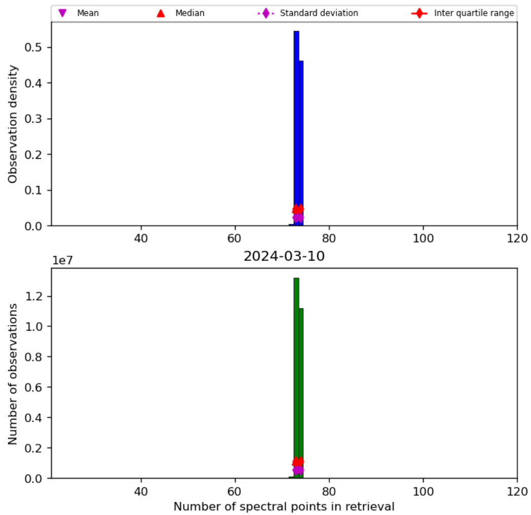
Figure 74: Histogram of “Number of spectral points in retrieval” for 2024-03-09 to 2024-03-11
