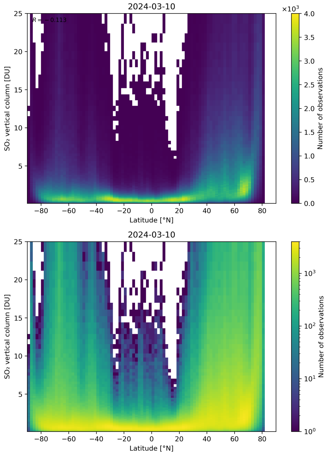
Figure 156: Scatter density plot of “Latitude” against “SO 2 vertical column” for 2024-03-09 to 2024-03-11.
