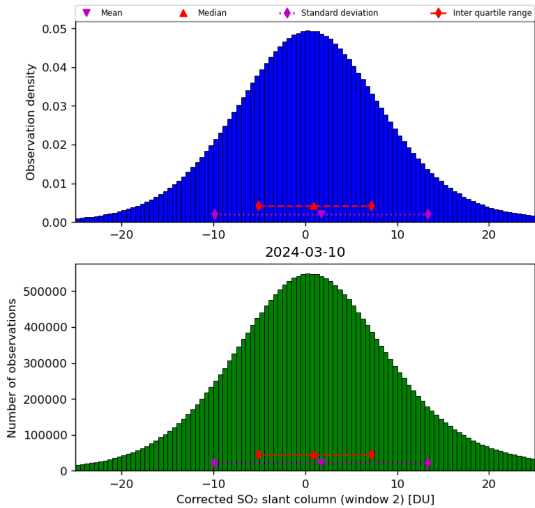
Figure 62: Histogram of "Corrected SO 2 slant column (window 2)" for 2024-03-09 to 2024-03-11
