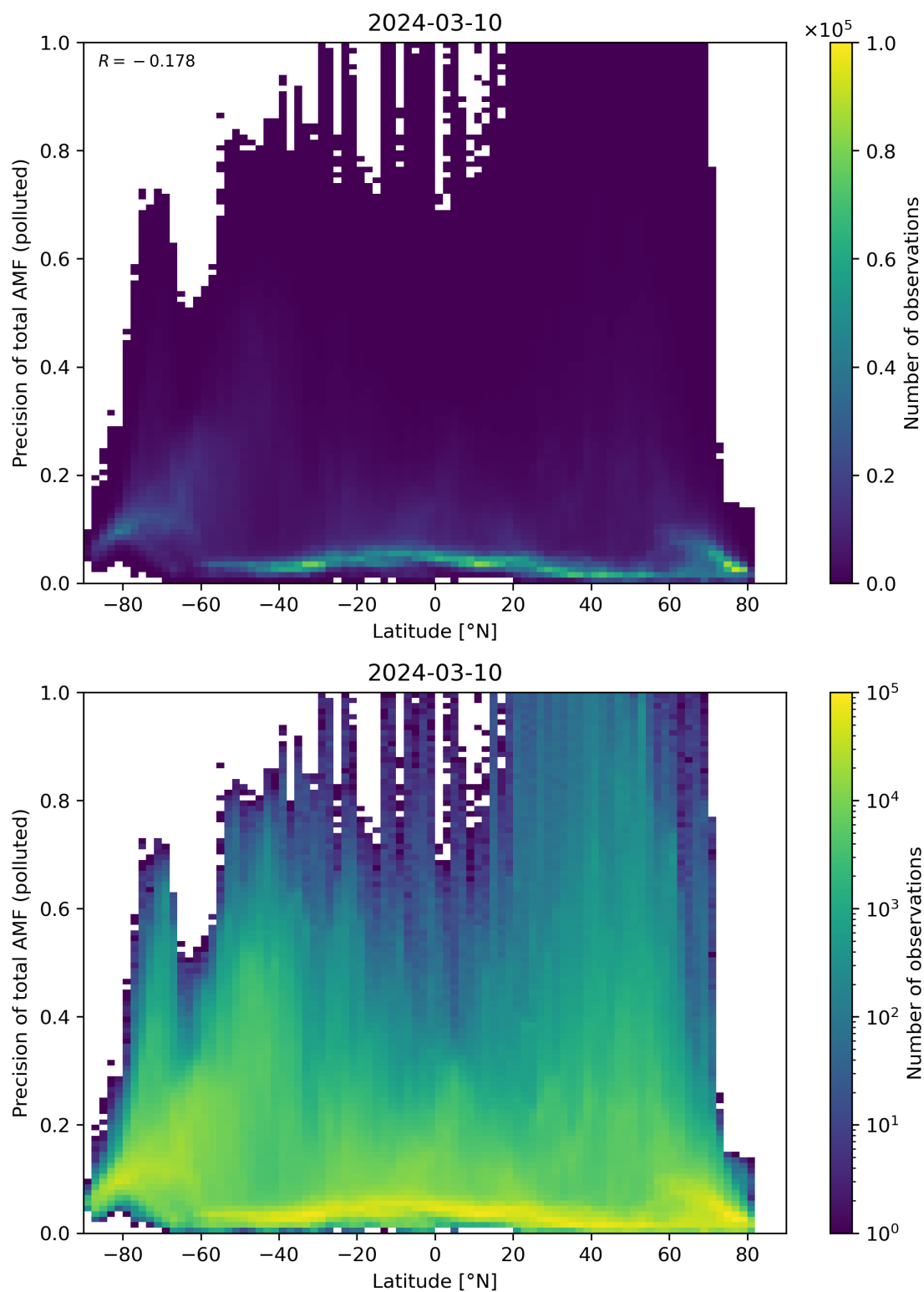
Figure 155: Scatter density plot of “Latitude” against “Precision of total AMF (polluted)” for 2024-03-09 to 2024-03-11.
