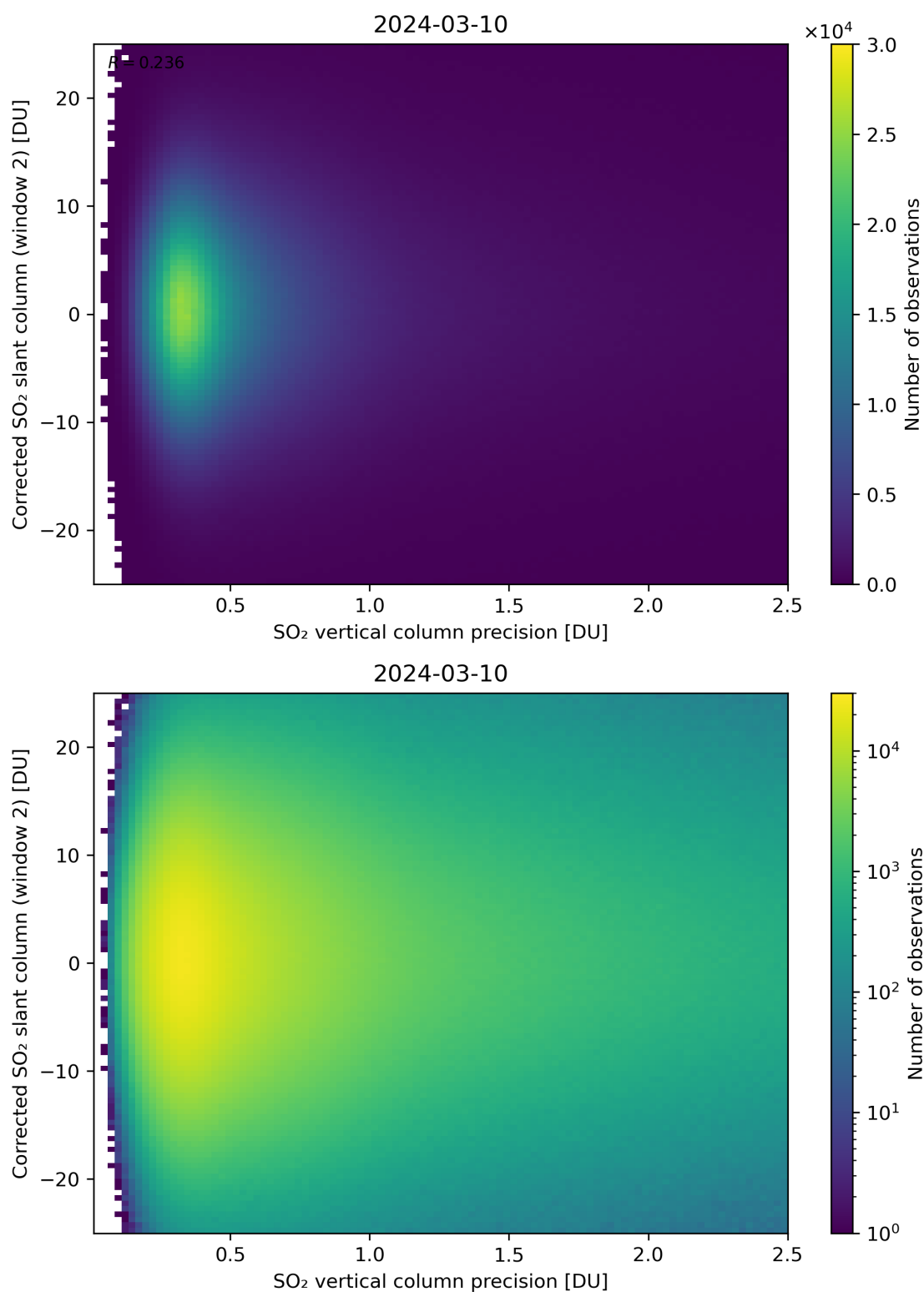
Figure 287: Scatter density plot of “SO 2 vertical column precision” against “Corrected SO 2 slant column (window 2)” for 2024-03-09 to 2024-03-11.
