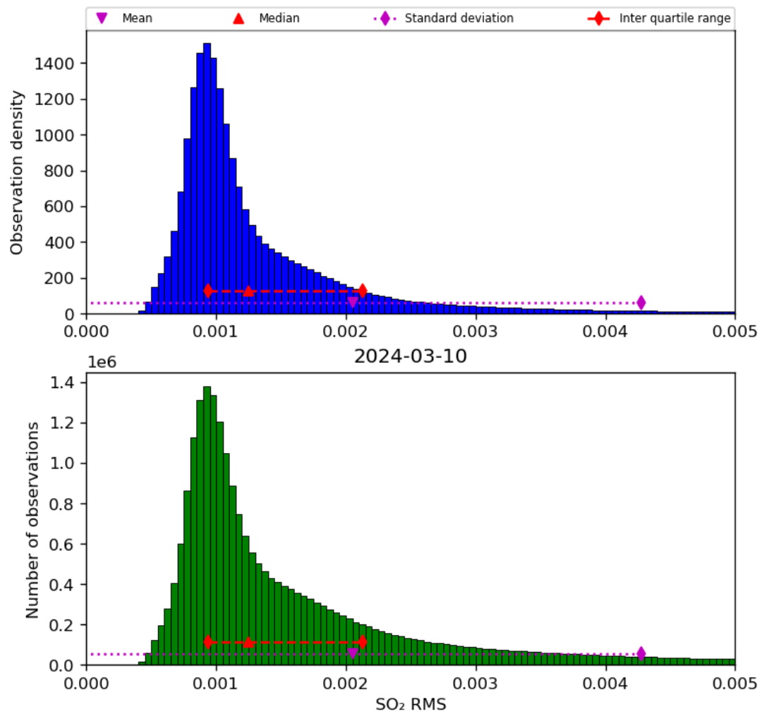
Figure 70: Histogram of “SO 2 RMS” for 2024-03-09 to 2024-03-11
