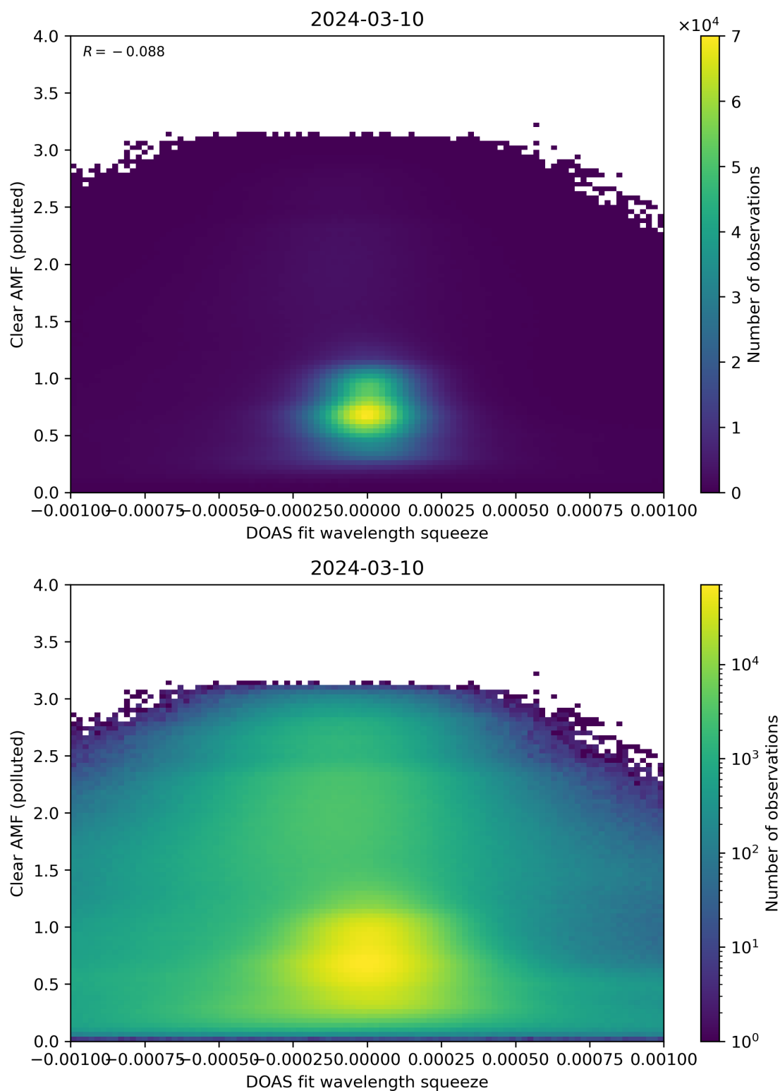
Figure 133: Scatter density plot of “DOAS fit wavelength squeeze” against “Clear AMF (polluted)” for 2024-03-09 to 2024-03-11.
