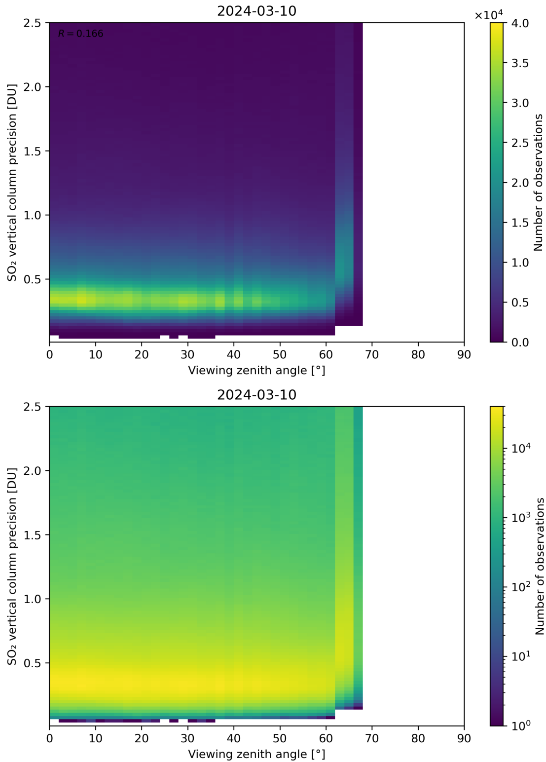
Figure 328: Scatter density plot of “Viewing zenith angle” against “SO 2 vertical column precision” for 2024-03-09 to 2024-03-11.
