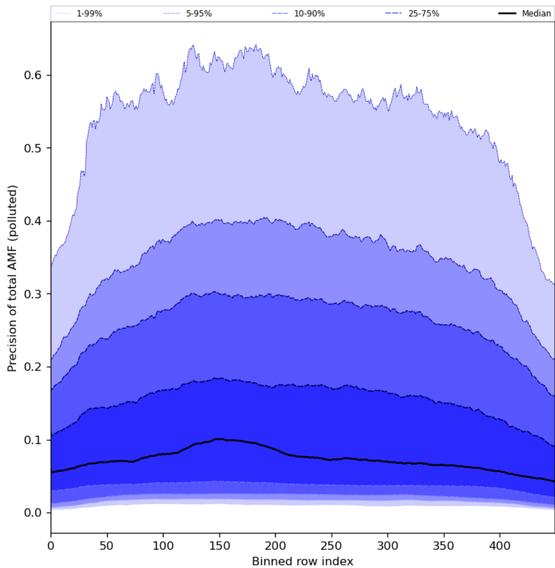
Figure 95: Along track statistics of “Precision of total AMF (polluted)” for 2024-03-09 to 2024-03-11
