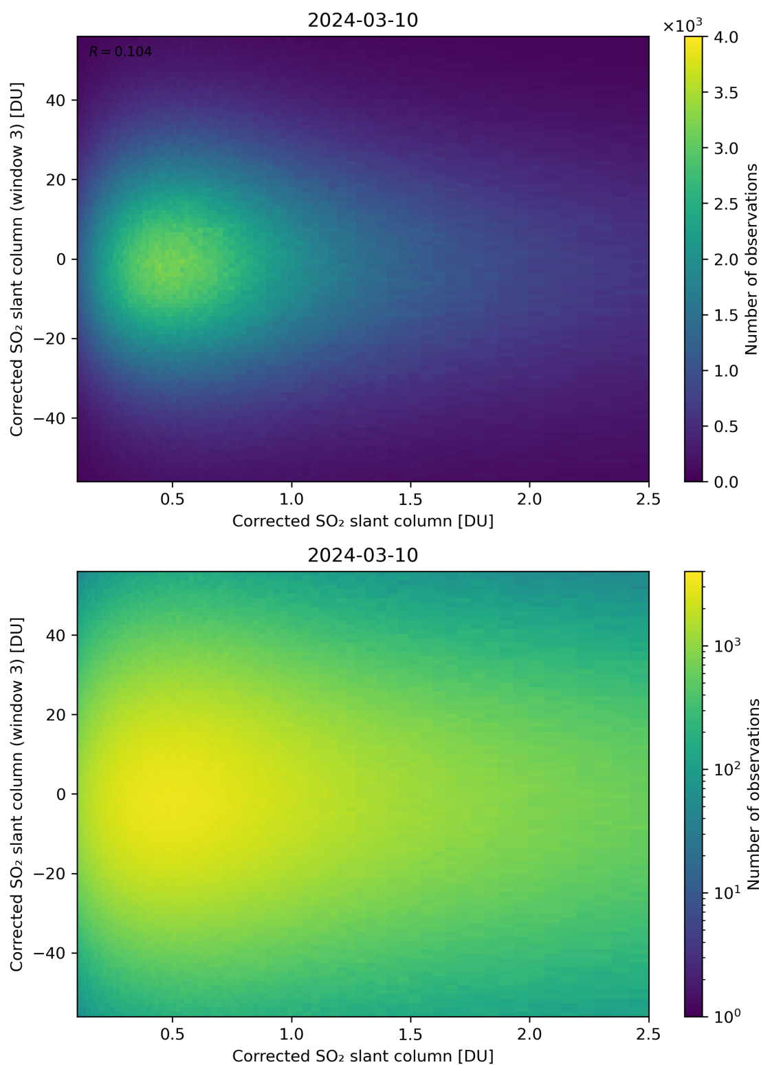
Figure 186: Scatter density plot of “Corrected SO 2 slant column” against “Corrected SO 2 slant column (window 3)” for 2024-03-09 to 2024-03-11.
