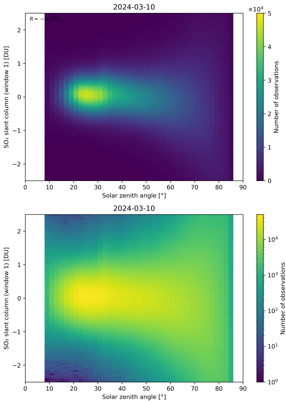
Figure 169: Scatter density plot of “Solar zenith angle” against “SO 2 slant column (window 1)” for 2024-03-09 to 2024-03-11.
