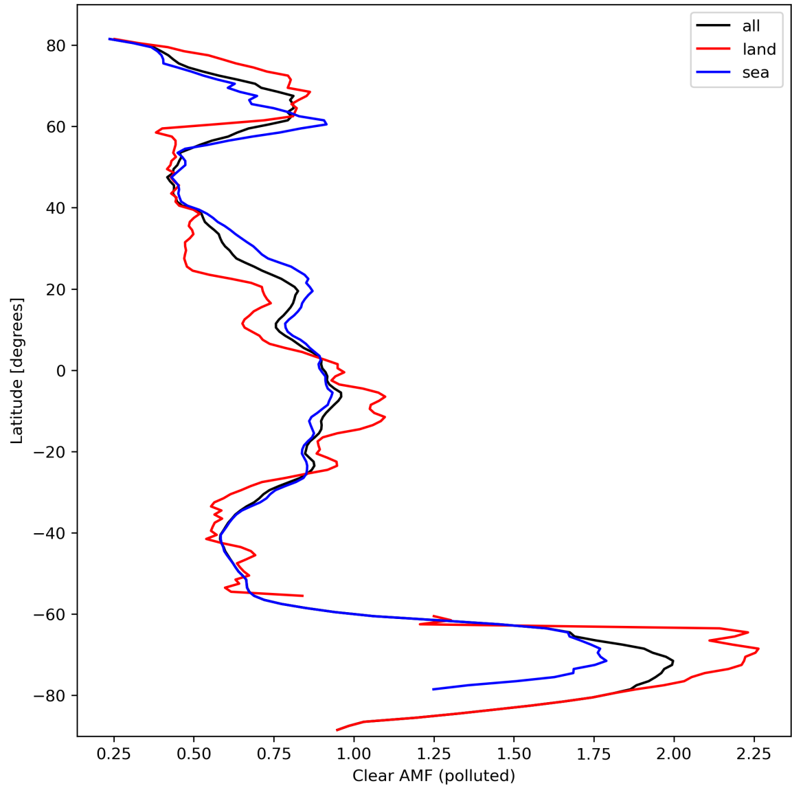
Figure 50: Zonal average of “Clear AMF (polluted)” for 2024-03-09 to 2024-03-11.
