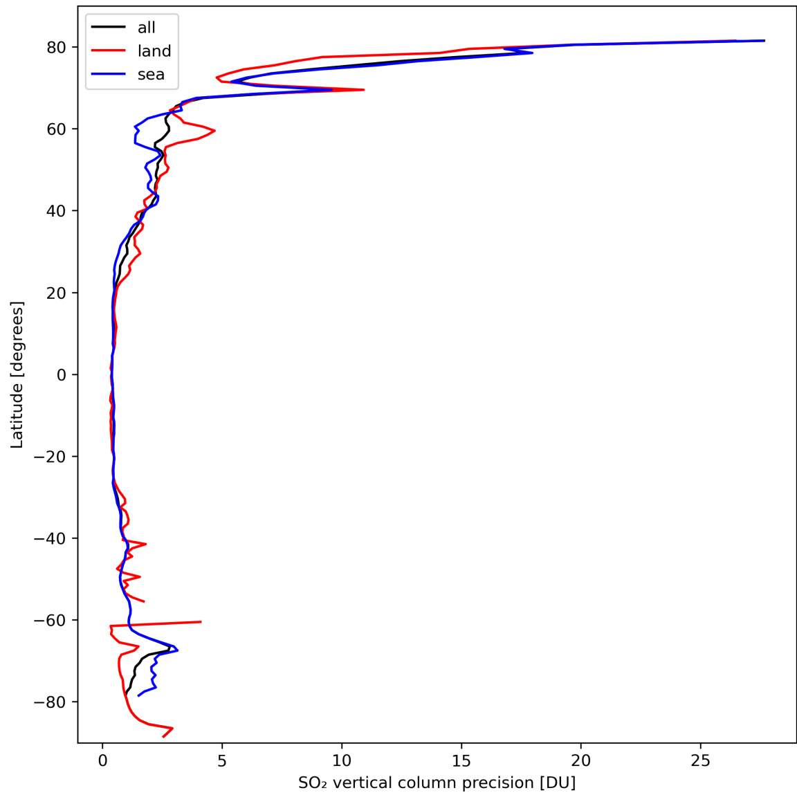
Figure 31: Zonal average of “SO 2 vertical column precision” for 2024-03-09 to 2024-03-11.
