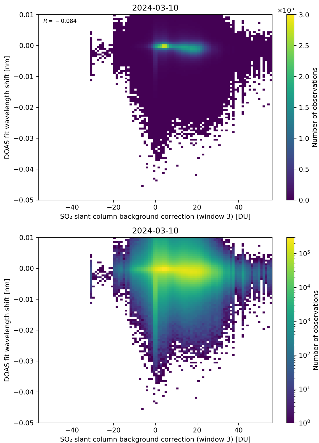
Figure 121: Scatter density plot of “SO 2 slant column background correction (window 3)” against “DOAS fit wavelength shift” for 2024-03-09 to 2024-03-11.
