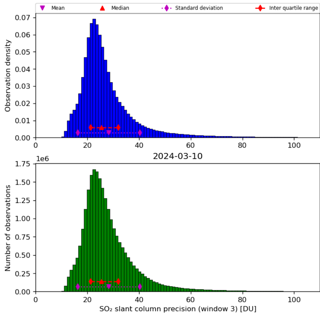
Figure 65: Histogram of “SO 2 slant column precision (window 3)” for 2024-03-09 to 2024-03-11
