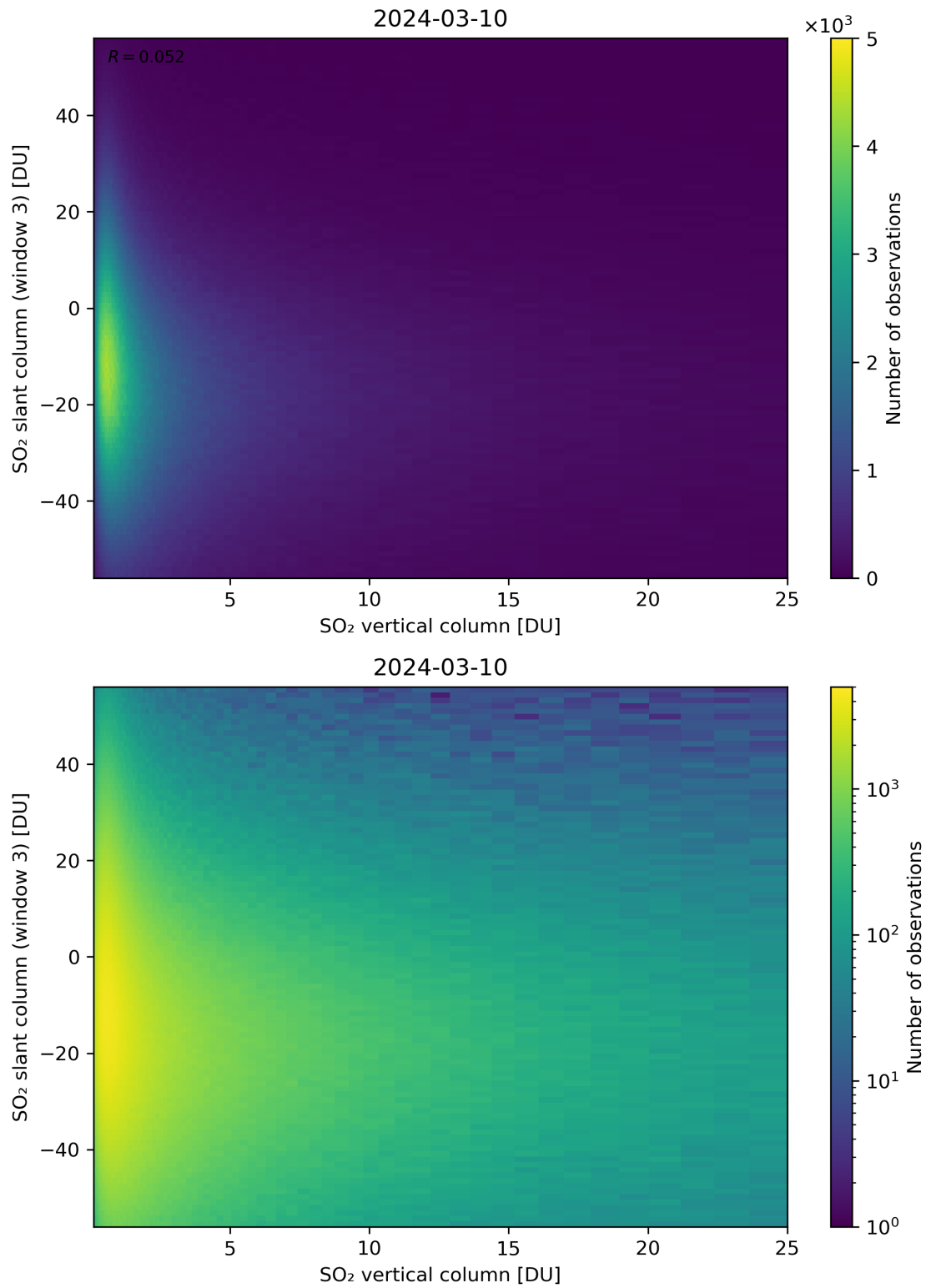
Figure 303: Scatter density plot of “SO 2 vertical column” against “SO 2 slant column (window 3)” for 2024-03-09 to 2024-03-11.
