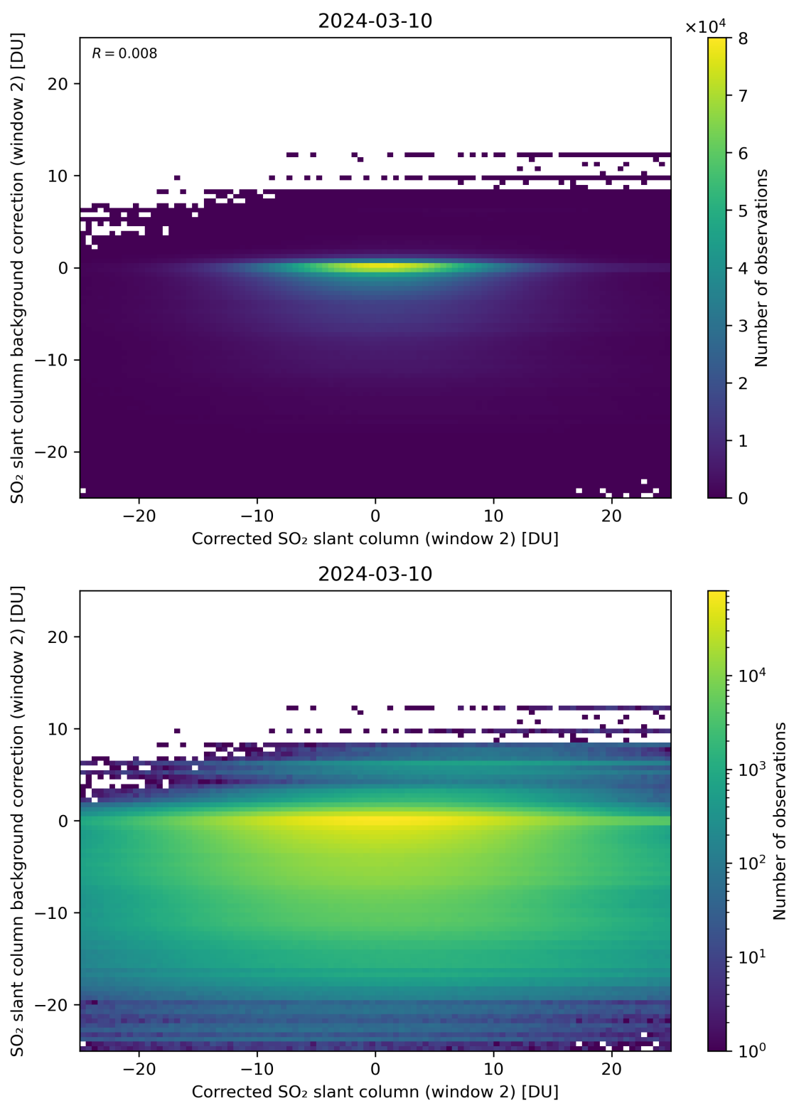
Figure 194: Scatter density plot of “Corrected SO 2 slant column (window 2)” against “SO 2 slant column background correction (window 2)” for 2024-03-09 to 2024-03-11.
