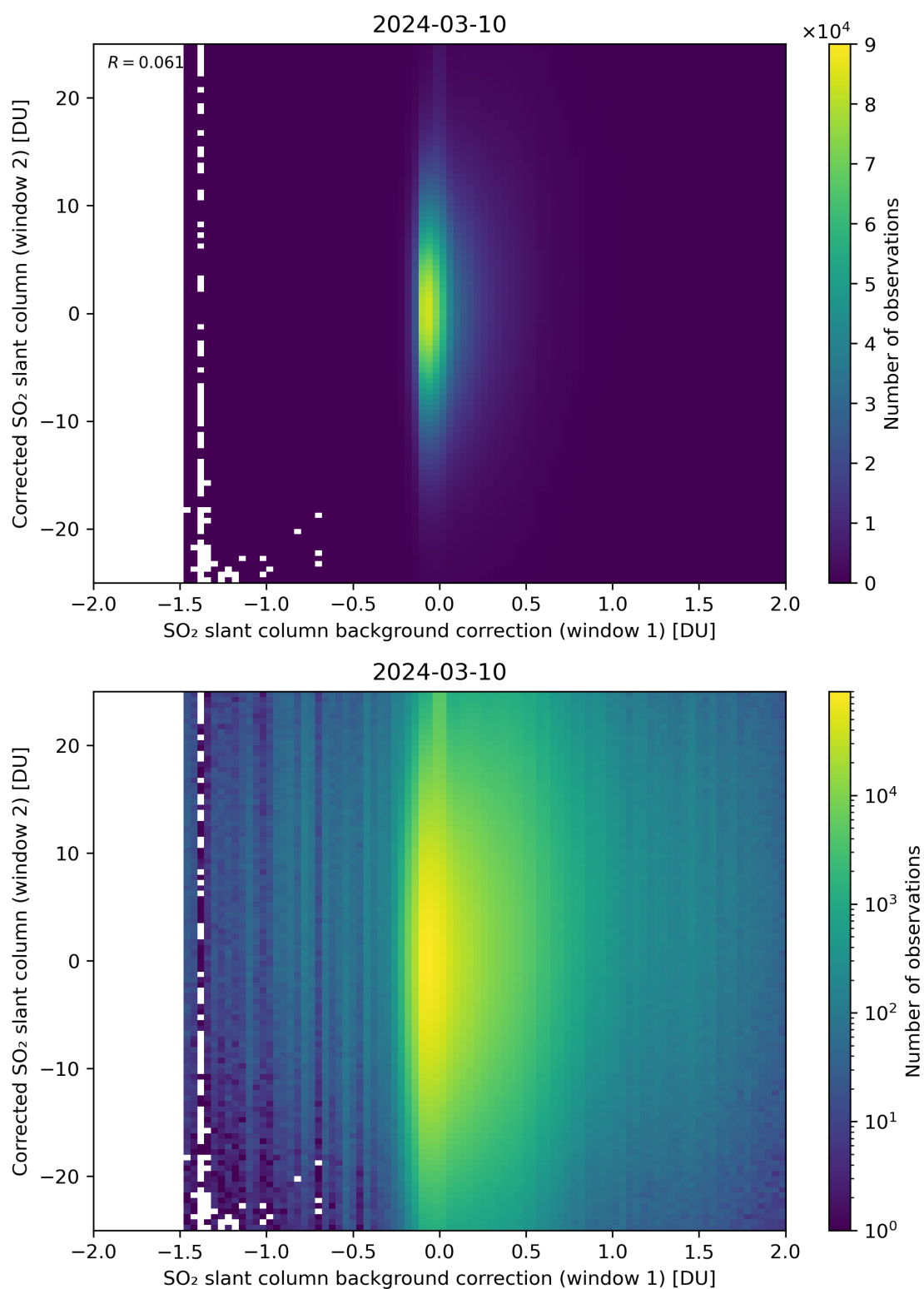
Figure 104: Scatter density plot of “SO 2 slant column background correction (window 1)” against “Corrected SO 2 slant column (window 2)” for 2024-03-09 to 2024-03-11.
