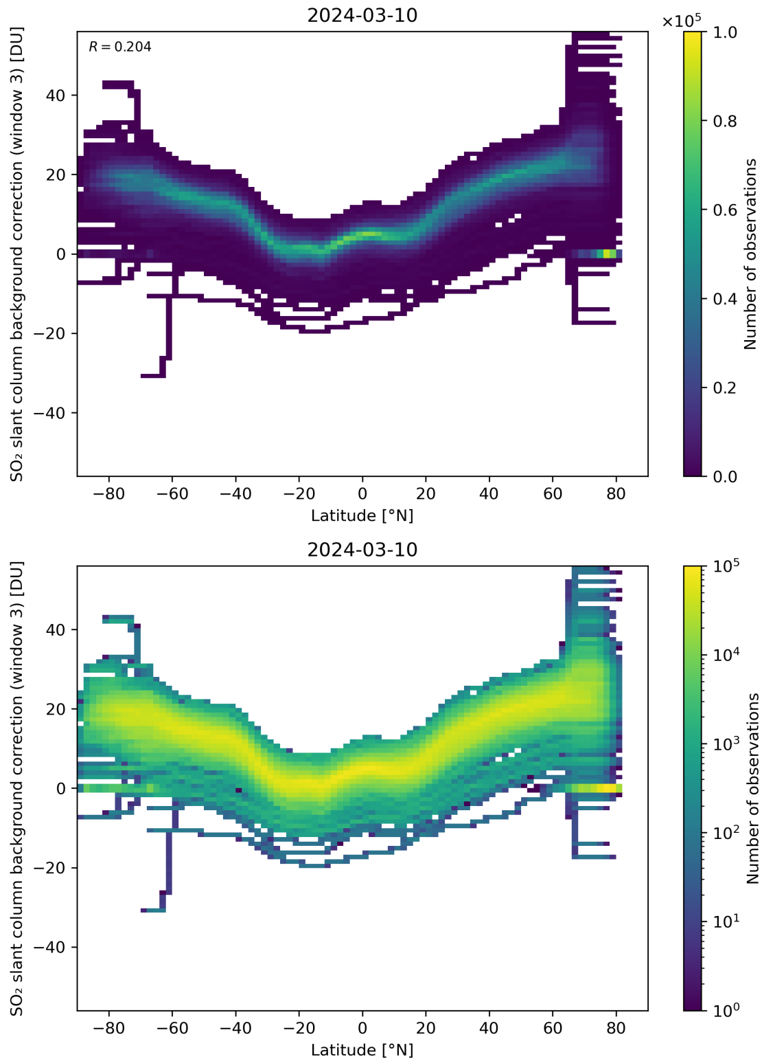
Figure 141: Scatter density plot of “Latitude” against “SO 2 slant column background correction (window 3)” for 2024-03-09 to 2024-03-11.
