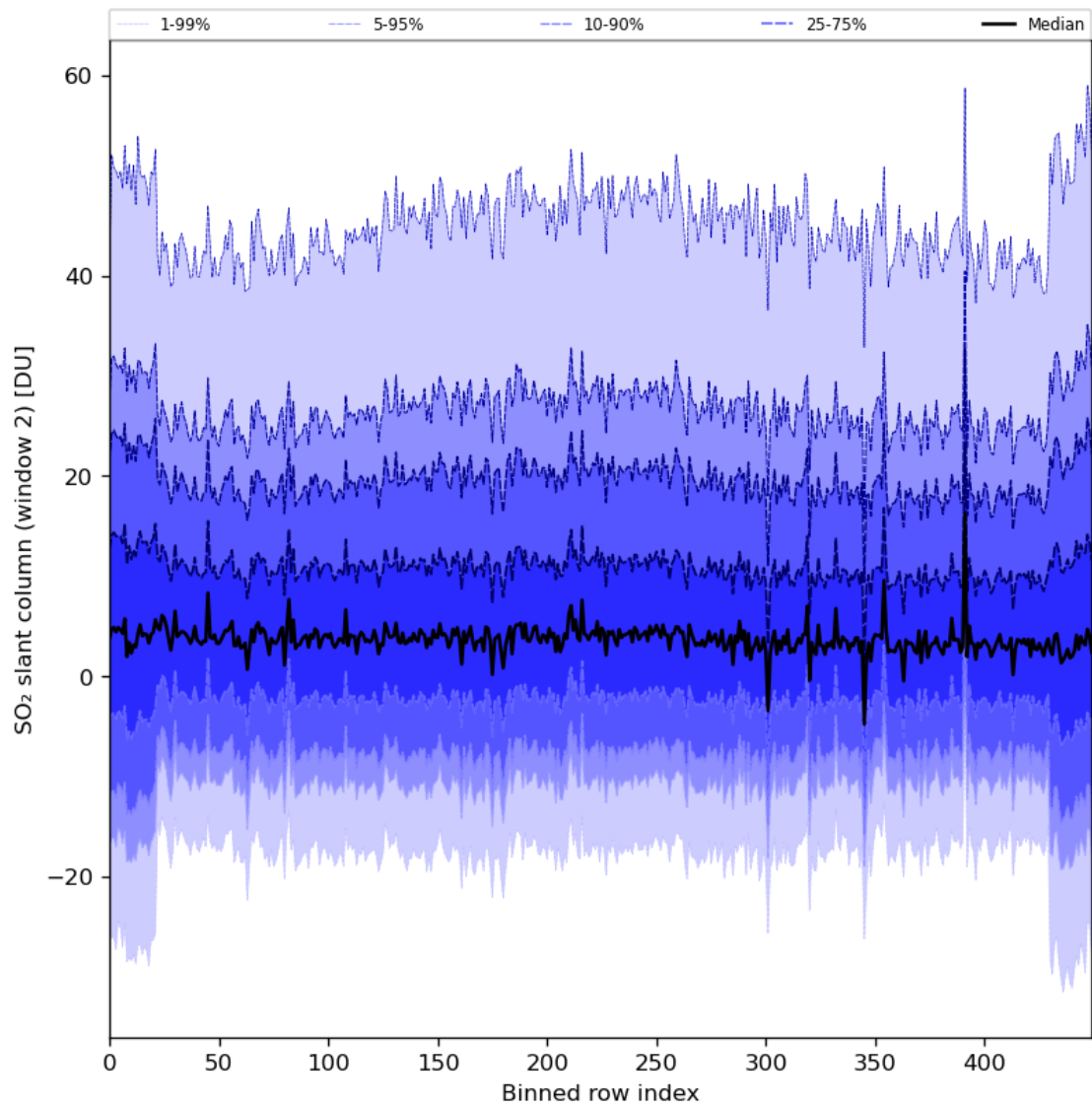
Figure 83: Along track statistics of “SO 2 slant column (window 2)” for 2024-03-09 to 2024-03-11
