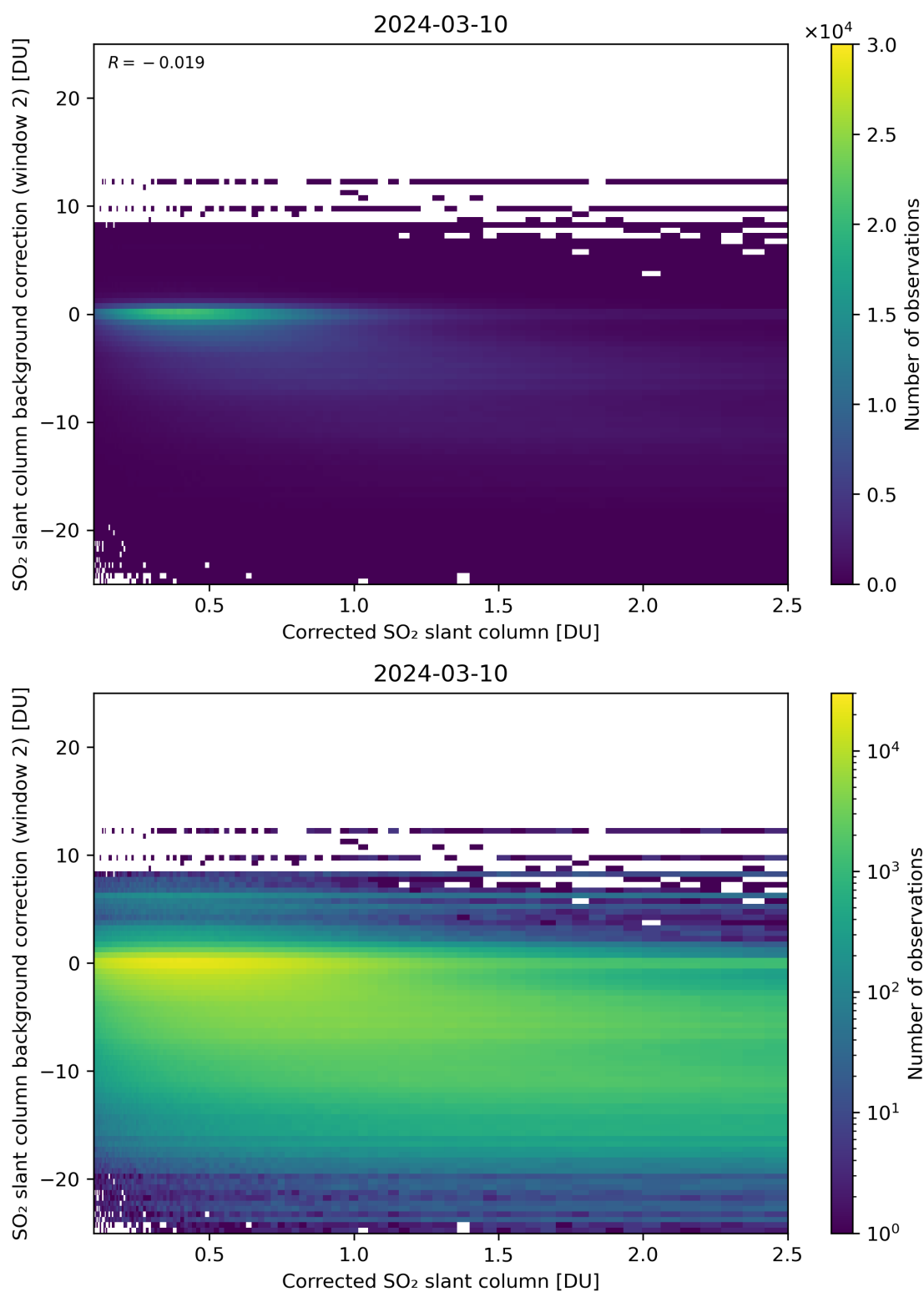
Figure 179: Scatter density plot of “Corrected SO 2 slant column” against “SO 2 slant column background correction (window 2)” for 2024-03-09 to 2024-03-11.
