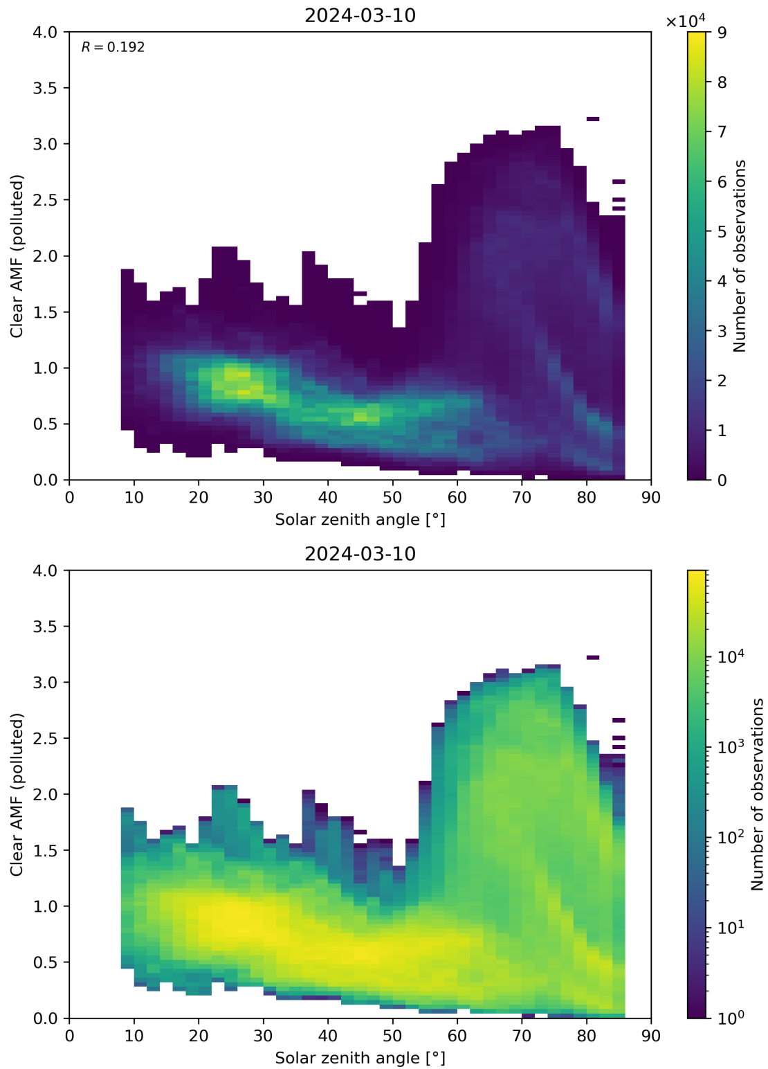
Figure 165: Scatter density plot of “Solar zenith angle” against “Clear AMF (polluted)” for 2024-03-09 to 2024-03-11.
