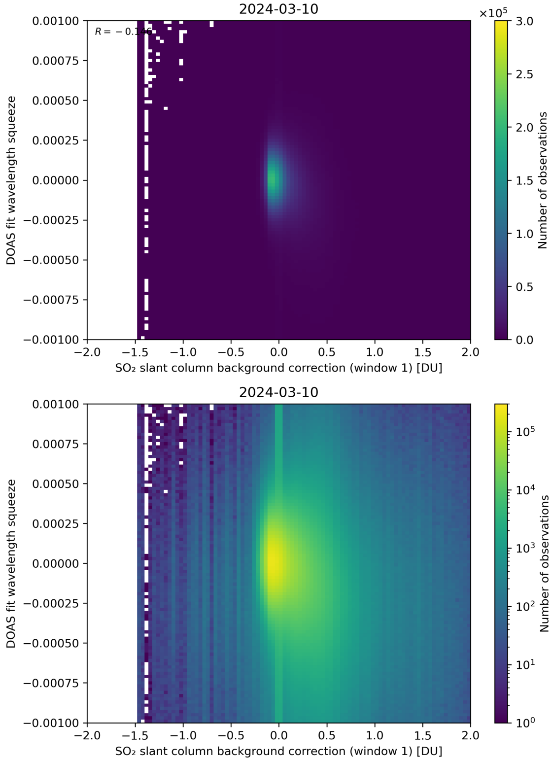
Figure 101: Scatter density plot of “SO 2 slant column background correction (window 1)” against “DOAS fit wavelength squeeze” for 2024-03-09 to 2024-03-11.
