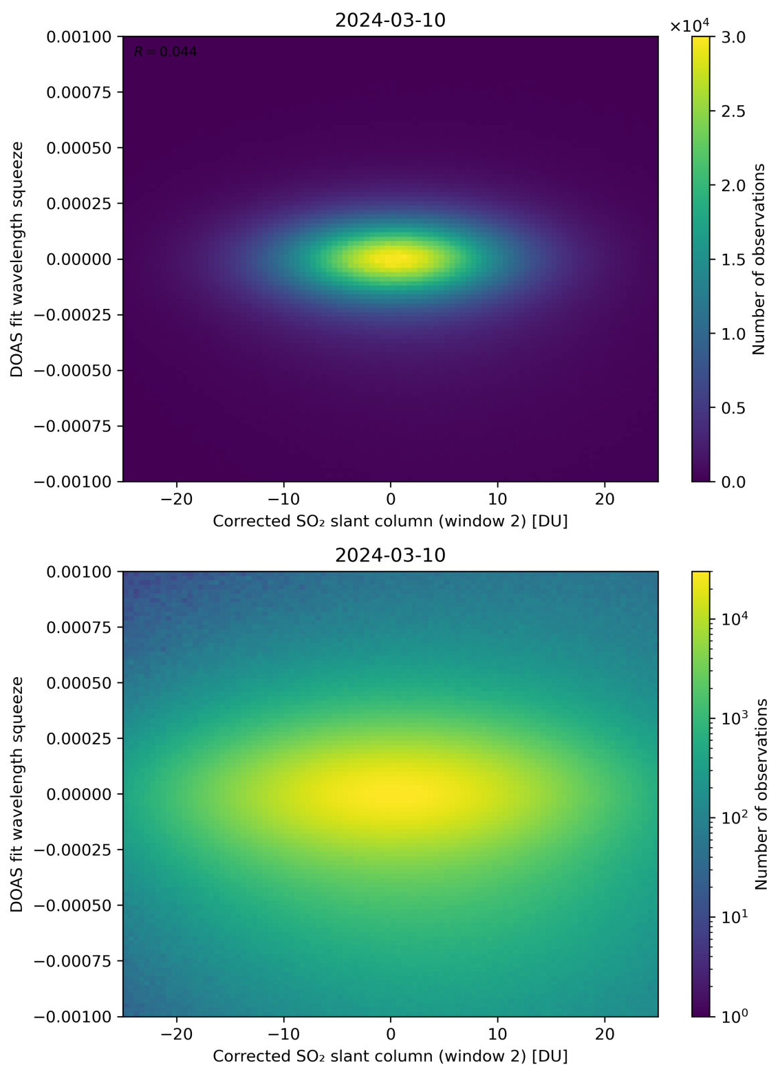
Figure 197: Scatter density plot of “Corrected SO 2 slant column (window 2)” against “DOAS fit wavelength squeeze” for 2024-03-09 to 2024-03-11.
