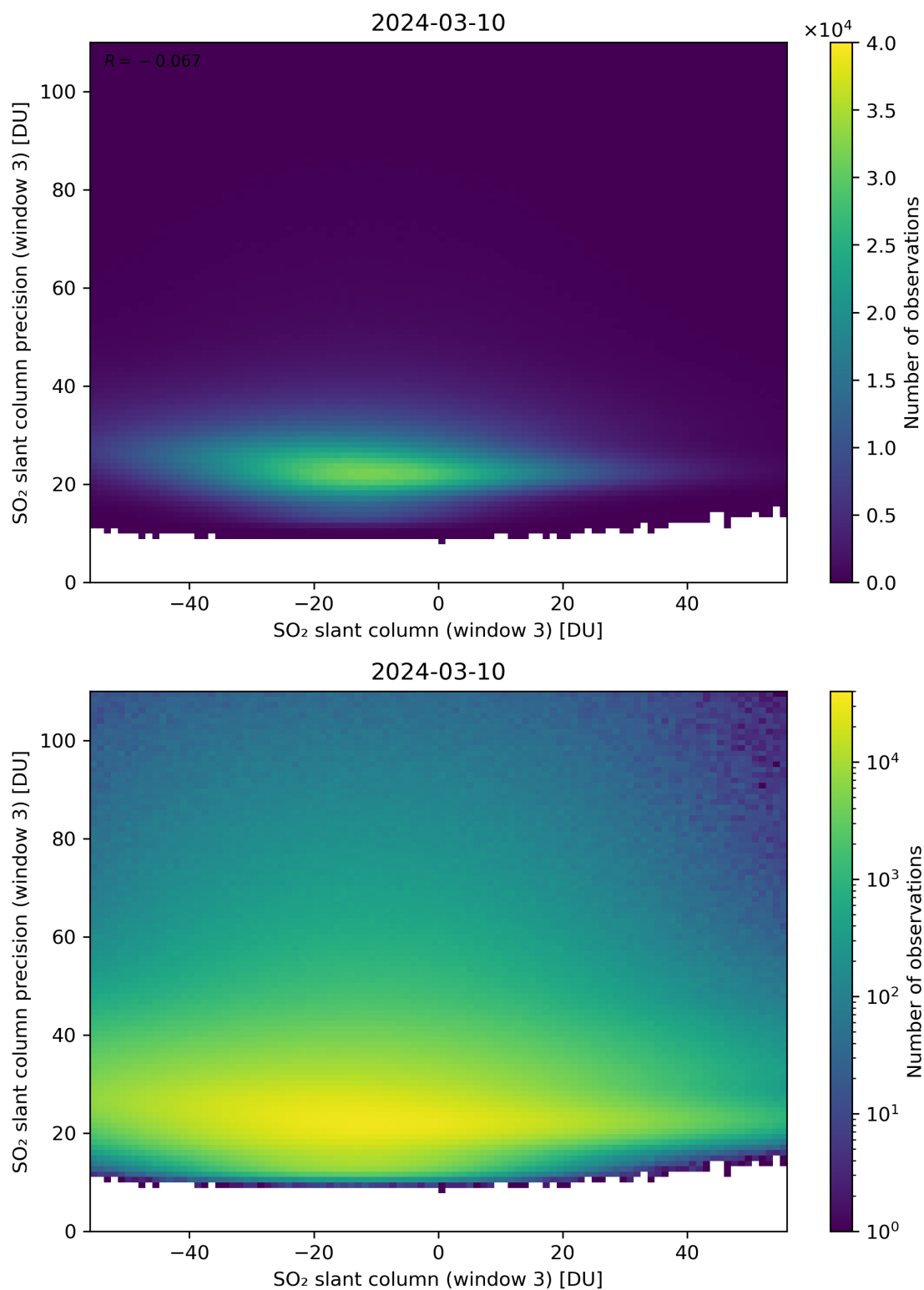
Figure 267: Scatter density plot of “SO 2 slant column (window 3)” against “SO 2 slant column precision (window 3)” for 2024-03-09 to 2024-03-11.
