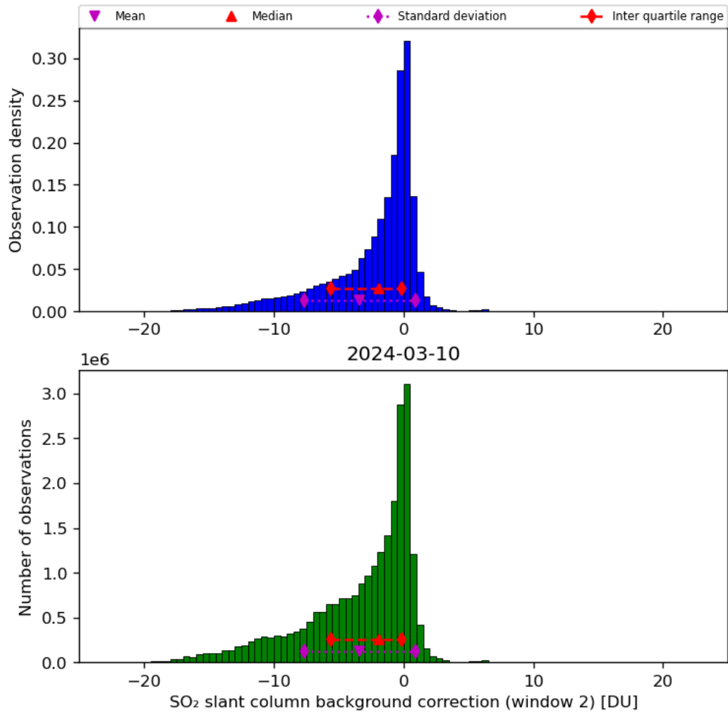
Figure 63: Histogram of “SO 2 slant column background correction (window 2)” for 2024-03-09 to 2024-03-11
