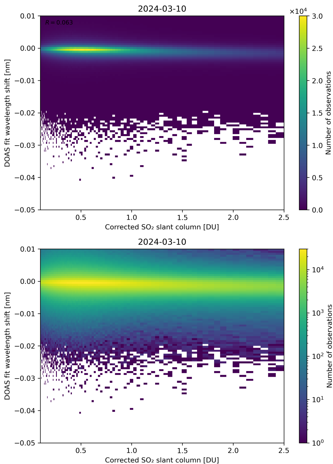
Figure 181: Scatter density plot of “Corrected SO 2 slant column” against “DOAS fit wavelength shift” for 2024-03-09 to 2024-03-11.
