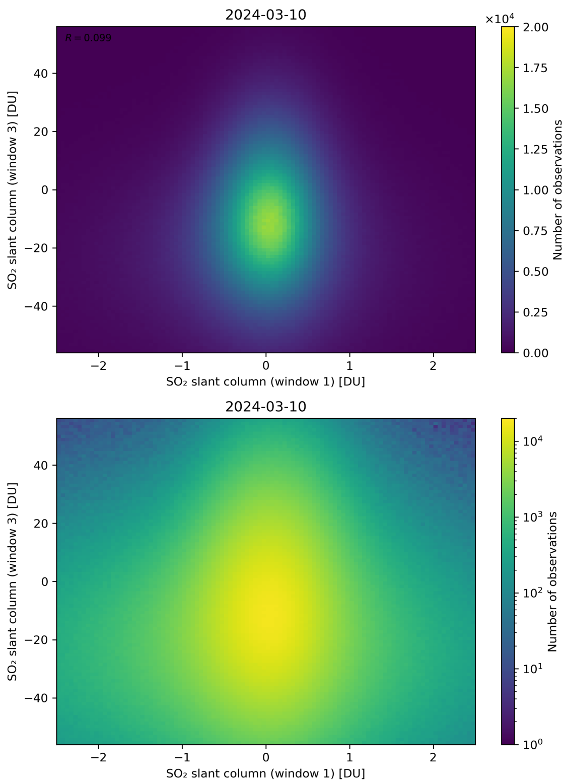
Figure 237: Scatter density plot of “SO 2 slant column (window 1)” against “SO 2 slant column (window 3)” for 2024-03-09 to 2024-03-11.
