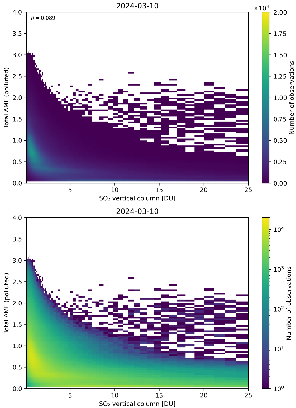
Figure 305: Scatter density plot of “SO 2 vertical column” against “Total AMF (polluted)” for 2024-03-09 to 2024-03-11.
