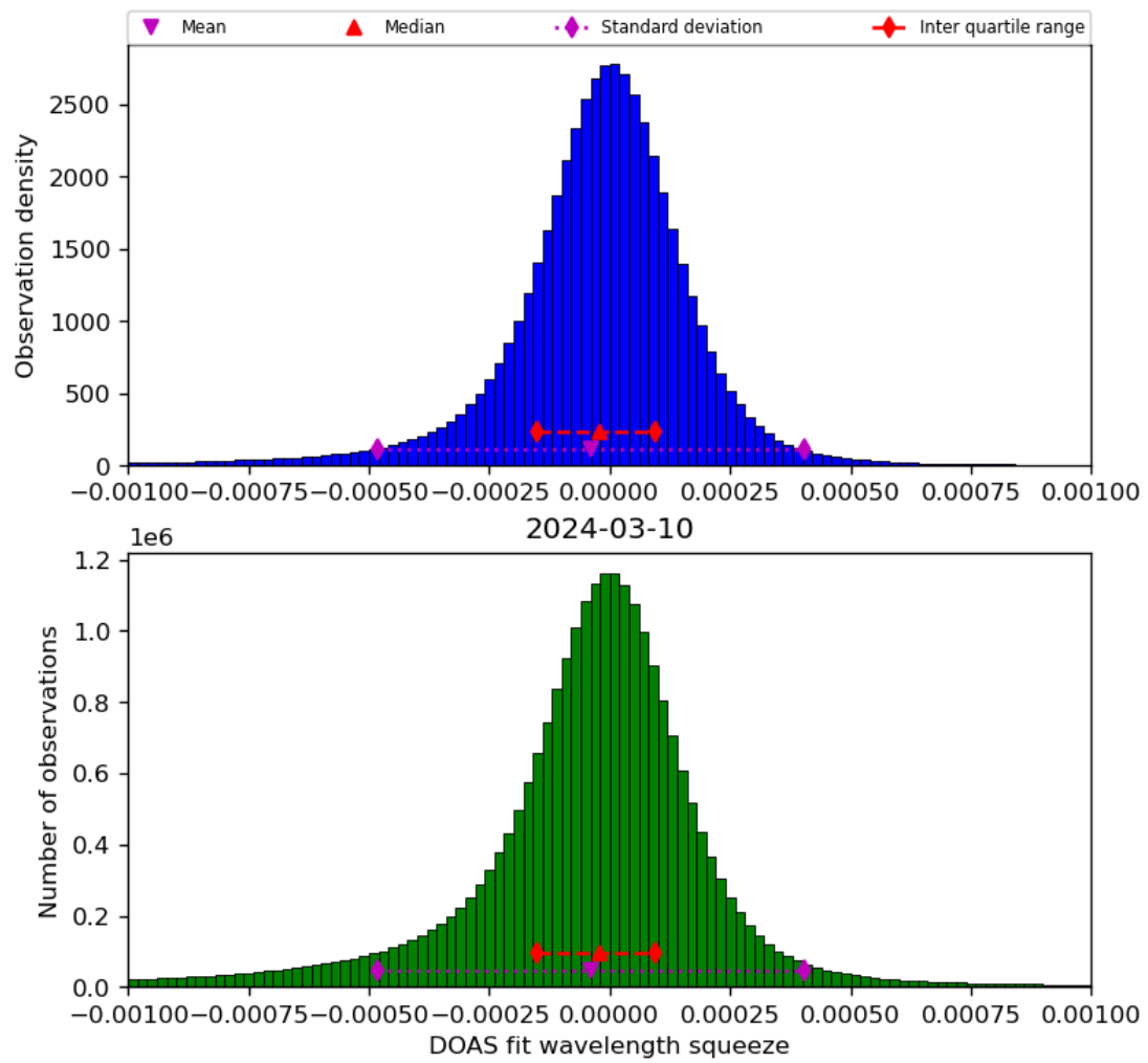
Figure 69: Histogram of “DOAS fit wavelength squeeze” for 2024-03-09 to 2024-03-11
