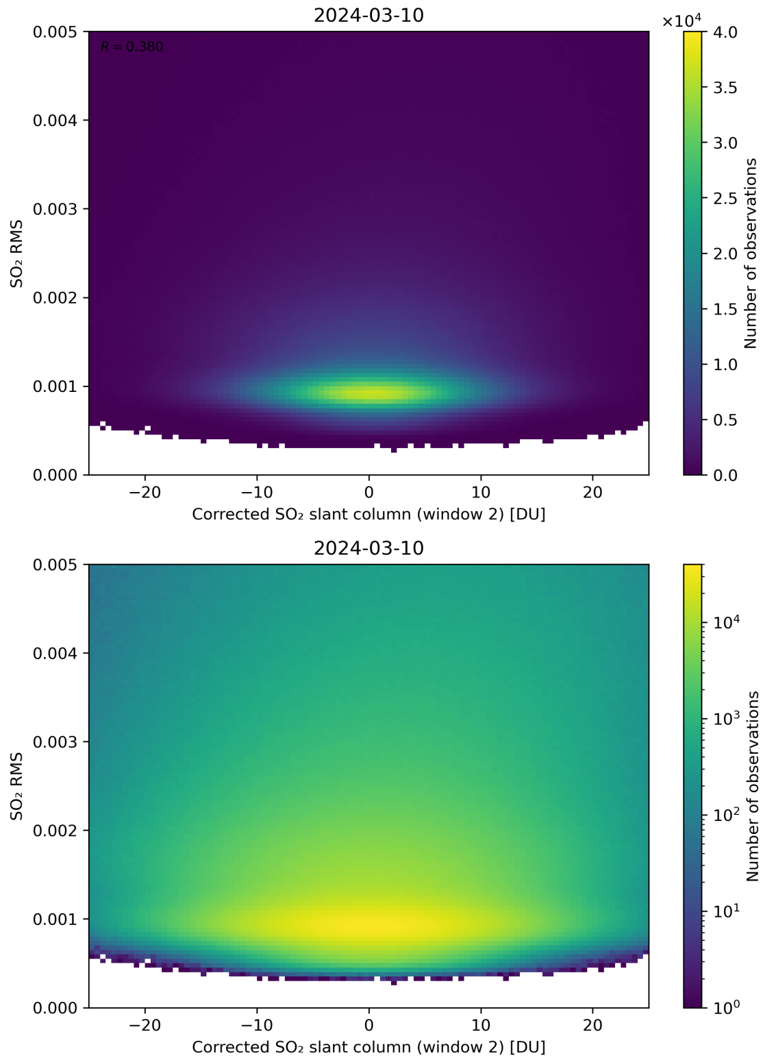
Figure 198: Scatter density plot of “Corrected SO 2 slant column (window 2)” against “SO 2 RMS” for 2024-03-09 to 2024-03-11.
