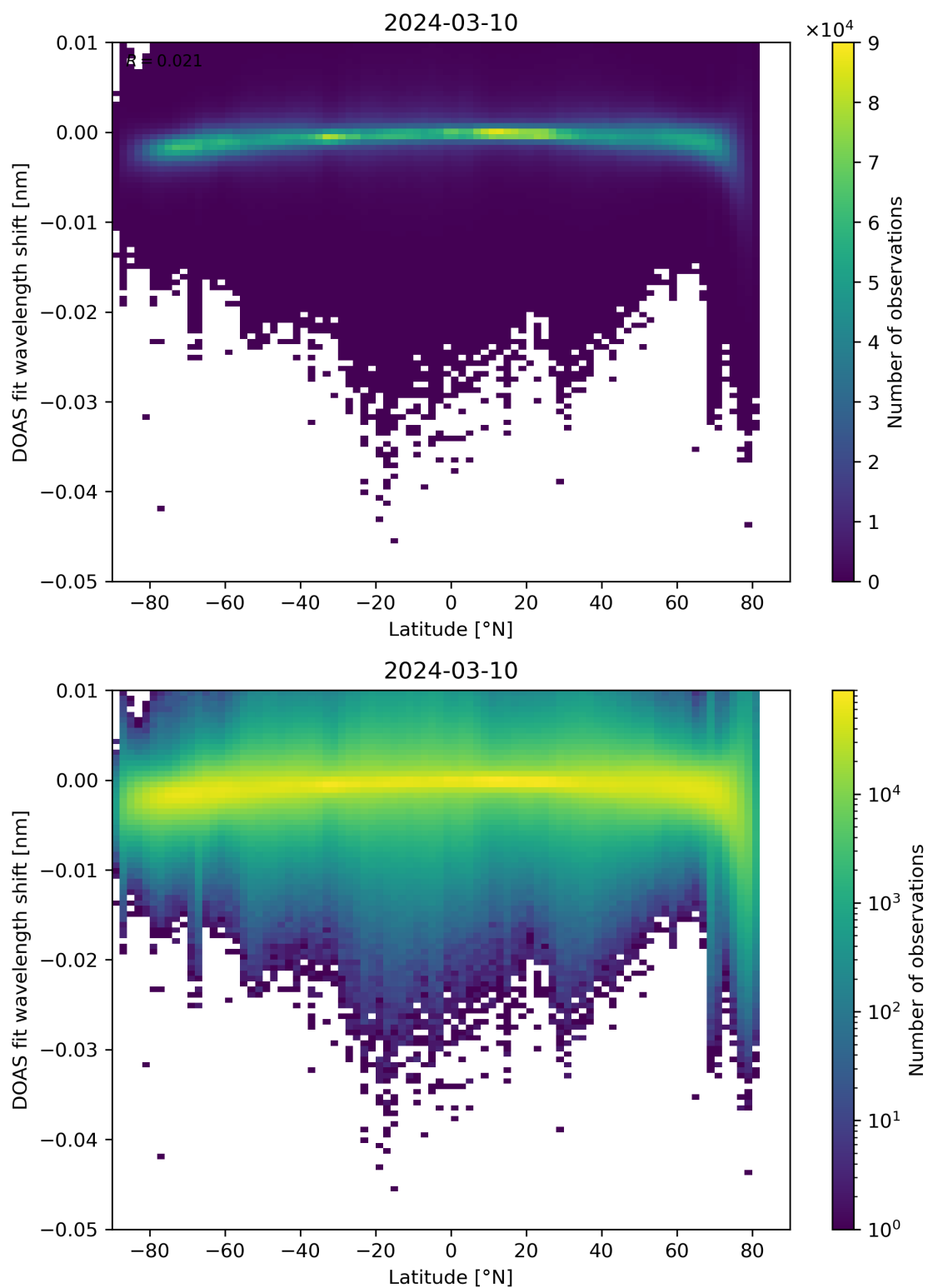
Figure 142: Scatter density plot of “Latitude” against “DOAS fit wavelength shift” for 2024-03-09 to 2024-03-11.
