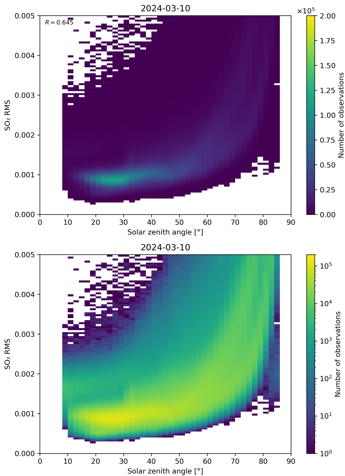
Figure 163: Scatter density plot of “Solar zenith angle” against “SO 2 RMS” for 2024-03-09 to 2024-03-11.
