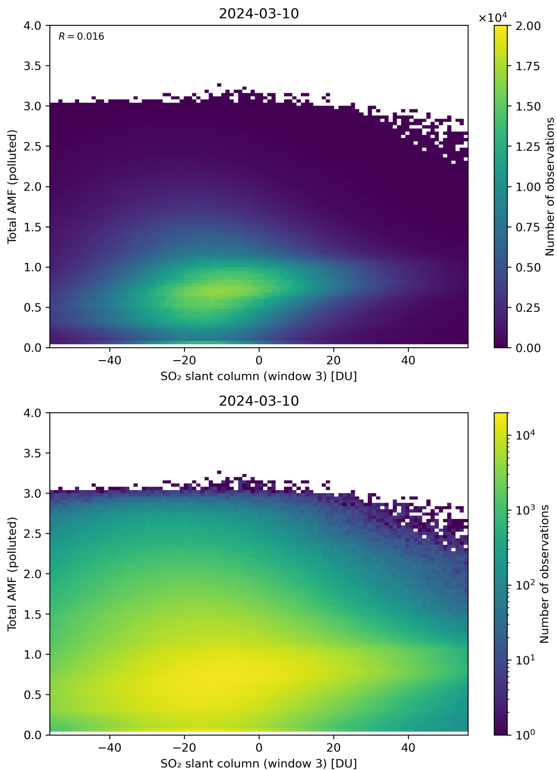
Figure 268: Scatter density plot of “SO 2 slant column (window 3)” against “Total AMF (polluted)” for 2024-03-09 to 2024-03-11.
