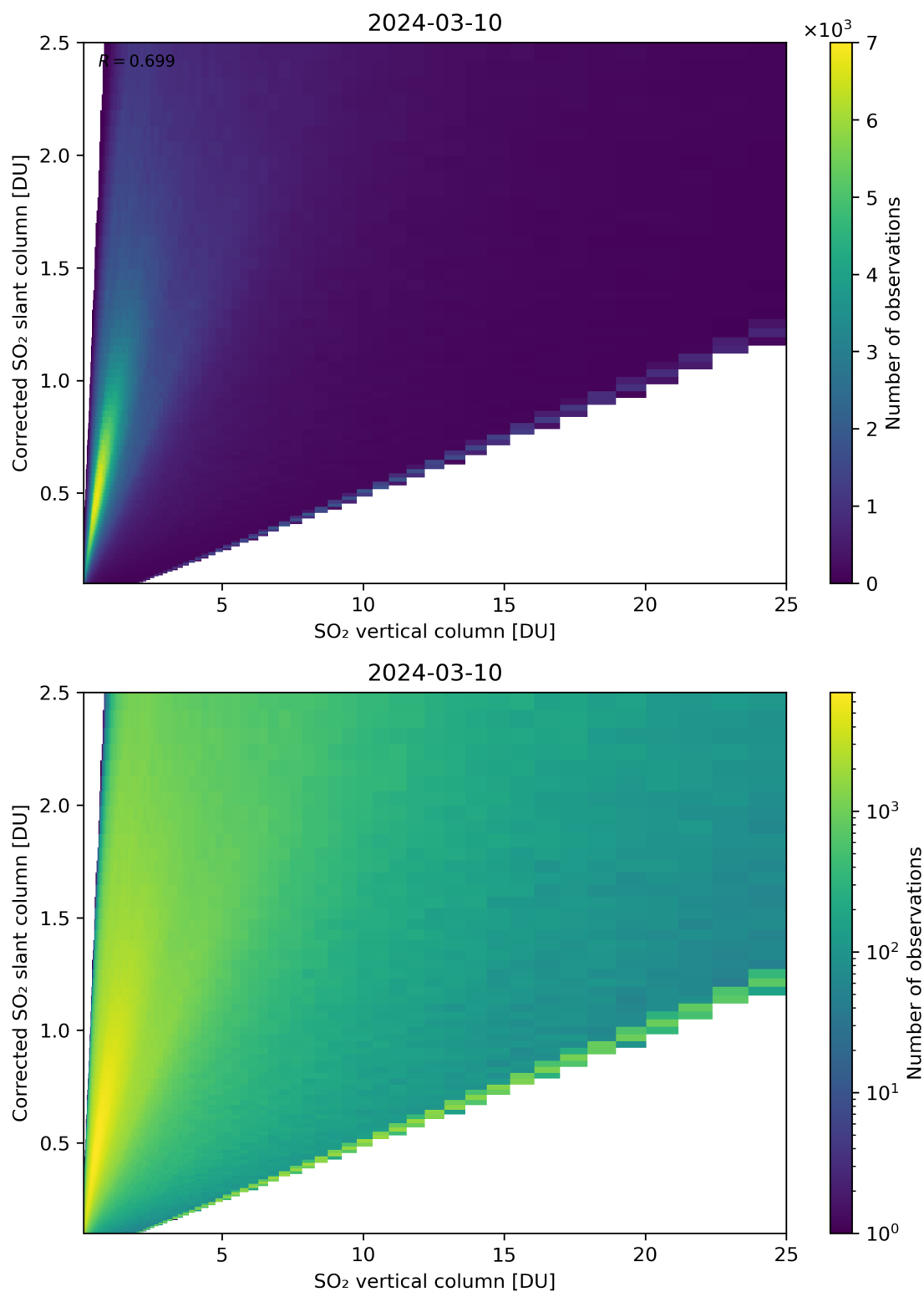
Figure 297: Scatter density plot of “SO 2 vertical column” against “Corrected SO 2 slant column” for 2024-03-09 to 2024-03-11.
