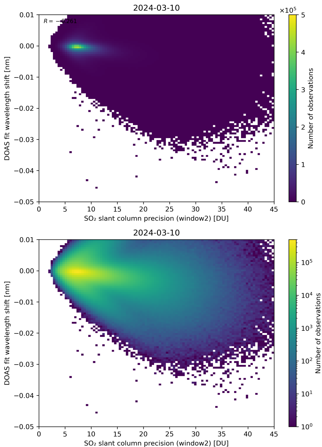
Figure 243: Scatter density plot of “SO 2 slant column precision (window2)” against “DOAS fit wavelength shift” for 2024-03-09 to 2024-03-11.
