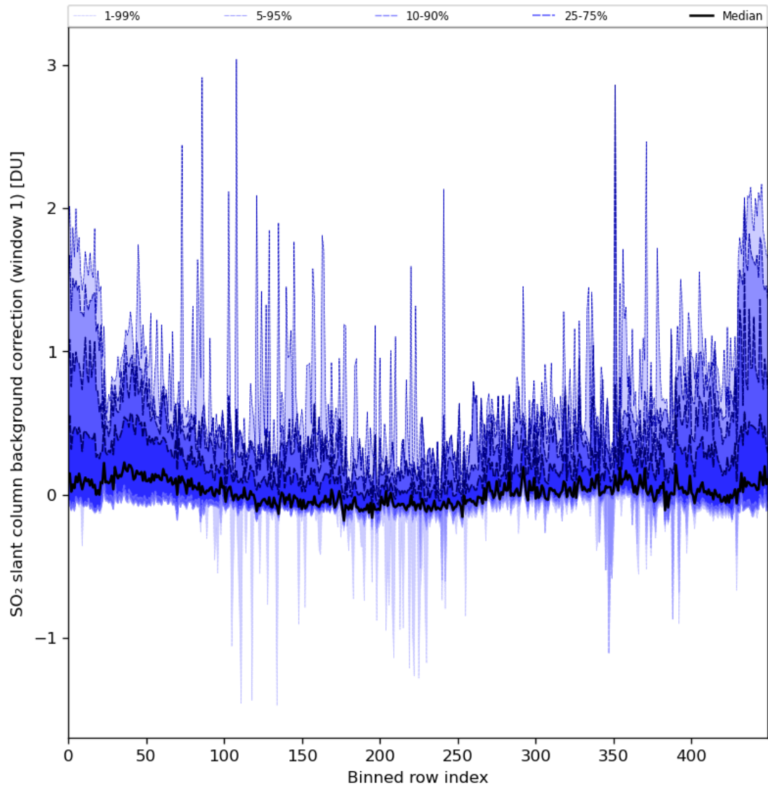
Figure 82: Along track statistics of “SO 2 slant column background correction (window 1)” for 2024-03-09 to 2024-03-11
