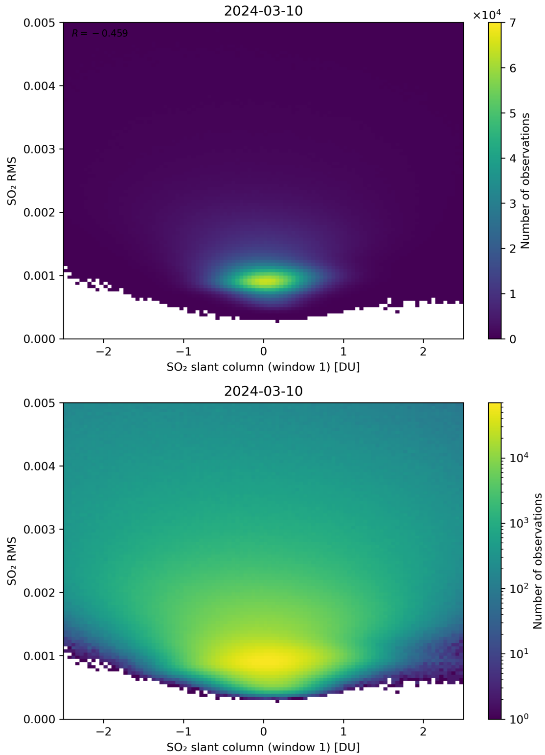
Figure 217: Scatter density plot of “SO 2 slant column (window 1)” against “SO 2 RMS” for 2024-03-09 to 2024-03-11.
