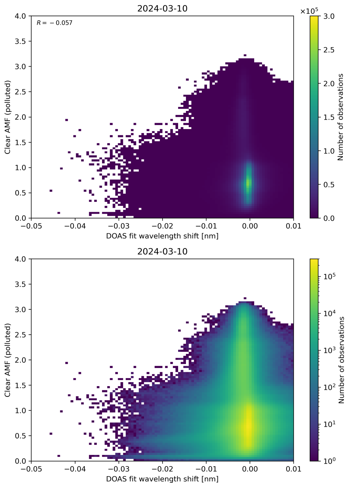
Figure 129: Scatter density plot of “DOAS fit wavelength shift” against “Clear AMF (polluted)” for 2024-03-09 to 2024-03-11.
