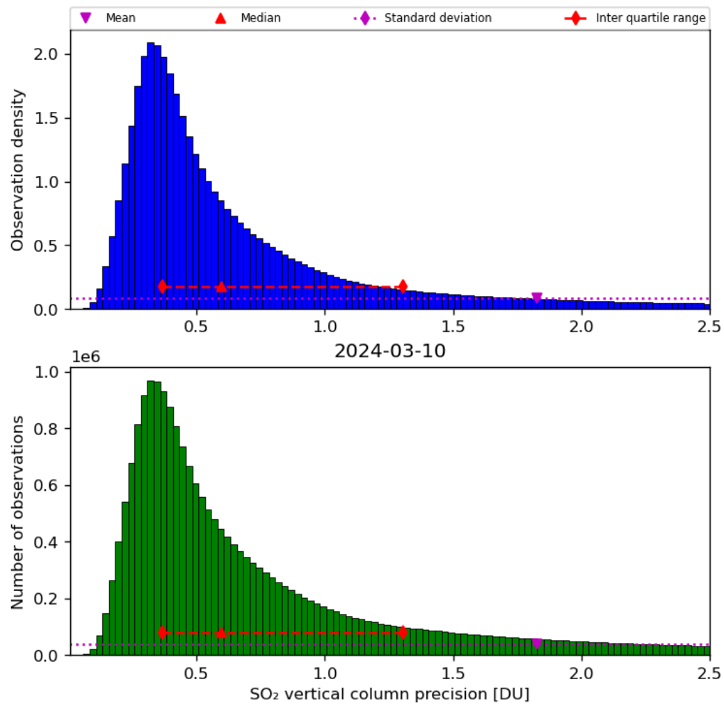
Figure 54: Histogram of “SO 2 vertical column precision” for 2024-03-09 to 2024-03-11
