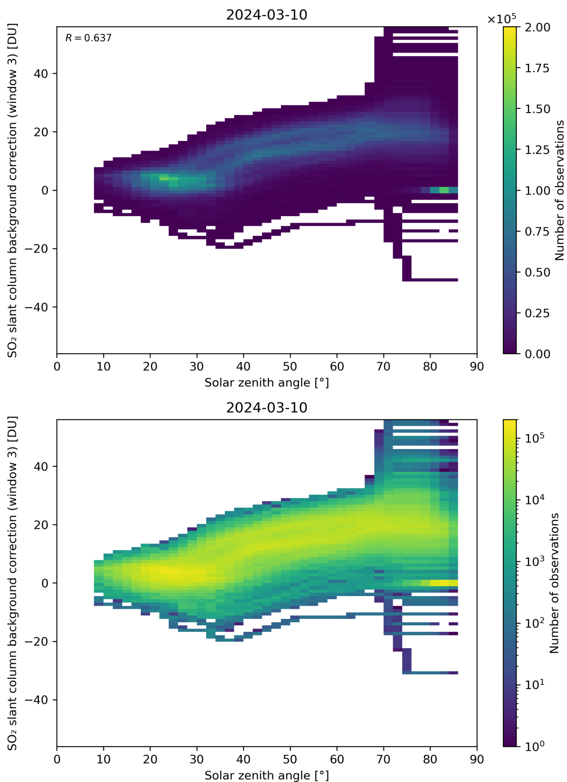
Figure 160: Scatter density plot of “Solar zenith angle” against “SO 2 slant column background correction (window 3)” for 2024-03-09 to 2024-03-11.
