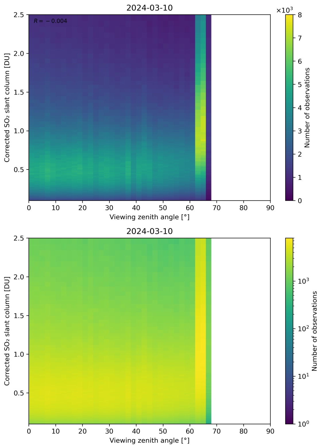
Figure 317: Scatter density plot of “Viewing zenith angle” against “Corrected SO 2 slant column” for 2024-03-09 to 2024-03-11.
