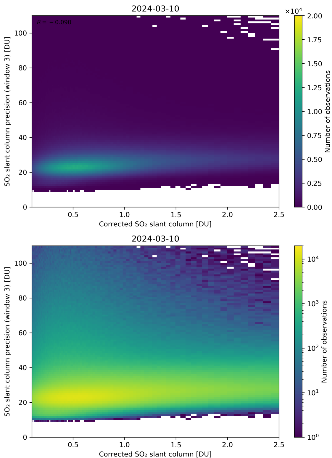
Figure 191: Scatter density plot of “Corrected SO 2 slant column” against “SO 2 slant column precision (window 3)” for 2024-03-09 to 2024-03-11.
