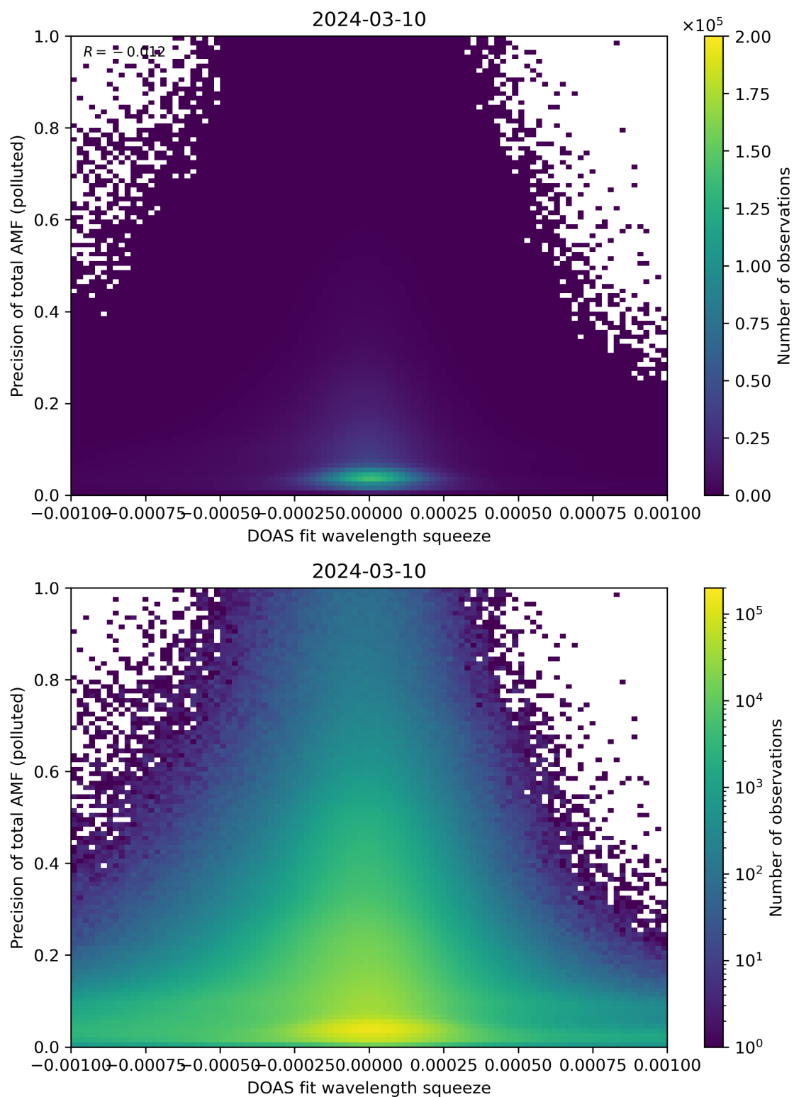
Figure 135: Scatter density plot of “DOAS fit wavelength squeeze” against “Precision of total AMF (polluted)” for 2024-03-09 to 2024-03-11.
