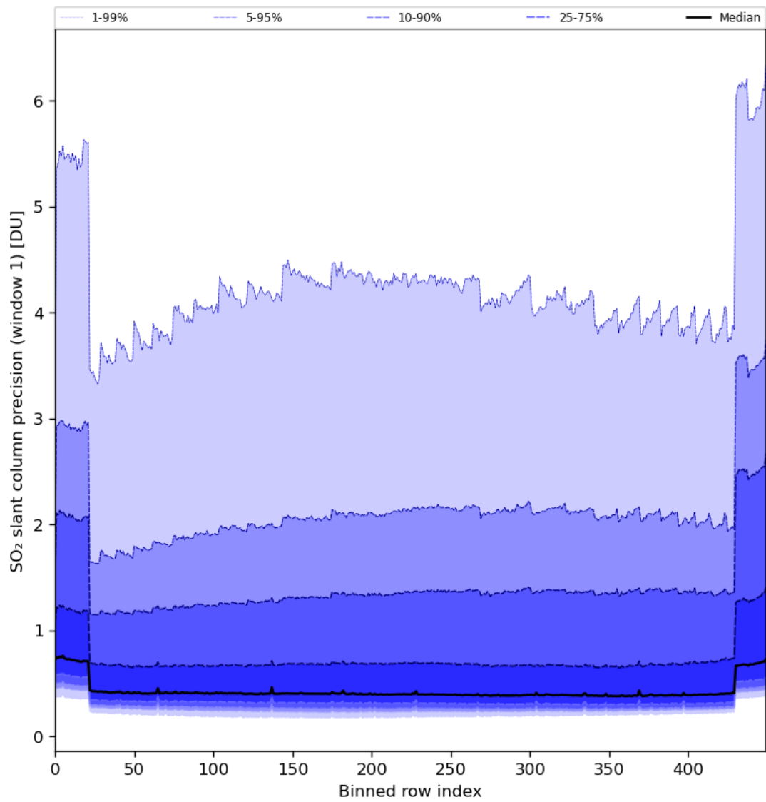
Figure 80: Along track statistics of “SO 2 slant column precision (window 1)” for 2024-03-09 to 2024-03-11
