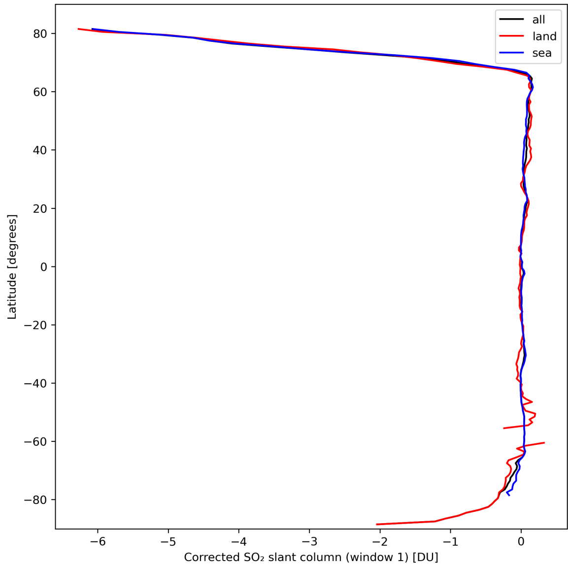
Figure 35: Zonal average of “Corrected SO 2 slant column (window 1)” for 2024-03-09 to 2024-03-11.
