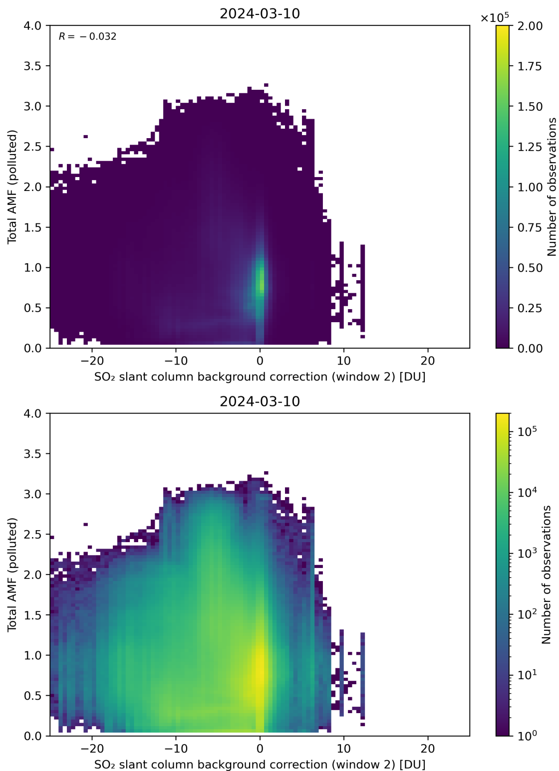
Figure 119: Scatter density plot of “SO 2 slant column background correction (window 2)” against “Total AMF (polluted)” for 2024-03-09 to 2024-03-11.
