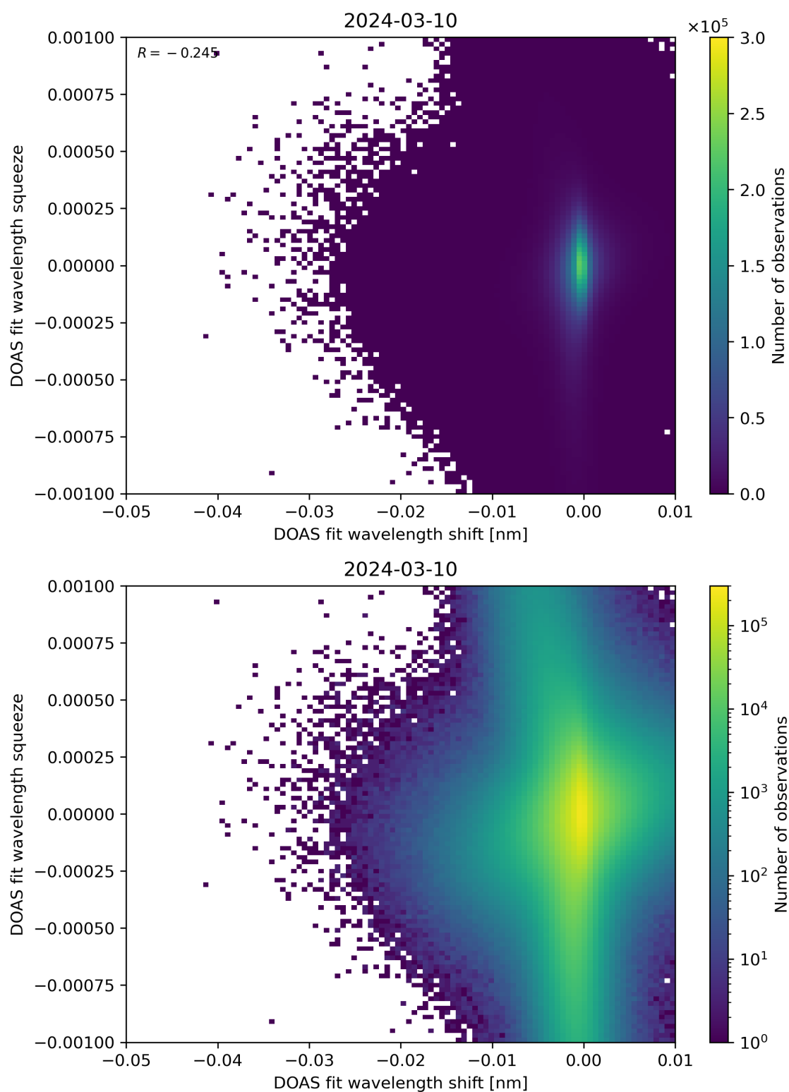
Figure 127: Scatter density plot of “DOAS fit wavelength shift” against “DOAS fit wavelength squeeze” for 2024-03-09 to 2024-03-11.
