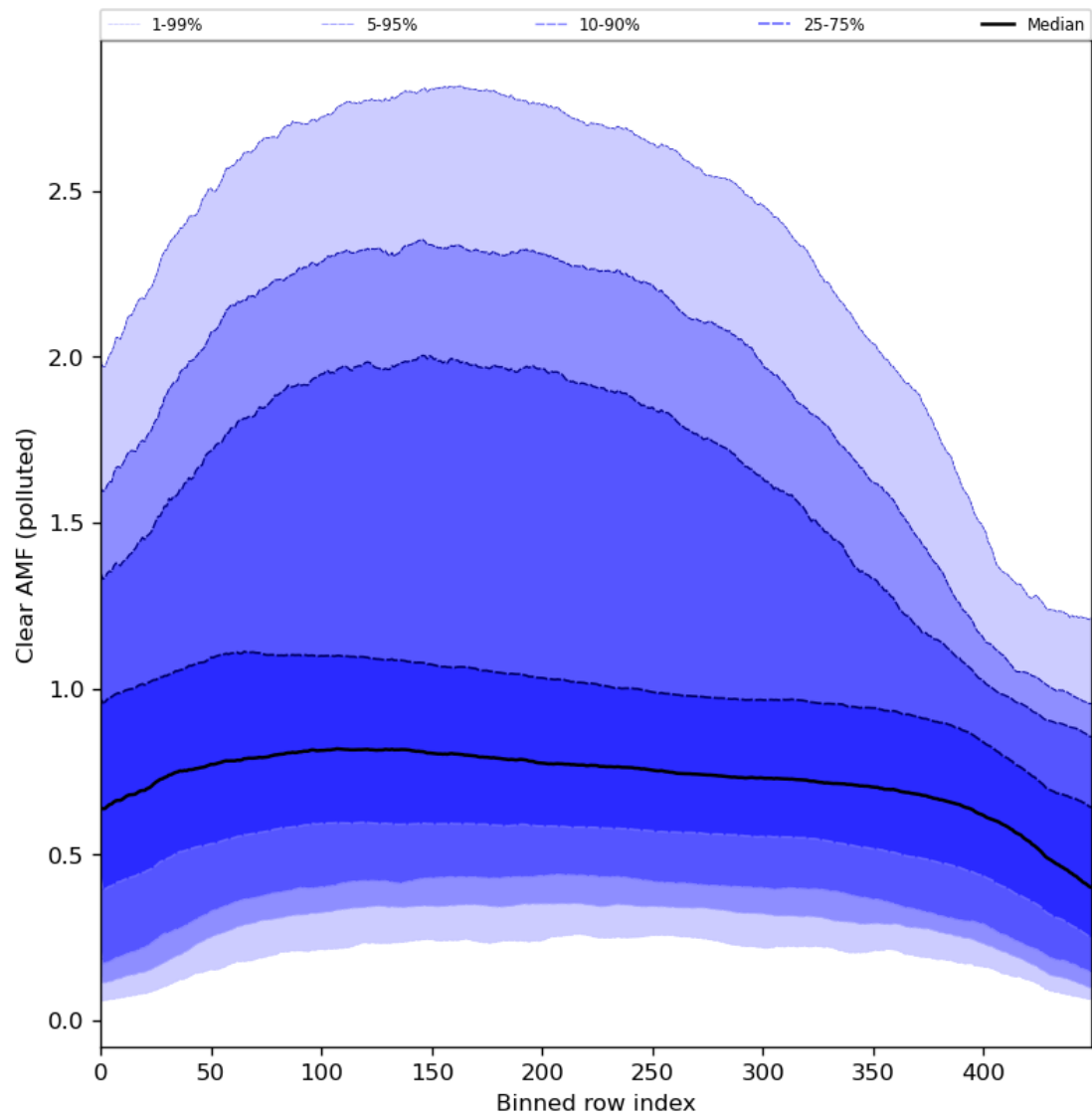
Figure 96: Along track statistics of “Clear AMF (polluted)” for 2024-03-09 to 2024-03-11
