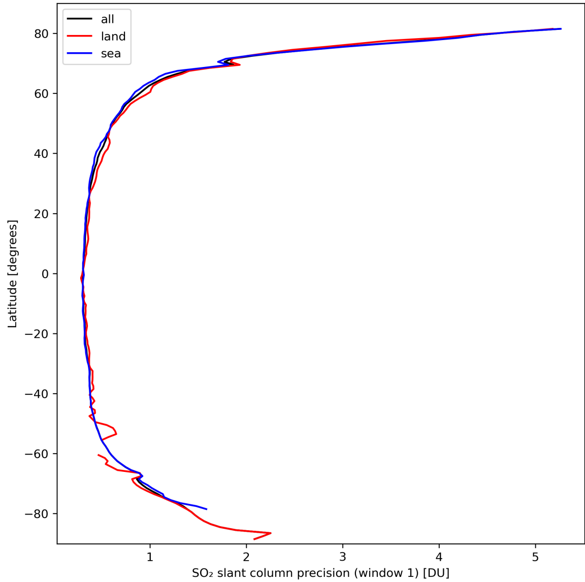
Figure 34: Zonal average of “SO 2 slant column precision (window 1)” for 2024-03-09 to 2024-03-11.
