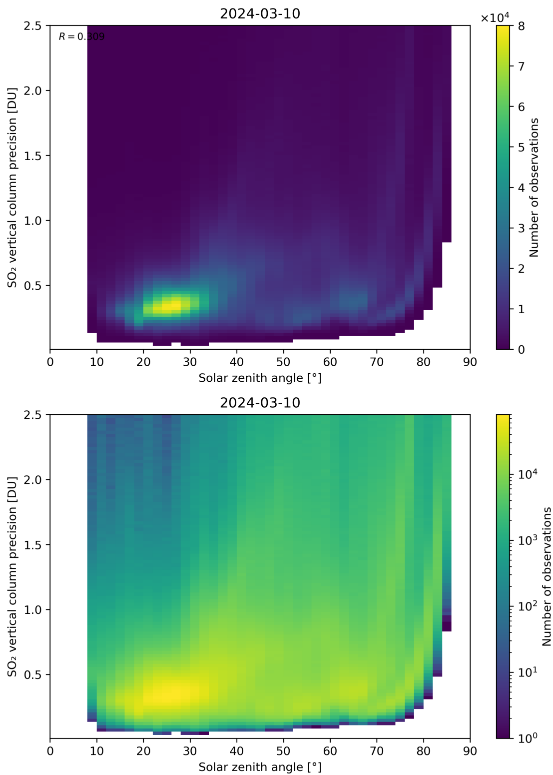
Figure 177: Scatter density plot of “Solar zenith angle” against “SO 2 vertical column precision” for 2024-03-09 to 2024-03-11.
