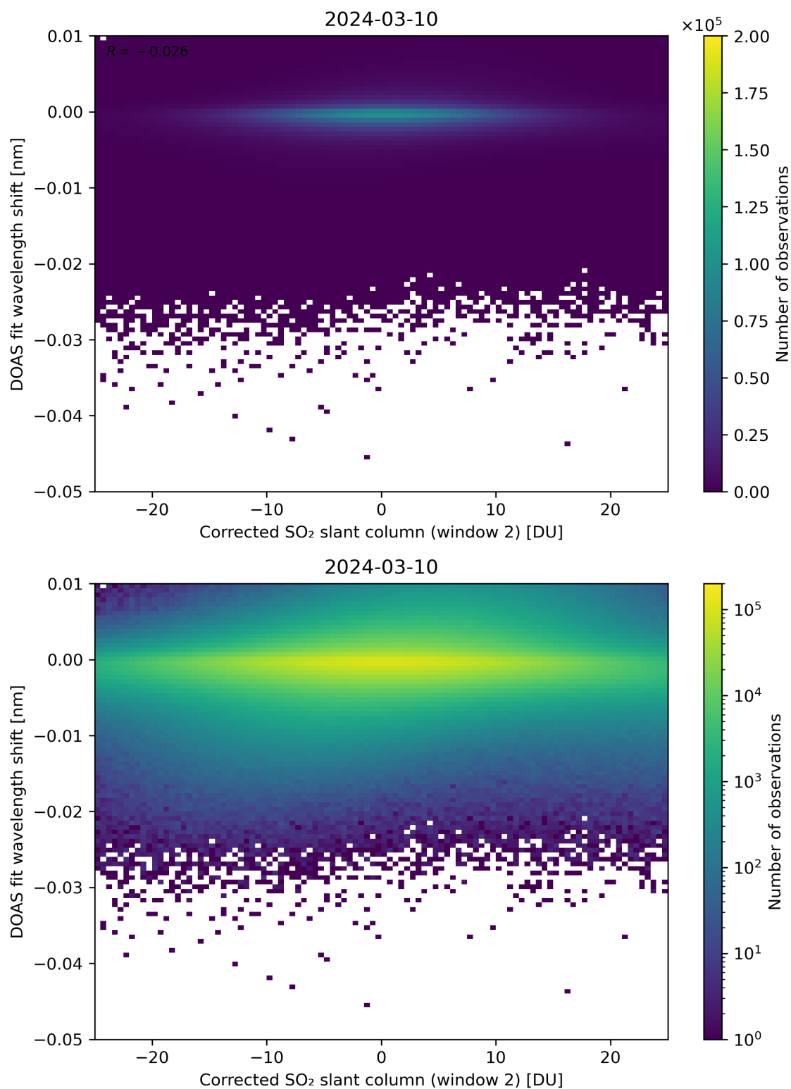
Figure 196: Scatter density plot of “Corrected SO 2 slant column (window 2)” against “DOAS fit wavelength shift” for 2024-03-09 to 2024-03-11.
