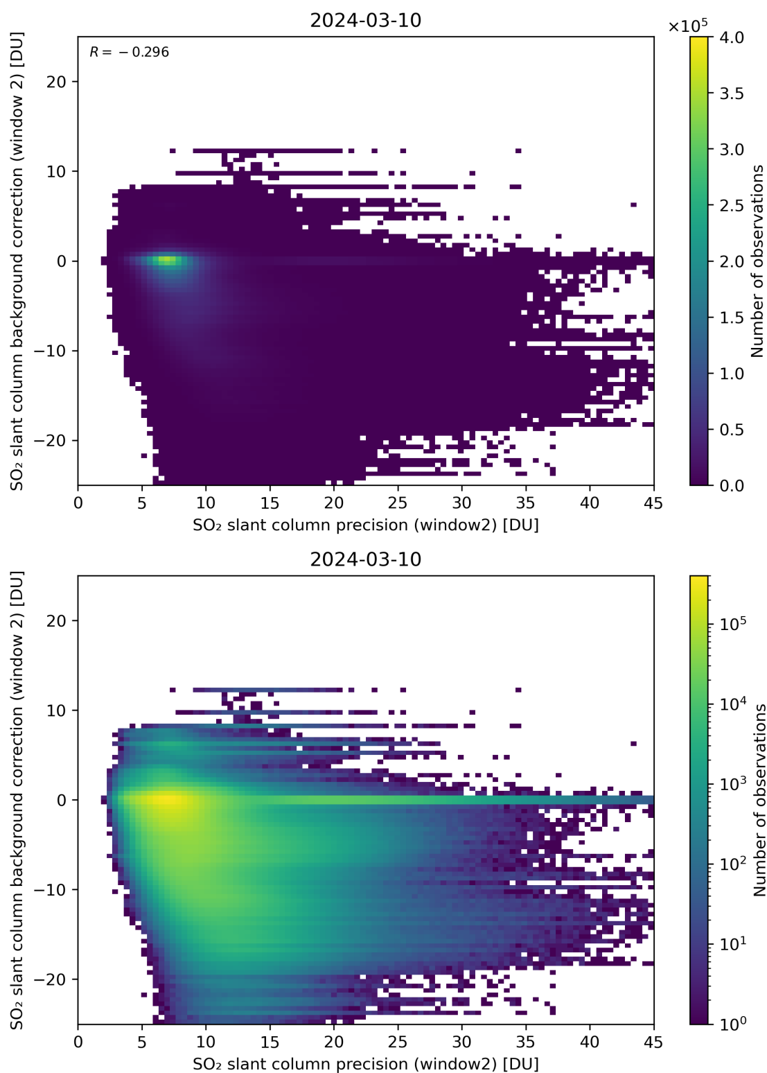
Figure 241: Scatter density plot of “SO 2 slant column precision (window2)” against “SO 2 slant column background correction (window 2)” for 2024-03-09 to 2024-03-11.
