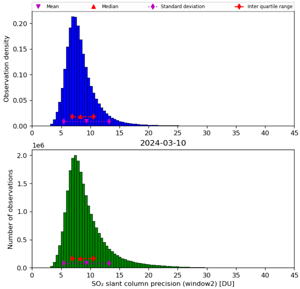
Figure 61: Histogram of “SO 2 slant column precision (window2)” for 2024-03-09 to 2024-03-11
