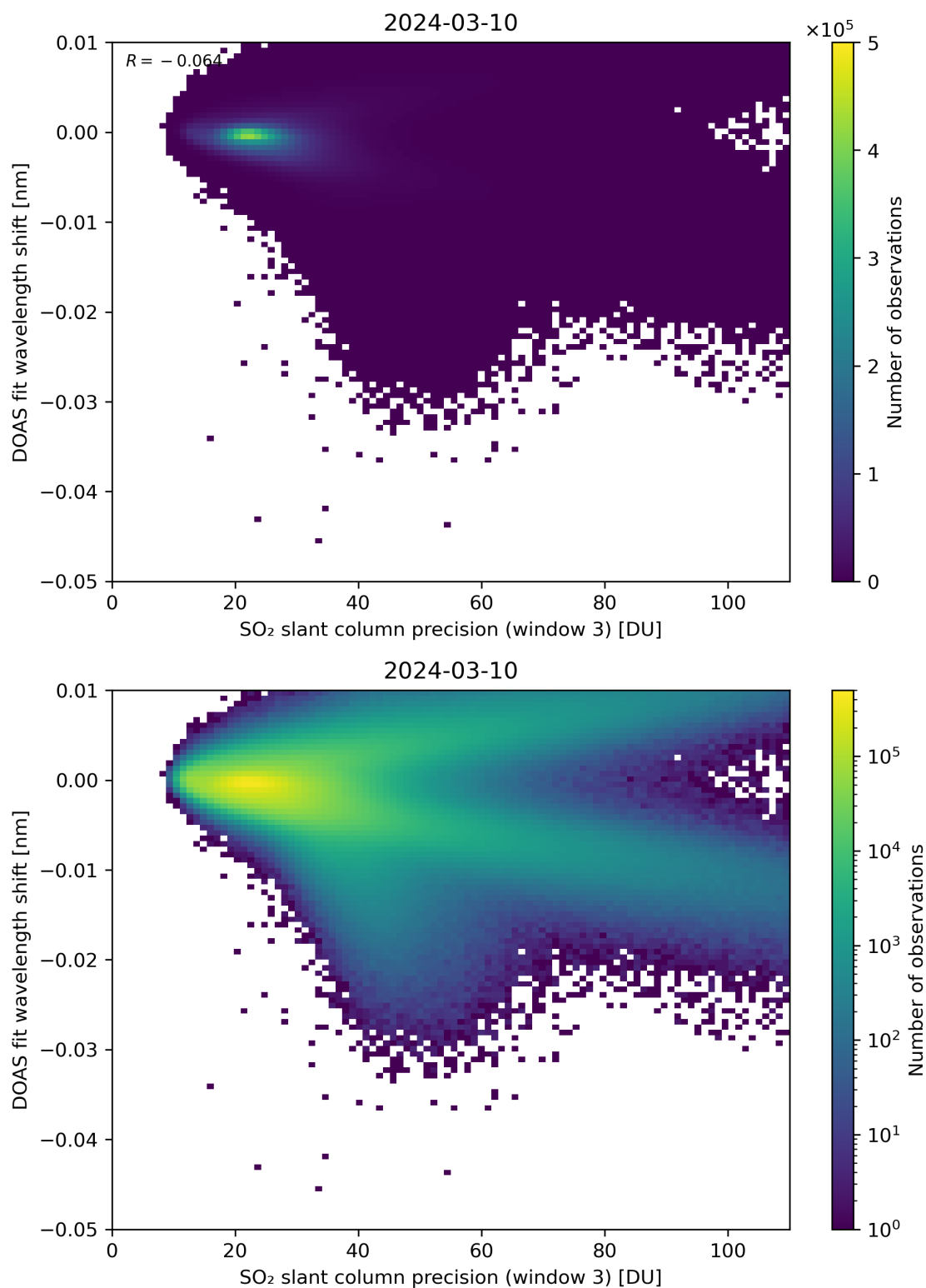
Figure 258: Scatter density plot of “SO 2 slant column precision (window 3)” against “DOAS fit wavelength shift” for 2024-03-09 to 2024-03-11.
