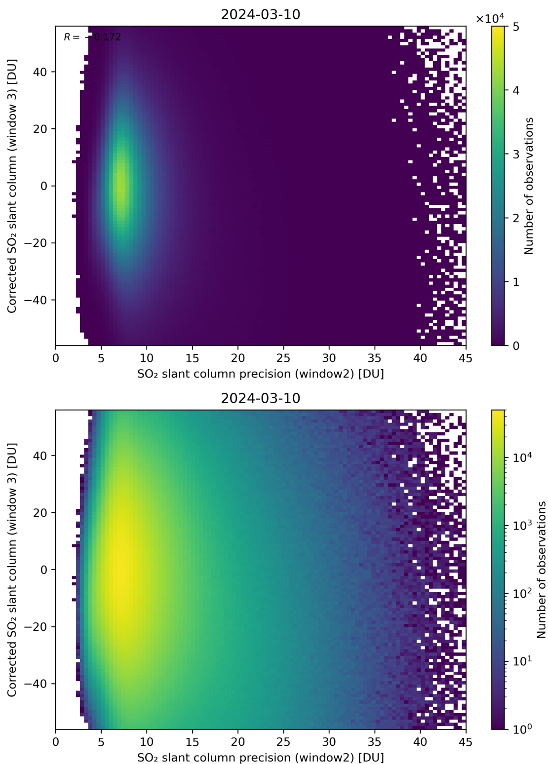
Figure 248: Scatter density plot of “SO 2 slant column precision (window2)” against “Corrected SO 2 slant column (window 3)” for 2024-03-09 to 2024-03-11.
