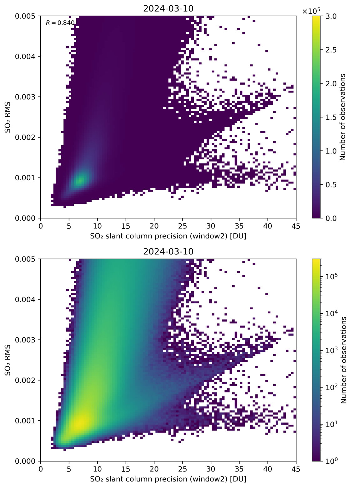
Figure 245: Scatter density plot of “SO 2 slant column precision (window2)” against “SO 2 RMS” for 2024-03-09 to 2024-03-11.
