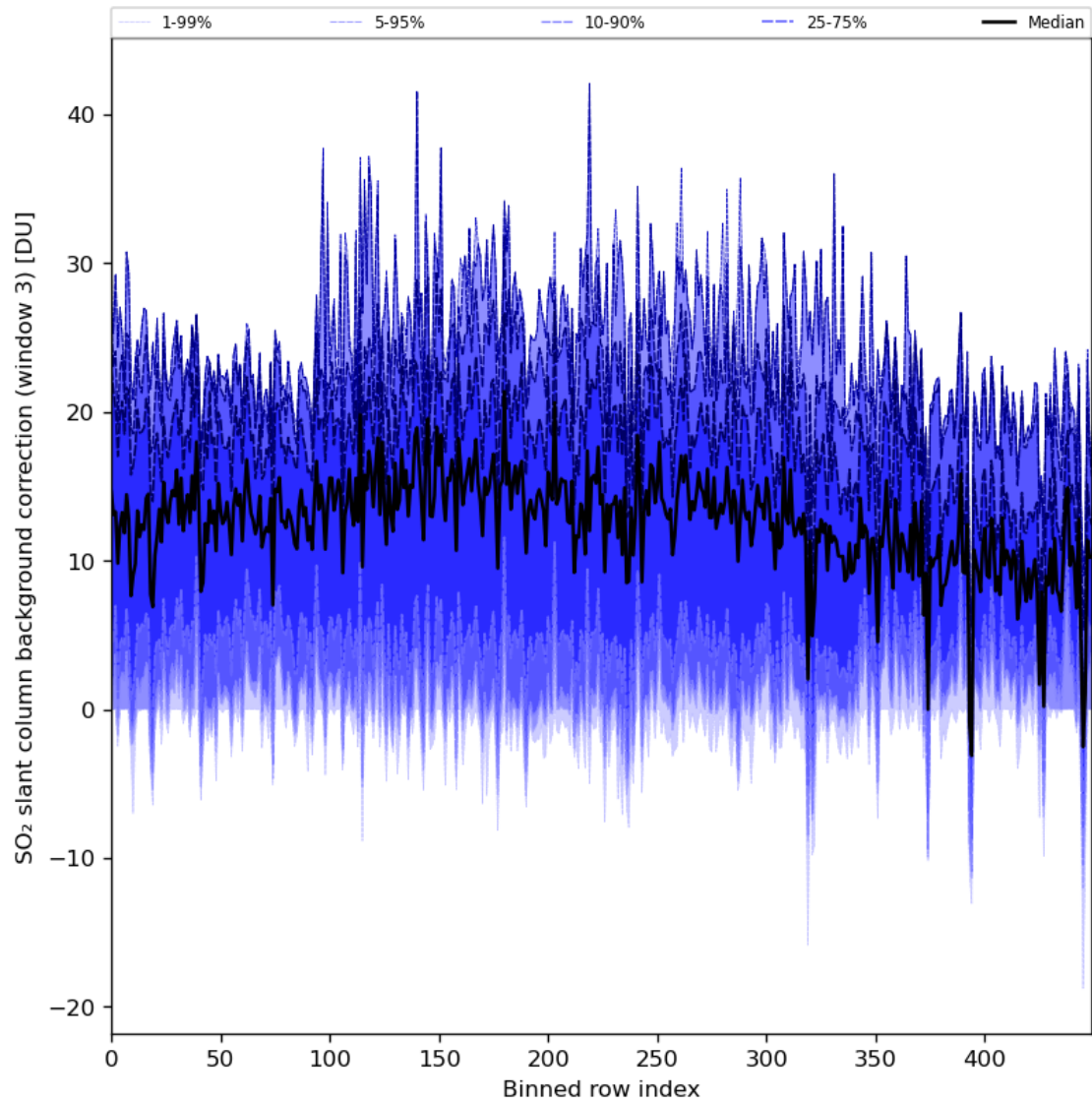
Figure 90: Along track statistics of “SO 2 slant column background correction (window 3)” for 2024-03-09 to 2024-03-11
