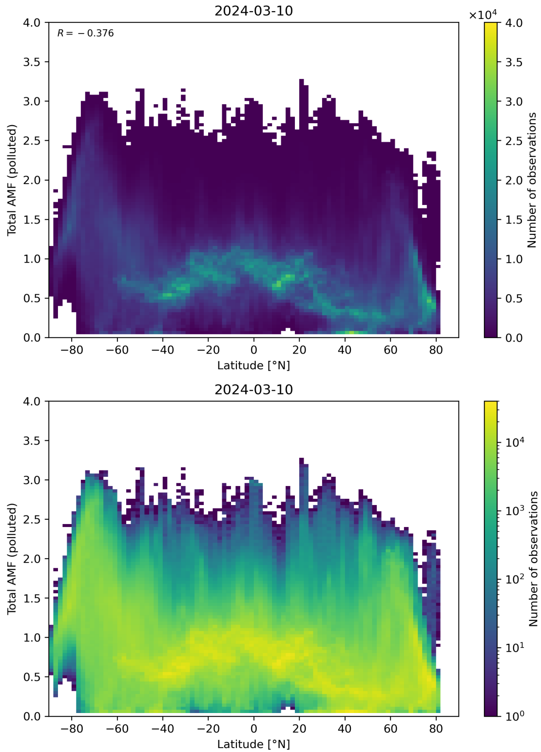
Figure 154: Scatter density plot of “Latitude” against “Total AMF (polluted)” for 2024-03-09 to 2024-03-11.
