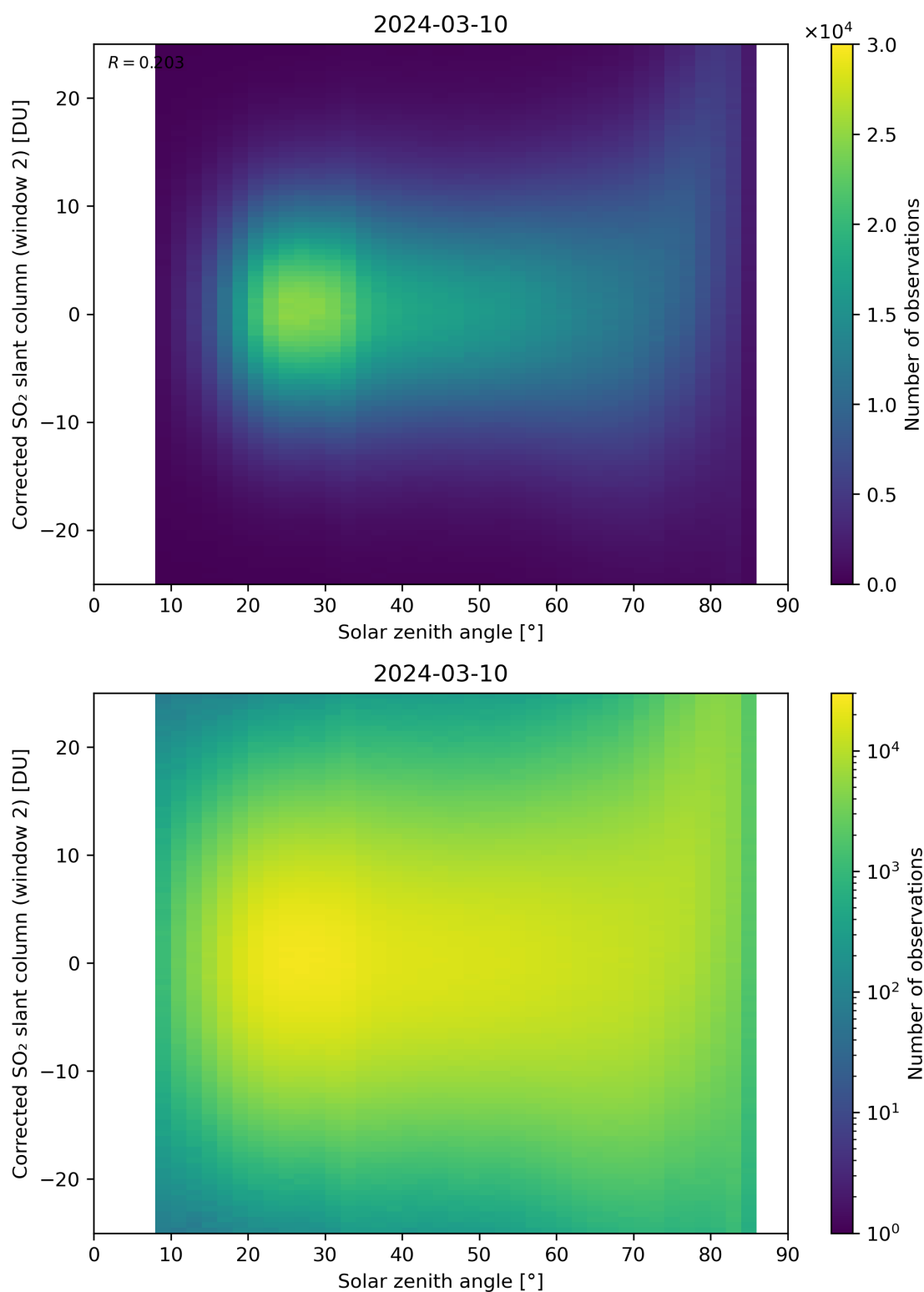
Figure 167: Scatter density plot of “Solar zenith angle” against “Corrected SO 2 slant column (window 2)” for 2024-03-09 to 2024-03-11.
