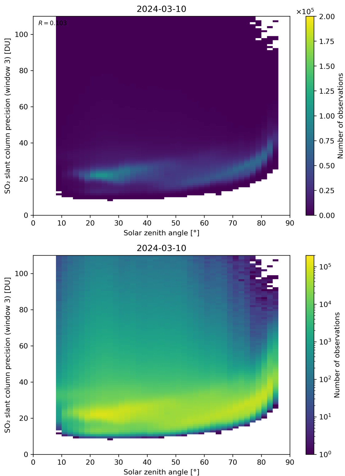
Figure 173: Scatter density plot of “Solar zenith angle” against “SO 2 slant column precision (window 3)” for 2024-03-09 to 2024-03-11.
