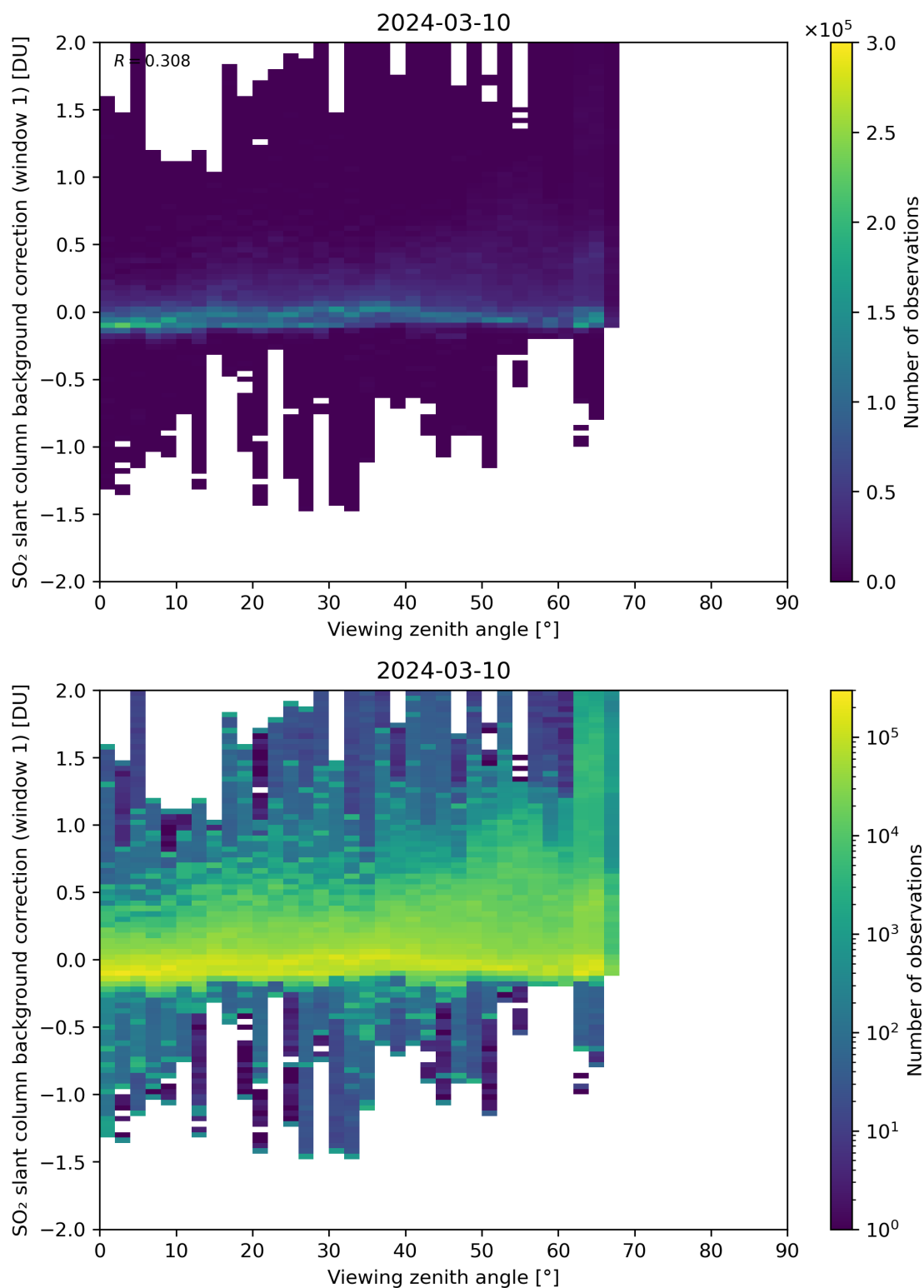
Figure 308: Scatter density plot of “Viewing zenith angle” against “SO 2 slant column background correction (window 1)” for 2024-03-09 to 2024-03-11.
