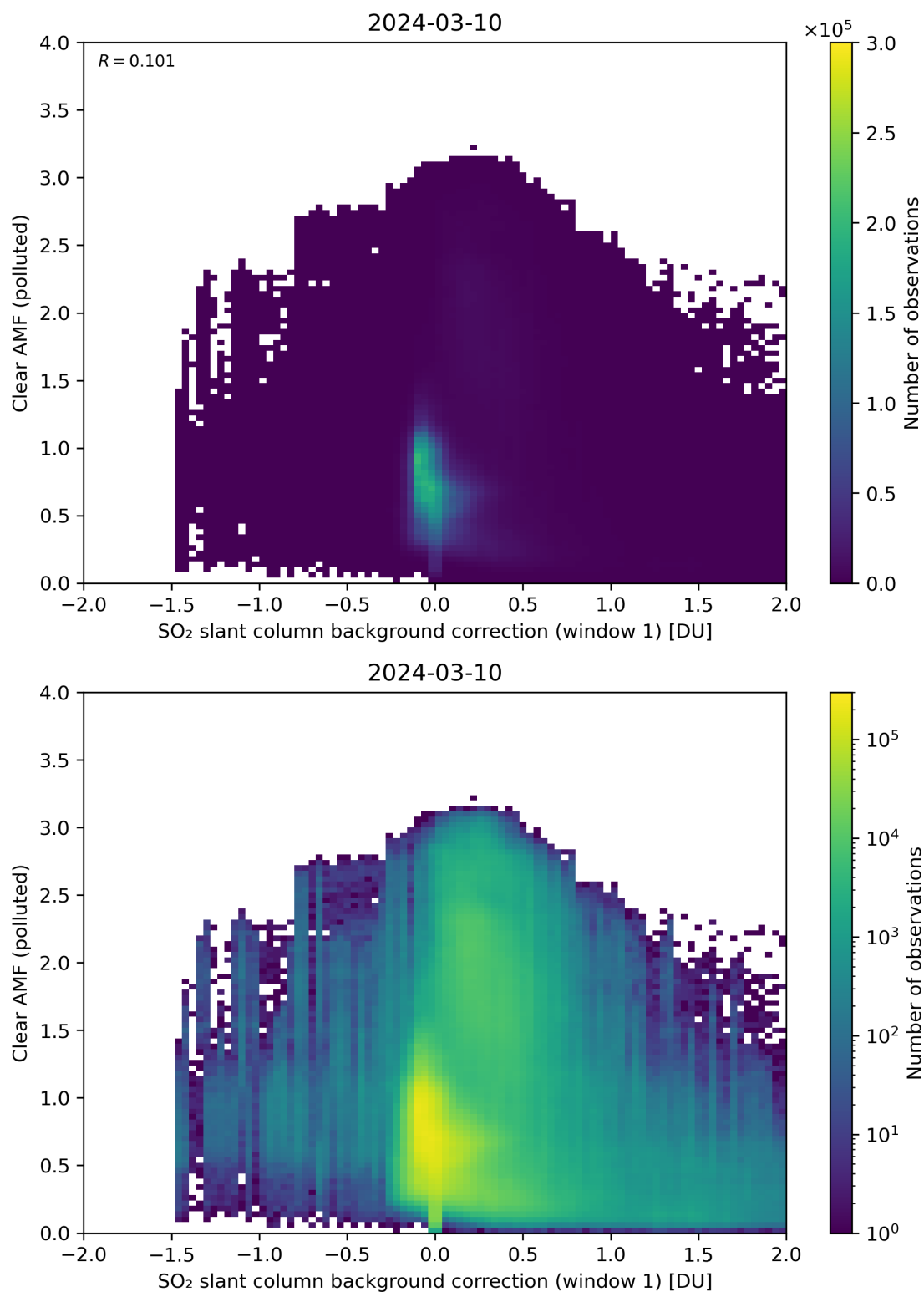
Figure 103: Scatter density plot of “SO 2 slant column background correction (window 1)” against “Clear AMF (polluted)” for 2024-03-09 to 2024-03-11.
