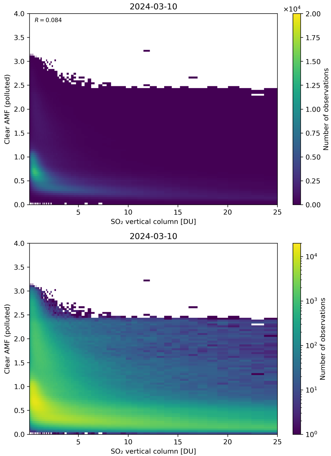
Figure 296: Scatter density plot of “SO 2 vertical column” against “Clear AMF (polluted)” for 2024-03-09 to 2024-03-11.
