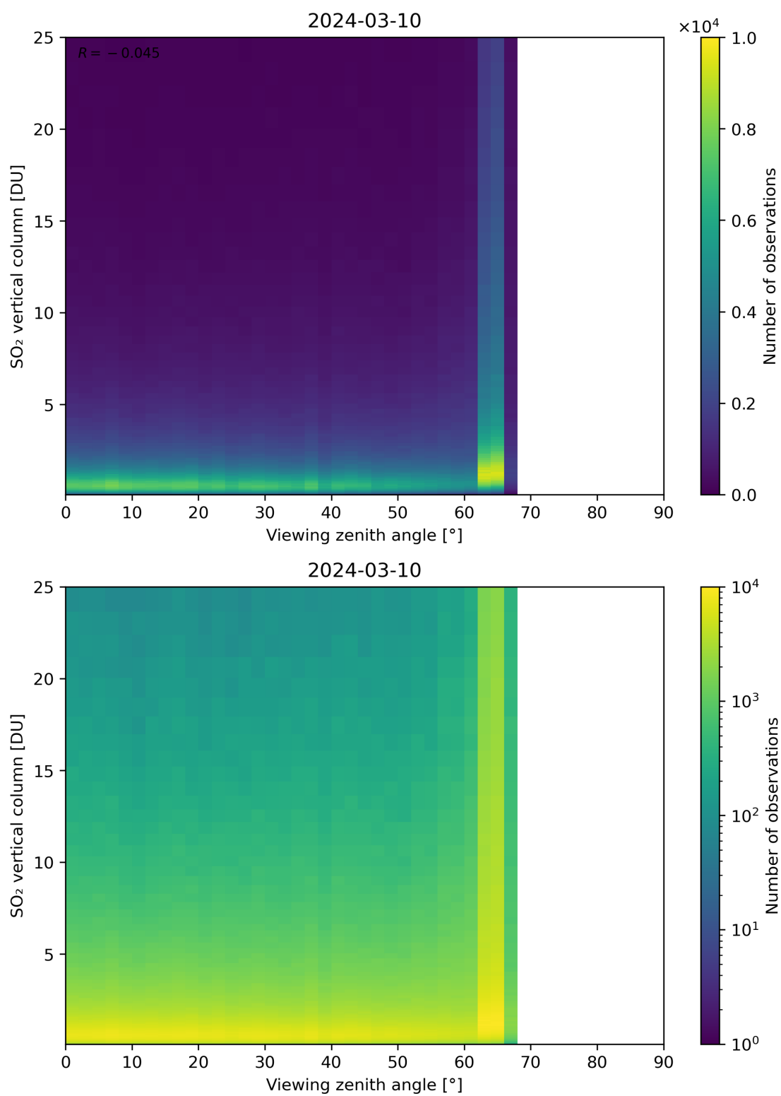
Figure 327: Scatter density plot of “Viewing zenith angle” against “SO 2 vertical column” for 2024-03-09 to 2024-03-11.
