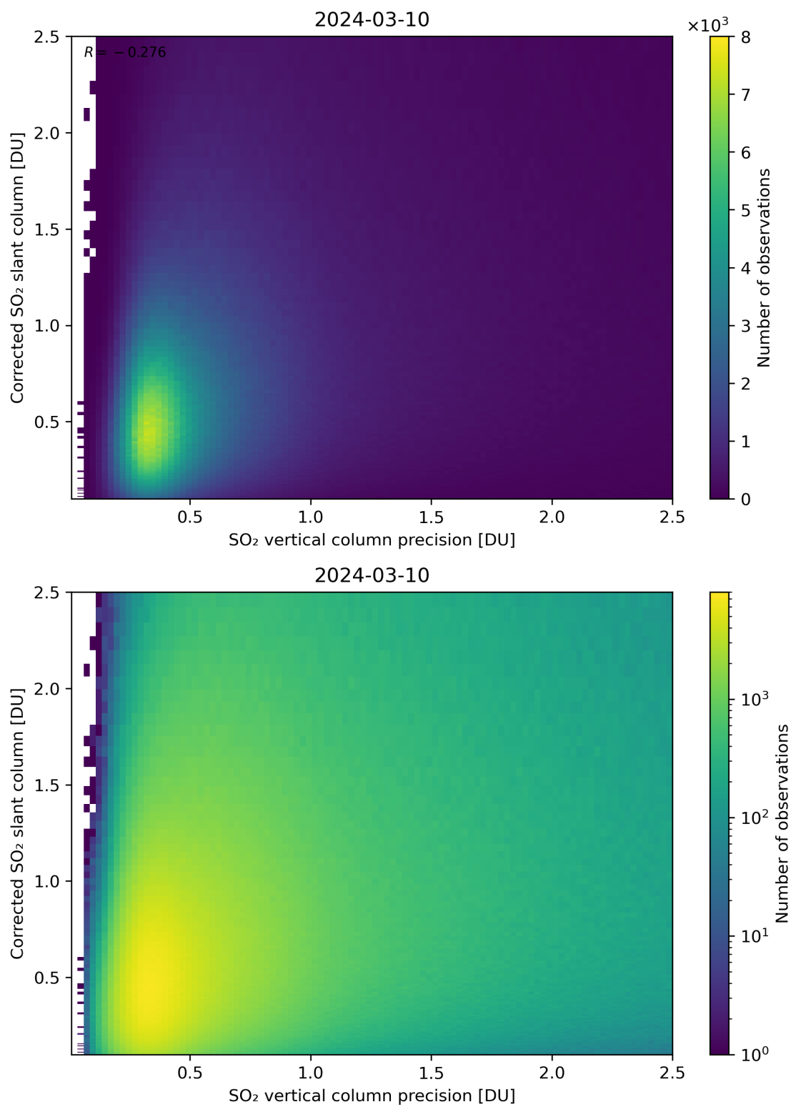
Figure 286: Scatter density plot of “SO 2 vertical column precision” against “Corrected SO 2 slant column” for 2024-03-09 to 2024-03-11.
