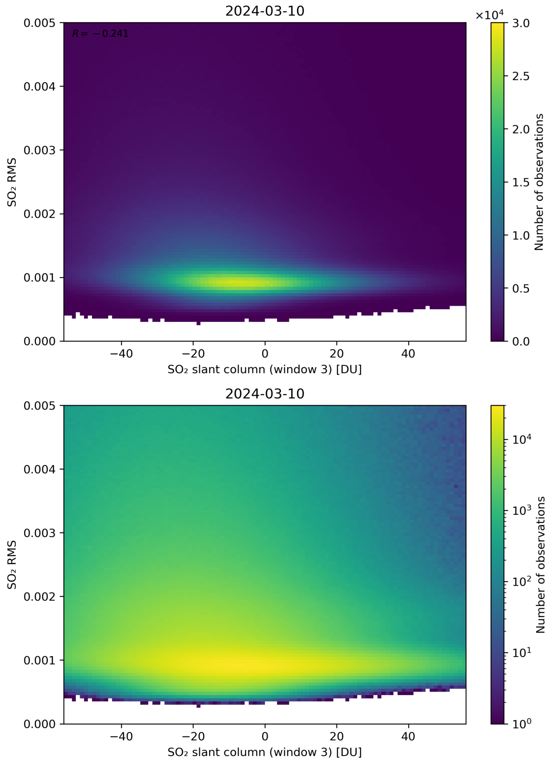
Figure 256: Scatter density plot of “SO 2 slant column (window 3)” against “SO 2 RMS” for 2024-03-09 to 2024-03-11.
