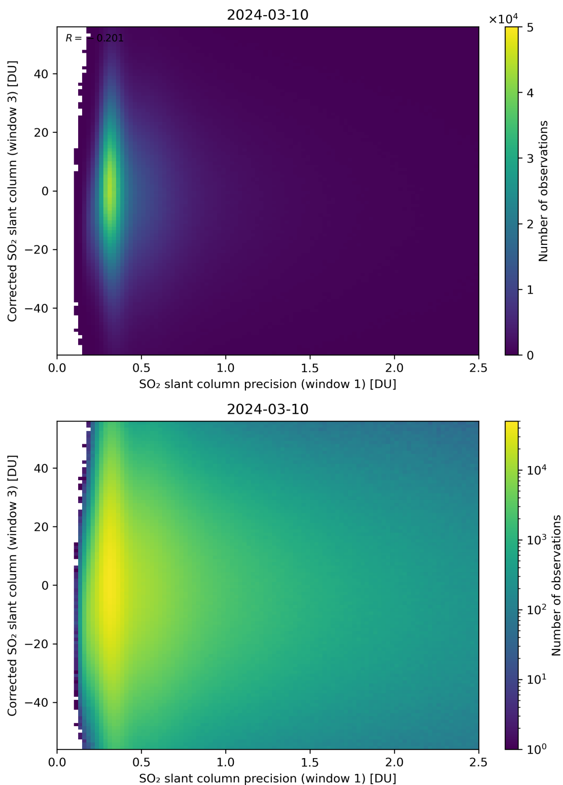
Figure 226: Scatter density plot of “SO 2 slant column precision (window 1)” against “Corrected SO 2 slant column (window 3)” for 2024-03-09 to 2024-03-11.
