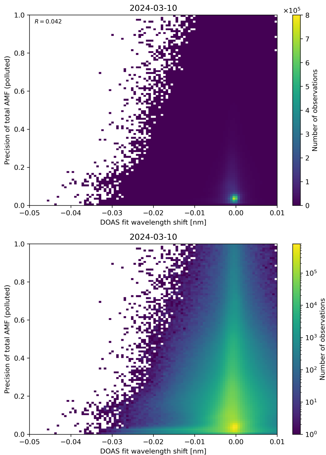
Figure 131: Scatter density plot of “DOAS fit wavelength shift” against “Precision of total AMF (polluted)” for 2024-03-09 to 2024-03-11.
