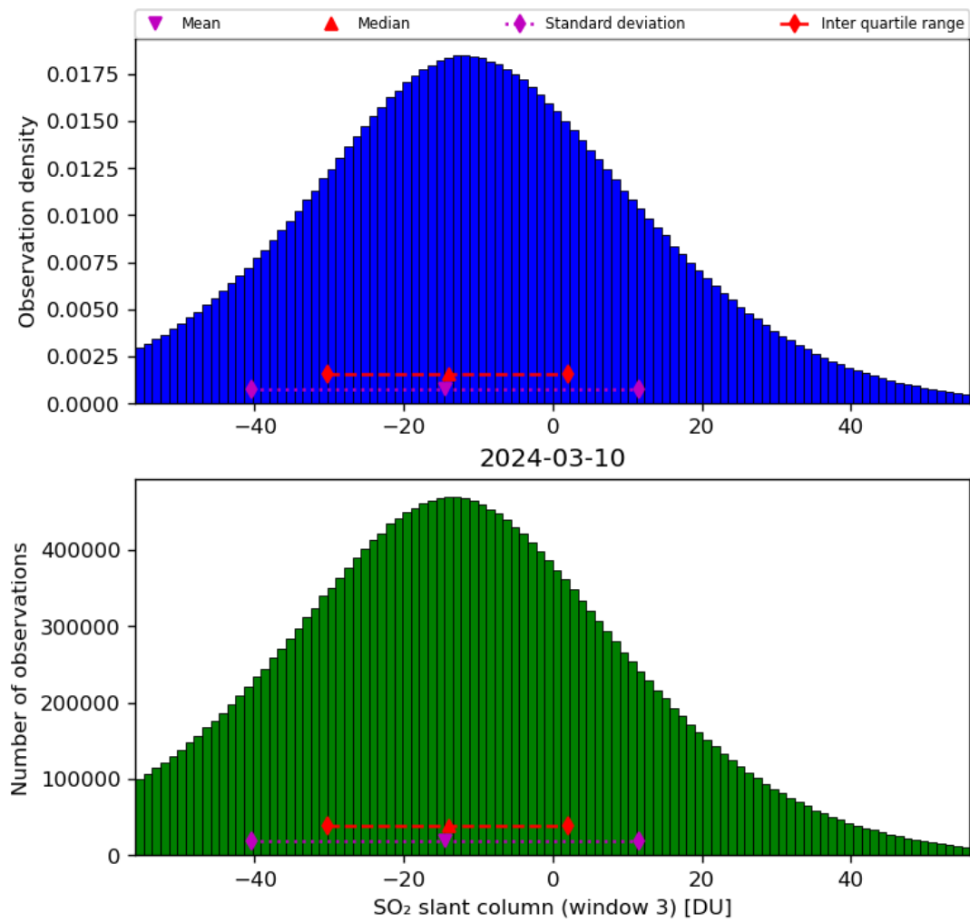
Figure 64: Histogram of “SO 2 slant column (window 3)” for 2024-03-09 to 2024-03-11
