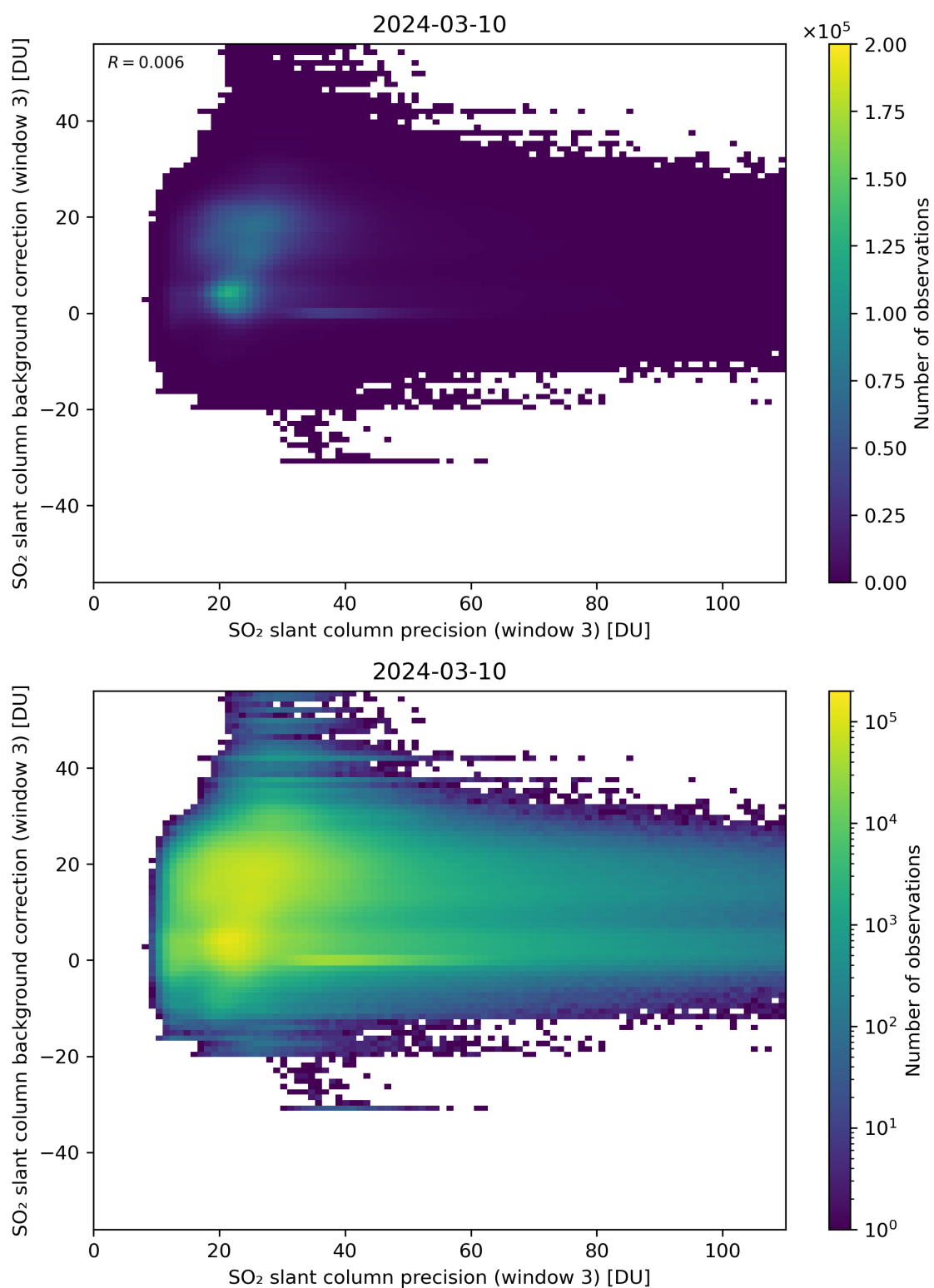
Figure 257: Scatter density plot of “SO 2 slant column precision (window 3)” against “SO 2 slant column background correction (window 3)” for 2024-03-09 to 2024-03-11.
