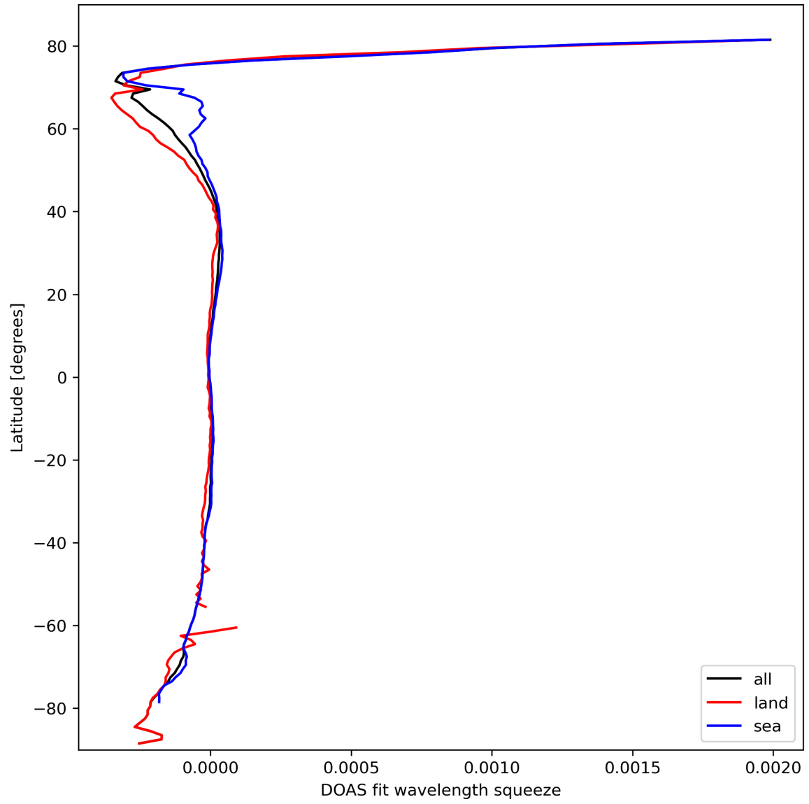
Figure 46: Zonal average of “DOAS fit wavelength squeeze” for 2024-03-09 to 2024-03-11.
