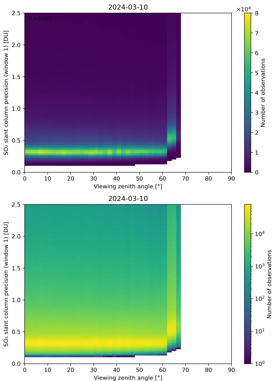
Figure 321: Scatter density plot of “Viewing zenith angle” against “SO 2 slant column precision (window 1)” for 2024-03-09 to 2024-03-11.
