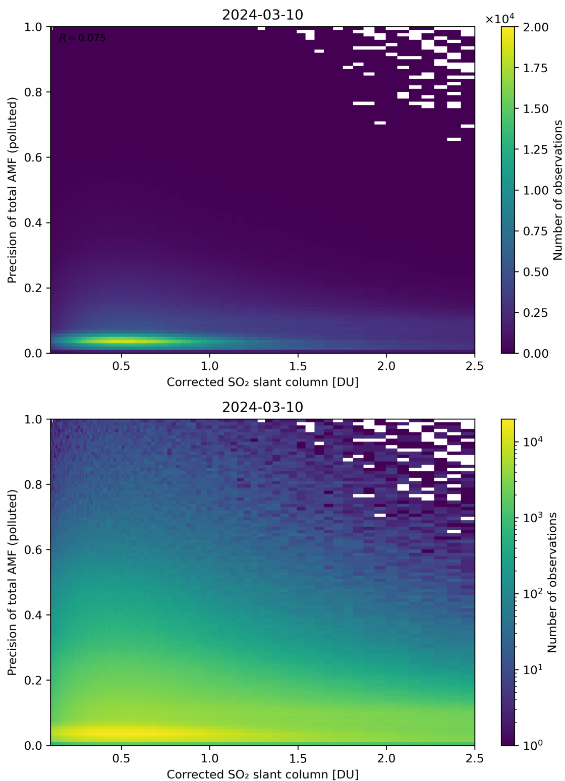
Figure 193: Scatter density plot of “Corrected SO 2 slant column” against “Precision of total AMF (polluted)” for 2024-03-09 to 2024-03-11.
