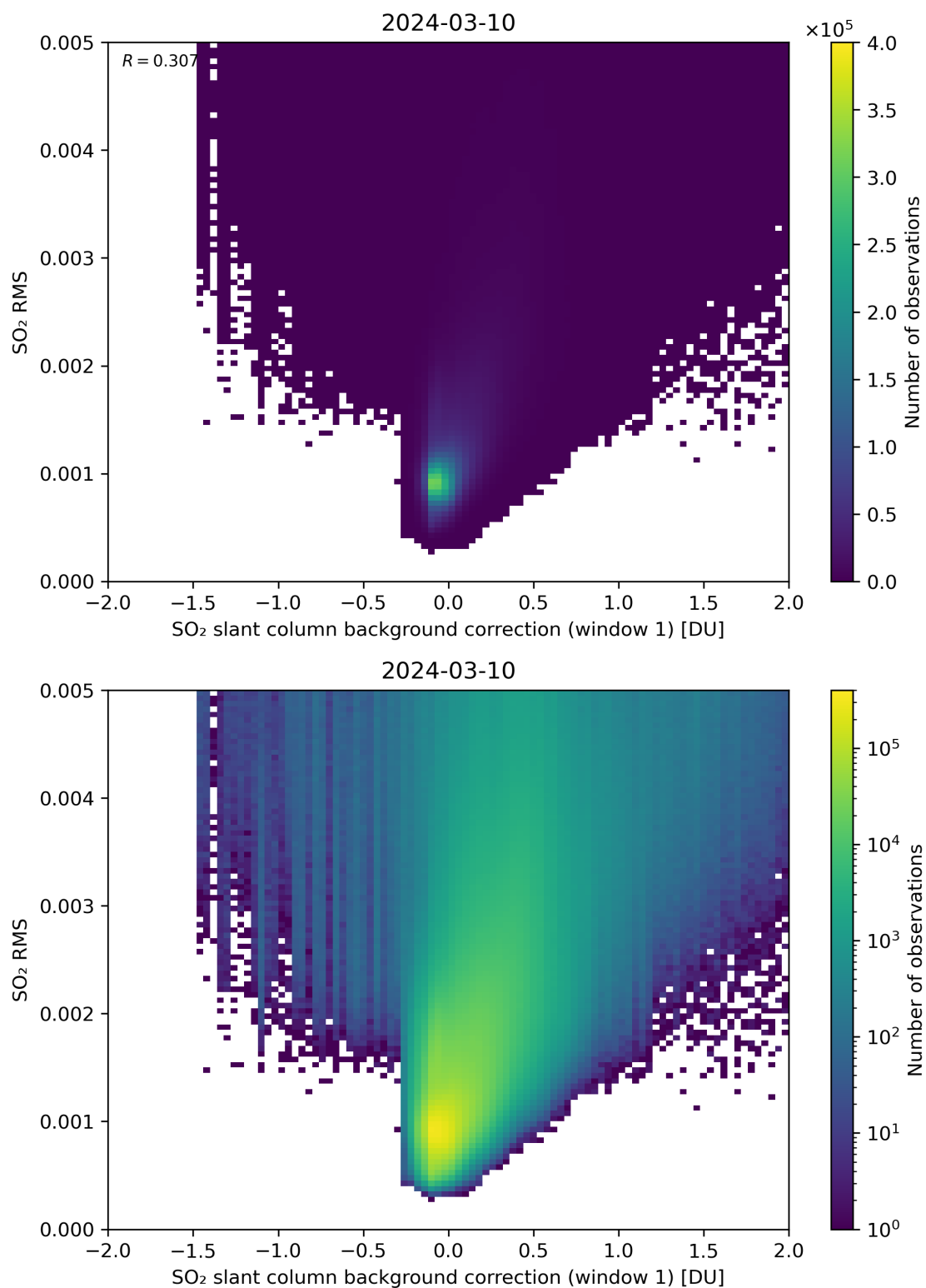
Figure 102: Scatter density plot of “SO 2 slant column background correction (window 1)” against “SO 2 RMS” for 2024-03-09 to 2024-03-11.
