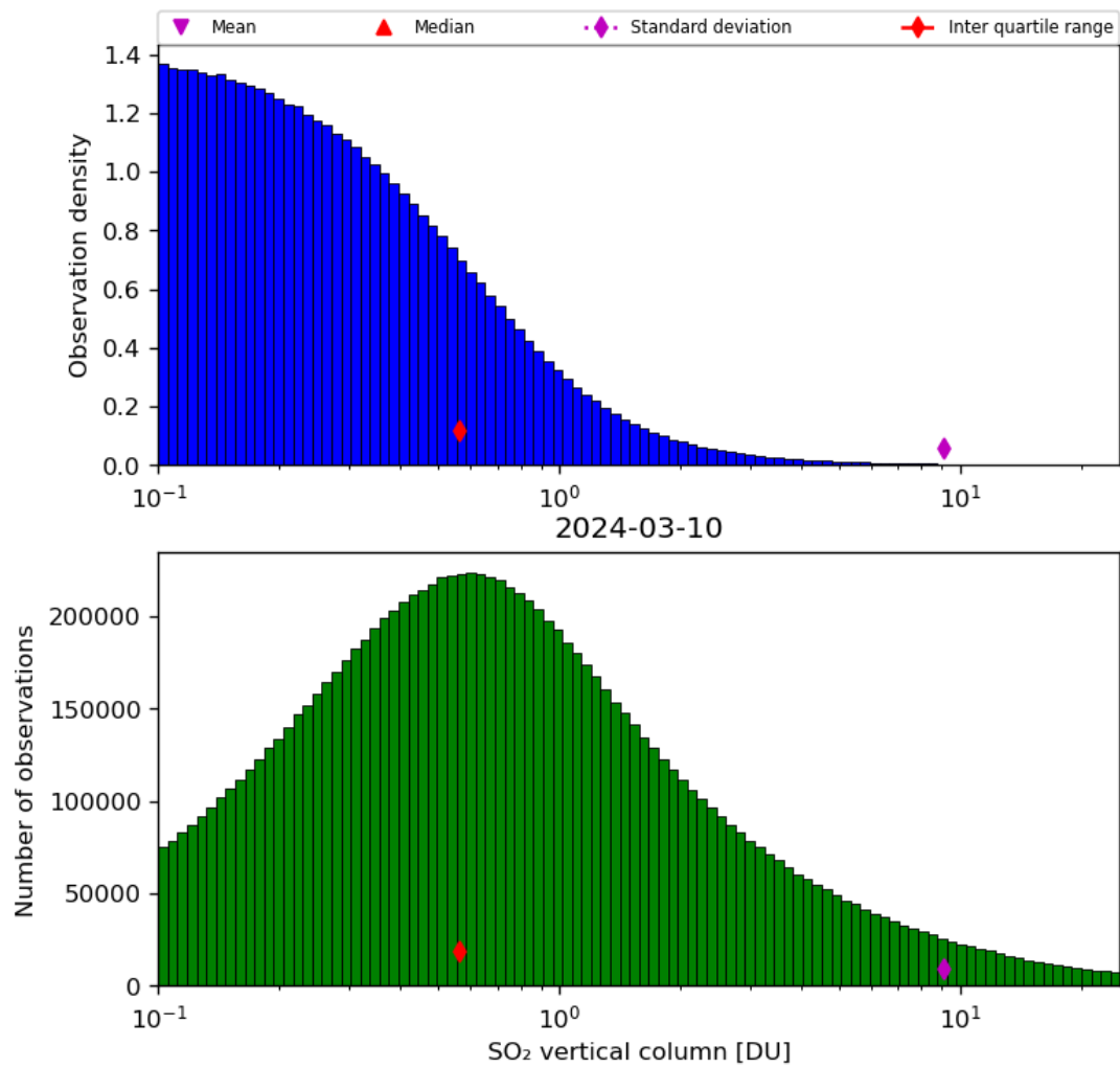
Figure 53: Histogram of “SO 2 vertical column” for 2024-03-09 to 2024-03-11
