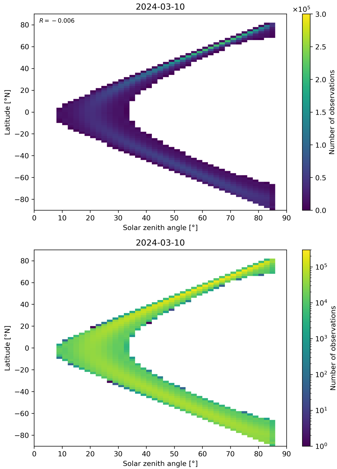
Figure 164: Scatter density plot of “Solar zenith angle” against “Latitude” for 2024-03-09 to 2024-03-11.
