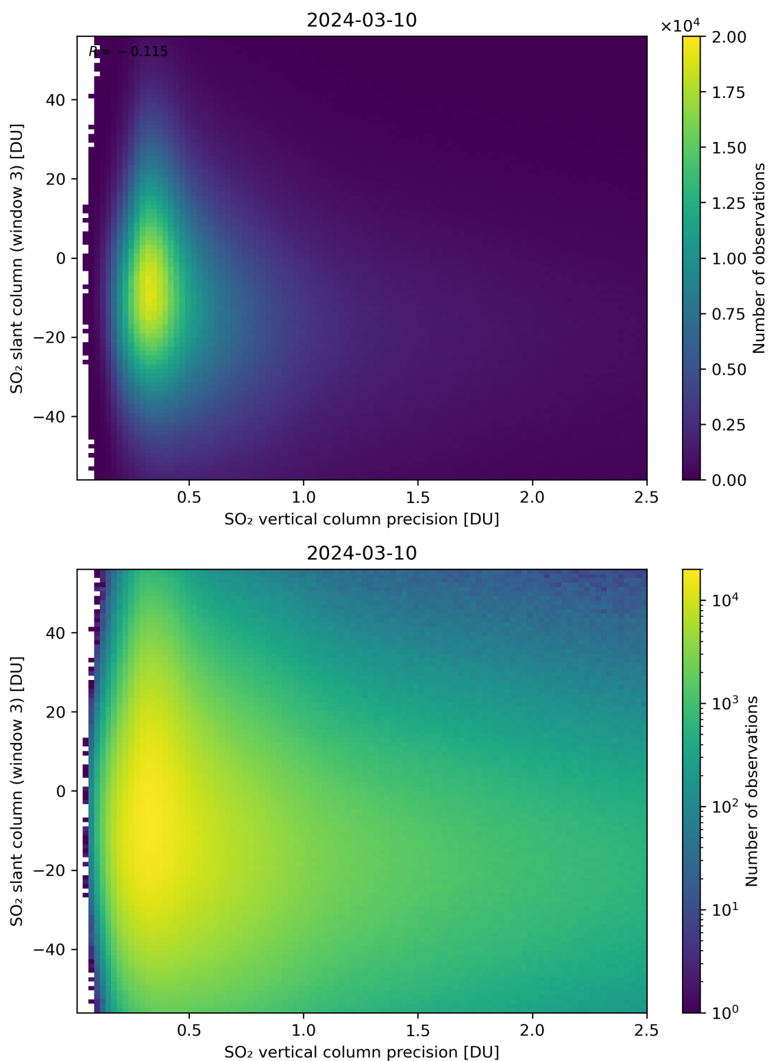
Figure 292: Scatter density plot of “SO 2 vertical column precision” against “SO 2 slant column (window 3)” for 2024-03-09 to 2024-03-11.
