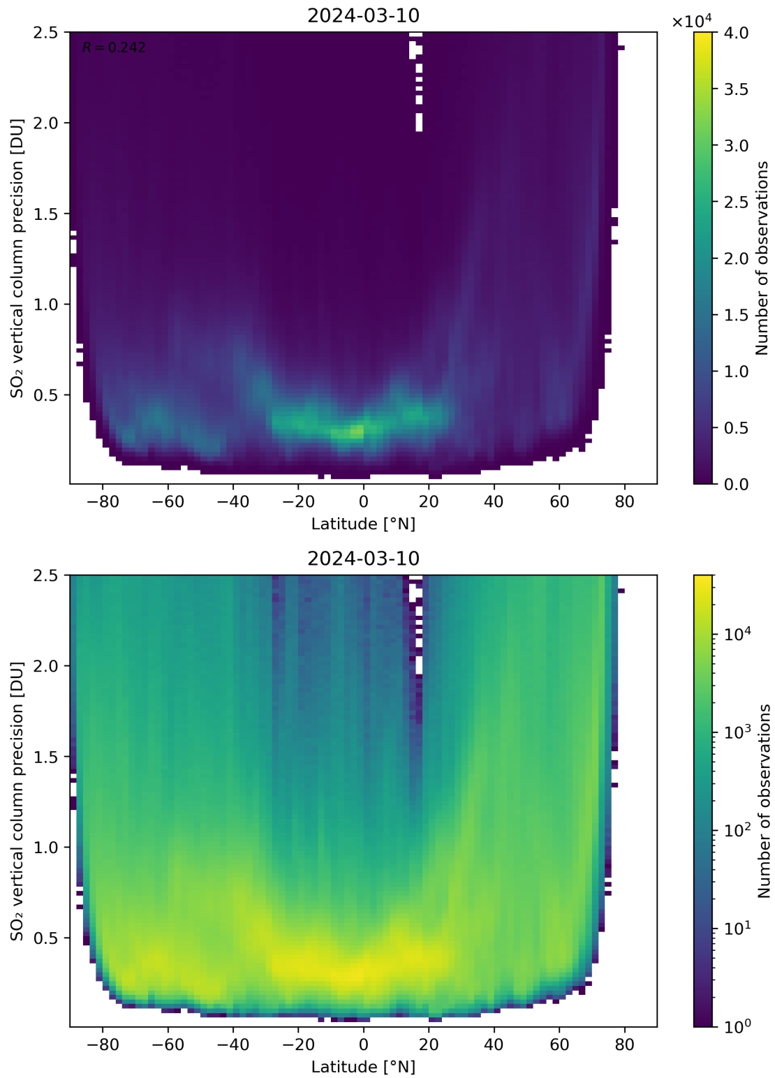
Figure 157: Scatter density plot of “Latitude” against “SO 2 vertical column precision” for 2024-03-09 to 2024-03-11.
