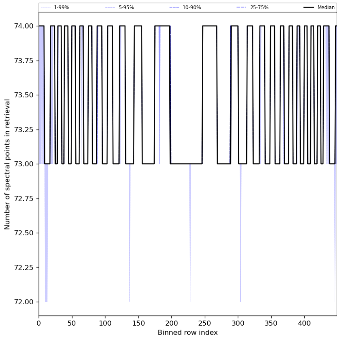
Figure 97: Along track statistics of “Number of spectral points in retrieval” for 2024-03-09 to 2024-03-11
