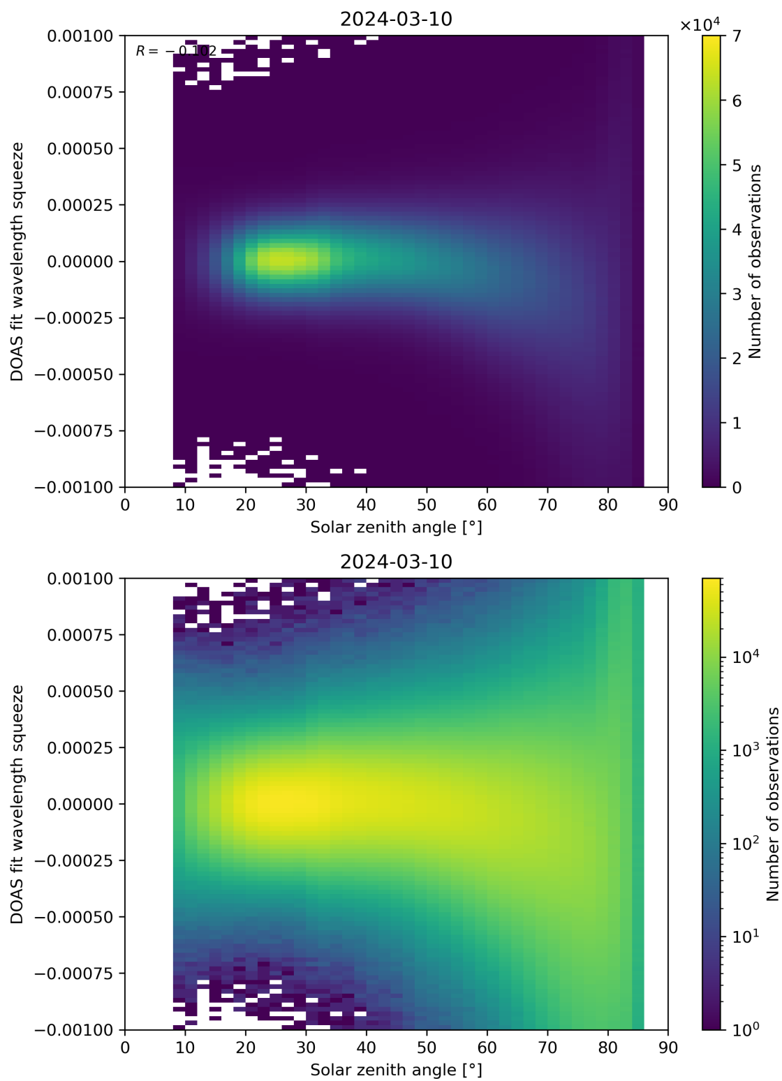
Figure 162: Scatter density plot of “Solar zenith angle” against “DOAS fit wavelength squeeze” for 2024-03-09 to 2024-03-11.
