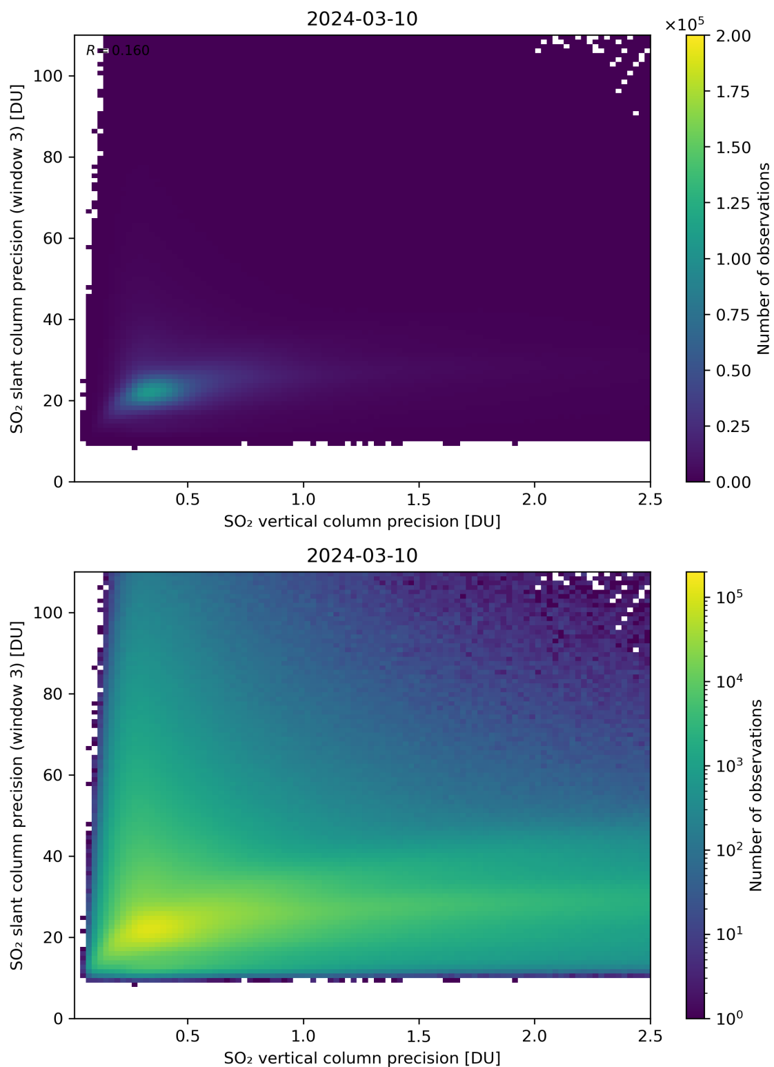
Figure 293: Scatter density plot of “SO 2 vertical column precision” against “SO 2 slant column precision (window 3)” for 2024-03-09 to 2024-03-11.
