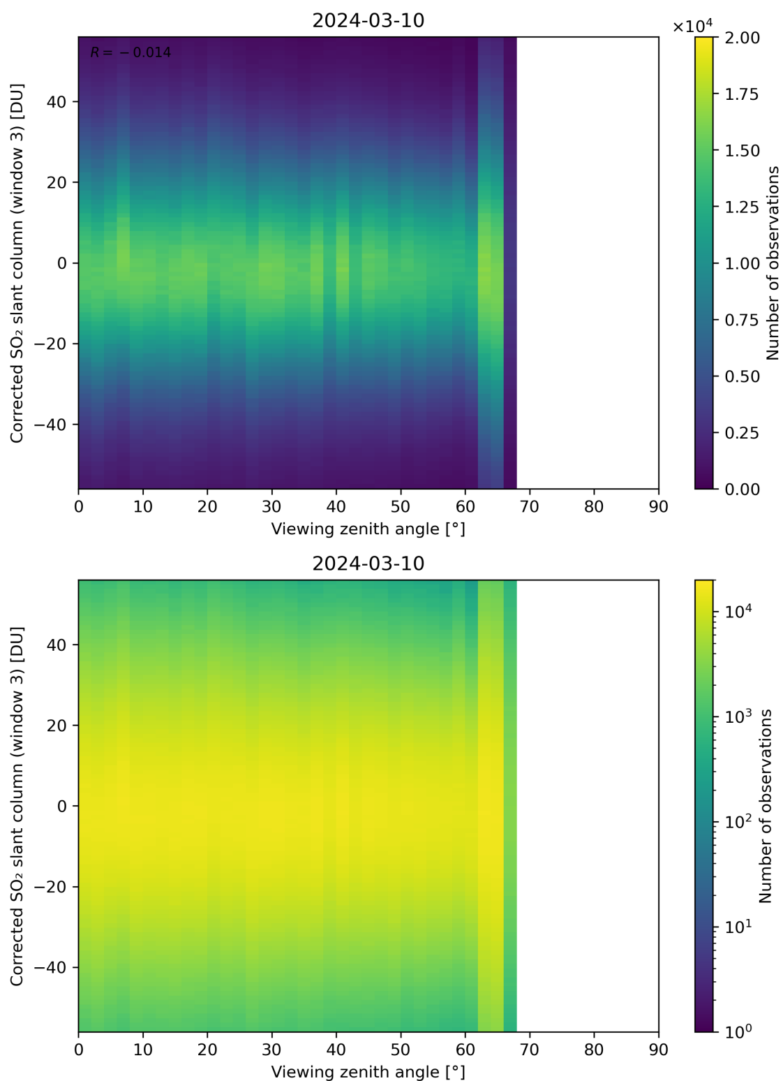
Figure 319: Scatter density plot of “Viewing zenith angle” against “Corrected SO 2 slant column (window 3)” for 2024-03-09 to 2024-03-11.
