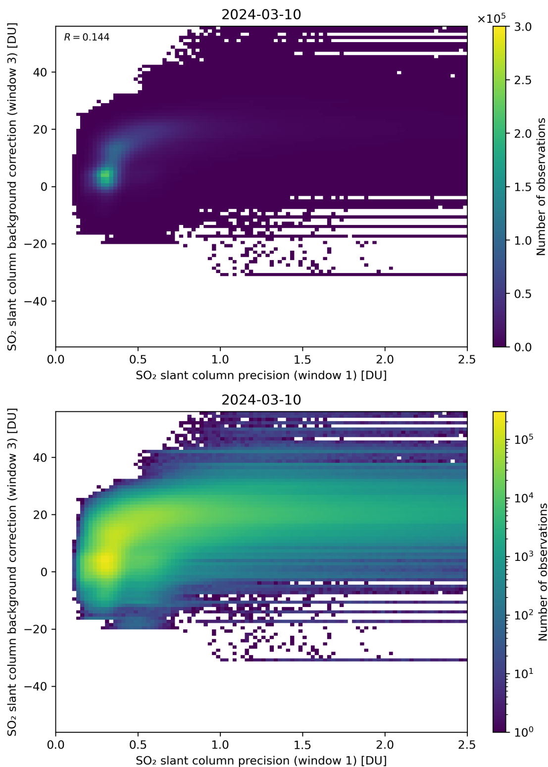
Figure 220: Scatter density plot of “SO 2 slant column precision (window 1)” against “SO 2 slant column background correction (window 3)” for 2024-03-09 to 2024-03-11.
