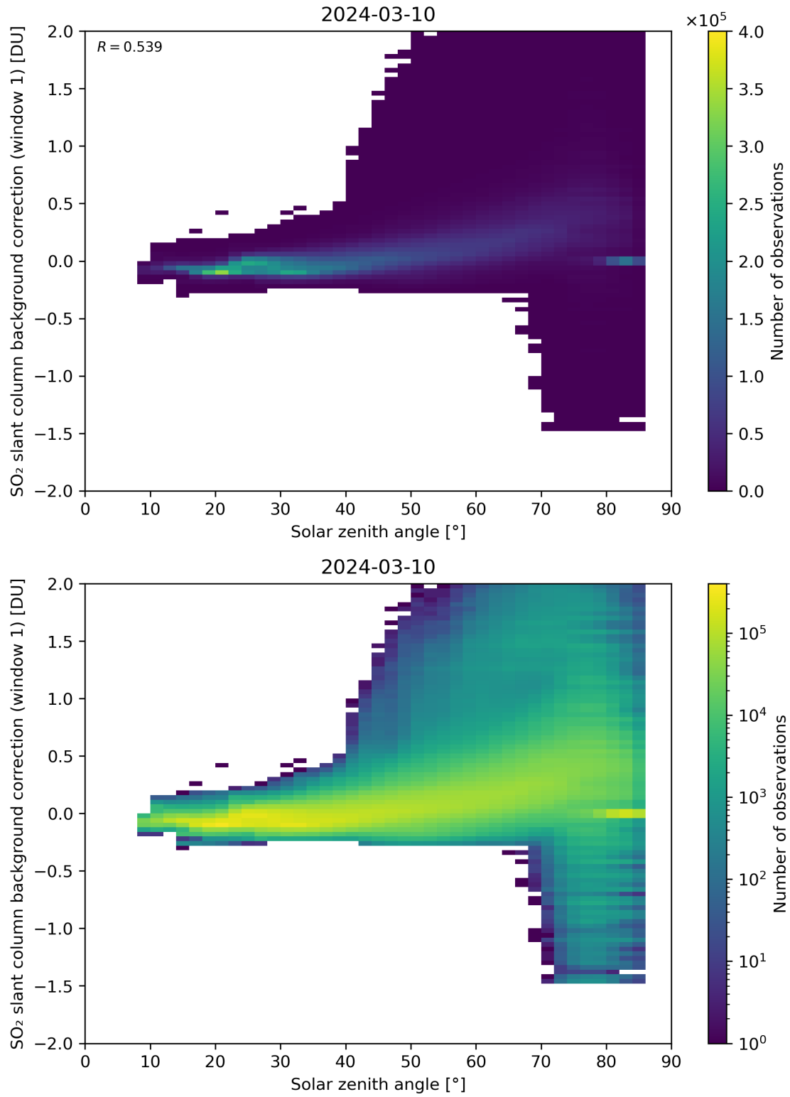
Figure 158: Scatter density plot of “Solar zenith angle” against “SO 2 slant column background correction (window 1)” for 2024-03-09 to 2024-03-11.
