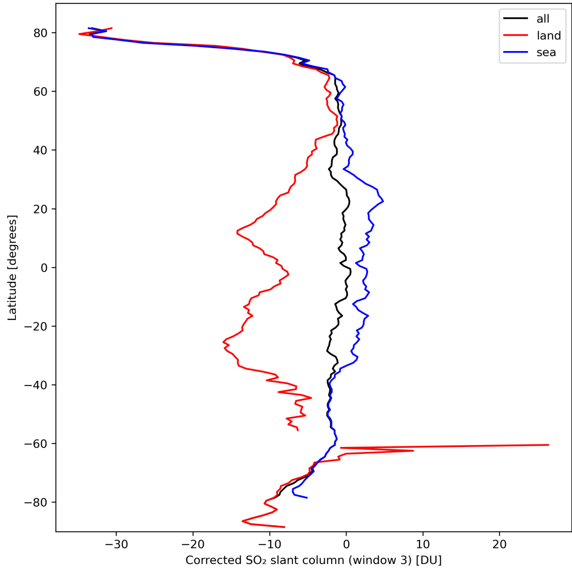
Figure 43: Zonal average of “Corrected SO 2 slant column (window 3)” for 2024-03-09 to 2024-03-11.
