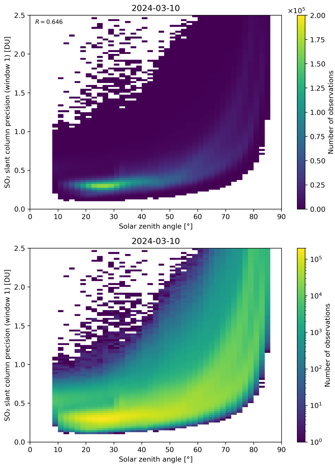
Figure 170: Scatter density plot of “Solar zenith angle” against “SO 2 slant column precision (window 1)” for 2024-03-09 to 2024-03-11.
