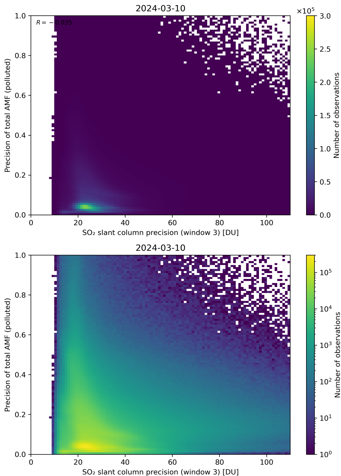
Figure 264: Scatter density plot of “SO 2 slant column precision (window 3)” against “Precision of total AMF (polluted)” for 2024-03-09 to 2024-03-11.
