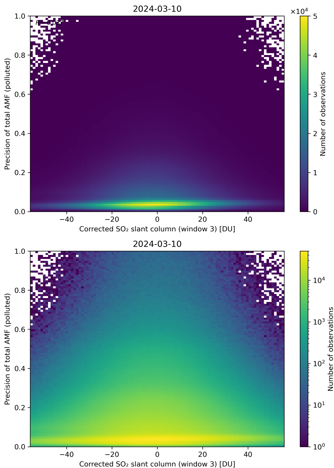
Figure 211: Scatter density plot of “Corrected SO 2 slant column (window 3)” against “Precision of total AMF (polluted)” for 2024-03-09 to 2024-03-11.
