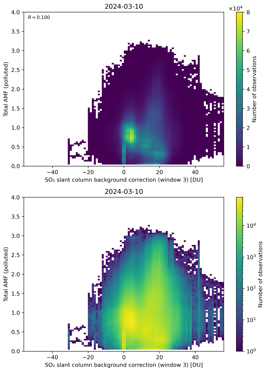
Figure 125: Scatter density plot of “SO 2 slant column background correction (window 3)” against “Total AMF (polluted)” for 2024-03-09 to 2024-03-11.
