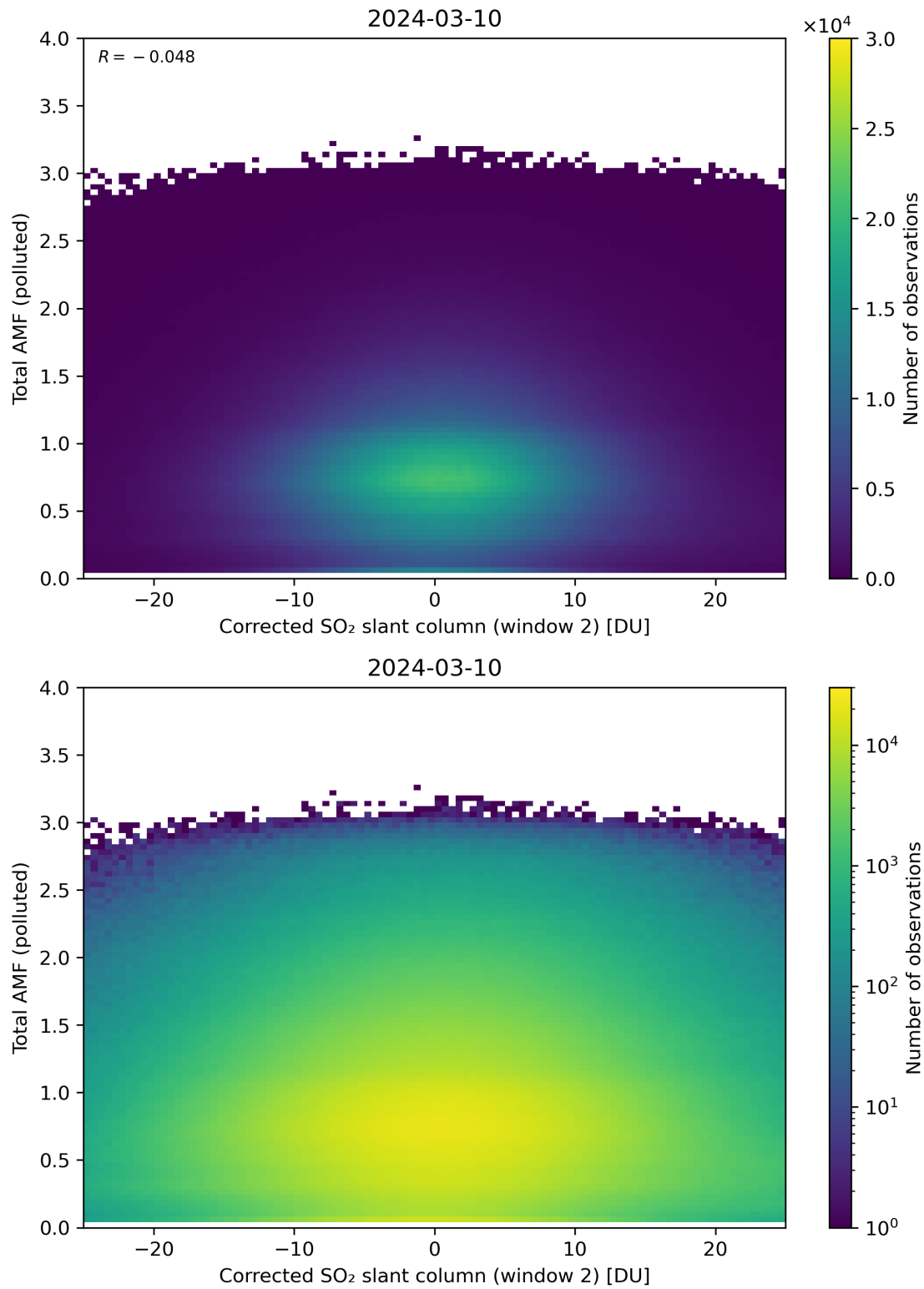
Figure 203: Scatter density plot of “Corrected SO 2 slant column (window 2)” against “Total AMF (polluted)” for 2024-03-09 to 2024-03-11.
