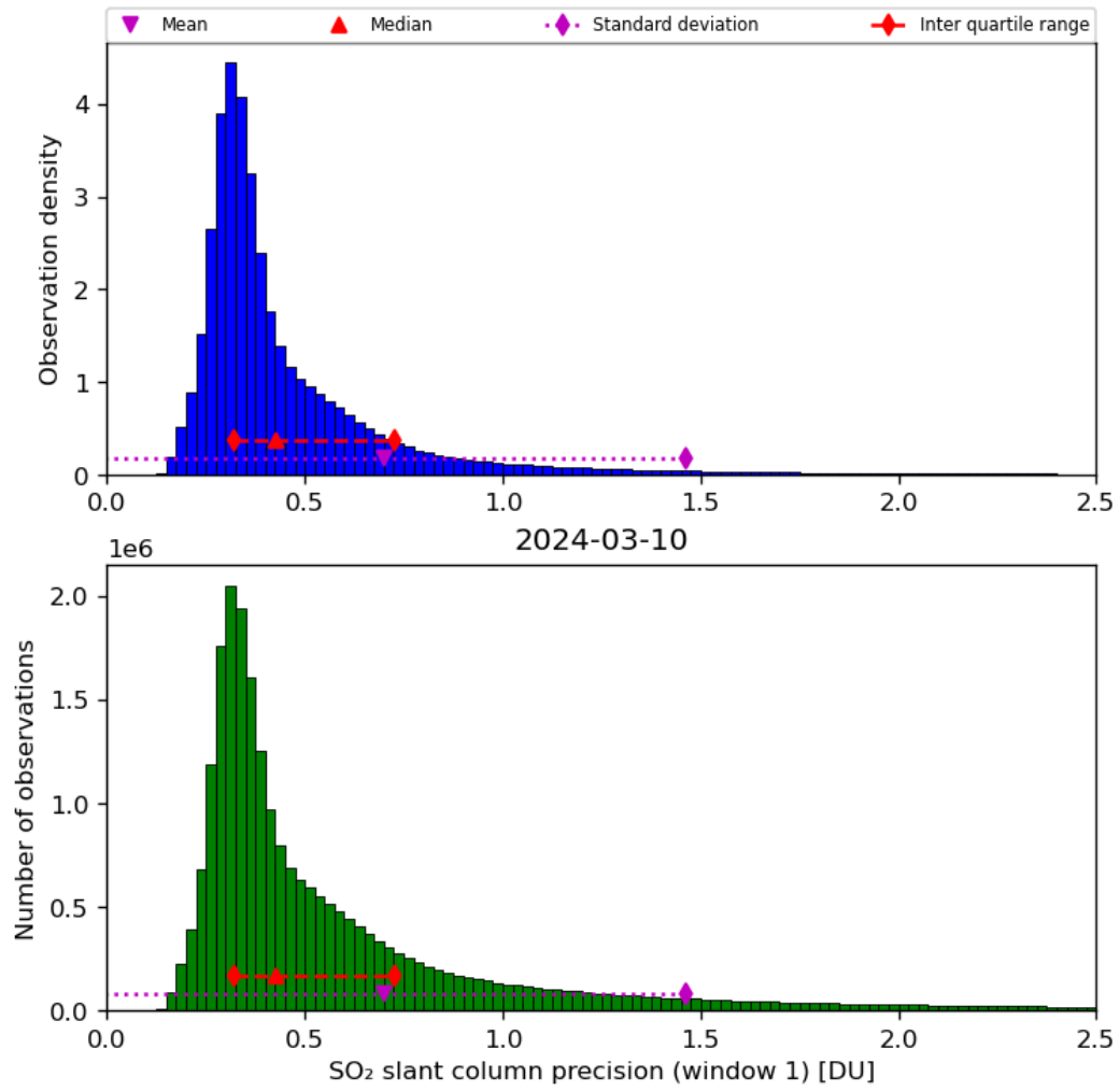
Figure 57: Histogram of “SO 2 slant column precision (window 1)” for 2024-03-09 to 2024-03-11
