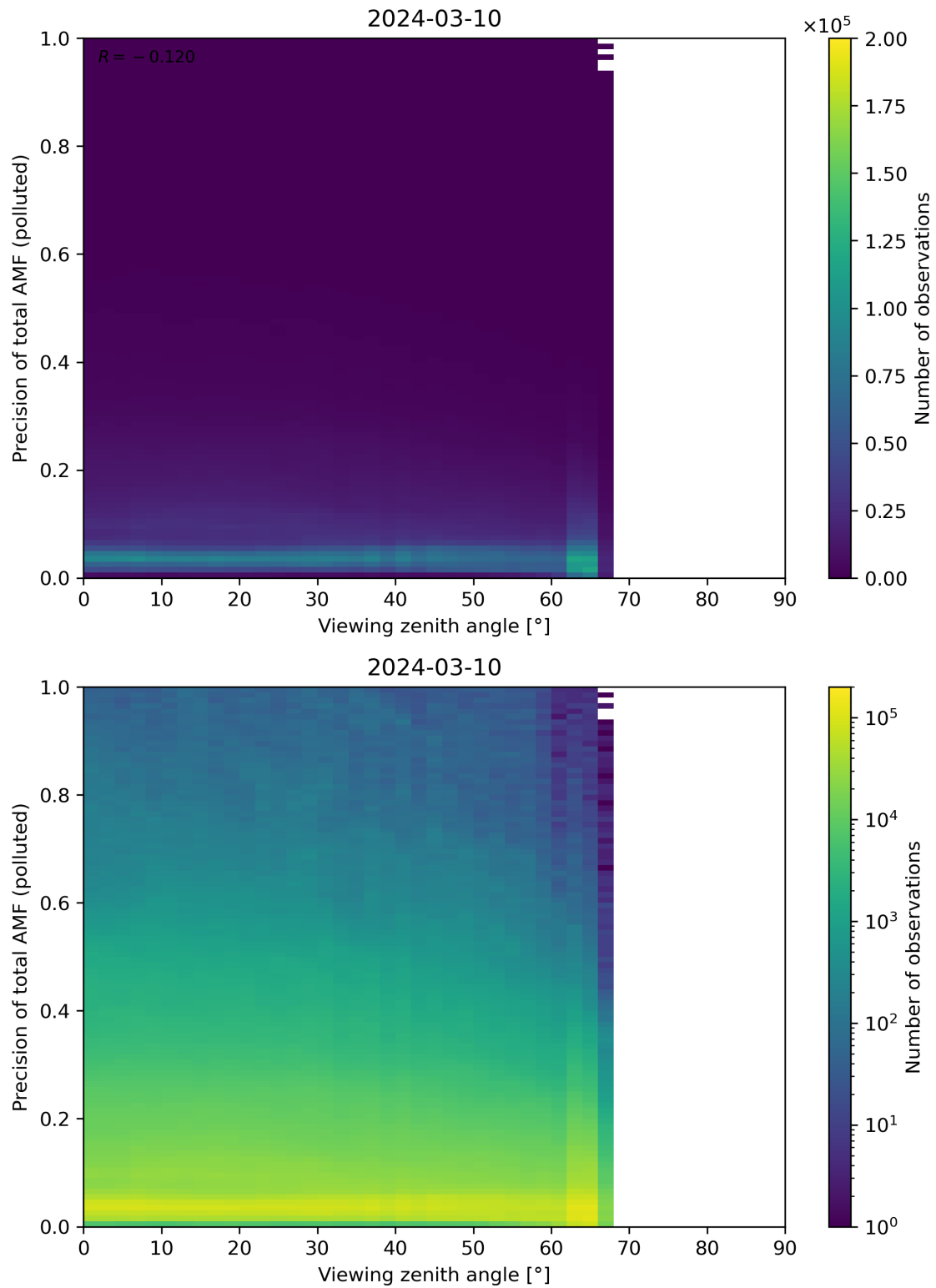
Figure 326: Scatter density plot of “Viewing zenith angle” against “Precision of total AMF (polluted)” for 2024-03-09 to 2024-03-11.
