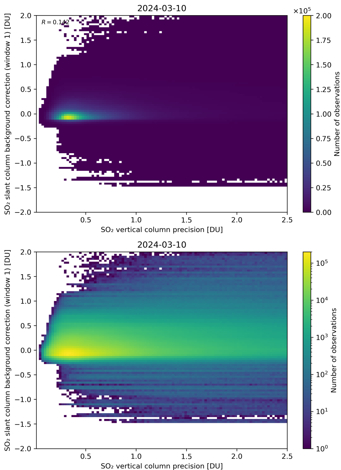
Figure 279: Scatter density plot of “SO 2 vertical column precision” against “SO 2 slant column background correction (window 1)” for 2024-03-09 to 2024-03-11.
