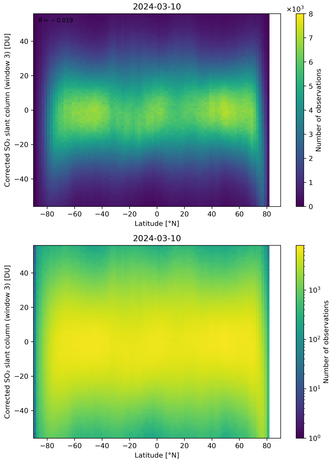
Figure 148: Scatter density plot of “Latitude” against “Corrected SO 2 slant column (window 3)” for 2024-03-09 to 2024-03-11.
