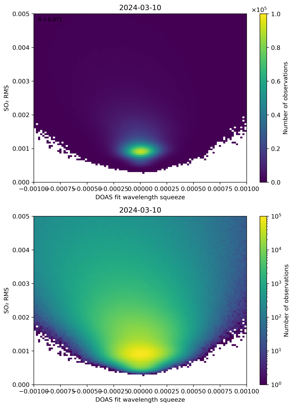
Figure 132: Scatter density plot of “DOAS fit wavelength squeeze” against “SO 2 RMS” for 2024-03-09 to 2024-03-11.
