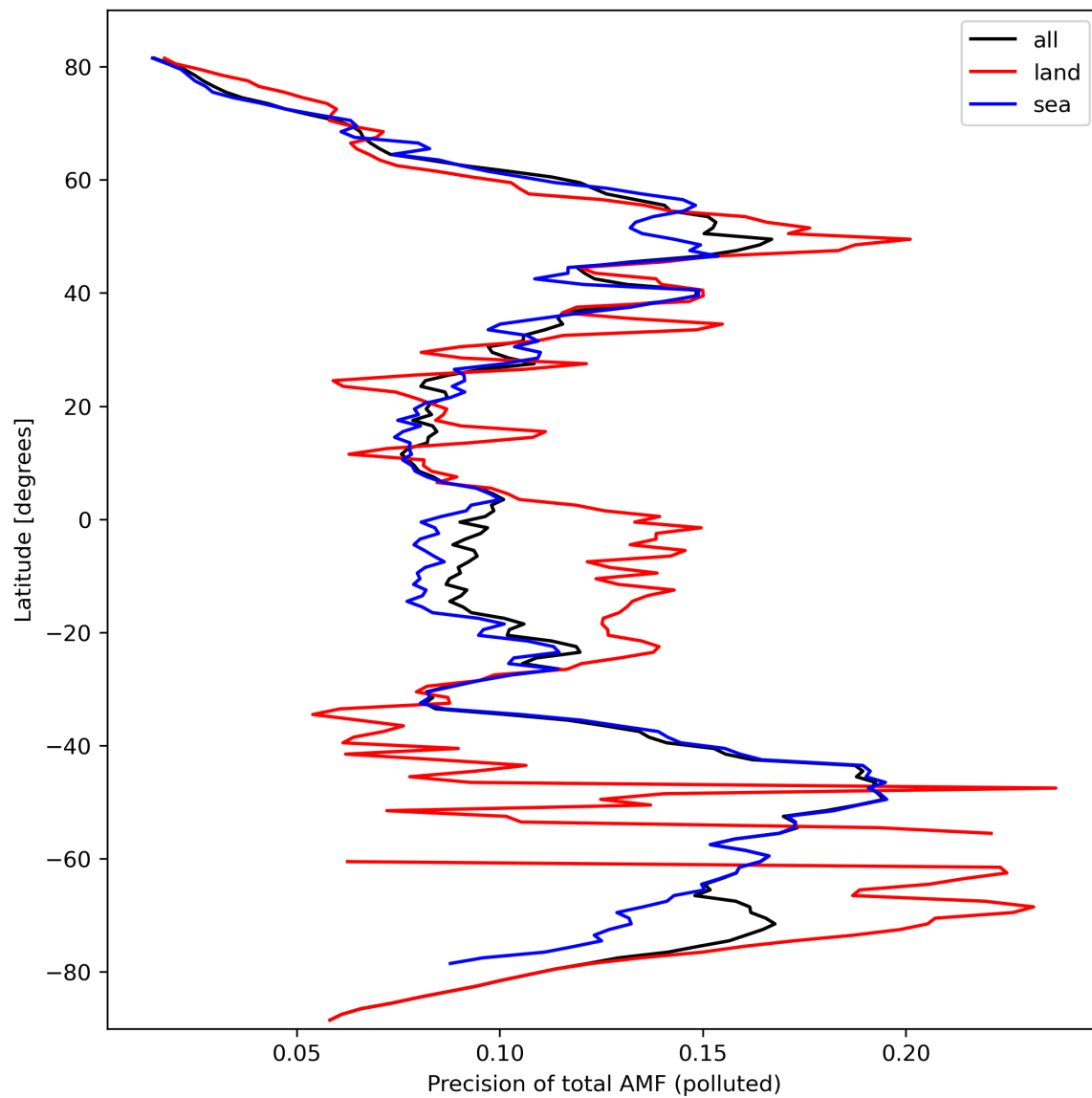
Figure 49: Zonal average of “Precision of total AMF (polluted)” for 2024-03-09 to 2024-03-11.
