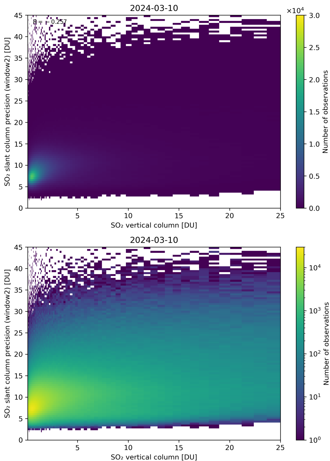
Figure 302: Scatter density plot of “SO 2 vertical column” against “SO 2 slant column precision (window2)” for 2024-03-09 to 2024-03-11.
