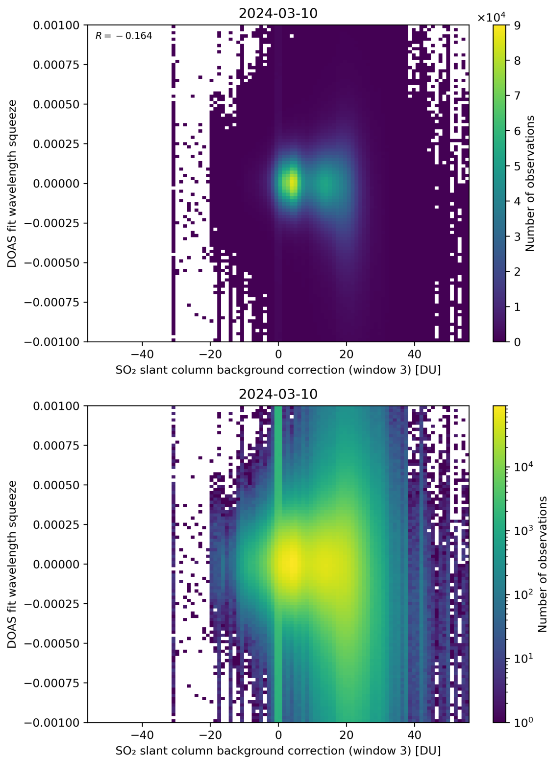
Figure 122: Scatter density plot of “SO 2 slant column background correction (window 3)” against “DOAS fit wavelength squeeze” for 2024-03-09 to 2024-03-11.
