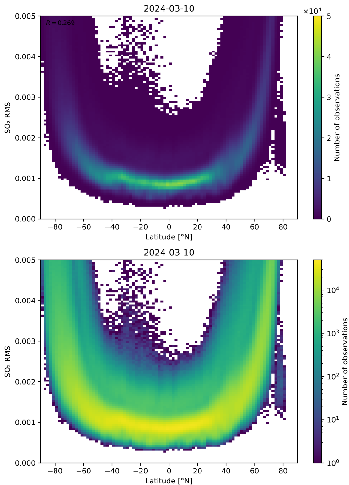
Figure 144: Scatter density plot of “Latitude” against “SO 2 RMS” for 2024-03-09 to 2024-03-11.
