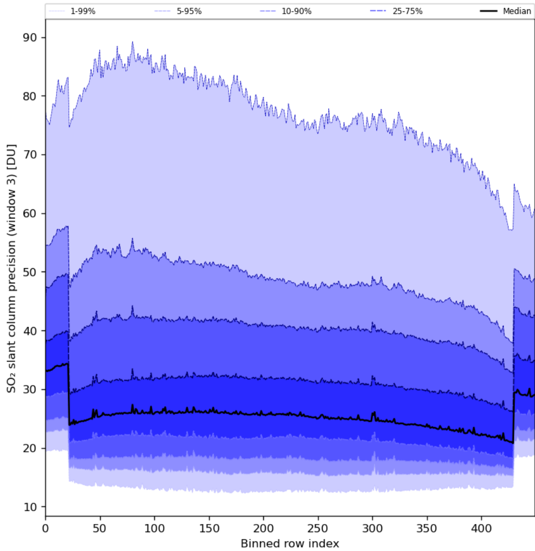
Figure 88: Along track statistics of “SO 2 slant column precision (window 3)” for 2024-03-09 to 2024-03-11
