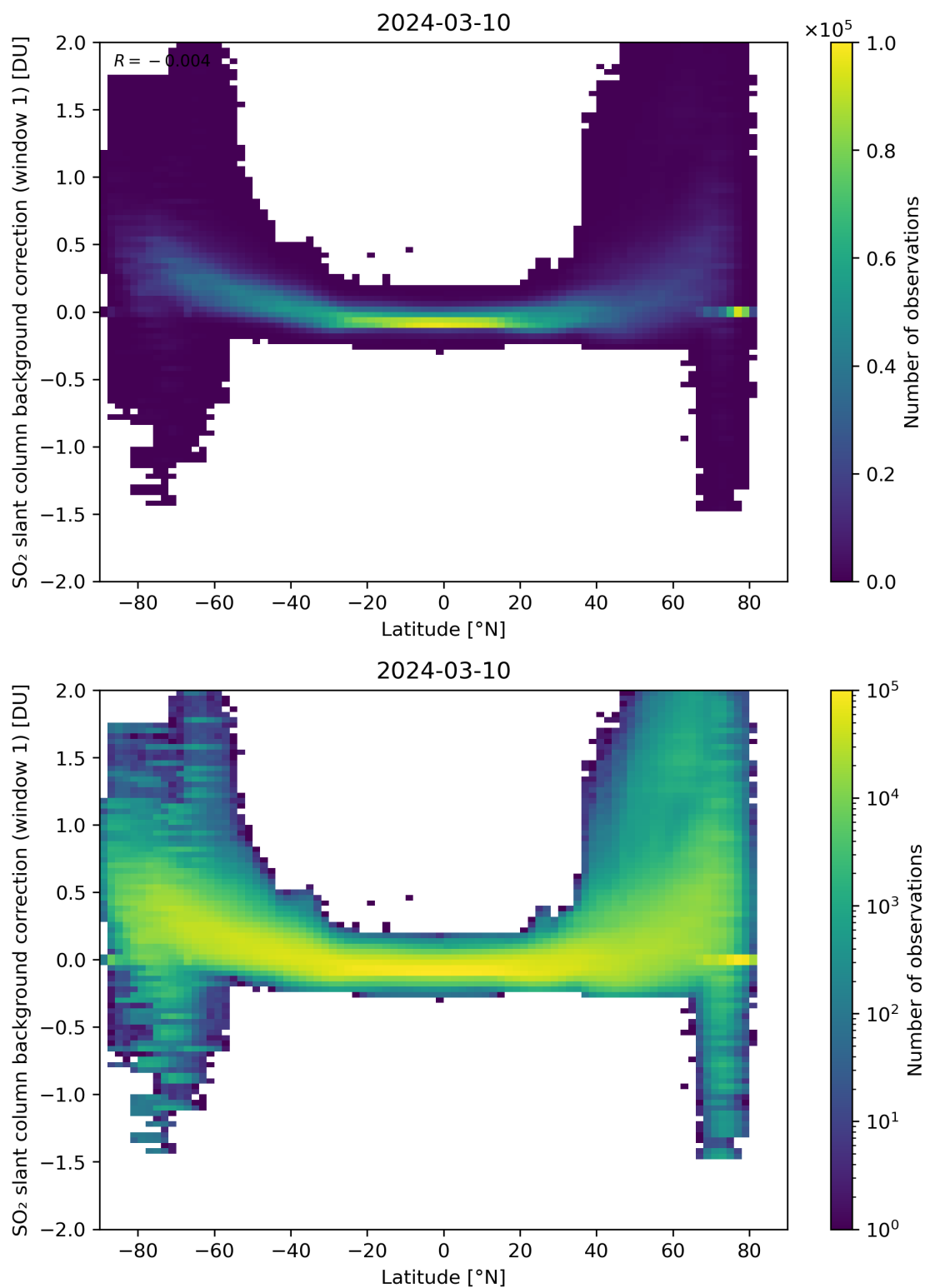
Figure 139: Scatter density plot of “Latitude” against “SO 2 slant column background correction (window 1)” for 2024-03-09 to 2024-03-11.
