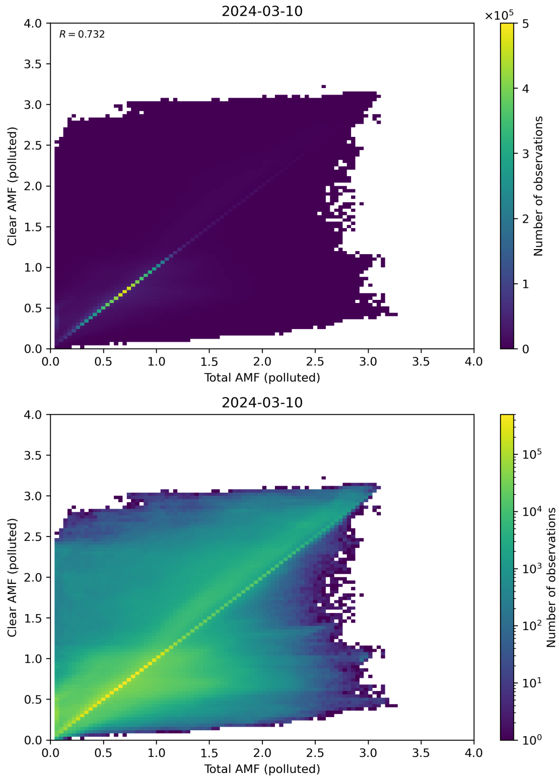
Figure 271: Scatter density plot of “Total AMF (polluted)” against “Clear AMF (polluted)” for 2024-03-09 to 2024-03-11.
