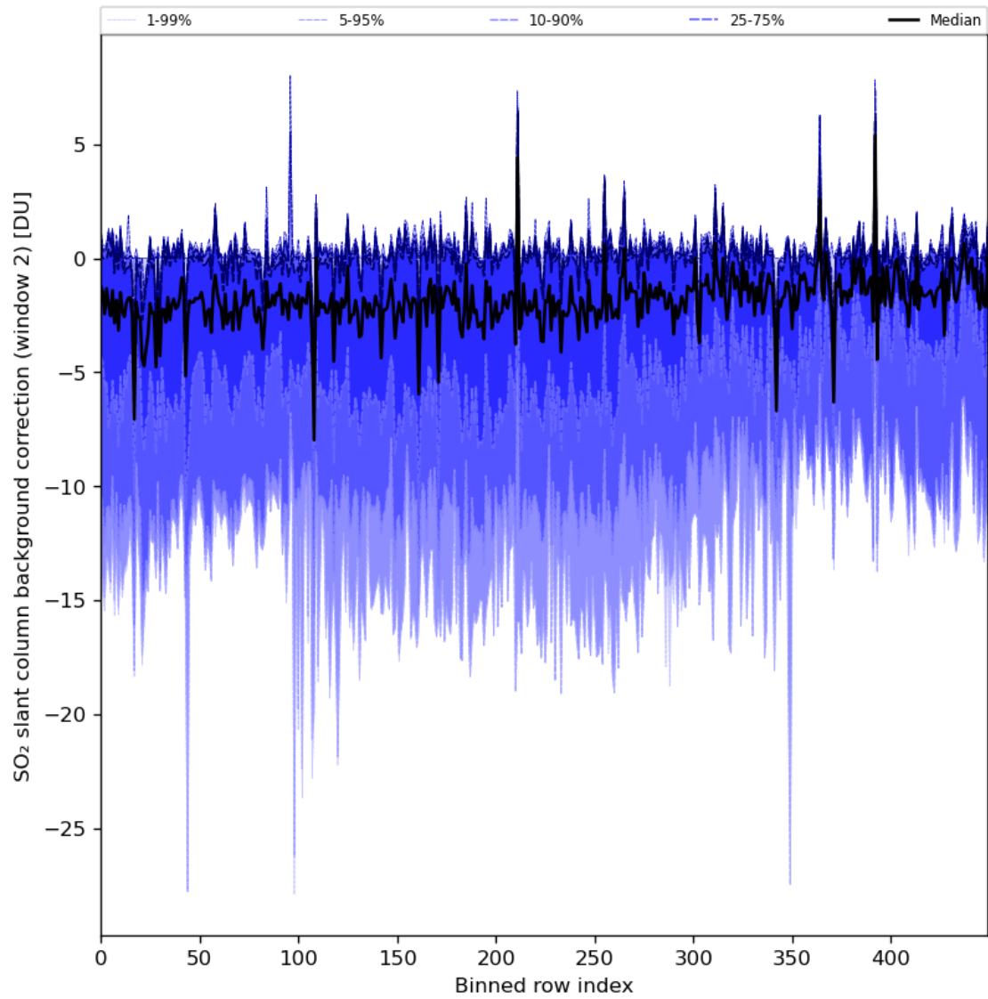
Figure 86: Along track statistics of “SO 2 slant column background correction (window 2)” for 2024-03-09 to 2024-03-11
