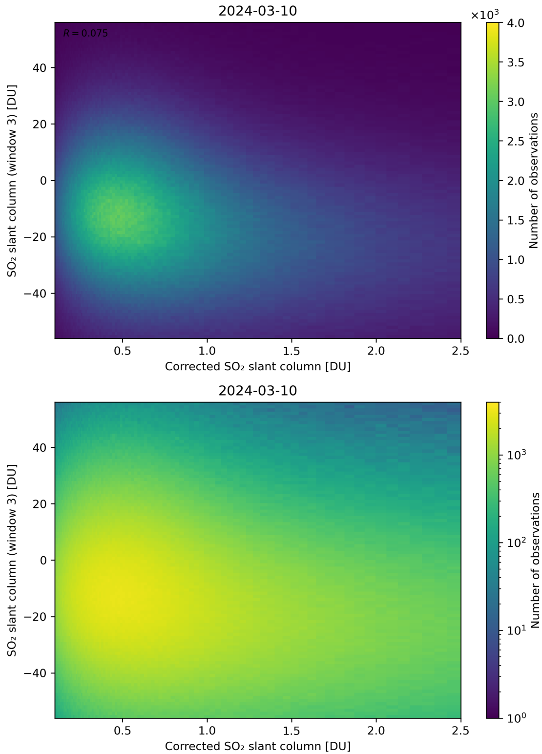
Figure 190: Scatter density plot of “Corrected SO 2 slant column” against “SO 2 slant column (window 3)” for 2024-03-09 to 2024-03-11.
