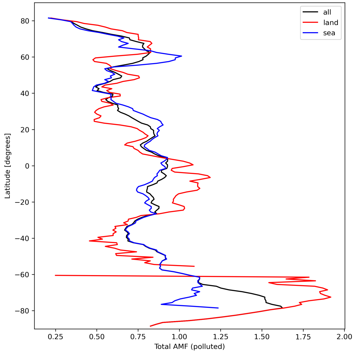
Figure 48: Zonal average of “Total AMF (polluted)” for 2024-03-09 to 2024-03-11.
