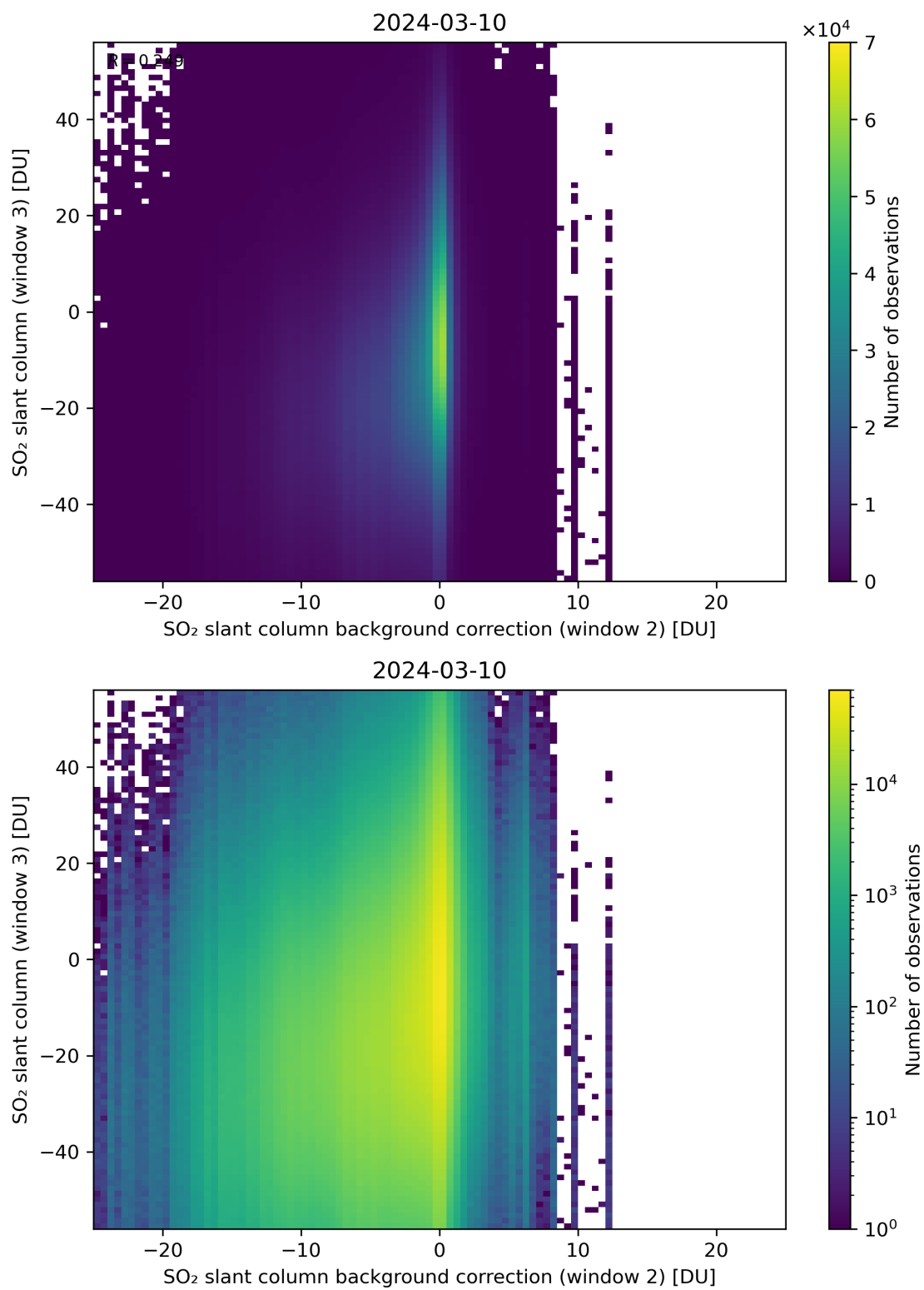
Figure 117: Scatter density plot of “SO 2 slant column background correction (window 2)” against “SO 2 slant column (window 3)” for 2024-03-09 to 2024-03-11.
