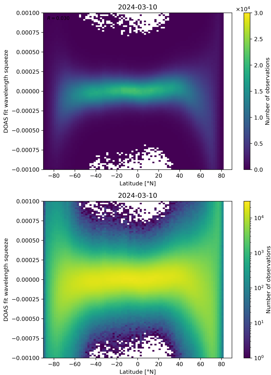
Figure 143: Scatter density plot of “Latitude” against “DOAS fit wavelength squeeze” for 2024-03-09 to 2024-03-11.
