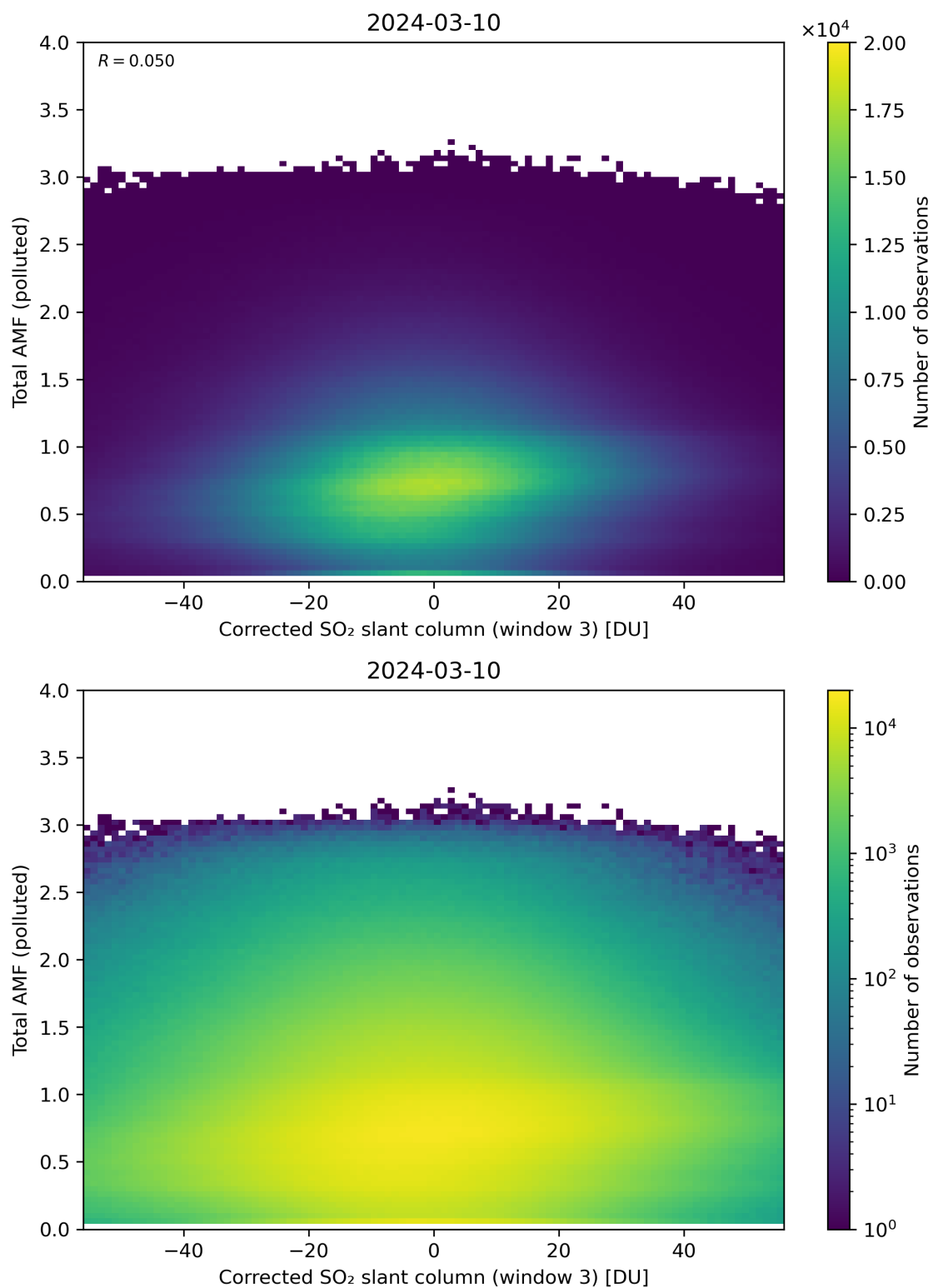
Figure 210: Scatter density plot of “Corrected SO 2 slant column (window 3)” against “Total AMF (polluted)” for 2024-03-09 to 2024-03-11.
