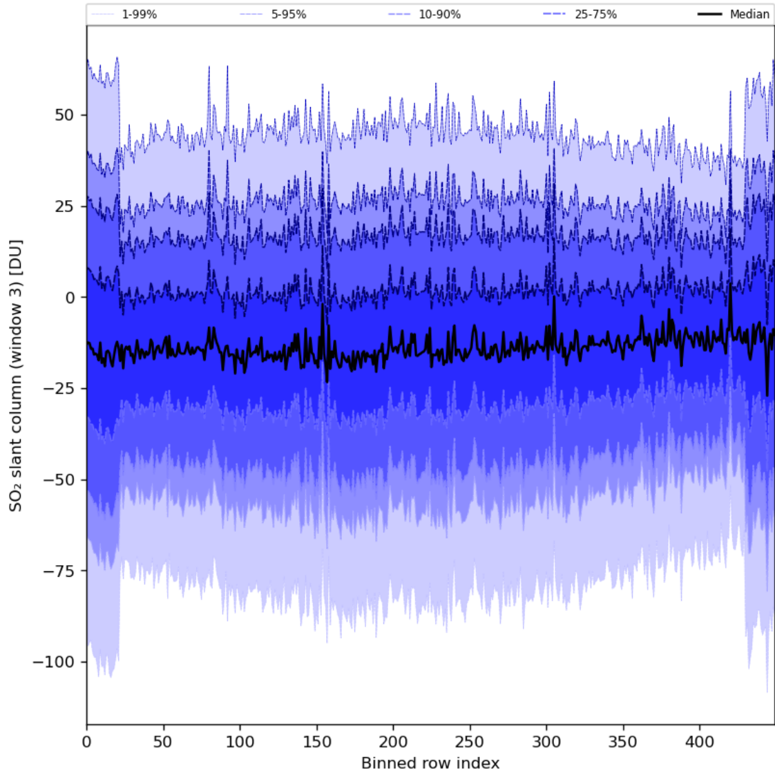
Figure 87: Along track statistics of “SO 2 slant column (window 3)” for 2024-03-09 to 2024-03-11
