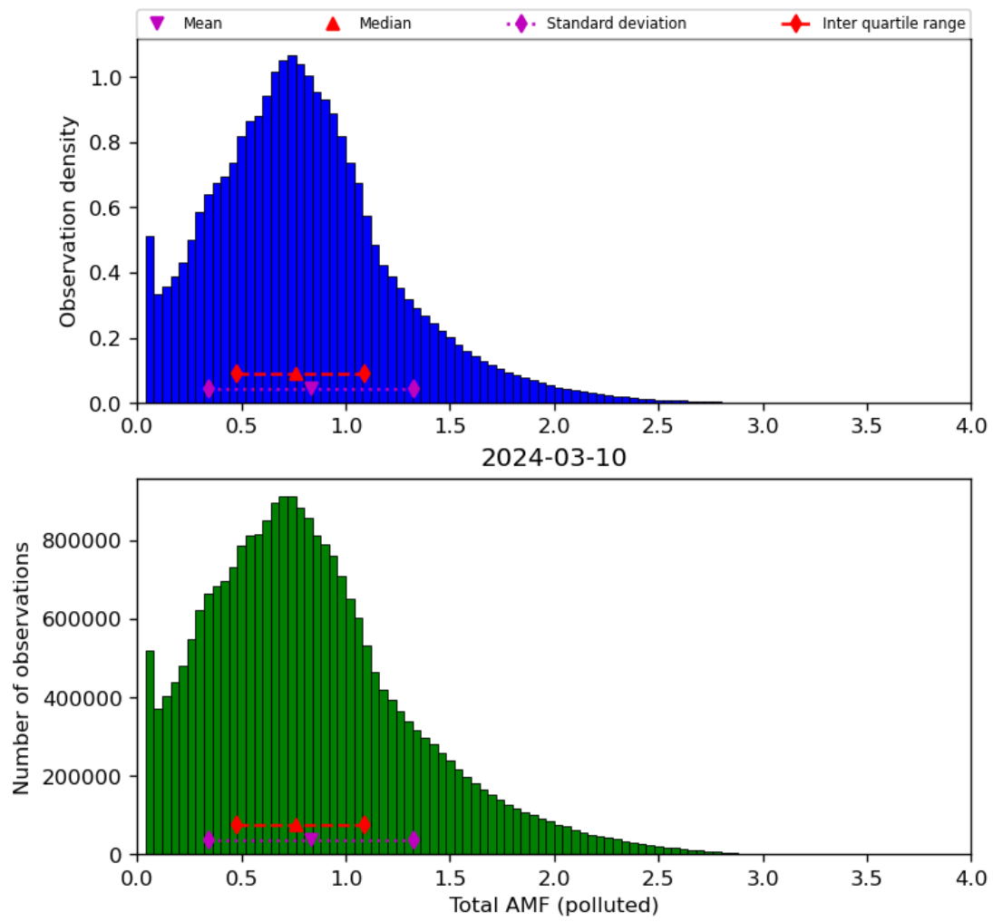
Figure 71: Histogram of “Total AMF (polluted)” for 2024-03-09 to 2024-03-11
