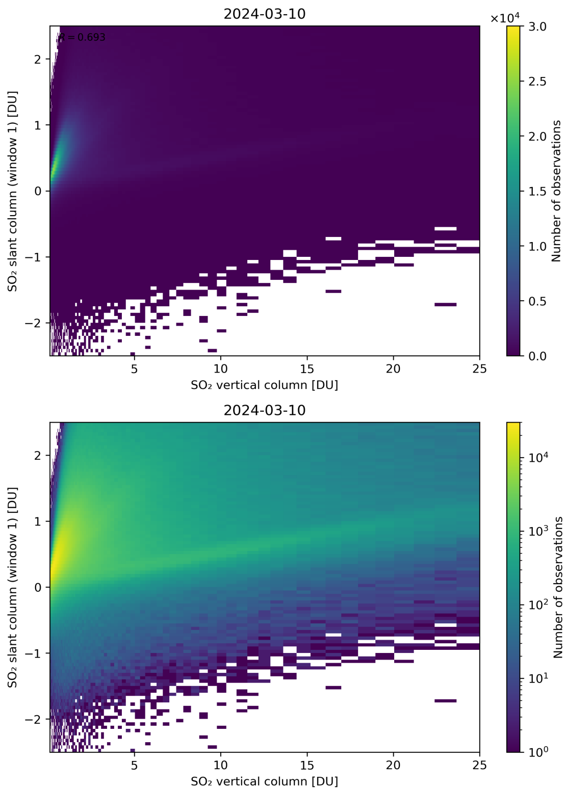
Figure 300: Scatter density plot of “SO 2 vertical column” against “SO 2 slant column (window 1)” for 2024-03-09 to 2024-03-11.
