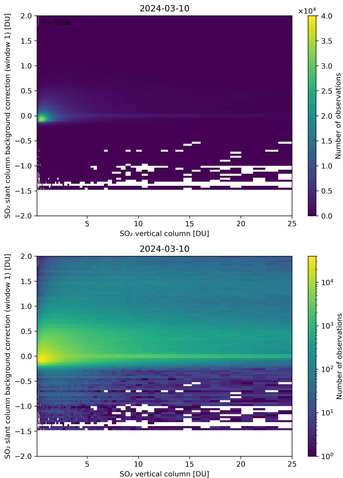
Figure 273: Scatter density plot of “SO 2 vertical column” against “SO 2 slant column background correction (window 1)” for 2024-03-09 to 2024-03-11.
