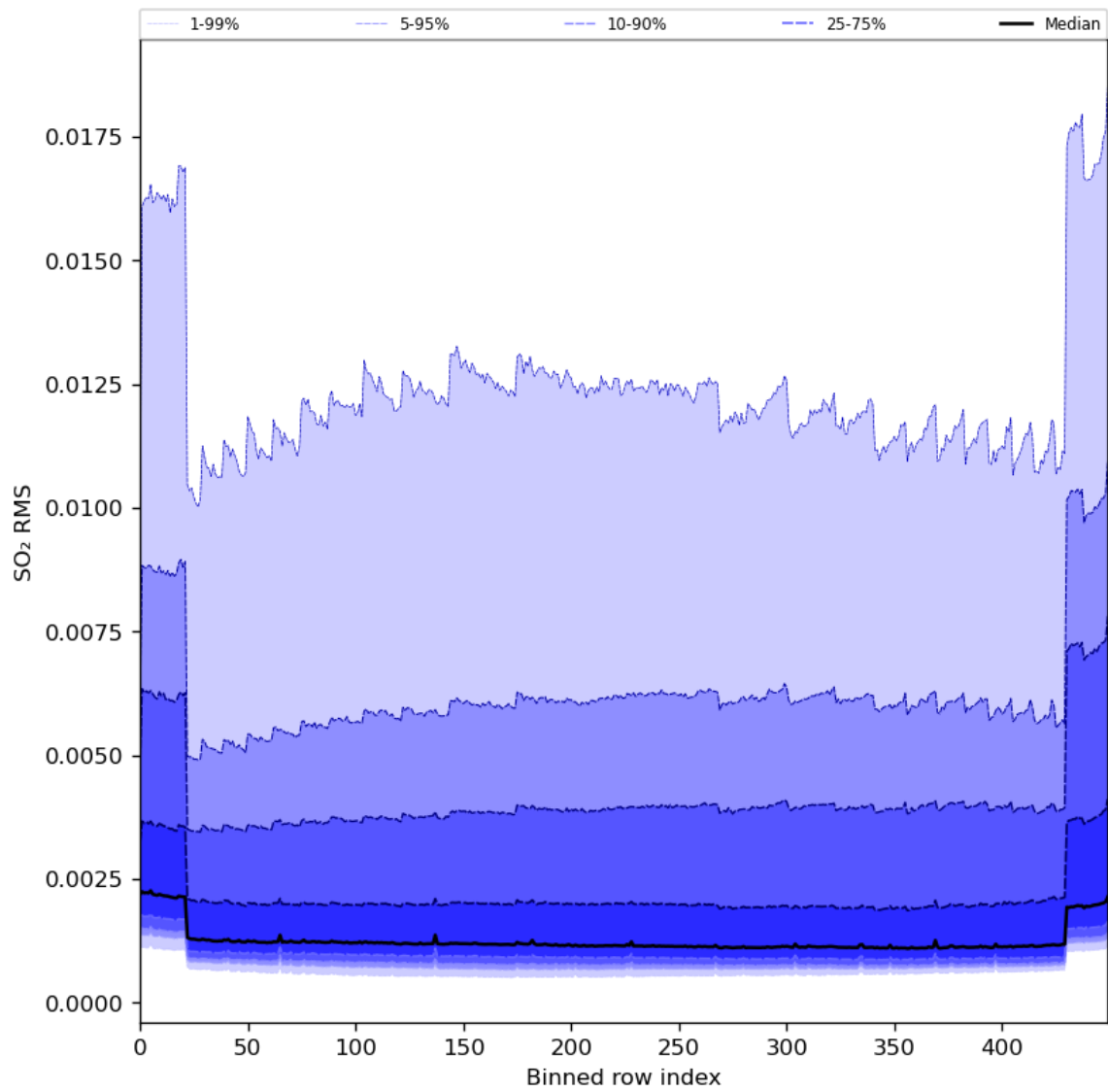
Figure 93: Along track statistics of “SO 2 RMS” for 2024-03-09 to 2024-03-11
