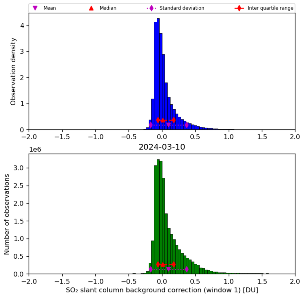
Figure 59: Histogram of “SO 2 slant column background correction (window 1)” for 2024-03-09 to 2024-03-11
