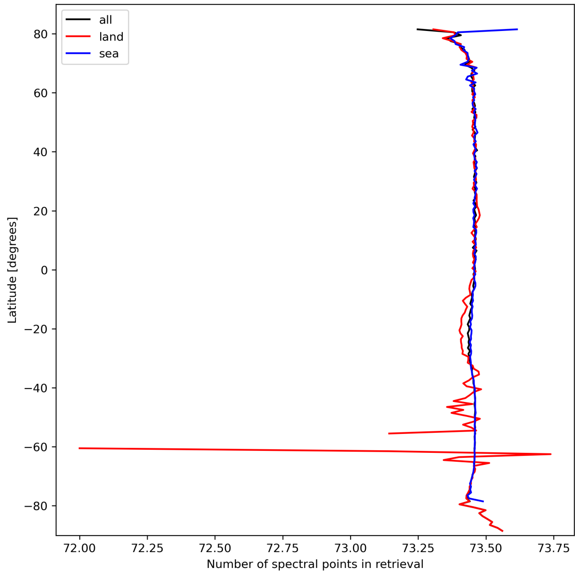
Figure 51: Zonal average of “Number of spectral points in retrieval” for 2024-03-09 to 2024-03-11.
