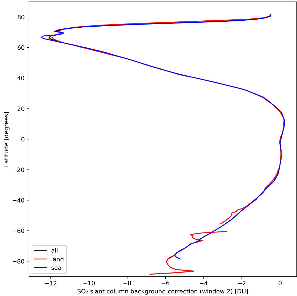
Figure 40: Zonal average of “SO 2 slant column background correction (window 2)” for 2024-03-09 to 2024-03-11.
