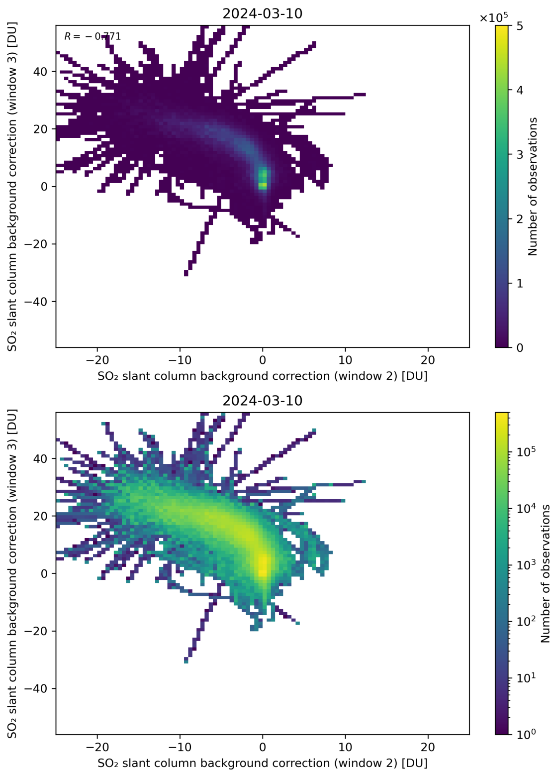
Figure 111: Scatter density plot of “SO 2 slant column background correction (window 2)” against “SO 2 slant column background correction (window 3)” for 2024-03-09 to 2024-03-11.
