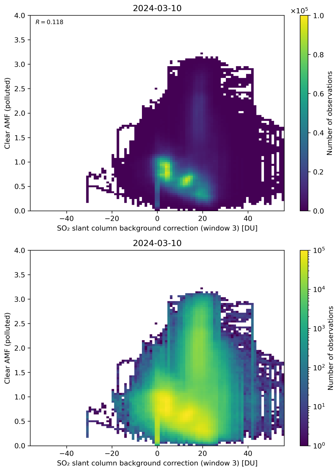
Figure 124: Scatter density plot of “SO 2 slant column background correction (window 3)” against “Clear AMF (polluted)” for 2024-03-09 to 2024-03-11.
