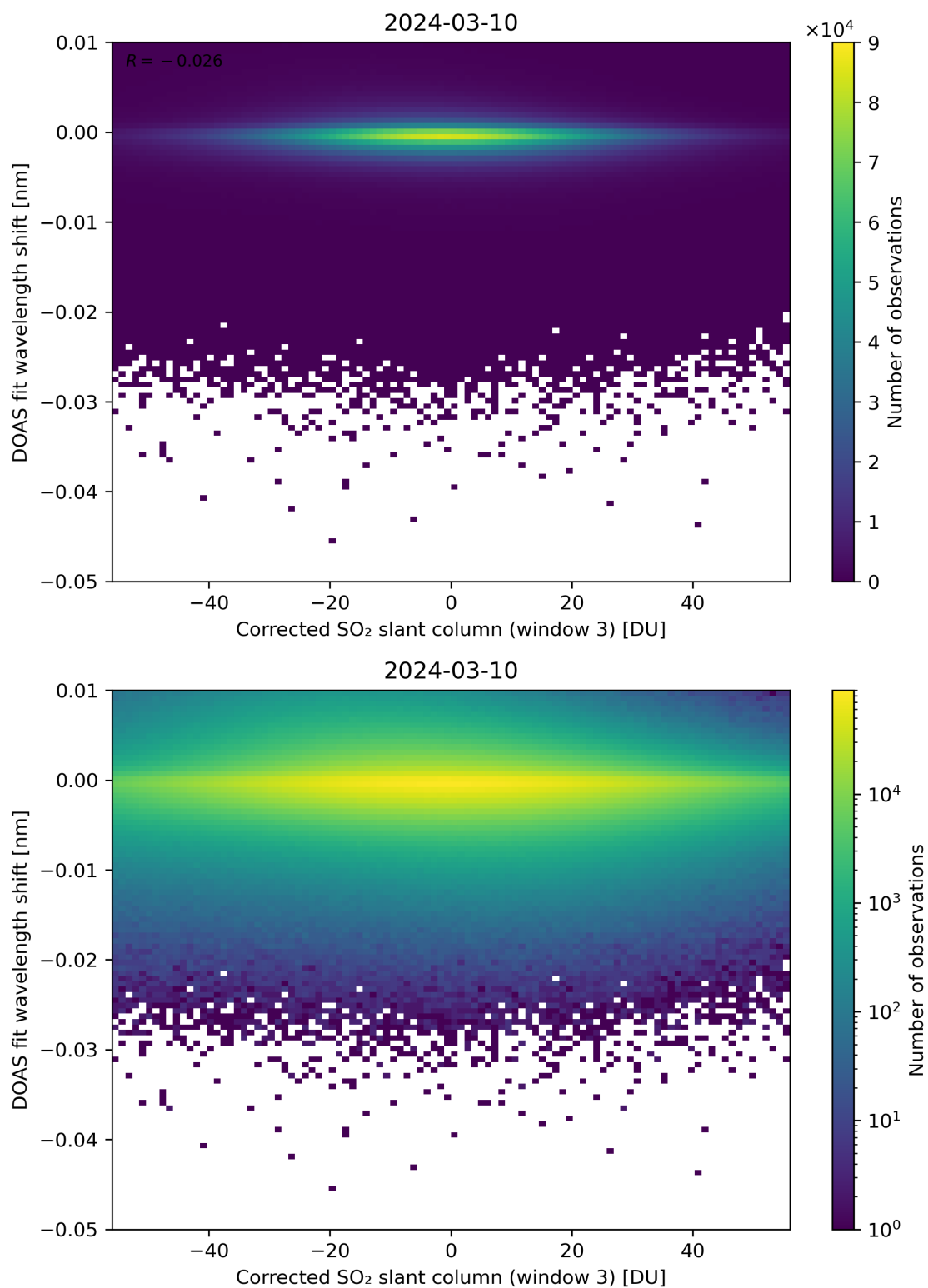
Figure 206: Scatter density plot of “Corrected SO 2 slant column (window 3)” against “DOAS fit wavelength shift” for 2024-03-09 to 2024-03-11.
