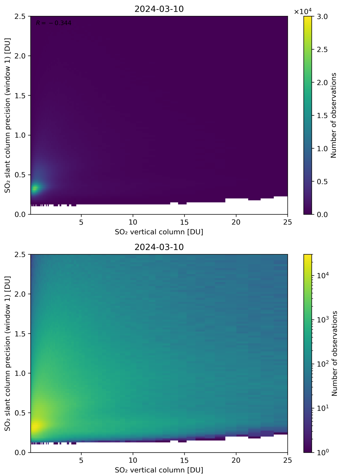
Figure 301: Scatter density plot of “SO 2 vertical column” against “SO 2 slant column precision (window 1)” for 2024-03-09 to 2024-03-11.
