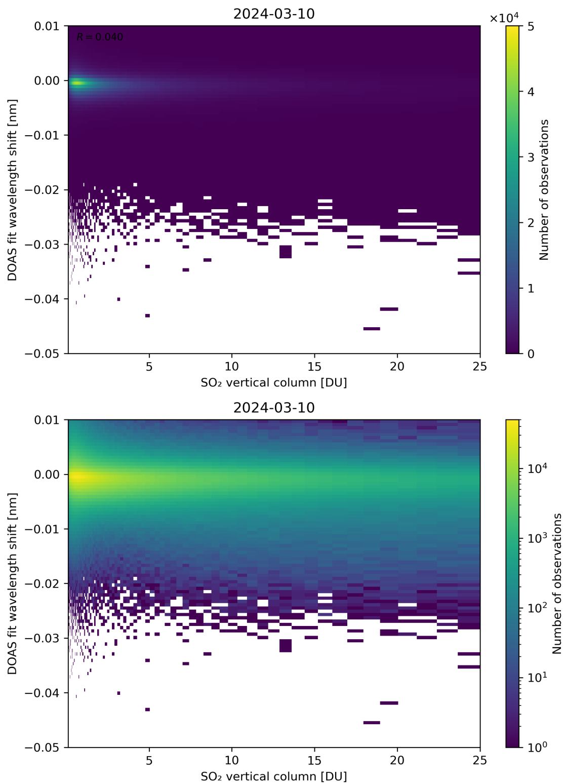
Figure 276: Scatter density plot of “SO 2 vertical column” against “DOAS fit wavelength shift” for 2024-03-09 to 2024-03-11.
