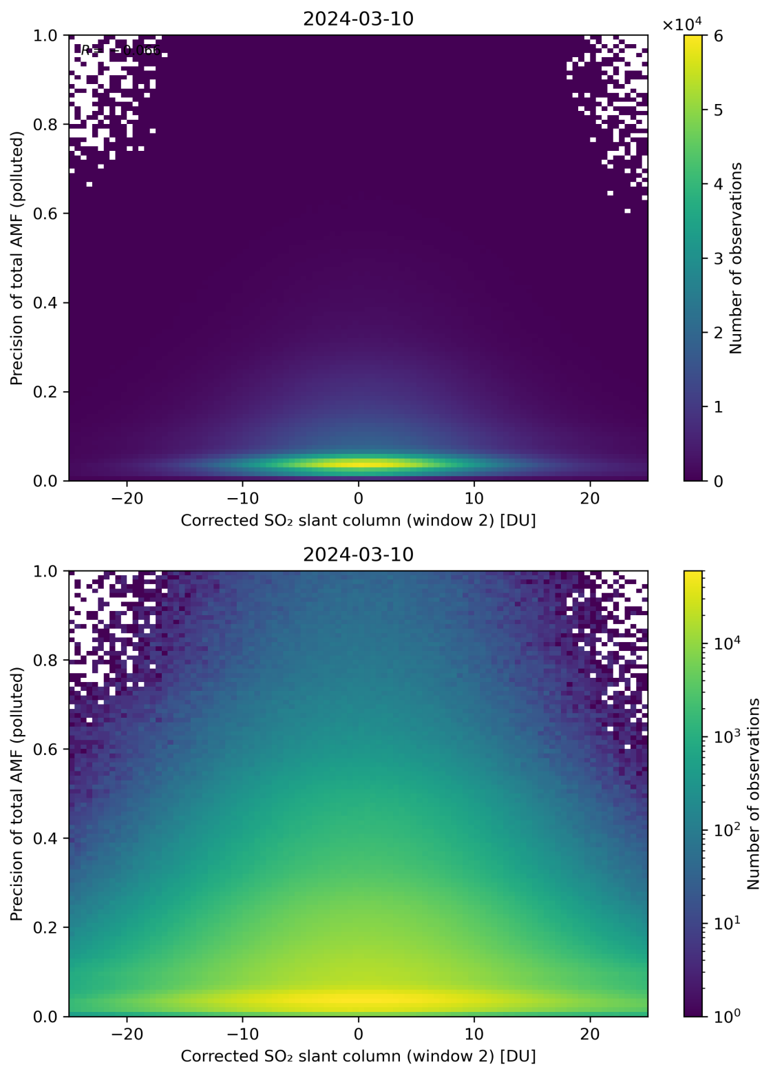
Figure 204: Scatter density plot of “Corrected SO 2 slant column (window 2)” against “Precision of total AMF (polluted)” for 2024-03-09 to 2024-03-11.
