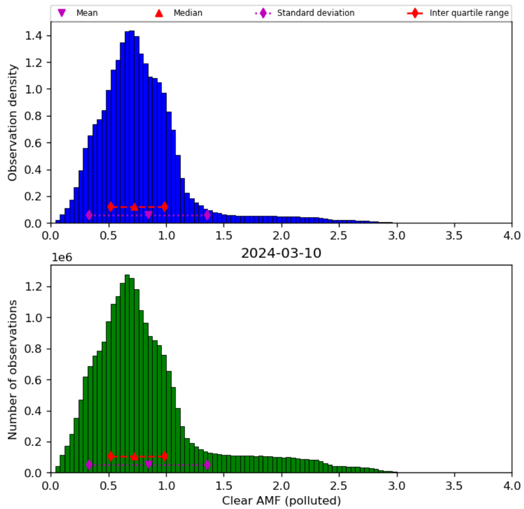
Figure 73: Histogram of “Clear AMF (polluted)” for 2024-03-09 to 2024-03-11
