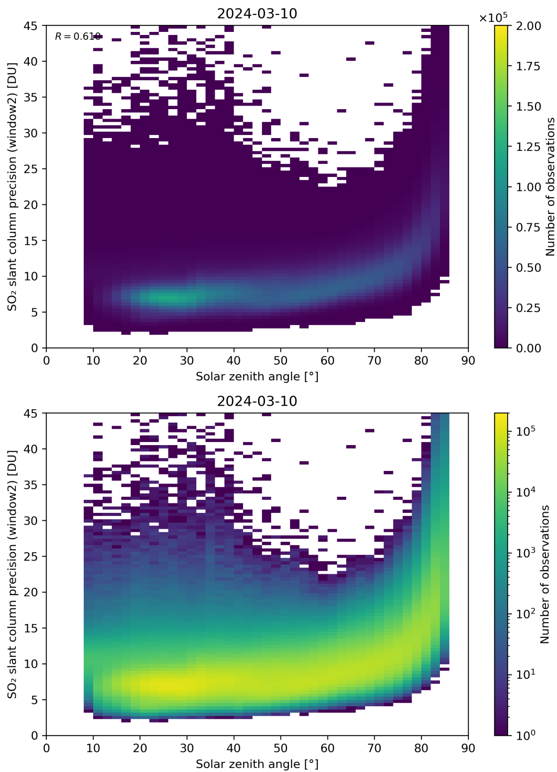
Figure 171: Scatter density plot of “Solar zenith angle” against “SO 2 slant column precision (window2)” for 2024-03-09 to 2024-03-11.
