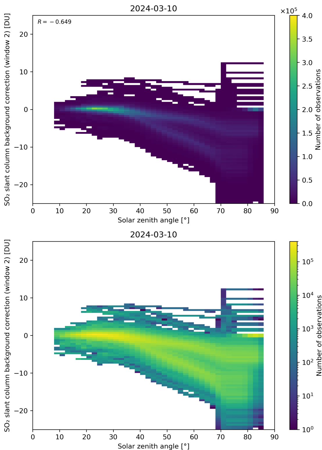
Figure 159: Scatter density plot of “Solar zenith angle” against “SO 2 slant column background correction (window 2)” for 2024-03-09 to 2024-03-11.
