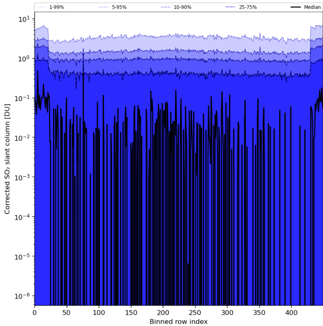
Figure 78: Along track statistics of “Corrected SO 2 slant column” for 2024-03-09 to 2024-03-11
