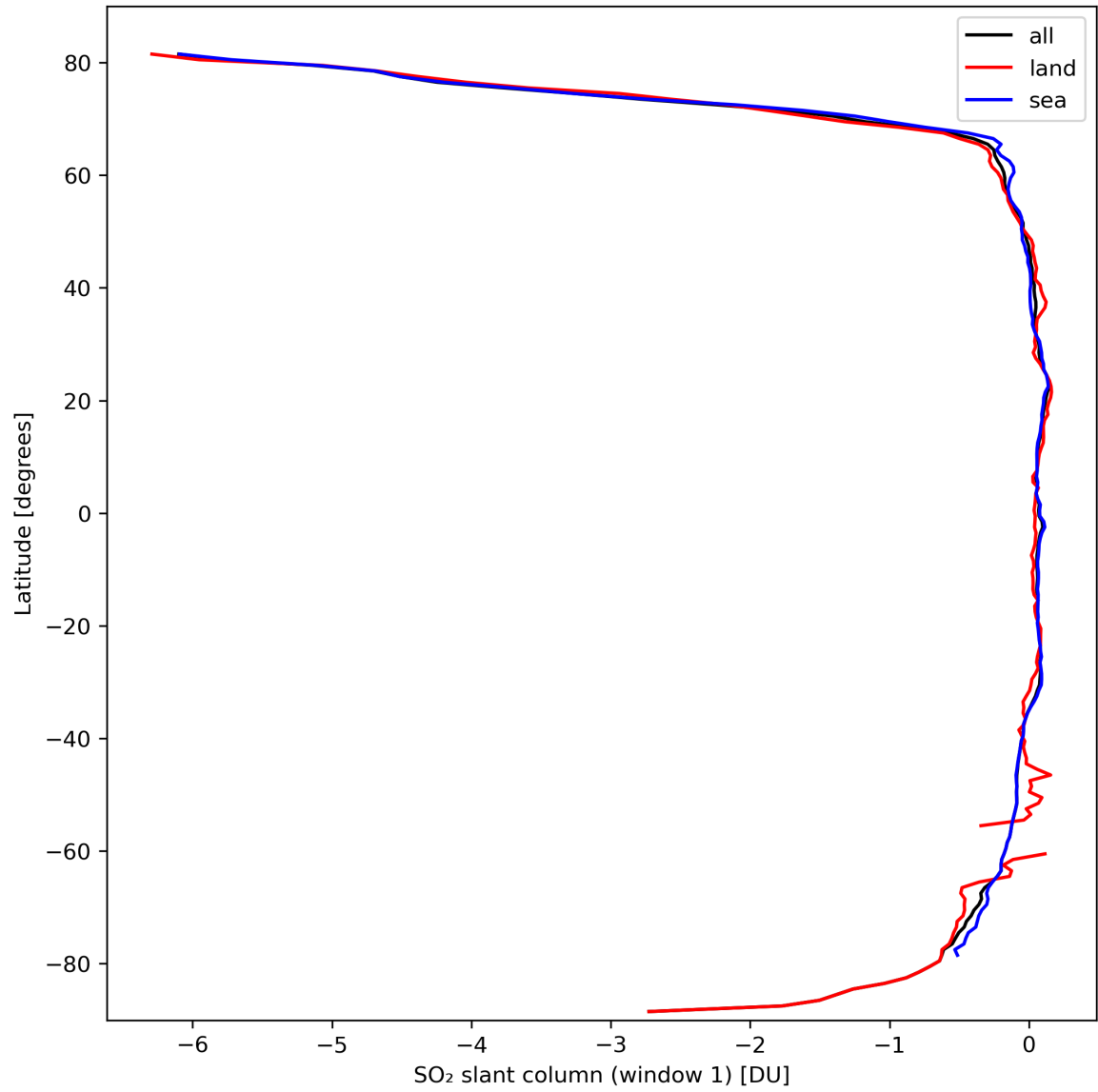
Figure 33: Zonal average of “SO 2 slant column (window 1)” for 2024-03-09 to 2024-03-11.
