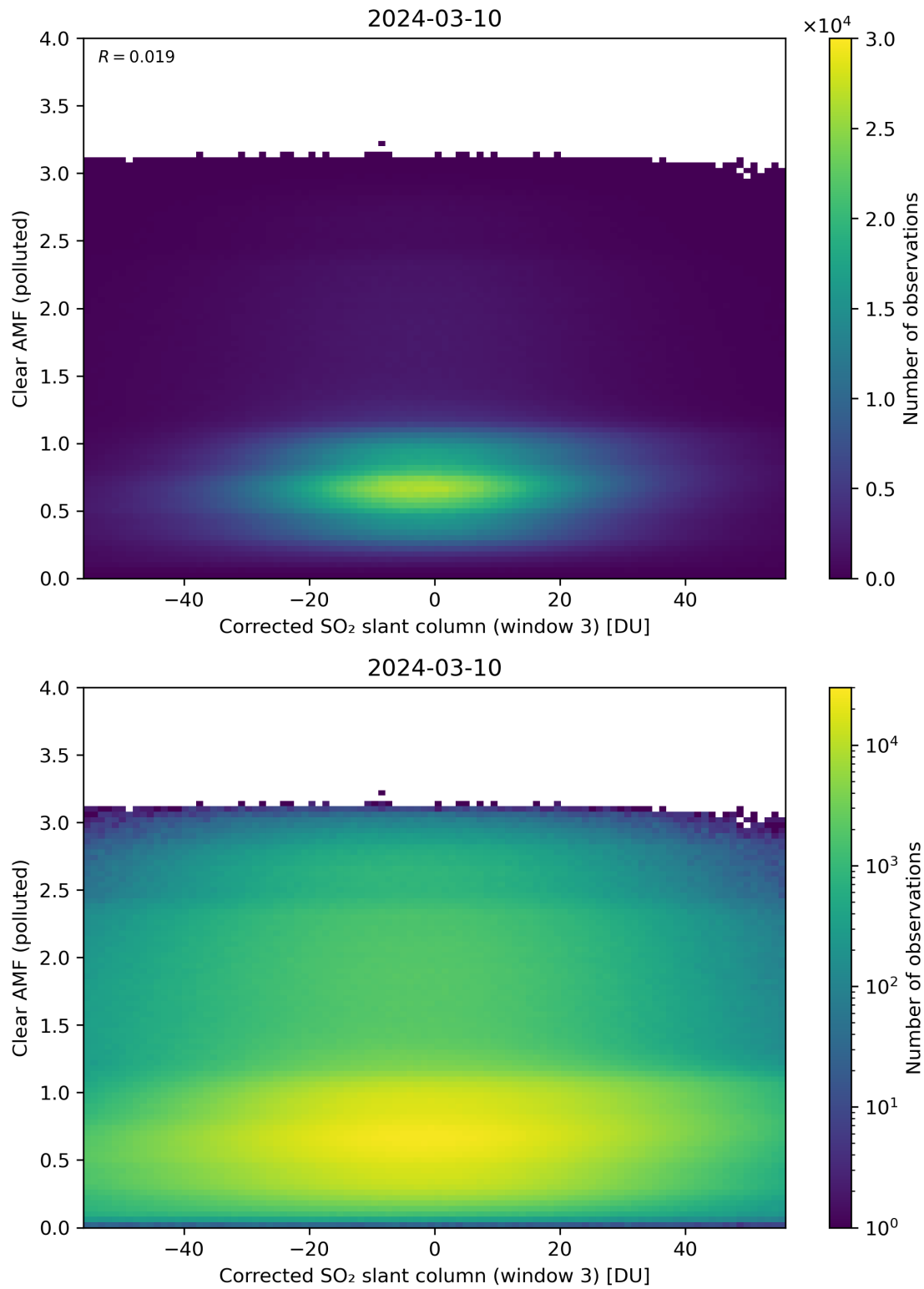
Figure 209: Scatter density plot of “Corrected SO 2 slant column (window 3)” against “Clear AMF (polluted)” for 2024-03-09 to 2024-03-11.
