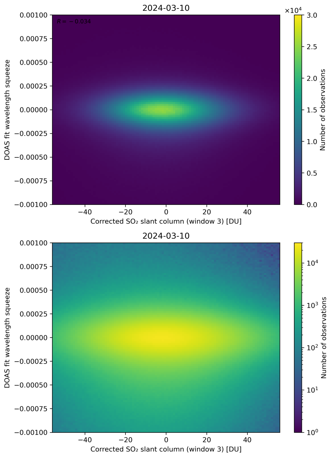
Figure 207: Scatter density plot of “Corrected SO 2 slant column (window 3)” against “DOAS fit wavelength squeeze” for 2024-03-09 to 2024-03-11.
