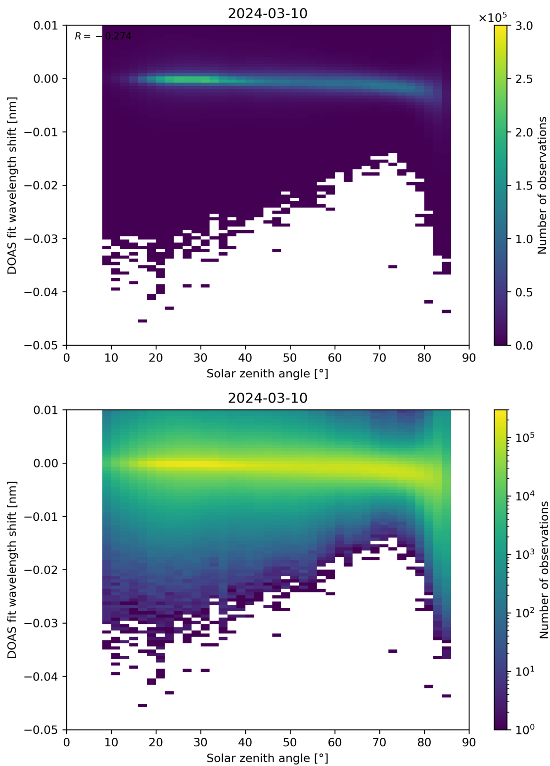
Figure 161: Scatter density plot of “Solar zenith angle” against “DOAS fit wavelength shift” for 2024-03-09 to 2024-03-11.
