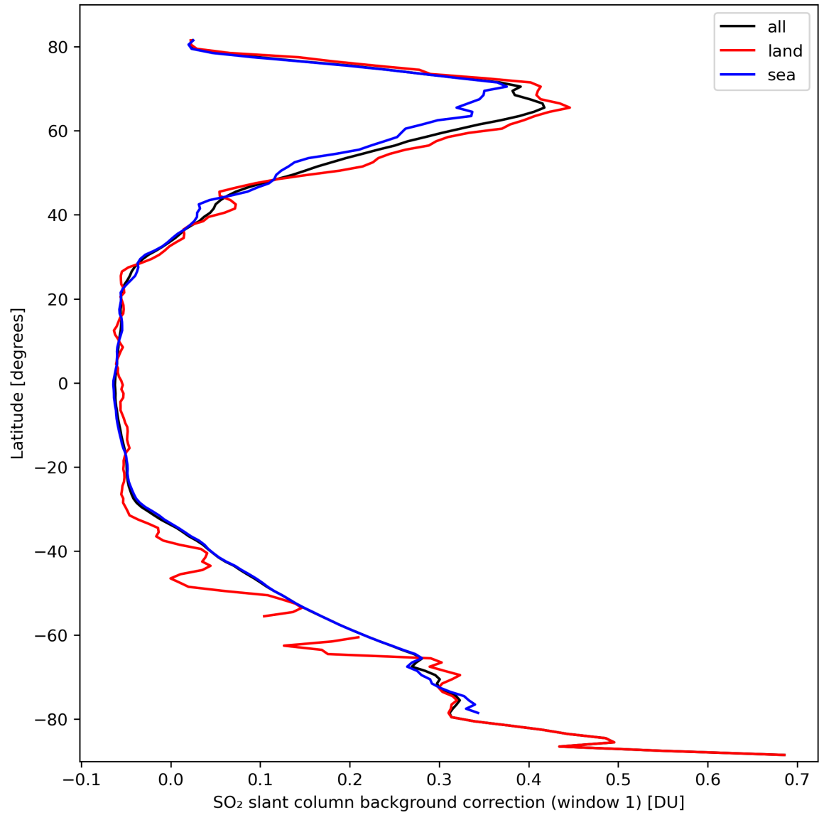
Figure 36: Zonal average of “SO 2 slant column background correction (window 1)” for 2024-03-09 to 2024-03-11.
