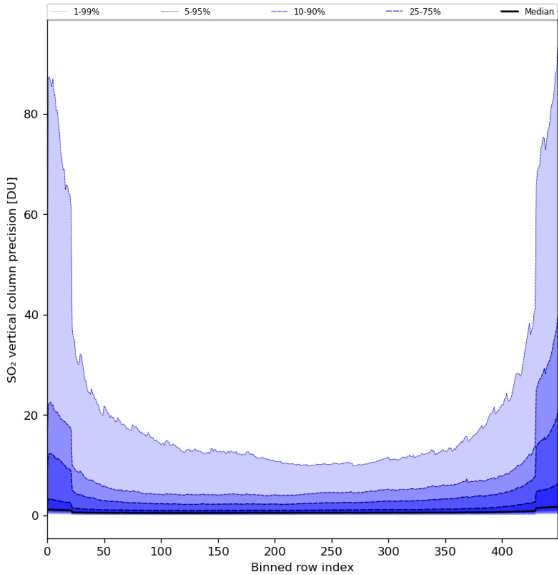
Figure 77: Along track statistics of “SO 2 vertical column precision” for 2024-03-09 to 2024-03-11
