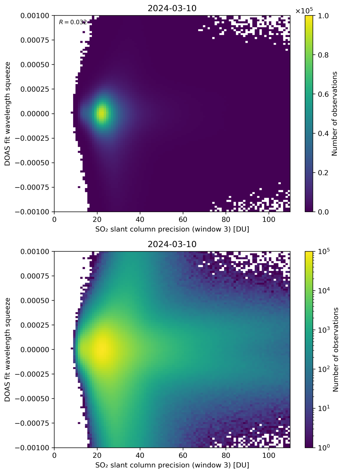
Figure 259: Scatter density plot of “SO 2 slant column precision (window 3)” against “DOAS fit wavelength squeeze” for 2024-03-09 to 2024-03-11.
