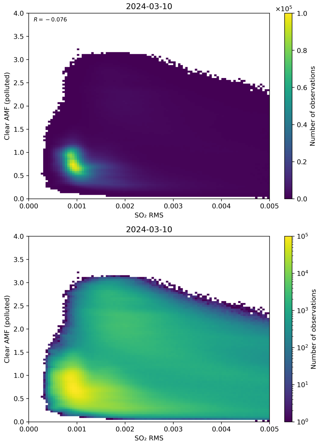
Figure 136: Scatter density plot of “SO 2 RMS” against “Clear AMF (polluted)” for 2024-03-09 to 2024-03-11.
