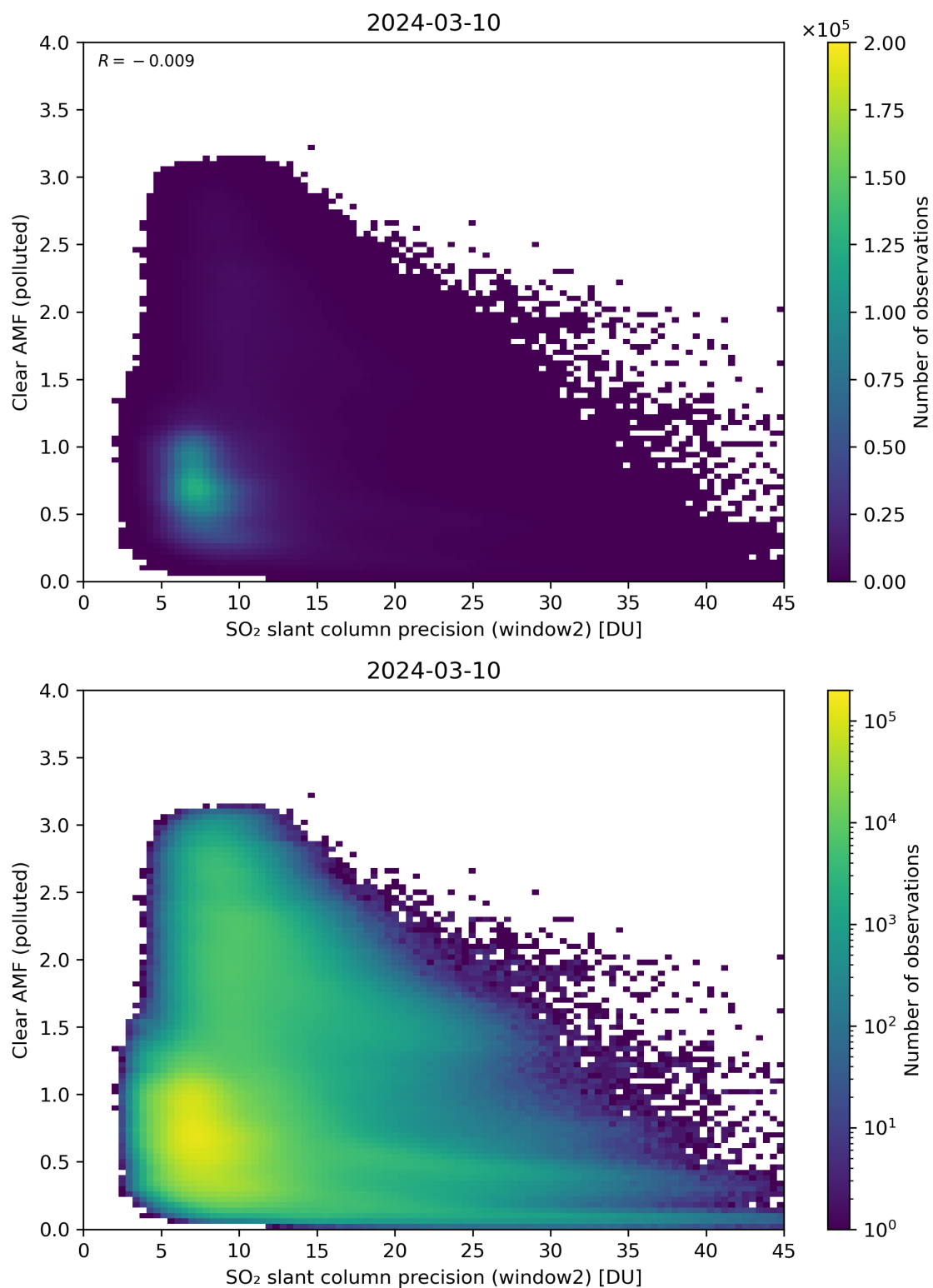
Figure 246: Scatter density plot of “SO 2 slant column precision (window2)” against “Clear AMF (polluted)” for 2024-03-09 to 2024-03-11.
