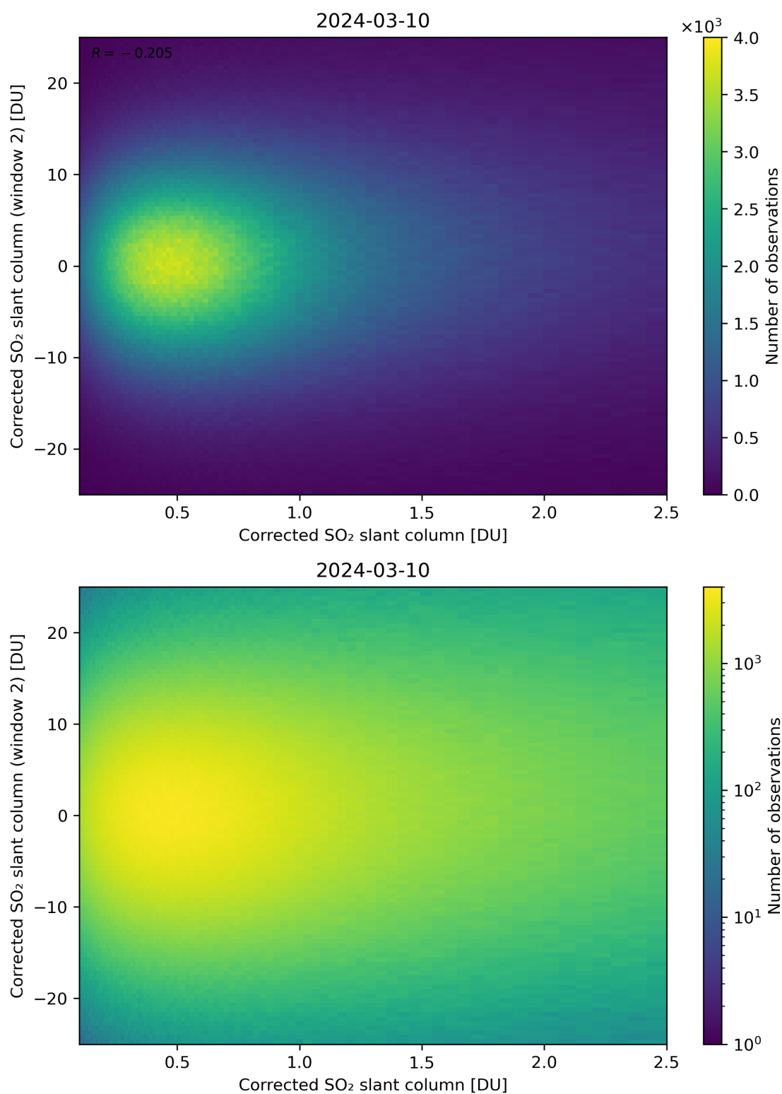
Figure 185: Scatter density plot of “Corrected SO 2 slant column” against “Corrected SO 2 slant column (window 2)” for 2024-03-09 to 2024-03-11.
