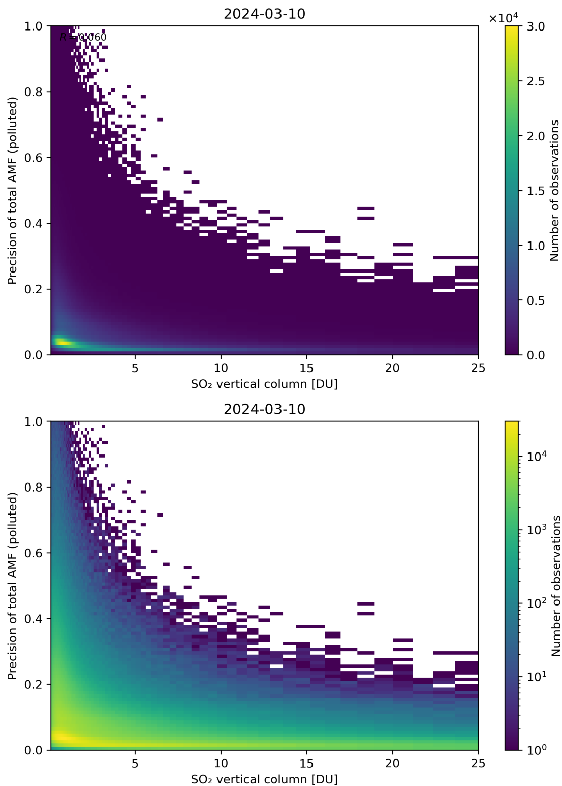
Figure 306: Scatter density plot of “SO 2 vertical column” against “Precision of total AMF (polluted)” for 2024-03-09 to 2024-03-11.
