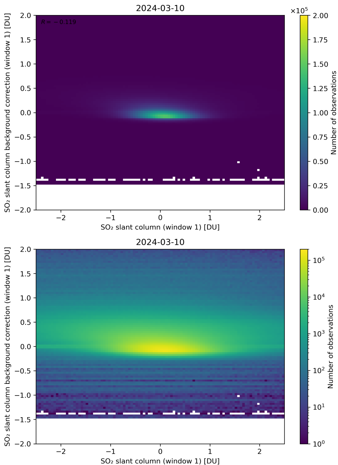
Figure 212: Scatter density plot of “SO 2 slant column (window 1)” against “SO 2 slant column background correction (window 1)” for 2024-03-09 to 2024-03-11.
