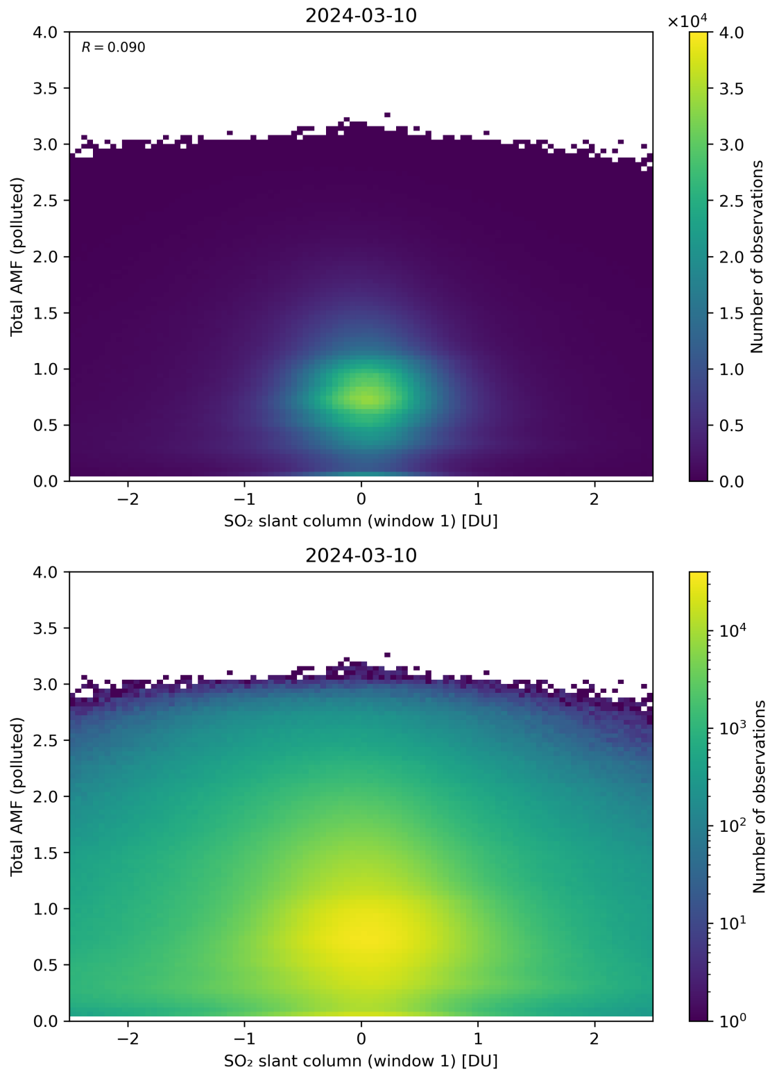
Figure 239: Scatter density plot of “SO 2 slant column (window 1)” against “Total AMF (polluted)” for 2024-03-09 to 2024-03-11.
