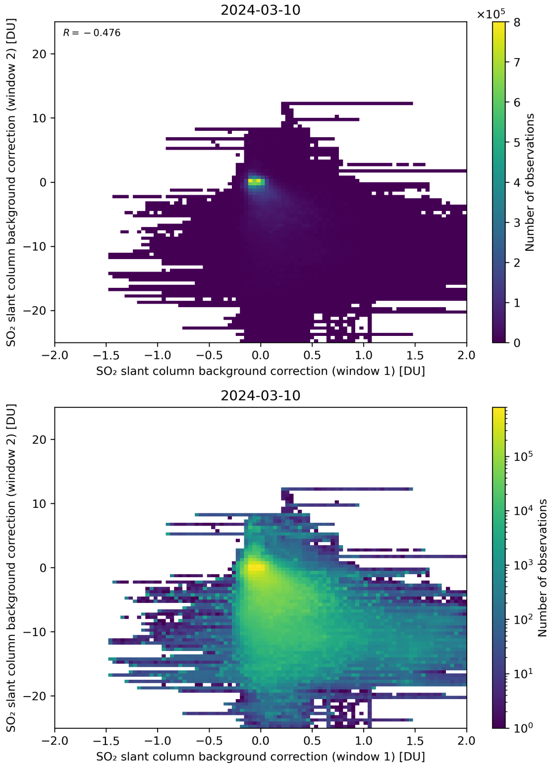
Figure 98: Scatter density plot of “SO 2 slant column background correction (window 1)” against “SO 2 slant column background correction (window 2)” for 2024-03-09 to 2024-03-11.
