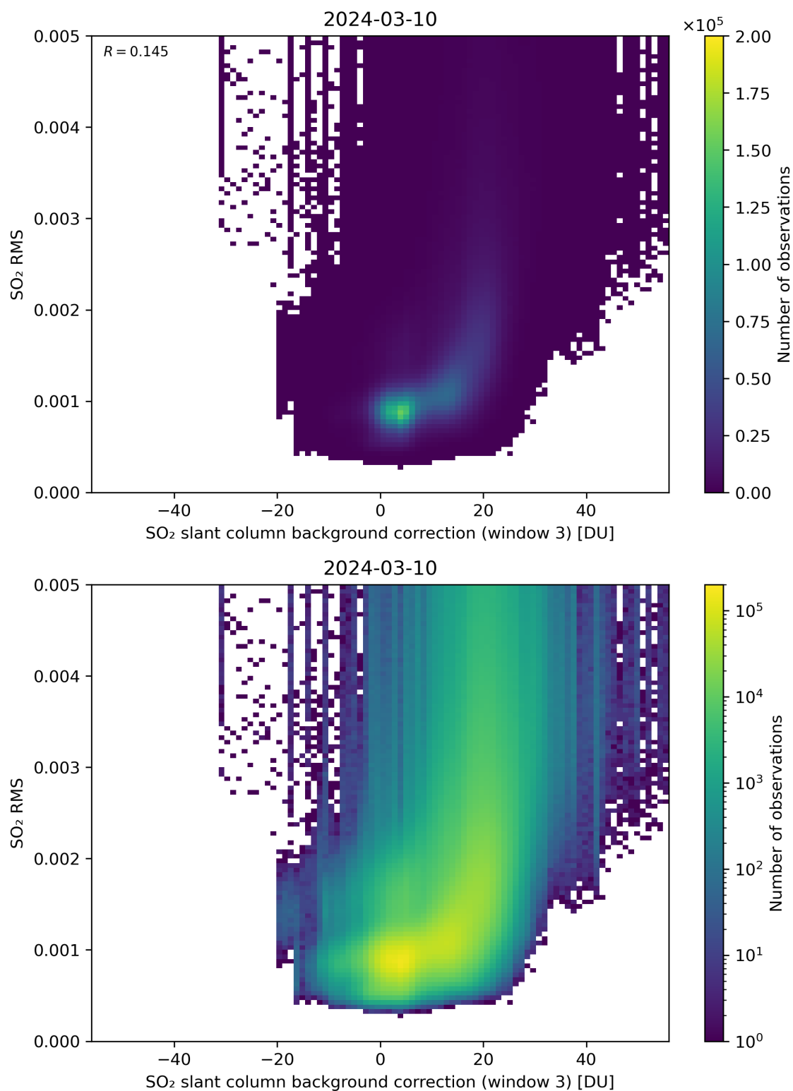
Figure 123: Scatter density plot of “SO 2 slant column background correction (window 3)” against “SO 2 RMS” for 2024-03-09 to 2024-03-11.
