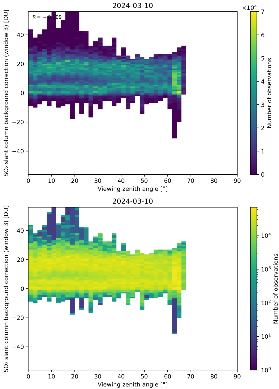
Figure 310: Scatter density plot of “Viewing zenith angle” against “SO 2 slant column background correction (window 3)” for 2024-03-09 to 2024-03-11.
