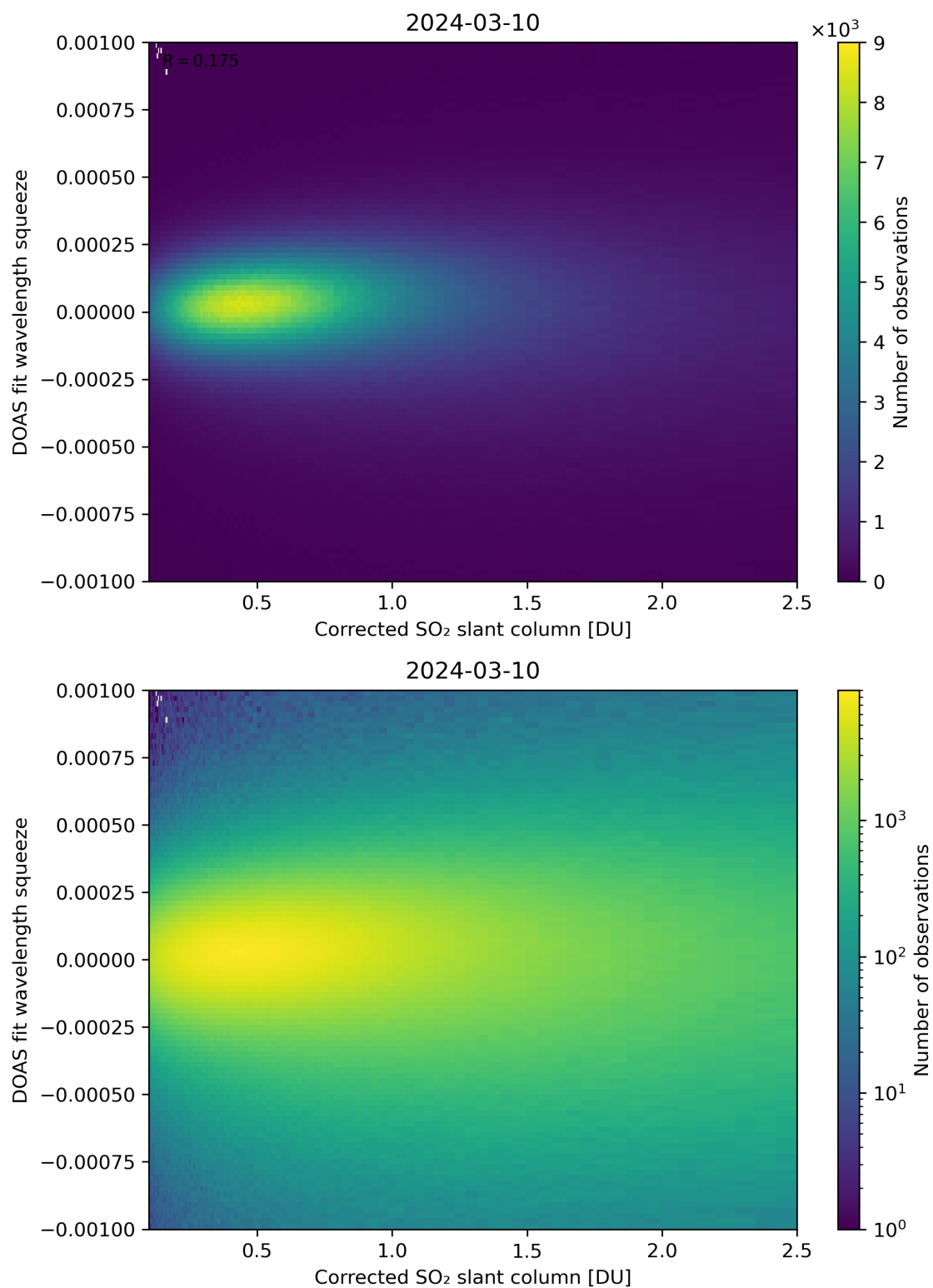
Figure 182: Scatter density plot of “Corrected SO 2 slant column” against “DOAS fit wavelength squeeze” for 2024-03-09 to 2024-03-11.
