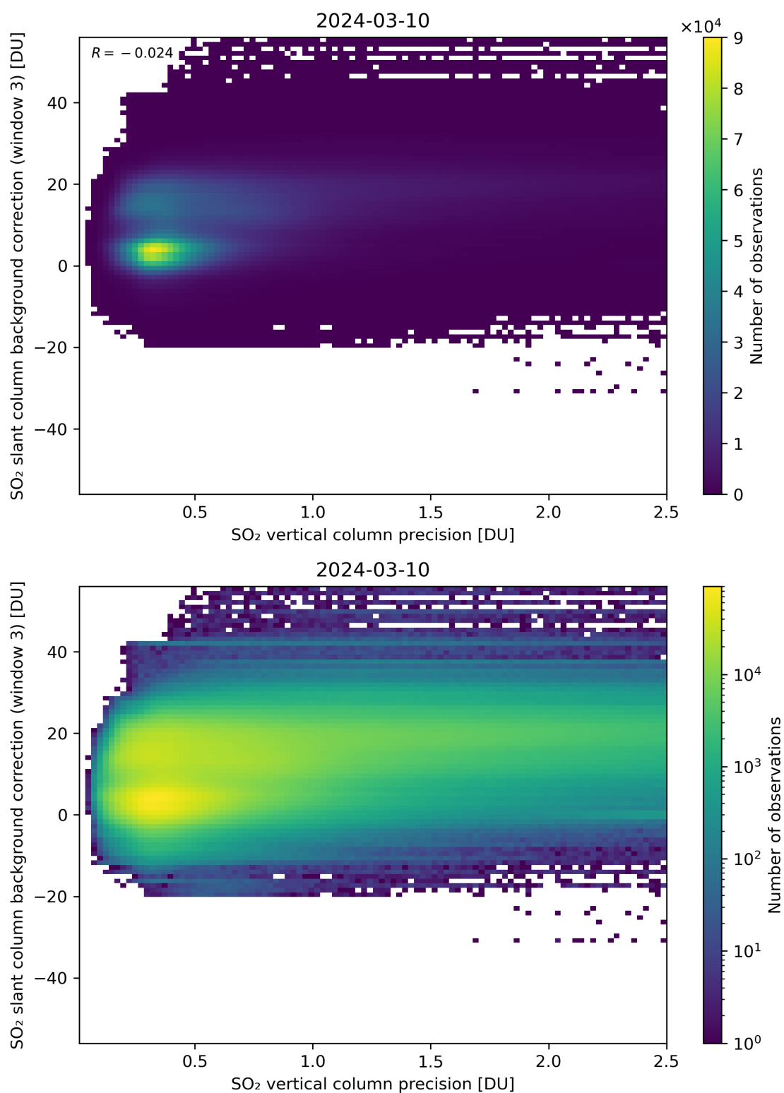
Figure 281: Scatter density plot of “SO 2 vertical column precision” against “SO 2 slant column background correction (window 3)” for 2024-03-09 to 2024-03-11.
