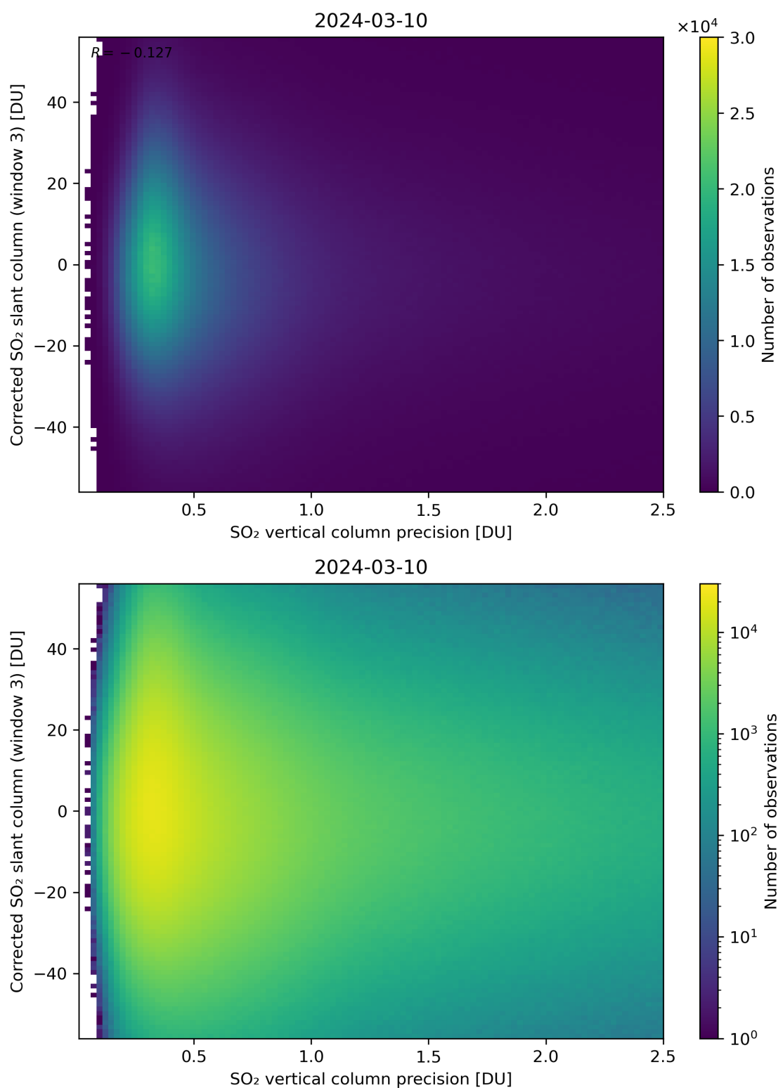
Figure 288: Scatter density plot of “SO 2 vertical column precision” against “Corrected SO 2 slant column (window 3)” for 2024-03-09 to 2024-03-11.
