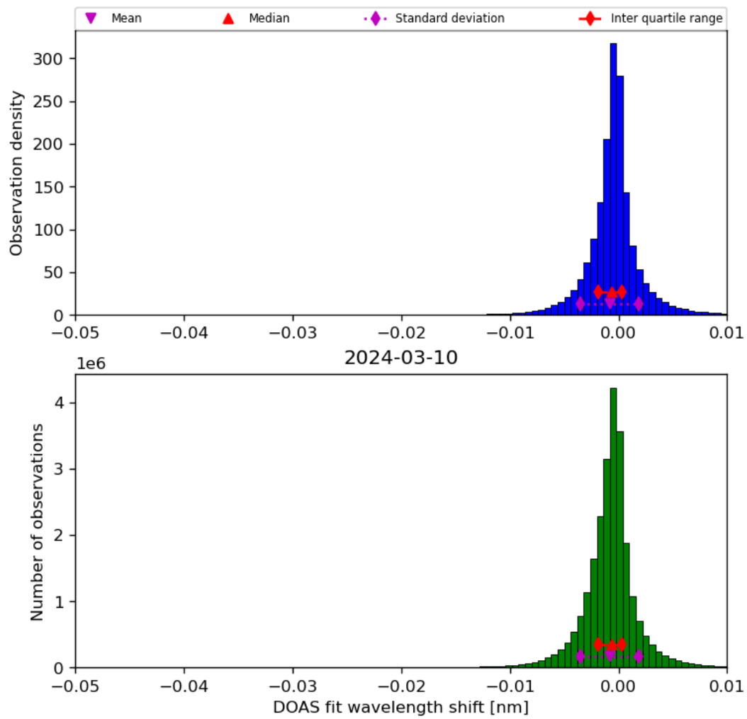
Figure 68: Histogram of “DOAS fit wavelength shift” for 2024-03-09 to 2024-03-11
