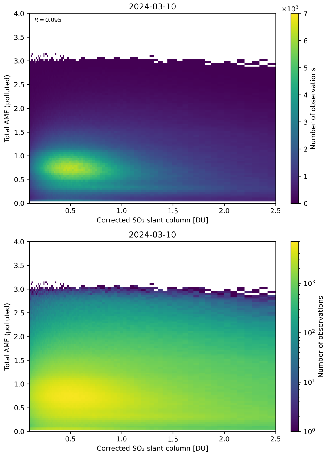
Figure 192: Scatter density plot of “Corrected SO 2 slant column” against “Total AMF (polluted)” for 2024-03-09 to 2024-03-11.
