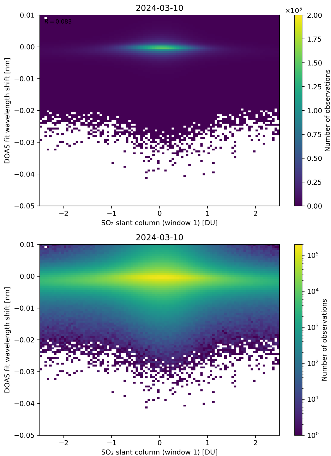
Figure 215: Scatter density plot of “SO 2 slant column (window 1)” against “DOAS fit wavelength shift” for 2024-03-09 to 2024-03-11.
