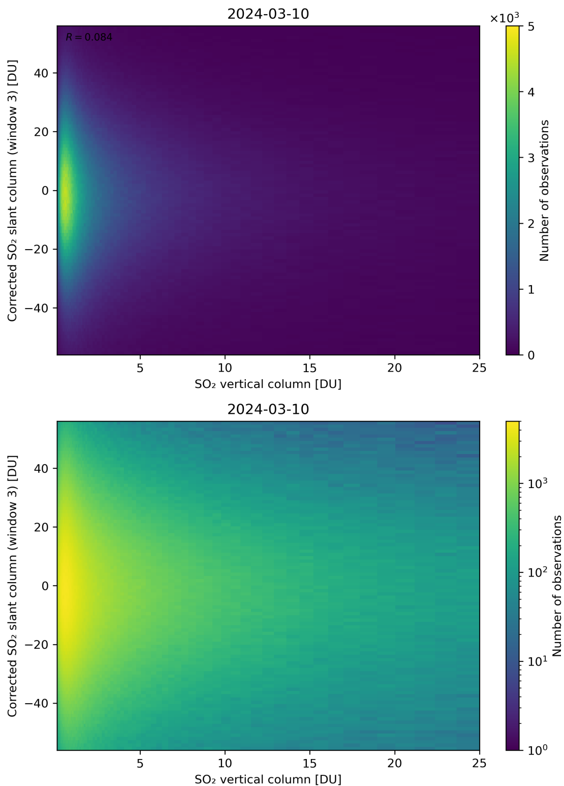
Figure 299: Scatter density plot of “SO 2 vertical column” against “Corrected SO 2 slant column (window 3)” for 2024-03-09 to 2024-03-11.
