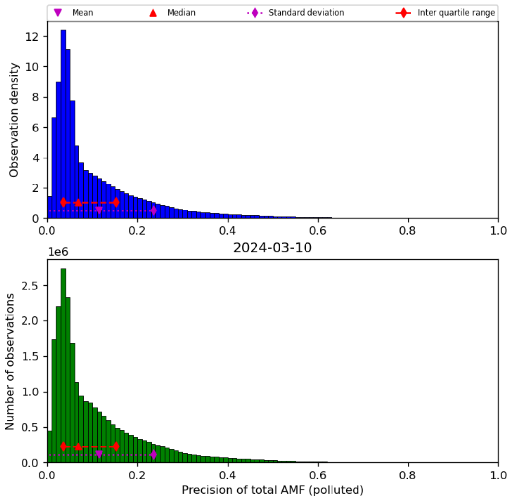
Figure 72: Histogram of “Precision of total AMF (polluted)” for 2024-03-09 to 2024-03-11
