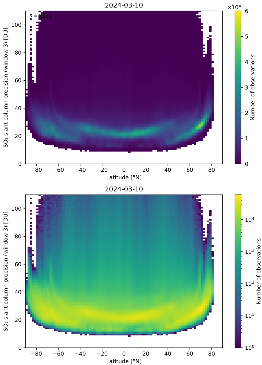
Figure 153: Scatter density plot of “Latitude” against “SO 2 slant column precision (window 3)” for 2024-03-09 to 2024-03-11.
