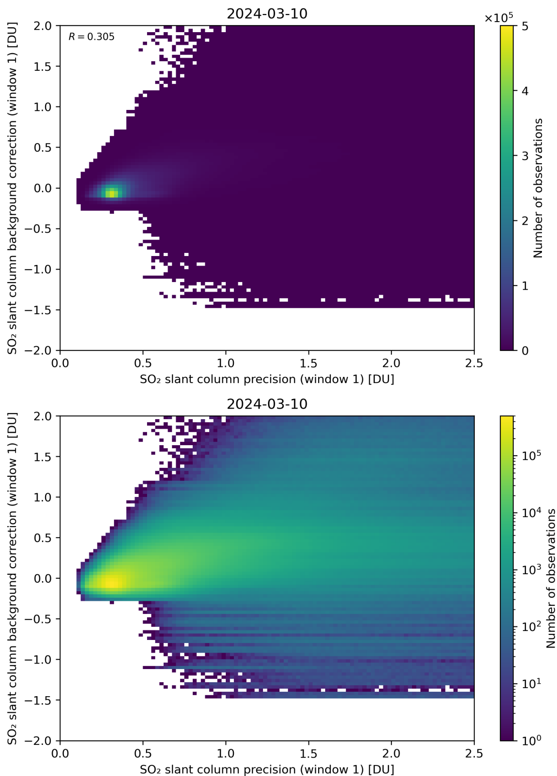
Figure 218: Scatter density plot of “SO 2 slant column precision (window 1)” against “SO 2 slant column background correction (window 1)” for 2024-03-09 to 2024-03-11.
