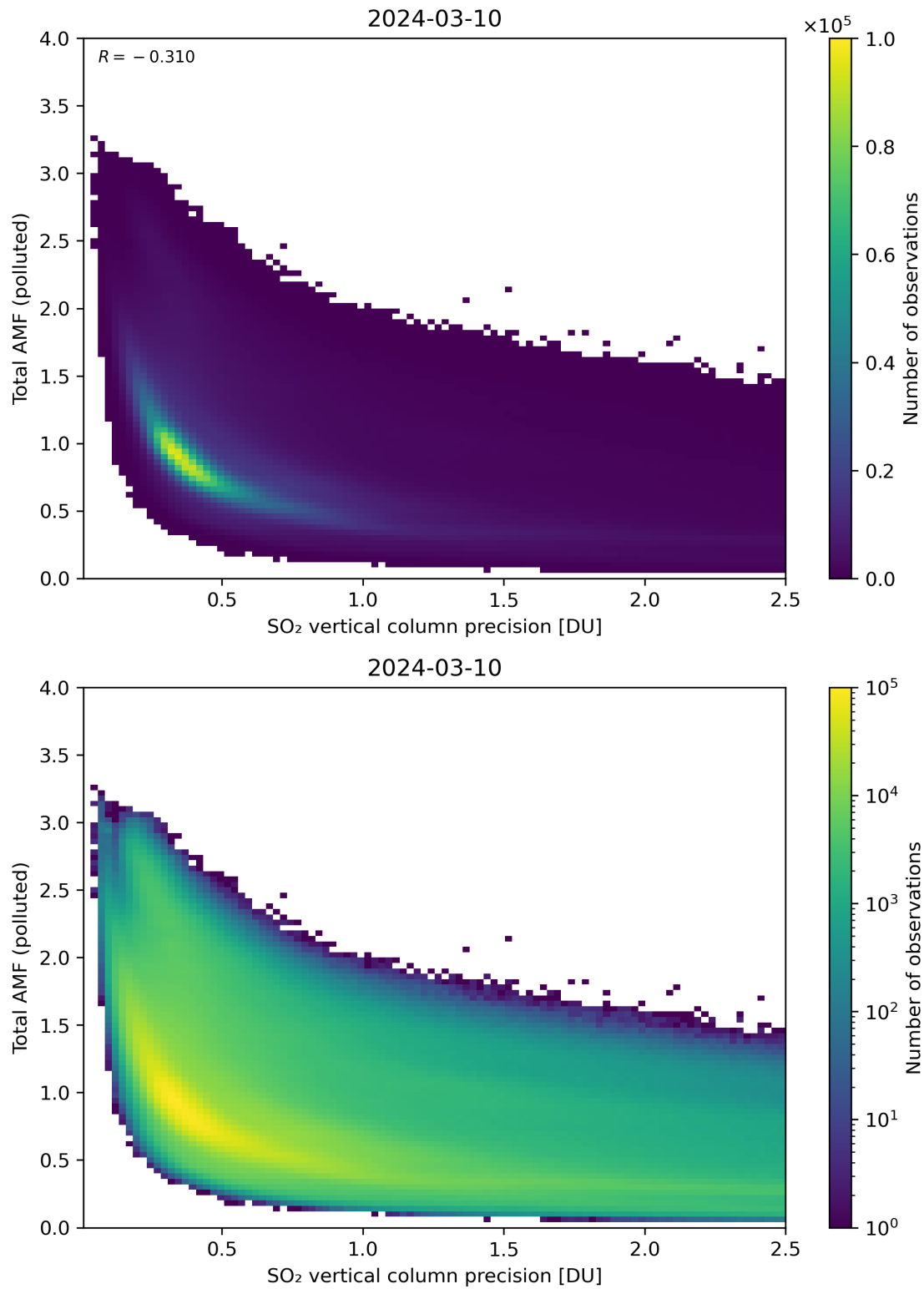
Figure 294: Scatter density plot of “SO 2 vertical column precision” against “Total AMF (polluted)” for 2024-03-09 to 2024-03-11.
