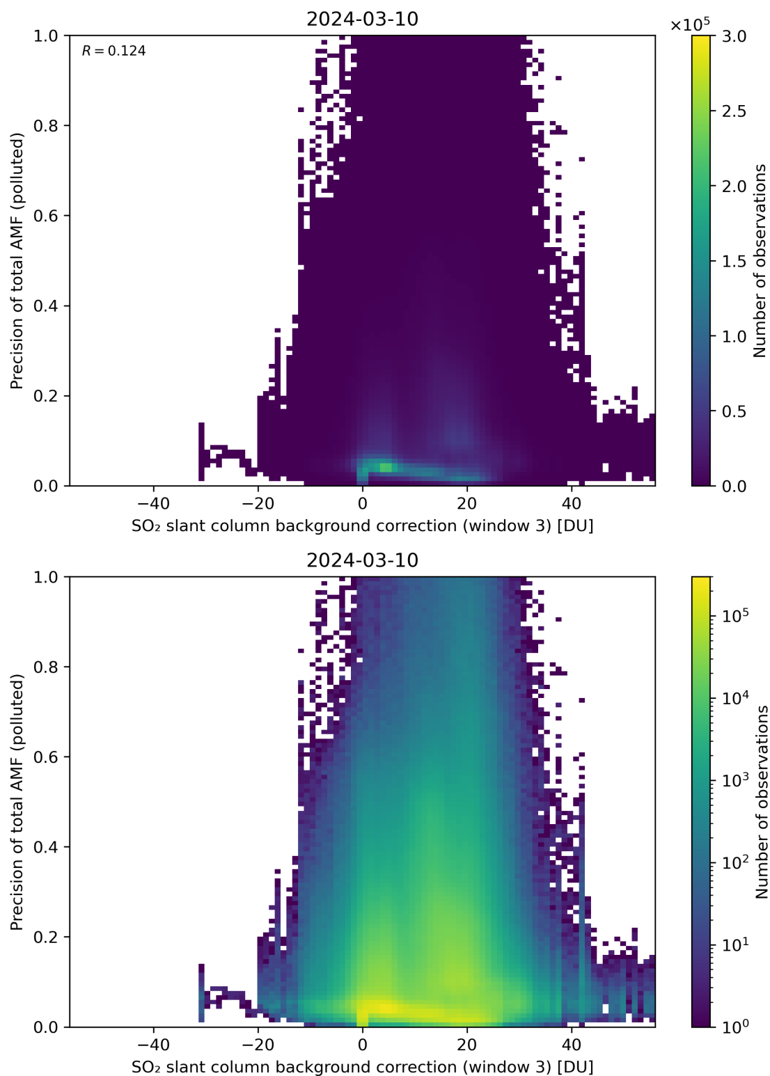
Figure 126: Scatter density plot of “SO 2 slant column background correction (window 3)” against “Precision of total AMF (polluted)” for 2024-03-09 to 2024-03-11.
