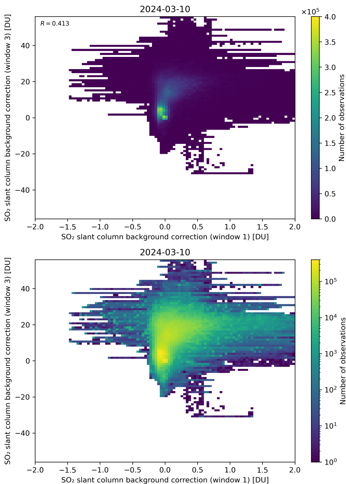
Figure 99: Scatter density plot of “SO 2 slant column background correction (window 1)” against “SO 2 slant column background correction (window 3)” for 2024-03-09 to 2024-03-11.
