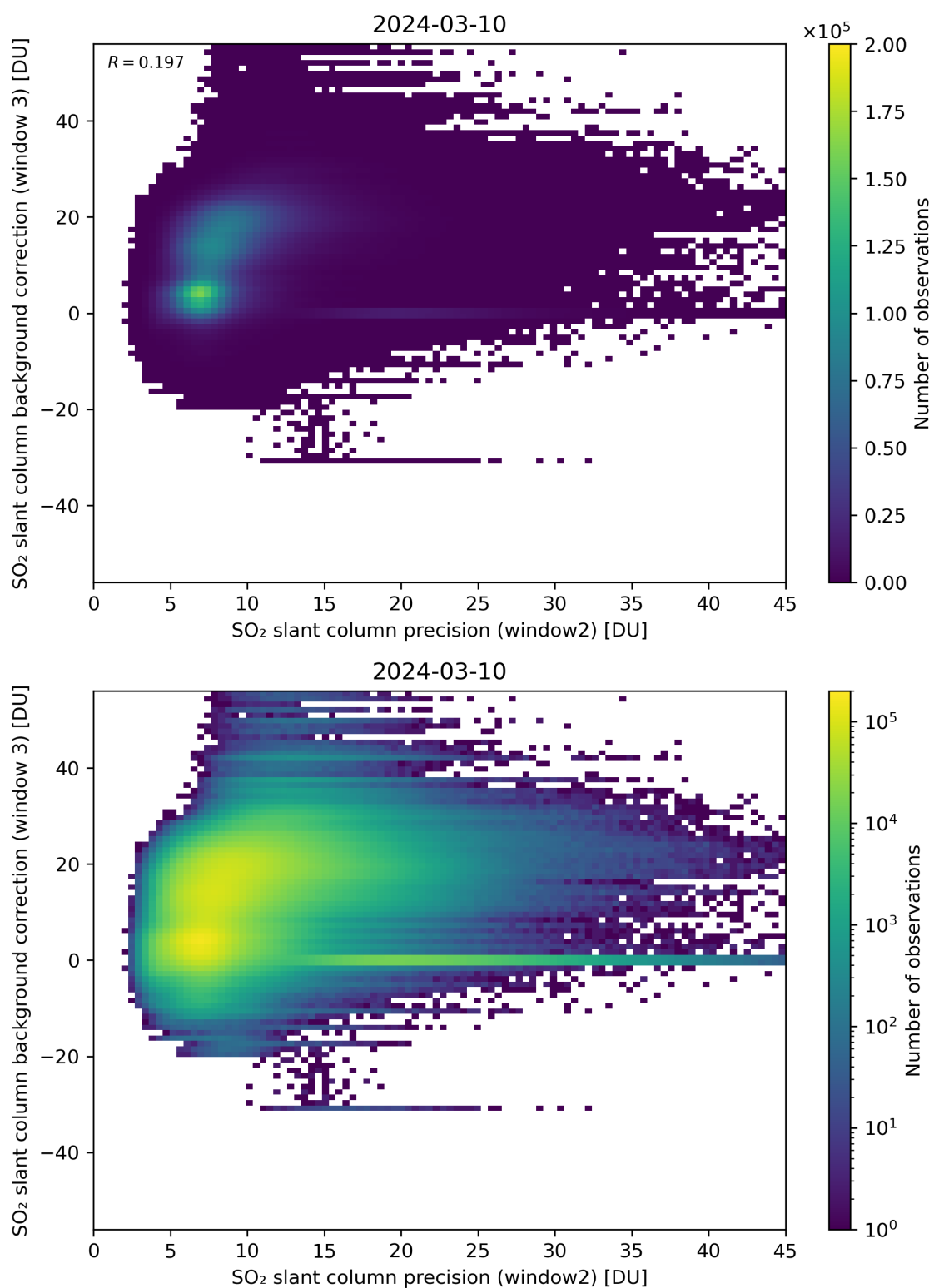
Figure 242: Scatter density plot of “SO 2 slant column precision (window2)” against “SO 2 slant column background correction (window 3)” for 2024-03-09 to 2024-03-11.
