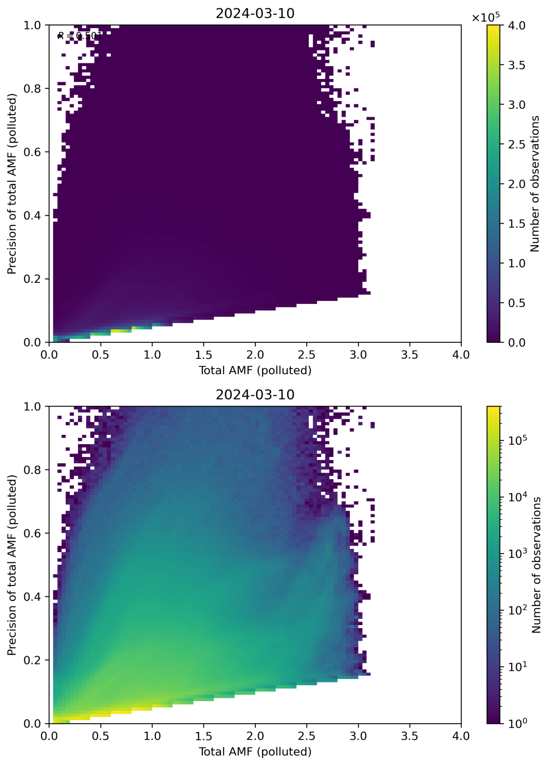
Figure 272: Scatter density plot of “Total AMF (polluted)” against “Precision of total AMF (polluted)” for 2024-03-09 to 2024-03-11.
