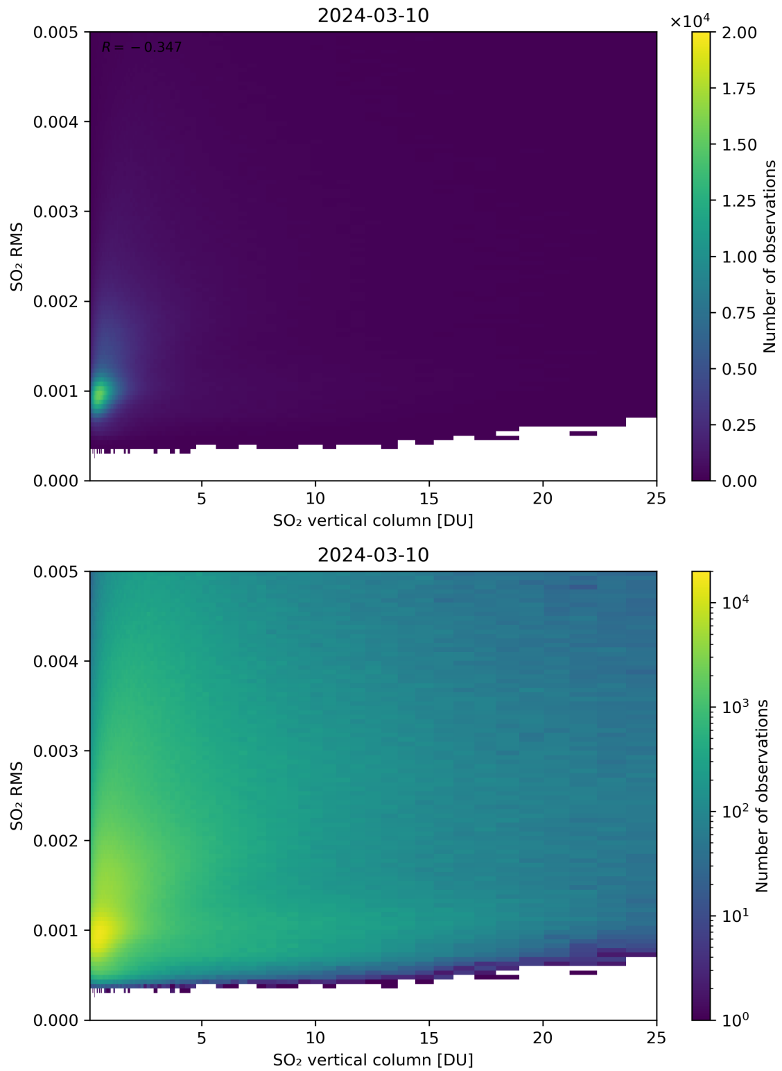
Figure 278: Scatter density plot of “SO 2 vertical column” against “SO 2 RMS” for 2024-03-09 to 2024-03-11.
