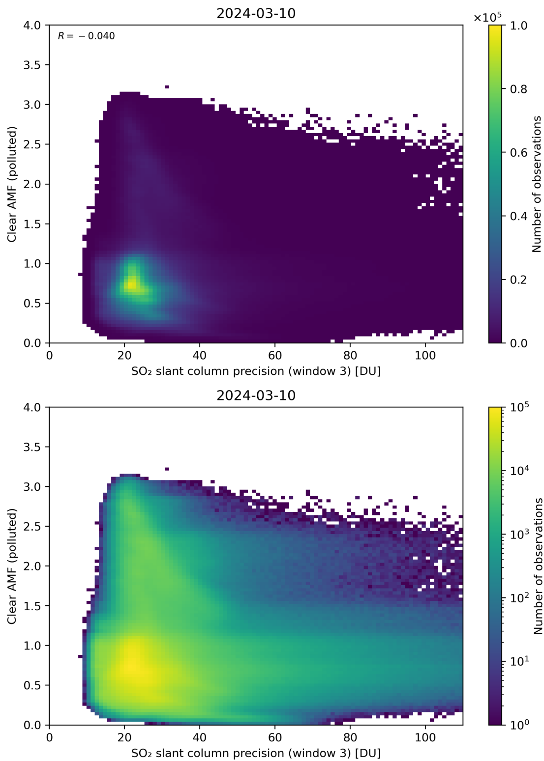
Figure 261: Scatter density plot of “SO 2 slant column precision (window 3)” against “Clear AMF (polluted)” for 2024-03-09 to 2024-03-11.
