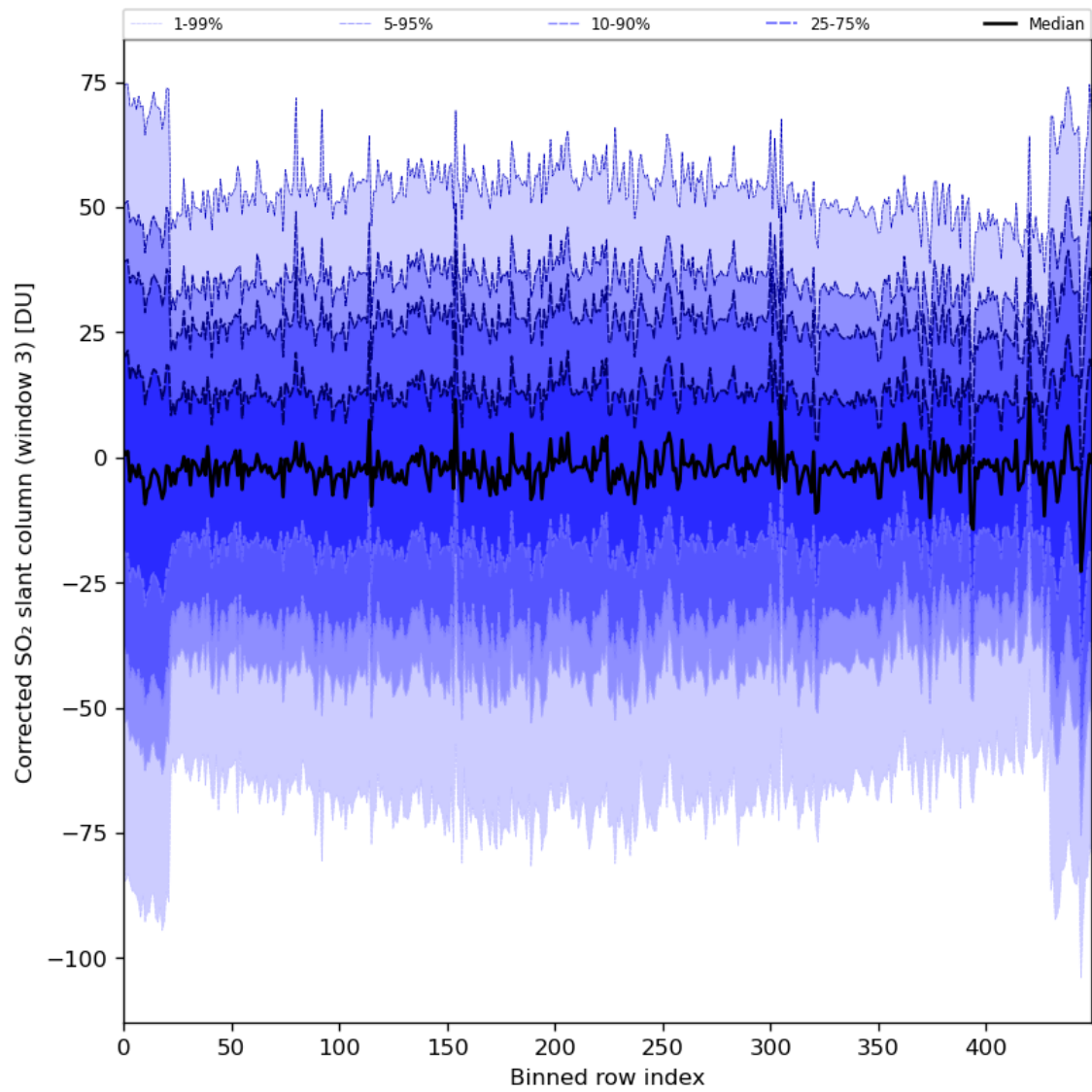
Figure 89: Along track statistics of “Corrected SO 2 slant column (window 3)” for 2024-03-09 to 2024-03-11
