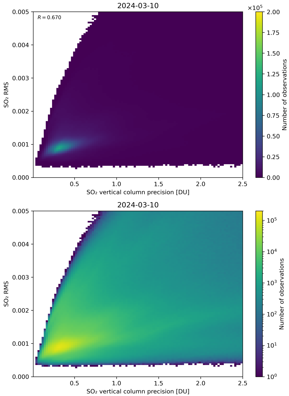
Figure 284: Scatter density plot of “SO 2 vertical column precision” against “SO 2 RMS” for 2024-03-09 to 2024-03-11.
