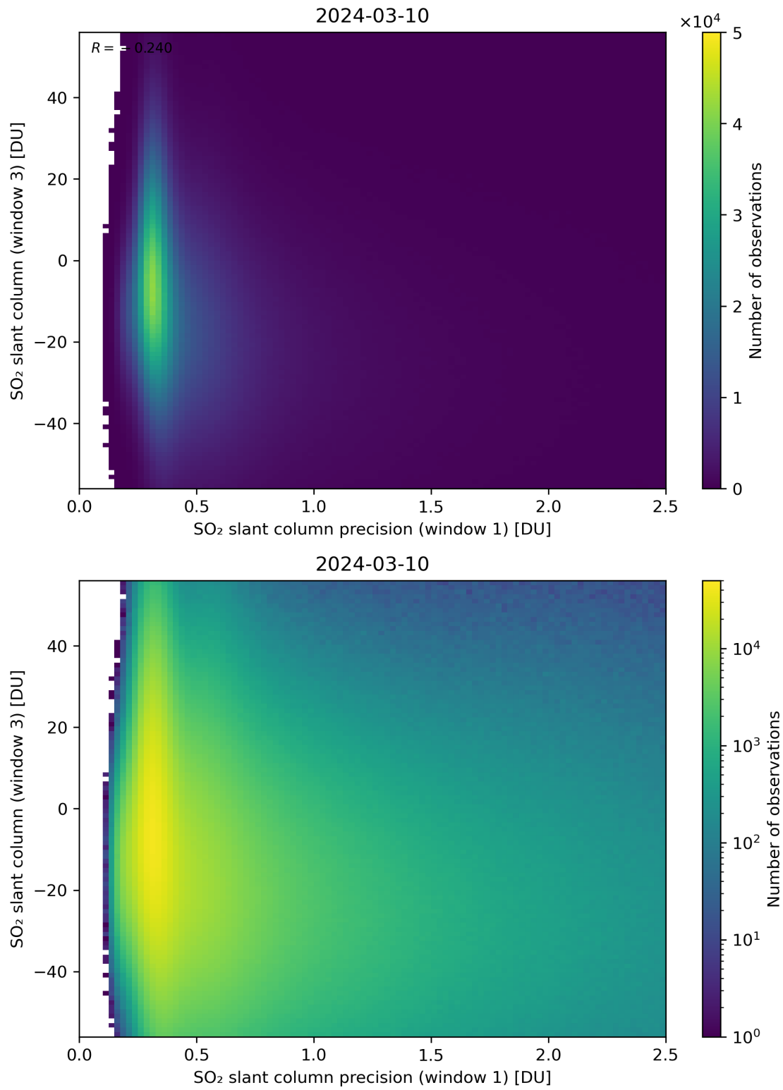
Figure 228: Scatter density plot of “SO 2 slant column precision (window 1)” against “SO 2 slant column (window 3)” for 2024-03-09 to 2024-03-11.
