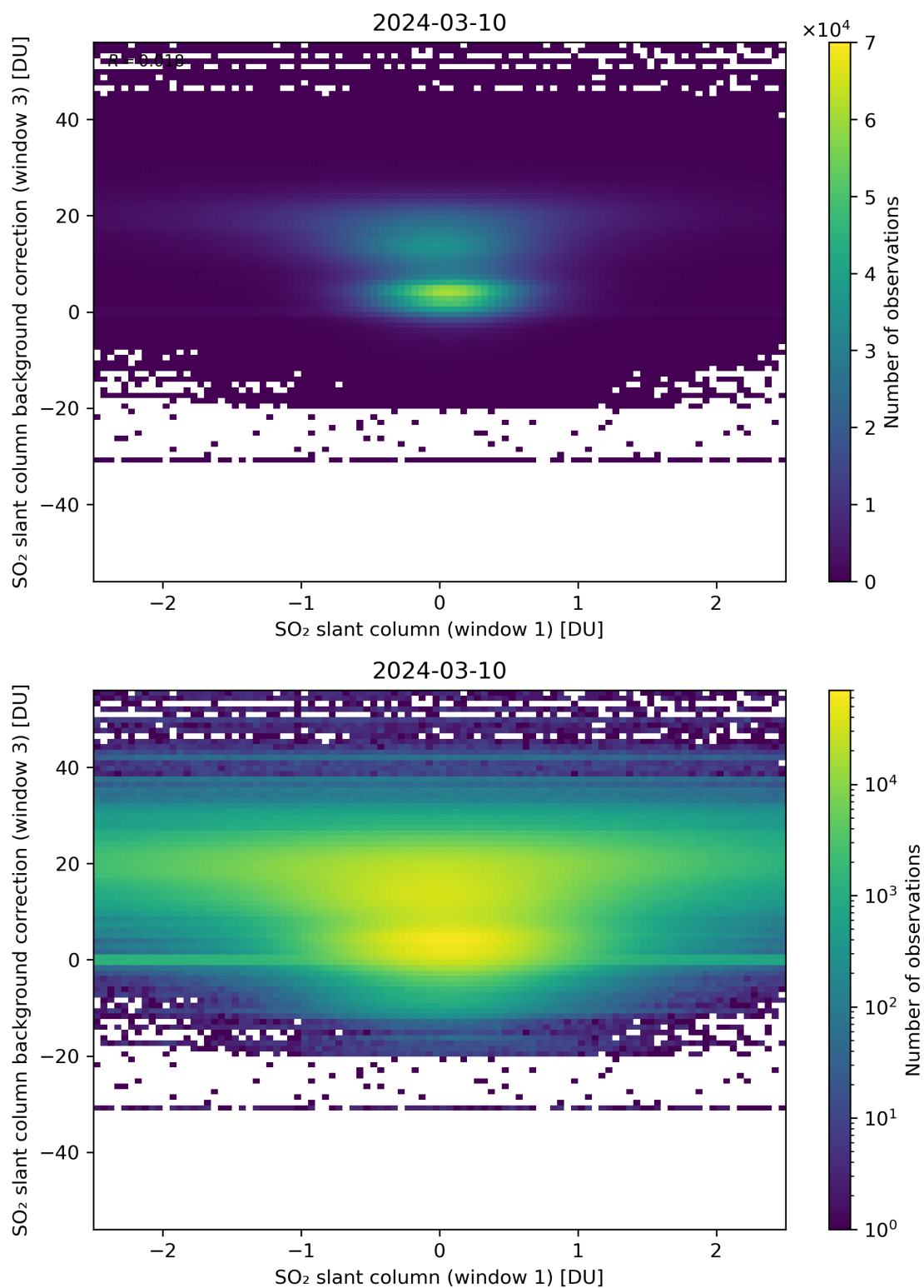
Figure 214: Scatter density plot of “SO 2 slant column (window 1)” against “SO 2 slant column background correction (window 3)” for 2024-03-09 to 2024-03-11.
