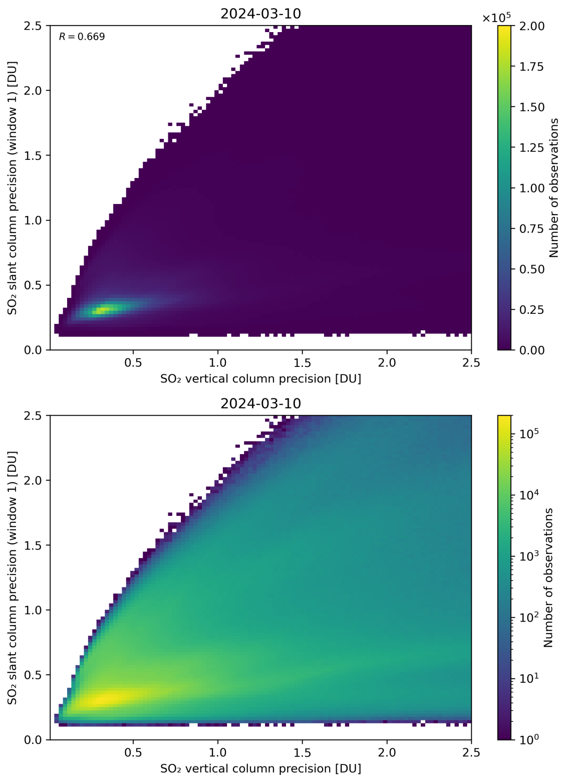
Figure 290: Scatter density plot of “SO 2 vertical column precision” against “SO 2 slant column precision (window 1)” for 2024-03-09 to 2024-03-11.
