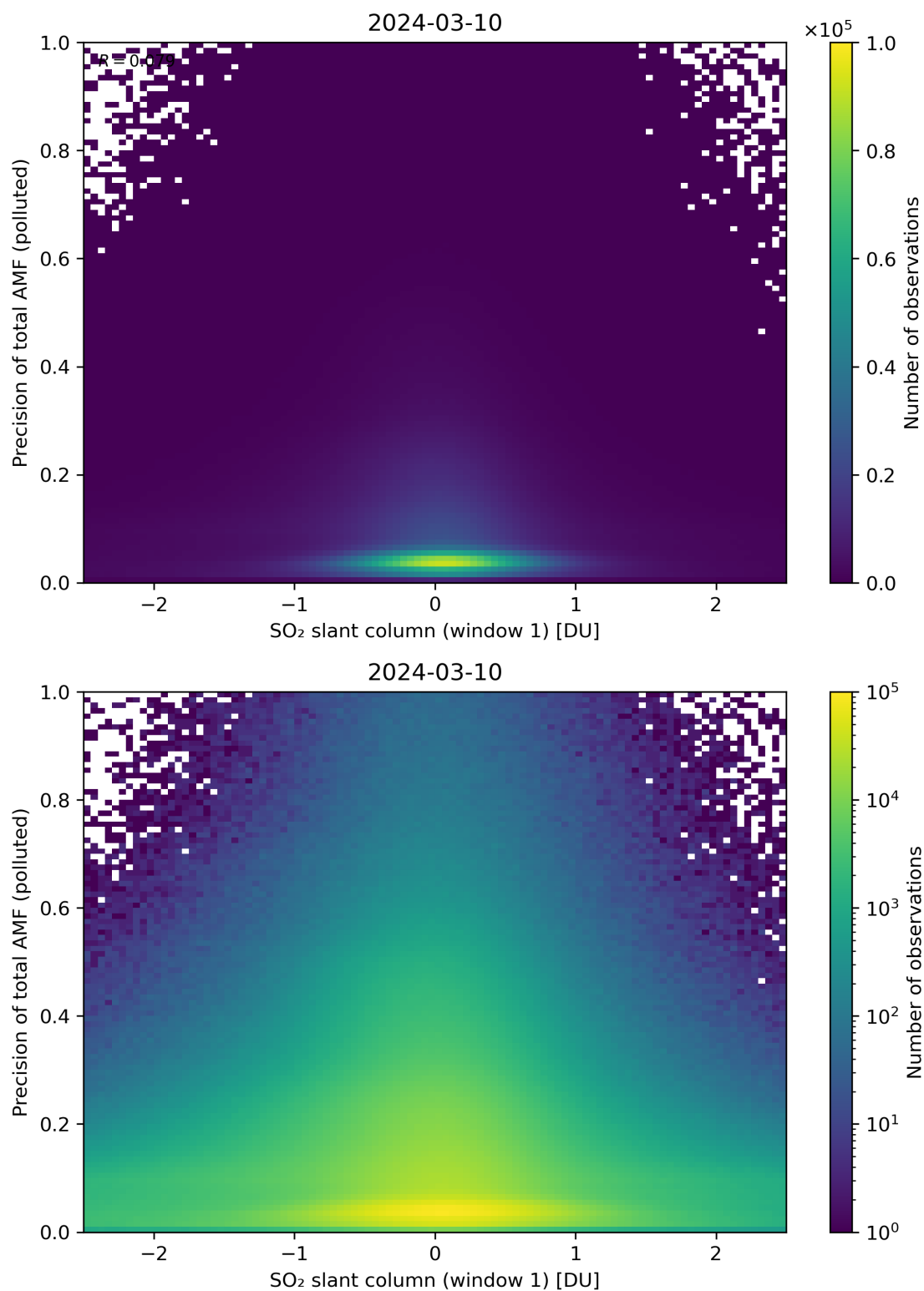
Figure 240: Scatter density plot of “SO 2 slant column (window 1)” against “Precision of total AMF (polluted)” for 2024-03-09 to 2024-03-11.
