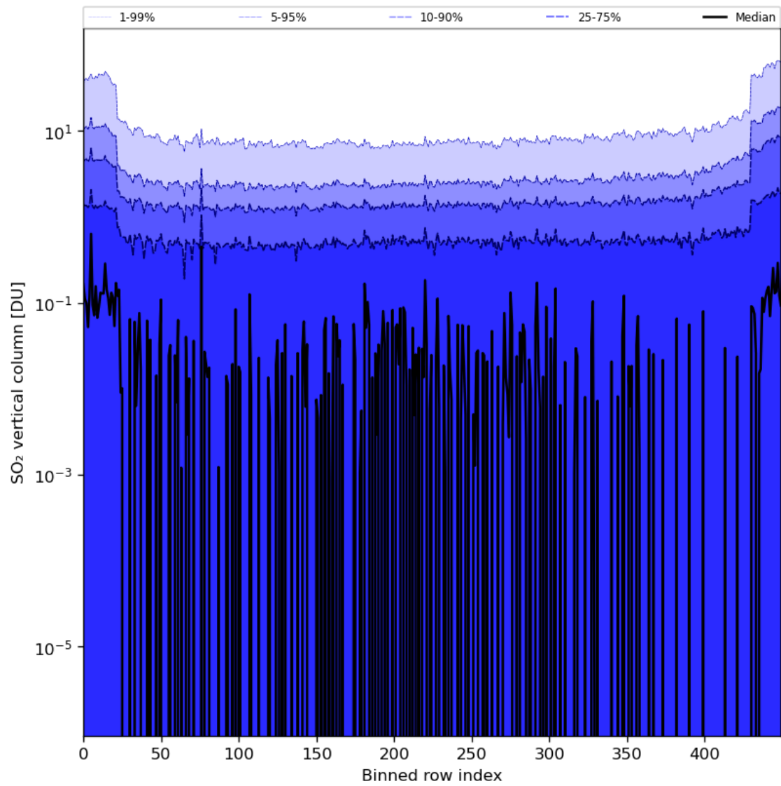
Figure 76: Along track statistics of “SO 2 vertical column” for 2024-03-09 to 2024-03-11
