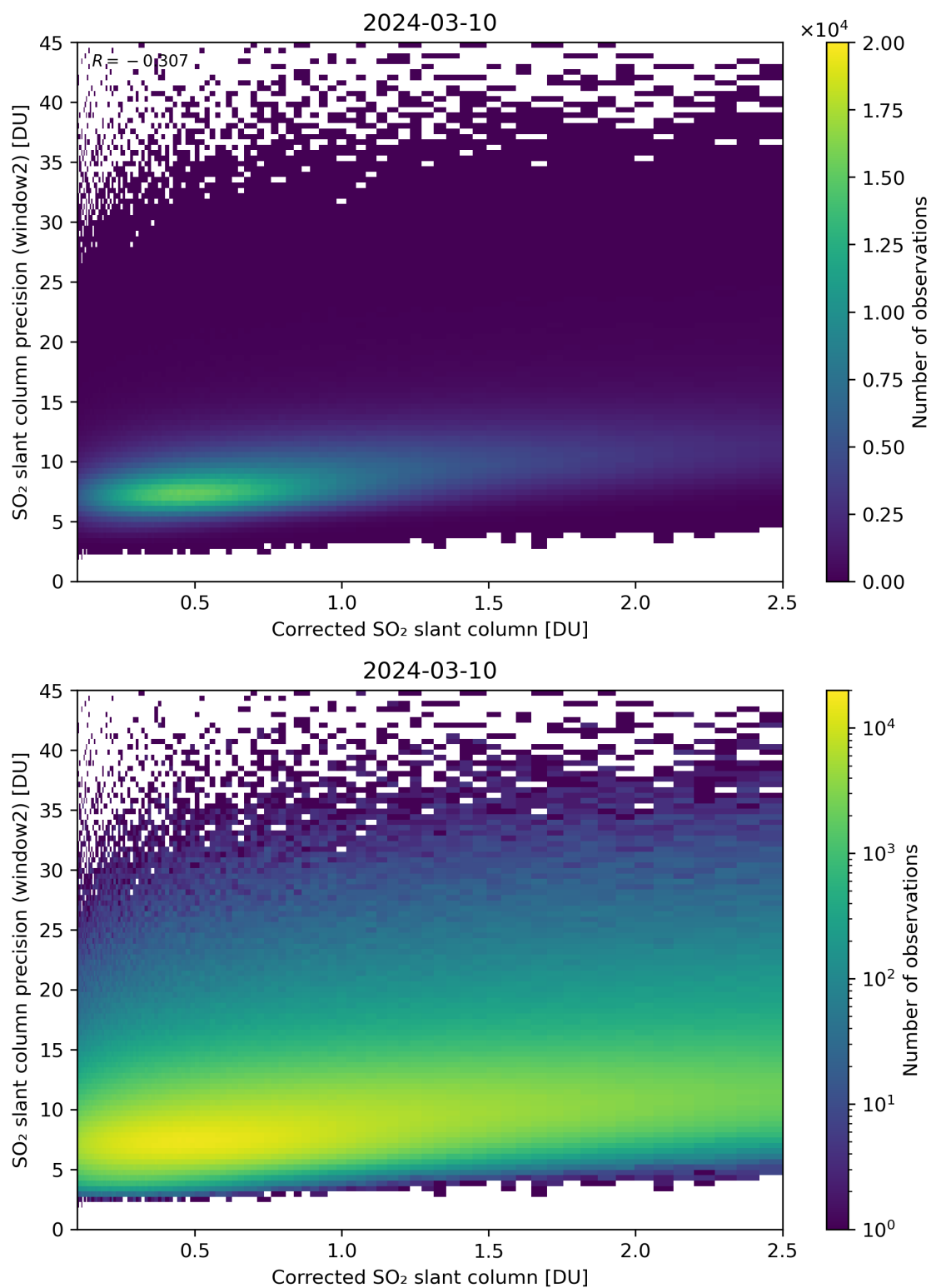
Figure 189: Scatter density plot of “Corrected SO 2 slant column” against “SO 2 slant column precision (window2)” for 2024-03-09 to 2024-03-11.
