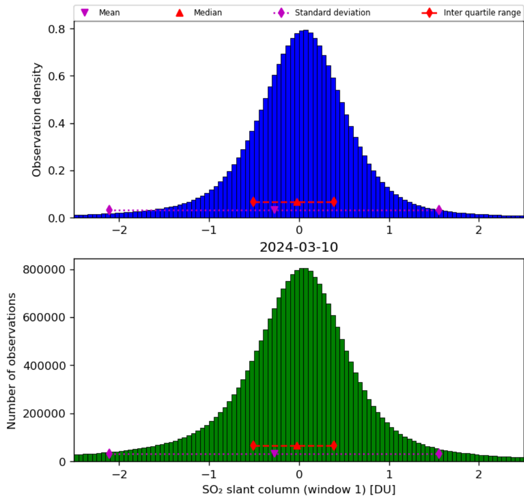
Figure 56: Histogram of “SO 2 slant column (window 1)” for 2024-03-09 to 2024-03-11
