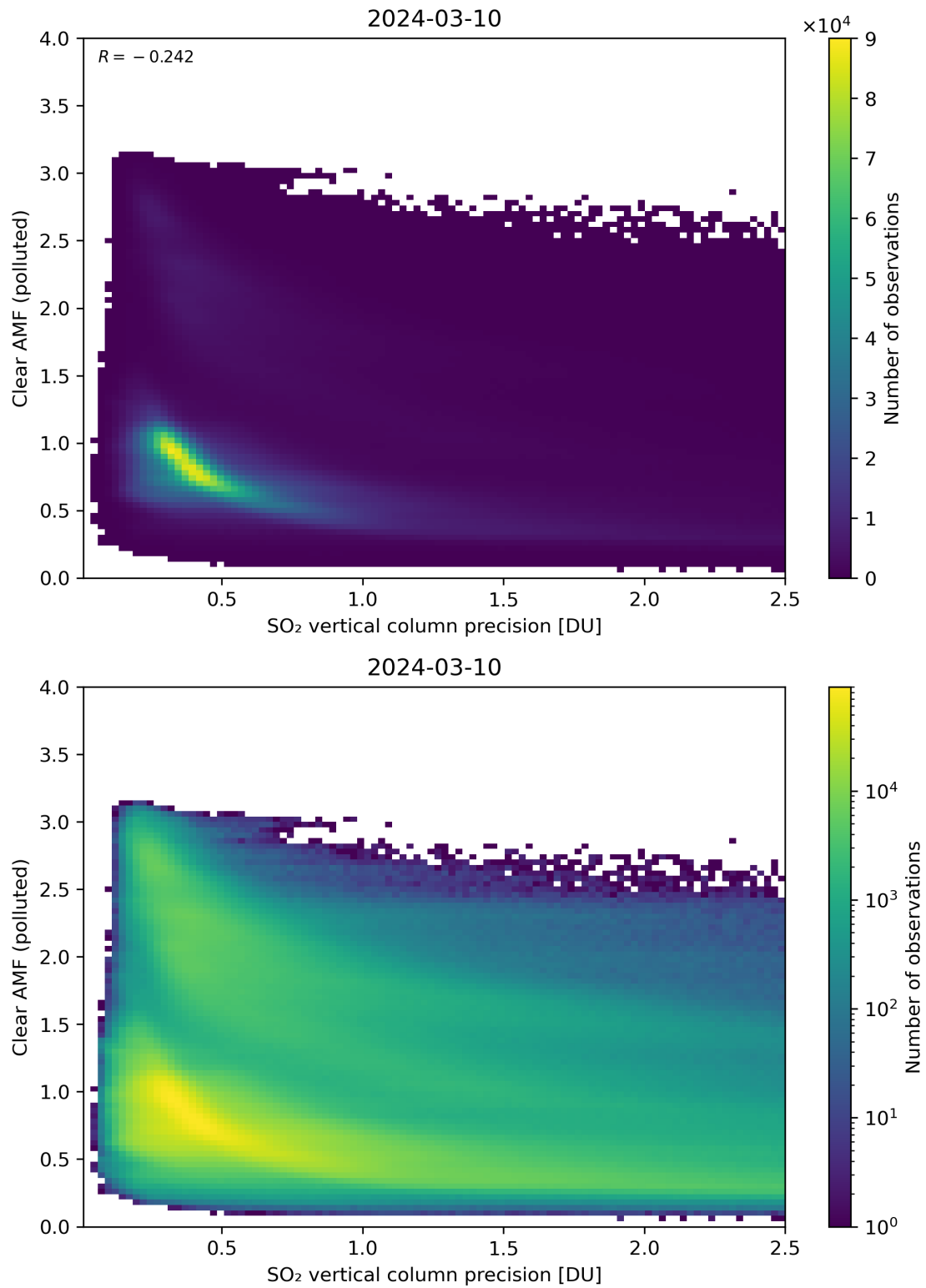
Figure 285: Scatter density plot of “SO 2 vertical column precision” against “Clear AMF (polluted)” for 2024-03-09 to 2024-03-11.
