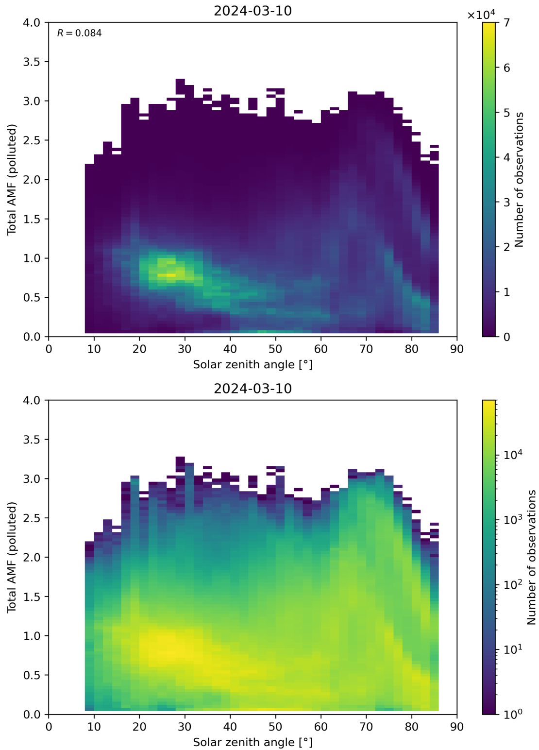
Figure 174: Scatter density plot of “Solar zenith angle” against “Total AMF (polluted)” for 2024-03-09 to 2024-03-11.
