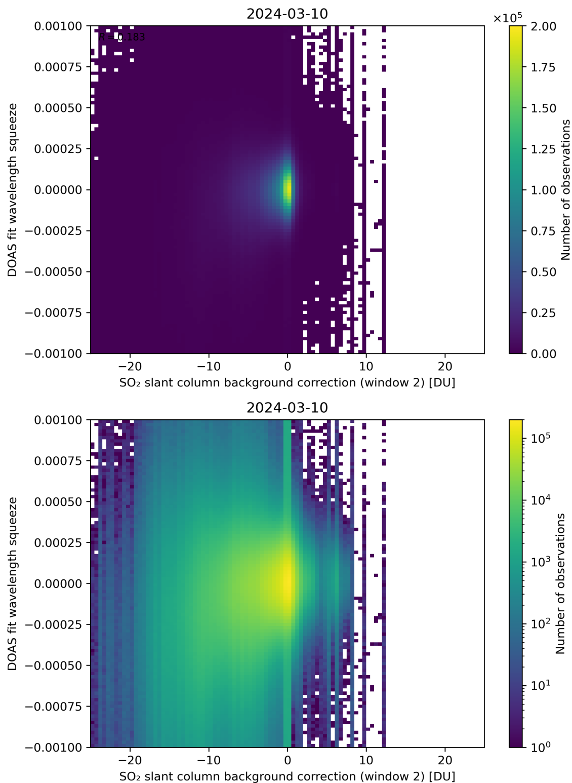
Figure 113: Scatter density plot of "SO 2 slant column background correction (window 2)" against "DOAS fit wavelength squeeze" for 2024-03-09 to 2024-03-11.
