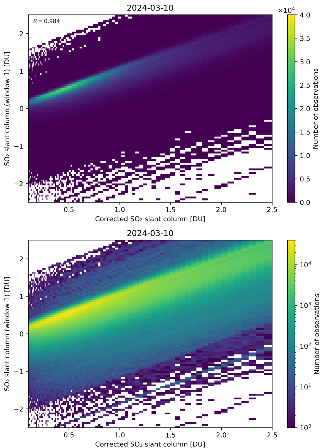
Figure 187: Scatter density plot of “Corrected SO 2 slant column” against “SO 2 slant column (window 1)” for 2024-03-09 to 2024-03-11.
