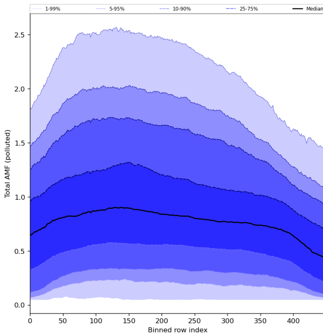
Figure 94: Along track statistics of “Total AMF (polluted)” for 2024-03-09 to 2024-03-11
