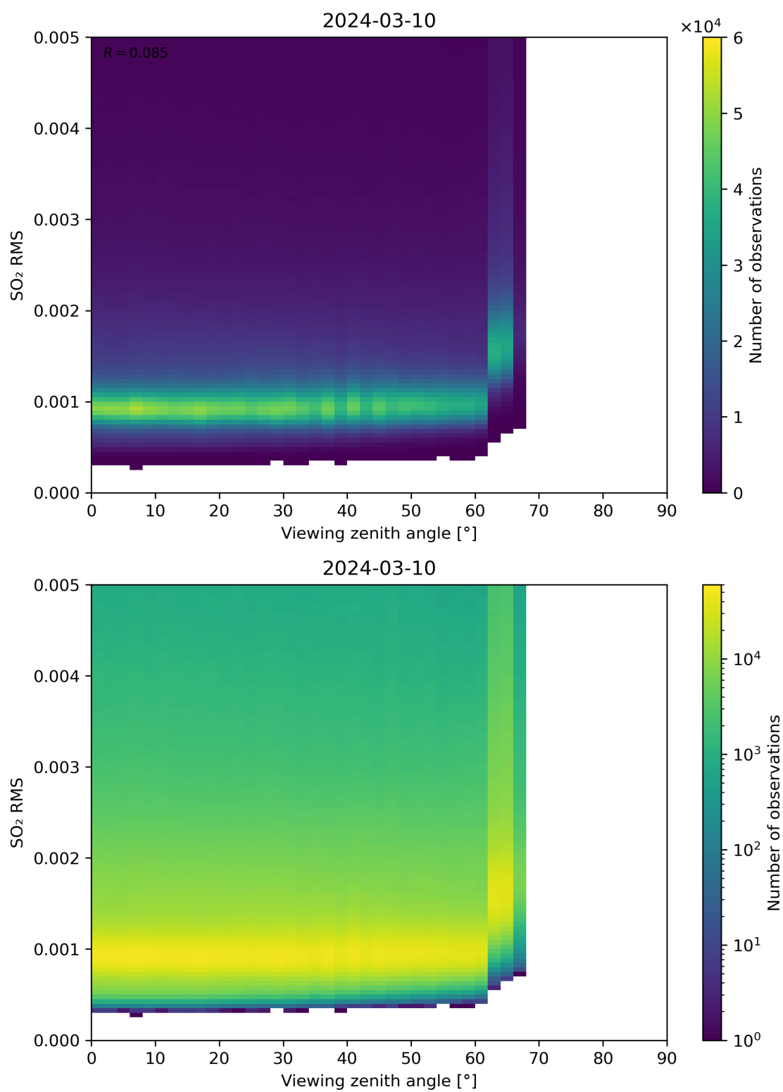
Figure 313: Scatter density plot of “Viewing zenith angle” against “SO 2 RMS” for 2024-03-09 to 2024-03-11.
