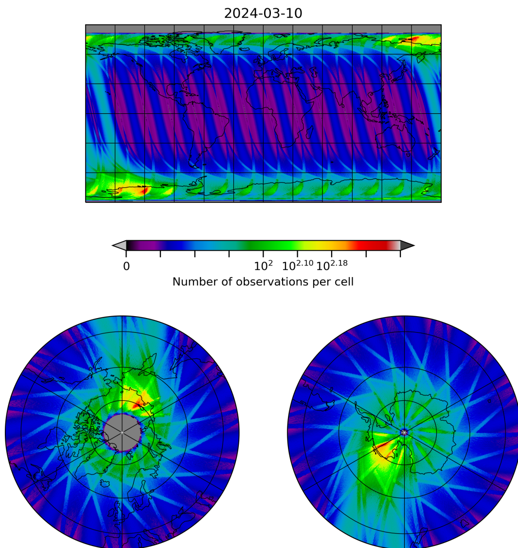
Figure 28: Map of the number of observations for 2024-03-09 to 2024-03-11
