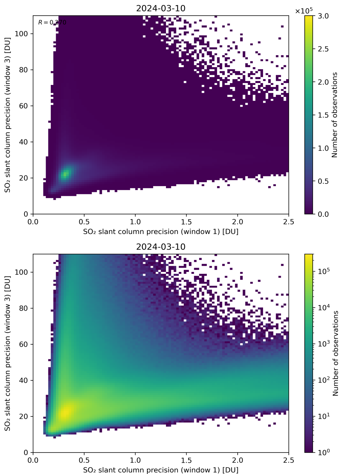
Figure 229: Scatter density plot of “SO 2 slant column precision (window 1)” against “SO 2 slant column precision (window 3)” for 2024-03-09 to 2024-03-11.
