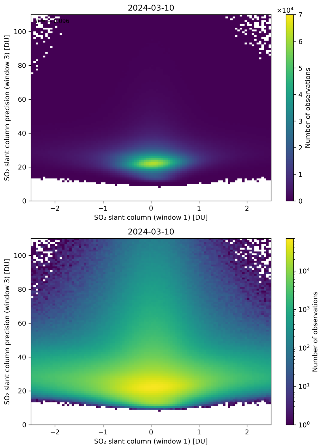
Figure 238: Scatter density plot of “SO 2 slant column (window 1)” against “SO 2 slant column precision (window 3)” for 2024-03-09 to 2024-03-11.
