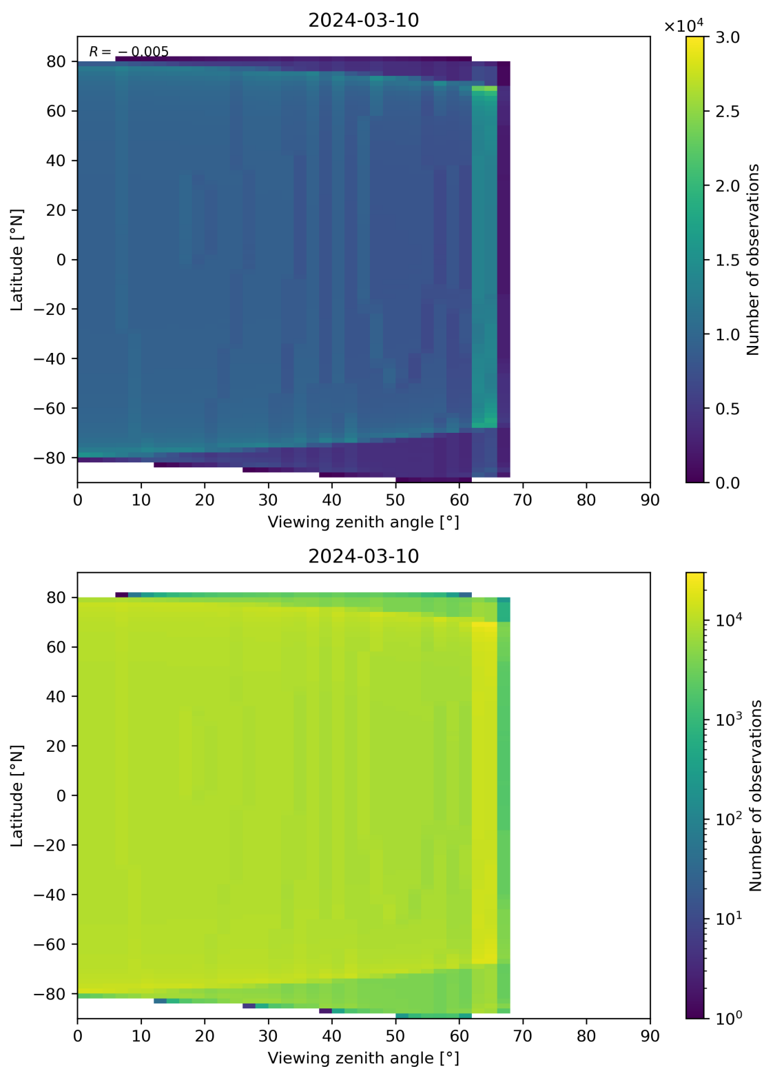
Figure 314: Scatter density plot of “Viewing zenith angle” against “Latitude” for 2024-03-09 to 2024-03-11.
