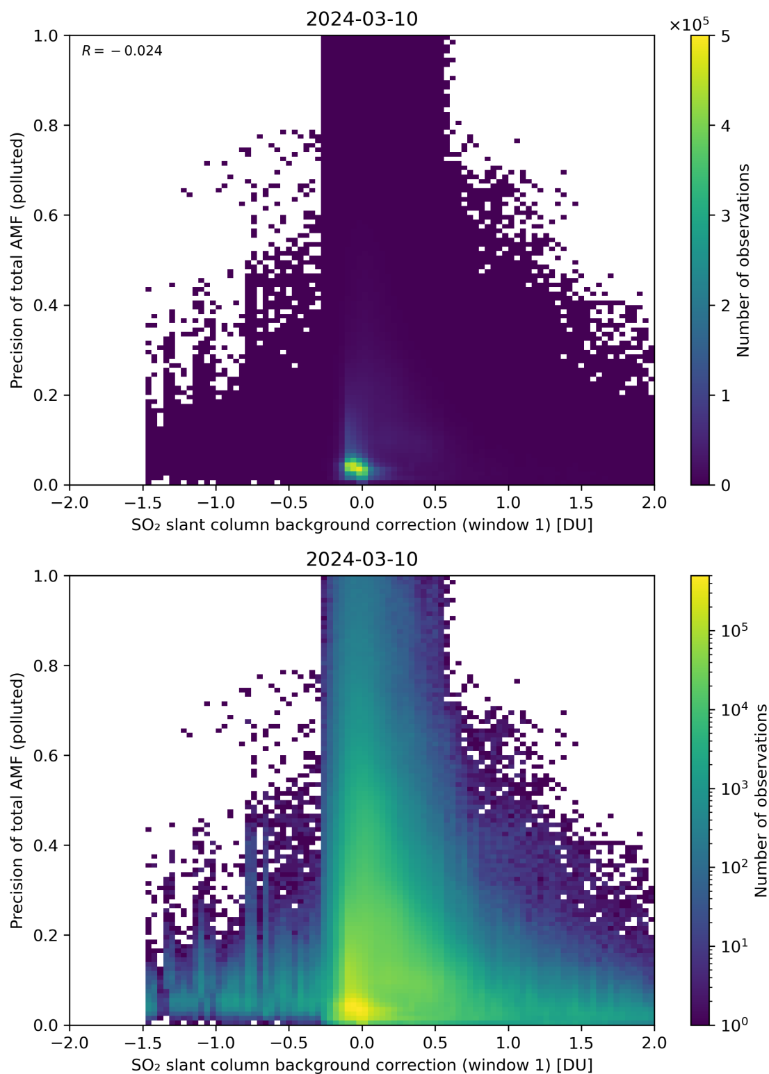
Figure 110: Scatter density plot of “SO 2 slant column background correction (window 1)” against “Precision of total AMF (polluted)” for 2024-03-09 to 2024-03-11.
