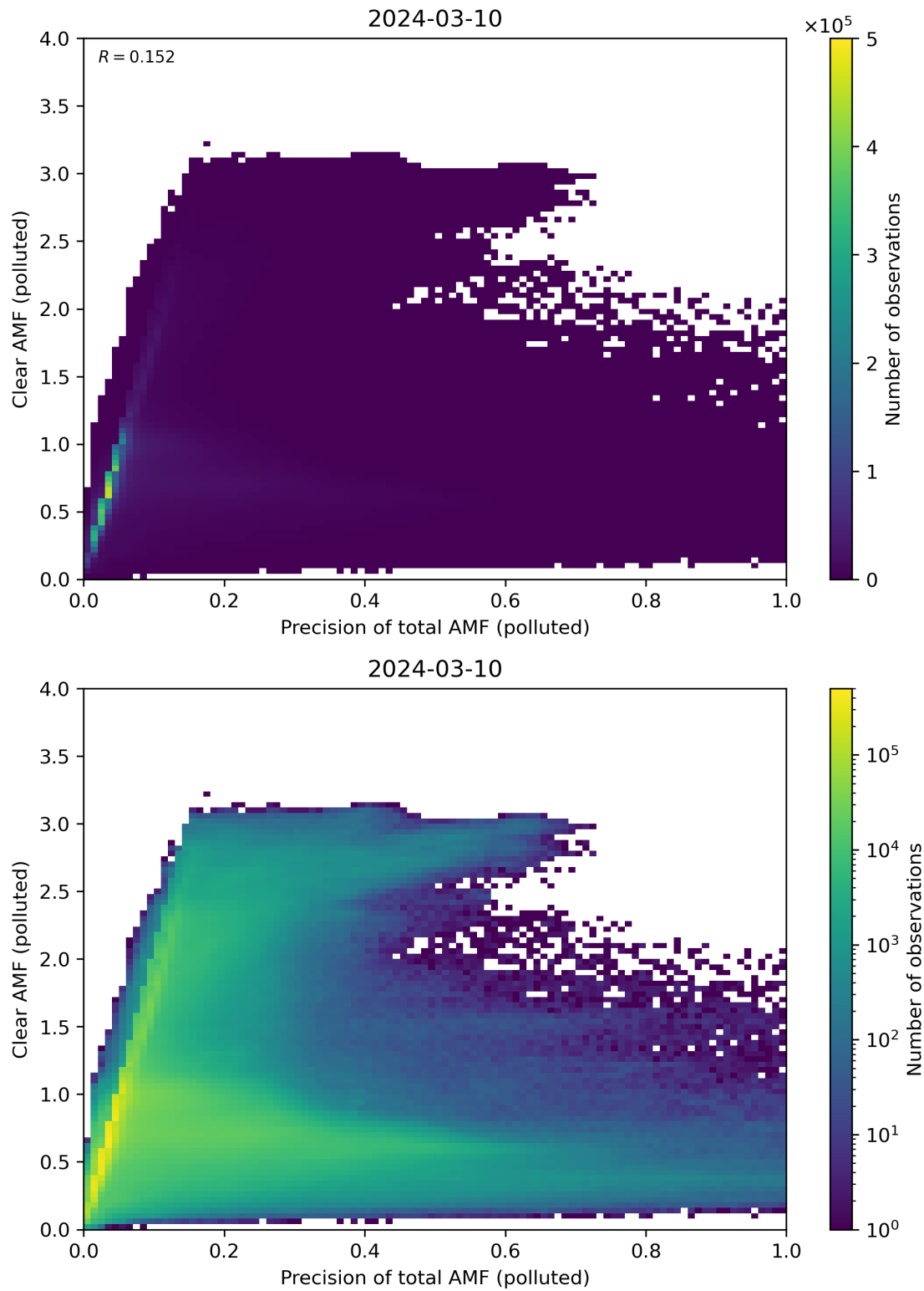
Figure 270: Scatter density plot of “Precision of total AMF (polluted)” against “Clear AMF (polluted)” for 2024-03-09 to 2024-03-11.
