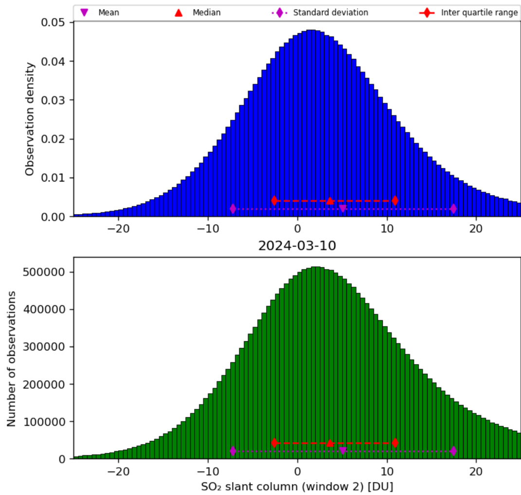
Figure 60: Histogram of “SO 2 slant column (window 2)” for 2024-03-09 to 2024-03-11
