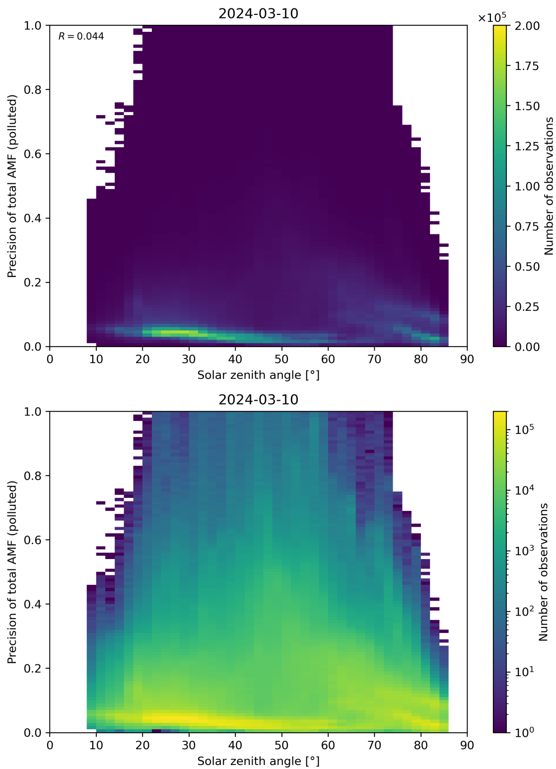
Figure 175: Scatter density plot of “Solar zenith angle” against “Precision of total AMF (polluted)” for 2024-03-09 to 2024-03-11.
