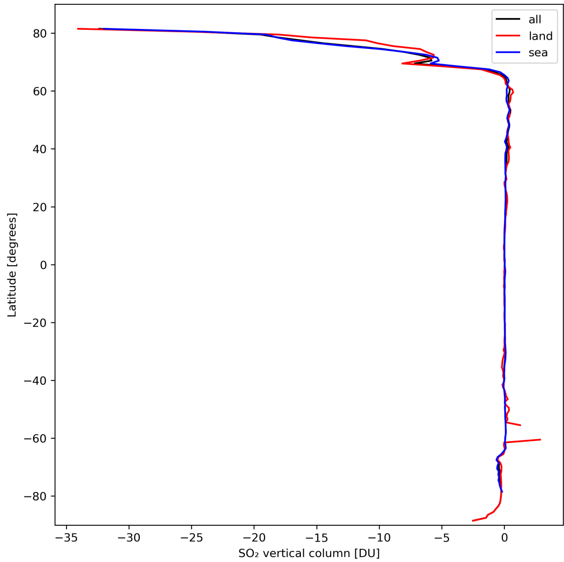
Figure 30: Zonal average of “SO 2 vertical column” for 2024-03-09 to 2024-03-11.
