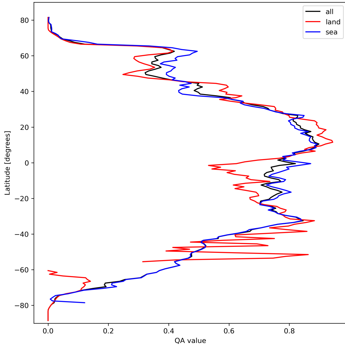
Figure 29: Zonal average of “QA value” for 2024-03-09 to 2024-03-11.
