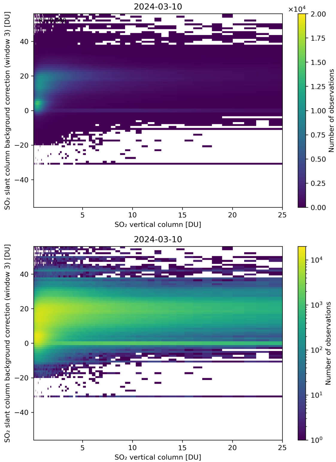
Figure 275: Scatter density plot of “SO 2 vertical column” against “SO 2 slant column background correction (window 3)” for 2024-03-09 to 2024-03-11.
