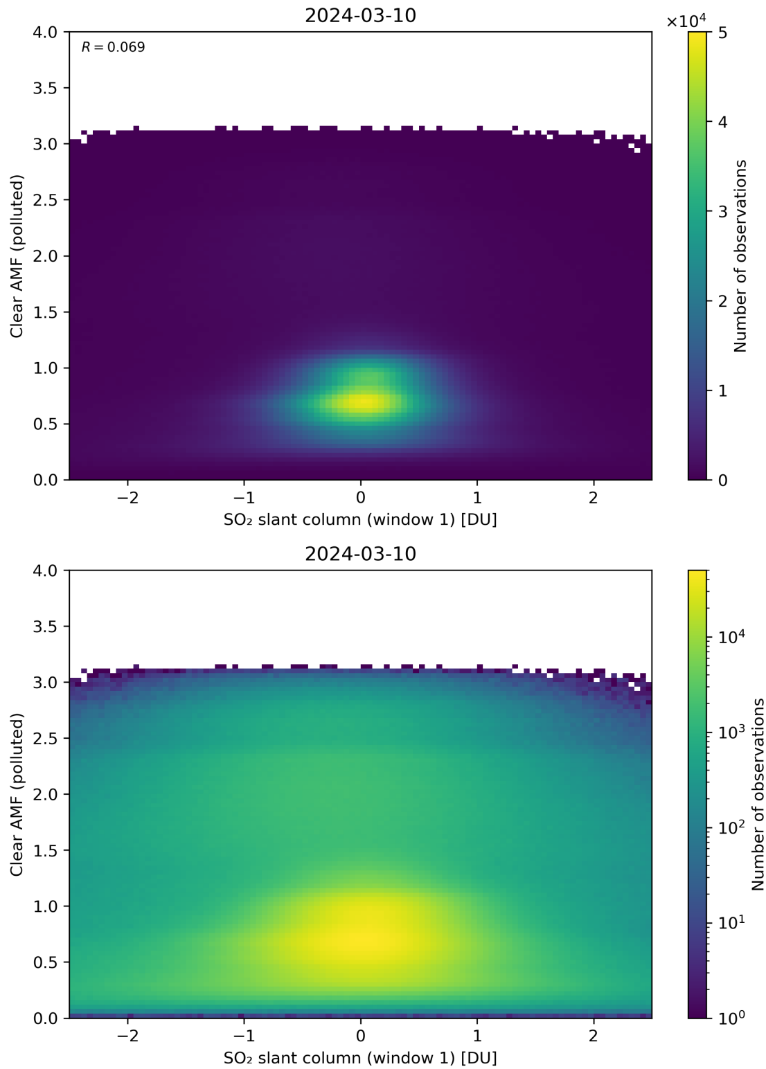
Figure 232: Scatter density plot of “SO 2 slant column (window 1)” against “Clear AMF (polluted)” for 2024-03-09 to 2024-03-11.
