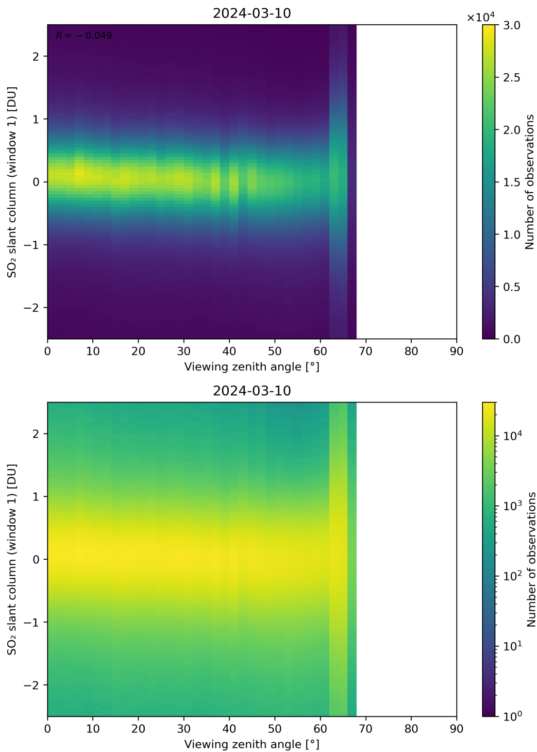
Figure 320: Scatter density plot of “Viewing zenith angle” against “SO 2 slant column (window 1)” for 2024-03-09 to 2024-03-11.
