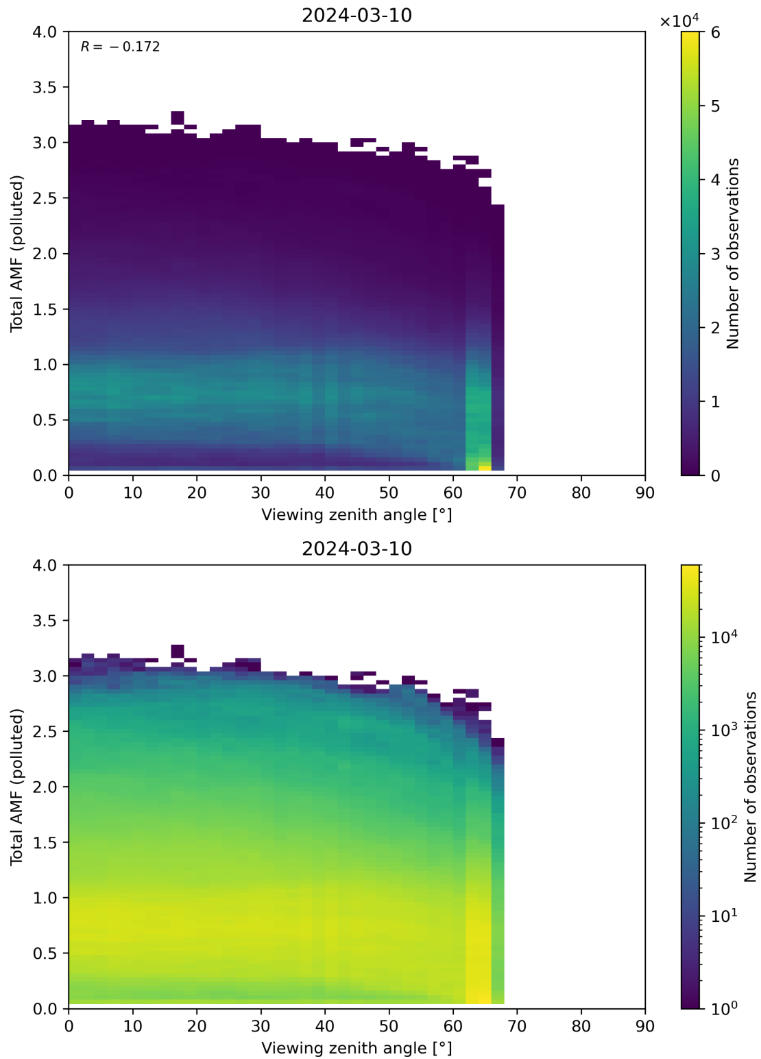
Figure 325: Scatter density plot of “Viewing zenith angle” against “Total AMF (polluted)” for 2024-03-09 to 2024-03-11.
