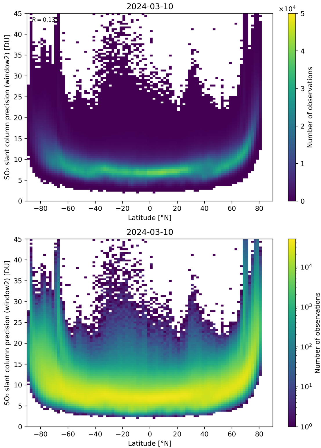
Figure 151: Scatter density plot of “Latitude” against “SO 2 slant column precision (window2)” for 2024-03-09 to 2024-03-11.
