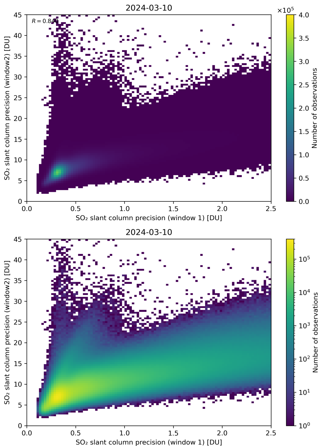
Figure 227: Scatter density plot of “SO 2 slant column precision (window 1)” against “SO 2 slant column precision (window2)” for 2024-03-09 to 2024-03-11.
