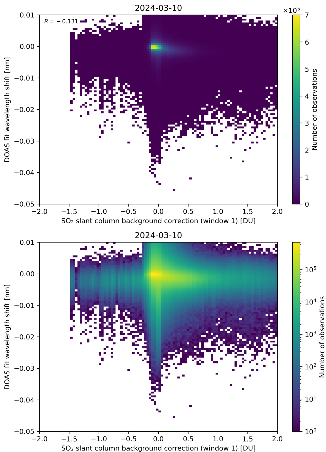
Figure 100: Scatter density plot of “SO 2 slant column background correction (window 1)” against “DOAS fit wavelength shift” for 2024-03-09 to 2024-03-11.
