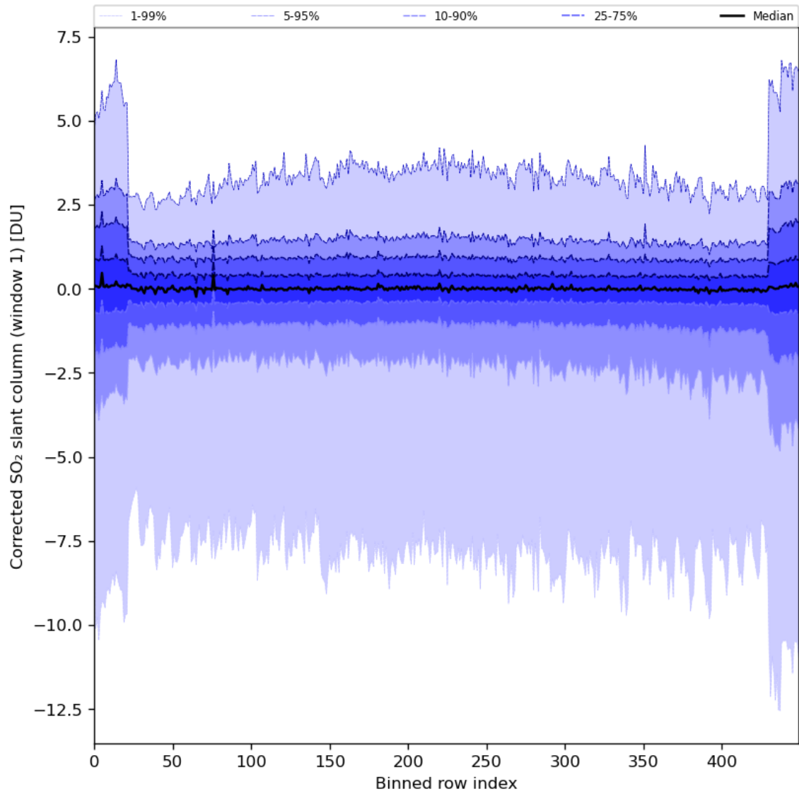
Figure 81: Along track statistics of “Corrected SO 2 slant column (window 1)” for 2024-03-09 to 2024-03-11
