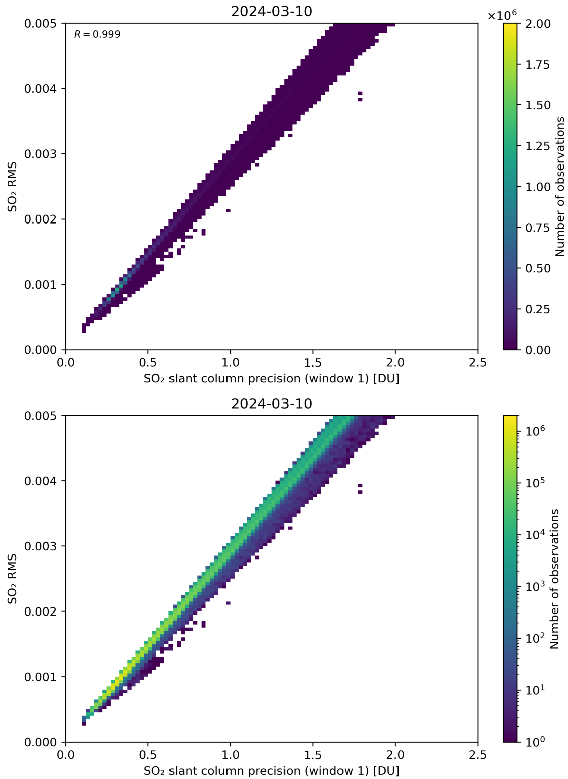
Figure 223: Scatter density plot of “SO 2 slant column precision (window 1)” against “SO 2 RMS” for 2024-03-09 to 2024-03-11.
