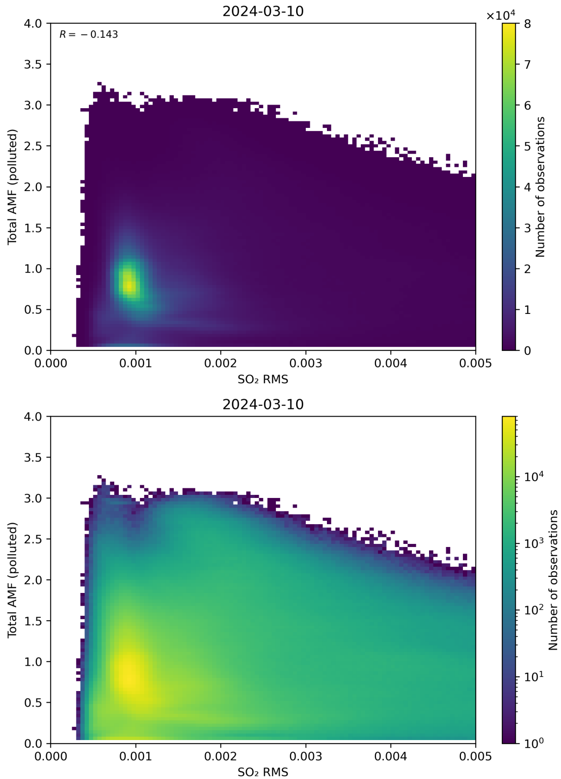
Figure 137: Scatter density plot of “SO 2 RMS” against “Total AMF (polluted)” for 2024-03-09 to 2024-03-11.
