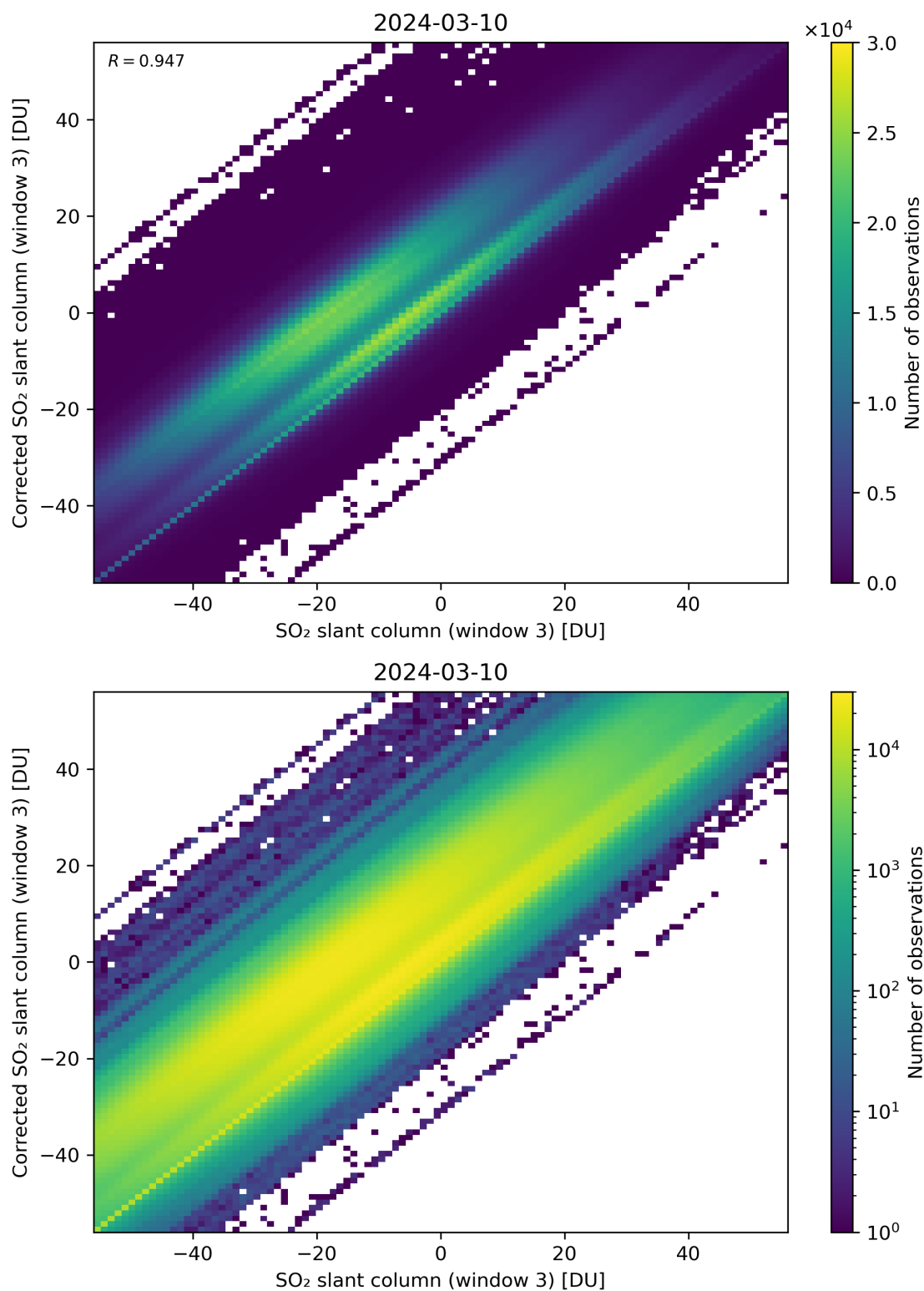
Figure 266: Scatter density plot of “SO 2 slant column (window 3)” against “Corrected SO 2 slant column (window 3)” for 2024-03-09 to 2024-03-11.
