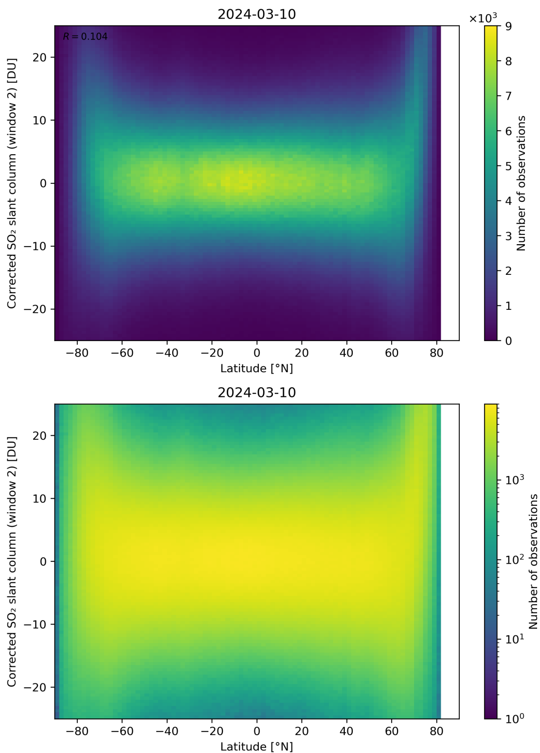
Figure 147: Scatter density plot of “Latitude” against “Corrected SO 2 slant column (window 2)” for 2024-03-09 to 2024-03-11.
