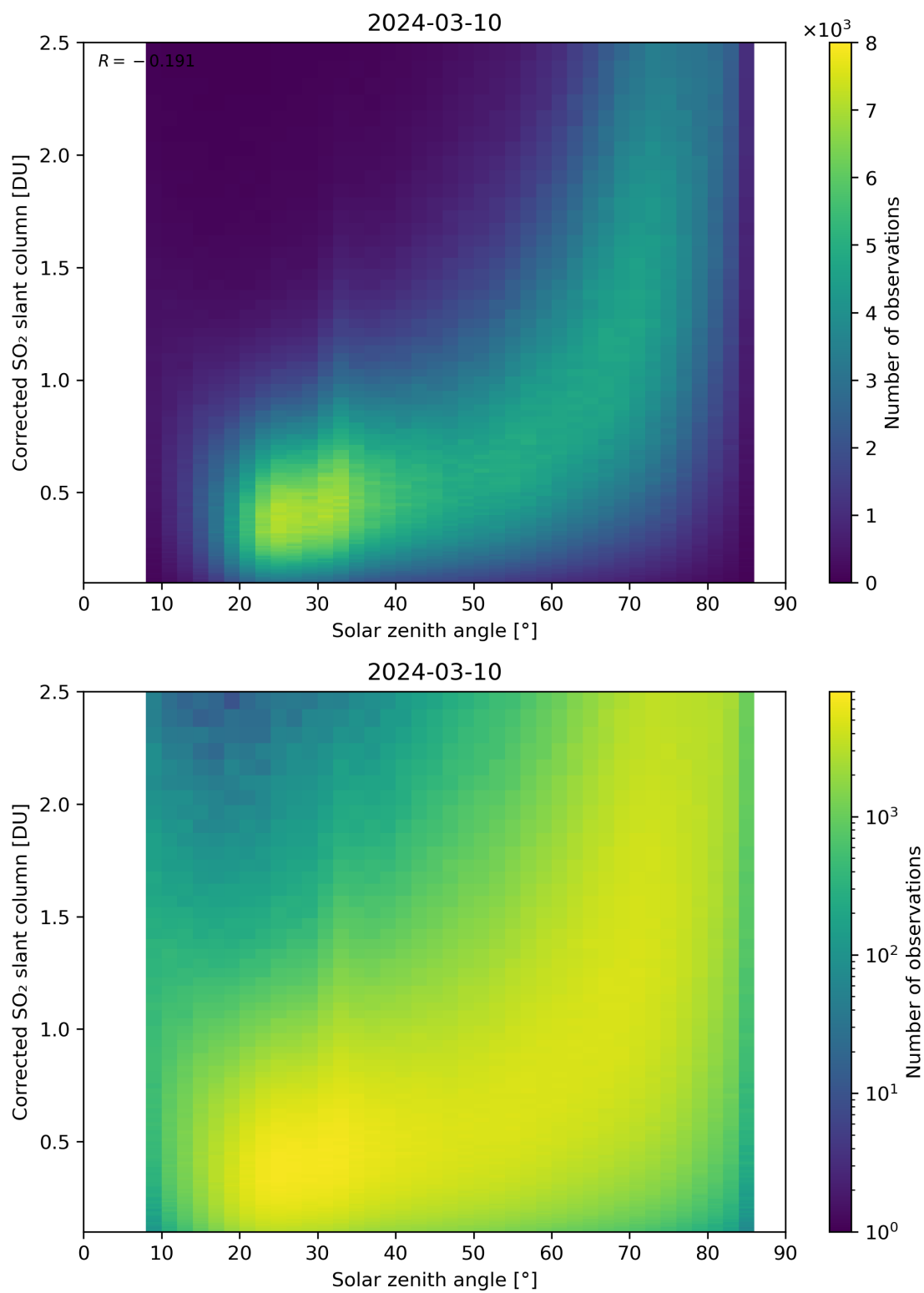
Figure 166: Scatter density plot of “Solar zenith angle” against “Corrected SO 2 slant column” for 2024-03-09 to 2024-03-11.
