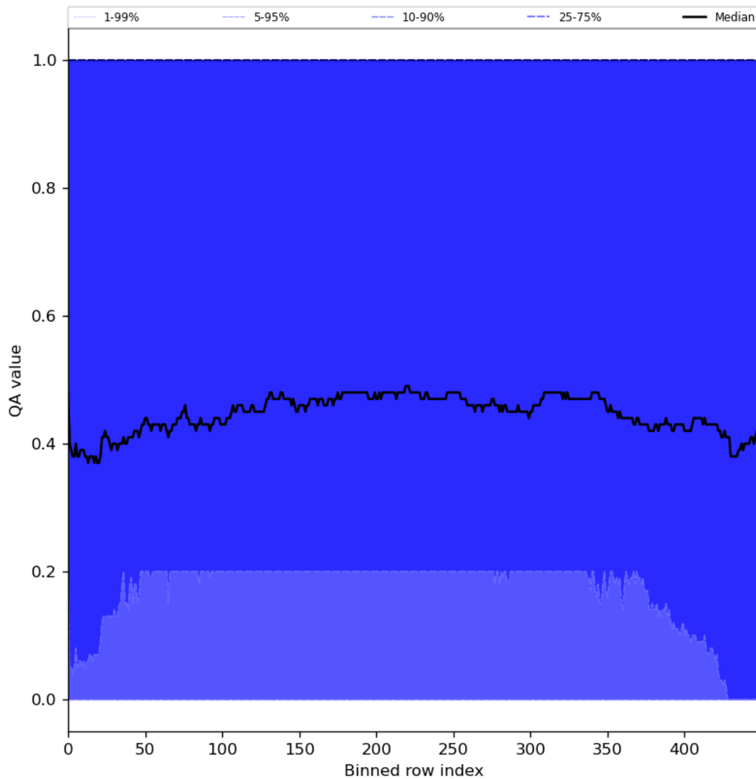
Figure 75: Along track statistics of “QA value” for 2024-03-09 to 2024-03-11
