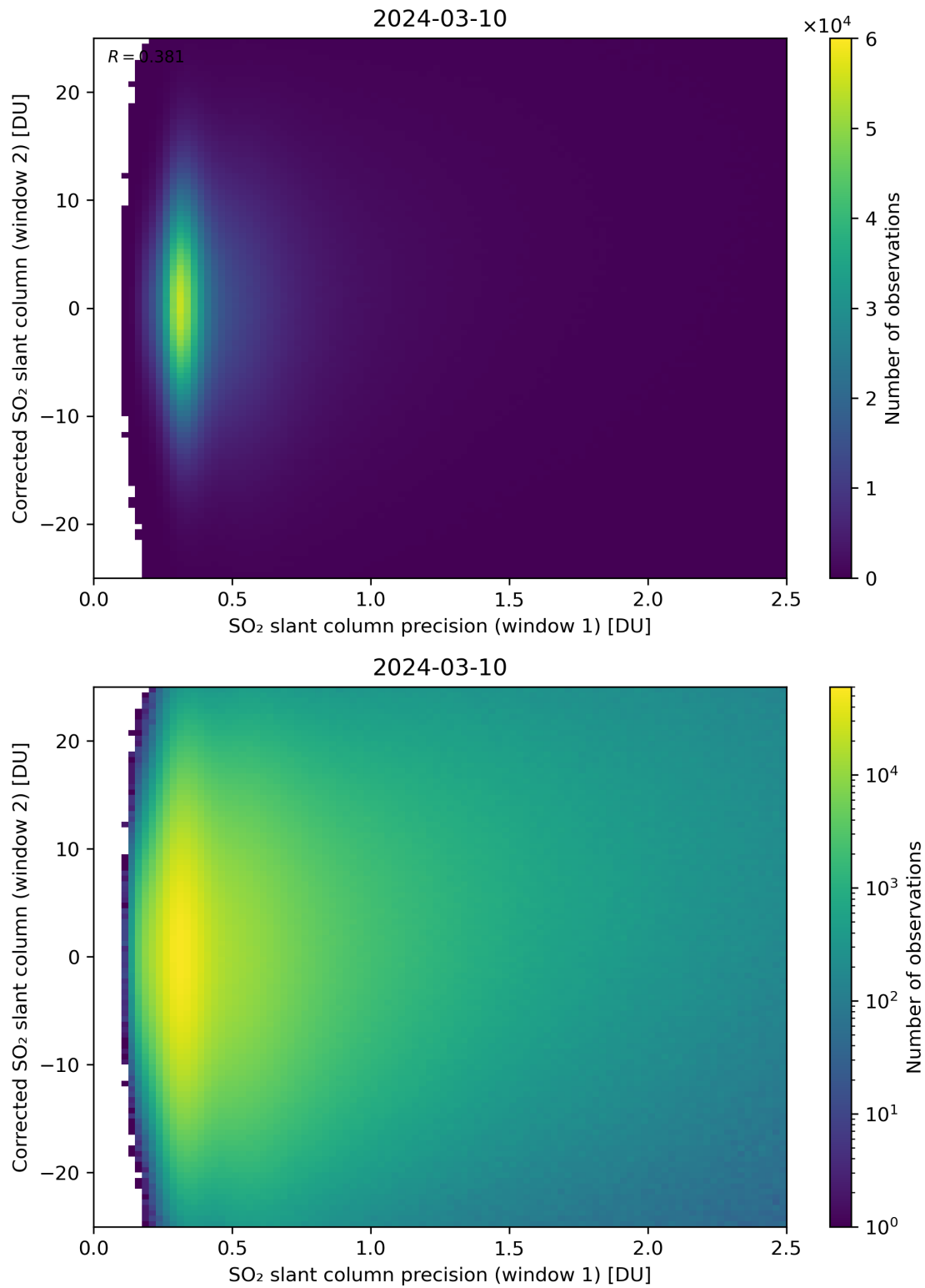
Figure 225: Scatter density plot of “SO 2 slant column precision (window 1)” against “Corrected SO 2 slant column (window 2)” for 2024-03-09 to 2024-03-11.
