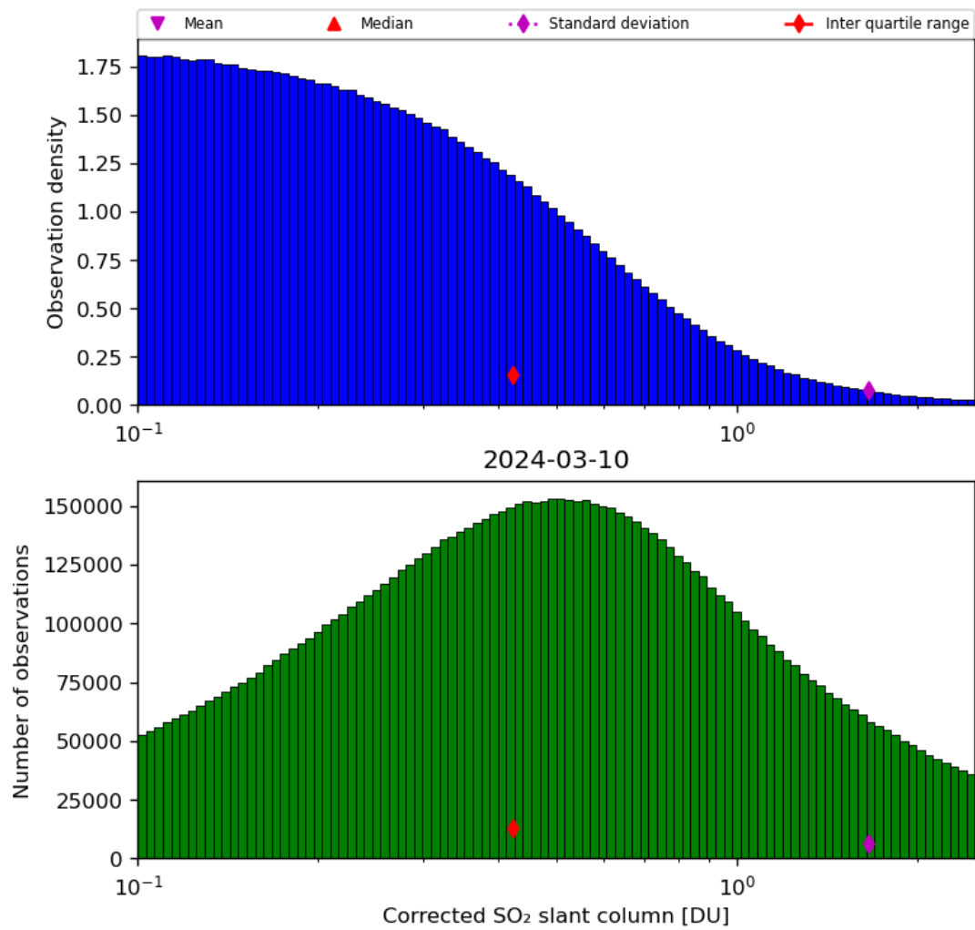
Figure 55: Histogram of “Corrected SO 2 slant column” for 2024-03-09 to 2024-03-11
