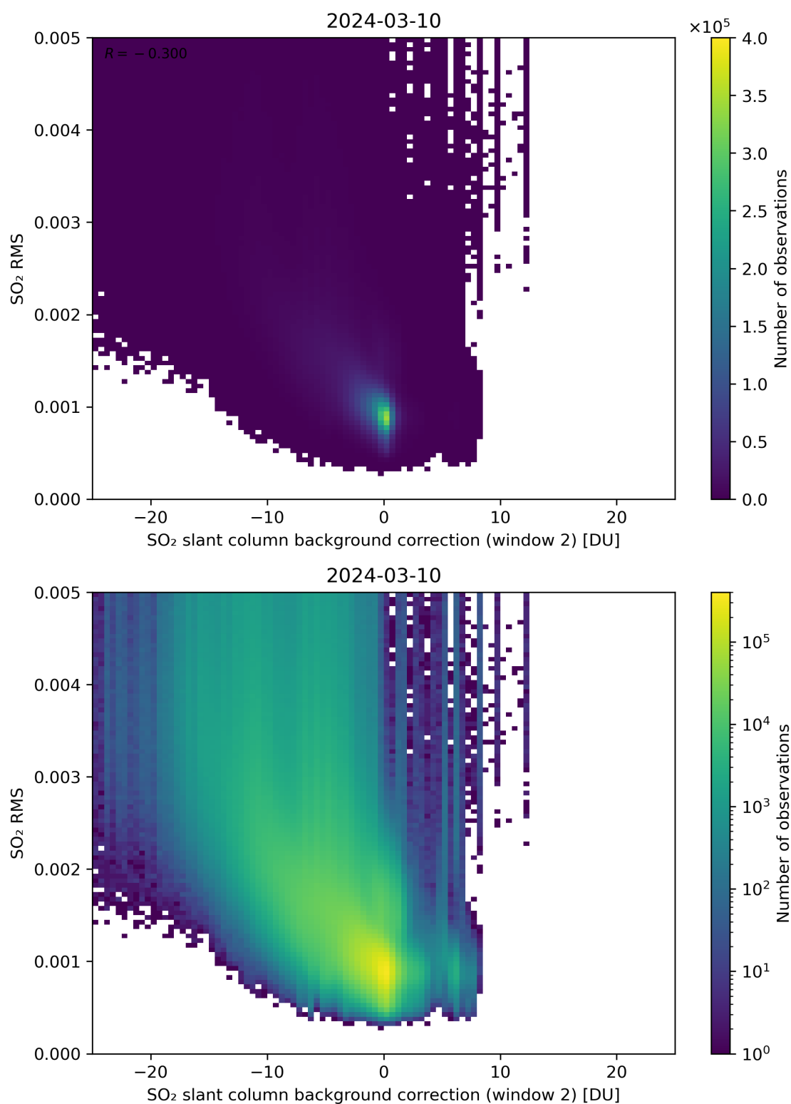
Figure 114: Scatter density plot of “SO 2 slant column background correction (window 2)” against “SO 2 RMS” for 2024-03-09 to 2024-03-11.
