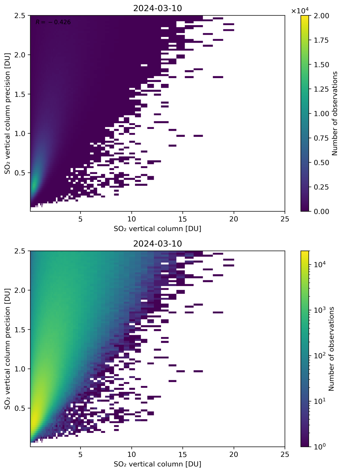
Figure 307: Scatter density plot of “SO 2 vertical column” against “SO 2 vertical column precision” for 2024-03-09 to 2024-03-11.
