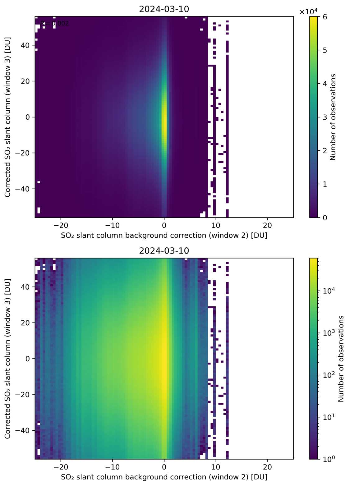
Figure 116: Scatter density plot of “SO 2 slant column background correction (window 2)” against “Corrected SO 2 slant column (window 3)” for 2024-03-09 to 2024-03-11.
