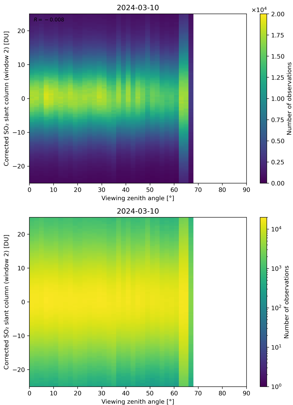
Figure 318: Scatter density plot of “Viewing zenith angle” against “Corrected SO 2 slant column (window 2)” for 2024-03-09 to 2024-03-11.
