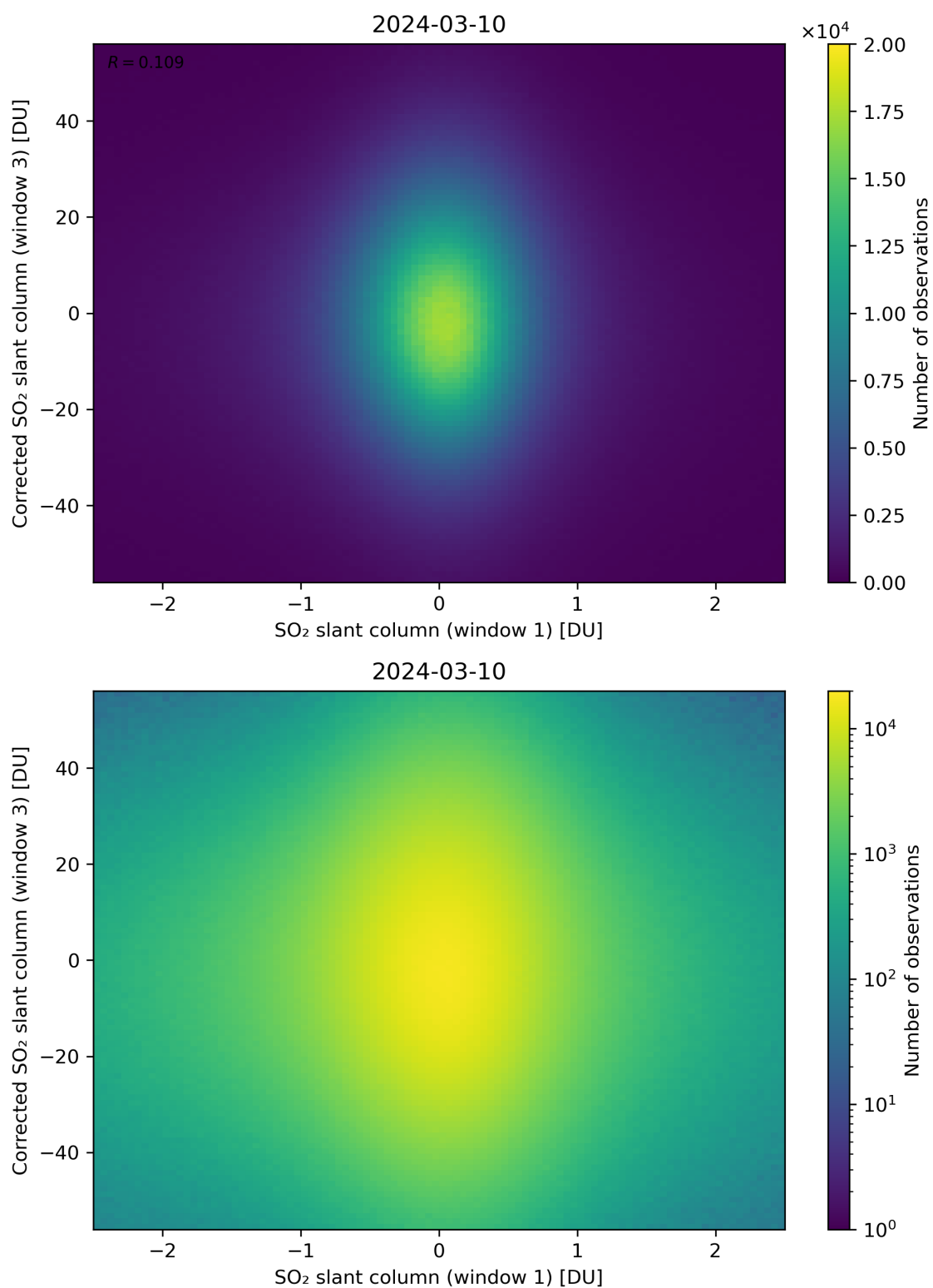
Figure 234: Scatter density plot of “SO 2 slant column (window 1)” against “Corrected SO 2 slant column (window 3)” for 2024-03-09 to 2024-03-11.
