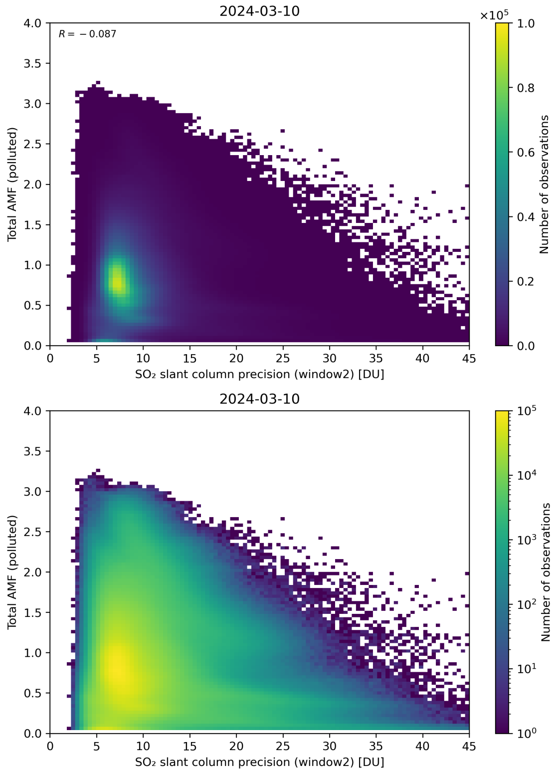
Figure 251: Scatter density plot of “SO 2 slant column precision (window2)” against “Total AMF (polluted)” for 2024-03-09 to 2024-03-11.
