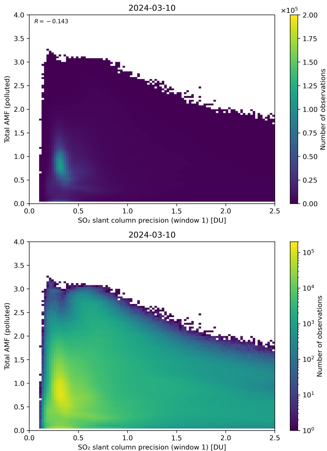
Figure 230: Scatter density plot of “SO 2 slant column precision (window 1)” against “Total AMF (polluted)” for 2024-03-09 to 2024-03-11.
