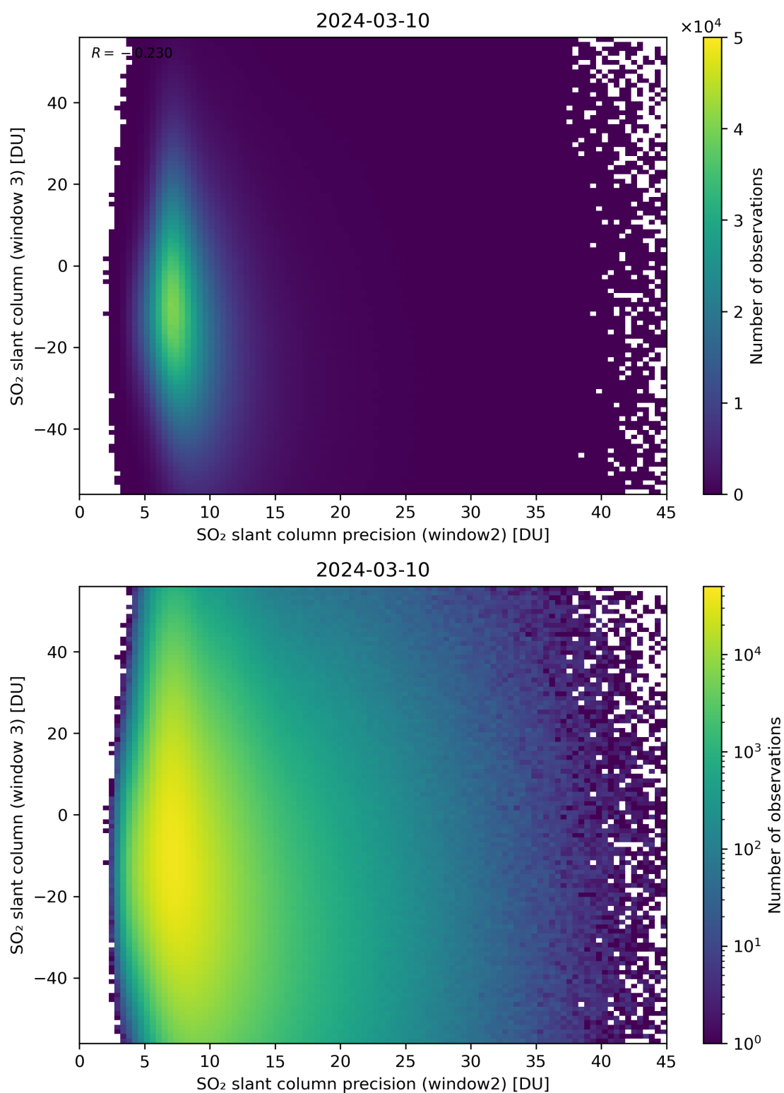
Figure 249: Scatter density plot of “SO 2 slant column precision (window2)” against “SO 2 slant column (window 3)” for 2024-03-09 to 2024-03-11.
