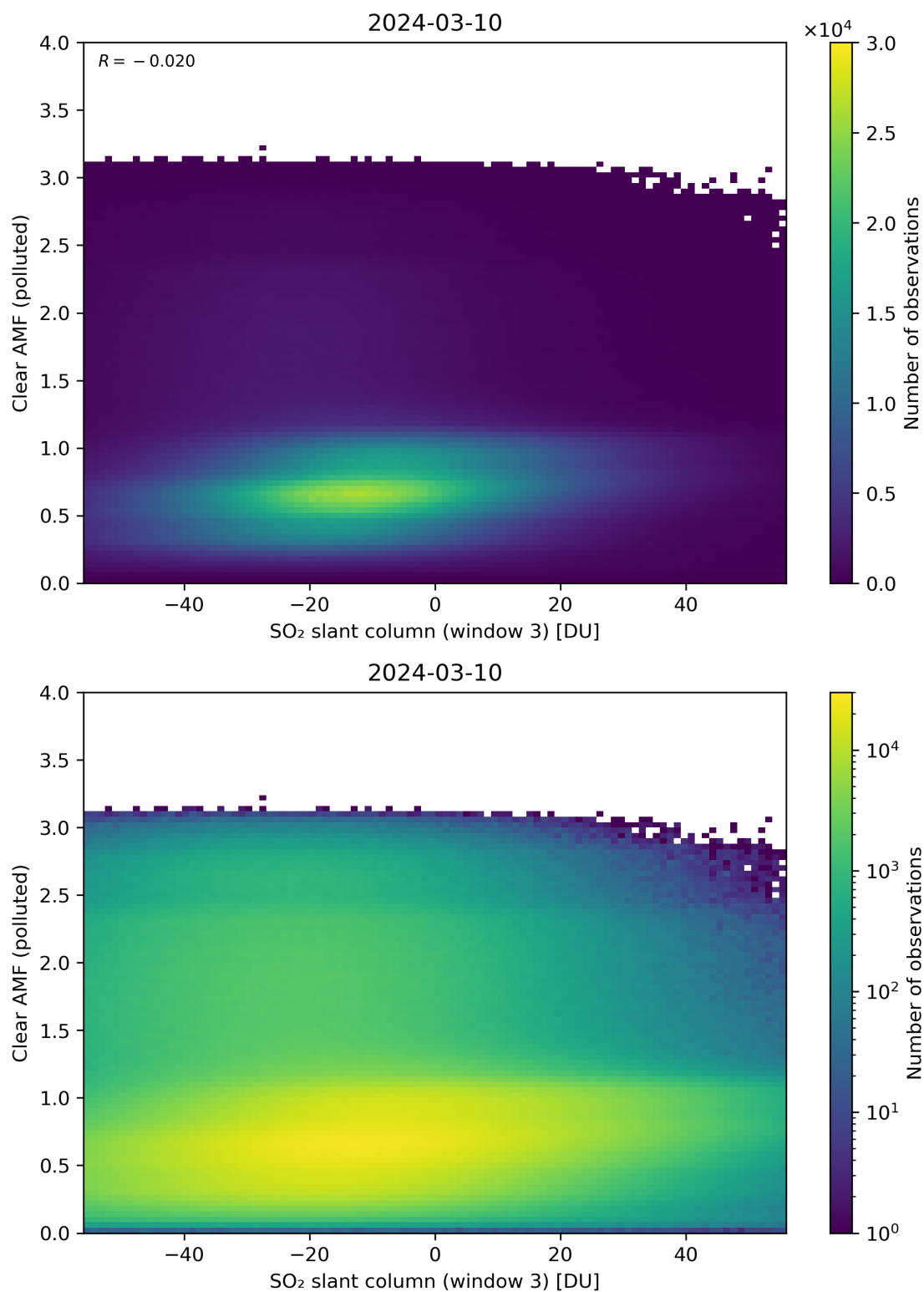
Figure 265: Scatter density plot of “SO 2 slant column (window 3)” against “Clear AMF (polluted)” for 2024-03-09 to 2024-03-11.
