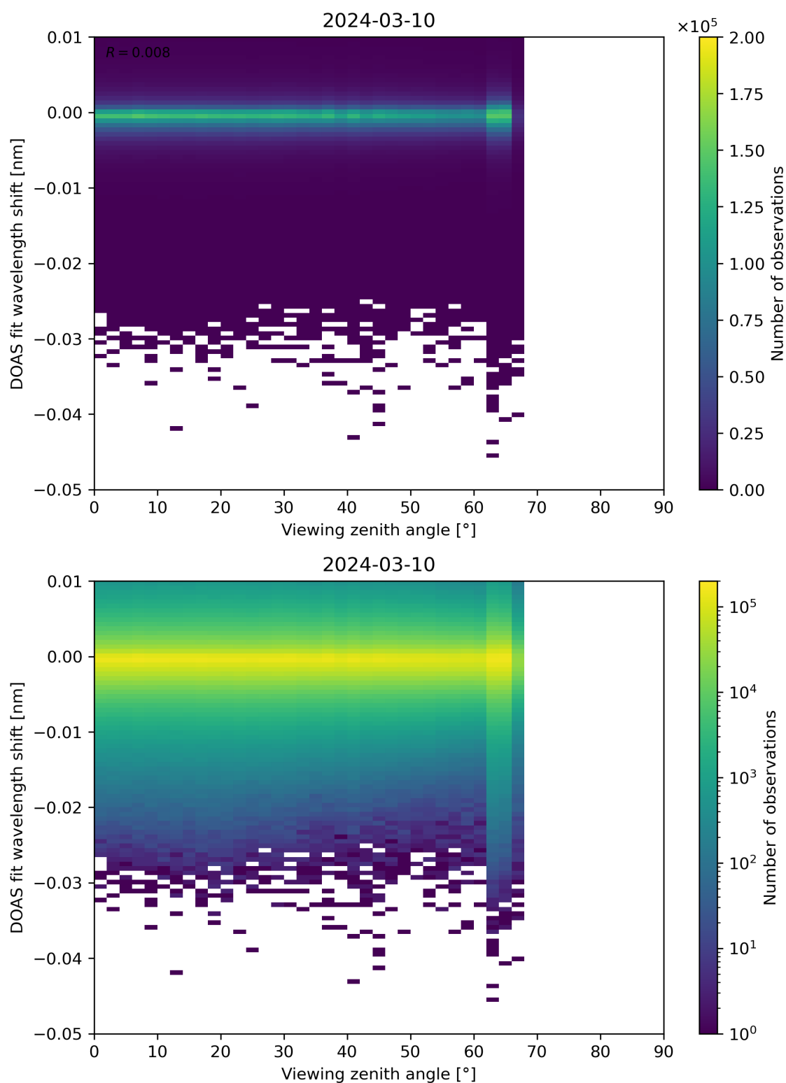
Figure 311: Scatter density plot of “Viewing zenith angle” against “DOAS fit wavelength shift” for 2024-03-09 to 2024-03-11.
