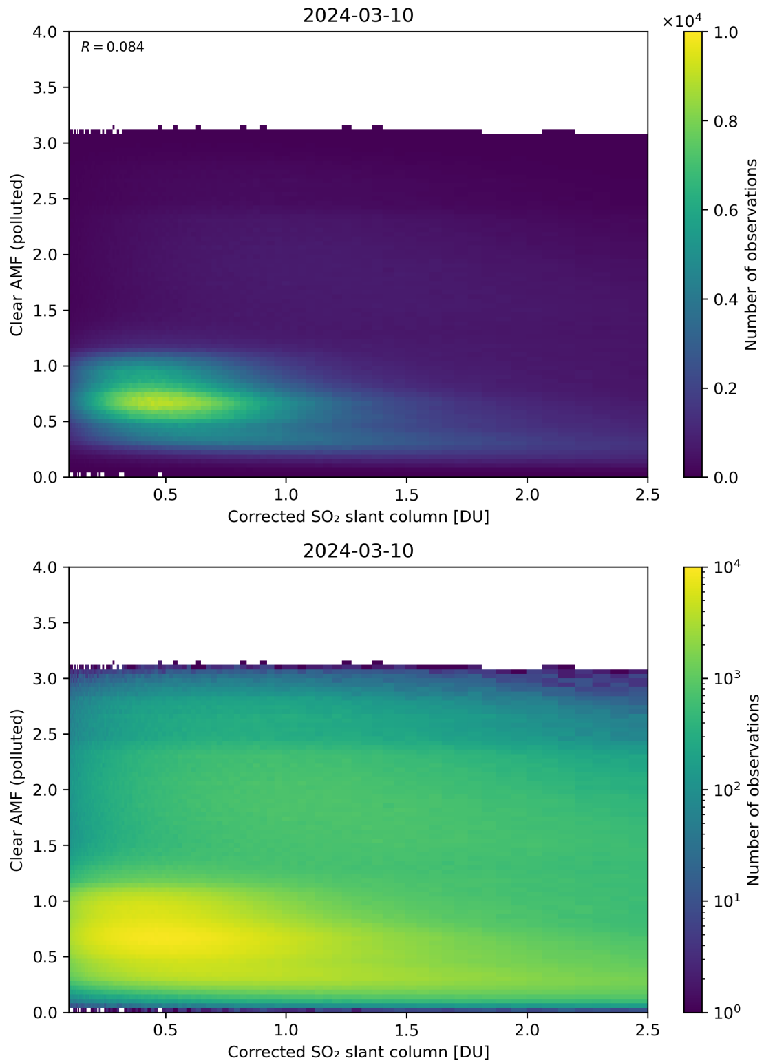
Figure 184: Scatter density plot of “Corrected SO 2 slant column” against “Clear AMF (polluted)” for 2024-03-09 to 2024-03-11.
