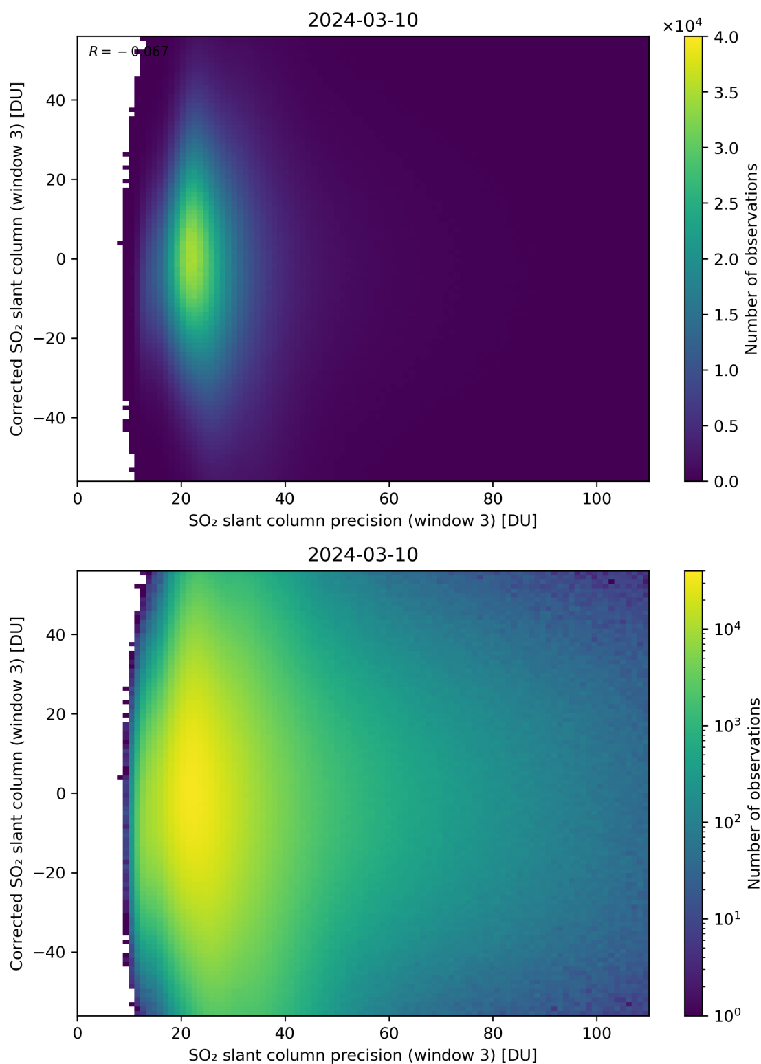
Figure 262: Scatter density plot of “SO 2 slant column precision (window 3)” against “Corrected SO 2 slant column (window 3)” for 2024-03-09 to 2024-03-11.
