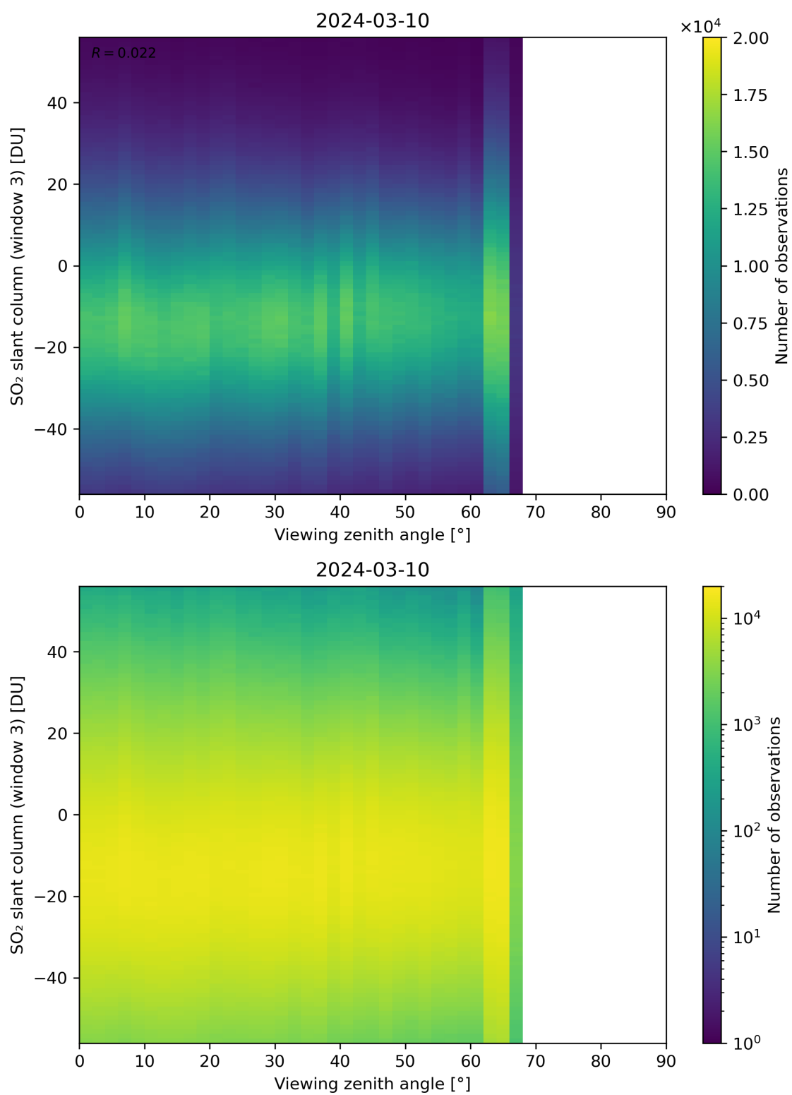
Figure 323: Scatter density plot of “Viewing zenith angle” against “SO 2 slant column (window 3)” for 2024-03-09 to 2024-03-11.
