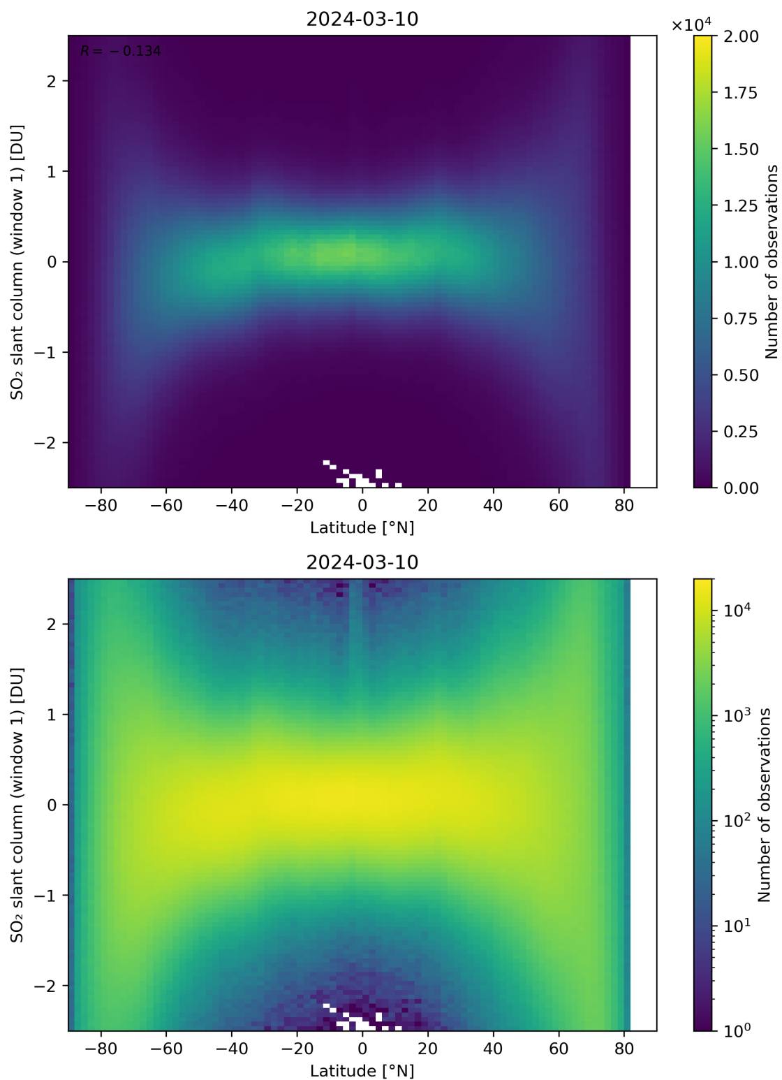
Figure 149: Scatter density plot of “Latitude” against “SO 2 slant column (window 1)” for 2024-03-09 to 2024-03-11.
