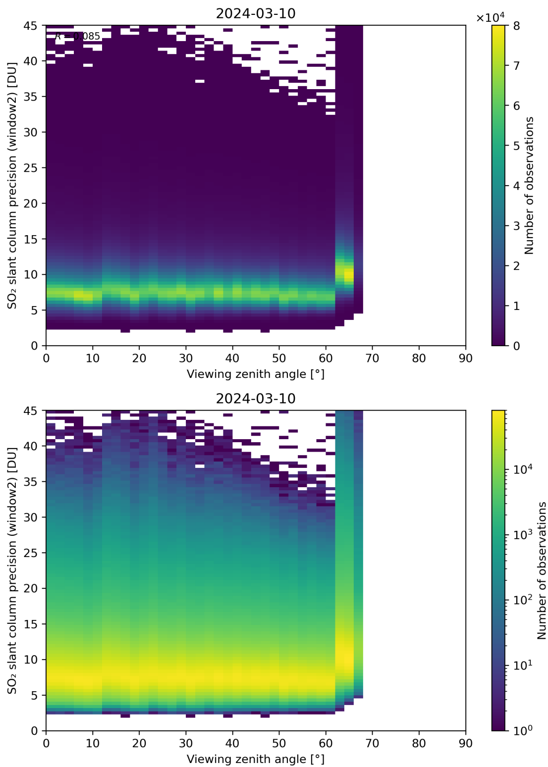
Figure 322: Scatter density plot of “Viewing zenith angle” against “SO 2 slant column precision (window2)” for 2024-03-09 to 2024-03-11.
