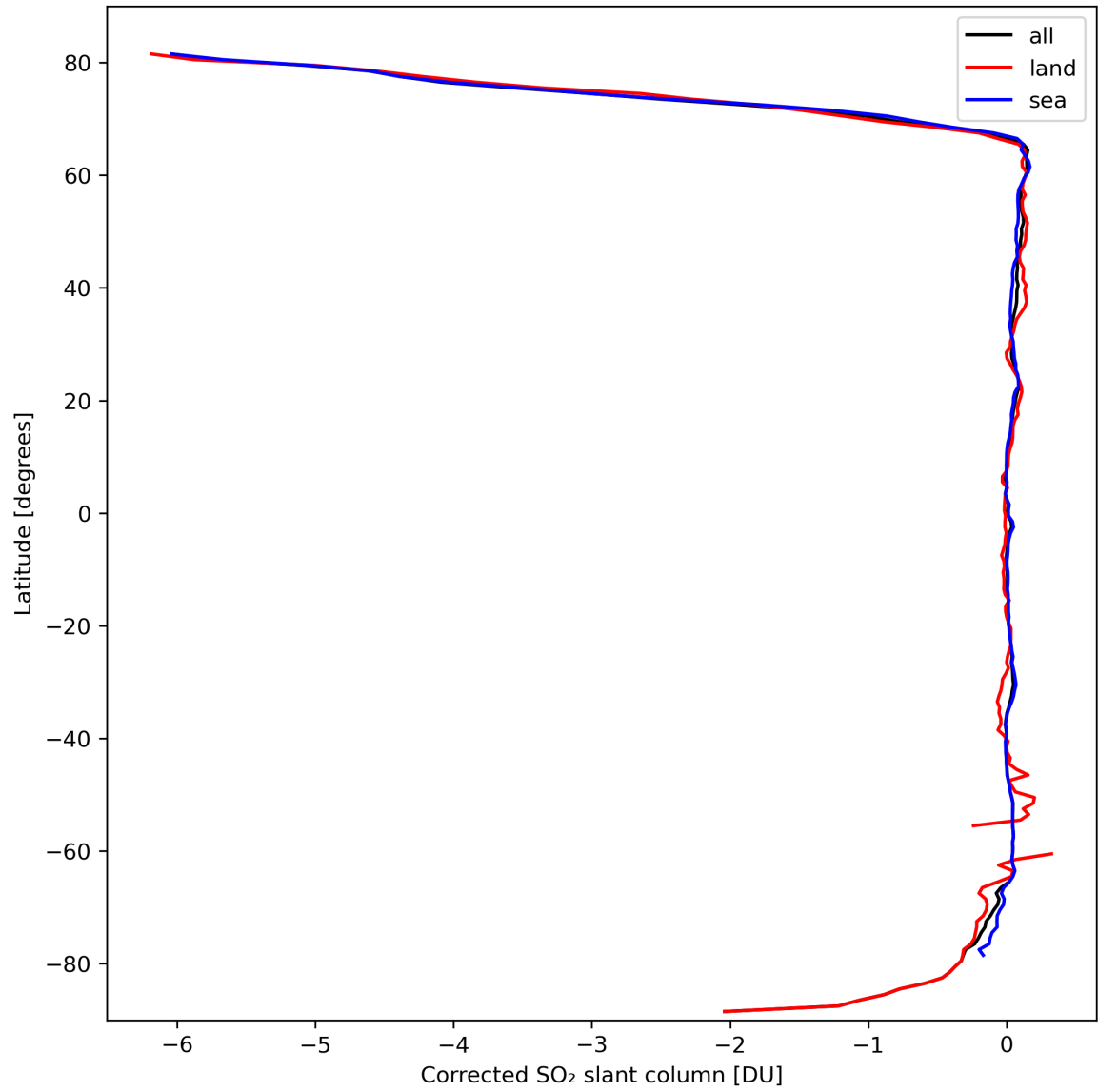
Figure 32: Zonal average of “Corrected SO 2 slant column” for 2024-03-09 to 2024-03-11.
