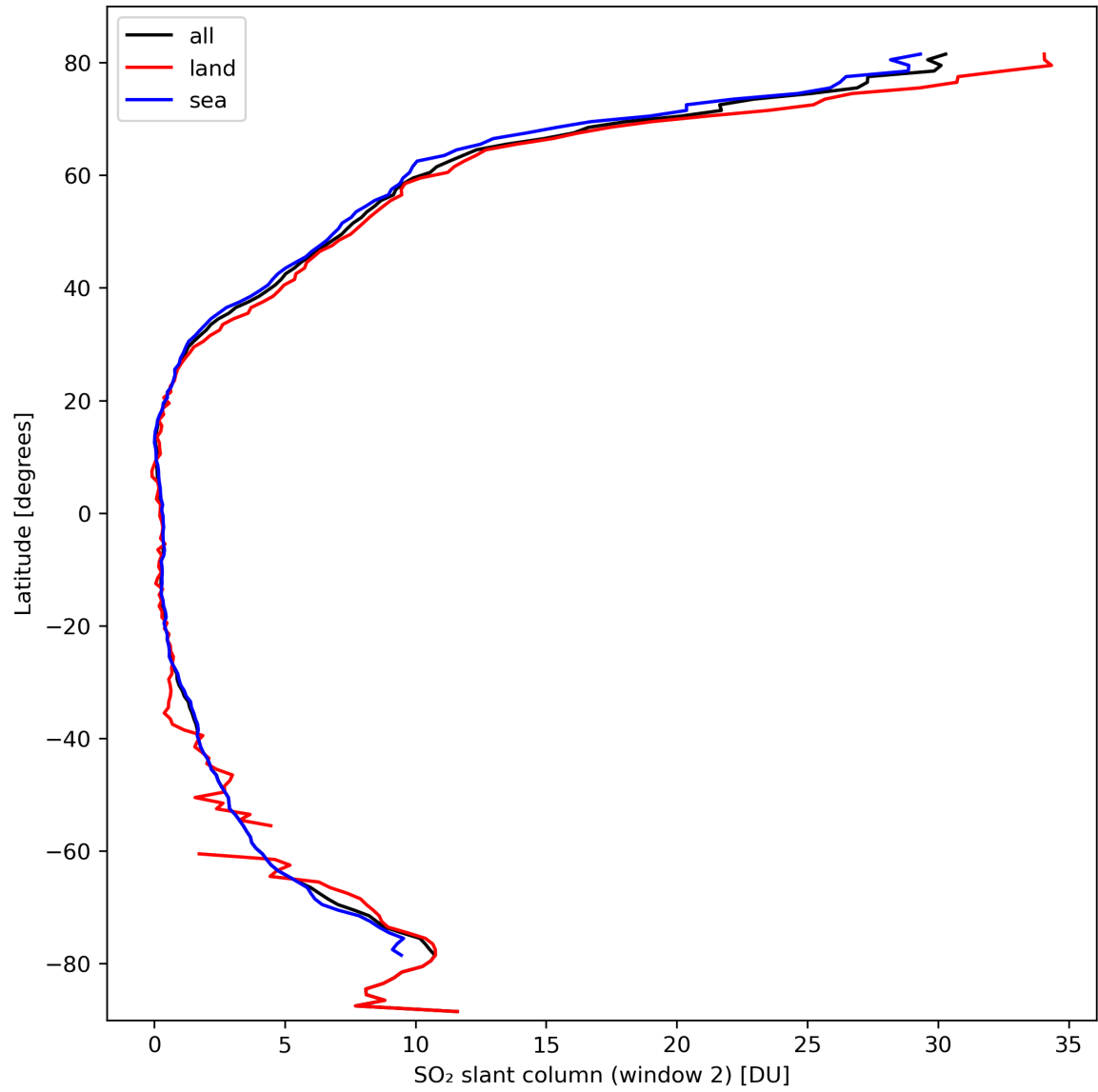
Figure 37: Zonal average of “SO 2 slant column (window 2)” for 2024-03-09 to 2024-03-11.
