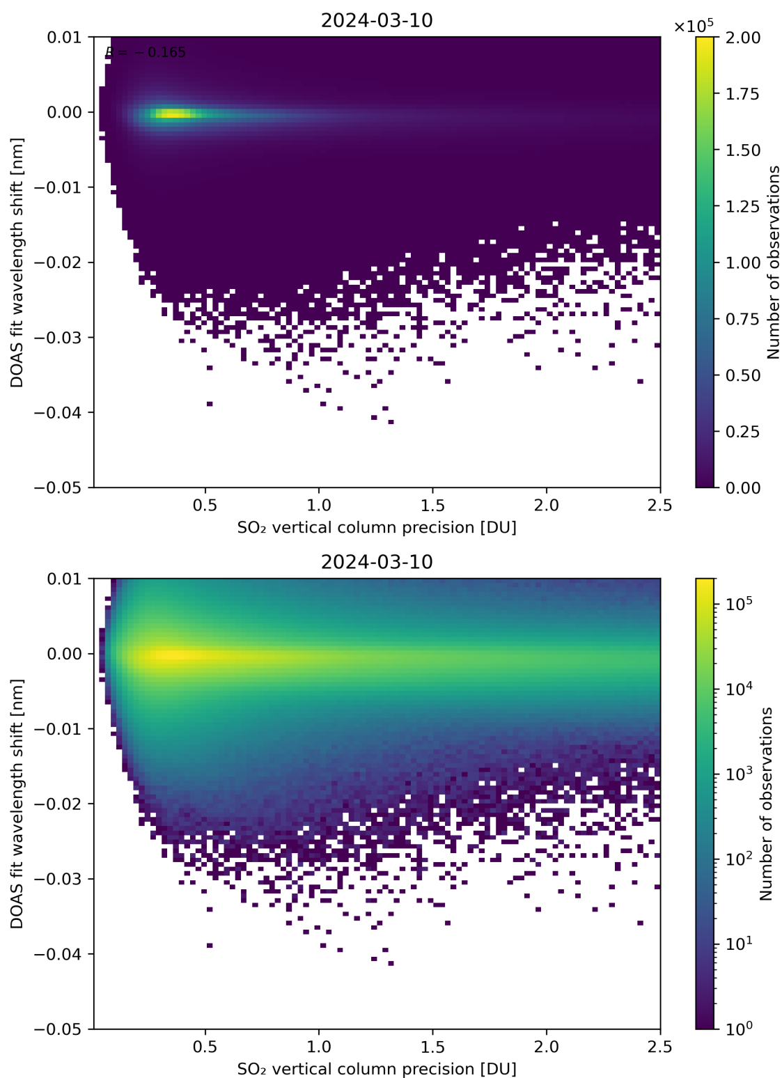
Figure 282: Scatter density plot of “SO 2 vertical column precision” against “DOAS fit wavelength shift” for 2024-03-09 to 2024-03-11.
