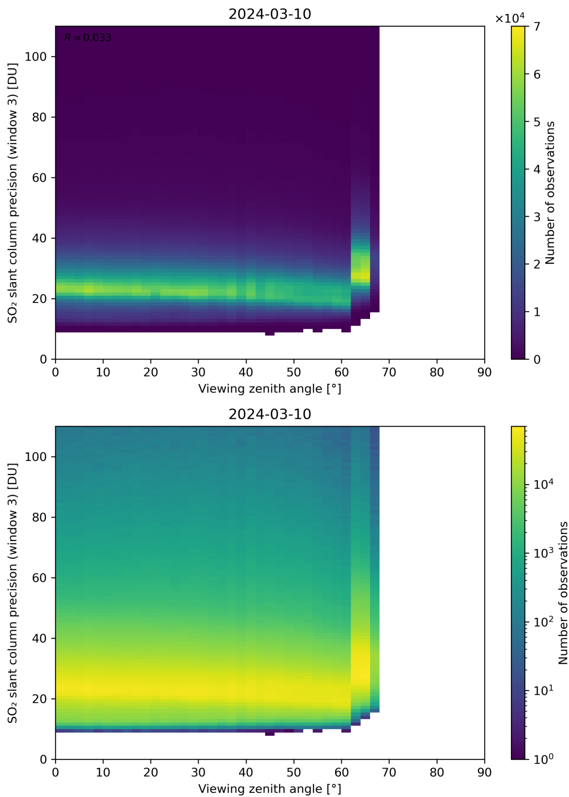
Figure 324: Scatter density plot of “Viewing zenith angle” against “SO 2 slant column precision (window 3)” for 2024-03-09 to 2024-03-11.
