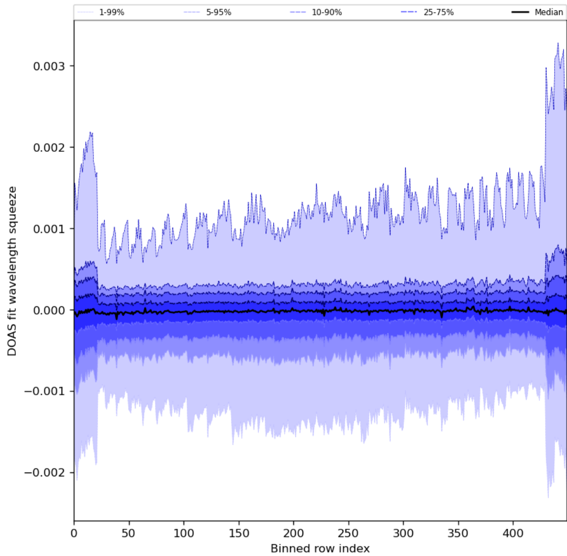
Figure 92: Along track statistics of “DOAS fit wavelength squeeze” for 2024-03-09 to 2024-03-11
