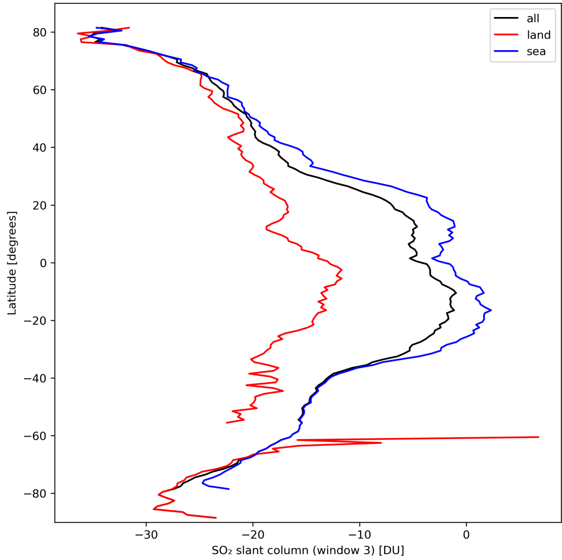
Figure 41: Zonal average of “SO 2 slant column (window 3)” for 2024-03-09 to 2024-03-11.
