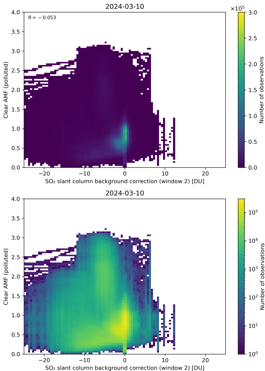
Figure 115: Scatter density plot of “SO 2 slant column background correction (window 2)” against “Clear AMF (polluted)” for 2024-03-09 to 2024-03-11.
