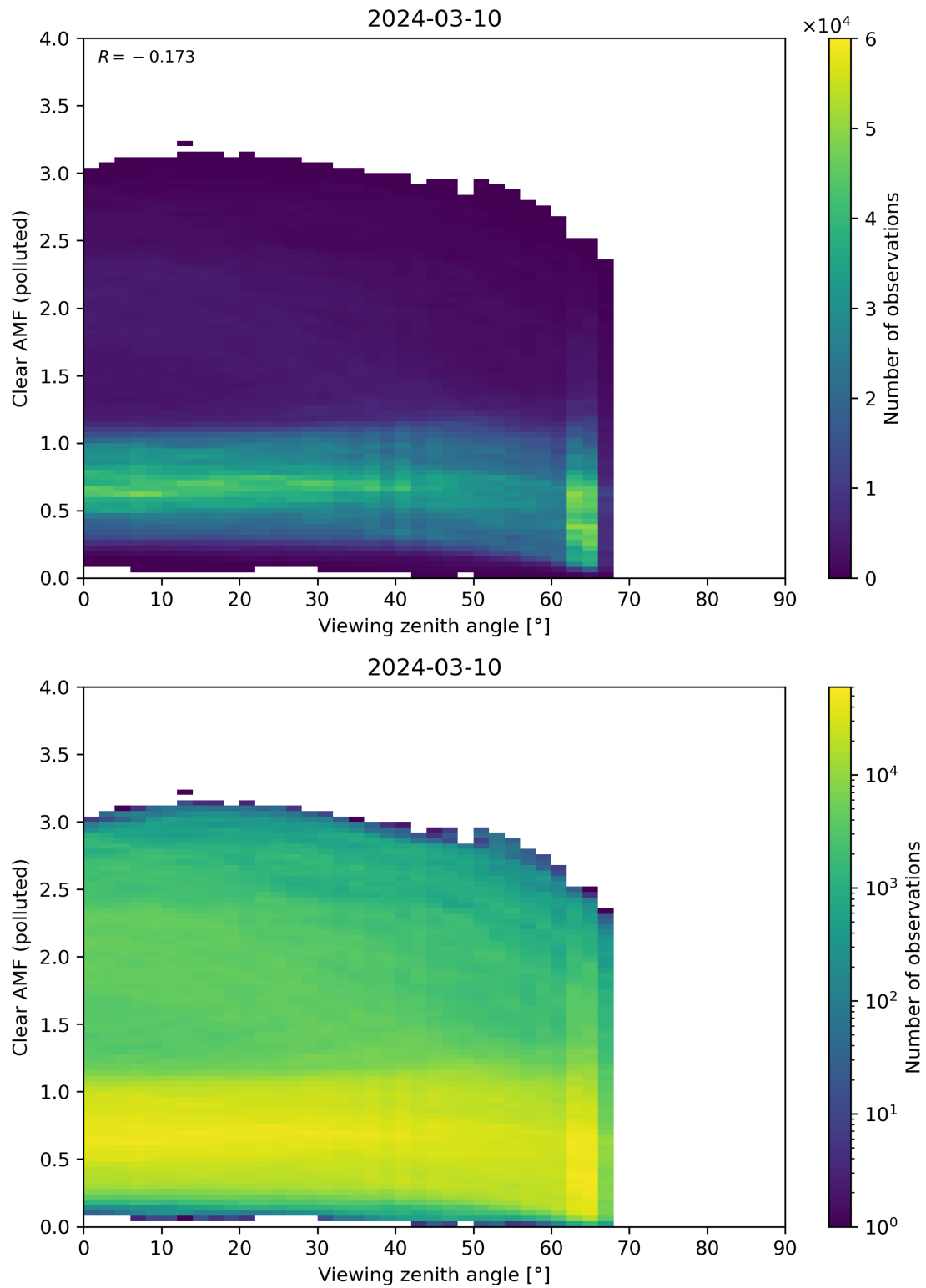
Figure 316: Scatter density plot of “Viewing zenith angle” against “Clear AMF (polluted)” for 2024-03-09 to 2024-03-11.
