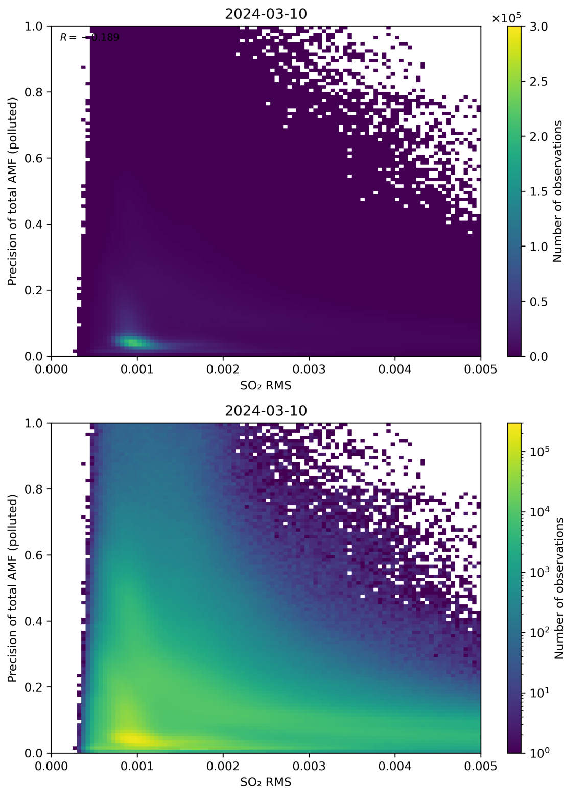
Figure 138: Scatter density plot of “SO 2 RMS” against “Precision of total AMF (polluted)” for 2024-03-09 to 2024-03-11.
