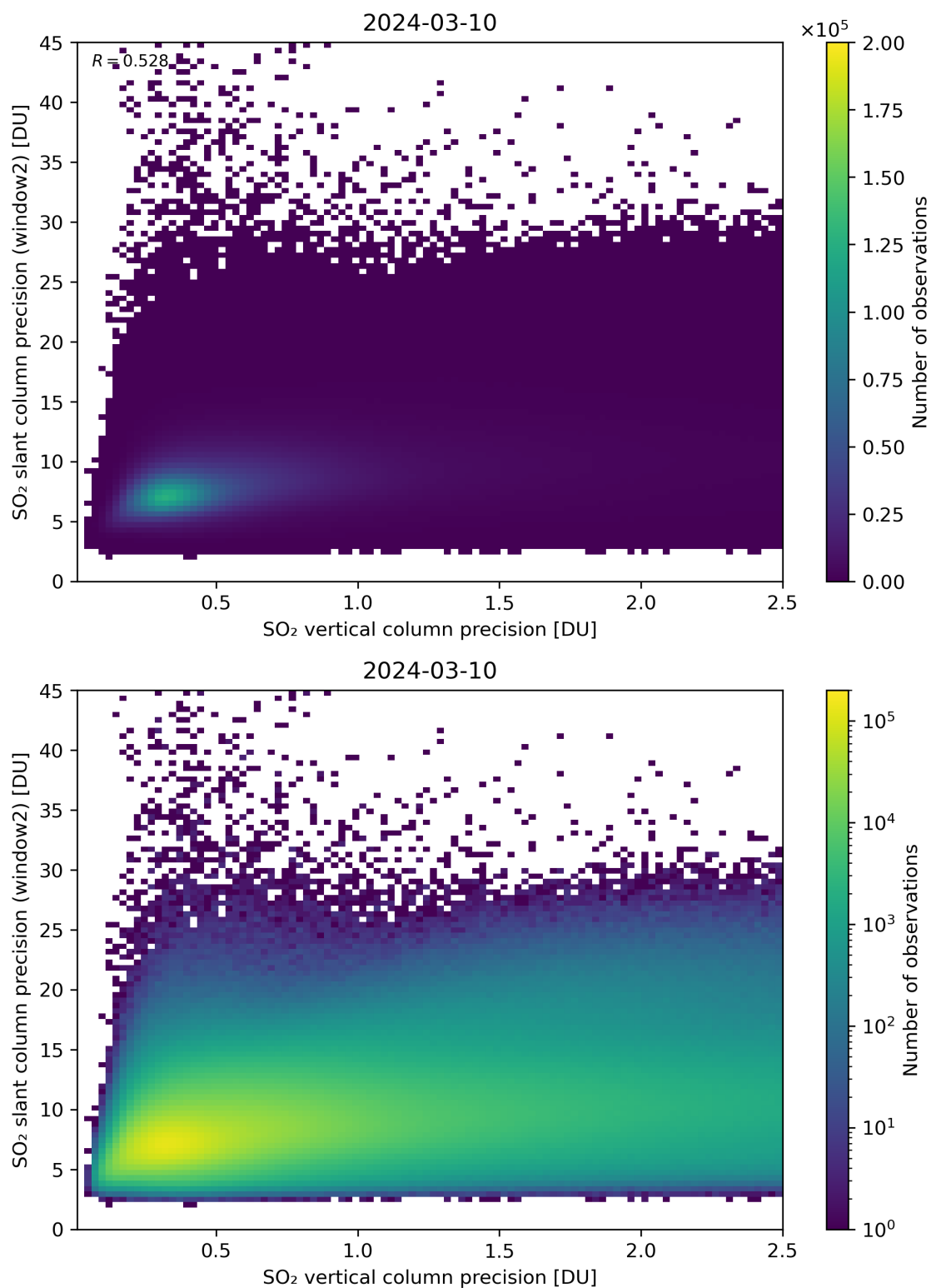
Figure 291: Scatter density plot of “SO 2 vertical column precision” against “SO 2 slant column precision (window2)” for 2024-03-09 to 2024-03-11.
