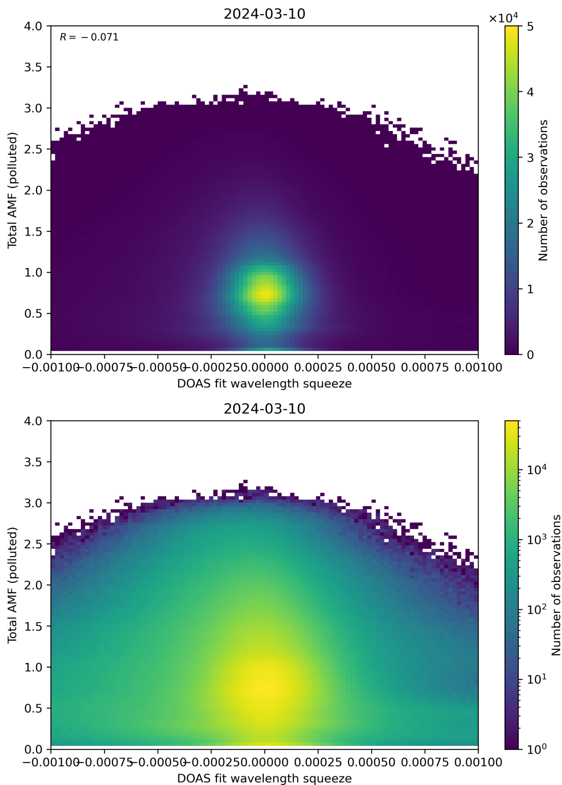
Figure 134: Scatter density plot of “DOAS fit wavelength squeeze” against “Total AMF (polluted)” for 2024-03-09 to 2024-03-11.
