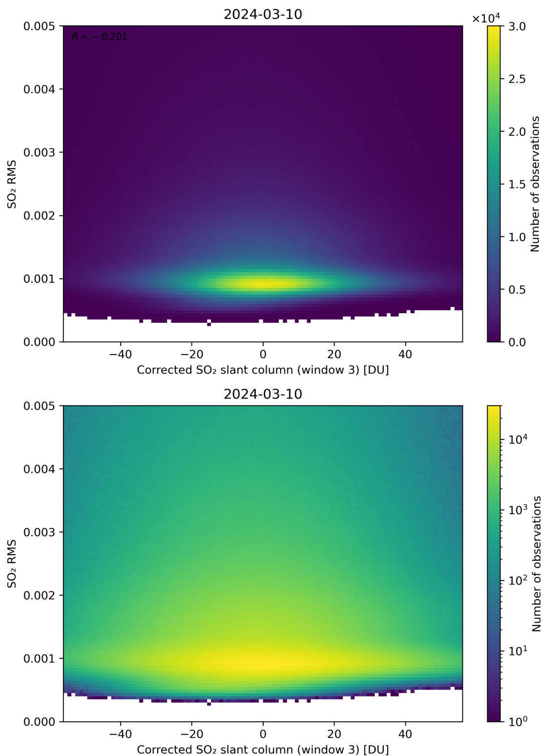
Figure 208: Scatter density plot of “Corrected SO 2 slant column (window 3)” against “SO 2 RMS” for 2024-03-09 to 2024-03-11.
