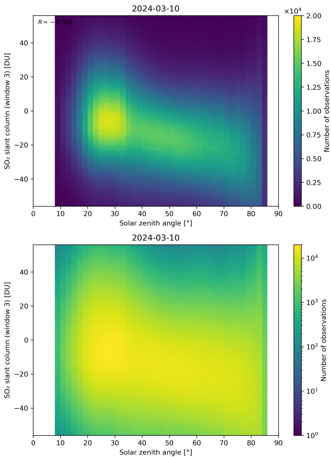
Figure 172: Scatter density plot of “Solar zenith angle” against “SO 2 slant column (window 3)” for 2024-03-09 to 2024-03-11.
