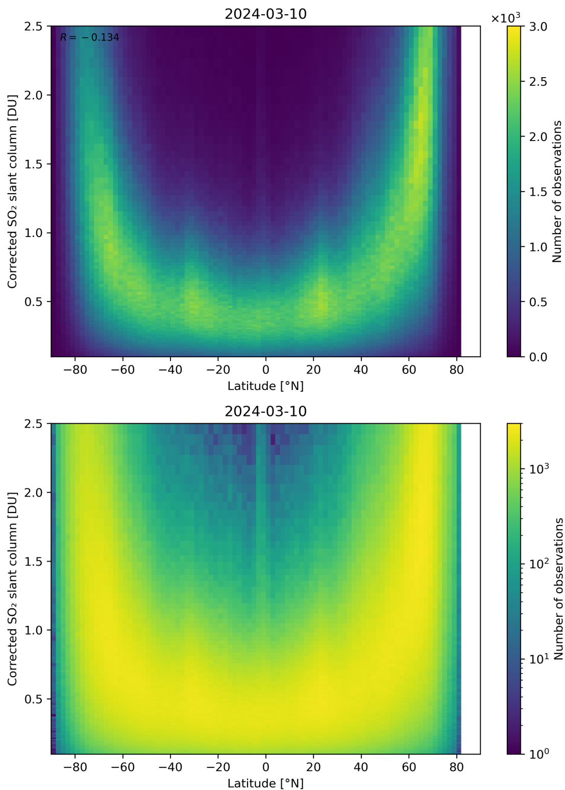
Figure 146: Scatter density plot of “Latitude” against “Corrected SO 2 slant column” for 2024-03-09 to 2024-03-11.
