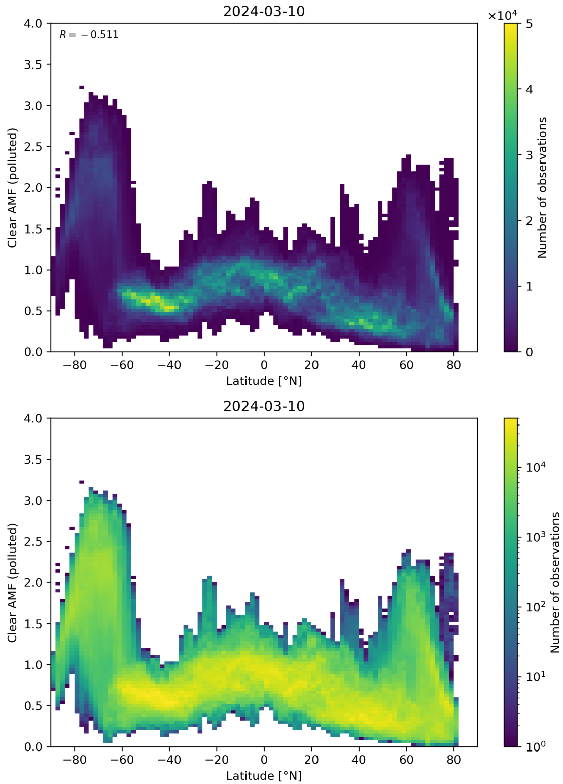
Figure 145: Scatter density plot of “Latitude” against “Clear AMF (polluted)” for 2024-03-09 to 2024-03-11.
