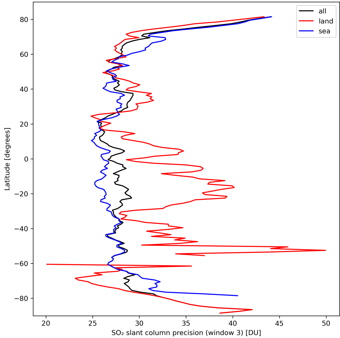
Figure 42: Zonal average of "SO 2 slant column precision (window 3)" for 2024-03-09 to 2024-03-11.
