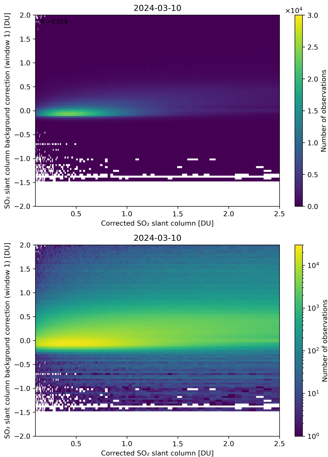
Figure 178: Scatter density plot of “Corrected SO 2 slant column” against “SO 2 slant column background correction (window 1)” for 2024-03-09 to 2024-03-11.
