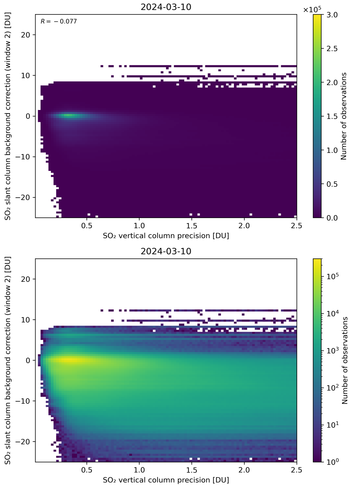
Figure 280: Scatter density plot of “SO 2 vertical column precision” against “SO 2 slant column background correction (window 2)” for 2024-03-09 to 2024-03-11.
