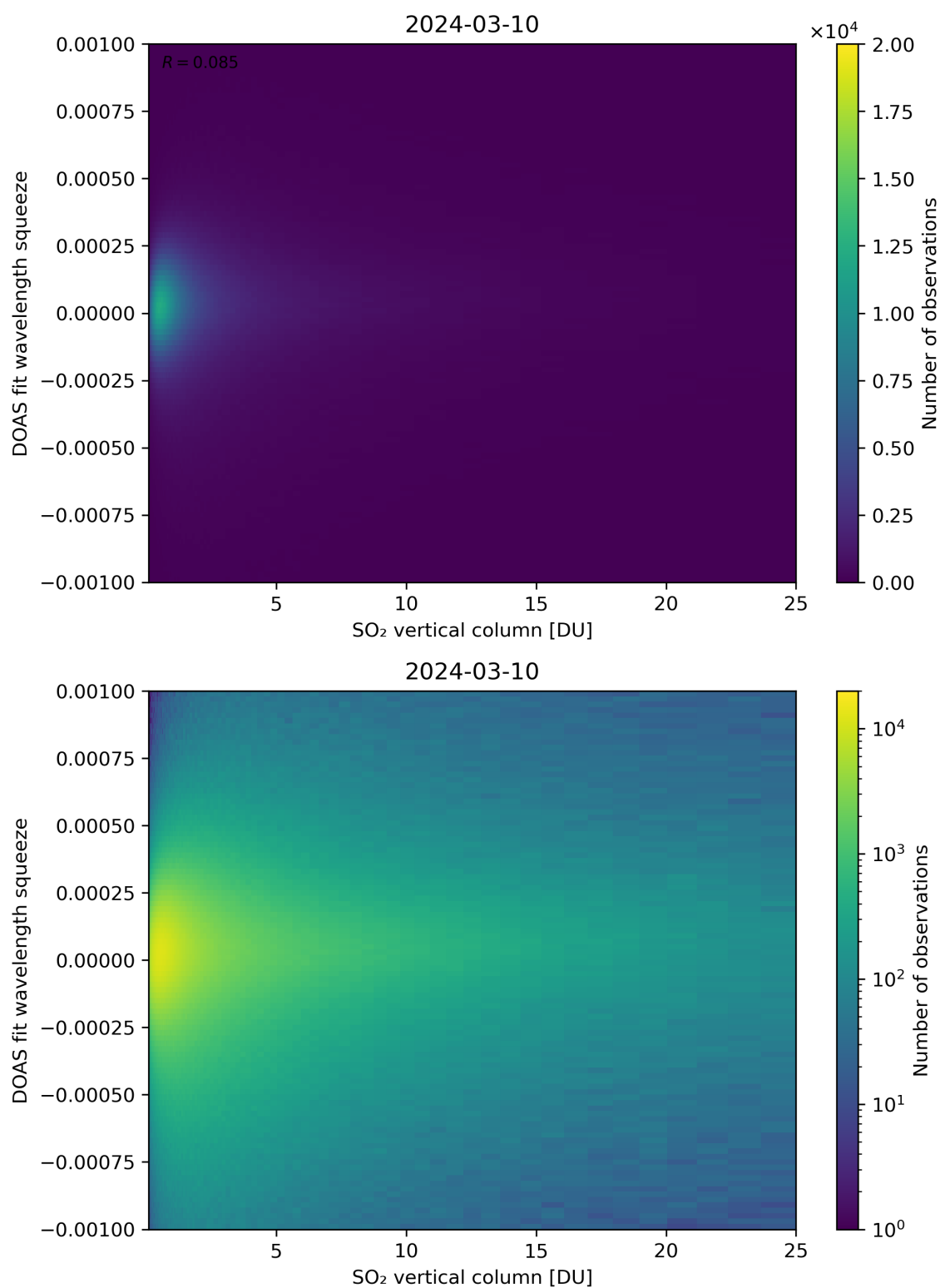
Figure 277: Scatter density plot of “SO 2 vertical column” against “DOAS fit wavelength squeeze” for 2024-03-09 to 2024-03-11.
