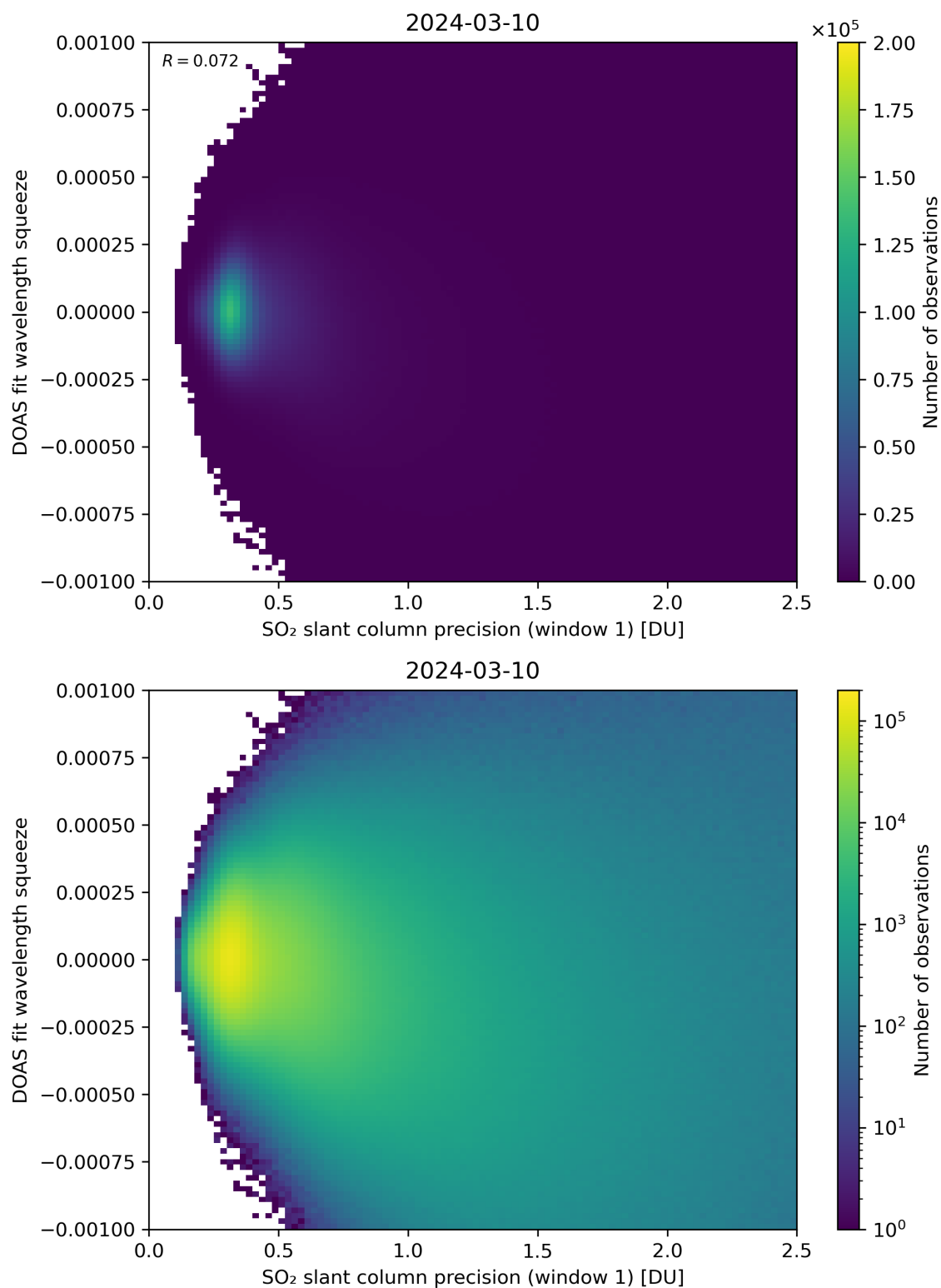
Figure 222: Scatter density plot of “SO 2 slant column precision (window 1)” against “DOAS fit wavelength squeeze” for 2024-03-09 to 2024-03-11.
