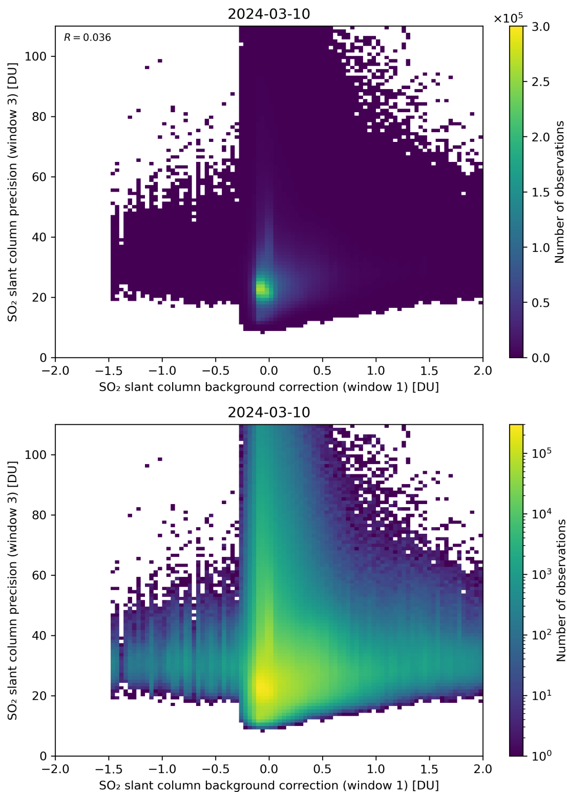
Figure 108: Scatter density plot of “SO 2 slant column background correction (window 1)” against “SO 2 slant column precision (window 3)” for 2024-03-09 to 2024-03-11.
