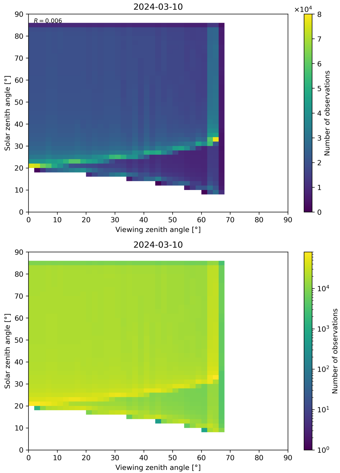
Figure 315: Scatter density plot of “Viewing zenith angle” against “Solar zenith angle” for 2024-03-09 to 2024-03-11.
