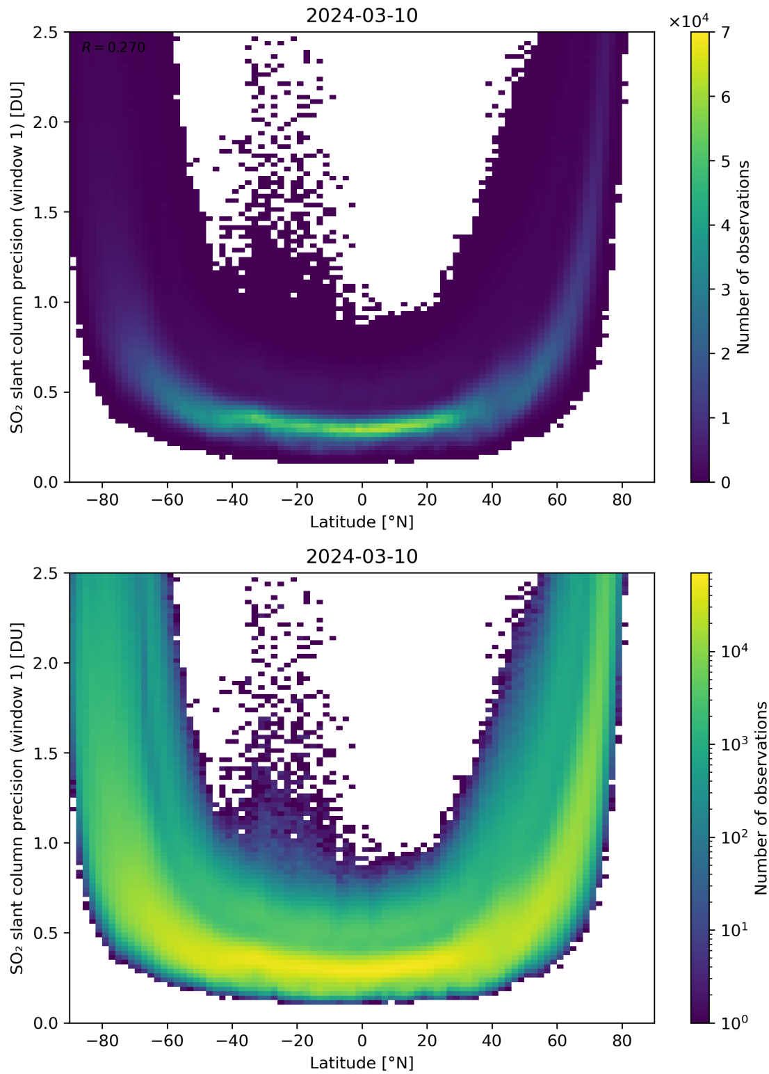
Figure 150: Scatter density plot of “Latitude” against “SO 2 slant column precision (window 1)” for 2024-03-09 to 2024-03-11.
