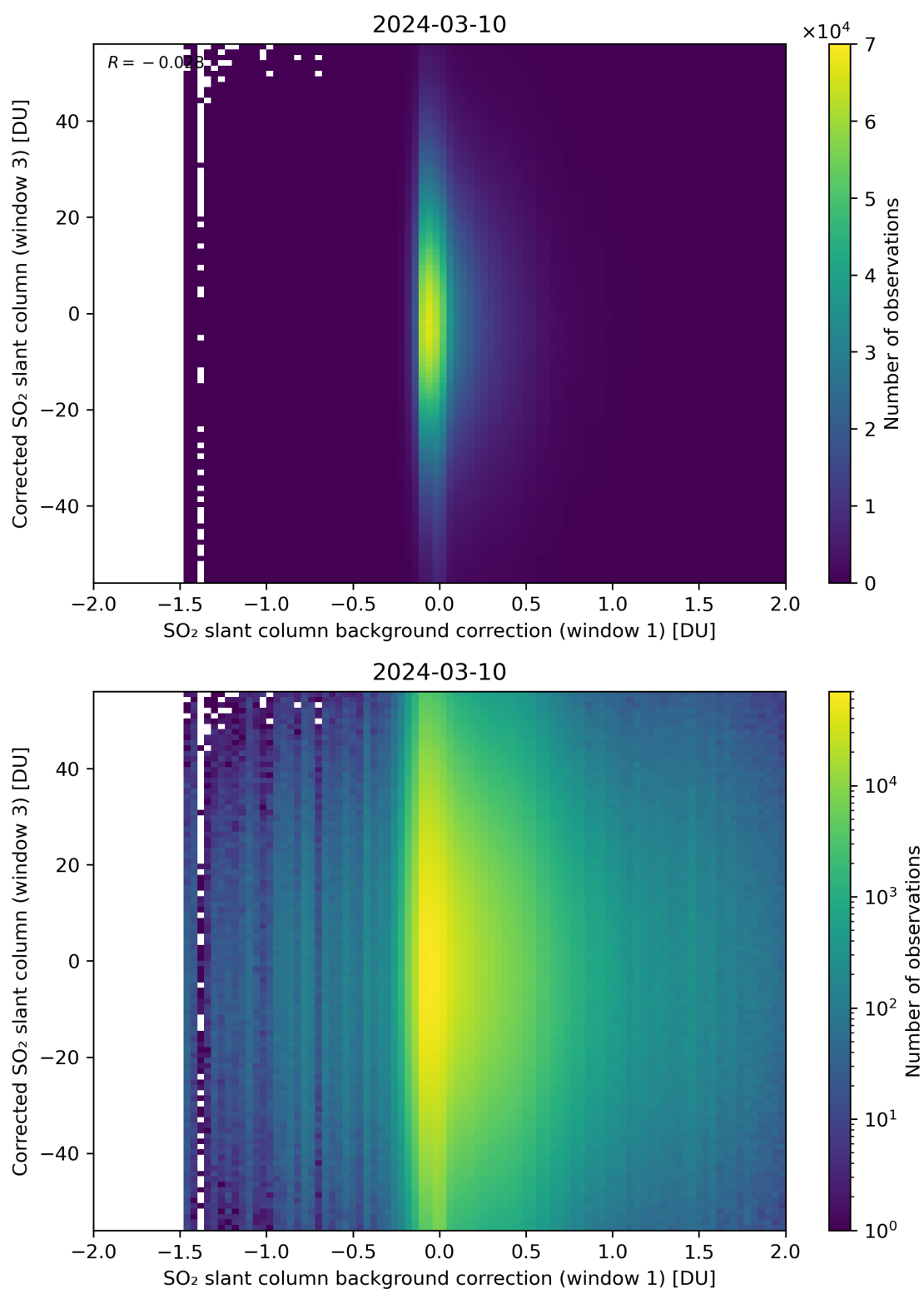
Figure 105: Scatter density plot of “SO 2 slant column background correction (window 1)” against “Corrected SO 2 slant column (window 3)” for 2024-03-09 to 2024-03-11.
