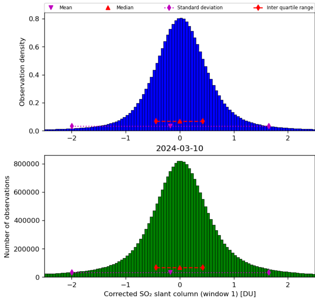
Figure 58: Histogram of “Corrected SO 2 slant column (window 1)” for 2024-03-09 to 2024-03-11
