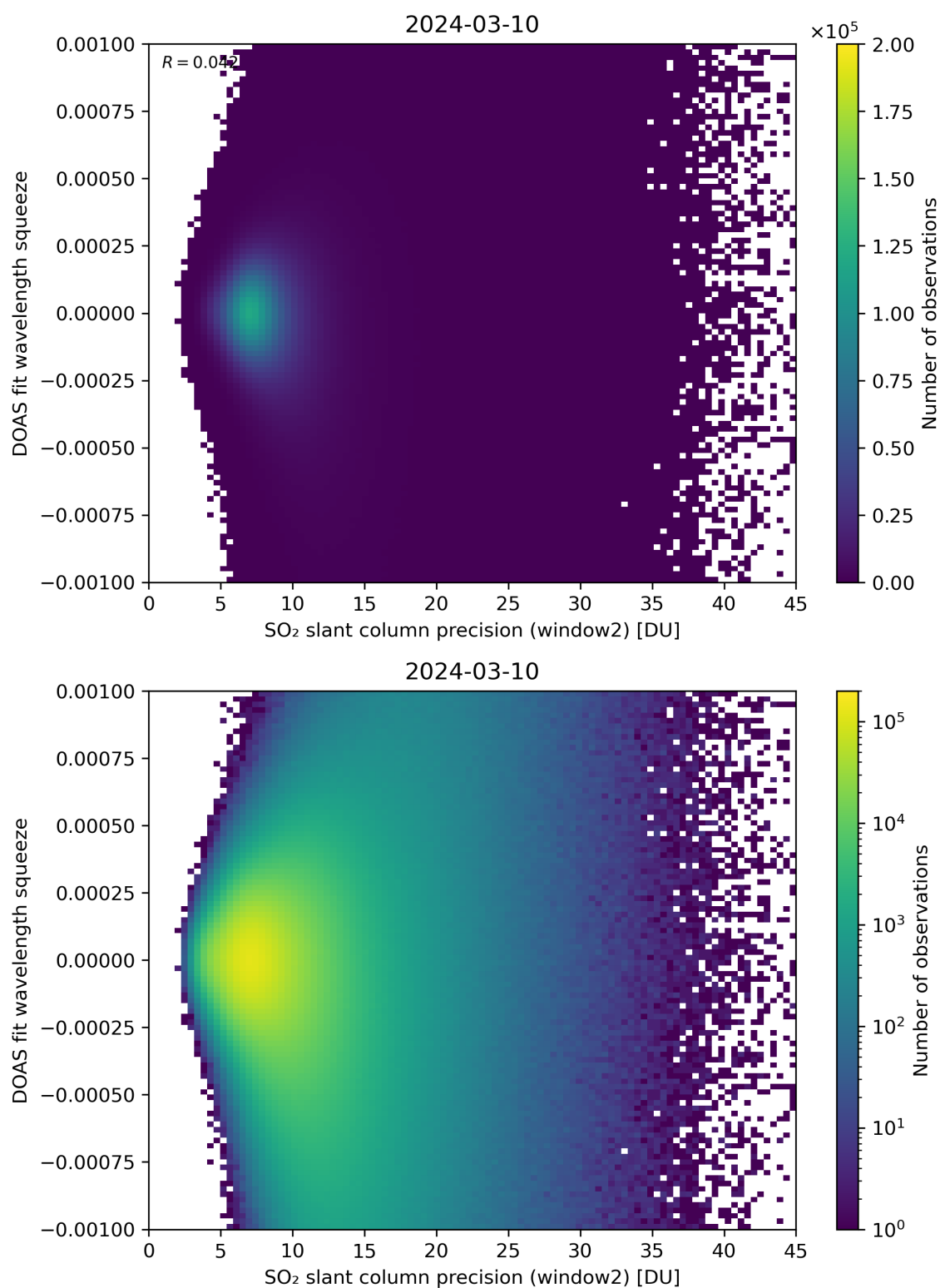
Figure 244: Scatter density plot of “SO 2 slant column precision (window2)” against “DOAS fit wavelength squeeze” for 2024-03-09 to 2024-03-11.
