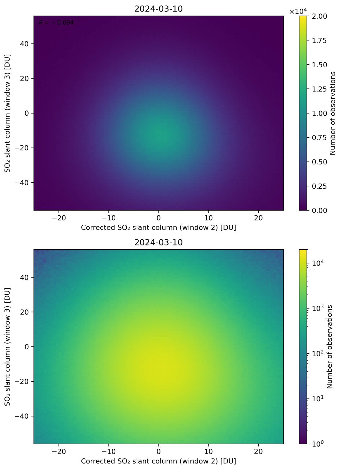
Figure 201: Scatter density plot of “Corrected SO 2 slant column (window 2)” against “SO 2 slant column (window 3)” for 2024-03-09 to 2024-03-11.
