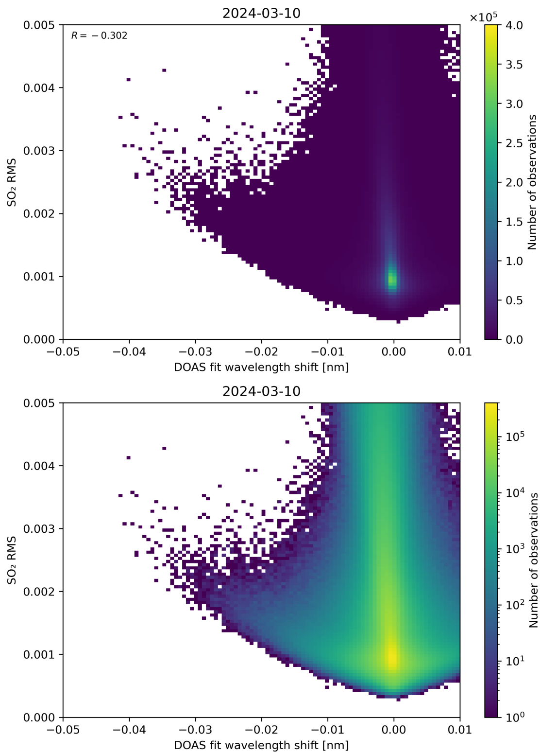
Figure 128: Scatter density plot of “DOAS fit wavelength shift” against “SO 2 RMS” for 2024-03-09 to 2024-03-11.
