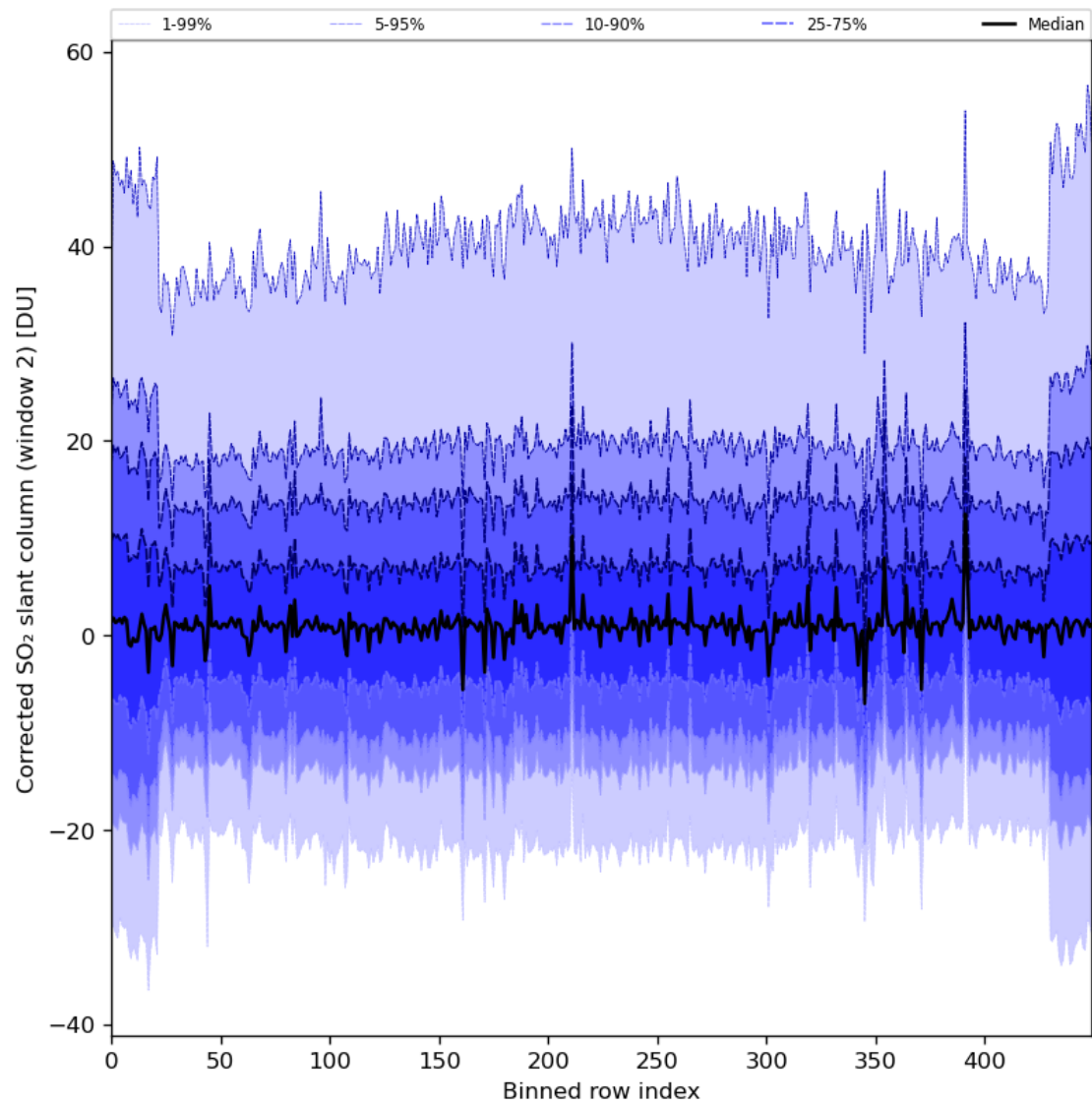
Figure 85: Along track statistics of “Corrected SO 2 slant column (window 2)” for 2024-03-09 to 2024-03-11
