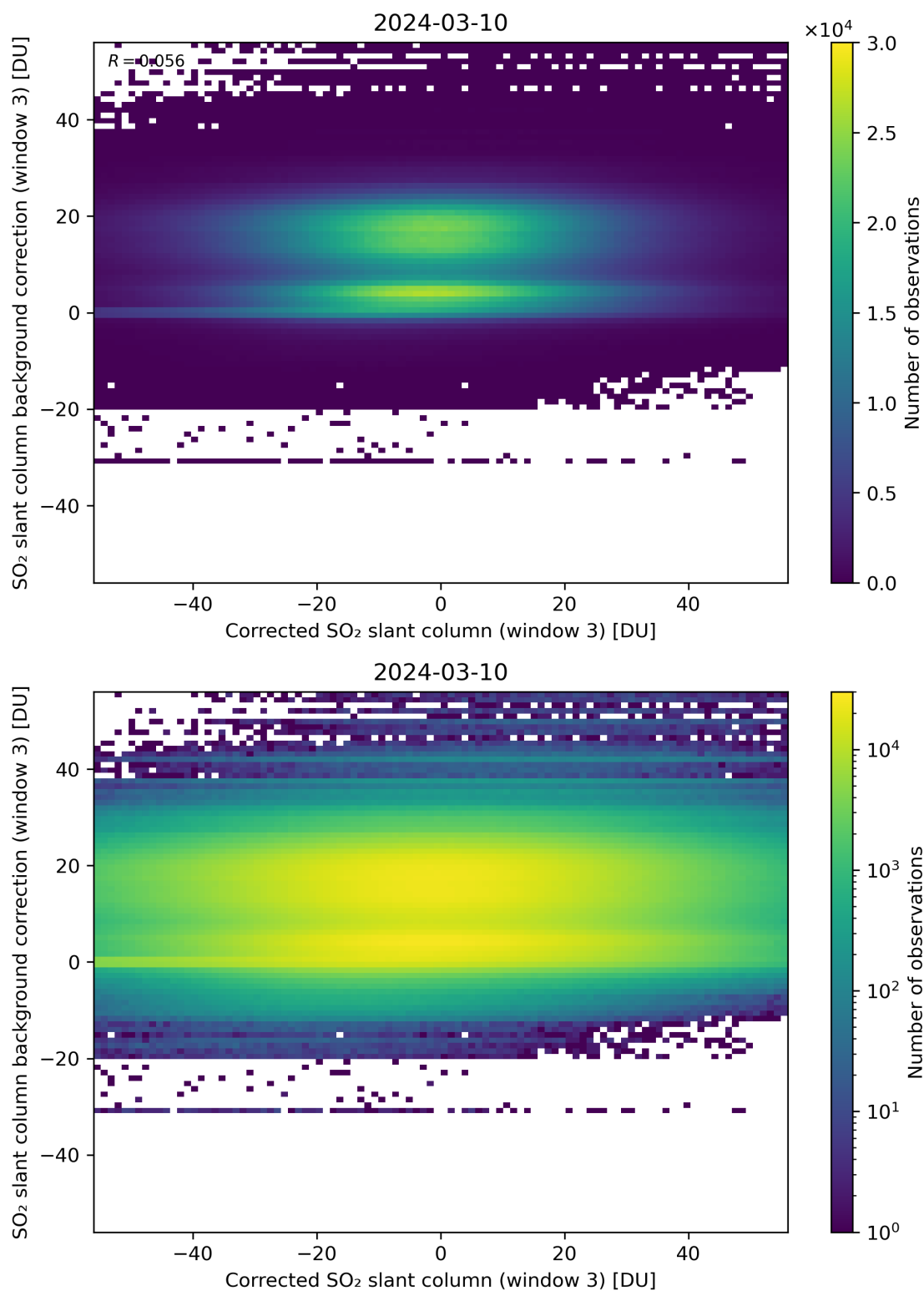
Figure 205: Scatter density plot of “Corrected SO 2 slant column (window 3)” against “SO 2 slant column background correction (window 3)” for 2024-03-09 to 2024-03-11.
