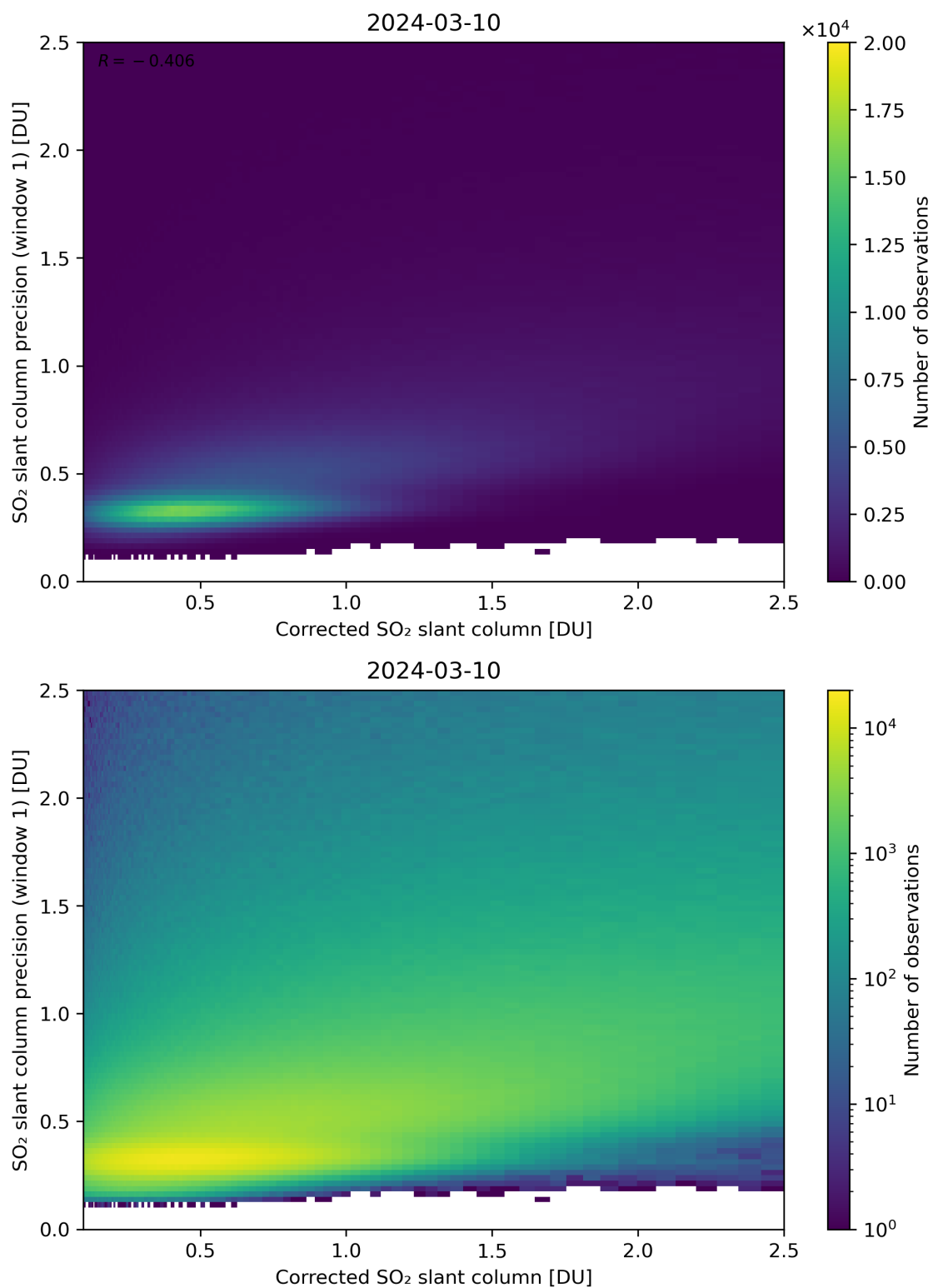
Figure 188: Scatter density plot of “Corrected SO 2 slant column” against “SO 2 slant column precision (window 1)” for 2024-03-09 to 2024-03-11.
