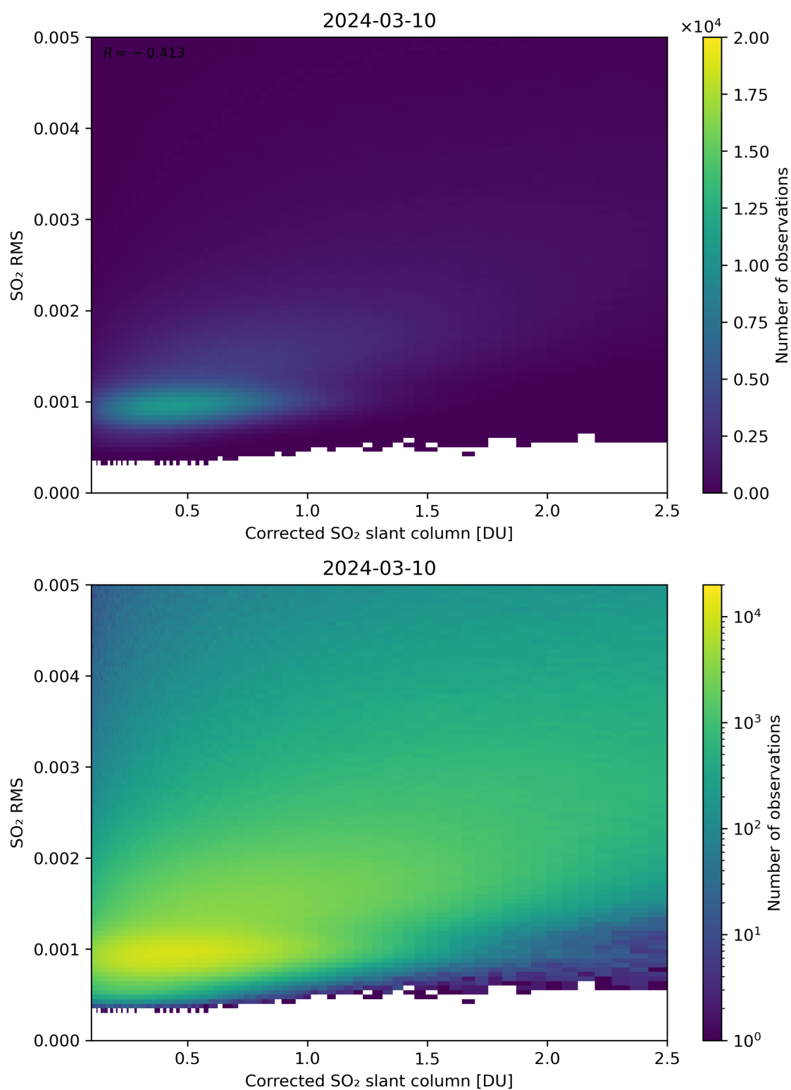
Figure 183: Scatter density plot of “Corrected SO 2 slant column” against “SO 2 RMS” for 2024-03-09 to 2024-03-11.
