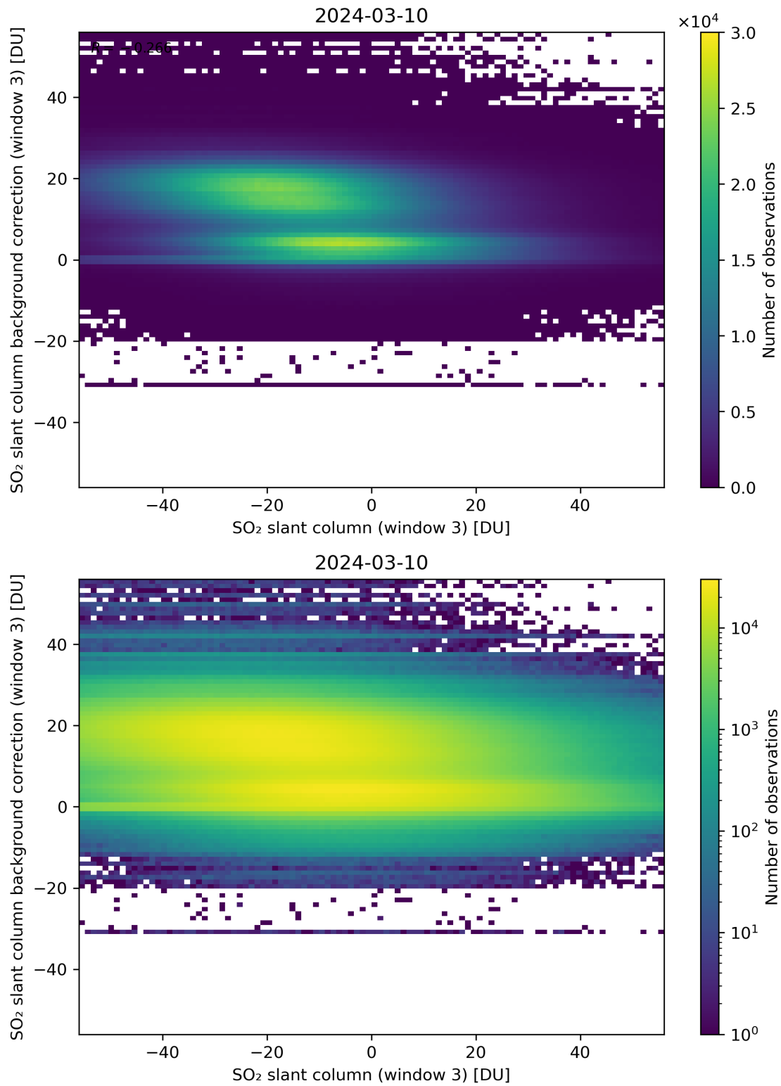
Figure 253: Scatter density plot of “SO 2 slant column (window 3)” against “SO 2 slant column background correction (window 3)” for 2024-03-09 to 2024-03-11.
