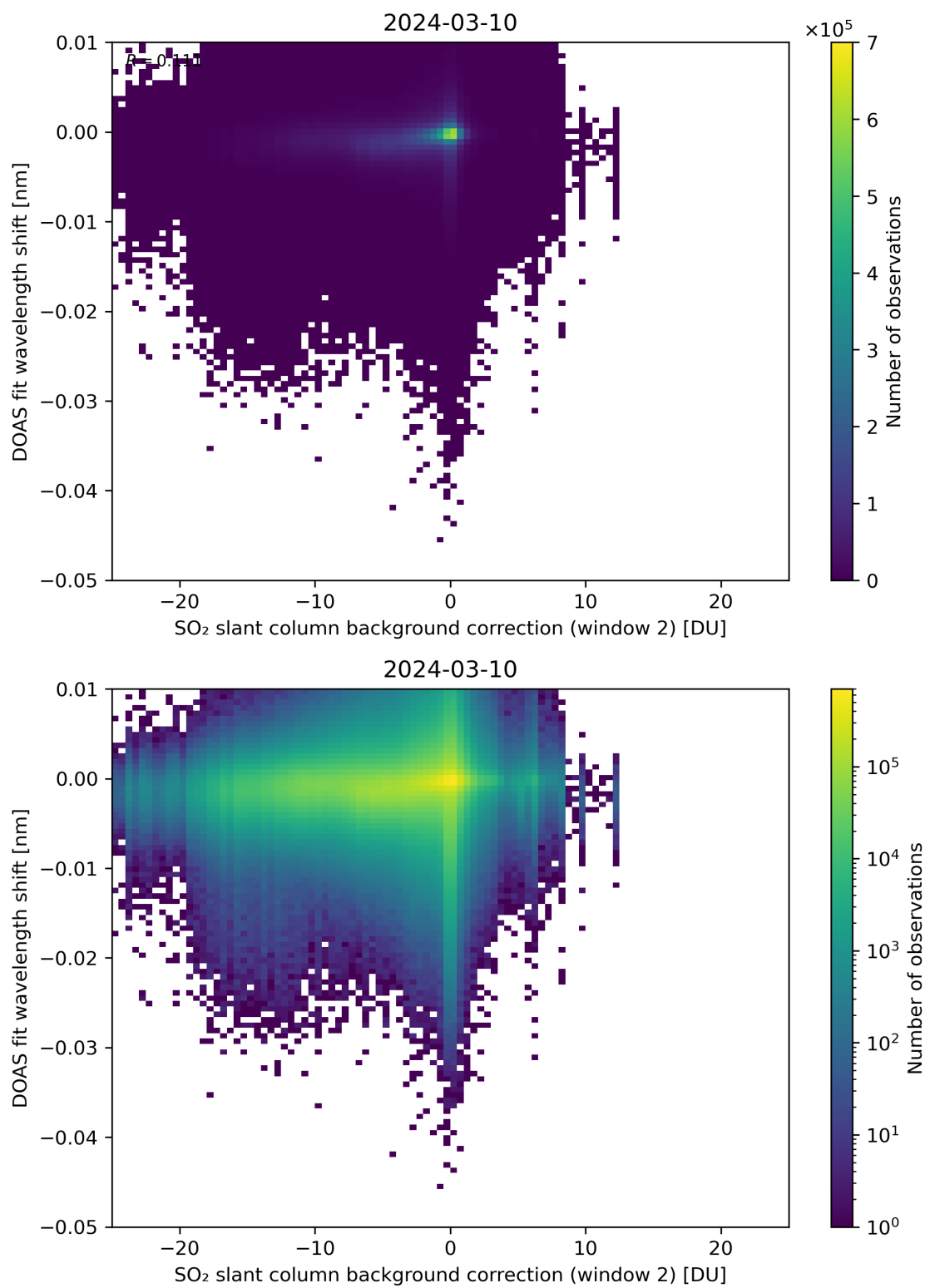
Figure 112: Scatter density plot of “SO 2 slant column background correction (window 2)” against “DOAS fit wavelength shift” for 2024-03-09 to 2024-03-11.
