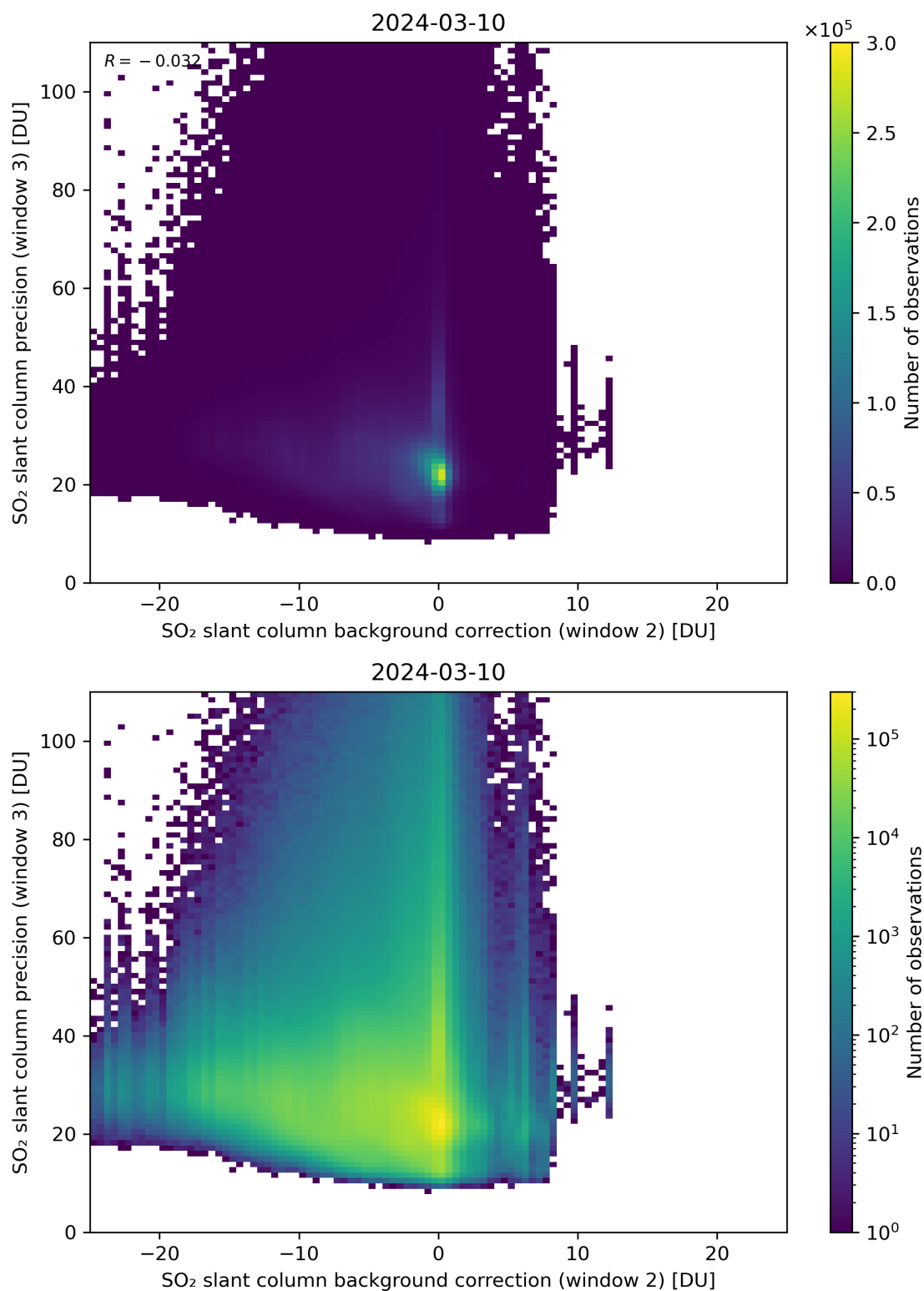
Figure 118: Scatter density plot of “SO 2 slant column background correction (window 2)” against “SO 2 slant column precision (window 3)” for 2024-03-09 to 2024-03-11.
