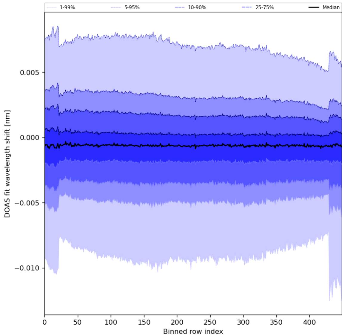
Figure 91: Along track statistics of “DOAS fit wavelength shift” for 2024-03-09 to 2024-03-11
