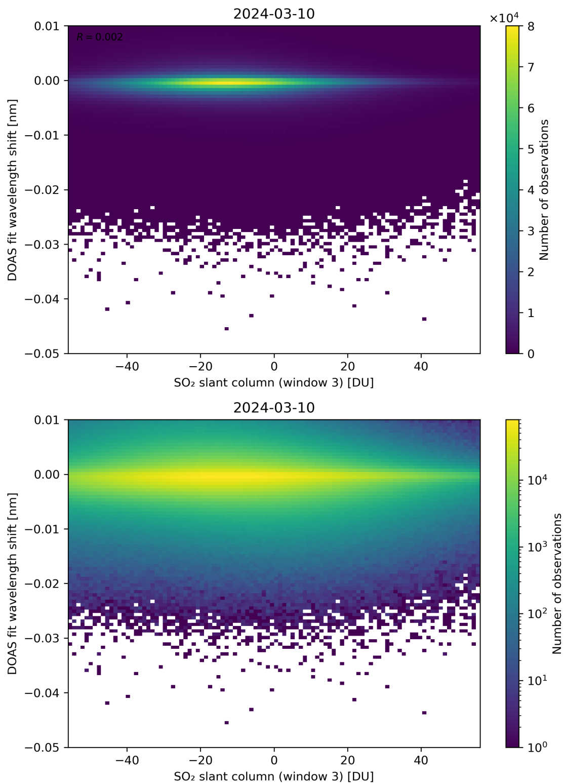
Figure 254: Scatter density plot of “SO 2 slant column (window 3)” against “DOAS fit wavelength shift” for 2024-03-09 to 2024-03-11.
