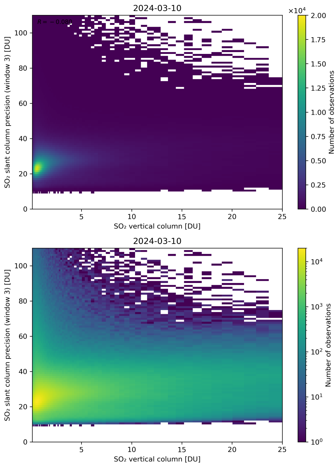
Figure 304: Scatter density plot of “SO 2 vertical column” against “SO 2 slant column precision (window 3)” for 2024-03-09 to 2024-03-11.
