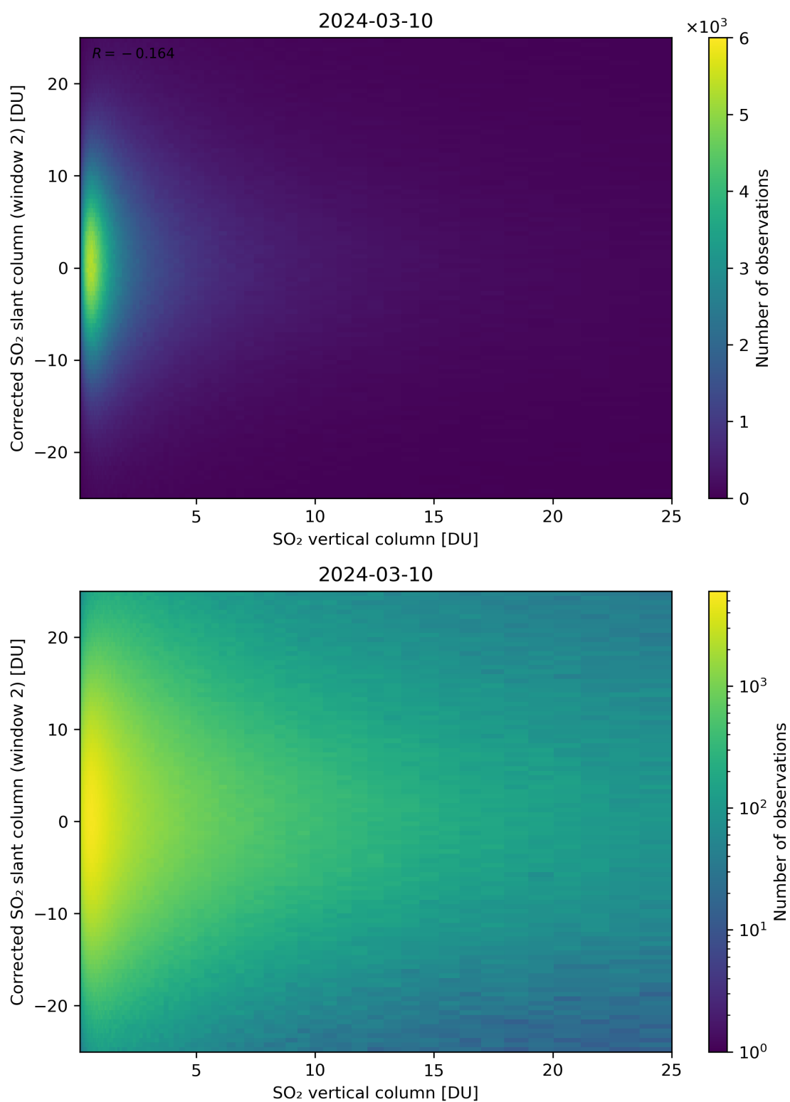
Figure 298: Scatter density plot of “SO 2 vertical column” against “Corrected SO 2 slant column (window 2)” for 2024-03-09 to 2024-03-11.
