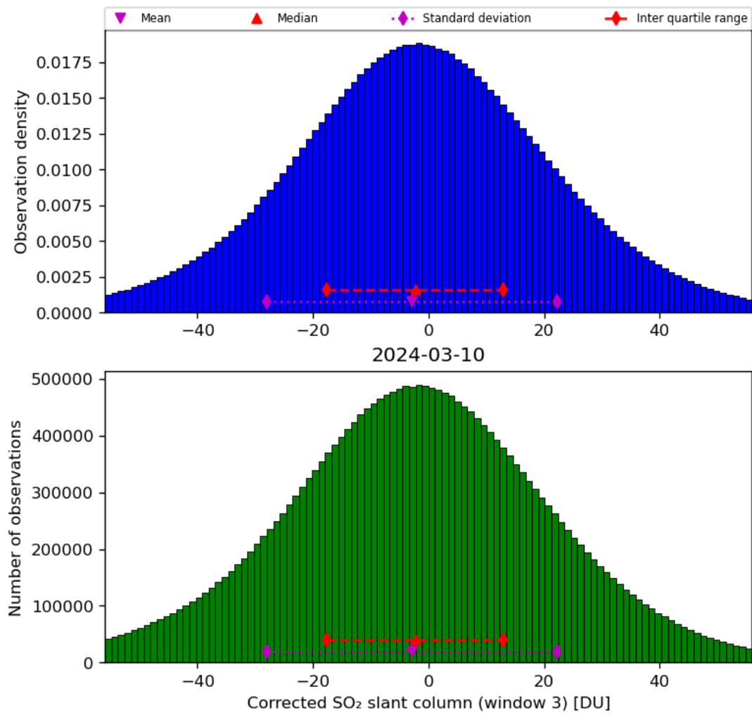
Figure 66: Histogram of “Corrected SO 2 slant column (window 3)” for 2024-03-09 to 2024-03-11
