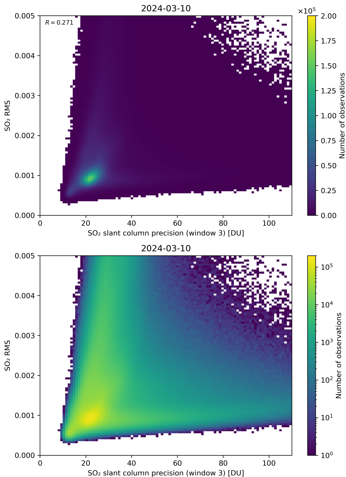
Figure 260: Scatter density plot of “SO 2 slant column precision (window 3)” against “SO 2 RMS” for 2024-03-09 to 2024-03-11.
