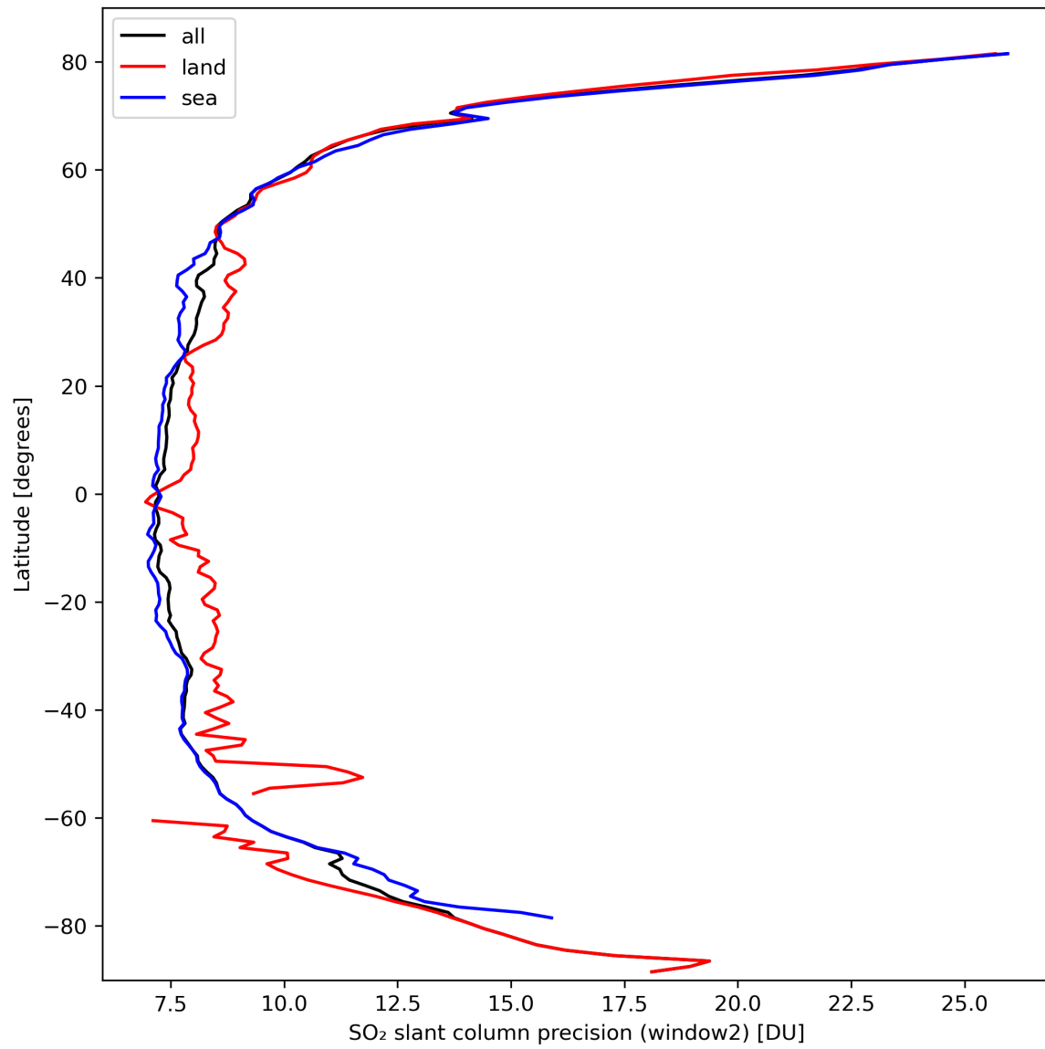
Figure 38: Zonal average of “SO 2 slant column precision (window2)” for 2024-03-09 to 2024-03-11.
