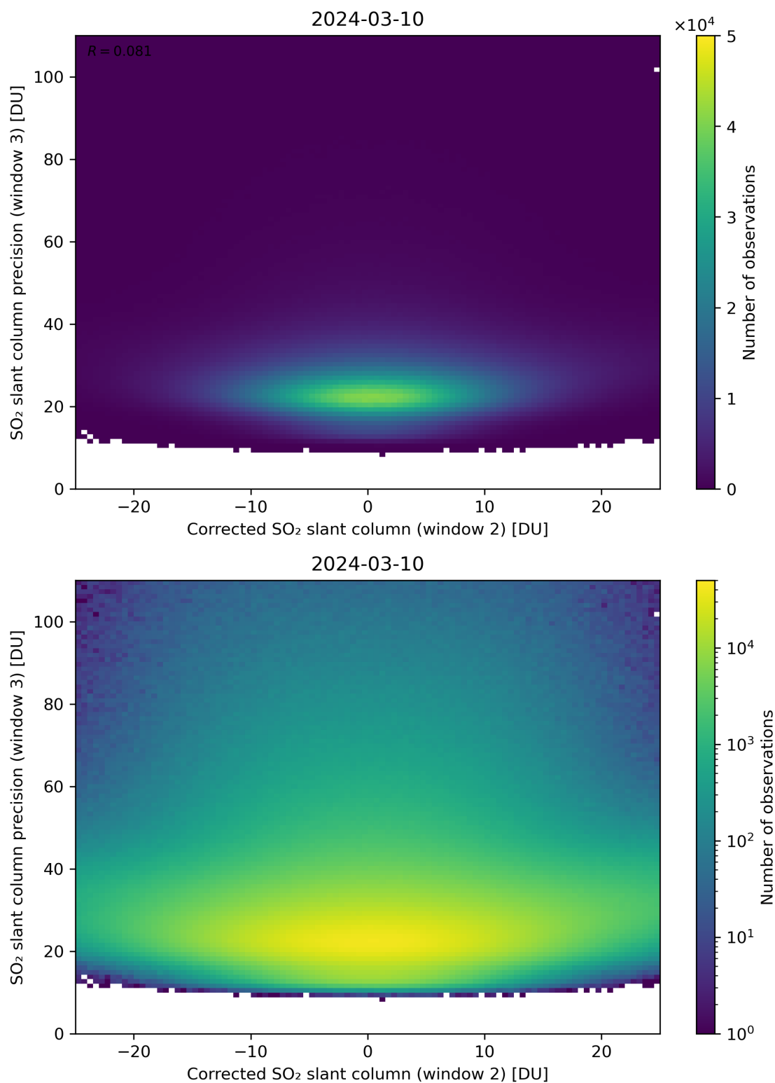
Figure 202: Scatter density plot of “Corrected SO 2 slant column (window 2)” against “SO 2 slant column precision (window 3)” for 2024-03-09 to 2024-03-11.
