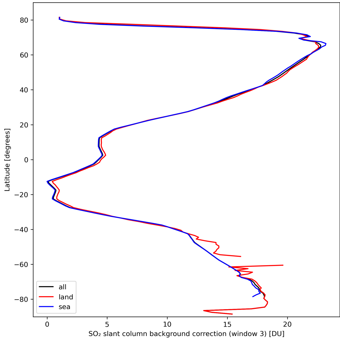
Figure 44: Zonal average of “SO 2 slant column background correction (window 3)” for 2024-03-09 to 2024-03-11.
