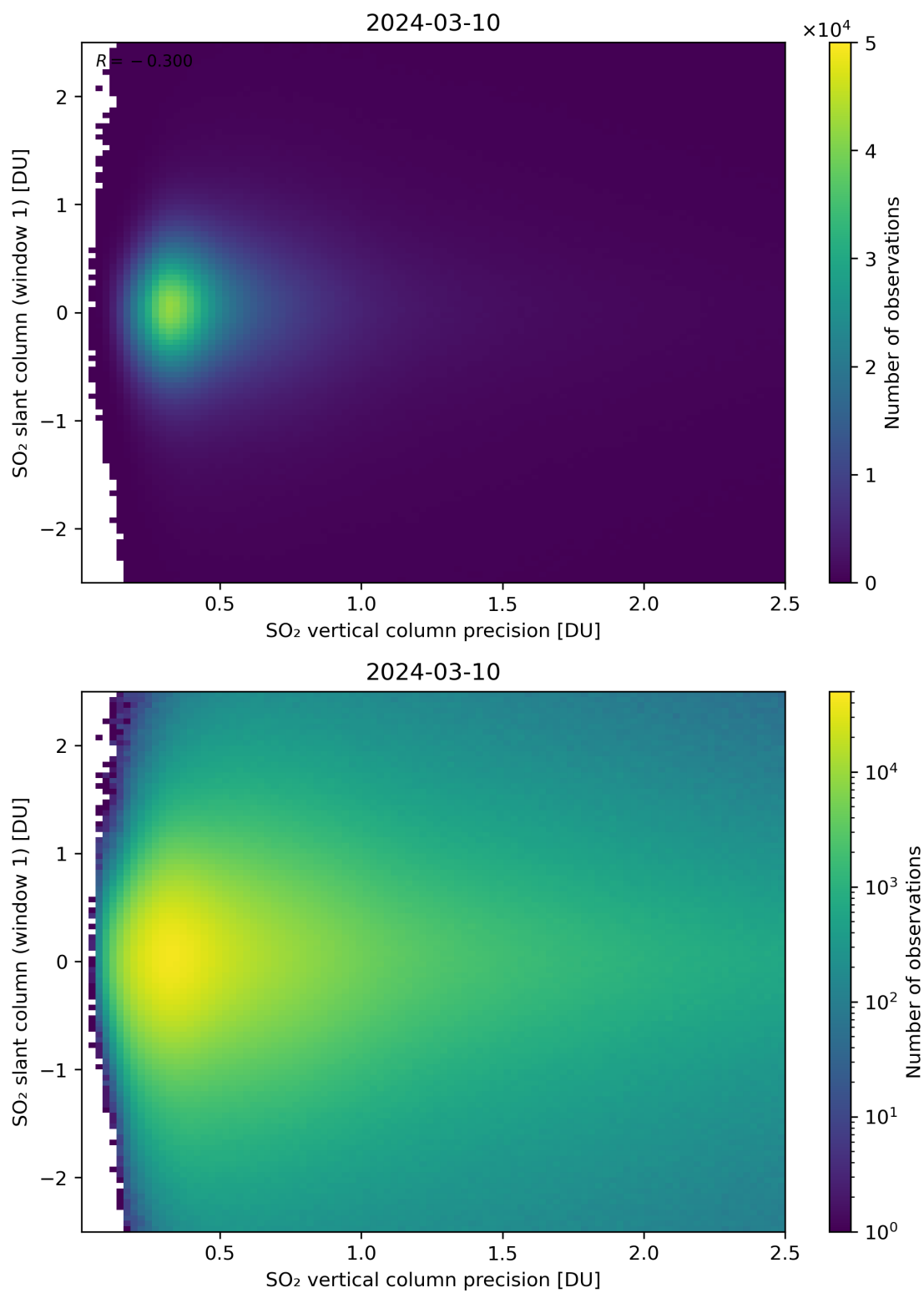
Figure 289: Scatter density plot of “SO 2 vertical column precision” against “SO 2 slant column (window 1)” for 2024-03-09 to 2024-03-11.
