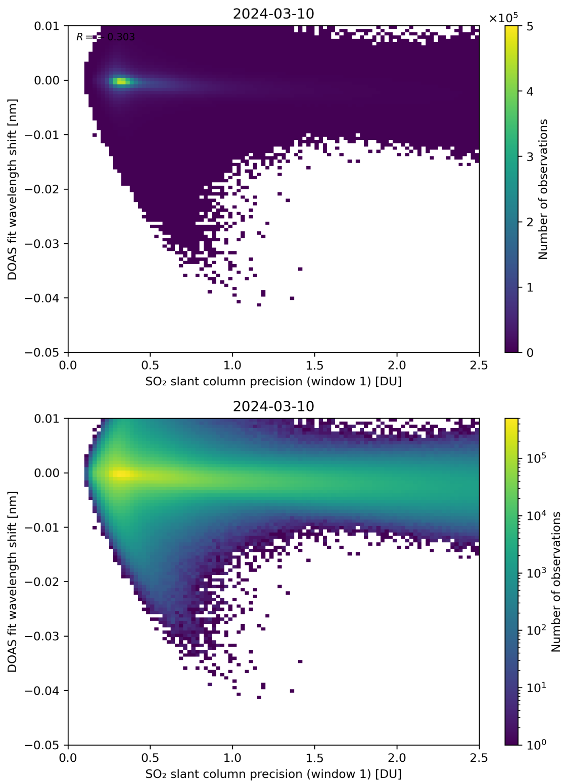
Figure 221: Scatter density plot of “SO 2 slant column precision (window 1)” against “DOAS fit wavelength shift” for 2024-03-09 to 2024-03-11.
