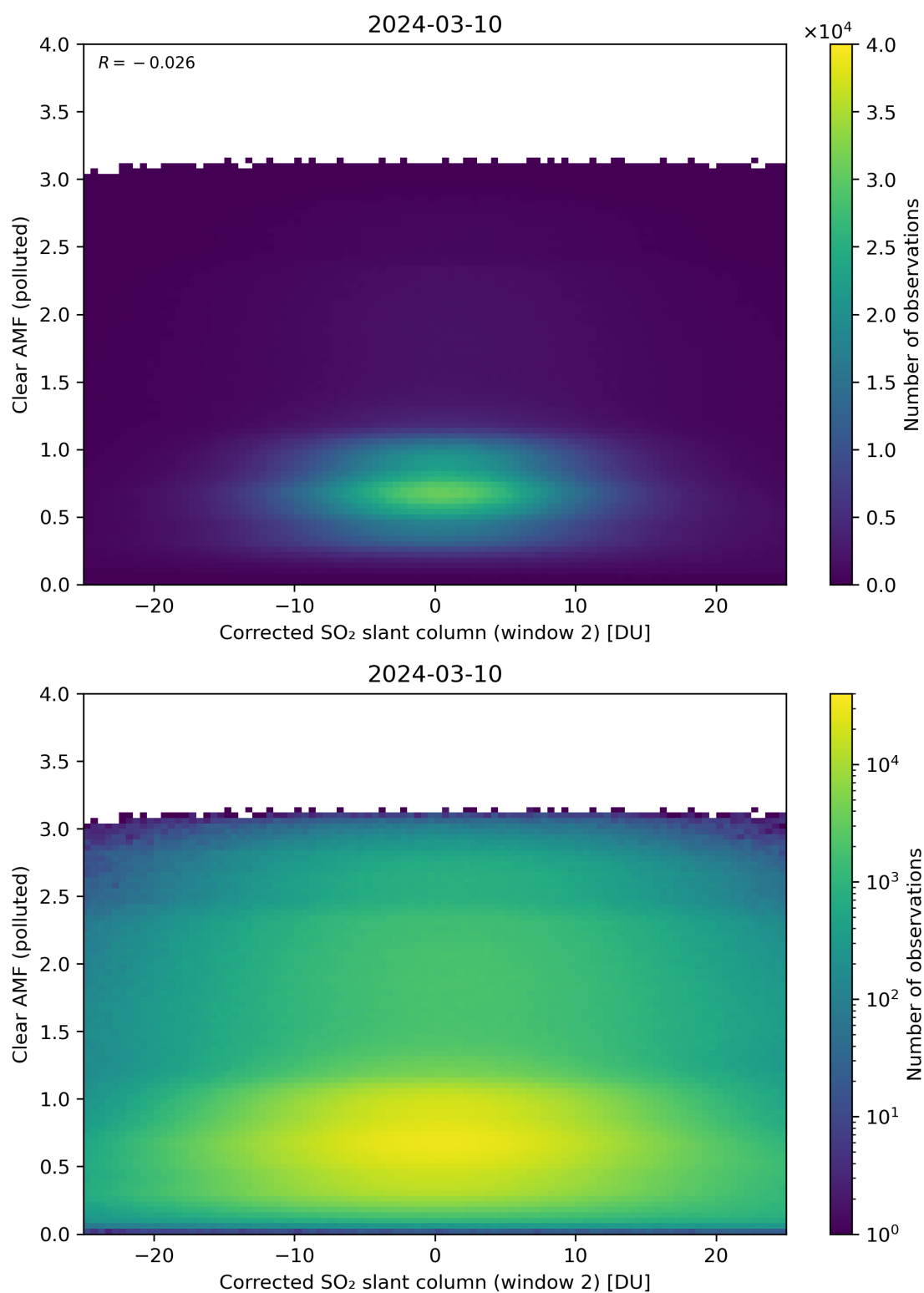
Figure 199: Scatter density plot of “Corrected SO 2 slant column (window 2)” against “Clear AMF (polluted)” for 2024-03-09 to 2024-03-11.
