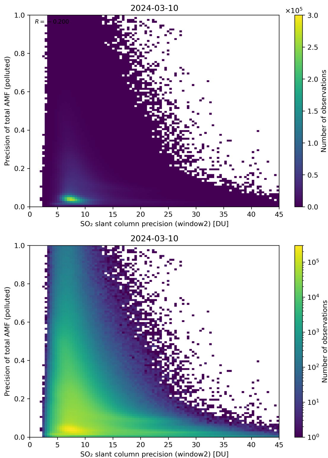
Figure 252: Scatter density plot of “SO 2 slant column precision (window2)” against “Precision of total AMF (polluted)” for 2024-03-09 to 2024-03-11.
