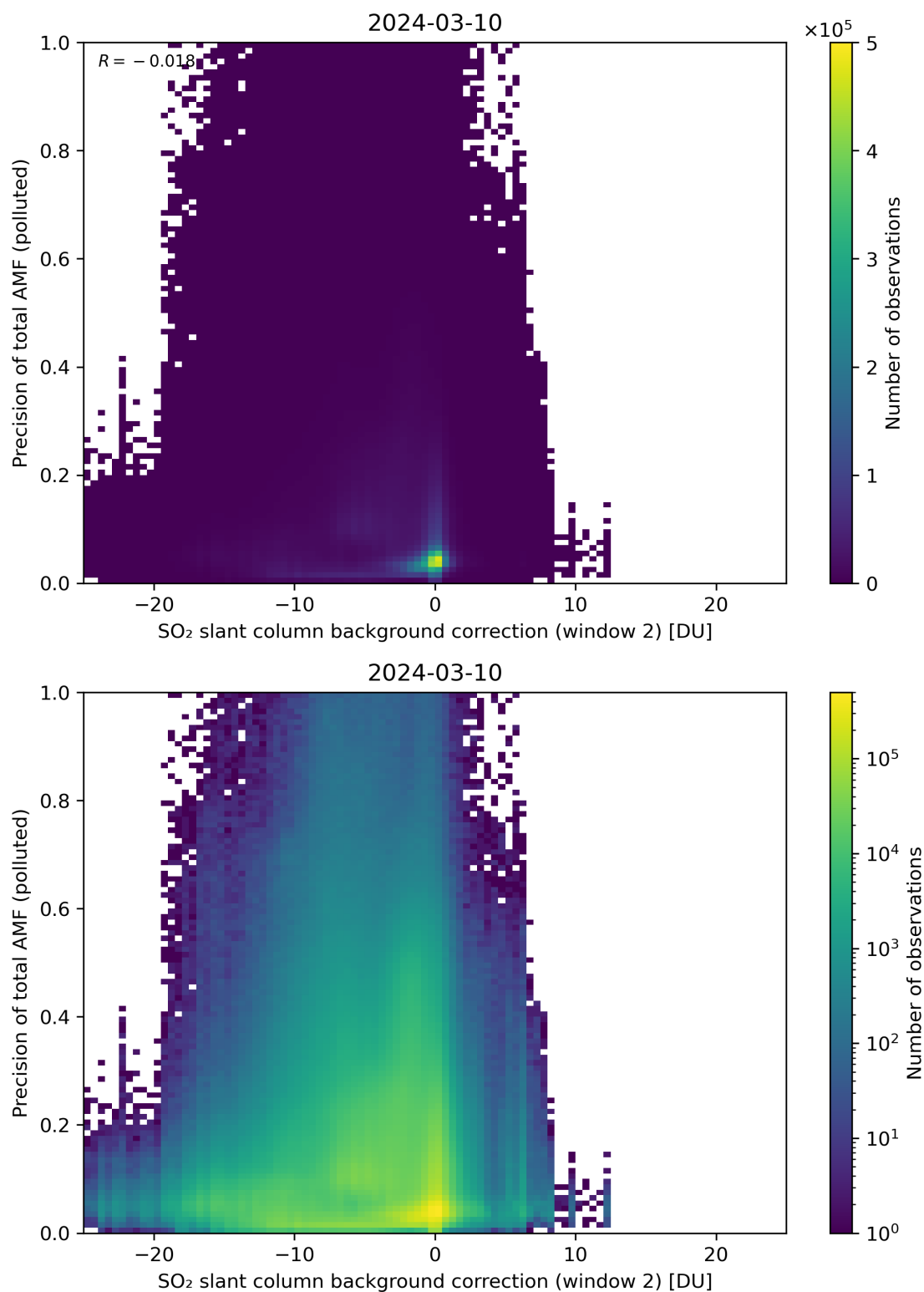
Figure 120: Scatter density plot of “SO 2 slant column background correction (window 2)” against “Precision of total AMF (polluted)” for 2024-03-09 to 2024-03-11.
