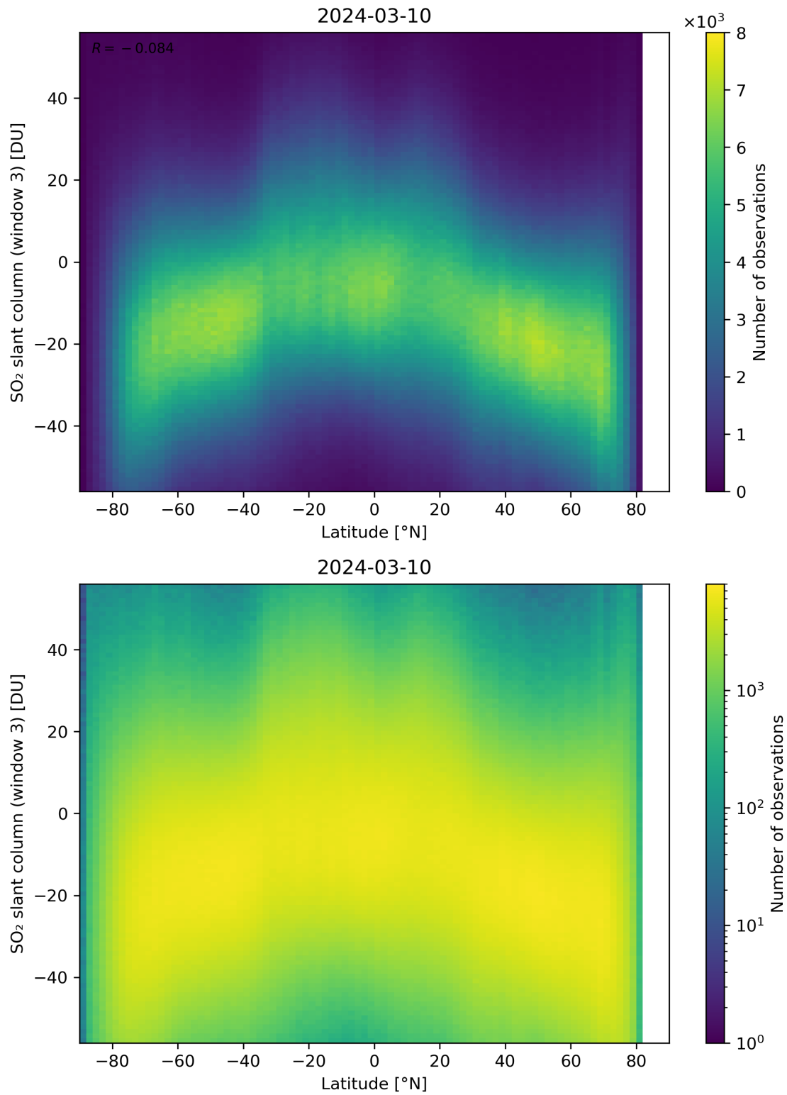
Figure 152: Scatter density plot of “Latitude” against “SO 2 slant column (window 3)” for 2024-03-09 to 2024-03-11.
