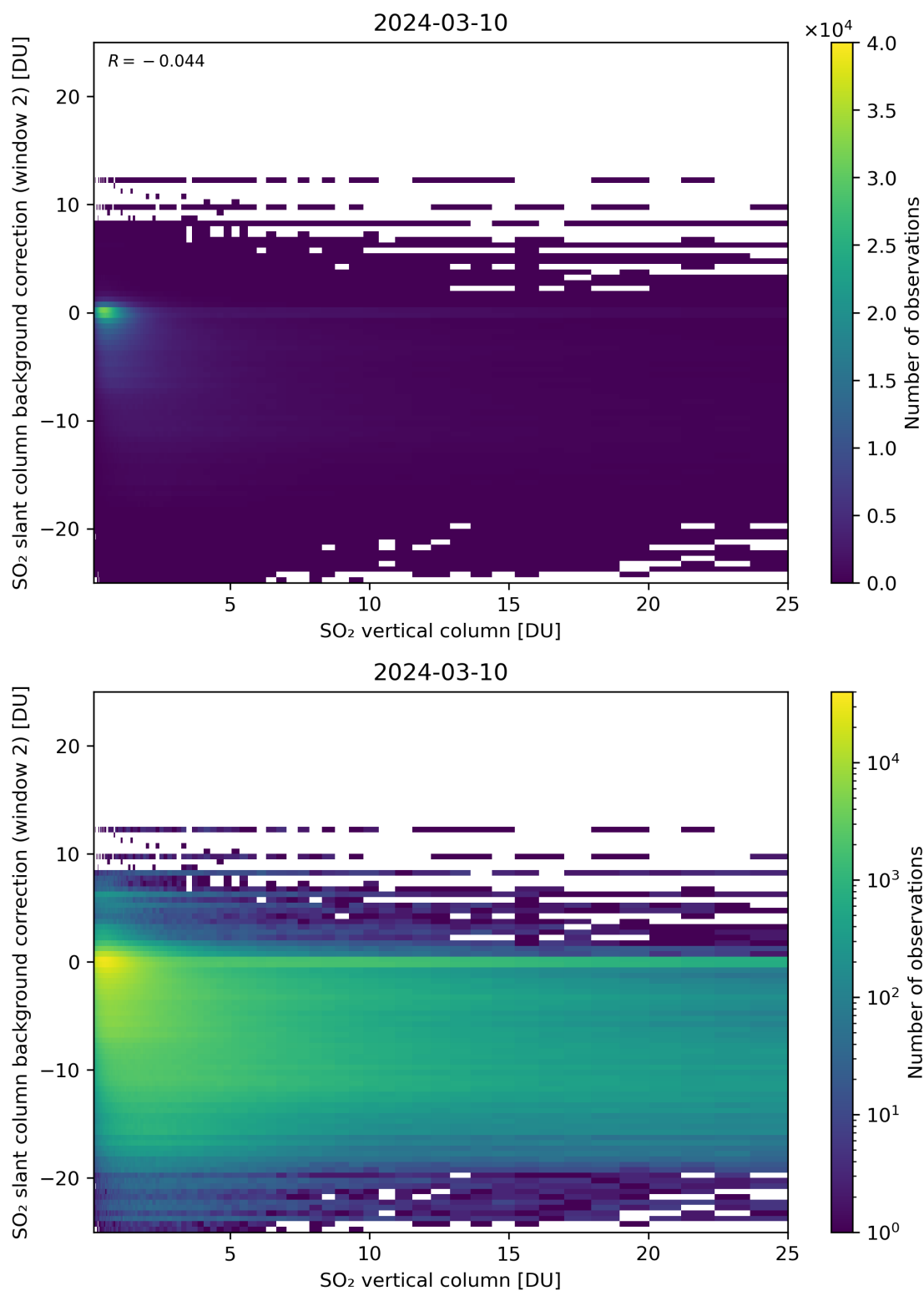
Figure 274: Scatter density plot of “SO 2 vertical column” against “SO 2 slant column background correction (window 2)” for 2024-03-09 to 2024-03-11.
