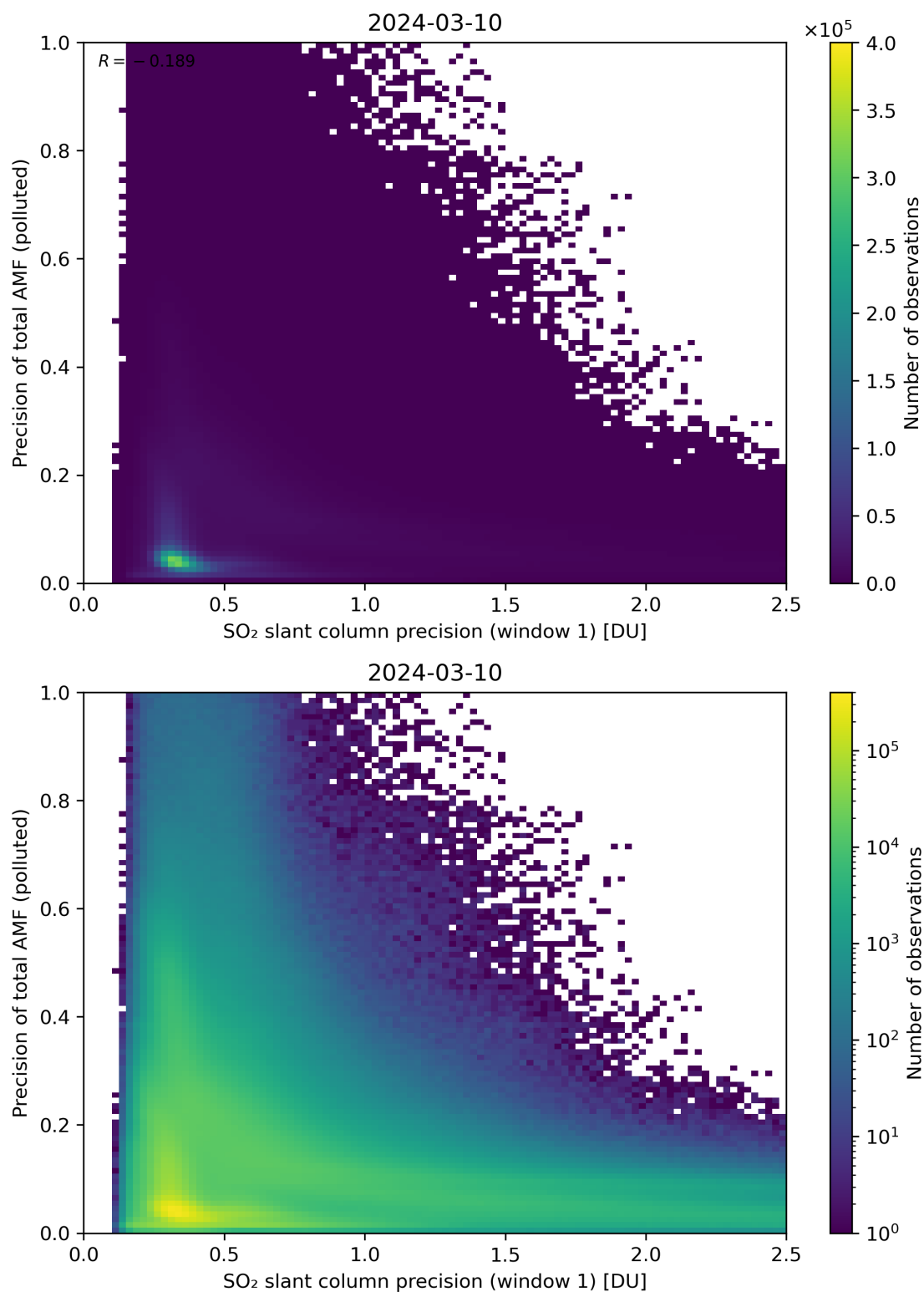
Figure 231: Scatter density plot of “SO 2 slant column precision (window 1)” against “Precision of total AMF (polluted)” for 2024-03-09 to 2024-03-11.
