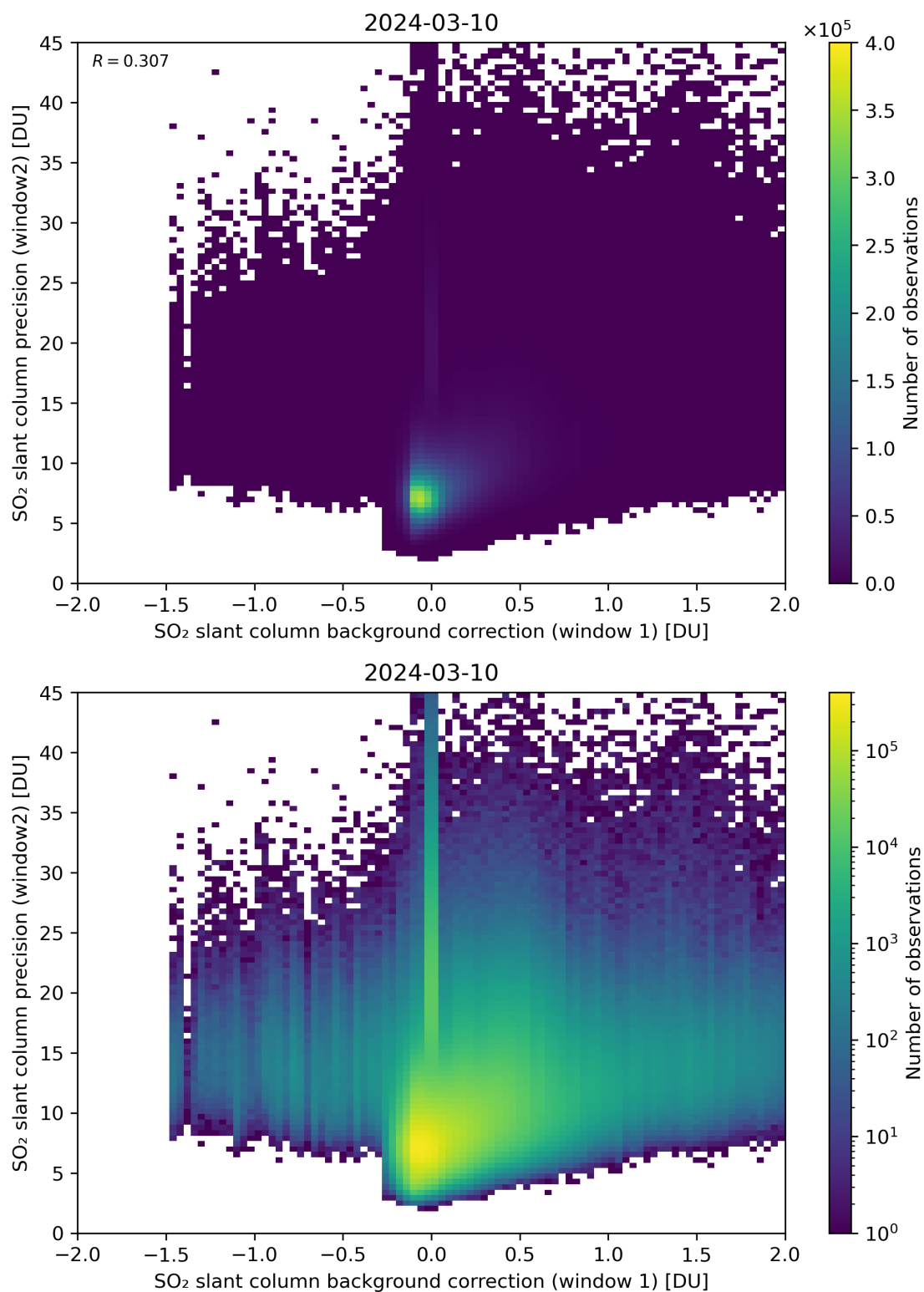
Figure 106: Scatter density plot of “SO 2 slant column background correction (window 1)” against “SO 2 slant column precision (window2)” for 2024-03-09 to 2024-03-11.
