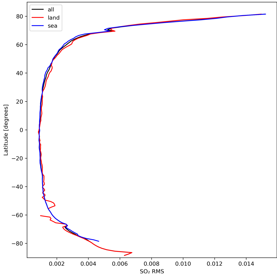
Figure 47: Zonal average of “SO 2 RMS” for 2024-03-09 to 2024-03-11.
