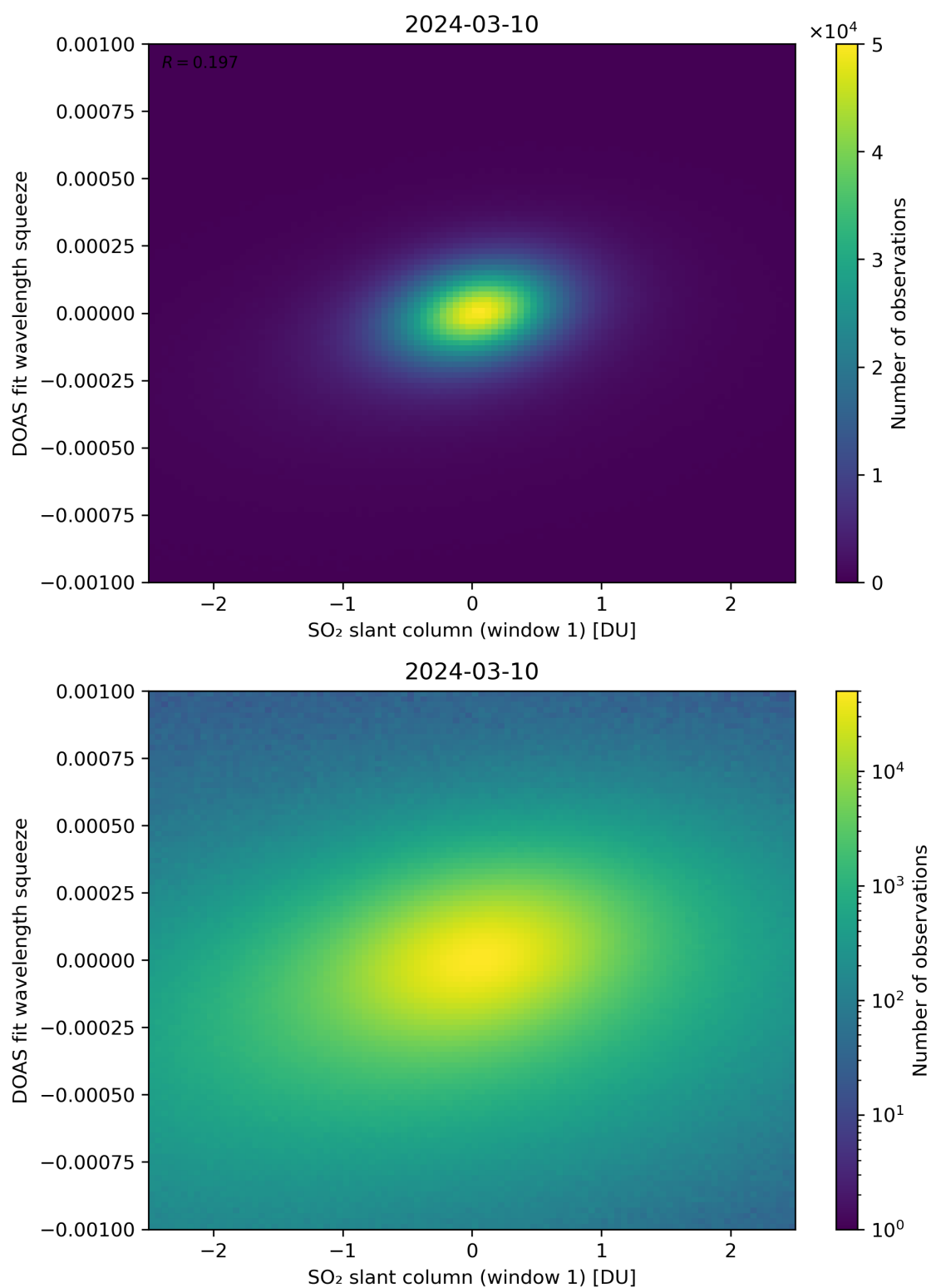
Figure 216: Scatter density plot of “SO 2 slant column (window 1)” against “DOAS fit wavelength squeeze” for 2024-03-09 to 2024-03-11.
