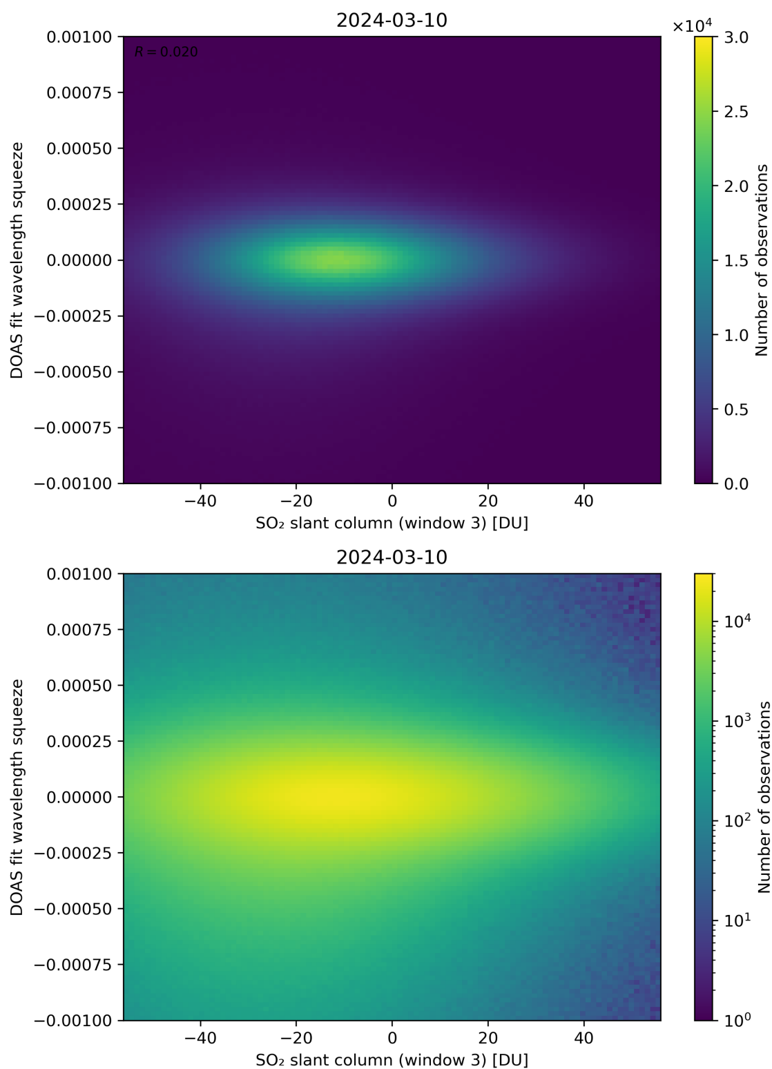
Figure 255: Scatter density plot of “SO 2 slant column (window 3)” against “DOAS fit wavelength squeeze” for 2024-03-09 to 2024-03-11.
