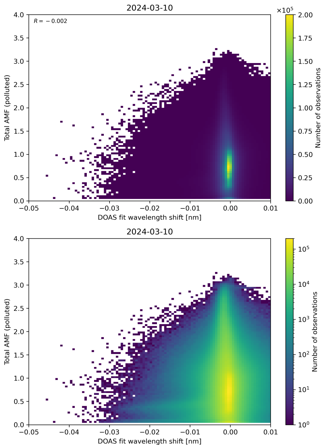
Figure 130: Scatter density plot of “DOAS fit wavelength shift” against “Total AMF (polluted)” for 2024-03-09 to 2024-03-11.
