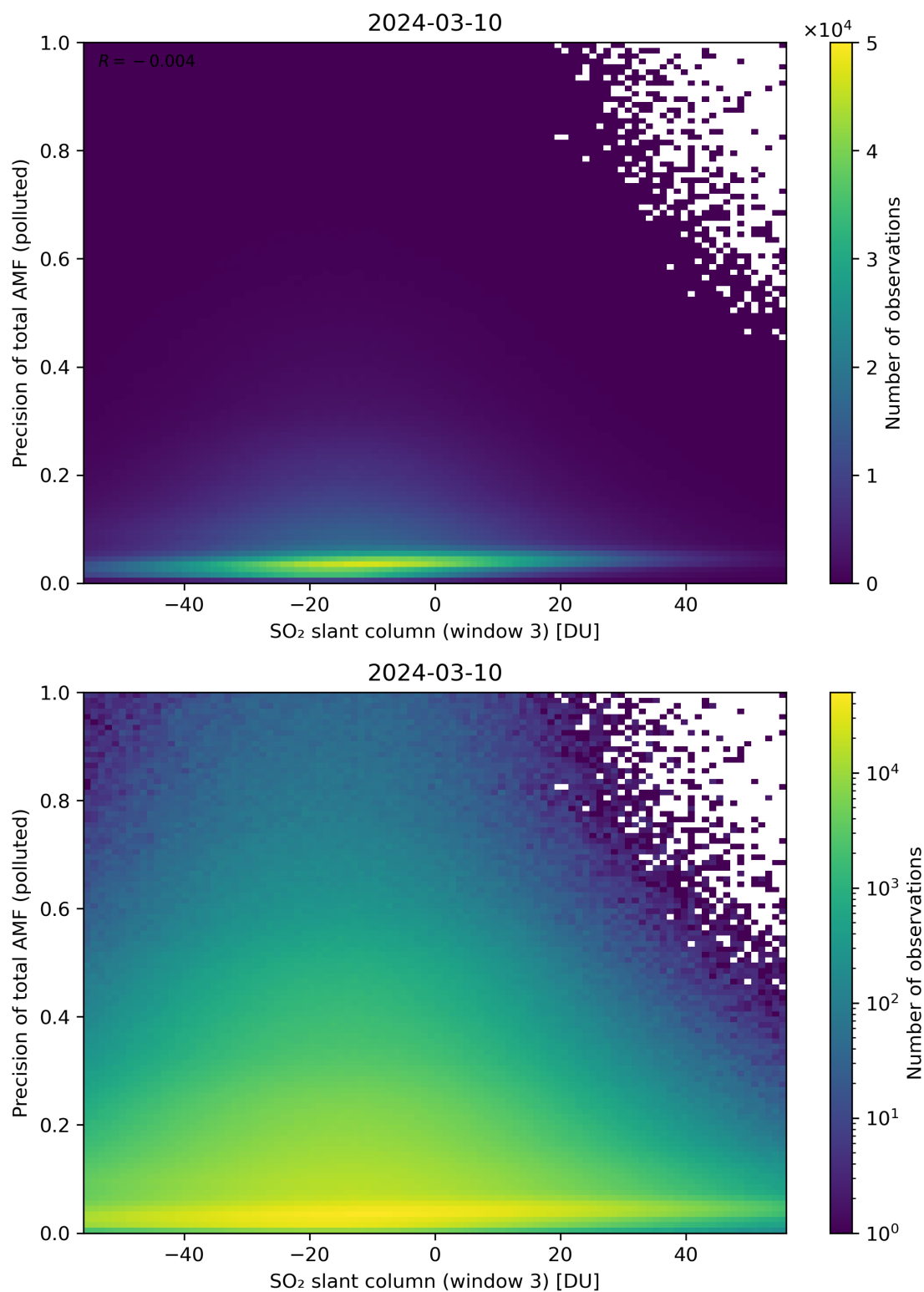
Figure 269: Scatter density plot of “SO 2 slant column (window 3)” against “Precision of total AMF (polluted)” for 2024-03-09 to 2024-03-11.
