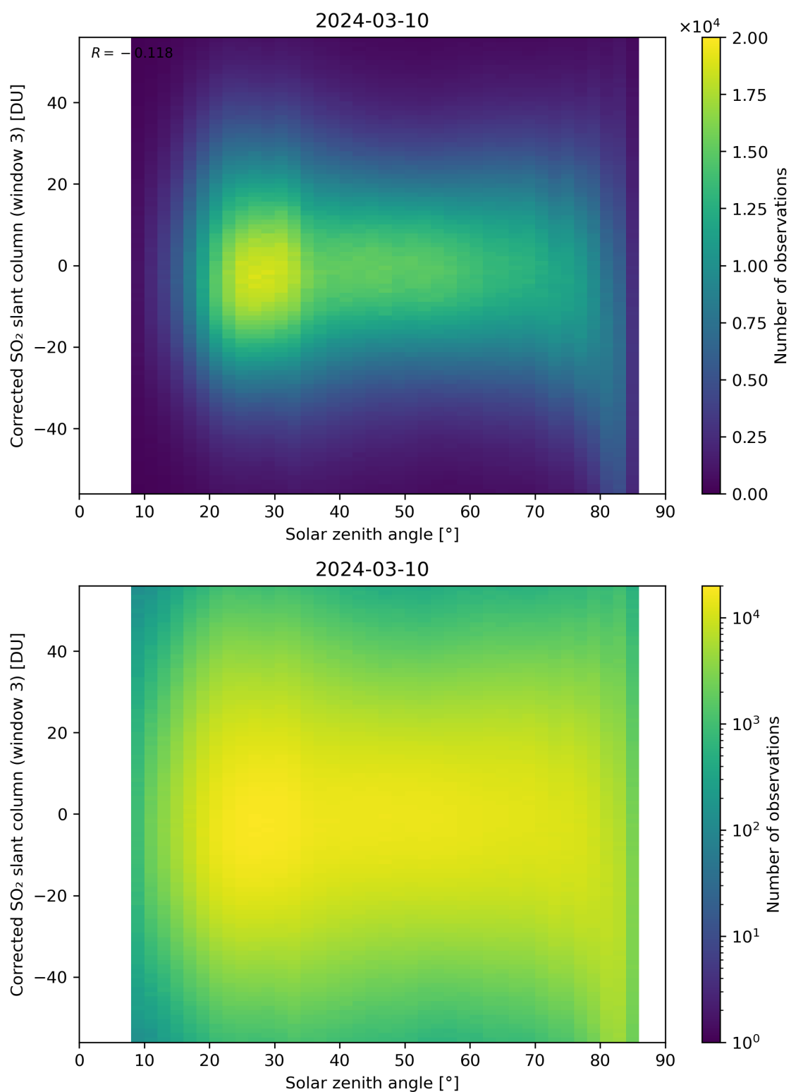
Figure 168: Scatter density plot of “Solar zenith angle” against “Corrected SO 2 slant column (window 3)” for 2024-03-09 to 2024-03-11.
