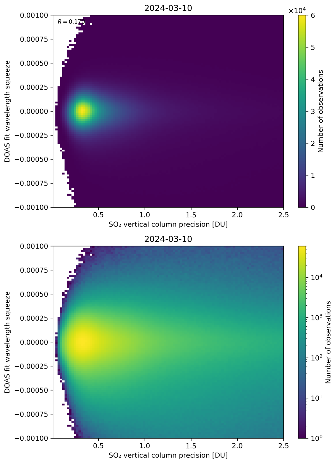
Figure 283: Scatter density plot of “SO 2 vertical column precision” against “DOAS fit wavelength squeeze” for 2024-03-09 to 2024-03-11.
