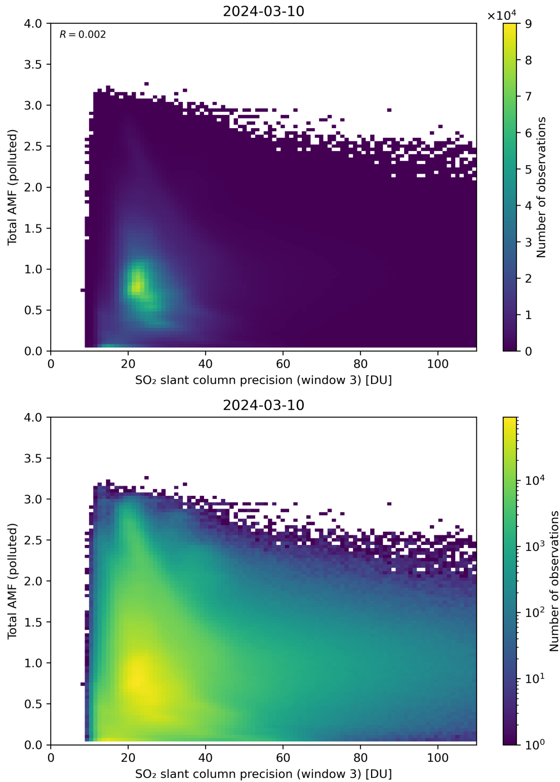
Figure 263: Scatter density plot of “SO 2 slant column precision (window 3)” against “Total AMF (polluted)” for 2024-03-09 to 2024-03-11.
