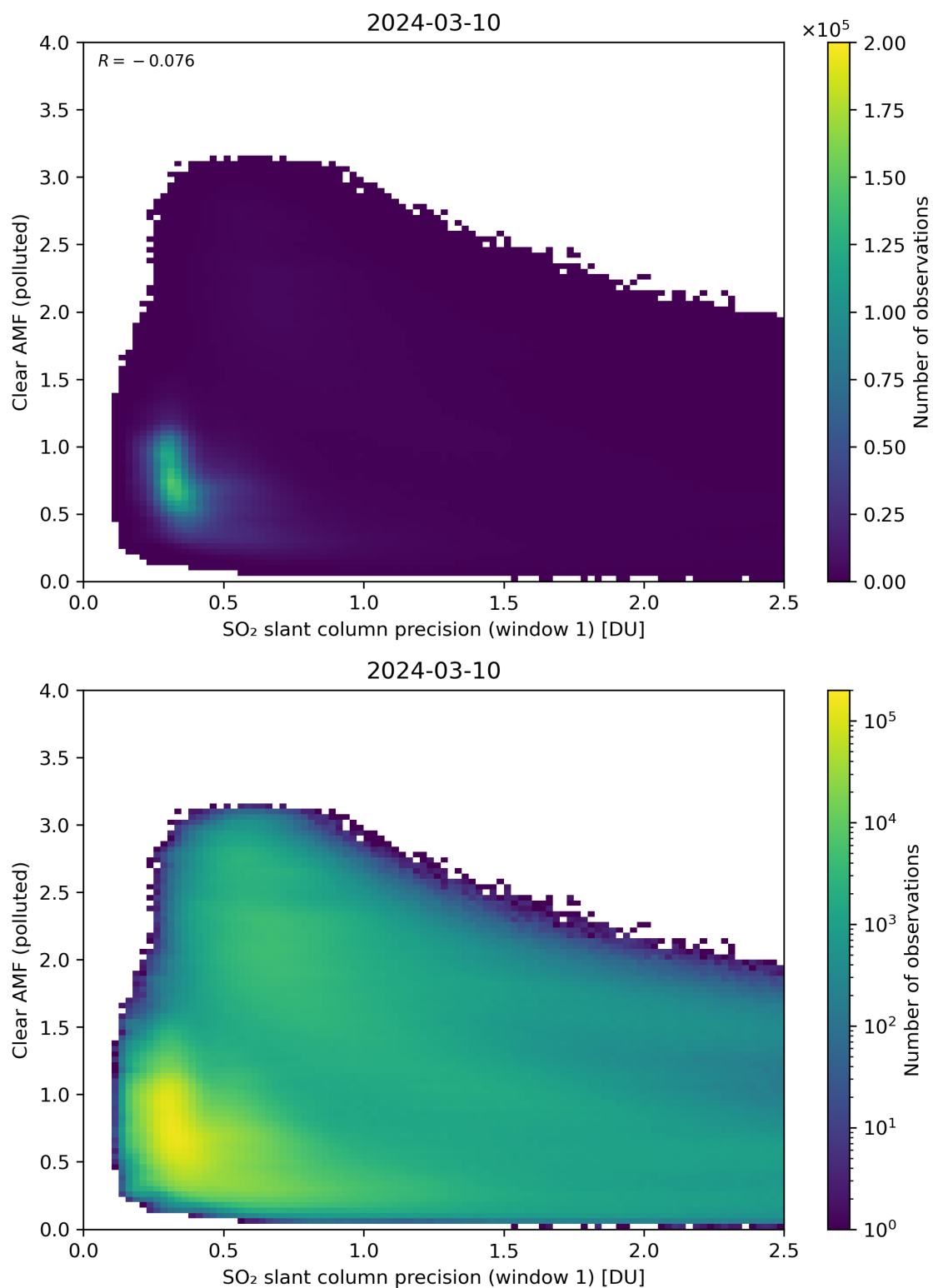
Figure 224: Scatter density plot of “SO 2 slant column precision (window 1)” against “Clear AMF (polluted)” for 2024-03-09 to 2024-03-11.
