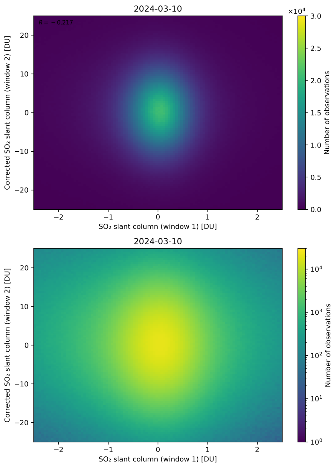
Figure 233: Scatter density plot of “SO 2 slant column (window 1)” against “Corrected SO 2 slant column (window 2)” for 2024-03-09 to 2024-03-11.
