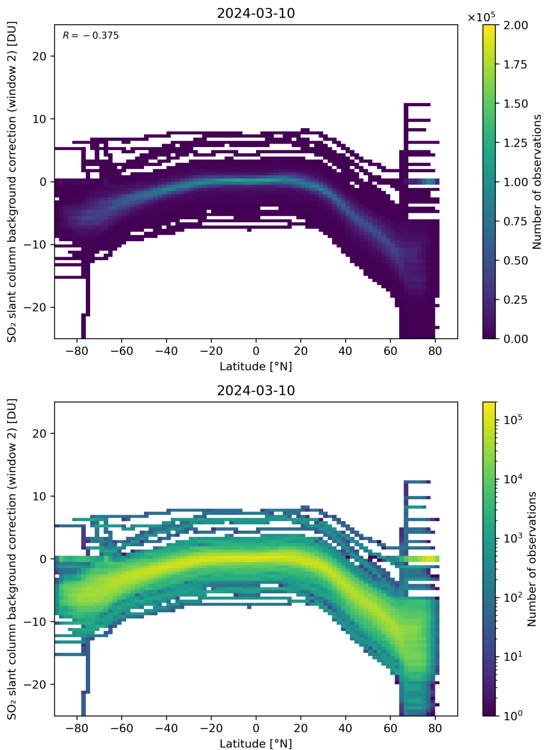
Figure 140: Scatter density plot of “Latitude” against “SO 2 slant column background correction (window 2)” for 2024-03-09 to 2024-03-11.
