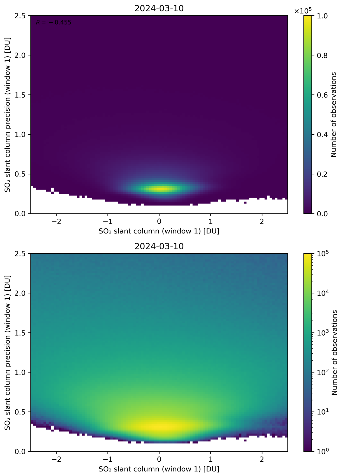
Figure 235: Scatter density plot of “SO 2 slant column (window 1)” against “SO 2 slant column precision (window 1)” for 2024-03-09 to 2024-03-11.
