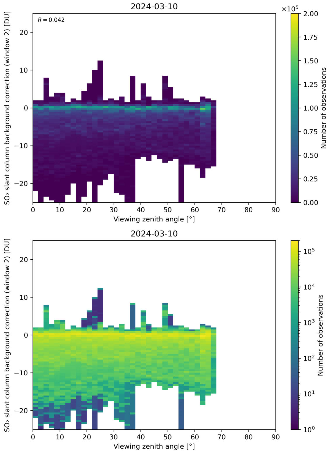
Figure 309: Scatter density plot of “Viewing zenith angle” against “SO 2 slant column background correction (window 2)” for 2024-03-09 to 2024-03-11.
